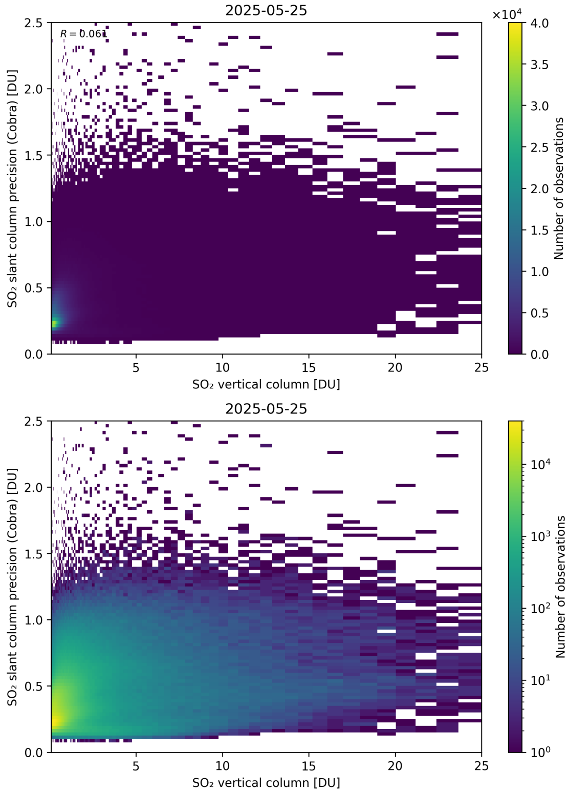
Figure 350: Scatter density plot of “SO 2 vertical column” against “SO 2 slant column precision (Cobra)” for 2025-05-24 to 2025-05-26.
