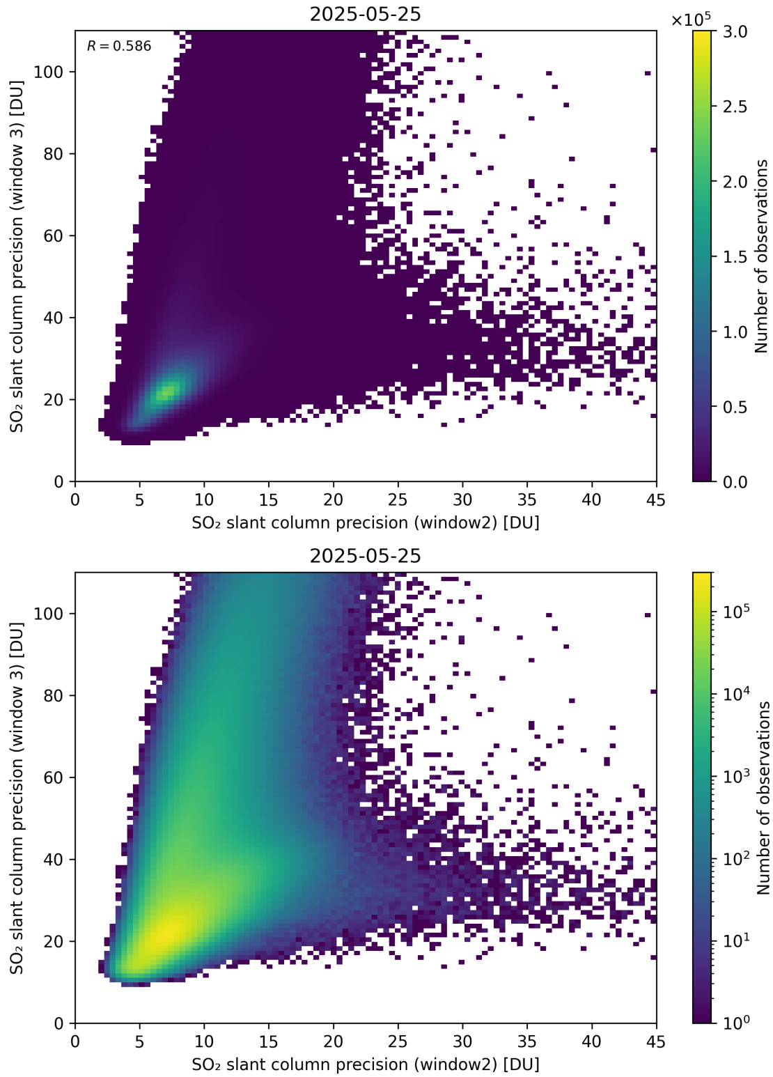
Figure 300: Scatter density plot of “SO 2 slant column precision (window2)” against “SO 2 slant column precision (window 3)” for 2025-05-24 to 2025-05-26.
