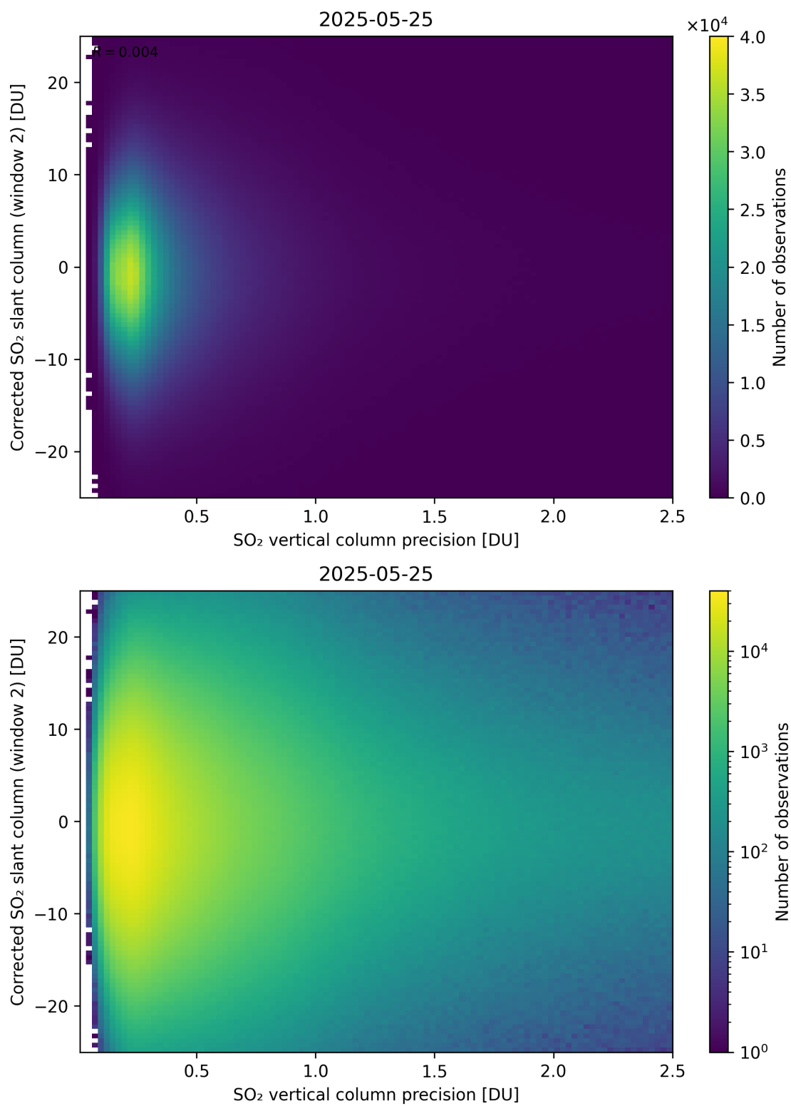
Figure 339: Scatter density plot of “SO 2 vertical column precision” against “Corrected SO 2 slant column (window 2)” for 2025-05-24 to 2025-05-26.
