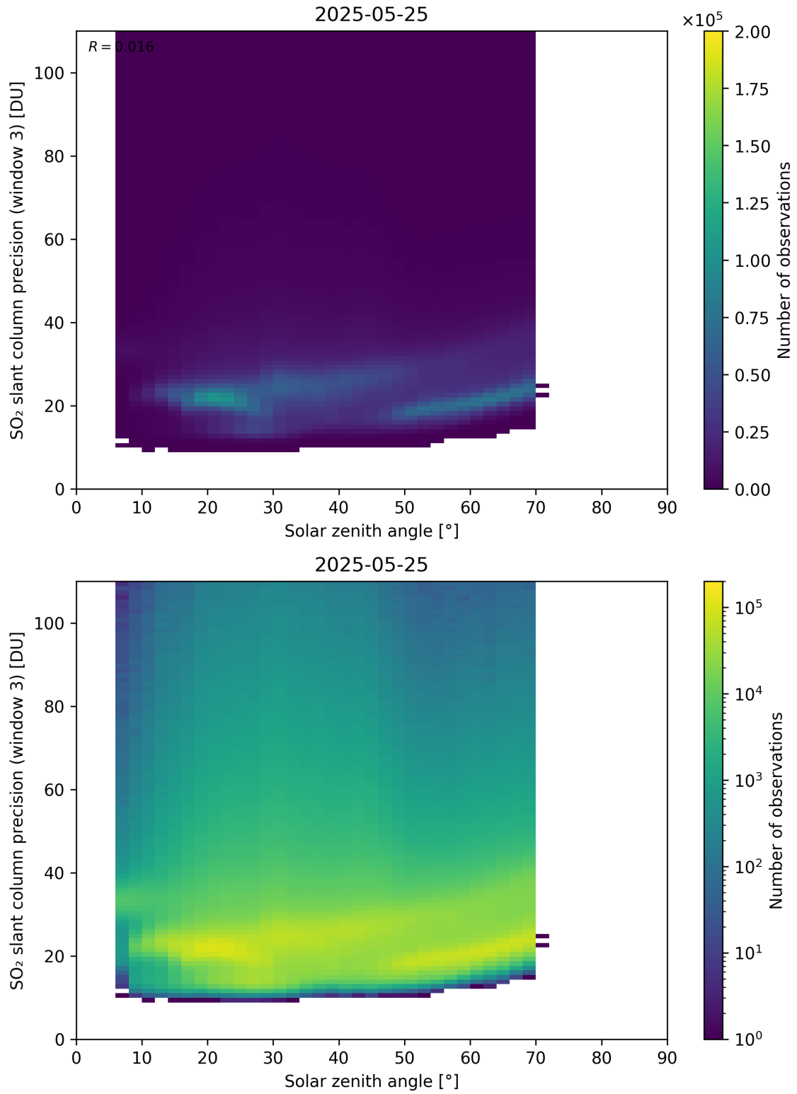
Figure 188: Scatter density plot of “Solar zenith angle” against “SO 2 slant column precision (window 3)” for 2025-05-24 to 2025-05-26.
