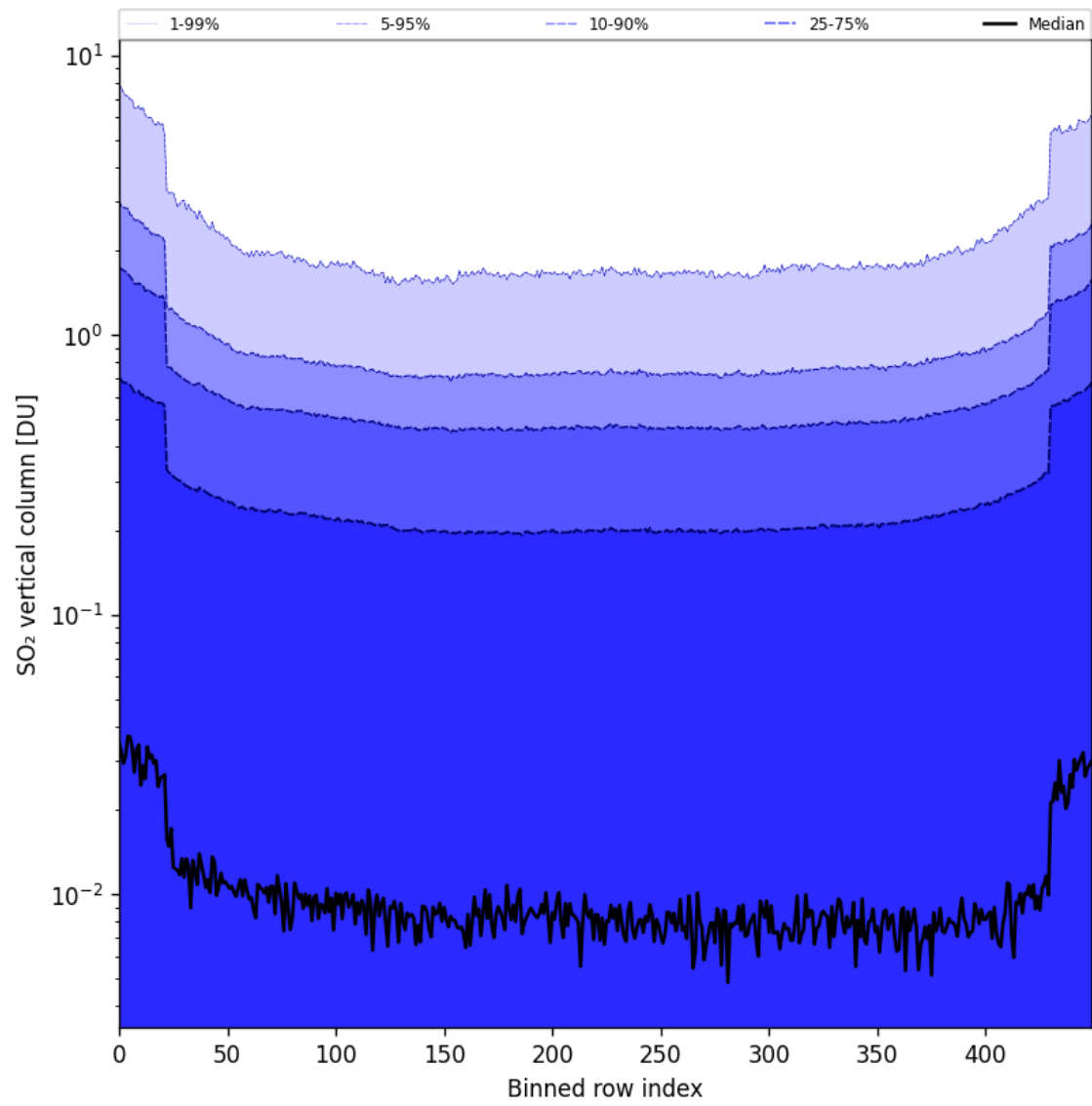
Figure 84: Along track statistics of “SO 2 vertical column” for 2025-05-24 to 2025-05-26
