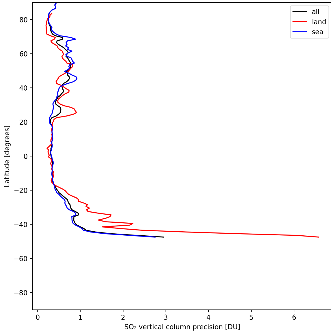
Figure 33: Zonal average of “SO 2 vertical column precision” for 2025-05-24 to 2025-05-26.
