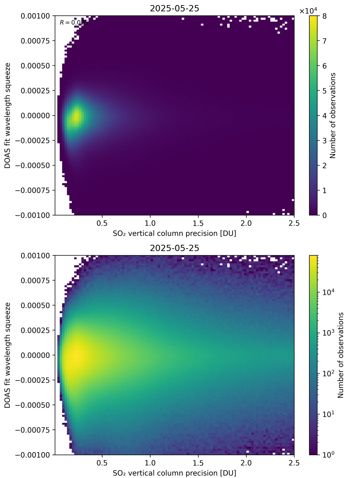
Figure 333: Scatter density plot of “SO 2 vertical column precision” against “DOAS fit wavelength squeeze” for 2025-05-24 to 2025-05-26.
