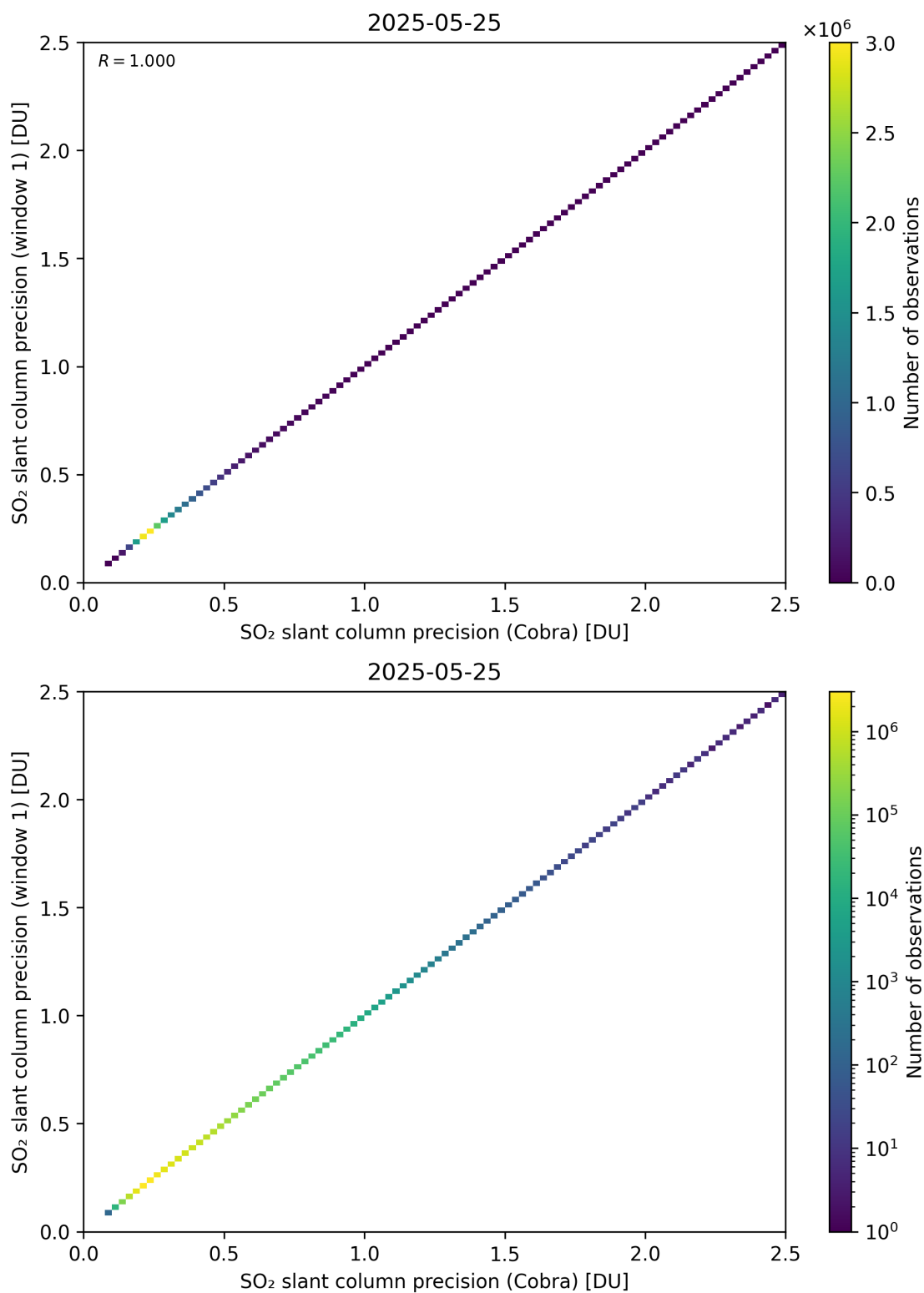
Figure 209: Scatter density plot of “SO 2 slant column precision (Cobra)” against “SO 2 slant column precision (window 1)” for 2025-05-24 to 2025-05-26.
