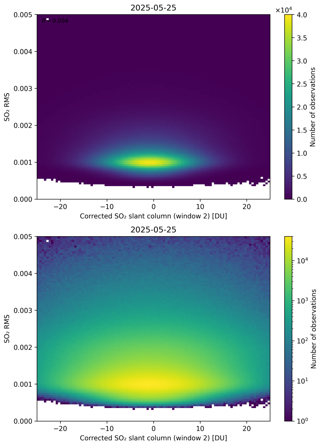
Figure 248: Scatter density plot of “Corrected SO 2 slant column (window 2)” against “SO 2 RMS” for 2025-05-24 to 2025-05-26.
