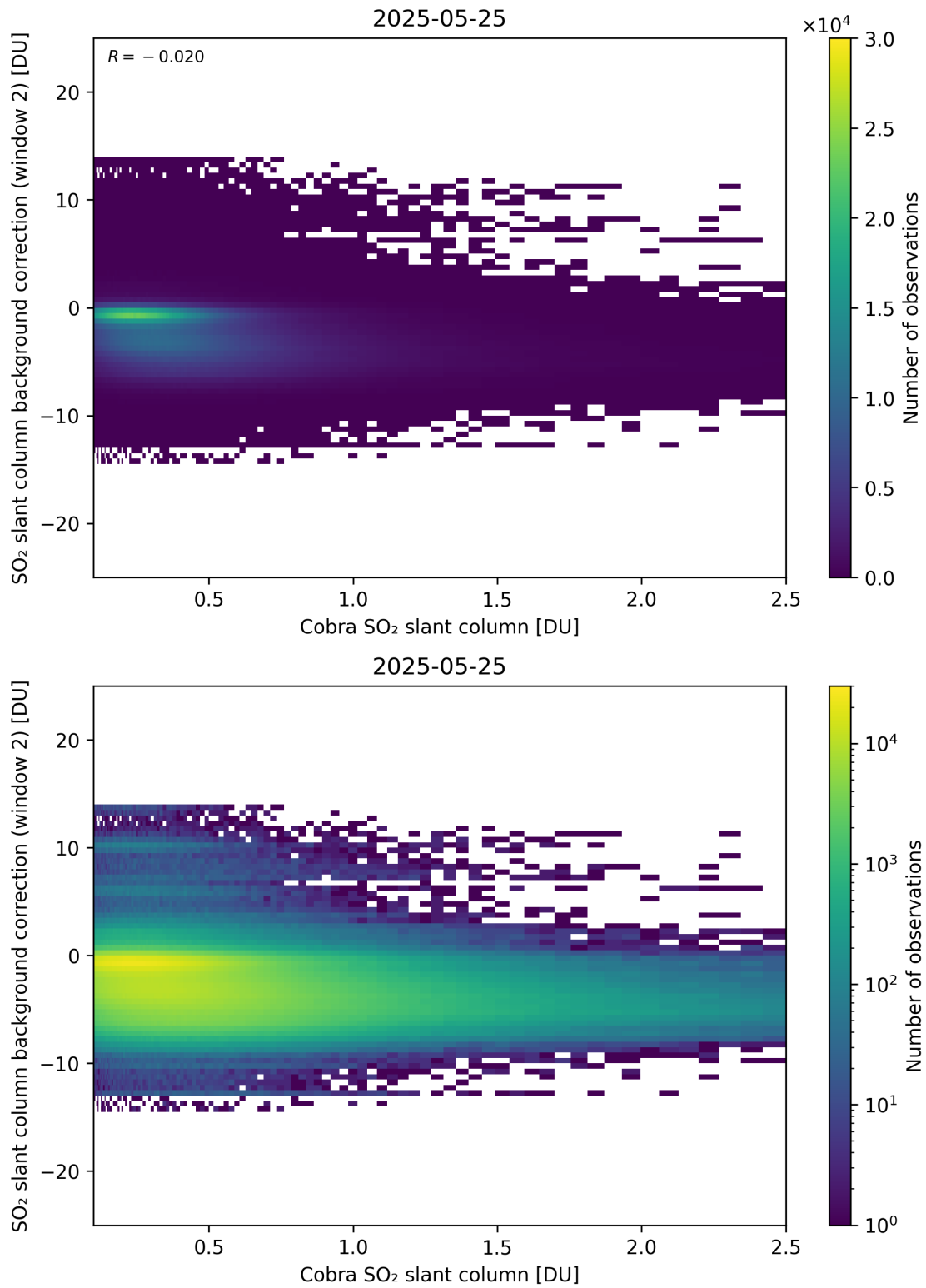
Figure 194: Scatter density plot of “Cobra SO 2 slant column” against “SO 2 slant column background correction (window 2)” for 2025-05-24 to 2025-05-26.
