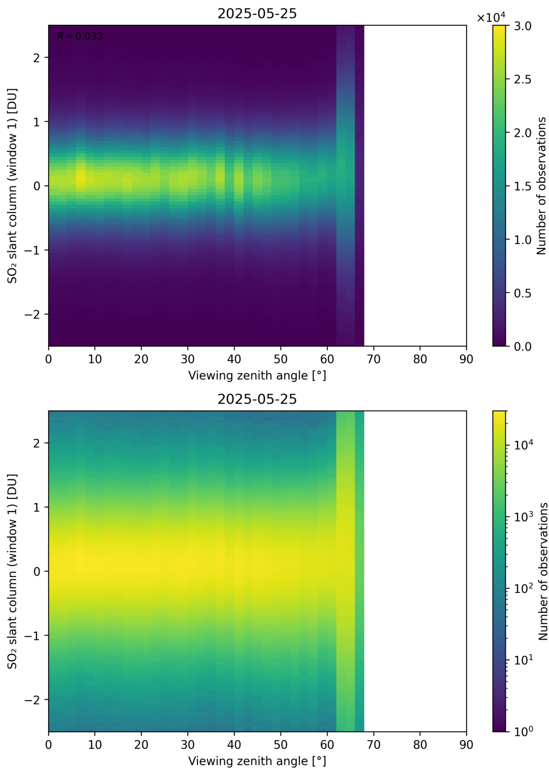
Figure 376: Scatter density plot of “Viewing zenith angle” against “SO 2 slant column (window 1)” for 2025-05-24 to 2025-05-26.
