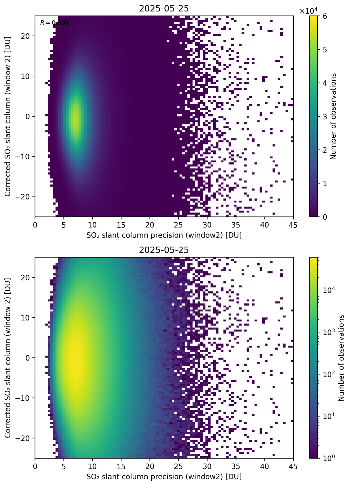
Figure 297: Scatter density plot of “SO 2 slant column precision (window2)” against “Corrected SO 2 slant column (window 2)” for 2025-05-24 to 2025-05-26.
