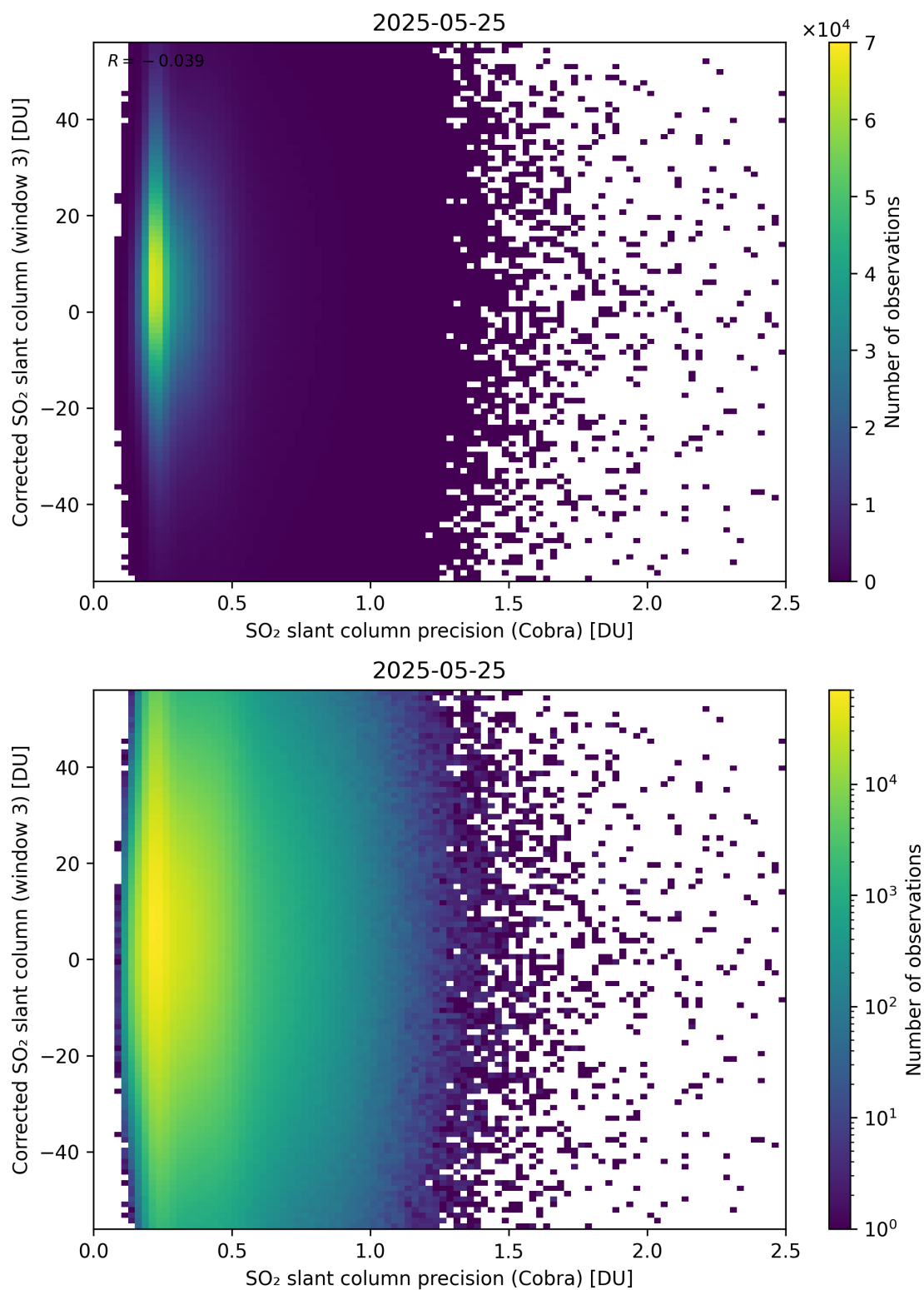
Figure 207: Scatter density plot of “SO 2 slant column precision (Cobra)” against “Corrected SO 2 slant column (window 3)” for 2025-05-24 to 2025-05-26.
