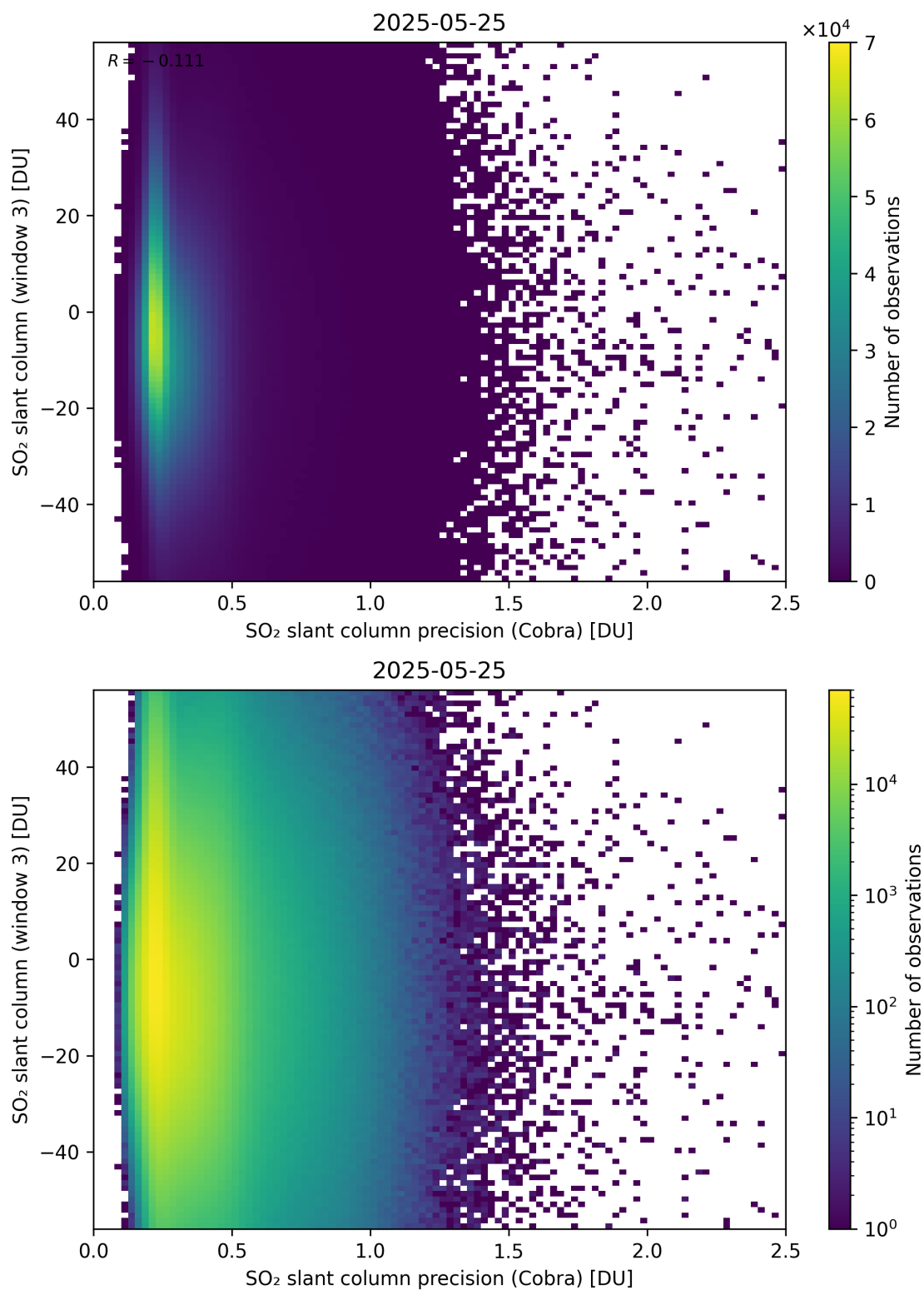
Figure 211: Scatter density plot of “SO 2 slant column precision (Cobra)” against “SO 2 slant column (window 3)” for 2025-05-24 to 2025-05-26.
