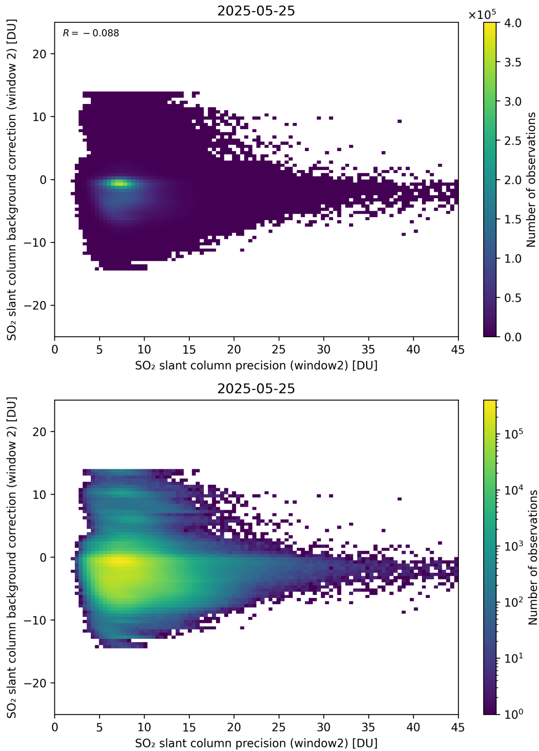
Figure 291: Scatter density plot of “SO 2 slant column precision (window2)” against “SO 2 slant column background correction (window 2)” for 2025-05-24 to 2025-05-26.
