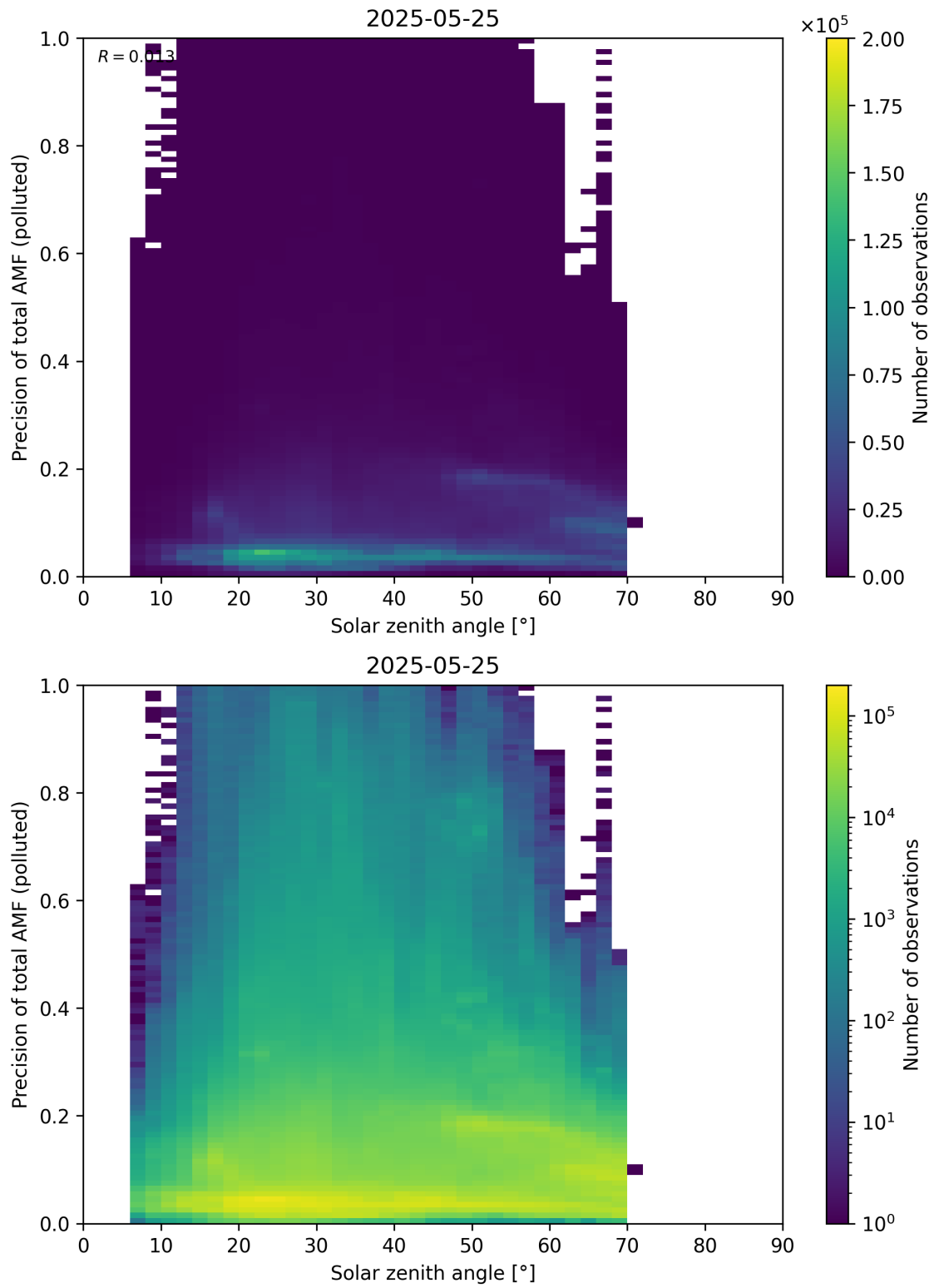
Figure 190: Scatter density plot of “Solar zenith angle” against “Precision of total AMF (polluted)” for 2025-05-24 to 2025-05-26.
