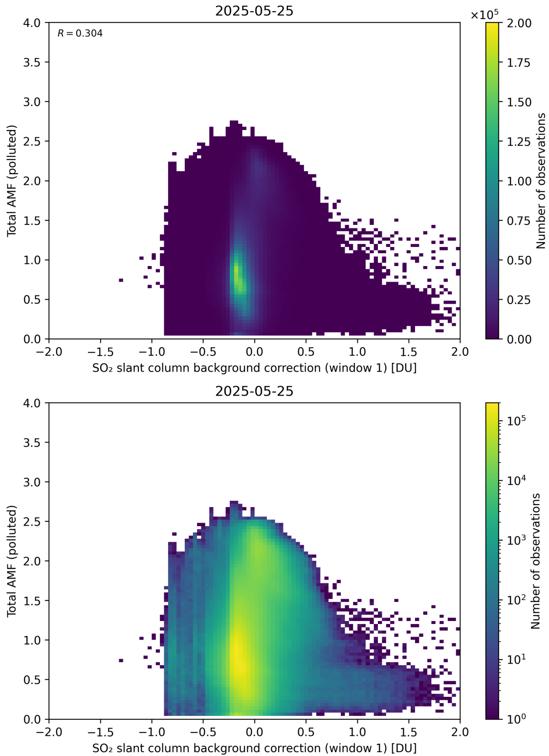
Figure 120: Scatter density plot of “SO 2 slant column background correction (window 1)” against “Total AMF (polluted)” for 2025-05-24 to 2025-05-26.
