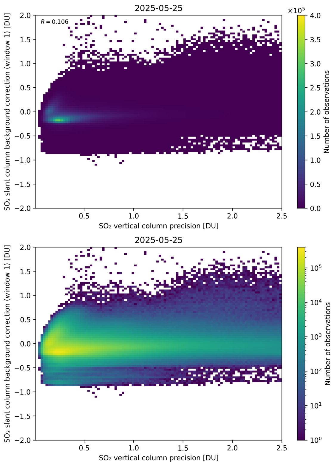
Figure 329: Scatter density plot of “SO 2 vertical column precision” against “SO 2 slant column background correction (window 1)” for 2025-05-24 to 2025-05-26.
