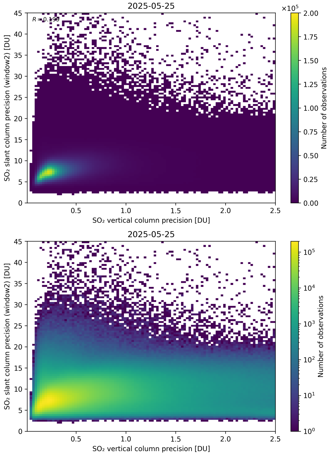
Figure 343: Scatter density plot of “SO 2 vertical column precision” against “SO 2 slant column precision (window2)” for 2025-05-24 to 2025-05-26.
