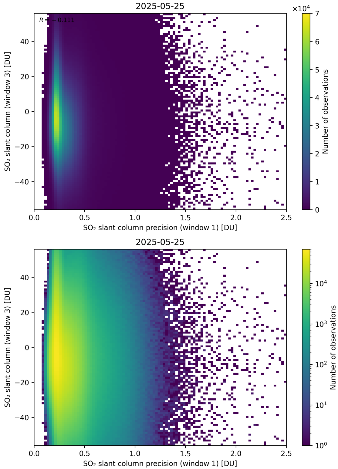
Figure 278: Scatter density plot of “SO 2 slant column precision (window 1)” against “SO 2 slant column (window 3)” for 2025-05-24 to 2025-05-26.
