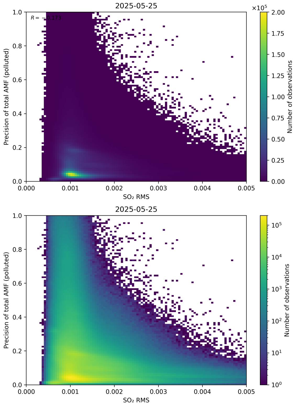
Figure 149: Scatter density plot of “SO 2 RMS” against “Precision of total AMF (polluted)” for 2025-05-24 to 2025-05-26.
