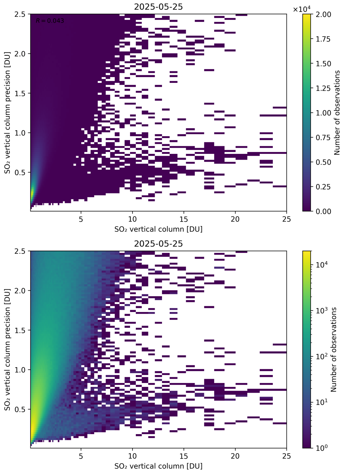
Figure 361: Scatter density plot of “SO 2 vertical column” against “SO 2 vertical column precision” for 2025-05-24 to 2025-05-26.
