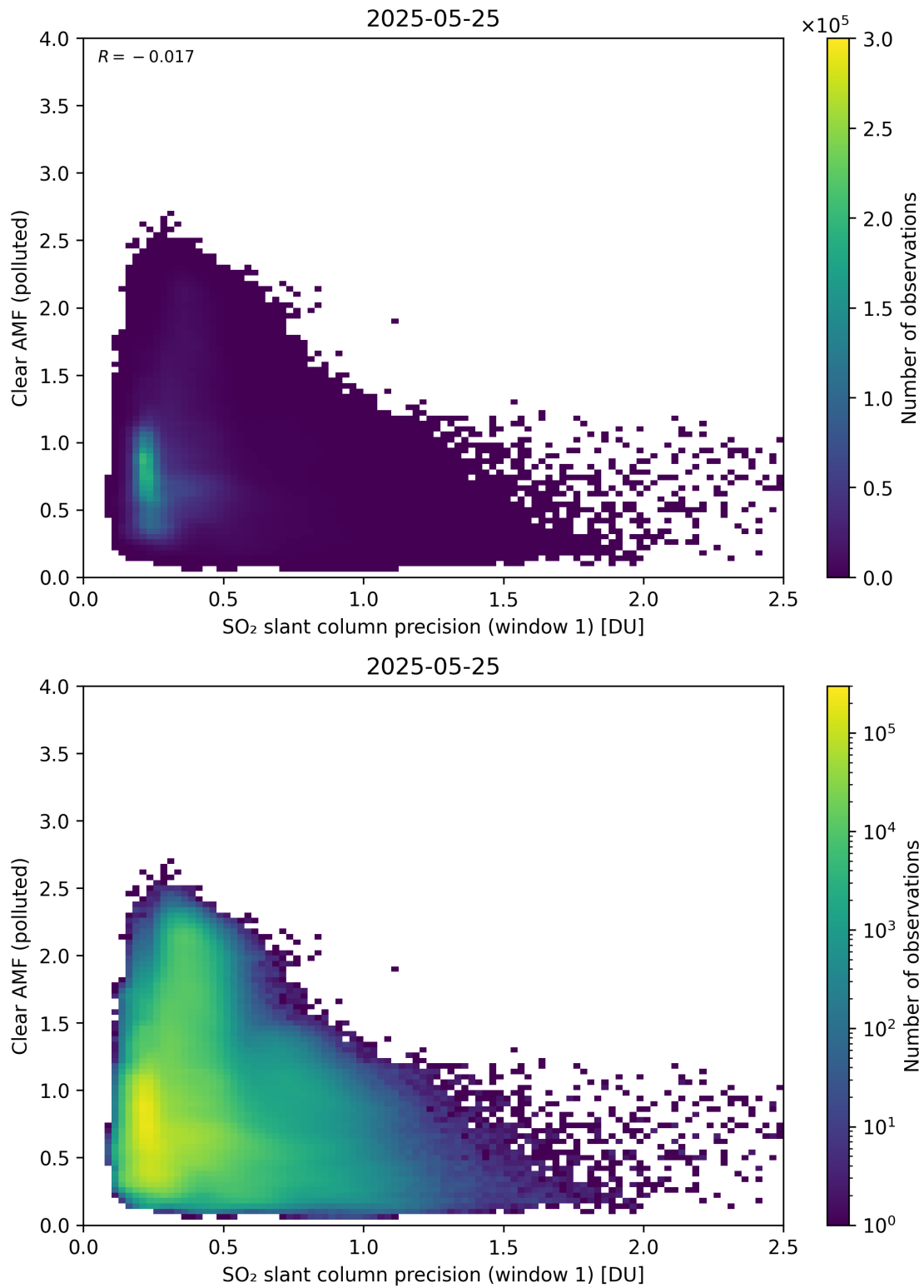
Figure 274: Scatter density plot of “SO 2 slant column precision (window 1)” against “Clear AMF (polluted)” for 2025-05-24 to 2025-05-26.
