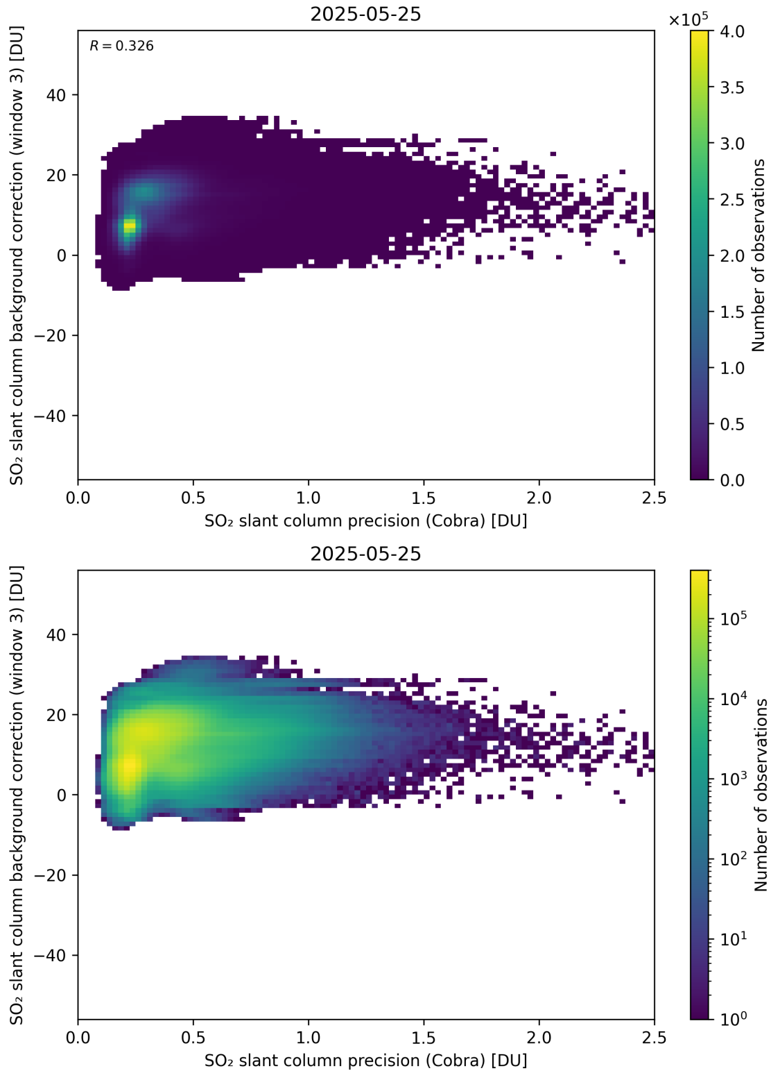
Figure 201: Scatter density plot of “SO 2 slant column precision (Cobra)” against “SO 2 slant column background correction (window 3)” for 2025-05-24 to 2025-05-26.
