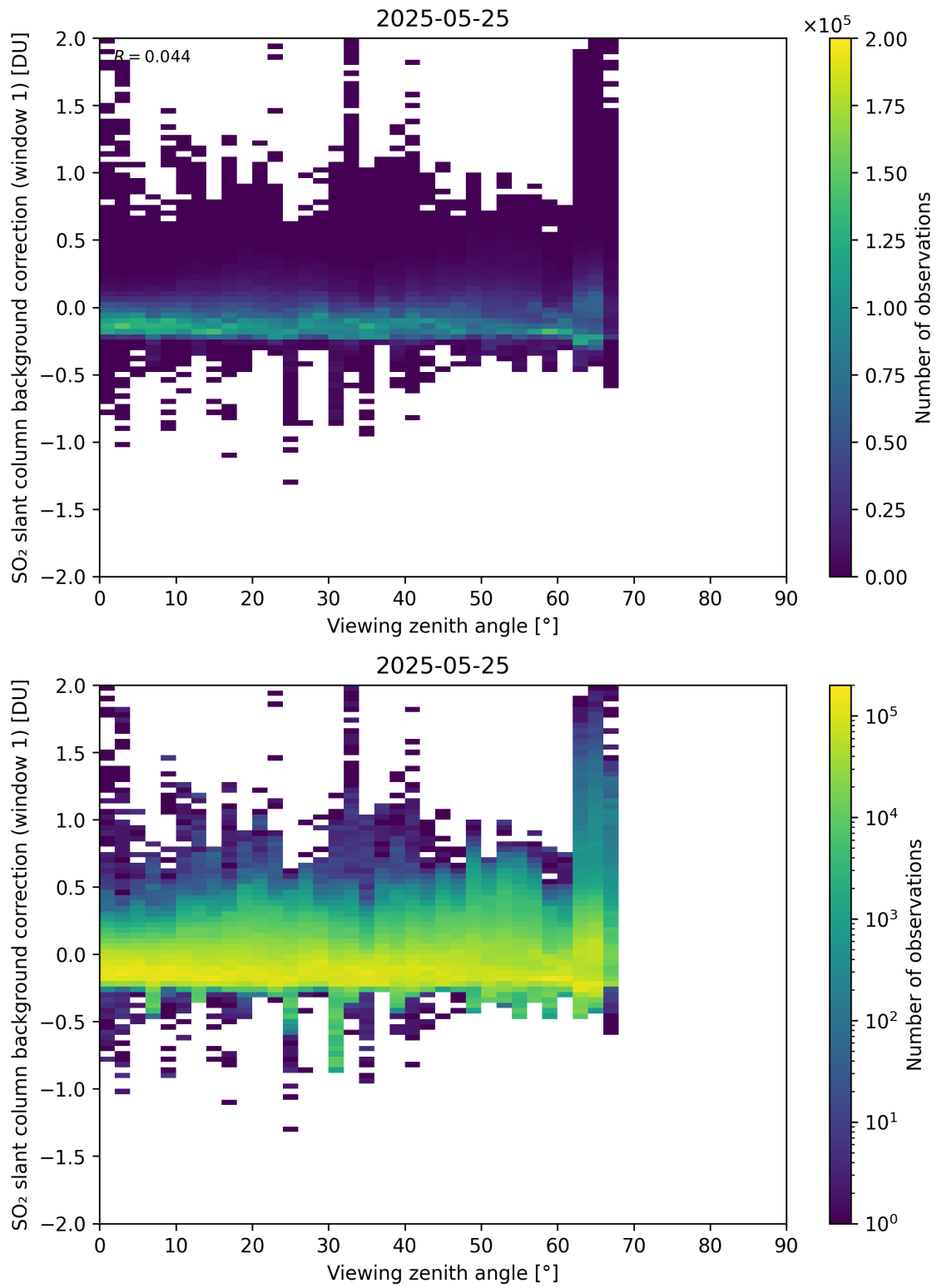
Figure 362: Scatter density plot of “Viewing zenith angle” against “SO 2 slant column background correction (window 1)” for 2025-05-24 to 2025-05-26.
