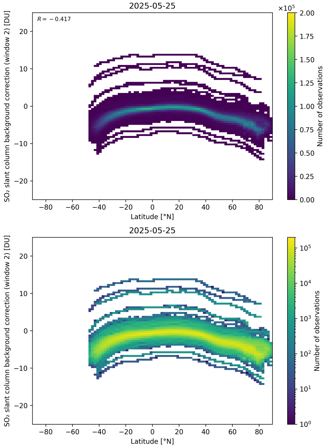
Figure 151: Scatter density plot of “Latitude” against “SO 2 slant column background correction (window 2)” for 2025-05-24 to 2025-05-26.
