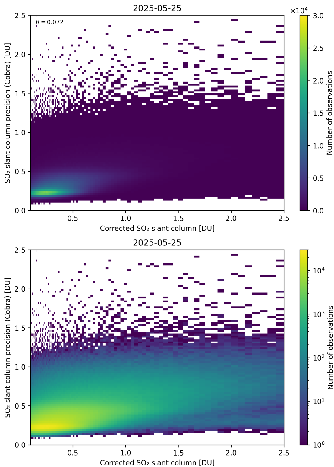
Figure 234: Scatter density plot of “Corrected SO 2 slant column” against “SO 2 slant column precision (Cobra)” for 2025-05-24 to 2025-05-26.
