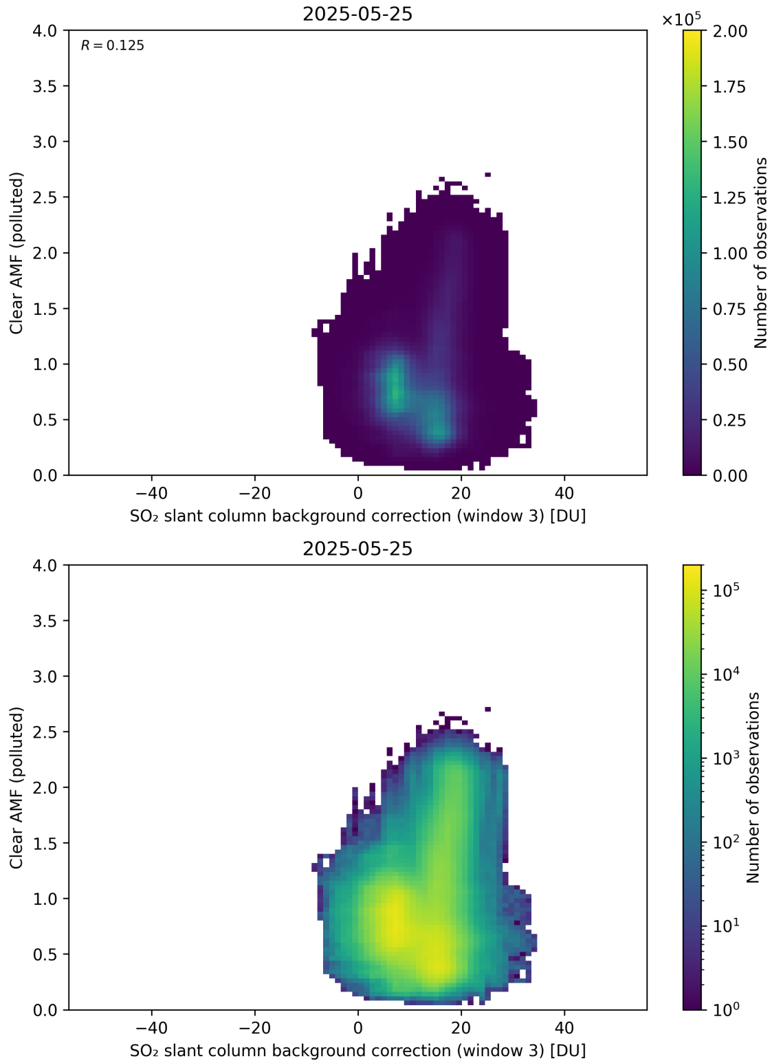
Figure 135: Scatter density plot of “SO 2 slant column background correction (window 3)” against “Clear AMF (polluted)” for 2025-05-24 to 2025-05-26.
