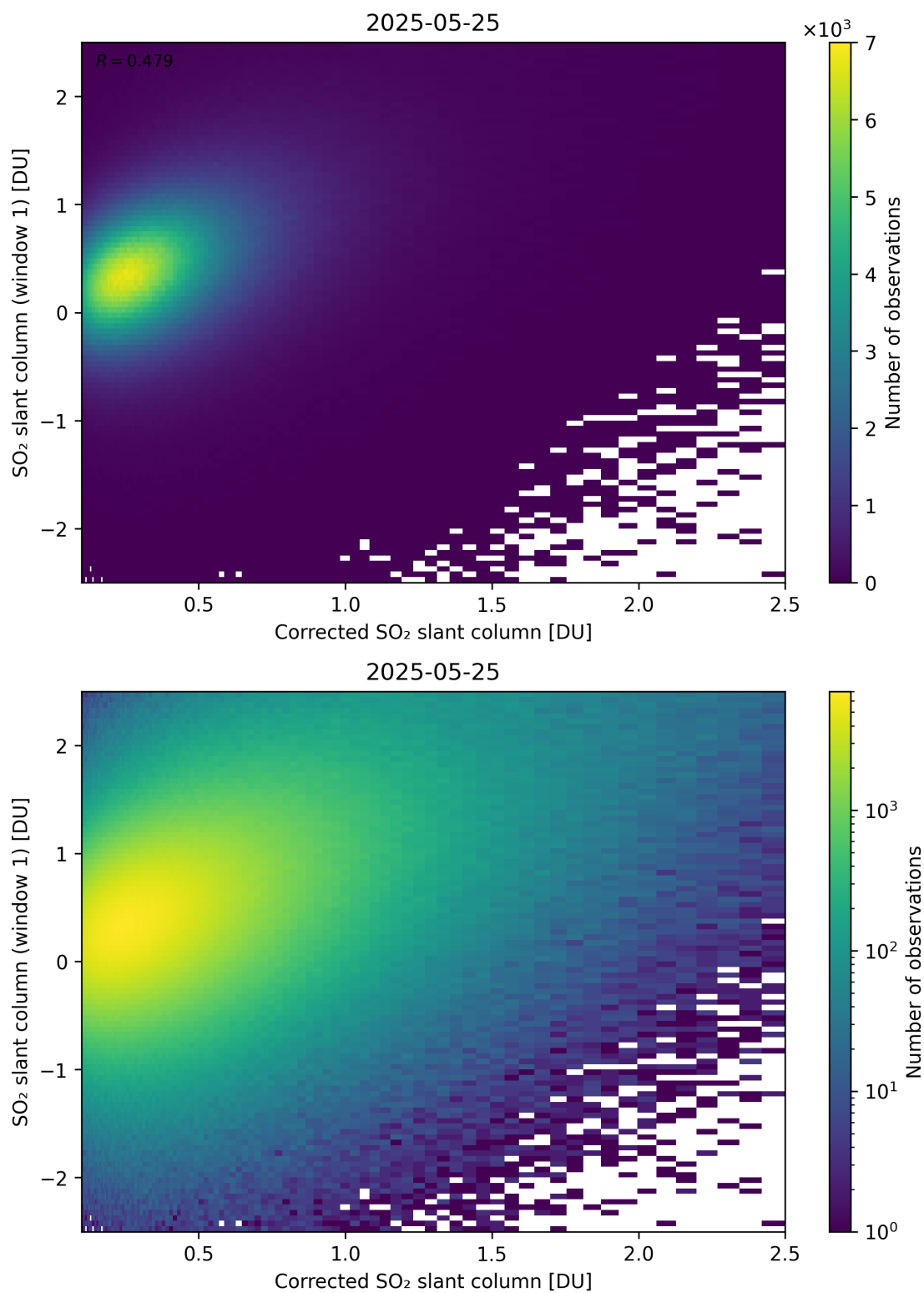
Figure 237: Scatter density plot of “Corrected SO 2 slant column” against “SO 2 slant column (window 1)” for 2025-05-24 to 2025-05-26.
