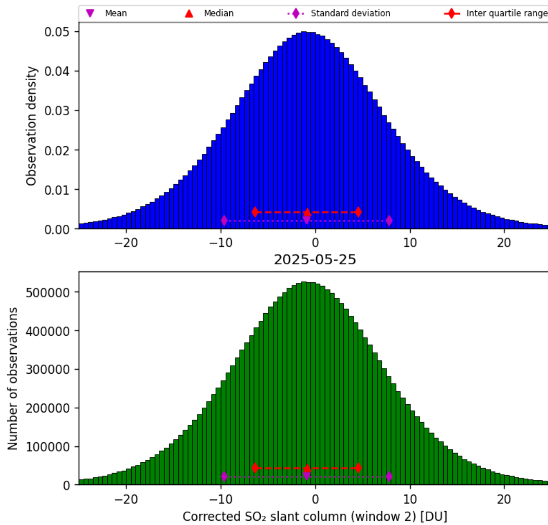
Figure 69: Histogram of “Corrected SO 2 slant column (window 2)” for 2025-05-24 to 2025-05-26
