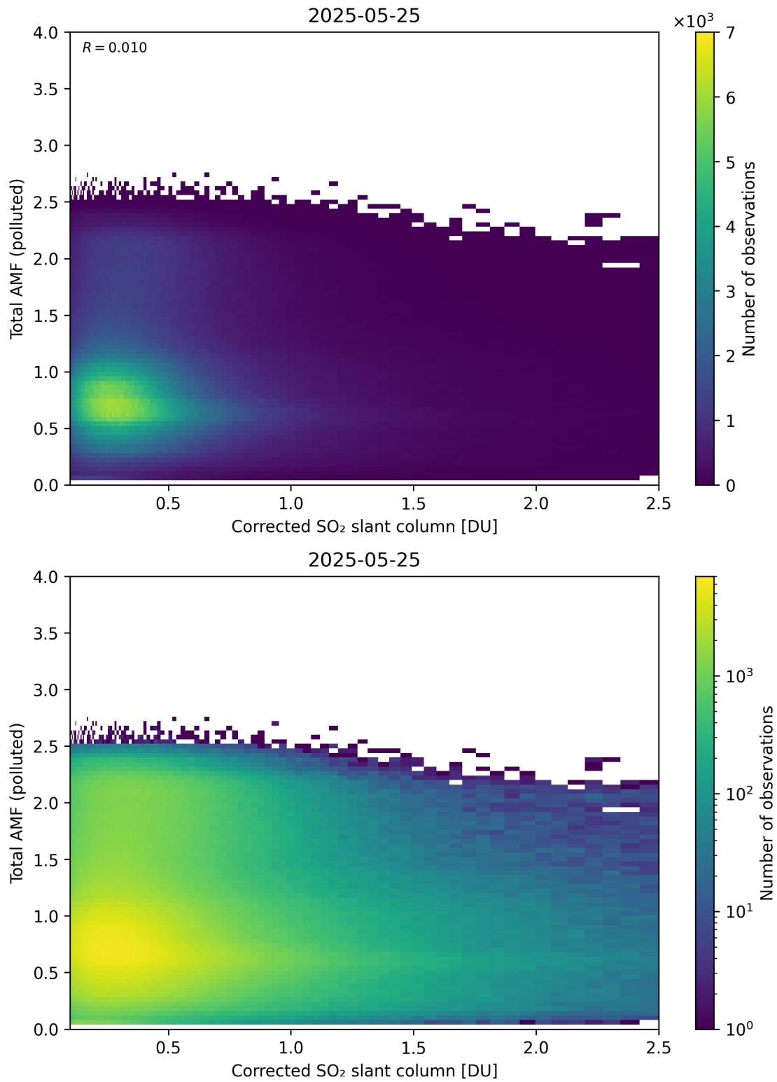
Figure 242: Scatter density plot of “Corrected SO 2 slant column” against “Total AMF (polluted)” for 2025-05-24 to 2025-05-26.
