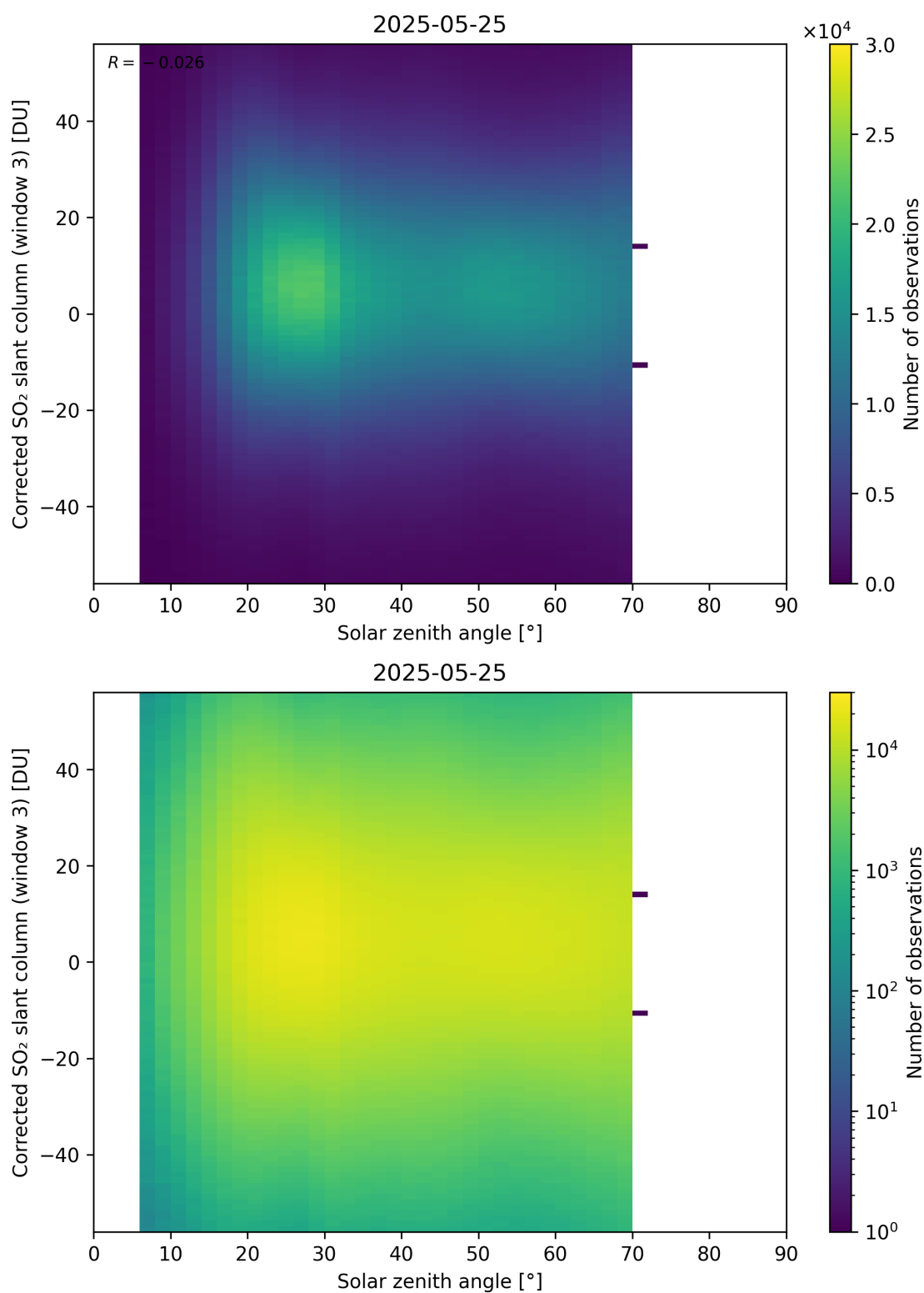
Figure 183: Scatter density plot of “Solar zenith angle” against “Corrected SO 2 slant column (window 3)” for 2025-05-24 to 2025-05-26.
