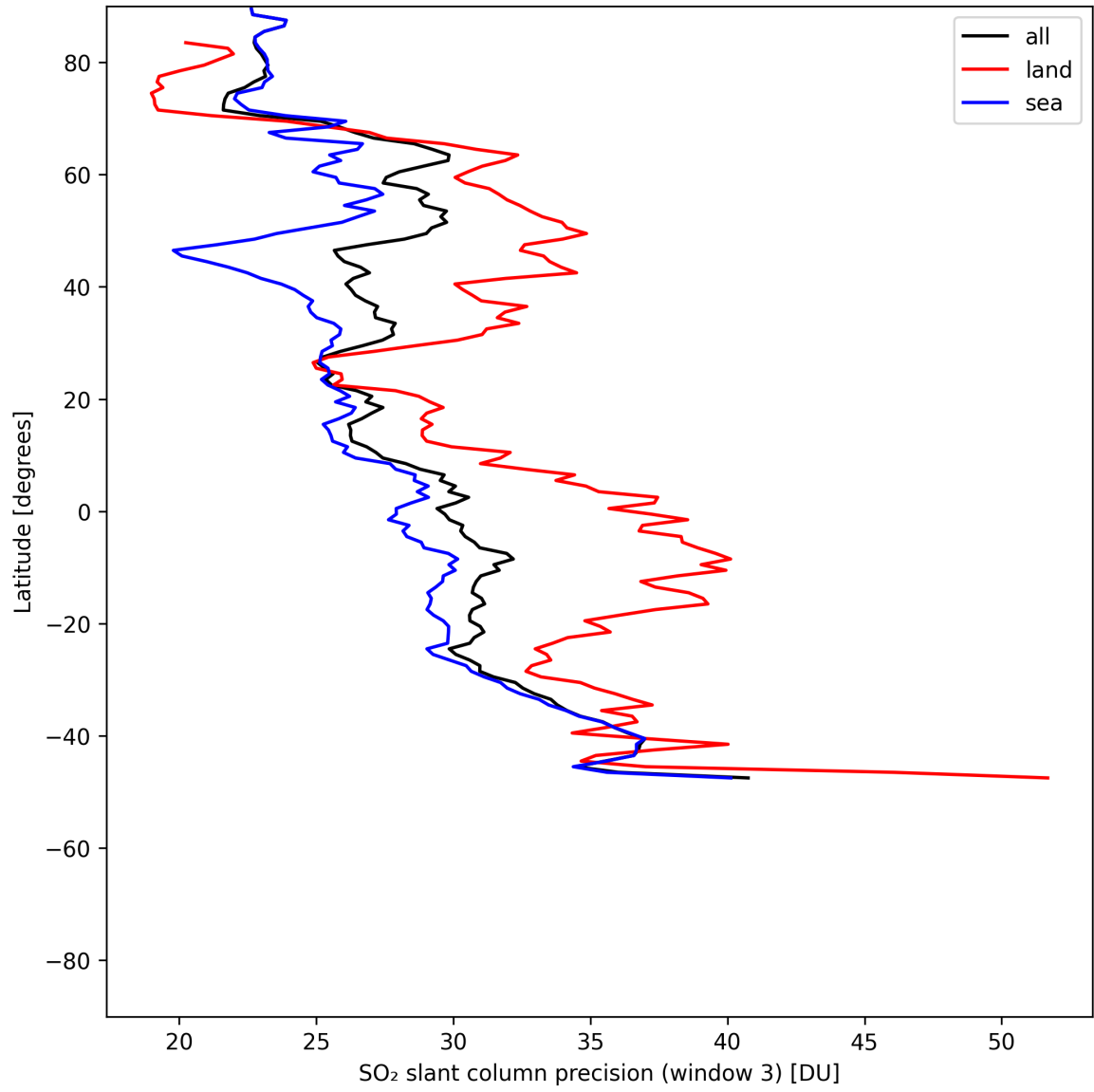
Figure 46: Zonal average of “SO 2 slant column precision (window 3)” for 2025-05-24 to 2025-05-26.
