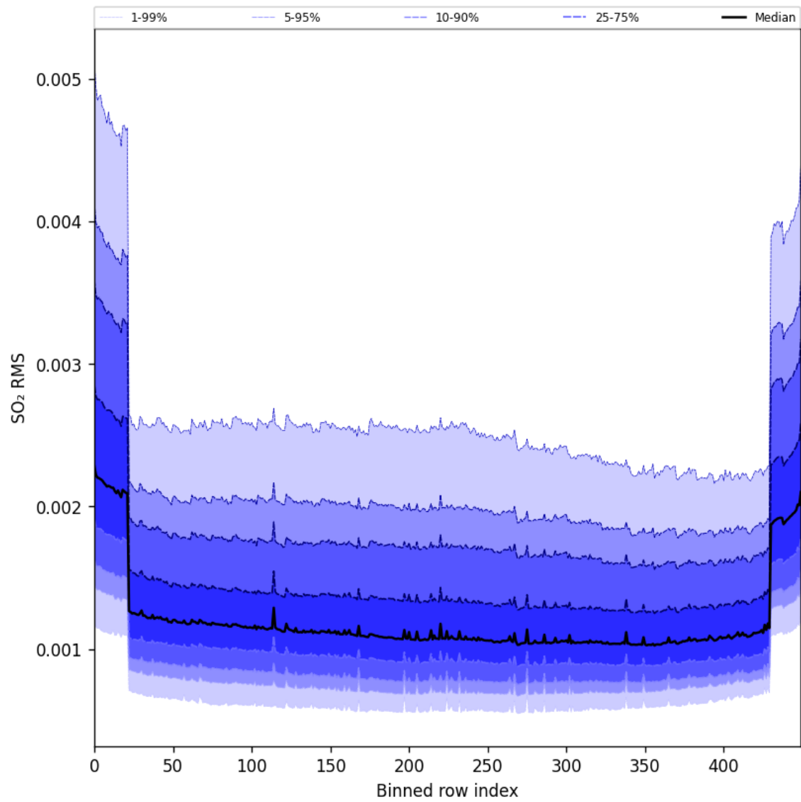
Figure 104: Along track statistics of “SO 2 RMS” for 2025-05-24 to 2025-05-26
