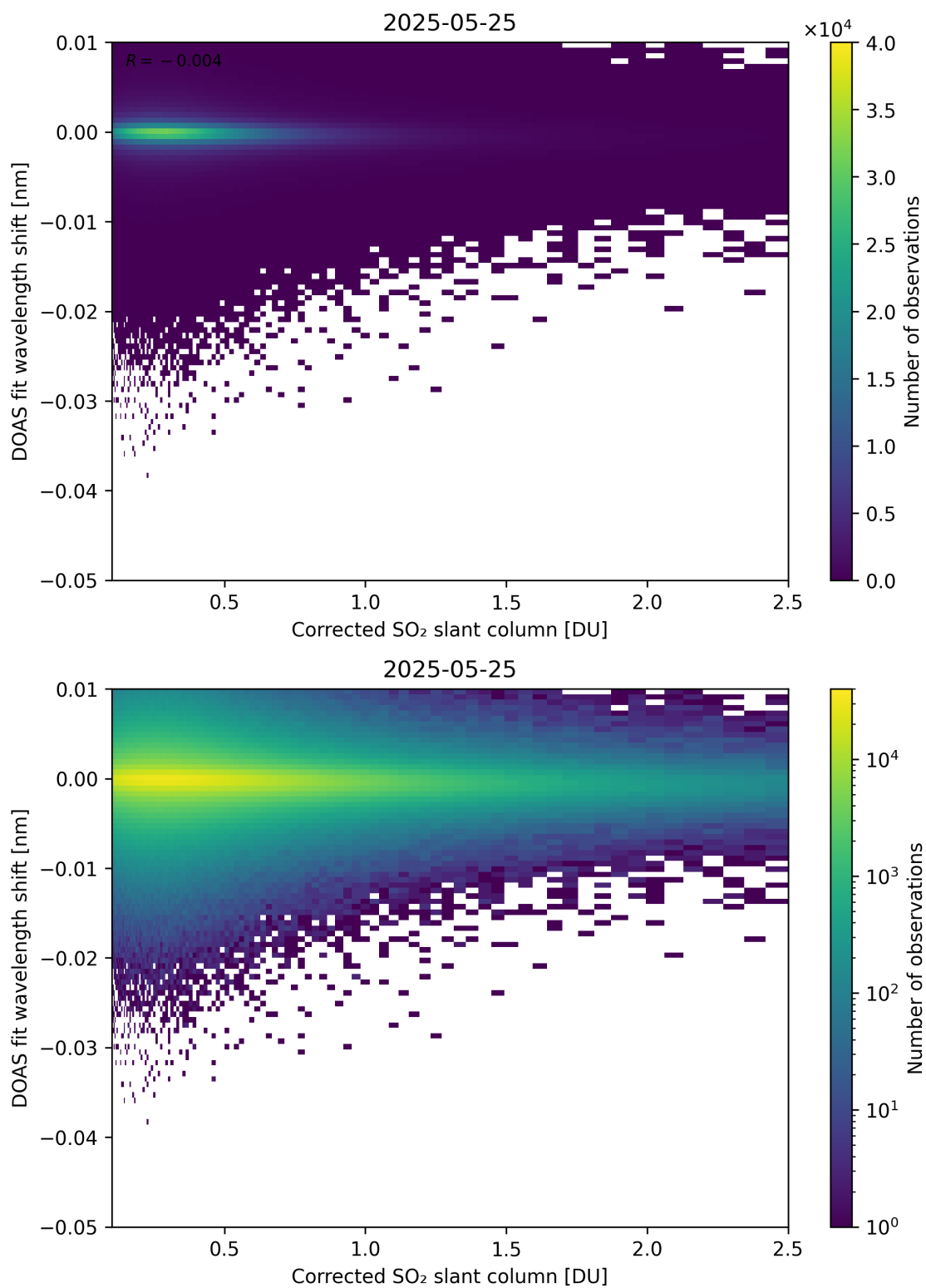
Figure 229: Scatter density plot of “Corrected SO 2 slant column” against “DOAS fit wavelength shift” for 2025-05-24 to 2025-05-26.
