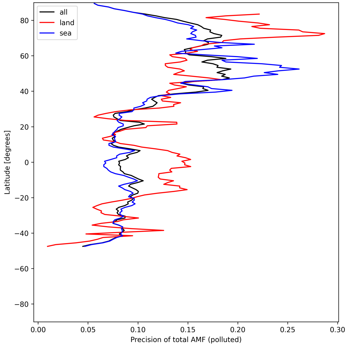
Figure 54: Zonal average of “Precision of total AMF (polluted)” for 2025-05-24 to 2025-05-26.
