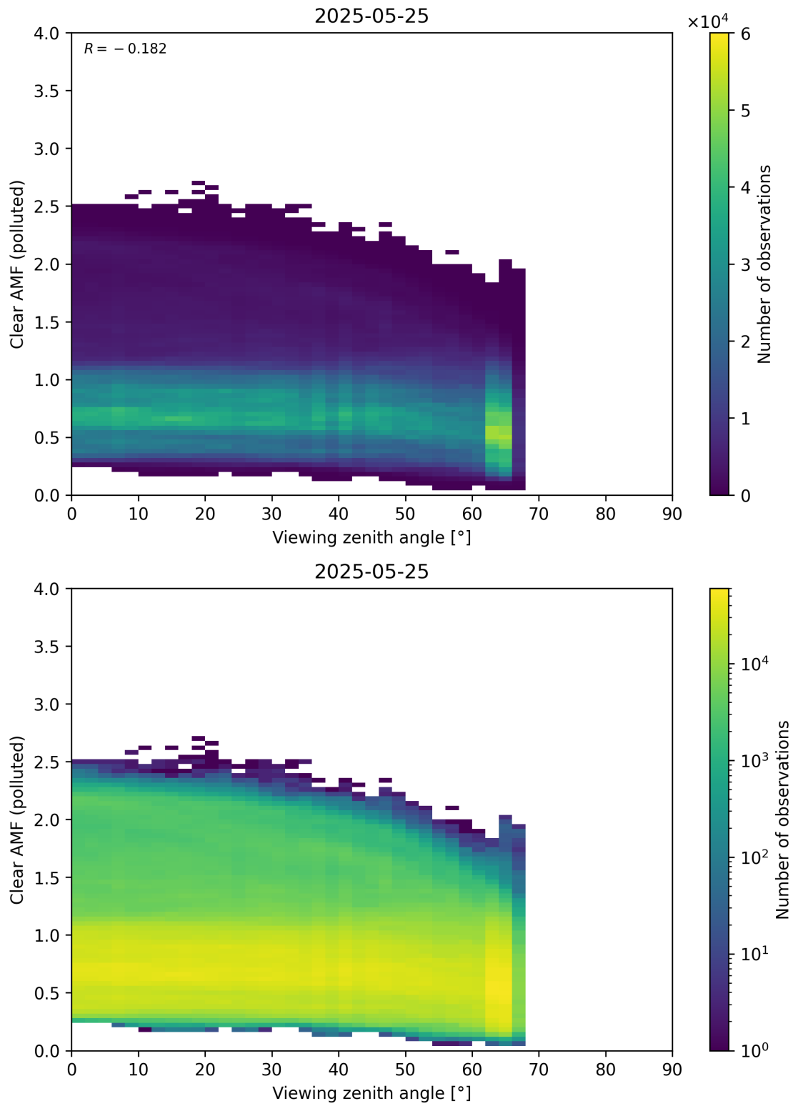
Figure 370: Scatter density plot of “Viewing zenith angle” against “Clear AMF (polluted)” for 2025-05-24 to 2025-05-26.
