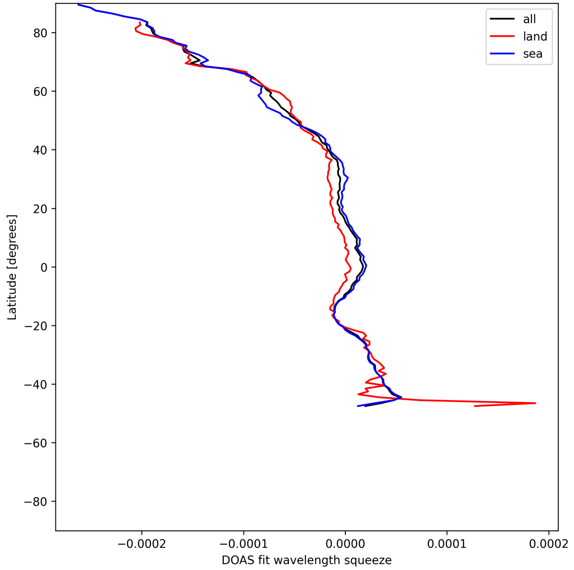
Figure 51: Zonal average of “DOAS fit wavelength squeeze” for 2025-05-24 to 2025-05-26.
