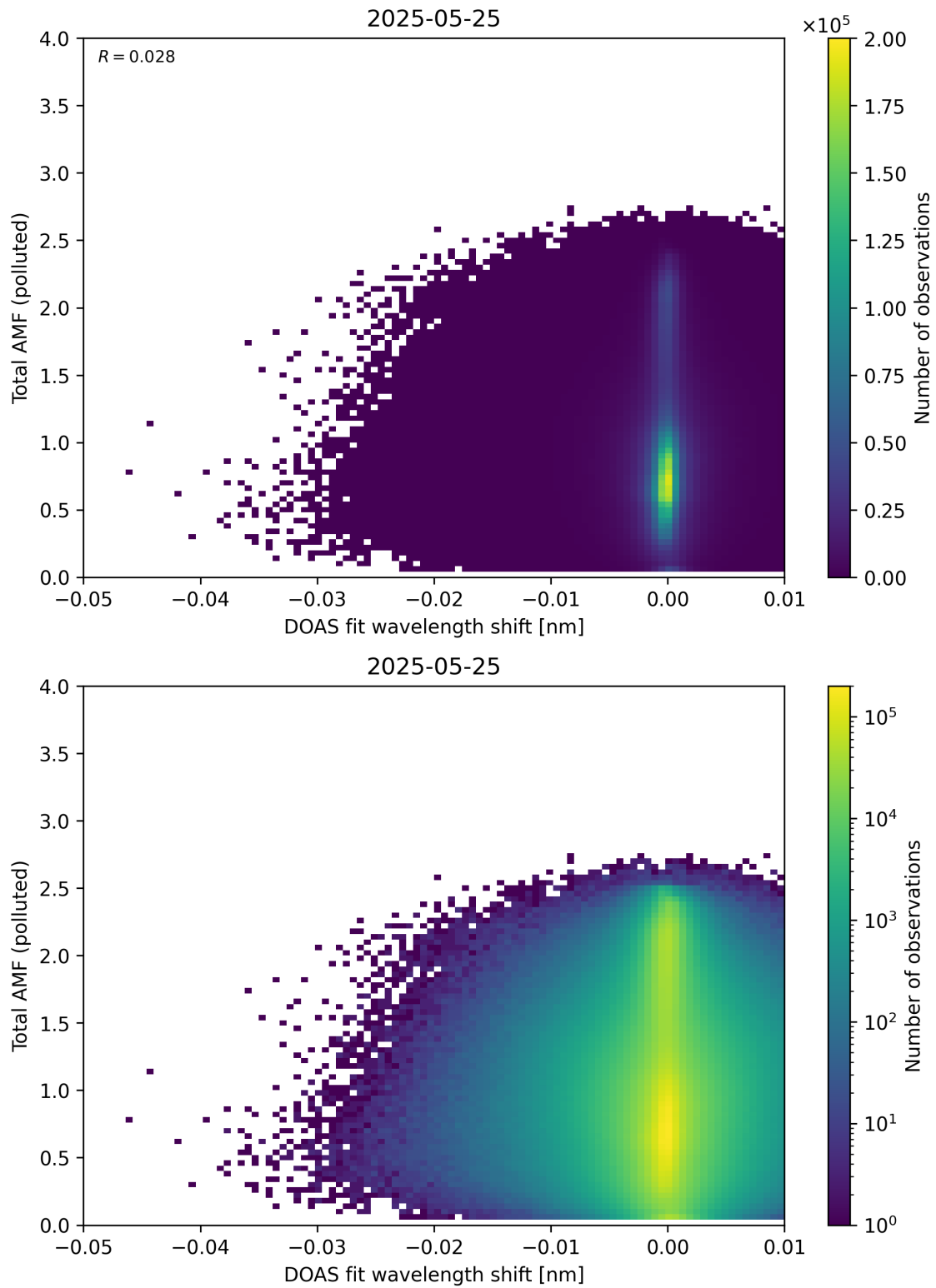
Figure 141: Scatter density plot of “DOAS fit wavelength shift” against “Total AMF (polluted)” for 2025-05-24 to 2025-05-26.
