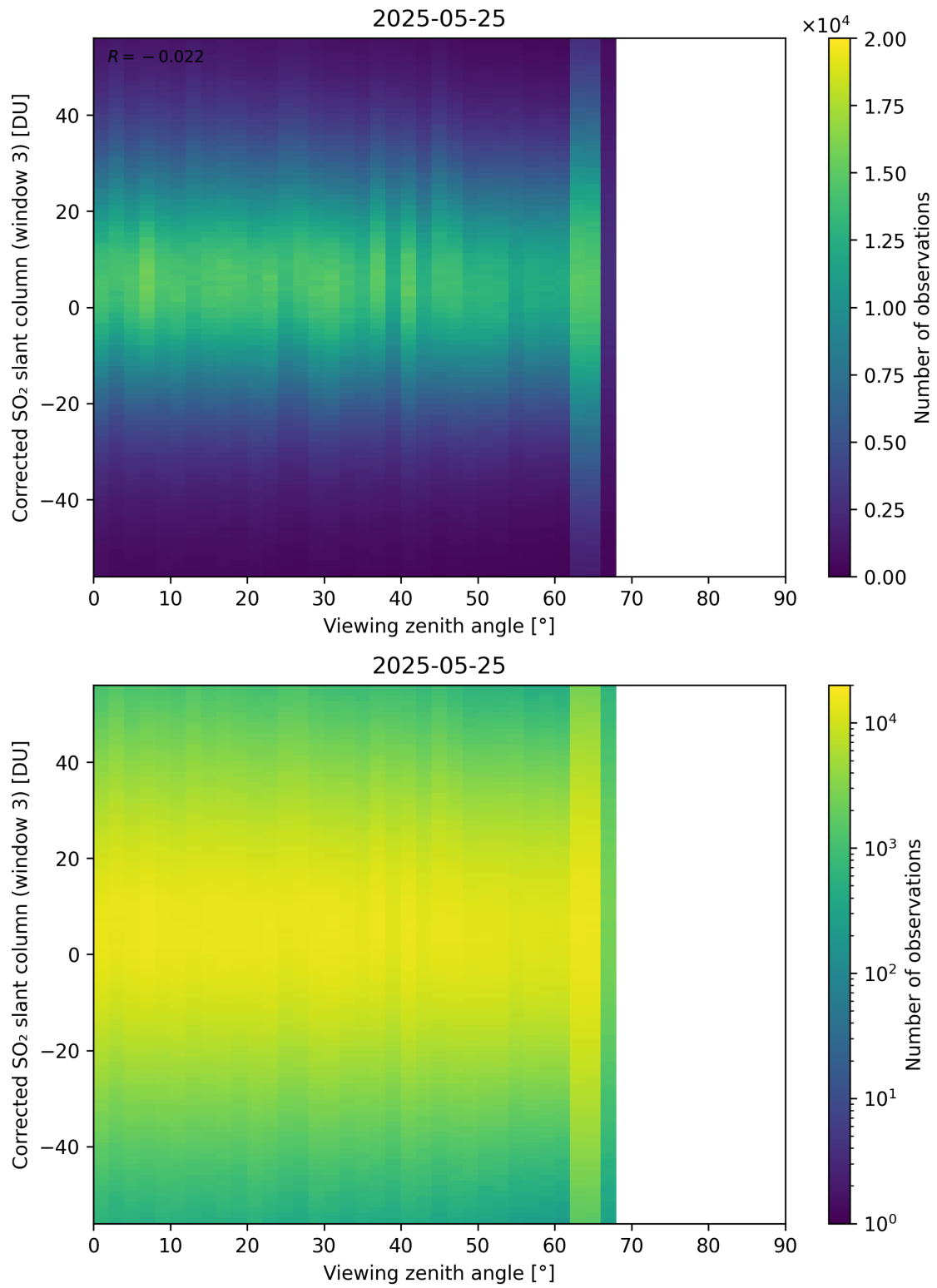
Figure 375: Scatter density plot of “Viewing zenith angle” against “Corrected SO 2 slant column (window 3)” for 2025-05-24 to 2025-05-26.
