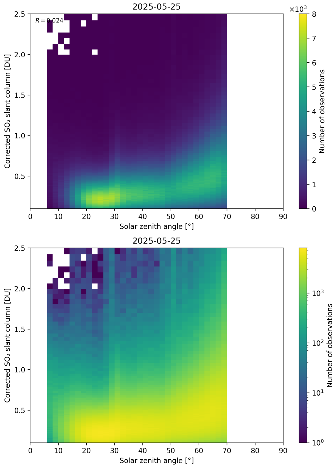
Figure 181: Scatter density plot of “Solar zenith angle” against “Corrected SO 2 slant column” for 2025-05-24 to 2025-05-26.
