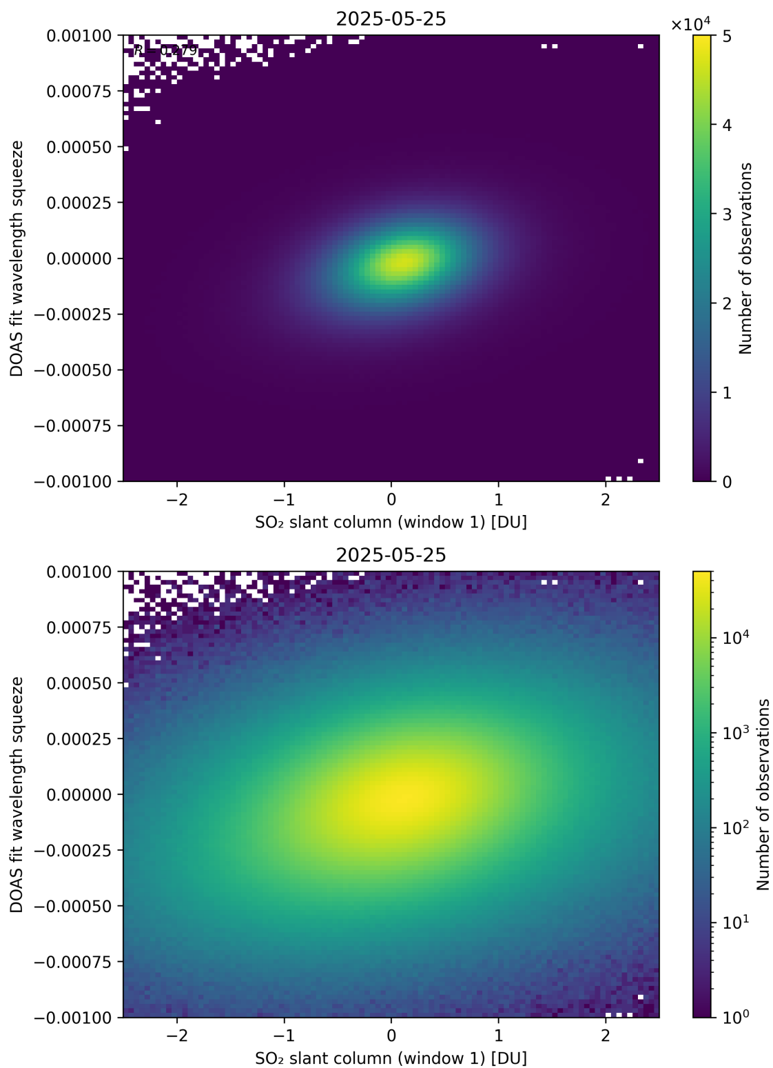
Figure 266: Scatter density plot of “SO 2 slant column (window 1)” against “DOAS fit wavelength squeeze” for 2025-05-24 to 2025-05-26.
