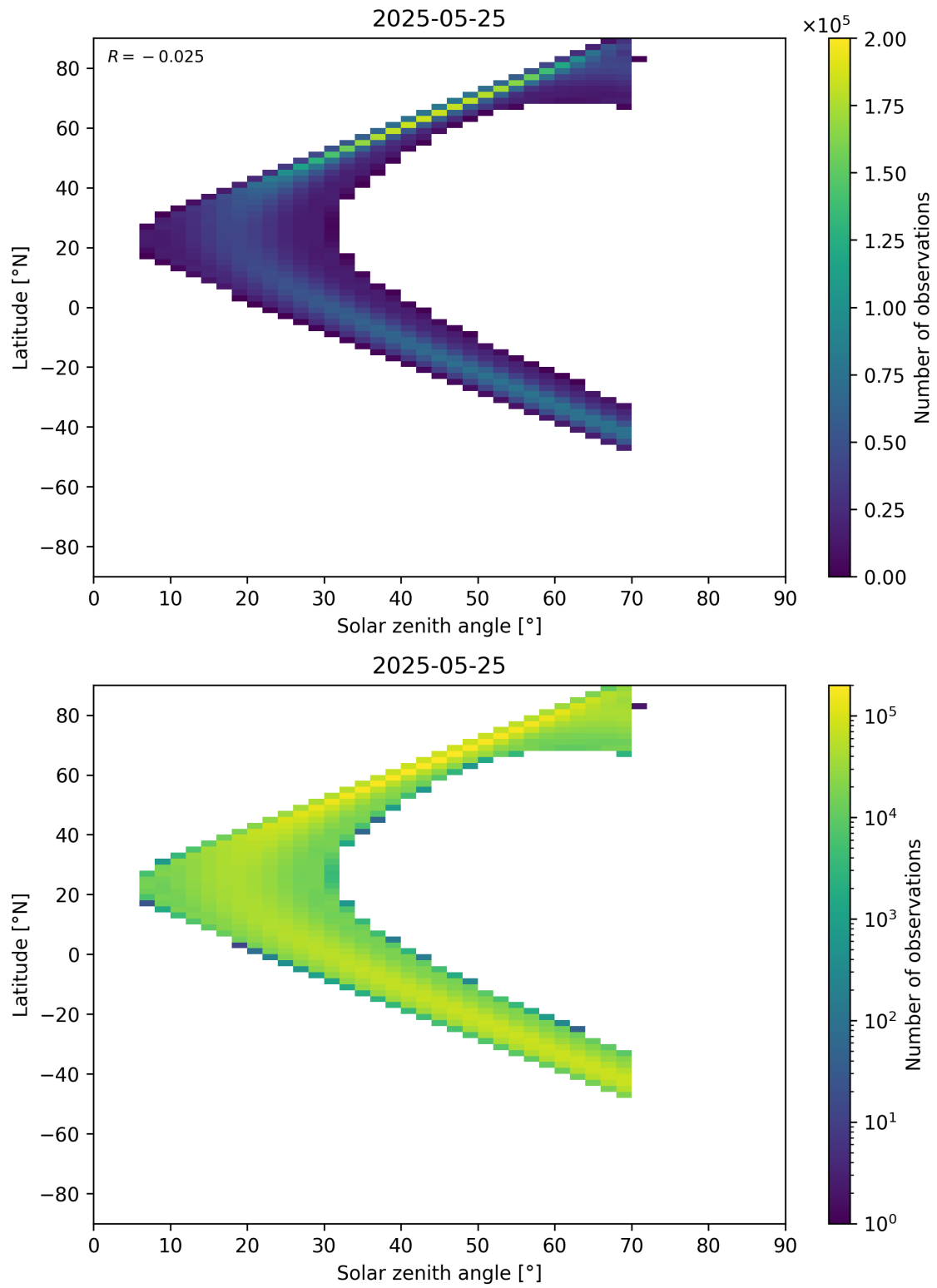
Figure 177: Scatter density plot of “Solar zenith angle” against “Latitude” for 2025-05-24 to 2025-05-26.
