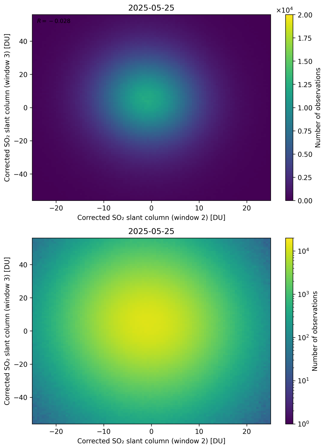
Figure 250: Scatter density plot of “Corrected SO 2 slant column (window 2)” against “Corrected SO 2 slant column (window 3)” for 2025-05-24 to 2025-05-26.
