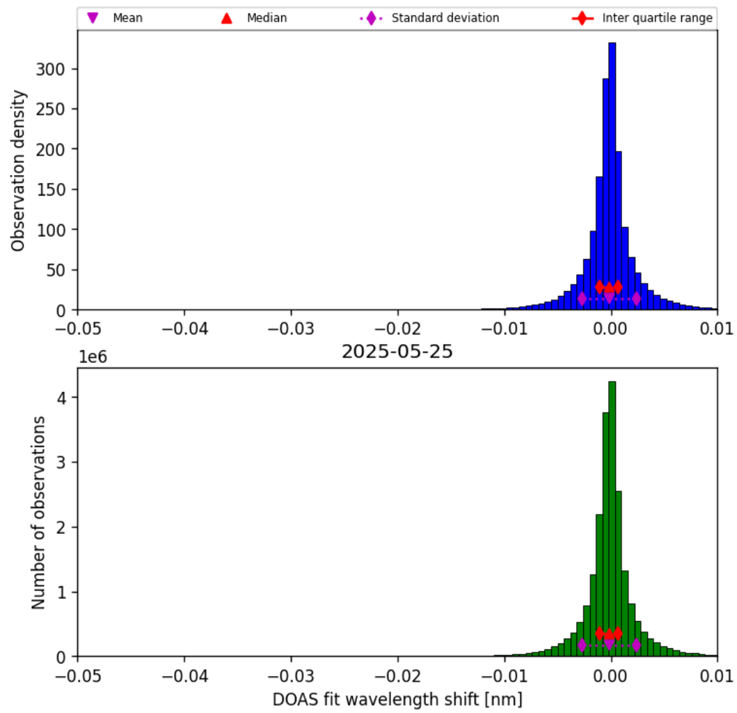
Figure 76: Histogram of “DOAS fit wavelength shift” for 2025-05-24 to 2025-05-26
