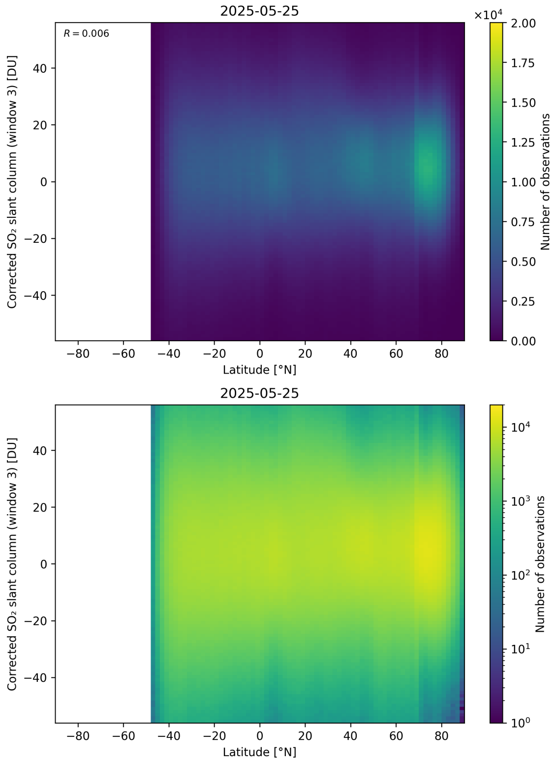
Figure 161: Scatter density plot of “Latitude” against “Corrected SO 2 slant column (window 3)” for 2025-05-24 to 2025-05-26.
