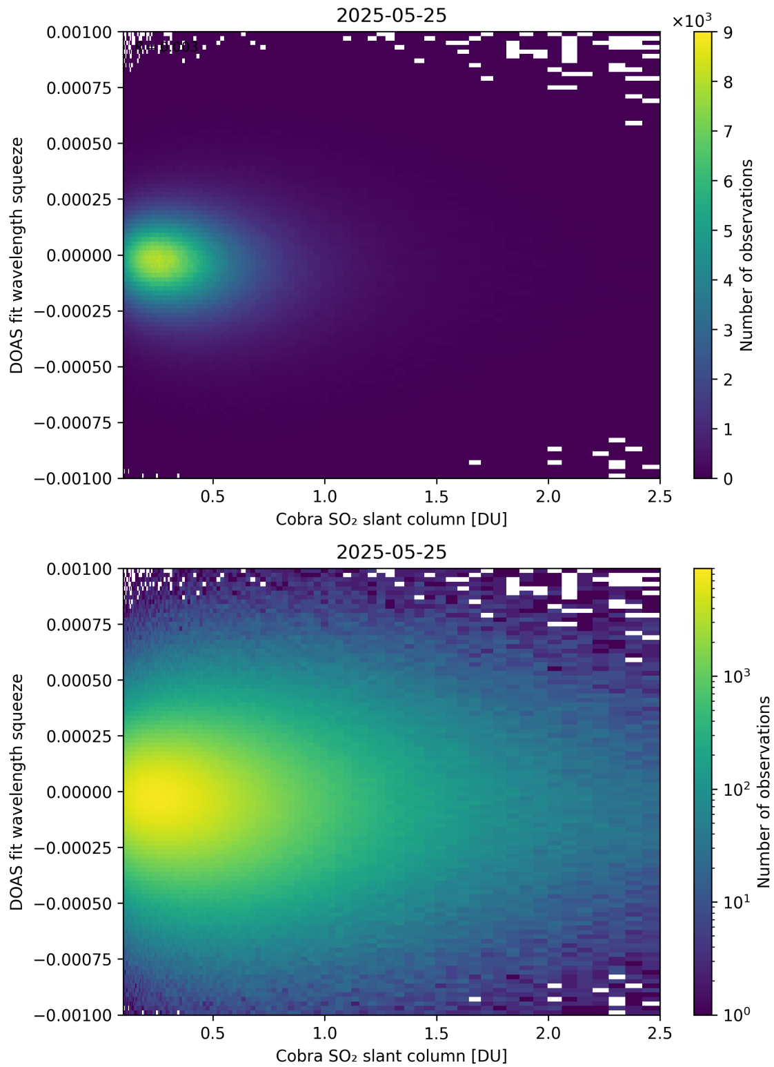
Figure 197: Scatter density plot of “Cobra SO 2 slant column” against “DOAS fit wavelength squeeze” for 2025-05-24 to 2025-05-26.
