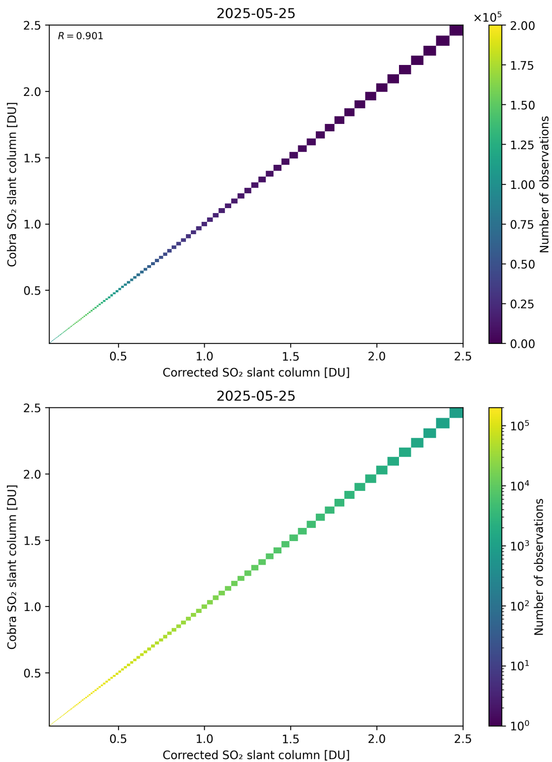
Figure 233: Scatter density plot of “Corrected SO 2 slant column” against “Cobra SO 2 slant column” for 2025-05-24 to 2025-05-26.
