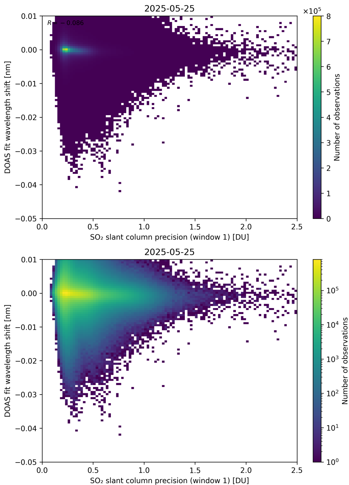
Figure 271: Scatter density plot of “SO 2 slant column precision (window 1)” against “DOAS fit wavelength shift” for 2025-05-24 to 2025-05-26.
