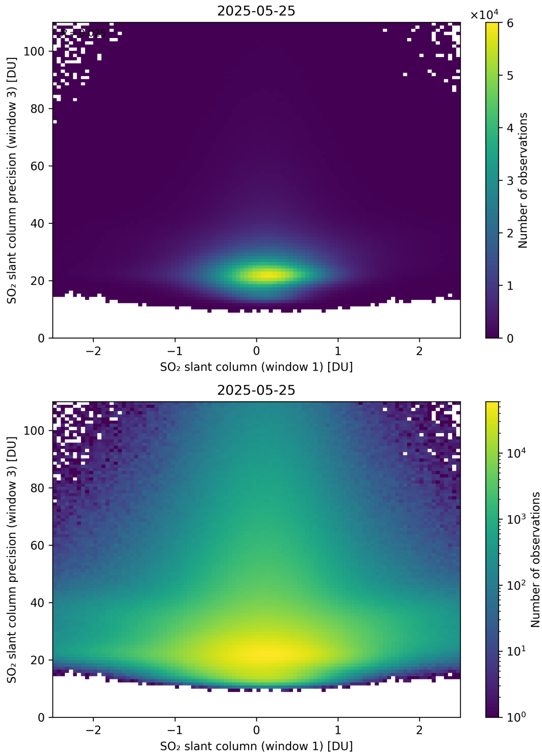
Figure 288: Scatter density plot of “SO 2 slant column (window 1)” against “SO 2 slant column precision (window 3)” for 2025-05-24 to 2025-05-26.
