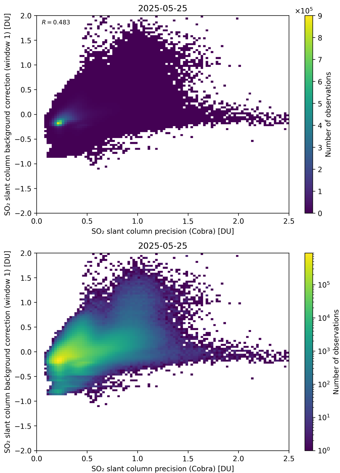
Figure 199: Scatter density plot of “SO 2 slant column precision (Cobra)” against “SO 2 slant column background correction (window 1)” for 2025-05-24 to 2025-05-26.
