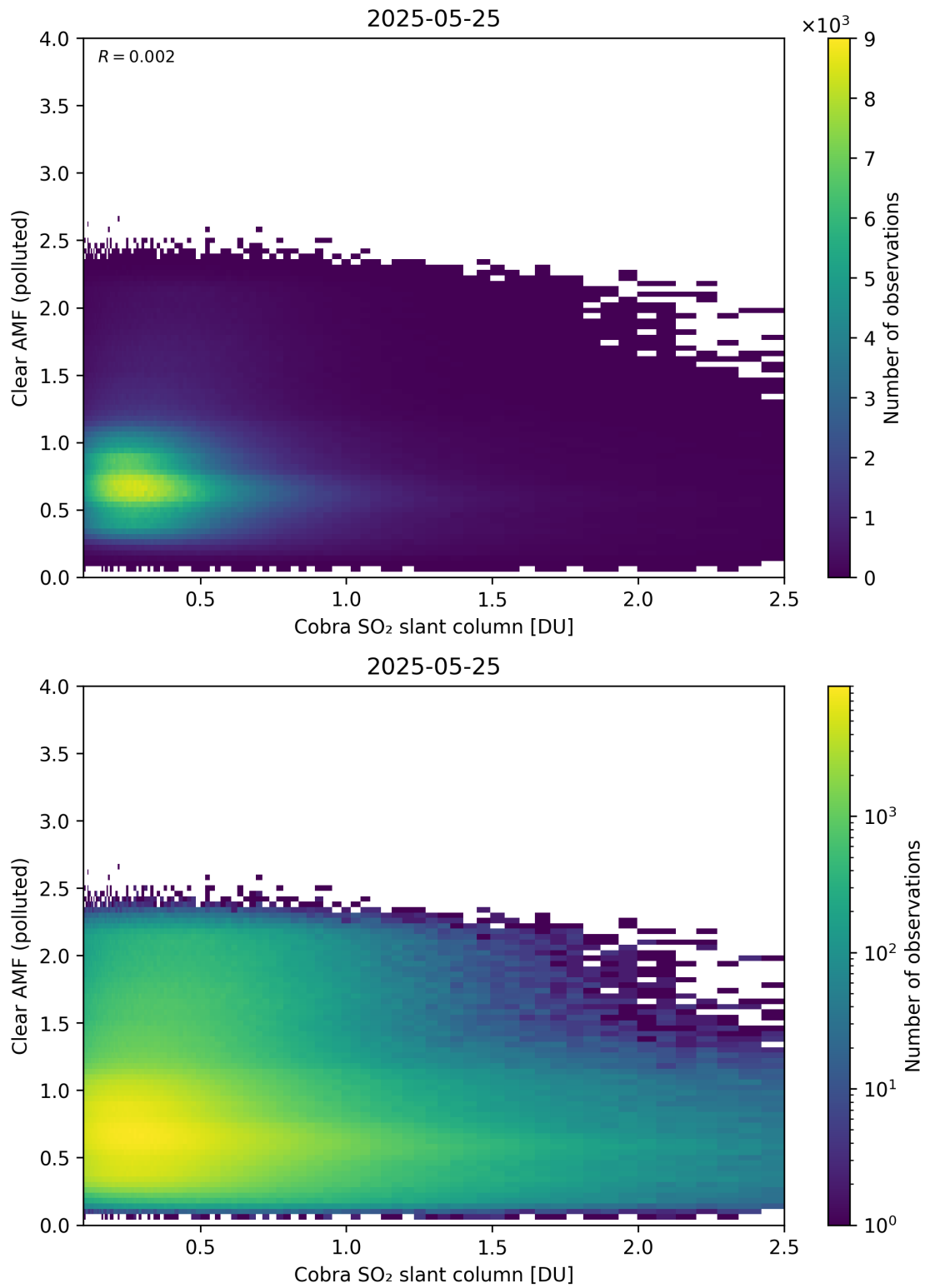
Figure 215: Scatter density plot of “Cobra SO 2 slant column” against “Clear AMF (polluted)” for 2025-05-24 to 2025-05-26.
