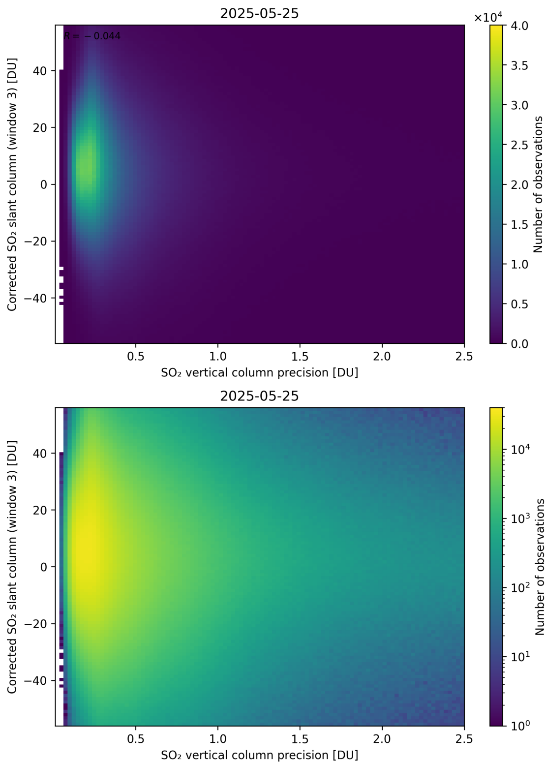
Figure 340: Scatter density plot of “SO 2 vertical column precision” against “Corrected SO 2 slant column (window 3)” for 2025-05-24 to 2025-05-26.
