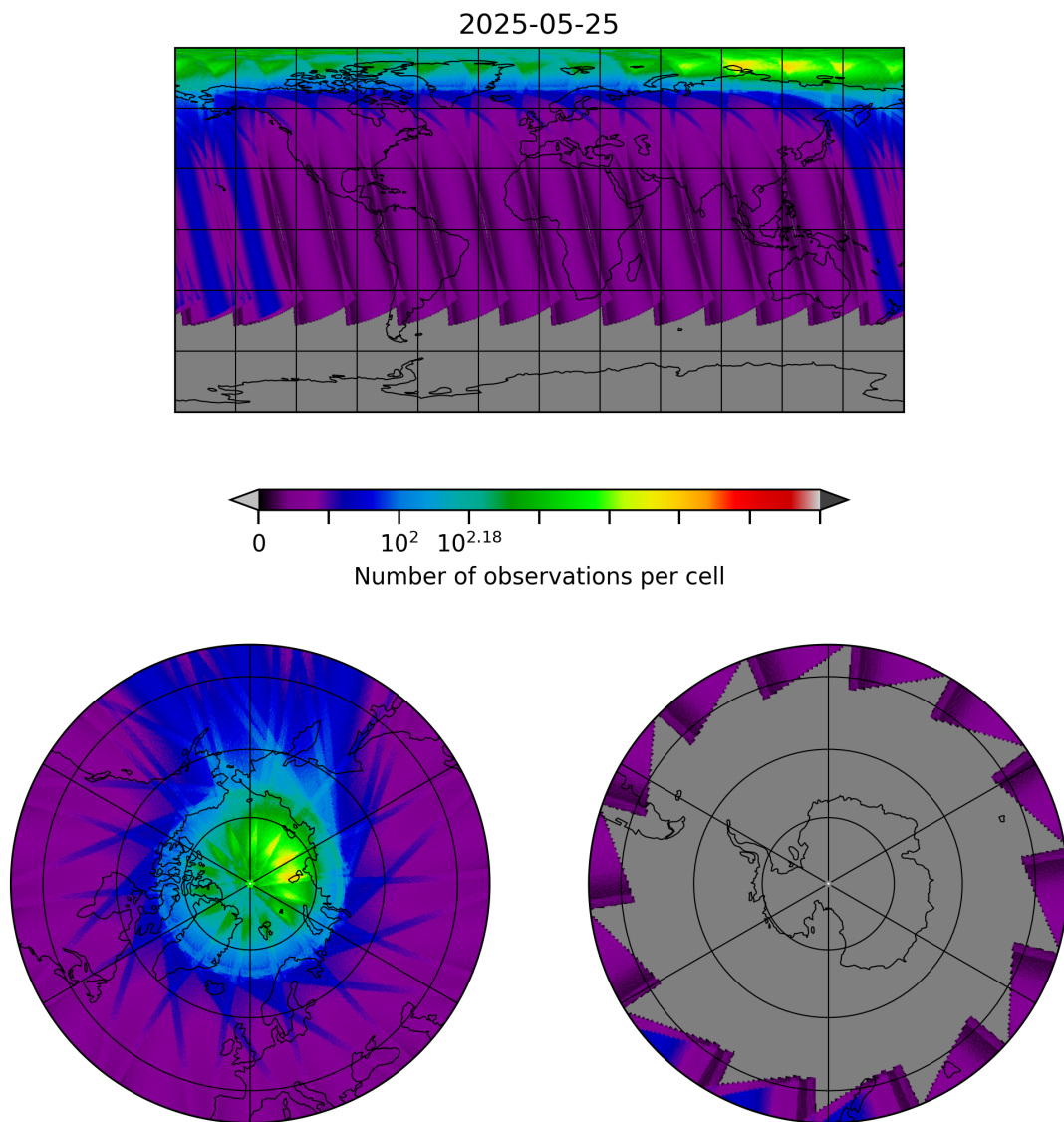
Figure 30: Map of the number of observations for 2025-05-24 to 2025-05-26
