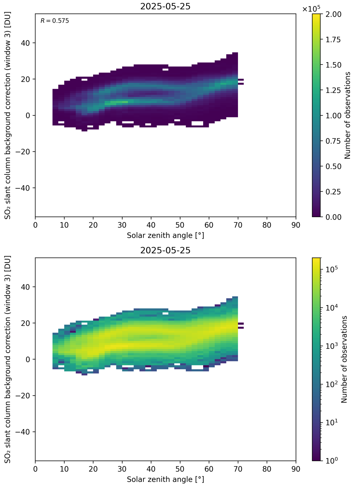
Figure 173: Scatter density plot of “Solar zenith angle” against “SO 2 slant column background correction (window 3)” for 2025-05-24 to 2025-05-26.
