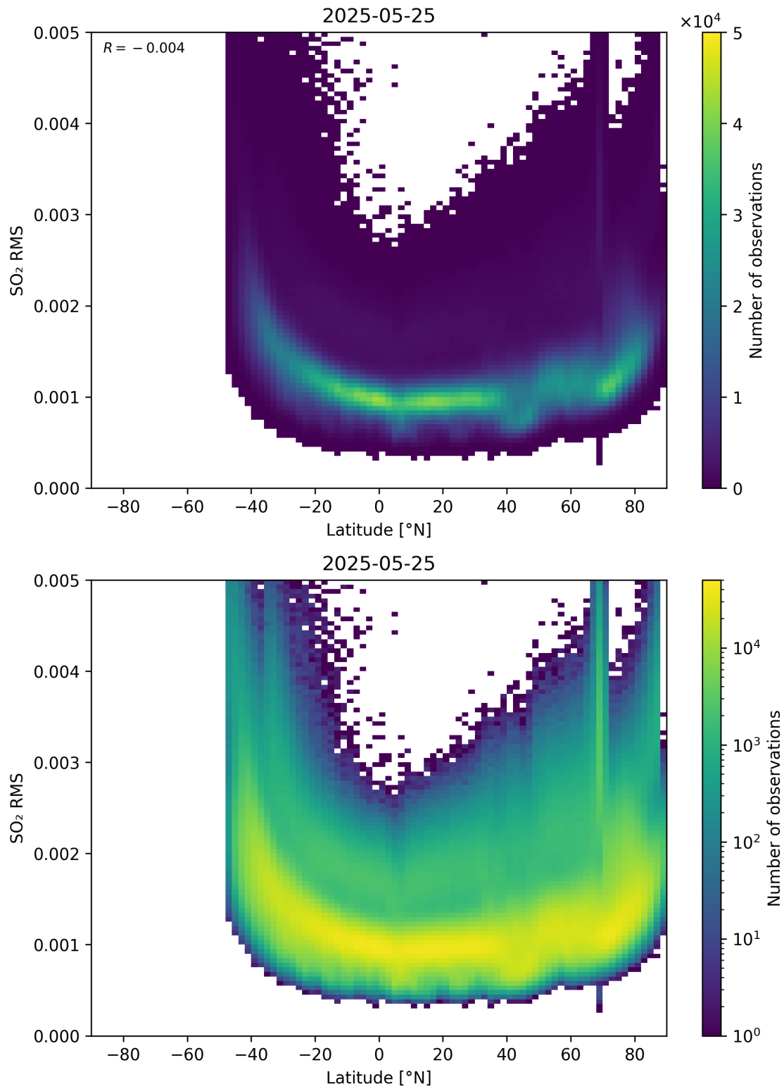
Figure 155: Scatter density plot of “Latitude” against “SO 2 RMS” for 2025-05-24 to 2025-05-26.
