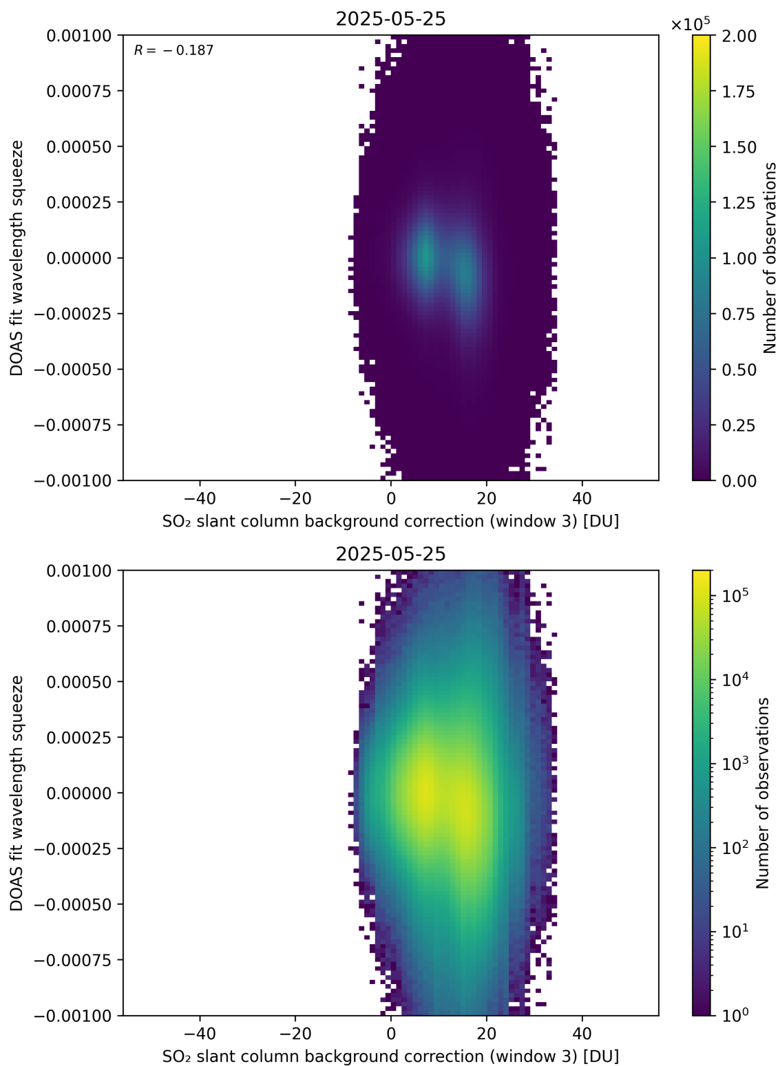
Figure 133: Scatter density plot of “SO 2 slant column background correction (window 3)” against “DOAS fit wavelength squeeze” for 2025-05-24 to 2025-05-26.
