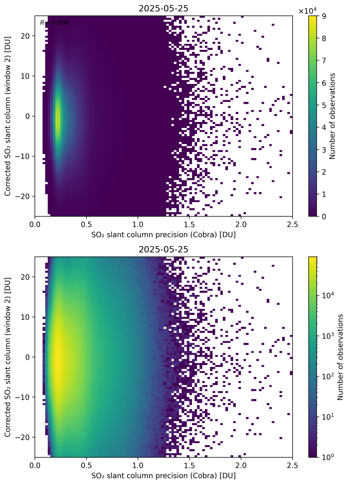
Figure 206: Scatter density plot of “SO 2 slant column precision (Cobra)” against “Corrected SO 2 slant column (window 2)” for 2025-05-24 to 2025-05-26.
