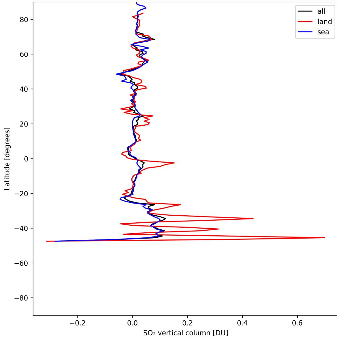
Figure 32: Zonal average of “SO 2 vertical column” for 2025-05-24 to 2025-05-26.
