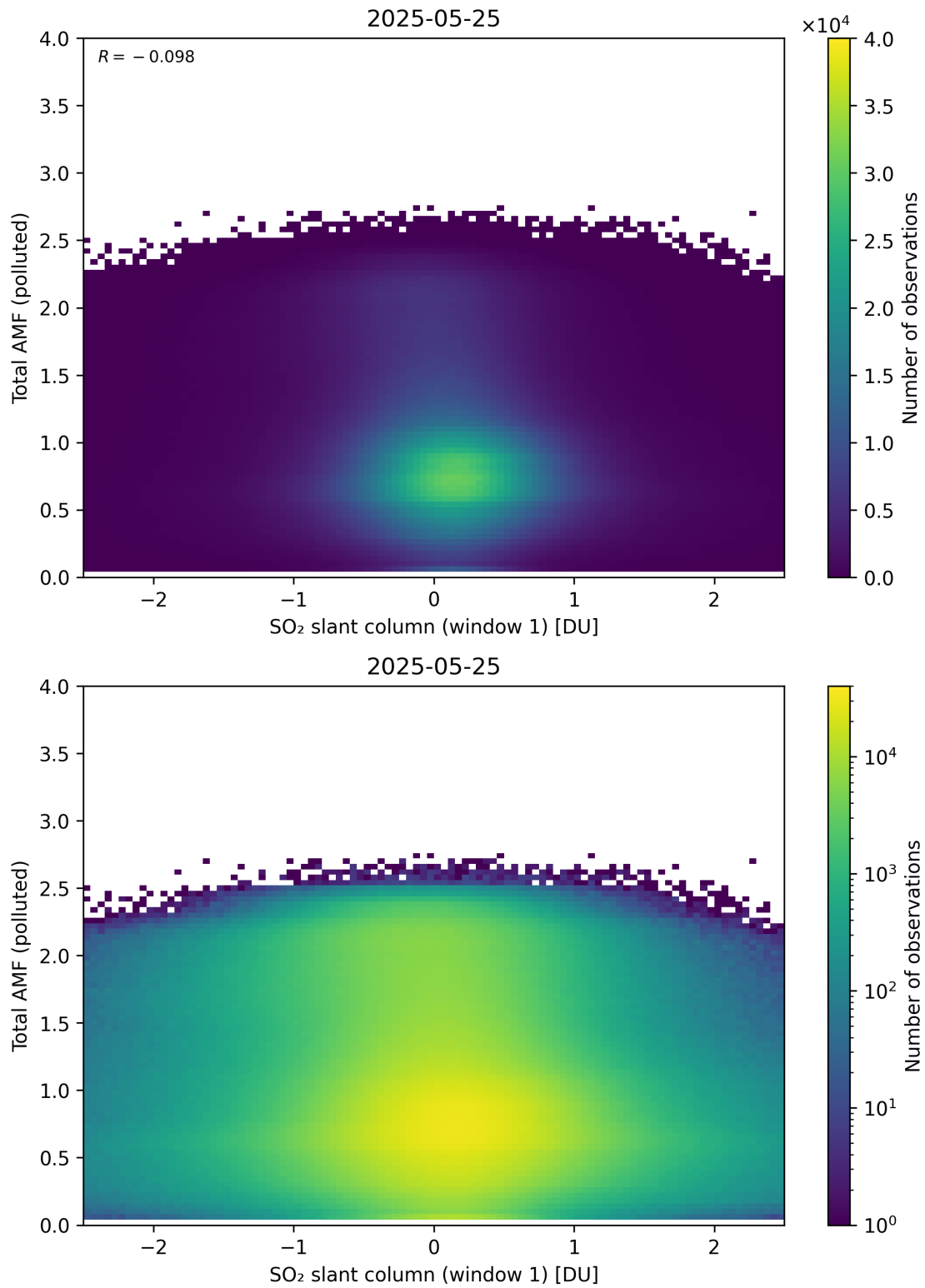
Figure 289: Scatter density plot of “SO 2 slant column (window 1)” against “Total AMF (polluted)” for 2025-05-24 to 2025-05-26.
