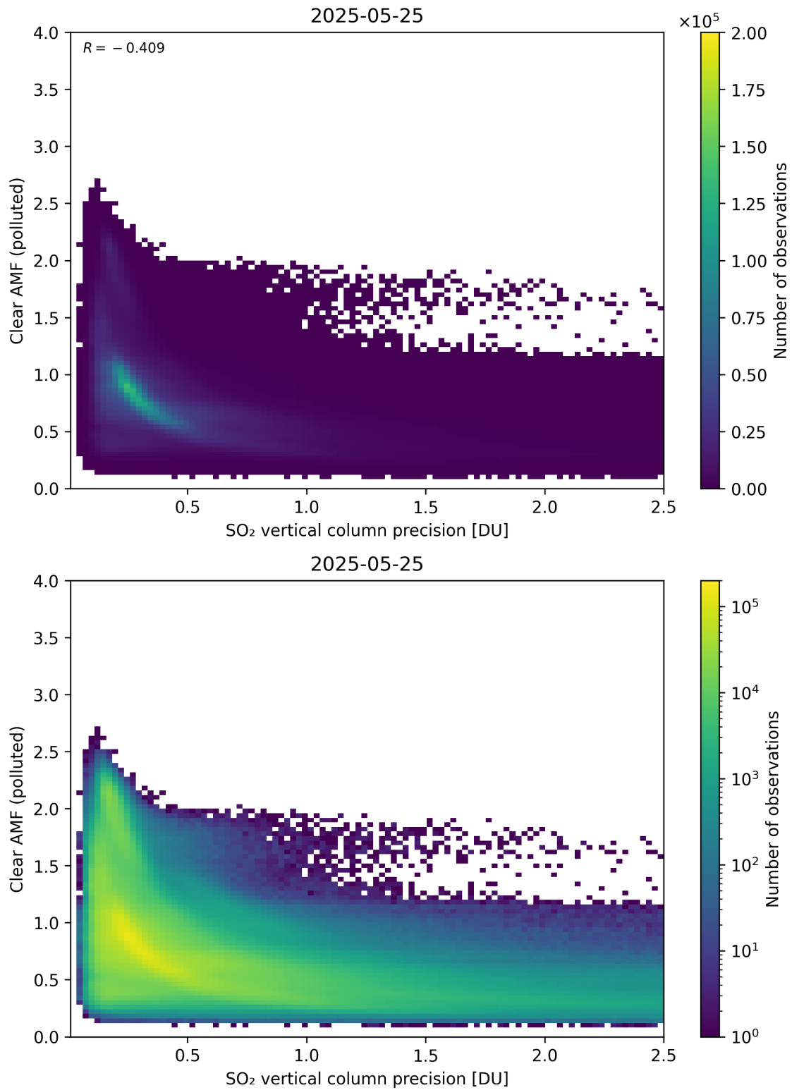
Figure 335: Scatter density plot of “SO 2 vertical column precision” against “Clear AMF (polluted)” for 2025-05-24 to 2025-05-26.
