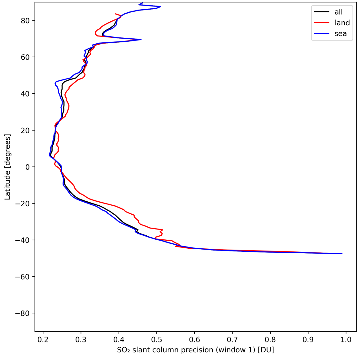
Figure 38: Zonal average of “SO 2 slant column precision (window 1)” for 2025-05-24 to 2025-05-26.
