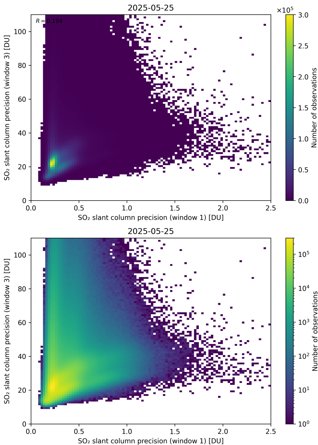
Figure 279: Scatter density plot of “SO 2 slant column precision (window 1)” against “SO 2 slant column precision (window 3)” for 2025-05-24 to 2025-05-26.
