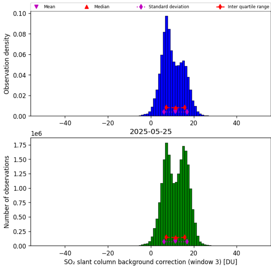
Figure 74: Histogram of “SO 2 slant column background correction (window 3)” for 2025-05-24 to 2025-05-26
