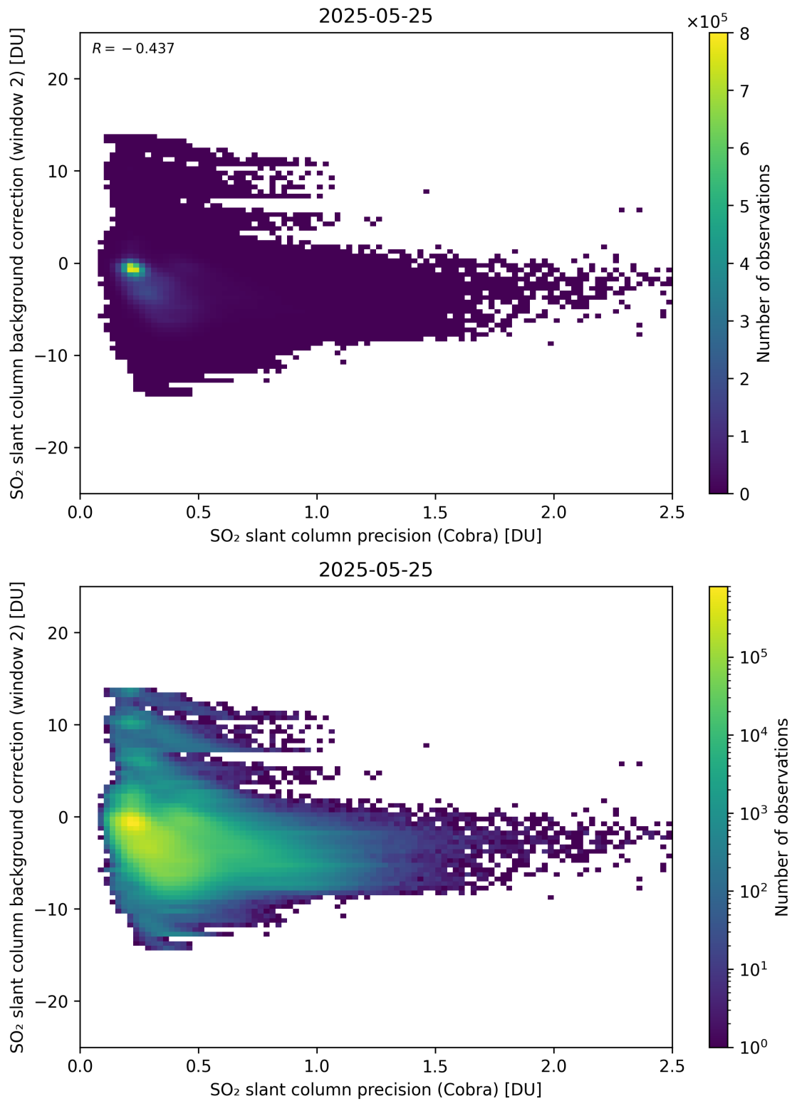
Figure 200: Scatter density plot of “SO 2 slant column precision (Cobra)” against “SO 2 slant column background correction (window 2)” for 2025-05-24 to 2025-05-26.
