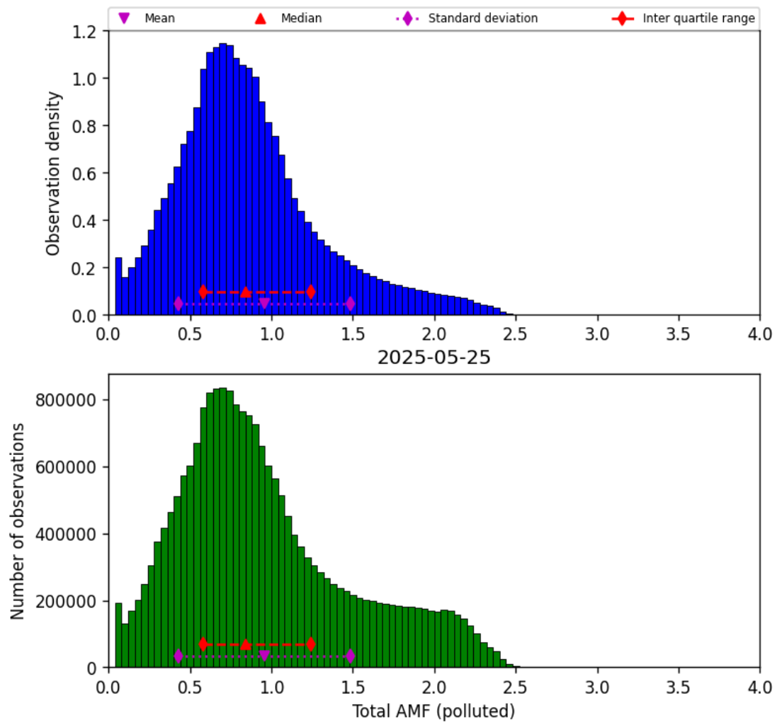
Figure 79: Histogram of “Total AMF (polluted)” for 2025-05-24 to 2025-05-26
