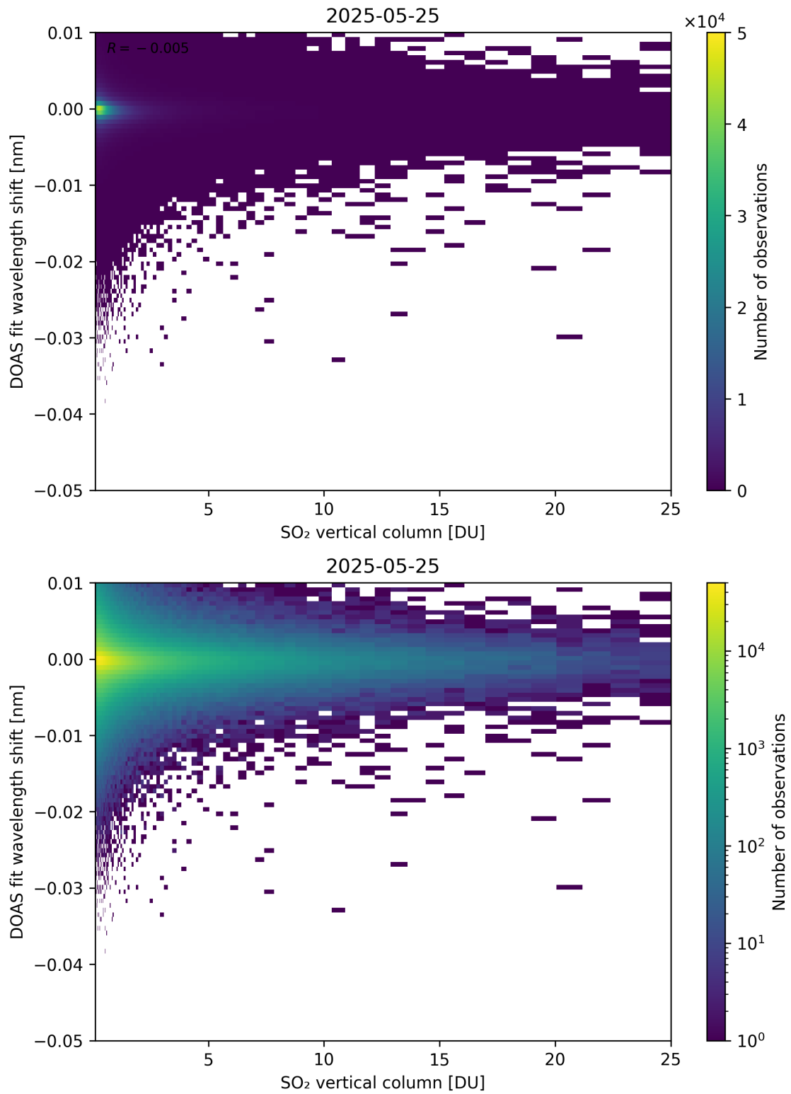
Figure 326: Scatter density plot of “SO 2 vertical column” against “DOAS fit wavelength shift” for 2025-05-24 to 2025-05-26.
