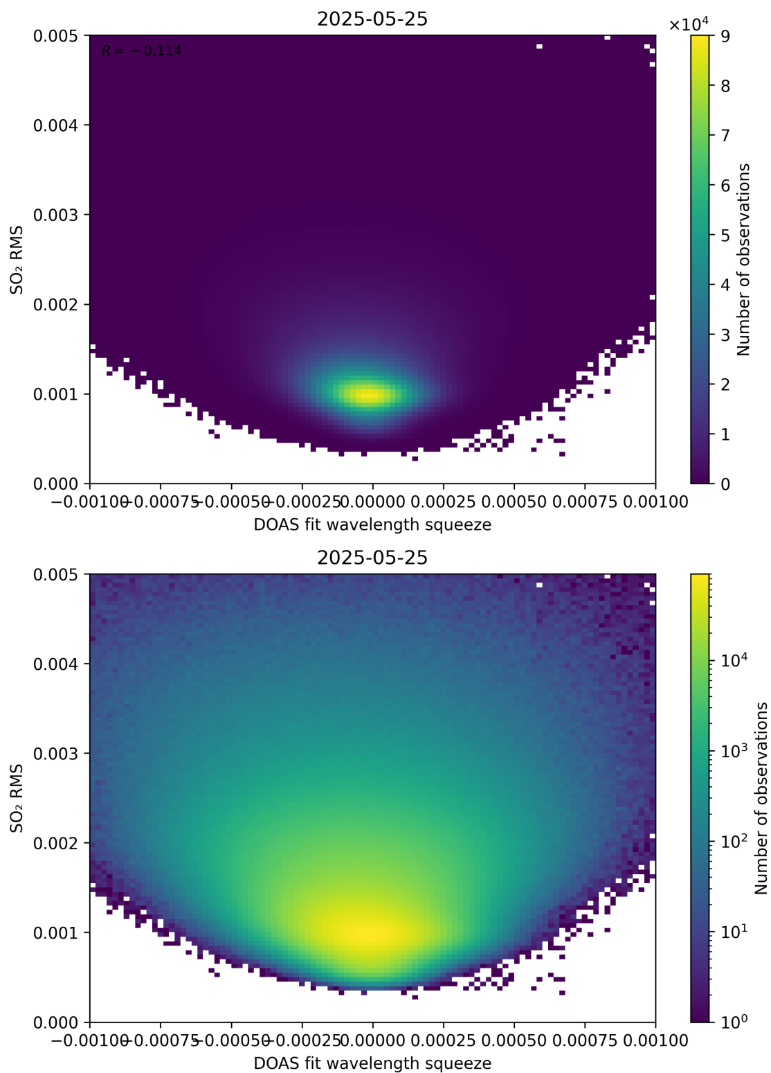
Figure 143: Scatter density plot of “DOAS fit wavelength squeeze” against “SO 2 RMS” for 2025-05-24 to 2025-05-26.
