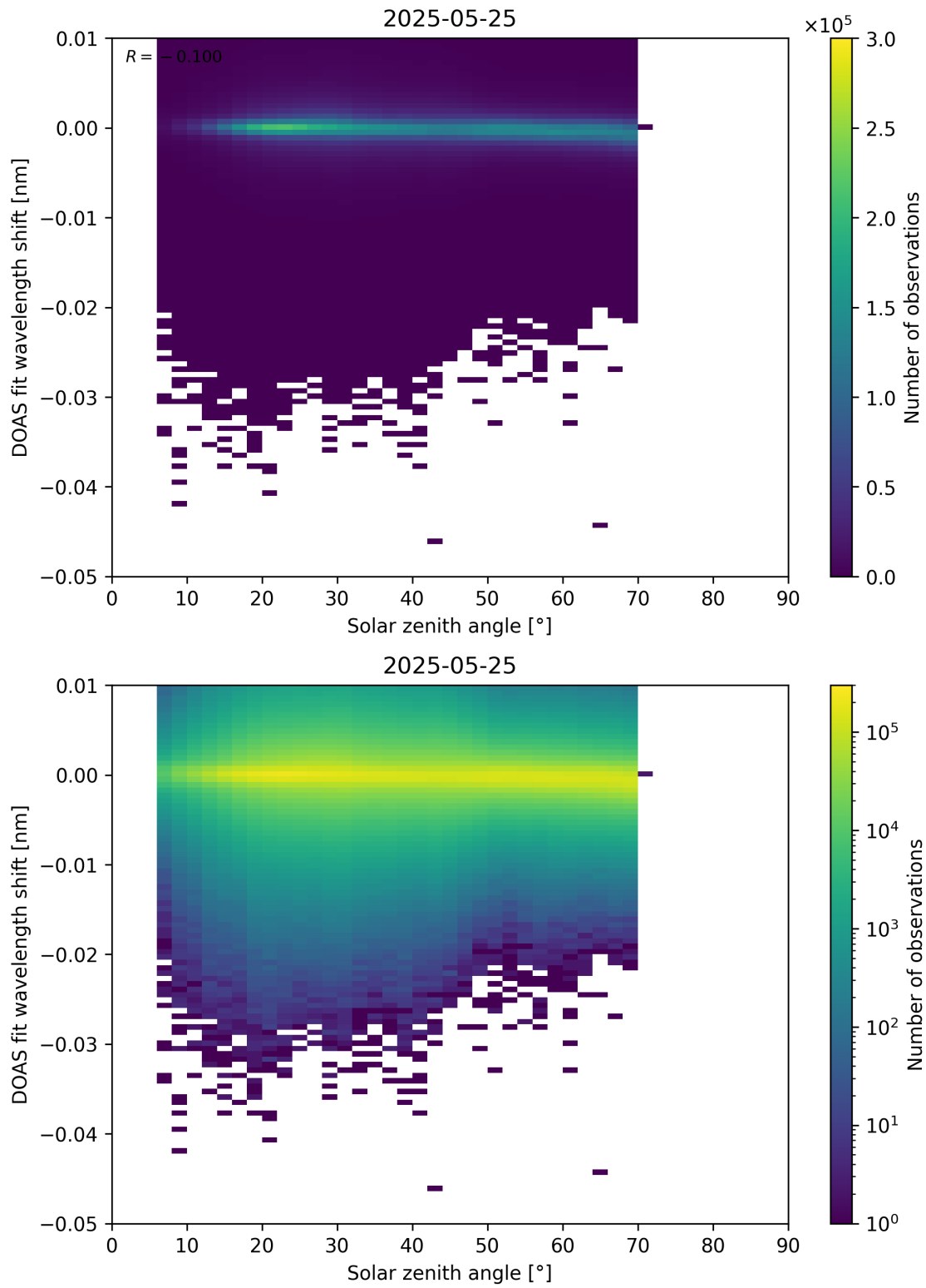
Figure 174: Scatter density plot of “Solar zenith angle” against “DOAS fit wavelength shift” for 2025-05-24 to 2025-05-26.
