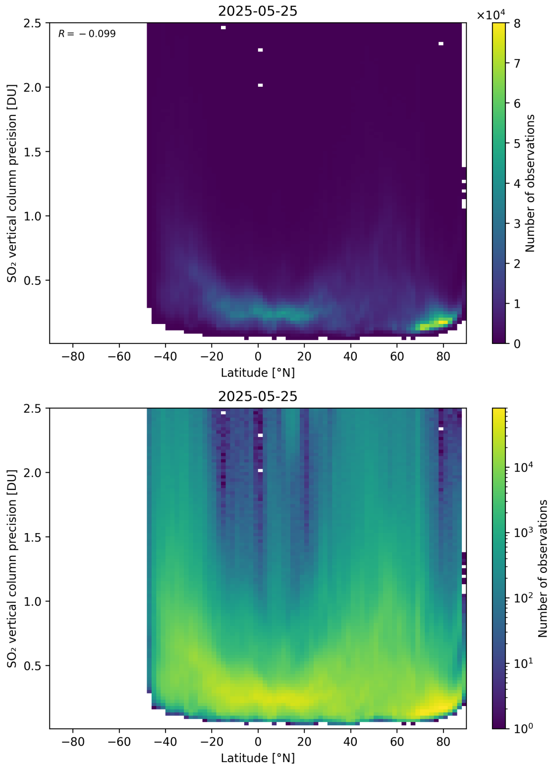
Figure 170: Scatter density plot of “Latitude” against “SO 2 vertical column precision” for 2025-05-24 to 2025-05-26.
