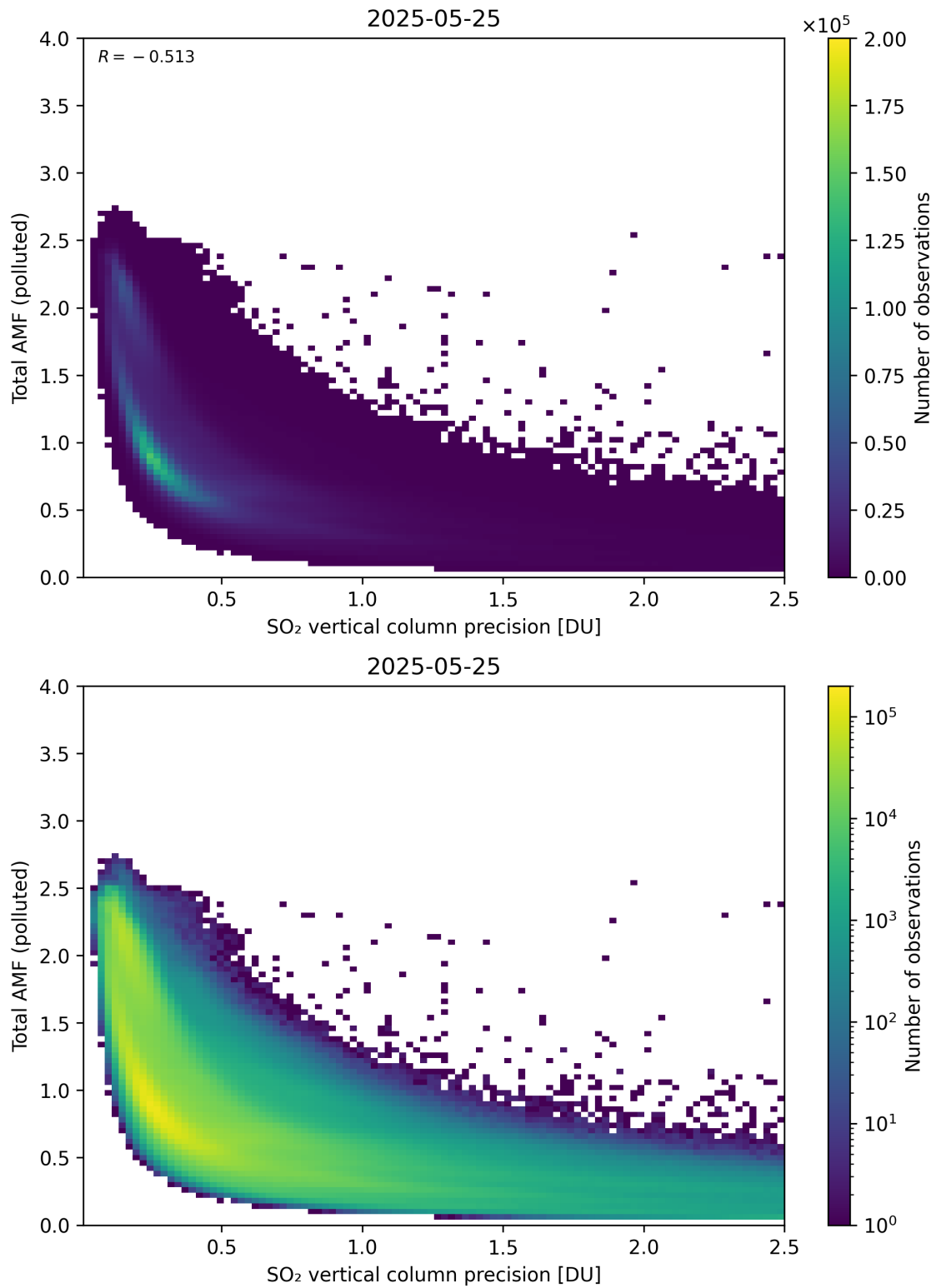
Figure 346: Scatter density plot of “SO 2 vertical column precision” against “Total AMF (polluted)” for 2025-05-24 to 2025-05-26.
