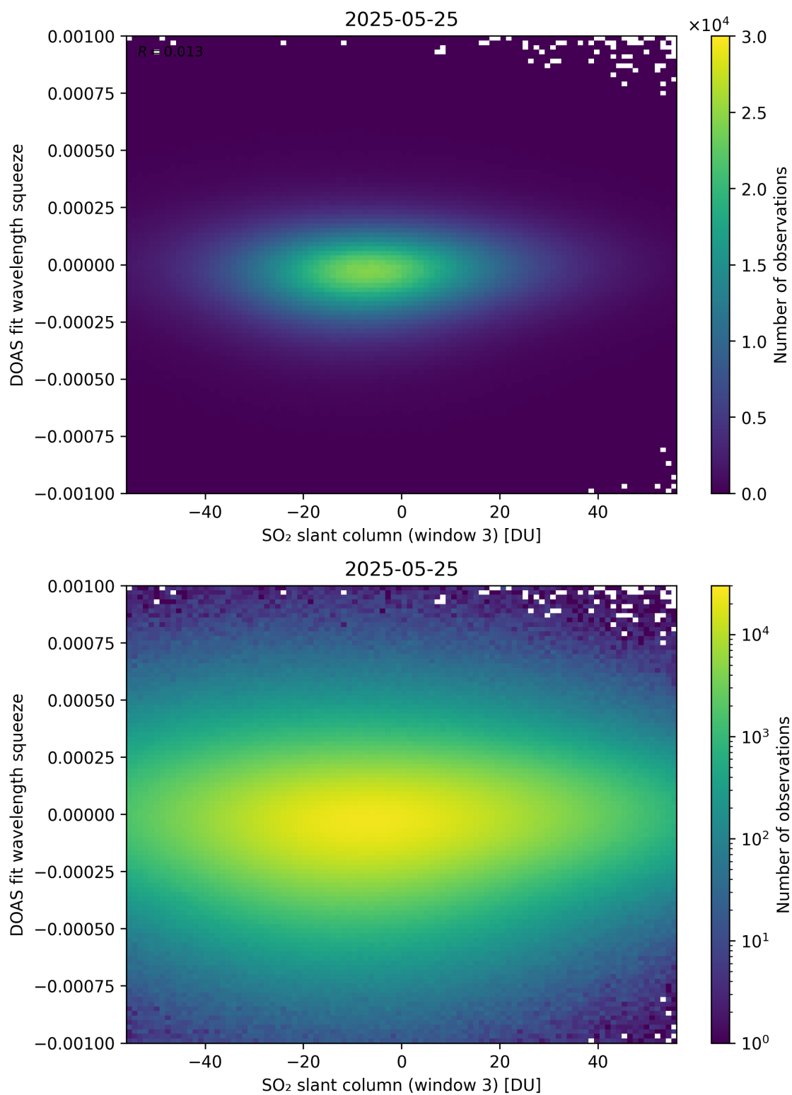
Figure 305: Scatter density plot of “SO 2 slant column (window 3)” against “DOAS fit wavelength squeeze” for 2025-05-24 to 2025-05-26.
