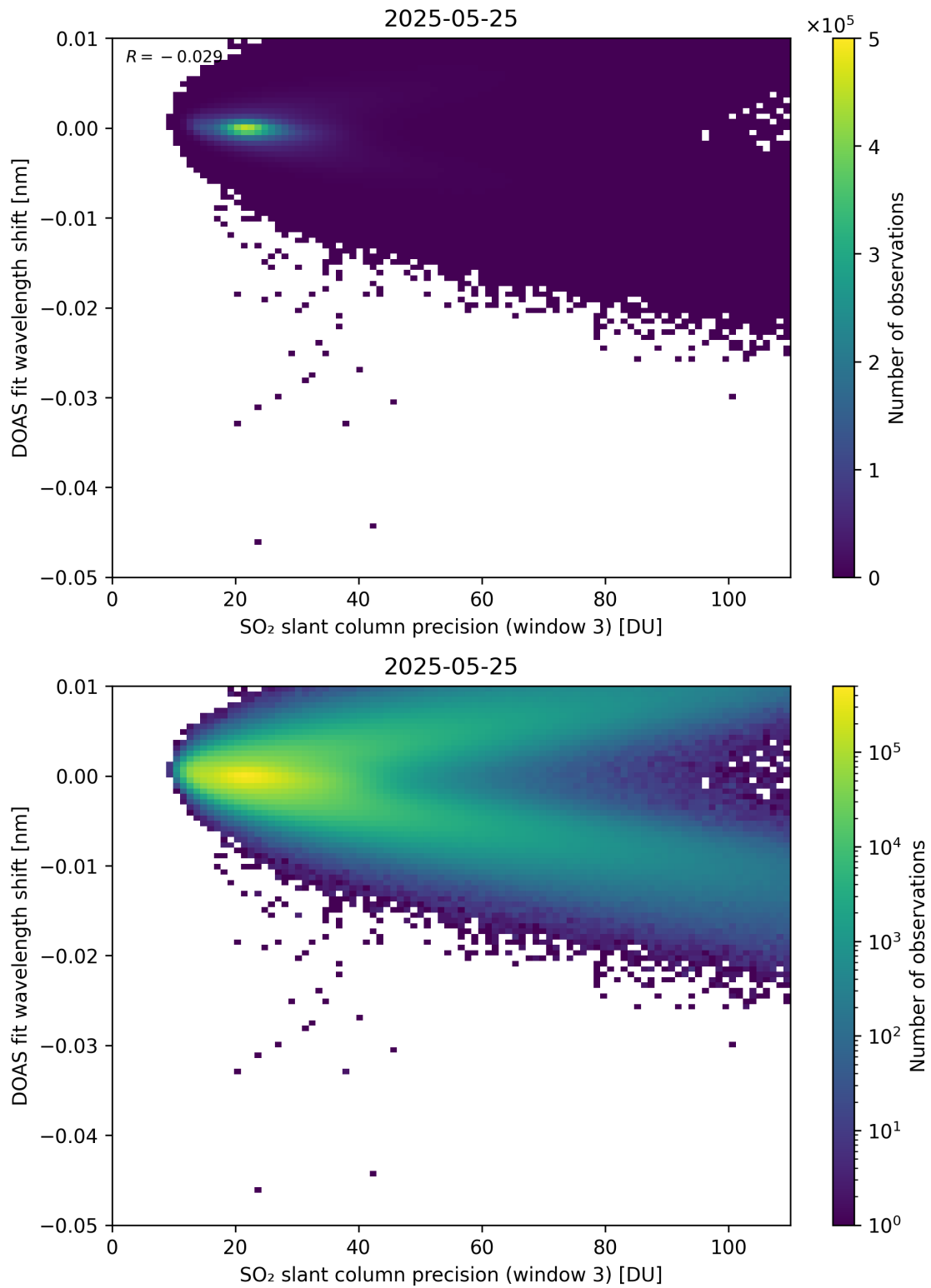
Figure 308: Scatter density plot of “SO 2 slant column precision (window 3)” against “DOAS fit wavelength shift” for 2025-05-24 to 2025-05-26.
