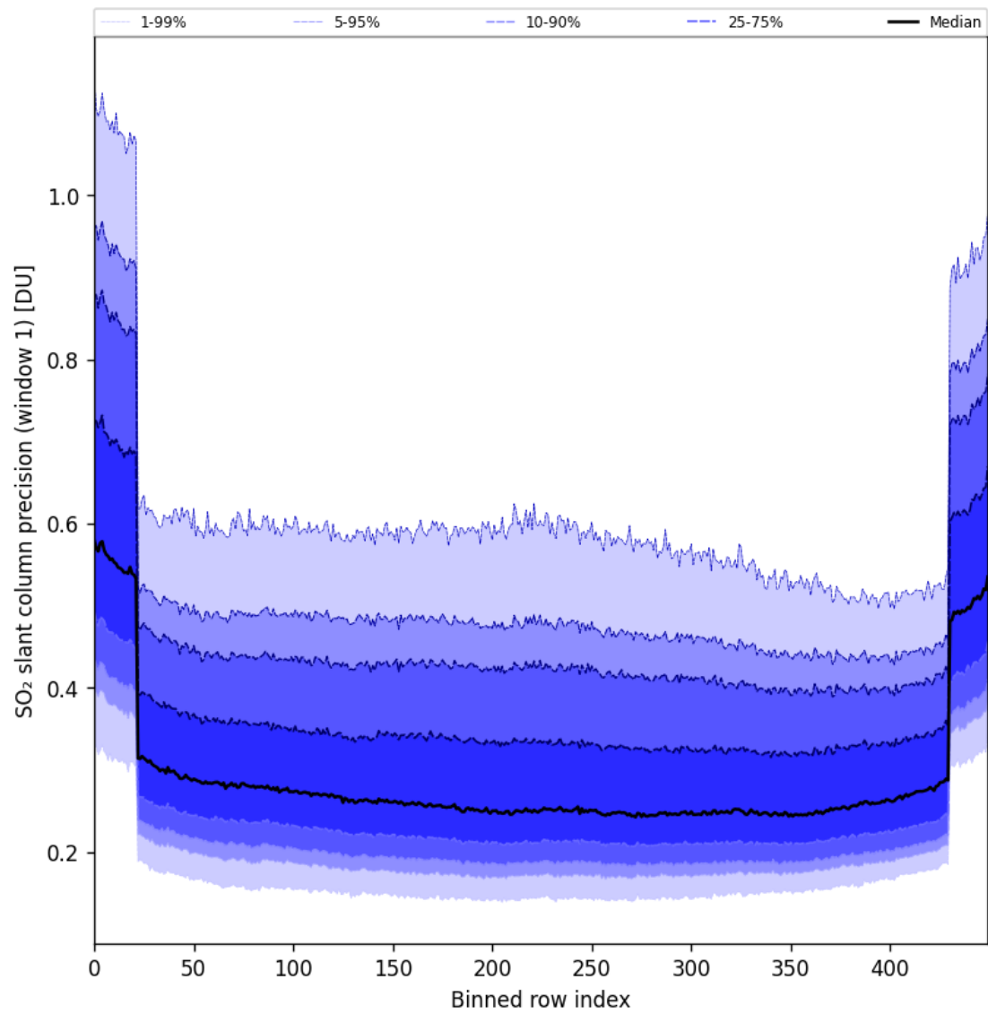
Figure 90: Along track statistics of “SO 2 slant column precision (window 1)” for 2025-05-24 to 2025-05-26
