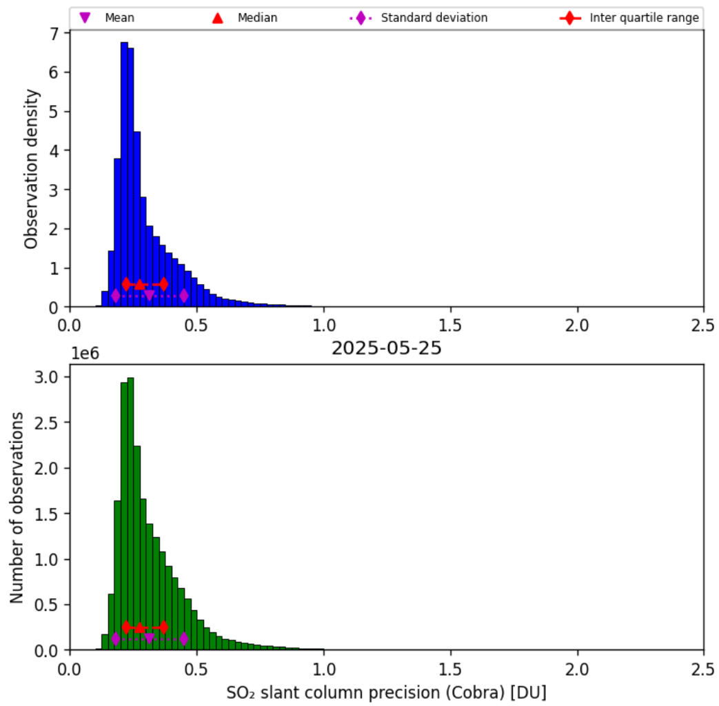
Figure 62: Histogram of “SO 2 slant column precision (Cobra)” for 2025-05-24 to 2025-05-26
