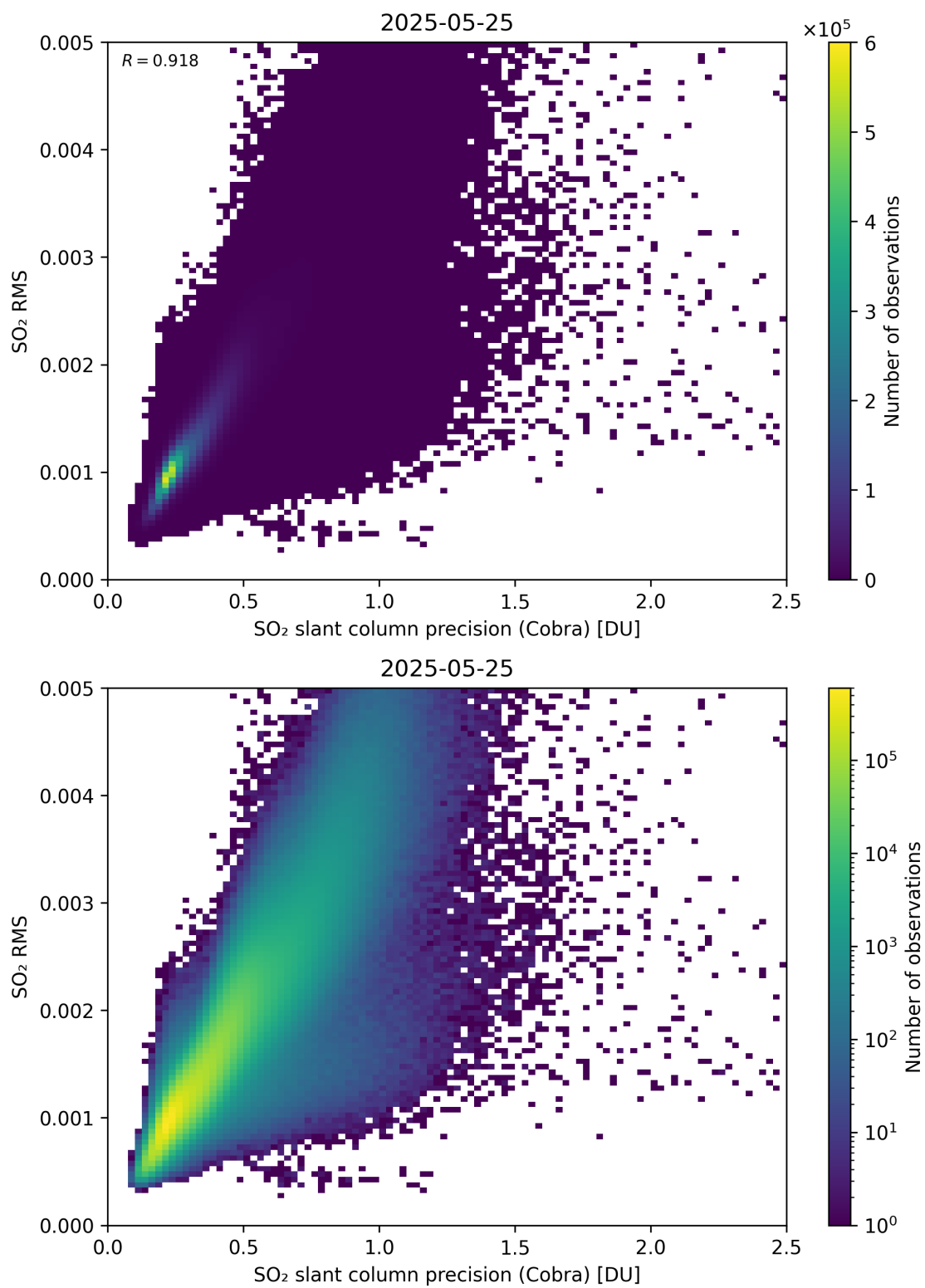
Figure 204: Scatter density plot of “SO 2 slant column precision (Cobra)” against “SO 2 RMS” for 2025-05-24 to 2025-05-26.
