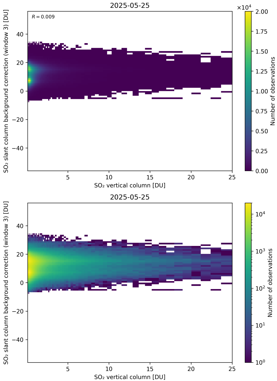
Figure 325: Scatter density plot of “SO 2 vertical column” against “SO 2 slant column background correction (window 3)” for 2025-05-24 to 2025-05-26.
