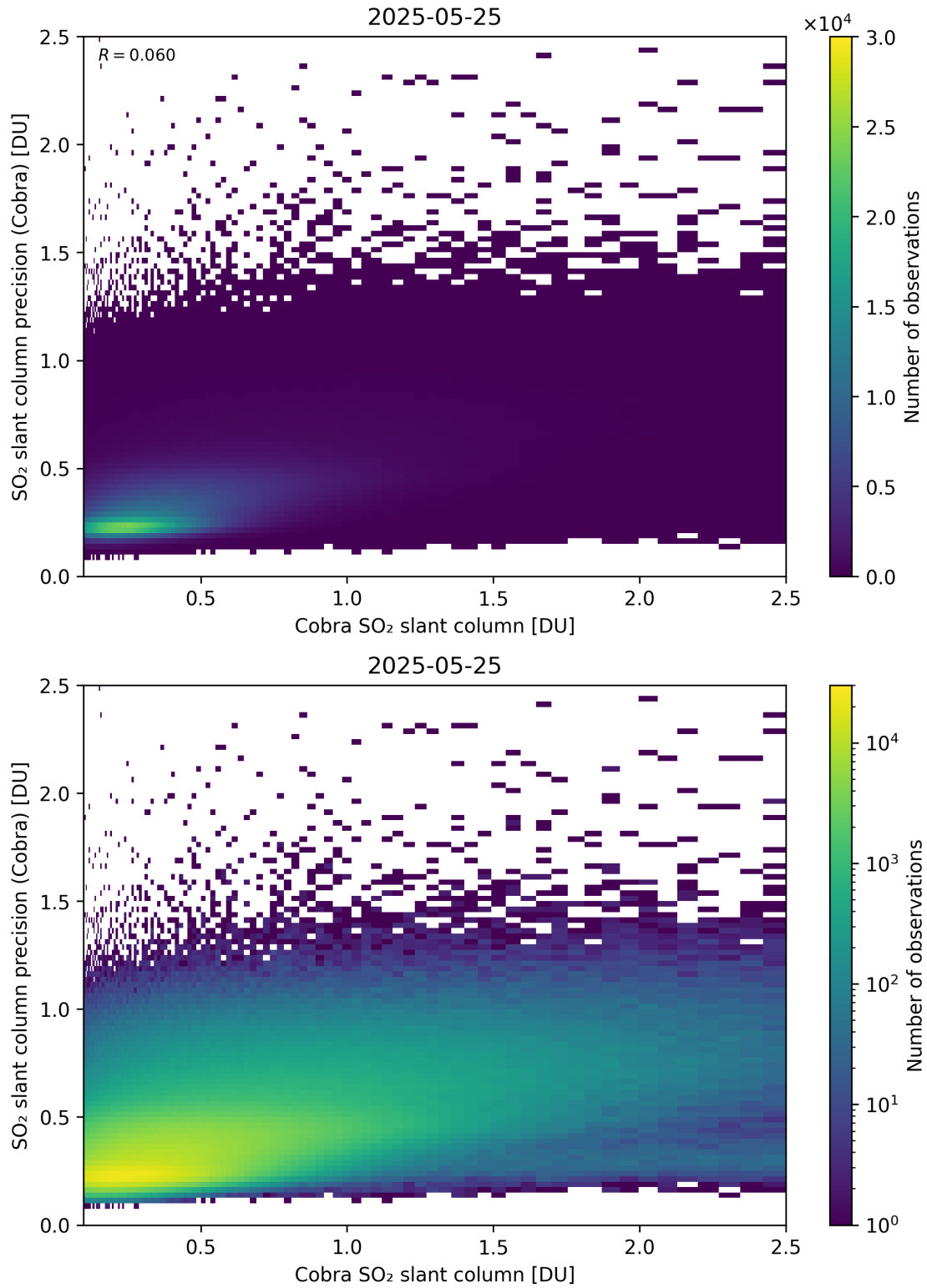
Figure 216: Scatter density plot of “Cobra SO 2 slant column” against “SO 2 slant column precision (Cobra)” for 2025-05-24 to 2025-05-26.
