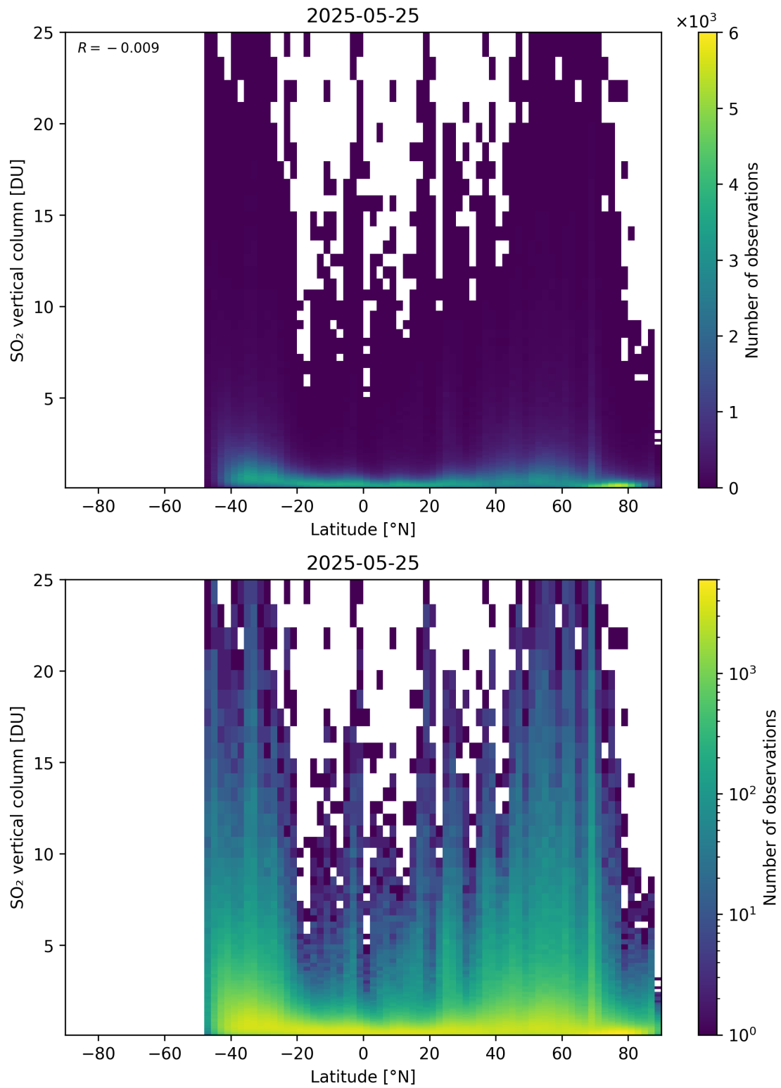
Figure 169: Scatter density plot of “Latitude” against “SO 2 vertical column” for 2025-05-24 to 2025-05-26.
