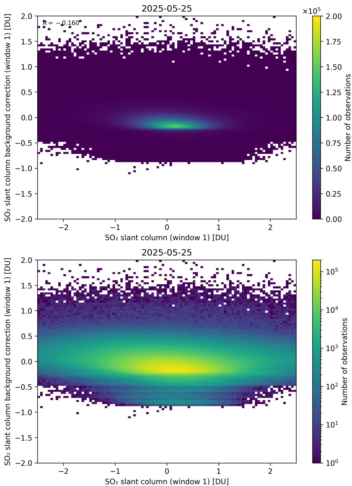
Figure 262: Scatter density plot of “SO 2 slant column (window 1)” against “SO 2 slant column background correction (window 1)” for 2025-05-24 to 2025-05-26.
