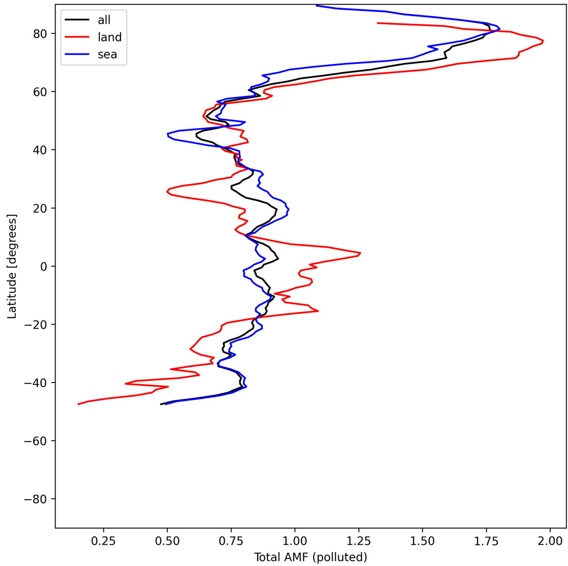
Figure 53: Zonal average of “Total AMF (polluted)” for 2025-05-24 to 2025-05-26.
