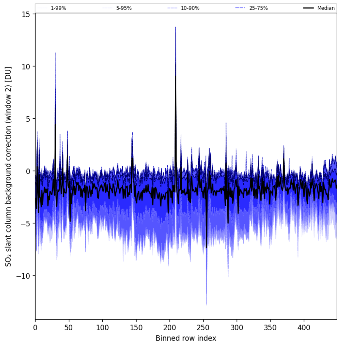
Figure 96: Along track statistics of “SO 2 slant column background correction (window 2)” for 2025-05-24 to 2025-05-26
