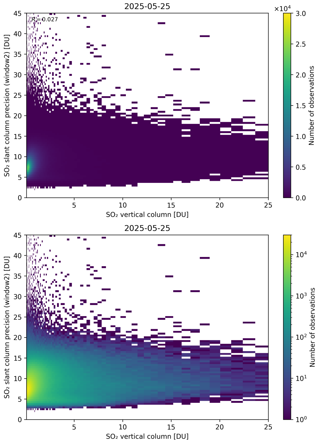
Figure 356: Scatter density plot of “SO 2 vertical column” against “SO 2 slant column precision (window2)” for 2025-05-24 to 2025-05-26.
