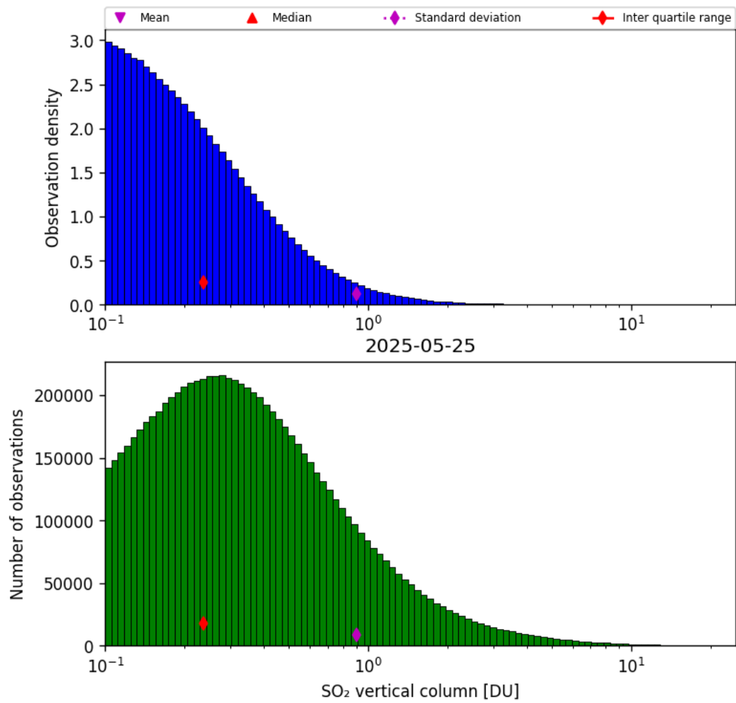
Figure 58: Histogram of “SO 2 vertical column” for 2025-05-24 to 2025-05-26
