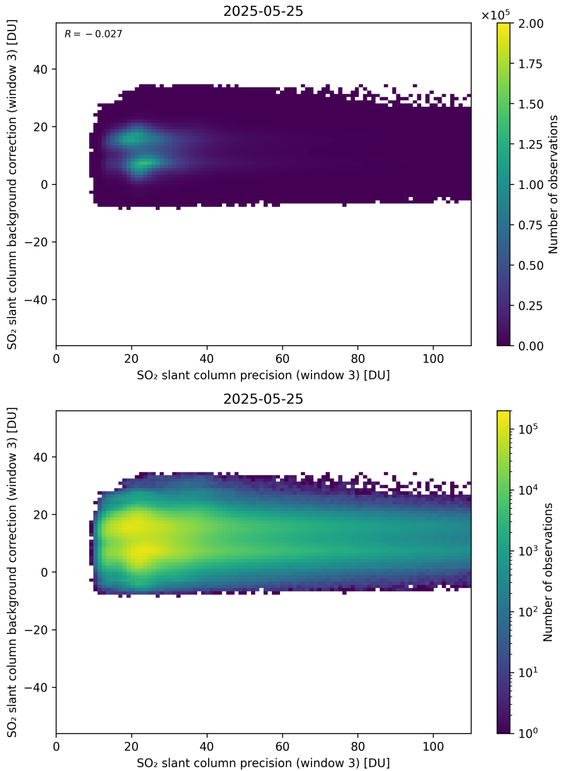
Figure 307: Scatter density plot of “SO 2 slant column precision (window 3)” against “SO 2 slant column background correction (window 3)” for 2025-05-24 to 2025-05-26.
