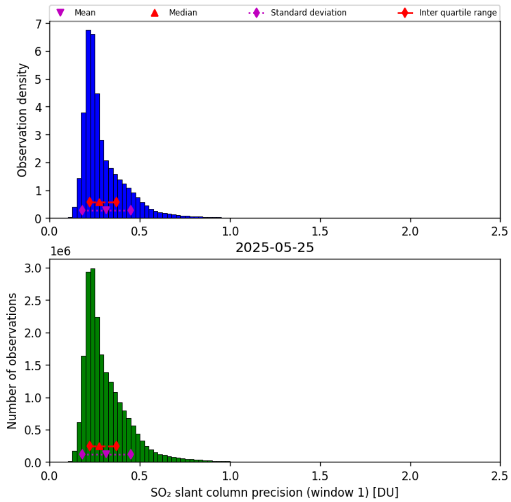
Figure 64: Histogram of “SO 2 slant column precision (window 1)” for 2025-05-24 to 2025-05-26
