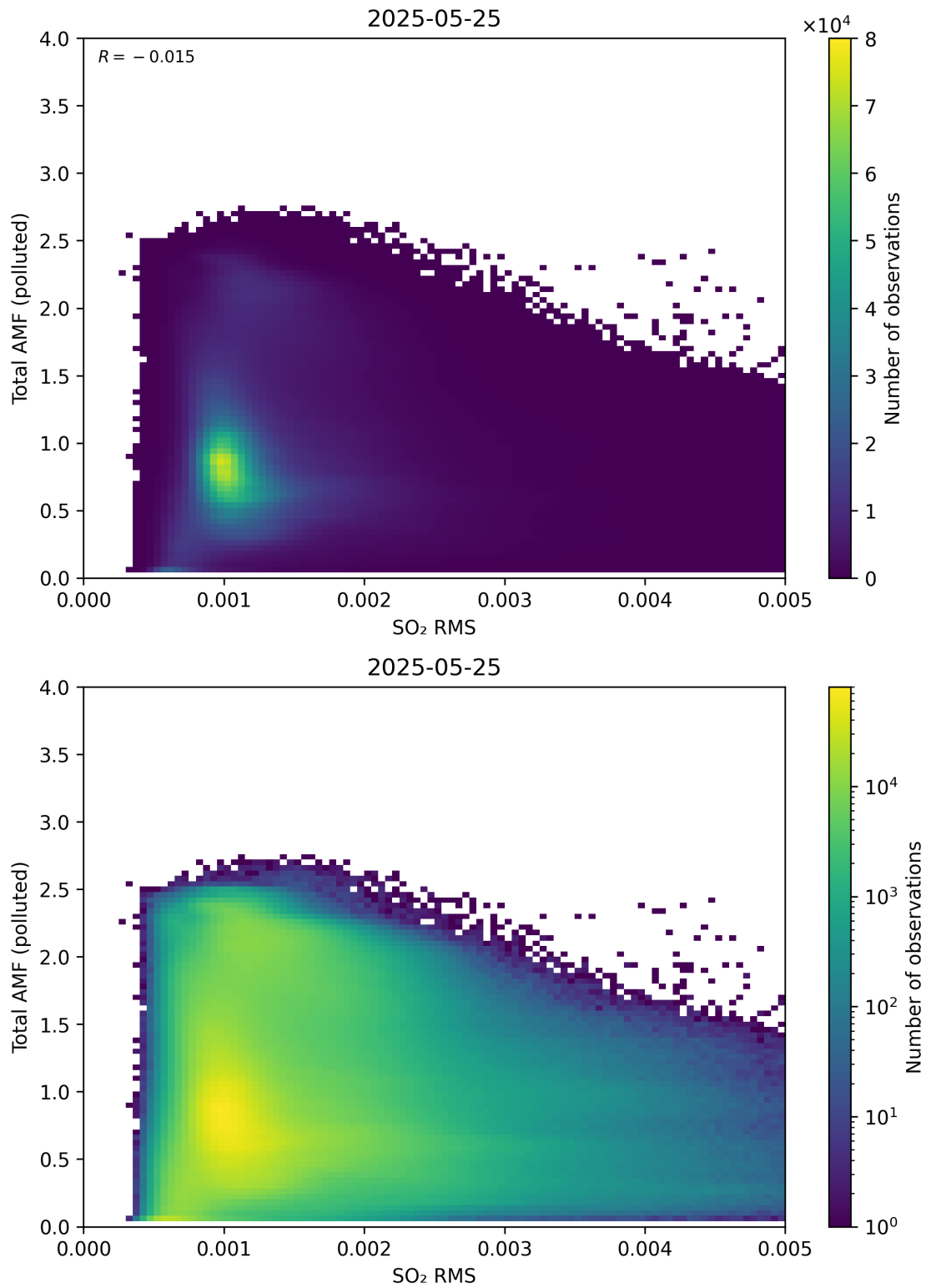
Figure 148: Scatter density plot of “SO 2 RMS” against “Total AMF (polluted)” for 2025-05-24 to 2025-05-26.
