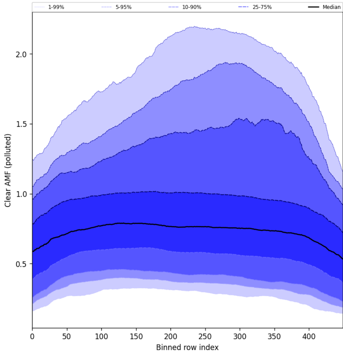
Figure 107: Along track statistics of “Clear AMF (polluted)” for 2025-05-24 to 2025-05-26
