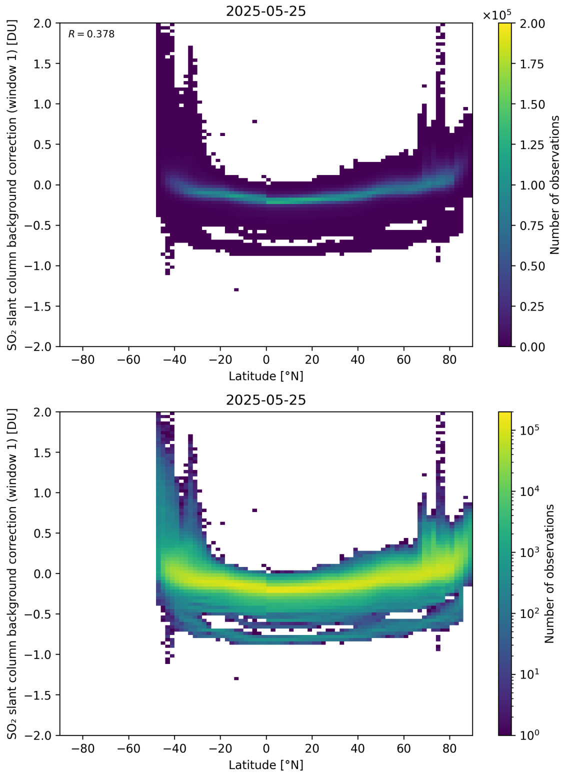
Figure 150: Scatter density plot of “Latitude” against “SO 2 slant column background correction (window 1)” for 2025-05-24 to 2025-05-26.
