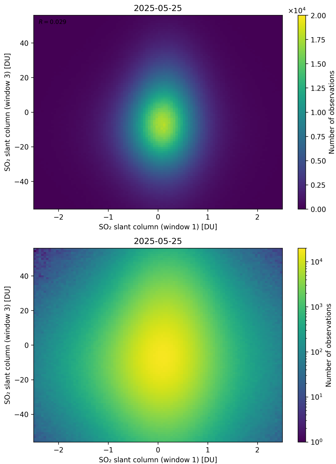
Figure 287: Scatter density plot of “SO 2 slant column (window 1)” against “SO 2 slant column (window 3)” for 2025-05-24 to 2025-05-26.
