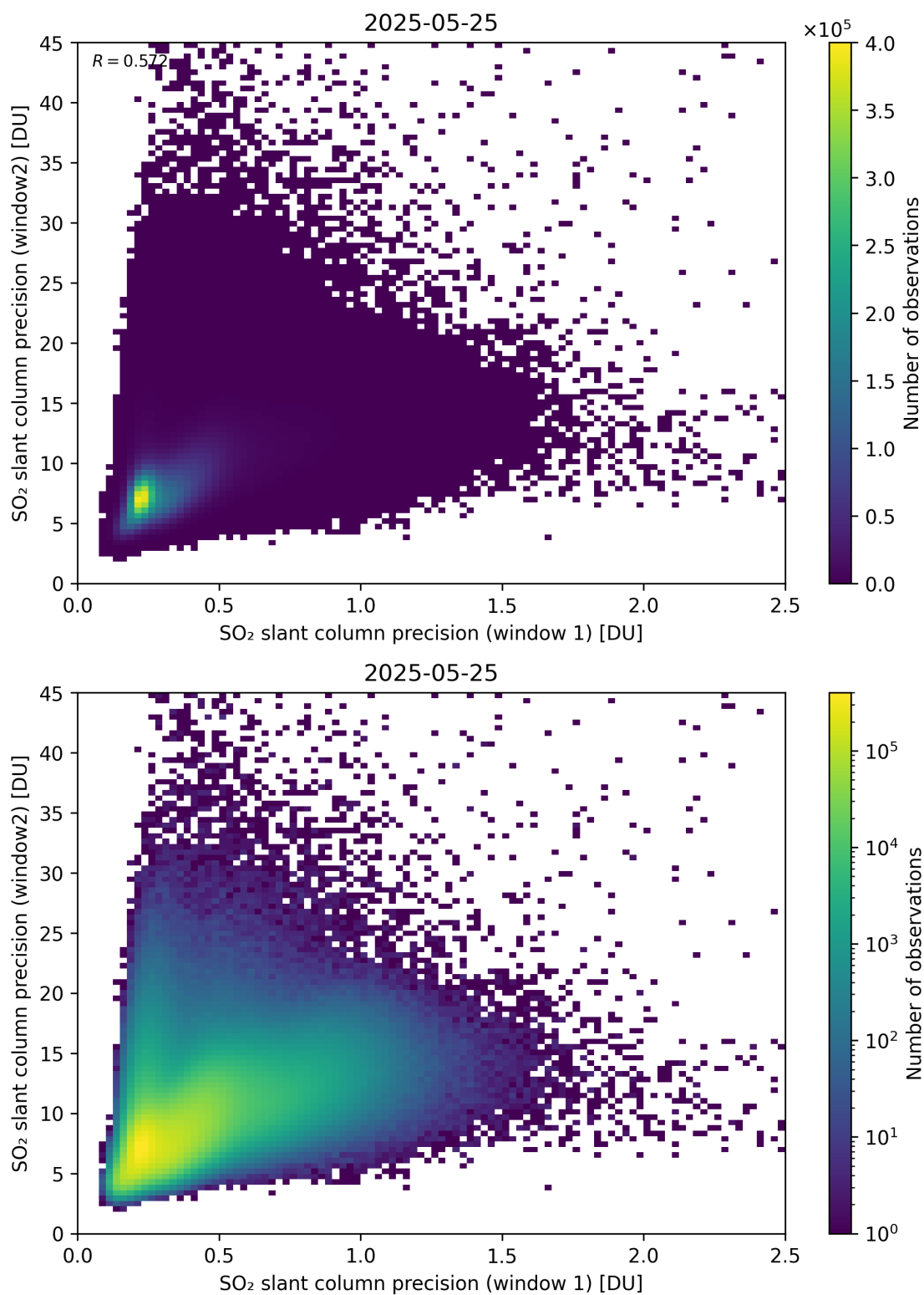
Figure 277: Scatter density plot of “SO 2 slant column precision (window 1)” against “SO 2 slant column precision (window2)” for 2025-05-24 to 2025-05-26.
