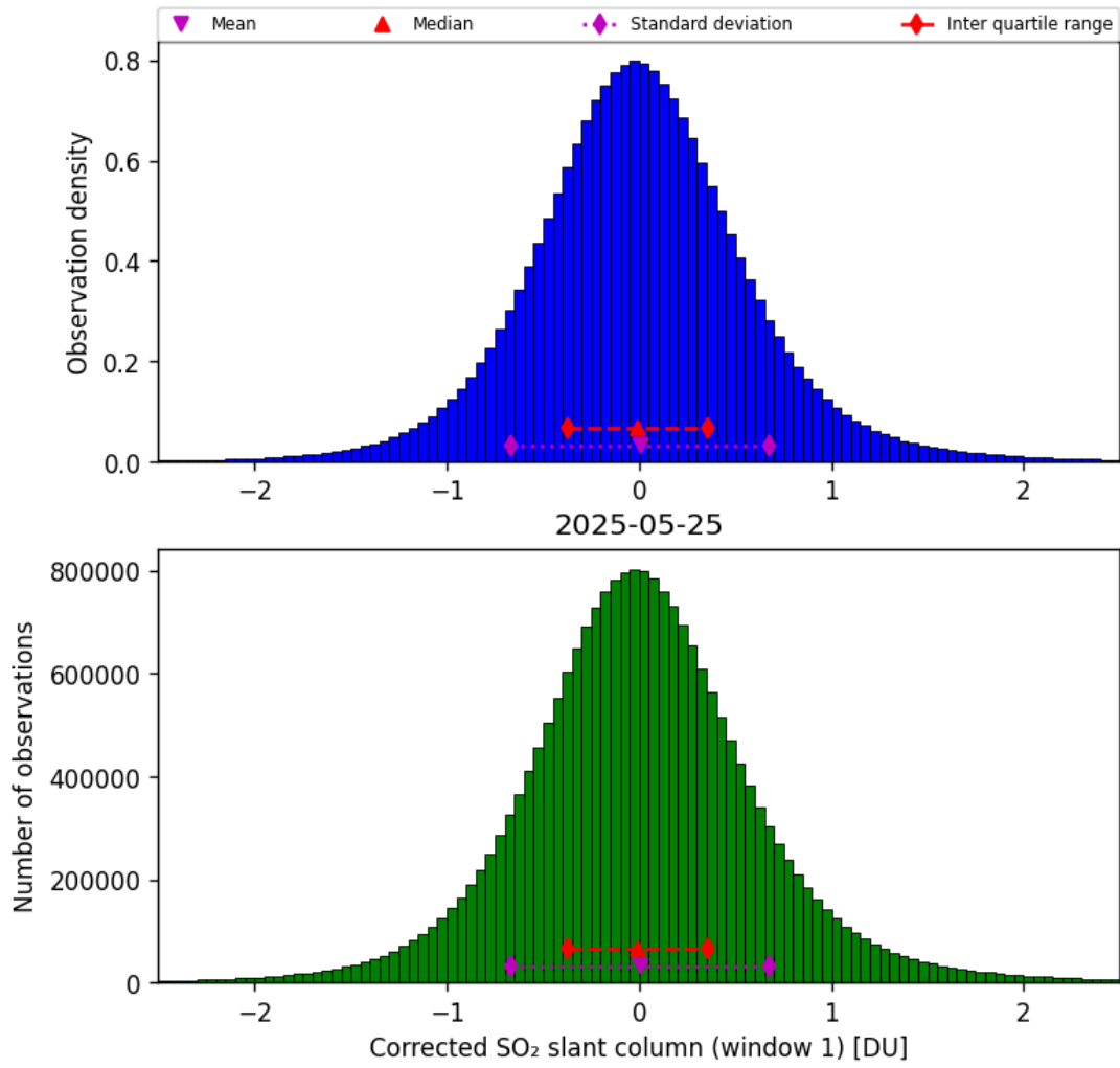
Figure 65: Histogram of “Corrected SO 2 slant column (window 1)” for 2025-05-24 to 2025-05-26
