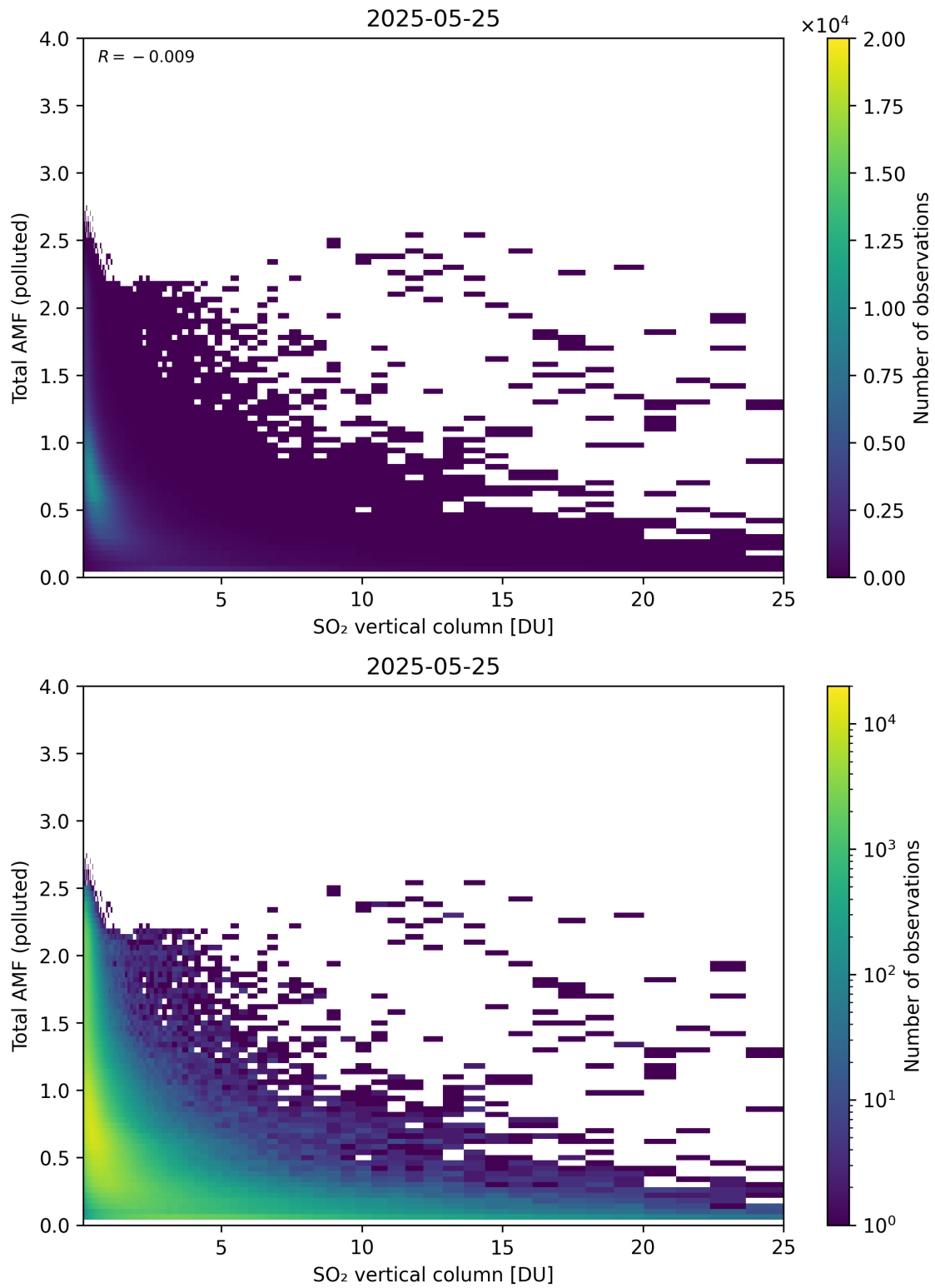
Figure 359: Scatter density plot of “SO 2 vertical column” against “Total AMF (polluted)” for 2025-05-24 to 2025-05-26.
