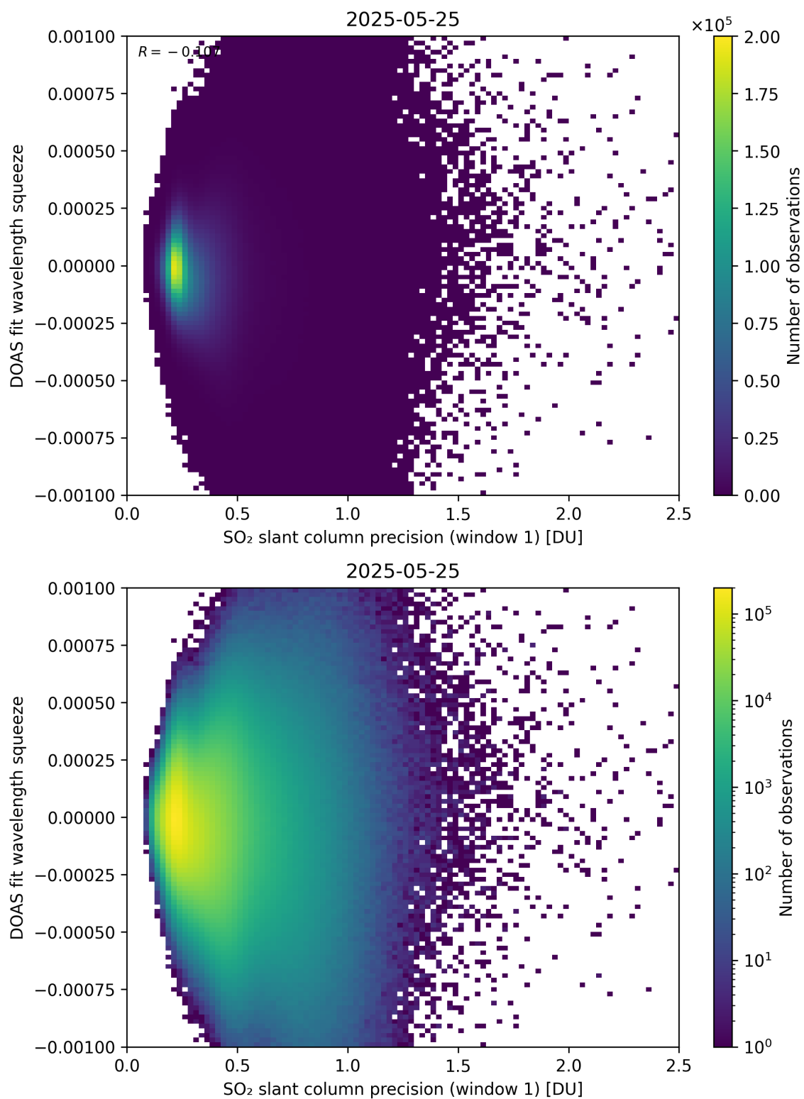
Figure 272: Scatter density plot of “SO 2 slant column precision (window 1)” against “DOAS fit wavelength squeeze” for 2025-05-24 to 2025-05-26.
