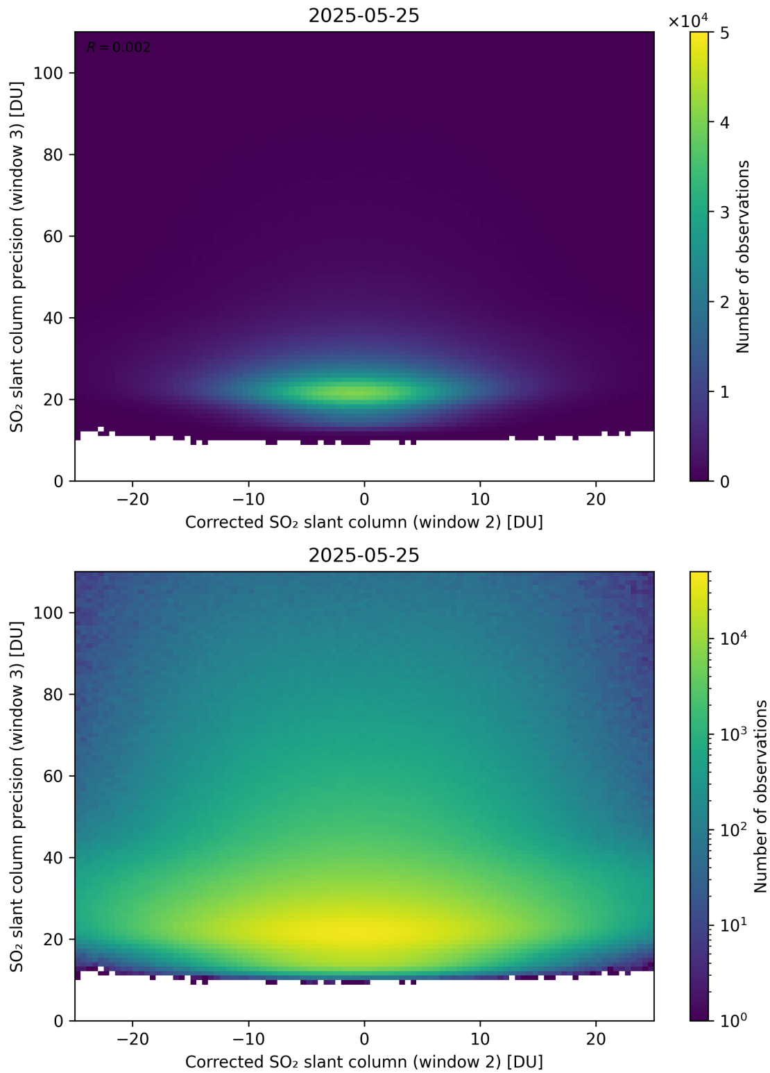
Figure 252: Scatter density plot of “Corrected SO 2 slant column (window 2)” against “SO 2 slant column precision (window 3)” for 2025-05-24 to 2025-05-26.
