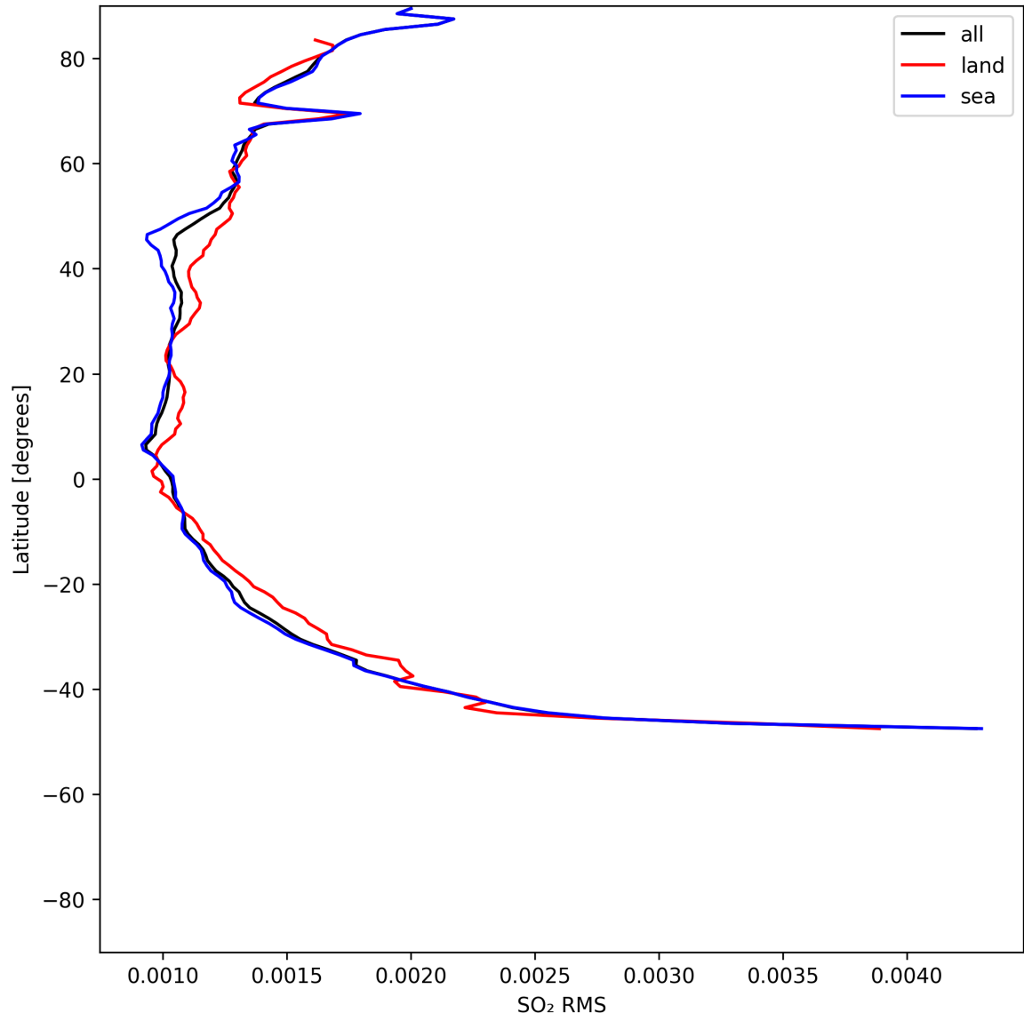
Figure 52: Zonal average of “SO 2 RMS” for 2025-05-24 to 2025-05-26.
