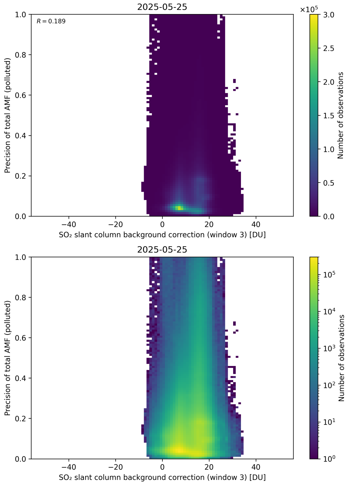
Figure 137: Scatter density plot of “SO 2 slant column background correction (window 3)” against “Precision of total AMF (polluted)” for 2025-05-24 to 2025-05-26.
