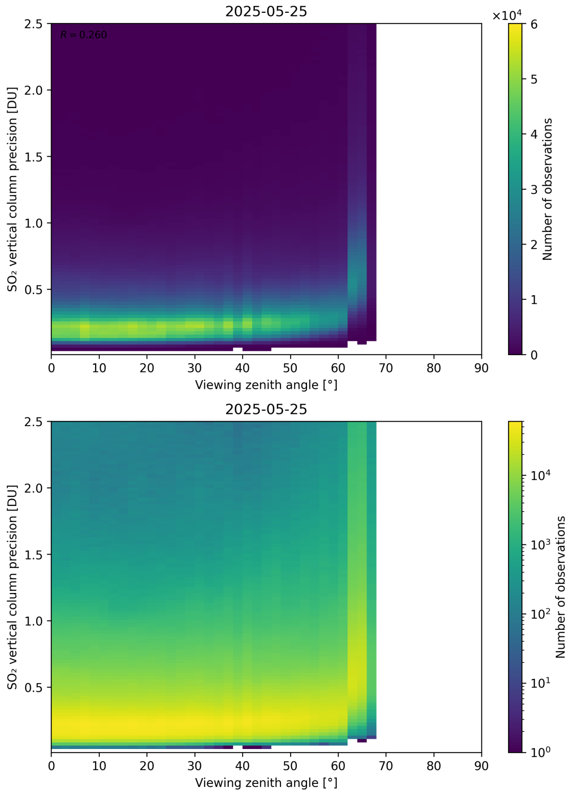
Figure 384: Scatter density plot of “Viewing zenith angle” against “SO 2 vertical column precision” for 2025-05-24 to 2025-05-26.
