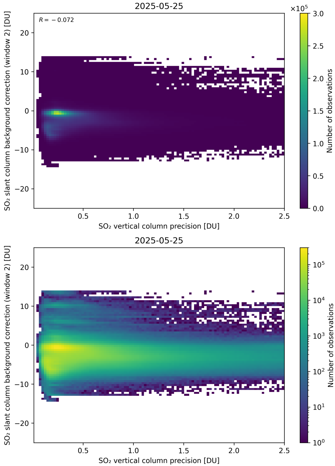
Figure 330: Scatter density plot of “SO 2 vertical column precision” against “SO 2 slant column background correction (window 2)” for 2025-05-24 to 2025-05-26.
