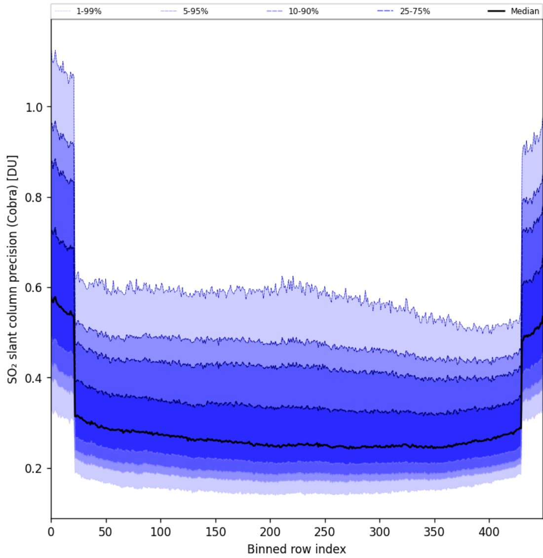
Figure 88: Along track statistics of “SO 2 slant column precision (Cobra)” for 2025-05-24 to 2025-05-26
