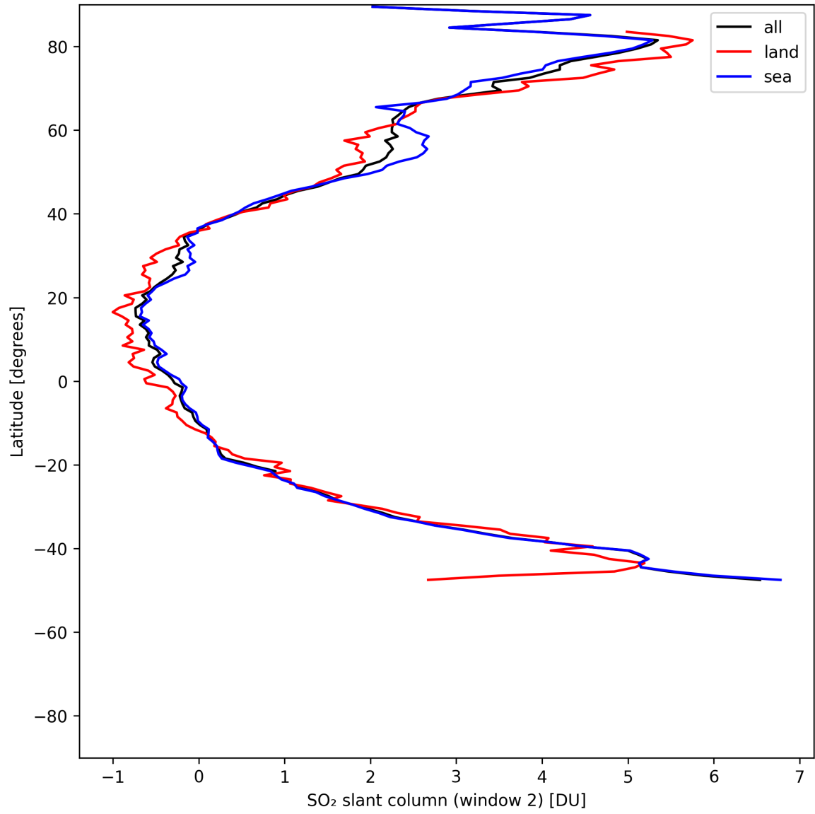
Figure 41: Zonal average of “SO 2 slant column (window 2)” for 2025-05-24 to 2025-05-26.
