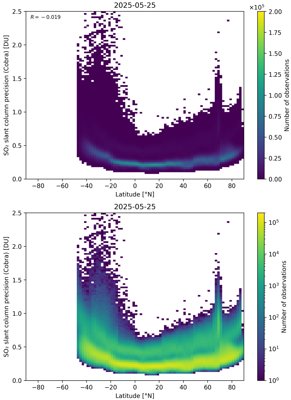
Figure 158: Scatter density plot of “Latitude” against “SO 2 slant column precision (Cobra)” for 2025-05-24 to 2025-05-26.
