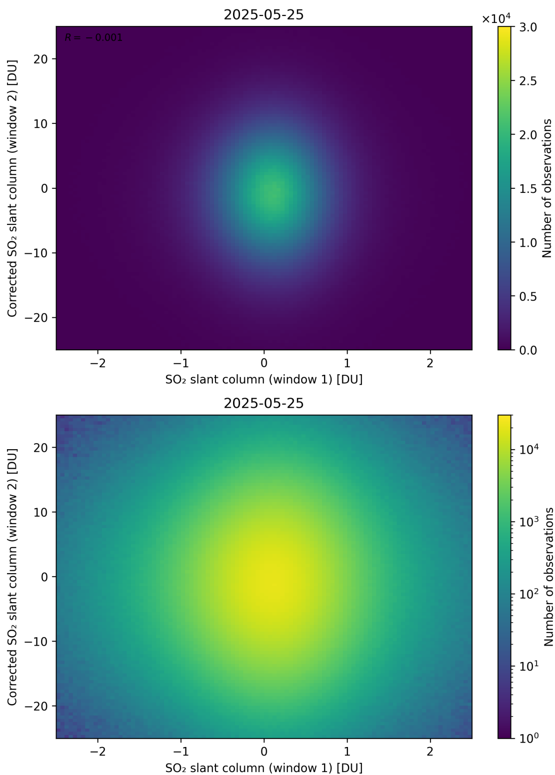
Figure 283: Scatter density plot of “SO 2 slant column (window 1)” against “Corrected SO 2 slant column (window 2)” for 2025-05-24 to 2025-05-26.
