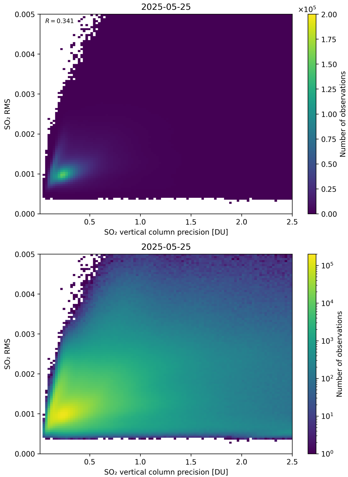
Figure 334: Scatter density plot of “SO 2 vertical column precision” against “SO 2 RMS” for 2025-05-24 to 2025-05-26.
