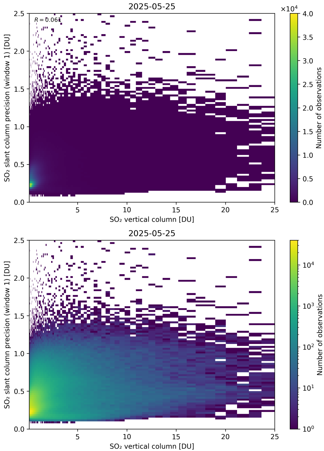
Figure 355: Scatter density plot of “SO 2 vertical column” against “SO 2 slant column precision (window 1)” for 2025-05-24 to 2025-05-26.
