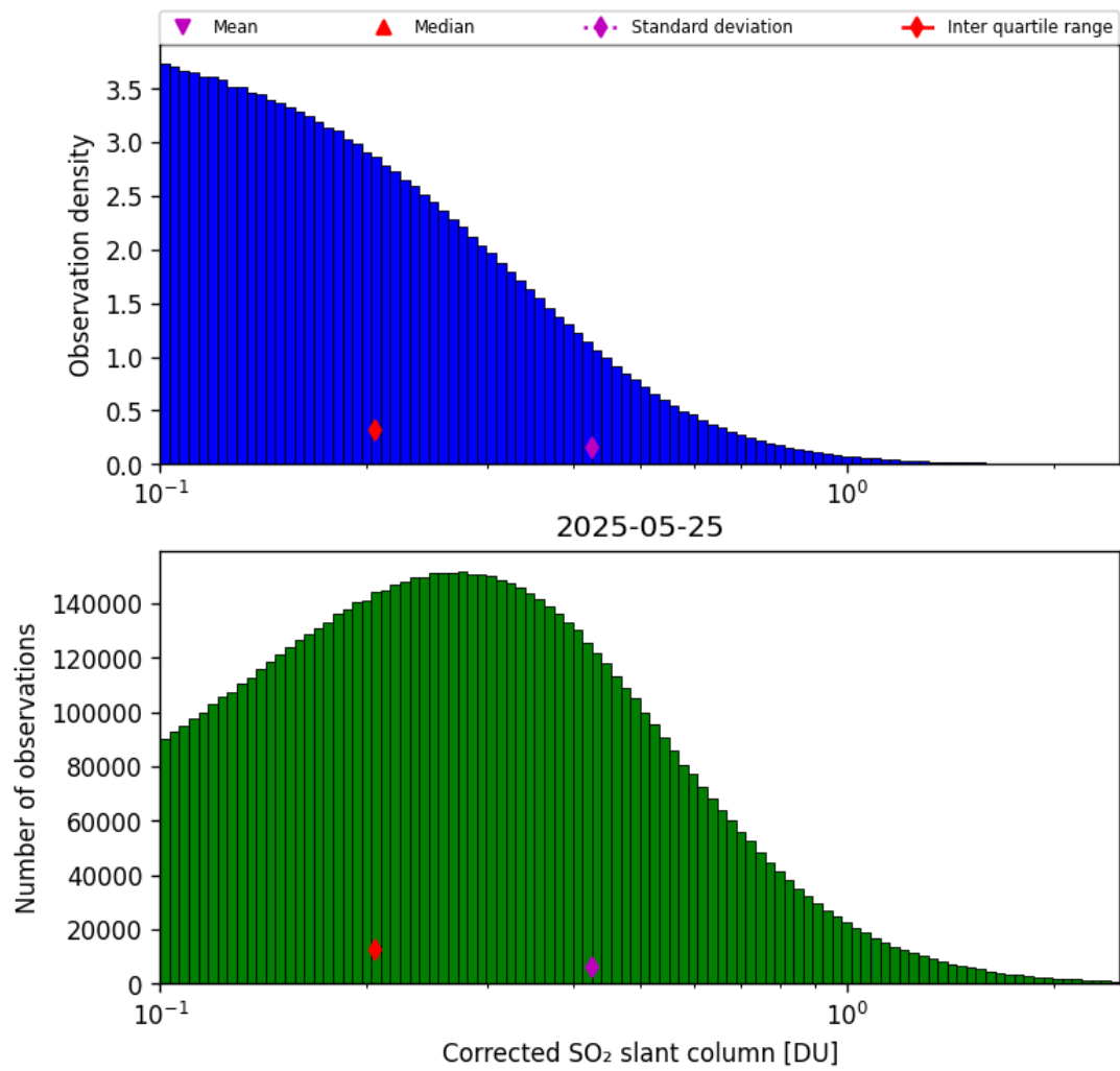
Figure 60: Histogram of "Corrected SO 2 slant column" for 2025-05-24 to 2025-05-26
