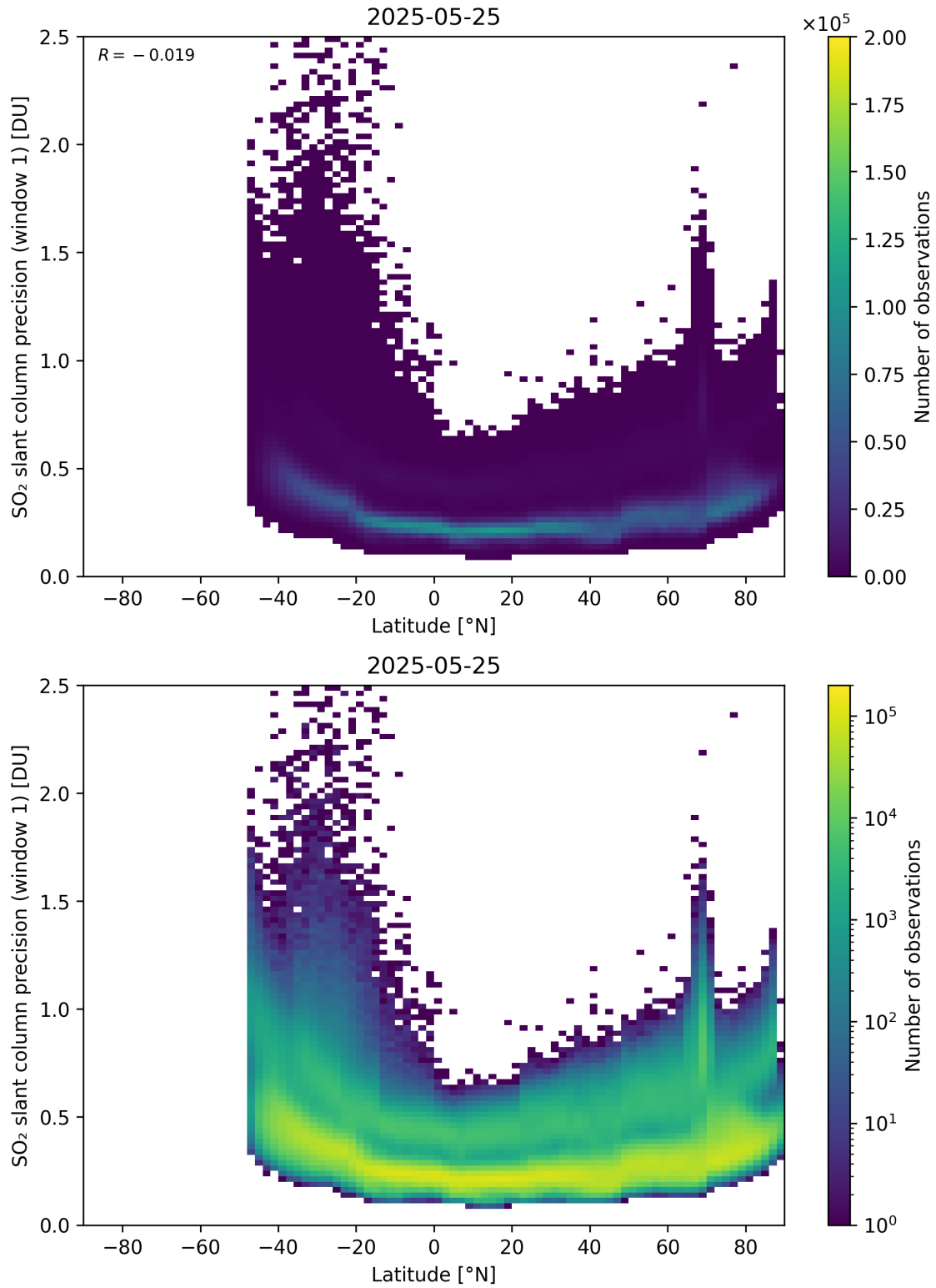
Figure 163: Scatter density plot of “Latitude” against “SO 2 slant column precision (window 1)” for 2025-05-24 to 2025-05-26.
