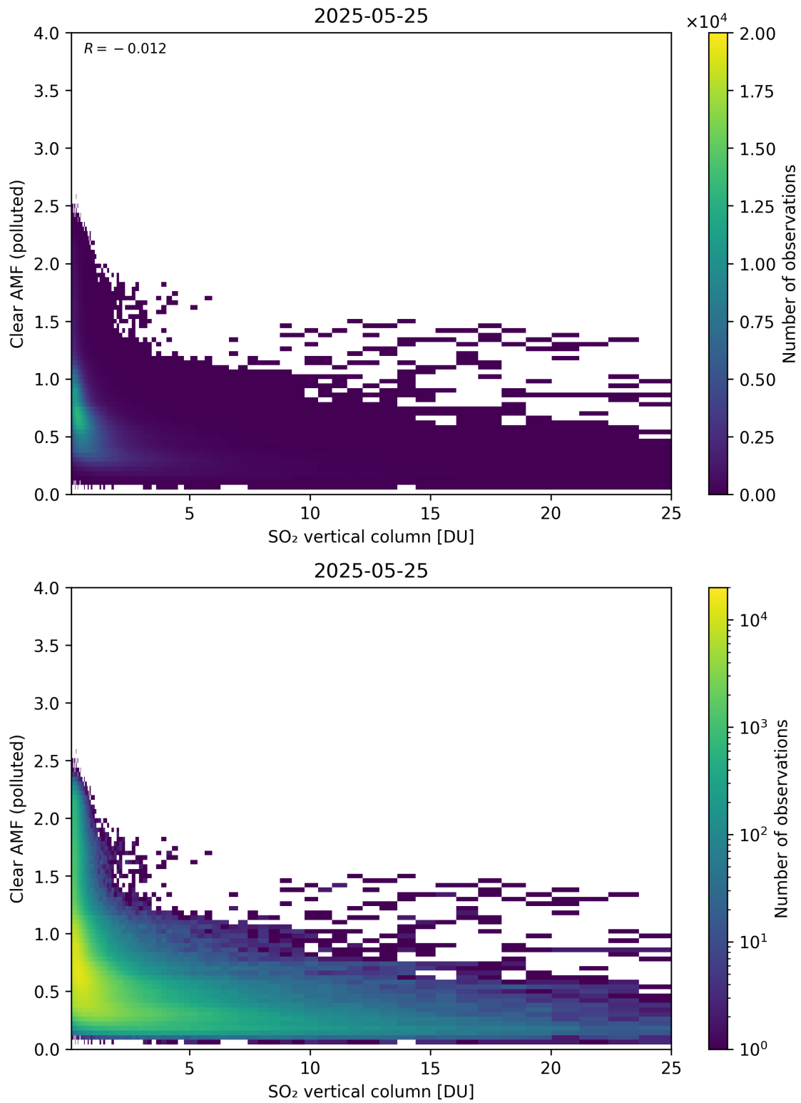
Figure 348: Scatter density plot of “SO 2 vertical column” against “Clear AMF (polluted)” for 2025-05-24 to 2025-05-26.
