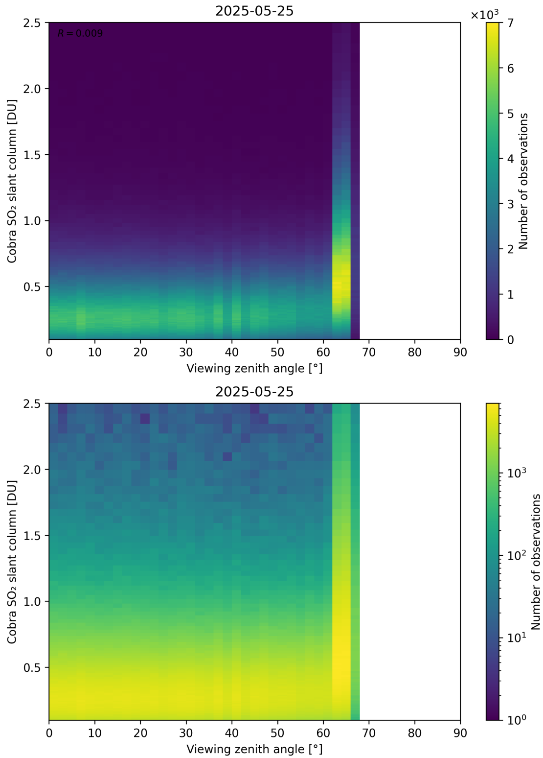
Figure 371: Scatter density plot of “Viewing zenith angle” against “Cobra SO 2 slant column” for 2025-05-24 to 2025-05-26.
