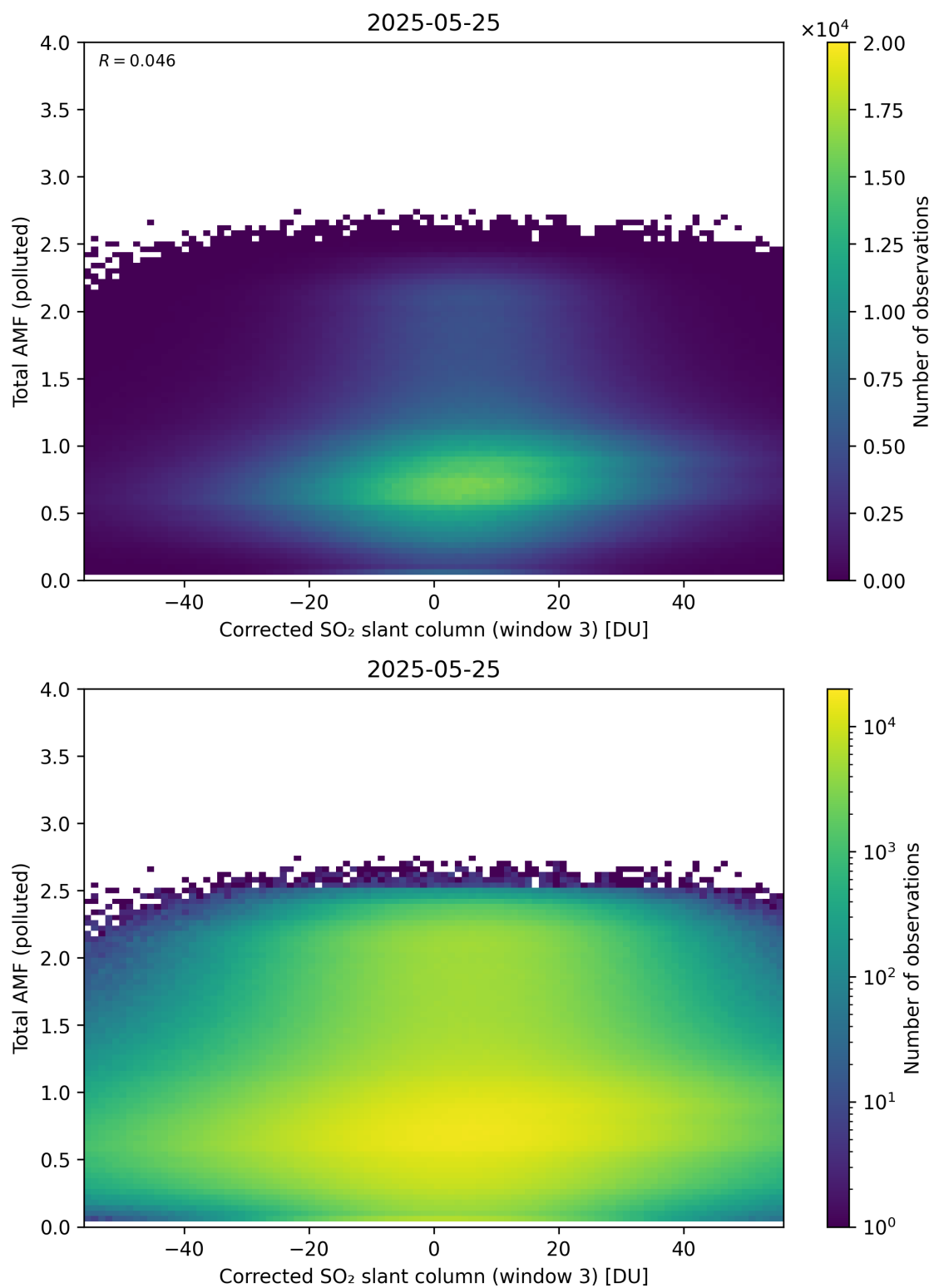
Figure 260: Scatter density plot of “Corrected SO 2 slant column (window 3)” against “Total AMF (polluted)” for 2025-05-24 to 2025-05-26.
