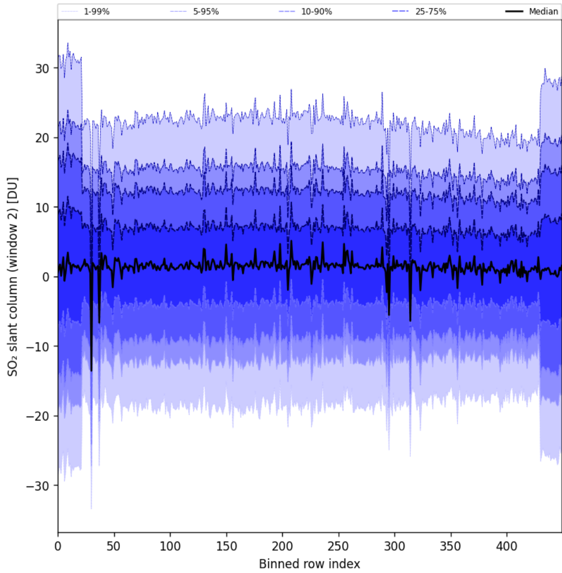
Figure 93: Along track statistics of “SO 2 slant column (window 2)” for 2025-05-24 to 2025-05-26
