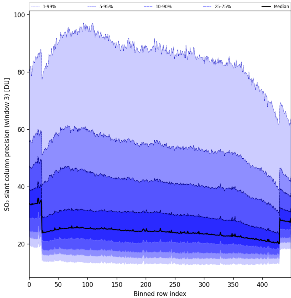
Figure 98: Along track statistics of “SO 2 slant column precision (window 3)” for 2025-05-24 to 2025-05-26
