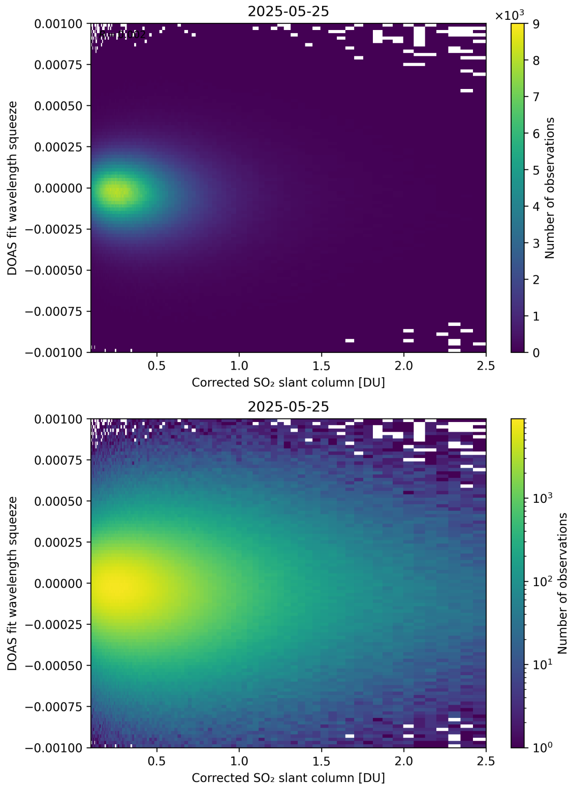
Figure 230: Scatter density plot of “Corrected SO 2 slant column” against “DOAS fit wavelength squeeze” for 2025-05-24 to 2025-05-26.
