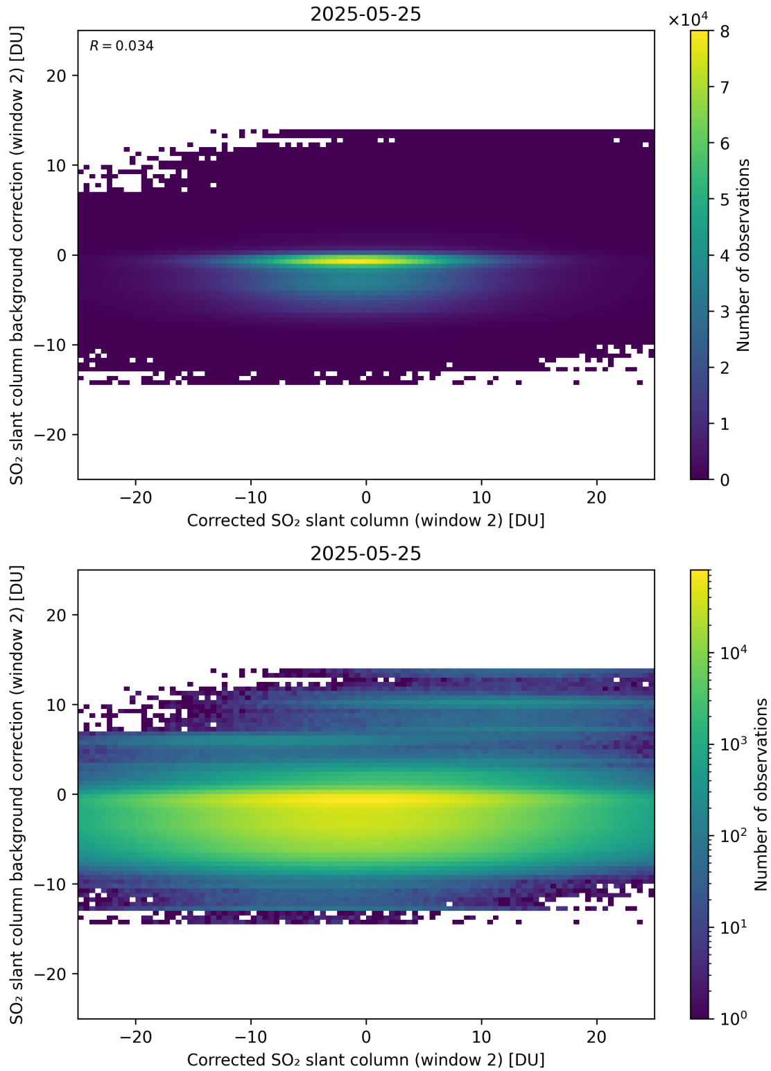
Figure 244: Scatter density plot of “Corrected SO 2 slant column (window 2)” against “SO 2 slant column background correction (window 2)” for 2025-05-24 to 2025-05-26.
