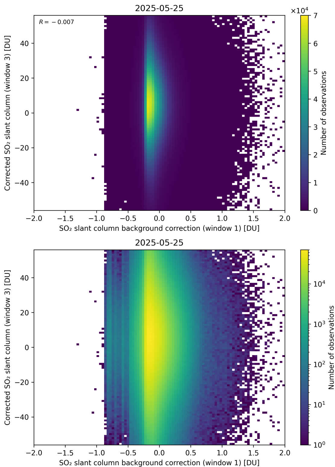
Figure 116: Scatter density plot of “SO 2 slant column background correction (window 1)” against “Corrected SO 2 slant column (window 3)” for 2025-05-24 to 2025-05-26.
