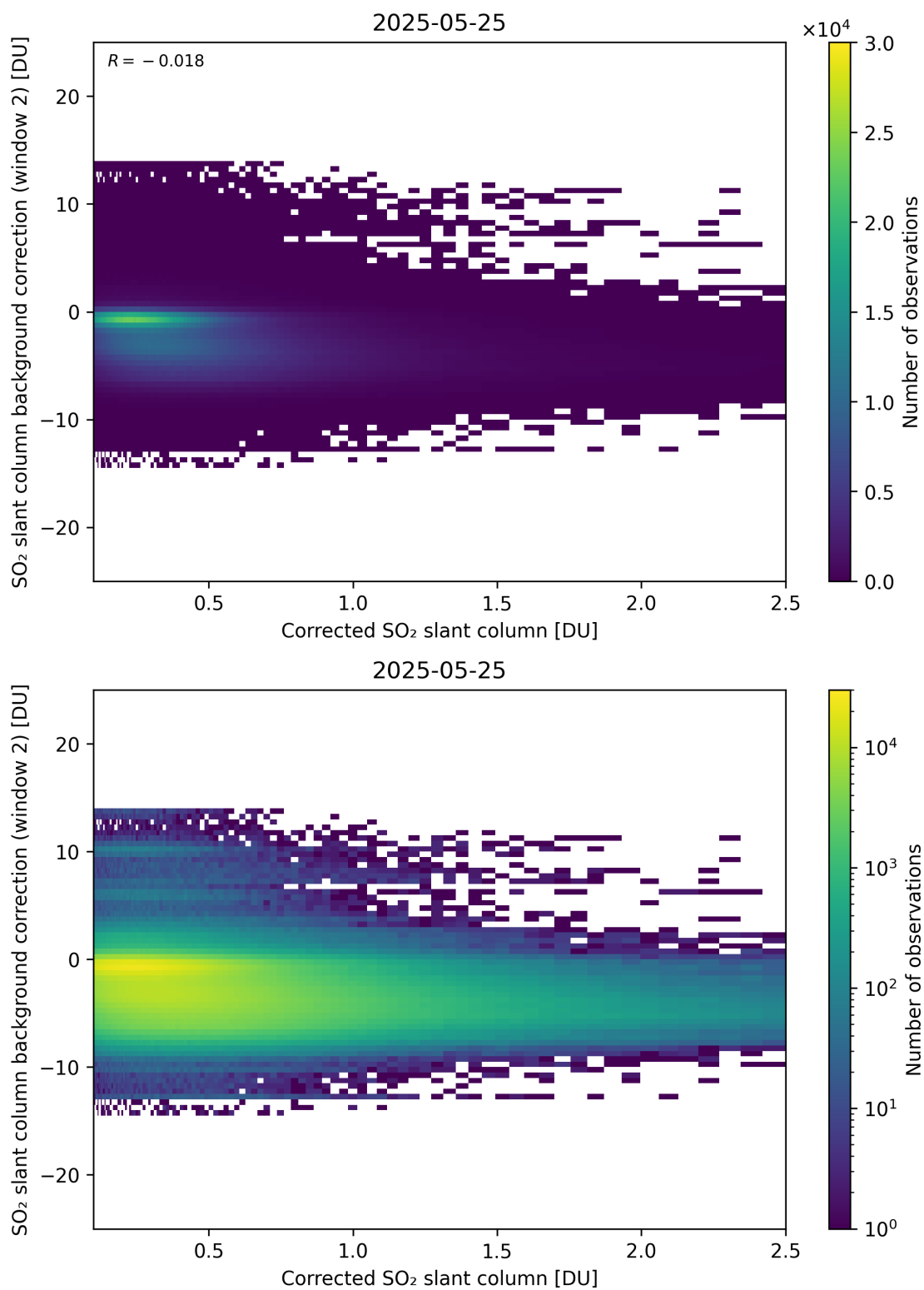
Figure 227: Scatter density plot of “Corrected SO 2 slant column” against “SO 2 slant column background correction (window 2)” for 2025-05-24 to 2025-05-26.
