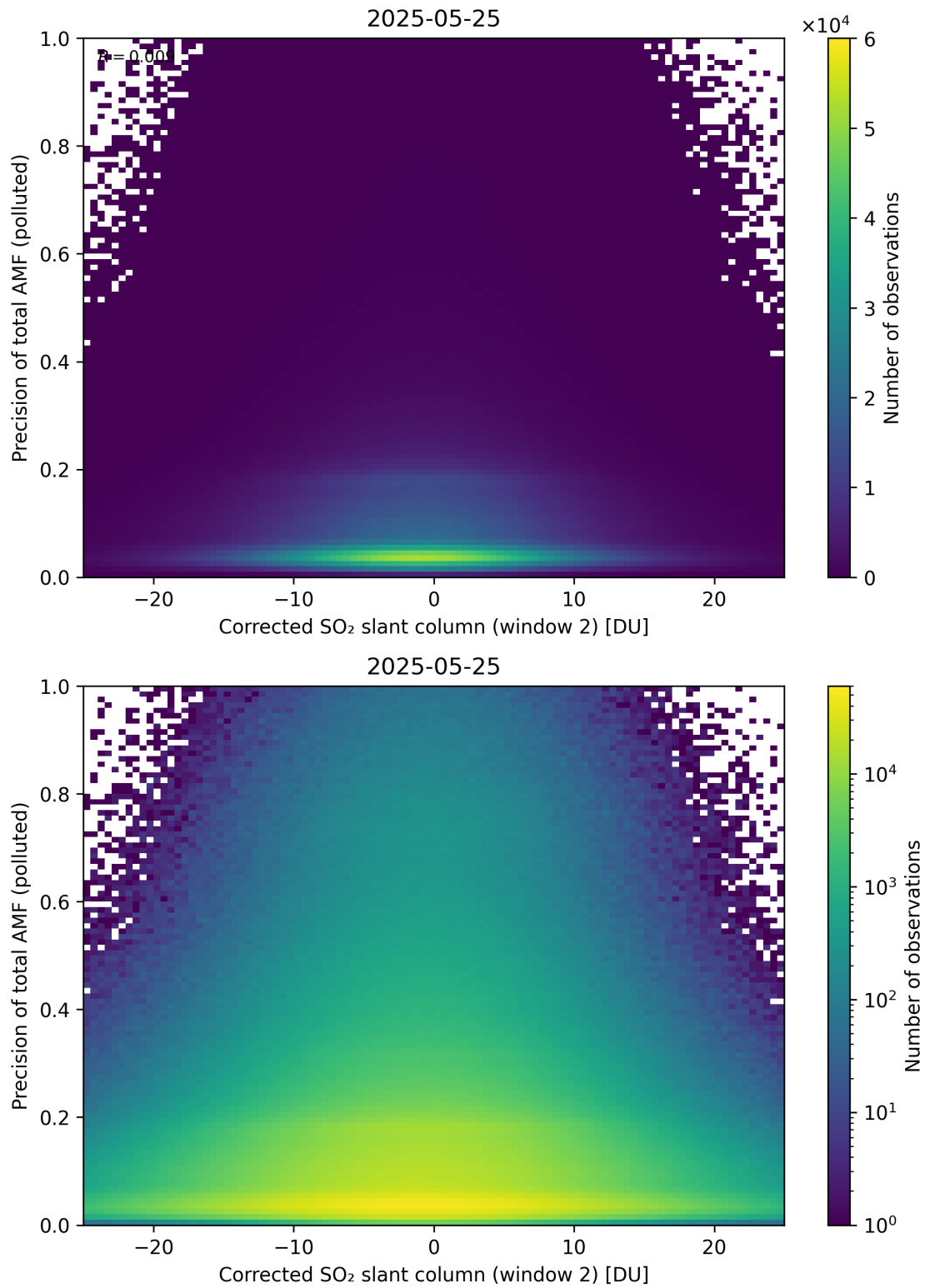
Figure 254: Scatter density plot of “Corrected SO 2 slant column (window 2)” against “Precision of total AMF (polluted)” for 2025-05-24 to 2025-05-26.
