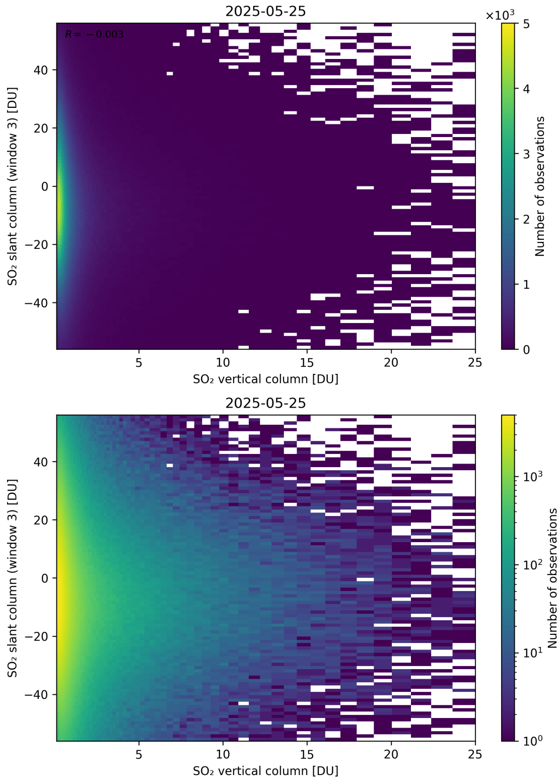
Figure 357: Scatter density plot of “SO 2 vertical column” against “SO 2 slant column (window 3)” for 2025-05-24 to 2025-05-26.
