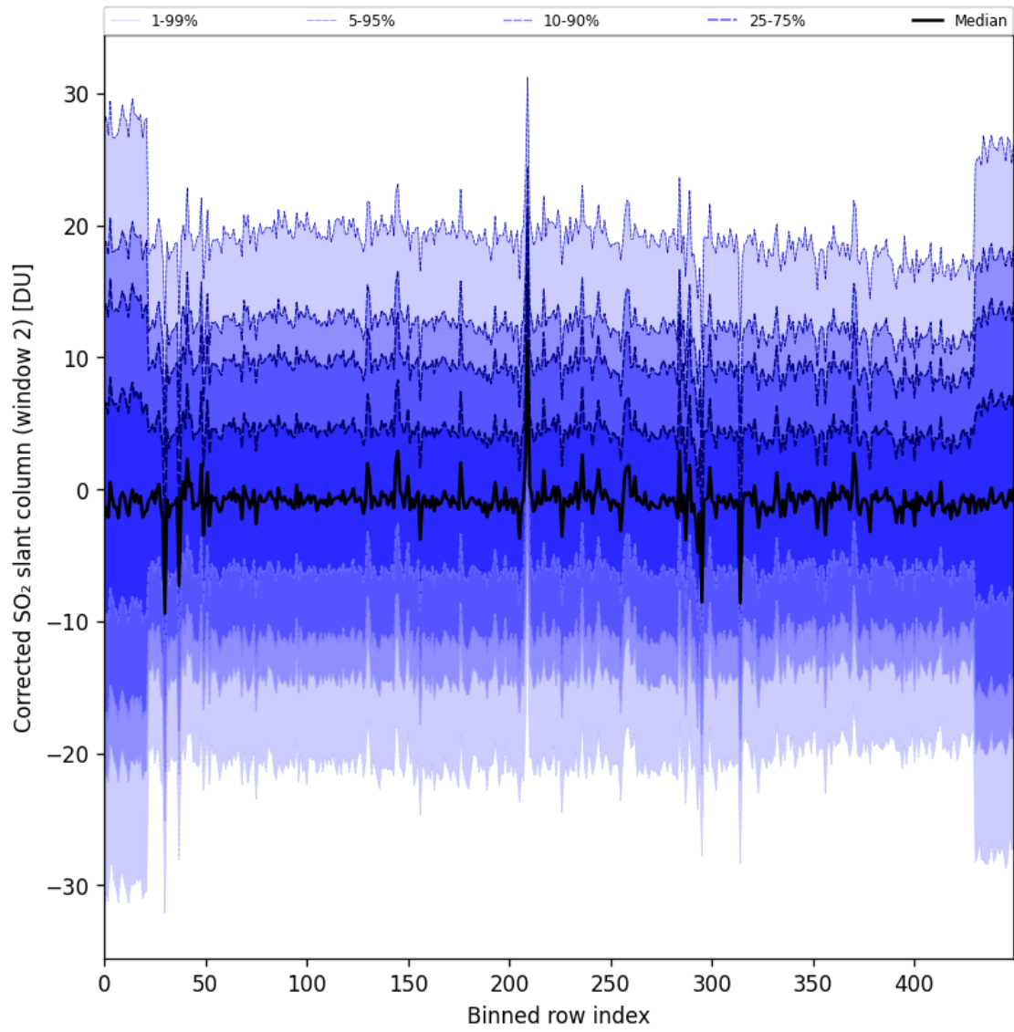
Figure 95: Along track statistics of “Corrected SO 2 slant column (window 2)” for 2025-05-24 to 2025-05-26
