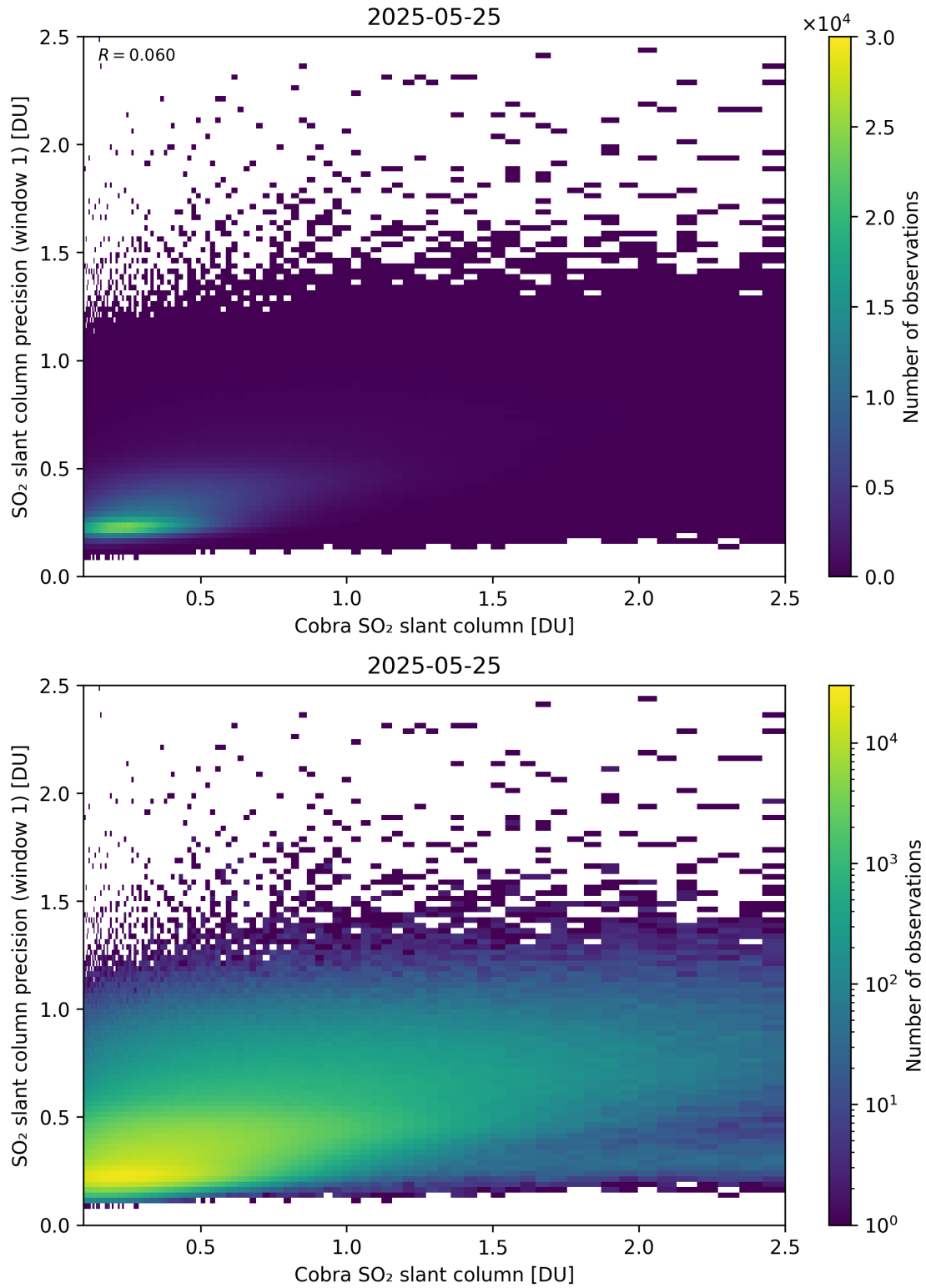
Figure 220: Scatter density plot of “Cobra SO 2 slant column” against “SO 2 slant column precision (window 1)” for 2025-05-24 to 2025-05-26.
