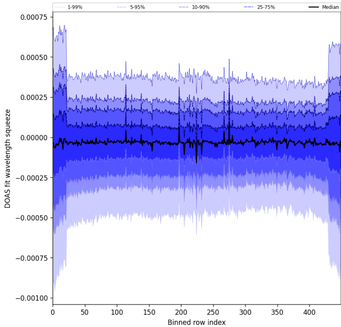
Figure 103: Along track statistics of “DOAS fit wavelength squeeze” for 2025-05-24 to 2025-05-26
