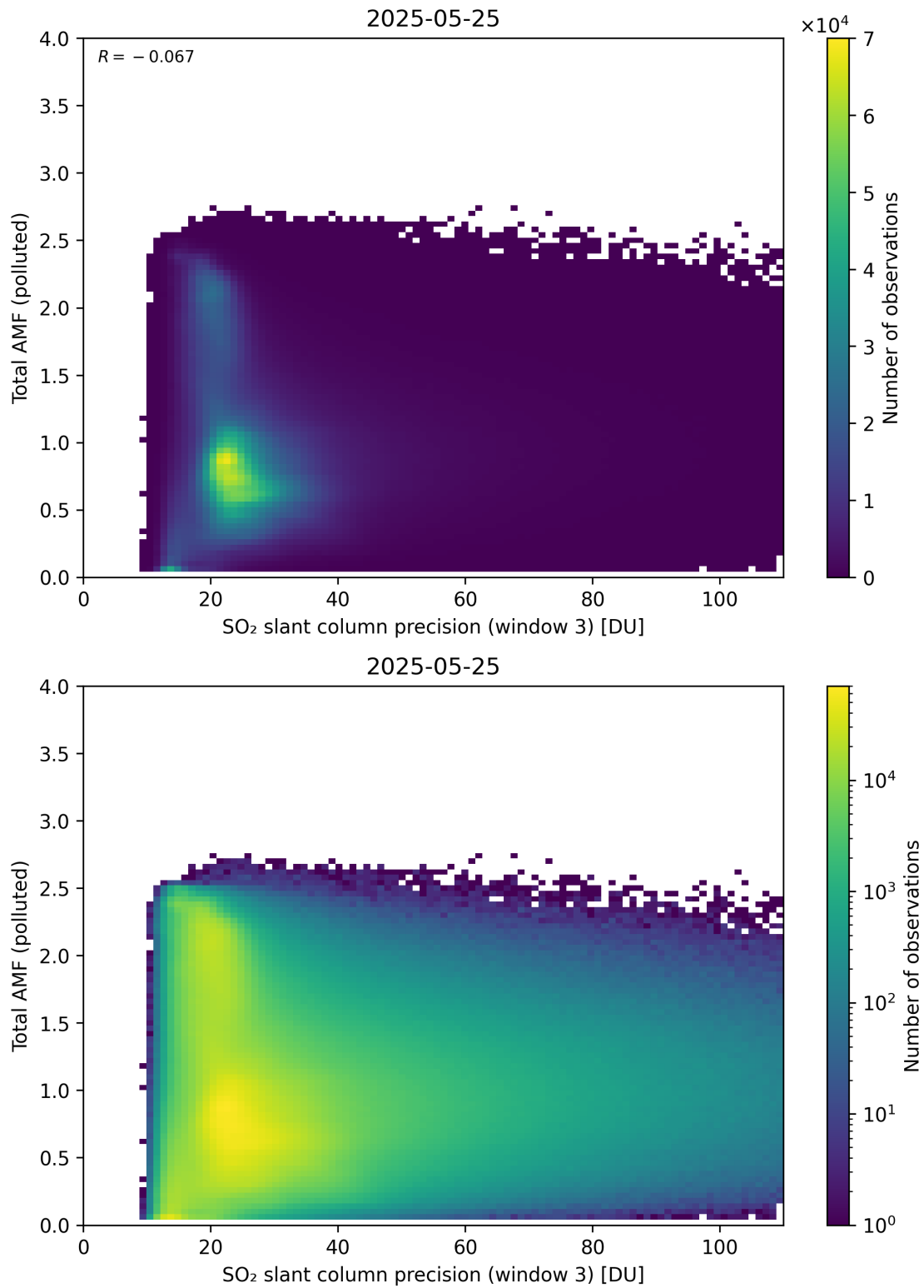
Figure 313: Scatter density plot of “SO 2 slant column precision (window 3)” against “Total AMF (polluted)” for 2025-05-24 to 2025-05-26.
