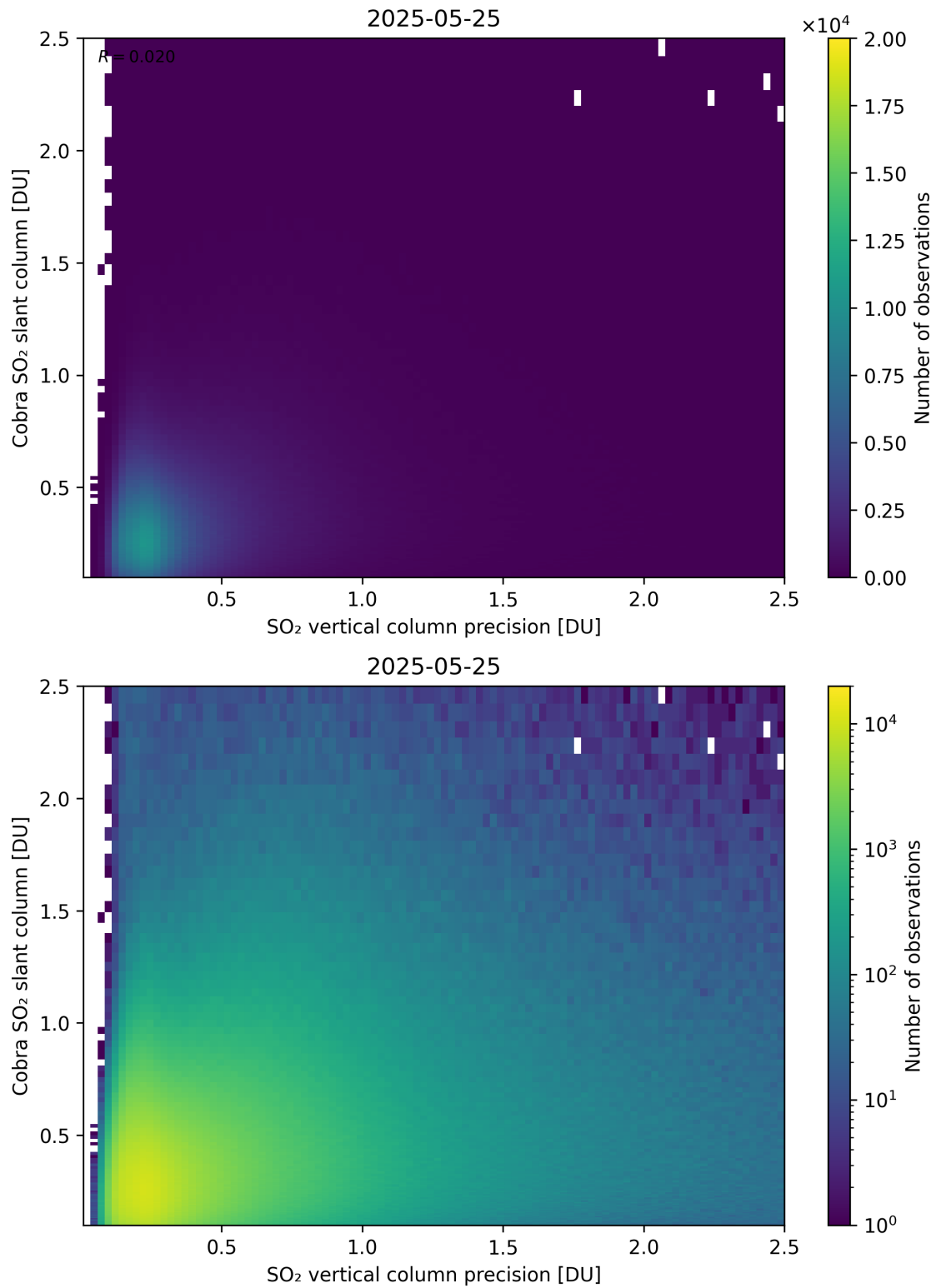
Figure 336: Scatter density plot of “SO 2 vertical column precision” against “Cobra SO 2 slant column” for 2025-05-24 to 2025-05-26.
