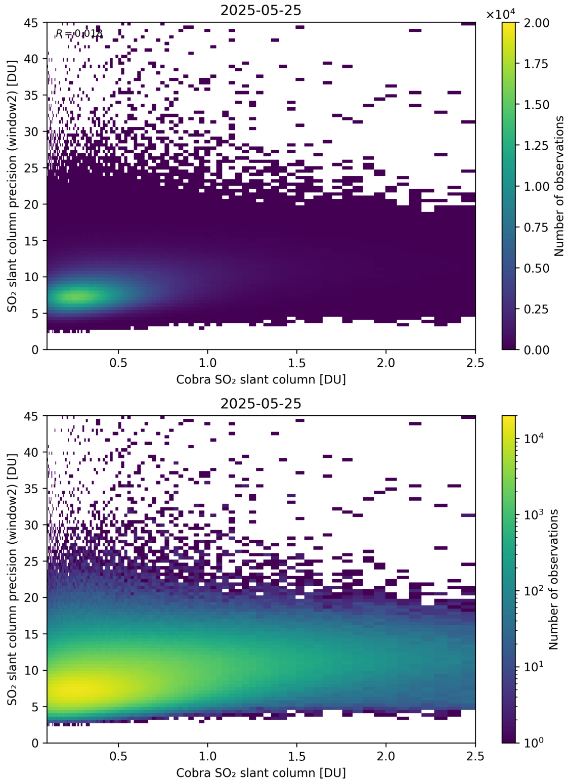
Figure 221: Scatter density plot of “Cobra SO 2 slant column” against “SO 2 slant column precision (window2)” for 2025-05-24 to 2025-05-26.
