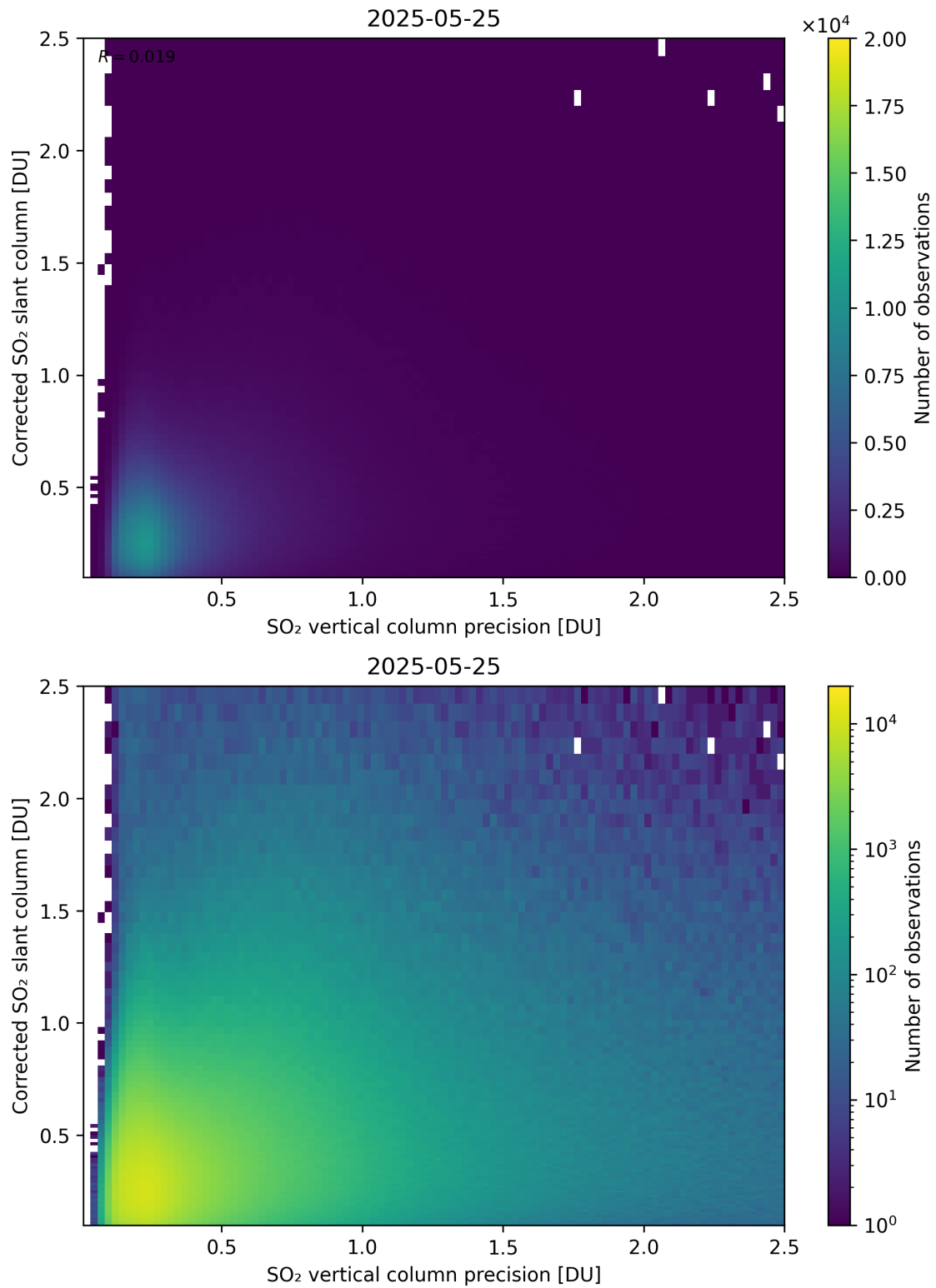
Figure 338: Scatter density plot of “SO 2 vertical column precision” against “Corrected SO 2 slant column” for 2025-05-24 to 2025-05-26.
