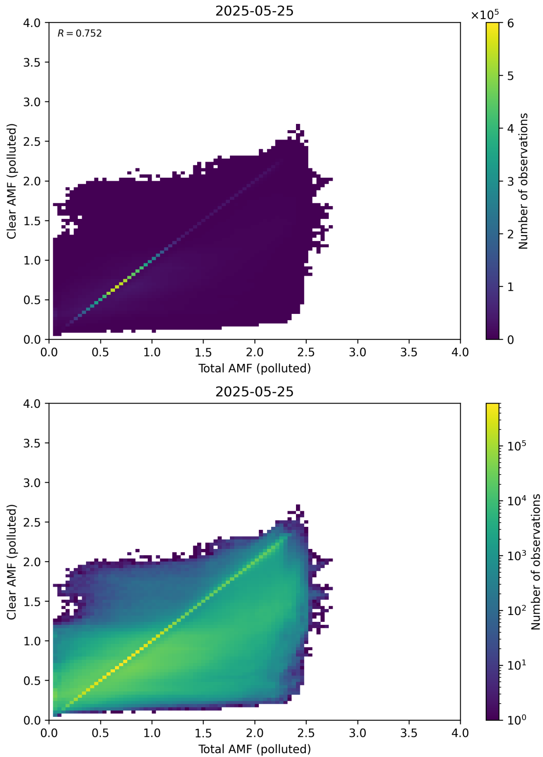
Figure 321: Scatter density plot of “Total AMF (polluted)” against “Clear AMF (polluted)” for 2025-05-24 to 2025-05-26.
