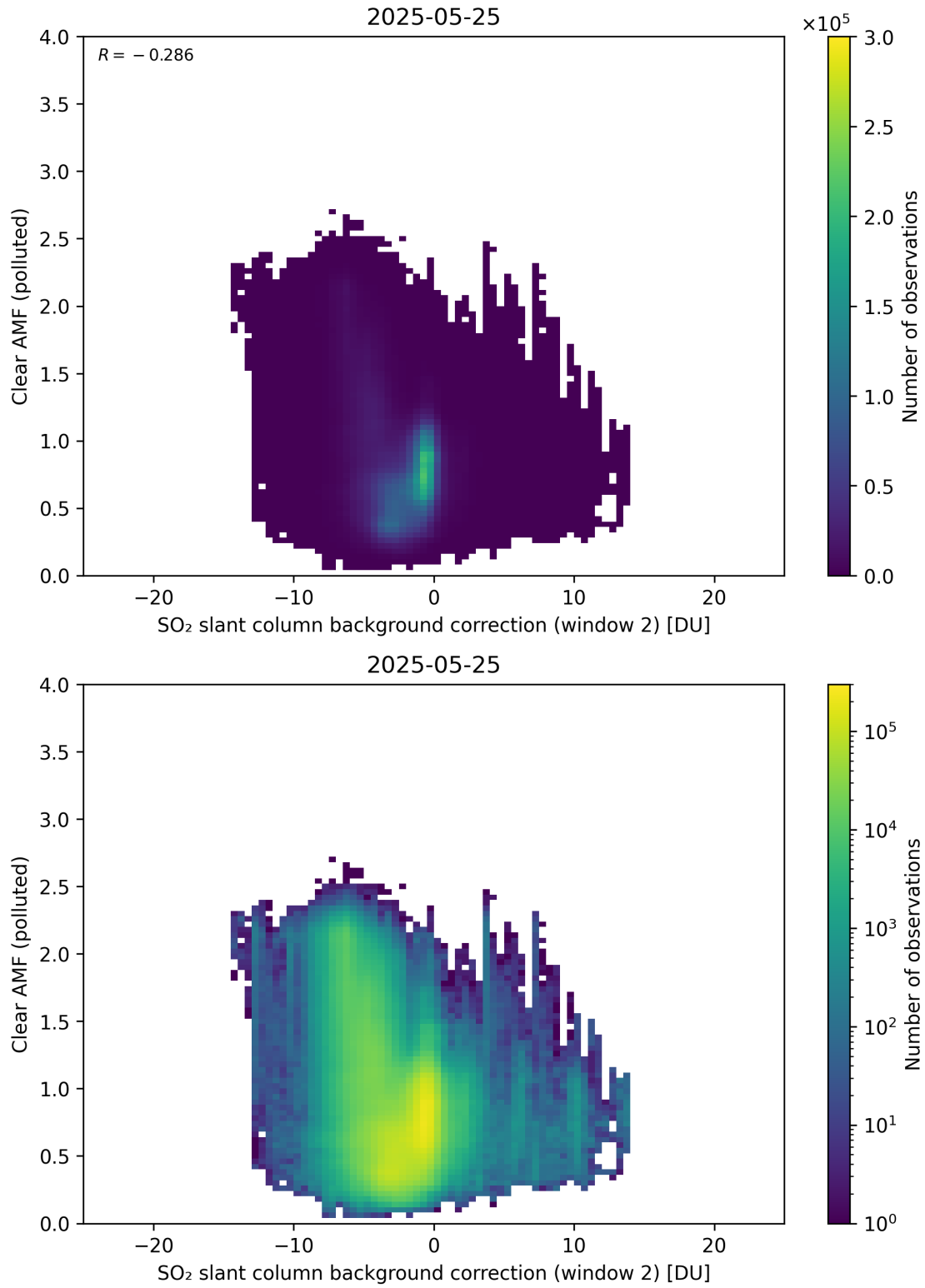
Figure 126: Scatter density plot of “SO 2 slant column background correction (window 2)” against “Clear AMF (polluted)” for 2025-05-24 to 2025-05-26.
