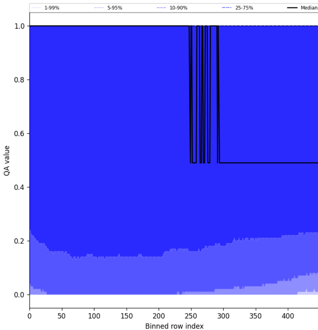
Figure 83: Along track statistics of “QA value” for 2025-05-24 to 2025-05-26
