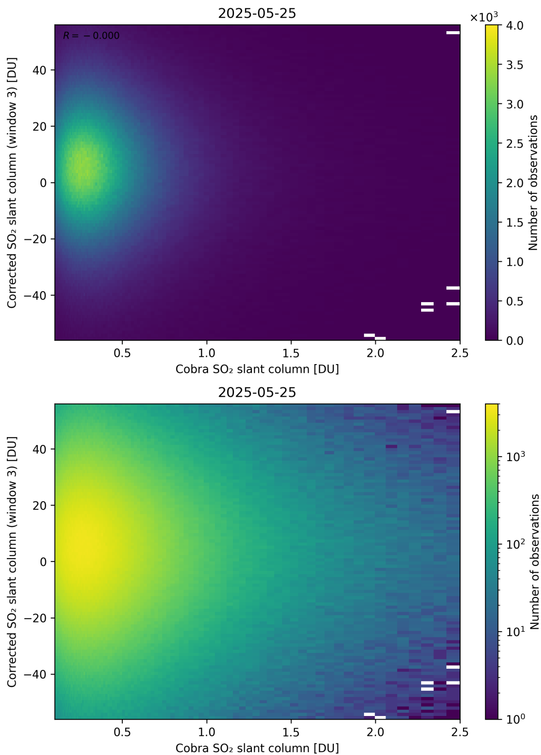
Figure 218: Scatter density plot of “Cobra SO 2 slant column” against “Corrected SO 2 slant column (window 3)” for 2025-05-24 to 2025-05-26.
