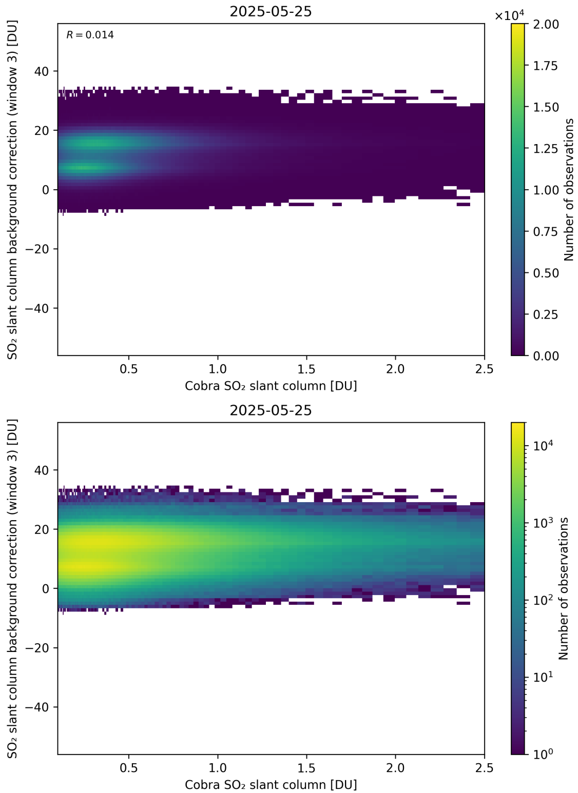
Figure 195: Scatter density plot of “Cobra SO 2 slant column” against “SO 2 slant column background correction (window 3)” for 2025-05-24 to 2025-05-26.
