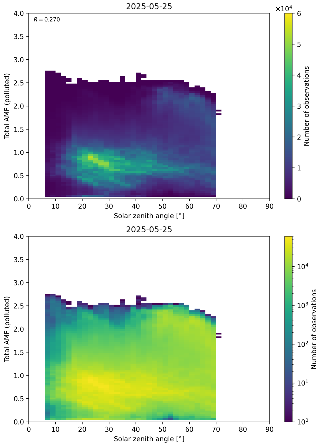
Figure 189: Scatter density plot of “Solar zenith angle” against “Total AMF (polluted)” for 2025-05-24 to 2025-05-26.
