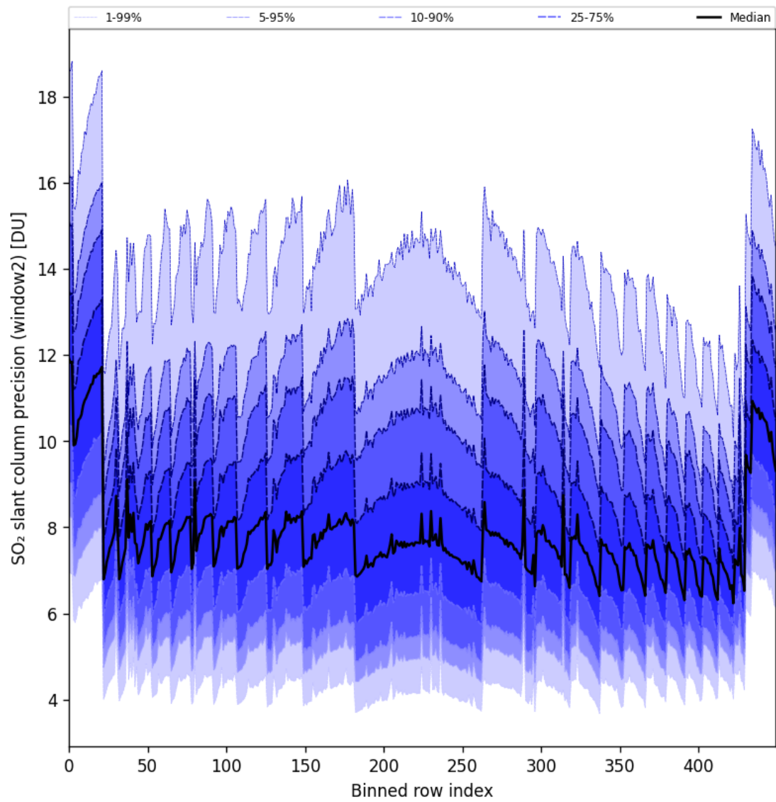
Figure 94: Along track statistics of “SO 2 slant column precision (window2)” for 2025-05-24 to 2025-05-26
