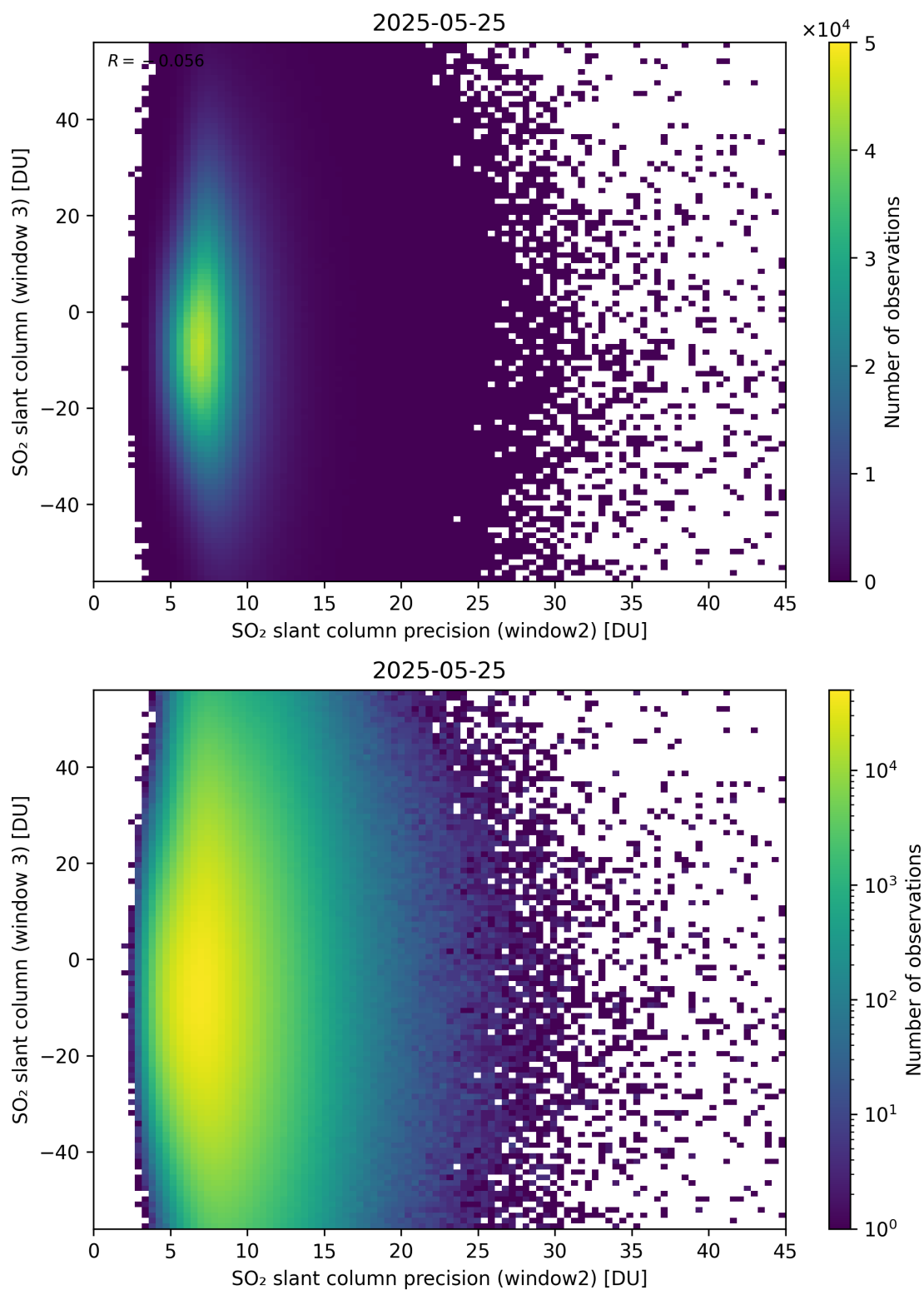
Figure 299: Scatter density plot of “SO 2 slant column precision (window2)” against “SO 2 slant column (window 3)” for 2025-05-24 to 2025-05-26.
