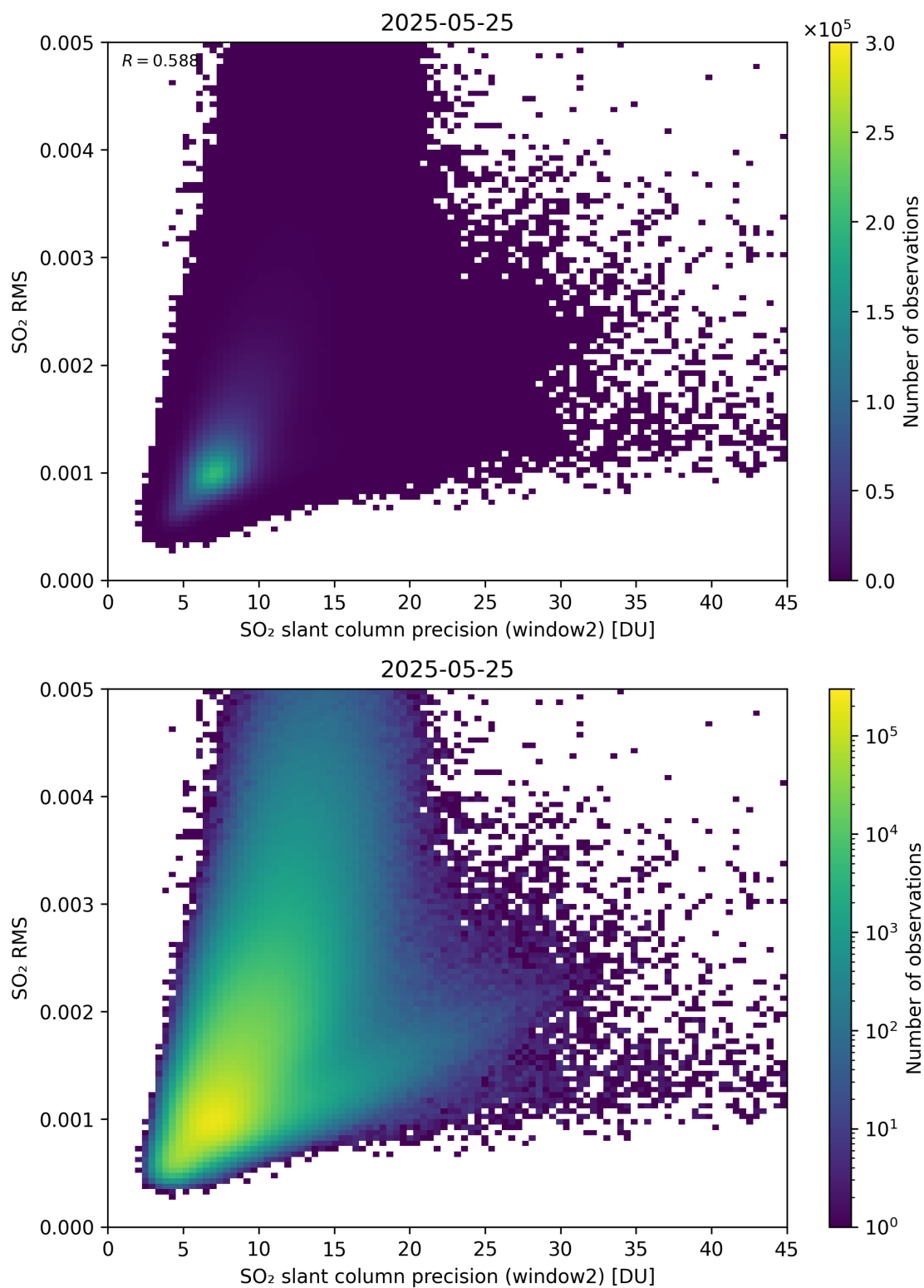
Figure 295: Scatter density plot of “SO 2 slant column precision (window2)” against “SO 2 RMS” for 2025-05-24 to 2025-05-26.
