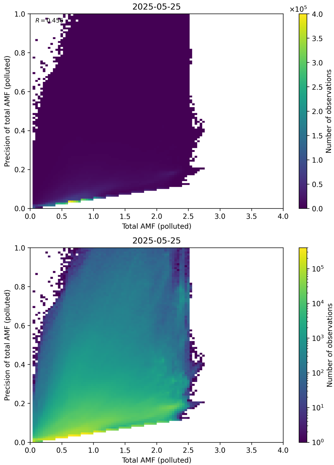
Figure 322: Scatter density plot of “Total AMF (polluted)” against “Precision of total AMF (polluted)” for 2025-05-24 to 2025-05-26.
