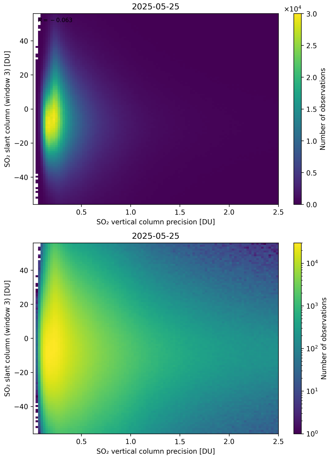
Figure 344: Scatter density plot of “SO 2 vertical column precision” against “SO 2 slant column (window 3)” for 2025-05-24 to 2025-05-26.
