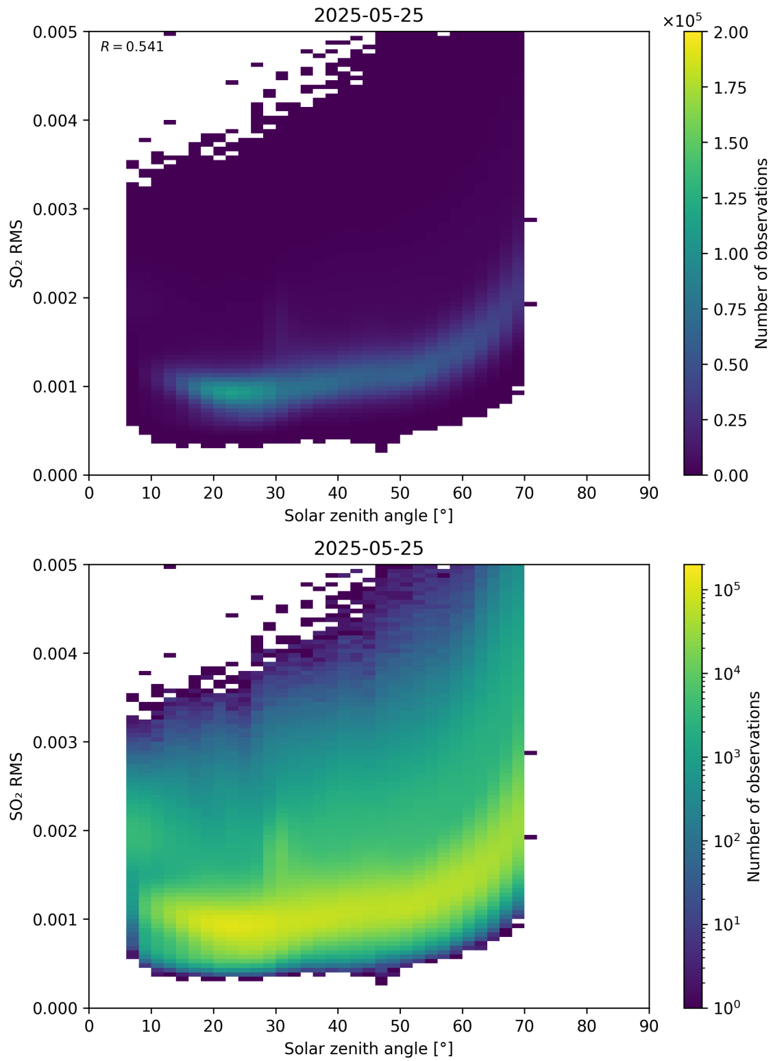
Figure 176: Scatter density plot of “Solar zenith angle” against “SO 2 RMS” for 2025-05-24 to 2025-05-26.
