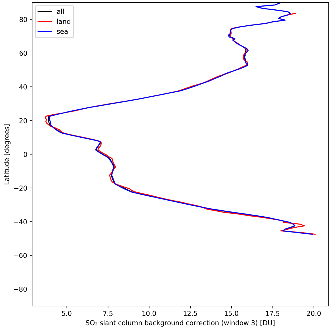
Figure 48: Zonal average of “SO 2 slant column background correction (window 3)” for 2025-05-24 to 2025-05-26.
