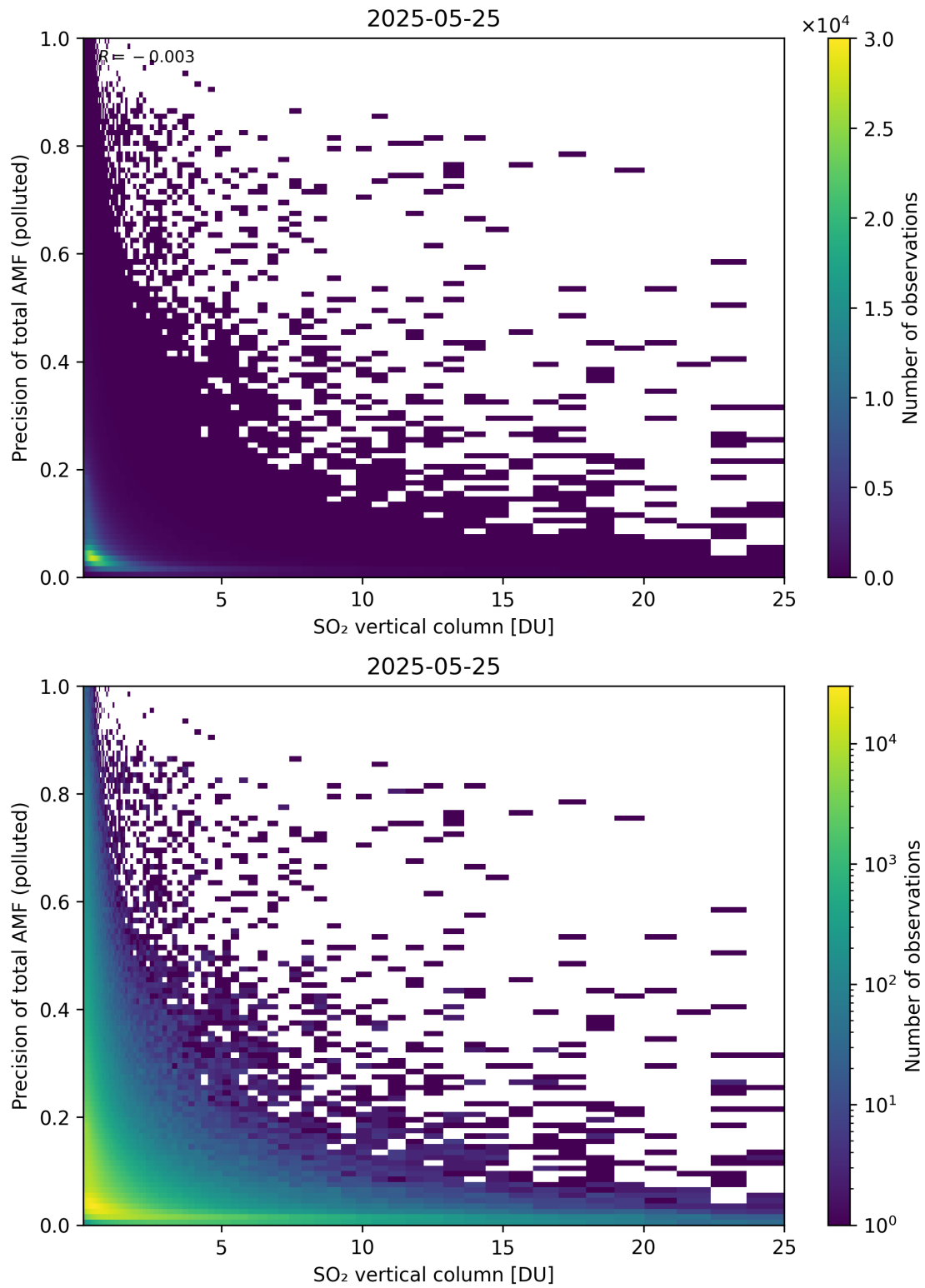
Figure 360: Scatter density plot of “SO 2 vertical column” against “Precision of total AMF (polluted)” for 2025-05-24 to 2025-05-26.
