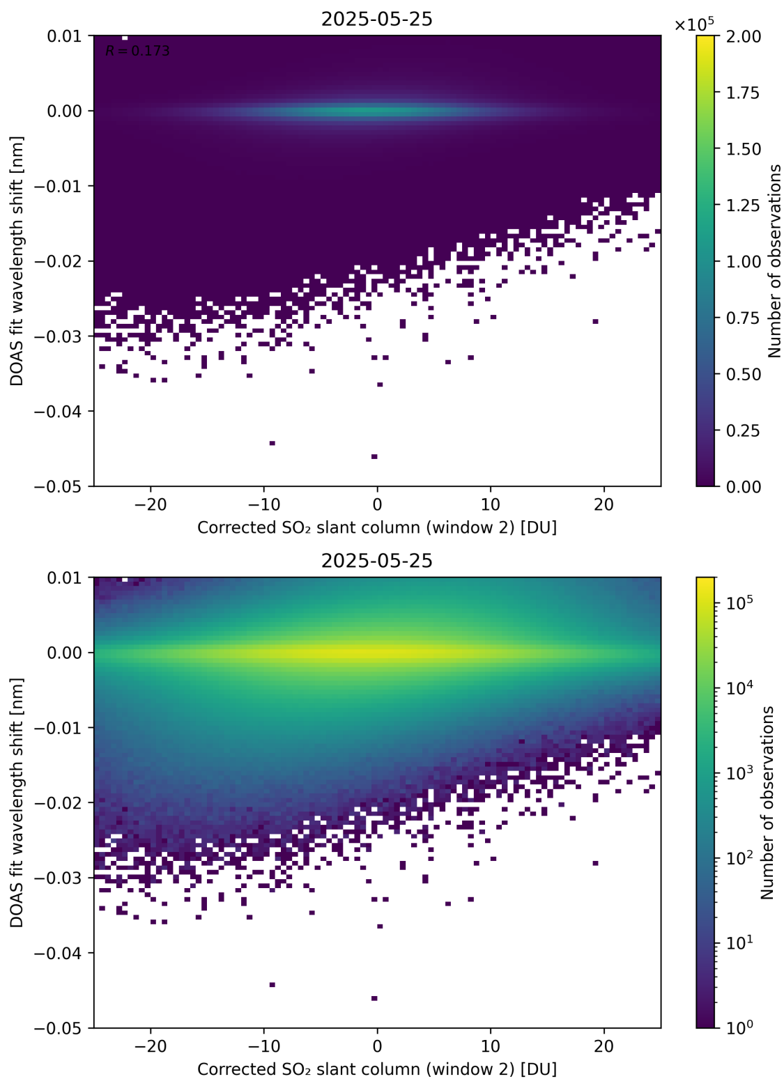
Figure 246: Scatter density plot of “Corrected SO 2 slant column (window 2)” against “DOAS fit wavelength shift” for 2025-05-24 to 2025-05-26.
