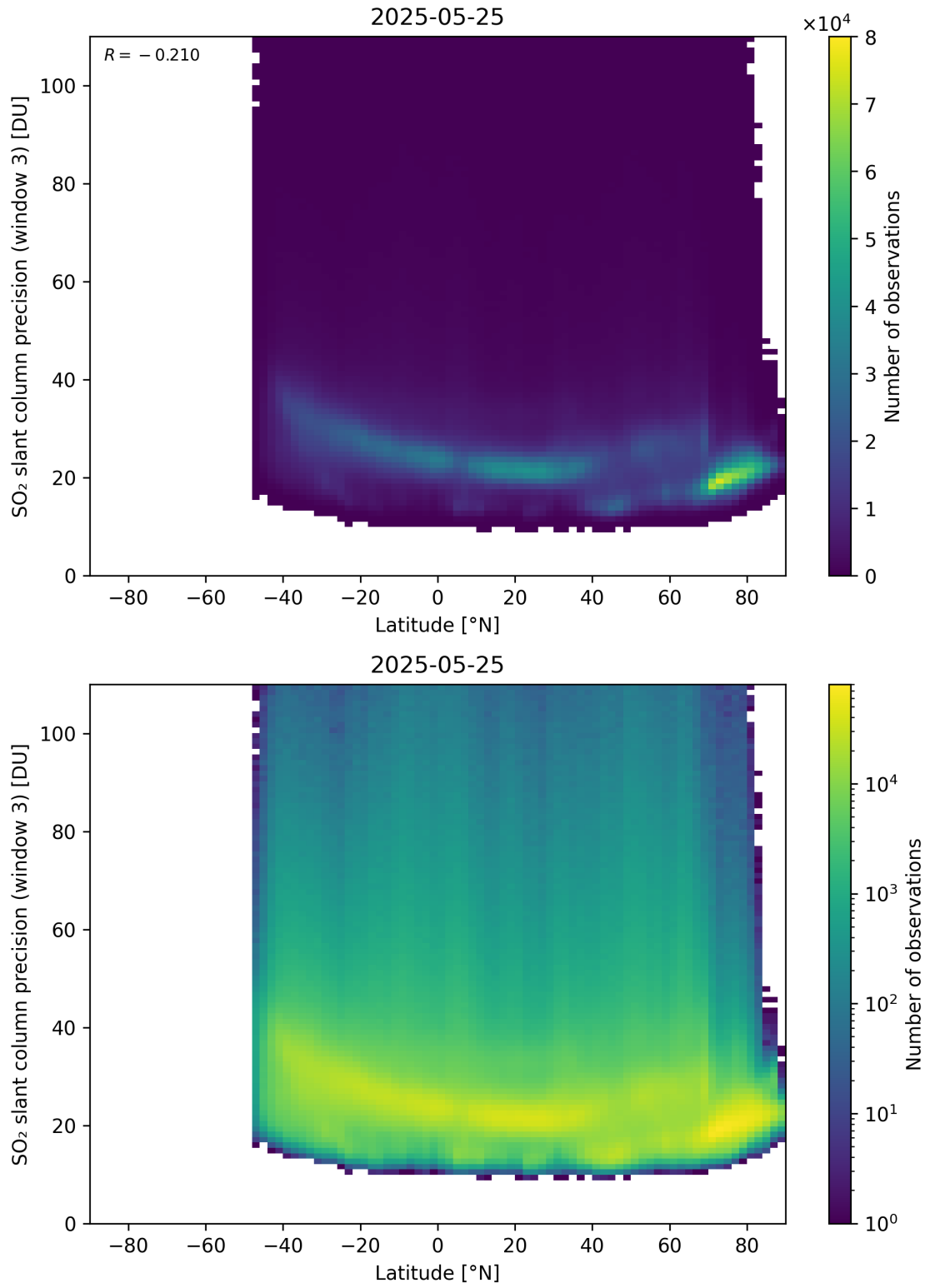
Figure 166: Scatter density plot of “Latitude” against “SO 2 slant column precision (window 3)” for 2025-05-24 to 2025-05-26.
