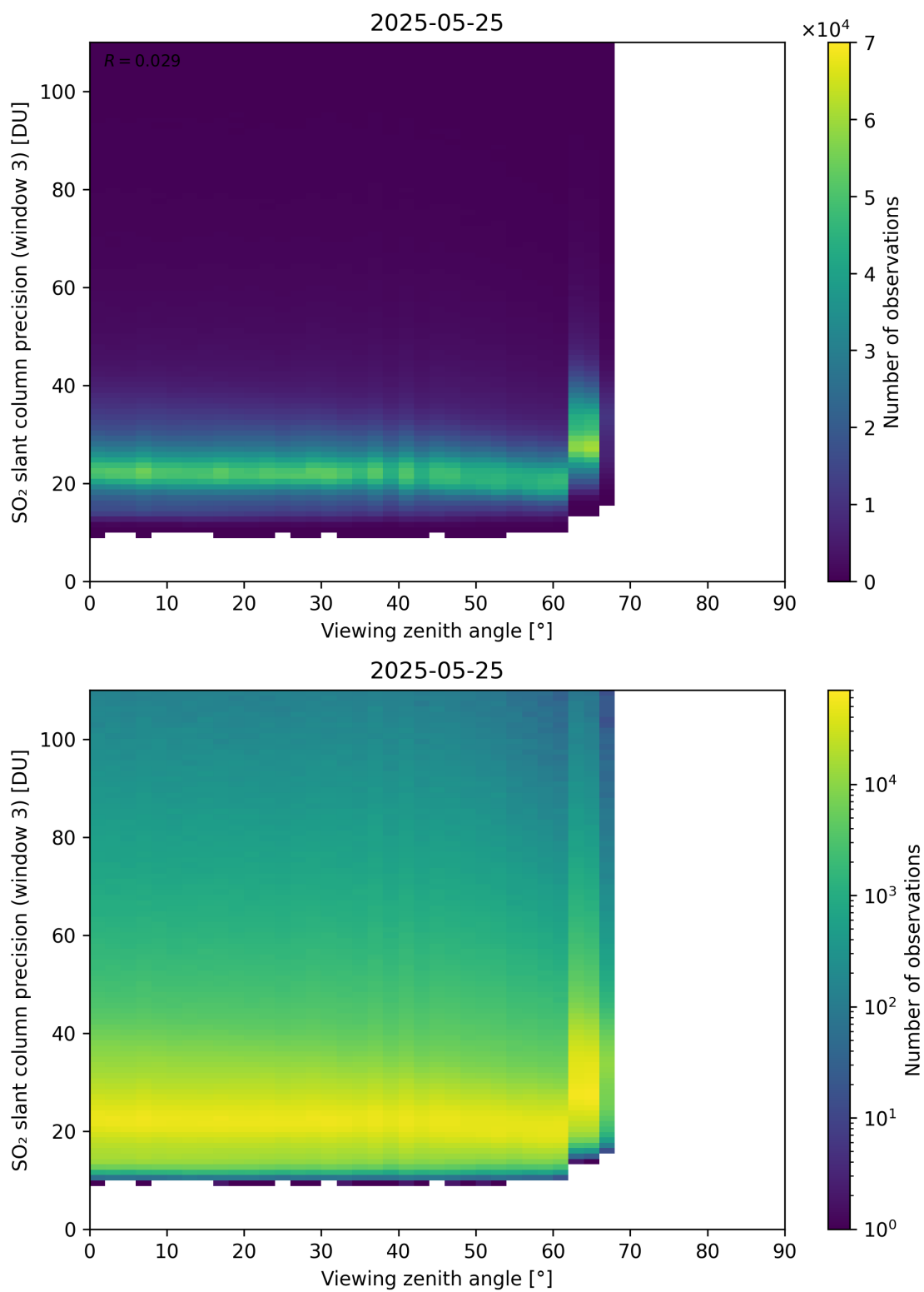
Figure 380: Scatter density plot of “Viewing zenith angle” against “SO 2 slant column precision (window 3)” for 2025-05-24 to 2025-05-26.
