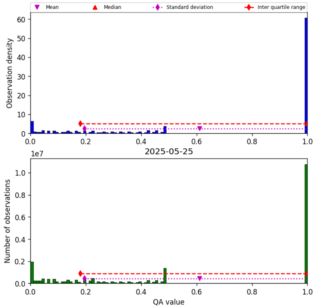
Figure 57: Histogram of “QA value” for 2025-05-24 to 2025-05-26
