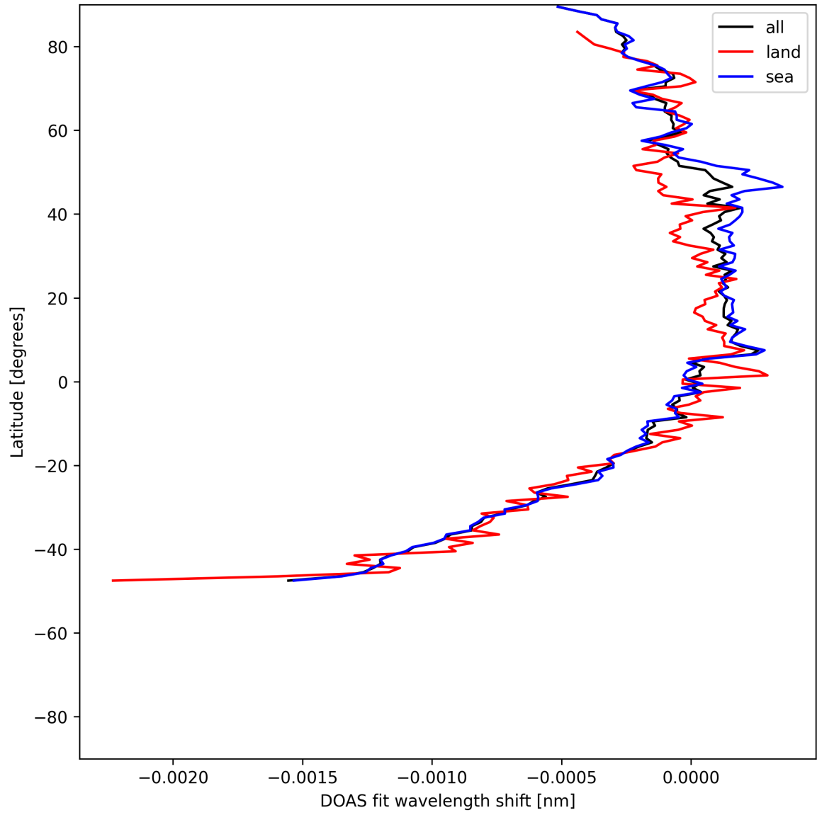
Figure 50: Zonal average of "DOAS fit wavelength shift" for 2025-05-24 to 2025-05-26.
