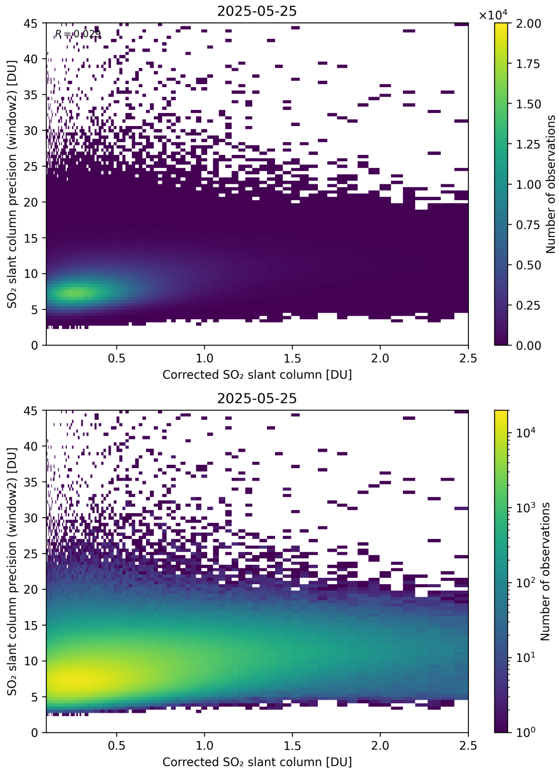
Figure 239: Scatter density plot of “Corrected SO 2 slant column” against “SO 2 slant column precision (window2)” for 2025-05-24 to 2025-05-26.
