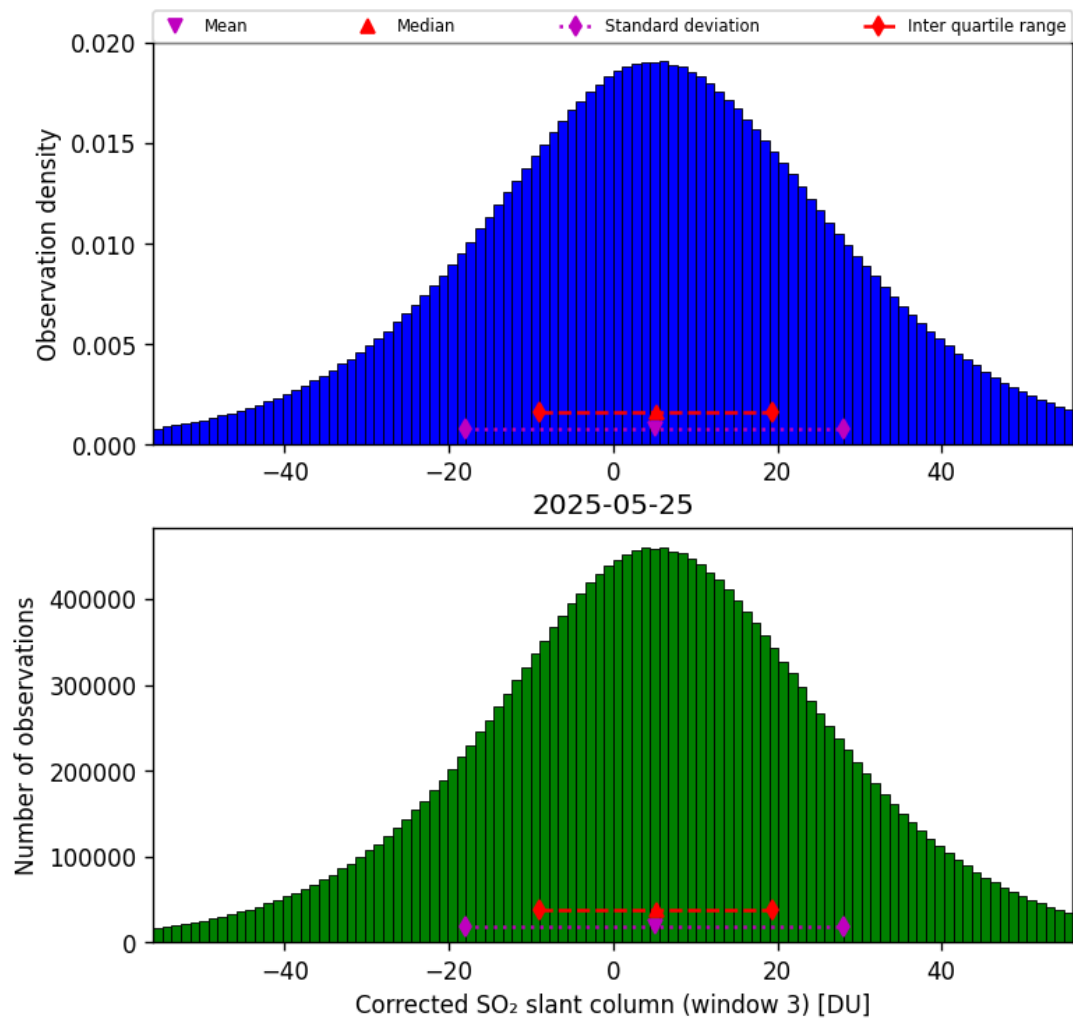
Figure 73: Histogram of “Corrected SO 2 slant column (window 3)” for 2025-05-24 to 2025-05-26
