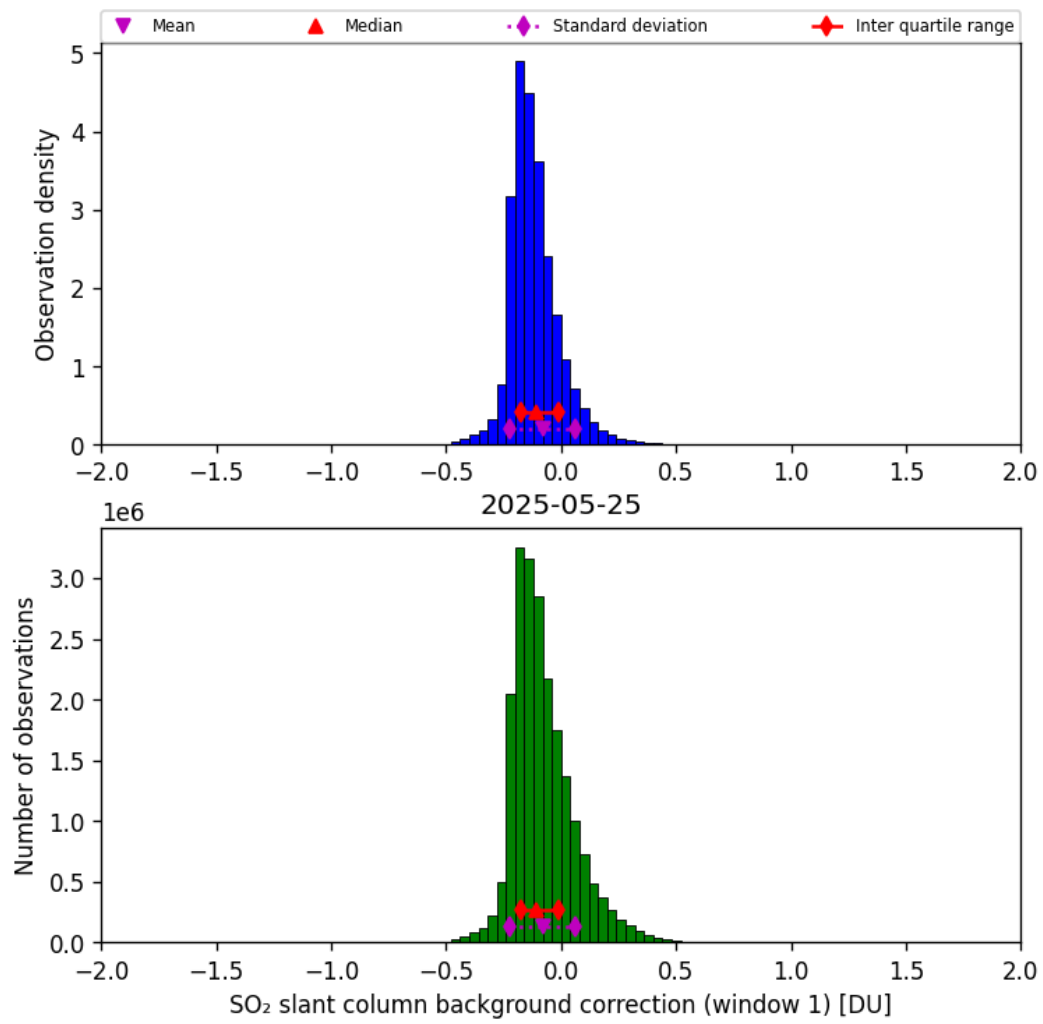
Figure 66: Histogram of “SO 2 slant column background correction (window 1)” for 2025-05-24 to 2025-05-26
