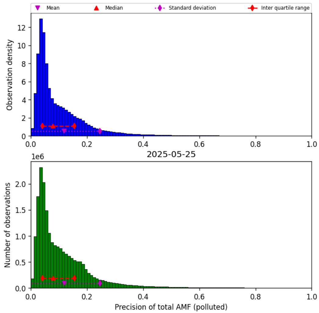
Figure 80: Histogram of “Precision of total AMF (polluted)” for 2025-05-24 to 2025-05-26
