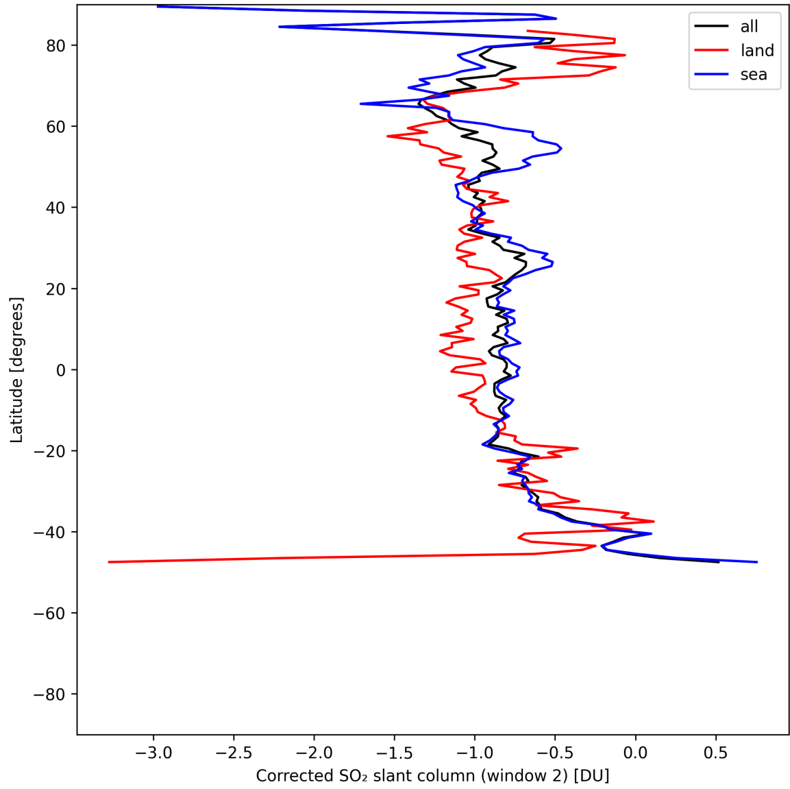
Figure 43: Zonal average of “Corrected SO 2 slant column (window 2)” for 2025-05-24 to 2025-05-26.
