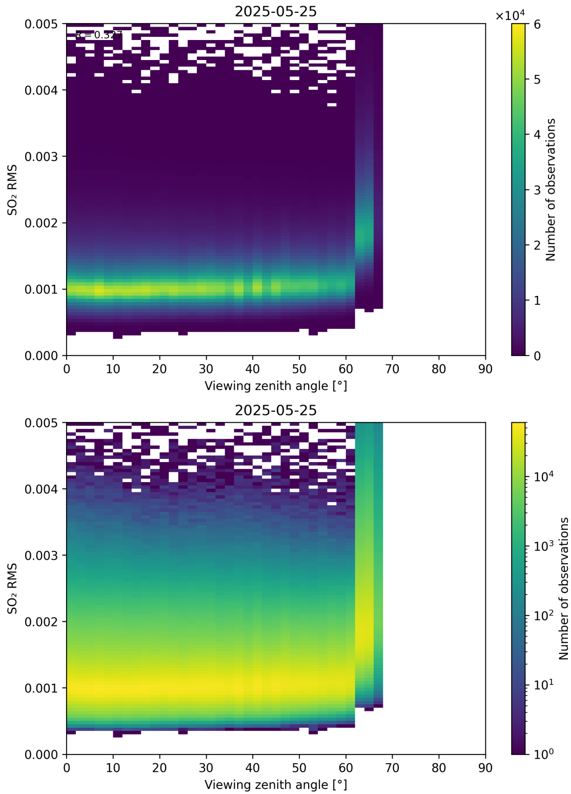
Figure 367: Scatter density plot of “Viewing zenith angle” against “SO 2 RMS” for 2025-05-24 to 2025-05-26.
