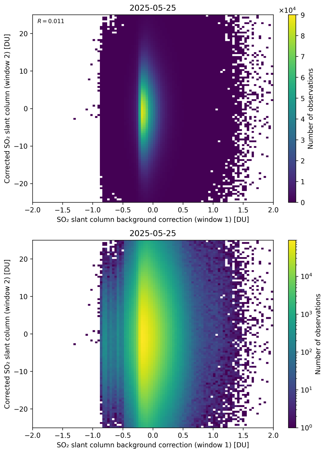
Figure 115: Scatter density plot of “SO 2 slant column background correction (window 1)” against “Corrected SO 2 slant column (window 2)” for 2025-05-24 to 2025-05-26.
