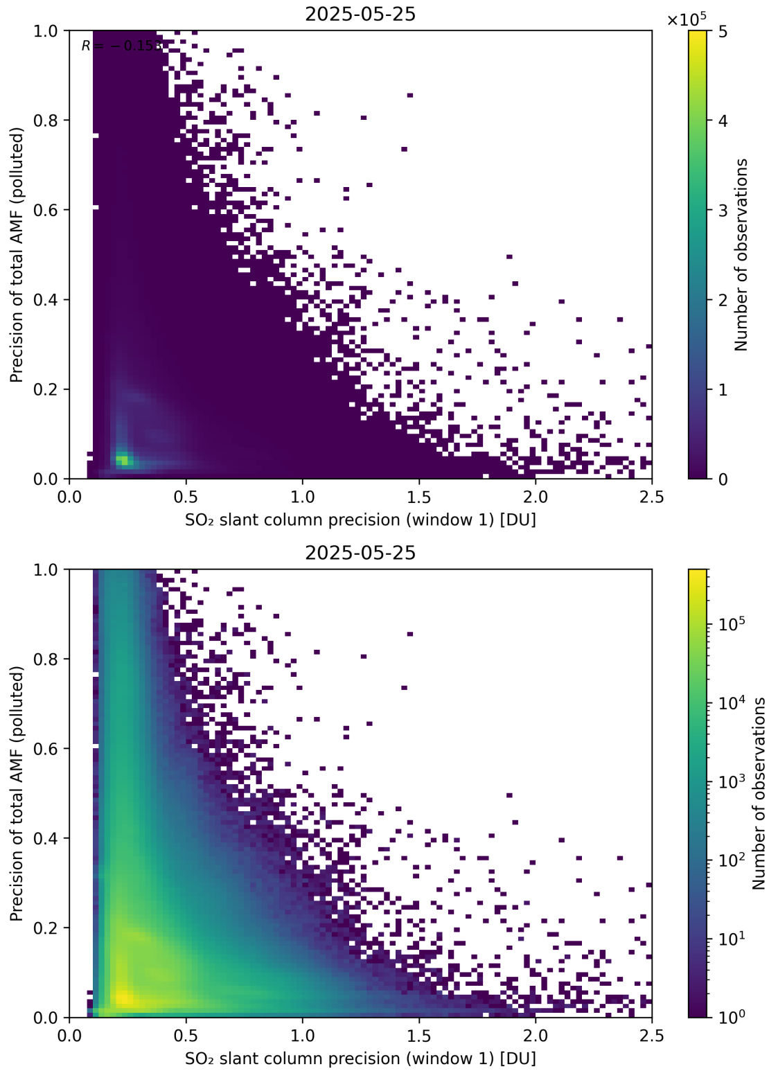
Figure 281: Scatter density plot of “SO 2 slant column precision (window 1)” against “Precision of total AMF (polluted)” for 2025-05-24 to 2025-05-26.
