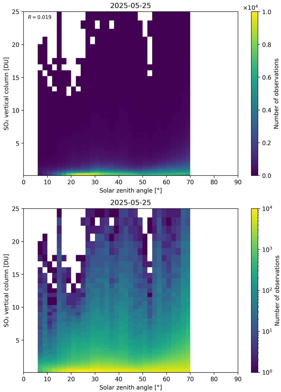
Figure 191: Scatter density plot of “Solar zenith angle” against “SO 2 vertical column” for 2025-05-24 to 2025-05-26.
