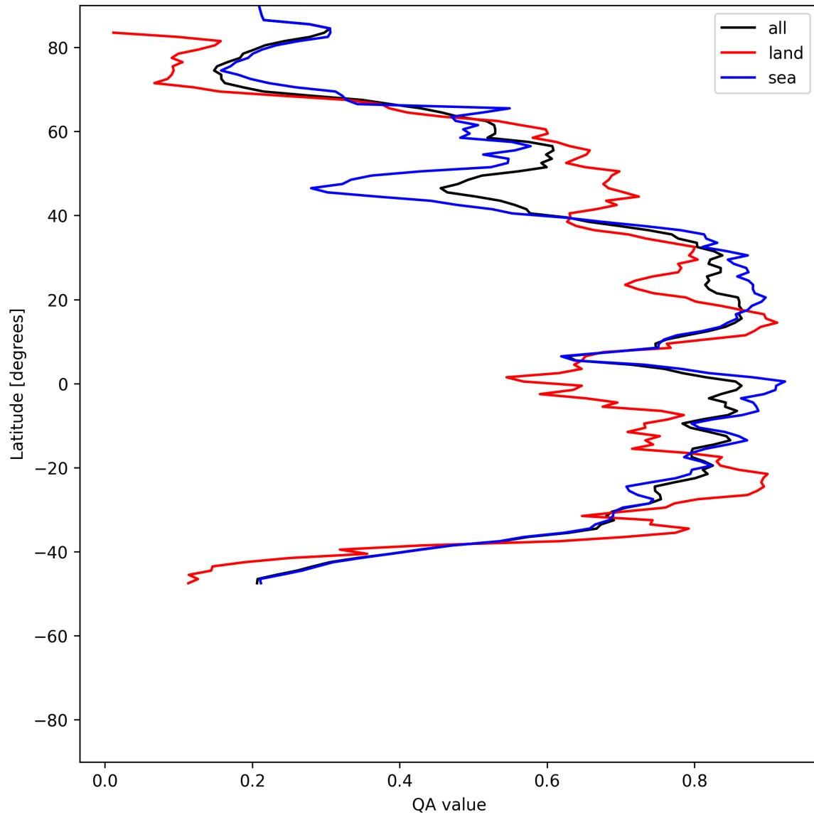
Figure 31: Zonal average of “QA value” for 2025-05-24 to 2025-05-26.
