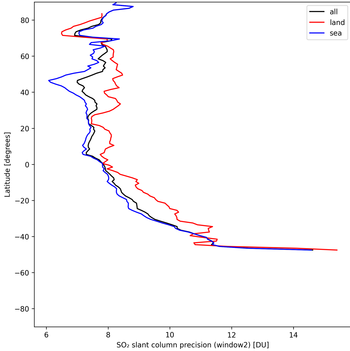
Figure 42: Zonal average of “SO 2 slant column precision (window2)” for 2025-05-24 to 2025-05-26.
