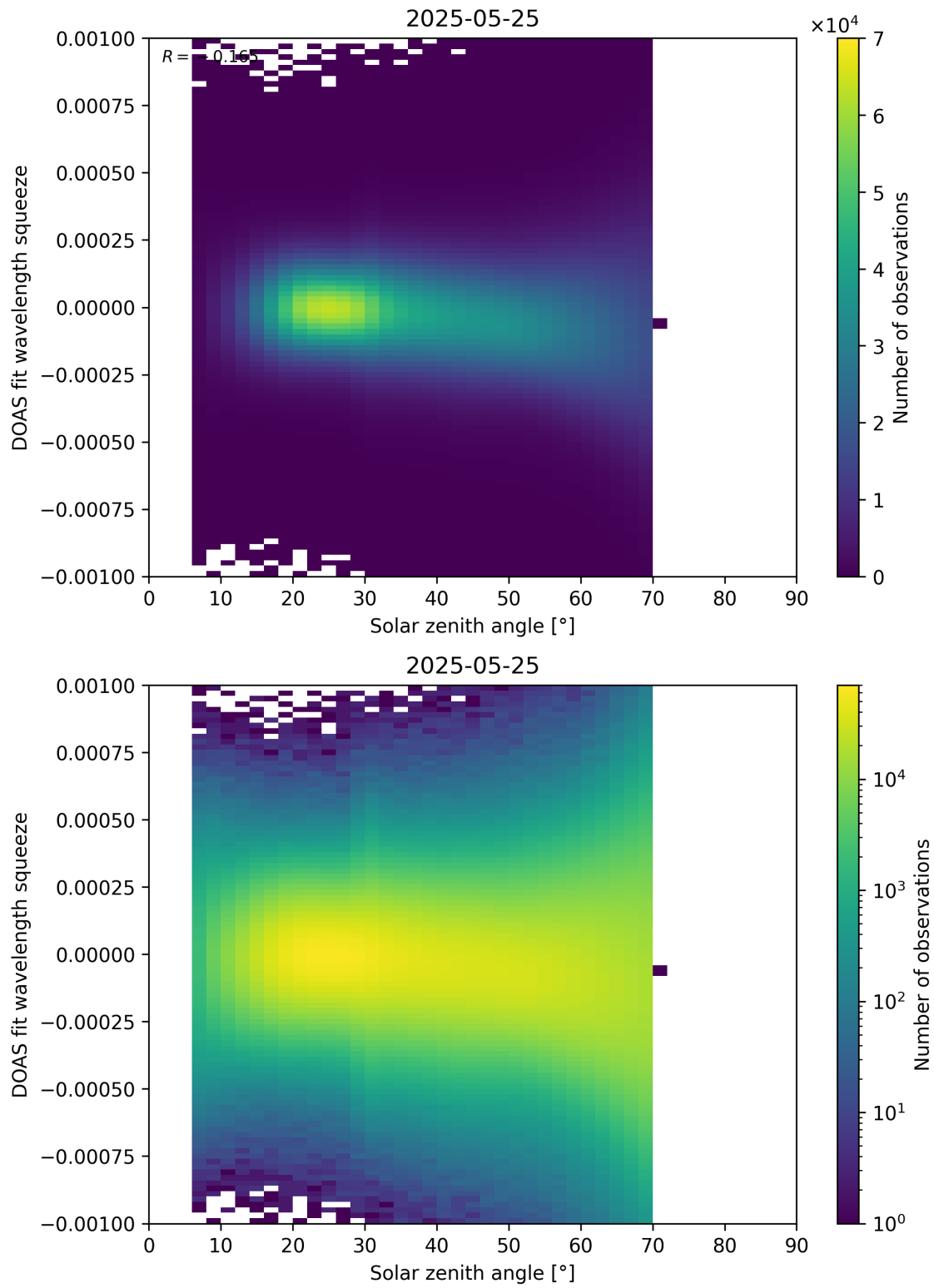
Figure 175: Scatter density plot of “Solar zenith angle” against “DOAS fit wavelength squeeze” for 2025-05-24 to 2025-05-26.
