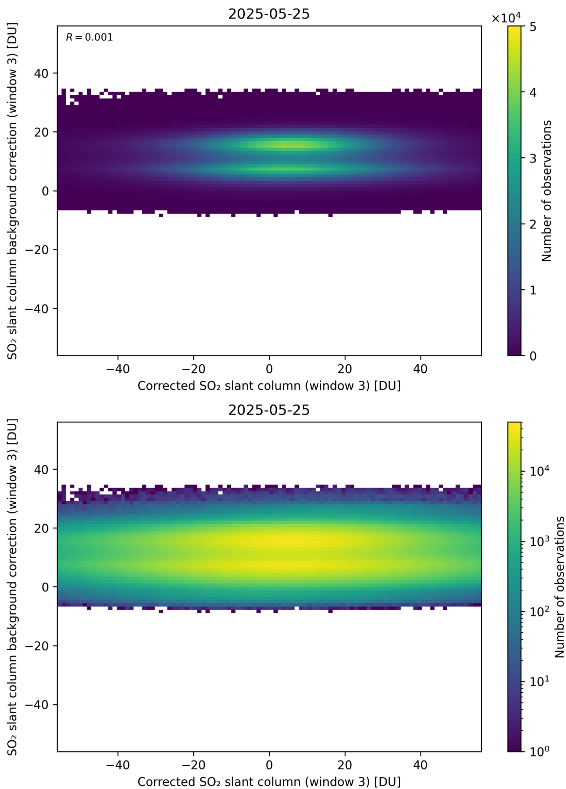
Figure 255: Scatter density plot of “Corrected SO 2 slant column (window 3)” against “SO 2 slant column background correction (window 3)” for 2025-05-24 to 2025-05-26.
