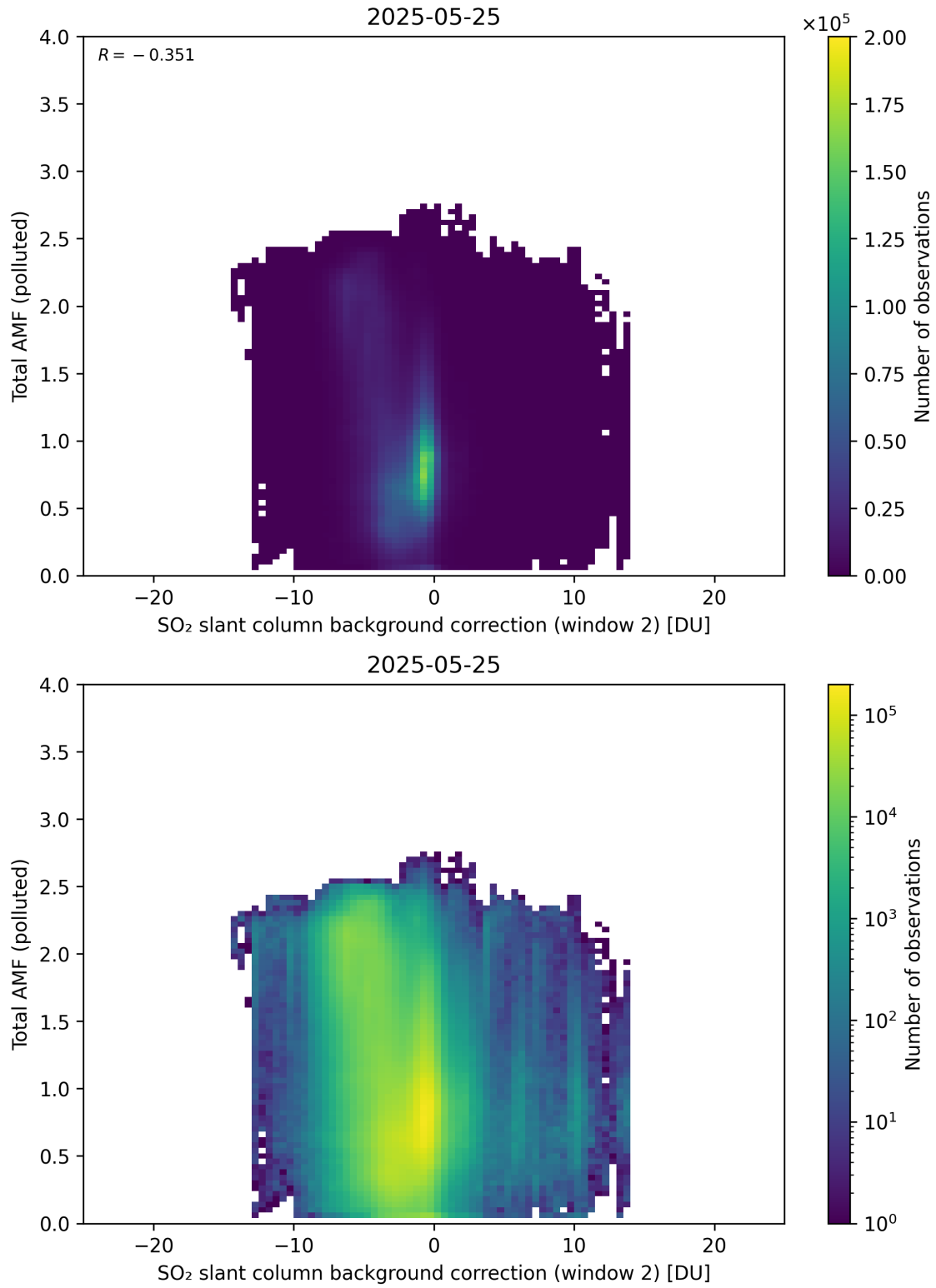
Figure 130: Scatter density plot of “SO 2 slant column background correction (window 2)” against “Total AMF (polluted)” for 2025-05-24 to 2025-05-26.
