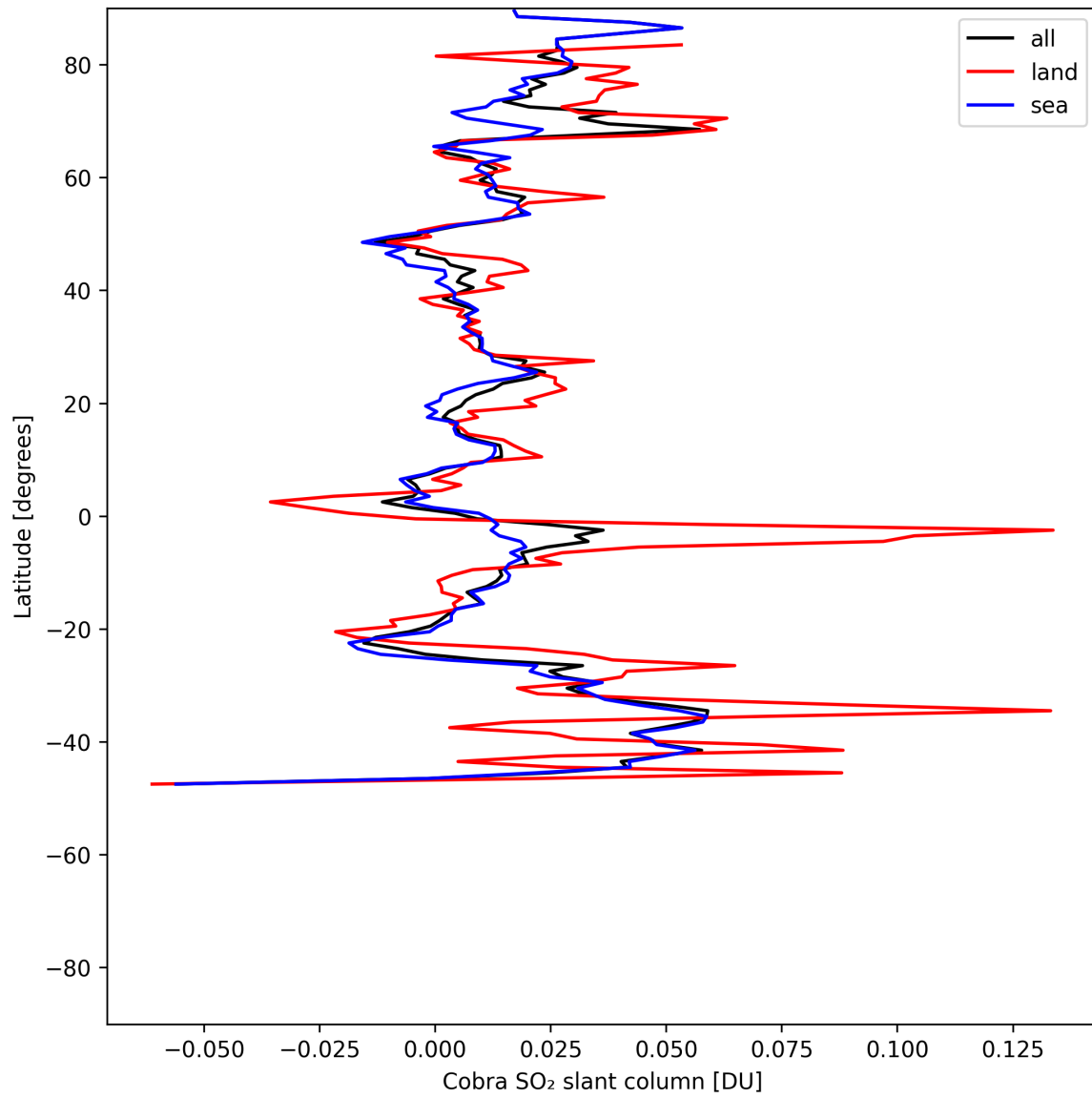
Figure 35: Zonal average of “Cobra SO 2 slant column” for 2025-05-24 to 2025-05-26.
