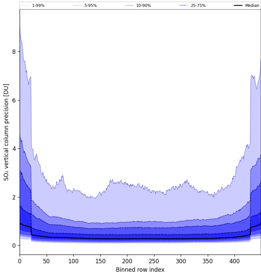
Figure 85: Along track statistics of “SO 2 vertical column precision” for 2025-05-24 to 2025-05-26
