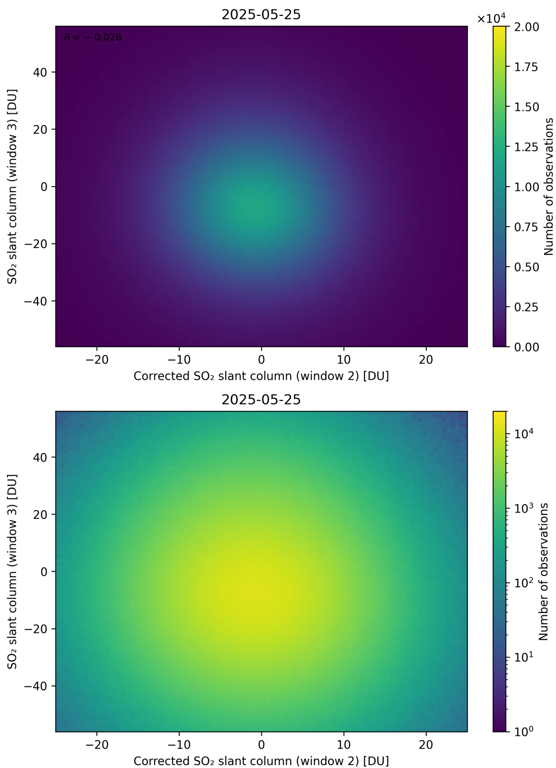
Figure 251: Scatter density plot of “Corrected SO 2 slant column (window 2)” against “SO 2 slant column (window 3)” for 2025-05-24 to 2025-05-26.
