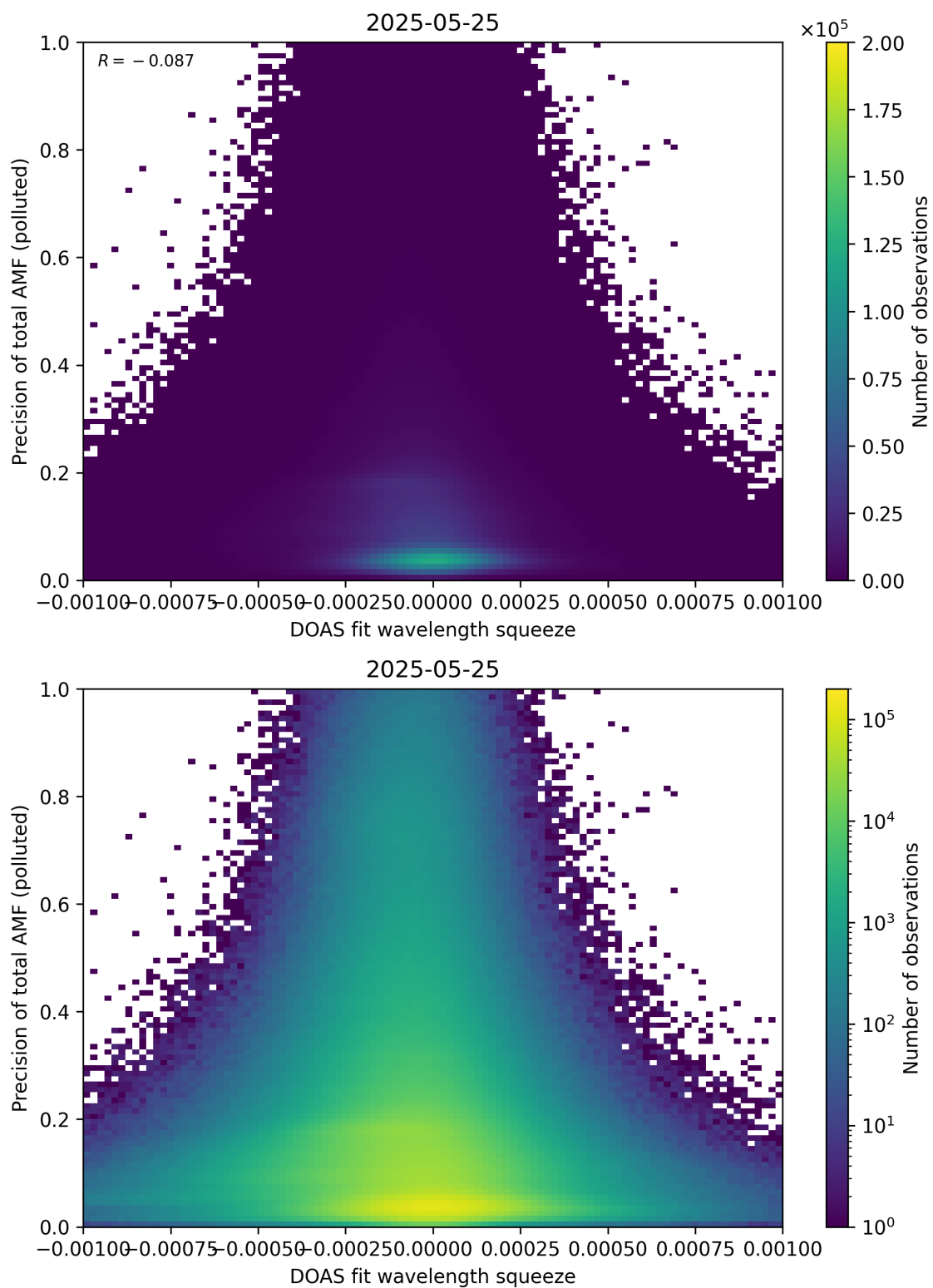
Figure 146: Scatter density plot of “DOAS fit wavelength squeeze” against “Precision of total AMF (polluted)” for 2025-05-24 to 2025-05-26.
