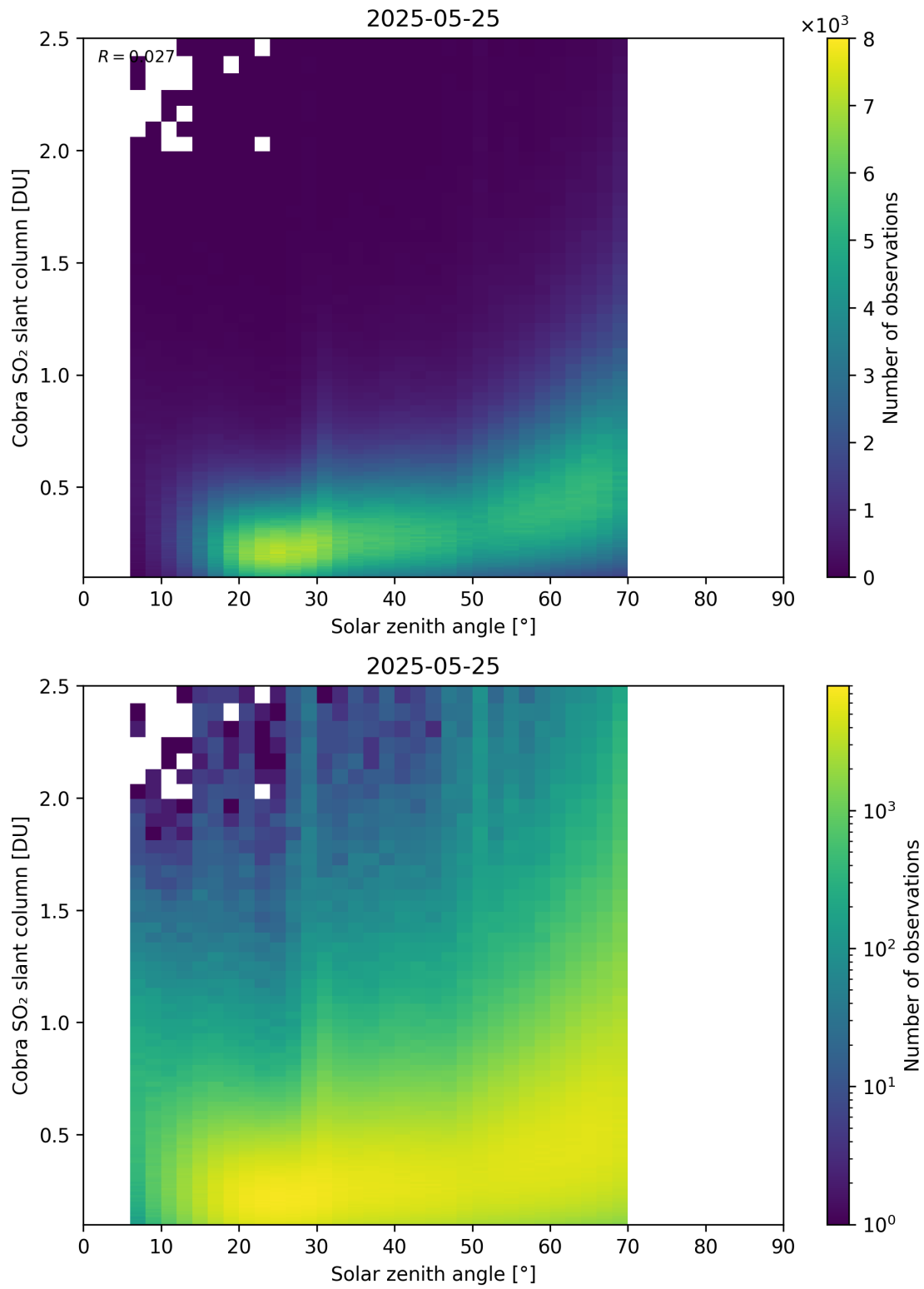
Figure 179: Scatter density plot of “Solar zenith angle” against “Cobra SO 2 slant column” for 2025-05-24 to 2025-05-26.
