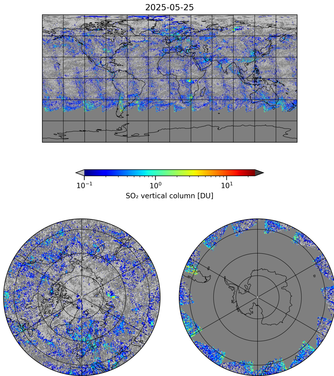
Figure 6: Map of “SO 2 vertical column” for 2025-05-24 to 2025-05-26
