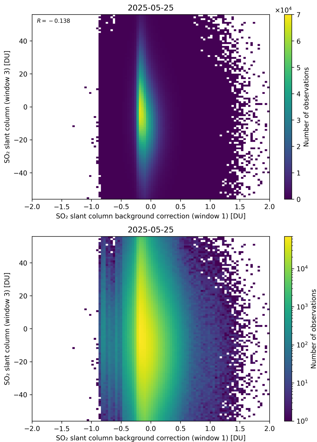
Figure 118: Scatter density plot of “SO 2 slant column background correction (window 1)” against “SO 2 slant column (window 3)” for 2025-05-24 to 2025-05-26.
