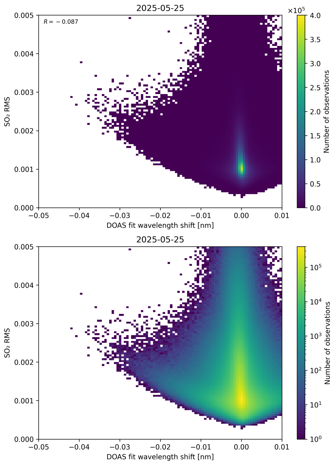
Figure 139: Scatter density plot of “DOAS fit wavelength shift” against “SO 2 RMS” for 2025-05-24 to 2025-05-26.
