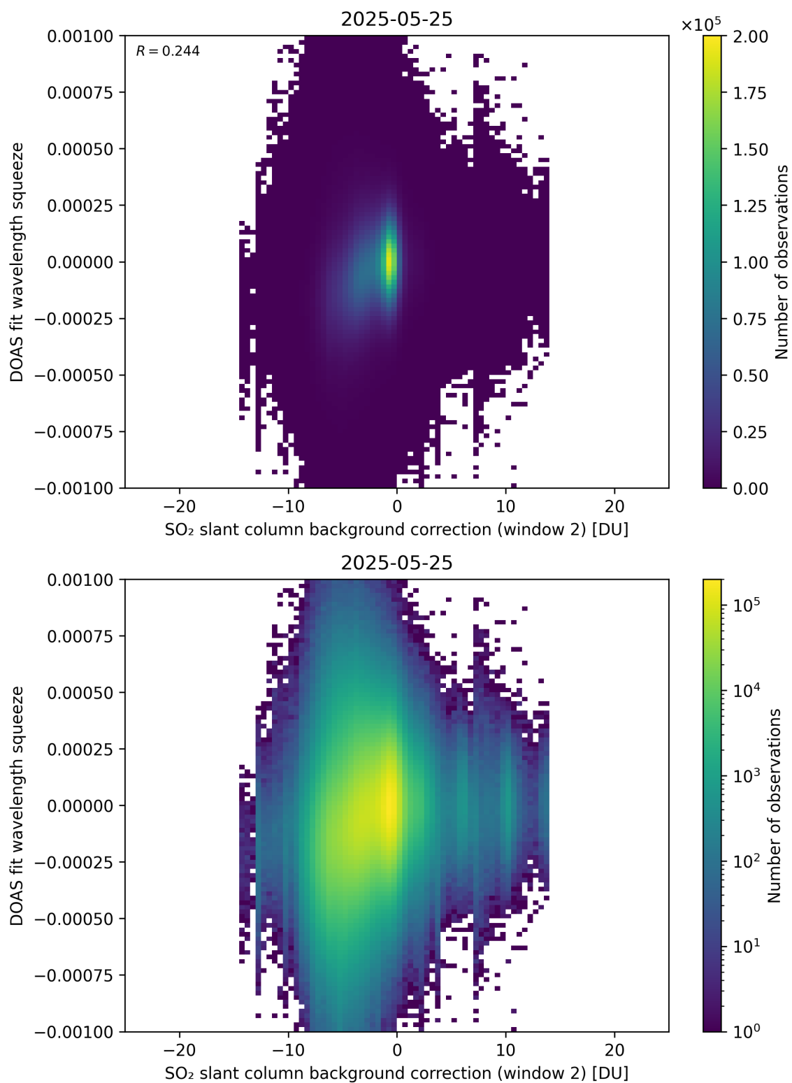
Figure 124: Scatter density plot of “SO 2 slant column background correction (window 2)” against “DOAS fit wavelength squeeze” for 2025-05-24 to 2025-05-26.
