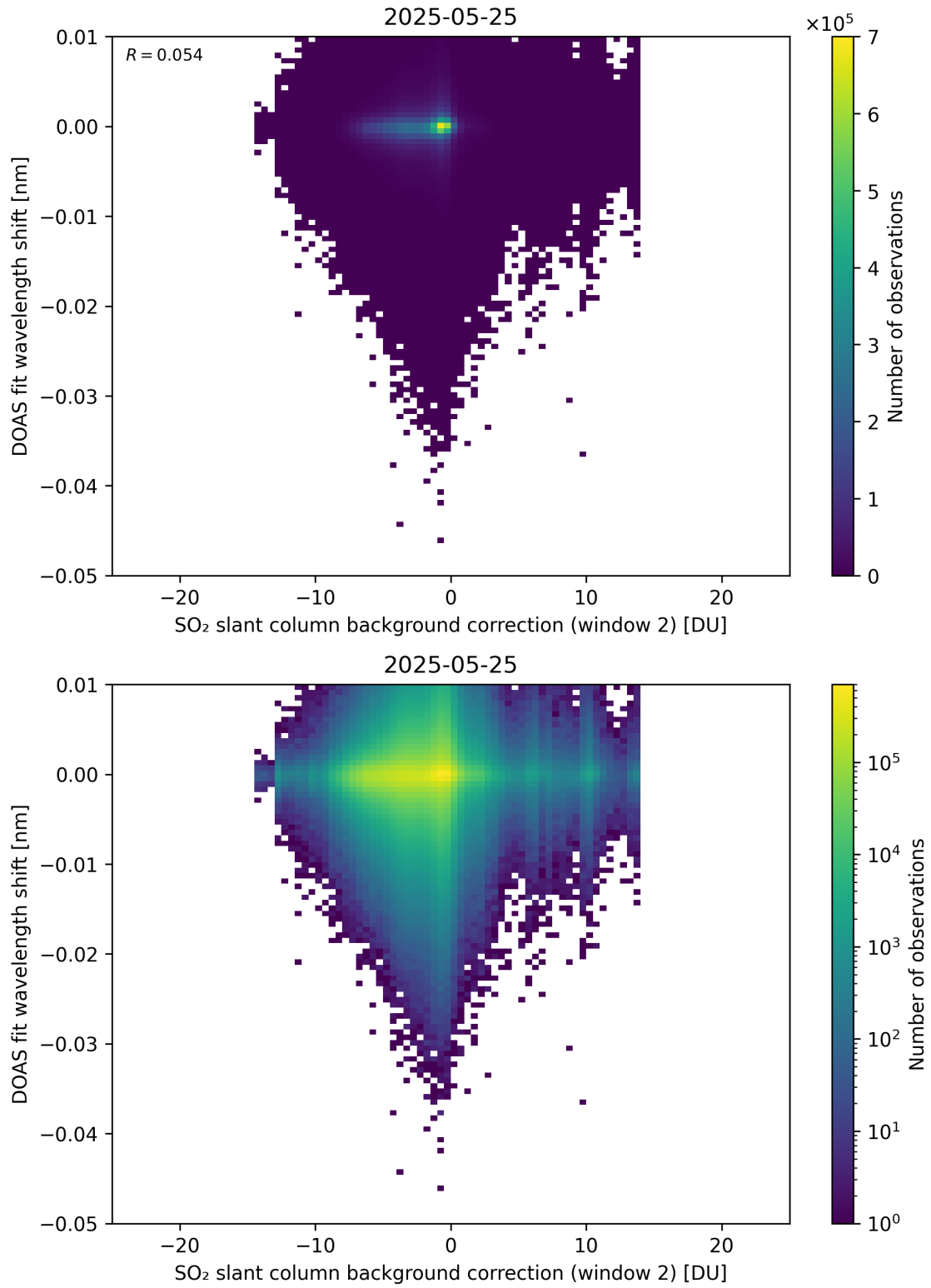
Figure 123: Scatter density plot of “SO 2 slant column background correction (window 2)” against “DOAS fit wavelength shift” for 2025-05-24 to 2025-05-26.
