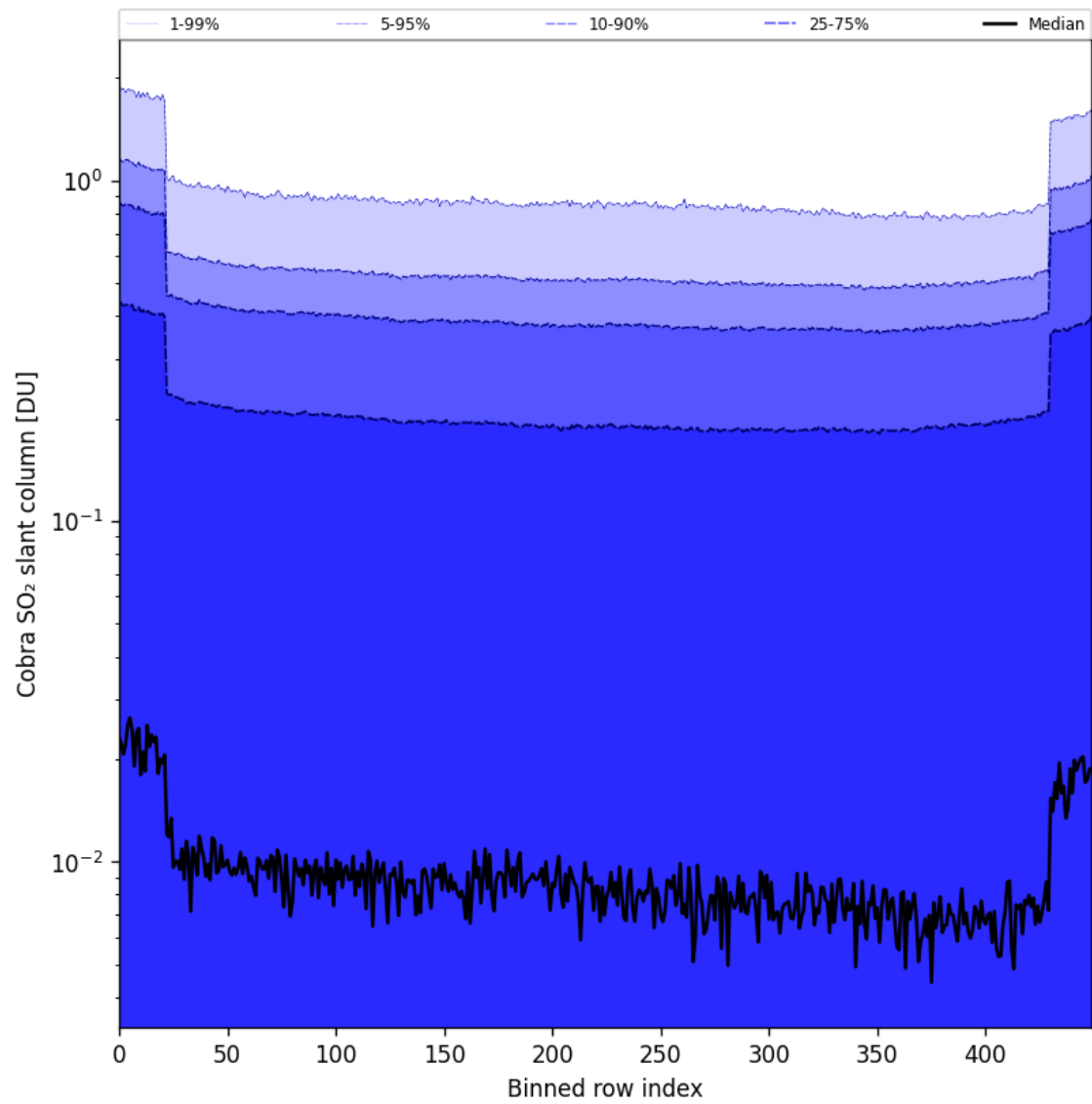
Figure 87: Along track statistics of “Cobra SO 2 slant column” for 2025-05-24 to 2025-05-26
