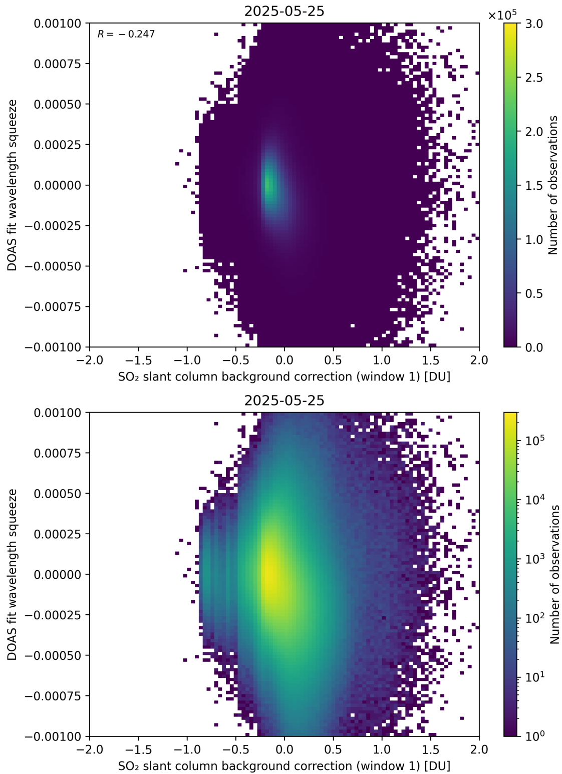
Figure 112: Scatter density plot of “SO 2 slant column background correction (window 1)” against “DOAS fit wavelength squeeze” for 2025-05-24 to 2025-05-26.
