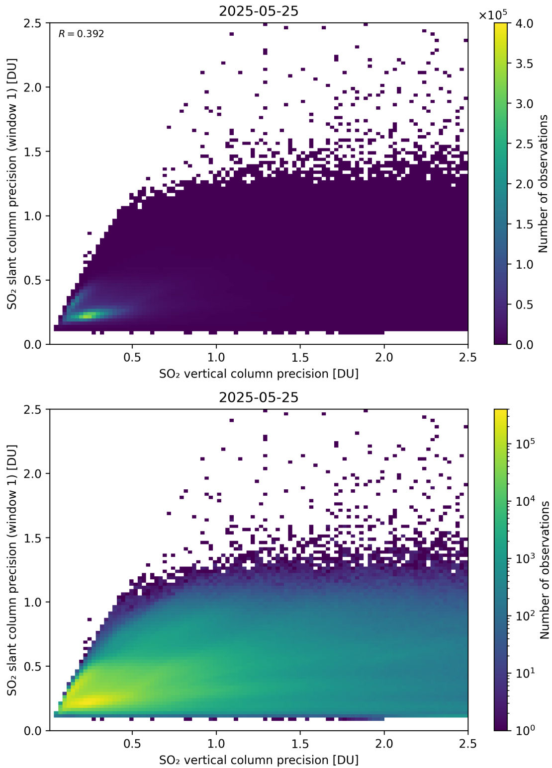
Figure 342: Scatter density plot of “SO 2 vertical column precision” against “SO 2 slant column precision (window 1)” for 2025-05-24 to 2025-05-26.
