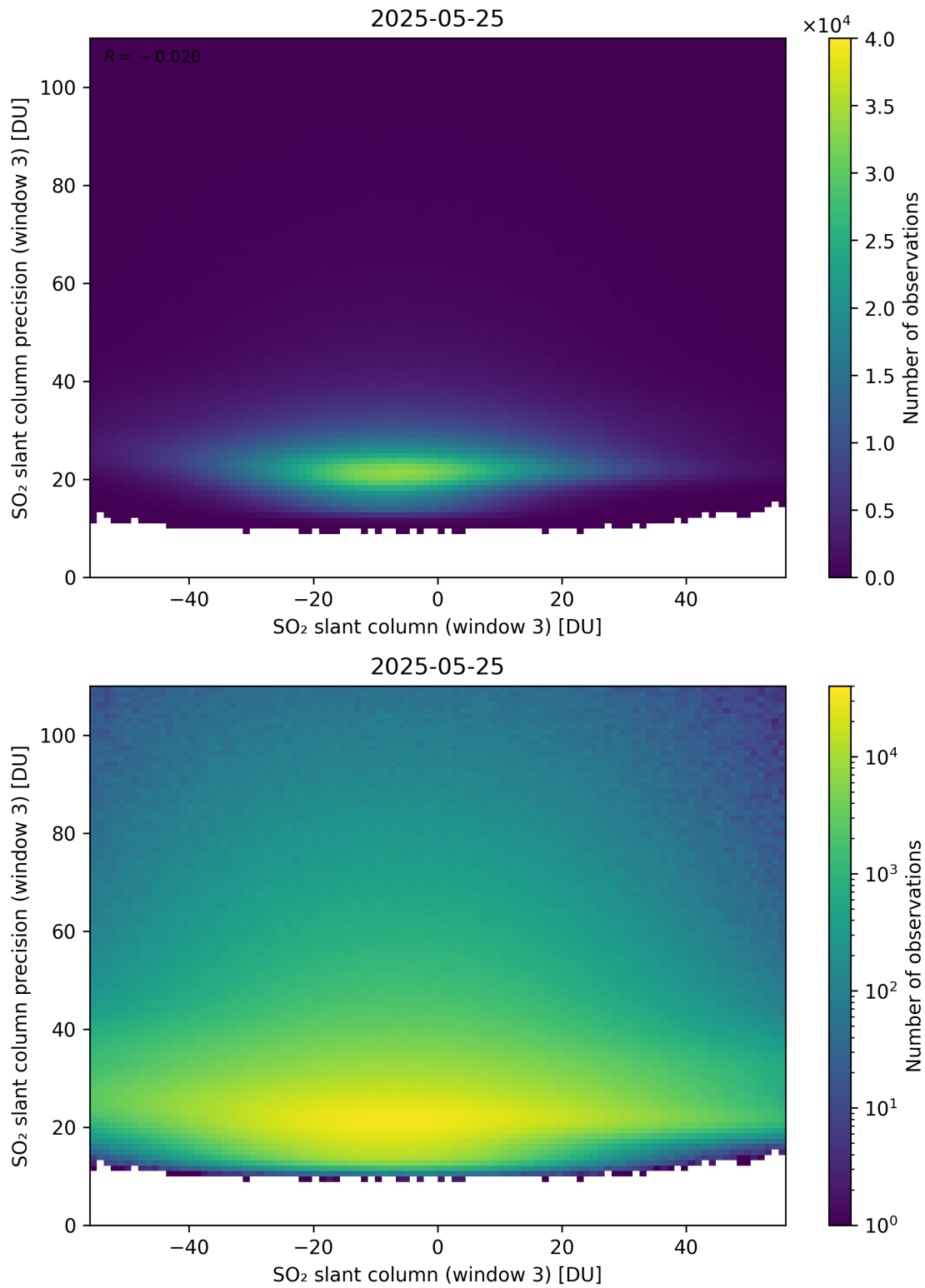
Figure 317: Scatter density plot of “SO 2 slant column (window 3)” against “SO 2 slant column precision (window 3)” for 2025-05-24 to 2025-05-26.
