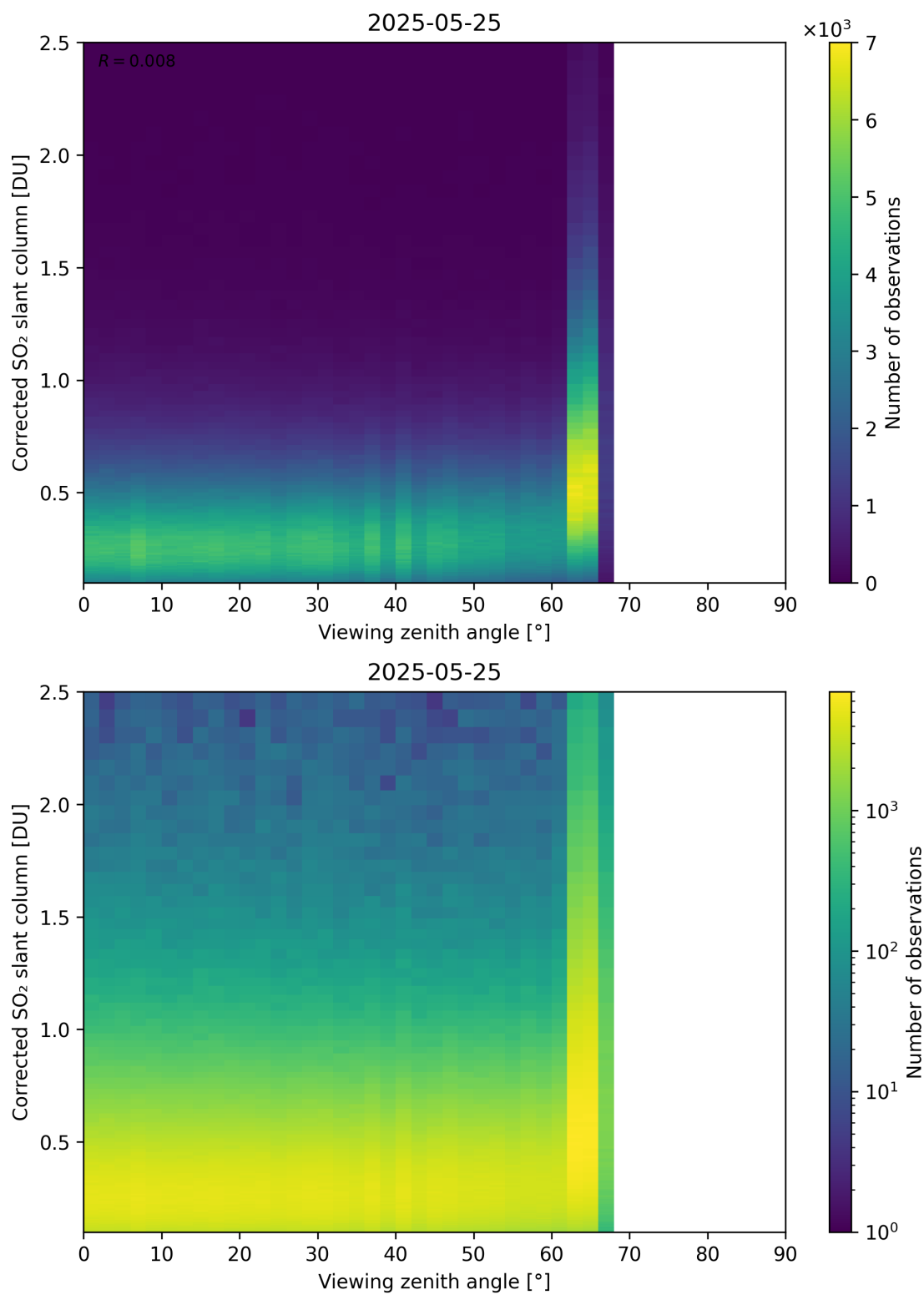
Figure 373: Scatter density plot of “Viewing zenith angle” against “Corrected SO 2 slant column” for 2025-05-24 to 2025-05-26.
