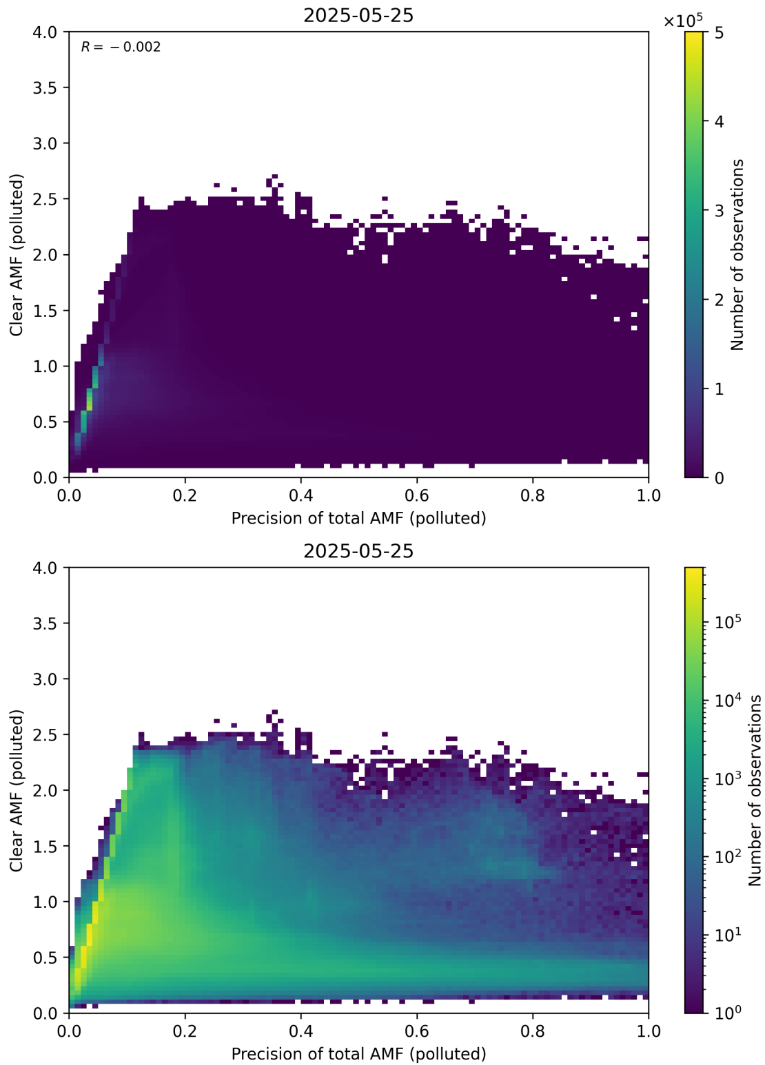
Figure 320: Scatter density plot of “Precision of total AMF (polluted)” against “Clear AMF (polluted)” for 2025-05-24 to 2025-05-26.
