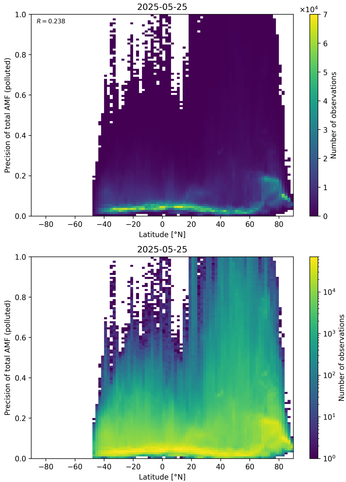
Figure 168: Scatter density plot of “Latitude” against “Precision of total AMF (polluted)” for 2025-05-24 to 2025-05-26.
