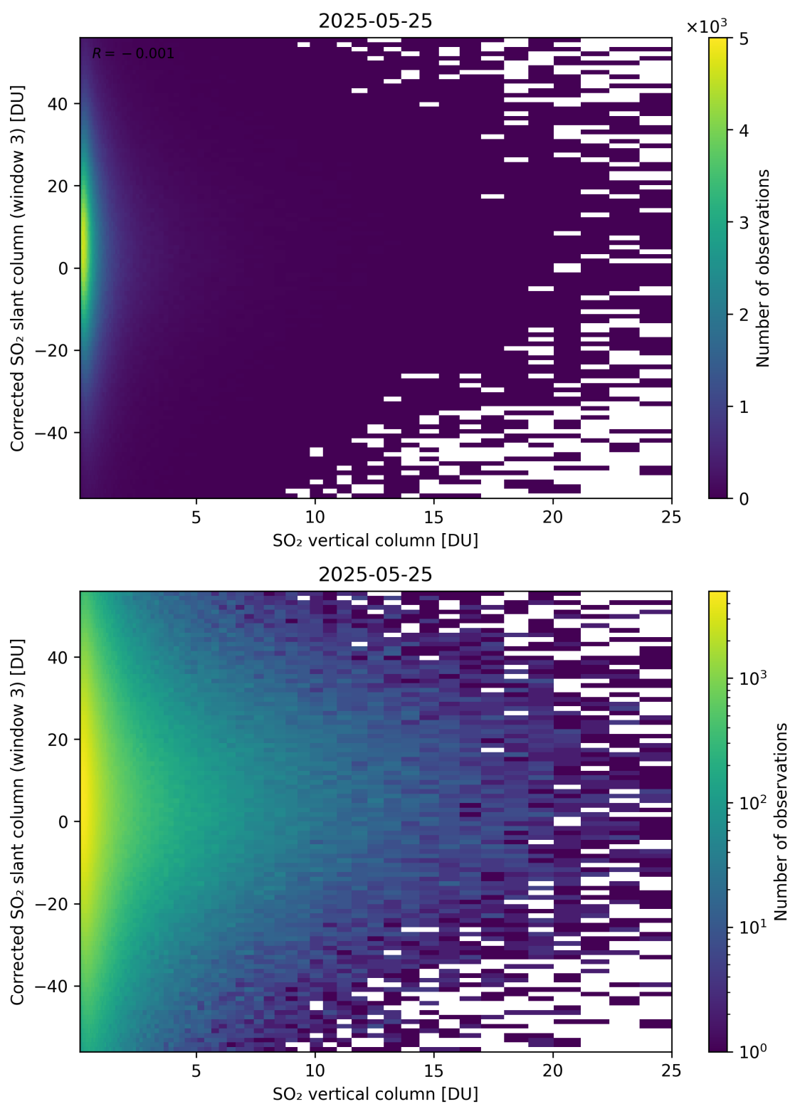
Figure 353: Scatter density plot of “SO 2 vertical column” against “Corrected SO 2 slant column (window 3)” for 2025-05-24 to 2025-05-26.
