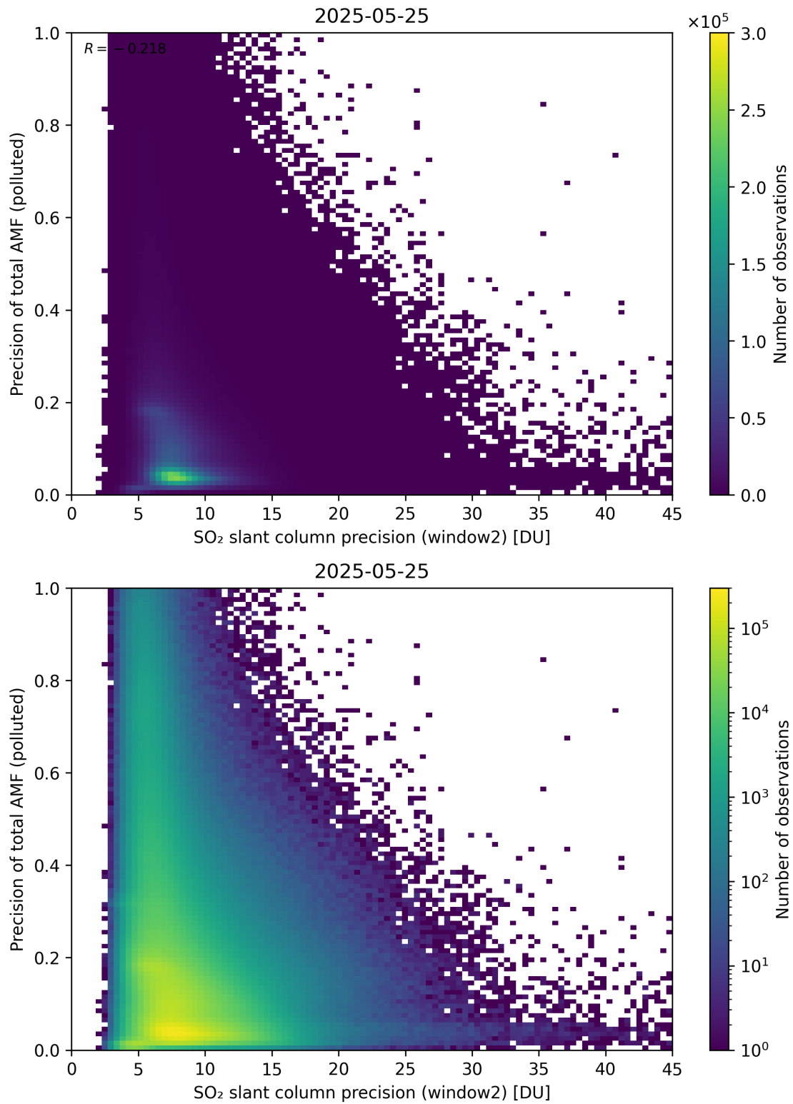
Figure 302: Scatter density plot of “SO 2 slant column precision (window2)” against “Precision of total AMF (polluted)” for 2025-05-24 to 2025-05-26.
