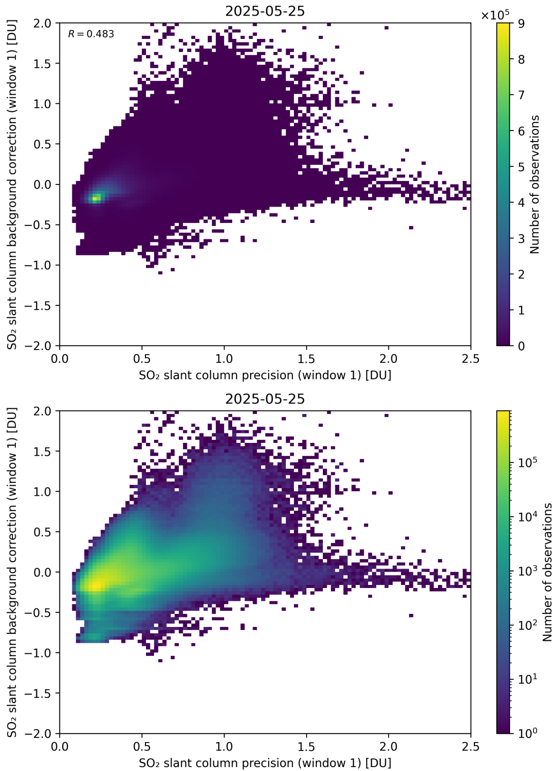
Figure 268: Scatter density plot of “SO 2 slant column precision (window 1)” against “SO 2 slant column background correction (window 1)” for 2025-05-24 to 2025-05-26.
