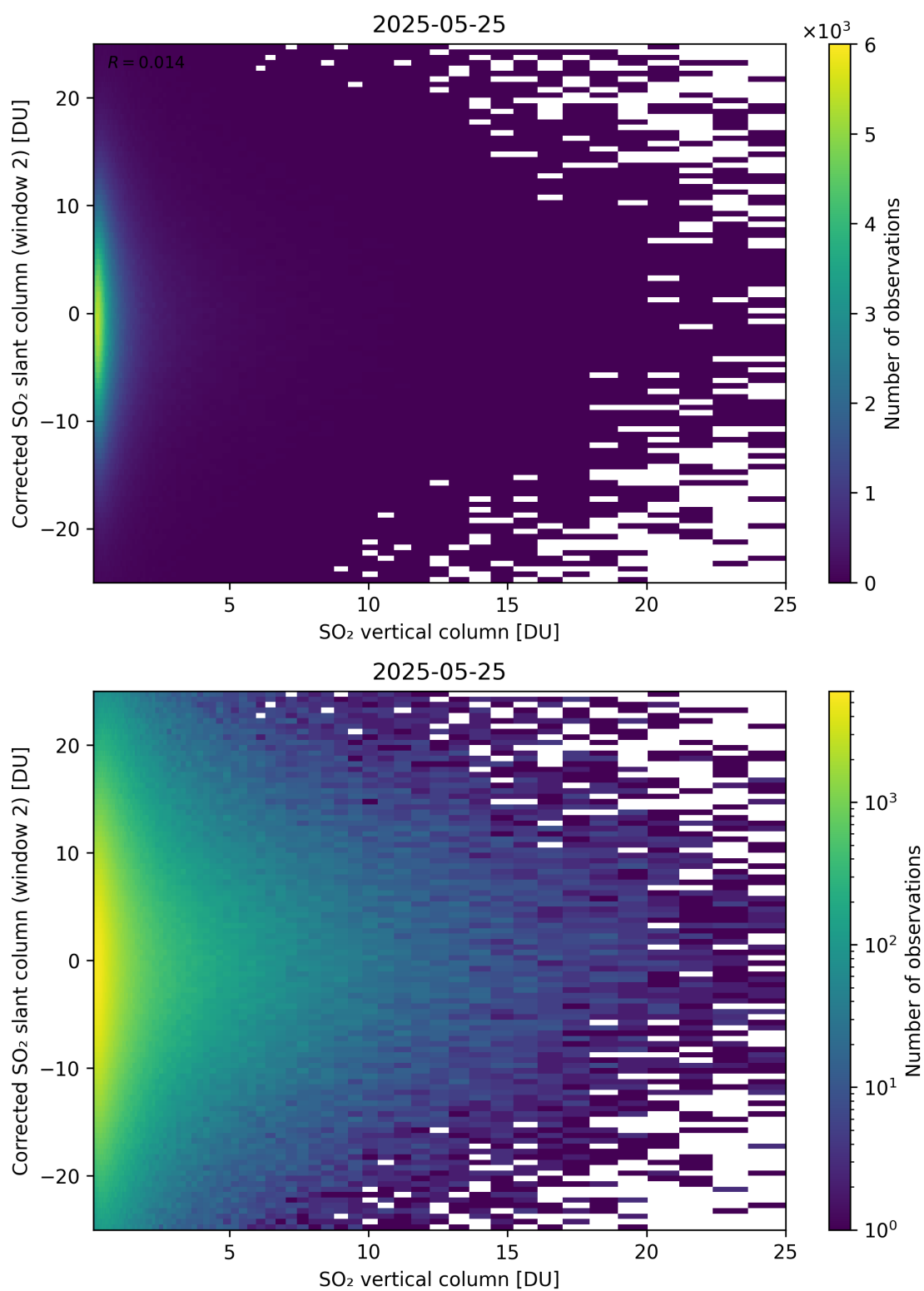
Figure 352: Scatter density plot of “SO 2 vertical column” against “Corrected SO 2 slant column (window 2)” for 2025-05-24 to 2025-05-26.
