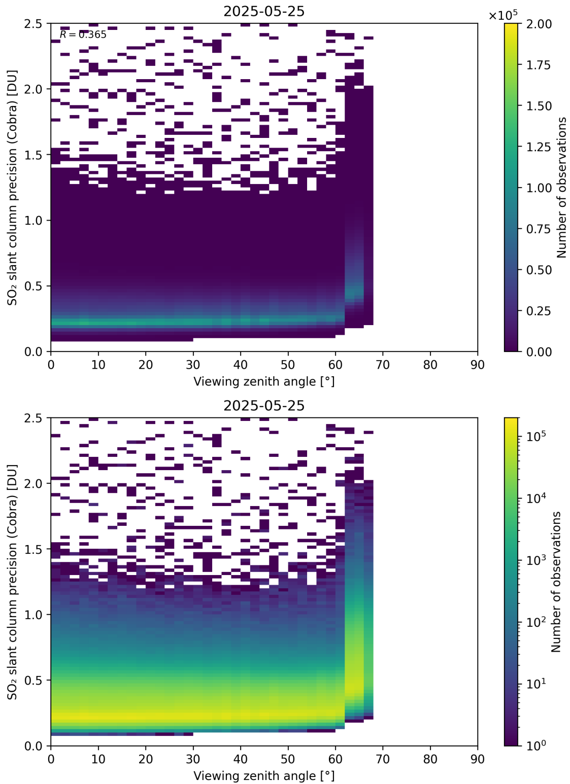
Figure 372: Scatter density plot of “Viewing zenith angle” against “SO 2 slant column precision (Cobra)” for 2025-05-24 to 2025-05-26.
