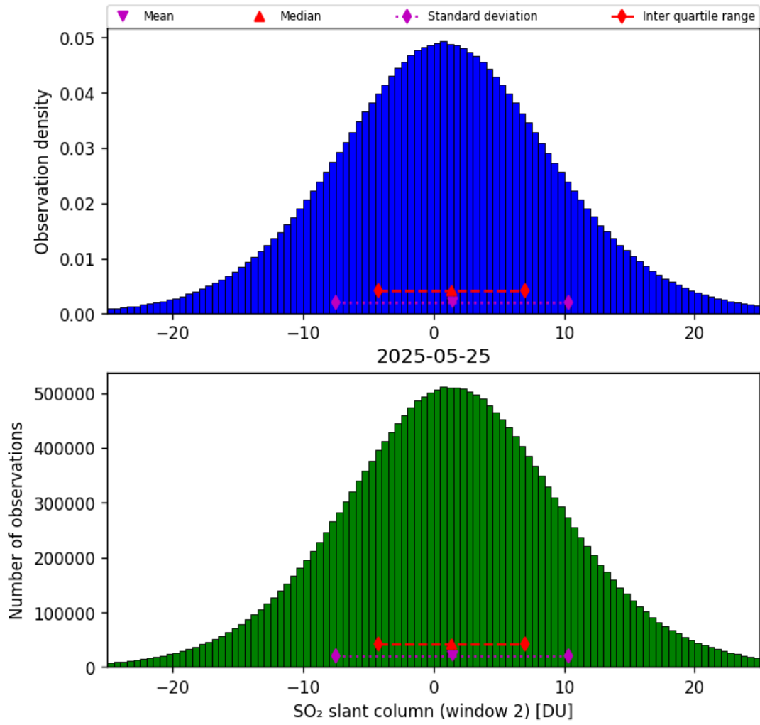
Figure 67: Histogram of “SO 2 slant column (window 2)” for 2025-05-24 to 2025-05-26
