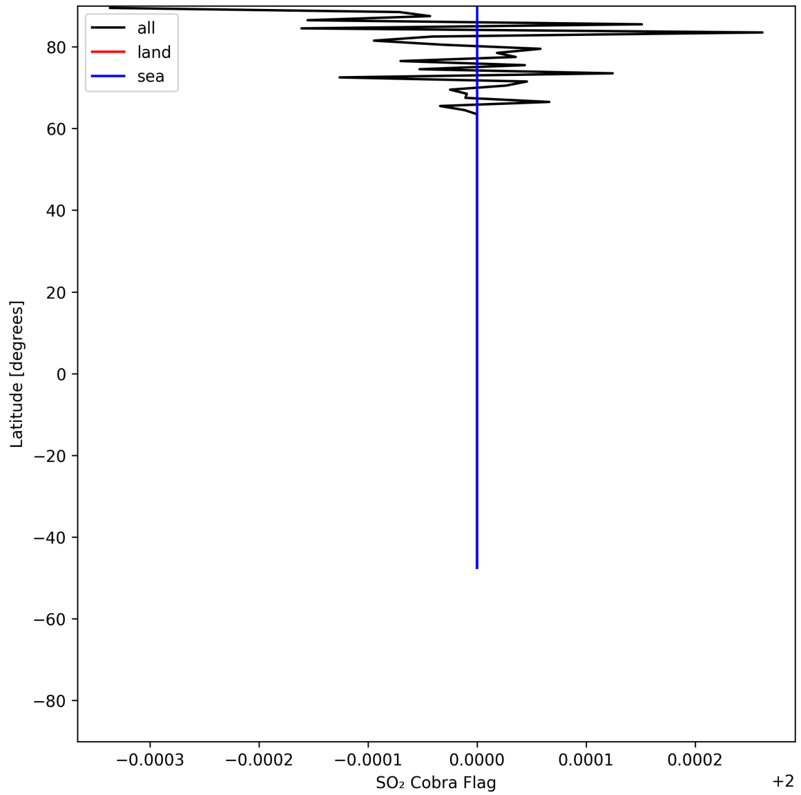
Figure 49: Zonal average of "SO 2 Cobra Flag" for 2025-05-24 to 2025-05-26.
