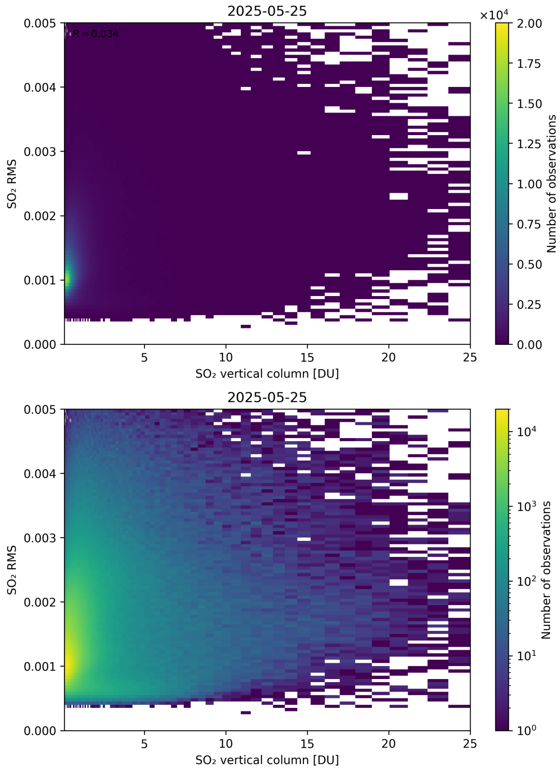
Figure 328: Scatter density plot of “SO 2 vertical column” against “SO 2 RMS” for 2025-05-24 to 2025-05-26.
