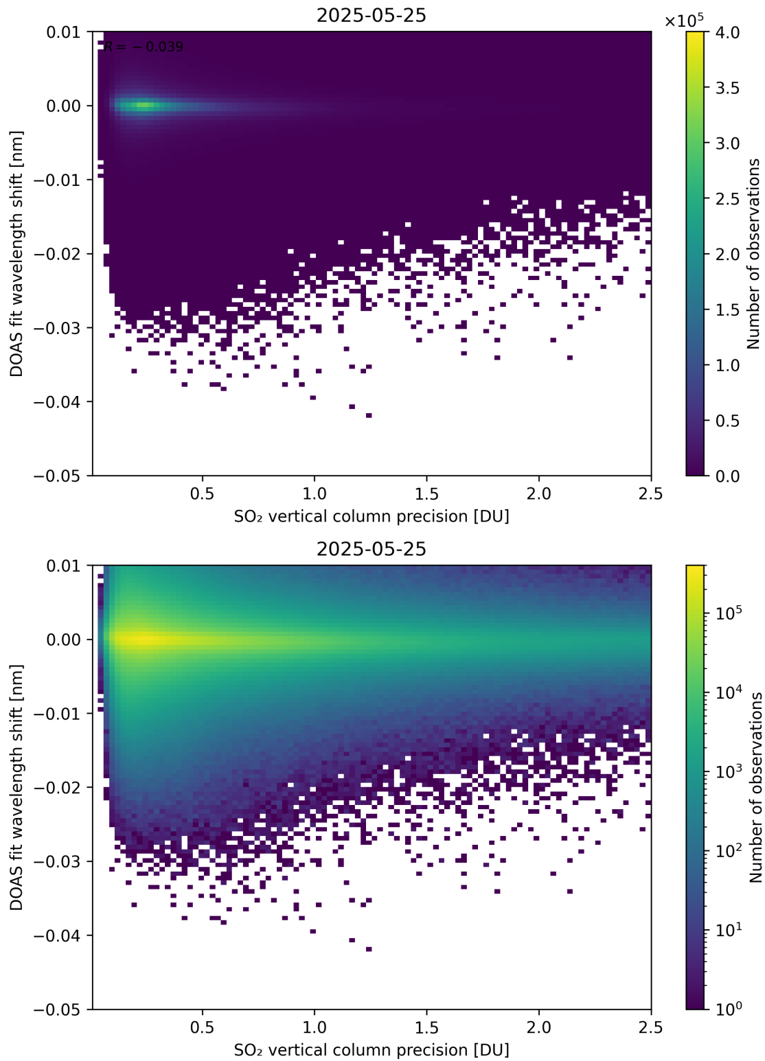
Figure 332: Scatter density plot of “SO 2 vertical column precision” against “DOAS fit wavelength shift” for 2025-05-24 to 2025-05-26.
