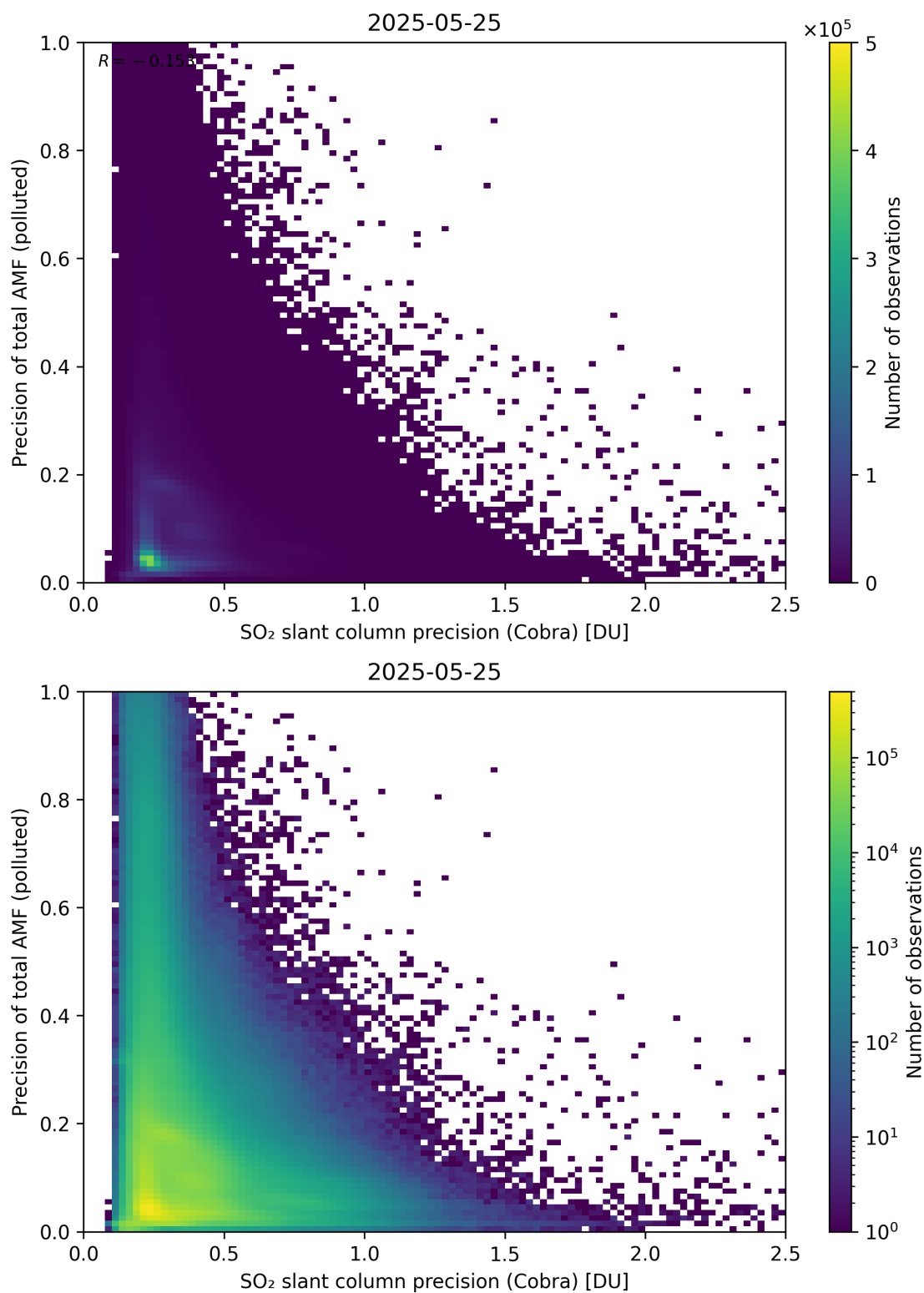
Figure 214: Scatter density plot of “SO 2 slant column precision (Cobra)” against “Precision of total AMF (polluted)” for 2025-05-24 to 2025-05-26.
