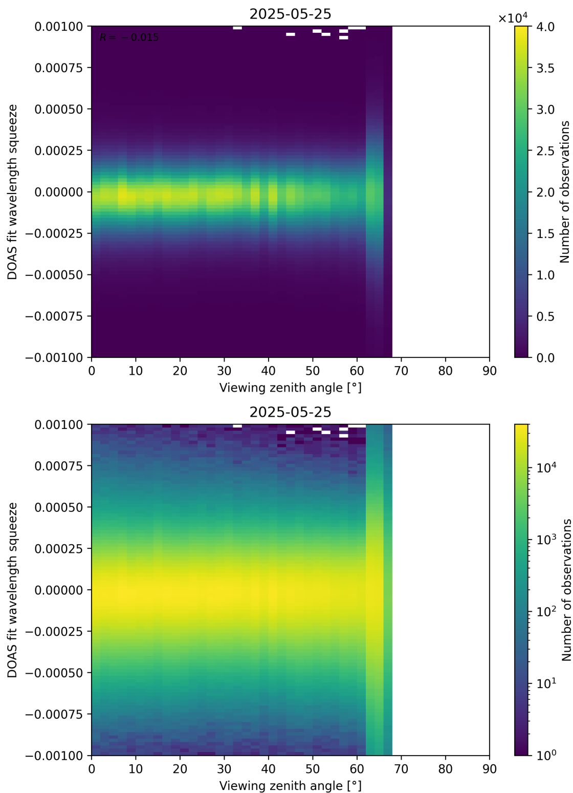
Figure 366: Scatter density plot of “Viewing zenith angle” against “DOAS fit wavelength squeeze” for 2025-05-24 to 2025-05-26.
