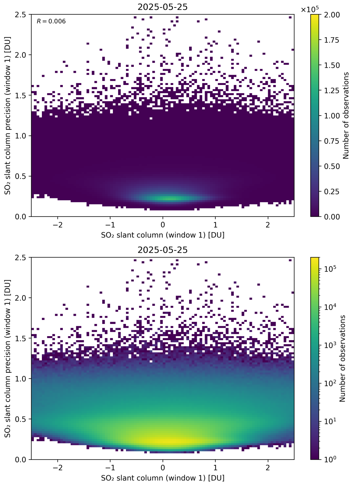
Figure 285: Scatter density plot of “SO 2 slant column (window 1)” against “SO 2 slant column precision (window 1)” for 2025-05-24 to 2025-05-26.
