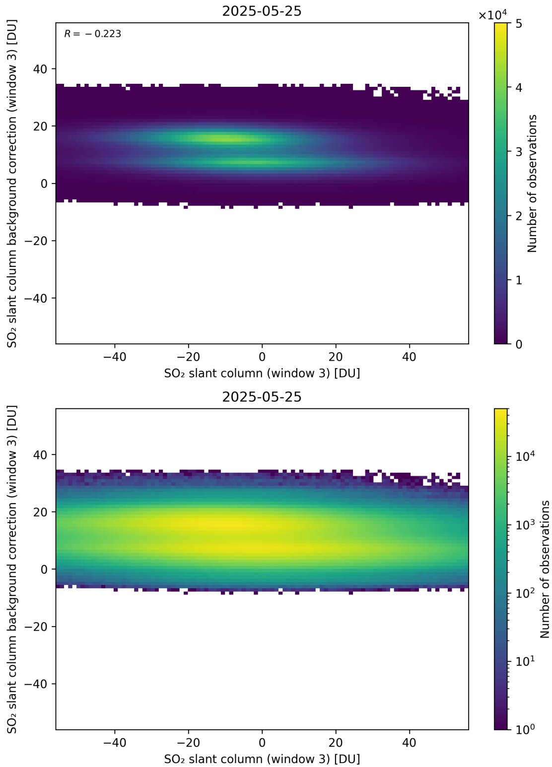
Figure 303: Scatter density plot of “SO 2 slant column (window 3)” against “SO 2 slant column background correction (window 3)” for 2025-05-24 to 2025-05-26.
