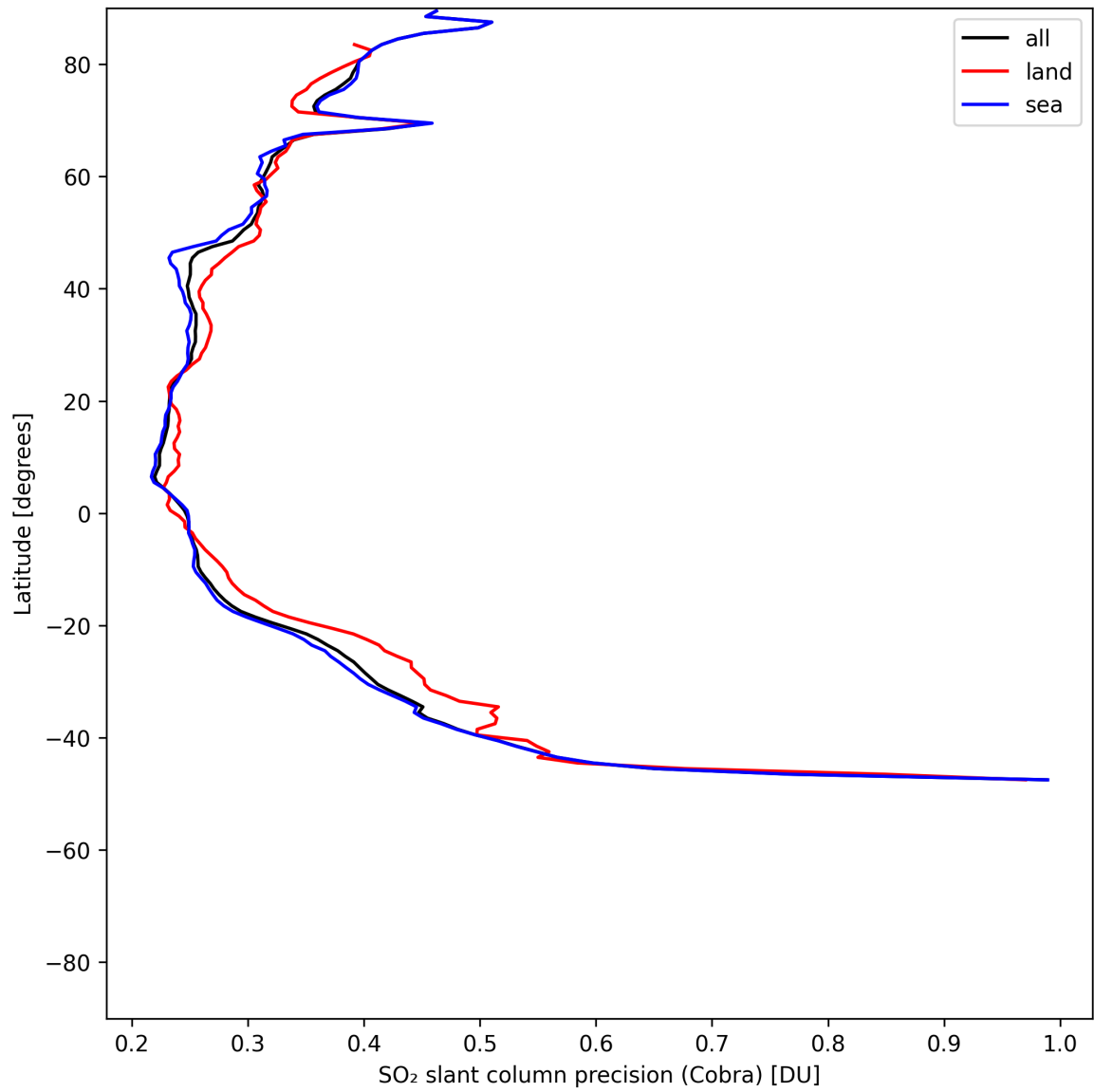
Figure 36: Zonal average of “SO 2 slant column precision (Cobra)” for 2025-05-24 to 2025-05-26.
