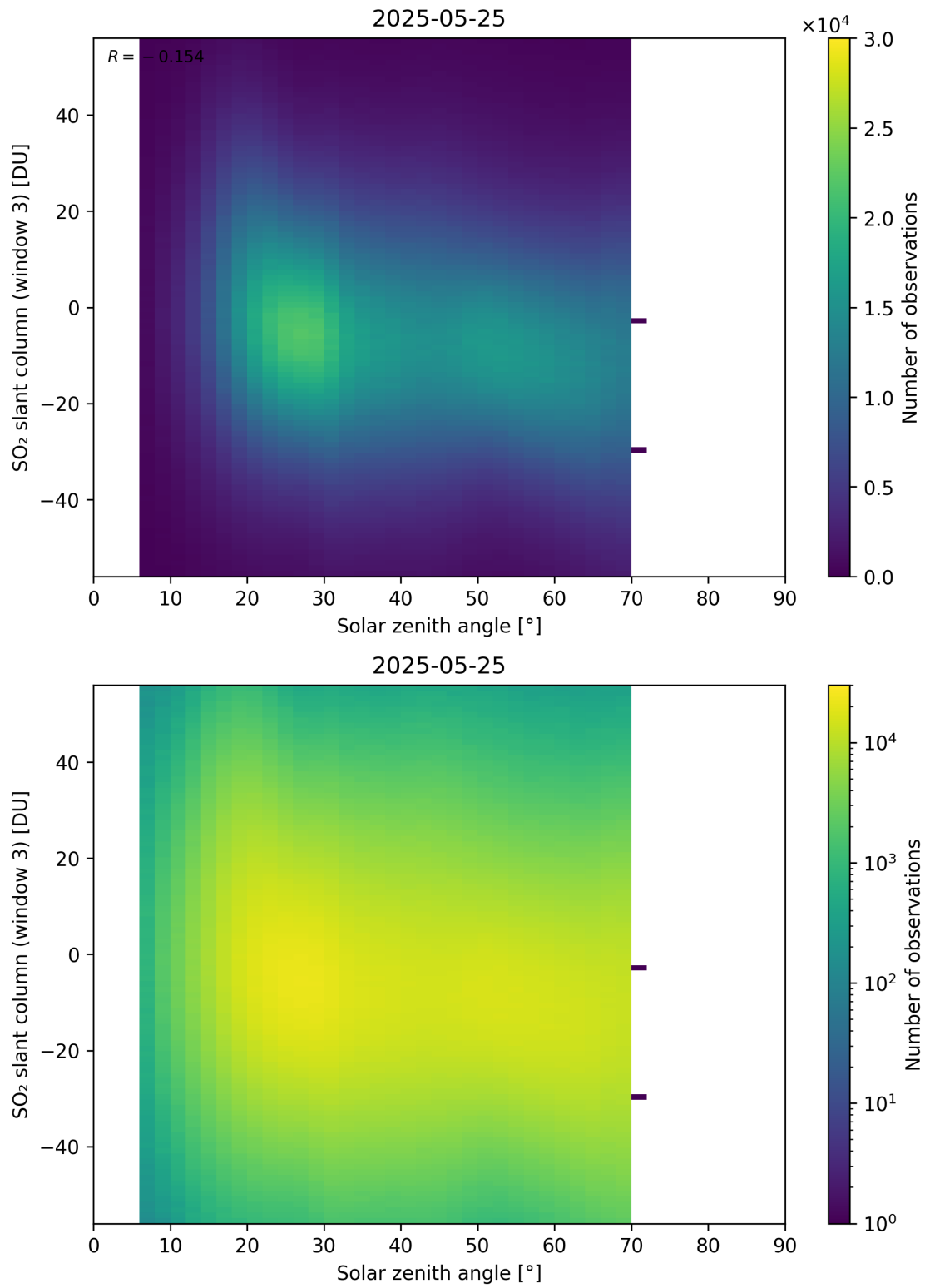
Figure 187: Scatter density plot of “Solar zenith angle” against “SO 2 slant column (window 3)” for 2025-05-24 to 2025-05-26.
