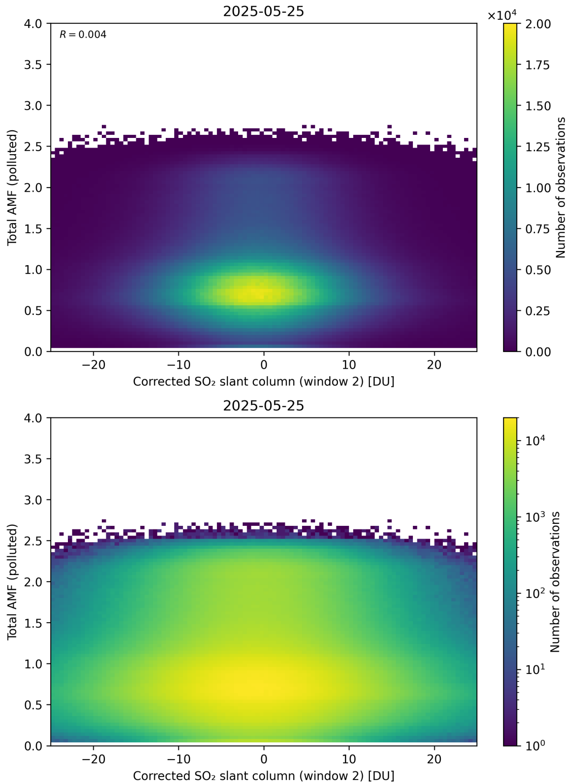
Figure 253: Scatter density plot of “Corrected SO 2 slant column (window 2)” against “Total AMF (polluted)” for 2025-05-24 to 2025-05-26.
