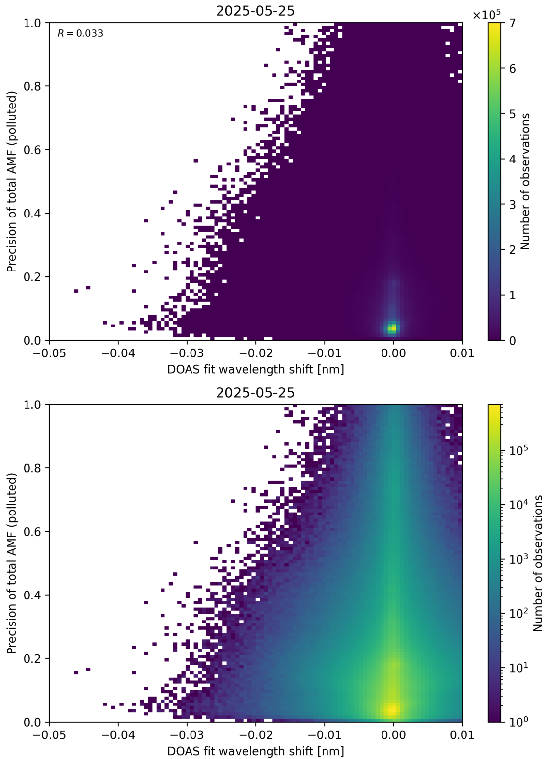
Figure 142: Scatter density plot of “DOAS fit wavelength shift” against “Precision of total AMF (polluted)” for 2025-05-24 to 2025-05-26.
