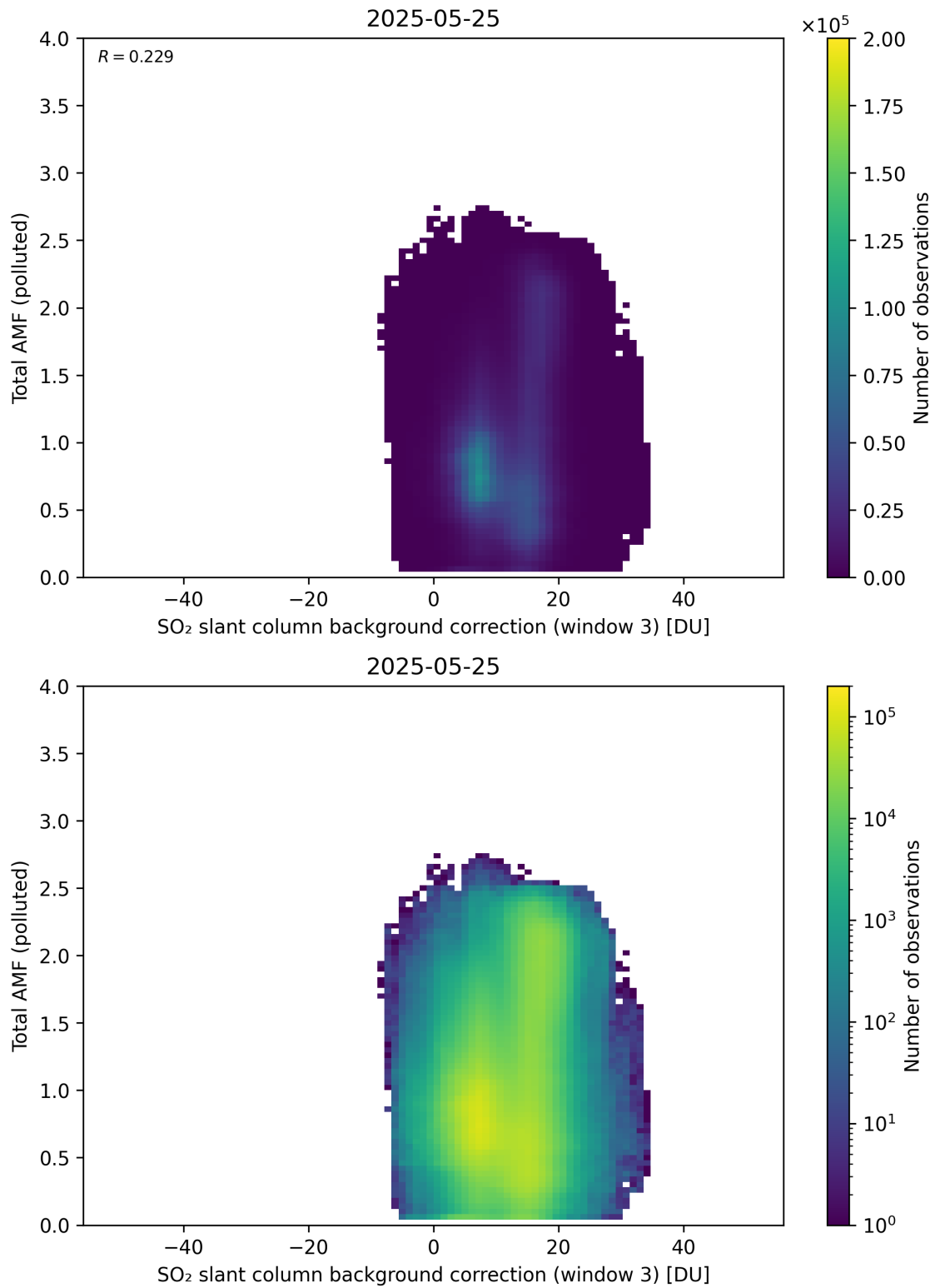
Figure 136: Scatter density plot of “SO 2 slant column background correction (window 3)” against “Total AMF (polluted)” for 2025-05-24 to 2025-05-26.
