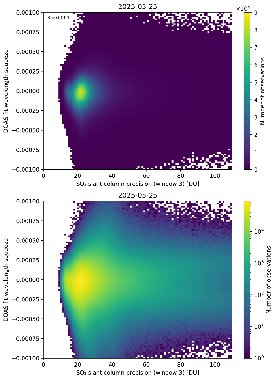
Figure 309: Scatter density plot of “SO 2 slant column precision (window 3)” against “DOAS fit wavelength squeeze” for 2025-05-24 to 2025-05-26.
