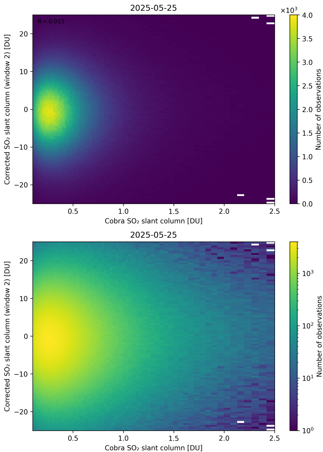
Figure 217: Scatter density plot of “Cobra SO 2 slant column” against “Corrected SO 2 slant column (window 2)” for 2025-05-24 to 2025-05-26.
