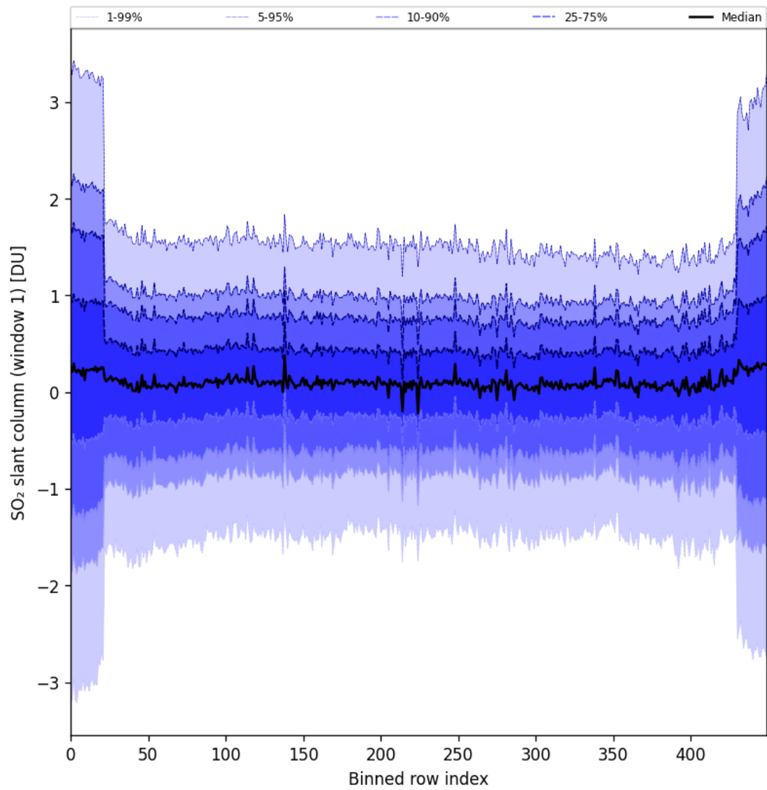
Figure 89: Along track statistics of “SO 2 slant column (window 1)” for 2025-05-24 to 2025-05-26
