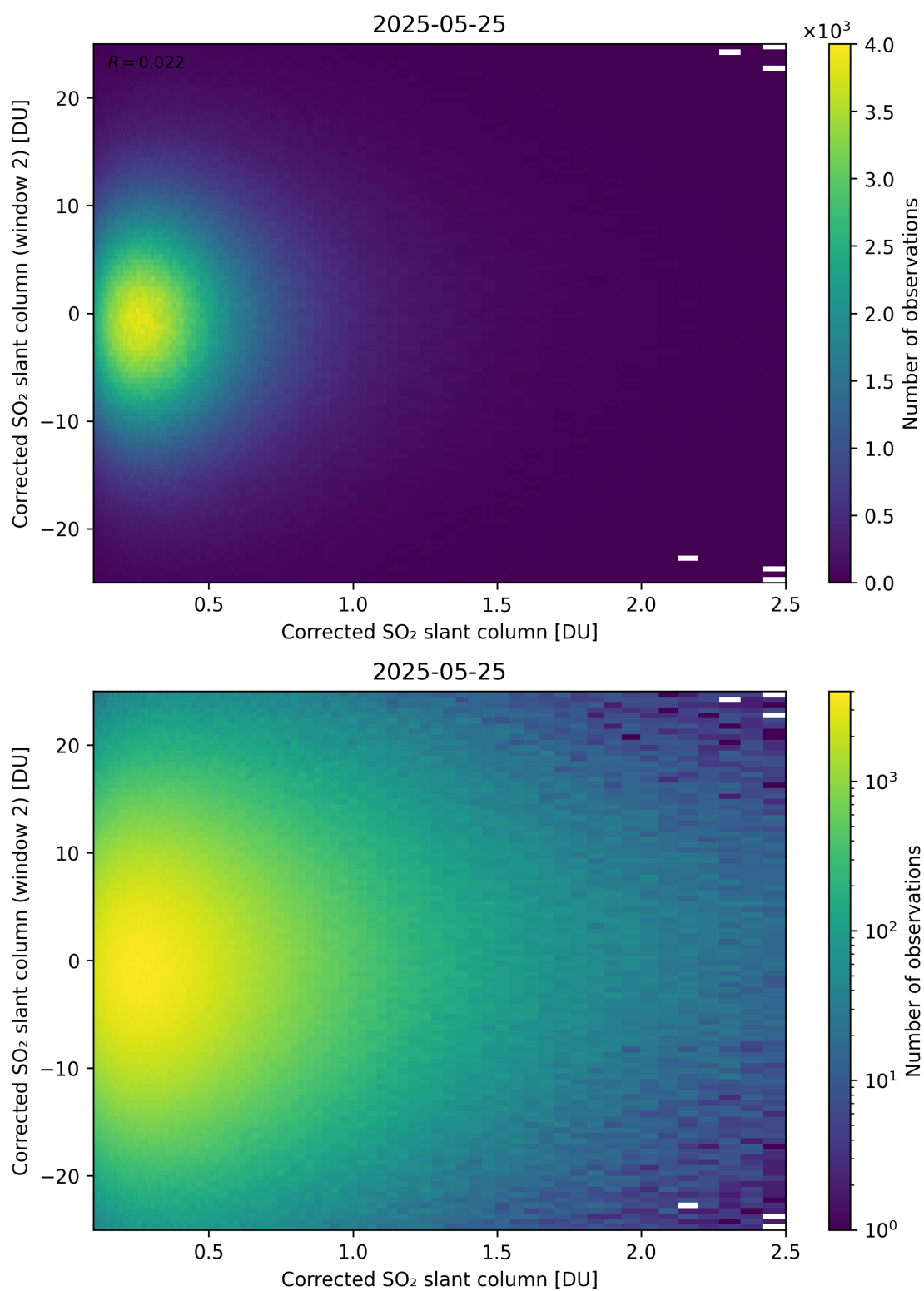
Figure 235: Scatter density plot of “Corrected SO 2 slant column” against “Corrected SO 2 slant column (window 2)” for 2025-05-24 to 2025-05-26.
