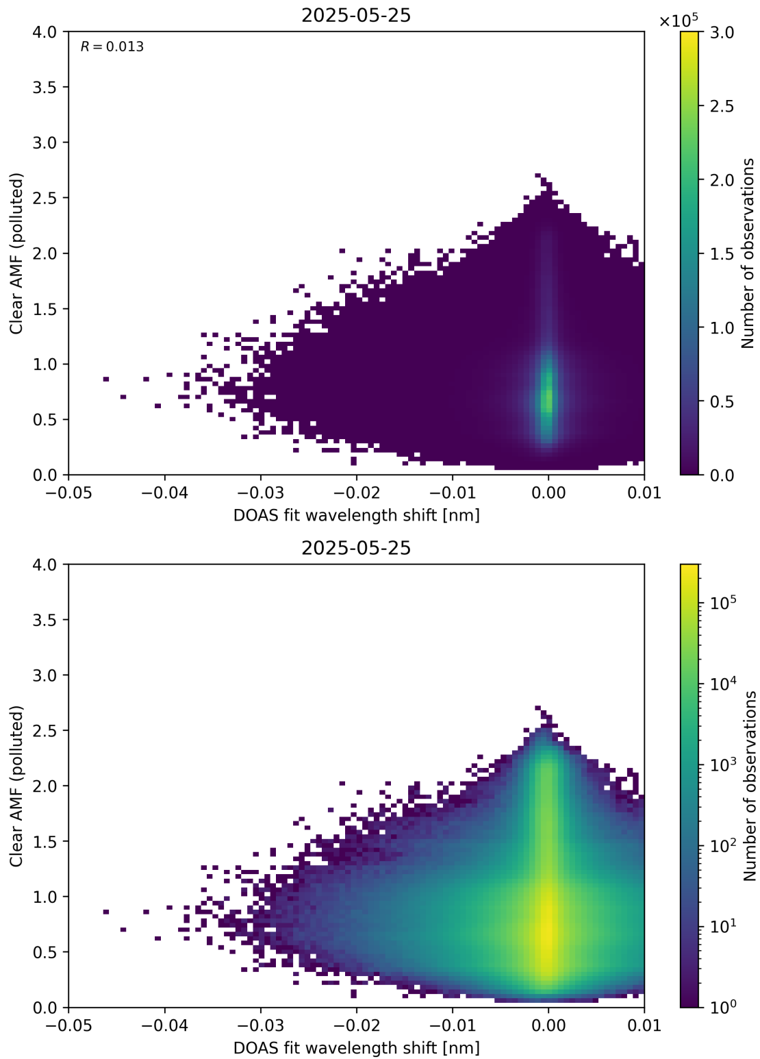
Figure 140: Scatter density plot of “DOAS fit wavelength shift” against “Clear AMF (polluted)” for 2025-05-24 to 2025-05-26.
