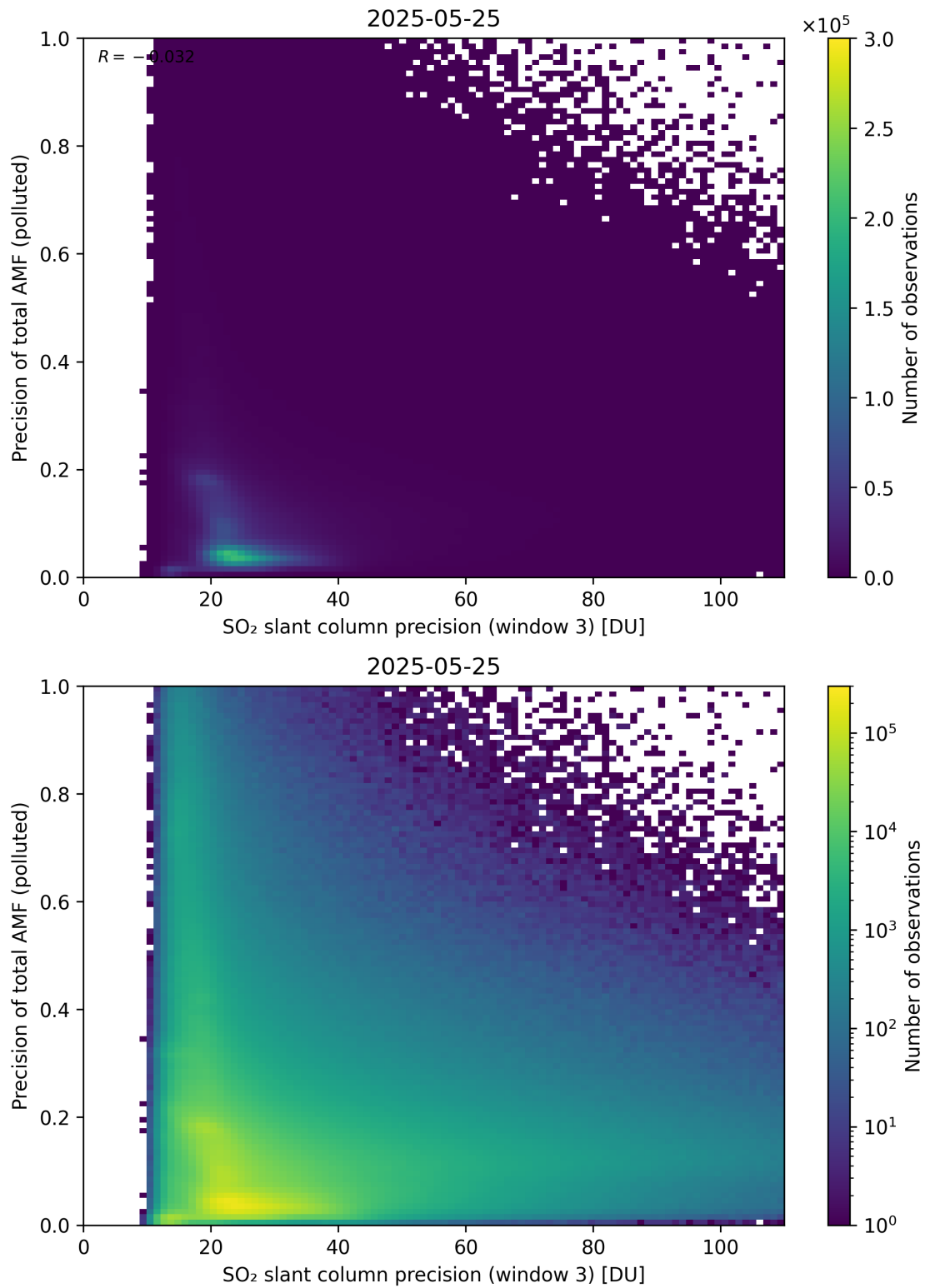
Figure 314: Scatter density plot of “SO 2 slant column precision (window 3)” against “Precision of total AMF (polluted)” for 2025-05-24 to 2025-05-26.
