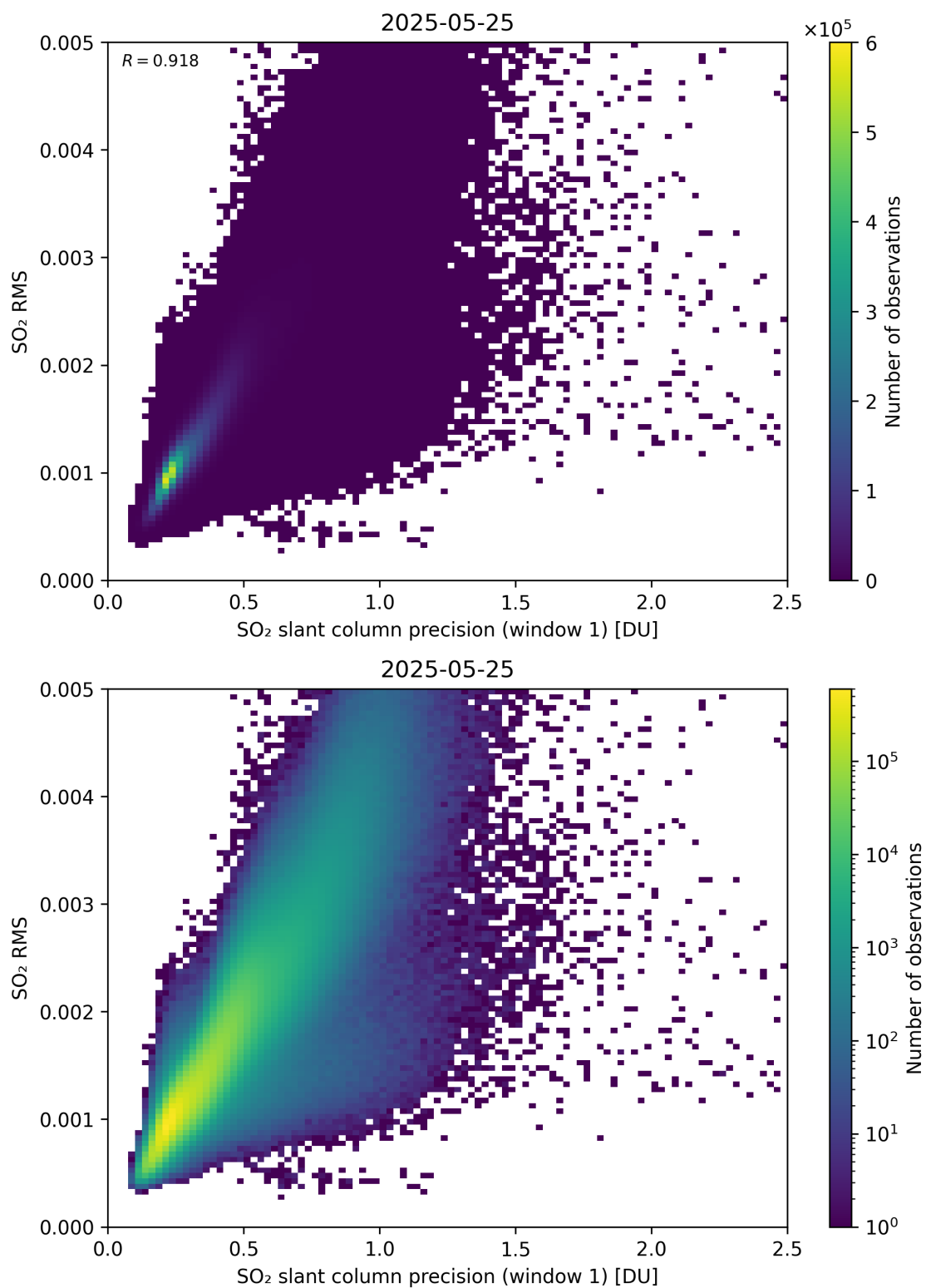
Figure 273: Scatter density plot of “SO 2 slant column precision (window 1)” against “SO 2 RMS” for 2025-05-24 to 2025-05-26.
