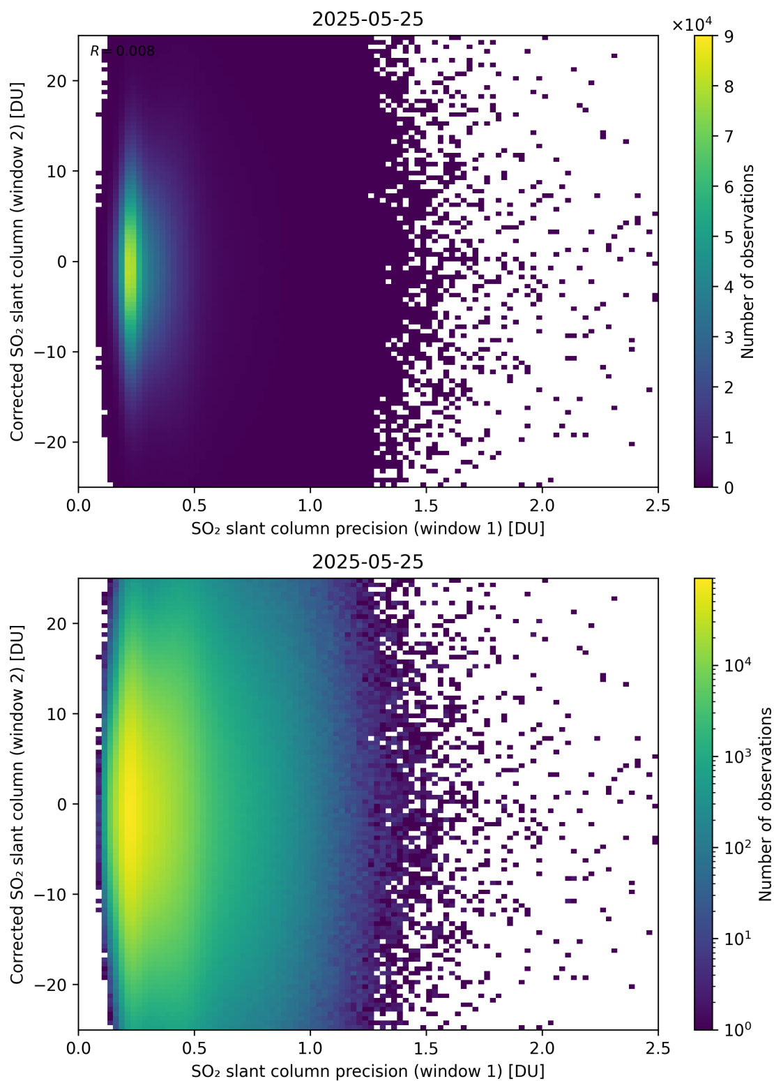
Figure 275: Scatter density plot of “SO 2 slant column precision (window 1)” against “Corrected SO 2 slant column (window 2)” for 2025-05-24 to 2025-05-26.
