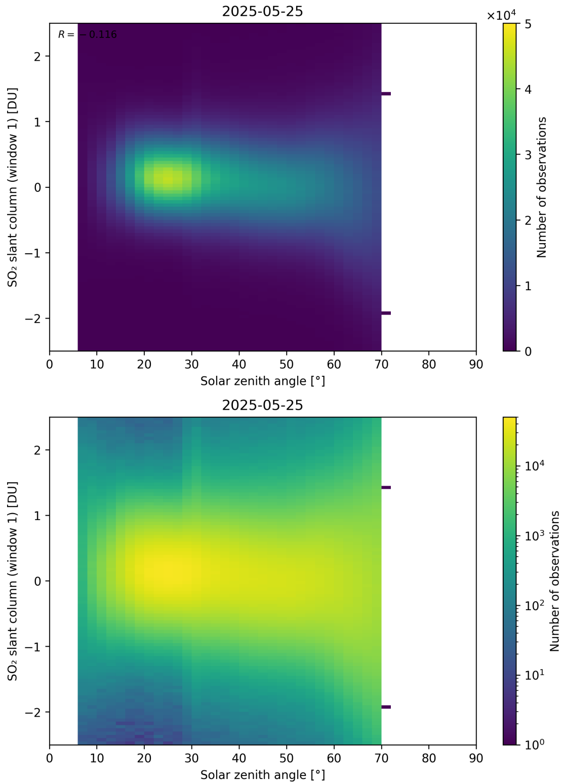
Figure 184: Scatter density plot of “Solar zenith angle” against “SO 2 slant column (window 1)” for 2025-05-24 to 2025-05-26.
