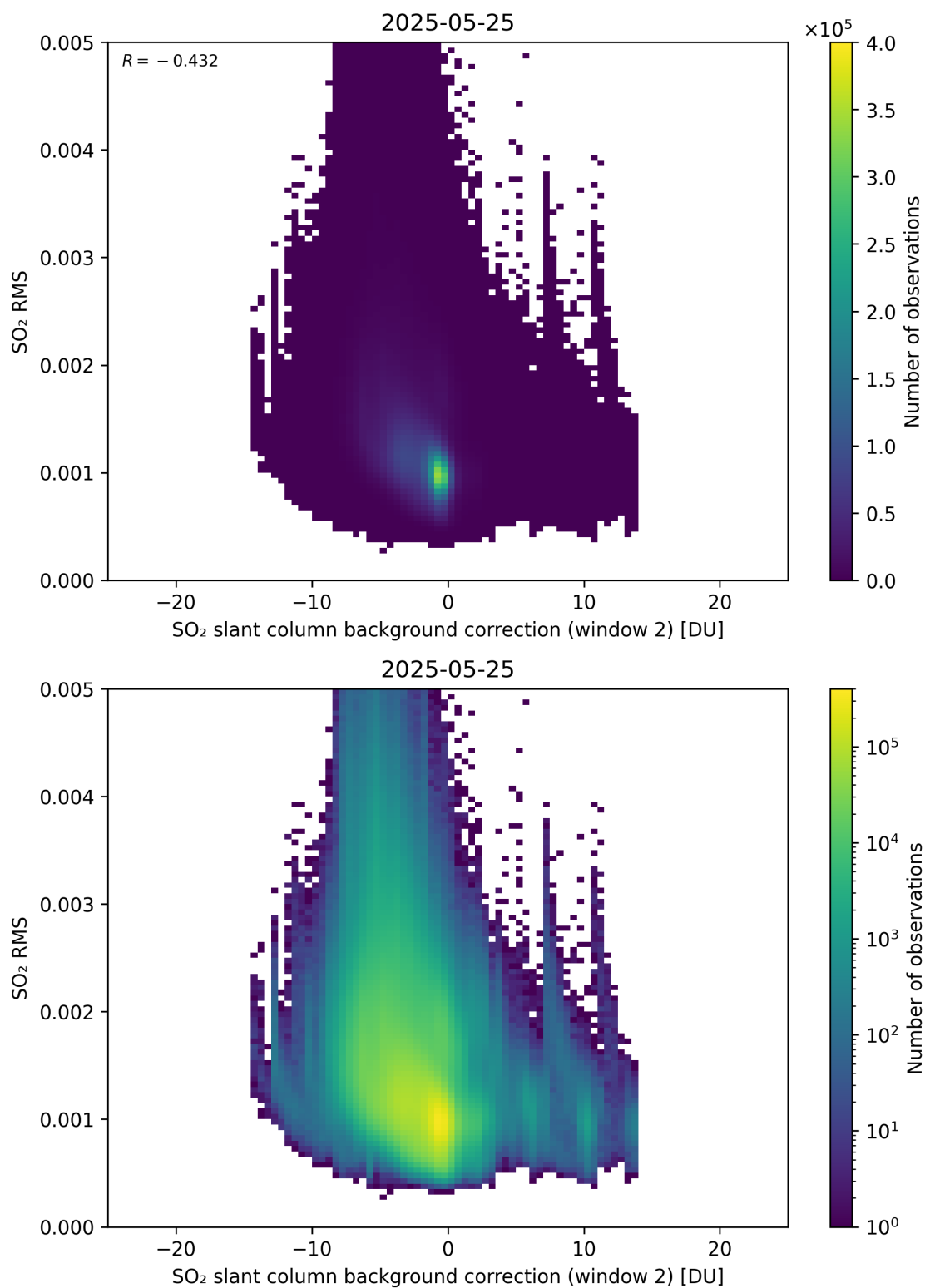
Figure 125: Scatter density plot of “SO 2 slant column background correction (window 2)” against “SO 2 RMS” for 2025-05-24 to 2025-05-26.
