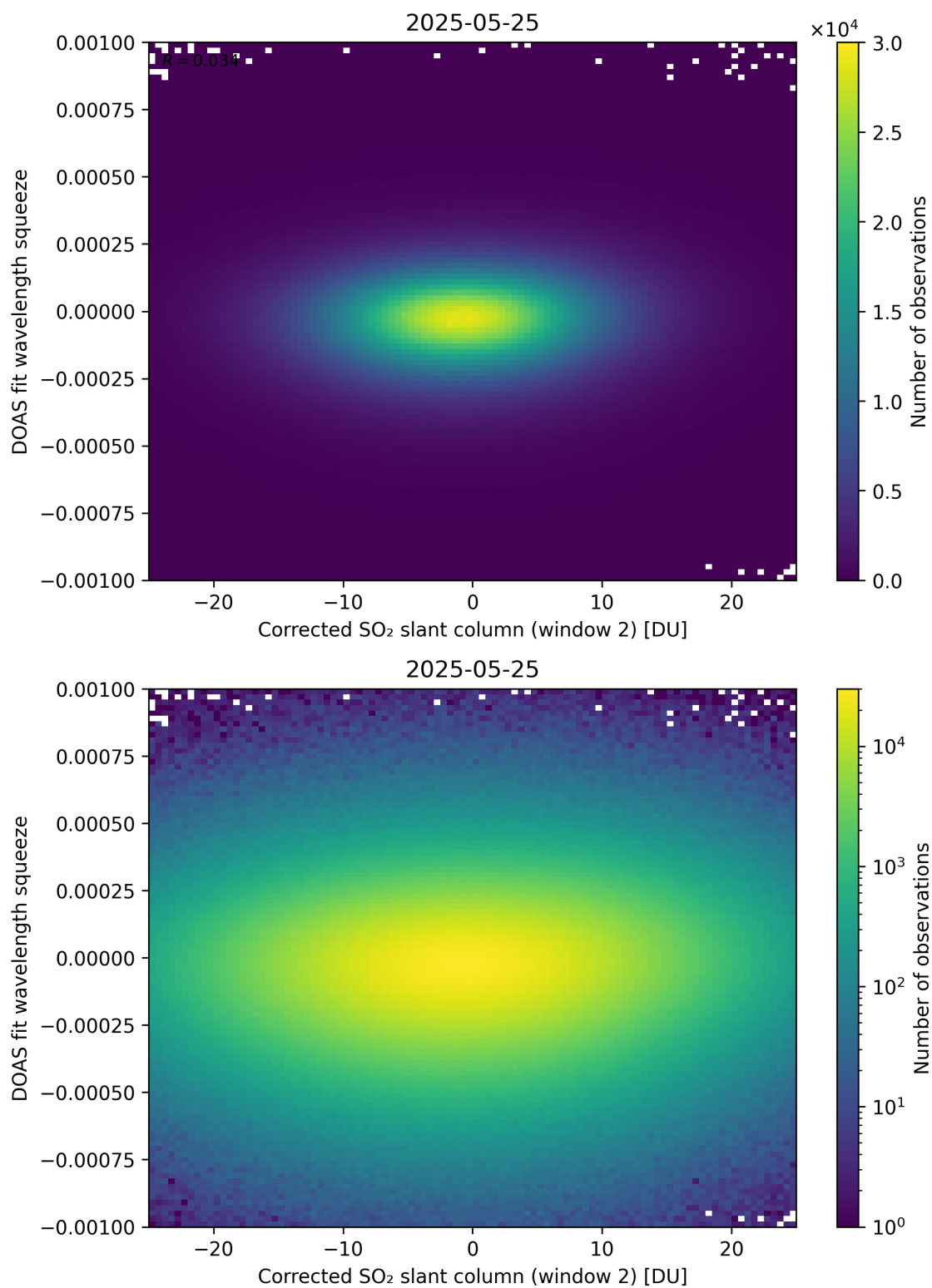
Figure 247: Scatter density plot of “Corrected SO 2 slant column (window 2)” against “DOAS fit wavelength squeeze” for 2025-05-24 to 2025-05-26.
