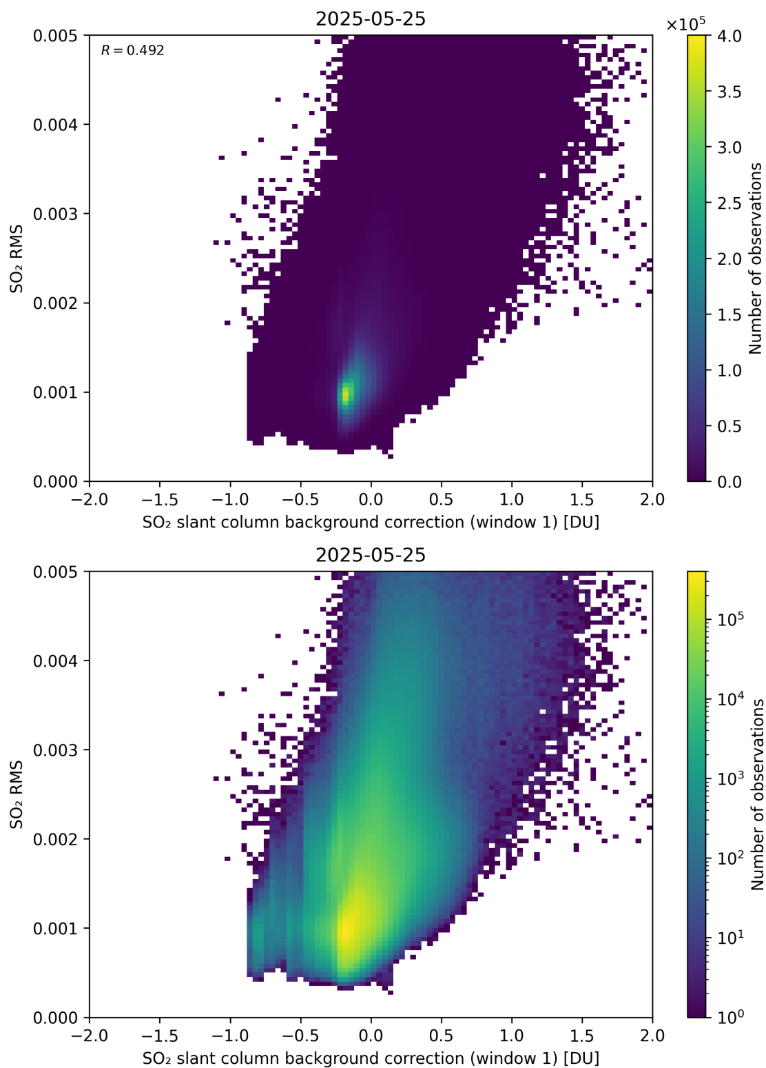
Figure 113: Scatter density plot of “SO 2 slant column background correction (window 1)” against “SO 2 RMS” for 2025-05-24 to 2025-05-26.
