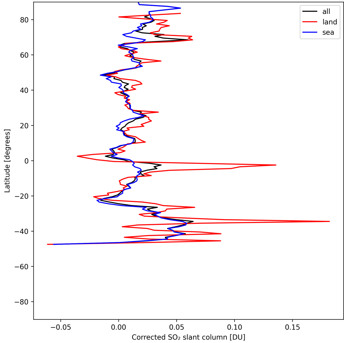
Figure 34: Zonal average of "Corrected SO 2 slant column" for 2025-05-24 to 2025-05-26.
