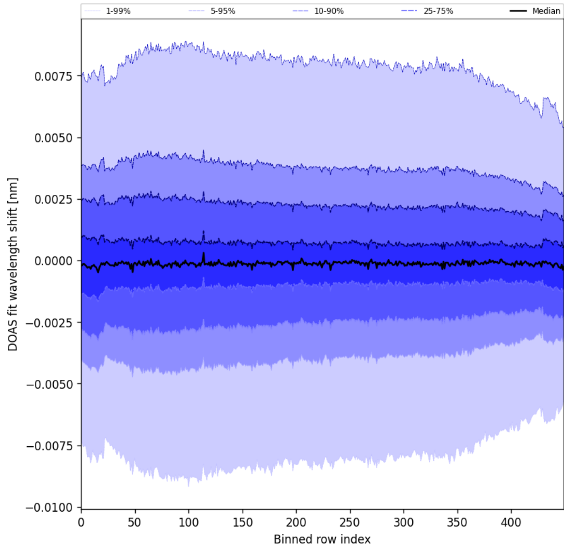
Figure 102: Along track statistics of “DOAS fit wavelength shift” for 2025-05-24 to 2025-05-26
