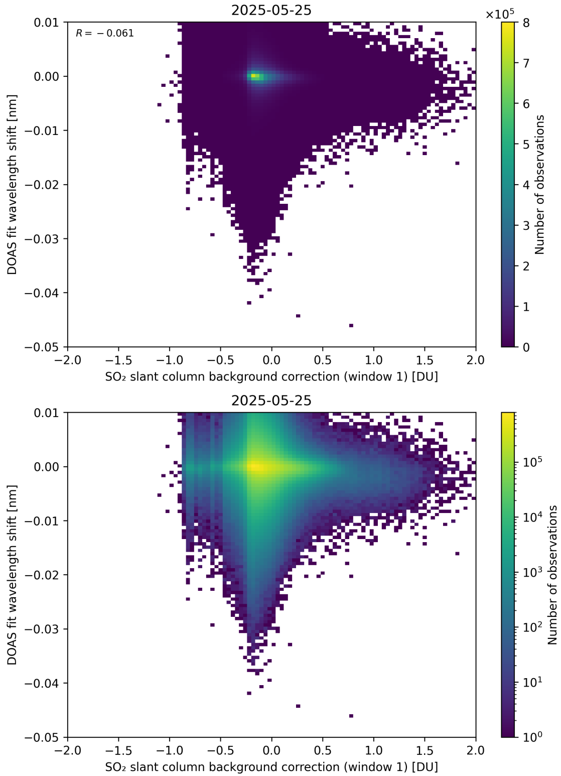
Figure 111: Scatter density plot of “SO 2 slant column background correction (window 1)” against “DOAS fit wavelength shift” for 2025-05-24 to 2025-05-26.
