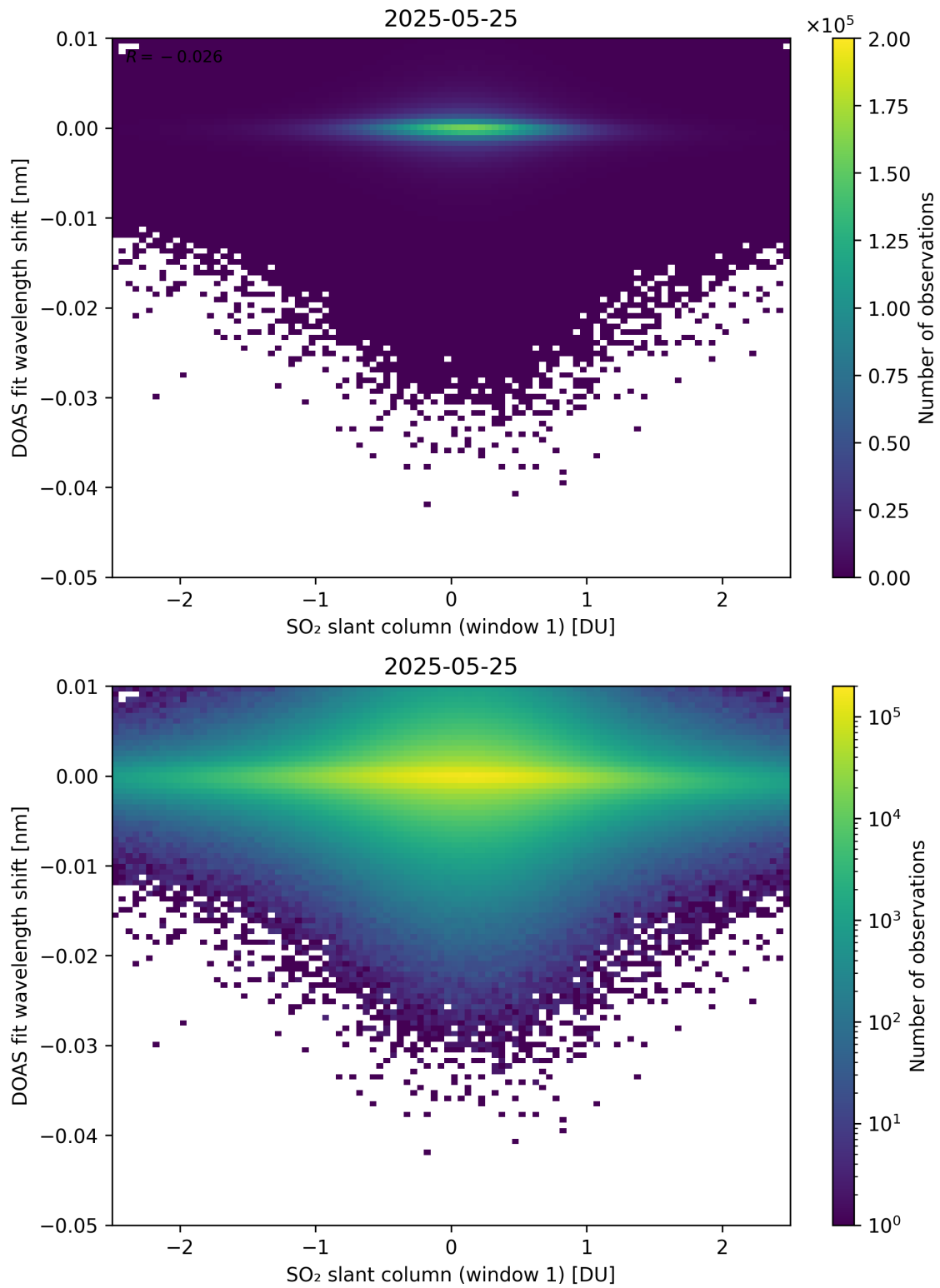
Figure 265: Scatter density plot of “SO 2 slant column (window 1)” against “DOAS fit wavelength shift” for 2025-05-24 to 2025-05-26.
