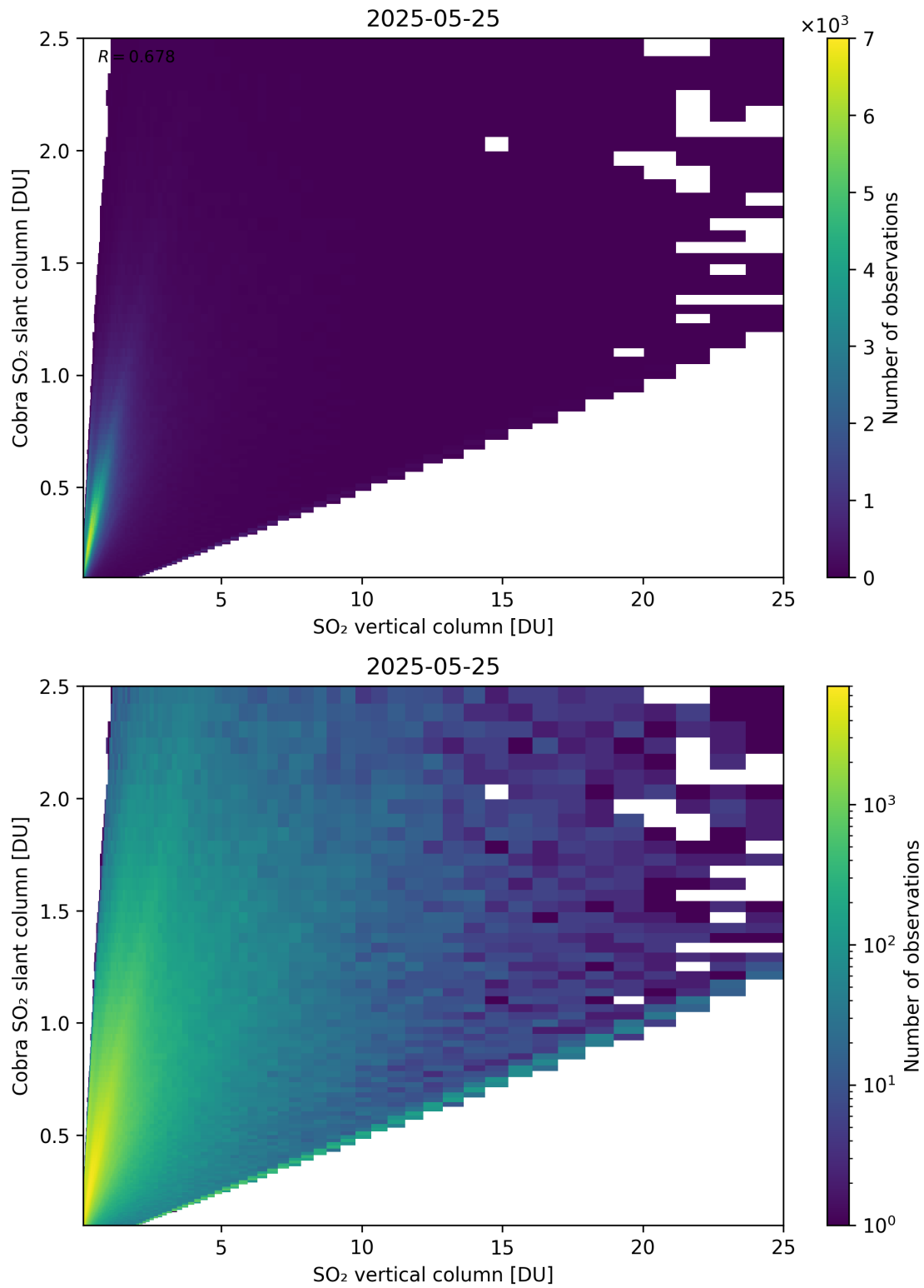
Figure 349: Scatter density plot of “SO 2 vertical column” against “Cobra SO 2 slant column” for 2025-05-24 to 2025-05-26.
