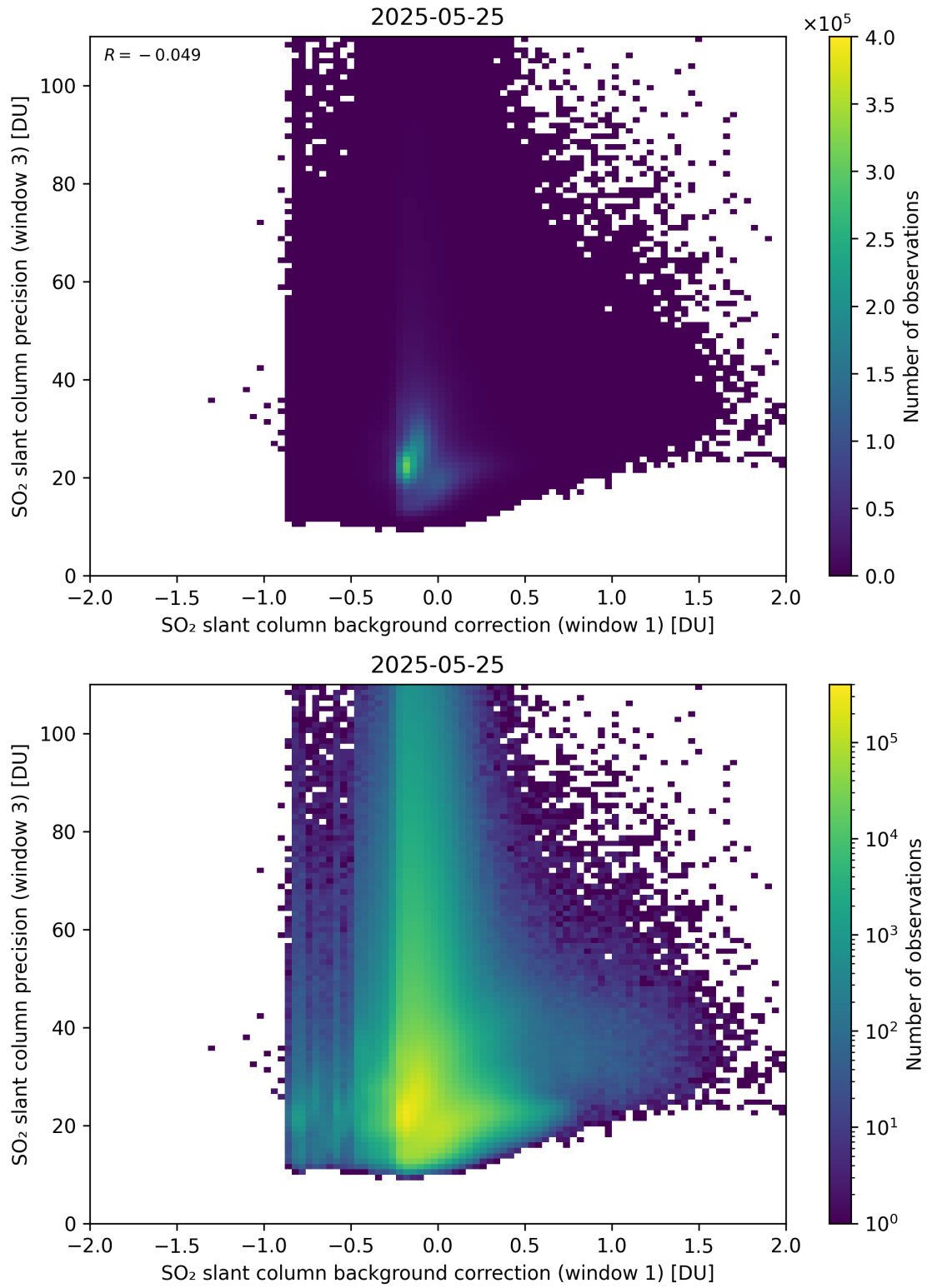
Figure 119: Scatter density plot of “SO 2 slant column background correction (window 1)” against “SO 2 slant column precision (window 3)” for 2025-05-24 to 2025-05-26.
