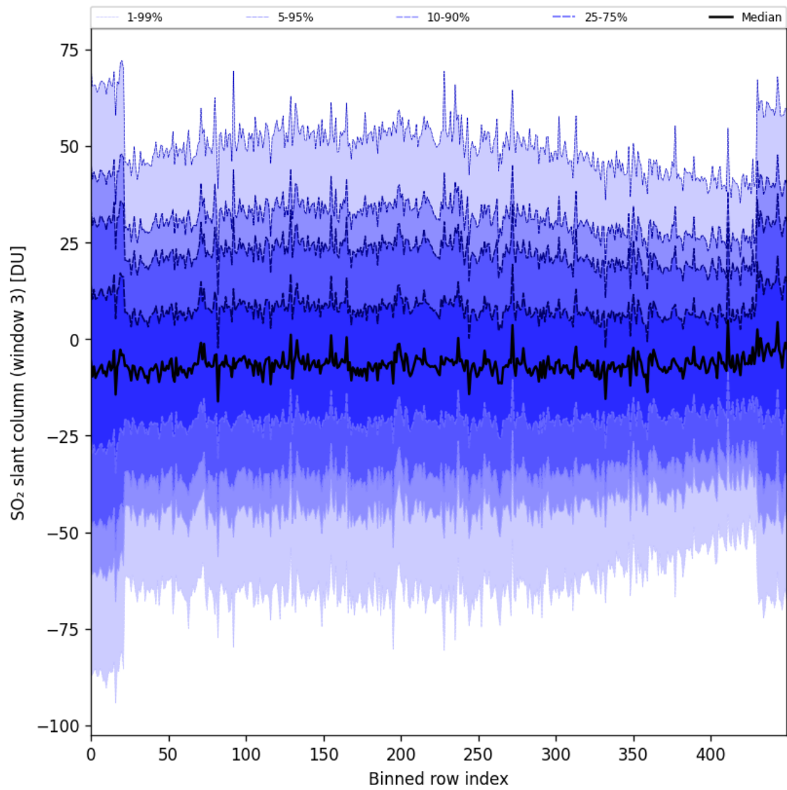
Figure 97: Along track statistics of “SO 2 slant column (window 3)” for 2025-05-24 to 2025-05-26
