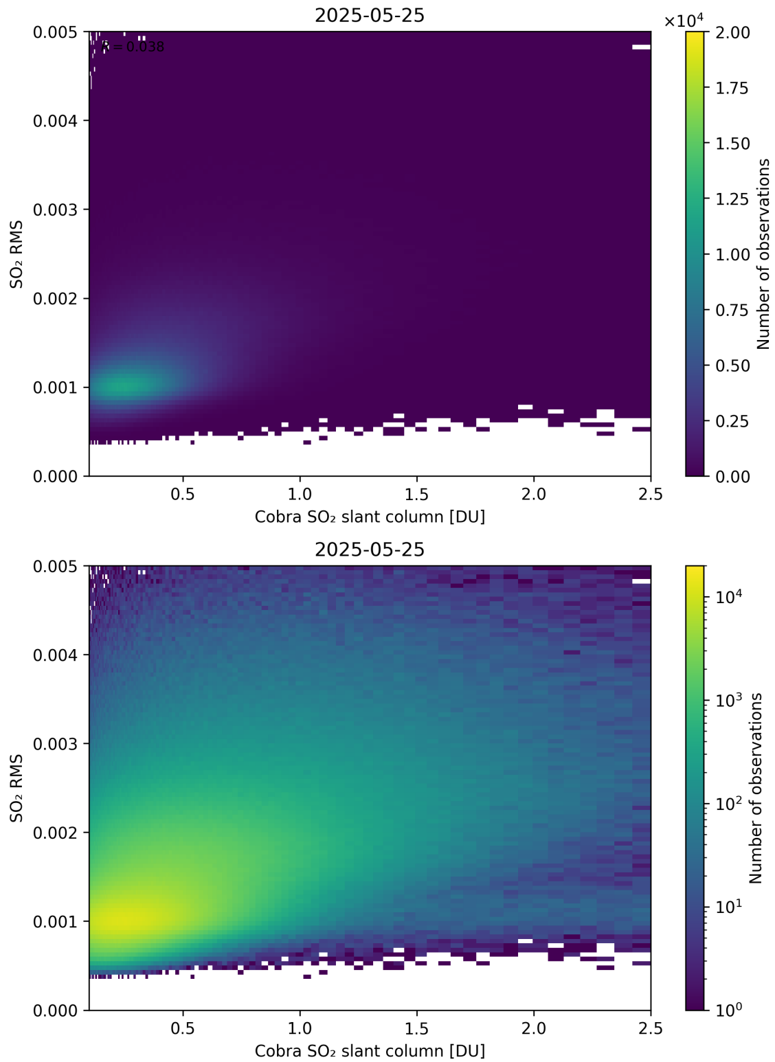
Figure 198: Scatter density plot of “Cobra SO 2 slant column” against “SO 2 RMS” for 2025-05-24 to 2025-05-26.
