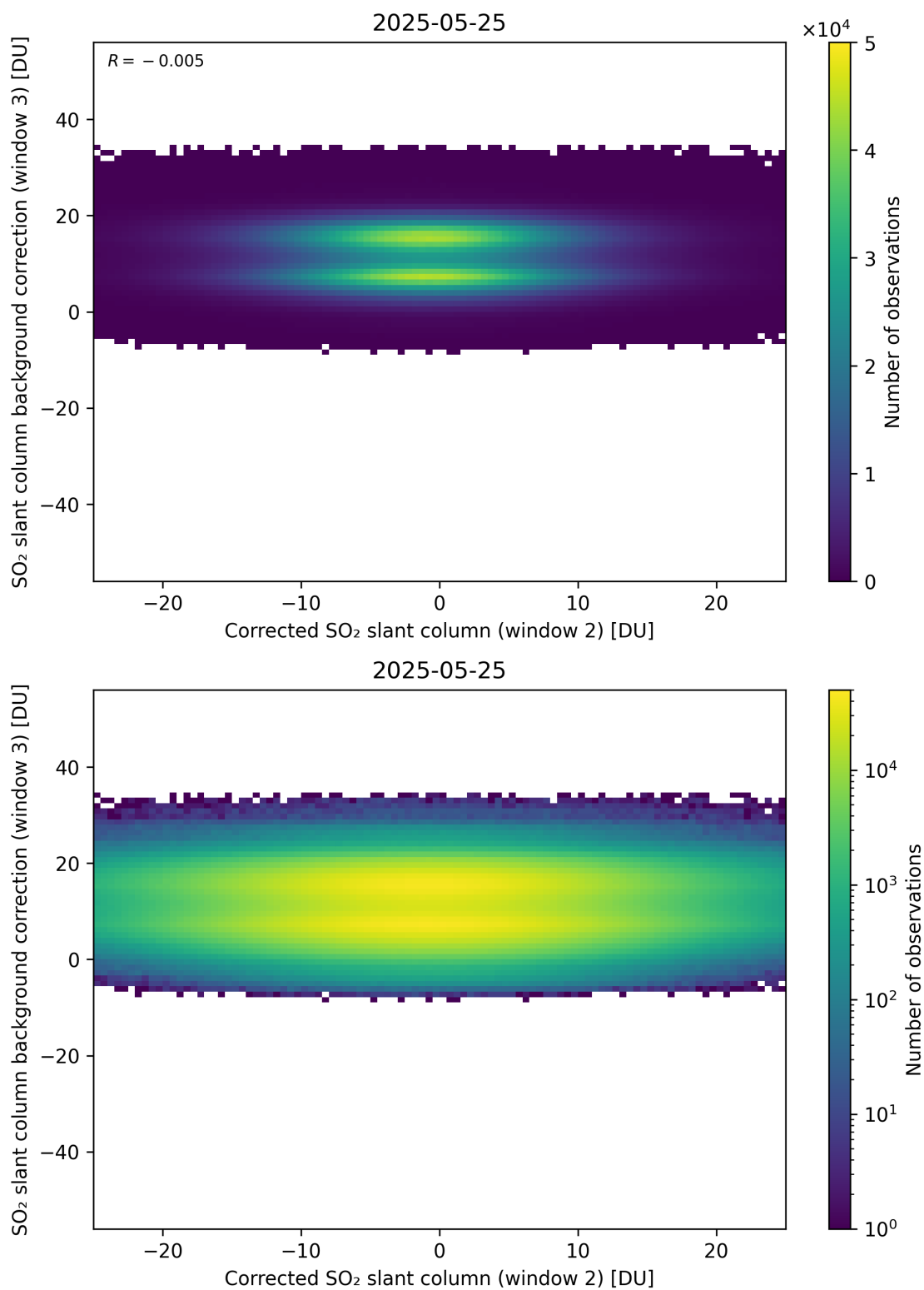
Figure 245: Scatter density plot of “Corrected SO 2 slant column (window 2)” against “SO 2 slant column background correction (window 3)” for 2025-05-24 to 2025-05-26.
