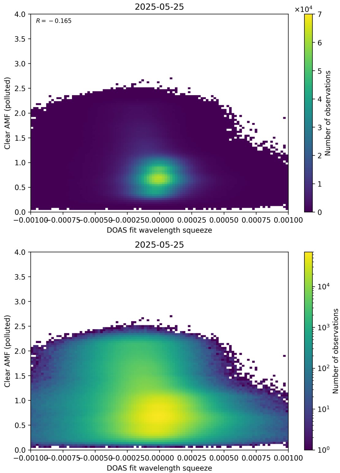
Figure 144: Scatter density plot of “DOAS fit wavelength squeeze” against “Clear AMF (polluted)” for 2025-05-24 to 2025-05-26.
