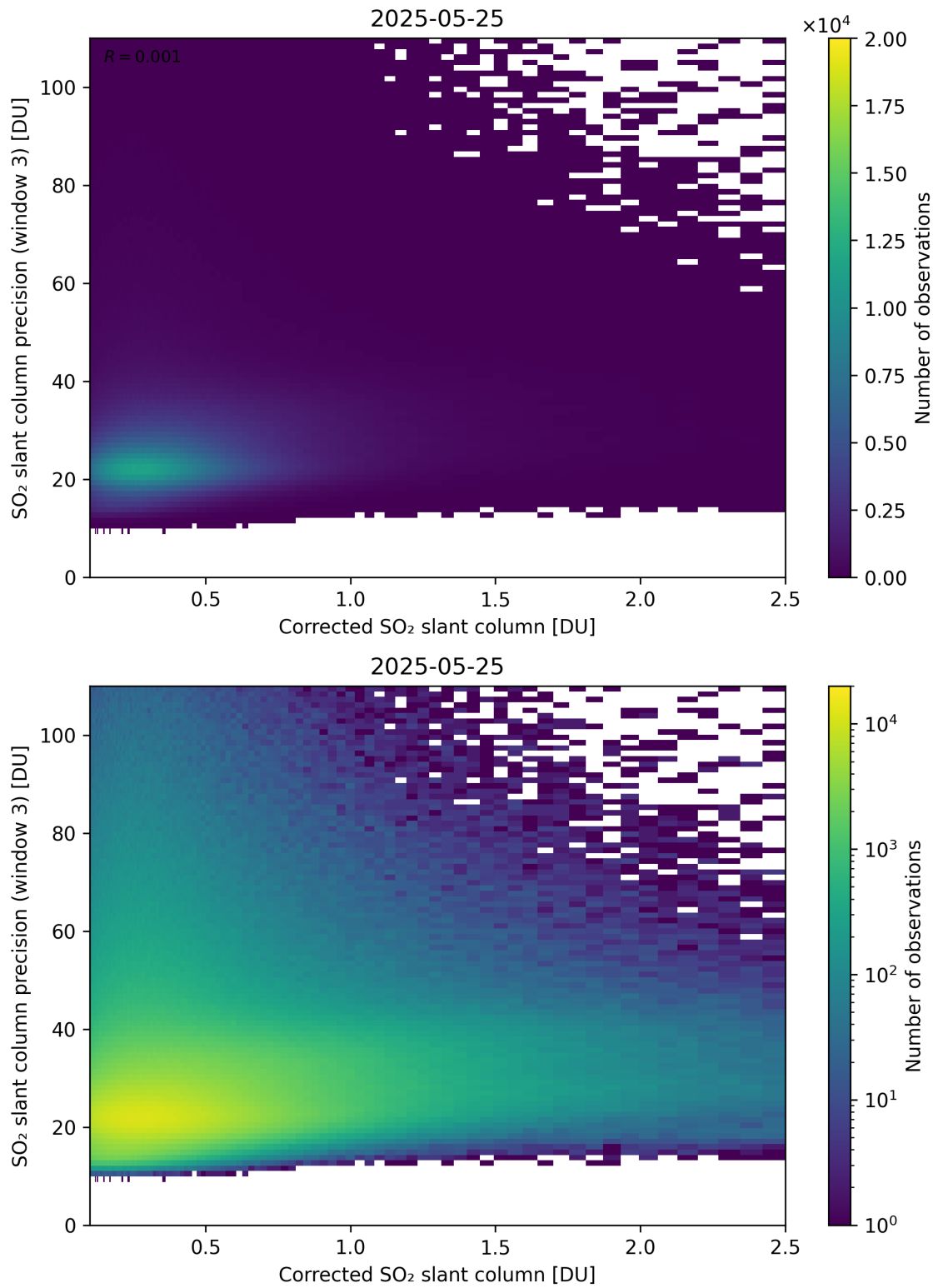
Figure 241: Scatter density plot of “Corrected SO 2 slant column” against “SO 2 slant column precision (window 3)” for 2025-05-24 to 2025-05-26.
