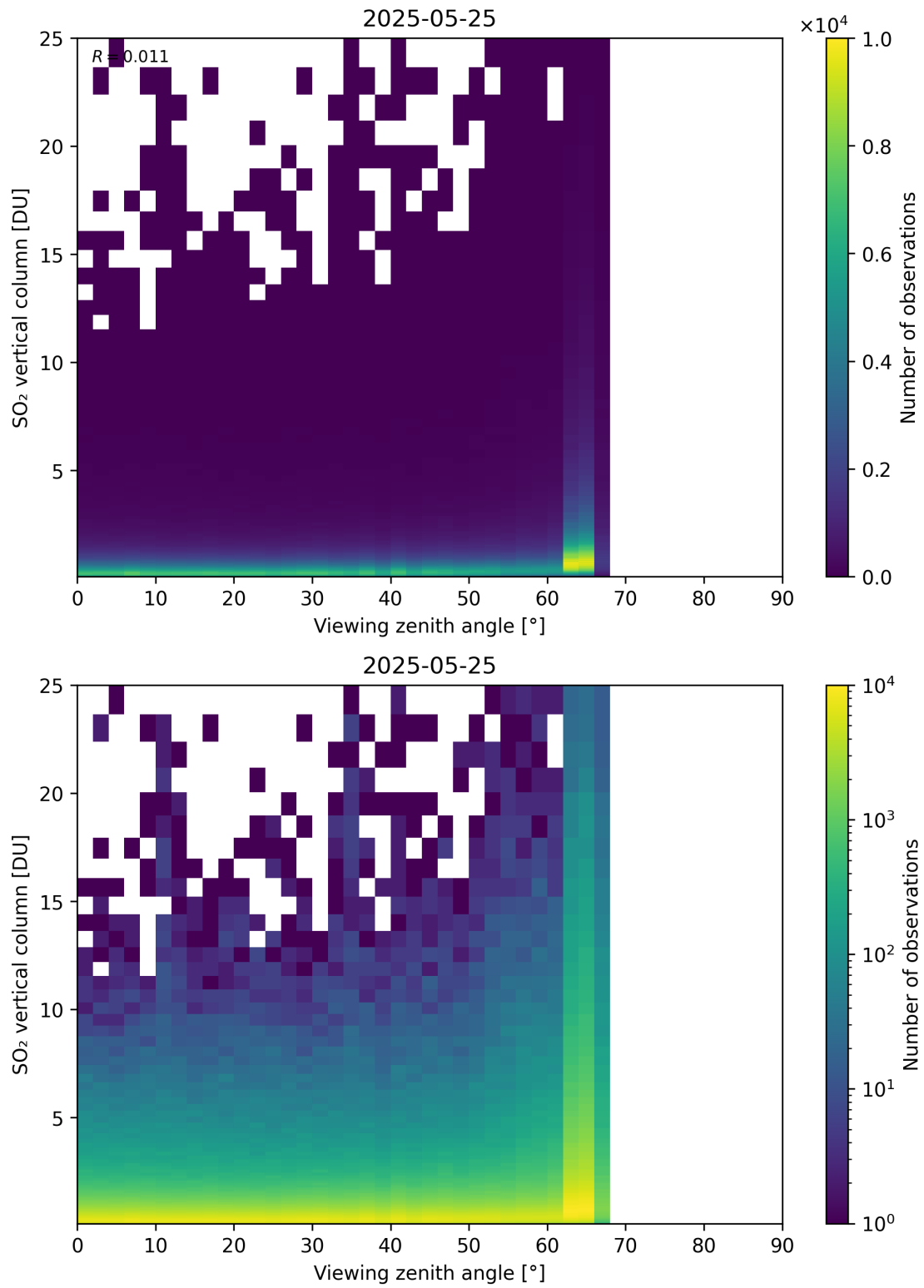
Figure 383: Scatter density plot of “Viewing zenith angle” against “SO 2 vertical column” for 2025-05-24 to 2025-05-26.
