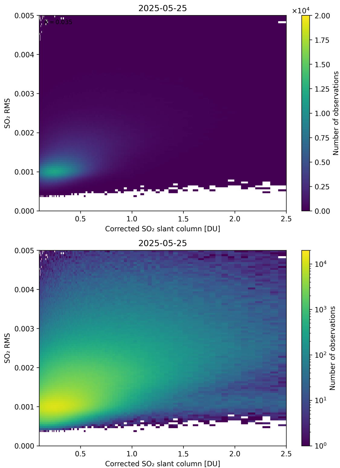
Figure 231: Scatter density plot of “Corrected SO 2 slant column” against “SO 2 RMS” for 2025-05-24 to 2025-05-26.
