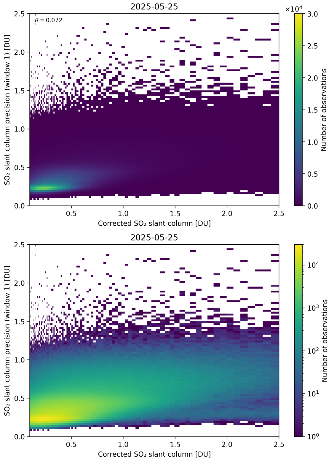
Figure 238: Scatter density plot of “Corrected SO 2 slant column” against “SO 2 slant column precision (window 1)” for 2025-05-24 to 2025-05-26.
