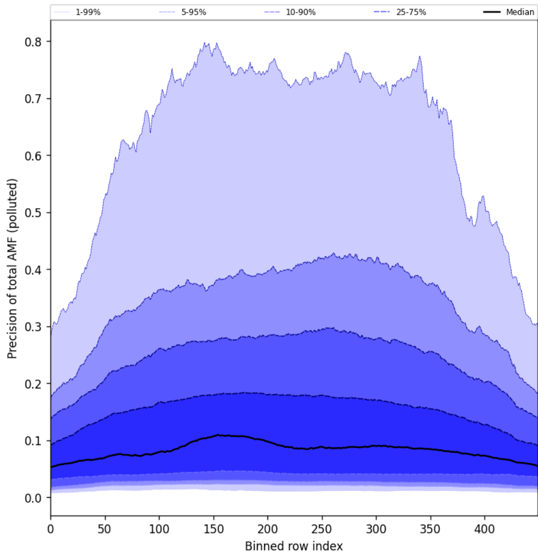
Figure 106: Along track statistics of “Precision of total AMF (polluted)” for 2025-05-24 to 2025-05-26
