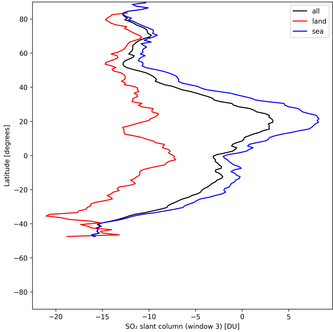
Figure 45: Zonal average of “SO 2 slant column (window 3)” for 2025-05-24 to 2025-05-26.
