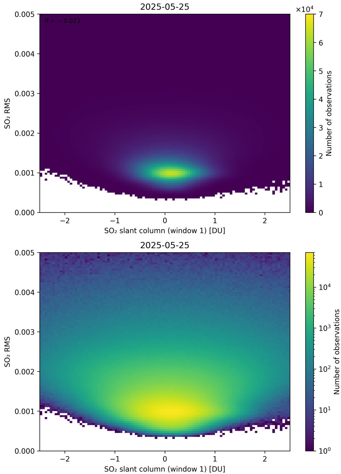
Figure 267: Scatter density plot of “SO 2 slant column (window 1)” against “SO 2 RMS” for 2025-05-24 to 2025-05-26.
