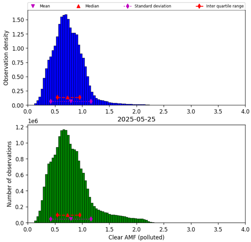
Figure 81: Histogram of “Clear AMF (polluted)” for 2025-05-24 to 2025-05-26
