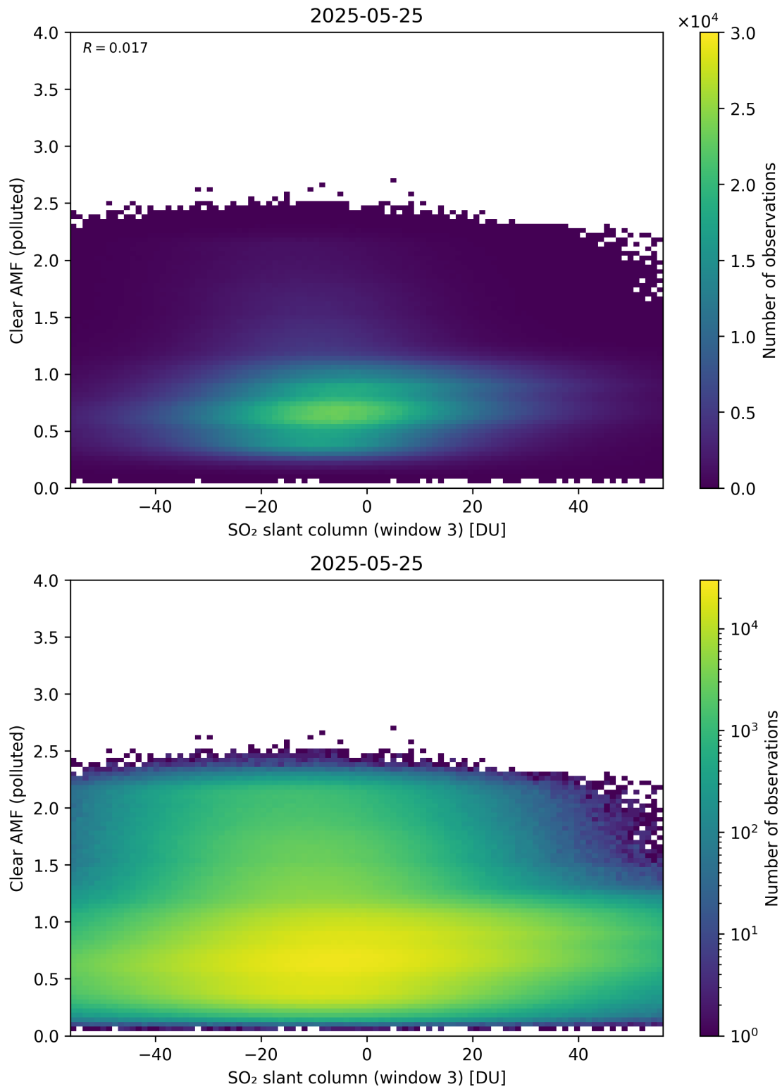
Figure 315: Scatter density plot of “SO 2 slant column (window 3)” against “Clear AMF (polluted)” for 2025-05-24 to 2025-05-26.
