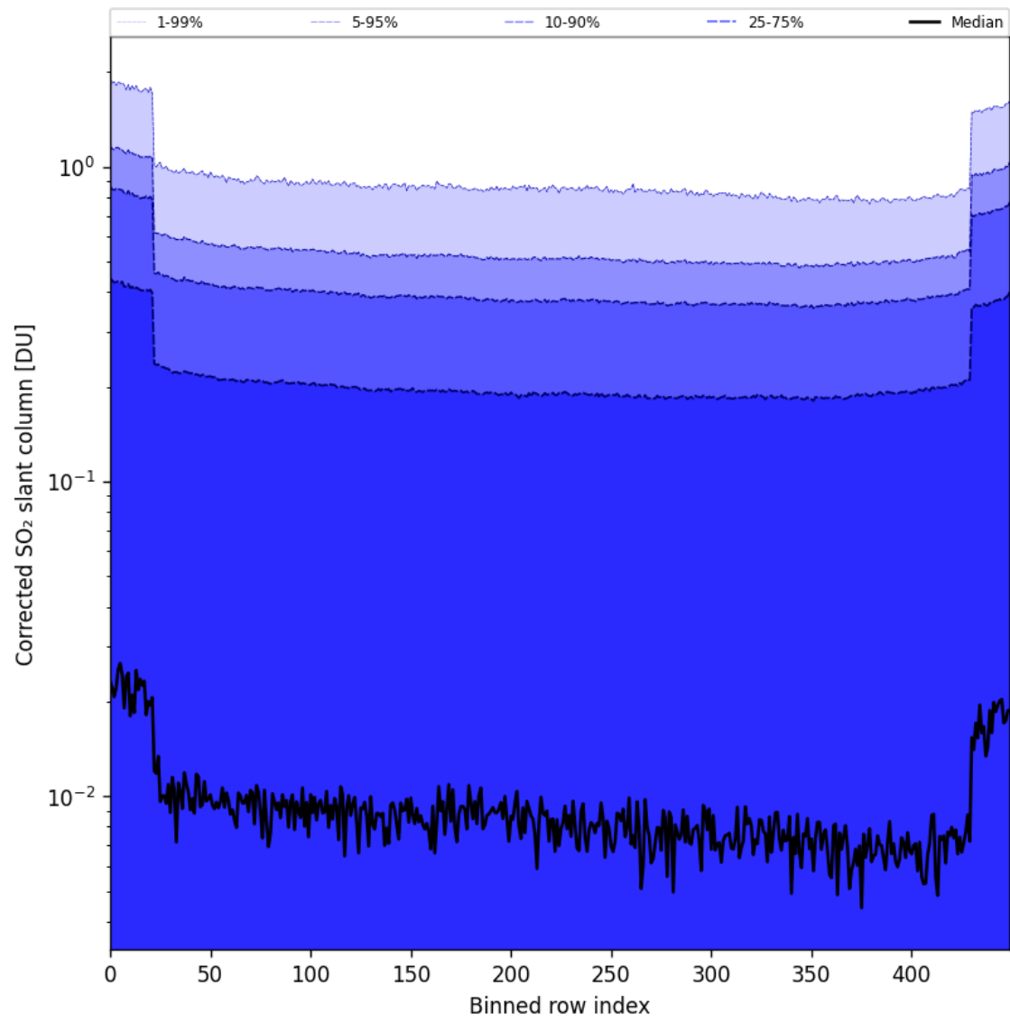
Figure 86: Along track statistics of “Corrected SO 2 slant column” for 2025-05-24 to 2025-05-26
