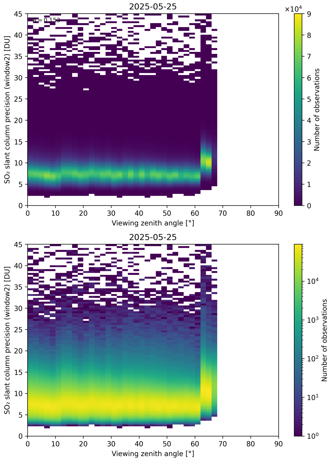
Figure 378: Scatter density plot of “Viewing zenith angle” against “SO 2 slant column precision (window2)” for 2025-05-24 to 2025-05-26.
