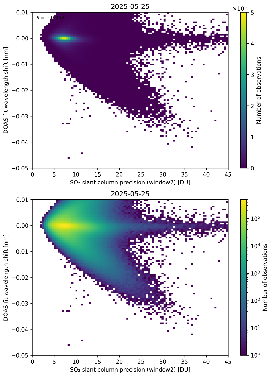
Figure 293: Scatter density plot of “SO 2 slant column precision (window2)” against “DOAS fit wavelength shift” for 2025-05-24 to 2025-05-26.
