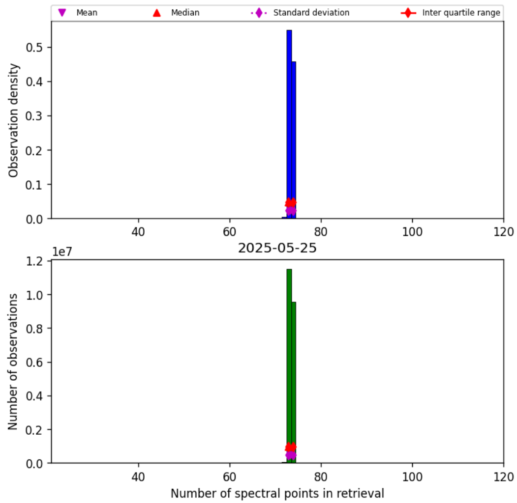
Figure 82: Histogram of “Number of spectral points in retrieval” for 2025-05-24 to 2025-05-26
