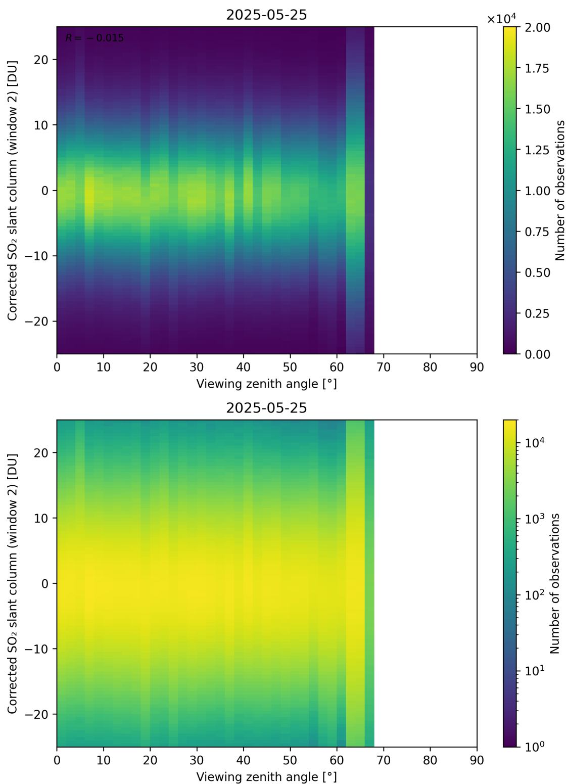
Figure 374: Scatter density plot of “Viewing zenith angle” against “Corrected SO 2 slant column (window 2)” for 2025-05-24 to 2025-05-26.
