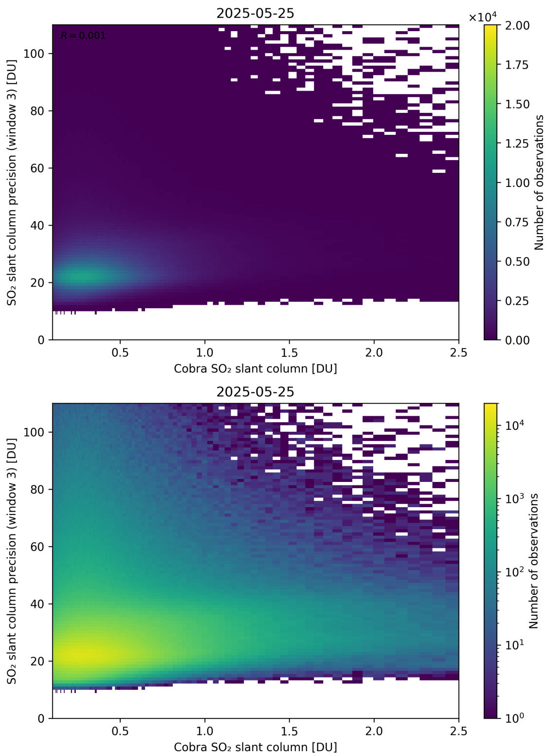
Figure 223: Scatter density plot of “Cobra SO 2 slant column” against “SO 2 slant column precision (window 3)” for 2025-05-24 to 2025-05-26.
