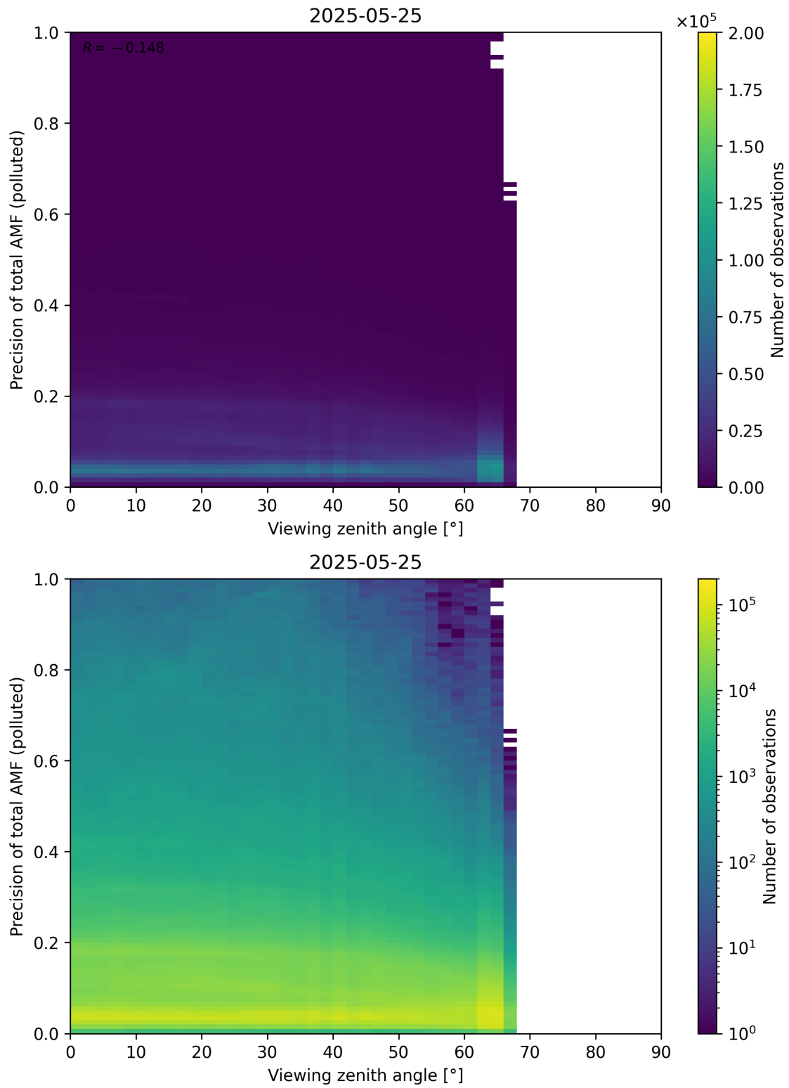
Figure 382: Scatter density plot of “Viewing zenith angle” against “Precision of total AMF (polluted)” for 2025-05-24 to 2025-05-26.
