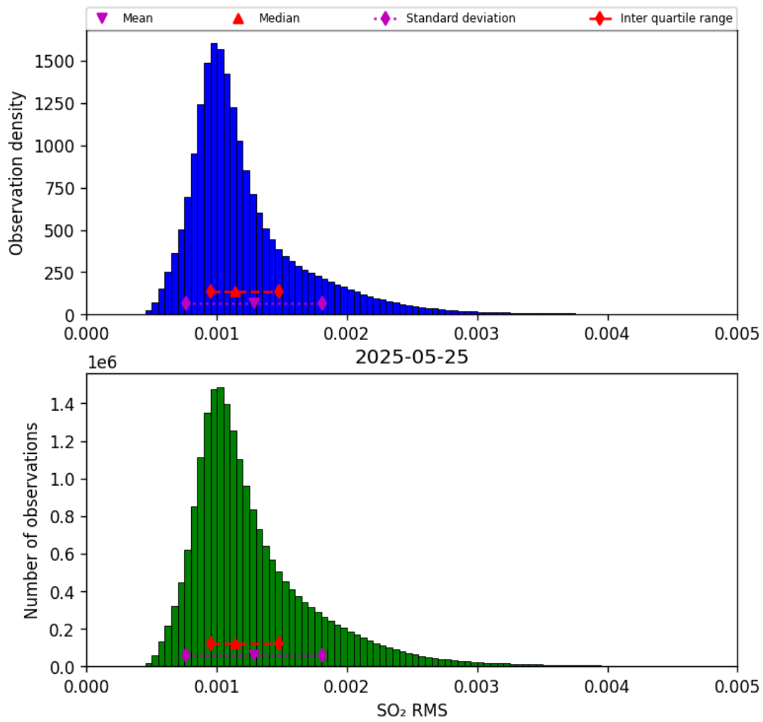
Figure 78: Histogram of “SO 2 RMS” for 2025-05-24 to 2025-05-26
