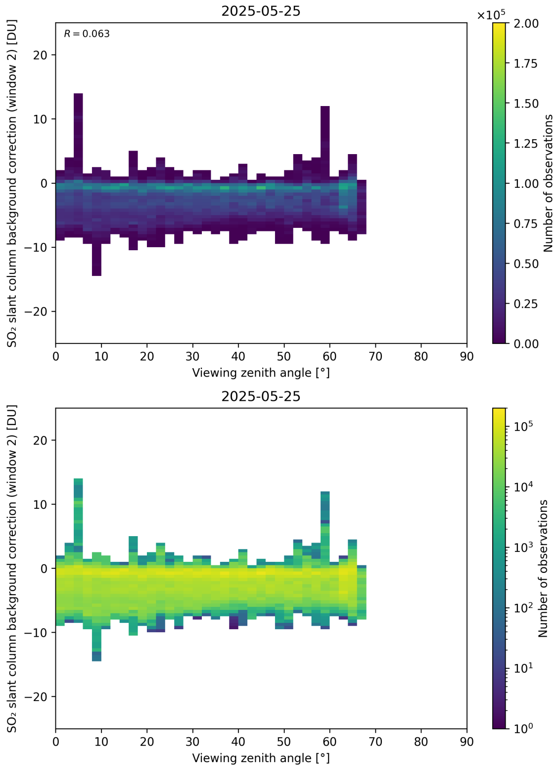
Figure 363: Scatter density plot of “Viewing zenith angle” against “SO 2 slant column background correction (window 2)” for 2025-05-24 to 2025-05-26.
