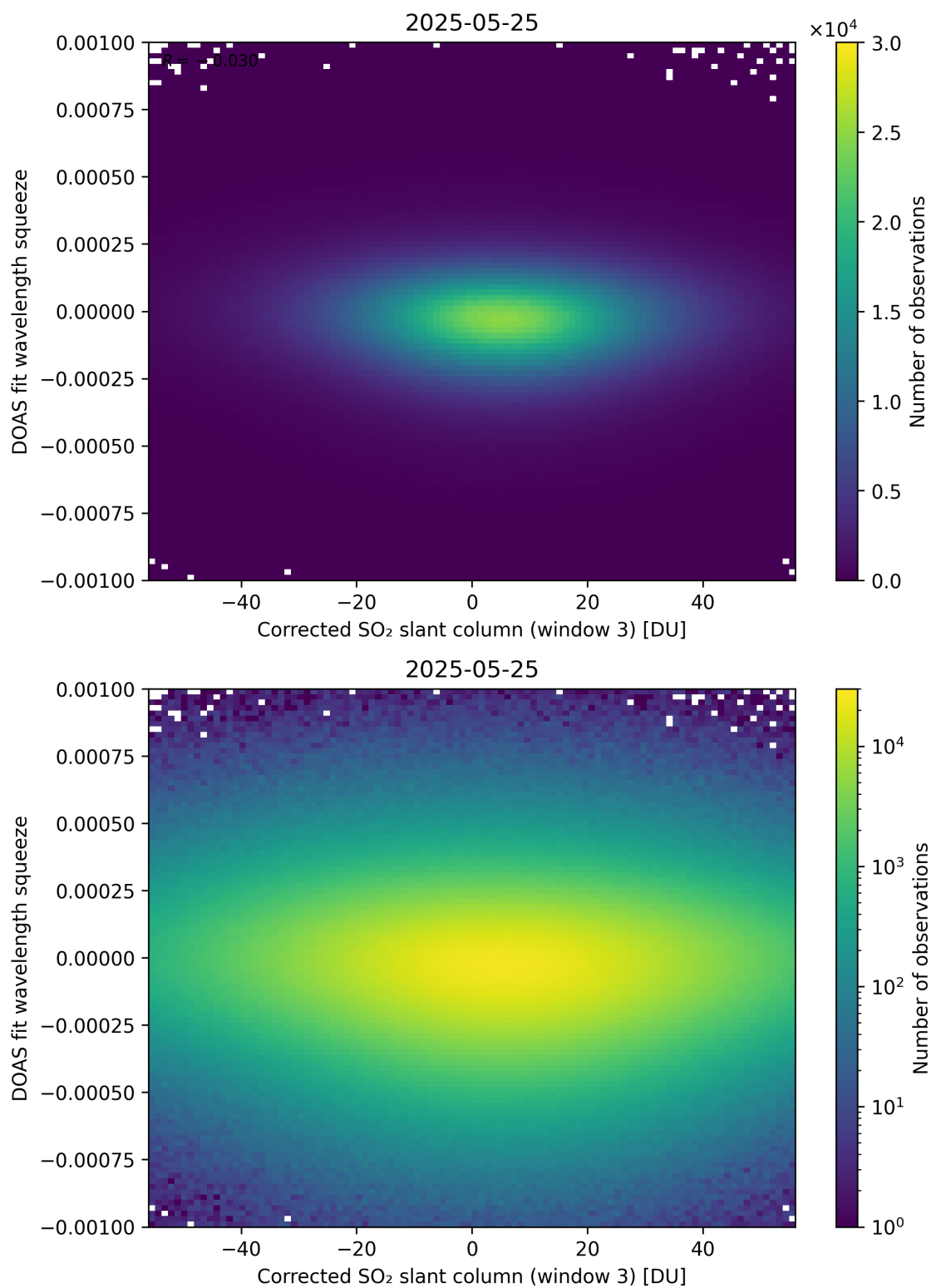
Figure 257: Scatter density plot of “Corrected SO 2 slant column (window 3)” against “DOAS fit wavelength squeeze” for 2025-05-24 to 2025-05-26.
