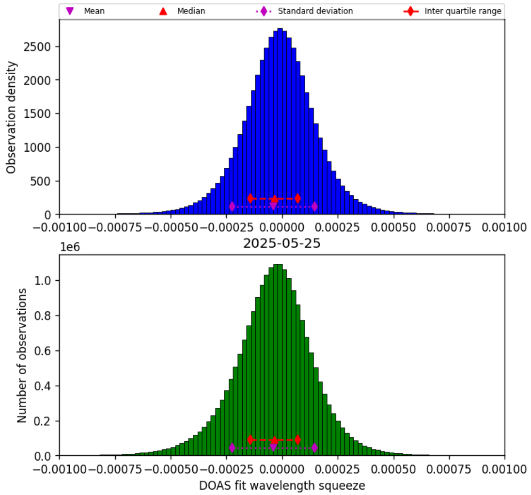
Figure 77: Histogram of “DOAS fit wavelength squeeze” for 2025-05-24 to 2025-05-26
