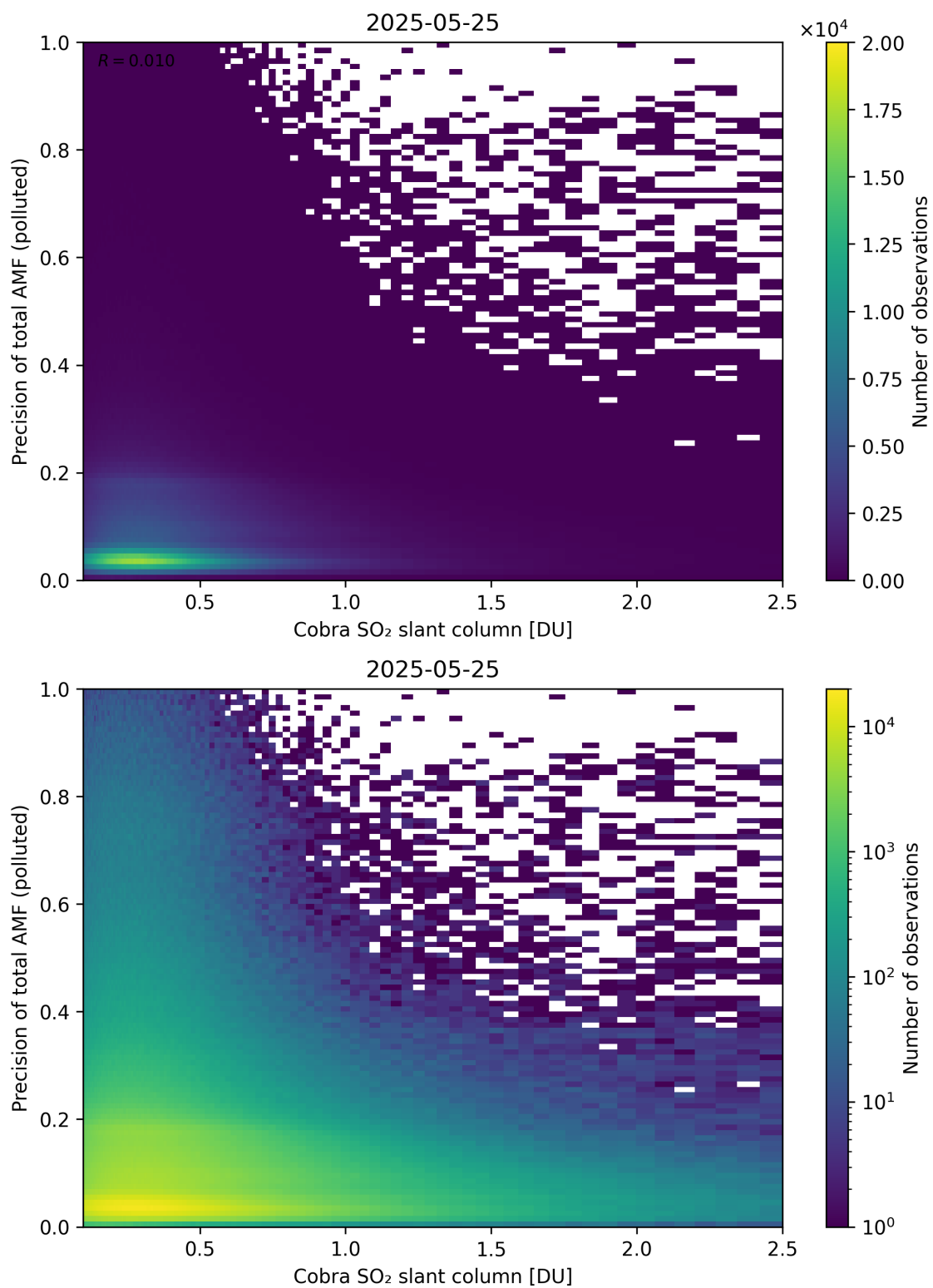
Figure 225: Scatter density plot of “Cobra SO 2 slant column” against “Precision of total AMF (polluted)” for 2025-05-24 to 2025-05-26.
