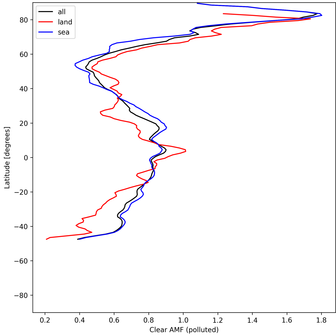
Figure 55: Zonal average of “Clear AMF (polluted)” for 2025-05-24 to 2025-05-26.
