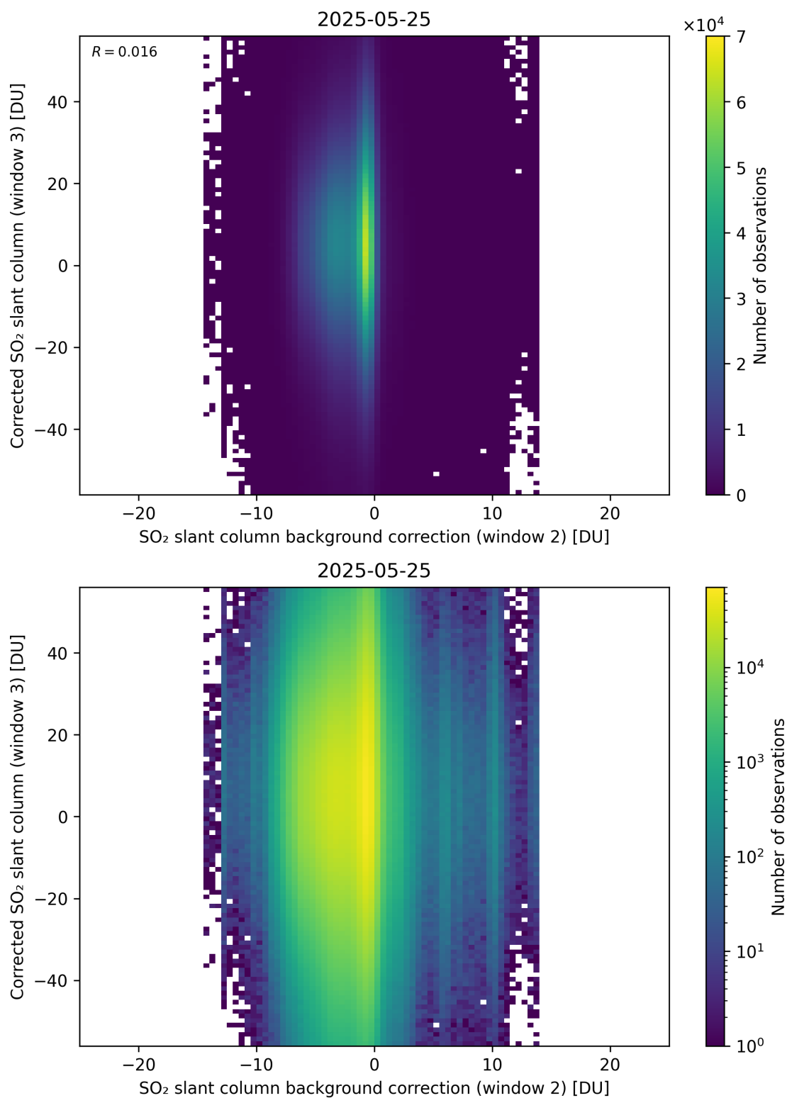
Figure 127: Scatter density plot of “SO 2 slant column background correction (window 2)” against “Corrected SO 2 slant column (window 3)” for 2025-05-24 to 2025-05-26.
