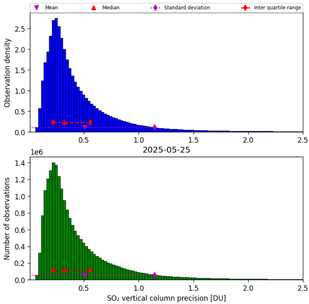
Figure 59: Histogram of “SO 2 vertical column precision” for 2025-05-24 to 2025-05-26
