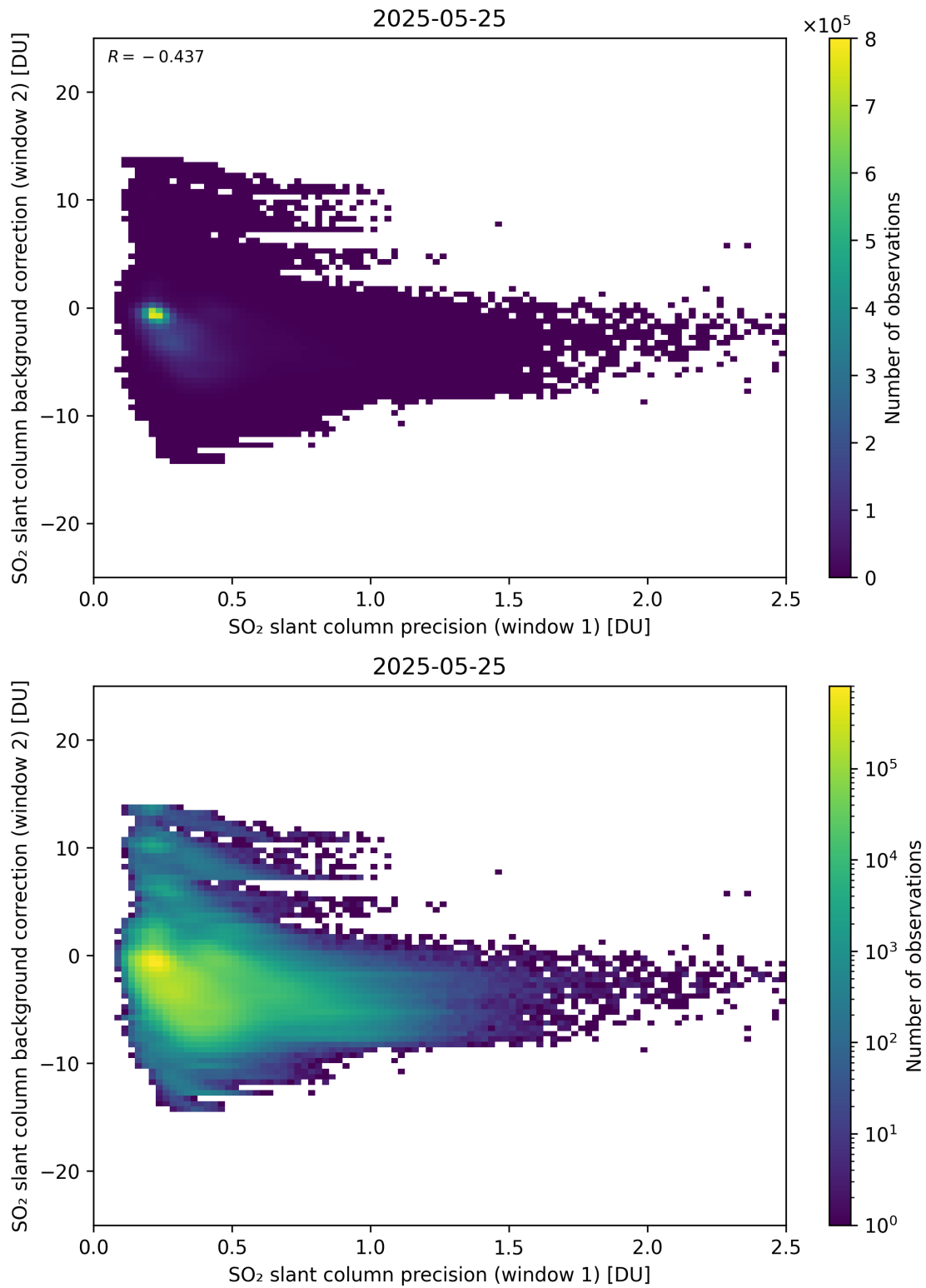
Figure 269: Scatter density plot of “SO 2 slant column precision (window 1)” against “SO 2 slant column background correction (window 2)” for 2025-05-24 to 2025-05-26.
