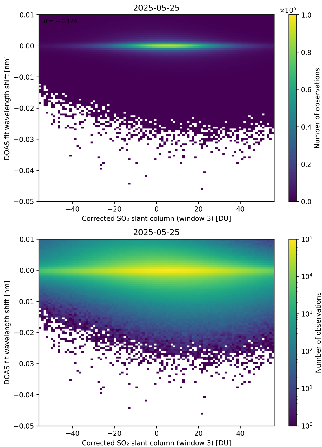
Figure 256: Scatter density plot of “Corrected SO 2 slant column (window 3)” against “DOAS fit wavelength shift” for 2025-05-24 to 2025-05-26.
