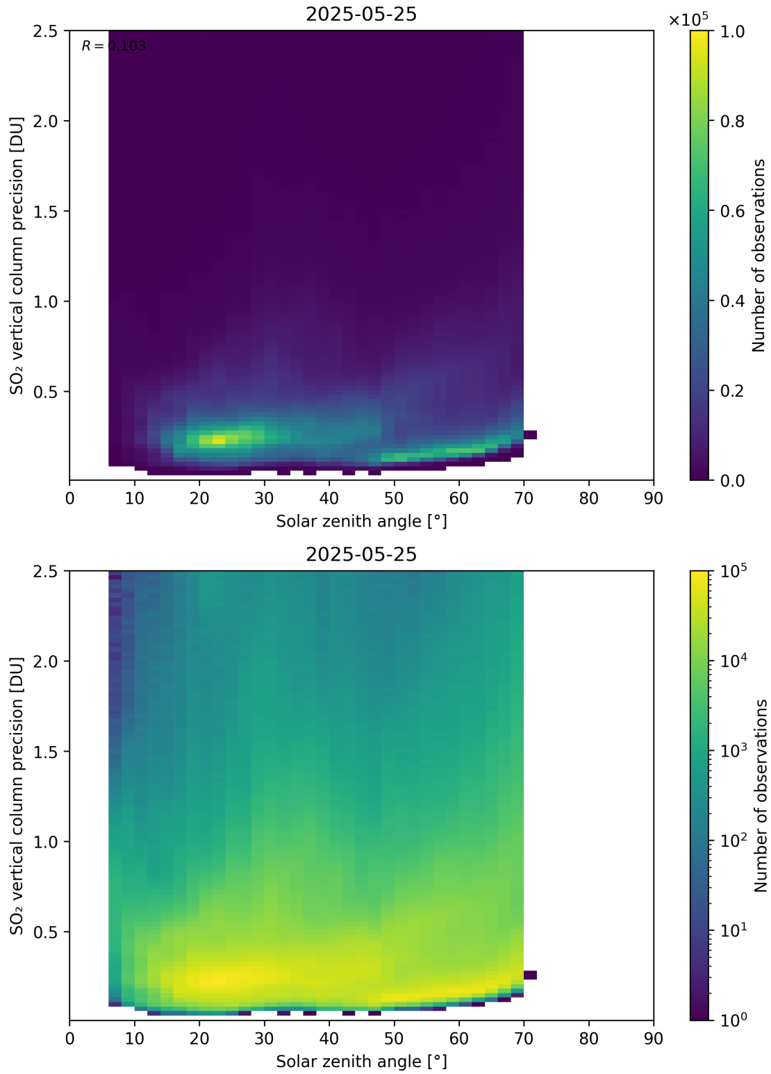
Figure 192: Scatter density plot of “Solar zenith angle” against “SO 2 vertical column precision” for 2025-05-24 to 2025-05-26.
