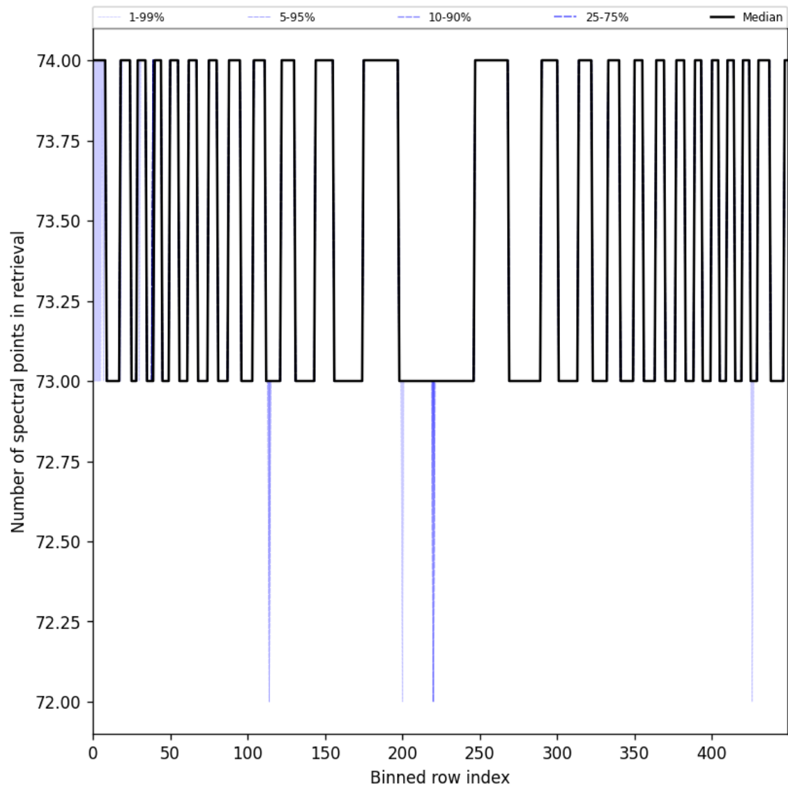
Figure 108: Along track statistics of “Number of spectral points in retrieval” for 2025-05-24 to 2025-05-26
