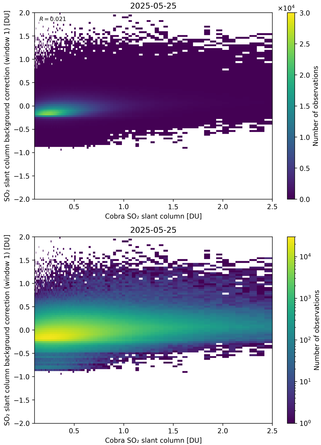
Figure 193: Scatter density plot of “Cobra SO 2 slant column” against “SO 2 slant column background correction (window 1)” for 2025-05-24 to 2025-05-26.
