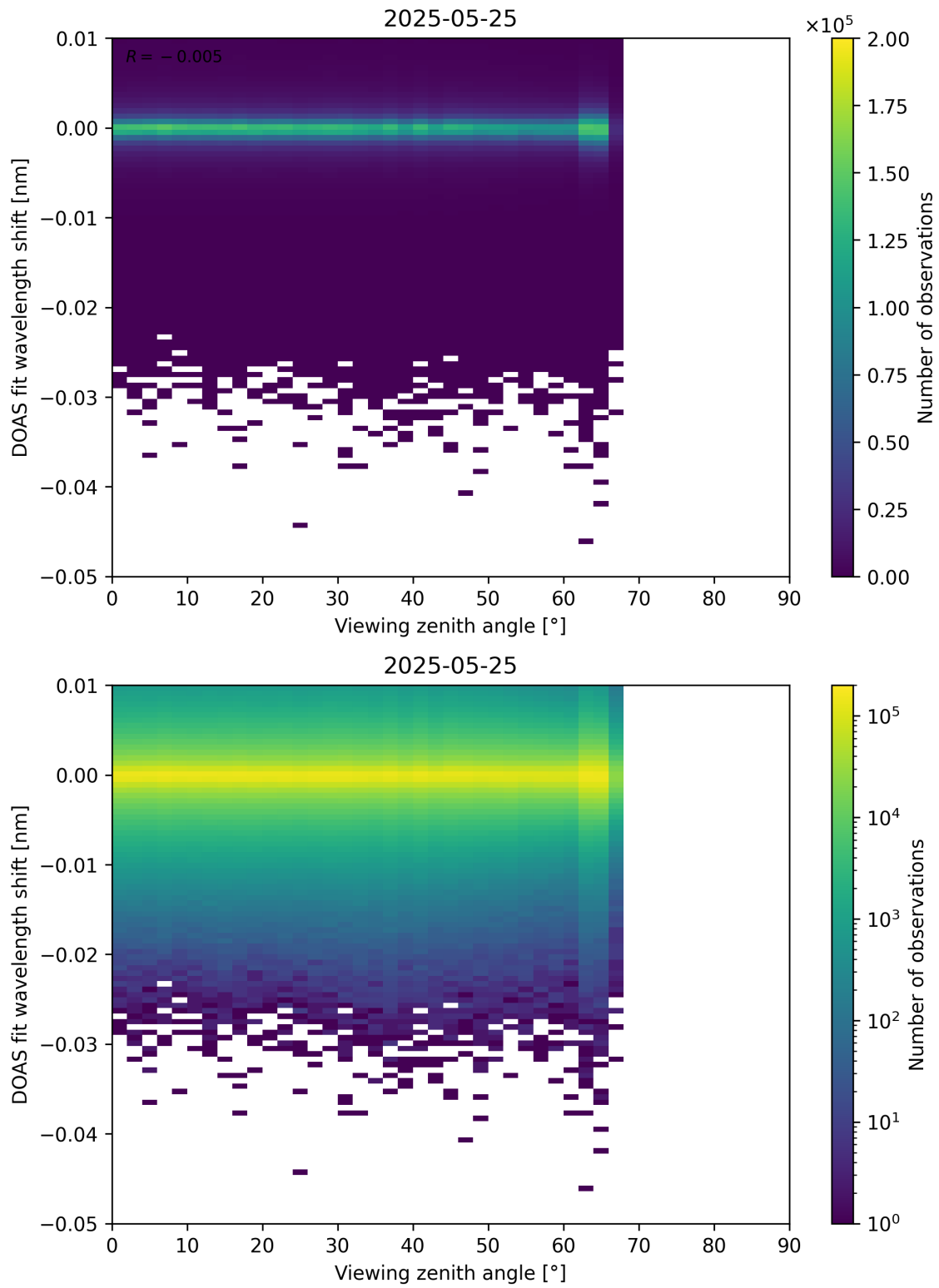
Figure 365: Scatter density plot of “Viewing zenith angle” against “DOAS fit wavelength shift” for 2025-05-24 to 2025-05-26.
