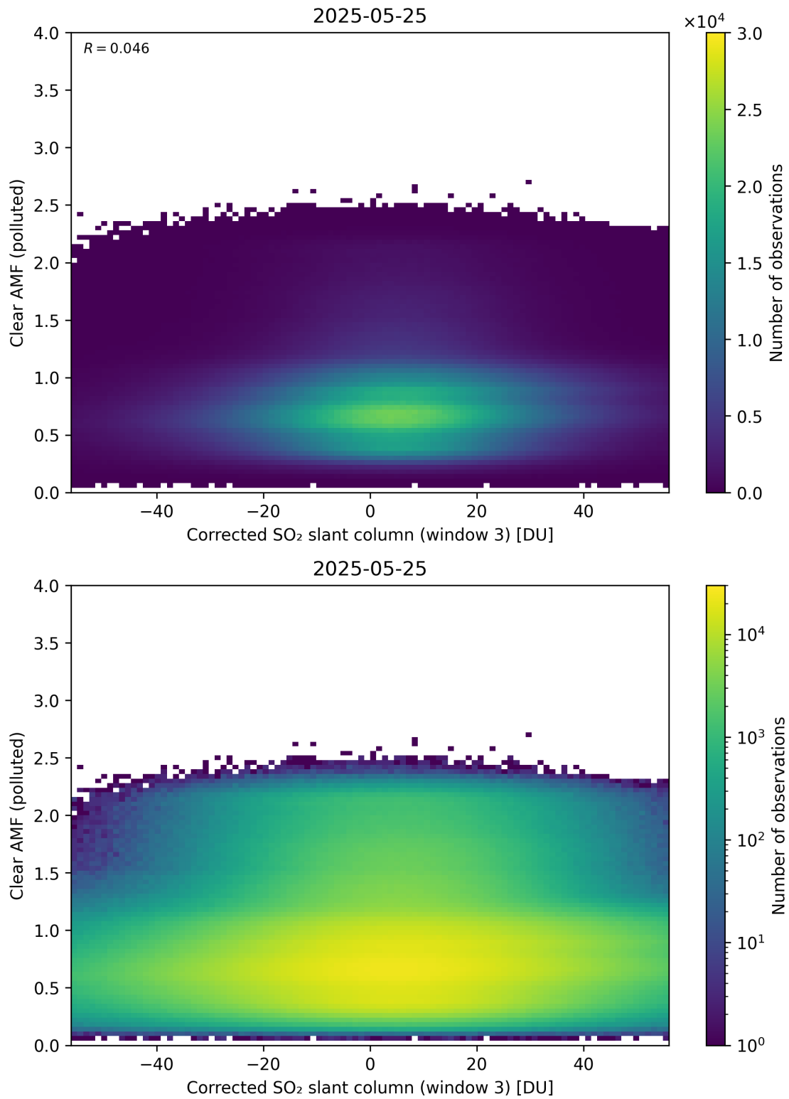
Figure 259: Scatter density plot of “Corrected SO 2 slant column (window 3)” against “Clear AMF (polluted)” for 2025-05-24 to 2025-05-26.
