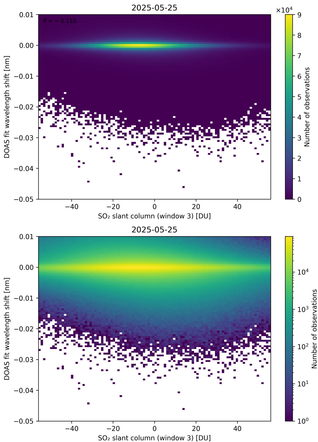
Figure 304: Scatter density plot of “SO 2 slant column (window 3)” against “DOAS fit wavelength shift” for 2025-05-24 to 2025-05-26.
