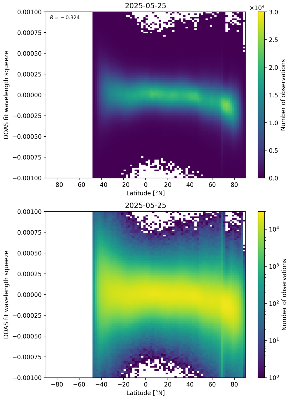
Figure 154: Scatter density plot of “Latitude” against “DOAS fit wavelength squeeze” for 2025-05-24 to 2025-05-26.
