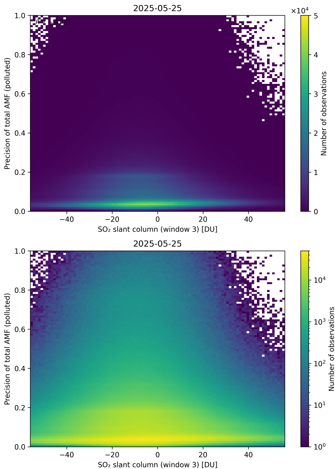
Figure 319: Scatter density plot of “SO 2 slant column (window 3)” against “Precision of total AMF (polluted)” for 2025-05-24 to 2025-05-26.
