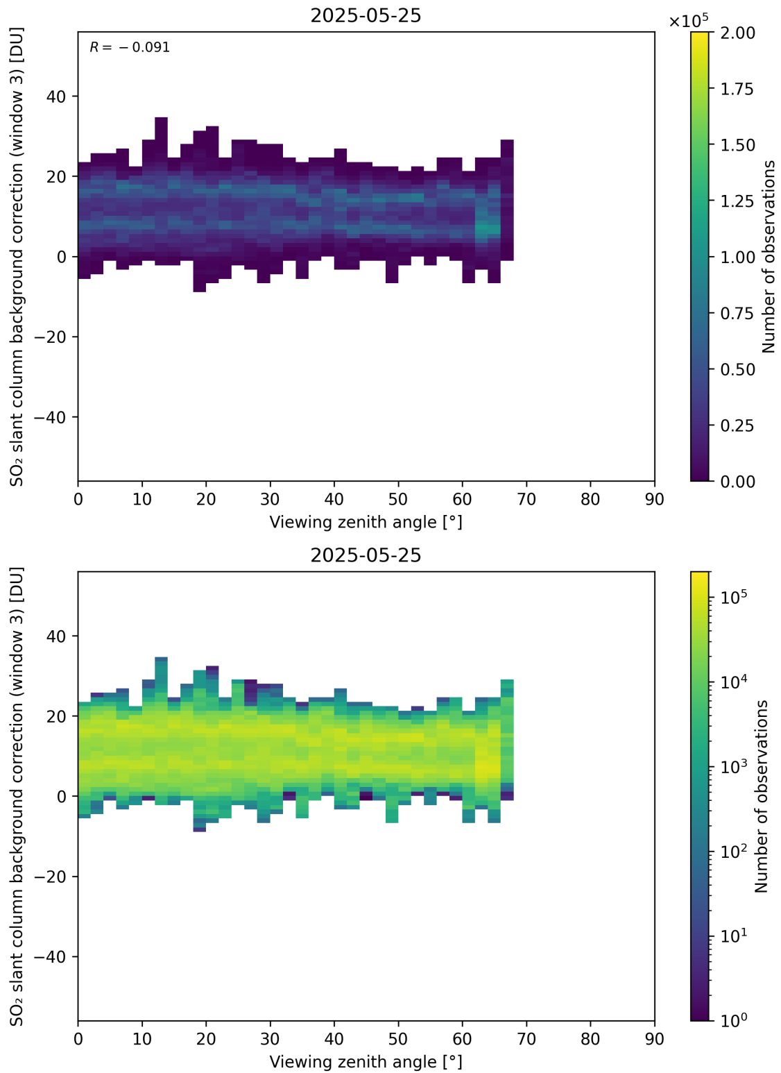
Figure 364: Scatter density plot of “Viewing zenith angle” against “SO 2 slant column background correction (window 3)” for 2025-05-24 to 2025-05-26.
