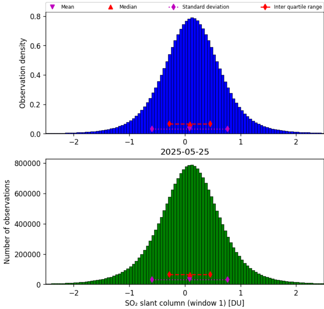
Figure 63: Histogram of “SO 2 slant column (window 1)” for 2025-05-24 to 2025-05-26
