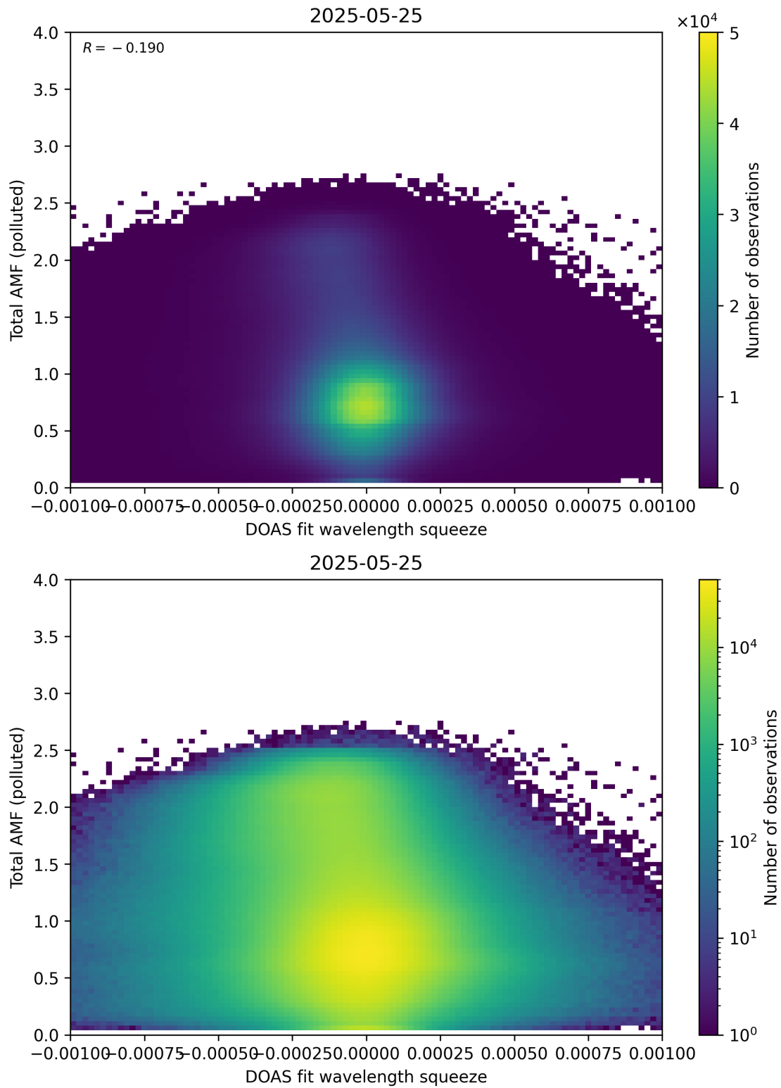
Figure 145: Scatter density plot of “DOAS fit wavelength squeeze” against “Total AMF (polluted)” for 2025-05-24 to 2025-05-26.
