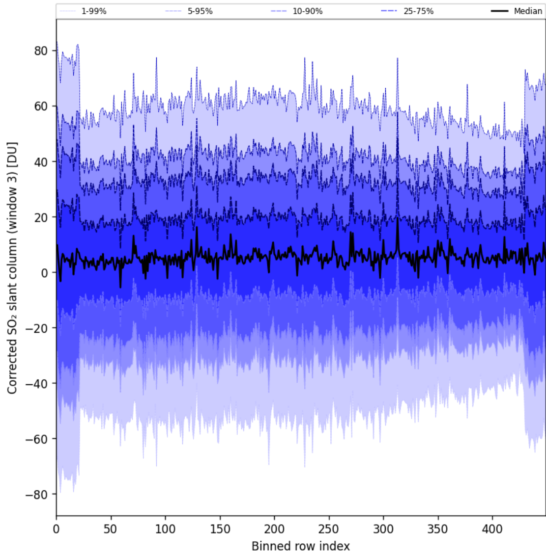
Figure 99: Along track statistics of “Corrected SO 2 slant column (window 3)” for 2025-05-24 to 2025-05-26
