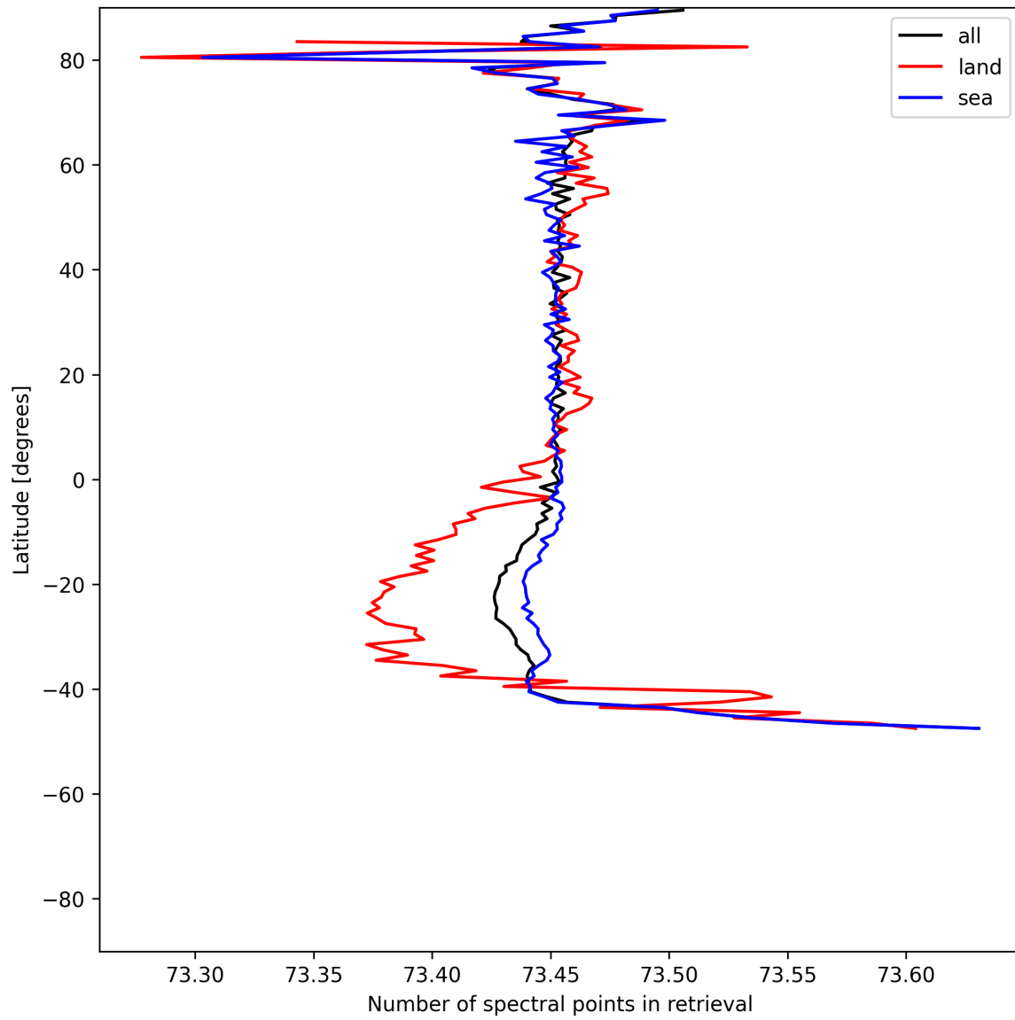
Figure 56: Zonal average of “Number of spectral points in retrieval” for 2025-05-24 to 2025-05-26.
