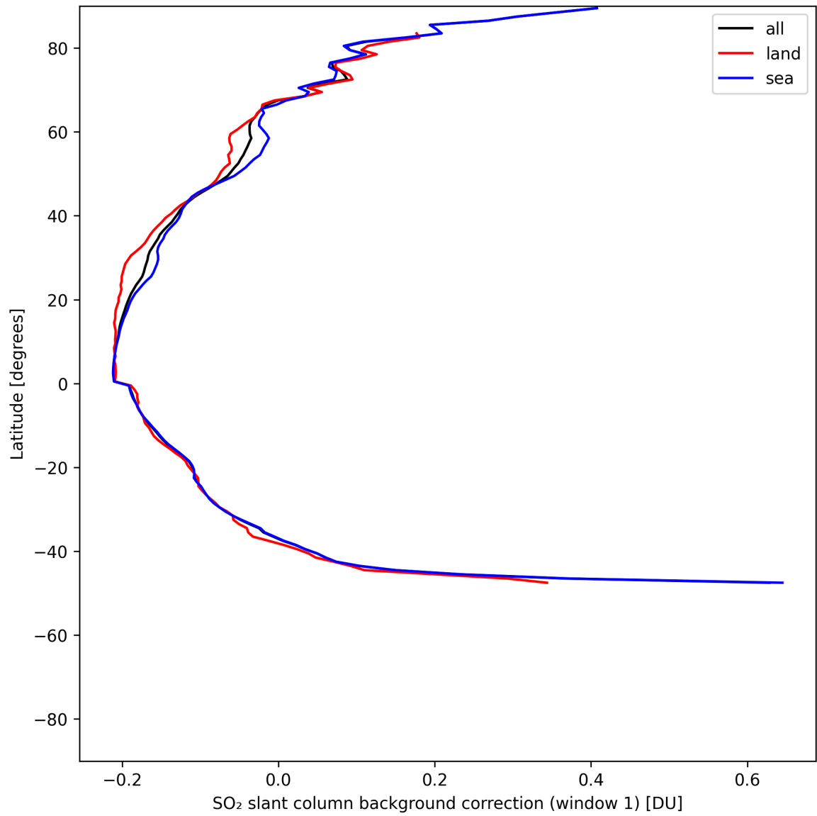
Figure 40: Zonal average of “SO 2 slant column background correction (window 1)” for 2025-05-24 to 2025-05-26.
