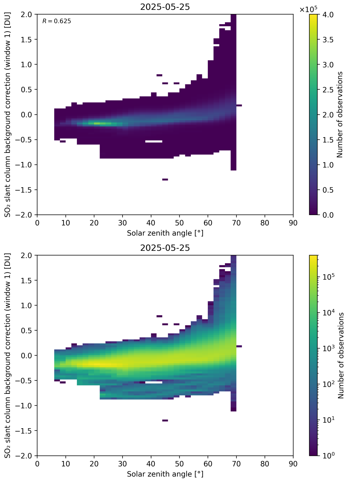
Figure 171: Scatter density plot of “Solar zenith angle” against “SO 2 slant column background correction (window 1)” for 2025-05-24 to 2025-05-26.
