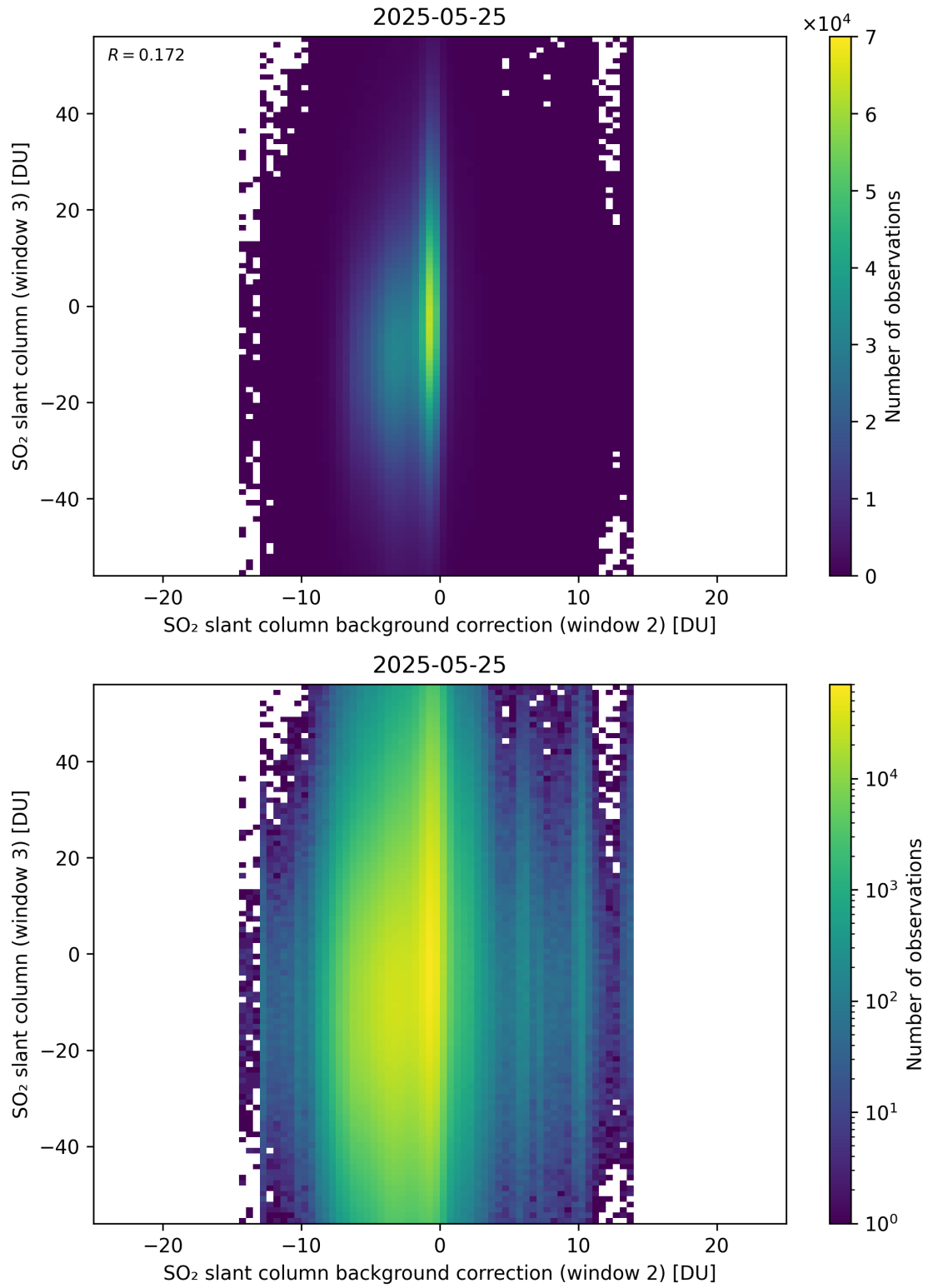
Figure 128: Scatter density plot of “SO 2 slant column background correction (window 2)” against “SO 2 slant column (window 3)” for 2025-05-24 to 2025-05-26.
