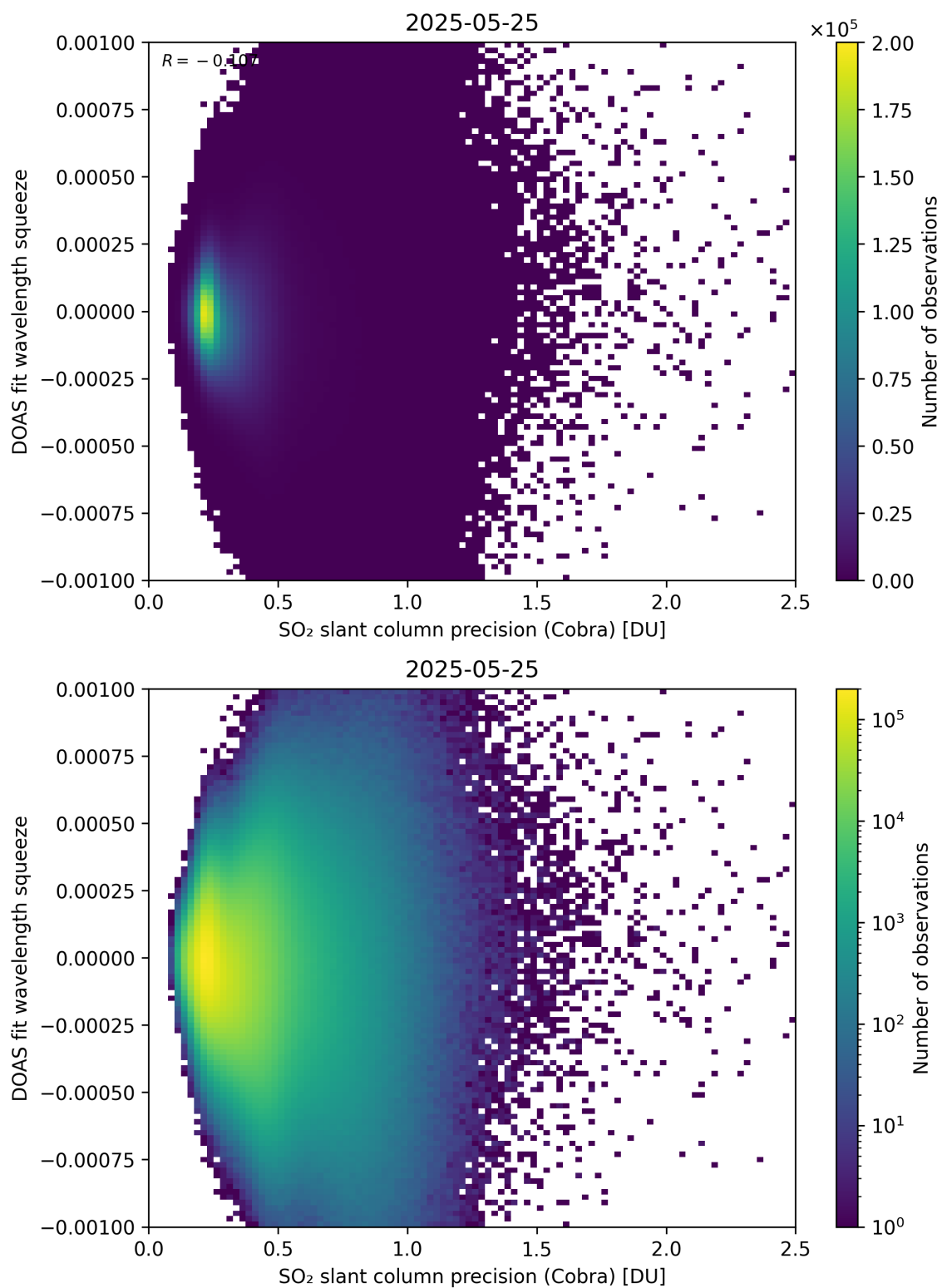
Figure 203: Scatter density plot of “SO 2 slant column precision (Cobra)” against “DOAS fit wavelength squeeze” for 2025-05-24 to 2025-05-26.
