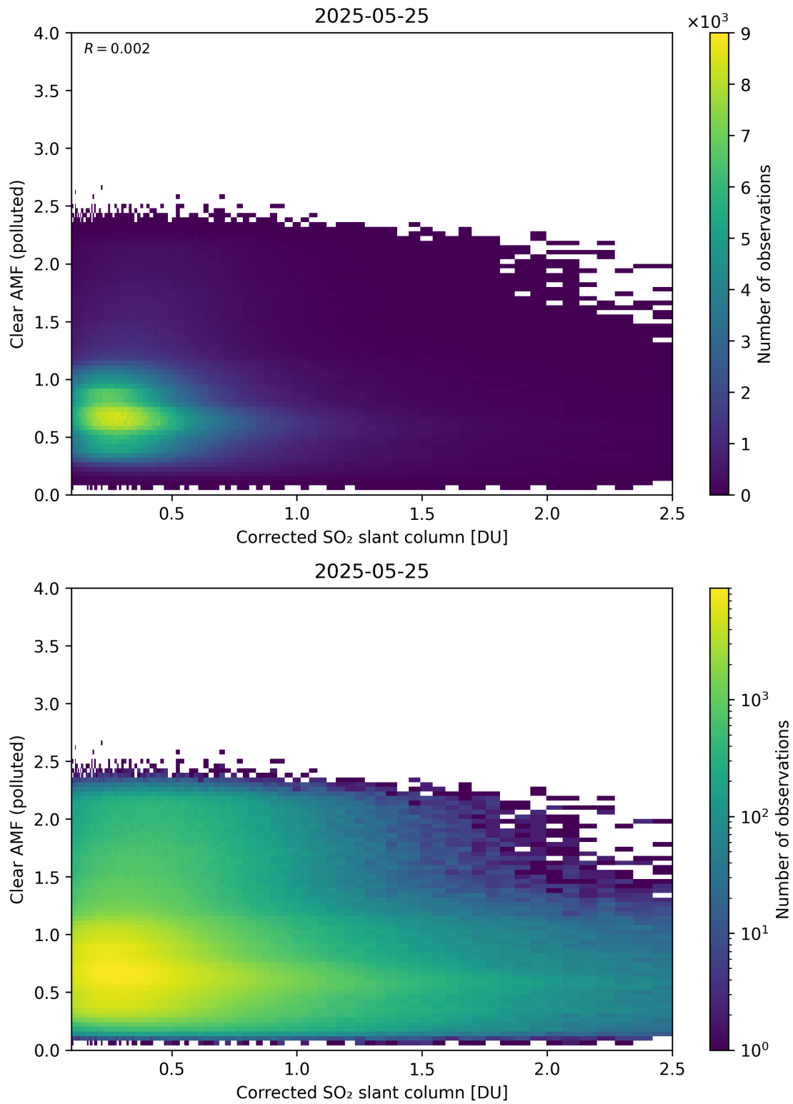
Figure 232: Scatter density plot of “Corrected SO 2 slant column” against “Clear AMF (polluted)” for 2025-05-24 to 2025-05-26.
