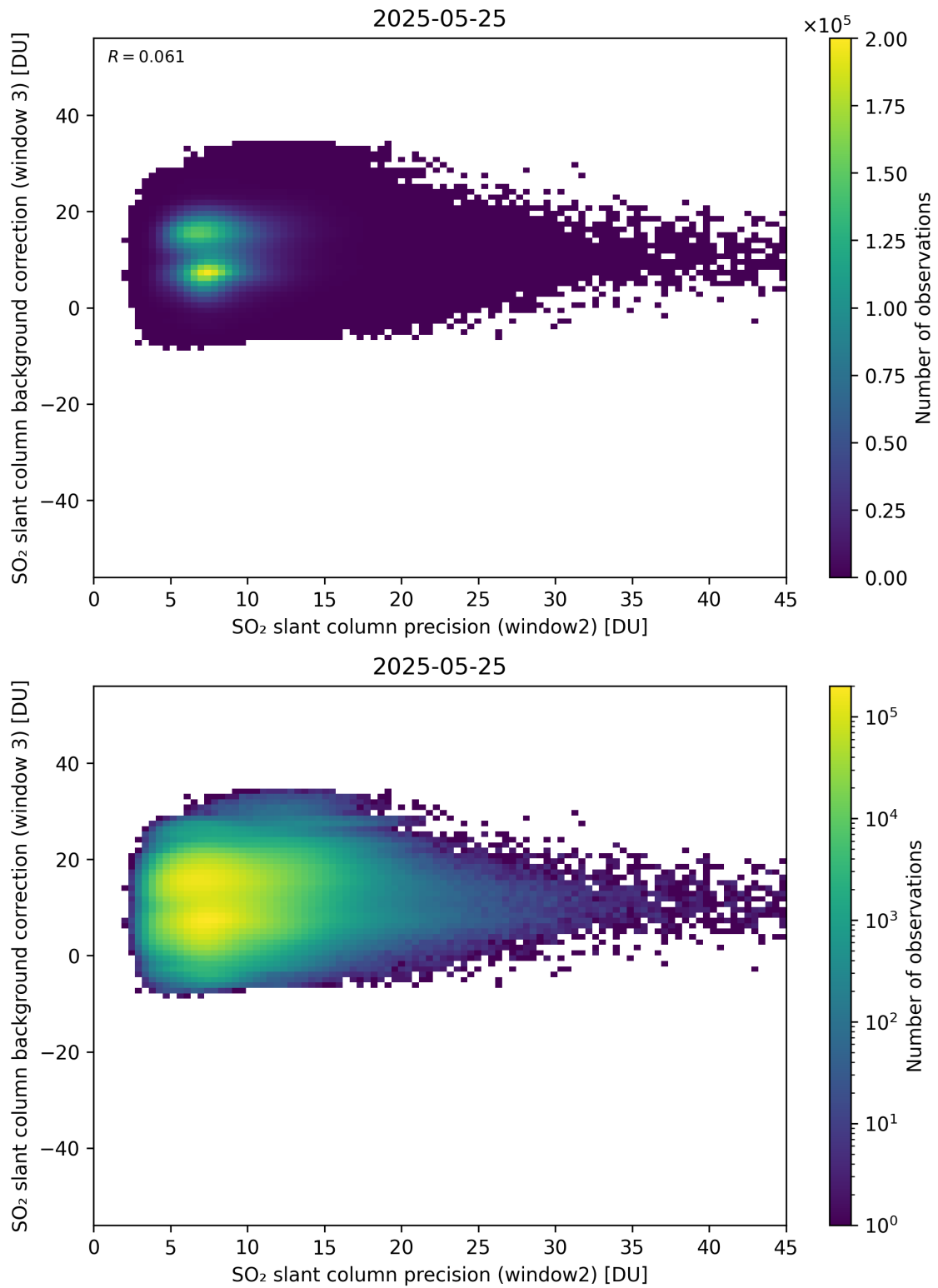
Figure 292: Scatter density plot of “SO 2 slant column precision (window2)” against “SO 2 slant column background correction (window 3)” for 2025-05-24 to 2025-05-26.
