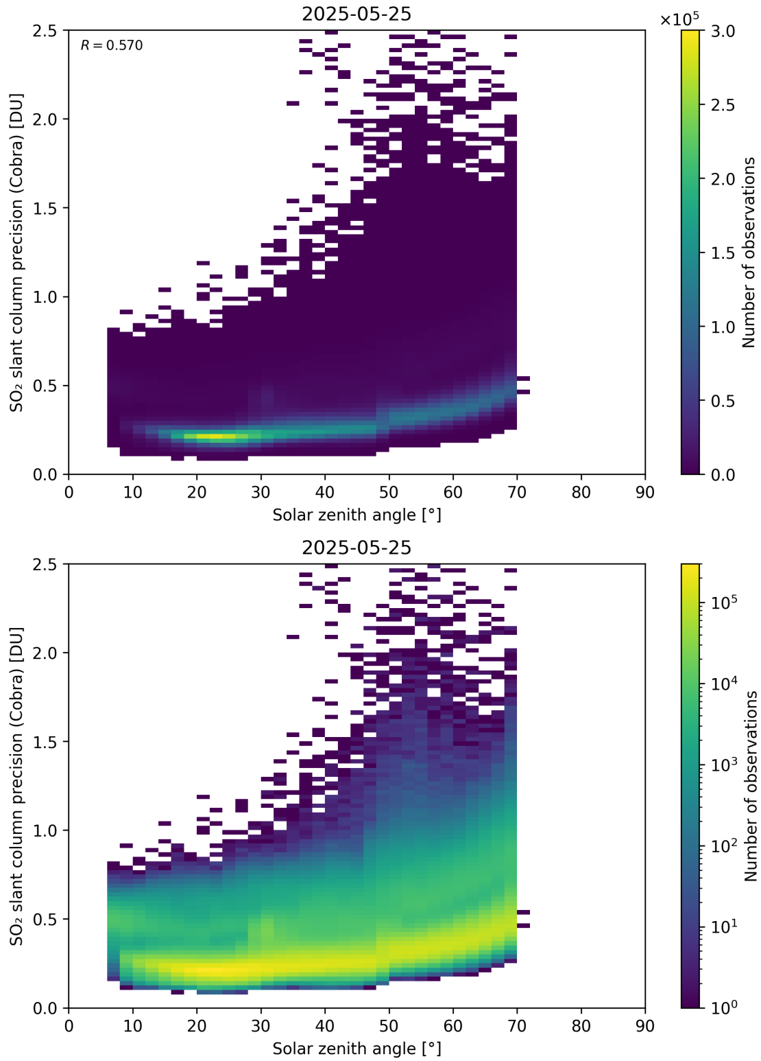
Figure 180: Scatter density plot of “Solar zenith angle” against “SO 2 slant column precision (Cobra)” for 2025-05-24 to 2025-05-26.
