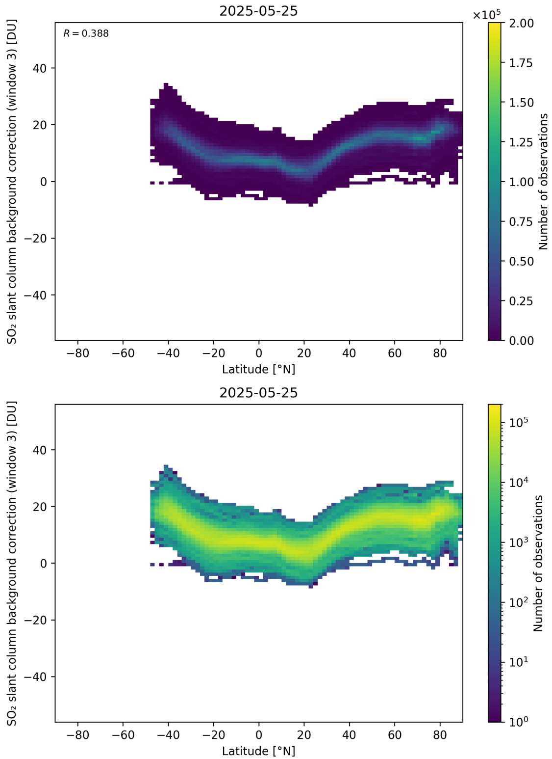
Figure 152: Scatter density plot of “Latitude” against “SO 2 slant column background correction (window 3)” for 2025-05-24 to 2025-05-26.
