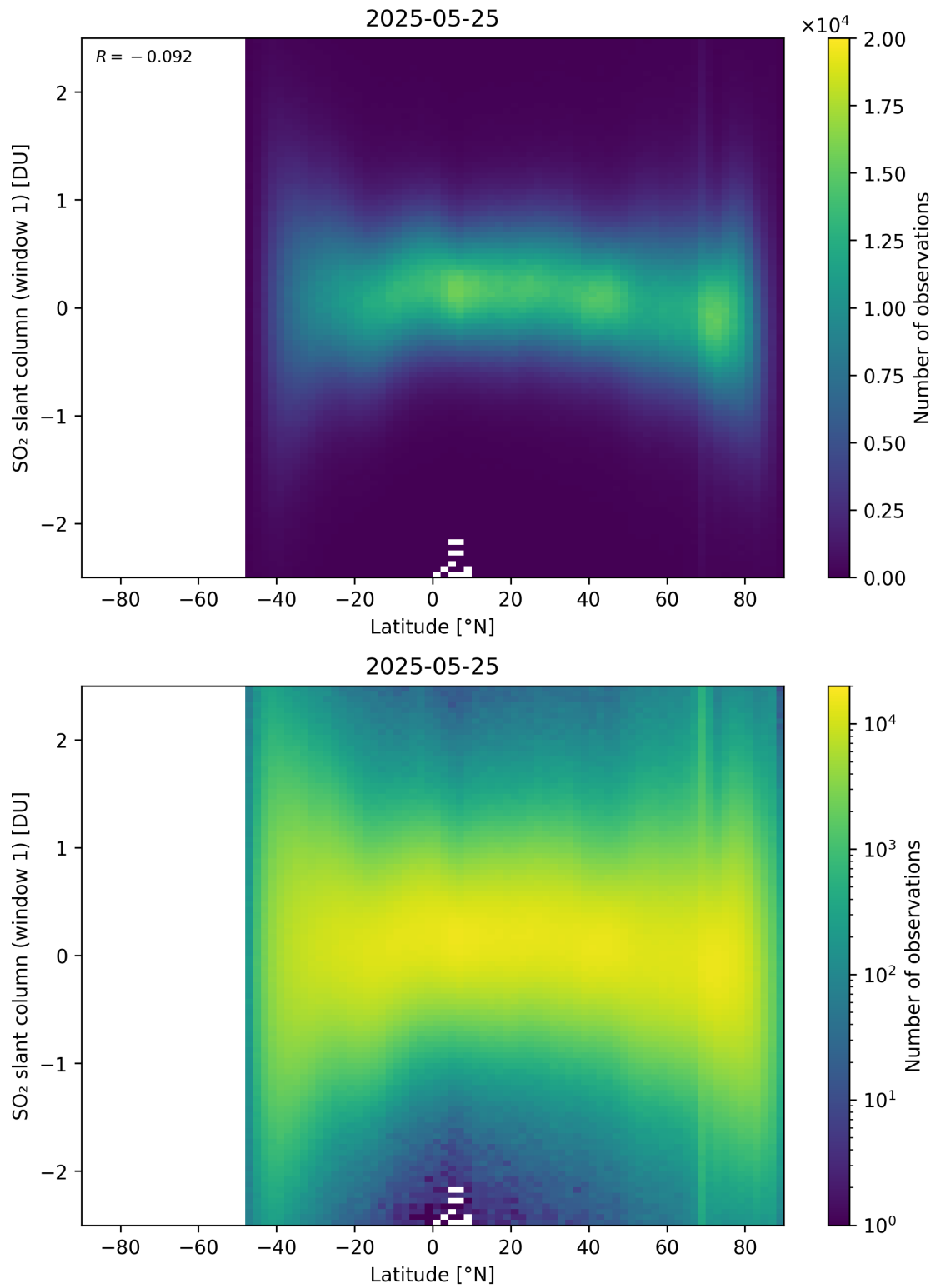
Figure 162: Scatter density plot of “Latitude” against “SO 2 slant column (window 1)” for 2025-05-24 to 2025-05-26.
