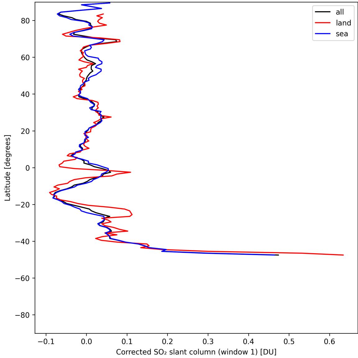
Figure 39: Zonal average of “Corrected SO 2 slant column (window 1)” for 2025-05-24 to 2025-05-26.
