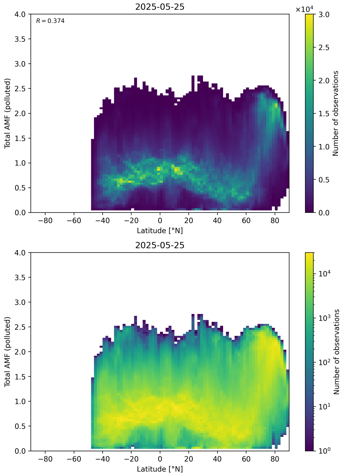
Figure 167: Scatter density plot of “Latitude” against “Total AMF (polluted)” for 2025-05-24 to 2025-05-26.
