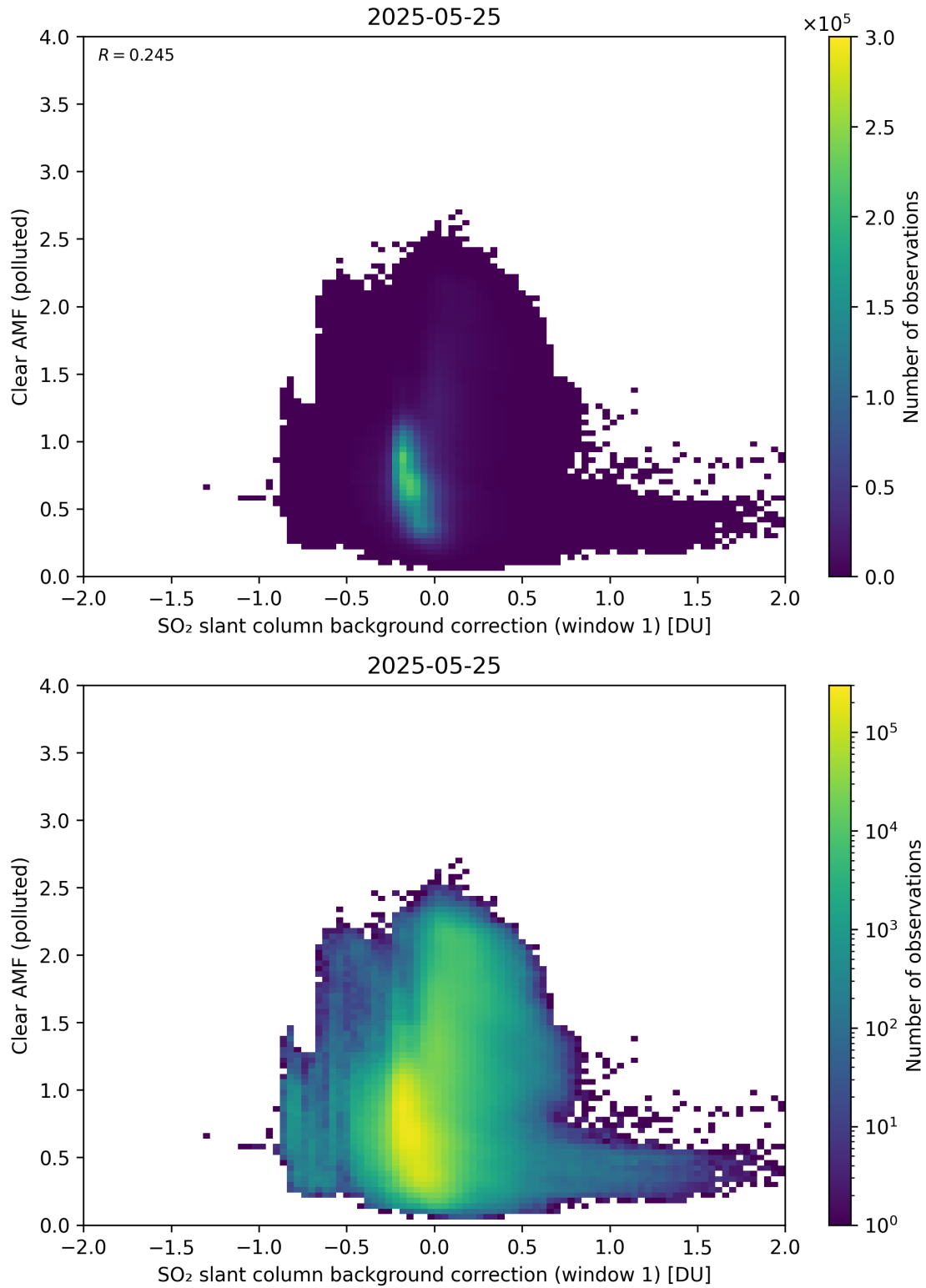
Figure 114: Scatter density plot of “SO 2 slant column background correction (window 1)” against “Clear AMF (polluted)” for 2025-05-24 to 2025-05-26.
