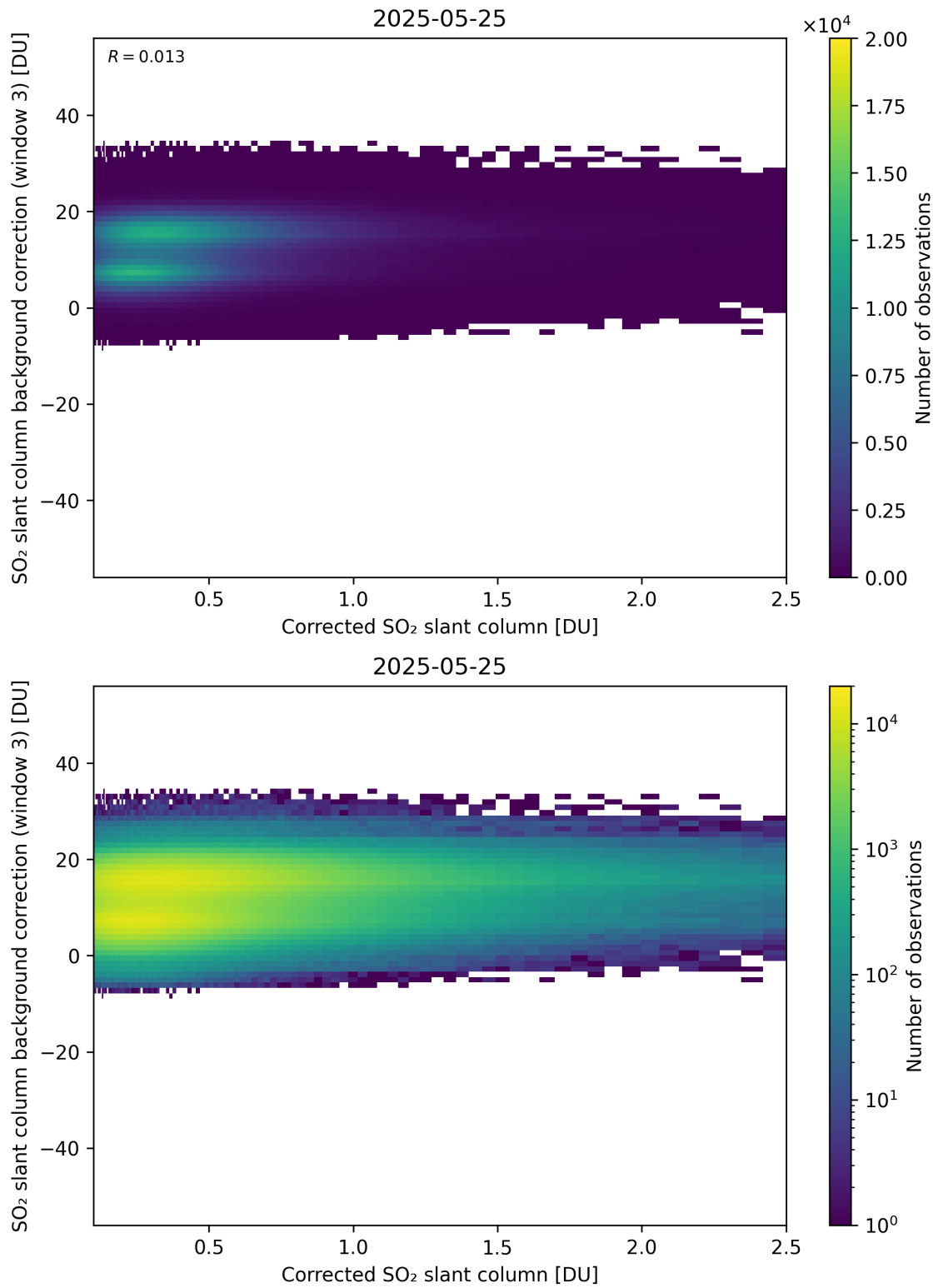
Figure 228: Scatter density plot of “Corrected SO 2 slant column” against “SO 2 slant column background correction (window 3)” for 2025-05-24 to 2025-05-26.
