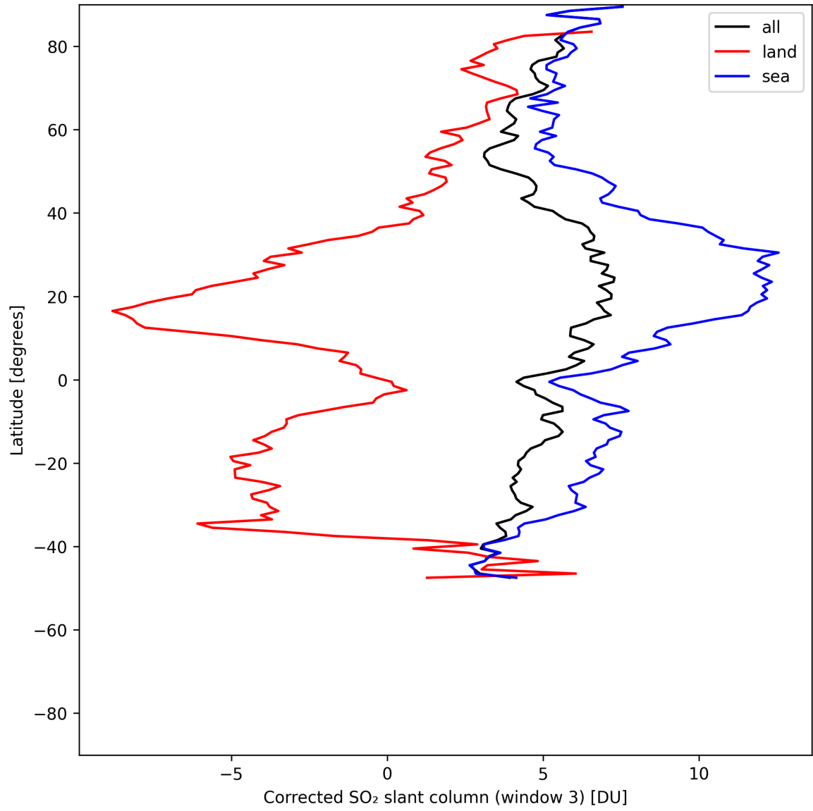
Figure 47: Zonal average of “Corrected SO 2 slant column (window 3)” for 2025-05-24 to 2025-05-26.
