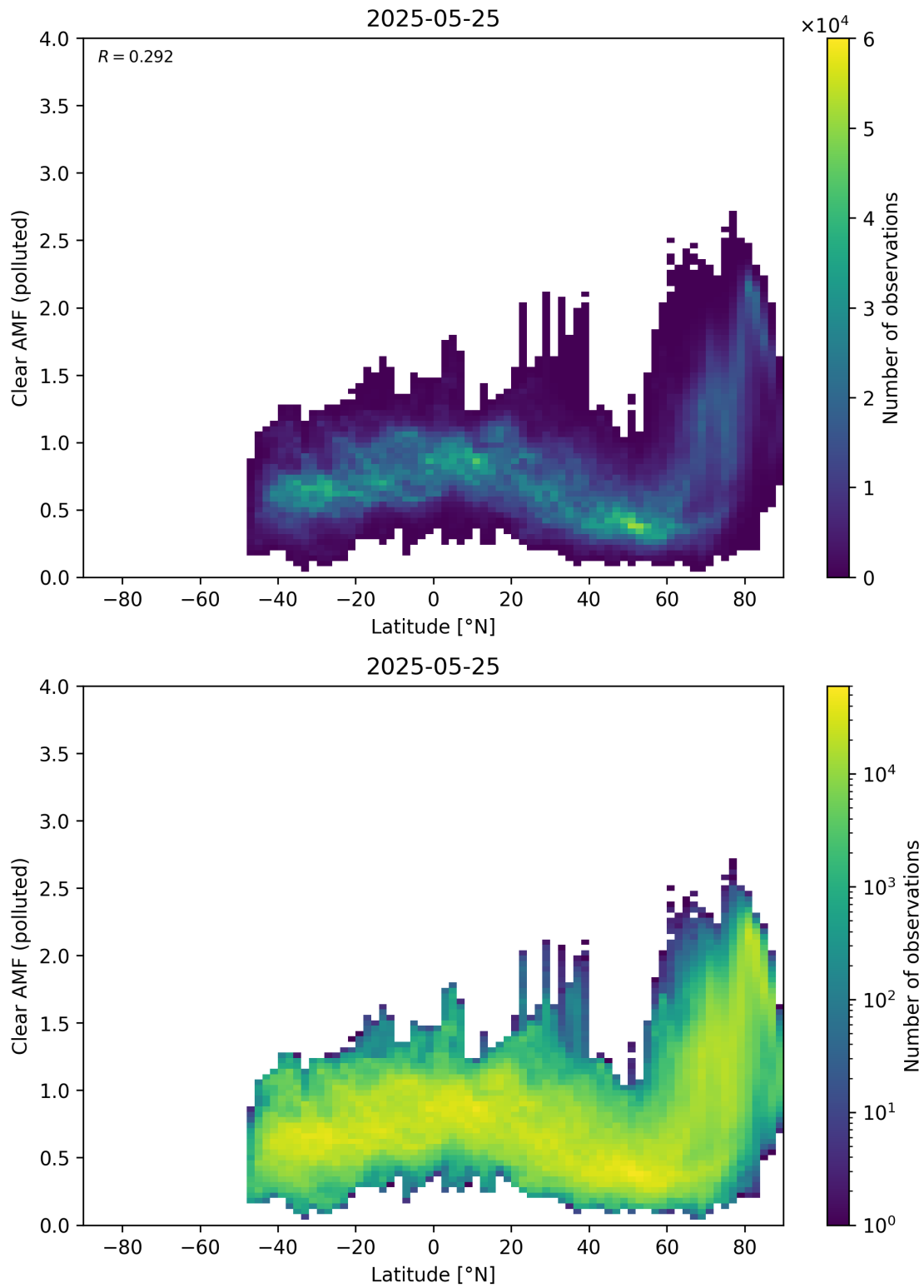
Figure 156: Scatter density plot of “Latitude” against “Clear AMF (polluted)” for 2025-05-24 to 2025-05-26.
