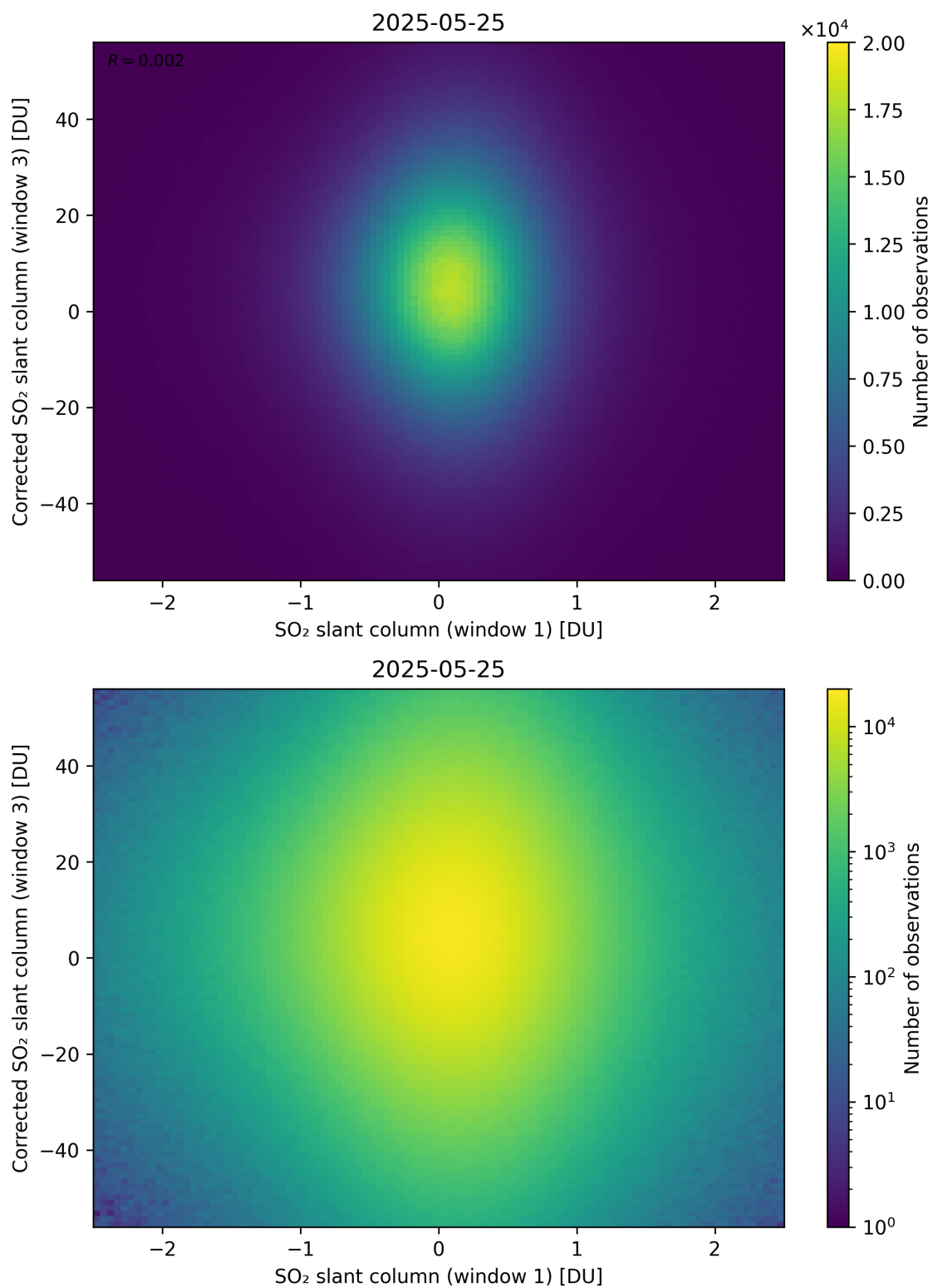
Figure 284: Scatter density plot of “SO 2 slant column (window 1)” against “Corrected SO 2 slant column (window 3)” for 2025-05-24 to 2025-05-26.
