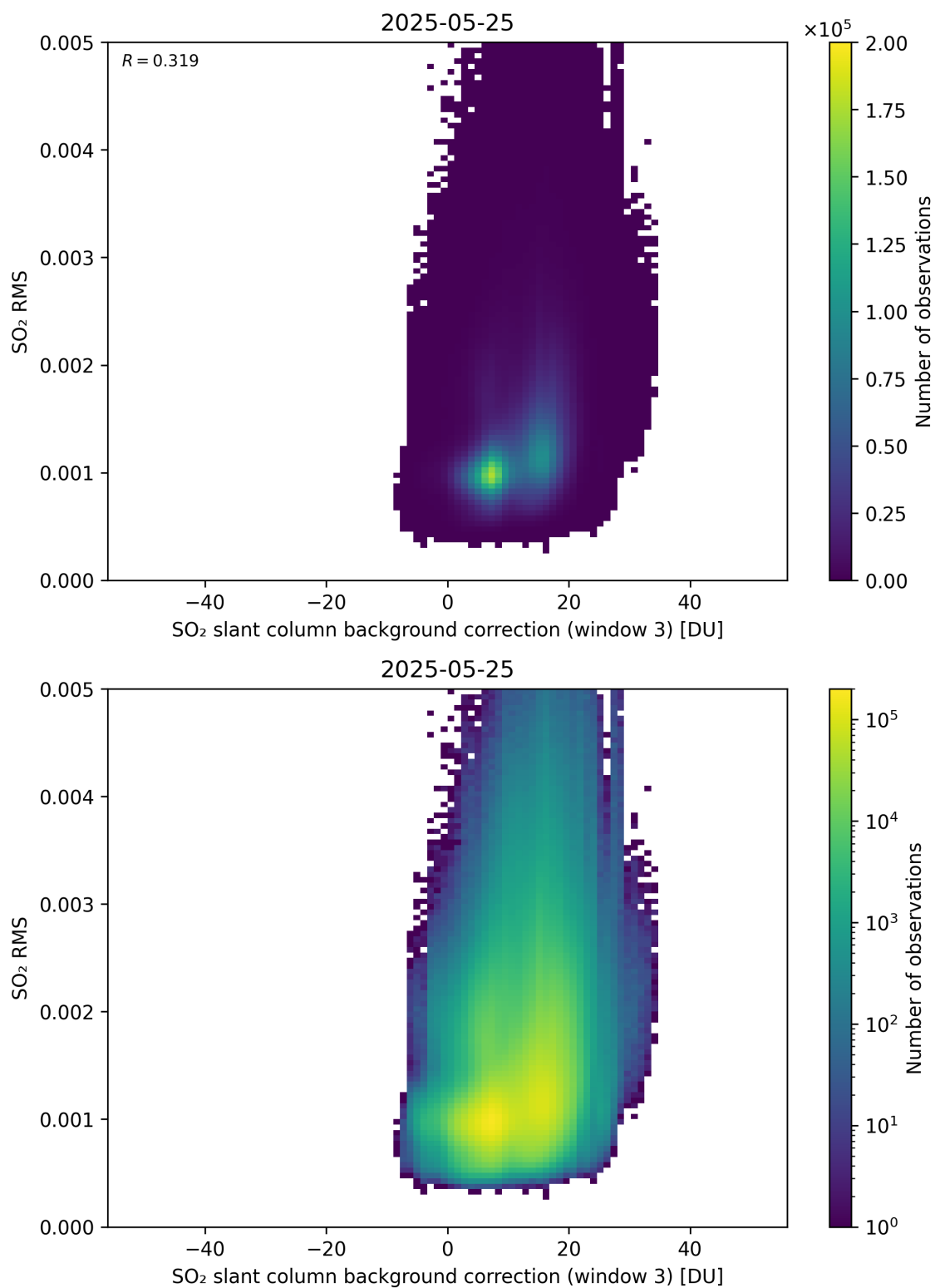
Figure 134: Scatter density plot of “SO 2 slant column background correction (window 3)” against “SO 2 RMS” for 2025-05-24 to 2025-05-26.
