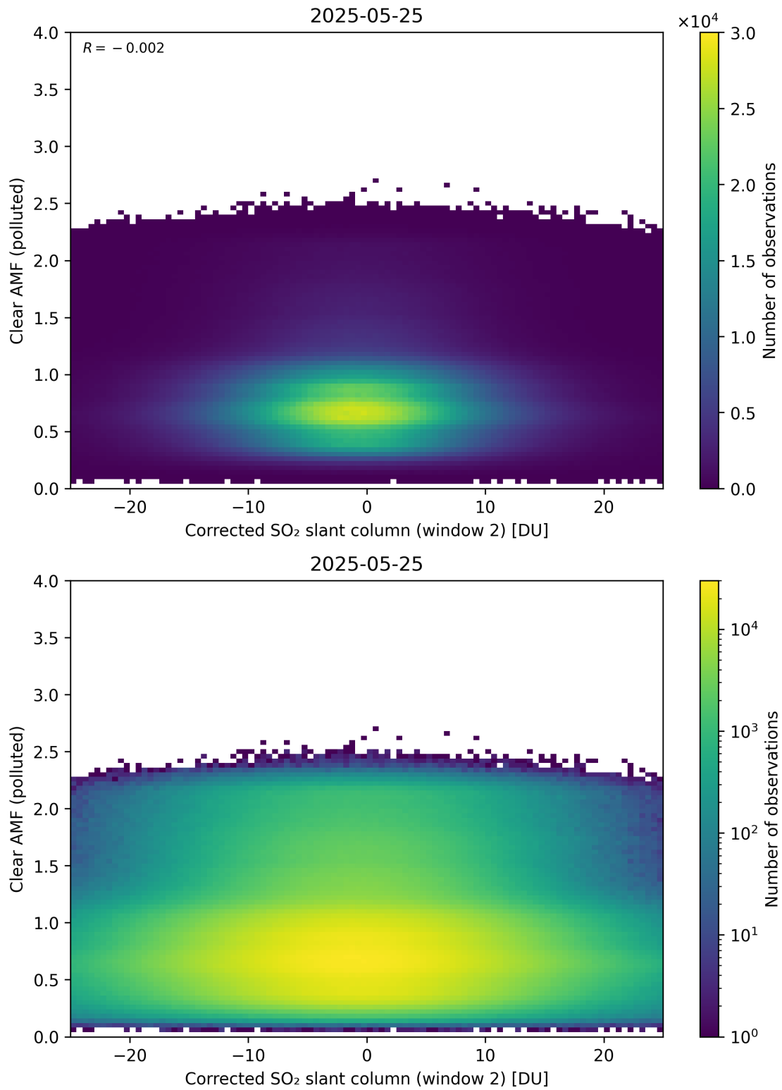
Figure 249: Scatter density plot of “Corrected SO 2 slant column (window 2)” against “Clear AMF (polluted)” for 2025-05-24 to 2025-05-26.
