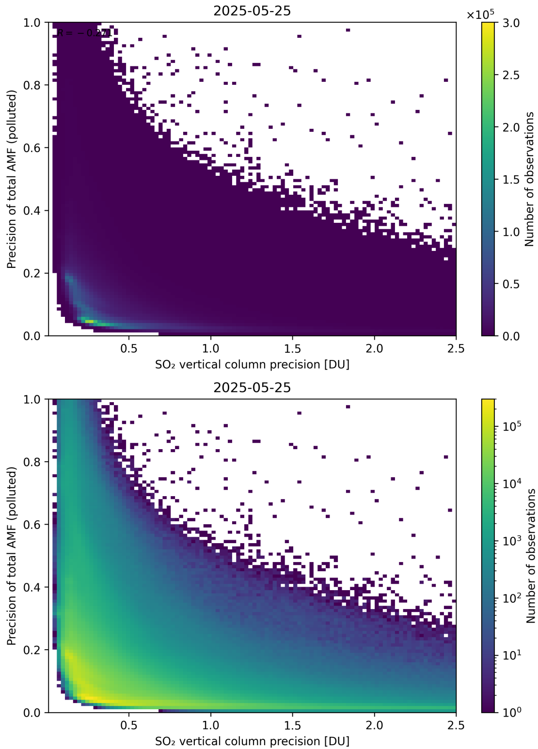
Figure 347: Scatter density plot of “SO 2 vertical column precision” against “Precision of total AMF (polluted)” for 2025-05-24 to 2025-05-26.
