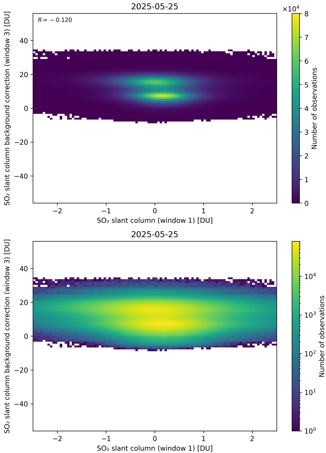
Figure 264: Scatter density plot of “SO 2 slant column (window 1)” against “SO 2 slant column background correction (window 3)” for 2025-05-24 to 2025-05-26.
