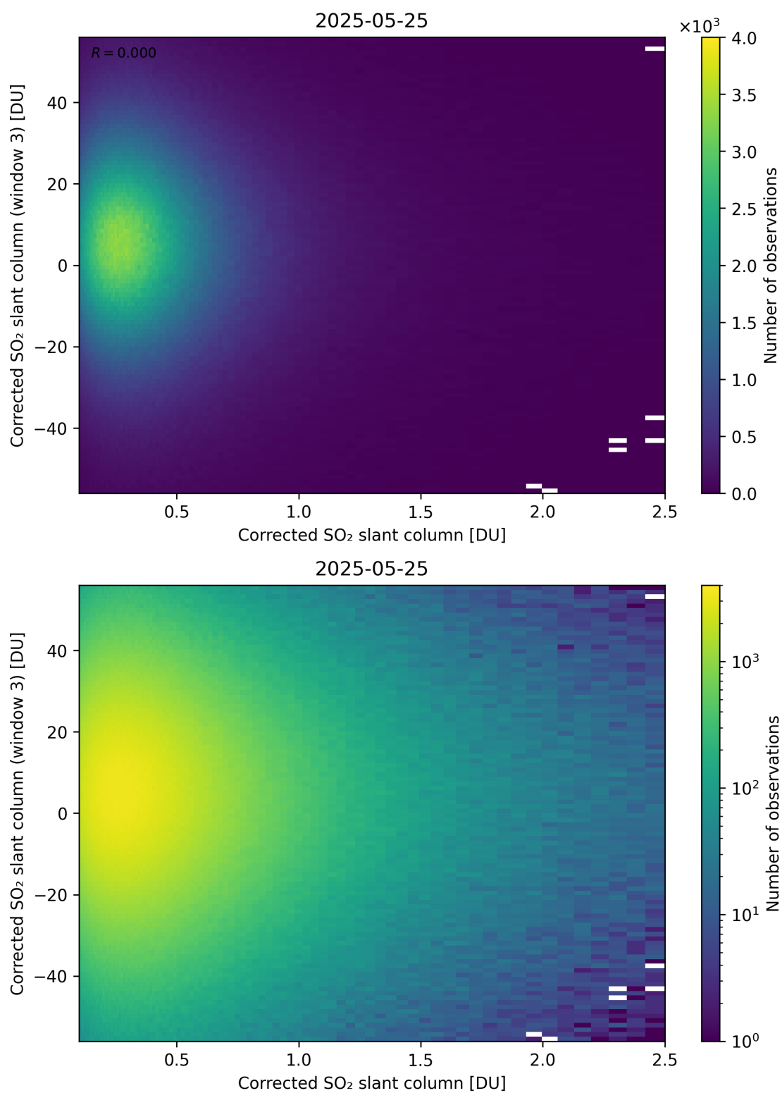
Figure 236: Scatter density plot of “Corrected SO 2 slant column” against “Corrected SO 2 slant column (window 3)” for 2025-05-24 to 2025-05-26.
