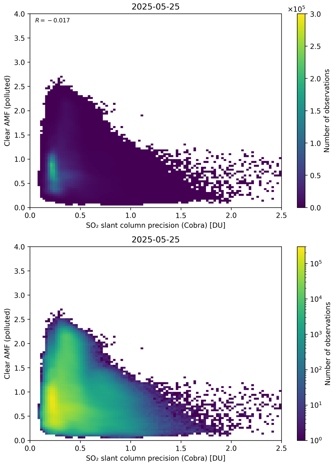
Figure 205: Scatter density plot of “SO 2 slant column precision (Cobra)” against “Clear AMF (polluted)” for 2025-05-24 to 2025-05-26.
