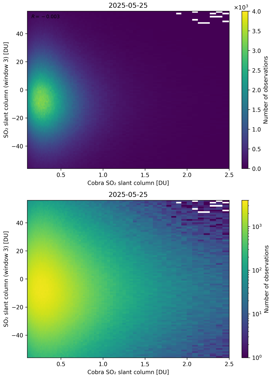
Figure 222: Scatter density plot of “Cobra SO 2 slant column” against “SO 2 slant column (window 3)” for 2025-05-24 to 2025-05-26.
