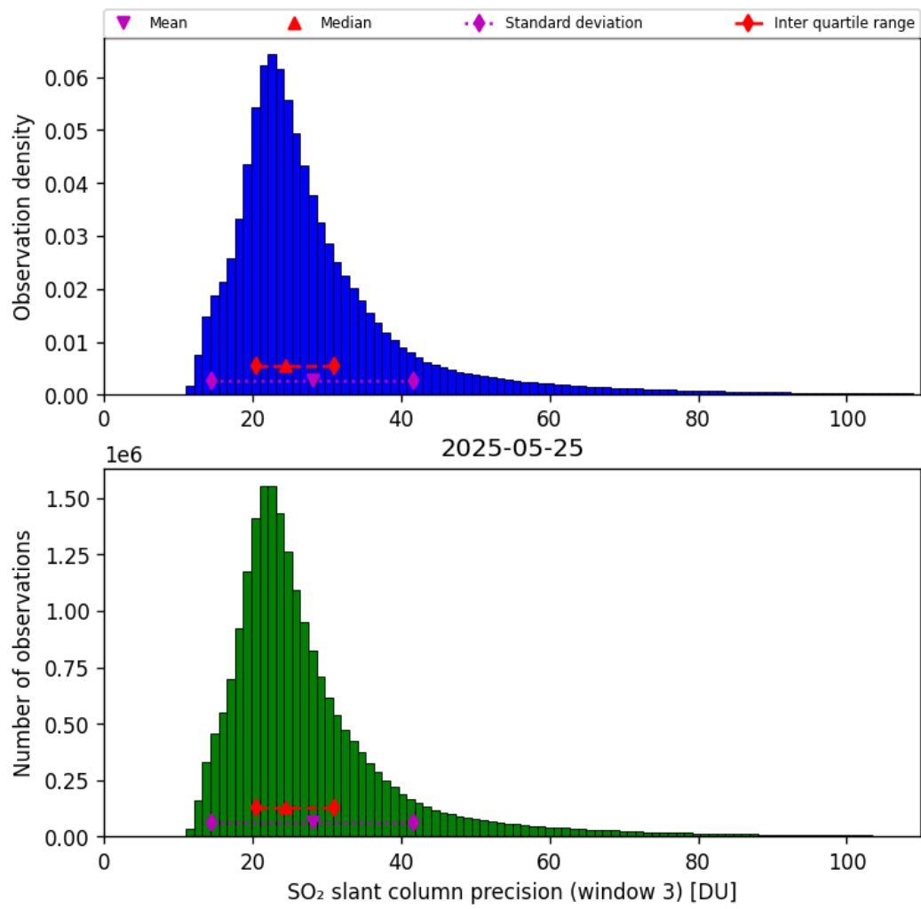
Figure 72: Histogram of “SO 2 slant column precision (window 3)” for 2025-05-24 to 2025-05-26
