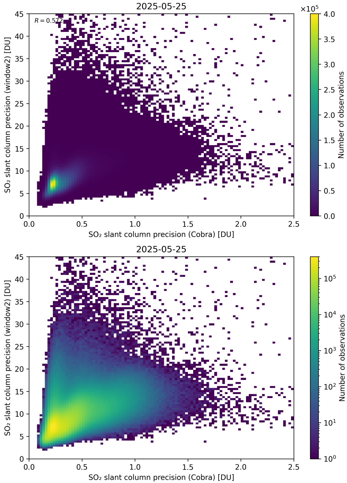
Figure 210: Scatter density plot of “SO 2 slant column precision (Cobra)” against “SO 2 slant column precision (window2)” for 2025-05-24 to 2025-05-26.
