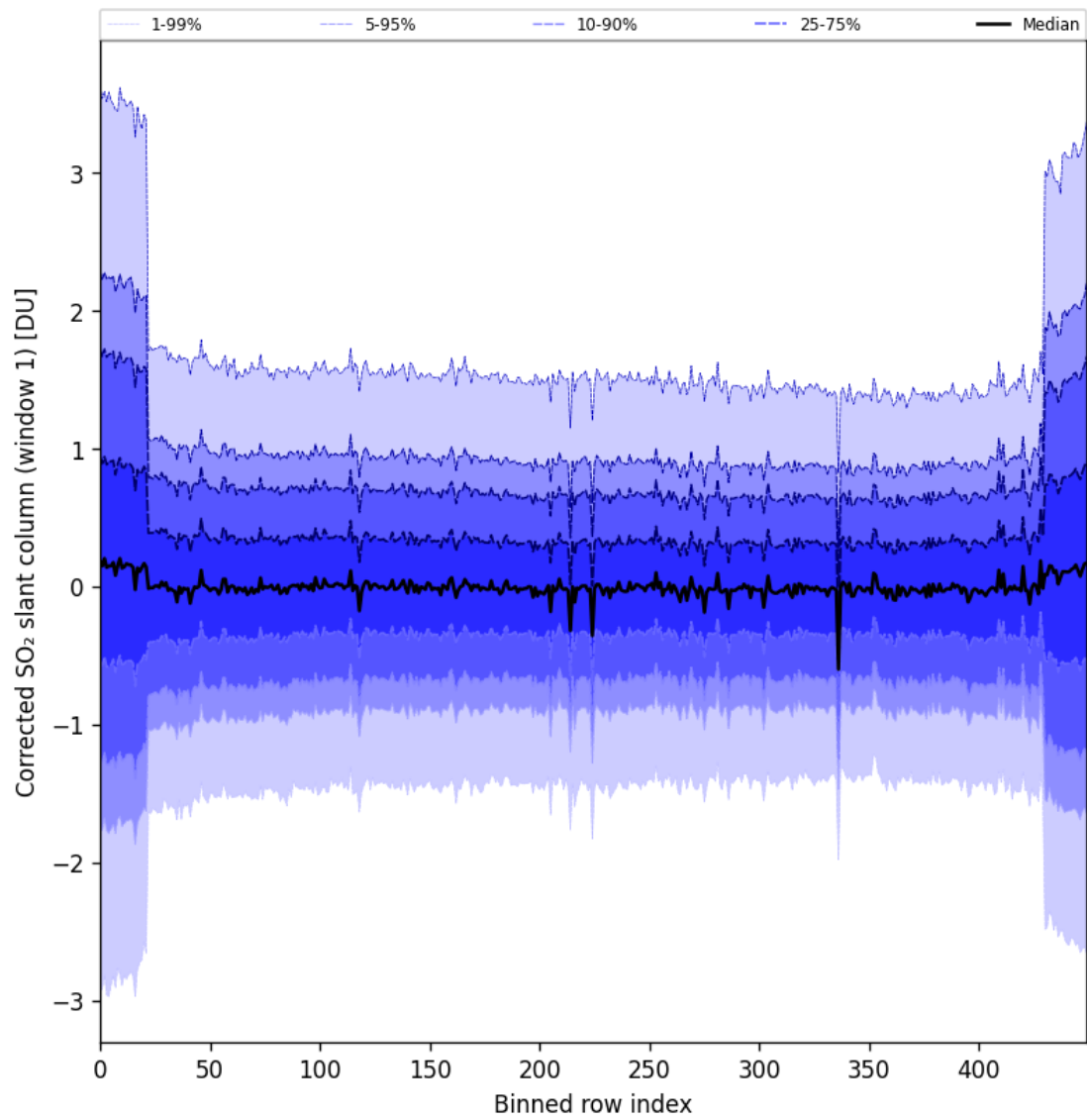
Figure 91: Along track statistics of “Corrected SO 2 slant column (window 1)” for 2025-05-24 to 2025-05-26
