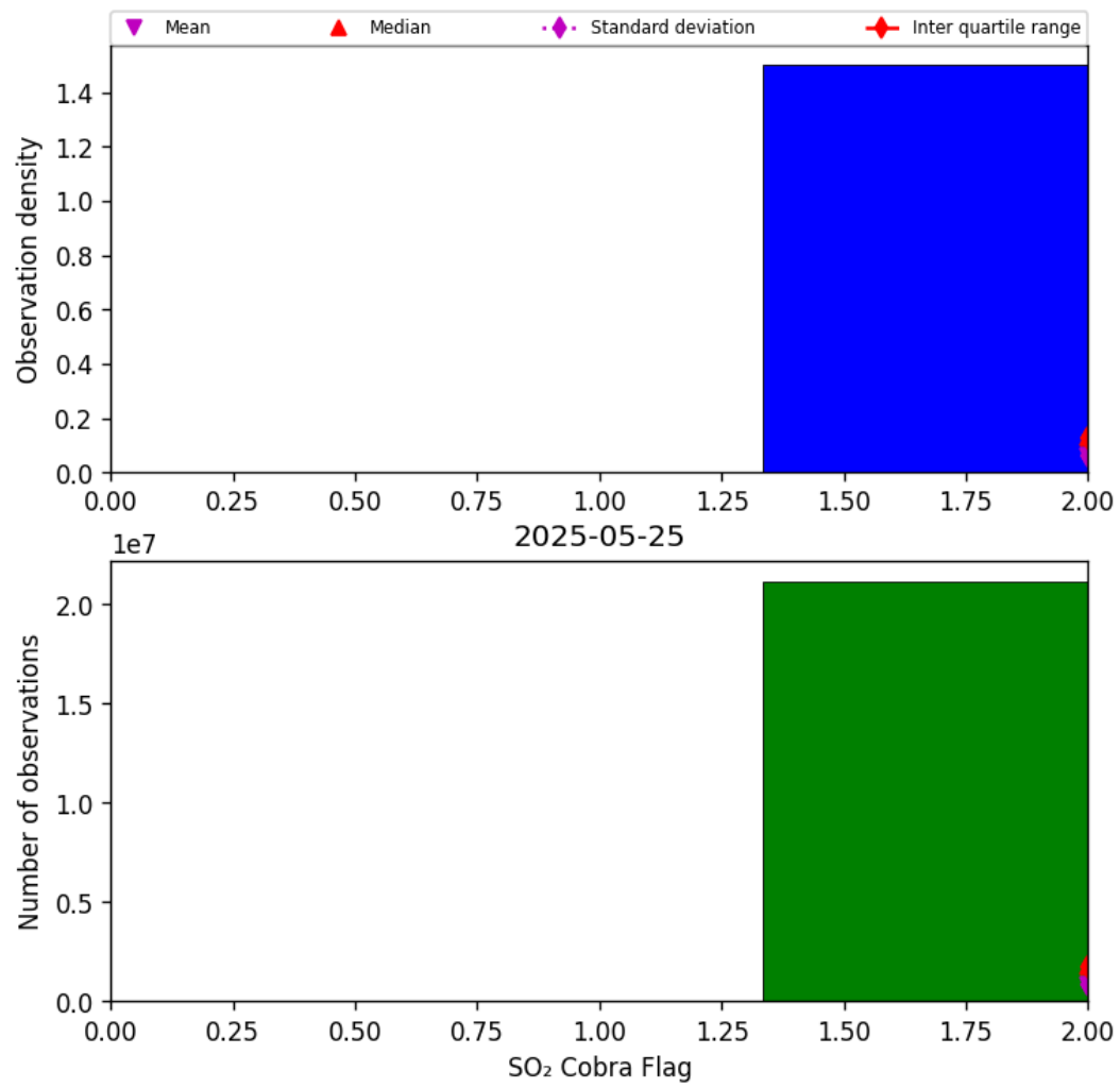
Figure 75: Histogram of “SO 2 Cobra Flag” for 2025-05-24 to 2025-05-26
