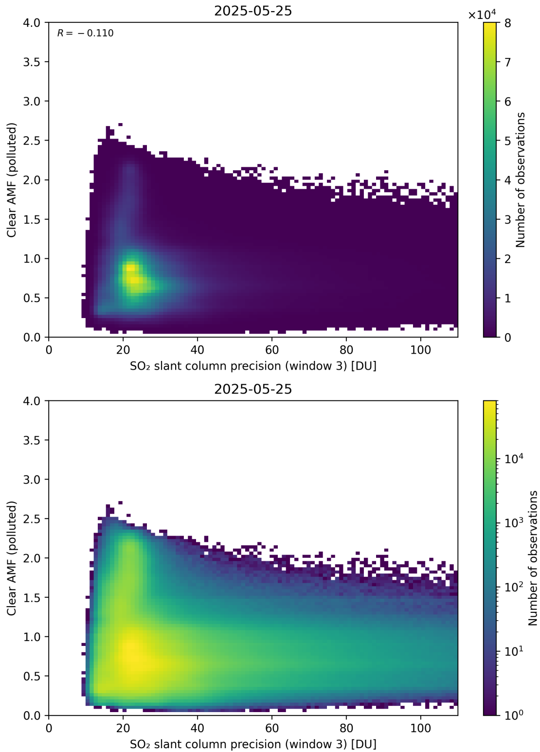
Figure 311: Scatter density plot of “SO 2 slant column precision (window 3)” against “Clear AMF (polluted)” for 2025-05-24 to 2025-05-26.
