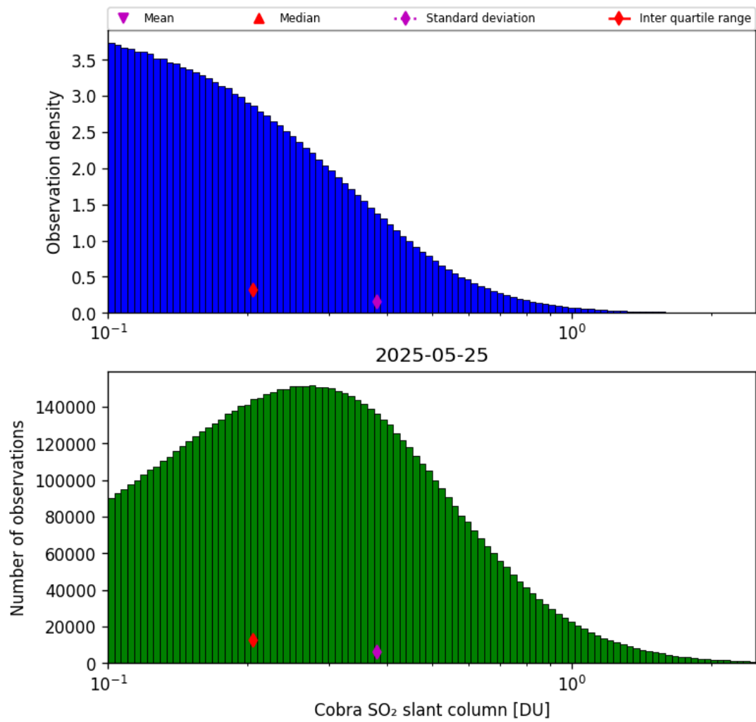
Figure 61: Histogram of “Cobra SO 2 slant column” for 2025-05-24 to 2025-05-26
