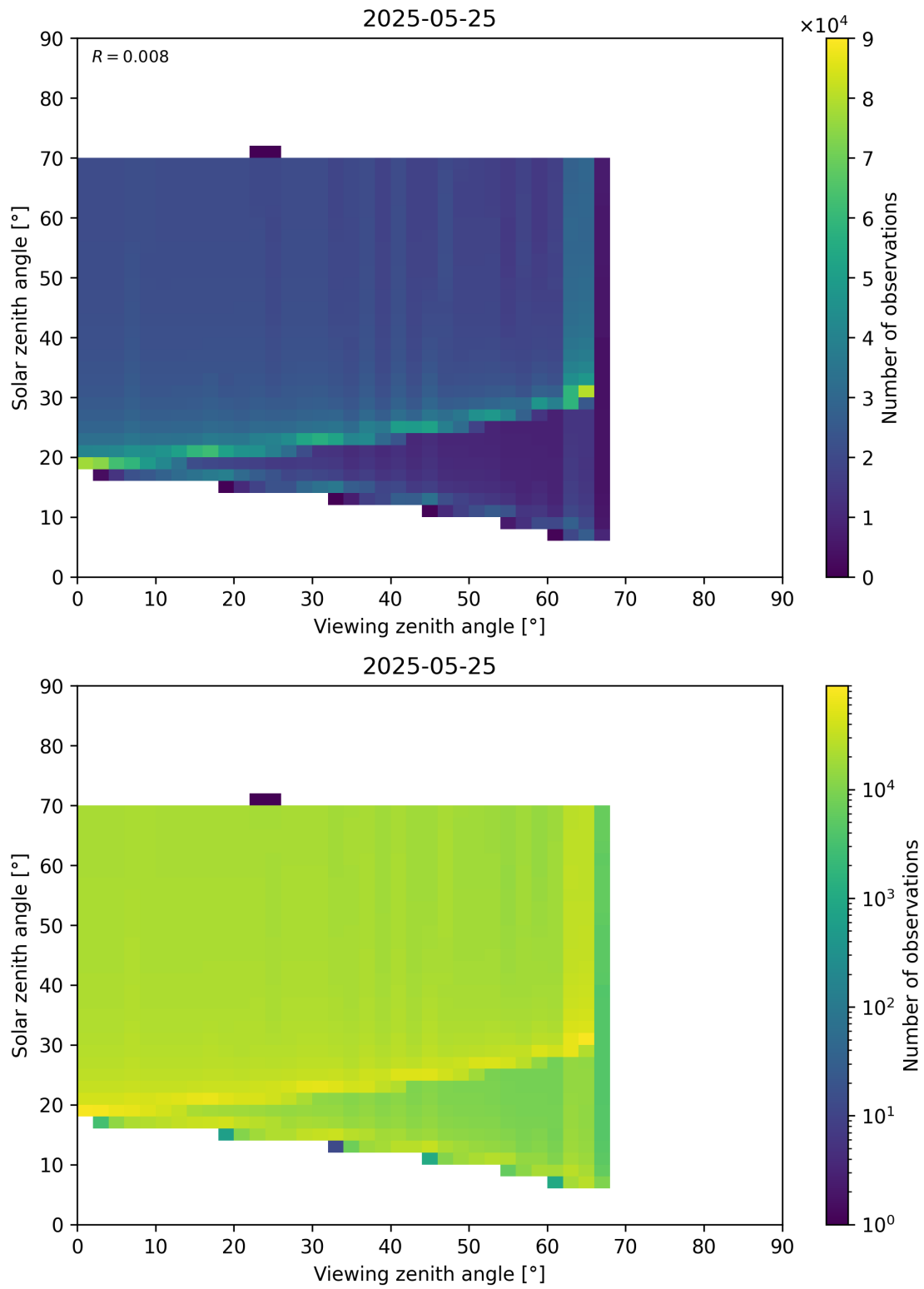
Figure 369: Scatter density plot of “Viewing zenith angle” against “Solar zenith angle” for 2025-05-24 to 2025-05-26.
