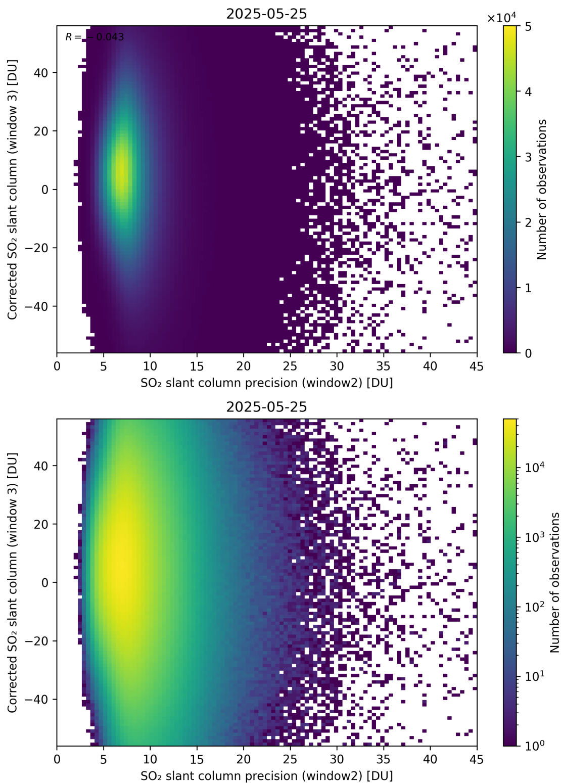
Figure 298: Scatter density plot of “SO 2 slant column precision (window2)” against “Corrected SO 2 slant column (window 3)” for 2025-05-24 to 2025-05-26.
