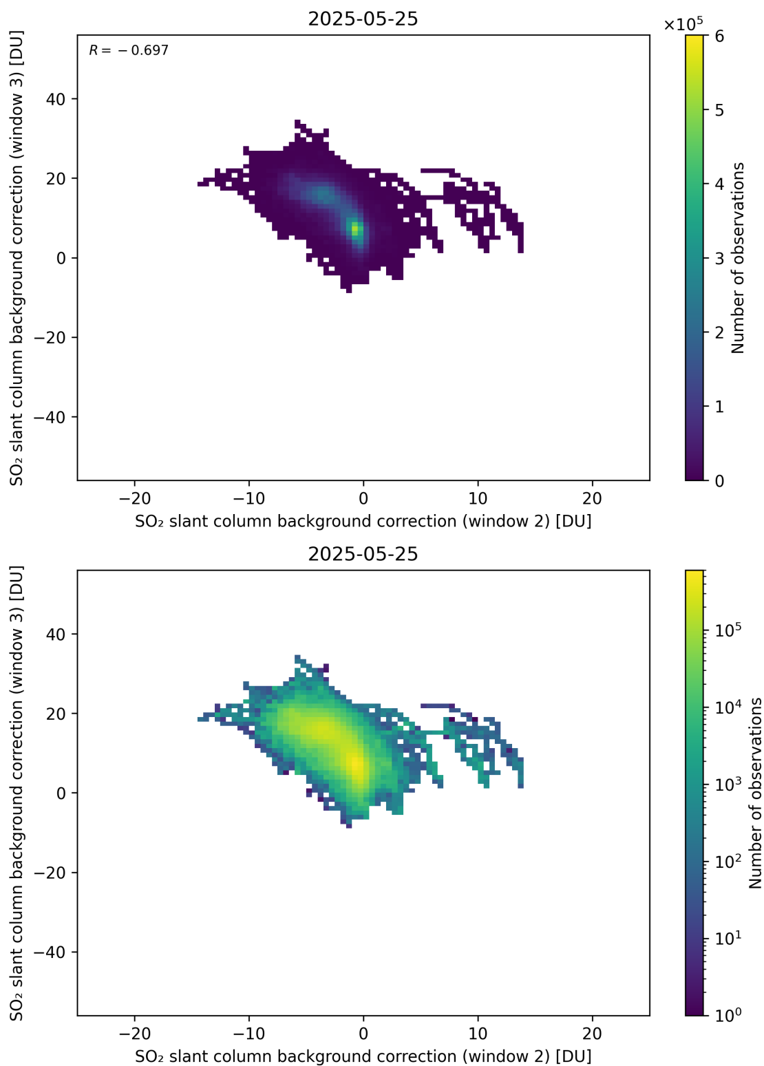
Figure 122: Scatter density plot of “SO 2 slant column background correction (window 2)” against “SO 2 slant column background correction (window 3)” for 2025-05-24 to 2025-05-26.
