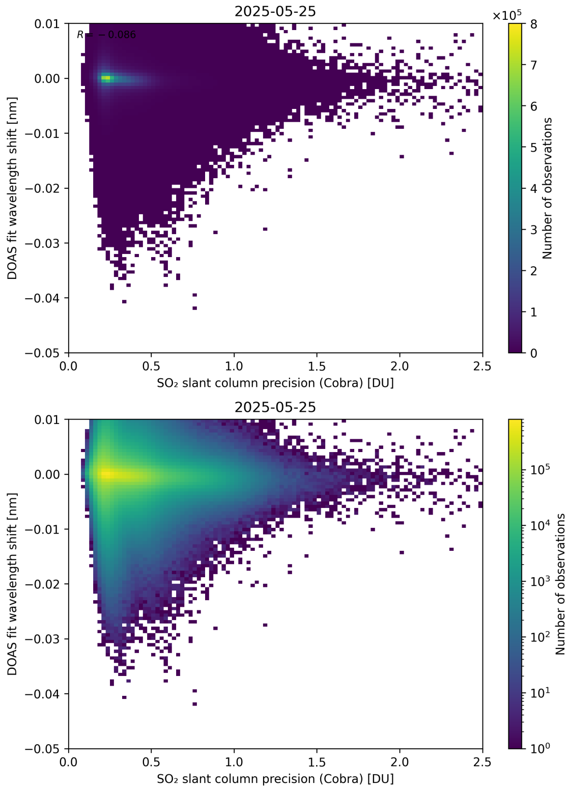
Figure 202: Scatter density plot of “SO 2 slant column precision (Cobra)” against “DOAS fit wavelength shift” for 2025-05-24 to 2025-05-26.
