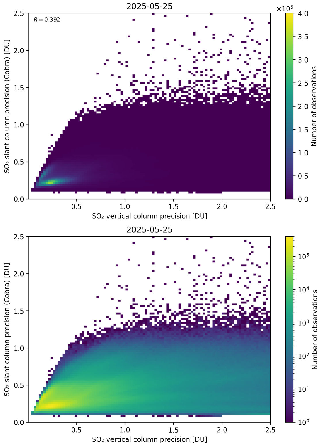
Figure 337: Scatter density plot of “SO 2 vertical column precision” against “SO 2 slant column precision (Cobra)” for 2025-05-24 to 2025-05-26.
