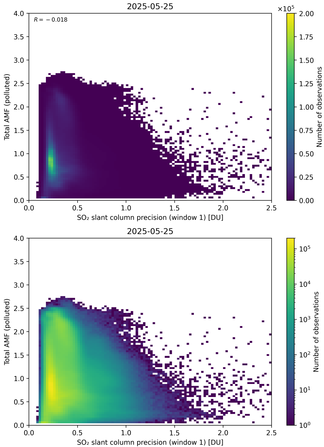
Figure 280: Scatter density plot of “SO 2 slant column precision (window 1)” against “Total AMF (polluted)” for 2025-05-24 to 2025-05-26.
