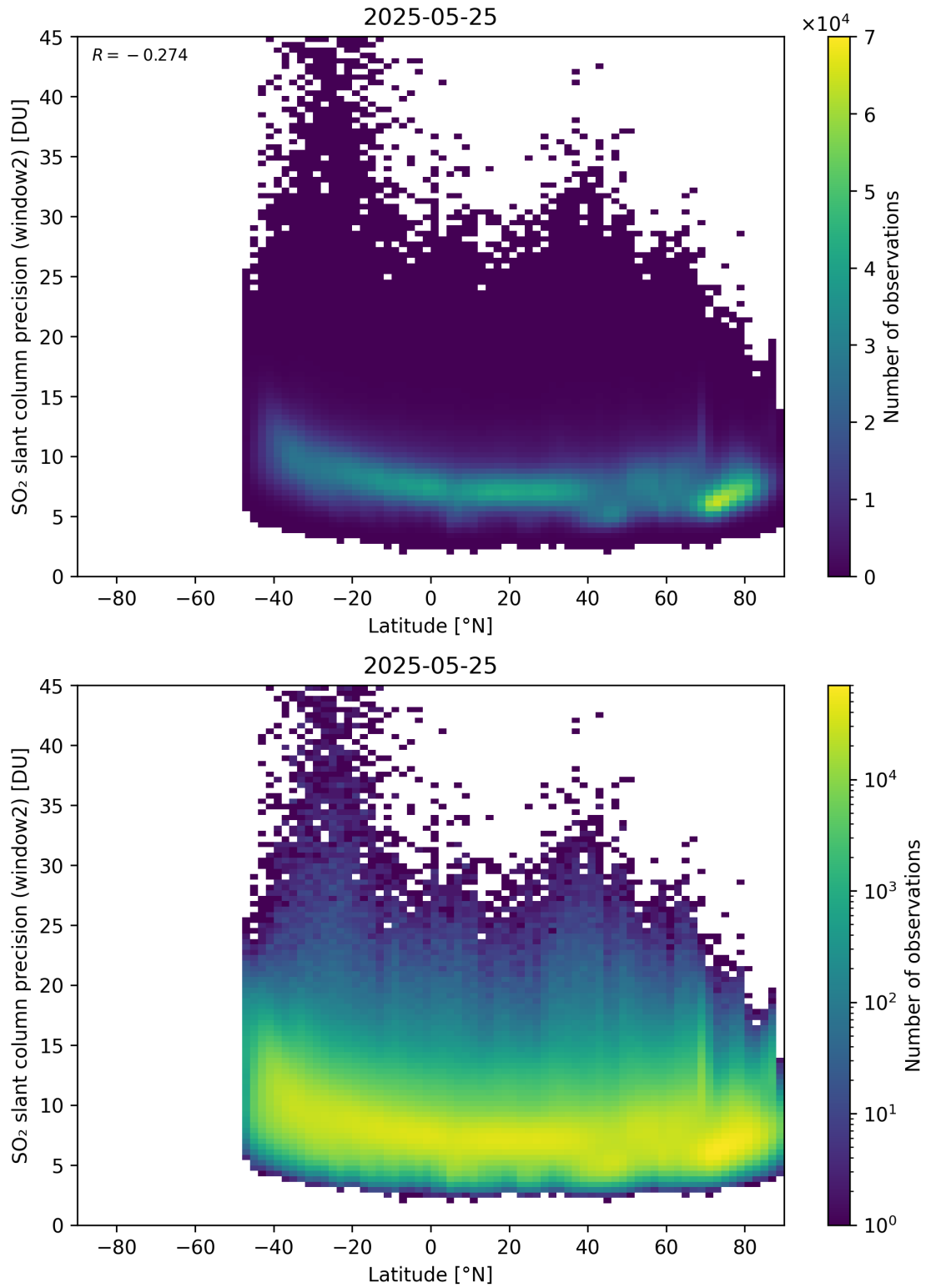
Figure 164: Scatter density plot of “Latitude” against “SO 2 slant column precision (window2)” for 2025-05-24 to 2025-05-26.
