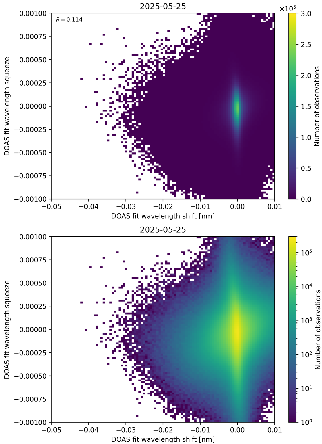
Figure 138: Scatter density plot of “DOAS fit wavelength shift” against “DOAS fit wavelength squeeze” for 2025-05-24 to 2025-05-26.
