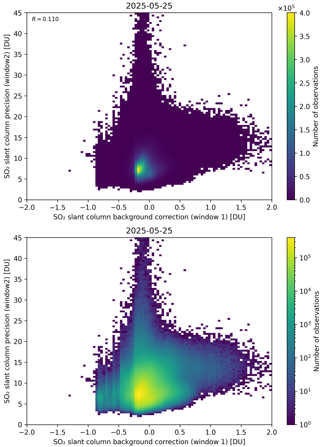
Figure 117: Scatter density plot of “SO 2 slant column background correction (window 1)” against “SO 2 slant column precision (window2)” for 2025-05-24 to 2025-05-26.
