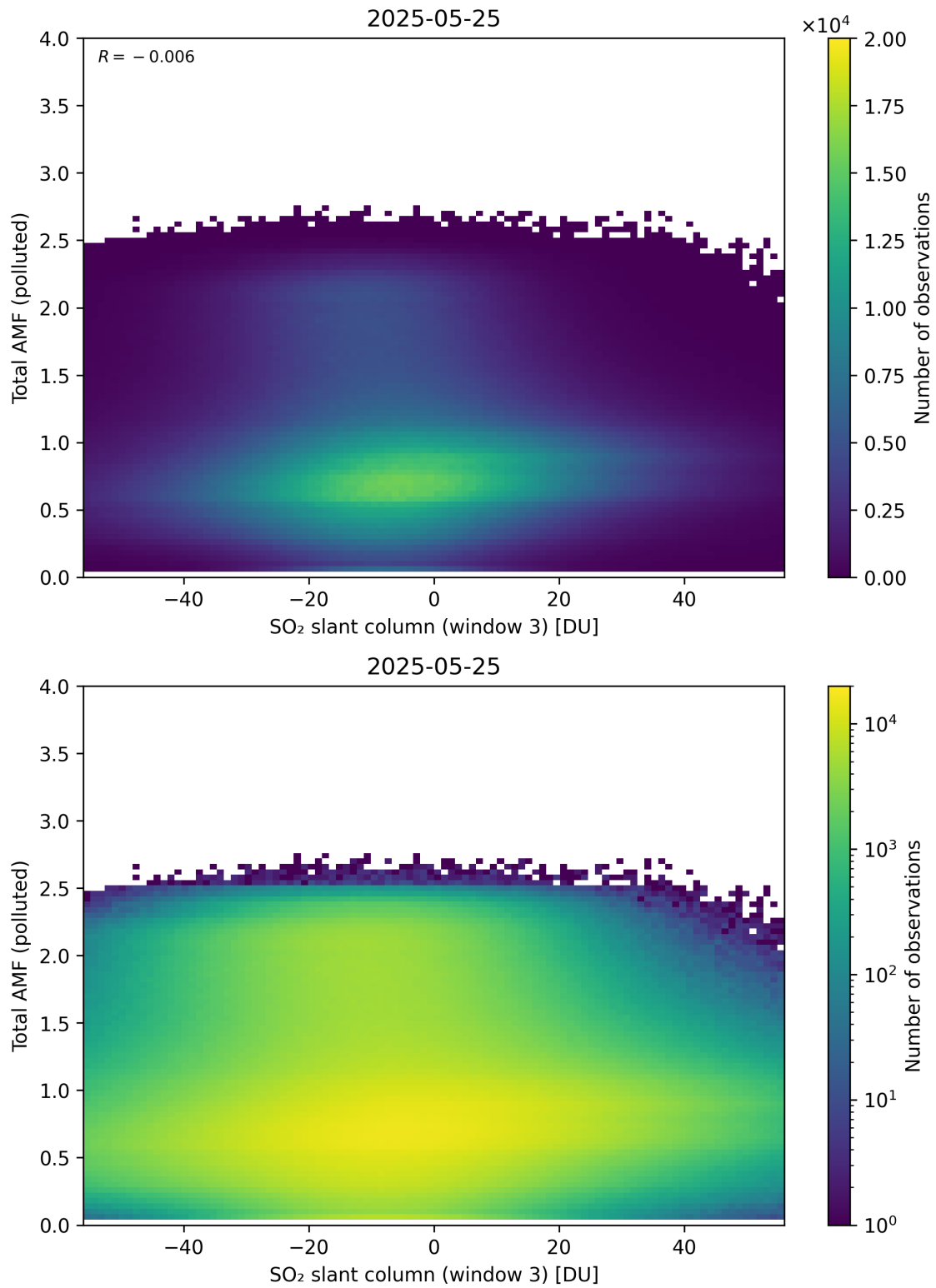
Figure 318: Scatter density plot of “SO 2 slant column (window 3)” against “Total AMF (polluted)” for 2025-05-24 to 2025-05-26.
