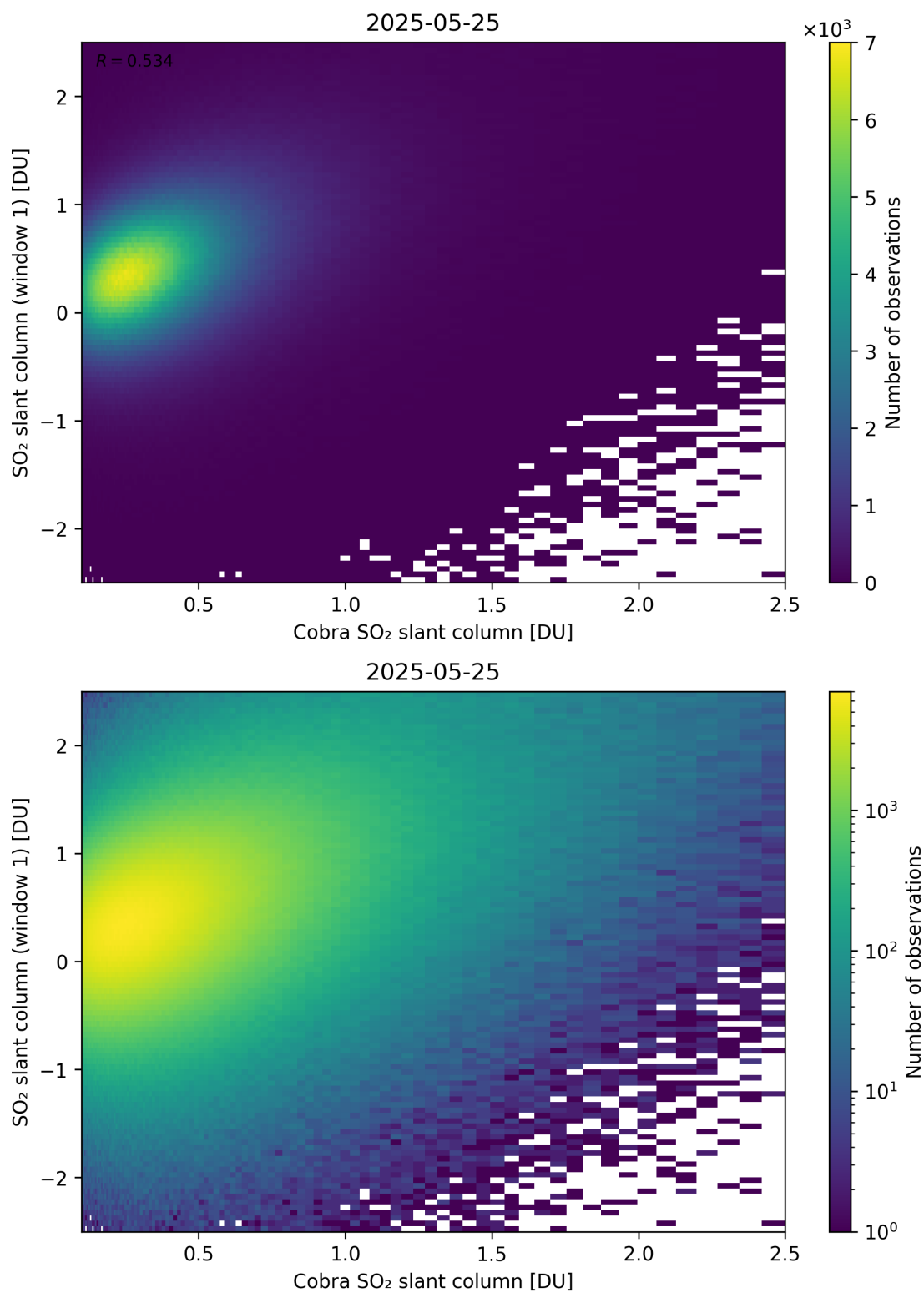
Figure 219: Scatter density plot of “Cobra SO 2 slant column” against “SO 2 slant column (window 1)” for 2025-05-24 to 2025-05-26.
