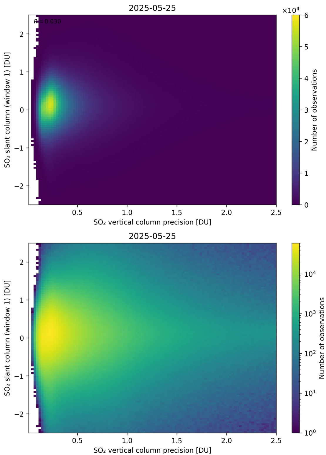
Figure 341: Scatter density plot of “SO 2 vertical column precision” against “SO 2 slant column (window 1)” for 2025-05-24 to 2025-05-26.
