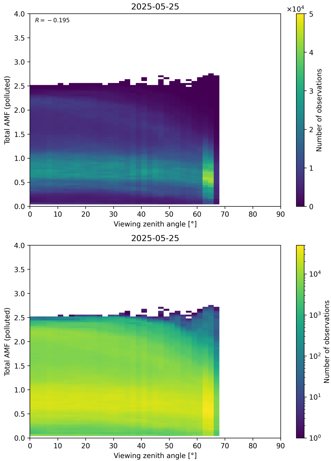
Figure 381: Scatter density plot of “Viewing zenith angle” against “Total AMF (polluted)” for 2025-05-24 to 2025-05-26.
