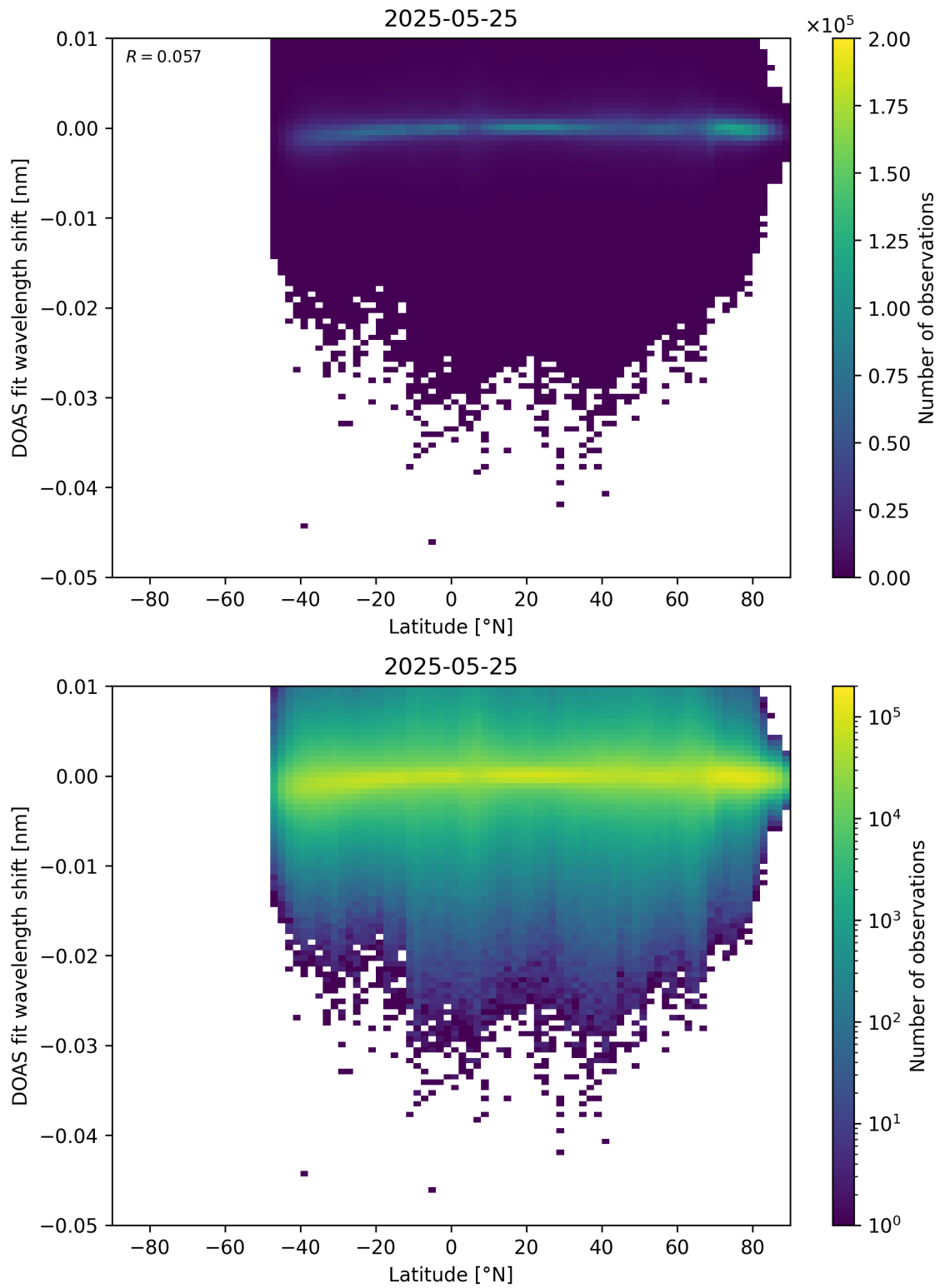
Figure 153: Scatter density plot of “Latitude” against “DOAS fit wavelength shift” for 2025-05-24 to 2025-05-26.
