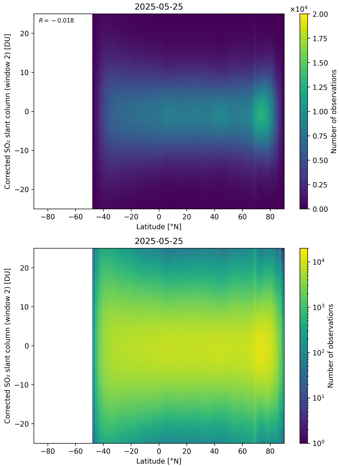
Figure 160: Scatter density plot of “Latitude” against “Corrected SO 2 slant column (window 2)” for 2025-05-24 to 2025-05-26.
