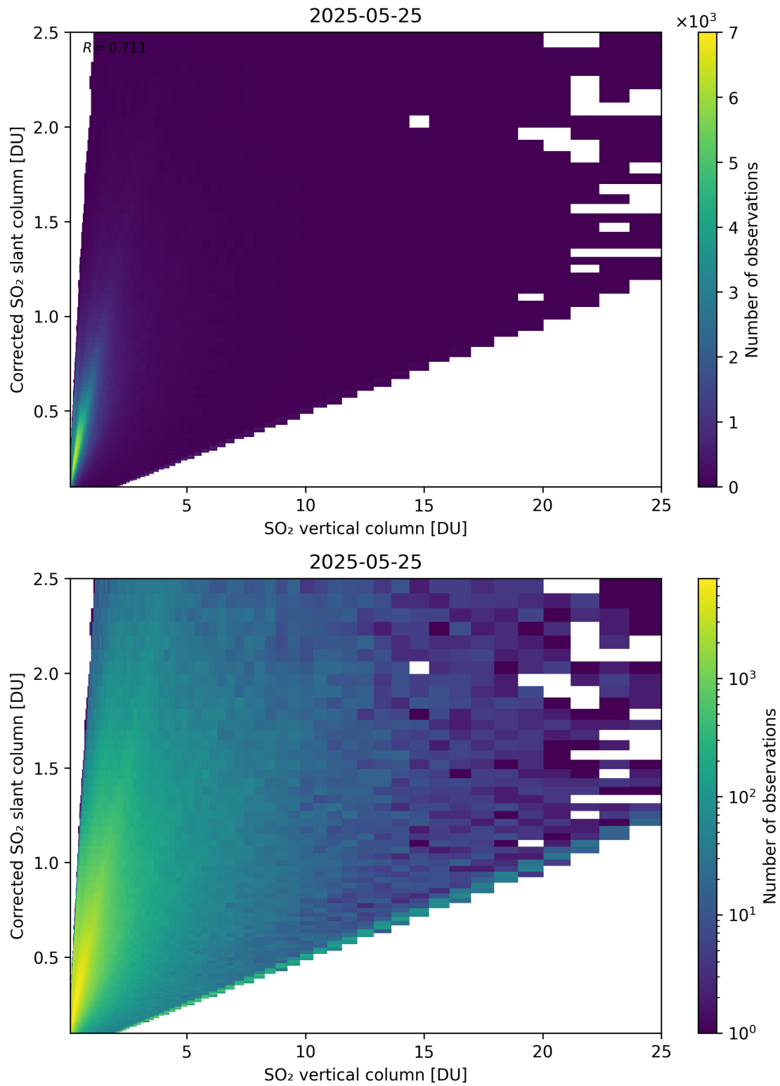
Figure 351: Scatter density plot of “SO 2 vertical column” against “Corrected SO 2 slant column” for 2025-05-24 to 2025-05-26.
