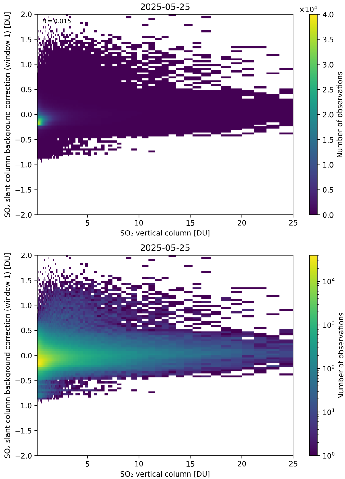
Figure 323: Scatter density plot of “SO 2 vertical column” against “SO 2 slant column background correction (window 1)” for 2025-05-24 to 2025-05-26.
