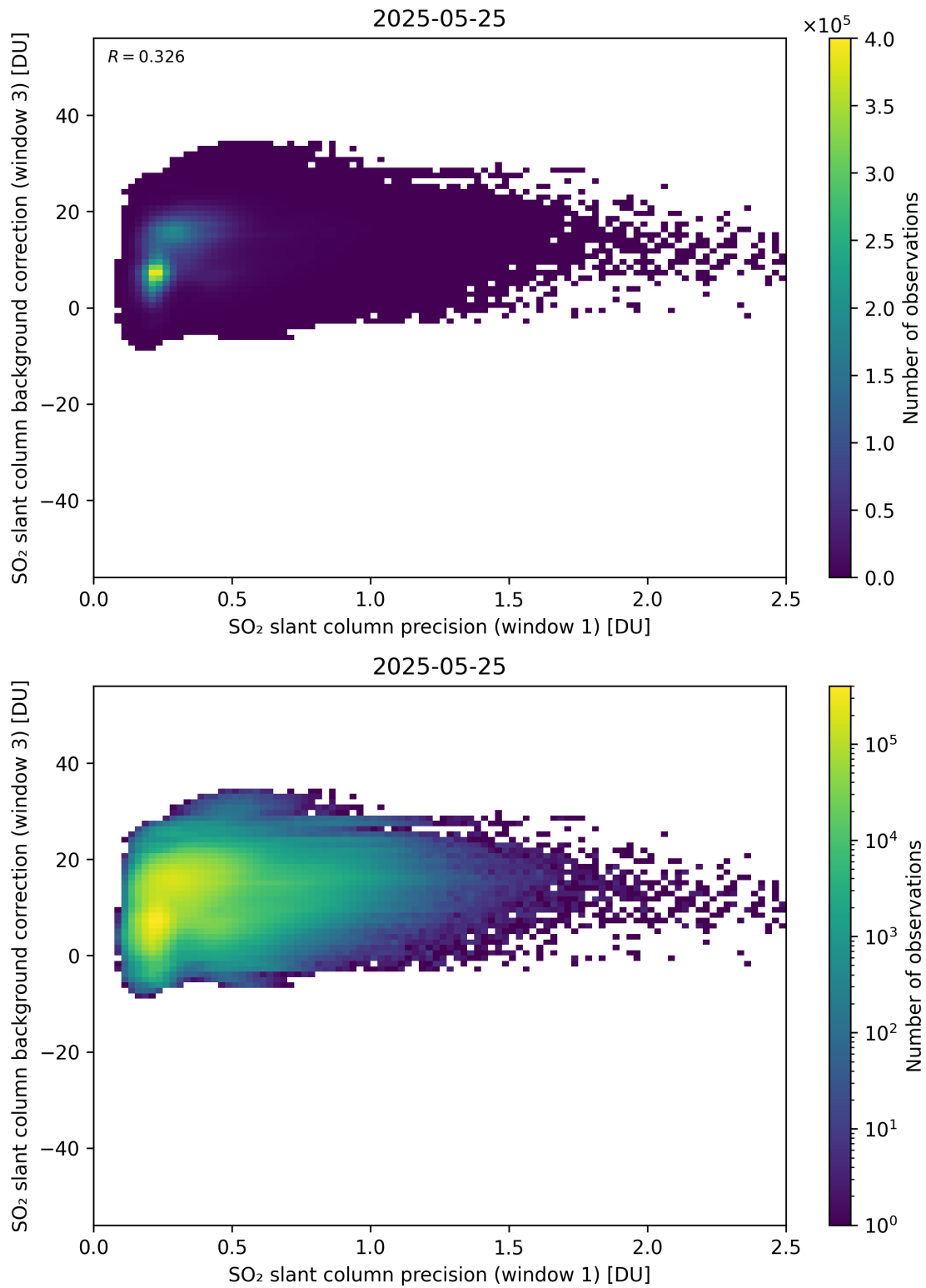
Figure 270: Scatter density plot of “SO 2 slant column precision (window 1)” against “SO 2 slant column background correction (window 3)” for 2025-05-24 to 2025-05-26.
