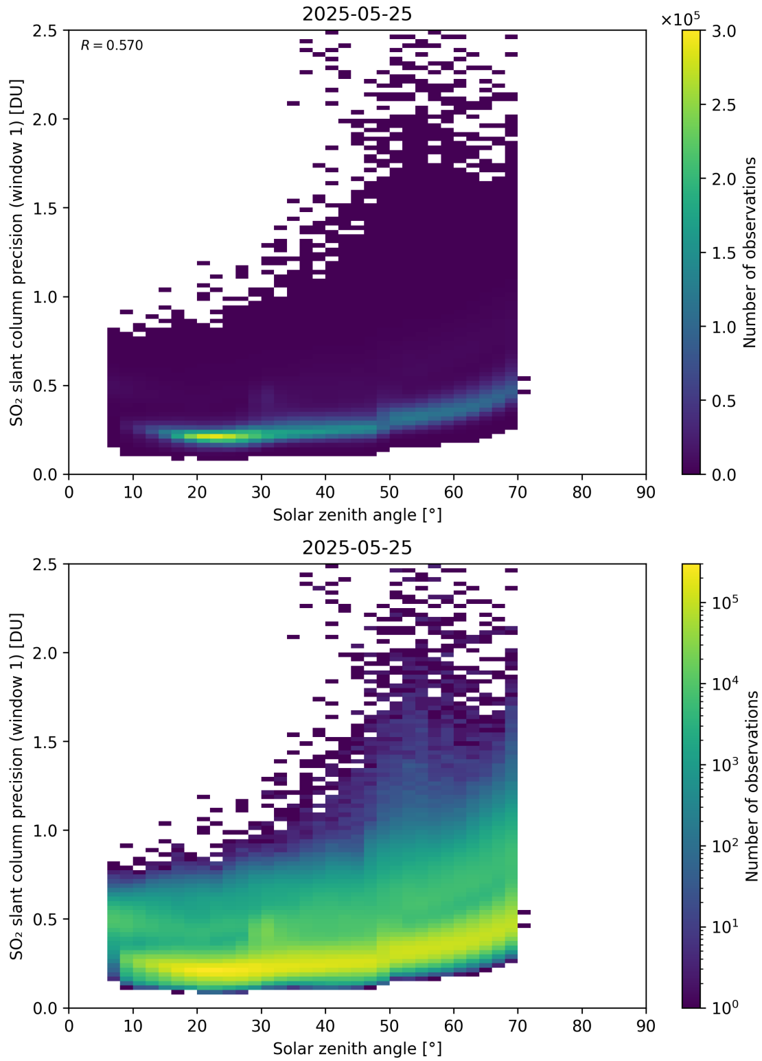
Figure 185: Scatter density plot of “Solar zenith angle” against “SO 2 slant column precision (window 1)” for 2025-05-24 to 2025-05-26.
