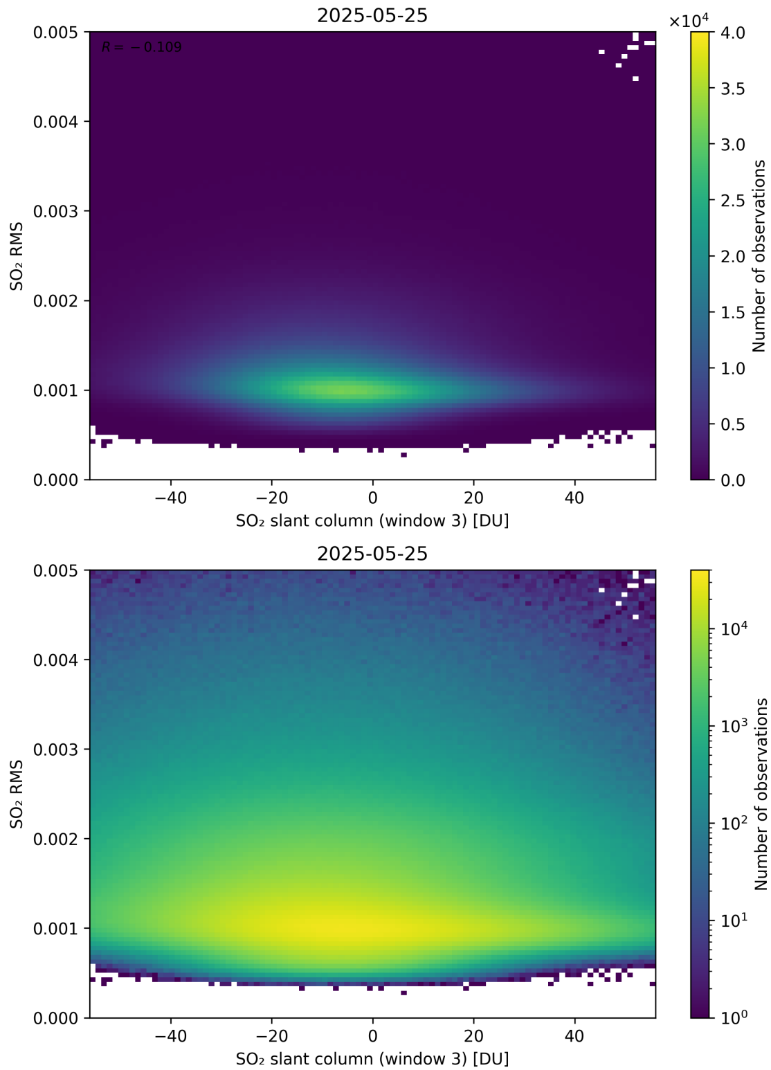
Figure 306: Scatter density plot of “SO 2 slant column (window 3)” against “SO 2 RMS” for 2025-05-24 to 2025-05-26.
