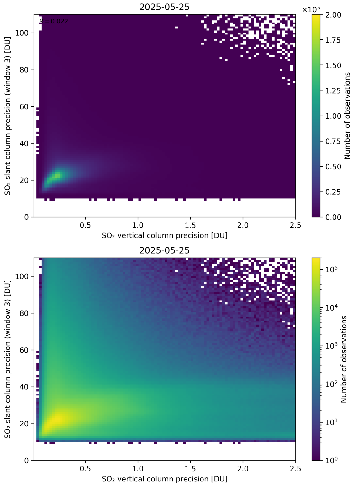
Figure 345: Scatter density plot of “SO 2 vertical column precision” against “SO 2 slant column precision (window 3)” for 2025-05-24 to 2025-05-26.
