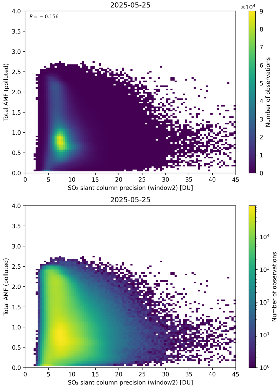
Figure 301: Scatter density plot of “SO 2 slant column precision (window2)” against “Total AMF (polluted)” for 2025-05-24 to 2025-05-26.
