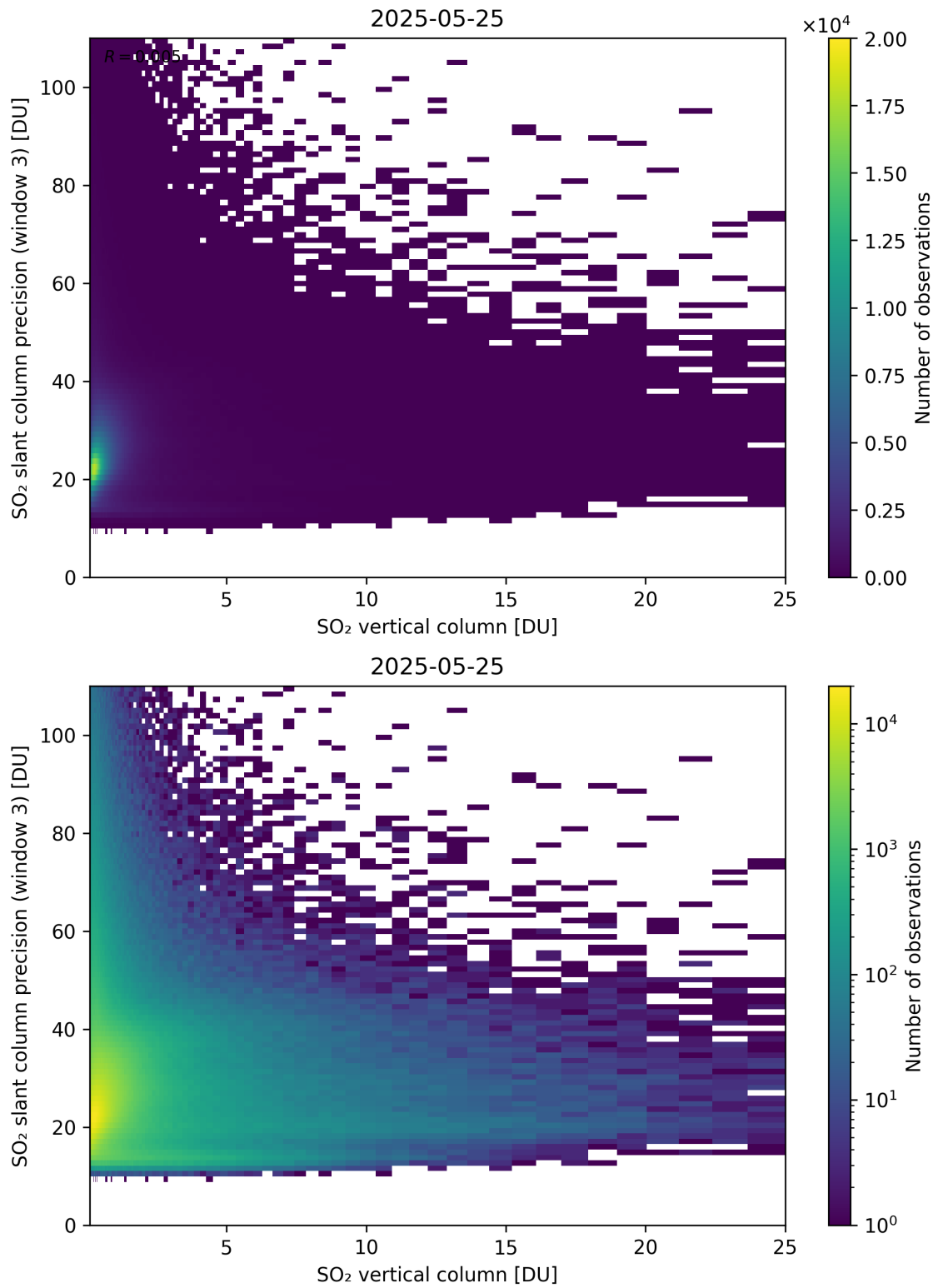
Figure 358: Scatter density plot of “SO 2 vertical column” against “SO 2 slant column precision (window 3)” for 2025-05-24 to 2025-05-26.
