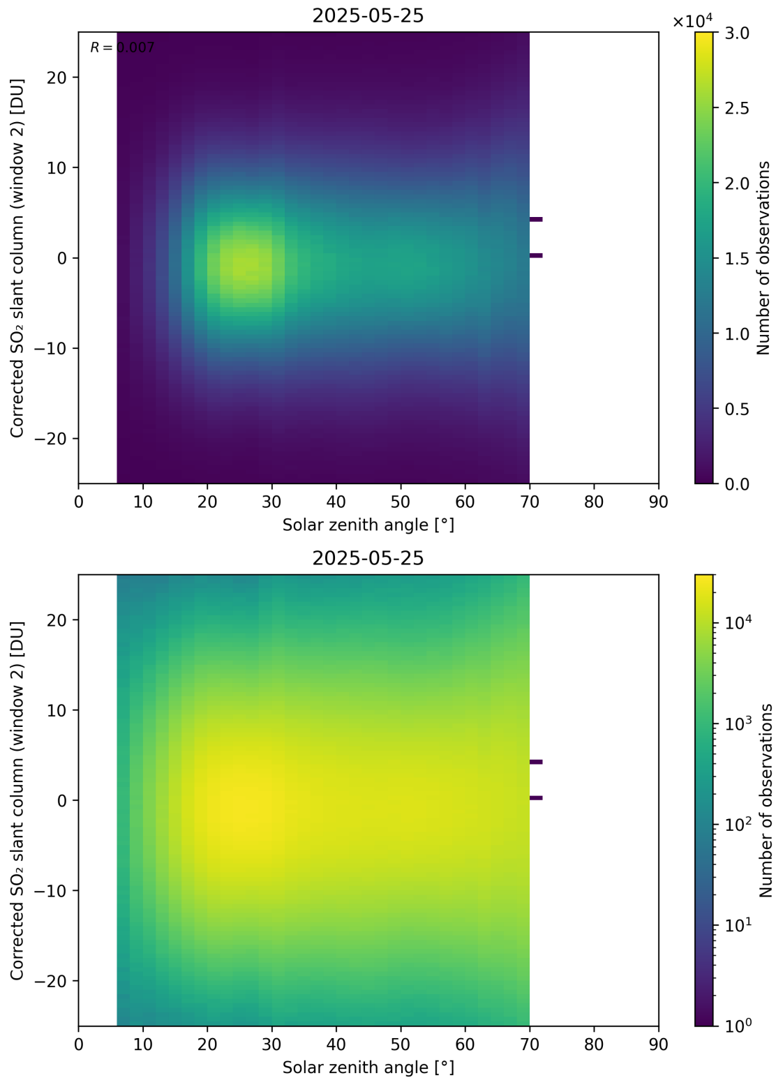
Figure 182: Scatter density plot of “Solar zenith angle” against “Corrected SO 2 slant column (window 2)” for 2025-05-24 to 2025-05-26.
