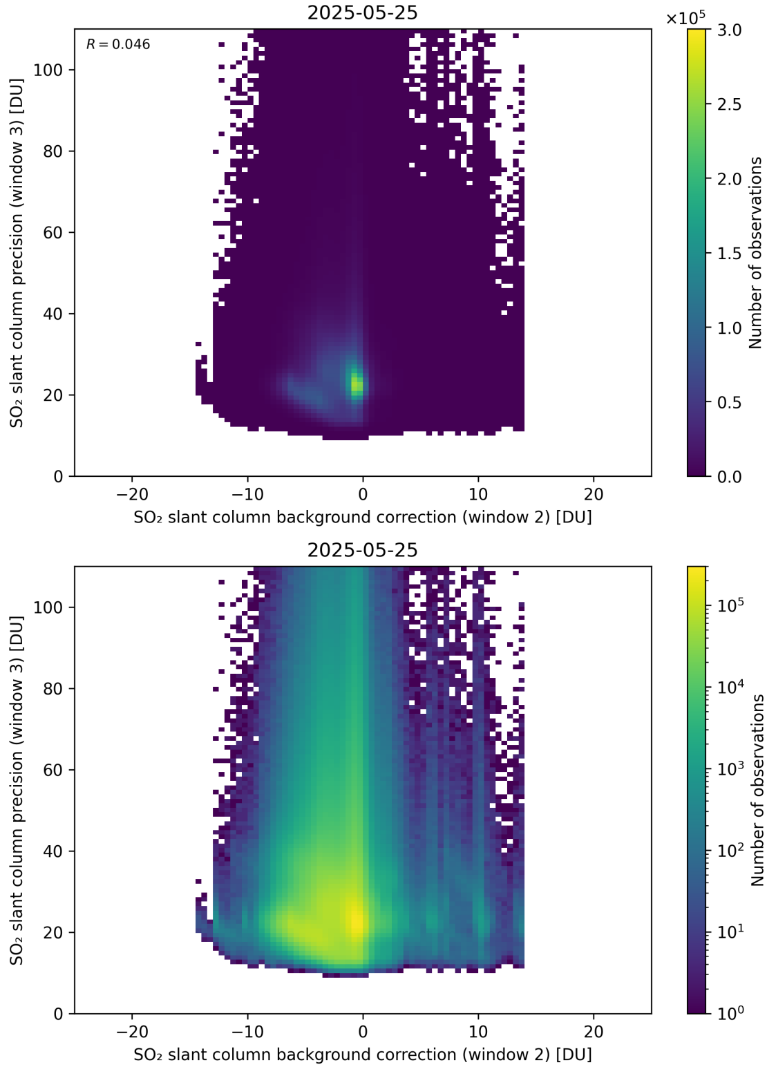
Figure 129: Scatter density plot of “SO 2 slant column background correction (window 2)” against “SO 2 slant column precision (window 3)” for 2025-05-24 to 2025-05-26.
