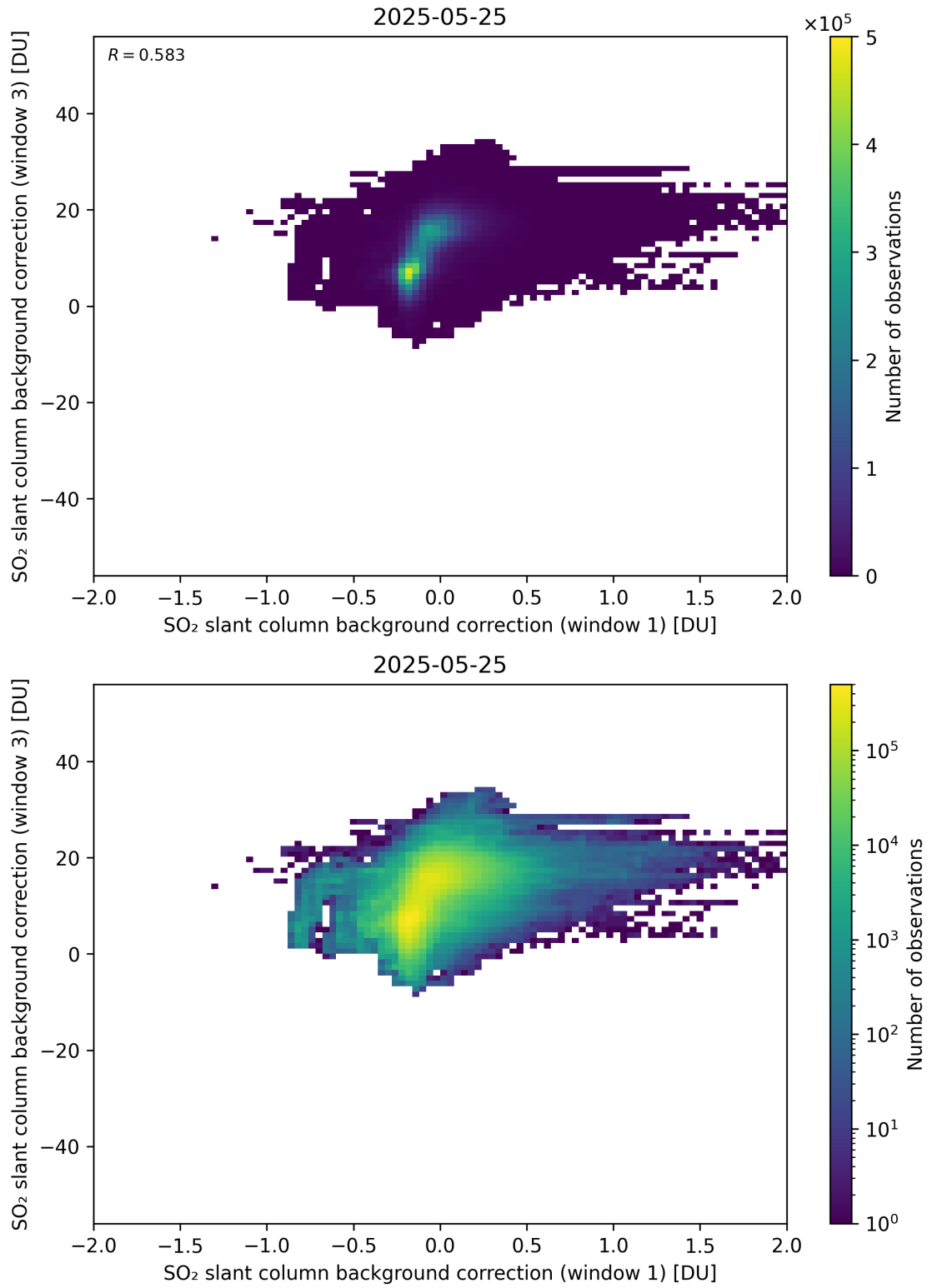
Figure 110: Scatter density plot of “SO 2 slant column background correction (window 1)” against “SO 2 slant column background correction (window 3)” for 2025-05-24 to 2025-05-26.
