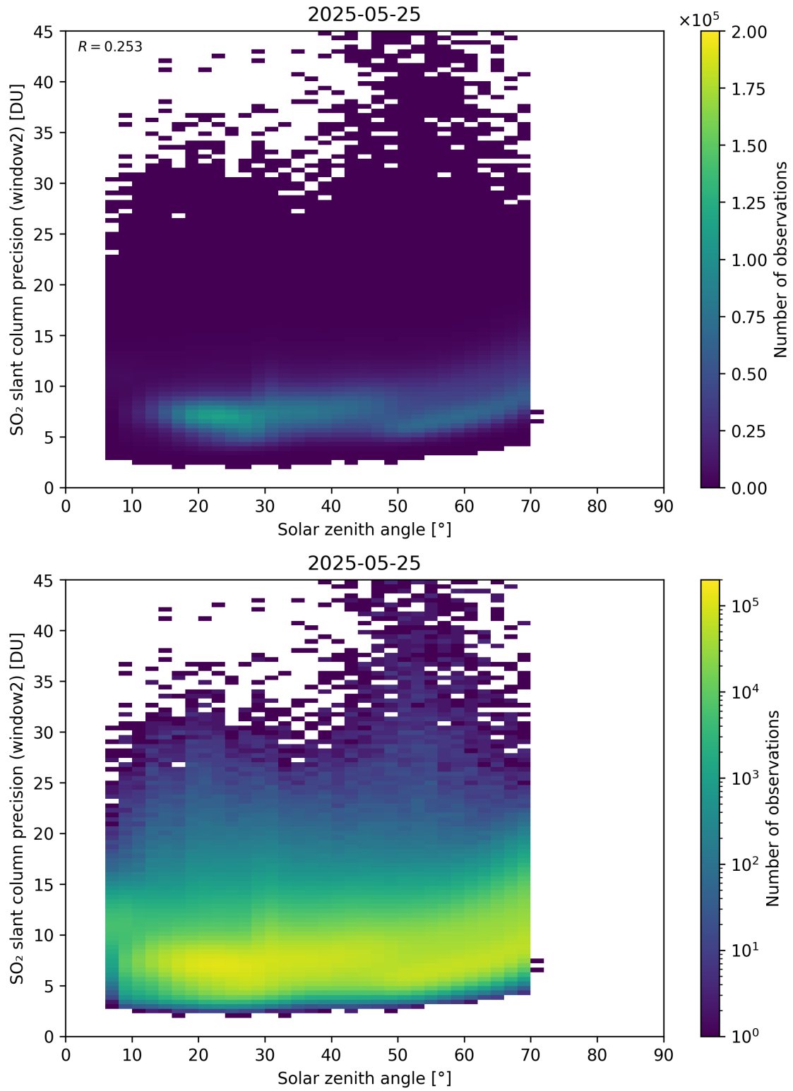
Figure 186: Scatter density plot of “Solar zenith angle” against “SO 2 slant column precision (window2)” for 2025-05-24 to 2025-05-26.
