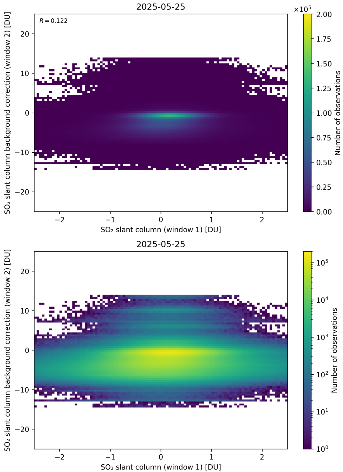
Figure 263: Scatter density plot of “SO 2 slant column (window 1)” against “SO 2 slant column background correction (window 2)” for 2025-05-24 to 2025-05-26.
