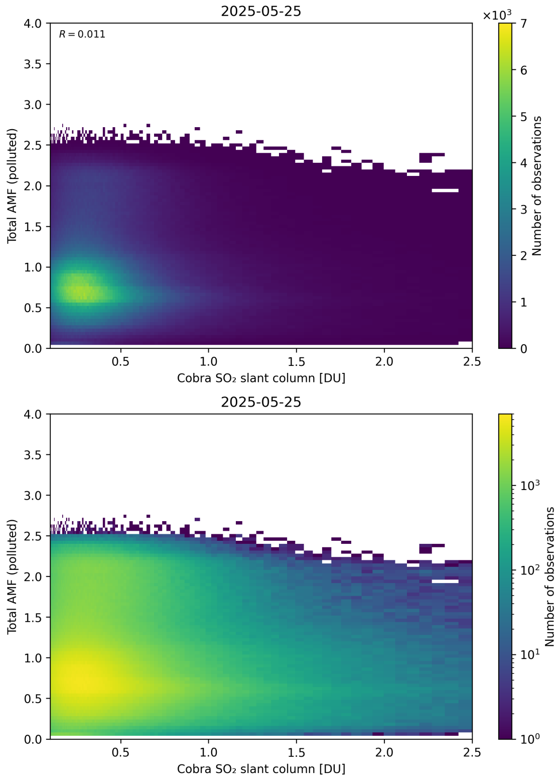
Figure 224: Scatter density plot of “Cobra SO 2 slant column” against “Total AMF (polluted)” for 2025-05-24 to 2025-05-26.
