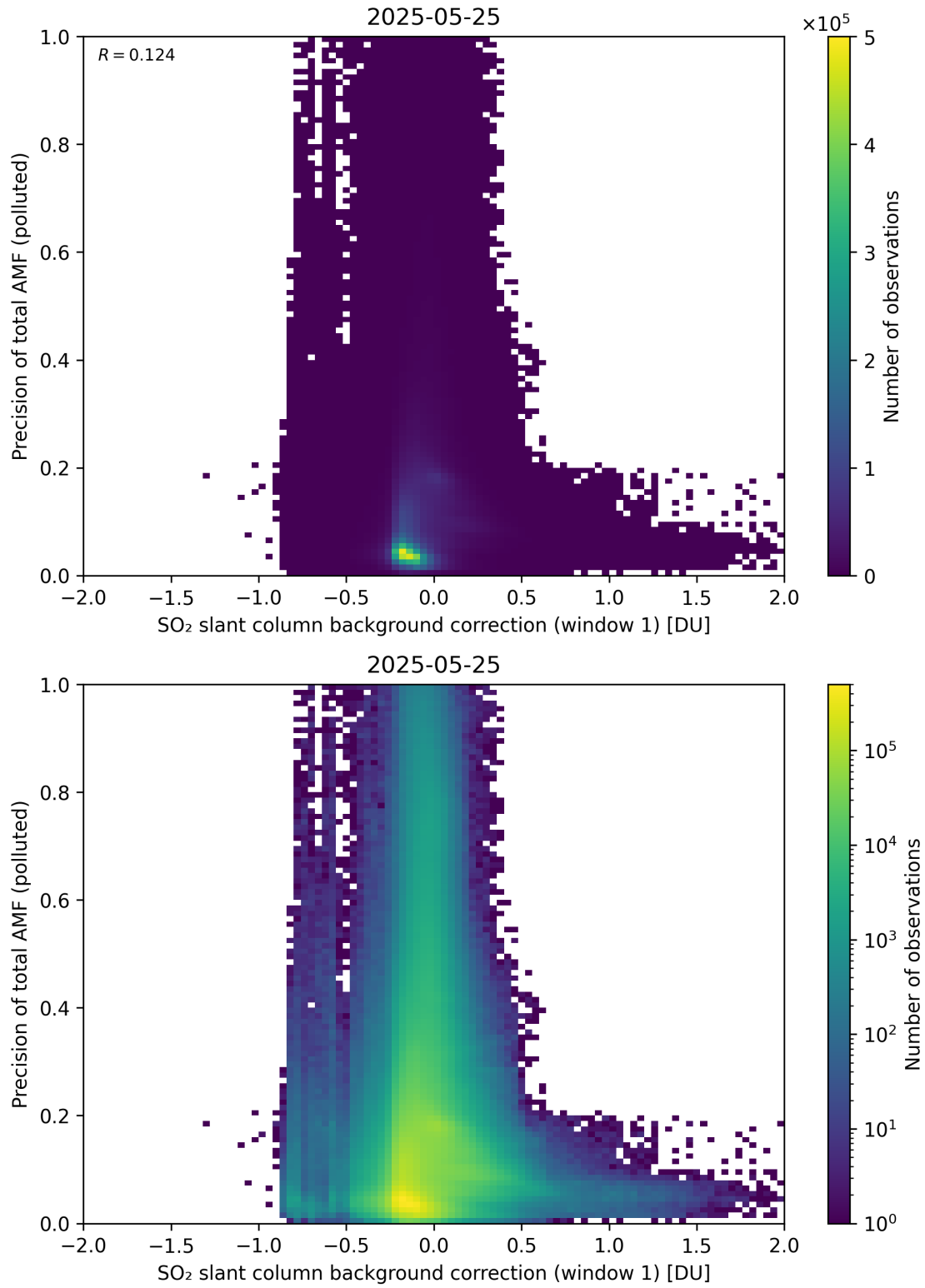
Figure 121: Scatter density plot of “SO 2 slant column background correction (window 1)” against “Precision of total AMF (polluted)” for 2025-05-24 to 2025-05-26.
