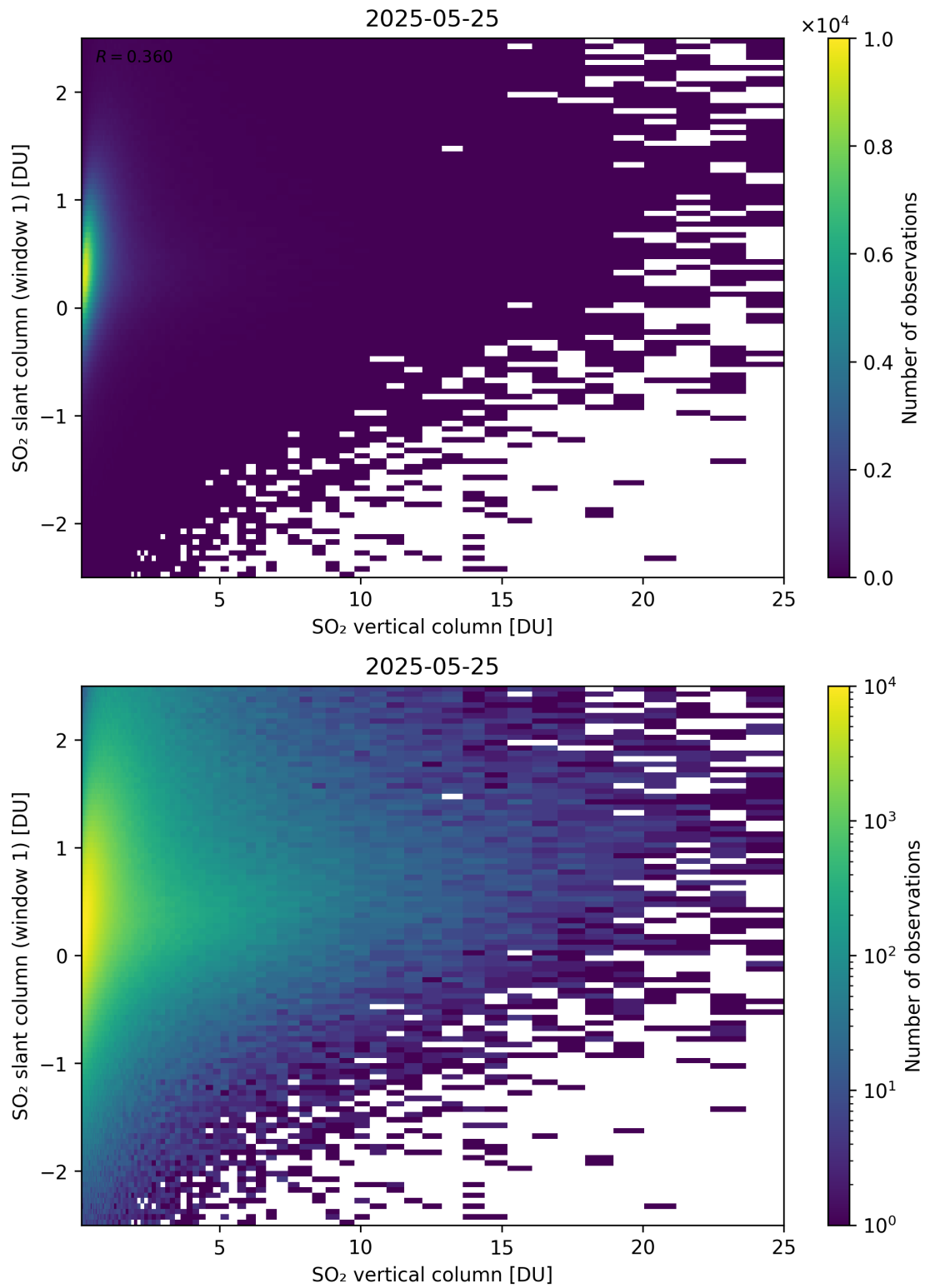
Figure 354: Scatter density plot of “SO 2 vertical column” against “SO 2 slant column (window 1)” for 2025-05-24 to 2025-05-26.
