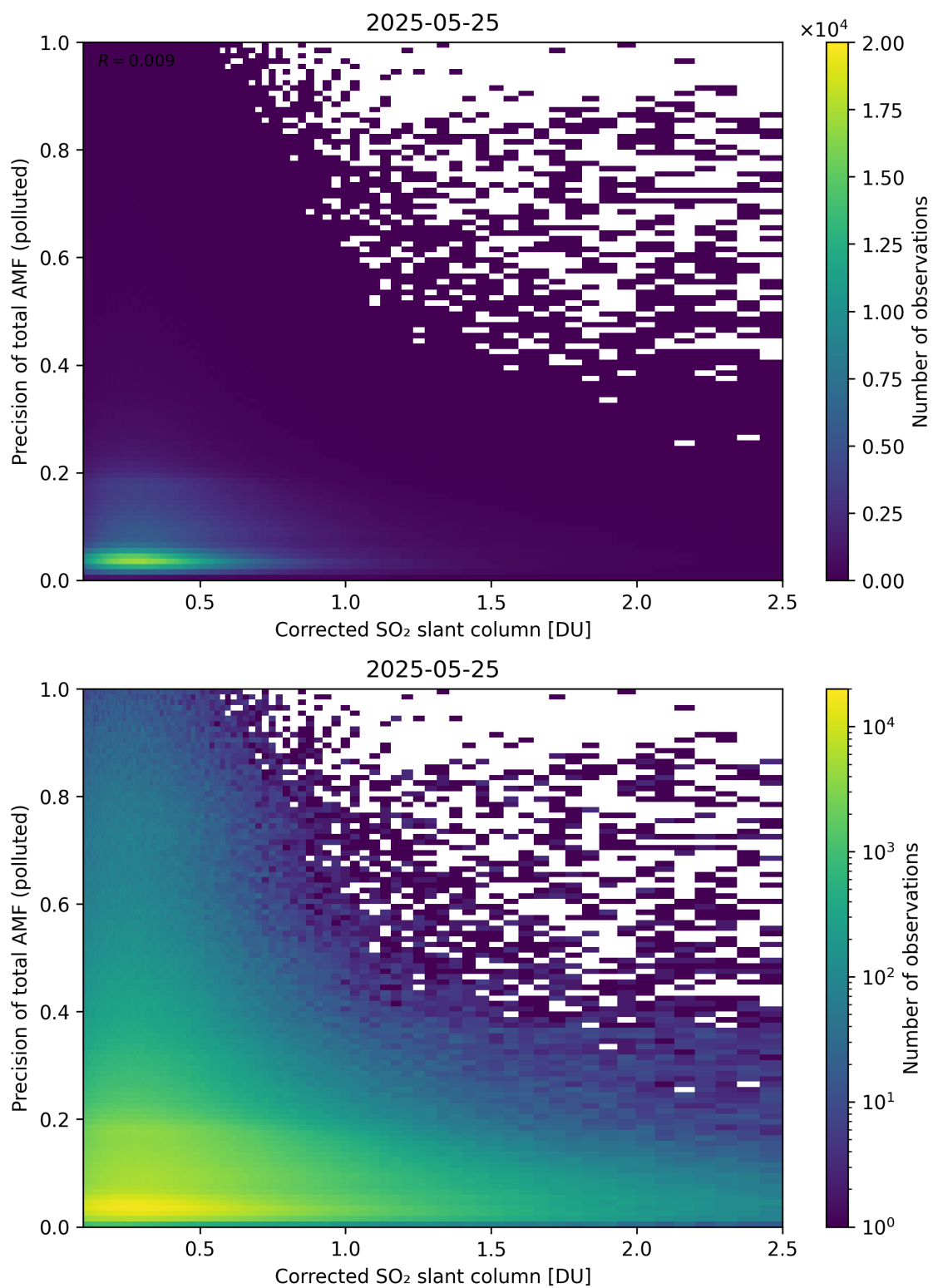
Figure 243: Scatter density plot of “Corrected SO 2 slant column” against “Precision of total AMF (polluted)” for 2025-05-24 to 2025-05-26.
