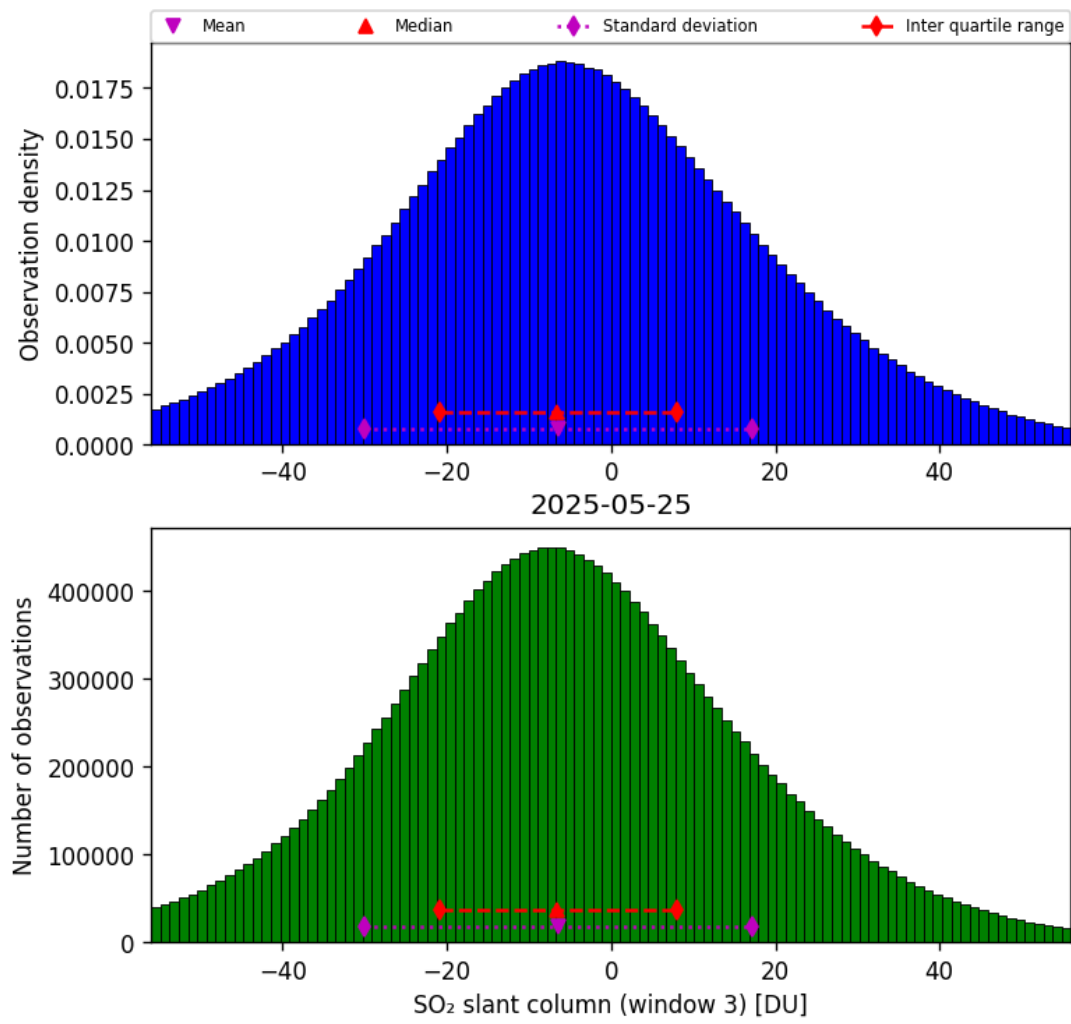
Figure 71: Histogram of “SO 2 slant column (window 3)” for 2025-05-24 to 2025-05-26
