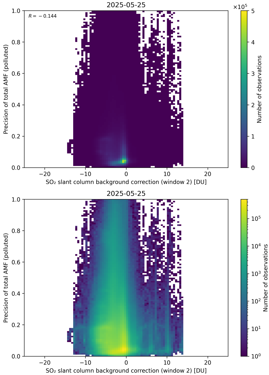
Figure 131: Scatter density plot of “SO 2 slant column background correction (window 2)” against “Precision of total AMF (polluted)” for 2025-05-24 to 2025-05-26.
