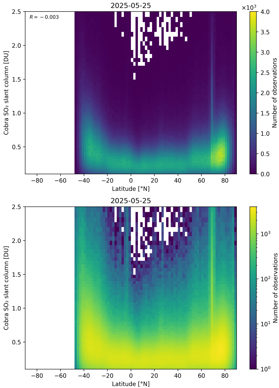
Figure 157: Scatter density plot of “Latitude” against “Cobra SO 2 slant column” for 2025-05-24 to 2025-05-26.
