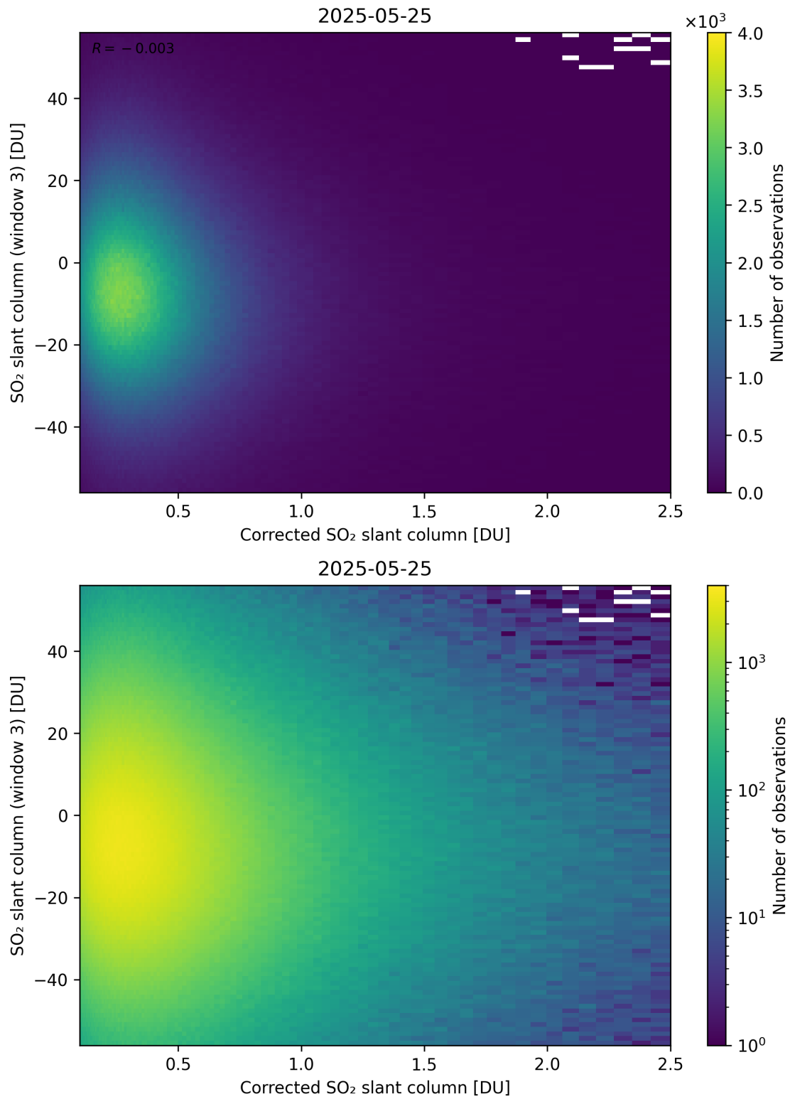
Figure 240: Scatter density plot of “Corrected SO 2 slant column” against “SO 2 slant column (window 3)” for 2025-05-24 to 2025-05-26.
