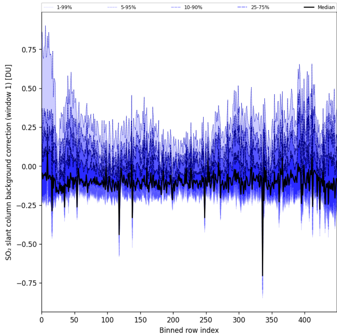
Figure 92: Along track statistics of “SO 2 slant column background correction (window 1)” for 2025-05-24 to 2025-05-26
