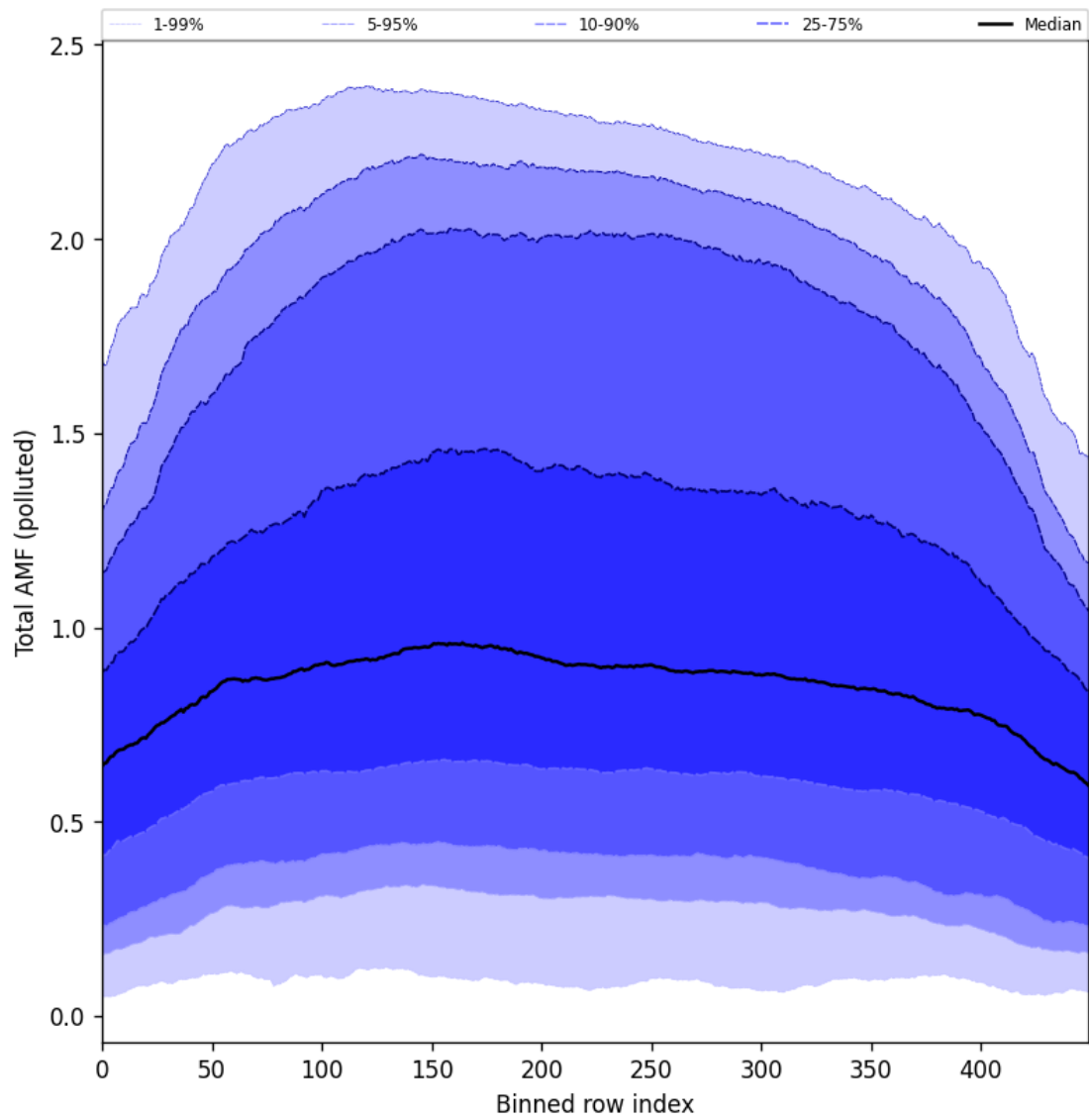
Figure 105: Along track statistics of “Total AMF (polluted)” for 2025-05-24 to 2025-05-26
