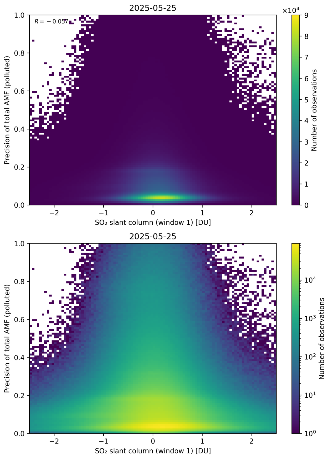
Figure 290: Scatter density plot of “SO 2 slant column (window 1)” against “Precision of total AMF (polluted)” for 2025-05-24 to 2025-05-26.
