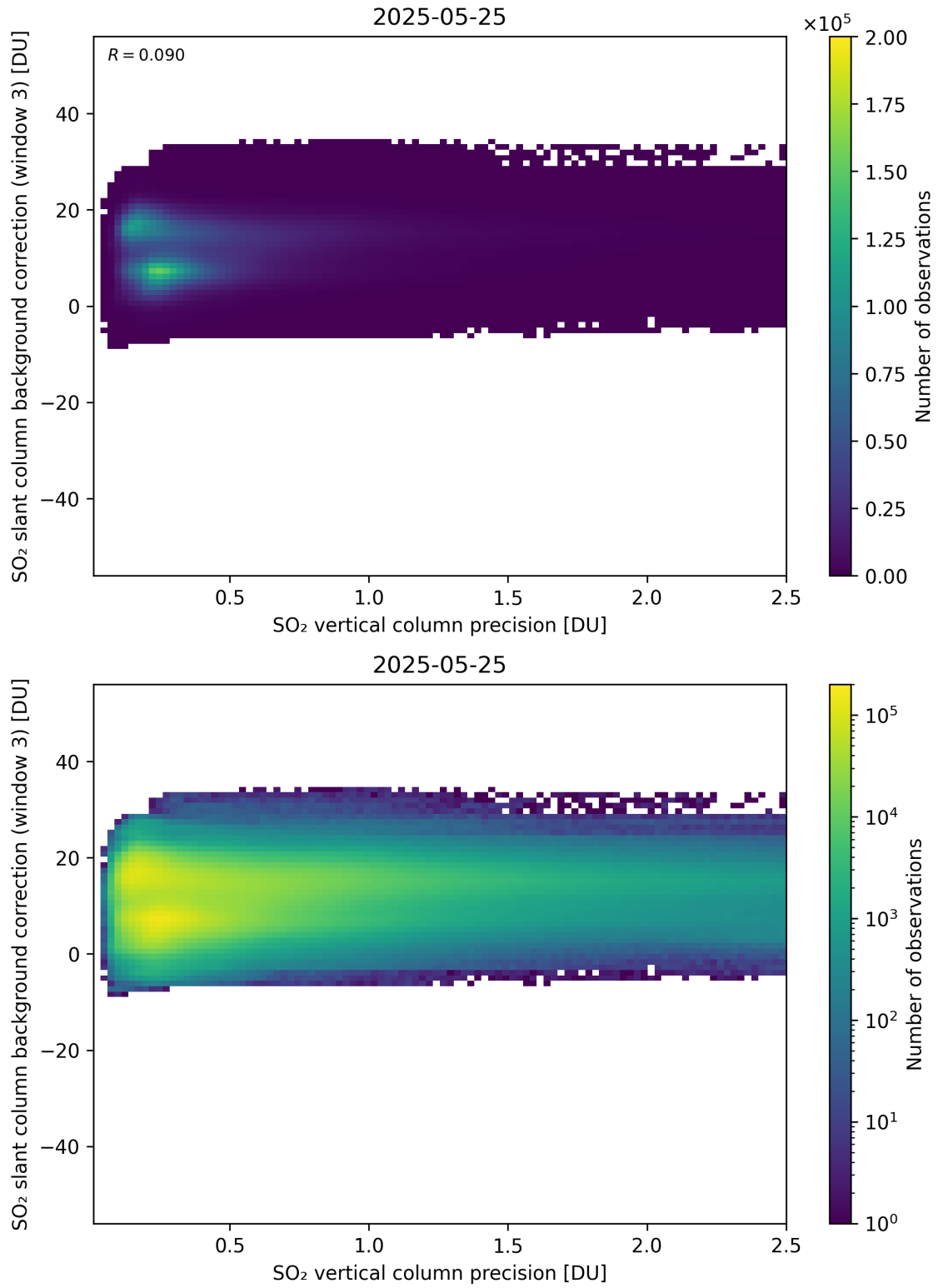
Figure 331: Scatter density plot of “SO 2 vertical column precision” against “SO 2 slant column background correction (window 3)” for 2025-05-24 to 2025-05-26.
