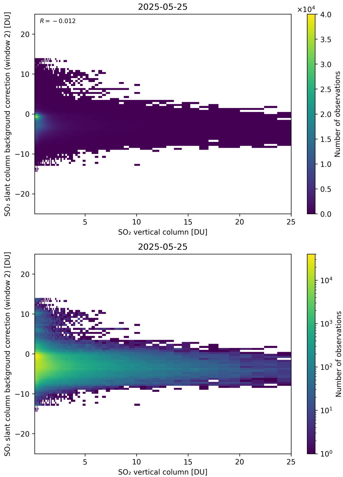
Figure 324: Scatter density plot of “SO 2 vertical column” against “SO 2 slant column background correction (window 2)” for 2025-05-24 to 2025-05-26.
