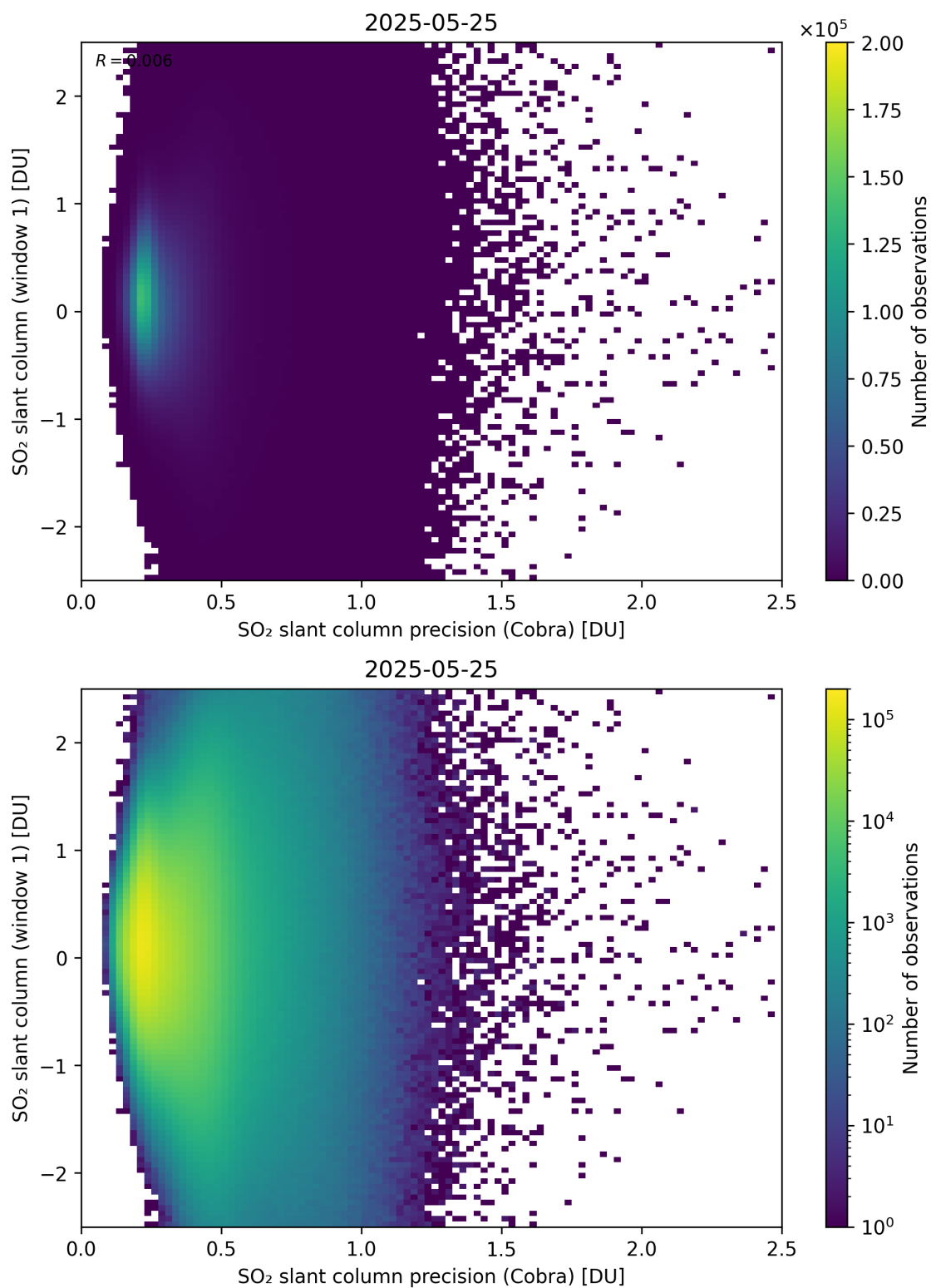
Figure 208: Scatter density plot of “SO 2 slant column precision (Cobra)” against “SO 2 slant column (window 1)” for 2025-05-24 to 2025-05-26.
