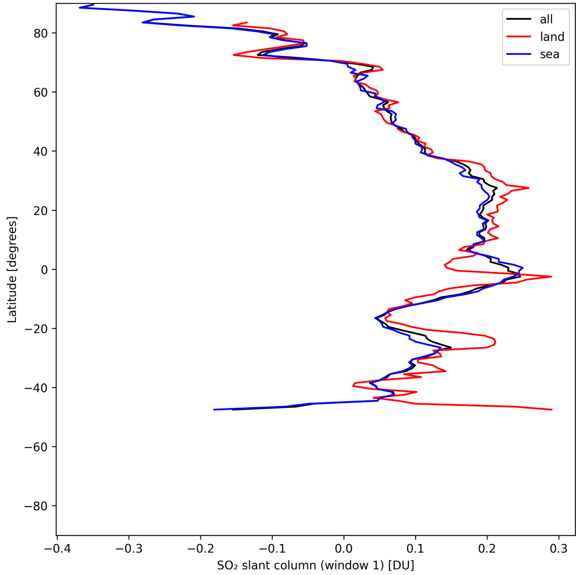
Figure 37: Zonal average of “SO 2 slant column (window 1)” for 2025-05-24 to 2025-05-26.
