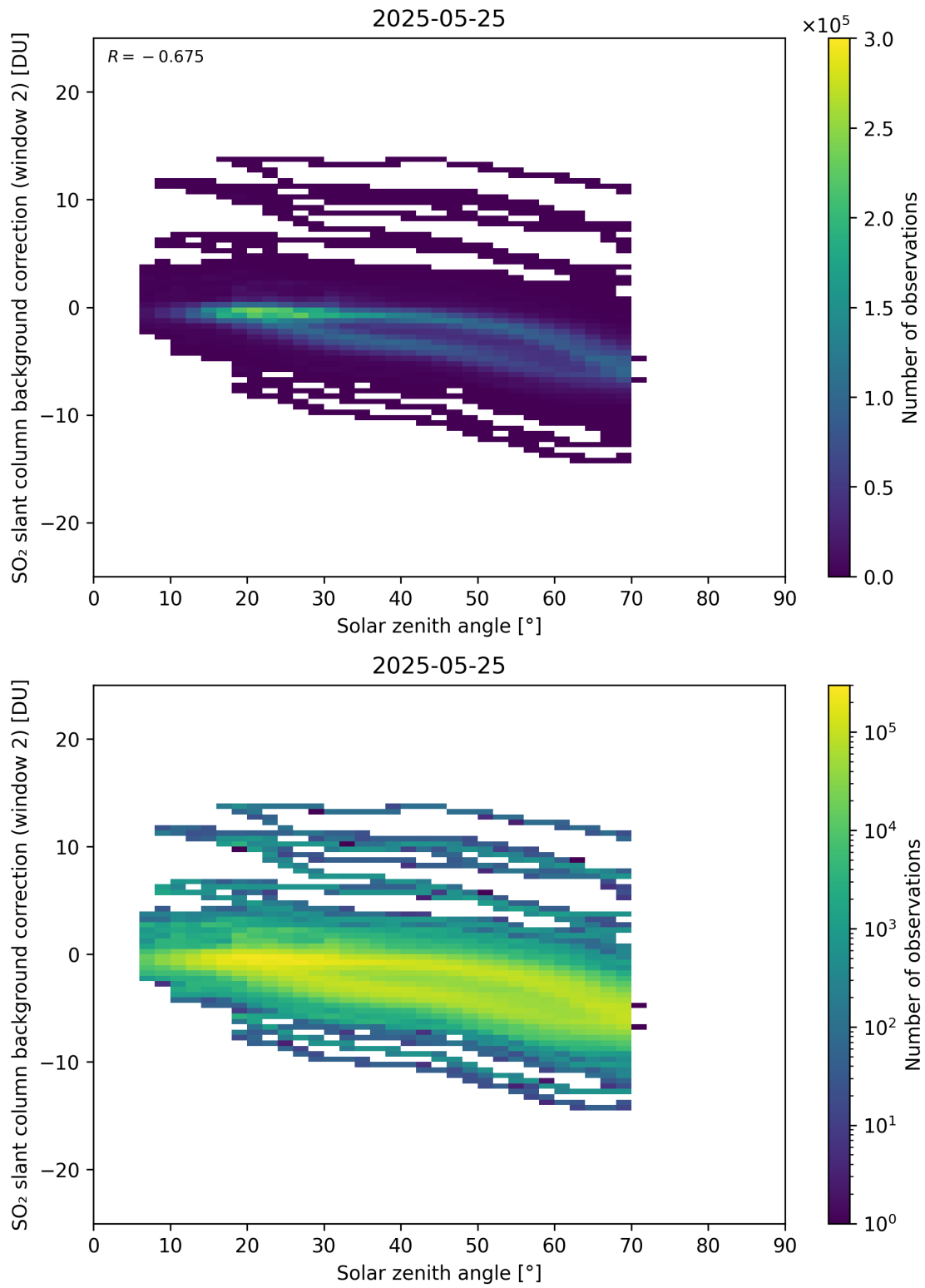
Figure 172: Scatter density plot of “Solar zenith angle” against “SO 2 slant column background correction (window 2)” for 2025-05-24 to 2025-05-26.
