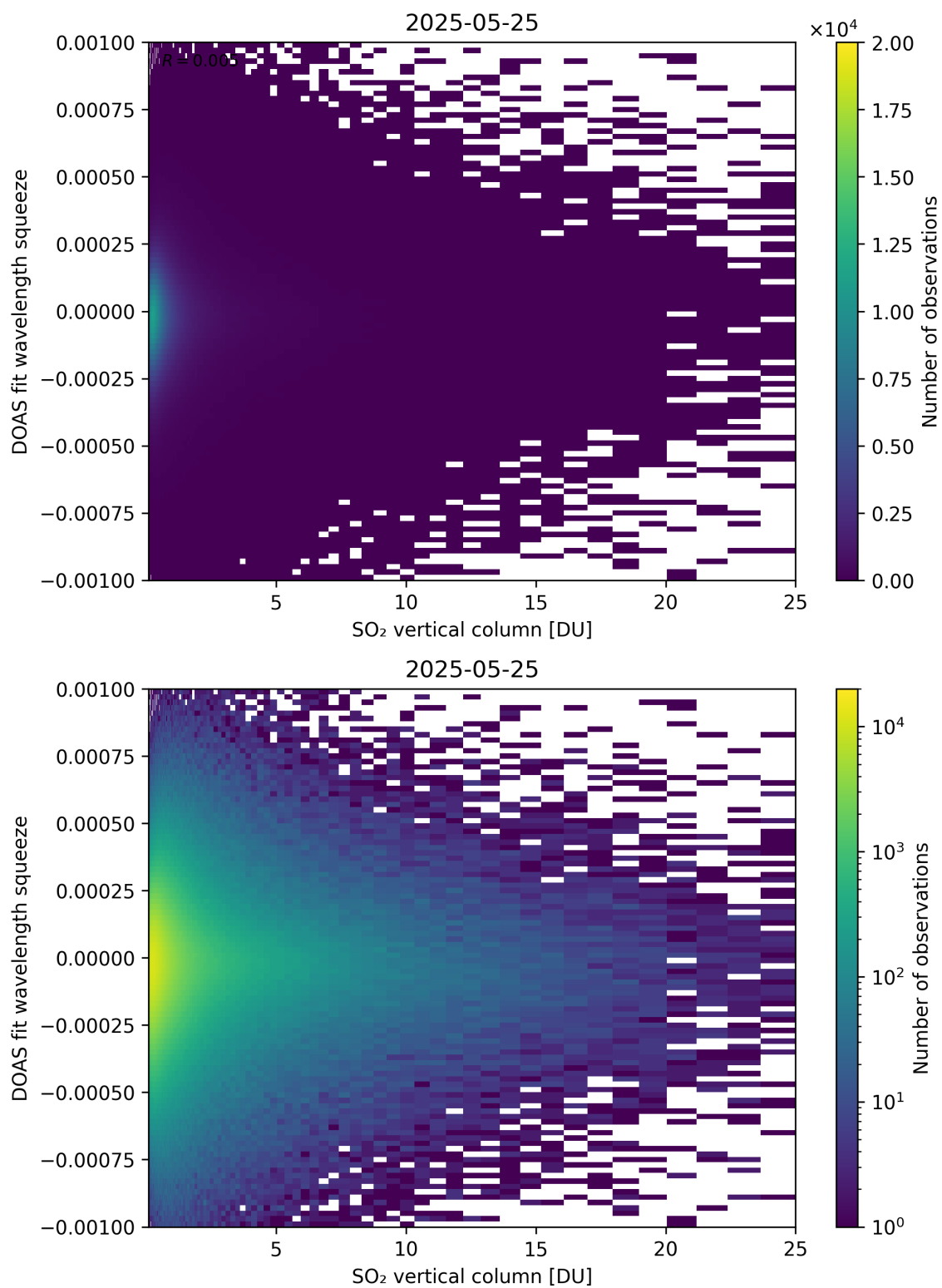
Figure 327: Scatter density plot of “SO 2 vertical column” against “DOAS fit wavelength squeeze” for 2025-05-24 to 2025-05-26.
