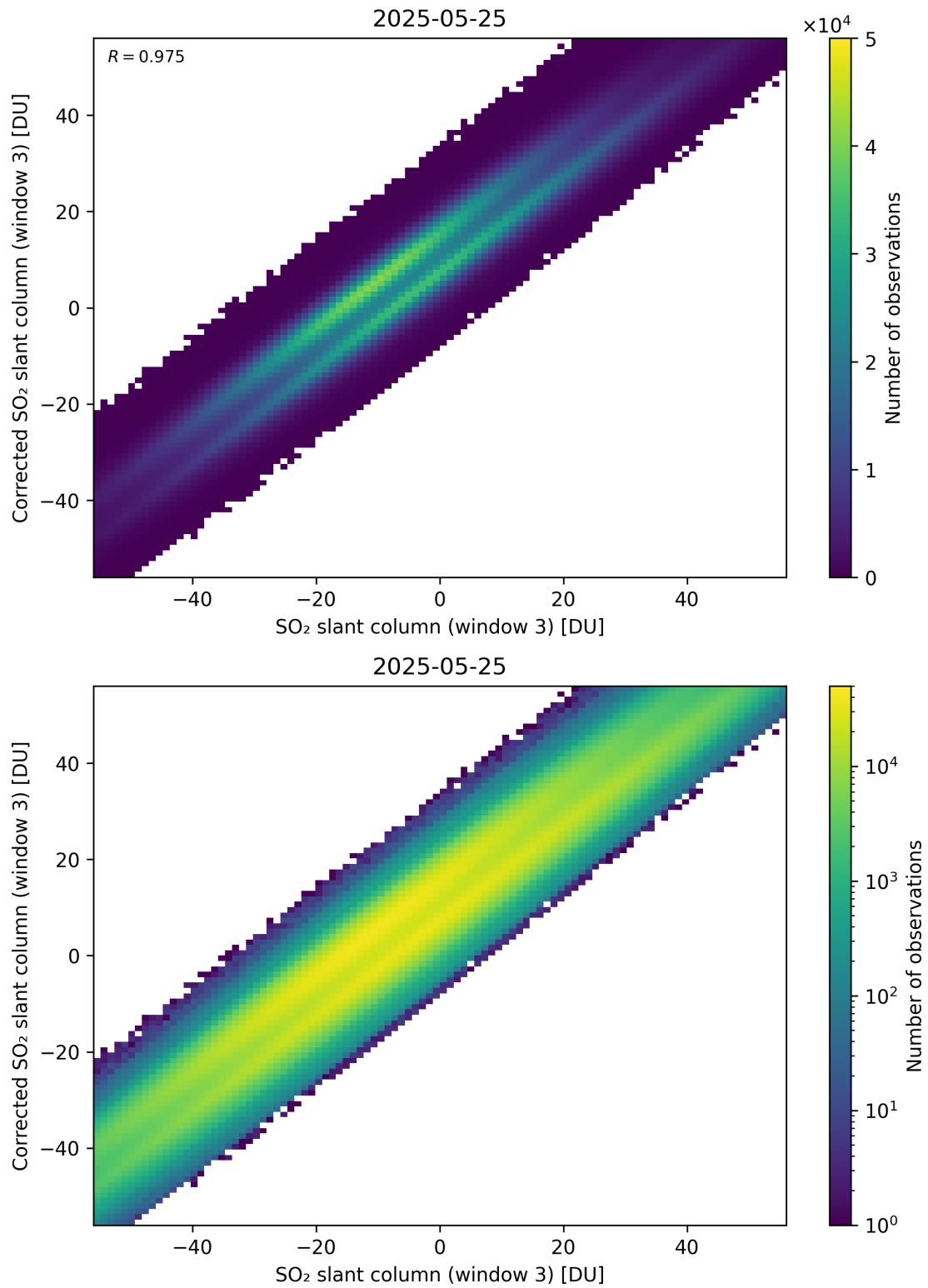
Figure 316: Scatter density plot of “SO 2 slant column (window 3)” against “Corrected SO 2 slant column (window 3)” for 2025-05-24 to 2025-05-26.
