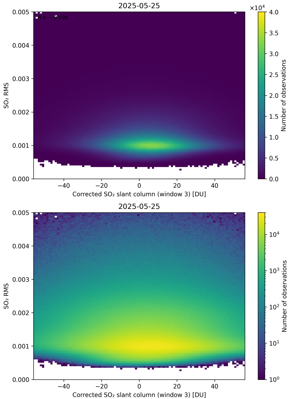
Figure 258: Scatter density plot of “Corrected SO 2 slant column (window 3)” against “SO 2 RMS” for 2025-05-24 to 2025-05-26.
