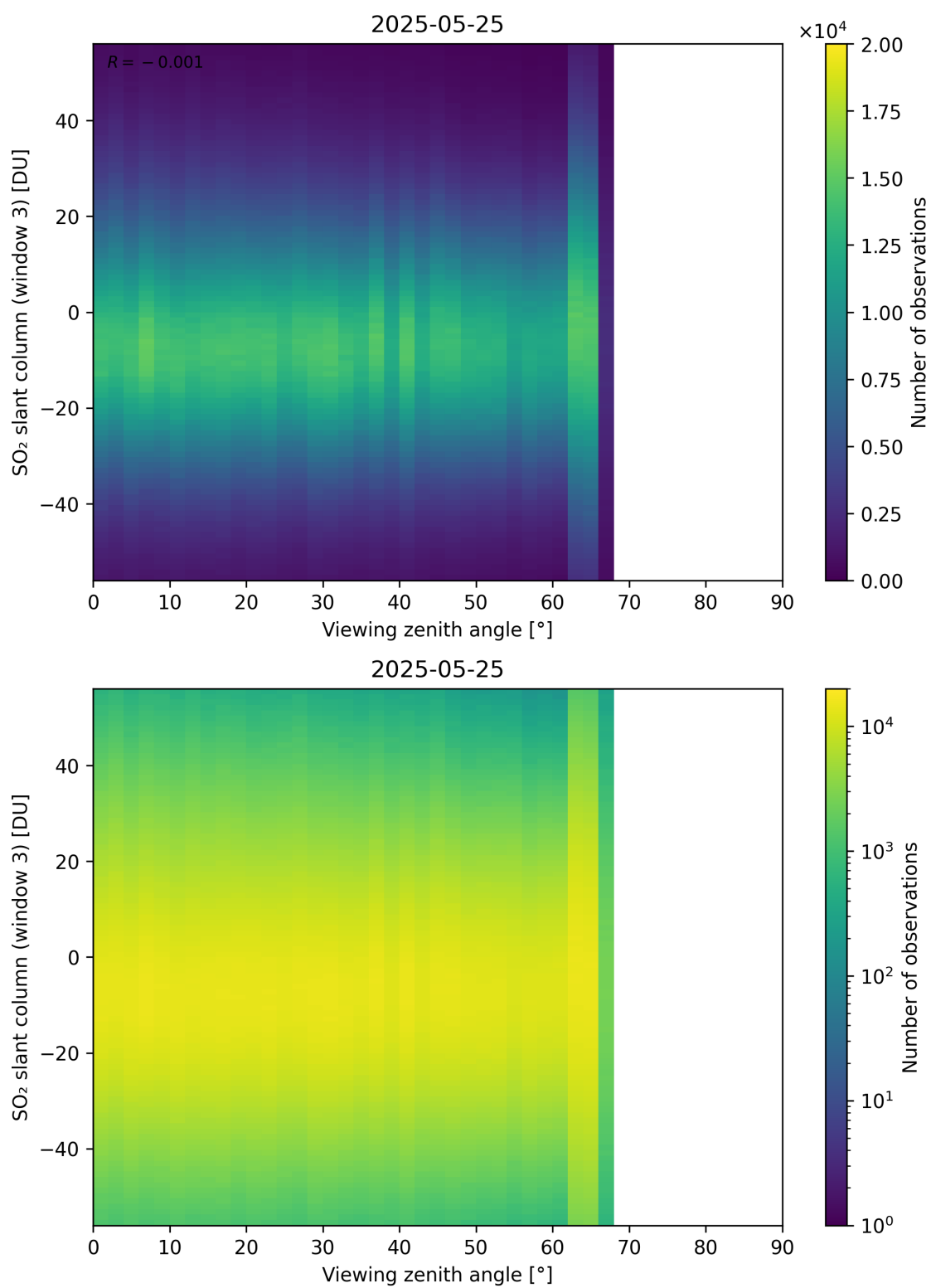
Figure 379: Scatter density plot of “Viewing zenith angle” against “SO 2 slant column (window 3)” for 2025-05-24 to 2025-05-26.
