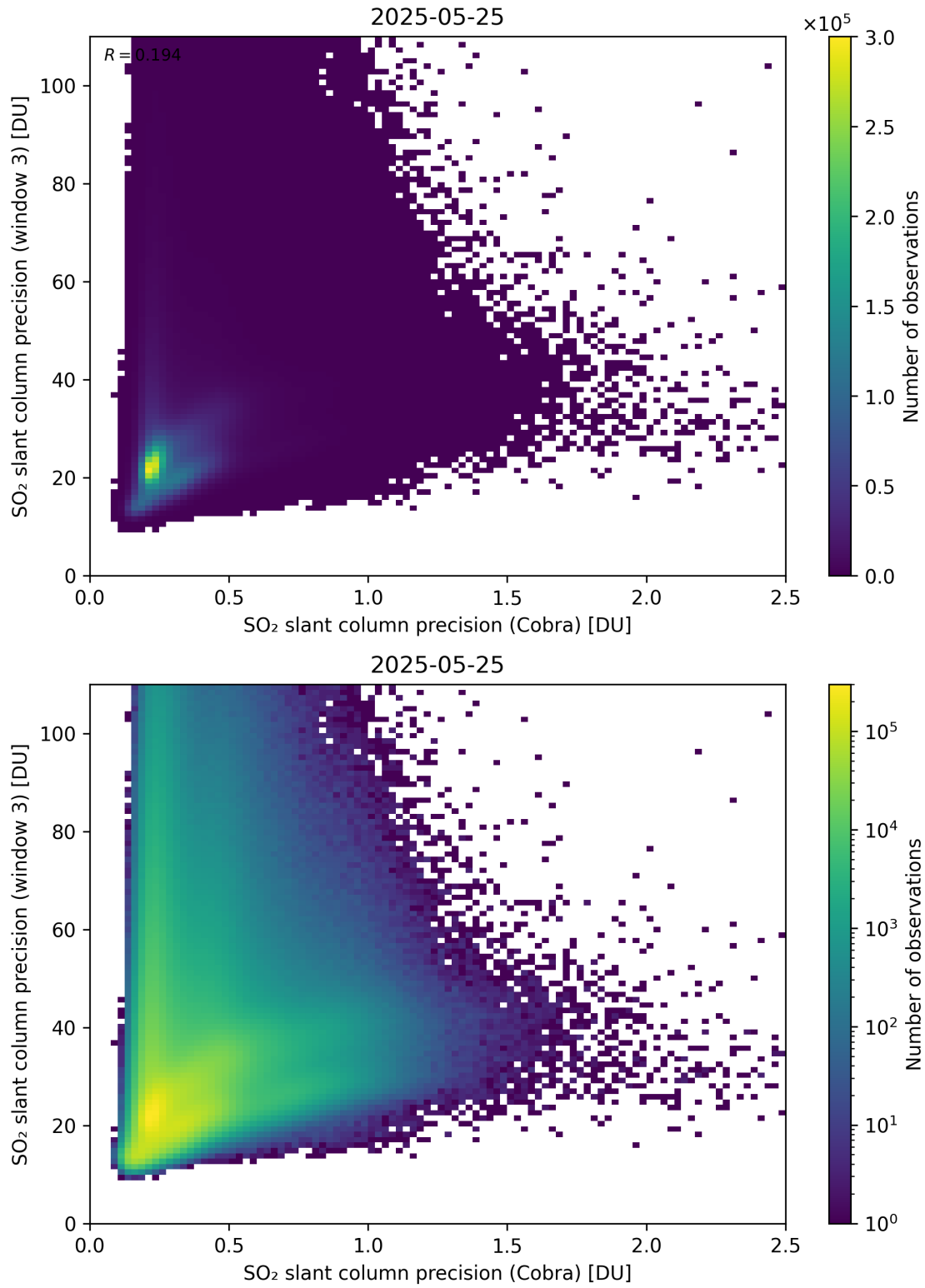
Figure 212: Scatter density plot of “SO 2 slant column precision (Cobra)” against “SO 2 slant column precision (window 3)” for 2025-05-24 to 2025-05-26.
