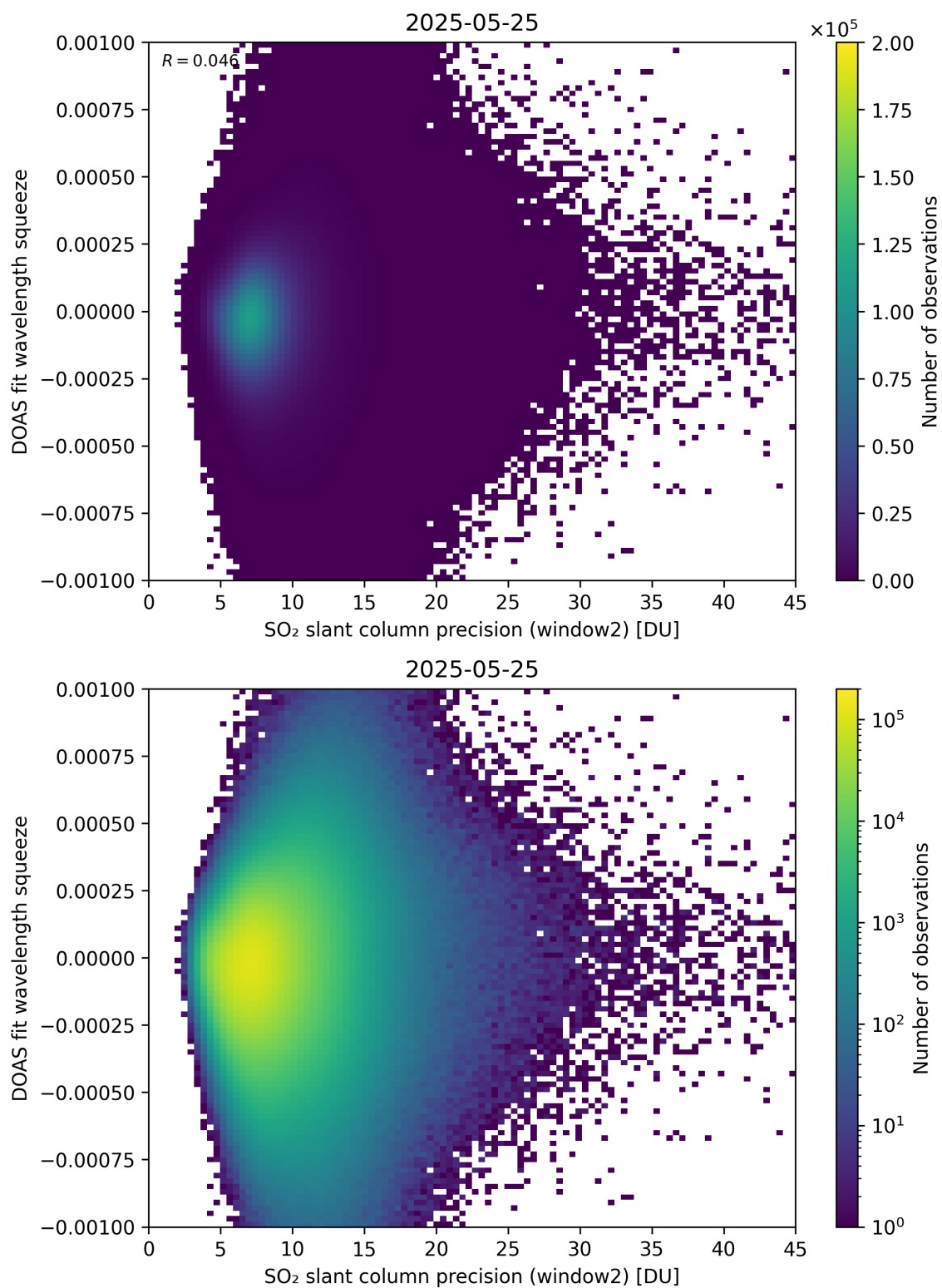
Figure 294: Scatter density plot of “SO 2 slant column precision (window2)” against “DOAS fit wavelength squeeze” for 2025-05-24 to 2025-05-26.
