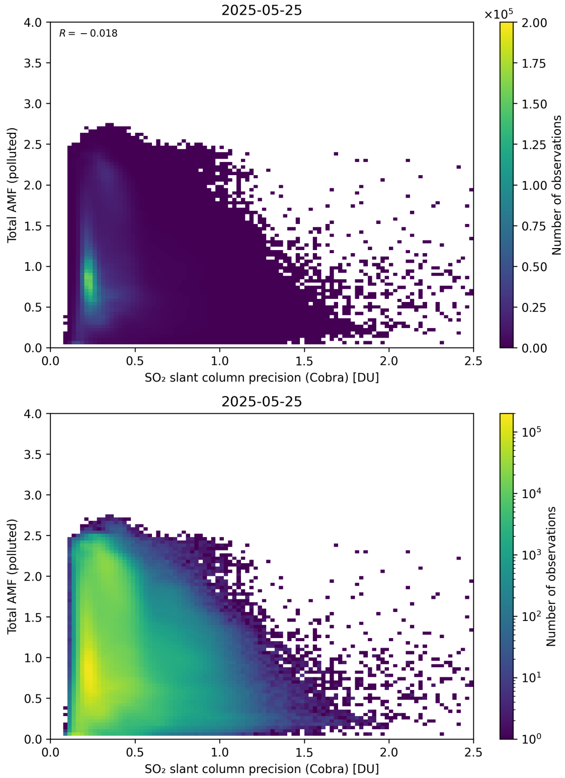
Figure 213: Scatter density plot of “SO 2 slant column precision (Cobra)” against “Total AMF (polluted)” for 2025-05-24 to 2025-05-26.
