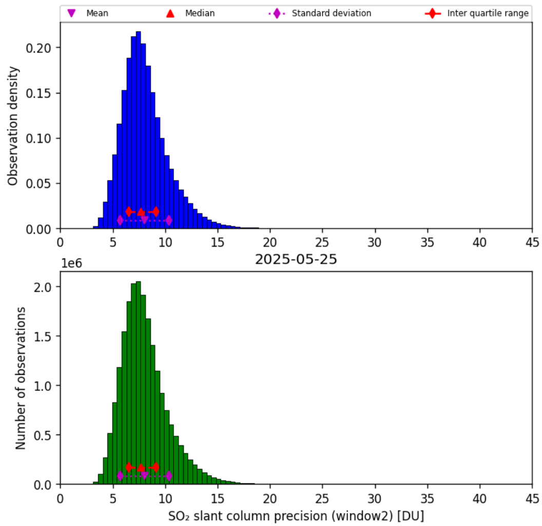
Figure 68: Histogram of “SO 2 slant column precision (window2)” for 2025-05-24 to 2025-05-26
