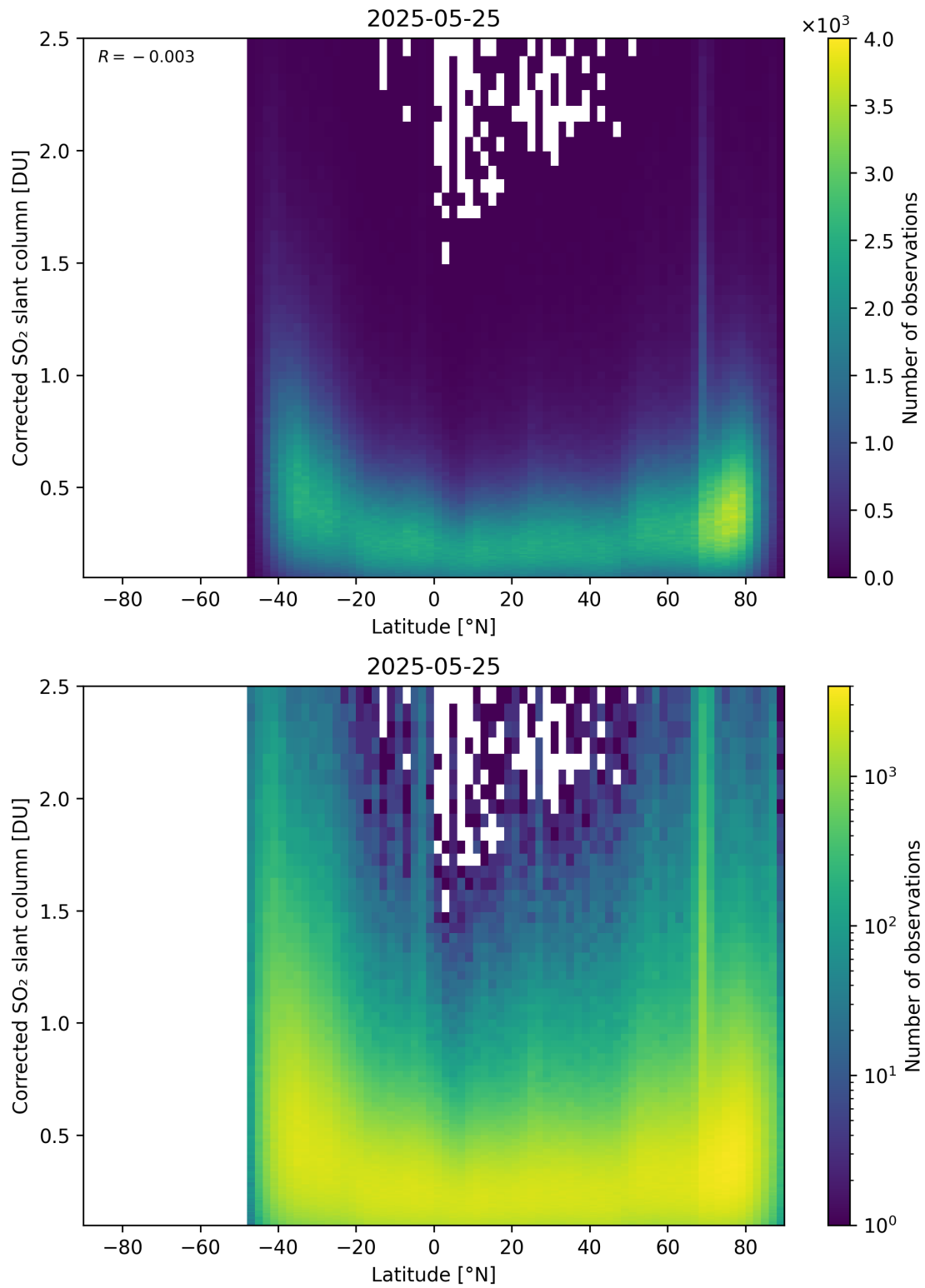
Figure 159: Scatter density plot of “Latitude” against “Corrected SO 2 slant column” for 2025-05-24 to 2025-05-26.
