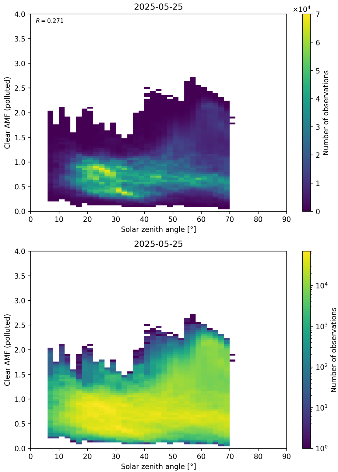
Figure 178: Scatter density plot of “Solar zenith angle” against “Clear AMF (polluted)” for 2025-05-24 to 2025-05-26.
