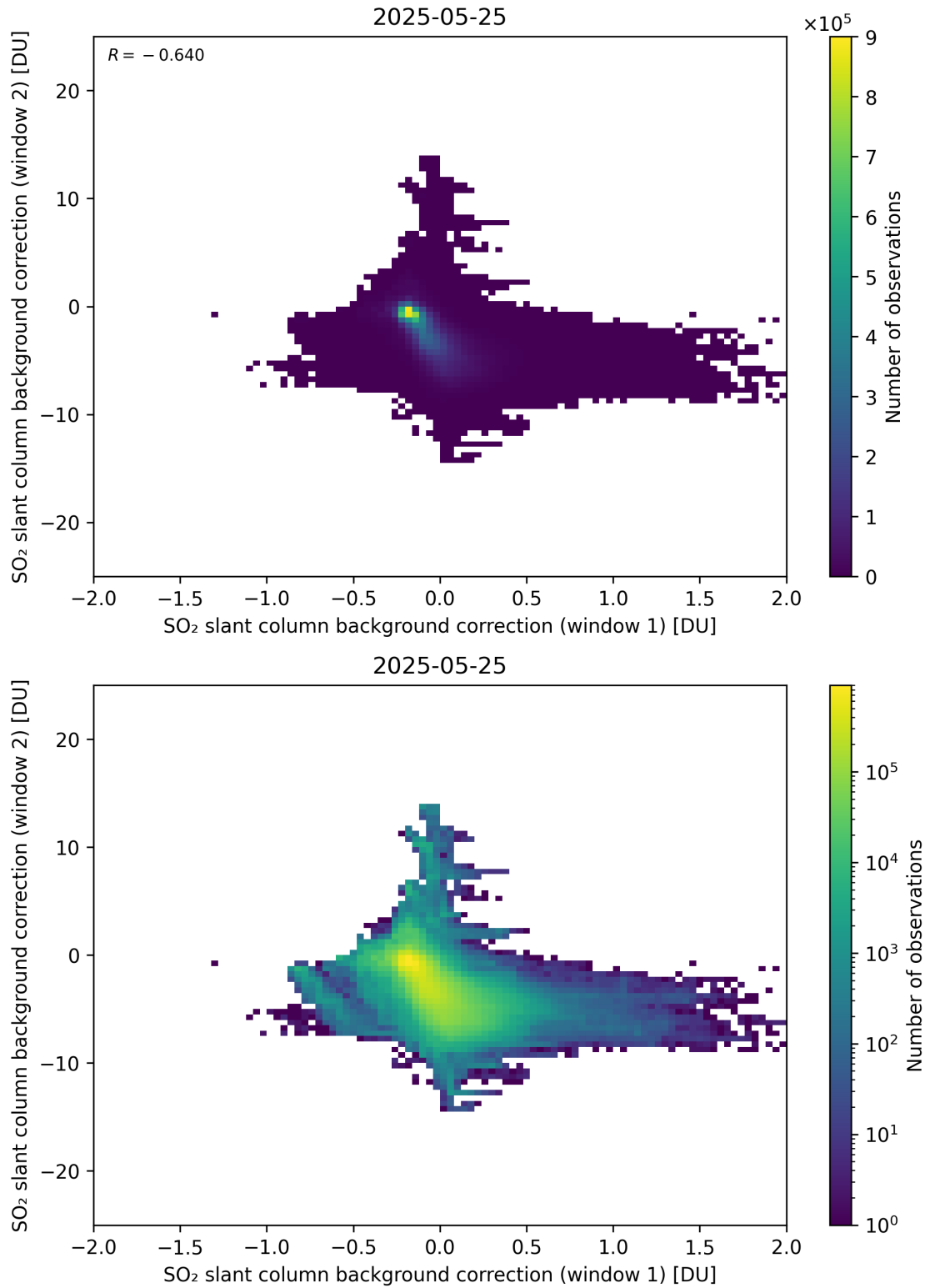
Figure 109: Scatter density plot of “SO 2 slant column background correction (window 1)” against “SO 2 slant column background correction (window 2)” for 2025-05-24 to 2025-05-26.
