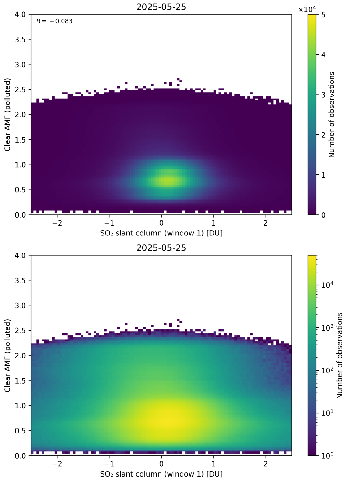
Figure 282: Scatter density plot of “SO 2 slant column (window 1)” against “Clear AMF (polluted)” for 2025-05-24 to 2025-05-26.
