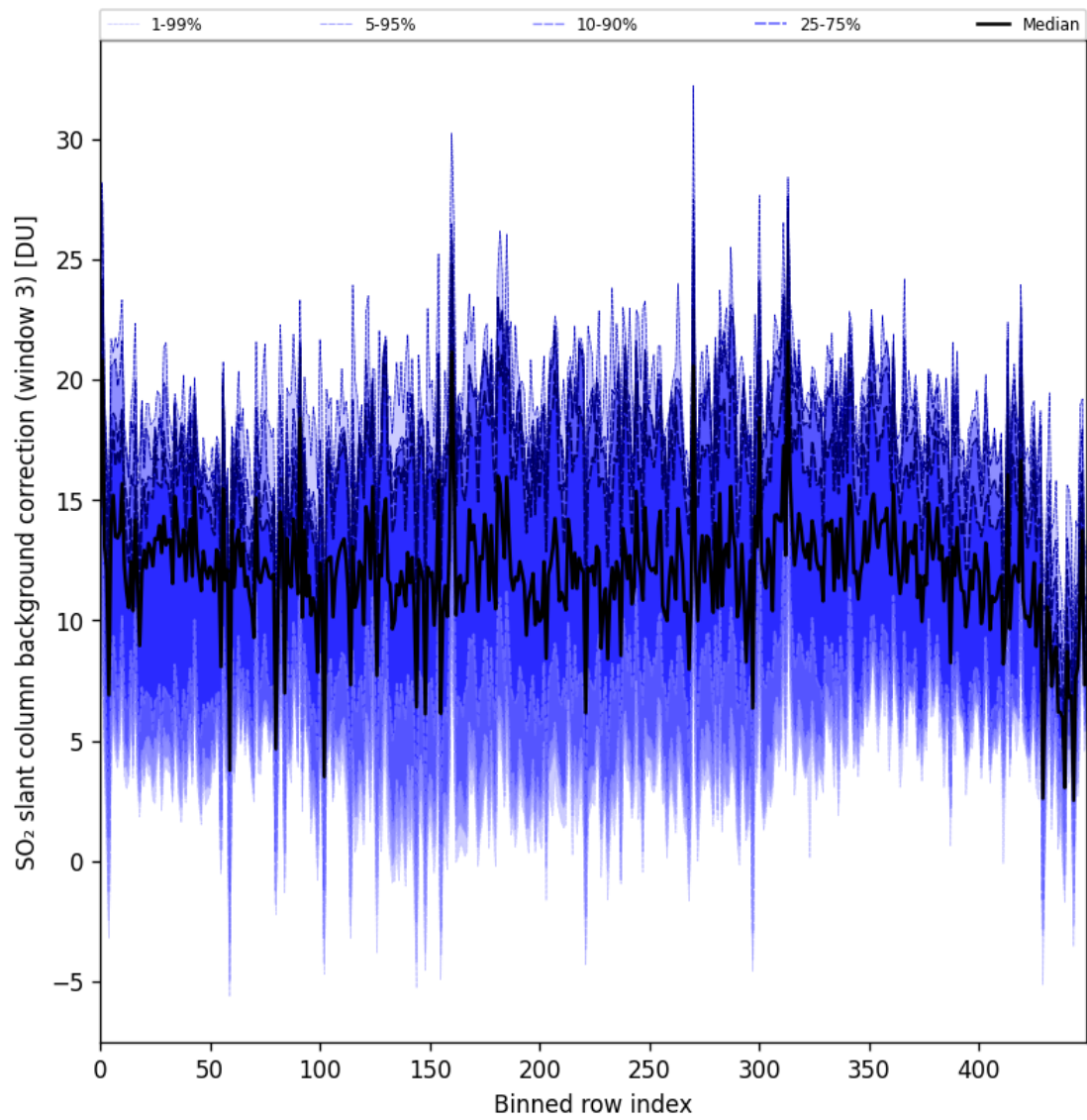
Figure 100: Along track statistics of “SO 2 slant column background correction (window 3)” for 2025-05-24 to 2025-05-26
