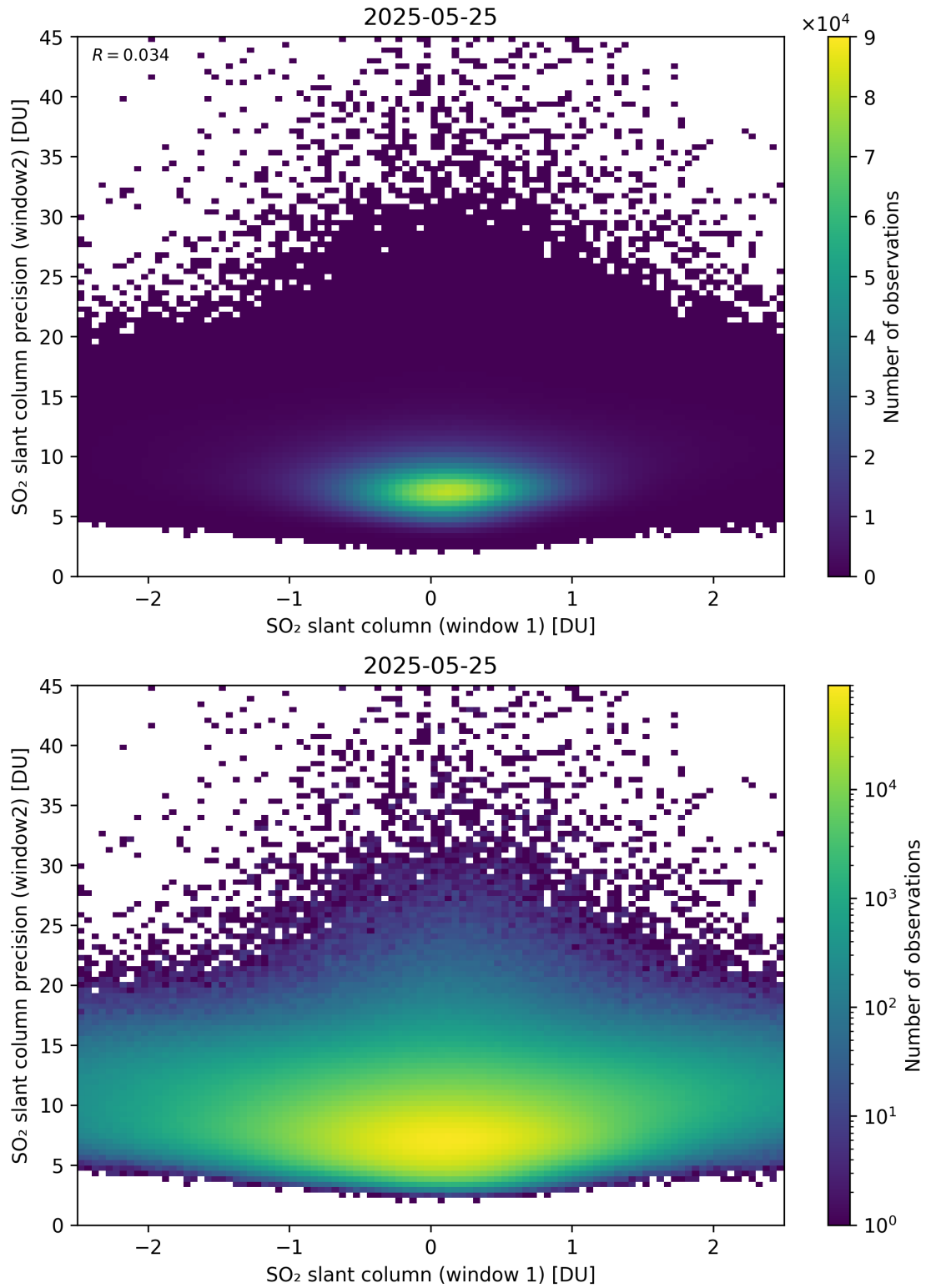
Figure 286: Scatter density plot of “SO 2 slant column (window 1)” against “SO 2 slant column precision (window2)” for 2025-05-24 to 2025-05-26.
