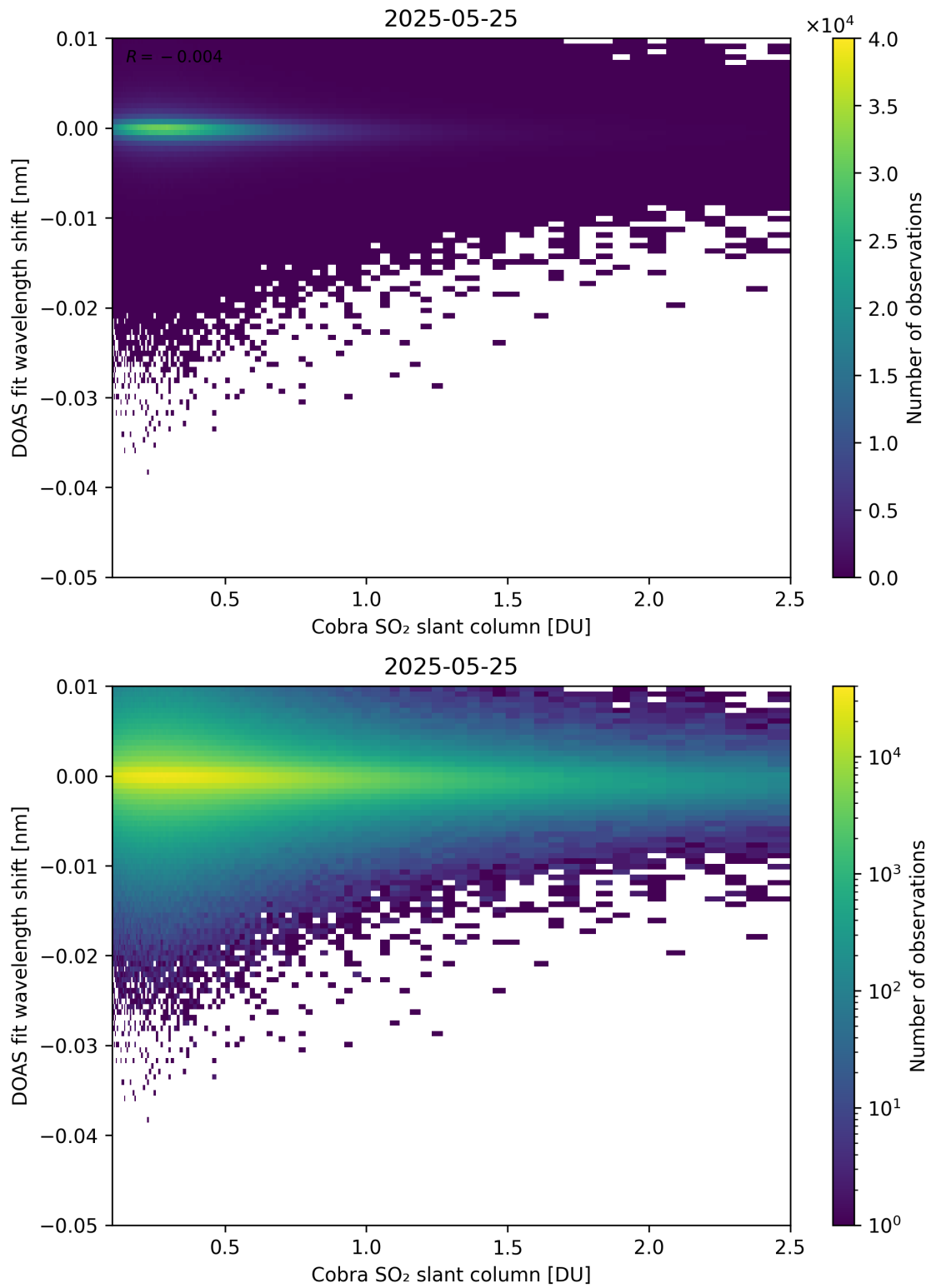
Figure 196: Scatter density plot of “Cobra SO 2 slant column” against “DOAS fit wavelength shift” for 2025-05-24 to 2025-05-26.
