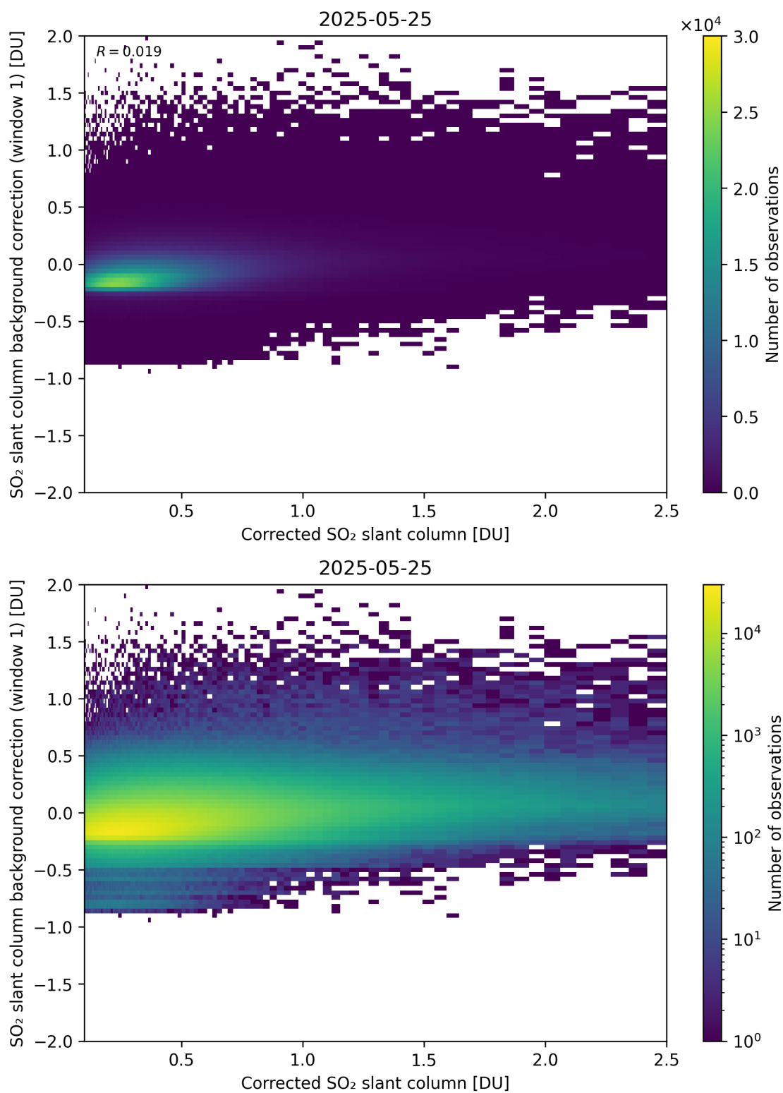
Figure 226: Scatter density plot of “Corrected SO 2 slant column” against “SO 2 slant column background correction (window 1)” for 2025-05-24 to 2025-05-26.
