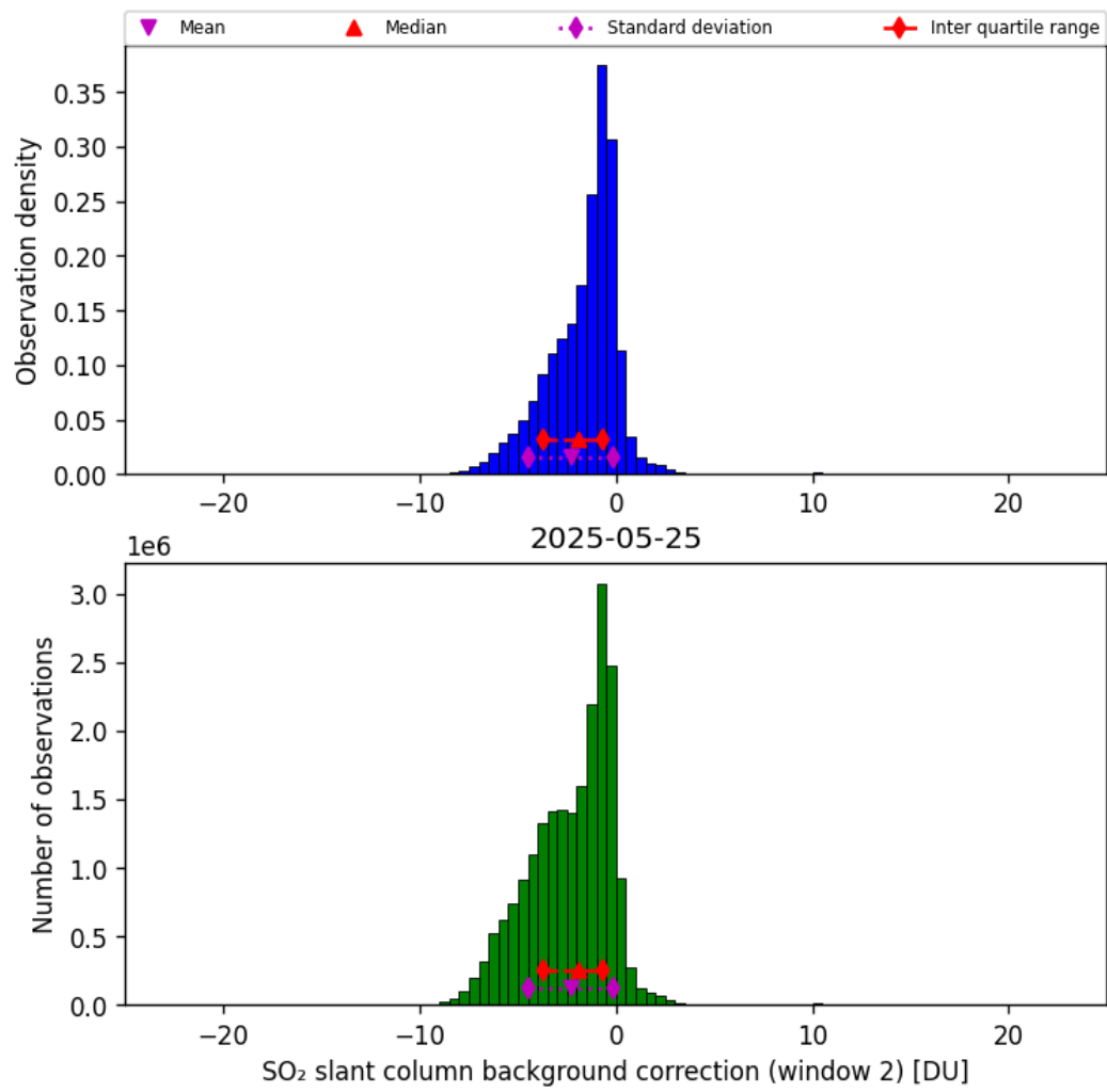
Figure 70: Histogram of “SO 2 slant column background correction (window 2)” for 2025-05-24 to 2025-05-26
