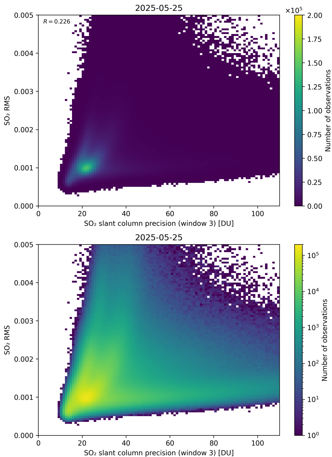
Figure 310: Scatter density plot of “SO 2 slant column precision (window 3)” against “SO 2 RMS” for 2025-05-24 to 2025-05-26.
