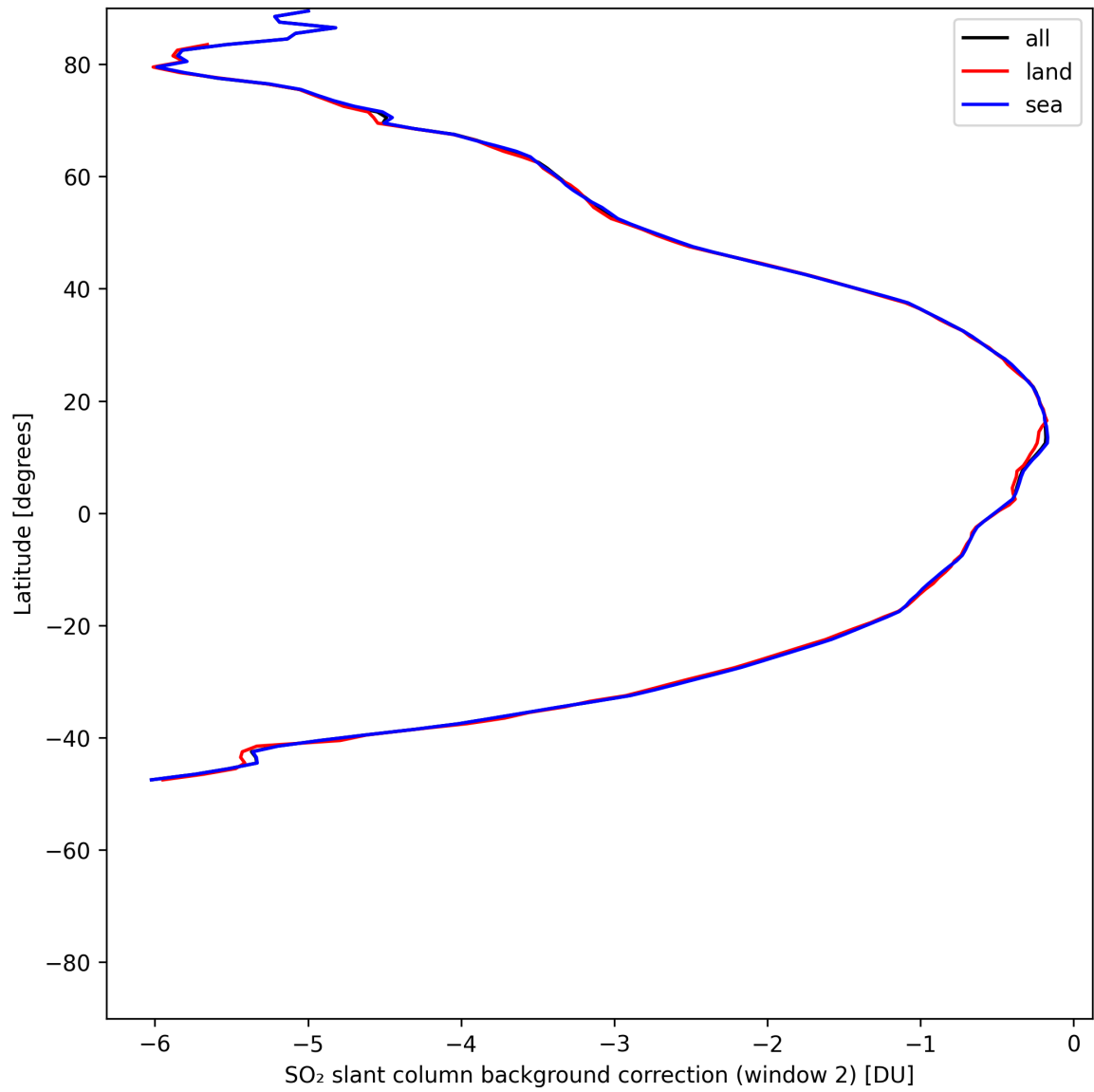
Figure 44: Zonal average of “SO 2 slant column background correction (window 2)” for 2025-05-24 to 2025-05-26.
