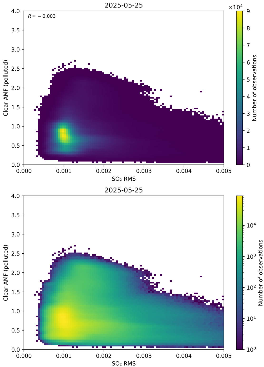
Figure 147: Scatter density plot of “SO 2 RMS” against “Clear AMF (polluted)” for 2025-05-24 to 2025-05-26.
