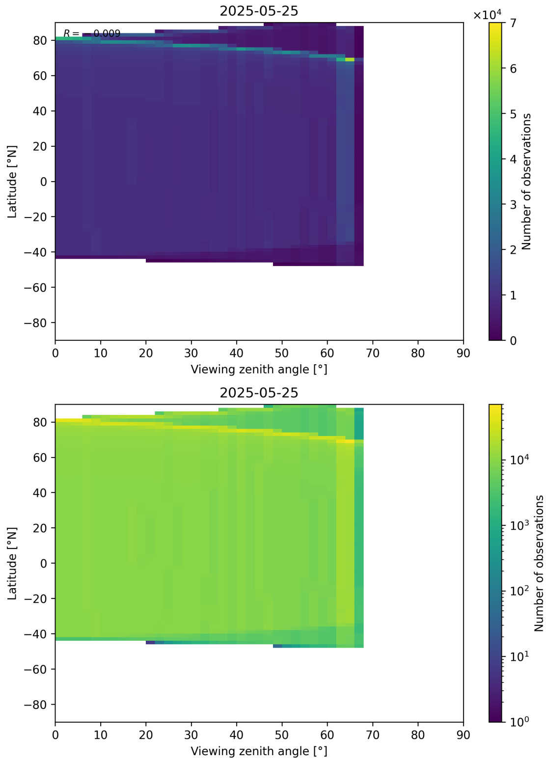
Figure 368: Scatter density plot of “Viewing zenith angle” against “Latitude” for 2025-05-24 to 2025-05-26.
