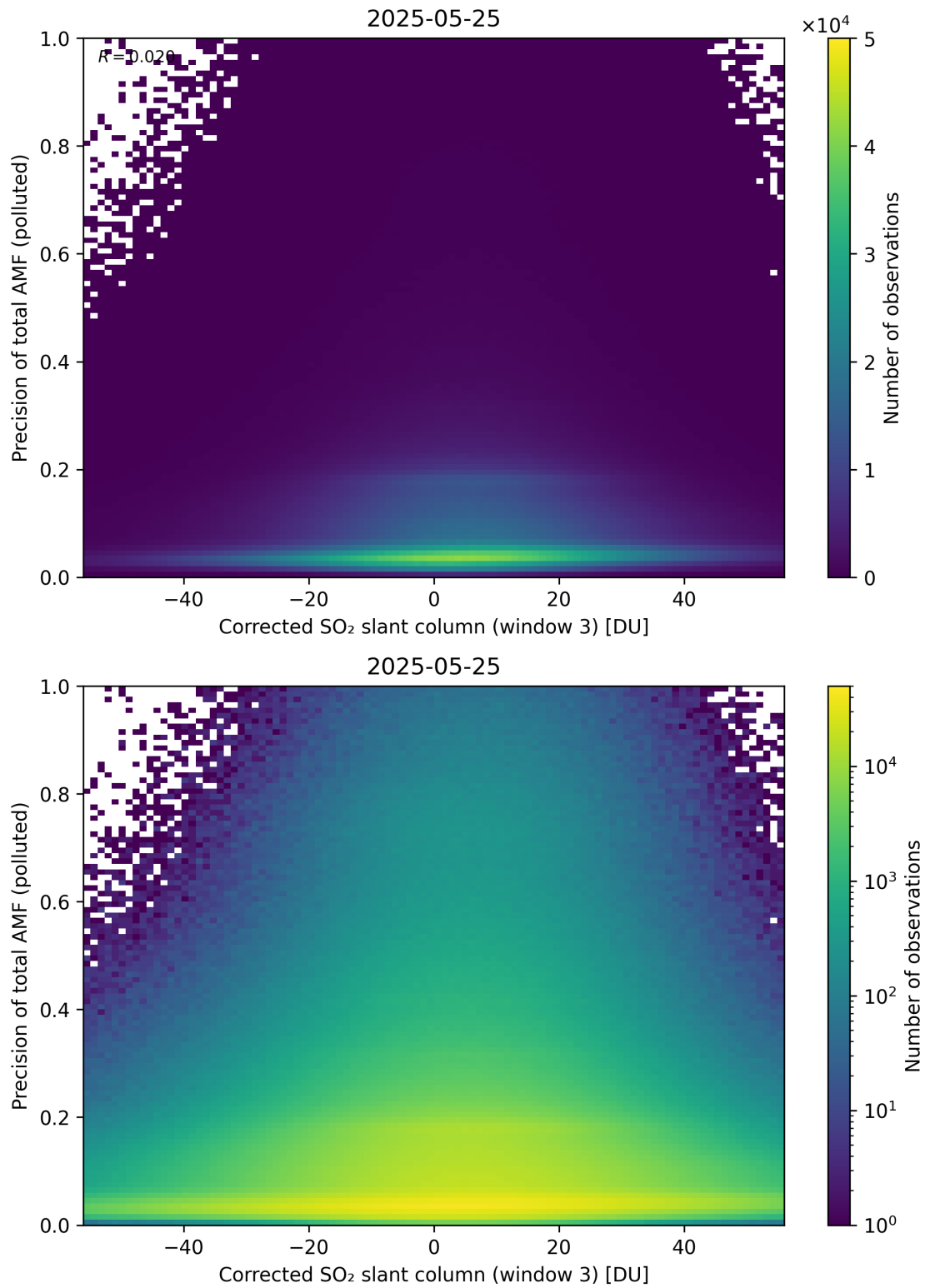
Figure 261: Scatter density plot of “Corrected SO 2 slant column (window 3)” against “Precision of total AMF (polluted)” for 2025-05-24 to 2025-05-26.
