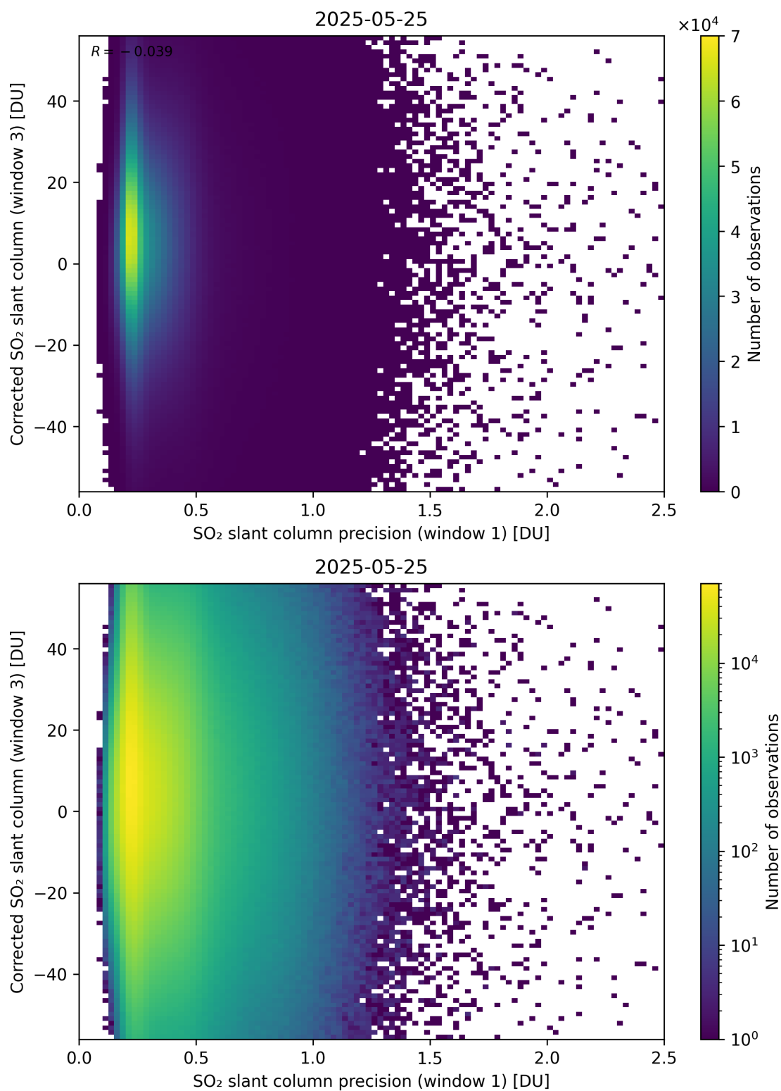
Figure 276: Scatter density plot of “SO 2 slant column precision (window 1)” against “Corrected SO 2 slant column (window 3)” for 2025-05-24 to 2025-05-26.
