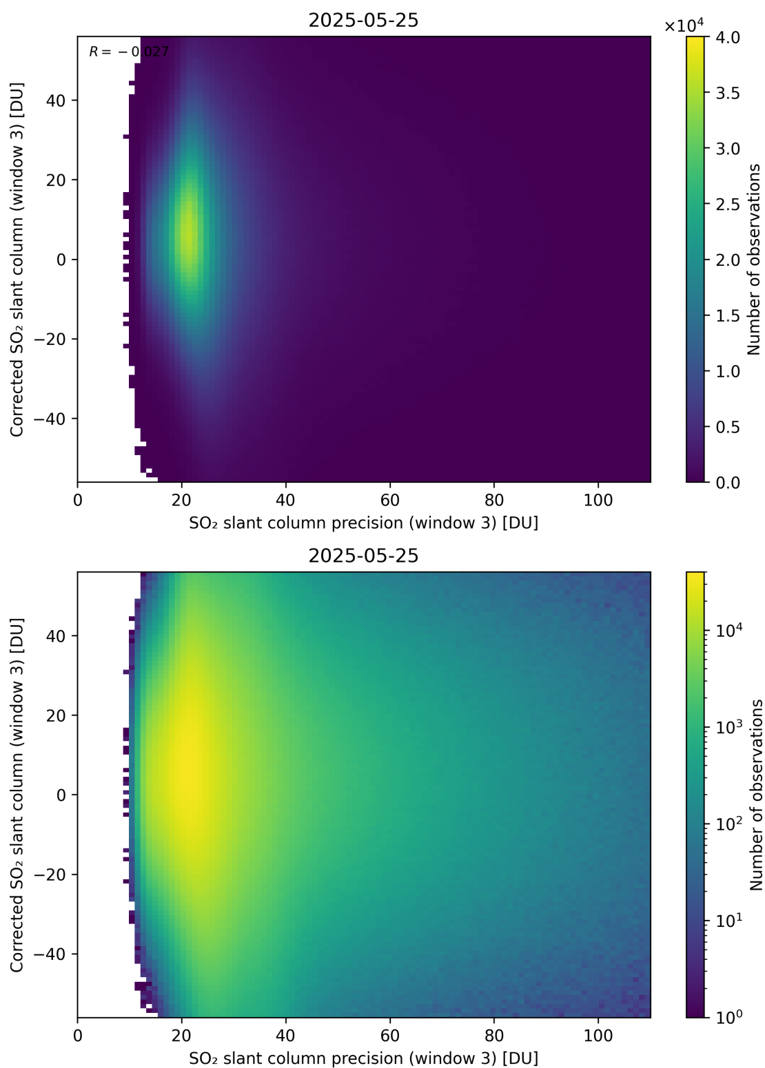
Figure 312: Scatter density plot of “SO 2 slant column precision (window 3)” against “Corrected SO 2 slant column (window 3)” for 2025-05-24 to 2025-05-26.
