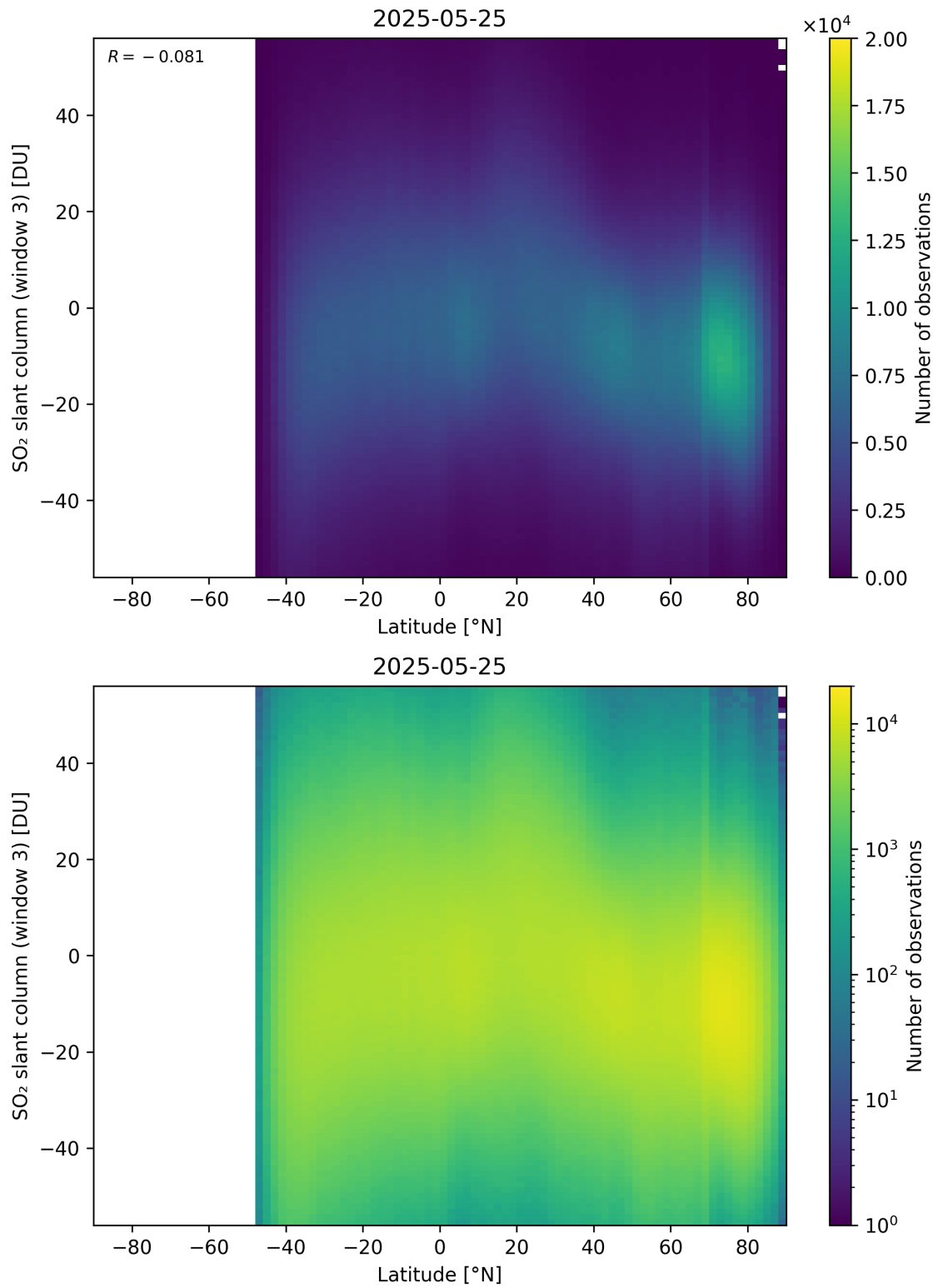
Figure 165: Scatter density plot of “Latitude” against “SO 2 slant column (window 3)” for 2025-05-24 to 2025-05-26.
