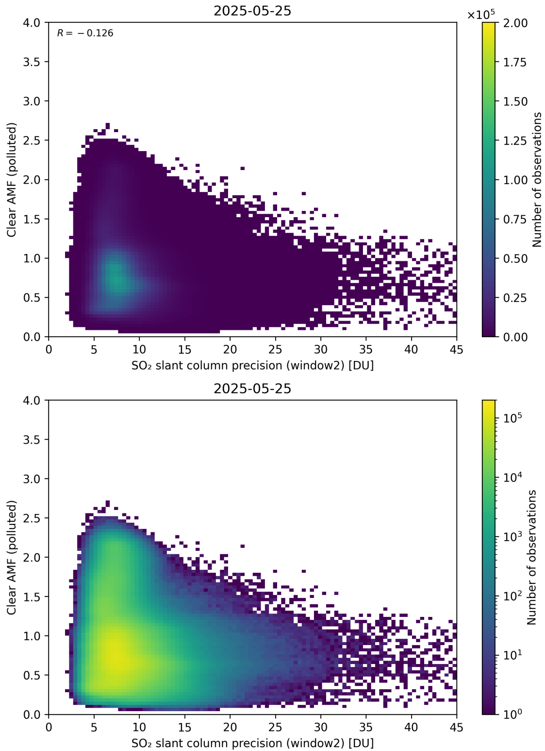
Figure 296: Scatter density plot of “SO 2 slant column precision (window2)” against “Clear AMF (polluted)” for 2025-05-24 to 2025-05-26.
