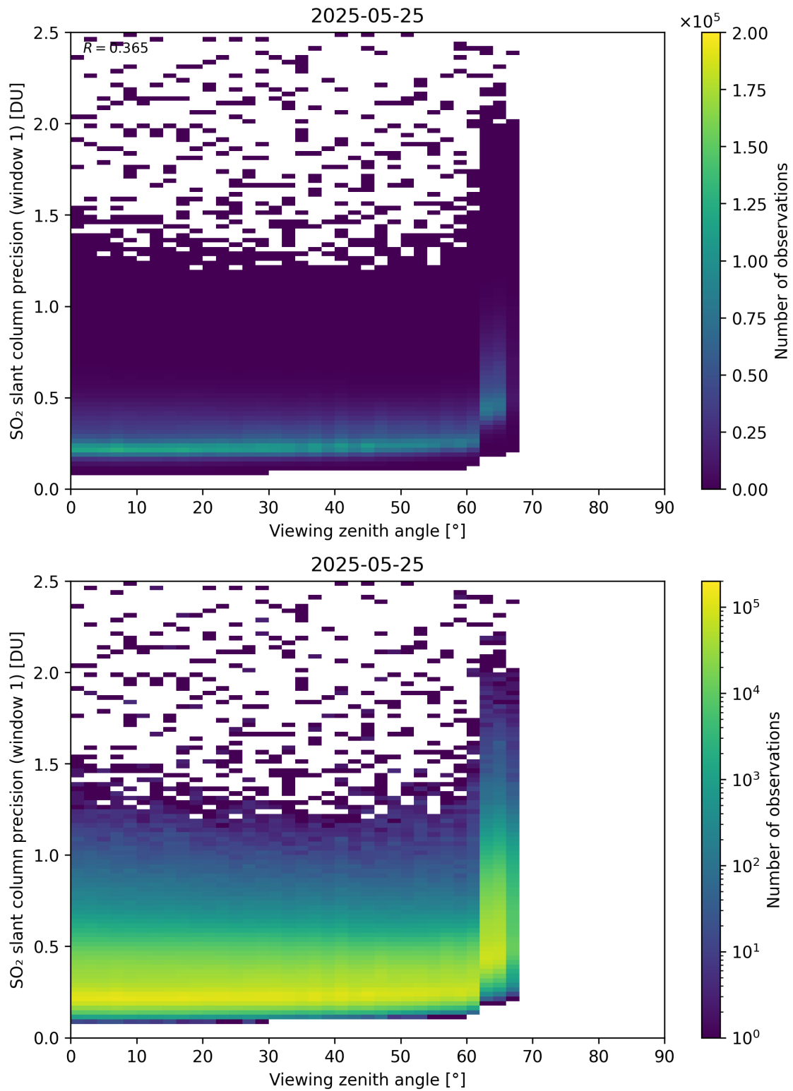
Figure 377: Scatter density plot of “Viewing zenith angle” against “SO 2 slant column precision (window 1)” for 2025-05-24 to 2025-05-26.
