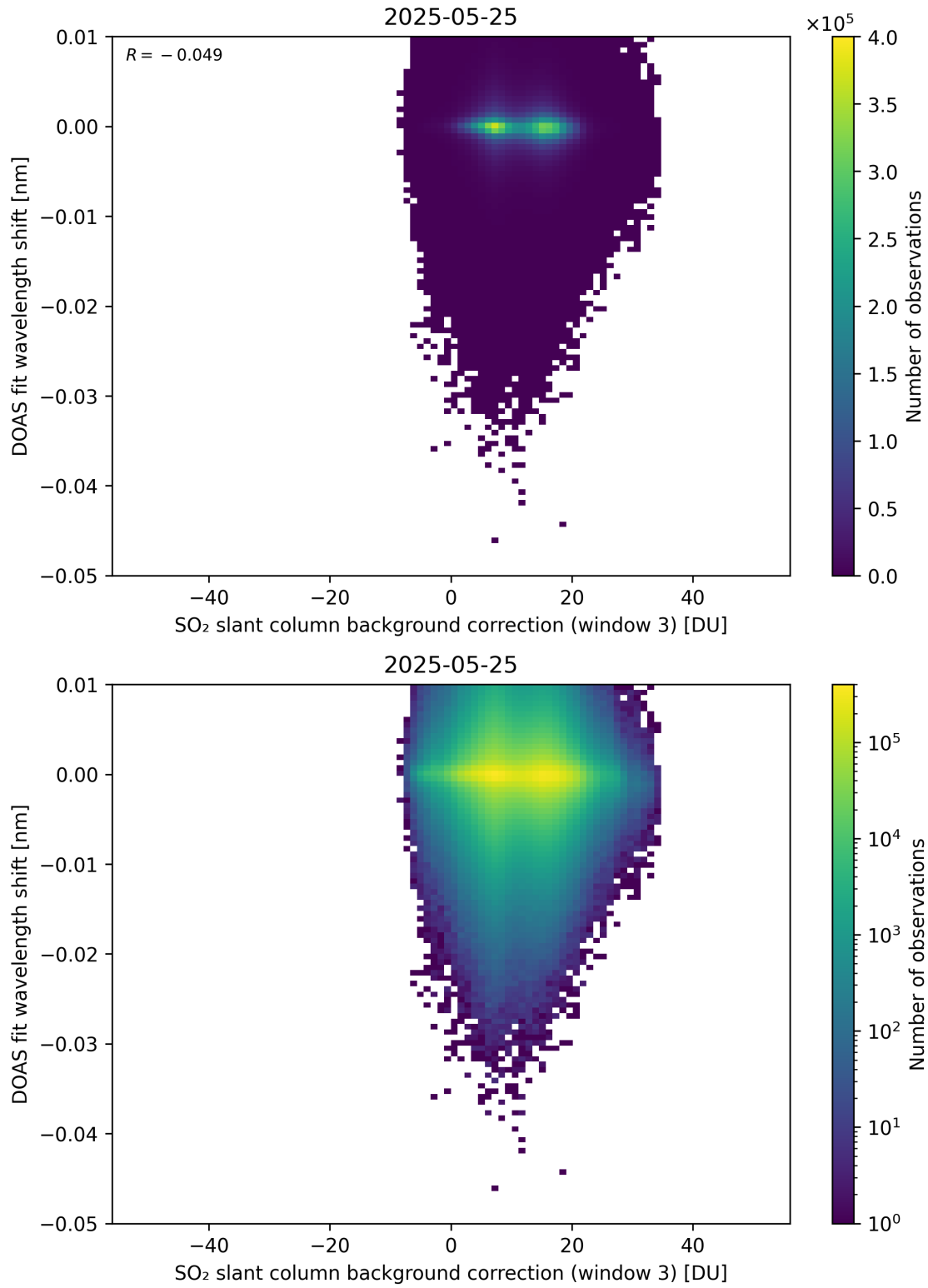
Figure 132: Scatter density plot of “SO 2 slant column background correction (window 3)” against “DOAS fit wavelength shift” for 2025-05-24 to 2025-05-26.
