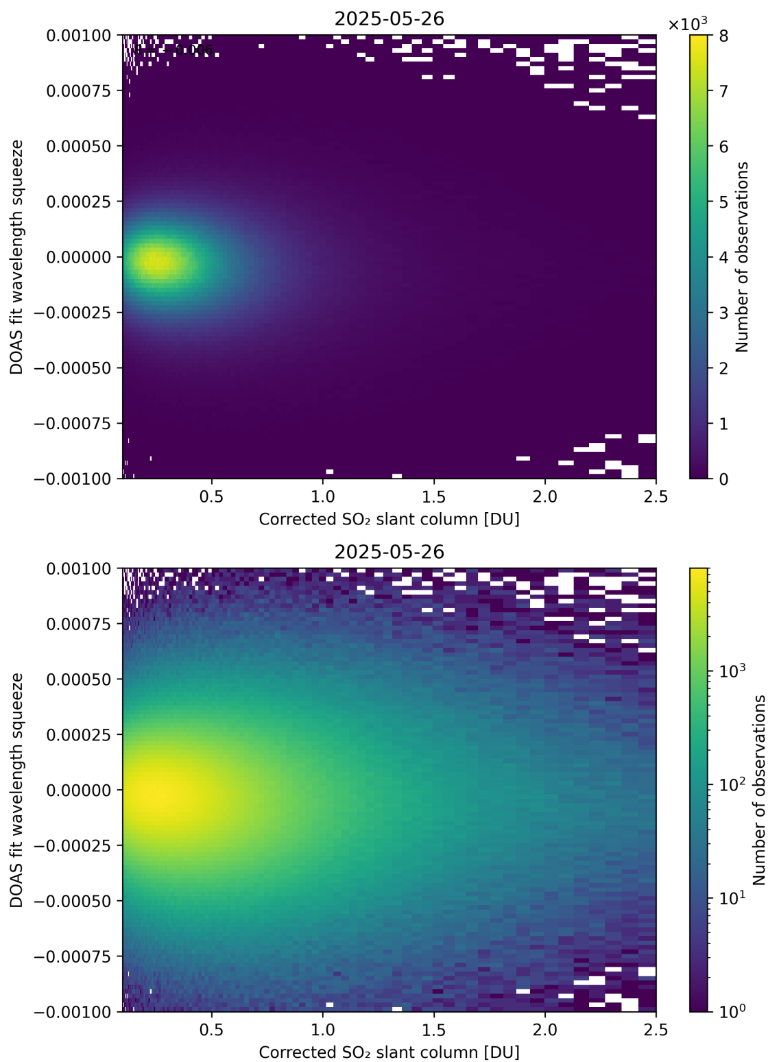
Figure 230: Scatter density plot of "Corrected SO 2 slant column" against "DOAS fit wavelength squeeze" for 2025-05-26 to 2025-05-27.
