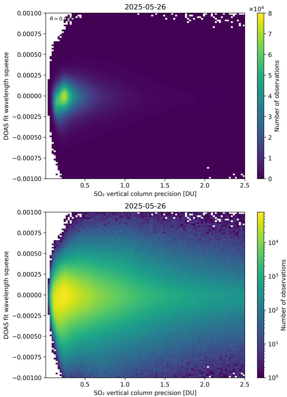
Figure 333: Scatter density plot of “SO 2 vertical column precision” against “DOAS fit wavelength squeeze” for 2025-05-26 to 2025-05-27.
