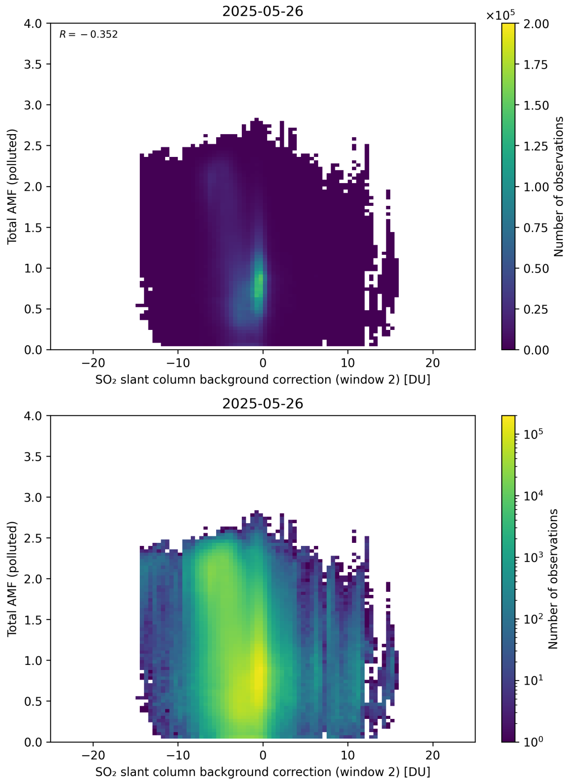
Figure 130: Scatter density plot of “SO 2 slant column background correction (window 2)” against “Total AMF (polluted)” for 2025-05-26 to 2025-05-27.
