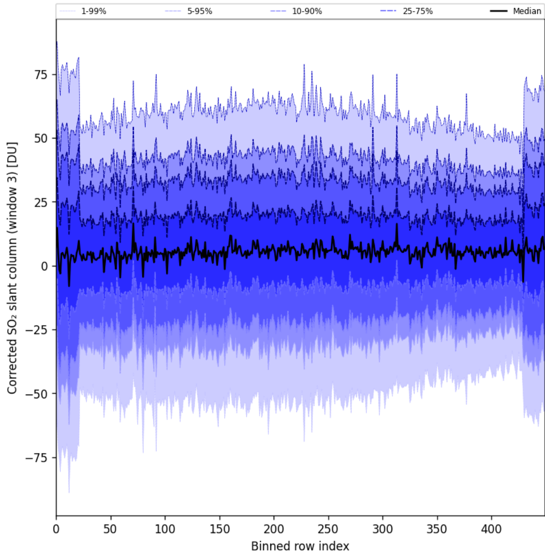
Figure 99: Along track statistics of “Corrected SO 2 slant column (window 3)” for 2025-05-26 to 2025-05-27
