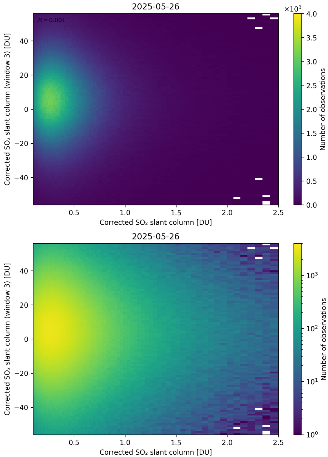
Figure 236: Scatter density plot of “Corrected SO 2 slant column” against “Corrected SO 2 slant column (window 3)” for 2025-05-26 to 2025-05-27.
