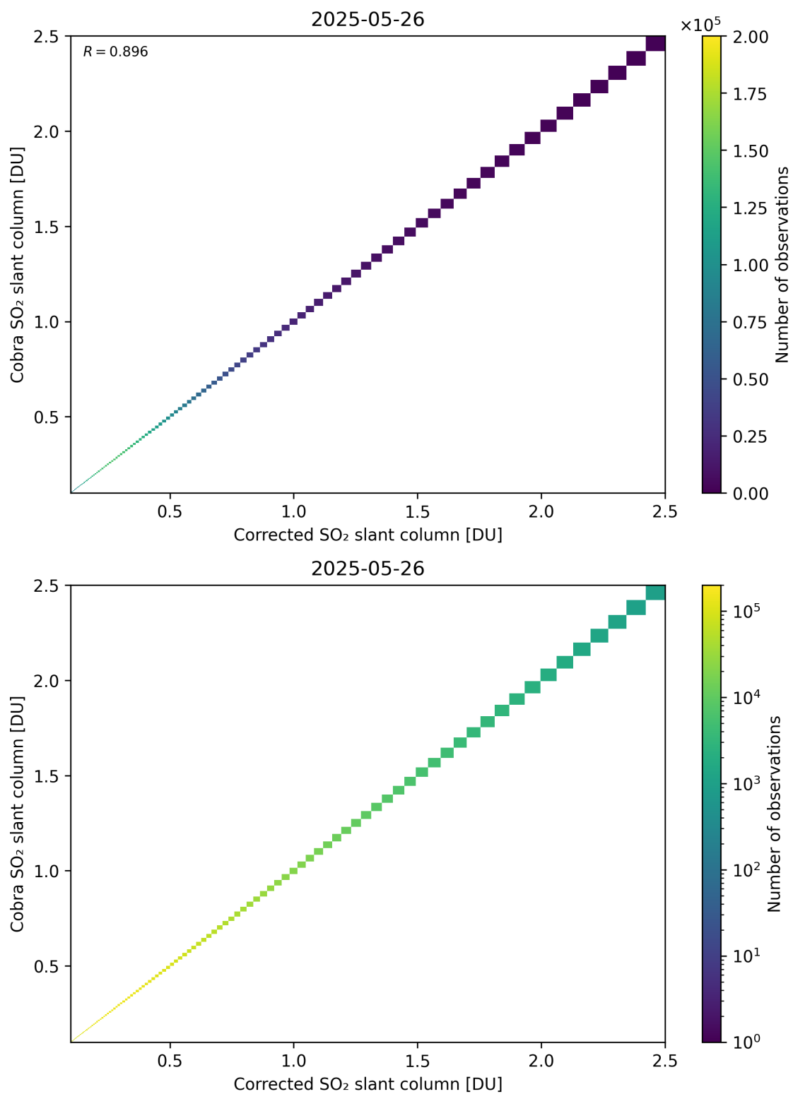
Figure 233: Scatter density plot of “Corrected SO 2 slant column” against “Cobra SO 2 slant column” for 2025-05-26 to 2025-05-27.
