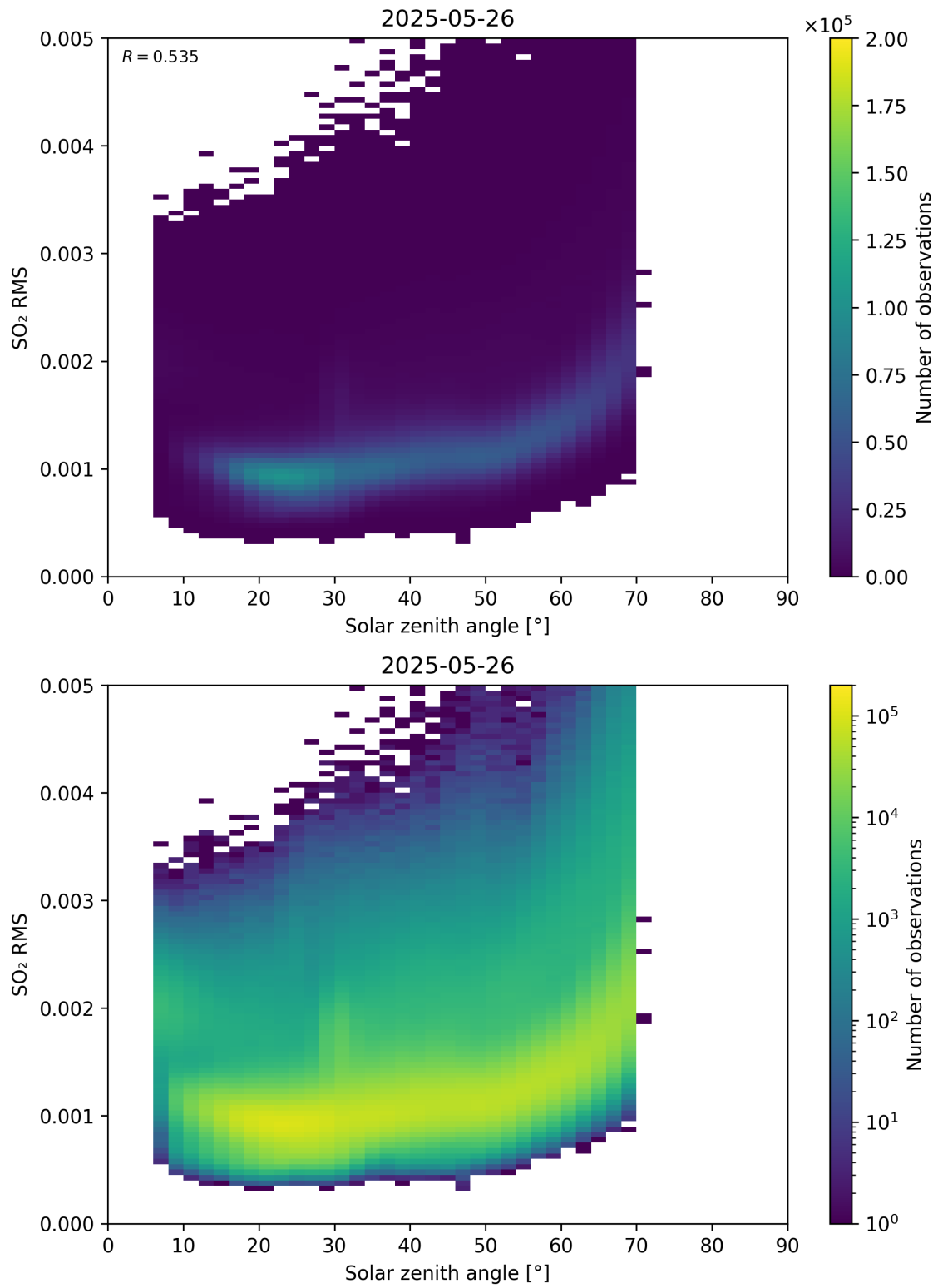
Figure 176: Scatter density plot of “Solar zenith angle” against “SO 2 RMS” for 2025-05-26 to 2025-05-27.
