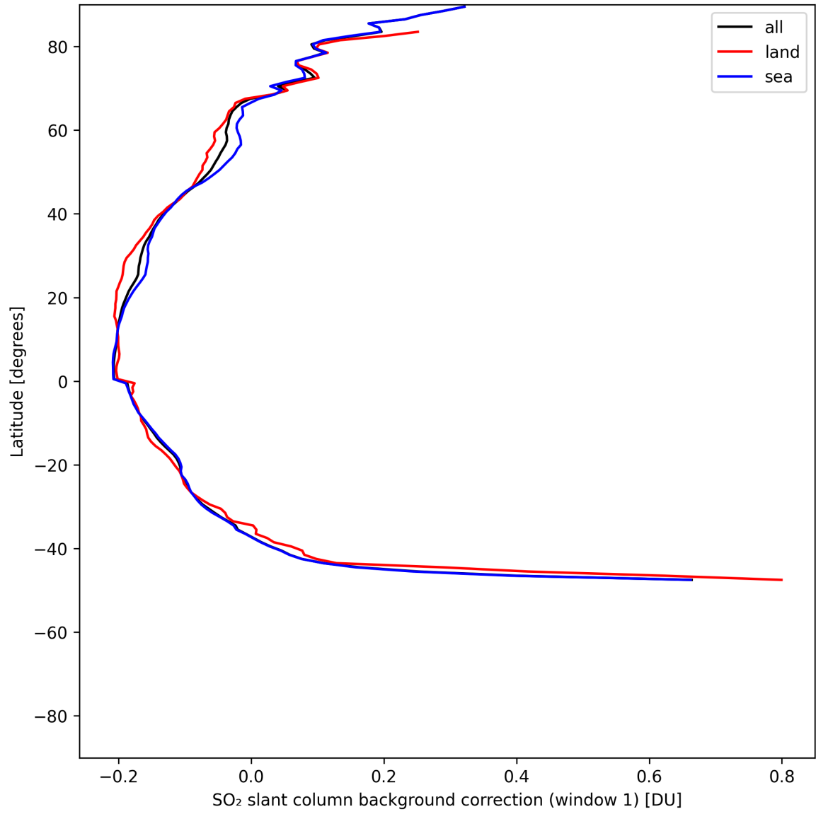
Figure 40: Zonal average of “SO 2 slant column background correction (window 1)” for 2025-05-26 to 2025-05-27.
