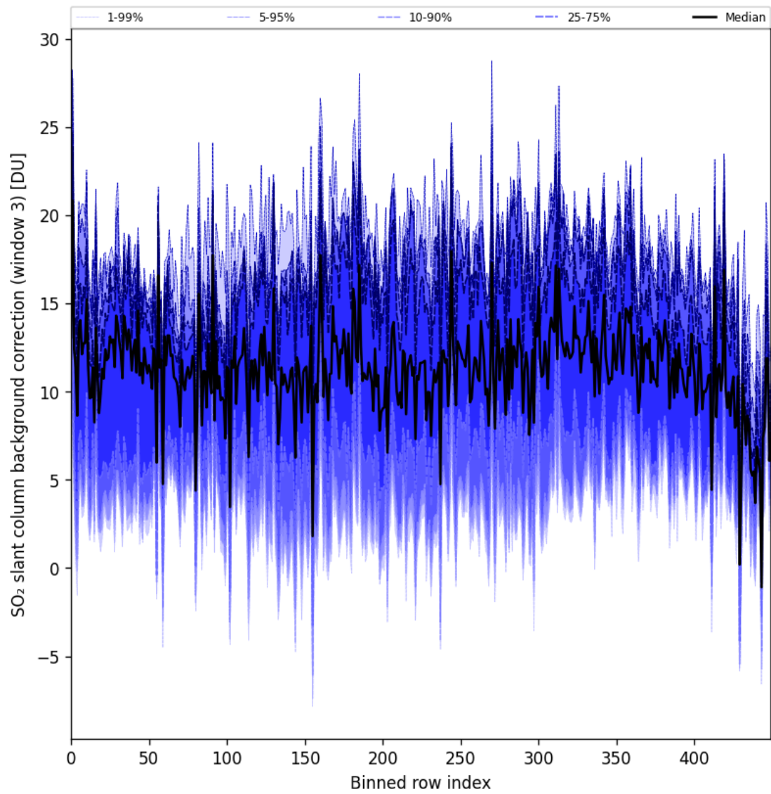
Figure 100: Along track statistics of “SO 2 slant column background correction (window 3)” for 2025-05-26 to 2025-05-27
