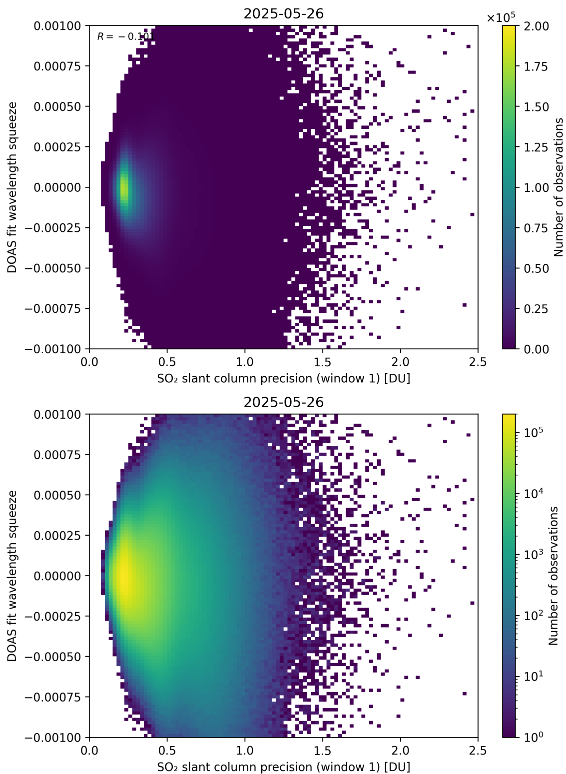
Figure 272: Scatter density plot of “SO 2 slant column precision (window 1)” against “DOAS fit wavelength squeeze” for 2025-05-26 to 2025-05-27.
