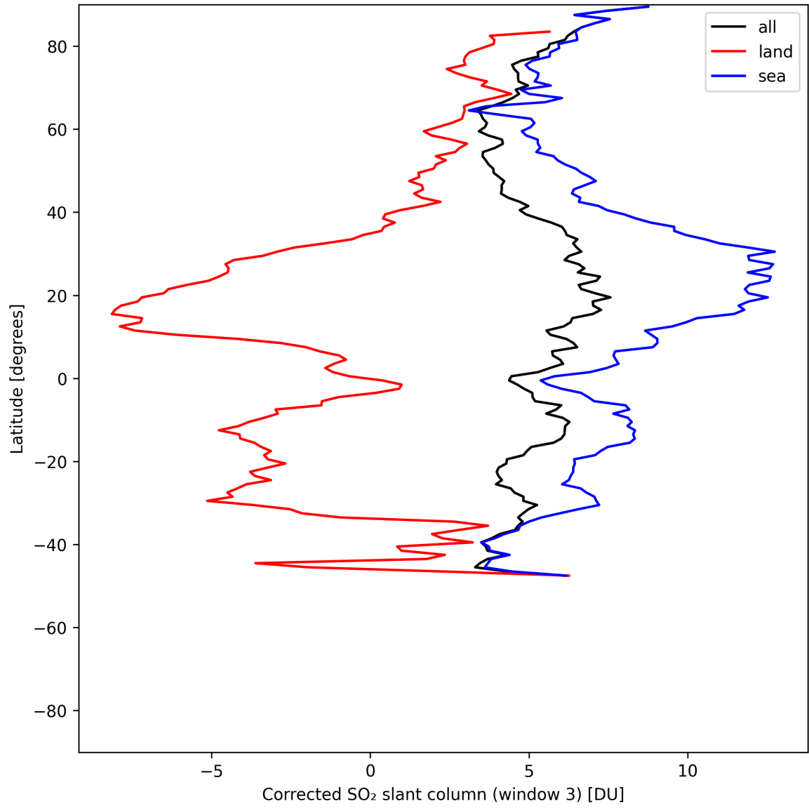
Figure 47: Zonal average of “Corrected SO 2 slant column (window 3)” for 2025-05-26 to 2025-05-27.
