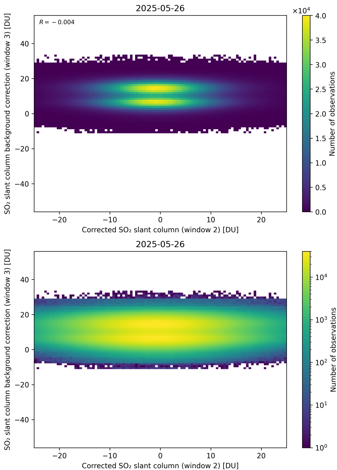
Figure 245: Scatter density plot of “Corrected SO 2 slant column (window 2)” against “SO 2 slant column background correction (window 3)” for 2025-05-26 to 2025-05-27.
