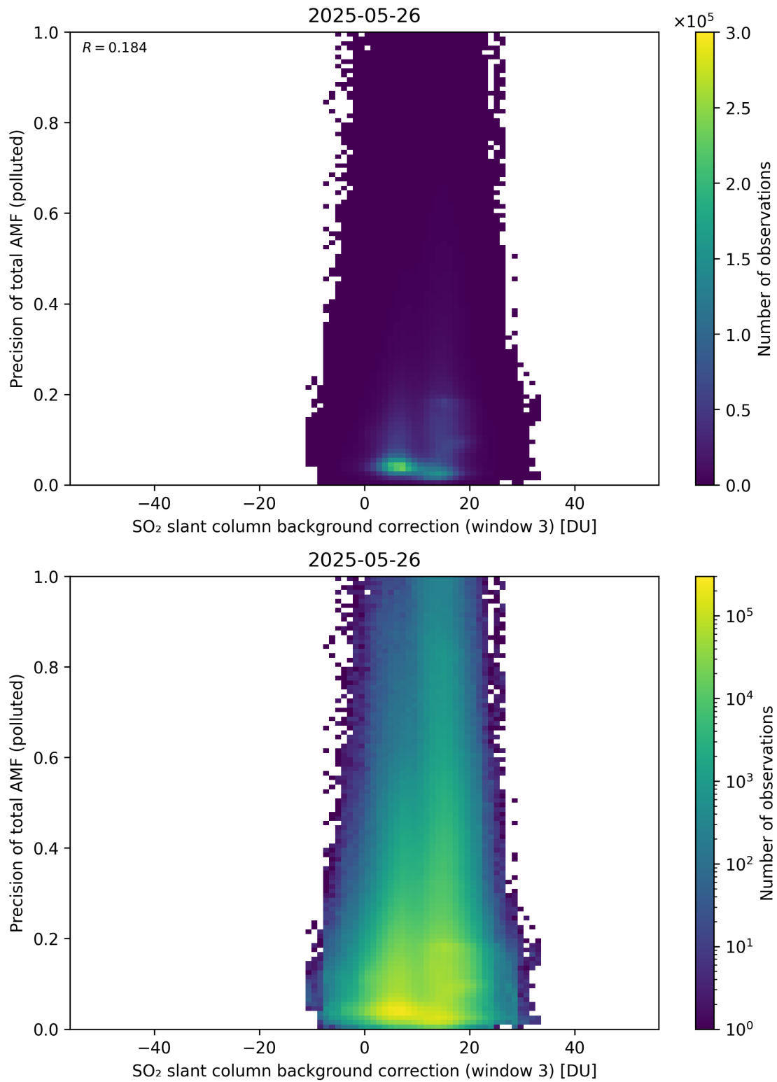
Figure 137: Scatter density plot of “SO 2 slant column background correction (window 3)” against “Precision of total AMF (polluted)” for 2025-05-26 to 2025-05-27.
