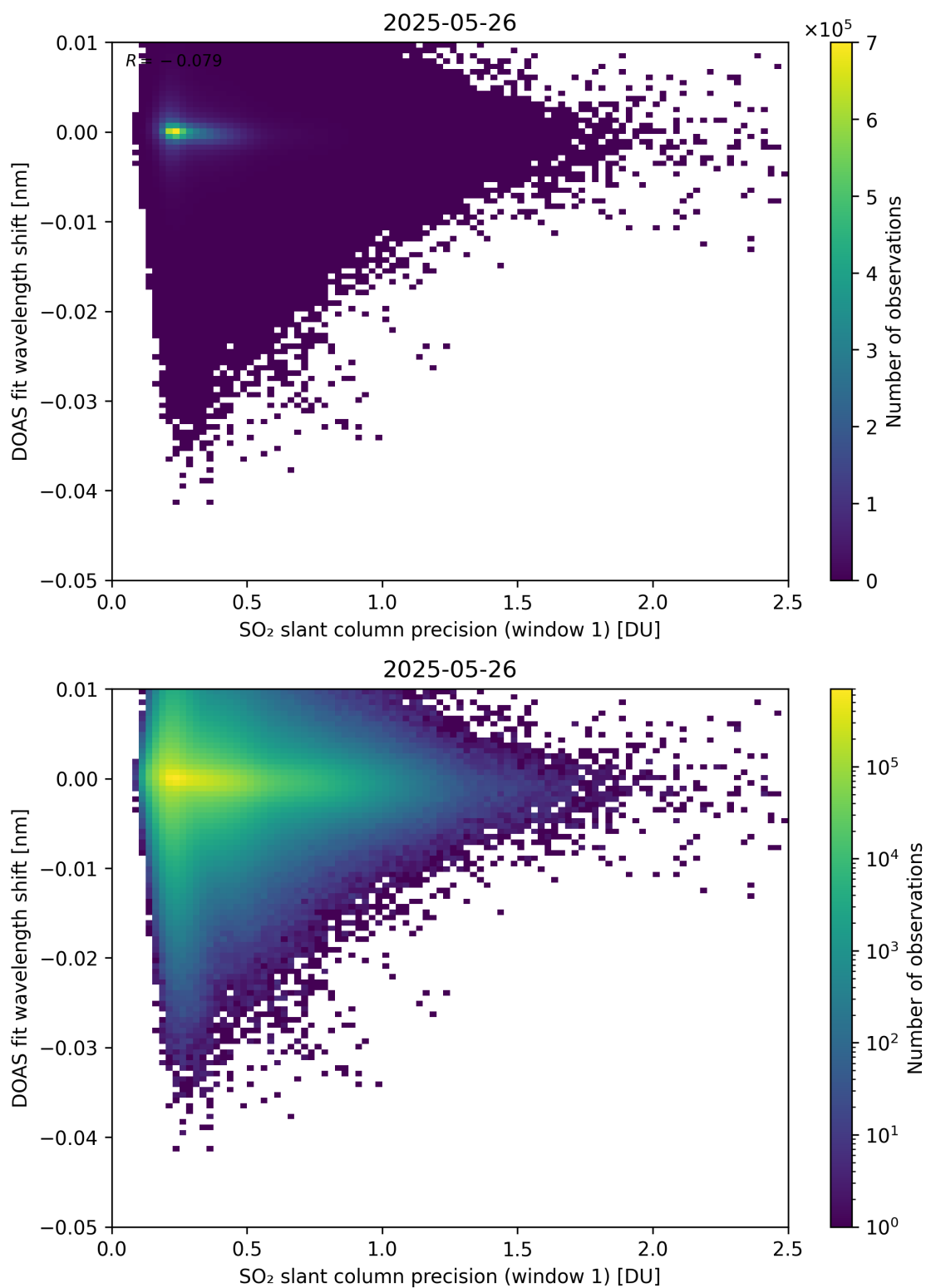
Figure 271: Scatter density plot of “SO 2 slant column precision (window 1)” against “DOAS fit wavelength shift” for 2025-05-26 to 2025-05-27.
