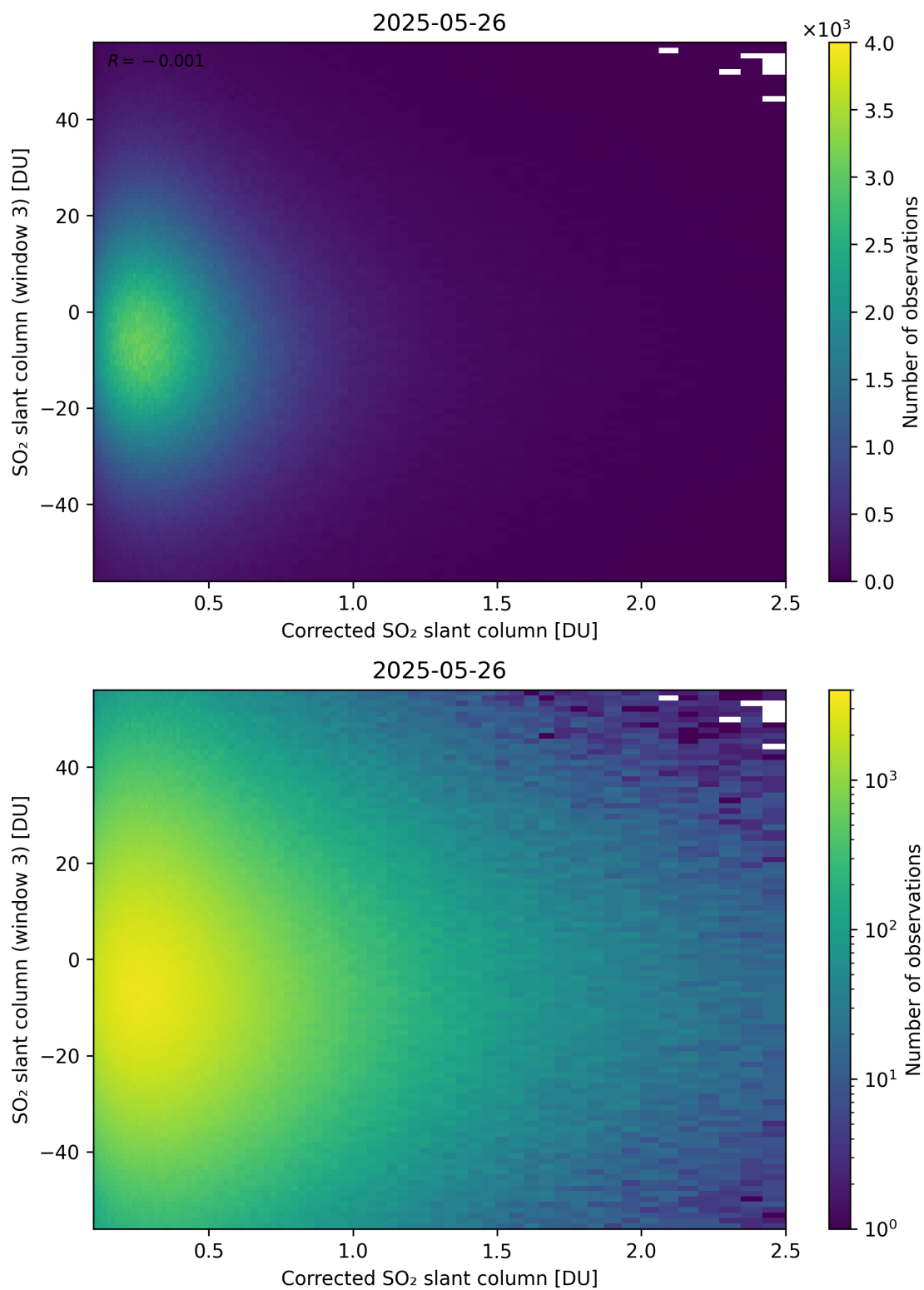
Figure 240: Scatter density plot of “Corrected SO 2 slant column” against “SO 2 slant column (window 3)” for 2025-05-26 to 2025-05-27.
