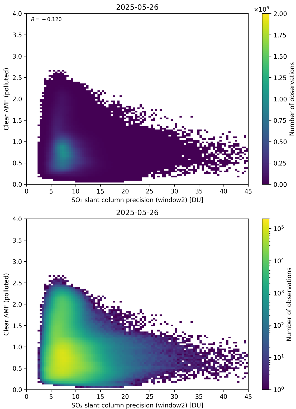
Figure 296: Scatter density plot of “SO 2 slant column precision (window2)” against “Clear AMF (polluted)” for 2025-05-26 to 2025-05-27.
