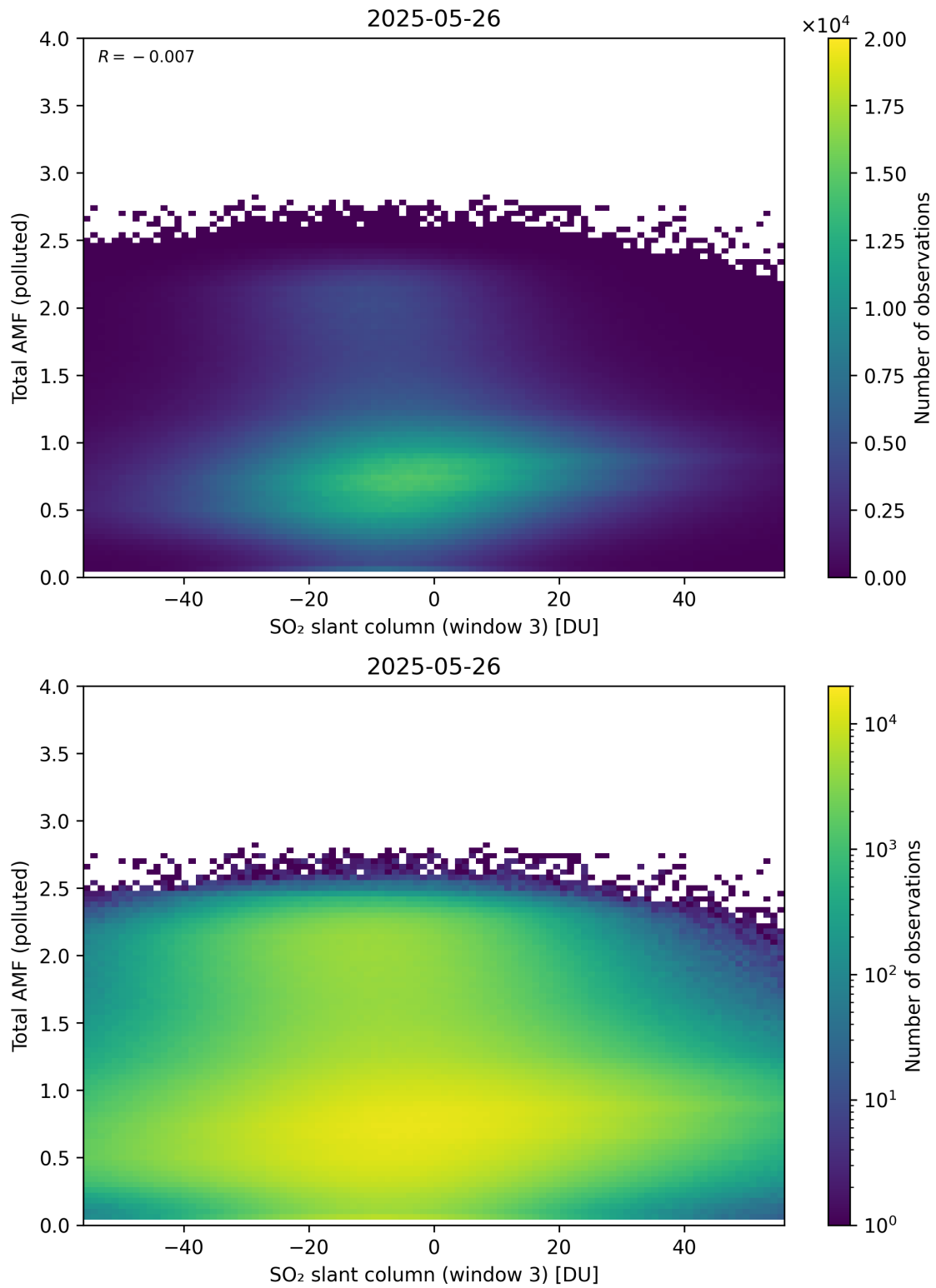
Figure 318: Scatter density plot of “SO 2 slant column (window 3)” against “Total AMF (polluted)” for 2025-05-26 to 2025-05-27.
