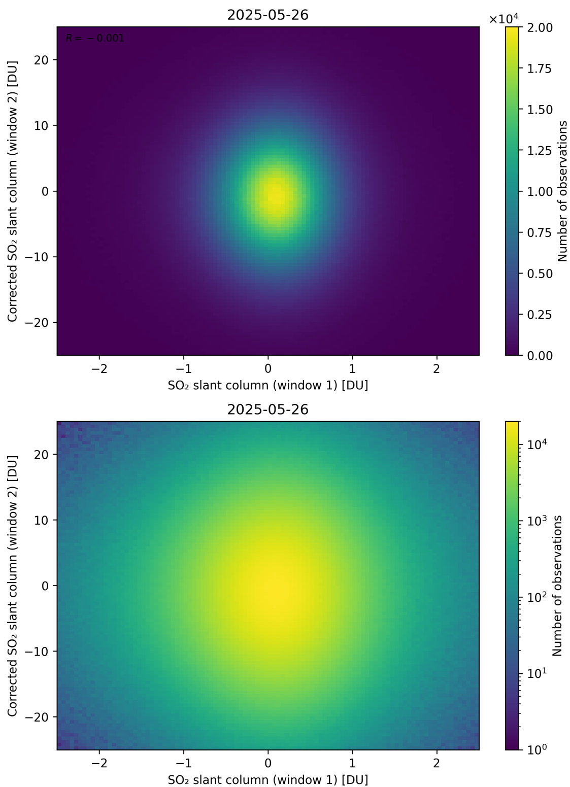
Figure 283: Scatter density plot of “SO 2 slant column (window 1)” against “Corrected SO 2 slant column (window 2)” for 2025-05-26 to 2025-05-27.
