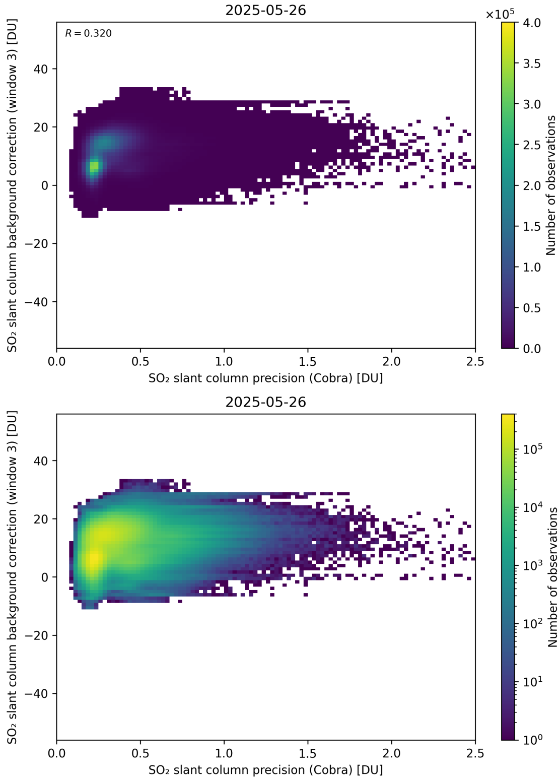
Figure 201: Scatter density plot of “SO 2 slant column precision (Cobra)” against “SO 2 slant column background correction (window 3)” for 2025-05-26 to 2025-05-27.
