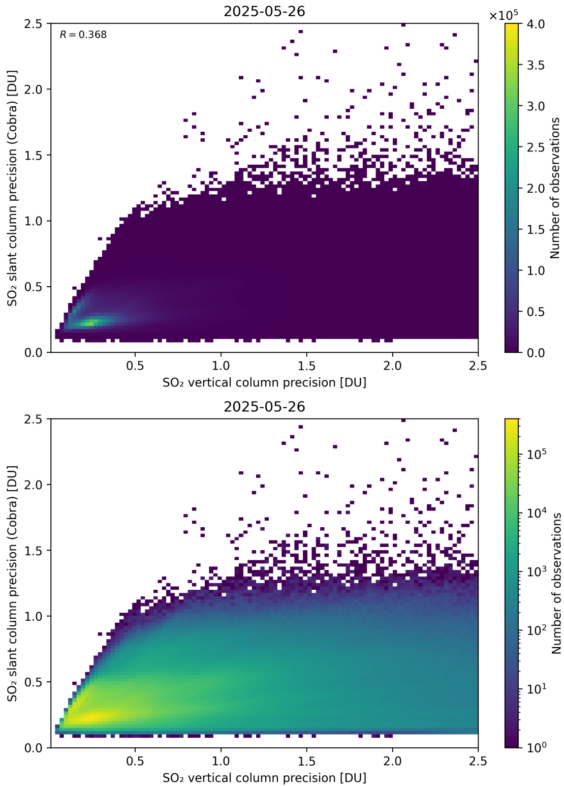
Figure 337: Scatter density plot of “SO 2 vertical column precision” against “SO 2 slant column precision (Cobra)” for 2025-05-26 to 2025-05-27.
