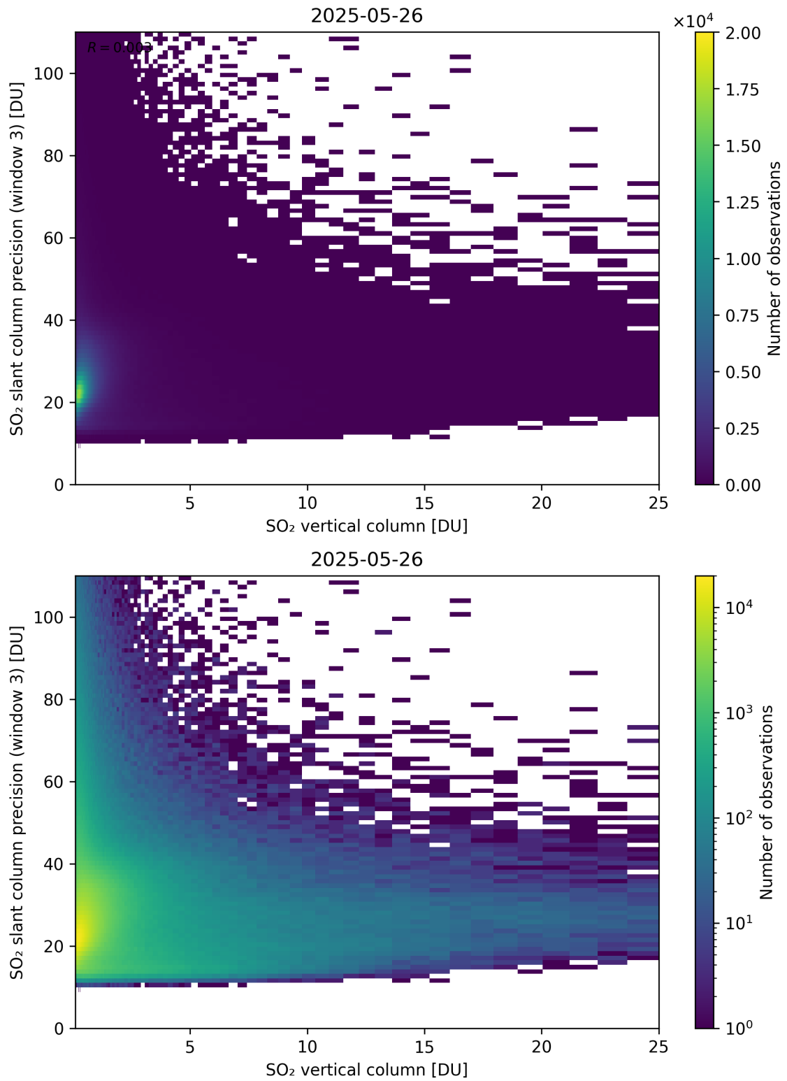
Figure 358: Scatter density plot of “SO 2 vertical column” against “SO 2 slant column precision (window 3)” for 2025-05-26 to 2025-05-27.
