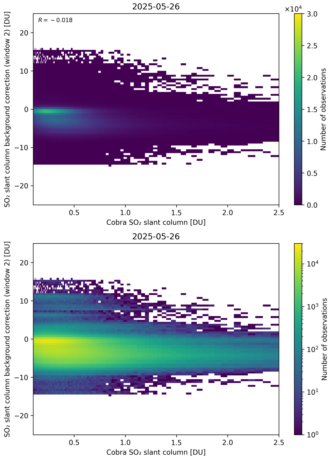
Figure 194: Scatter density plot of “Cobra SO 2 slant column” against “SO 2 slant column background correction (window 2)” for 2025-05-26 to 2025-05-27.
