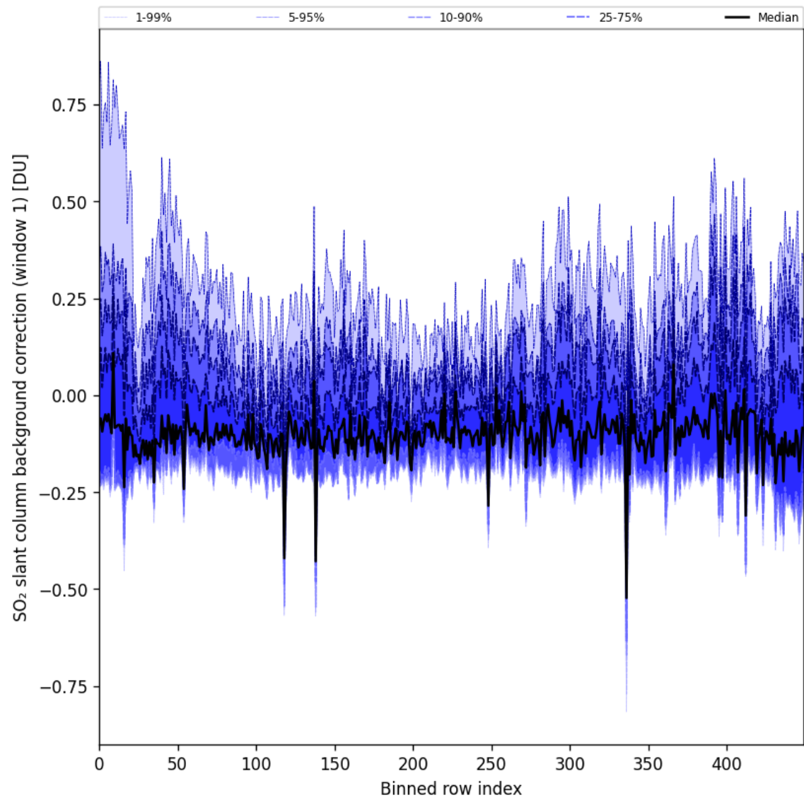
Figure 92: Along track statistics of “SO 2 slant column background correction (window 1)” for 2025-05-26 to 2025-05-27
