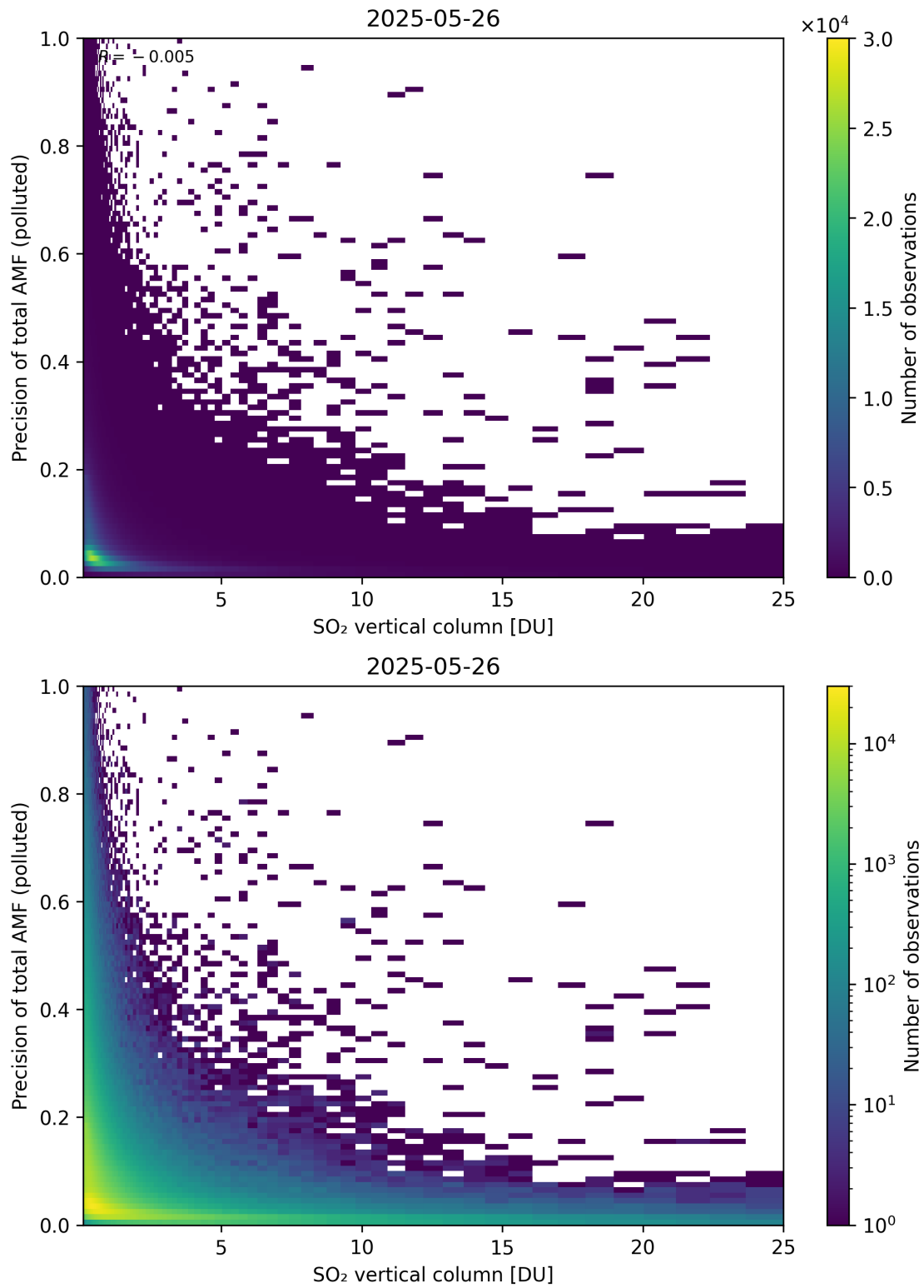
Figure 360: Scatter density plot of “SO 2 vertical column” against “Precision of total AMF (polluted)” for 2025-05-26 to 2025-05-27.
