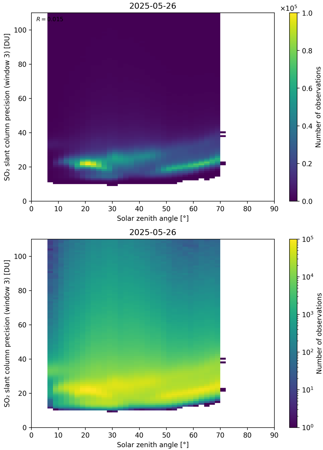
Figure 188: Scatter density plot of “Solar zenith angle” against “SO 2 slant column precision (window 3)” for 2025-05-26 to 2025-05-27.
