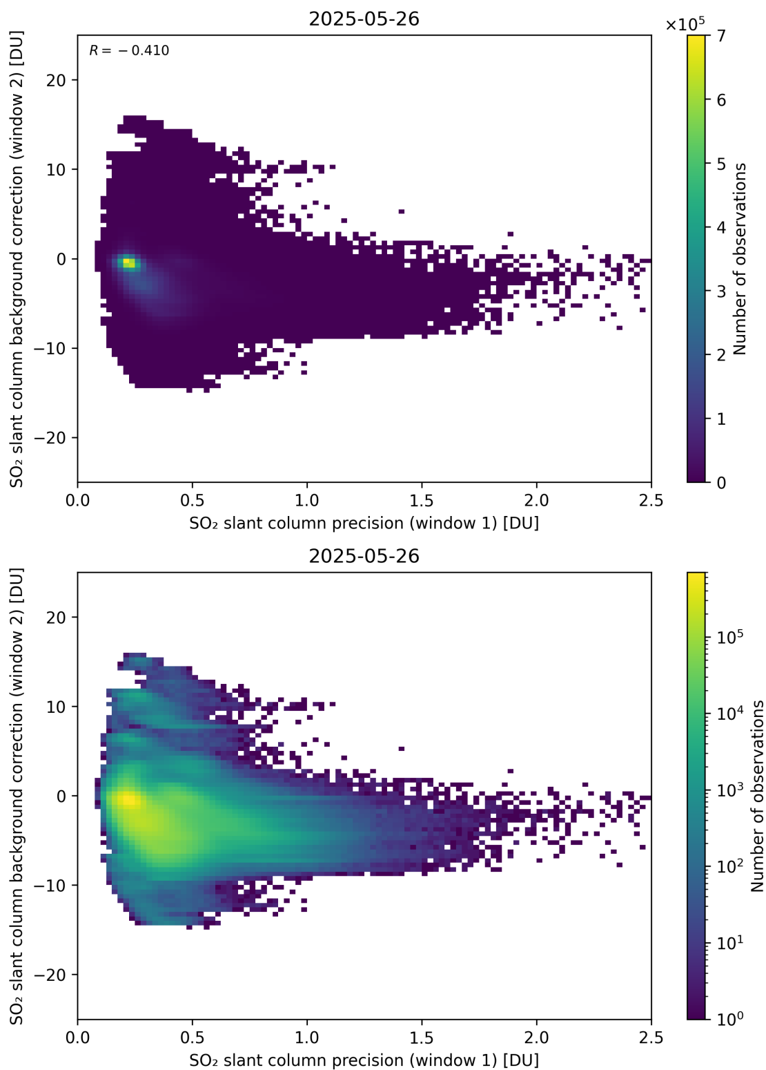
Figure 269: Scatter density plot of “SO 2 slant column precision (window 1)” against “SO 2 slant column background correction (window 2)” for 2025-05-26 to 2025-05-27.
