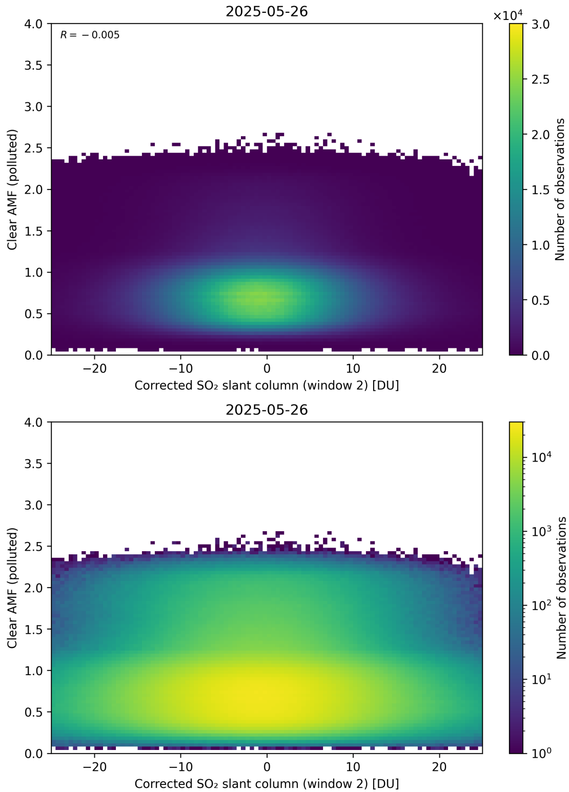
Figure 249: Scatter density plot of “Corrected SO 2 slant column (window 2)” against “Clear AMF (polluted)” for 2025-05-26 to 2025-05-27.
