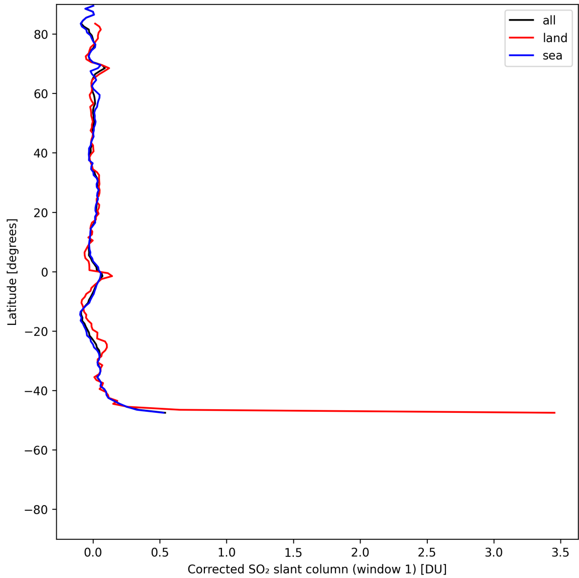
Figure 39: Zonal average of “Corrected SO 2 slant column (window 1)” for 2025-05-26 to 2025-05-27.
