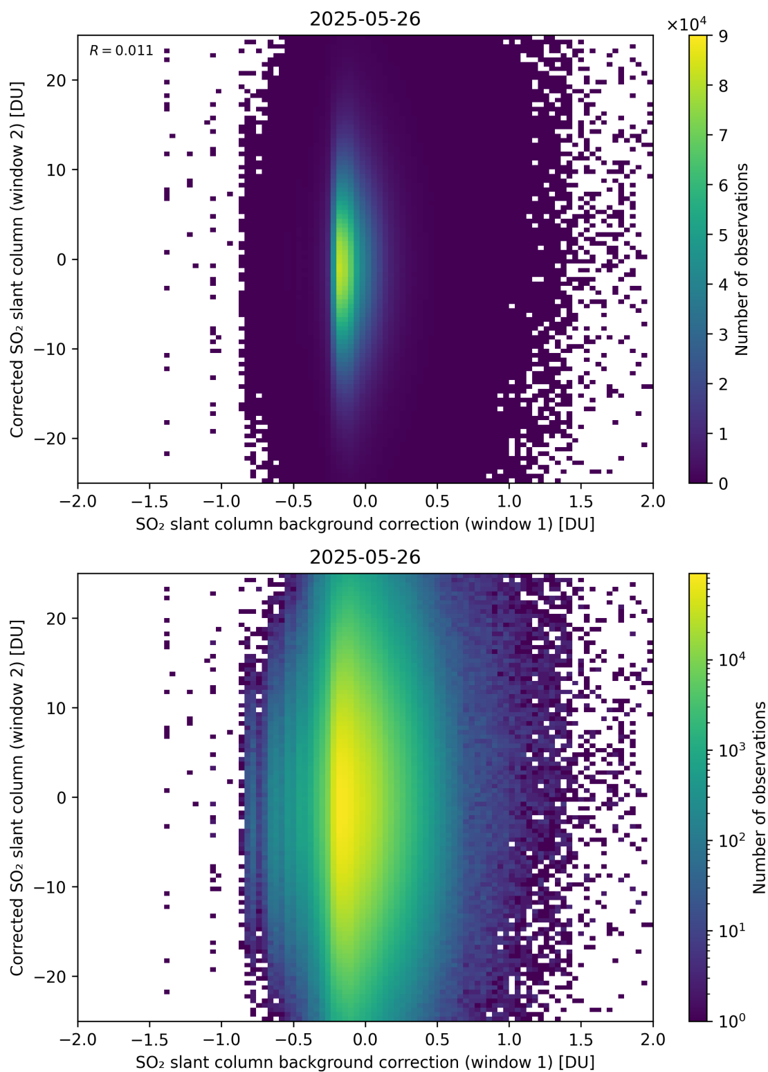
Figure 115: Scatter density plot of “SO 2 slant column background correction (window 1)” against “Corrected SO 2 slant column (window 2)” for 2025-05-26 to 2025-05-27.
