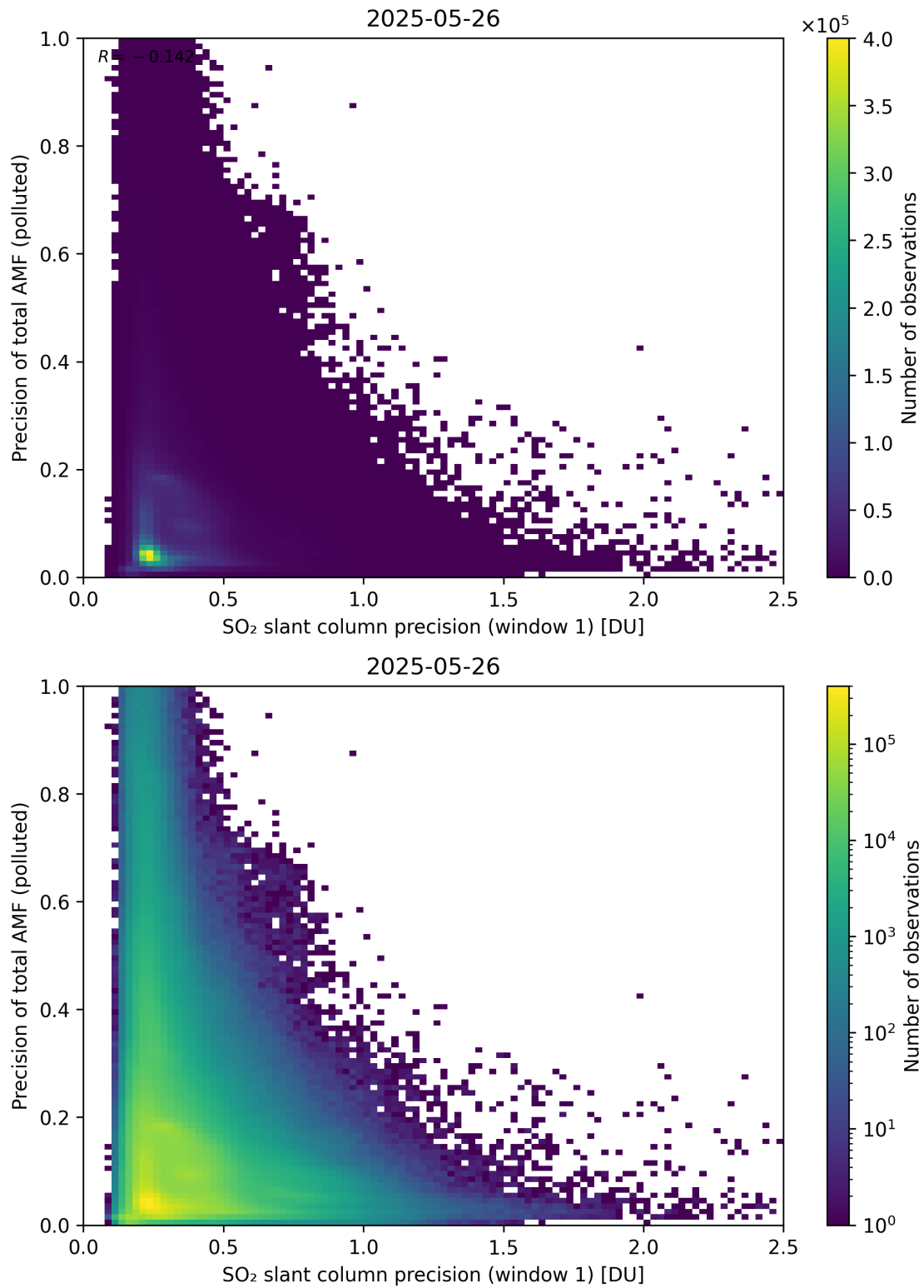
Figure 281: Scatter density plot of “SO 2 slant column precision (window 1)” against “Precision of total AMF (polluted)” for 2025-05-26 to 2025-05-27.
