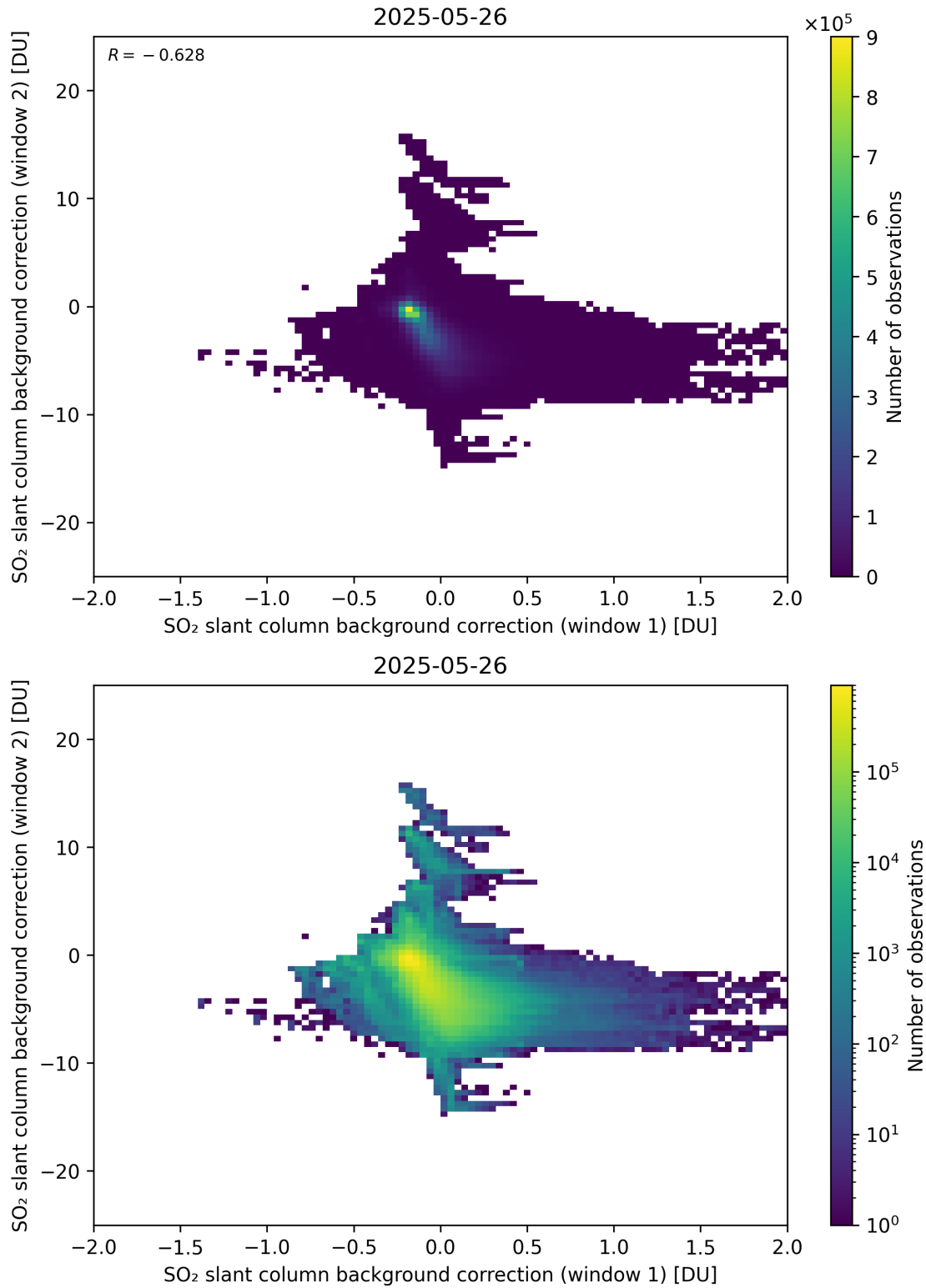
Figure 109: Scatter density plot of “SO 2 slant column background correction (window 1)” against “SO 2 slant column background correction (window 2)” for 2025-05-26 to 2025-05-27.
