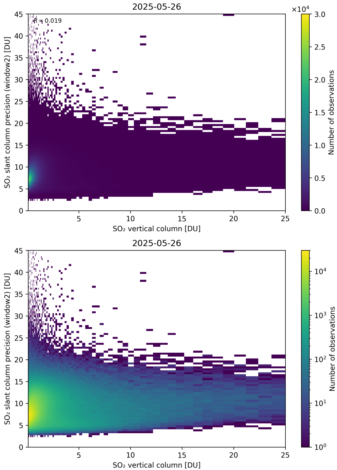
Figure 356: Scatter density plot of “SO 2 vertical column” against “SO 2 slant column precision (window2)” for 2025-05-26 to 2025-05-27.
