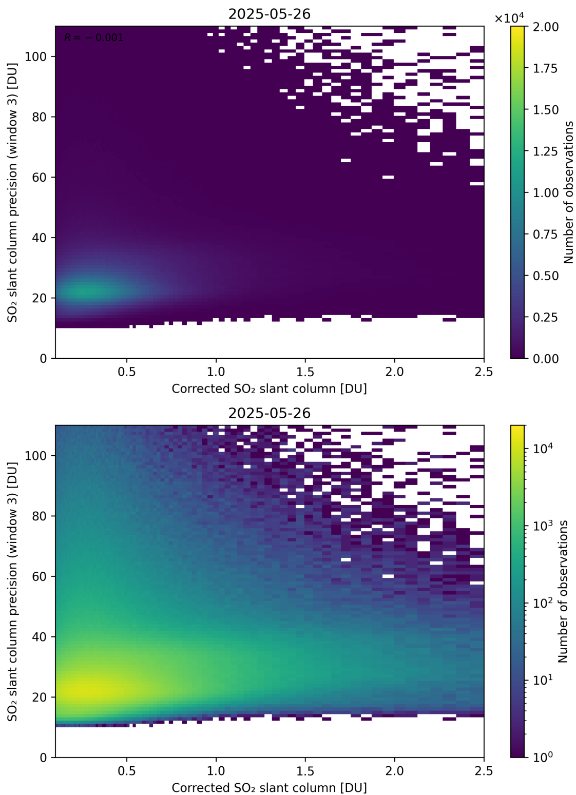
Figure 241: Scatter density plot of “Corrected SO 2 slant column” against “SO 2 slant column precision (window 3)” for 2025-05-26 to 2025-05-27.
