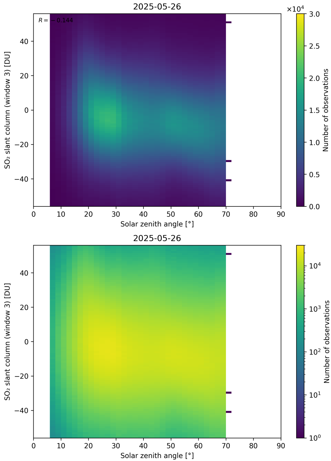
Figure 187: Scatter density plot of “Solar zenith angle” against “SO 2 slant column (window 3)” for 2025-05-26 to 2025-05-27.
