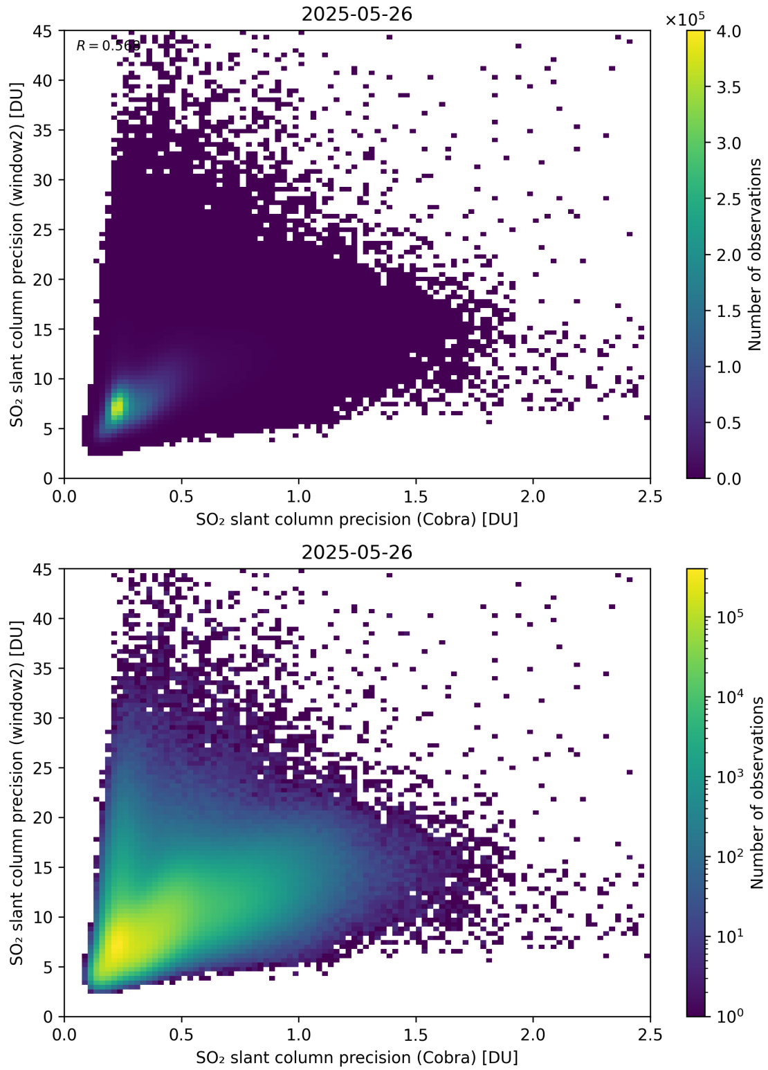
Figure 210: Scatter density plot of “SO 2 slant column precision (Cobra)” against “SO 2 slant column precision (window2)” for 2025-05-26 to 2025-05-27.
