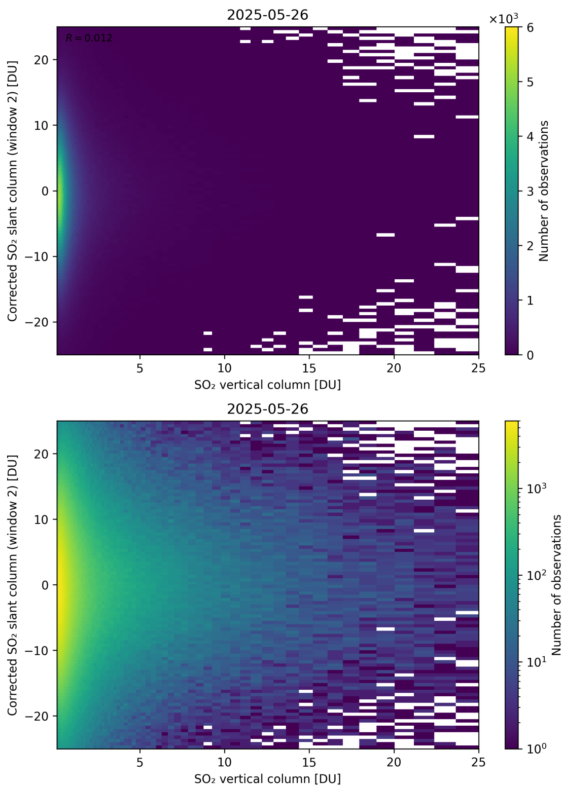
Figure 352: Scatter density plot of “SO 2 vertical column” against “Corrected SO 2 slant column (window 2)” for 2025-05-26 to 2025-05-27.
