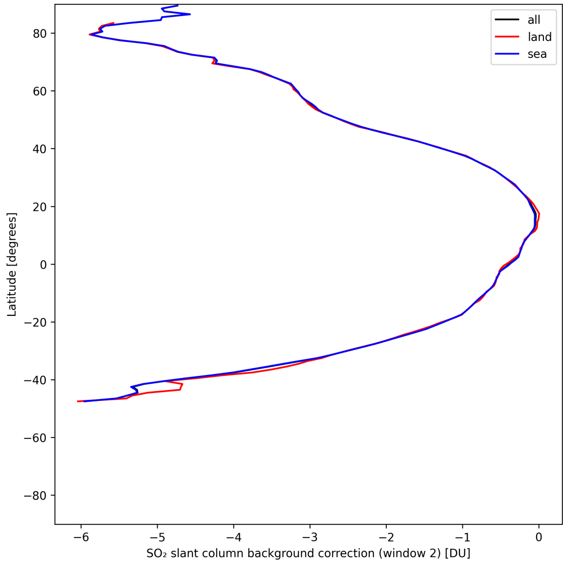
Figure 44: Zonal average of “SO 2 slant column background correction (window 2)” for 2025-05-26 to 2025-05-27.
