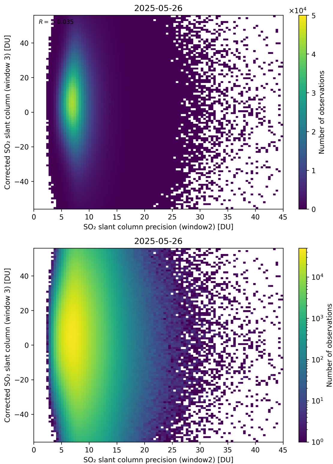
Figure 298: Scatter density plot of “SO 2 slant column precision (window2)” against “Corrected SO 2 slant column (window 3)” for 2025-05-26 to 2025-05-27.
