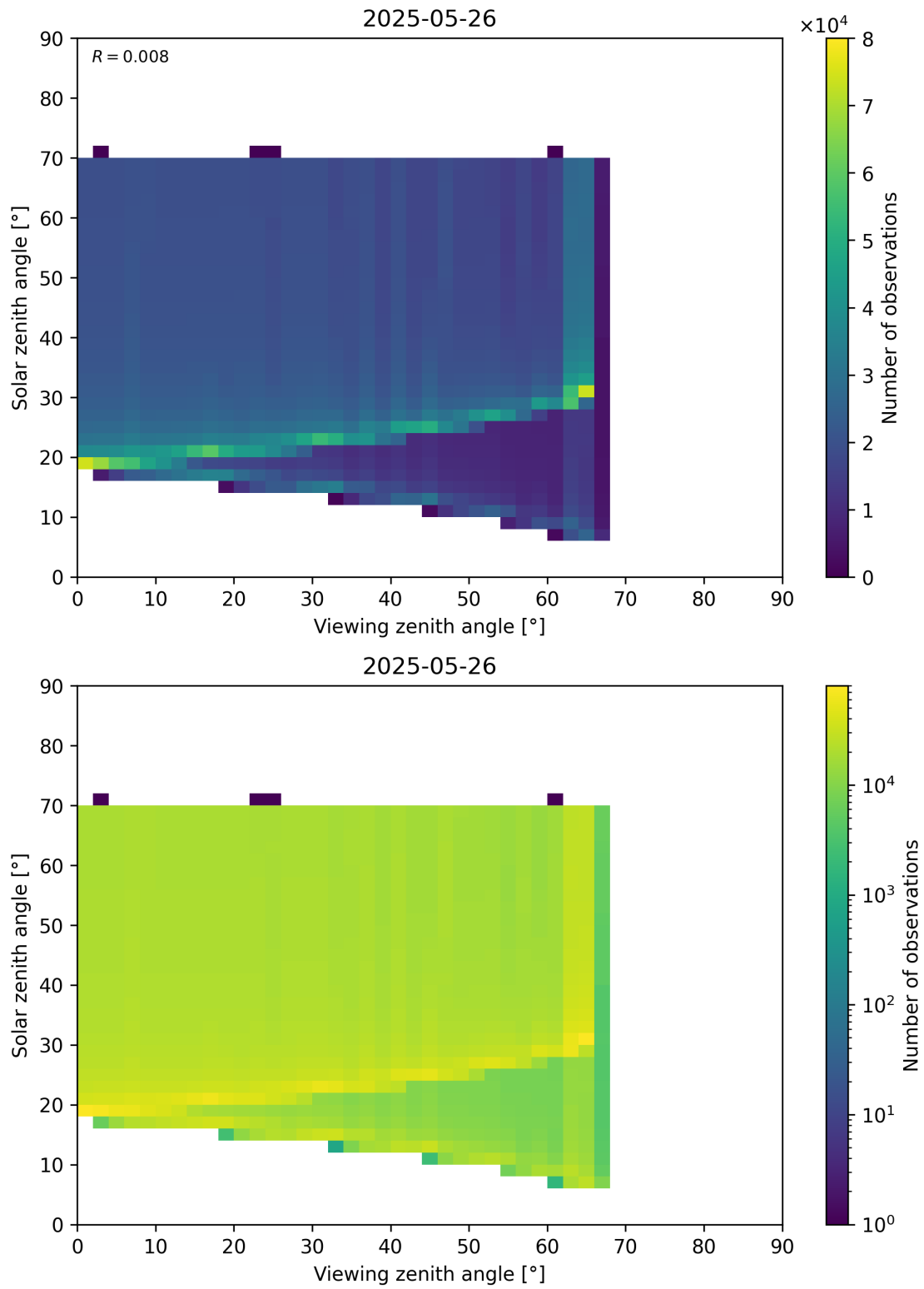
Figure 369: Scatter density plot of “Viewing zenith angle” against “Solar zenith angle” for 2025-05-26 to 2025-05-27.
