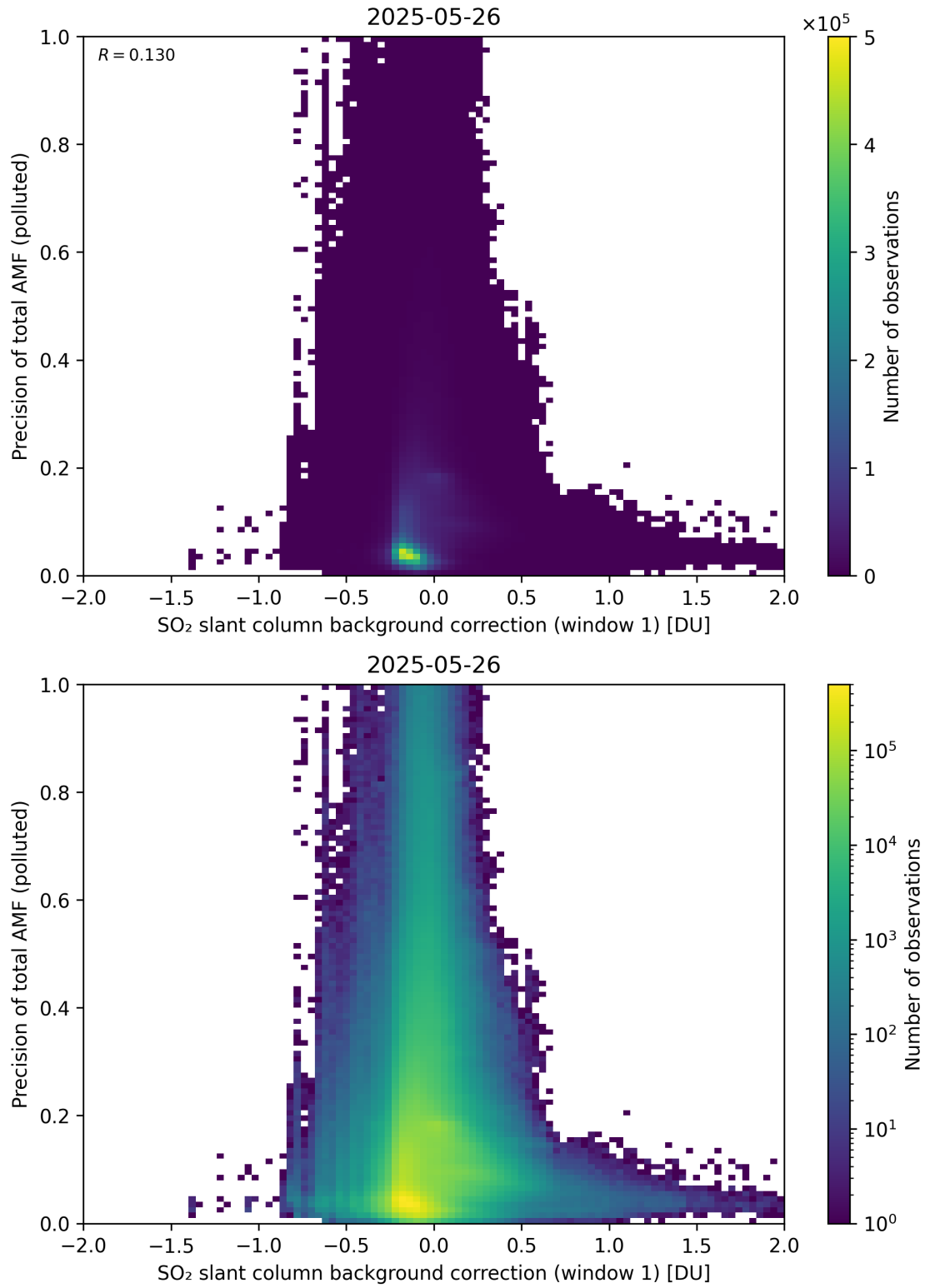
Figure 121: Scatter density plot of “SO 2 slant column background correction (window 1)” against “Precision of total AMF (polluted)” for 2025-05-26 to 2025-05-27.
