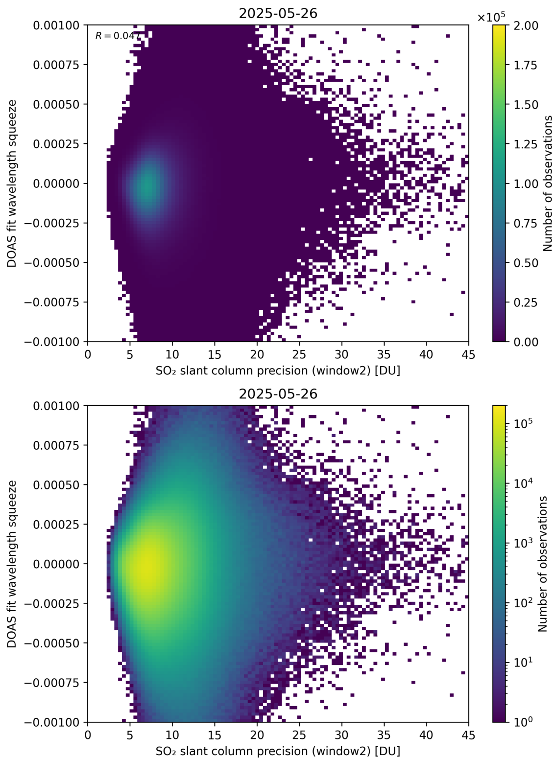
Figure 294: Scatter density plot of “SO 2 slant column precision (window2)” against “DOAS fit wavelength squeeze” for 2025-05-26 to 2025-05-27.
