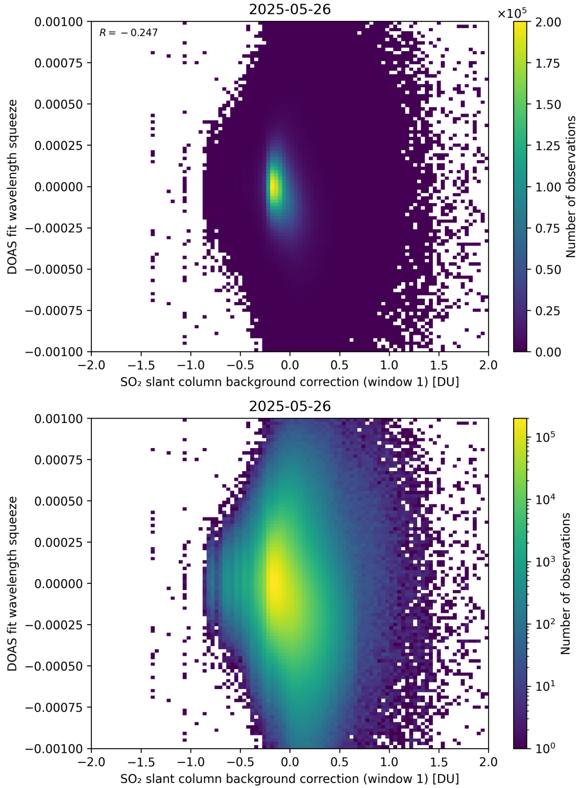
Figure 112: Scatter density plot of “SO 2 slant column background correction (window 1)” against “DOAS fit wavelength squeeze” for 2025-05-26 to 2025-05-27.
