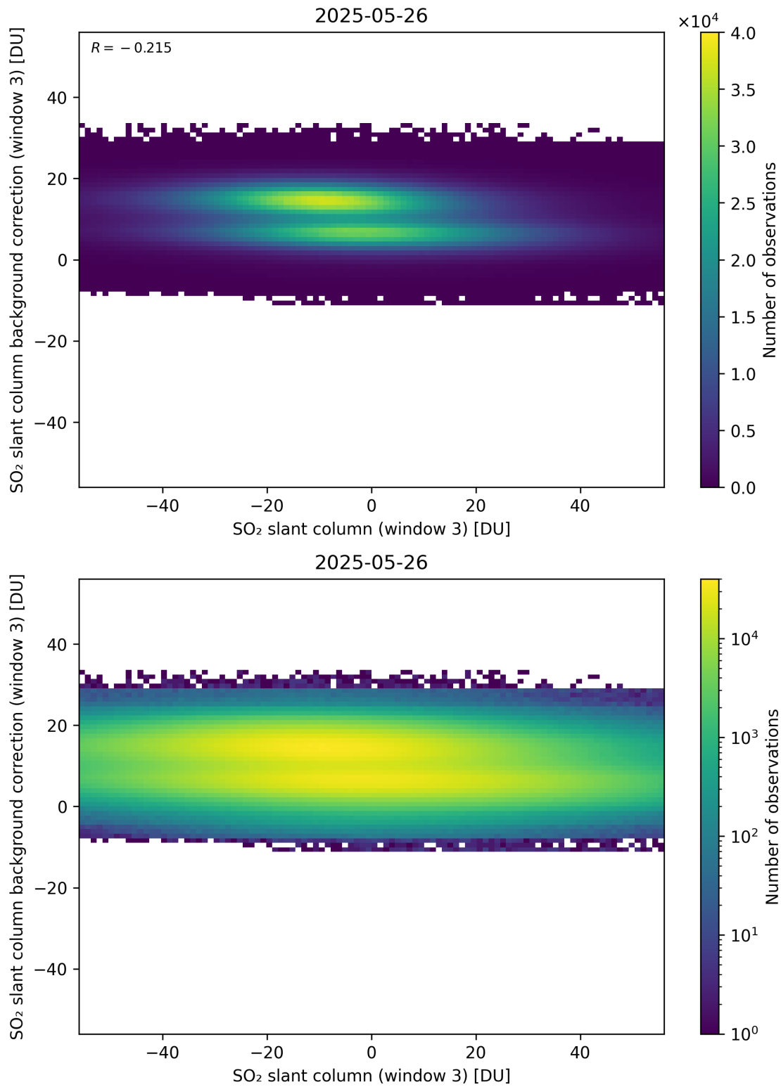
Figure 303: Scatter density plot of “SO 2 slant column (window 3)” against “SO 2 slant column background correction (window 3)” for 2025-05-26 to 2025-05-27.
