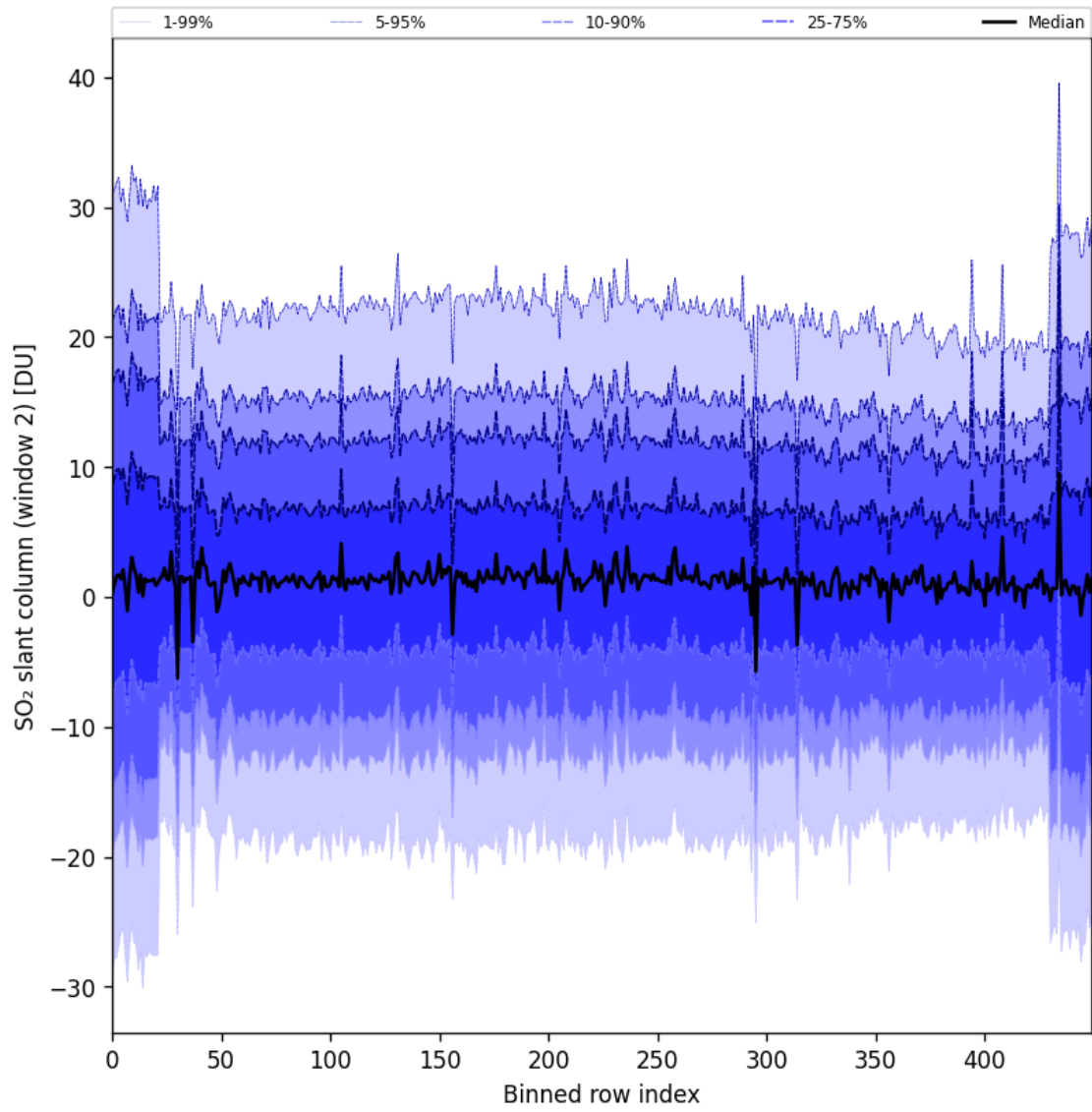
Figure 93: Along track statistics of "SO 2 slant column (window 2)" for 2025-05-26 to 2025-05-27
