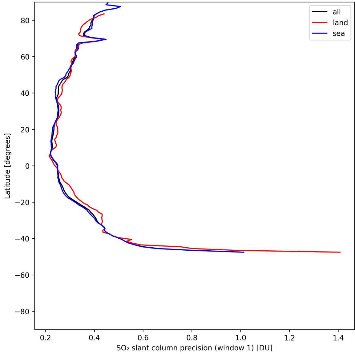
Figure 38: Zonal average of “SO 2 slant column precision (window 1)” for 2025-05-26 to 2025-05-27.
