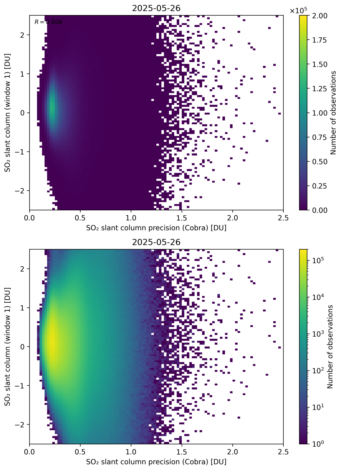
Figure 208: Scatter density plot of “SO 2 slant column precision (Cobra)” against “SO 2 slant column (window 1)” for 2025-05-26 to 2025-05-27.
