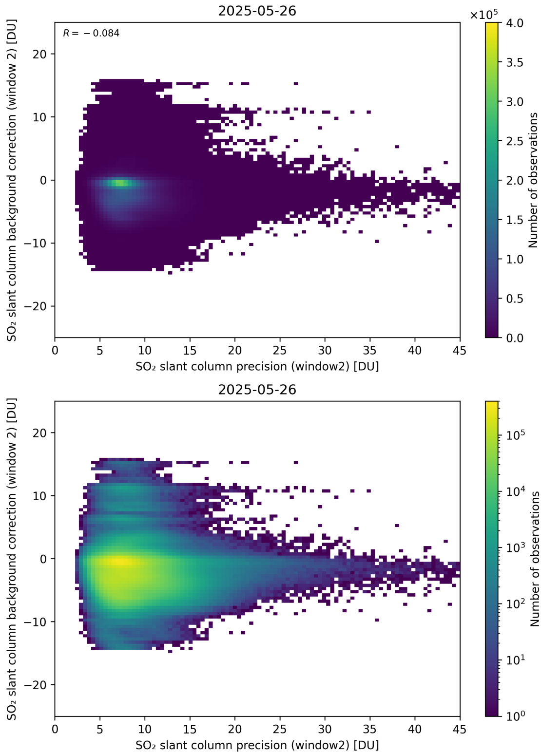
Figure 291: Scatter density plot of “SO 2 slant column precision (window2)” against “SO 2 slant column background correction (window 2)” for 2025-05-26 to 2025-05-27.
