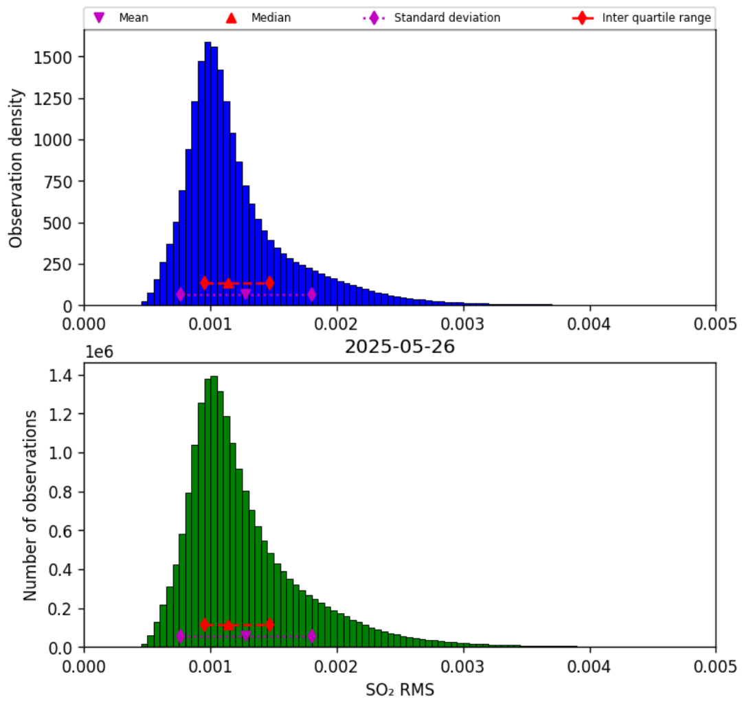
Figure 78: Histogram of “SO 2 RMS” for 2025-05-26 to 2025-05-27
