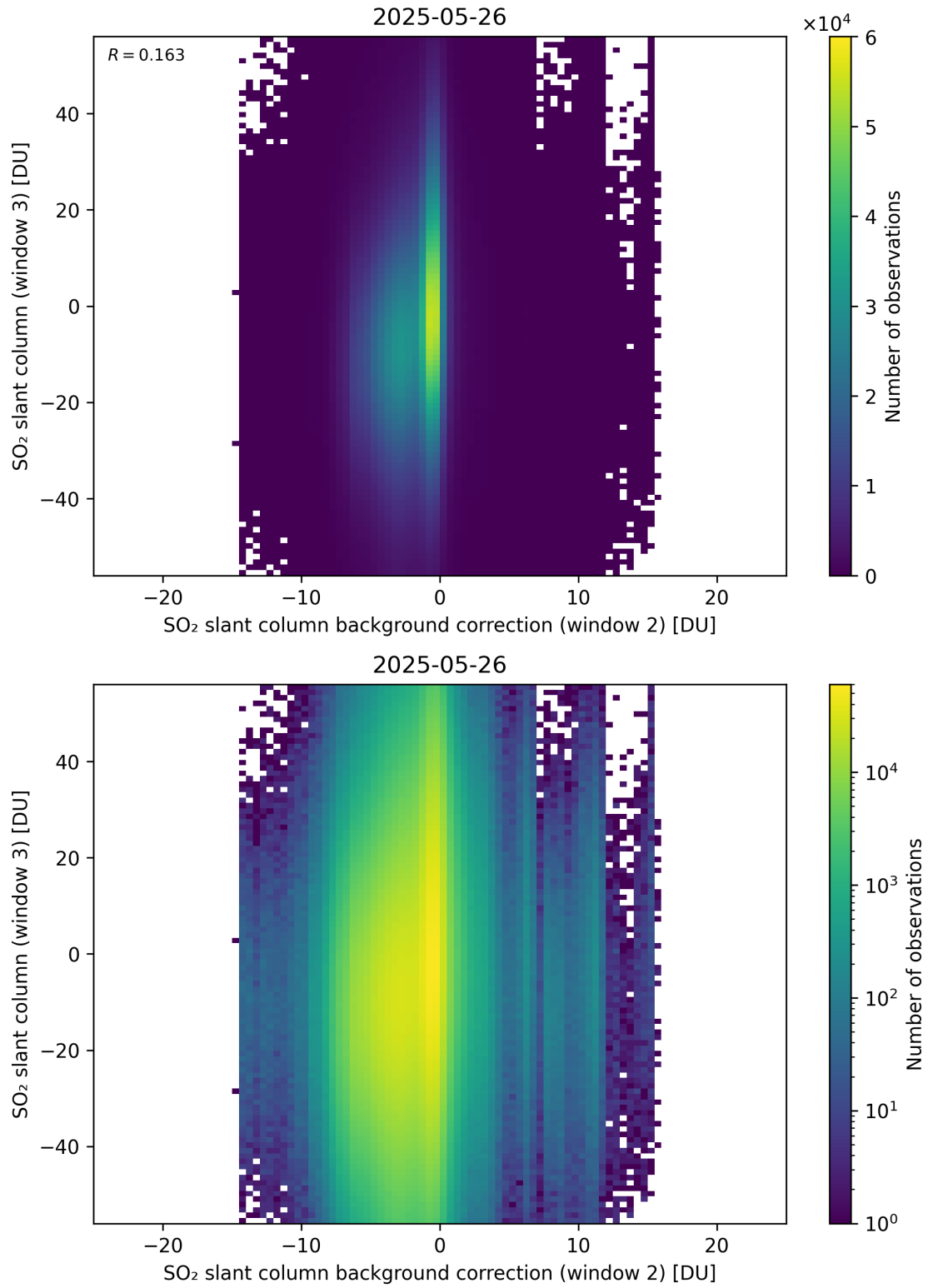
Figure 128: Scatter density plot of “SO 2 slant column background correction (window 2)” against “SO 2 slant column (window 3)” for 2025-05-26 to 2025-05-27.
