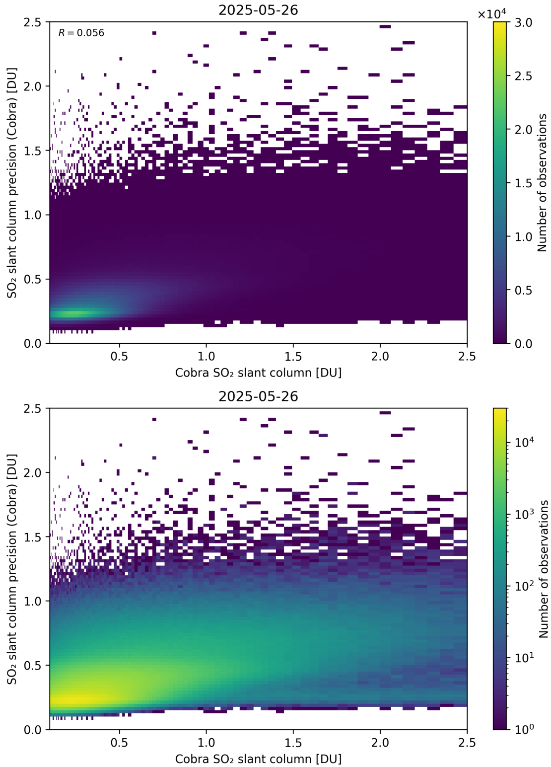
Figure 216: Scatter density plot of “Cobra SO 2 slant column” against “SO 2 slant column precision (Cobra)” for 2025-05-26 to 2025-05-27.
