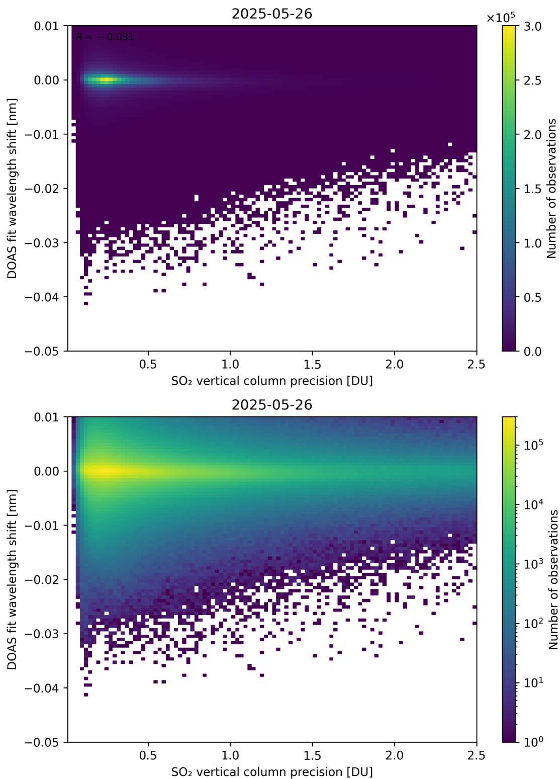
Figure 332: Scatter density plot of “SO 2 vertical column precision” against “DOAS fit wavelength shift” for 2025-05-26 to 2025-05-27.
