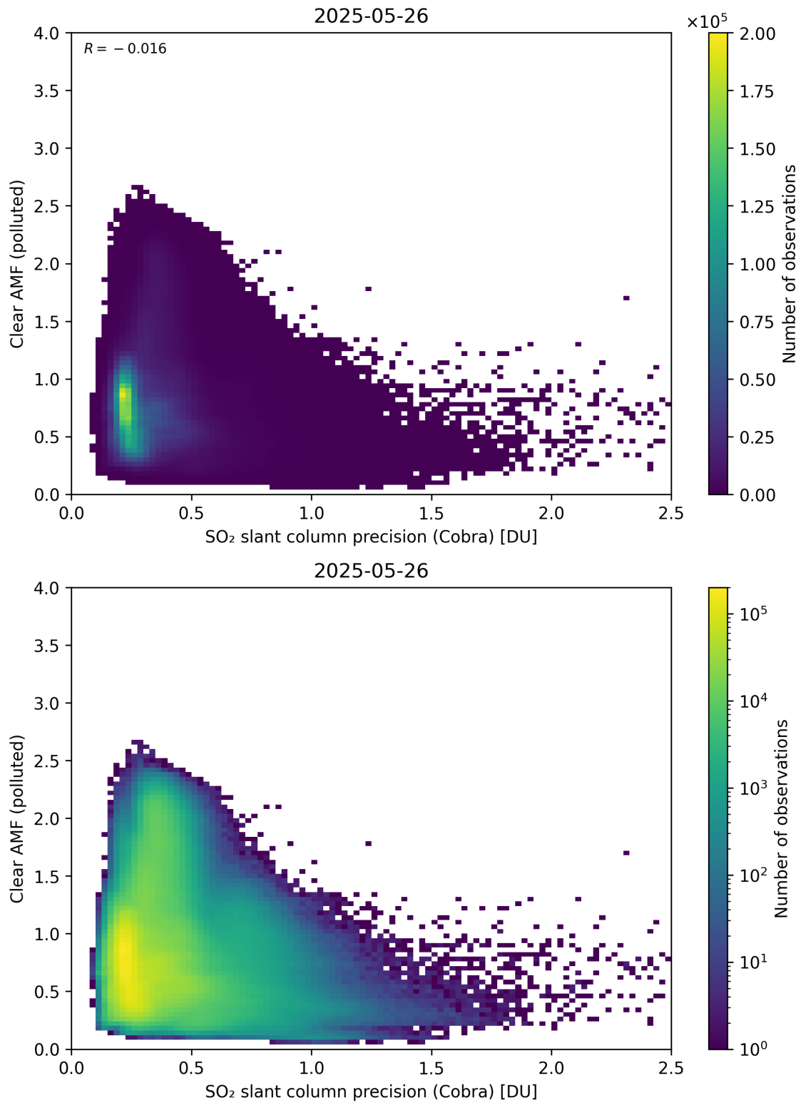
Figure 205: Scatter density plot of “SO 2 slant column precision (Cobra)” against “Clear AMF (polluted)” for 2025-05-26 to 2025-05-27.
