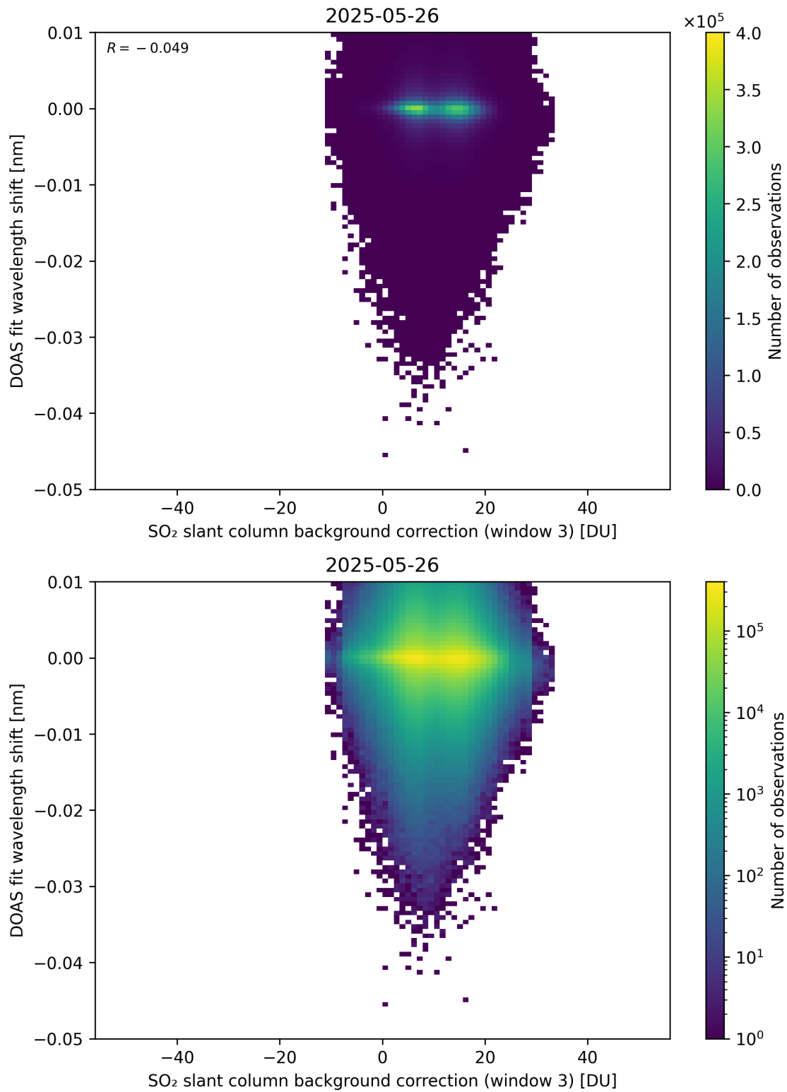
Figure 132: Scatter density plot of “SO 2 slant column background correction (window 3)” against “DOAS fit wavelength shift” for 2025-05-26 to 2025-05-27.
