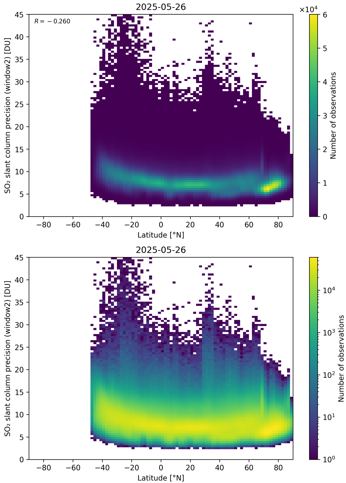
Figure 164: Scatter density plot of “Latitude” against “SO 2 slant column precision (window2)” for 2025-05-26 to 2025-05-27.
