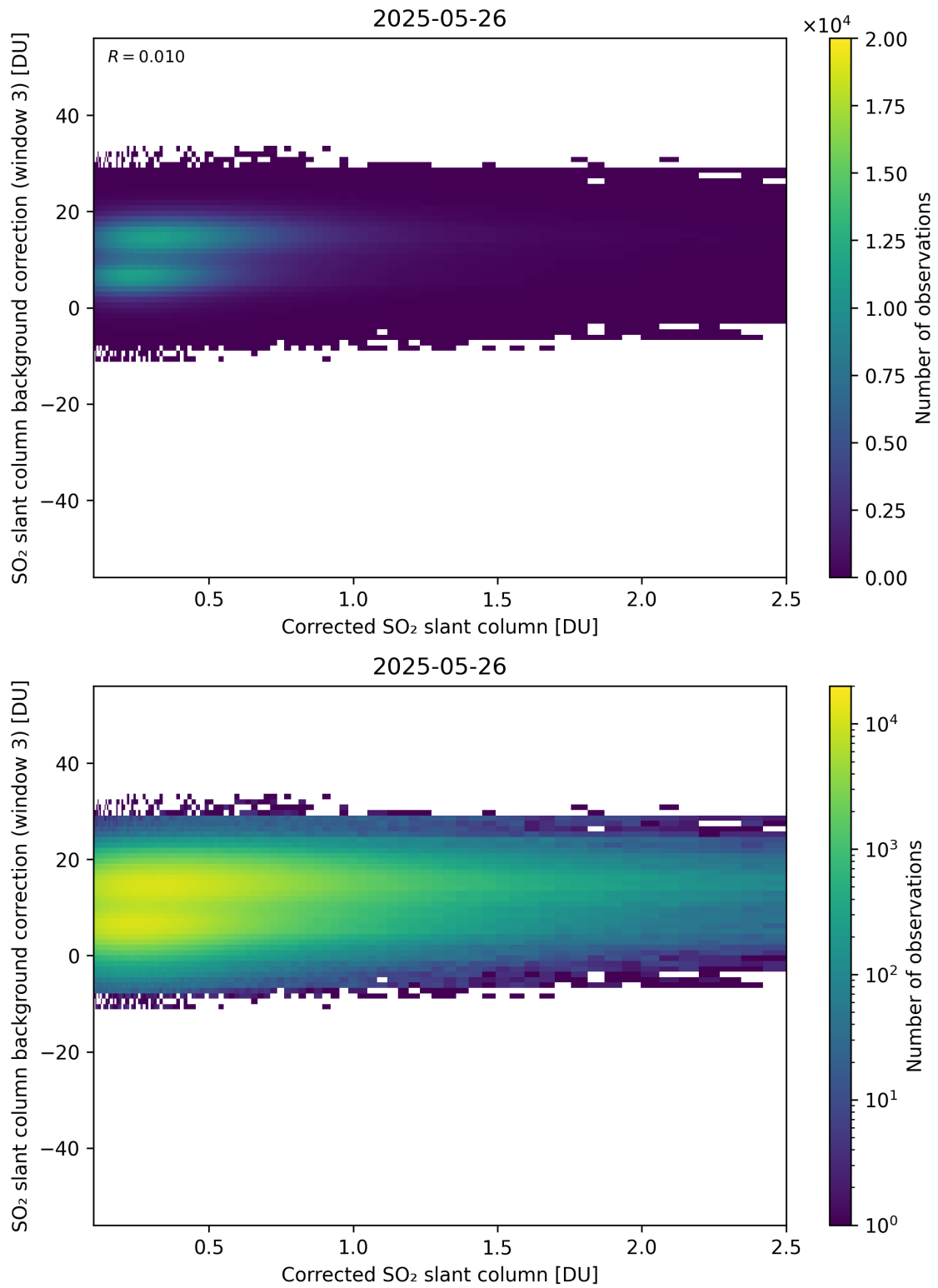
Figure 228: Scatter density plot of “Corrected SO 2 slant column” against “SO 2 slant column background correction (window 3)” for 2025-05-26 to 2025-05-27.
