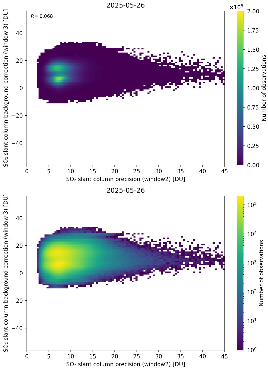
Figure 292: Scatter density plot of “SO 2 slant column precision (window2)” against “SO 2 slant column background correction (window 3)” for 2025-05-26 to 2025-05-27.
