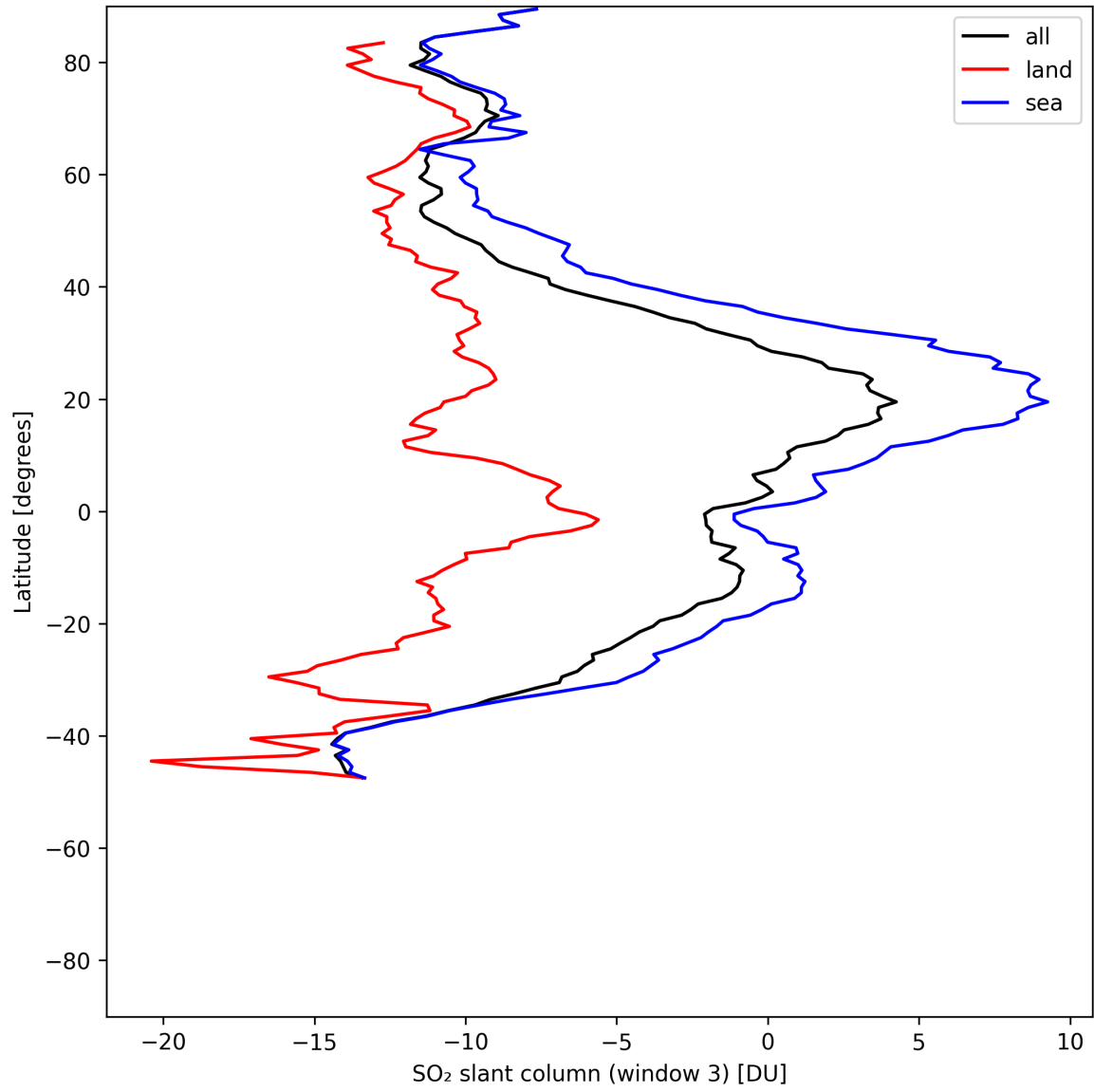
Figure 45: Zonal average of “SO 2 slant column (window 3)” for 2025-05-26 to 2025-05-27.
