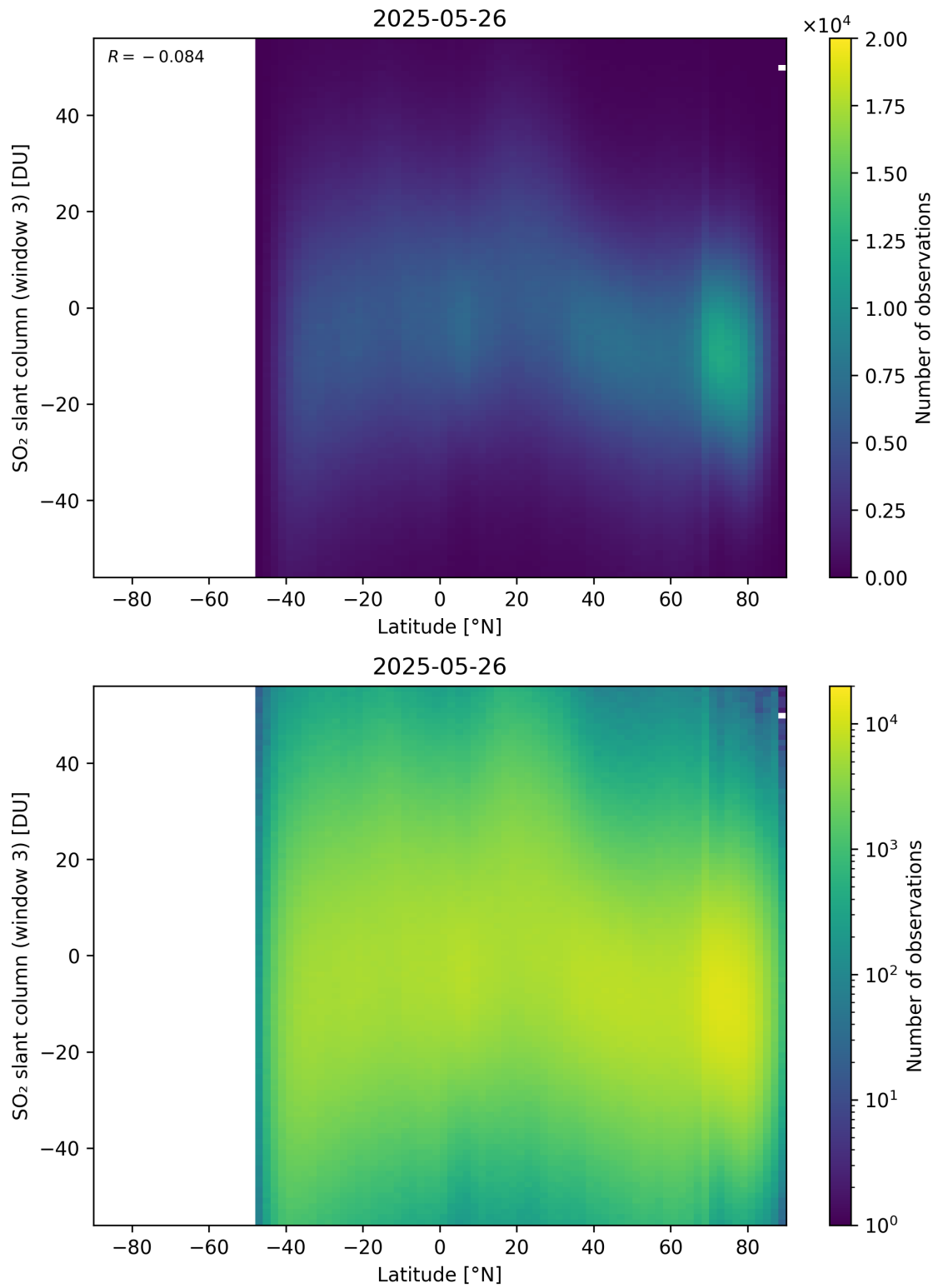
Figure 165: Scatter density plot of “Latitude” against “SO 2 slant column (window 3)” for 2025-05-26 to 2025-05-27.
