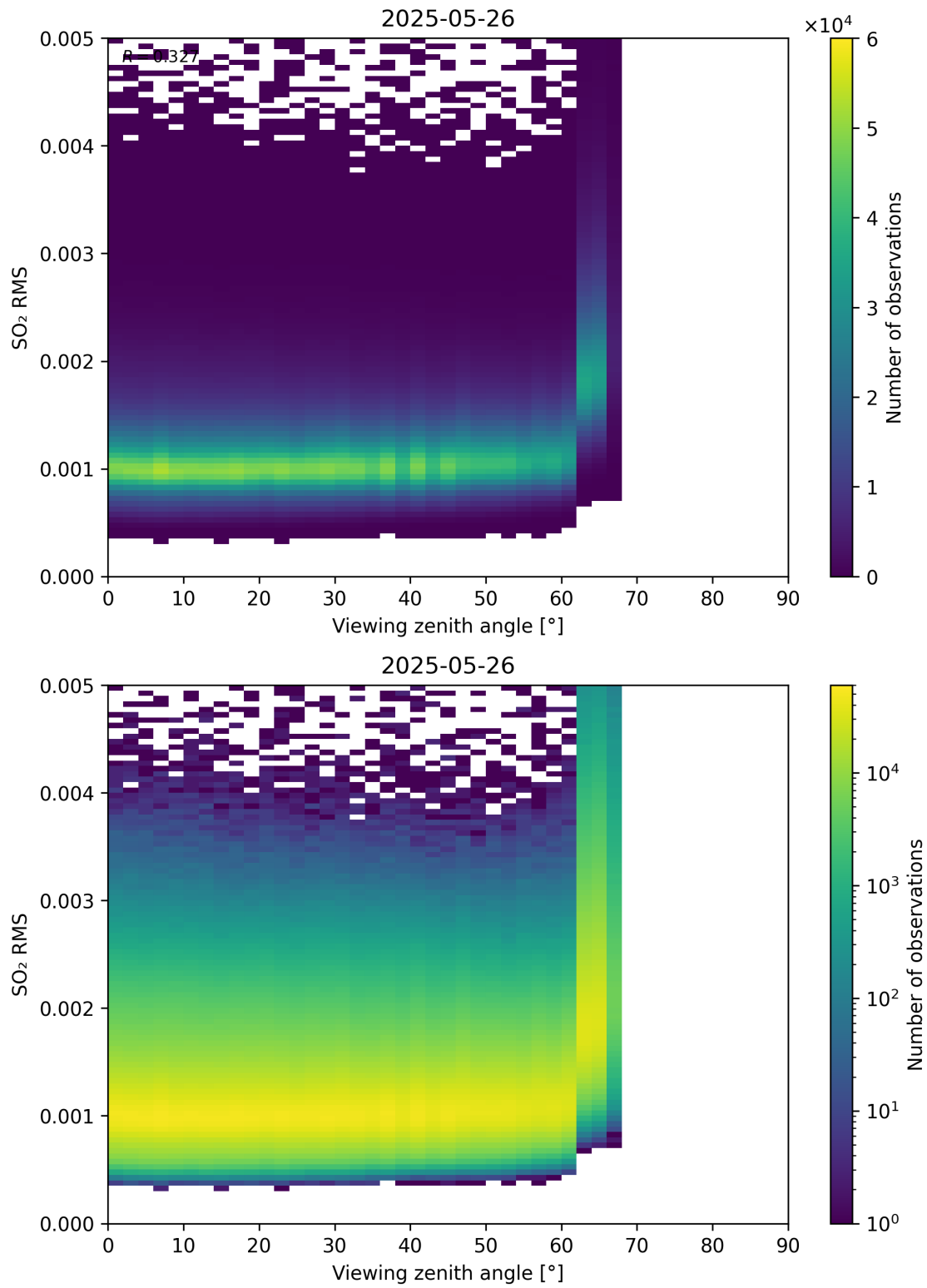
Figure 367: Scatter density plot of “Viewing zenith angle” against “SO 2 RMS” for 2025-05-26 to 2025-05-27.
