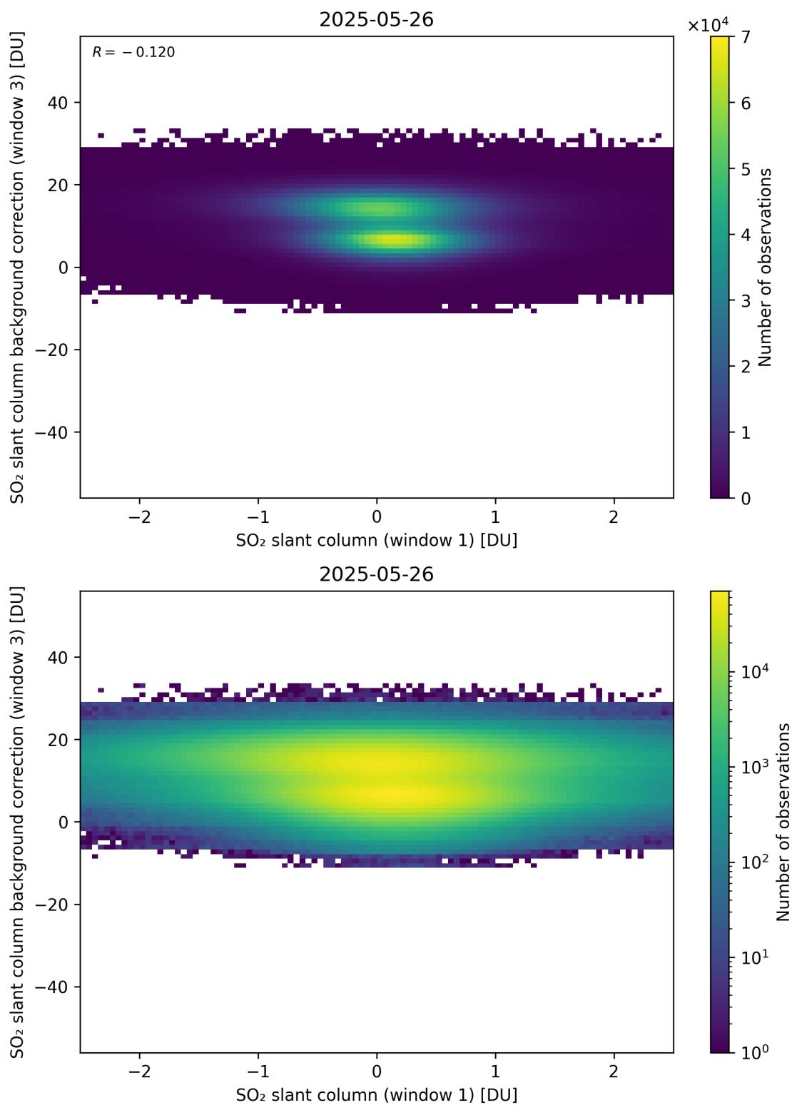
Figure 264: Scatter density plot of “SO 2 slant column (window 1)” against “SO 2 slant column background correction (window 3)” for 2025-05-26 to 2025-05-27.
