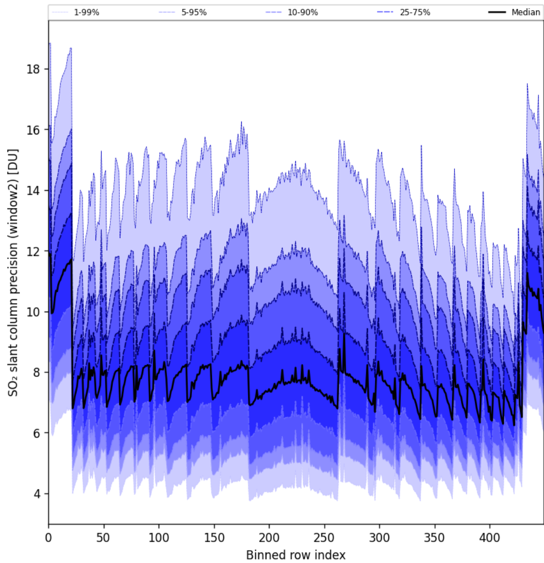
Figure 94: Along track statistics of “SO 2 slant column precision (window2)” for 2025-05-26 to 2025-05-27
