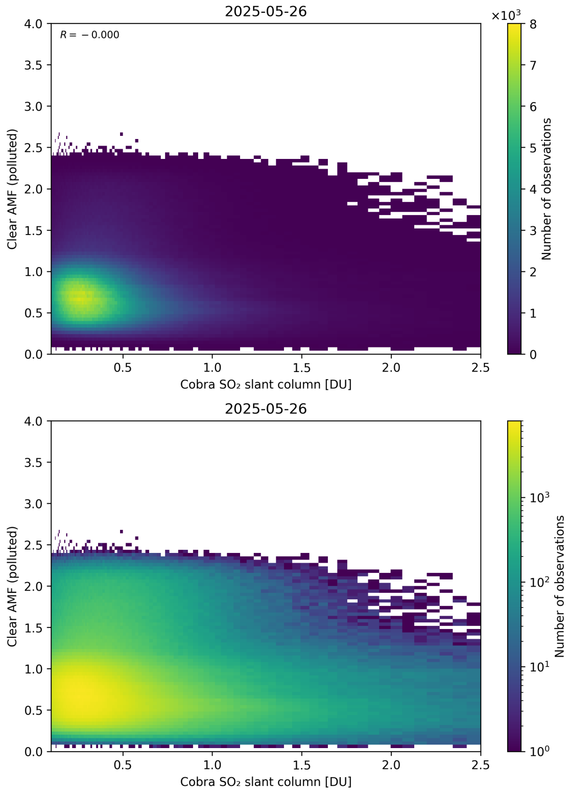
Figure 215: Scatter density plot of “Cobra SO 2 slant column” against “Clear AMF (polluted)” for 2025-05-26 to 2025-05-27.
