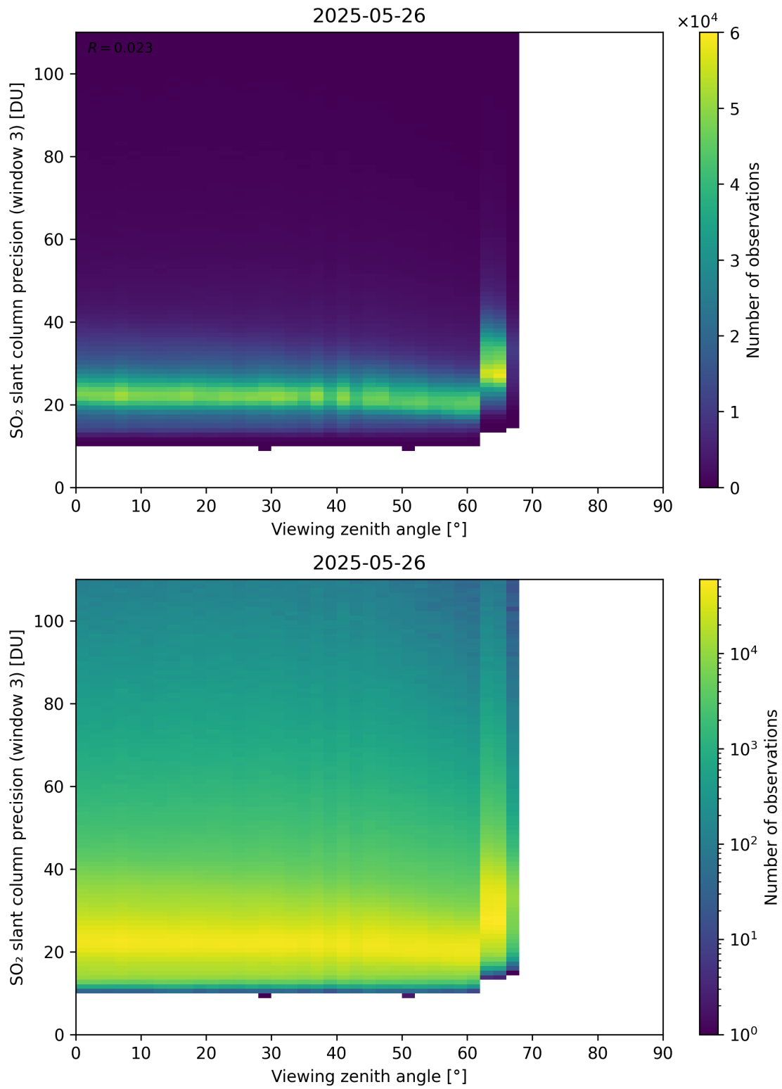
Figure 380: Scatter density plot of “Viewing zenith angle” against “SO 2 slant column precision (window 3)” for 2025-05-26 to 2025-05-27.
