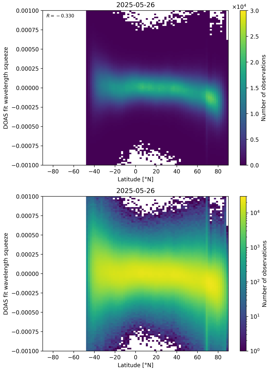
Figure 154: Scatter density plot of “Latitude” against “DOAS fit wavelength squeeze” for 2025-05-26 to 2025-05-27.
