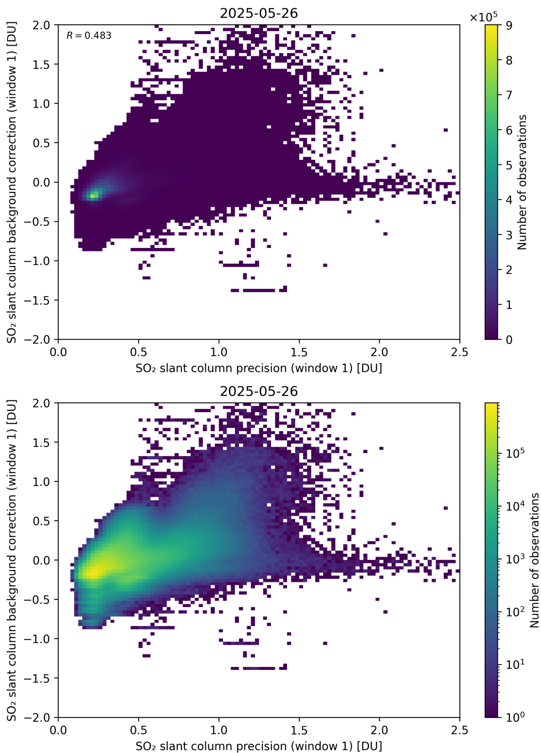
Figure 268: Scatter density plot of “SO 2 slant column precision (window 1)” against “SO 2 slant column background correction (window 1)” for 2025-05-26 to 2025-05-27.
