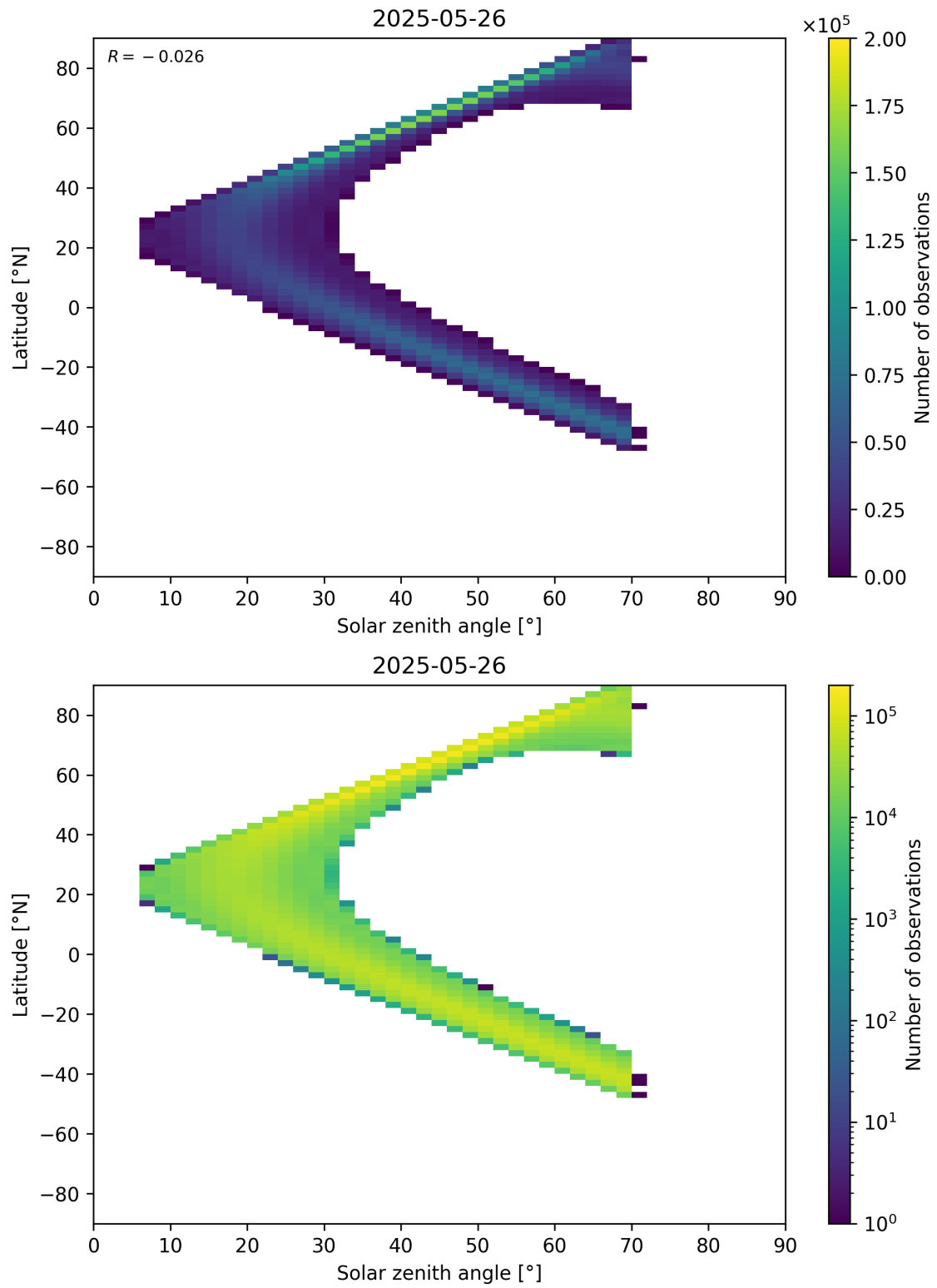
Figure 177: Scatter density plot of “Solar zenith angle” against “Latitude” for 2025-05-26 to 2025-05-27.
