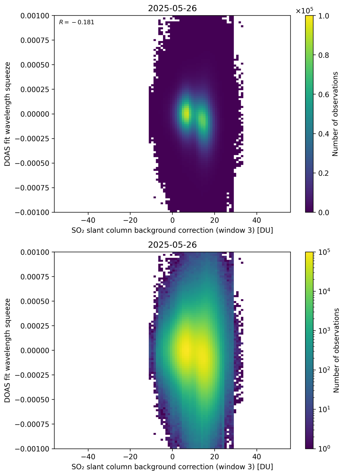
Figure 133: Scatter density plot of “SO 2 slant column background correction (window 3)” against “DOAS fit wavelength squeeze” for 2025-05-26 to 2025-05-27.
