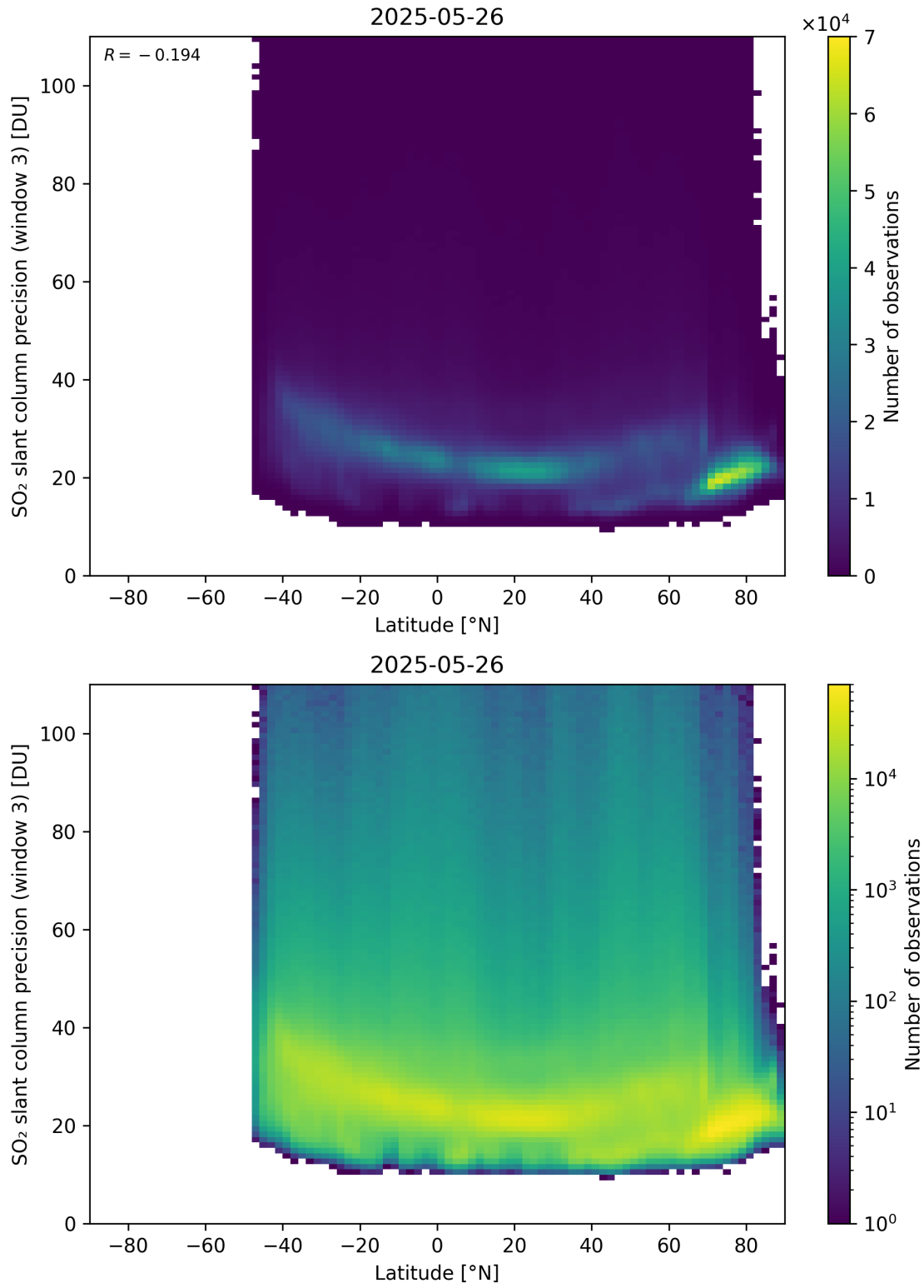
Figure 166: Scatter density plot of “Latitude” against “SO 2 slant column precision (window 3)” for 2025-05-26 to 2025-05-27.
