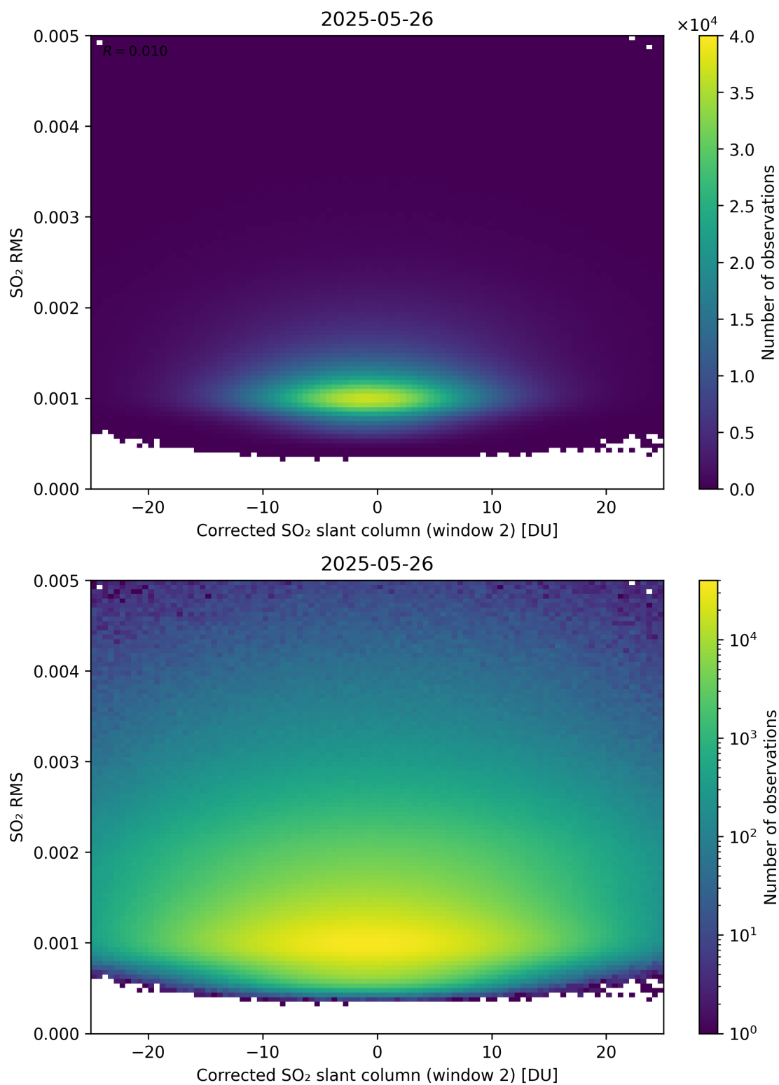
Figure 248: Scatter density plot of “Corrected SO 2 slant column (window 2)” against “SO 2 RMS” for 2025-05-26 to 2025-05-27.
