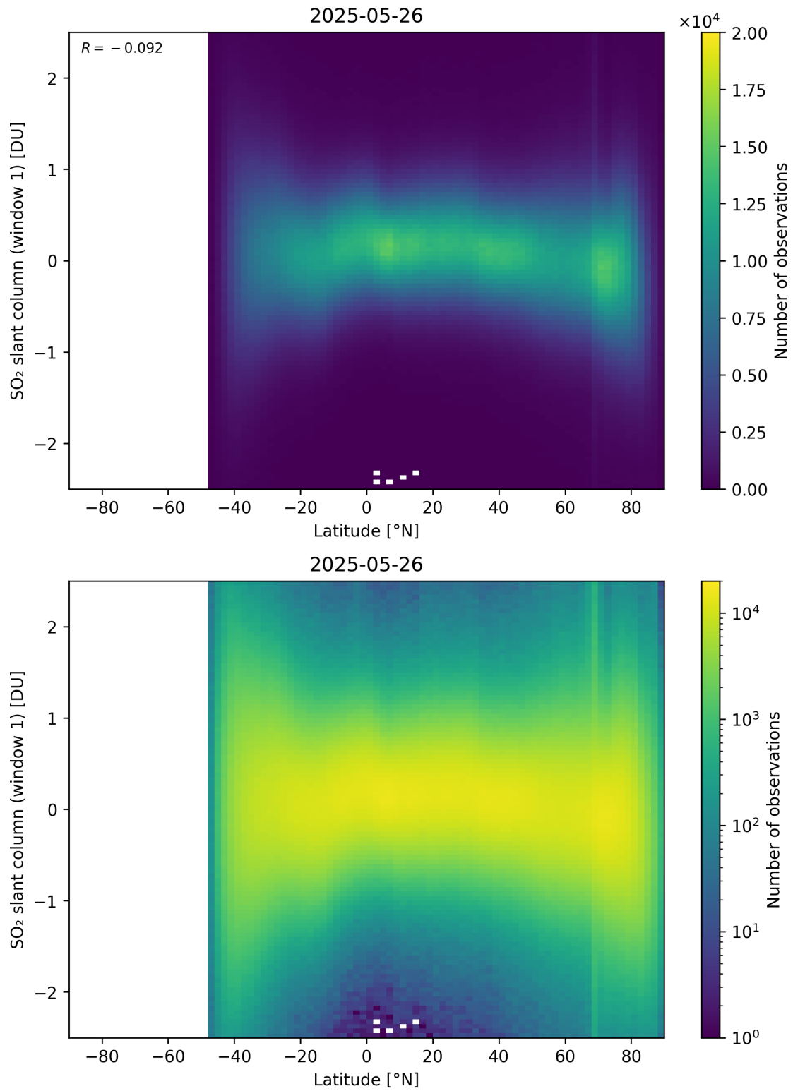
Figure 162: Scatter density plot of “Latitude” against “SO 2 slant column (window 1)” for 2025-05-26 to 2025-05-27.
