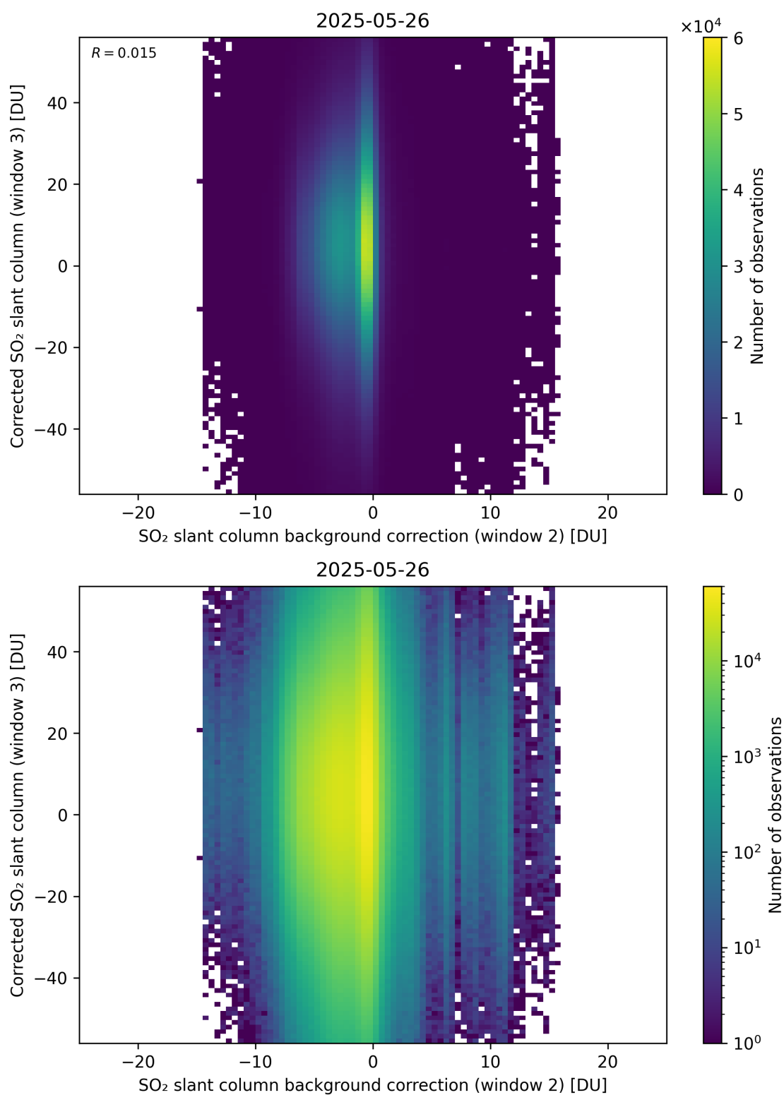
Figure 127: Scatter density plot of “SO 2 slant column background correction (window 2)” against “Corrected SO 2 slant column (window 3)” for 2025-05-26 to 2025-05-27.
