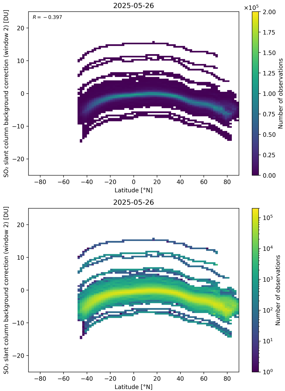
Figure 151: Scatter density plot of “Latitude” against “SO 2 slant column background correction (window 2)” for 2025-05-26 to 2025-05-27.
