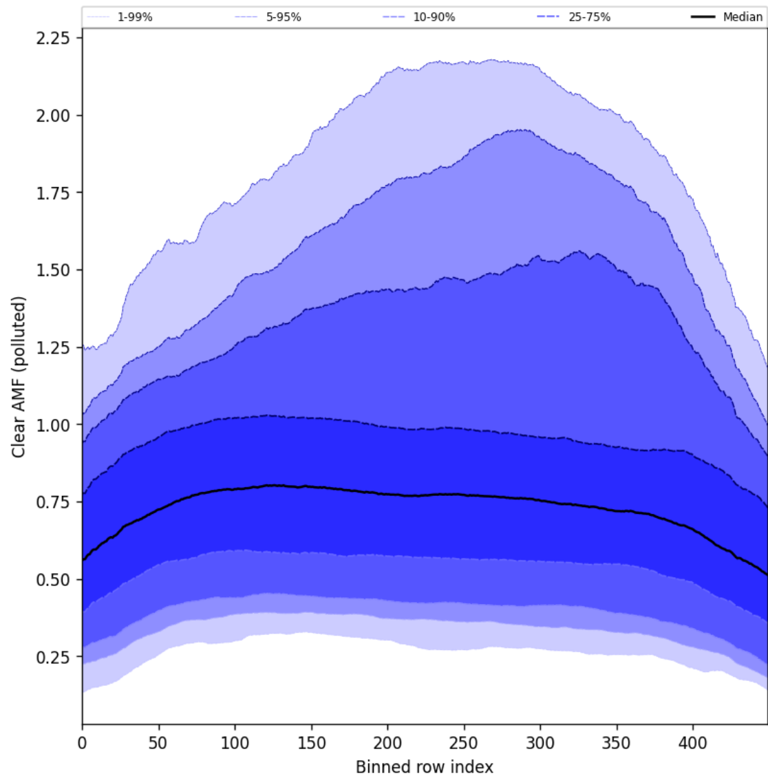
Figure 107: Along track statistics of “Clear AMF (polluted)” for 2025-05-26 to 2025-05-27
