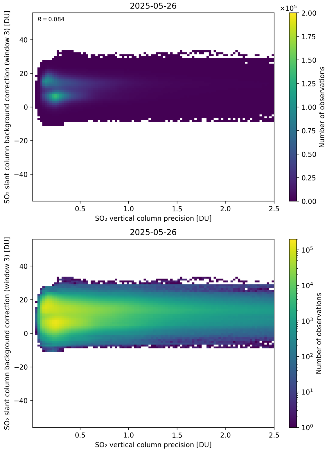
Figure 331: Scatter density plot of “SO 2 vertical column precision” against “SO 2 slant column background correction (window 3)” for 2025-05-26 to 2025-05-27.
