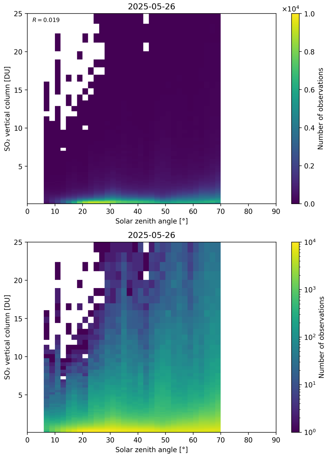
Figure 191: Scatter density plot of “Solar zenith angle” against “SO 2 vertical column” for 2025-05-26 to 2025-05-27.
