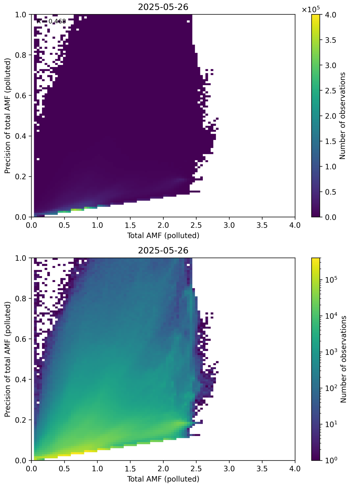
Figure 322: Scatter density plot of “Total AMF (polluted)” against “Precision of total AMF (polluted)” for 2025-05-26 to 2025-05-27.
