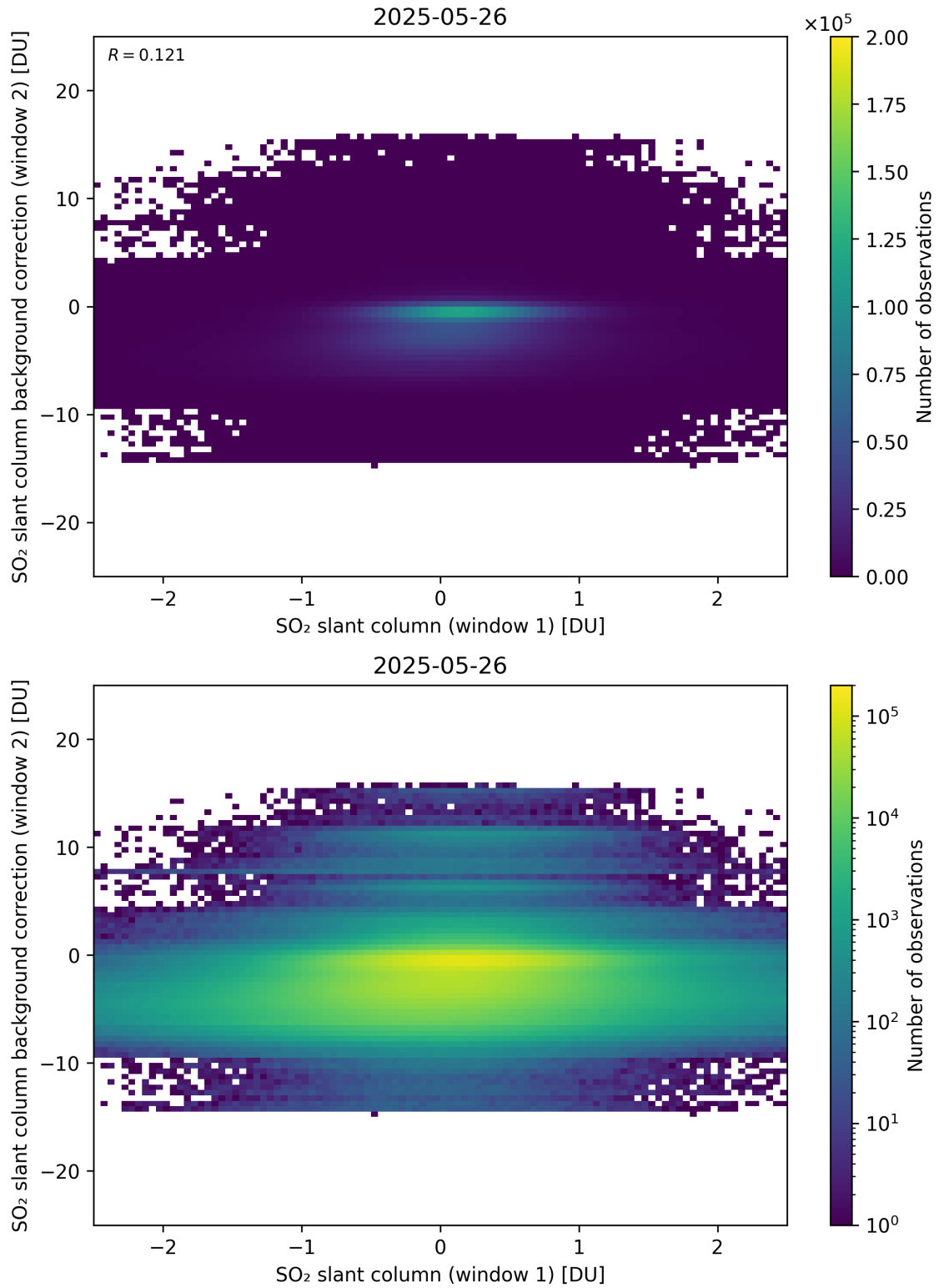
Figure 263: Scatter density plot of “SO 2 slant column (window 1)” against “SO 2 slant column background correction (window 2)” for 2025-05-26 to 2025-05-27.
