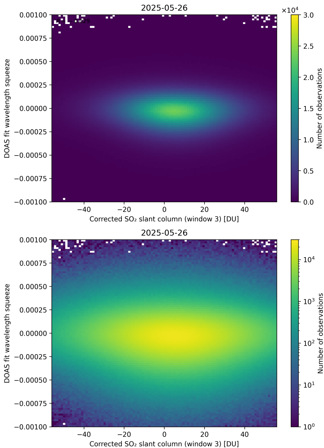
Figure 257: Scatter density plot of “Corrected SO 2 slant column (window 3)” against “DOAS fit wavelength squeeze” for 2025-05-26 to 2025-05-27.
