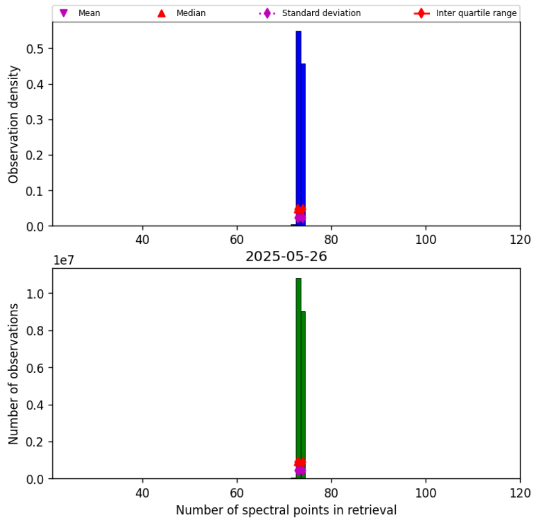
Figure 82: Histogram of “Number of spectral points in retrieval” for 2025-05-26 to 2025-05-27
