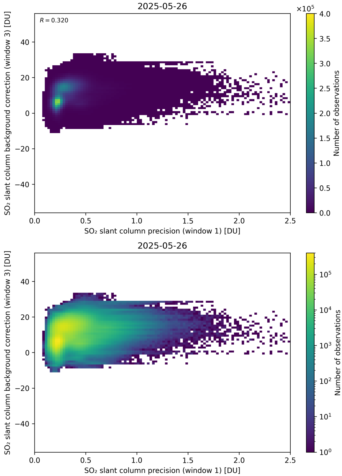
Figure 270: Scatter density plot of “SO 2 slant column precision (window 1)” against “SO 2 slant column background correction (window 3)” for 2025-05-26 to 2025-05-27.
