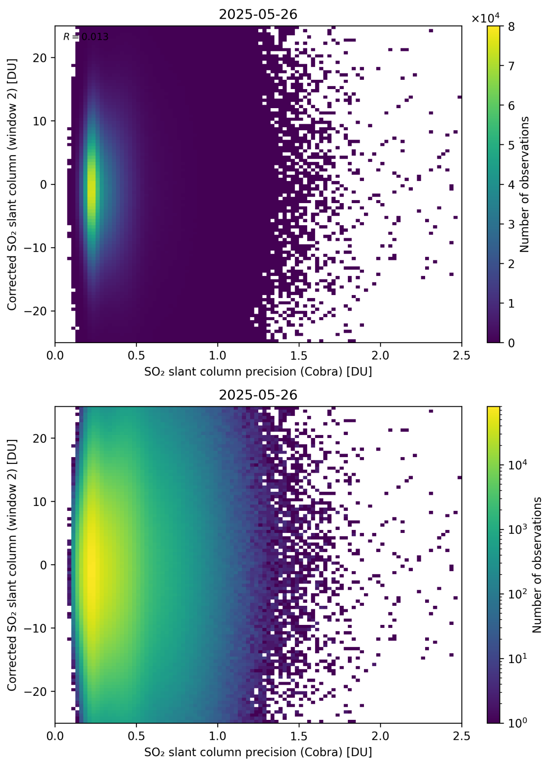
Figure 206: Scatter density plot of “SO 2 slant column precision (Cobra)” against “Corrected SO 2 slant column (window 2)” for 2025-05-26 to 2025-05-27.
