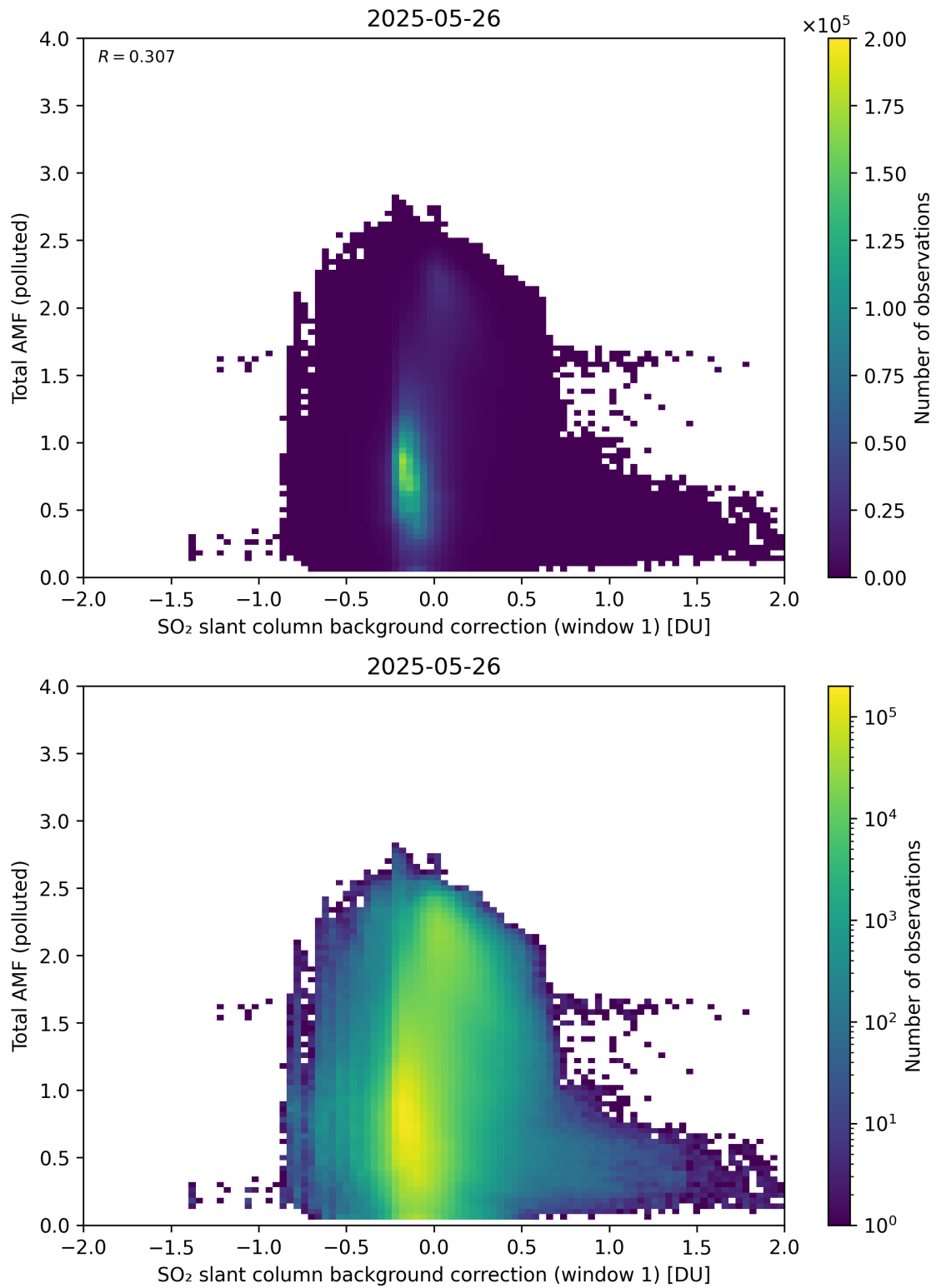
Figure 120: Scatter density plot of “SO 2 slant column background correction (window 1)” against “Total AMF (polluted)” for 2025-05-26 to 2025-05-27.
