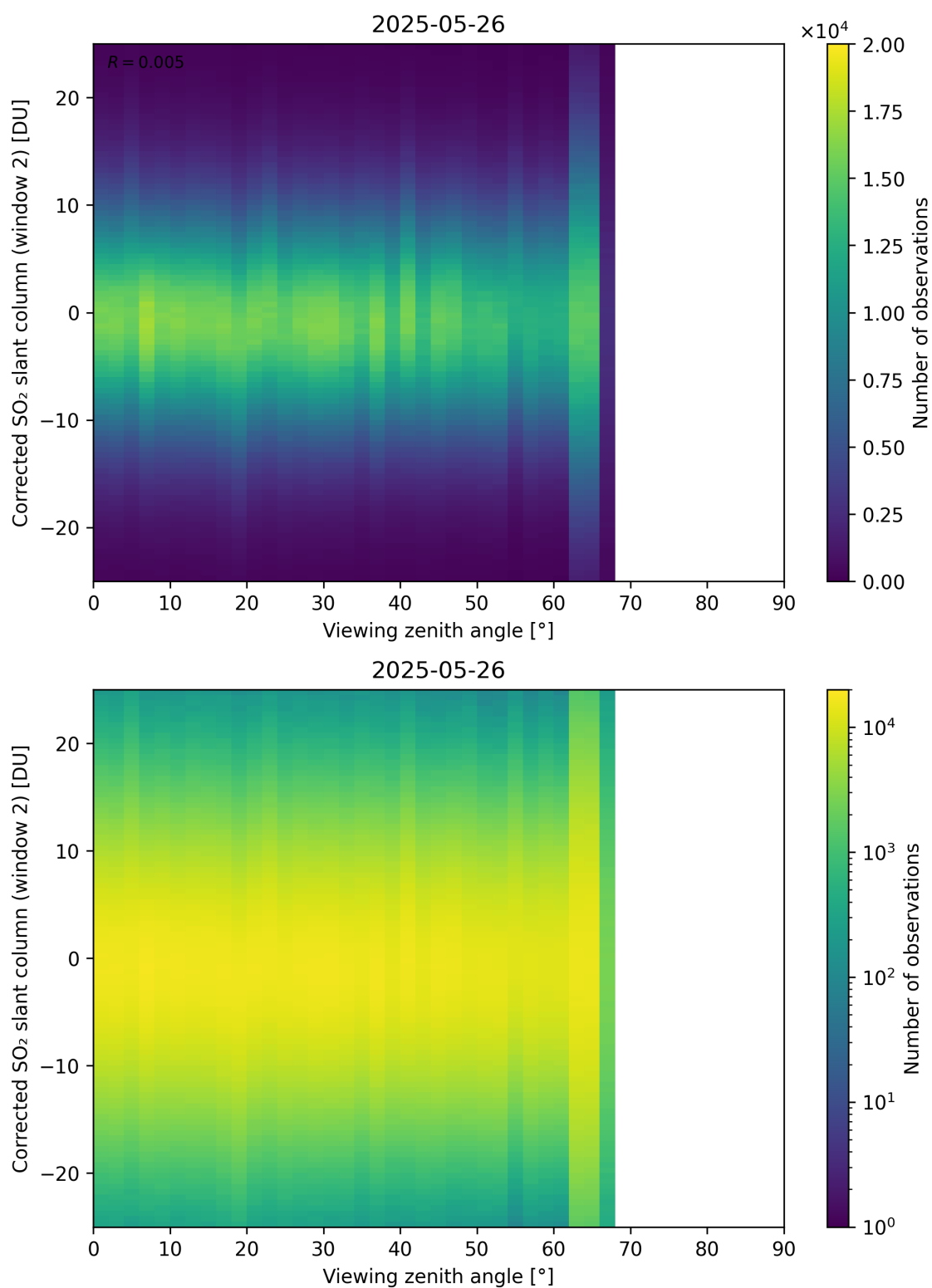
Figure 374: Scatter density plot of “Viewing zenith angle” against “Corrected SO 2 slant column (window 2)” for 2025-05-26 to 2025-05-27.
