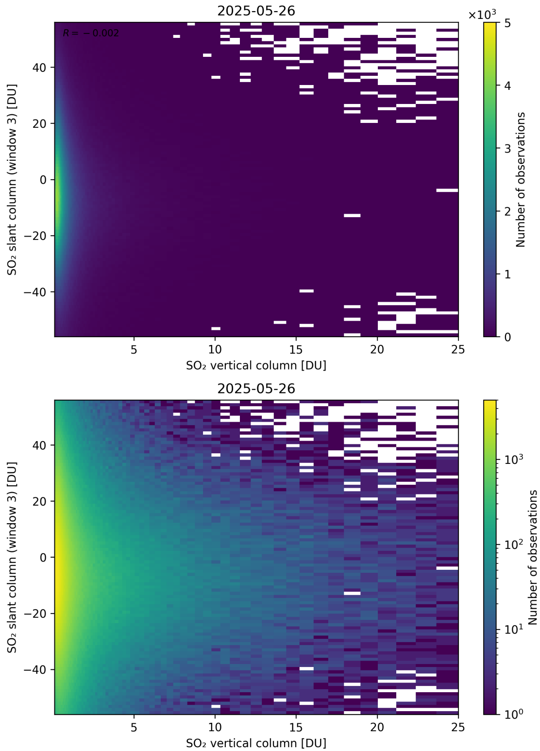
Figure 357: Scatter density plot of “SO 2 vertical column” against “SO 2 slant column (window 3)” for 2025-05-26 to 2025-05-27.
