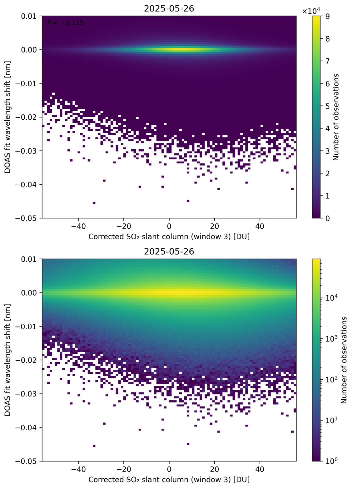
Figure 256: Scatter density plot of “Corrected SO 2 slant column (window 3)” against “DOAS fit wavelength shift” for 2025-05-26 to 2025-05-27.
