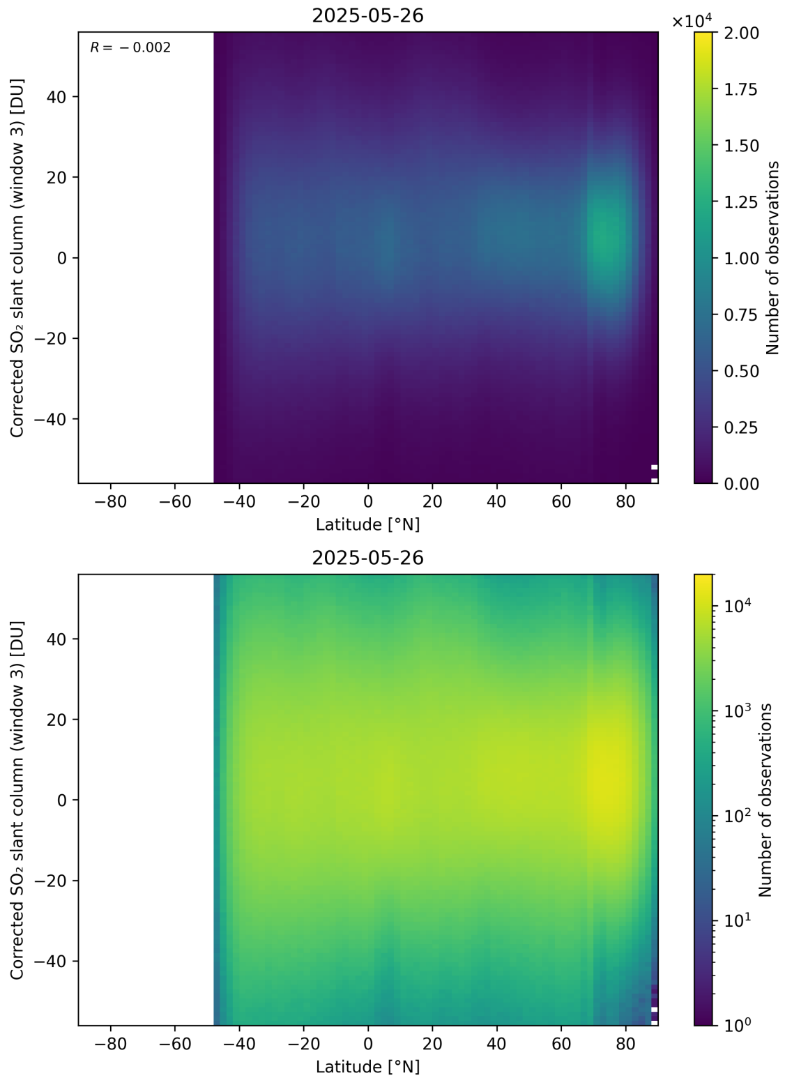
Figure 161: Scatter density plot of “Latitude” against “Corrected SO 2 slant column (window 3)” for 2025-05-26 to 2025-05-27.
