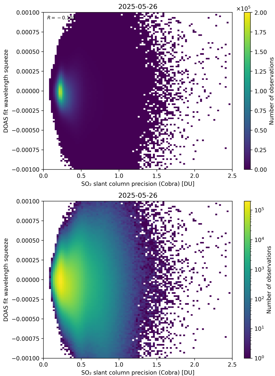
Figure 203: Scatter density plot of “SO 2 slant column precision (Cobra)” against “DOAS fit wavelength squeeze” for 2025-05-26 to 2025-05-27.
