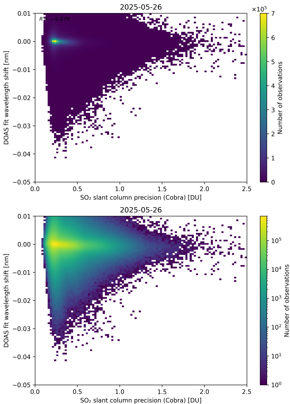
Figure 202: Scatter density plot of “SO 2 slant column precision (Cobra)” against “DOAS fit wavelength shift” for 2025-05-26 to 2025-05-27.
