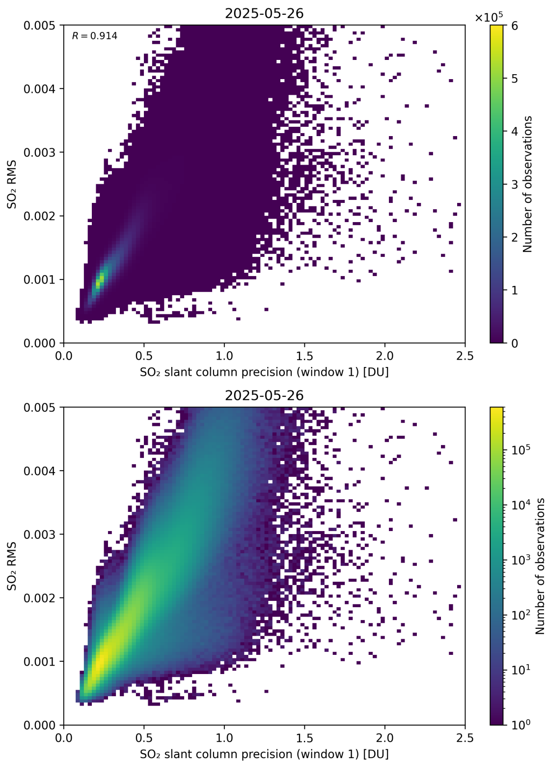
Figure 273: Scatter density plot of “SO 2 slant column precision (window 1)” against “SO 2 RMS” for 2025-05-26 to 2025-05-27.
