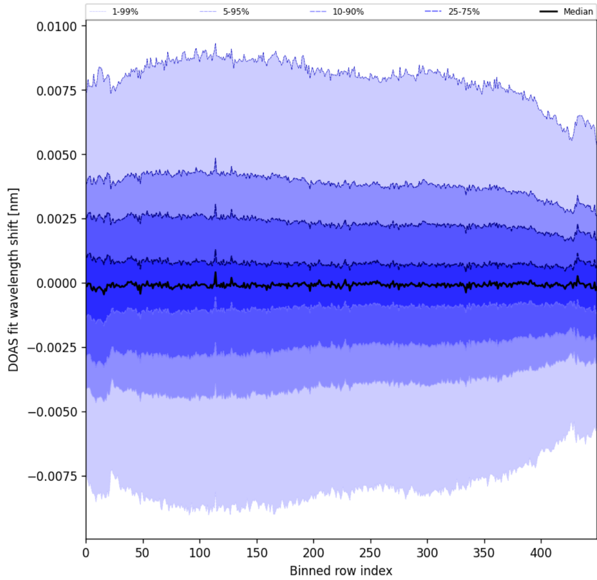
Figure 102: Along track statistics of “DOAS fit wavelength shift” for 2025-05-26 to 2025-05-27
