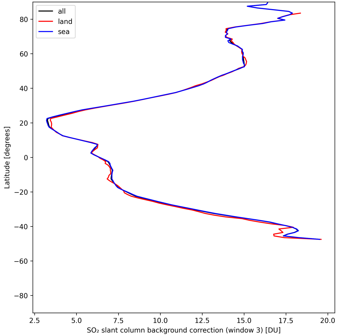
Figure 48: Zonal average of “SO 2 slant column background correction (window 3)” for 2025-05-26 to 2025-05-27.
