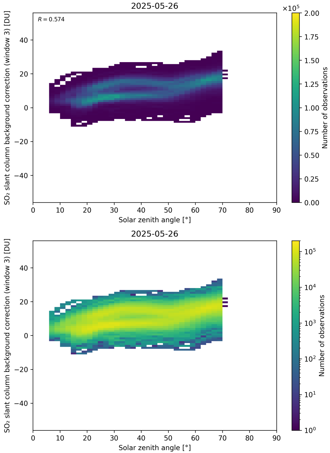
Figure 173: Scatter density plot of “Solar zenith angle” against “SO 2 slant column background correction (window 3)” for 2025-05-26 to 2025-05-27.
