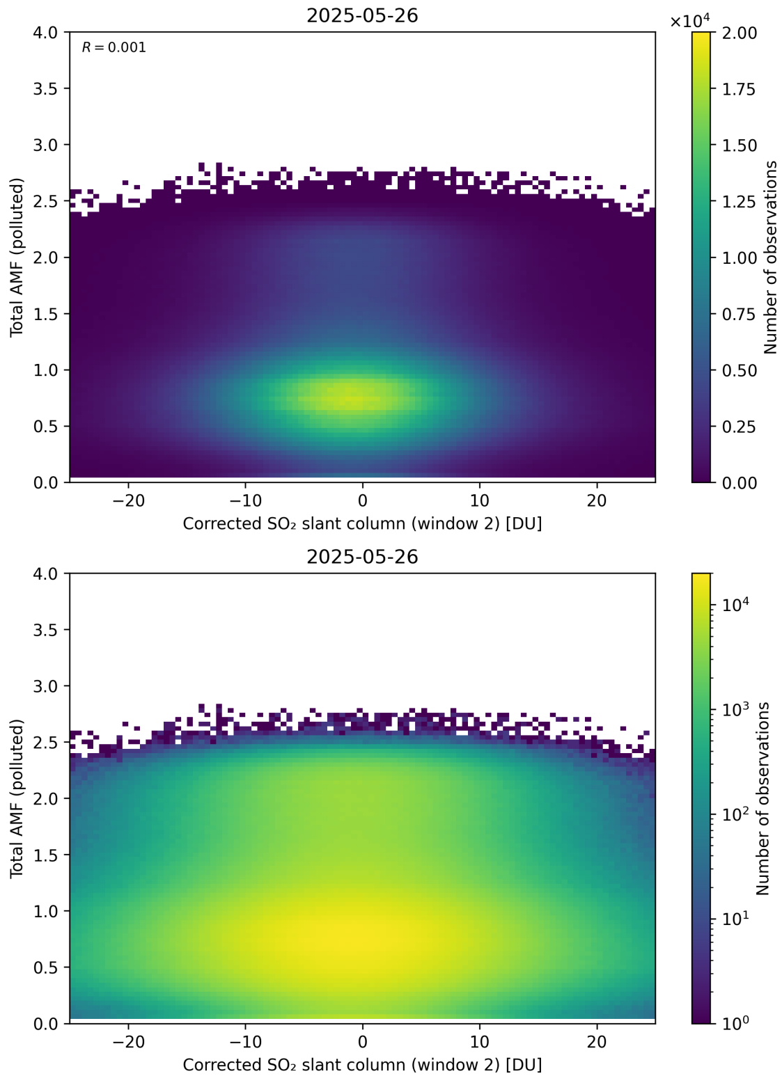
Figure 253: Scatter density plot of “Corrected SO 2 slant column (window 2)” against “Total AMF (polluted)” for 2025-05-26 to 2025-05-27.
