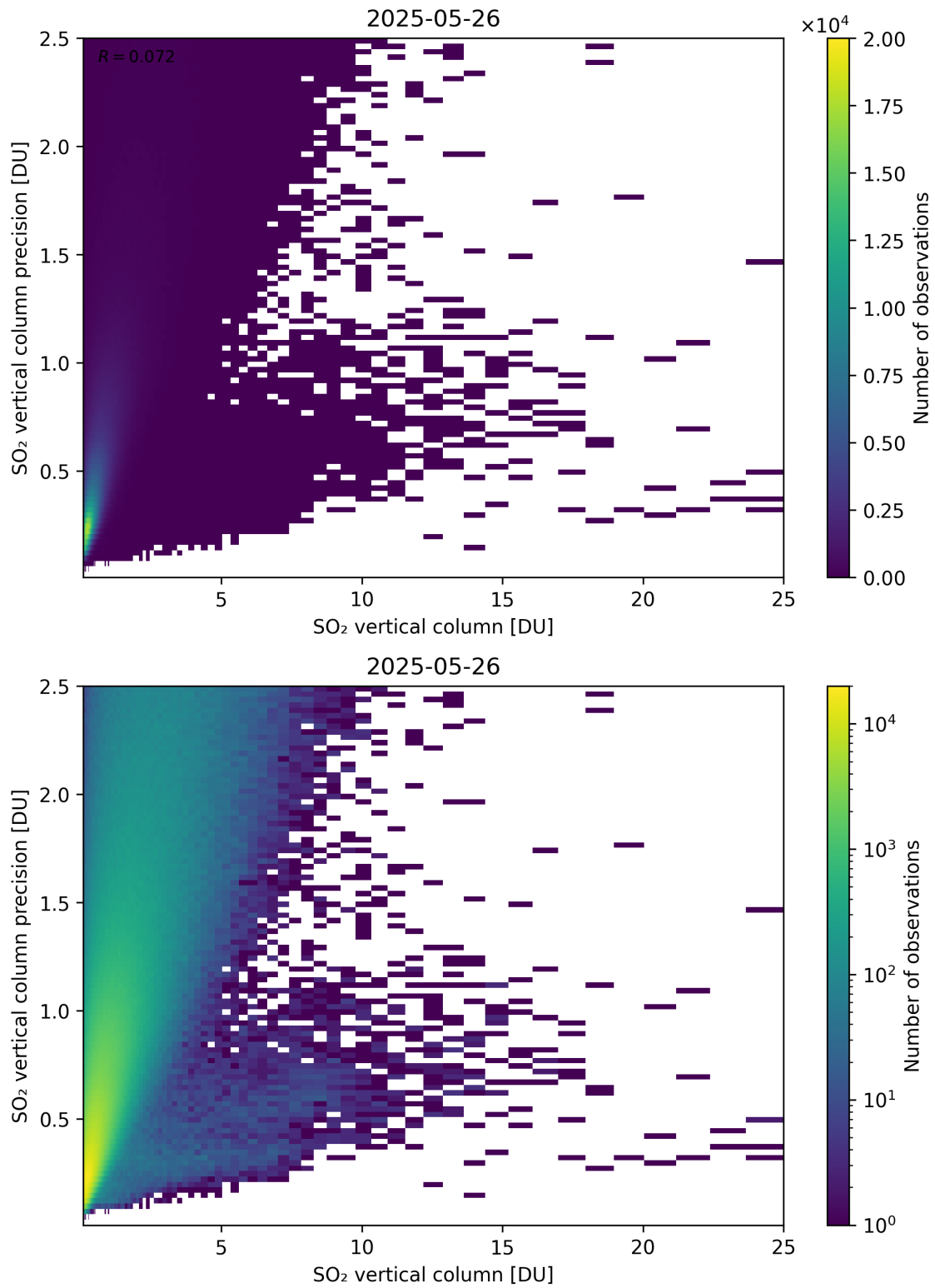
Figure 361: Scatter density plot of “SO 2 vertical column” against “SO 2 vertical column precision” for 2025-05-26 to 2025-05-27.
