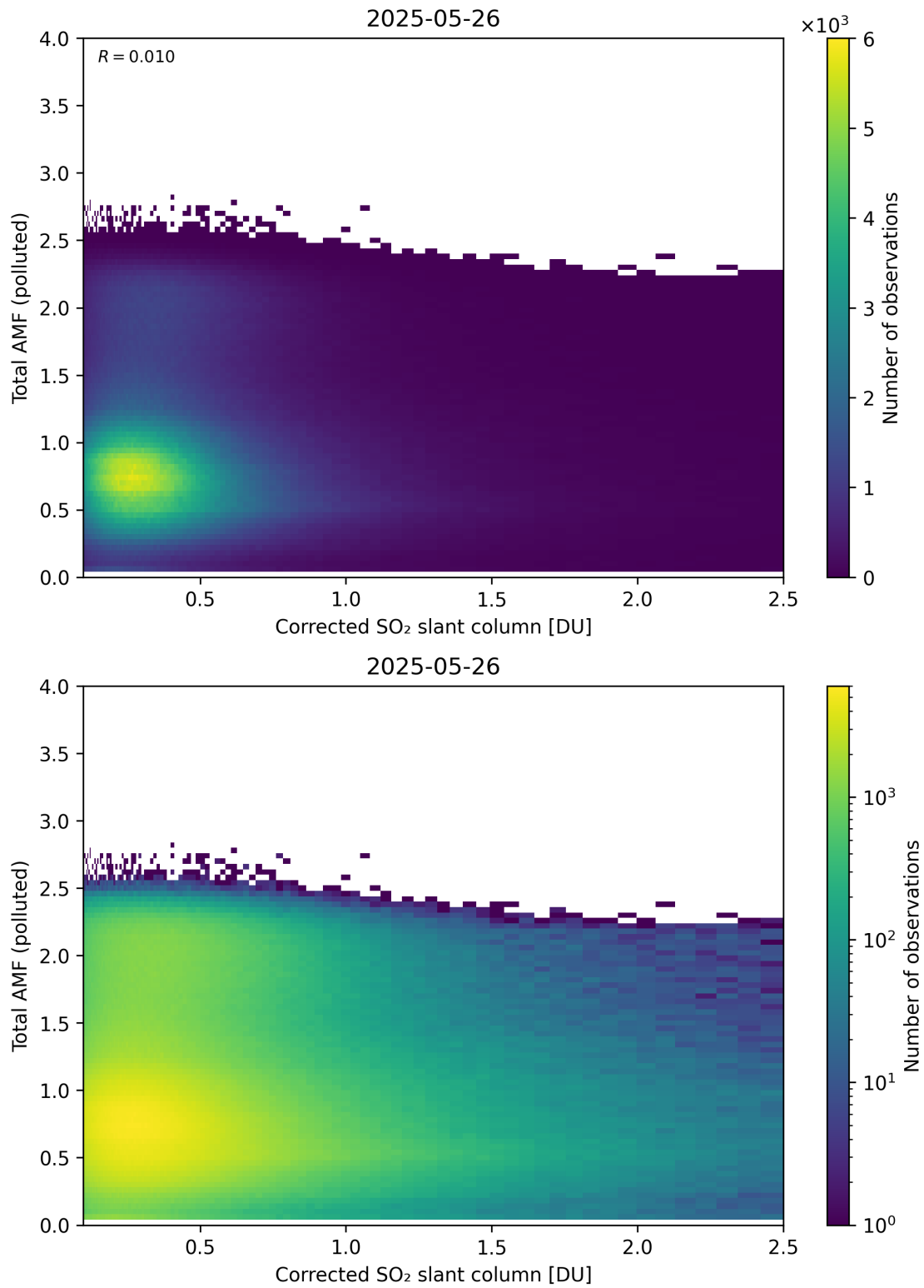
Figure 242: Scatter density plot of “Corrected SO 2 slant column” against “Total AMF (polluted)” for 2025-05-26 to 2025-05-27.
