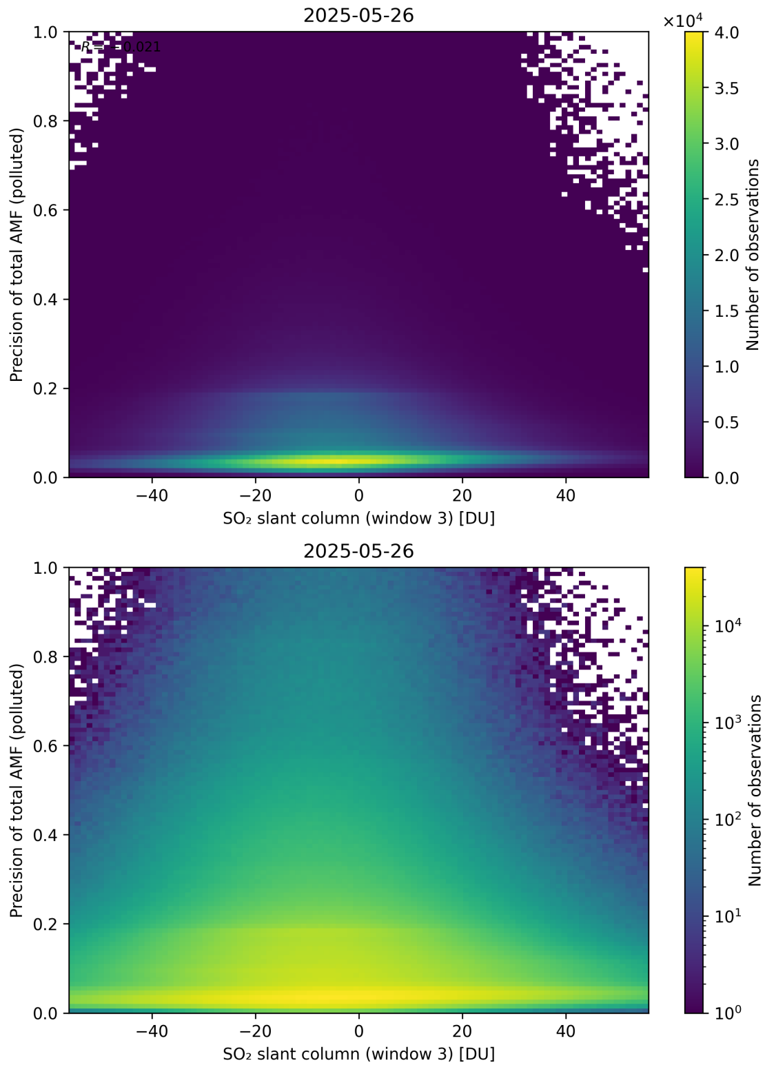
Figure 319: Scatter density plot of “SO 2 slant column (window 3)” against “Precision of total AMF (polluted)” for 2025-05-26 to 2025-05-27.
