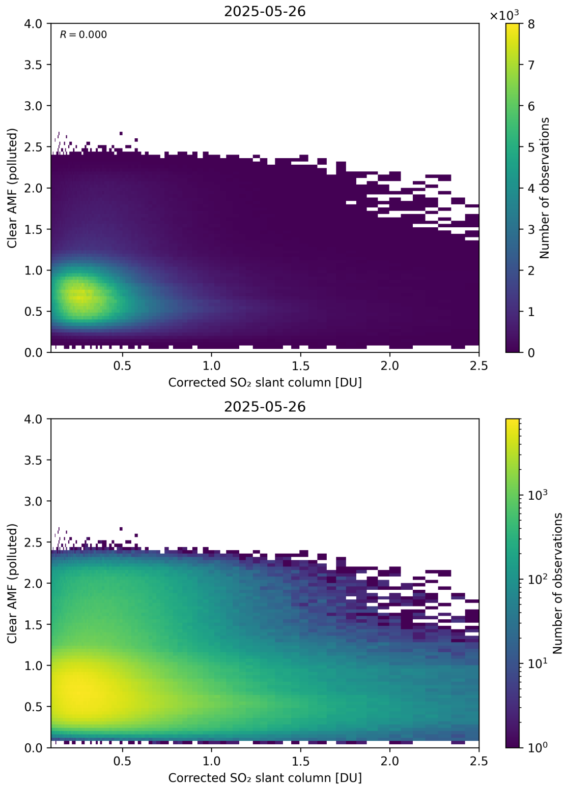
Figure 232: Scatter density plot of “Corrected SO 2 slant column” against “Clear AMF (polluted)” for 2025-05-26 to 2025-05-27.
