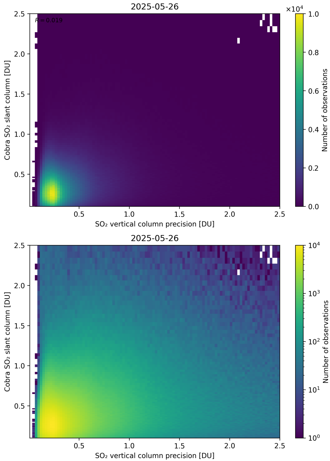
Figure 336: Scatter density plot of “SO 2 vertical column precision” against “Cobra SO 2 slant column” for 2025-05-26 to 2025-05-27.
