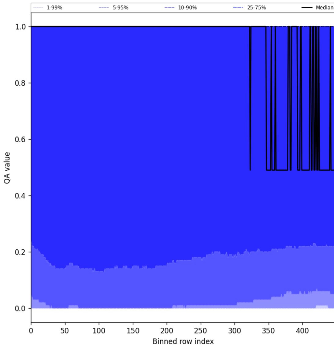
Figure 83: Along track statistics of “QA value” for 2025-05-26 to 2025-05-27
