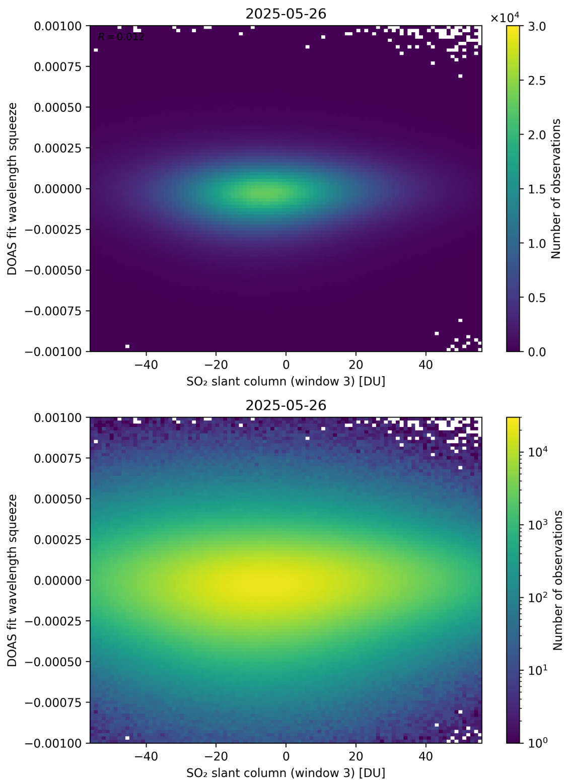
Figure 305: Scatter density plot of “SO 2 slant column (window 3)” against “DOAS fit wavelength squeeze” for 2025-05-26 to 2025-05-27.
