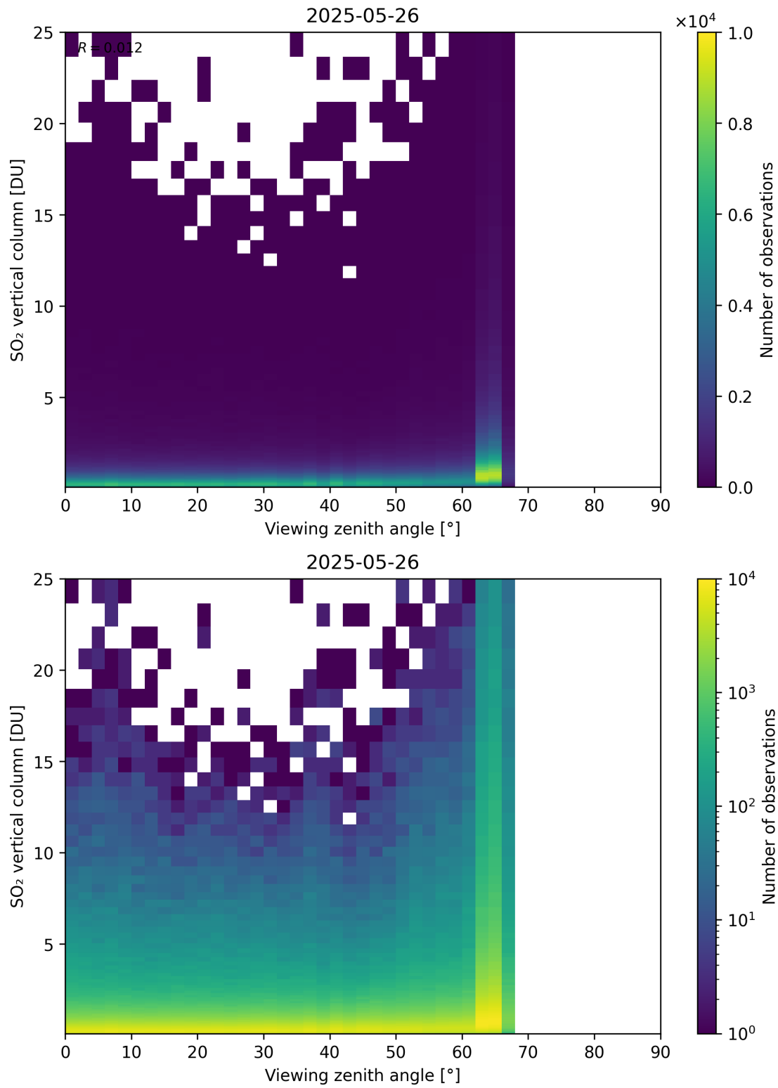
Figure 383: Scatter density plot of “Viewing zenith angle” against “SO 2 vertical column” for 2025-05-26 to 2025-05-27.
