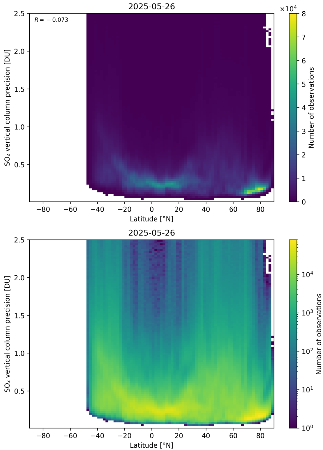
Figure 170: Scatter density plot of “Latitude” against “SO 2 vertical column precision” for 2025-05-26 to 2025-05-27.
