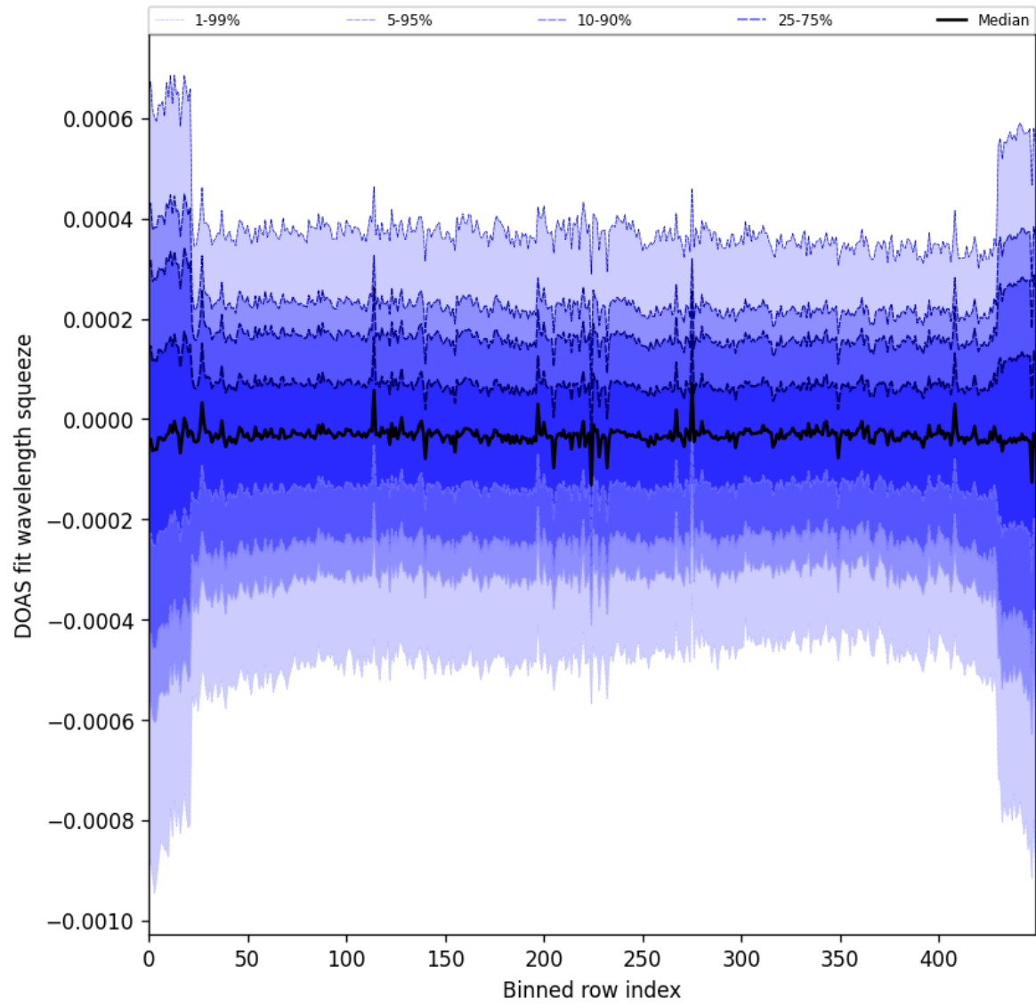
Figure 103: Along track statistics of “DOAS fit wavelength squeeze” for 2025-05-26 to 2025-05-27
