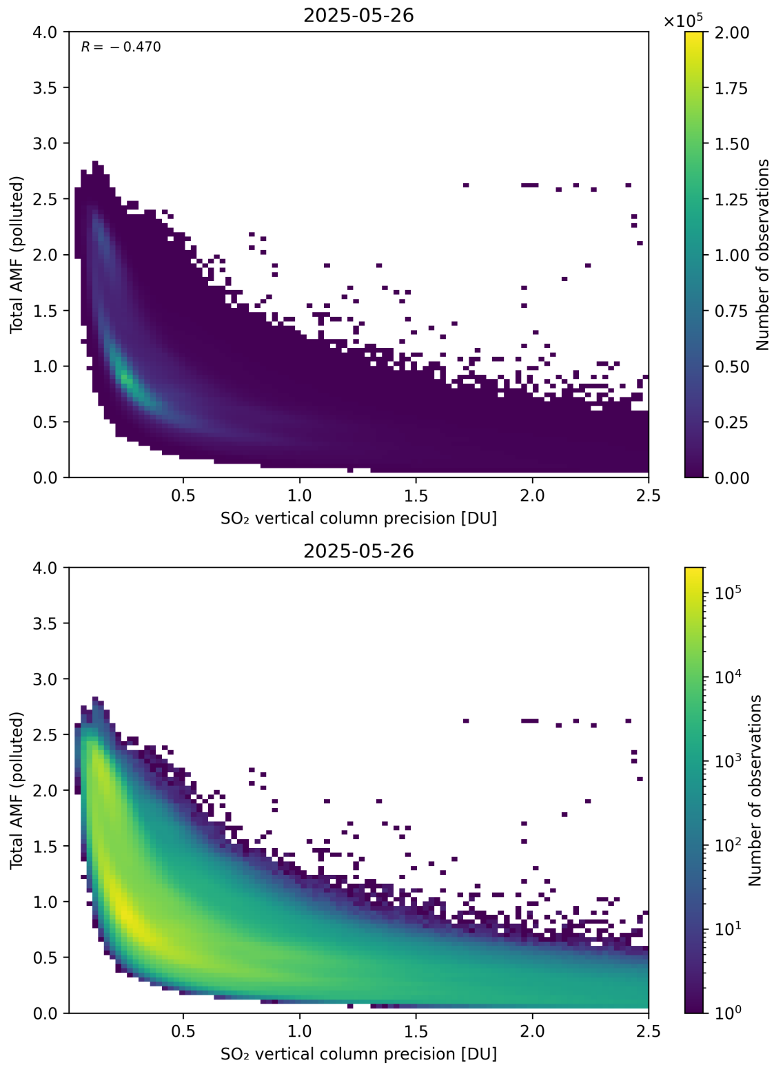
Figure 346: Scatter density plot of “SO 2 vertical column precision” against “Total AMF (polluted)” for 2025-05-26 to 2025-05-27.
