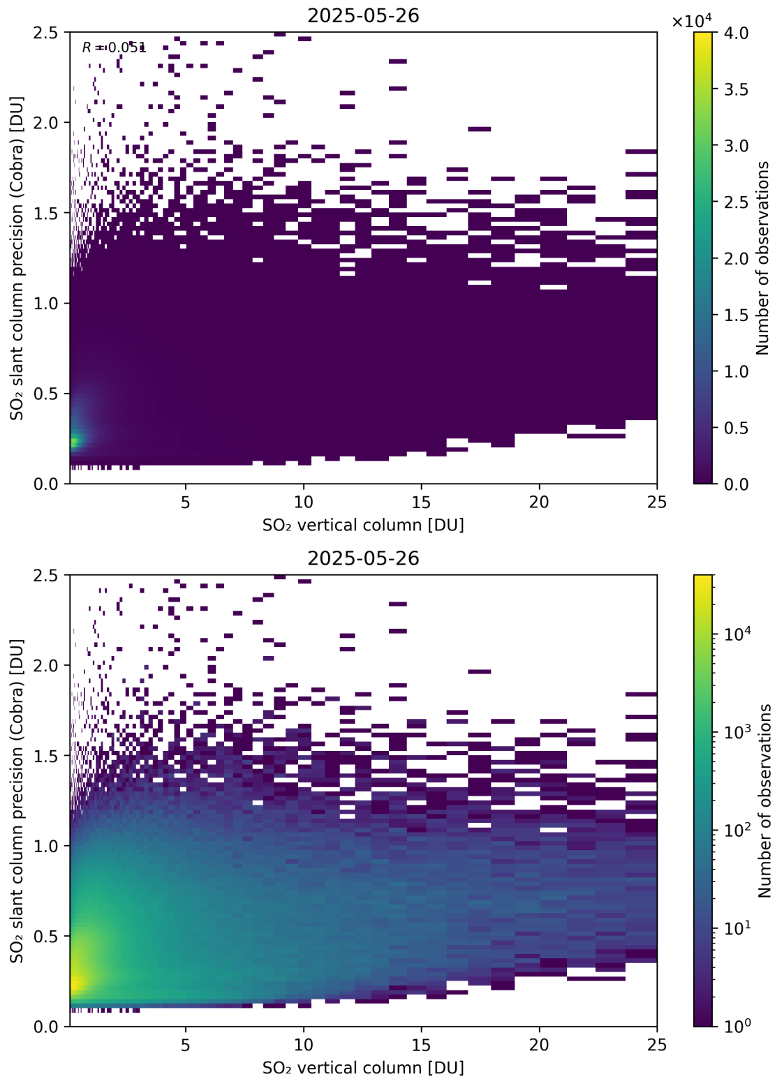
Figure 350: Scatter density plot of “SO 2 vertical column” against “SO 2 slant column precision (Cobra)” for 2025-05-26 to 2025-05-27.
