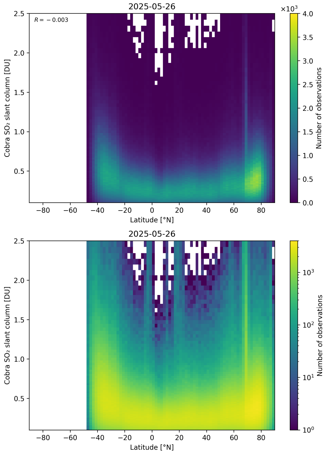
Figure 157: Scatter density plot of “Latitude” against “Cobra SO 2 slant column” for 2025-05-26 to 2025-05-27.
