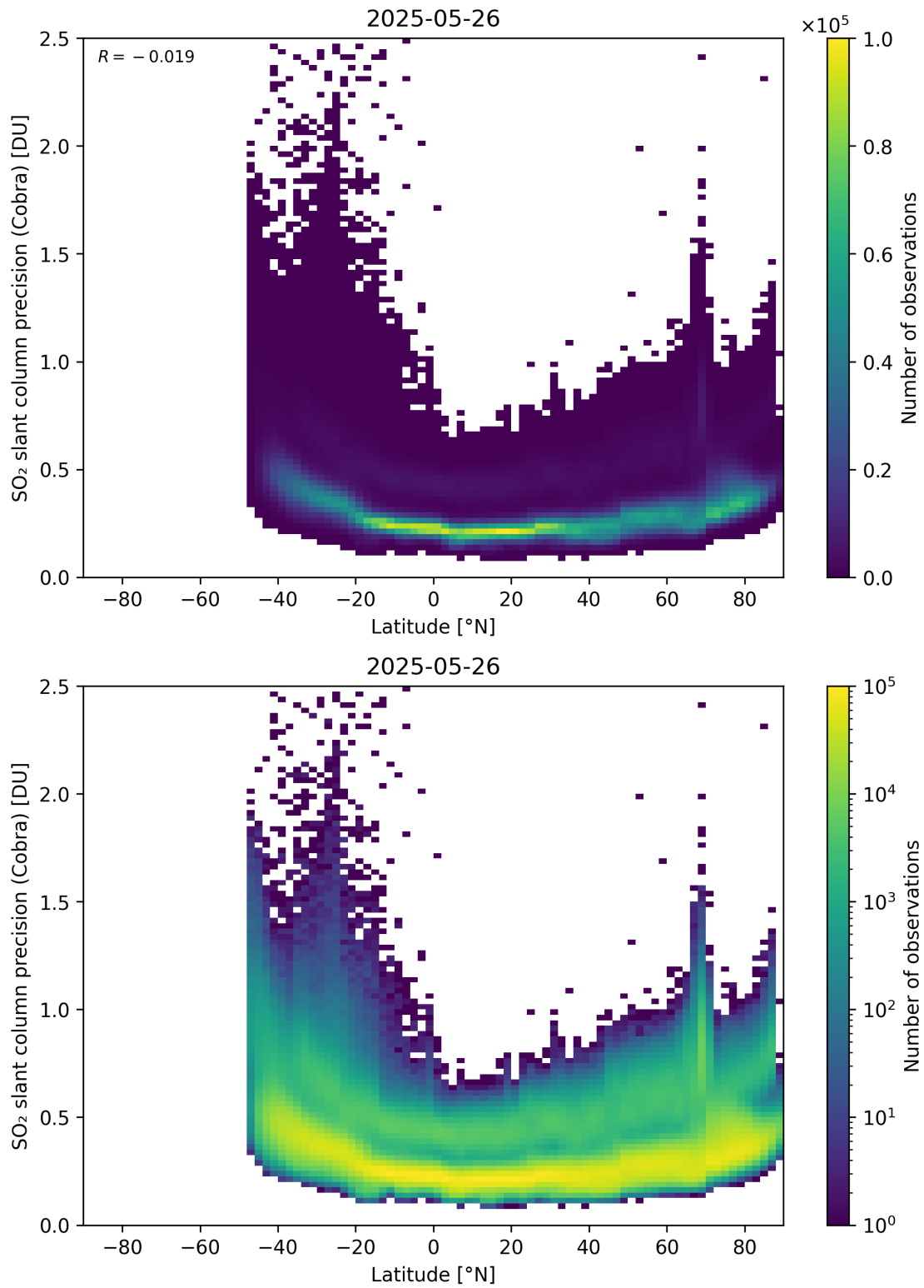
Figure 158: Scatter density plot of “Latitude” against “SO 2 slant column precision (Cobra)” for 2025-05-26 to 2025-05-27.
