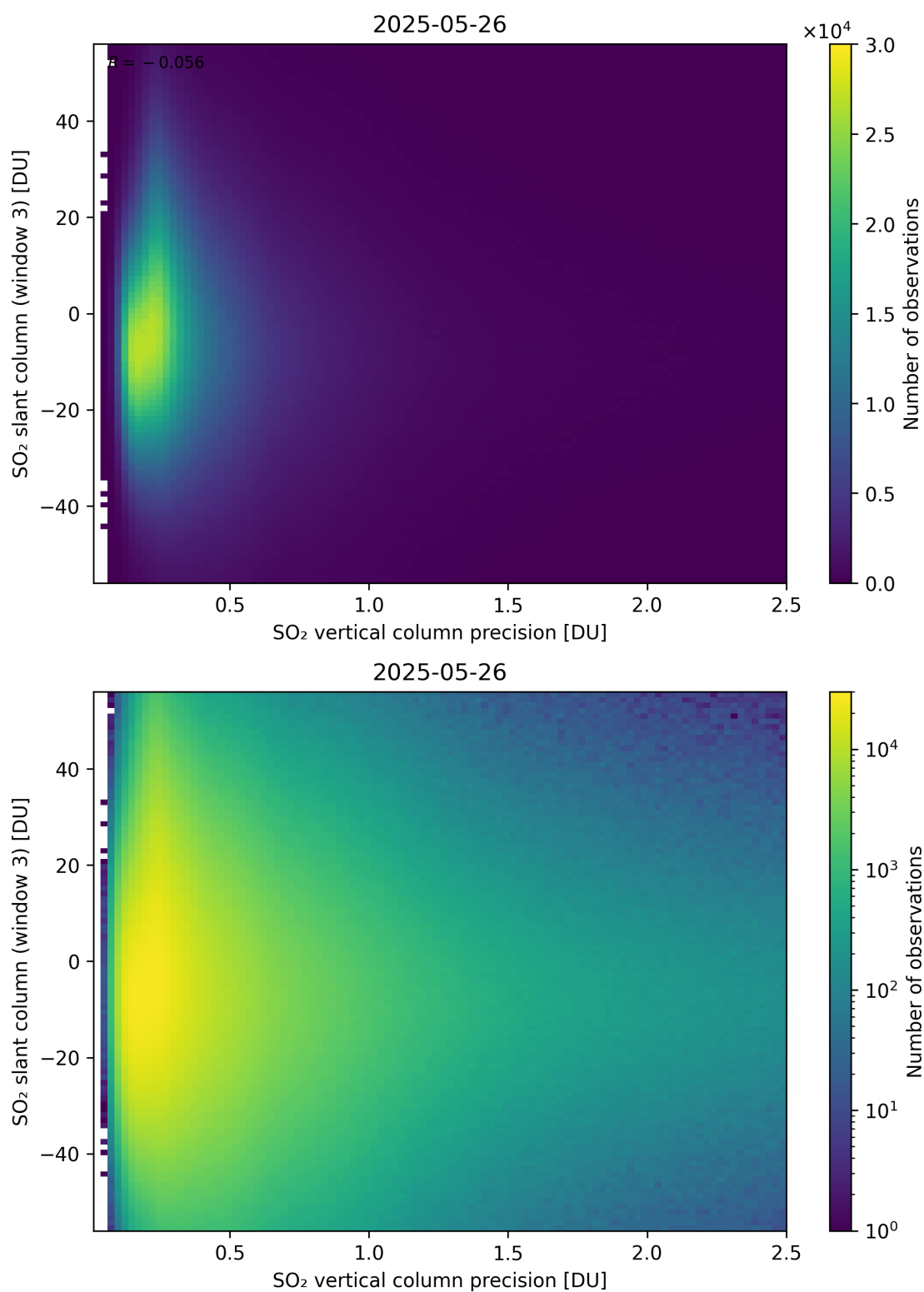
Figure 344: Scatter density plot of “SO 2 vertical column precision” against “SO 2 slant column (window 3)” for 2025-05-26 to 2025-05-27.
