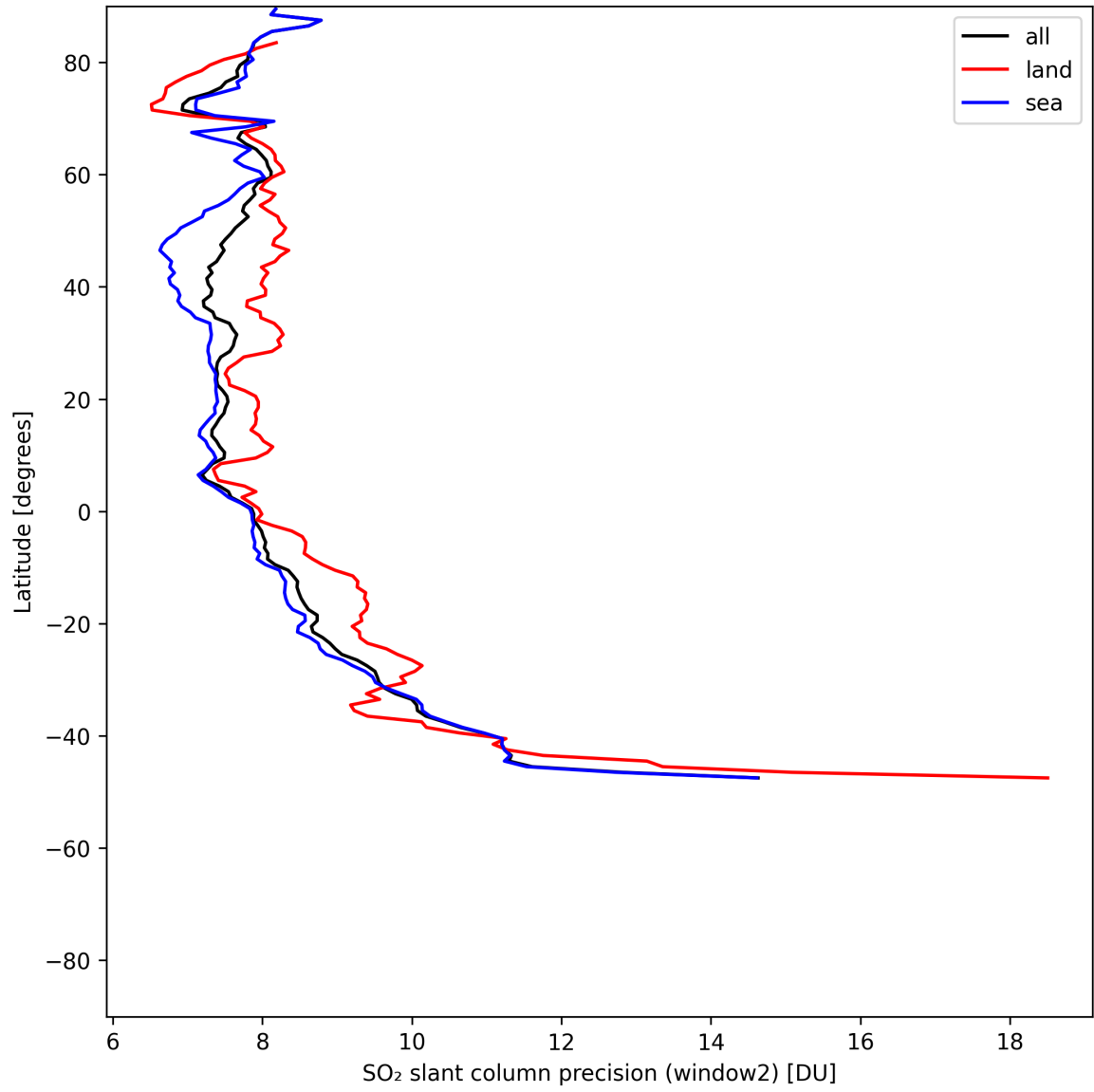
Figure 42: Zonal average of “SO 2 slant column precision (window2)” for 2025-05-26 to 2025-05-27.
