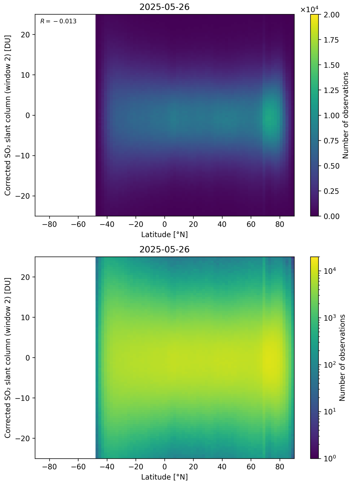
Figure 160: Scatter density plot of “Latitude” against “Corrected SO 2 slant column (window 2)” for 2025-05-26 to 2025-05-27.
