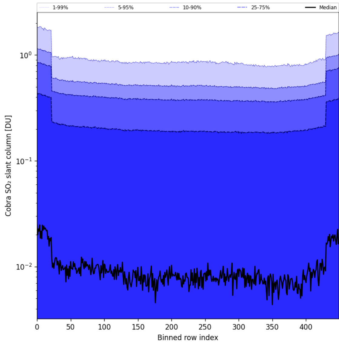
Figure 87: Along track statistics of “Cobra SO 2 slant column” for 2025-05-26 to 2025-05-27
