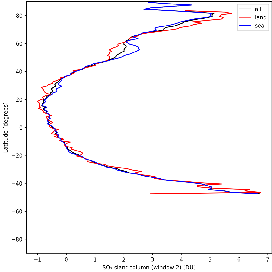
Figure 41: Zonal average of “SO 2 slant column (window 2)” for 2025-05-26 to 2025-05-27.
