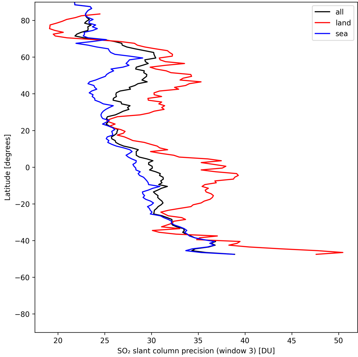
Figure 46: Zonal average of “SO 2 slant column precision (window 3)” for 2025-05-26 to 2025-05-27.
