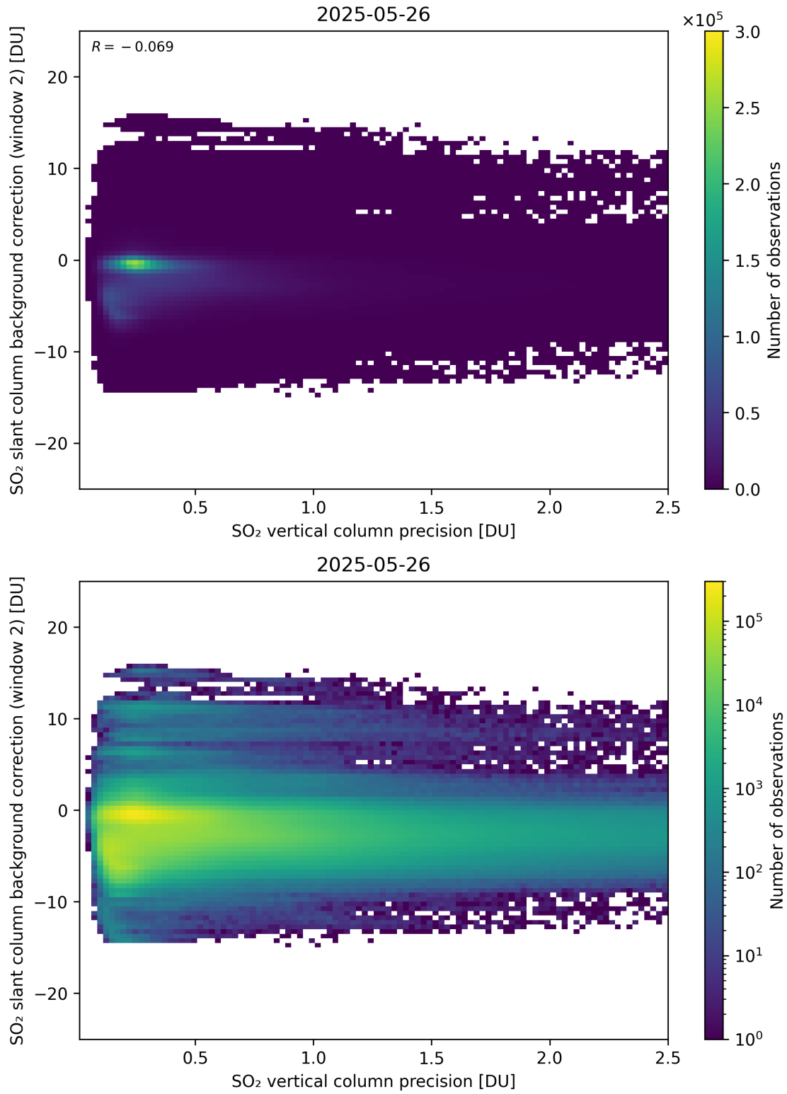
Figure 330: Scatter density plot of “SO 2 vertical column precision” against “SO 2 slant column background correction (window 2)” for 2025-05-26 to 2025-05-27.
