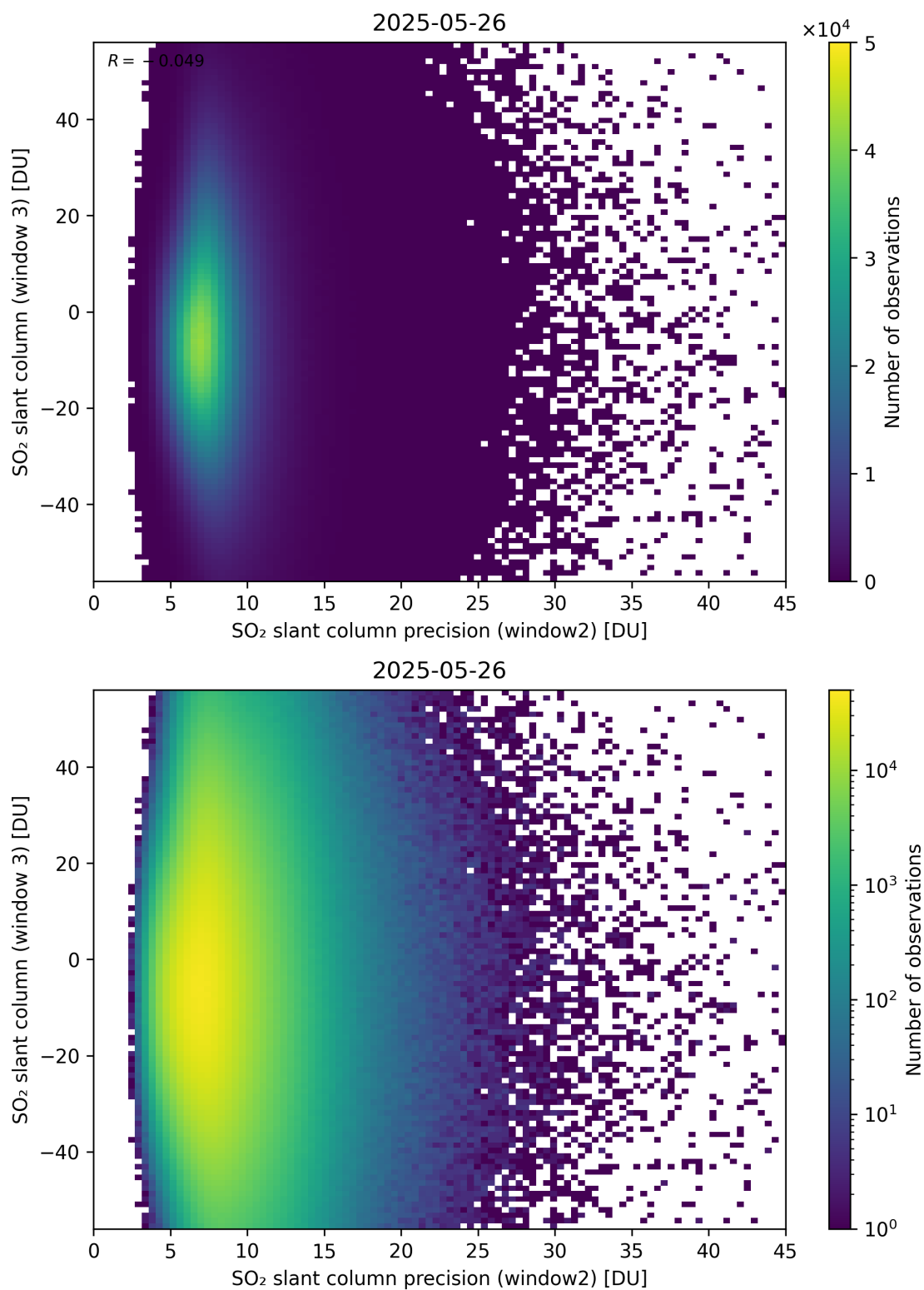
Figure 299: Scatter density plot of “SO 2 slant column precision (window2)” against “SO 2 slant column (window 3)” for 2025-05-26 to 2025-05-27.
