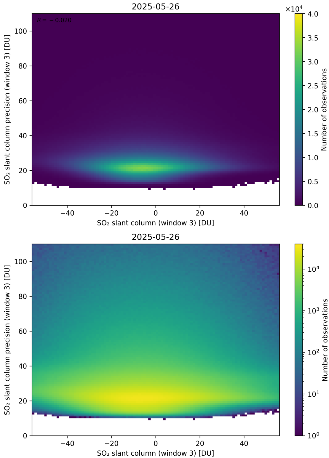
Figure 317: Scatter density plot of “SO 2 slant column (window 3)” against “SO 2 slant column precision (window 3)” for 2025-05-26 to 2025-05-27.
