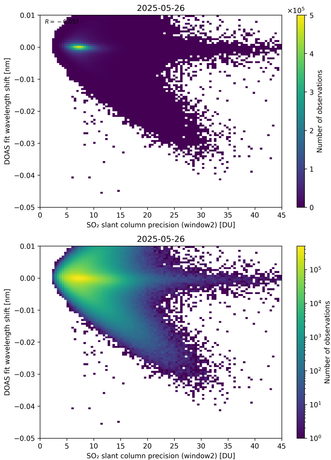
Figure 293: Scatter density plot of “SO 2 slant column precision (window2)” against “DOAS fit wavelength shift” for 2025-05-26 to 2025-05-27.
