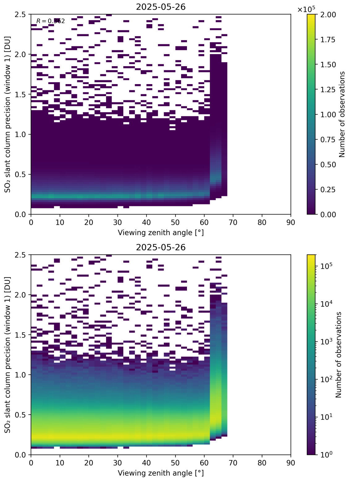
Figure 377: Scatter density plot of “Viewing zenith angle” against “SO 2 slant column precision (window 1)” for 2025-05-26 to 2025-05-27.
