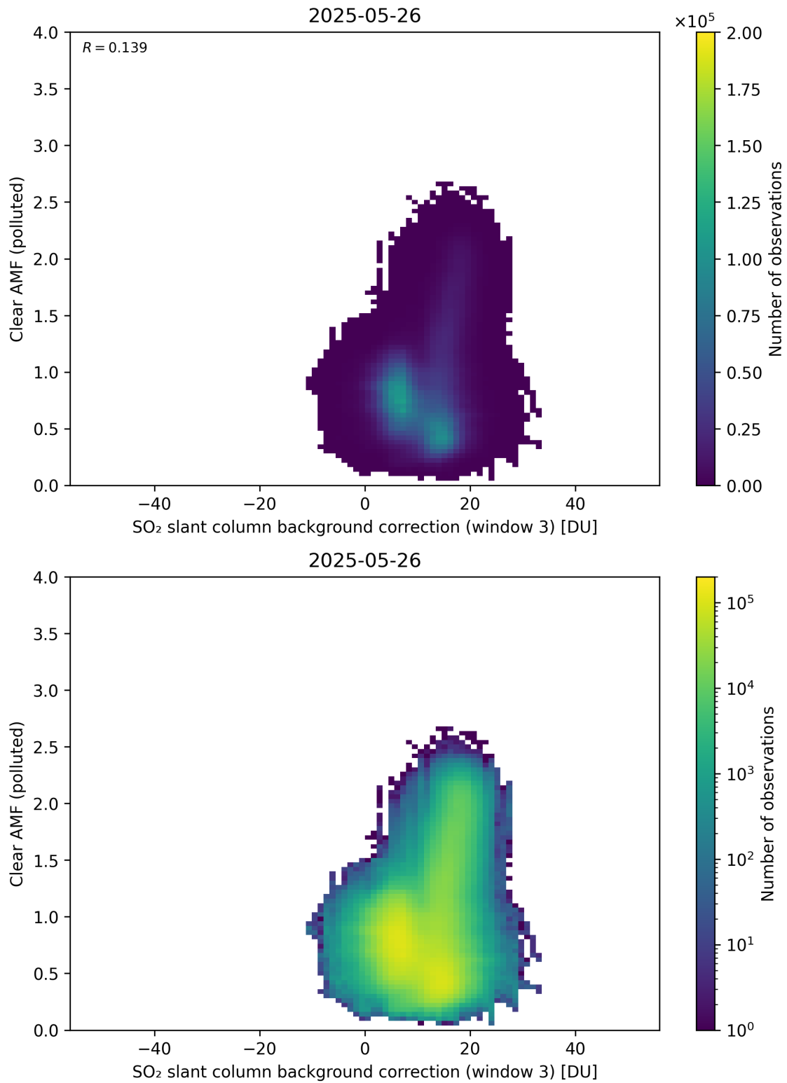
Figure 135: Scatter density plot of “SO 2 slant column background correction (window 3)” against “Clear AMF (polluted)” for 2025-05-26 to 2025-05-27.
