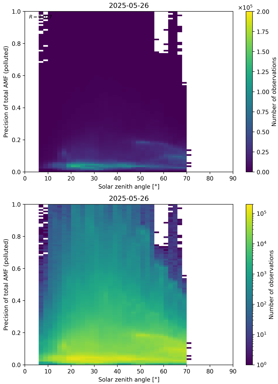
Figure 190: Scatter density plot of “Solar zenith angle” against “Precision of total AMF (polluted)” for 2025-05-26 to 2025-05-27.
