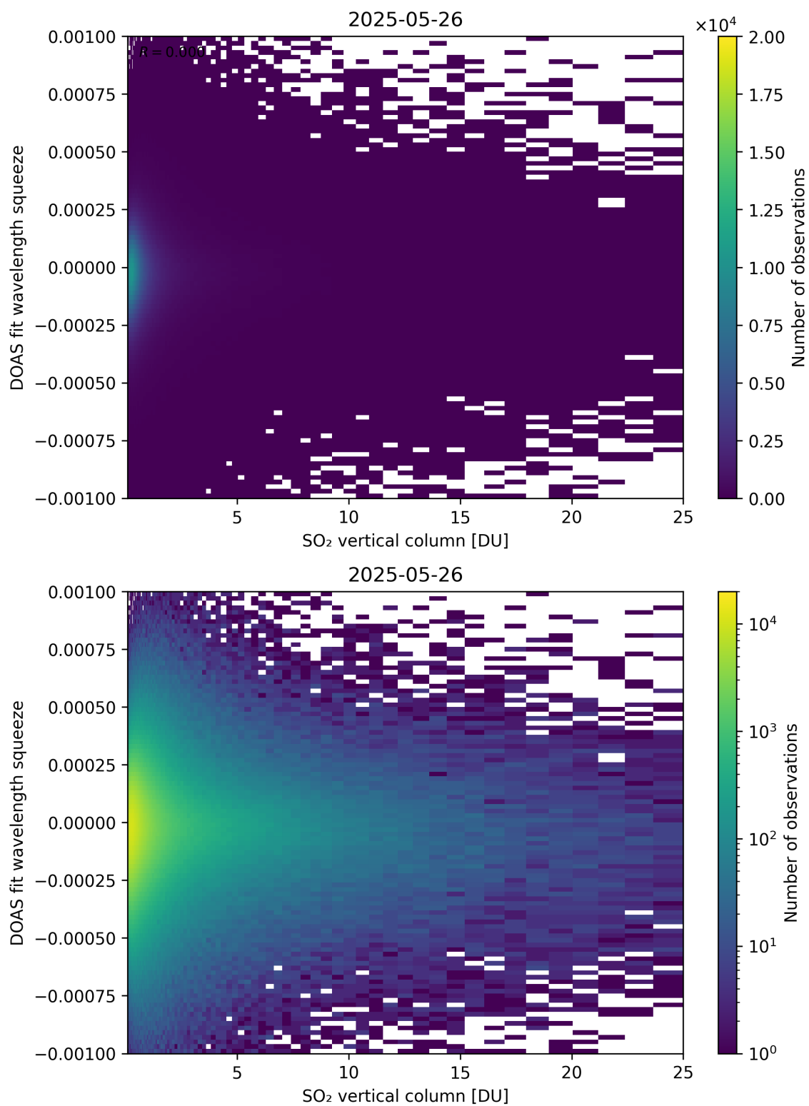
Figure 327: Scatter density plot of “SO 2 vertical column” against “DOAS fit wavelength squeeze” for 2025-05-26 to 2025-05-27.
