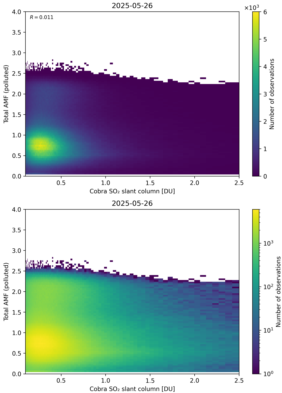
Figure 224: Scatter density plot of “Cobra SO 2 slant column” against “Total AMF (polluted)” for 2025-05-26 to 2025-05-27.
