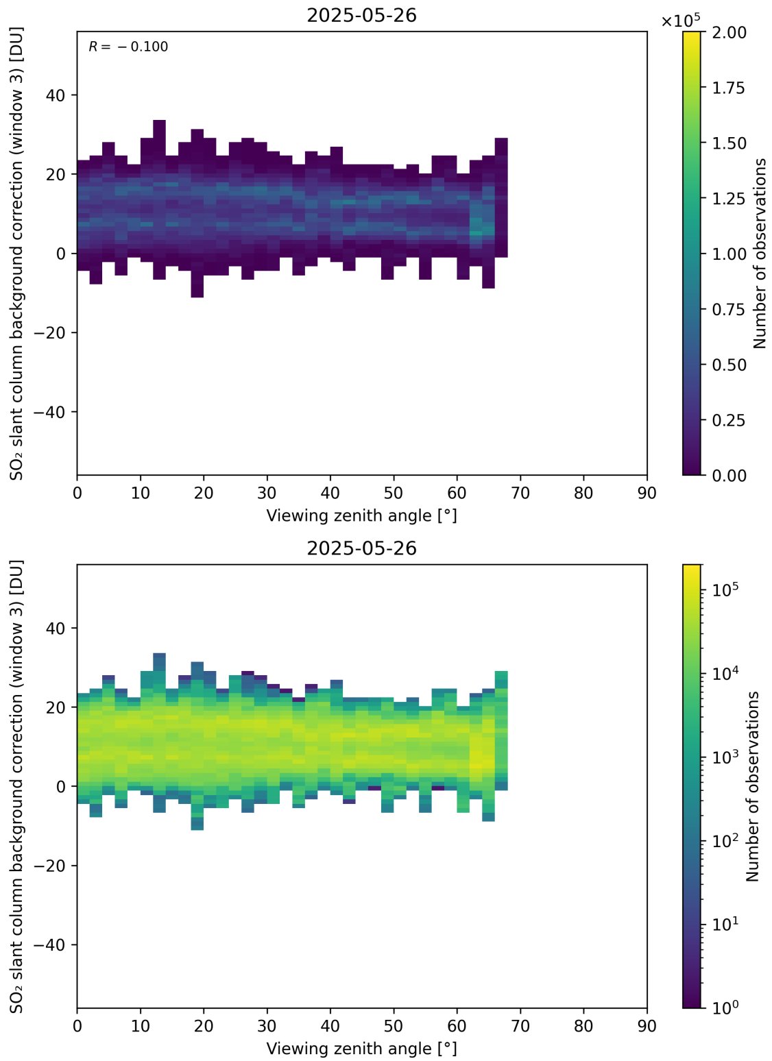
Figure 364: Scatter density plot of “Viewing zenith angle” against “SO 2 slant column background correction (window 3)” for 2025-05-26 to 2025-05-27.
