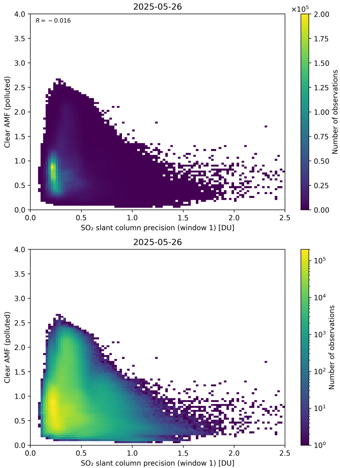
Figure 274: Scatter density plot of “SO 2 slant column precision (window 1)” against “Clear AMF (polluted)” for 2025-05-26 to 2025-05-27.
