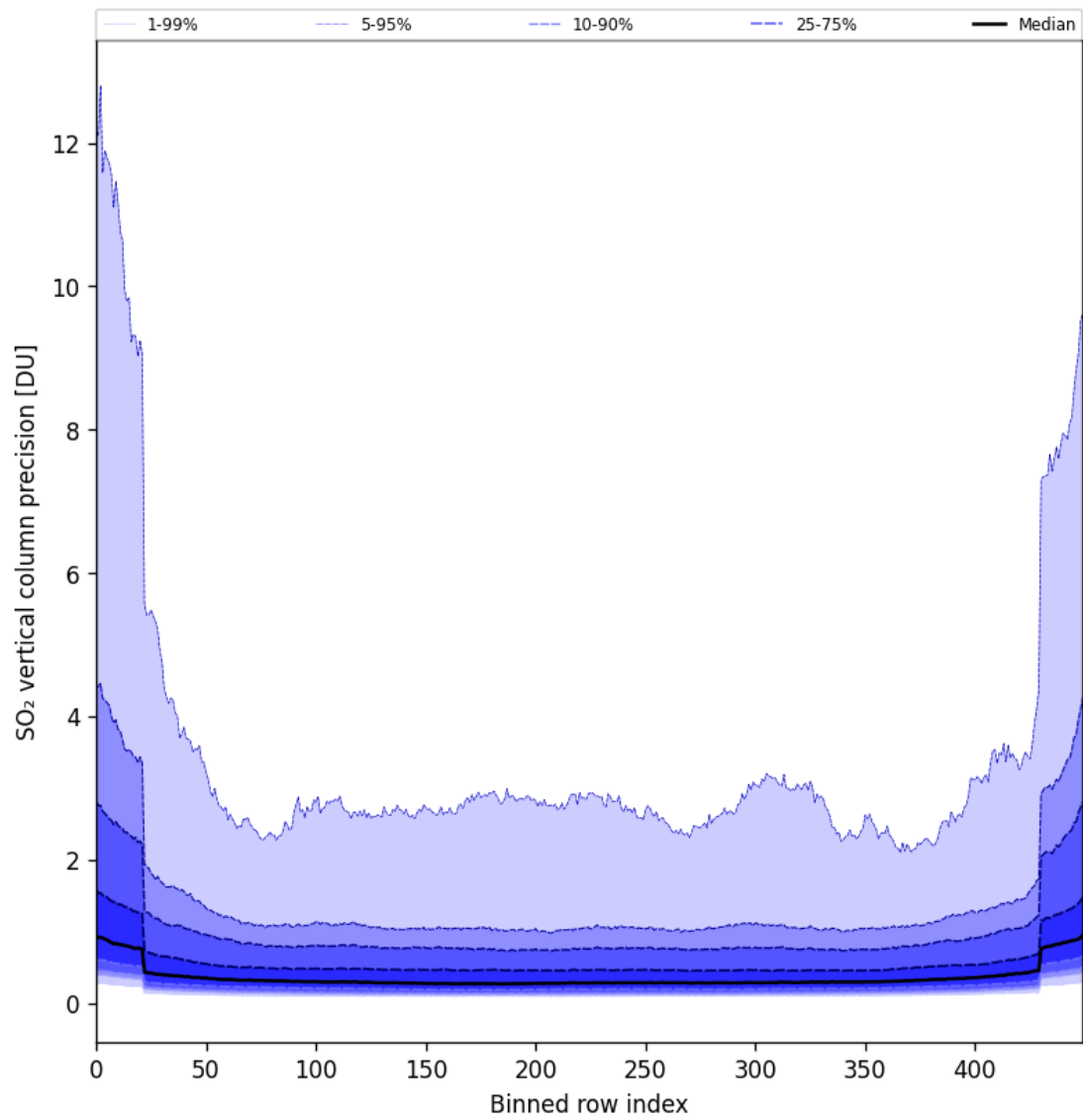
Figure 85: Along track statistics of “SO 2 vertical column precision” for 2025-05-26 to 2025-05-27
