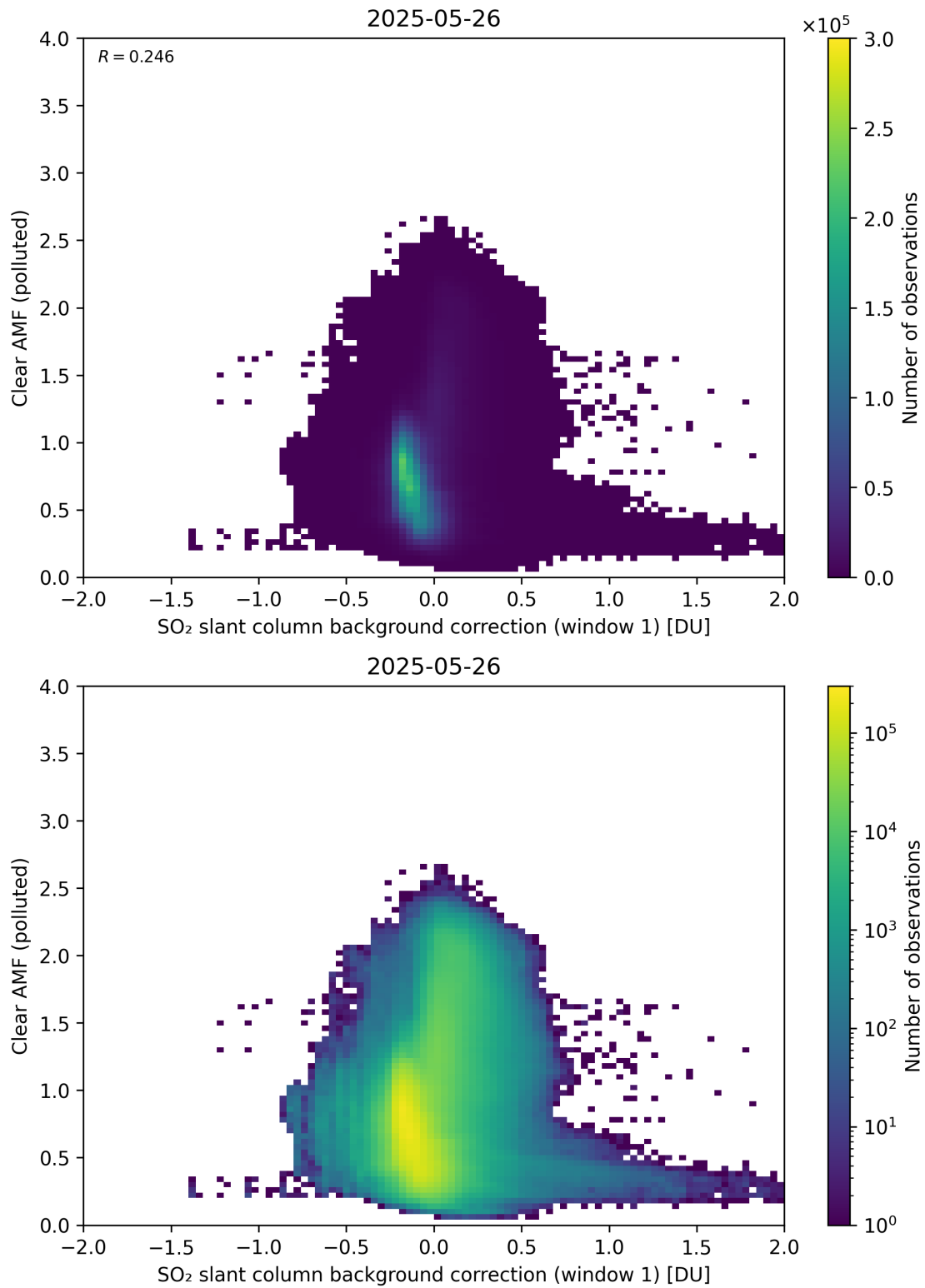
Figure 114: Scatter density plot of “SO 2 slant column background correction (window 1)” against “Clear AMF (polluted)” for 2025-05-26 to 2025-05-27.
