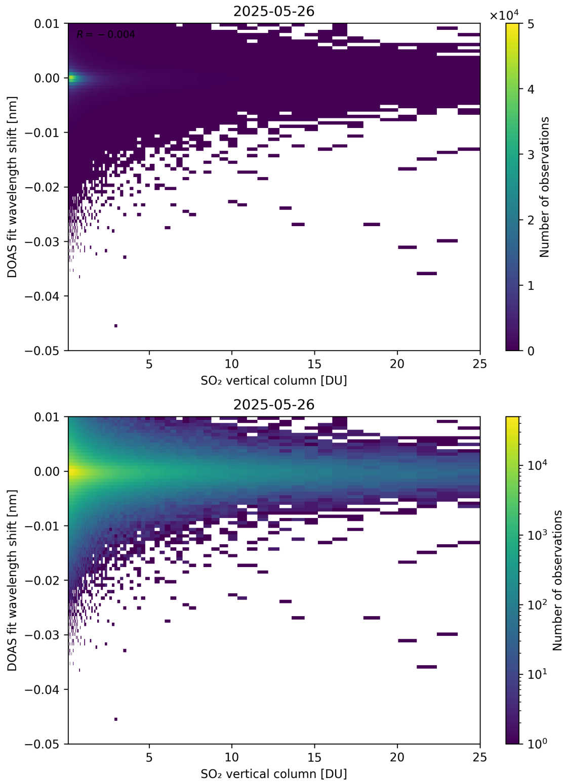
Figure 326: Scatter density plot of “SO 2 vertical column” against “DOAS fit wavelength shift” for 2025-05-26 to 2025-05-27.
