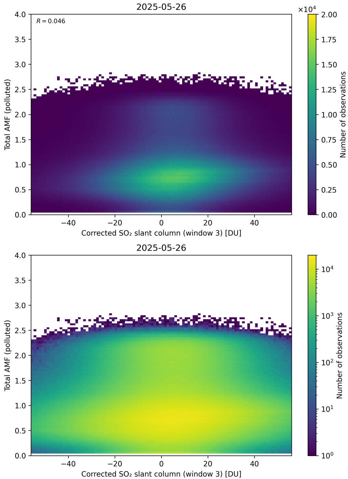
Figure 260: Scatter density plot of “Corrected SO 2 slant column (window 3)” against “Total AMF (polluted)” for 2025-05-26 to 2025-05-27.
