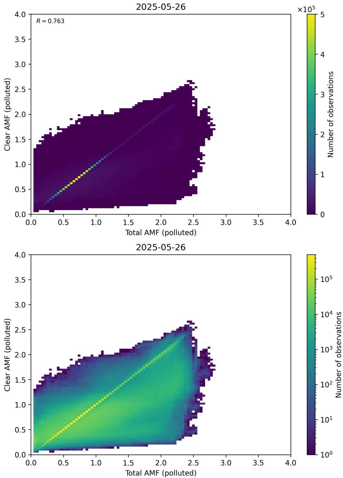
Figure 321: Scatter density plot of “Total AMF (polluted)” against “Clear AMF (polluted)” for 2025-05-26 to 2025-05-27.
