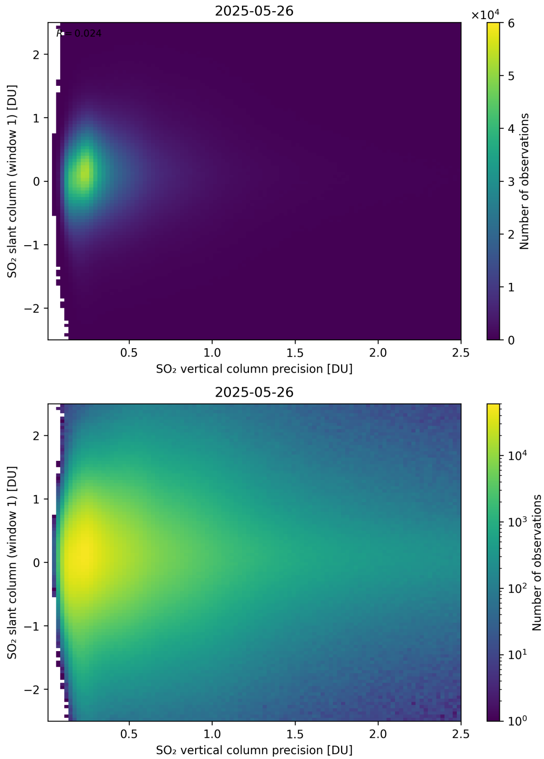
Figure 341: Scatter density plot of “SO 2 vertical column precision” against “SO 2 slant column (window 1)” for 2025-05-26 to 2025-05-27.
