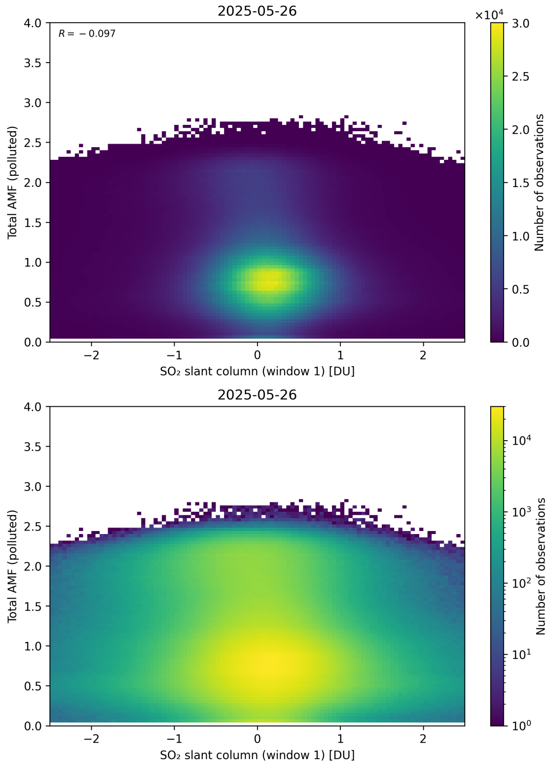
Figure 289: Scatter density plot of “SO 2 slant column (window 1)” against “Total AMF (polluted)” for 2025-05-26 to 2025-05-27.
