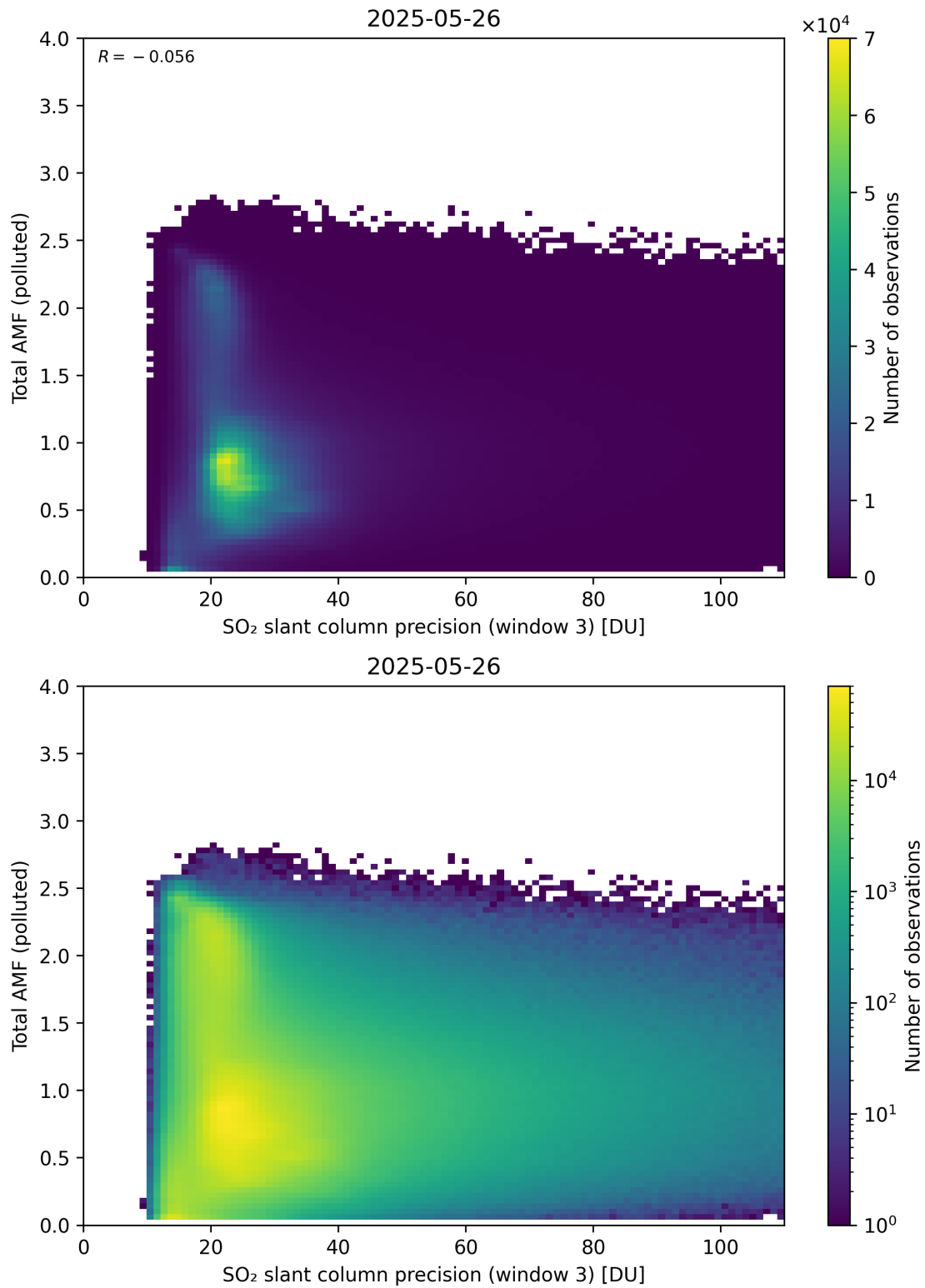
Figure 313: Scatter density plot of “SO 2 slant column precision (window 3)” against “Total AMF (polluted)” for 2025-05-26 to 2025-05-27.
