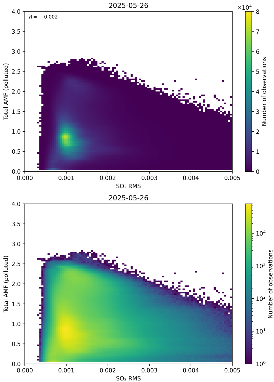
Figure 148: Scatter density plot of “SO 2 RMS” against “Total AMF (polluted)” for 2025-05-26 to 2025-05-27.
