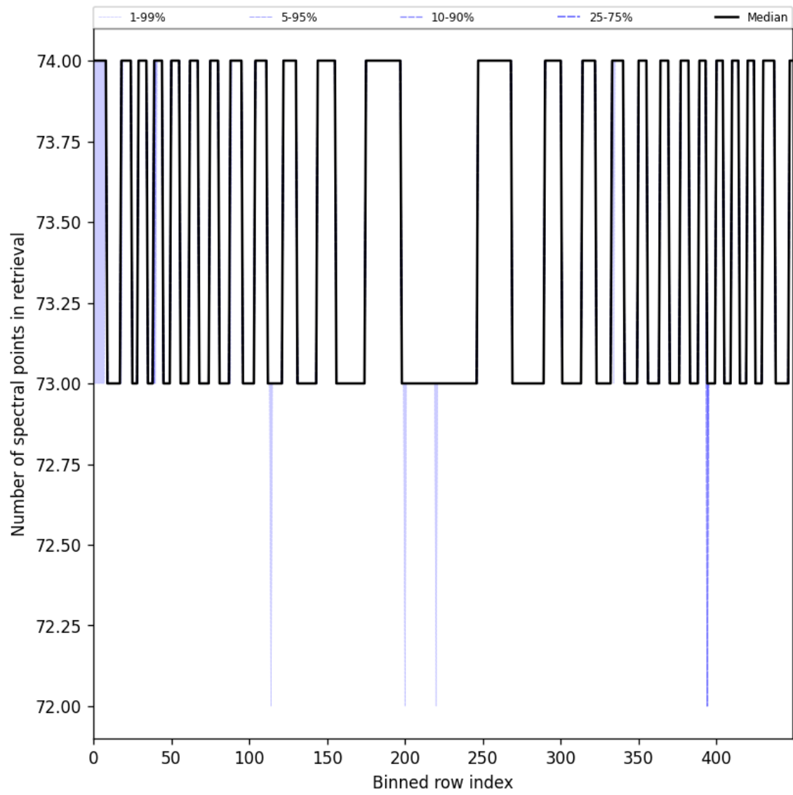
Figure 108: Along track statistics of “Number of spectral points in retrieval” for 2025-05-26 to 2025-05-27
