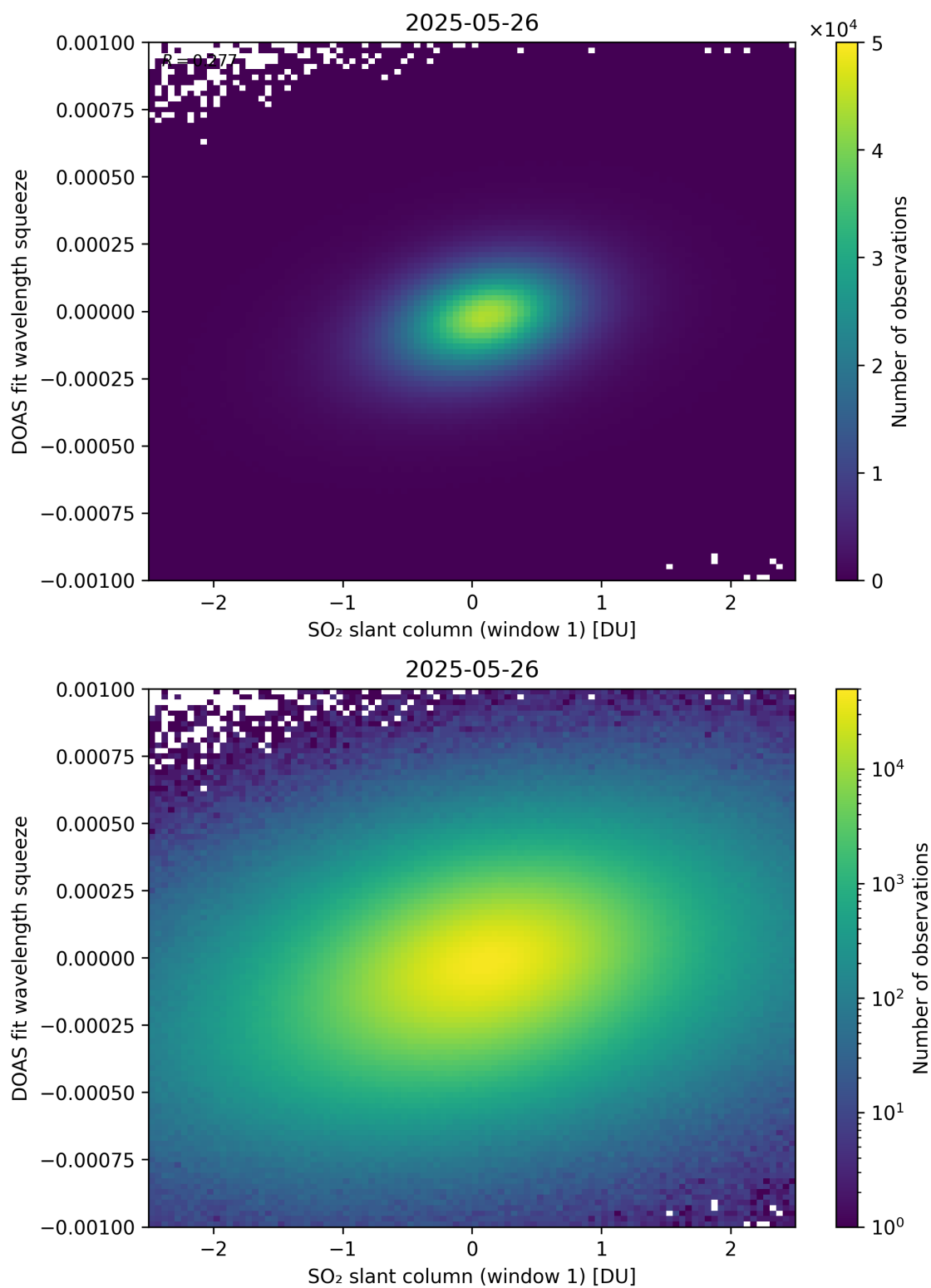
Figure 266: Scatter density plot of “SO 2 slant column (window 1)” against “DOAS fit wavelength squeeze” for 2025-05-26 to 2025-05-27.
