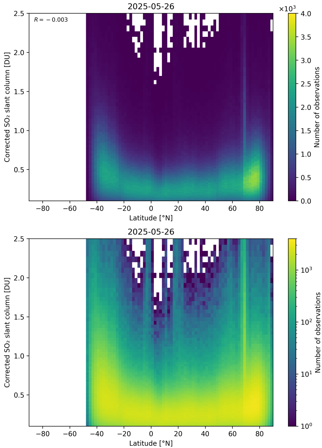
Figure 159: Scatter density plot of “Latitude” against “Corrected SO 2 slant column” for 2025-05-26 to 2025-05-27.
