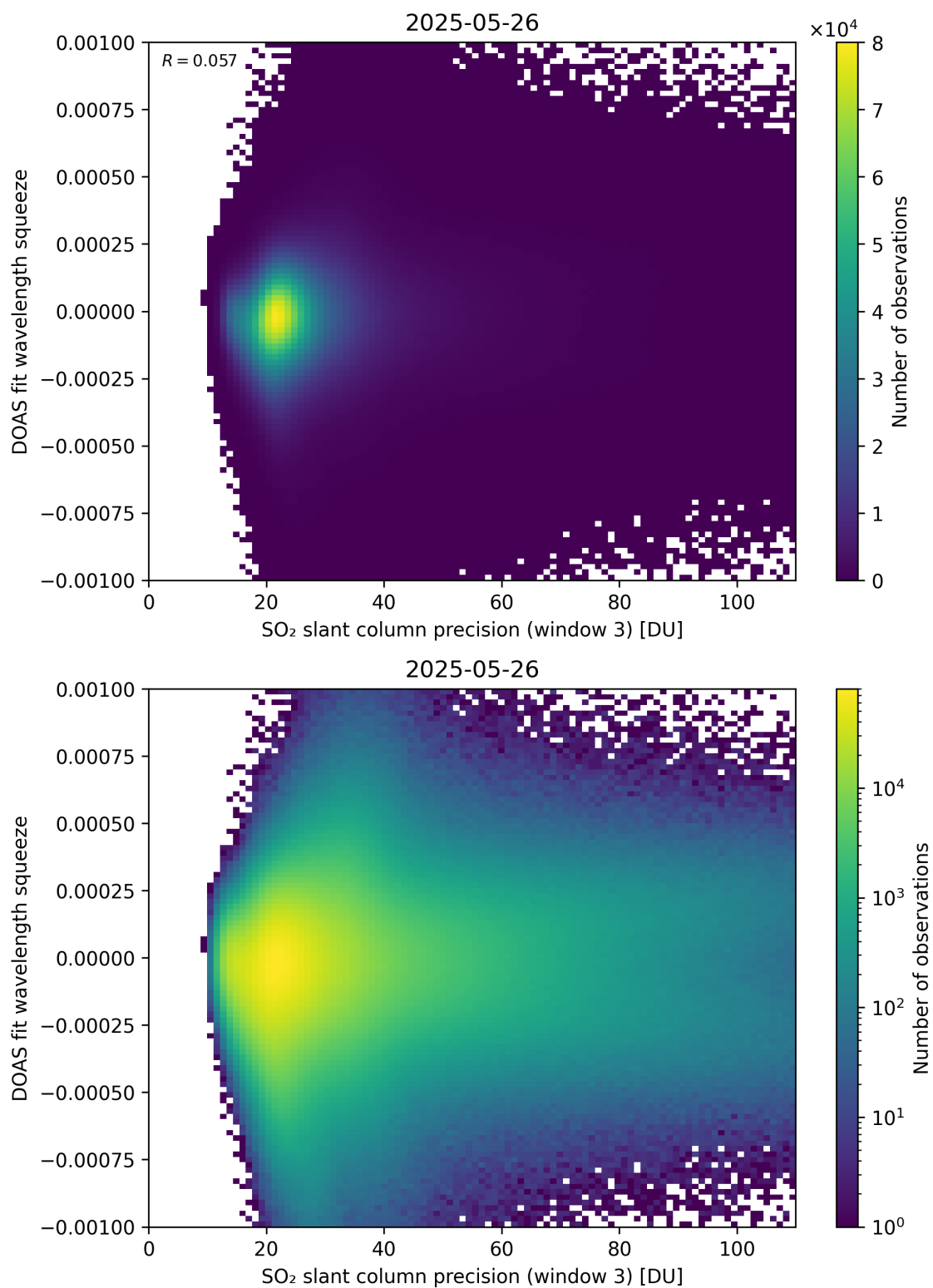
Figure 309: Scatter density plot of “SO 2 slant column precision (window 3)” against “DOAS fit wavelength squeeze” for 2025-05-26 to 2025-05-27.
