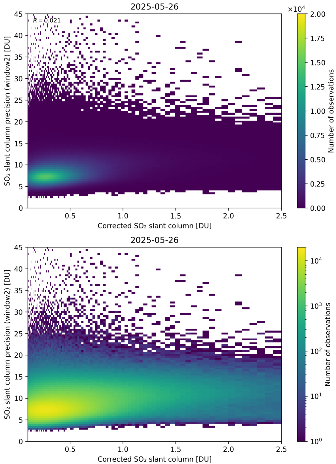
Figure 239: Scatter density plot of “Corrected SO 2 slant column” against “SO 2 slant column precision (window2)” for 2025-05-26 to 2025-05-27.
