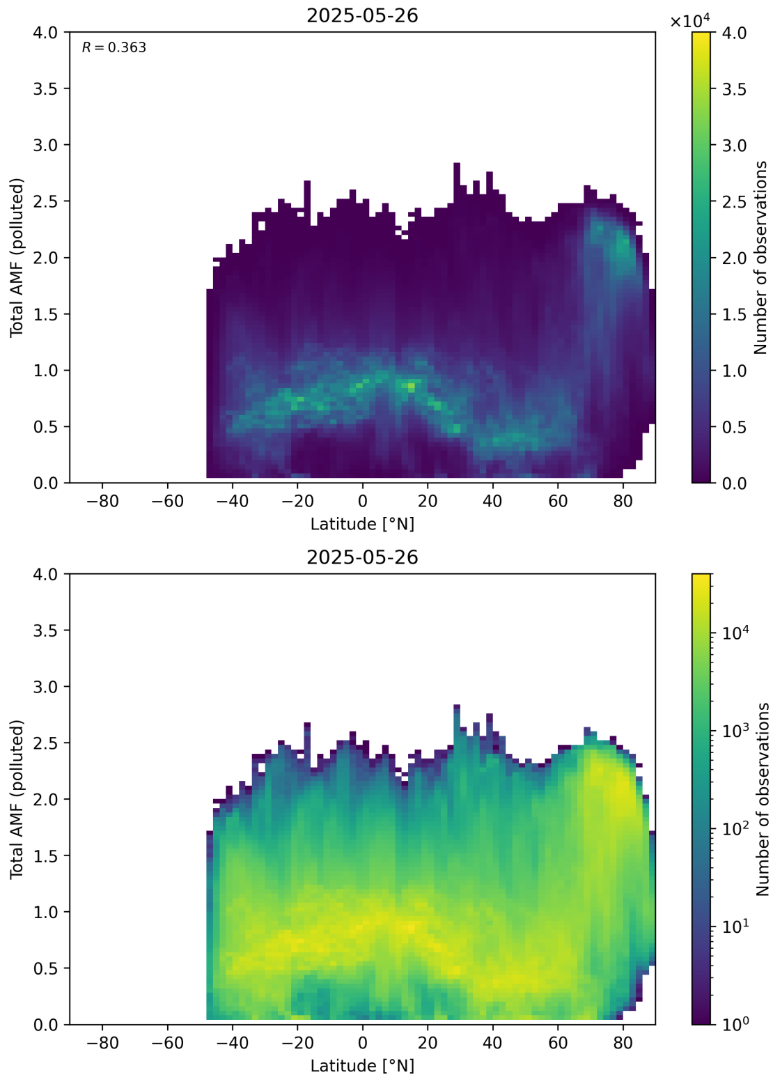
Figure 167: Scatter density plot of “Latitude” against “Total AMF (polluted)” for 2025-05-26 to 2025-05-27.
