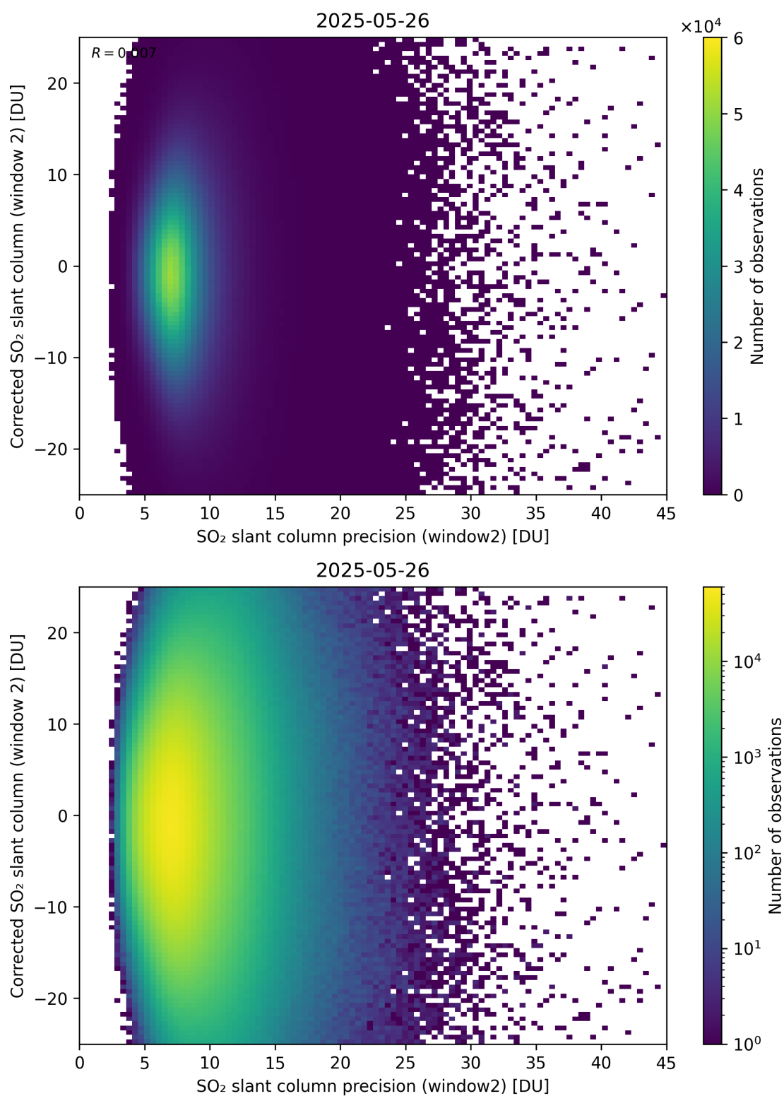
Figure 297: Scatter density plot of “SO 2 slant column precision (window2)” against “Corrected SO 2 slant column (window 2)” for 2025-05-26 to 2025-05-27.
