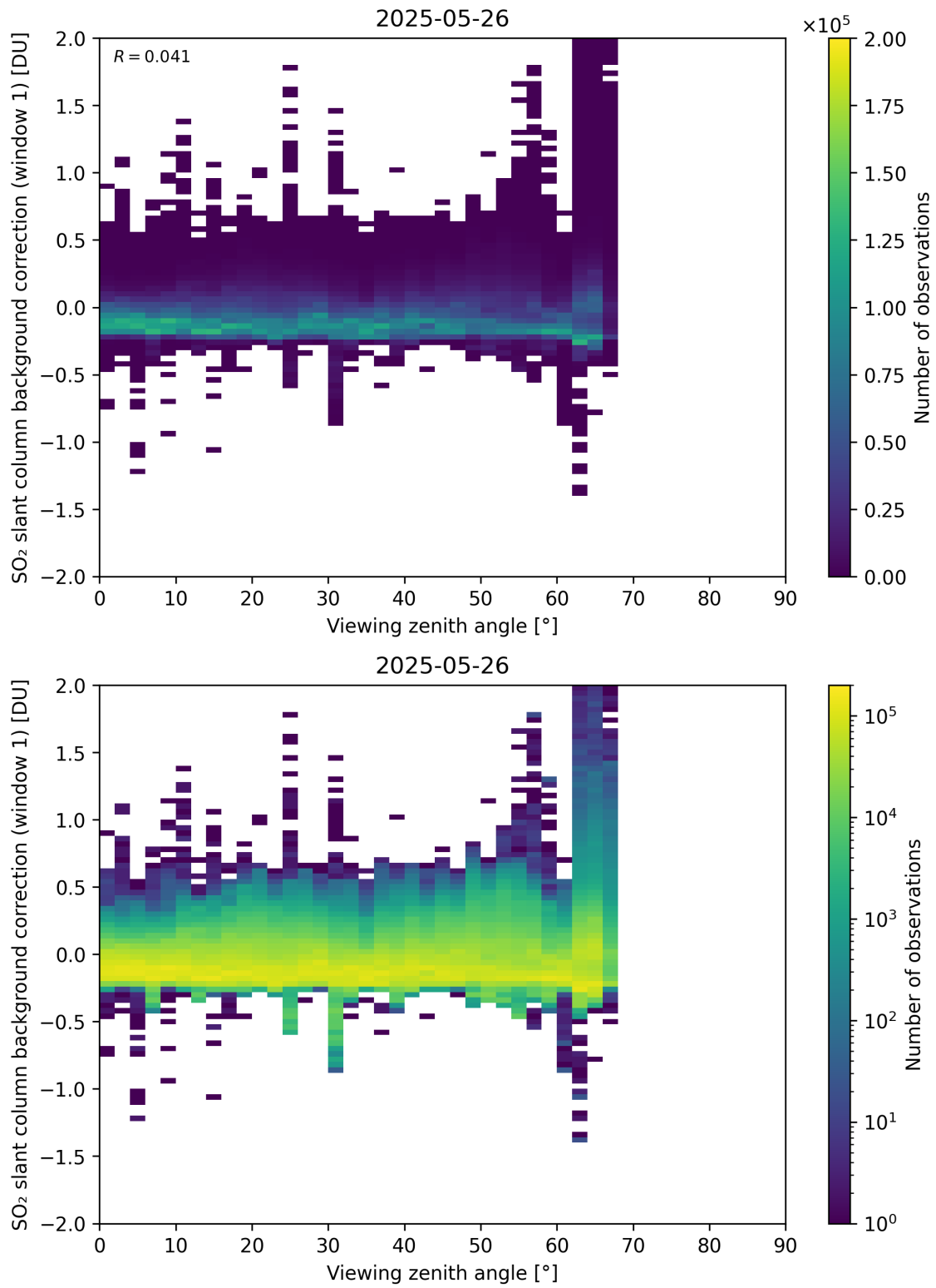
Figure 362: Scatter density plot of “Viewing zenith angle” against “SO 2 slant column background correction (window 1)” for 2025-05-26 to 2025-05-27.
