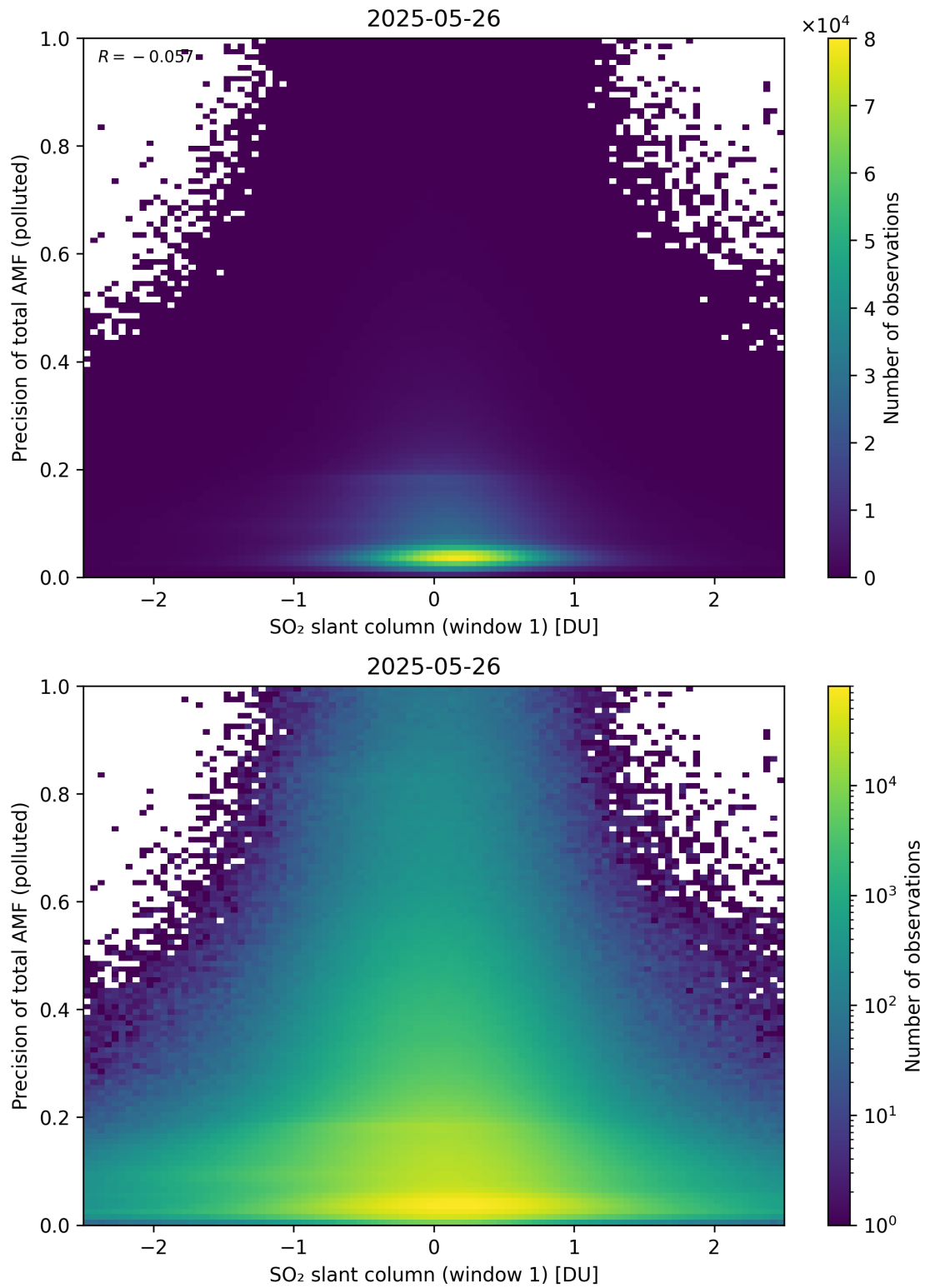
Figure 290: Scatter density plot of “SO 2 slant column (window 1)” against “Precision of total AMF (polluted)” for 2025-05-26 to 2025-05-27.
