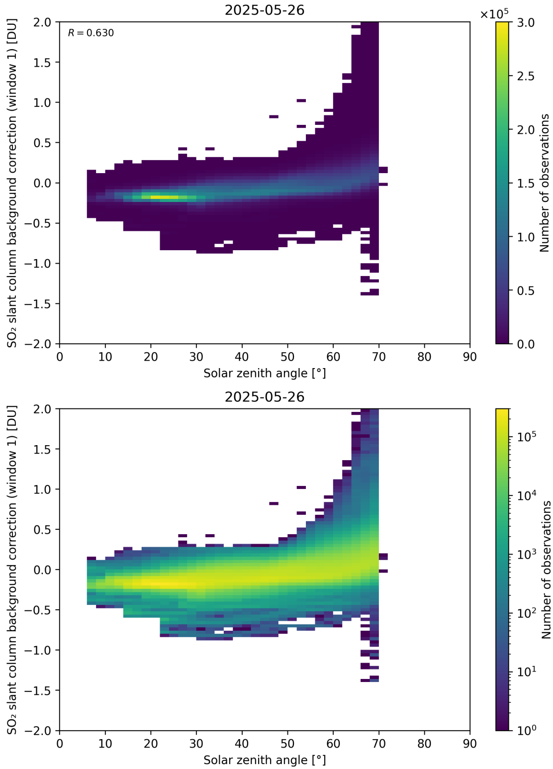
Figure 171: Scatter density plot of “Solar zenith angle” against “SO 2 slant column background correction (window 1)” for 2025-05-26 to 2025-05-27.
