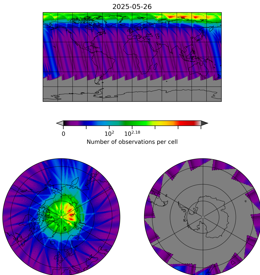
Figure 30: Map of the number of observations for 2025-05-26 to 2025-05-27
