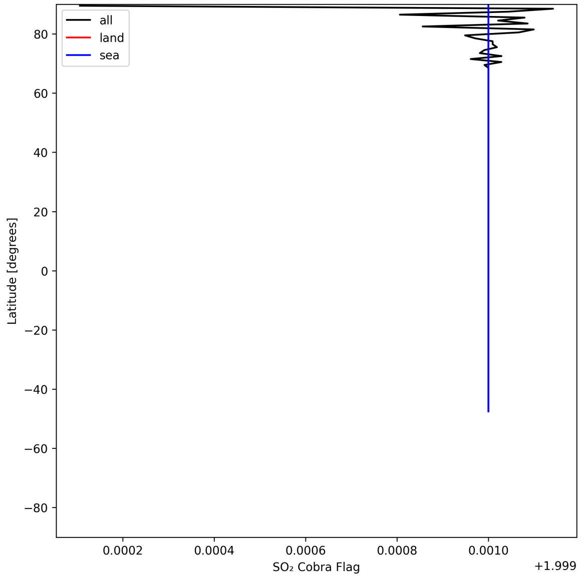
Figure 49: Zonal average of “SO 2 Cobra Flag” for 2025-05-26 to 2025-05-27.
