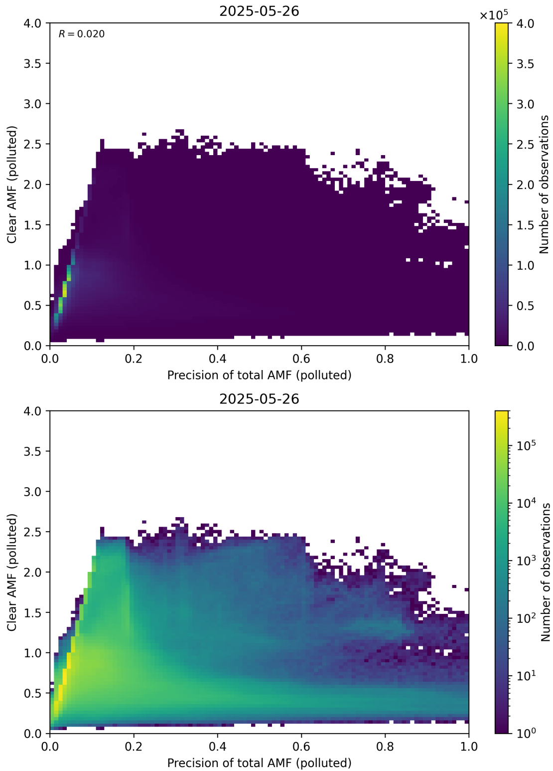
Figure 320: Scatter density plot of “Precision of total AMF (polluted)” against “Clear AMF (polluted)” for 2025-05-26 to 2025-05-27.
