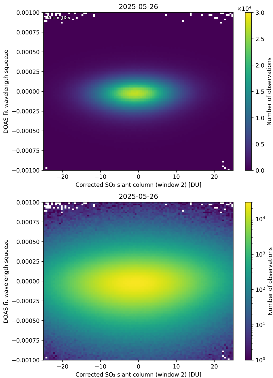
Figure 247: Scatter density plot of “Corrected SO 2 slant column (window 2)” against “DOAS fit wavelength squeeze” for 2025-05-26 to 2025-05-27.
