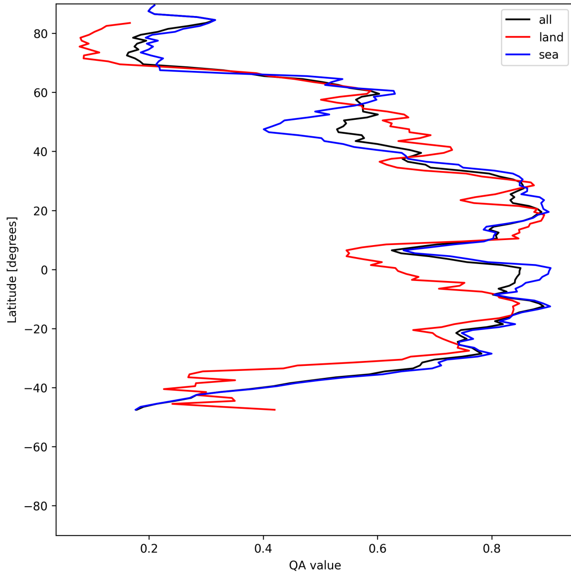
Figure 31: Zonal average of “QA value” for 2025-05-26 to 2025-05-27.
