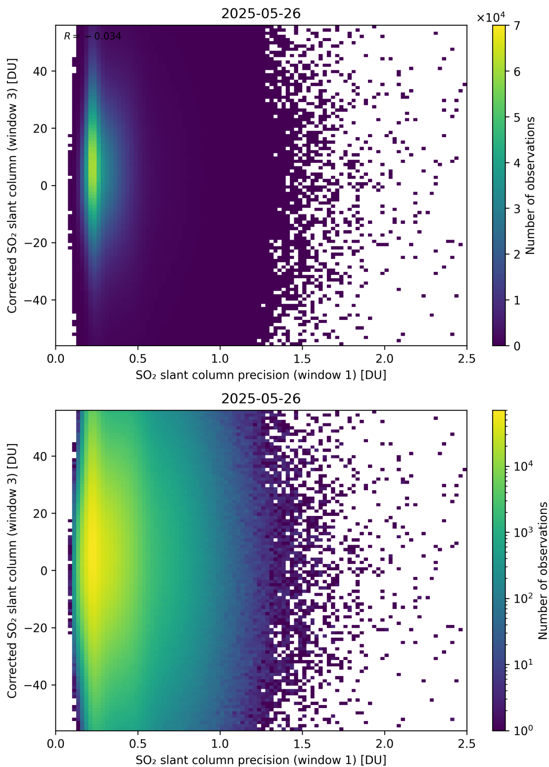
Figure 276: Scatter density plot of “SO 2 slant column precision (window 1)” against “Corrected SO 2 slant column (window 3)” for 2025-05-26 to 2025-05-27.
