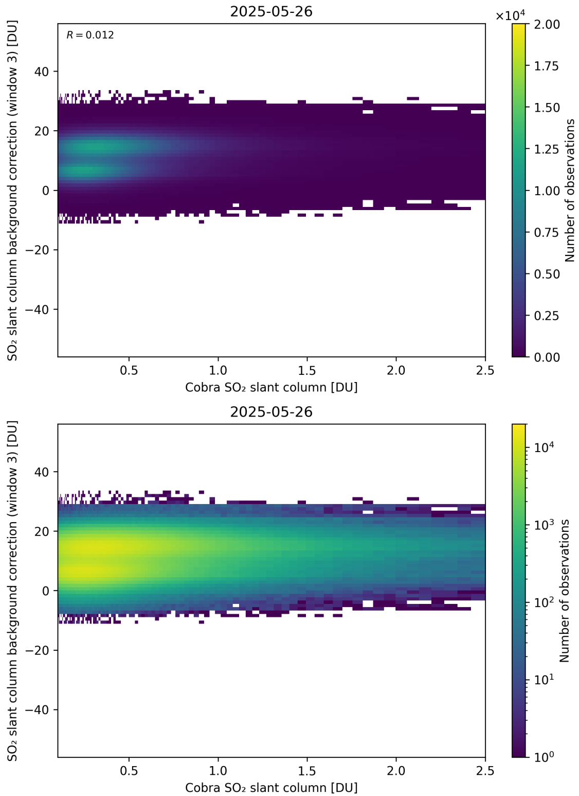
Figure 195: Scatter density plot of “Cobra SO 2 slant column” against “SO 2 slant column background correction (window 3)” for 2025-05-26 to 2025-05-27.
