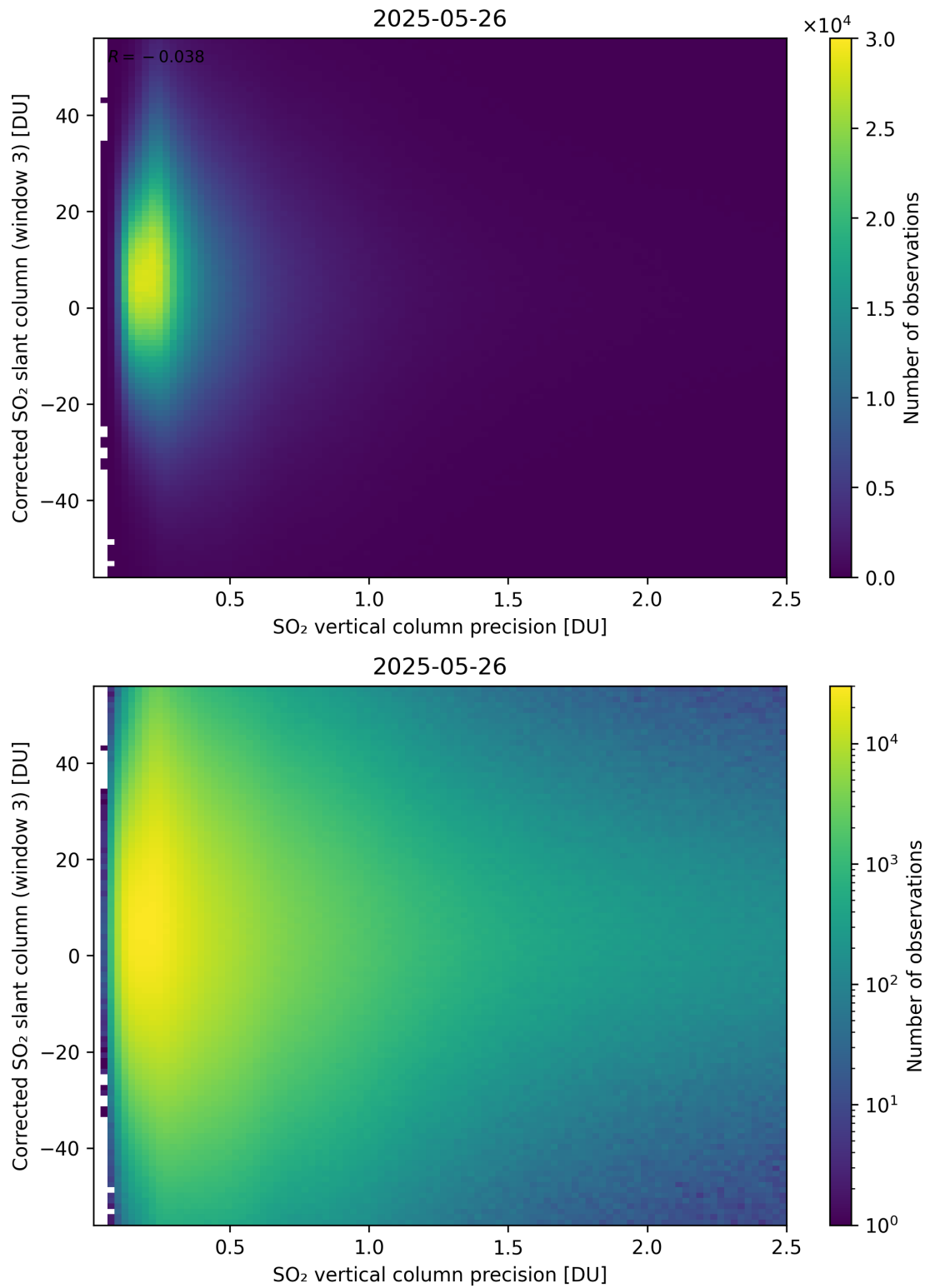
Figure 340: Scatter density plot of “SO 2 vertical column precision” against “Corrected SO 2 slant column (window 3)” for 2025-05-26 to 2025-05-27.
