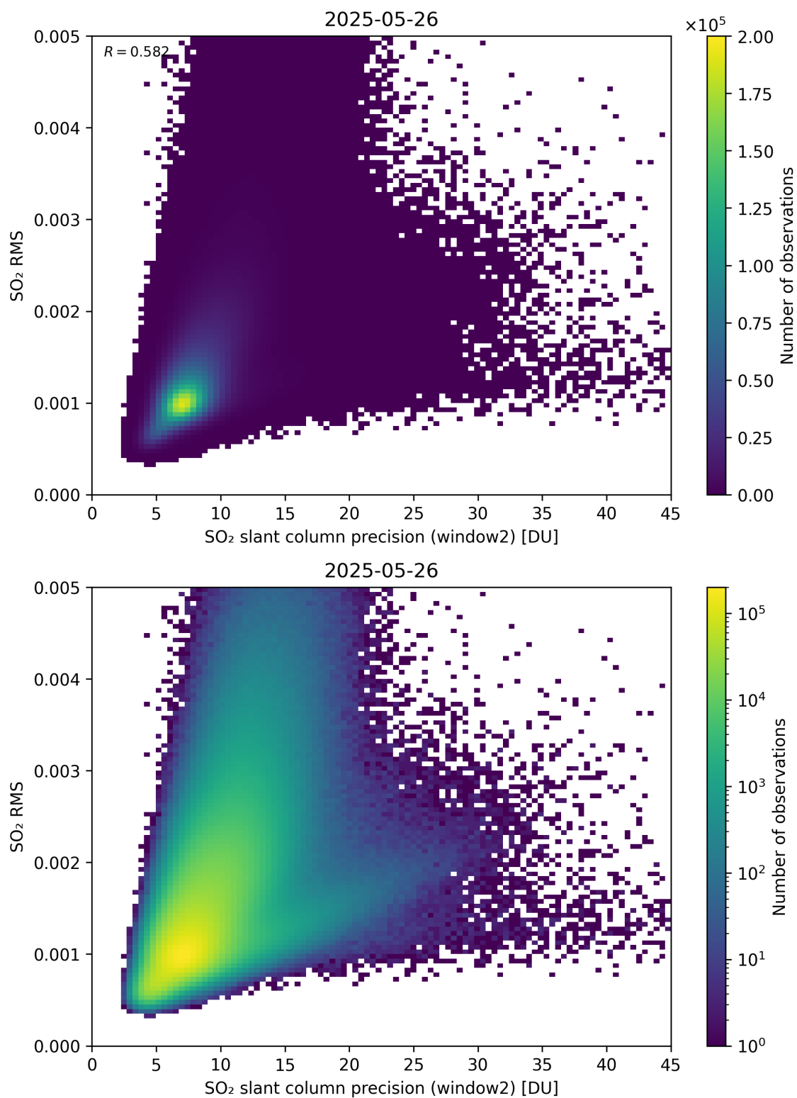
Figure 295: Scatter density plot of “SO 2 slant column precision (window2)” against “SO 2 RMS” for 2025-05-26 to 2025-05-27.
