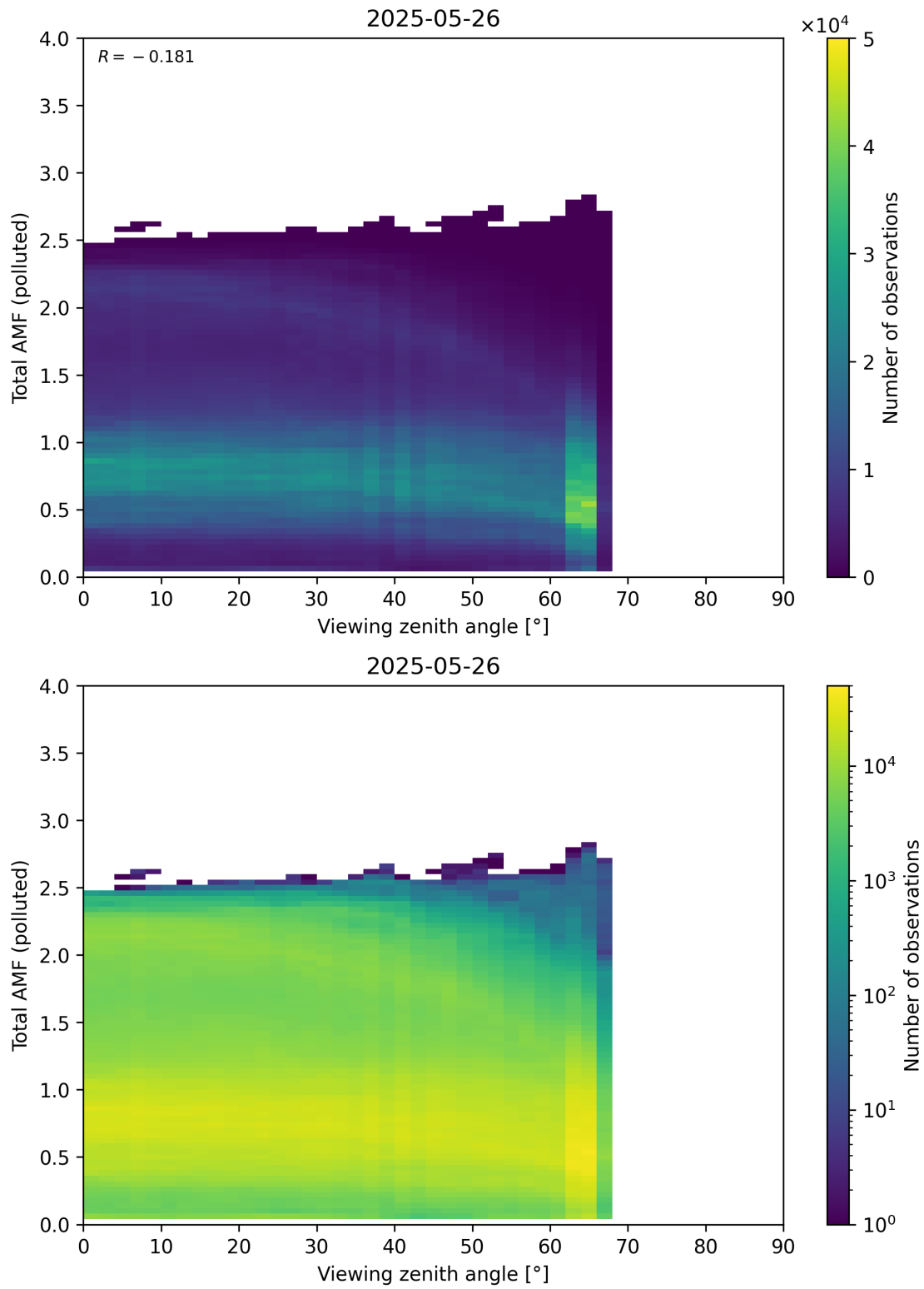
Figure 381: Scatter density plot of “Viewing zenith angle” against “Total AMF (polluted)” for 2025-05-26 to 2025-05-27.
