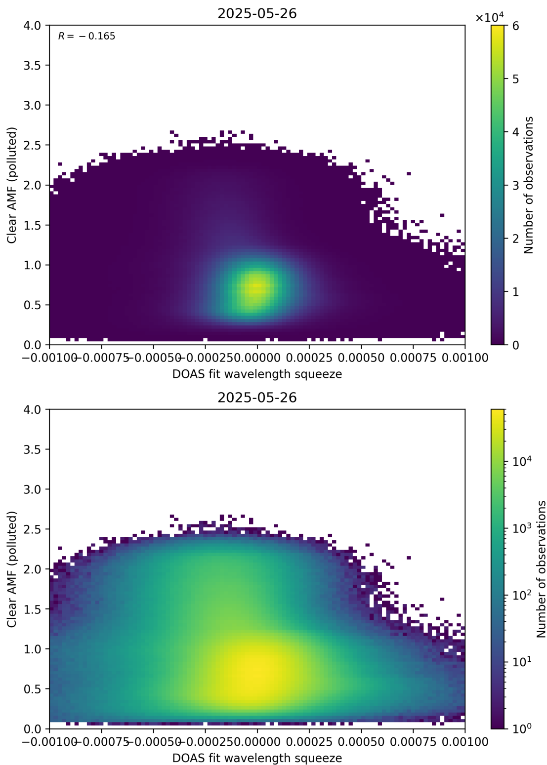
Figure 144: Scatter density plot of “DOAS fit wavelength squeeze” against “Clear AMF (polluted)” for 2025-05-26 to 2025-05-27.
