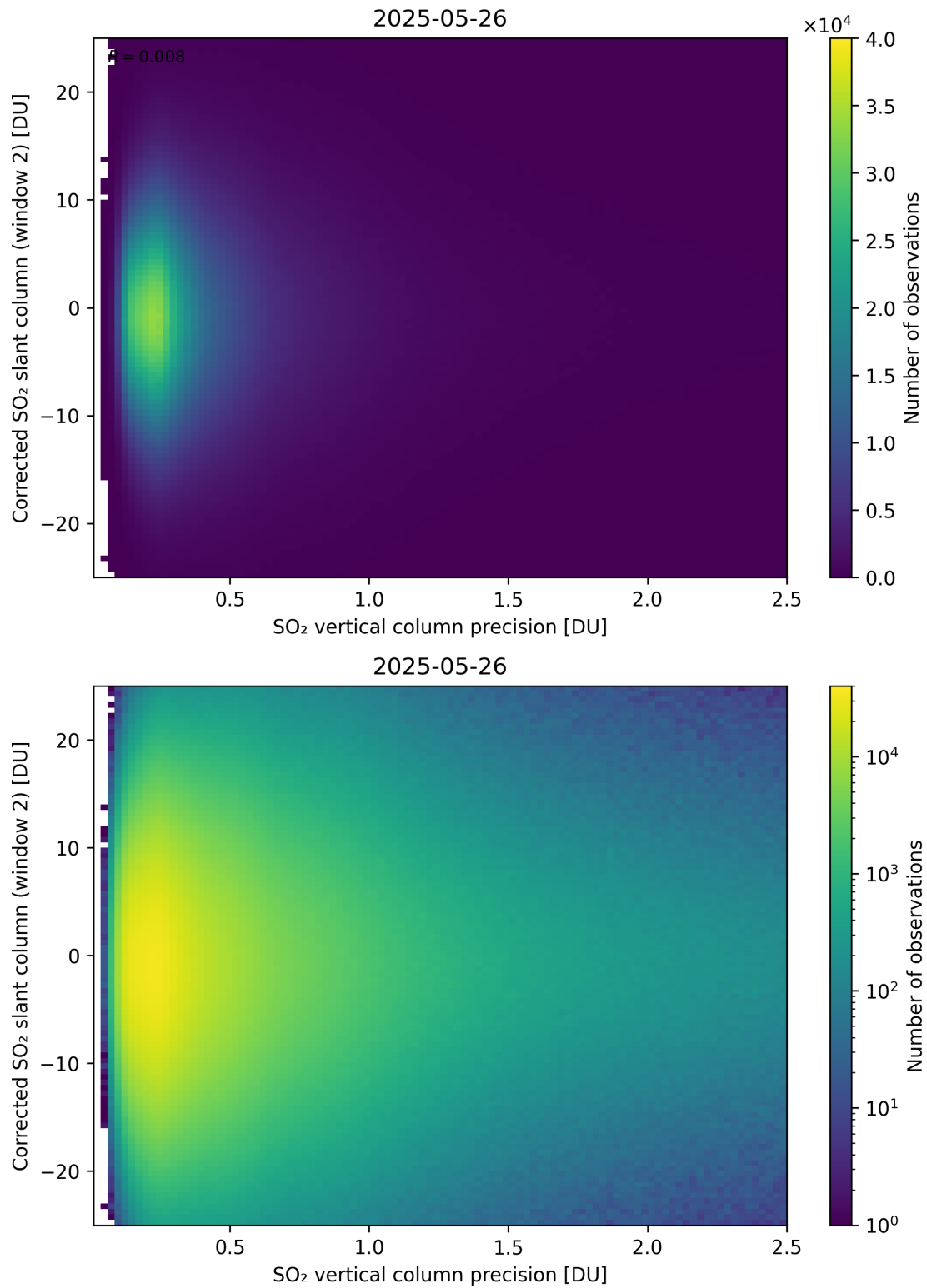
Figure 339: Scatter density plot of “SO 2 vertical column precision” against “Corrected SO 2 slant column (window 2)” for 2025-05-26 to 2025-05-27.
