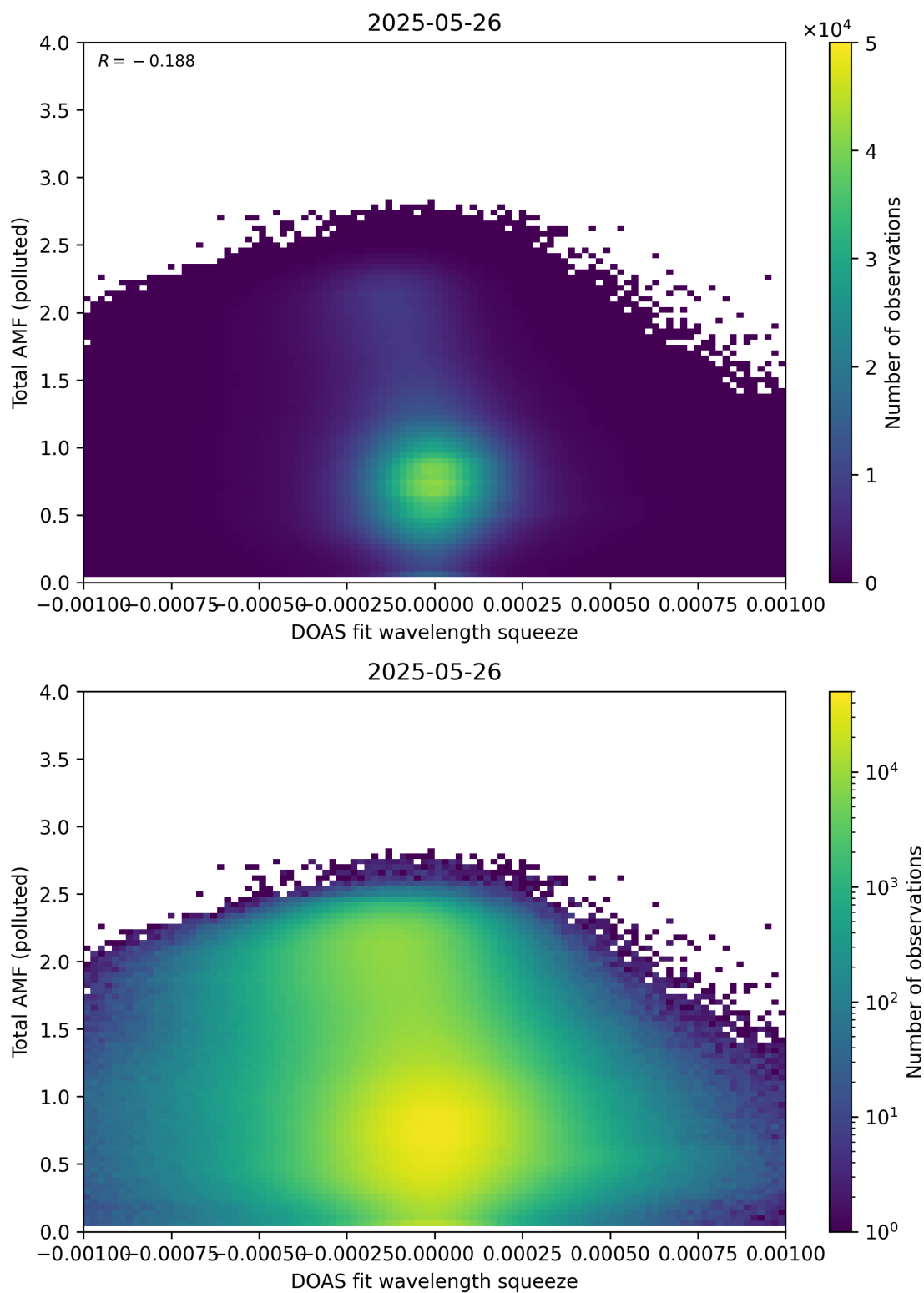
Figure 145: Scatter density plot of “DOAS fit wavelength squeeze” against “Total AMF (polluted)” for 2025-05-26 to 2025-05-27.
