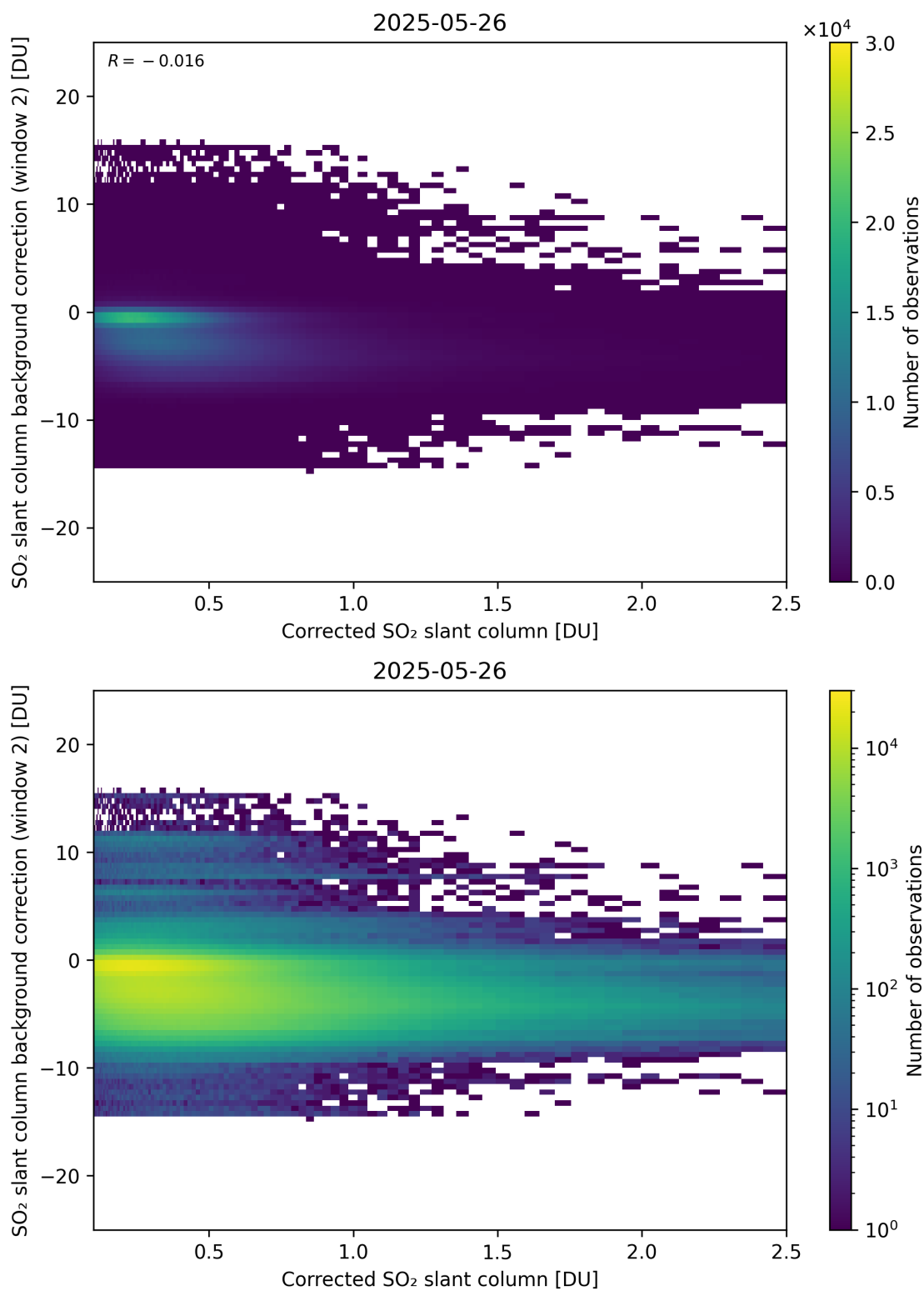
Figure 227: Scatter density plot of “Corrected SO 2 slant column” against “SO 2 slant column background correction (window 2)” for 2025-05-26 to 2025-05-27.
