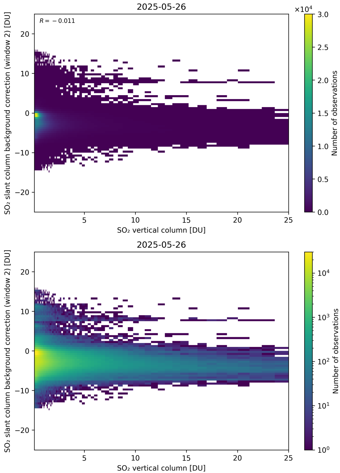
Figure 324: Scatter density plot of “SO 2 vertical column” against “SO 2 slant column background correction (window 2)” for 2025-05-26 to 2025-05-27.
