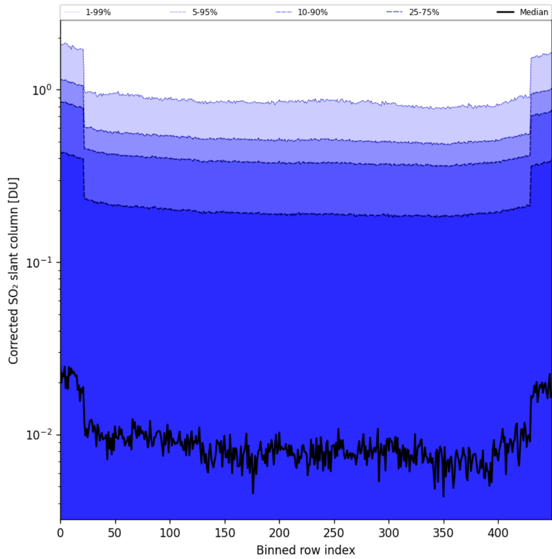
Figure 86: Along track statistics of “Corrected SO 2 slant column” for 2025-05-26 to 2025-05-27
