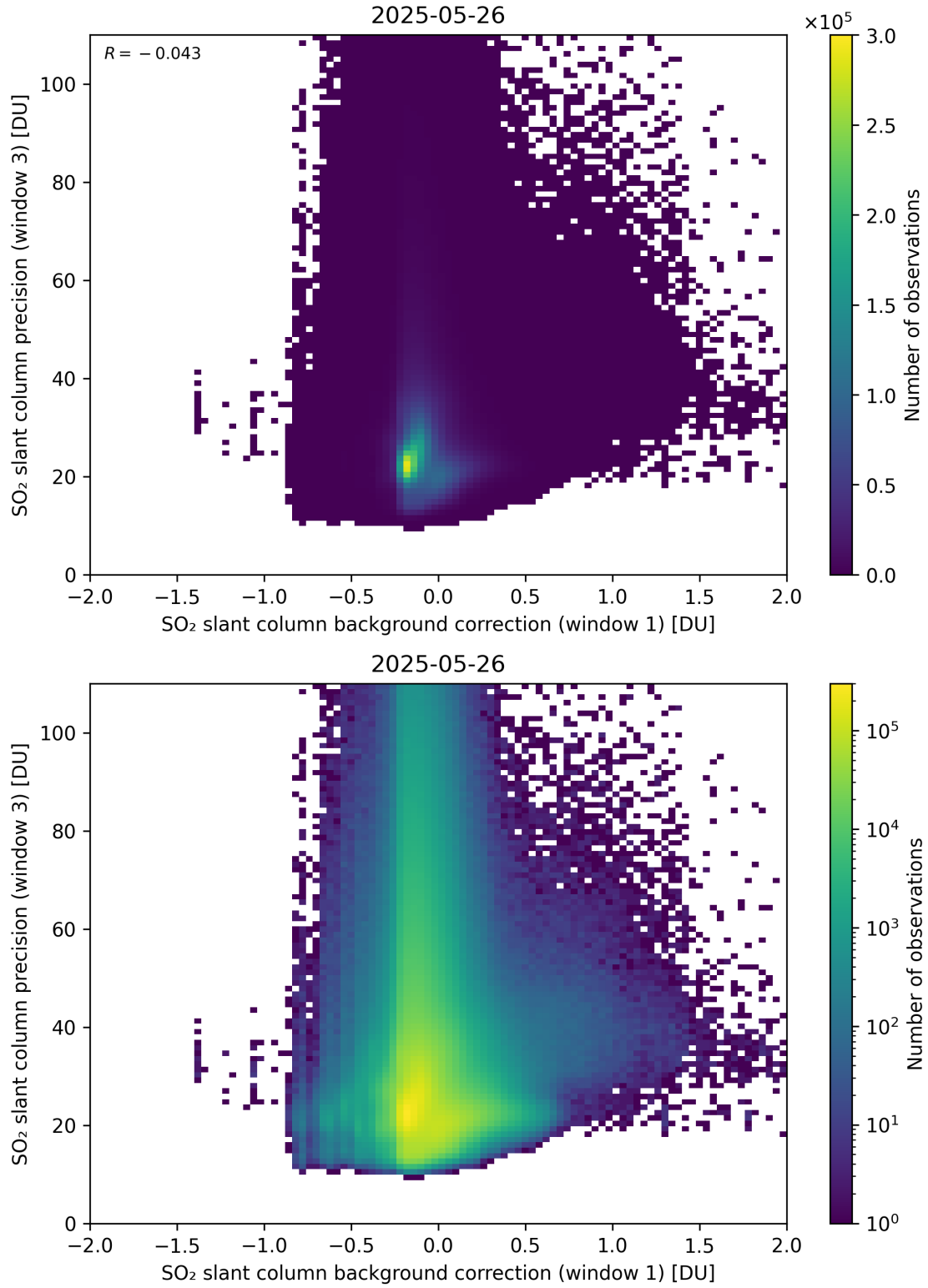
Figure 119: Scatter density plot of “SO 2 slant column background correction (window 1)” against “SO 2 slant column precision (window 3)” for 2025-05-26 to 2025-05-27.
