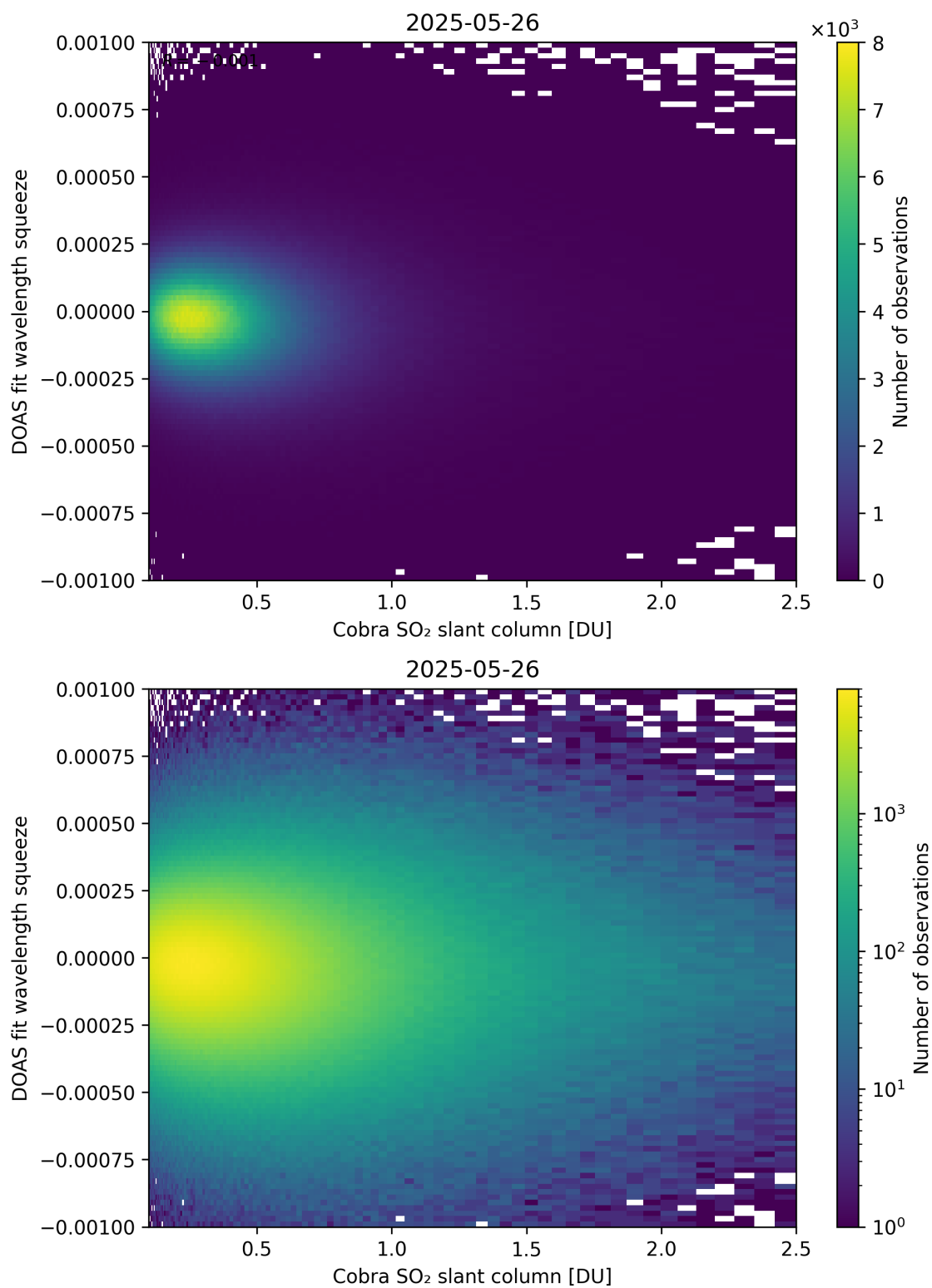
Figure 197: Scatter density plot of “Cobra SO 2 slant column” against “DOAS fit wavelength squeeze” for 2025-05-26 to 2025-05-27.
