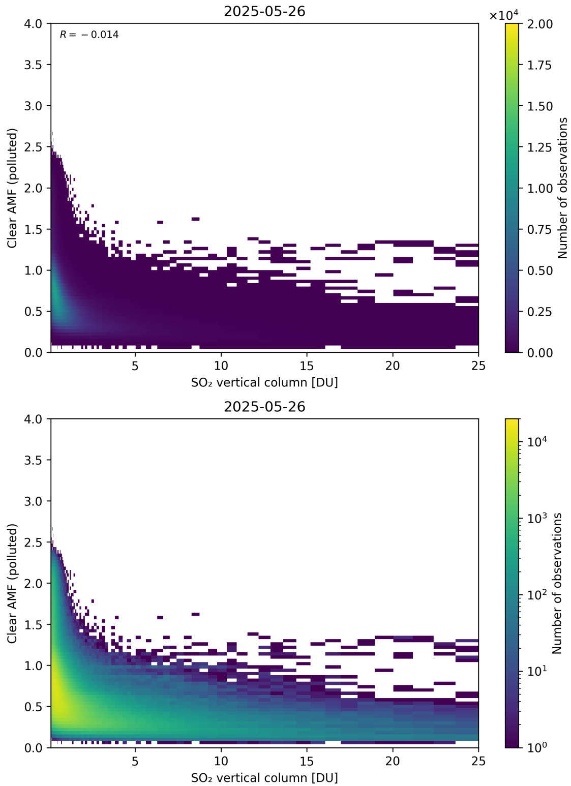
Figure 348: Scatter density plot of “SO 2 vertical column” against “Clear AMF (polluted)” for 2025-05-26 to 2025-05-27.
