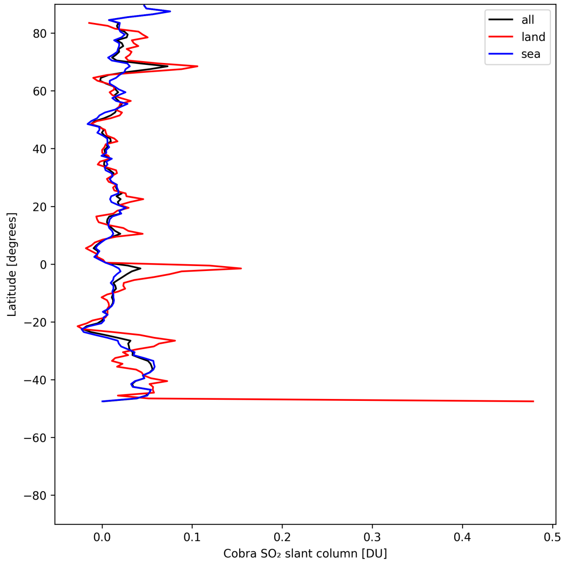
Figure 35: Zonal average of “Cobra SO 2 slant column” for 2025-05-26 to 2025-05-27.
