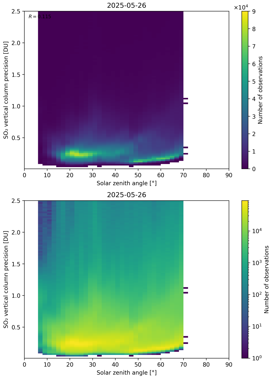
Figure 192: Scatter density plot of “Solar zenith angle” against “SO 2 vertical column precision” for 2025-05-26 to 2025-05-27.
