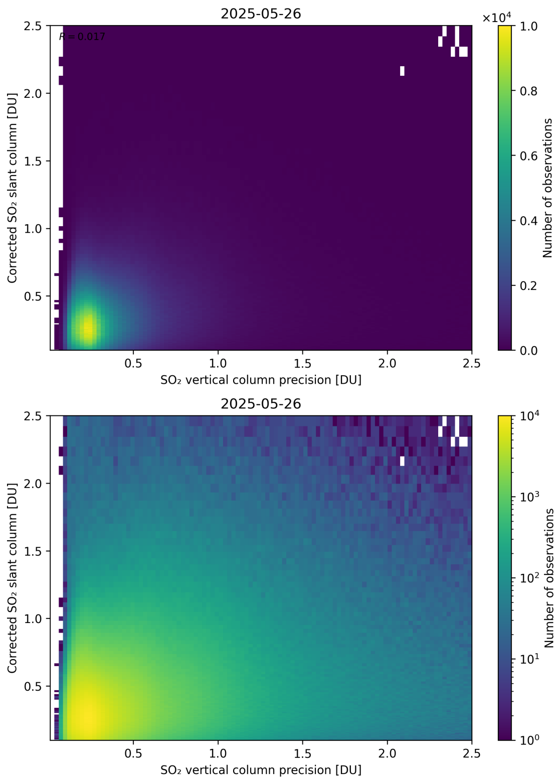
Figure 338: Scatter density plot of “SO 2 vertical column precision” against “Corrected SO 2 slant column” for 2025-05-26 to 2025-05-27.
