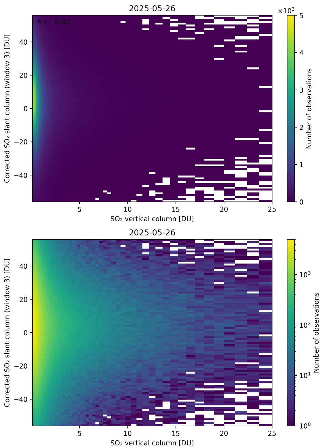
Figure 353: Scatter density plot of “SO 2 vertical column” against “Corrected SO 2 slant column (window 3)” for 2025-05-26 to 2025-05-27.
