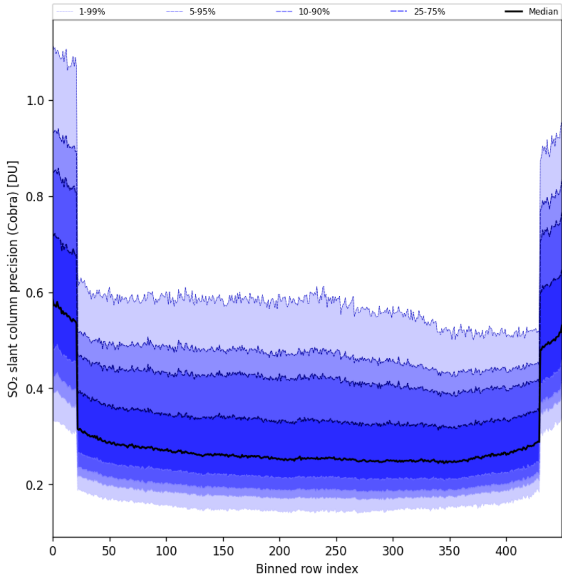
Figure 88: Along track statistics of “SO 2 slant column precision (Cobra)” for 2025-05-26 to 2025-05-27
