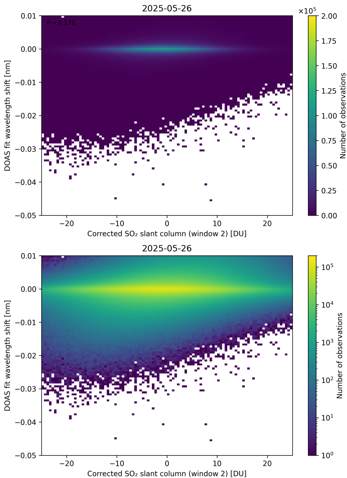
Figure 246: Scatter density plot of “Corrected SO 2 slant column (window 2)” against “DOAS fit wavelength shift” for 2025-05-26 to 2025-05-27.
