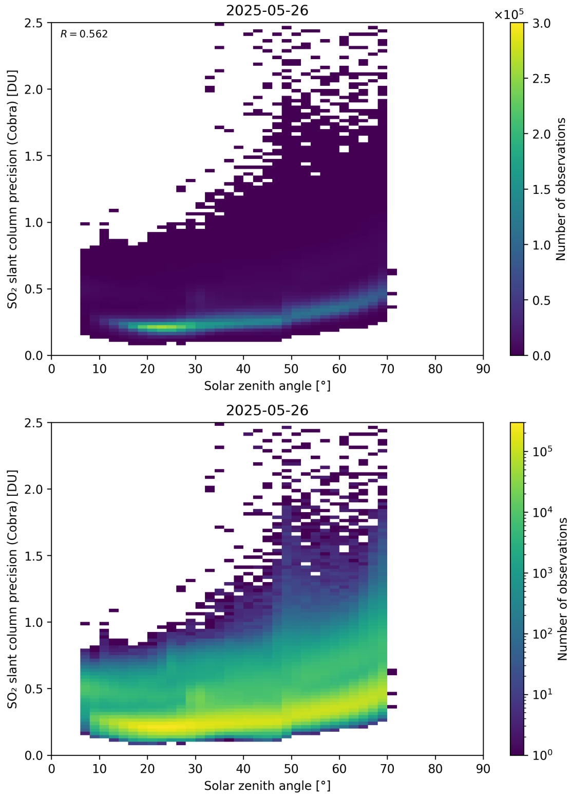
Figure 180: Scatter density plot of “Solar zenith angle” against “SO 2 slant column precision (Cobra)” for 2025-05-26 to 2025-05-27.
