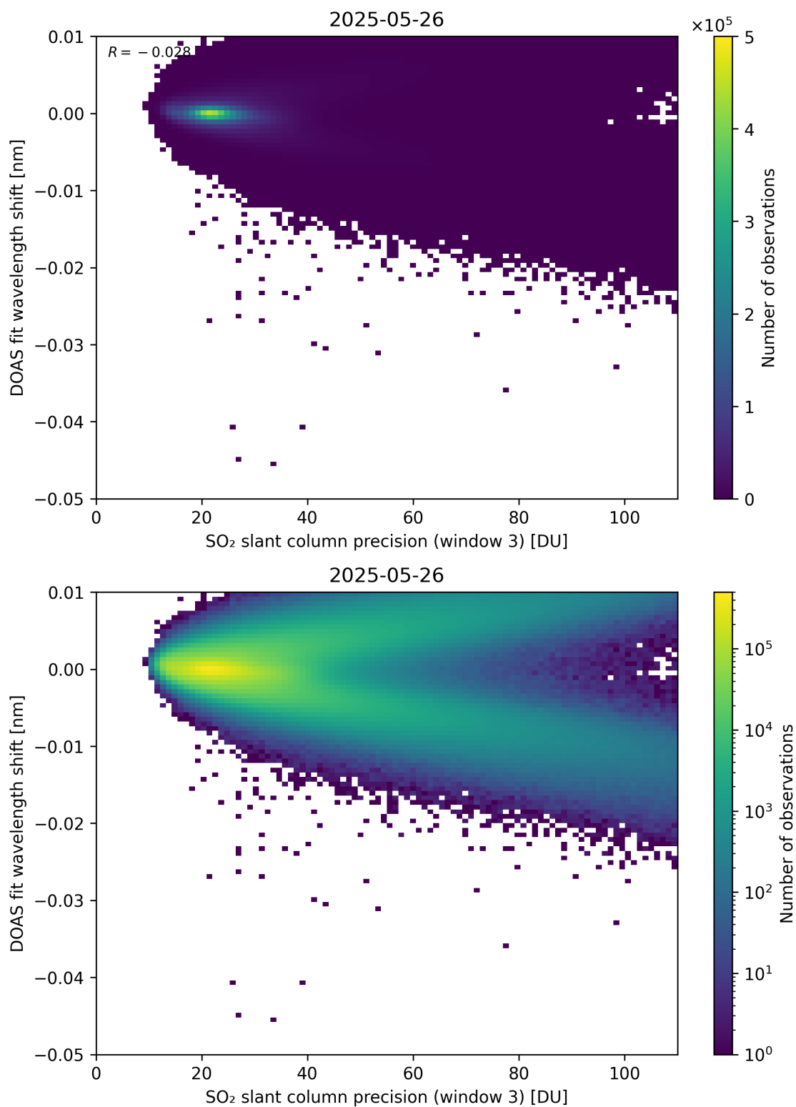
Figure 308: Scatter density plot of “SO 2 slant column precision (window 3)” against “DOAS fit wavelength shift” for 2025-05-26 to 2025-05-27.
