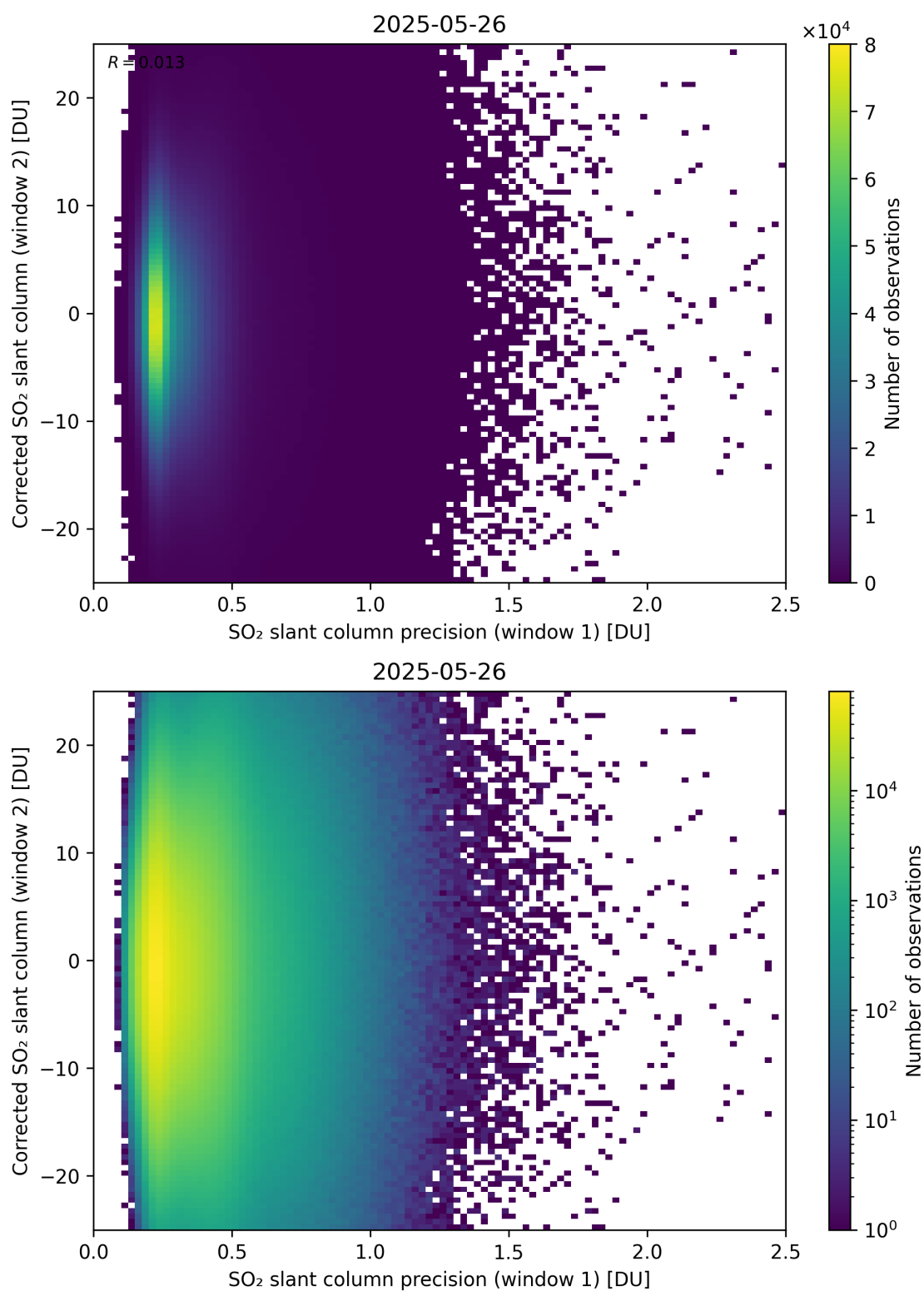
Figure 275: Scatter density plot of “SO 2 slant column precision (window 1)” against “Corrected SO 2 slant column (window 2)” for 2025-05-26 to 2025-05-27.
