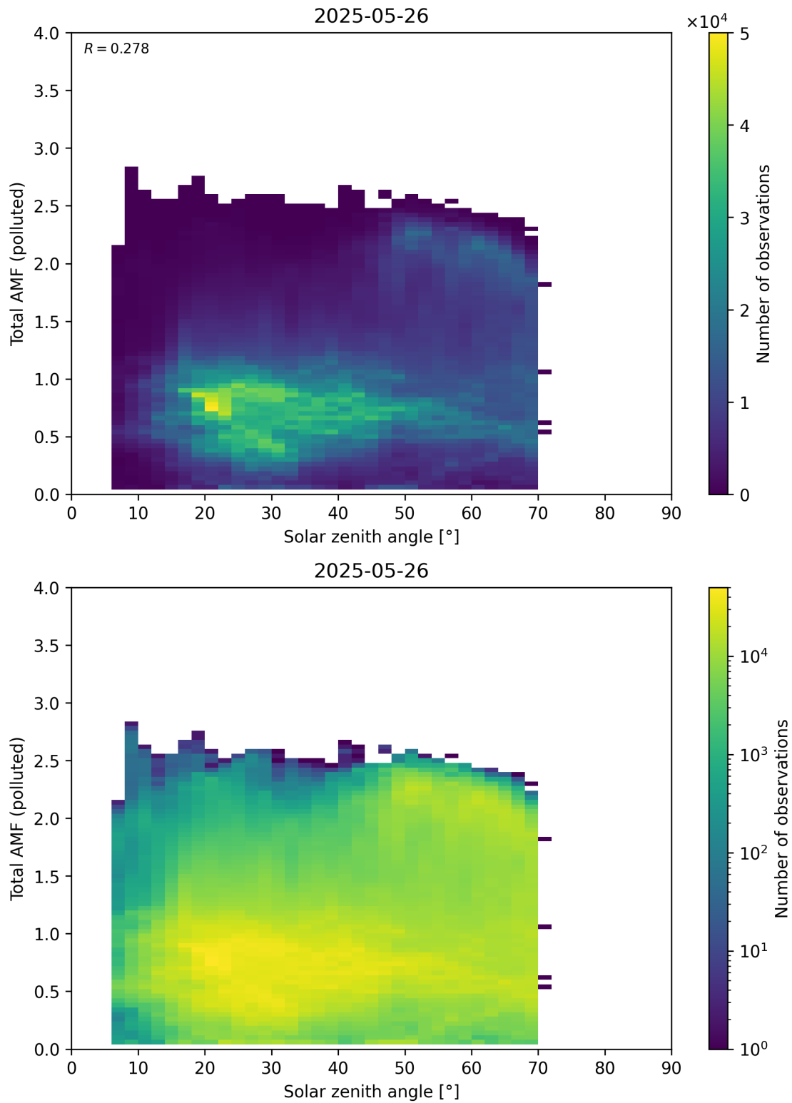
Figure 189: Scatter density plot of “Solar zenith angle” against “Total AMF (polluted)” for 2025-05-26 to 2025-05-27.
