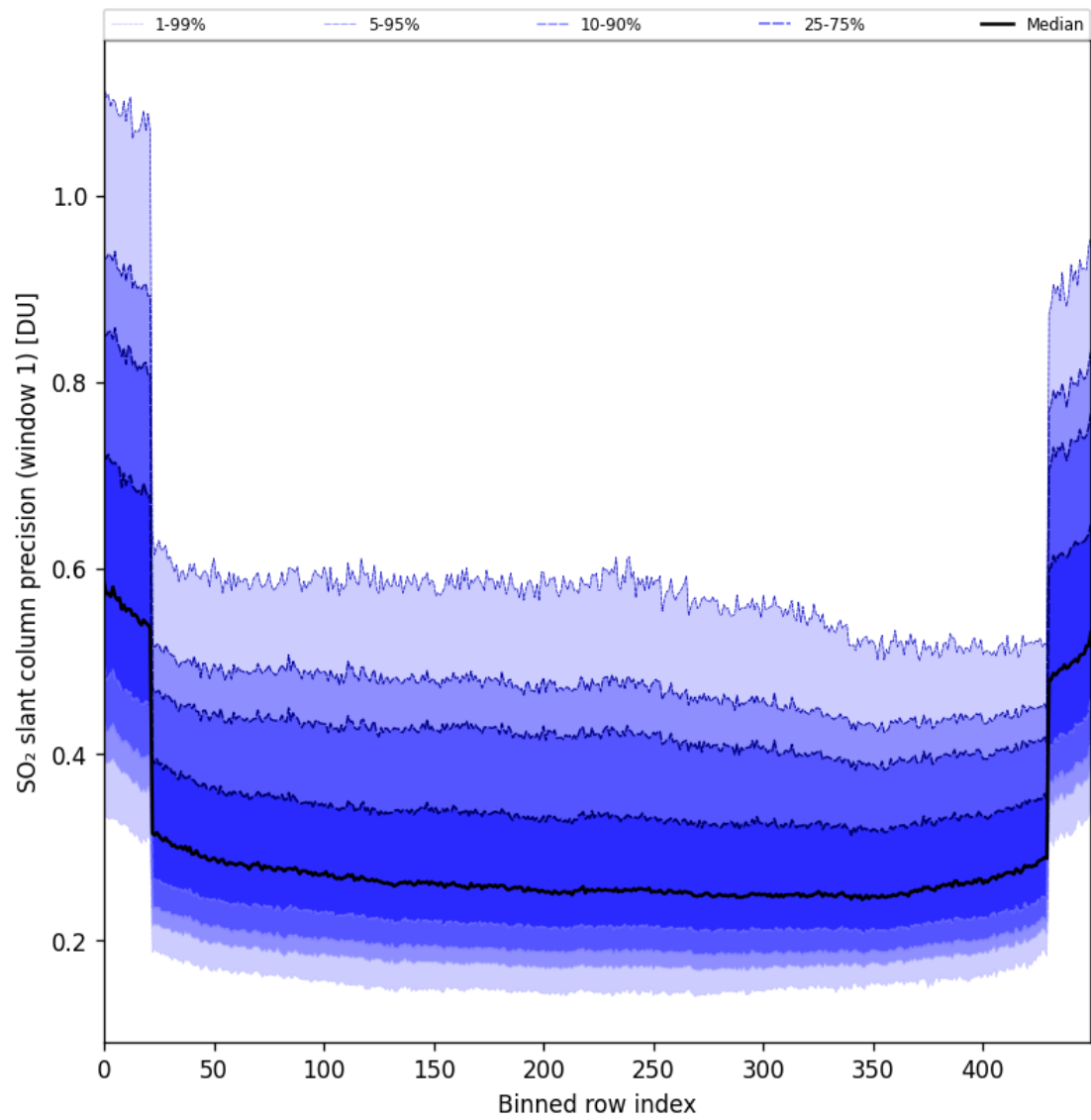
Figure 90: Along track statistics of “SO 2 slant column precision (window 1)” for 2025-05-26 to 2025-05-27
