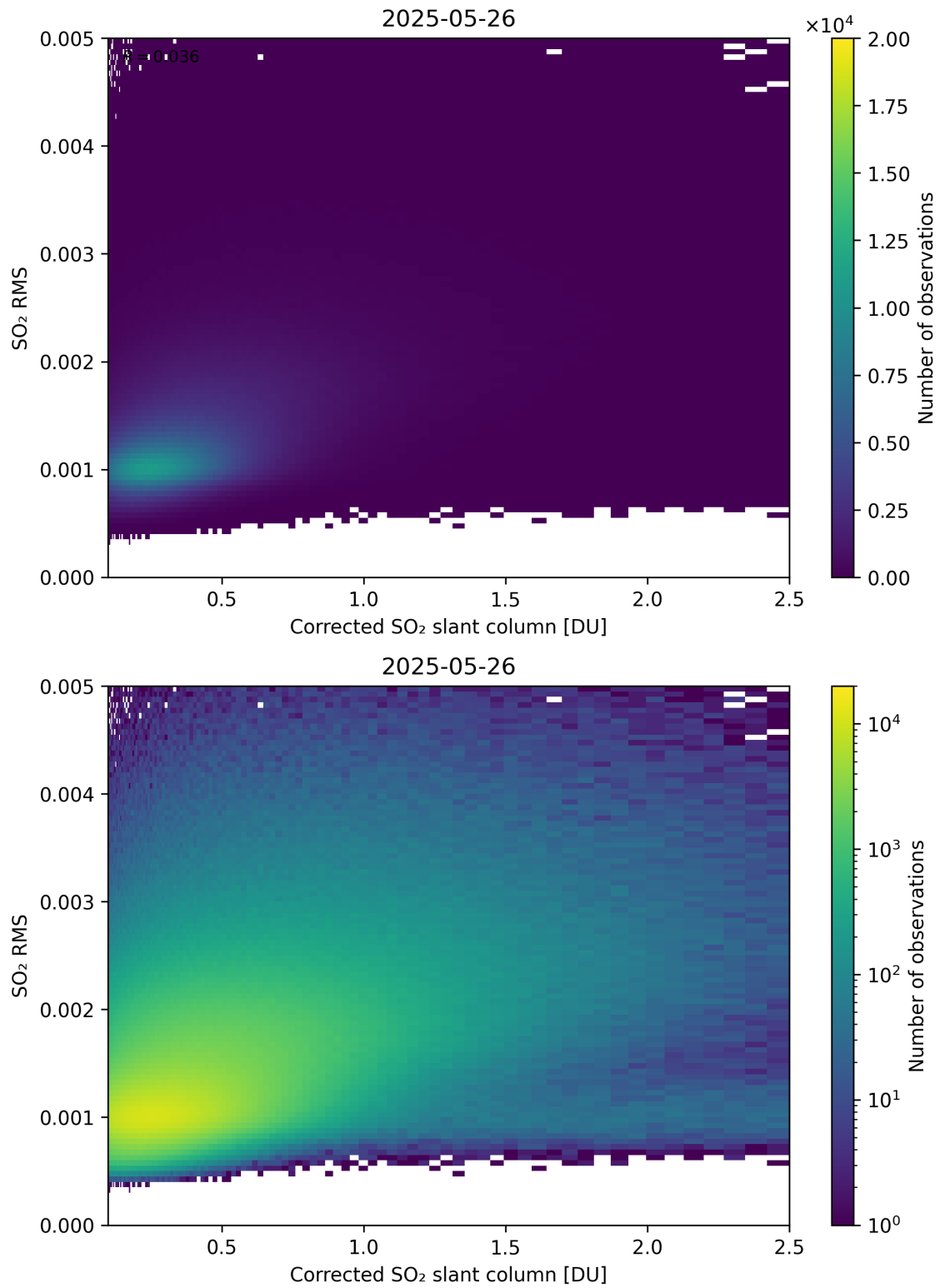
Figure 231: Scatter density plot of “Corrected SO 2 slant column” against “SO 2 RMS” for 2025-05-26 to 2025-05-27.
