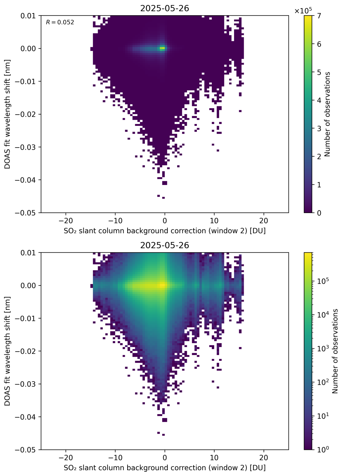
Figure 123: Scatter density plot of “SO 2 slant column background correction (window 2)” against “DOAS fit wavelength shift” for 2025-05-26 to 2025-05-27.
