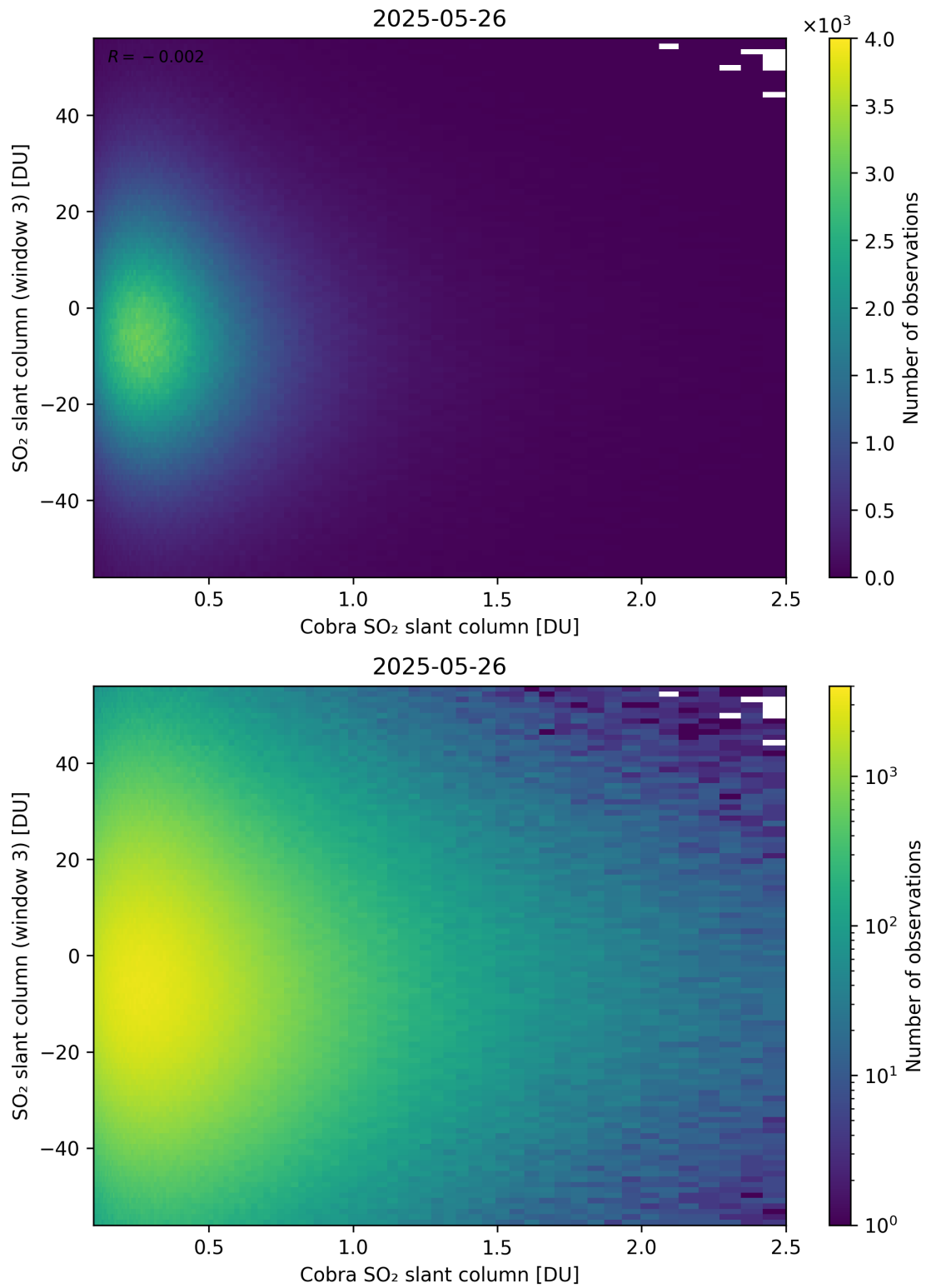
Figure 222: Scatter density plot of “Cobra SO 2 slant column” against “SO 2 slant column (window 3)” for 2025-05-26 to 2025-05-27.
