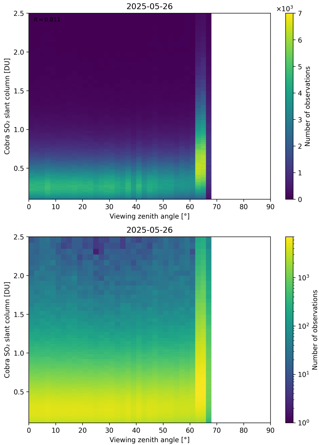
Figure 371: Scatter density plot of “Viewing zenith angle” against “Cobra SO 2 slant column” for 2025-05-26 to 2025-05-27.
