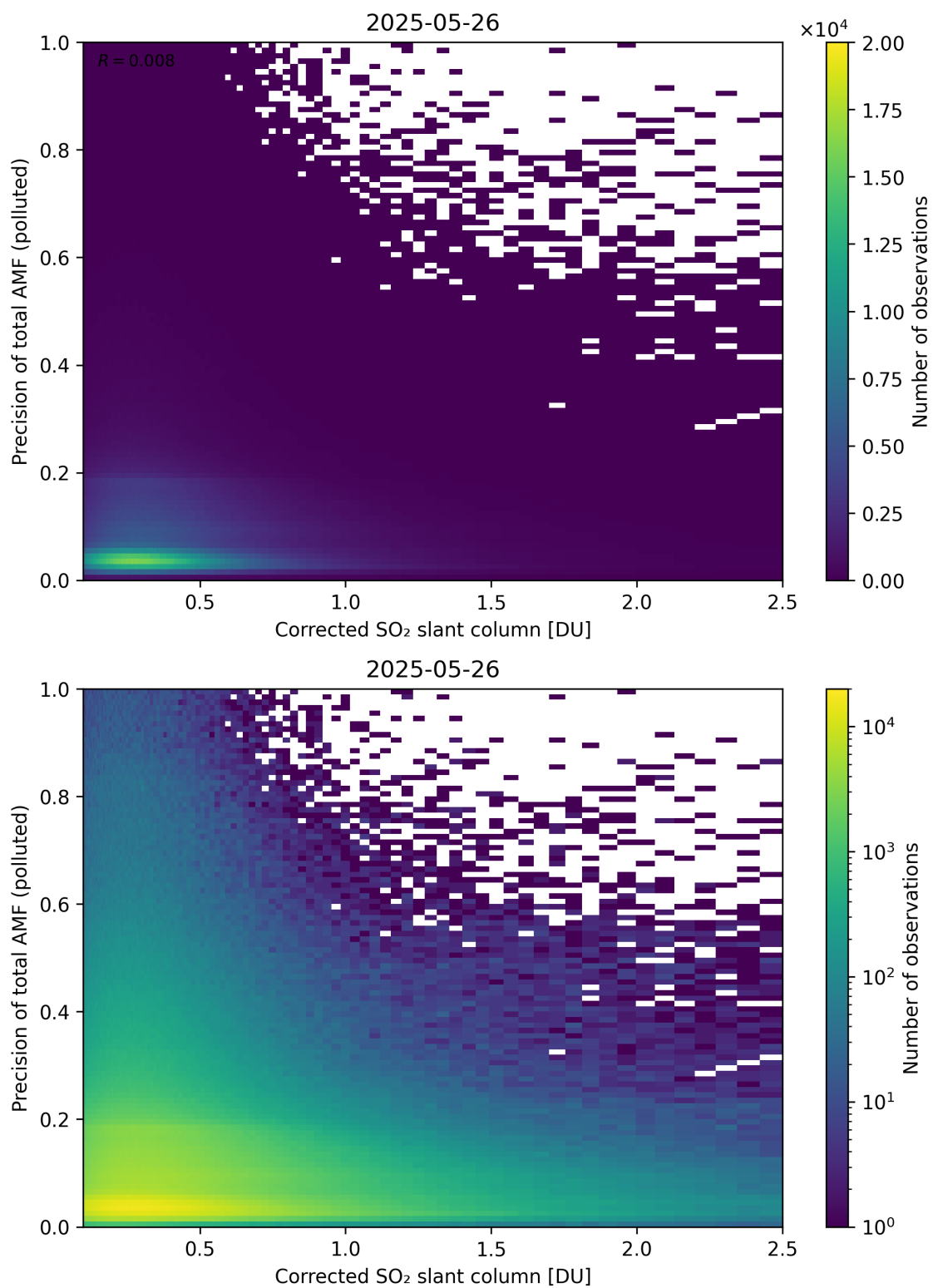
Figure 243: Scatter density plot of “Corrected SO 2 slant column” against “Precision of total AMF (polluted)” for 2025-05-26 to 2025-05-27.
