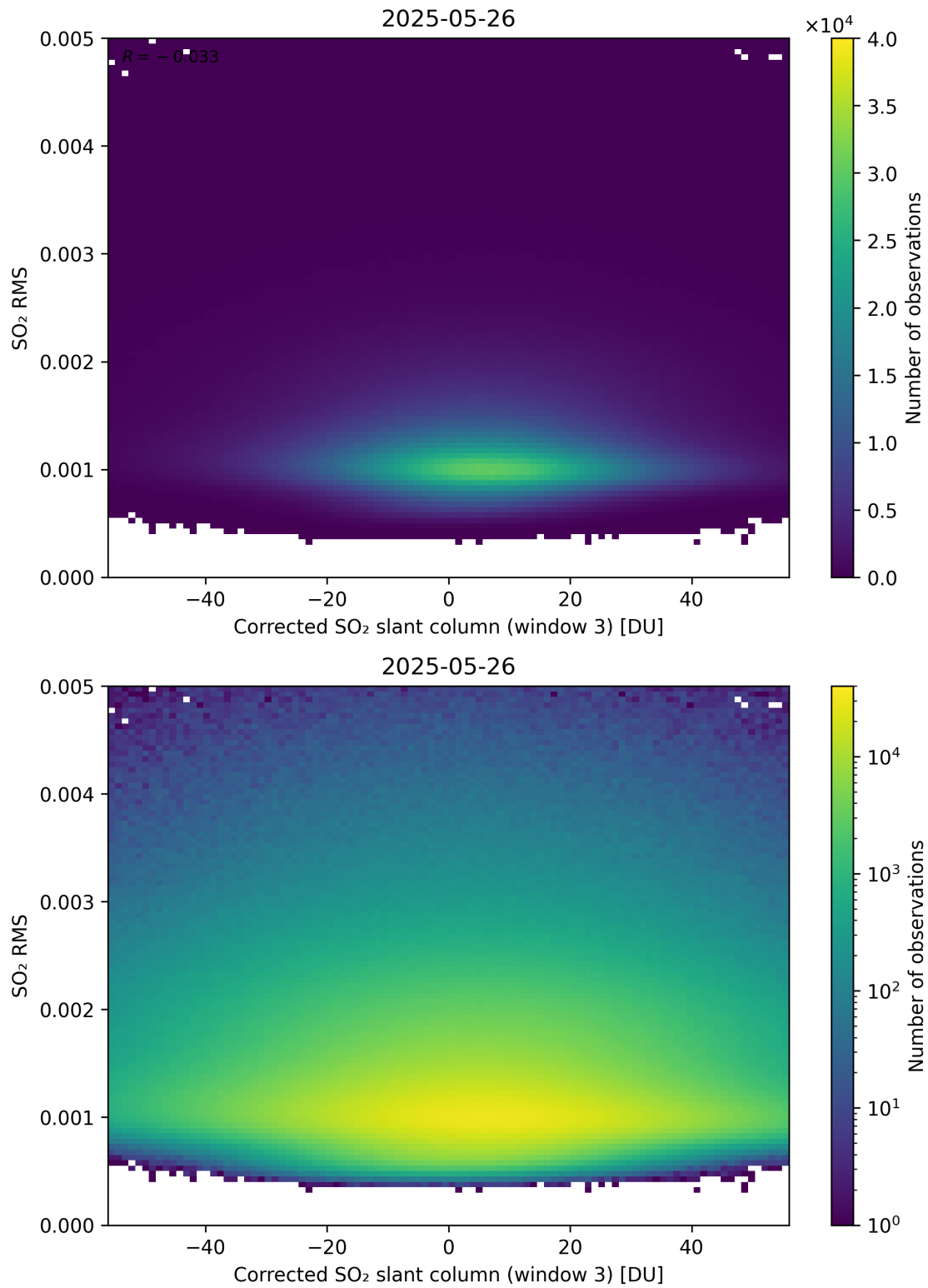
Figure 258: Scatter density plot of “Corrected SO 2 slant column (window 3)” against “SO 2 RMS” for 2025-05-26 to 2025-05-27.
