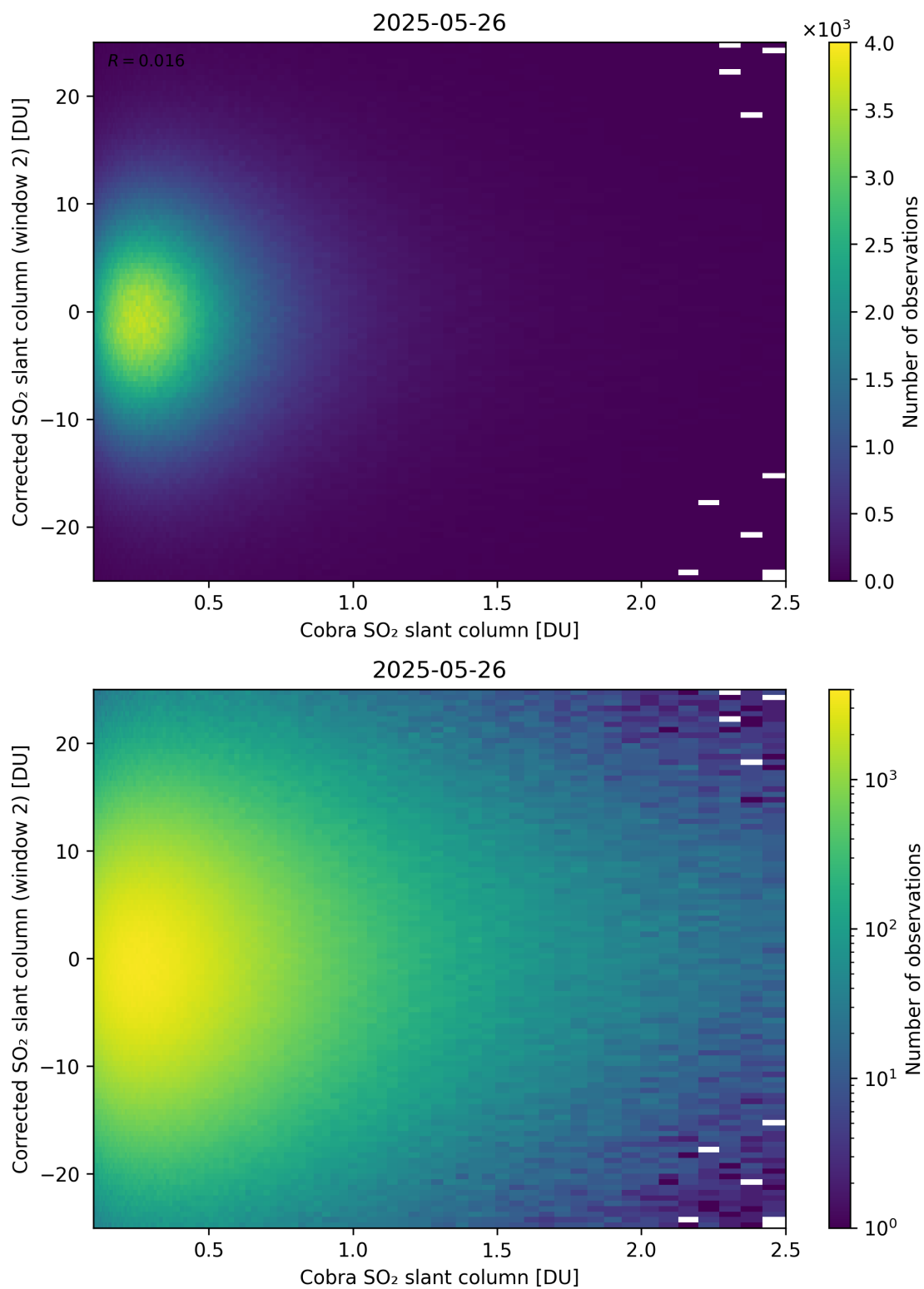
Figure 217: Scatter density plot of “Cobra SO 2 slant column” against “Corrected SO 2 slant column (window 2)” for 2025-05-26 to 2025-05-27.
