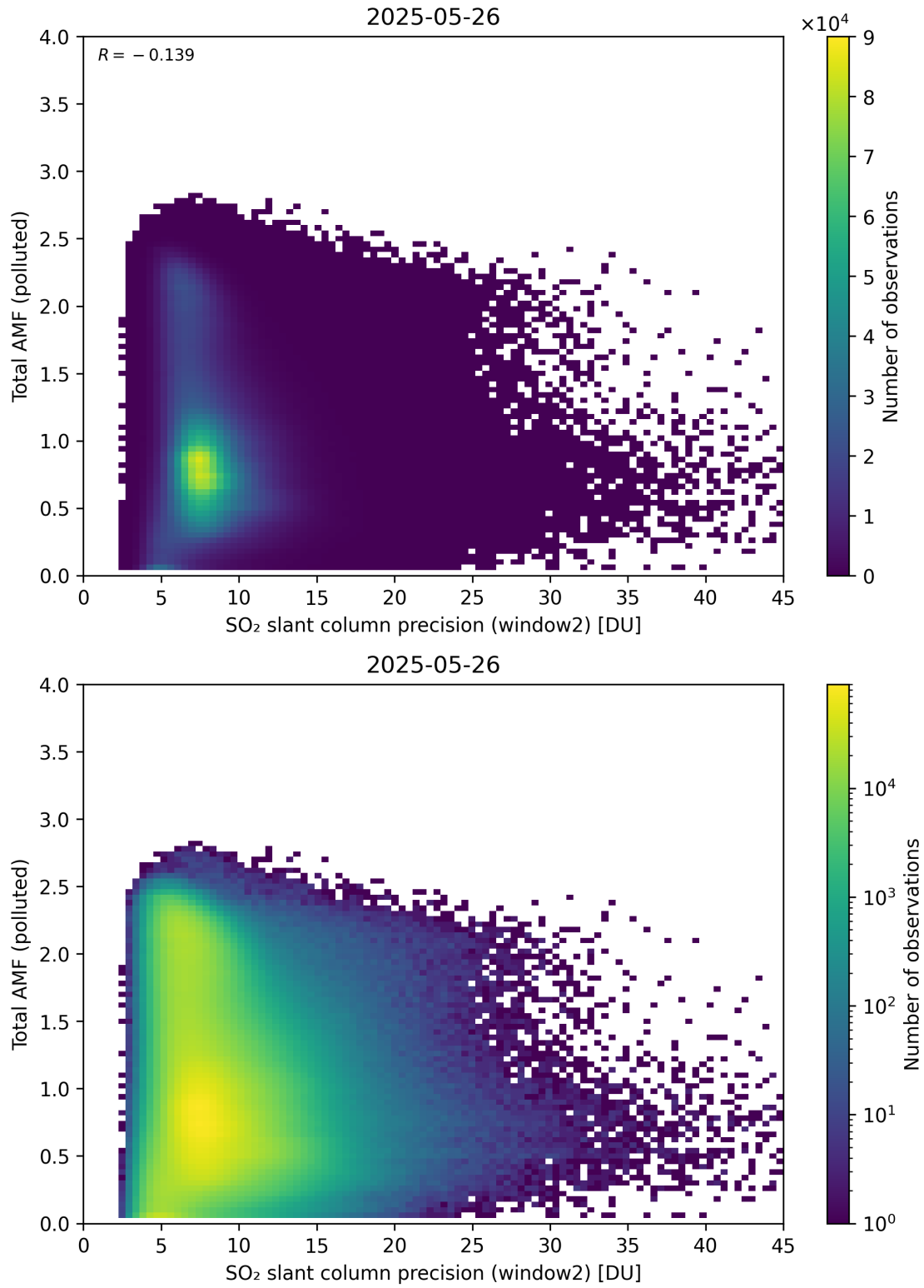
Figure 301: Scatter density plot of “SO 2 slant column precision (window2)” against “Total AMF (polluted)” for 2025-05-26 to 2025-05-27.
