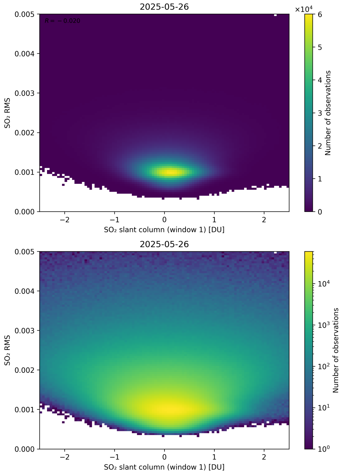
Figure 267: Scatter density plot of “SO 2 slant column (window 1)” against “SO 2 RMS” for 2025-05-26 to 2025-05-27.
