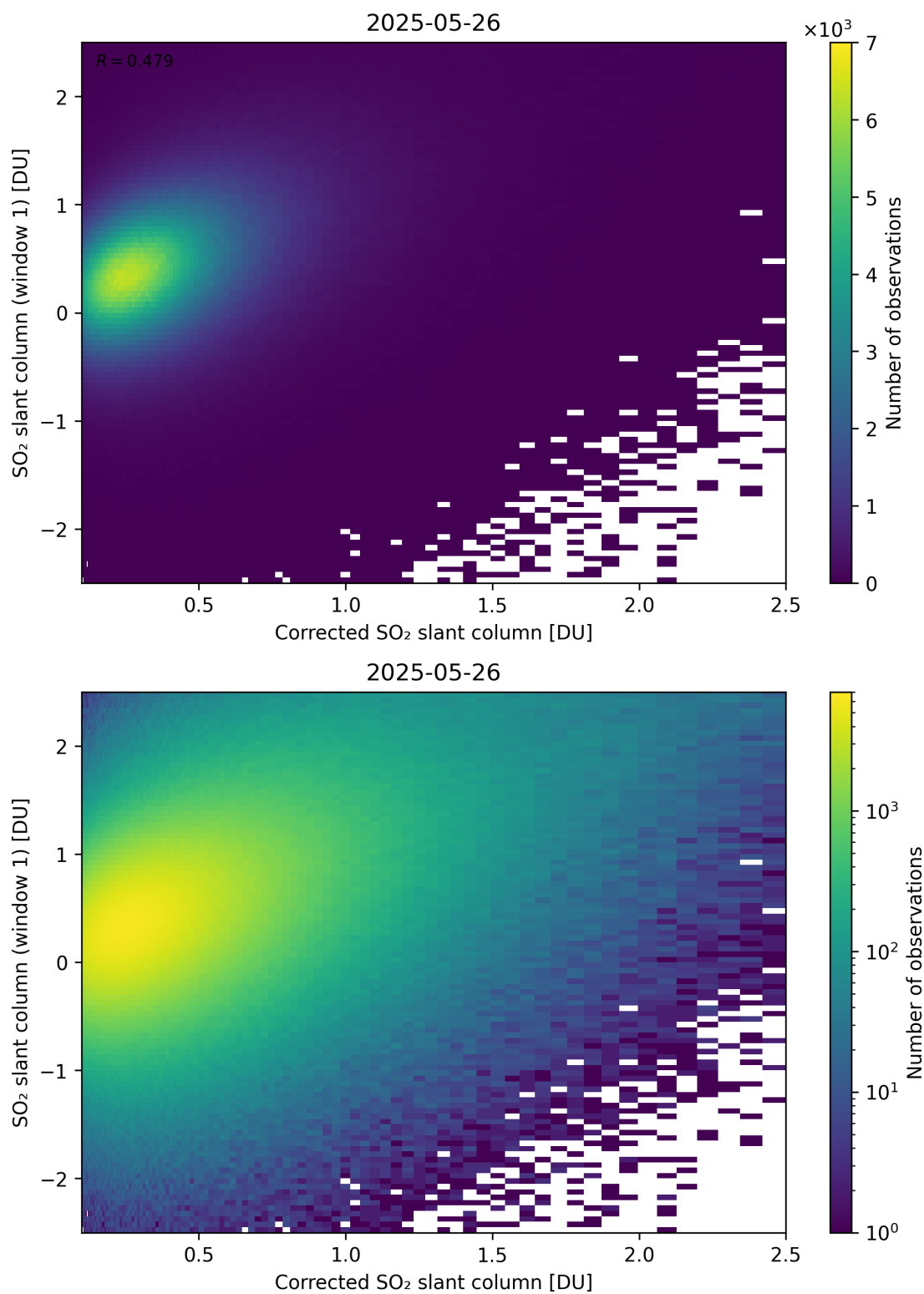
Figure 237: Scatter density plot of “Corrected SO 2 slant column” against “SO 2 slant column (window 1)” for 2025-05-26 to 2025-05-27.
