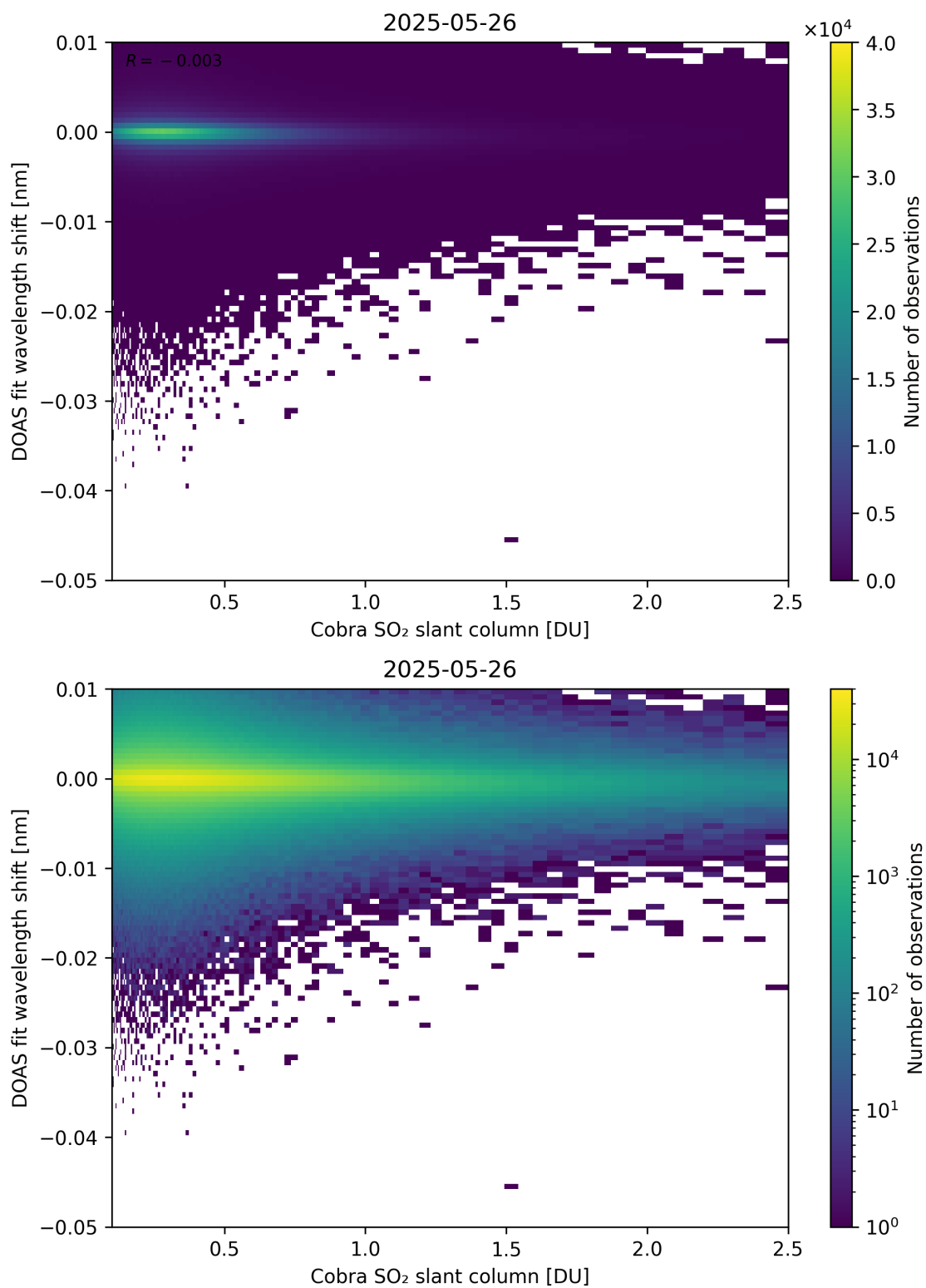
Figure 196: Scatter density plot of “Cobra SO 2 slant column” against “DOAS fit wavelength shift” for 2025-05-26 to 2025-05-27.
