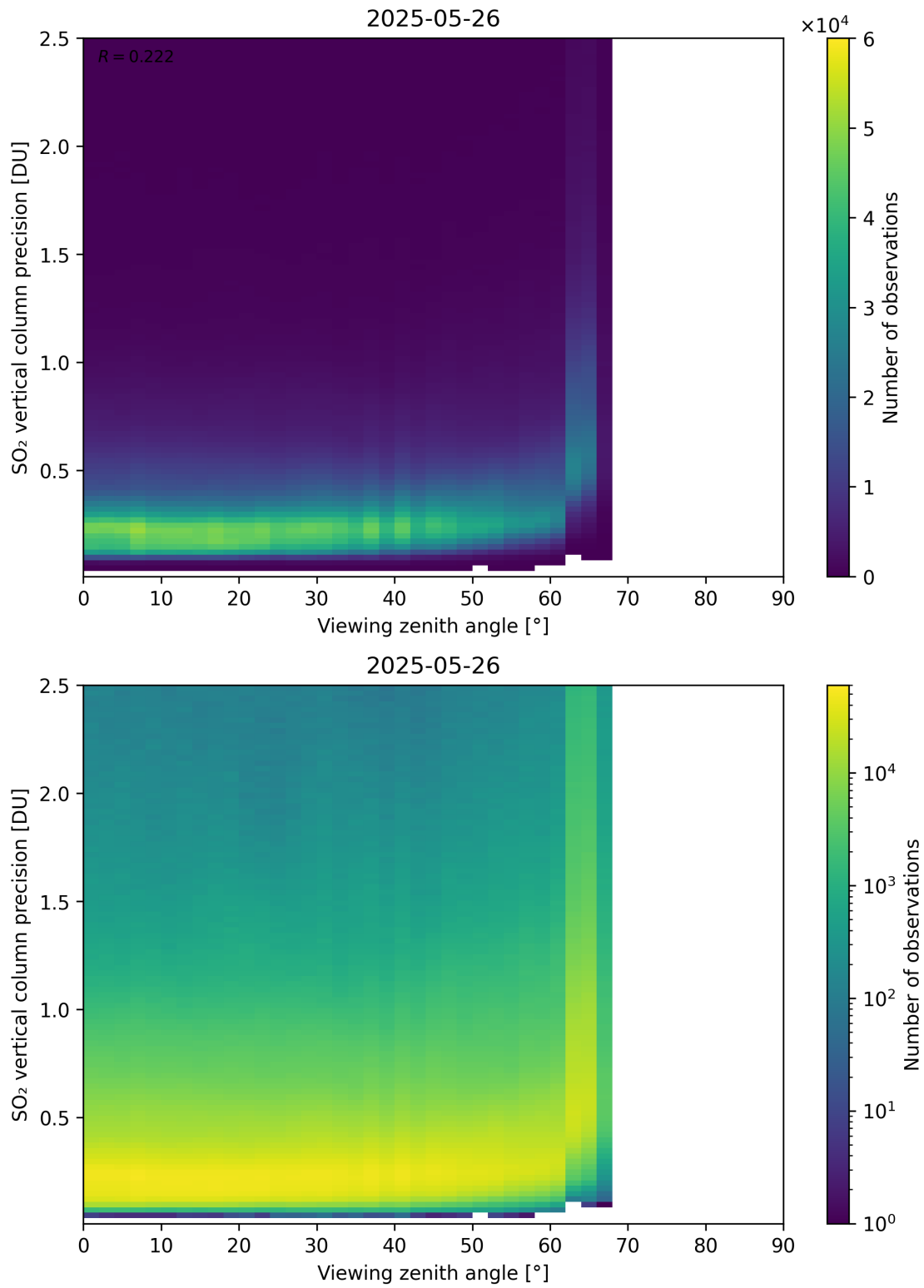
Figure 384: Scatter density plot of “Viewing zenith angle” against “SO 2 vertical column precision” for 2025-05-26 to 2025-05-27.
