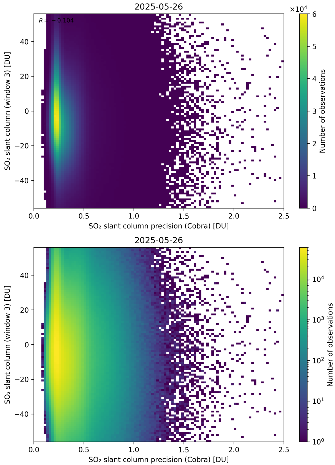
Figure 211: Scatter density plot of “SO 2 slant column precision (Cobra)” against “SO 2 slant column (window 3)” for 2025-05-26 to 2025-05-27.
