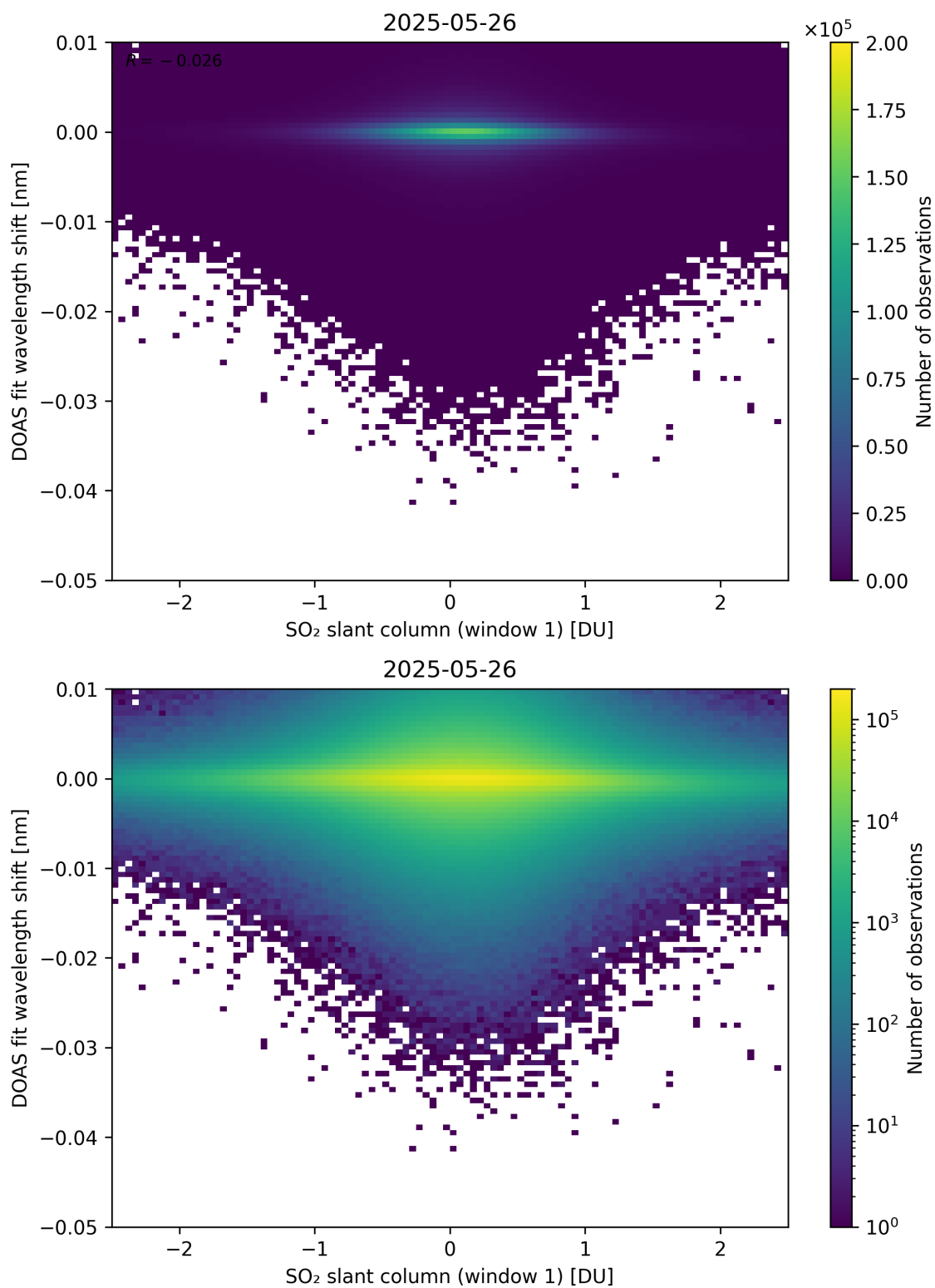
Figure 265: Scatter density plot of “SO 2 slant column (window 1)” against “DOAS fit wavelength shift” for 2025-05-26 to 2025-05-27.
