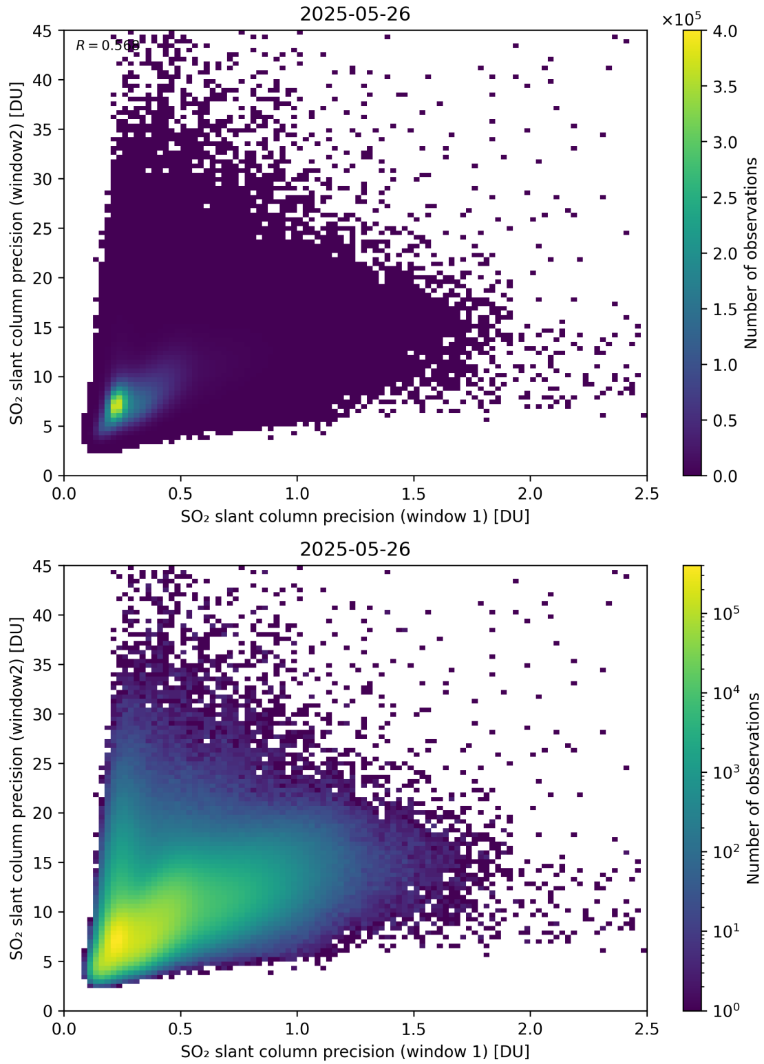
Figure 277: Scatter density plot of “SO 2 slant column precision (window 1)” against “SO 2 slant column precision (window 2)” for 2025-05-26 to 2025-05-27.
