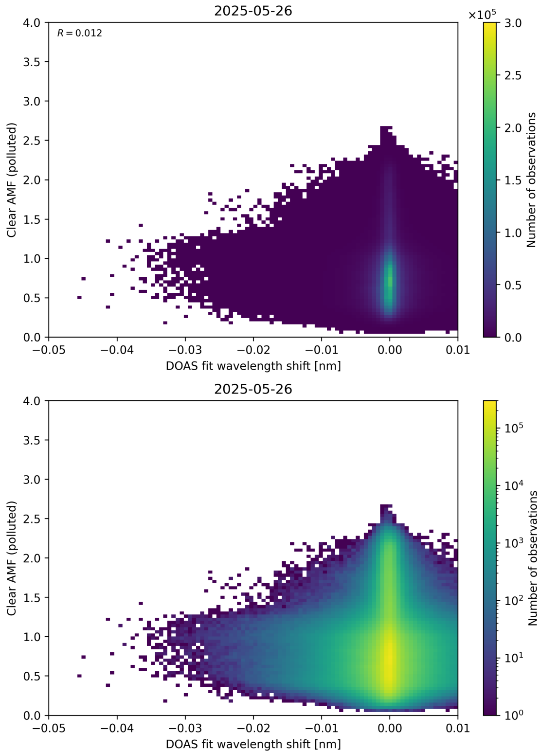
Figure 140: Scatter density plot of “DOAS fit wavelength shift” against “Clear AMF (polluted)” for 2025-05-26 to 2025-05-27.
