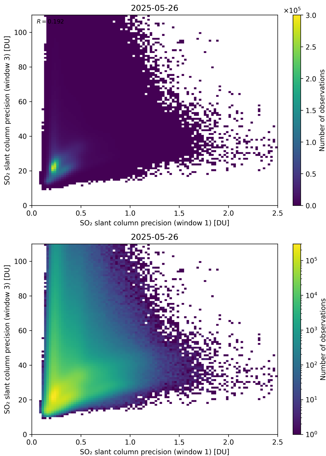
Figure 279: Scatter density plot of “SO 2 slant column precision (window 1)” against “SO 2 slant column precision (window 3)” for 2025-05-26 to 2025-05-27.
