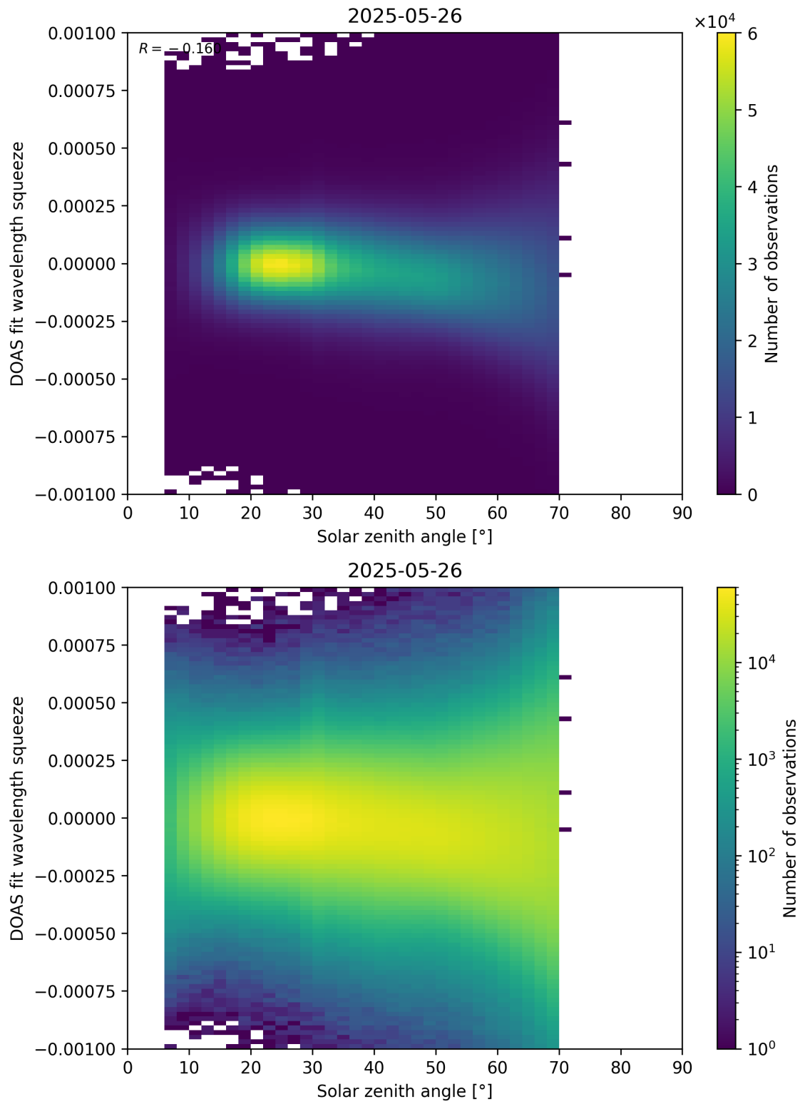
Figure 175: Scatter density plot of “Solar zenith angle” against “DOAS fit wavelength squeeze” for 2025-05-26 to 2025-05-27.
