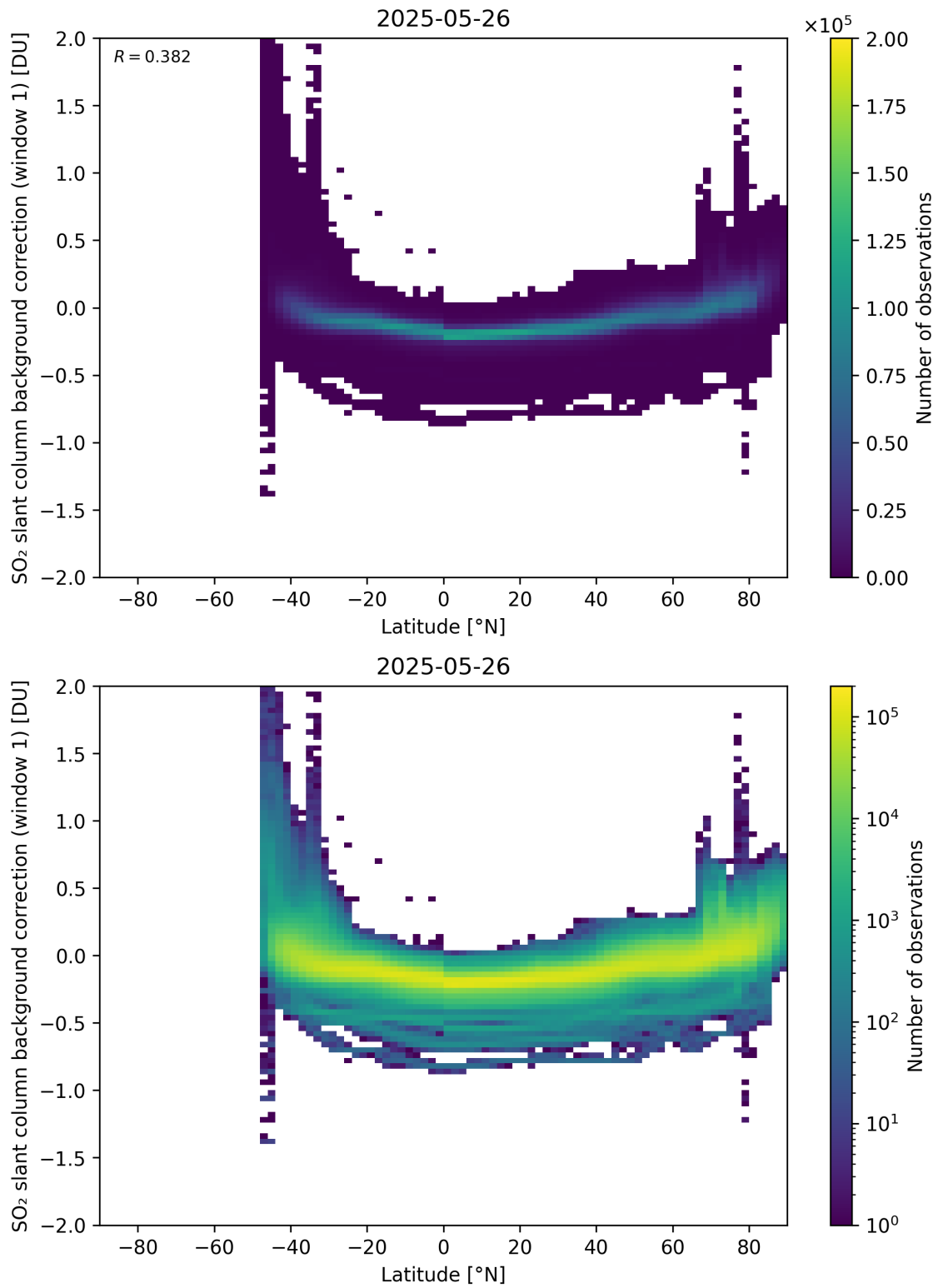
Figure 150: Scatter density plot of “Latitude” against “SO 2 slant column background correction (window 1)” for 2025-05-26 to 2025-05-27.
