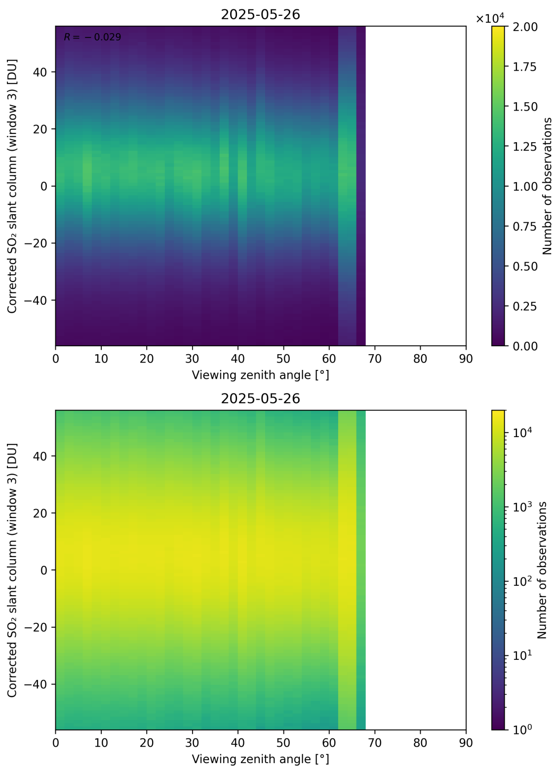
Figure 375: Scatter density plot of “Viewing zenith angle” against “Corrected SO 2 slant column (window 3)” for 2025-05-26 to 2025-05-27.
