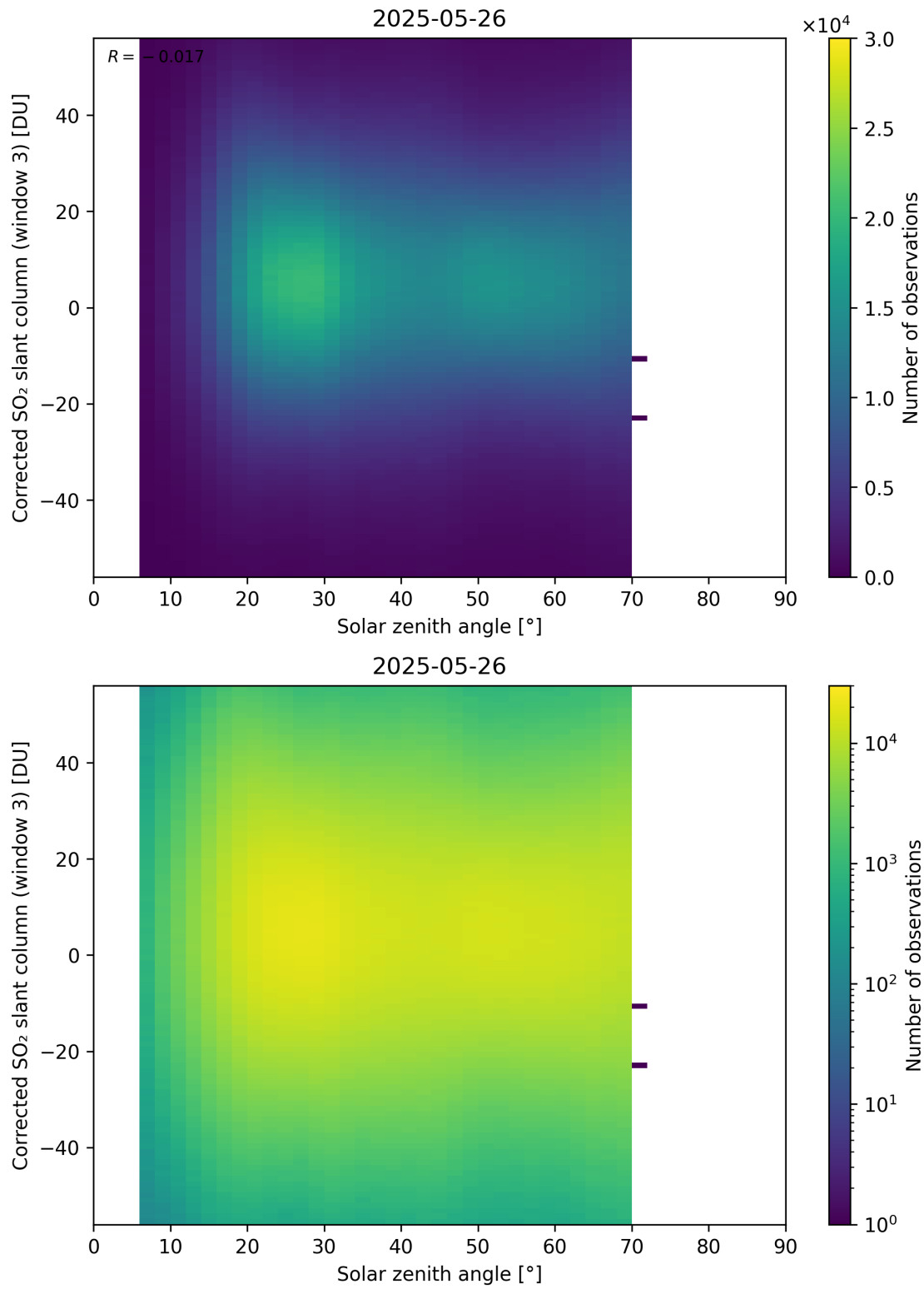
Figure 183: Scatter density plot of “Solar zenith angle” against “Corrected SO 2 slant column (window 3)” for 2025-05-26 to 2025-05-27.
