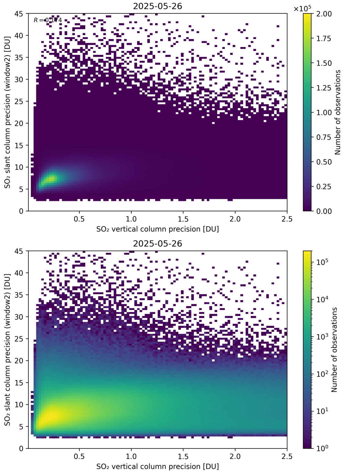
Figure 343: Scatter density plot of “SO 2 vertical column precision” against “SO 2 slant column precision (window2)” for 2025-05-26 to 2025-05-27.
