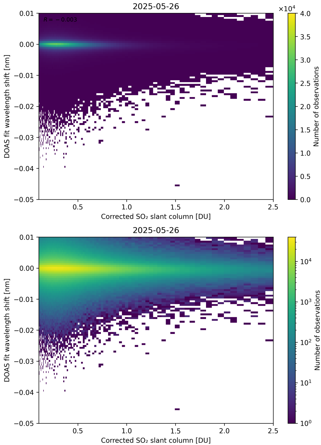
Figure 229: Scatter density plot of “Corrected SO 2 slant column” against “DOAS fit wavelength shift” for 2025-05-26 to 2025-05-27.
