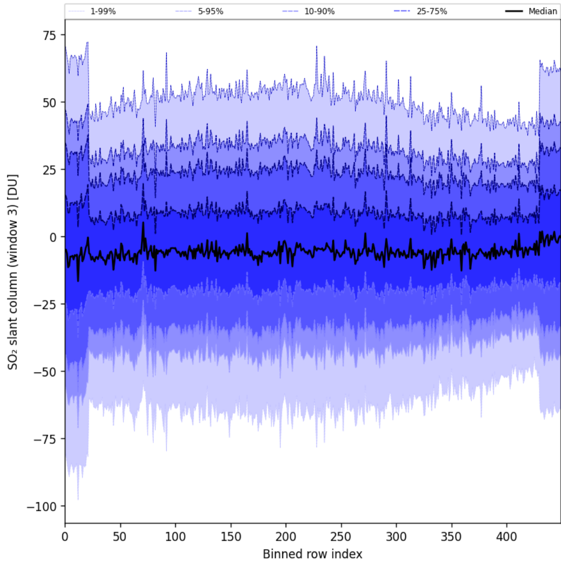
Figure 97: Along track statistics of “SO 2 slant column (window 3)” for 2025-05-26 to 2025-05-27
