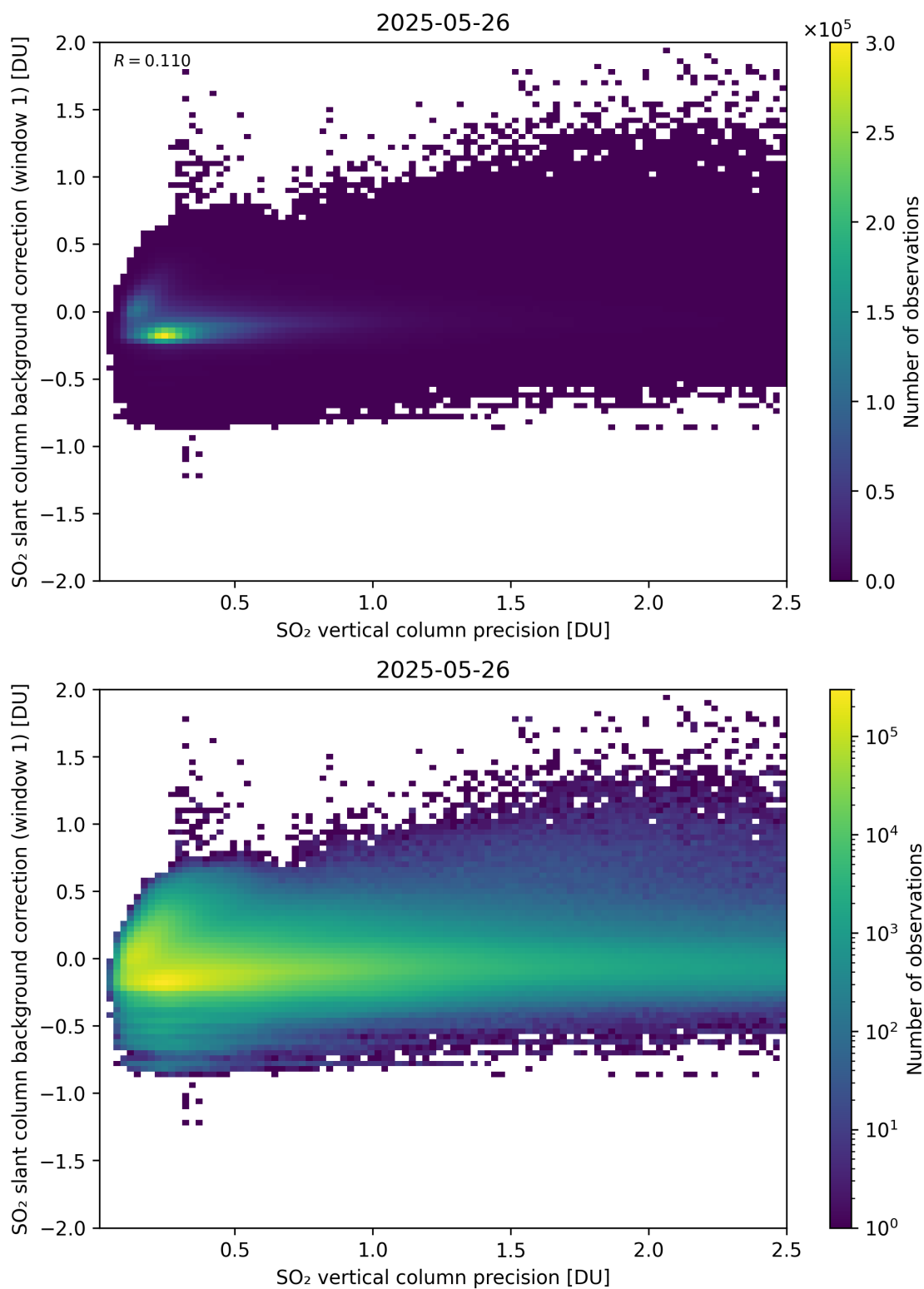
Figure 329: Scatter density plot of “SO 2 vertical column precision” against “SO 2 slant column background correction (window 1)” for 2025-05-26 to 2025-05-27.
