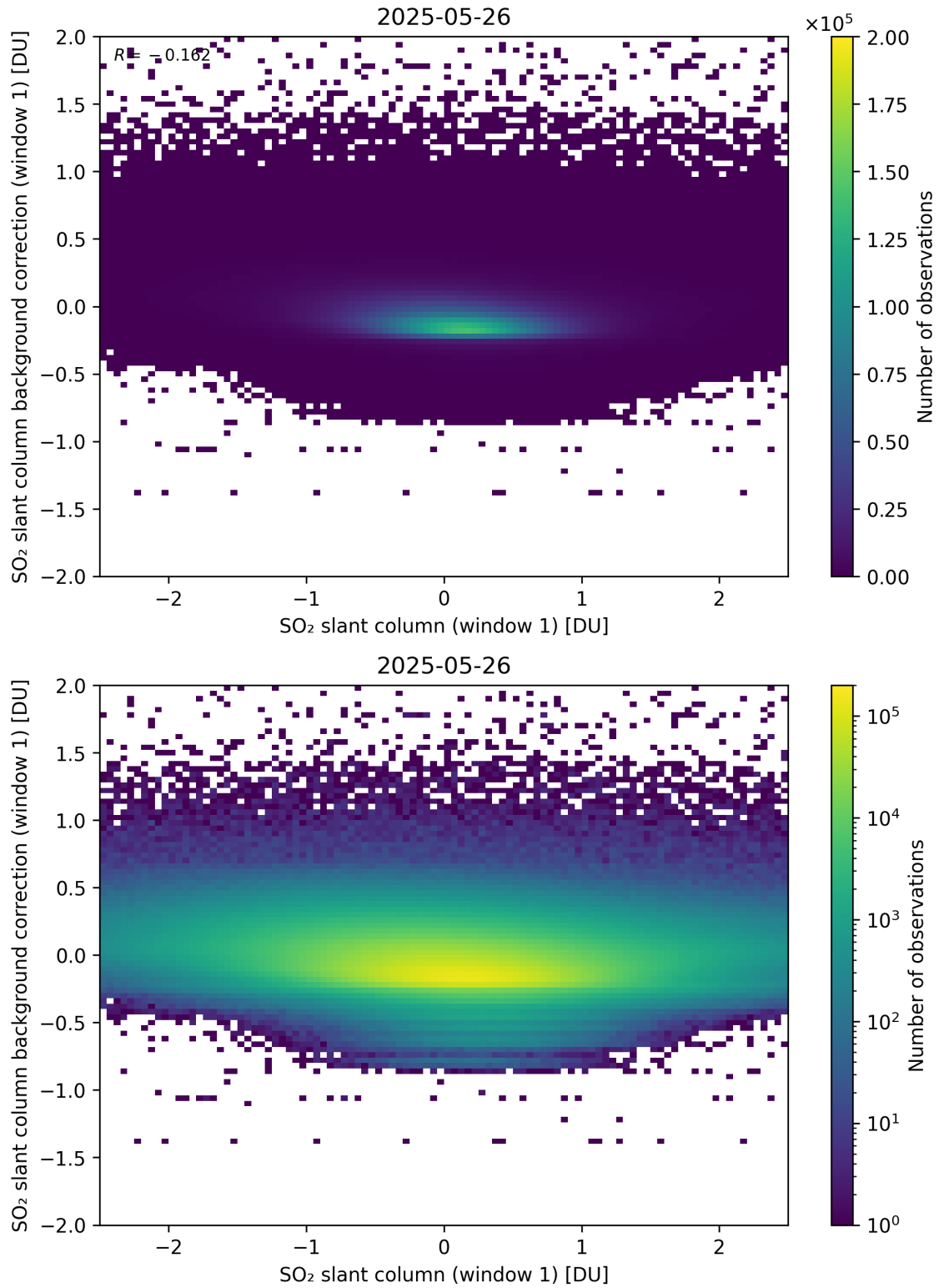
Figure 262: Scatter density plot of “SO 2 slant column (window 1)” against “SO 2 slant column background correction (window 1)” for 2025-05-26 to 2025-05-27.
