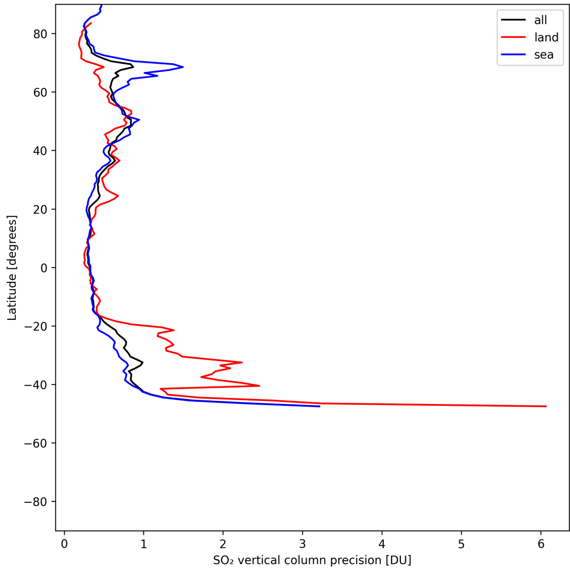
Figure 33: Zonal average of “SO 2 vertical column precision” for 2025-05-26 to 2025-05-27.
