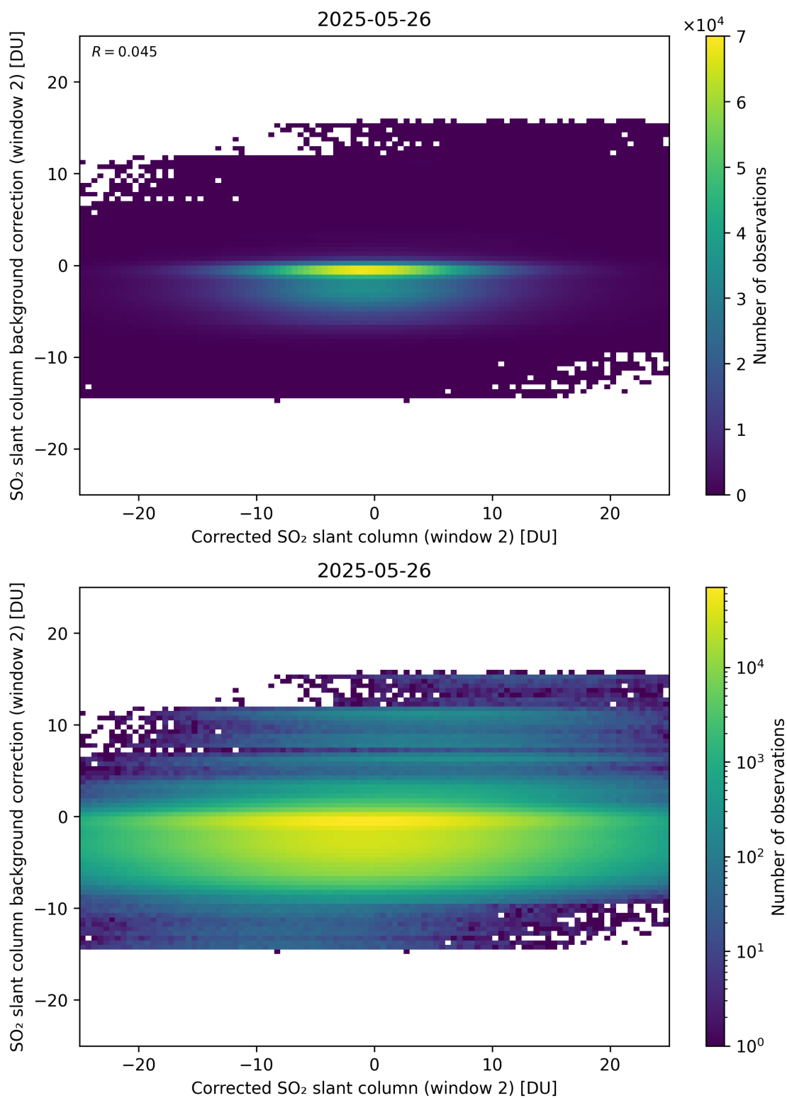
Figure 244: Scatter density plot of “Corrected SO 2 slant column (window 2)” against “SO 2 slant column background correction (window 2)” for 2025-05-26 to 2025-05-27.
