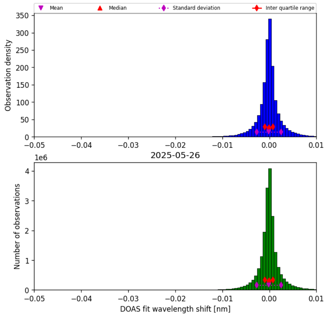
Figure 76: Histogram of “DOAS fit wavelength shift” for 2025-05-26 to 2025-05-27
