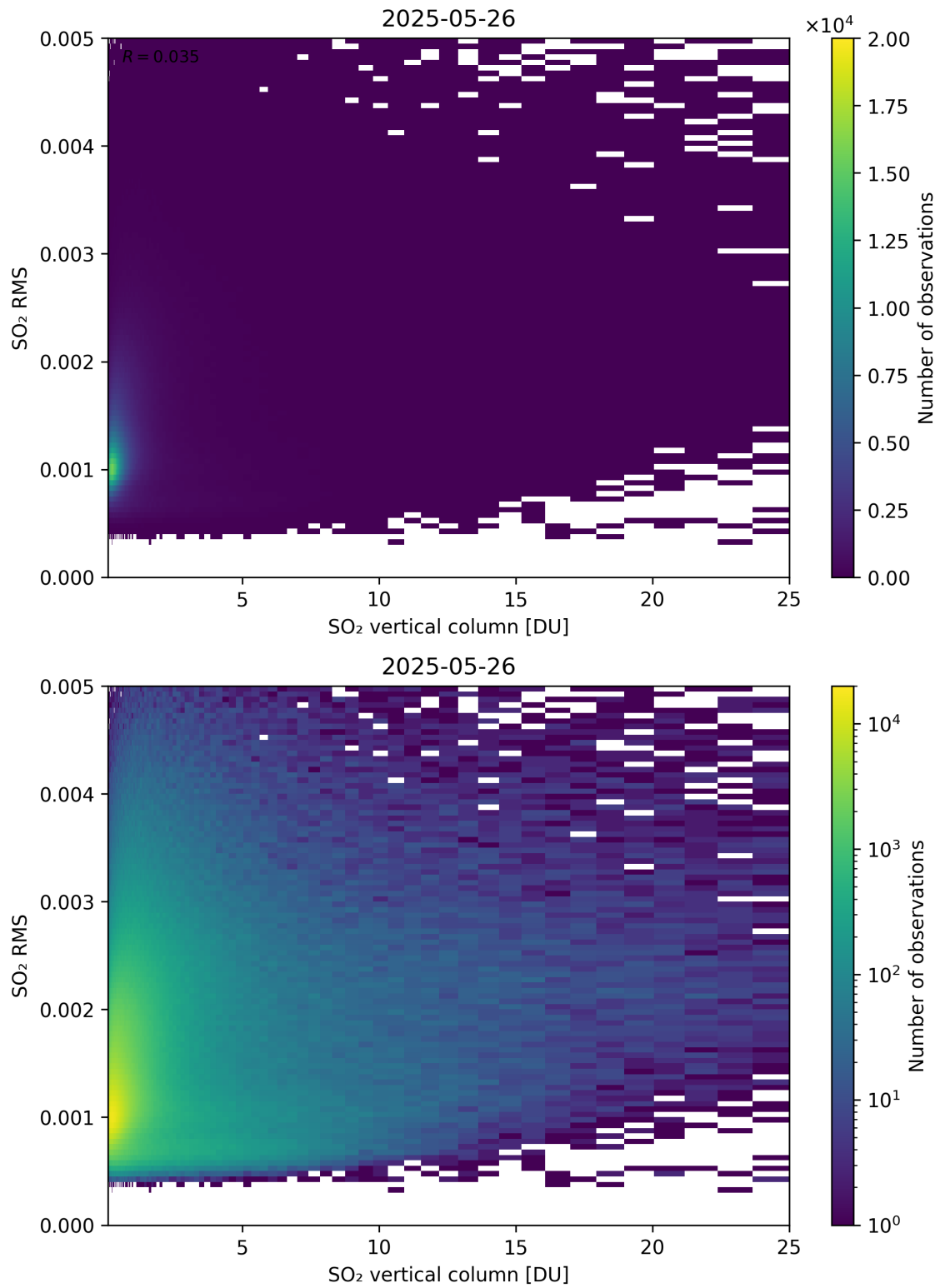
Figure 328: Scatter density plot of “SO 2 vertical column” against “SO 2 RMS” for 2025-05-26 to 2025-05-27.
