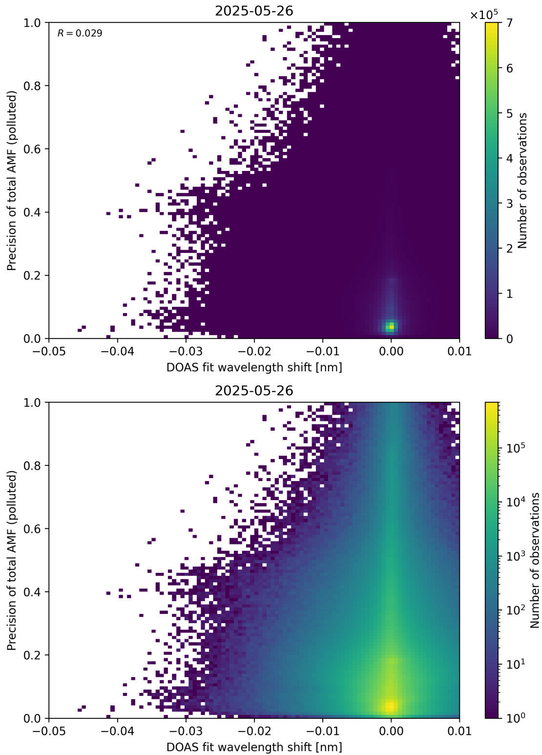
Figure 142: Scatter density plot of “DOAS fit wavelength shift” against “Precision of total AMF (polluted)” for 2025-05-26 to 2025-05-27.
