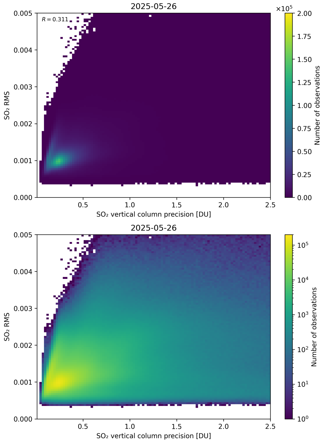
Figure 334: Scatter density plot of “SO 2 vertical column precision” against “SO 2 RMS” for 2025-05-26 to 2025-05-27.
