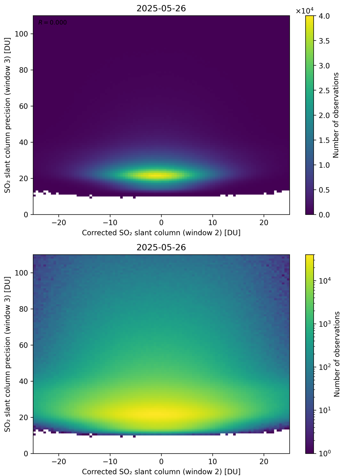
Figure 252: Scatter density plot of “Corrected SO 2 slant column (window 2)” against “SO 2 slant column precision (window 3)” for 2025-05-26 to 2025-05-27.
