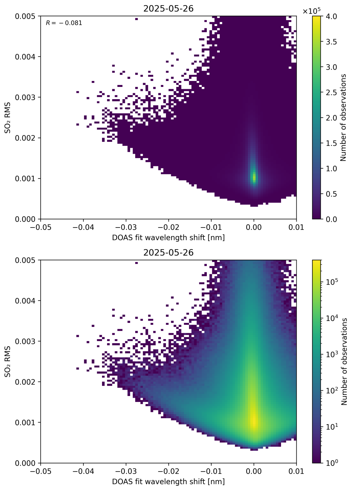
Figure 139: Scatter density plot of “DOAS fit wavelength shift” against “SO 2 RMS” for 2025-05-26 to 2025-05-27.
