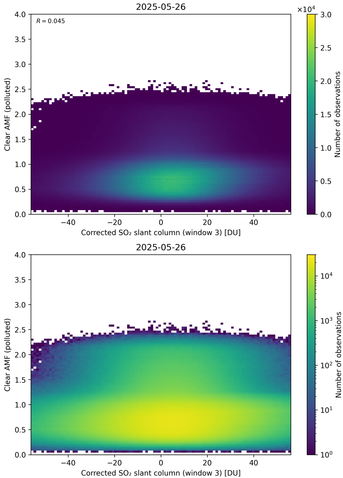
Figure 259: Scatter density plot of “Corrected SO 2 slant column (window 3)” against “Clear AMF (polluted)” for 2025-05-26 to 2025-05-27.
