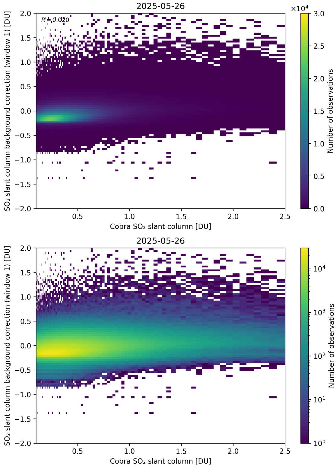
Figure 193: Scatter density plot of “Cobra SO 2 slant column” against “SO 2 slant column background correction (window 1)” for 2025-05-26 to 2025-05-27.
