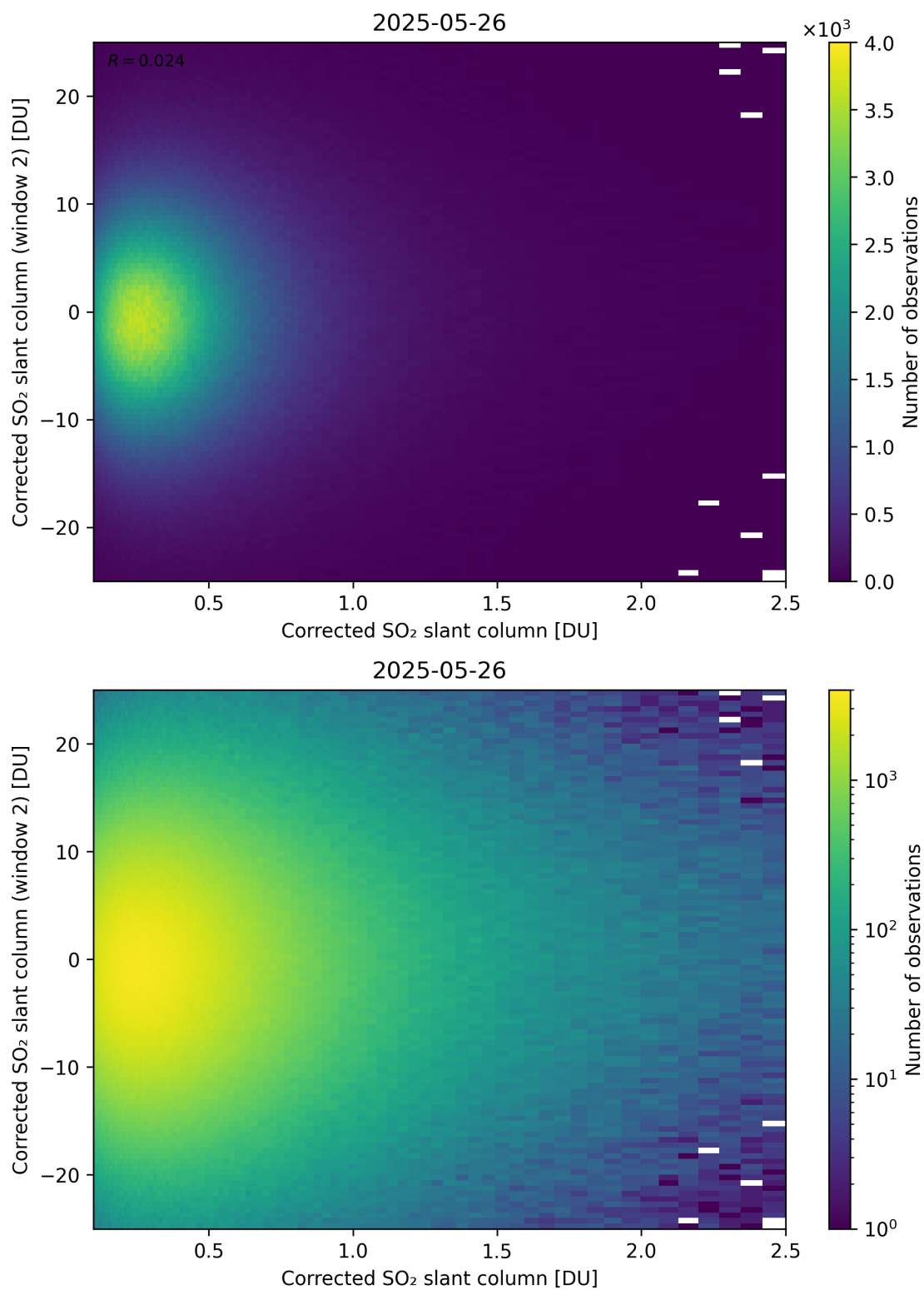
Figure 235: Scatter density plot of “Corrected SO 2 slant column” against “Corrected SO 2 slant column (window 2)” for 2025-05-26 to 2025-05-27.
