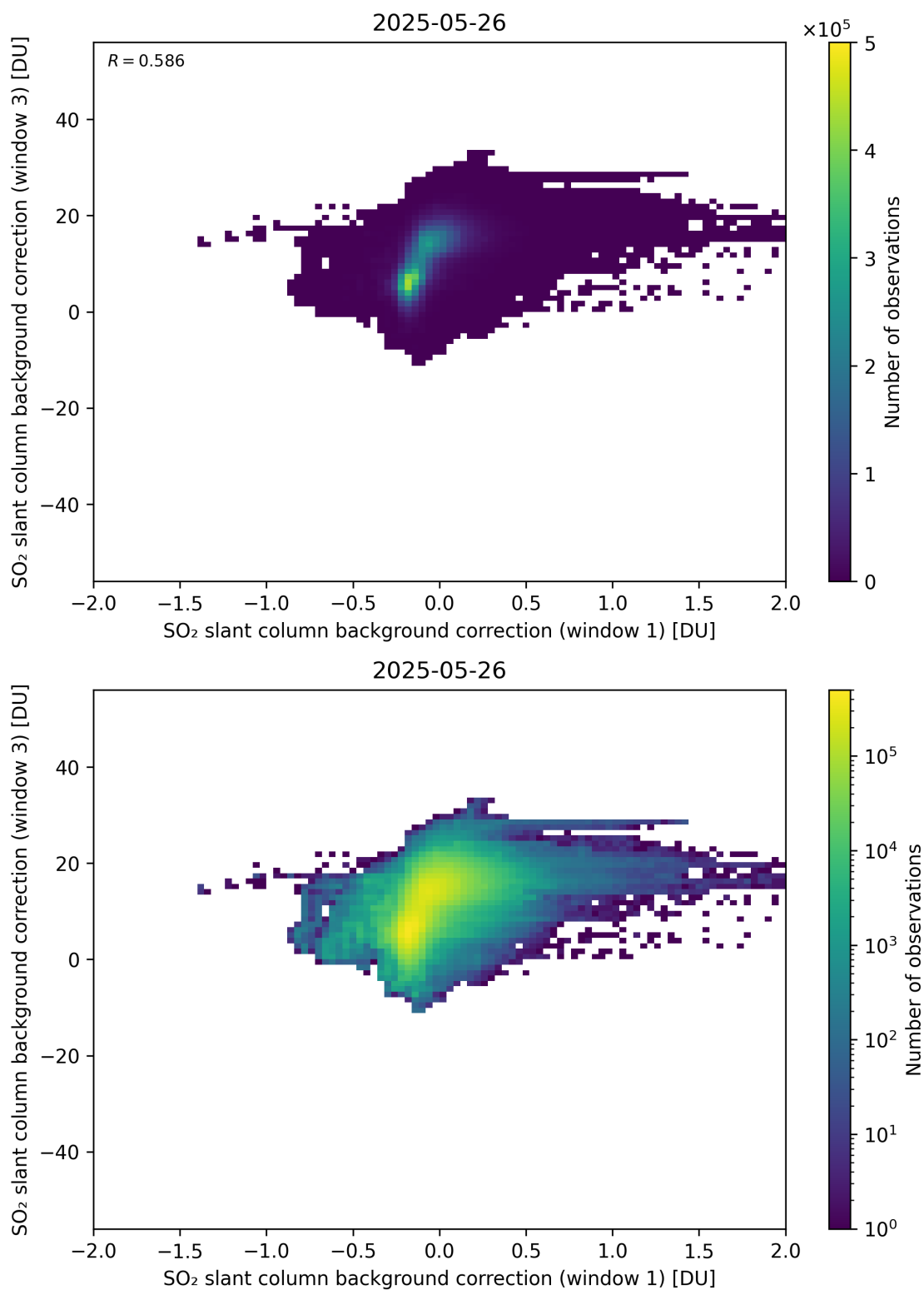
Figure 110: Scatter density plot of “SO 2 slant column background correction (window 1)” against “SO 2 slant column background correction (window 3)” for 2025-05-26 to 2025-05-27.
