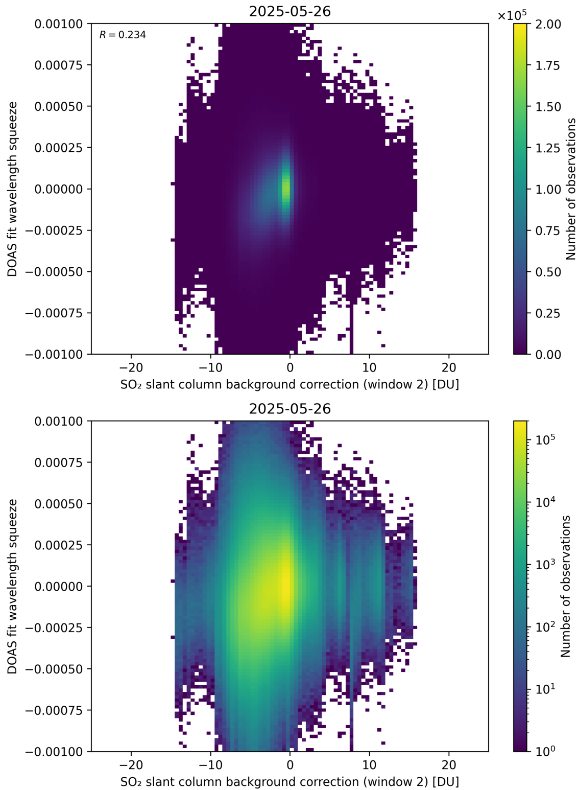
Figure 124: Scatter density plot of “SO 2 slant column background correction (window 2)” against “DOAS fit wavelength squeeze” for 2025-05-26 to 2025-05-27.
