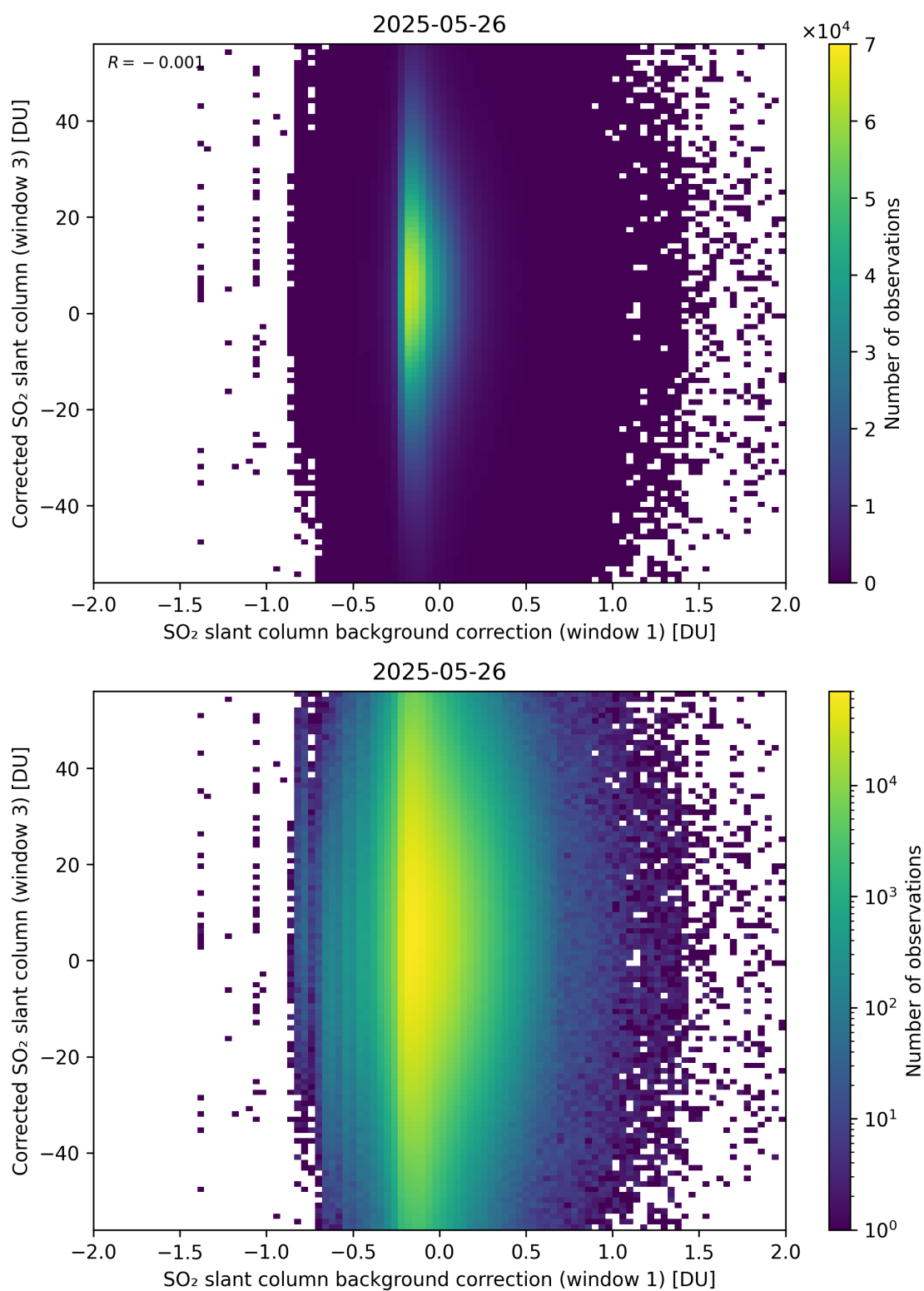
Figure 116: Scatter density plot of “SO 2 slant column background correction (window 1)” against “Corrected SO 2 slant column (window 3)” for 2025-05-26 to 2025-05-27.
