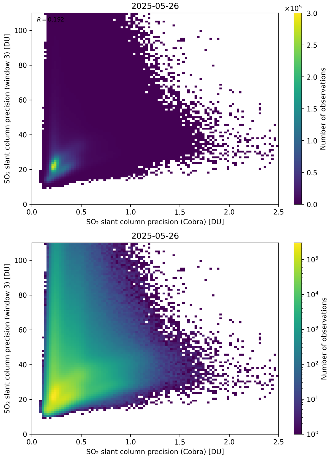
Figure 212: Scatter density plot of “SO 2 slant column precision (Cobra)” against “SO 2 slant column precision (window 3)” for 2025-05-26 to 2025-05-27.
