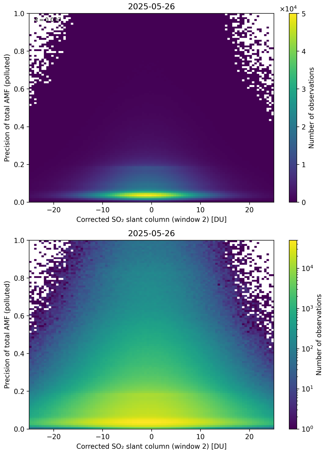
Figure 254: Scatter density plot of “Corrected SO 2 slant column (window 2)” against “Precision of total AMF (polluted)” for 2025-05-26 to 2025-05-27.
