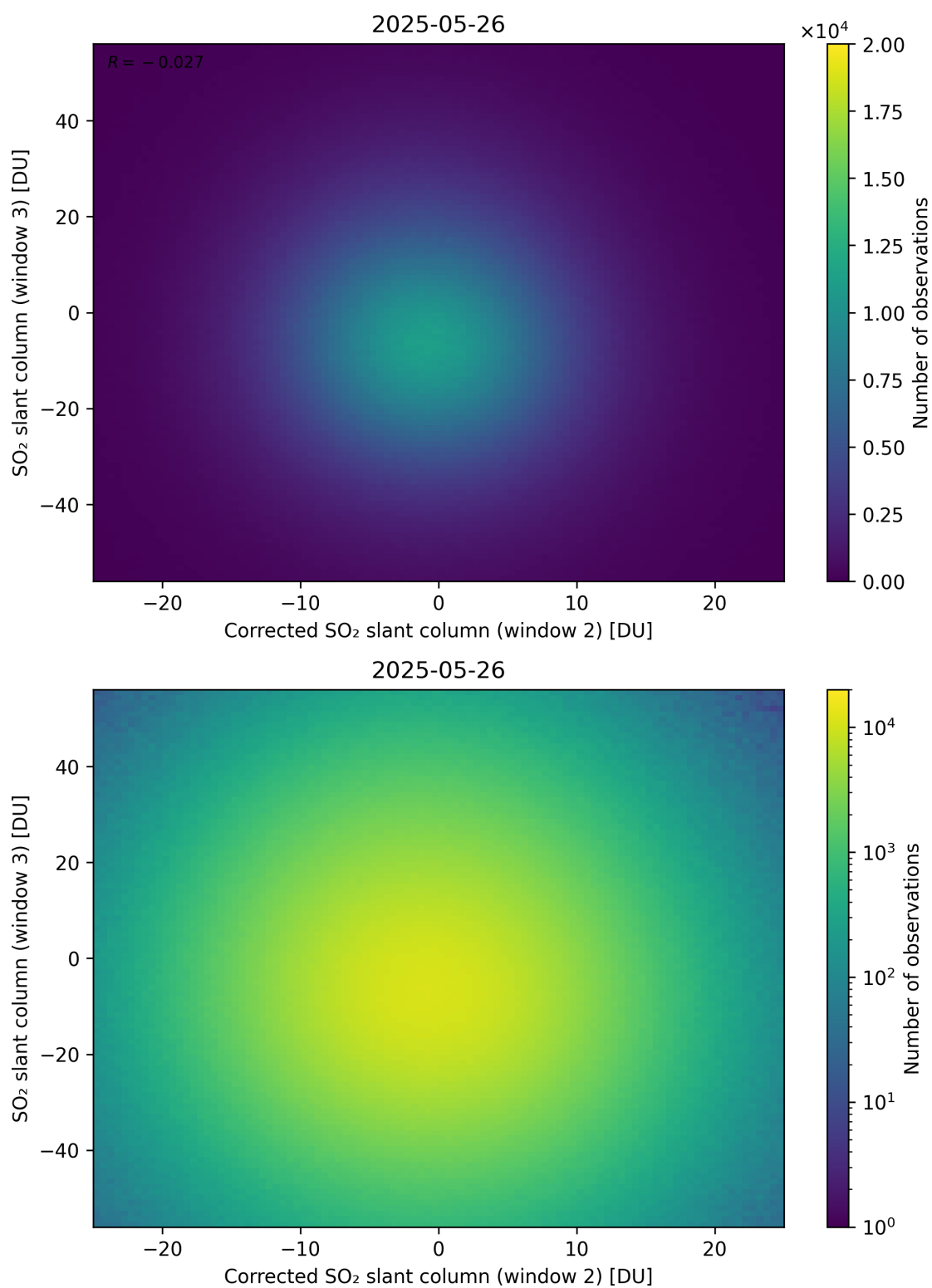
Figure 251: Scatter density plot of “Corrected SO 2 slant column (window 2)” against “SO 2 slant column (window 3)” for 2025-05-26 to 2025-05-27.
