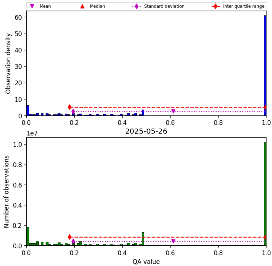
Figure 57: Histogram of “QA value” for 2025-05-26 to 2025-05-27
