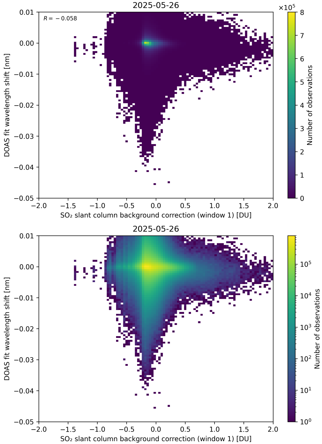
Figure 111: Scatter density plot of “SO 2 slant column background correction (window 1)” against “DOAS fit wavelength shift” for 2025-05-26 to 2025-05-27.
