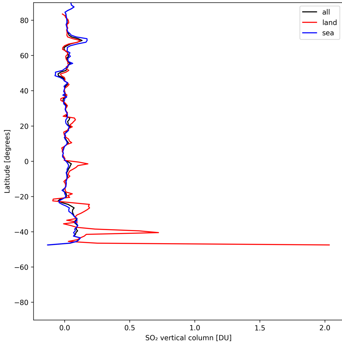
Figure 32: Zonal average of “SO 2 vertical column” for 2025-05-26 to 2025-05-27.
