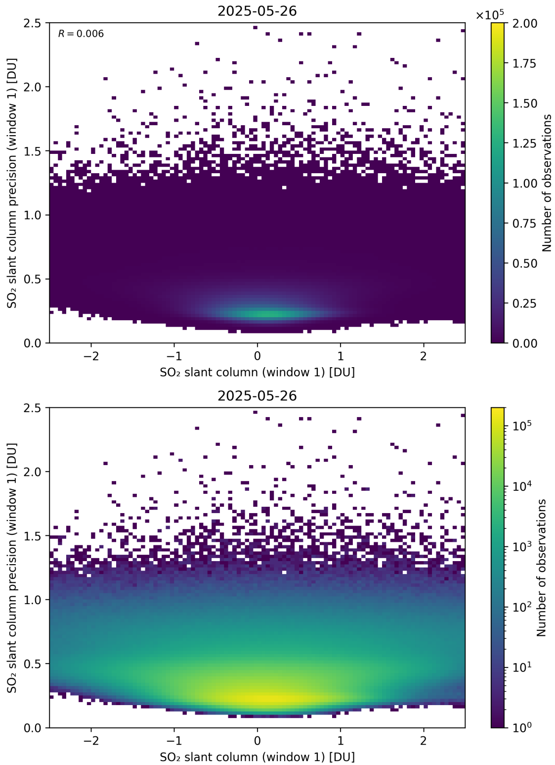
Figure 285: Scatter density plot of “SO 2 slant column (window 1)” against “SO 2 slant column precision (window 1)” for 2025-05-26 to 2025-05-27.
