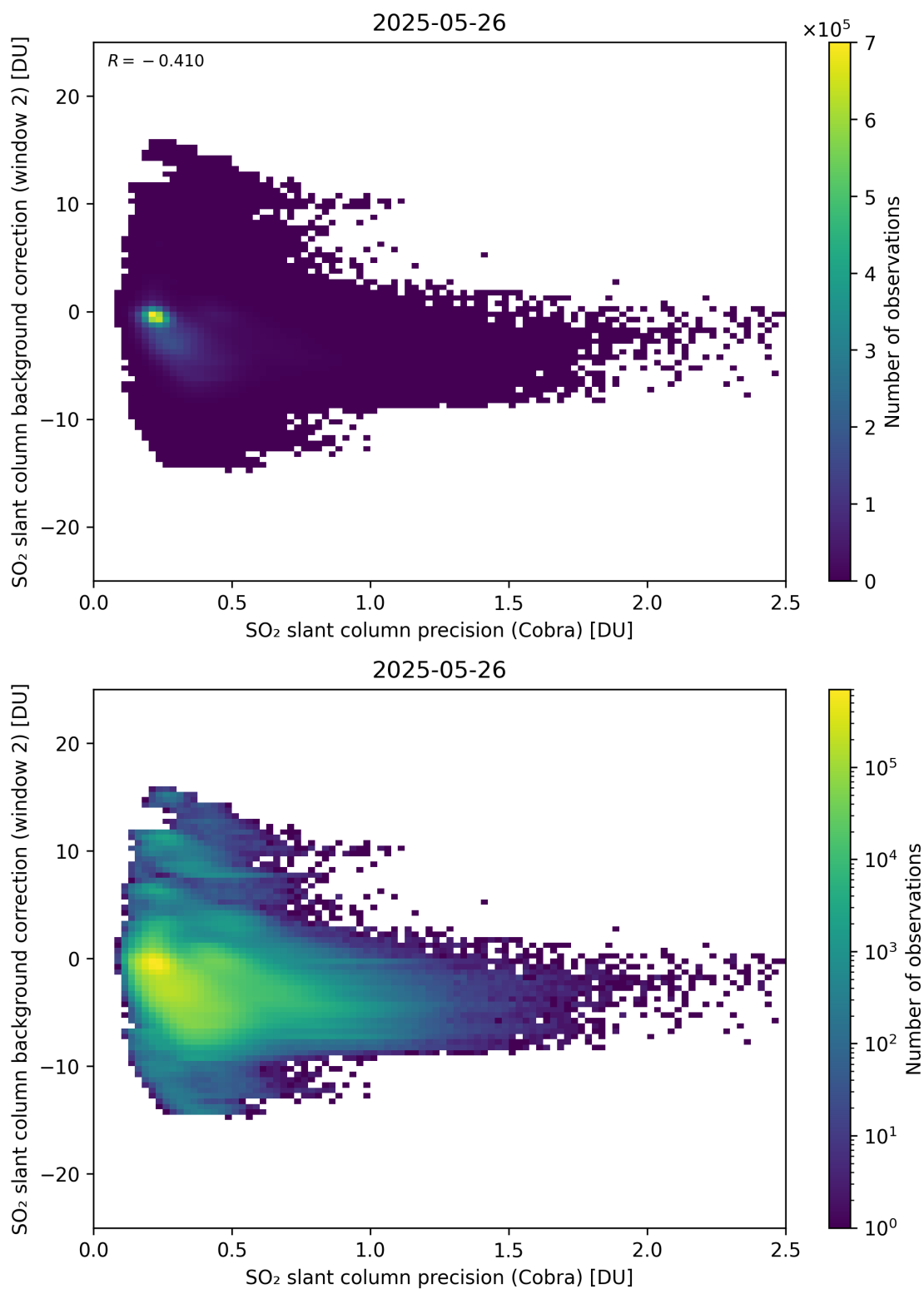
Figure 200: Scatter density plot of “SO 2 slant column precision (Cobra)” against “SO 2 slant column background correction (window 2)” for 2025-05-26 to 2025-05-27.
