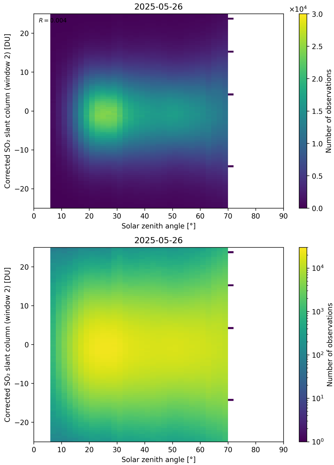
Figure 182: Scatter density plot of “Solar zenith angle” against “Corrected SO 2 slant column (window 2)” for 2025-05-26 to 2025-05-27.
