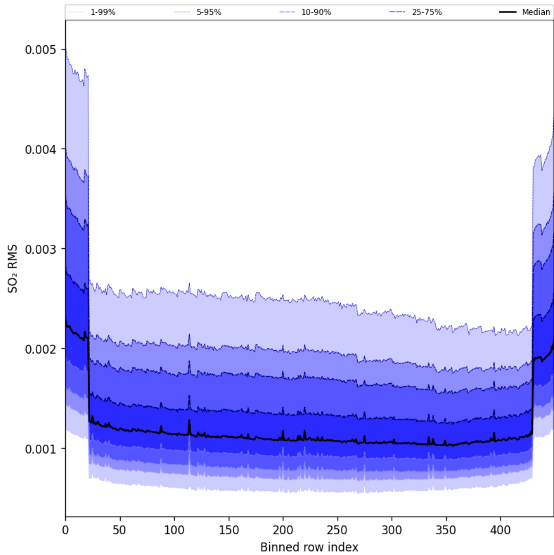
Figure 104: Along track statistics of “SO 2 RMS” for 2025-05-26 to 2025-05-27
