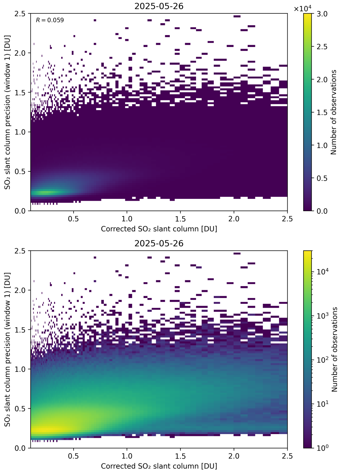
Figure 238: Scatter density plot of “Corrected SO 2 slant column” against “SO 2 slant column precision (window 1)” for 2025-05-26 to 2025-05-27.
