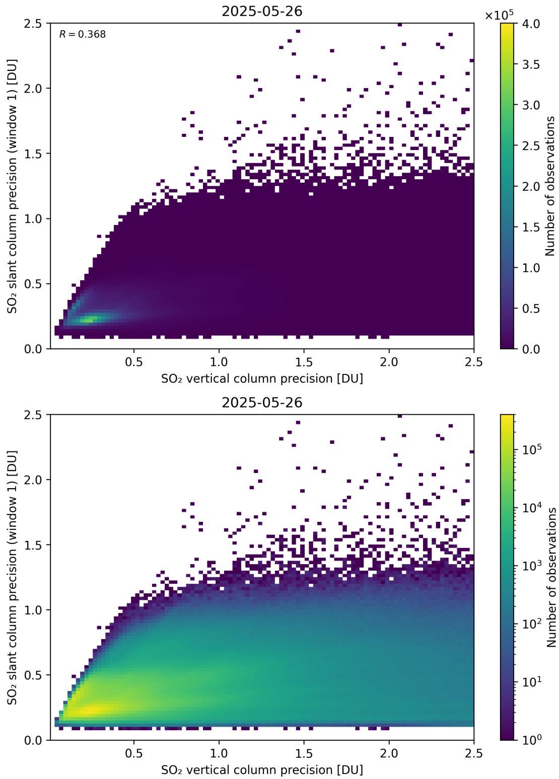
Figure 342: Scatter density plot of “SO 2 vertical column precision” against “SO 2 slant column precision (window 1)” for 2025-05-26 to 2025-05-27.
