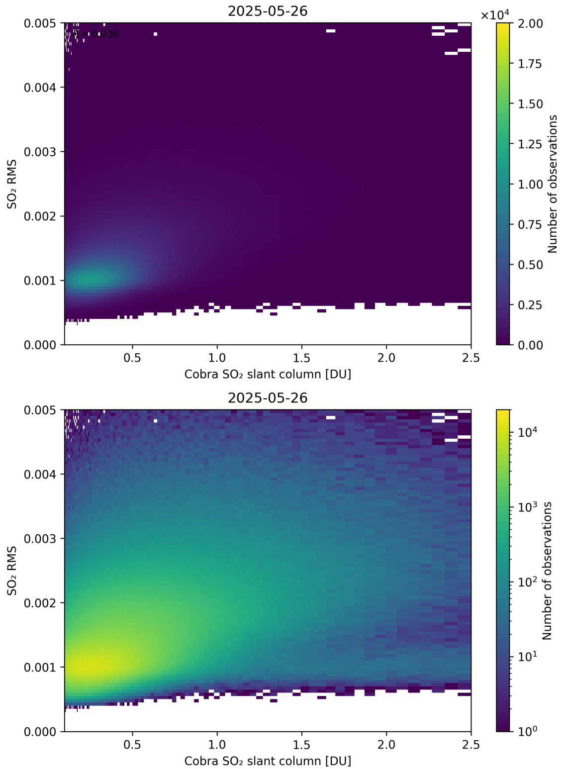
Figure 198: Scatter density plot of “Cobra SO 2 slant column” against “SO 2 RMS” for 2025-05-26 to 2025-05-27.
