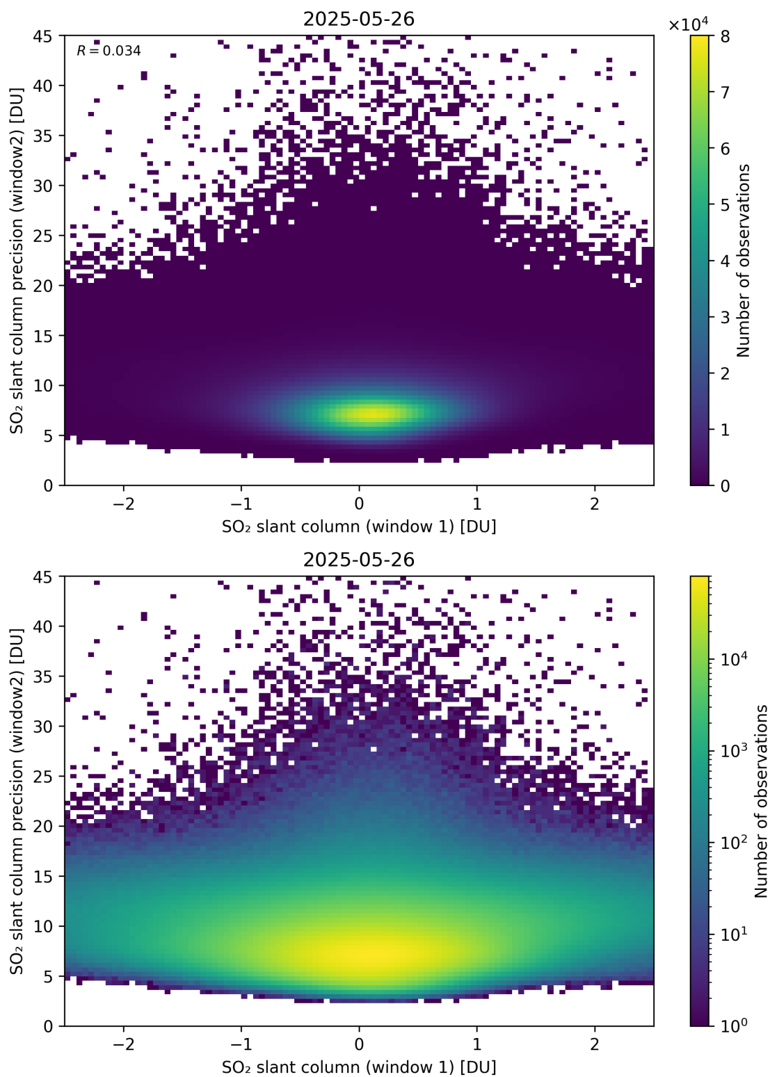
Figure 286: Scatter density plot of “SO 2 slant column (window 1)” against “SO 2 slant column precision (window2)” for 2025-05-26 to 2025-05-27.
