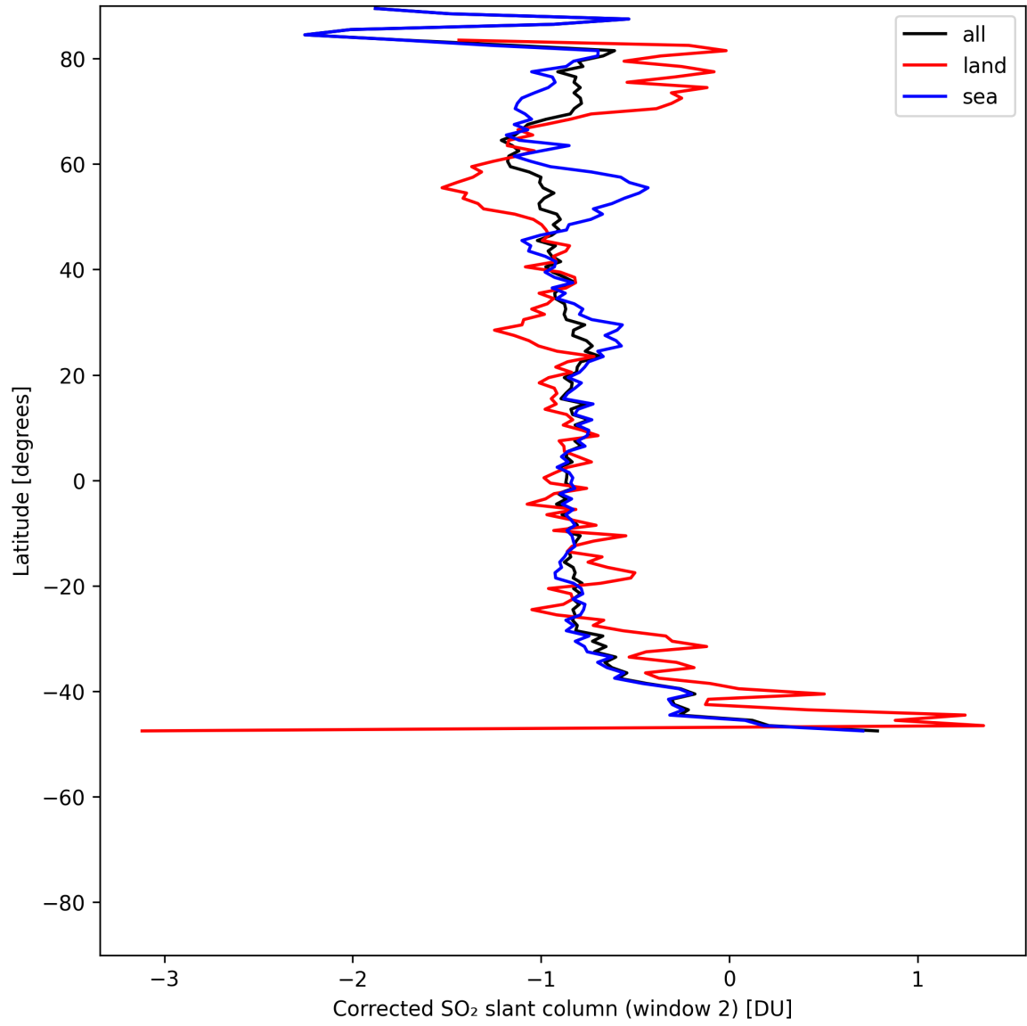
Figure 43: Zonal average of “Corrected SO 2 slant column (window 2)” for 2025-05-26 to 2025-05-27.
