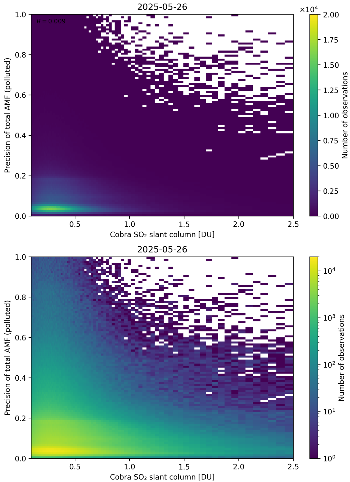
Figure 225: Scatter density plot of “Cobra SO 2 slant column” against “Precision of total AMF (polluted)” for 2025-05-26 to 2025-05-27.
