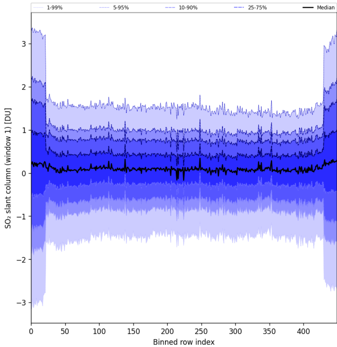
Figure 89: Along track statistics of “SO 2 slant column (window 1)” for 2025-05-26 to 2025-05-27
