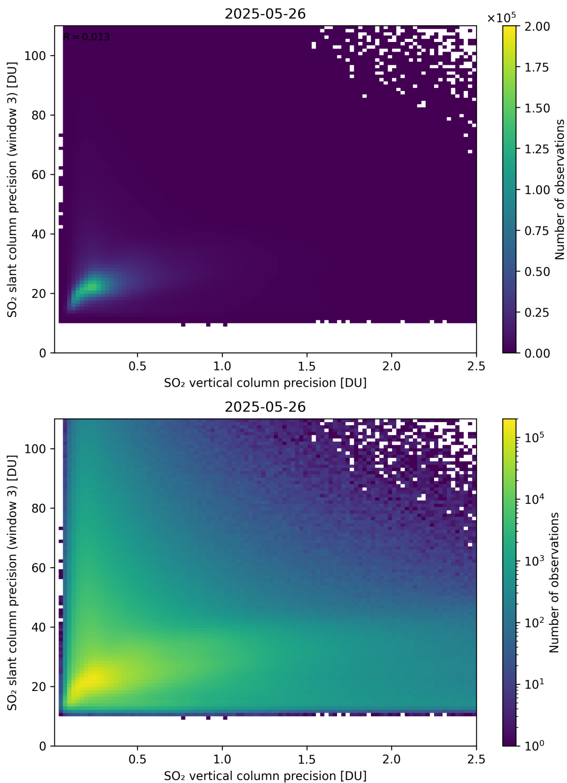
Figure 345: Scatter density plot of “SO 2 vertical column precision” against “SO 2 slant column precision (window 3)” for 2025-05-26 to 2025-05-27.
