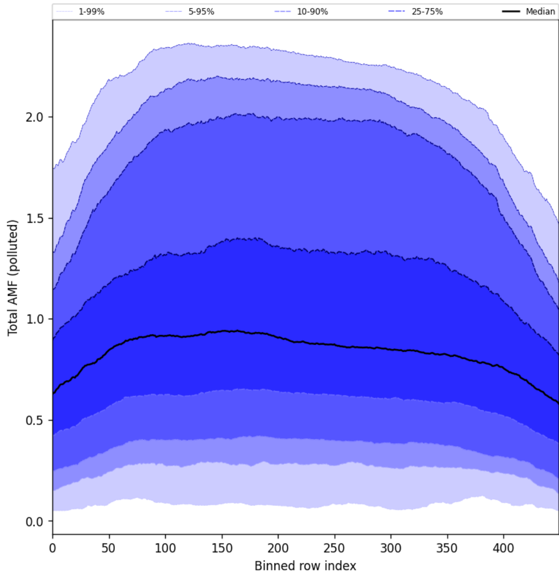
Figure 105: Along track statistics of “Total AMF (polluted)” for 2025-05-26 to 2025-05-27
