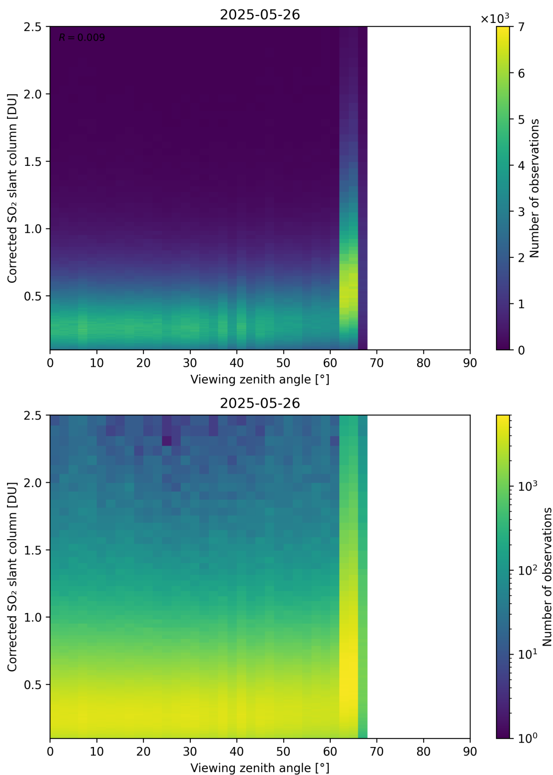
Figure 373: Scatter density plot of “Viewing zenith angle” against “Corrected SO 2 slant column” for 2025-05-26 to 2025-05-27.
