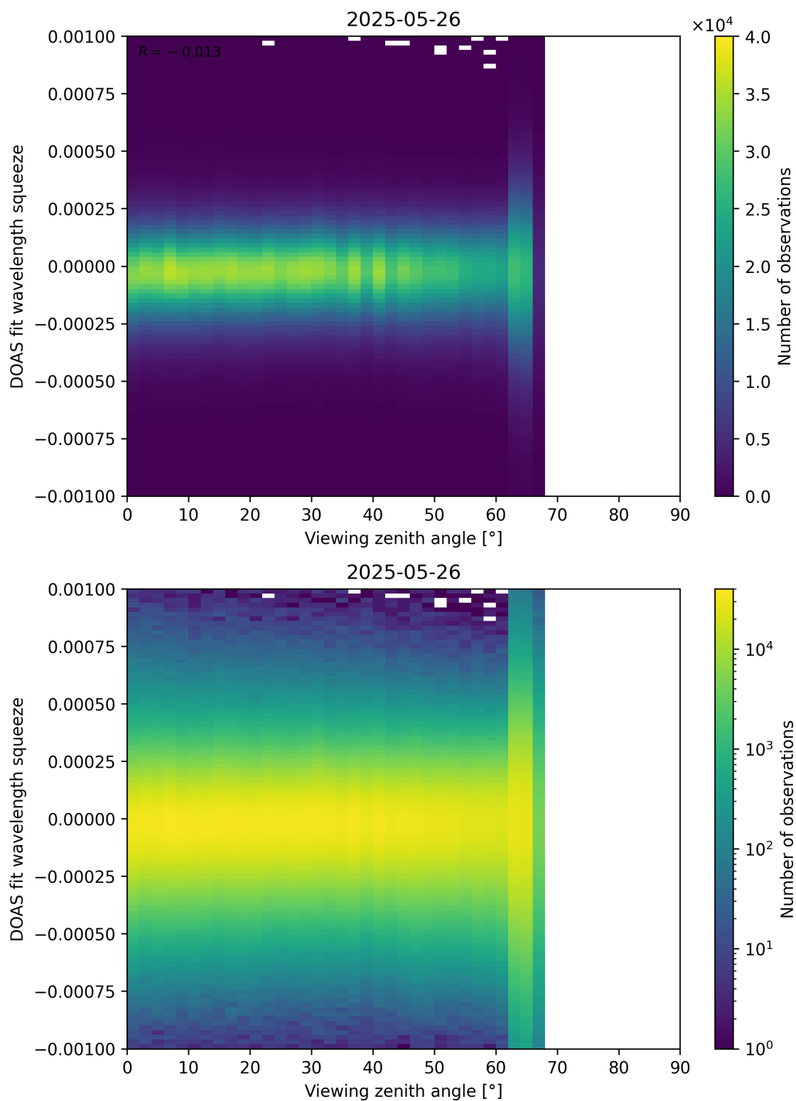
Figure 366: Scatter density plot of “Viewing zenith angle” against “DOAS fit wavelength squeeze” for 2025-05-26 to 2025-05-27.
