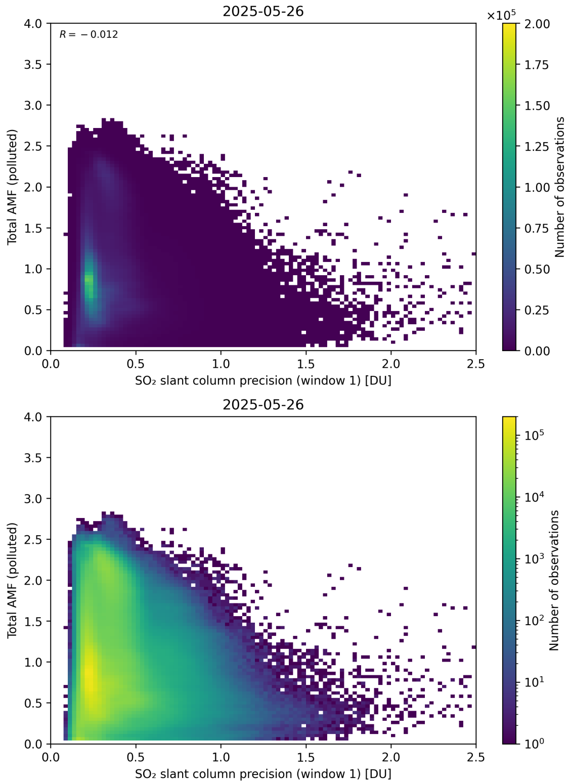
Figure 280: Scatter density plot of “SO 2 slant column precision (window 1)” against “Total AMF (polluted)” for 2025-05-26 to 2025-05-27.
