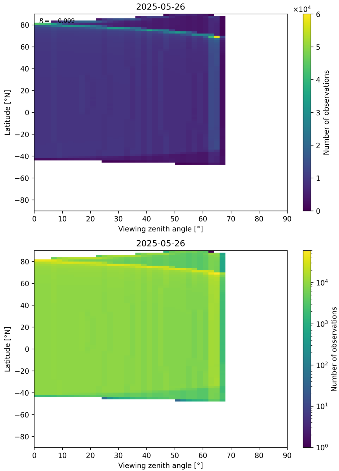
Figure 368: Scatter density plot of “Viewing zenith angle” against “Latitude” for 2025-05-26 to 2025-05-27.
