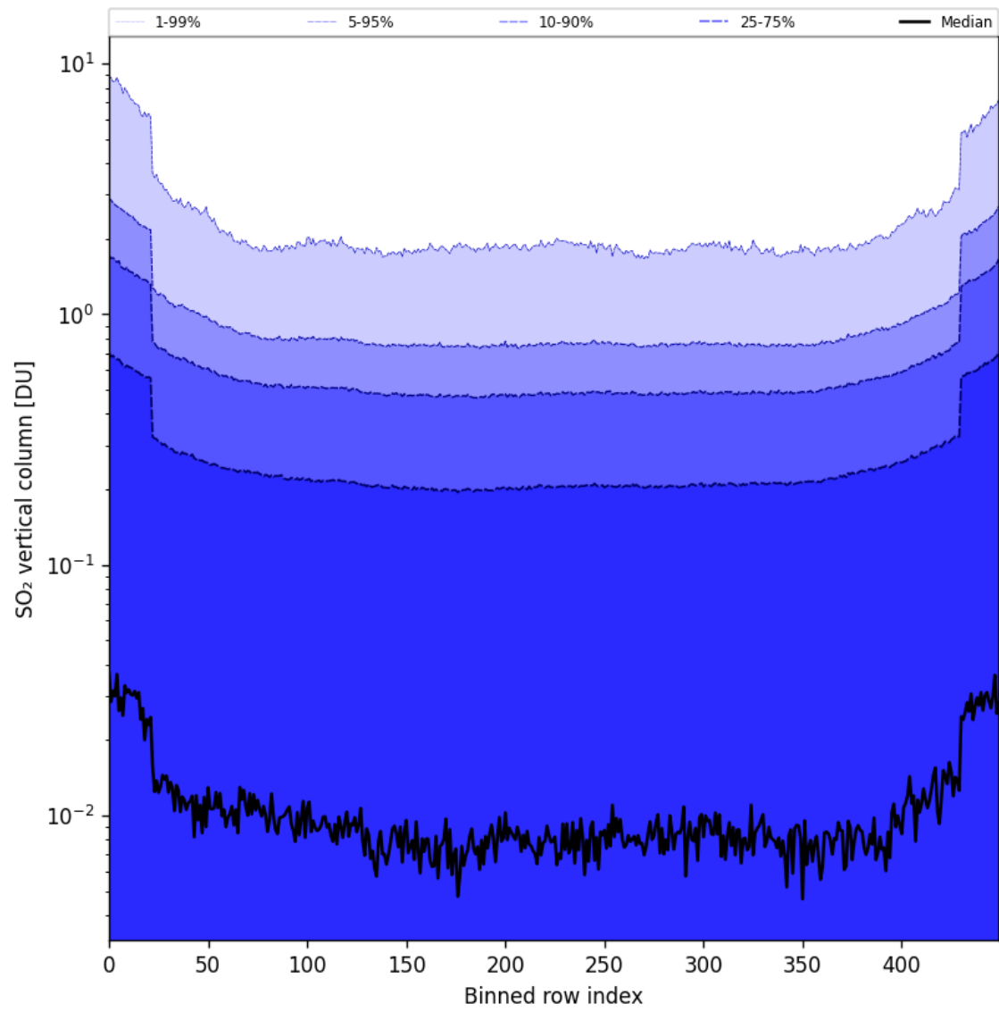
Figure 84: Along track statistics of “SO 2 vertical column” for 2025-05-26 to 2025-05-27
