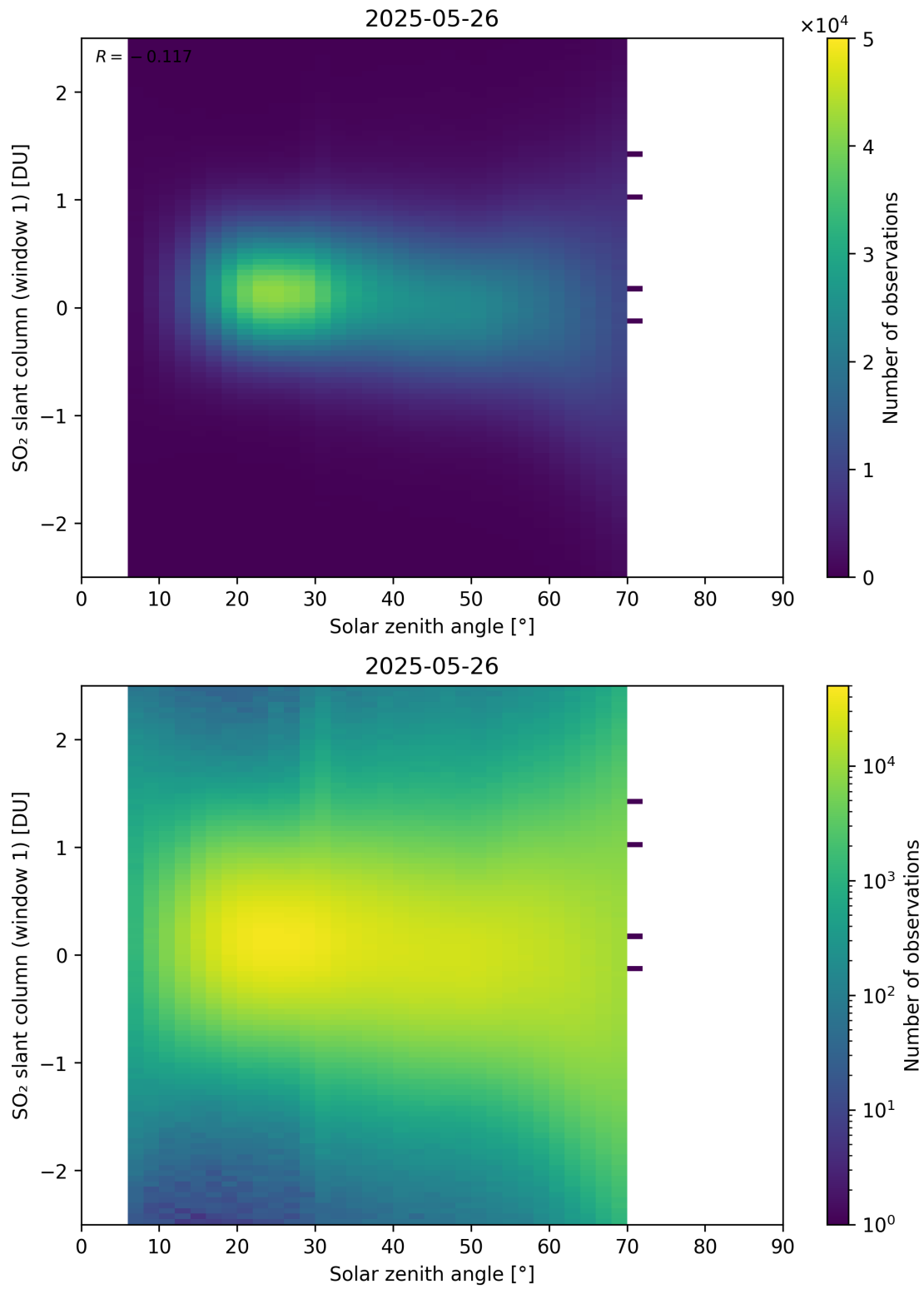
Figure 184: Scatter density plot of “Solar zenith angle” against “SO 2 slant column (window 1)” for 2025-05-26 to 2025-05-27.
