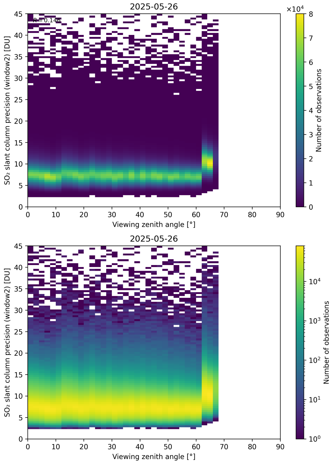
Figure 378: Scatter density plot of “Viewing zenith angle” against “SO 2 slant column precision (window2)” for 2025-05-26 to 2025-05-27.
