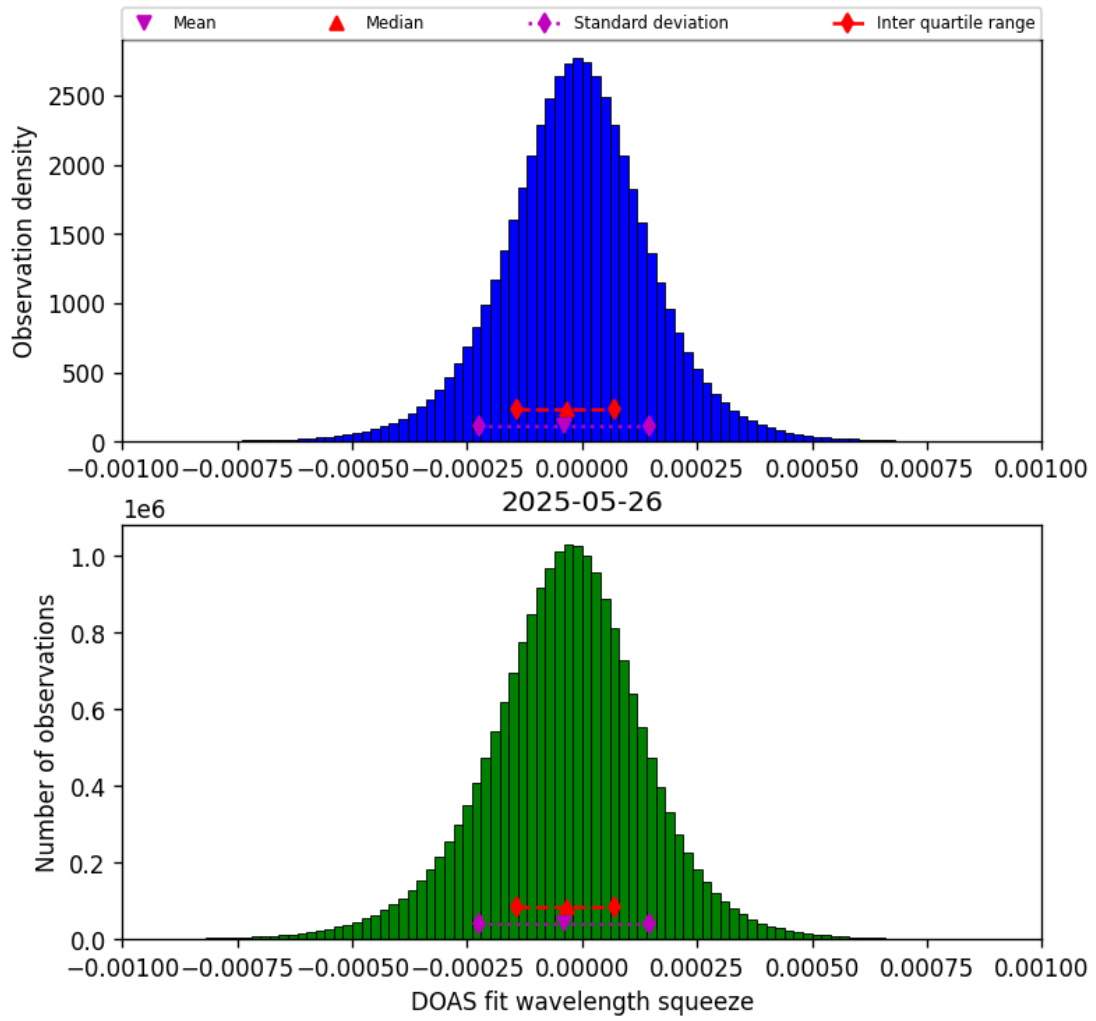
Figure 77: Histogram of “DOAS fit wavelength squeeze” for 2025-05-26 to 2025-05-27
