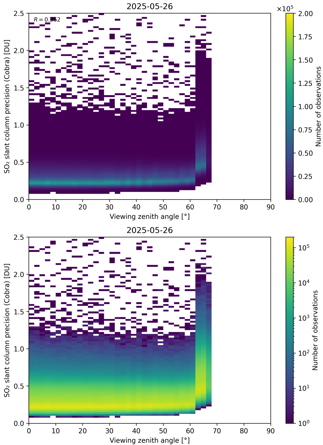
Figure 372: Scatter density plot of “Viewing zenith angle” against “SO 2 slant column precision (Cobra)” for 2025-05-26 to 2025-05-27.
