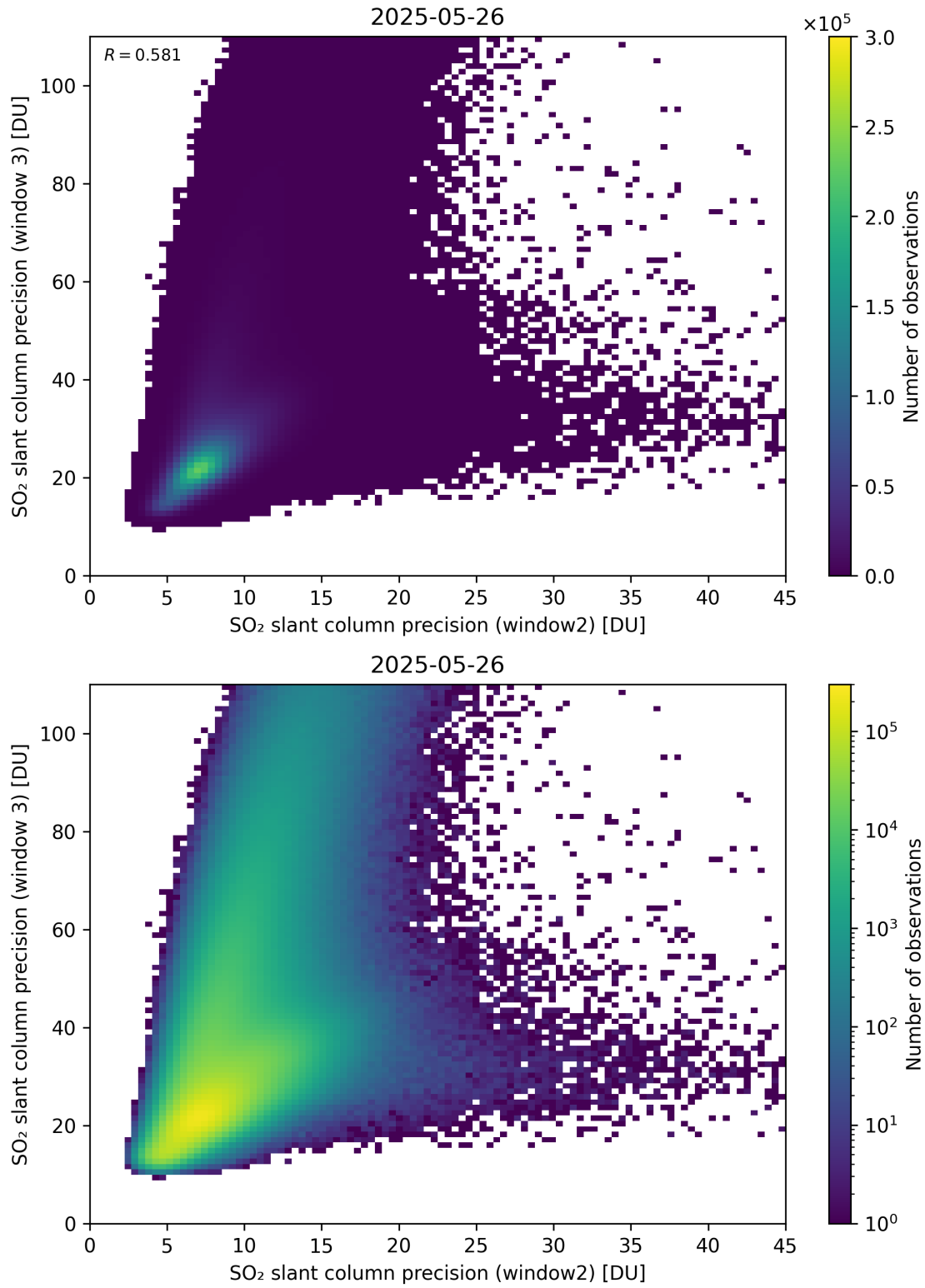
Figure 300: Scatter density plot of “SO 2 slant column precision (window2)” against “SO 2 slant column precision (window 3)” for 2025-05-26 to 2025-05-27.
