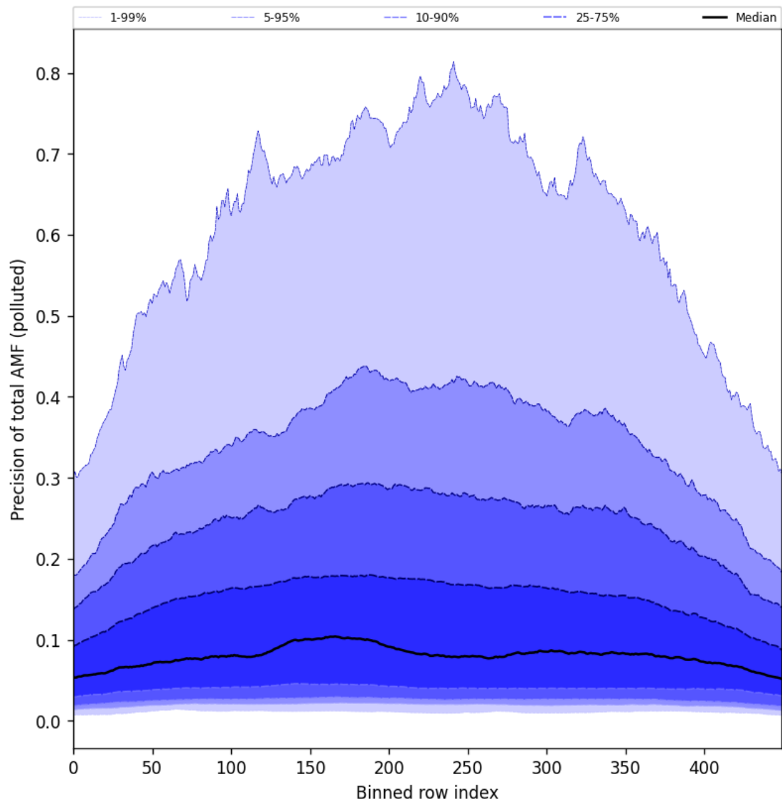
Figure 106: Along track statistics of “Precision of total AMF (polluted)” for 2025-05-26 to 2025-05-27
