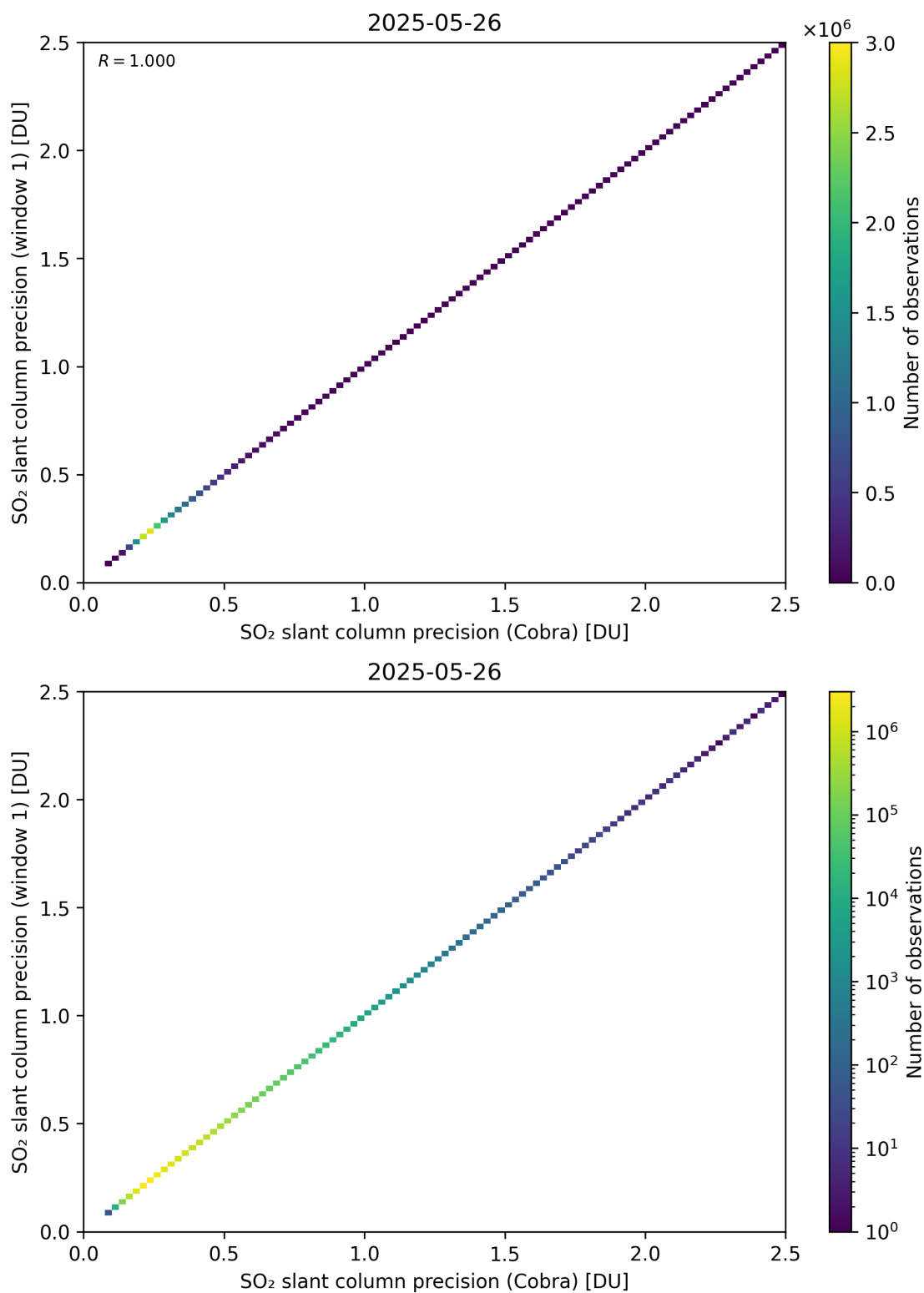
Figure 209: Scatter density plot of “SO 2 slant column precision (Cobra)” against “SO 2 slant column precision (window 1)” for 2025-05-26 to 2025-05-27.
