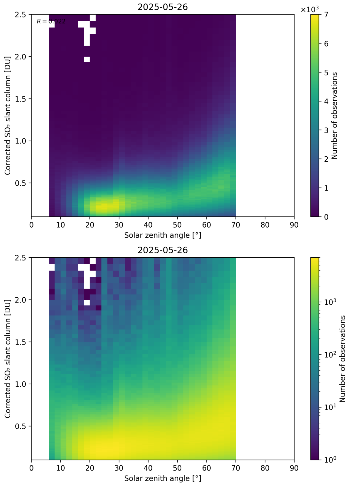
Figure 181: Scatter density plot of “Solar zenith angle” against “Corrected SO 2 slant column” for 2025-05-26 to 2025-05-27.
