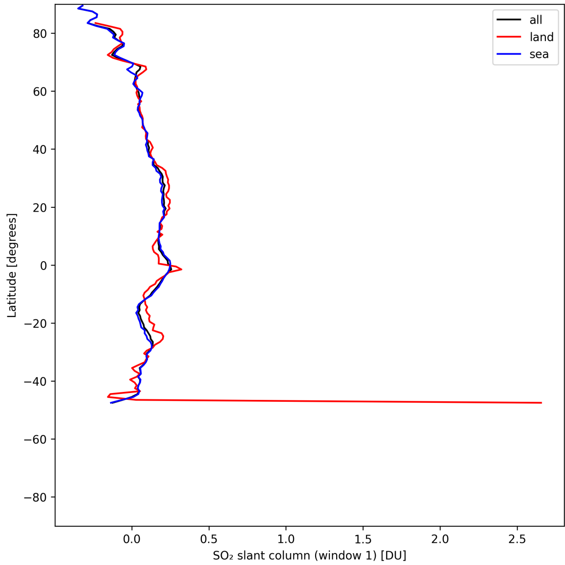
Figure 37: Zonal average of “SO 2 slant column (window 1)” for 2025-05-26 to 2025-05-27.
