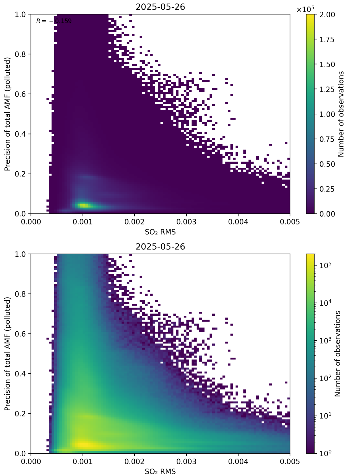
Figure 149: Scatter density plot of “SO 2 RMS” against “Precision of total AMF (polluted)” for 2025-05-26 to 2025-05-27.
