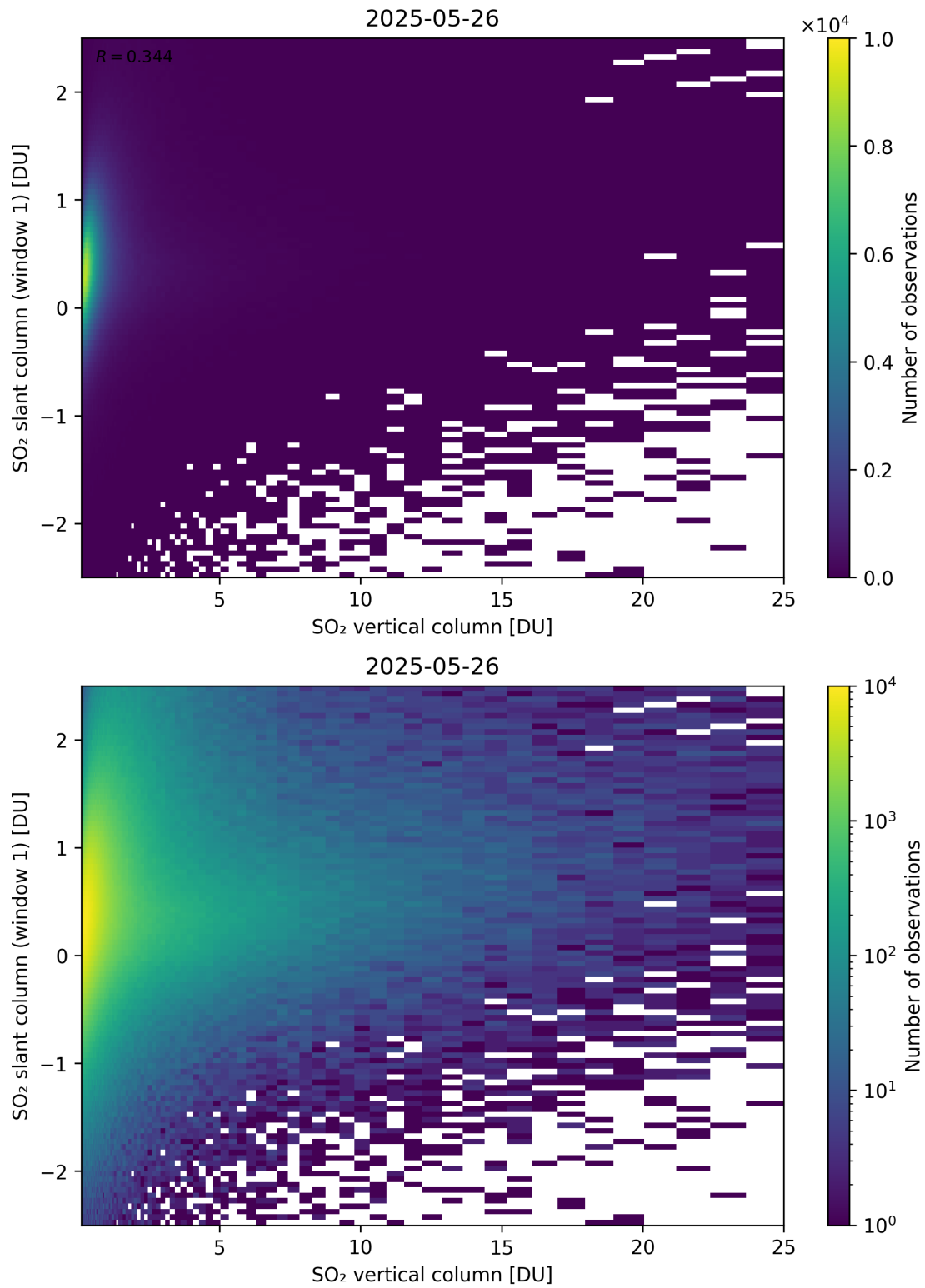
Figure 354: Scatter density plot of “SO 2 vertical column” against “SO 2 slant column (window 1)” for 2025-05-26 to 2025-05-27.
