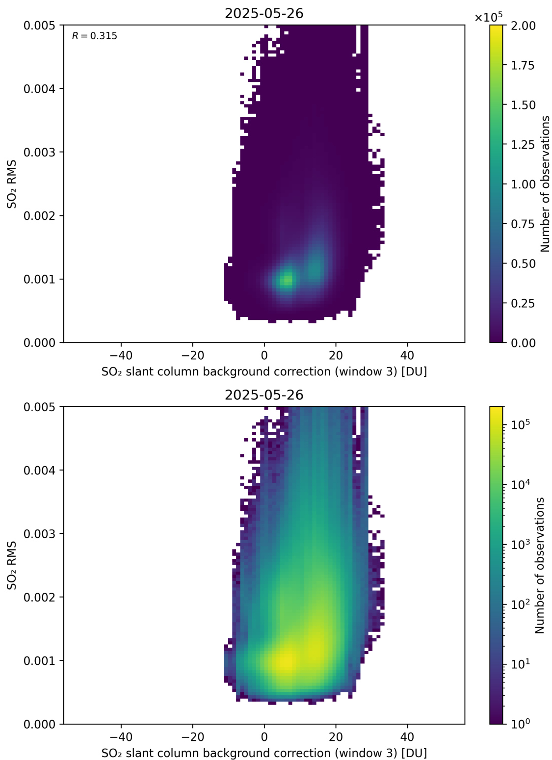
Figure 134: Scatter density plot of “SO 2 slant column background correction (window 3)” against “SO 2 RMS” for 2025-05-26 to 2025-05-27.
