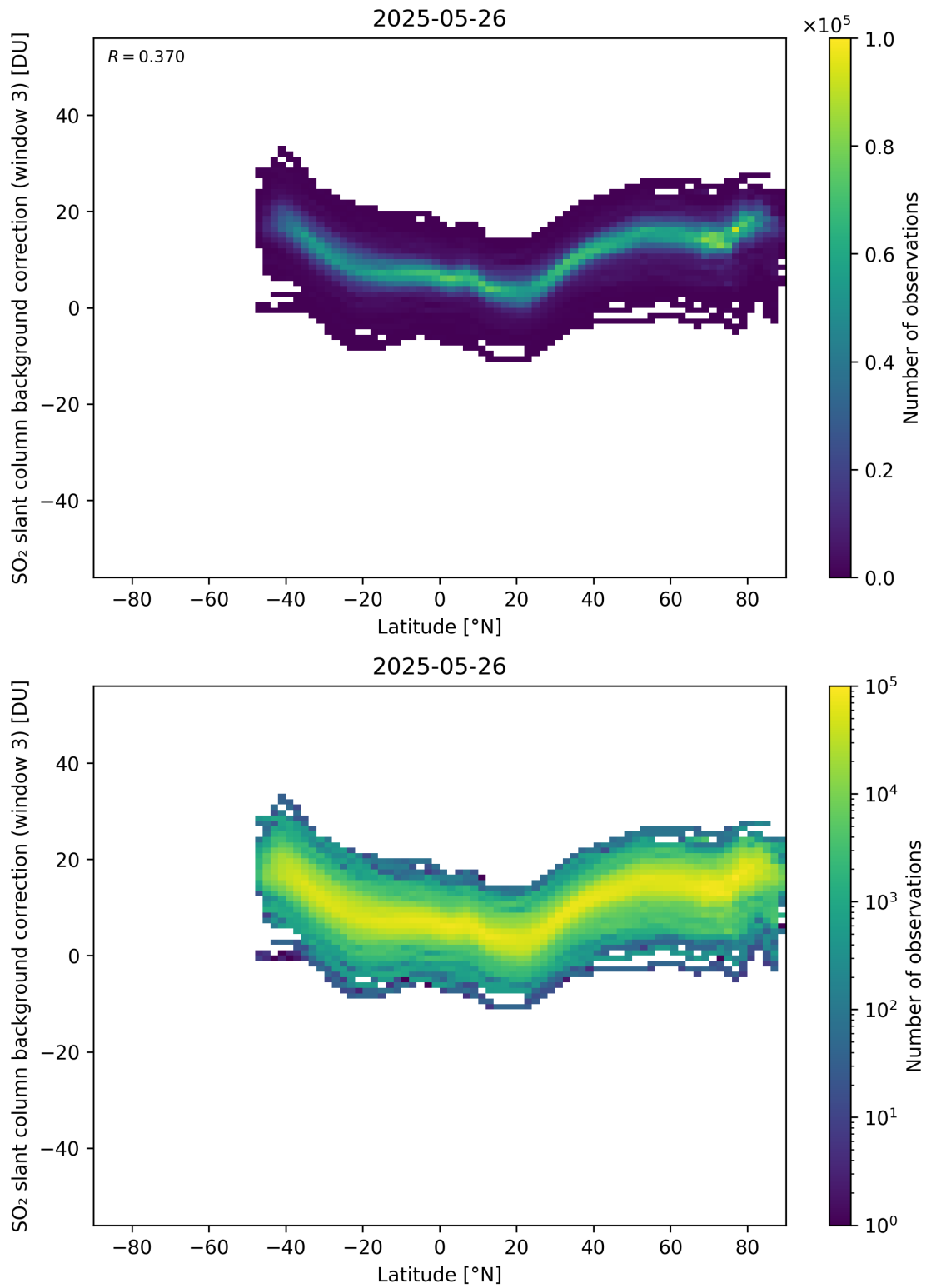
Figure 152: Scatter density plot of “Latitude” against “SO 2 slant column background correction (window 3)” for 2025-05-26 to 2025-05-27.
