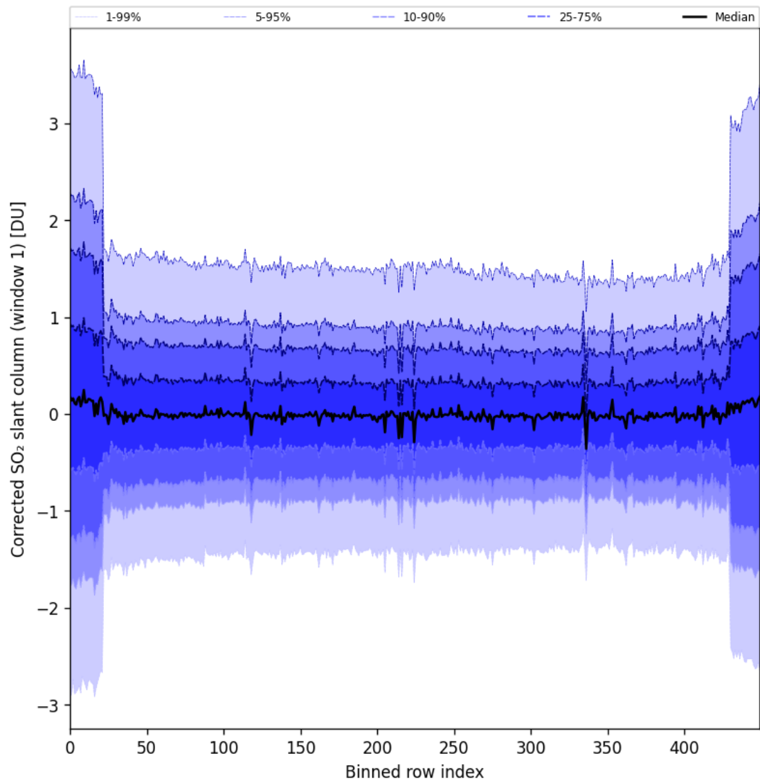
Figure 91: Along track statistics of “Corrected SO 2 slant column (window 1)” for 2025-05-26 to 2025-05-27
