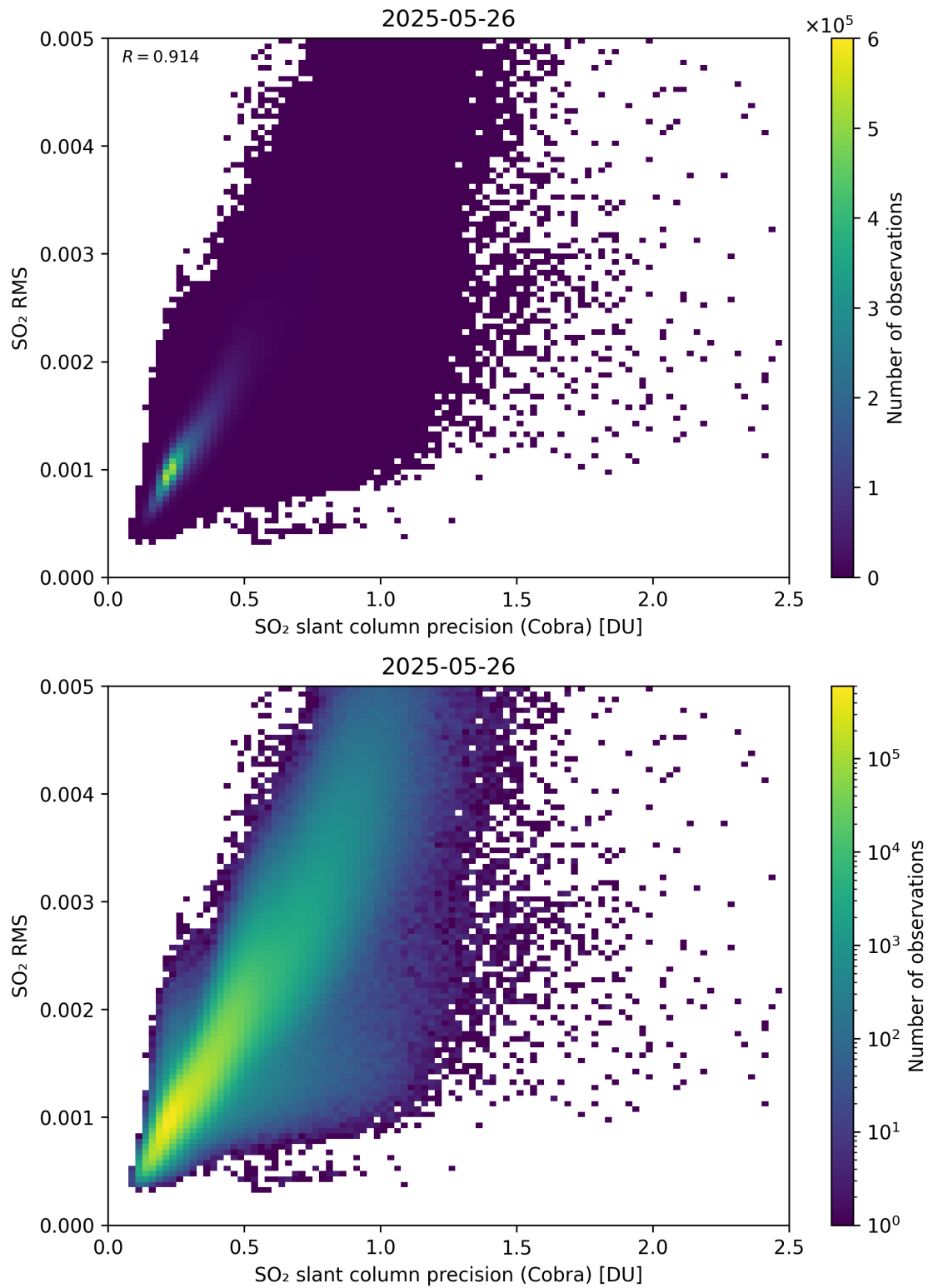
Figure 204: Scatter density plot of “SO 2 slant column precision (Cobra)” against “SO 2 RMS” for 2025-05-26 to 2025-05-27.
