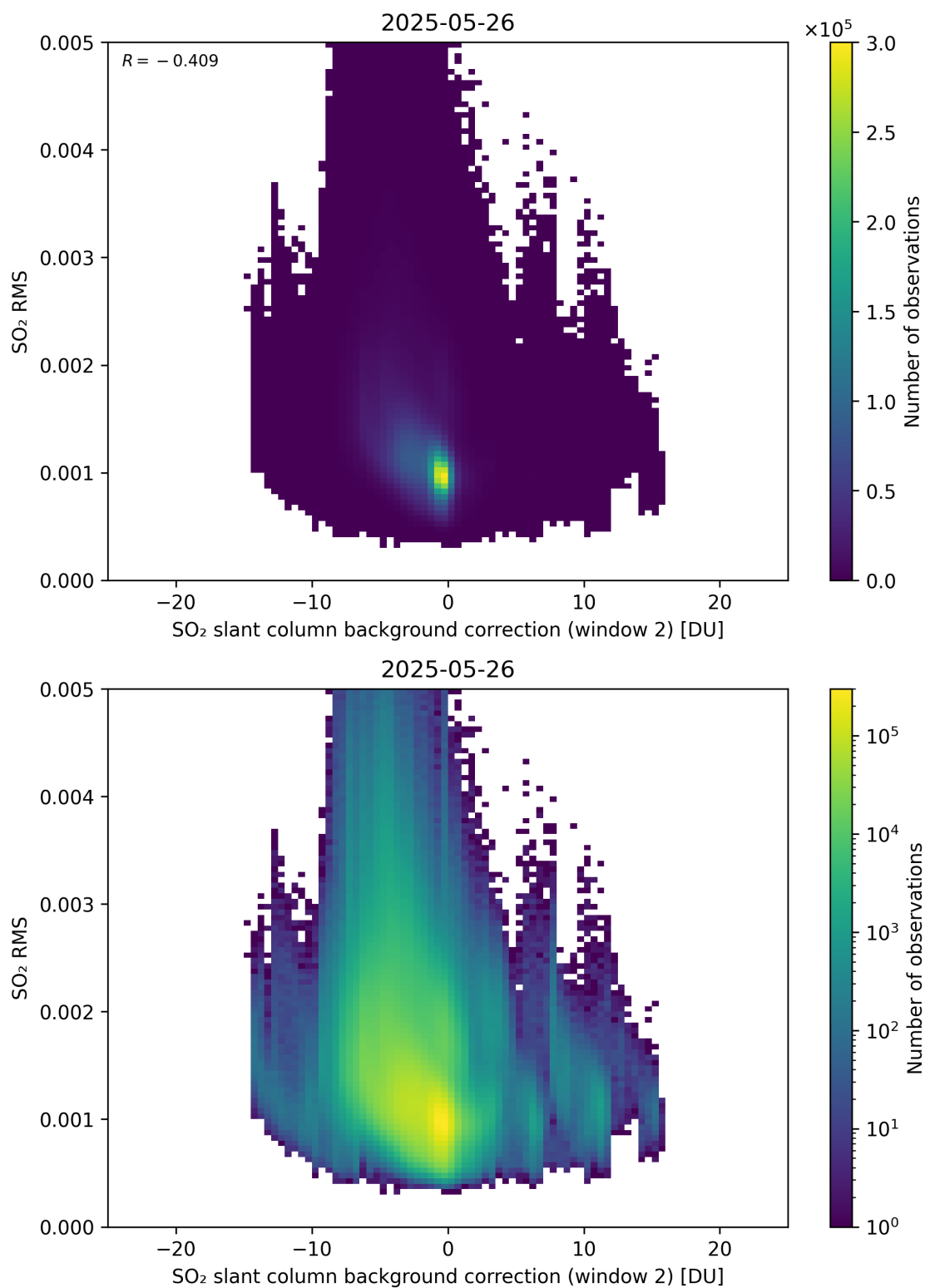
Figure 125: Scatter density plot of “SO 2 slant column background correction (window 2)” against “SO 2 RMS” for 2025-05-26 to 2025-05-27.
