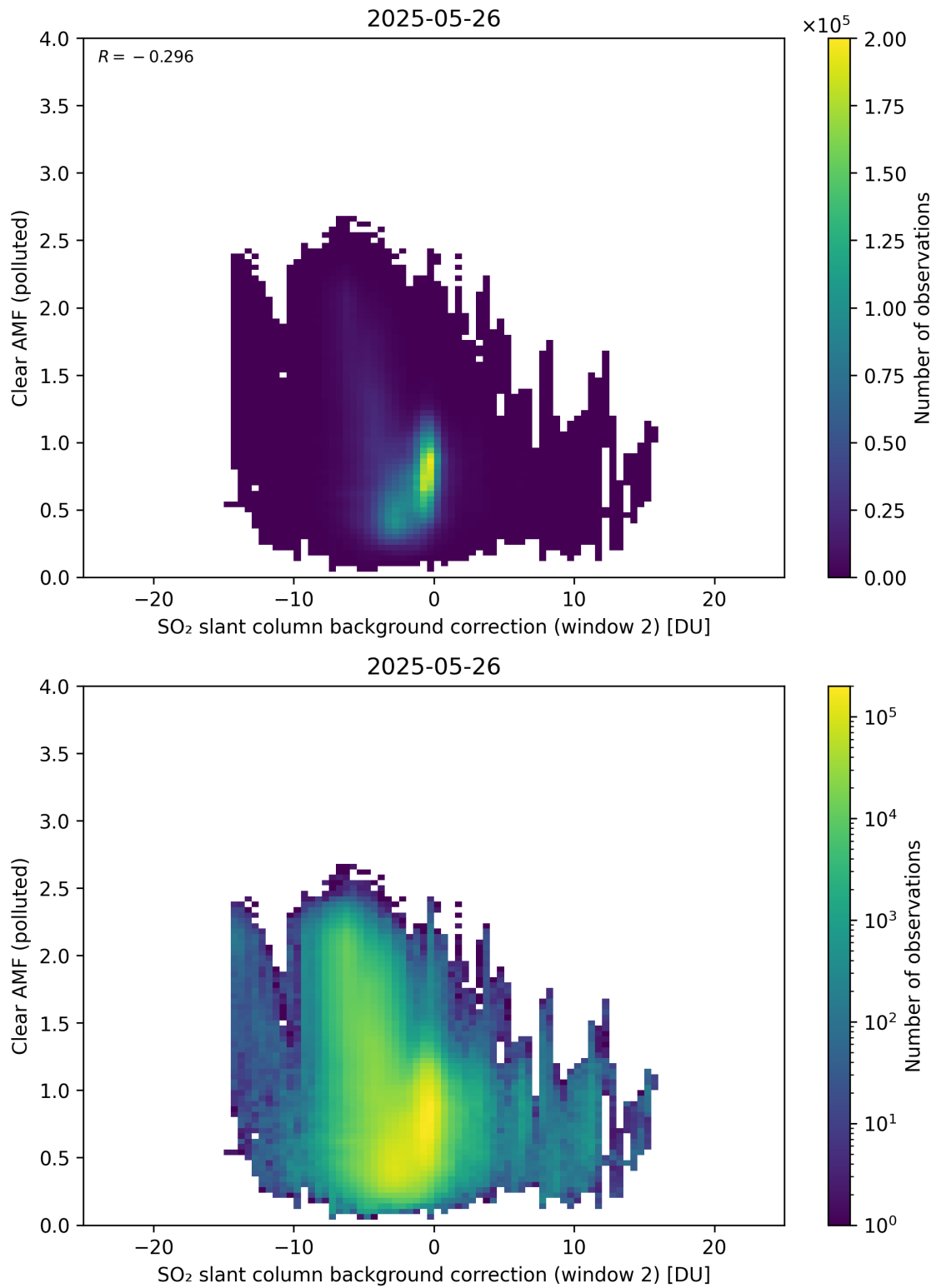
Figure 126: Scatter density plot of “SO 2 slant column background correction (window 2)” against “Clear AMF (polluted)” for 2025-05-26 to 2025-05-27.
