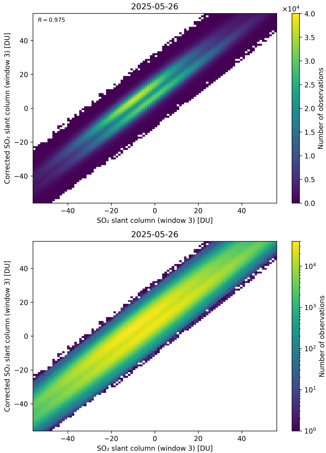
Figure 316: Scatter density plot of “SO 2 slant column (window 3)” against “Corrected SO 2 slant column (window 3)” for 2025-05-26 to 2025-05-27.
