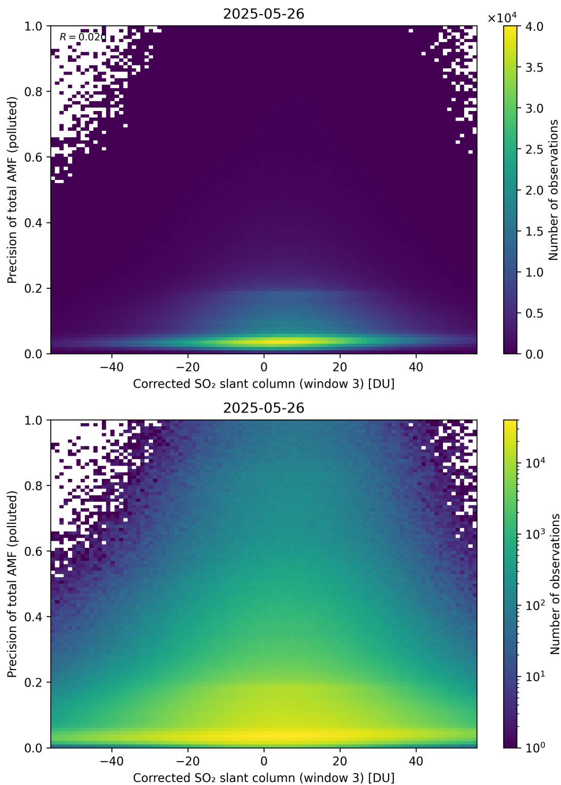
Figure 261: Scatter density plot of “Corrected SO 2 slant column (window 3)” against “Precision of total AMF (polluted)” for 2025-05-26 to 2025-05-27.
