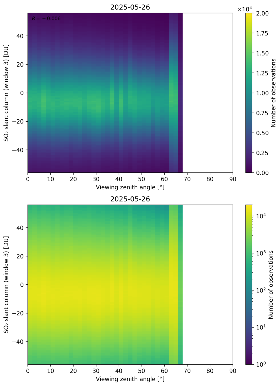
Figure 379: Scatter density plot of “Viewing zenith angle” against “SO 2 slant column (window 3)” for 2025-05-26 to 2025-05-27.
