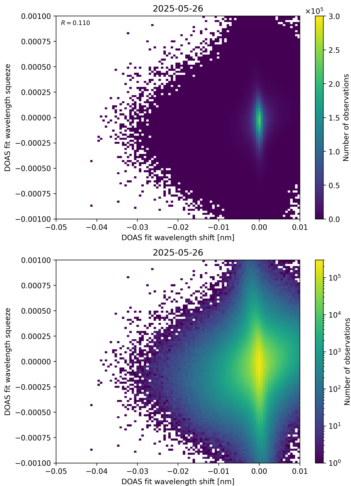
Figure 138: Scatter density plot of “DOAS fit wavelength shift” against “DOAS fit wavelength squeeze” for 2025-05-26 to 2025-05-27.
