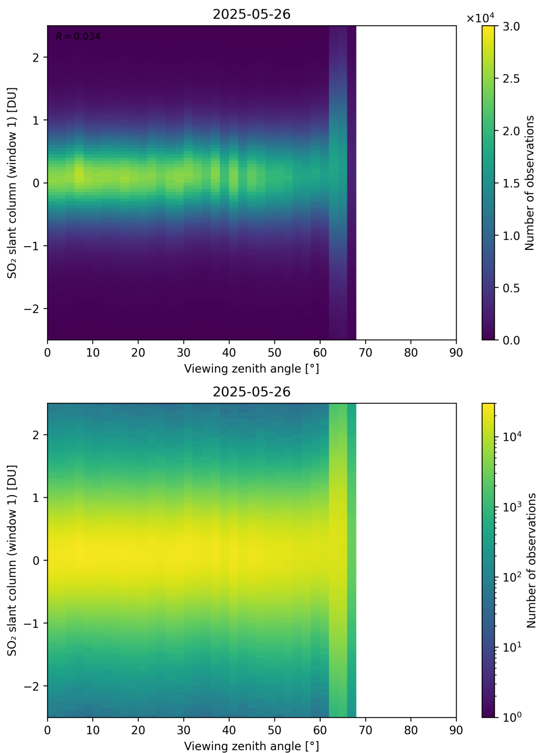
Figure 376: Scatter density plot of “Viewing zenith angle” against “SO 2 slant column (window 1)” for 2025-05-26 to 2025-05-27.
