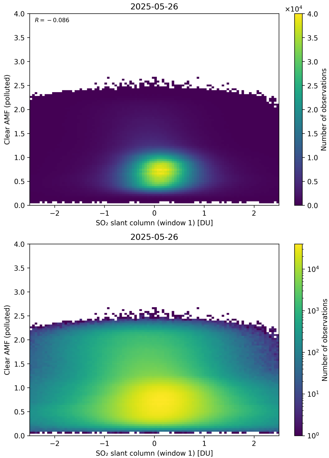
Figure 282: Scatter density plot of “SO 2 slant column (window 1)” against “Clear AMF (polluted)” for 2025-05-26 to 2025-05-27.
