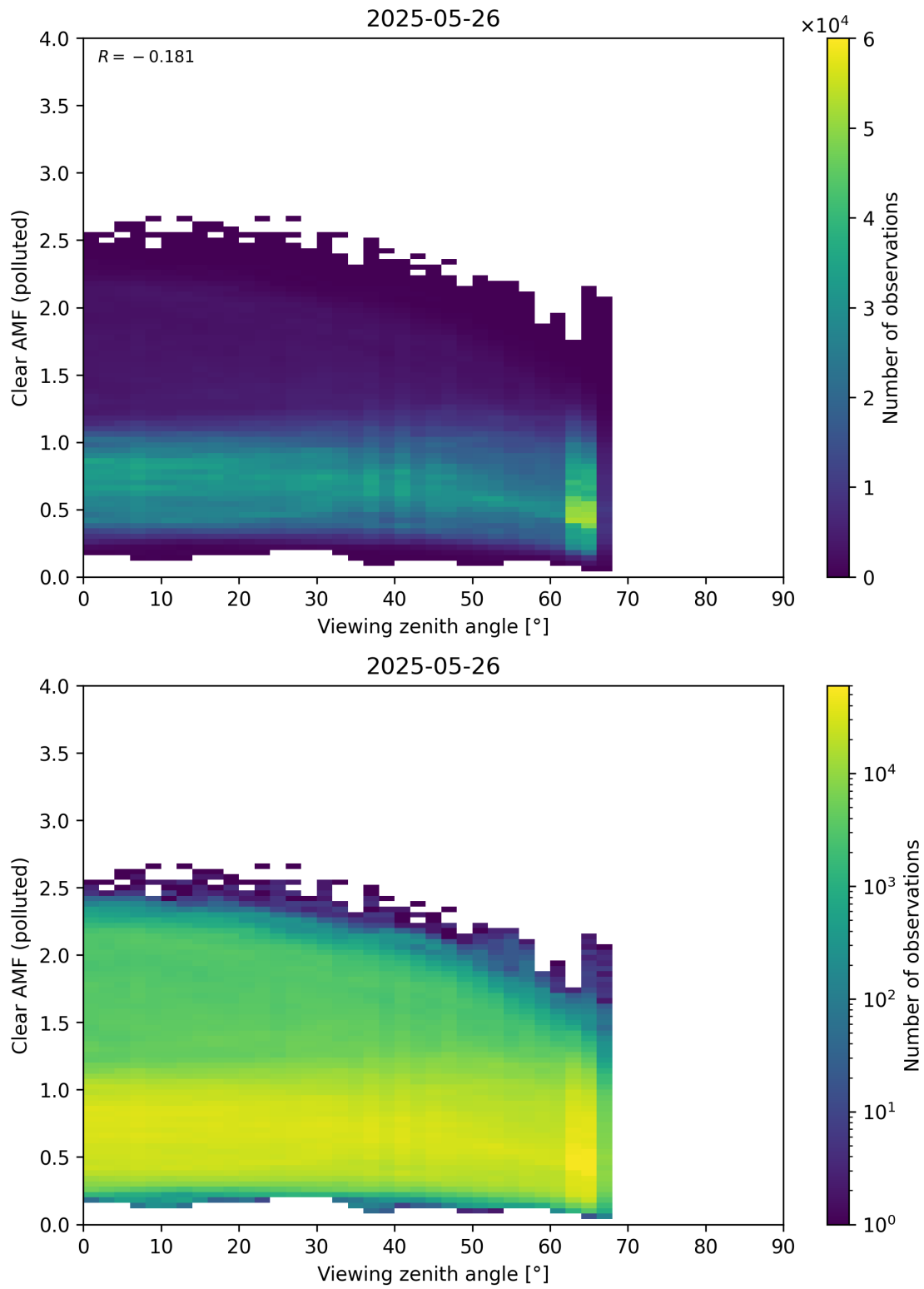
Figure 370: Scatter density plot of “Viewing zenith angle” against “Clear AMF (polluted)” for 2025-05-26 to 2025-05-27.
