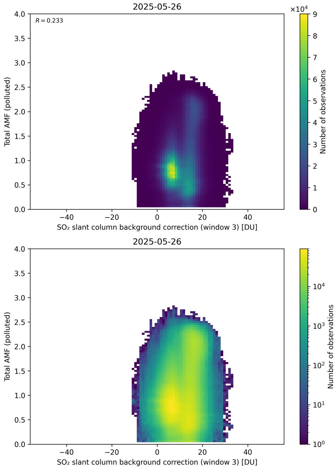
Figure 136: Scatter density plot of “SO 2 slant column background correction (window 3)” against “Total AMF (polluted)” for 2025-05-26 to 2025-05-27.
