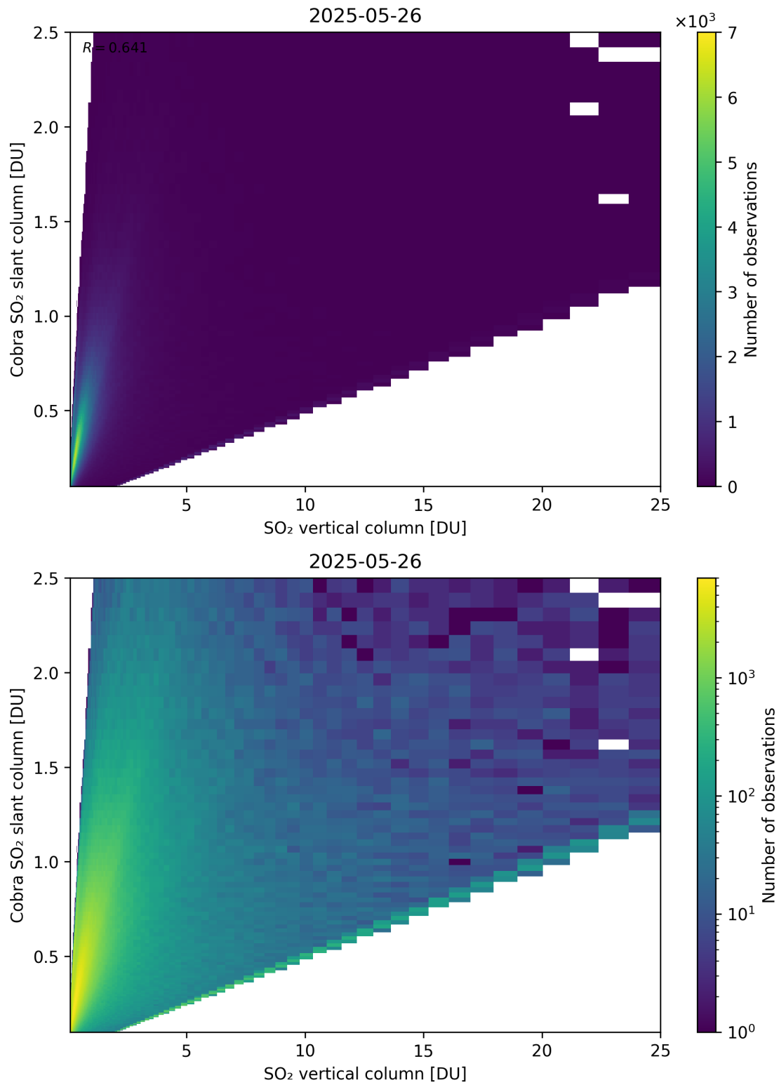
Figure 349: Scatter density plot of “SO 2 vertical column” against “Cobra SO 2 slant column” for 2025-05-26 to 2025-05-27.
