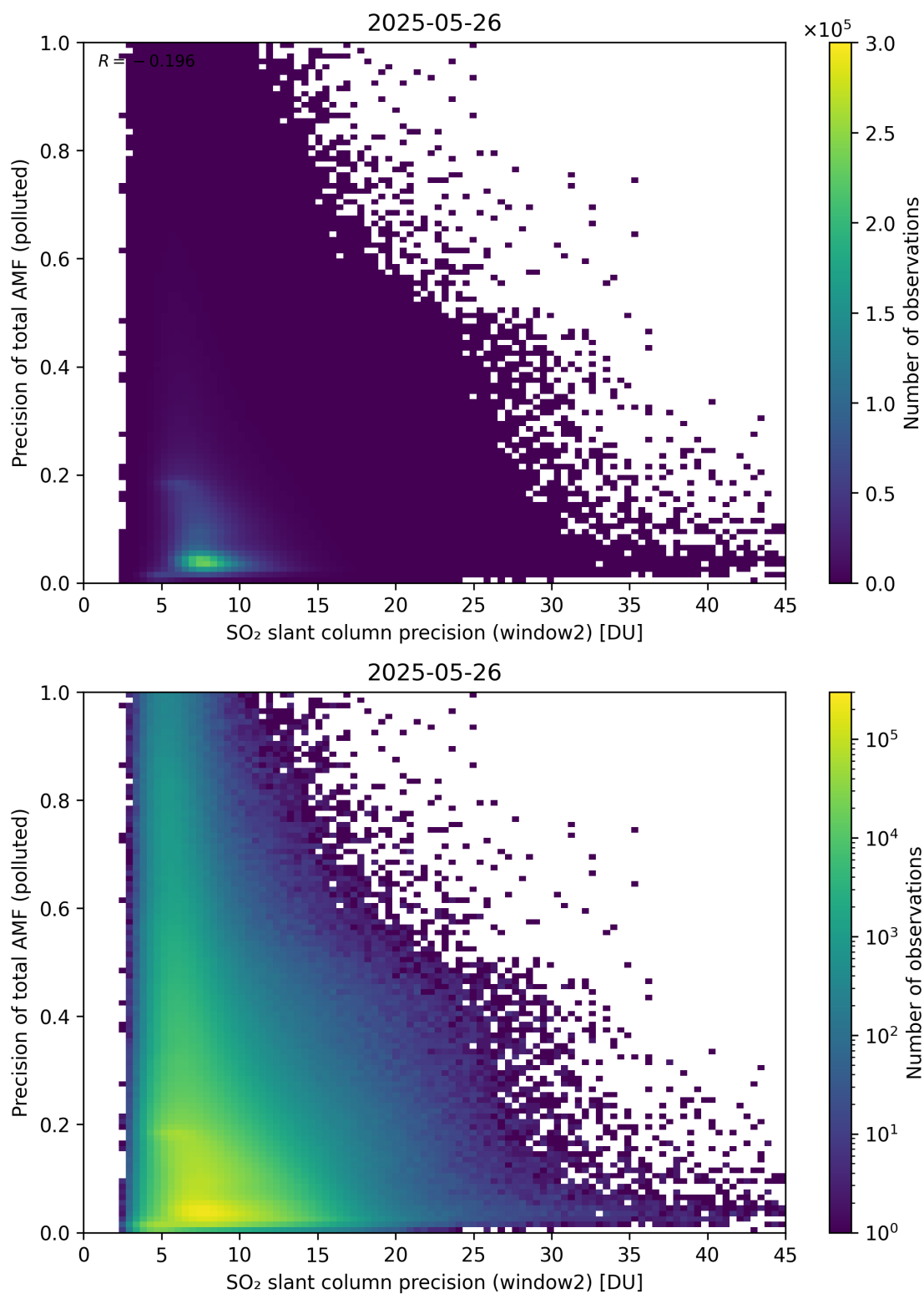
Figure 302: Scatter density plot of “SO 2 slant column precision (window2)” against “Precision of total AMF (polluted)” for 2025-05-26 to 2025-05-27.
