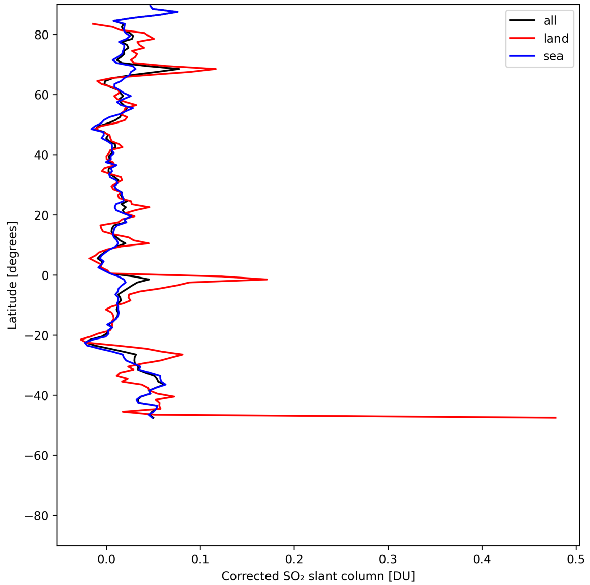
Figure 34: Zonal average of “Corrected SO 2 slant column” for 2025-05-26 to 2025-05-27.
