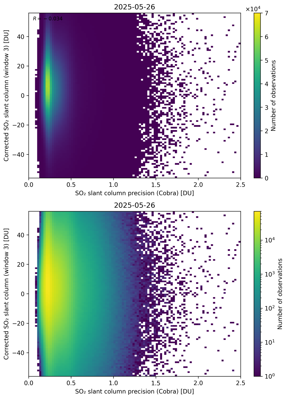
Figure 207: Scatter density plot of “SO 2 slant column precision (Cobra)” against “Corrected SO 2 slant column (window 3)” for 2025-05-26 to 2025-05-27.
