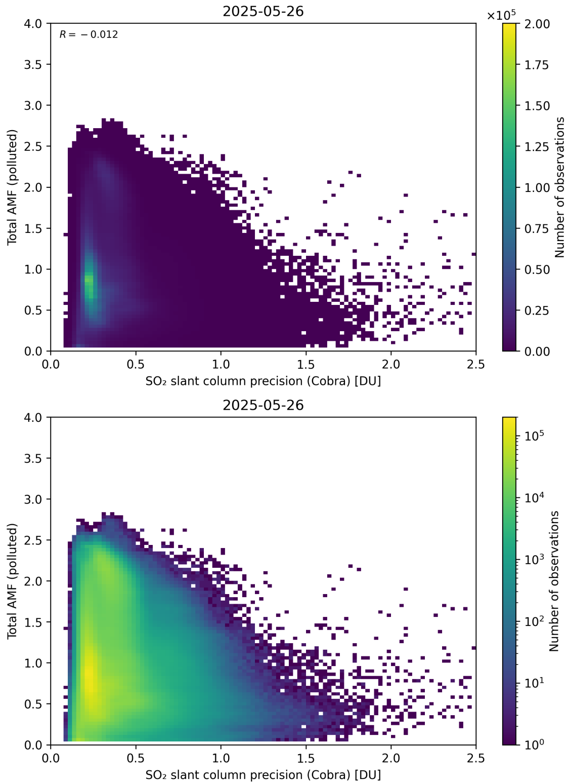
Figure 213: Scatter density plot of “SO 2 slant column precision (Cobra)” against “Total AMF (polluted)” for 2025-05-26 to 2025-05-27.
