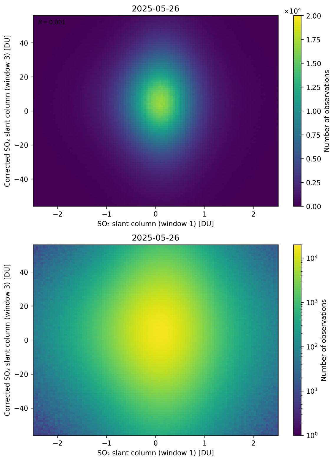
Figure 284: Scatter density plot of “SO 2 slant column (window 1)” against “Corrected SO 2 slant column (window 3)” for 2025-05-26 to 2025-05-27.
