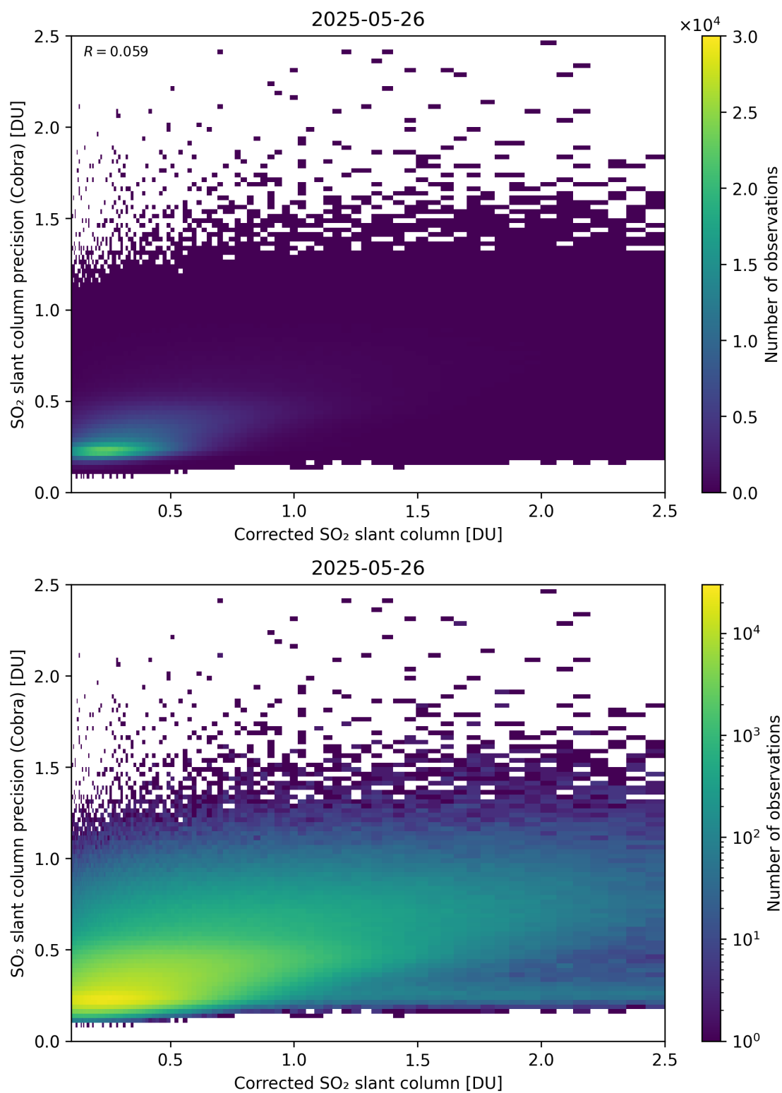
Figure 234: Scatter density plot of “Corrected SO 2 slant column” against “SO 2 slant column precision (Cobra)” for 2025-05-26 to 2025-05-27.
