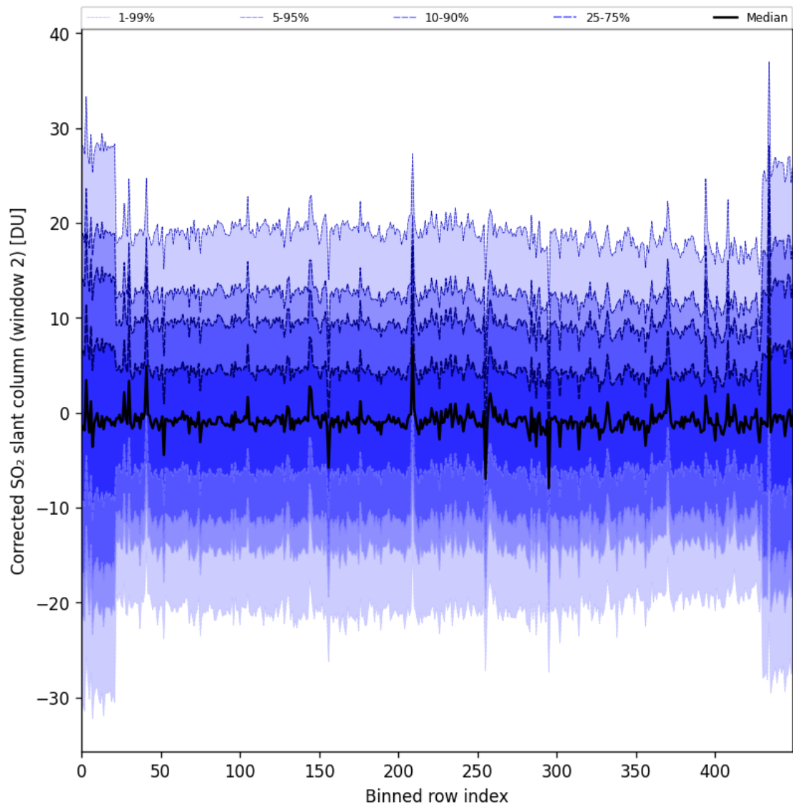
Figure 95: Along track statistics of “Corrected SO 2 slant column (window 2)” for 2025-05-26 to 2025-05-27
