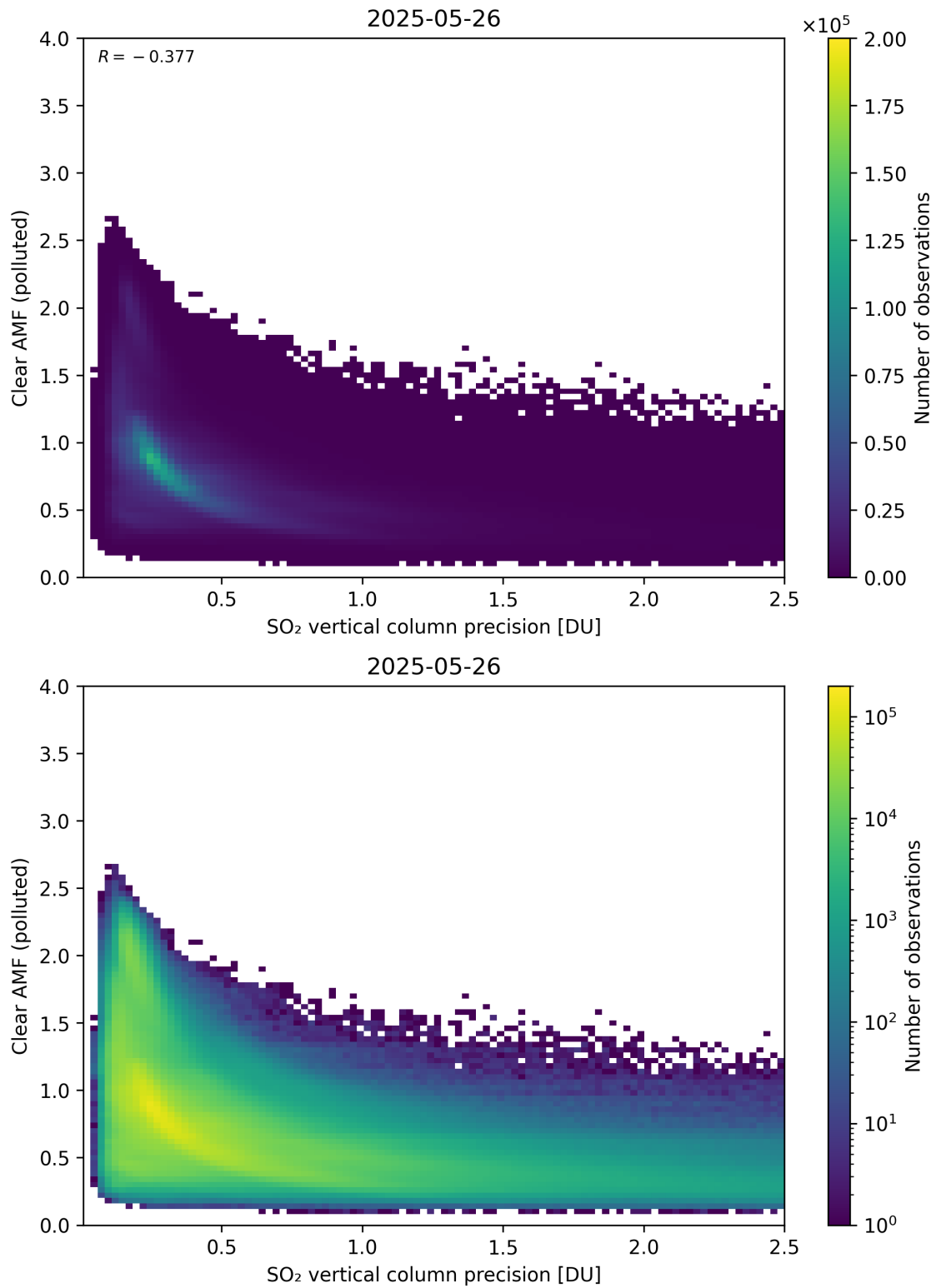
Figure 335: Scatter density plot of “SO 2 vertical column precision” against “Clear AMF (polluted)” for 2025-05-26 to 2025-05-27.
