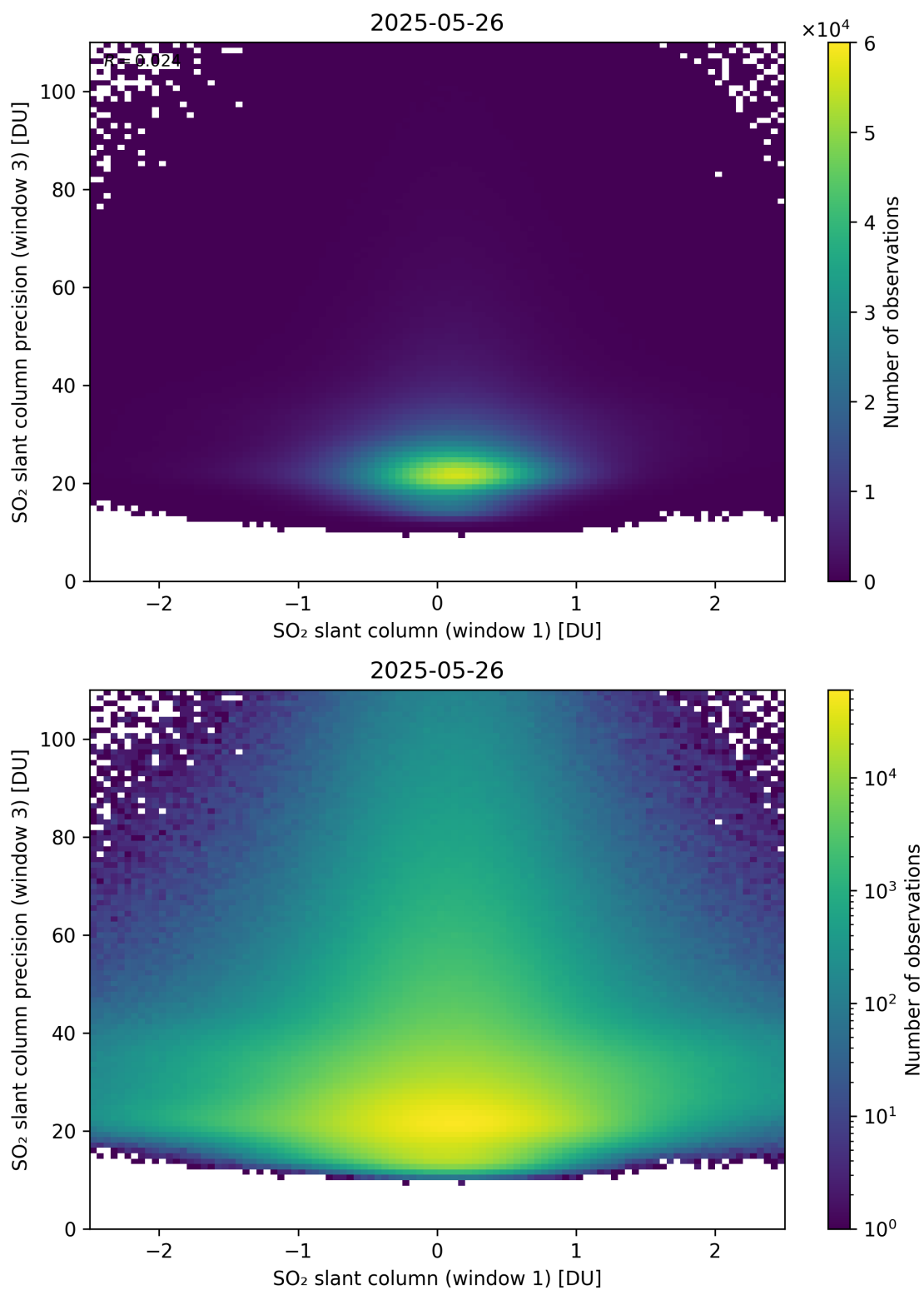
Figure 288: Scatter density plot of “SO 2 slant column (window 1)” against “SO 2 slant column precision (window 3)” for 2025-05-26 to 2025-05-27.
