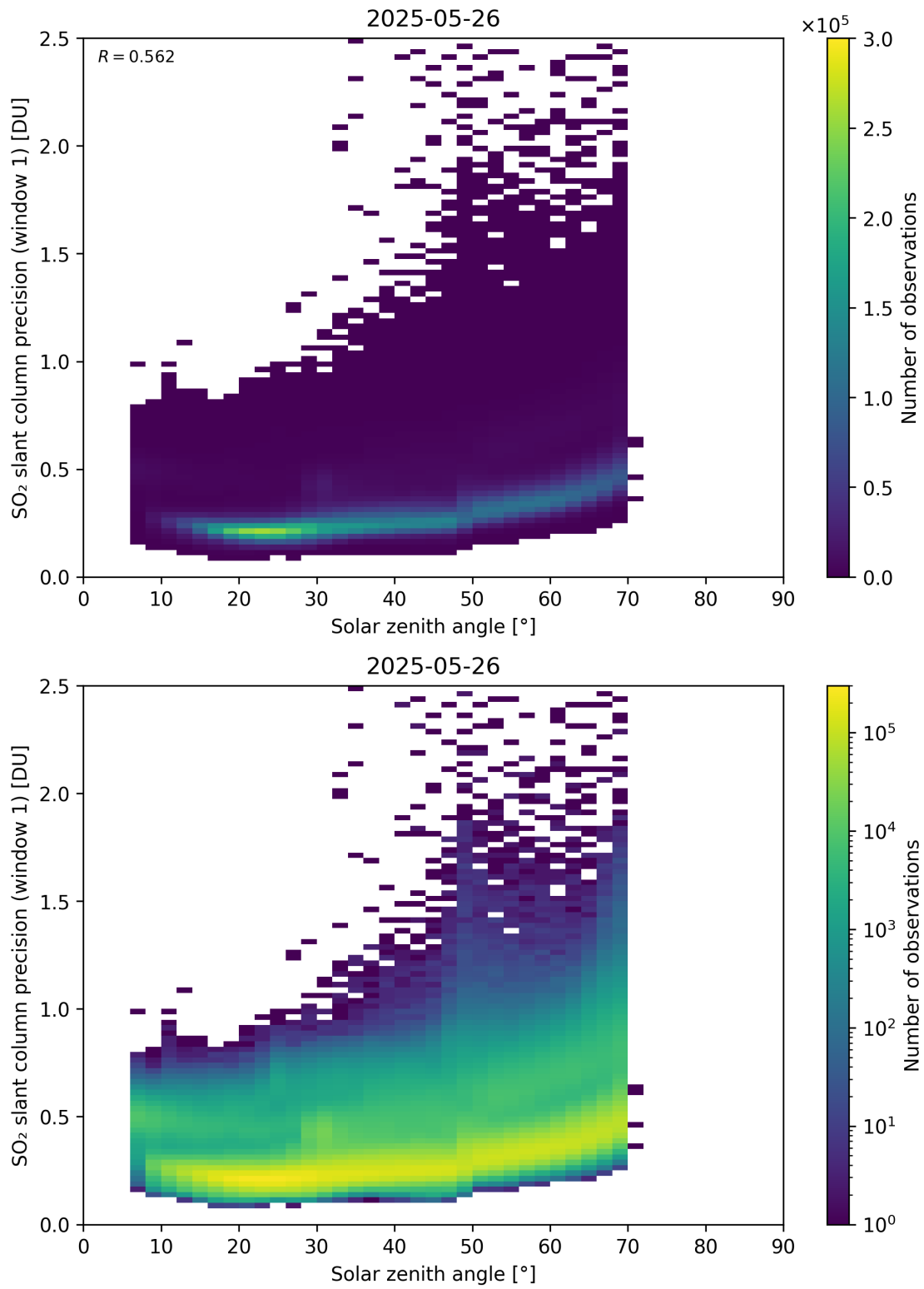
Figure 185: Scatter density plot of “Solar zenith angle” against “SO 2 slant column precision (window 1)” for 2025-05-26 to 2025-05-27.
