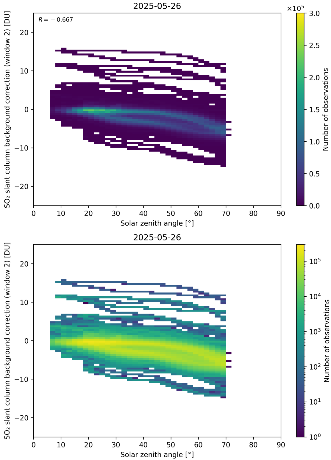
Figure 172: Scatter density plot of “Solar zenith angle” against “SO 2 slant column background correction (window 2)” for 2025-05-26 to 2025-05-27.
