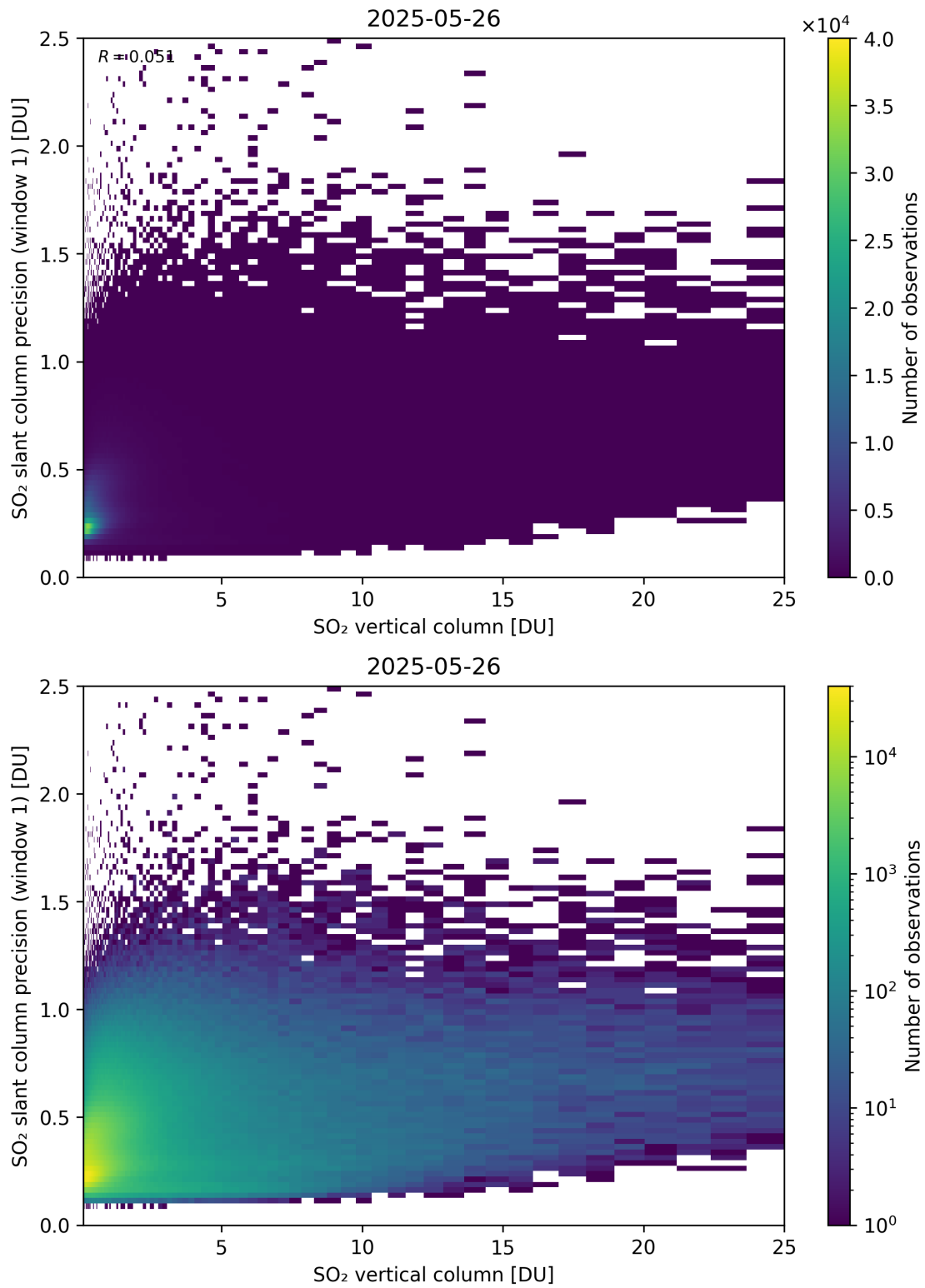
Figure 355: Scatter density plot of “SO 2 vertical column” against “SO 2 slant column precision (window 1)” for 2025-05-26 to 2025-05-27.
