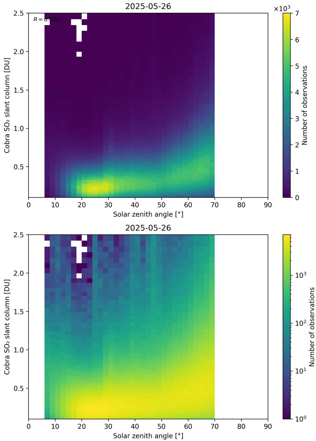
Figure 179: Scatter density plot of “Solar zenith angle” against “Cobra SO 2 slant column” for 2025-05-26 to 2025-05-27.
