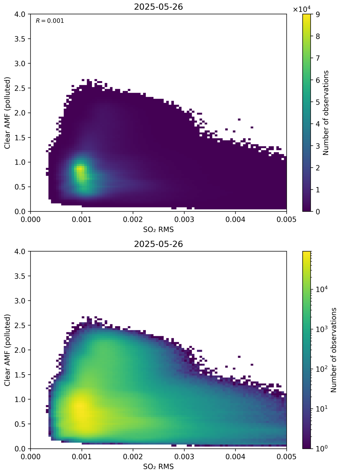
Figure 147: Scatter density plot of “SO 2 RMS” against “Clear AMF (polluted)” for 2025-05-26 to 2025-05-27.
