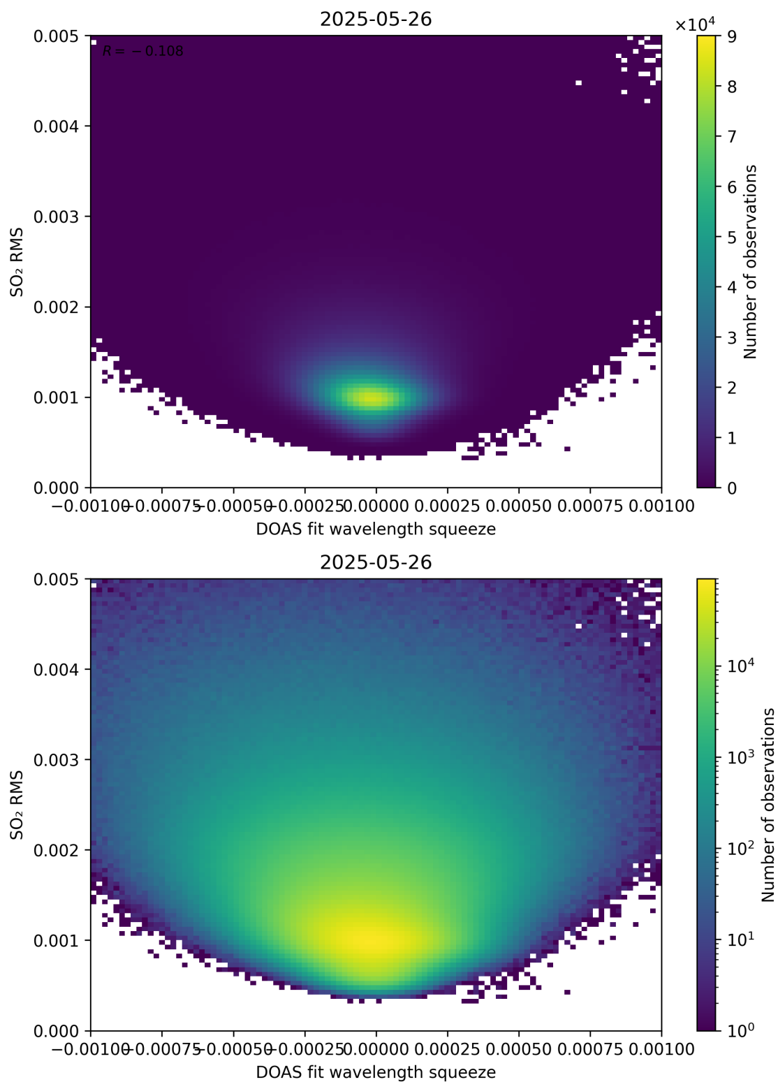
Figure 143: Scatter density plot of “DOAS fit wavelength squeeze” against “SO 2 RMS” for 2025-05-26 to 2025-05-27.
