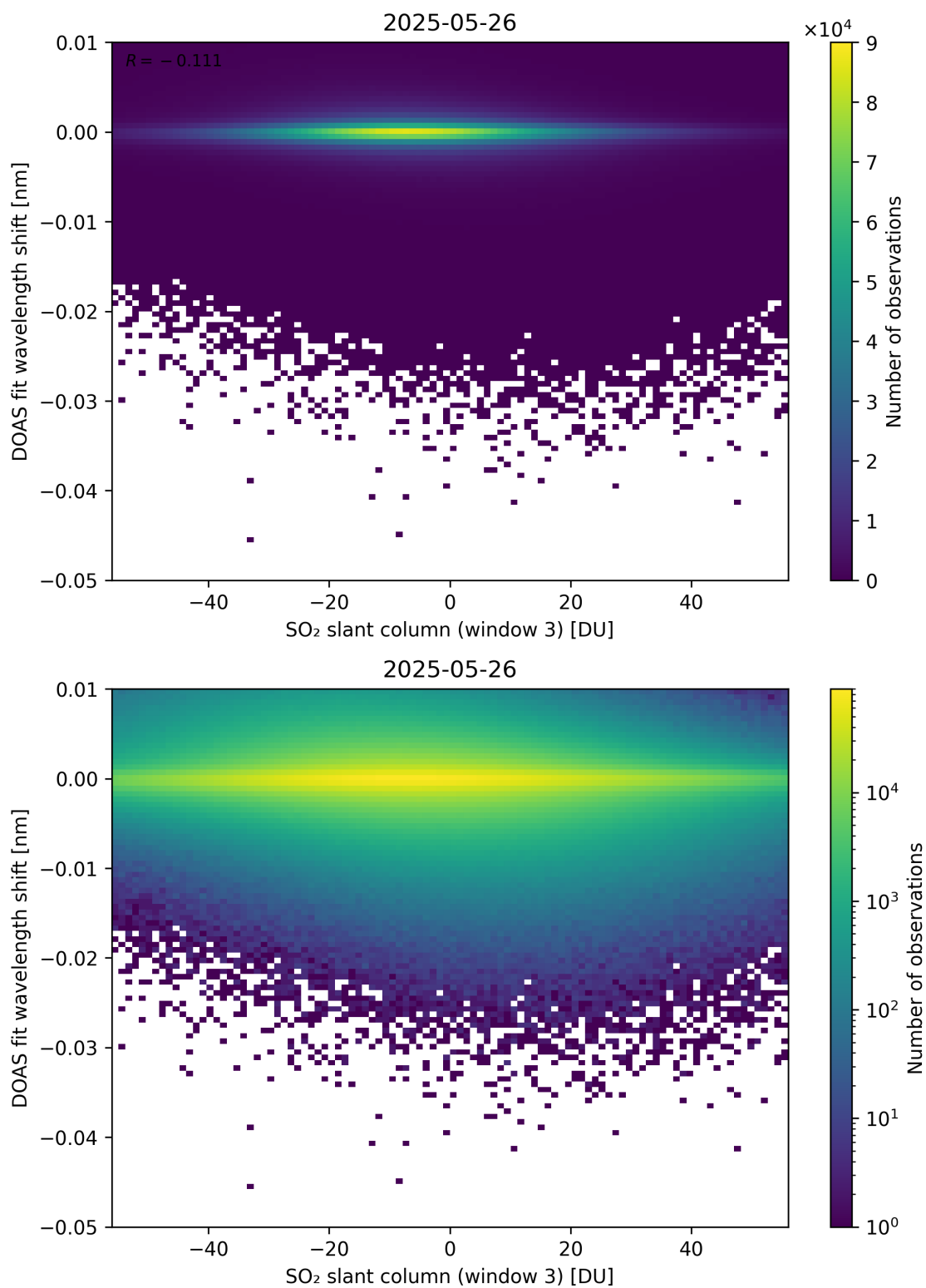
Figure 304: Scatter density plot of “SO 2 slant column (window 3)” against “DOAS fit wavelength shift” for 2025-05-26 to 2025-05-27.
