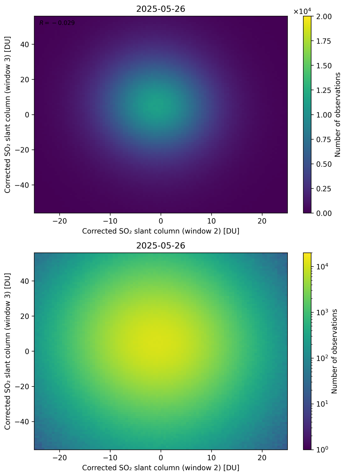
Figure 250: Scatter density plot of “Corrected SO 2 slant column (window 2)” against “Corrected SO 2 slant column (window 3)” for 2025-05-26 to 2025-05-27.
