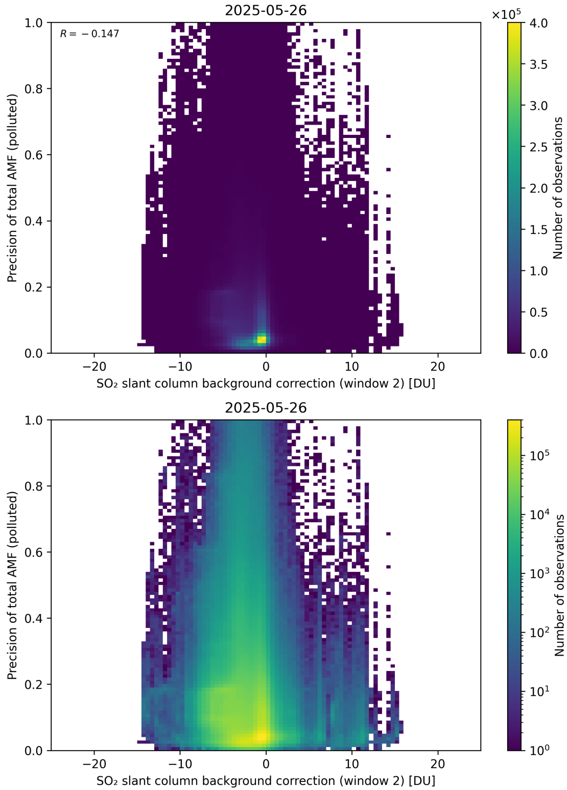
Figure 131: Scatter density plot of “SO 2 slant column background correction (window 2)” against “Precision of total AMF (polluted)” for 2025-05-26 to 2025-05-27.
