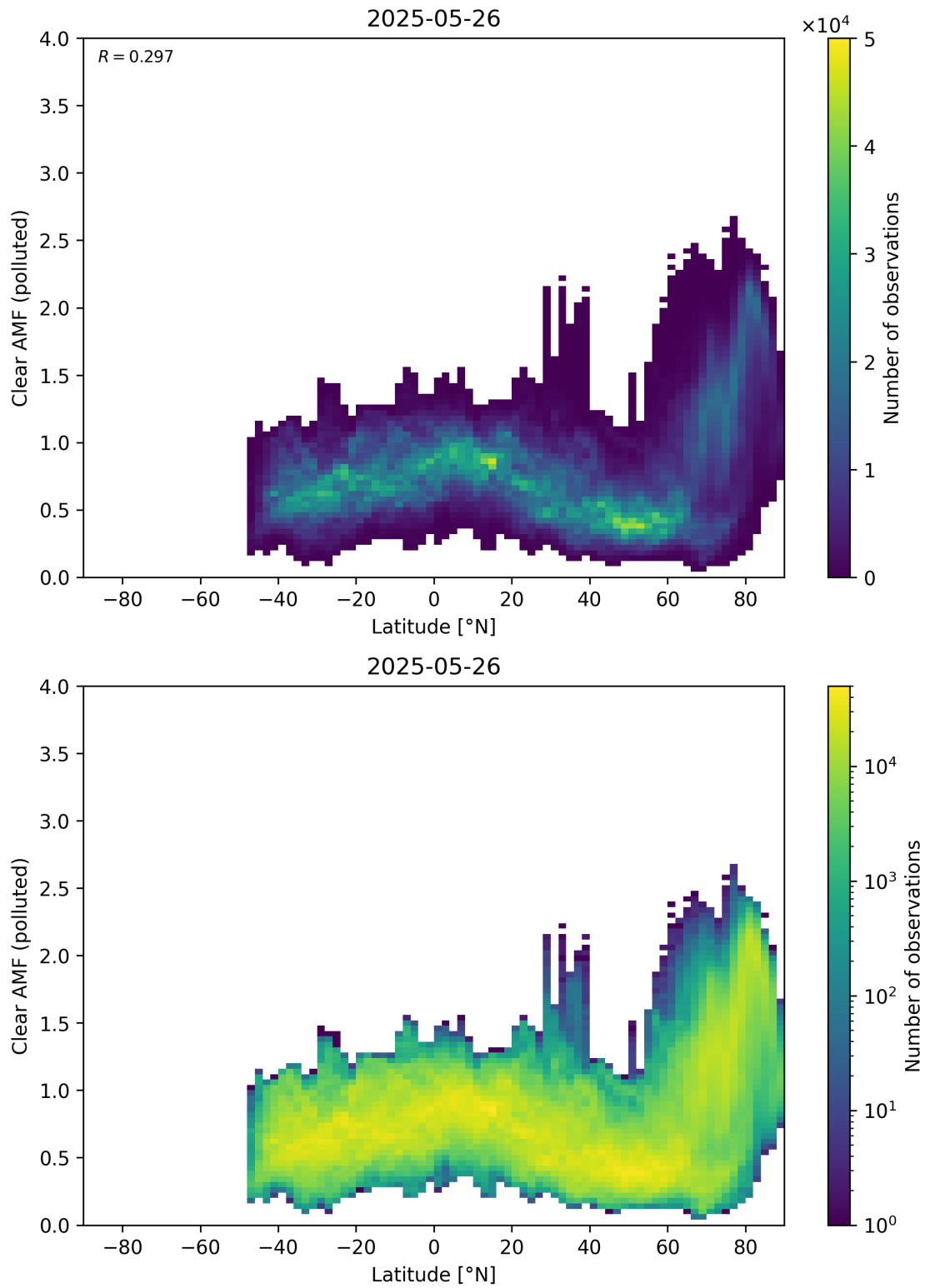
Figure 156: Scatter density plot of “Latitude” against “Clear AMF (polluted)” for 2025-05-26 to 2025-05-27.
