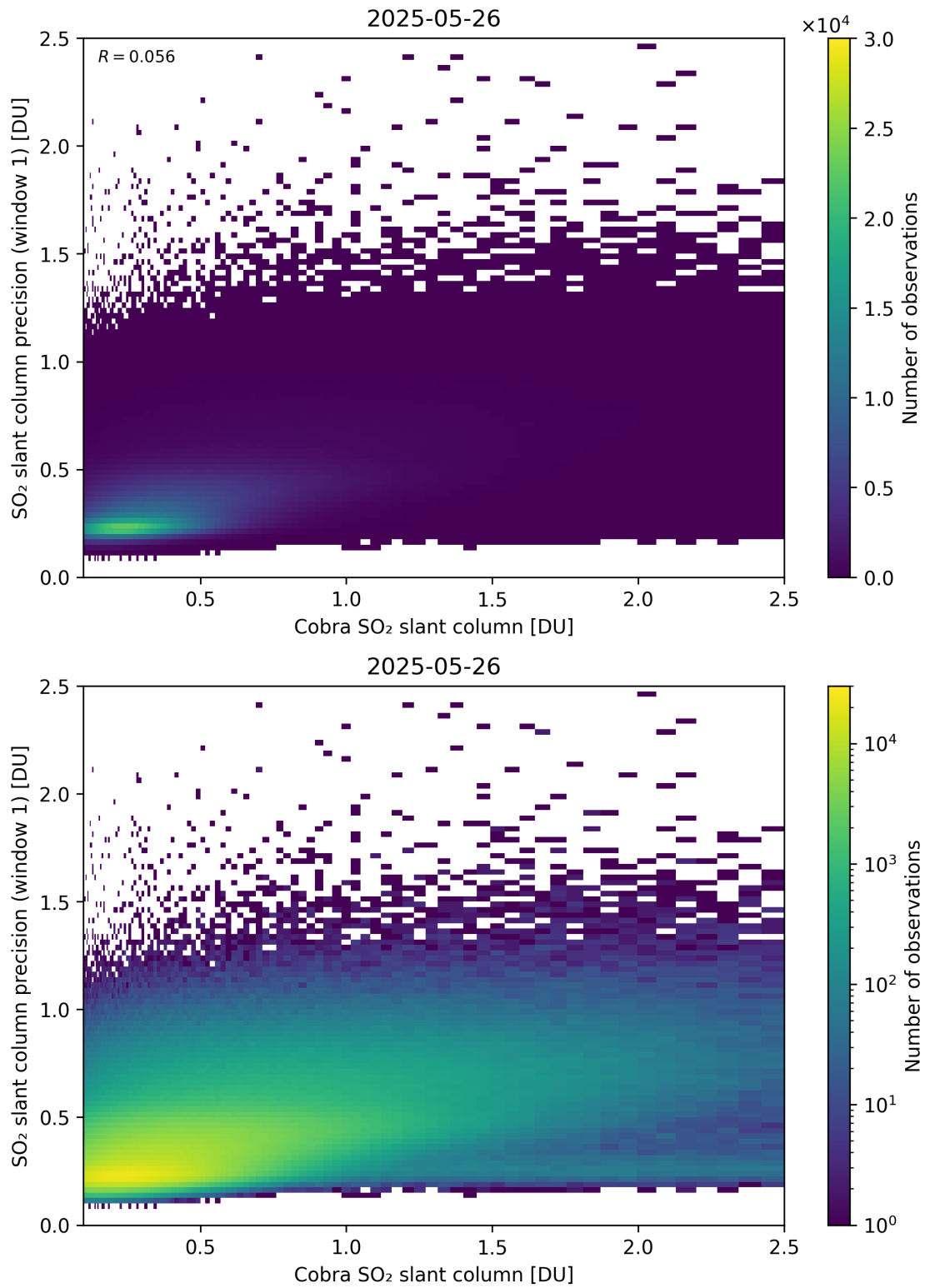
Figure 220: Scatter density plot of “Cobra SO 2 slant column” against “SO 2 slant column precision (window 1)” for 2025-05-26 to 2025-05-27.
