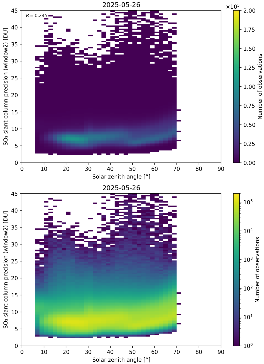
Figure 186: Scatter density plot of “Solar zenith angle” against “SO 2 slant column precision (window2)” for 2025-05-26 to 2025-05-27.
