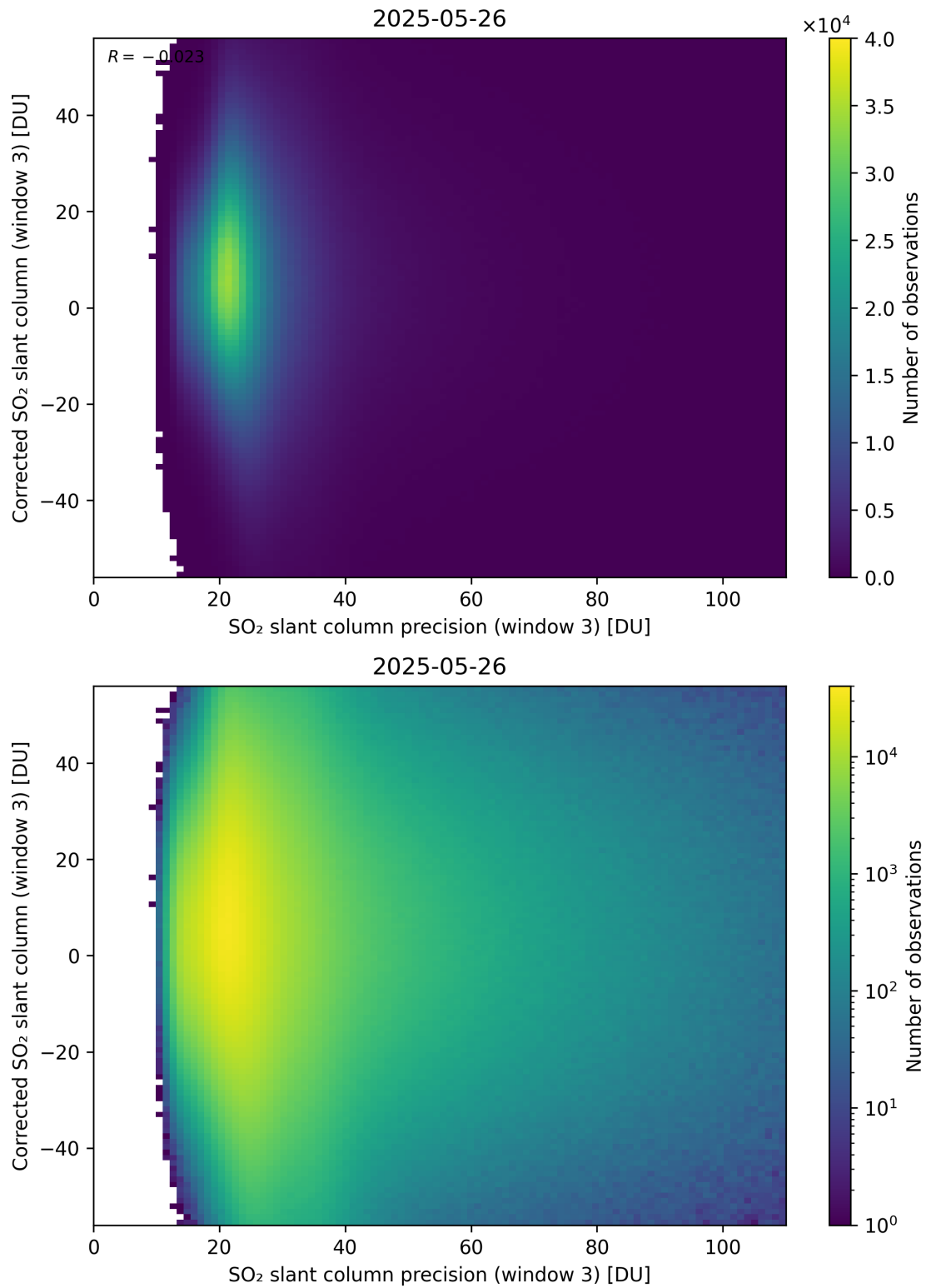
Figure 312: Scatter density plot of “SO 2 slant column precision (window 3)” against “Corrected SO 2 slant column (window 3)” for 2025-05-26 to 2025-05-27.
