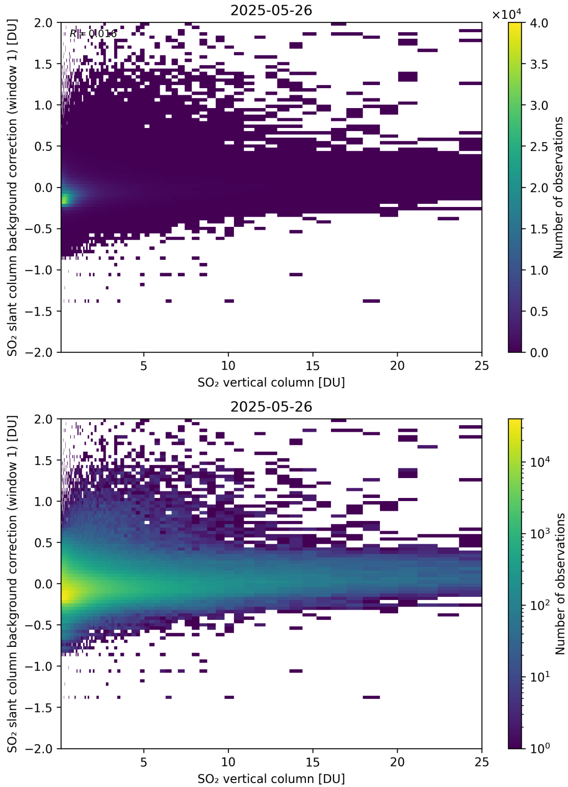
Figure 323: Scatter density plot of “SO 2 vertical column” against “SO 2 slant column background correction (window 1)” for 2025-05-26 to 2025-05-27.
