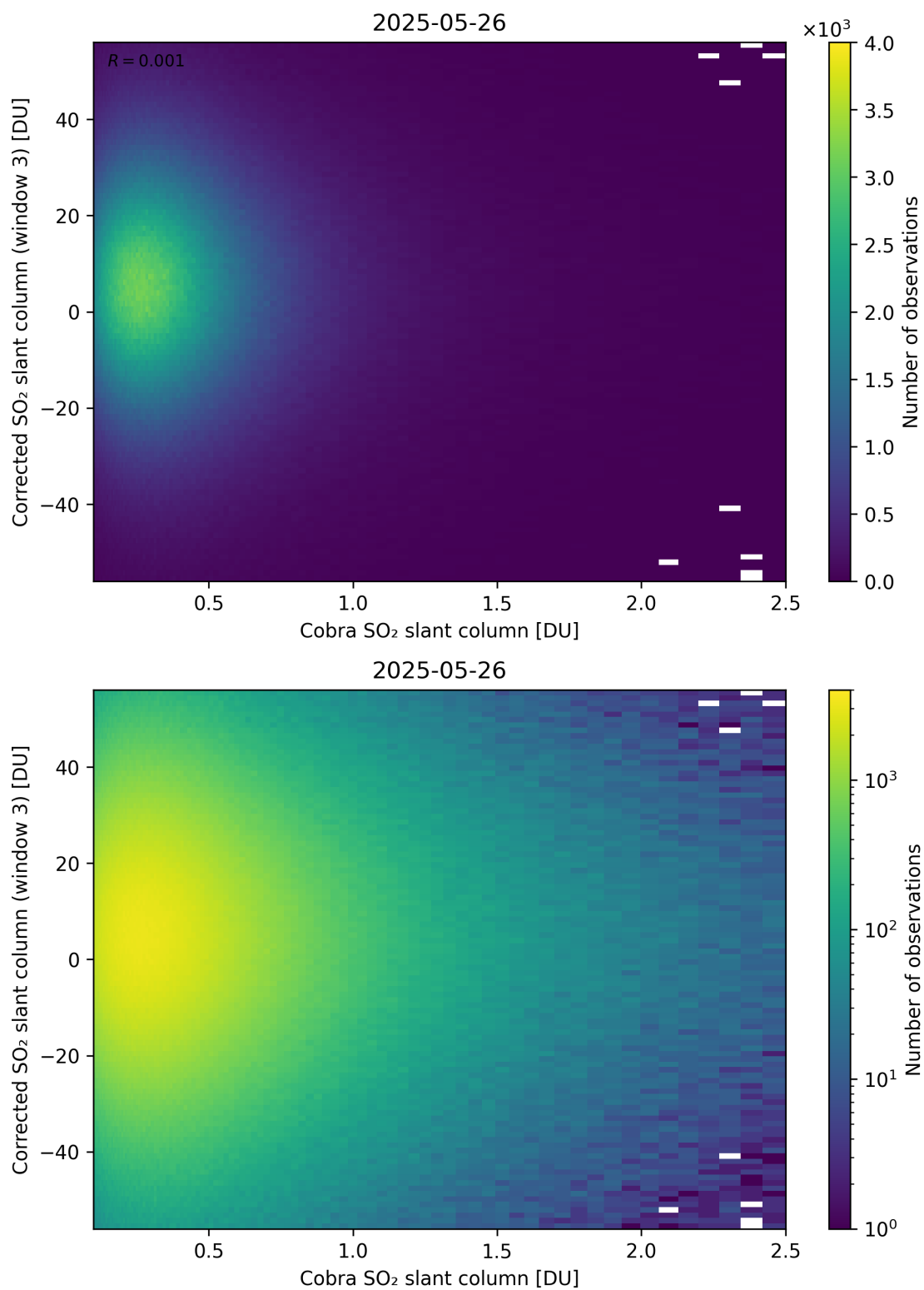
Figure 218: Scatter density plot of “Cobra SO 2 slant column” against “Corrected SO 2 slant column (window 3)” for 2025-05-26 to 2025-05-27.
