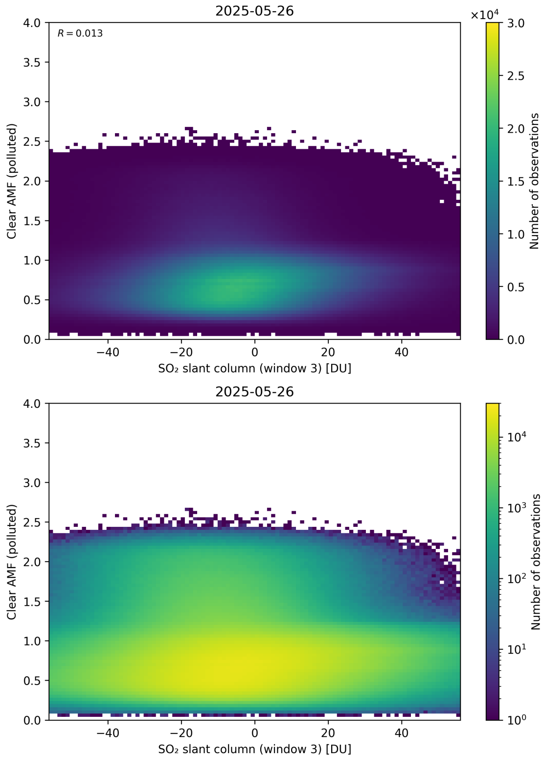
Figure 315: Scatter density plot of “SO 2 slant column (window 3)” against “Clear AMF (polluted)” for 2025-05-26 to 2025-05-27.
