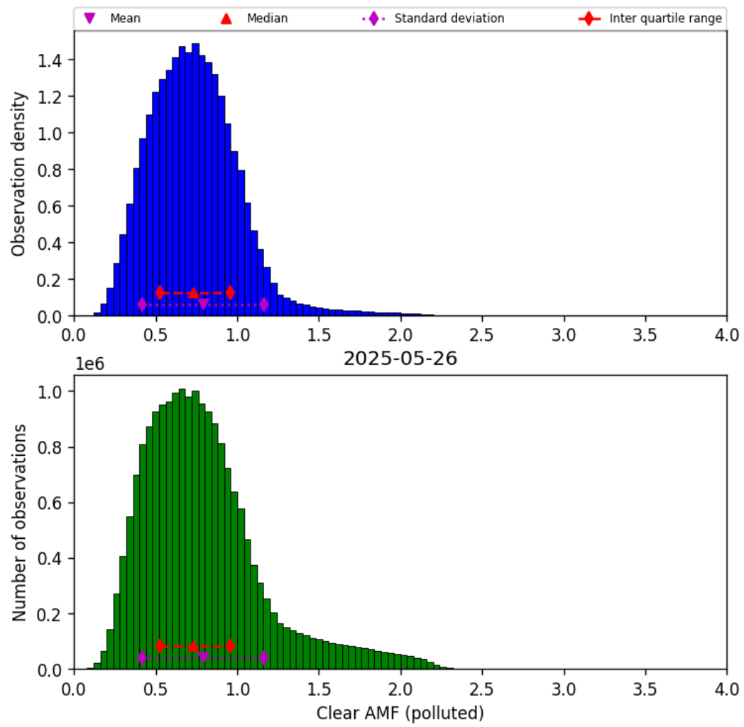
Figure 81: Histogram of “Clear AMF (polluted)” for 2025-05-26 to 2025-05-27
