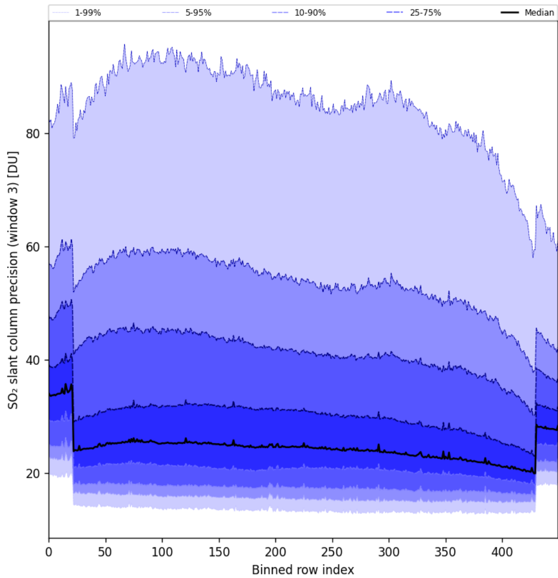
Figure 98: Along track statistics of “SO 2 slant column precision (window 3)” for 2025-05-26 to 2025-05-27
