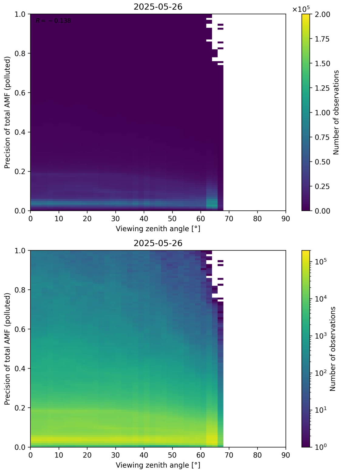
Figure 382: Scatter density plot of “Viewing zenith angle” against “Precision of total AMF (polluted)” for 2025-05-26 to 2025-05-27.
