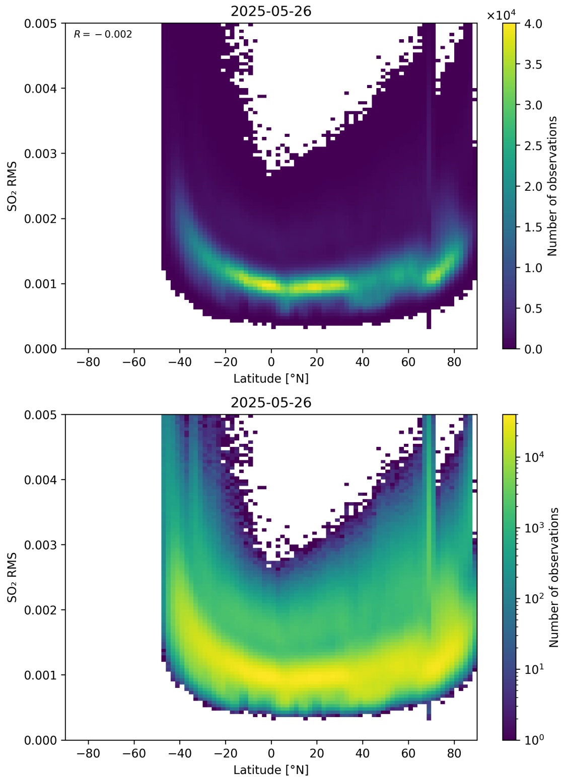
Figure 155: Scatter density plot of “Latitude” against “SO 2 RMS” for 2025-05-26 to 2025-05-27.
