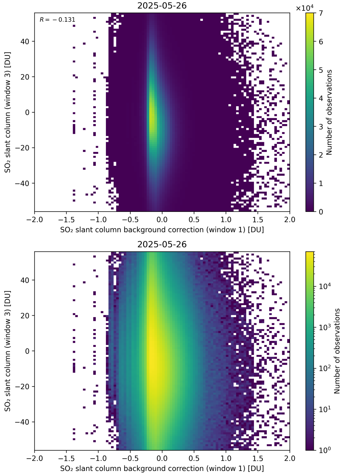
Figure 118: Scatter density plot of “SO 2 slant column background correction (window 1)” against “SO 2 slant column (window 3)” for 2025-05-26 to 2025-05-27.
