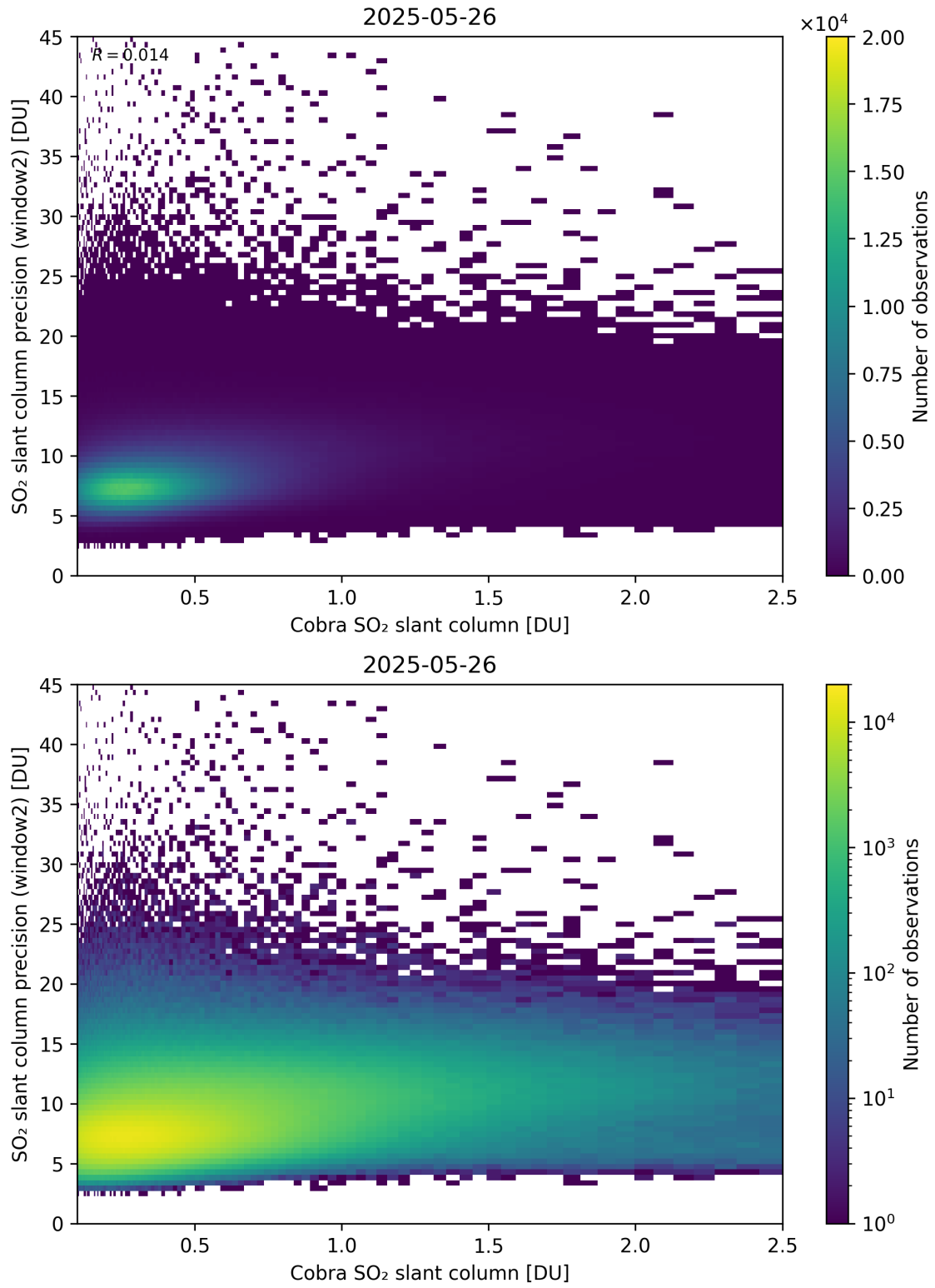
Figure 221: Scatter density plot of “Cobra SO 2 slant column” against “SO 2 slant column precision (window2)” for 2025-05-26 to 2025-05-27.
