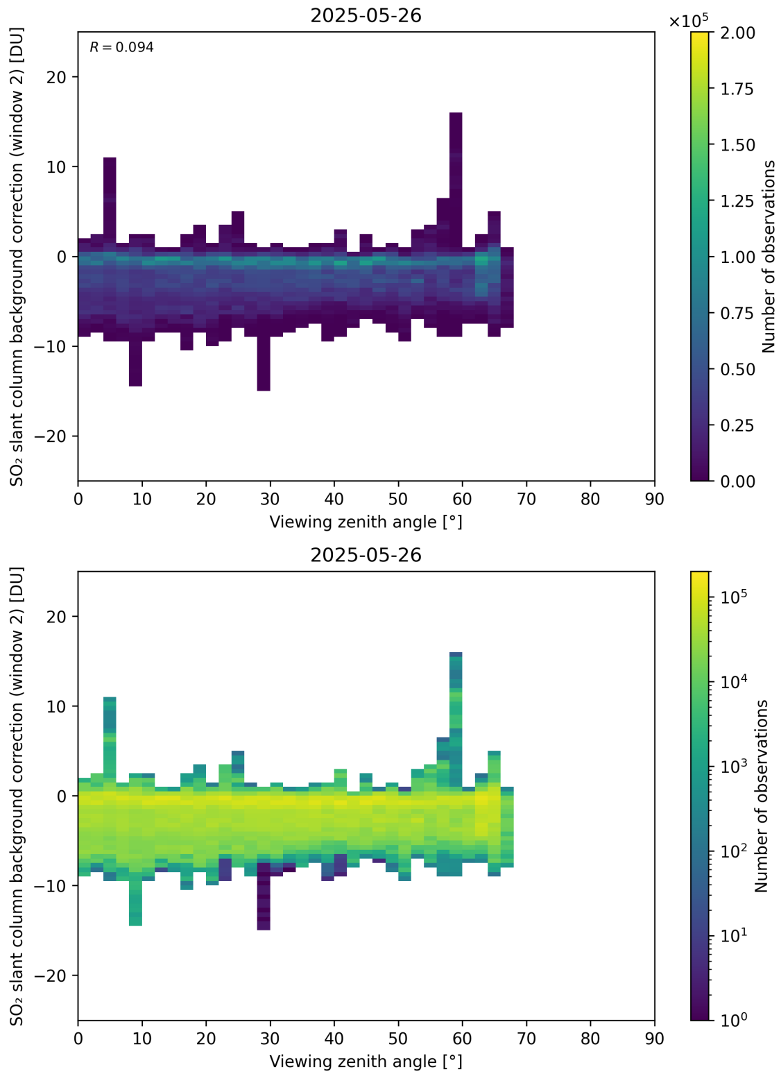
Figure 363: Scatter density plot of “Viewing zenith angle” against “SO 2 slant column background correction (window 2)” for 2025-05-26 to 2025-05-27.
