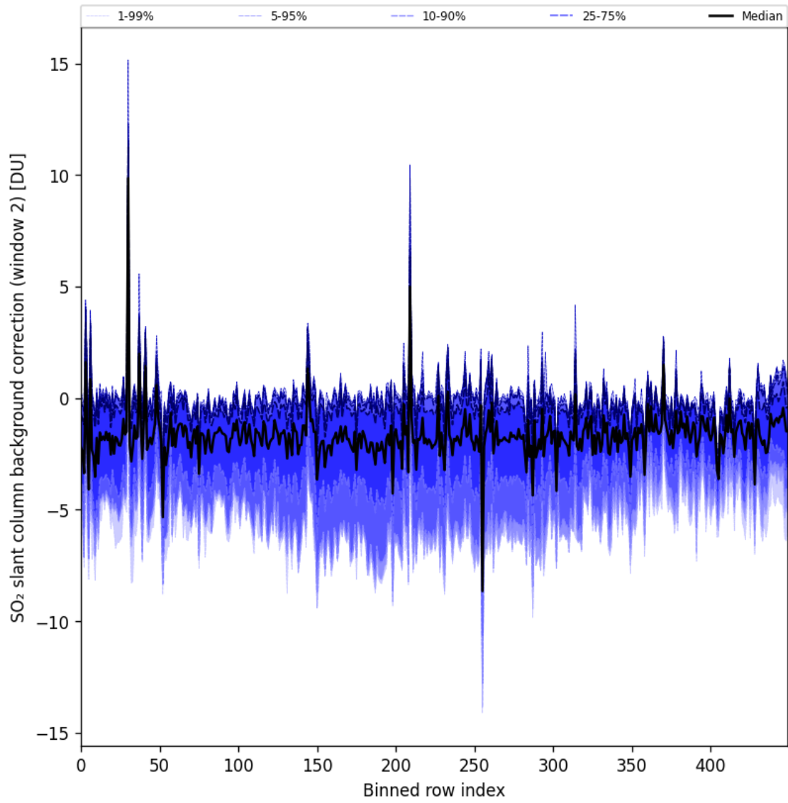
Figure 96: Along track statistics of “SO 2 slant column background correction (window 2)” for 2025-05-26 to 2025-05-27
