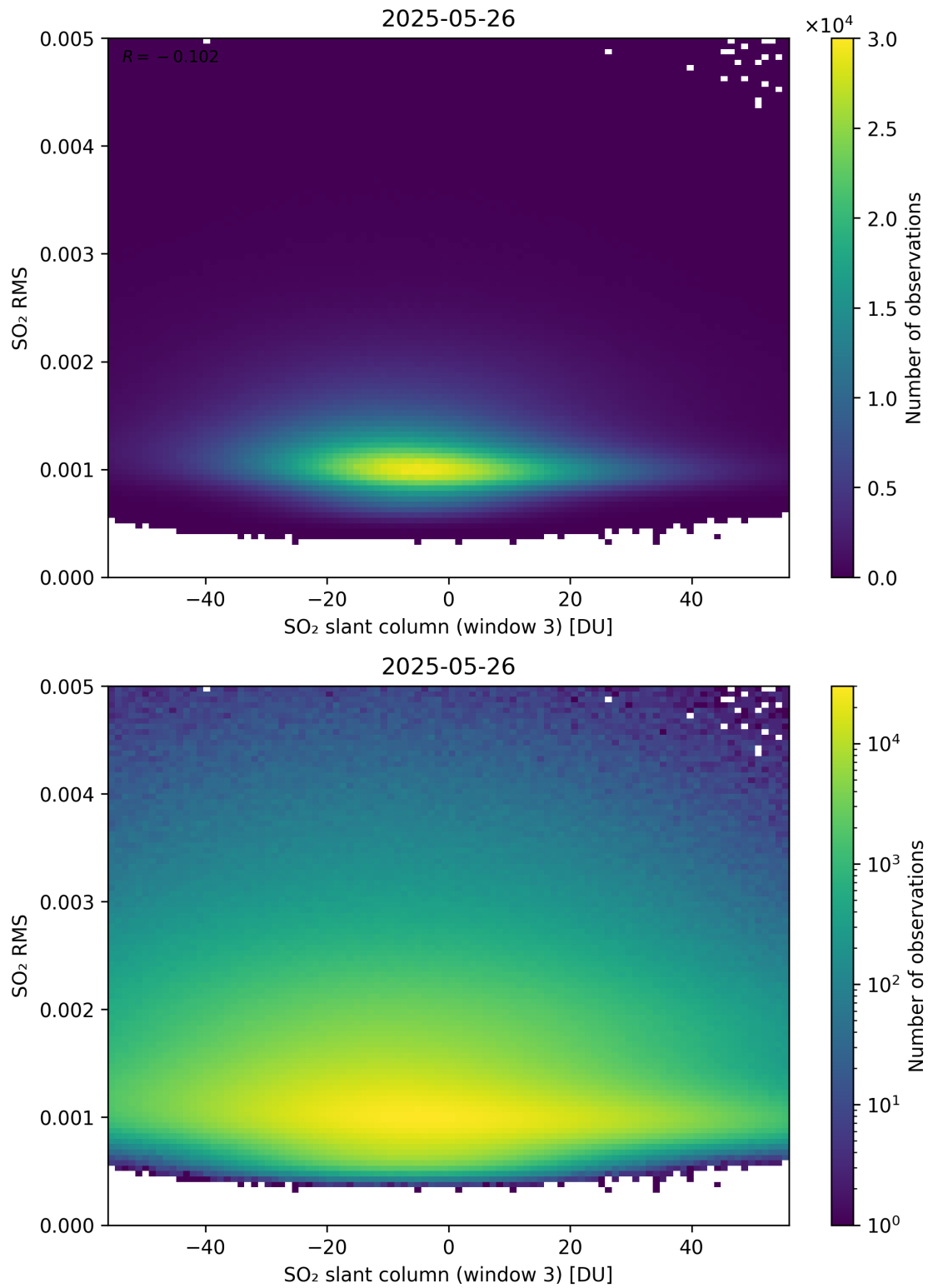
Figure 306: Scatter density plot of “SO 2 slant column (window 3)” against “SO 2 RMS” for 2025-05-26 to 2025-05-27.
