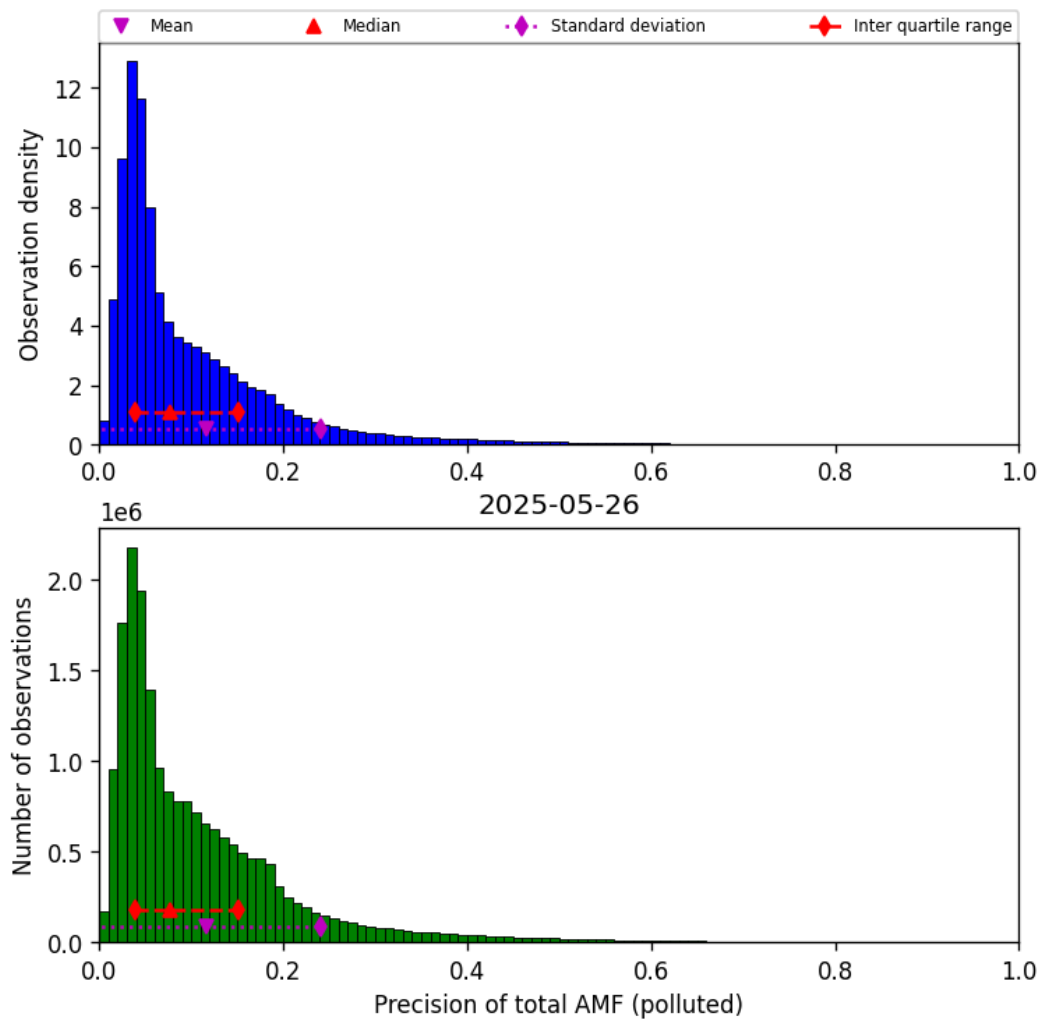
Figure 80: Histogram of “Precision of total AMF (polluted)” for 2025-05-26 to 2025-05-27
