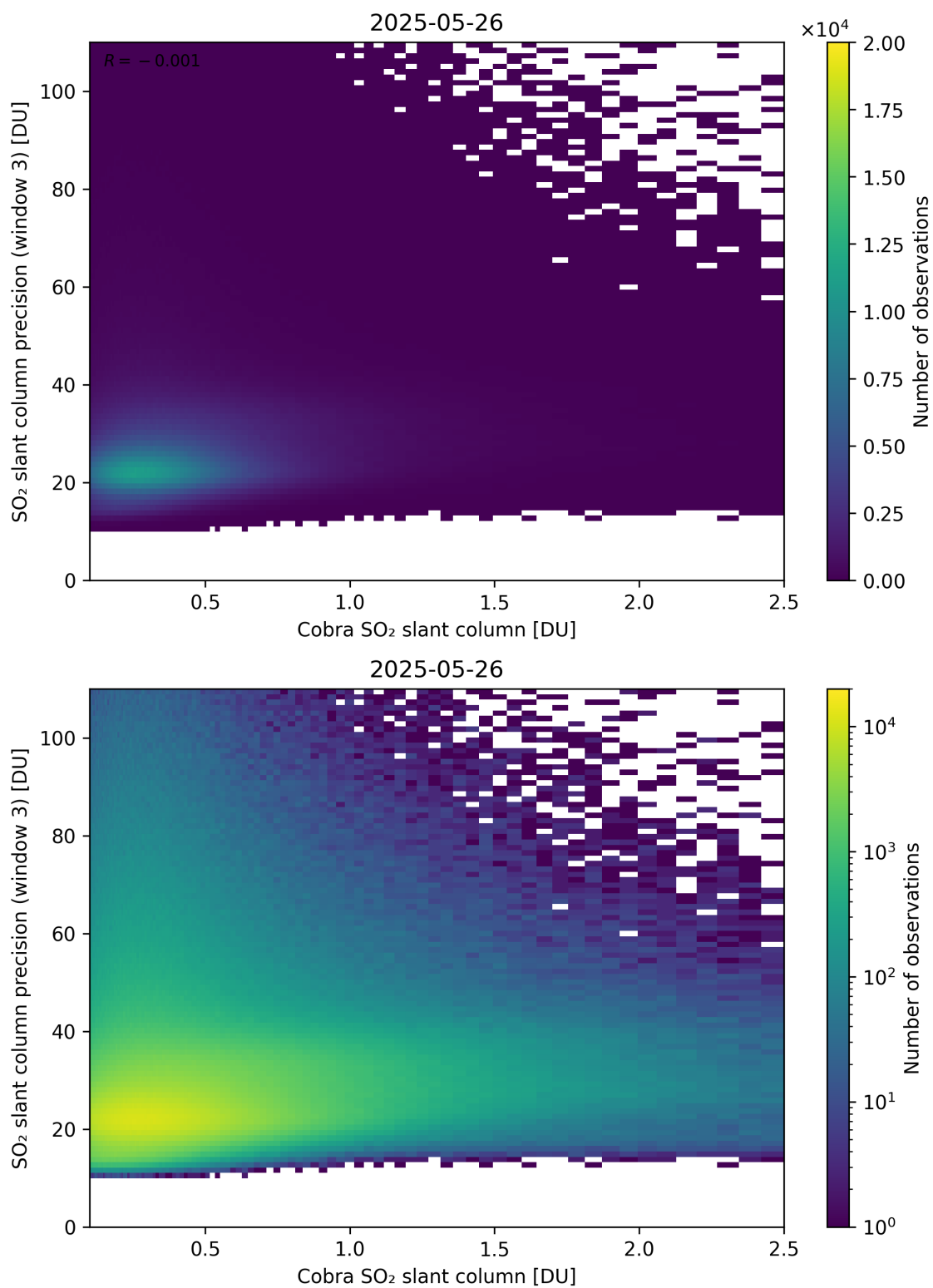
Figure 223: Scatter density plot of “Cobra SO 2 slant column” against “SO 2 slant column precision (window 3)” for 2025-05-26 to 2025-05-27.
