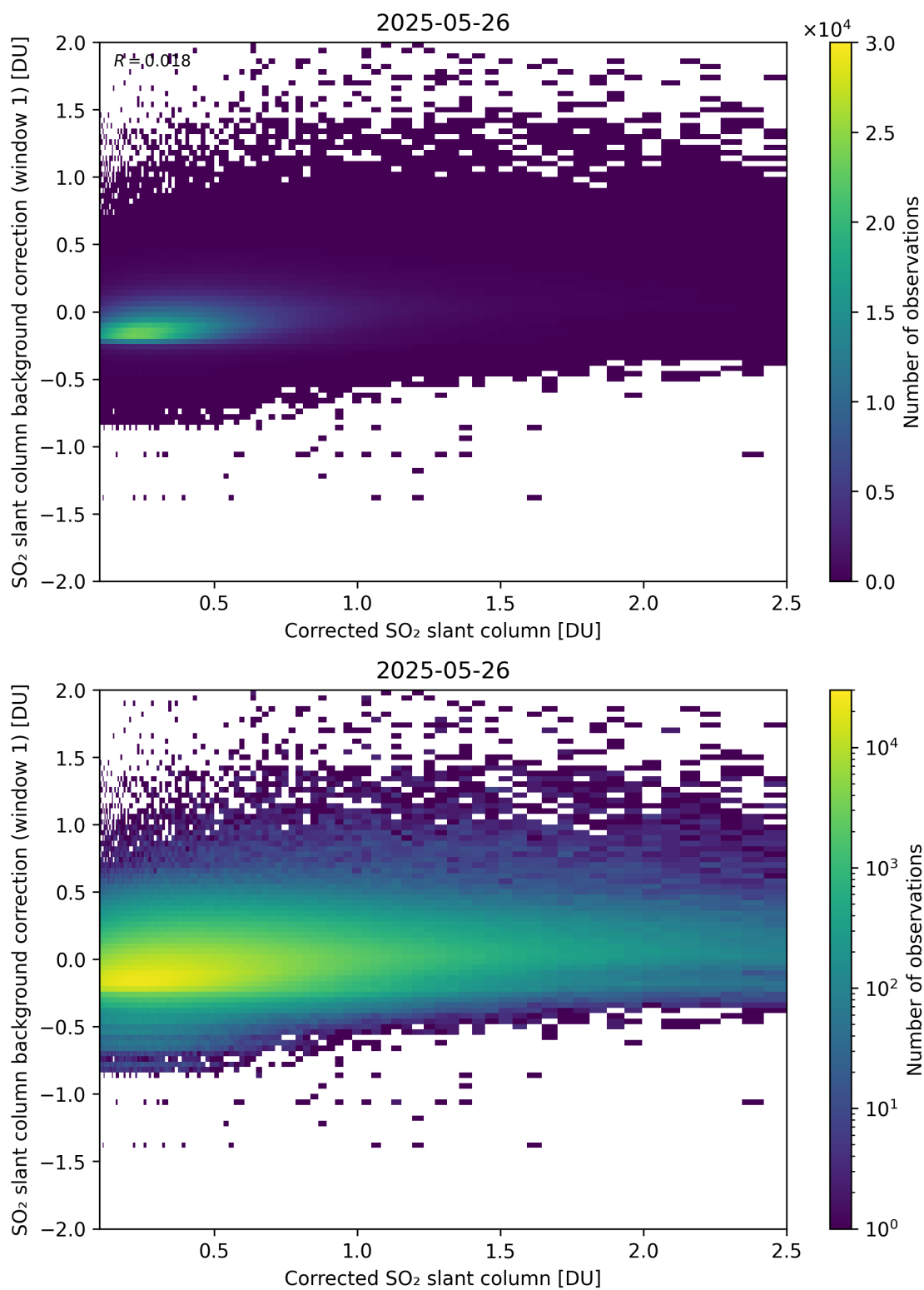
Figure 226: Scatter density plot of “Corrected SO 2 slant column” against “SO 2 slant column background correction (window 1)” for 2025-05-26 to 2025-05-27.
