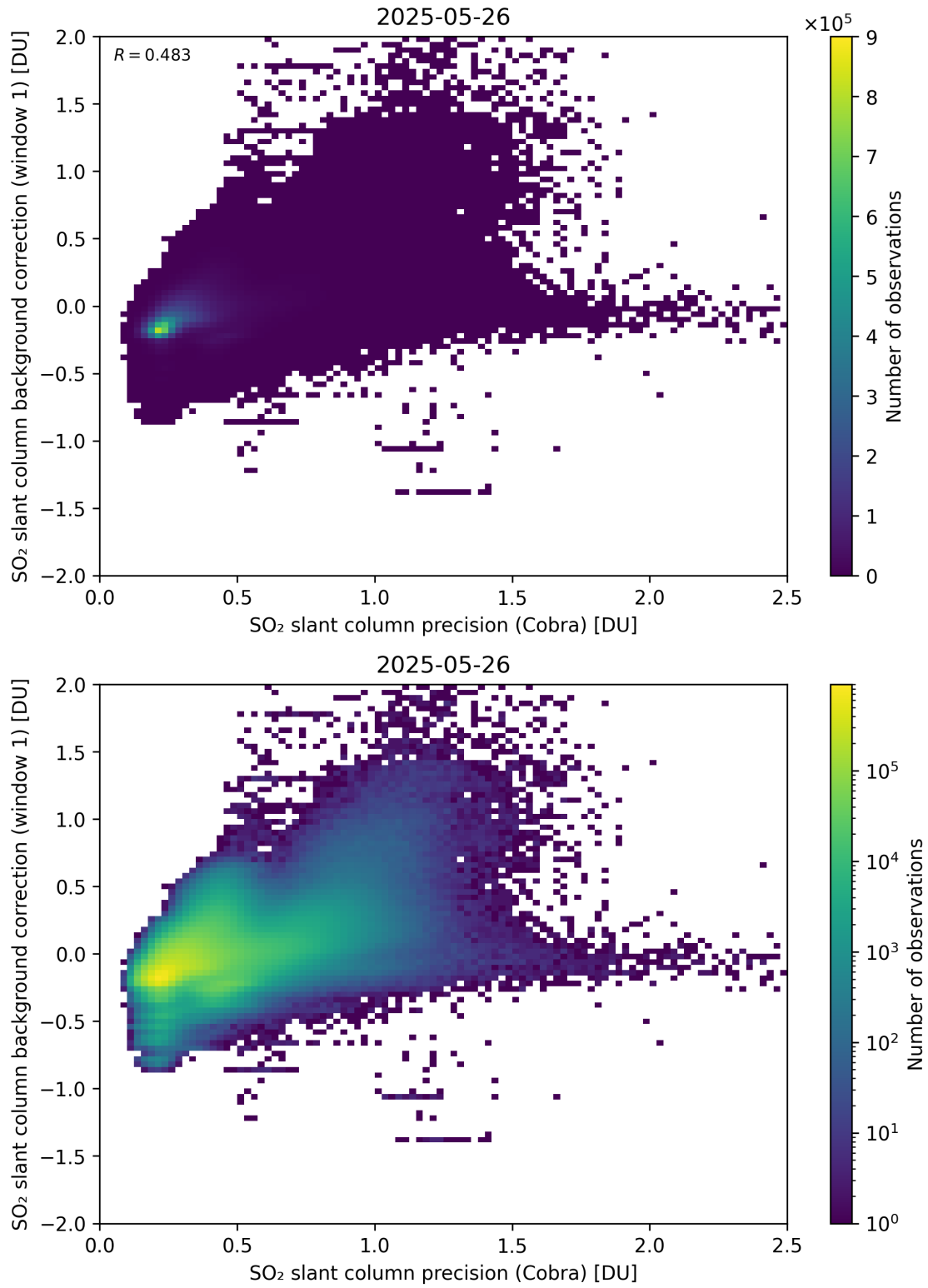
Figure 199: Scatter density plot of “SO 2 slant column precision (Cobra)” against “SO 2 slant column background correction (window 1)” for 2025-05-26 to 2025-05-27.
