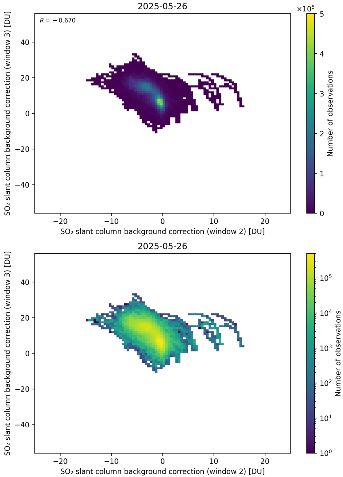
Figure 122: Scatter density plot of “SO 2 slant column background correction (window 2)” against “SO 2 slant column background correction (window 3)” for 2025-05-26 to 2025-05-27.
