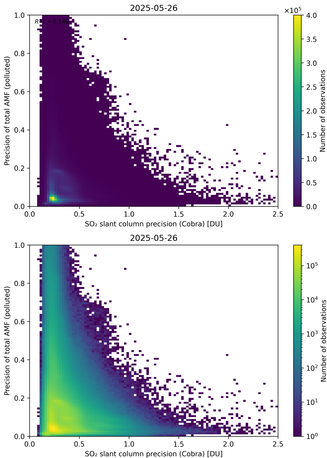
Figure 214: Scatter density plot of “SO 2 slant column precision (Cobra)” against “Precision of total AMF (polluted)” for 2025-05-26 to 2025-05-27.
