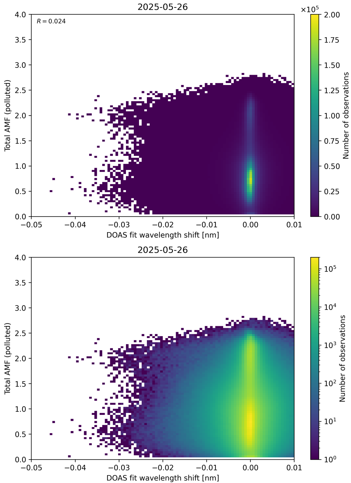
Figure 141: Scatter density plot of “DOAS fit wavelength shift” against “Total AMF (polluted)” for 2025-05-26 to 2025-05-27.
