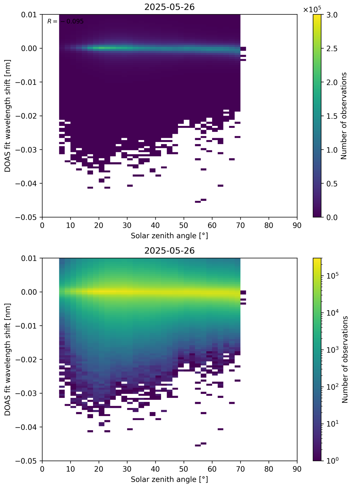
Figure 174: Scatter density plot of “Solar zenith angle” against “DOAS fit wavelength shift” for 2025-05-26 to 2025-05-27.
