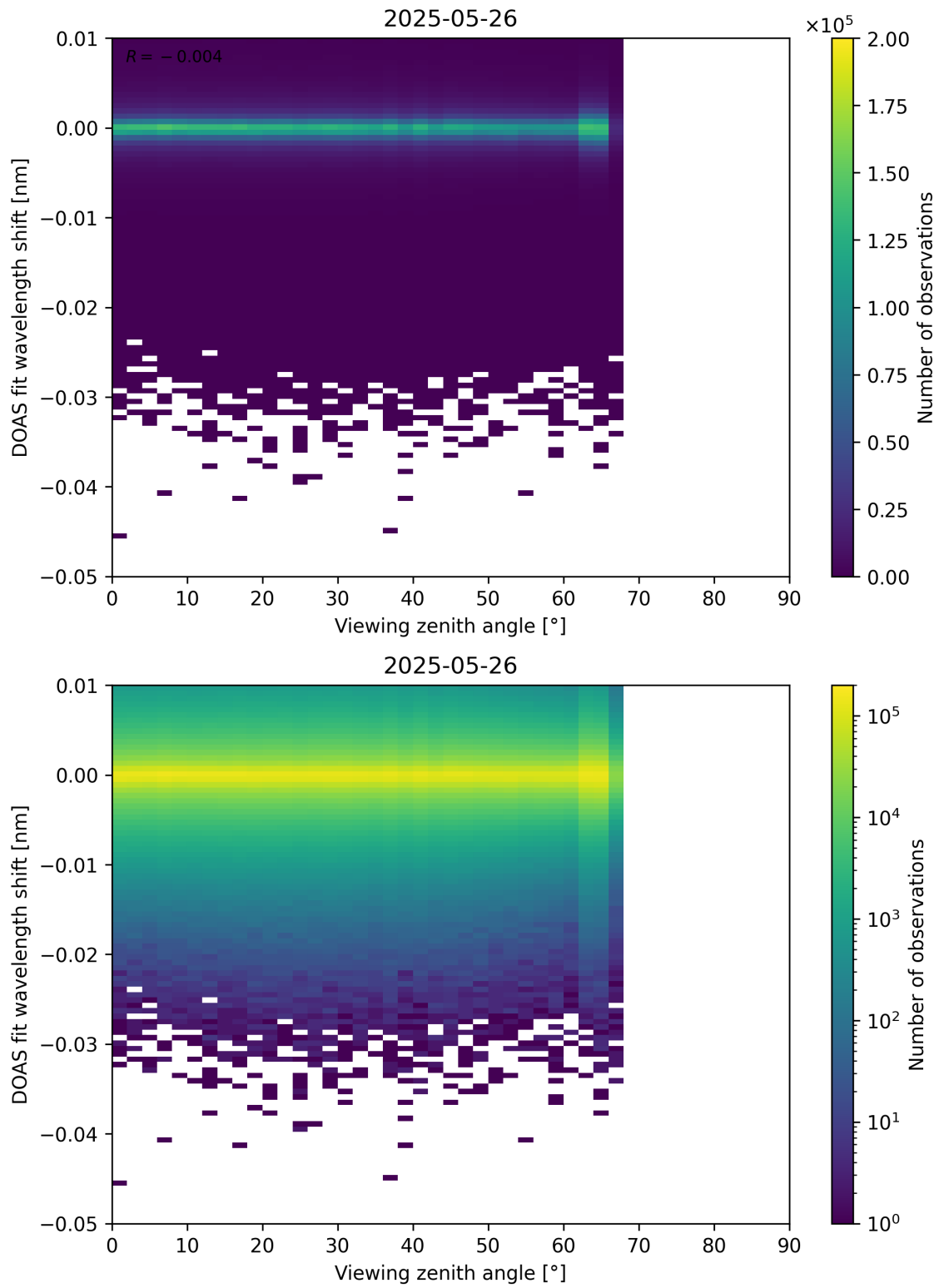
Figure 365: Scatter density plot of “Viewing zenith angle” against “DOAS fit wavelength shift” for 2025-05-26 to 2025-05-27.
