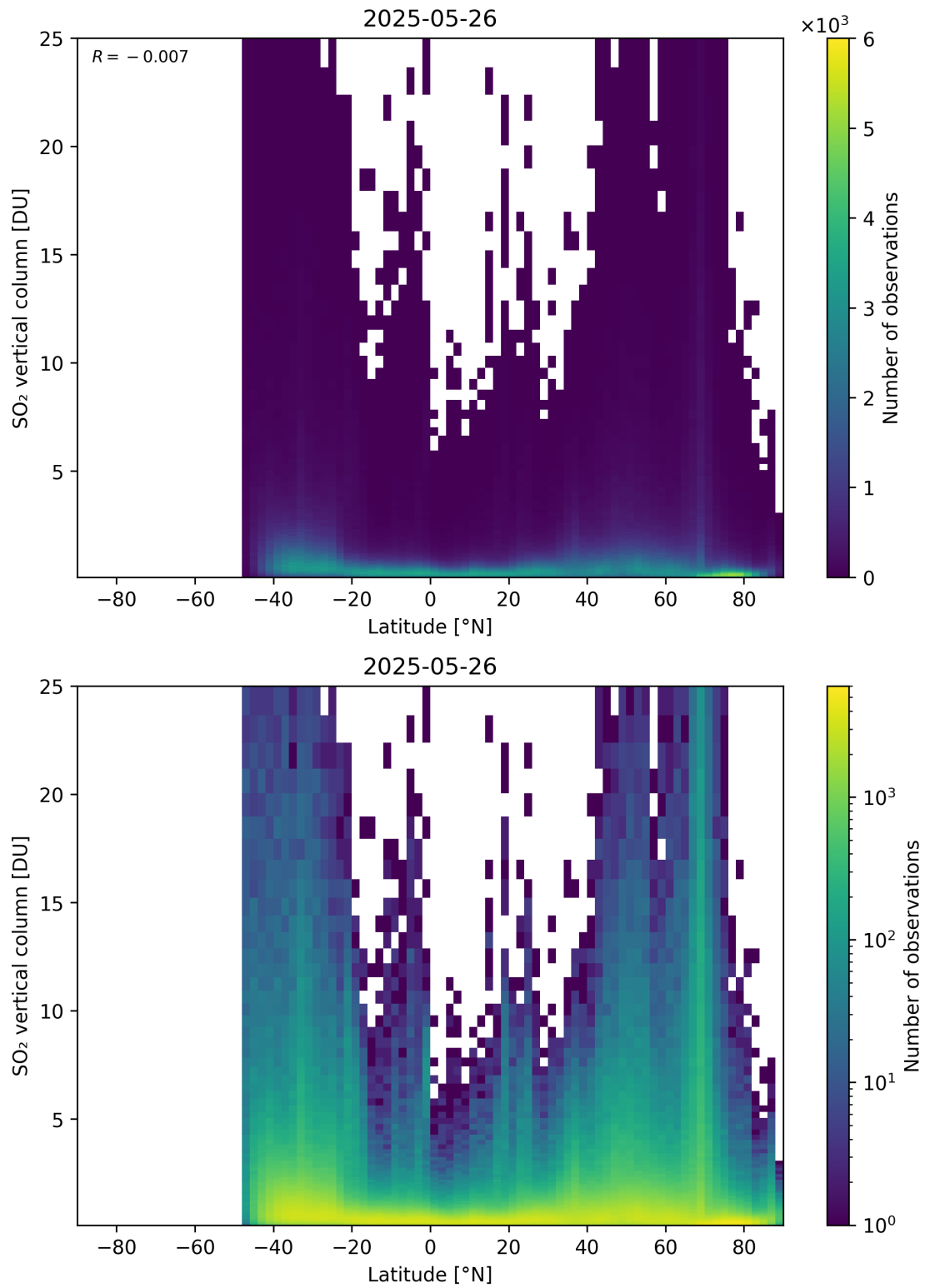
Figure 169: Scatter density plot of “Latitude” against “SO 2 vertical column” for 2025-05-26 to 2025-05-27.
