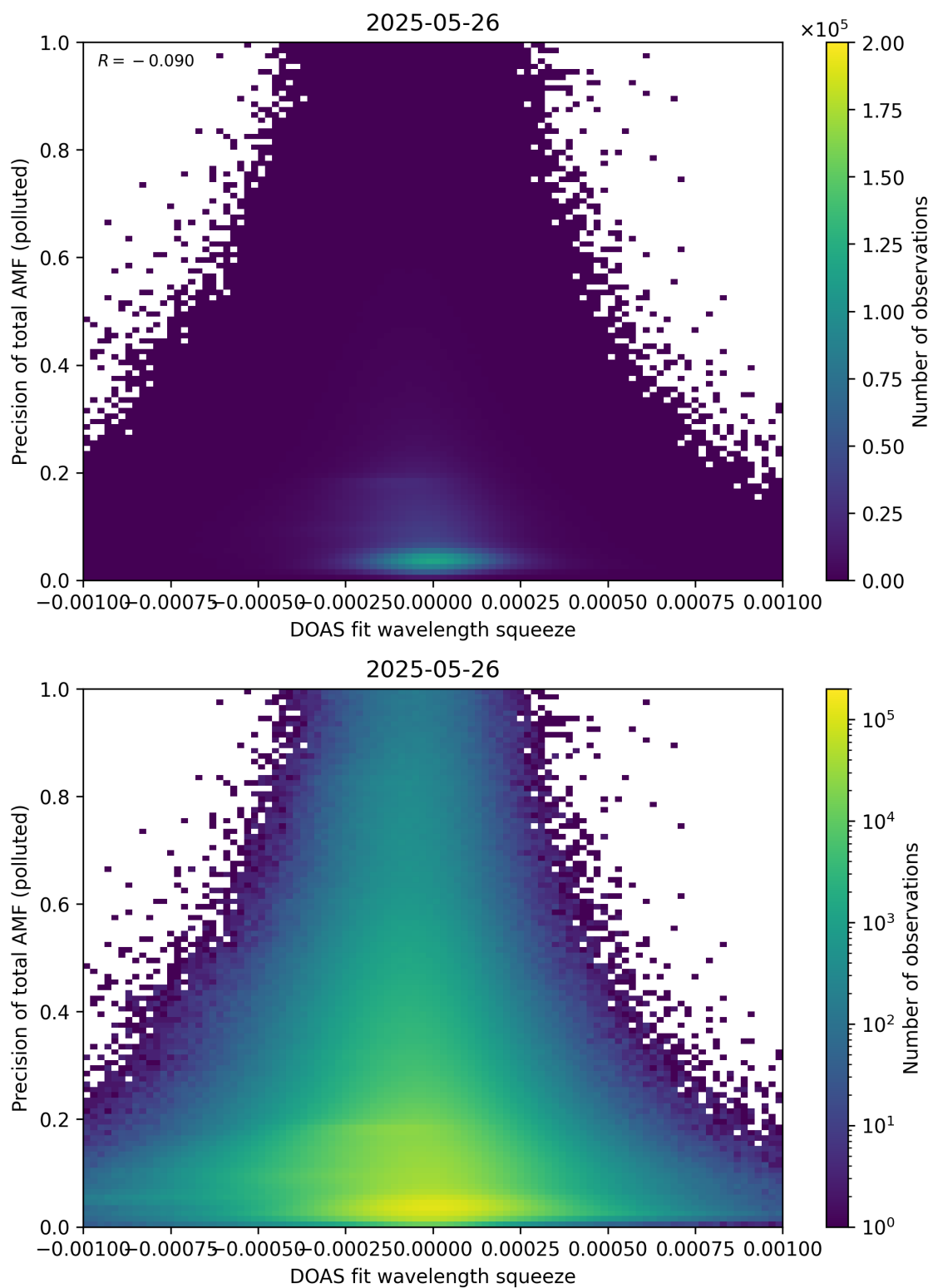
Figure 146: Scatter density plot of “DOAS fit wavelength squeeze” against “Precision of total AMF (polluted)” for 2025-05-26 to 2025-05-27.
