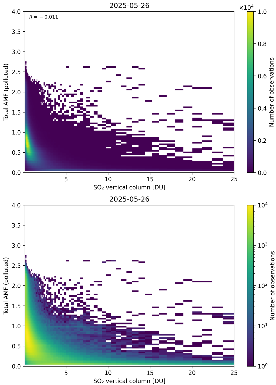
Figure 359: Scatter density plot of “SO 2 vertical column” against “Total AMF (polluted)” for 2025-05-26 to 2025-05-27.
