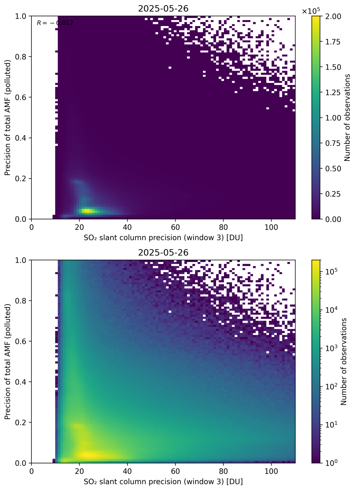
Figure 314: Scatter density plot of “SO 2 slant column precision (window 3)” against “Precision of total AMF (polluted)” for 2025-05-26 to 2025-05-27.
