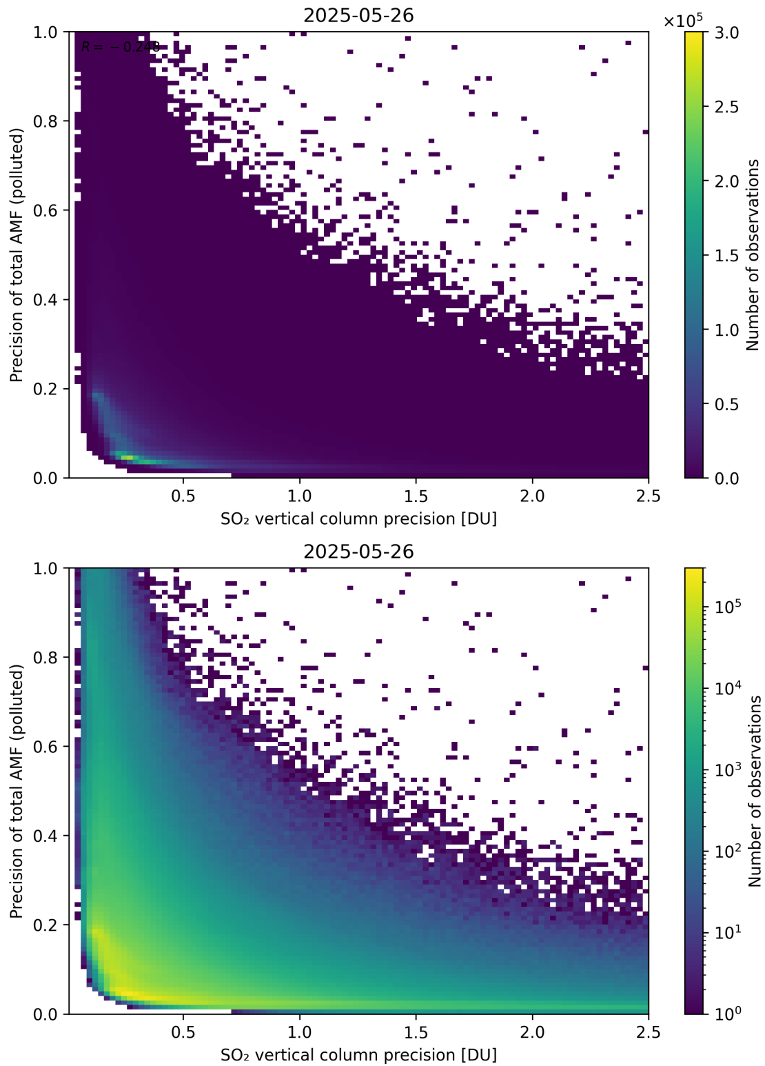
Figure 347: Scatter density plot of “SO 2 vertical column precision” against “Precision of total AMF (polluted)” for 2025-05-26 to 2025-05-27.
