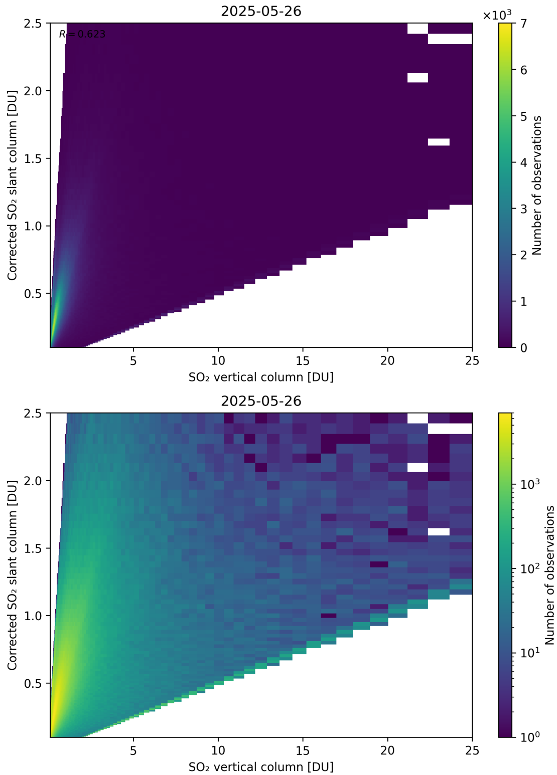
Figure 351: Scatter density plot of “SO 2 vertical column” against “Corrected SO 2 slant column” for 2025-05-26 to 2025-05-27.
