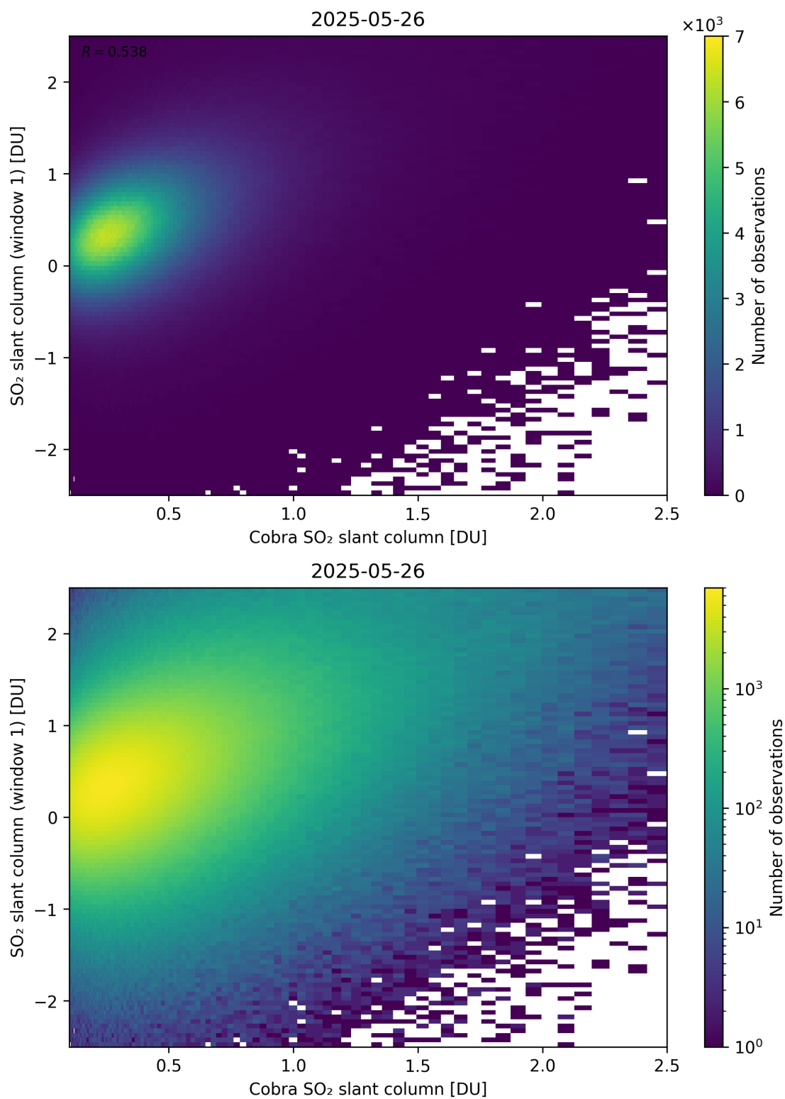
Figure 219: Scatter density plot of “Cobra SO 2 slant column” against “SO 2 slant column (window 1)” for 2025-05-26 to 2025-05-27.
