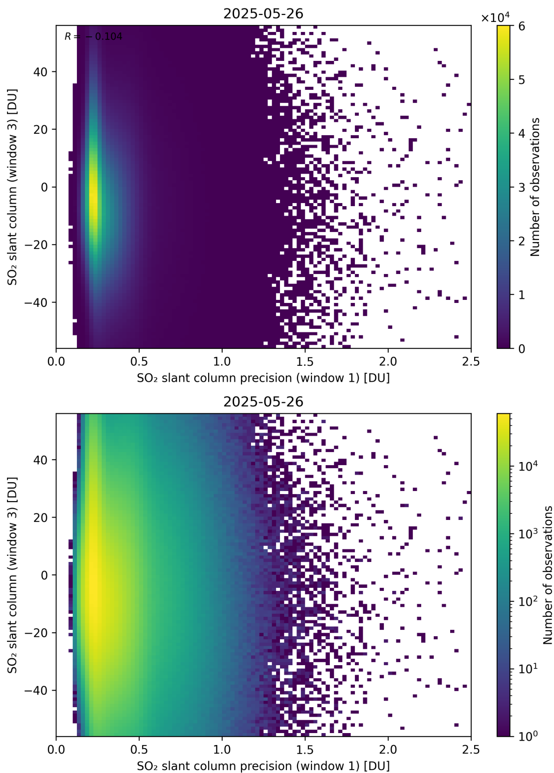
Figure 278: Scatter density plot of “SO 2 slant column precision (window 1)” against “SO 2 slant column (window 3)” for 2025-05-26 to 2025-05-27.
