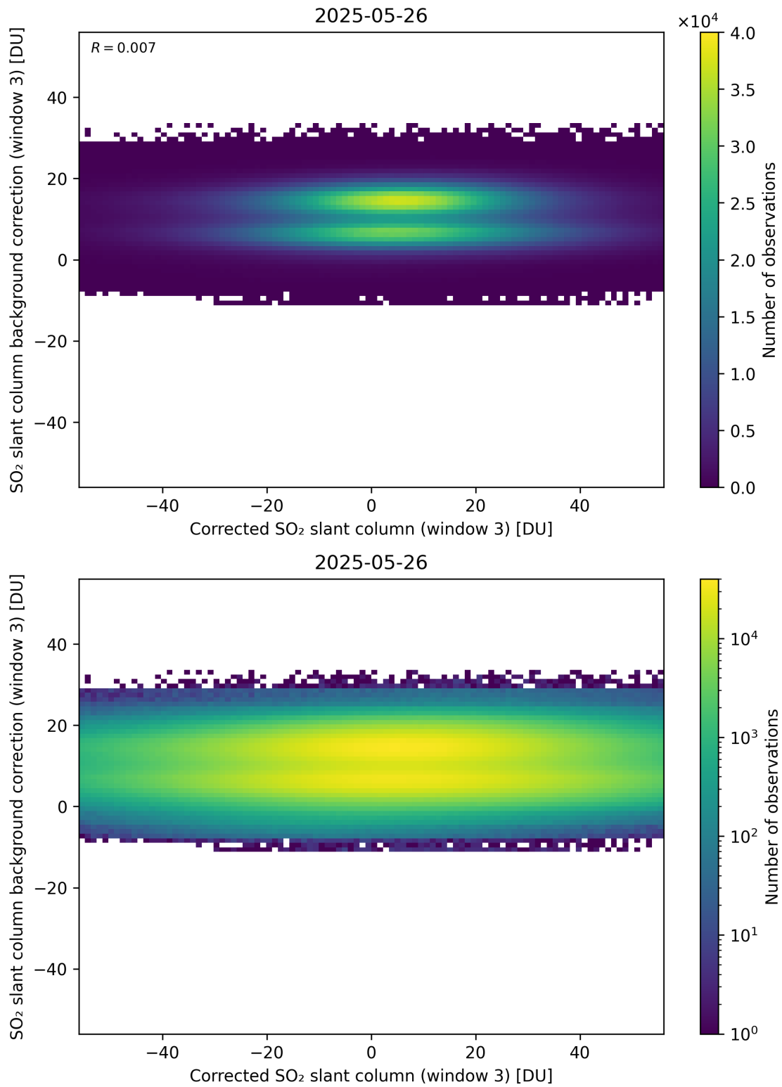
Figure 255: Scatter density plot of “Corrected SO 2 slant column (window 3)” against “SO 2 slant column background correction (window 3)” for 2025-05-26 to 2025-05-27.
