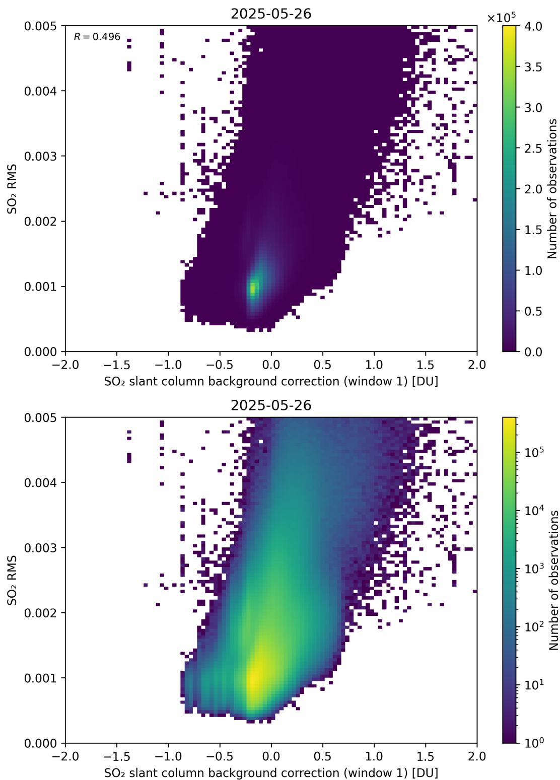
Figure 113: Scatter density plot of “SO 2 slant column background correction (window 1)” against “SO 2 RMS” for 2025-05-26 to 2025-05-27.
