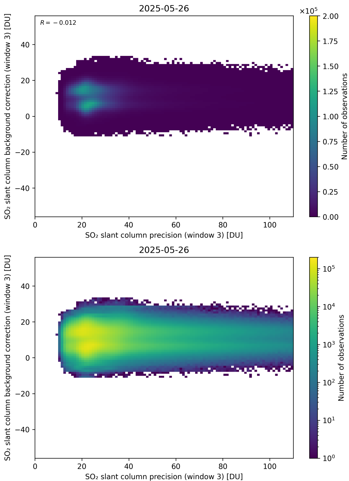
Figure 307: Scatter density plot of “SO 2 slant column precision (window 3)” against “SO 2 slant column background correction (window 3)” for 2025-05-26 to 2025-05-27.
