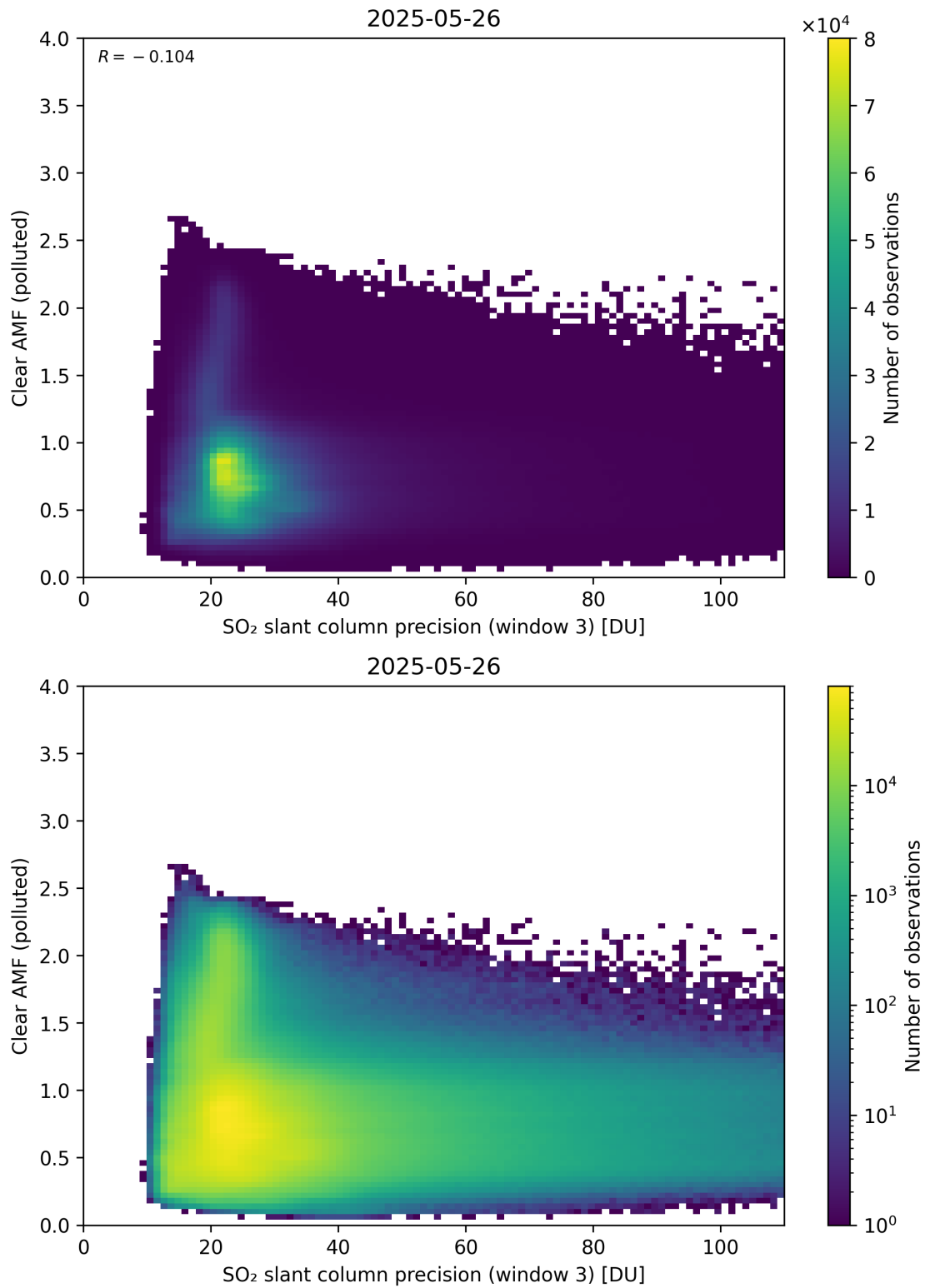
Figure 311: Scatter density plot of “SO 2 slant column precision (window 3)” against “Clear AMF (polluted)” for 2025-05-26 to 2025-05-27.
