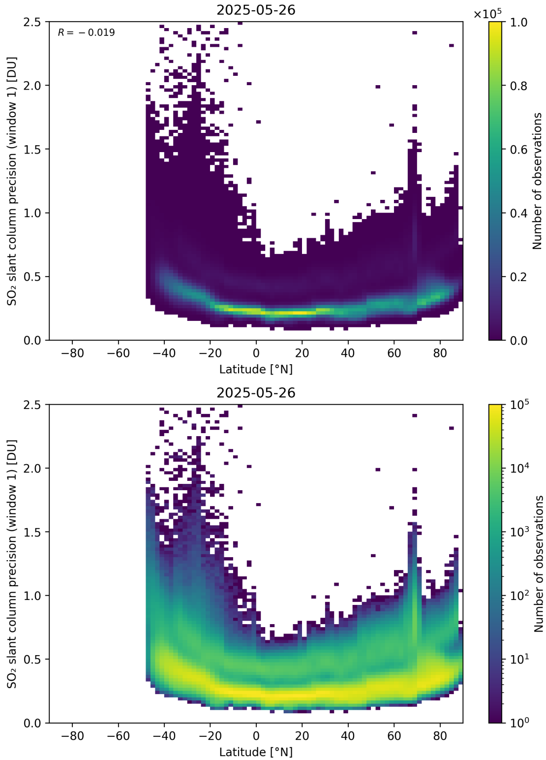
Figure 163: Scatter density plot of “Latitude” against “SO 2 slant column precision (window 1)” for 2025-05-26 to 2025-05-27.
