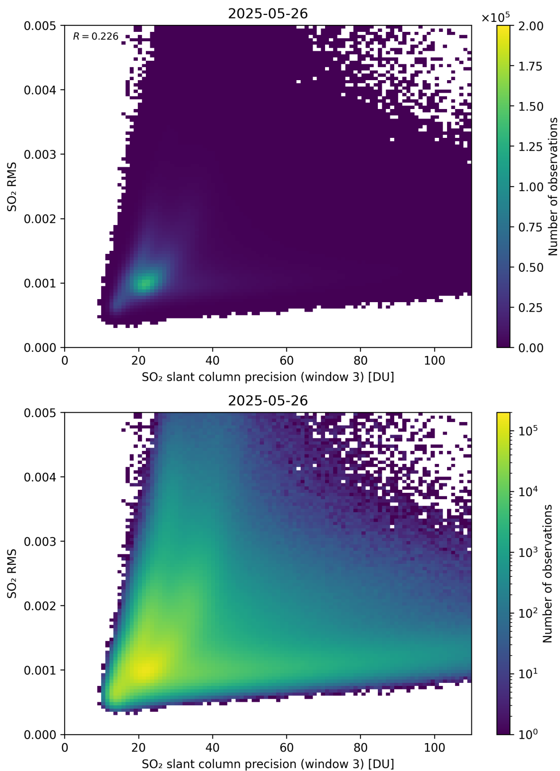
Figure 310: Scatter density plot of “SO 2 slant column precision (window 3)” against “SO 2 RMS” for 2025-05-26 to 2025-05-27.
