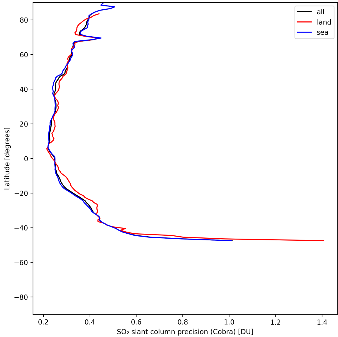
Figure 36: Zonal average of “SO 2 slant column precision (Cobra)” for 2025-05-26 to 2025-05-27.
