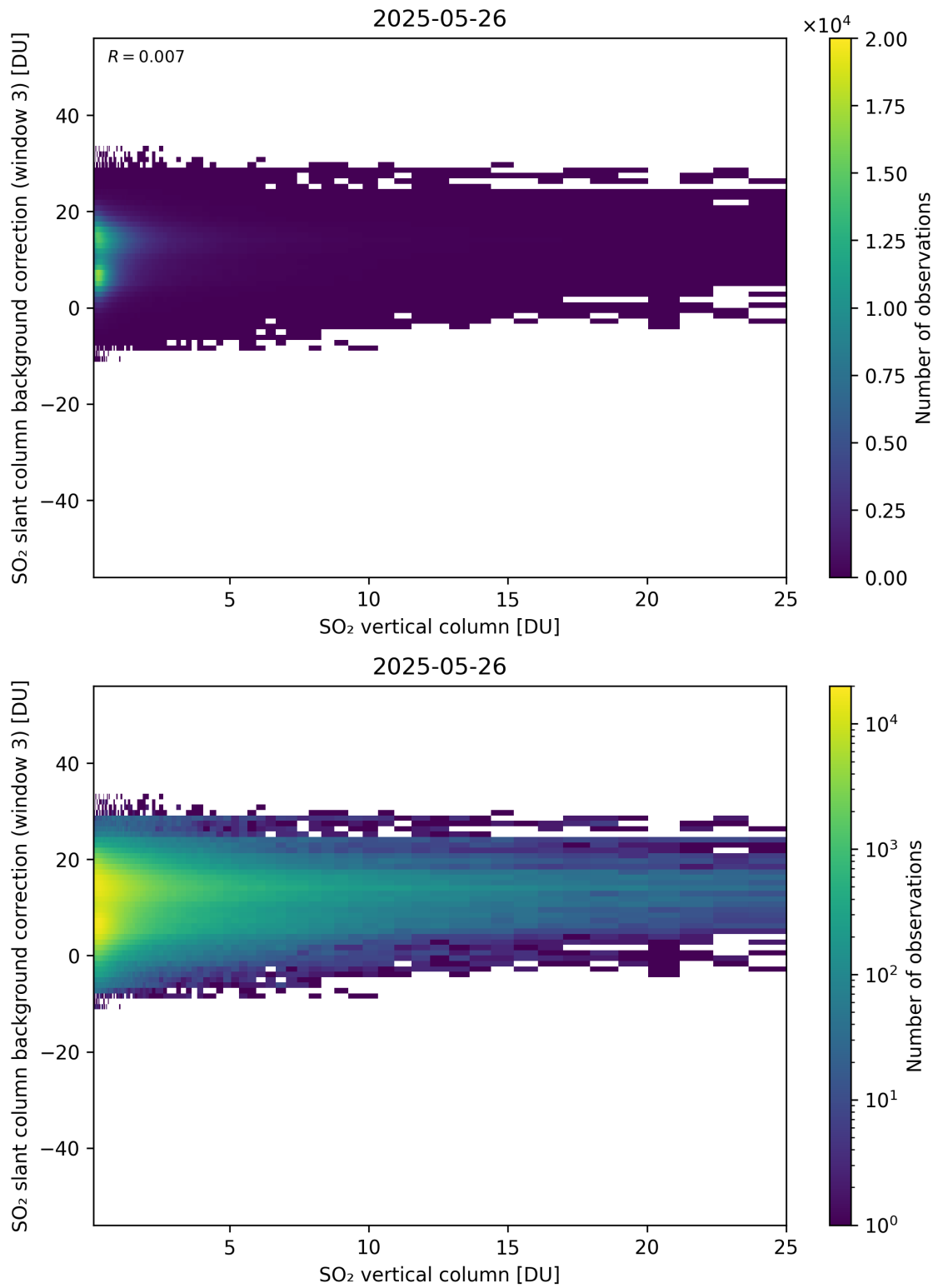
Figure 325: Scatter density plot of “SO 2 vertical column” against “SO 2 slant column background correction (window 3)” for 2025-05-26 to 2025-05-27.
