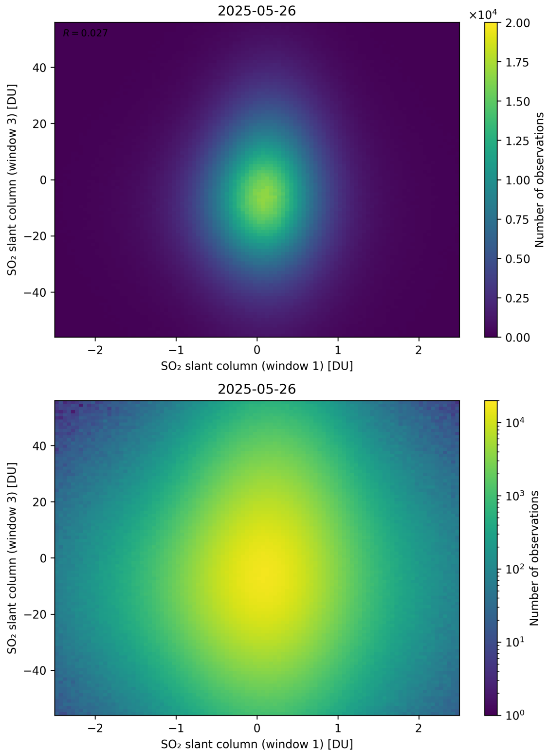
Figure 287: Scatter density plot of “SO 2 slant column (window 1)” against “SO 2 slant column (window 3)” for 2025-05-26 to 2025-05-27.
