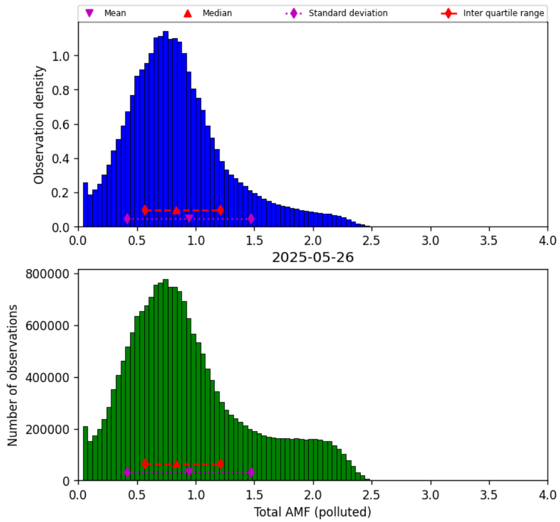
Figure 79: Histogram of “Total AMF (polluted)” for 2025-05-26 to 2025-05-27
