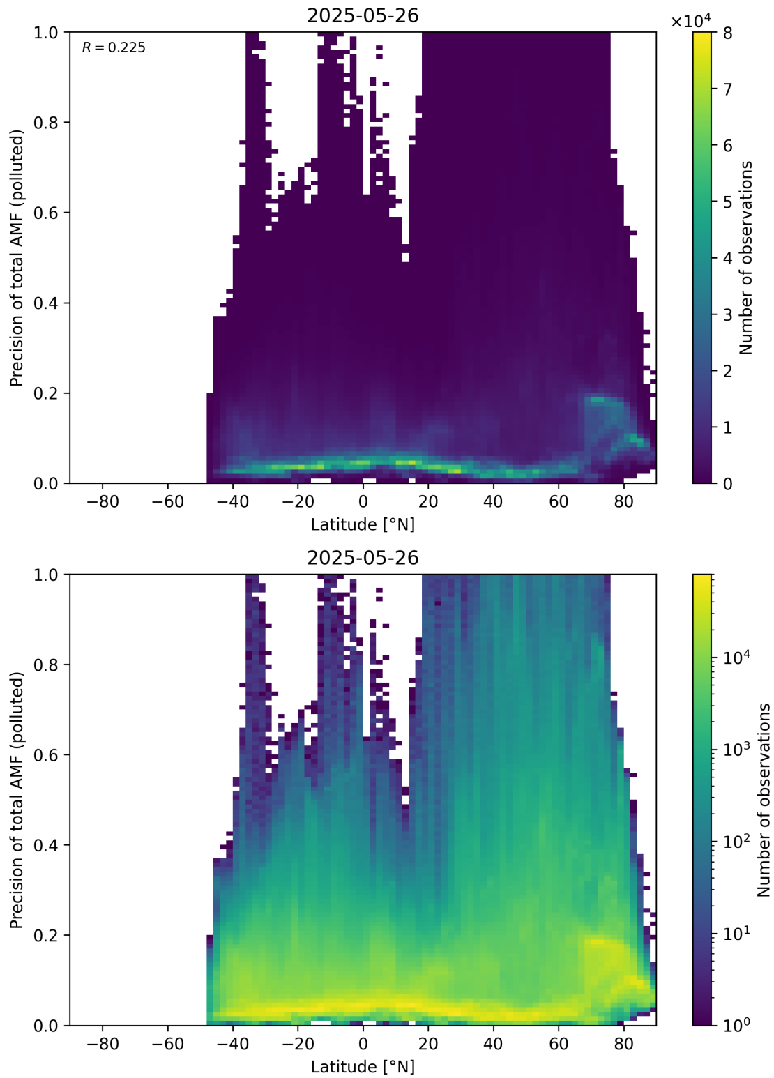
Figure 168: Scatter density plot of “Latitude” against “Precision of total AMF (polluted)” for 2025-05-26 to 2025-05-27.
