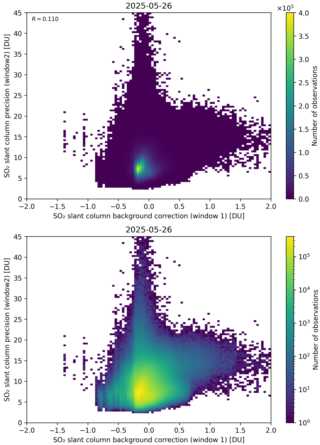
Figure 117: Scatter density plot of “SO 2 slant column background correction (window 1)” against “SO 2 slant column precision (window2)” for 2025-05-26 to 2025-05-27.
