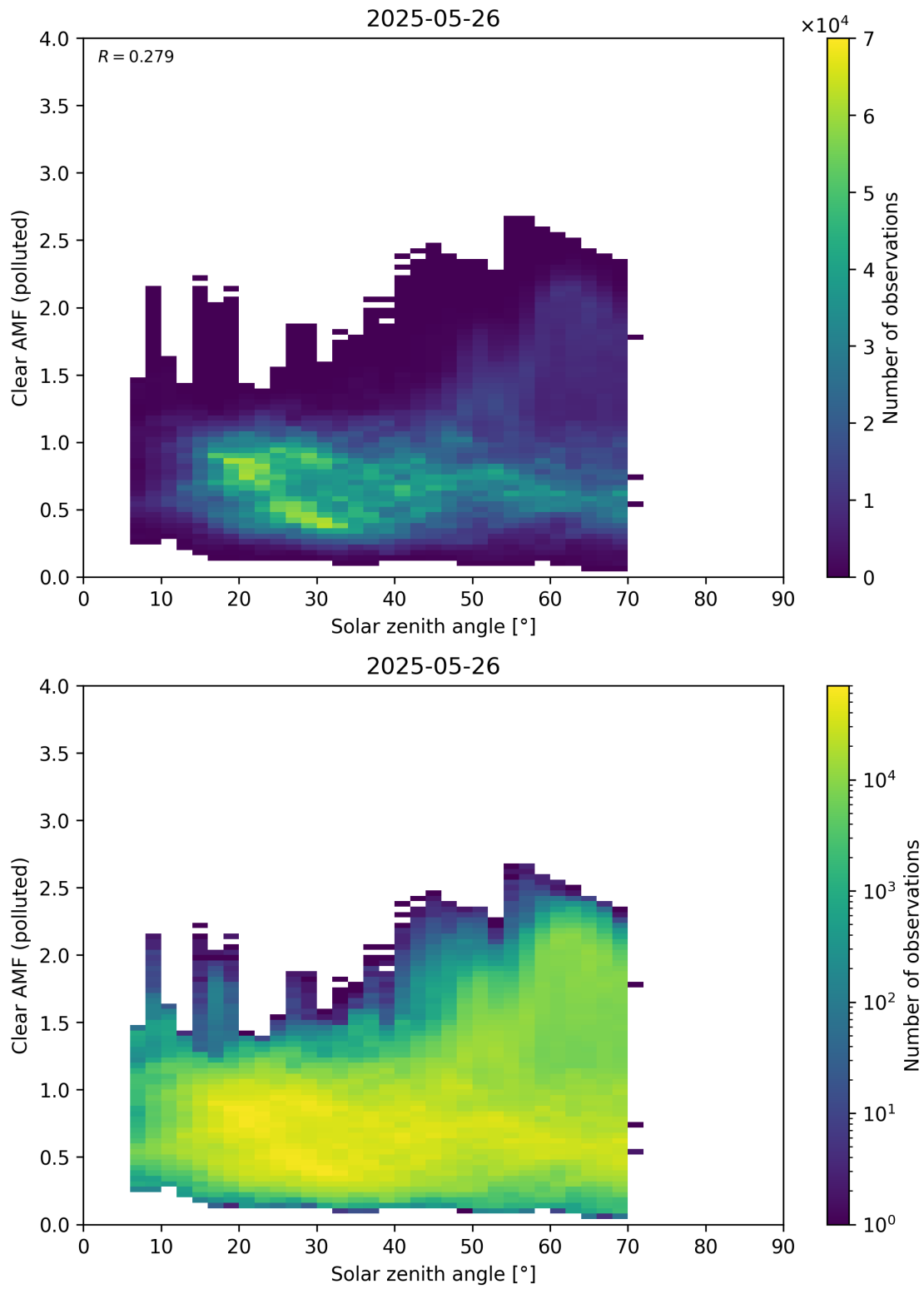
Figure 178: Scatter density plot of “Solar zenith angle” against “Clear AMF (polluted)” for 2025-05-26 to 2025-05-27.
