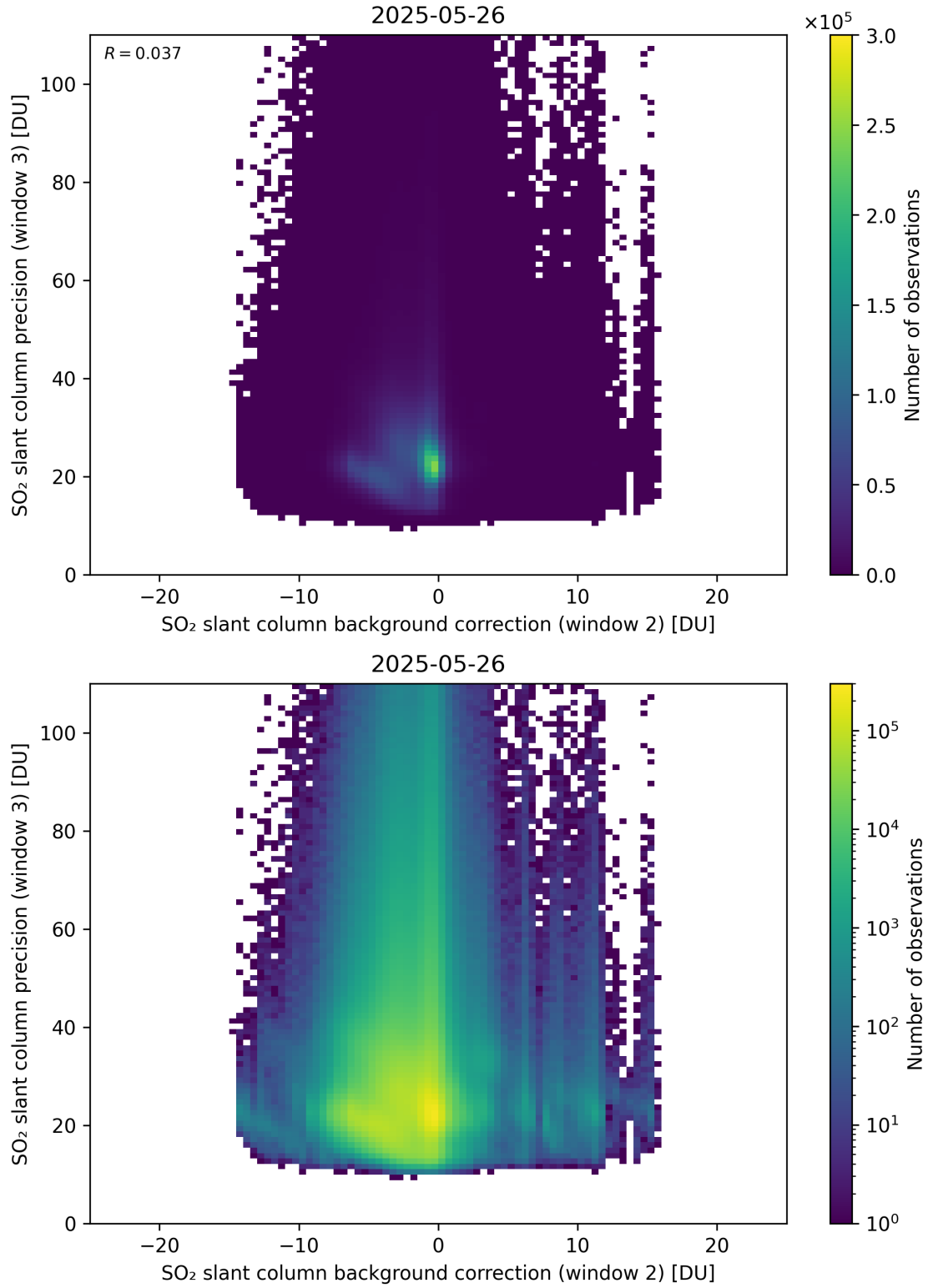
Figure 129: Scatter density plot of “SO 2 slant column background correction (window 2)” against “SO 2 slant column precision (window 3)” for 2025-05-26 to 2025-05-27.
