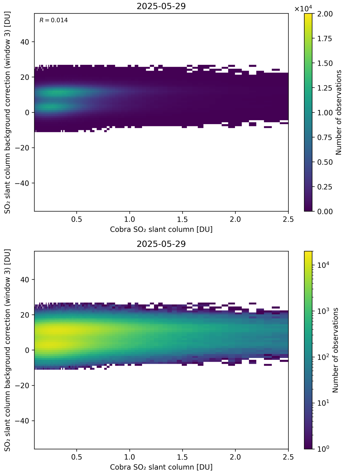
Figure 195: Scatter density plot of “Cobra SO 2 slant column” against “SO 2 slant column background correction (window 3)” for 2025-05-28 to 2025-05-30.
