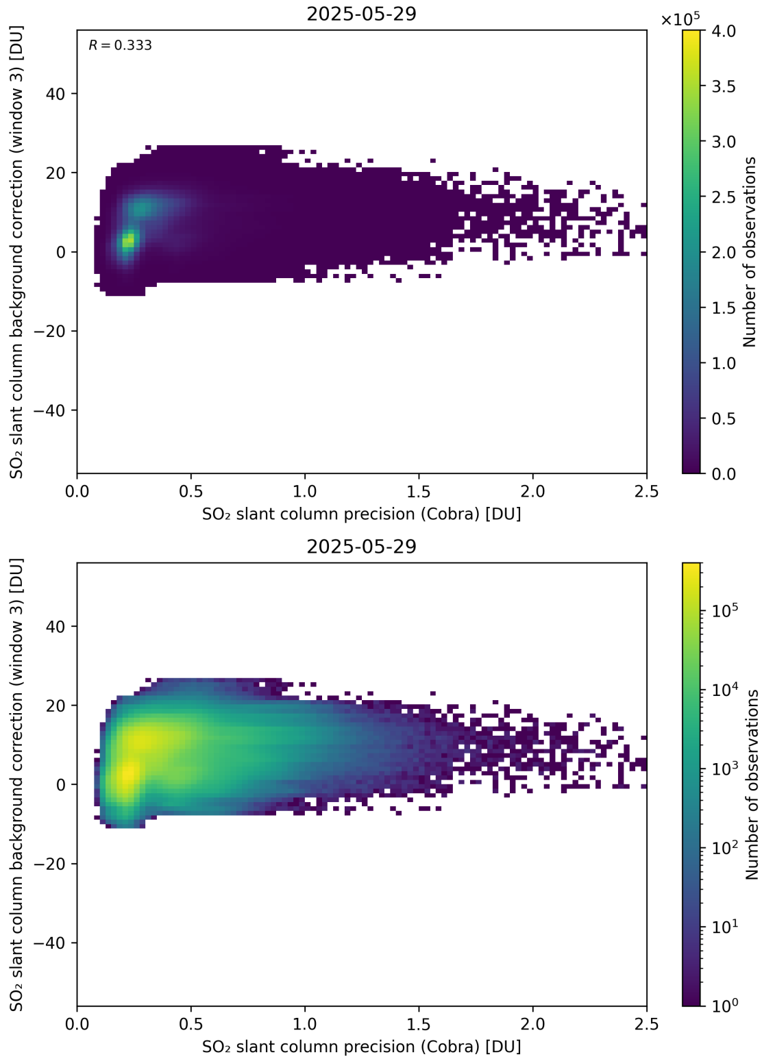
Figure 201: Scatter density plot of “SO 2 slant column precision (Cobra)” against “SO 2 slant column background correction (window 3)” for 2025-05-28 to 2025-05-30.
