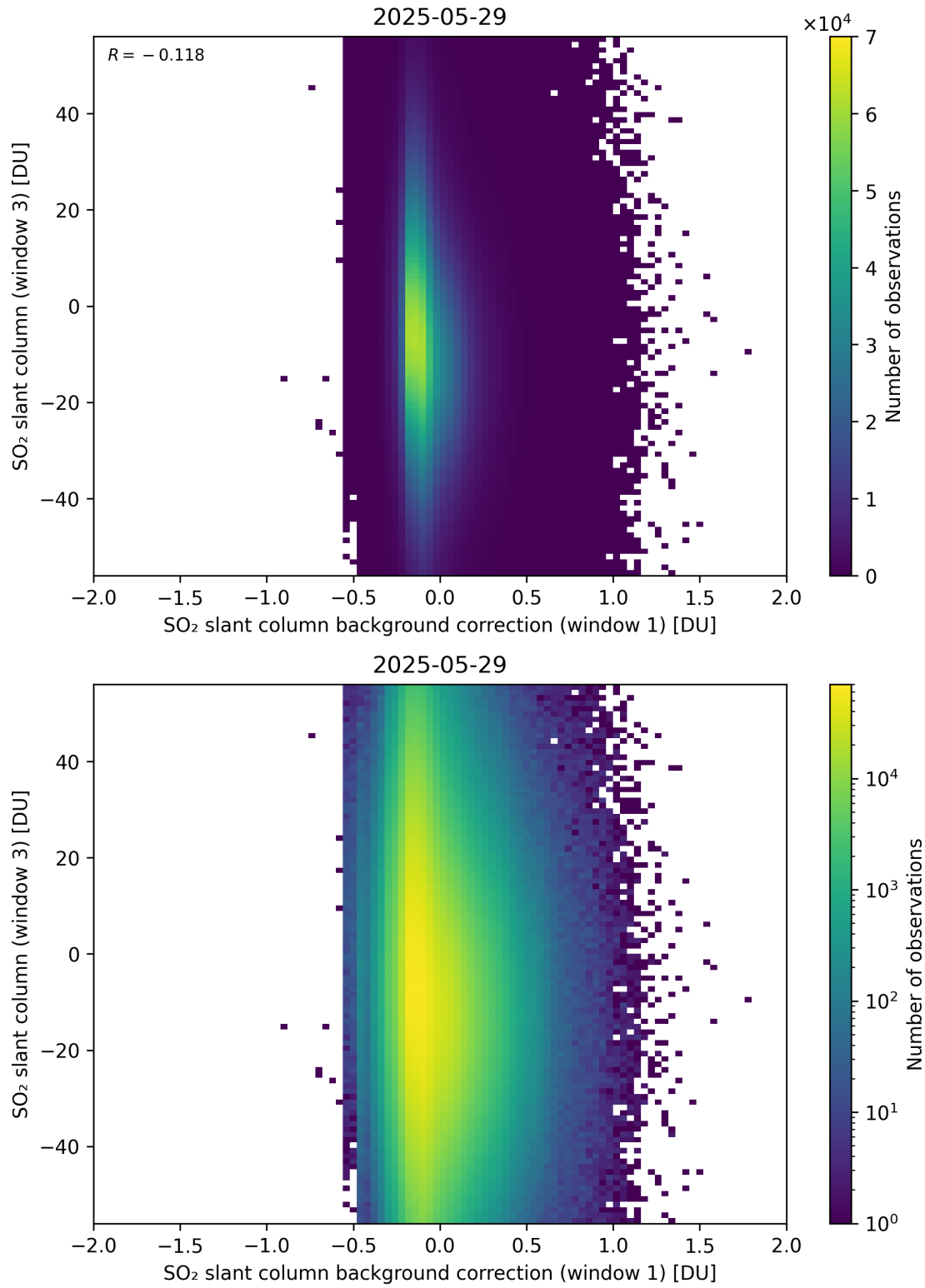
Figure 118: Scatter density plot of “SO 2 slant column background correction (window 1)” against “SO 2 slant column (window 3)” for 2025-05-28 to 2025-05-30.
