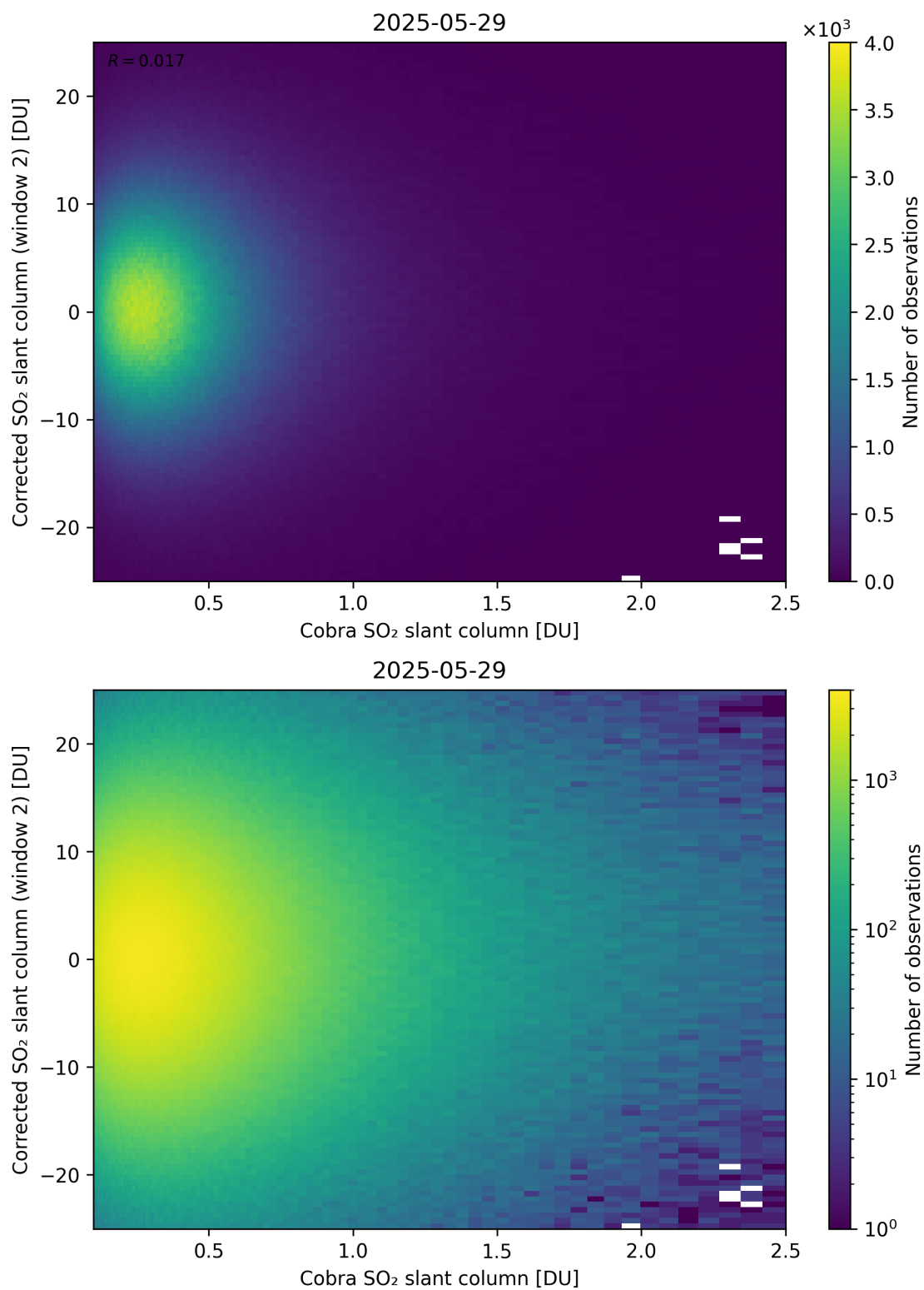
Figure 217: Scatter density plot of “Cobra SO 2 slant column” against “Corrected SO 2 slant column (window 2)” for 2025-05-28 to 2025-05-30.
