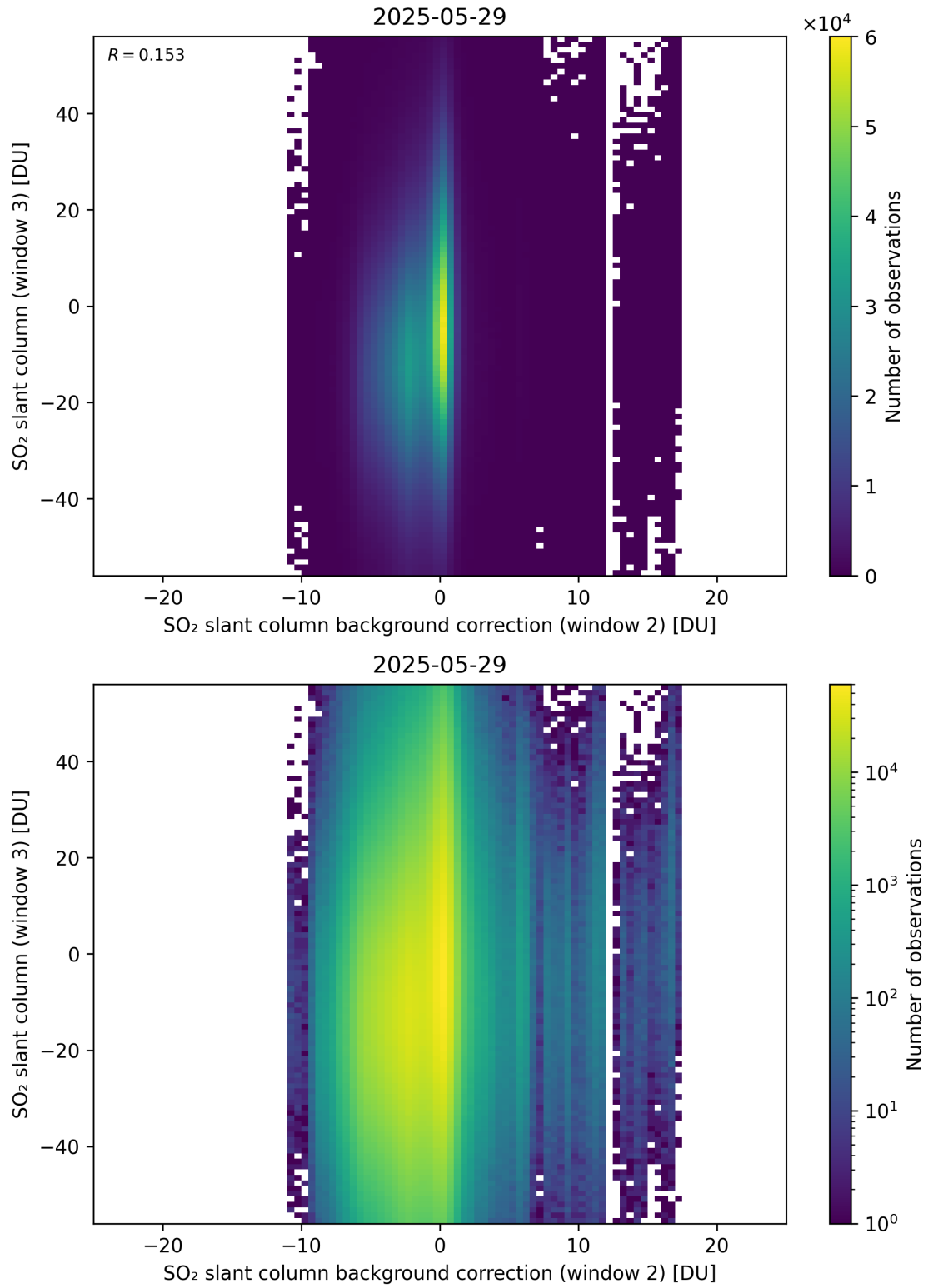
Figure 128: Scatter density plot of “SO 2 slant column background correction (window 2)” against “SO 2 slant column (window 3)” for 2025-05-28 to 2025-05-30.
