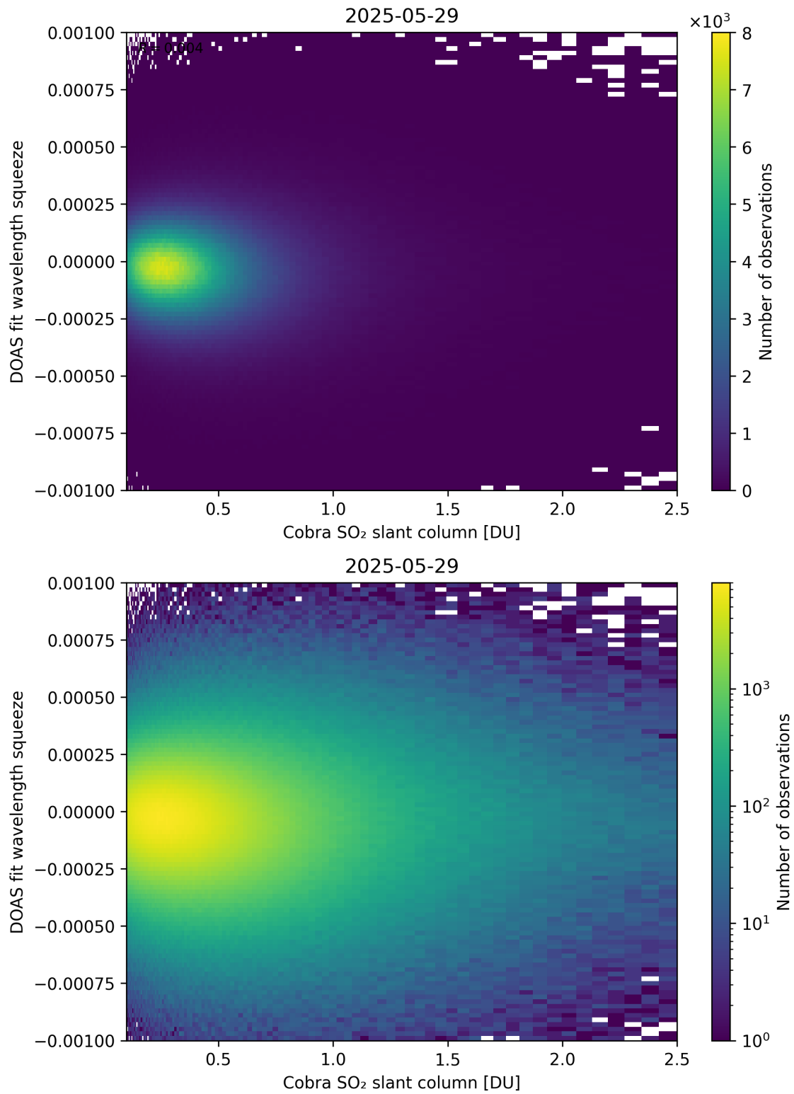
Figure 197: Scatter density plot of “Cobra SO 2 slant column” against “DOAS fit wavelength squeeze” for 2025-05-28 to 2025-05-30.
