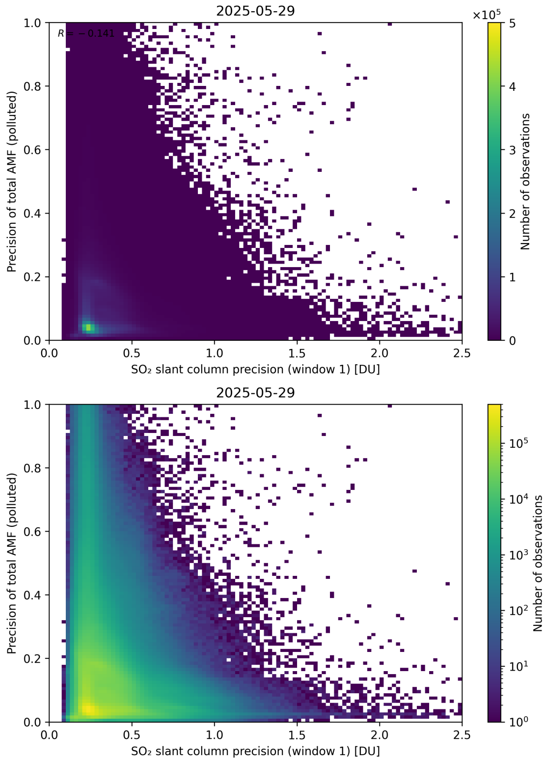
Figure 281: Scatter density plot of “SO 2 slant column precision (window 1)” against “Precision of total AMF (polluted)” for 2025-05-28 to 2025-05-30.
