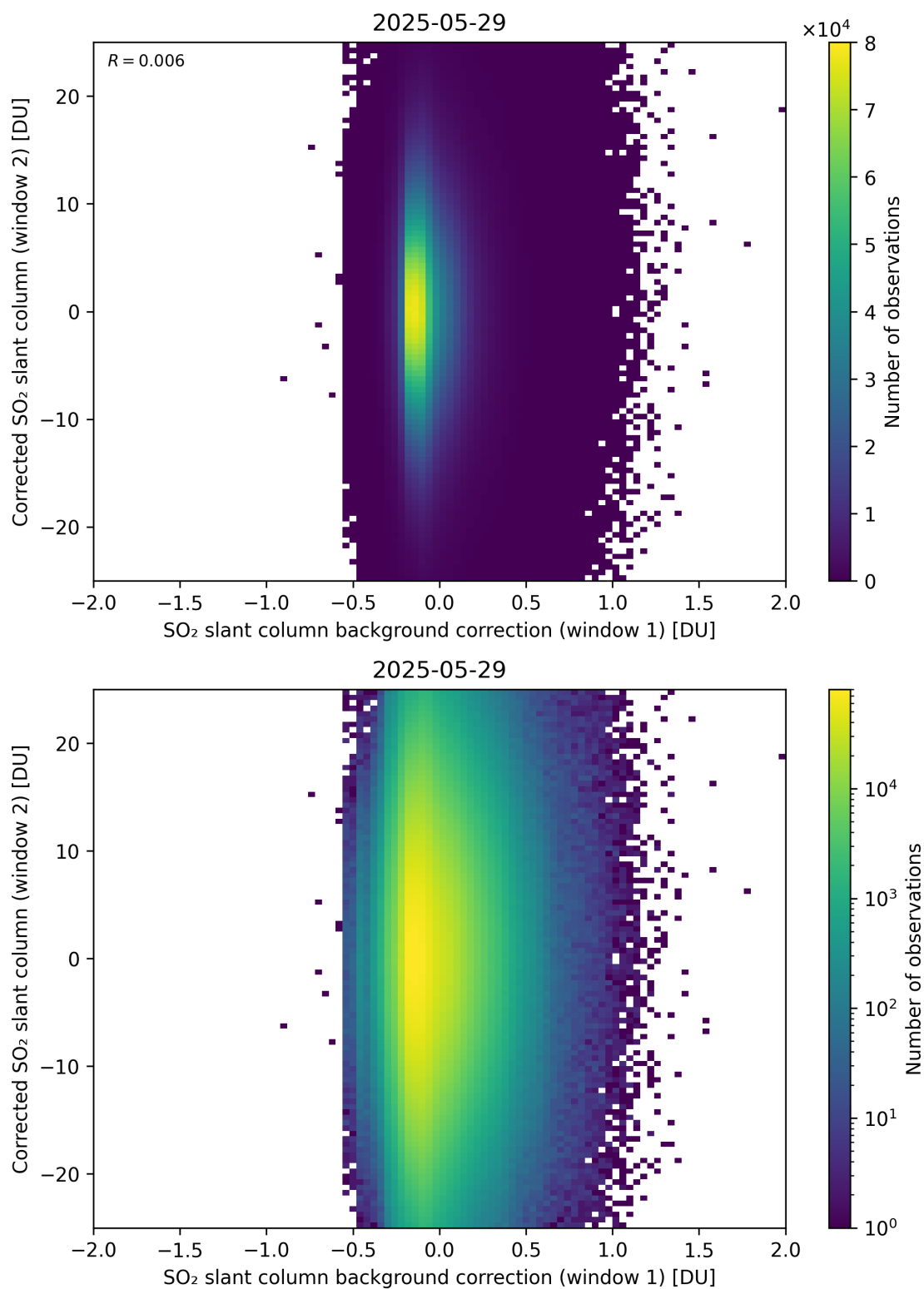
Figure 115: Scatter density plot of “SO 2 slant column background correction (window 1)” against “Corrected SO 2 slant column (window 2)” for 2025-05-28 to 2025-05-30.
