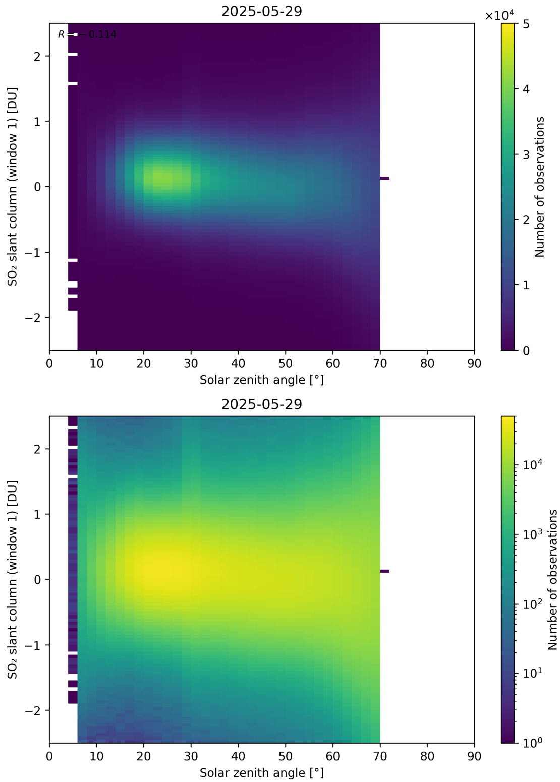
Figure 184: Scatter density plot of “Solar zenith angle” against “SO 2 slant column (window 1)” for 2025-05-28 to 2025-05-30.
