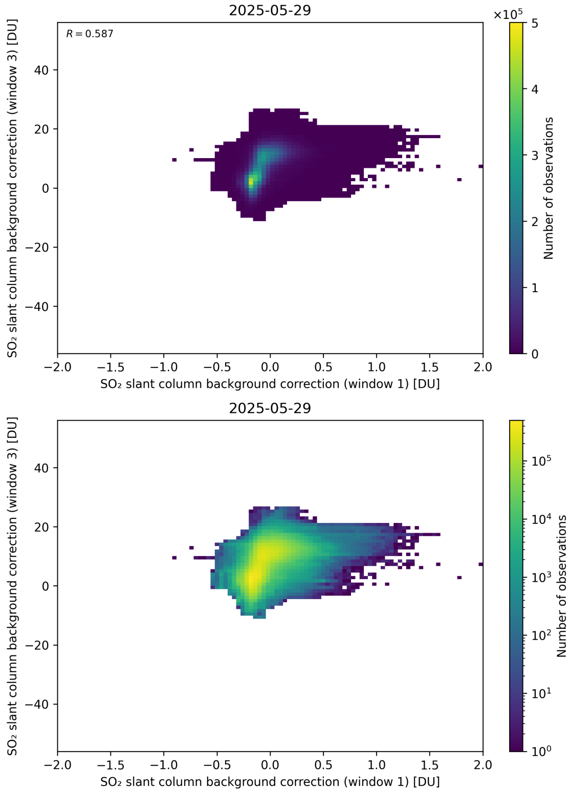
Figure 110: Scatter density plot of “SO 2 slant column background correction (window 1)” against “SO 2 slant column background correction (window 3)” for 2025-05-28 to 2025-05-30.
