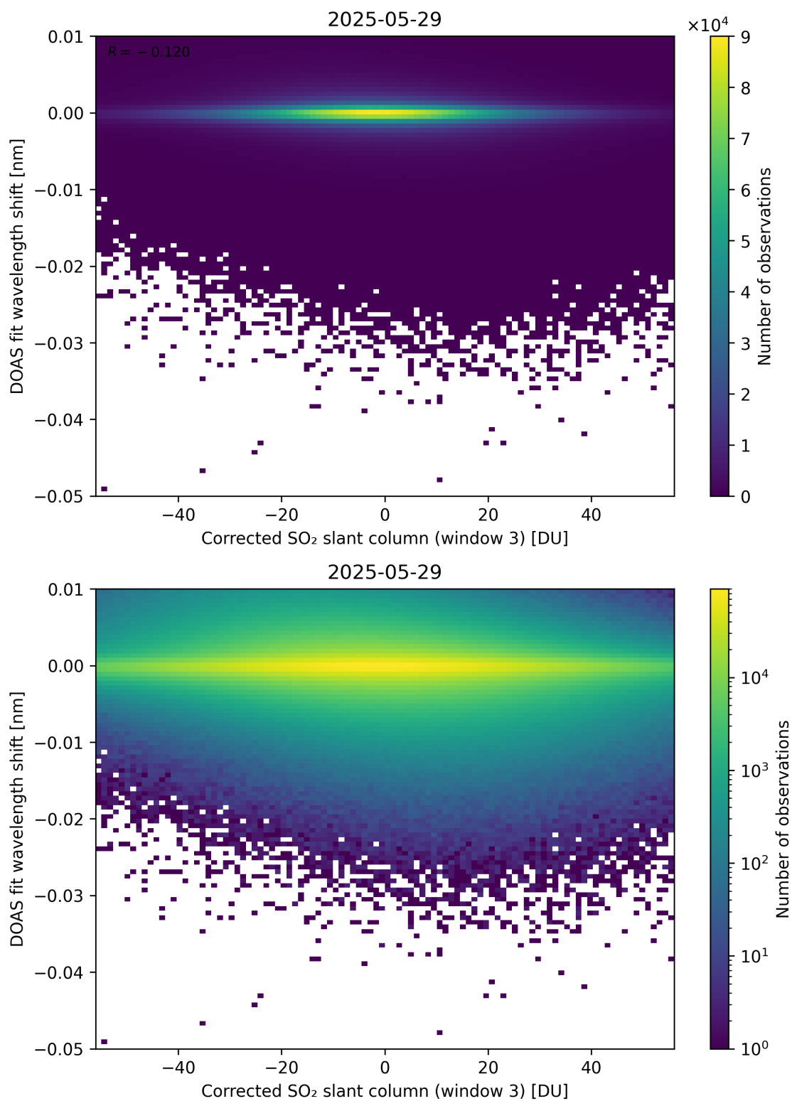
Figure 256: Scatter density plot of “Corrected SO 2 slant column (window 3)” against “DOAS fit wavelength shift” for 2025-05-28 to 2025-05-30.
