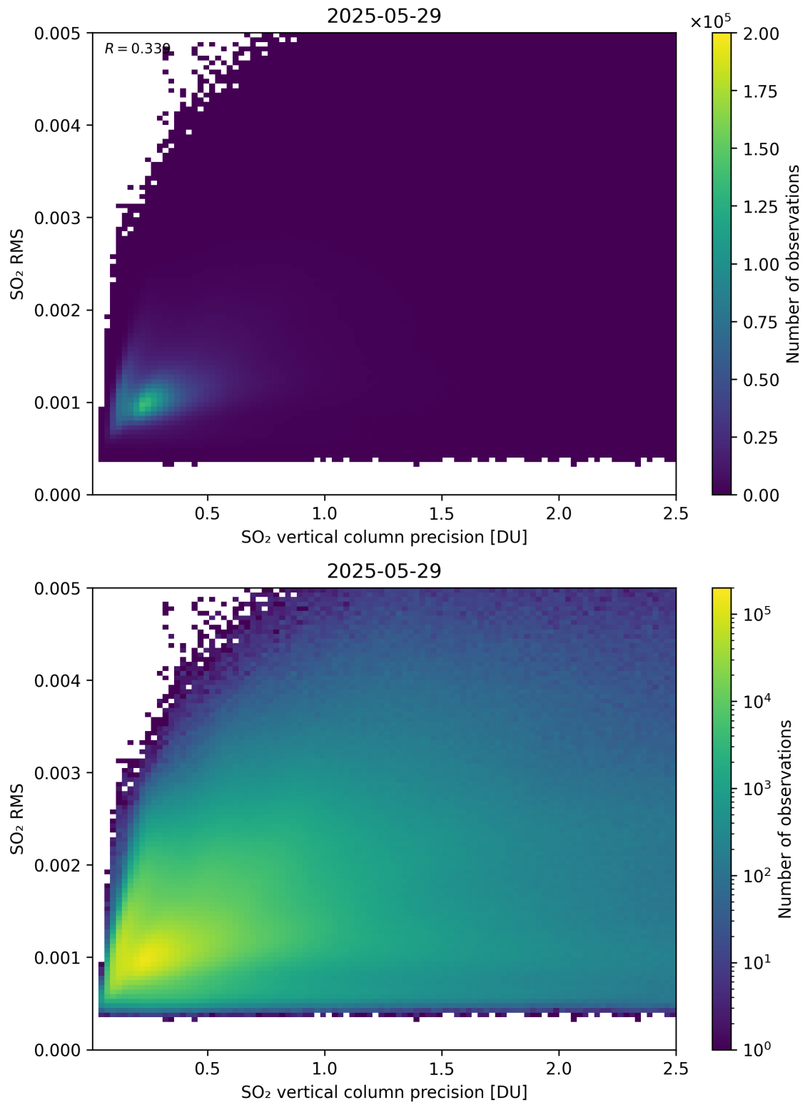
Figure 334: Scatter density plot of “SO 2 vertical column precision” against “SO 2 RMS” for 2025-05-28 to 2025-05-30.
