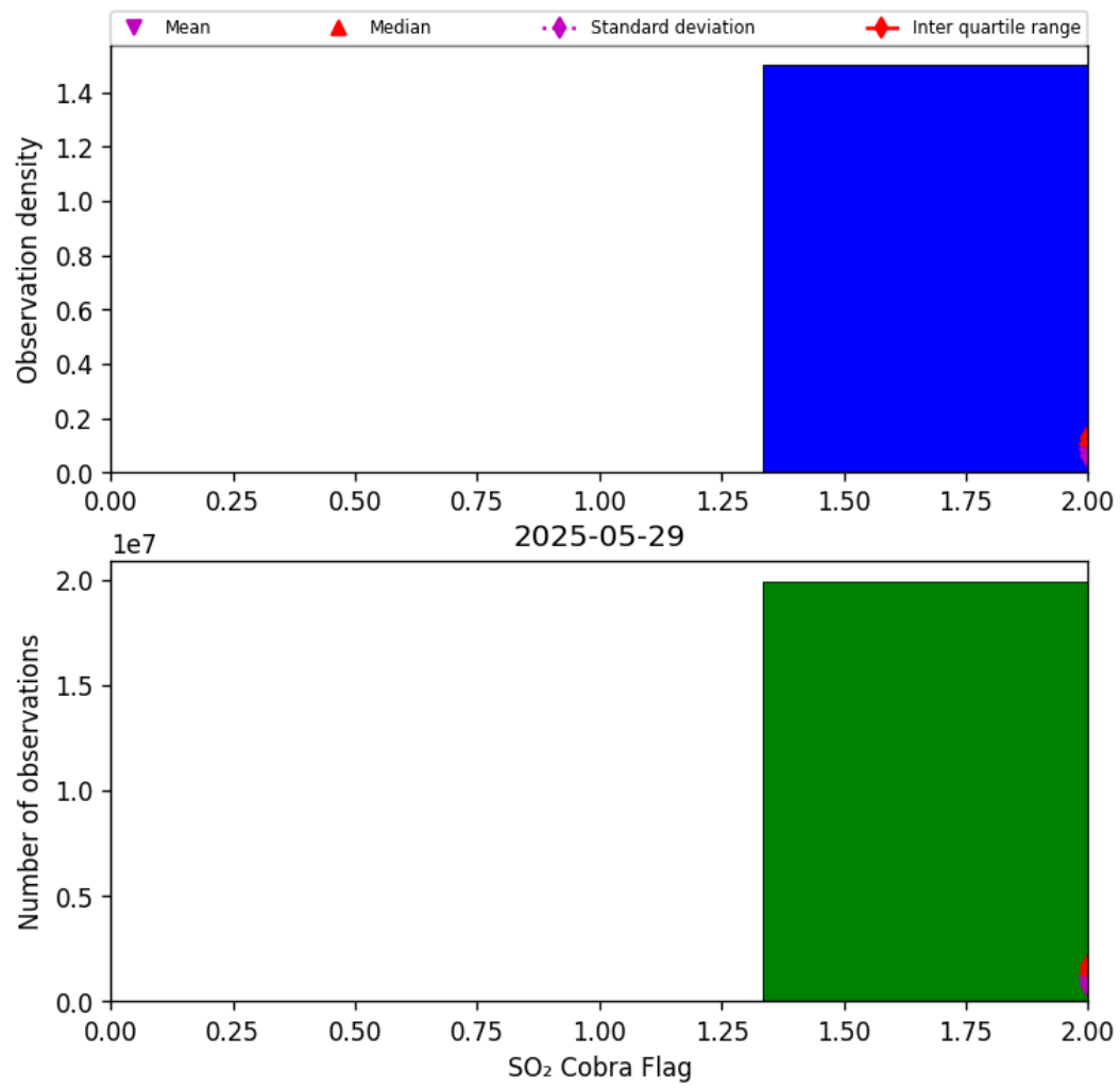
Figure 75: Histogram of “SO 2 Cobra Flag” for 2025-05-28 to 2025-05-30
