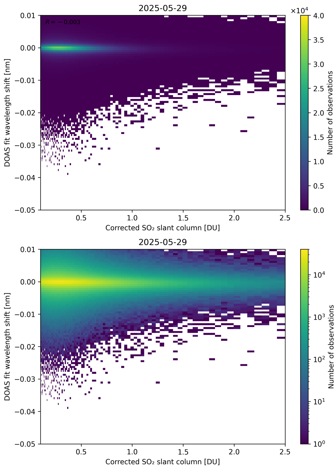
Figure 229: Scatter density plot of “Corrected SO 2 slant column” against “DOAS fit wavelength shift” for 2025-05-28 to 2025-05-30.
