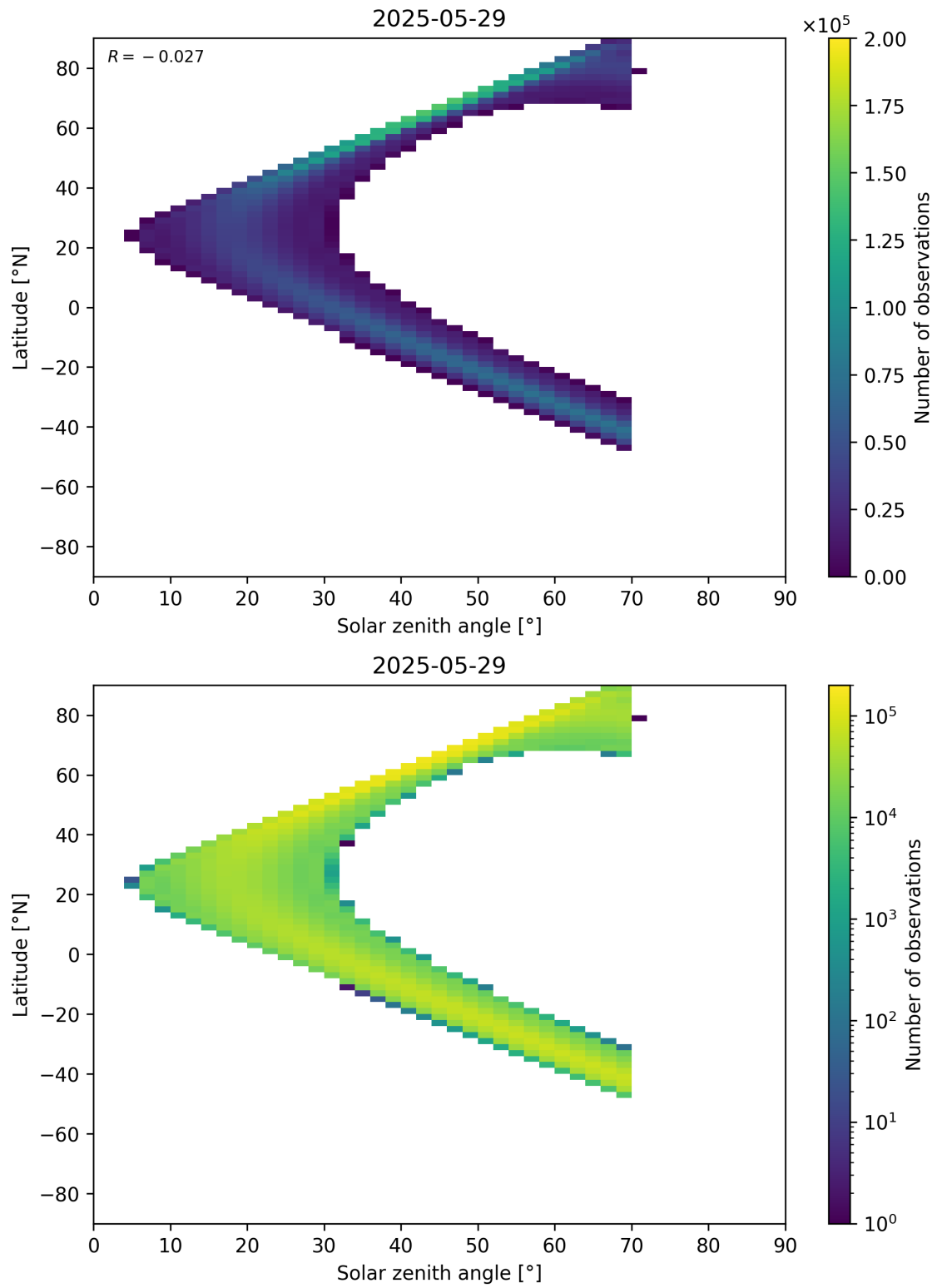
Figure 177: Scatter density plot of “Solar zenith angle” against “Latitude” for 2025-05-28 to 2025-05-30.
