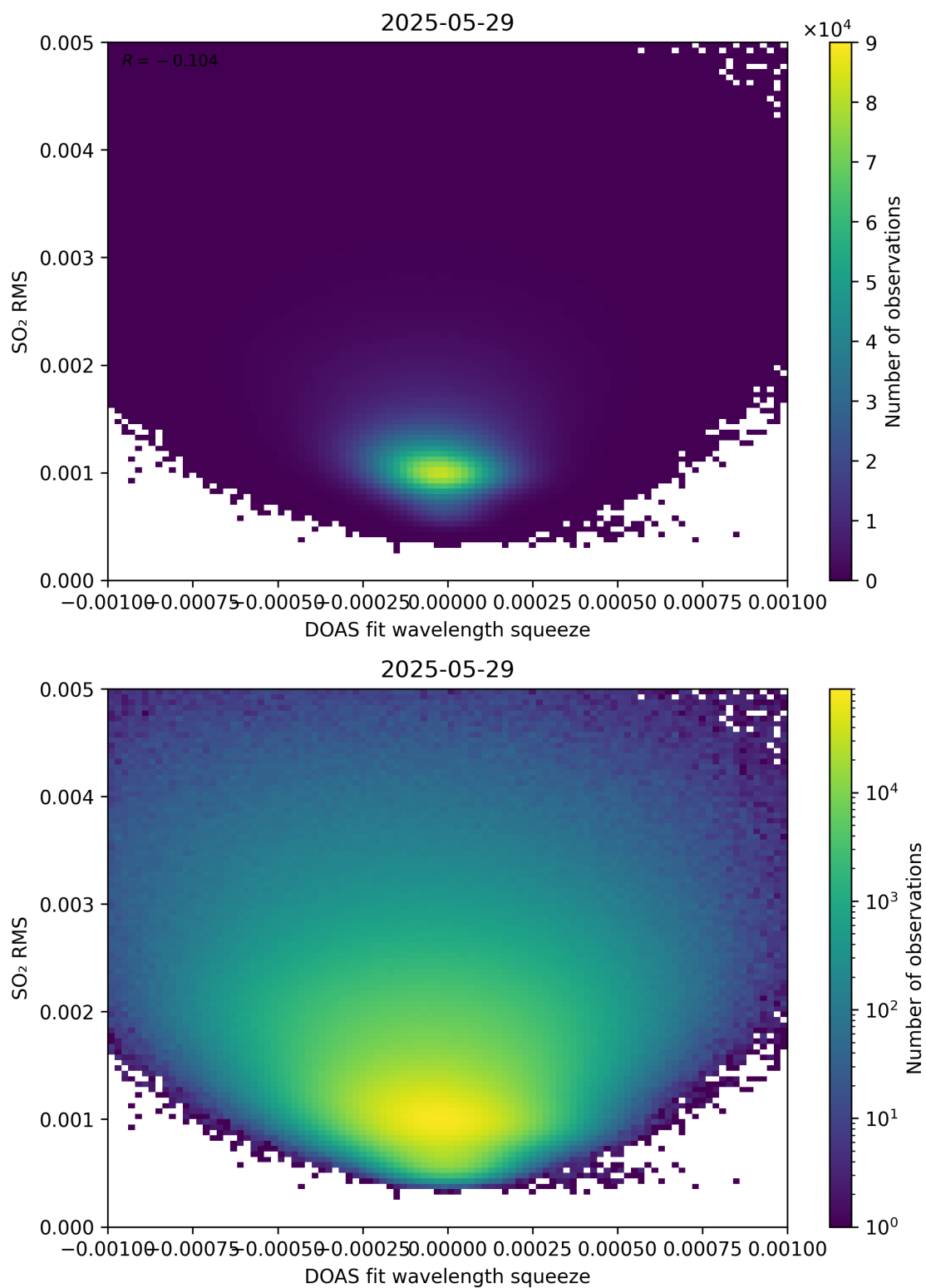
Figure 143: Scatter density plot of “DOAS fit wavelength squeeze” against “SO 2 RMS” for 2025-05-28 to 2025-05-30.
