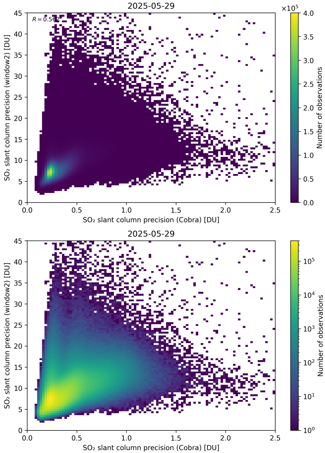
Figure 210: Scatter density plot of “SO 2 slant column precision (Cobra)” against “SO 2 slant column precision (window2)” for 2025-05-28 to 2025-05-30.
