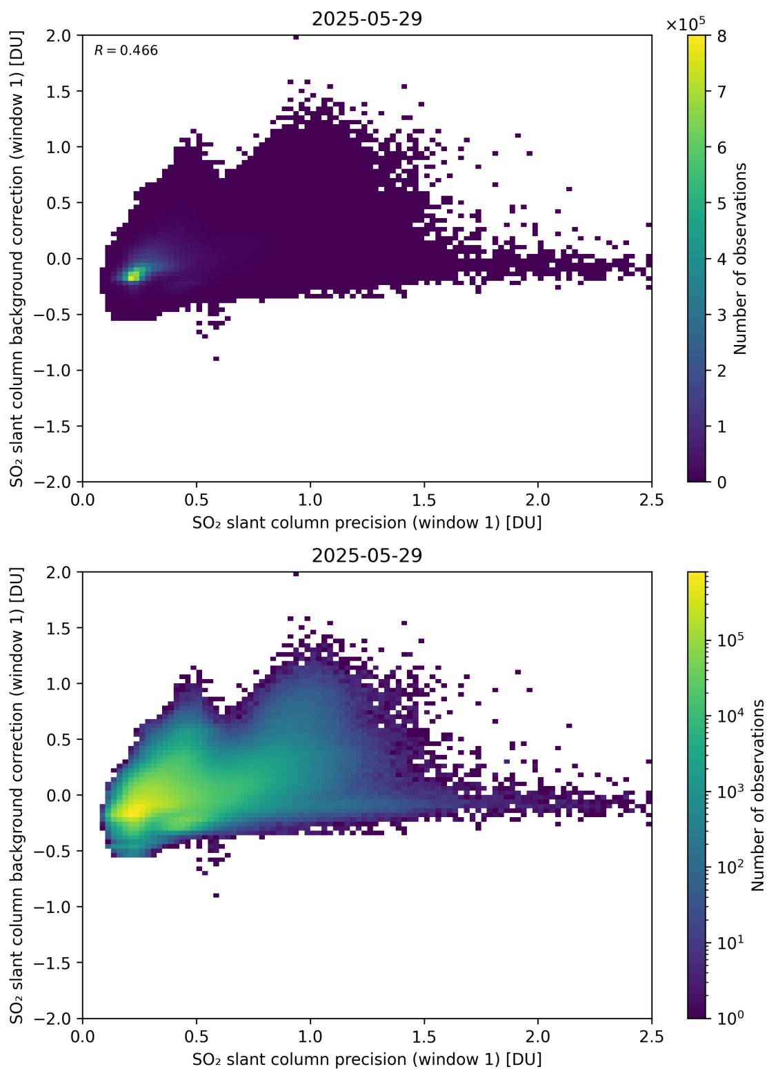
Figure 268: Scatter density plot of “SO 2 slant column precision (window 1)” against “SO 2 slant column background correction (window 1)” for 2025-05-28 to 2025-05-30.
