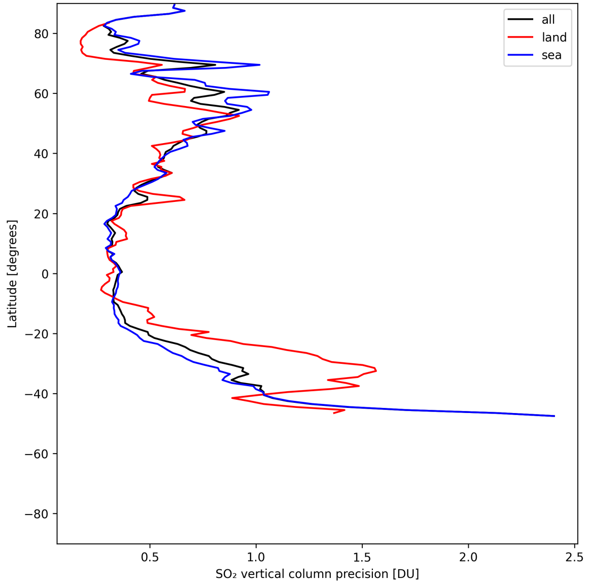
Figure 33: Zonal average of “SO 2 vertical column precision” for 2025-05-28 to 2025-05-30.
