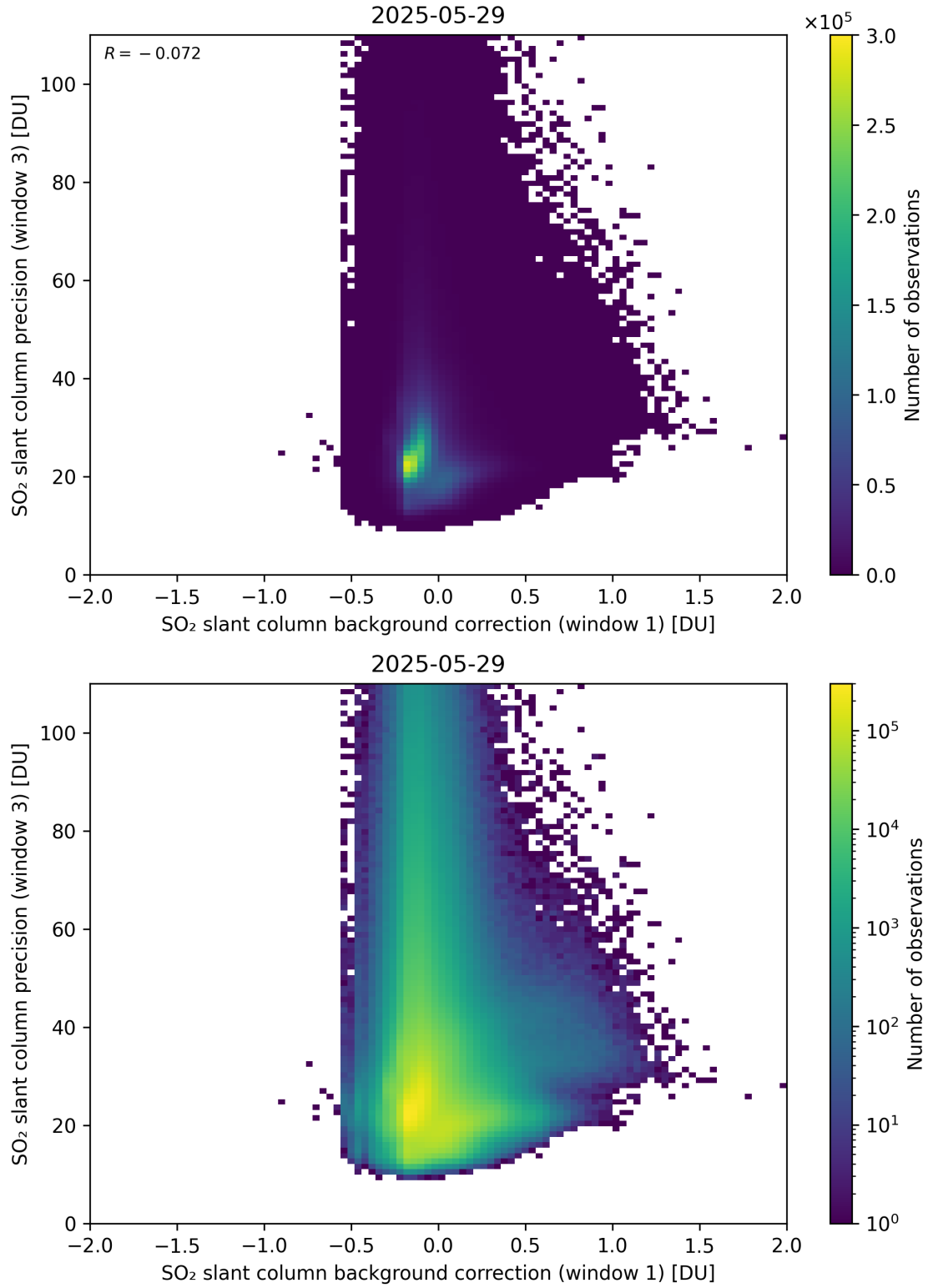
Figure 119: Scatter density plot of “SO 2 slant column background correction (window 1)” against “SO 2 slant column precision (window 3)” for 2025-05-28 to 2025-05-30.
