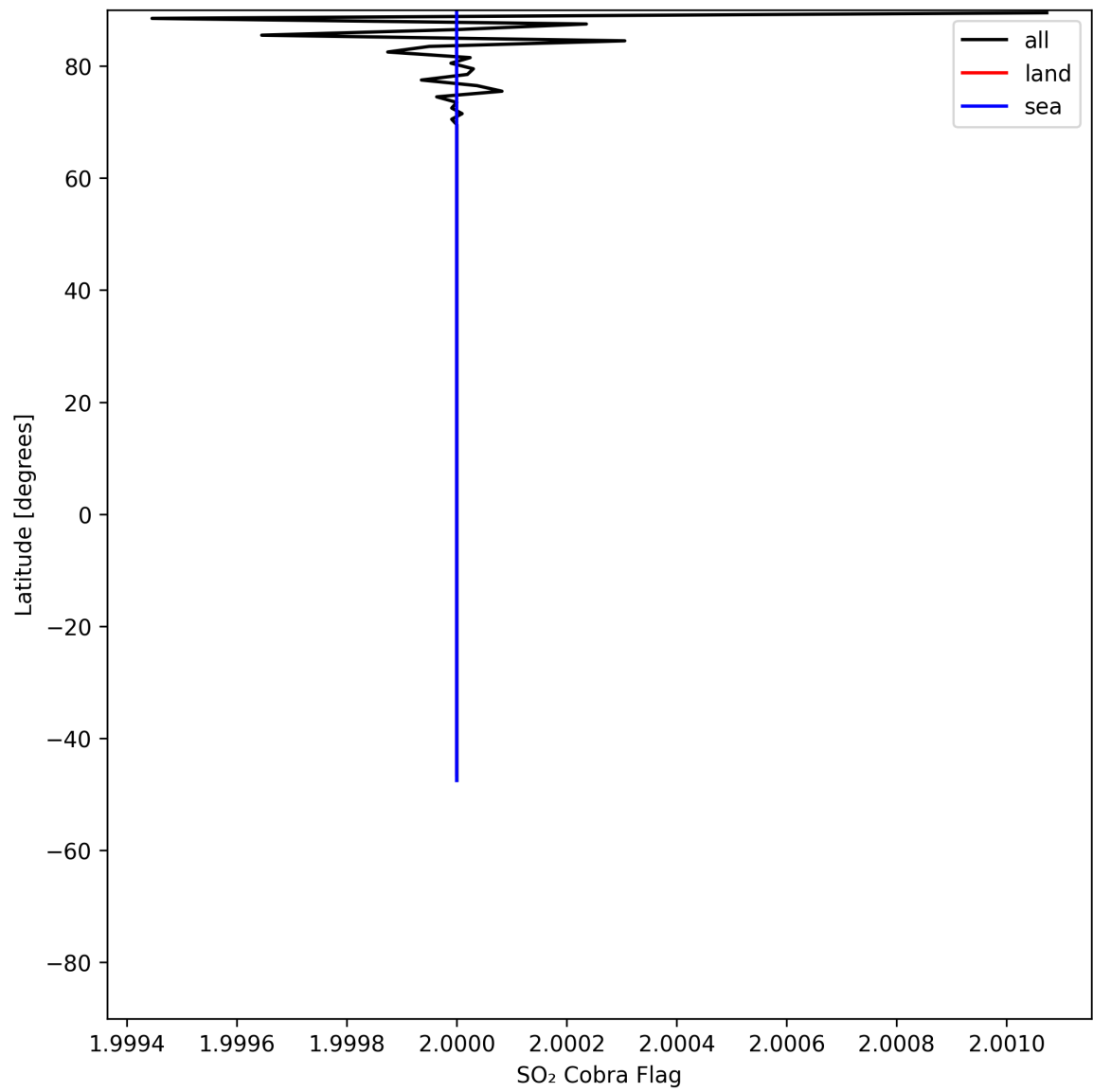
Figure 49: Zonal average of "SO 2 Cobra Flag" for 2025-05-28 to 2025-05-30.
