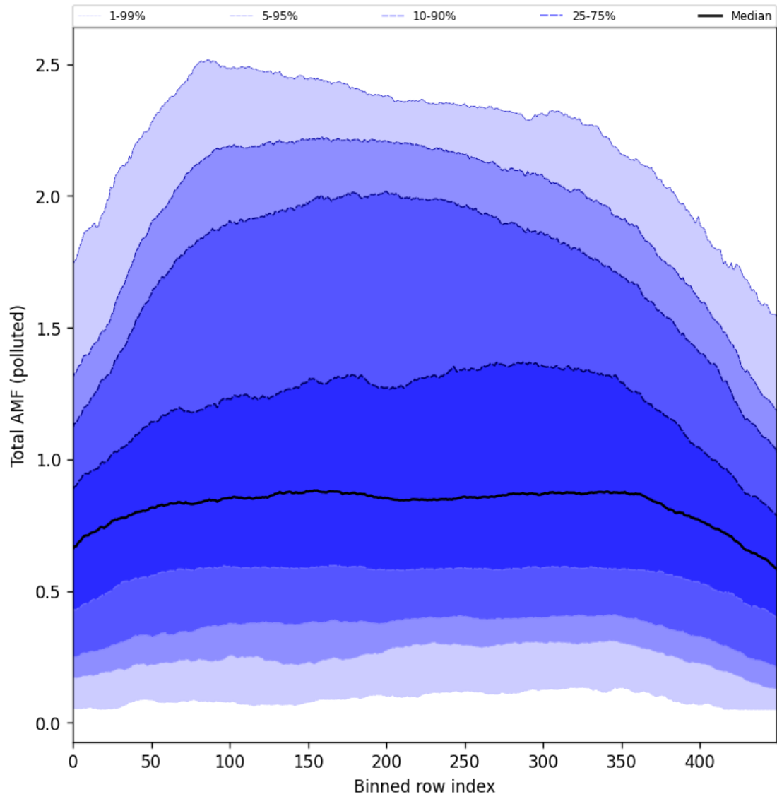
Figure 105: Along track statistics of “Total AMF (polluted)” for 2025-05-28 to 2025-05-30
