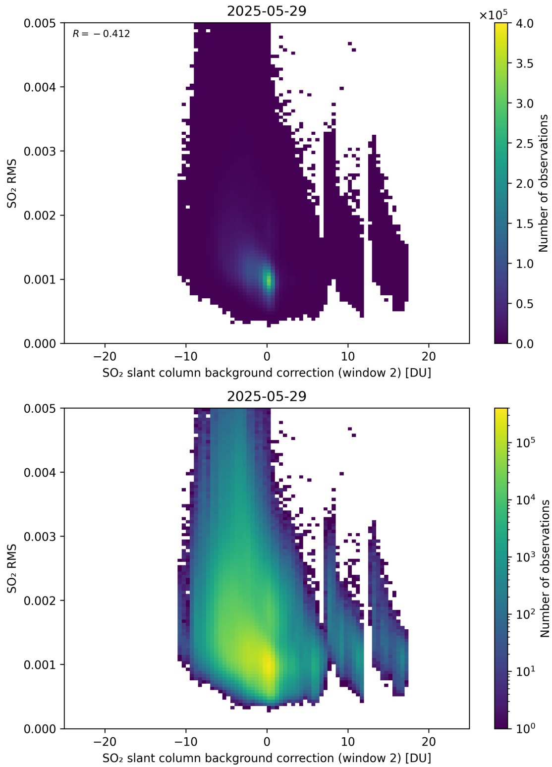
Figure 125: Scatter density plot of “SO 2 slant column background correction (window 2)” against “SO 2 RMS” for 2025-05-28 to 2025-05-30.
