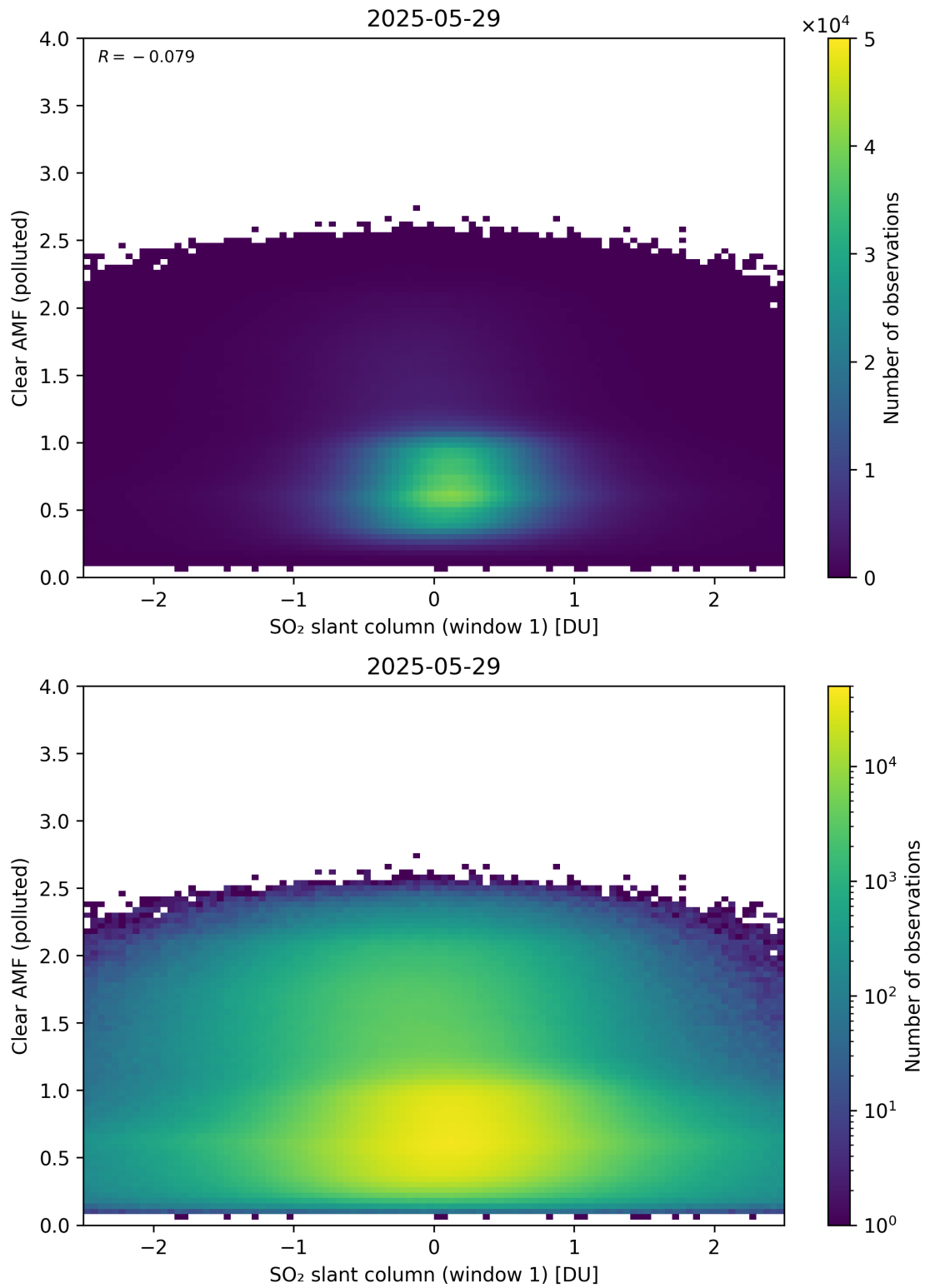
Figure 282: Scatter density plot of “SO 2 slant column (window 1)” against “Clear AMF (polluted)” for 2025-05-28 to 2025-05-30.
