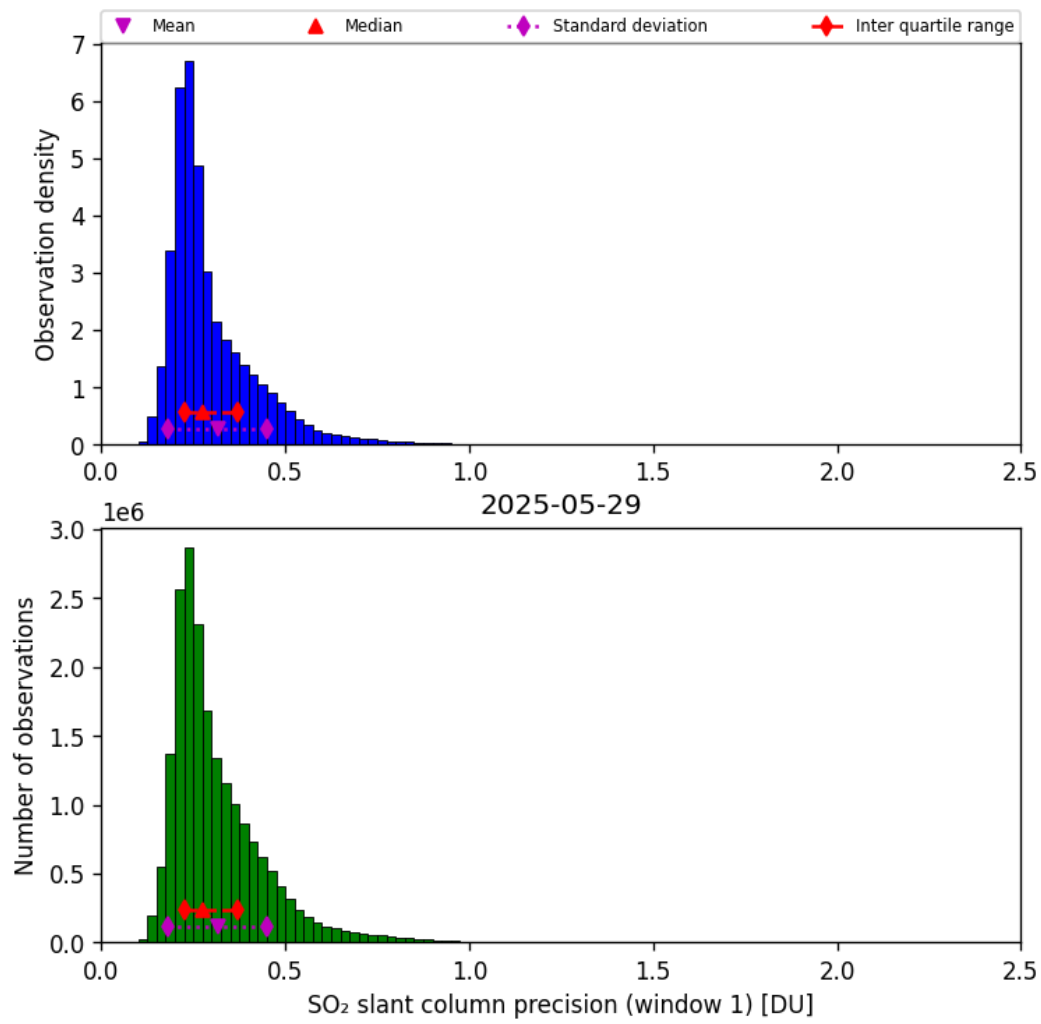
Figure 64: Histogram of “SO 2 slant column precision (window 1)” for 2025-05-28 to 2025-05-30
