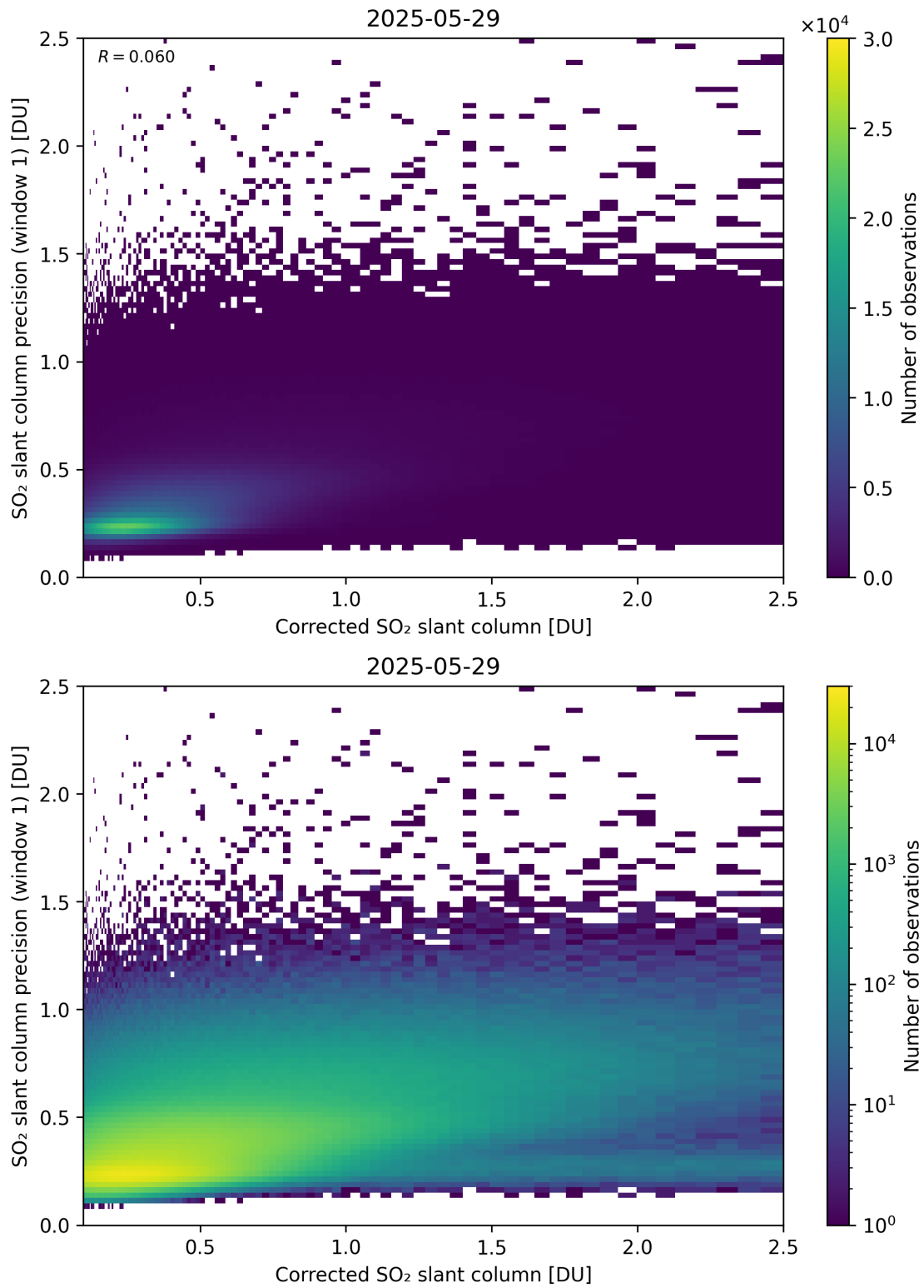
Figure 238: Scatter density plot of “Corrected SO 2 slant column” against “SO 2 slant column precision (window 1)” for 2025-05-28 to 2025-05-30.
