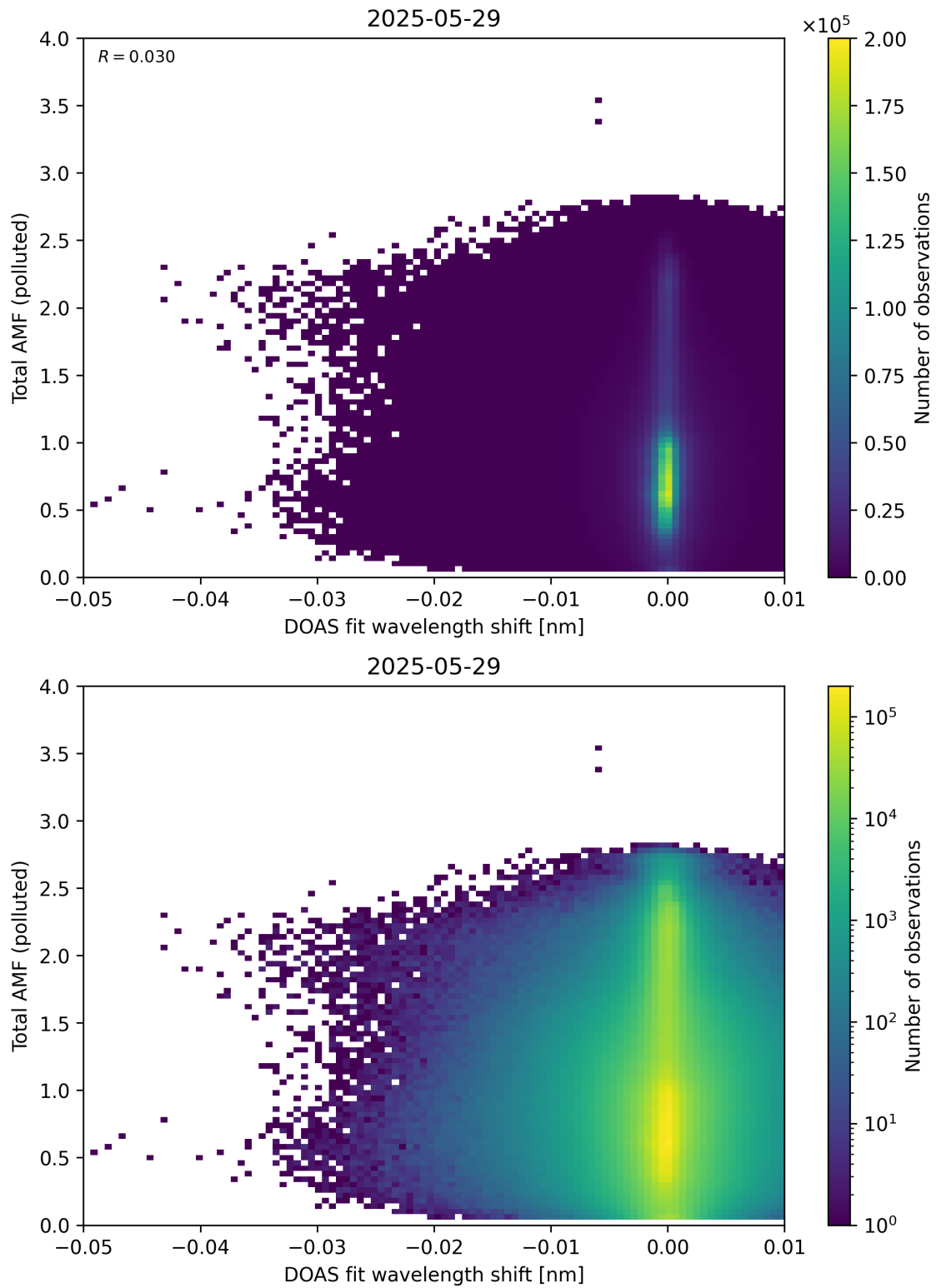
Figure 141: Scatter density plot of “DOAS fit wavelength shift” against “Total AMF (polluted)” for 2025-05-28 to 2025-05-30.
