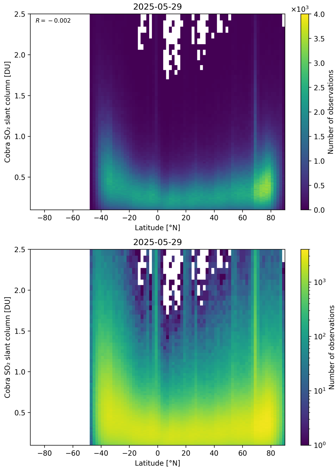
Figure 157: Scatter density plot of “Latitude” against “Cobra SO 2 slant column” for 2025-05-28 to 2025-05-30.
