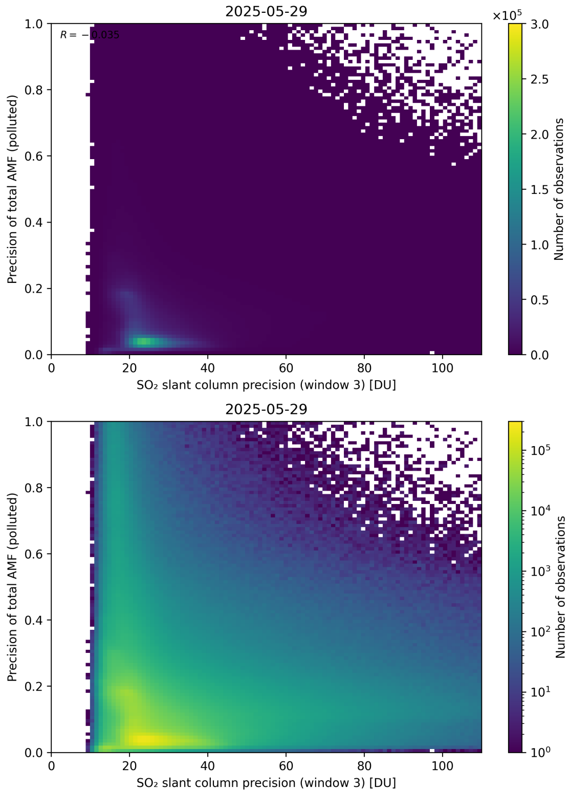
Figure 314: Scatter density plot of “SO 2 slant column precision (window 3)” against “Precision of total AMF (polluted)” for 2025-05-28 to 2025-05-30.
