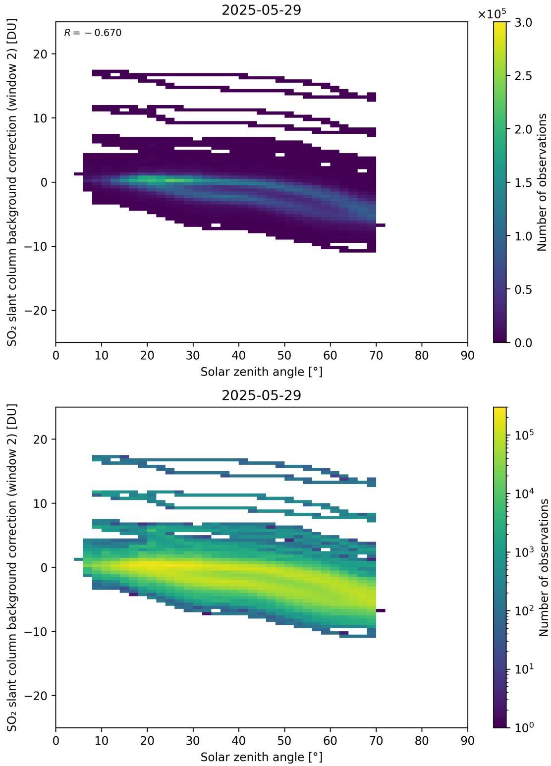
Figure 172: Scatter density plot of “Solar zenith angle” against “SO 2 slant column background correction (window 2)” for 2025-05-28 to 2025-05-30.
