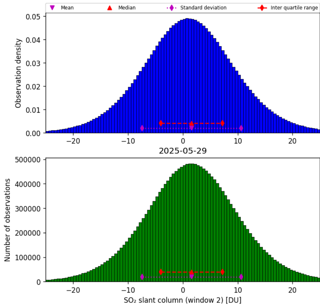
Figure 67: Histogram of “SO 2 slant column (window 2)” for 2025-05-28 to 2025-05-30
