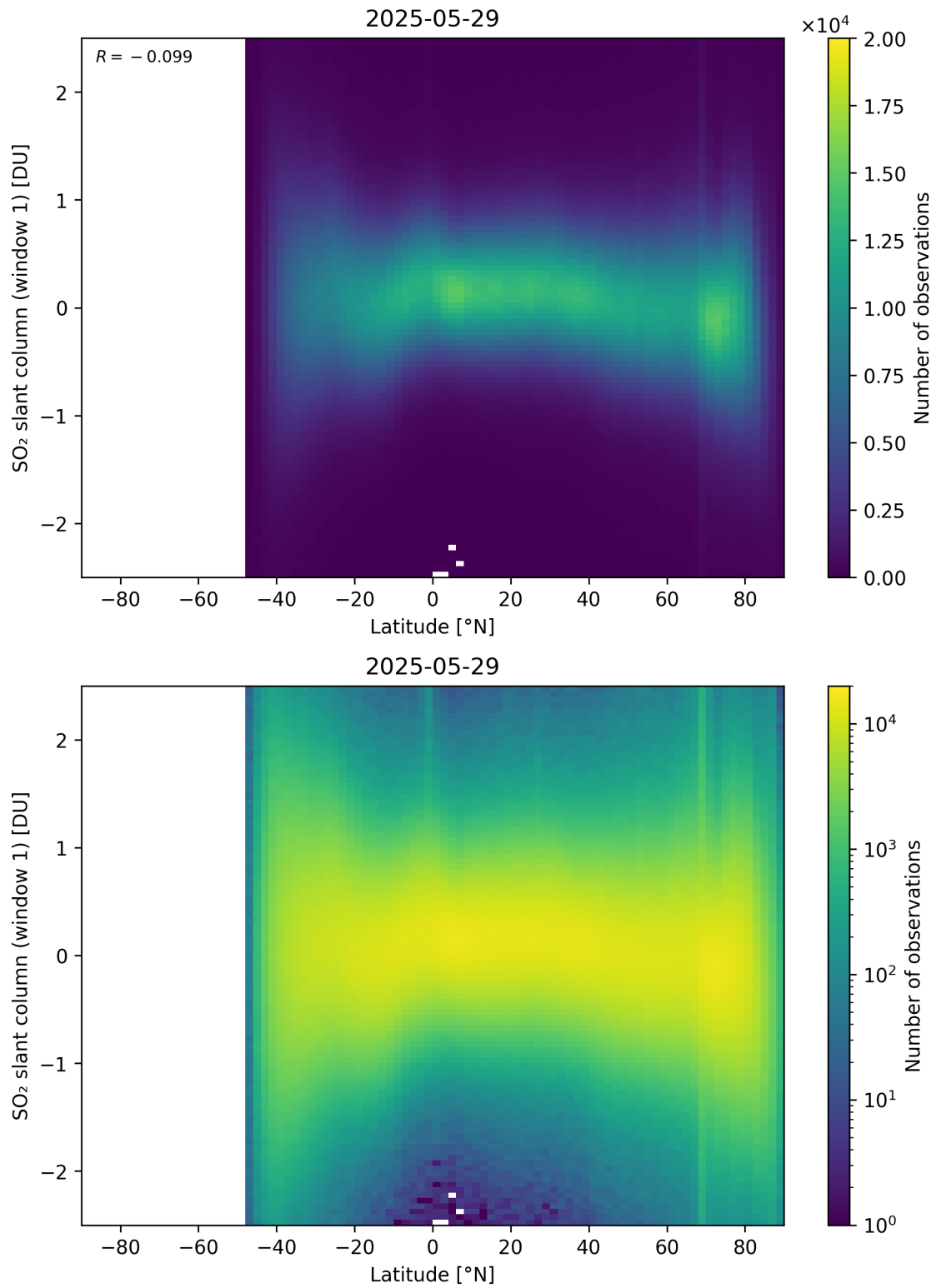
Figure 162: Scatter density plot of “Latitude” against “SO 2 slant column (window 1)” for 2025-05-28 to 2025-05-30.
