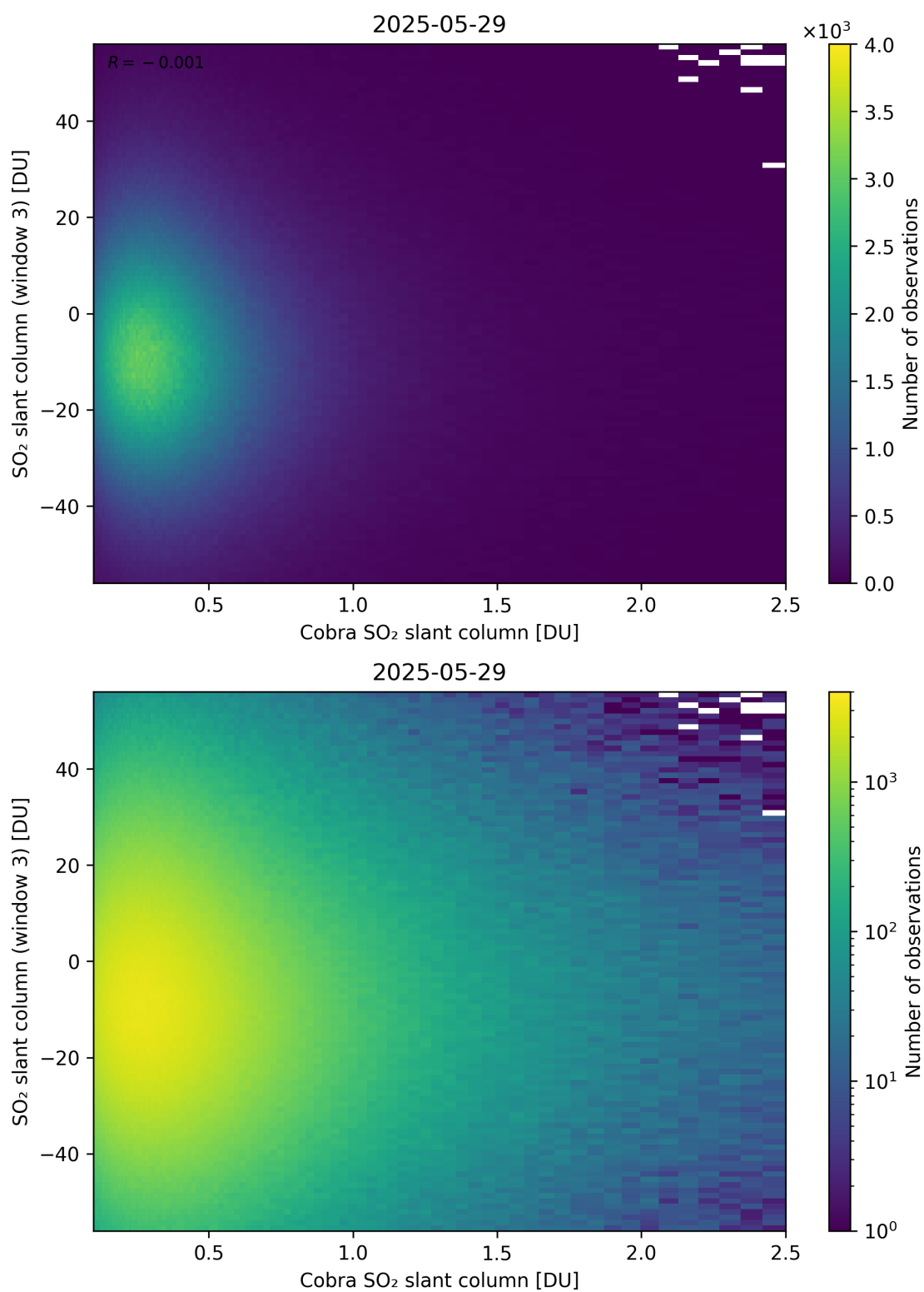
Figure 222: Scatter density plot of “Cobra SO 2 slant column” against “SO 2 slant column (window 3)” for 2025-05-28 to 2025-05-30.
