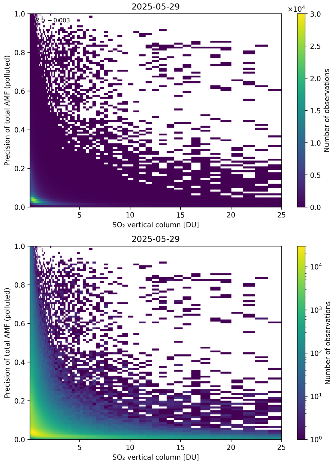
Figure 360: Scatter density plot of “SO 2 vertical column” against “Precision of total AMF (polluted)” for 2025-05-28 to 2025-05-30.
