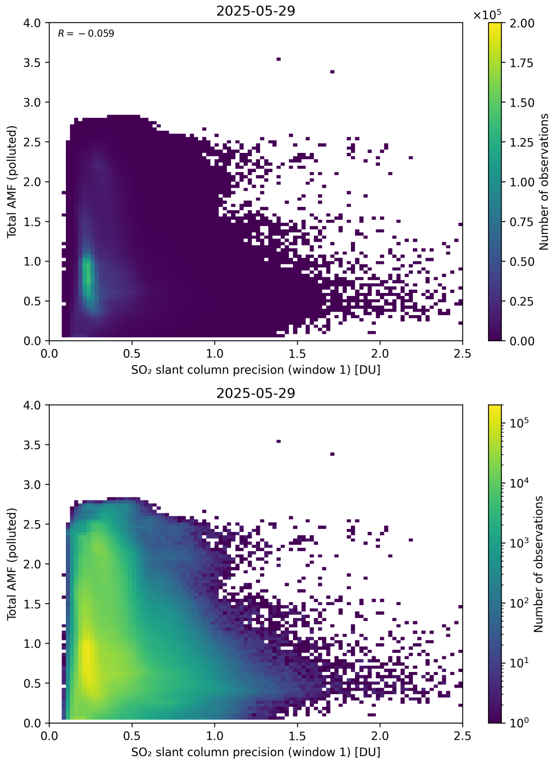
Figure 280: Scatter density plot of “SO 2 slant column precision (window 1)” against “Total AMF (polluted)” for 2025-05-28 to 2025-05-30.
