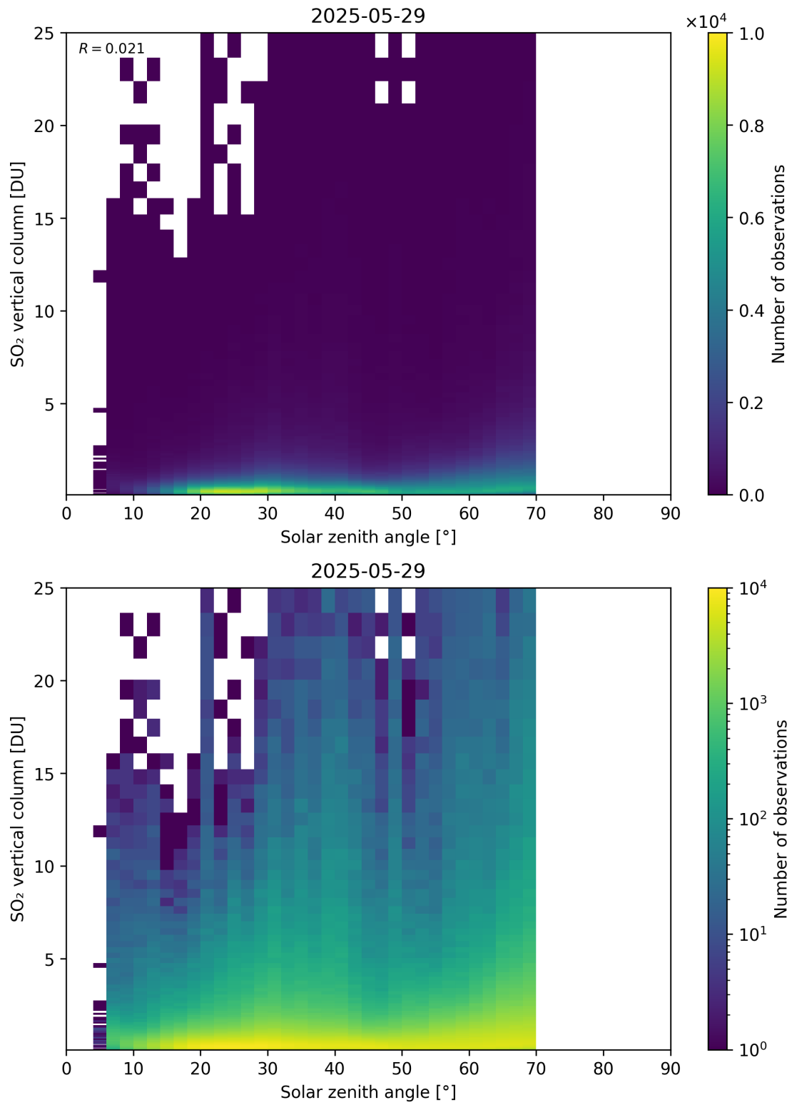
Figure 191: Scatter density plot of “Solar zenith angle” against “SO 2 vertical column” for 2025-05-28 to 2025-05-30.
