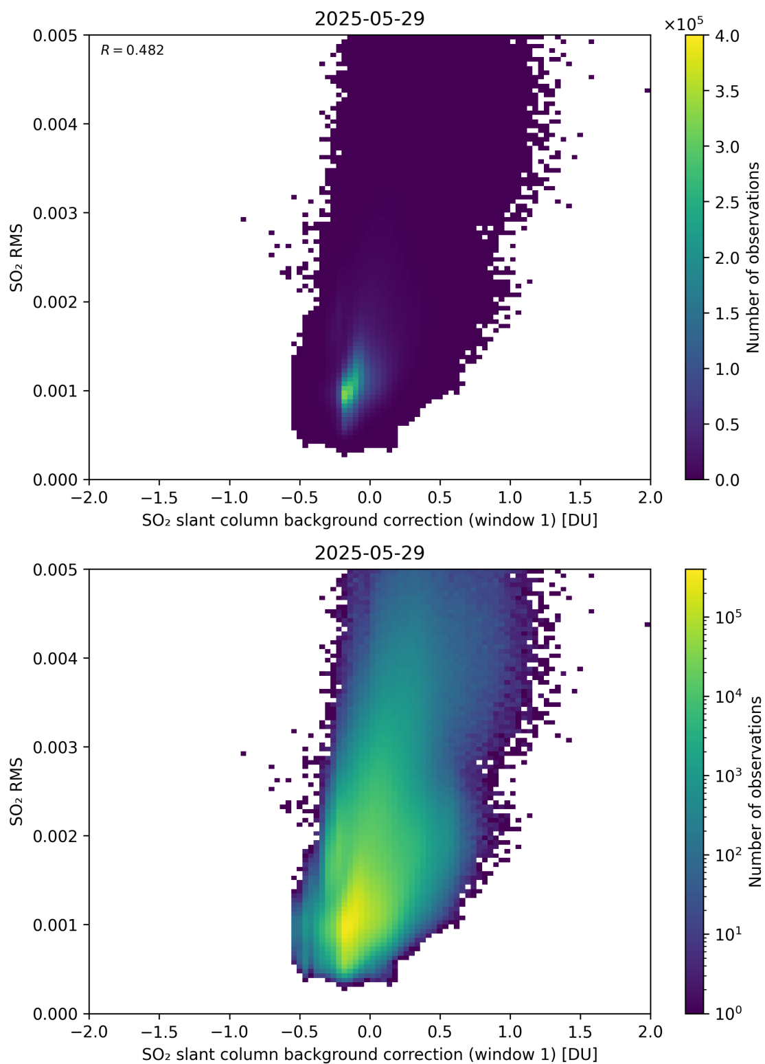
Figure 113: Scatter density plot of “SO 2 slant column background correction (window 1)” against “SO 2 RMS” for 2025-05-28 to 2025-05-30.
