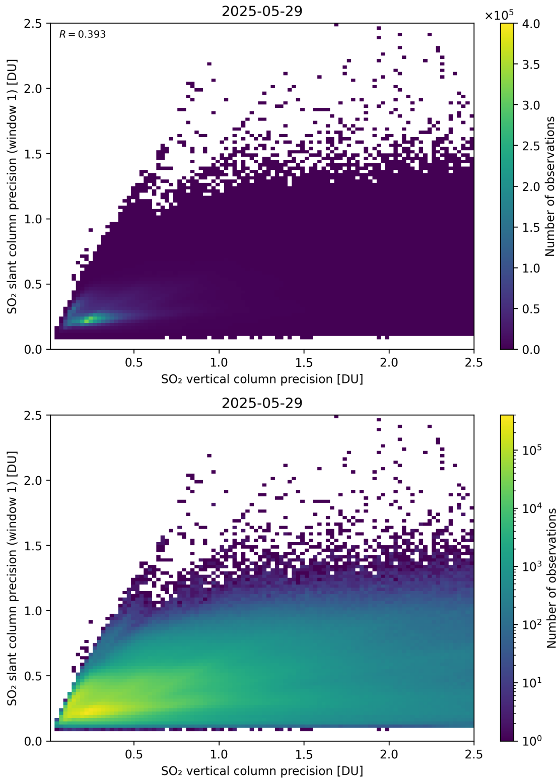
Figure 342: Scatter density plot of “SO 2 vertical column precision” against “SO 2 slant column precision (window 1)” for 2025-05-28 to 2025-05-30.
