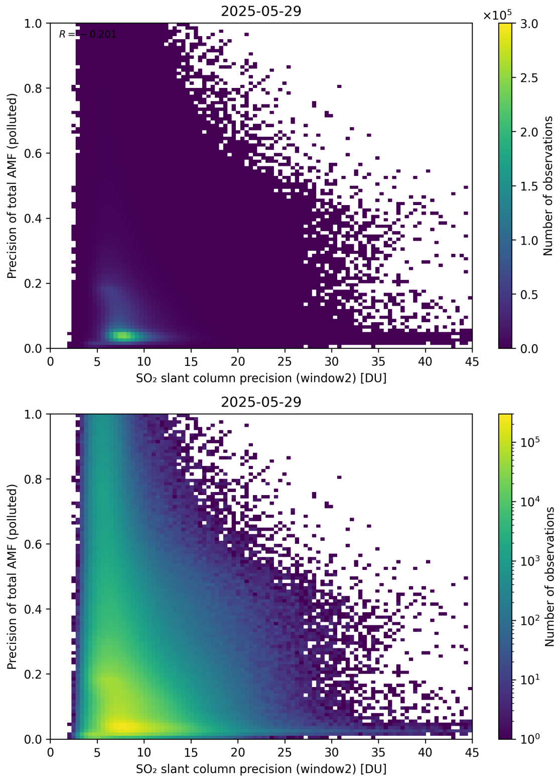
Figure 302: Scatter density plot of “SO 2 slant column precision (window2)” against “Precision of total AMF (polluted)” for 2025-05-28 to 2025-05-30.
