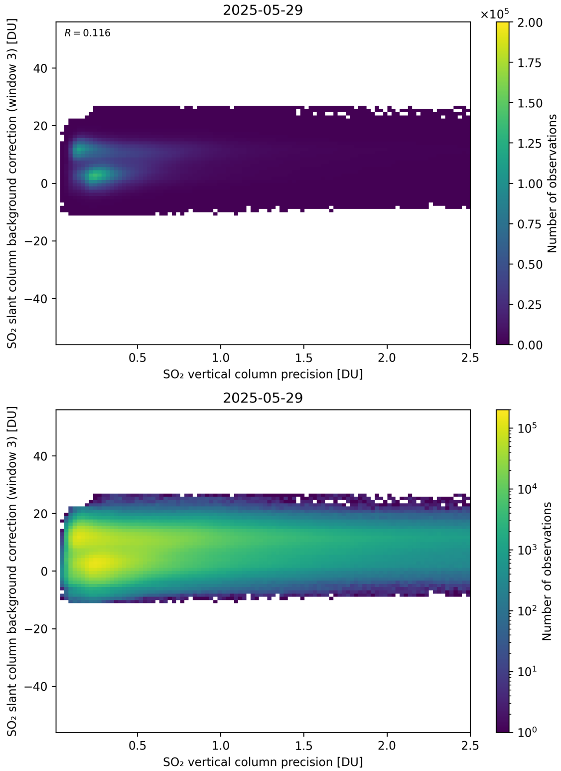
Figure 331: Scatter density plot of “SO 2 vertical column precision” against “SO 2 slant column background correction (window 3)” for 2025-05-28 to 2025-05-30.
