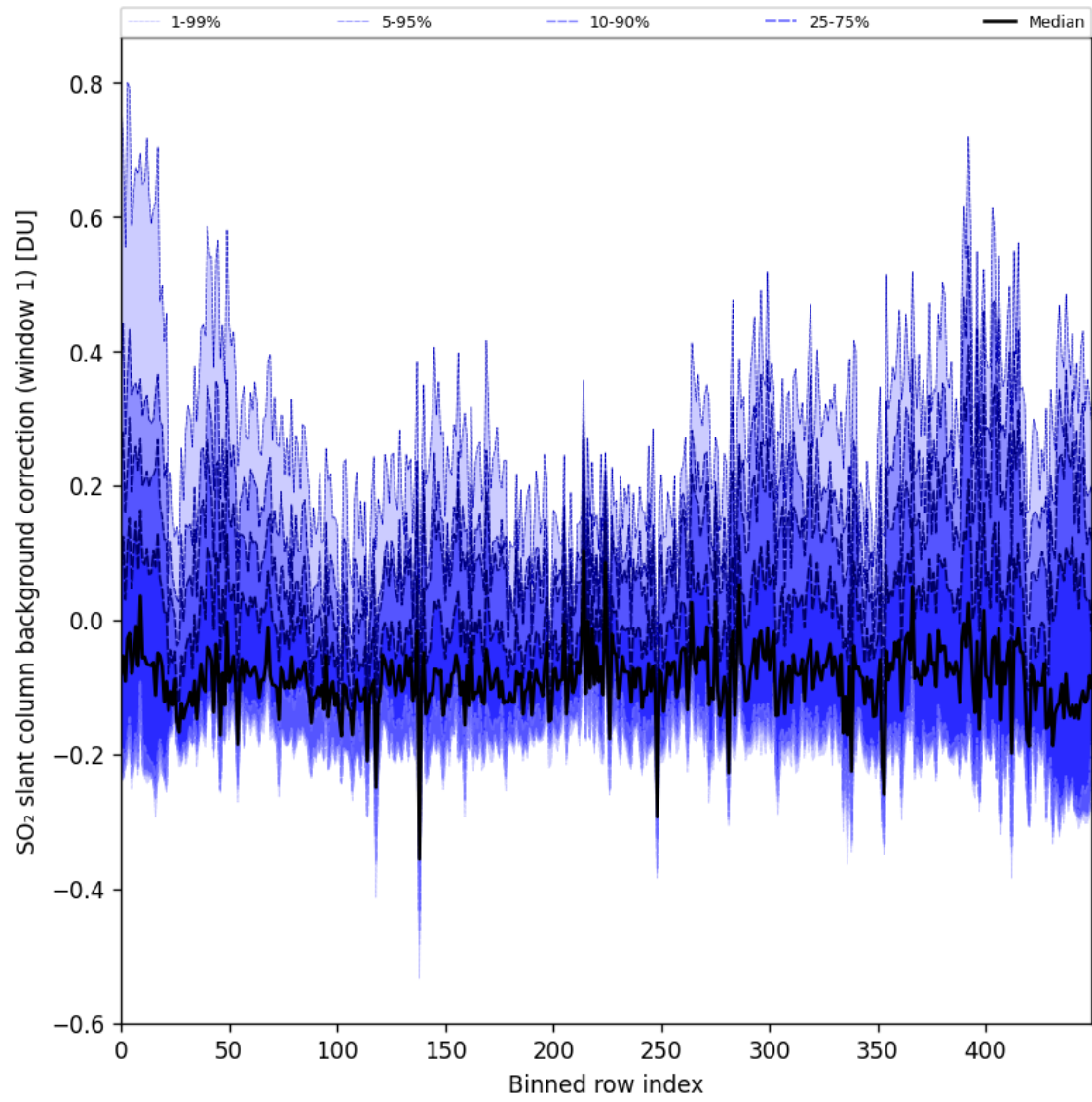
Figure 92: Along track statistics of “SO 2 slant column background correction (window 1)” for 2025-05-28 to 2025-05-30
