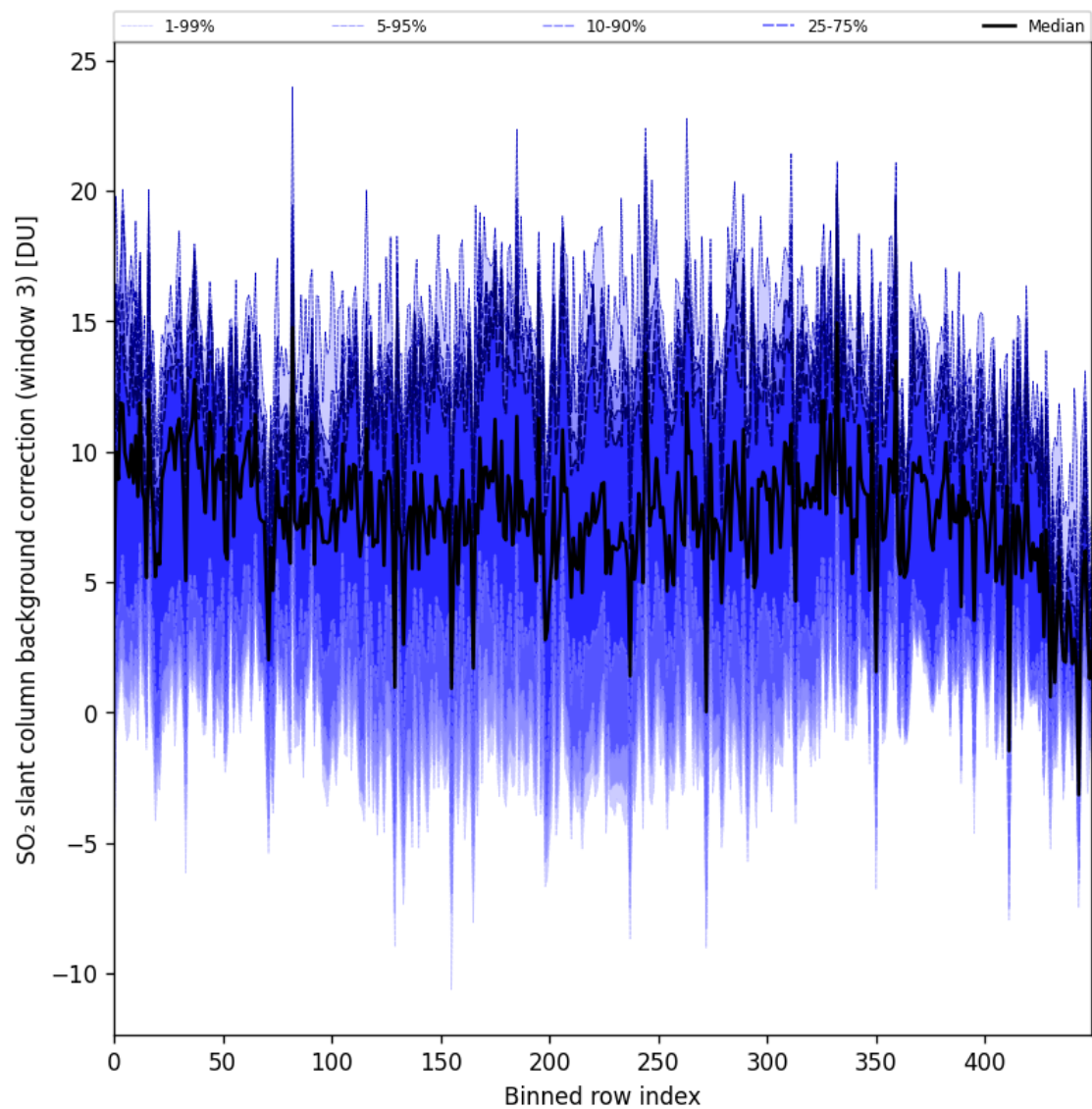
Figure 100: Along track statistics of “SO 2 slant column background correction (window 3)” for 2025-05-28 to 2025-05-30
