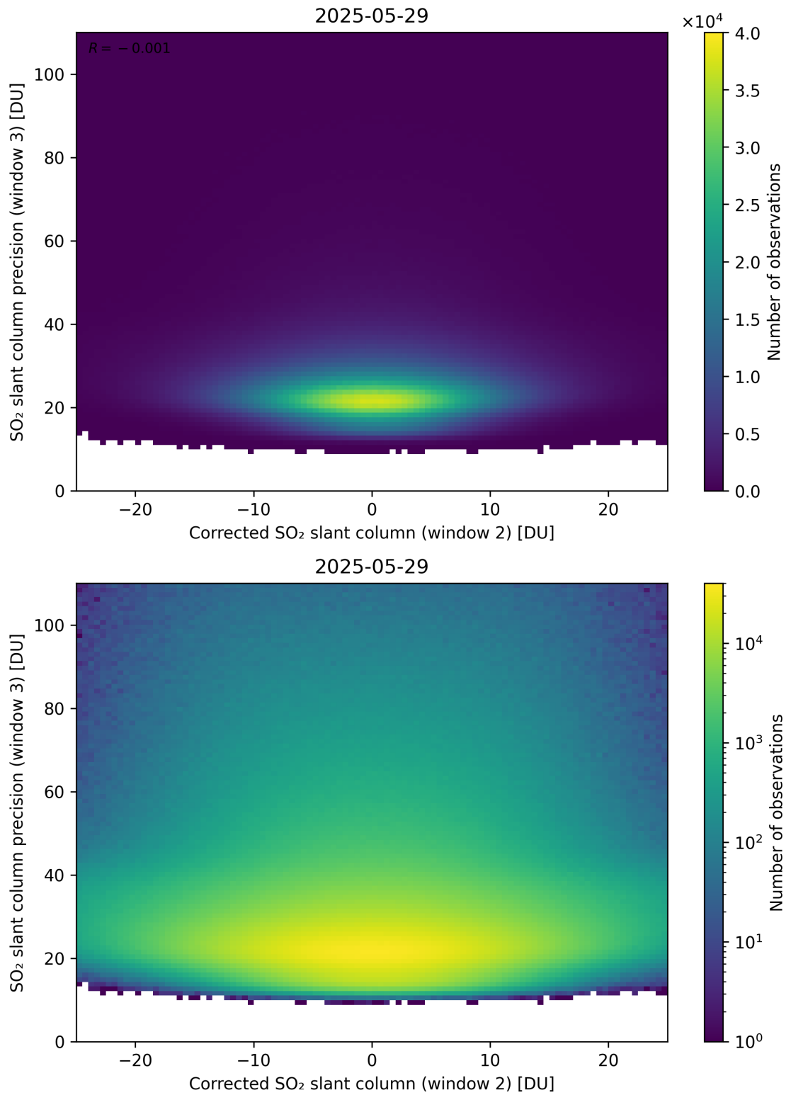
Figure 252: Scatter density plot of “Corrected SO 2 slant column (window 2)” against “SO 2 slant column precision (window 3)” for 2025-05-28 to 2025-05-30.
