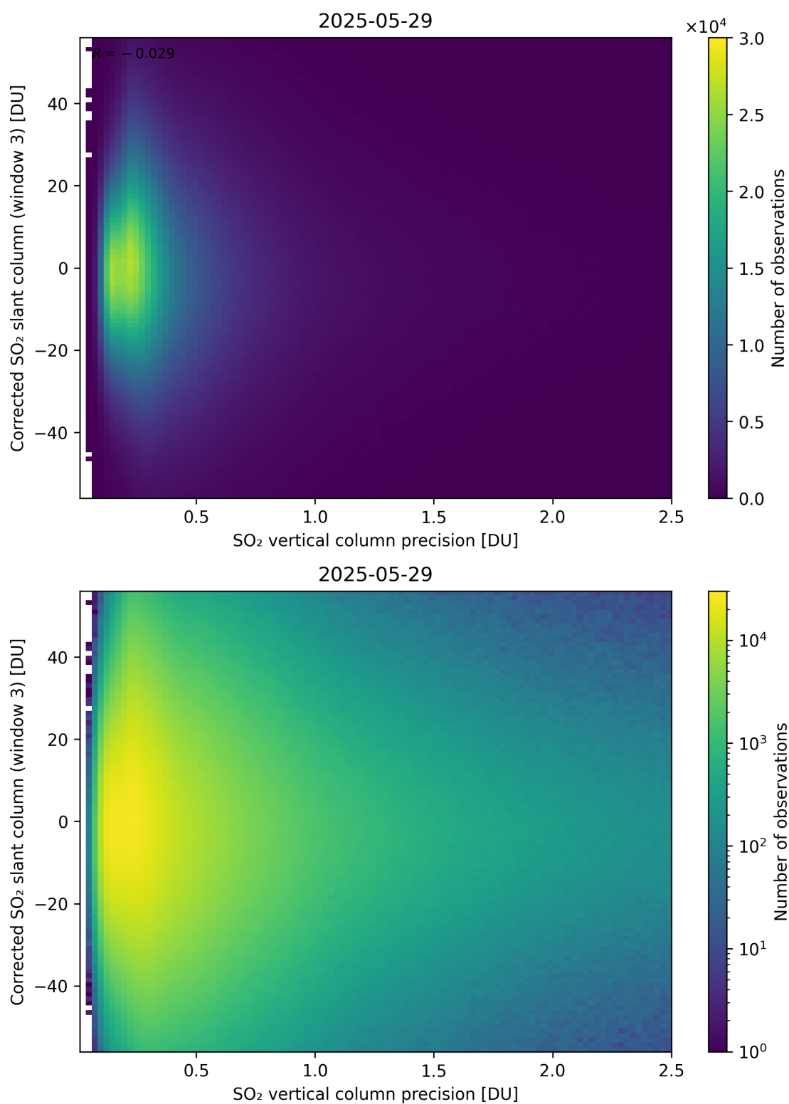
Figure 340: Scatter density plot of “SO 2 vertical column precision” against “Corrected SO 2 slant column (window 3)” for 2025-05-28 to 2025-05-30.
