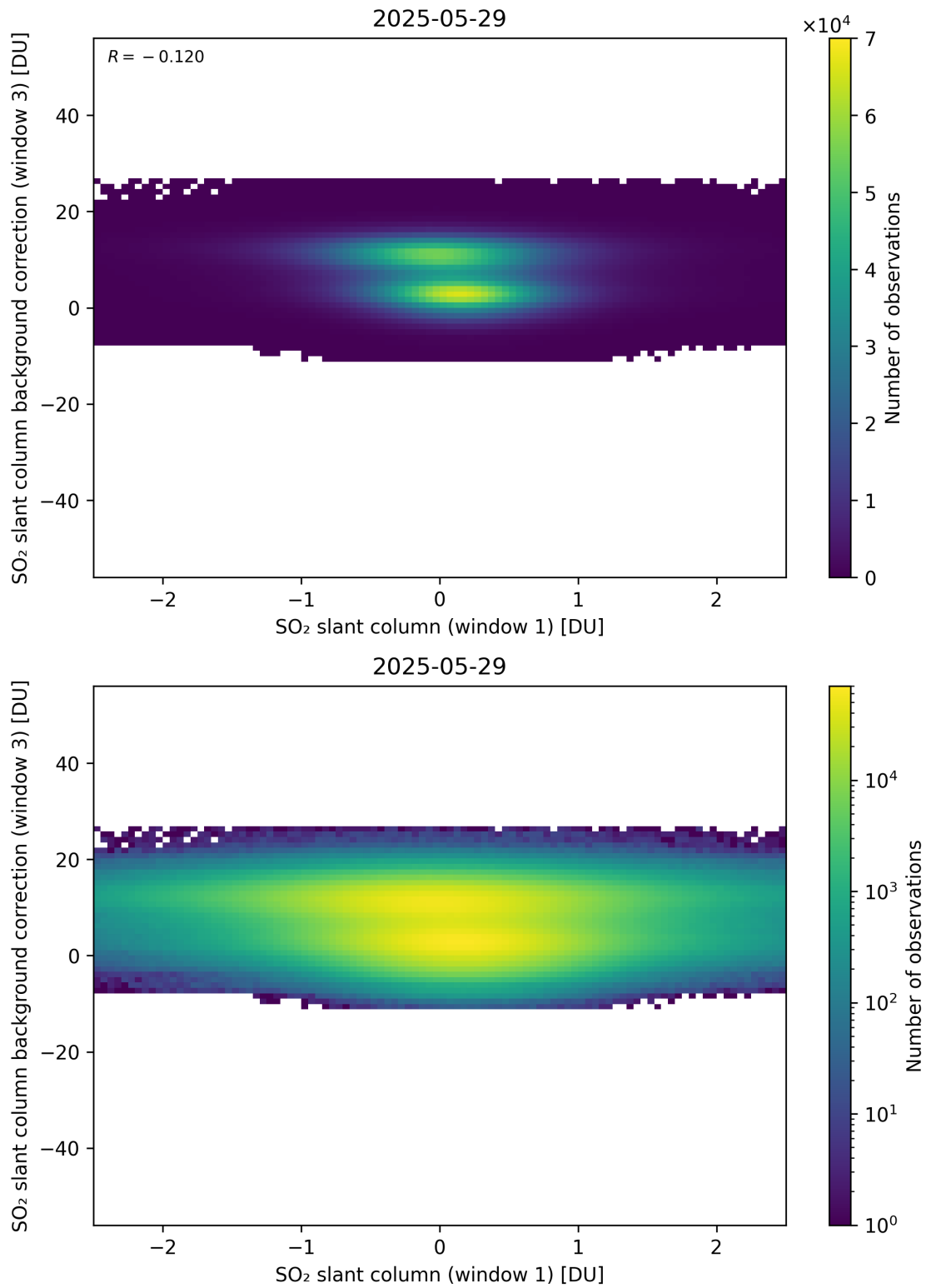
Figure 264: Scatter density plot of “SO 2 slant column (window 1)” against “SO 2 slant column background correction (window 3)” for 2025-05-28 to 2025-05-30.
