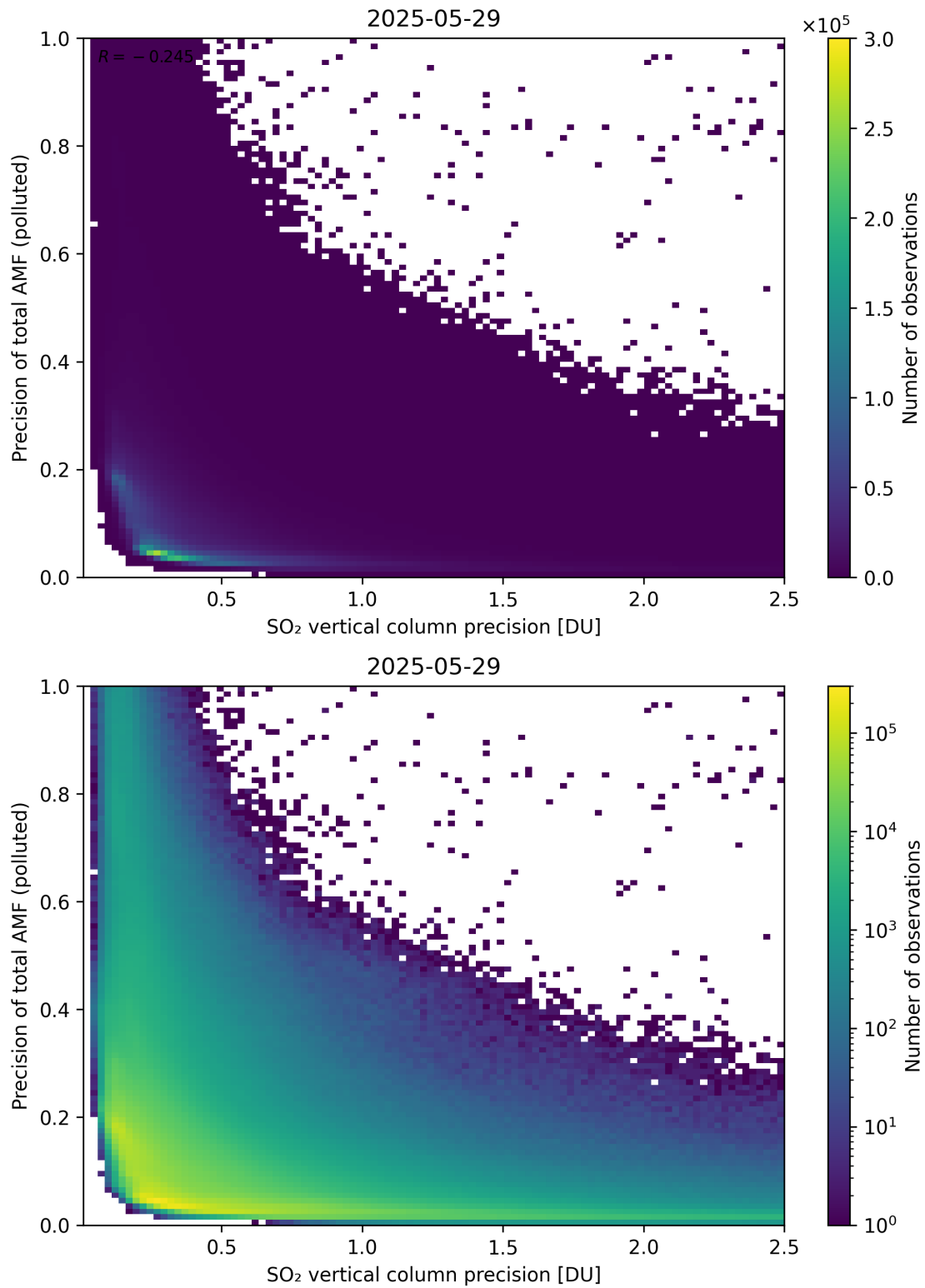
Figure 347: Scatter density plot of “SO 2 vertical column precision” against “Precision of total AMF (polluted)” for 2025-05-28 to 2025-05-30.
