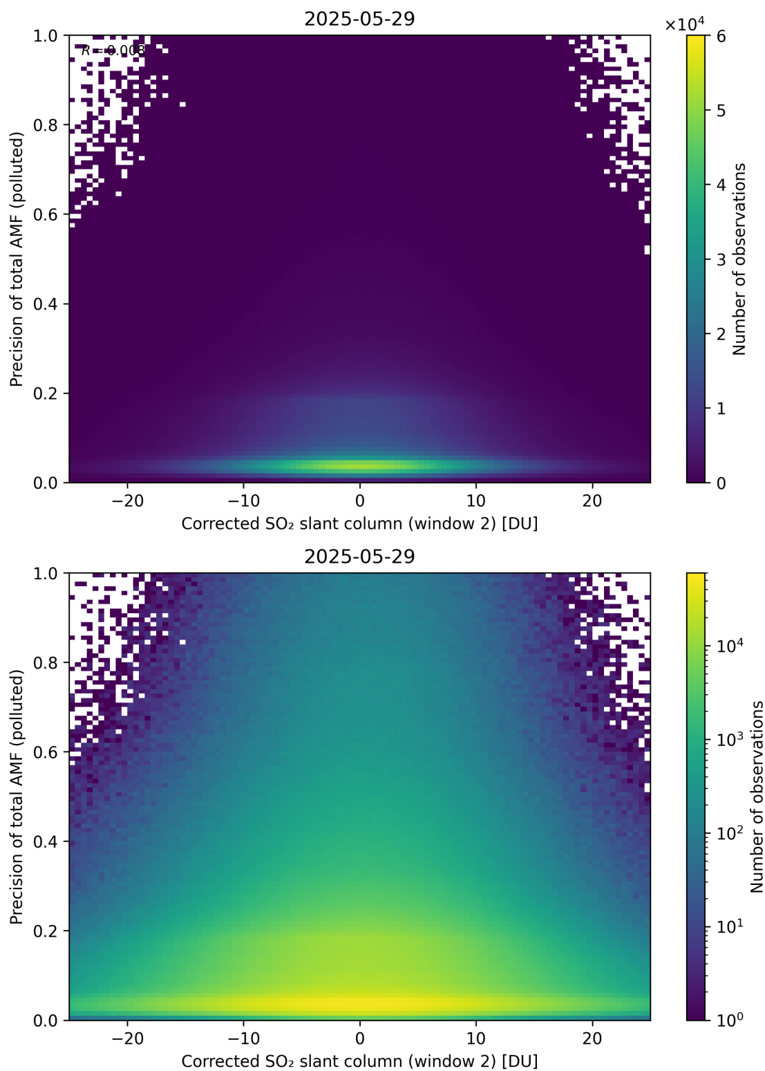
Figure 254: Scatter density plot of “Corrected SO 2 slant column (window 2)” against “Precision of total AMF (polluted)” for 2025-05-28 to 2025-05-30.
