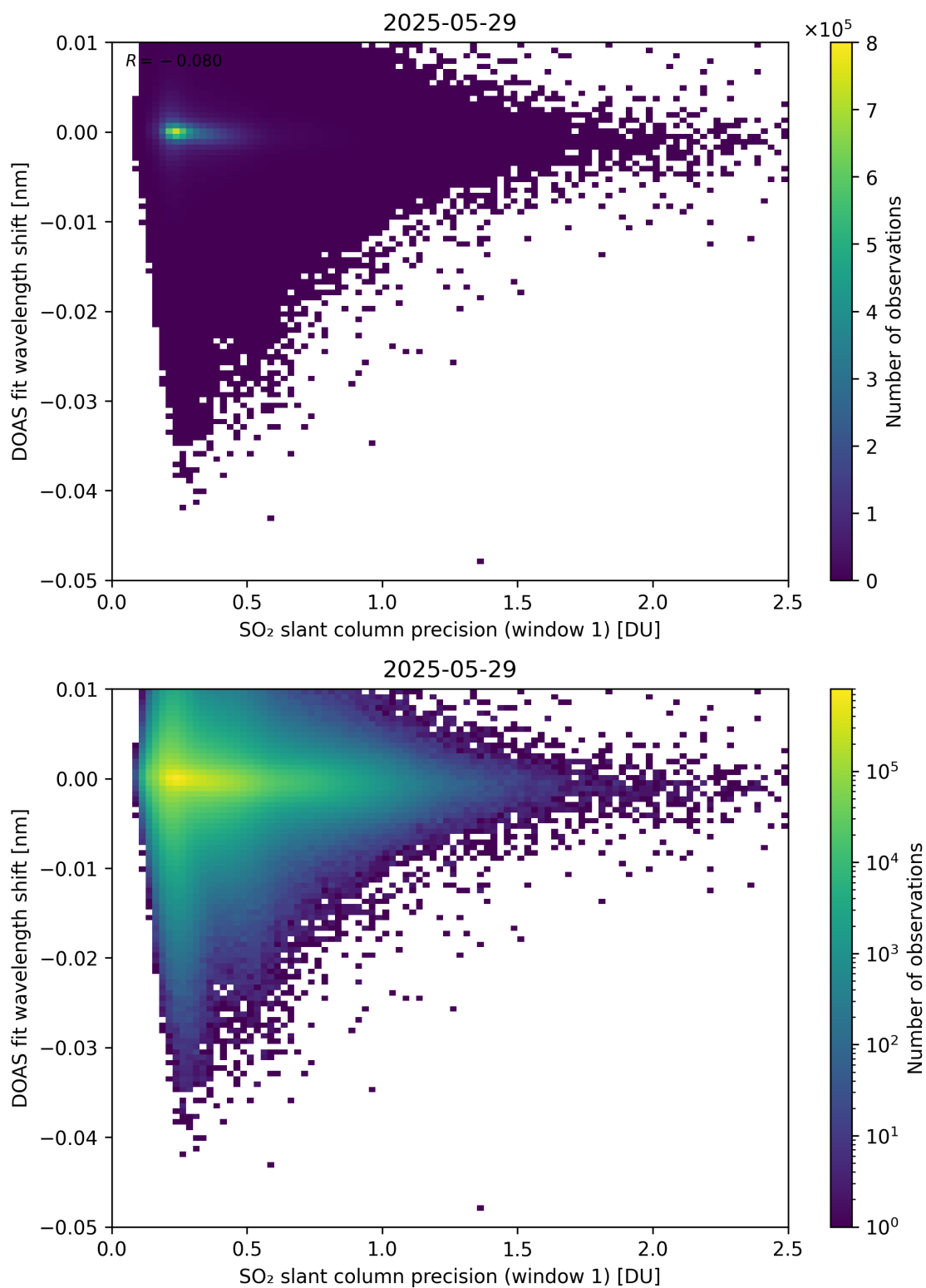
Figure 271: Scatter density plot of “SO 2 slant column precision (window 1)” against “DOAS fit wavelength shift” for 2025-05-28 to 2025-05-30.
