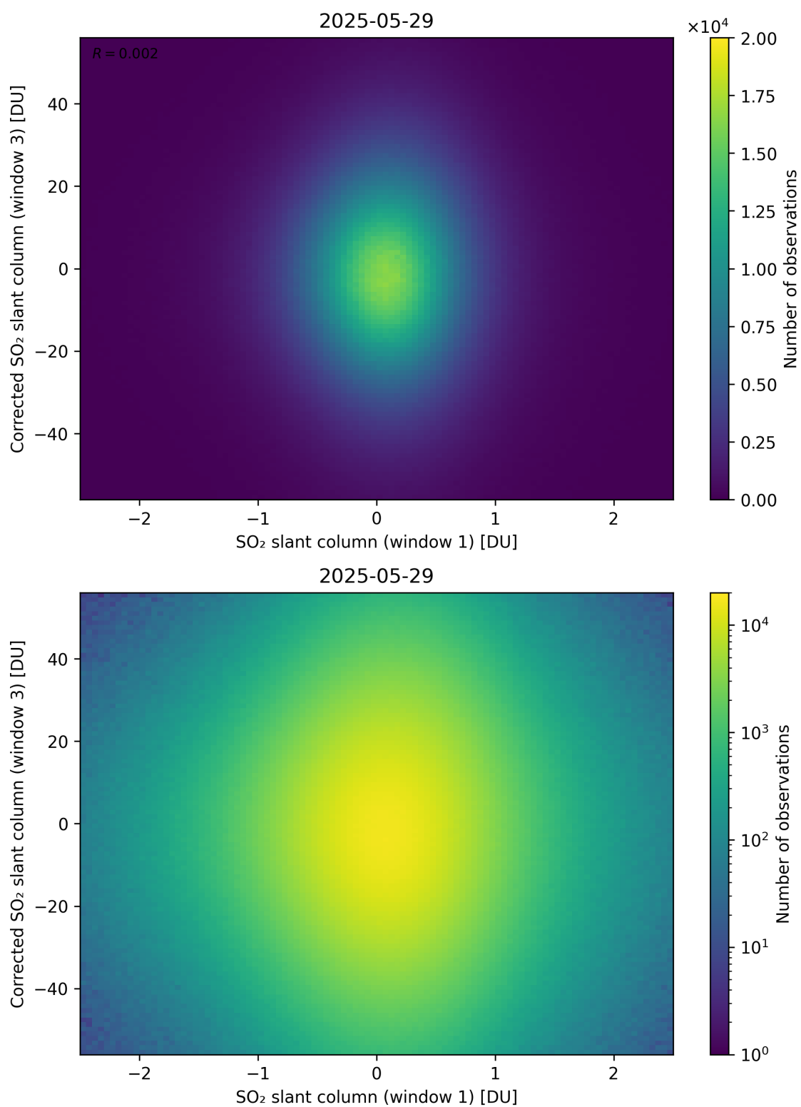
Figure 284: Scatter density plot of “SO 2 slant column (window 1)” against “Corrected SO 2 slant column (window 3)” for 2025-05-28 to 2025-05-30.
