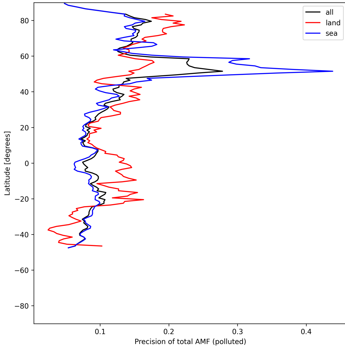
Figure 54: Zonal average of “Precision of total AMF (polluted)” for 2025-05-28 to 2025-05-30.
