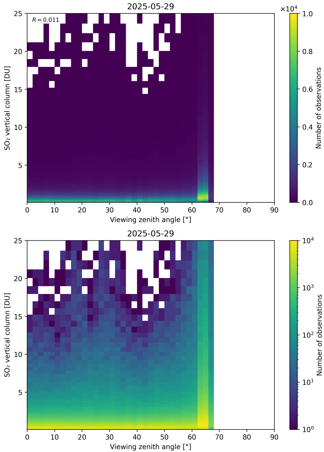
Figure 383: Scatter density plot of “Viewing zenith angle” against “SO 2 vertical column” for 2025-05-28 to 2025-05-30.
