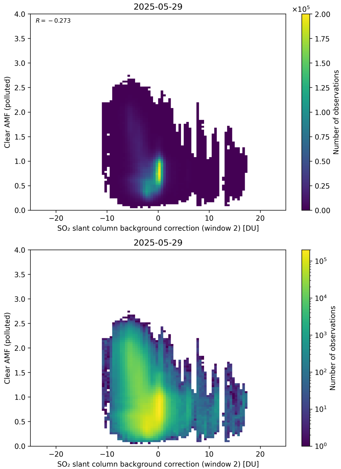
Figure 126: Scatter density plot of “SO 2 slant column background correction (window 2)” against “Clear AMF (polluted)” for 2025-05-28 to 2025-05-30.
