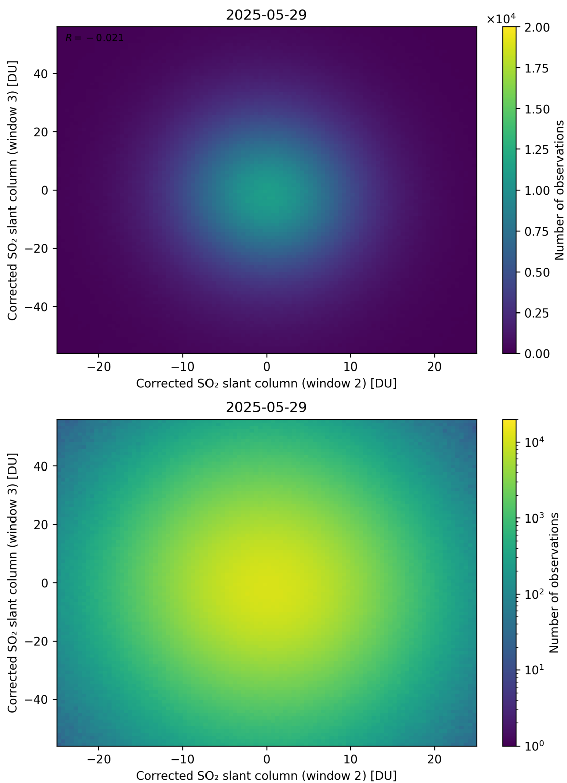
Figure 250: Scatter density plot of “Corrected SO 2 slant column (window 2)” against “Corrected SO 2 slant column (window 3)” for 2025-05-28 to 2025-05-30.
