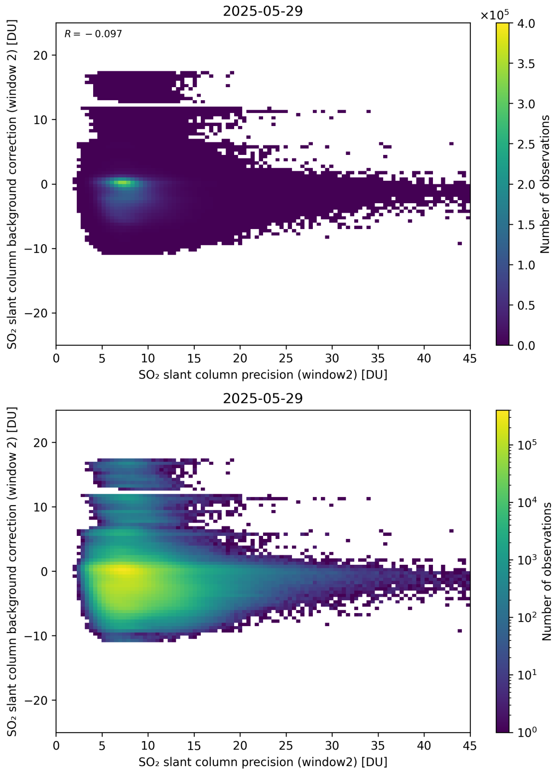
Figure 291: Scatter density plot of “SO 2 slant column precision (window2)” against “SO 2 slant column background correction (window 2)” for 2025-05-28 to 2025-05-30.
