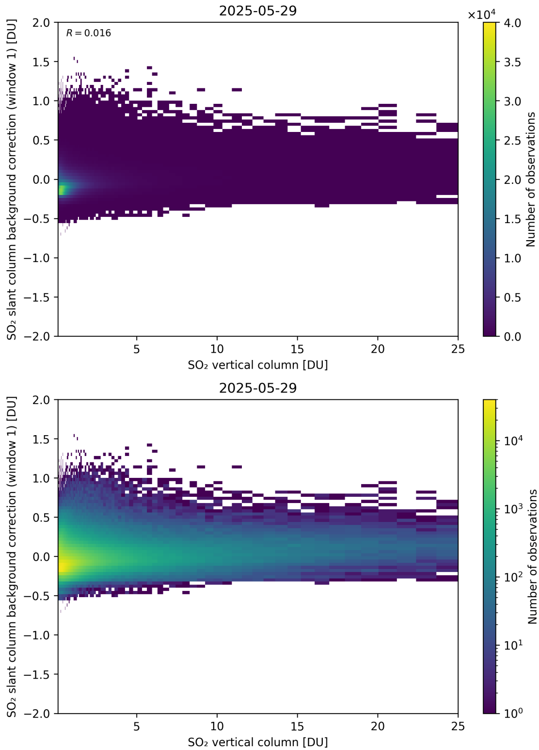
Figure 323: Scatter density plot of “SO 2 vertical column” against “SO 2 slant column background correction (window 1)” for 2025-05-28 to 2025-05-30.
