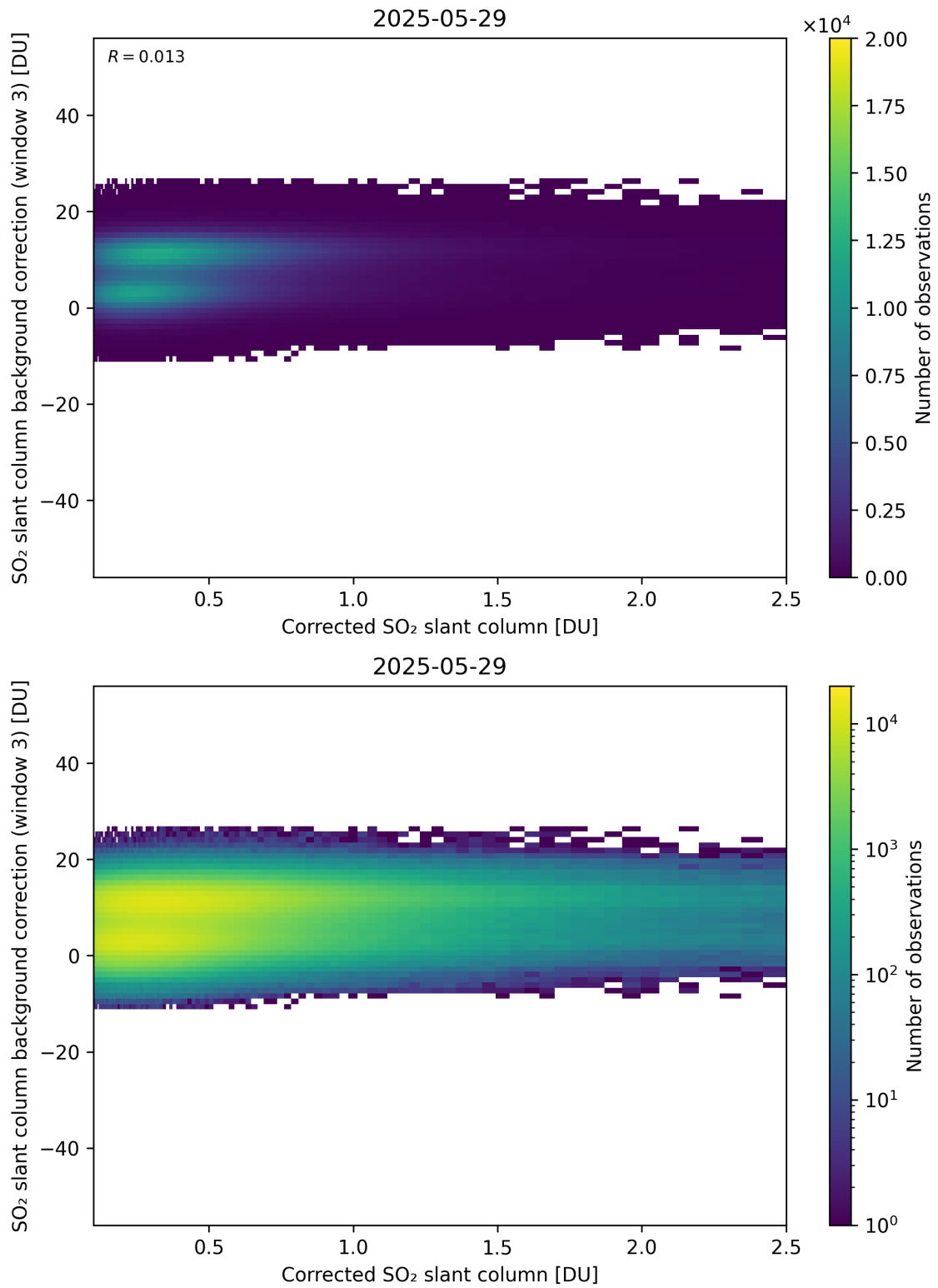
Figure 228: Scatter density plot of “Corrected SO 2 slant column” against “SO 2 slant column background correction (window 3)” for 2025-05-28 to 2025-05-30.
