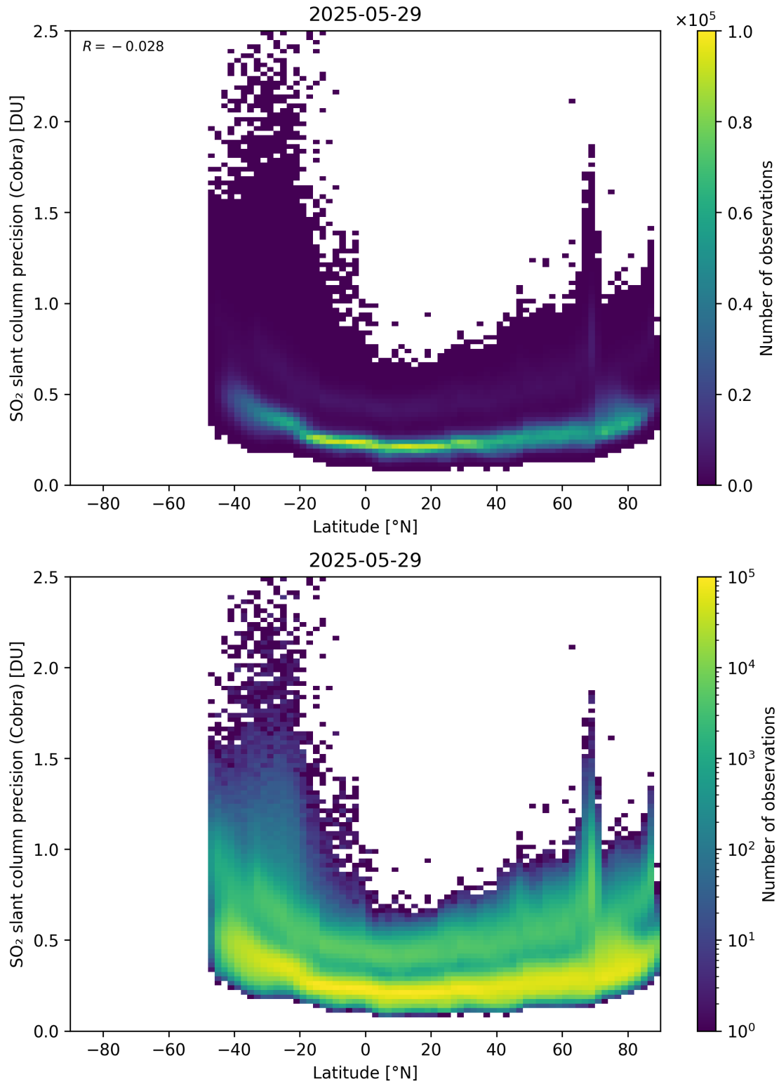
Figure 158: Scatter density plot of “Latitude” against “SO 2 slant column precision (Cobra)” for 2025-05-28 to 2025-05-30.
