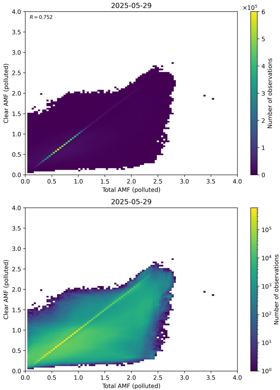
Figure 321: Scatter density plot of “Total AMF (polluted)” against “Clear AMF (polluted)” for 2025-05-28 to 2025-05-30.
