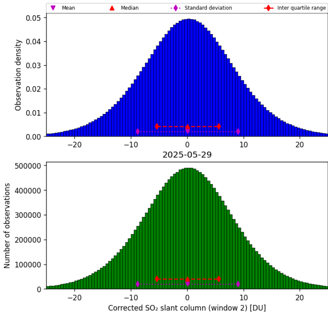
Figure 69: Histogram of “Corrected SO 2 slant column (window 2)” for 2025-05-28 to 2025-05-30
