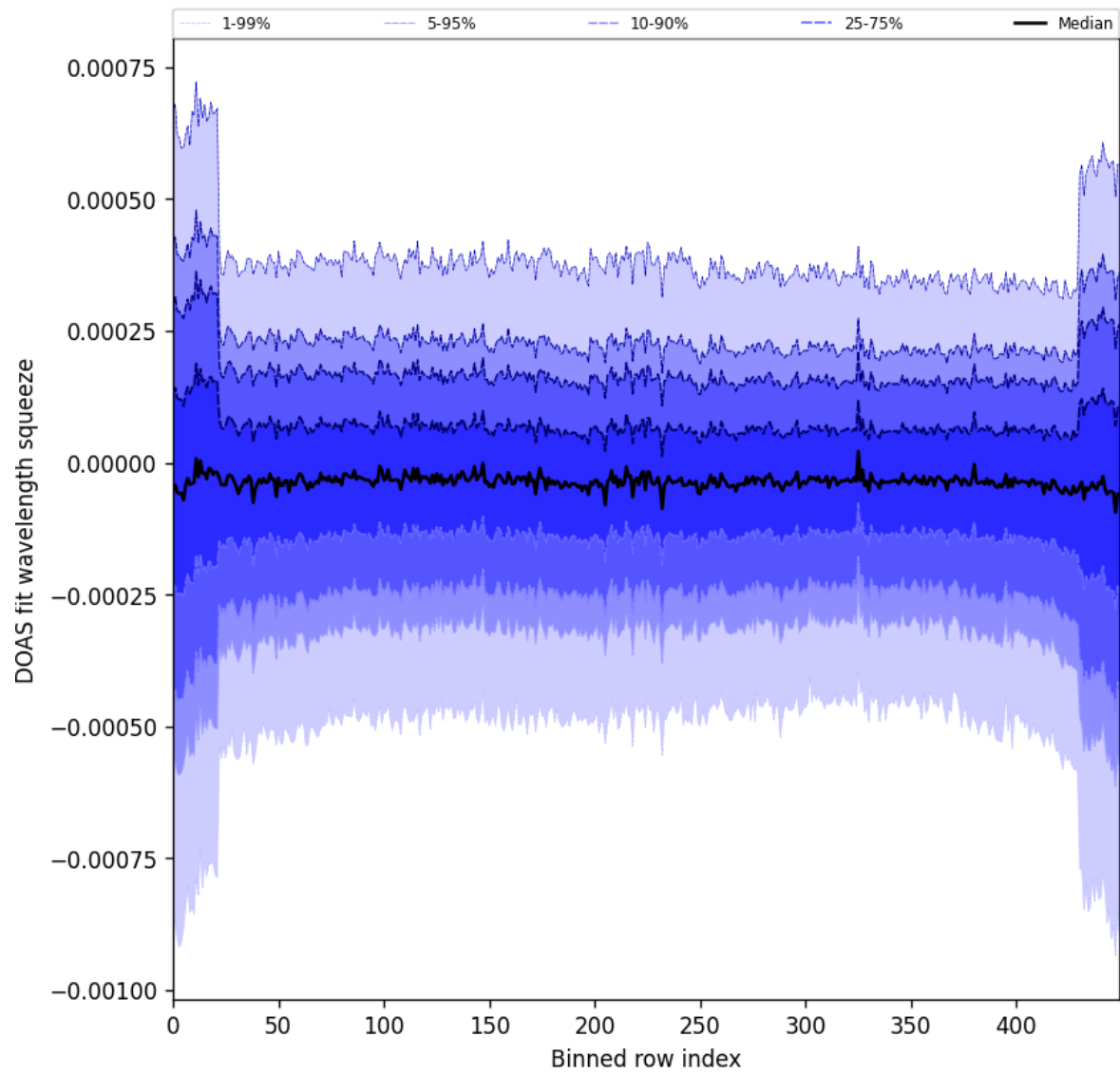
Figure 103: Along track statistics of “DOAS fit wavelength squeeze” for 2025-05-28 to 2025-05-30
