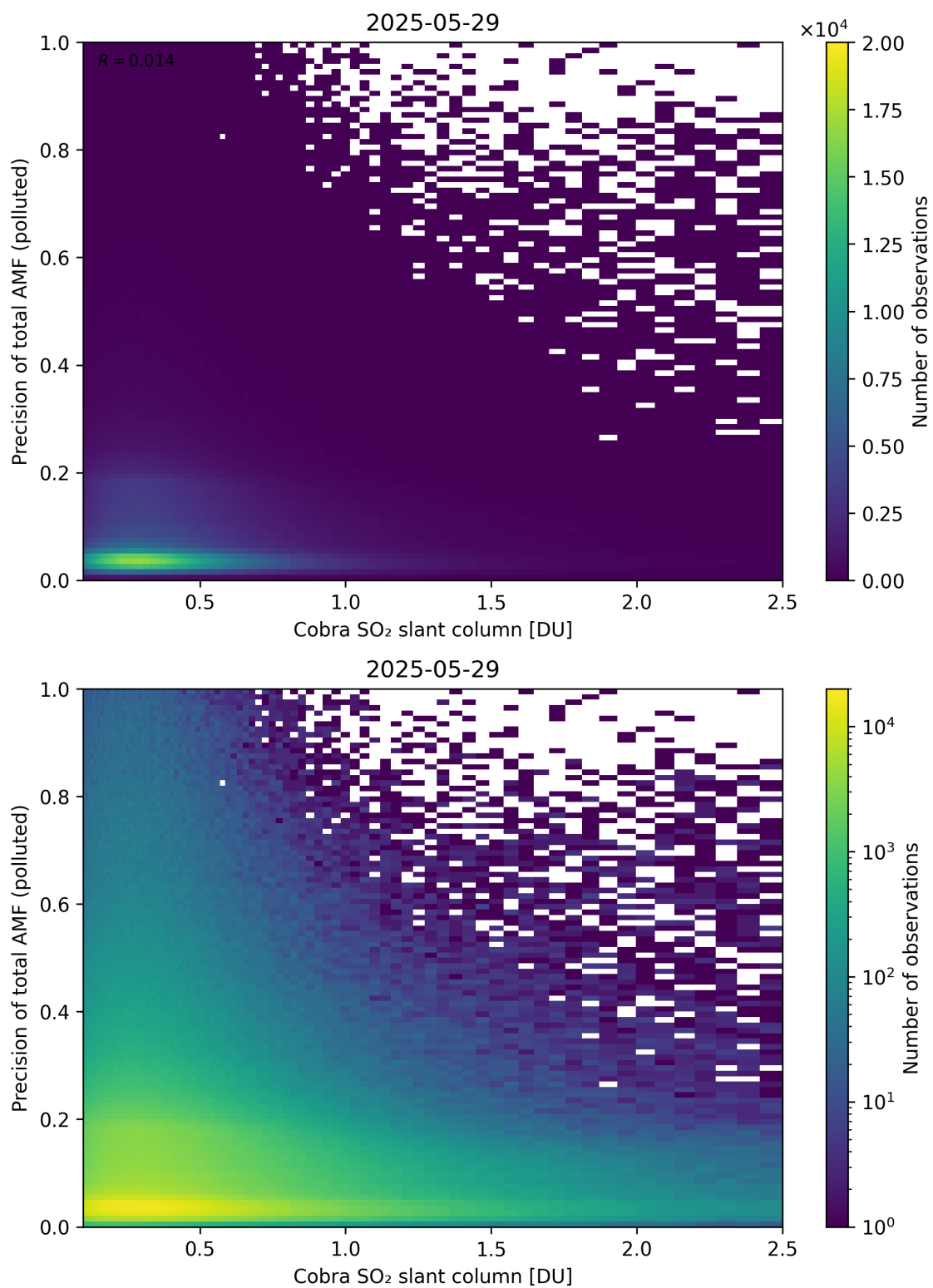
Figure 225: Scatter density plot of “Cobra SO 2 slant column” against “Precision of total AMF (polluted)” for 2025-05-28 to 2025-05-30.
