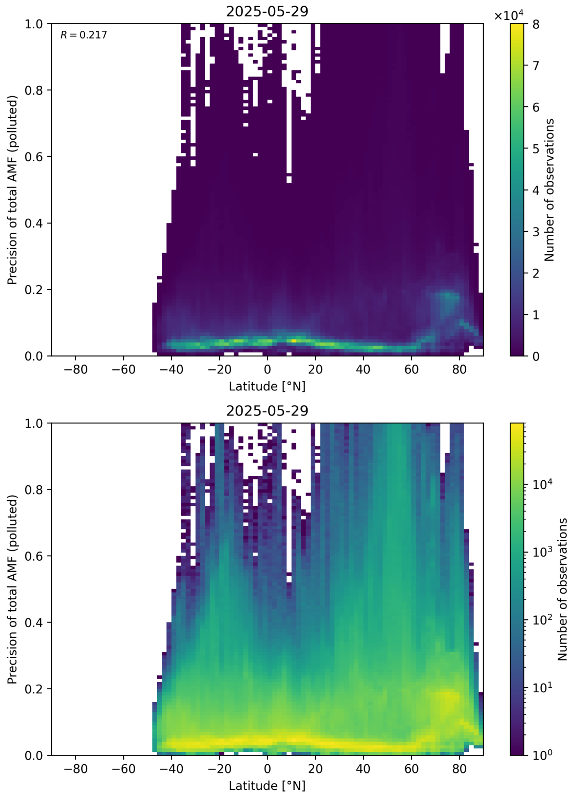
Figure 168: Scatter density plot of “Latitude” against “Precision of total AMF (polluted)” for 2025-05-28 to 2025-05-30.
