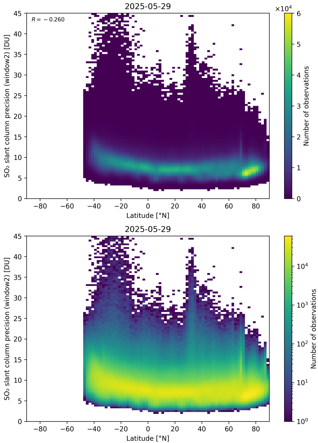
Figure 164: Scatter density plot of “Latitude” against “SO 2 slant column precision (window2)” for 2025-05-28 to 2025-05-30.
