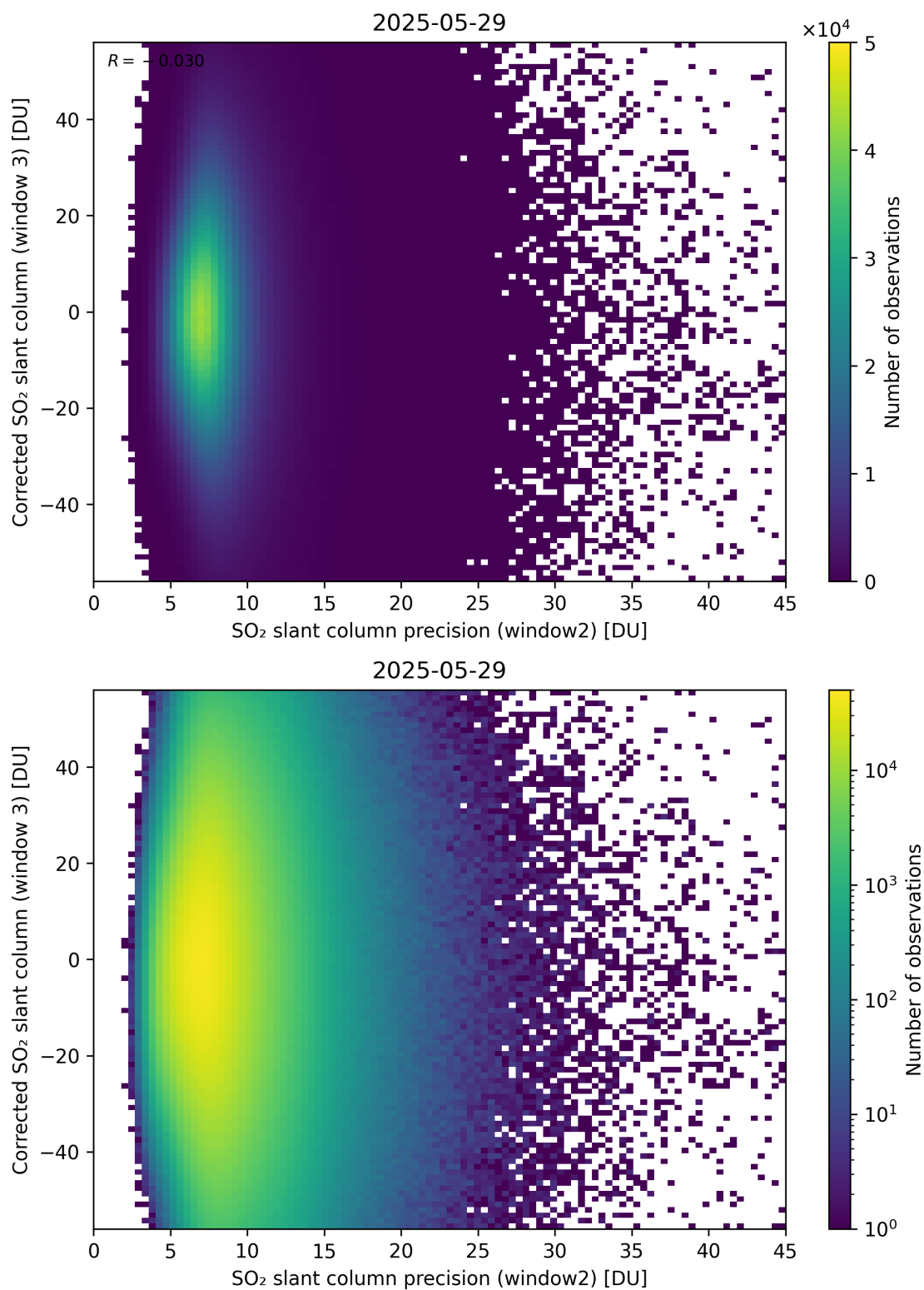
Figure 298: Scatter density plot of “SO 2 slant column precision (window2)” against “Corrected SO 2 slant column (window 3)” for 2025-05-28 to 2025-05-30.
