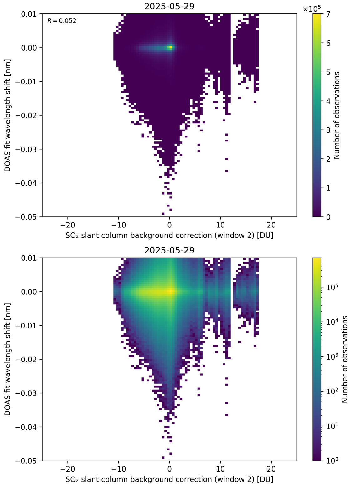
Figure 123: Scatter density plot of “SO 2 slant column background correction (window 2)” against “DOAS fit wavelength shift” for 2025-05-28 to 2025-05-30.
