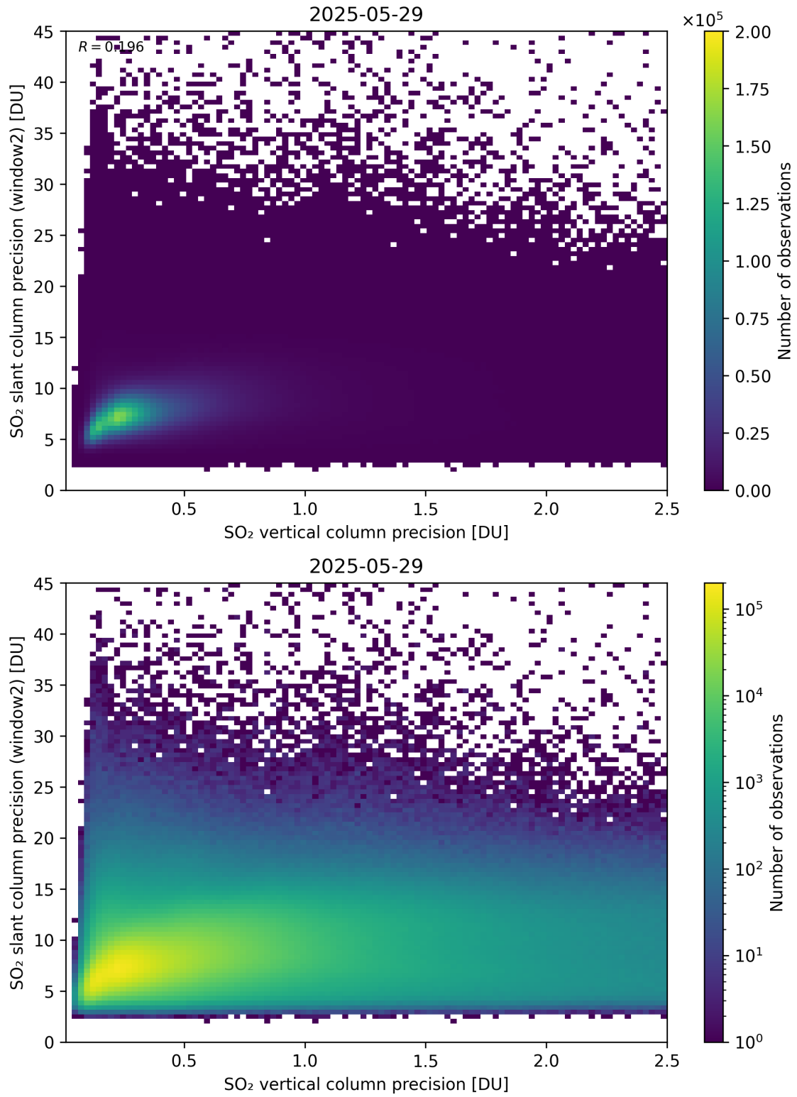
Figure 343: Scatter density plot of “SO 2 vertical column precision” against “SO 2 slant column precision (window2)” for 2025-05-28 to 2025-05-30.
