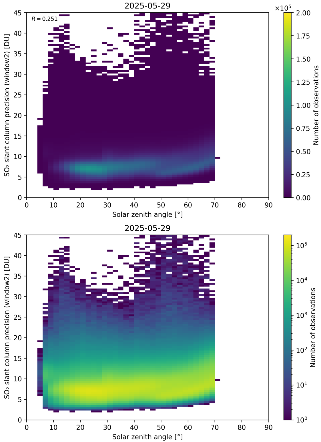
Figure 186: Scatter density plot of “Solar zenith angle” against “SO 2 slant column precision (window2)” for 2025-05-28 to 2025-05-30.
