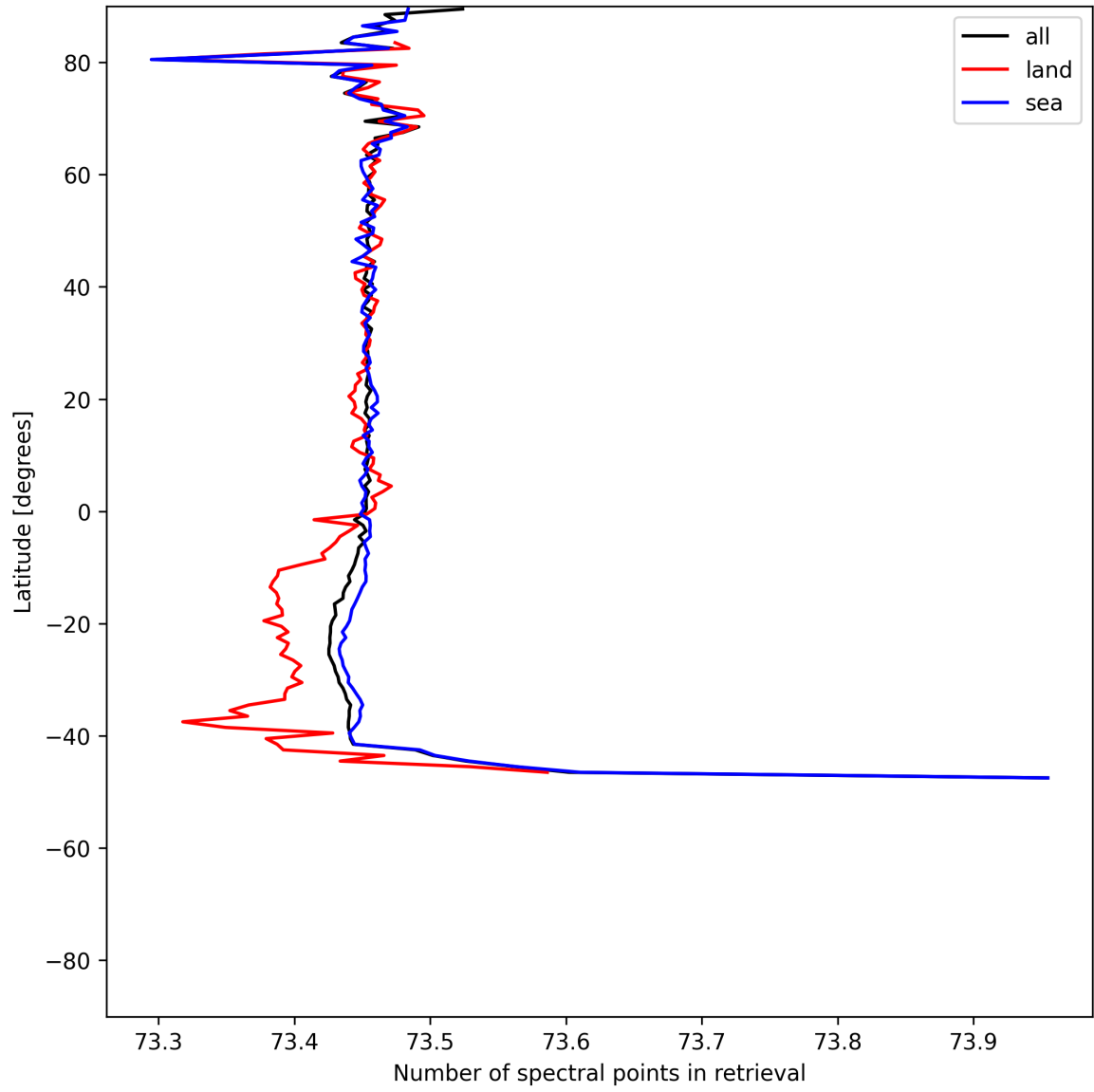
Figure 56: Zonal average of “Number of spectral points in retrieval” for 2025-05-28 to 2025-05-30.
