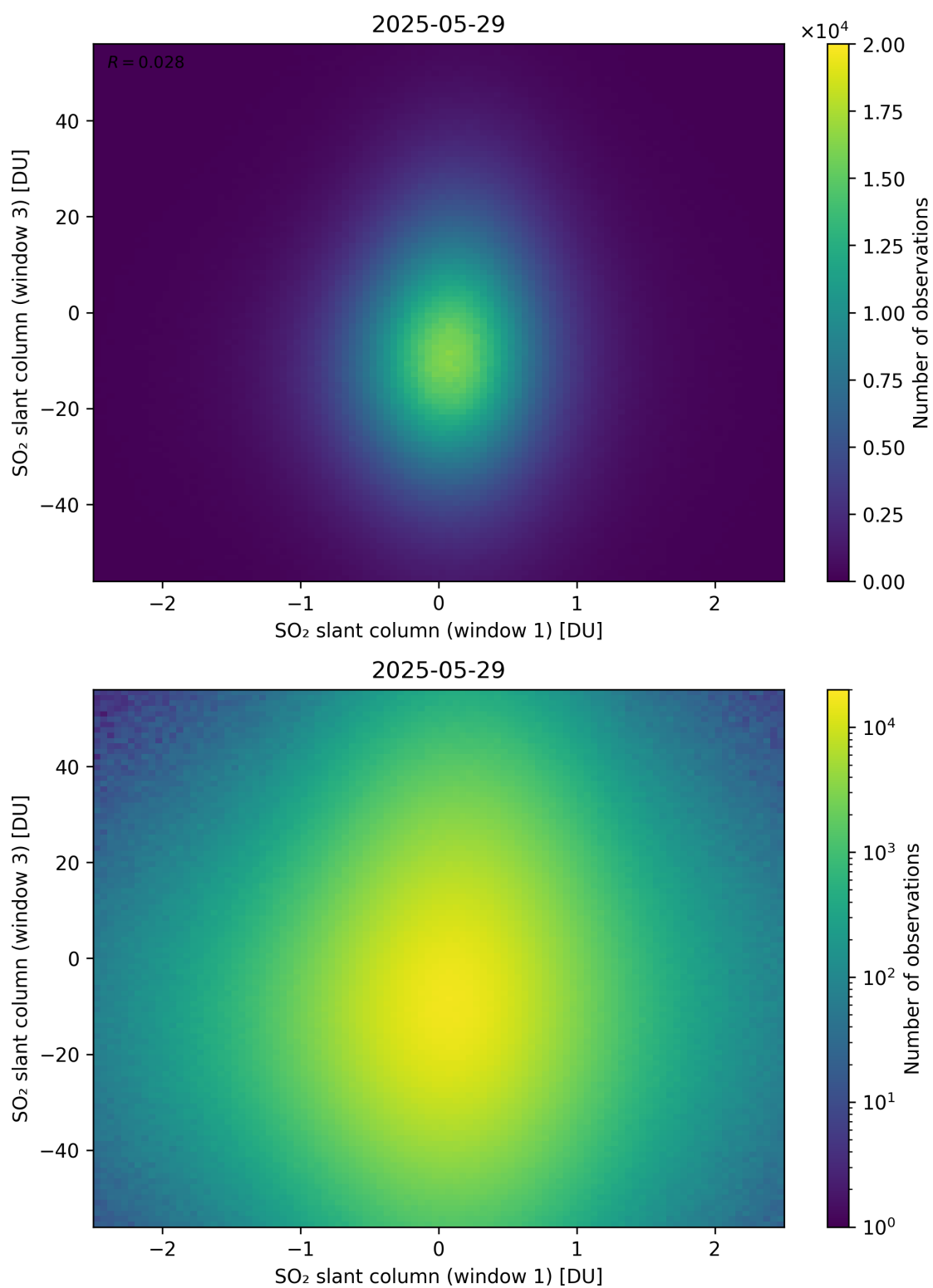
Figure 287: Scatter density plot of “SO 2 slant column (window 1)” against “SO 2 slant column (window 3)” for 2025-05-28 to 2025-05-30.
