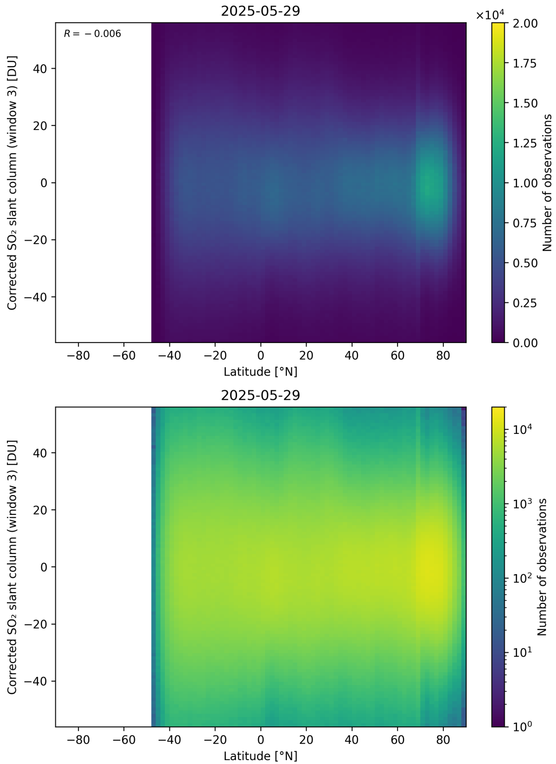
Figure 161: Scatter density plot of “Latitude” against “Corrected SO 2 slant column (window 3)” for 2025-05-28 to 2025-05-30.
