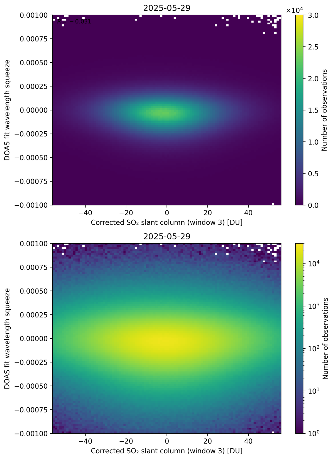
Figure 257: Scatter density plot of “Corrected SO 2 slant column (window 3)” against “DOAS fit wavelength squeeze” for 2025-05-28 to 2025-05-30.
