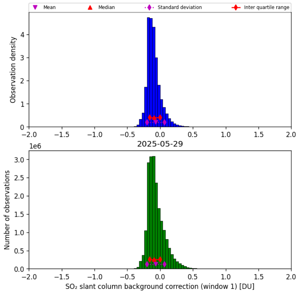
Figure 66: Histogram of “SO 2 slant column background correction (window 1)” for 2025-05-28 to 2025-05-30
