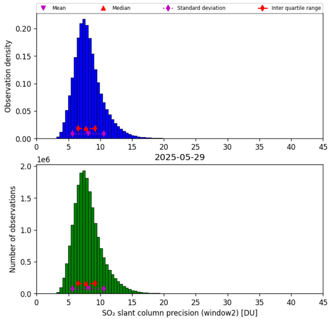
Figure 68: Histogram of “SO 2 slant column precision (window2)” for 2025-05-28 to 2025-05-30
