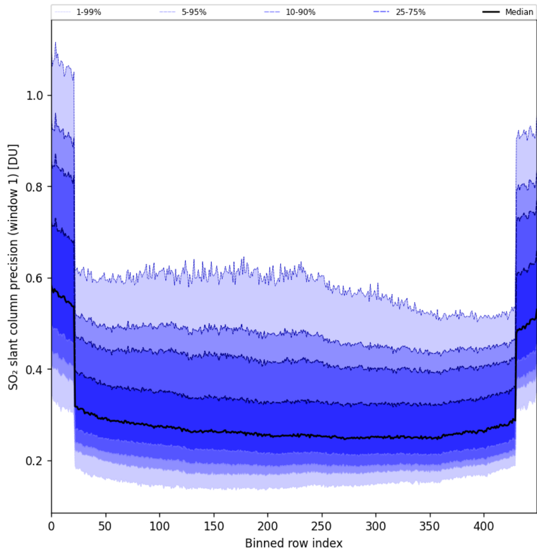
Figure 90: Along track statistics of “SO 2 slant column precision (window 1)” for 2025-05-28 to 2025-05-30
