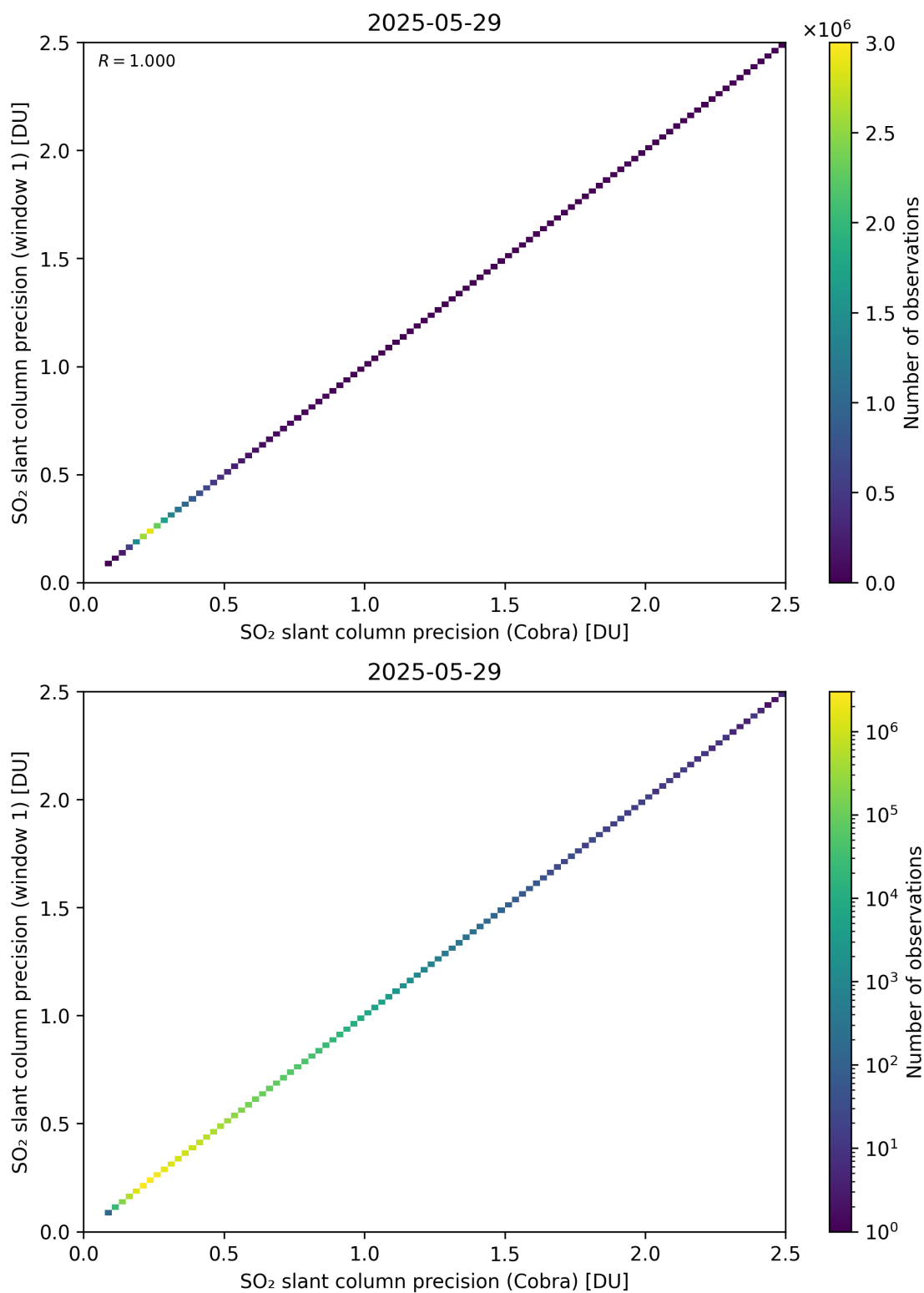
Figure 209: Scatter density plot of “SO 2 slant column precision (Cobra)” against “SO 2 slant column precision (window 1)” for 2025-05-28 to 2025-05-30.
