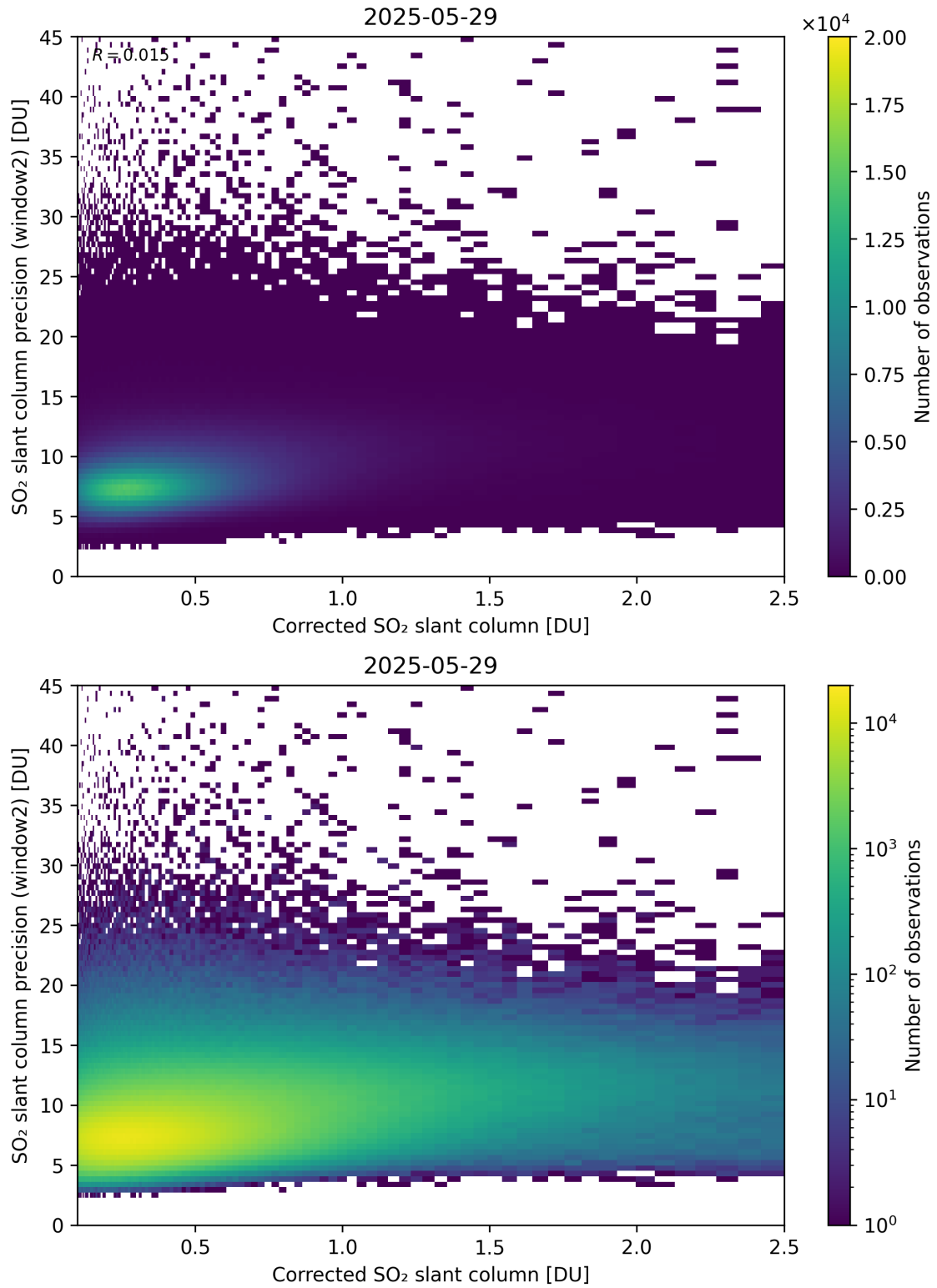
Figure 239: Scatter density plot of “Corrected SO 2 slant column” against “SO 2 slant column precision (window2)” for 2025-05-28 to 2025-05-30.
