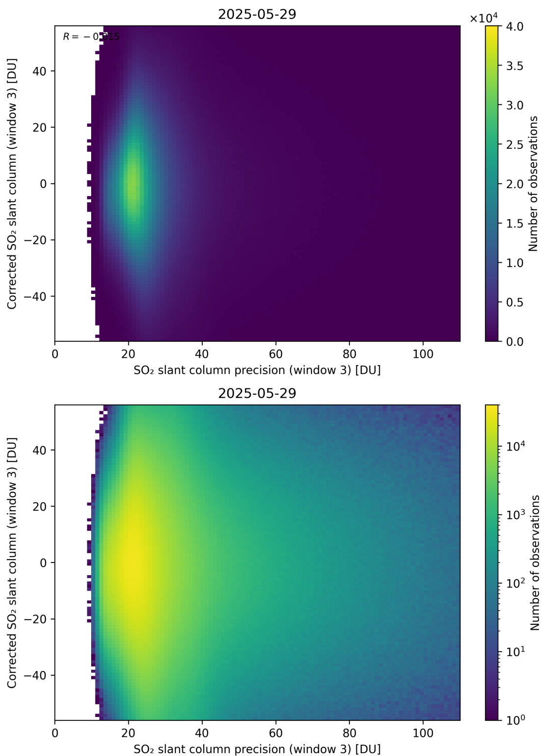
Figure 312: Scatter density plot of “SO 2 slant column precision (window 3)” against “Corrected SO 2 slant column (window 3)” for 2025-05-28 to 2025-05-30.
