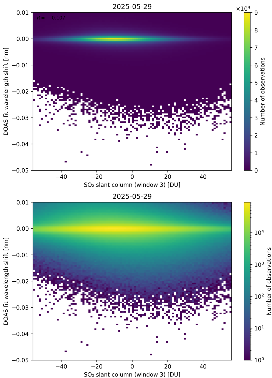
Figure 304: Scatter density plot of “SO 2 slant column (window 3)” against “DOAS fit wavelength shift” for 2025-05-28 to 2025-05-30.
