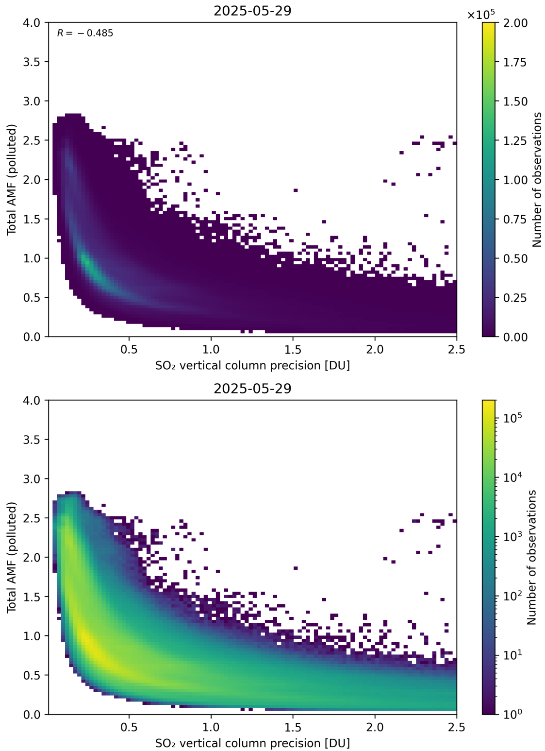
Figure 346: Scatter density plot of “SO 2 vertical column precision” against “Total AMF (polluted)” for 2025-05-28 to 2025-05-30.
