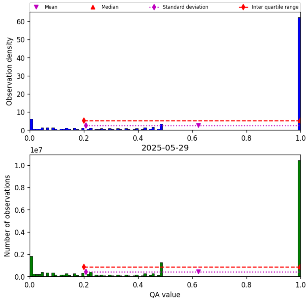
Figure 57: Histogram of “QA value” for 2025-05-28 to 2025-05-30
