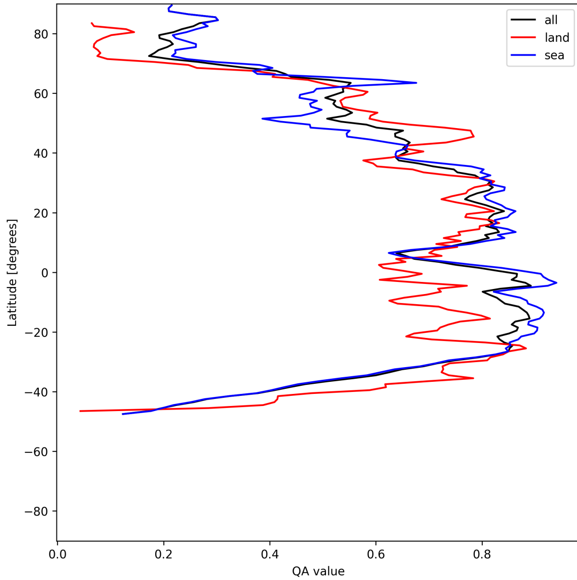
Figure 31: Zonal average of “QA value” for 2025-05-28 to 2025-05-30.
