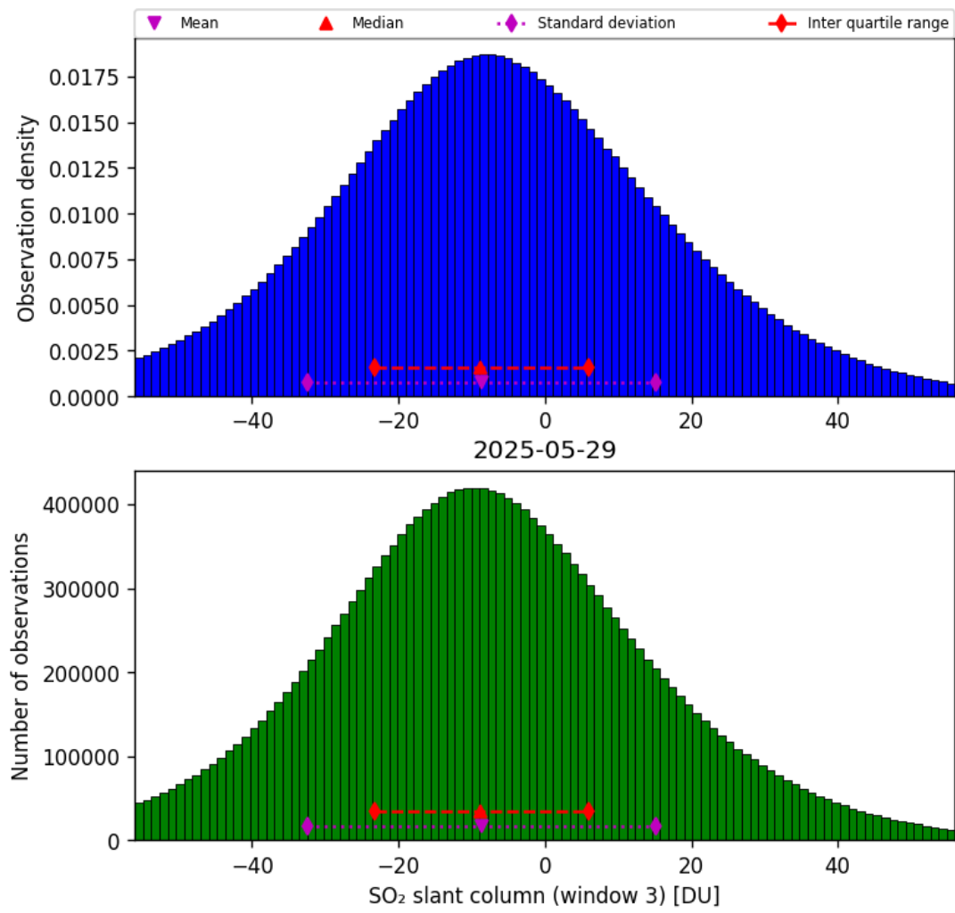
Figure 71: Histogram of “SO 2 slant column (window 3)” for 2025-05-28 to 2025-05-30
