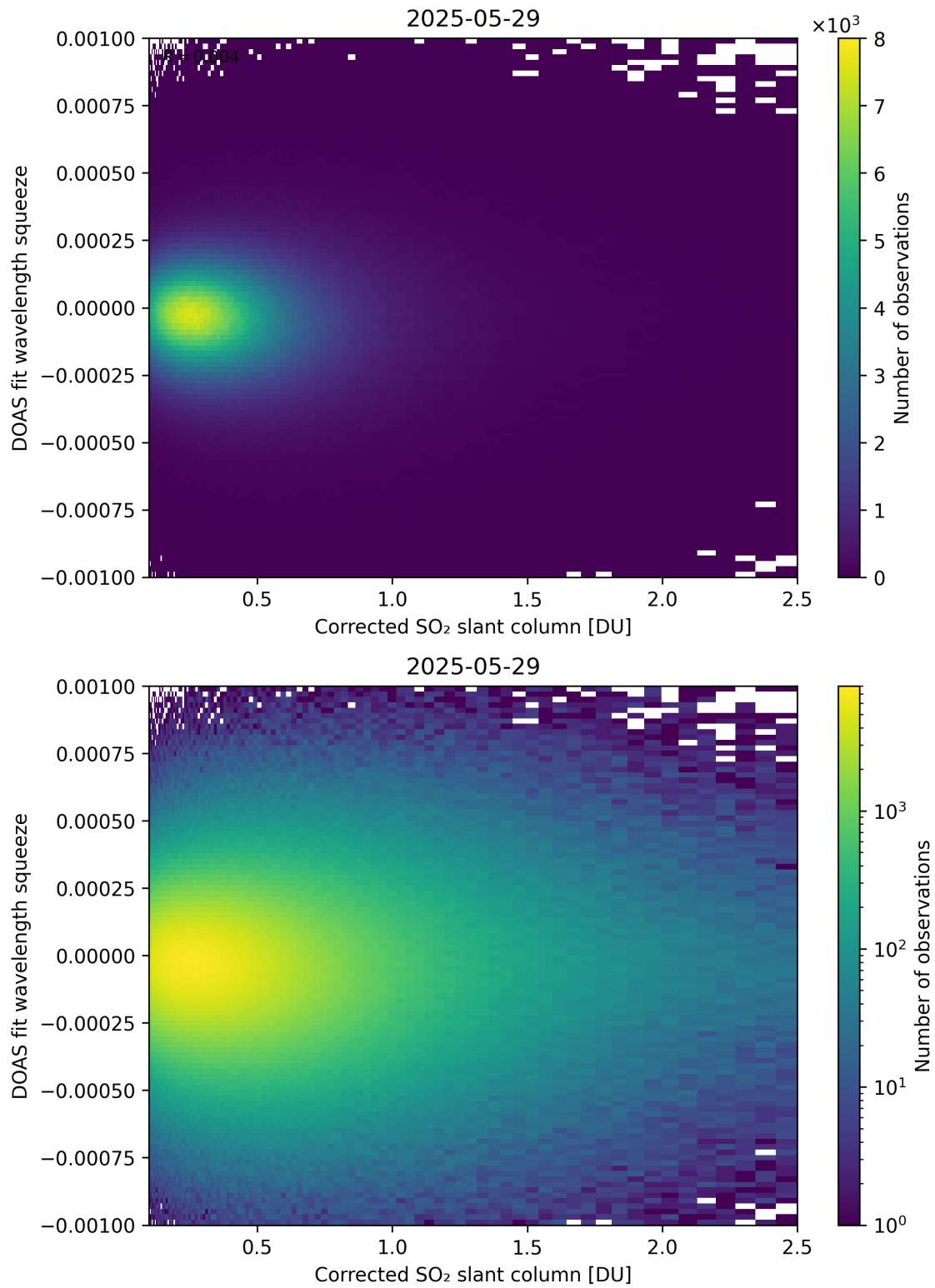
Figure 230: Scatter density plot of “Corrected SO 2 slant column” against “DOAS fit wavelength squeeze” for 2025-05-28 to 2025-05-30.
