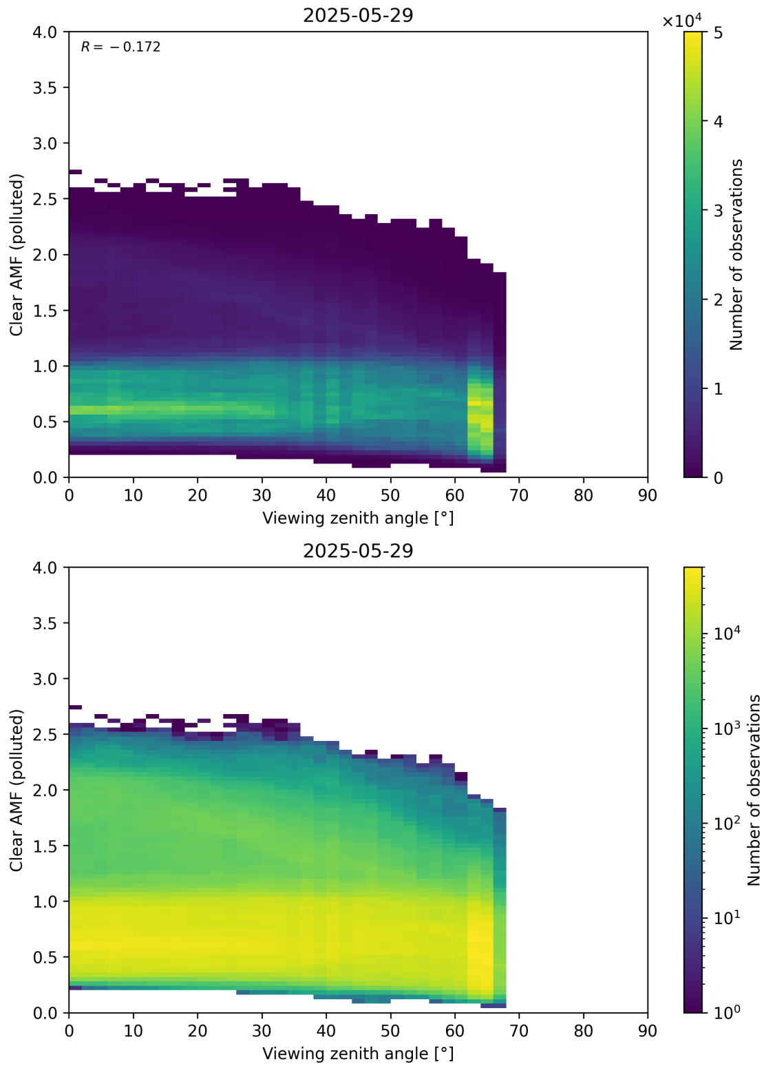
Figure 370: Scatter density plot of “Viewing zenith angle” against “Clear AMF (polluted)” for 2025-05-28 to 2025-05-30.
