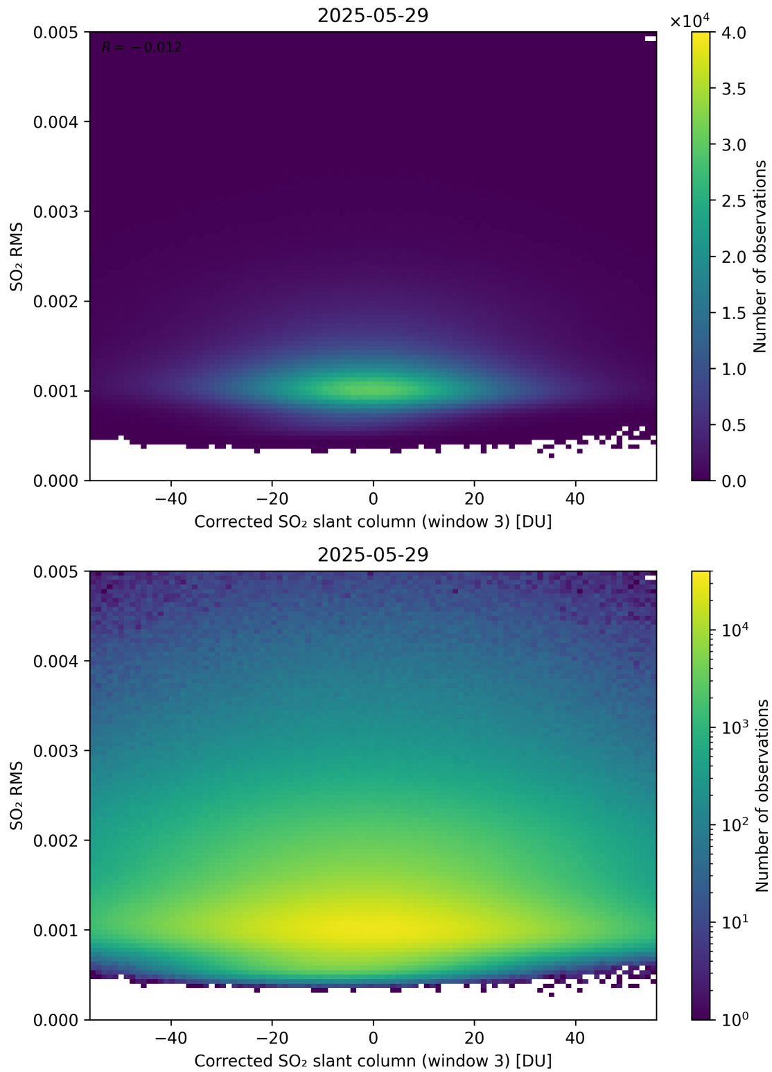
Figure 258: Scatter density plot of “Corrected SO 2 slant column (window 3)” against “SO 2 RMS” for 2025-05-28 to 2025-05-30.
