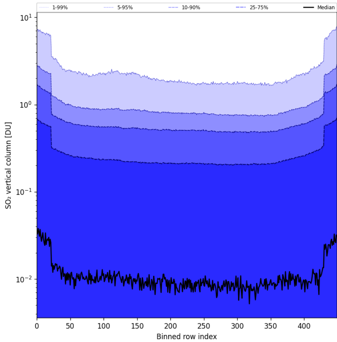
Figure 84: Along track statistics of “SO 2 vertical column” for 2025-05-28 to 2025-05-30
