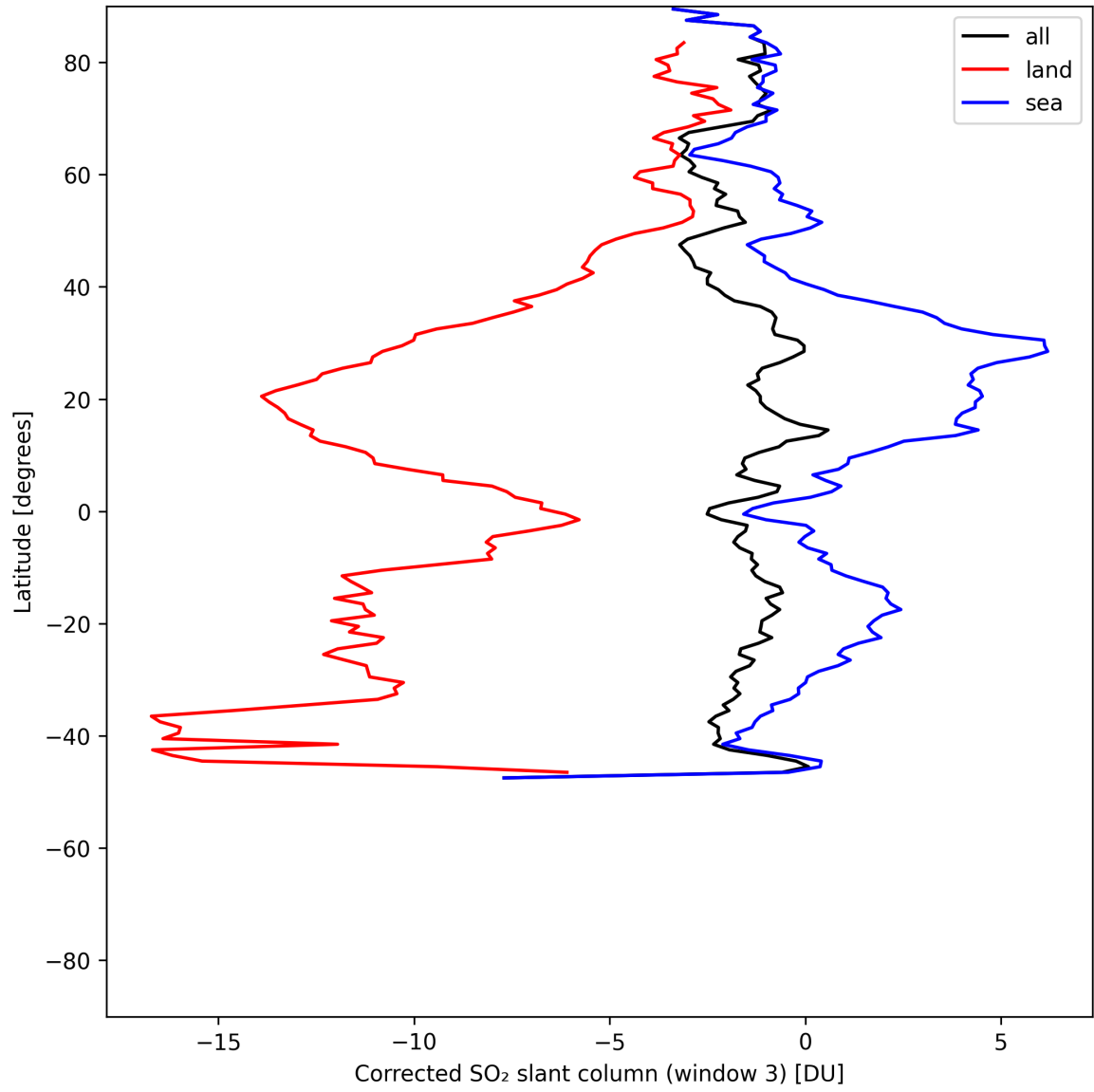
Figure 47: Zonal average of “Corrected SO 2 slant column (window 3)” for 2025-05-28 to 2025-05-30.
