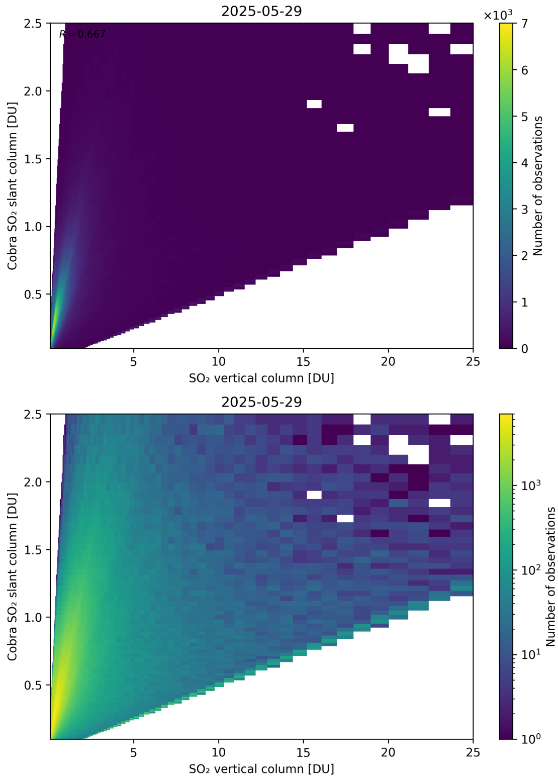
Figure 349: Scatter density plot of “SO 2 vertical column” against “Cobra SO 2 slant column” for 2025-05-28 to 2025-05-30.
