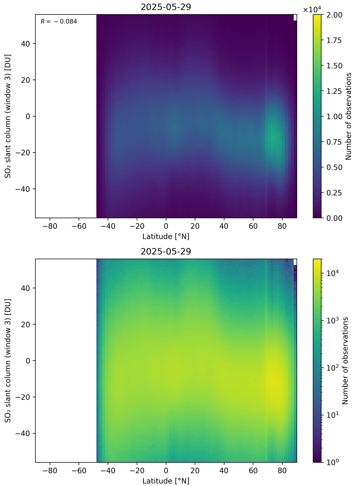
Figure 165: Scatter density plot of “Latitude” against “SO 2 slant column (window 3)” for 2025-05-28 to 2025-05-30.
