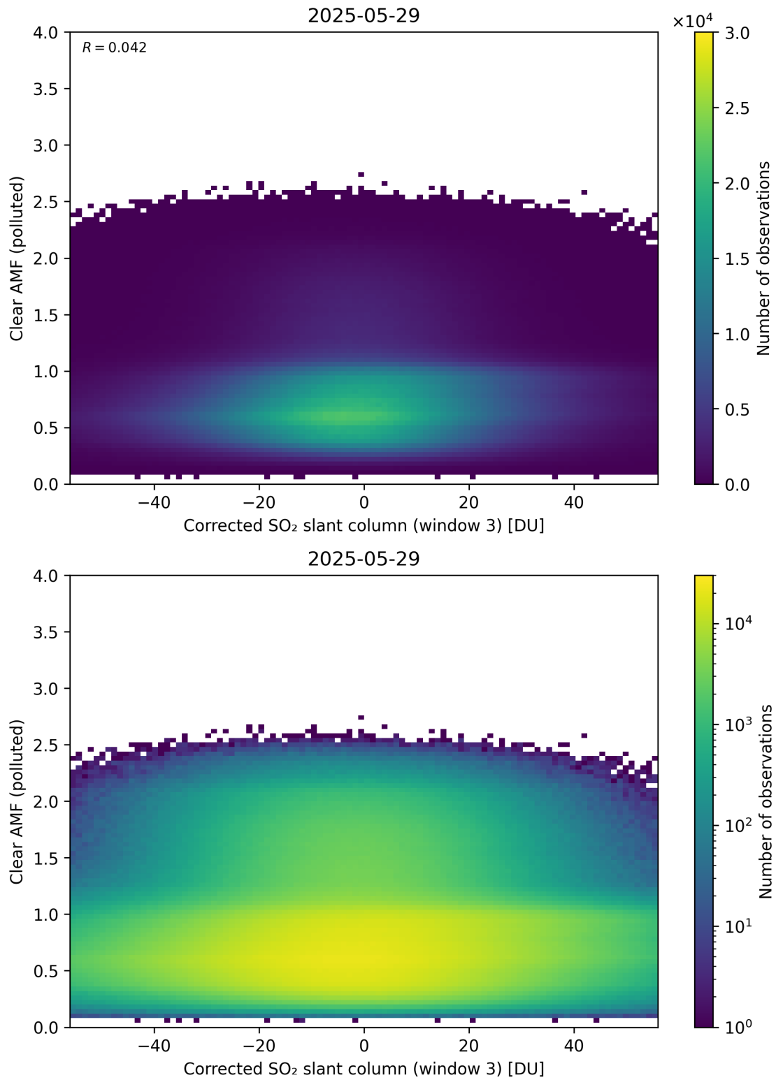
Figure 259: Scatter density plot of “Corrected SO 2 slant column (window 3)” against “Clear AMF (polluted)” for 2025-05-28 to 2025-05-30.
