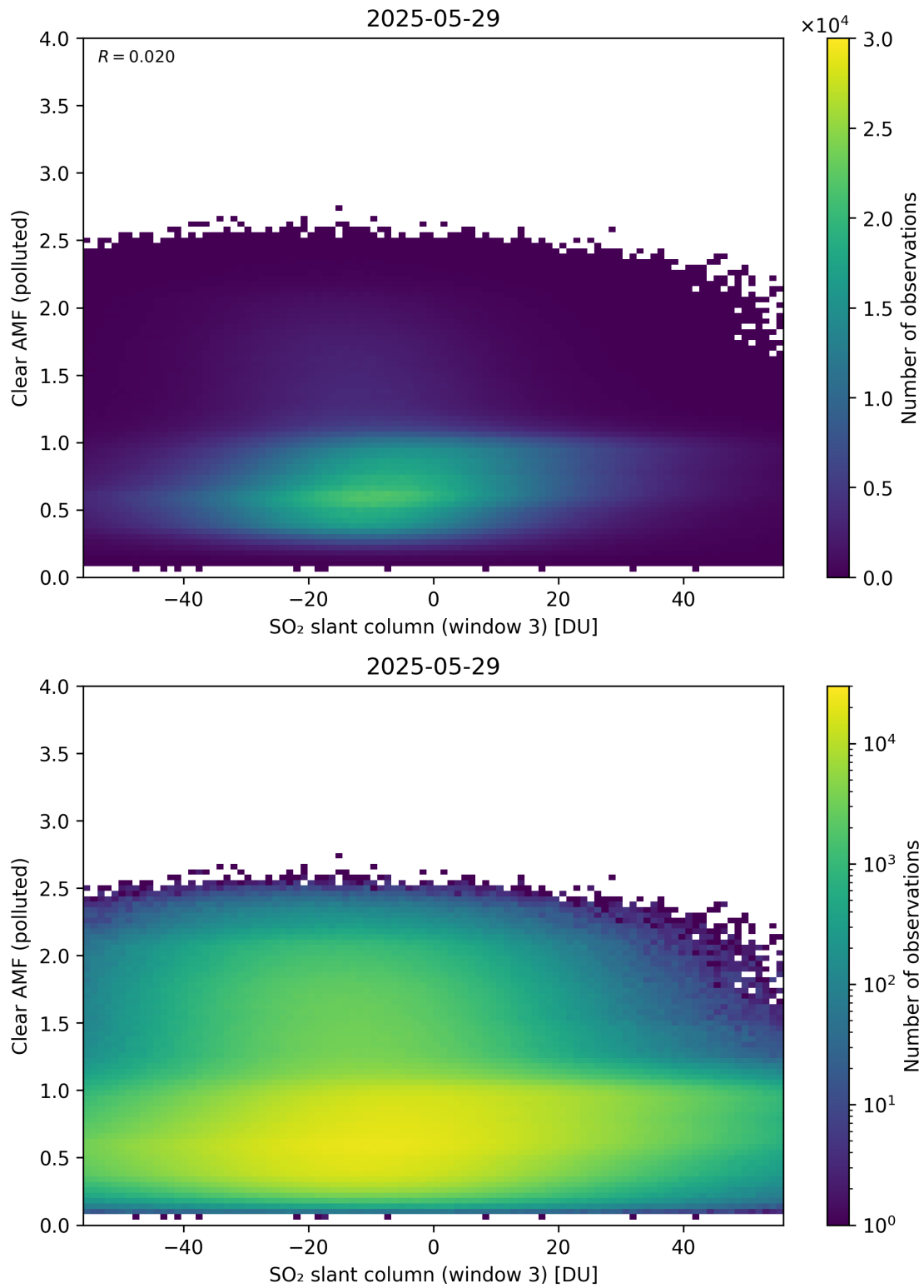
Figure 315: Scatter density plot of “SO 2 slant column (window 3)” against “Clear AMF (polluted)” for 2025-05-28 to 2025-05-30.
