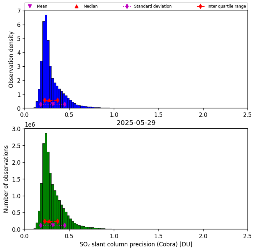
Figure 62: Histogram of “SO 2 slant column precision (Cobra)” for 2025-05-28 to 2025-05-30
