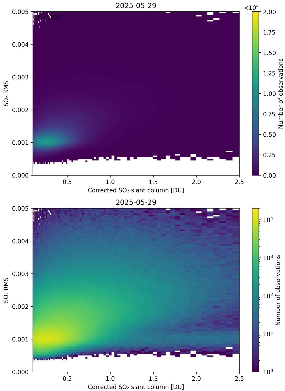
Figure 231: Scatter density plot of “Corrected SO 2 slant column” against “SO 2 RMS” for 2025-05-28 to 2025-05-30.
