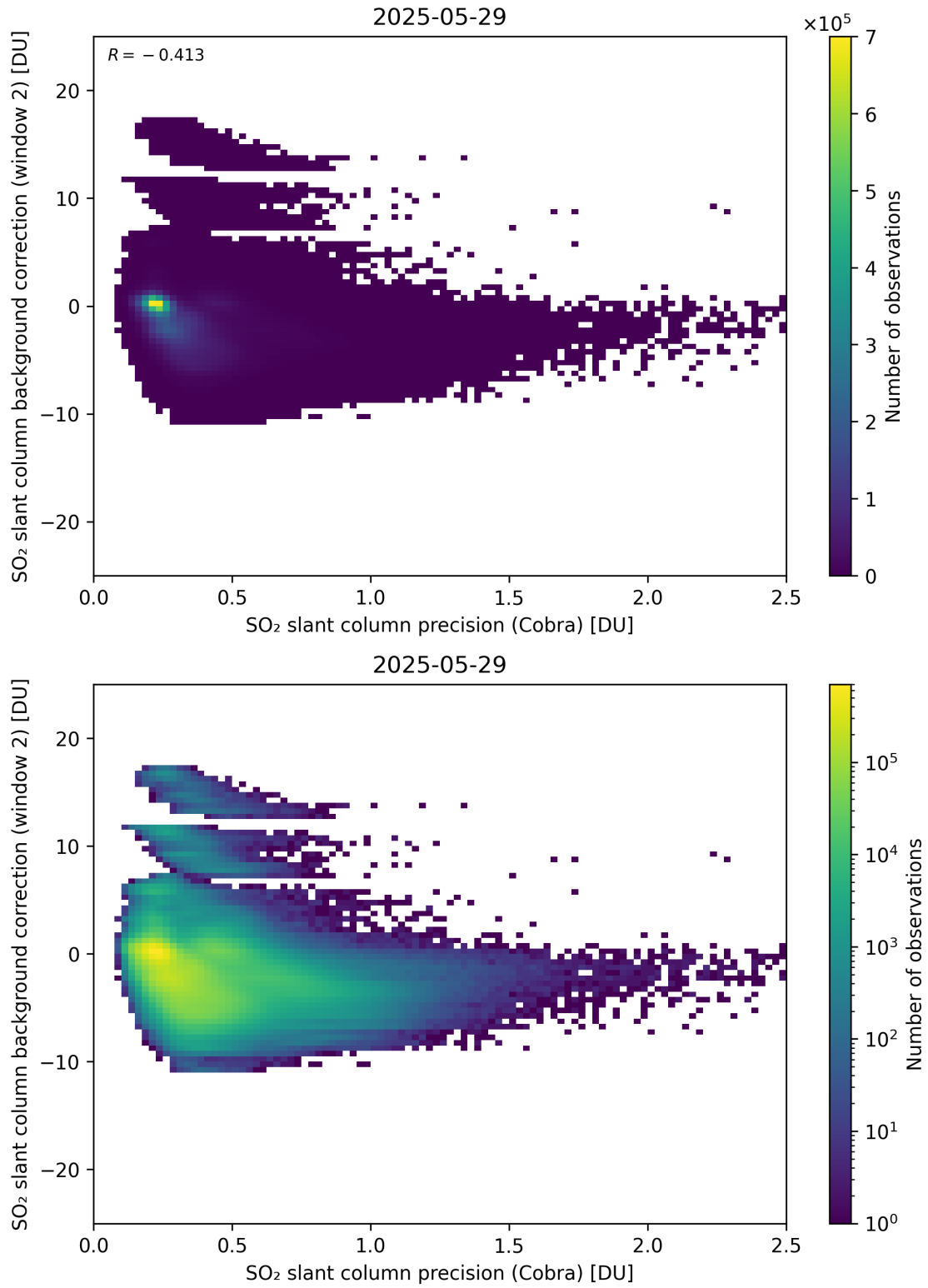
Figure 200: Scatter density plot of “SO 2 slant column precision (Cobra)” against “SO 2 slant column background correction (window 2)” for 2025-05-28 to 2025-05-30.
