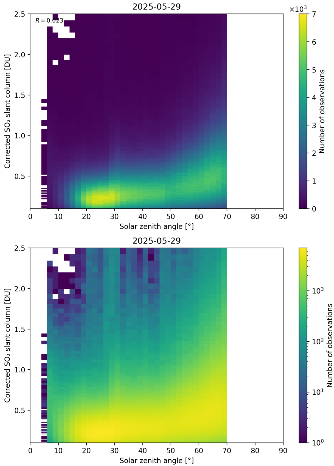
Figure 181: Scatter density plot of “Solar zenith angle” against “Corrected SO 2 slant column” for 2025-05-28 to 2025-05-30.
