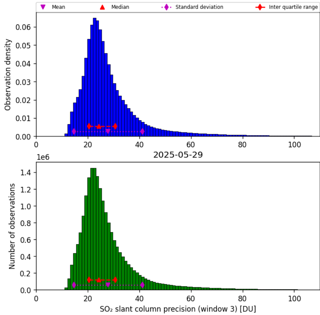
Figure 72: Histogram of “SO 2 slant column precision (window 3)” for 2025-05-28 to 2025-05-30
