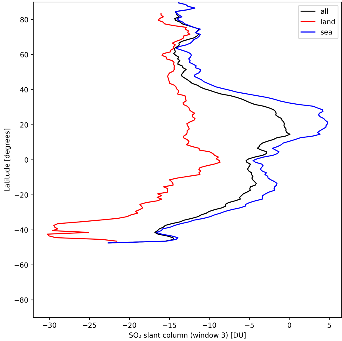
Figure 45: Zonal average of “SO 2 slant column (window 3)” for 2025-05-28 to 2025-05-30.
