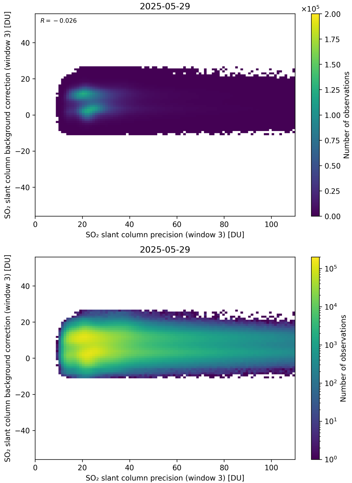
Figure 307: Scatter density plot of “SO 2 slant column precision (window 3)” against “SO 2 slant column background correction (window 3)” for 2025-05-28 to 2025-05-30.
