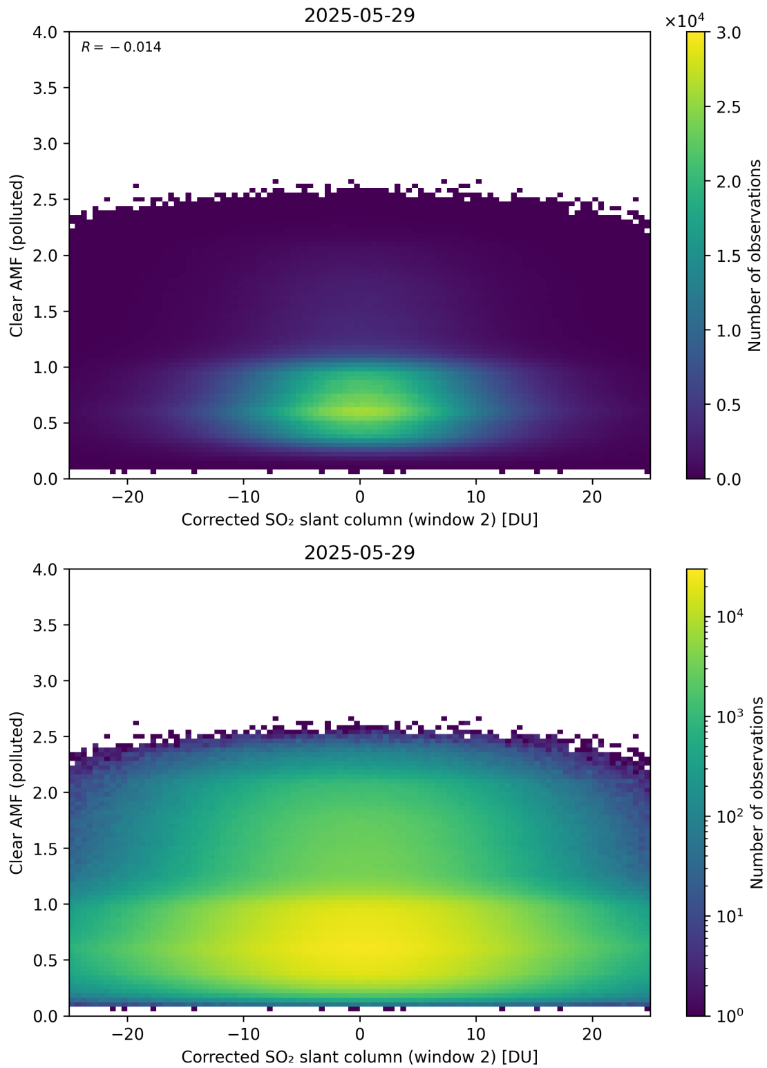
Figure 249: Scatter density plot of “Corrected SO 2 slant column (window 2)” against “Clear AMF (polluted)” for 2025-05-28 to 2025-05-30.
