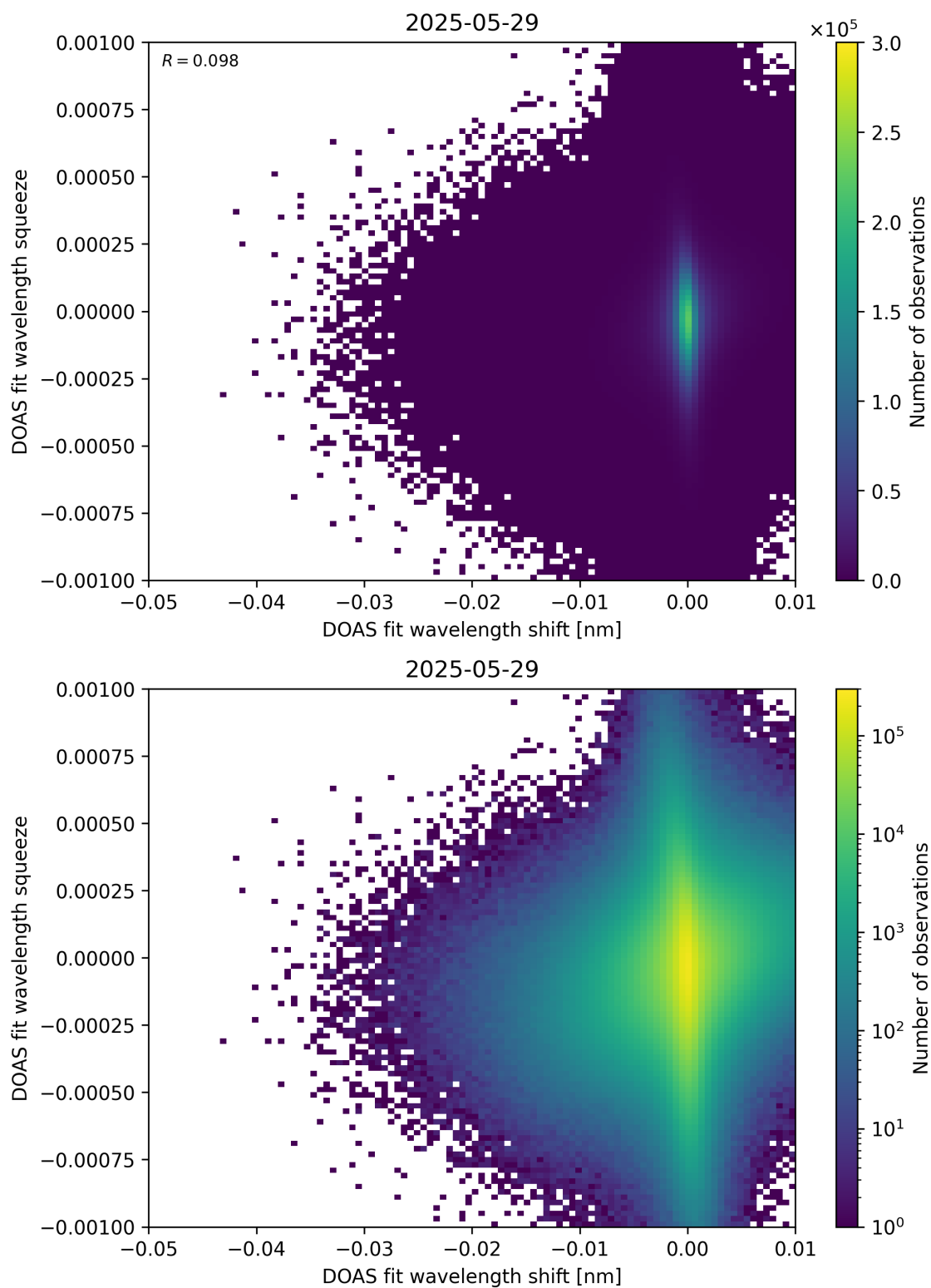
Figure 138: Scatter density plot of “DOAS fit wavelength shift” against “DOAS fit wavelength squeeze” for 2025-05-28 to 2025-05-30.
