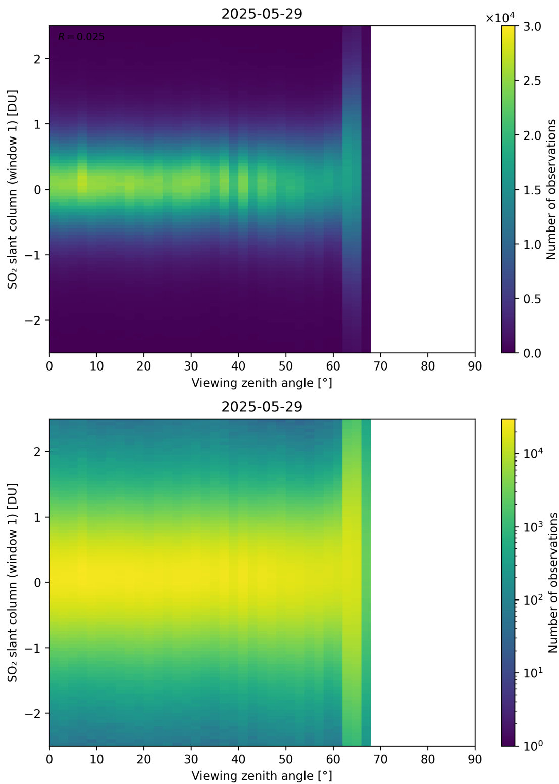
Figure 376: Scatter density plot of “Viewing zenith angle” against “SO 2 slant column (window 1)” for 2025-05-28 to 2025-05-30.
