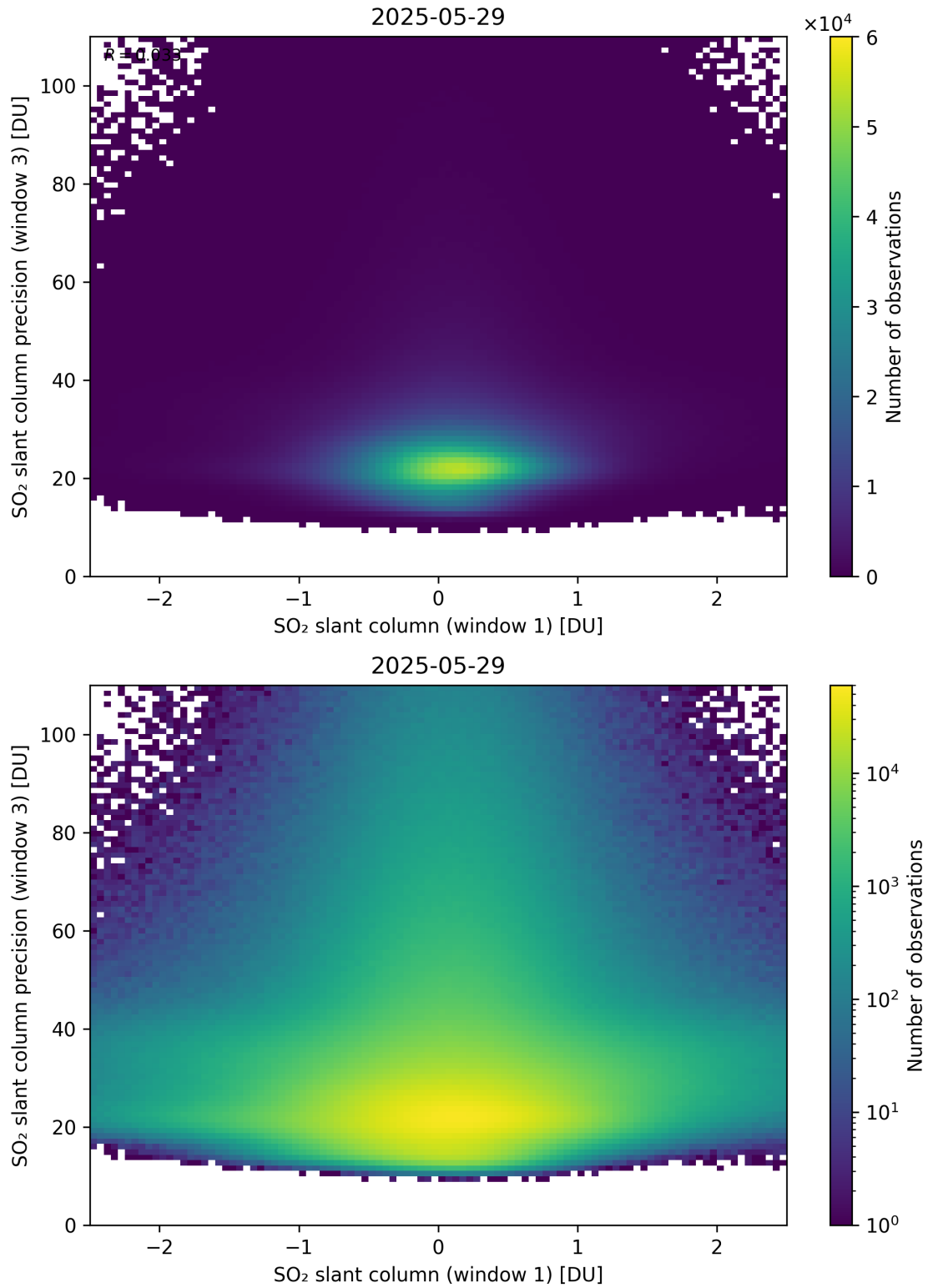
Figure 288: Scatter density plot of “SO 2 slant column (window 1)” against “SO 2 slant column precision (window 3)” for 2025-05-28 to 2025-05-30.
