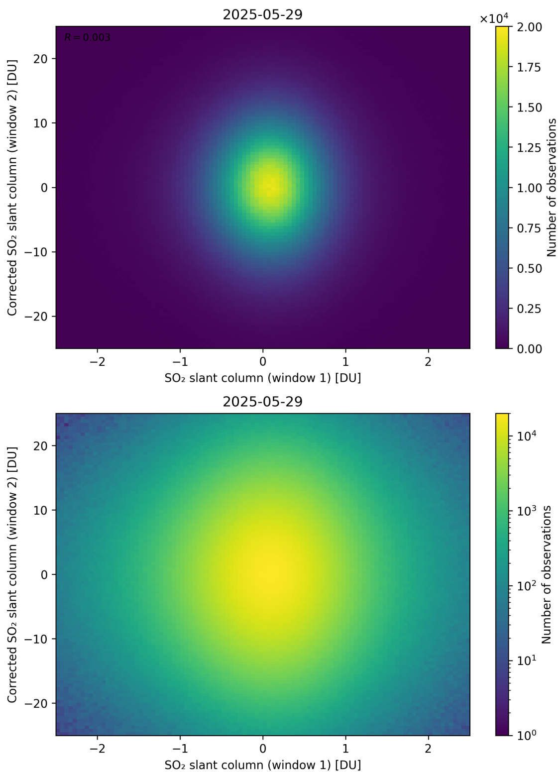
Figure 283: Scatter density plot of “SO 2 slant column (window 1)” against “Corrected SO 2 slant column (window 2)” for 2025-05-28 to 2025-05-30.
