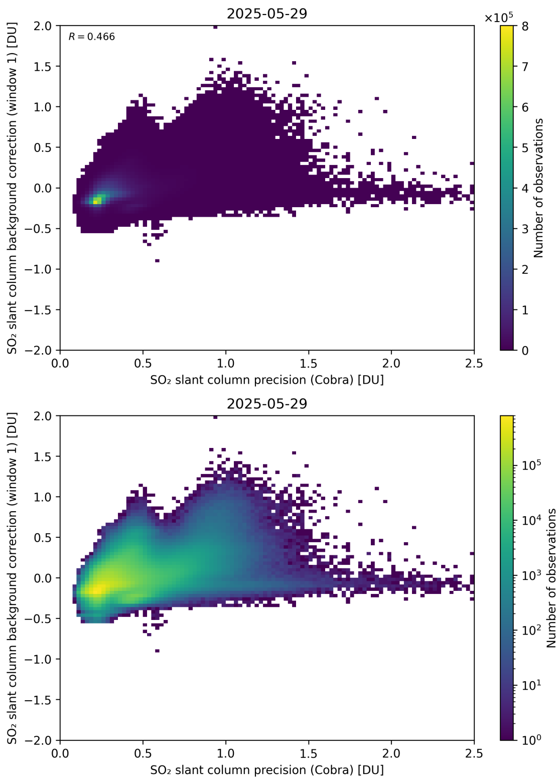
Figure 199: Scatter density plot of “SO 2 slant column precision (Cobra)” against “SO 2 slant column background correction (window 1)” for 2025-05-28 to 2025-05-30.
