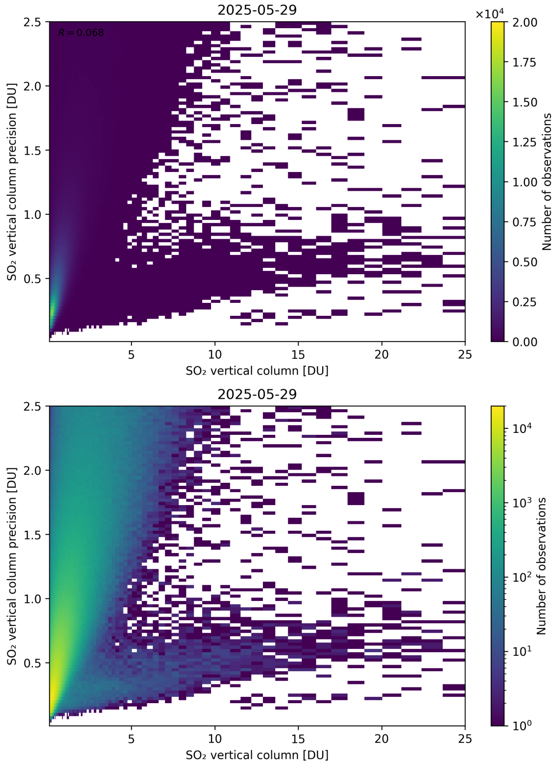
Figure 361: Scatter density plot of “SO 2 vertical column” against “SO 2 vertical column precision” for 2025-05-28 to 2025-05-30.
