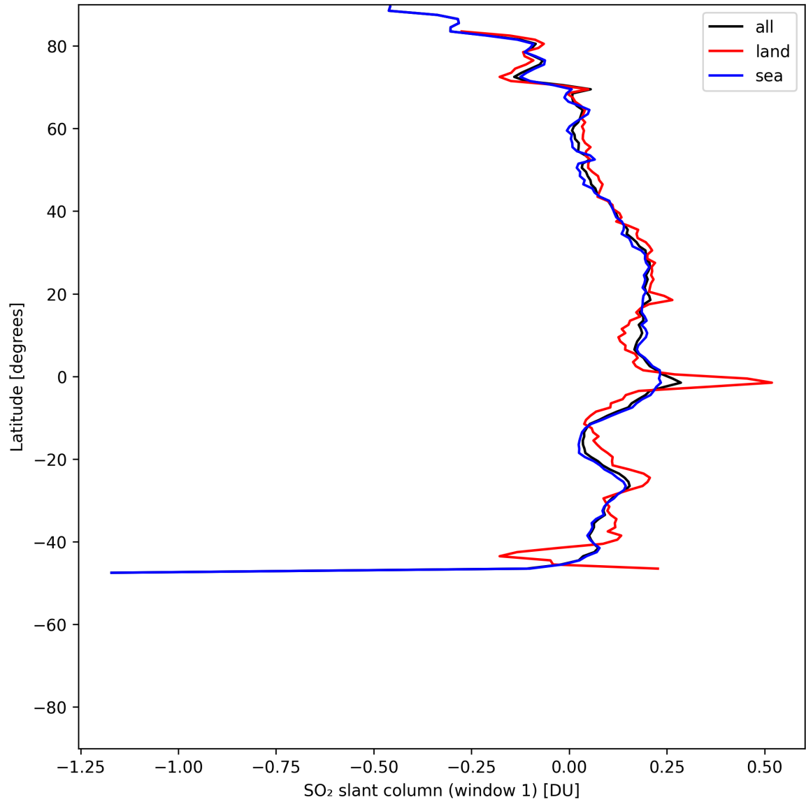
Figure 37: Zonal average of “SO 2 slant column (window 1)” for 2025-05-28 to 2025-05-30.
