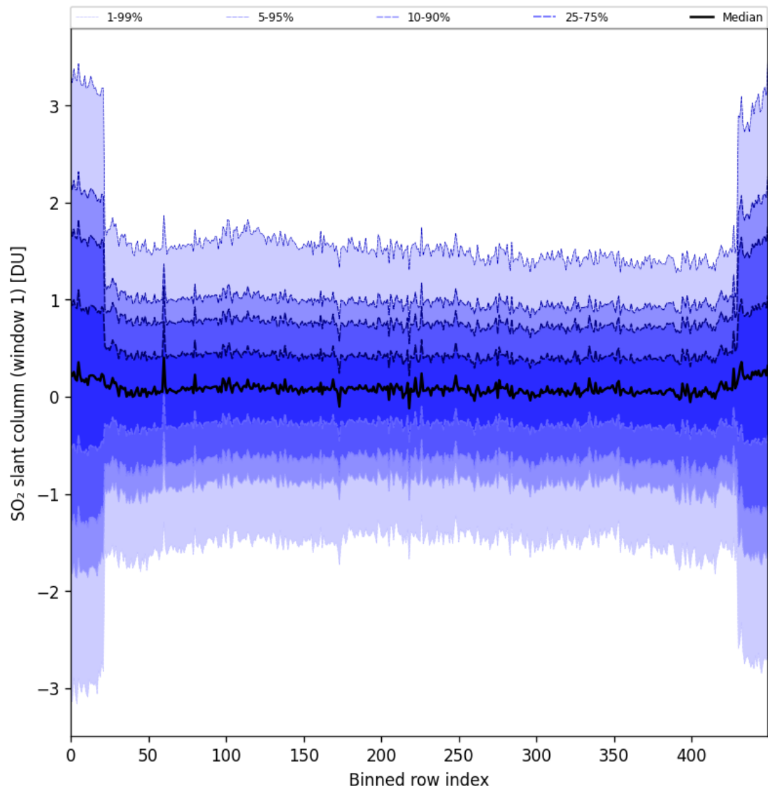
Figure 89: Along track statistics of “SO 2 slant column (window 1)” for 2025-05-28 to 2025-05-30
