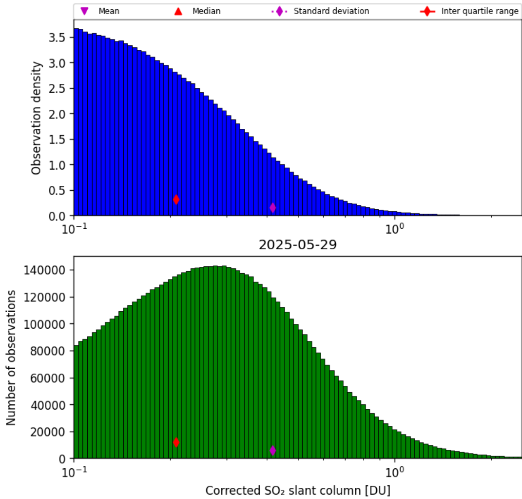
Figure 60: Histogram of “Corrected SO 2 slant column” for 2025-05-28 to 2025-05-30
