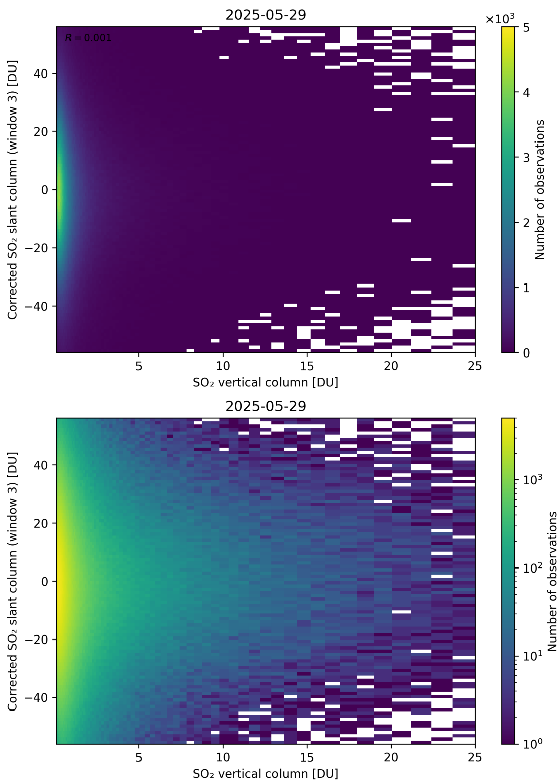
Figure 353: Scatter density plot of “SO 2 vertical column” against “Corrected SO 2 slant column (window 3)” for 2025-05-28 to 2025-05-30.
