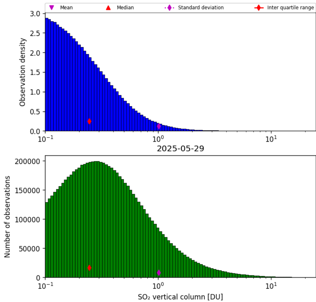
Figure 58: Histogram of “SO 2 vertical column” for 2025-05-28 to 2025-05-30
