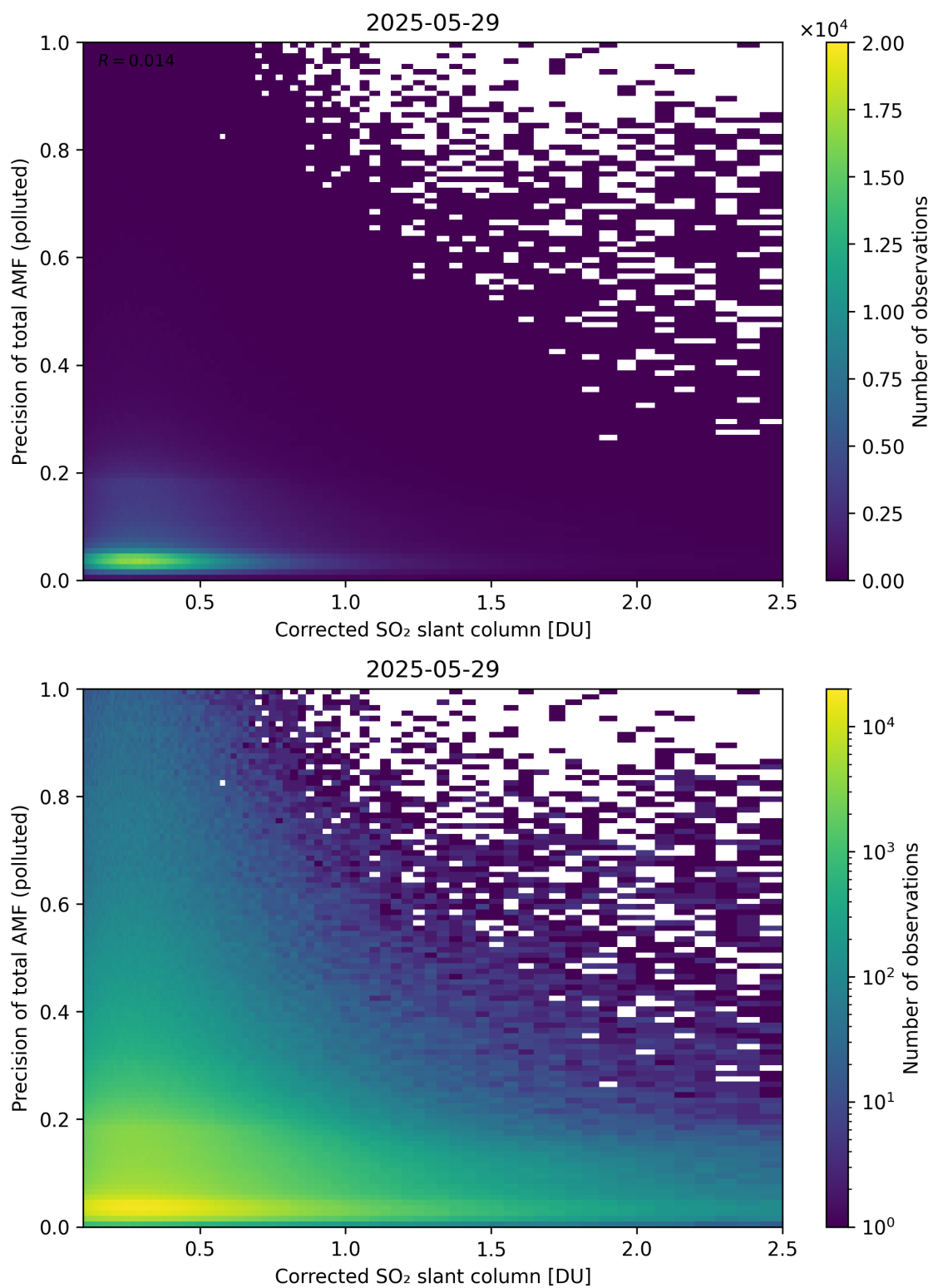
Figure 243: Scatter density plot of “Corrected SO 2 slant column” against “Precision of total AMF (polluted)” for 2025-05-28 to 2025-05-30.
