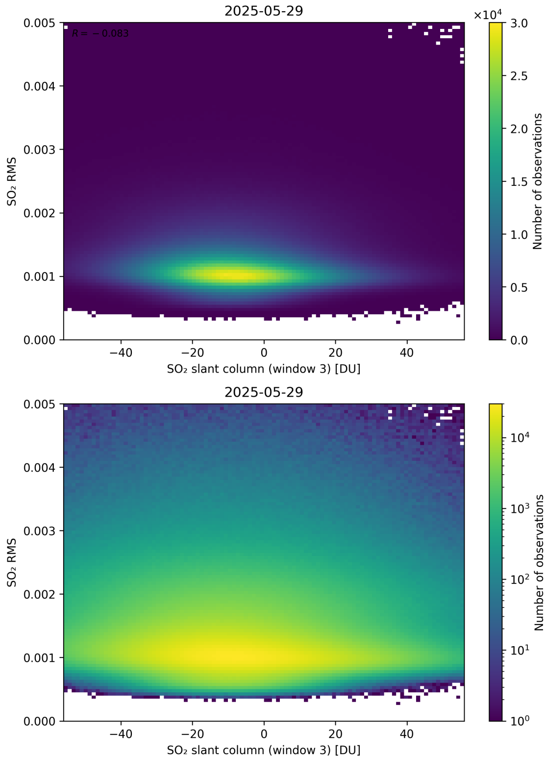
Figure 306: Scatter density plot of “SO 2 slant column (window 3)” against “SO 2 RMS” for 2025-05-28 to 2025-05-30.
