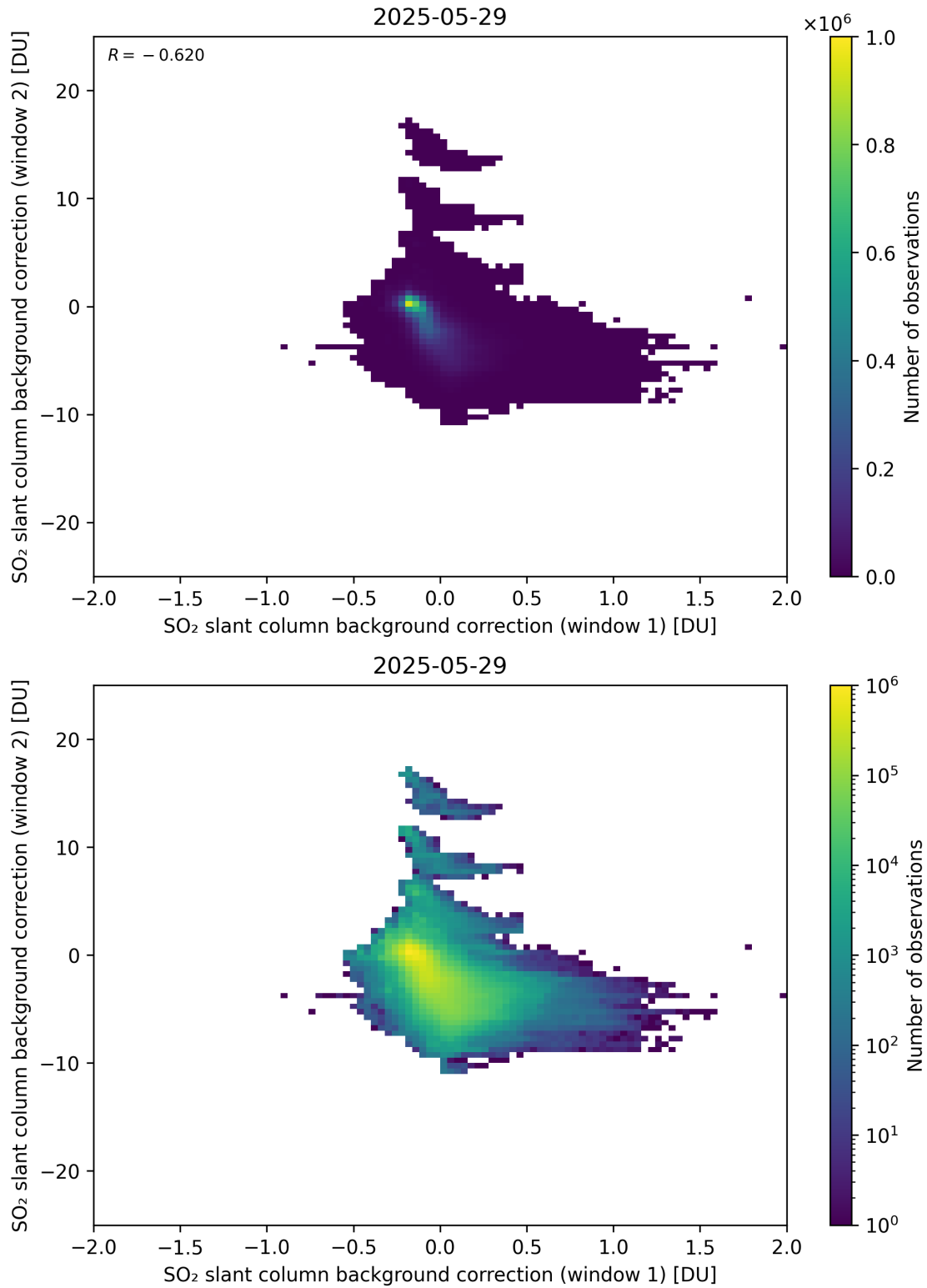
Figure 109: Scatter density plot of “SO 2 slant column background correction (window 1)” against “SO 2 slant column background correction (window 2)” for 2025-05-28 to 2025-05-30.
