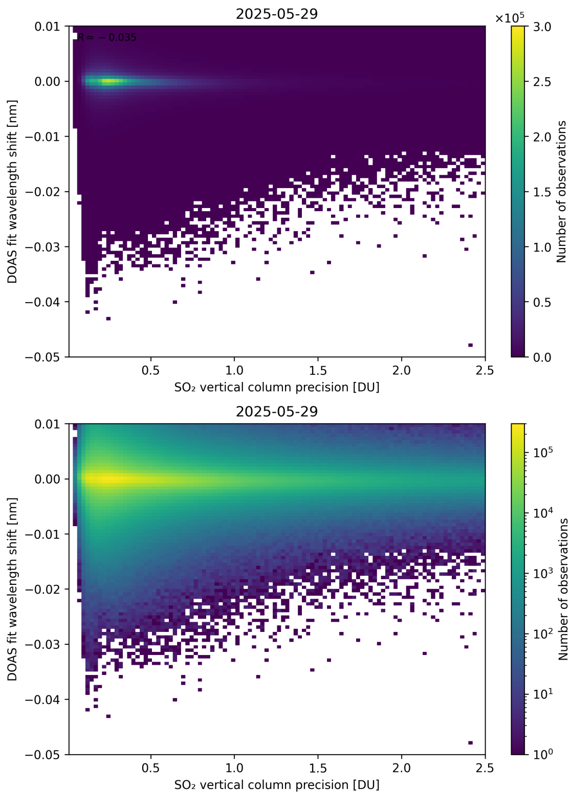
Figure 332: Scatter density plot of “SO 2 vertical column precision” against “DOAS fit wavelength shift” for 2025-05-28 to 2025-05-30.
