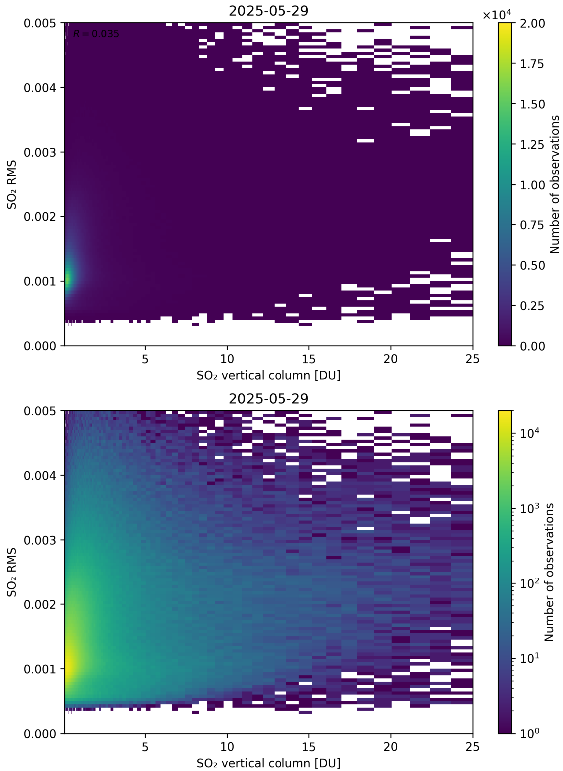
Figure 328: Scatter density plot of “SO 2 vertical column” against “SO 2 RMS” for 2025-05-28 to 2025-05-30.
