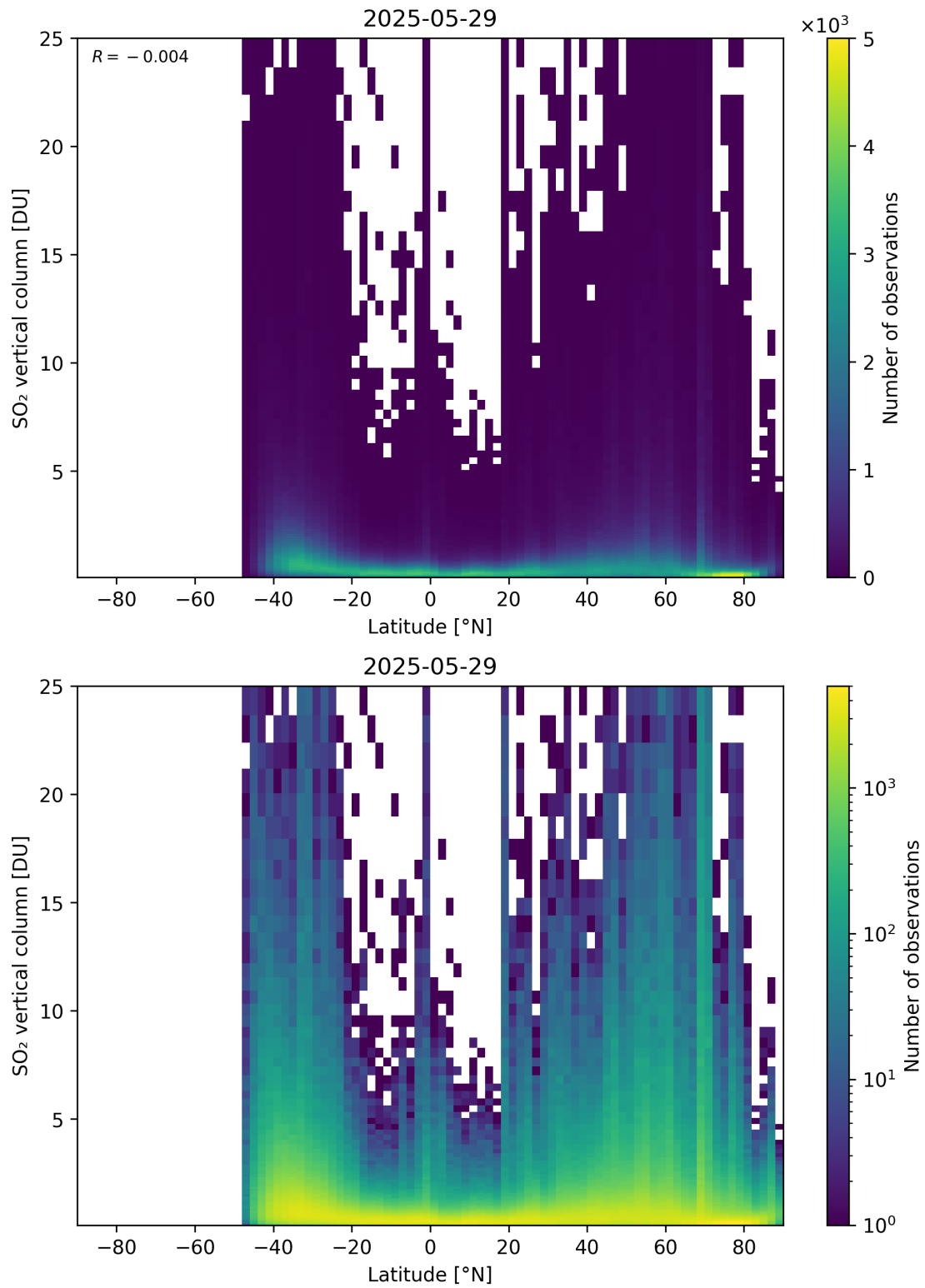
Figure 169: Scatter density plot of “Latitude” against “SO 2 vertical column” for 2025-05-28 to 2025-05-30.
