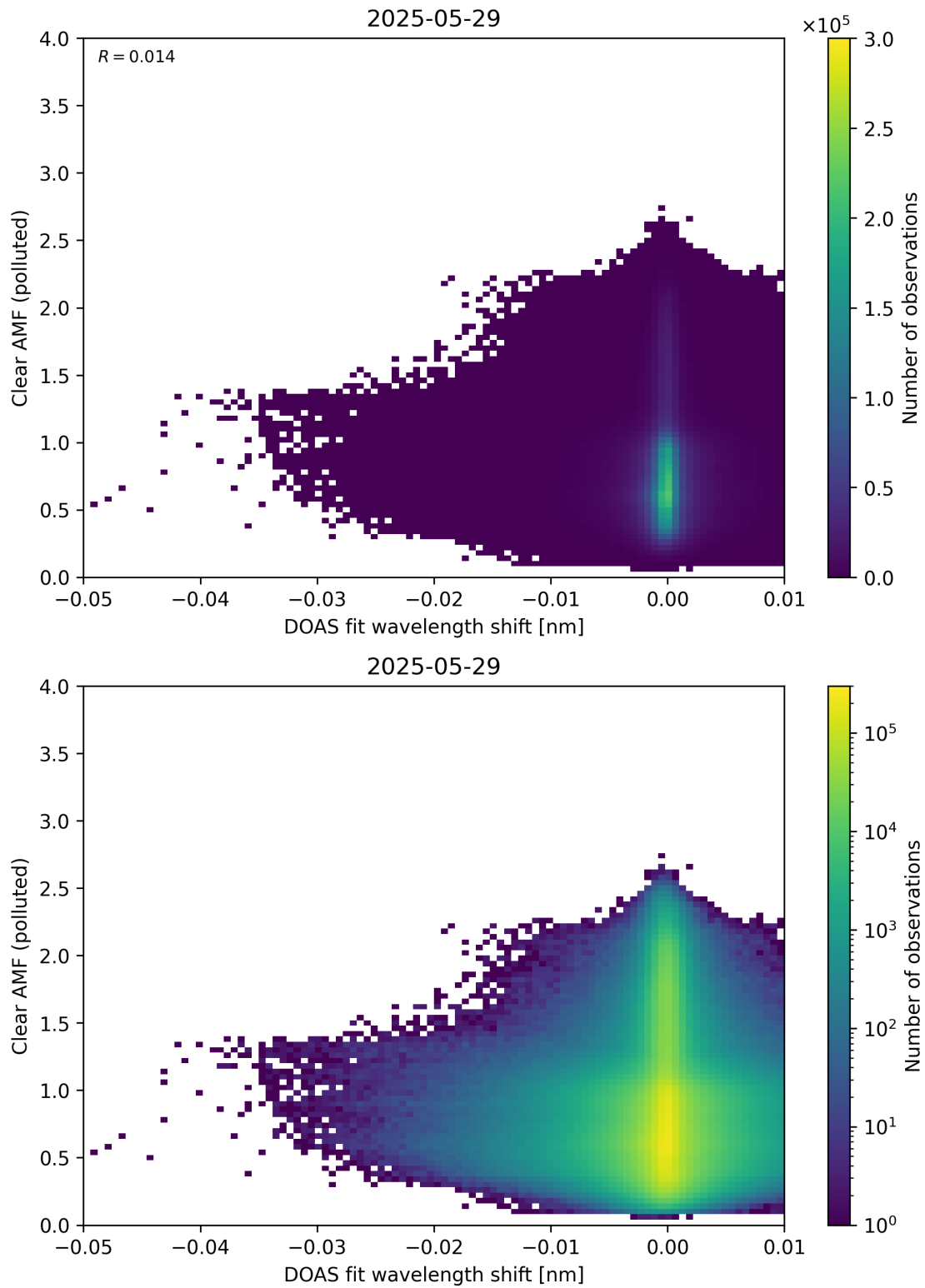
Figure 140: Scatter density plot of “DOAS fit wavelength shift” against “Clear AMF (polluted)” for 2025-05-28 to 2025-05-30.
