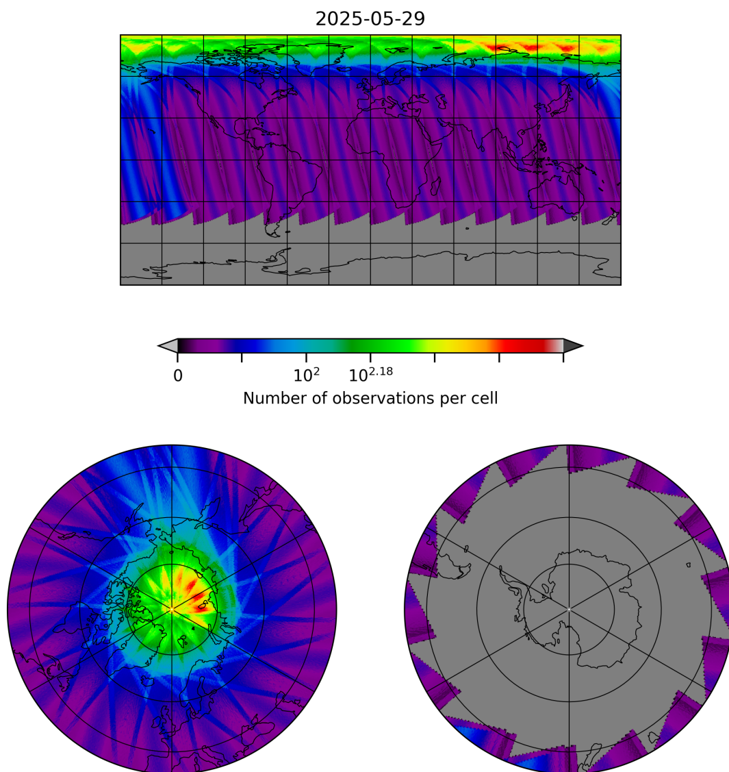
Figure 30: Map of the number of observations for 2025-05-28 to 2025-05-30
