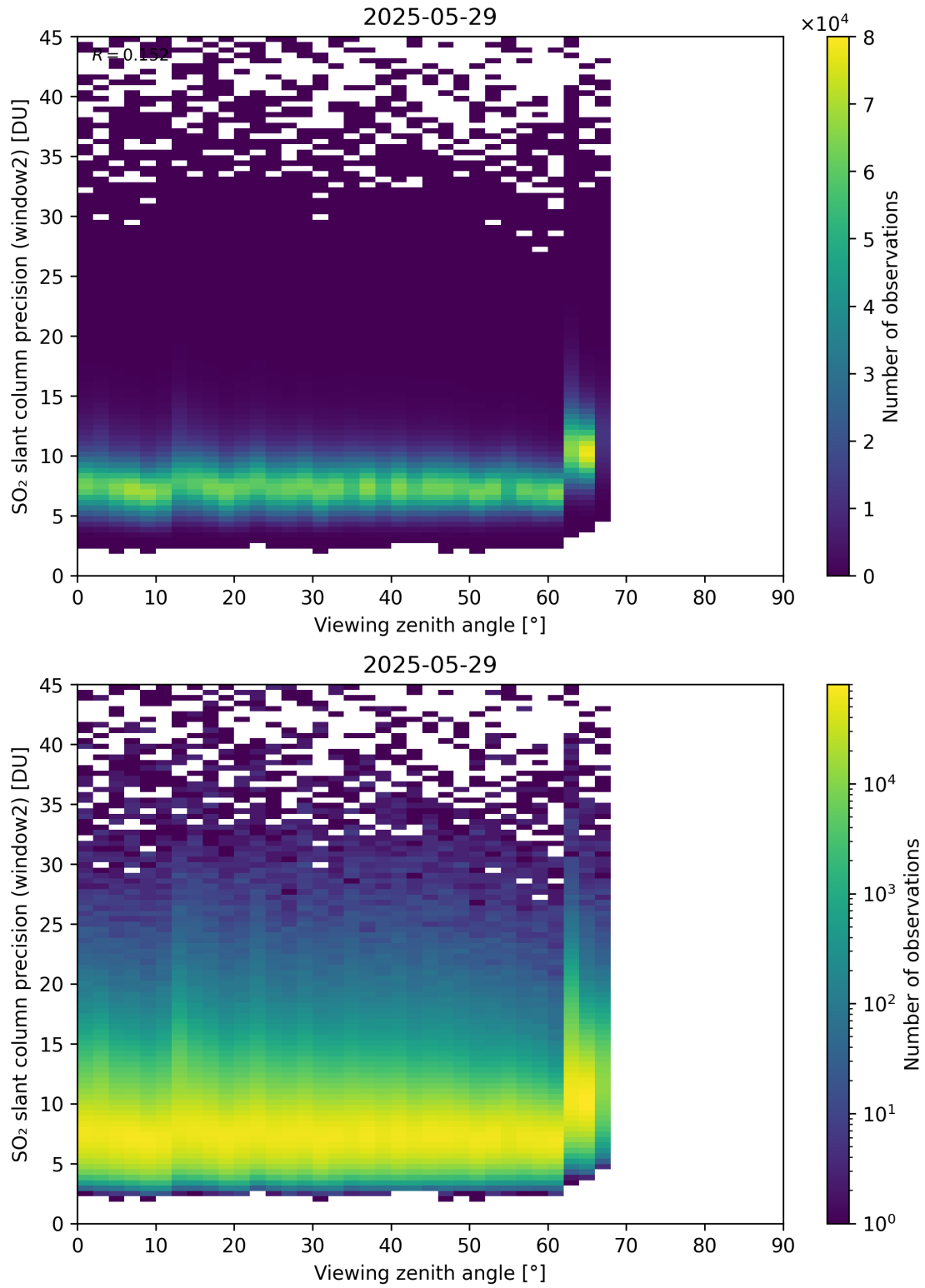
Figure 378: Scatter density plot of “Viewing zenith angle” against “SO 2 slant column precision (window2)” for 2025-05-28 to 2025-05-30.
