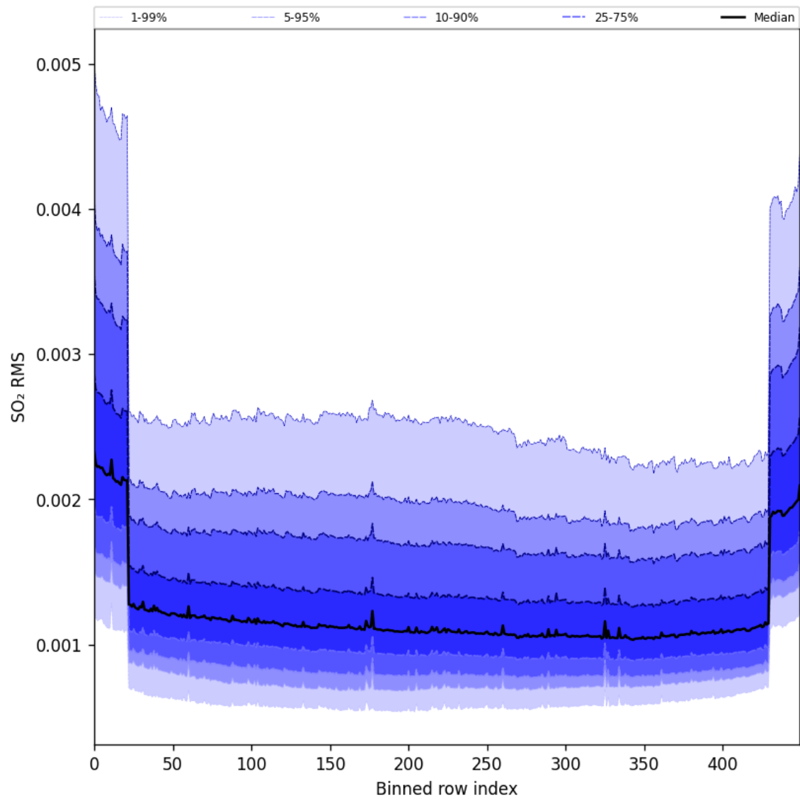
Figure 104: Along track statistics of “SO 2 RMS” for 2025-05-28 to 2025-05-30
