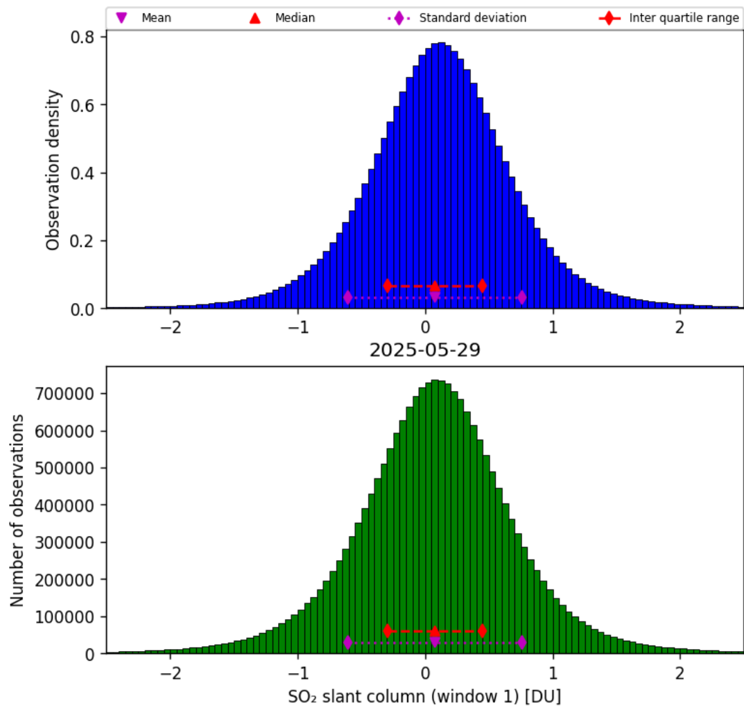
Figure 63: Histogram of “SO 2 slant column (window 1)” for 2025-05-28 to 2025-05-30
