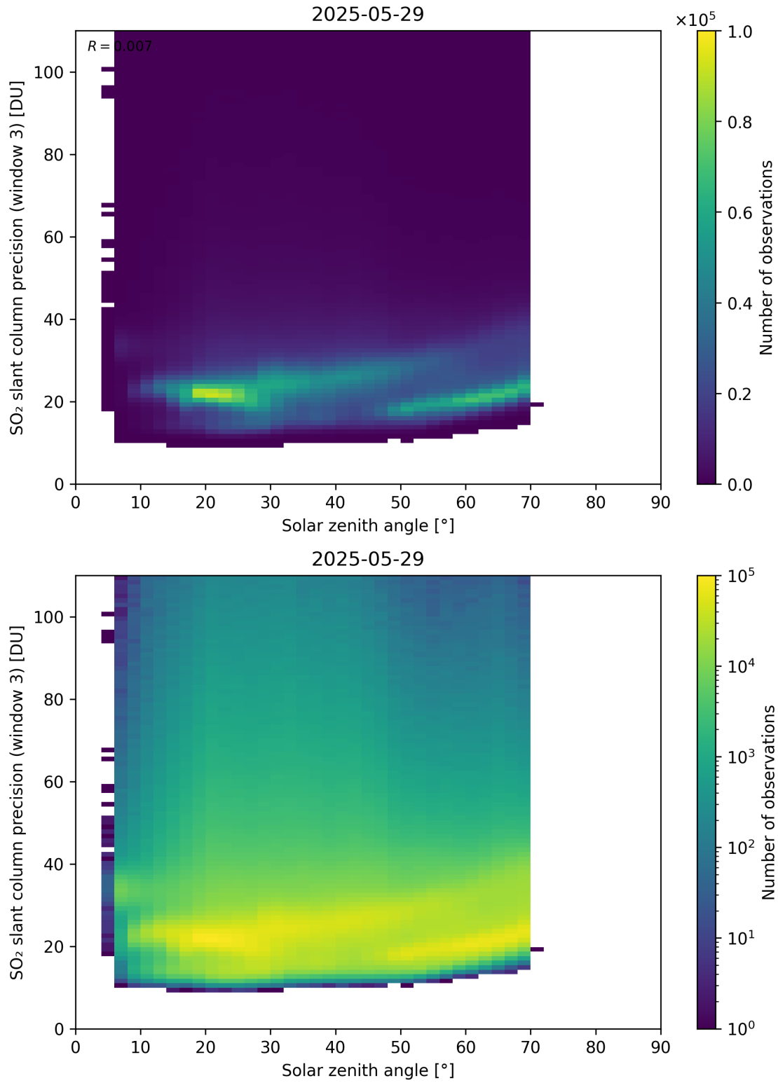
Figure 188: Scatter density plot of “Solar zenith angle” against “SO 2 slant column precision (window 3)” for 2025-05-28 to 2025-05-30.
