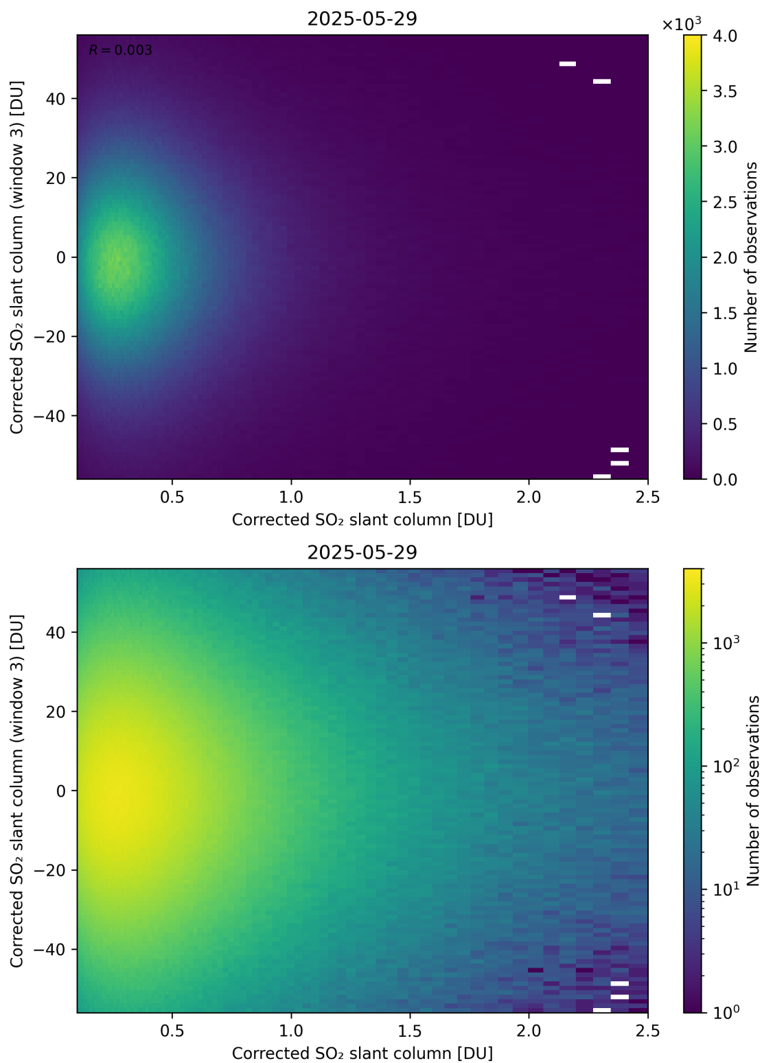
Figure 236: Scatter density plot of “Corrected SO 2 slant column” against “Corrected SO 2 slant column (window 3)” for 2025-05-28 to 2025-05-30.
