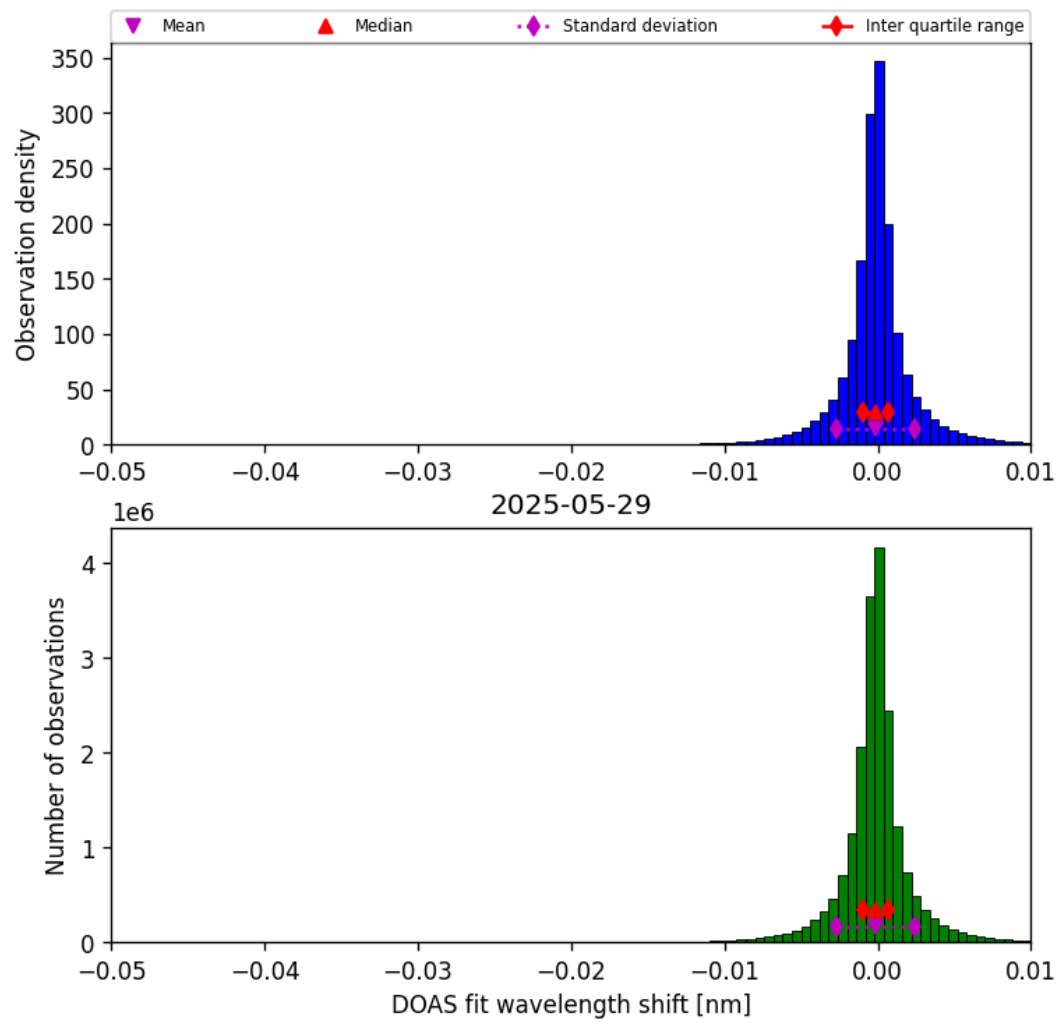
Figure 76: Histogram of “DOAS fit wavelength shift” for 2025-05-28 to 2025-05-30
