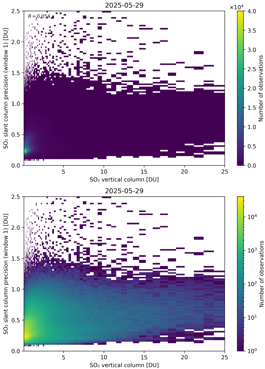
Figure 355: Scatter density plot of “SO 2 vertical column” against “SO 2 slant column precision (window 1)” for 2025-05-28 to 2025-05-30.
