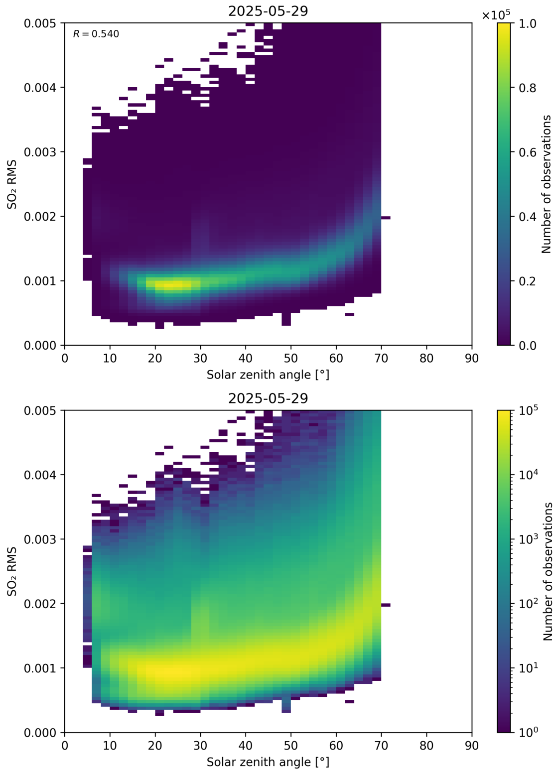
Figure 176: Scatter density plot of “Solar zenith angle” against “SO 2 RMS” for 2025-05-28 to 2025-05-30.
