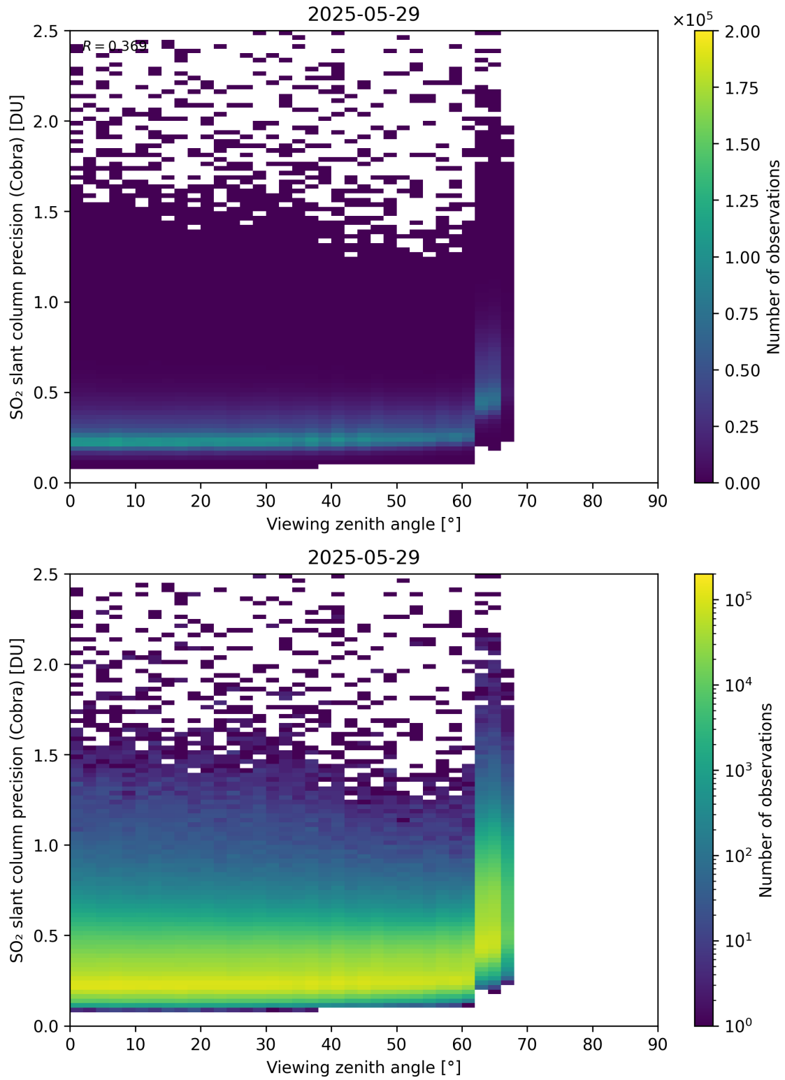
Figure 372: Scatter density plot of “Viewing zenith angle” against “SO 2 slant column precision (Cobra)” for 2025-05-28 to 2025-05-30.
