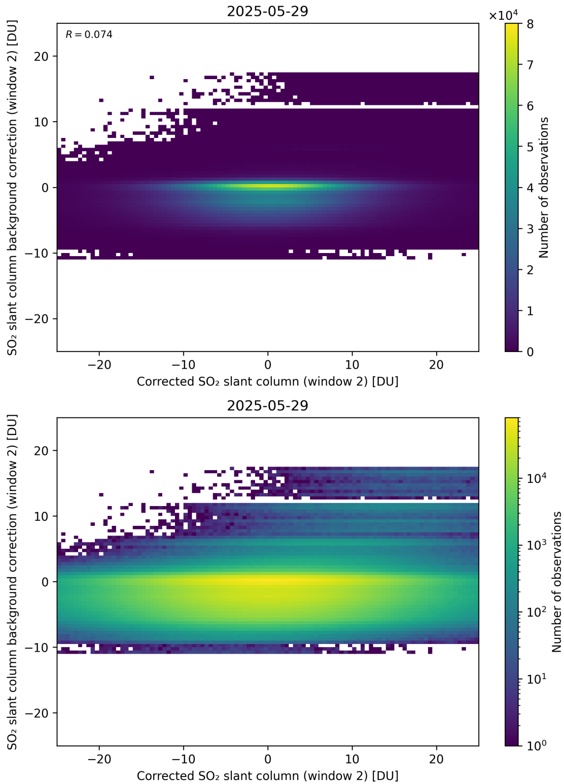
Figure 244: Scatter density plot of “Corrected SO 2 slant column (window 2)” against “SO 2 slant column background correction (window 2)” for 2025-05-28 to 2025-05-30.
