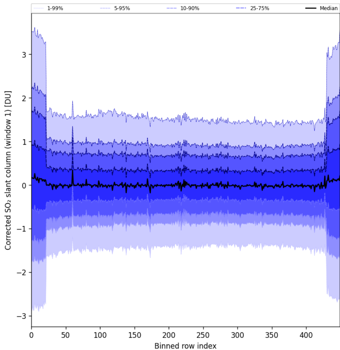
Figure 91: Along track statistics of “Corrected SO 2 slant column (window 1)” for 2025-05-28 to 2025-05-30
