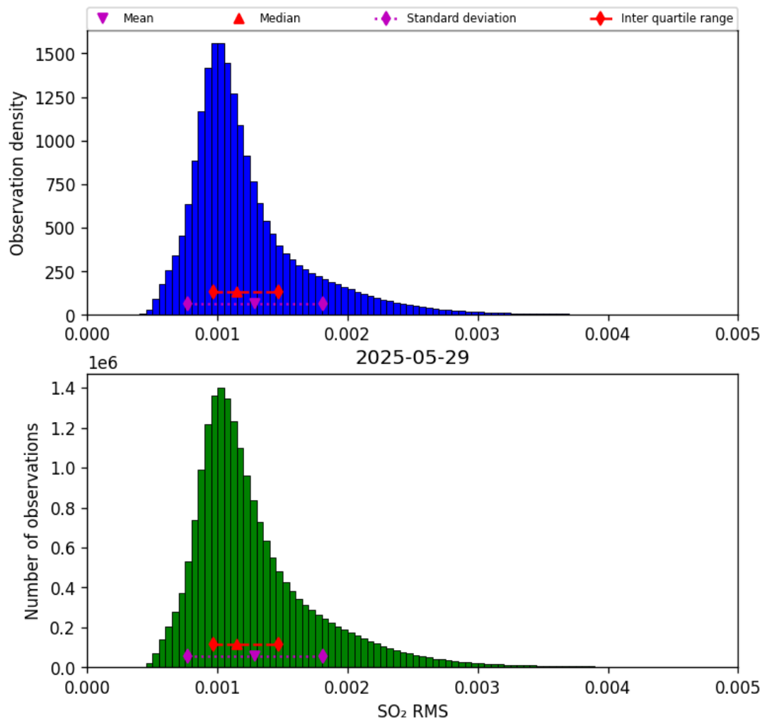
Figure 78: Histogram of “SO 2 RMS” for 2025-05-28 to 2025-05-30
