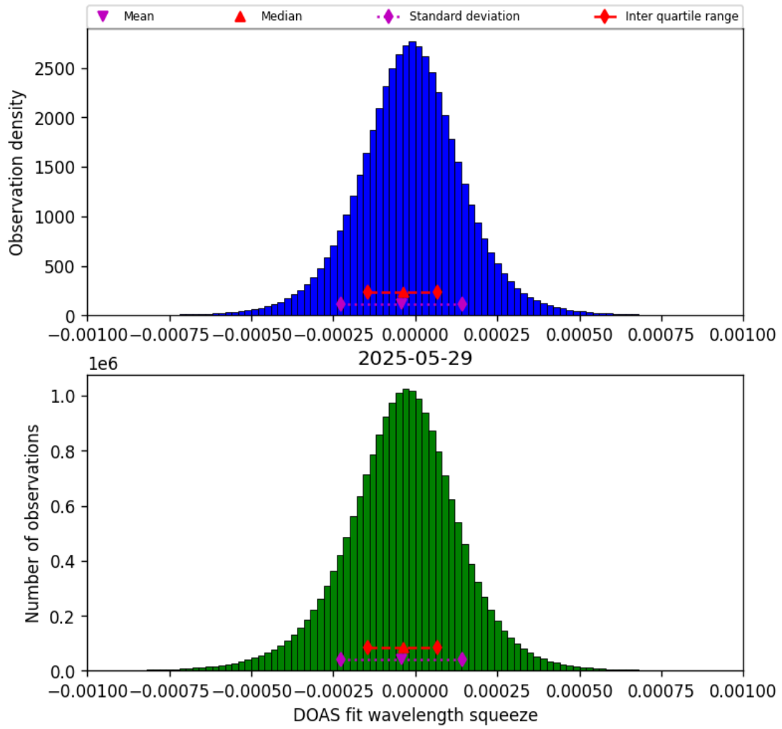
Figure 77: Histogram of “DOAS fit wavelength squeeze” for 2025-05-28 to 2025-05-30
