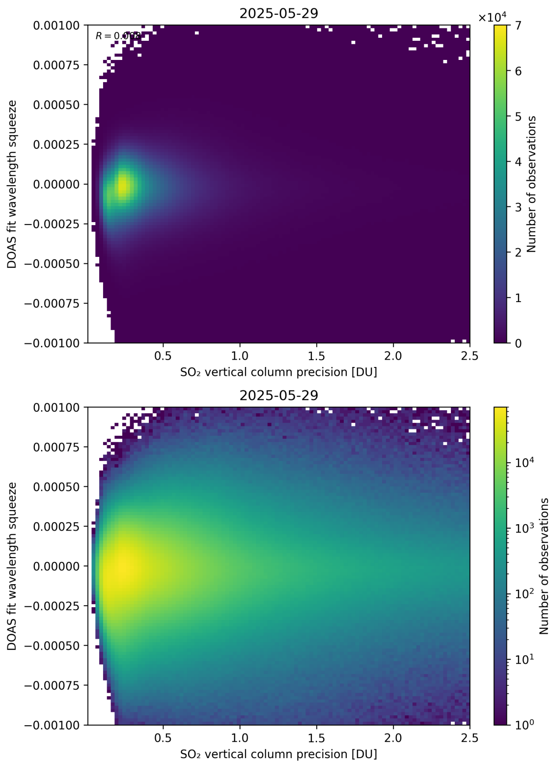
Figure 333: Scatter density plot of “SO 2 vertical column precision” against “DOAS fit wavelength squeeze” for 2025-05-28 to 2025-05-30.
