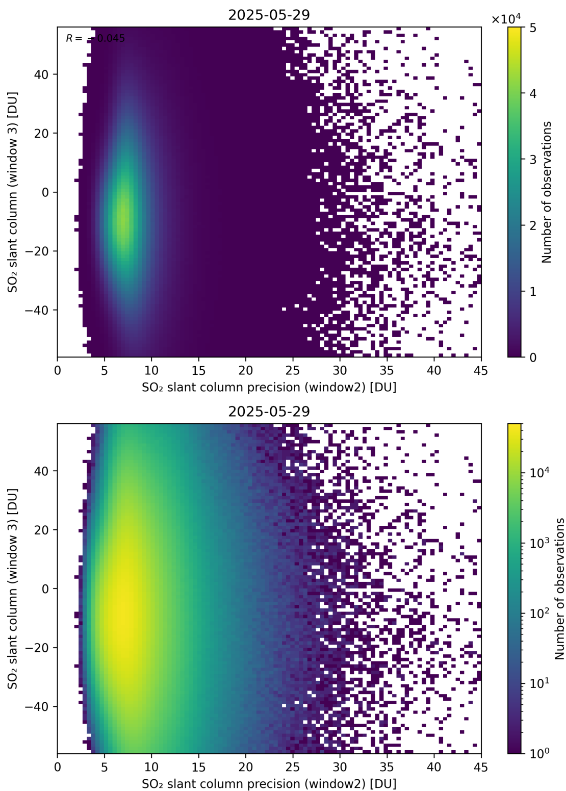
Figure 299: Scatter density plot of “SO 2 slant column precision (window2)” against “SO 2 slant column (window 3)” for 2025-05-28 to 2025-05-30.
