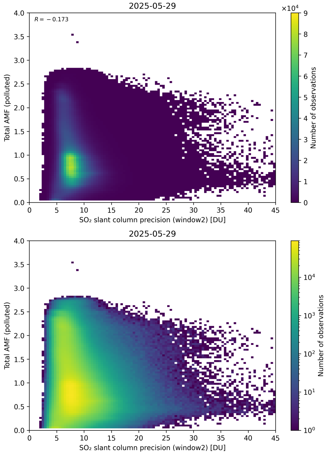
Figure 301: Scatter density plot of “SO 2 slant column precision (window2)” against “Total AMF (polluted)” for 2025-05-28 to 2025-05-30.
