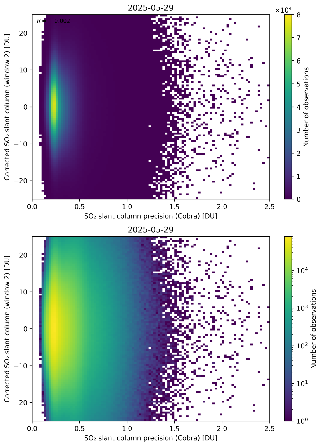
Figure 206: Scatter density plot of “SO 2 slant column precision (Cobra)” against “Corrected SO 2 slant column (window 2)” for 2025-05-28 to 2025-05-30.
