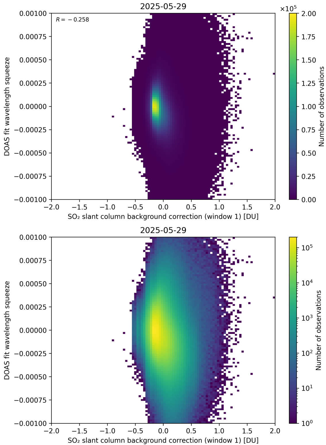
Figure 112: Scatter density plot of “SO 2 slant column background correction (window 1)” against “DOAS fit wavelength squeeze” for 2025-05-28 to 2025-05-30.
