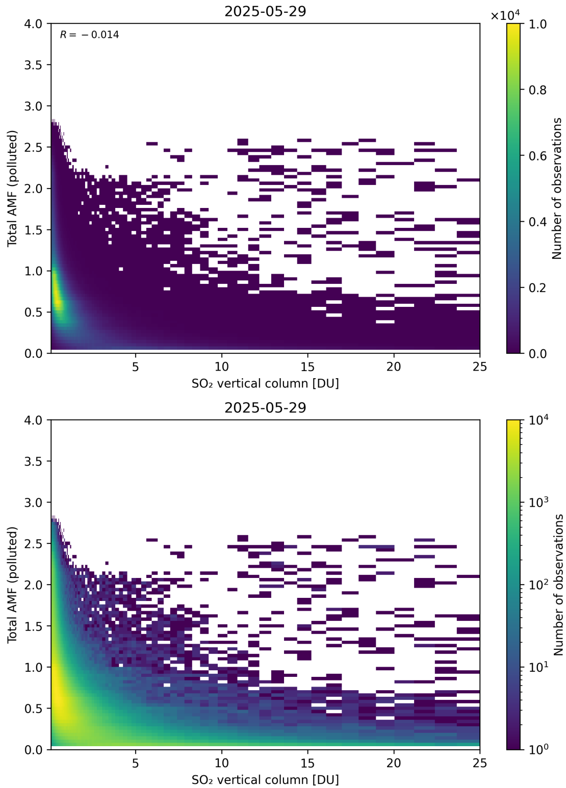
Figure 359: Scatter density plot of “SO 2 vertical column” against “Total AMF (polluted)” for 2025-05-28 to 2025-05-30.
