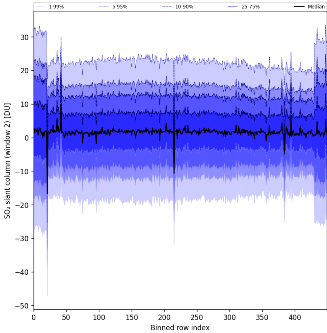
Figure 93: Along track statistics of “SO 2 slant column (window 2)” for 2025-05-28 to 2025-05-30
