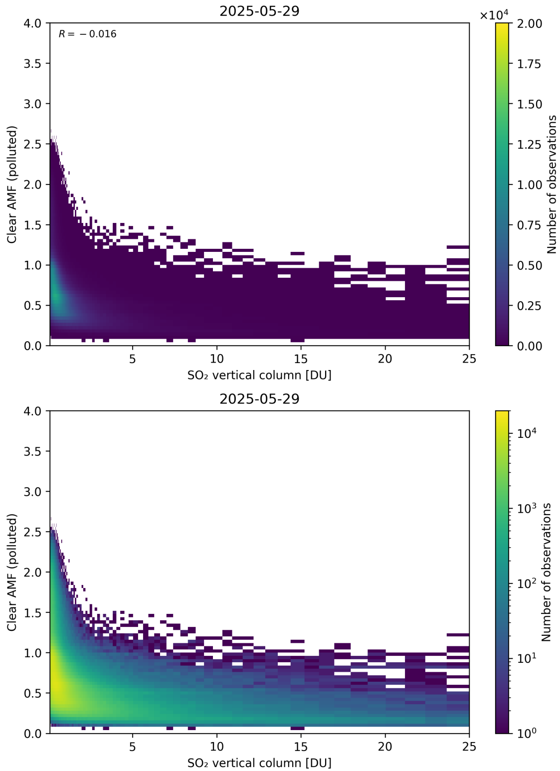
Figure 348: Scatter density plot of “SO 2 vertical column” against “Clear AMF (polluted)” for 2025-05-28 to 2025-05-30.
