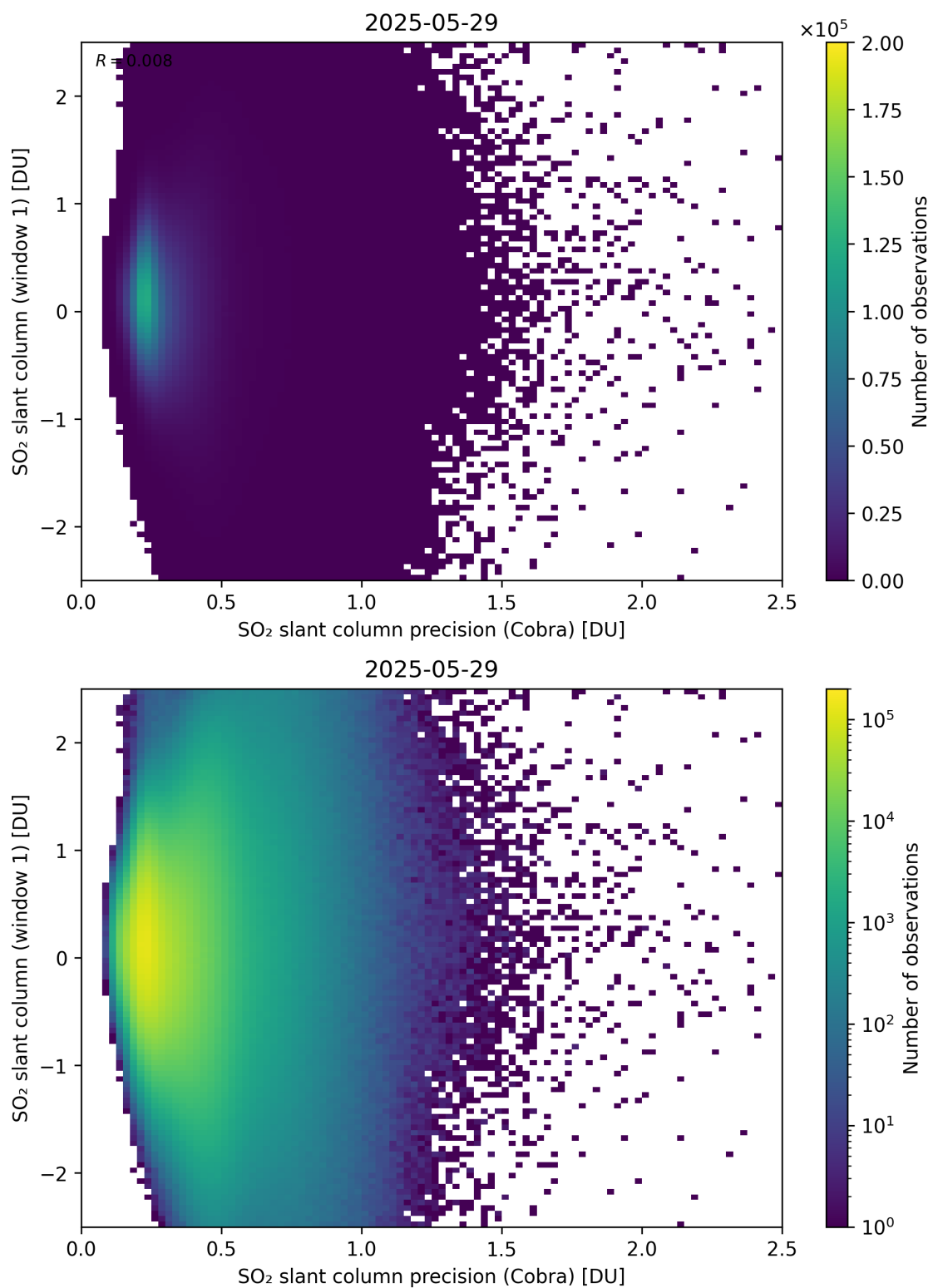
Figure 208: Scatter density plot of “SO 2 slant column precision (Cobra)” against “SO 2 slant column (window 1)” for 2025-05-28 to 2025-05-30.
