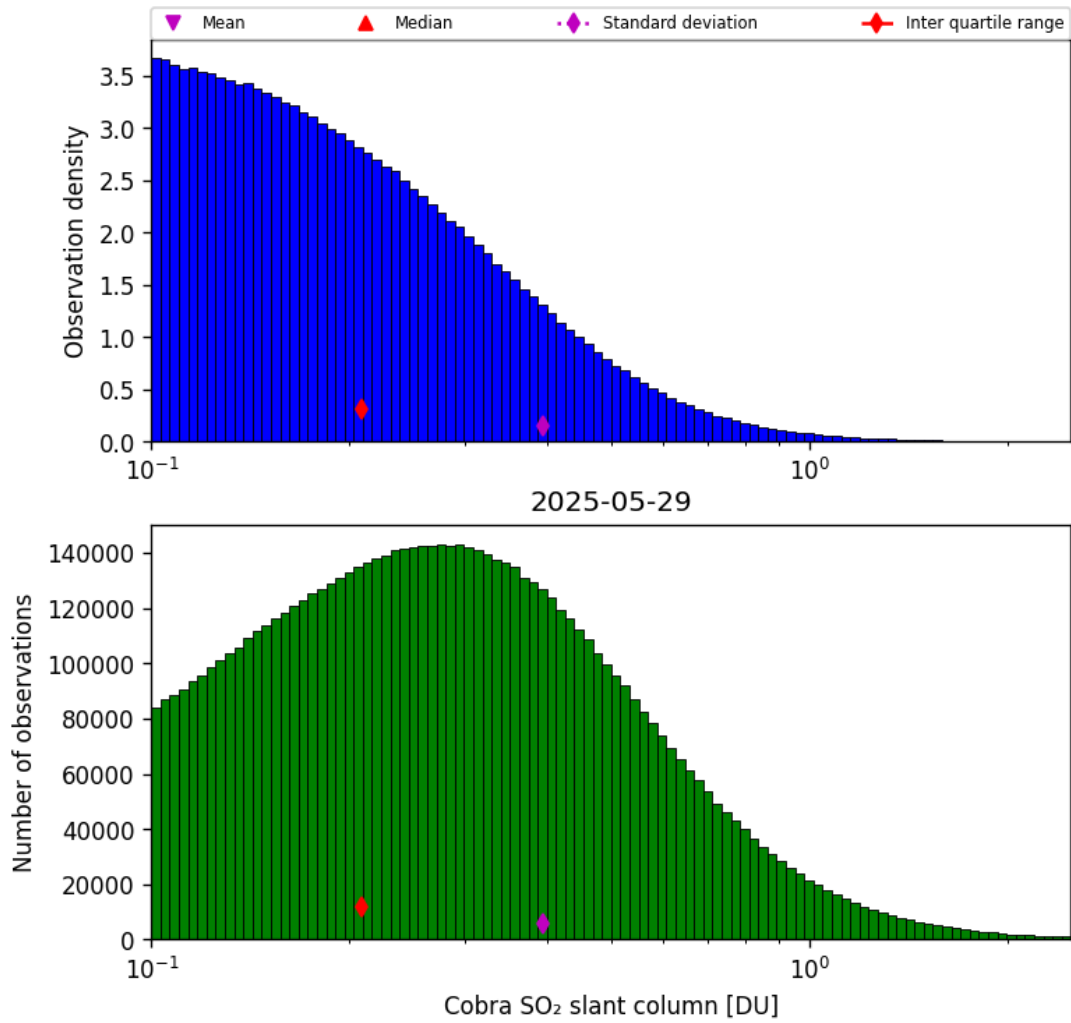
Figure 61: Histogram of “Cobra SO 2 slant column” for 2025-05-28 to 2025-05-30
