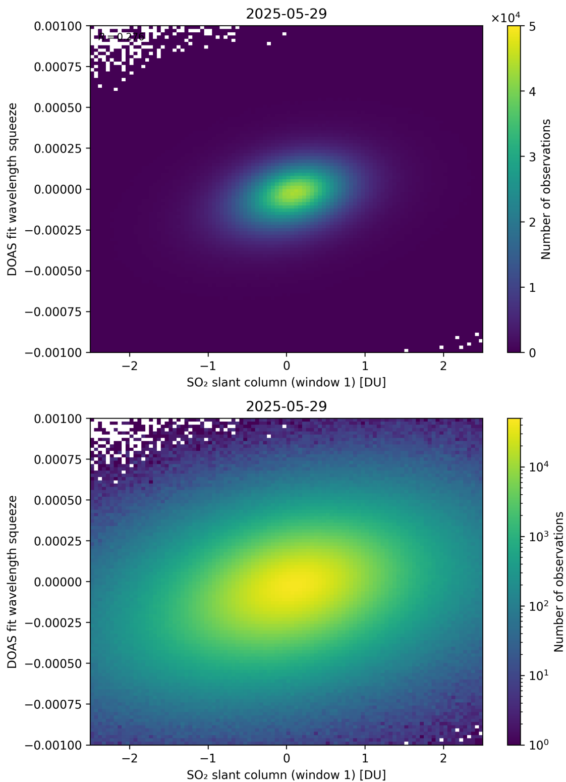
Figure 266: Scatter density plot of “SO 2 slant column (window 1)” against “DOAS fit wavelength squeeze” for 2025-05-28 to 2025-05-30.
