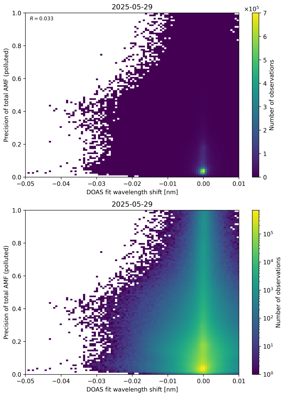
Figure 142: Scatter density plot of “DOAS fit wavelength shift” against “Precision of total AMF (polluted)” for 2025-05-28 to 2025-05-30.
