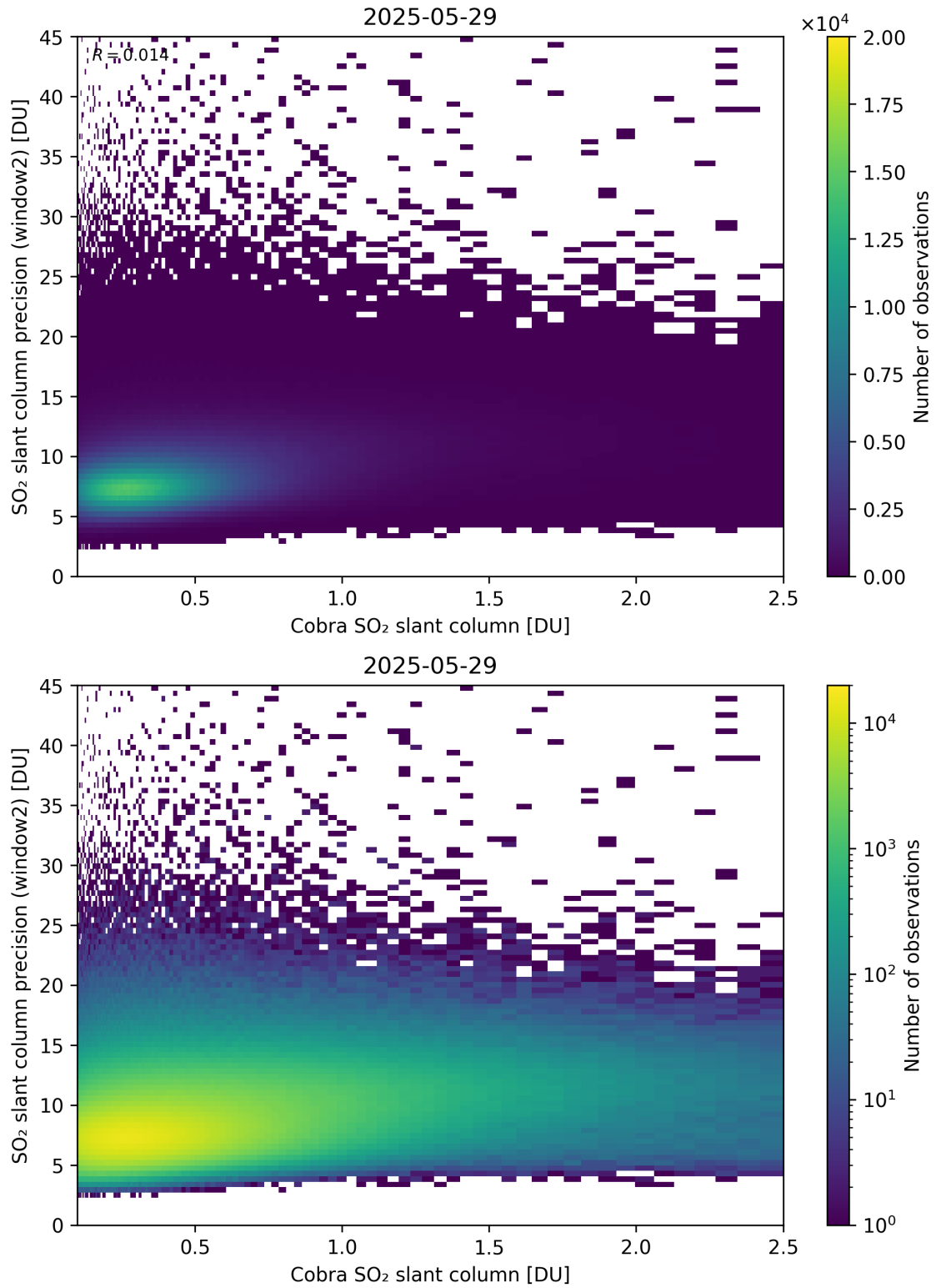
Figure 221: Scatter density plot of “Cobra SO 2 slant column” against “SO 2 slant column precision (window2)” for 2025-05-28 to 2025-05-30.
