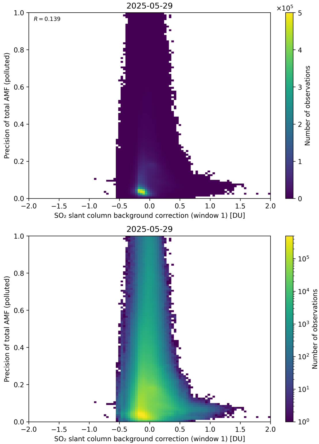
Figure 121: Scatter density plot of “SO 2 slant column background correction (window 1)” against “Precision of total AMF (polluted)” for 2025-05-28 to 2025-05-30.
