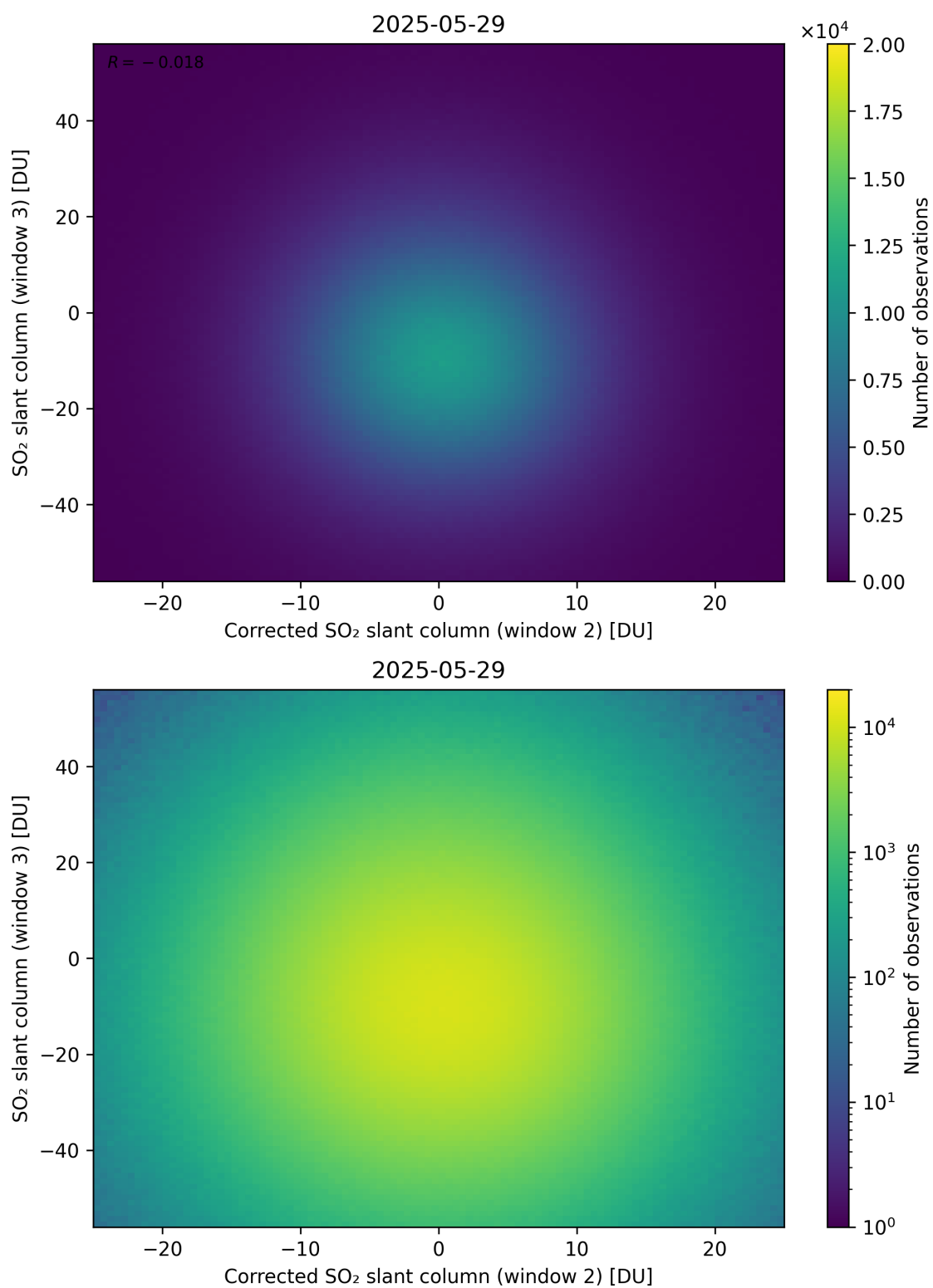
Figure 251: Scatter density plot of “Corrected SO 2 slant column (window 2)” against “SO 2 slant column (window 3)” for 2025-05-28 to 2025-05-30.
