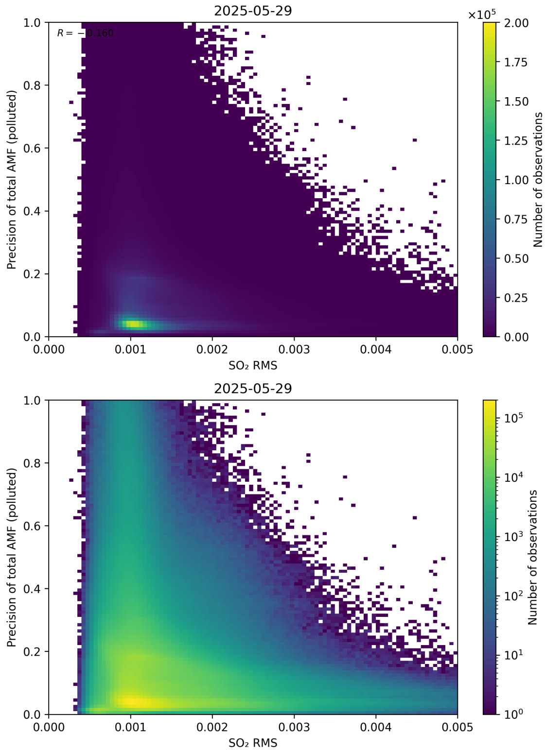
Figure 149: Scatter density plot of “SO 2 RMS” against “Precision of total AMF (polluted)” for 2025-05-28 to 2025-05-30.
