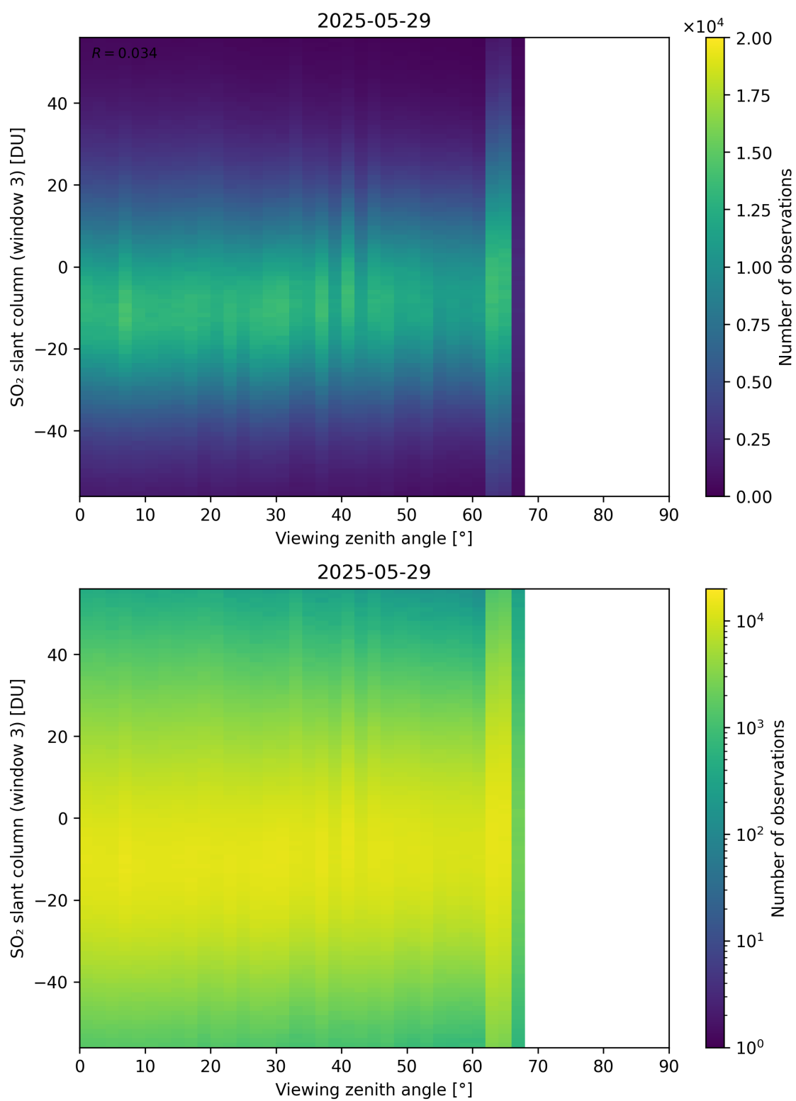
Figure 379: Scatter density plot of “Viewing zenith angle” against “SO 2 slant column (window 3)” for 2025-05-28 to 2025-05-30.
