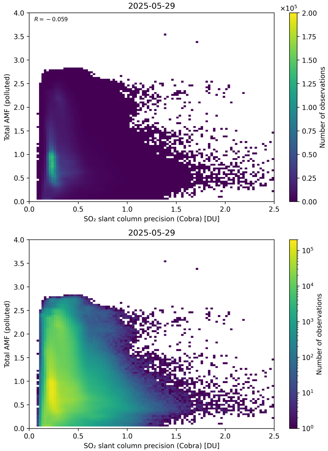
Figure 213: Scatter density plot of “SO 2 slant column precision (Cobra)” against “Total AMF (polluted)” for 2025-05-28 to 2025-05-30.
