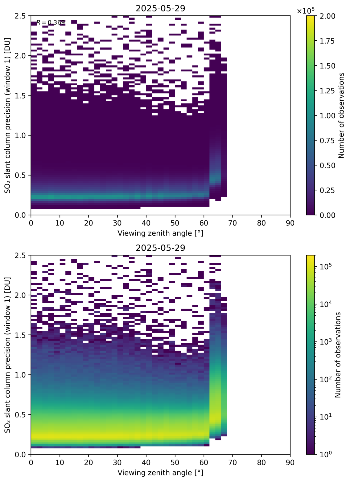
Figure 377: Scatter density plot of “Viewing zenith angle” against “SO 2 slant column precision (window 1)” for 2025-05-28 to 2025-05-30.
