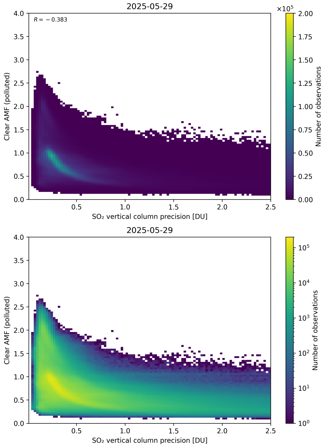
Figure 335: Scatter density plot of “SO 2 vertical column precision” against “Clear AMF (polluted)” for 2025-05-28 to 2025-05-30.
