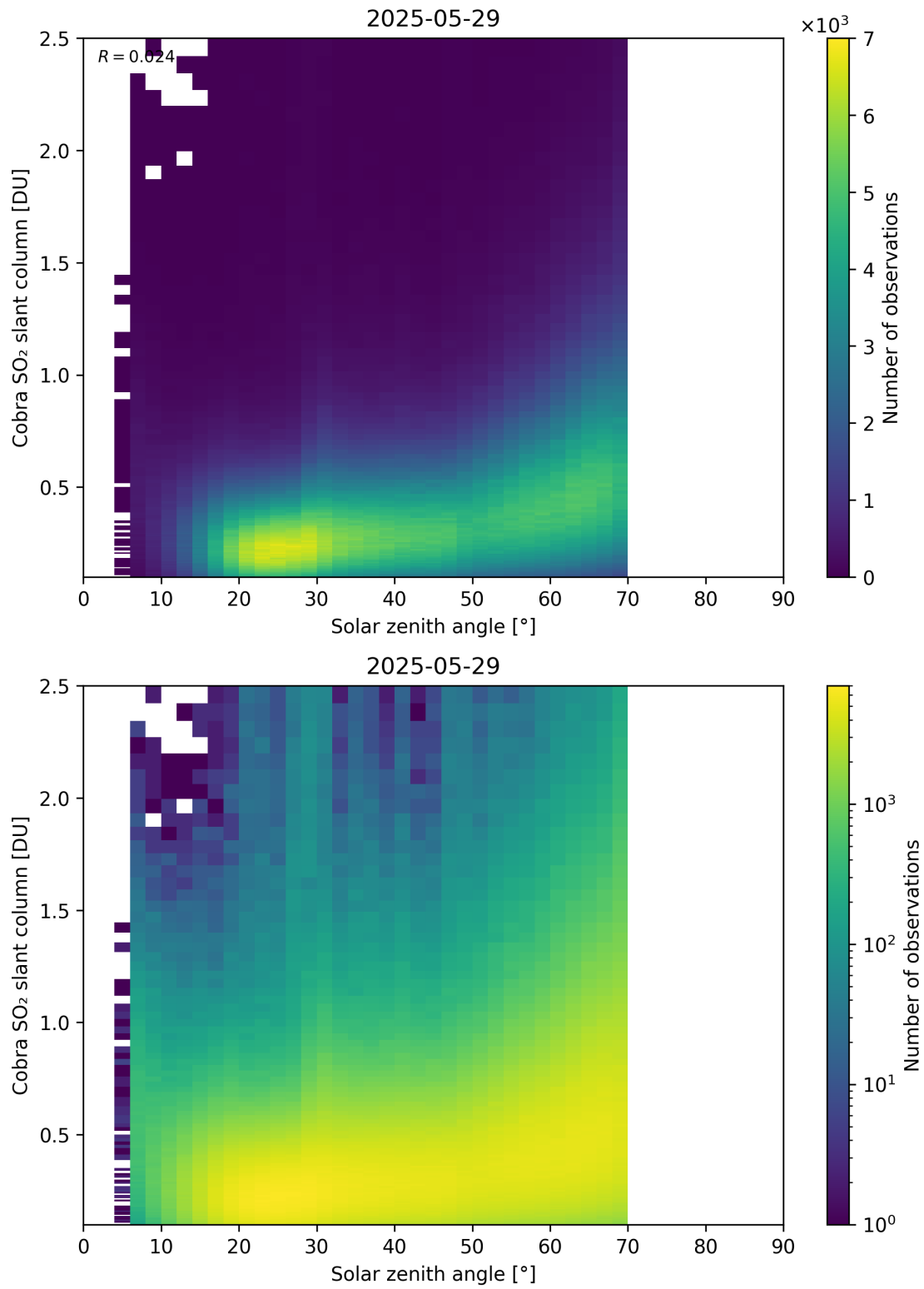
Figure 179: Scatter density plot of “Solar zenith angle” against “Cobra SO 2 slant column” for 2025-05-28 to 2025-05-30.
