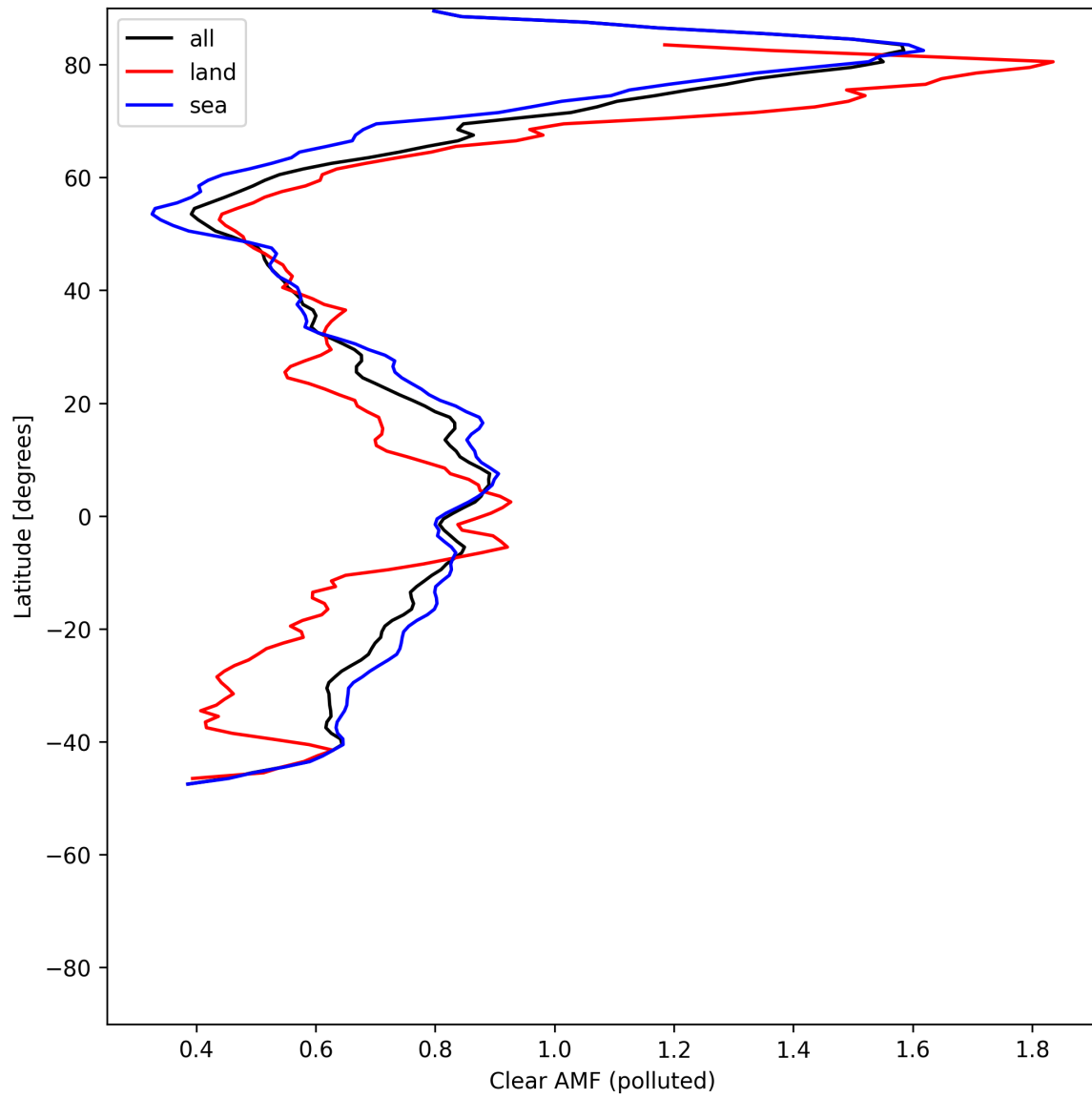
Figure 55: Zonal average of “Clear AMF (polluted)” for 2025-05-28 to 2025-05-30.
