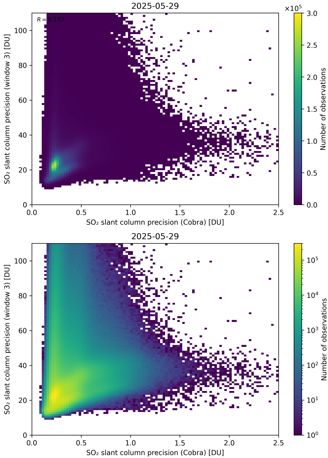
Figure 212: Scatter density plot of “SO 2 slant column precision (Cobra)” against “SO 2 slant column precision (window 3)” for 2025-05-28 to 2025-05-30.
