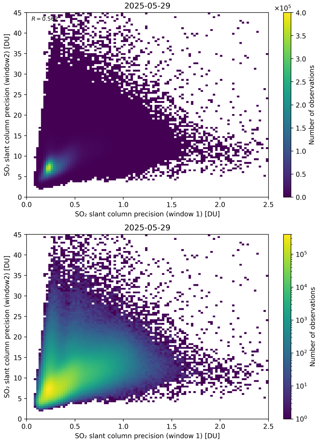
Figure 277: Scatter density plot of “SO 2 slant column precision (window 1)” against “SO 2 slant column precision (window 2)” for 2025-05-28 to 2025-05-30.
