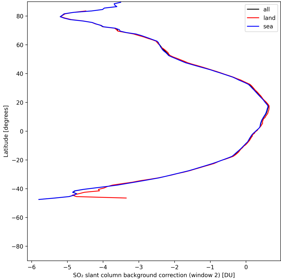
Figure 44: Zonal average of “SO 2 slant column background correction (window 2)” for 2025-05-28 to 2025-05-30.
