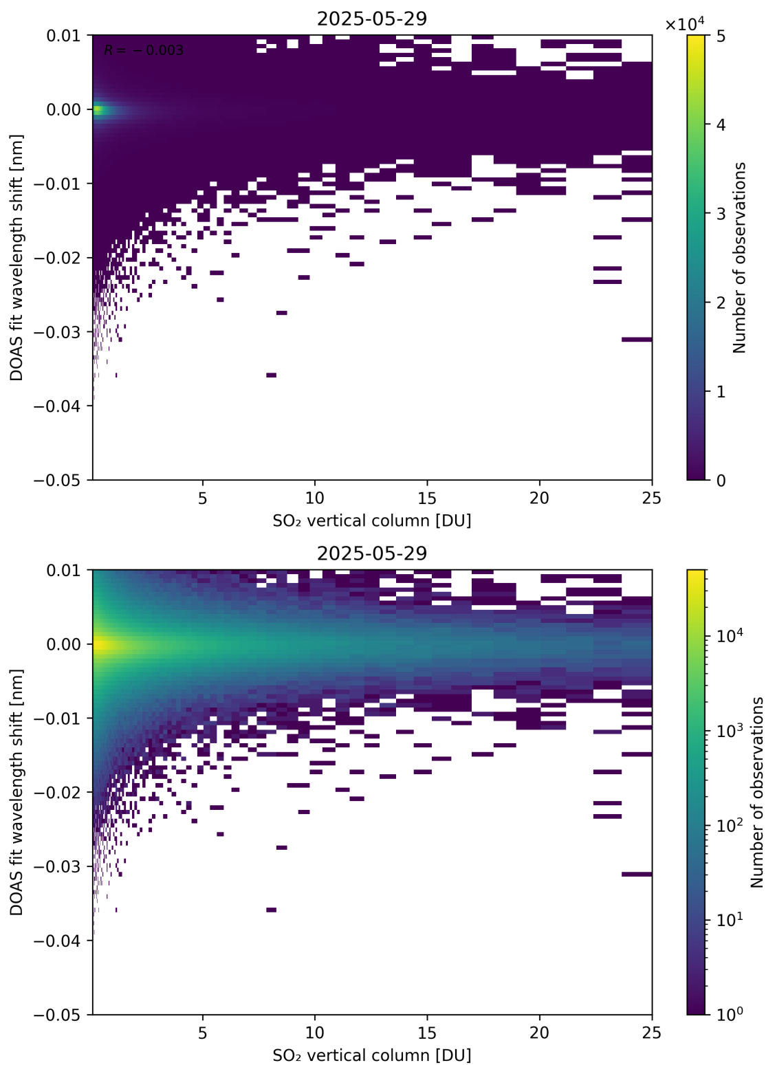
Figure 326: Scatter density plot of “SO 2 vertical column” against “DOAS fit wavelength shift” for 2025-05-28 to 2025-05-30.
