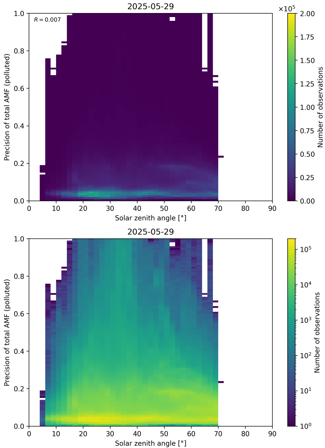
Figure 190: Scatter density plot of “Solar zenith angle” against “Precision of total AMF (polluted)” for 2025-05-28 to 2025-05-30.
