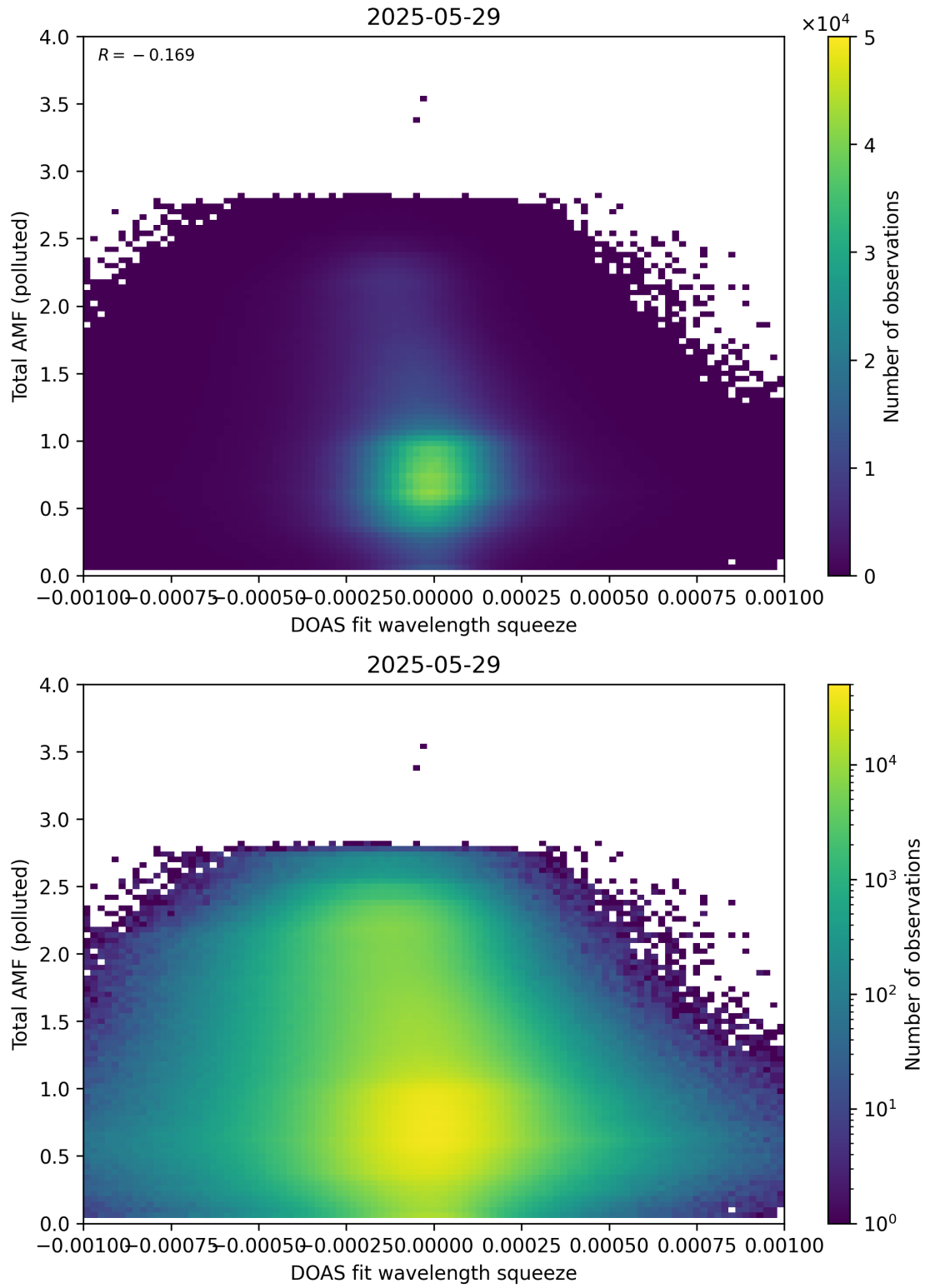
Figure 145: Scatter density plot of “DOAS fit wavelength squeeze” against “Total AMF (polluted)” for 2025-05-28 to 2025-05-30.
