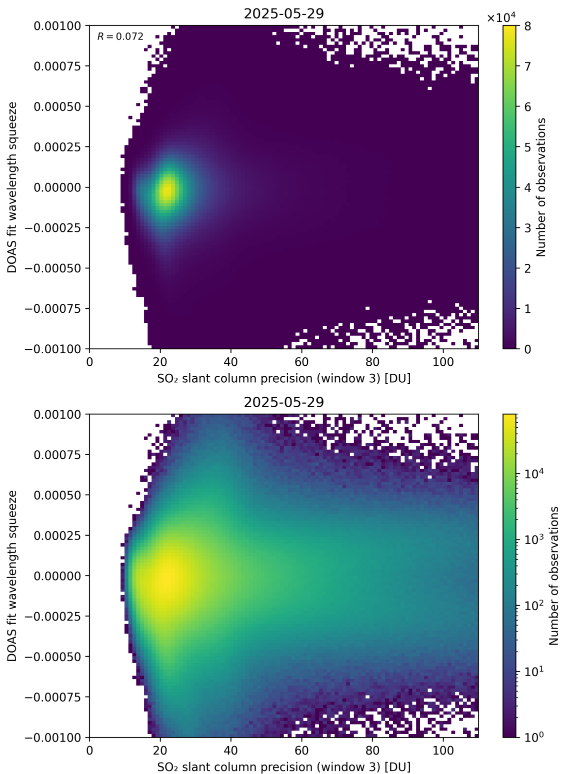
Figure 309: Scatter density plot of “SO 2 slant column precision (window 3)” against “DOAS fit wavelength squeeze” for 2025-05-28 to 2025-05-30.
