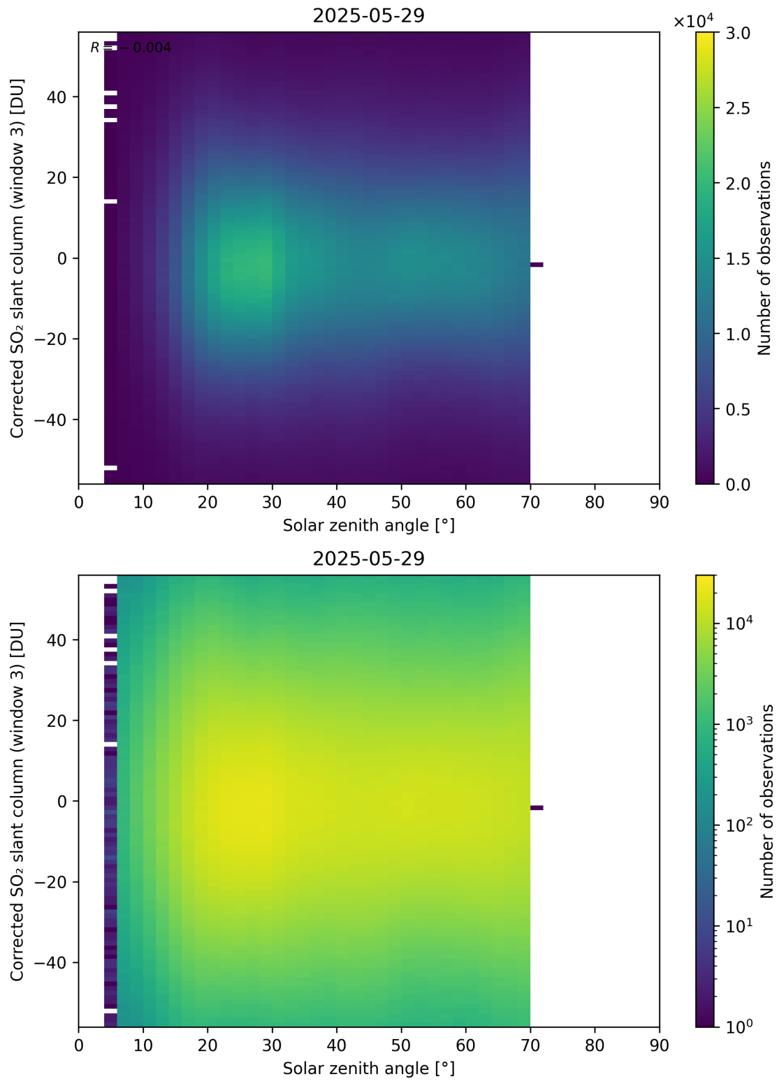
Figure 183: Scatter density plot of “Solar zenith angle” against “Corrected SO 2 slant column (window 3)” for 2025-05-28 to 2025-05-30.
