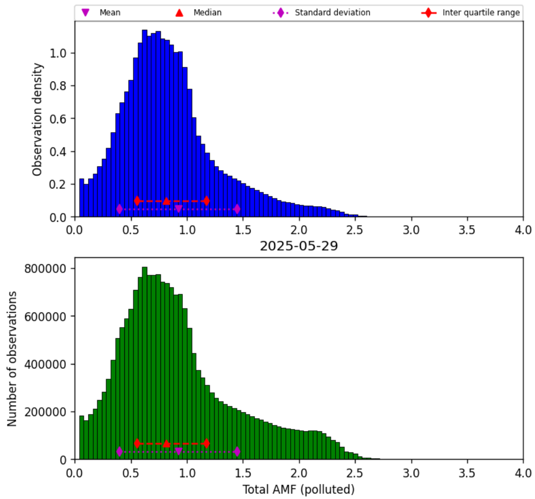
Figure 79: Histogram of “Total AMF (polluted)” for 2025-05-28 to 2025-05-30
