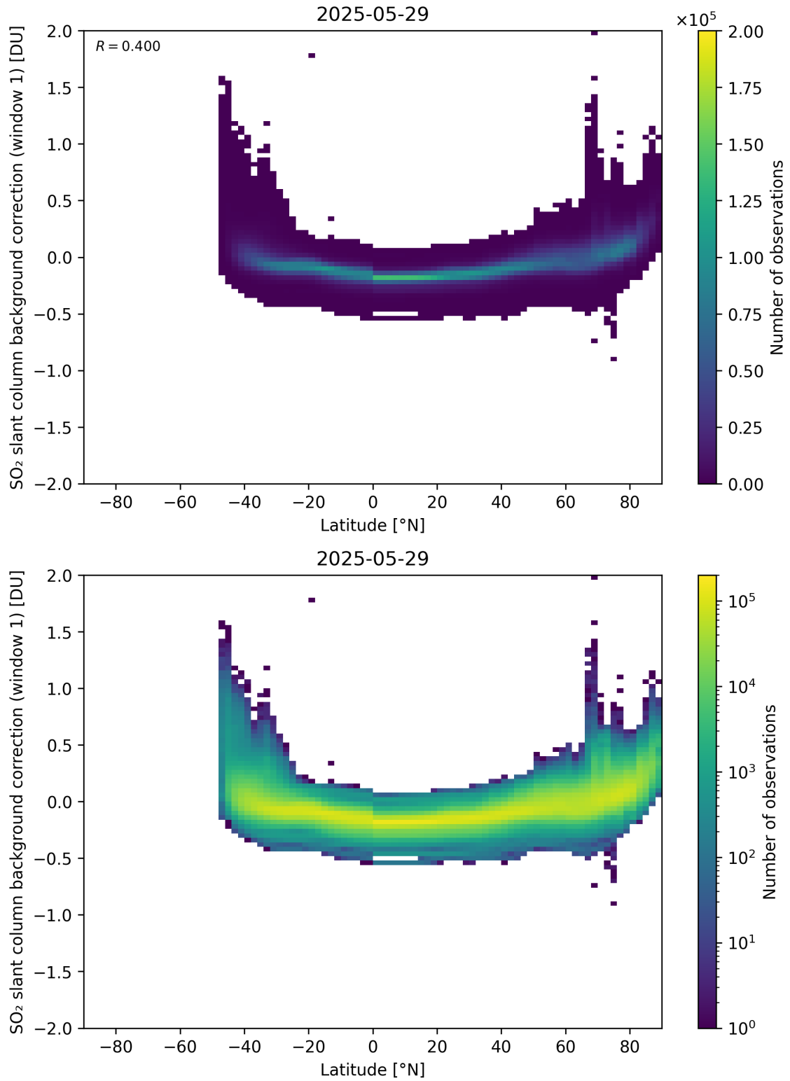
Figure 150: Scatter density plot of “Latitude” against “SO 2 slant column background correction (window 1)” for 2025-05-28 to 2025-05-30.
