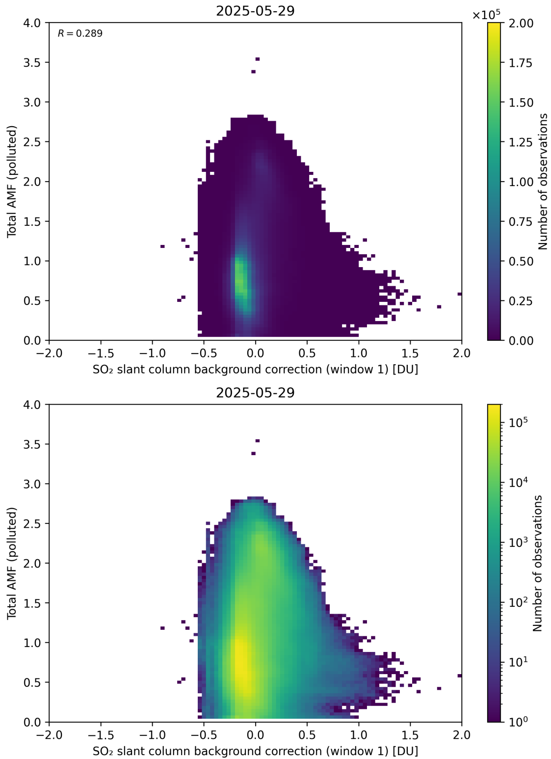
Figure 120: Scatter density plot of “SO 2 slant column background correction (window 1)” against “Total AMF (polluted)” for 2025-05-28 to 2025-05-30.
