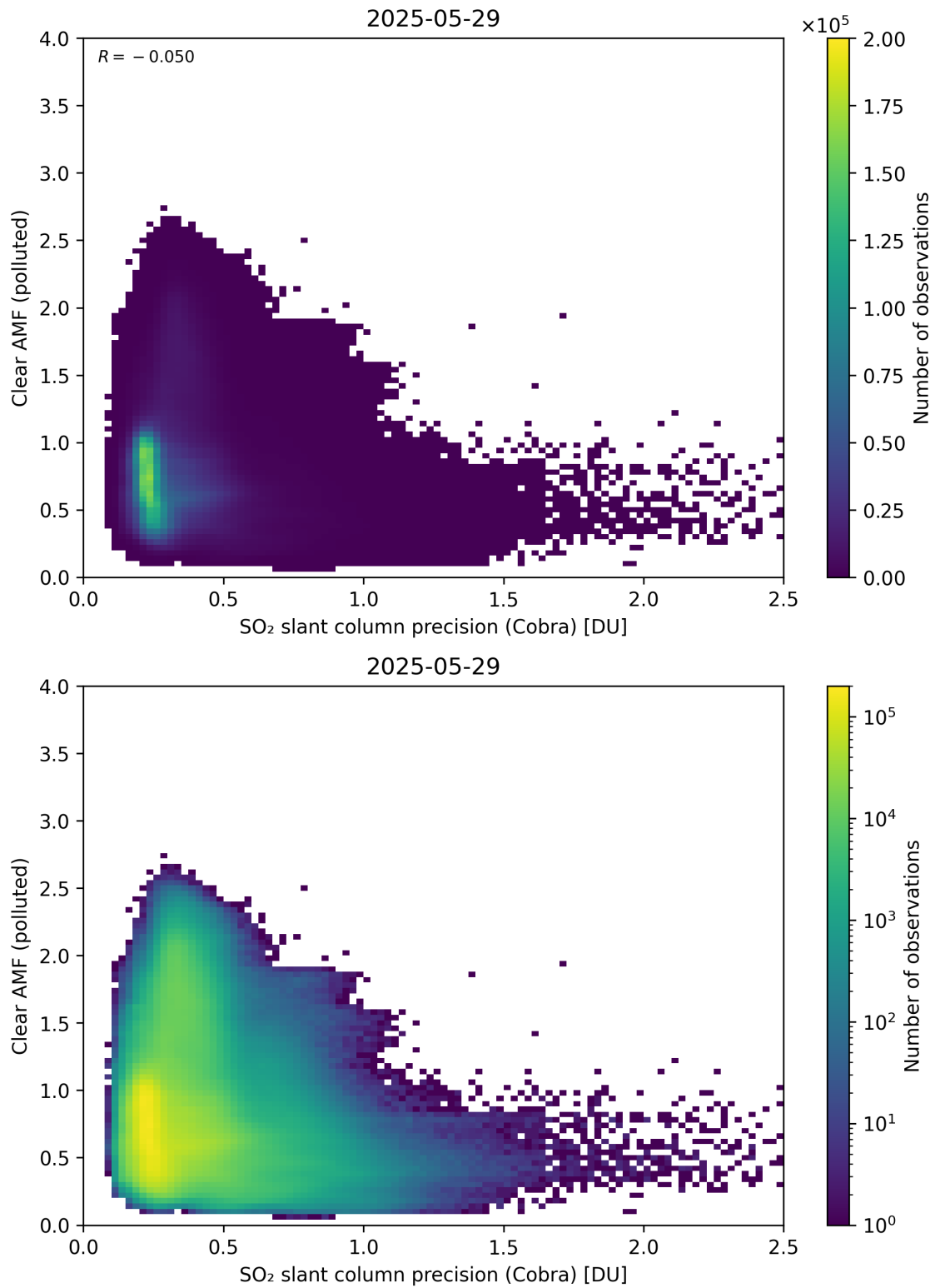
Figure 205: Scatter density plot of “SO 2 slant column precision (Cobra)” against “Clear AMF (polluted)” for 2025-05-28 to 2025-05-30.
