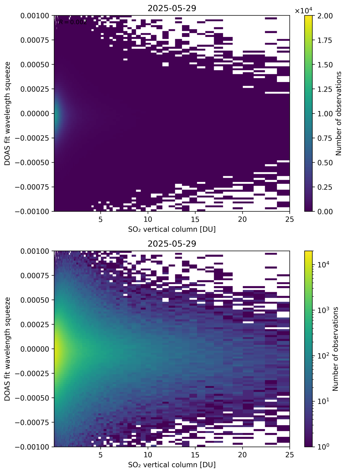
Figure 327: Scatter density plot of “SO 2 vertical column” against “DOAS fit wavelength squeeze” for 2025-05-28 to 2025-05-30.
