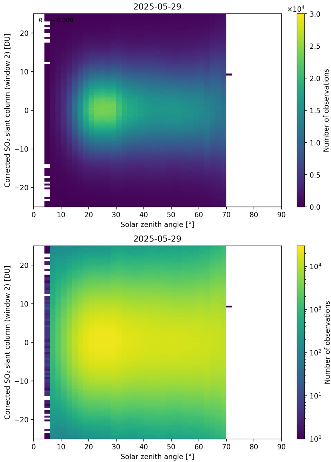
Figure 182: Scatter density plot of “Solar zenith angle” against “Corrected SO 2 slant column (window 2)” for 2025-05-28 to 2025-05-30.
