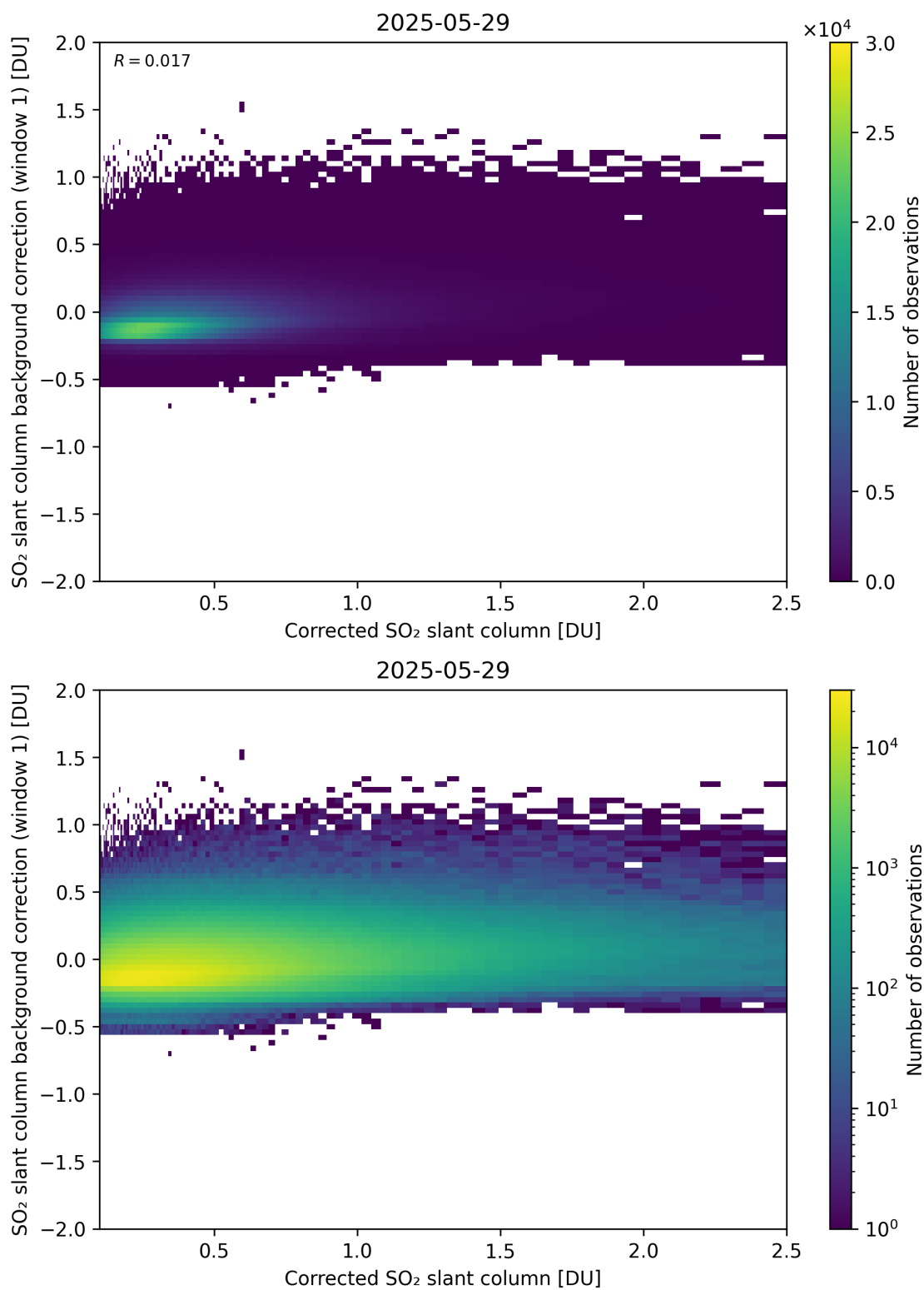
Figure 226: Scatter density plot of “Corrected SO 2 slant column” against “SO 2 slant column background correction (window 1)” for 2025-05-28 to 2025-05-30.
