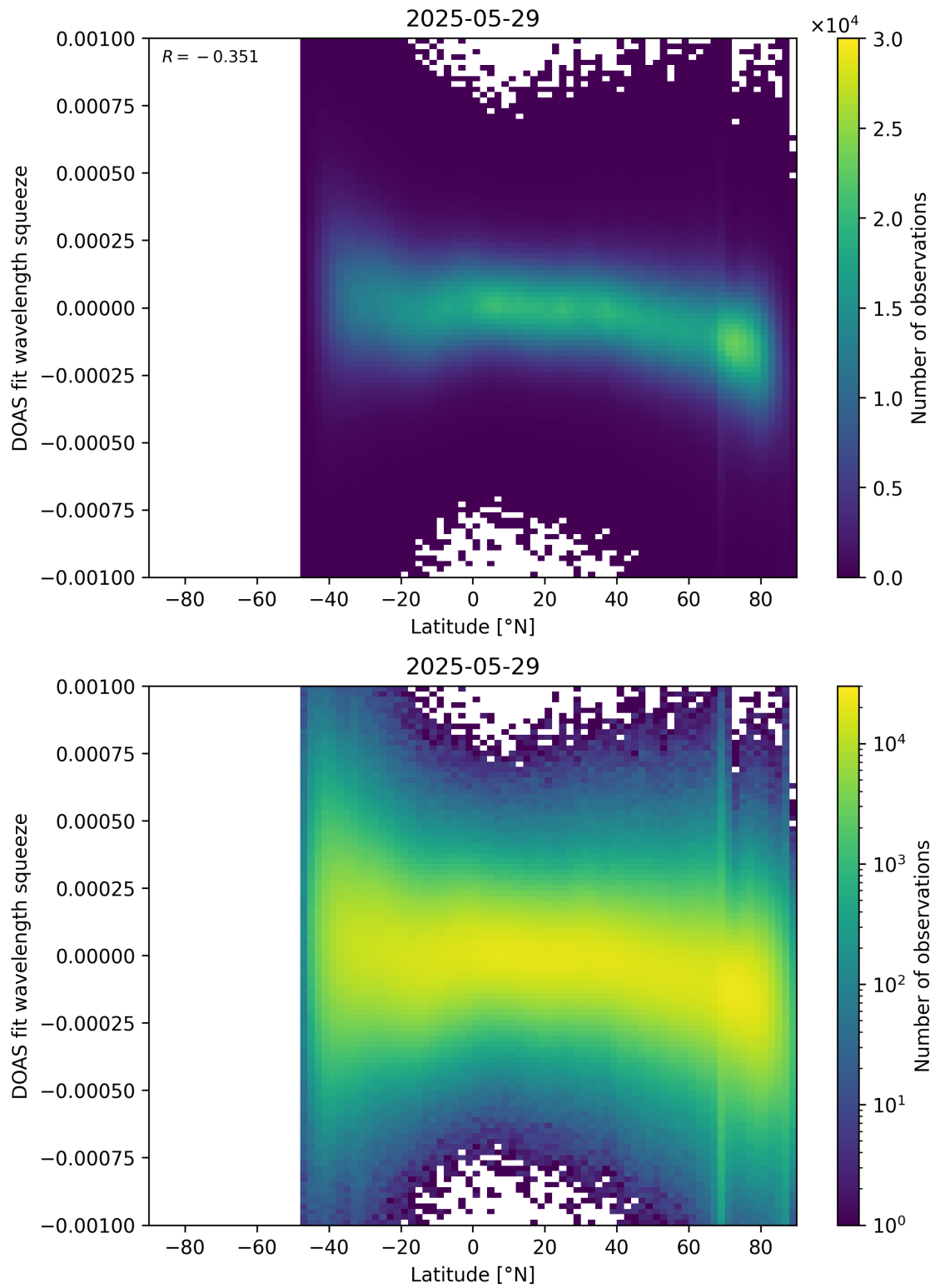
Figure 154: Scatter density plot of “Latitude” against “DOAS fit wavelength squeeze” for 2025-05-28 to 2025-05-30.
