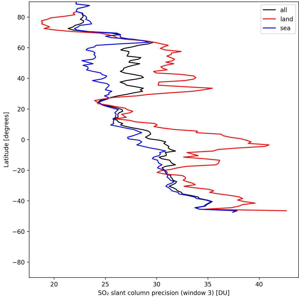
Figure 46: Zonal average of “SO 2 slant column precision (window 3)” for 2025-05-28 to 2025-05-30.
