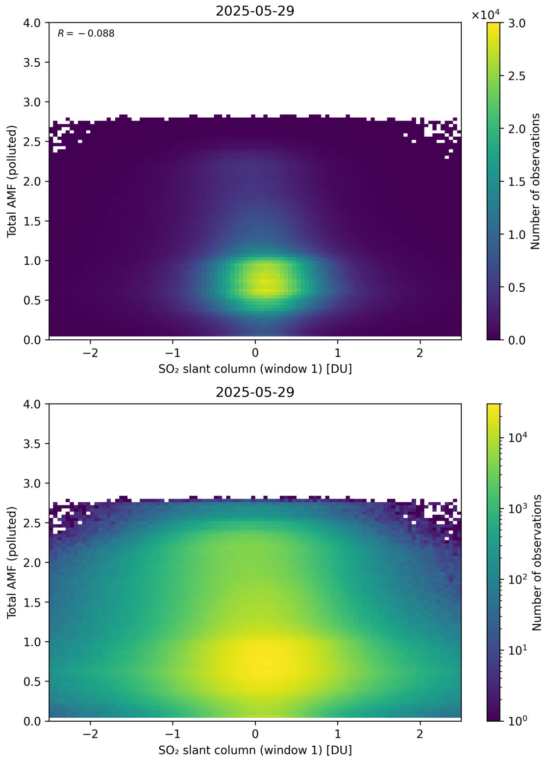
Figure 289: Scatter density plot of “SO 2 slant column (window 1)” against “Total AMF (polluted)” for 2025-05-28 to 2025-05-30.
