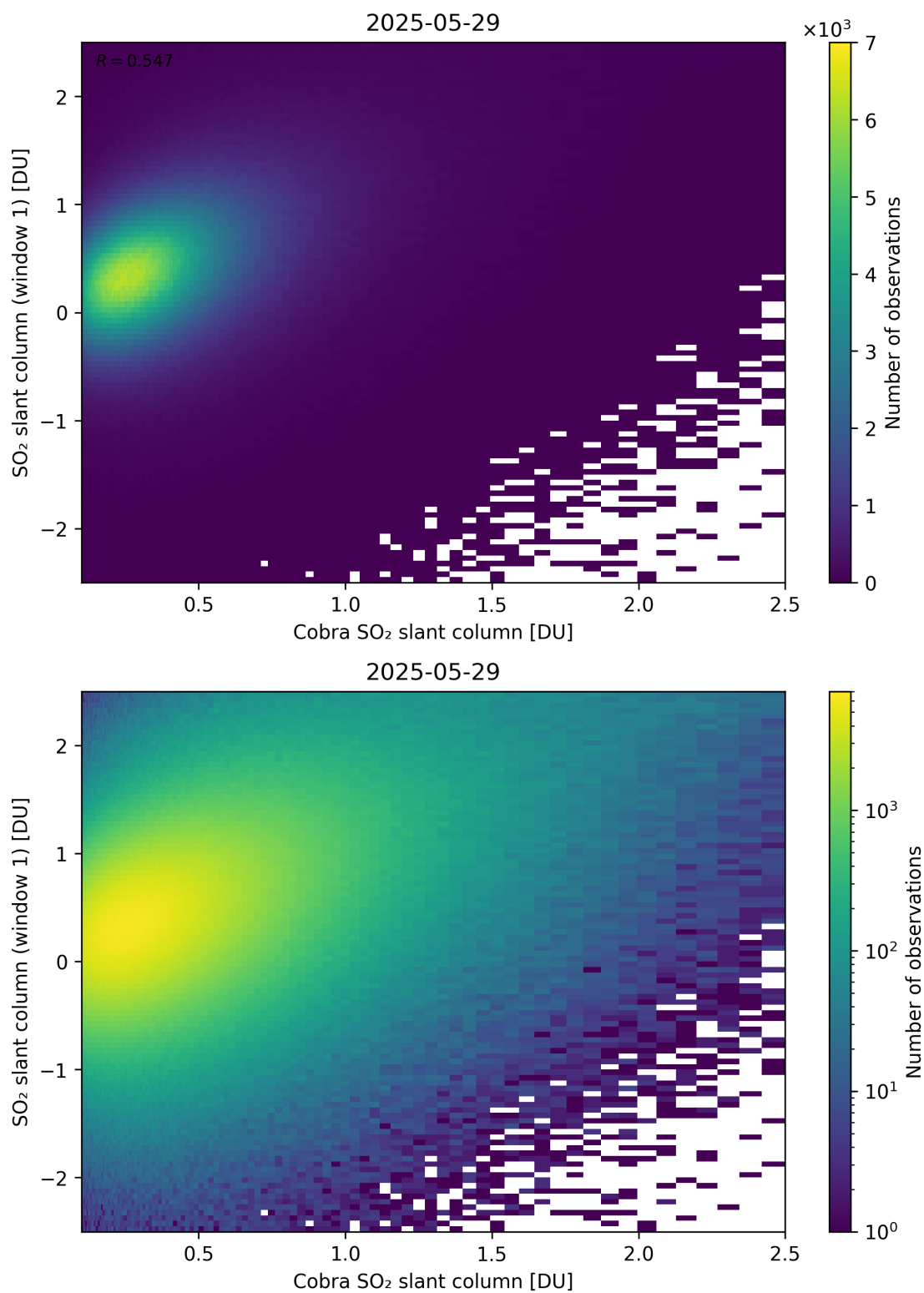
Figure 219: Scatter density plot of “Cobra SO 2 slant column” against “SO 2 slant column (window 1)” for 2025-05-28 to 2025-05-30.
