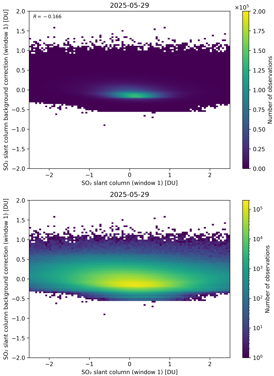
Figure 262: Scatter density plot of “SO 2 slant column (window 1)” against “SO 2 slant column background correction (window 1)” for 2025-05-28 to 2025-05-30.
