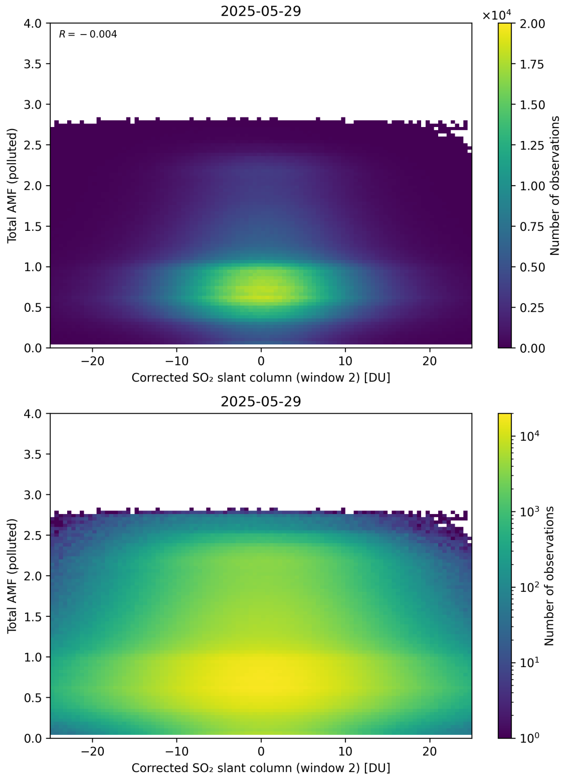
Figure 253: Scatter density plot of “Corrected SO 2 slant column (window 2)” against “Total AMF (polluted)” for 2025-05-28 to 2025-05-30.
