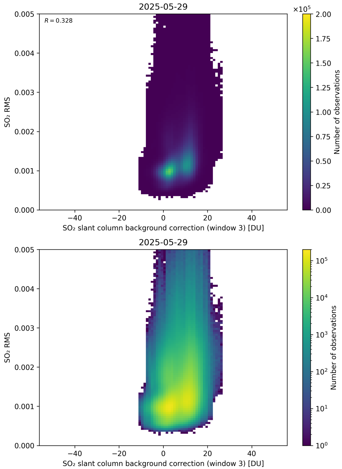
Figure 134: Scatter density plot of “SO 2 slant column background correction (window 3)” against “SO 2 RMS” for 2025-05-28 to 2025-05-30.
