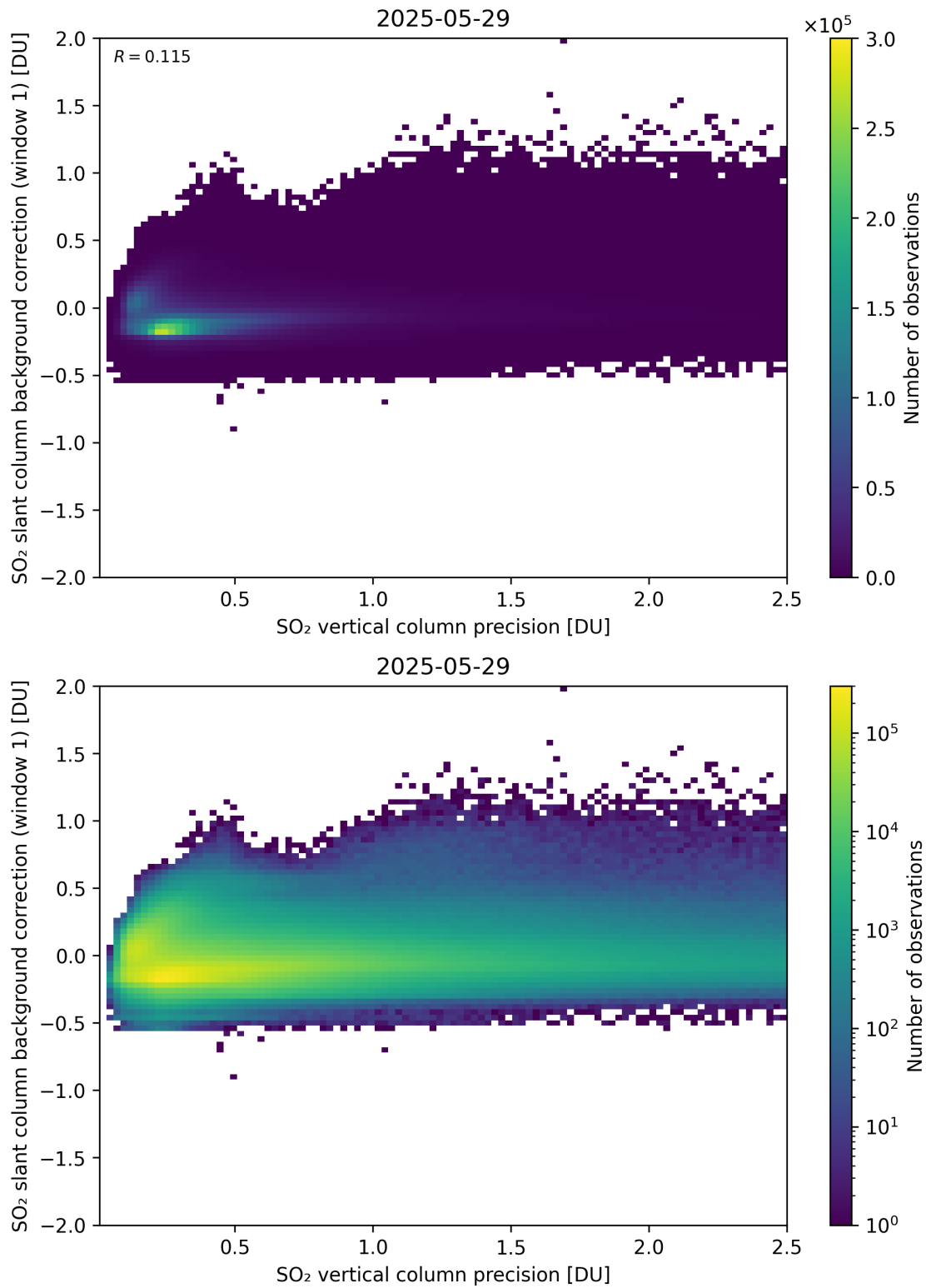
Figure 329: Scatter density plot of “SO 2 vertical column precision” against “SO 2 slant column background correction (window 1)” for 2025-05-28 to 2025-05-30.
