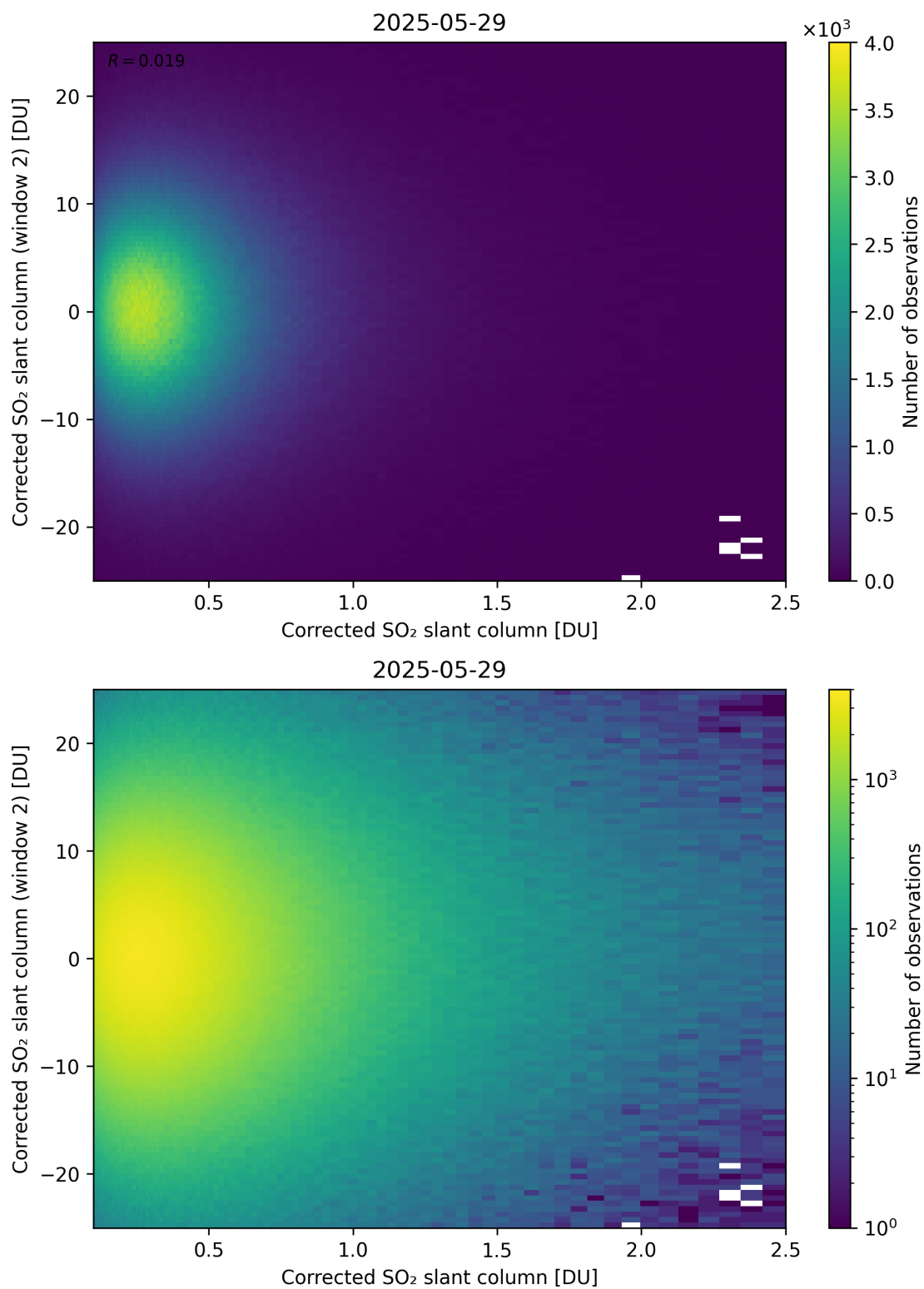
Figure 235: Scatter density plot of “Corrected SO 2 slant column” against “Corrected SO 2 slant column (window 2)” for 2025-05-28 to 2025-05-30.
