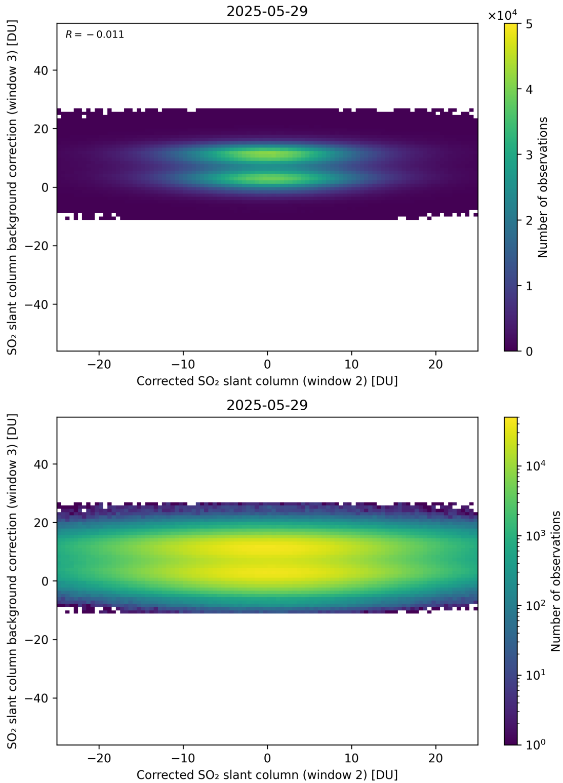
Figure 245: Scatter density plot of “Corrected SO 2 slant column (window 2)” against “SO 2 slant column background correction (window 3)” for 2025-05-28 to 2025-05-30.
