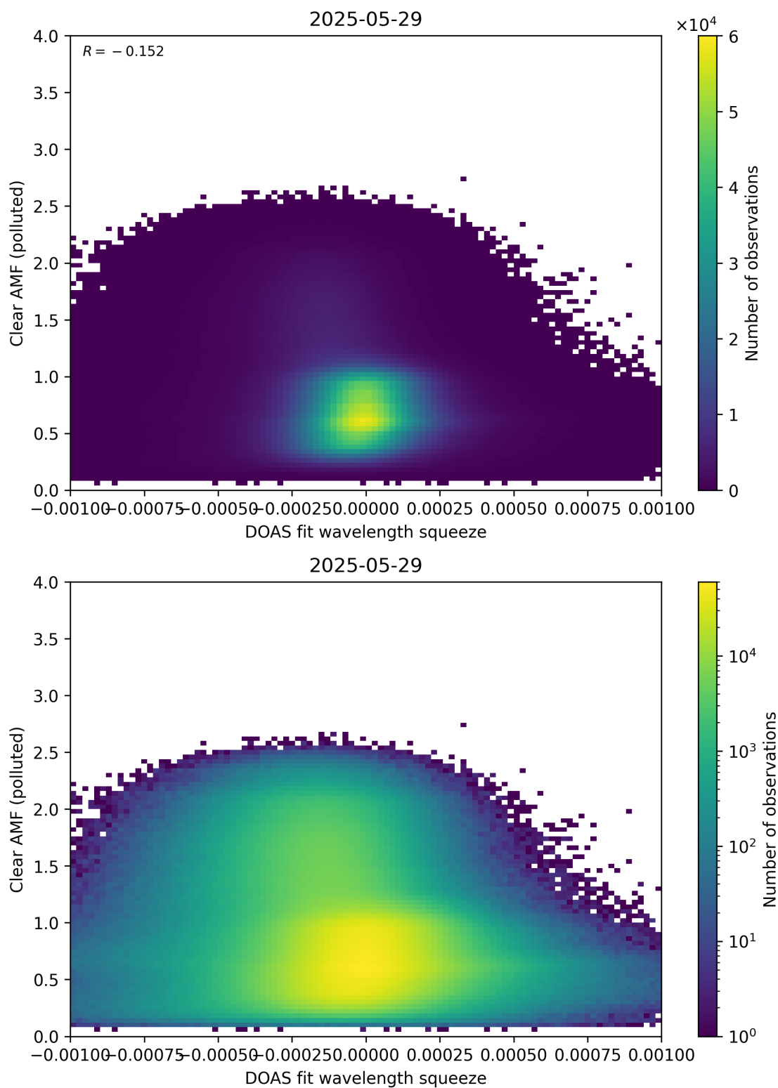
Figure 144: Scatter density plot of “DOAS fit wavelength squeeze” against “Clear AMF (polluted)” for 2025-05-28 to 2025-05-30.
