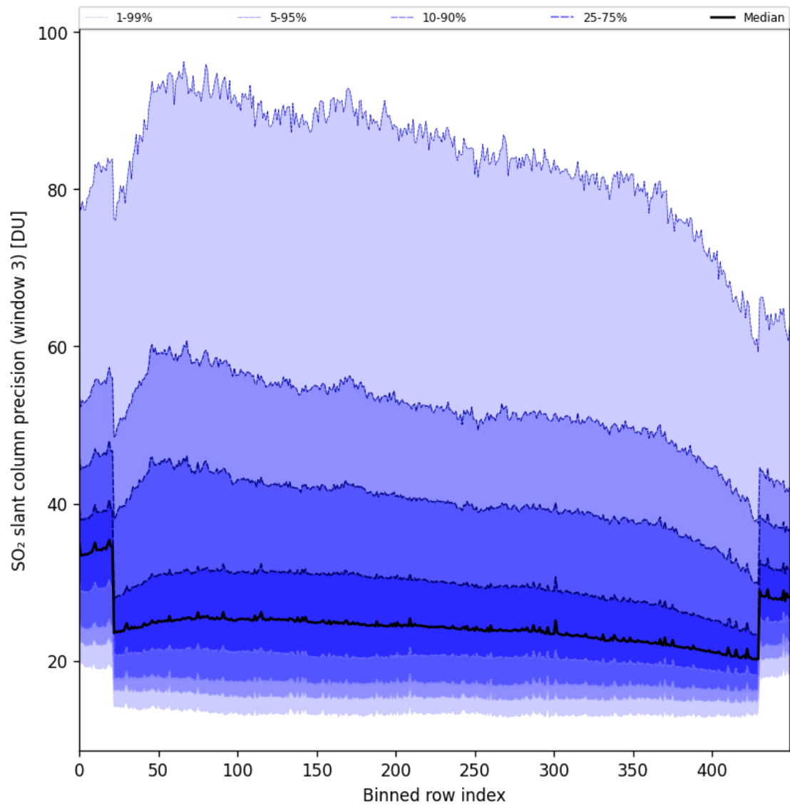
Figure 98: Along track statistics of “SO 2 slant column precision (window 3)” for 2025-05-28 to 2025-05-30
