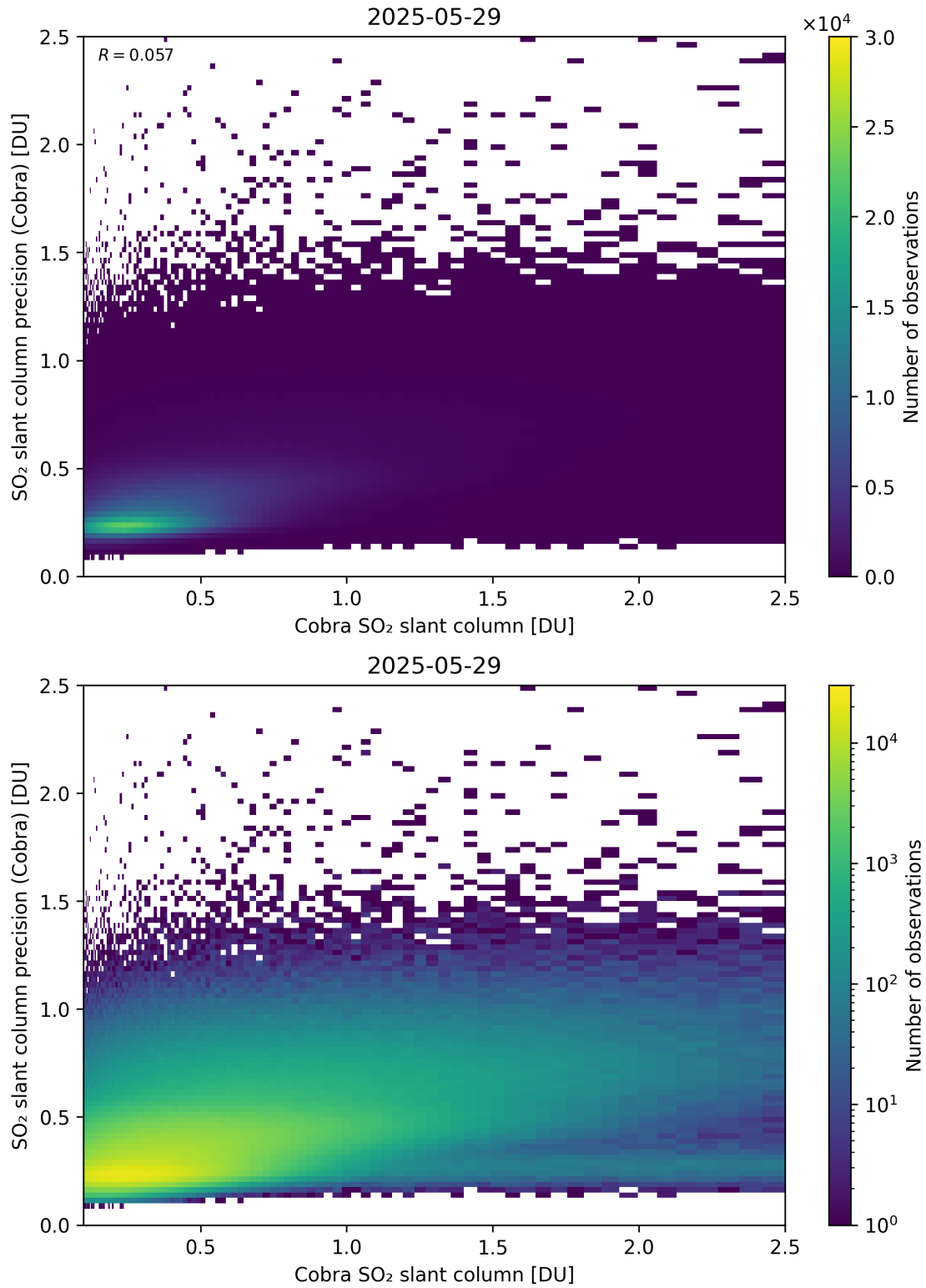
Figure 216: Scatter density plot of “Cobra SO 2 slant column” against “SO 2 slant column precision (Cobra)” for 2025-05-28 to 2025-05-30.
