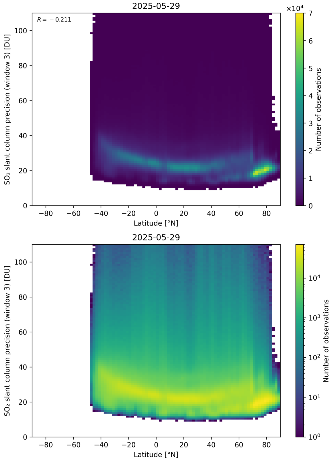
Figure 166: Scatter density plot of “Latitude” against “SO 2 slant column precision (window 3)” for 2025-05-28 to 2025-05-30.
