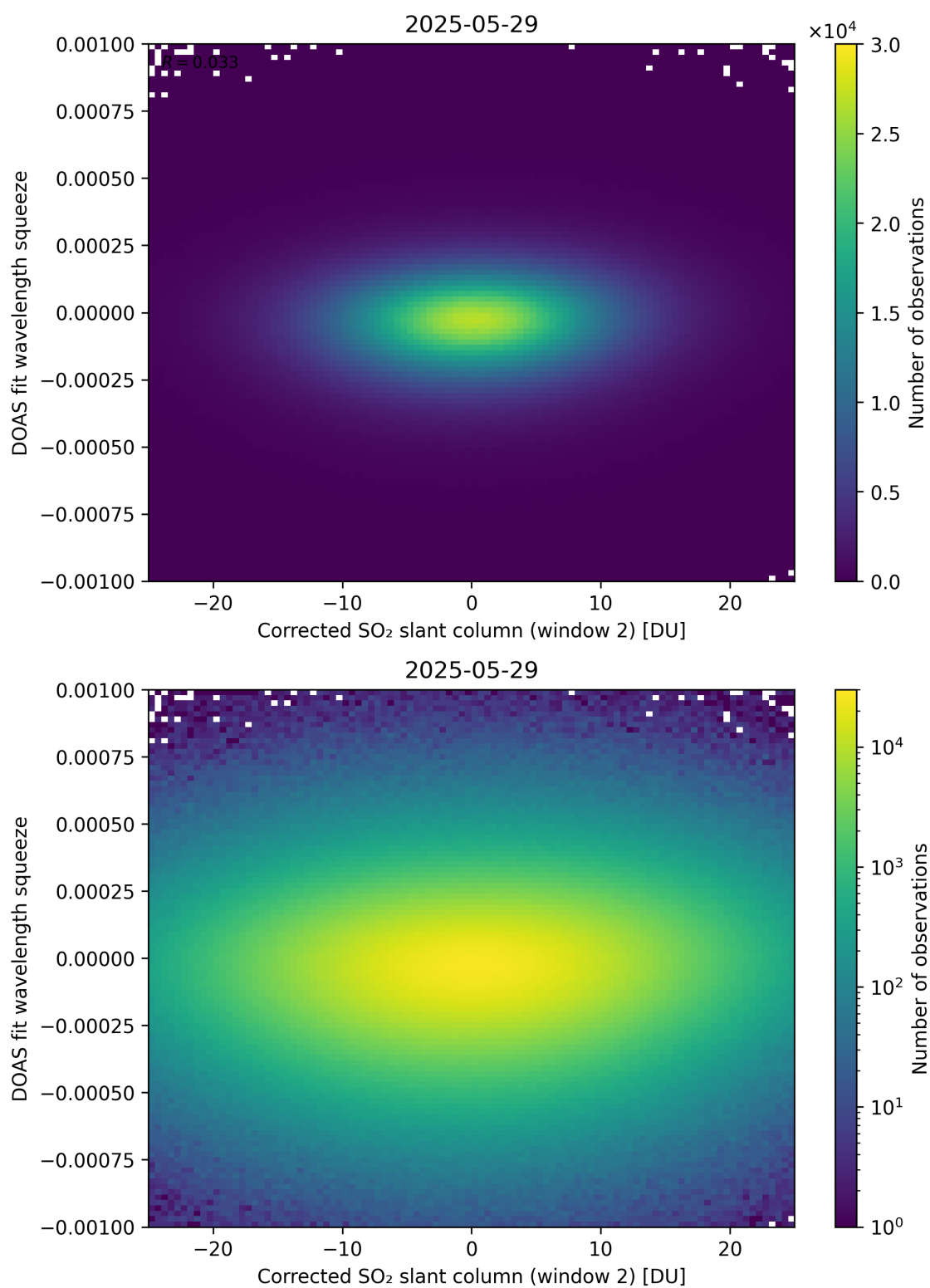
Figure 247: Scatter density plot of “Corrected SO 2 slant column (window 2)” against “DOAS fit wavelength squeeze” for 2025-05-28 to 2025-05-30.
