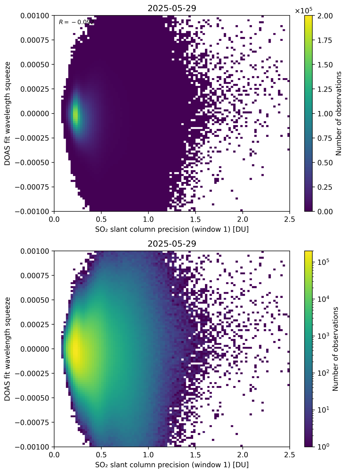
Figure 272: Scatter density plot of “SO 2 slant column precision (window 1)” against “DOAS fit wavelength squeeze” for 2025-05-28 to 2025-05-30.
