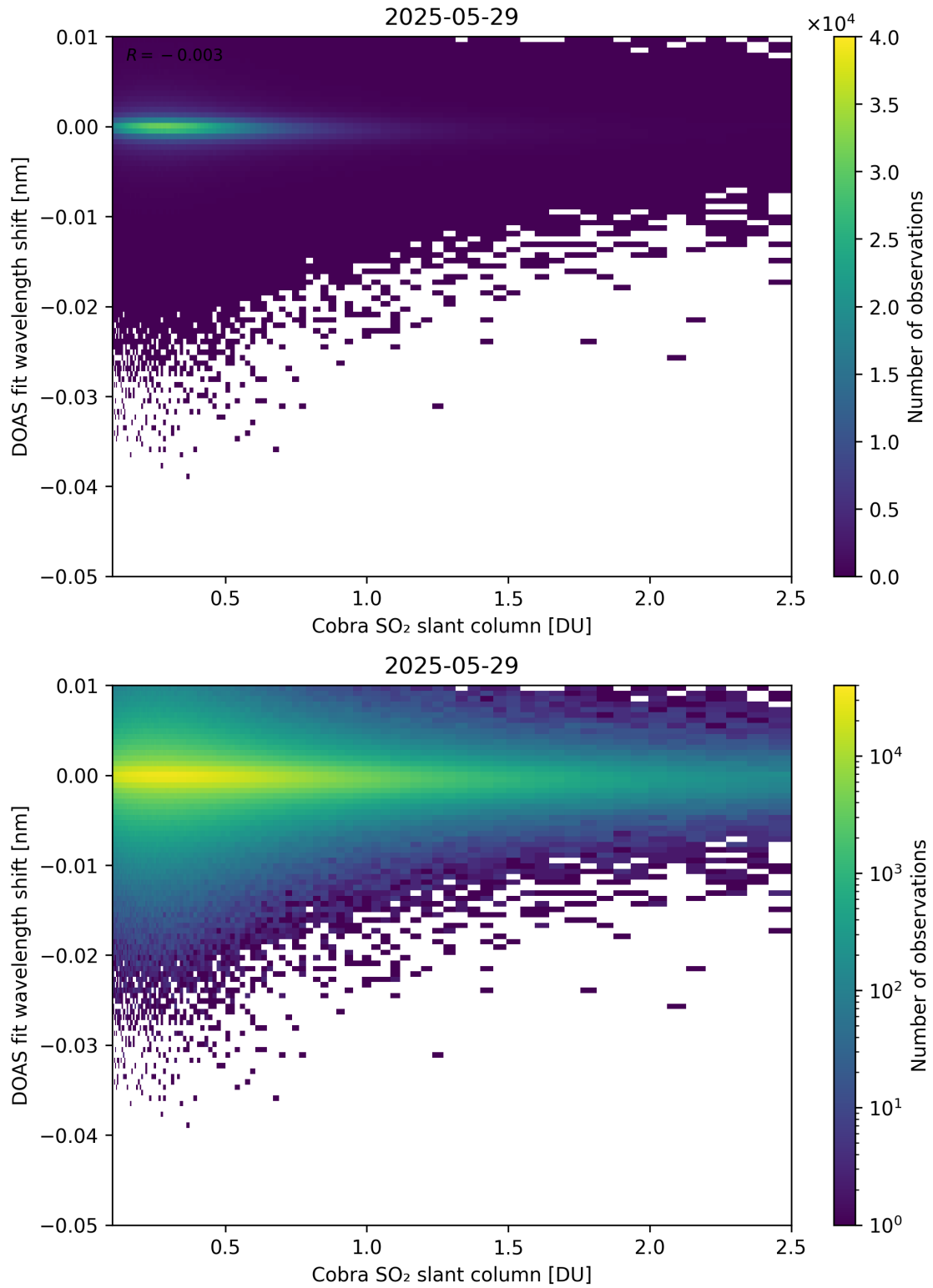
Figure 196: Scatter density plot of “Cobra SO 2 slant column” against “DOAS fit wavelength shift” for 2025-05-28 to 2025-05-30.
