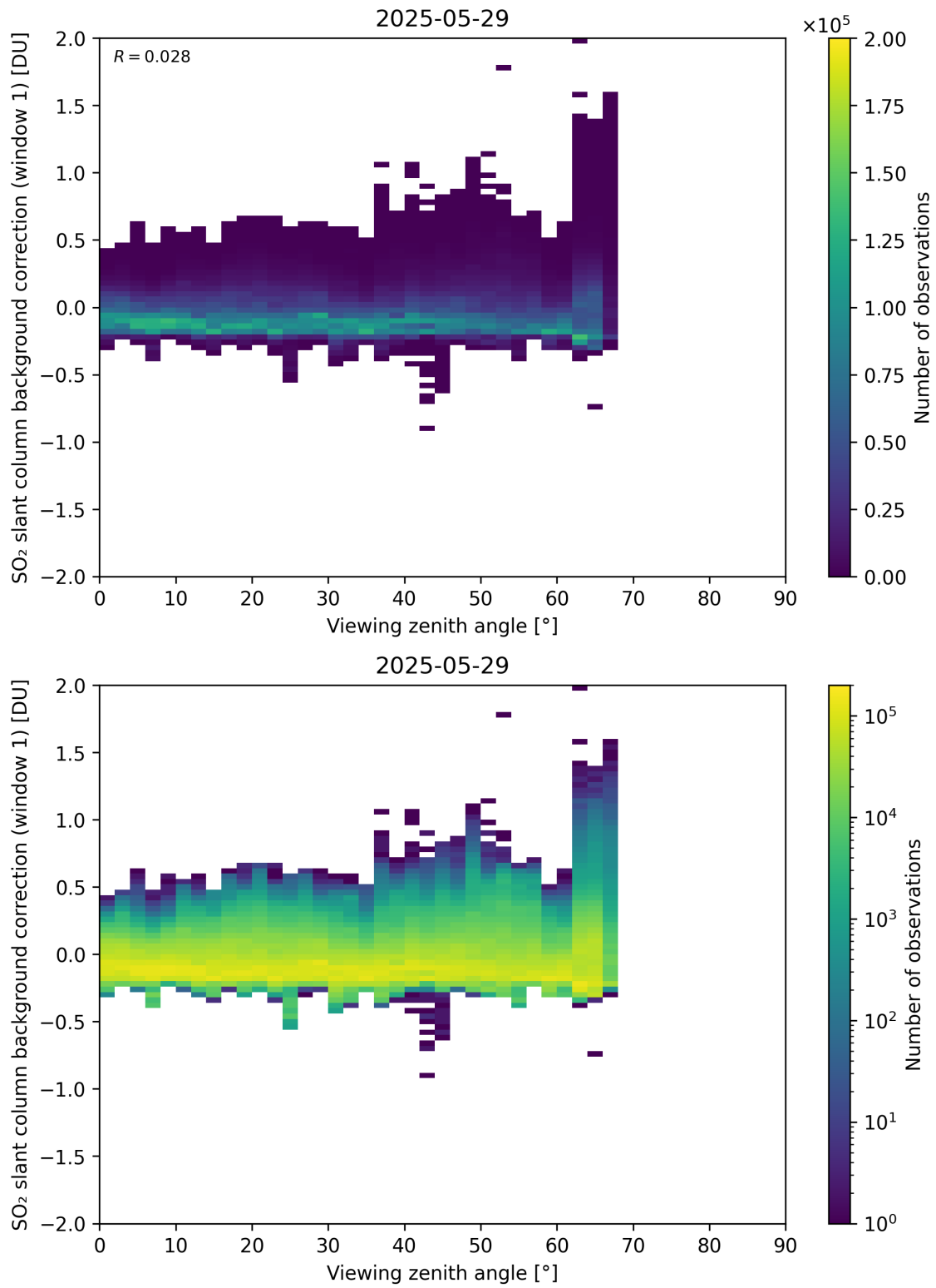
Figure 362: Scatter density plot of “Viewing zenith angle” against “SO 2 slant column background correction (window 1)” for 2025-05-28 to 2025-05-30.
