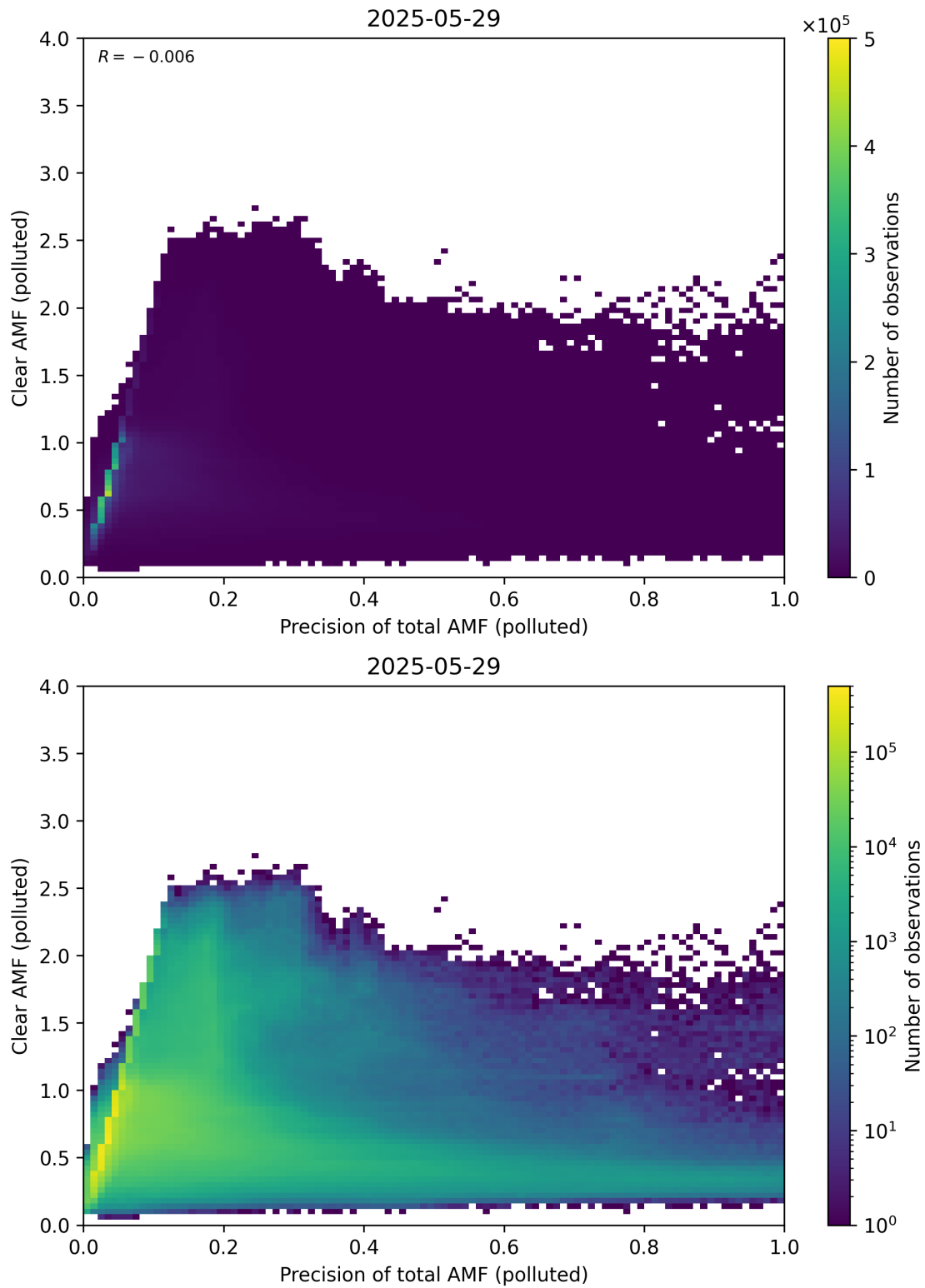
Figure 320: Scatter density plot of “Precision of total AMF (polluted)” against “Clear AMF (polluted)” for 2025-05-28 to 2025-05-30.
