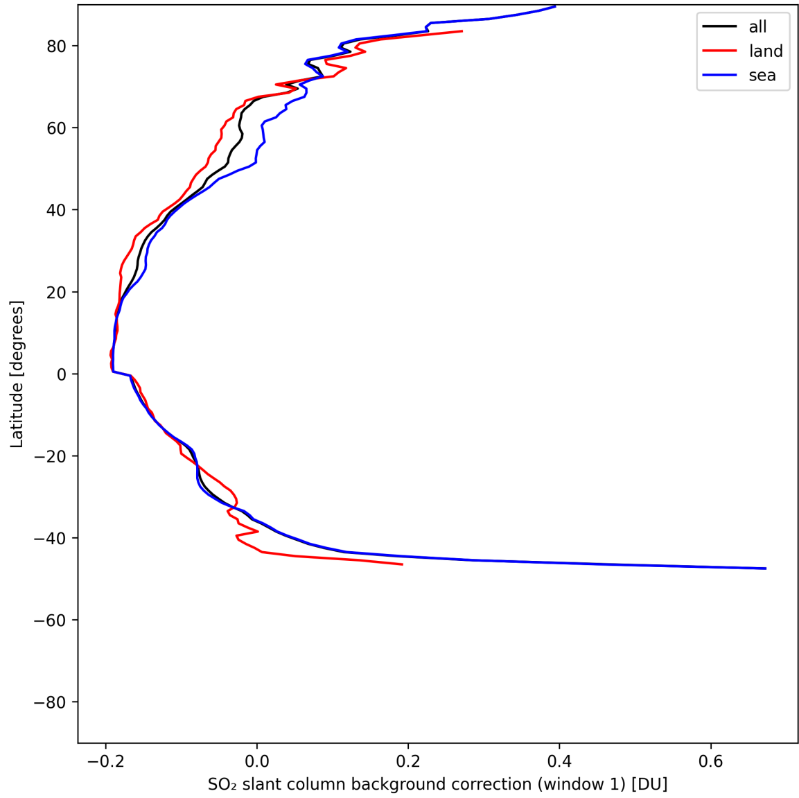
Figure 40: Zonal average of "SO 2 slant column background correction (window 1)" for 2025-05-28 to 2025-05-30.
