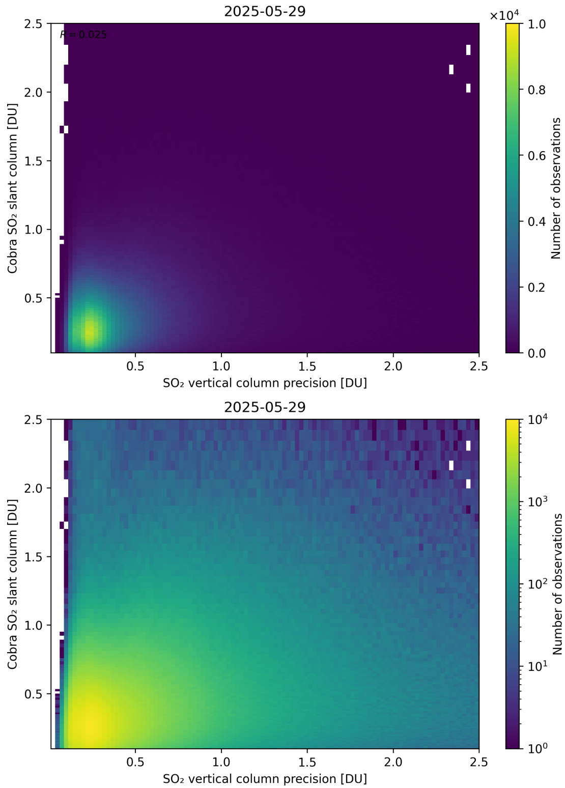
Figure 336: Scatter density plot of “SO 2 vertical column precision” against “Cobra SO 2 slant column” for 2025-05-28 to 2025-05-30.
