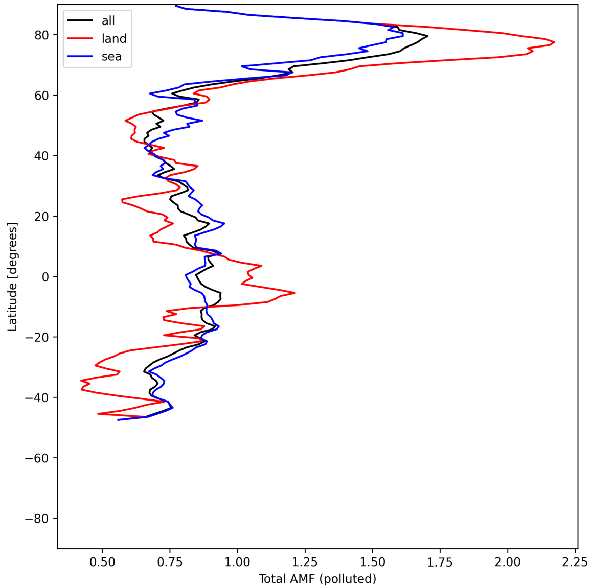
Figure 53: Zonal average of “Total AMF (polluted)” for 2025-05-28 to 2025-05-30.
