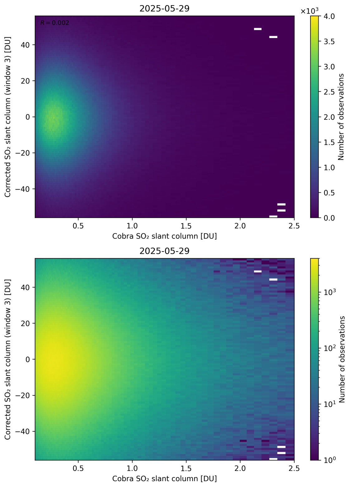
Figure 218: Scatter density plot of “Cobra SO 2 slant column” against “Corrected SO 2 slant column (window 3)” for 2025-05-28 to 2025-05-30.
