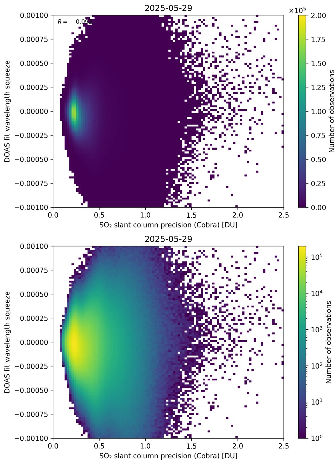
Figure 203: Scatter density plot of “SO 2 slant column precision (Cobra)” against “DOAS fit wavelength squeeze” for 2025-05-28 to 2025-05-30.
