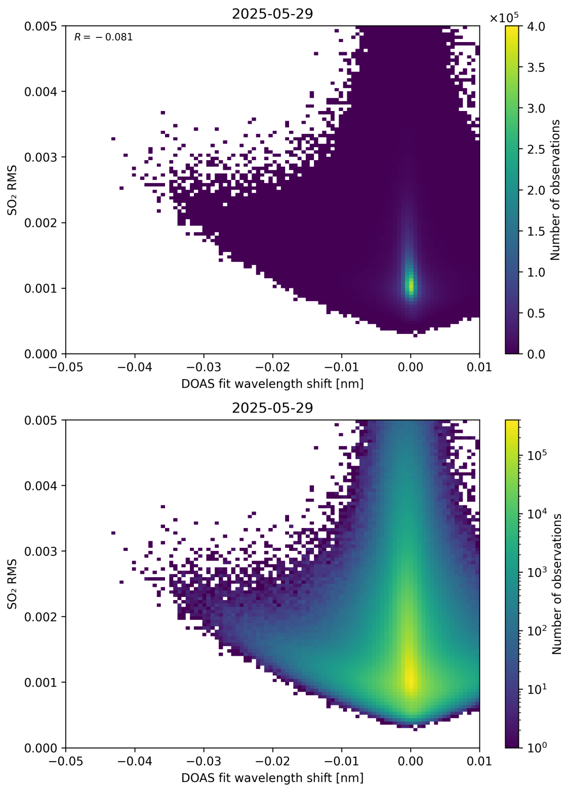
Figure 139: Scatter density plot of “DOAS fit wavelength shift” against “SO 2 RMS” for 2025-05-28 to 2025-05-30.
