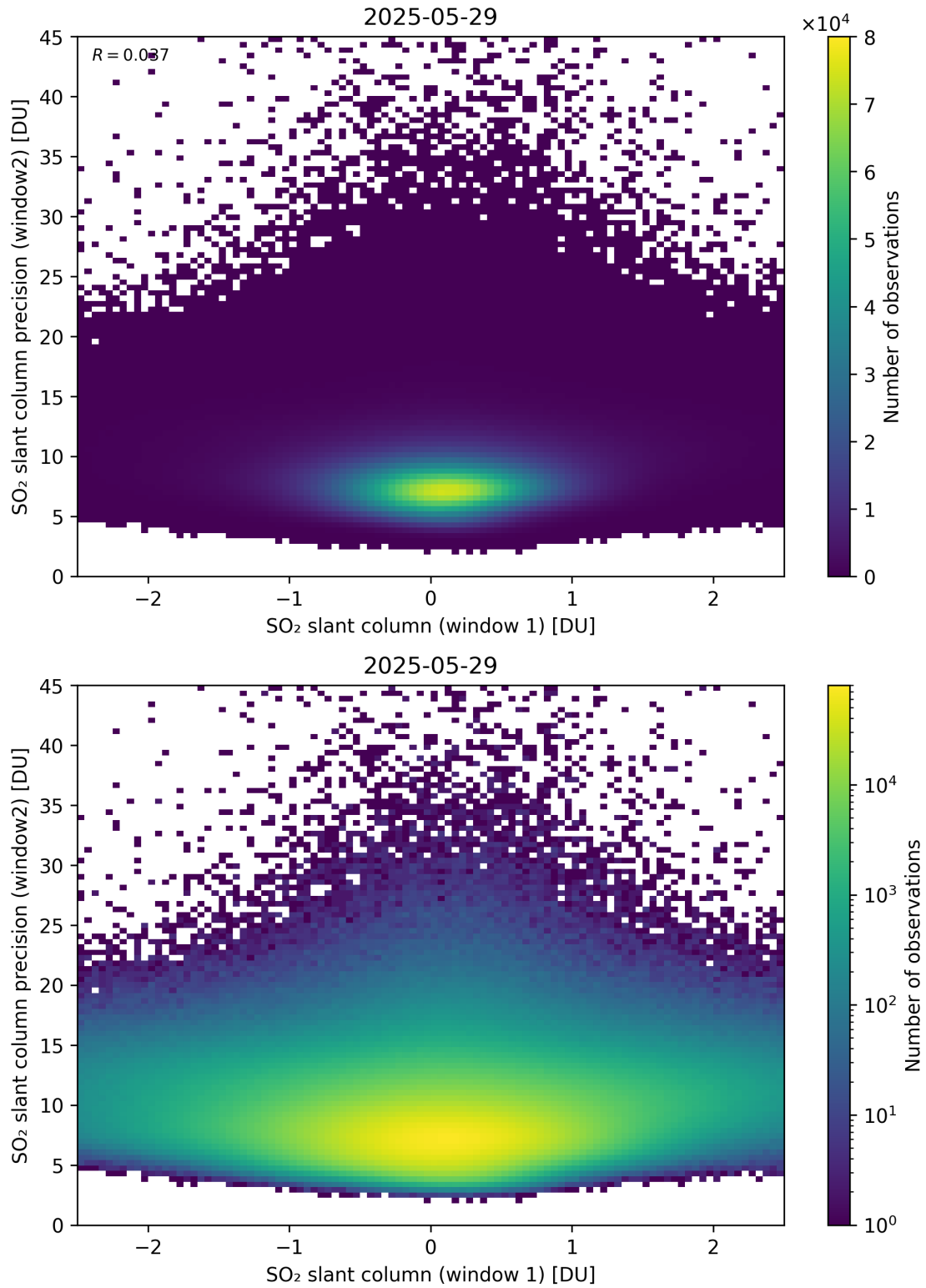
Figure 286: Scatter density plot of “SO 2 slant column (window 1)” against “SO 2 slant column precision (window2)” for 2025-05-28 to 2025-05-30.
