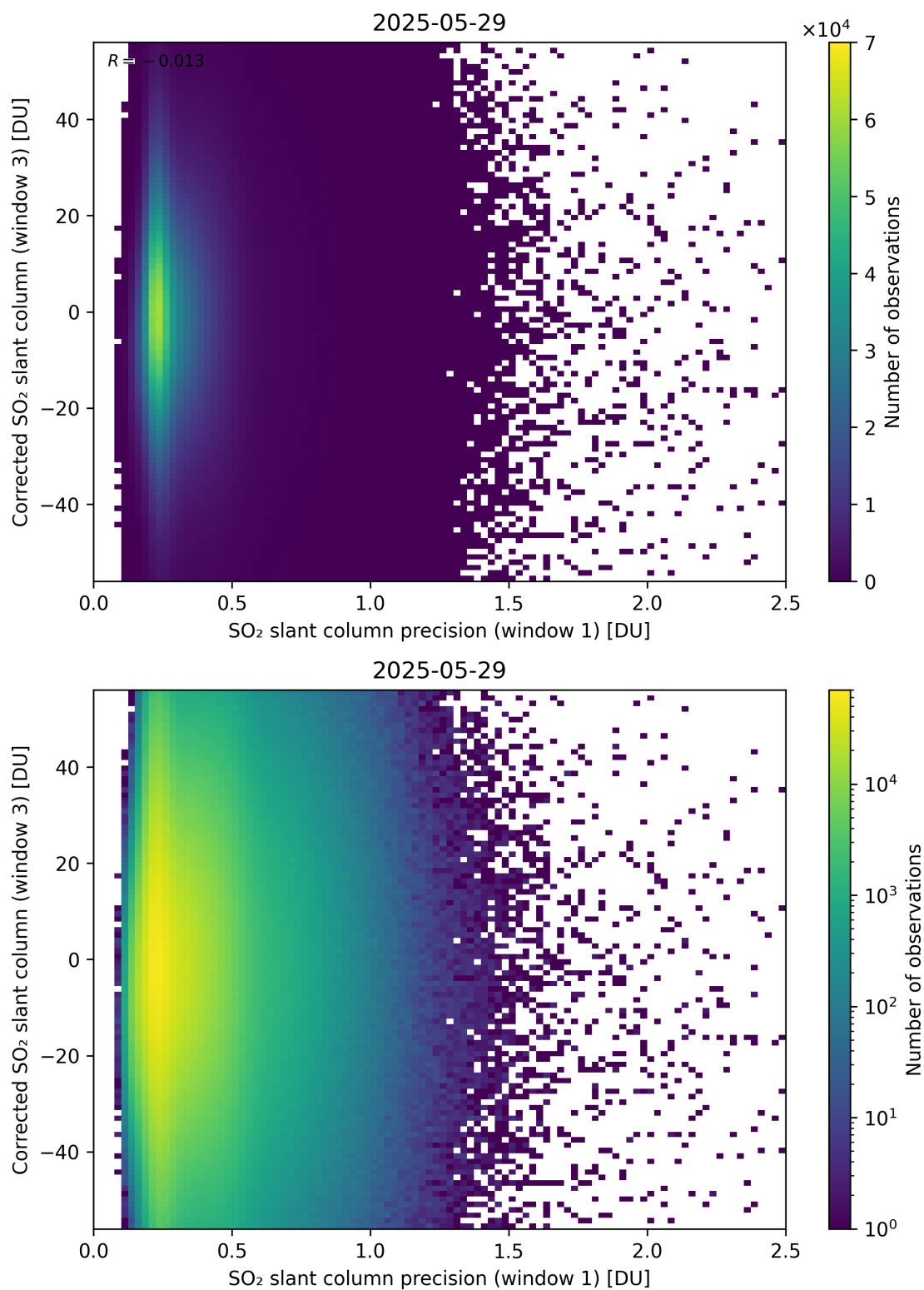
Figure 276: Scatter density plot of “SO 2 slant column precision (window 1)” against “Corrected SO 2 slant column (window 3)” for 2025-05-28 to 2025-05-30.
