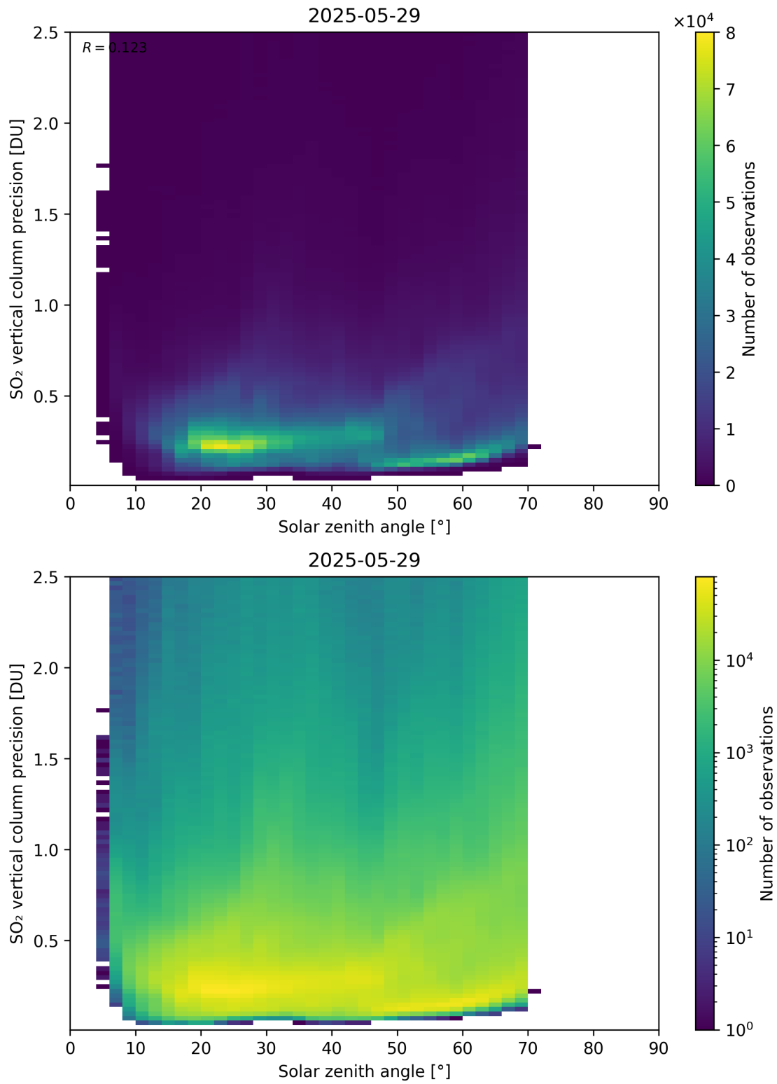
Figure 192: Scatter density plot of “Solar zenith angle” against “SO 2 vertical column precision” for 2025-05-28 to 2025-05-30.
