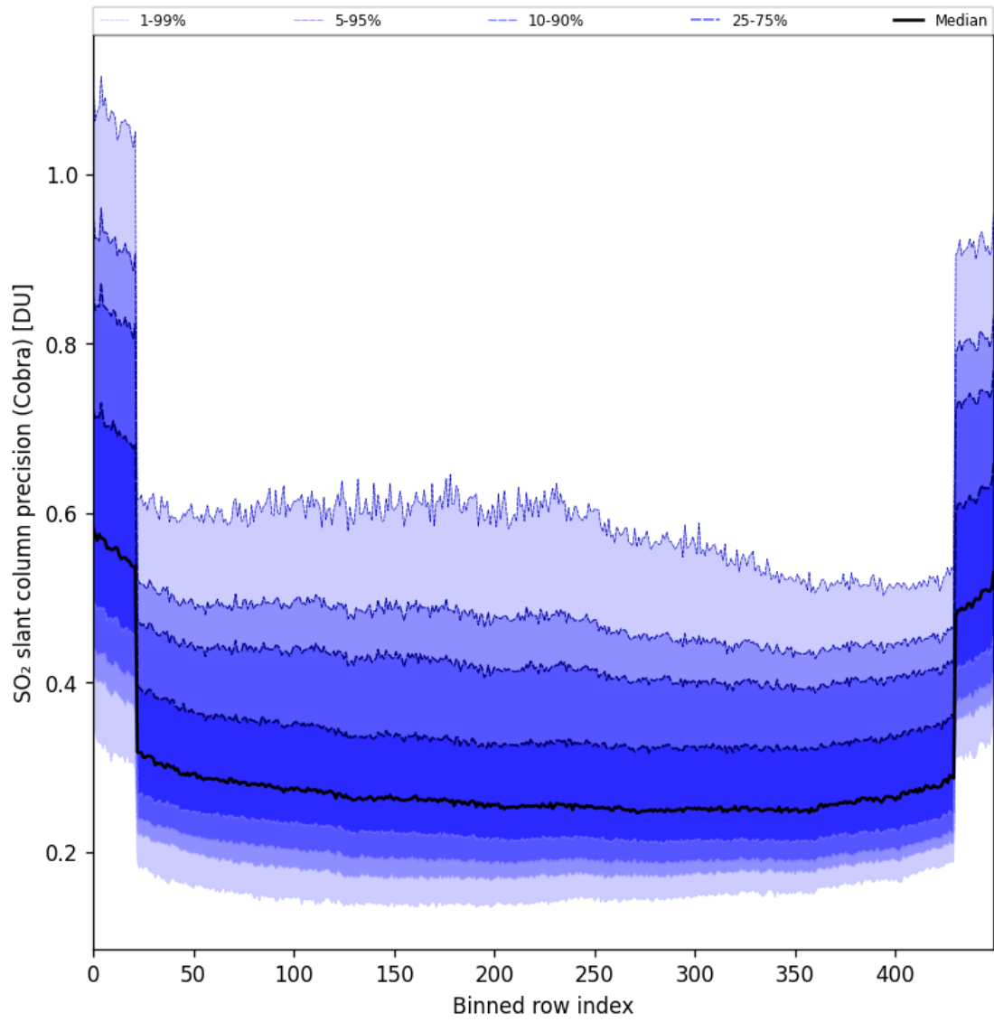
Figure 88: Along track statistics of “SO 2 slant column precision (Cobra)” for 2025-05-28 to 2025-05-30
