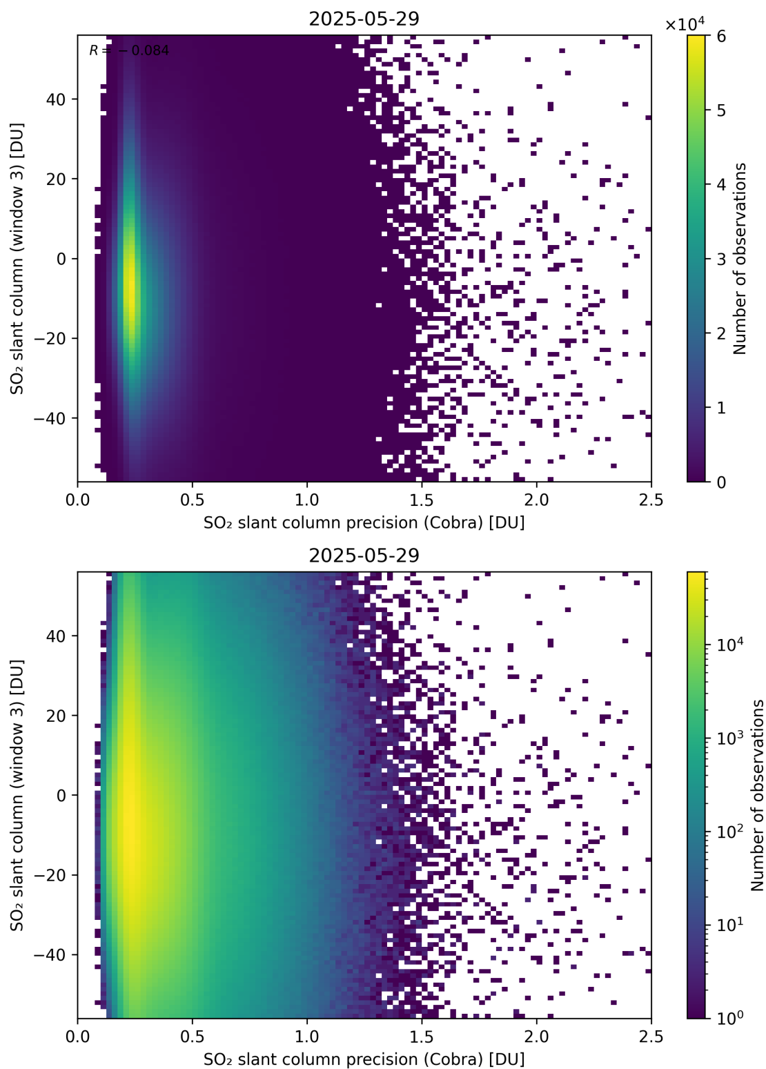
Figure 211: Scatter density plot of “SO 2 slant column precision (Cobra)” against “SO 2 slant column (window 3)” for 2025-05-28 to 2025-05-30.
