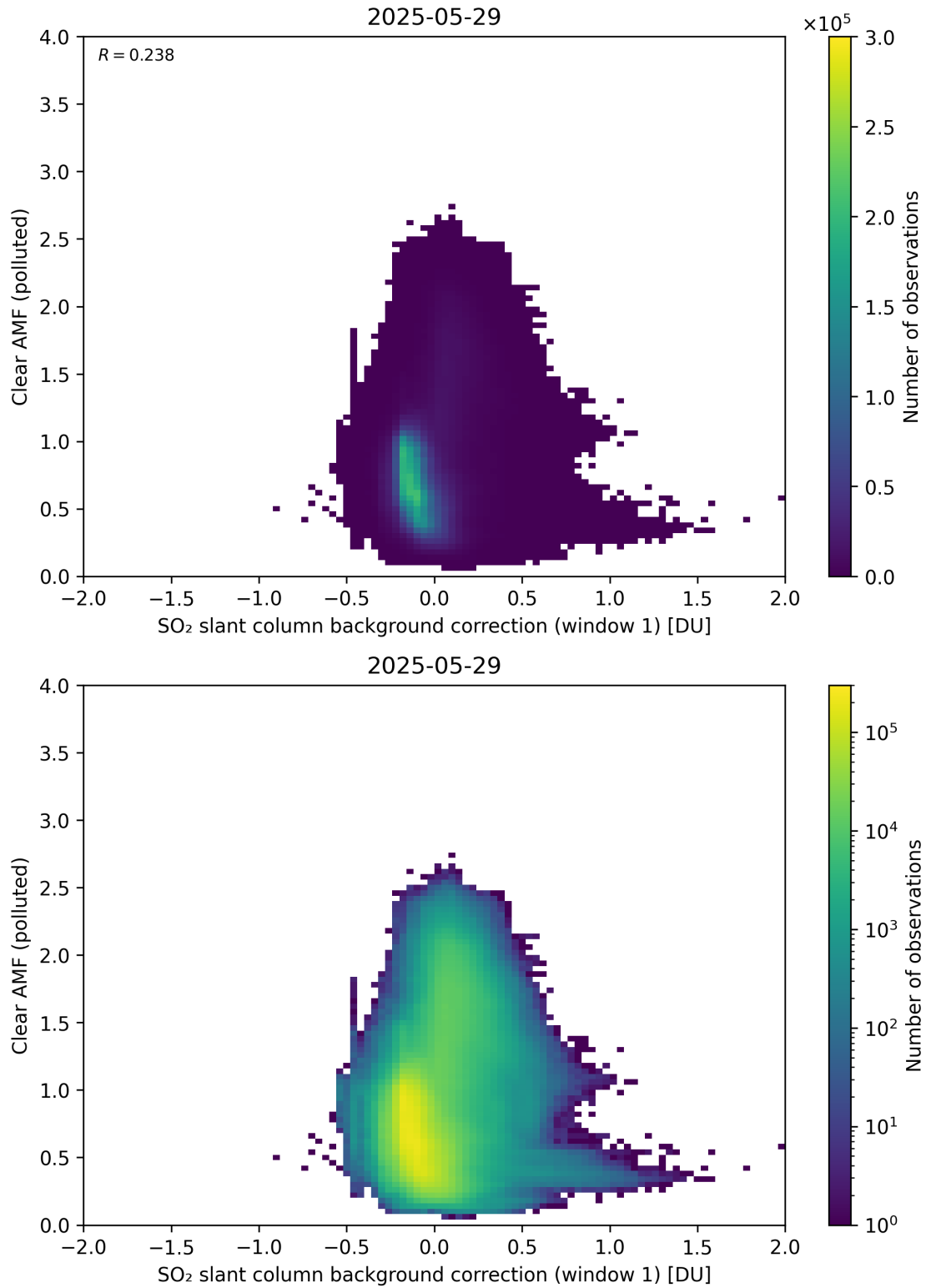
Figure 114: Scatter density plot of “SO 2 slant column background correction (window 1)” against “Clear AMF (polluted)” for 2025-05-28 to 2025-05-30.
