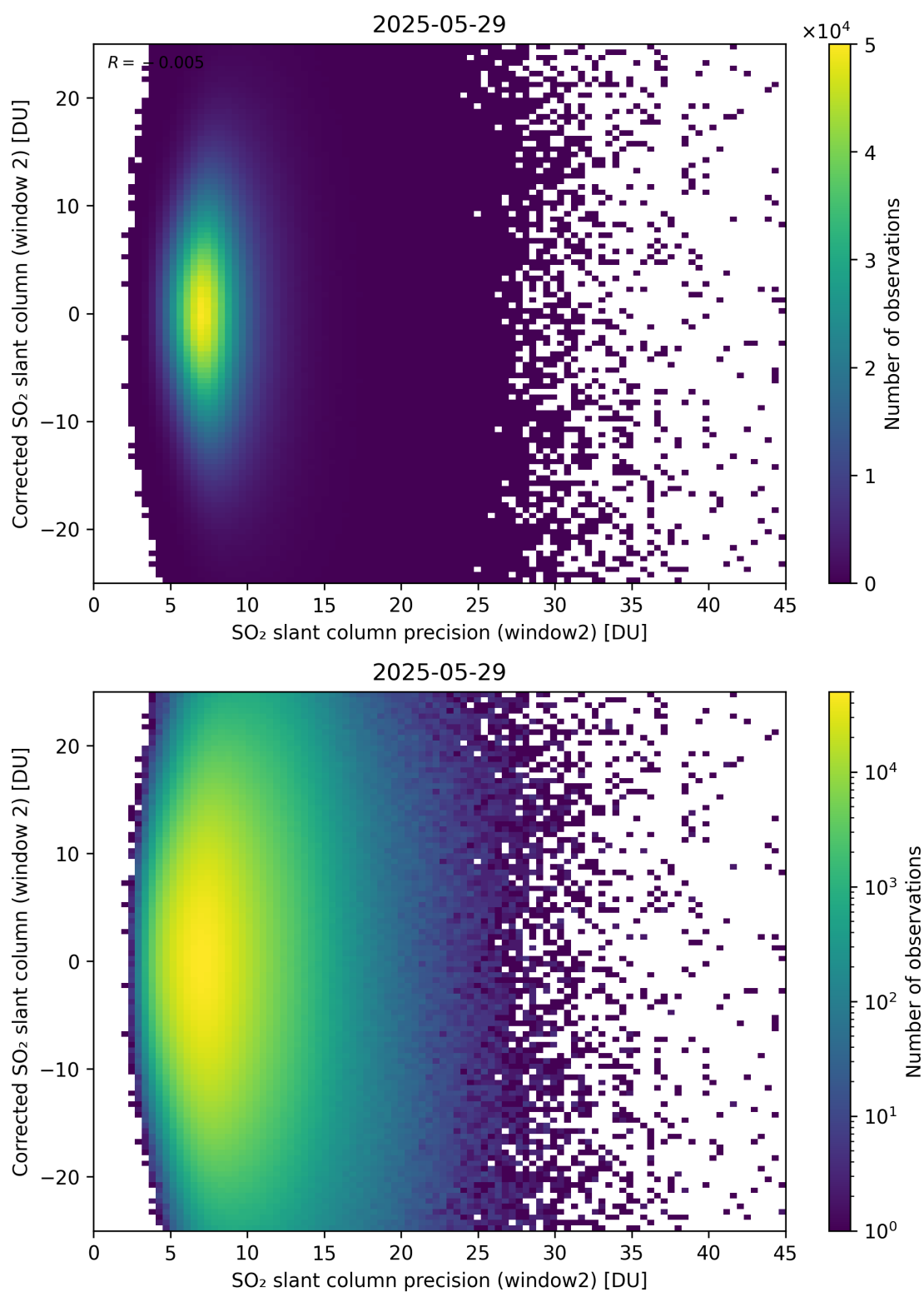
Figure 297: Scatter density plot of “SO 2 slant column precision (window2)” against “Corrected SO 2 slant column (window 2)” for 2025-05-28 to 2025-05-30.
