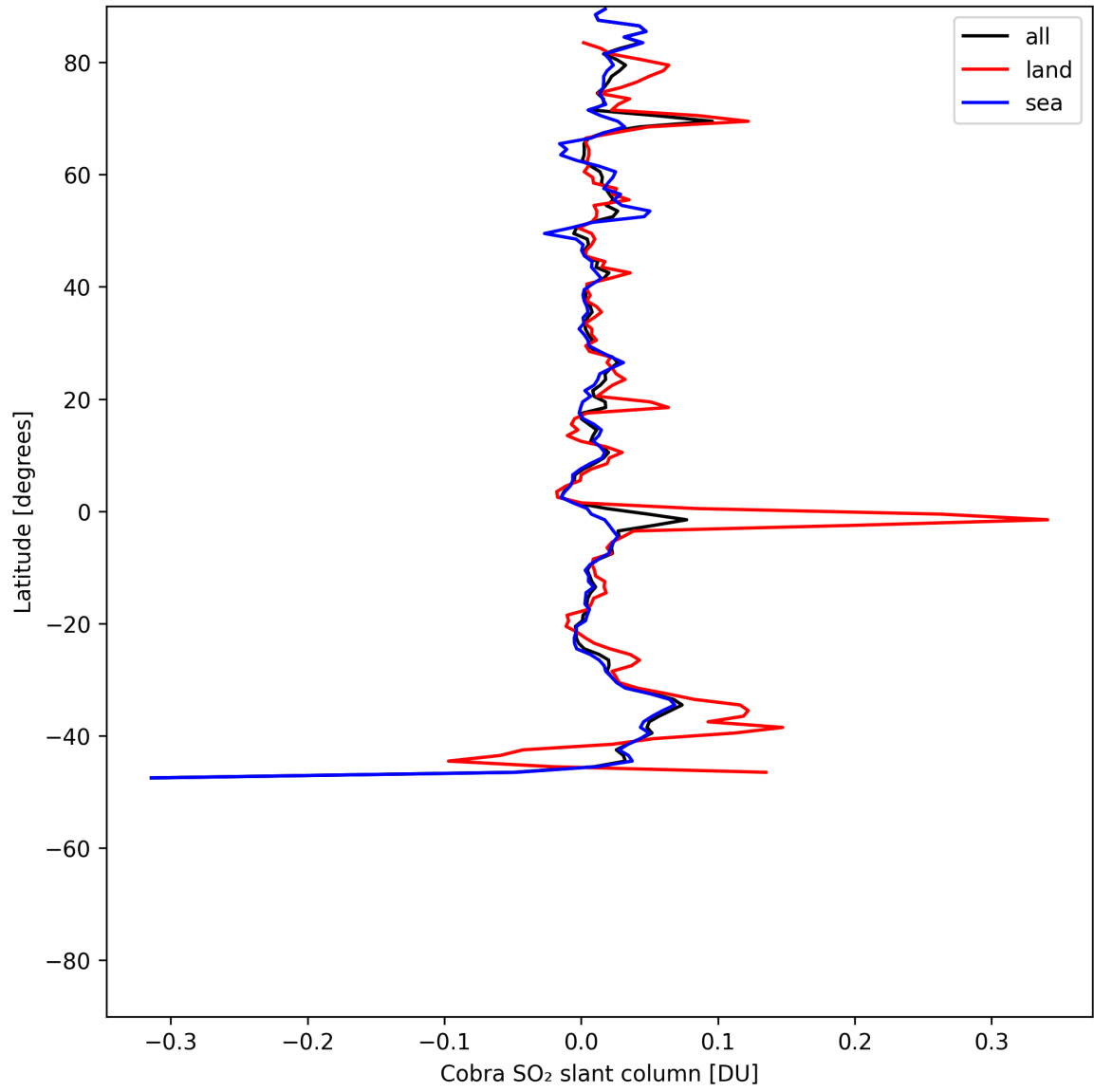
Figure 35: Zonal average of “Cobra SO 2 slant column” for 2025-05-28 to 2025-05-30.
