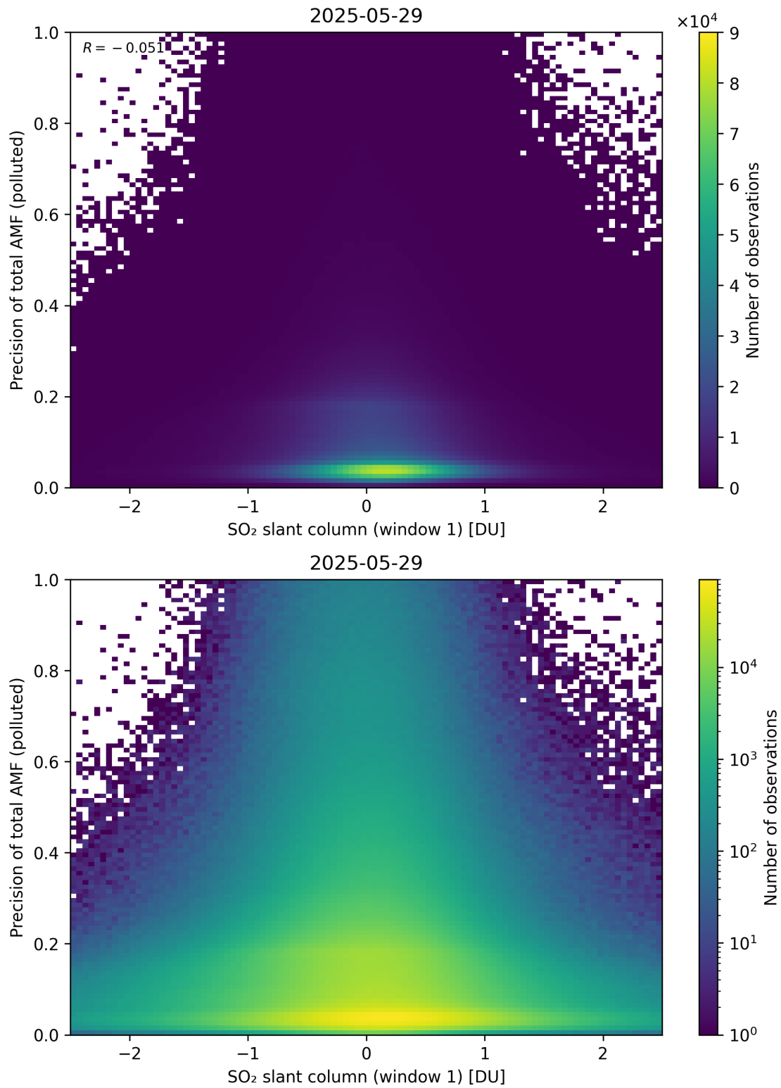
Figure 290: Scatter density plot of “SO 2 slant column (window 1)” against “Precision of total AMF (polluted)” for 2025-05-28 to 2025-05-30.
