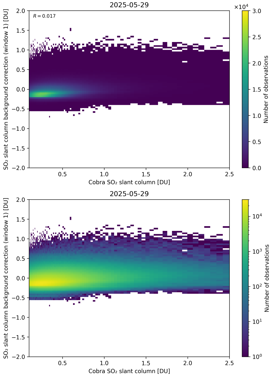
Figure 193: Scatter density plot of “Cobra SO 2 slant column” against “SO 2 slant column background correction (window 1)” for 2025-05-28 to 2025-05-30.
