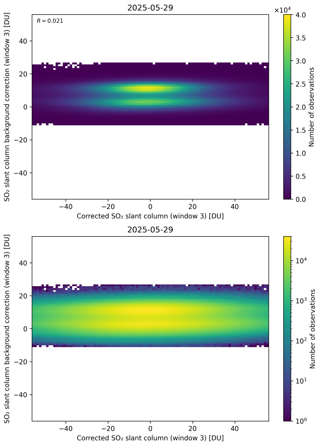
Figure 255: Scatter density plot of “Corrected SO 2 slant column (window 3)” against “SO 2 slant column background correction (window 3)” for 2025-05-28 to 2025-05-30.
