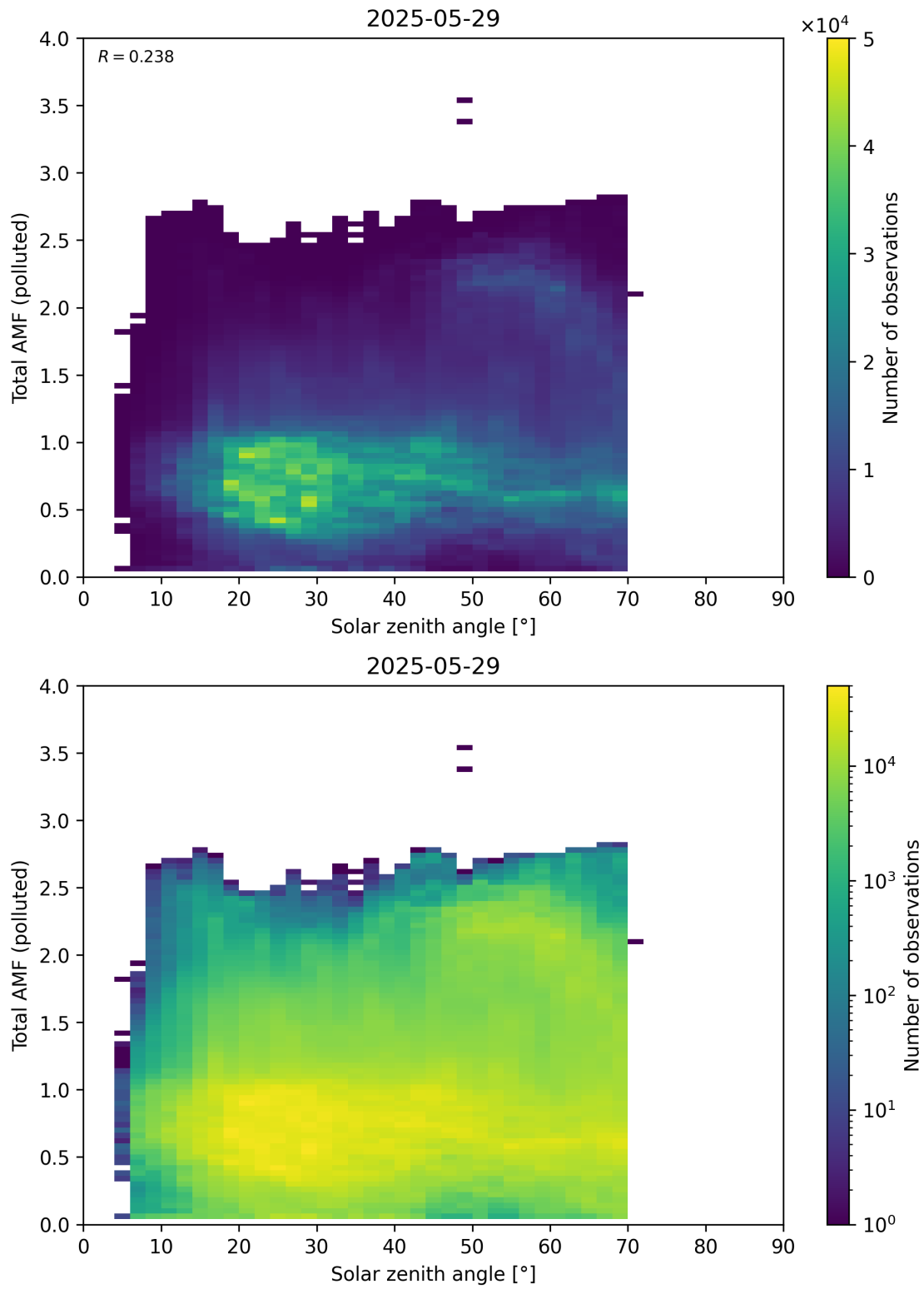
Figure 189: Scatter density plot of “Solar zenith angle” against “Total AMF (polluted)” for 2025-05-28 to 2025-05-30.
