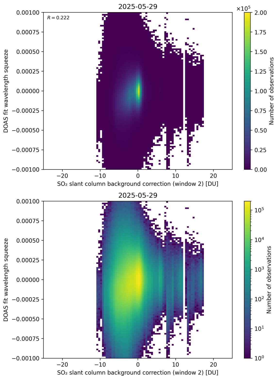
Figure 124: Scatter density plot of “SO 2 slant column background correction (window 2)” against “DOAS fit wavelength squeeze” for 2025-05-28 to 2025-05-30.
