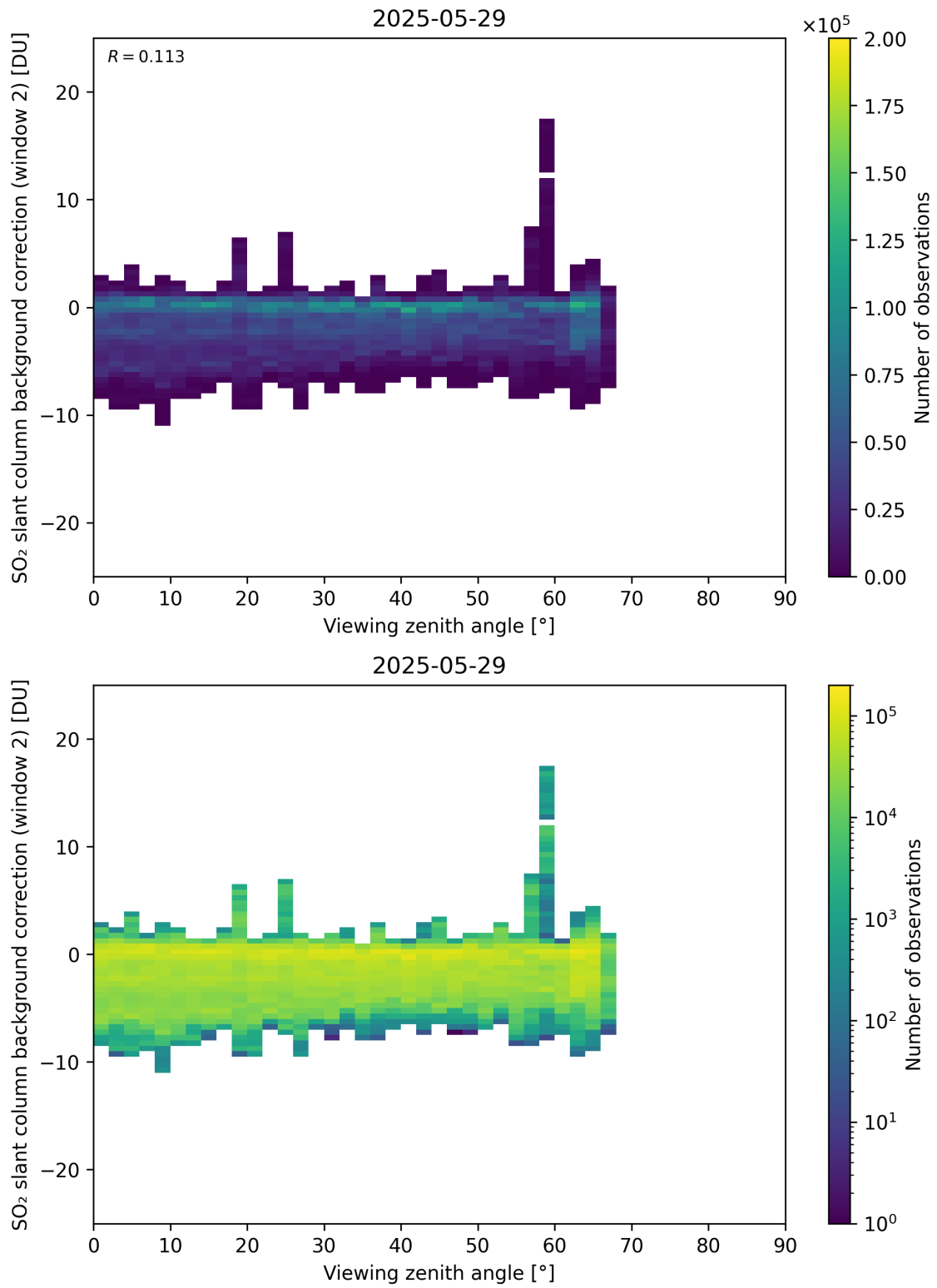
Figure 363: Scatter density plot of “Viewing zenith angle” against “SO 2 slant column background correction (window 2)” for 2025-05-28 to 2025-05-30.
