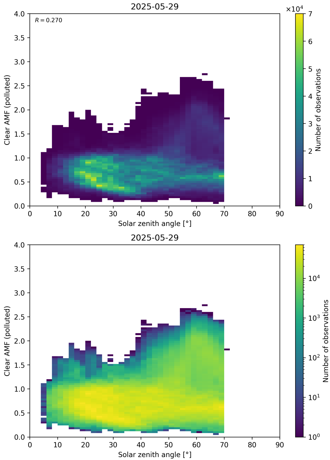
Figure 178: Scatter density plot of “Solar zenith angle” against “Clear AMF (polluted)” for 2025-05-28 to 2025-05-30.
