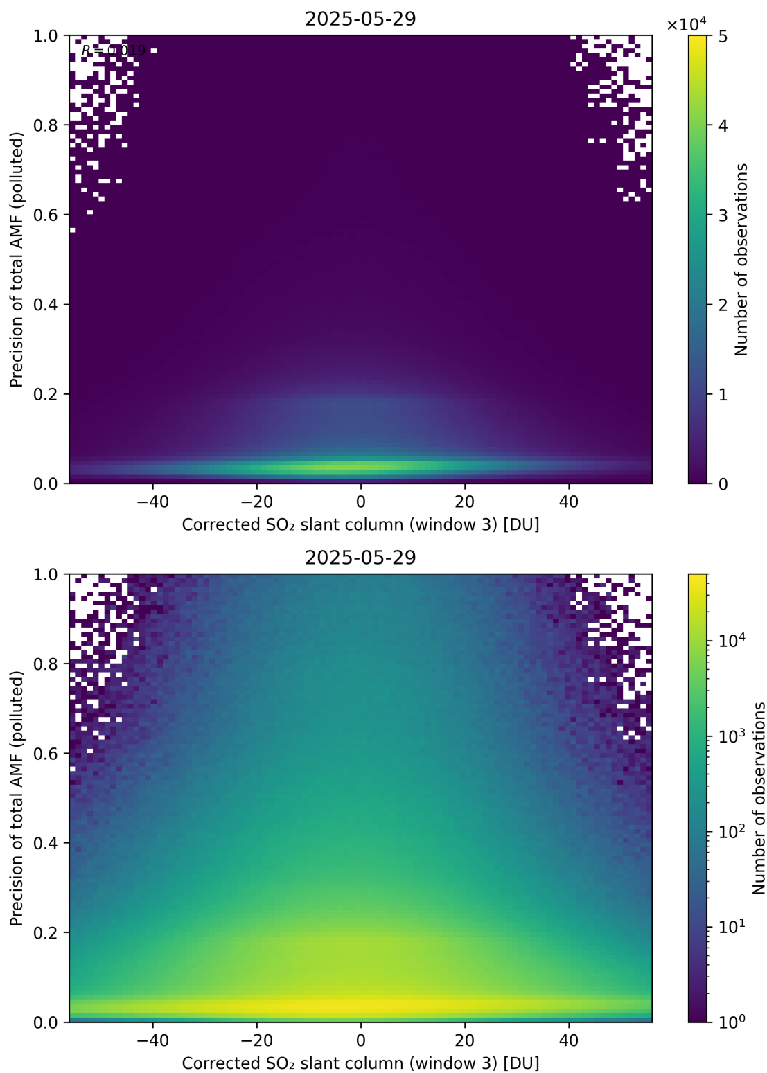
Figure 261: Scatter density plot of “Corrected SO 2 slant column (window 3)” against “Precision of total AMF (polluted)” for 2025-05-28 to 2025-05-30.
