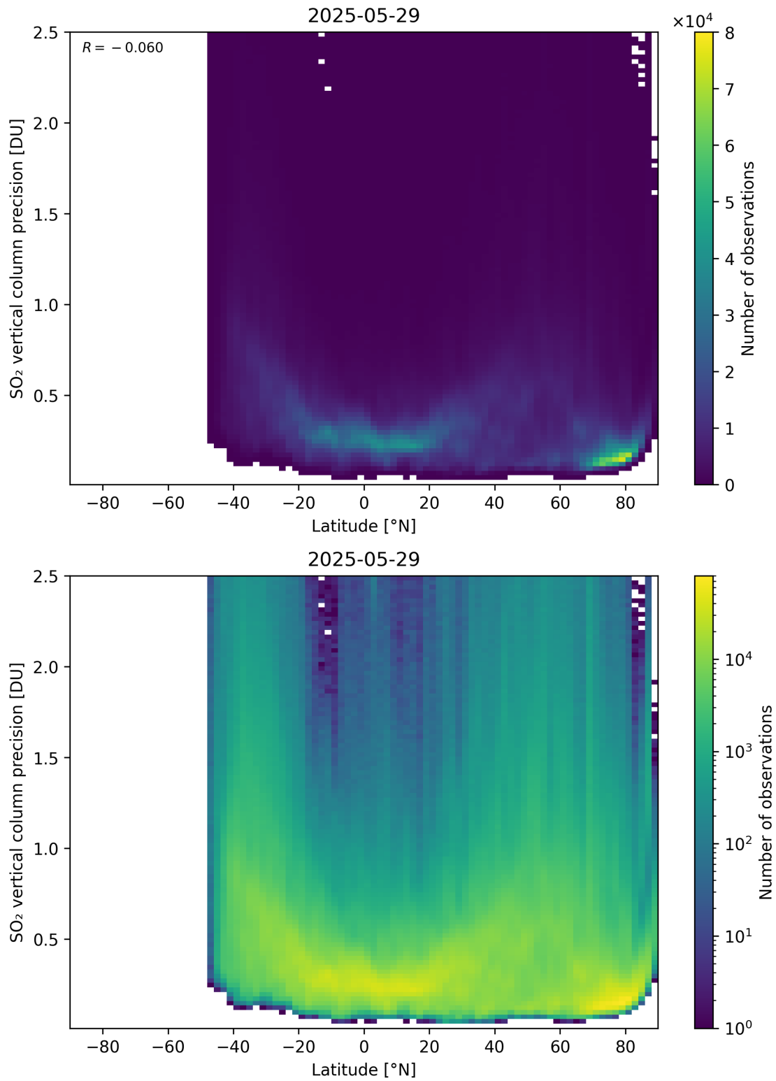
Figure 170: Scatter density plot of “Latitude” against “SO 2 vertical column precision” for 2025-05-28 to 2025-05-30.
