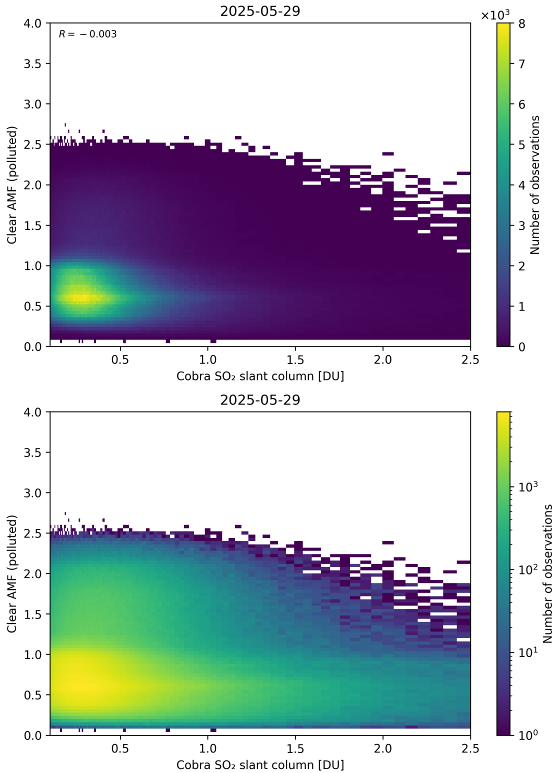
Figure 215: Scatter density plot of “Cobra SO 2 slant column” against “Clear AMF (polluted)” for 2025-05-28 to 2025-05-30.
