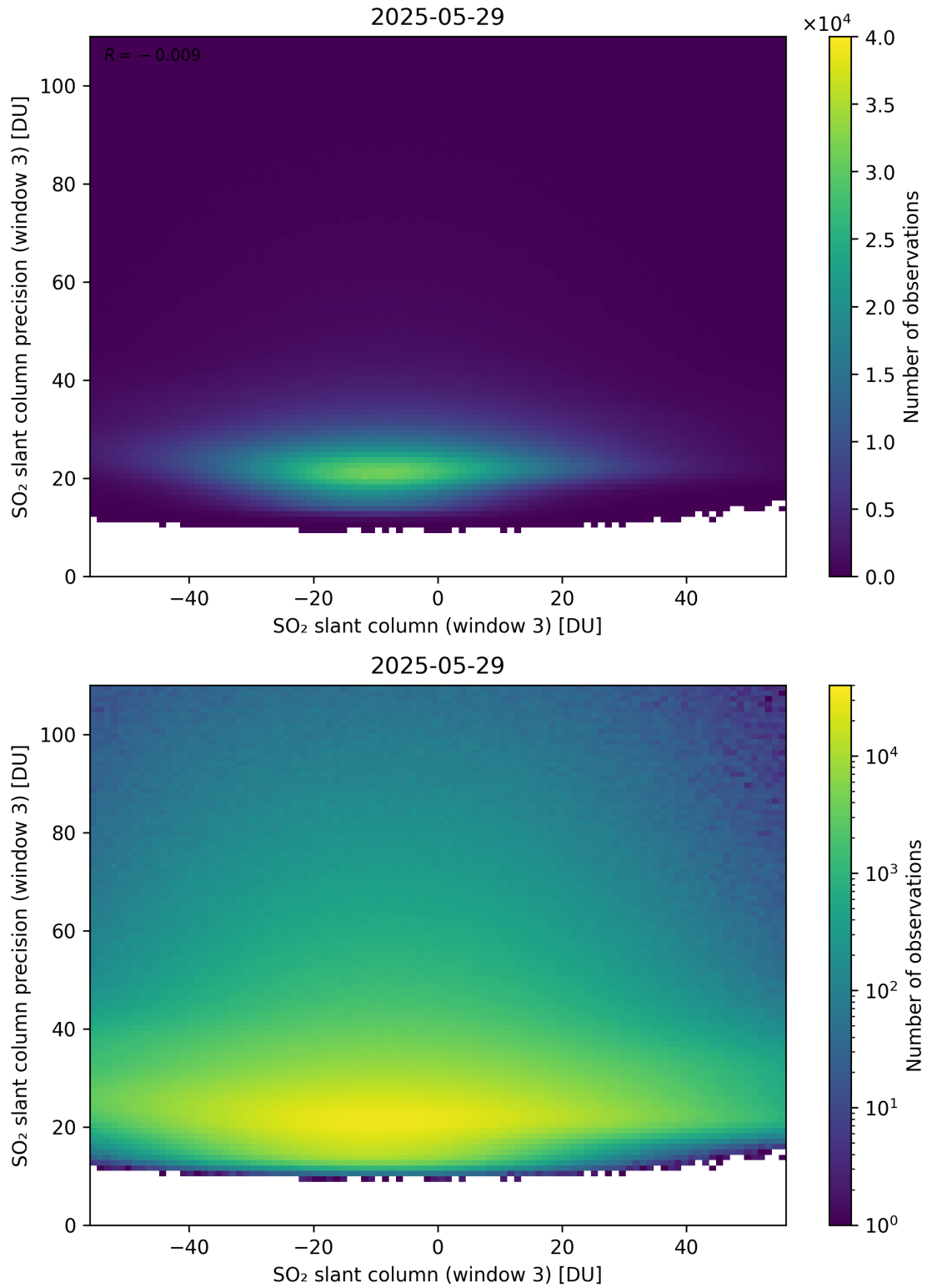
Figure 317: Scatter density plot of “SO 2 slant column (window 3)” against “SO 2 slant column precision (window 3)” for 2025-05-28 to 2025-05-30.
