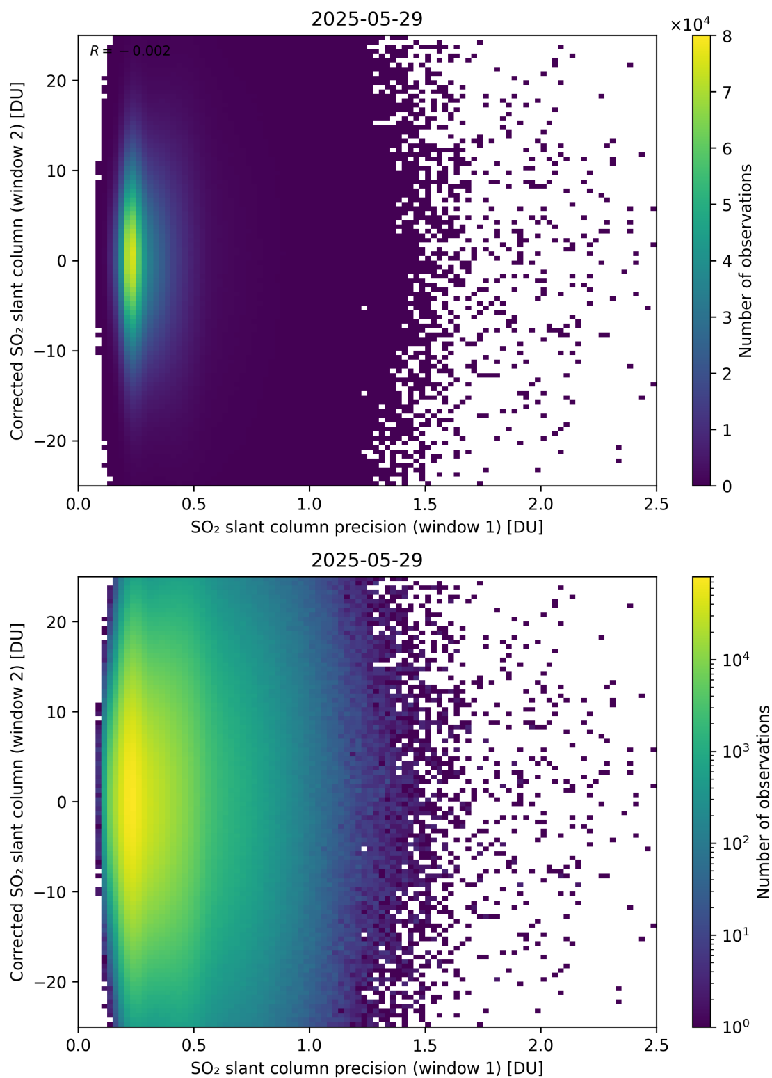
Figure 275: Scatter density plot of “SO 2 slant column precision (window 1)” against “Corrected SO 2 slant column (window 2)” for 2025-05-28 to 2025-05-30.
