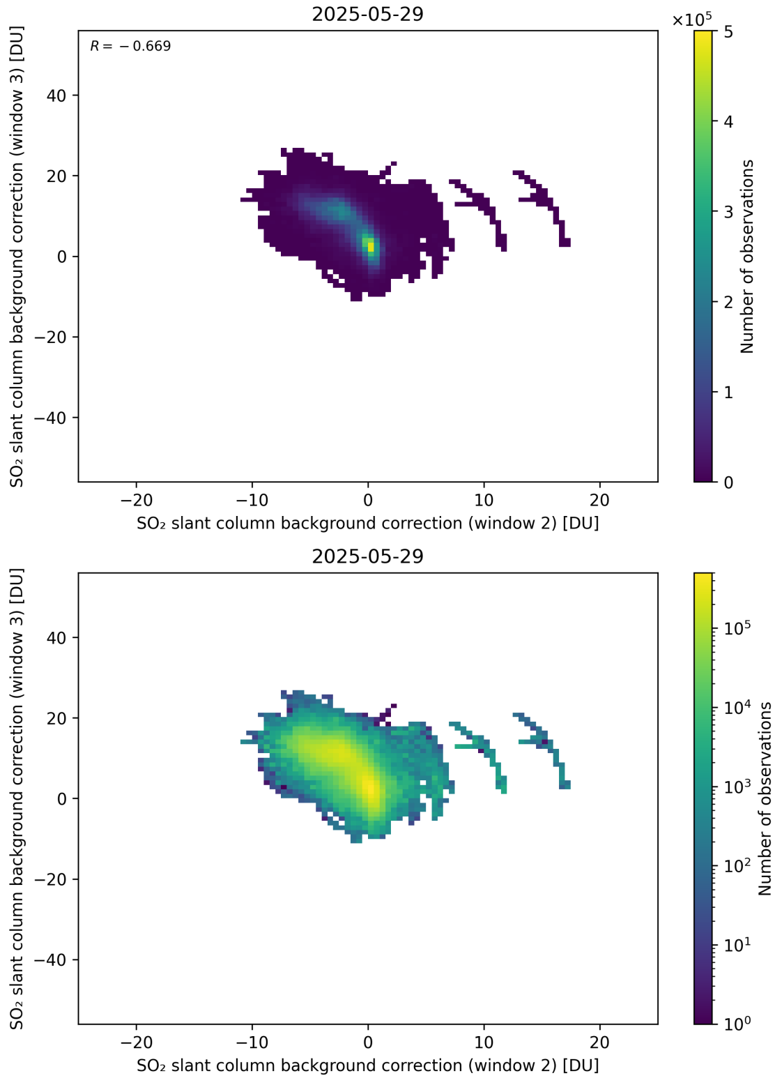
Figure 122: Scatter density plot of “SO 2 slant column background correction (window 2)” against “SO 2 slant column background correction (window 3)” for 2025-05-28 to 2025-05-30.
