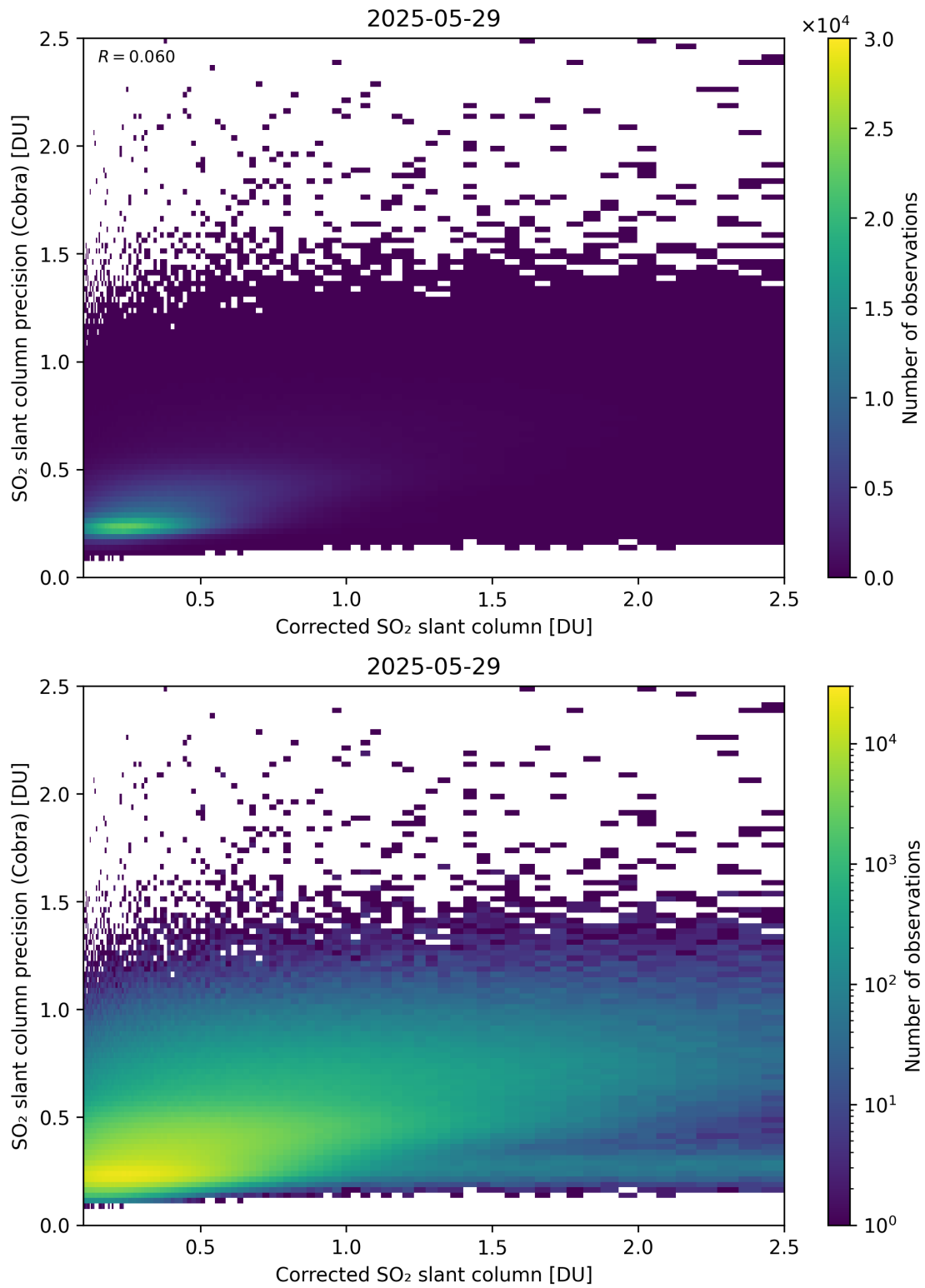
Figure 234: Scatter density plot of “Corrected SO 2 slant column” against “SO 2 slant column precision (Cobra)” for 2025-05-28 to 2025-05-30.
