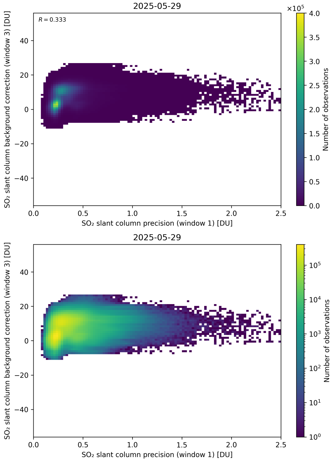
Figure 270: Scatter density plot of “SO 2 slant column precision (window 1)” against “SO 2 slant column background correction (window 3)” for 2025-05-28 to 2025-05-30.
