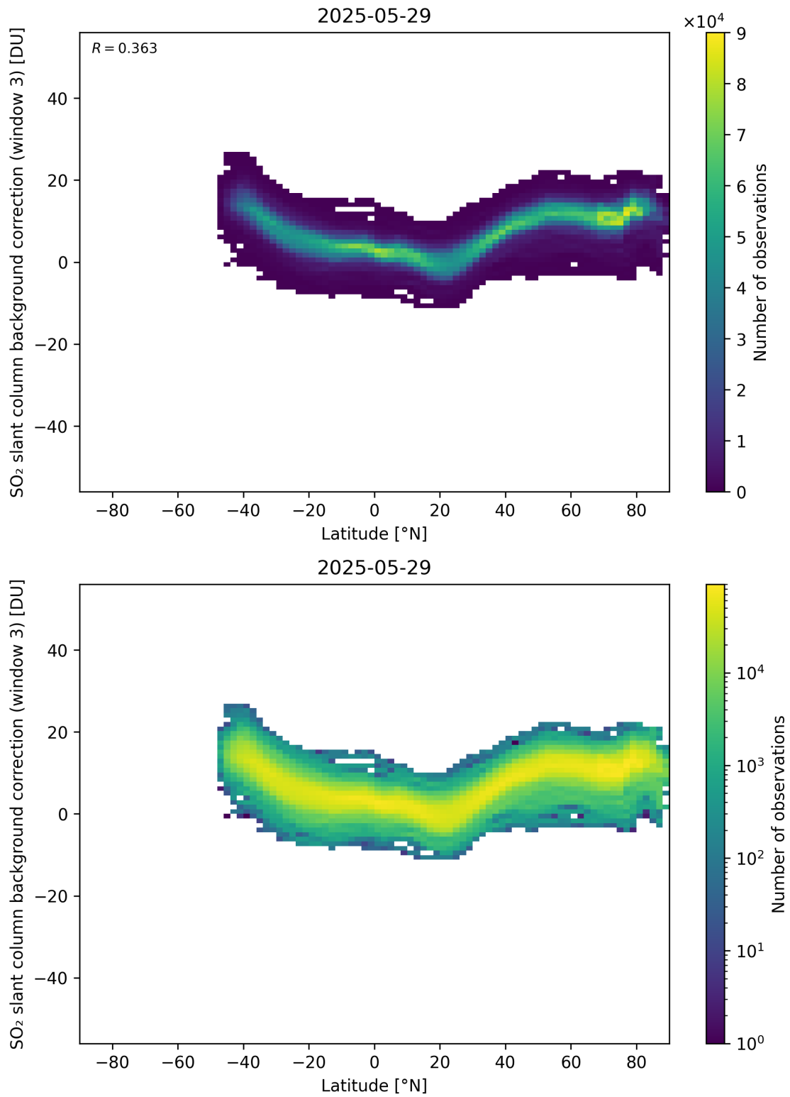
Figure 152: Scatter density plot of “Latitude” against “SO 2 slant column background correction (window 3)” for 2025-05-28 to 2025-05-30.
