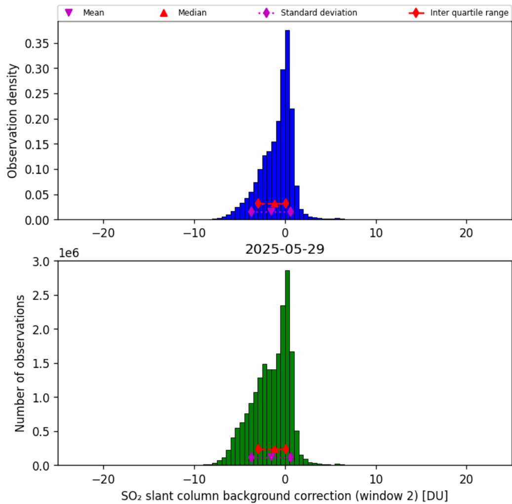
Figure 70: Histogram of “SO 2 slant column background correction (window 2)” for 2025-05-28 to 2025-05-30
