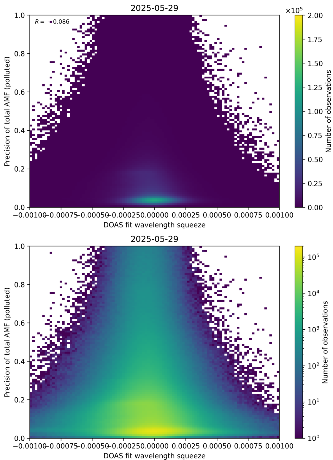
Figure 146: Scatter density plot of “DOAS fit wavelength squeeze” against “Precision of total AMF (polluted)” for 2025-05-28 to 2025-05-30.
