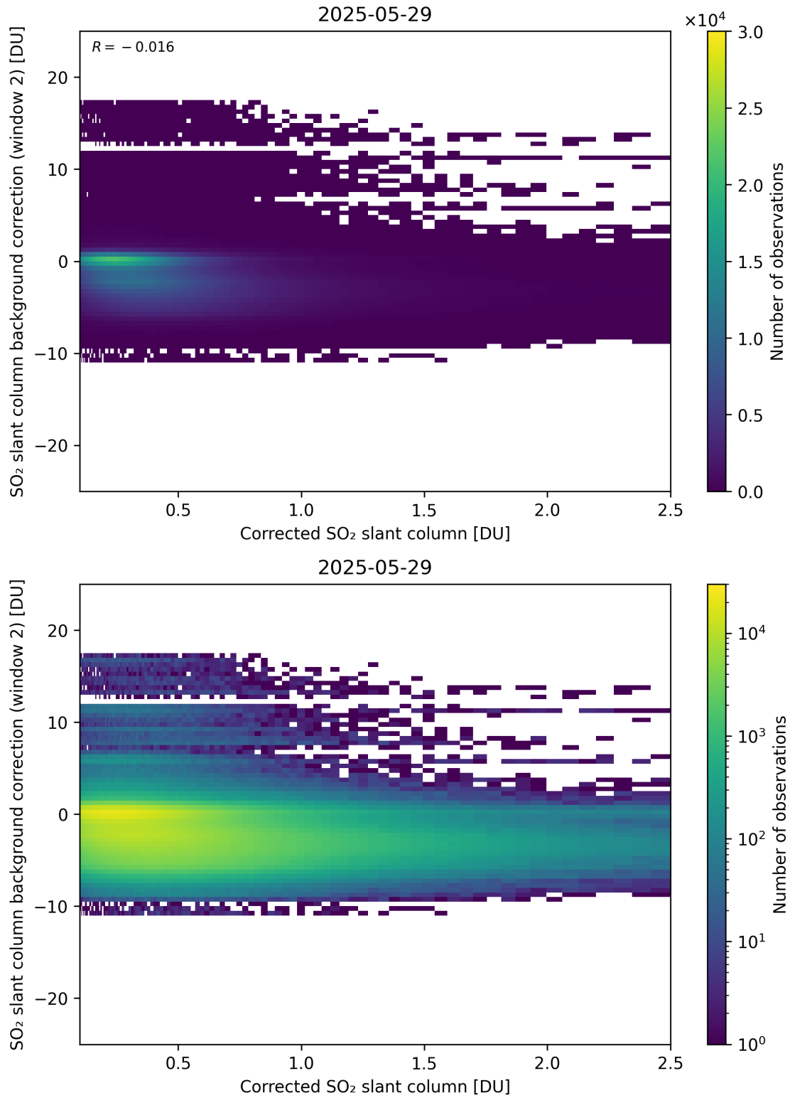
Figure 227: Scatter density plot of “Corrected SO 2 slant column” against “SO 2 slant column background correction (window 2)” for 2025-05-28 to 2025-05-30.
