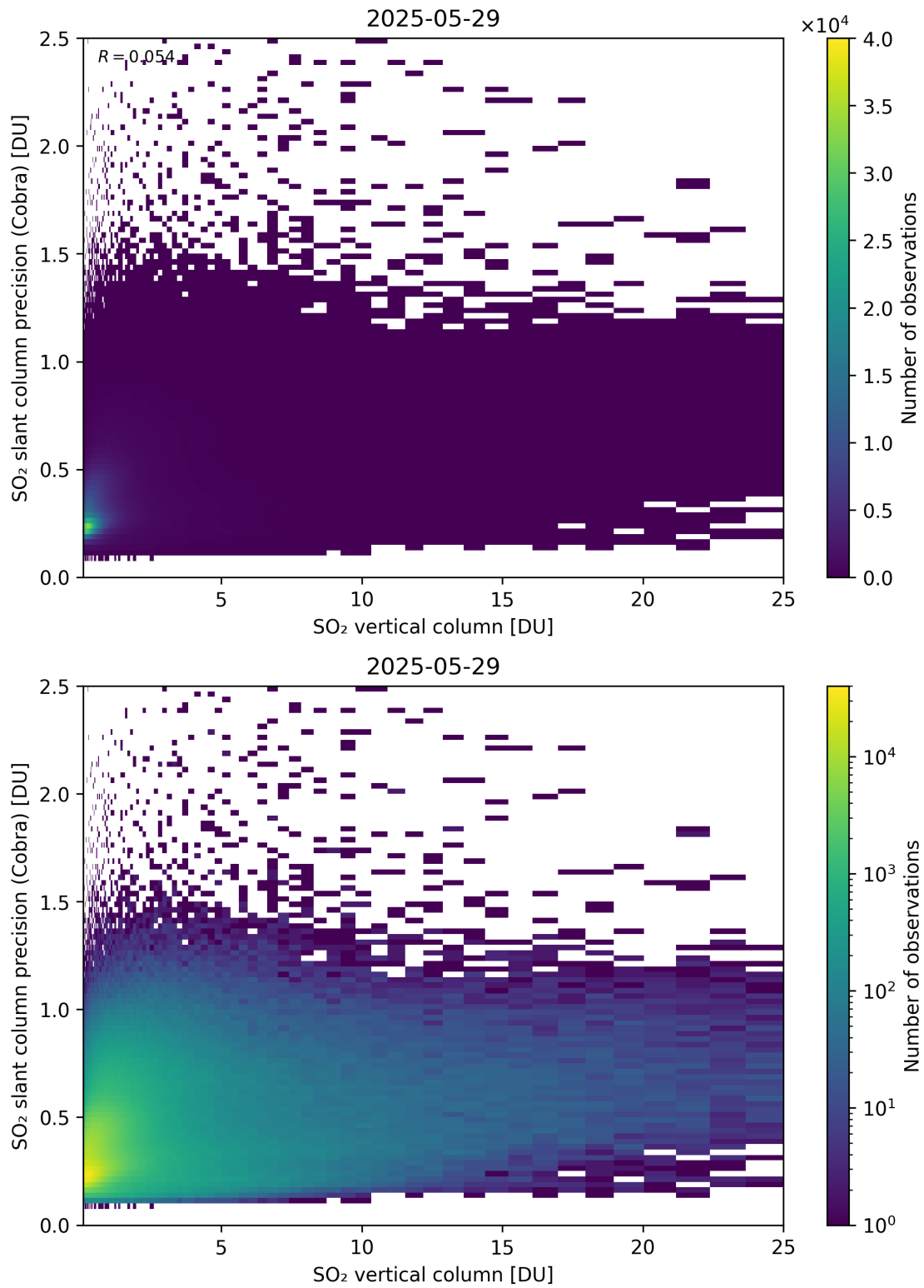
Figure 350: Scatter density plot of “SO 2 vertical column” against “SO 2 slant column precision (Cobra)” for 2025-05-28 to 2025-05-30.
