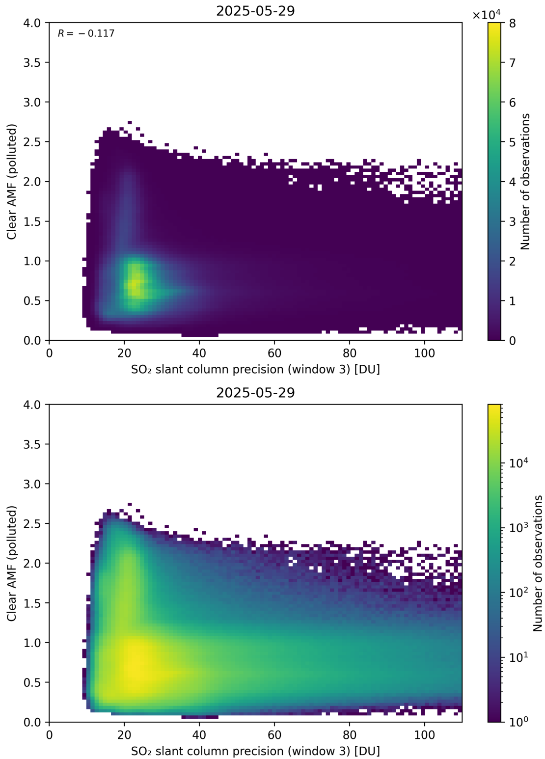
Figure 311: Scatter density plot of “SO 2 slant column precision (window 3)” against “Clear AMF (polluted)” for 2025-05-28 to 2025-05-30.
