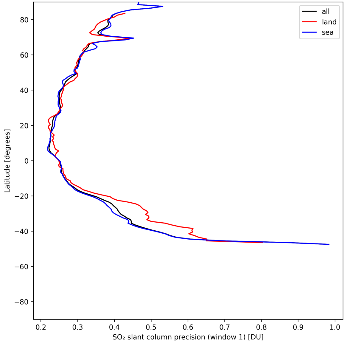
Figure 38: Zonal average of “SO 2 slant column precision (window 1)” for 2025-05-28 to 2025-05-30.
