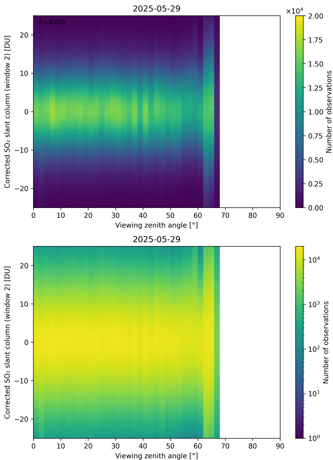
Figure 374: Scatter density plot of “Viewing zenith angle” against “Corrected SO 2 slant column (window 2)” for 2025-05-28 to 2025-05-30.
