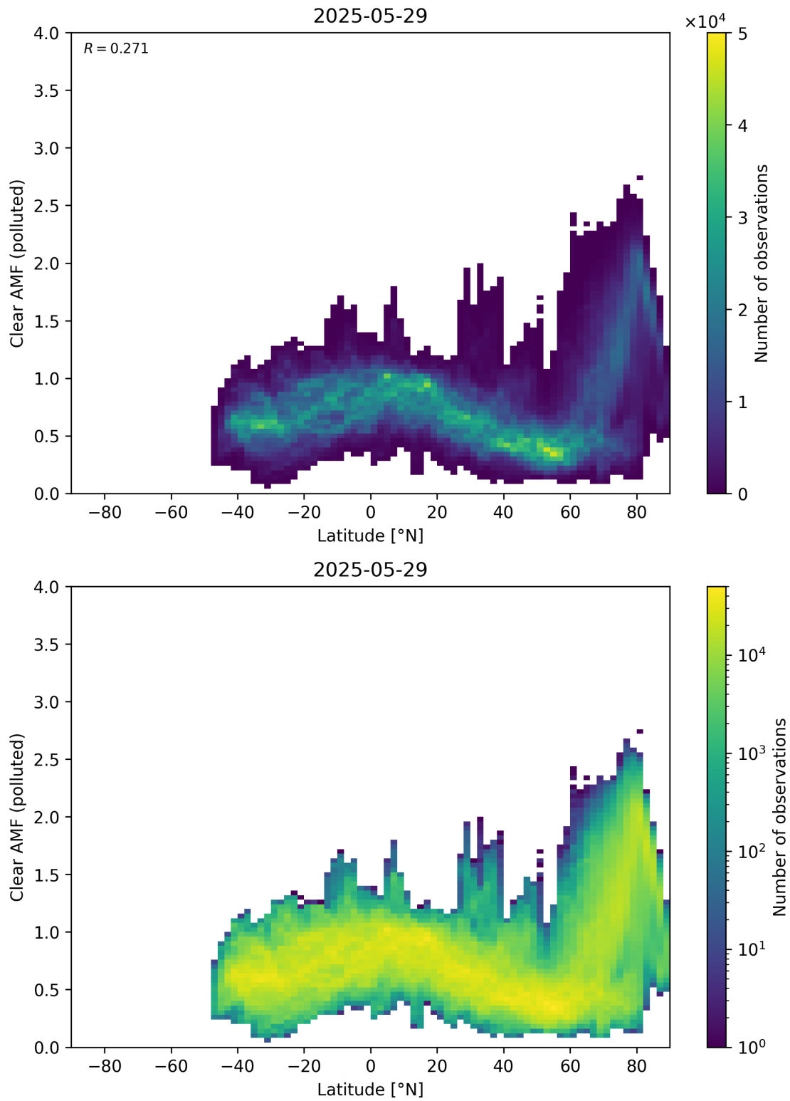
Figure 156: Scatter density plot of “Latitude” against “Clear AMF (polluted)” for 2025-05-28 to 2025-05-30.
