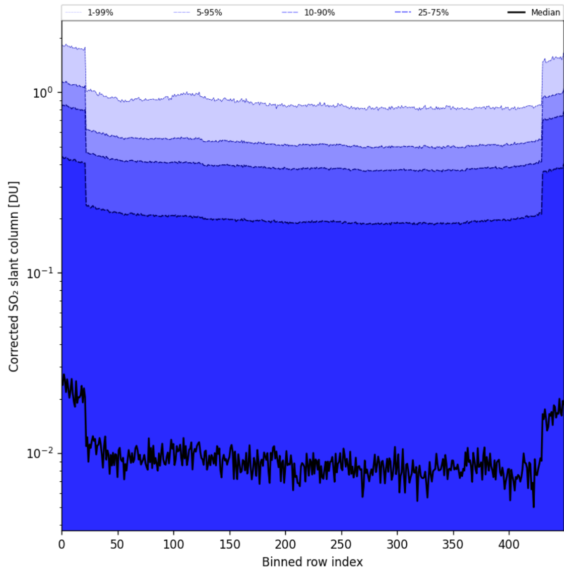
Figure 86: Along track statistics of “Corrected SO 2 slant column” for 2025-05-28 to 2025-05-30
