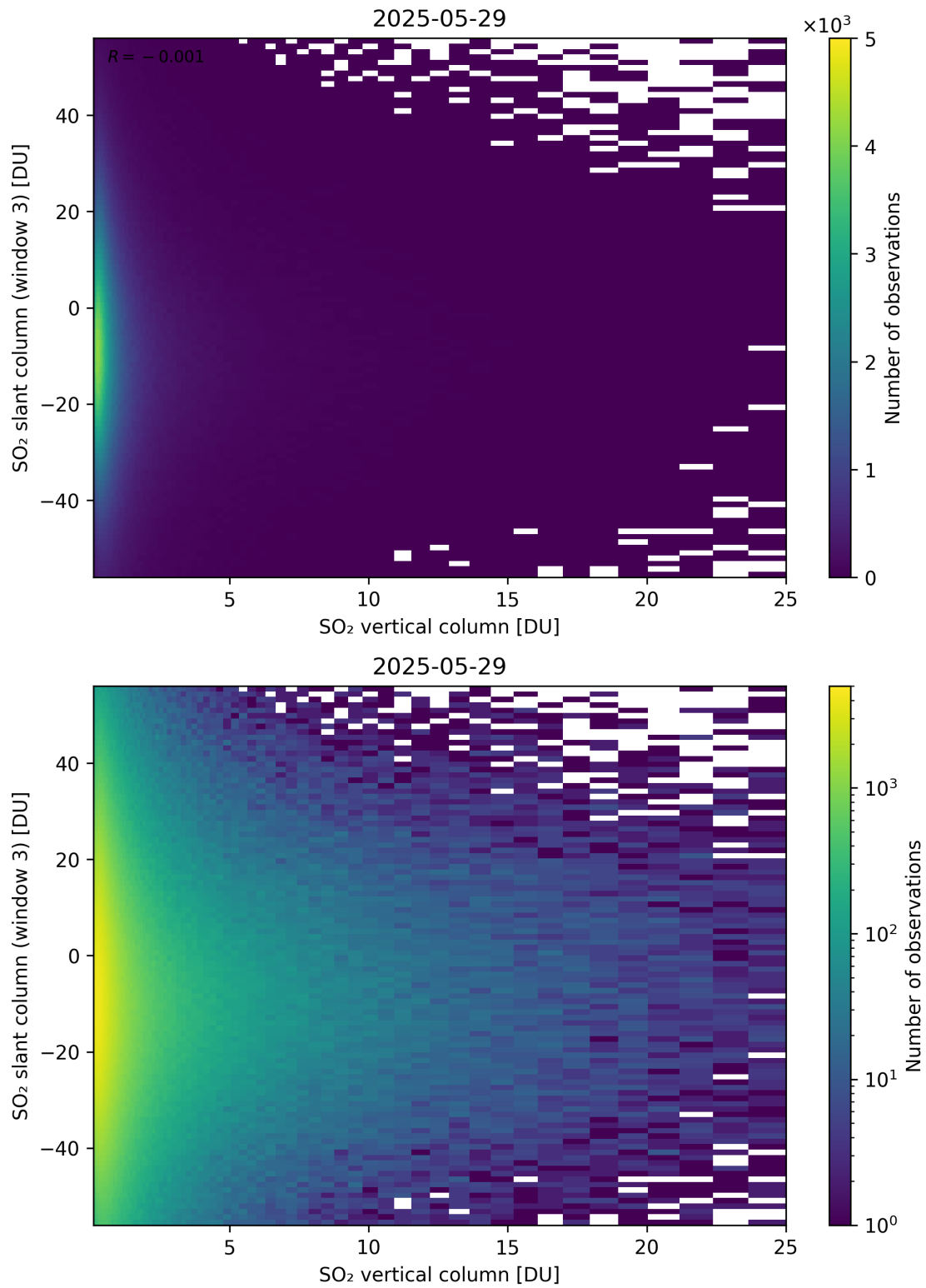
Figure 357: Scatter density plot of “SO 2 vertical column” against “SO 2 slant column (window 3)” for 2025-05-28 to 2025-05-30.
