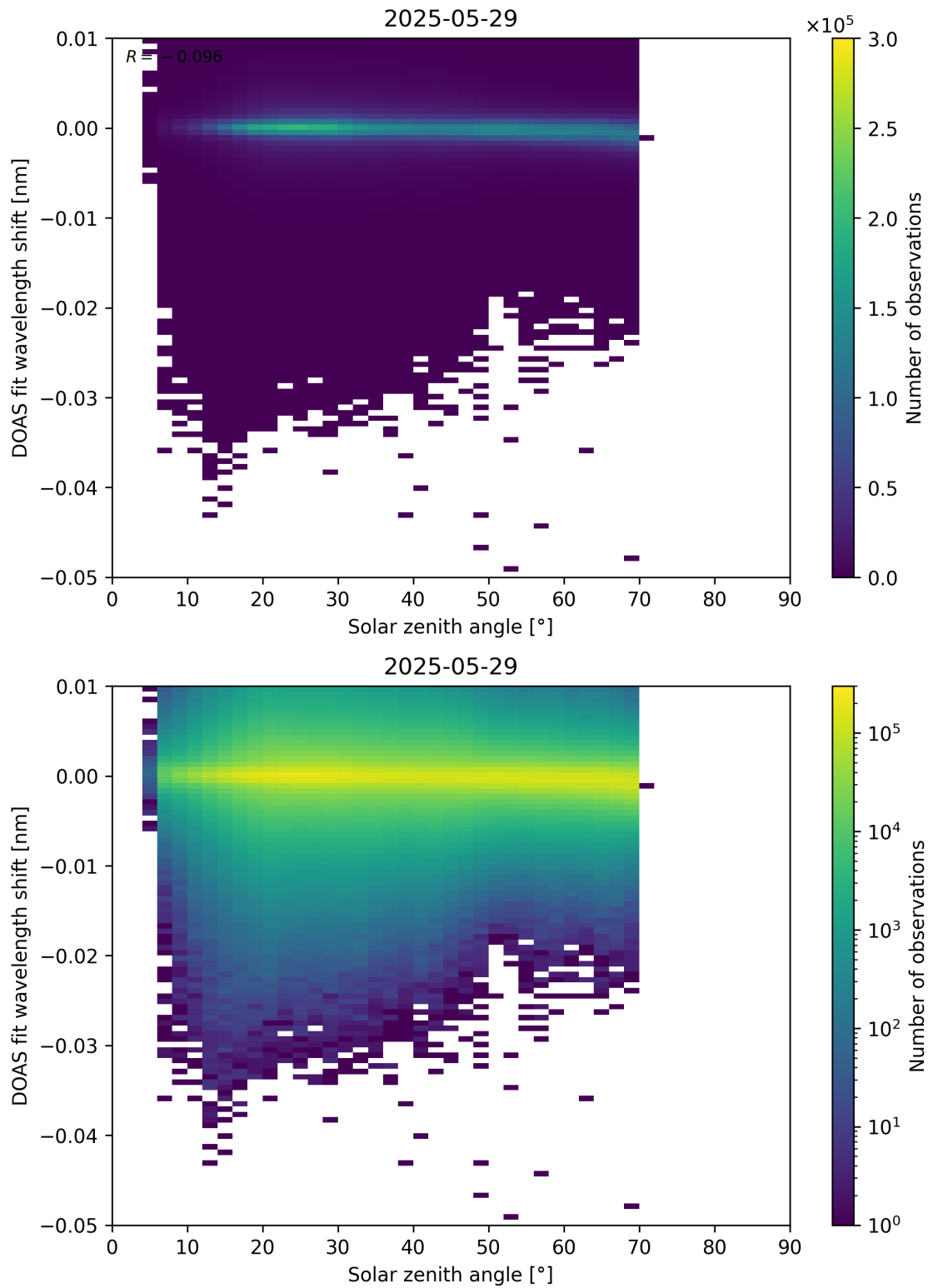
Figure 174: Scatter density plot of “Solar zenith angle” against “DOAS fit wavelength shift” for 2025-05-28 to 2025-05-30.
