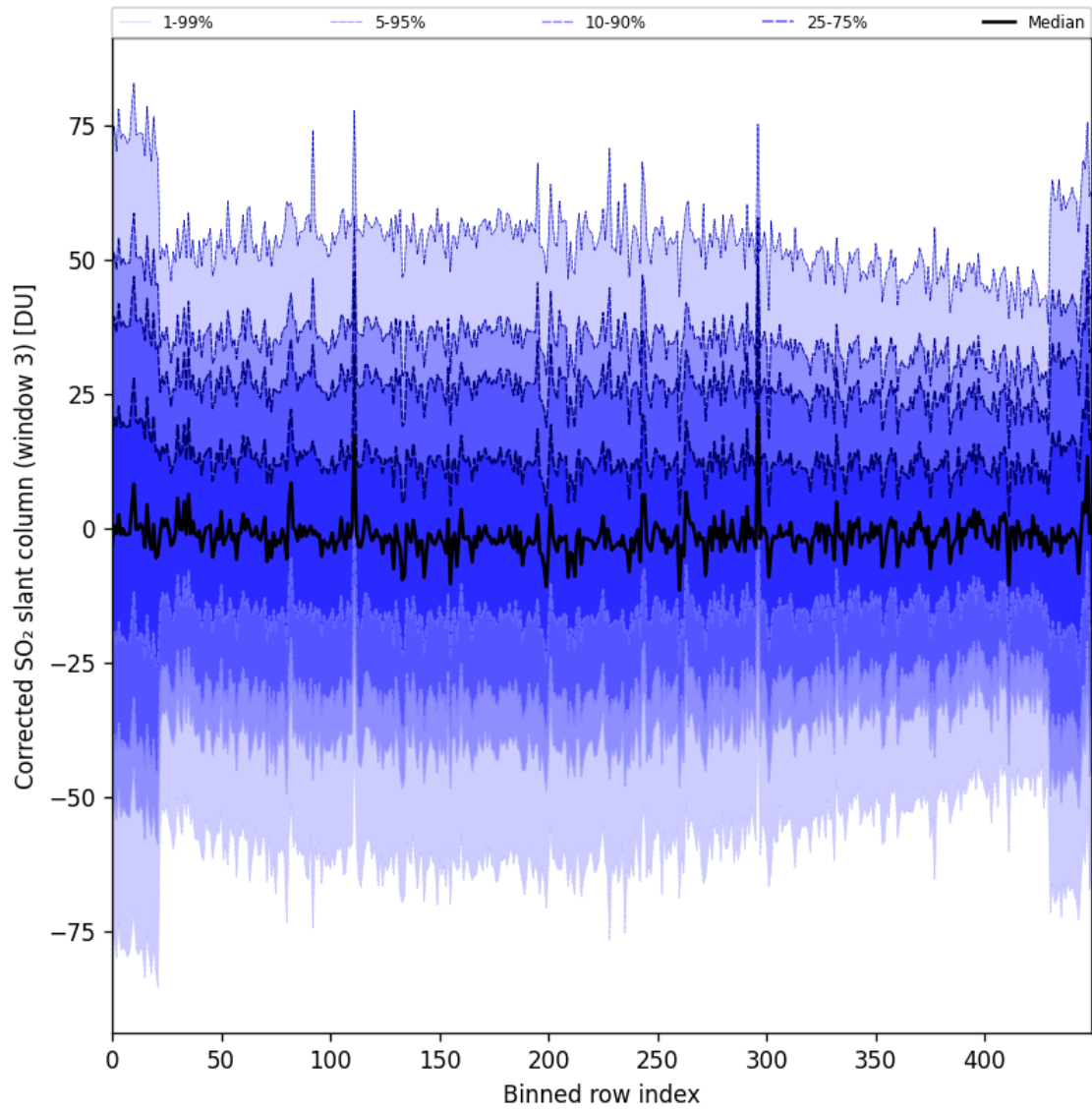
Figure 99: Along track statistics of “Corrected SO 2 slant column (window 3)” for 2025-05-28 to 2025-05-30
