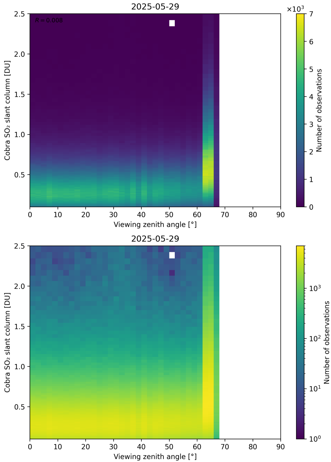
Figure 371: Scatter density plot of “Viewing zenith angle” against “Cobra SO 2 slant column” for 2025-05-28 to 2025-05-30.
