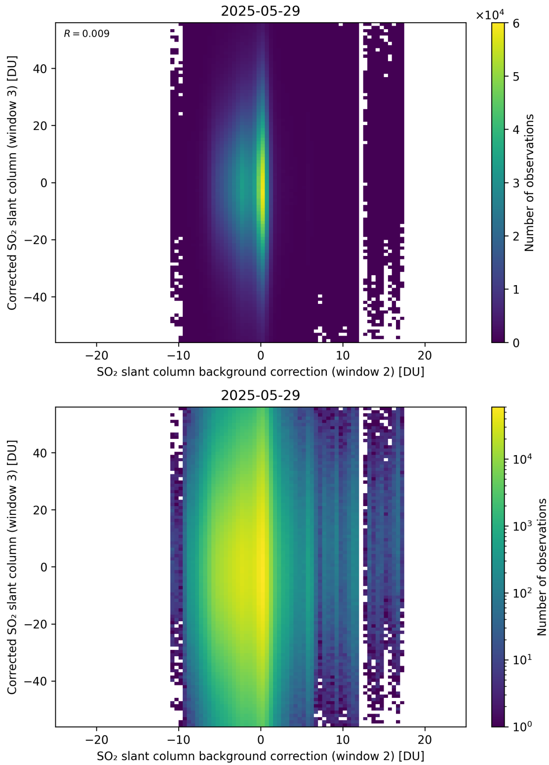
Figure 127: Scatter density plot of “SO 2 slant column background correction (window 2)” against “Corrected SO 2 slant column (window 3)” for 2025-05-28 to 2025-05-30.
