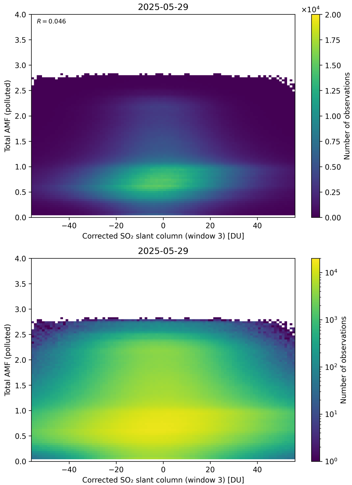
Figure 260: Scatter density plot of “Corrected SO 2 slant column (window 3)” against “Total AMF (polluted)” for 2025-05-28 to 2025-05-30.
