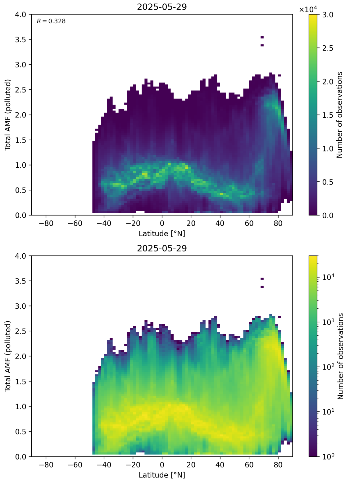
Figure 167: Scatter density plot of “Latitude” against “Total AMF (polluted)” for 2025-05-28 to 2025-05-30.
