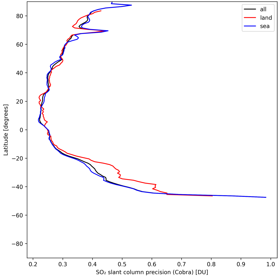
Figure 36: Zonal average of “SO 2 slant column precision (Cobra)” for 2025-05-28 to 2025-05-30.
