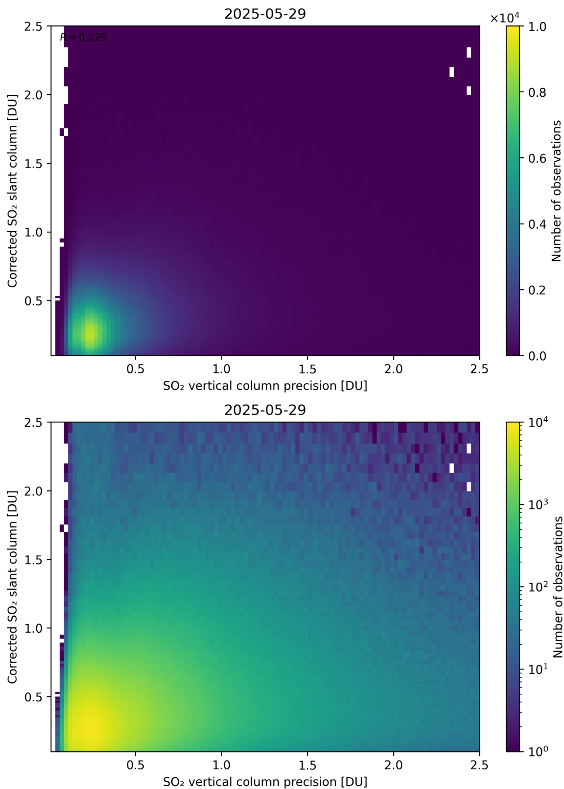
Figure 338: Scatter density plot of “SO 2 vertical column precision” against “Corrected SO 2 slant column” for 2025-05-28 to 2025-05-30.
