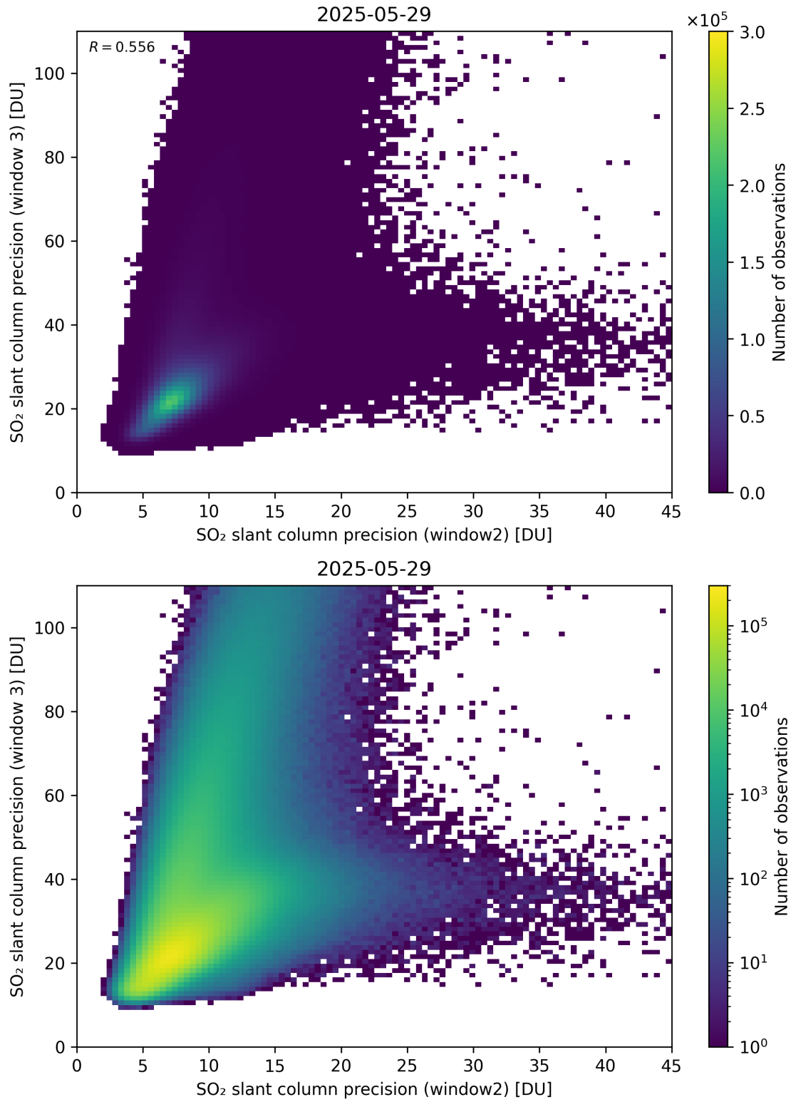
Figure 300: Scatter density plot of “SO 2 slant column precision (window2)” against “SO 2 slant column precision (window 3)” for 2025-05-28 to 2025-05-30.
