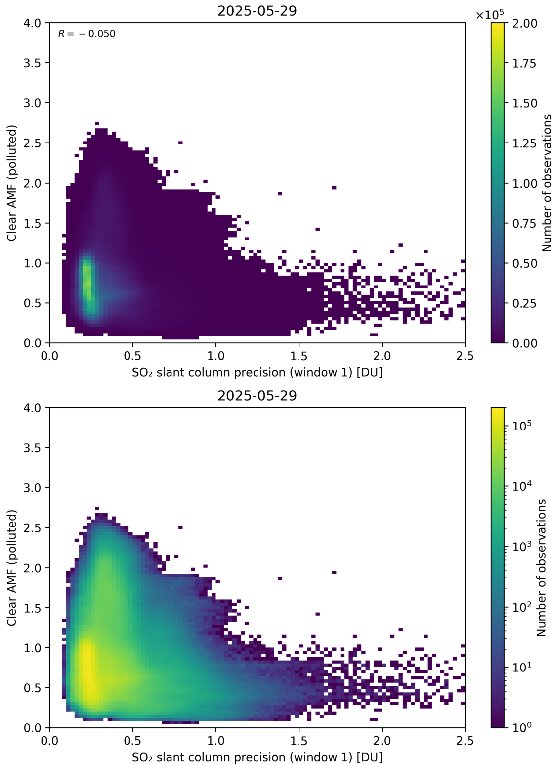
Figure 274: Scatter density plot of “SO 2 slant column precision (window 1)” against “Clear AMF (polluted)” for 2025-05-28 to 2025-05-30.
