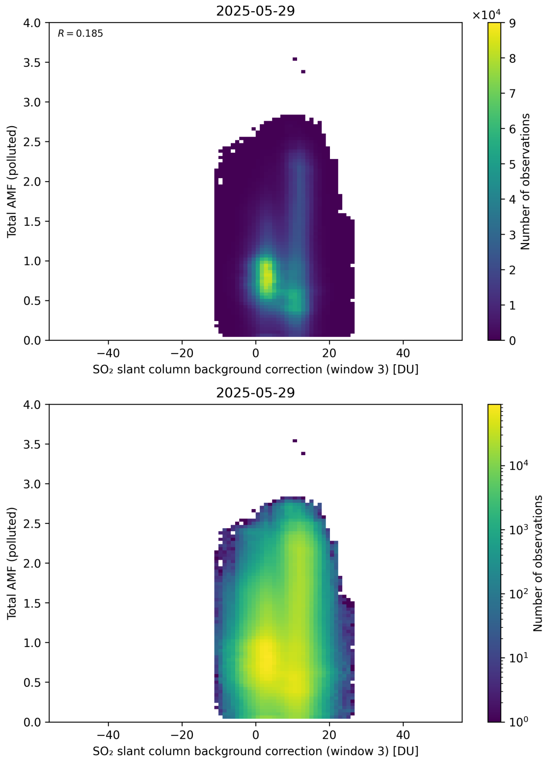
Figure 136: Scatter density plot of “SO 2 slant column background correction (window 3)” against “Total AMF (polluted)” for 2025-05-28 to 2025-05-30.
