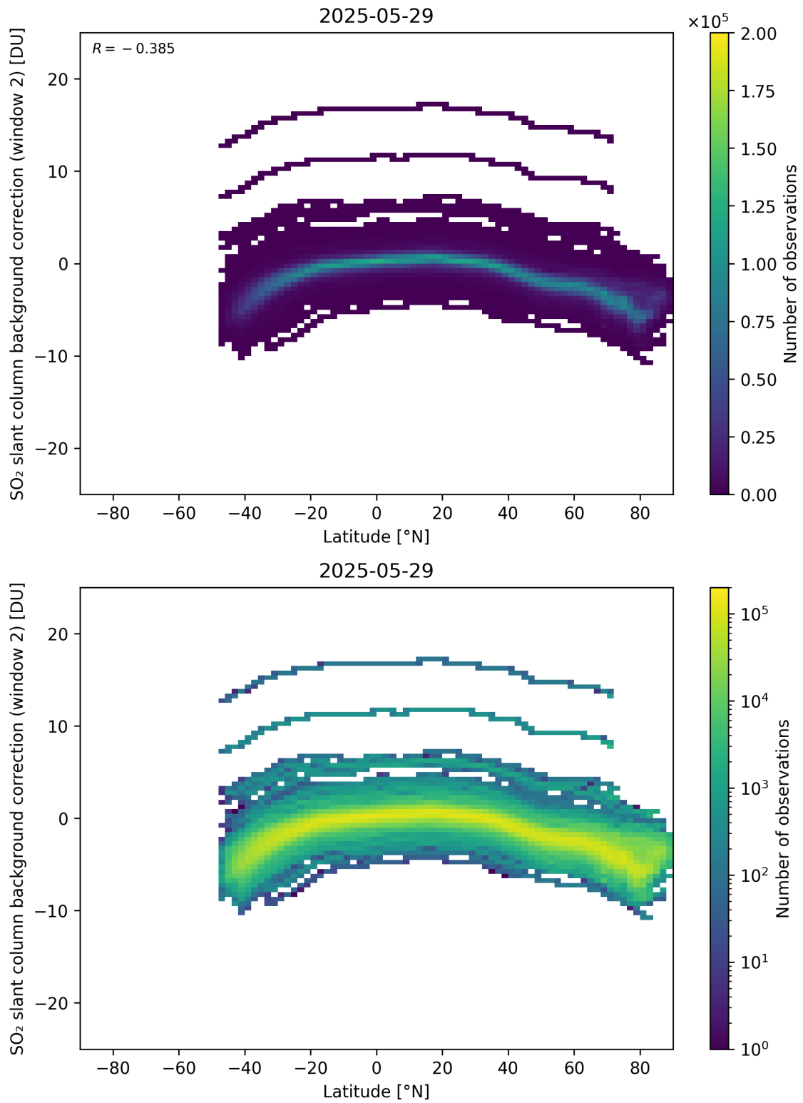
Figure 151: Scatter density plot of “Latitude” against “SO 2 slant column background correction (window 2)” for 2025-05-28 to 2025-05-30.
