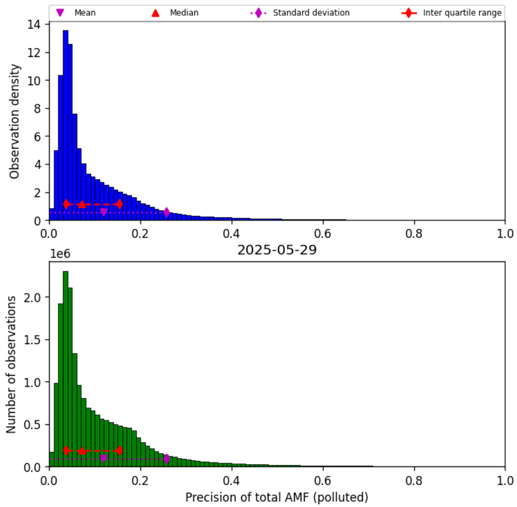
Figure 80: Histogram of “Precision of total AMF (polluted)” for 2025-05-28 to 2025-05-30
