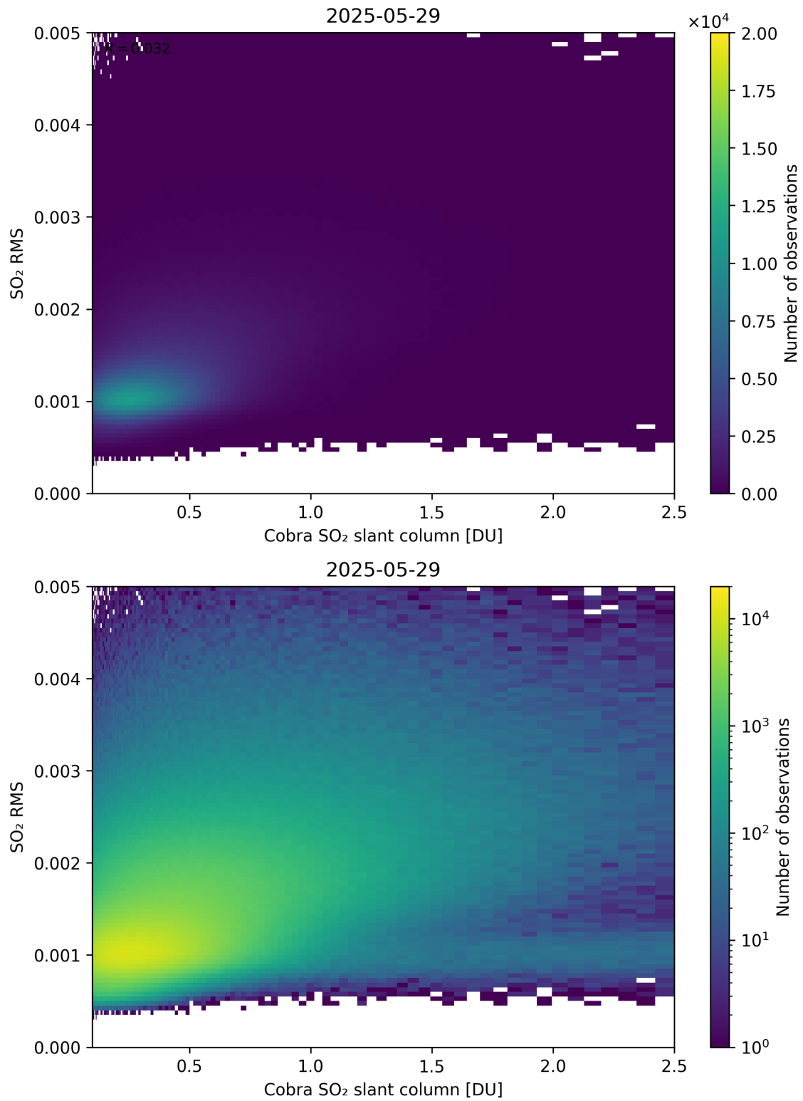
Figure 198: Scatter density plot of “Cobra SO 2 slant column” against “SO 2 RMS” for 2025-05-28 to 2025-05-30.
