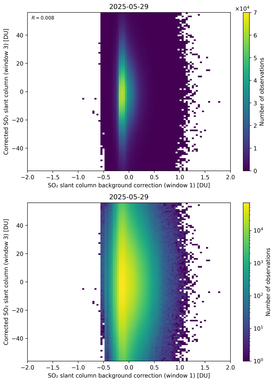
Figure 116: Scatter density plot of “SO 2 slant column background correction (window 1)” against “Corrected SO 2 slant column (window 3)” for 2025-05-28 to 2025-05-30.
