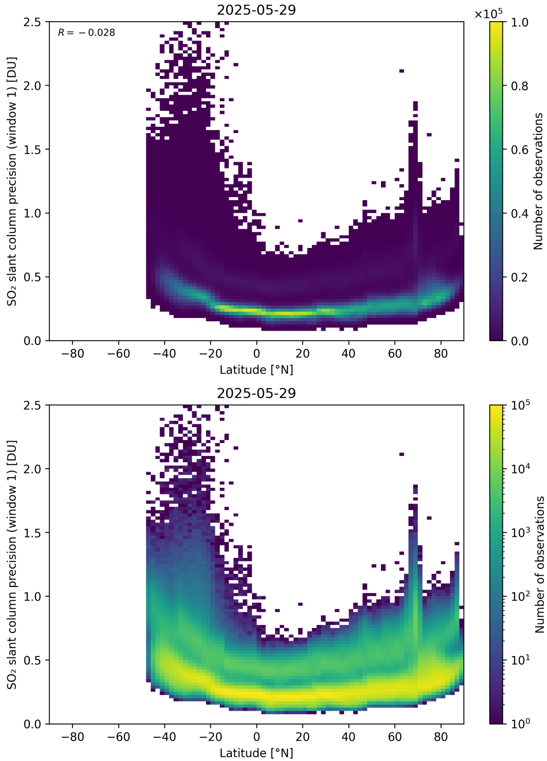
Figure 163: Scatter density plot of “Latitude” against “SO 2 slant column precision (window 1)” for 2025-05-28 to 2025-05-30.
