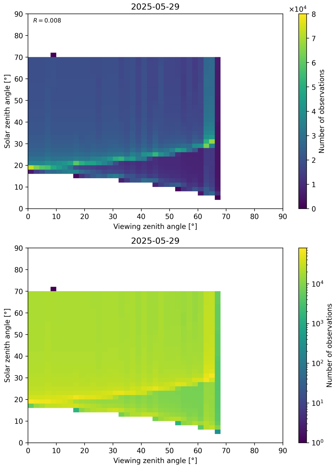
Figure 369: Scatter density plot of “Viewing zenith angle” against “Solar zenith angle” for 2025-05-28 to 2025-05-30.
