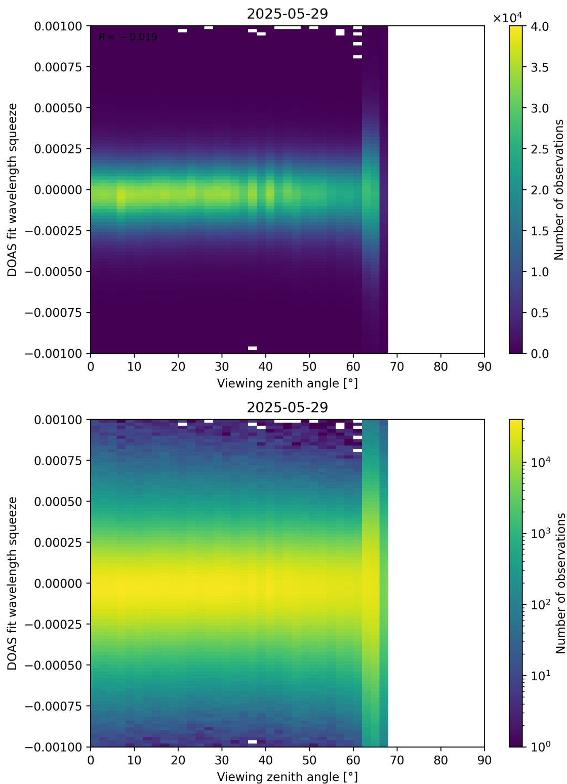
Figure 366: Scatter density plot of “Viewing zenith angle” against “DOAS fit wavelength squeeze” for 2025-05-28 to 2025-05-30.
