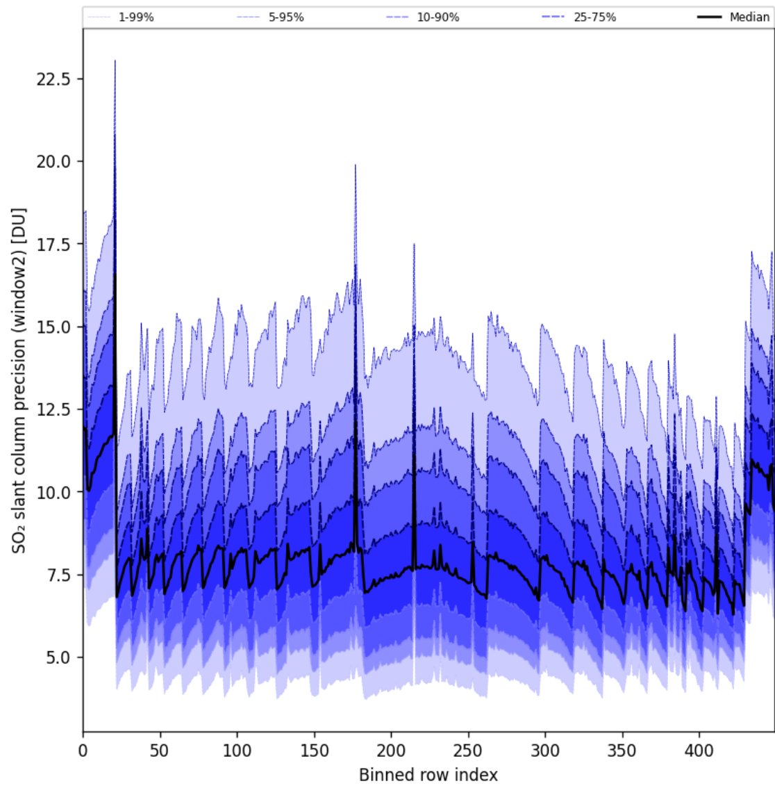
Figure 94: Along track statistics of “SO 2 slant column precision (window2)” for 2025-05-28 to 2025-05-30
