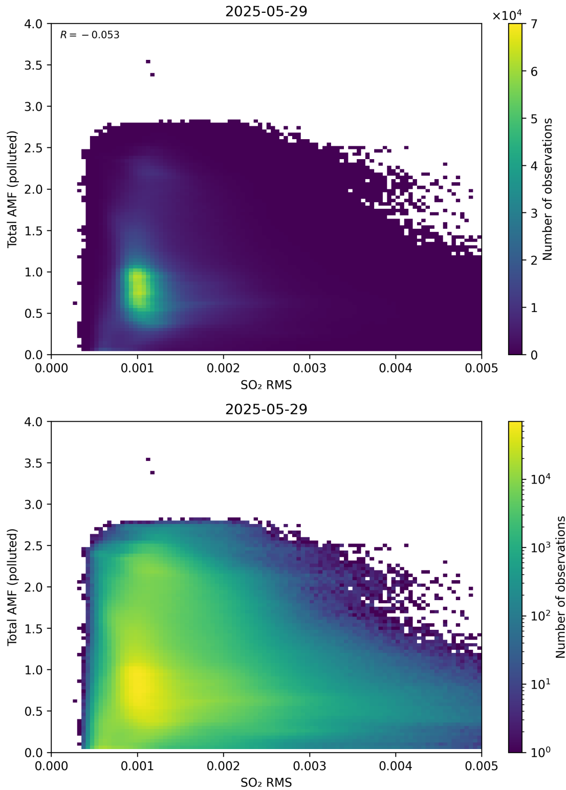
Figure 148: Scatter density plot of “SO 2 RMS” against “Total AMF (polluted)” for 2025-05-28 to 2025-05-30.
