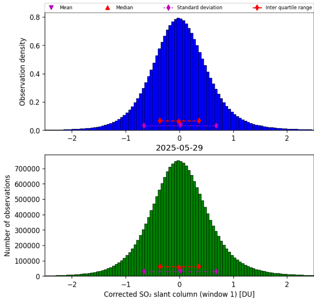
Figure 65: Histogram of “Corrected SO 2 slant column (window 1)” for 2025-05-28 to 2025-05-30
