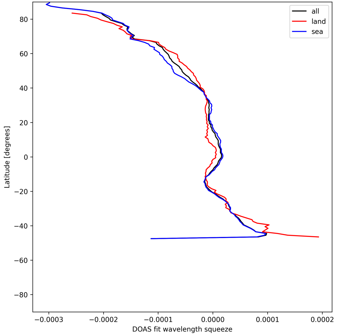
Figure 51: Zonal average of “DOAS fit wavelength squeeze” for 2025-05-28 to 2025-05-30.
