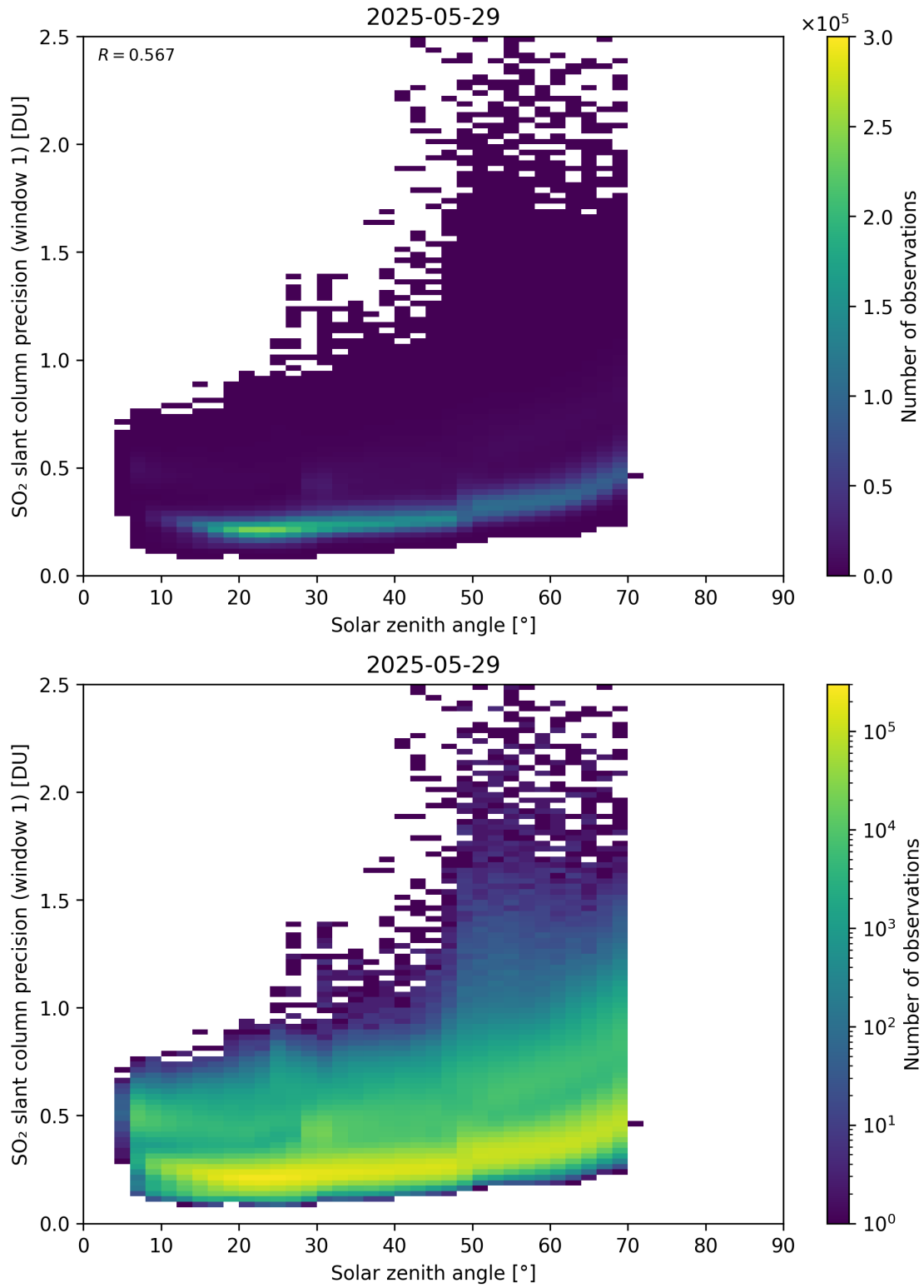
Figure 185: Scatter density plot of “Solar zenith angle” against “SO 2 slant column precision (window 1)” for 2025-05-28 to 2025-05-30.
