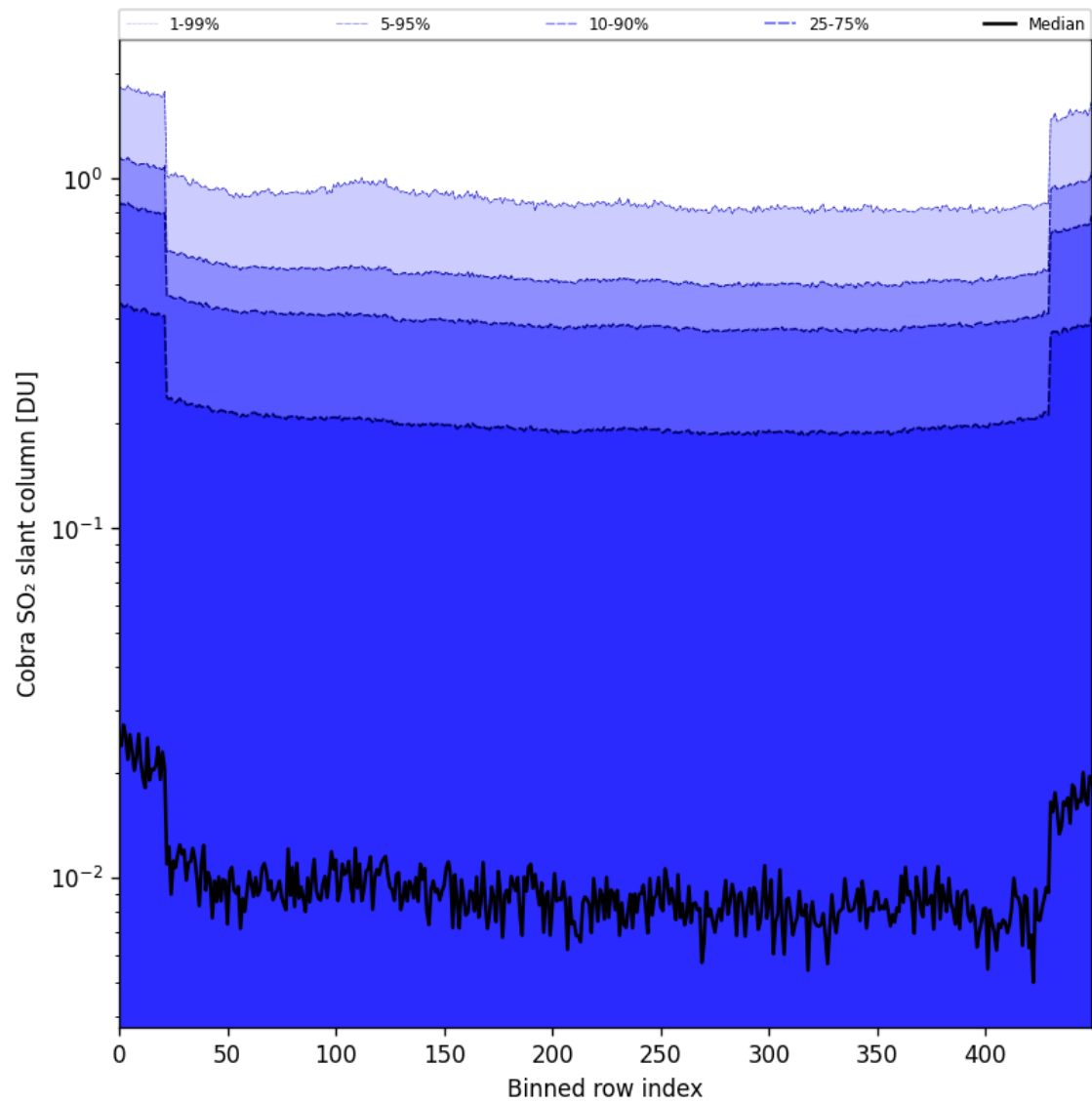
Figure 87: Along track statistics of “Cobra SO 2 slant column” for 2025-05-28 to 2025-05-30
