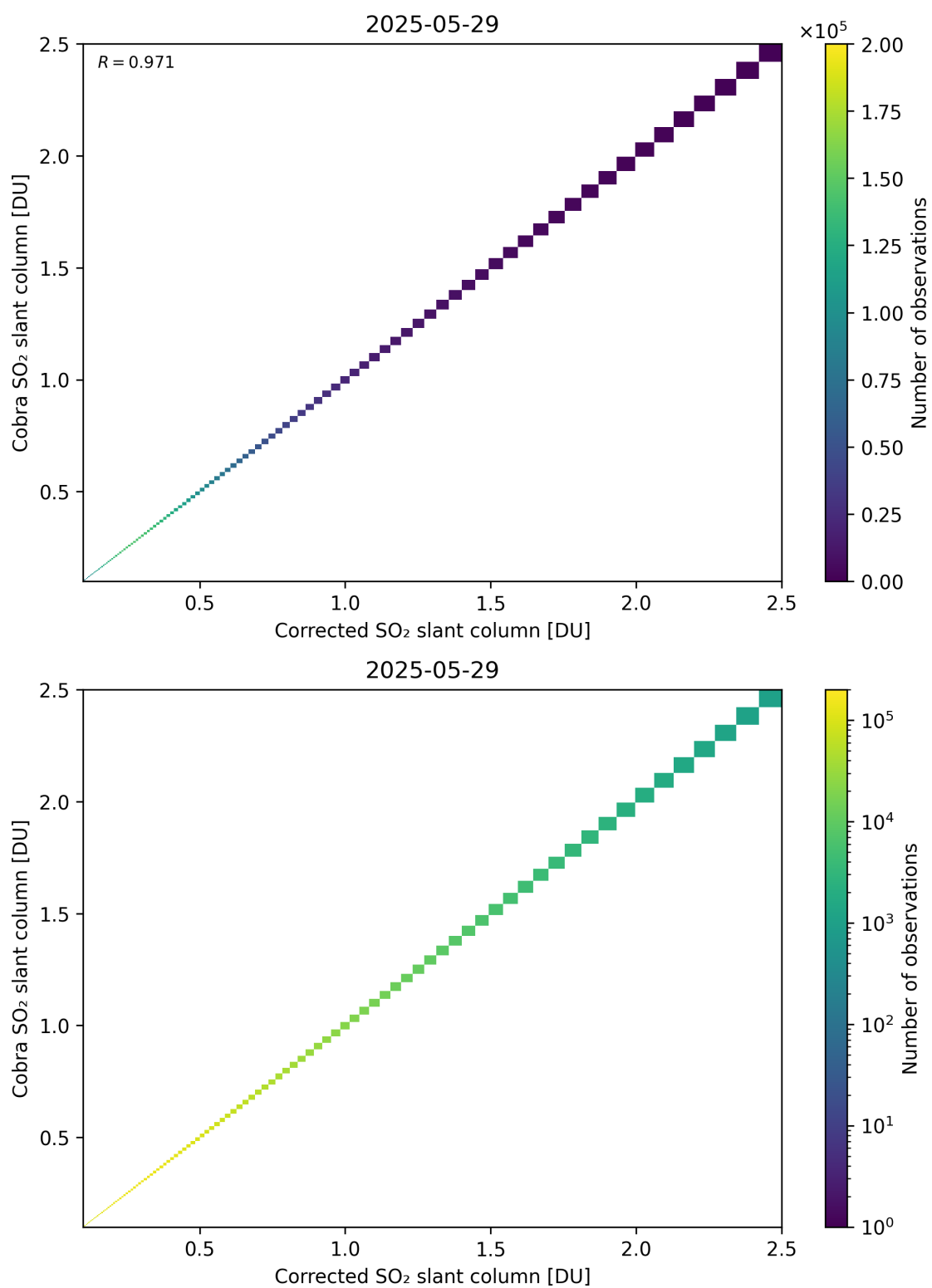
Figure 233: Scatter density plot of “Corrected SO 2 slant column” against “Cobra SO 2 slant column” for 2025-05-28 to 2025-05-30.
