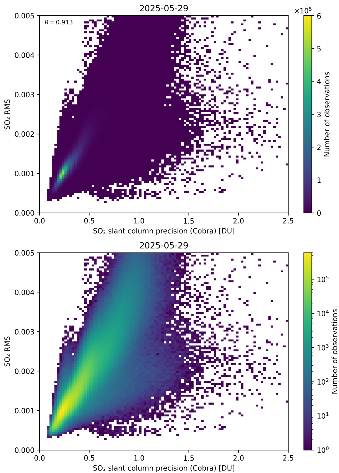
Figure 204: Scatter density plot of “SO 2 slant column precision (Cobra)” against “SO 2 RMS” for 2025-05-28 to 2025-05-30.
