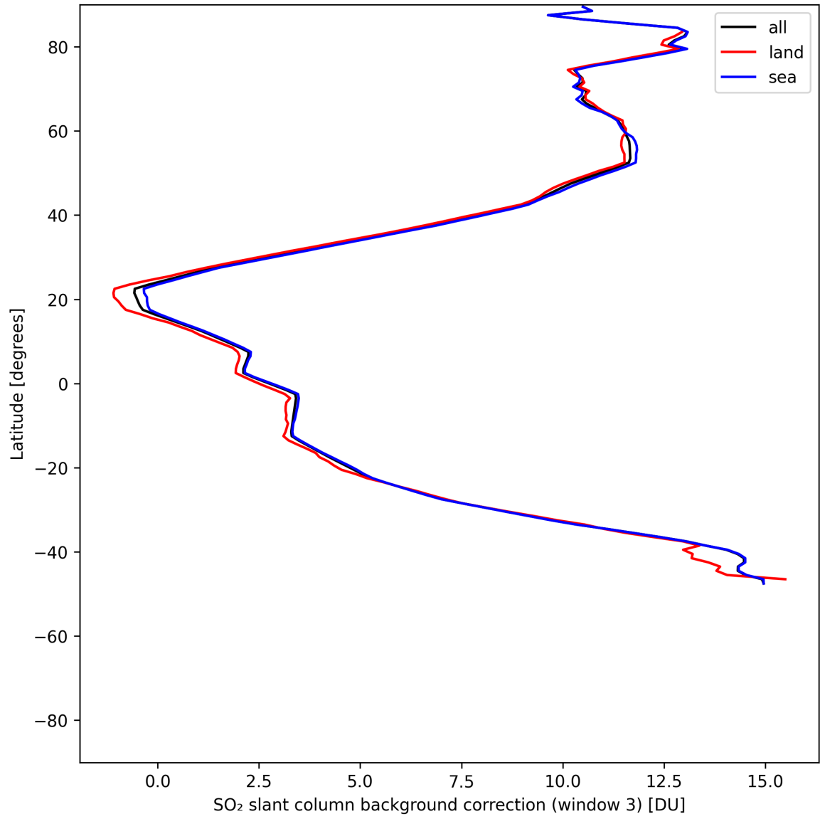
Figure 48: Zonal average of “SO 2 slant column background correction (window 3)” for 2025-05-28 to 2025-05-30.
