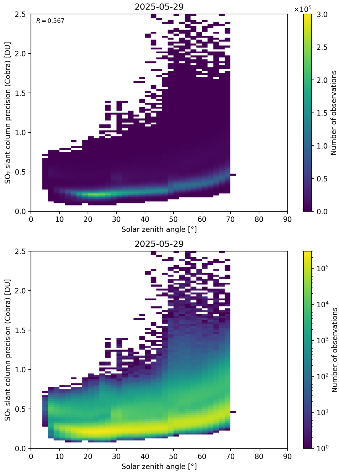
Figure 180: Scatter density plot of “Solar zenith angle” against “SO 2 slant column precision (Cobra)” for 2025-05-28 to 2025-05-30.
