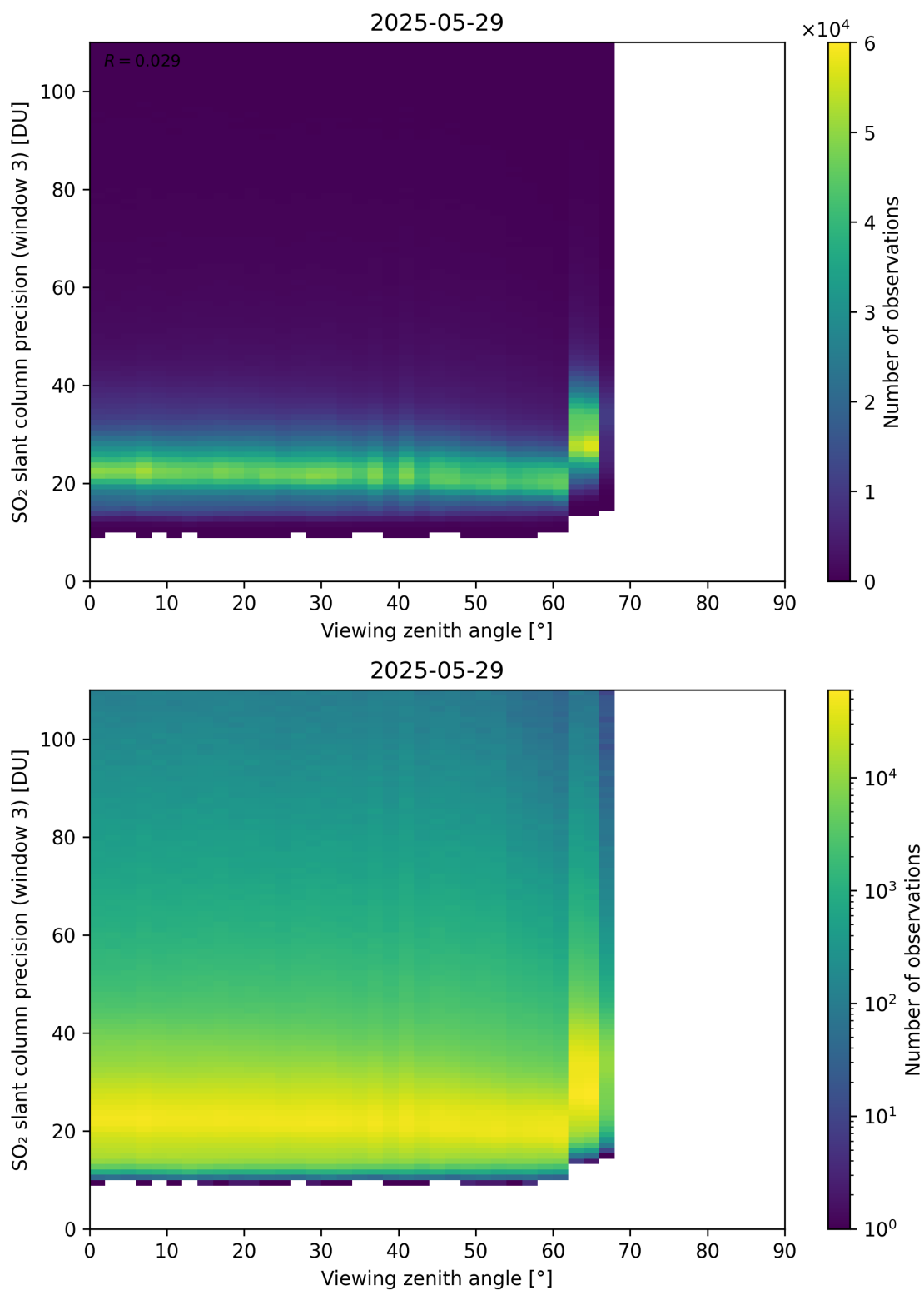
Figure 380: Scatter density plot of “Viewing zenith angle” against “SO 2 slant column precision (window 3)” for 2025-05-28 to 2025-05-30.
