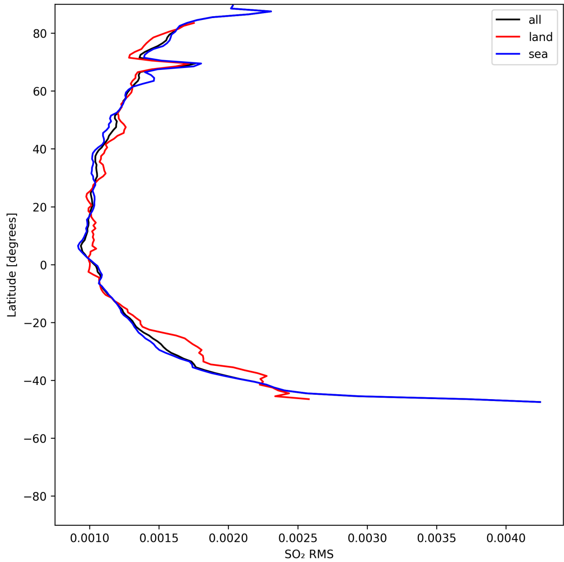
Figure 52: Zonal average of “SO 2 RMS” for 2025-05-28 to 2025-05-30.
