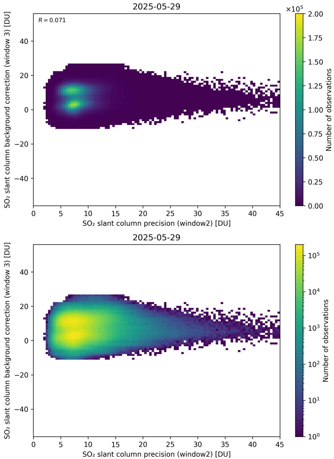
Figure 292: Scatter density plot of “SO 2 slant column precision (window2)” against “SO 2 slant column background correction (window 3)” for 2025-05-28 to 2025-05-30.
