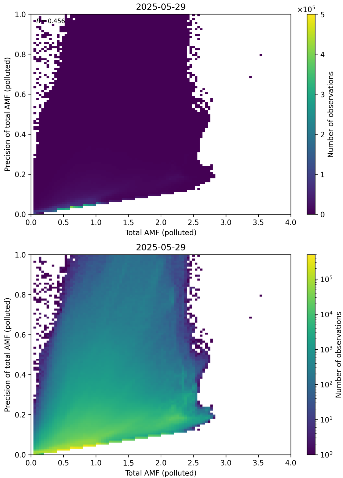
Figure 322: Scatter density plot of “Total AMF (polluted)” against “Precision of total AMF (polluted)” for 2025-05-28 to 2025-05-30.
