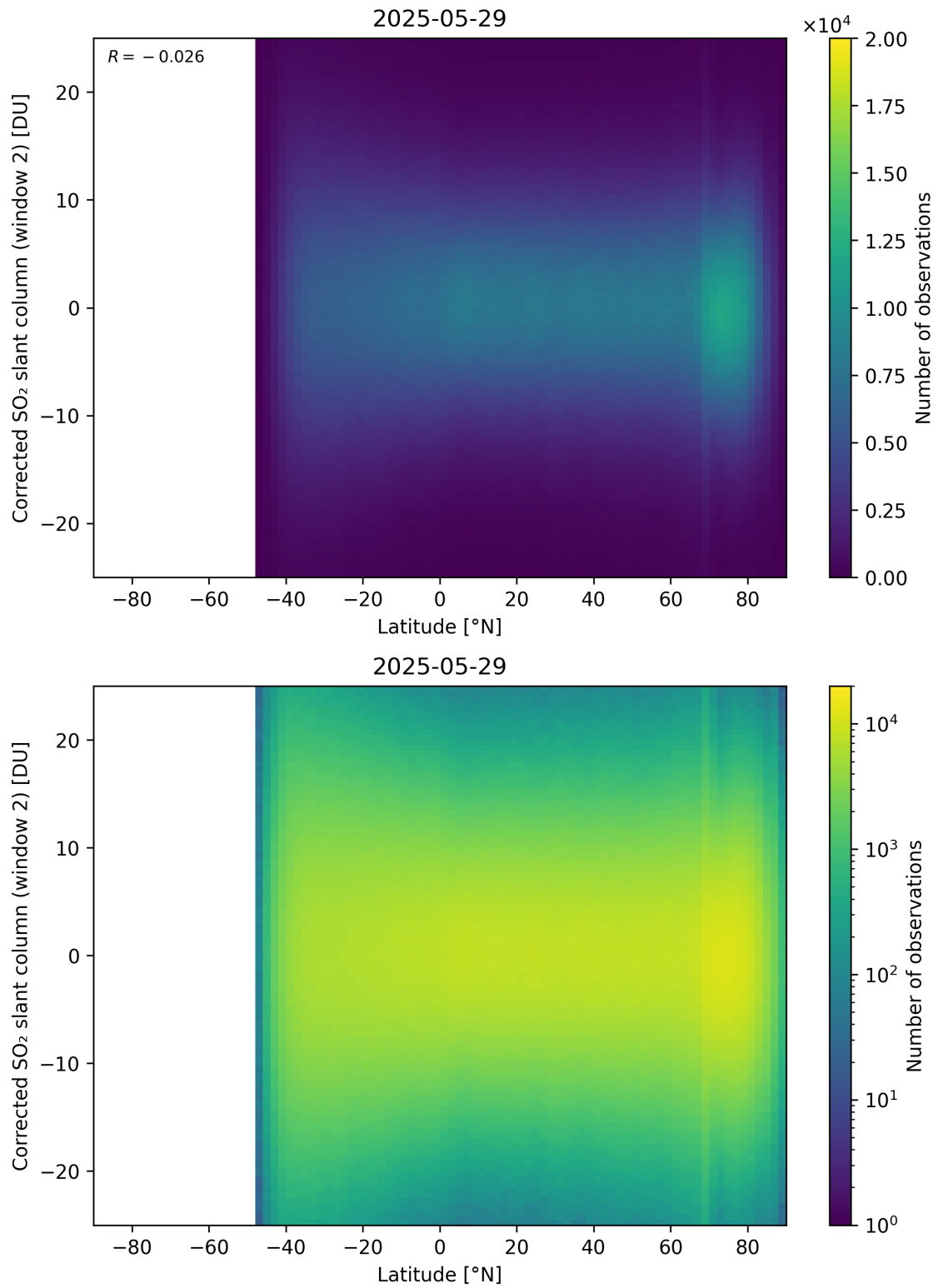
Figure 160: Scatter density plot of “Latitude” against “Corrected SO 2 slant column (window 2)” for 2025-05-28 to 2025-05-30.
