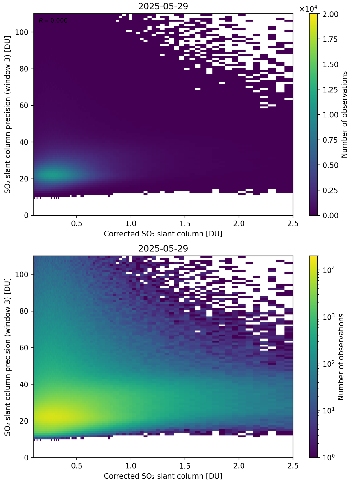
Figure 241: Scatter density plot of “Corrected SO 2 slant column” against “SO 2 slant column precision (window 3)” for 2025-05-28 to 2025-05-30.
