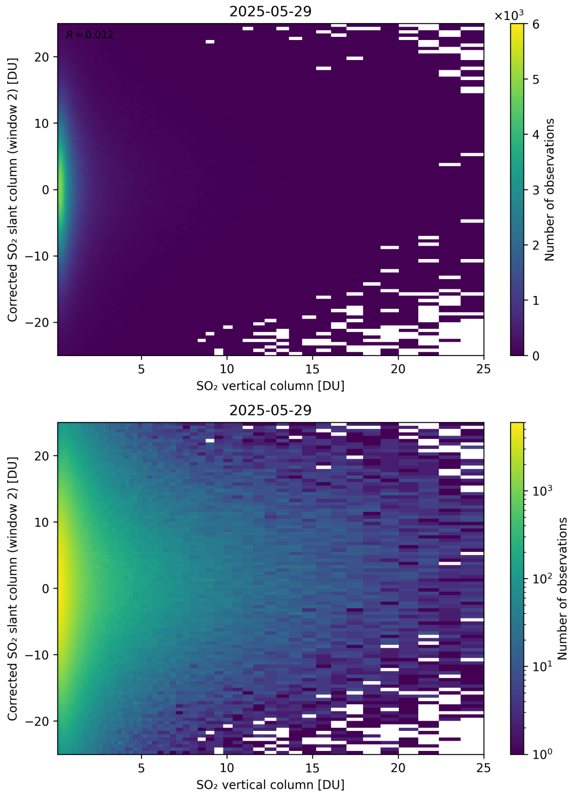
Figure 352: Scatter density plot of “SO 2 vertical column” against “Corrected SO 2 slant column (window 2)” for 2025-05-28 to 2025-05-30.
