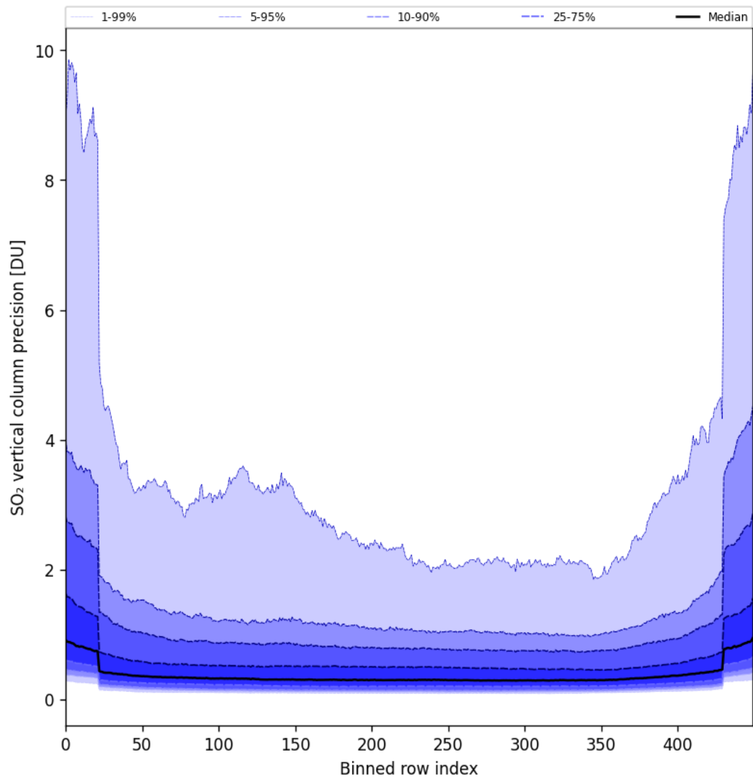
Figure 85: Along track statistics of “SO 2 vertical column precision” for 2025-05-28 to 2025-05-30
