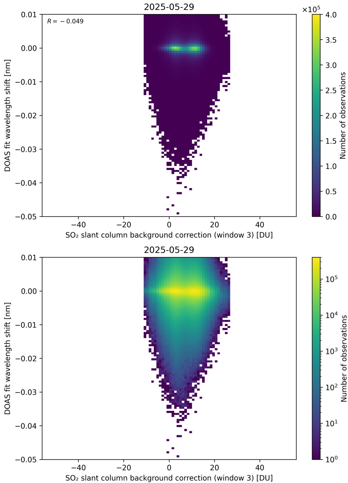
Figure 132: Scatter density plot of “SO 2 slant column background correction (window 3)” against “DOAS fit wavelength shift” for 2025-05-28 to 2025-05-30.
