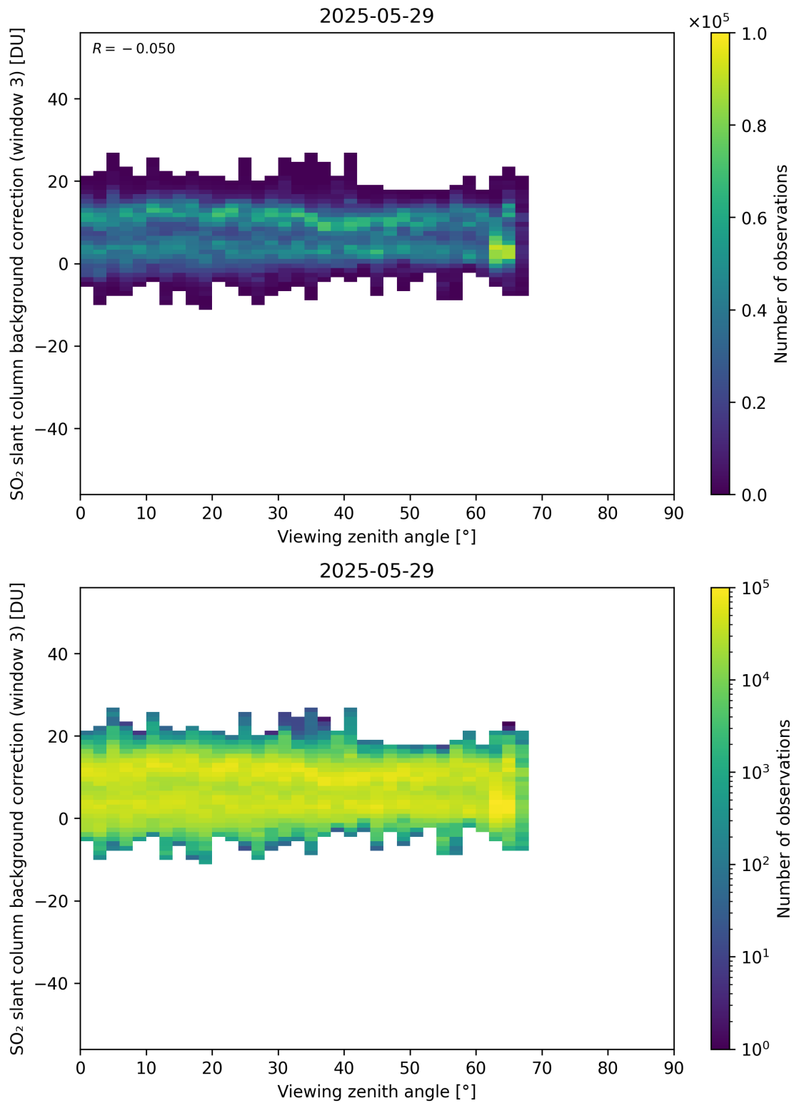
Figure 364: Scatter density plot of “Viewing zenith angle” against “SO 2 slant column background correction (window 3)” for 2025-05-28 to 2025-05-30.
