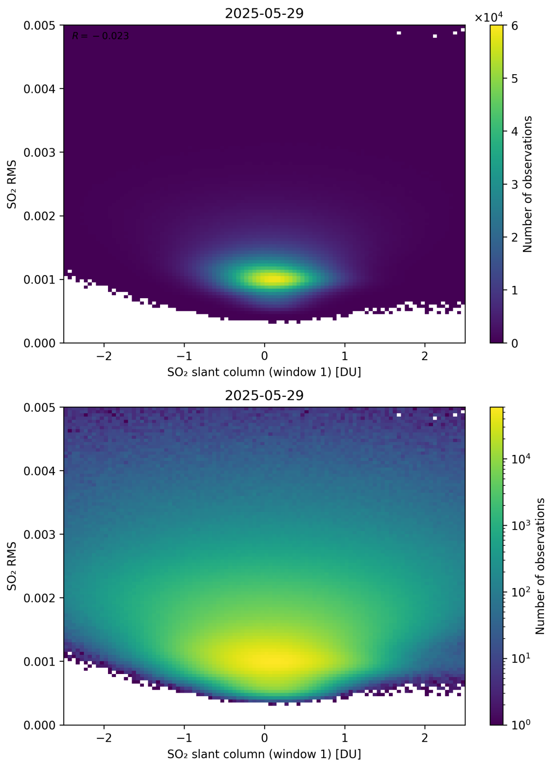
Figure 267: Scatter density plot of “SO 2 slant column (window 1)” against “SO 2 RMS” for 2025-05-28 to 2025-05-30.
