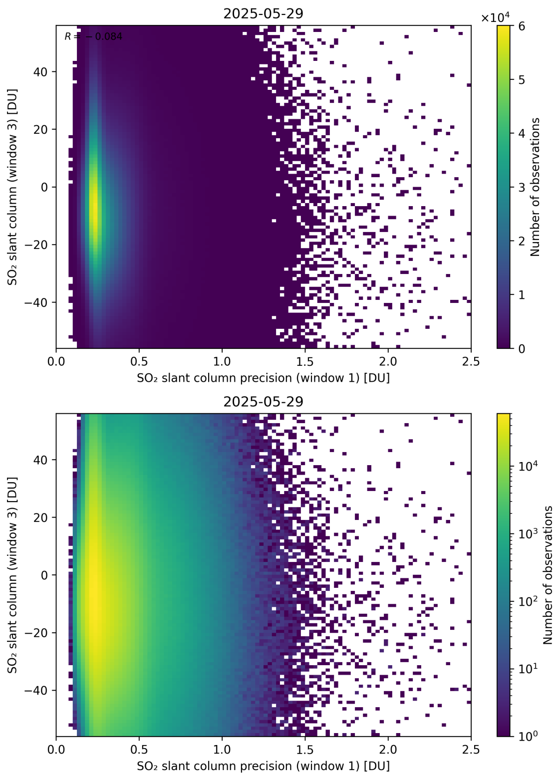
Figure 278: Scatter density plot of “SO 2 slant column precision (window 1)” against “SO 2 slant column (window 3)” for 2025-05-28 to 2025-05-30.
