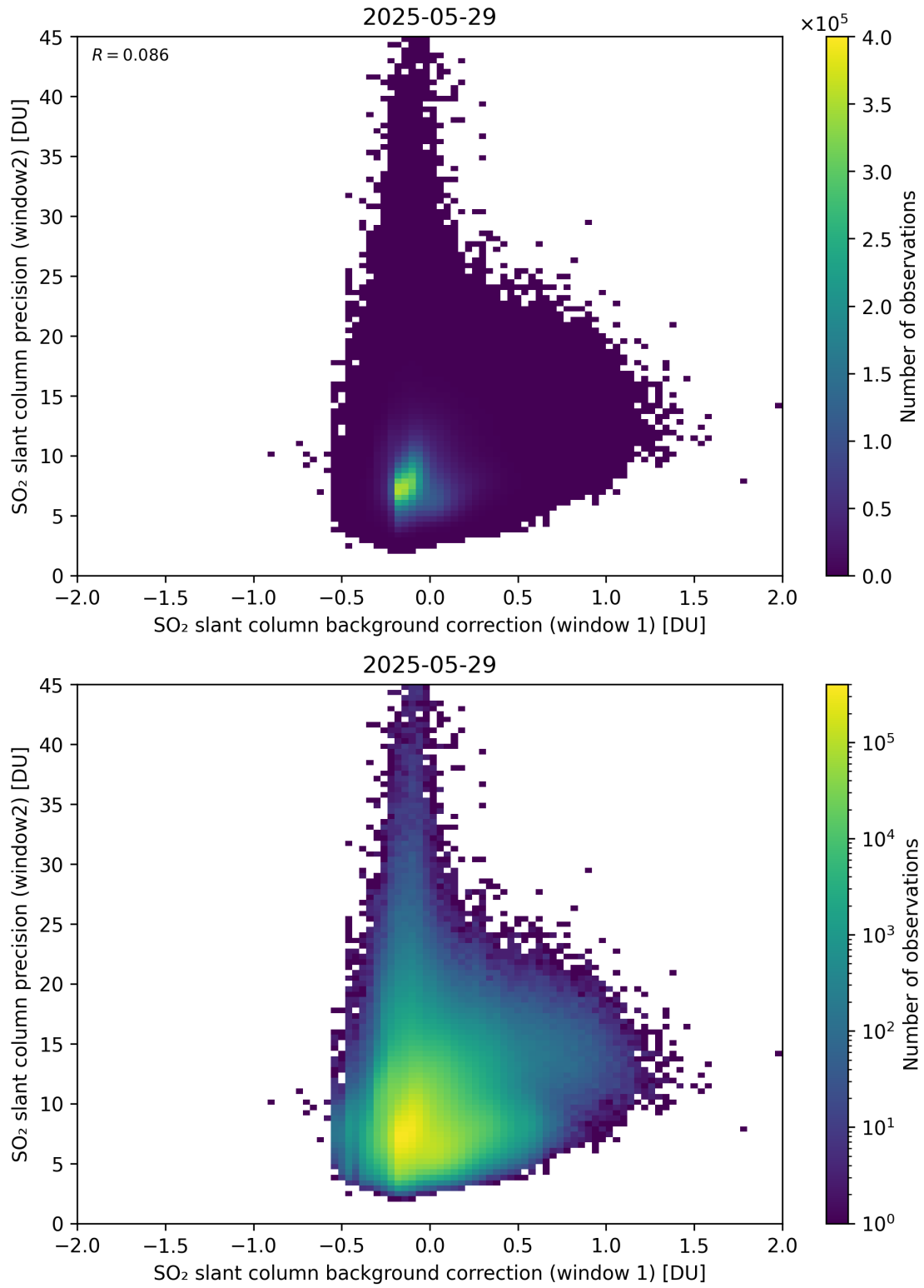
Figure 117: Scatter density plot of “SO 2 slant column background correction (window 1)” against “SO 2 slant column precision (window2)” for 2025-05-28 to 2025-05-30.
