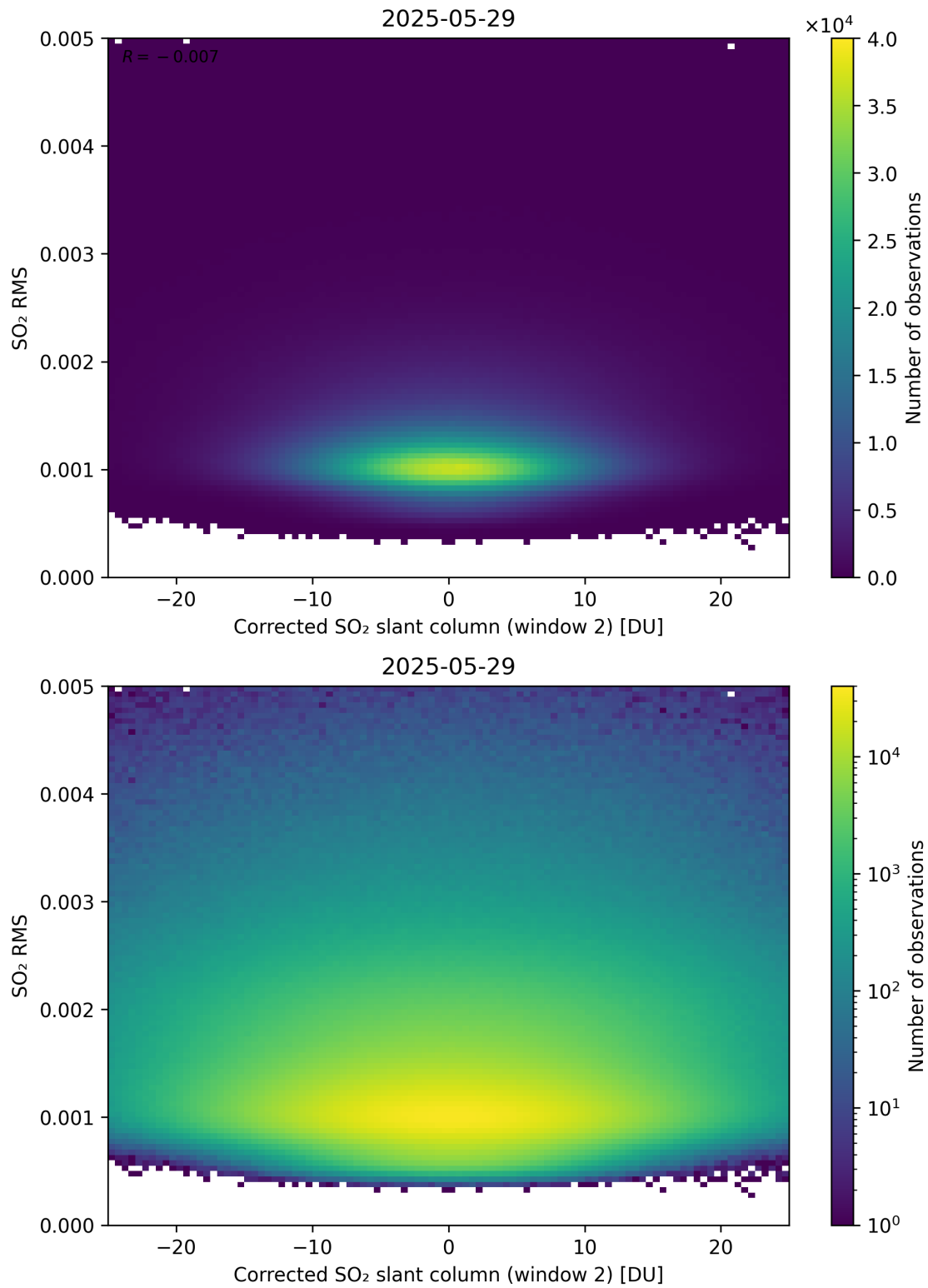
Figure 248: Scatter density plot of “Corrected SO 2 slant column (window 2)” against “SO 2 RMS” for 2025-05-28 to 2025-05-30.
