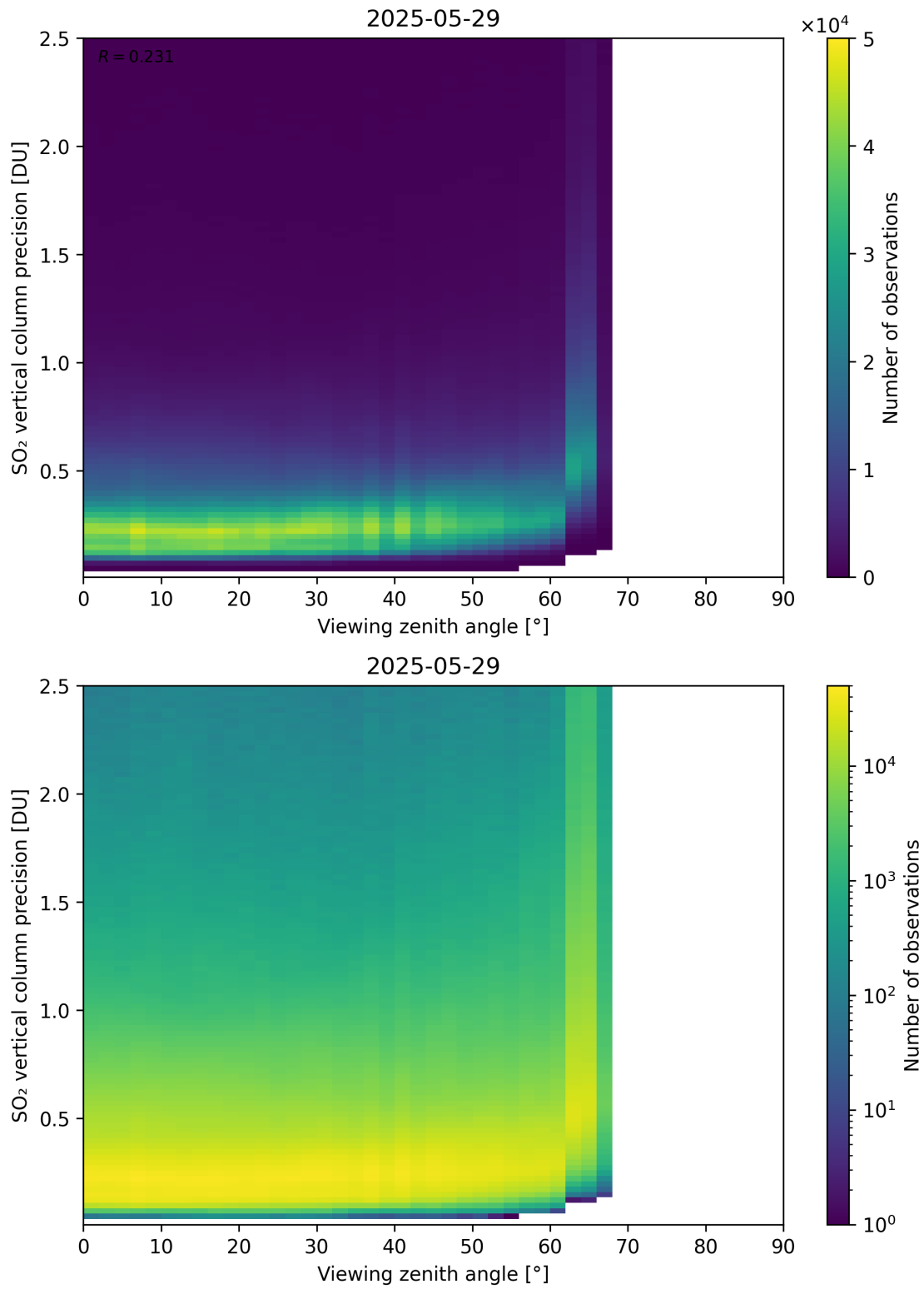
Figure 384: Scatter density plot of “Viewing zenith angle” against “SO 2 vertical column precision” for 2025-05-28 to 2025-05-30.
