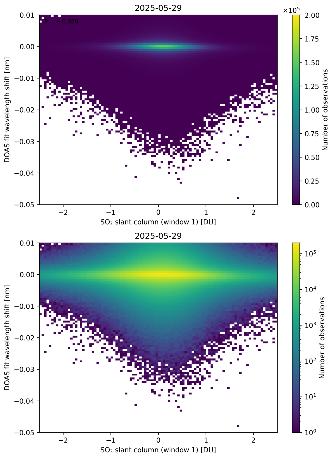
Figure 265: Scatter density plot of “SO 2 slant column (window 1)” against “DOAS fit wavelength shift” for 2025-05-28 to 2025-05-30.
