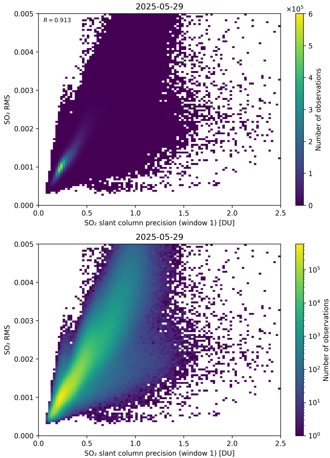
Figure 273: Scatter density plot of “SO 2 slant column precision (window 1)” against “SO 2 RMS” for 2025-05-28 to 2025-05-30.
