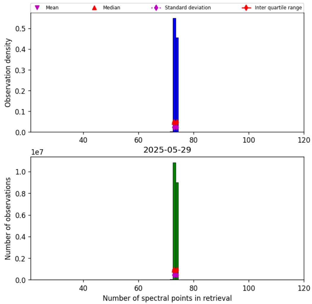
Figure 82: Histogram of “Number of spectral points in retrieval” for 2025-05-28 to 2025-05-30
