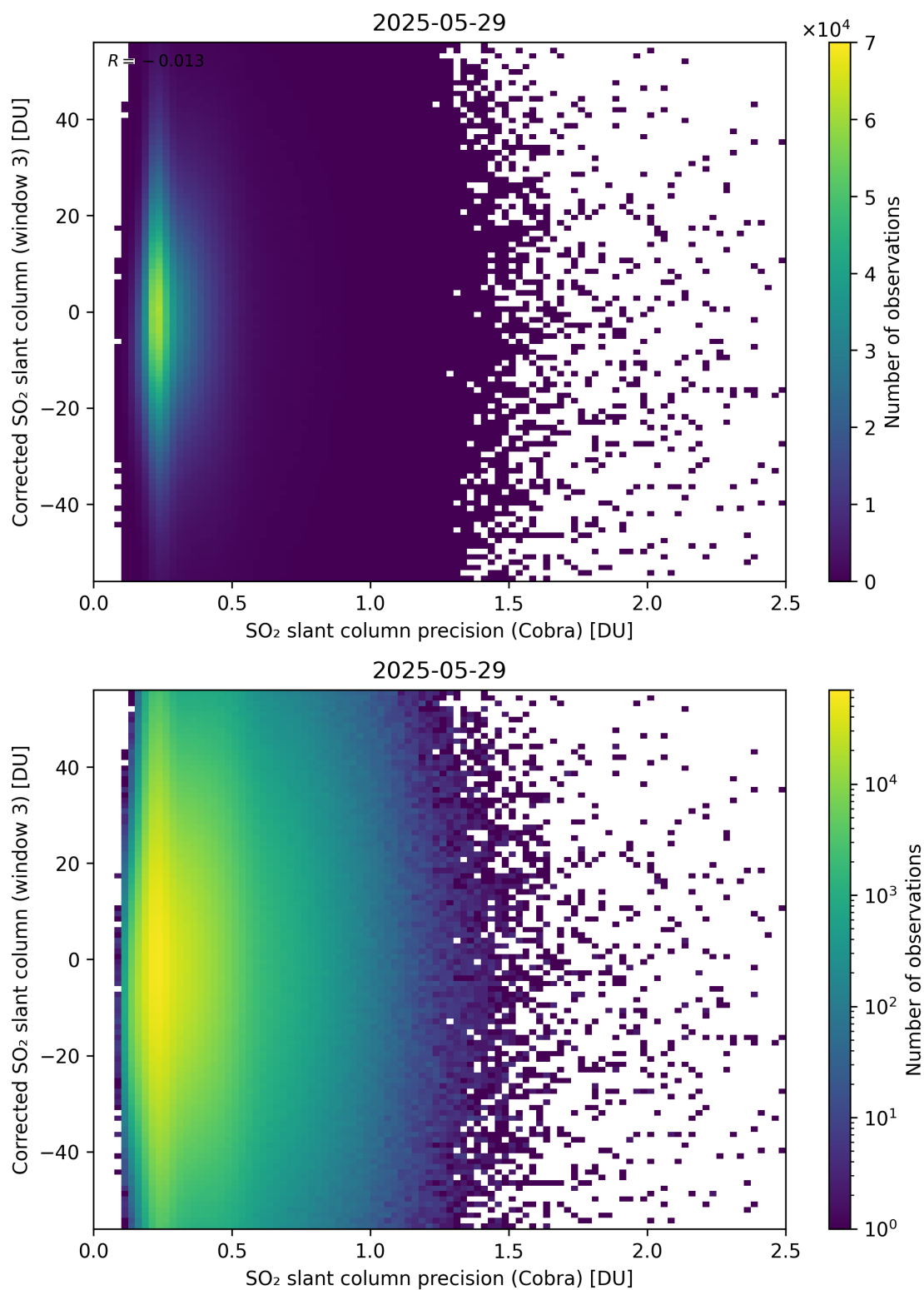
Figure 207: Scatter density plot of “SO 2 slant column precision (Cobra)” against “Corrected SO 2 slant column (window 3)” for 2025-05-28 to 2025-05-30.
