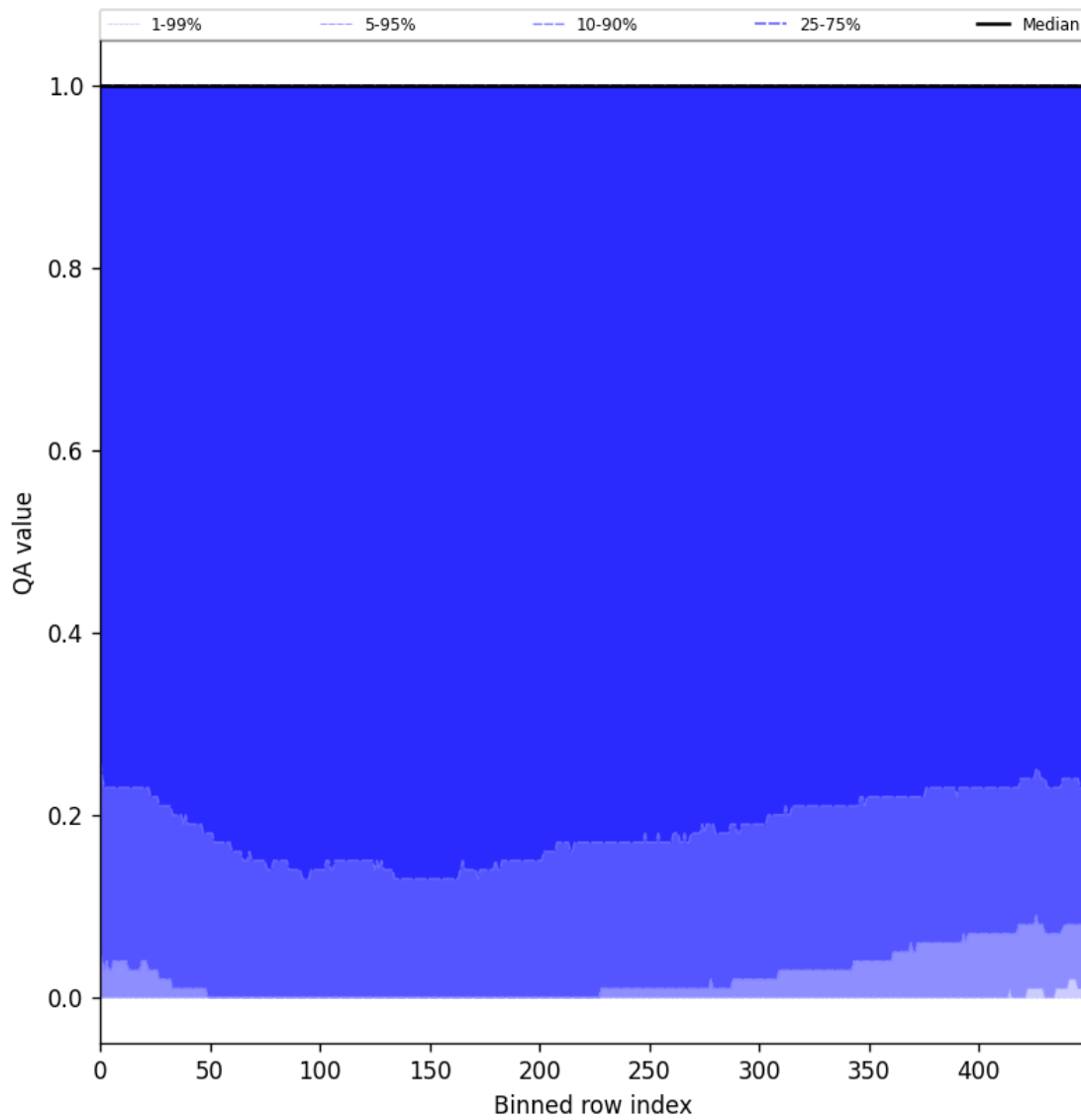
Figure 83: Along track statistics of “QA value” for 2025-05-28 to 2025-05-30
