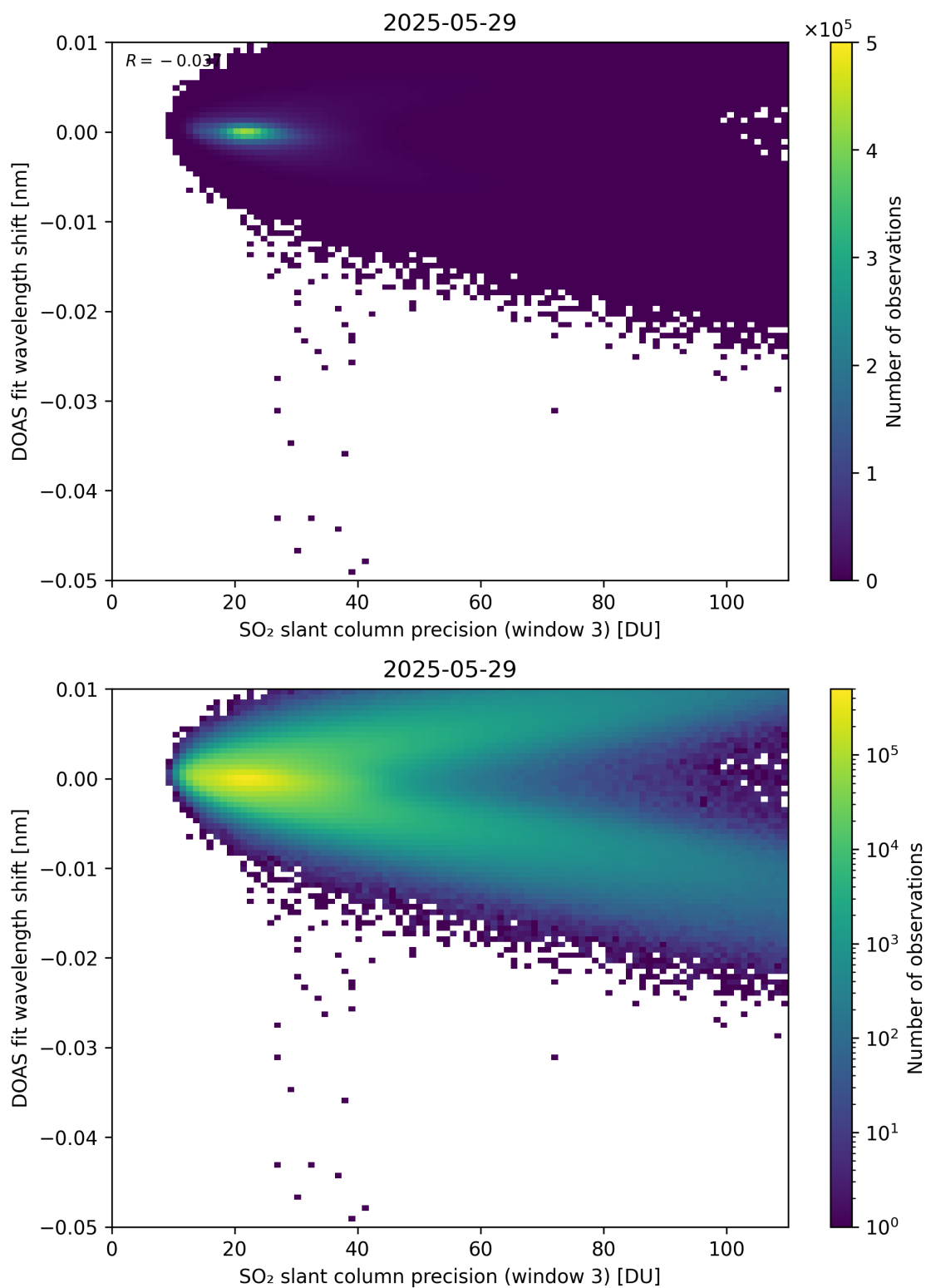
Figure 308: Scatter density plot of “SO 2 slant column precision (window 3)” against “DOAS fit wavelength shift” for 2025-05-28 to 2025-05-30.
