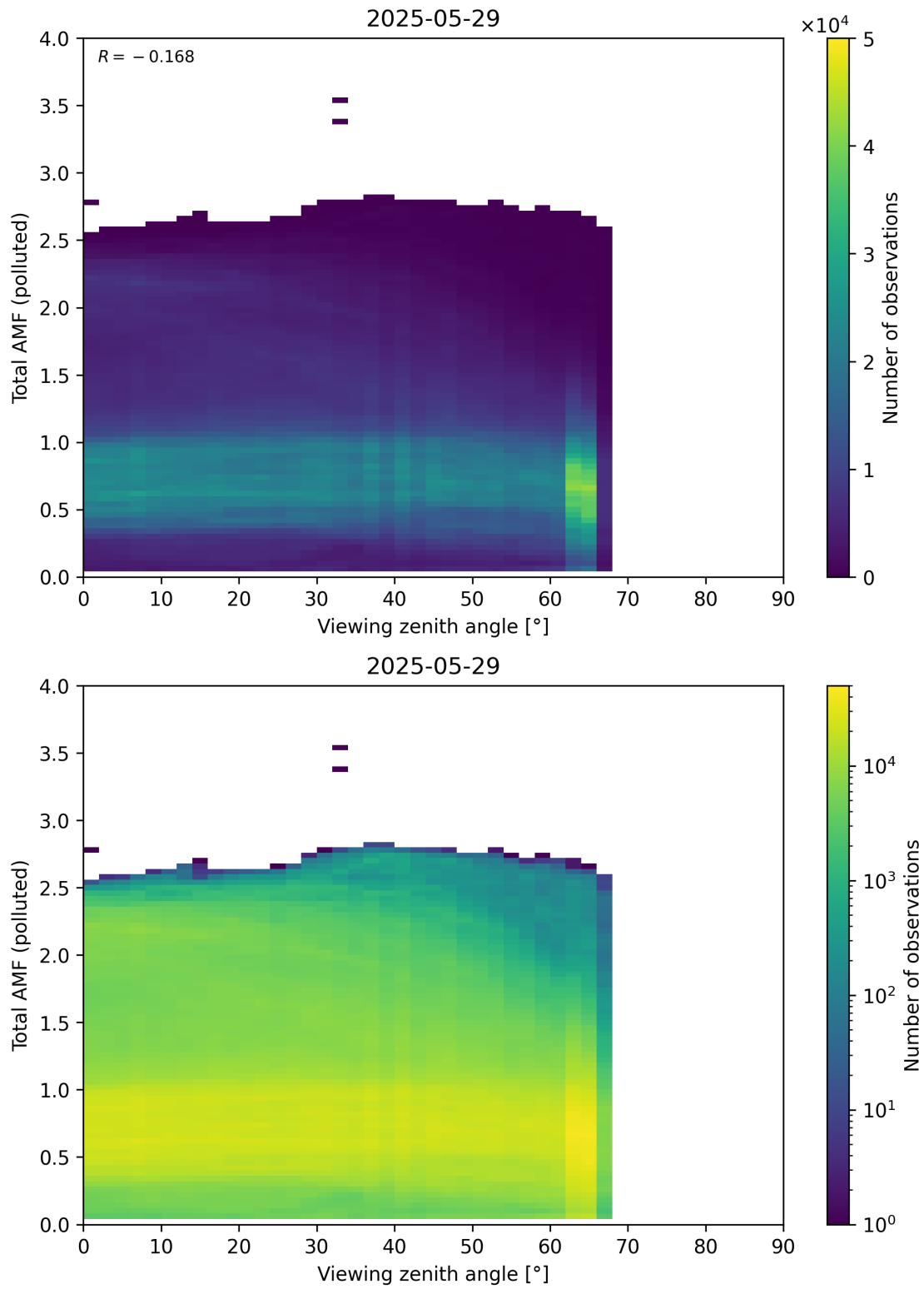
Figure 381: Scatter density plot of “Viewing zenith angle” against “Total AMF (polluted)” for 2025-05-28 to 2025-05-30.
