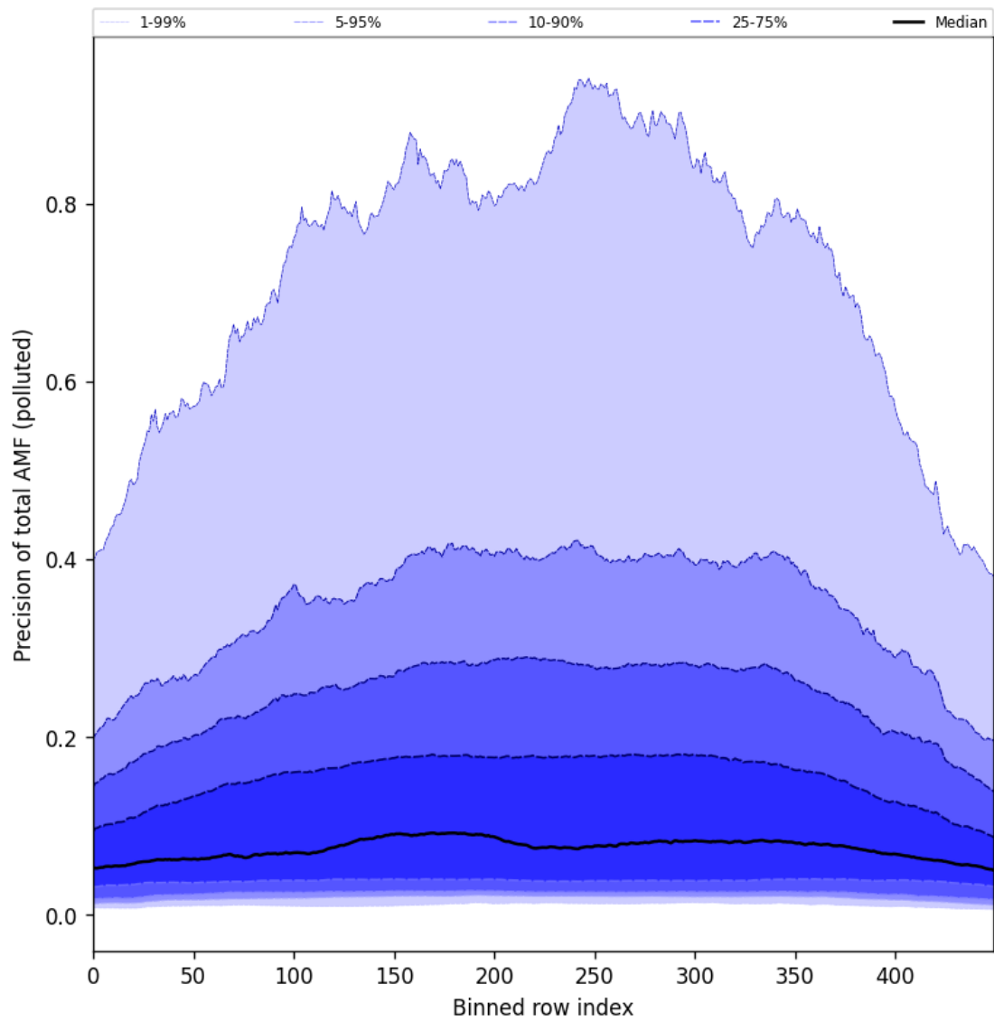
Figure 106: Along track statistics of “Precision of total AMF (polluted)” for 2025-05-28 to 2025-05-30
