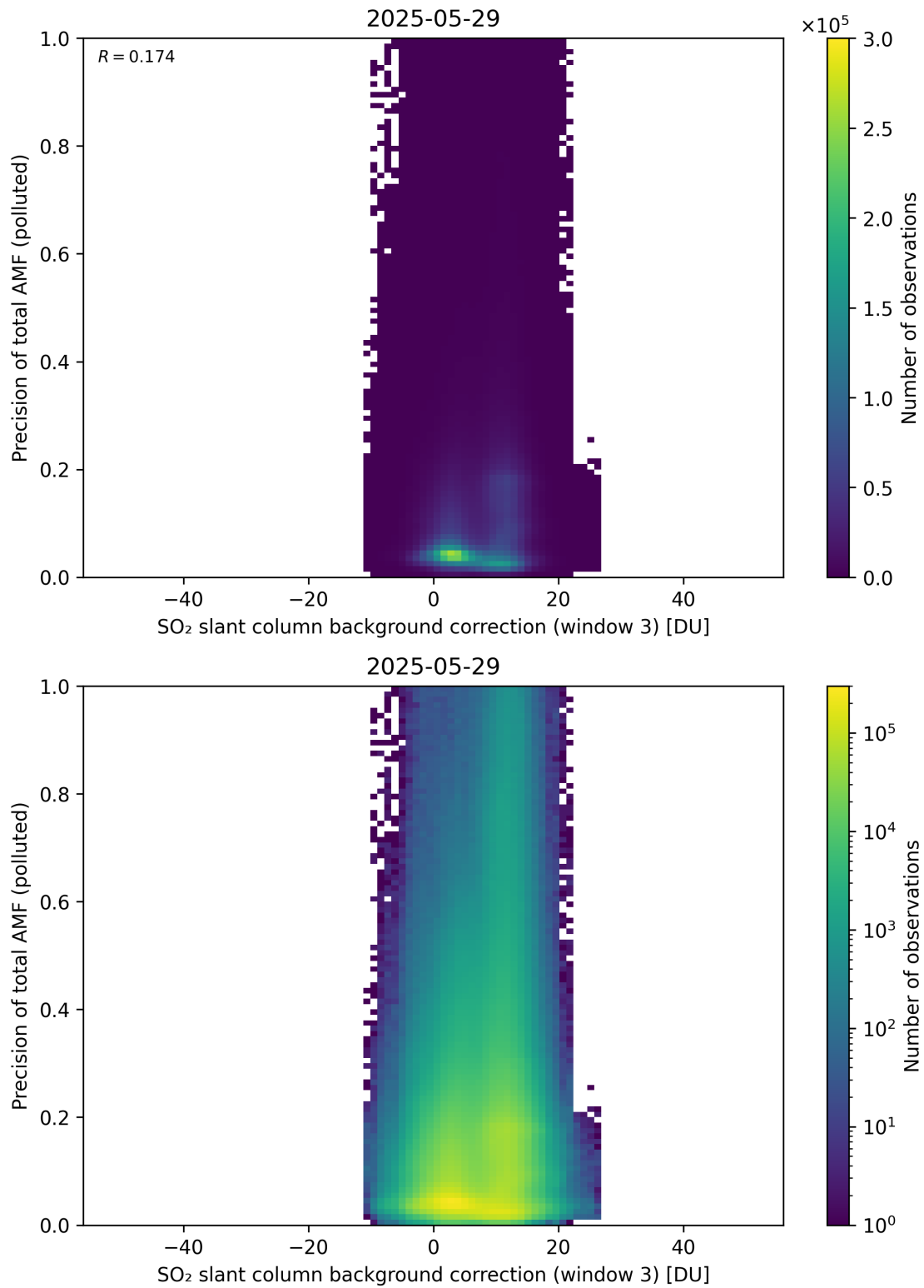
Figure 137: Scatter density plot of “SO 2 slant column background correction (window 3)” against “Precision of total AMF (polluted)” for 2025-05-28 to 2025-05-30.
