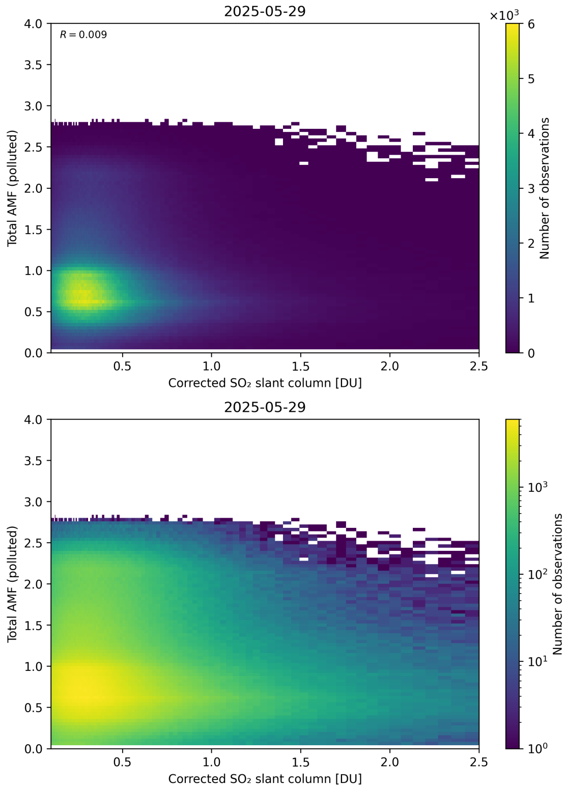
Figure 242: Scatter density plot of “Corrected SO 2 slant column” against “Total AMF (polluted)” for 2025-05-28 to 2025-05-30.
