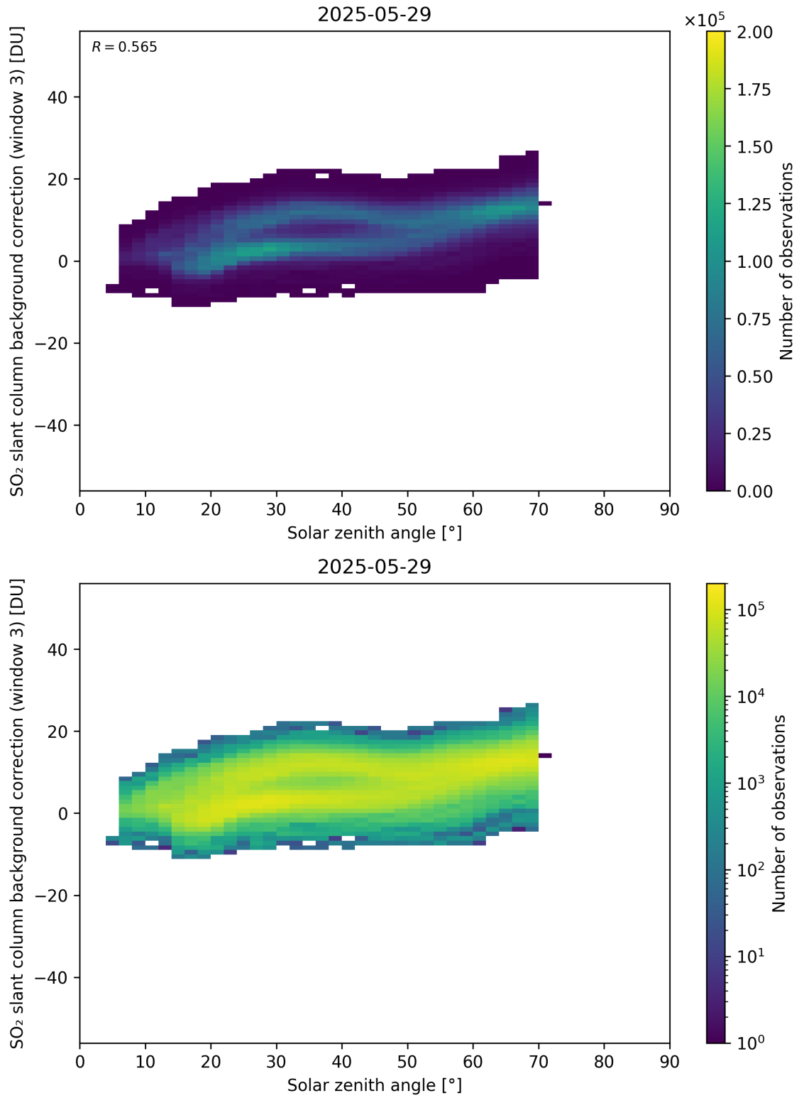
Figure 173: Scatter density plot of “Solar zenith angle” against “SO 2 slant column background correction (window 3)” for 2025-05-28 to 2025-05-30.
