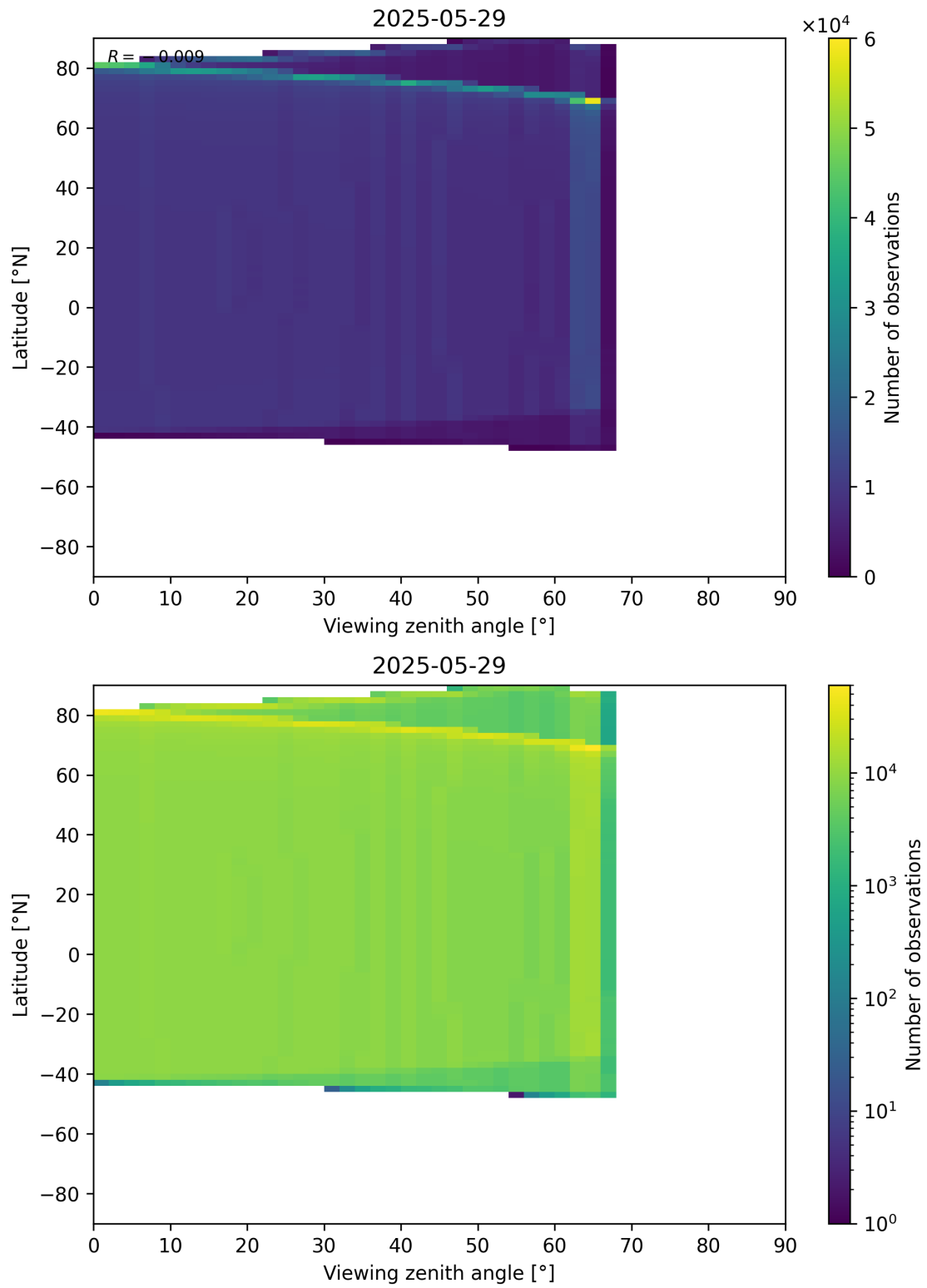
Figure 368: Scatter density plot of “Viewing zenith angle” against “Latitude” for 2025-05-28 to 2025-05-30.
