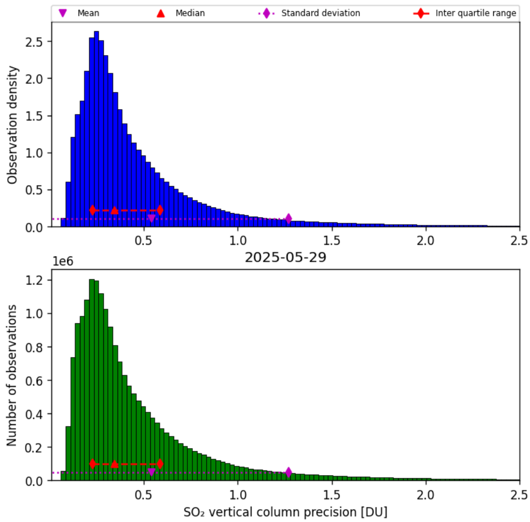
Figure 59: Histogram of “SO 2 vertical column precision” for 2025-05-28 to 2025-05-30
