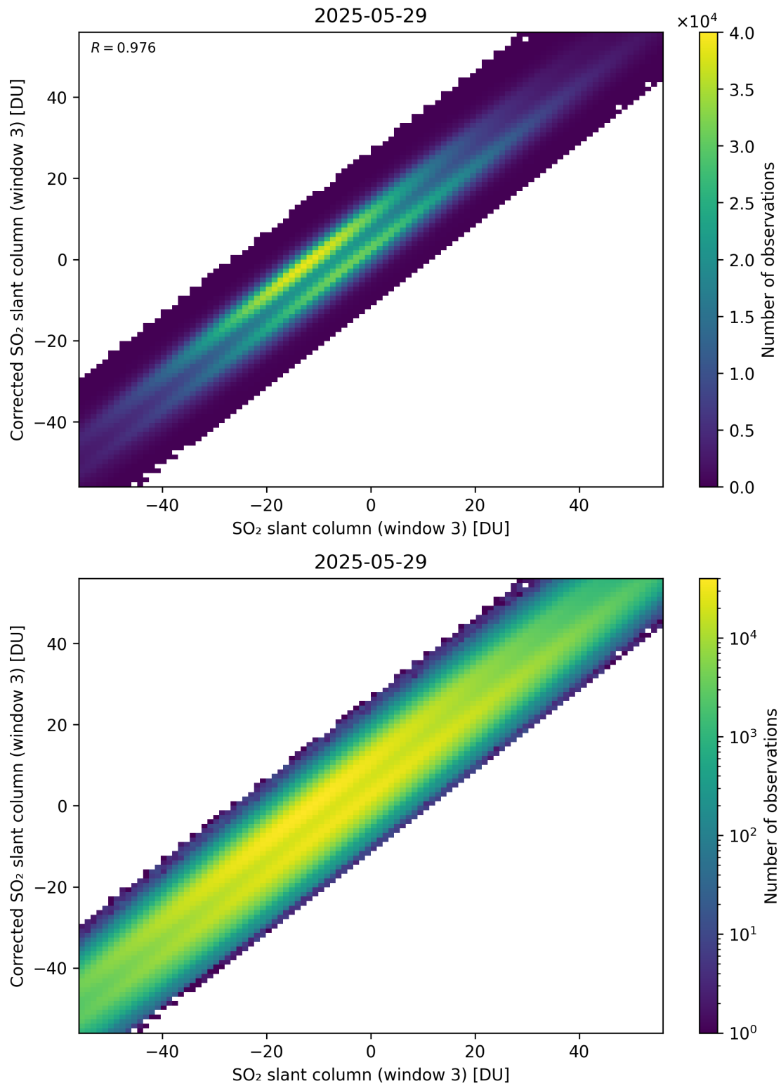
Figure 316: Scatter density plot of “SO 2 slant column (window 3)” against “Corrected SO 2 slant column (window 3)” for 2025-05-28 to 2025-05-30.
