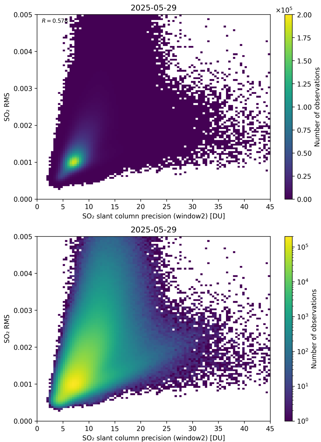
Figure 295: Scatter density plot of “SO 2 slant column precision (window2)” against “SO 2 RMS” for 2025-05-28 to 2025-05-30.
