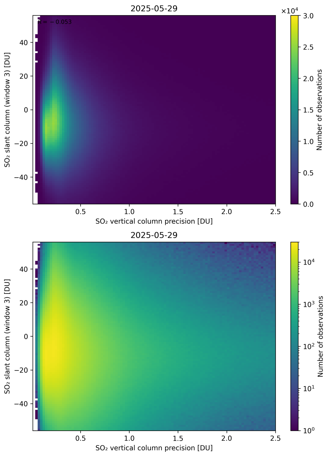
Figure 344: Scatter density plot of “SO 2 vertical column precision” against “SO 2 slant column (window 3)” for 2025-05-28 to 2025-05-30.
