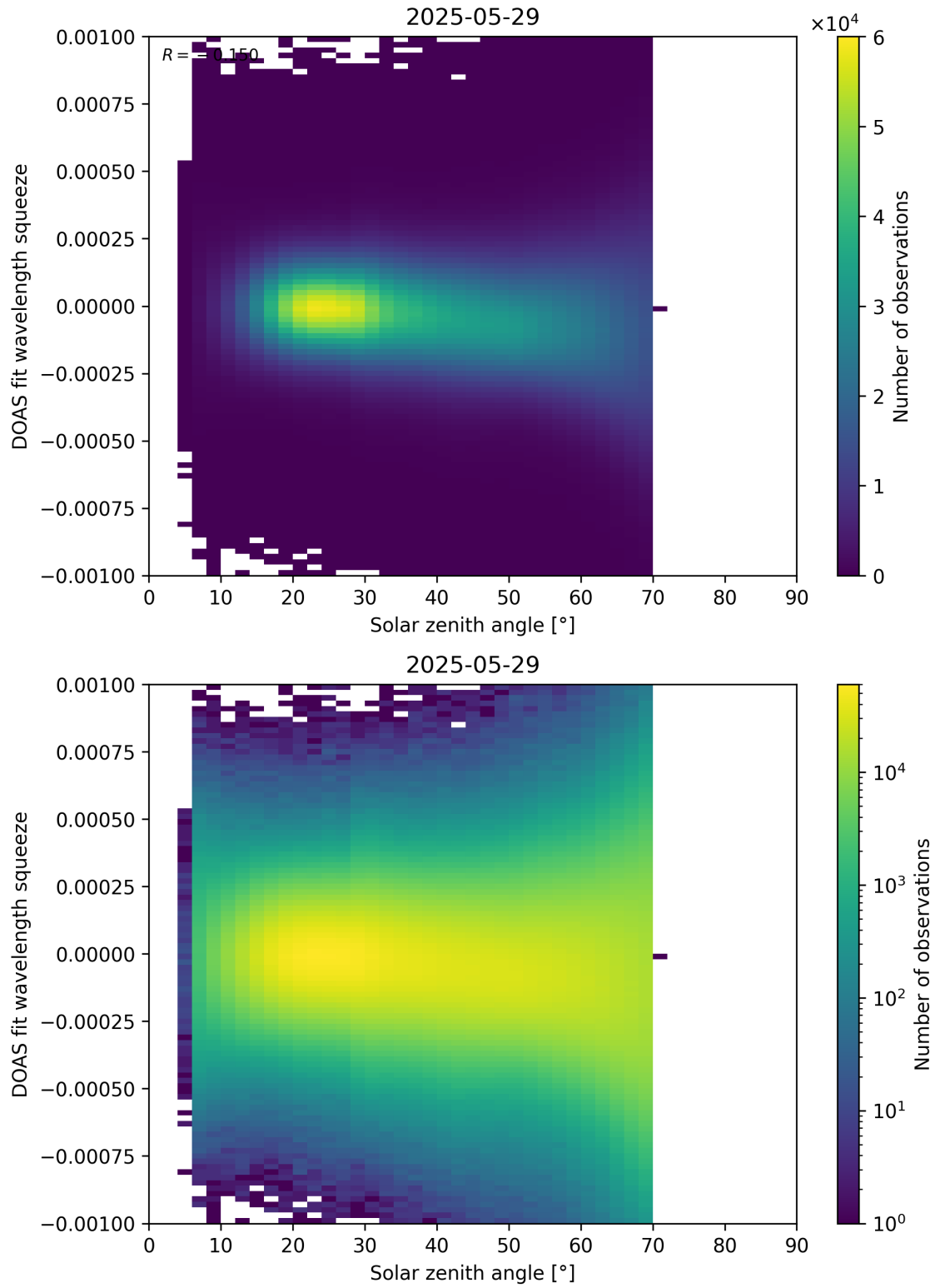
Figure 175: Scatter density plot of “Solar zenith angle” against “DOAS fit wavelength squeeze” for 2025-05-28 to 2025-05-30.
