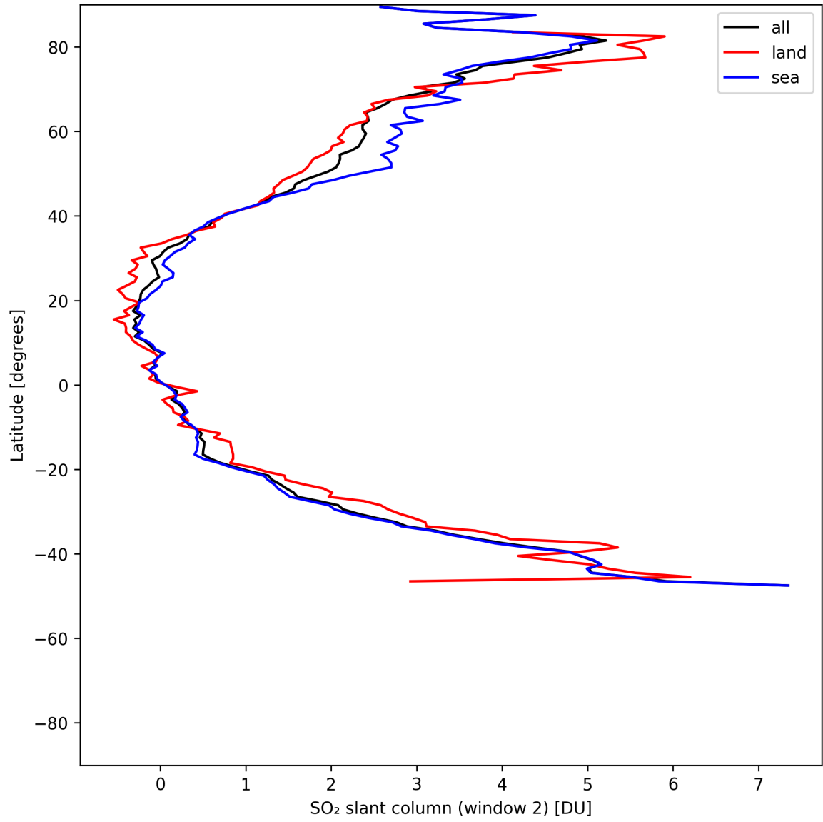
Figure 41: Zonal average of “SO 2 slant column (window 2)” for 2025-05-28 to 2025-05-30.
