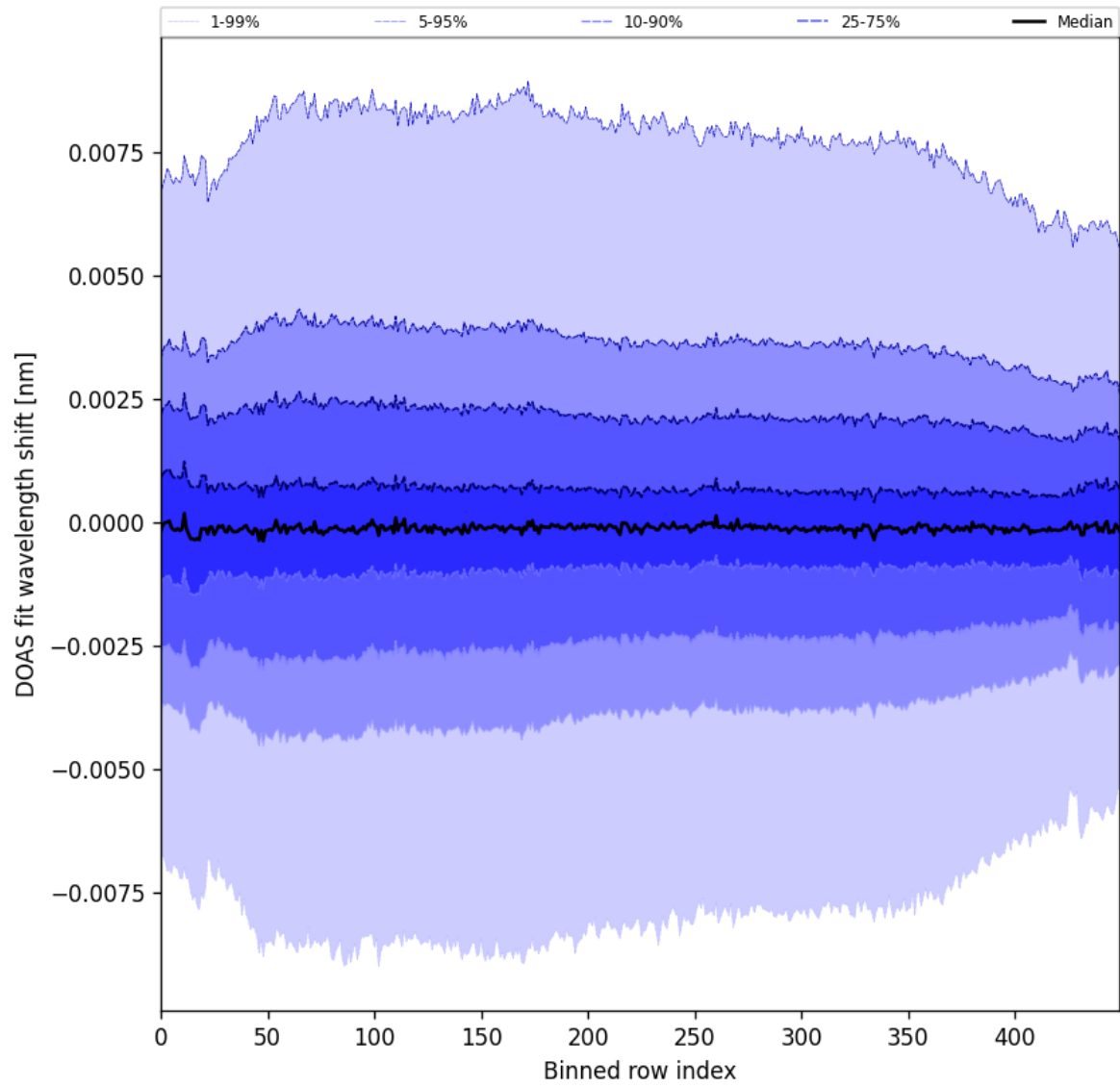
Figure 102: Along track statistics of “DOAS fit wavelength shift” for 2025-05-28 to 2025-05-30
