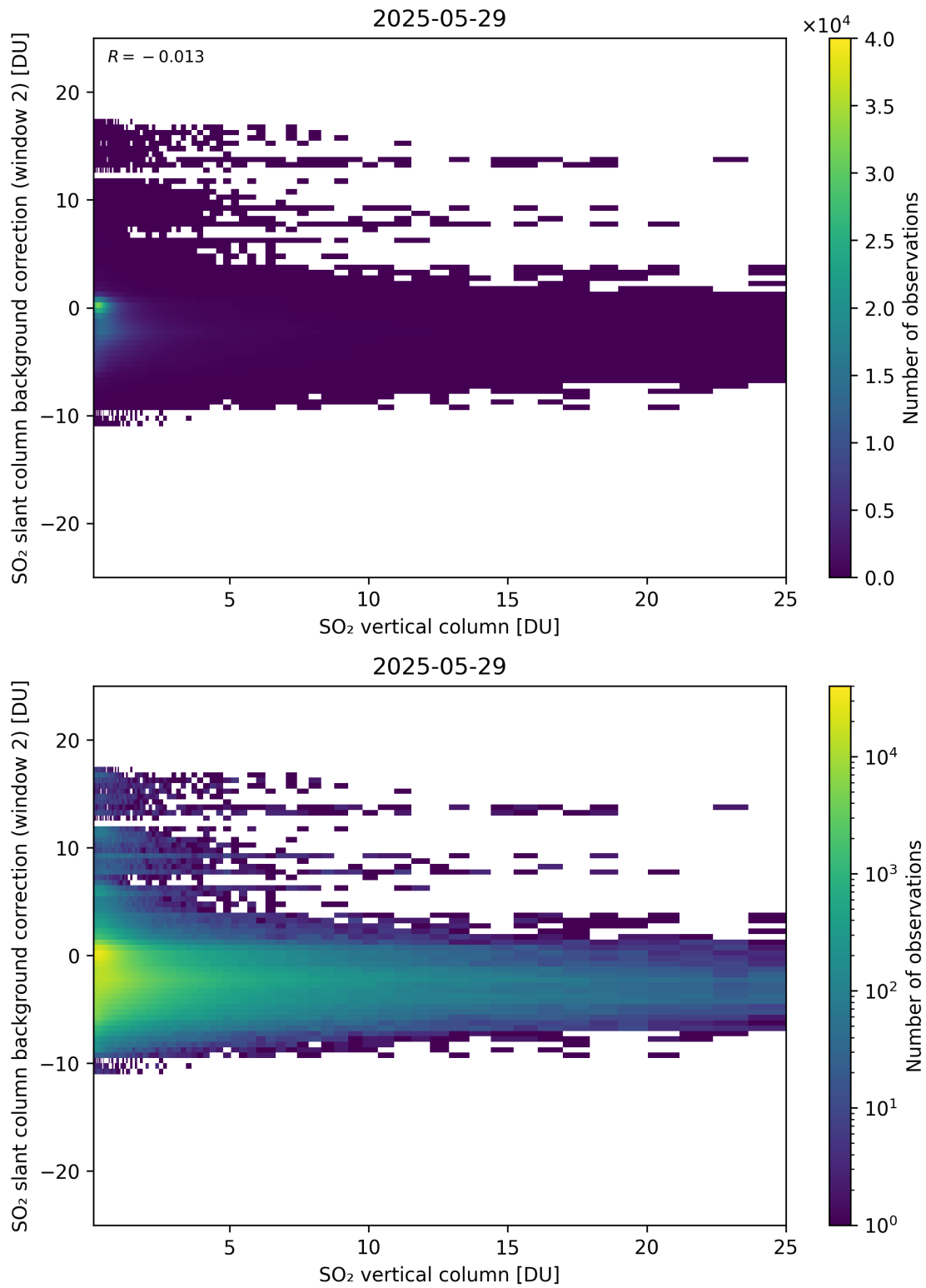
Figure 324: Scatter density plot of “SO 2 vertical column” against “SO 2 slant column background correction (window 2)” for 2025-05-28 to 2025-05-30.
