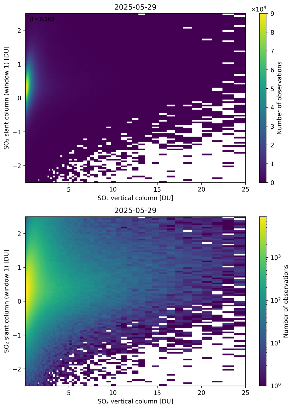
Figure 354: Scatter density plot of “SO 2 vertical column” against “SO 2 slant column (window 1)” for 2025-05-28 to 2025-05-30.
