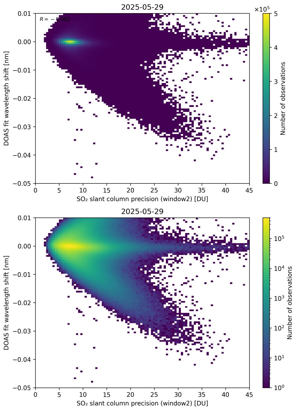
Figure 293: Scatter density plot of “SO 2 slant column precision (window2)” against “DOAS fit wavelength shift” for 2025-05-28 to 2025-05-30.
