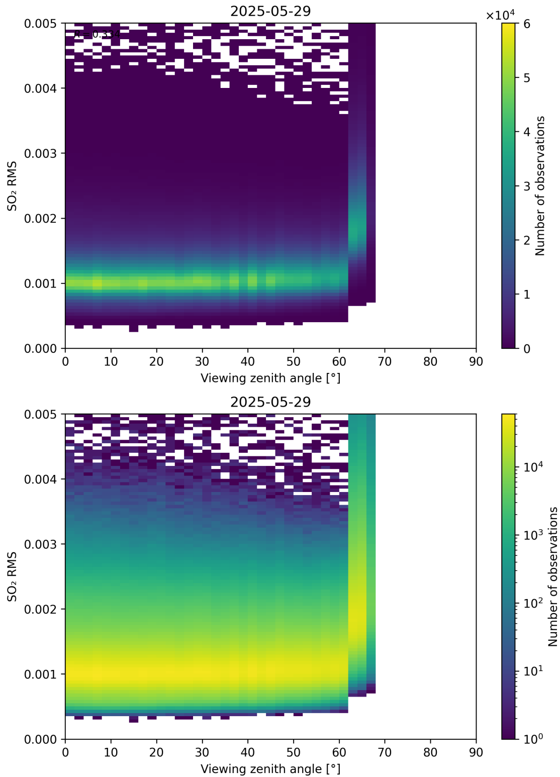
Figure 367: Scatter density plot of “Viewing zenith angle” against “SO 2 RMS” for 2025-05-28 to 2025-05-30.
