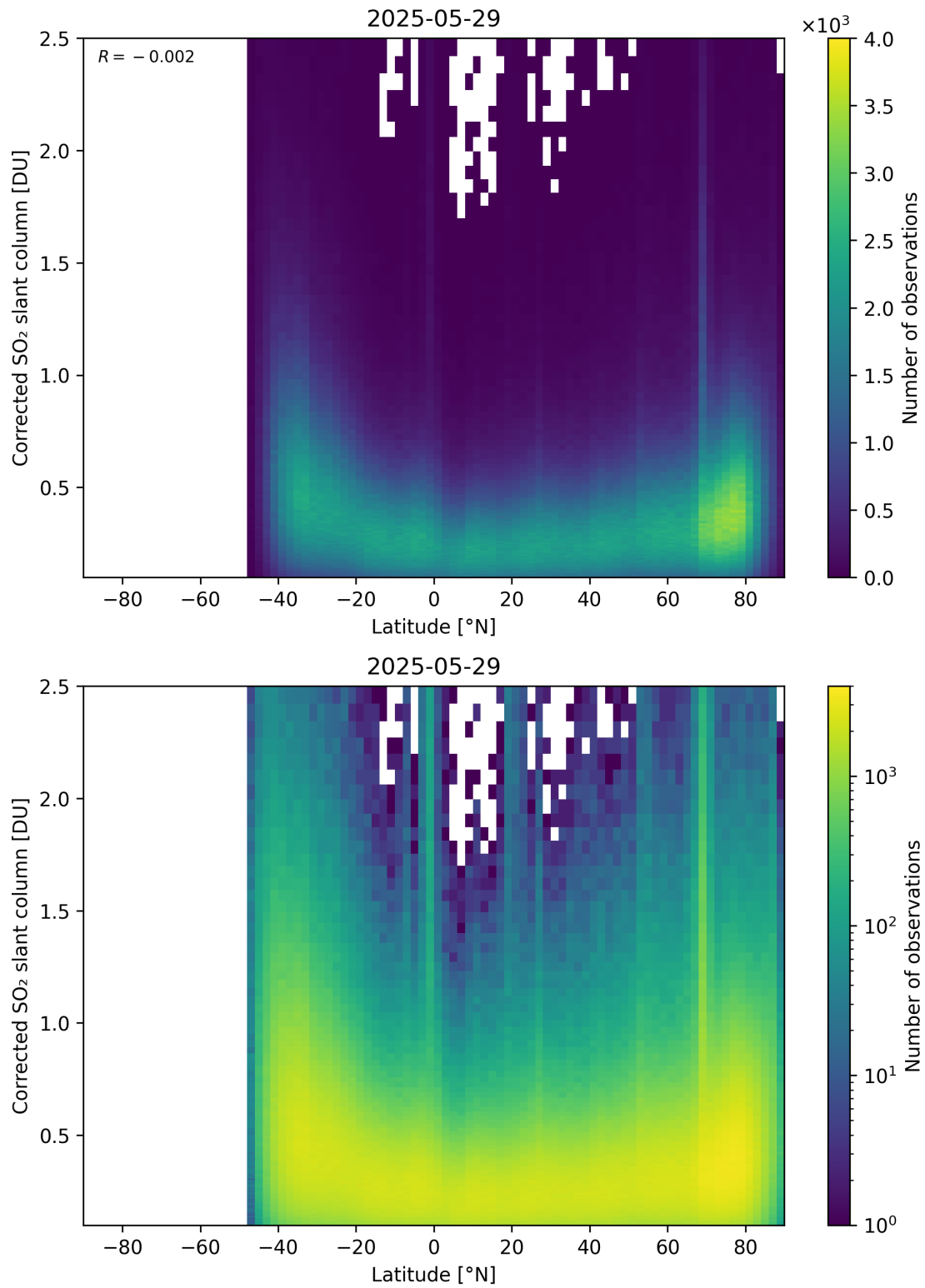
Figure 159: Scatter density plot of “Latitude” against “Corrected SO 2 slant column” for 2025-05-28 to 2025-05-30.
