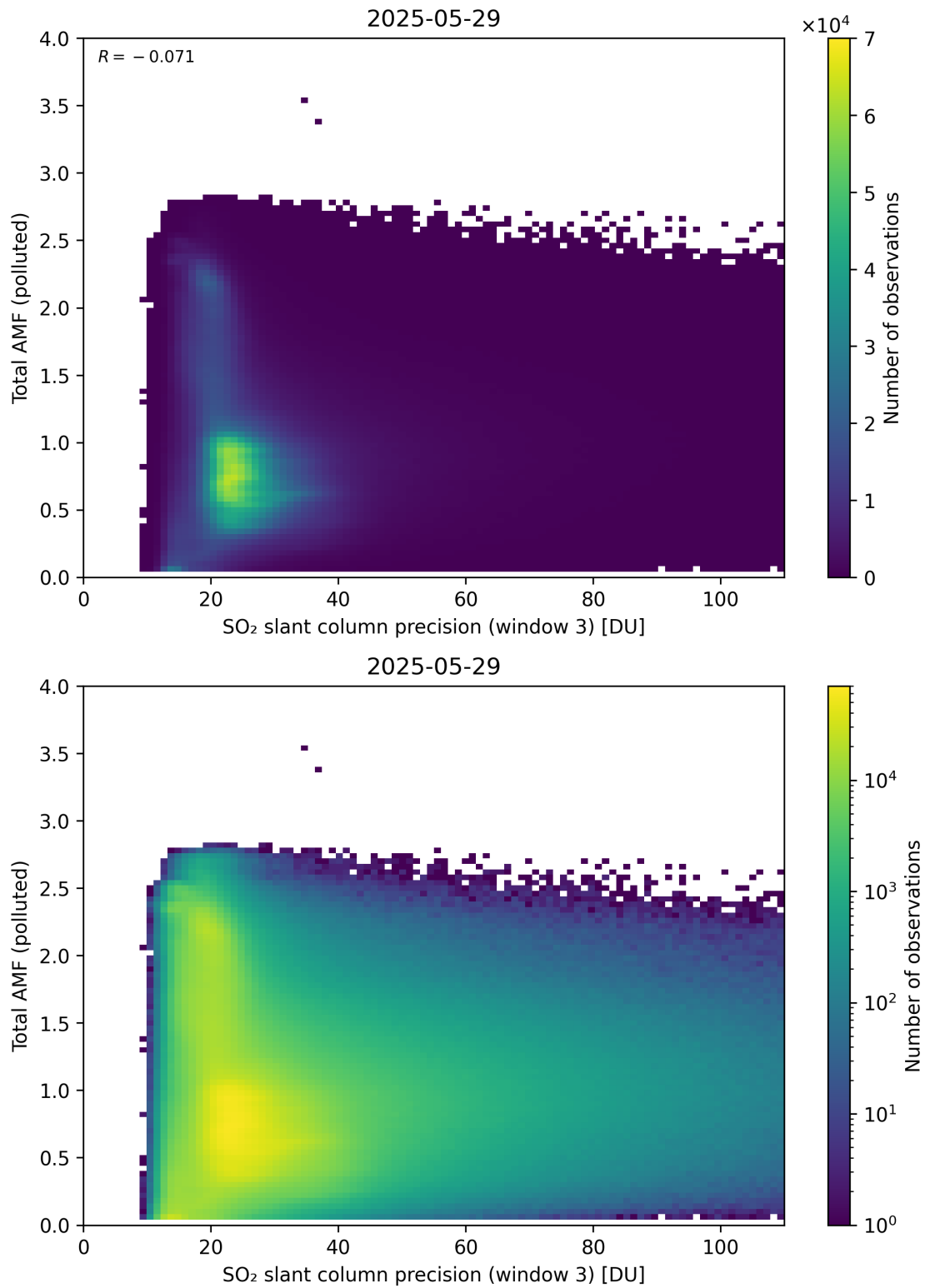
Figure 313: Scatter density plot of “SO 2 slant column precision (window 3)” against “Total AMF (polluted)” for 2025-05-28 to 2025-05-30.
