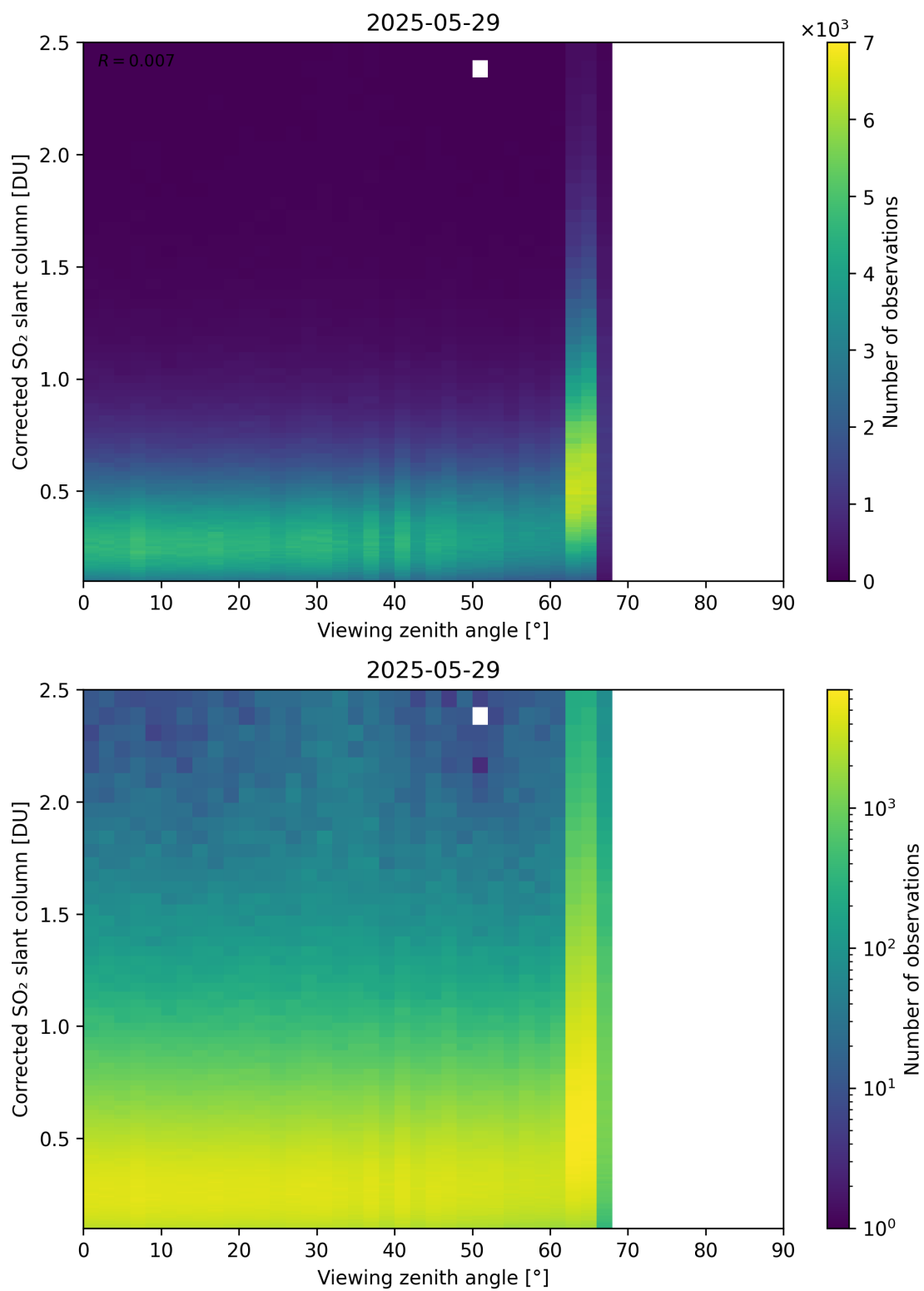
Figure 373: Scatter density plot of “Viewing zenith angle” against “Corrected SO 2 slant column” for 2025-05-28 to 2025-05-30.
