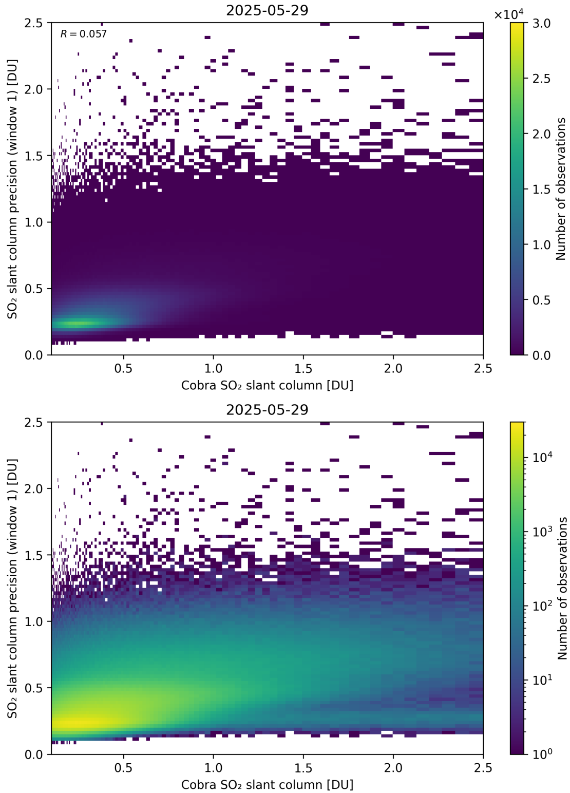
Figure 220: Scatter density plot of “Cobra SO 2 slant column” against “SO 2 slant column precision (window 1)” for 2025-05-28 to 2025-05-30.
