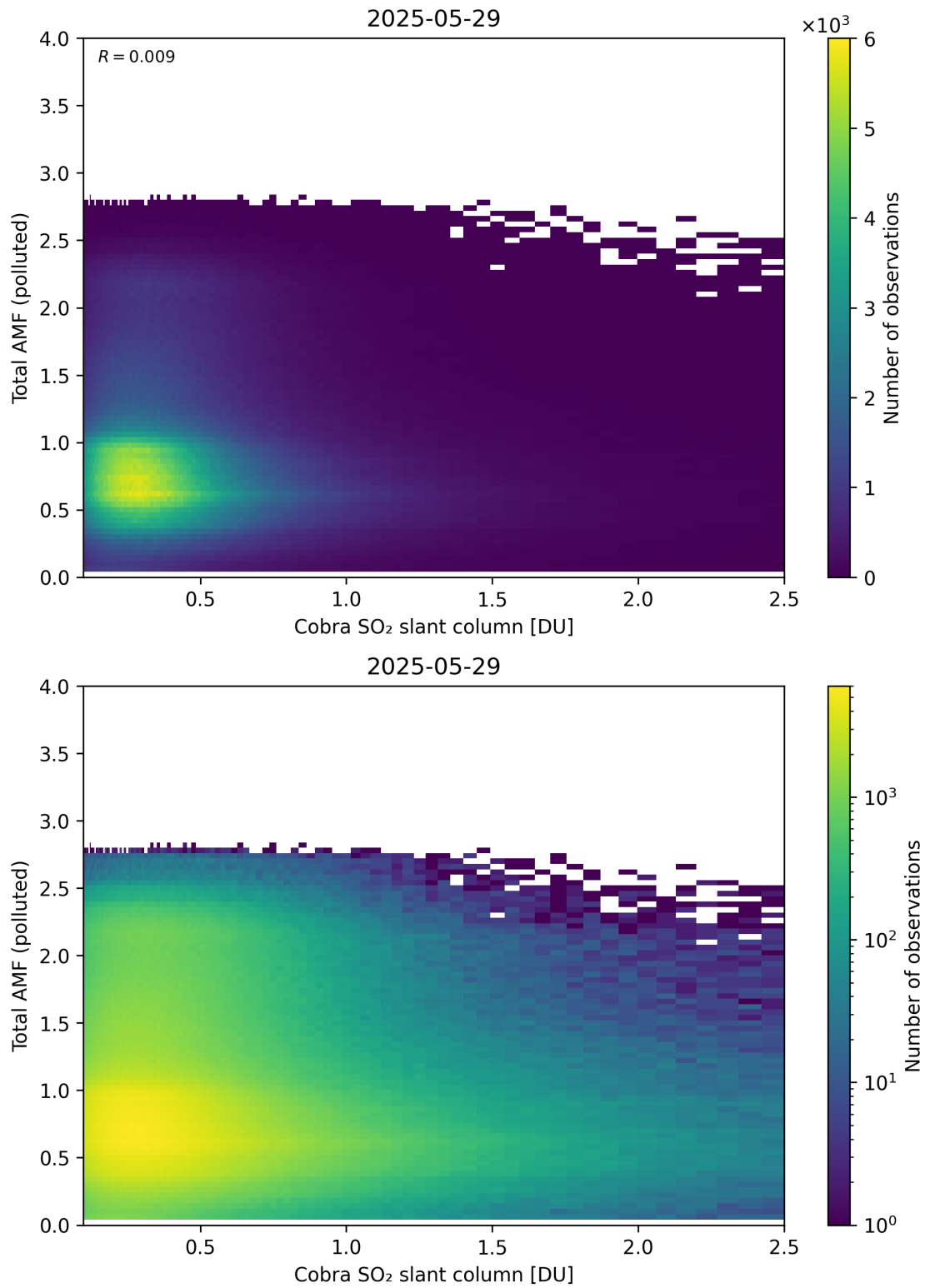
Figure 224: Scatter density plot of “Cobra SO 2 slant column” against “Total AMF (polluted)” for 2025-05-28 to 2025-05-30.
