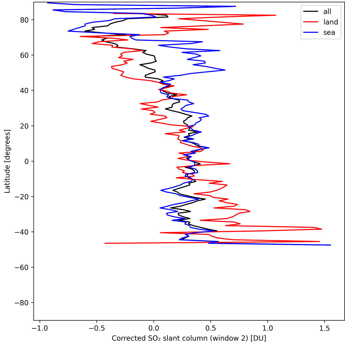
Figure 43: Zonal average of “Corrected SO 2 slant column (window 2)” for 2025-05-28 to 2025-05-30.
