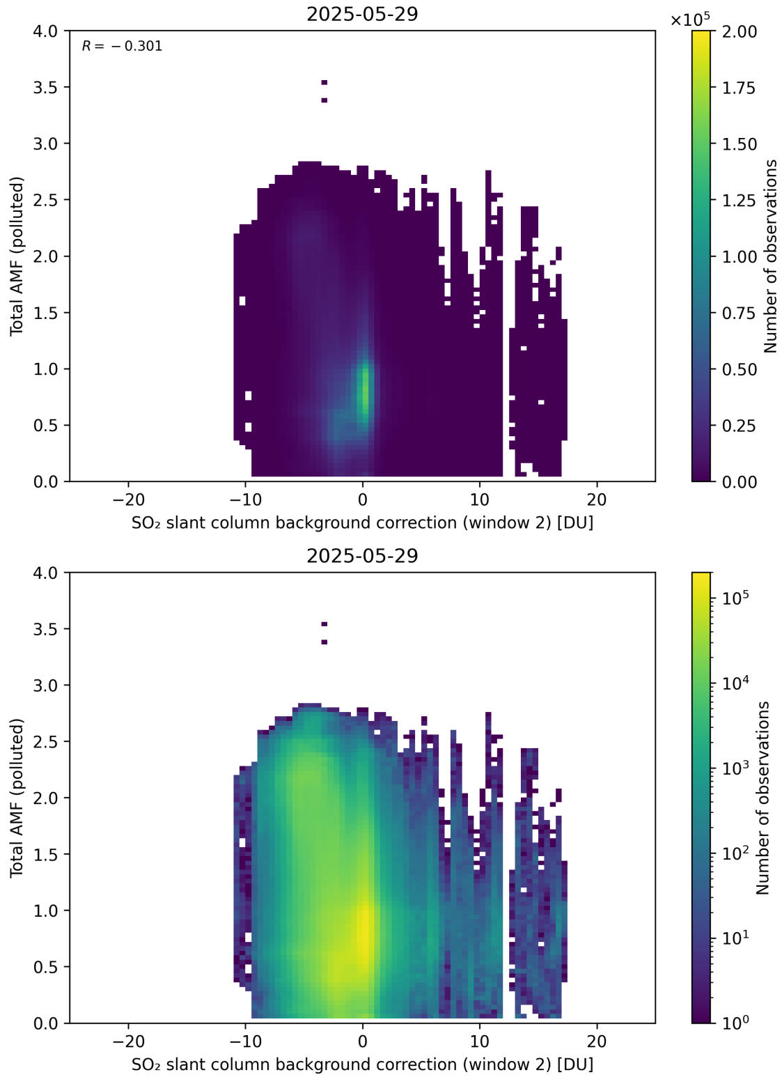
Figure 130: Scatter density plot of “SO 2 slant column background correction (window 2)” against “Total AMF (polluted)” for 2025-05-28 to 2025-05-30.
