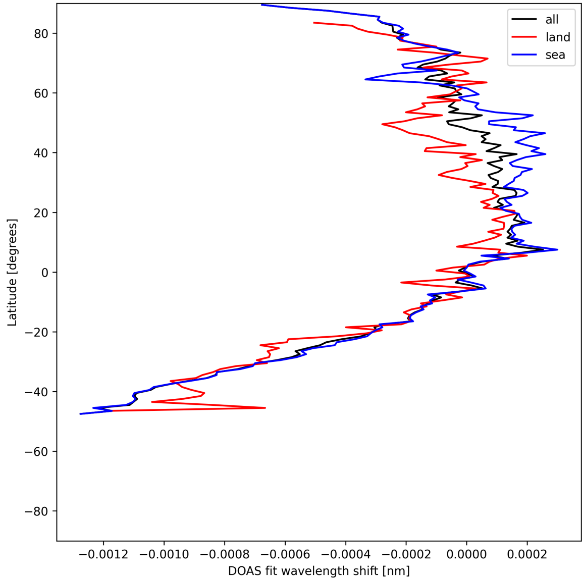
Figure 50: Zonal average of “DOAS fit wavelength shift” for 2025-05-28 to 2025-05-30.
