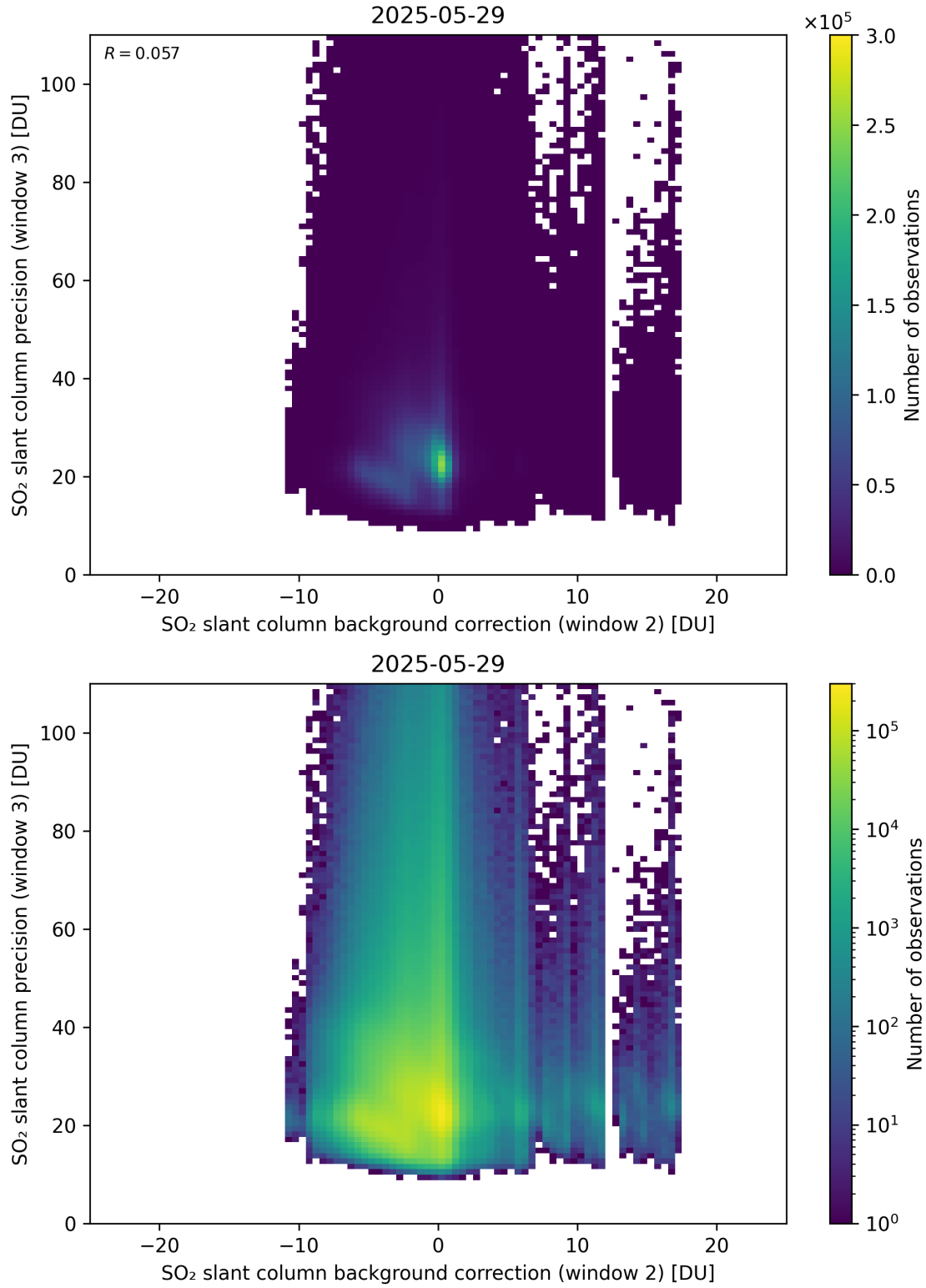
Figure 129: Scatter density plot of “SO 2 slant column background correction (window 2)” against “SO 2 slant column precision (window 3)” for 2025-05-28 to 2025-05-30.
