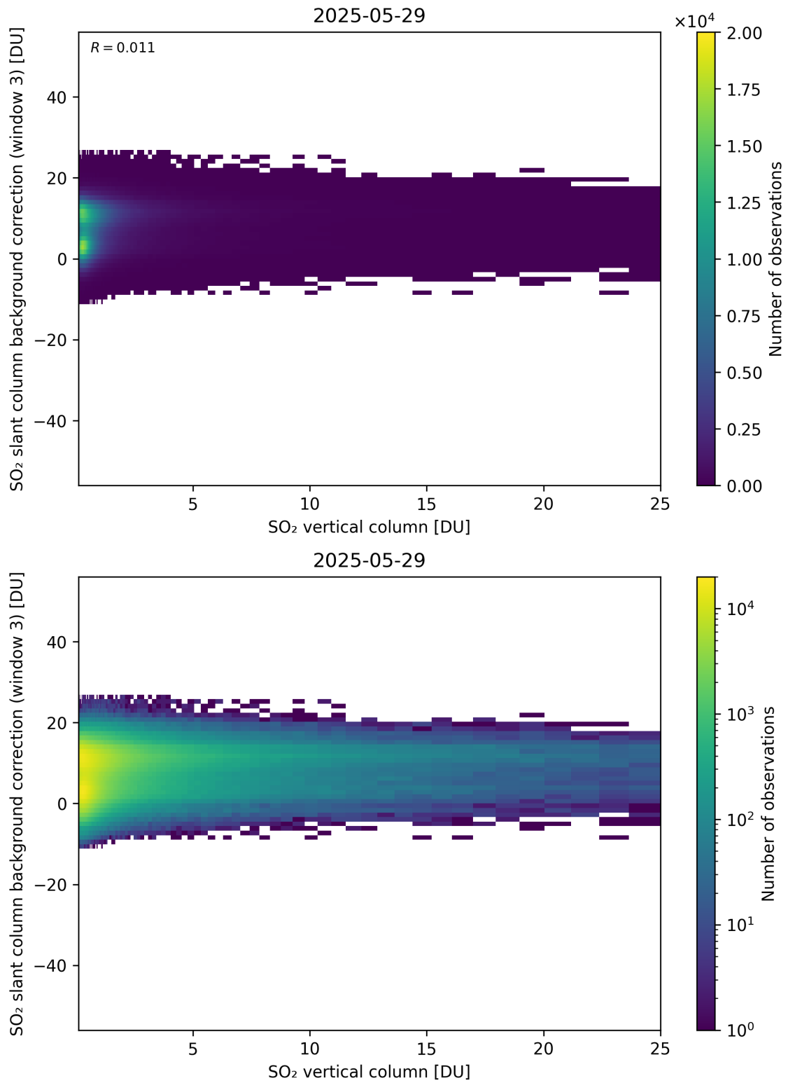
Figure 325: Scatter density plot of “SO 2 vertical column” against “SO 2 slant column background correction (window 3)” for 2025-05-28 to 2025-05-30.
