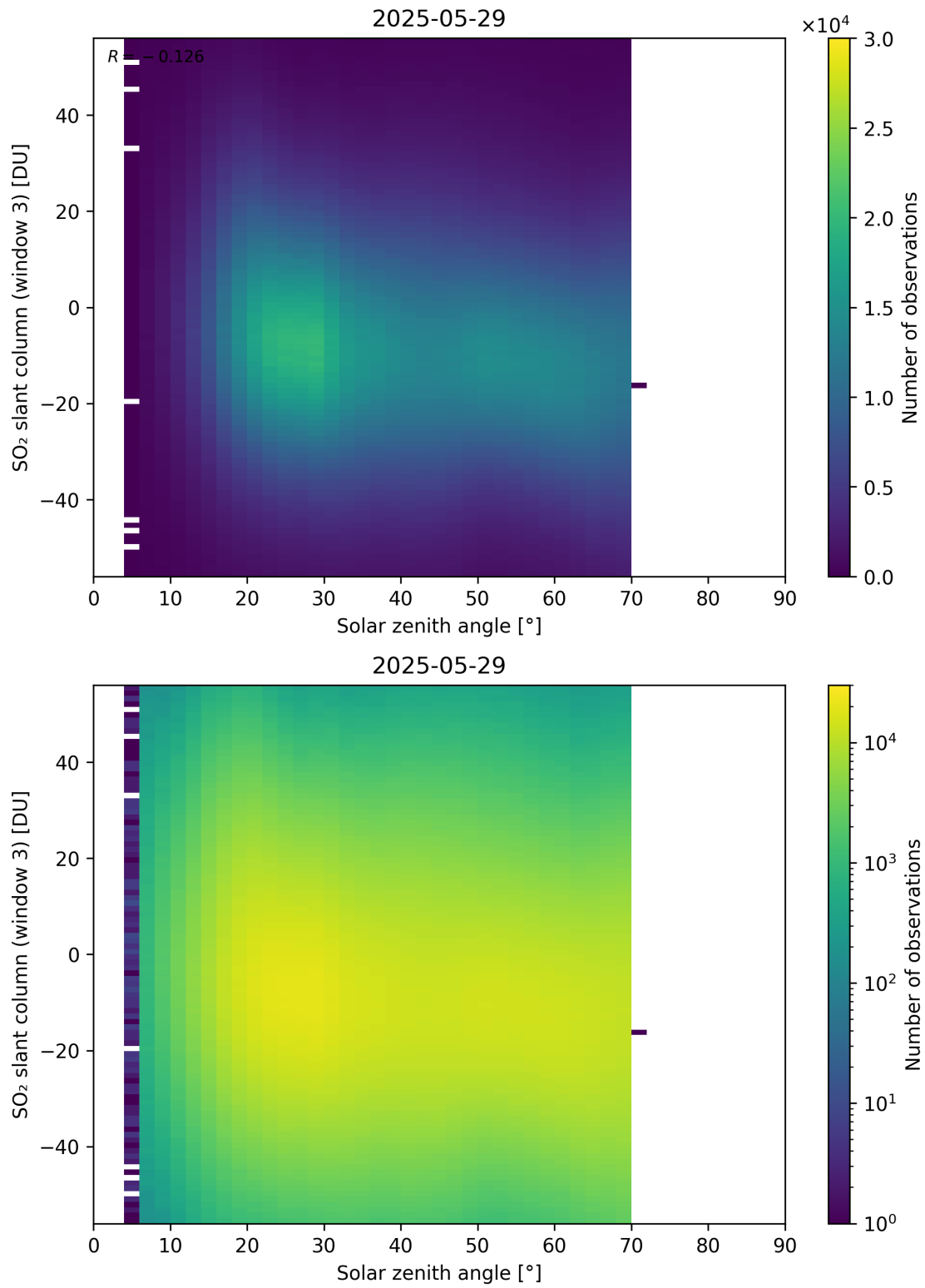
Figure 187: Scatter density plot of “Solar zenith angle” against “SO 2 slant column (window 3)” for 2025-05-28 to 2025-05-30.
