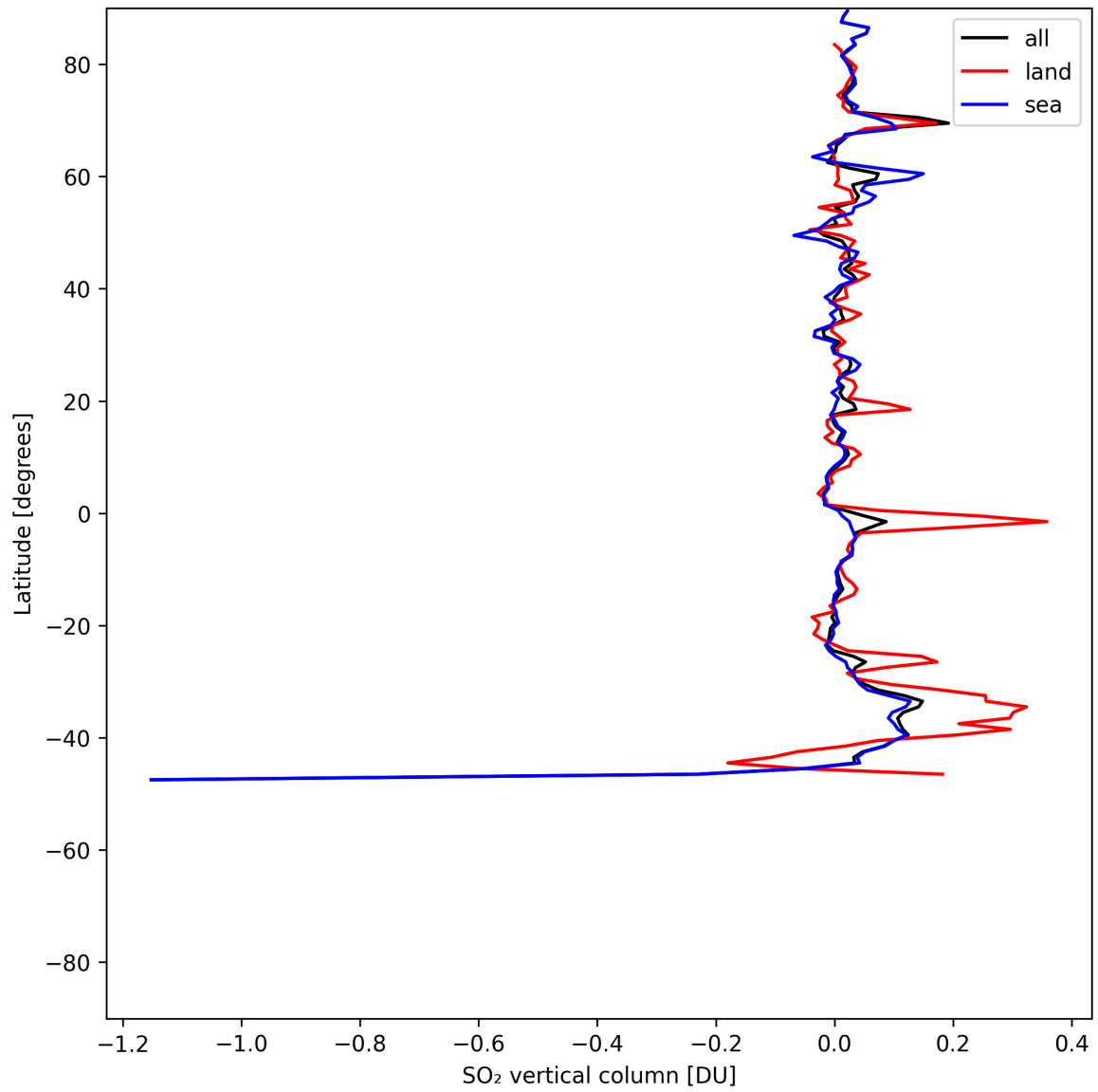
Figure 32: Zonal average of “SO 2 vertical column” for 2025-05-28 to 2025-05-30.
