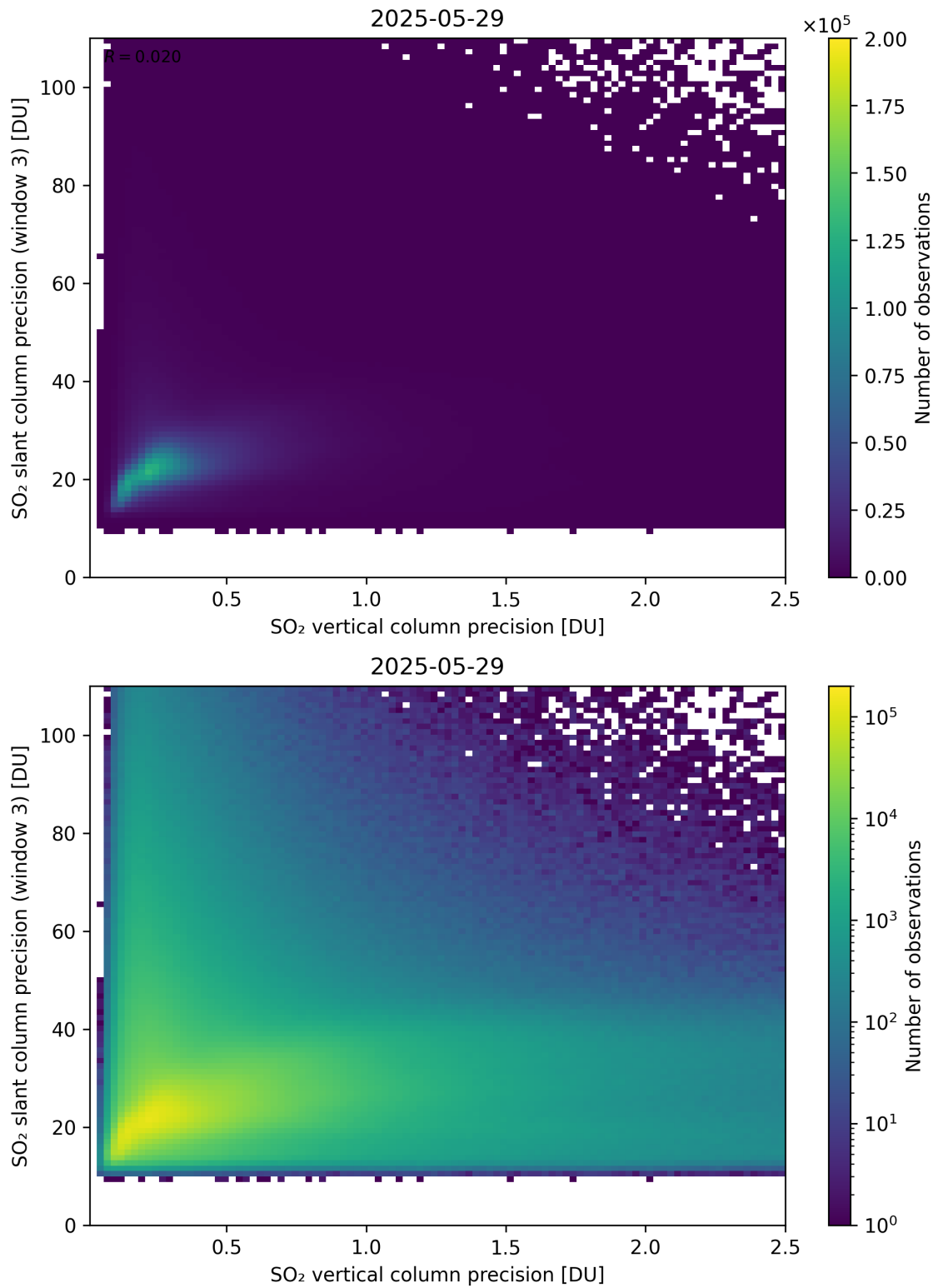
Figure 345: Scatter density plot of “SO 2 vertical column precision” against “SO 2 slant column precision (window 3)” for 2025-05-28 to 2025-05-30.
