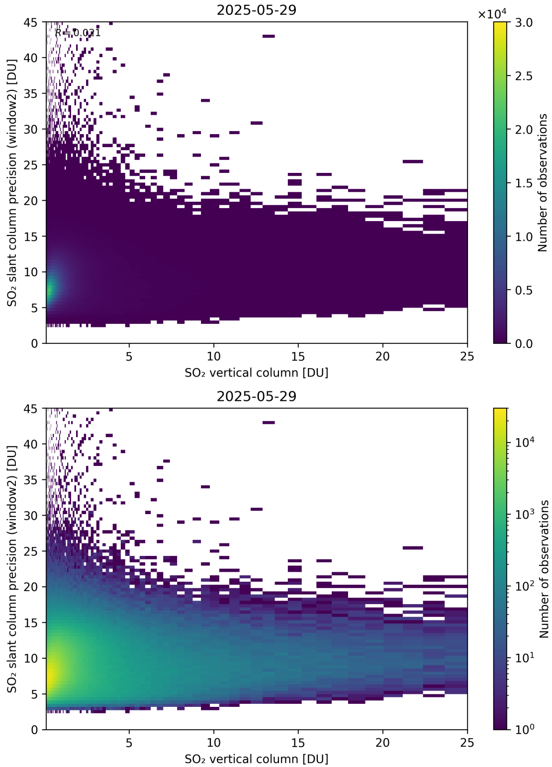
Figure 356: Scatter density plot of “SO 2 vertical column” against “SO 2 slant column precision (window2)” for 2025-05-28 to 2025-05-30.
