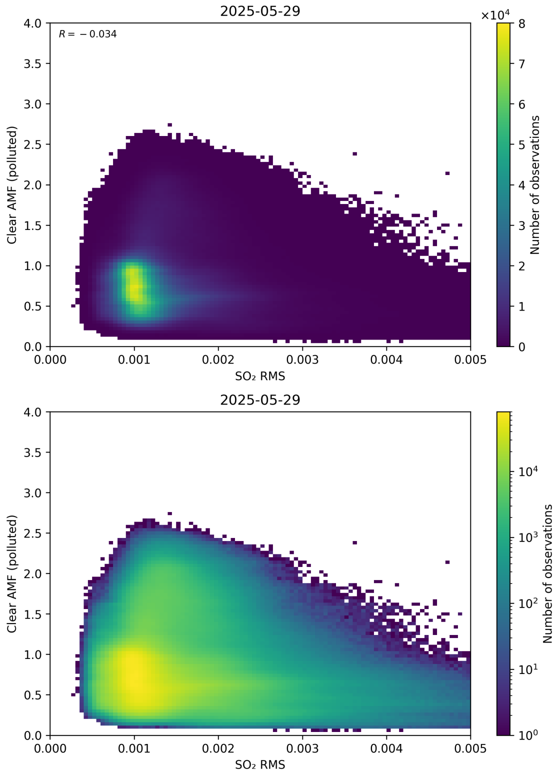
Figure 147: Scatter density plot of “SO 2 RMS” against “Clear AMF (polluted)” for 2025-05-28 to 2025-05-30.
