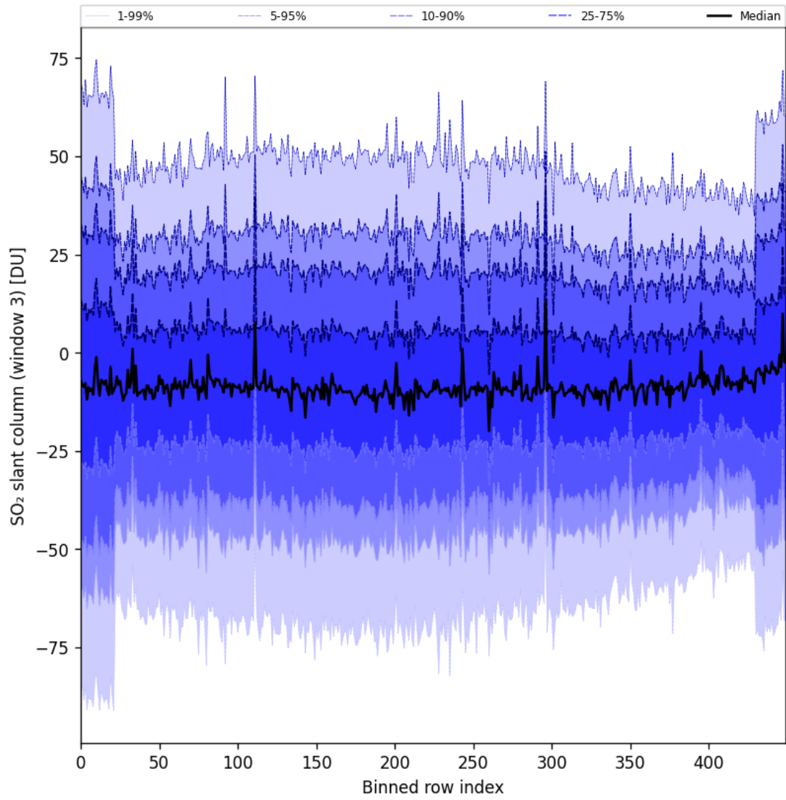
Figure 97: Along track statistics of “SO 2 slant column (window 3)” for 2025-05-28 to 2025-05-30
