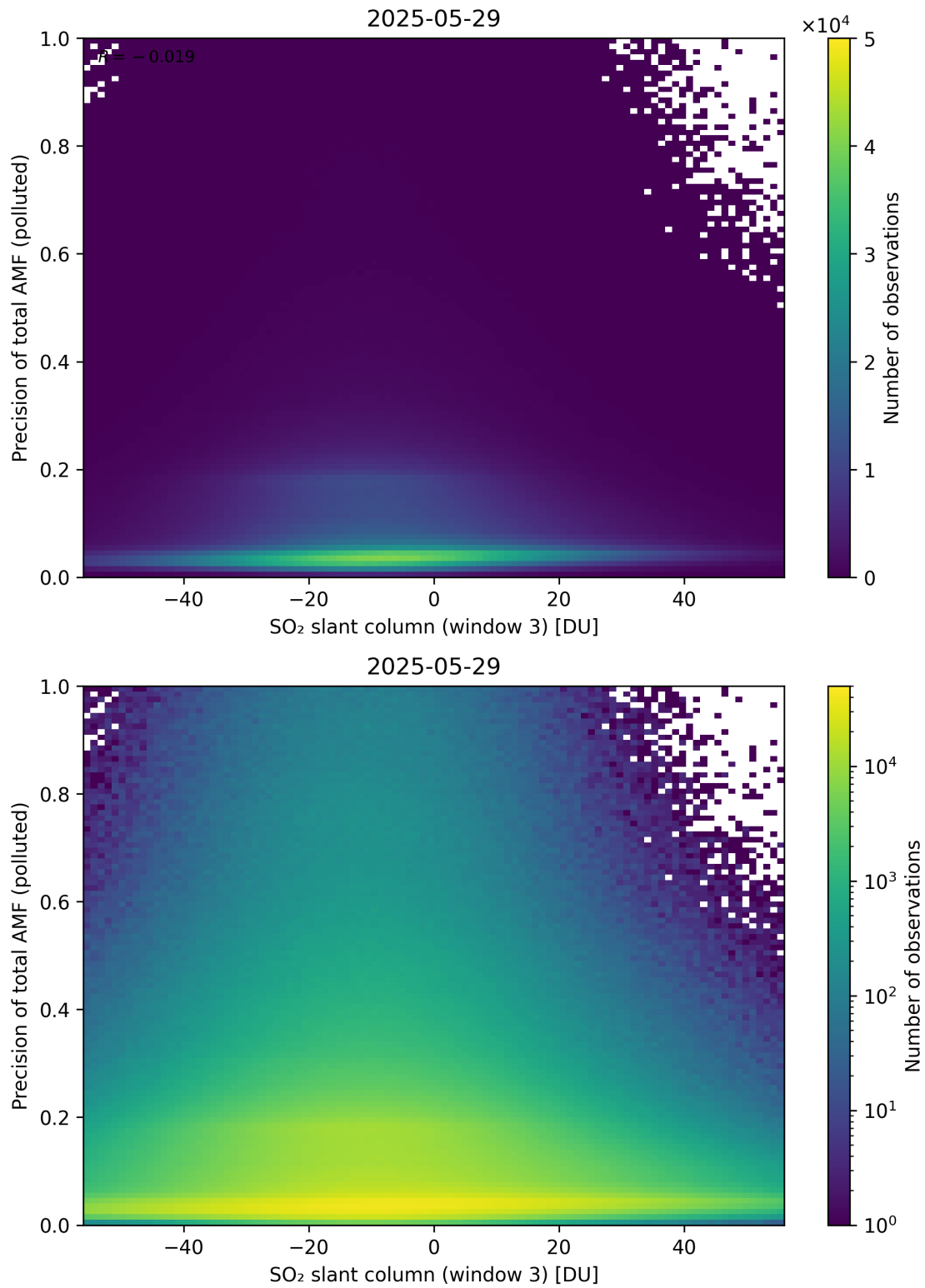
Figure 319: Scatter density plot of “SO 2 slant column (window 3)” against “Precision of total AMF (polluted)” for 2025-05-28 to 2025-05-30.
