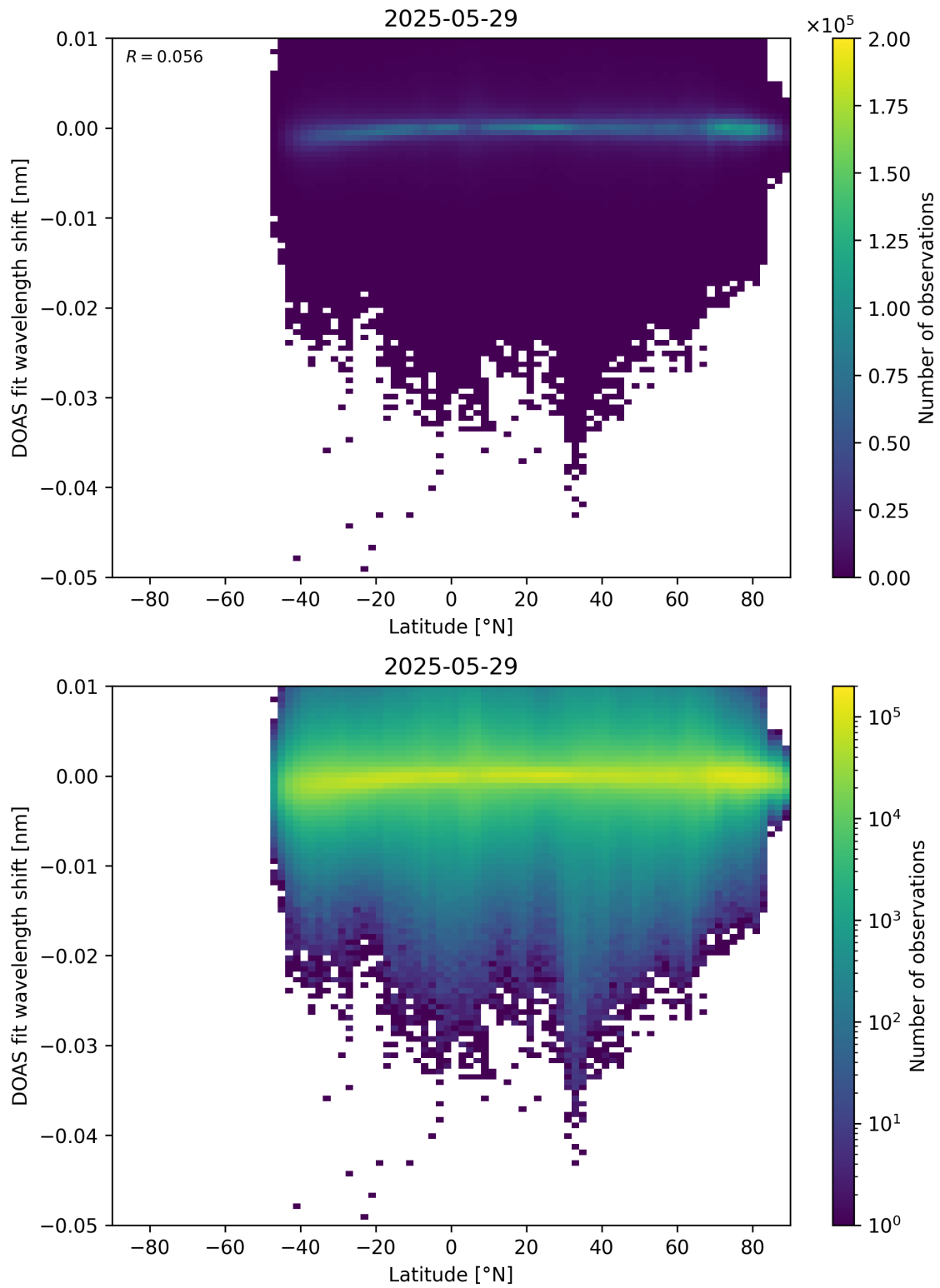
Figure 153: Scatter density plot of “Latitude” against “DOAS fit wavelength shift” for 2025-05-28 to 2025-05-30.
