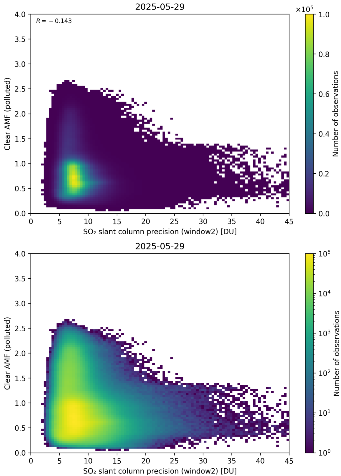
Figure 296: Scatter density plot of “SO 2 slant column precision (window2)” against “Clear AMF (polluted)” for 2025-05-28 to 2025-05-30.
