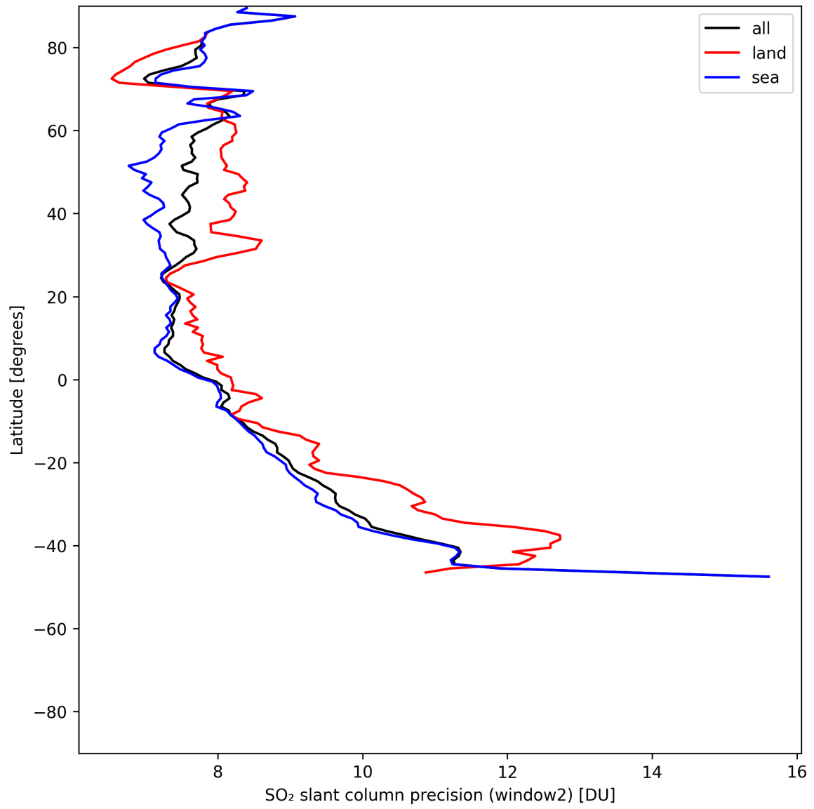
Figure 42: Zonal average of “SO 2 slant column precision (window2)” for 2025-05-28 to 2025-05-30.
