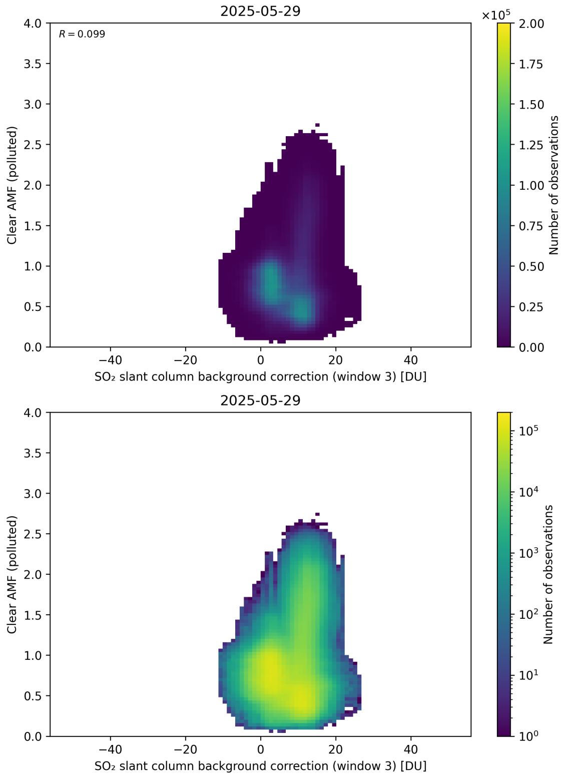
Figure 135: Scatter density plot of “SO 2 slant column background correction (window 3)” against “Clear AMF (polluted)” for 2025-05-28 to 2025-05-30.
