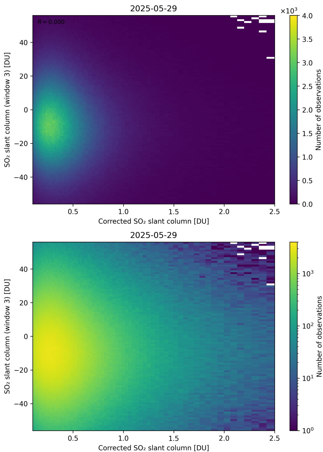
Figure 240: Scatter density plot of “Corrected SO 2 slant column” against “SO 2 slant column (window 3)” for 2025-05-28 to 2025-05-30.
