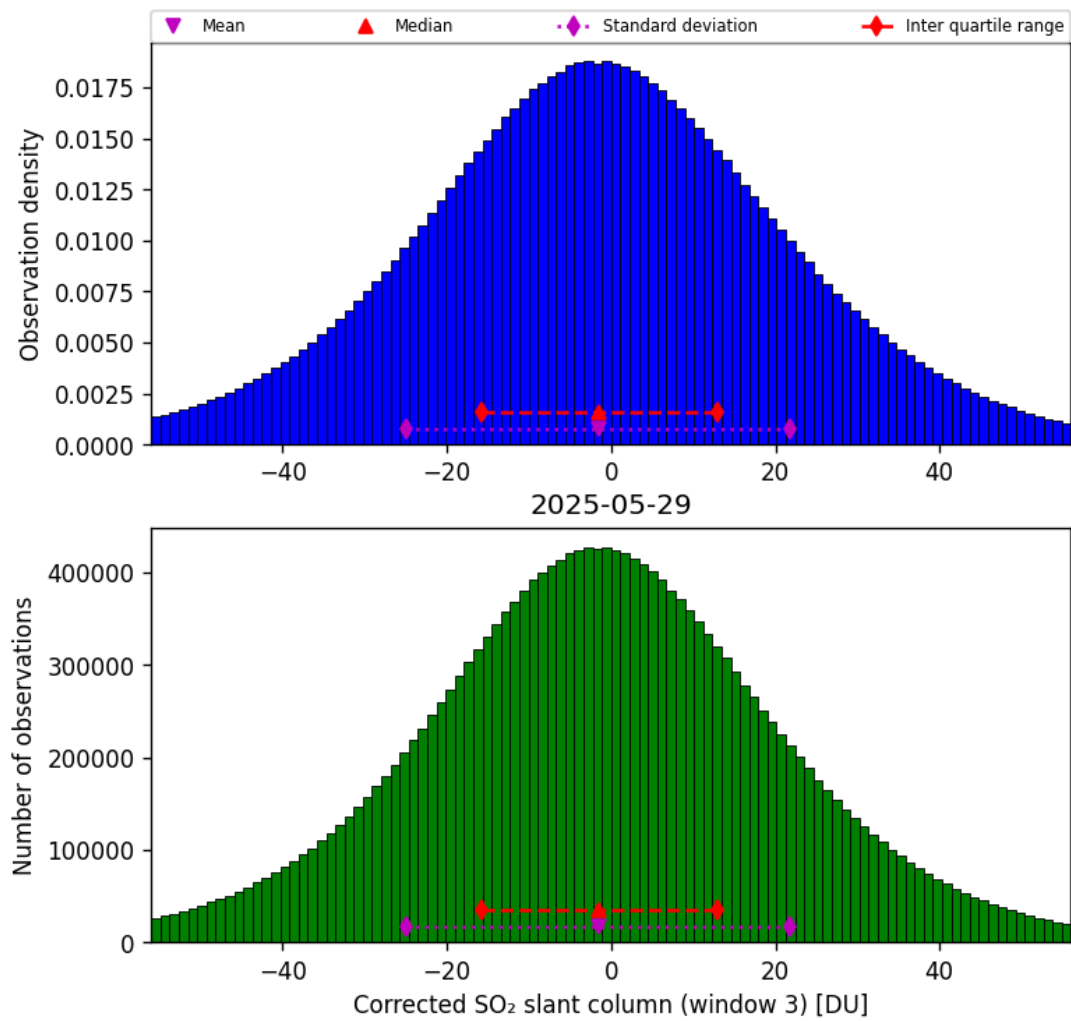
Figure 73: Histogram of “Corrected SO 2 slant column (window 3)” for 2025-05-28 to 2025-05-30
