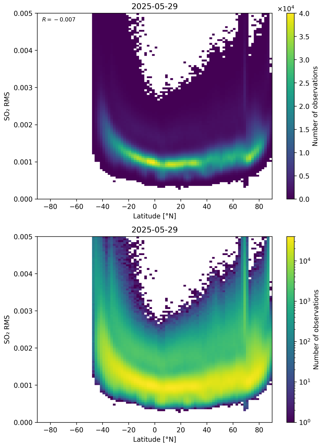
Figure 155: Scatter density plot of “Latitude” against “SO 2 RMS” for 2025-05-28 to 2025-05-30.
