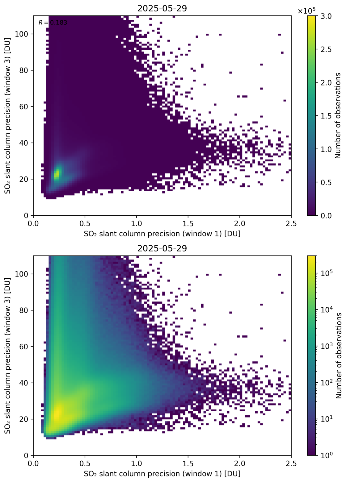
Figure 279: Scatter density plot of “SO 2 slant column precision (window 1)” against “SO 2 slant column precision (window 3)” for 2025-05-28 to 2025-05-30.
