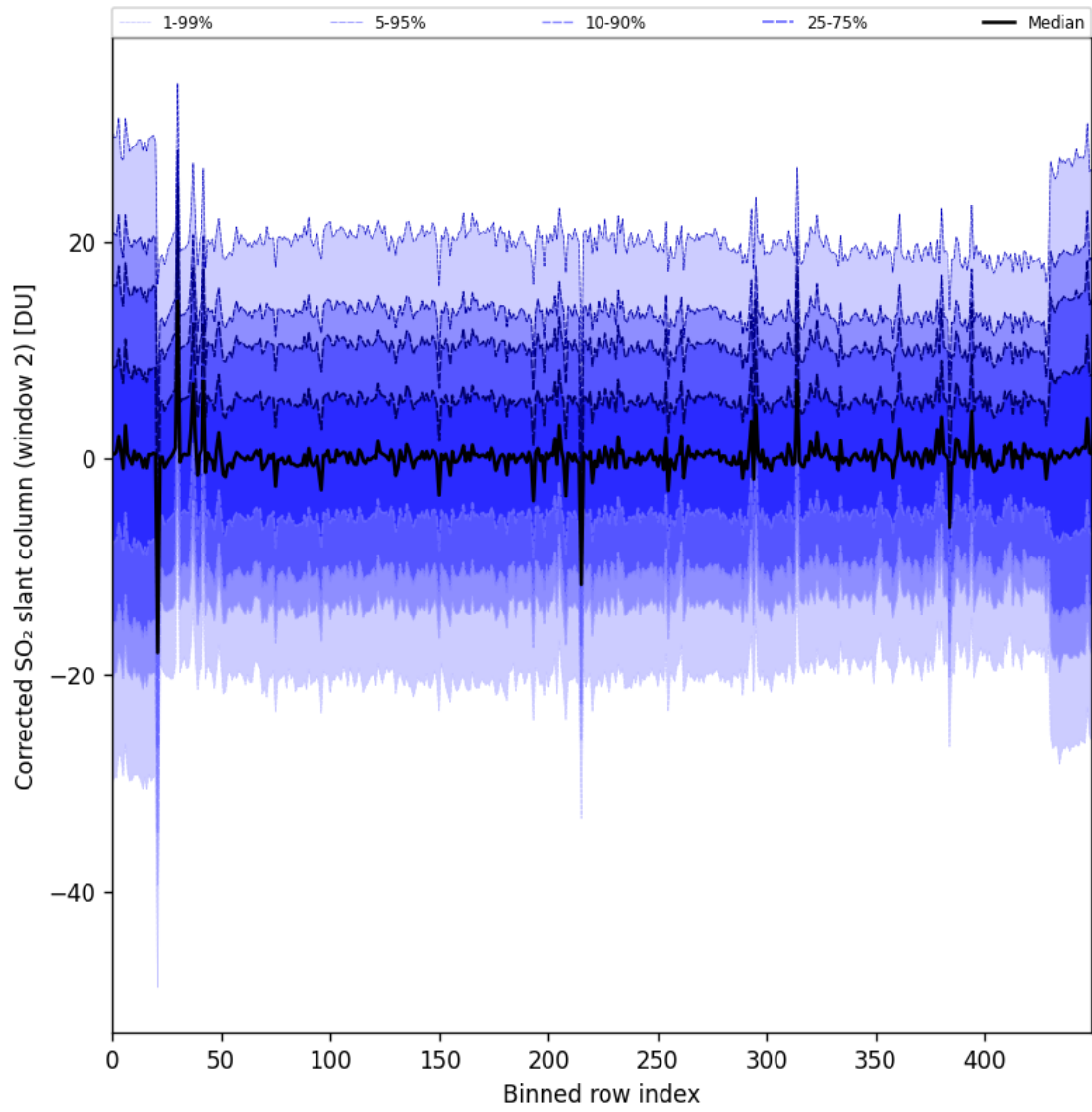
Figure 95: Along track statistics of “Corrected SO 2 slant column (window 2)” for 2025-05-28 to 2025-05-30
