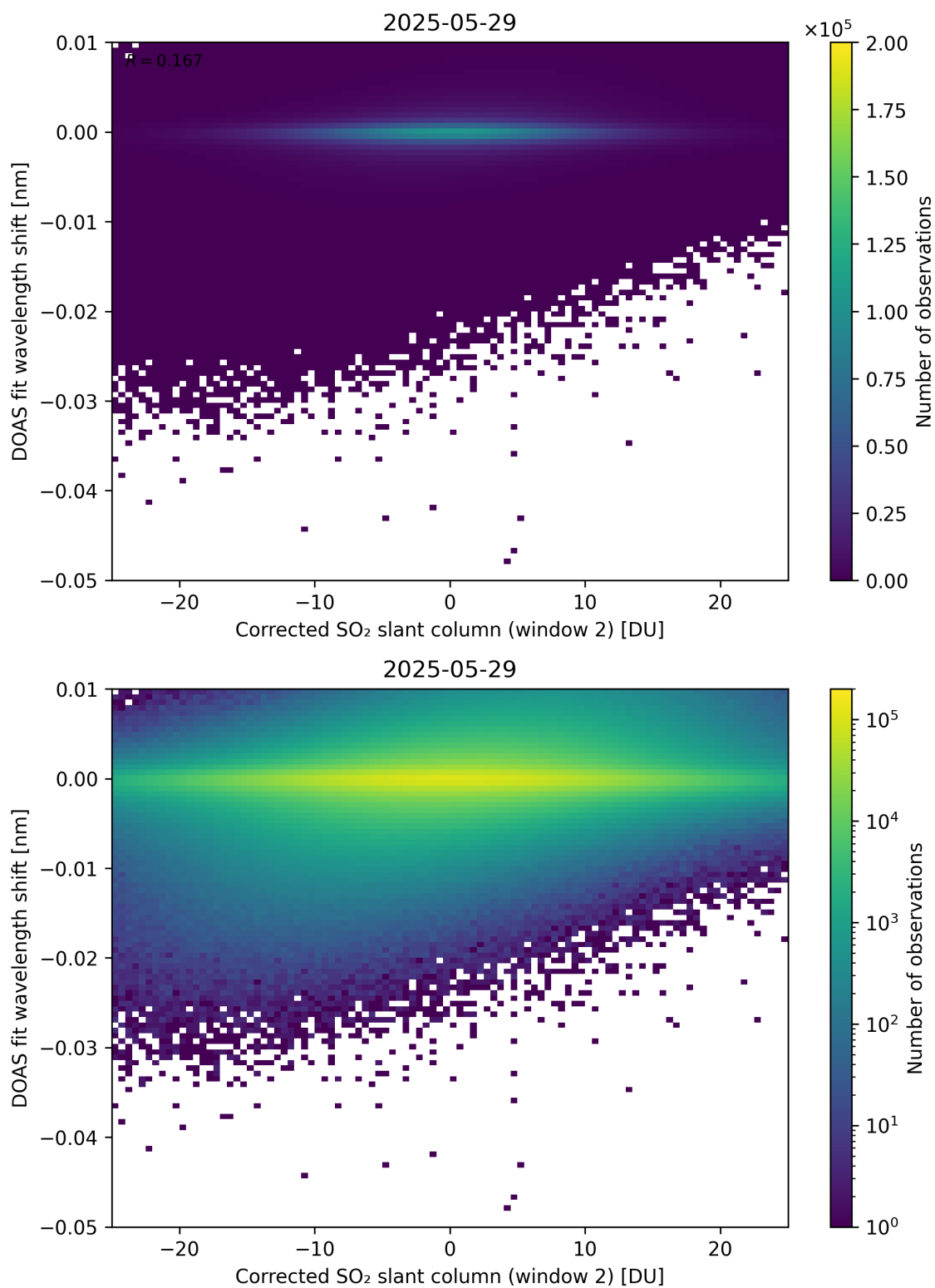
Figure 246: Scatter density plot of “Corrected SO 2 slant column (window 2)” against “DOAS fit wavelength shift” for 2025-05-28 to 2025-05-30.
