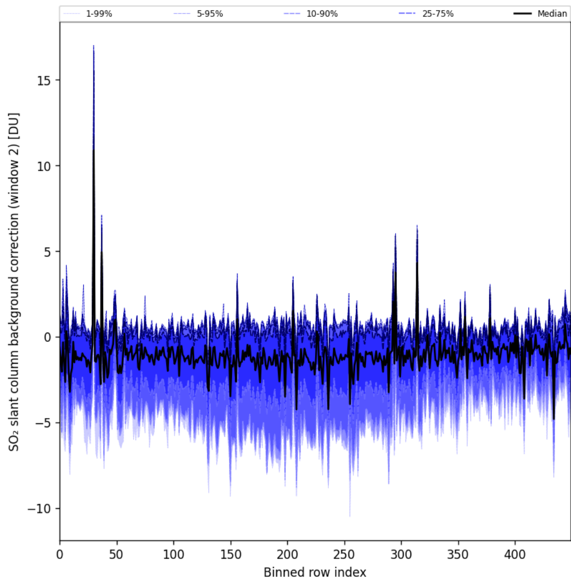
Figure 96: Along track statistics of “SO 2 slant column background correction (window 2)” for 2025-05-28 to 2025-05-30
