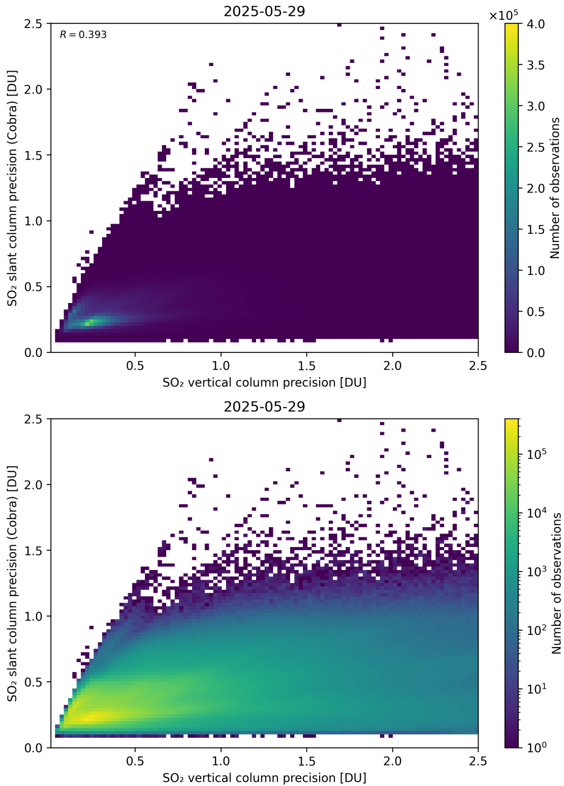
Figure 337: Scatter density plot of “SO 2 vertical column precision” against “SO 2 slant column precision (Cobra)” for 2025-05-28 to 2025-05-30.
