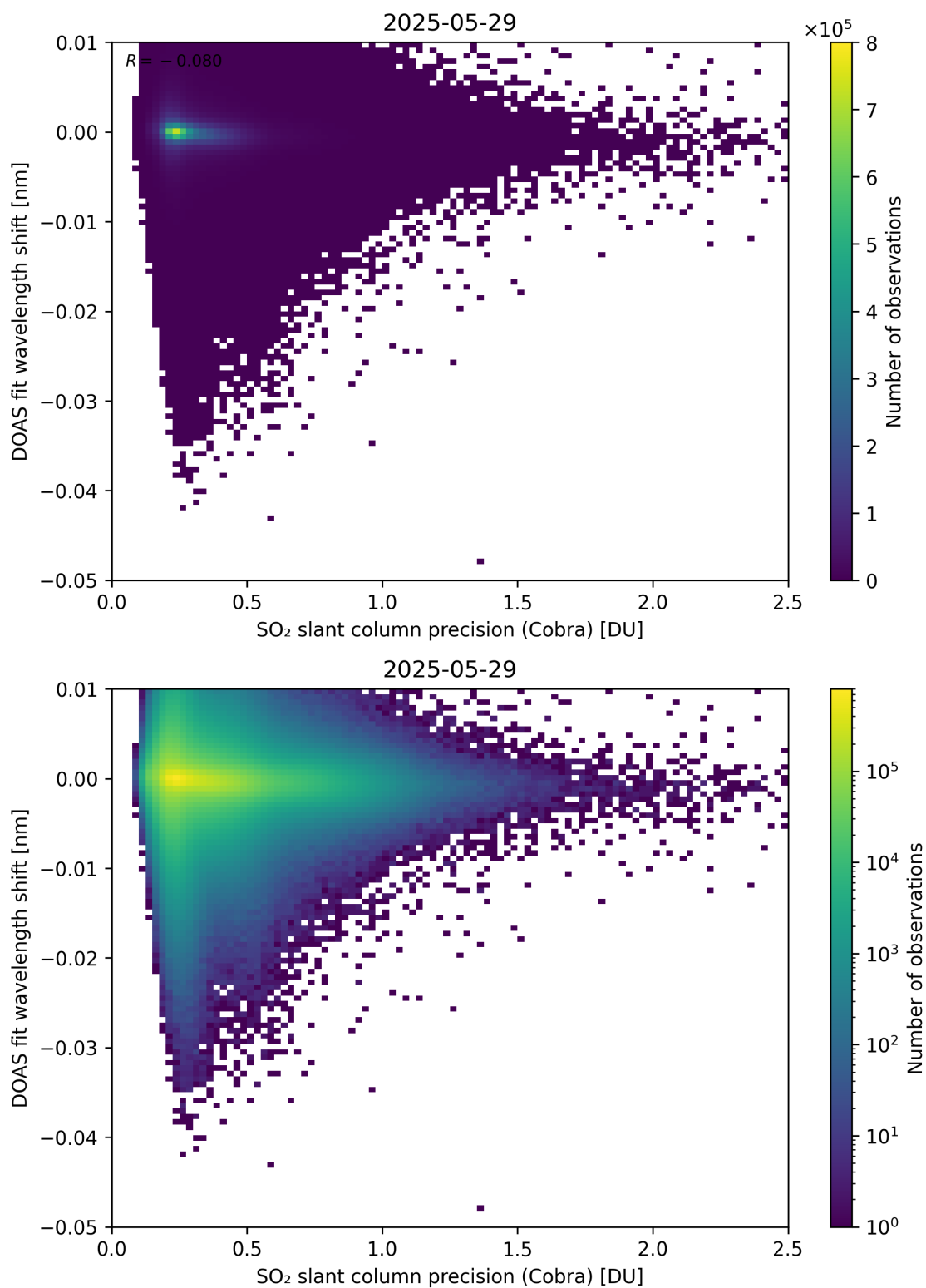
Figure 202: Scatter density plot of “SO 2 slant column precision (Cobra)” against “DOAS fit wavelength shift” for 2025-05-28 to 2025-05-30.
