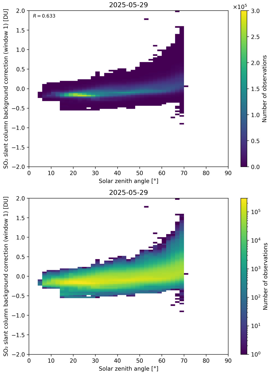
Figure 171: Scatter density plot of “Solar zenith angle” against “SO 2 slant column background correction (window 1)” for 2025-05-28 to 2025-05-30.
