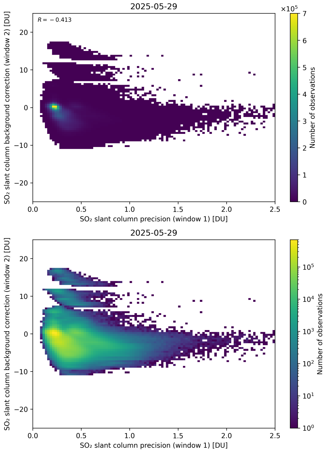
Figure 269: Scatter density plot of “SO 2 slant column precision (window 1)” against “SO 2 slant column background correction (window 2)” for 2025-05-28 to 2025-05-30.
