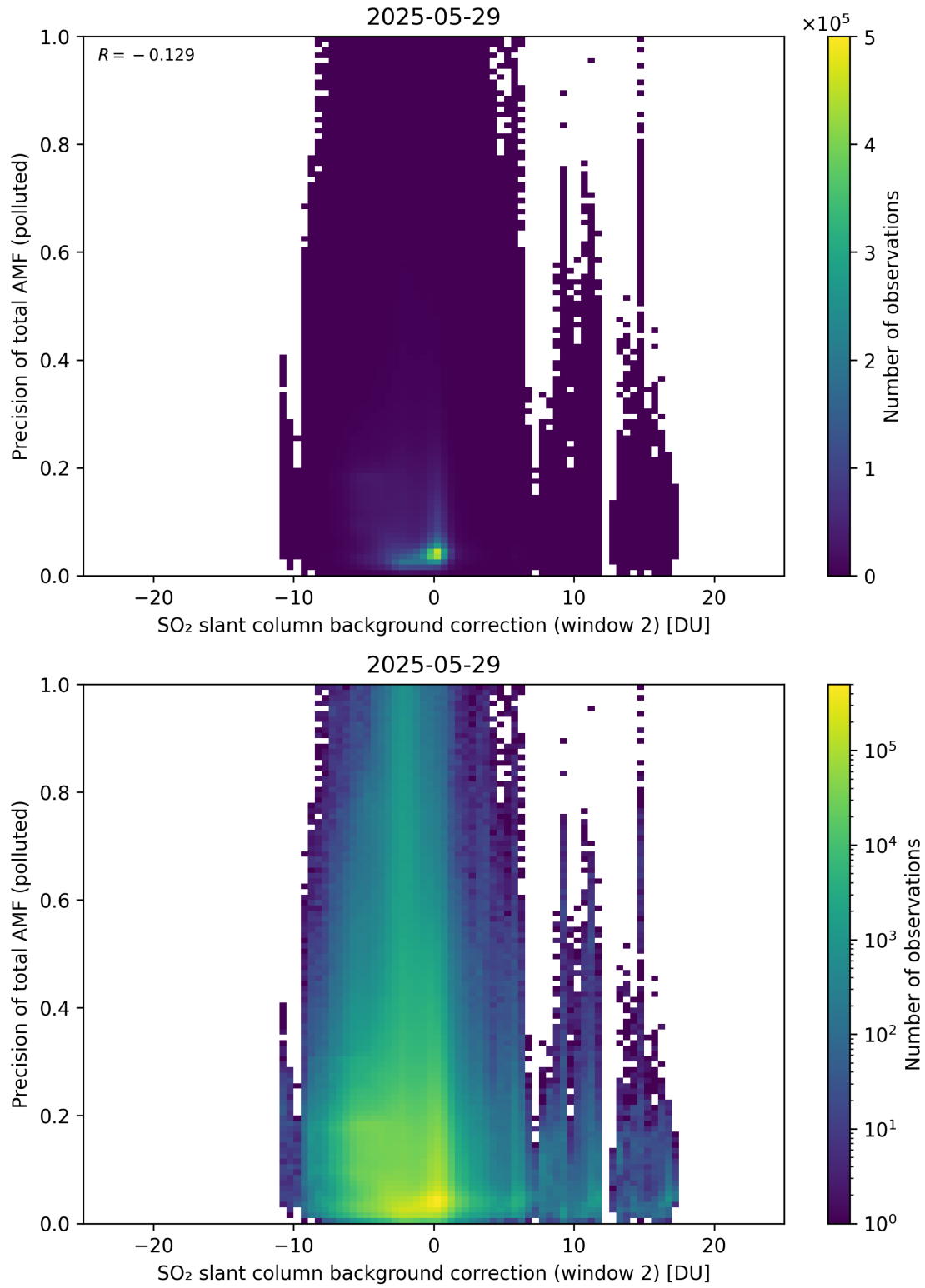
Figure 131: Scatter density plot of “SO 2 slant column background correction (window 2)” against “Precision of total AMF (polluted)” for 2025-05-28 to 2025-05-30.
