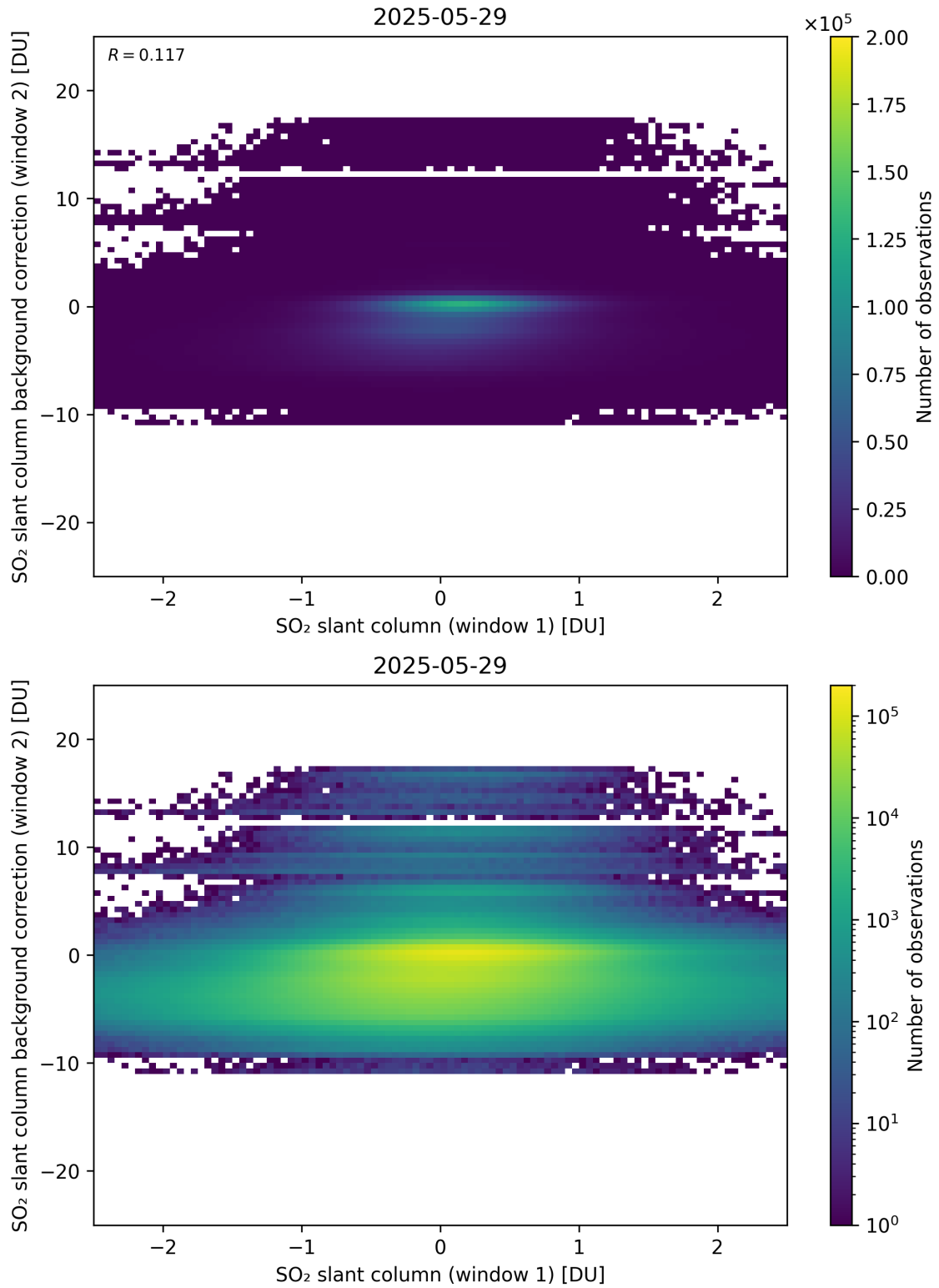
Figure 263: Scatter density plot of “SO 2 slant column (window 1)” against “SO 2 slant column background correction (window 2)” for 2025-05-28 to 2025-05-30.
