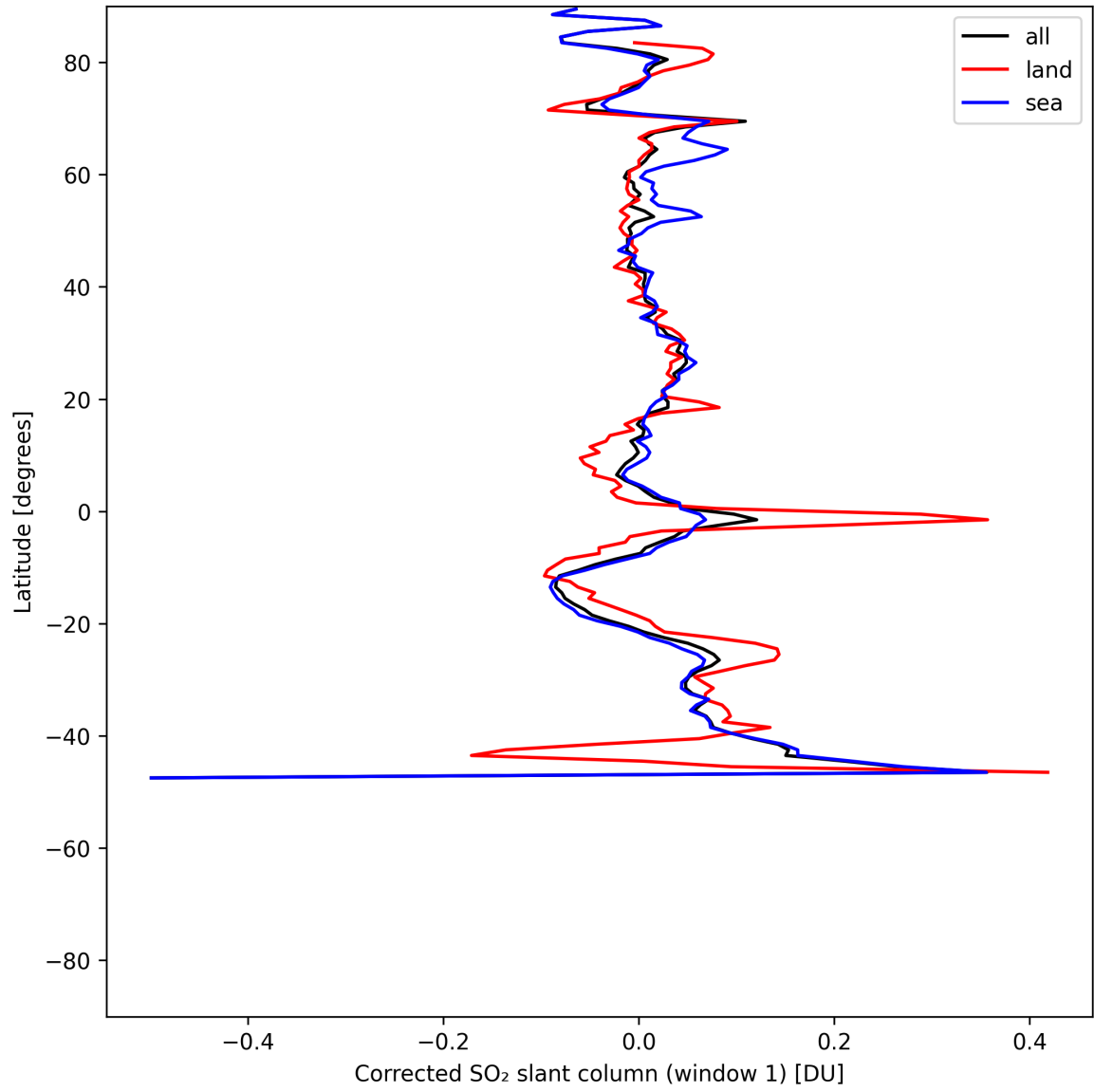
Figure 39: Zonal average of “Corrected SO 2 slant column (window 1)” for 2025-05-28 to 2025-05-30.
