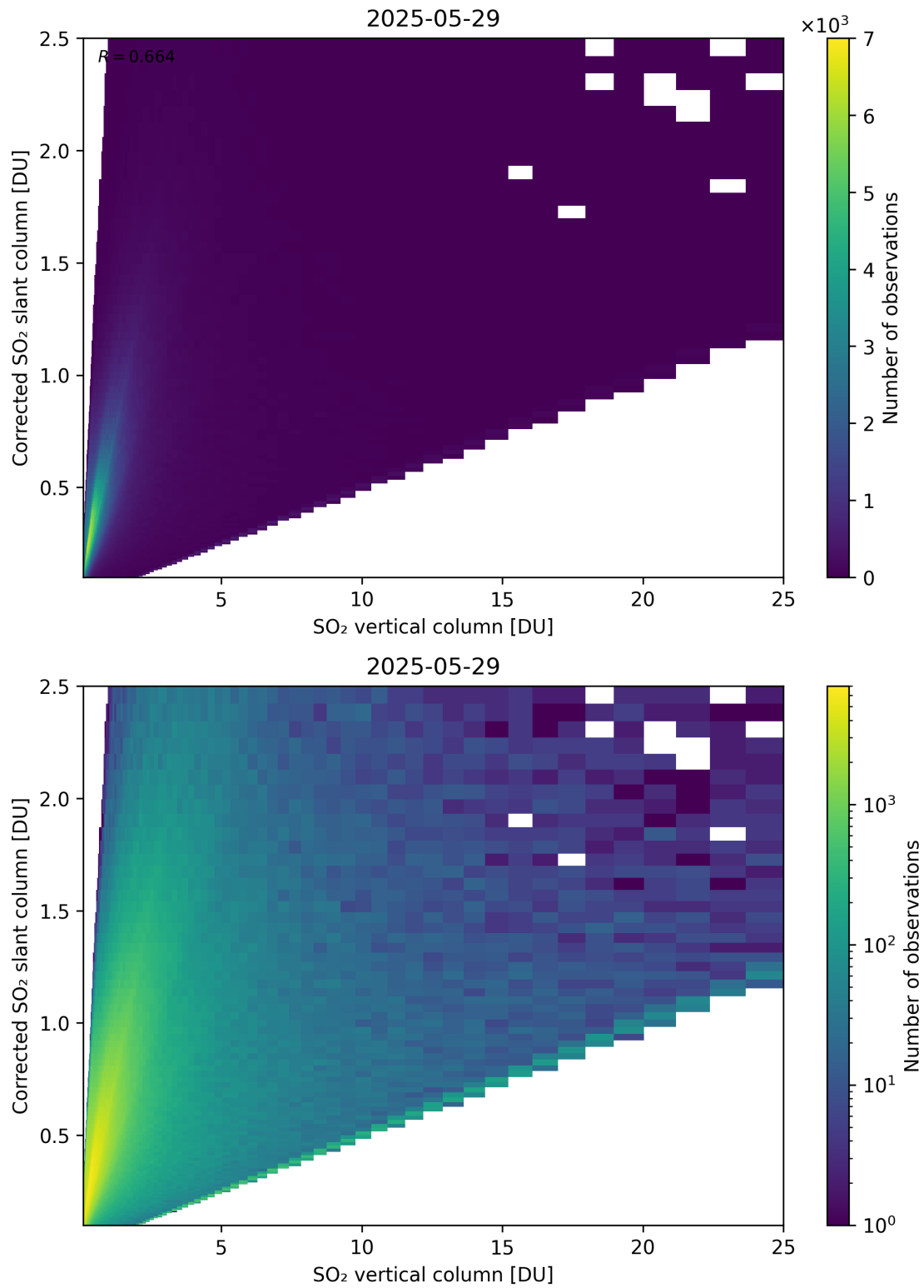
Figure 351: Scatter density plot of “SO 2 vertical column” against “Corrected SO 2 slant column” for 2025-05-28 to 2025-05-30.
