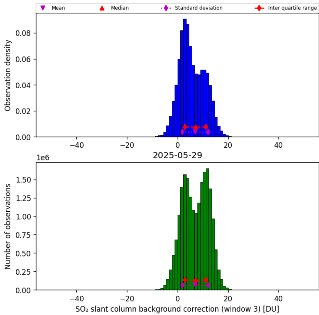
Figure 74: Histogram of “SO 2 slant column background correction (window 3)” for 2025-05-28 to 2025-05-30
