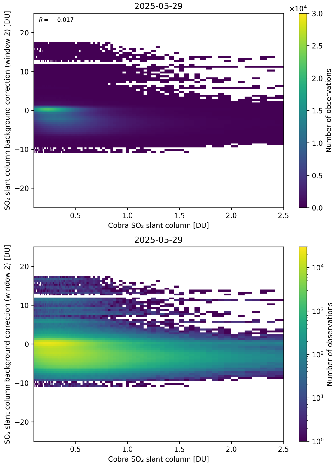
Figure 194: Scatter density plot of “Cobra SO 2 slant column” against “SO 2 slant column background correction (window 2)” for 2025-05-28 to 2025-05-30.
