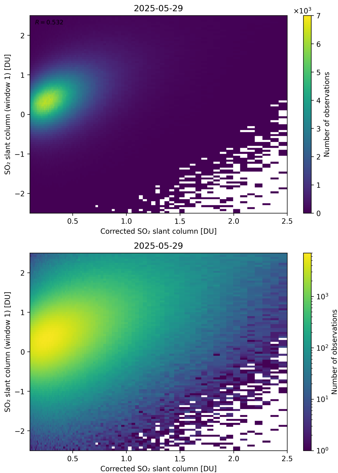
Figure 237: Scatter density plot of “Corrected SO 2 slant column” against “SO 2 slant column (window 1)” for 2025-05-28 to 2025-05-30.
