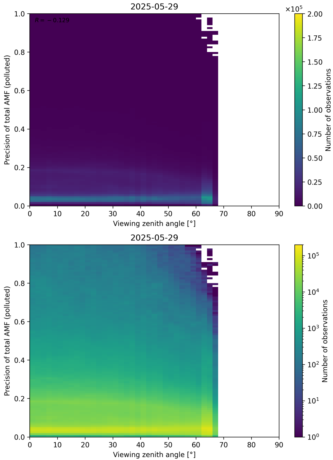
Figure 382: Scatter density plot of “Viewing zenith angle” against “Precision of total AMF (polluted)” for 2025-05-28 to 2025-05-30.
