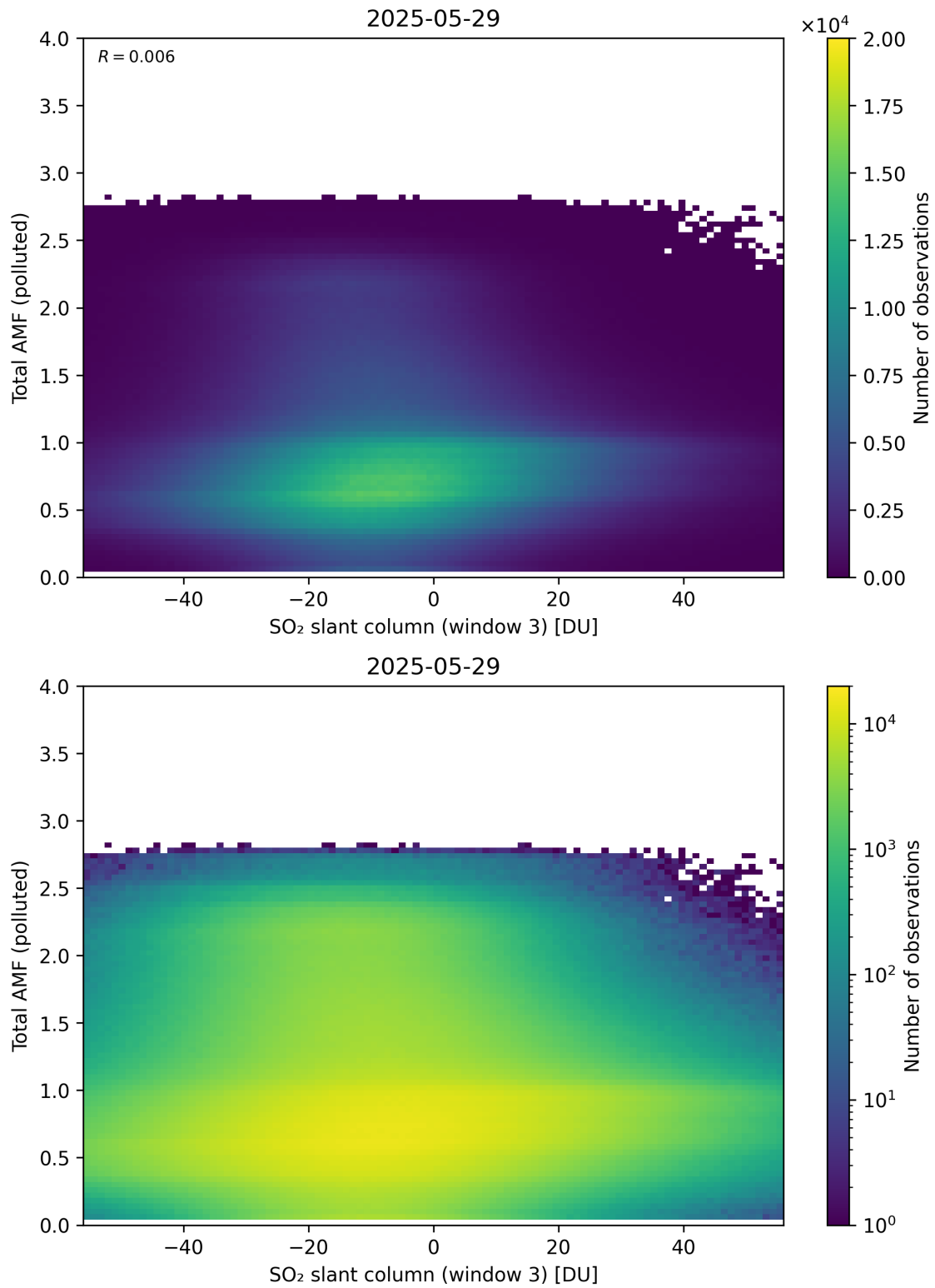
Figure 318: Scatter density plot of “SO 2 slant column (window 3)” against “Total AMF (polluted)” for 2025-05-28 to 2025-05-30.
