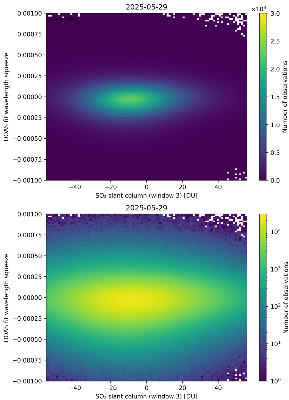
Figure 305: Scatter density plot of “SO 2 slant column (window 3)” against “DOAS fit wavelength squeeze” for 2025-05-28 to 2025-05-30.
