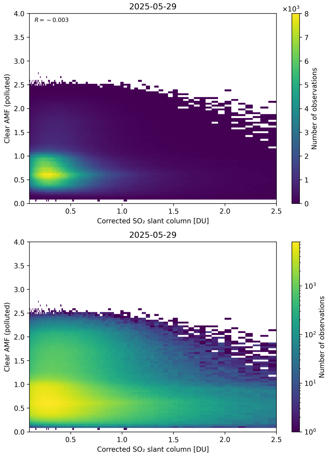
Figure 232: Scatter density plot of “Corrected SO 2 slant column” against “Clear AMF (polluted)” for 2025-05-28 to 2025-05-30.
