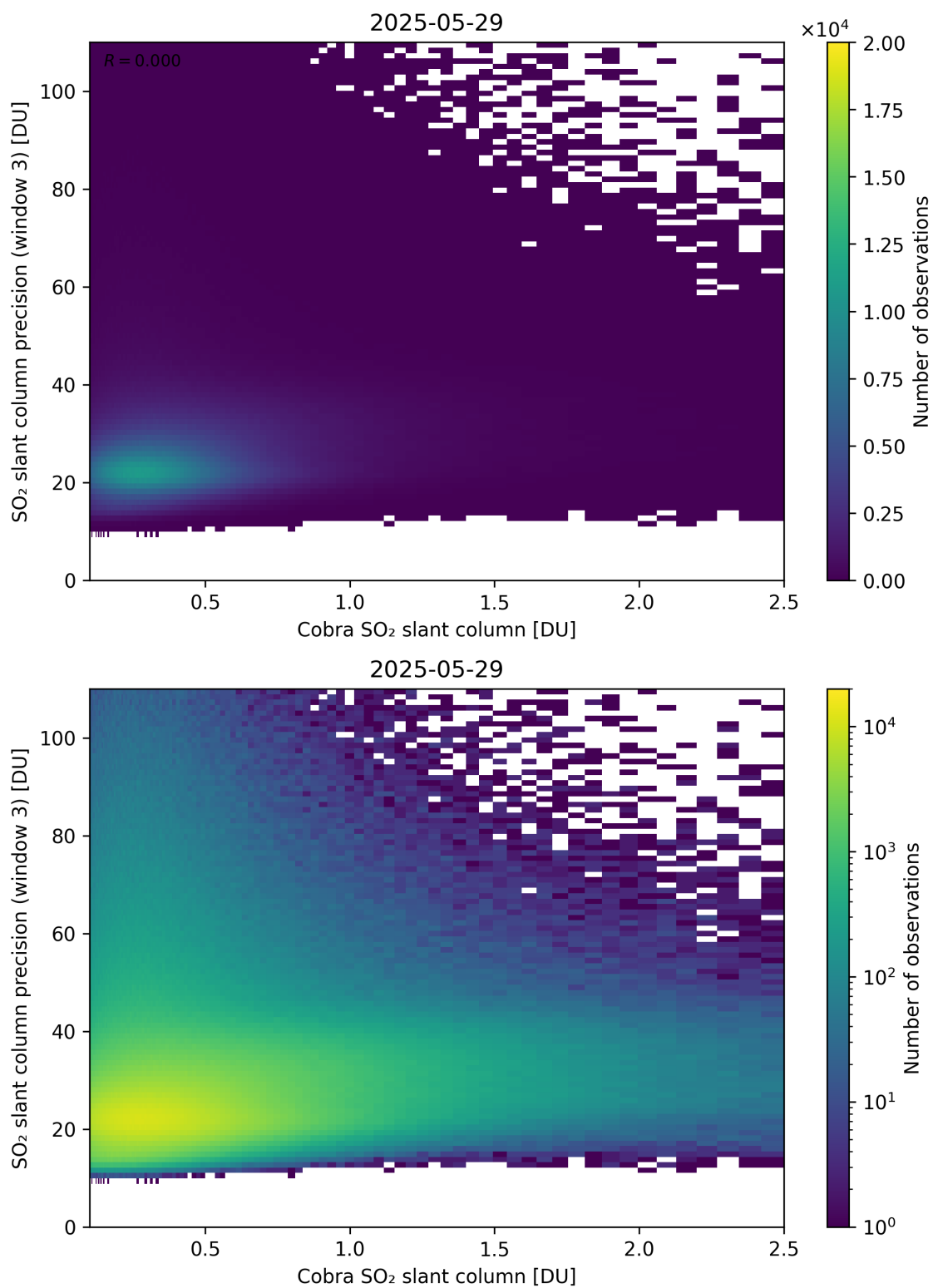
Figure 223: Scatter density plot of “Cobra SO 2 slant column” against “SO 2 slant column precision (window 3)” for 2025-05-28 to 2025-05-30.
