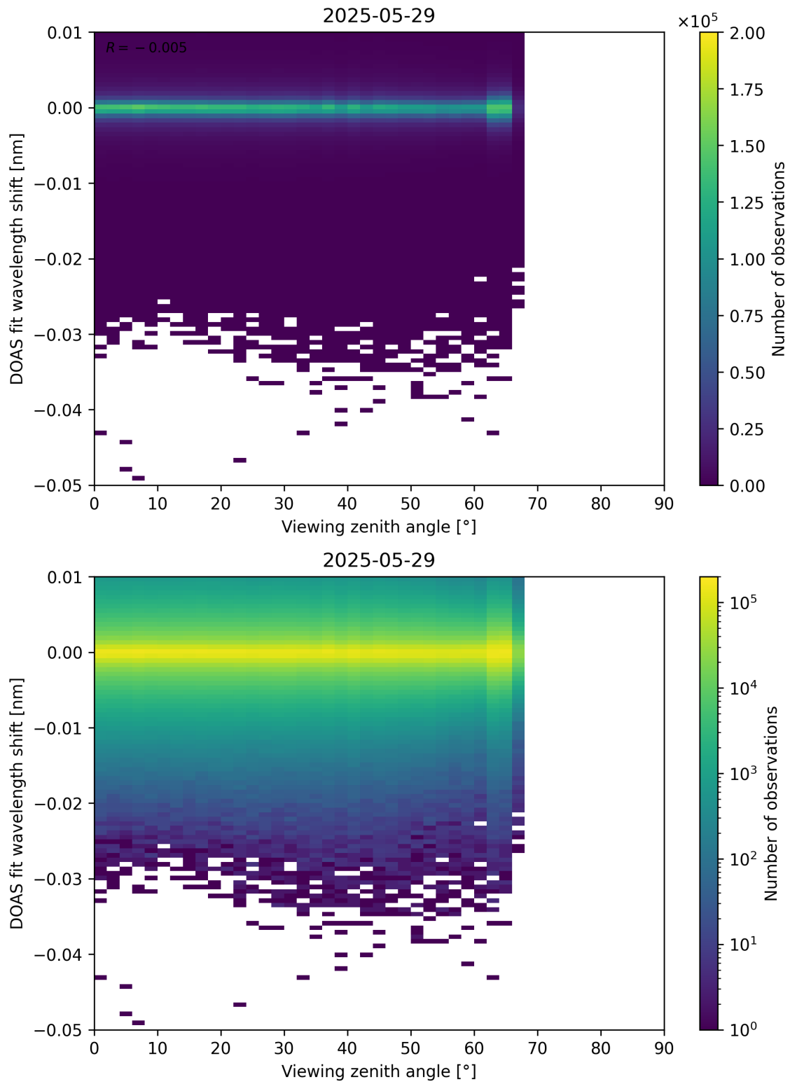
Figure 365: Scatter density plot of “Viewing zenith angle” against “DOAS fit wavelength shift” for 2025-05-28 to 2025-05-30.
