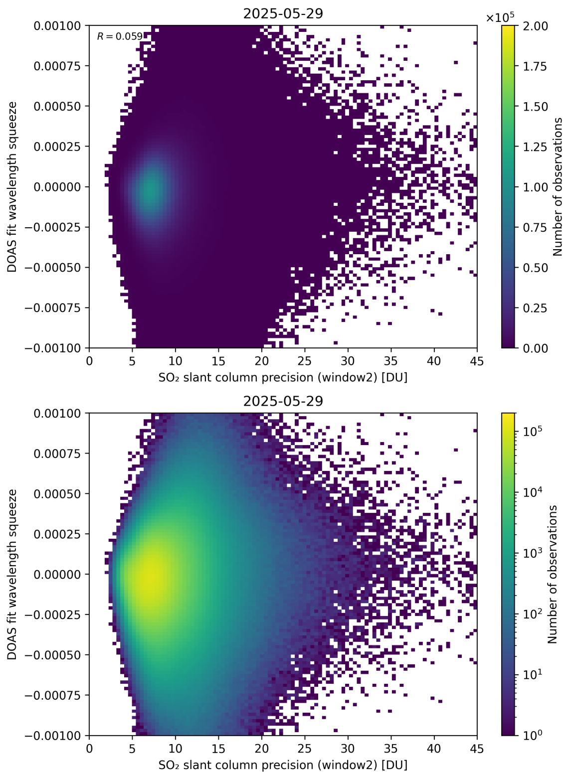
Figure 294: Scatter density plot of “SO 2 slant column precision (window2)” against “DOAS fit wavelength squeeze” for 2025-05-28 to 2025-05-30.
