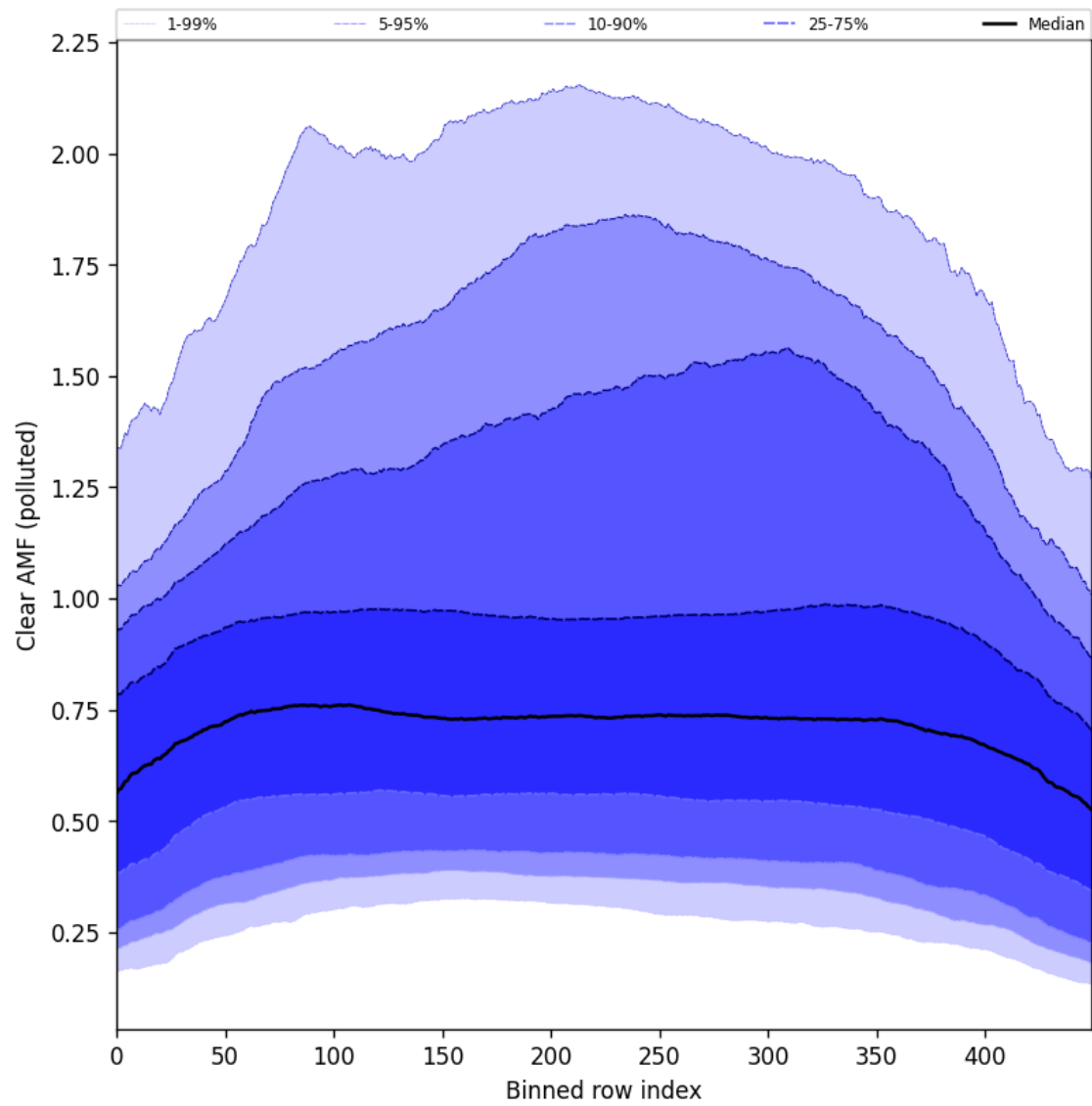
Figure 107: Along track statistics of “Clear AMF (polluted)” for 2025-05-28 to 2025-05-30
