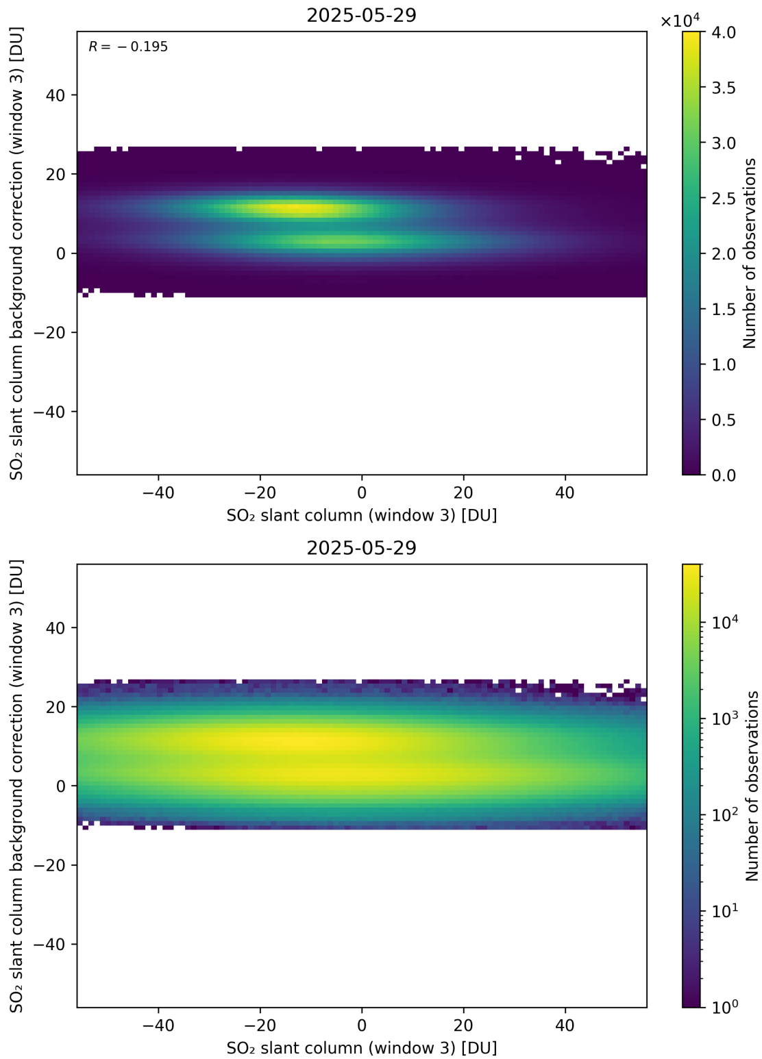
Figure 303: Scatter density plot of “SO 2 slant column (window 3)” against “SO 2 slant column background correction (window 3)” for 2025-05-28 to 2025-05-30.
