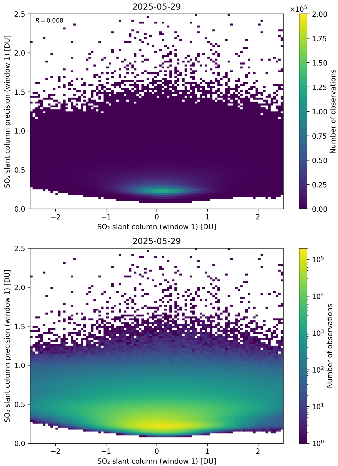
Figure 285: Scatter density plot of “SO 2 slant column (window 1)” against “SO 2 slant column precision (window 1)” for 2025-05-28 to 2025-05-30.
