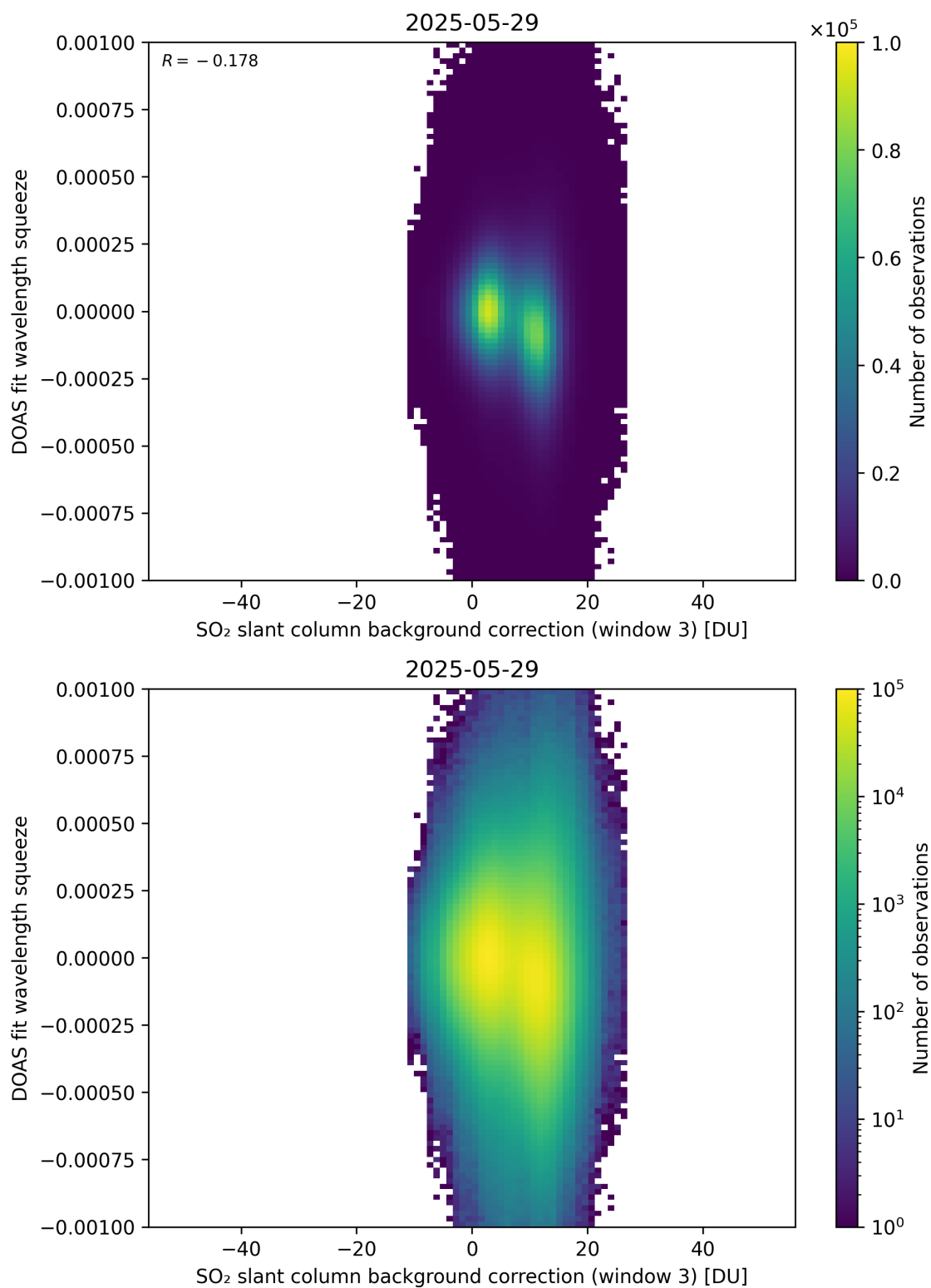
Figure 133: Scatter density plot of “SO 2 slant column background correction (window 3)” against “DOAS fit wavelength squeeze” for 2025-05-28 to 2025-05-30.
