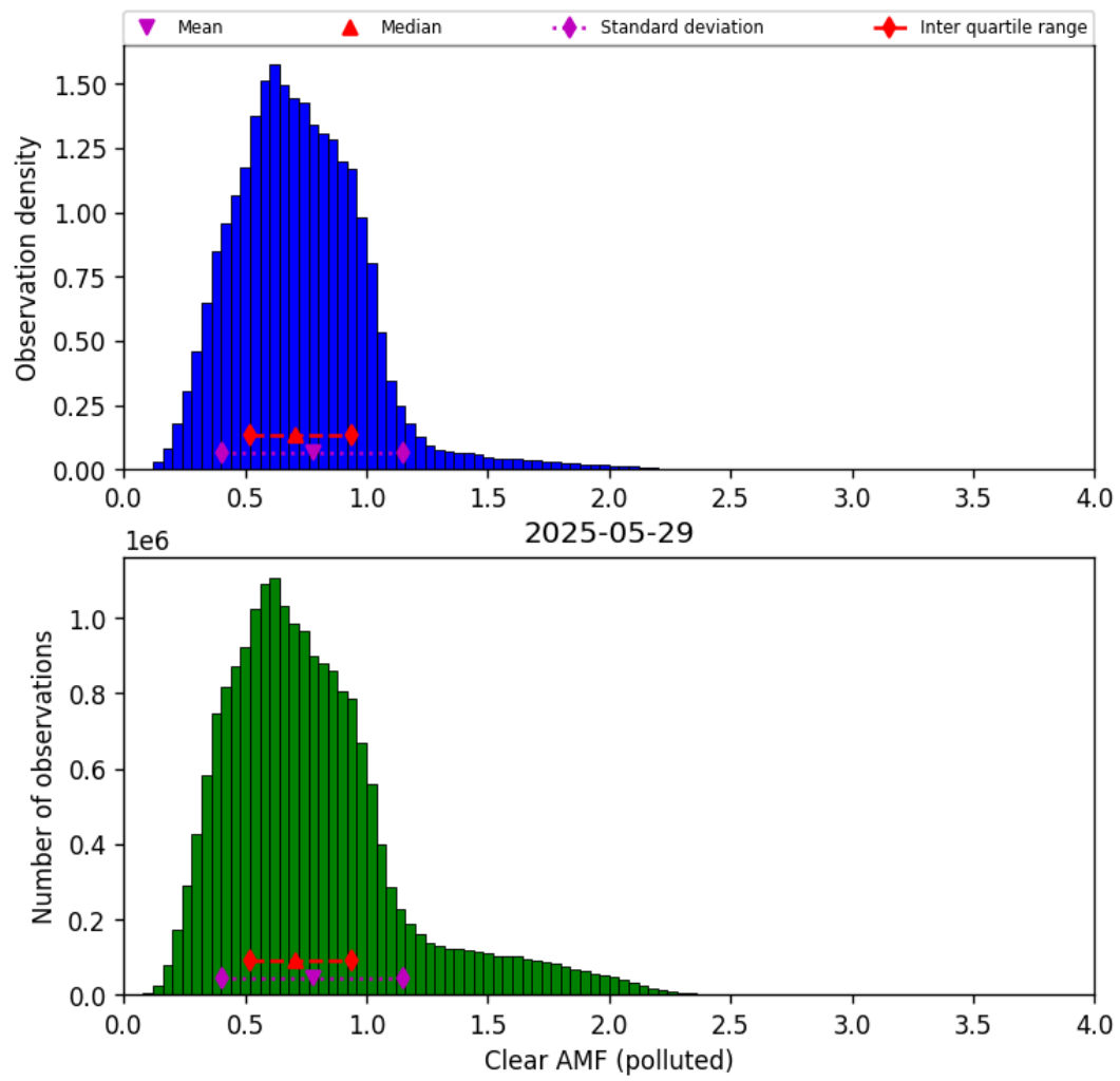
Figure 81: Histogram of “Clear AMF (polluted)” for 2025-05-28 to 2025-05-30
