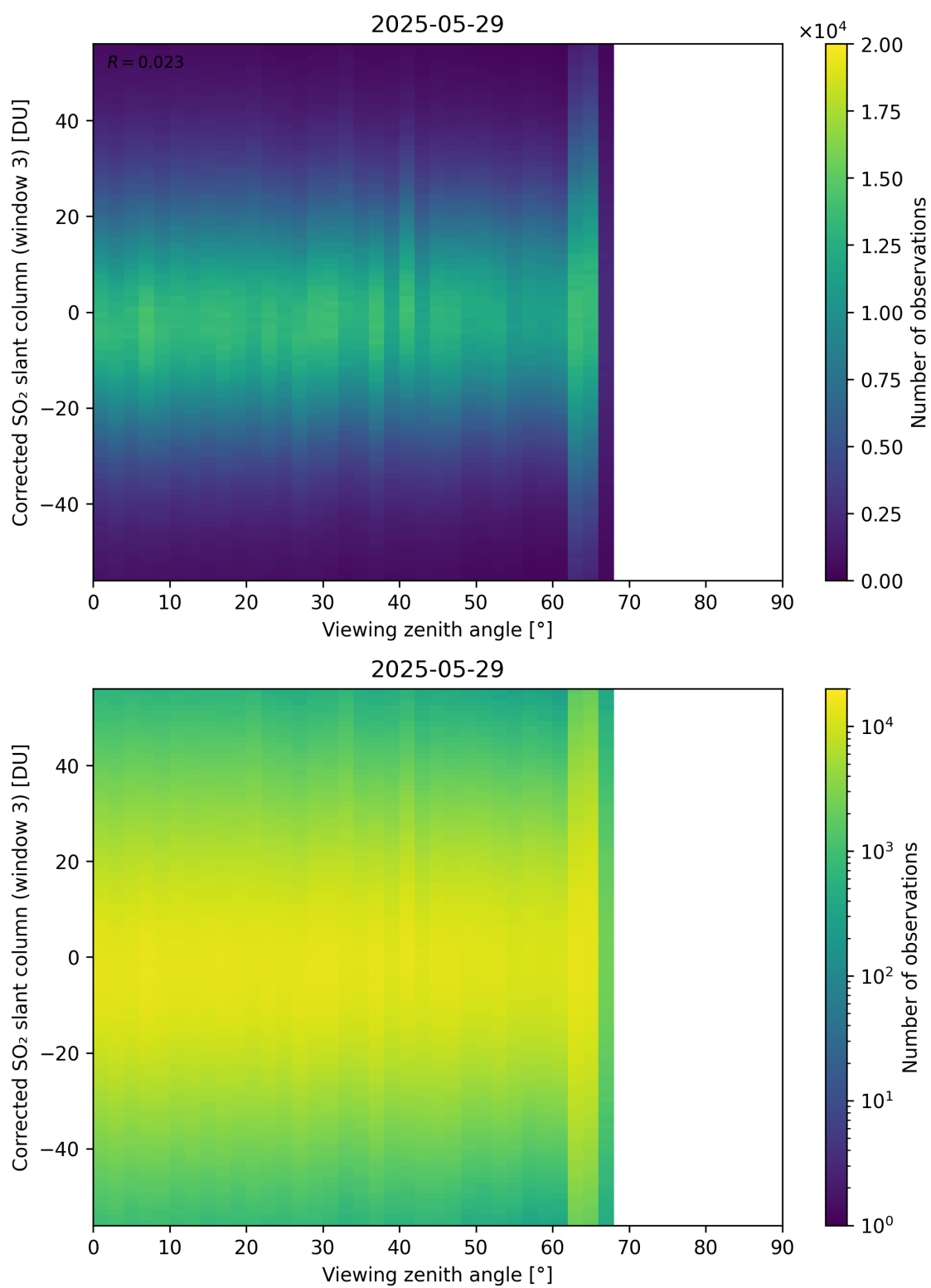
Figure 375: Scatter density plot of “Viewing zenith angle” against “Corrected SO 2 slant column (window 3)” for 2025-05-28 to 2025-05-30.
