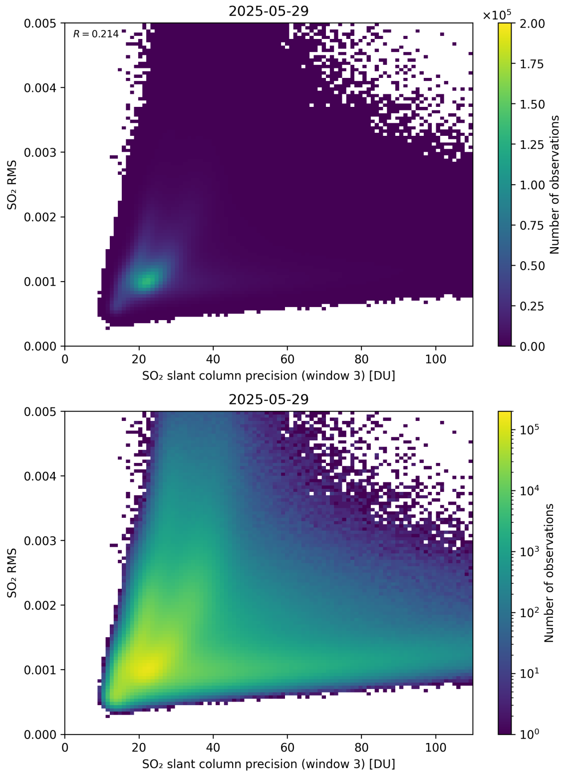
Figure 310: Scatter density plot of “SO 2 slant column precision (window 3)” against “SO 2 RMS” for 2025-05-28 to 2025-05-30.
