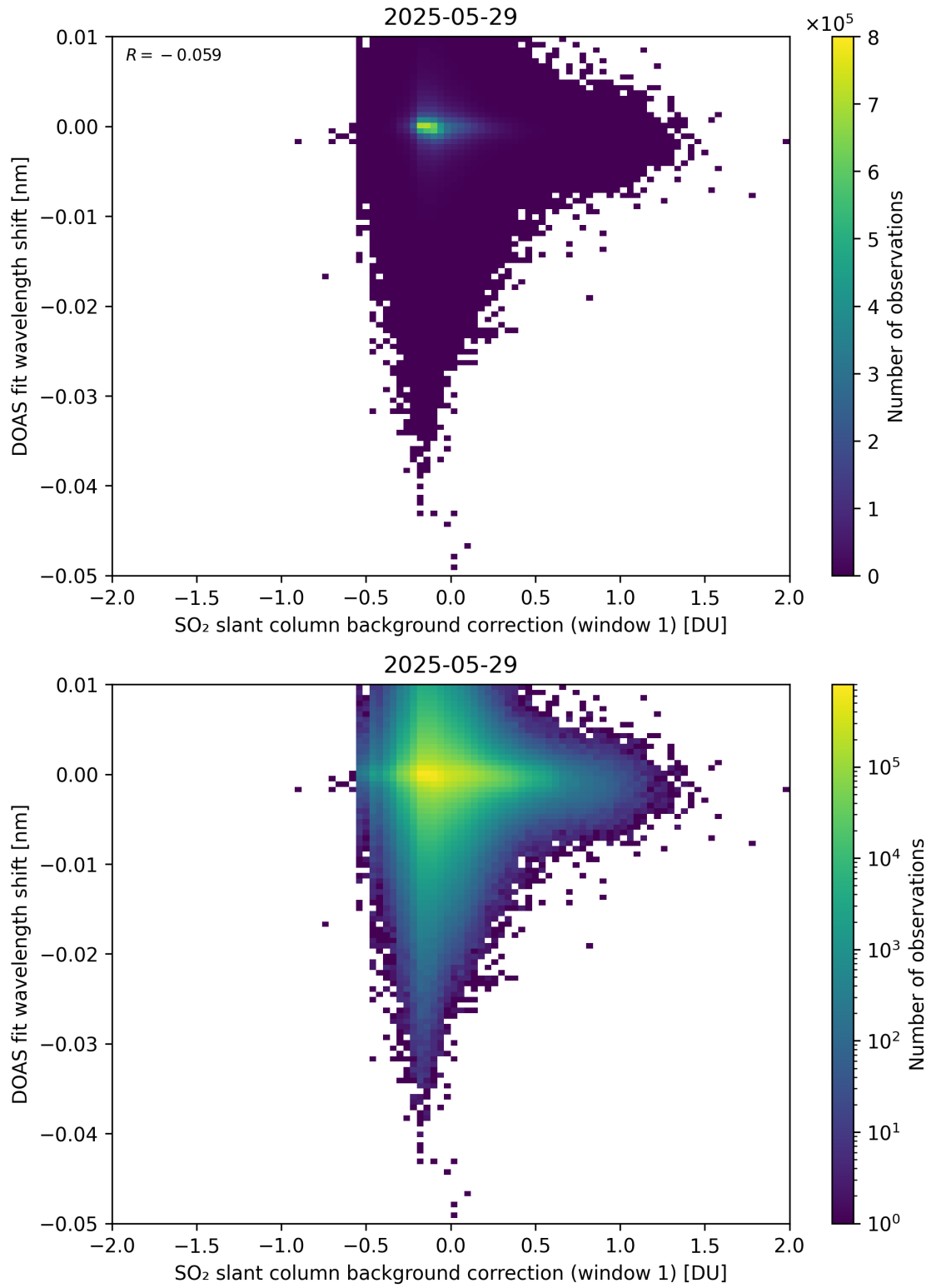
Figure 111: Scatter density plot of “SO 2 slant column background correction (window 1)” against “DOAS fit wavelength shift” for 2025-05-28 to 2025-05-30.
