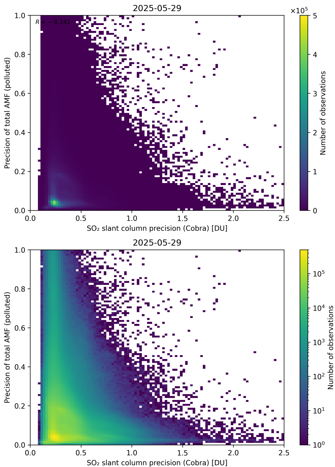
Figure 214: Scatter density plot of “SO 2 slant column precision (Cobra)” against “Precision of total AMF (polluted)” for 2025-05-28 to 2025-05-30.
