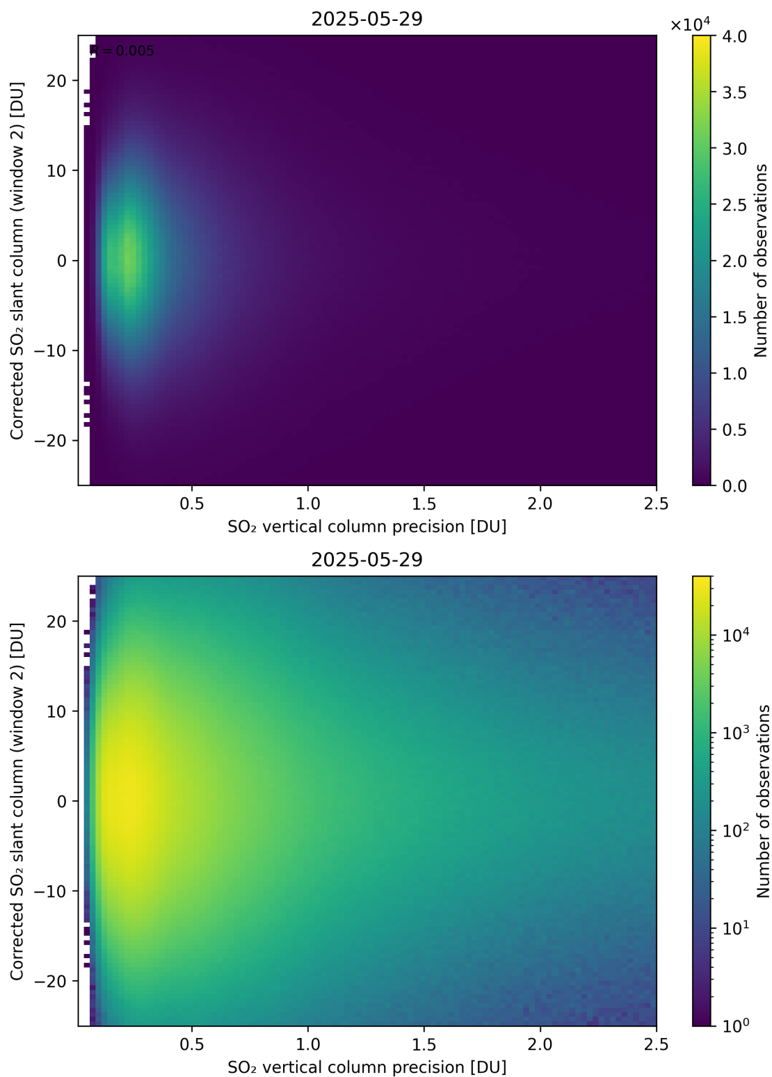
Figure 339: Scatter density plot of “SO 2 vertical column precision” against “Corrected SO 2 slant column (window 2)” for 2025-05-28 to 2025-05-30.
