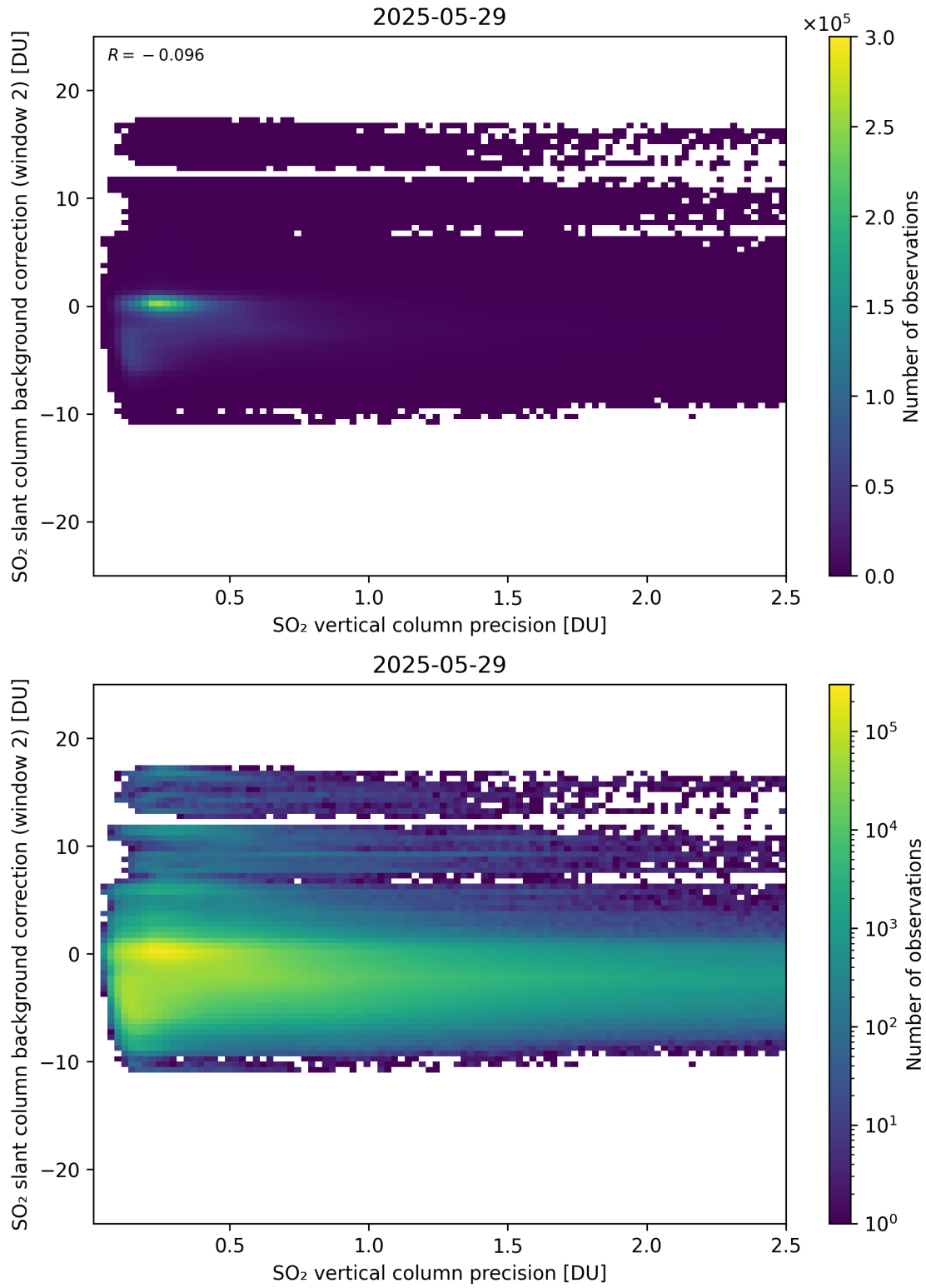
Figure 330: Scatter density plot of “SO 2 vertical column precision” against “SO 2 slant column background correction (window 2)” for 2025-05-28 to 2025-05-30.
