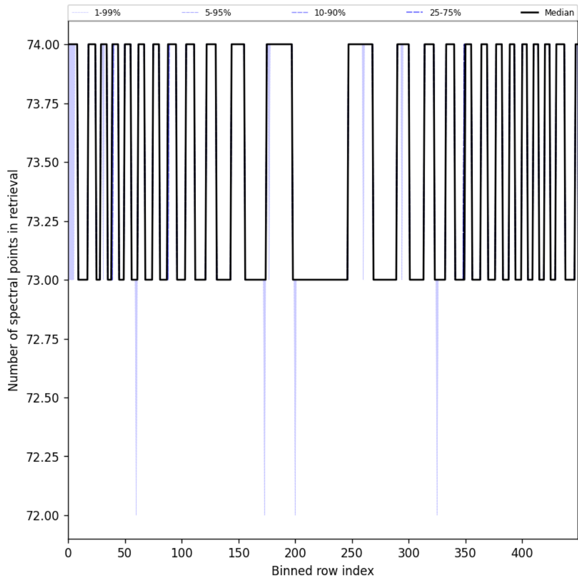
Figure 108: Along track statistics of “Number of spectral points in retrieval” for 2025-05-28 to 2025-05-30
