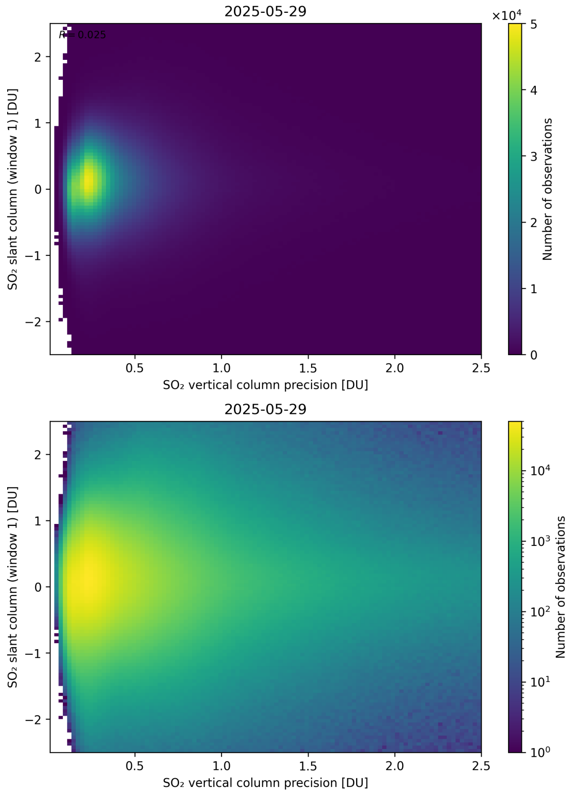
Figure 341: Scatter density plot of “SO 2 vertical column precision” against “SO 2 slant column (window 1)” for 2025-05-28 to 2025-05-30.
