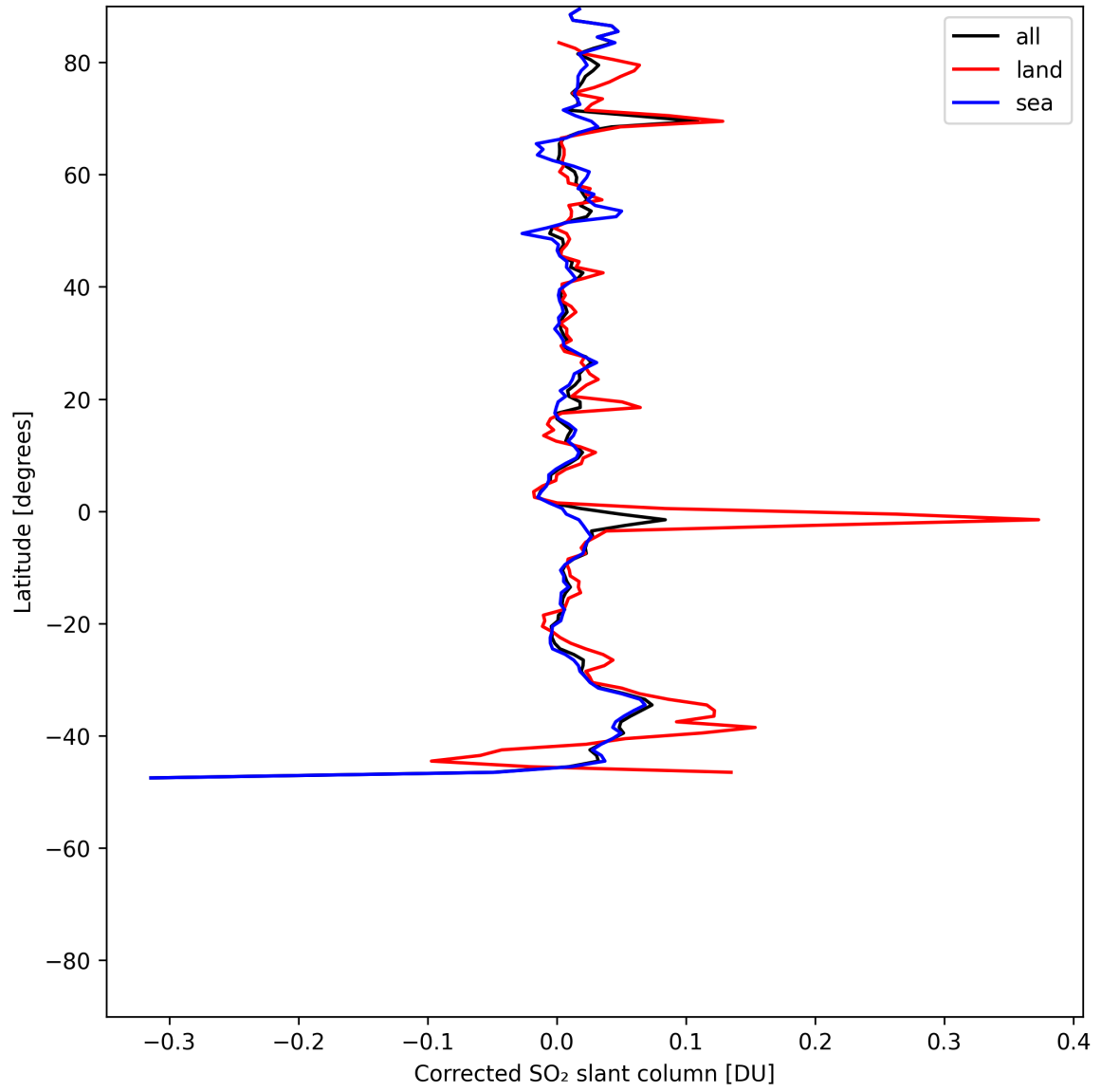
Figure 34: Zonal average of “Corrected SO 2 slant column” for 2025-05-28 to 2025-05-30.
