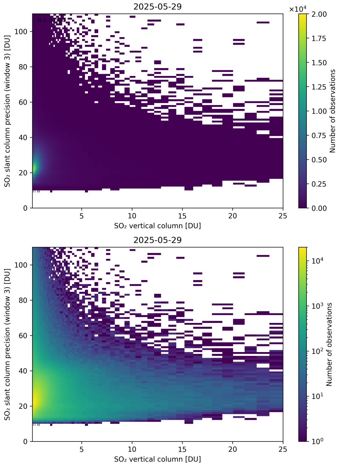
Figure 358: Scatter density plot of “SO 2 vertical column” against “SO 2 slant column precision (window 3)” for 2025-05-28 to 2025-05-30.
