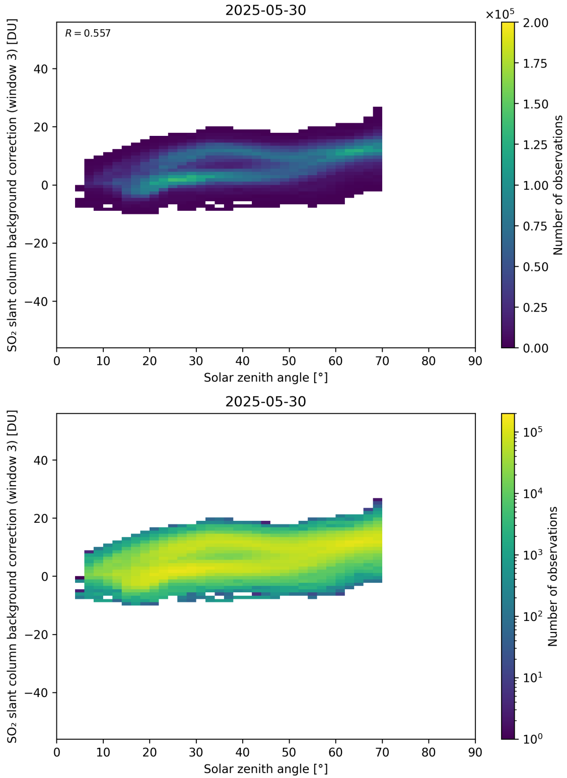
Figure 173: Scatter density plot of “Solar zenith angle” against “SO 2 slant column background correction (window 3)” for 2025-05-29 to 2025-05-31.
