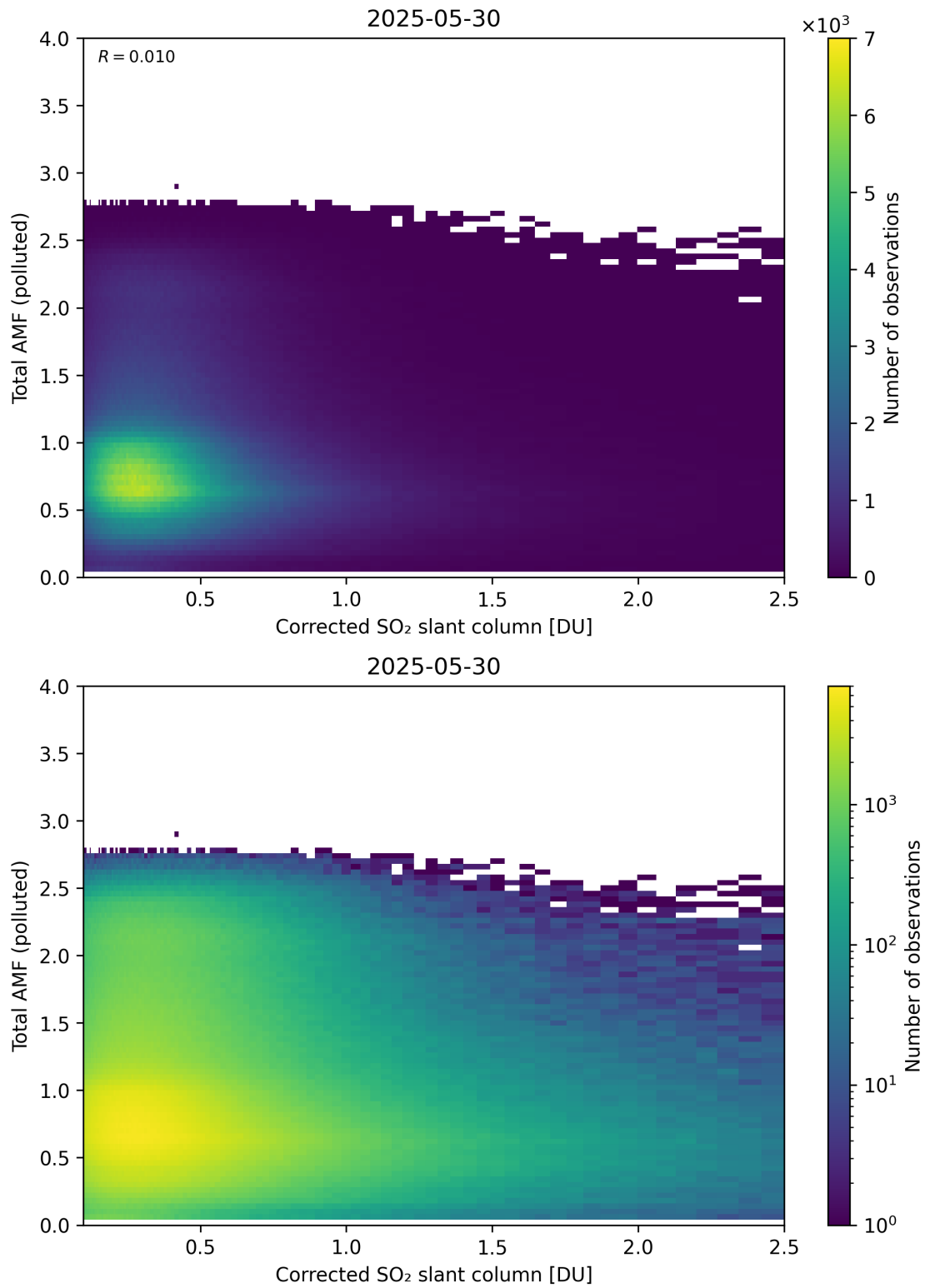
Figure 242: Scatter density plot of “Corrected SO 2 slant column” against “Total AMF (polluted)” for 2025-05-29 to 2025-05-31.
