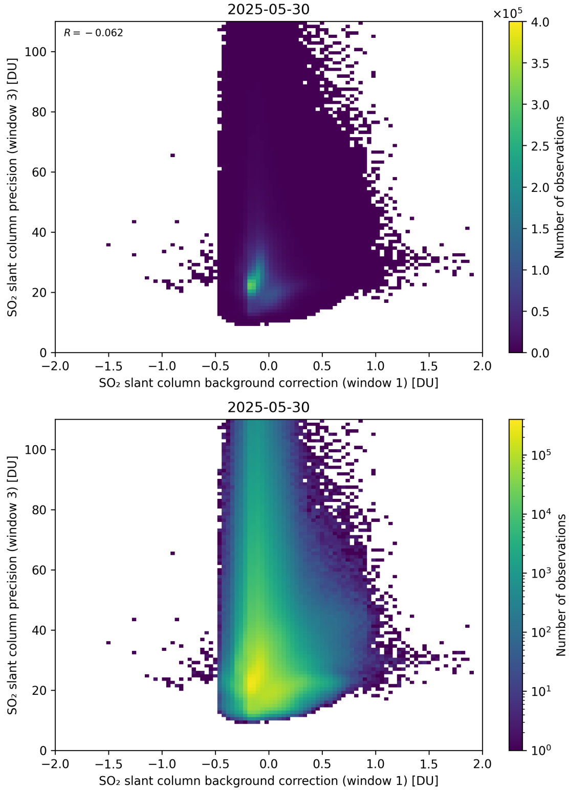
Figure 119: Scatter density plot of “SO 2 slant column background correction (window 1)” against “SO 2 slant column precision (window 3)” for 2025-05-29 to 2025-05-31.
