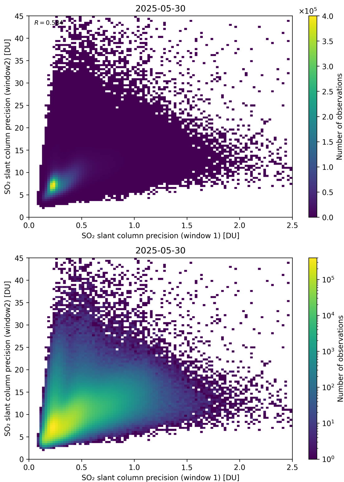
Figure 277: Scatter density plot of “SO 2 slant column precision (window 1)” against “SO 2 slant column precision (window 2)” for 2025-05-29 to 2025-05-31.
