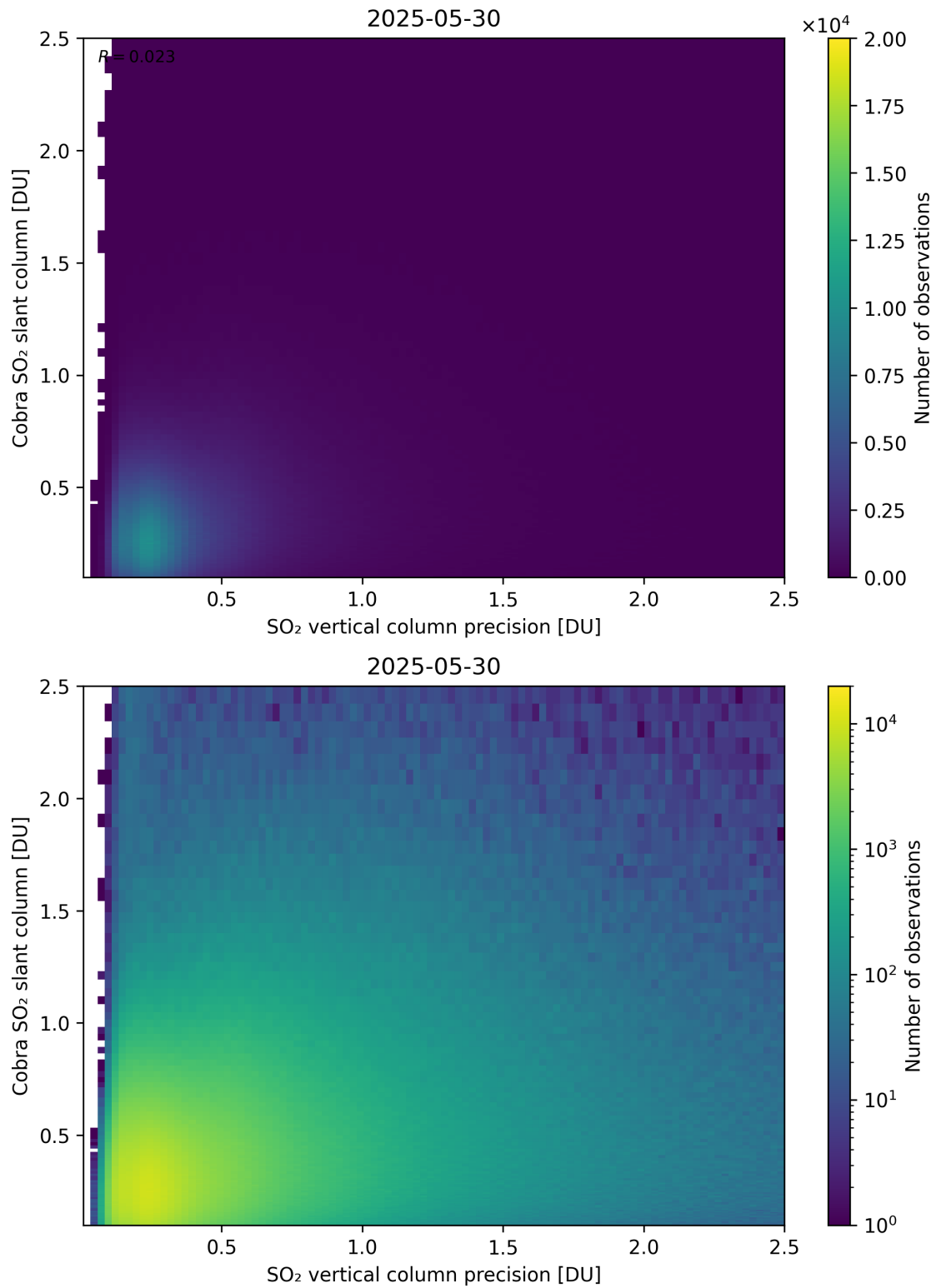
Figure 336: Scatter density plot of “SO 2 vertical column precision” against “Cobra SO 2 slant column” for 2025-05-29 to 2025-05-31.
