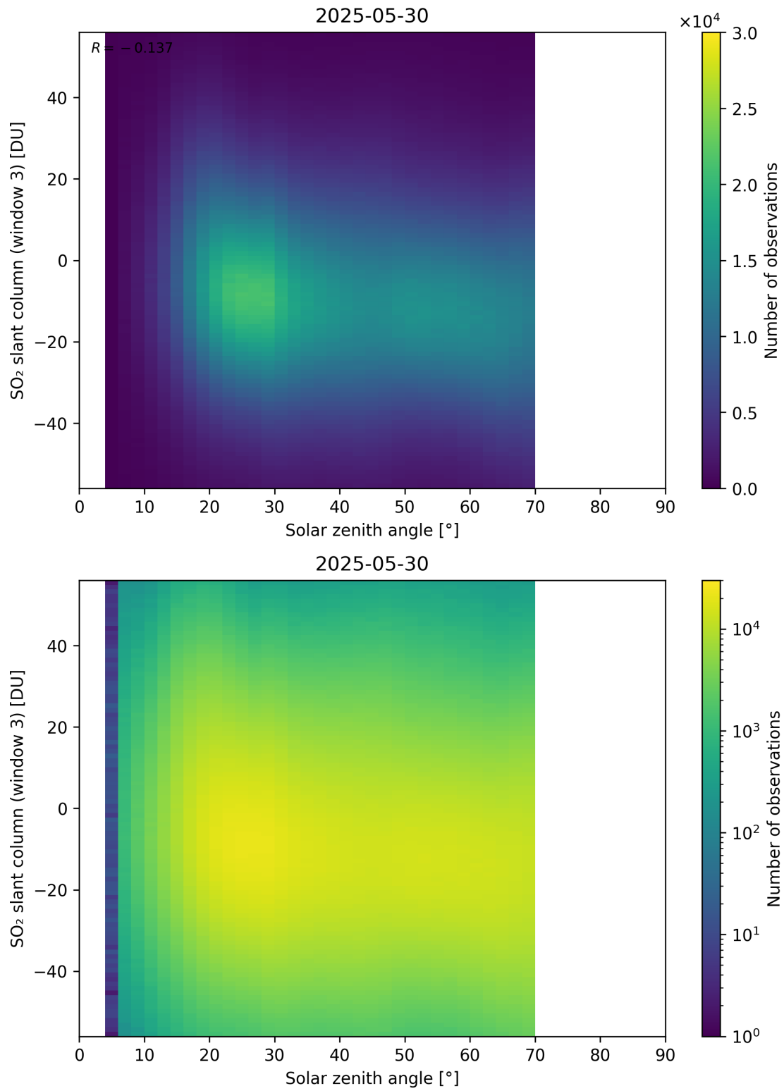
Figure 187: Scatter density plot of “Solar zenith angle” against “SO 2 slant column (window 3)” for 2025-05-29 to 2025-05-31.
