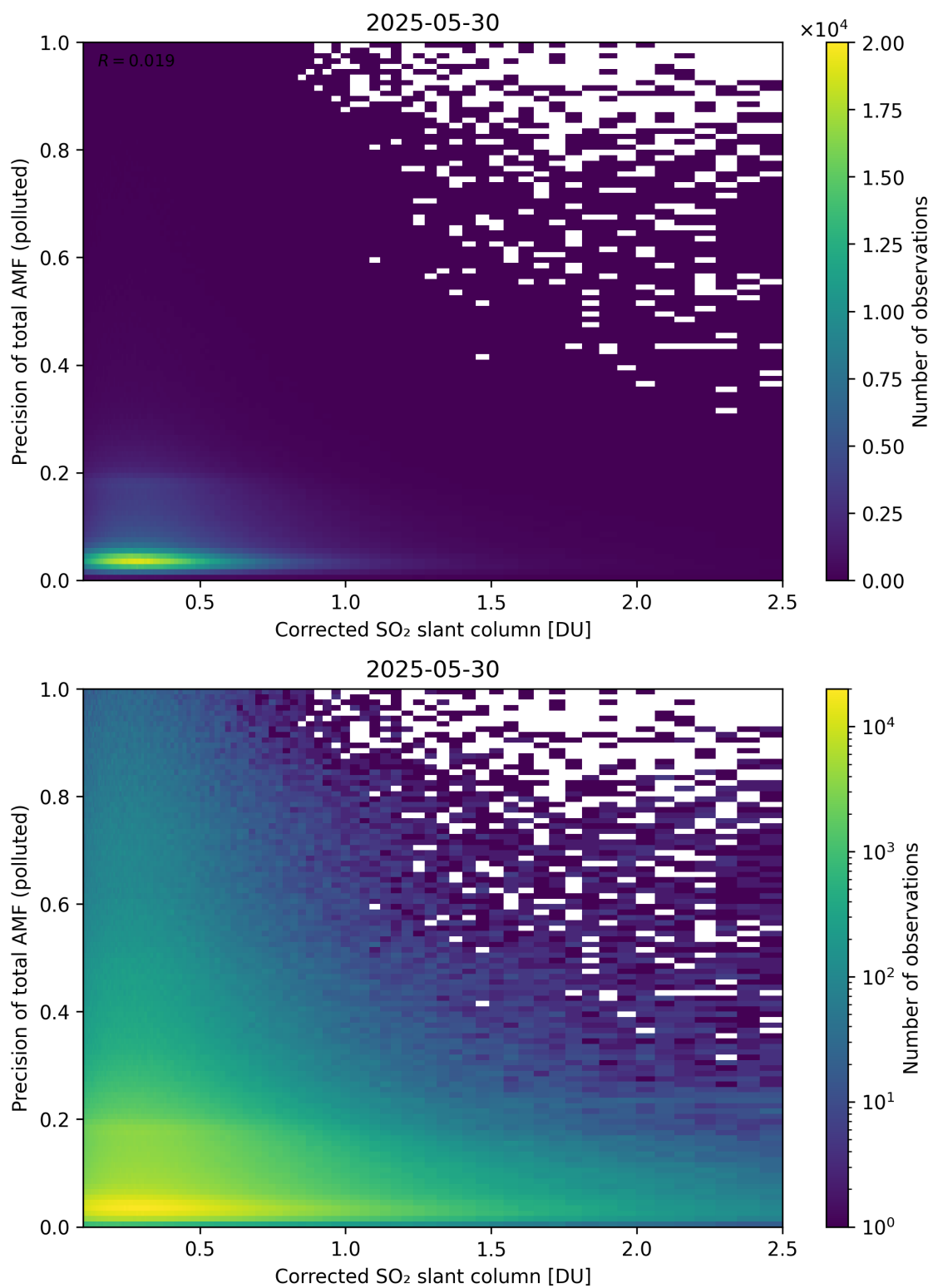
Figure 243: Scatter density plot of “Corrected SO 2 slant column” against “Precision of total AMF (polluted)” for 2025-05-29 to 2025-05-31.
