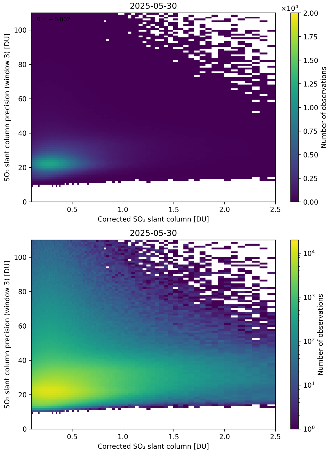
Figure 241: Scatter density plot of “Corrected SO 2 slant column” against “SO 2 slant column precision (window 3)” for 2025-05-29 to 2025-05-31.
