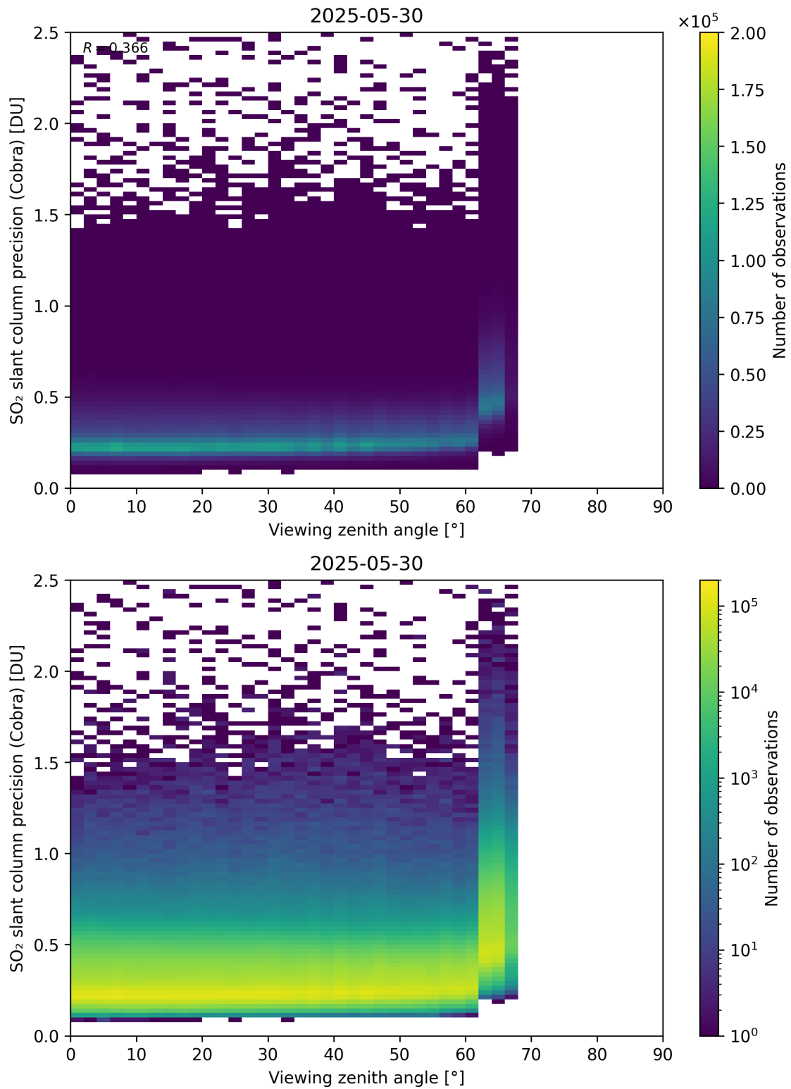
Figure 372: Scatter density plot of “Viewing zenith angle” against “SO 2 slant column precision (Cobra)” for 2025-05-29 to 2025-05-31.
