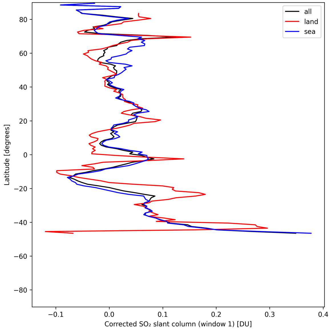
Figure 39: Zonal average of "Corrected SO 2 slant column (window 1)" for 2025-05-29 to 2025-05-31.
