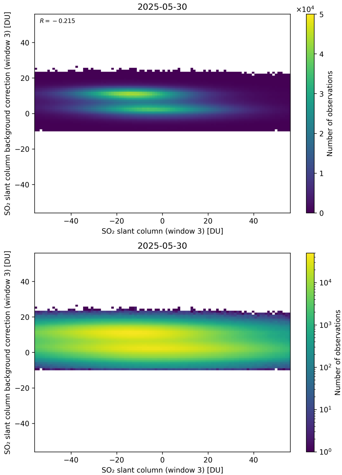
Figure 303: Scatter density plot of “SO 2 slant column (window 3)” against “SO 2 slant column background correction (window 3)” for 2025-05-29 to 2025-05-31.
