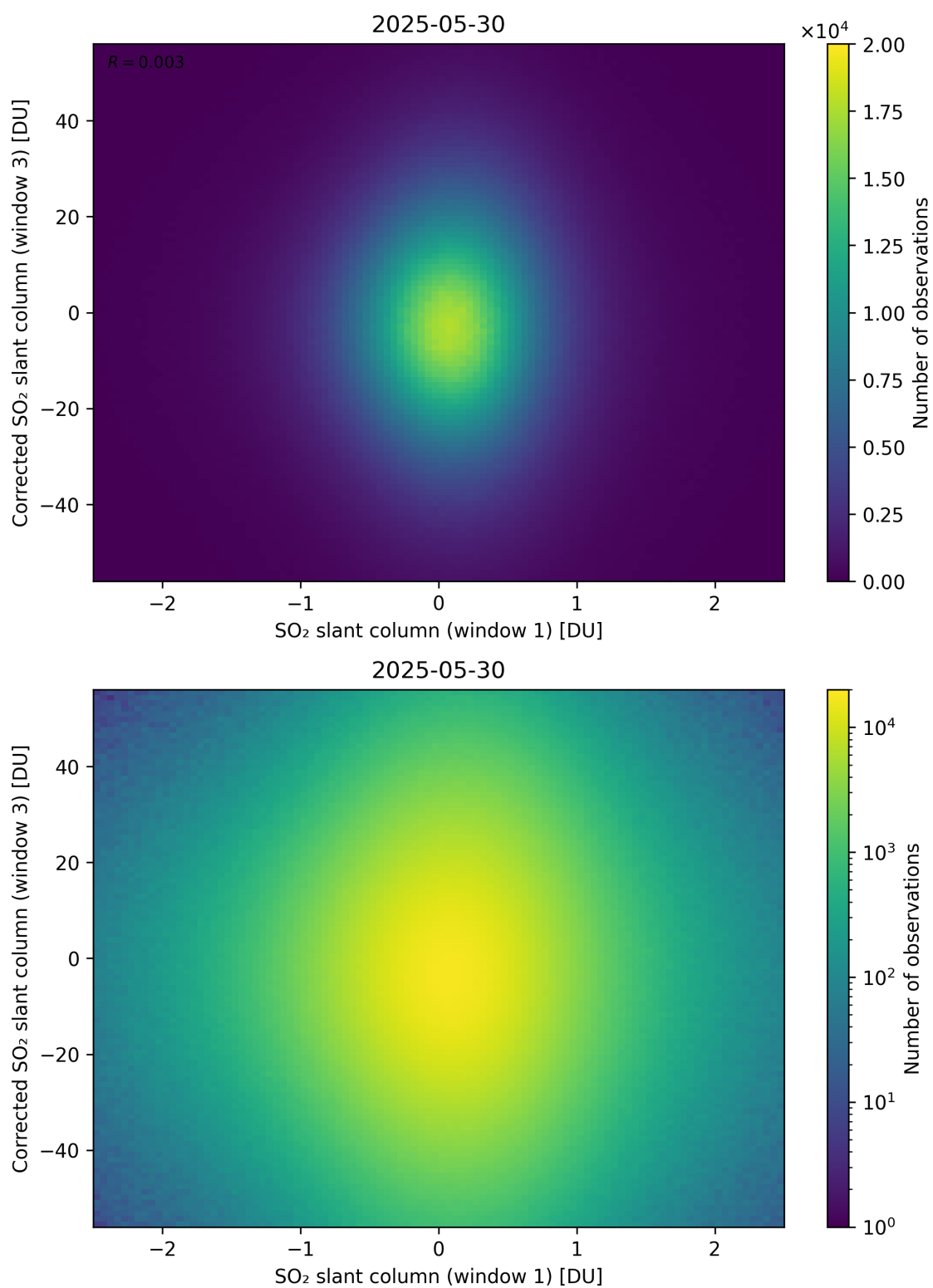
Figure 284: Scatter density plot of “SO 2 slant column (window 1)” against “Corrected SO 2 slant column (window 3)” for 2025-05-29 to 2025-05-31.
