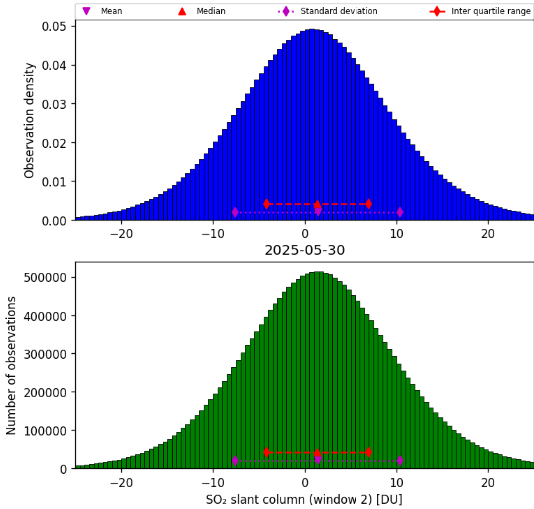
Figure 67: Histogram of “SO 2 slant column (window 2)” for 2025-05-29 to 2025-05-31
