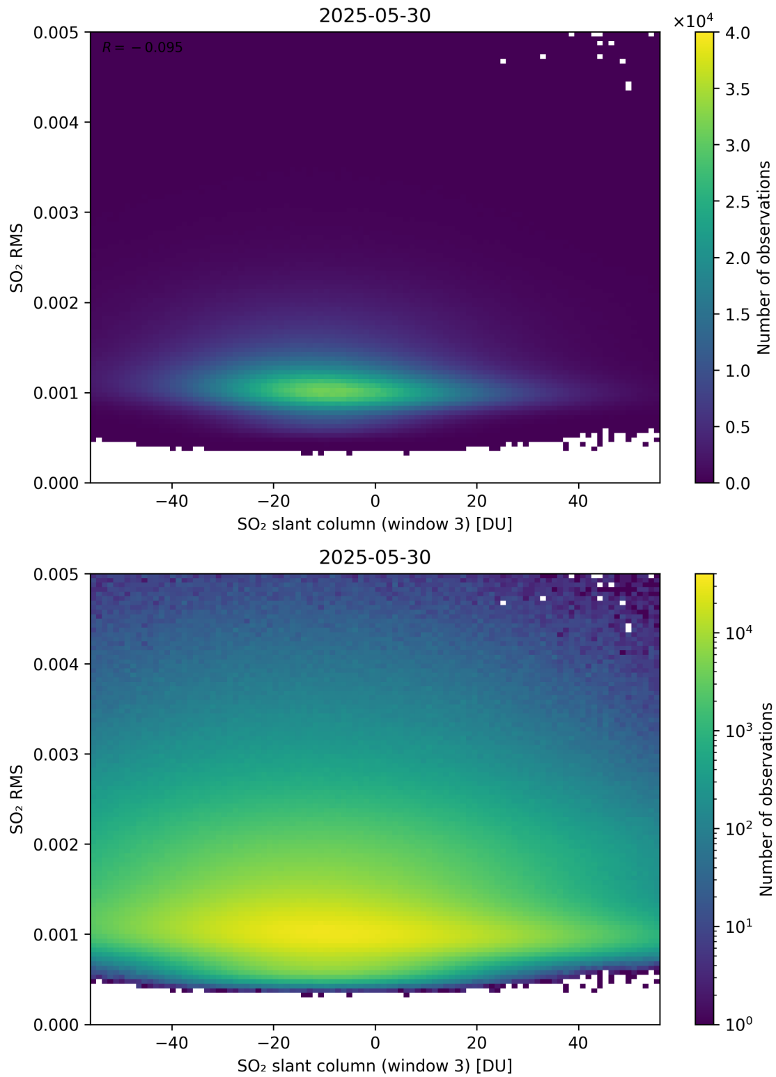
Figure 306: Scatter density plot of “SO 2 slant column (window 3)” against “SO 2 RMS” for 2025-05-29 to 2025-05-31.
