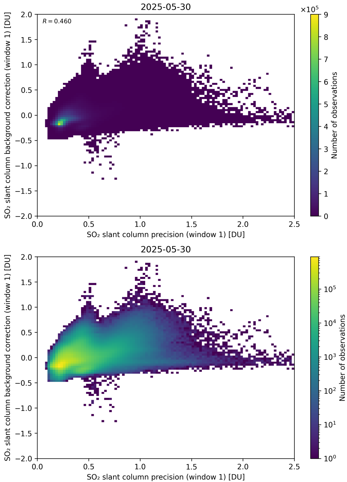
Figure 268: Scatter density plot of “SO 2 slant column precision (window 1)” against “SO 2 slant column background correction (window 1)” for 2025-05-29 to 2025-05-31.
