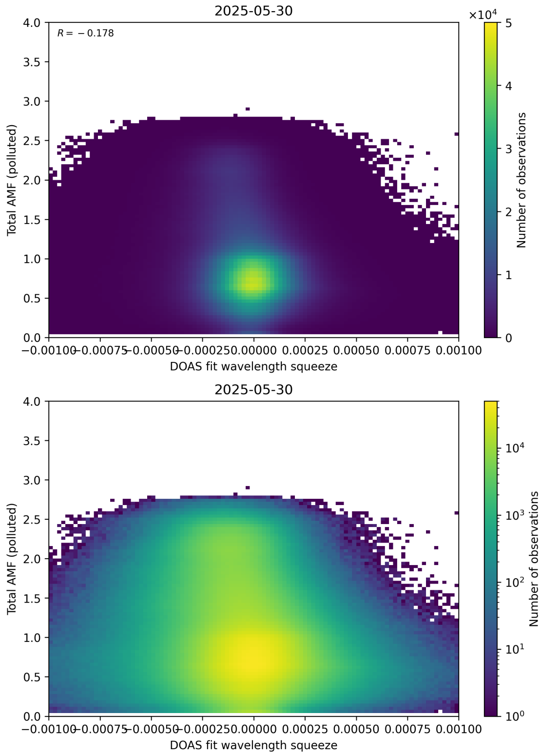
Figure 145: Scatter density plot of “DOAS fit wavelength squeeze” against “Total AMF (polluted)” for 2025-05-29 to 2025-05-31.
