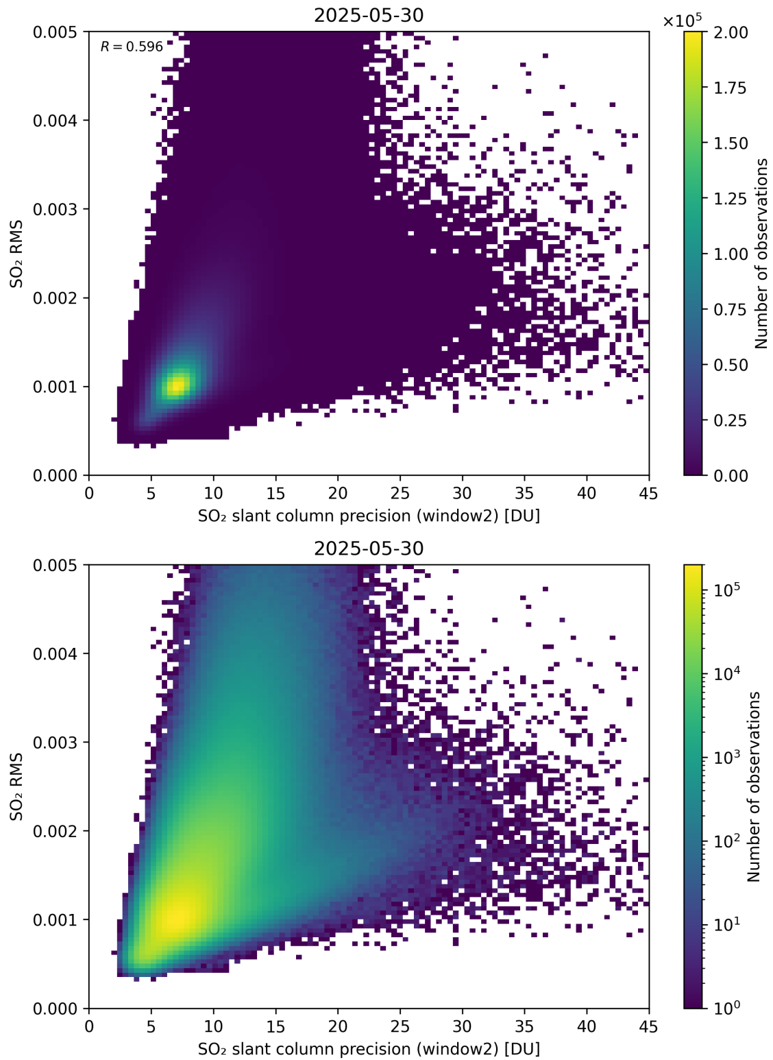
Figure 295: Scatter density plot of “SO 2 slant column precision (window2)” against “SO 2 RMS” for 2025-05-29 to 2025-05-31.
