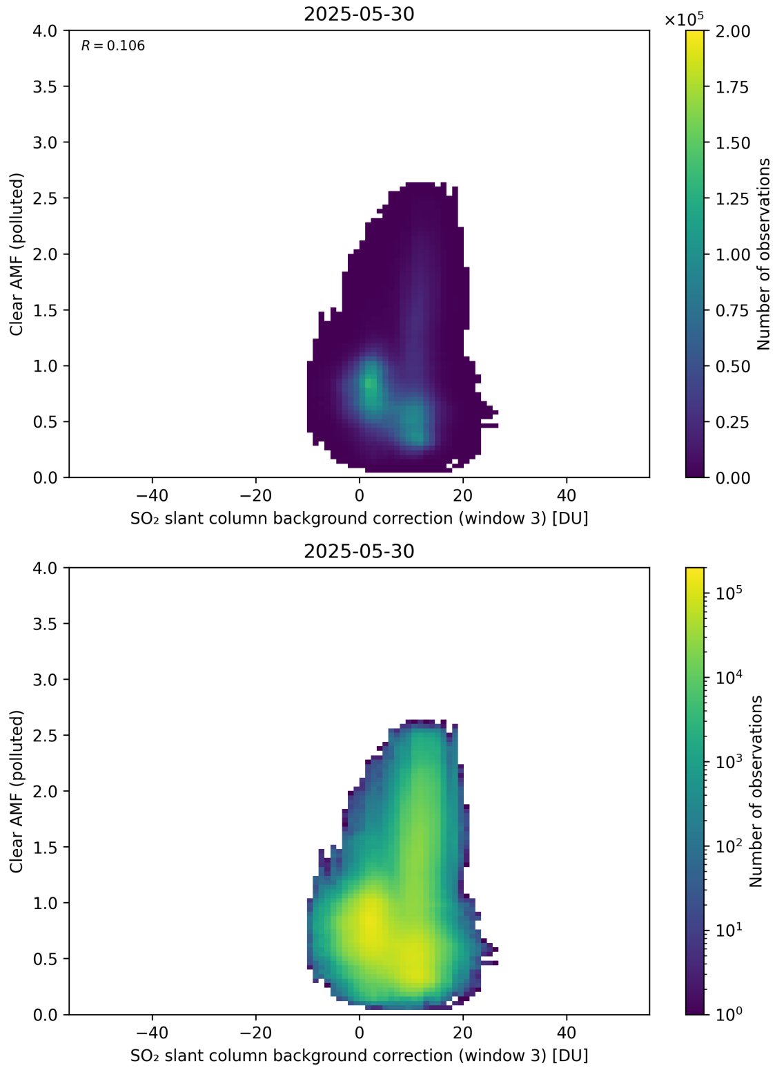
Figure 135: Scatter density plot of “SO 2 slant column background correction (window 3)” against “Clear AMF (polluted)” for 2025-05-29 to 2025-05-31.
