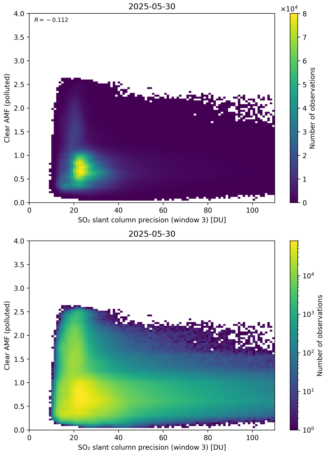
Figure 311: Scatter density plot of “SO 2 slant column precision (window 3)” against “Clear AMF (polluted)” for 2025-05-29 to 2025-05-31.
