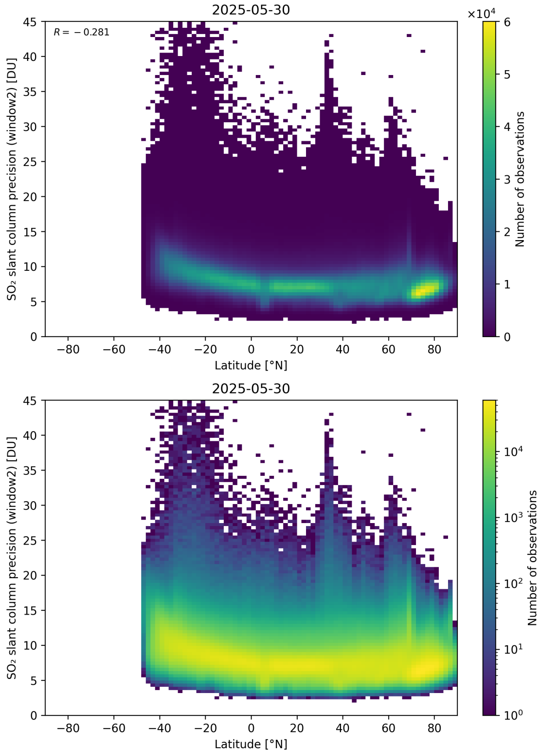
Figure 164: Scatter density plot of “Latitude” against “SO 2 slant column precision (window2)” for 2025-05-29 to 2025-05-31.
