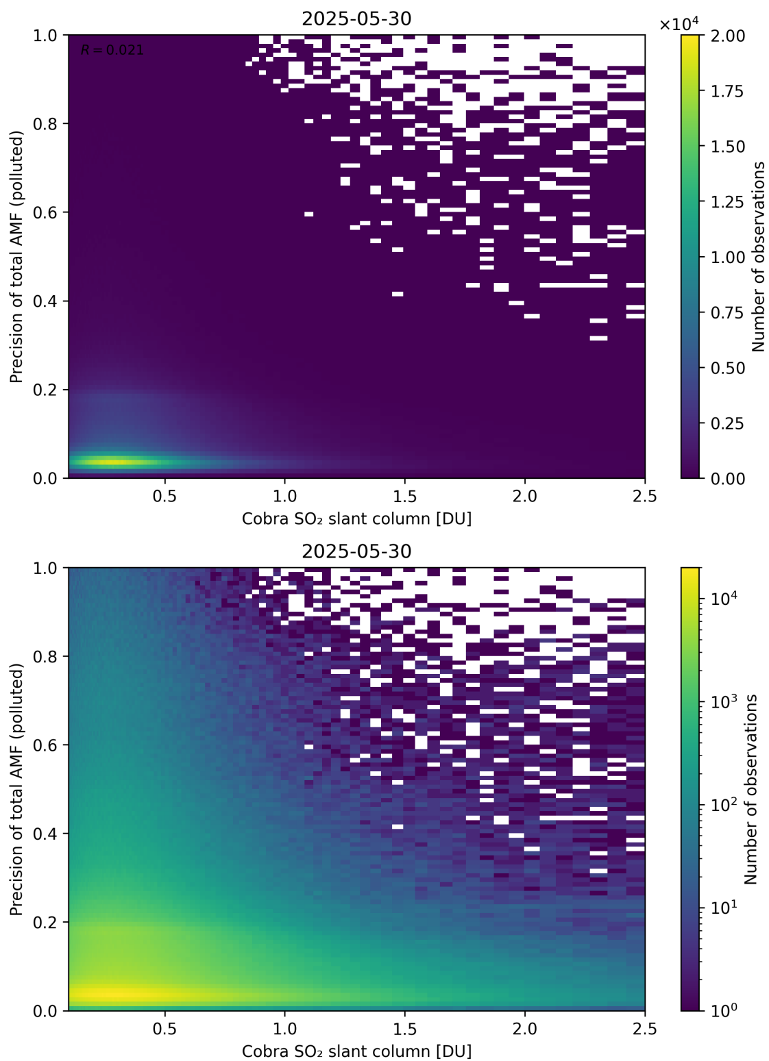
Figure 225: Scatter density plot of “Cobra SO 2 slant column” against “Precision of total AMF (polluted)” for 2025-05-29 to 2025-05-31.
