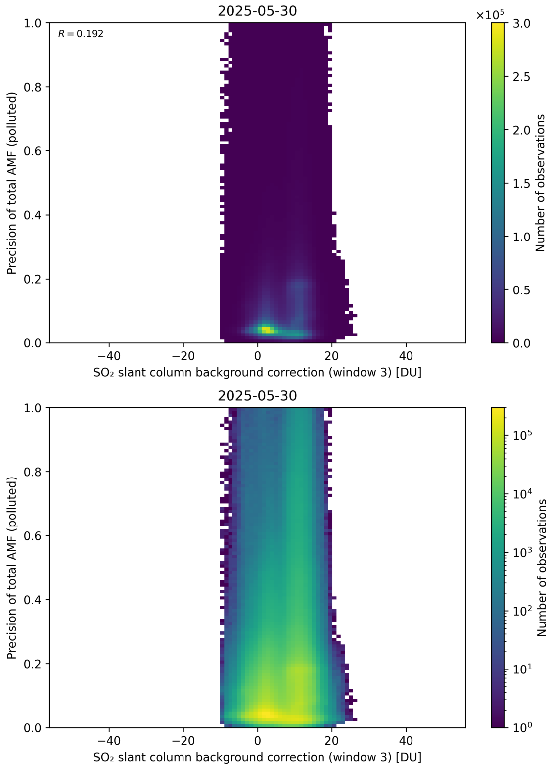
Figure 137: Scatter density plot of “SO 2 slant column background correction (window 3)” against “Precision of total AMF (polluted)” for 2025-05-29 to 2025-05-31.
