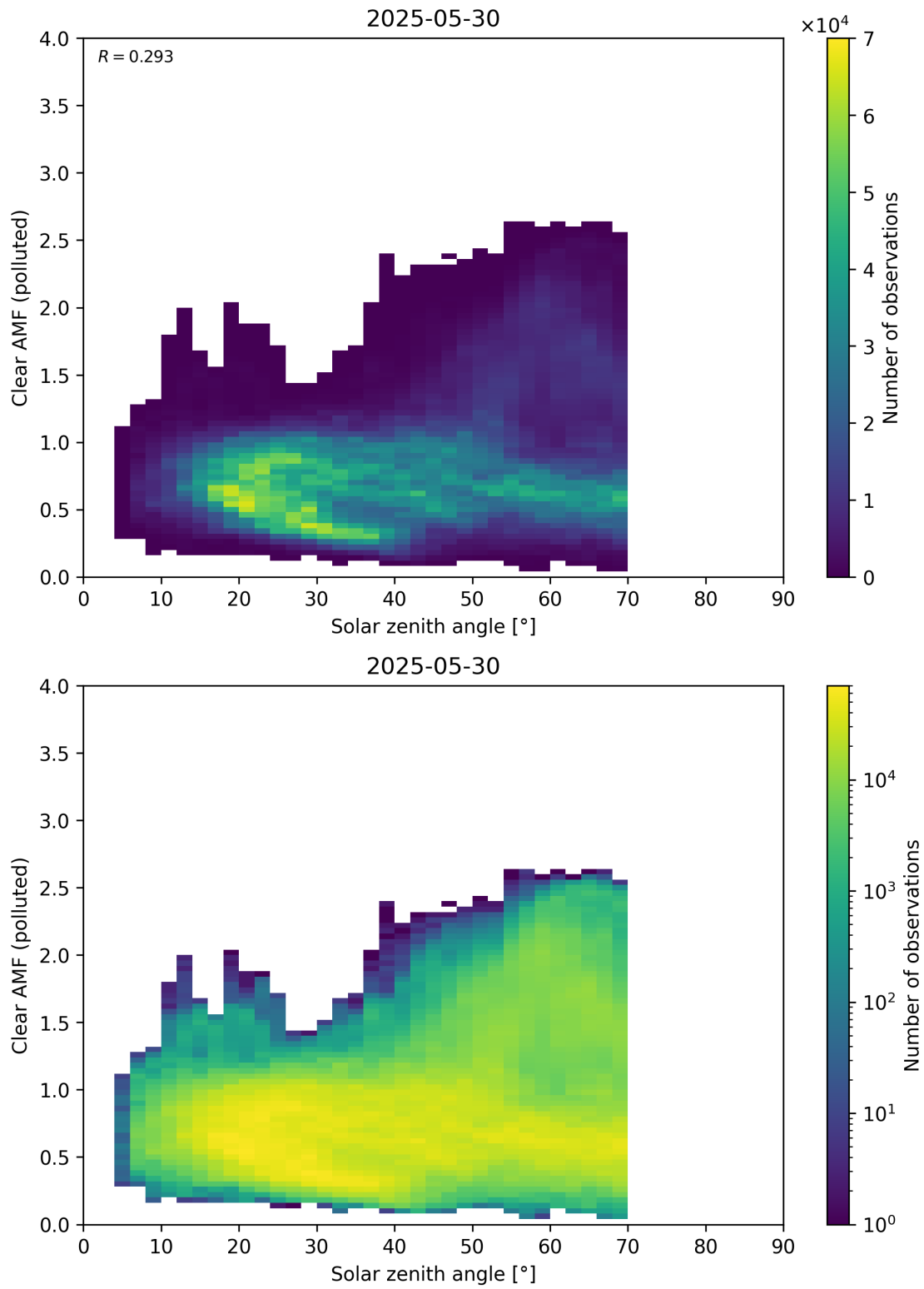
Figure 178: Scatter density plot of “Solar zenith angle” against “Clear AMF (polluted)” for 2025-05-29 to 2025-05-31.
