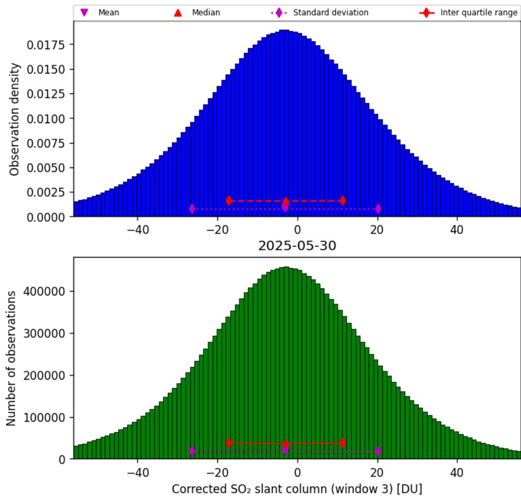
Figure 73: Histogram of “Corrected SO 2 slant column (window 3)” for 2025-05-29 to 2025-05-31
