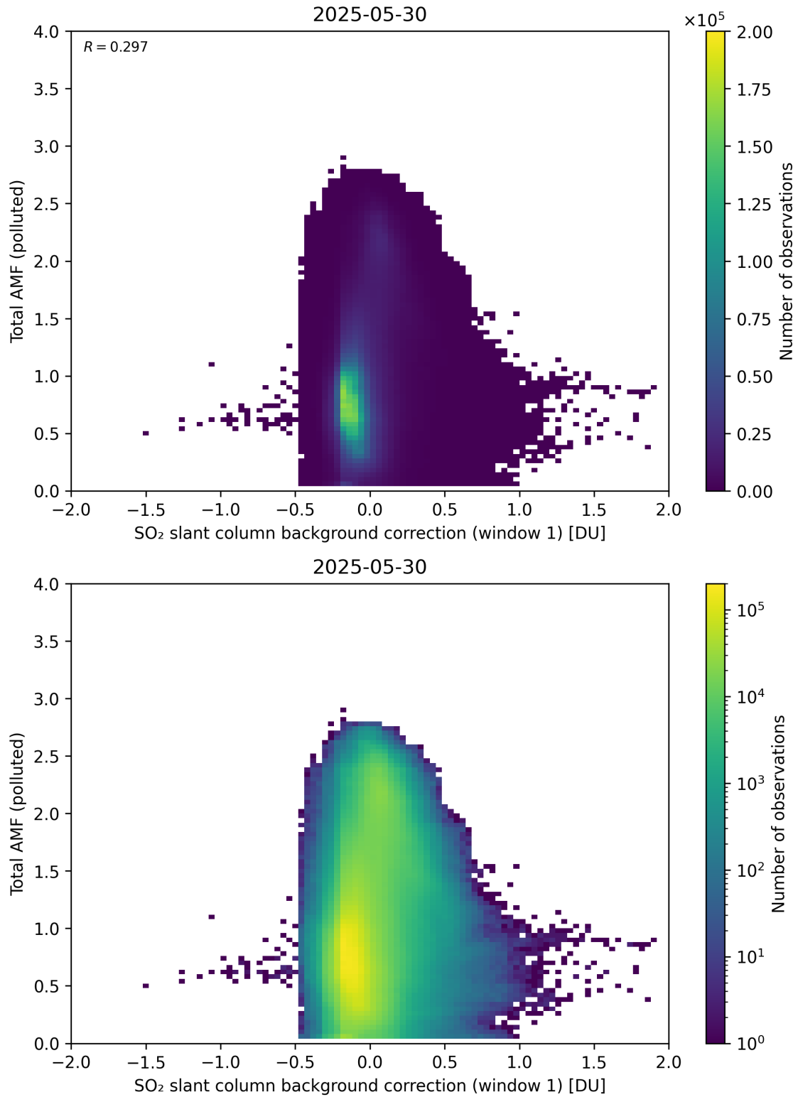
Figure 120: Scatter density plot of “SO 2 slant column background correction (window 1)” against “Total AMF (polluted)” for 2025-05-29 to 2025-05-31.
