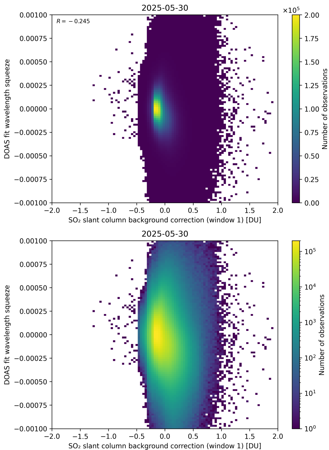
Figure 112: Scatter density plot of “SO 2 slant column background correction (window 1)” against “DOAS fit wavelength squeeze” for 2025-05-29 to 2025-05-31.
