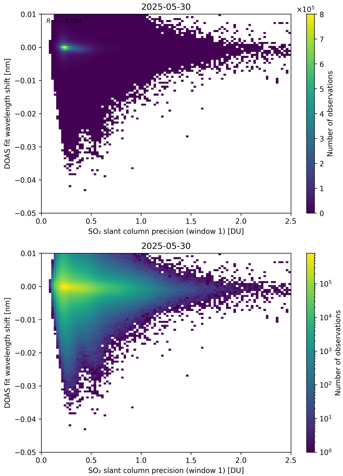
Figure 271: Scatter density plot of “SO 2 slant column precision (window 1)” against “DOAS fit wavelength shift” for 2025-05-29 to 2025-05-31.
