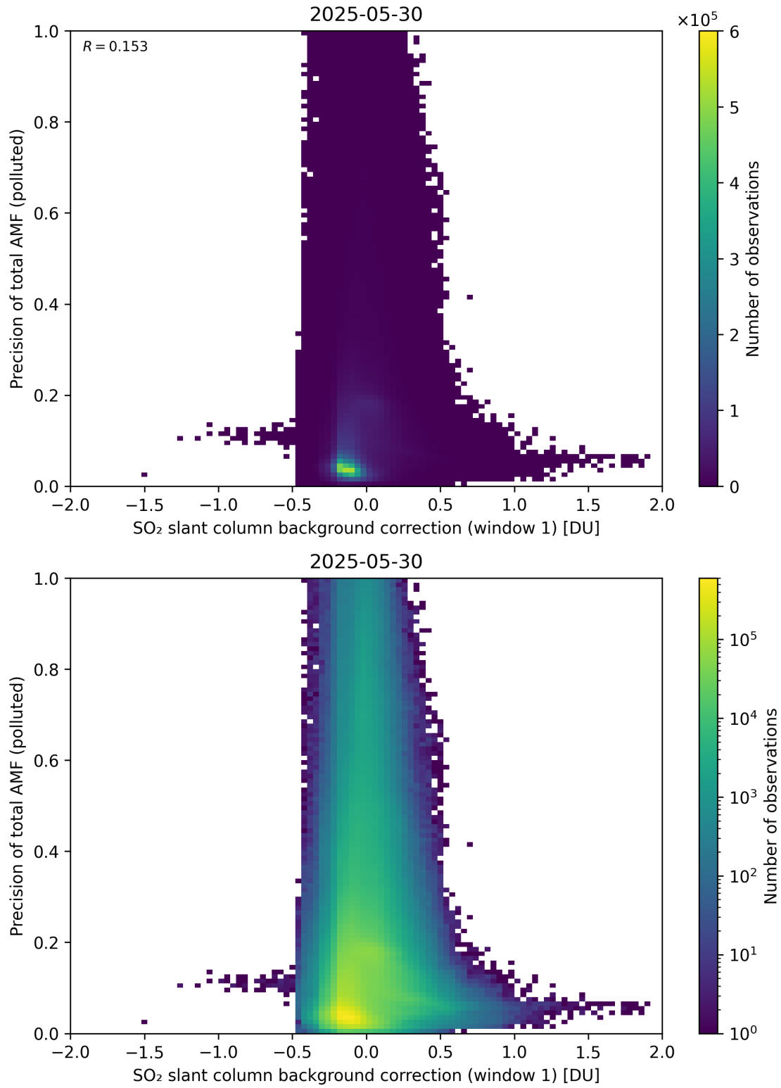
Figure 121: Scatter density plot of “SO 2 slant column background correction (window 1)” against “Precision of total AMF (polluted)” for 2025-05-29 to 2025-05-31.
