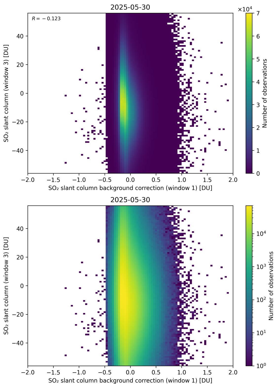
Figure 118: Scatter density plot of “SO 2 slant column background correction (window 1)” against “SO 2 slant column (window 3)” for 2025-05-29 to 2025-05-31.
