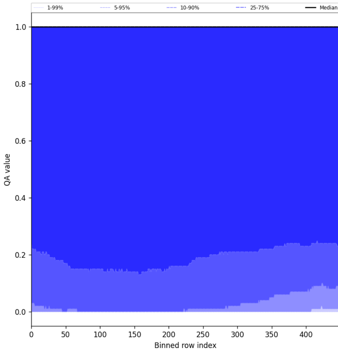
Figure 83: Along track statistics of “QA value” for 2025-05-29 to 2025-05-31
