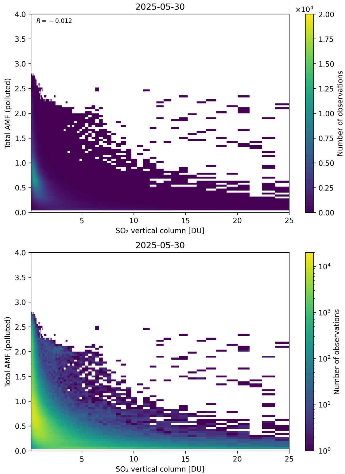
Figure 359: Scatter density plot of “SO 2 vertical column” against “Total AMF (polluted)” for 2025-05-29 to 2025-05-31.
