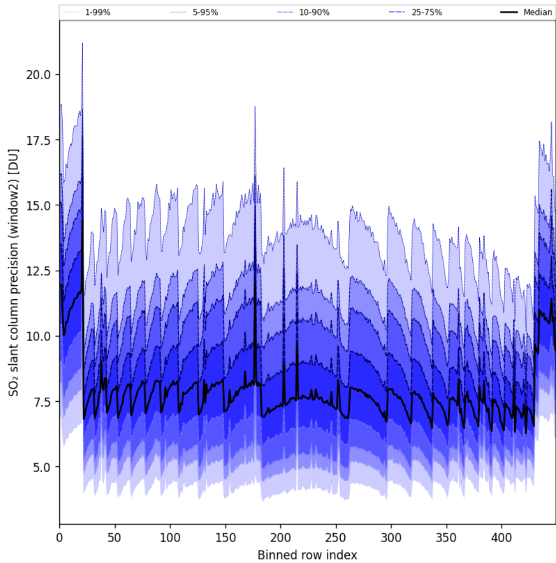
Figure 94: Along track statistics of “SO 2 slant column precision (window2)” for 2025-05-29 to 2025-05-31
