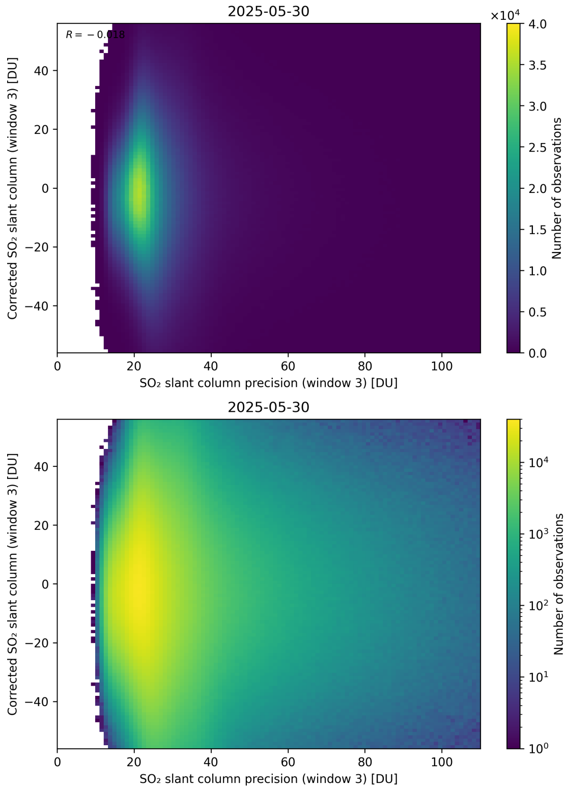
Figure 312: Scatter density plot of “SO 2 slant column precision (window 3)” against “Corrected SO 2 slant column (window 3)” for 2025-05-29 to 2025-05-31.
