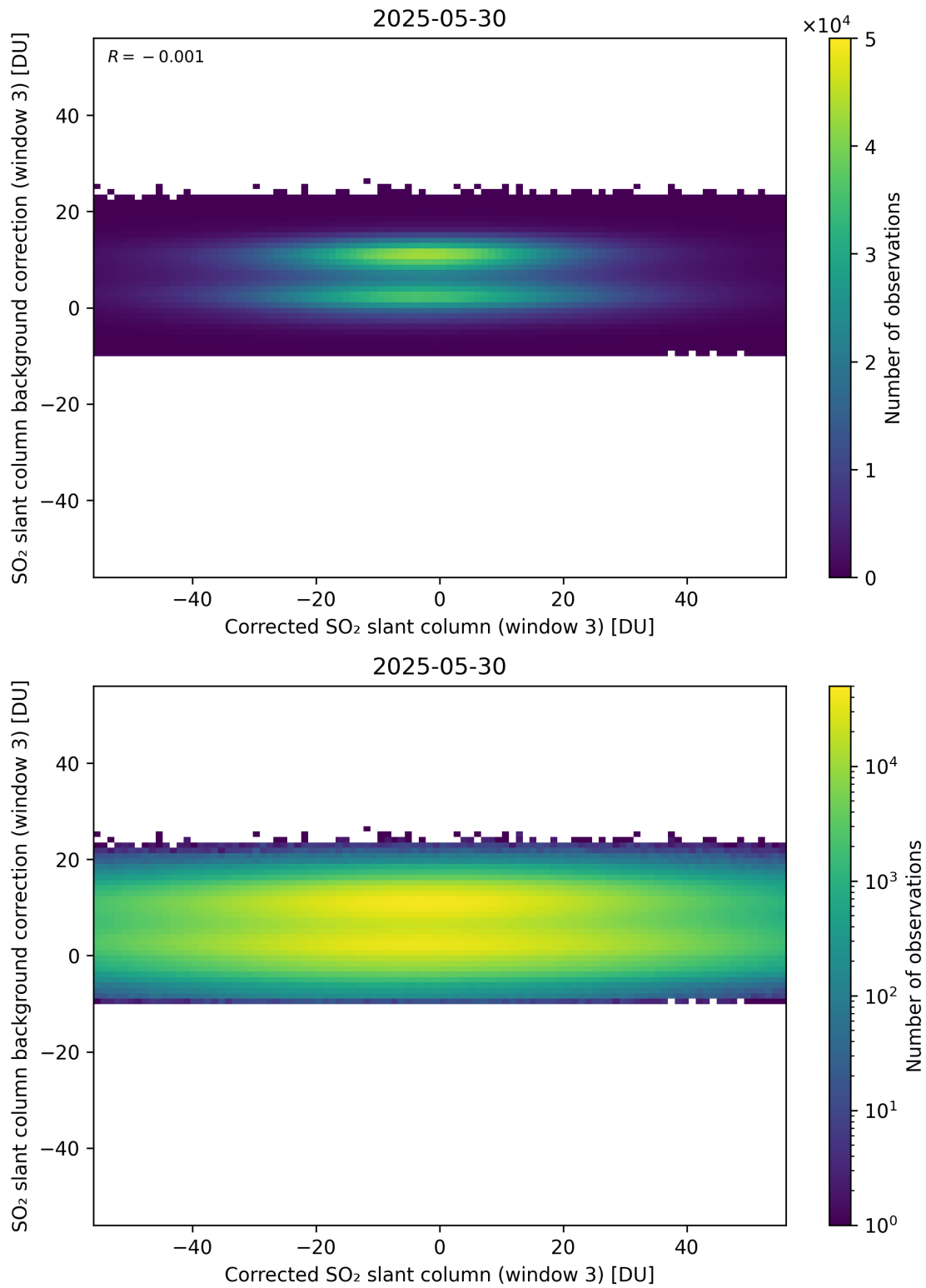
Figure 255: Scatter density plot of “Corrected SO 2 slant column (window 3)” against “SO 2 slant column background correction (window 3)” for 2025-05-29 to 2025-05-31.
