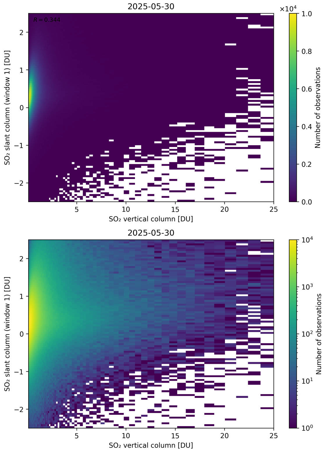
Figure 354: Scatter density plot of “SO 2 vertical column” against “SO 2 slant column (window 1)” for 2025-05-29 to 2025-05-31.
