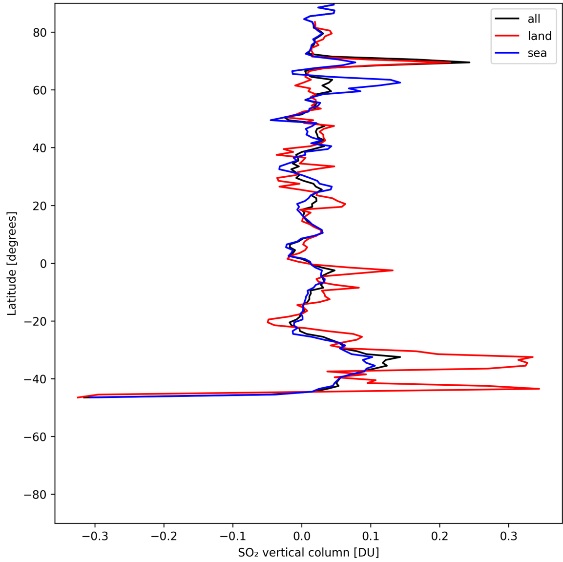
Figure 32: Zonal average of “SO 2 vertical column” for 2025-05-29 to 2025-05-31.
