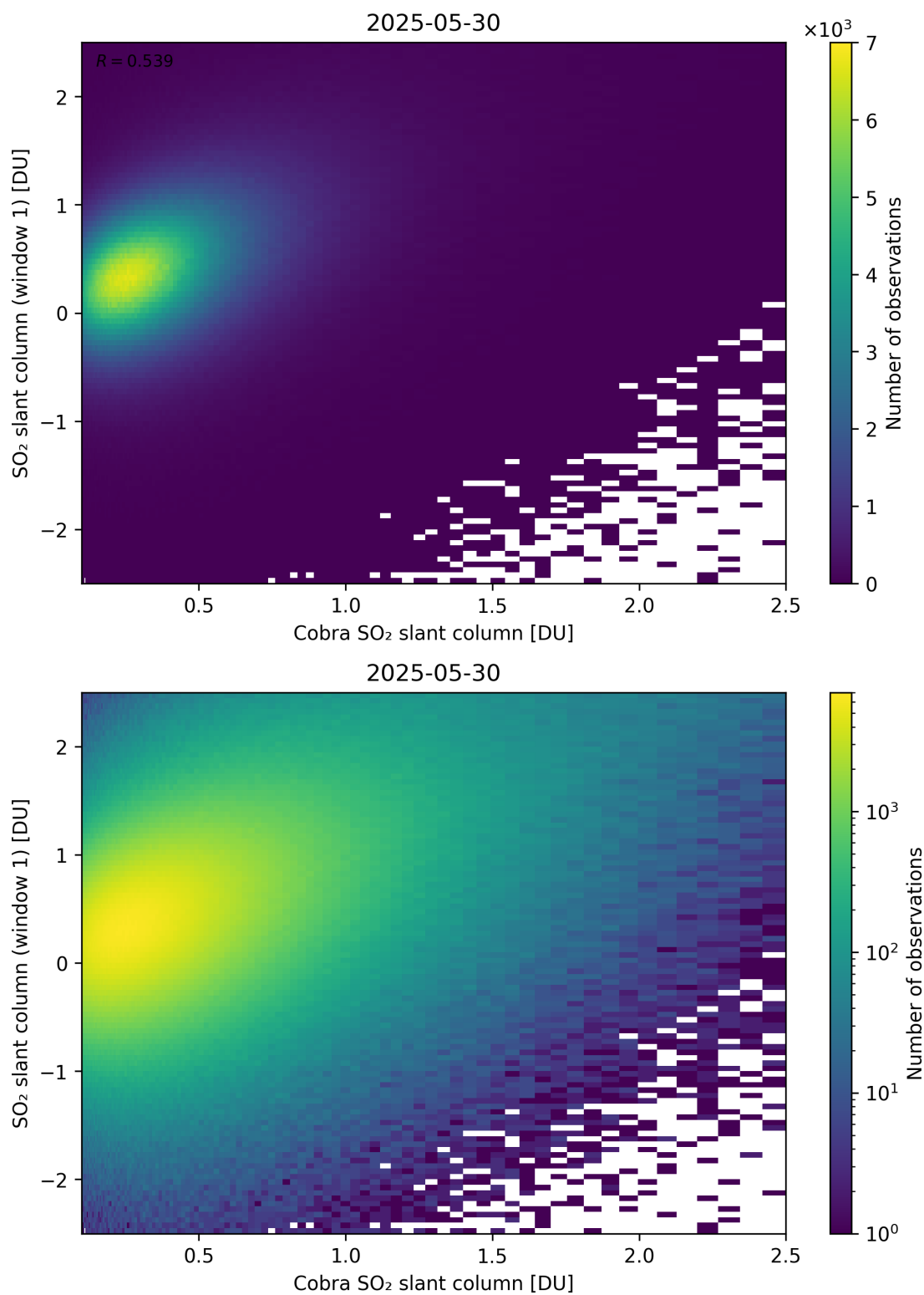
Figure 219: Scatter density plot of “Cobra SO 2 slant column” against “SO 2 slant column (window 1)” for 2025-05-29 to 2025-05-31.
