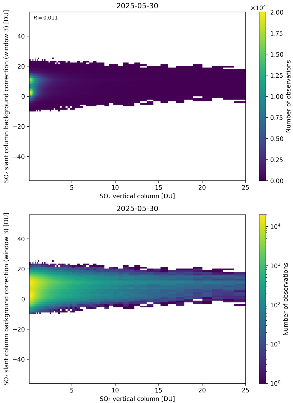
Figure 325: Scatter density plot of “SO 2 vertical column” against “SO 2 slant column background correction (window 3)” for 2025-05-29 to 2025-05-31.
