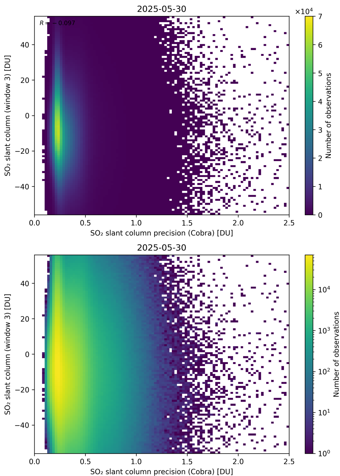
Figure 211: Scatter density plot of “SO 2 slant column precision (Cobra)” against “SO 2 slant column (window 3)” for 2025-05-29 to 2025-05-31.
