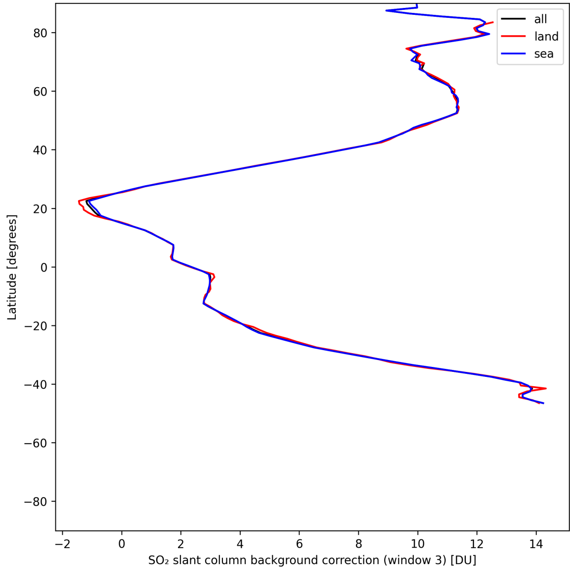
Figure 48: Zonal average of “SO 2 slant column background correction (window 3)” for 2025-05-29 to 2025-05-31.
