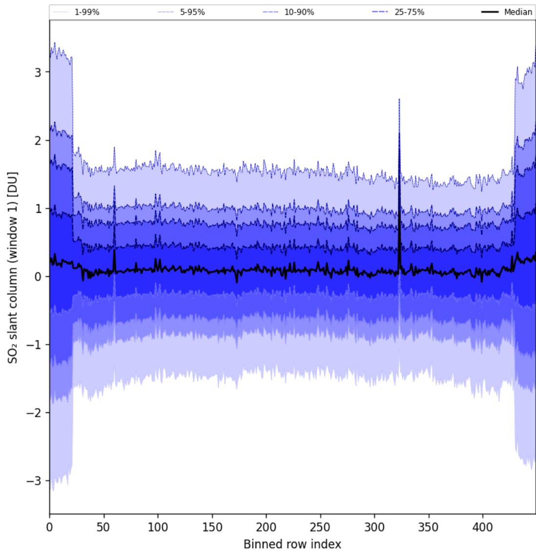
Figure 89: Along track statistics of “SO 2 slant column (window 1)” for 2025-05-29 to 2025-05-31
