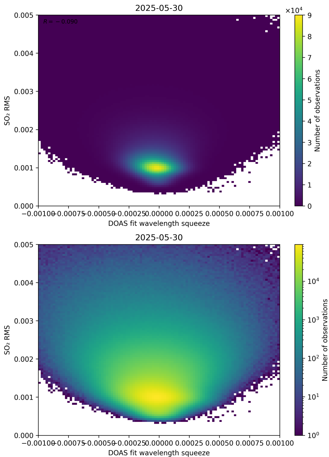
Figure 143: Scatter density plot of “DOAS fit wavelength squeeze” against “SO 2 RMS” for 2025-05-29 to 2025-05-31.
