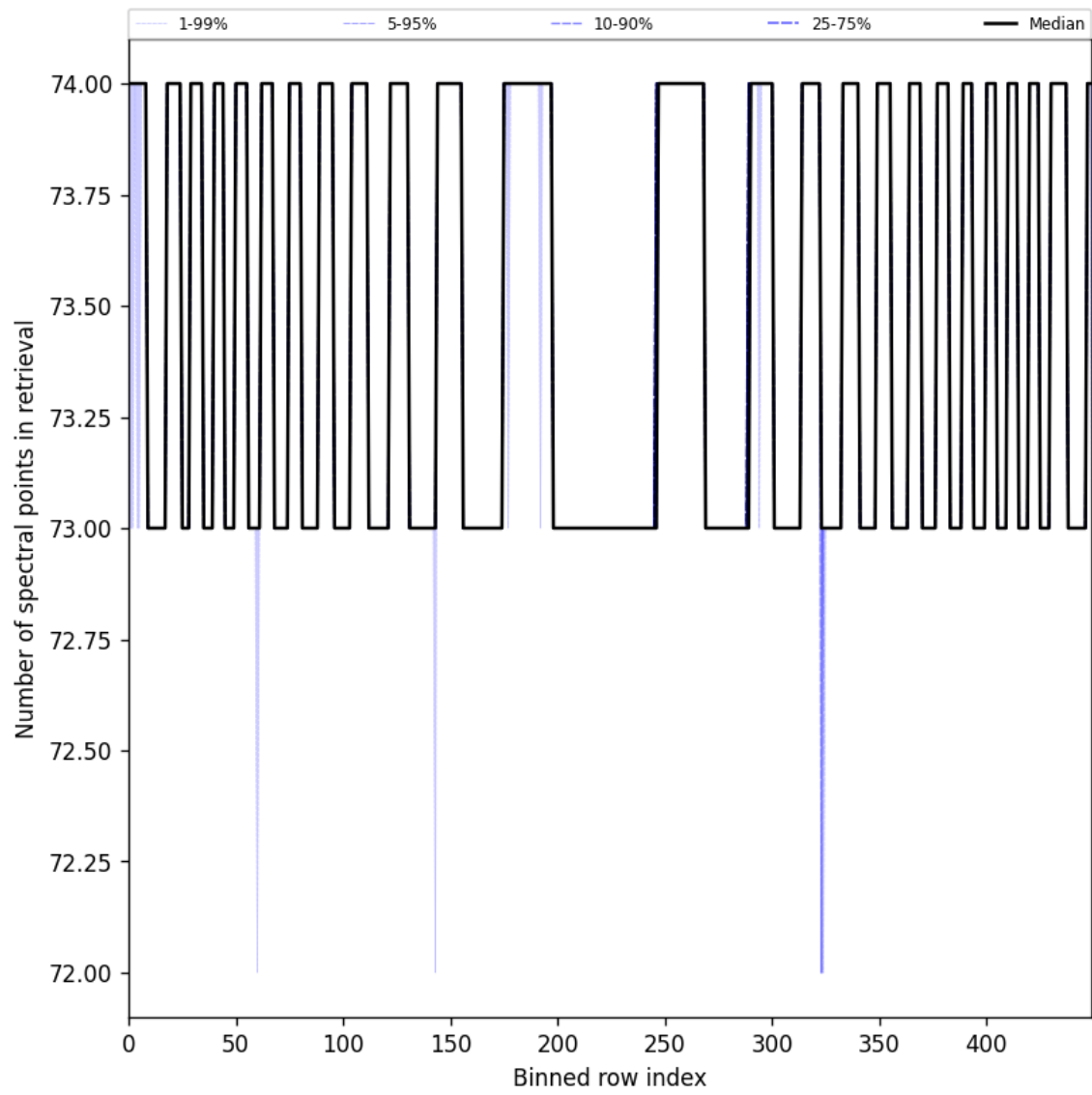
Figure 108: Along track statistics of “Number of spectral points in retrieval” for 2025-05-29 to 2025-05-31
