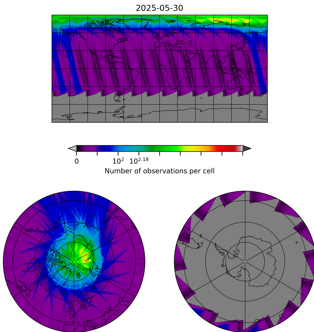
Figure 30: Map of the number of observations for 2025-05-29 to 2025-05-31
