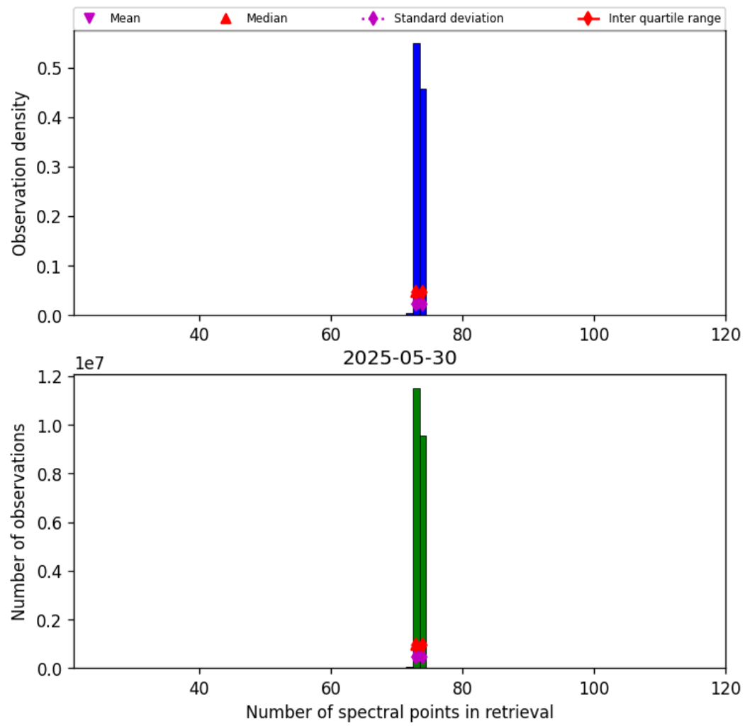
Figure 82: Histogram of “Number of spectral points in retrieval” for 2025-05-29 to 2025-05-31
