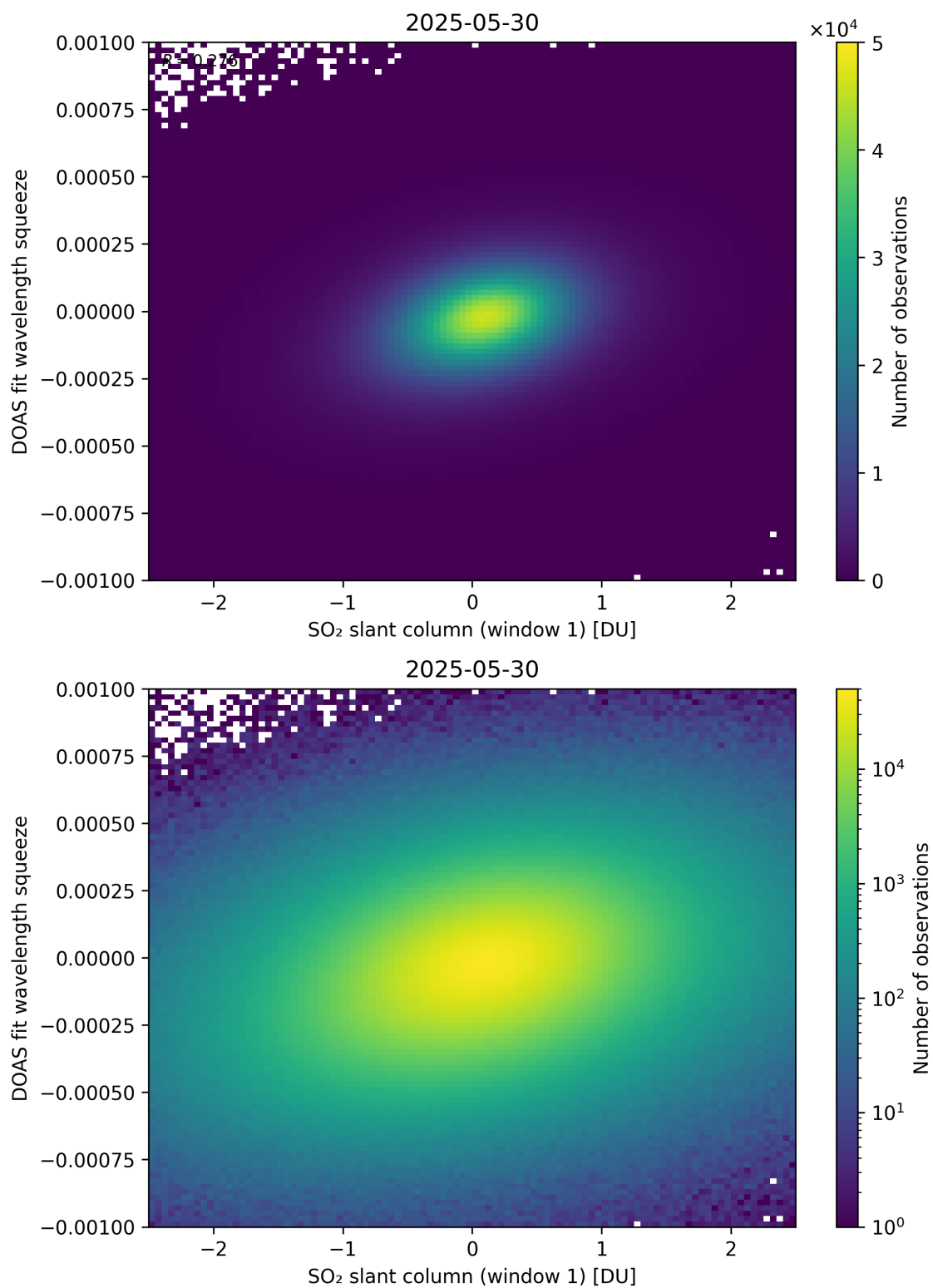
Figure 266: Scatter density plot of “SO 2 slant column (window 1)” against “DOAS fit wavelength squeeze” for 2025-05-29 to 2025-05-31.
