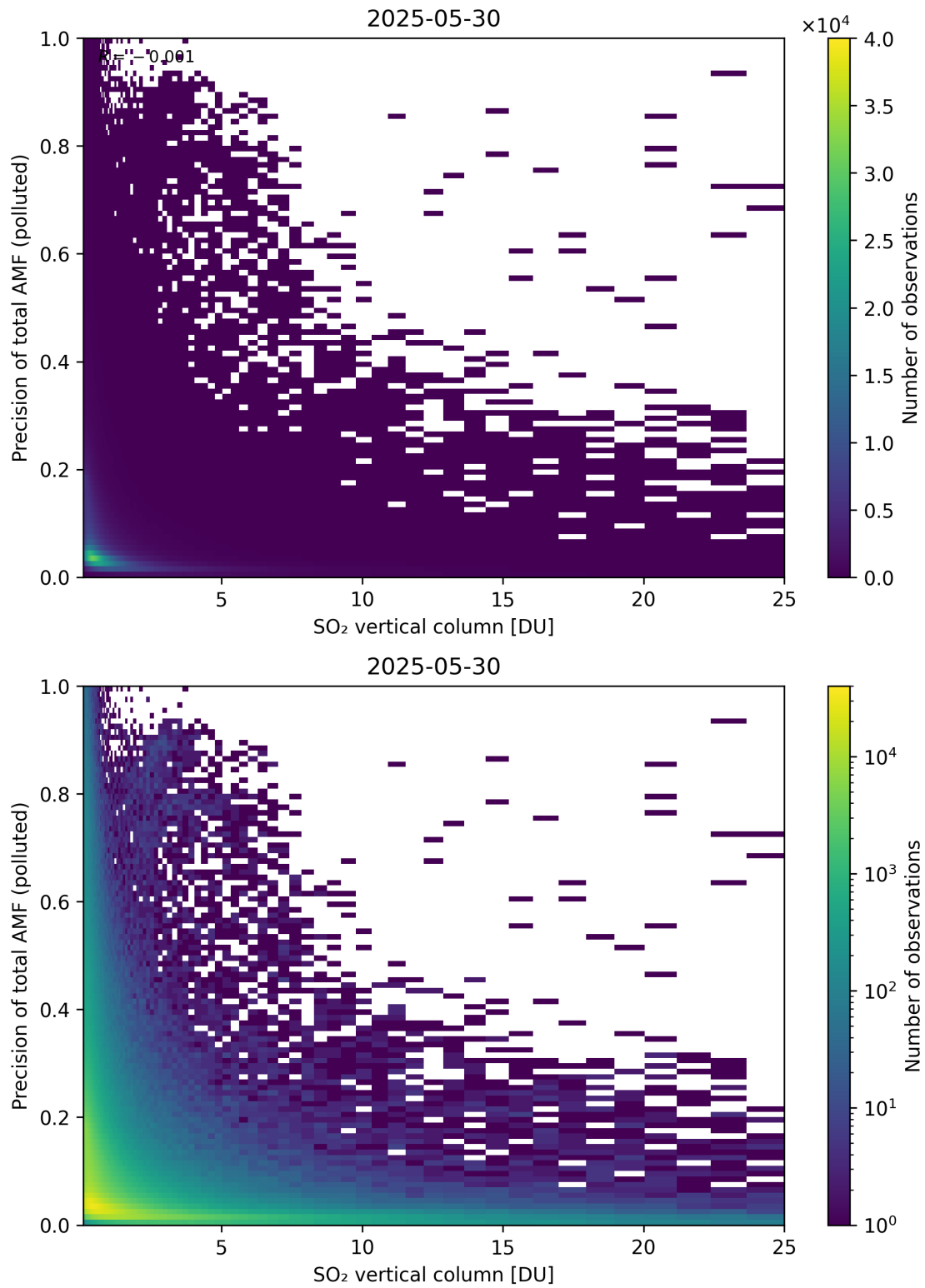
Figure 360: Scatter density plot of “SO 2 vertical column” against “Precision of total AMF (polluted)” for 2025-05-29 to 2025-05-31.
