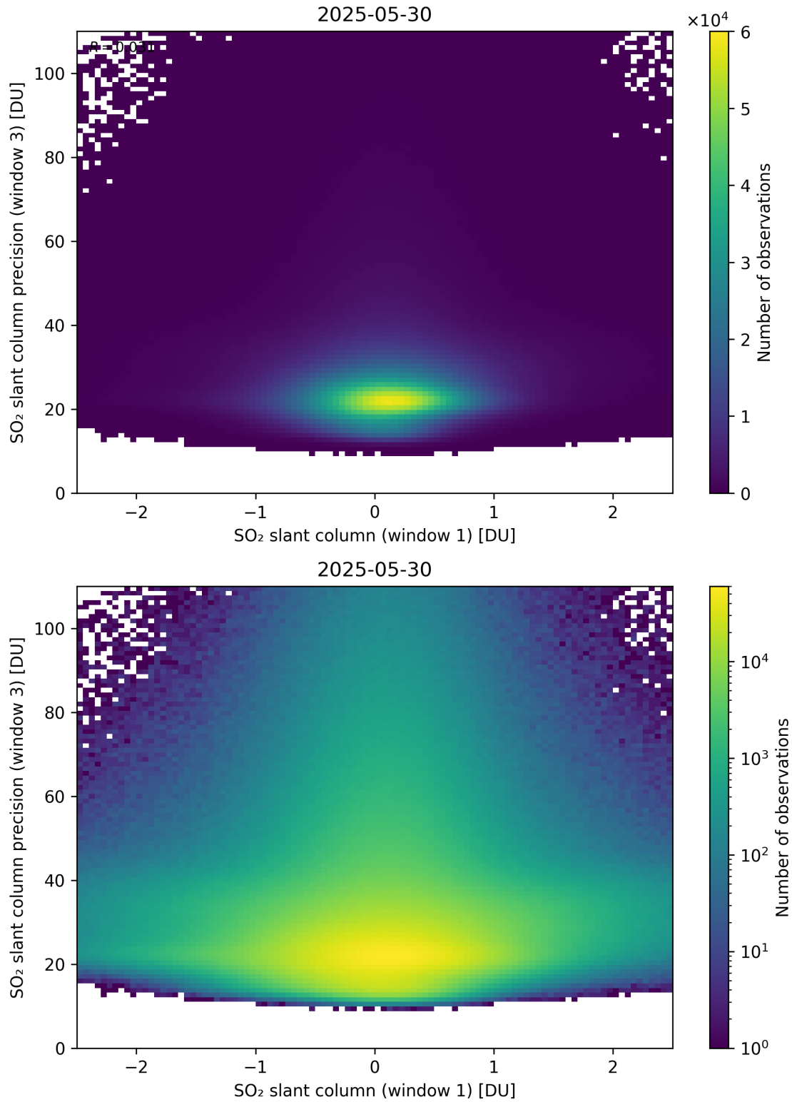
Figure 288: Scatter density plot of “SO 2 slant column (window 1)” against “SO 2 slant column precision (window 3)” for 2025-05-29 to 2025-05-31.
