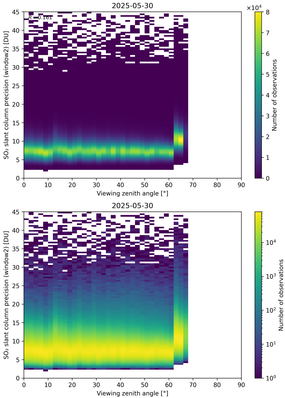
Figure 378: Scatter density plot of “Viewing zenith angle” against “SO 2 slant column precision (window2)” for 2025-05-29 to 2025-05-31.
