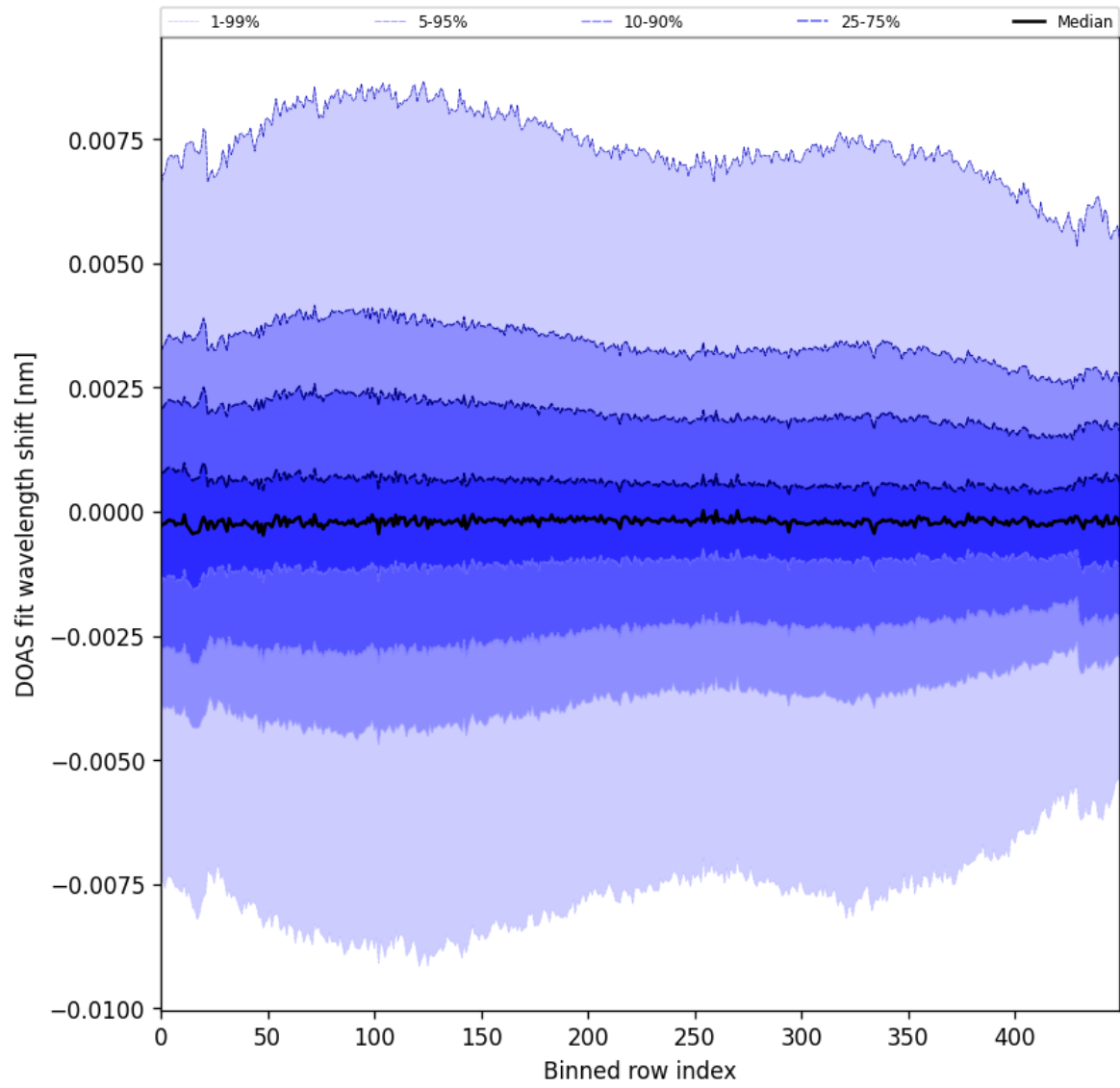
Figure 102: Along track statistics of “DOAS fit wavelength shift” for 2025-05-29 to 2025-05-31
