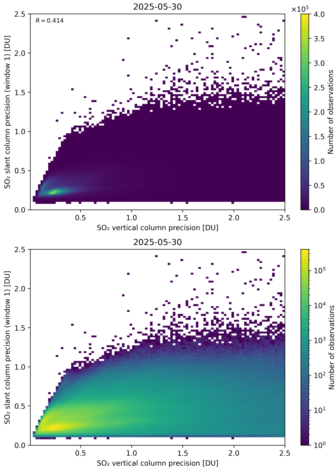
Figure 342: Scatter density plot of “SO 2 vertical column precision” against “SO 2 slant column precision (window 1)” for 2025-05-29 to 2025-05-31.
