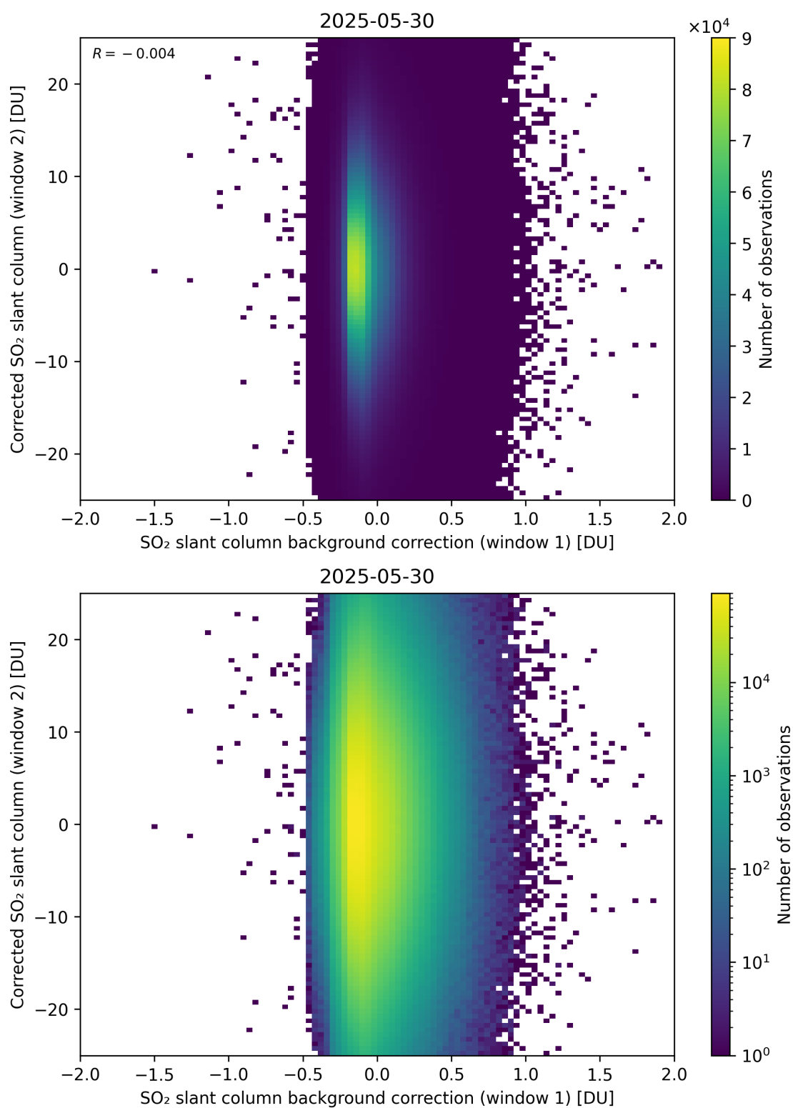
Figure 115: Scatter density plot of “SO 2 slant column background correction (window 1)” against “Corrected SO 2 slant column (window 2)” for 2025-05-29 to 2025-05-31.
