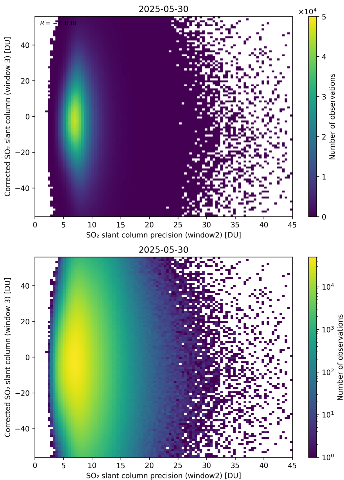
Figure 298: Scatter density plot of “SO 2 slant column precision (window2)” against “Corrected SO 2 slant column (window 3)” for 2025-05-29 to 2025-05-31.
