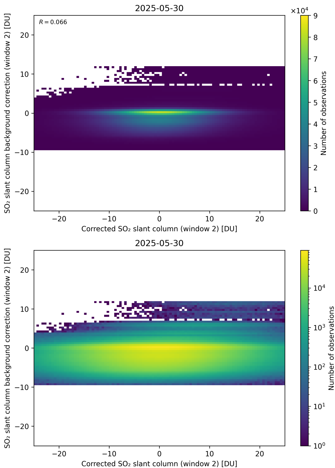
Figure 244: Scatter density plot of “Corrected SO 2 slant column (window 2)” against “SO 2 slant column background correction (window 2)” for 2025-05-29 to 2025-05-31.
