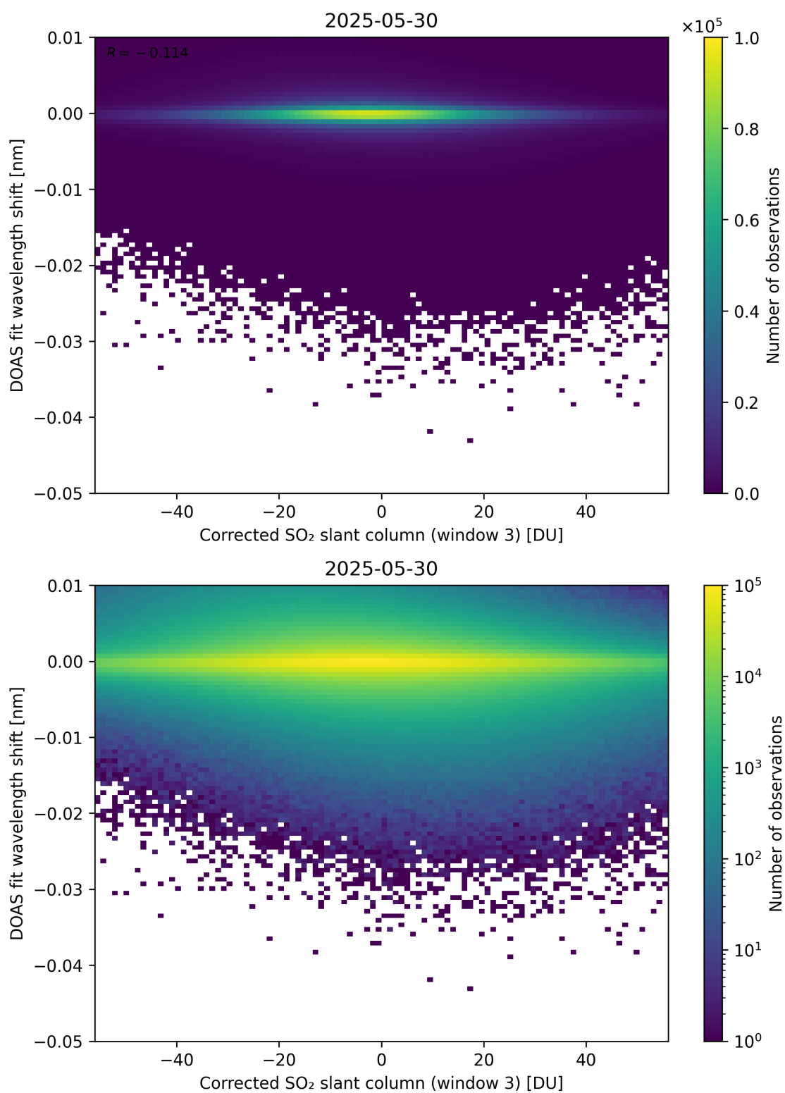
Figure 256: Scatter density plot of “Corrected SO 2 slant column (window 3)” against “DOAS fit wavelength shift” for 2025-05-29 to 2025-05-31.
