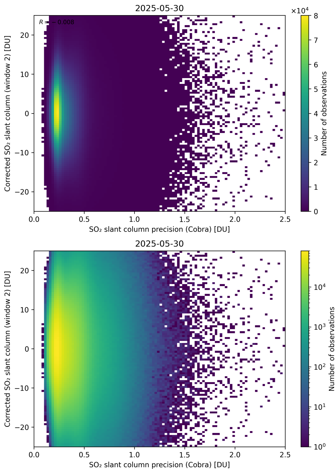
Figure 206: Scatter density plot of “SO 2 slant column precision (Cobra)” against “Corrected SO 2 slant column (window 2)” for 2025-05-29 to 2025-05-31.
