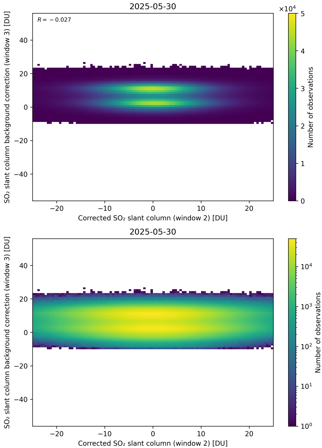
Figure 245: Scatter density plot of “Corrected SO 2 slant column (window 2)” against “SO 2 slant column background correction (window 3)” for 2025-05-29 to 2025-05-31.
