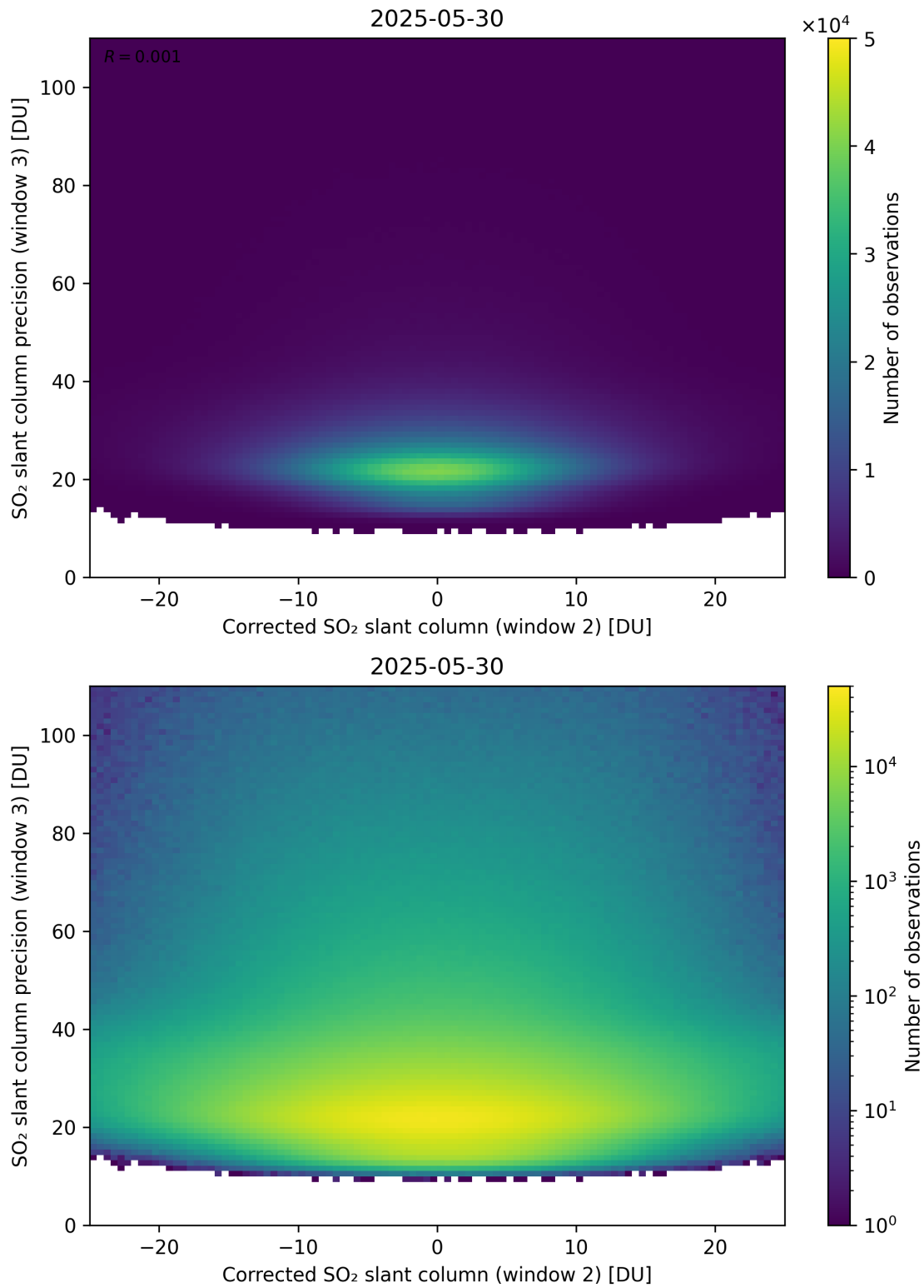
Figure 252: Scatter density plot of “Corrected SO 2 slant column (window 2)” against “SO 2 slant column precision (window 3)” for 2025-05-29 to 2025-05-31.
