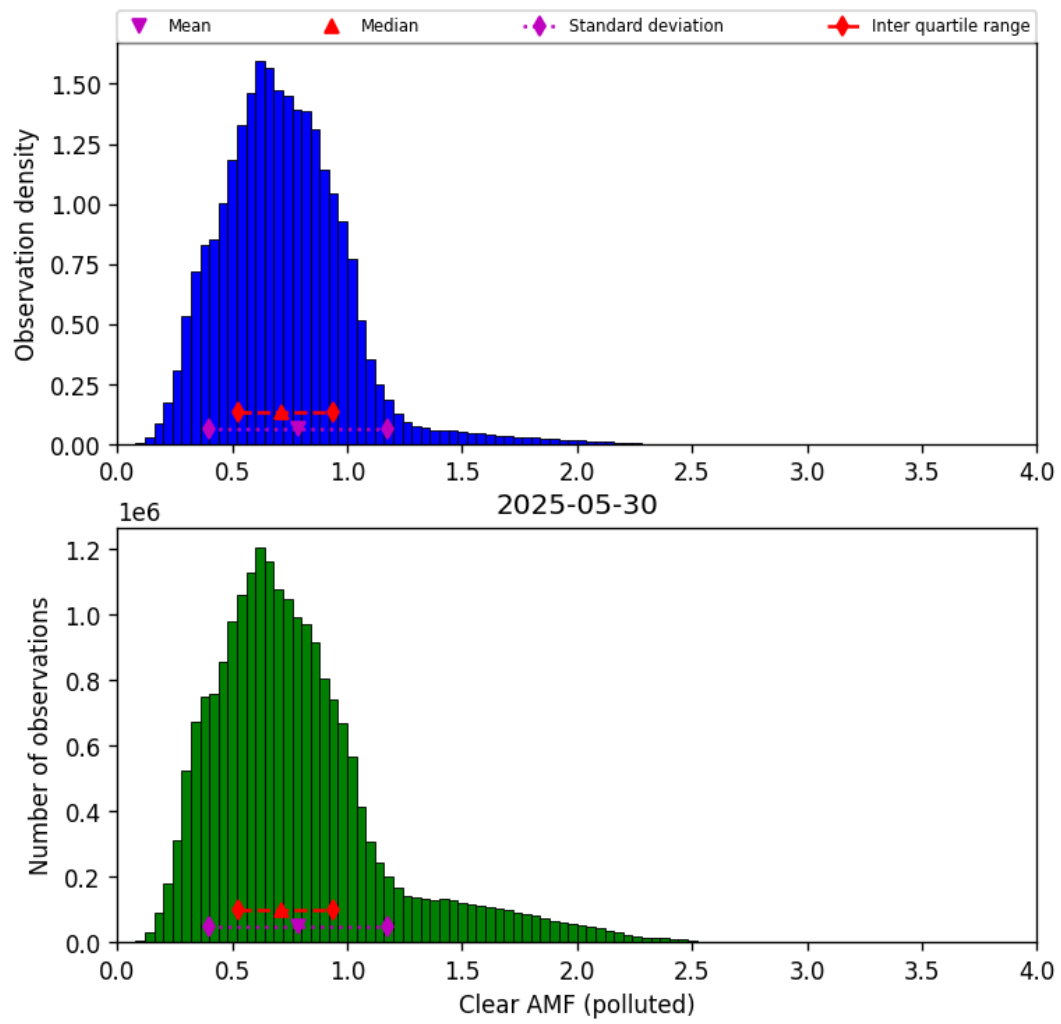
Figure 81: Histogram of “Clear AMF (polluted)” for 2025-05-29 to 2025-05-31
