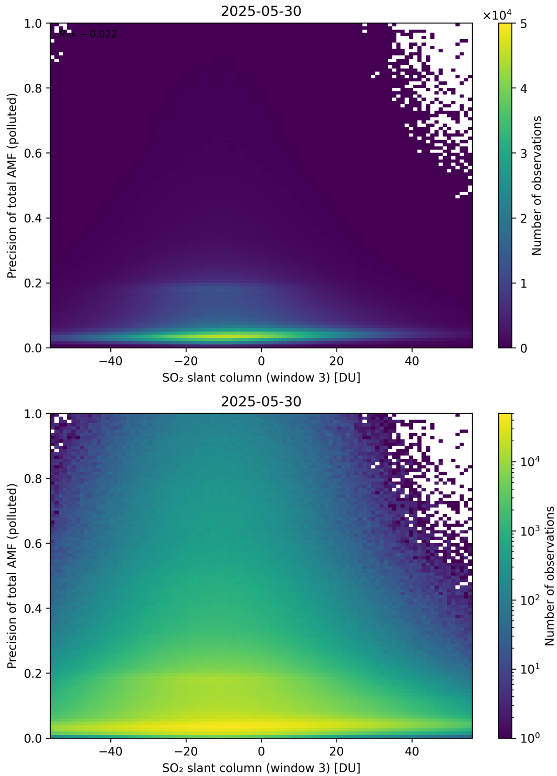
Figure 319: Scatter density plot of “SO 2 slant column (window 3)” against “Precision of total AMF (polluted)” for 2025-05-29 to 2025-05-31.
