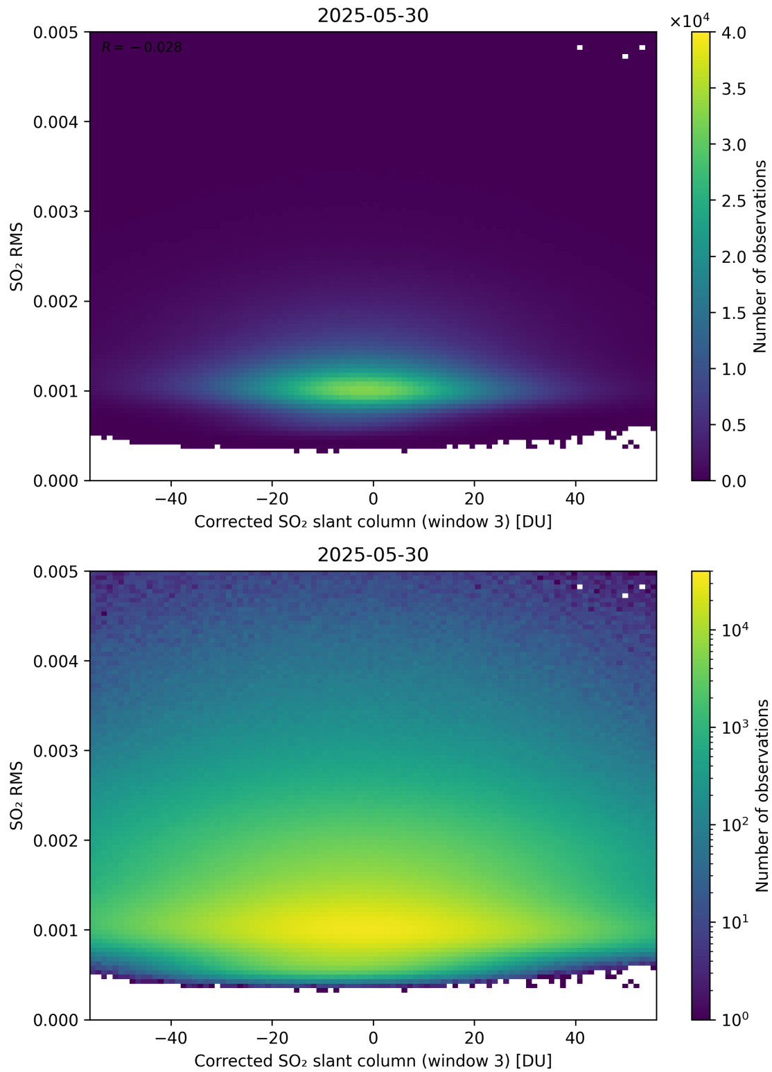
Figure 258: Scatter density plot of “Corrected SO 2 slant column (window 3)” against “SO 2 RMS” for 2025-05-29 to 2025-05-31.
