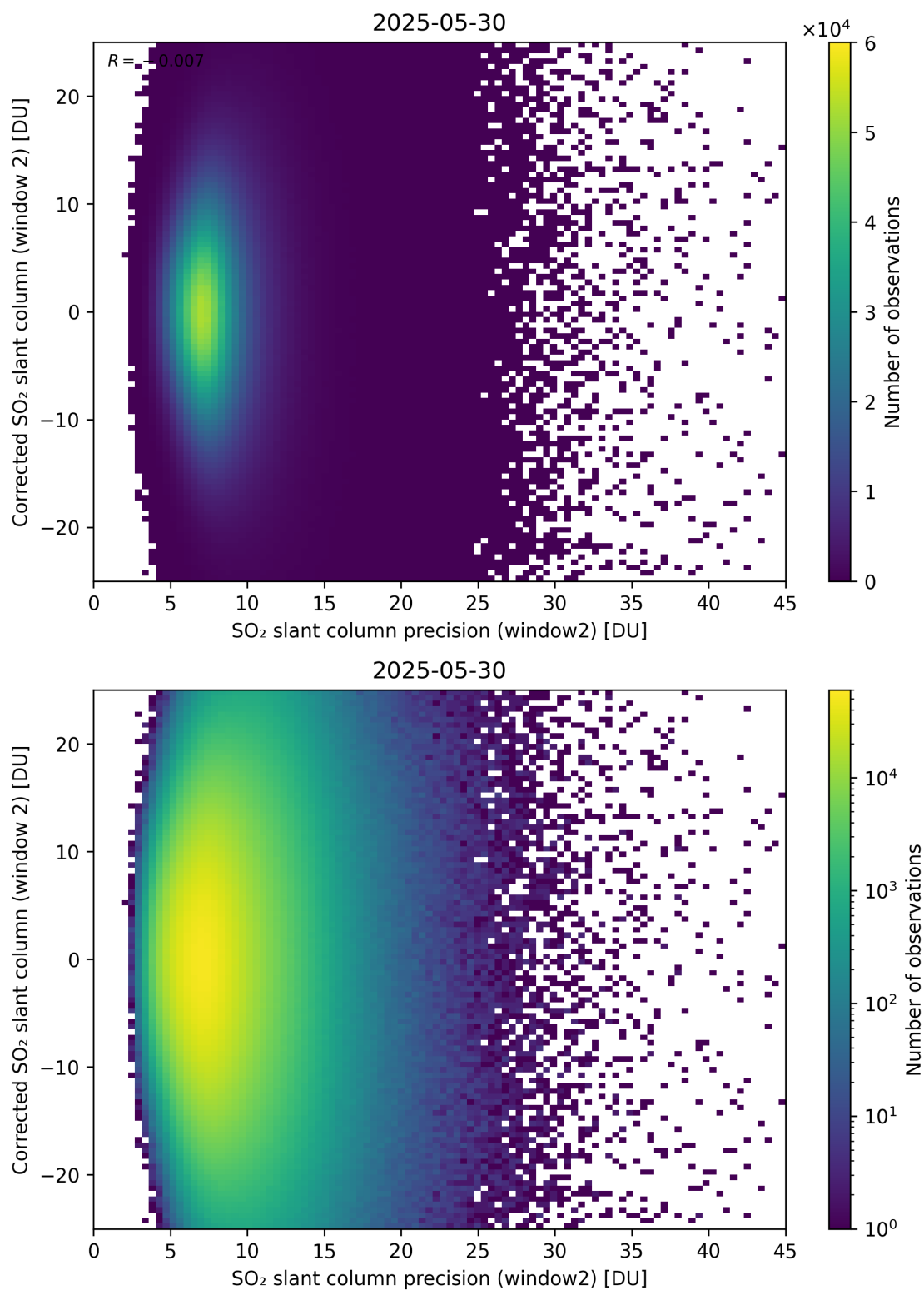
Figure 297: Scatter density plot of “SO 2 slant column precision (window2)” against “Corrected SO 2 slant column (window 2)” for 2025-05-29 to 2025-05-31.
