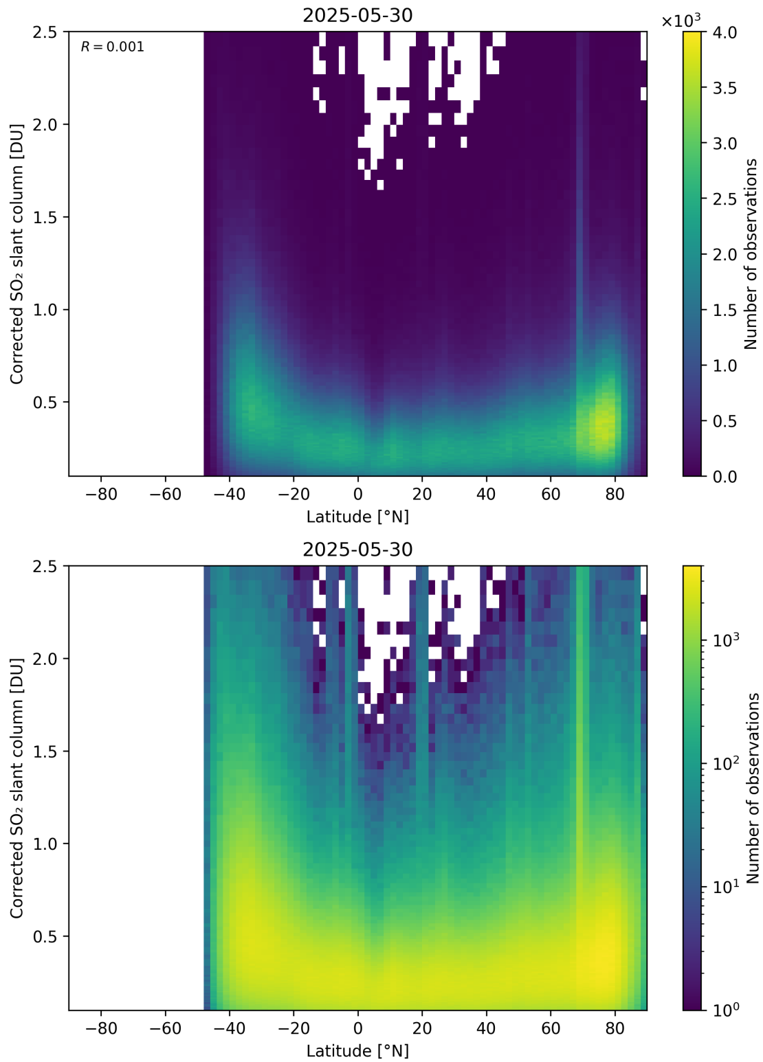
Figure 159: Scatter density plot of “Latitude” against “Corrected SO 2 slant column” for 2025-05-29 to 2025-05-31.
