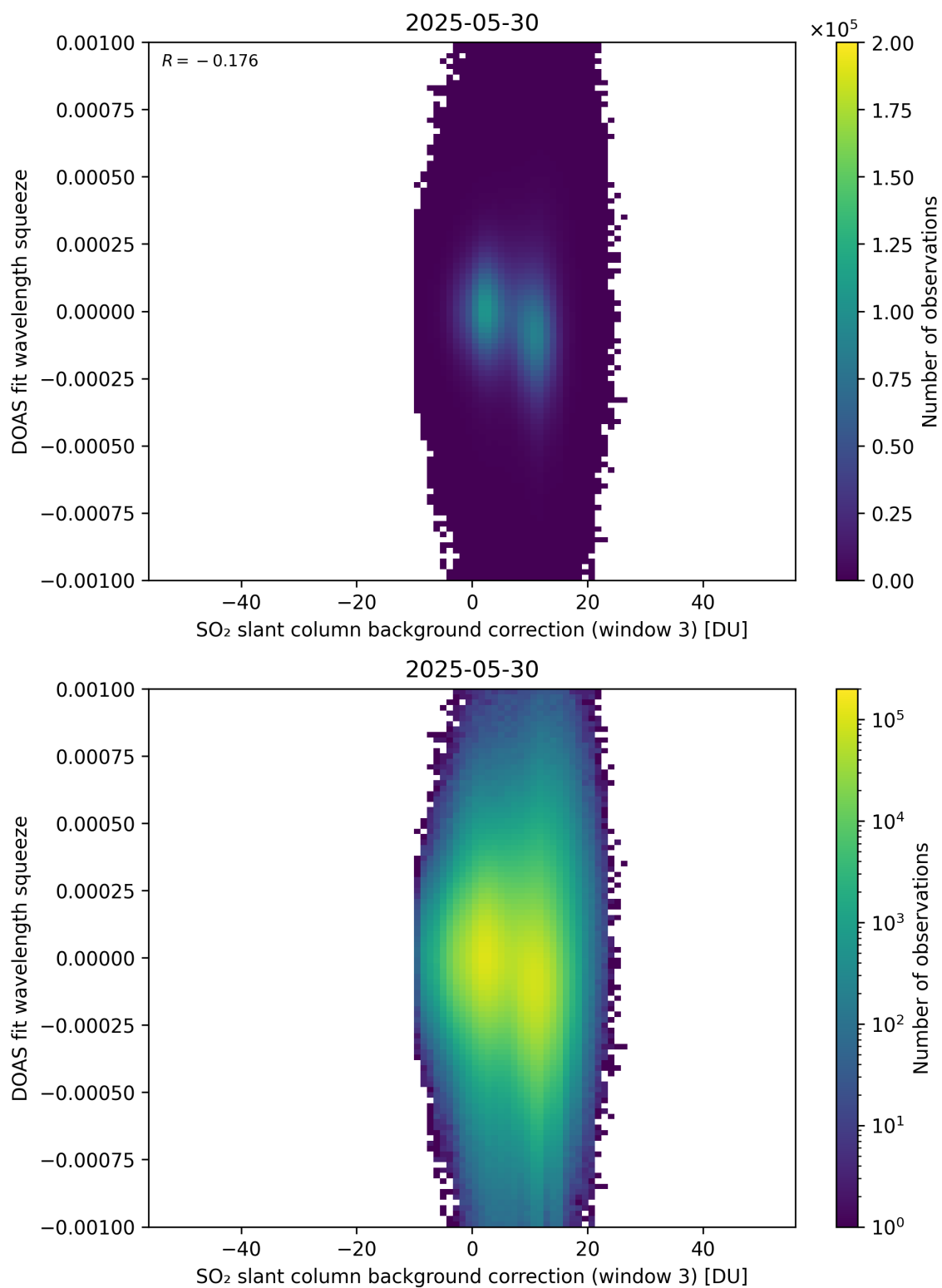
Figure 133: Scatter density plot of “SO 2 slant column background correction (window 3)” against “DOAS fit wavelength squeeze” for 2025-05-29 to 2025-05-31.
