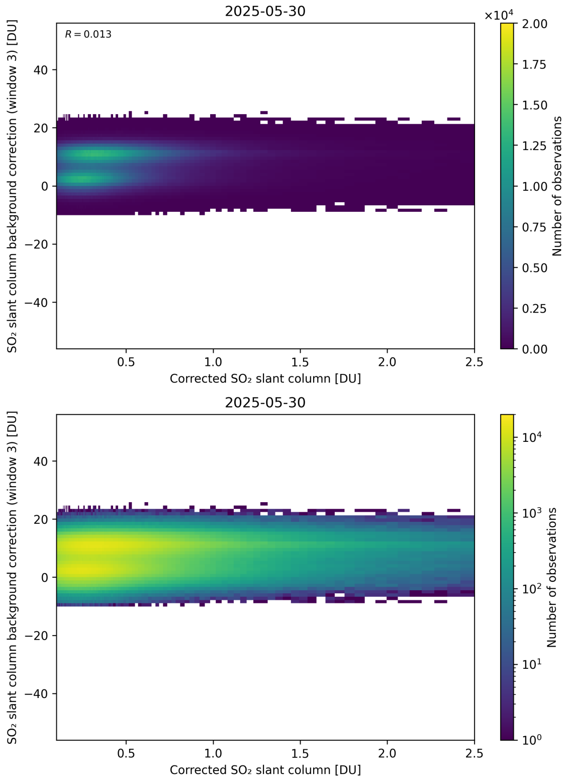
Figure 228: Scatter density plot of “Corrected SO 2 slant column” against “SO 2 slant column background correction (window 3)” for 2025-05-29 to 2025-05-31.
