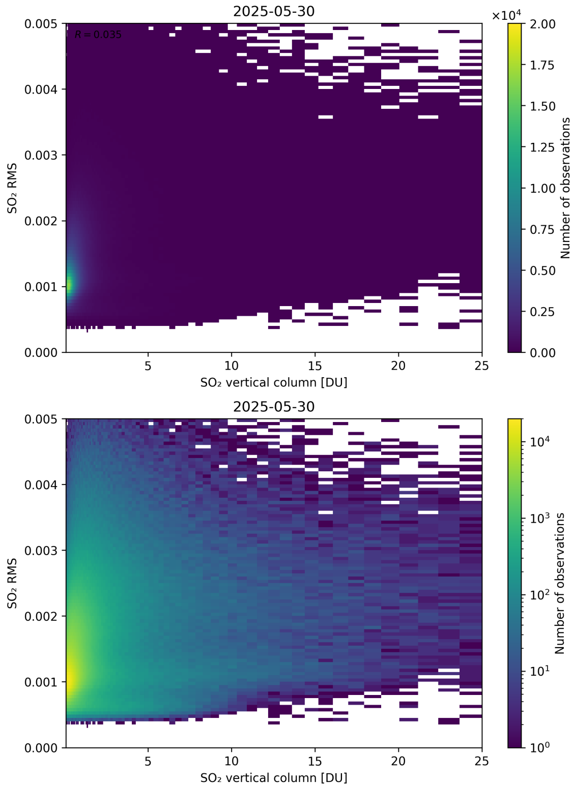
Figure 328: Scatter density plot of “SO 2 vertical column” against “SO 2 RMS” for 2025-05-29 to 2025-05-31.
