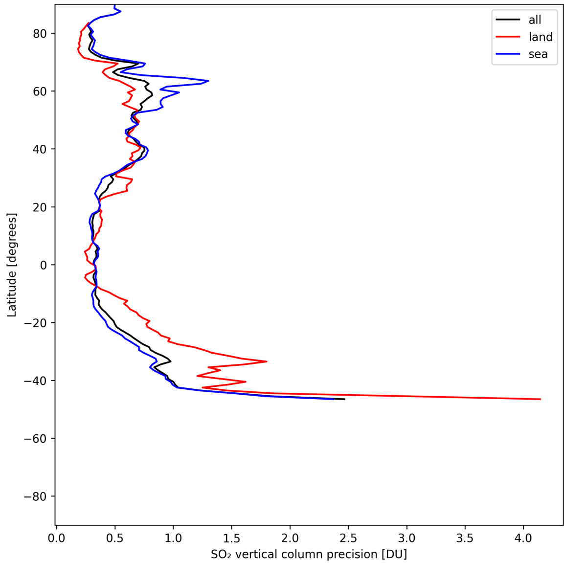
Figure 33: Zonal average of “SO 2 vertical column precision” for 2025-05-29 to 2025-05-31.
