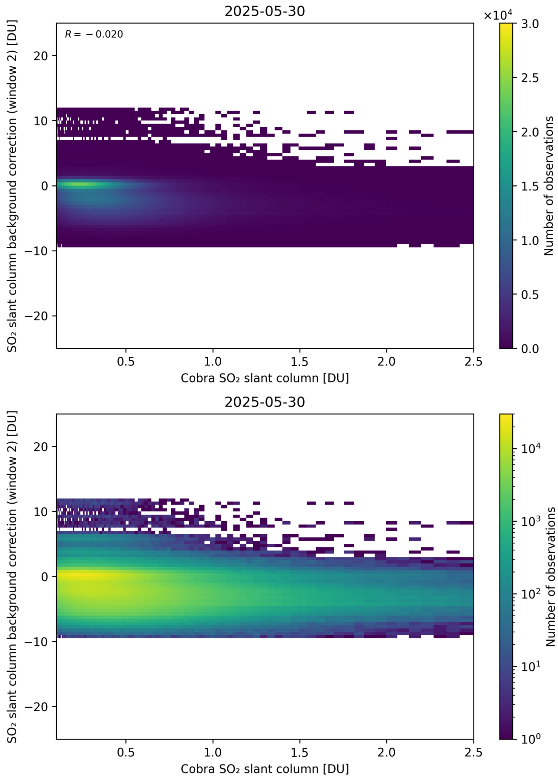
Figure 194: Scatter density plot of “Cobra SO 2 slant column” against “SO 2 slant column background correction (window 2)” for 2025-05-29 to 2025-05-31.
