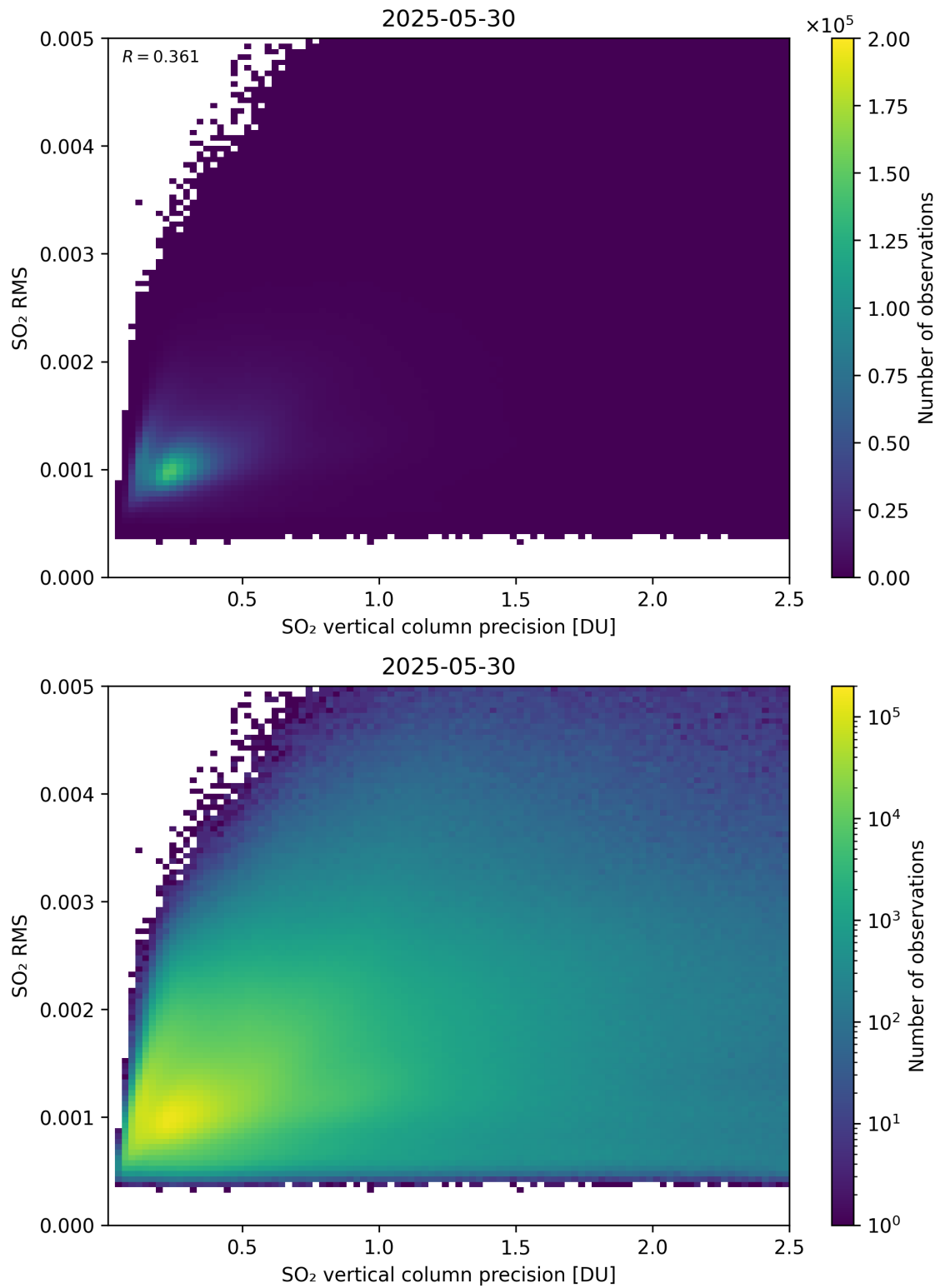
Figure 334: Scatter density plot of “SO 2 vertical column precision” against “SO 2 RMS” for 2025-05-29 to 2025-05-31.
