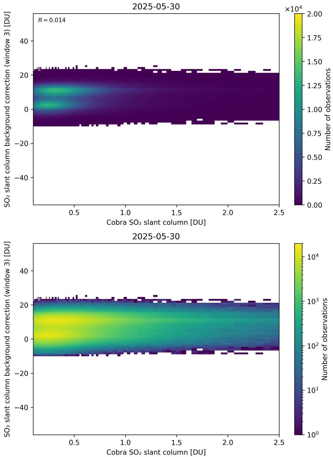
Figure 195: Scatter density plot of “Cobra SO 2 slant column” against “SO 2 slant column background correction (window 3)” for 2025-05-29 to 2025-05-31.
