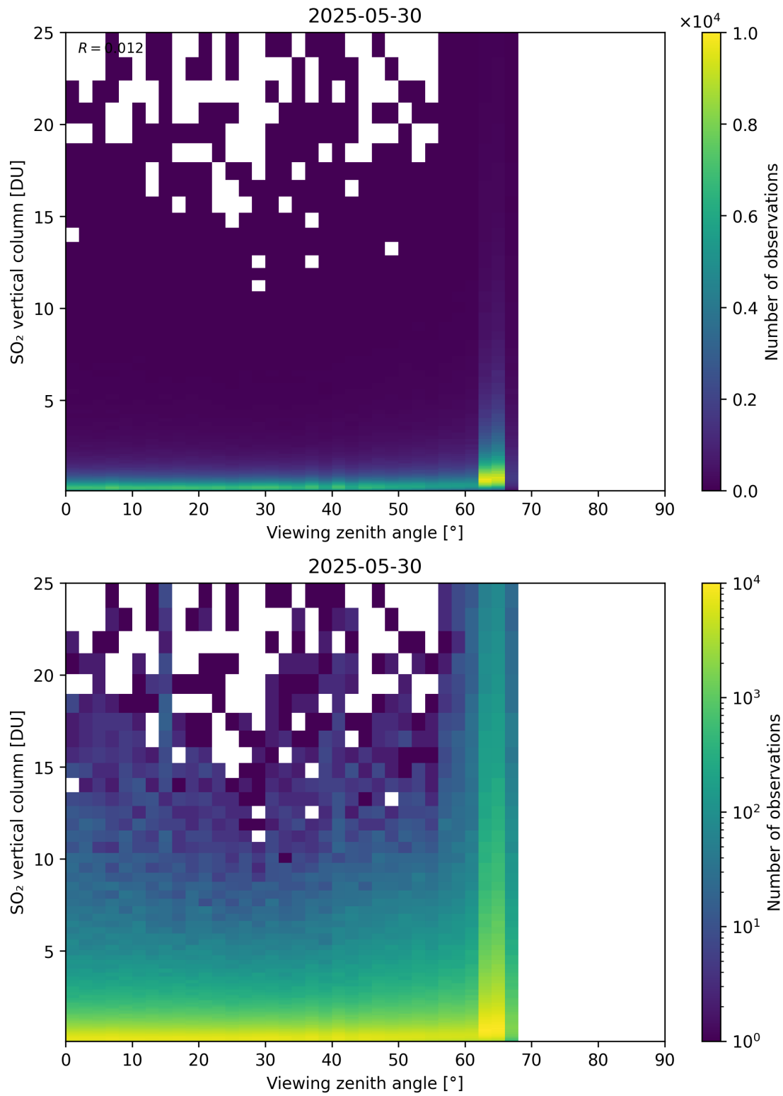
Figure 383: Scatter density plot of “Viewing zenith angle” against “SO 2 vertical column” for 2025-05-29 to 2025-05-31.
