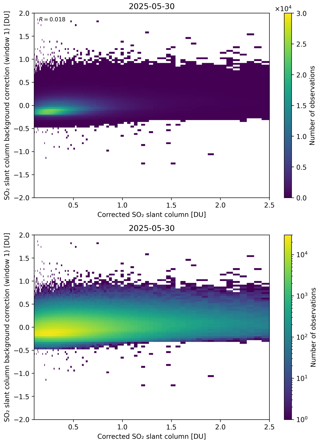
Figure 226: Scatter density plot of “Corrected SO 2 slant column” against “SO 2 slant column background correction (window 1)” for 2025-05-29 to 2025-05-31.
