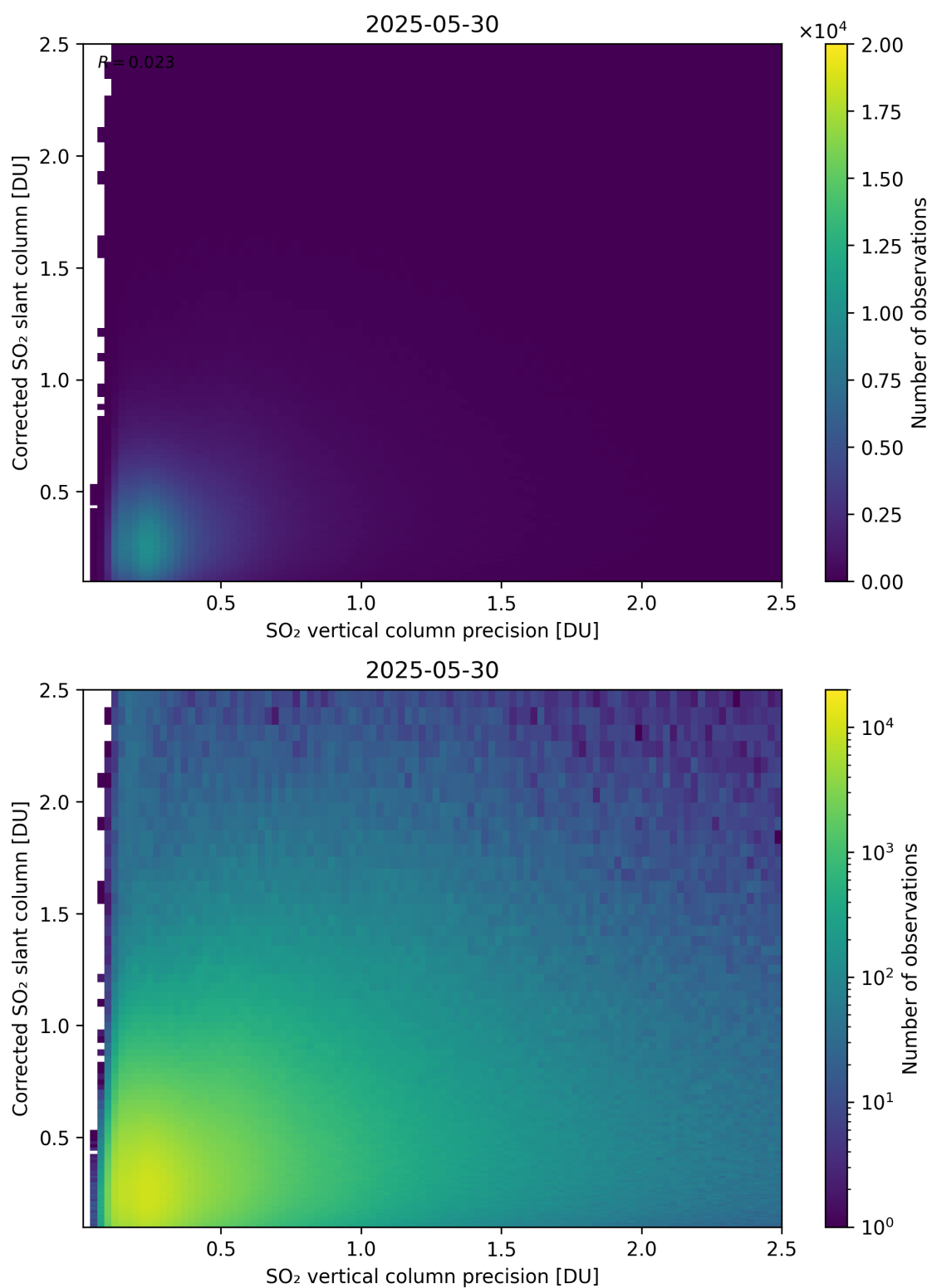
Figure 338: Scatter density plot of “SO 2 vertical column precision” against “Corrected SO 2 slant column” for 2025-05-29 to 2025-05-31.
