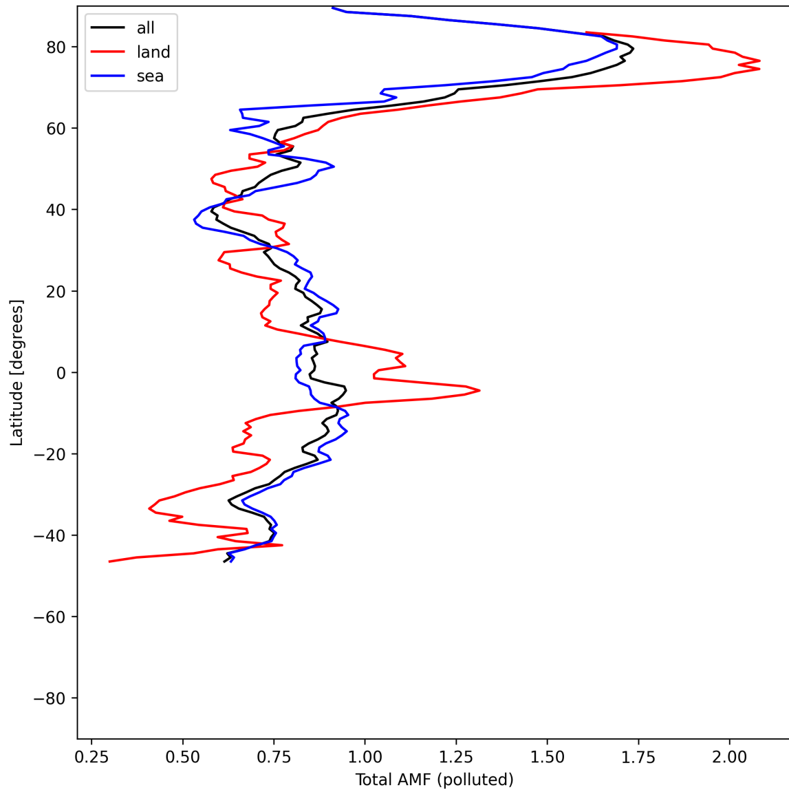
Figure 53: Zonal average of “Total AMF (polluted)” for 2025-05-29 to 2025-05-31.
