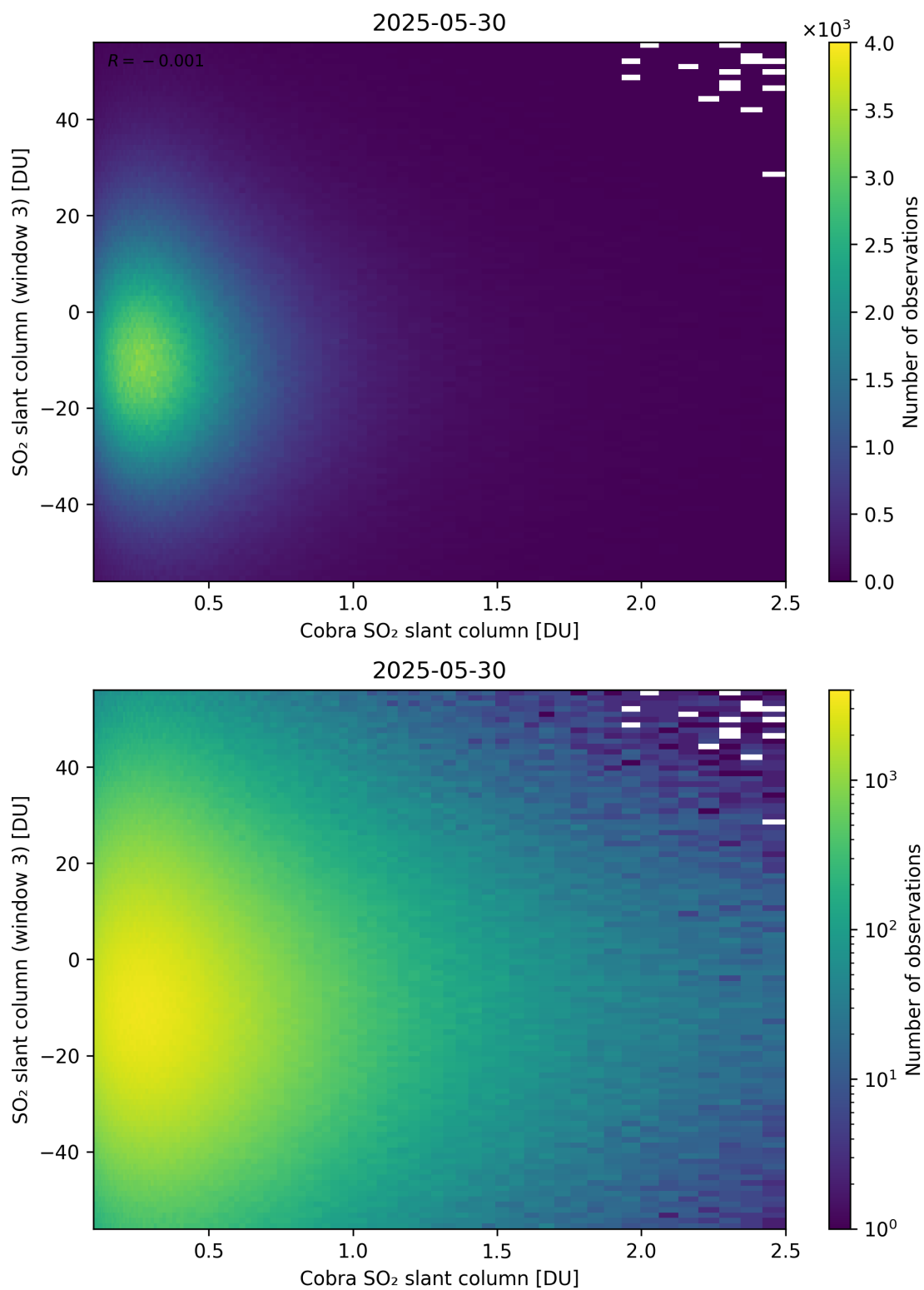
Figure 222: Scatter density plot of “Cobra SO 2 slant column” against “SO 2 slant column (window 3)” for 2025-05-29 to 2025-05-31.
