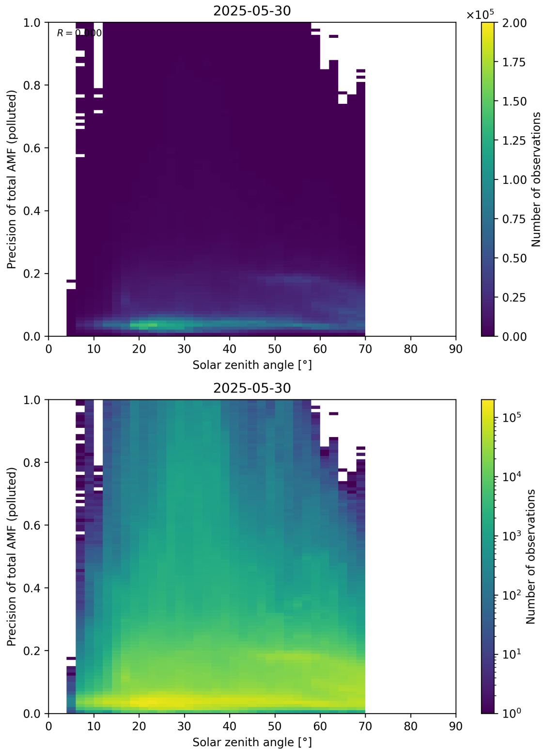
Figure 190: Scatter density plot of “Solar zenith angle” against “Precision of total AMF (polluted)” for 2025-05-29 to 2025-05-31.
