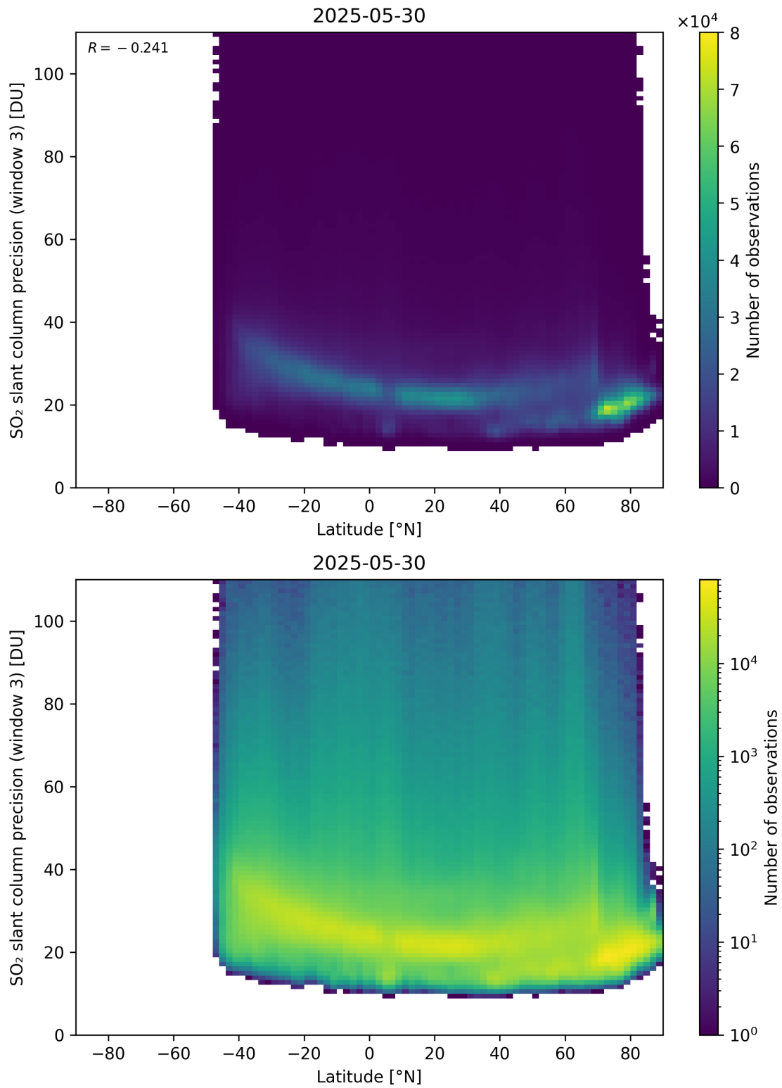
Figure 166: Scatter density plot of “Latitude” against “SO 2 slant column precision (window 3)” for 2025-05-29 to 2025-05-31.
