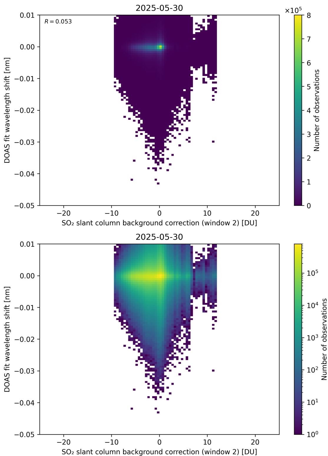
Figure 123: Scatter density plot of “SO 2 slant column background correction (window 2)” against “DOAS fit wavelength shift” for 2025-05-29 to 2025-05-31.
