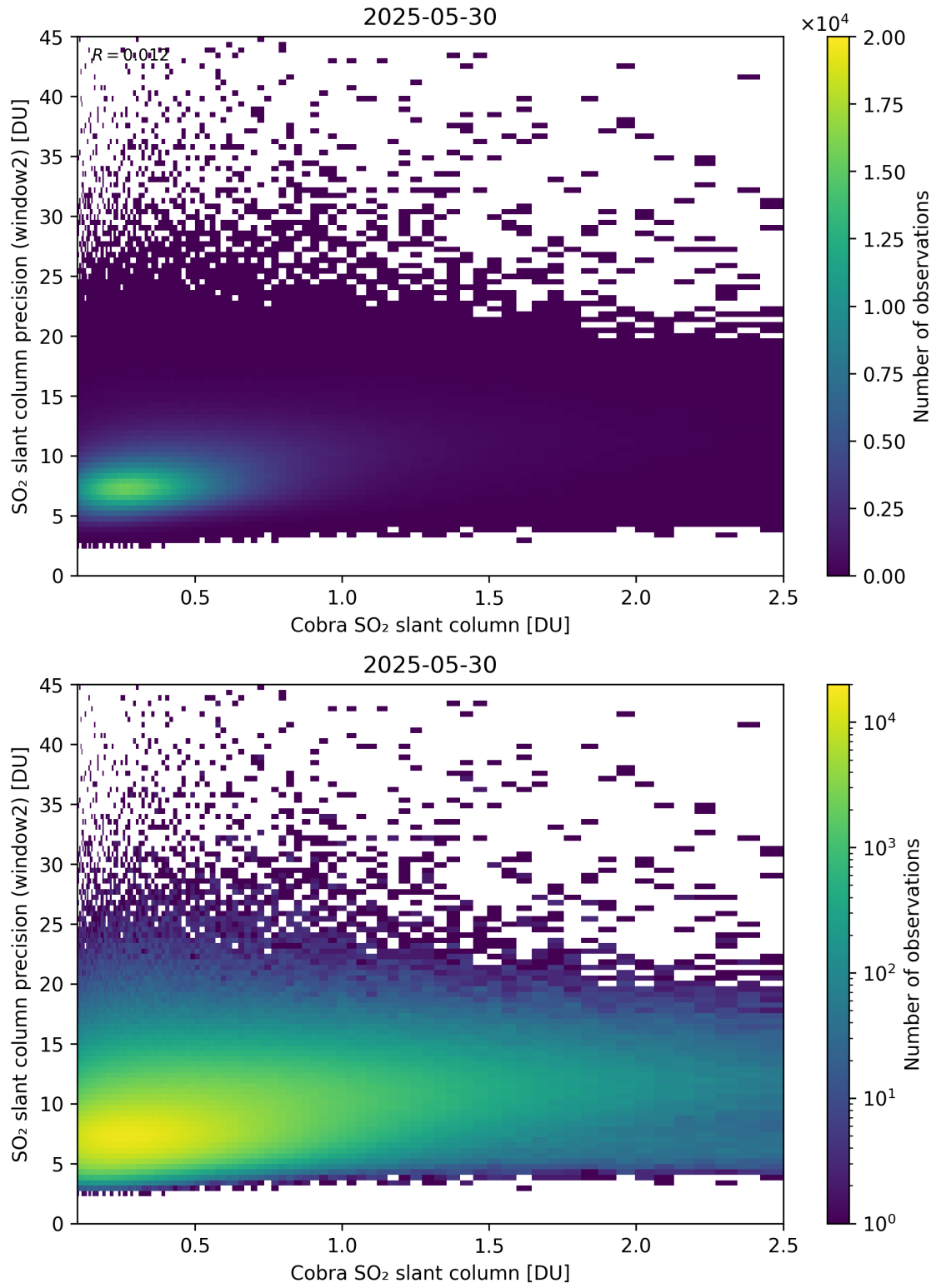
Figure 221: Scatter density plot of “Cobra SO 2 slant column” against “SO 2 slant column precision (window2)” for 2025-05-29 to 2025-05-31.
