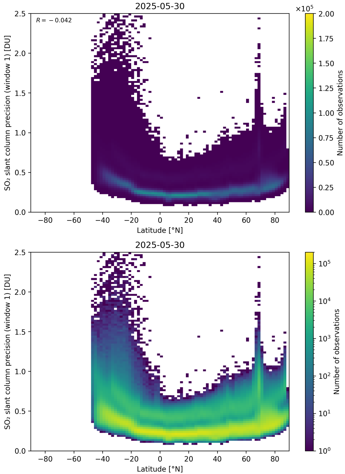
Figure 163: Scatter density plot of “Latitude” against “SO 2 slant column precision (window 1)” for 2025-05-29 to 2025-05-31.
