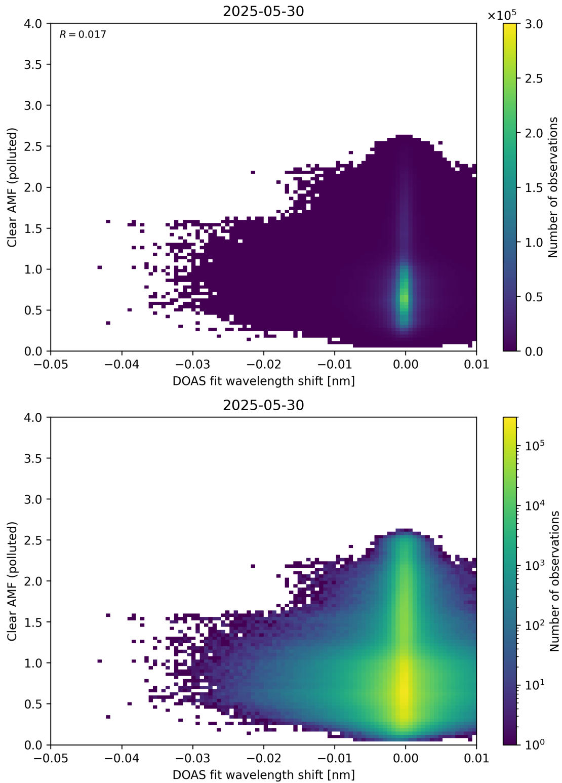
Figure 140: Scatter density plot of “DOAS fit wavelength shift” against “Clear AMF (polluted)” for 2025-05-29 to 2025-05-31.
