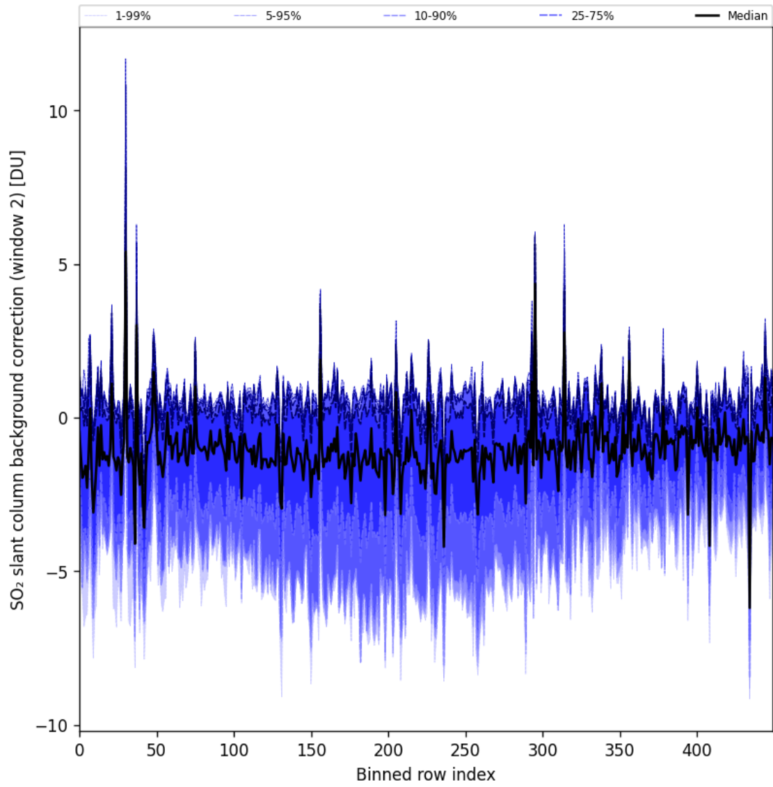
Figure 96: Along track statistics of “SO 2 slant column background correction (window 2)” for 2025-05-29 to 2025-05-31
