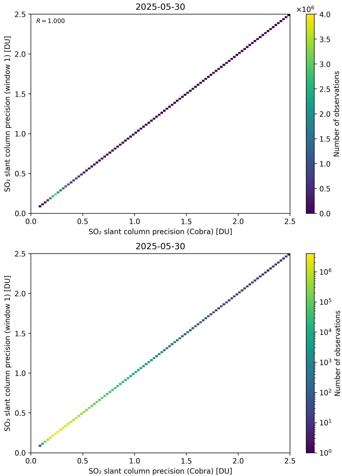
Figure 209: Scatter density plot of “SO 2 slant column precision (Cobra)” against “SO 2 slant column precision (window 1)” for 2025-05-29 to 2025-05-31.
