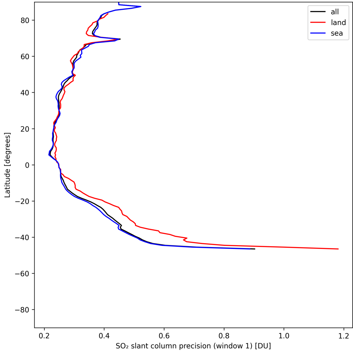
Figure 38: Zonal average of “SO 2 slant column precision (window 1)” for 2025-05-29 to 2025-05-31.
