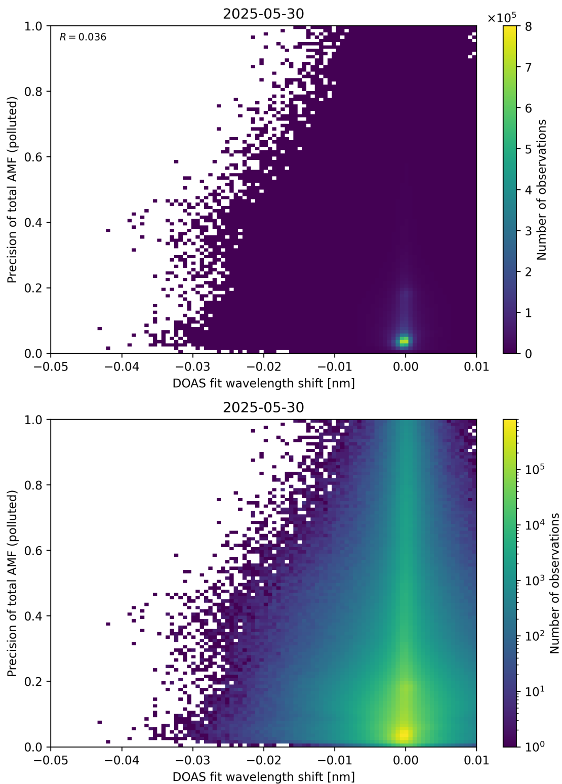
Figure 142: Scatter density plot of “DOAS fit wavelength shift” against “Precision of total AMF (polluted)” for 2025-05-29 to 2025-05-31.
