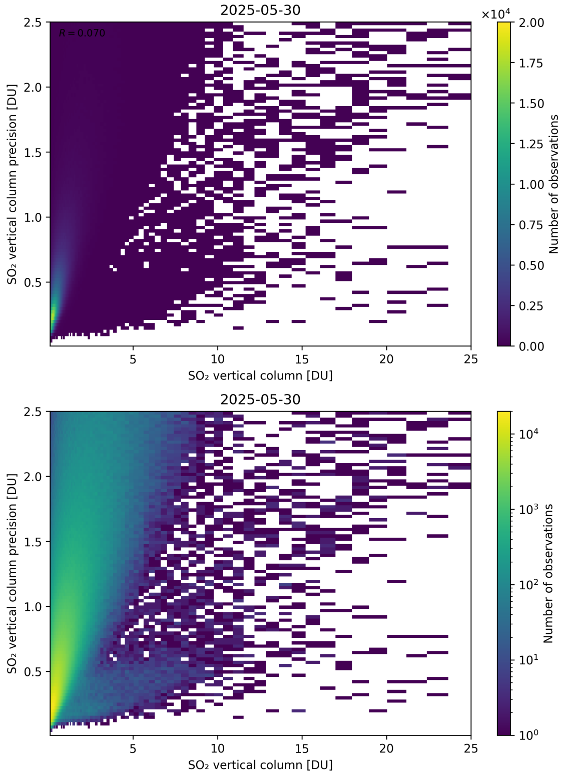
Figure 361: Scatter density plot of “SO 2 vertical column” against “SO 2 vertical column precision” for 2025-05-29 to 2025-05-31.
