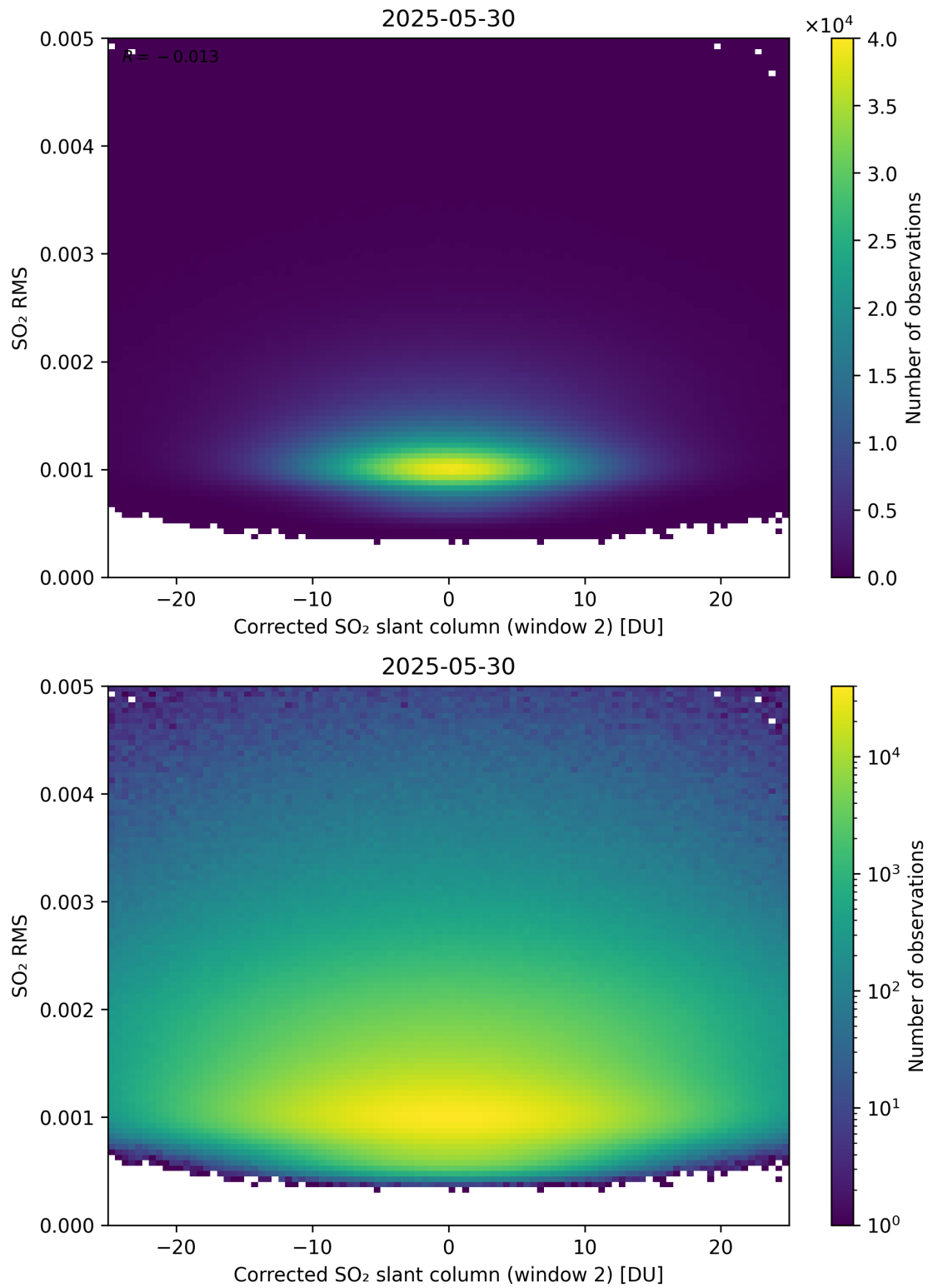
Figure 248: Scatter density plot of “Corrected SO 2 slant column (window 2)” against “SO 2 RMS” for 2025-05-29 to 2025-05-31.
