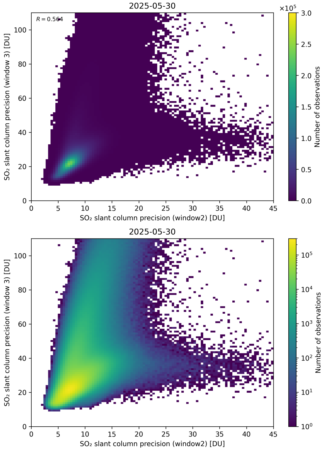
Figure 300: Scatter density plot of “SO 2 slant column precision (window2)” against “SO 2 slant column precision (window 3)” for 2025-05-29 to 2025-05-31.
