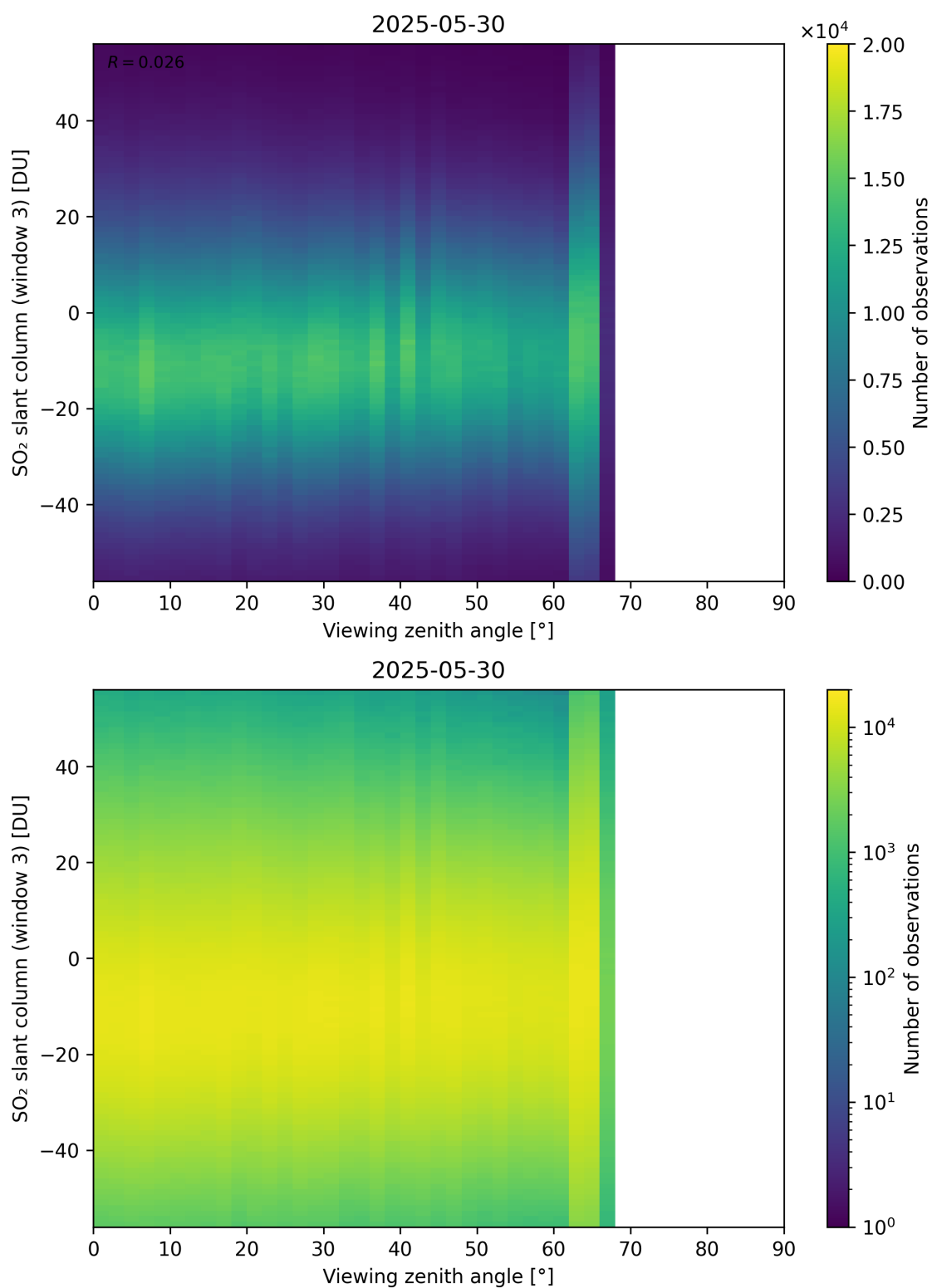
Figure 379: Scatter density plot of “Viewing zenith angle” against “SO 2 slant column (window 3)” for 2025-05-29 to 2025-05-31.
