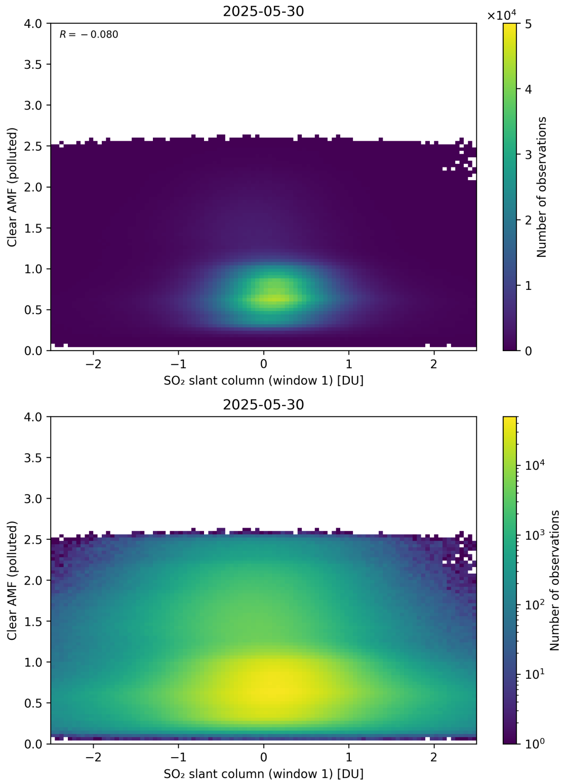
Figure 282: Scatter density plot of “SO 2 slant column (window 1)” against “Clear AMF (polluted)” for 2025-05-29 to 2025-05-31.
