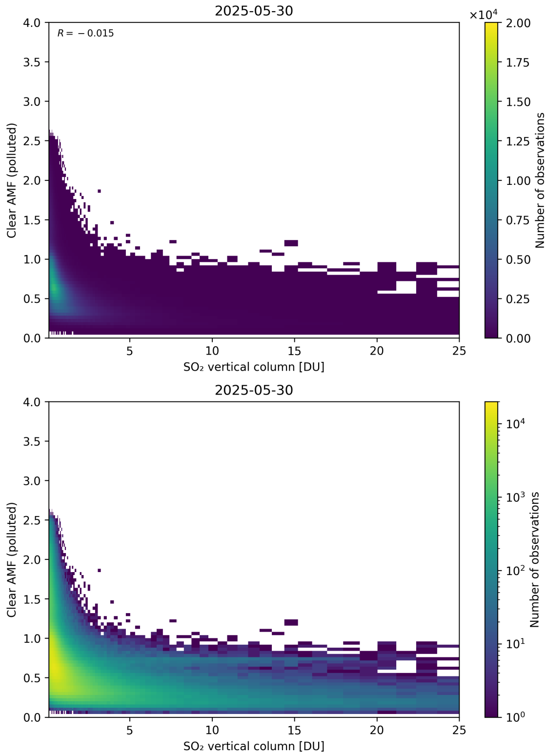
Figure 348: Scatter density plot of “SO 2 vertical column” against “Clear AMF (polluted)” for 2025-05-29 to 2025-05-31.
