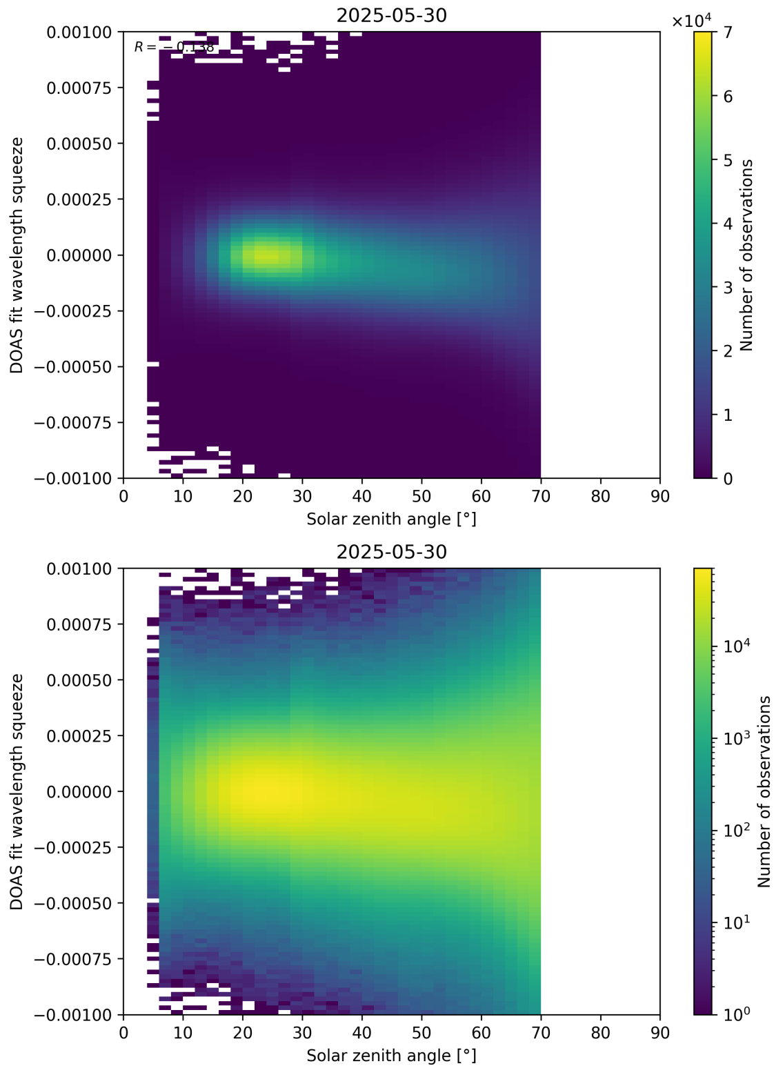
Figure 175: Scatter density plot of “Solar zenith angle” against “DOAS fit wavelength squeeze” for 2025-05-29 to 2025-05-31.
