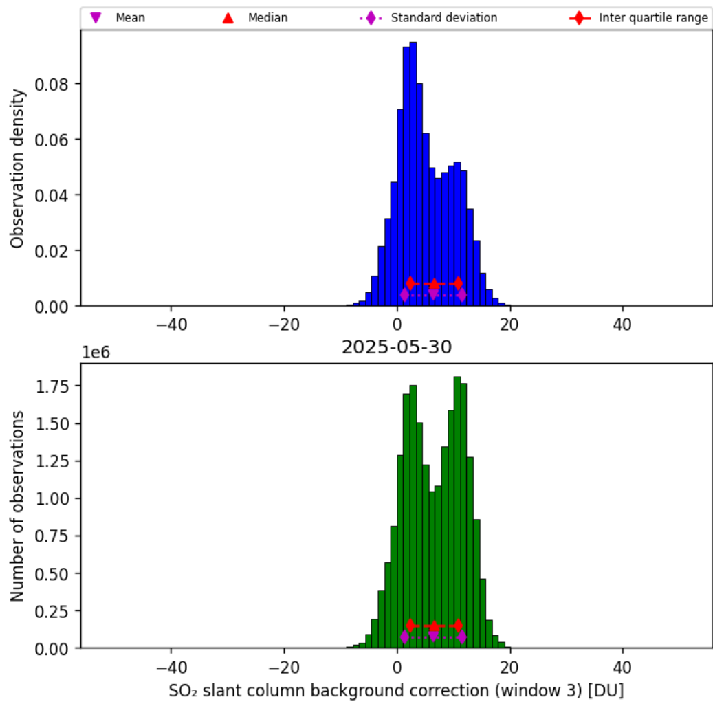
Figure 74: Histogram of “SO 2 slant column background correction (window 3)” for 2025-05-29 to 2025-05-31
