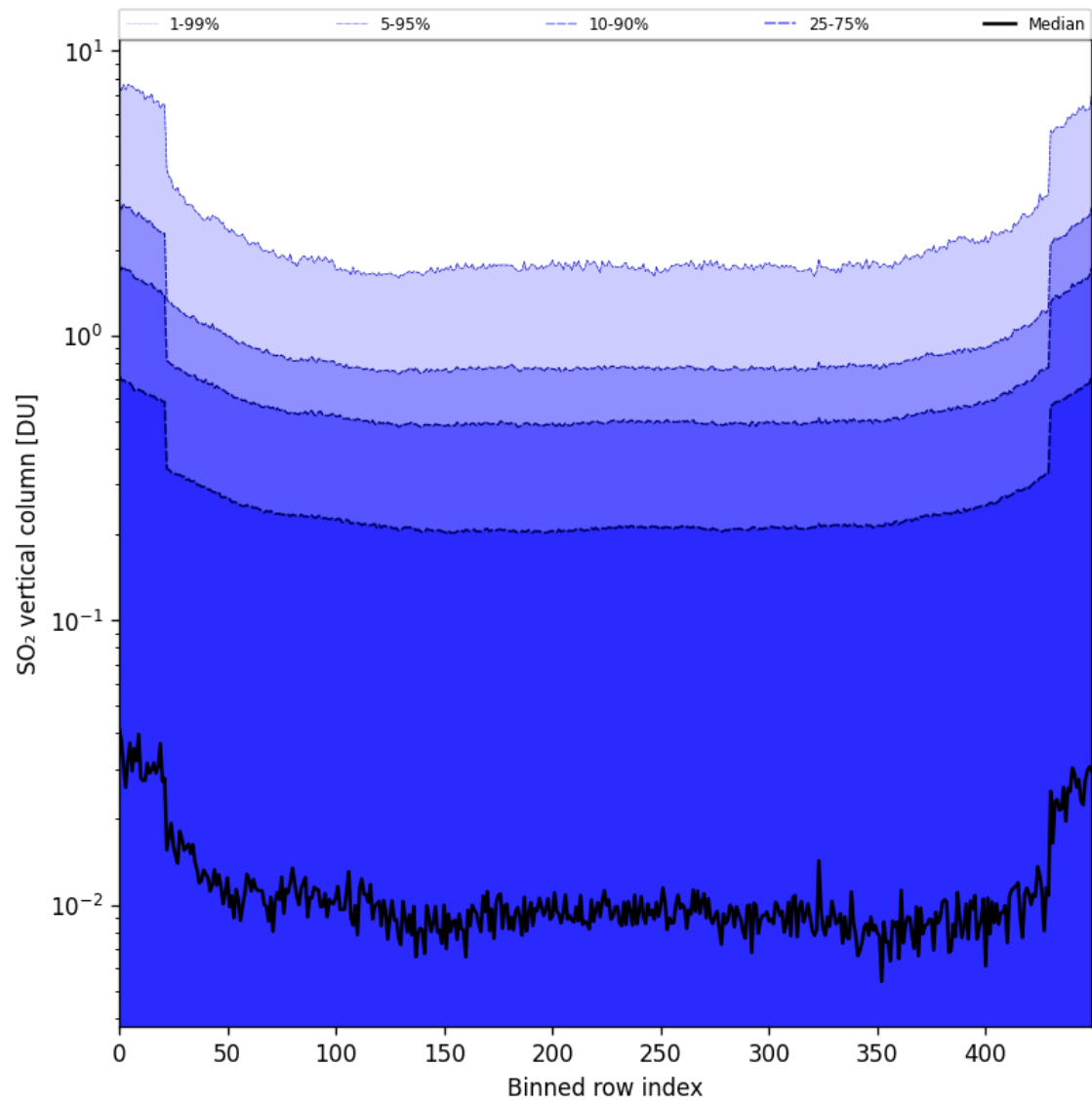
Figure 84: Along track statistics of “SO 2 vertical column” for 2025-05-29 to 2025-05-31
