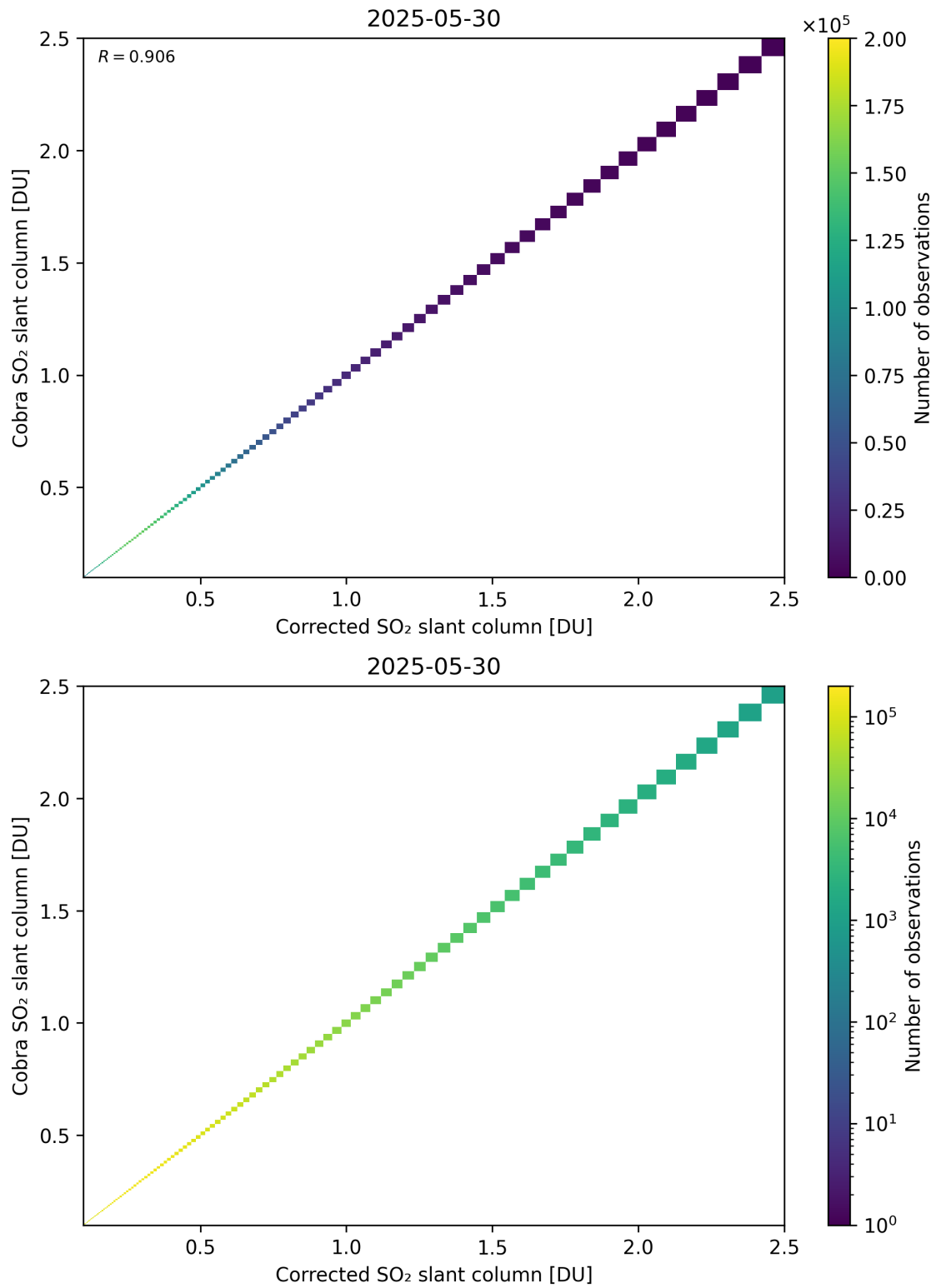
Figure 233: Scatter density plot of “Corrected SO 2 slant column” against “Cobra SO 2 slant column” for 2025-05-29 to 2025-05-31.
