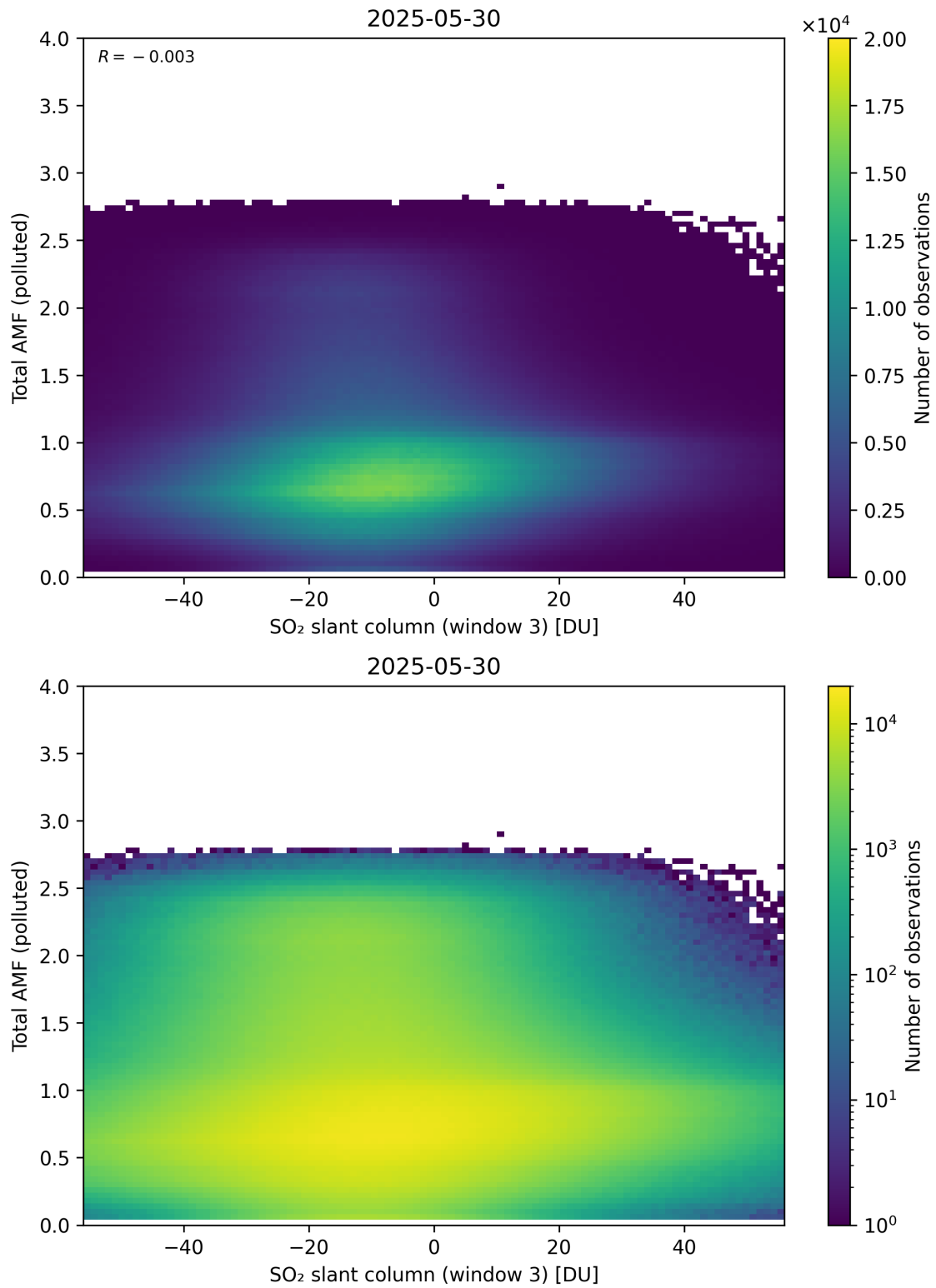
Figure 318: Scatter density plot of “SO 2 slant column (window 3)” against “Total AMF (polluted)” for 2025-05-29 to 2025-05-31.
