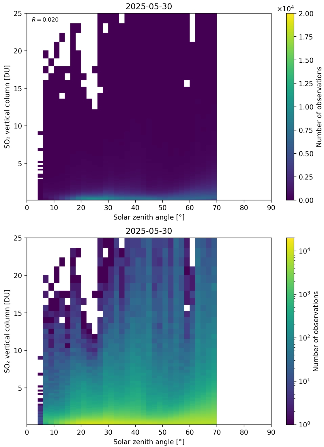
Figure 191: Scatter density plot of “Solar zenith angle” against “SO 2 vertical column” for 2025-05-29 to 2025-05-31.
