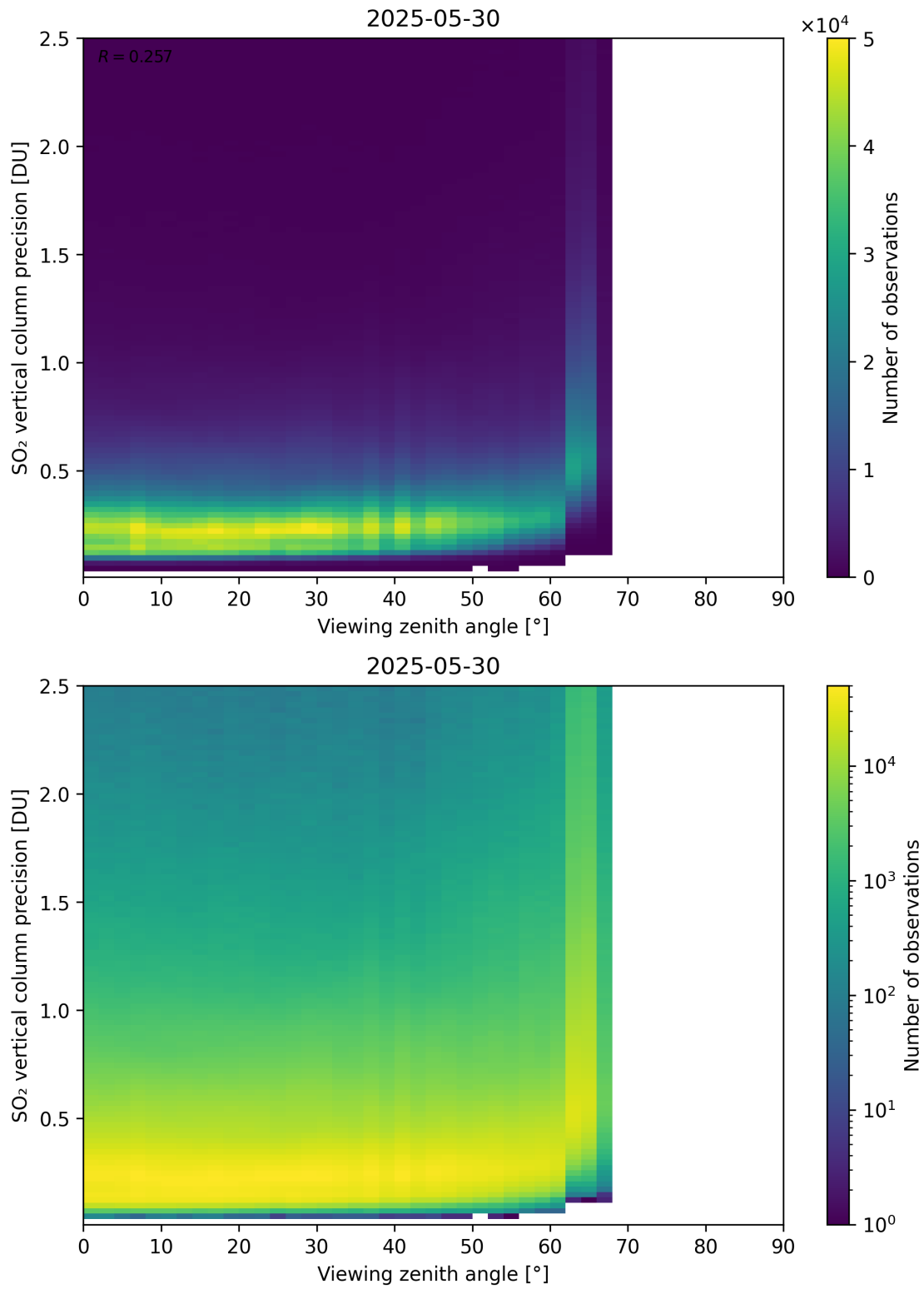
Figure 384: Scatter density plot of “Viewing zenith angle” against “SO 2 vertical column precision” for 2025-05-29 to 2025-05-31.
