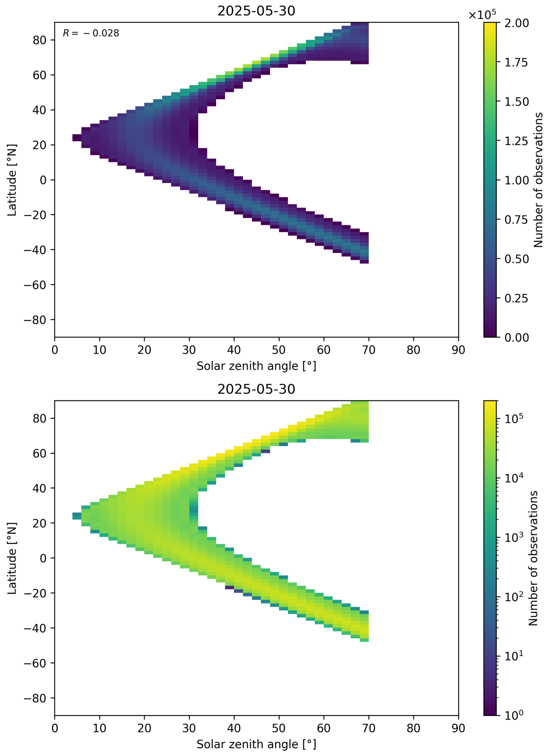
Figure 177: Scatter density plot of “Solar zenith angle” against “Latitude” for 2025-05-29 to 2025-05-31.
