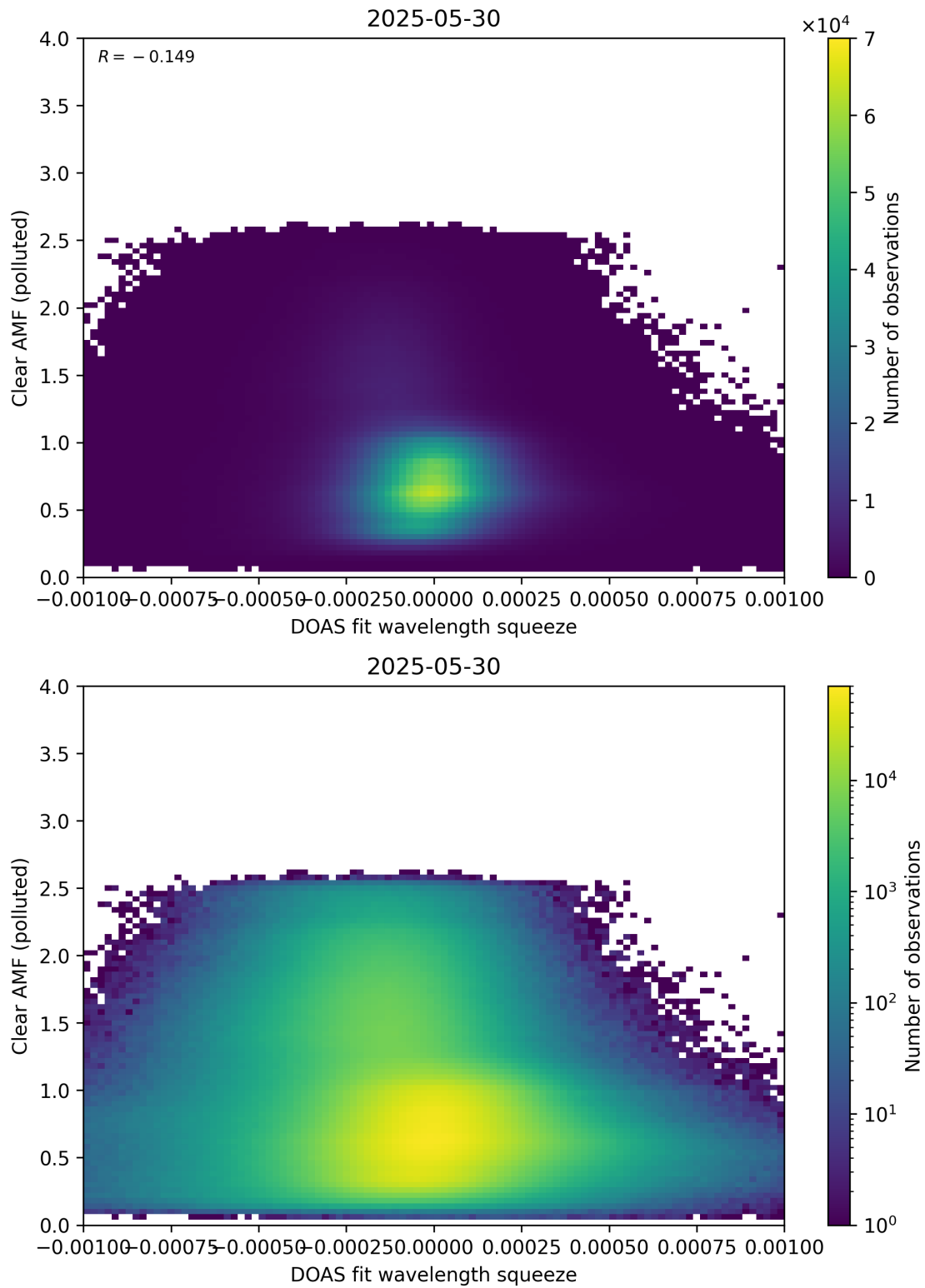
Figure 144: Scatter density plot of “DOAS fit wavelength squeeze” against “Clear AMF (polluted)” for 2025-05-29 to 2025-05-31.
