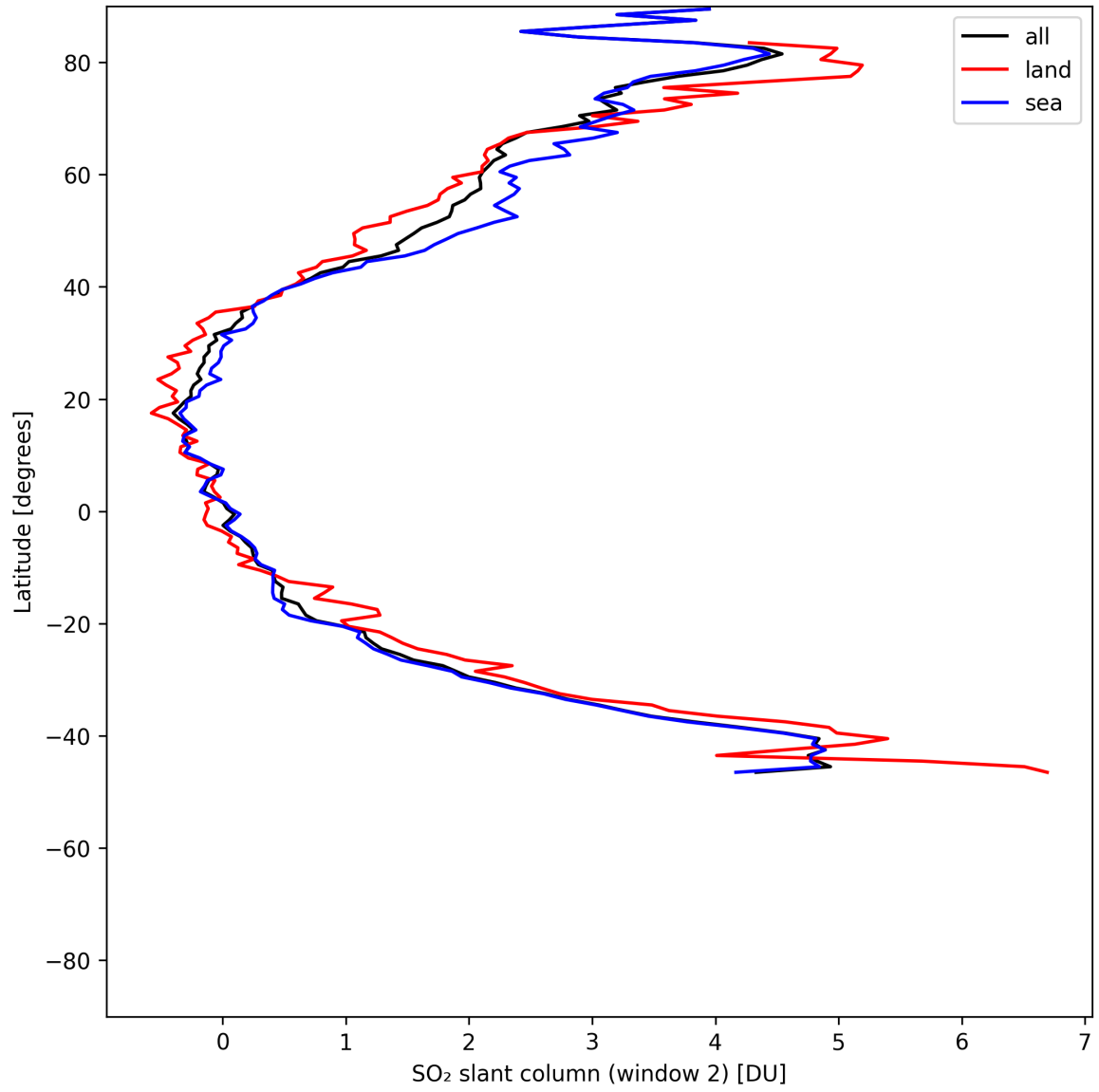
Figure 41: Zonal average of “SO 2 slant column (window 2)” for 2025-05-29 to 2025-05-31.
