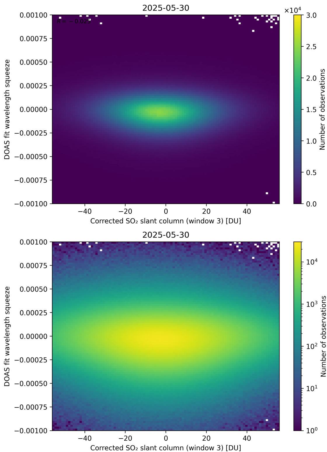
Figure 257: Scatter density plot of “Corrected SO 2 slant column (window 3)” against “DOAS fit wavelength squeeze” for 2025-05-29 to 2025-05-31.
