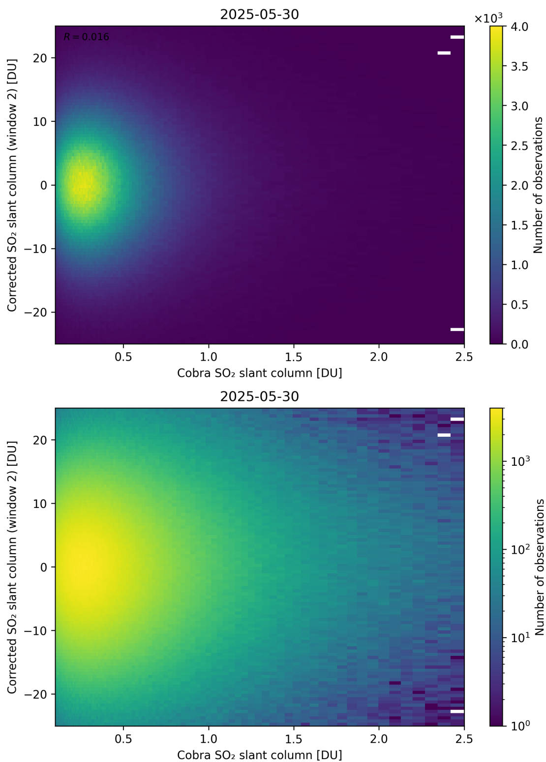
Figure 217: Scatter density plot of “Cobra SO 2 slant column” against “Corrected SO 2 slant column (window 2)” for 2025-05-29 to 2025-05-31.
