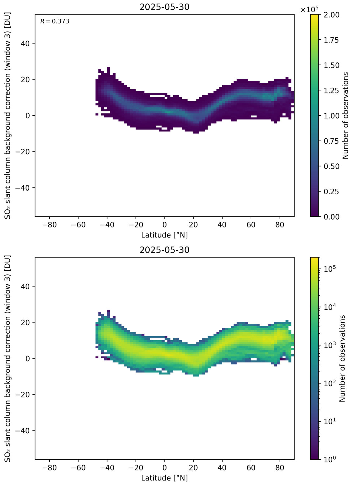
Figure 152: Scatter density plot of “Latitude” against “SO 2 slant column background correction (window 3)” for 2025-05-29 to 2025-05-31.
