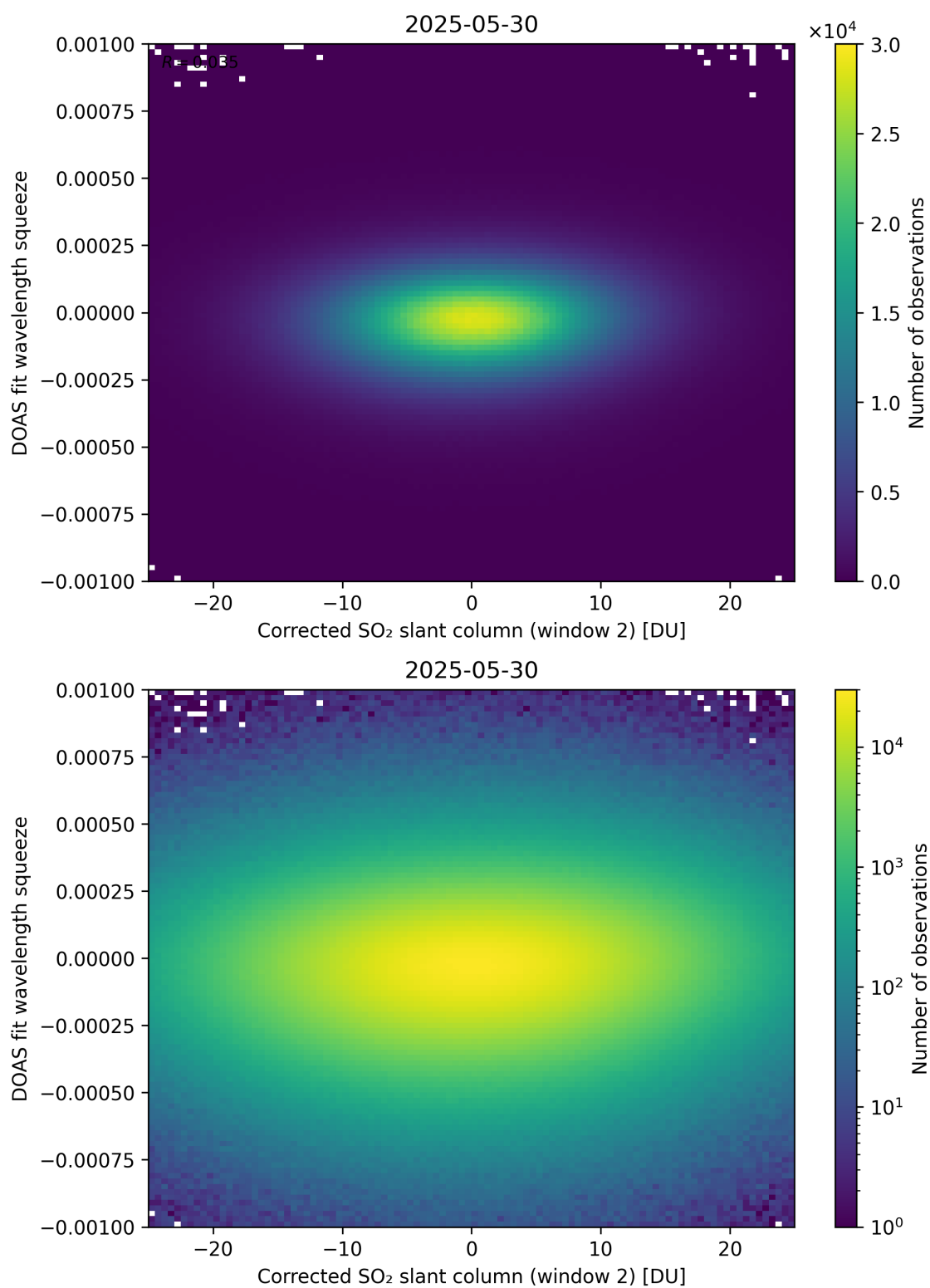
Figure 247: Scatter density plot of “Corrected SO 2 slant column (window 2)” against “DOAS fit wavelength squeeze” for 2025-05-29 to 2025-05-31.
