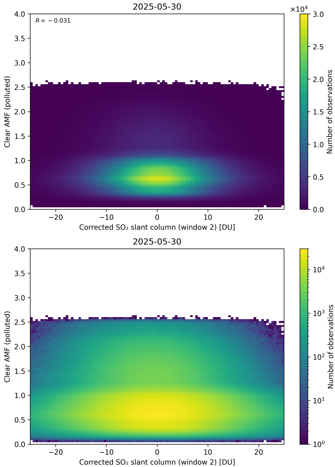
Figure 249: Scatter density plot of “Corrected SO 2 slant column (window 2)” against “Clear AMF (polluted)” for 2025-05-29 to 2025-05-31.
