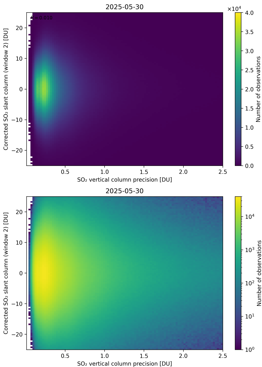
Figure 339: Scatter density plot of “SO 2 vertical column precision” against “Corrected SO 2 slant column (window 2)” for 2025-05-29 to 2025-05-31.
