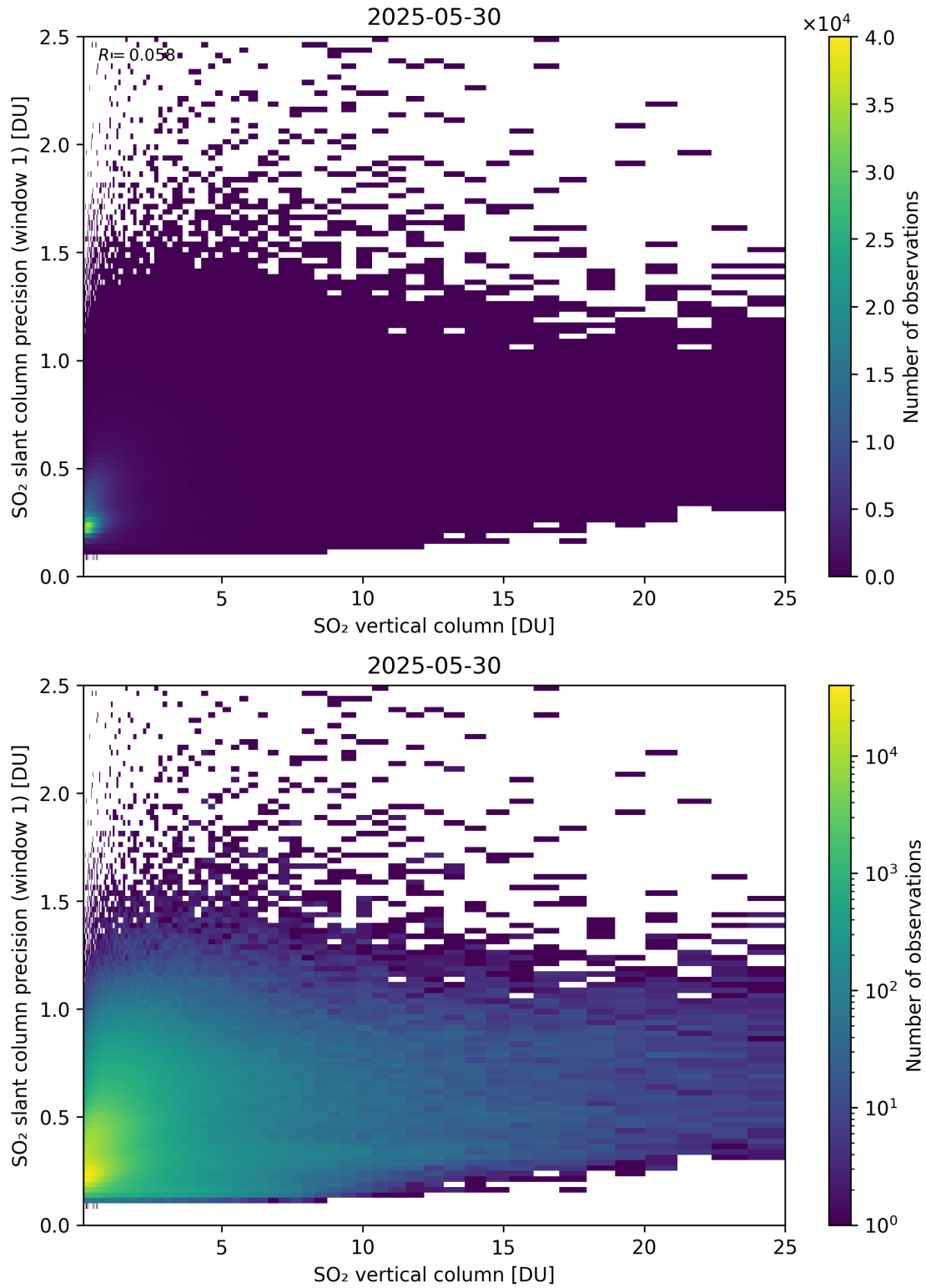
Figure 355: Scatter density plot of “SO 2 vertical column” against “SO 2 slant column precision (window 1)” for 2025-05-29 to 2025-05-31.
