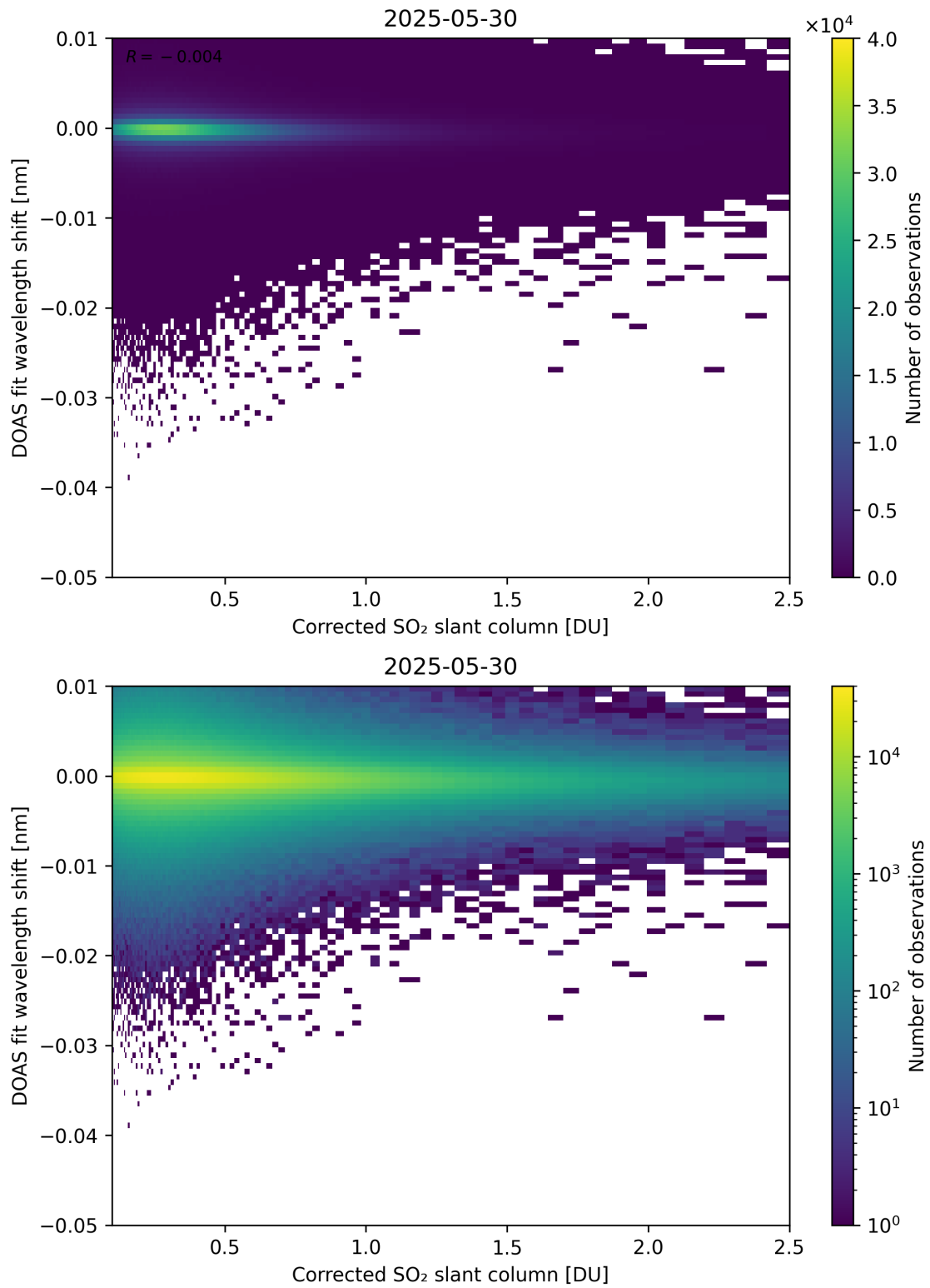
Figure 229: Scatter density plot of “Corrected SO 2 slant column” against “DOAS fit wavelength shift” for 2025-05-29 to 2025-05-31.
