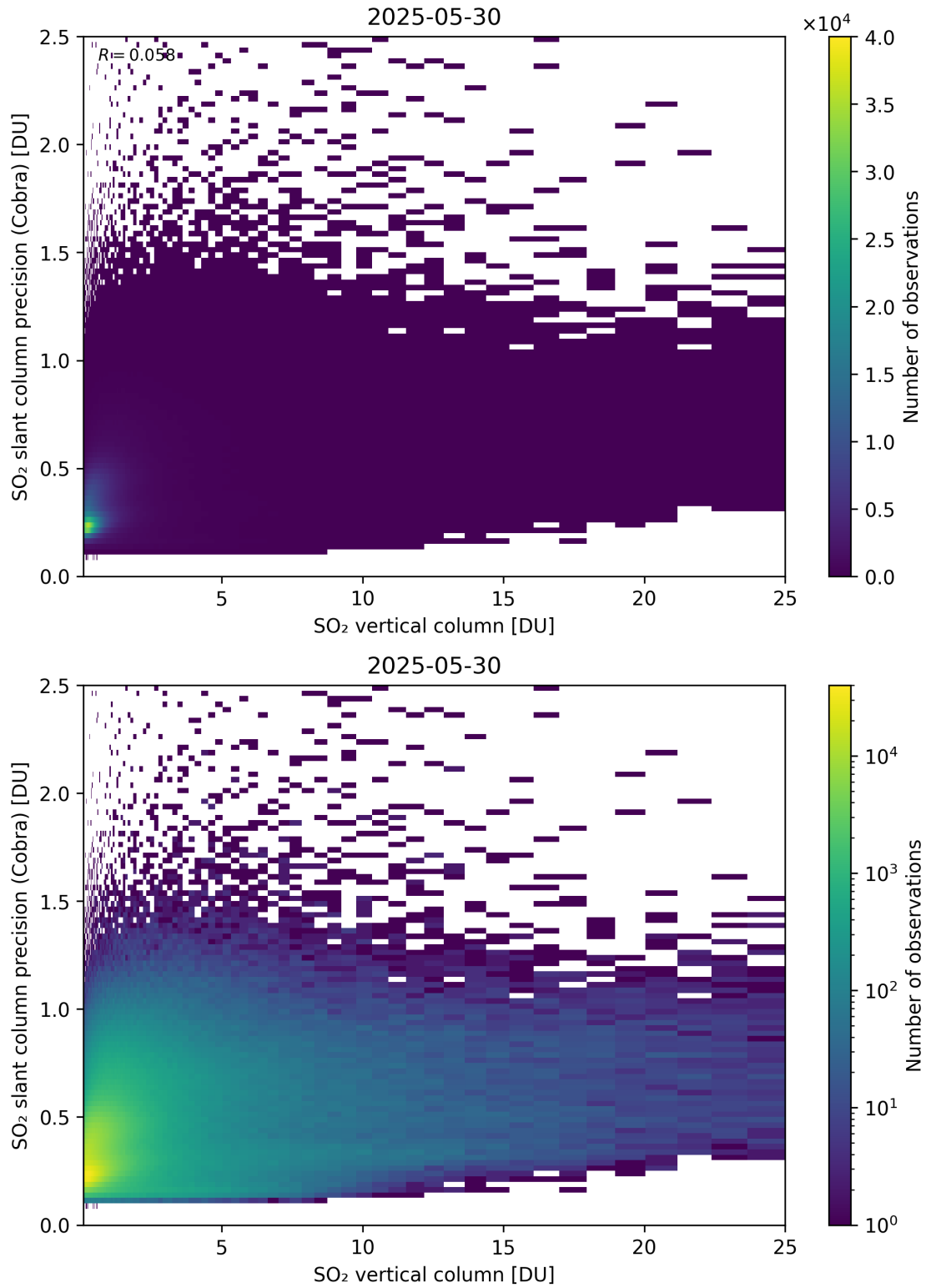
Figure 350: Scatter density plot of “SO 2 vertical column” against “SO 2 slant column precision (Cobra)” for 2025-05-29 to 2025-05-31.
