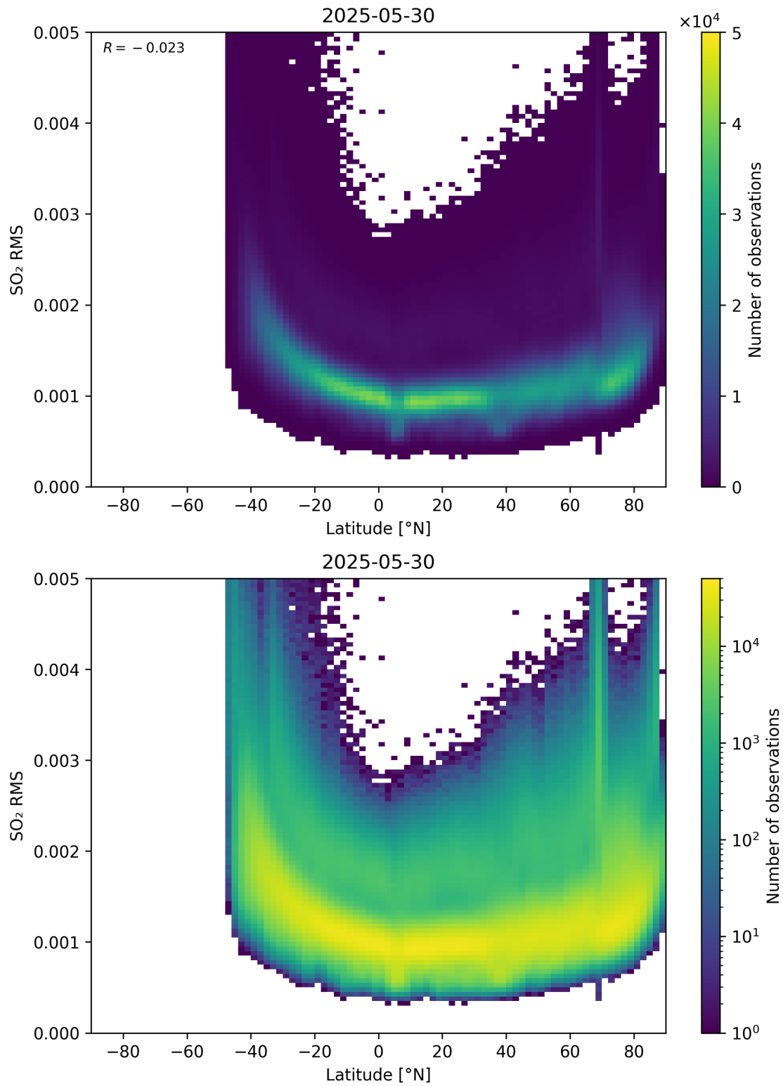
Figure 155: Scatter density plot of “Latitude” against “SO 2 RMS” for 2025-05-29 to 2025-05-31.
