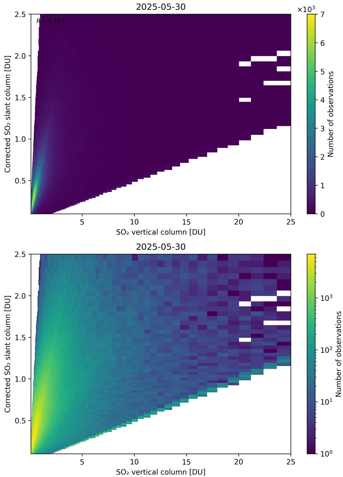
Figure 351: Scatter density plot of “SO 2 vertical column” against “Corrected SO 2 slant column” for 2025-05-29 to 2025-05-31.
