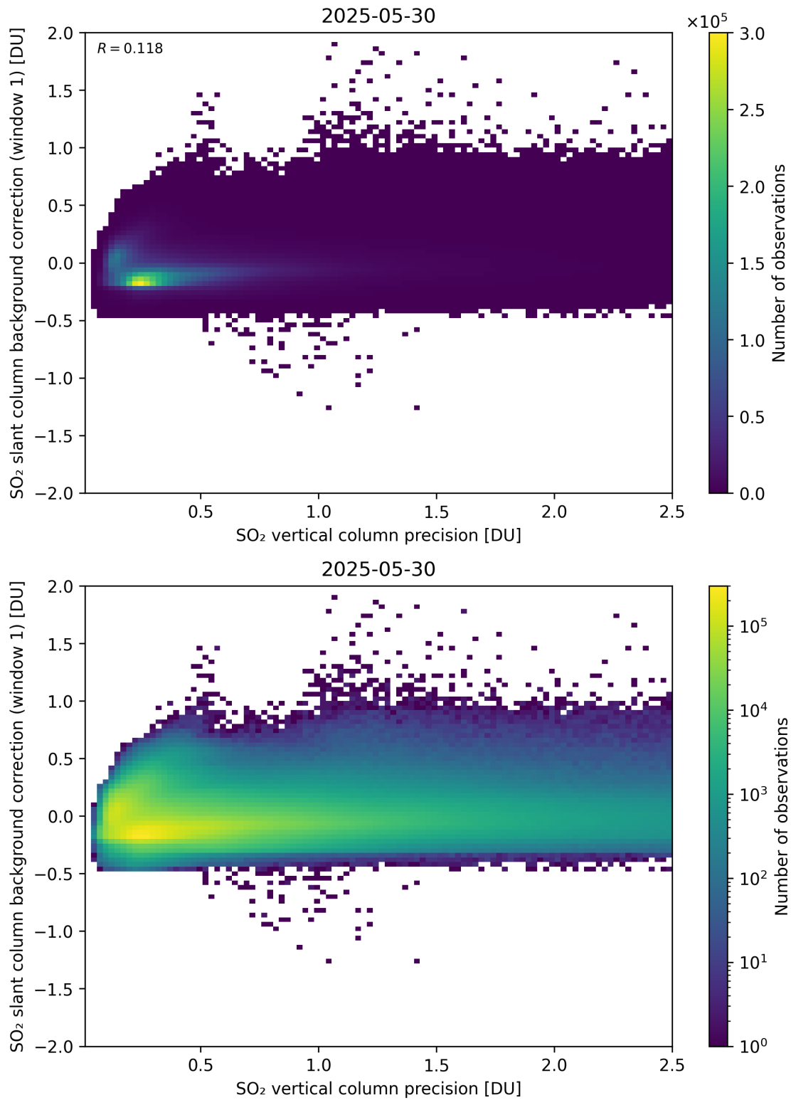
Figure 329: Scatter density plot of “SO 2 vertical column precision” against “SO 2 slant column background correction (window 1)” for 2025-05-29 to 2025-05-31.
