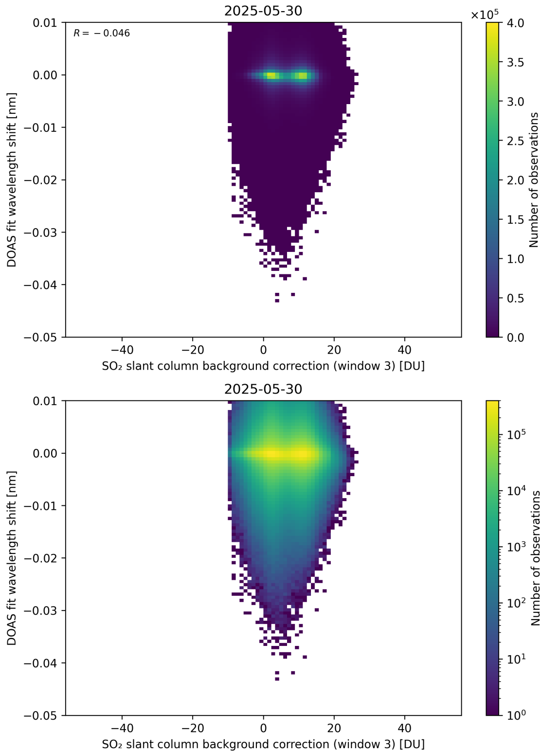
Figure 132: Scatter density plot of “SO 2 slant column background correction (window 3)” against “DOAS fit wavelength shift” for 2025-05-29 to 2025-05-31.
