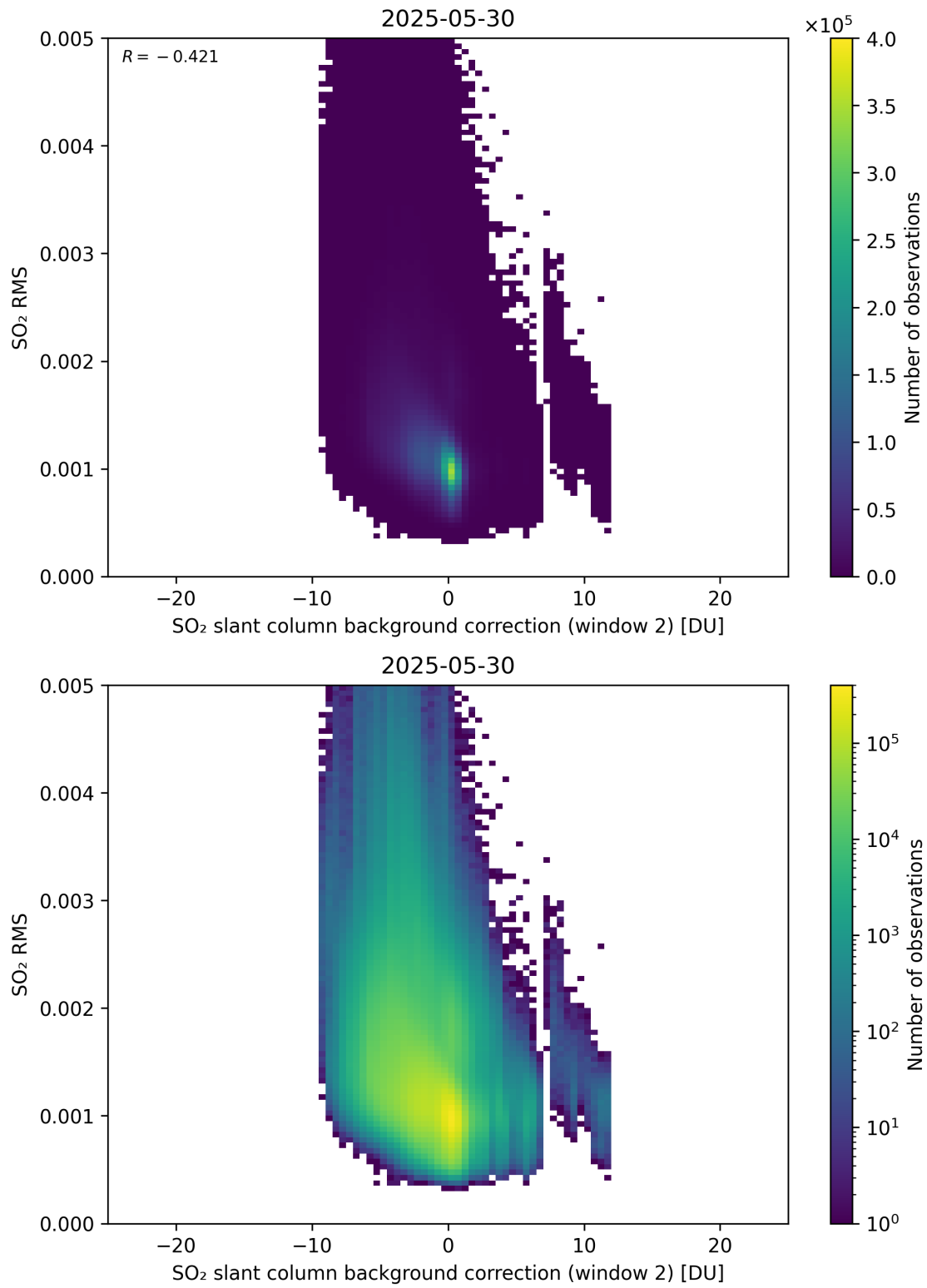
Figure 125: Scatter density plot of “SO 2 slant column background correction (window 2)” against “SO 2 RMS” for 2025-05-29 to 2025-05-31.
