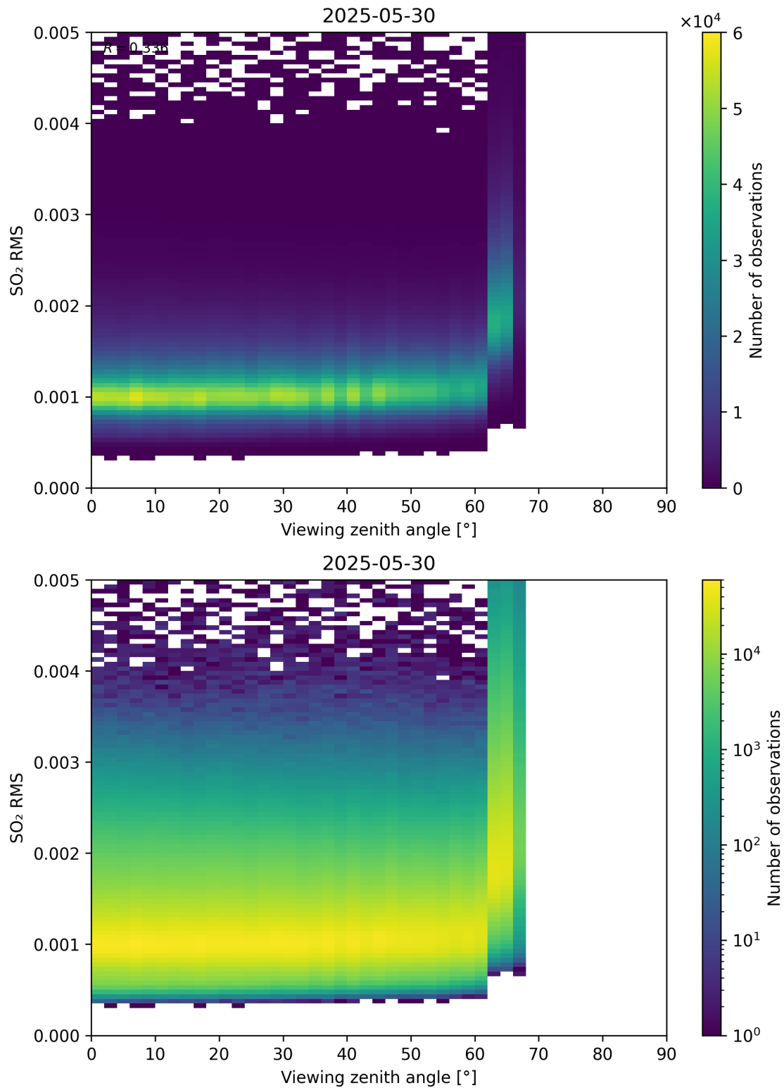
Figure 367: Scatter density plot of “Viewing zenith angle” against “SO 2 RMS” for 2025-05-29 to 2025-05-31.
