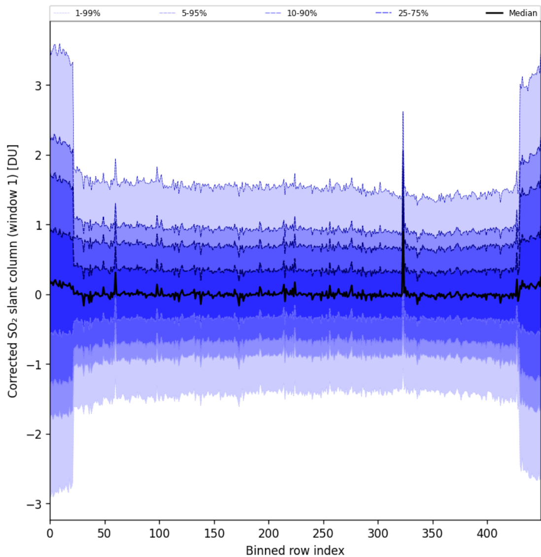
Figure 91: Along track statistics of “Corrected SO 2 slant column (window 1)” for 2025-05-29 to 2025-05-31
