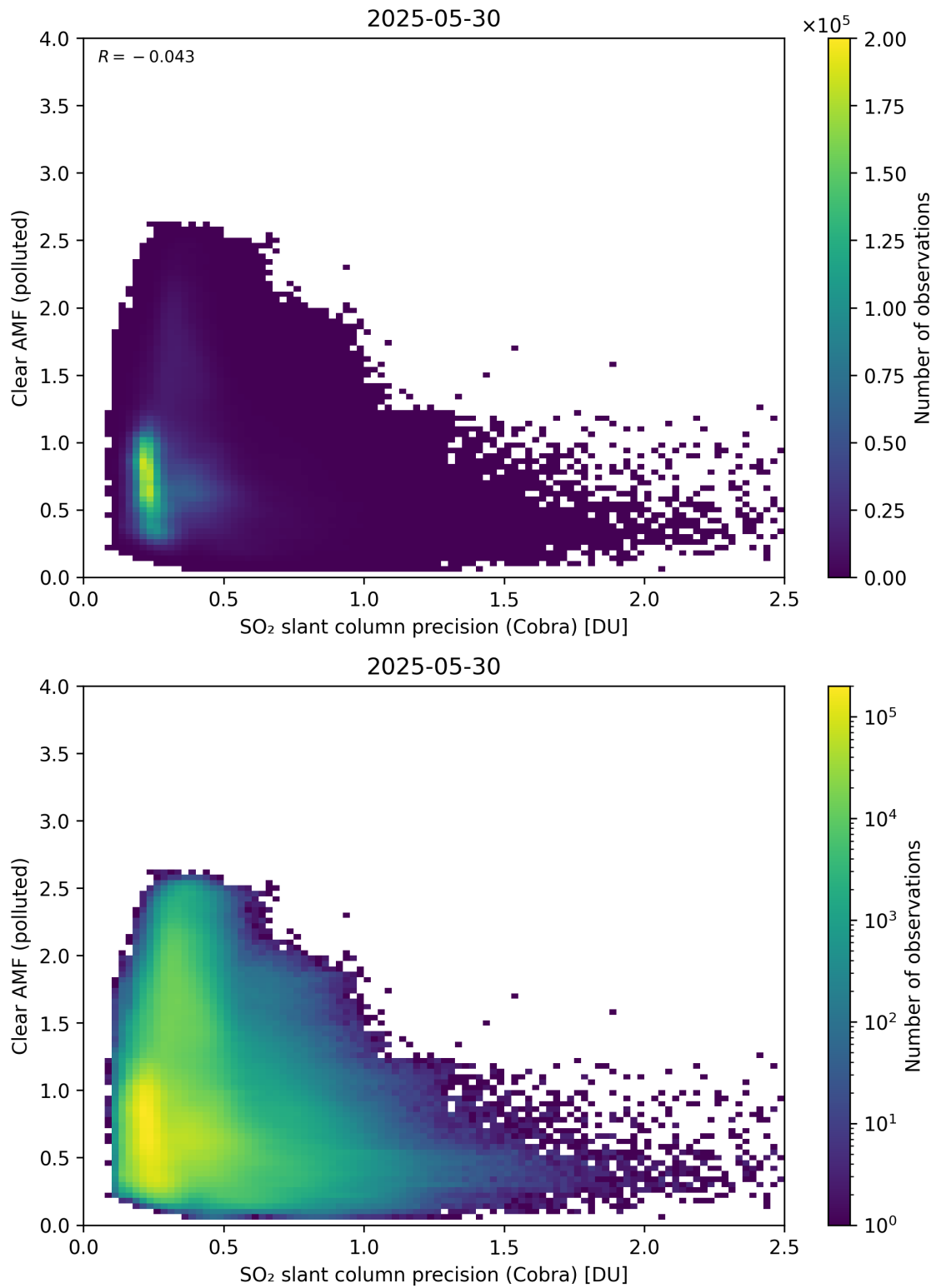
Figure 205: Scatter density plot of “SO 2 slant column precision (Cobra)” against “Clear AMF (polluted)” for 2025-05-29 to 2025-05-31.
