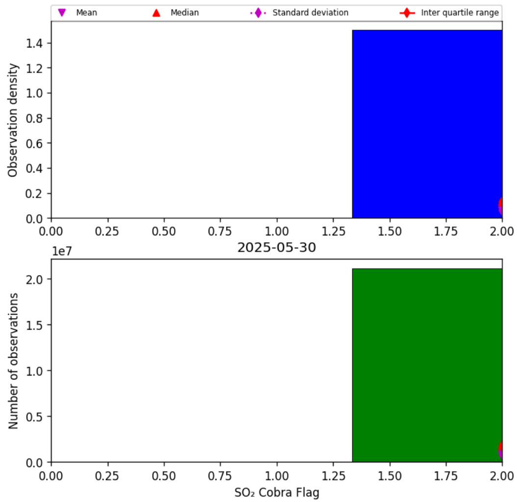
Figure 75: Histogram of “SO 2 Cobra Flag” for 2025-05-29 to 2025-05-31
