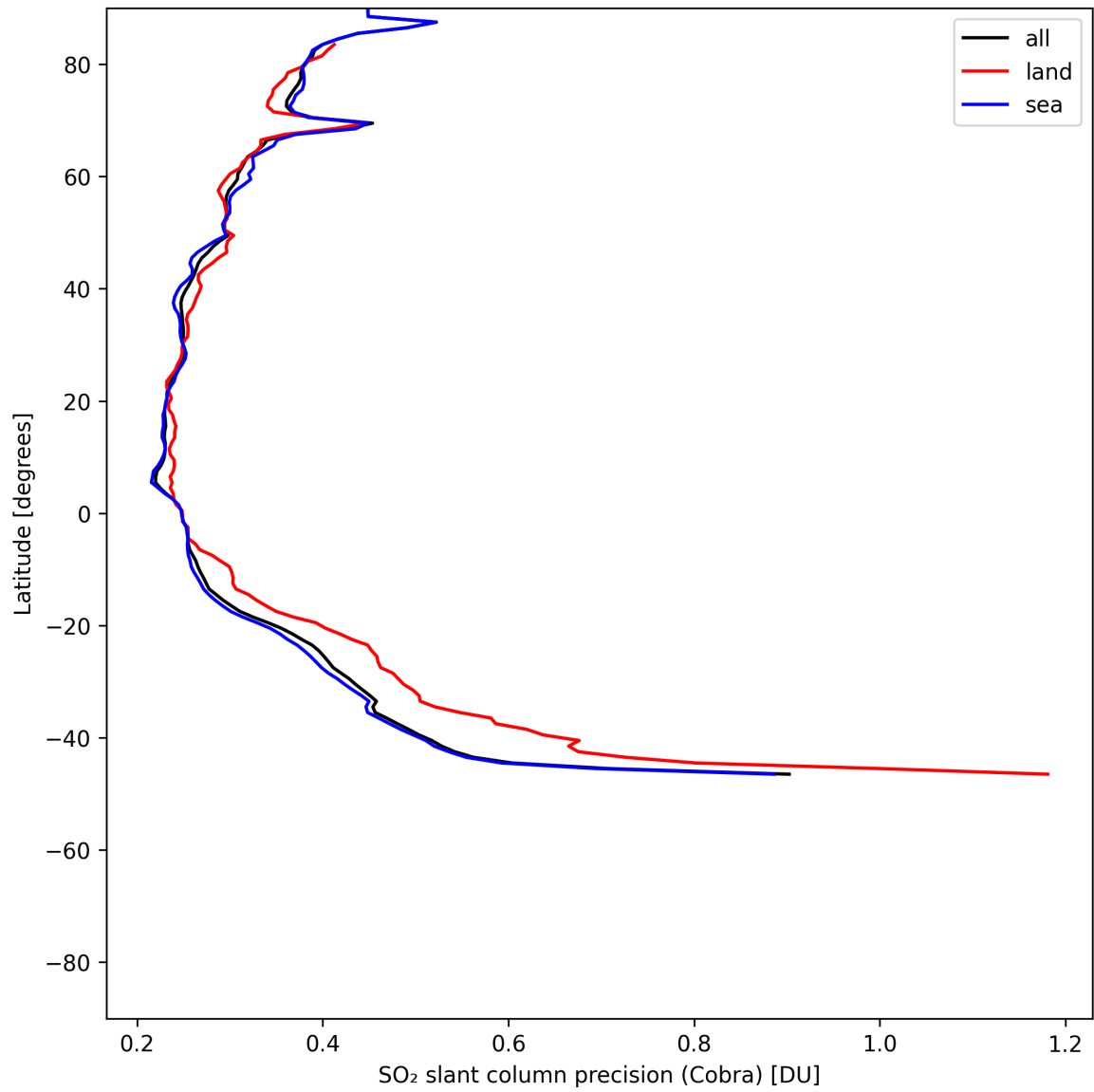
Figure 36: Zonal average of “SO 2 slant column precision (Cobra)” for 2025-05-29 to 2025-05-31.
