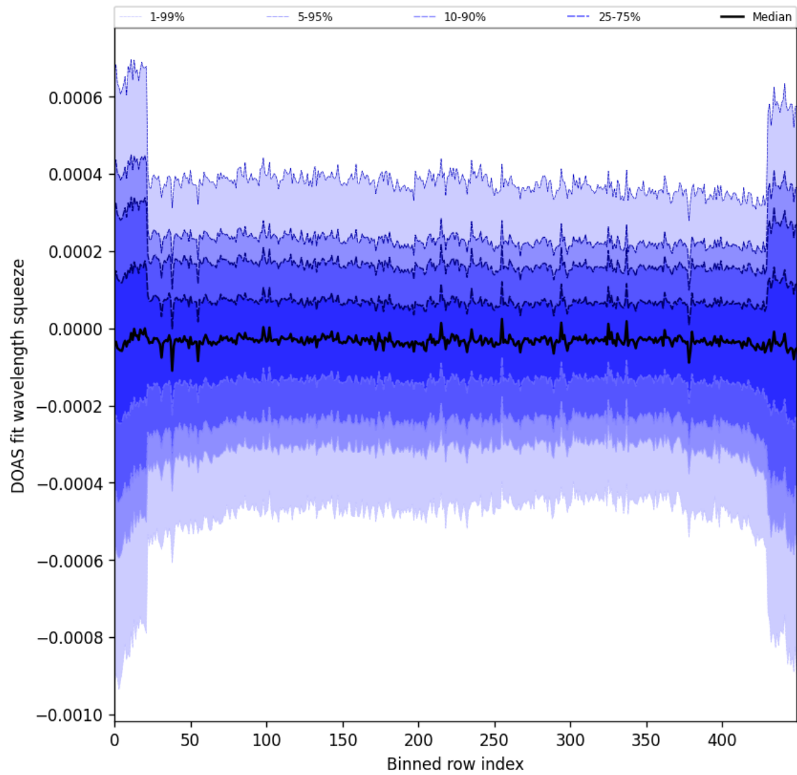
Figure 103: Along track statistics of “DOAS fit wavelength squeeze” for 2025-05-29 to 2025-05-31
