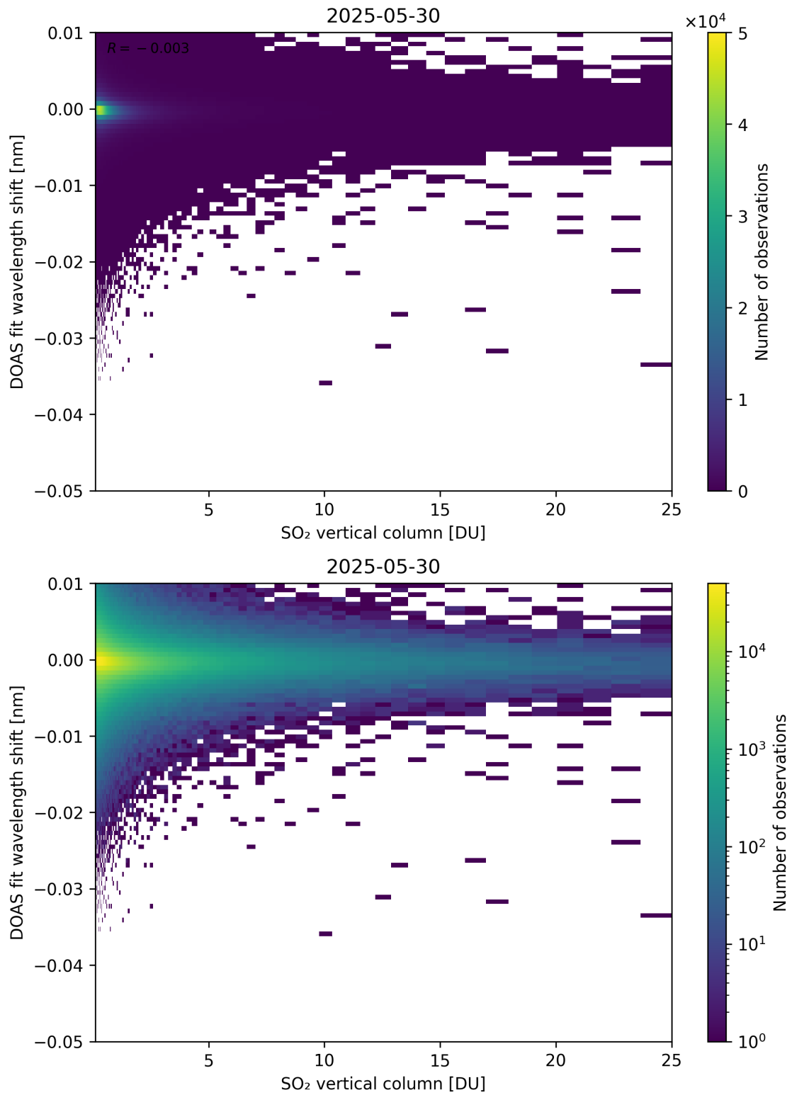
Figure 326: Scatter density plot of “SO 2 vertical column” against “DOAS fit wavelength shift” for 2025-05-29 to 2025-05-31.
