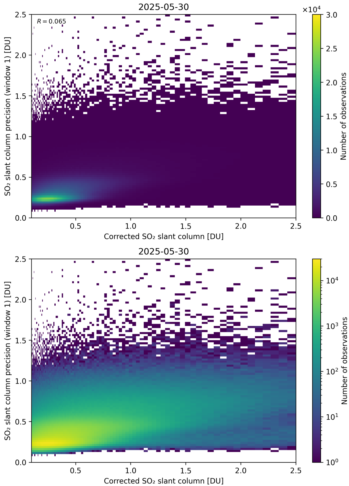
Figure 238: Scatter density plot of “Corrected SO 2 slant column” against “SO 2 slant column precision (window 1)” for 2025-05-29 to 2025-05-31.
