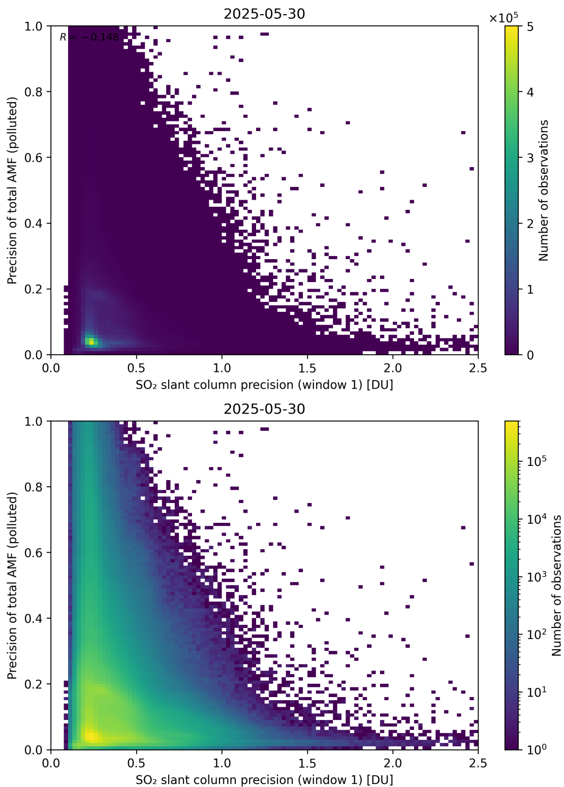
Figure 281: Scatter density plot of “SO 2 slant column precision (window 1)” against “Precision of total AMF (polluted)” for 2025-05-29 to 2025-05-31.
