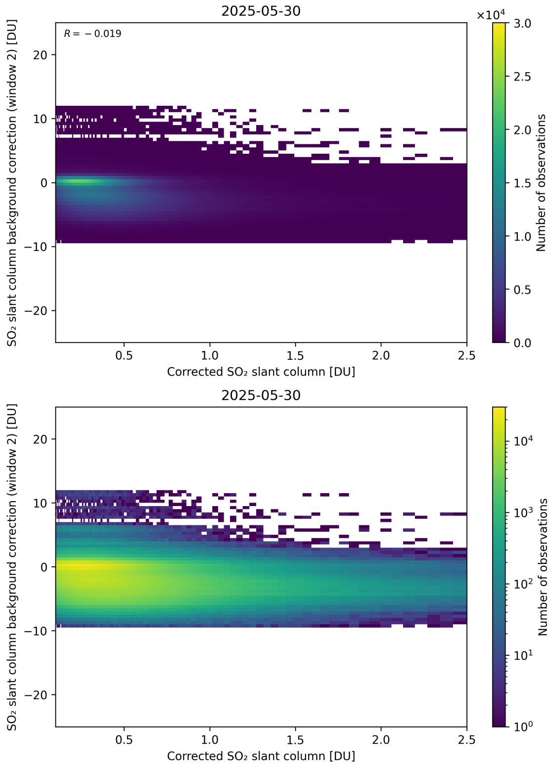
Figure 227: Scatter density plot of “Corrected SO 2 slant column” against “SO 2 slant column background correction (window 2)” for 2025-05-29 to 2025-05-31.
