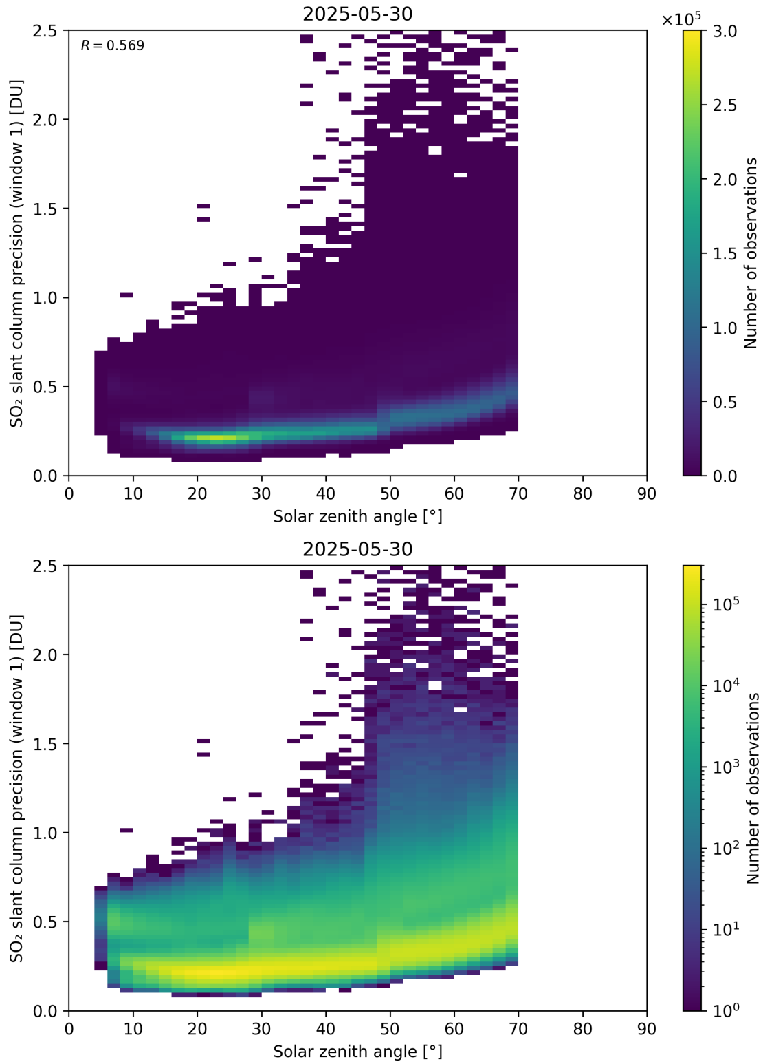
Figure 185: Scatter density plot of “Solar zenith angle” against “SO 2 slant column precision (window 1)” for 2025-05-29 to 2025-05-31.
