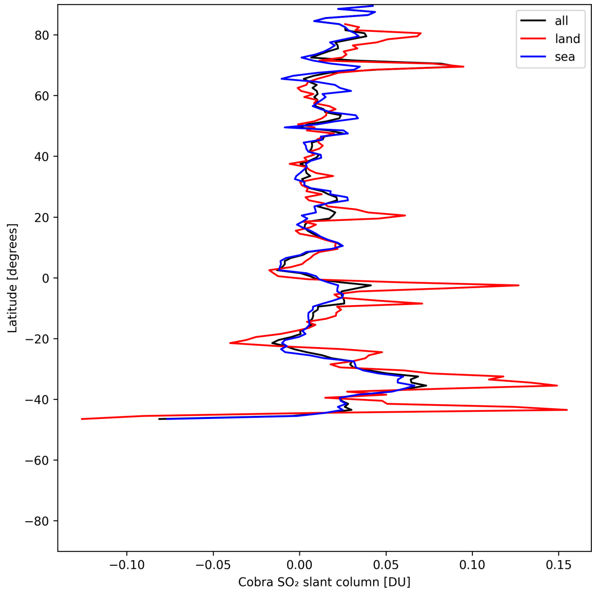
Figure 35: Zonal average of “Cobra SO 2 slant column” for 2025-05-29 to 2025-05-31.
