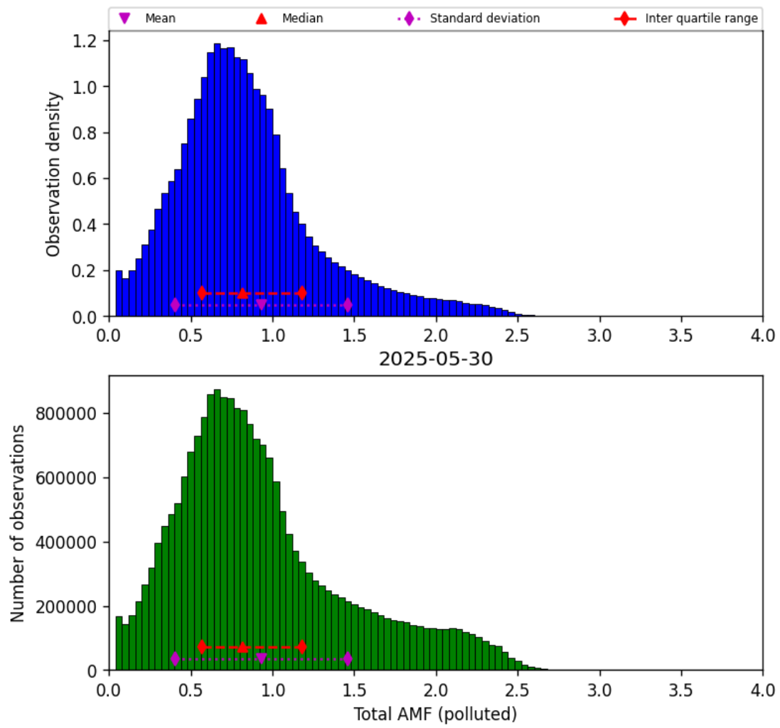
Figure 79: Histogram of “Total AMF (polluted)” for 2025-05-29 to 2025-05-31
