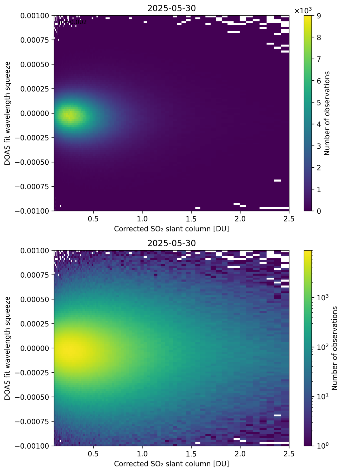
Figure 230: Scatter density plot of “Corrected SO 2 slant column” against “DOAS fit wavelength squeeze” for 2025-05-29 to 2025-05-31.
