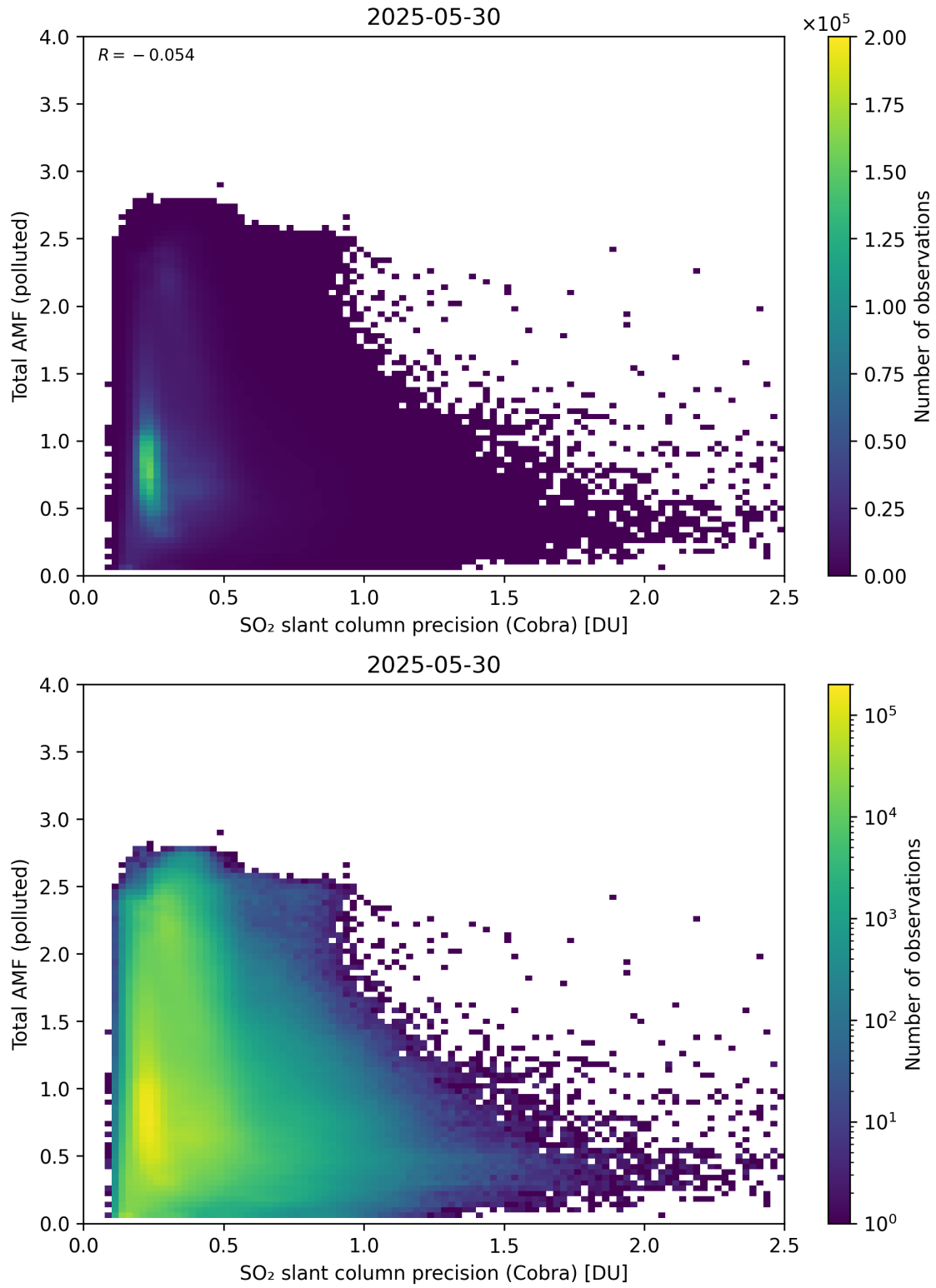
Figure 213: Scatter density plot of “SO 2 slant column precision (Cobra)” against “Total AMF (polluted)” for 2025-05-29 to 2025-05-31.
