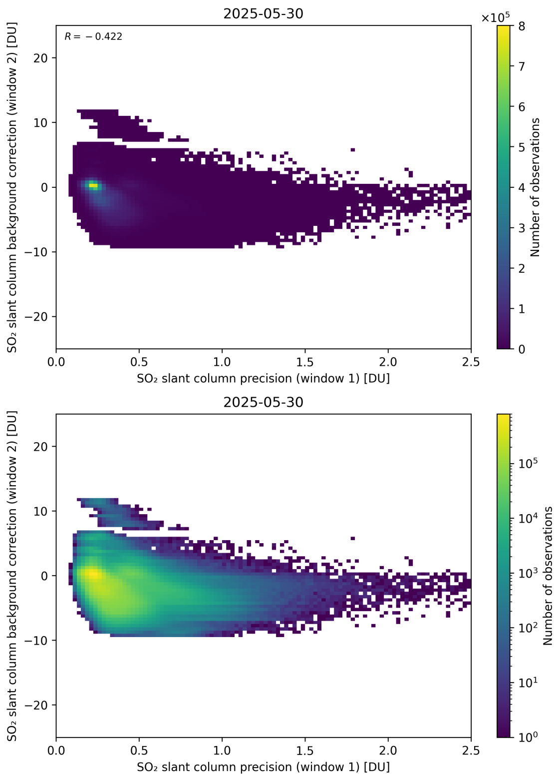
Figure 269: Scatter density plot of “SO 2 slant column precision (window 1)” against “SO 2 slant column background correction (window 2)” for 2025-05-29 to 2025-05-31.
