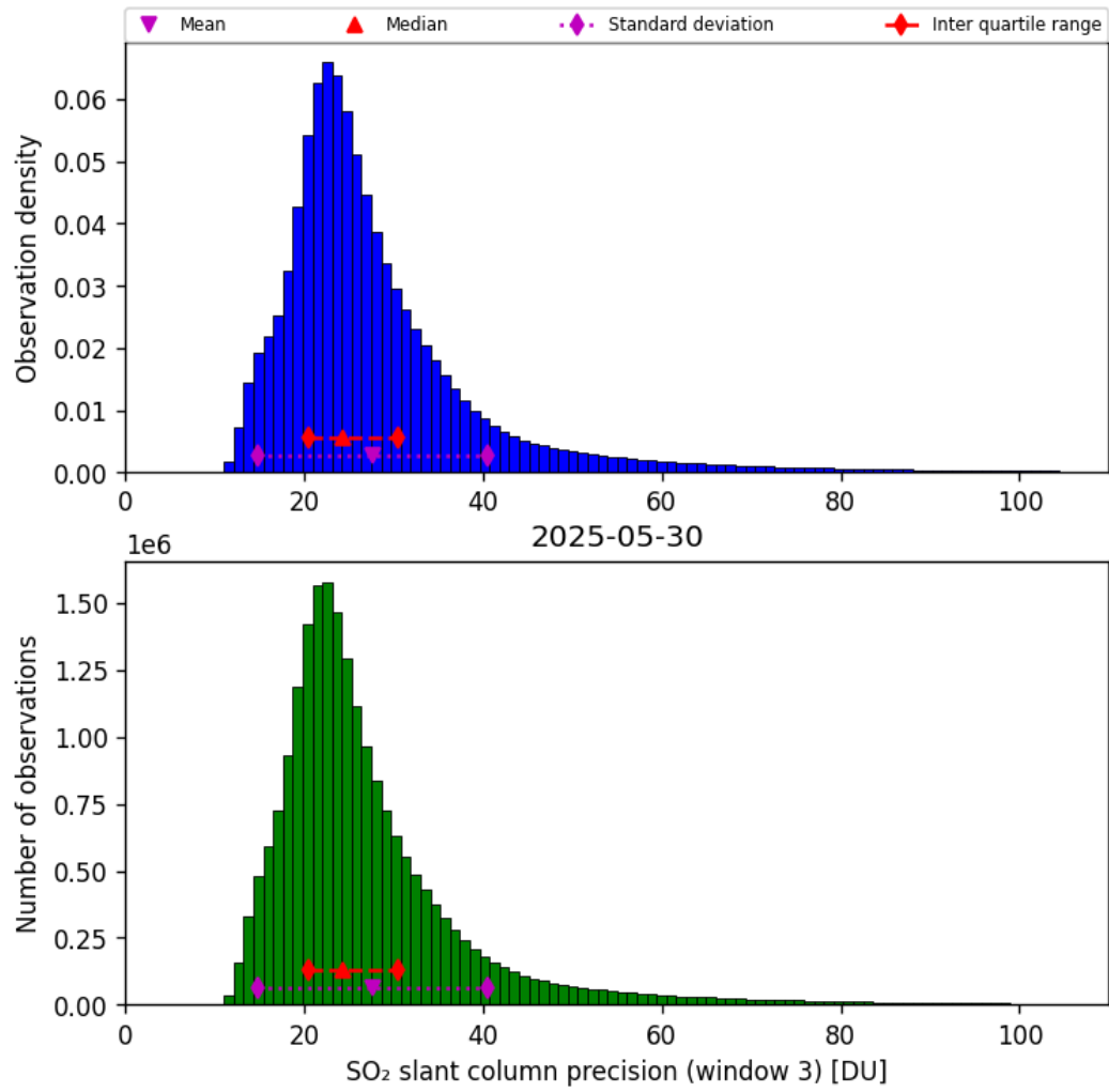
Figure 72: Histogram of “SO 2 slant column precision (window 3)” for 2025-05-29 to 2025-05-31
