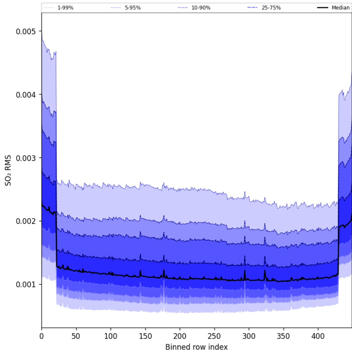
Figure 104: Along track statistics of “SO 2 RMS” for 2025-05-29 to 2025-05-31
