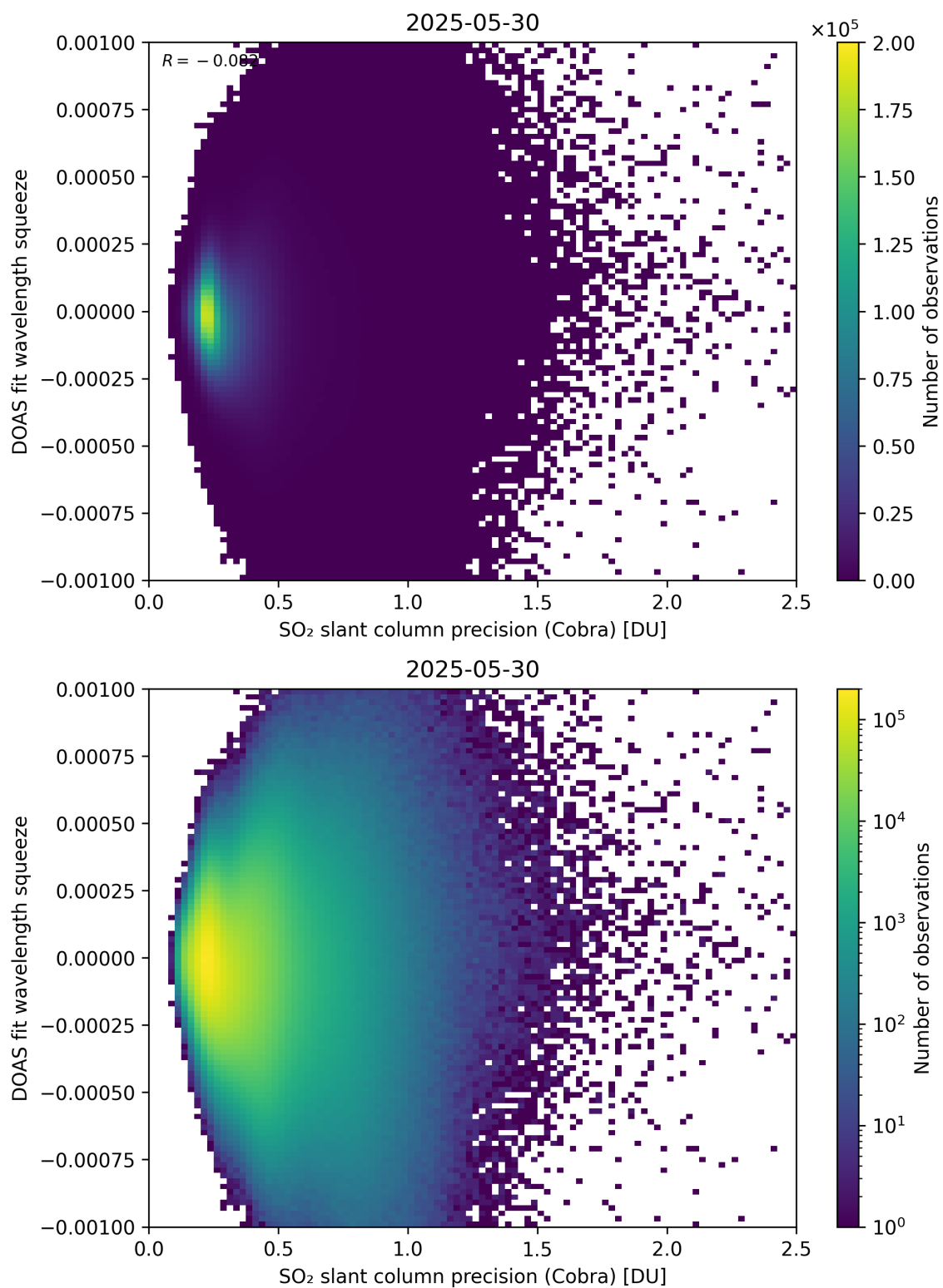
Figure 203: Scatter density plot of “SO 2 slant column precision (Cobra)” against “DOAS fit wavelength squeeze” for 2025-05-29 to 2025-05-31.
