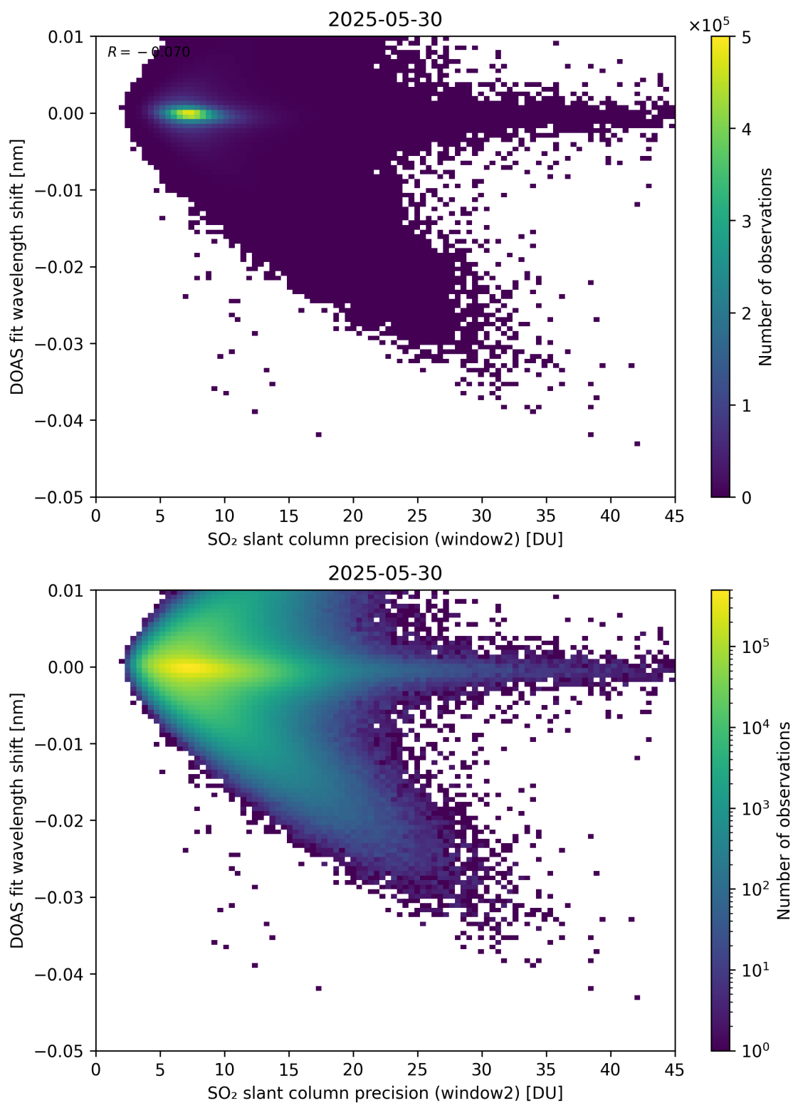
Figure 293: Scatter density plot of “SO 2 slant column precision (window2)” against “DOAS fit wavelength shift” for 2025-05-29 to 2025-05-31.
