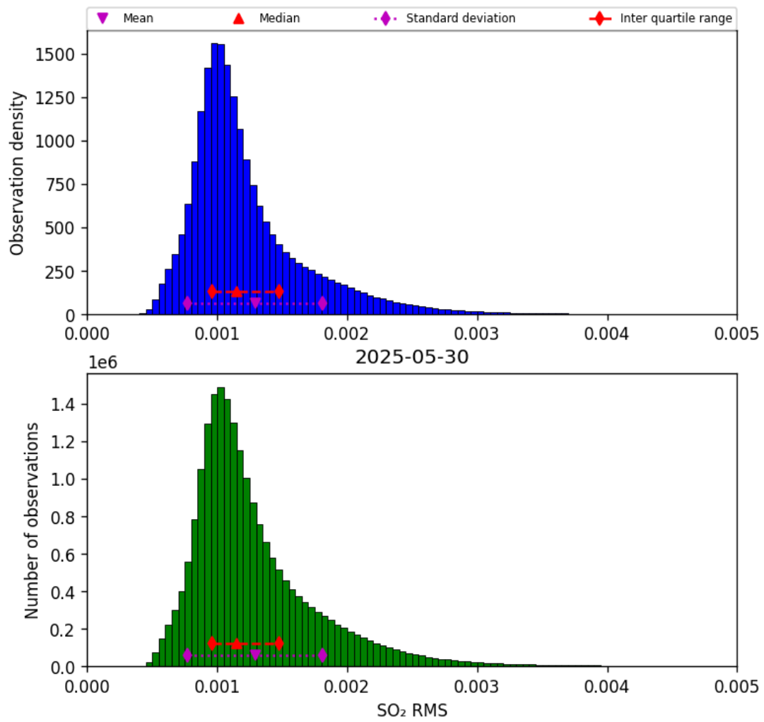
Figure 78: Histogram of “SO 2 RMS” for 2025-05-29 to 2025-05-31
