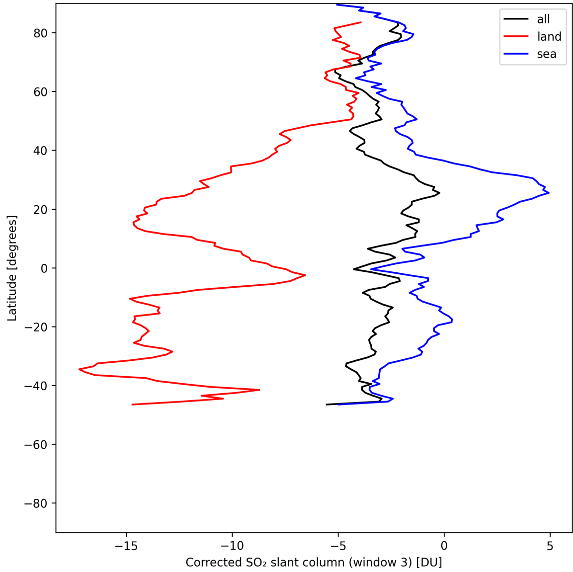
Figure 47: Zonal average of “Corrected SO 2 slant column (window 3)” for 2025-05-29 to 2025-05-31.
