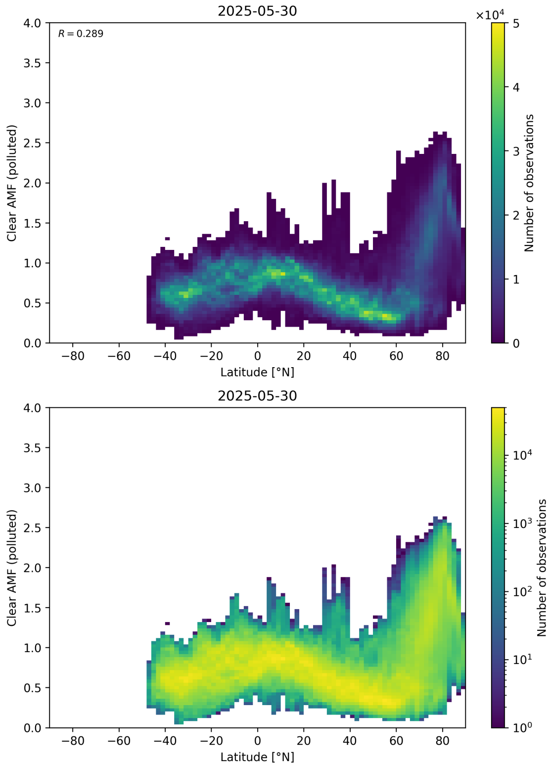
Figure 156: Scatter density plot of “Latitude” against “Clear AMF (polluted)” for 2025-05-29 to 2025-05-31.
