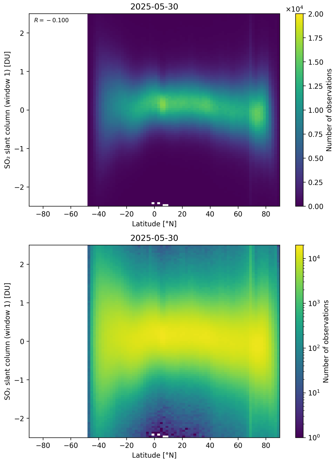
Figure 162: Scatter density plot of “Latitude” against “SO 2 slant column (window 1)” for 2025-05-29 to 2025-05-31.
