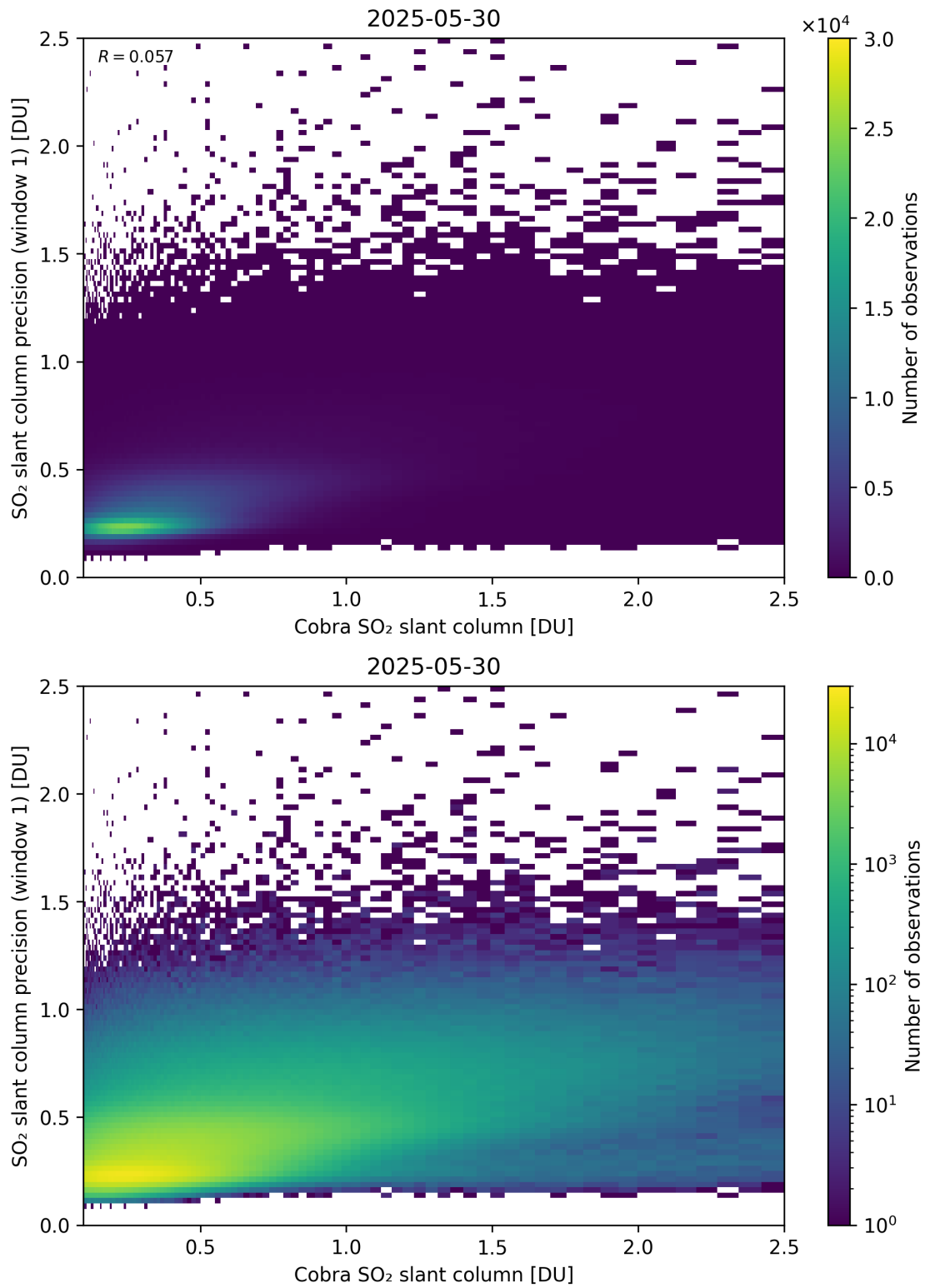
Figure 220: Scatter density plot of “Cobra SO 2 slant column” against “SO 2 slant column precision (window 1)” for 2025-05-29 to 2025-05-31.
