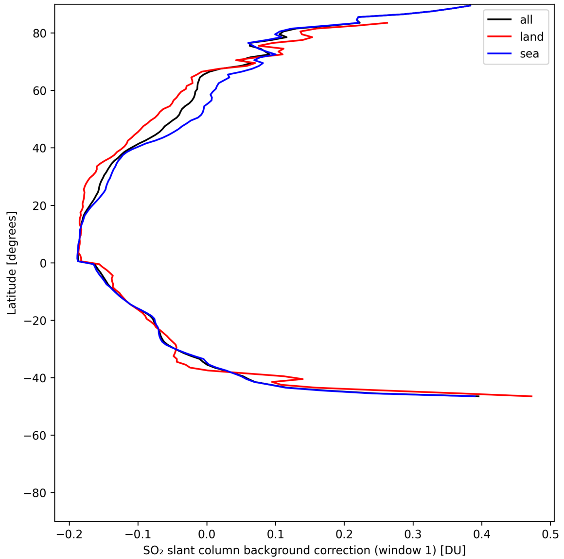
Figure 40: Zonal average of “SO 2 slant column background correction (window 1)” for 2025-05-29 to 2025-05-31.
