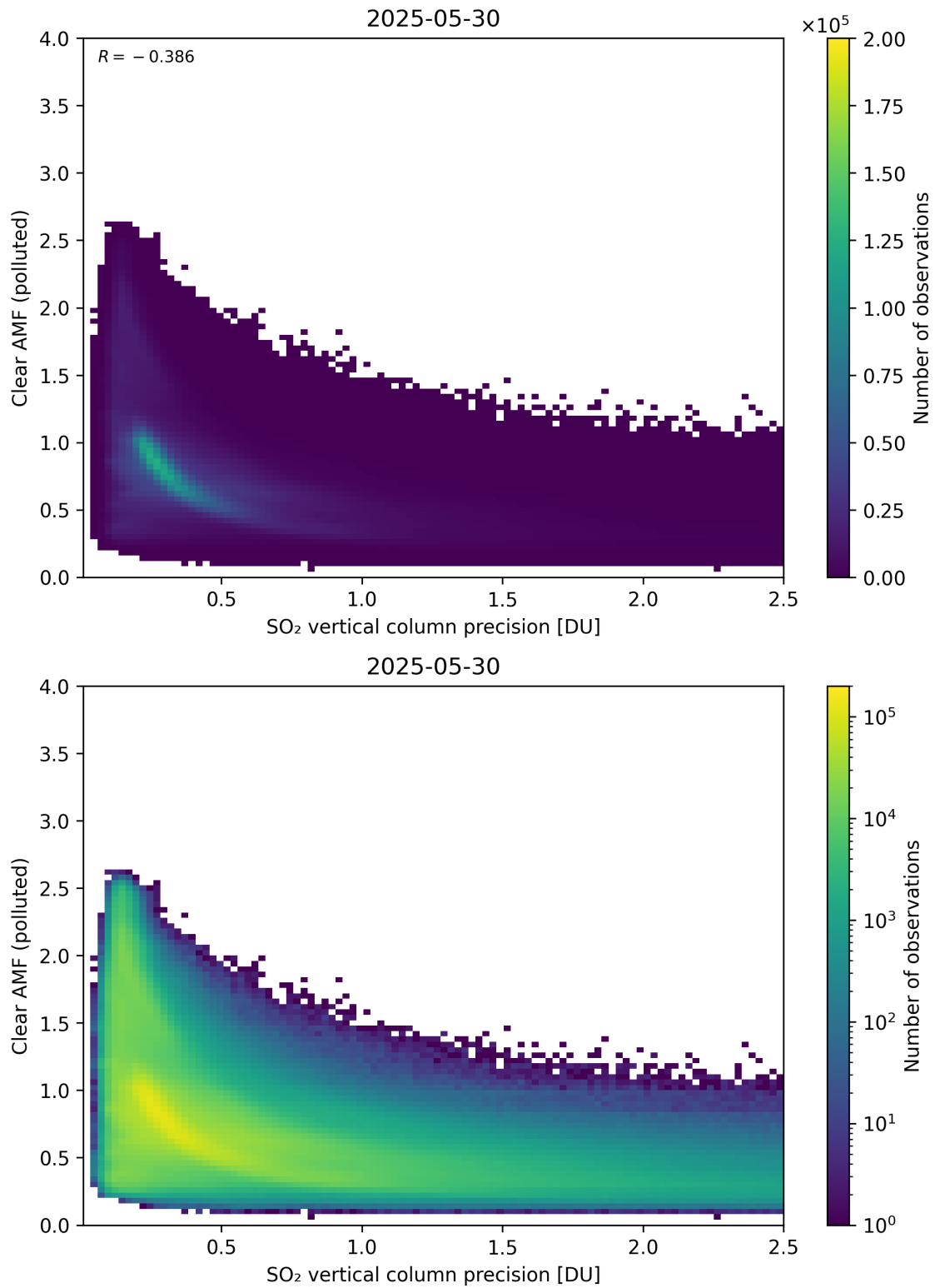
Figure 335: Scatter density plot of “SO 2 vertical column precision” against “Clear AMF (polluted)” for 2025-05-29 to 2025-05-31.
