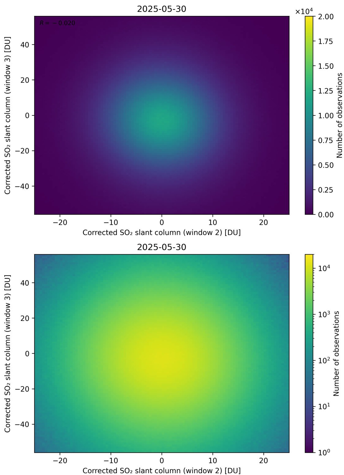
Figure 250: Scatter density plot of “Corrected SO 2 slant column (window 2)” against “Corrected SO 2 slant column (window 3)” for 2025-05-29 to 2025-05-31.
