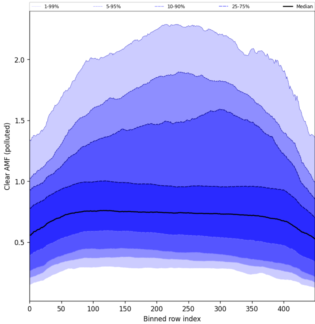
Figure 107: Along track statistics of “Clear AMF (polluted)” for 2025-05-29 to 2025-05-31
