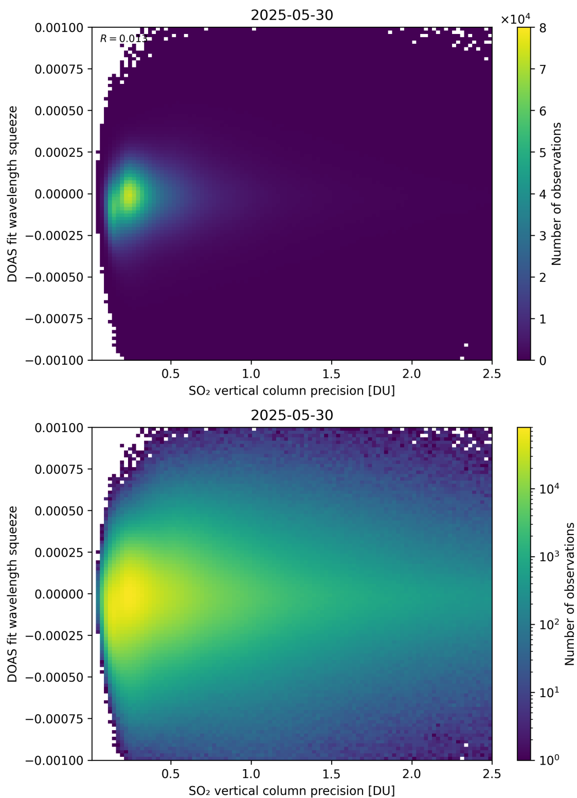
Figure 333: Scatter density plot of “SO 2 vertical column precision” against “DOAS fit wavelength squeeze” for 2025-05-29 to 2025-05-31.
