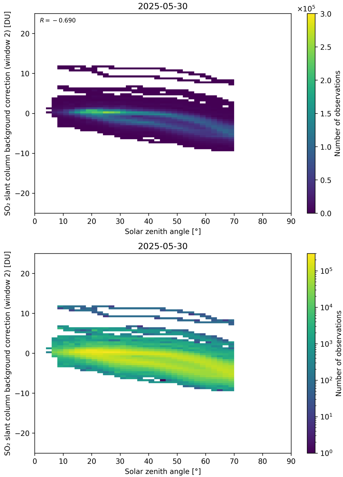
Figure 172: Scatter density plot of “Solar zenith angle” against “SO 2 slant column background correction (window 2)” for 2025-05-29 to 2025-05-31.
