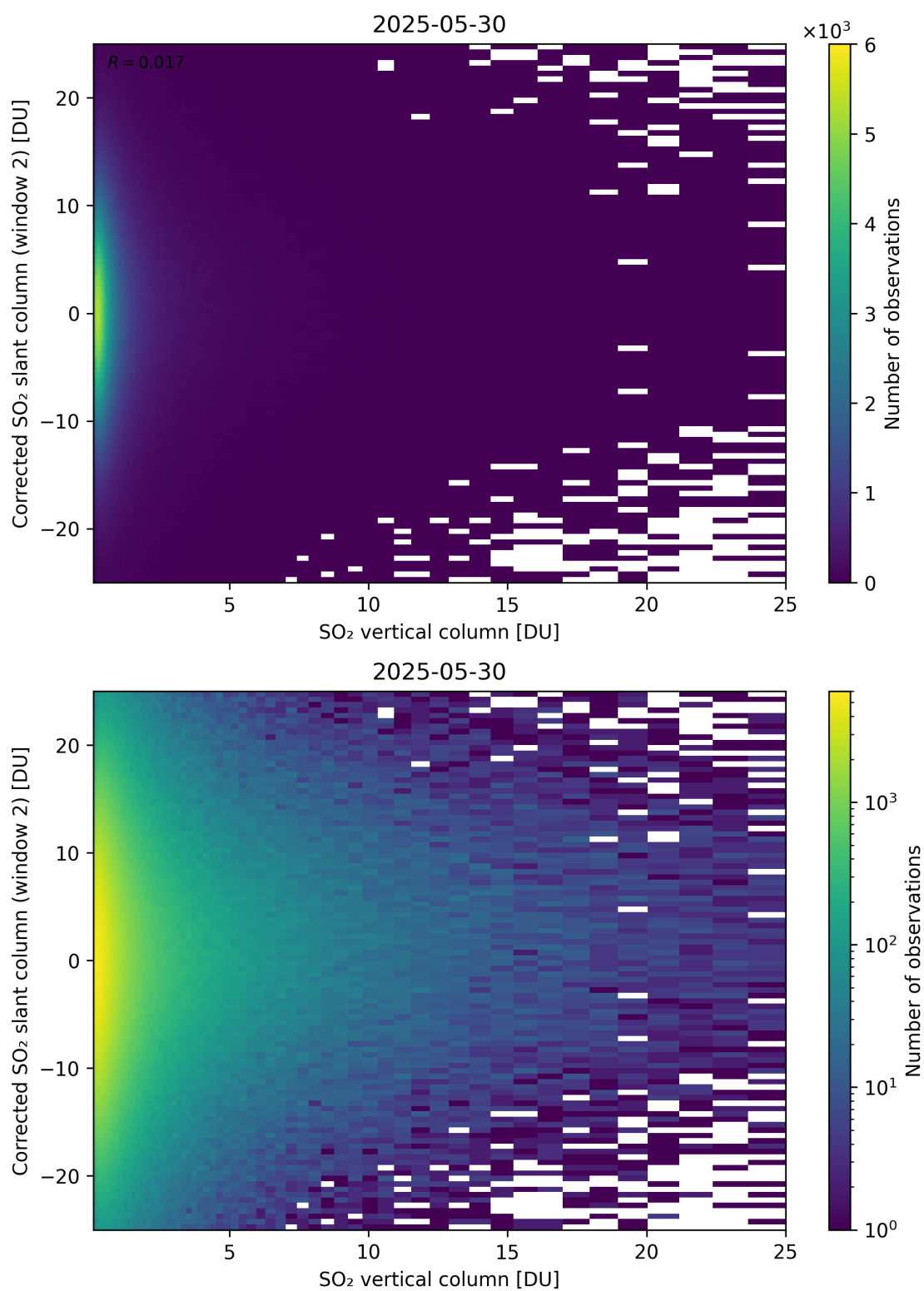
Figure 352: Scatter density plot of “SO 2 vertical column” against “Corrected SO 2 slant column (window 2)” for 2025-05-29 to 2025-05-31.
