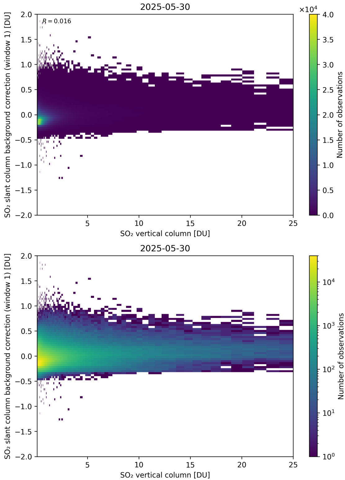
Figure 323: Scatter density plot of “SO 2 vertical column” against “SO 2 slant column background correction (window 1)” for 2025-05-29 to 2025-05-31.
