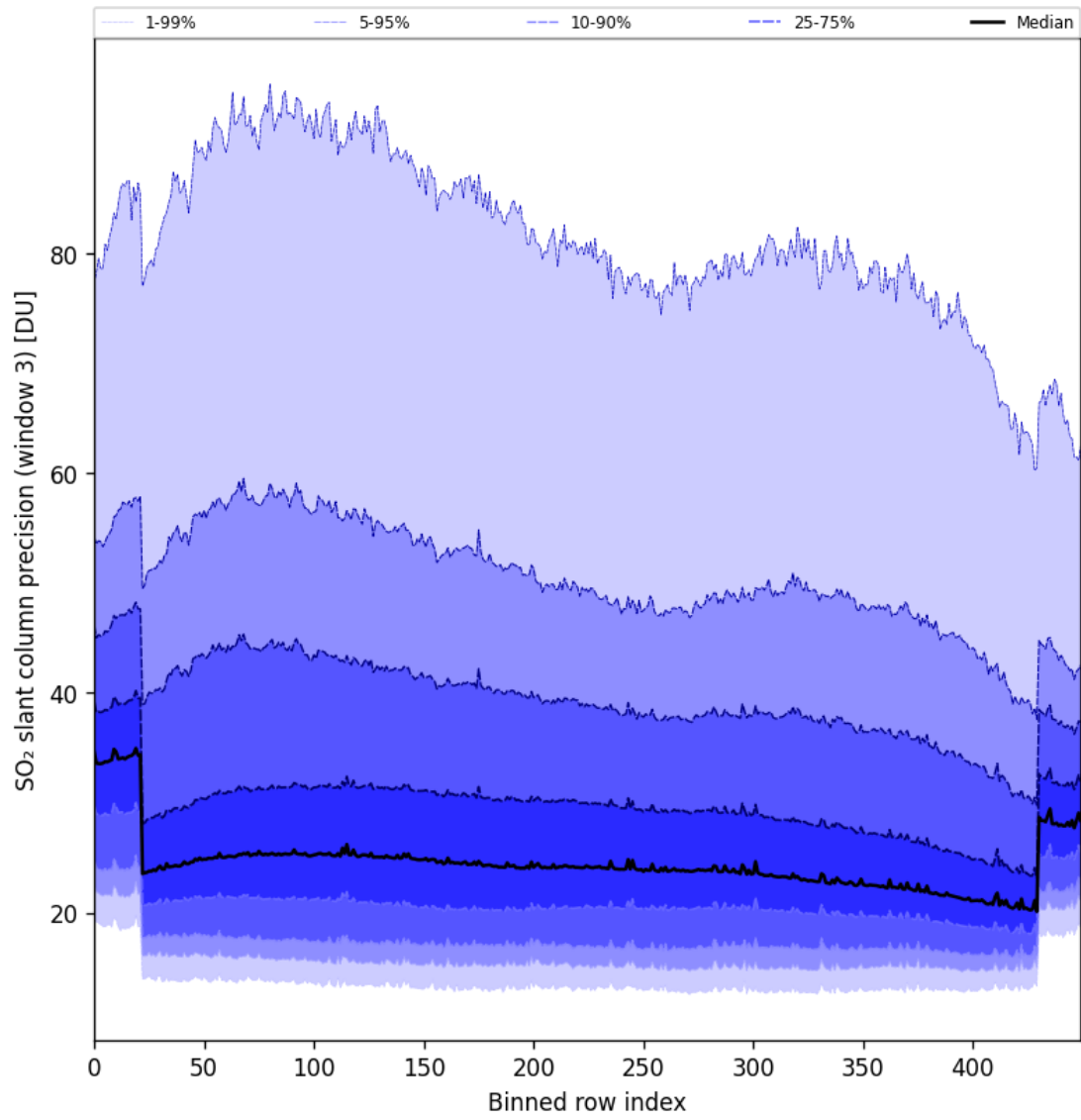
Figure 98: Along track statistics of “SO 2 slant column precision (window 3)” for 2025-05-29 to 2025-05-31
