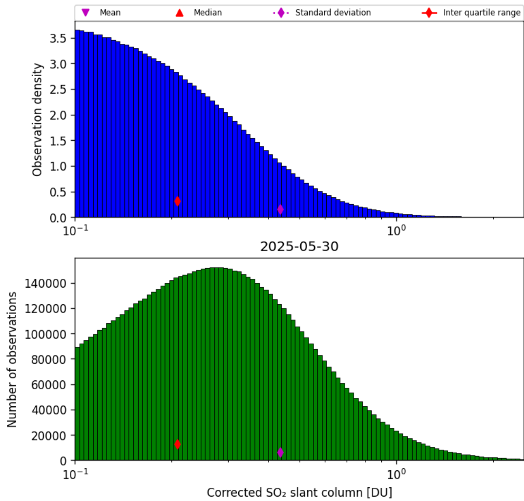
Figure 60: Histogram of "Corrected SO 2 slant column" for 2025-05-29 to 2025-05-31
