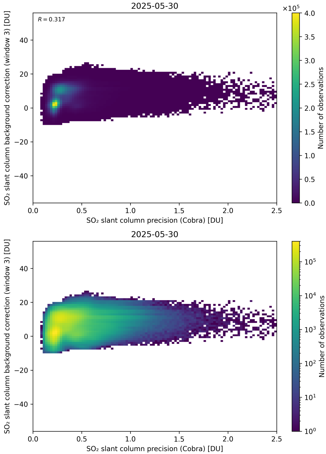
Figure 201: Scatter density plot of “SO 2 slant column precision (Cobra)” against “SO 2 slant column background correction (window 3)” for 2025-05-29 to 2025-05-31.
