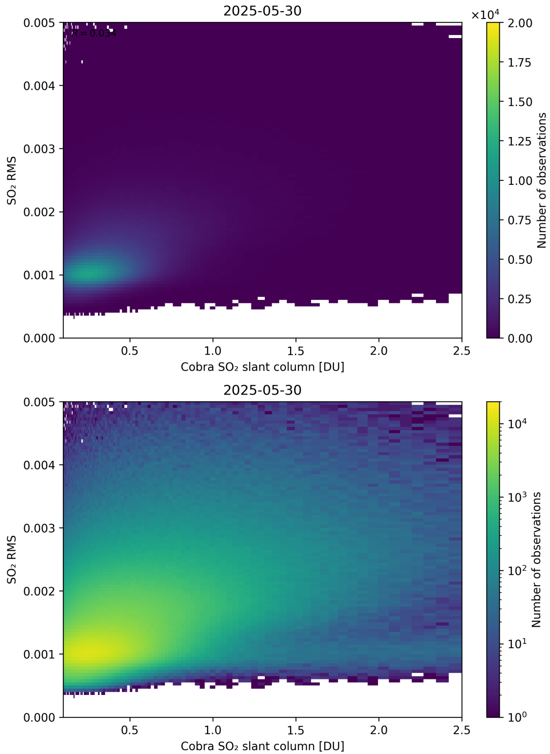
Figure 198: Scatter density plot of “Cobra SO 2 slant column” against “SO 2 RMS” for 2025-05-29 to 2025-05-31.
