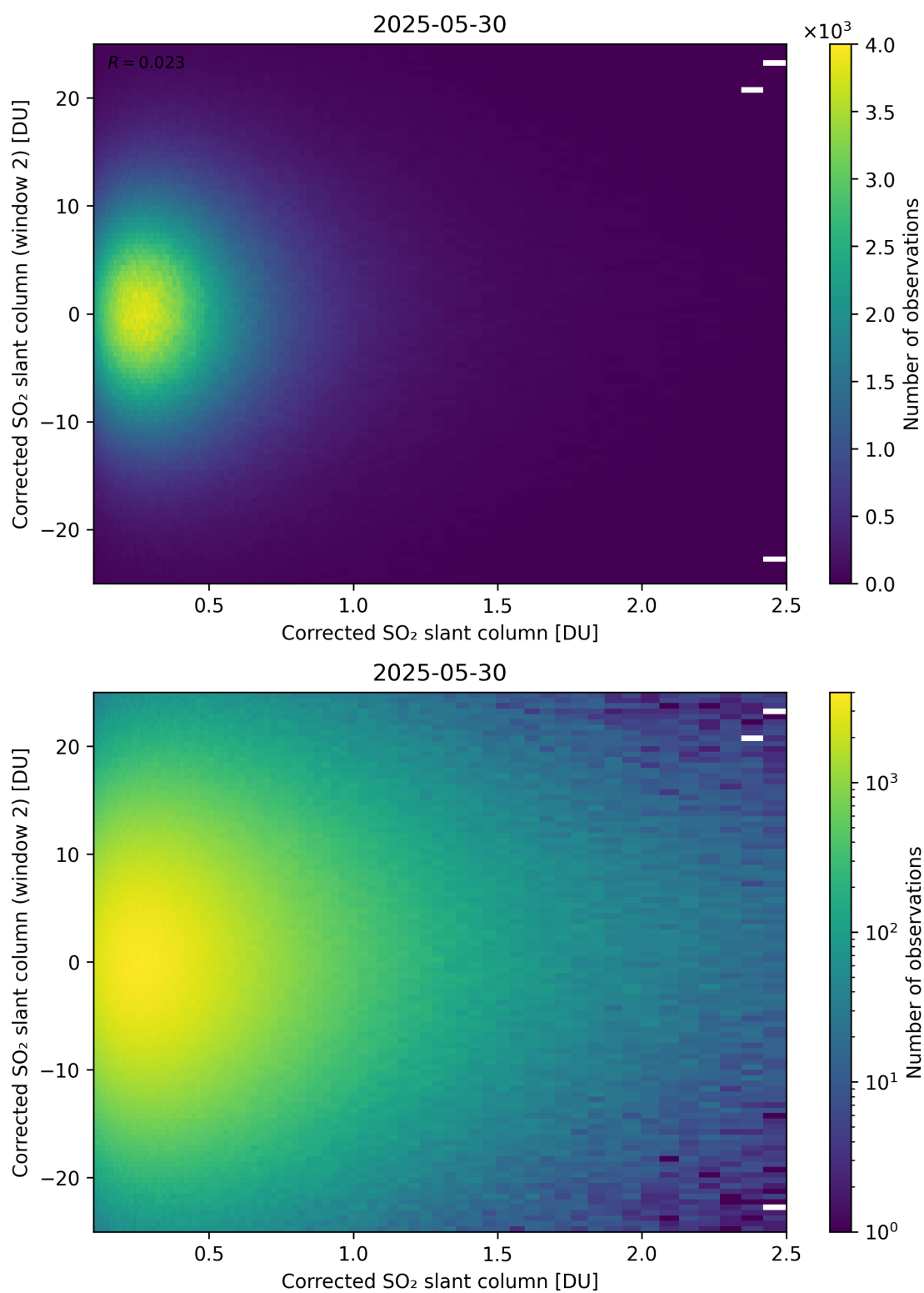
Figure 235: Scatter density plot of “Corrected SO 2 slant column” against “Corrected SO 2 slant column (window 2)” for 2025-05-29 to 2025-05-31.
