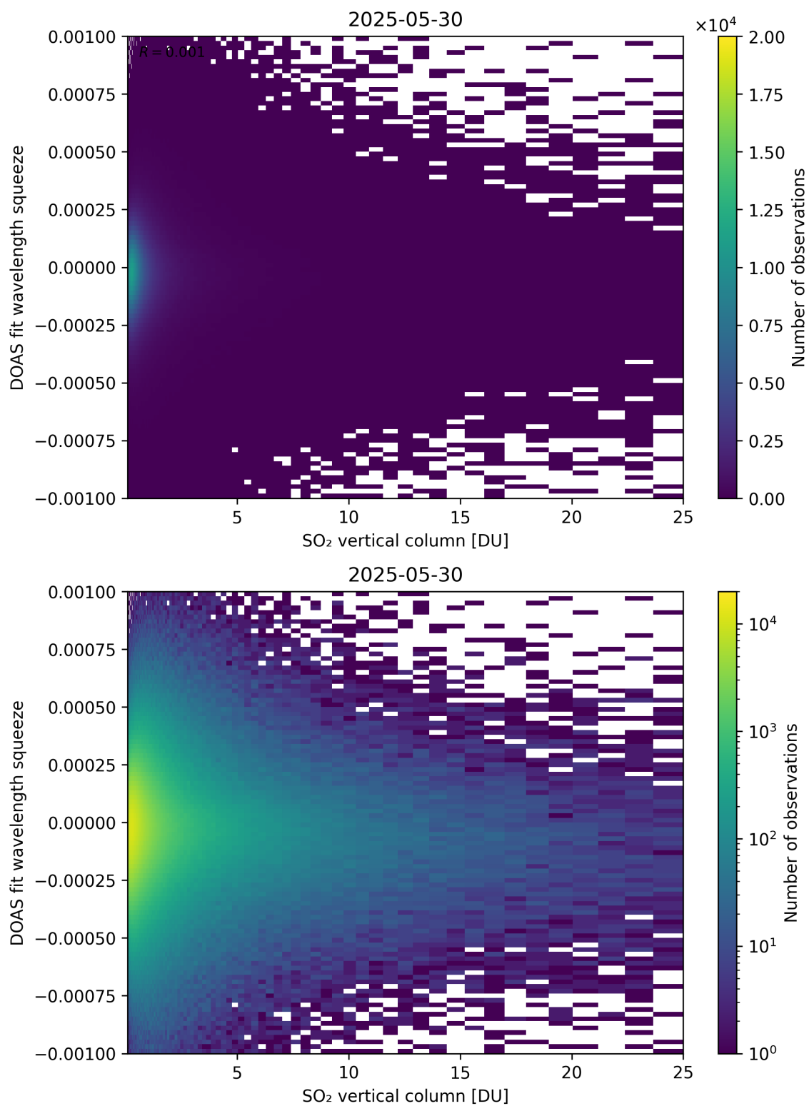
Figure 327: Scatter density plot of “SO 2 vertical column” against “DOAS fit wavelength squeeze” for 2025-05-29 to 2025-05-31.
