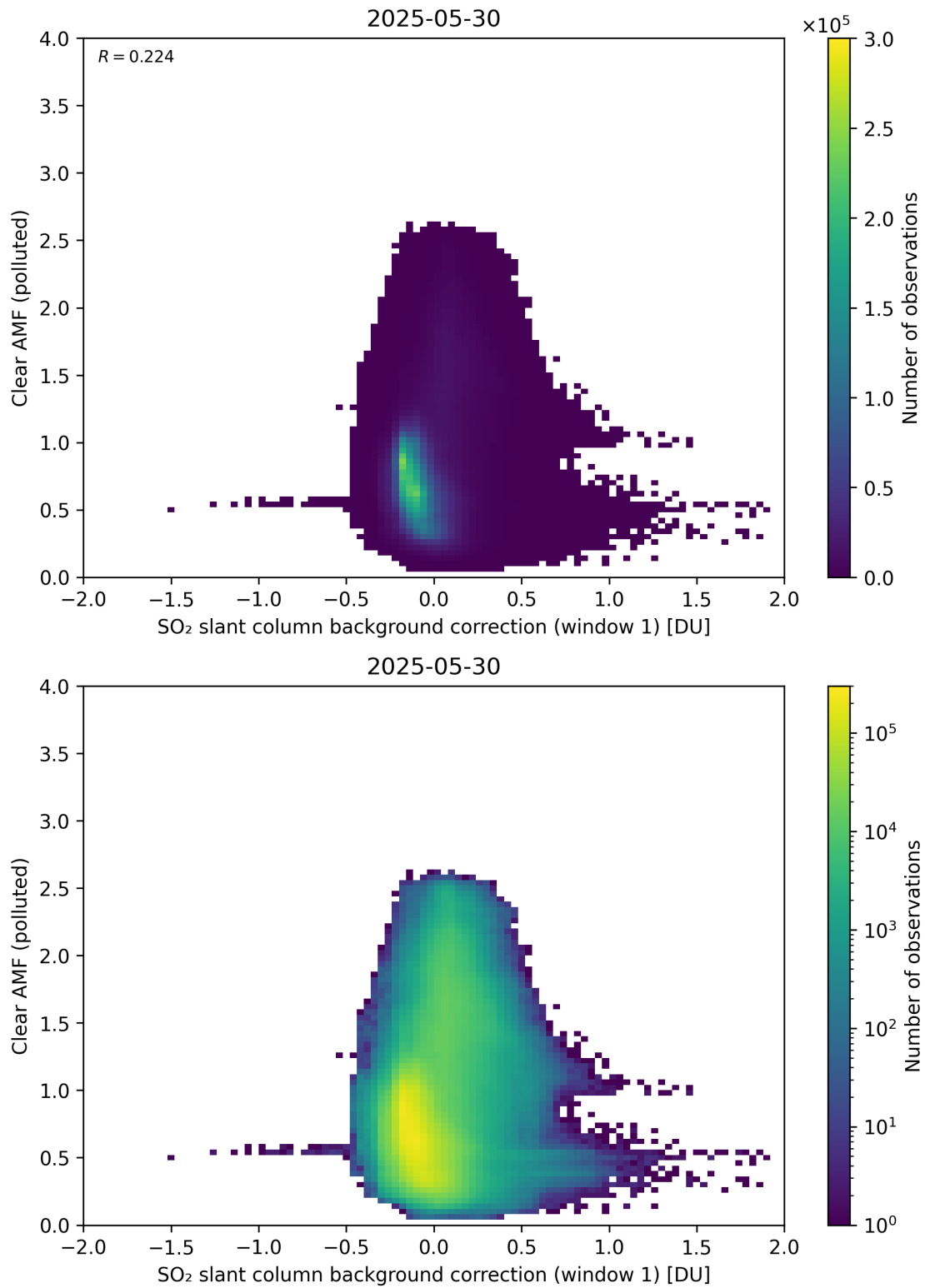
Figure 114: Scatter density plot of “SO 2 slant column background correction (window 1)” against “Clear AMF (polluted)” for 2025-05-29 to 2025-05-31.
