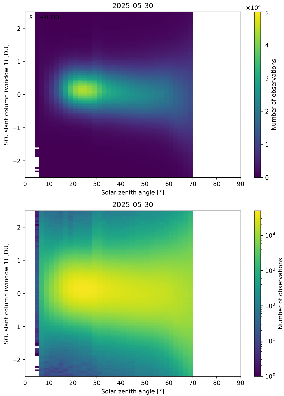
Figure 184: Scatter density plot of “Solar zenith angle” against “SO 2 slant column (window 1)” for 2025-05-29 to 2025-05-31.
