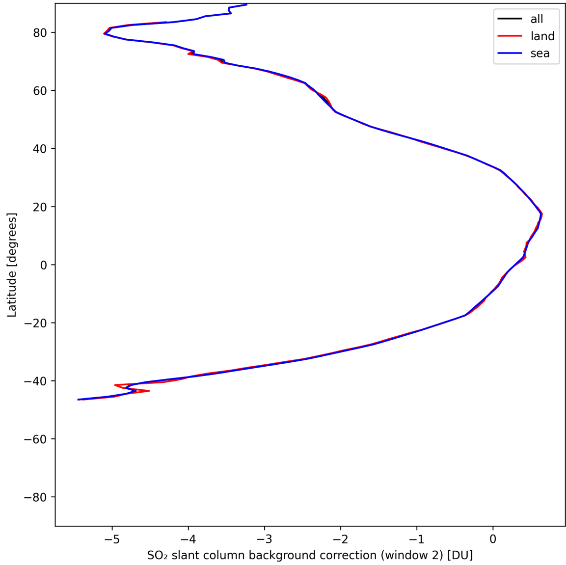
Figure 44: Zonal average of “SO 2 slant column background correction (window 2)” for 2025-05-29 to 2025-05-31.
