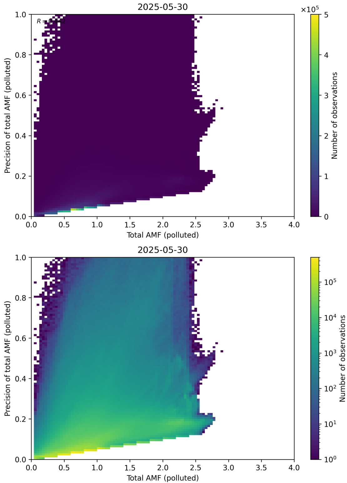
Figure 322: Scatter density plot of “Total AMF (polluted)” against “Precision of total AMF (polluted)” for 2025-05-29 to 2025-05-31.
