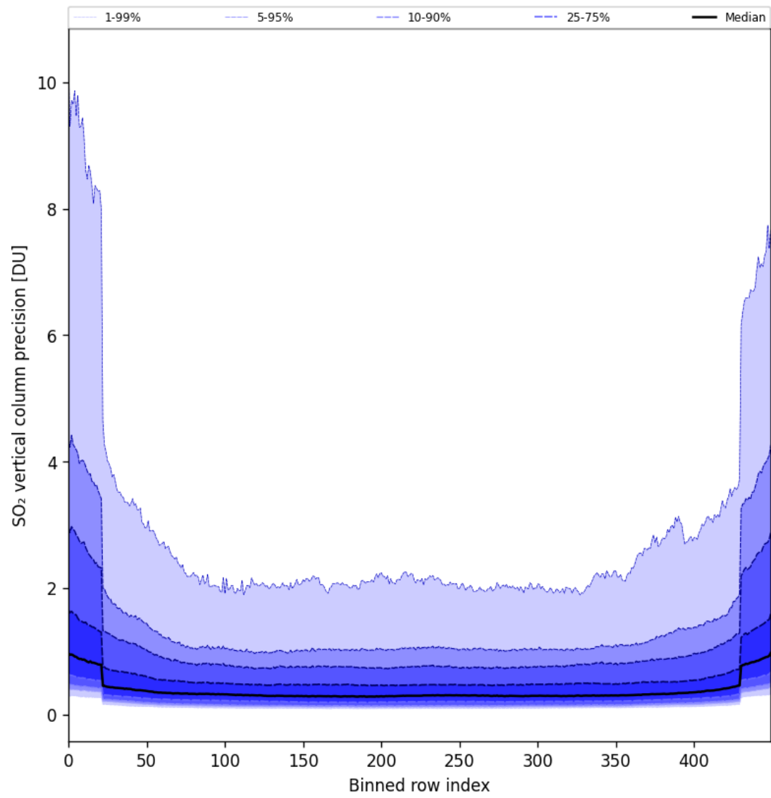
Figure 85: Along track statistics of “SO 2 vertical column precision” for 2025-05-29 to 2025-05-31
