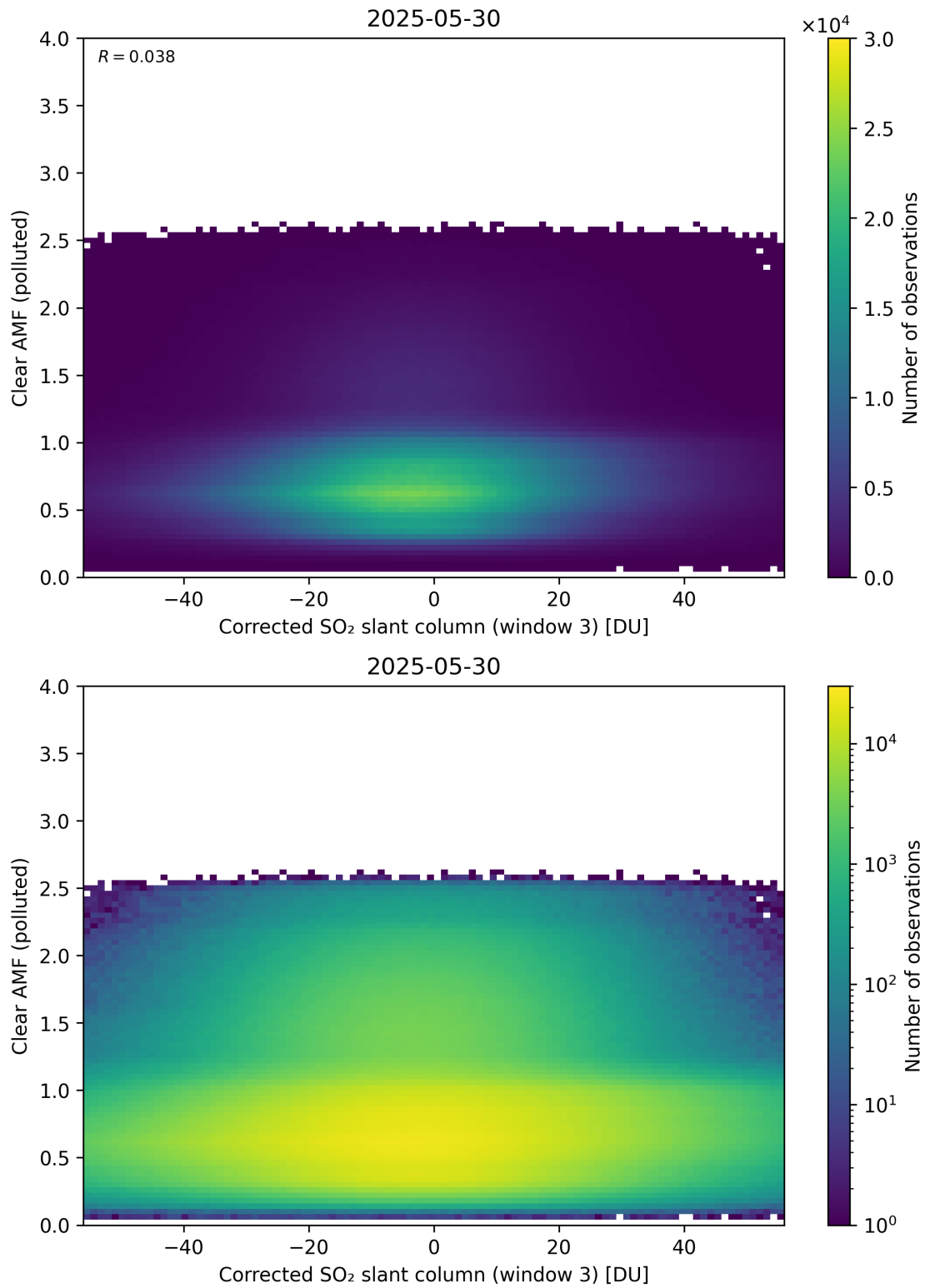
Figure 259: Scatter density plot of “Corrected SO 2 slant column (window 3)” against “Clear AMF (polluted)” for 2025-05-29 to 2025-05-31.
