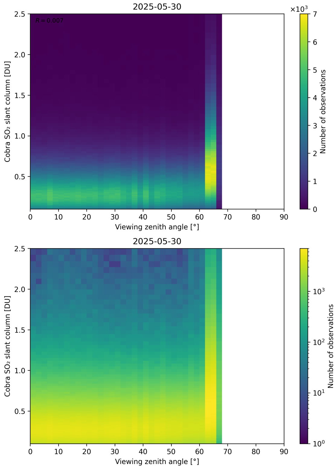
Figure 371: Scatter density plot of “Viewing zenith angle” against “Cobra SO 2 slant column” for 2025-05-29 to 2025-05-31.
