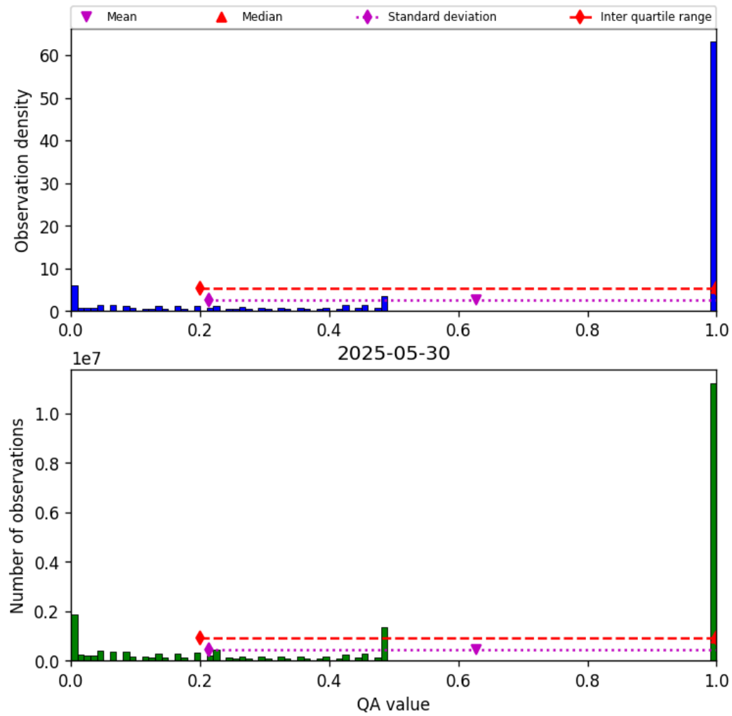
Figure 57: Histogram of “QA value” for 2025-05-29 to 2025-05-31
