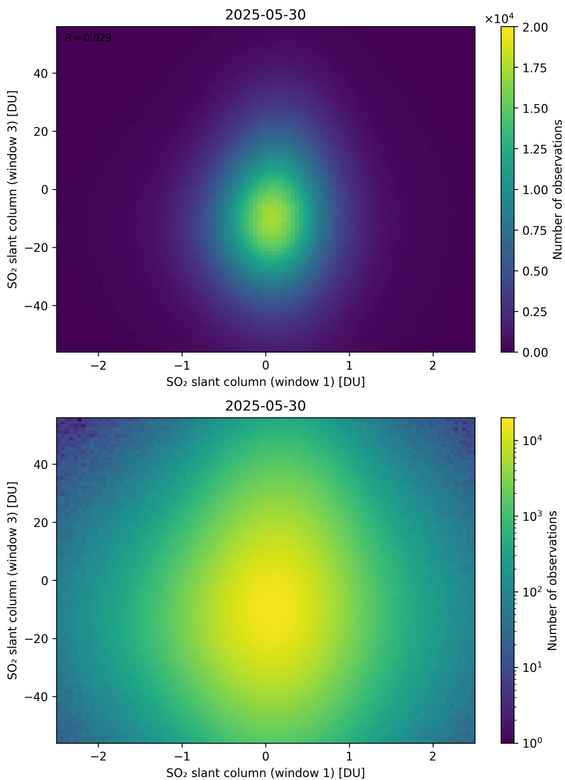
Figure 287: Scatter density plot of “SO 2 slant column (window 1)” against “SO 2 slant column (window 3)” for 2025-05-29 to 2025-05-31.
