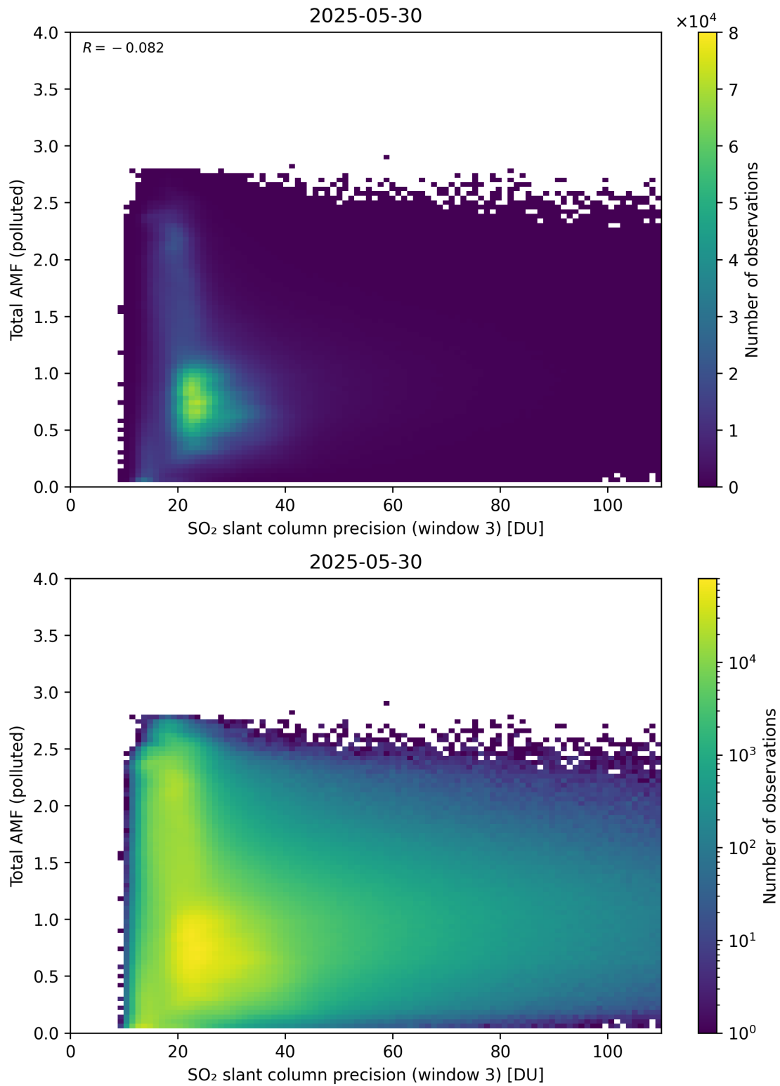
Figure 313: Scatter density plot of “SO 2 slant column precision (window 3)” against “Total AMF (polluted)” for 2025-05-29 to 2025-05-31.
