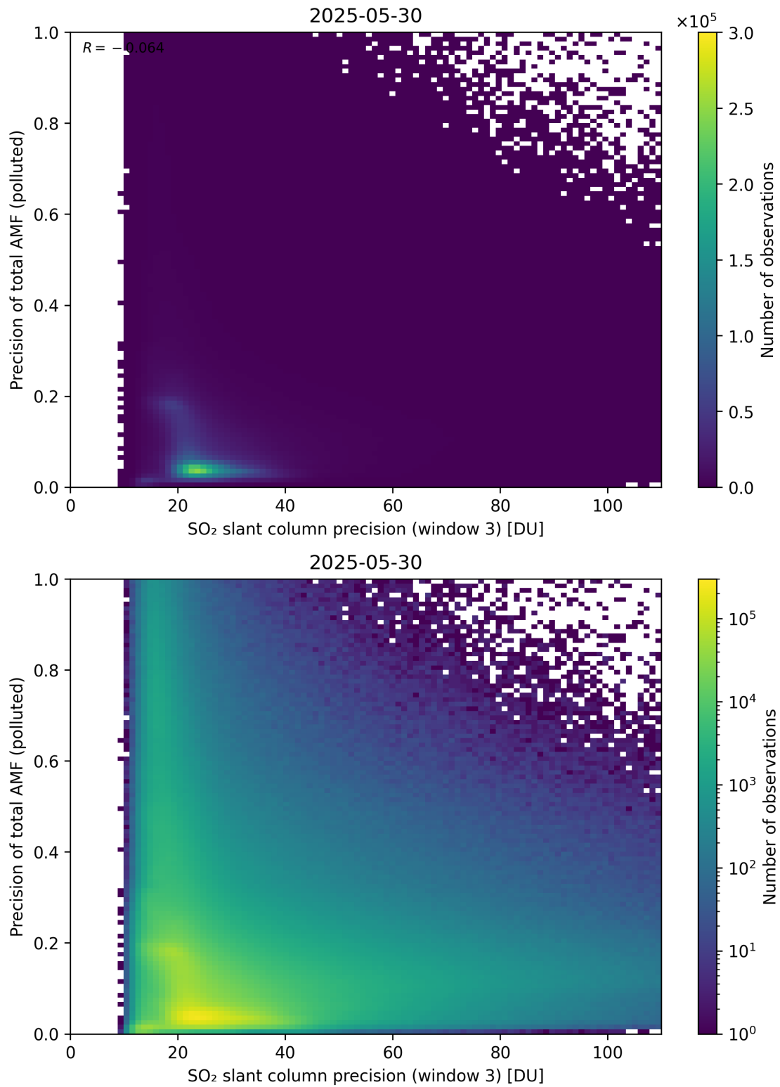
Figure 314: Scatter density plot of “SO 2 slant column precision (window 3)” against “Precision of total AMF (polluted)” for 2025-05-29 to 2025-05-31.
