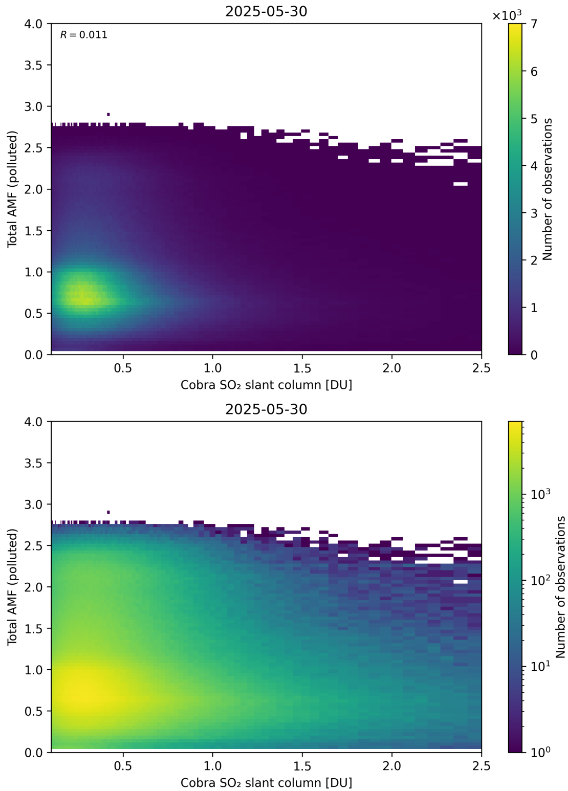
Figure 224: Scatter density plot of “Cobra SO 2 slant column” against “Total AMF (polluted)” for 2025-05-29 to 2025-05-31.
