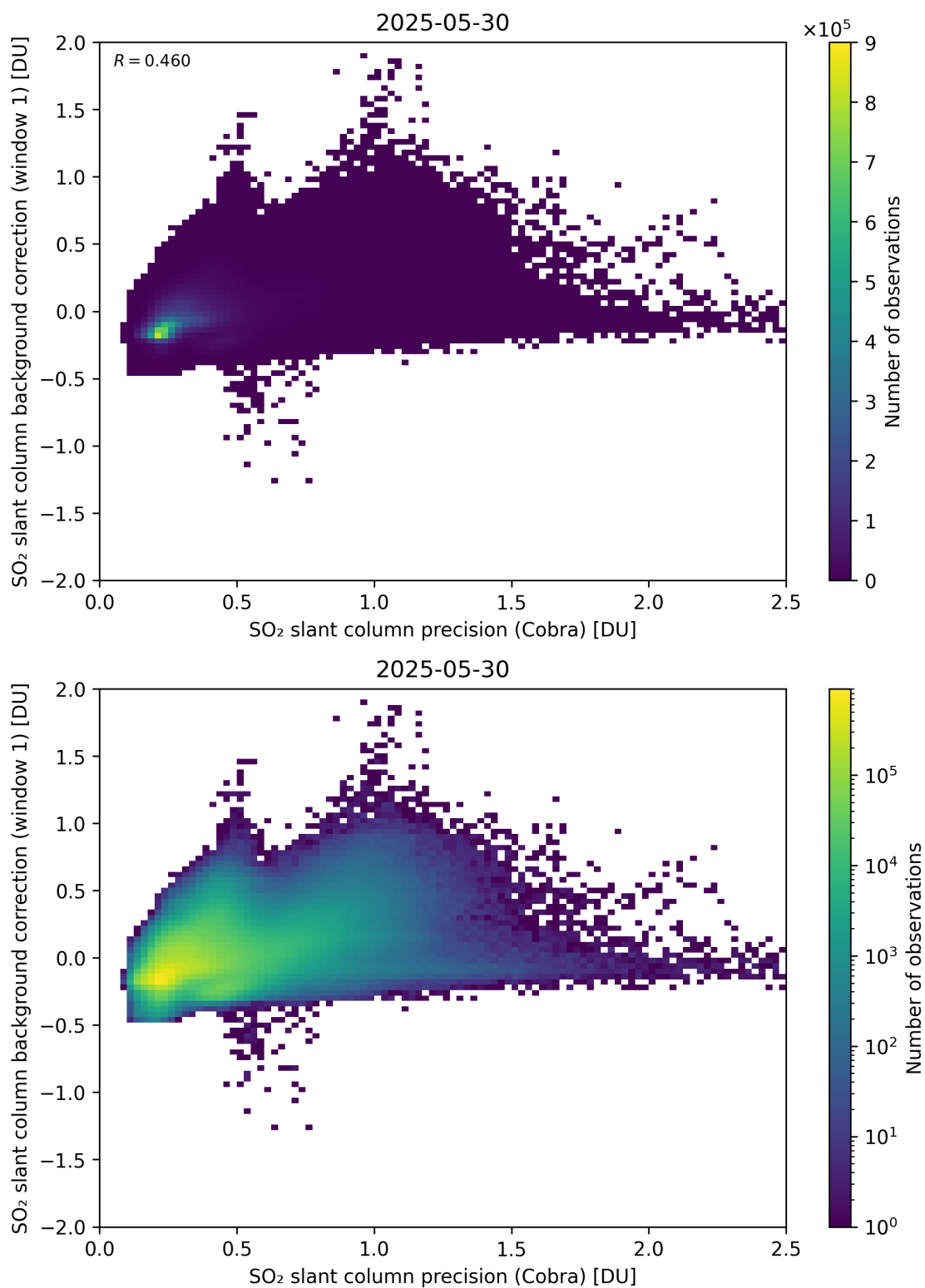
Figure 199: Scatter density plot of “SO 2 slant column precision (Cobra)” against “SO 2 slant column background correction (window 1)” for 2025-05-29 to 2025-05-31.
