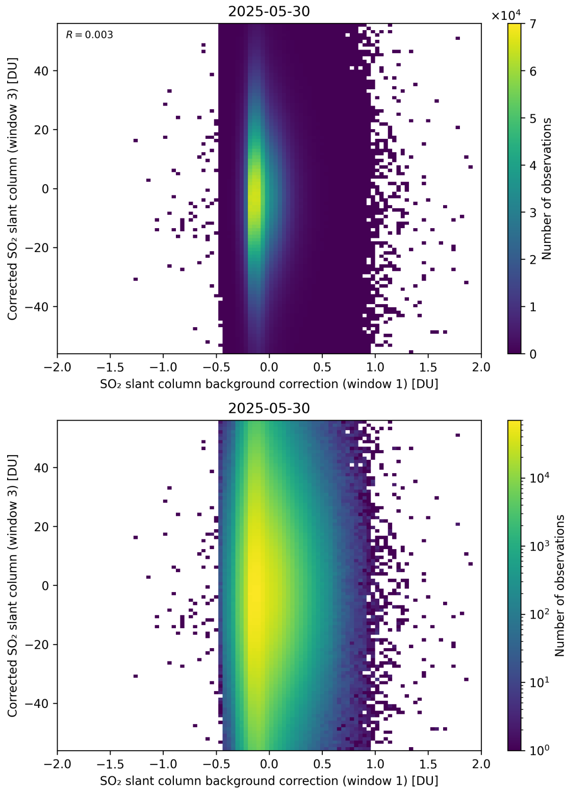
Figure 116: Scatter density plot of “SO 2 slant column background correction (window 1)” against “Corrected SO 2 slant column (window 3)” for 2025-05-29 to 2025-05-31.
