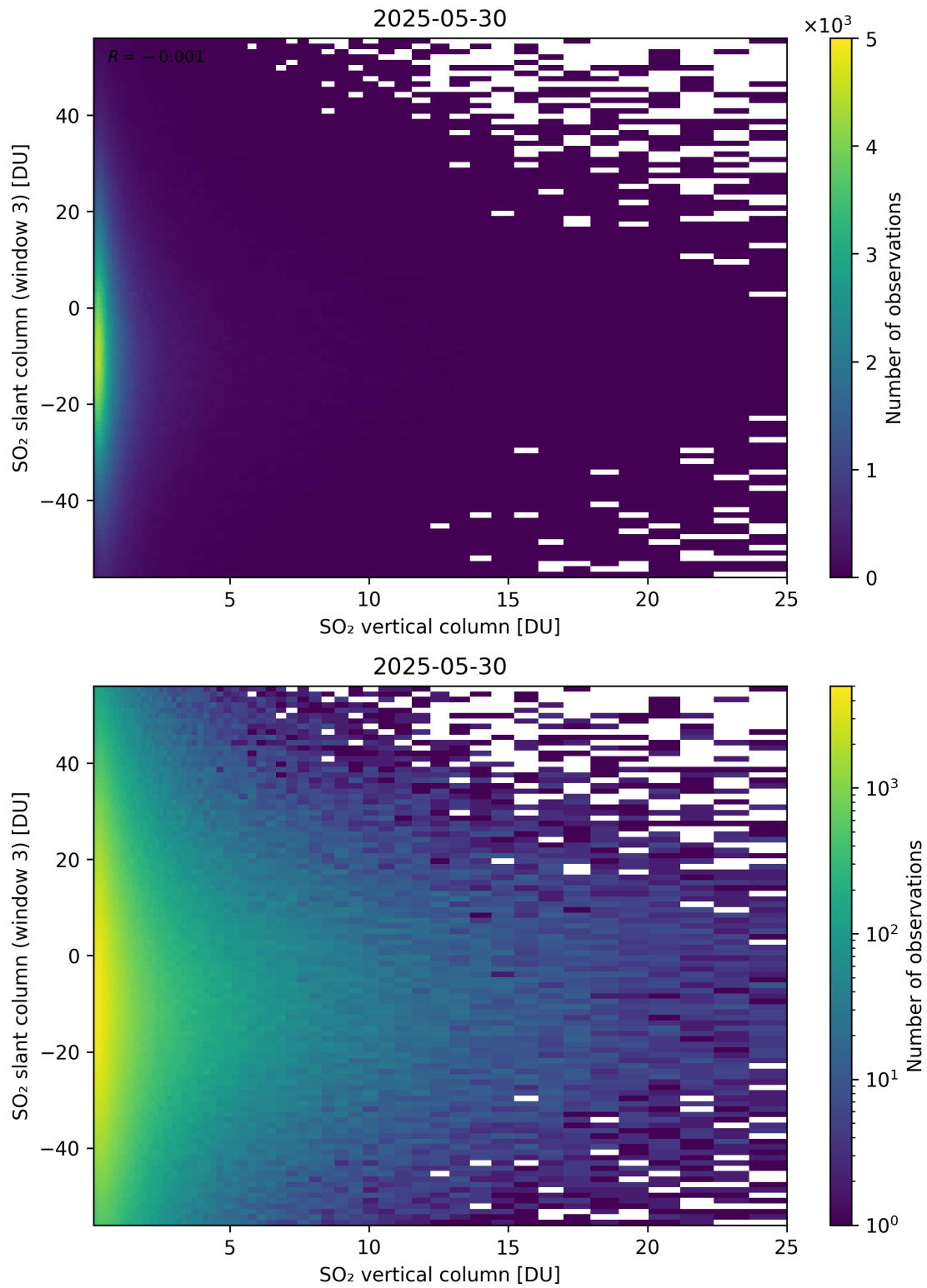
Figure 357: Scatter density plot of “SO 2 vertical column” against “SO 2 slant column (window 3)” for 2025-05-29 to 2025-05-31.
