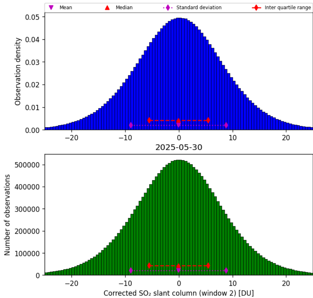
Figure 69: Histogram of “Corrected SO 2 slant column (window 2)” for 2025-05-29 to 2025-05-31
