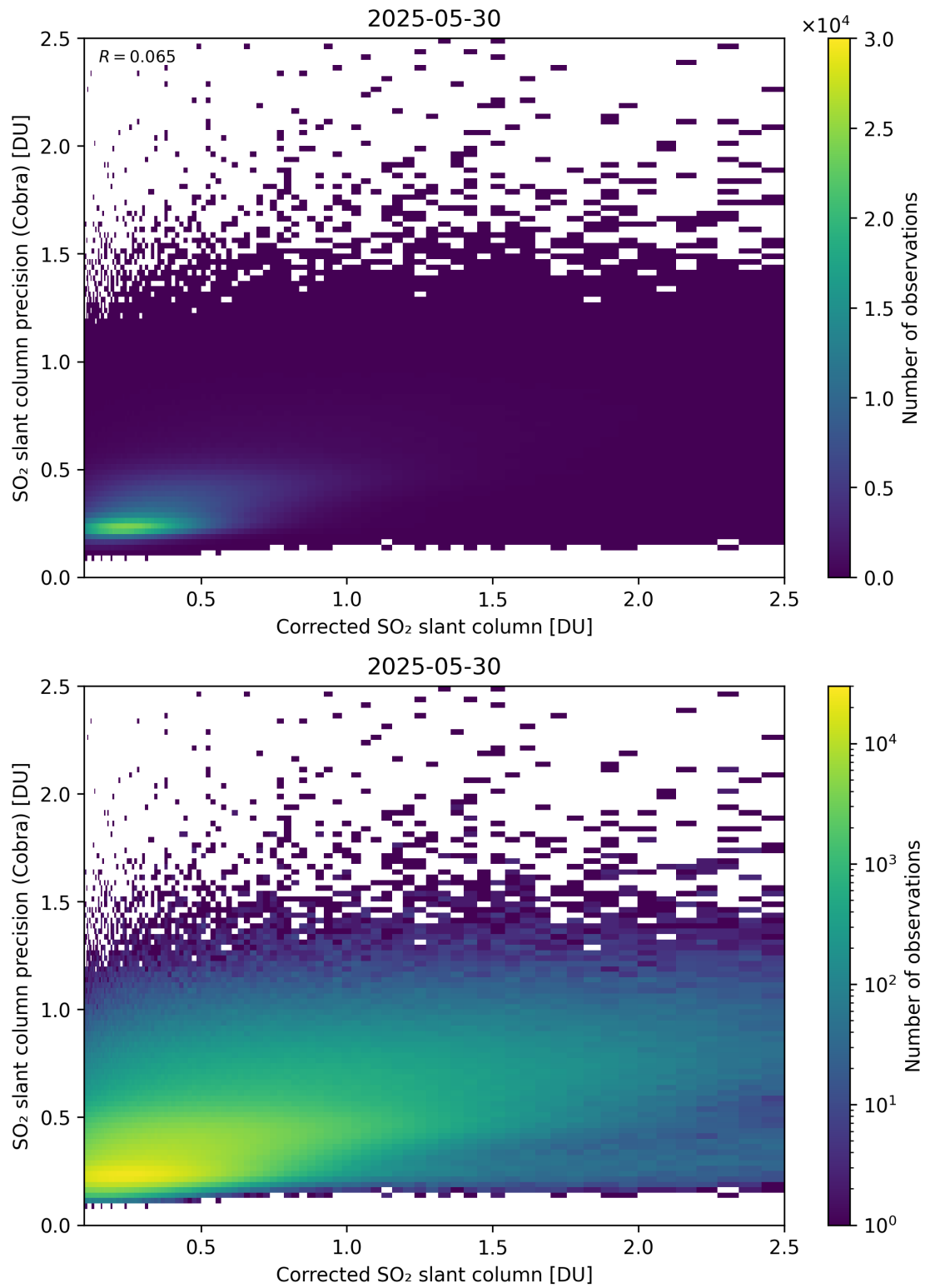
Figure 234: Scatter density plot of “Corrected SO 2 slant column” against “SO 2 slant column precision (Cobra)” for 2025-05-29 to 2025-05-31.
