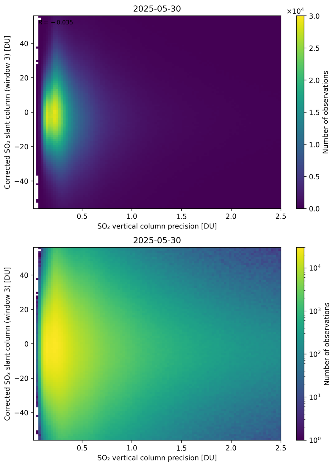
Figure 340: Scatter density plot of “SO 2 vertical column precision” against “Corrected SO 2 slant column (window 3)” for 2025-05-29 to 2025-05-31.
