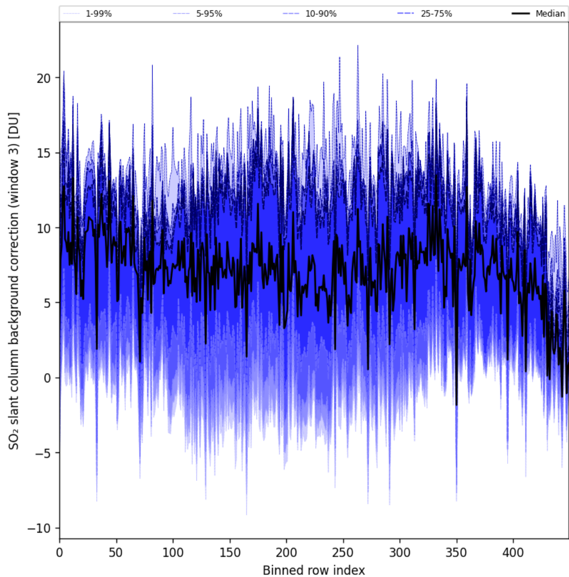
Figure 100: Along track statistics of “SO 2 slant column background correction (window 3)” for 2025-05-29 to 2025-05-31
