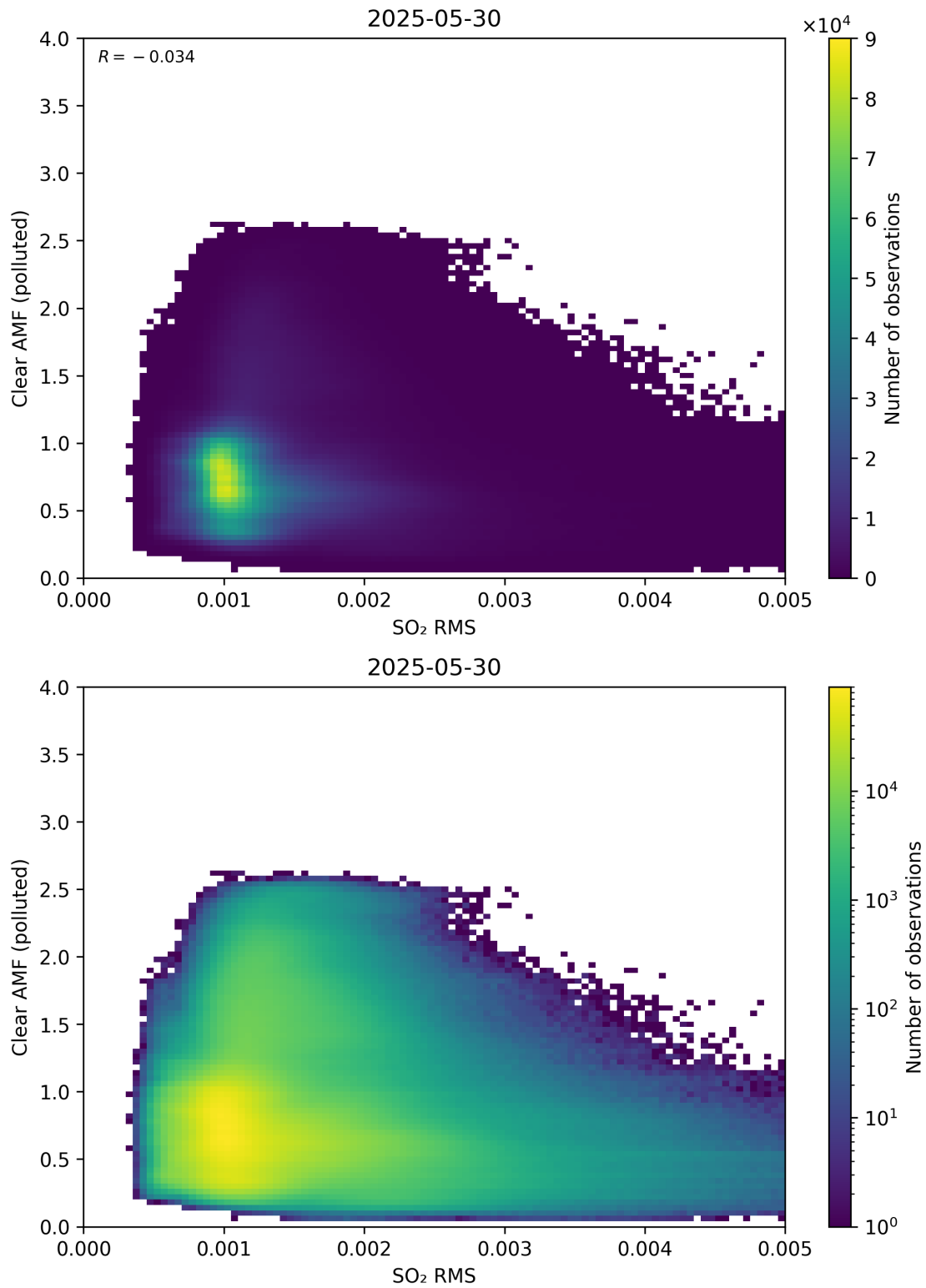
Figure 147: Scatter density plot of “SO 2 RMS” against “Clear AMF (polluted)” for 2025-05-29 to 2025-05-31.
