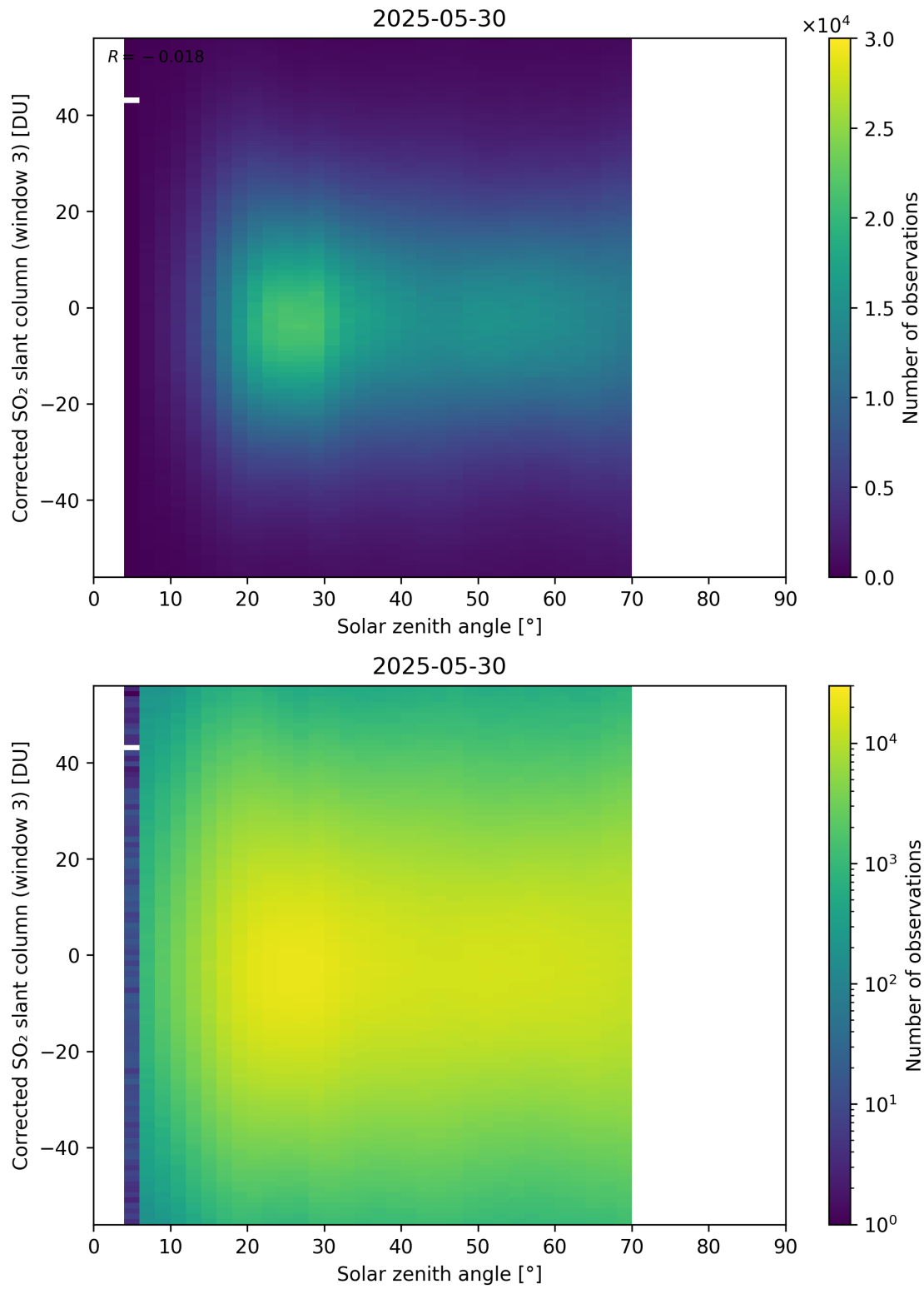
Figure 183: Scatter density plot of “Solar zenith angle” against “Corrected SO 2 slant column (window 3)” for 2025-05-29 to 2025-05-31.
