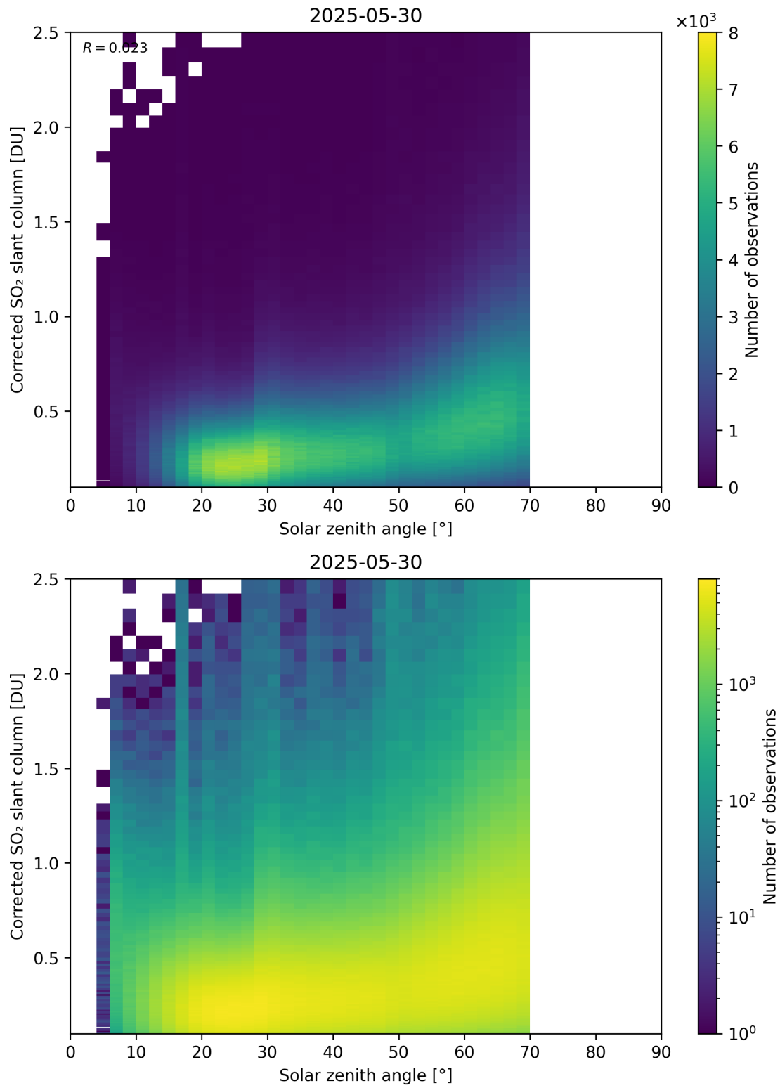
Figure 181: Scatter density plot of “Solar zenith angle” against “Corrected SO 2 slant column” for 2025-05-29 to 2025-05-31.
