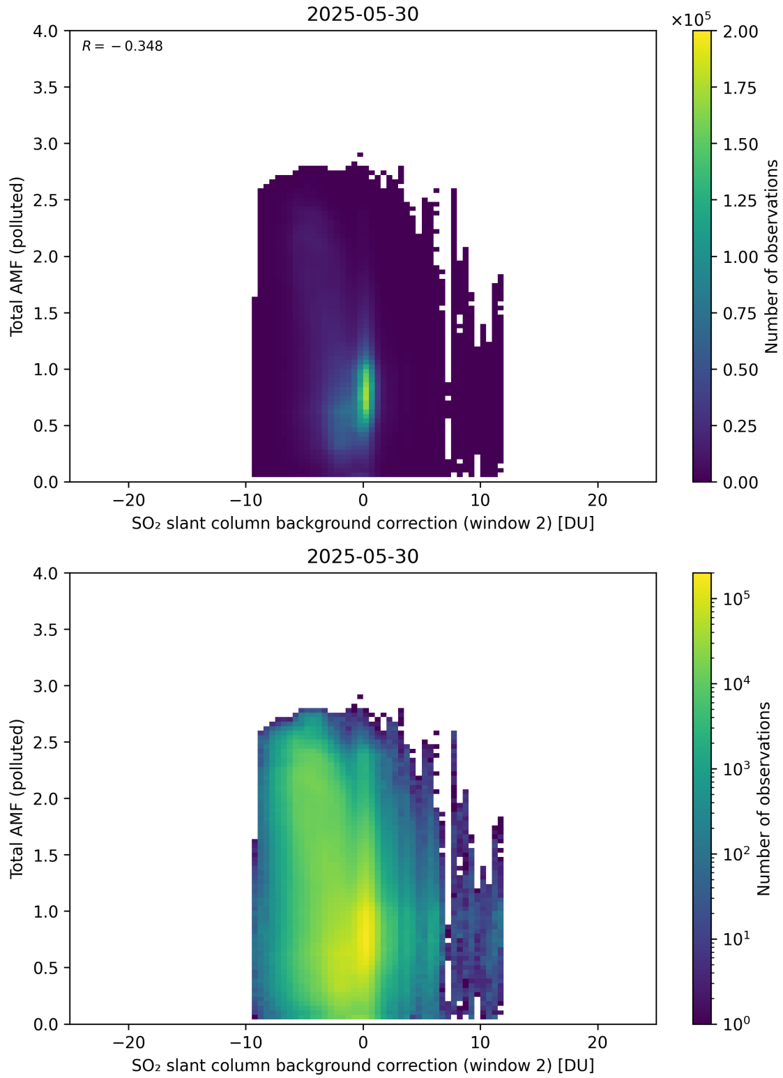
Figure 130: Scatter density plot of “SO 2 slant column background correction (window 2)” against “Total AMF (polluted)” for 2025-05-29 to 2025-05-31.
