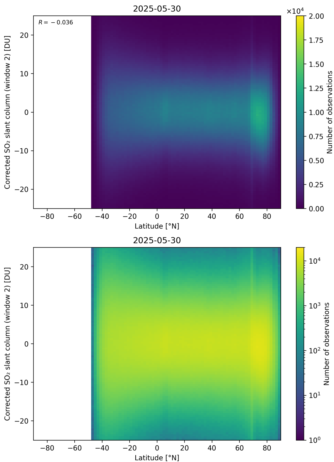
Figure 160: Scatter density plot of “Latitude” against “Corrected SO 2 slant column (window 2)” for 2025-05-29 to 2025-05-31.
