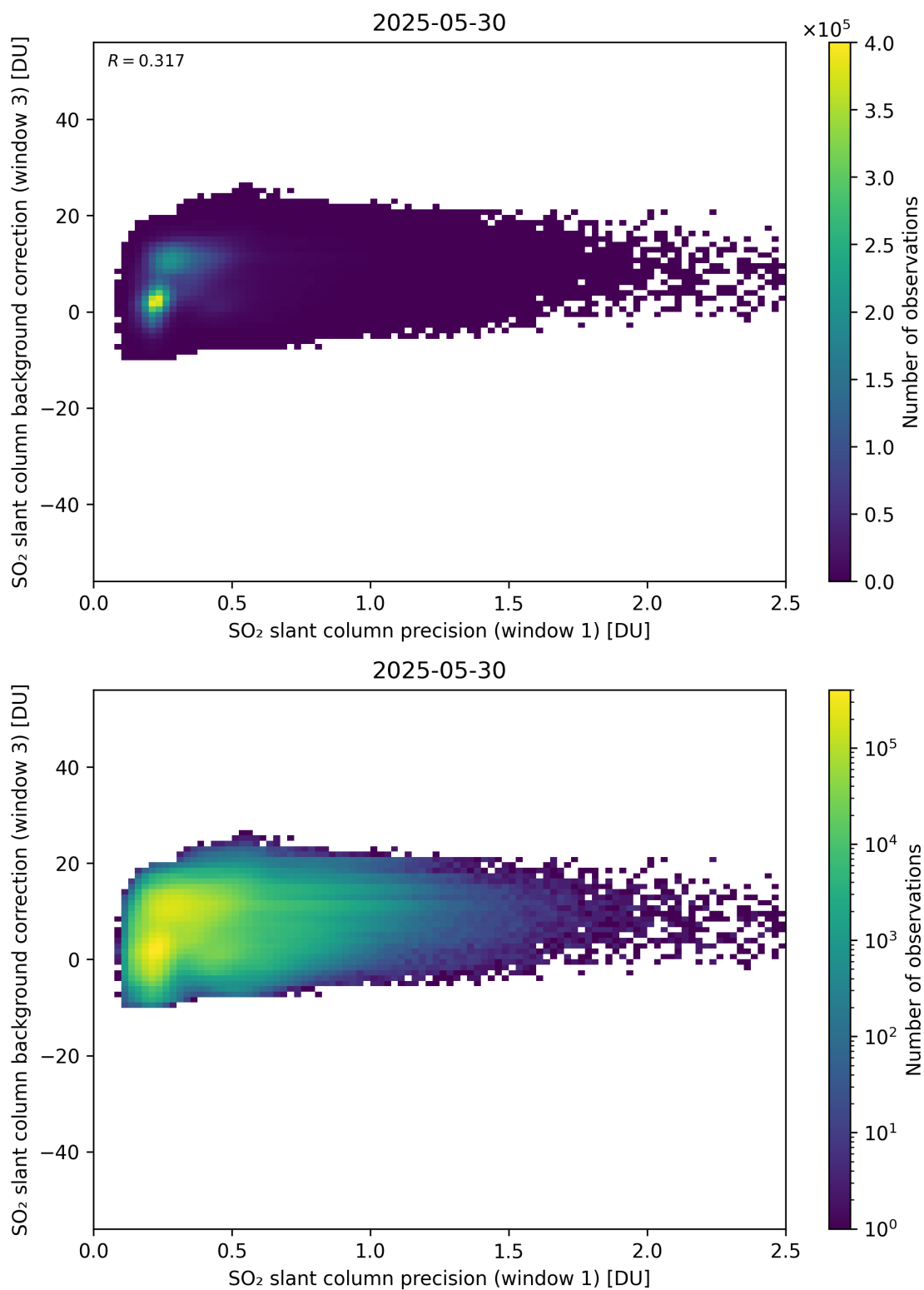
Figure 270: Scatter density plot of “SO 2 slant column precision (window 1)” against “SO 2 slant column background correction (window 3)” for 2025-05-29 to 2025-05-31.
