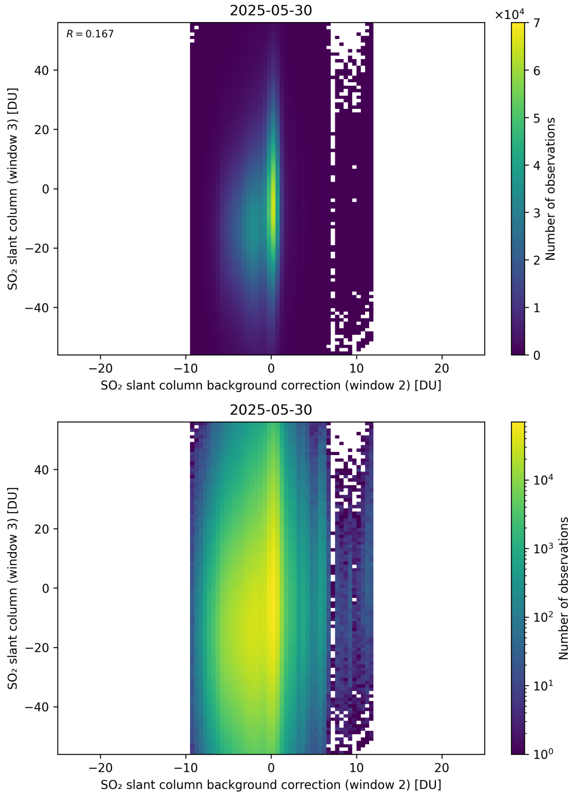
Figure 128: Scatter density plot of “SO 2 slant column background correction (window 2)” against “SO 2 slant column (window 3)” for 2025-05-29 to 2025-05-31.
