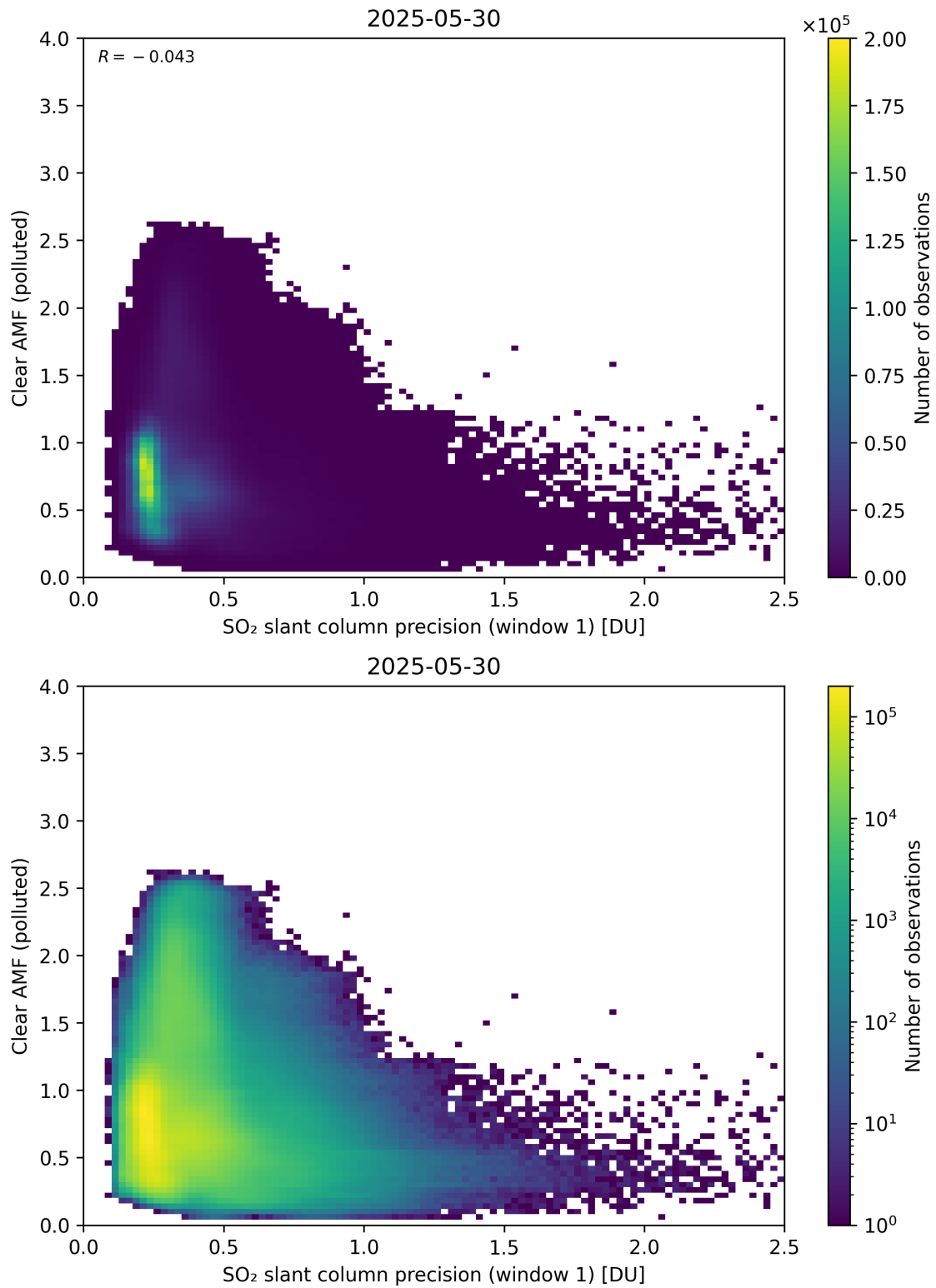
Figure 274: Scatter density plot of “SO 2 slant column precision (window 1)” against “Clear AMF (polluted)” for 2025-05-29 to 2025-05-31.
