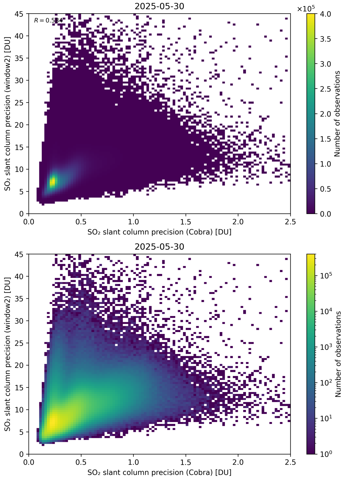
Figure 210: Scatter density plot of “SO 2 slant column precision (Cobra)” against “SO 2 slant column precision (window2)” for 2025-05-29 to 2025-05-31.
