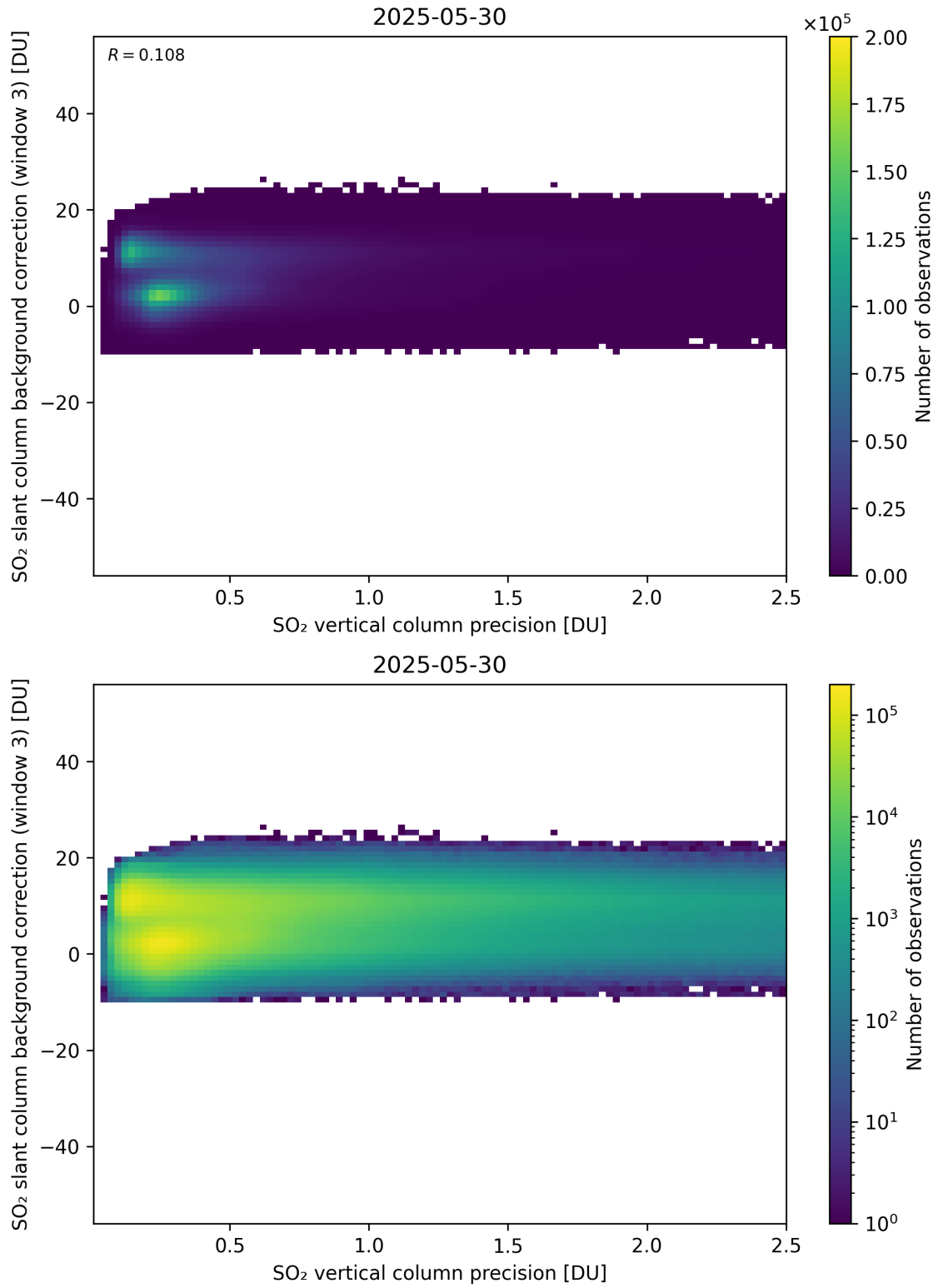
Figure 331: Scatter density plot of “SO 2 vertical column precision” against “SO 2 slant column background correction (window 3)” for 2025-05-29 to 2025-05-31.
