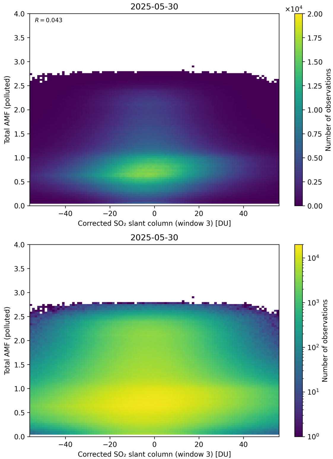
Figure 260: Scatter density plot of “Corrected SO 2 slant column (window 3)” against “Total AMF (polluted)” for 2025-05-29 to 2025-05-31.
