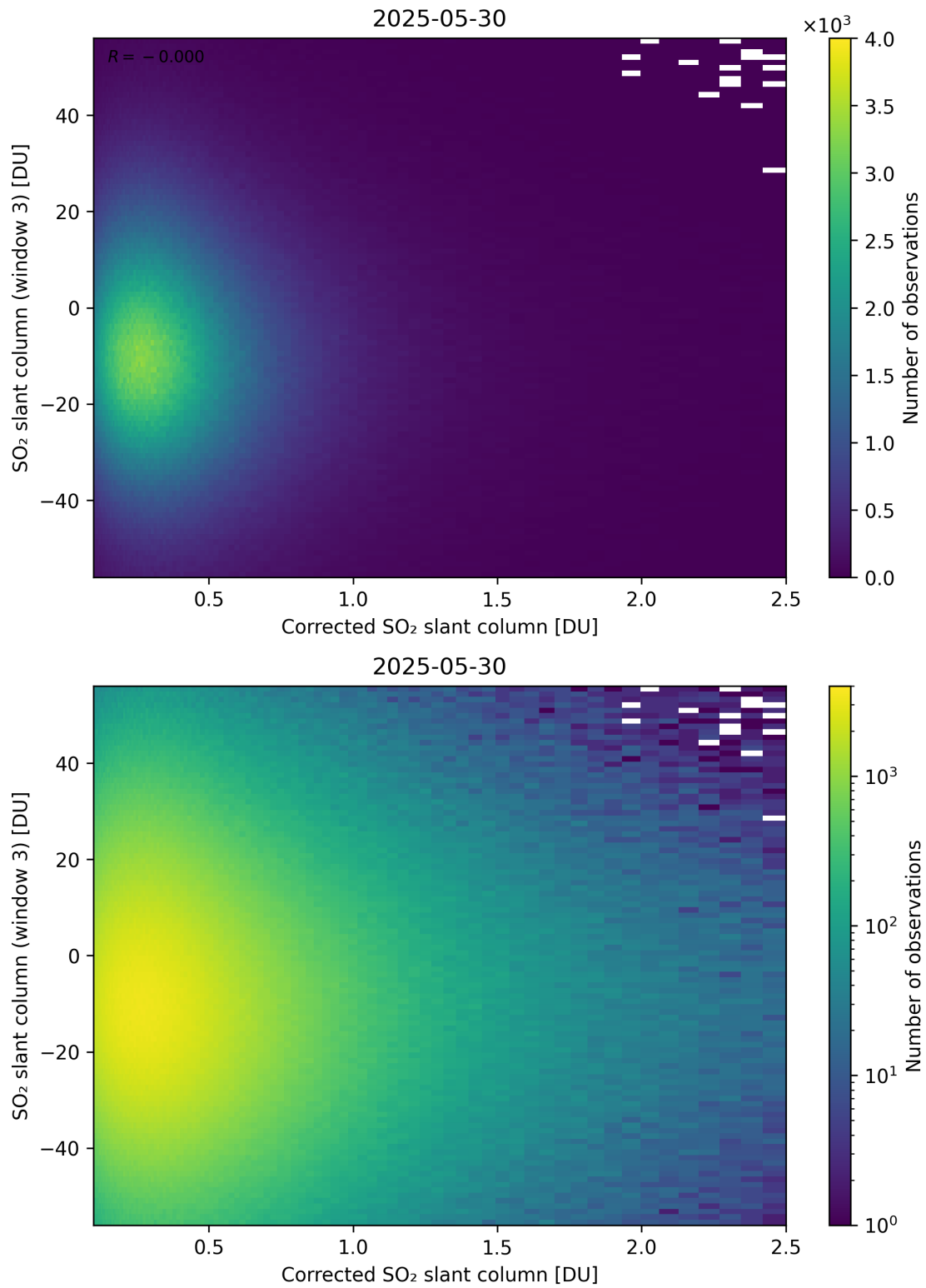
Figure 240: Scatter density plot of “Corrected SO 2 slant column” against “SO 2 slant column (window 3)” for 2025-05-29 to 2025-05-31.
