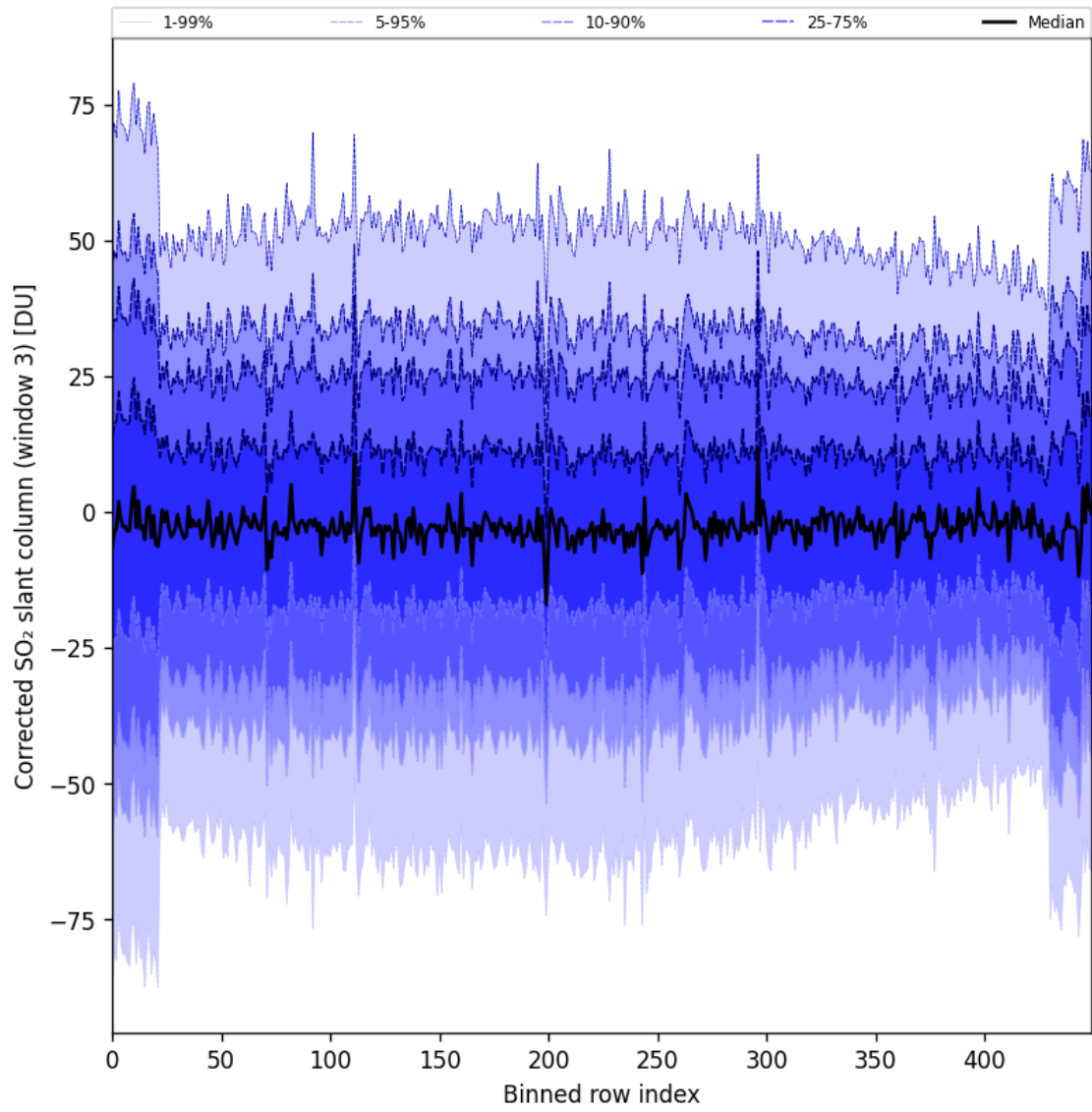
Figure 99: Along track statistics of “Corrected SO 2 slant column (window 3)” for 2025-05-29 to 2025-05-31
