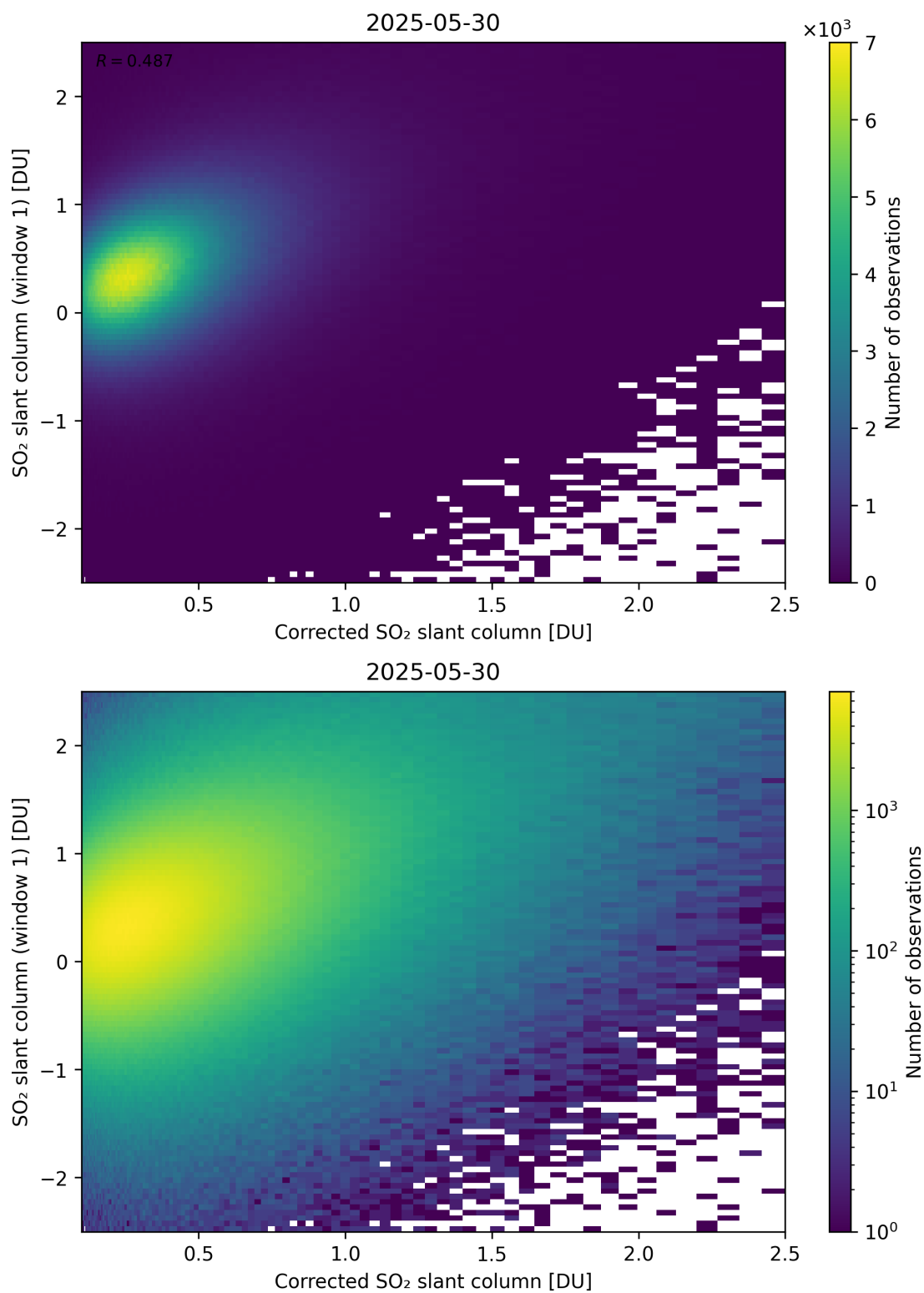
Figure 237: Scatter density plot of “Corrected SO 2 slant column” against “SO 2 slant column (window 1)” for 2025-05-29 to 2025-05-31.
