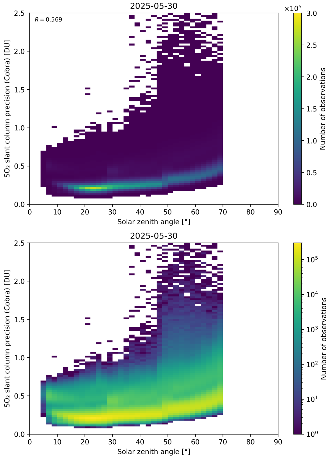
Figure 180: Scatter density plot of “Solar zenith angle” against “SO 2 slant column precision (Cobra)” for 2025-05-29 to 2025-05-31.
