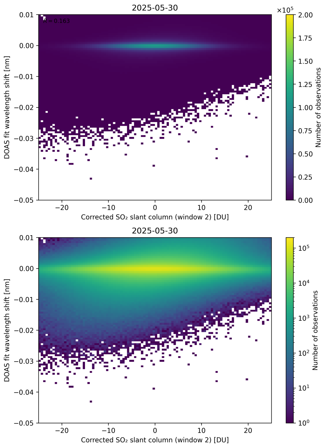
Figure 246: Scatter density plot of “Corrected SO 2 slant column (window 2)” against “DOAS fit wavelength shift” for 2025-05-29 to 2025-05-31.
