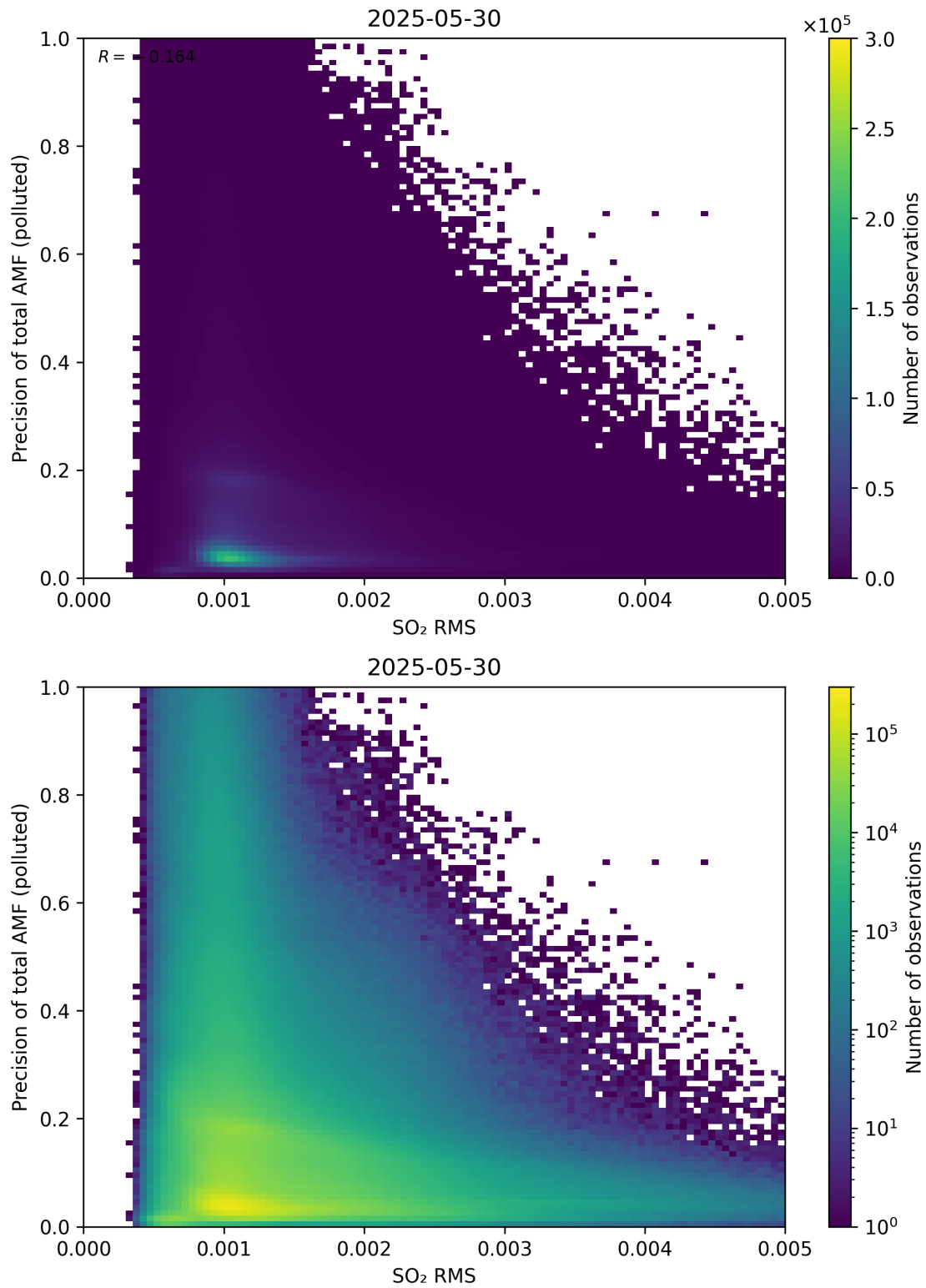
Figure 149: Scatter density plot of “SO 2 RMS” against “Precision of total AMF (polluted)” for 2025-05-29 to 2025-05-31.
