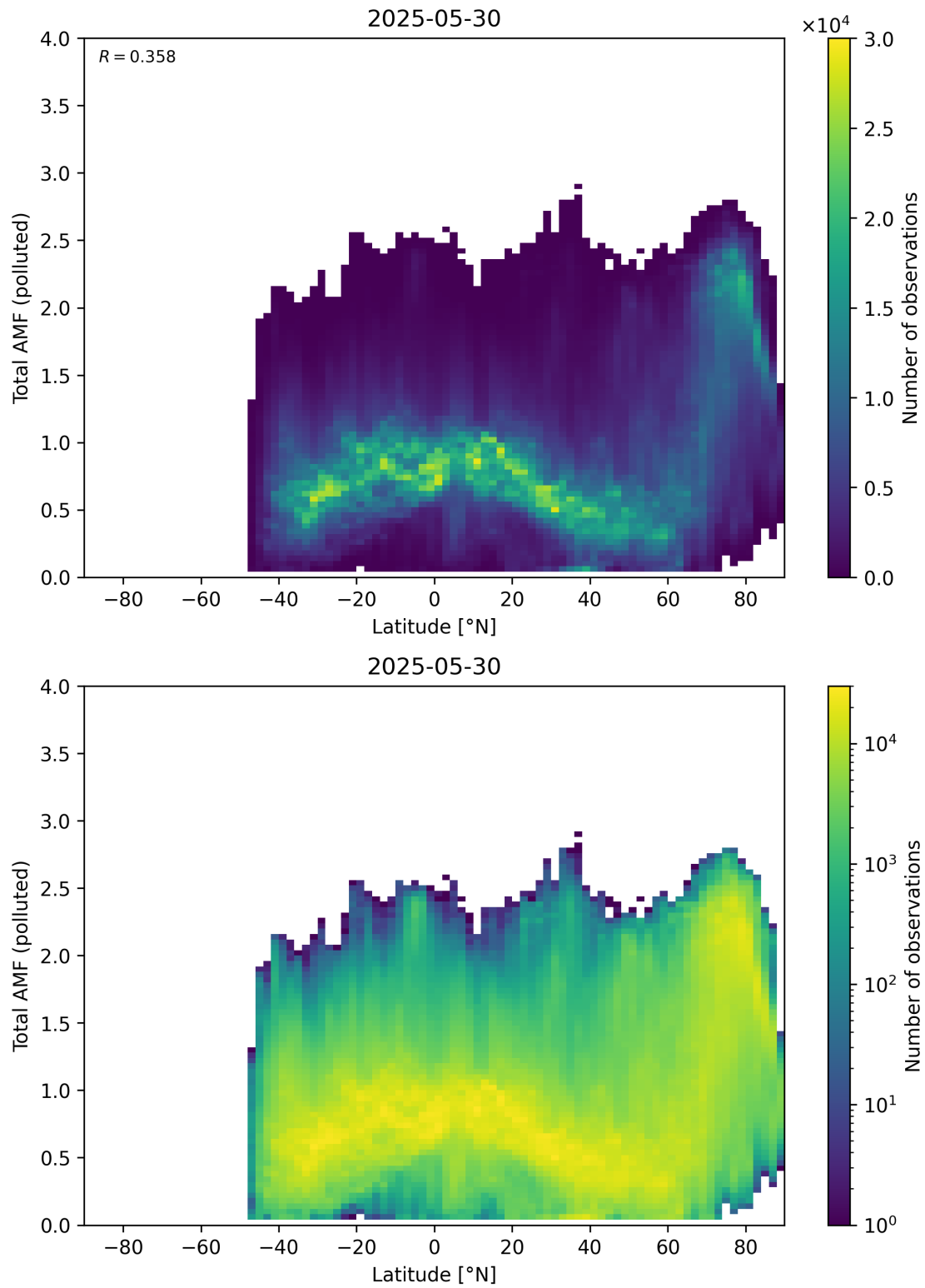
Figure 167: Scatter density plot of “Latitude” against “Total AMF (polluted)” for 2025-05-29 to 2025-05-31.
