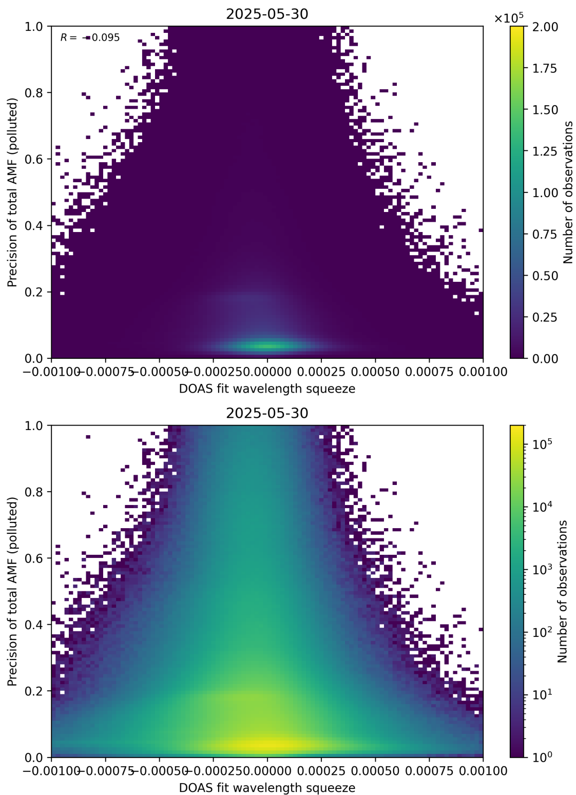
Figure 146: Scatter density plot of “DOAS fit wavelength squeeze” against “Precision of total AMF (polluted)” for 2025-05-29 to 2025-05-31.
