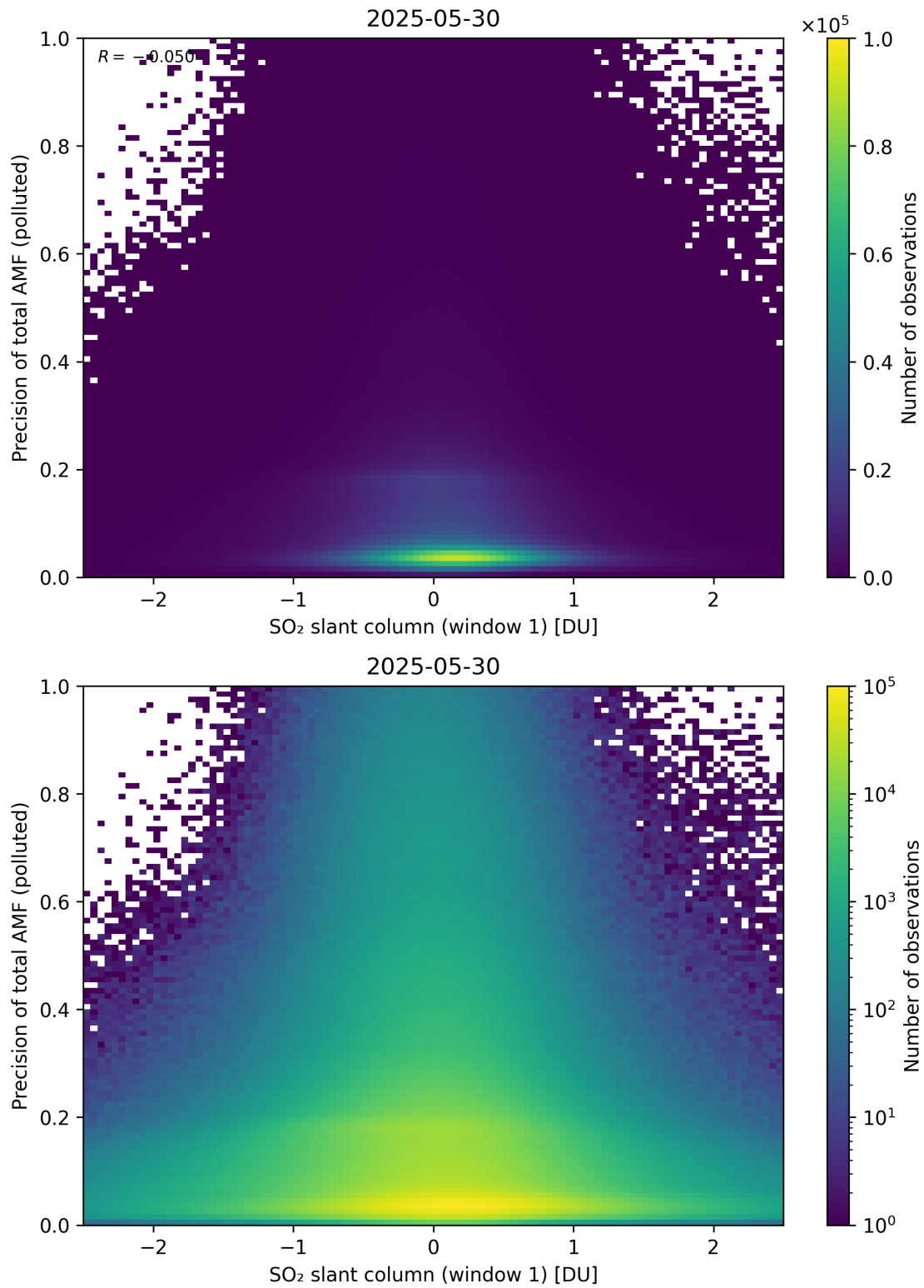
Figure 290: Scatter density plot of “SO 2 slant column (window 1)” against “Precision of total AMF (polluted)” for 2025-05-29 to 2025-05-31.
