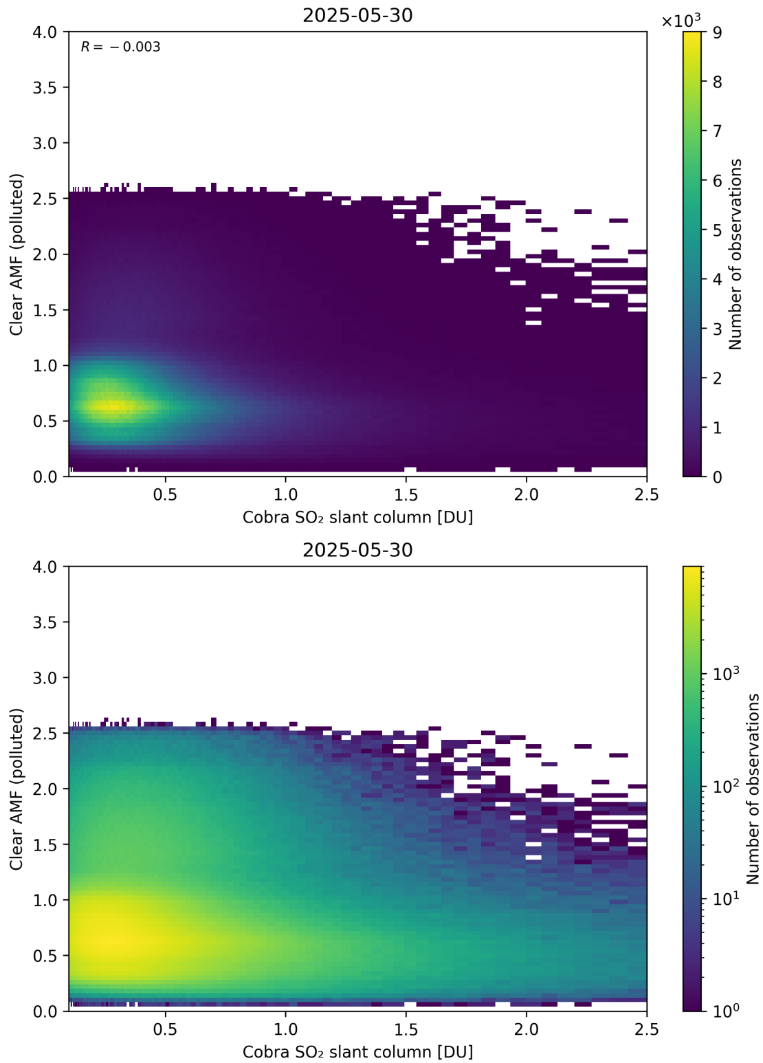
Figure 215: Scatter density plot of “Cobra SO 2 slant column” against “Clear AMF (polluted)” for 2025-05-29 to 2025-05-31.
