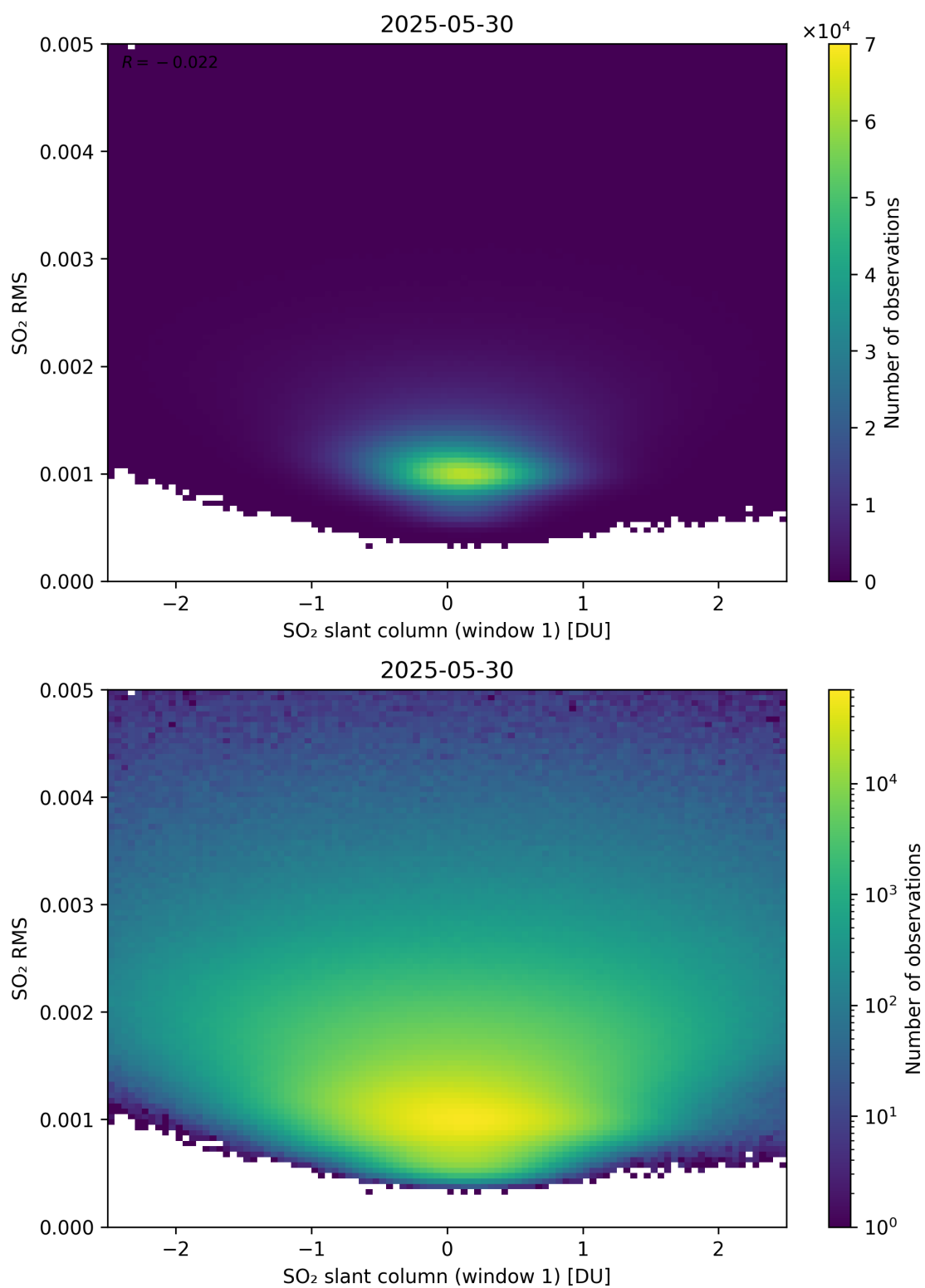
Figure 267: Scatter density plot of “SO 2 slant column (window 1)” against “SO 2 RMS” for 2025-05-29 to 2025-05-31.
