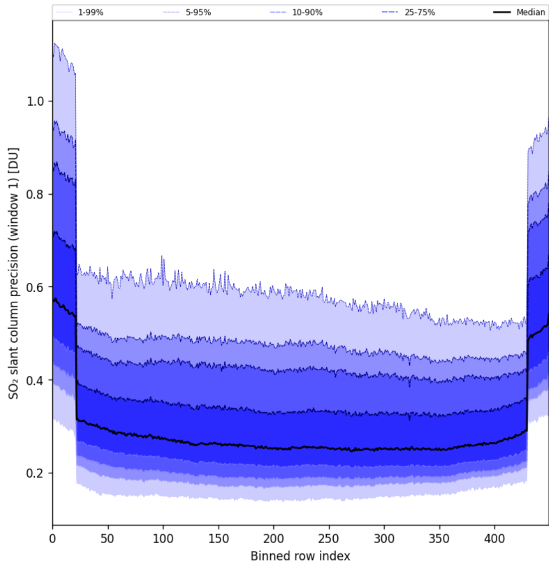
Figure 90: Along track statistics of “SO 2 slant column precision (window 1)” for 2025-05-29 to 2025-05-31
