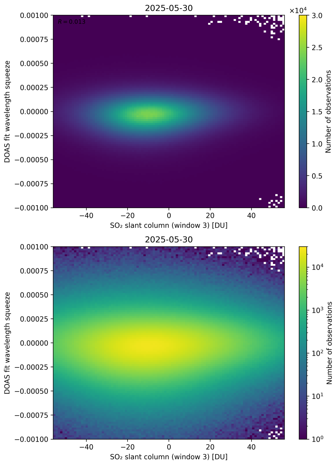
Figure 305: Scatter density plot of “SO 2 slant column (window 3)” against “DOAS fit wavelength squeeze” for 2025-05-29 to 2025-05-31.
