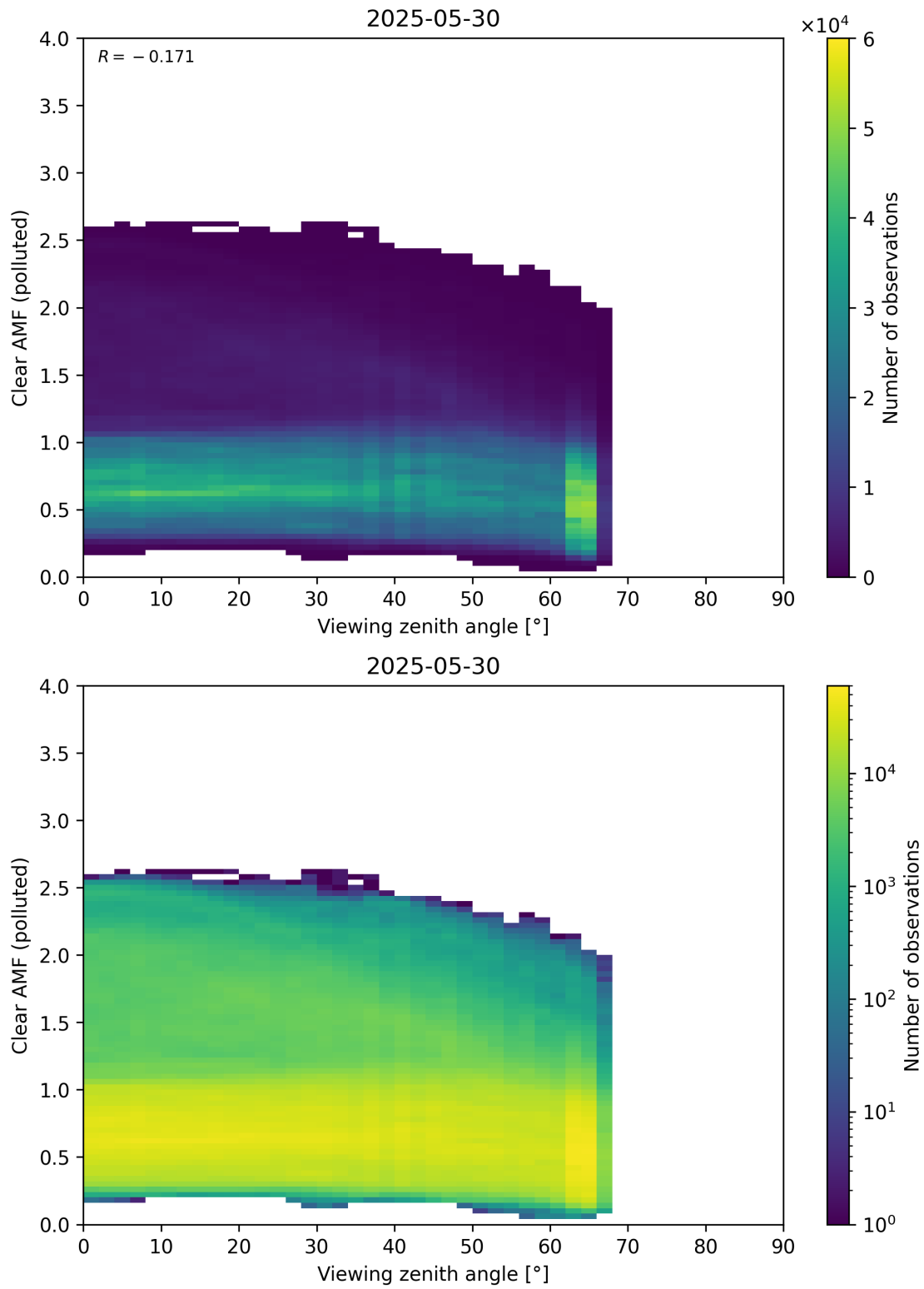
Figure 370: Scatter density plot of “Viewing zenith angle” against “Clear AMF (polluted)” for 2025-05-29 to 2025-05-31.
