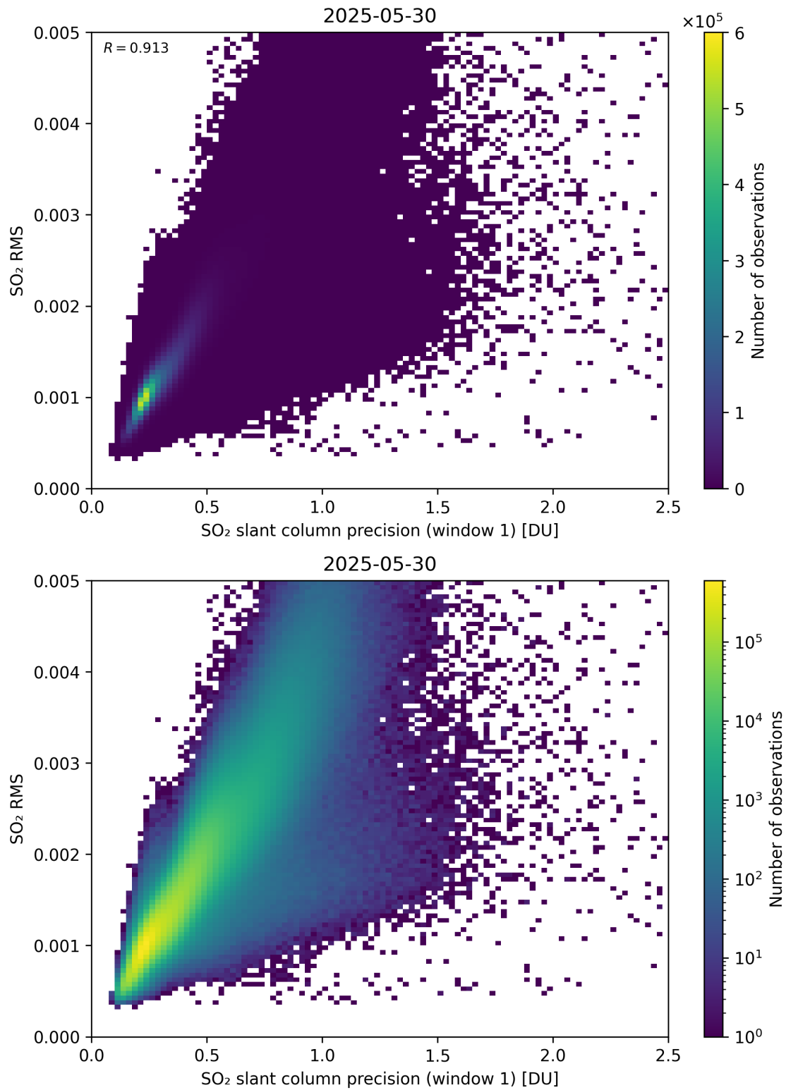
Figure 273: Scatter density plot of “SO 2 slant column precision (window 1)” against “SO 2 RMS” for 2025-05-29 to 2025-05-31.
