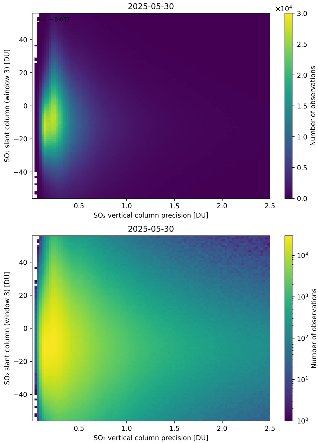
Figure 344: Scatter density plot of “SO 2 vertical column precision” against “SO 2 slant column (window 3)” for 2025-05-29 to 2025-05-31.
