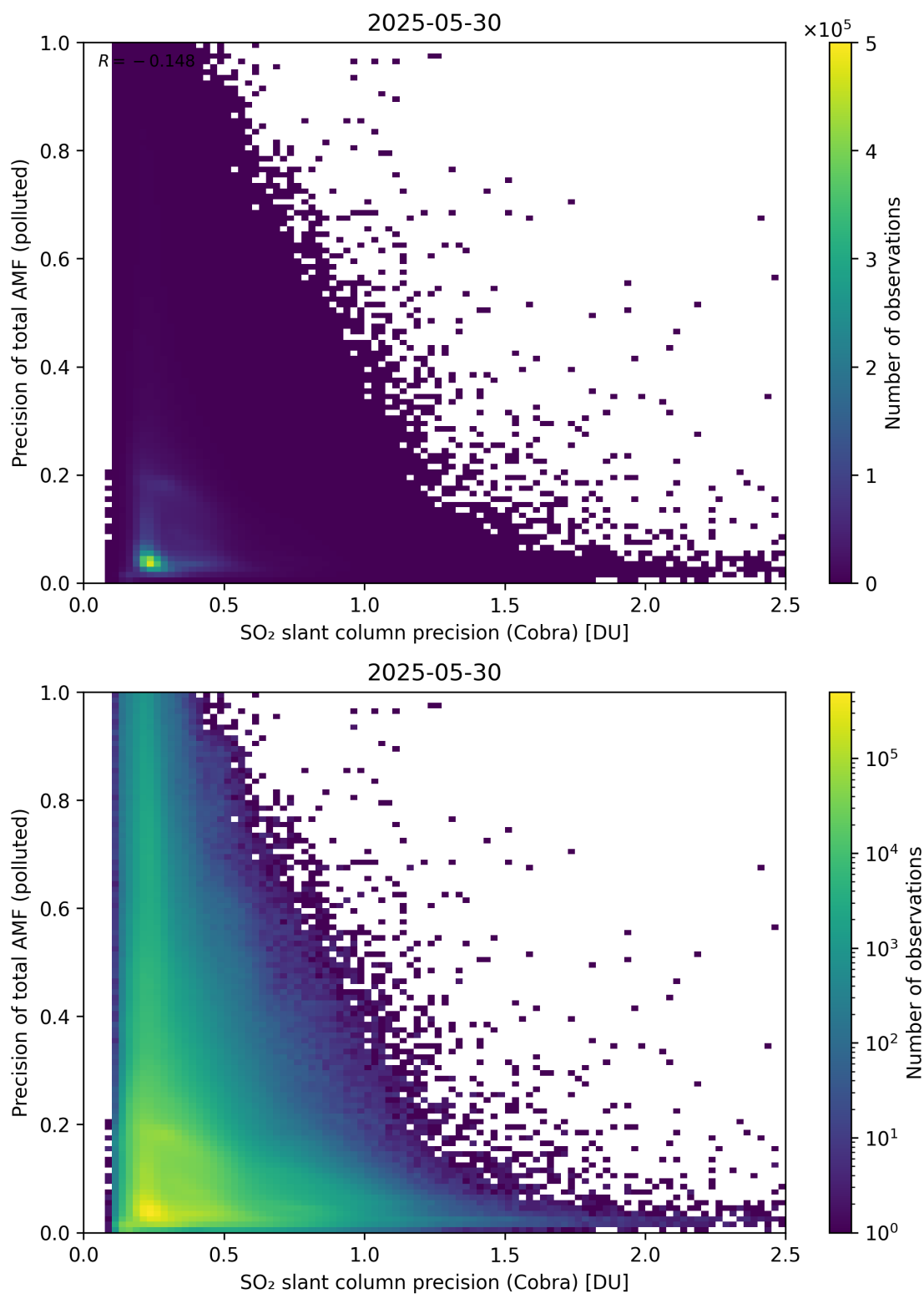
Figure 214: Scatter density plot of “SO 2 slant column precision (Cobra)” against “Precision of total AMF (polluted)” for 2025-05-29 to 2025-05-31.
