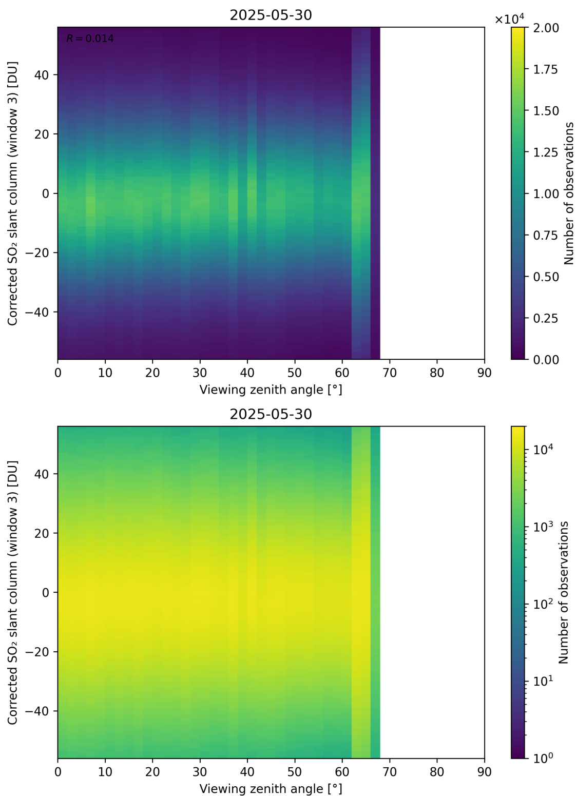
Figure 375: Scatter density plot of “Viewing zenith angle” against “Corrected SO 2 slant column (window 3)” for 2025-05-29 to 2025-05-31.
