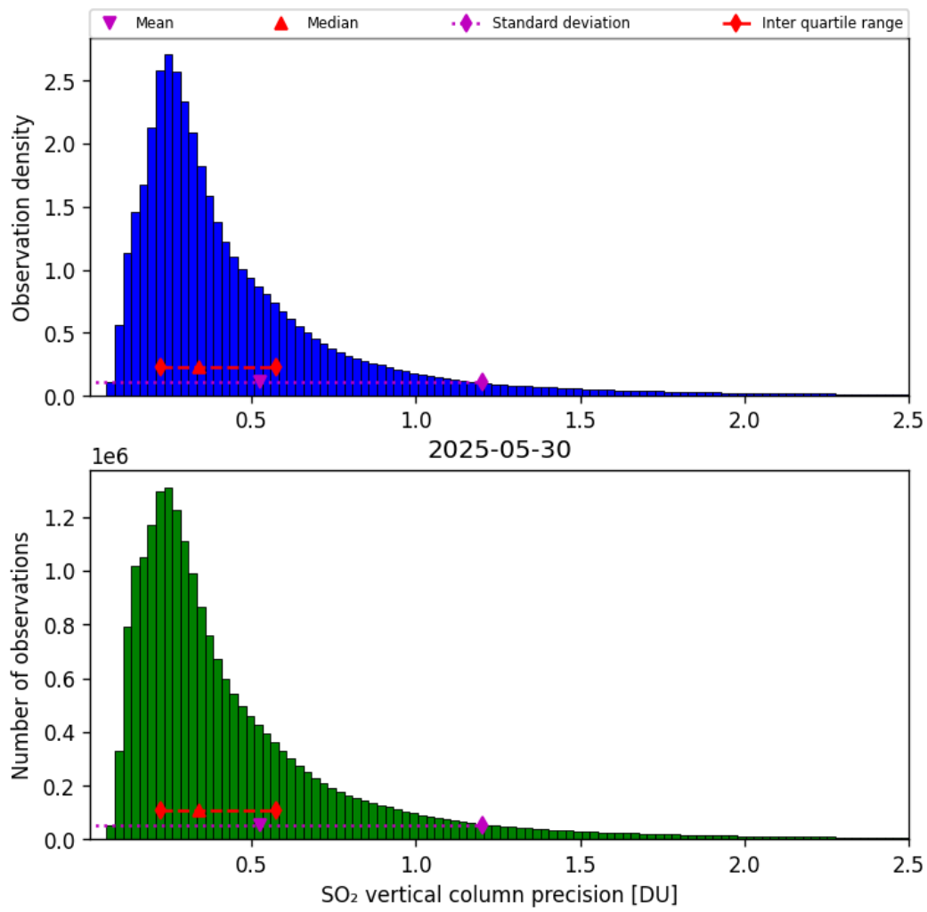
Figure 59: Histogram of “SO 2 vertical column precision” for 2025-05-29 to 2025-05-31
