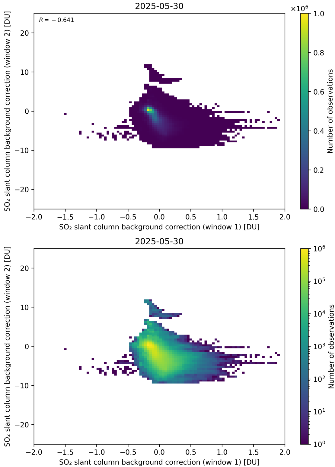
Figure 109: Scatter density plot of “SO 2 slant column background correction (window 1)” against “SO 2 slant column background correction (window 2)” for 2025-05-29 to 2025-05-31.
