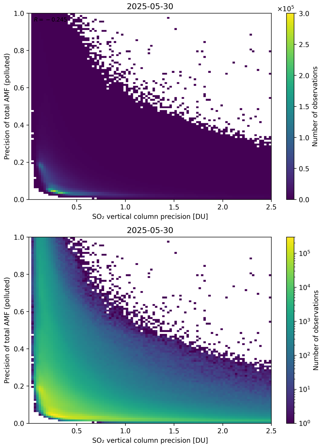
Figure 347: Scatter density plot of “SO 2 vertical column precision” against “Precision of total AMF (polluted)” for 2025-05-29 to 2025-05-31.
