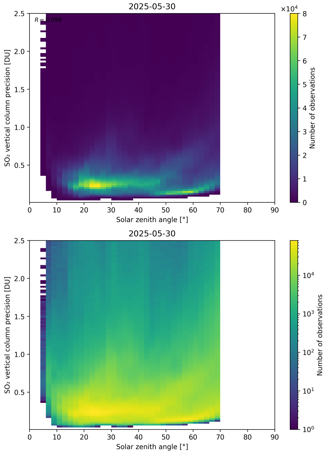
Figure 192: Scatter density plot of “Solar zenith angle” against “SO 2 vertical column precision” for 2025-05-29 to 2025-05-31.
