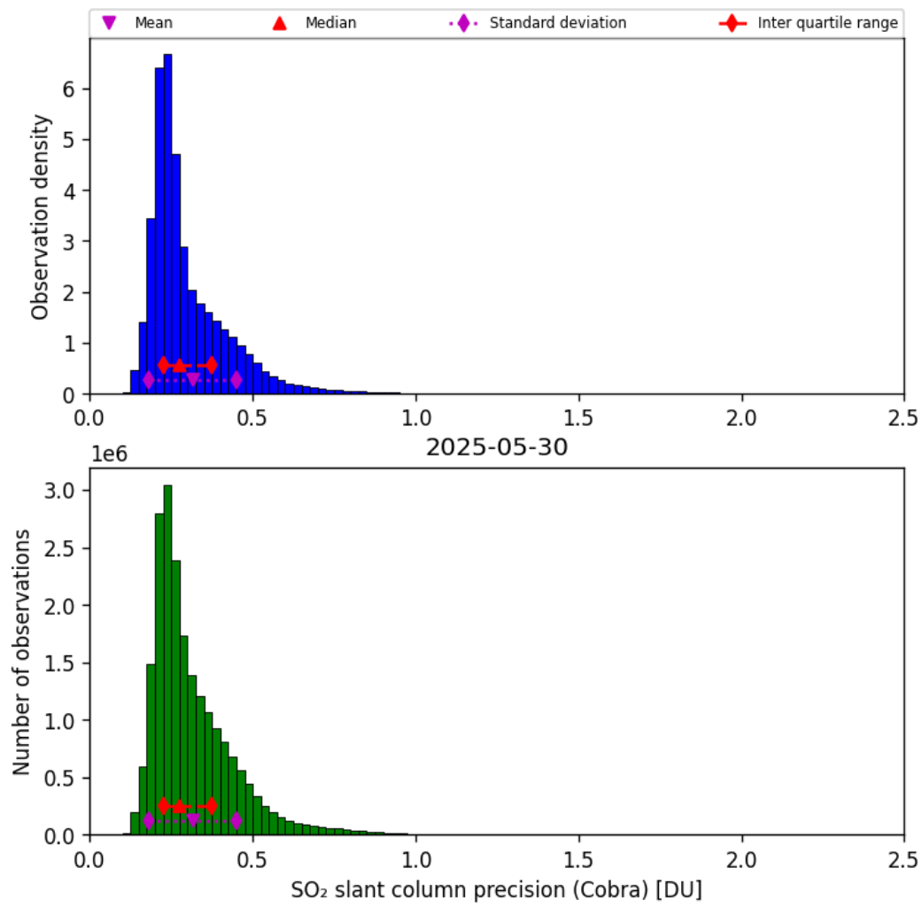
Figure 62: Histogram of “SO 2 slant column precision (Cobra)” for 2025-05-29 to 2025-05-31
