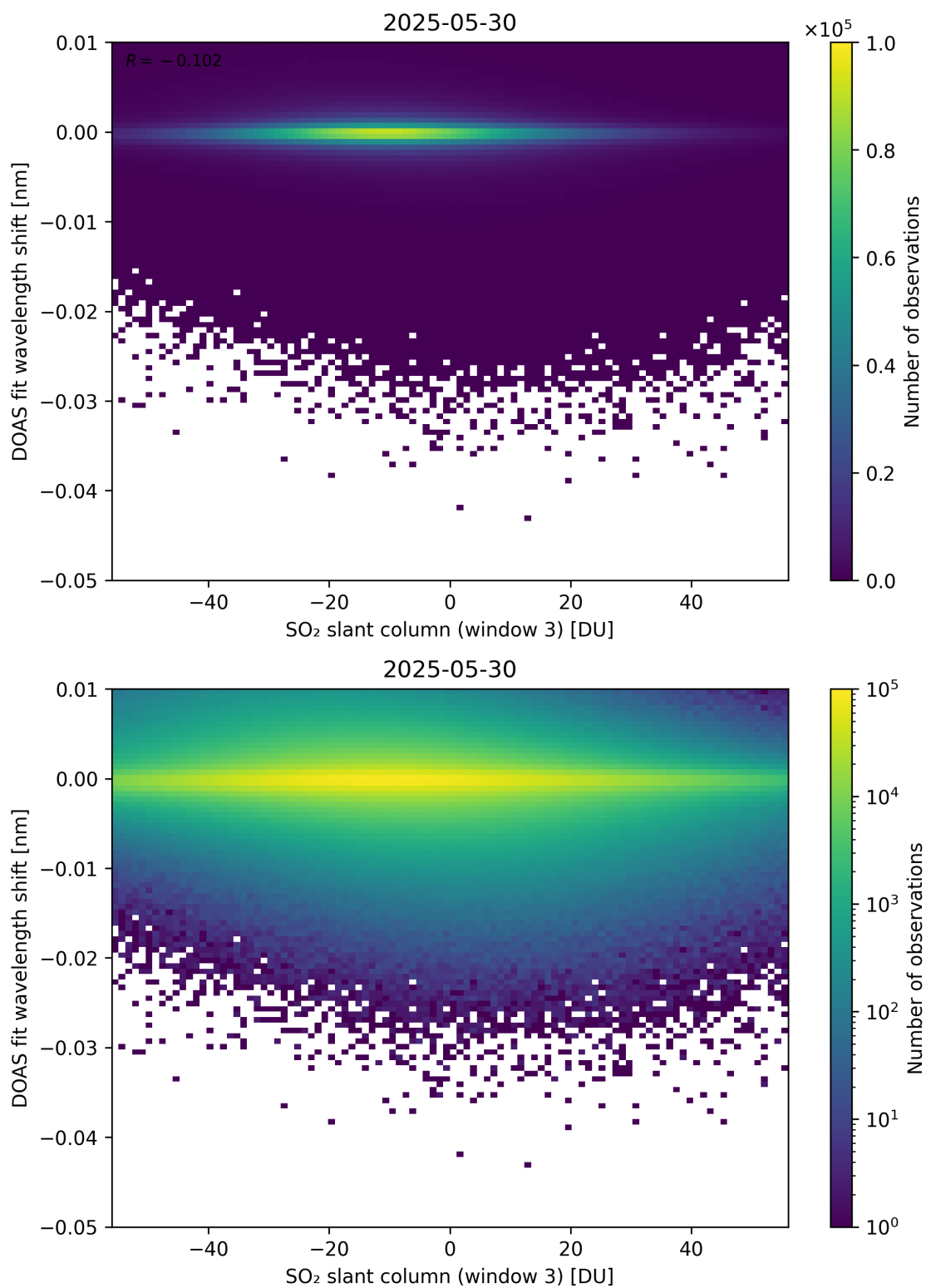
Figure 304: Scatter density plot of “SO 2 slant column (window 3)” against “DOAS fit wavelength shift” for 2025-05-29 to 2025-05-31.
