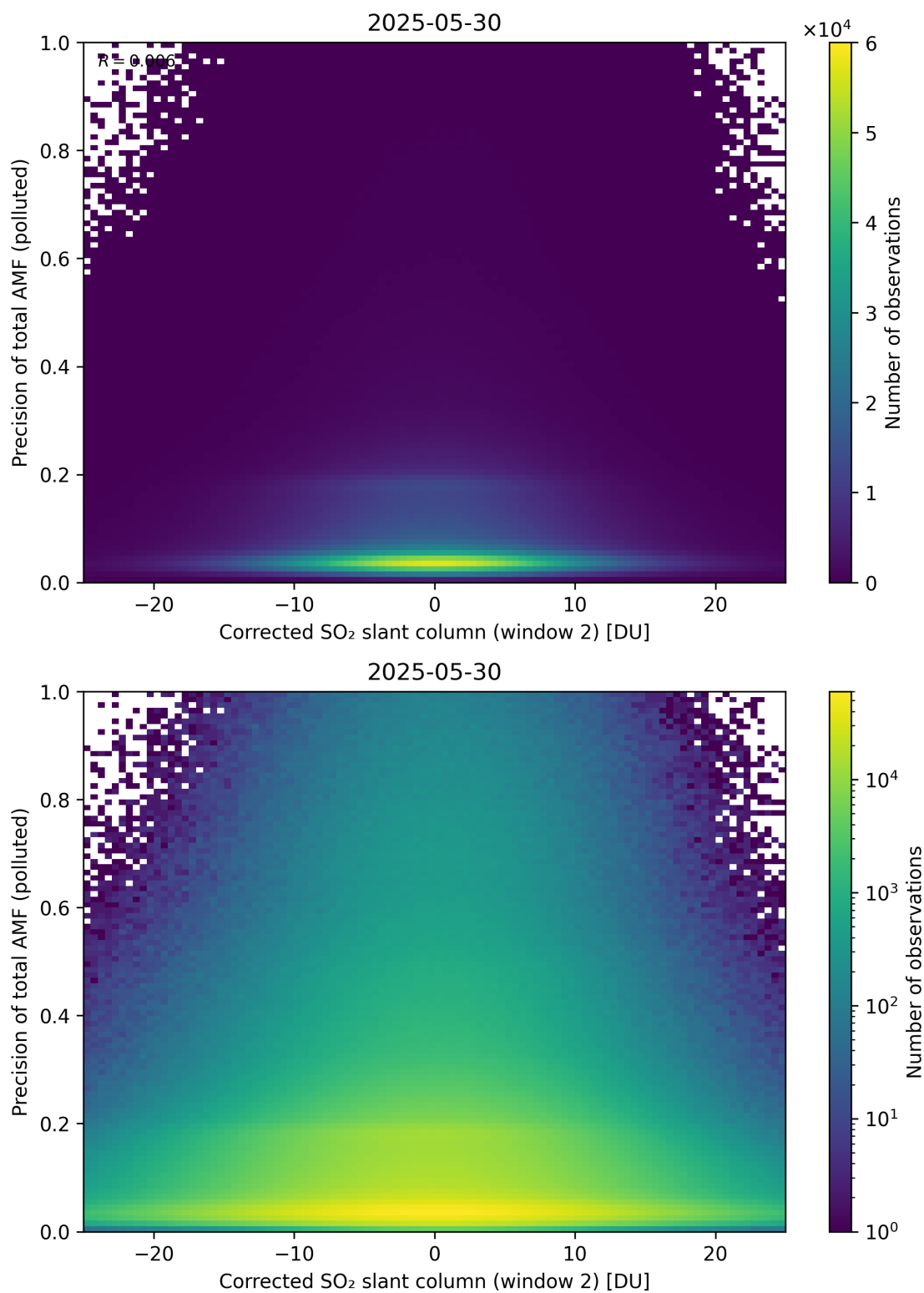
Figure 254: Scatter density plot of “Corrected SO 2 slant column (window 2)” against “Precision of total AMF (polluted)” for 2025-05-29 to 2025-05-31.
