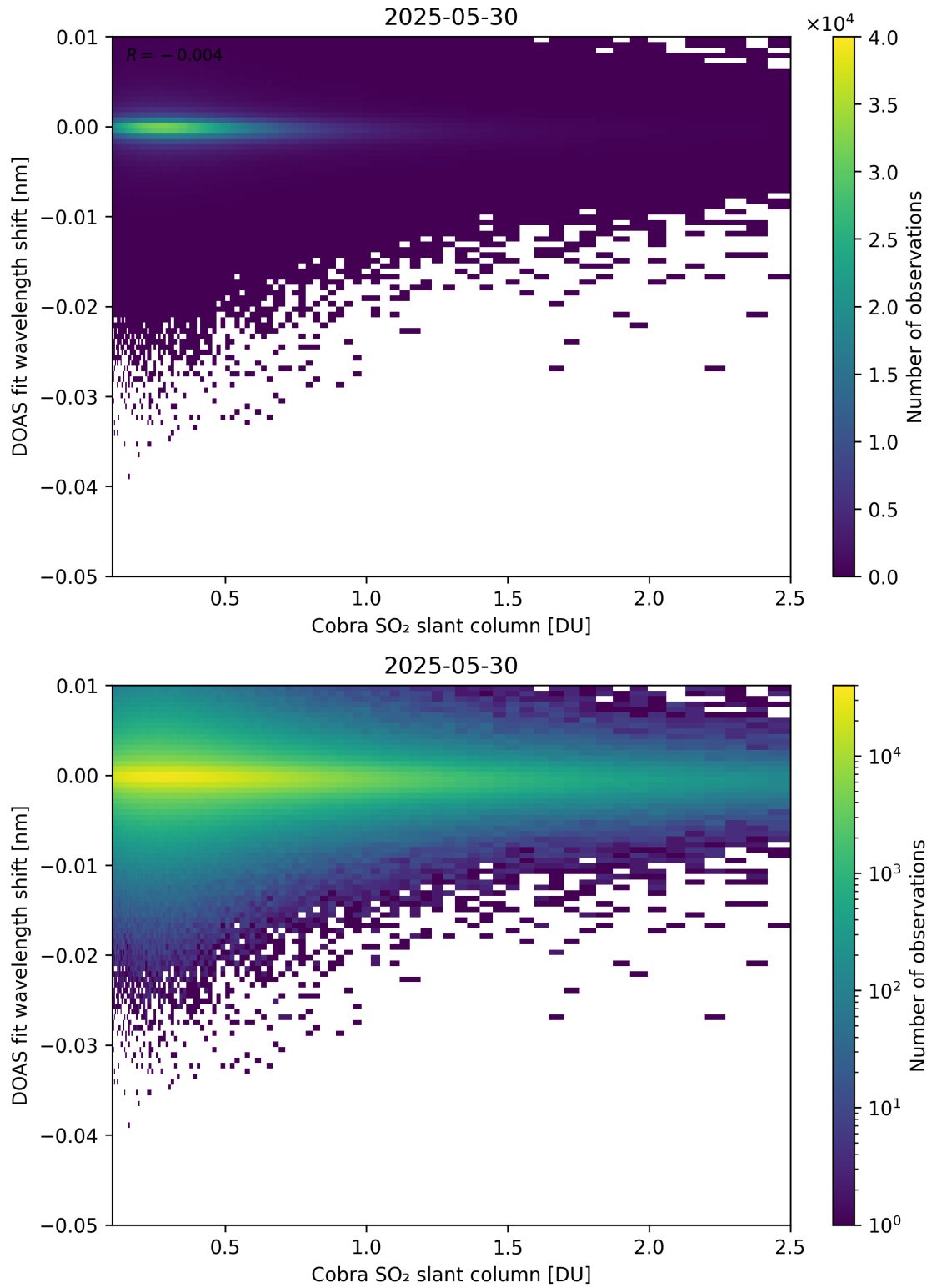
Figure 196: Scatter density plot of “Cobra SO 2 slant column” against “DOAS fit wavelength shift” for 2025-05-29 to 2025-05-31.
