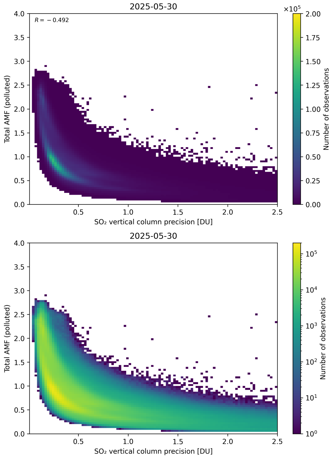
Figure 346: Scatter density plot of “SO 2 vertical column precision” against “Total AMF (polluted)” for 2025-05-29 to 2025-05-31.
