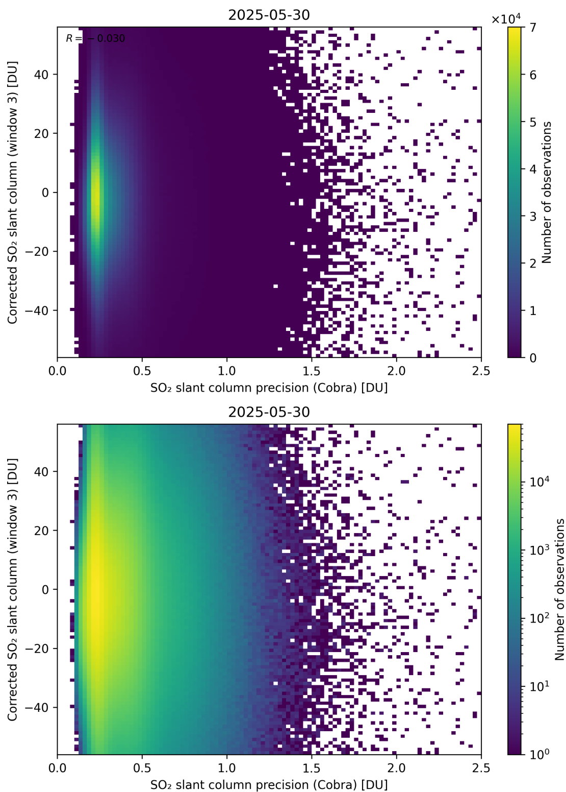
Figure 207: Scatter density plot of “SO 2 slant column precision (Cobra)” against “Corrected SO 2 slant column (window 3)” for 2025-05-29 to 2025-05-31.
