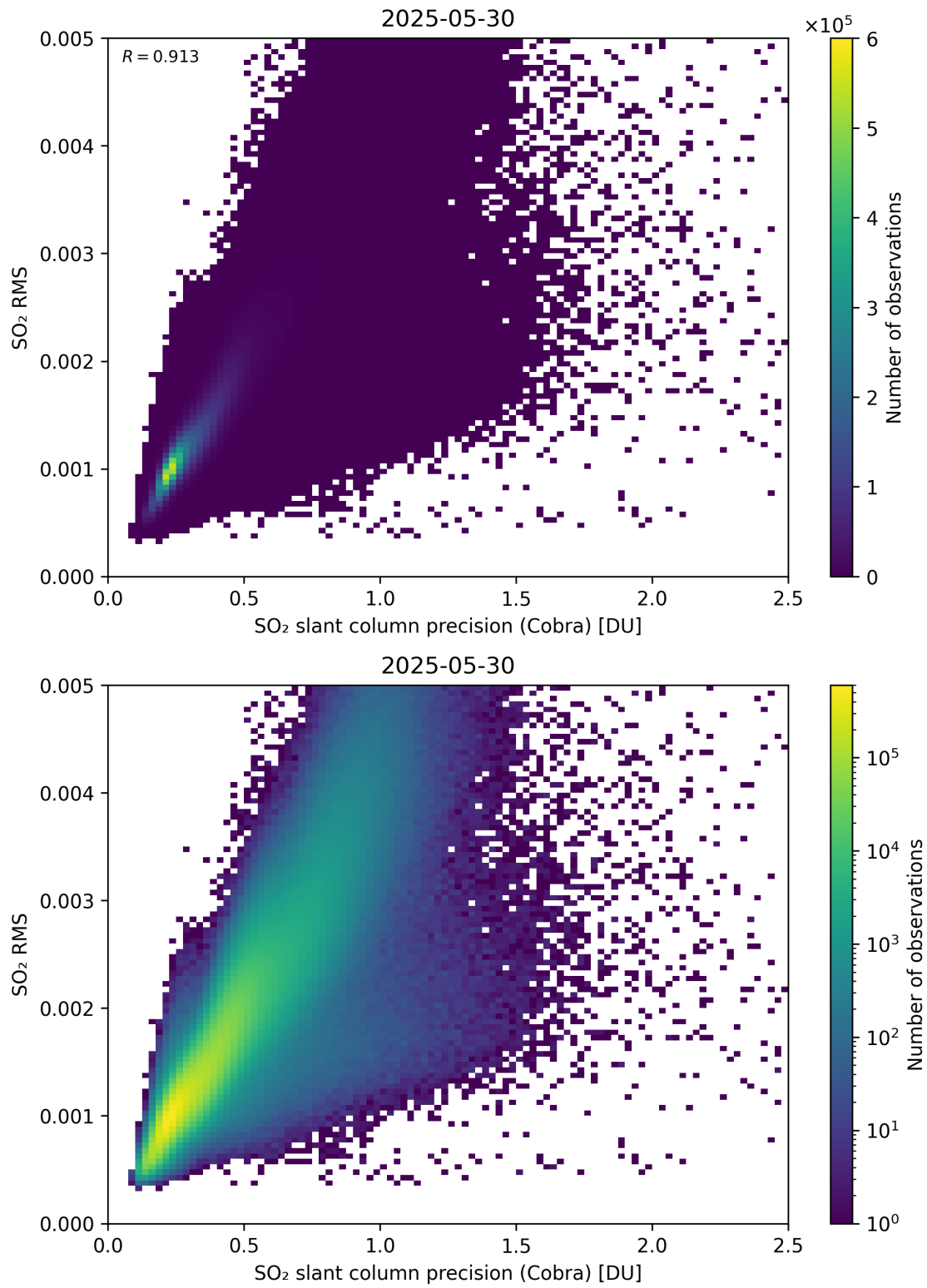
Figure 204: Scatter density plot of “SO 2 slant column precision (Cobra)” against “SO 2 RMS” for 2025-05-29 to 2025-05-31.
