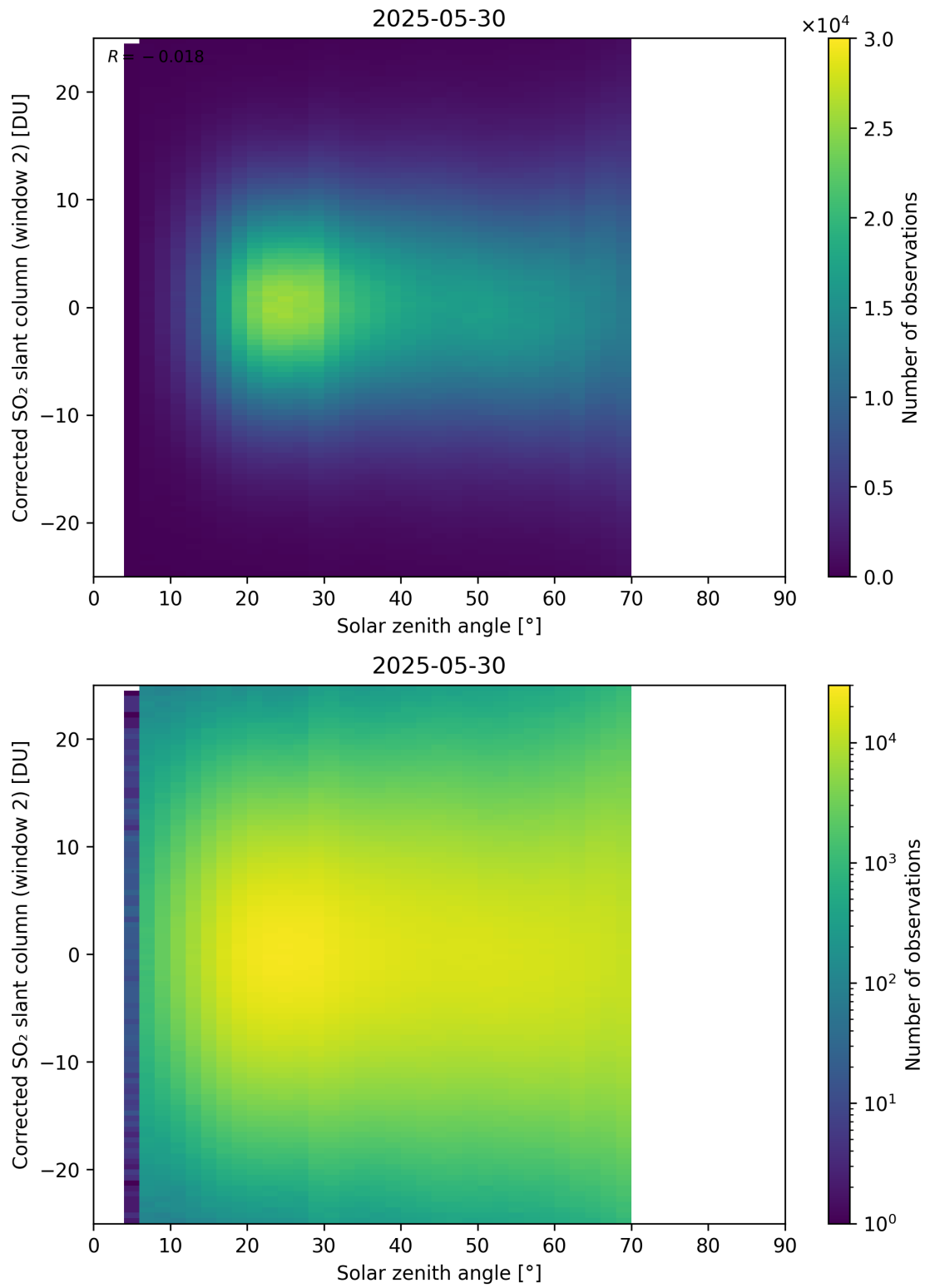
Figure 182: Scatter density plot of “Solar zenith angle” against “Corrected SO 2 slant column (window 2)” for 2025-05-29 to 2025-05-31.
