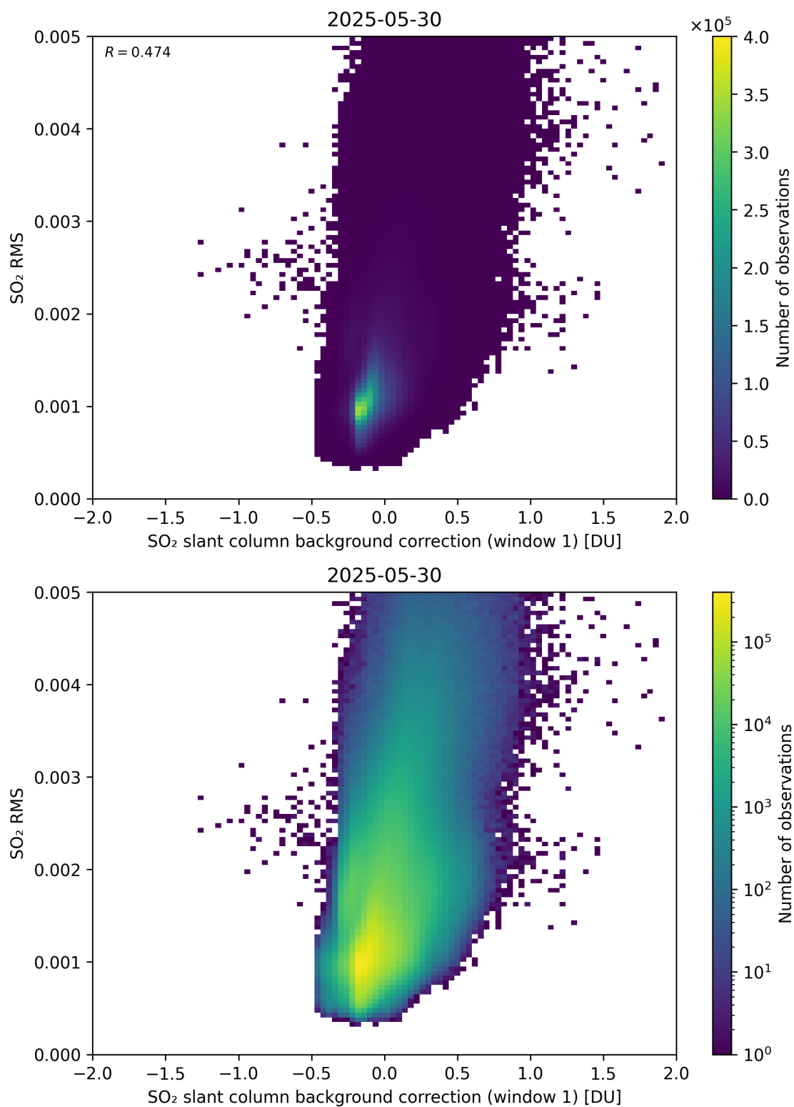
Figure 113: Scatter density plot of “SO 2 slant column background correction (window 1)” against “SO 2 RMS” for 2025-05-29 to 2025-05-31.
