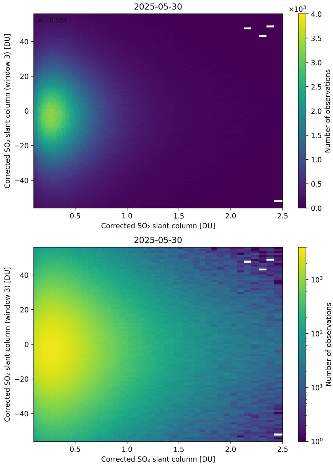
Figure 236: Scatter density plot of “Corrected SO 2 slant column” against “Corrected SO 2 slant column (window 3)” for 2025-05-29 to 2025-05-31.
