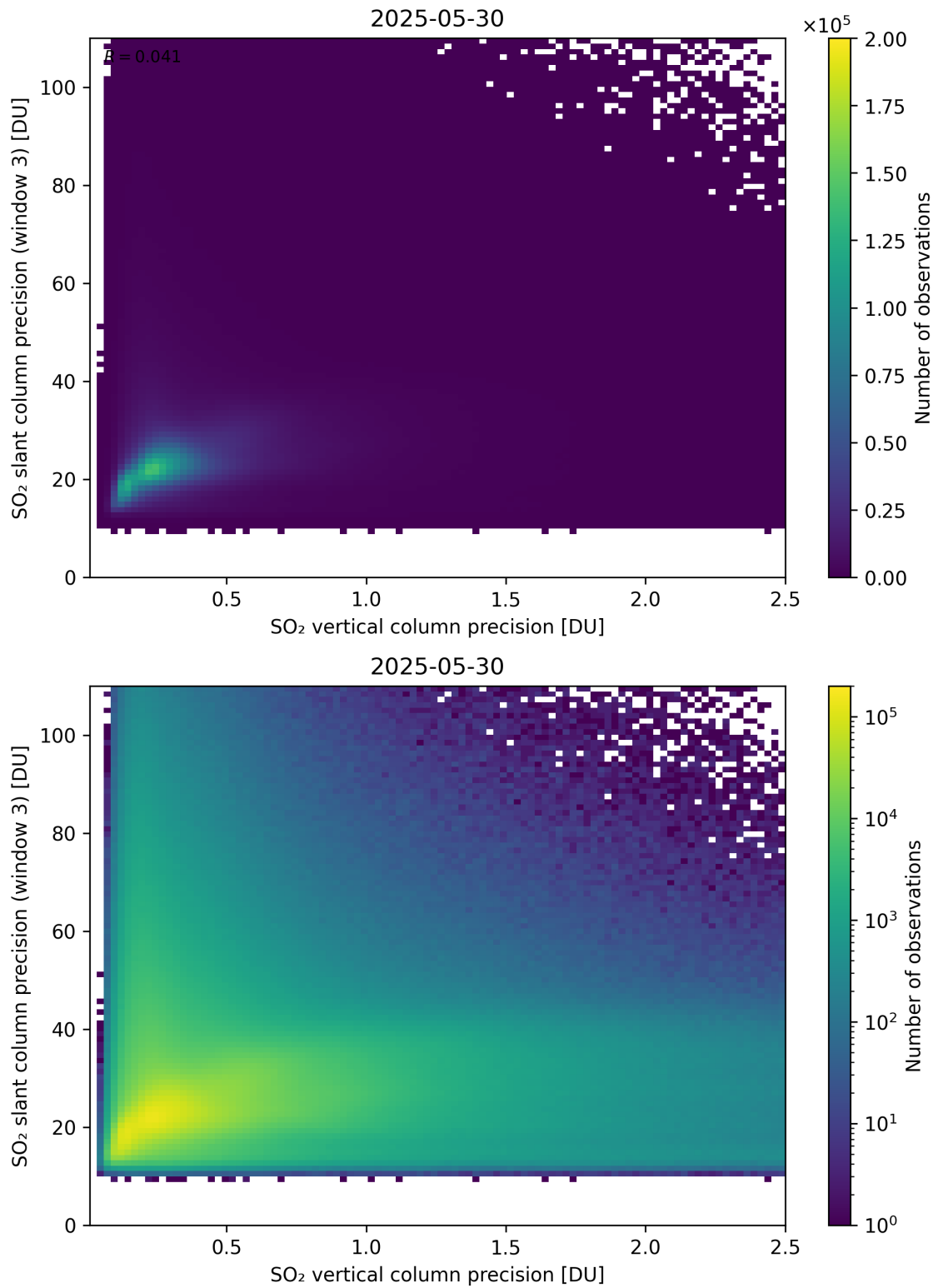
Figure 345: Scatter density plot of “SO 2 vertical column precision” against “SO 2 slant column precision (window 3)” for 2025-05-29 to 2025-05-31.
