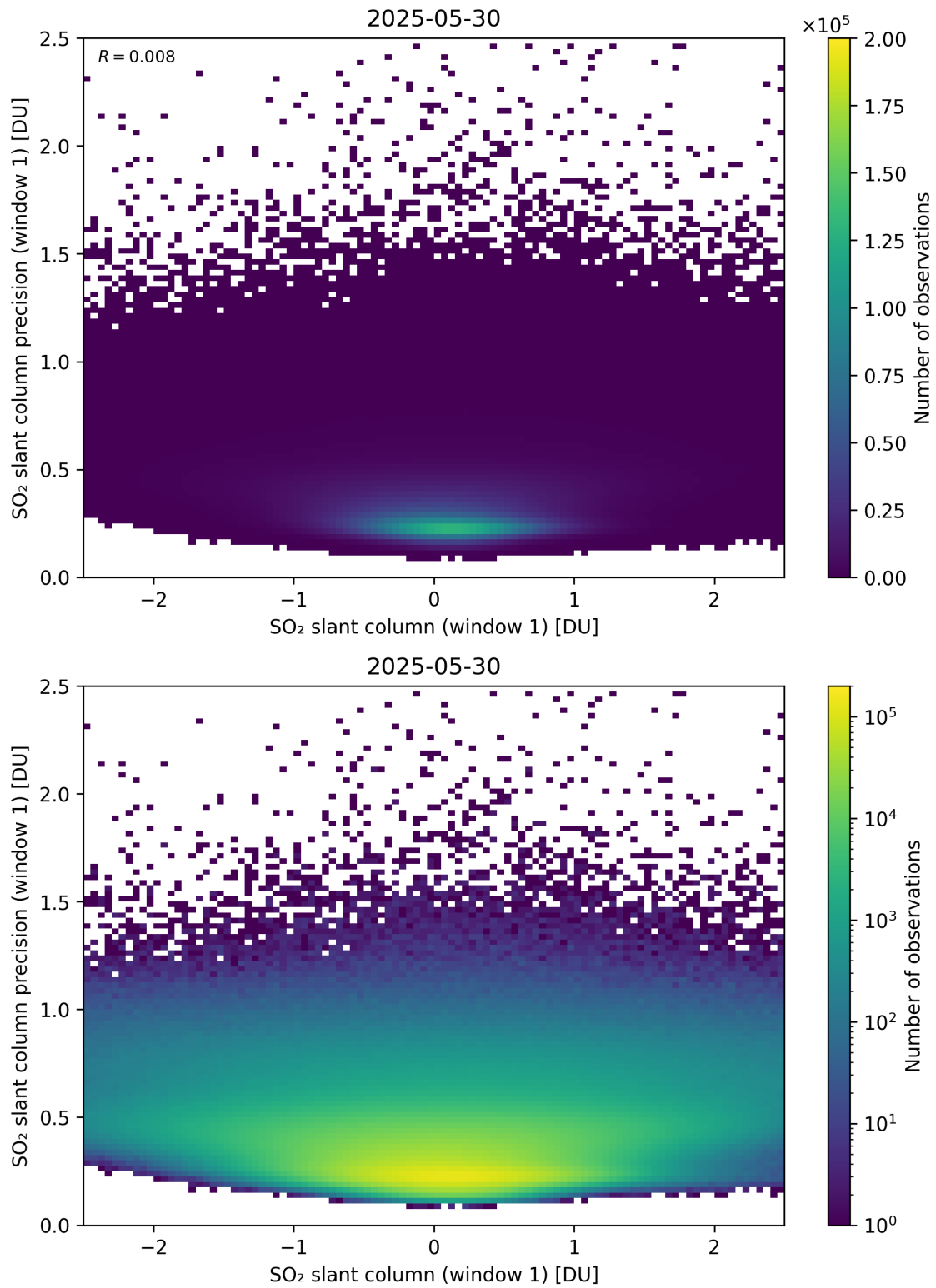
Figure 285: Scatter density plot of “SO 2 slant column (window 1)” against “SO 2 slant column precision (window 1)” for 2025-05-29 to 2025-05-31.
