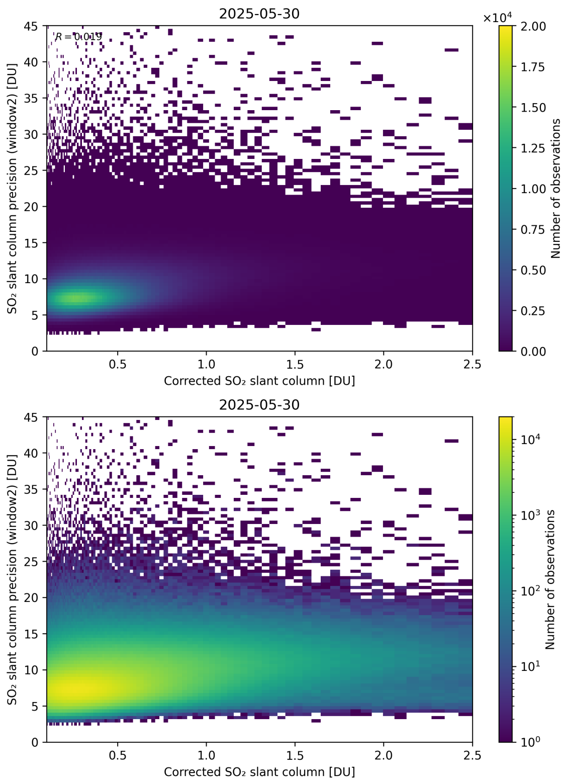
Figure 239: Scatter density plot of “Corrected SO 2 slant column” against “SO 2 slant column precision (window2)” for 2025-05-29 to 2025-05-31.
