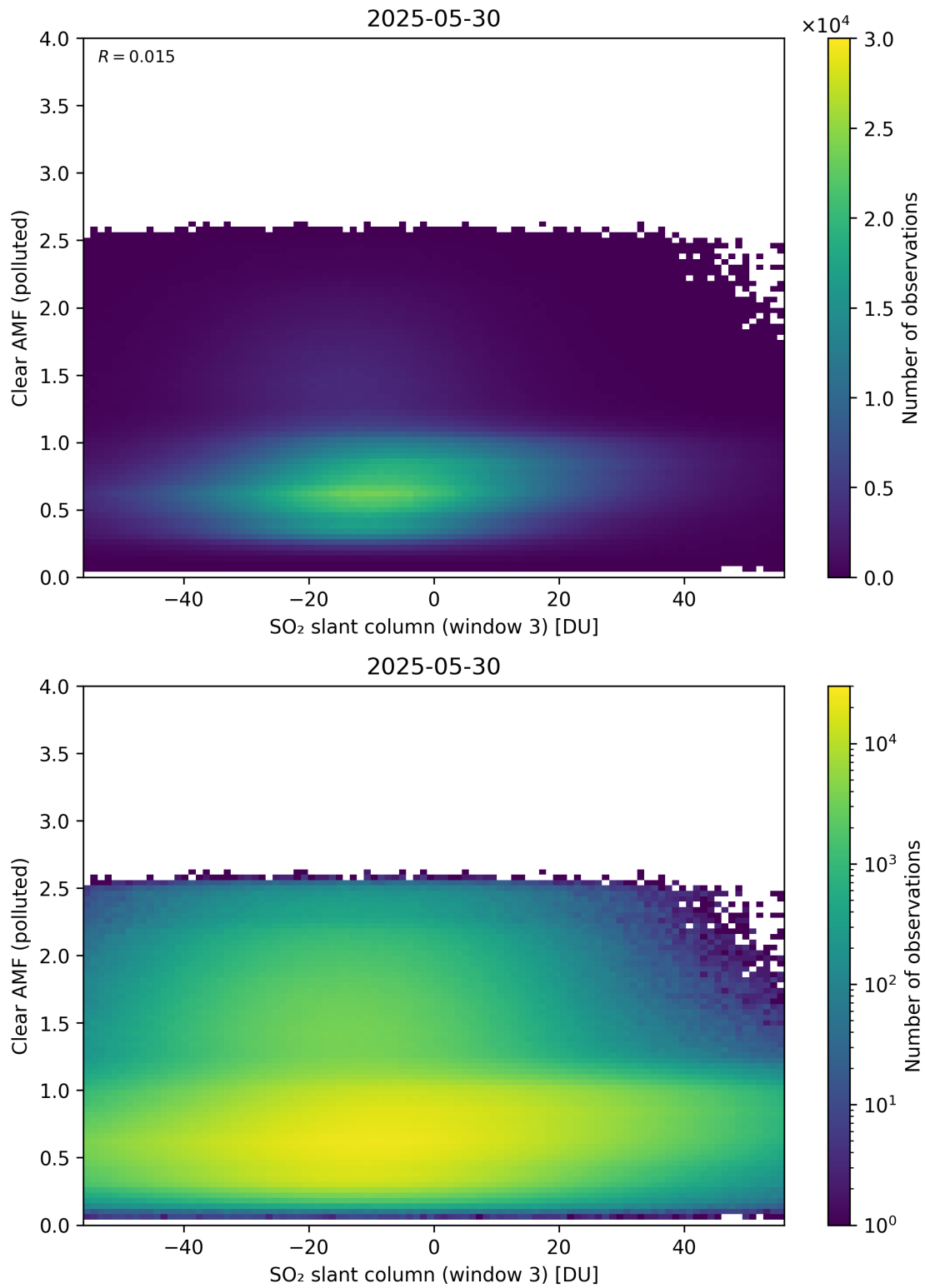
Figure 315: Scatter density plot of “SO 2 slant column (window 3)” against “Clear AMF (polluted)” for 2025-05-29 to 2025-05-31.
