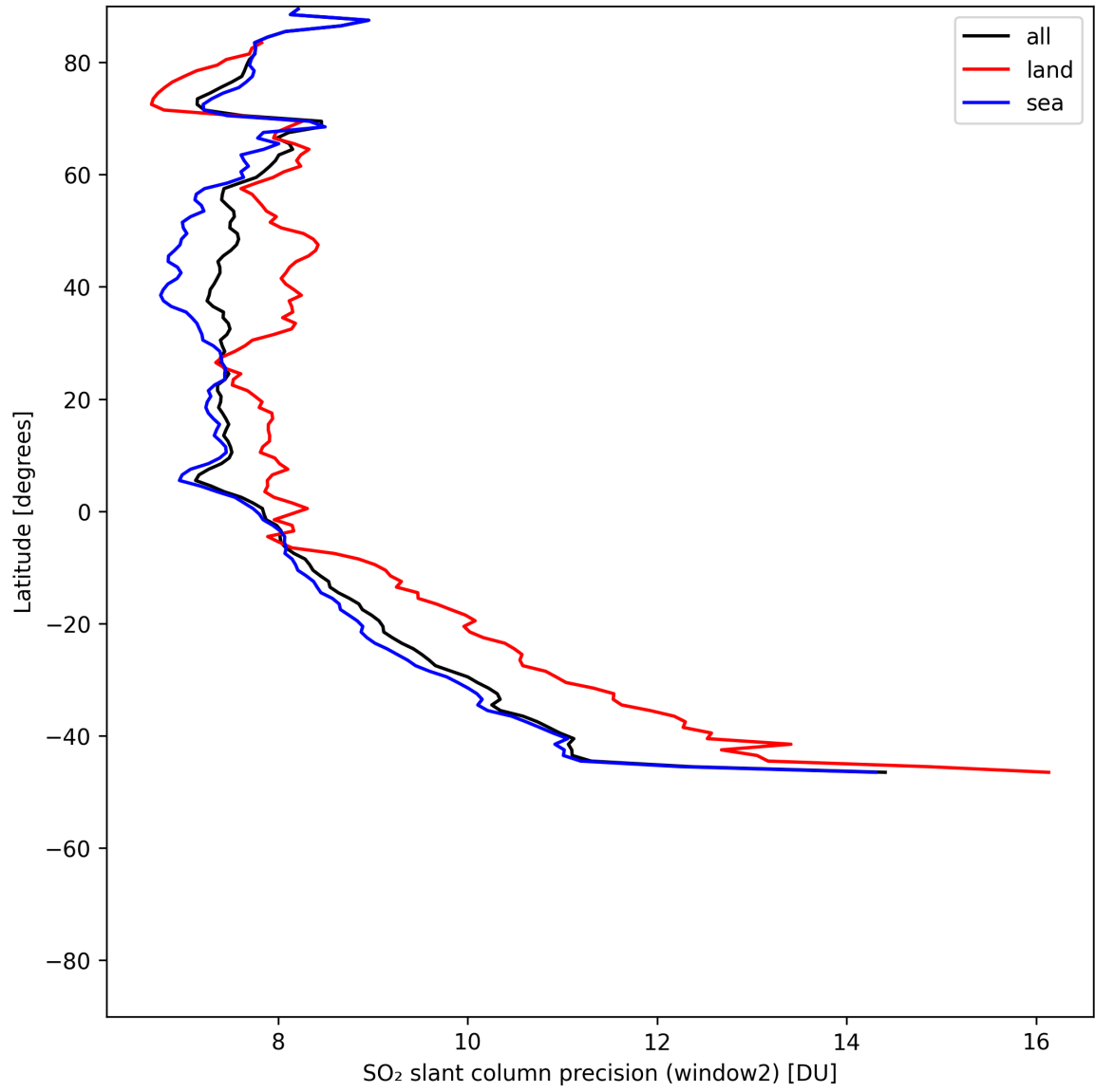
Figure 42: Zonal average of “SO 2 slant column precision (window2)” for 2025-05-29 to 2025-05-31.
