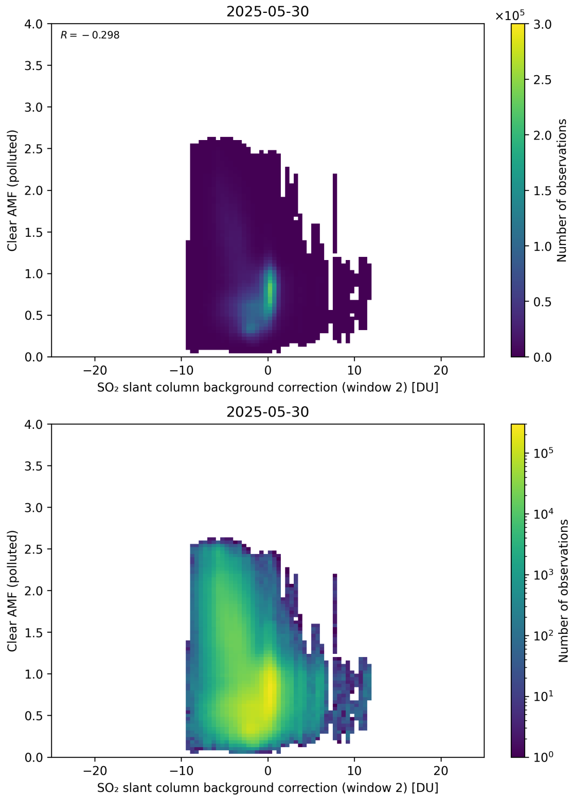
Figure 126: Scatter density plot of “SO 2 slant column background correction (window 2)” against “Clear AMF (polluted)” for 2025-05-29 to 2025-05-31.
