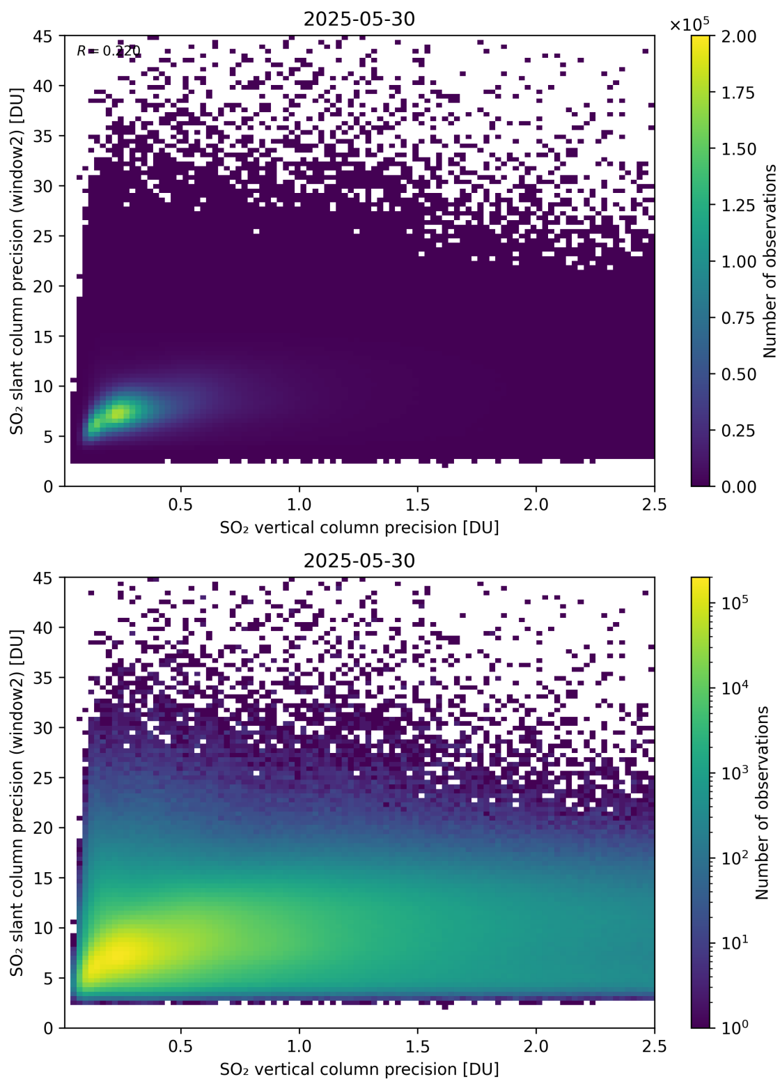
Figure 343: Scatter density plot of “SO 2 vertical column precision” against “SO 2 slant column precision (window2)” for 2025-05-29 to 2025-05-31.
