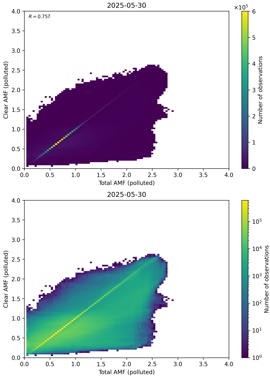
Figure 321: Scatter density plot of “Total AMF (polluted)” against “Clear AMF (polluted)” for 2025-05-29 to 2025-05-31.
