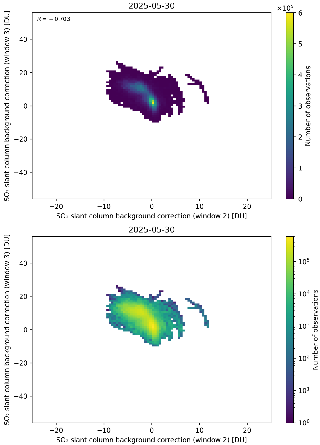
Figure 122: Scatter density plot of “SO 2 slant column background correction (window 2)” against “SO 2 slant column background correction (window 3)” for 2025-05-29 to 2025-05-31.
