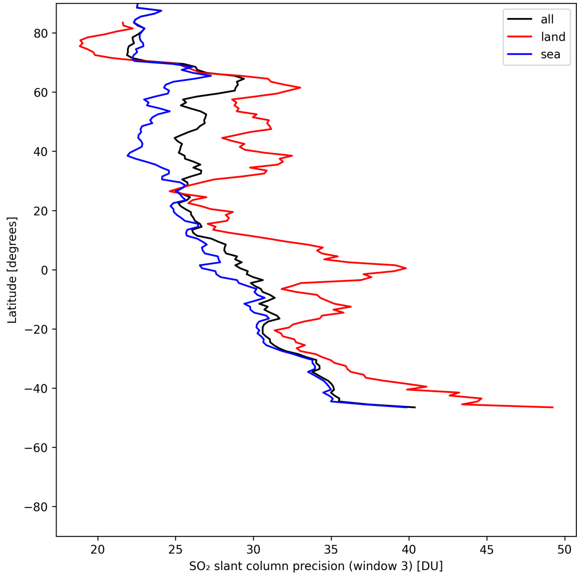
Figure 46: Zonal average of “SO 2 slant column precision (window 3)” for 2025-05-29 to 2025-05-31.
