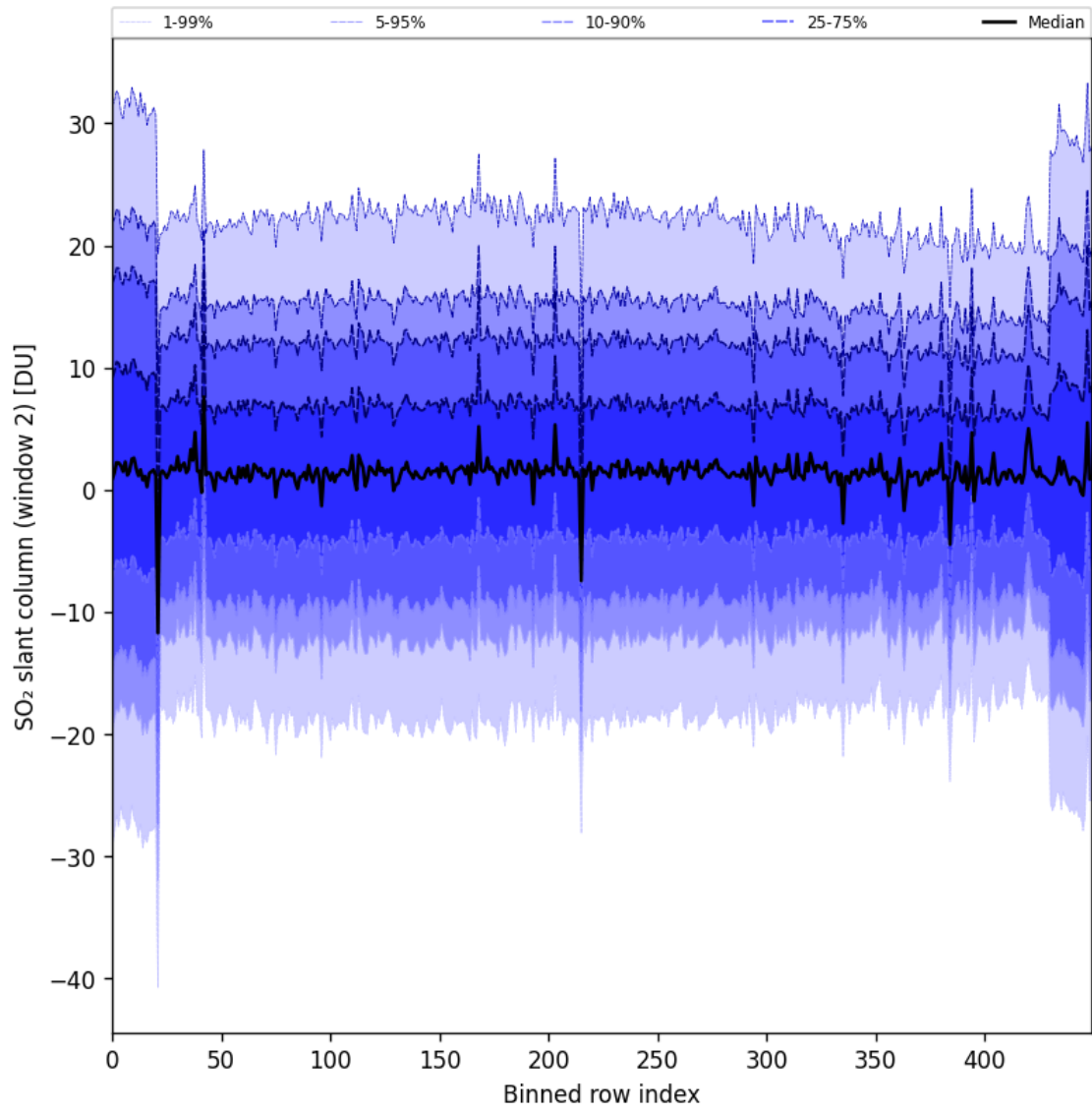
Figure 93: Along track statistics of “SO 2 slant column (window 2)” for 2025-05-29 to 2025-05-31
