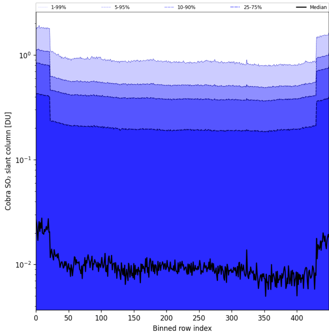
Figure 87: Along track statistics of “Cobra SO 2 slant column” for 2025-05-29 to 2025-05-31
