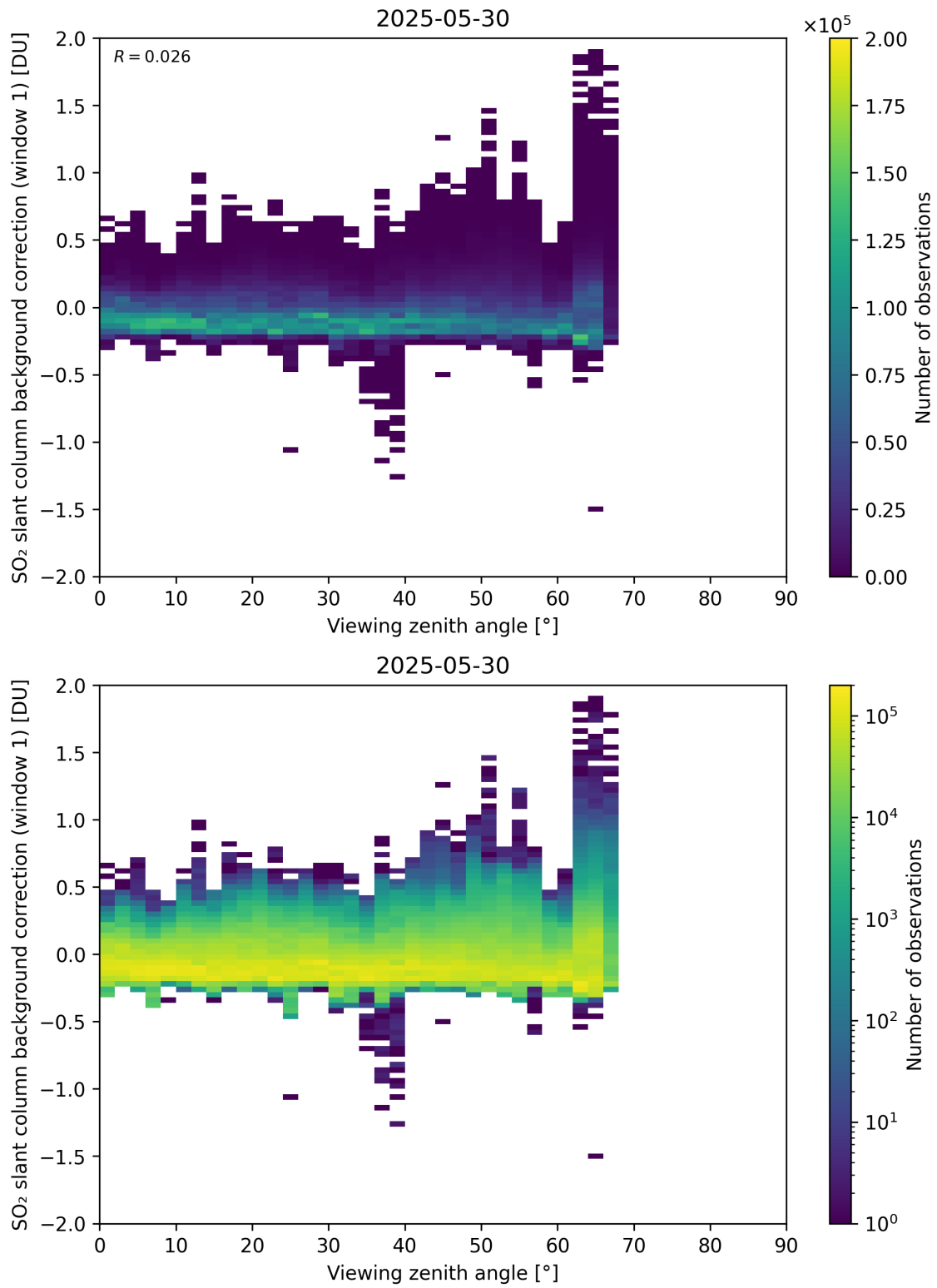
Figure 362: Scatter density plot of “Viewing zenith angle” against “SO 2 slant column background correction (window 1)” for 2025-05-29 to 2025-05-31.
