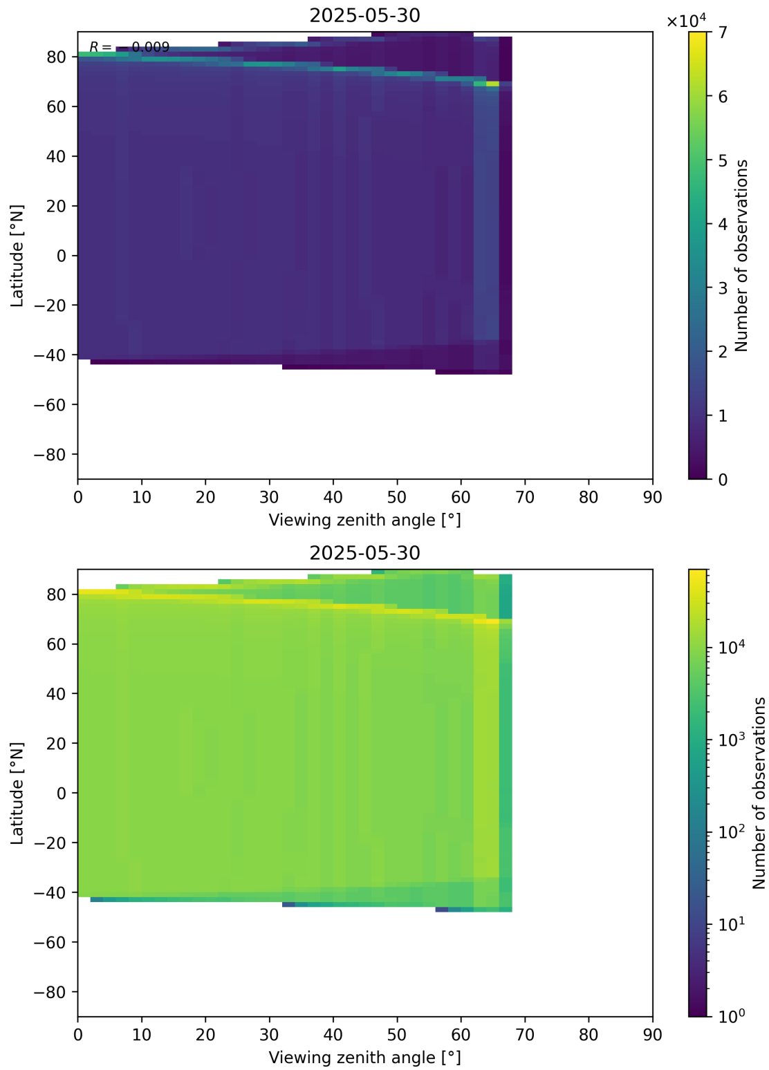
Figure 368: Scatter density plot of “Viewing zenith angle” against “Latitude” for 2025-05-29 to 2025-05-31.
