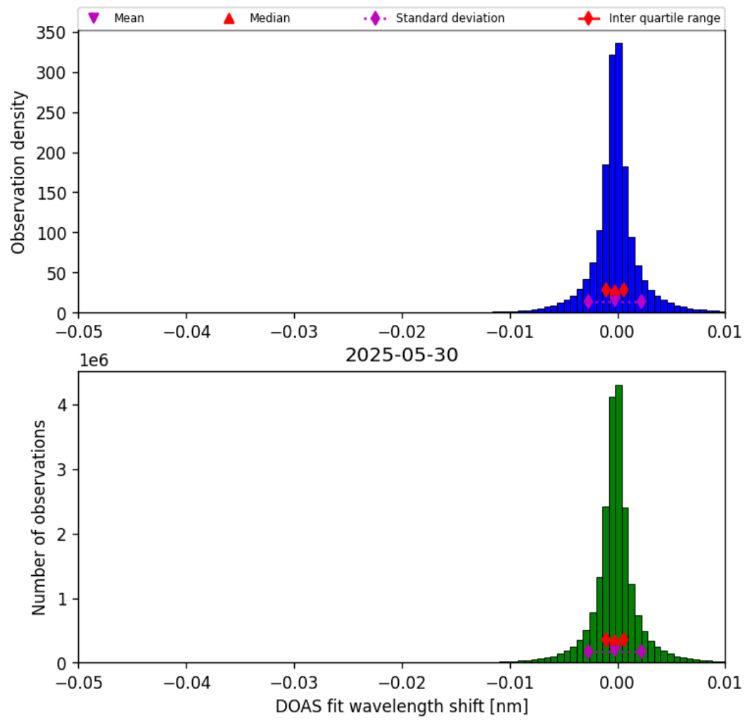
Figure 76: Histogram of “DOAS fit wavelength shift” for 2025-05-29 to 2025-05-31
