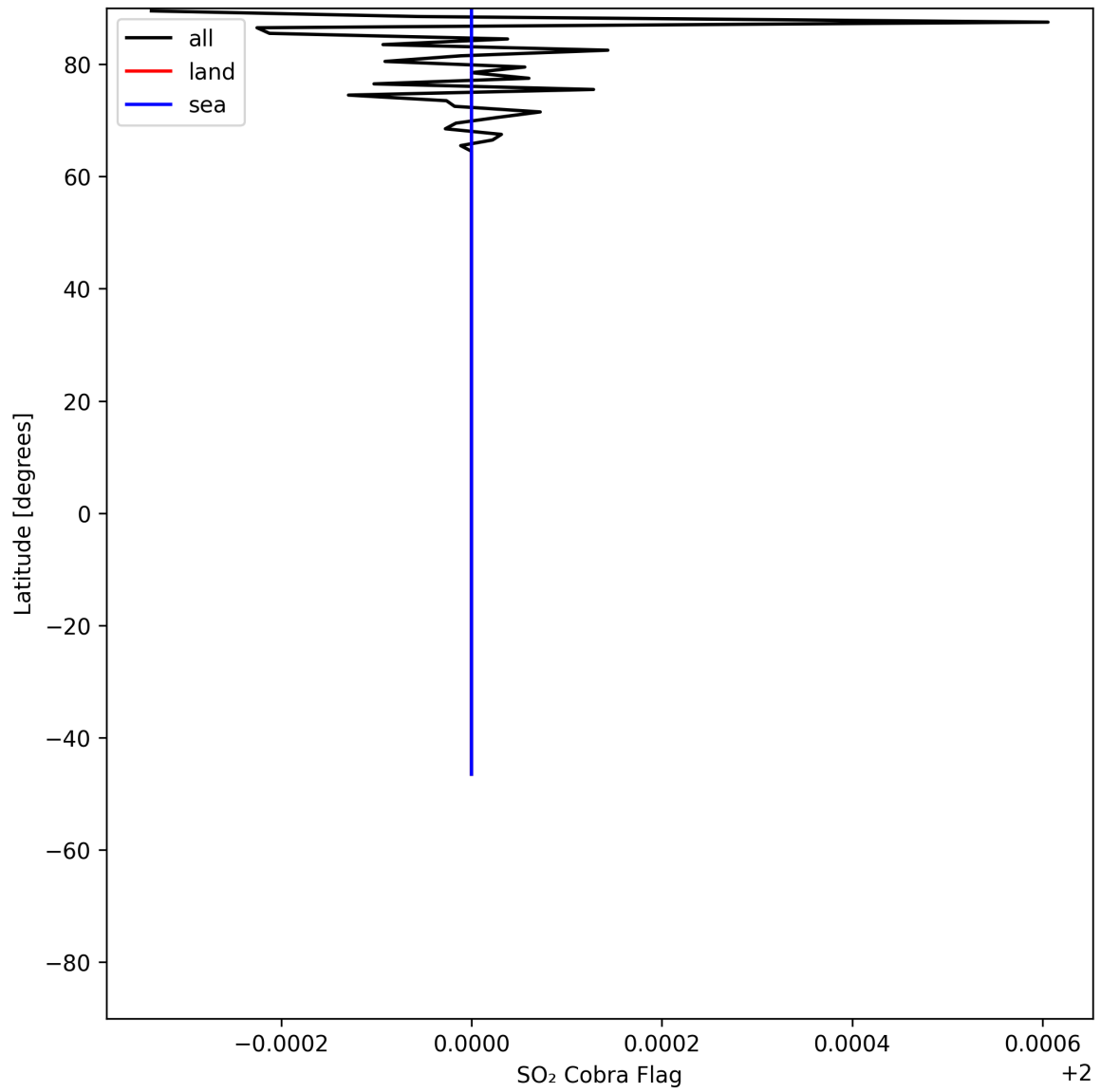
Figure 49: Zonal average of “SO 2 Cobra Flag” for 2025-05-29 to 2025-05-31.
