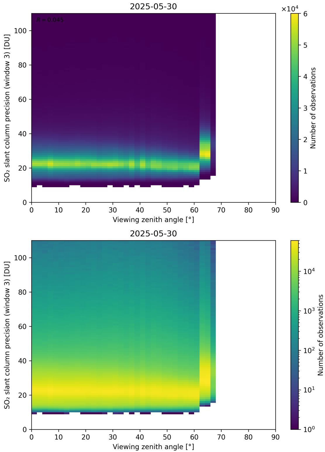
Figure 380: Scatter density plot of “Viewing zenith angle” against “SO 2 slant column precision (window 3)” for 2025-05-29 to 2025-05-31.
