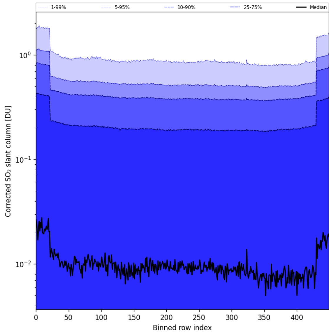
Figure 86: Along track statistics of "Corrected SO 2 slant column" for 2025-05-29 to 2025-05-31
