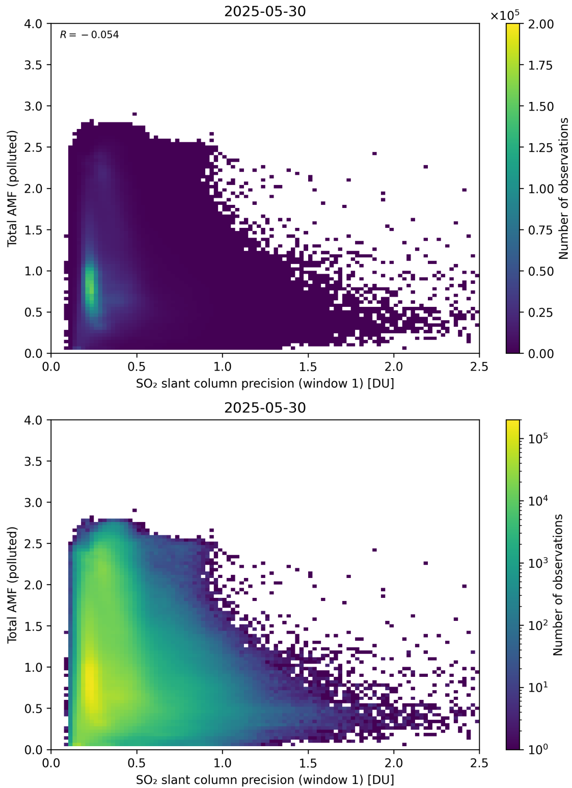
Figure 280: Scatter density plot of “SO 2 slant column precision (window 1)” against “Total AMF (polluted)” for 2025-05-29 to 2025-05-31.
