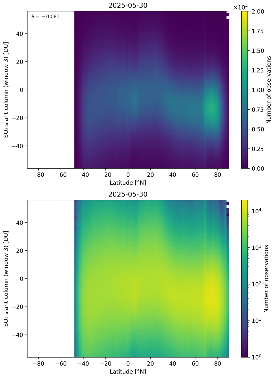
Figure 165: Scatter density plot of “Latitude” against “SO 2 slant column (window 3)” for 2025-05-29 to 2025-05-31.
