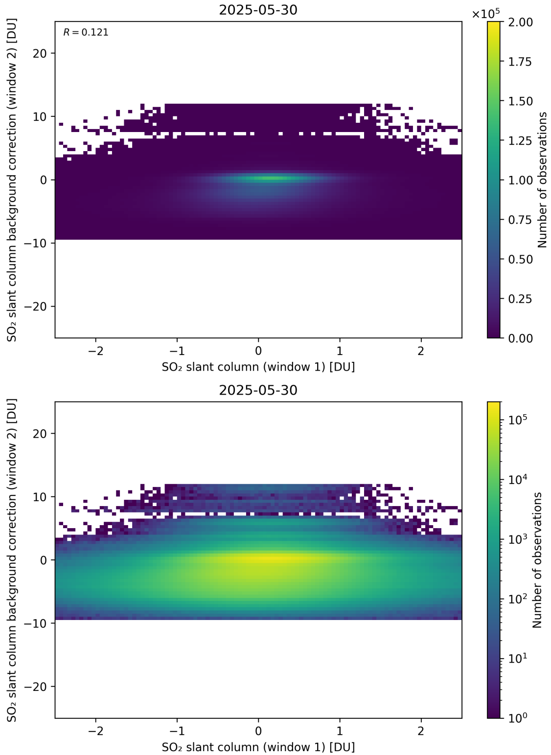
Figure 263: Scatter density plot of “SO 2 slant column (window 1)” against “SO 2 slant column background correction (window 2)” for 2025-05-29 to 2025-05-31.
