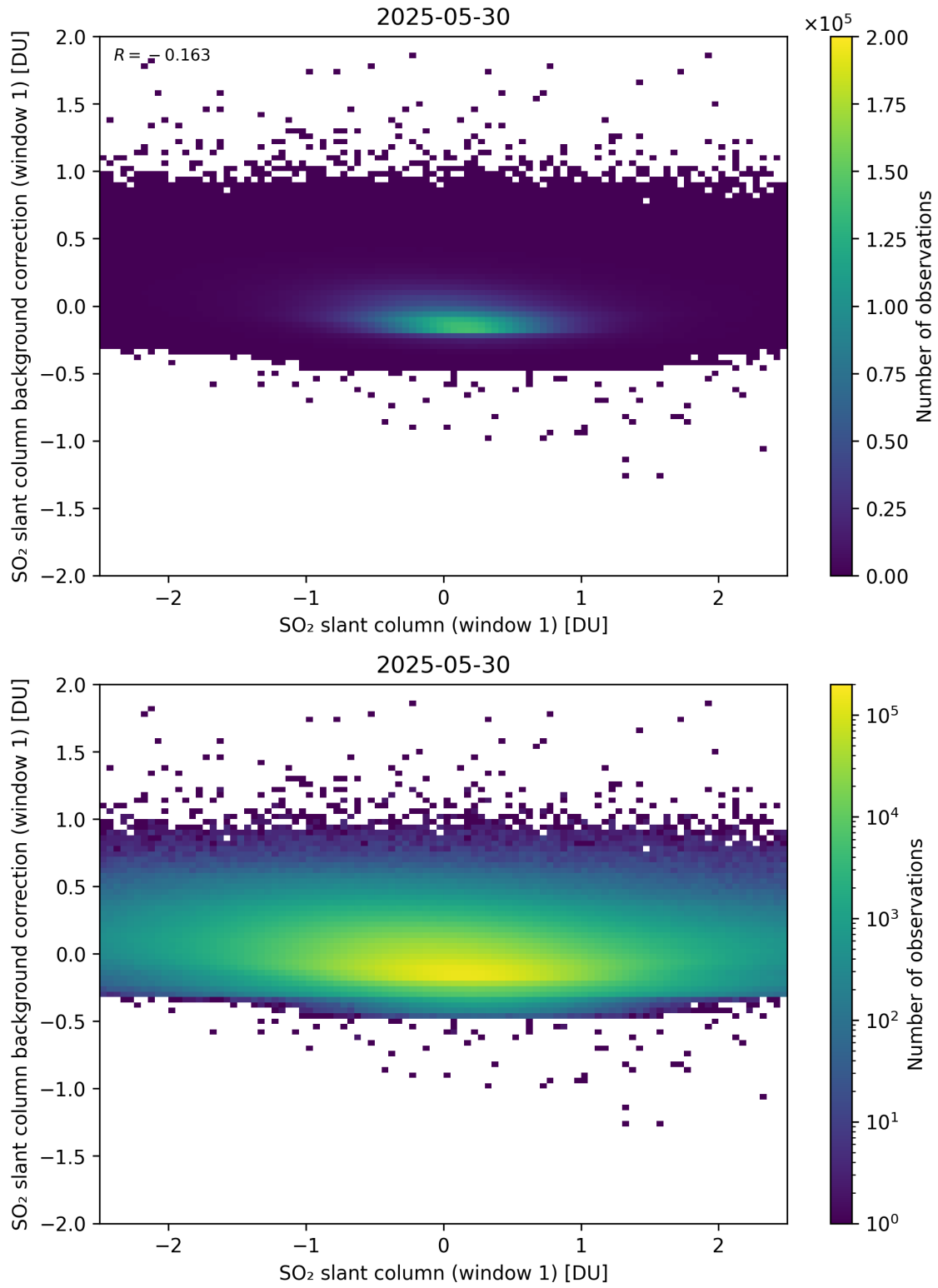
Figure 262: Scatter density plot of “SO 2 slant column (window 1)” against “SO 2 slant column background correction (window 1)” for 2025-05-29 to 2025-05-31.
