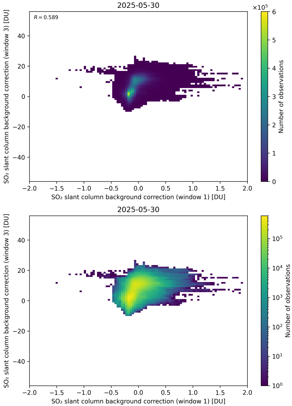
Figure 110: Scatter density plot of “SO 2 slant column background correction (window 1)” against “SO 2 slant column background correction (window 3)” for 2025-05-29 to 2025-05-31.
