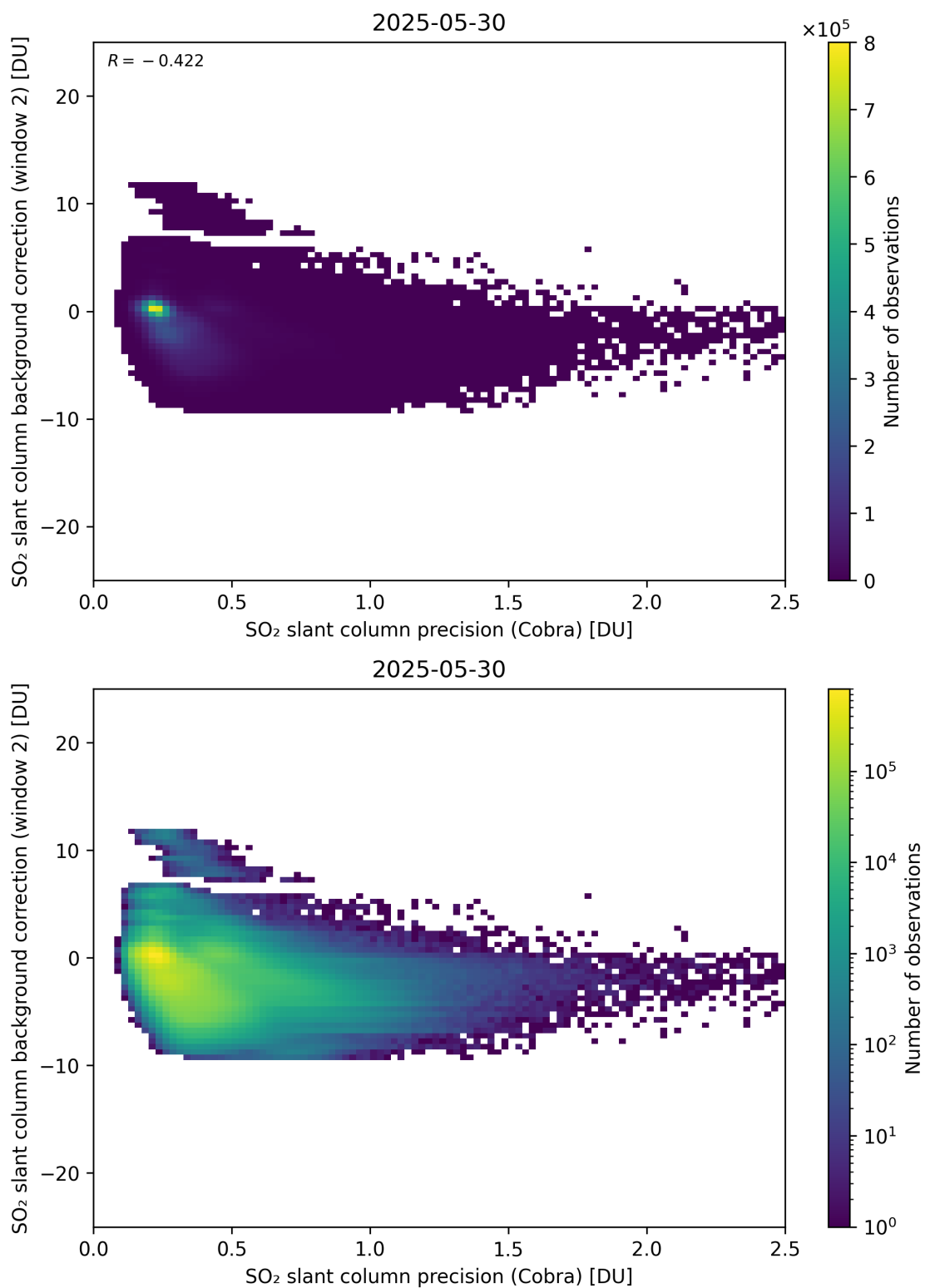
Figure 200: Scatter density plot of “SO 2 slant column precision (Cobra)” against “SO 2 slant column background correction (window 2)” for 2025-05-29 to 2025-05-31.
