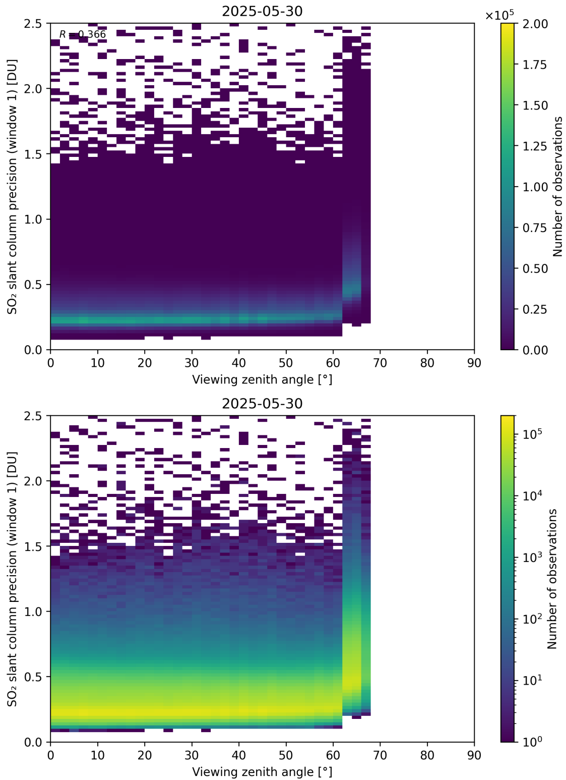
Figure 377: Scatter density plot of “Viewing zenith angle” against “SO 2 slant column precision (window 1)” for 2025-05-29 to 2025-05-31.
