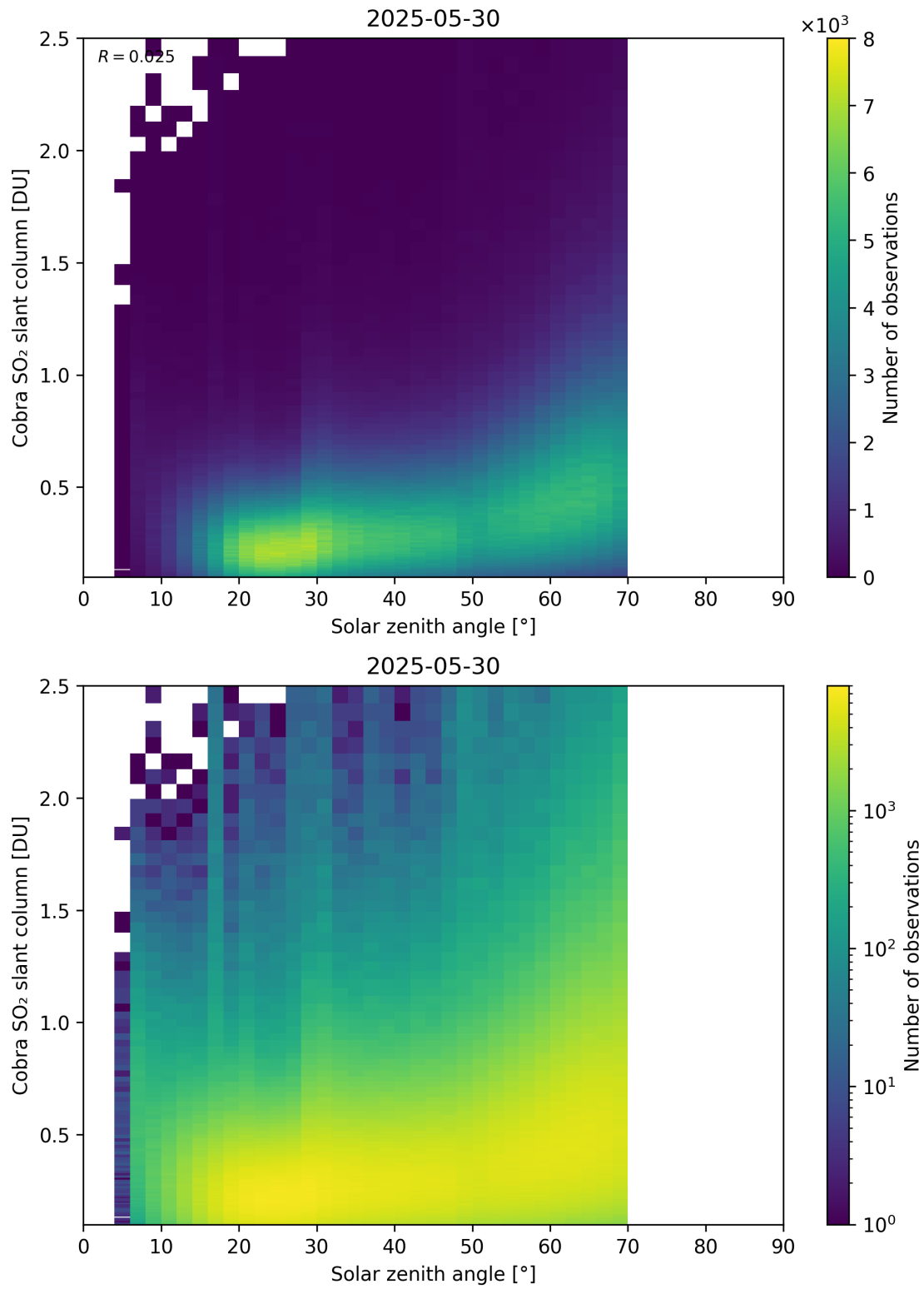
Figure 179: Scatter density plot of “Solar zenith angle” against “Cobra SO 2 slant column” for 2025-05-29 to 2025-05-31.
