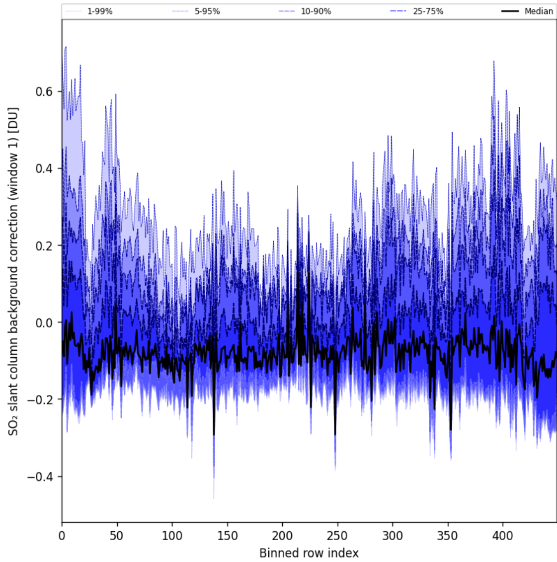
Figure 92: Along track statistics of “SO 2 slant column background correction (window 1)” for 2025-05-29 to 2025-05-31
