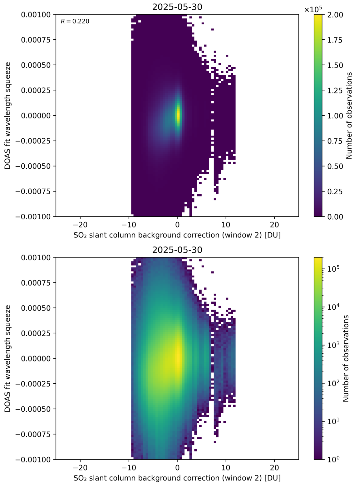
Figure 124: Scatter density plot of “SO 2 slant column background correction (window 2)” against “DOAS fit wavelength squeeze” for 2025-05-29 to 2025-05-31.
