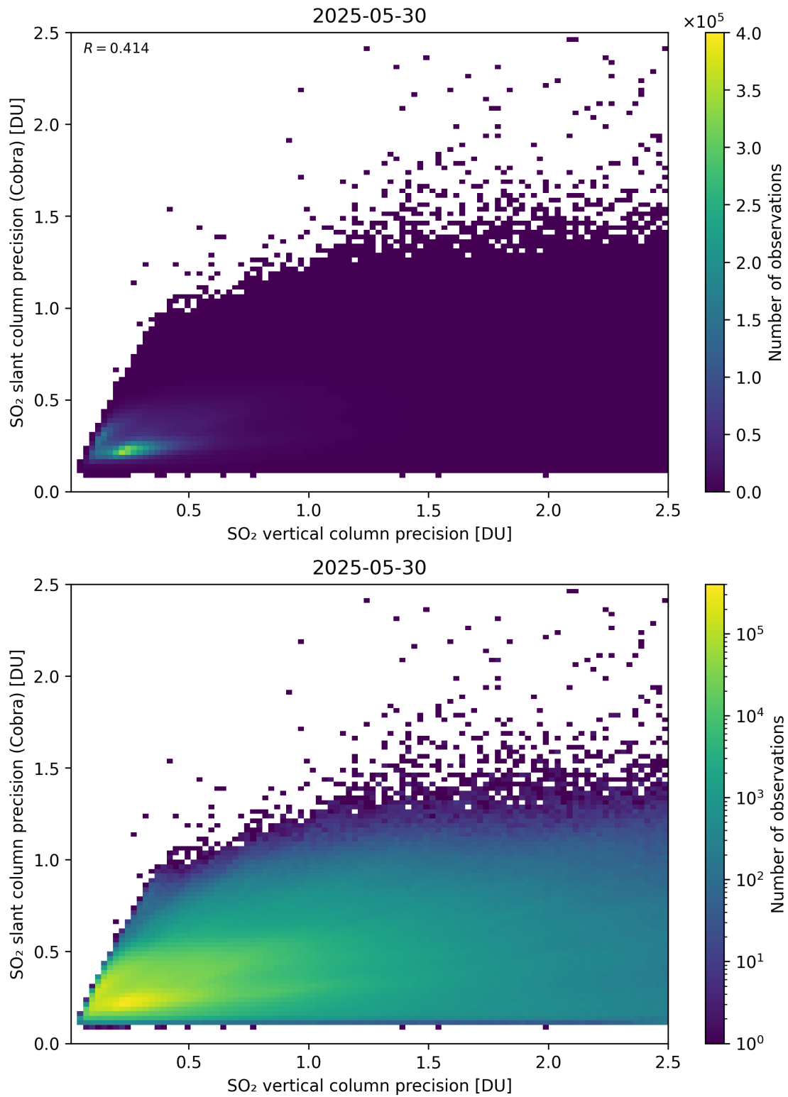
Figure 337: Scatter density plot of “SO 2 vertical column precision” against “SO 2 slant column precision (Cobra)” for 2025-05-29 to 2025-05-31.
