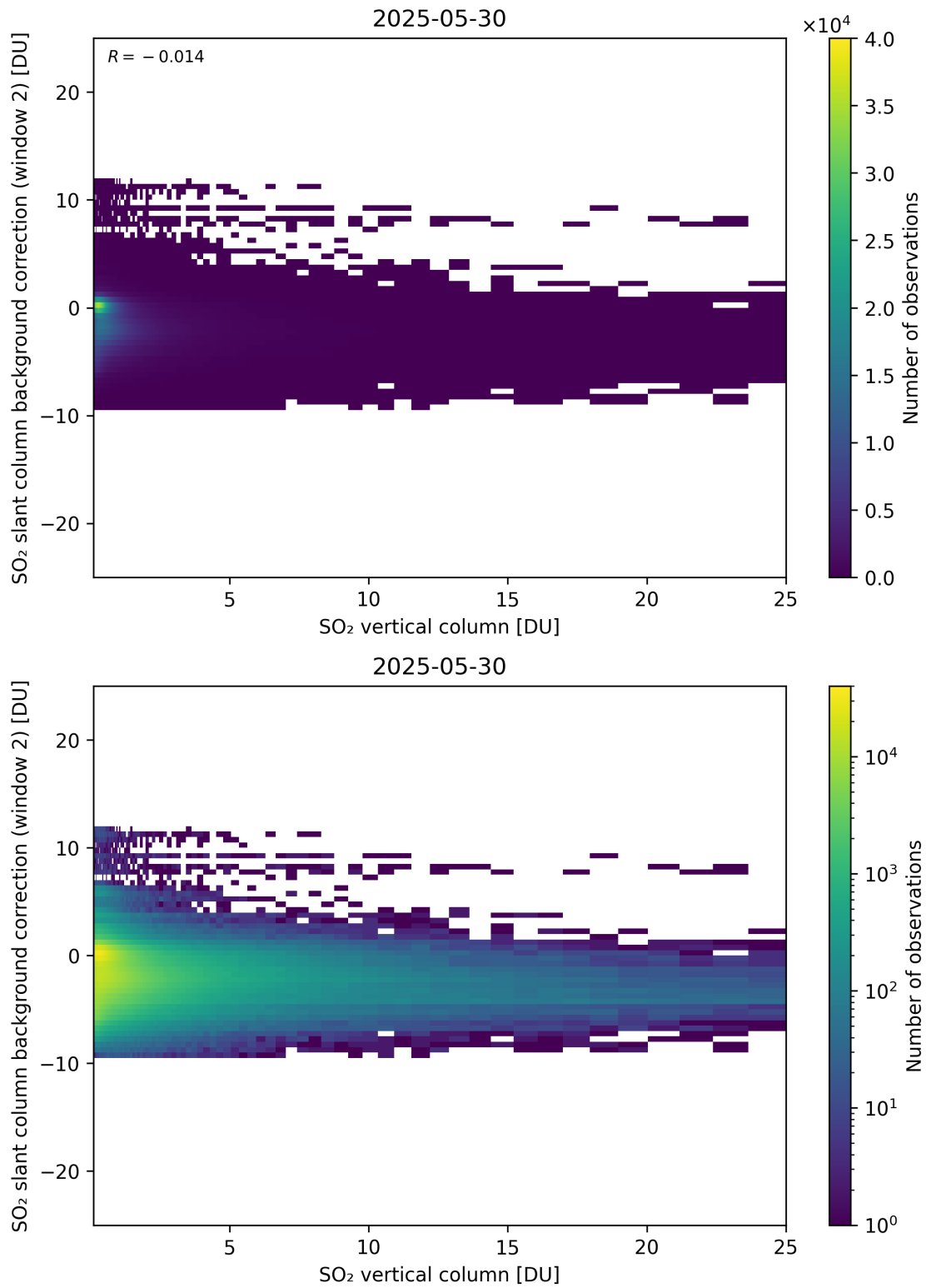
Figure 324: Scatter density plot of “SO 2 vertical column” against “SO 2 slant column background correction (window 2)” for 2025-05-29 to 2025-05-31.
