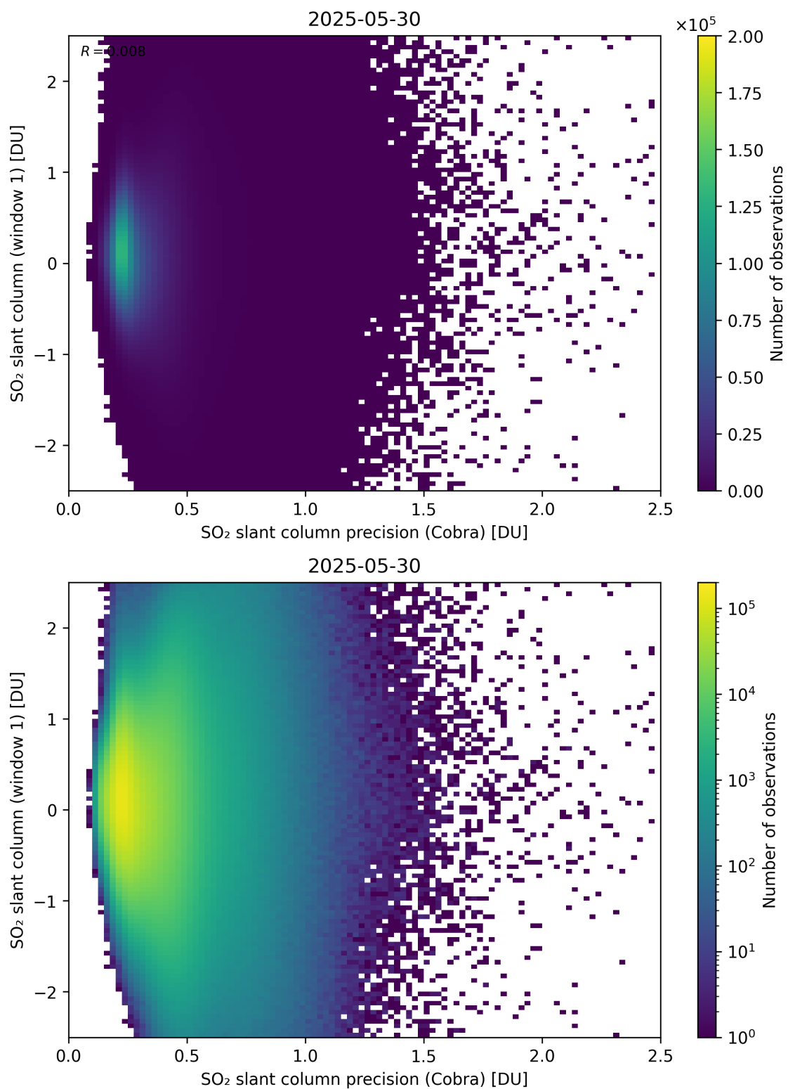
Figure 208: Scatter density plot of “SO 2 slant column precision (Cobra)” against “SO 2 slant column (window 1)” for 2025-05-29 to 2025-05-31.
