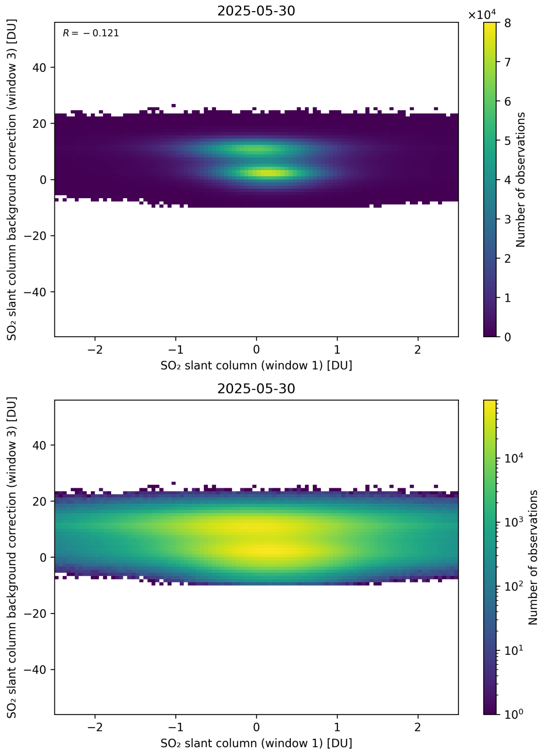
Figure 264: Scatter density plot of “SO 2 slant column (window 1)” against “SO 2 slant column background correction (window 3)” for 2025-05-29 to 2025-05-31.
