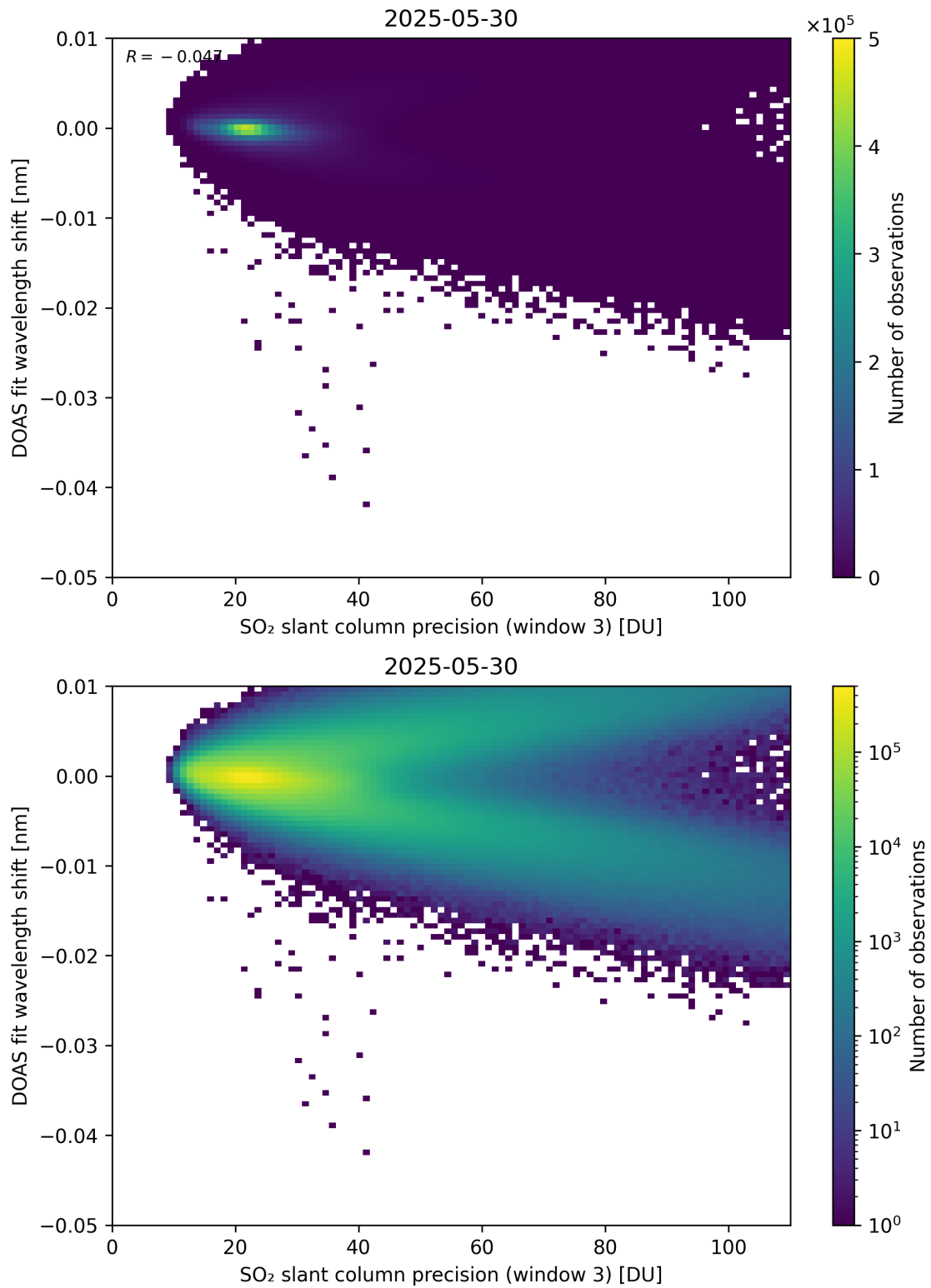
Figure 308: Scatter density plot of “SO 2 slant column precision (window 3)” against “DOAS fit wavelength shift” for 2025-05-29 to 2025-05-31.
