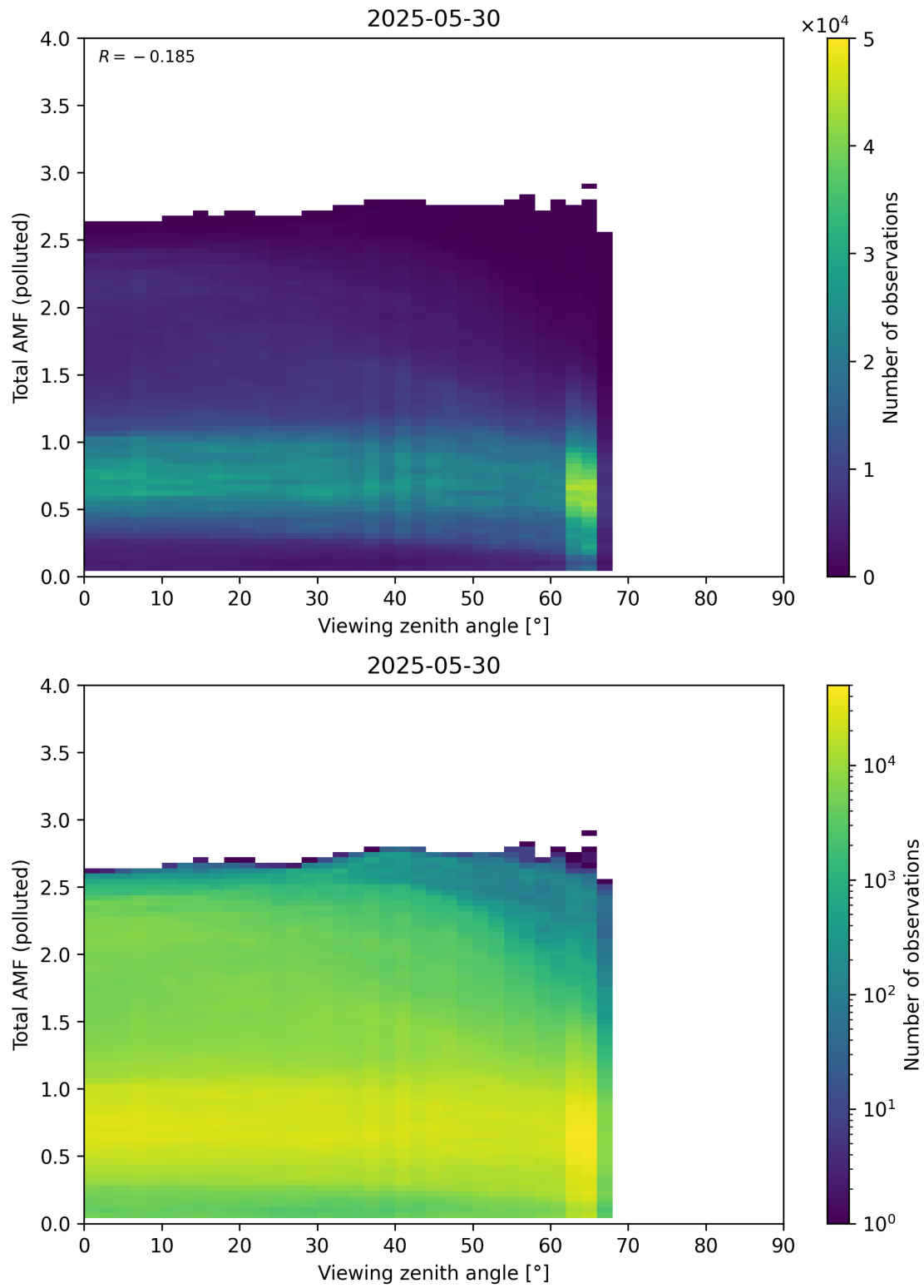
Figure 381: Scatter density plot of “Viewing zenith angle” against “Total AMF (polluted)” for 2025-05-29 to 2025-05-31.
