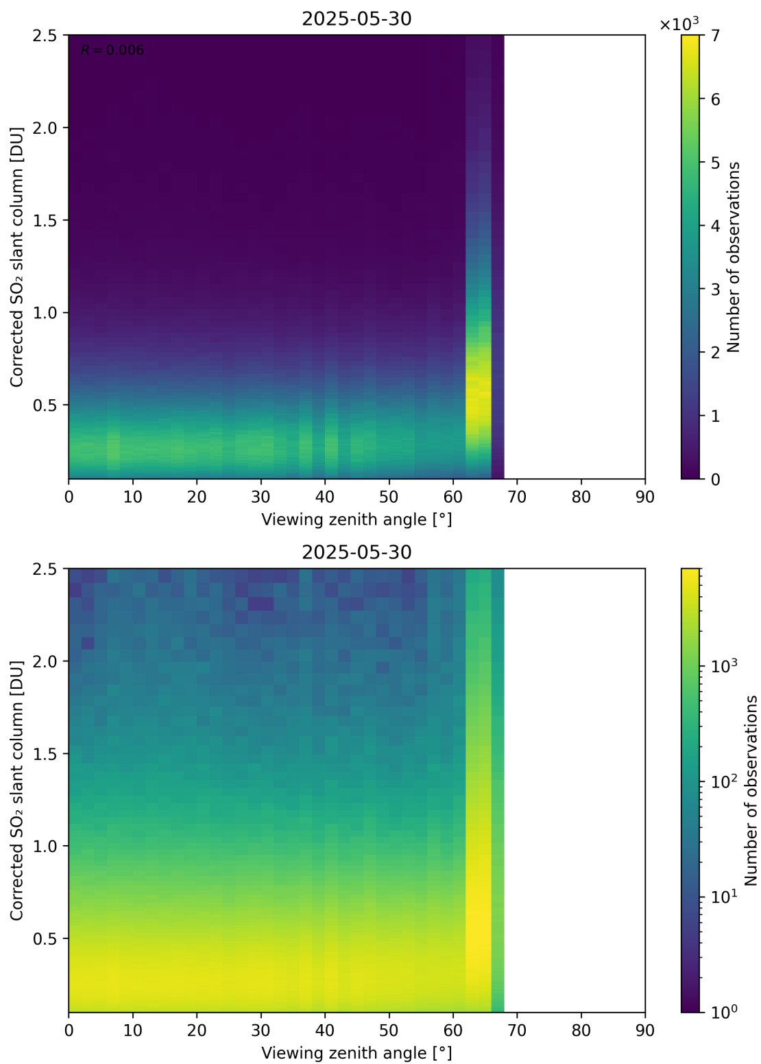
Figure 373: Scatter density plot of “Viewing zenith angle” against “Corrected SO 2 slant column” for 2025-05-29 to 2025-05-31.
