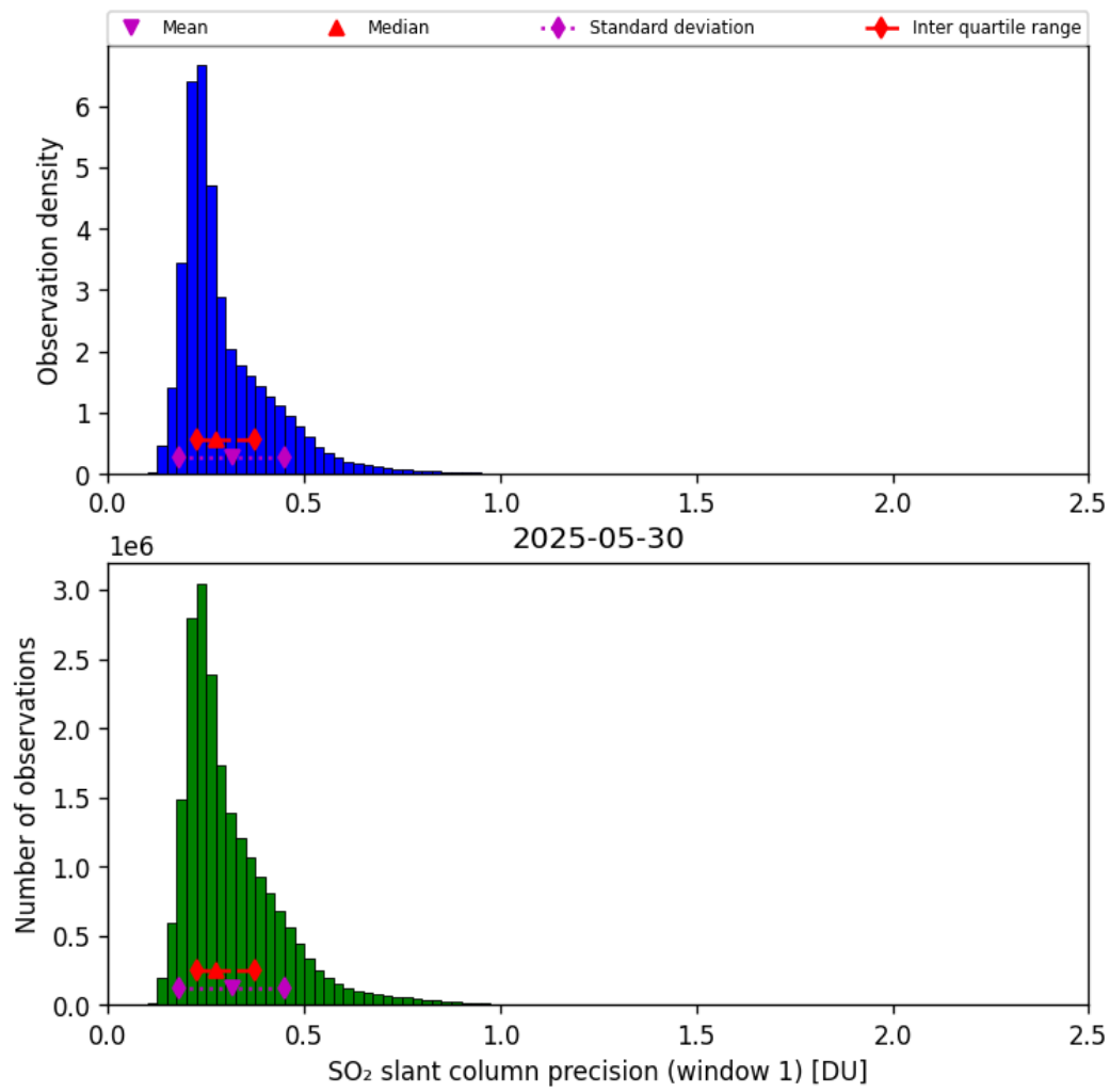
Figure 64: Histogram of “SO 2 slant column precision (window 1)” for 2025-05-29 to 2025-05-31
