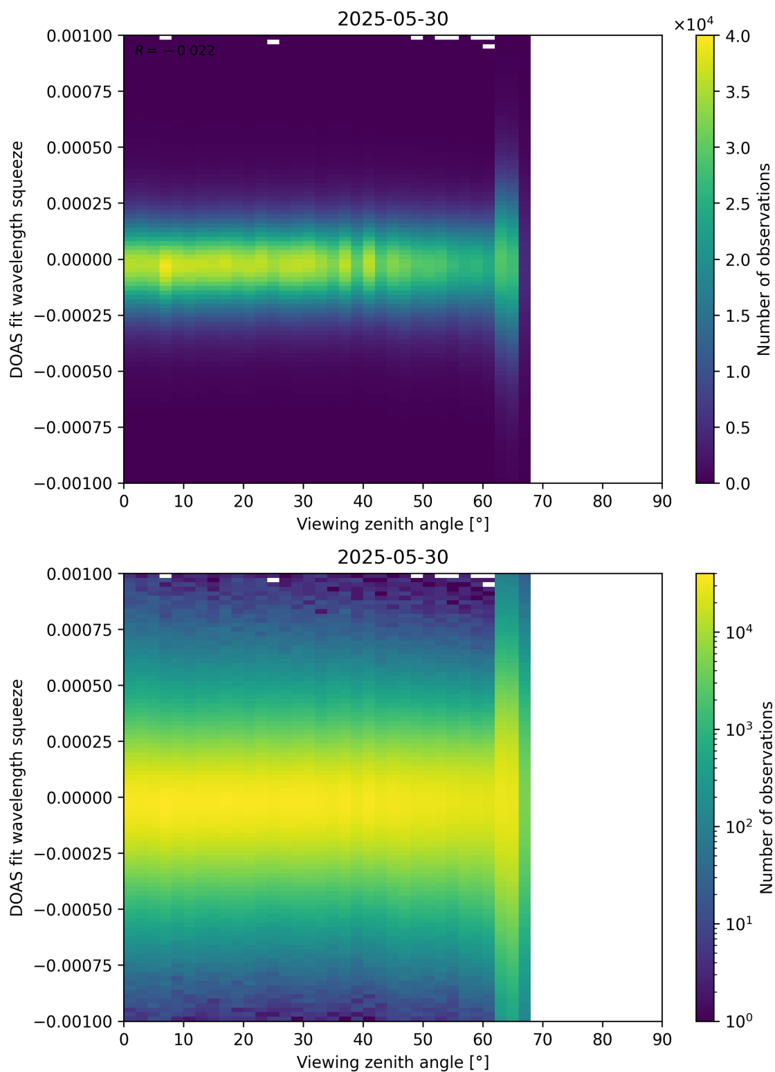
Figure 366: Scatter density plot of “Viewing zenith angle” against “DOAS fit wavelength squeeze” for 2025-05-29 to 2025-05-31.
