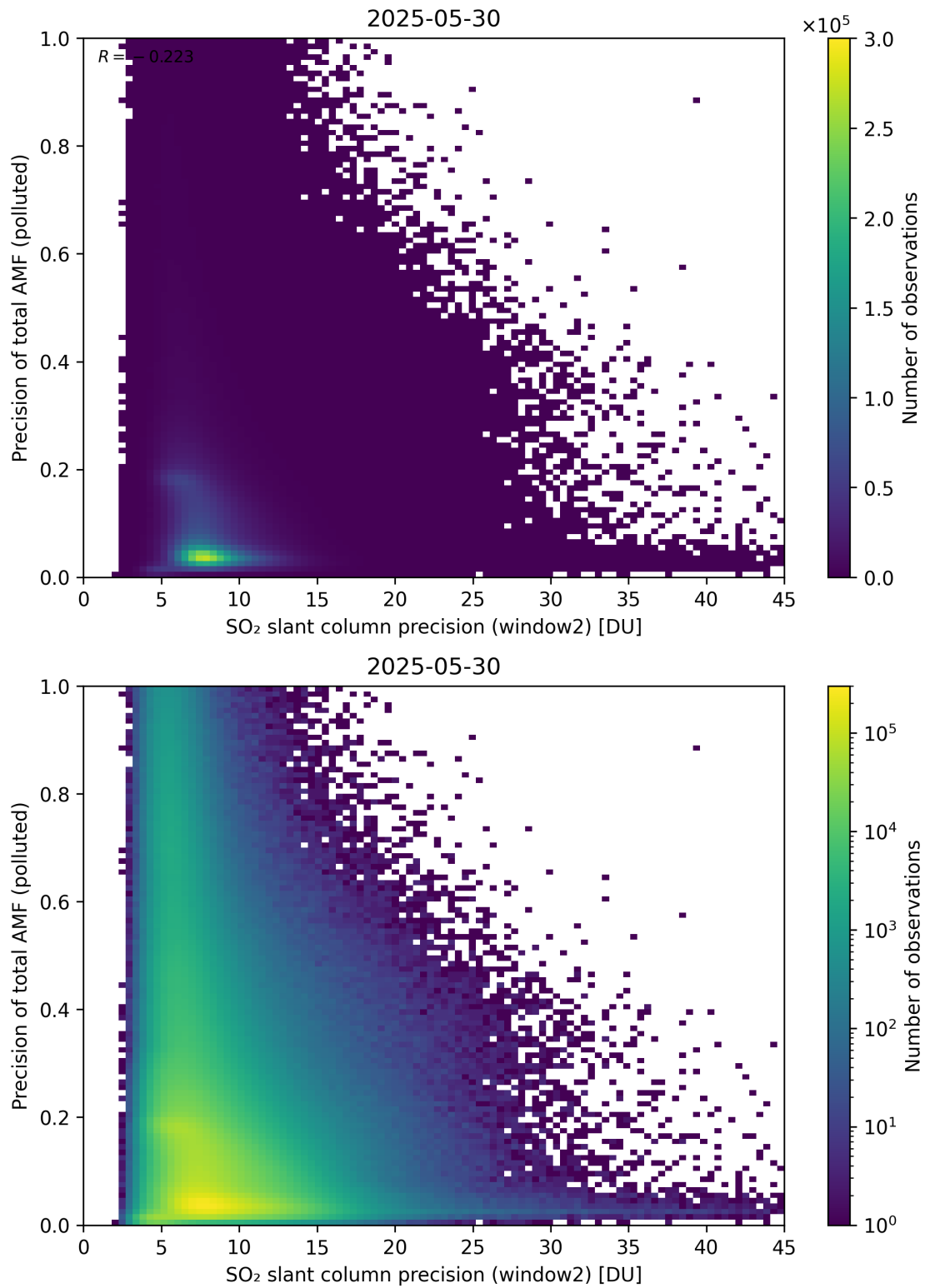
Figure 302: Scatter density plot of “SO 2 slant column precision (window2)” against “Precision of total AMF (polluted)” for 2025-05-29 to 2025-05-31.
