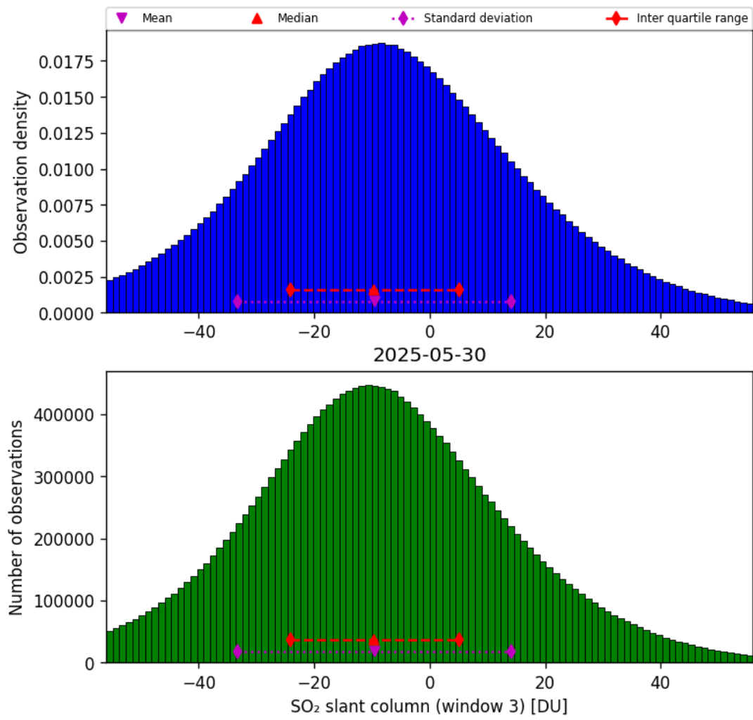
Figure 71: Histogram of “SO 2 slant column (window 3)” for 2025-05-29 to 2025-05-31
