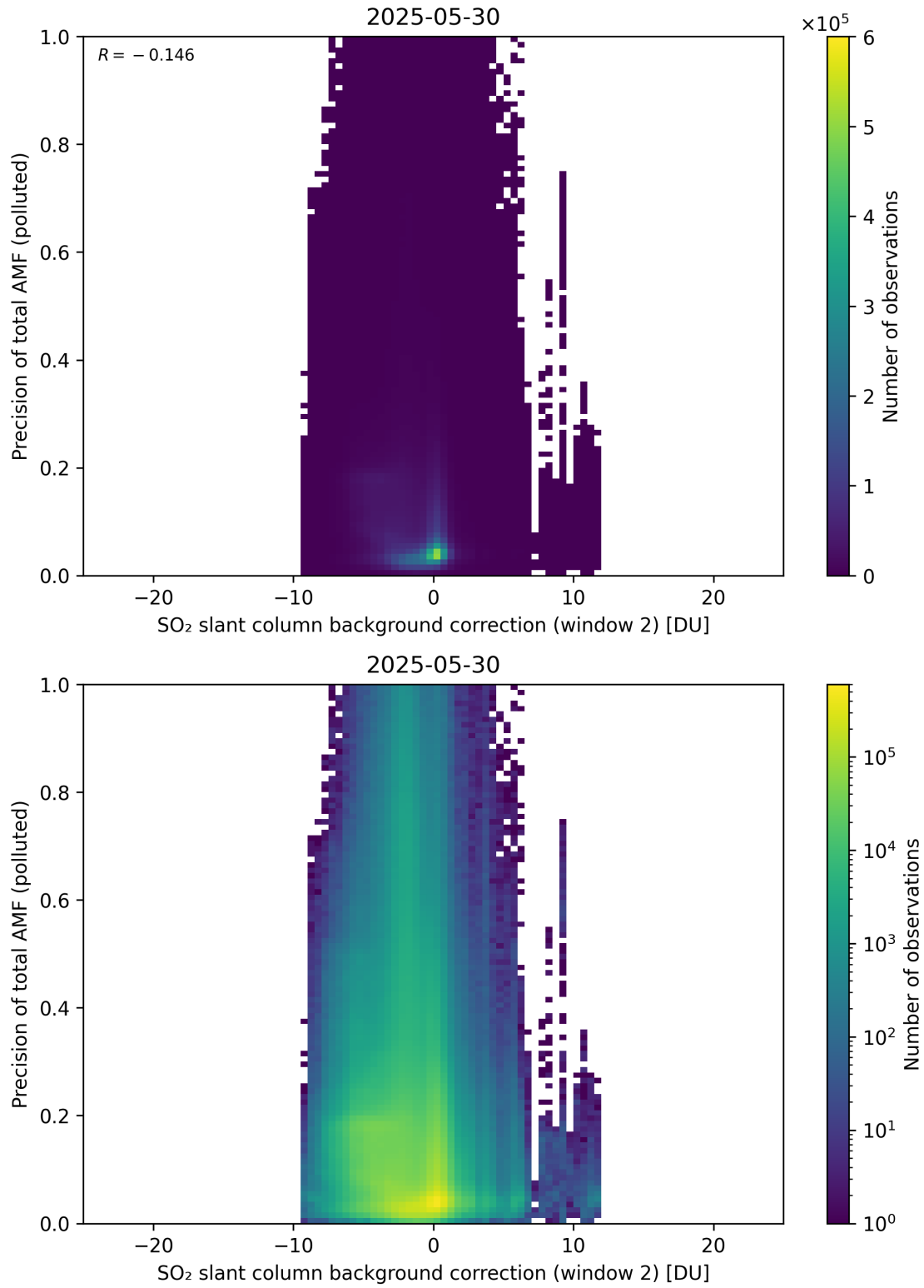
Figure 131: Scatter density plot of “SO 2 slant column background correction (window 2)” against “Precision of total AMF (polluted)” for 2025-05-29 to 2025-05-31.
