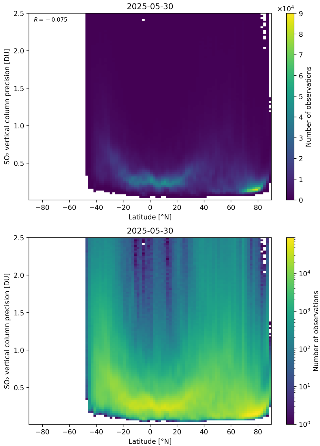
Figure 170: Scatter density plot of “Latitude” against “SO 2 vertical column precision” for 2025-05-29 to 2025-05-31.
