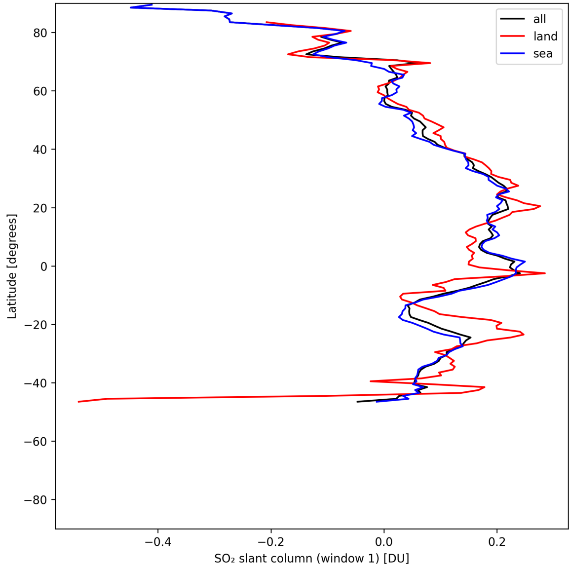
Figure 37: Zonal average of “SO 2 slant column (window 1)” for 2025-05-29 to 2025-05-31.
