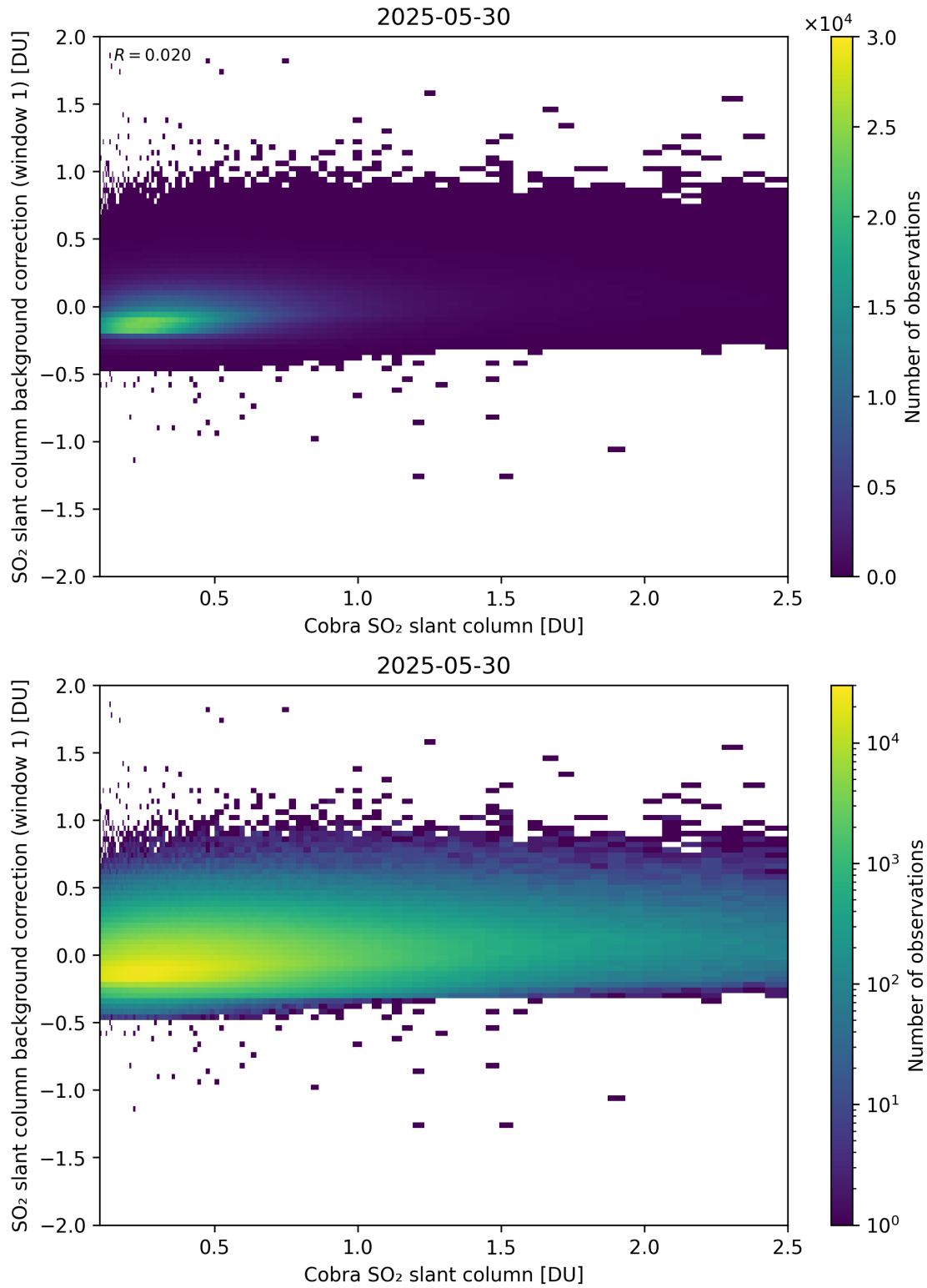
Figure 193: Scatter density plot of “Cobra SO 2 slant column” against “SO 2 slant column background correction (window 1)” for 2025-05-29 to 2025-05-31.
