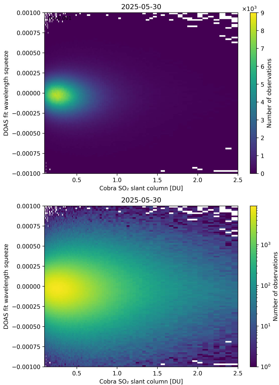
Figure 197: Scatter density plot of “Cobra SO 2 slant column” against “DOAS fit wavelength squeeze” for 2025-05-29 to 2025-05-31.
