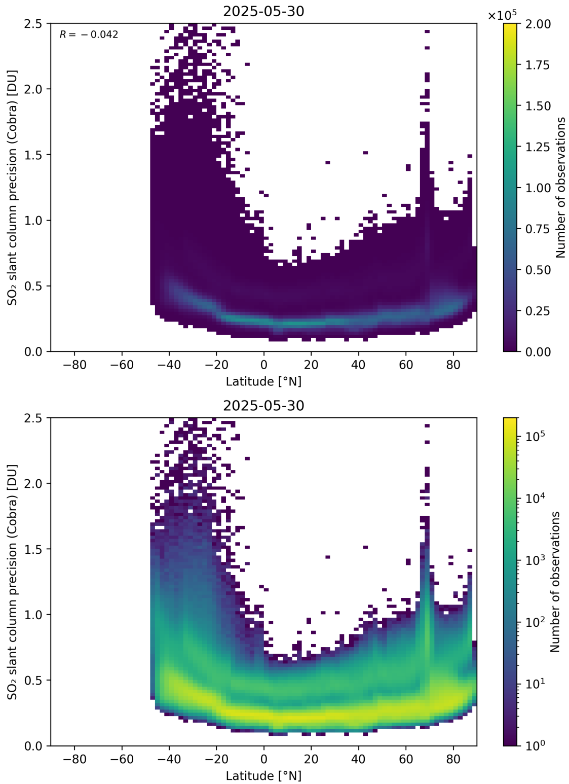
Figure 158: Scatter density plot of “Latitude” against “SO 2 slant column precision (Cobra)” for 2025-05-29 to 2025-05-31.
