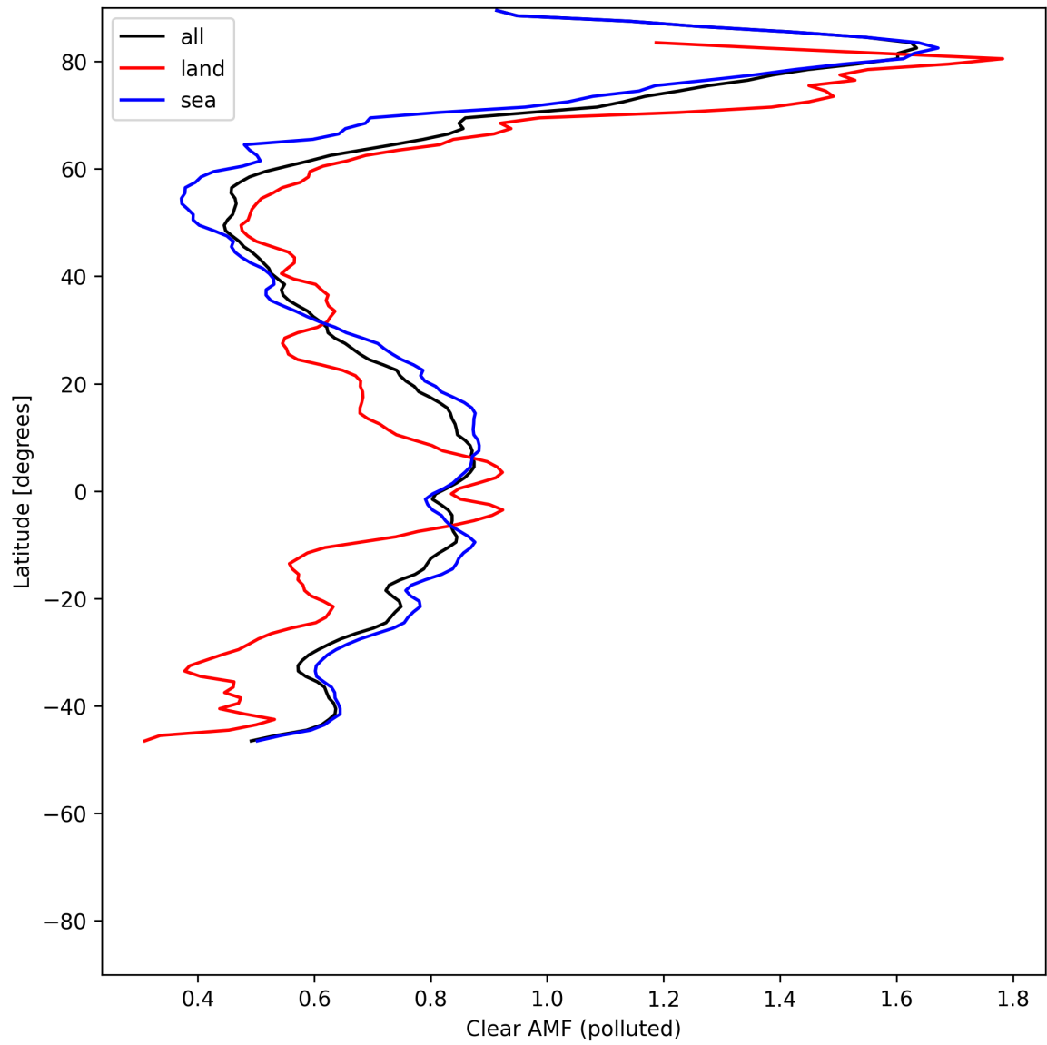
Figure 55: Zonal average of “Clear AMF (polluted)” for 2025-05-29 to 2025-05-31.
