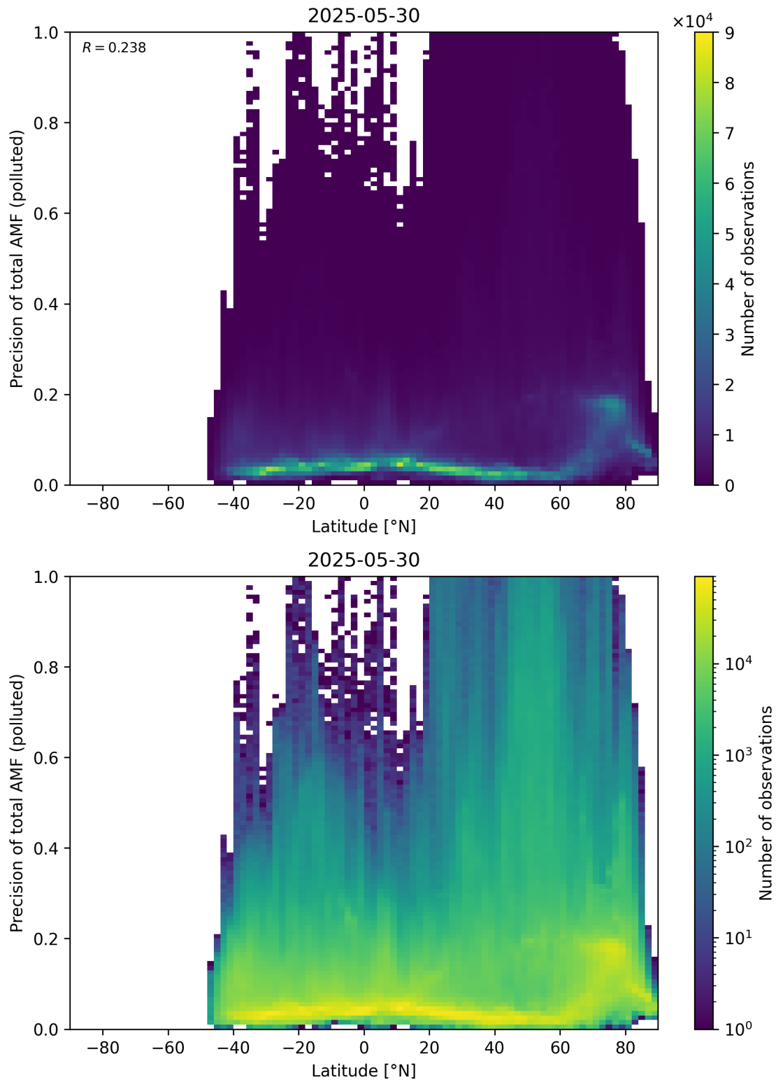
Figure 168: Scatter density plot of “Latitude” against “Precision of total AMF (polluted)” for 2025-05-29 to 2025-05-31.
