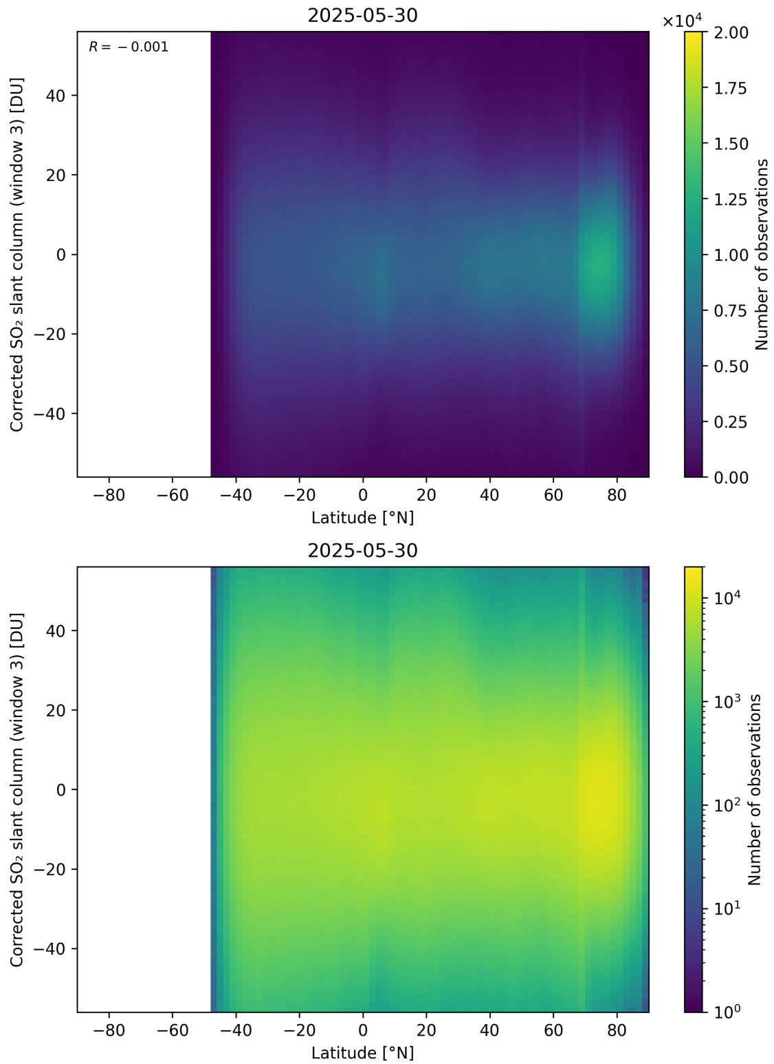
Figure 161: Scatter density plot of “Latitude” against “Corrected SO 2 slant column (window 3)” for 2025-05-29 to 2025-05-31.
