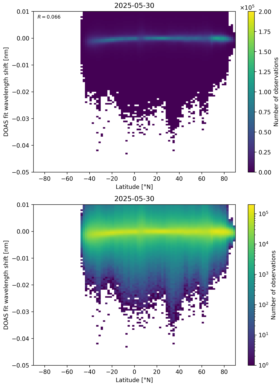
Figure 153: Scatter density plot of “Latitude” against “DOAS fit wavelength shift” for 2025-05-29 to 2025-05-31.
