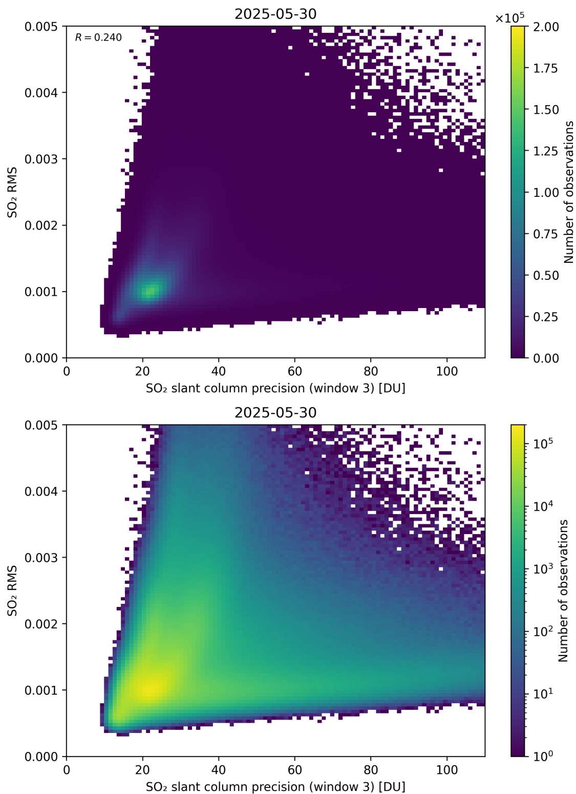
Figure 310: Scatter density plot of “SO 2 slant column precision (window 3)” against “SO 2 RMS” for 2025-05-29 to 2025-05-31.
