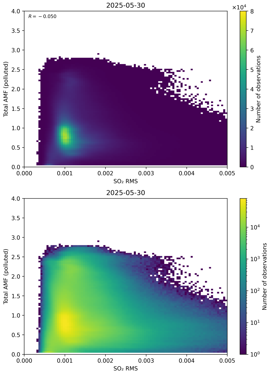
Figure 148: Scatter density plot of “SO 2 RMS” against “Total AMF (polluted)” for 2025-05-29 to 2025-05-31.
