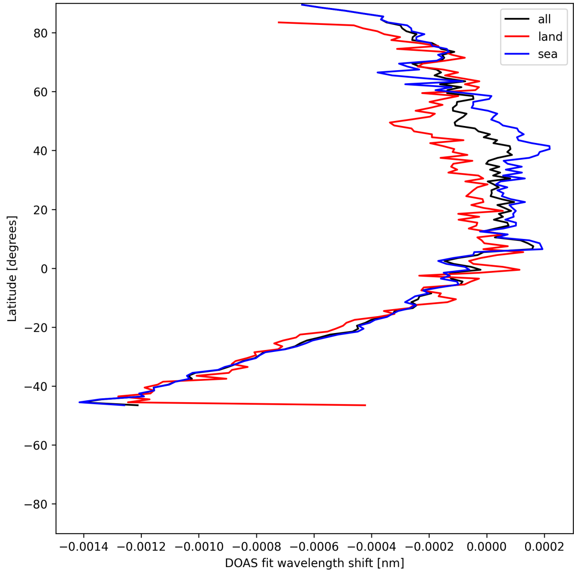
Figure 50: Zonal average of "DOAS fit wavelength shift" for 2025-05-29 to 2025-05-31.
