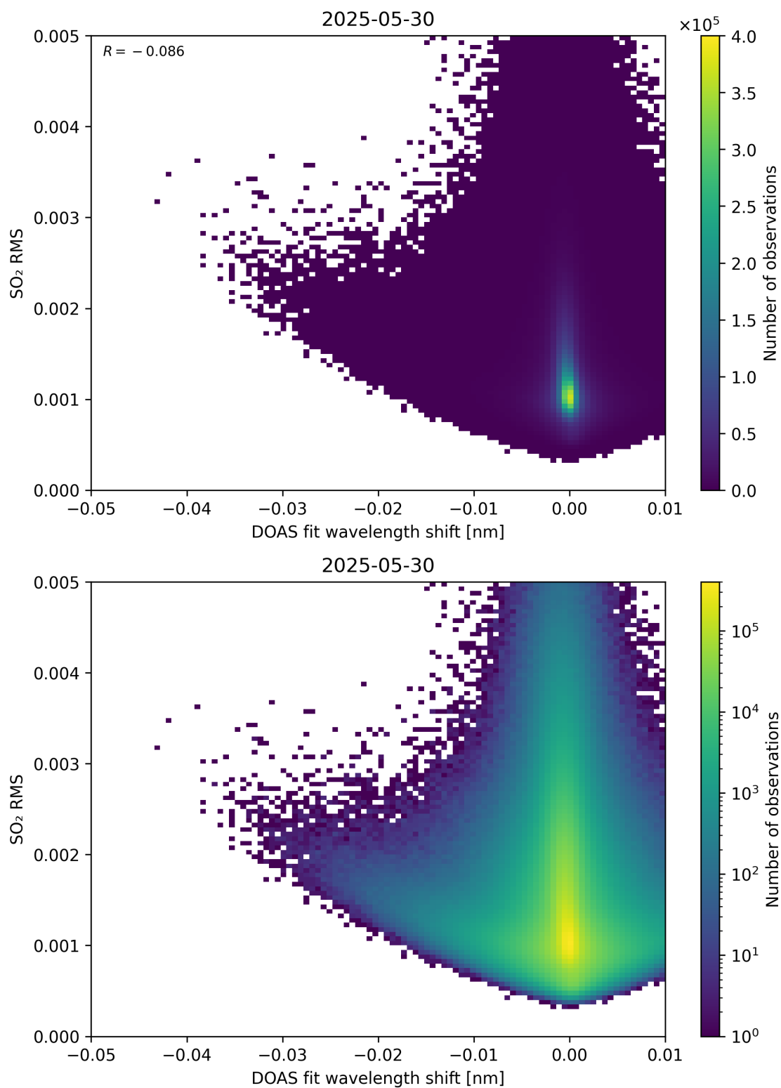
Figure 139: Scatter density plot of “DOAS fit wavelength shift” against “SO 2 RMS” for 2025-05-29 to 2025-05-31.
