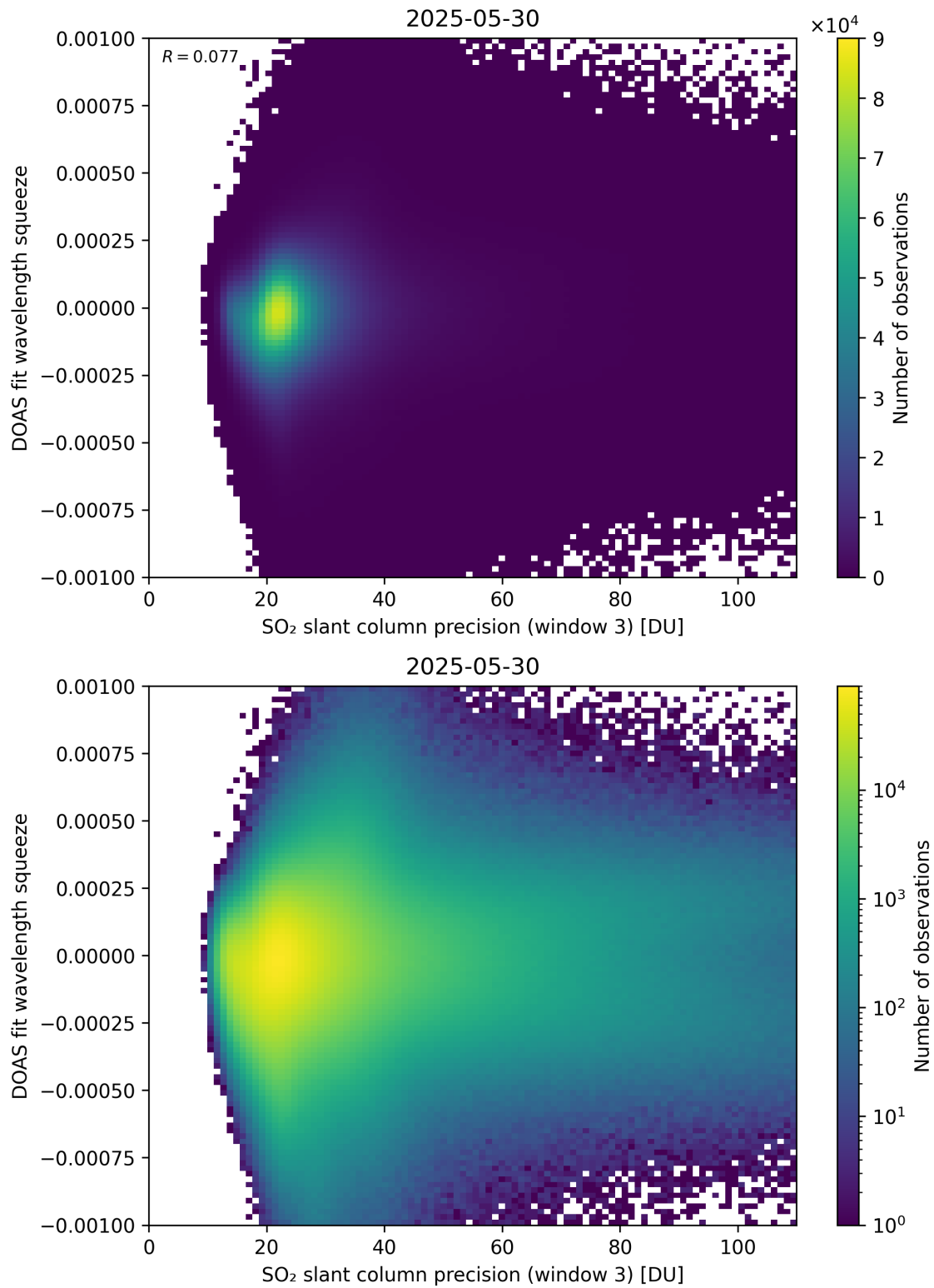
Figure 309: Scatter density plot of “SO 2 slant column precision (window 3)” against “DOAS fit wavelength squeeze” for 2025-05-29 to 2025-05-31.
