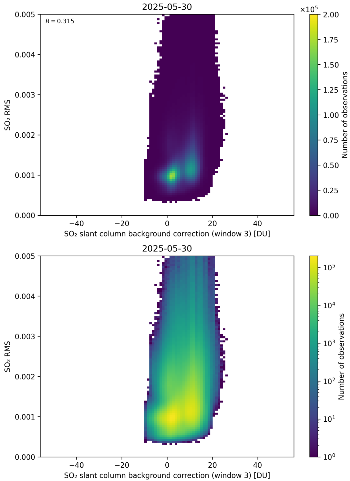
Figure 134: Scatter density plot of “SO 2 slant column background correction (window 3)” against “SO 2 RMS” for 2025-05-29 to 2025-05-31.
