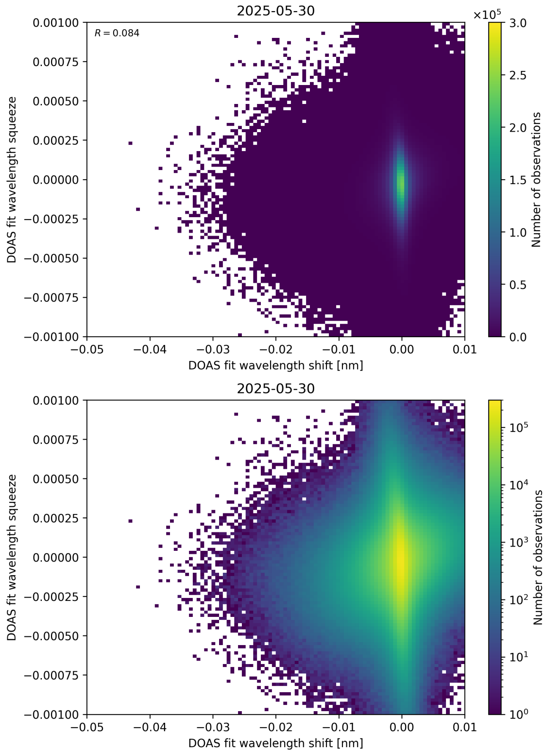
Figure 138: Scatter density plot of “DOAS fit wavelength shift” against “DOAS fit wavelength squeeze” for 2025-05-29 to 2025-05-31.
