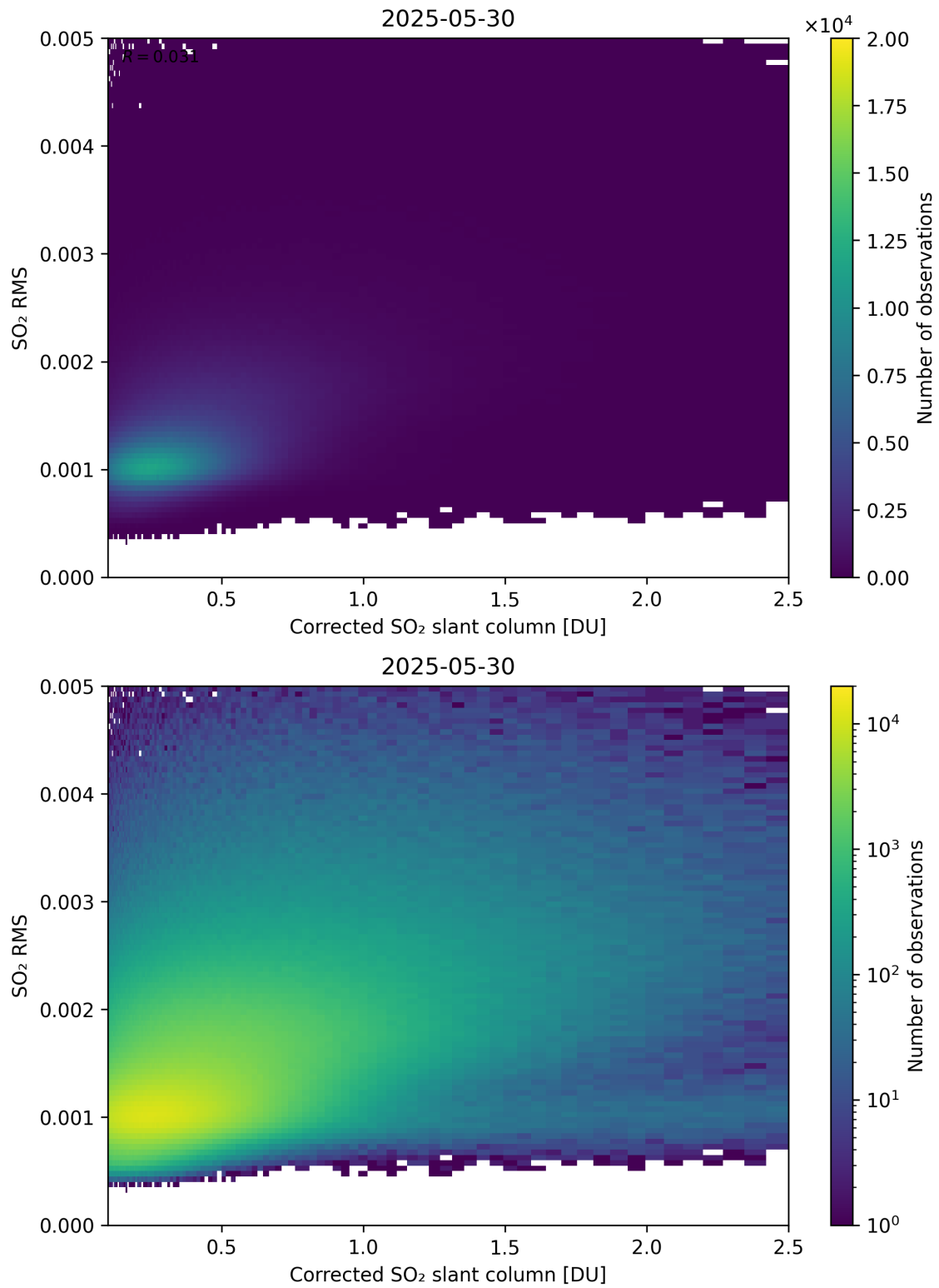
Figure 231: Scatter density plot of “Corrected SO 2 slant column” against “SO 2 RMS” for 2025-05-29 to 2025-05-31.
