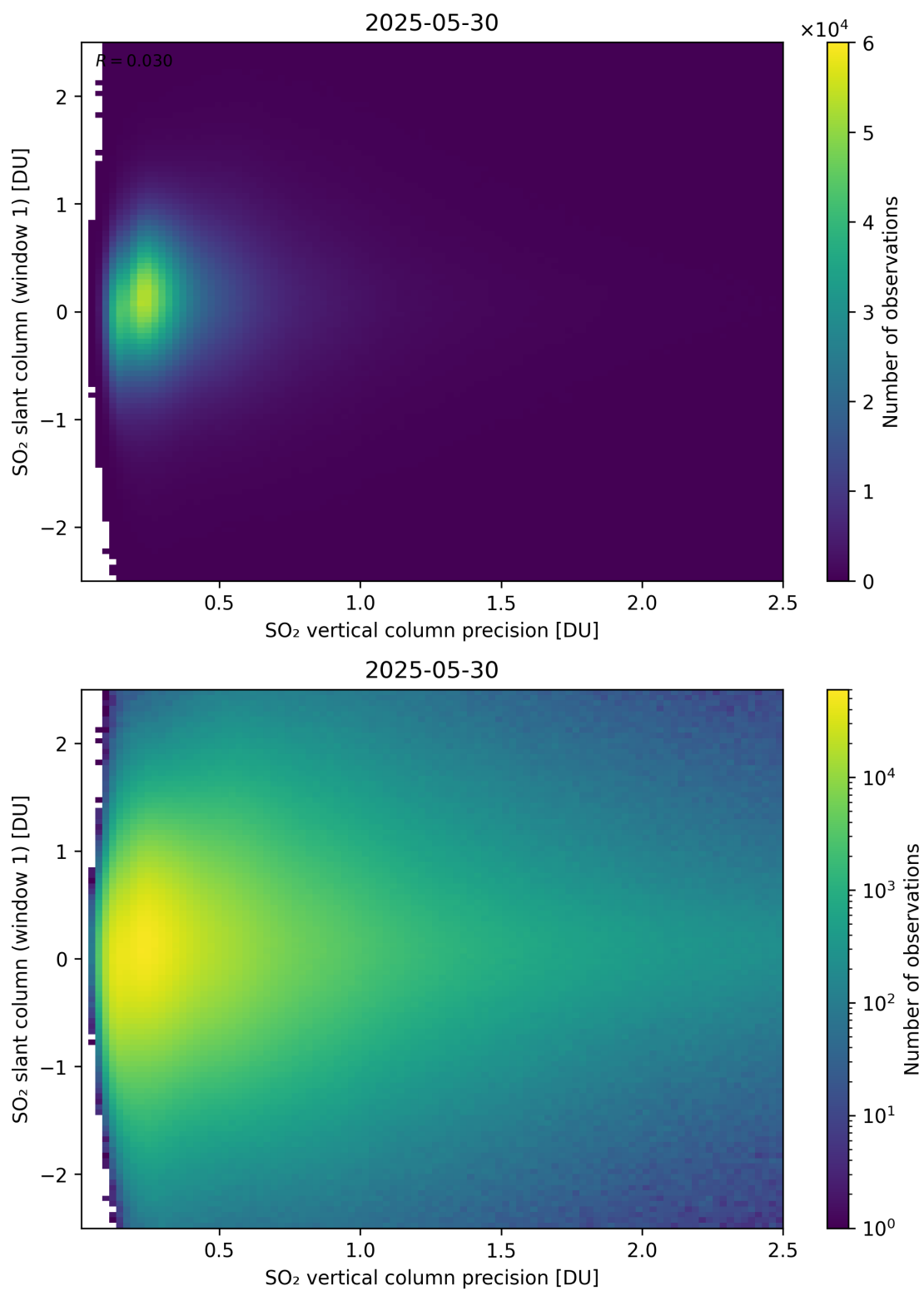
Figure 341: Scatter density plot of “SO 2 vertical column precision” against “SO 2 slant column (window 1)” for 2025-05-29 to 2025-05-31.
