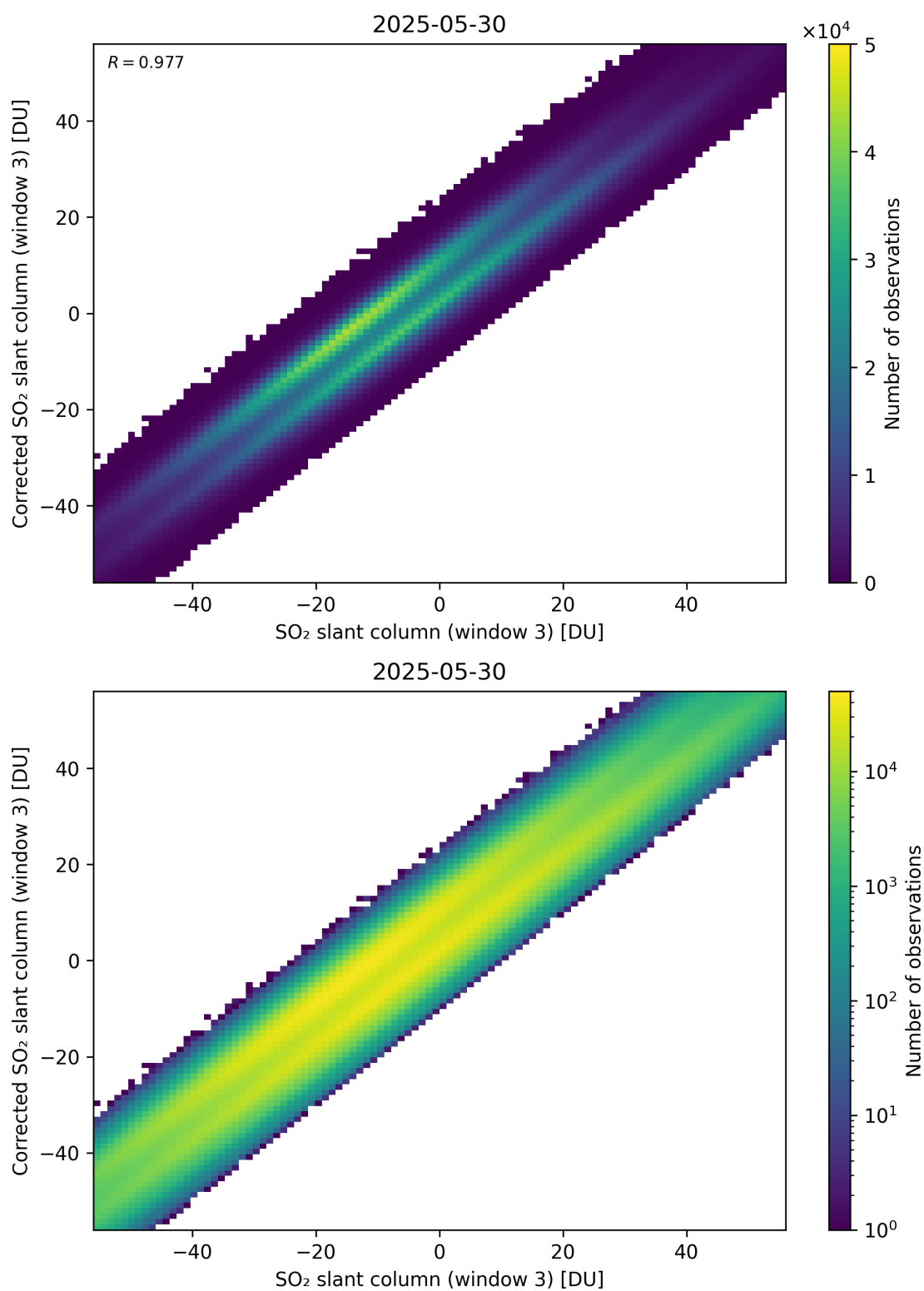
Figure 316: Scatter density plot of “SO 2 slant column (window 3)” against “Corrected SO 2 slant column (window 3)” for 2025-05-29 to 2025-05-31.
