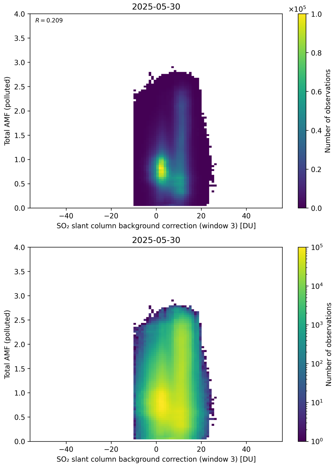
Figure 136: Scatter density plot of “SO 2 slant column background correction (window 3)” against “Total AMF (polluted)” for 2025-05-29 to 2025-05-31.
