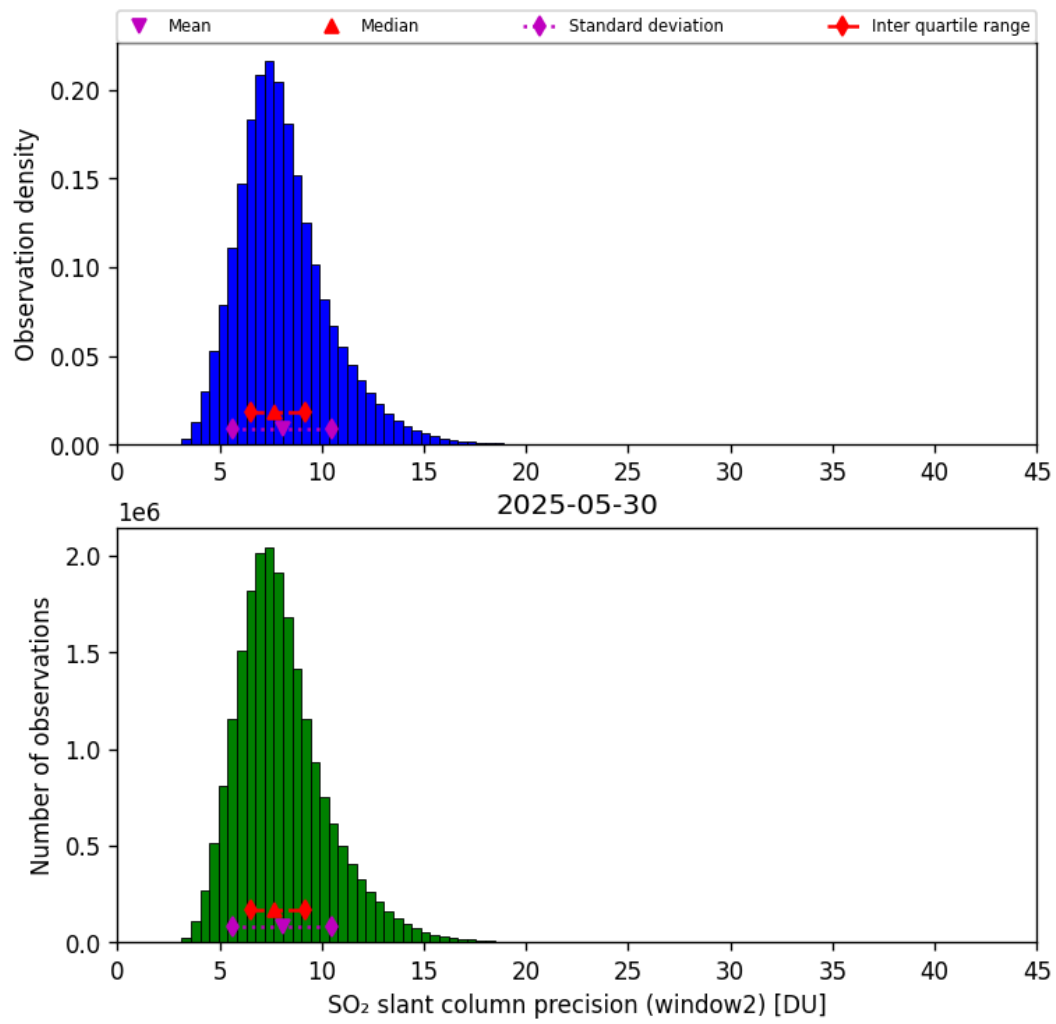
Figure 68: Histogram of “SO 2 slant column precision (window2)” for 2025-05-29 to 2025-05-31
