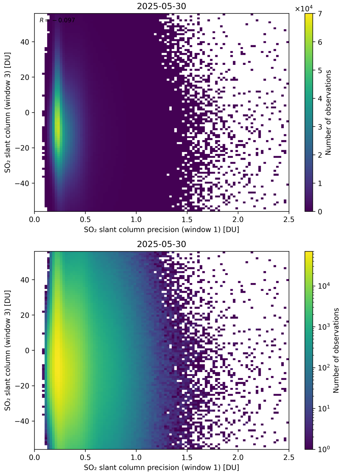
Figure 278: Scatter density plot of “SO 2 slant column precision (window 1)” against “SO 2 slant column (window 3)” for 2025-05-29 to 2025-05-31.
