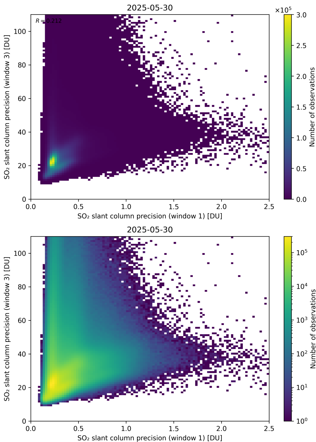
Figure 279: Scatter density plot of “SO 2 slant column precision (window 1)” against “SO 2 slant column precision (window 3)” for 2025-05-29 to 2025-05-31.
