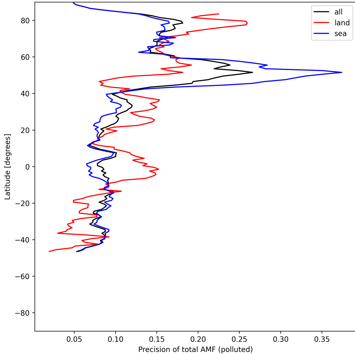
Figure 54: Zonal average of “Precision of total AMF (polluted)” for 2025-05-29 to 2025-05-31.
