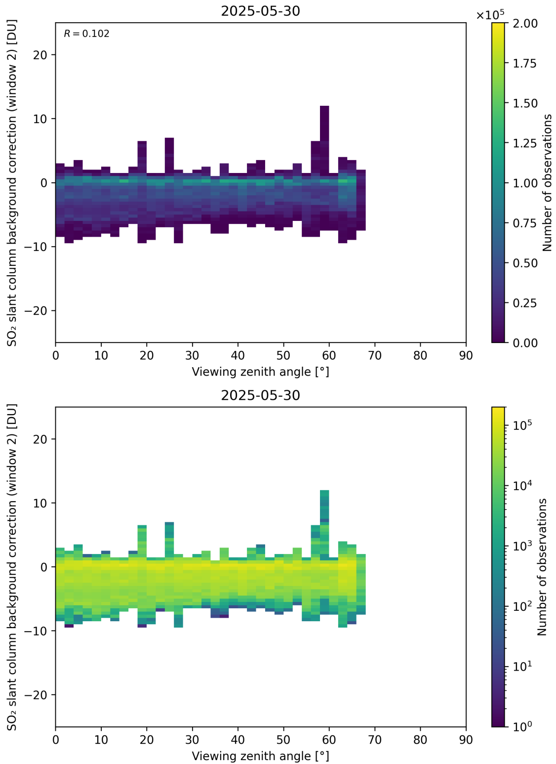
Figure 363: Scatter density plot of “Viewing zenith angle” against “SO 2 slant column background correction (window 2)” for 2025-05-29 to 2025-05-31.
