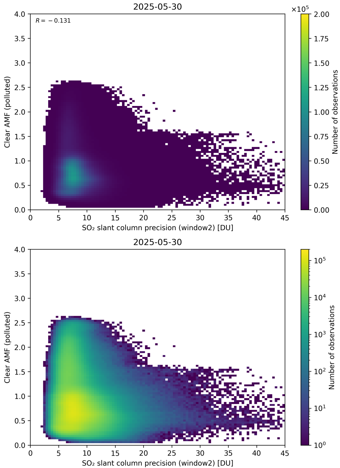
Figure 296: Scatter density plot of “SO 2 slant column precision (window2)” against “Clear AMF (polluted)” for 2025-05-29 to 2025-05-31.
