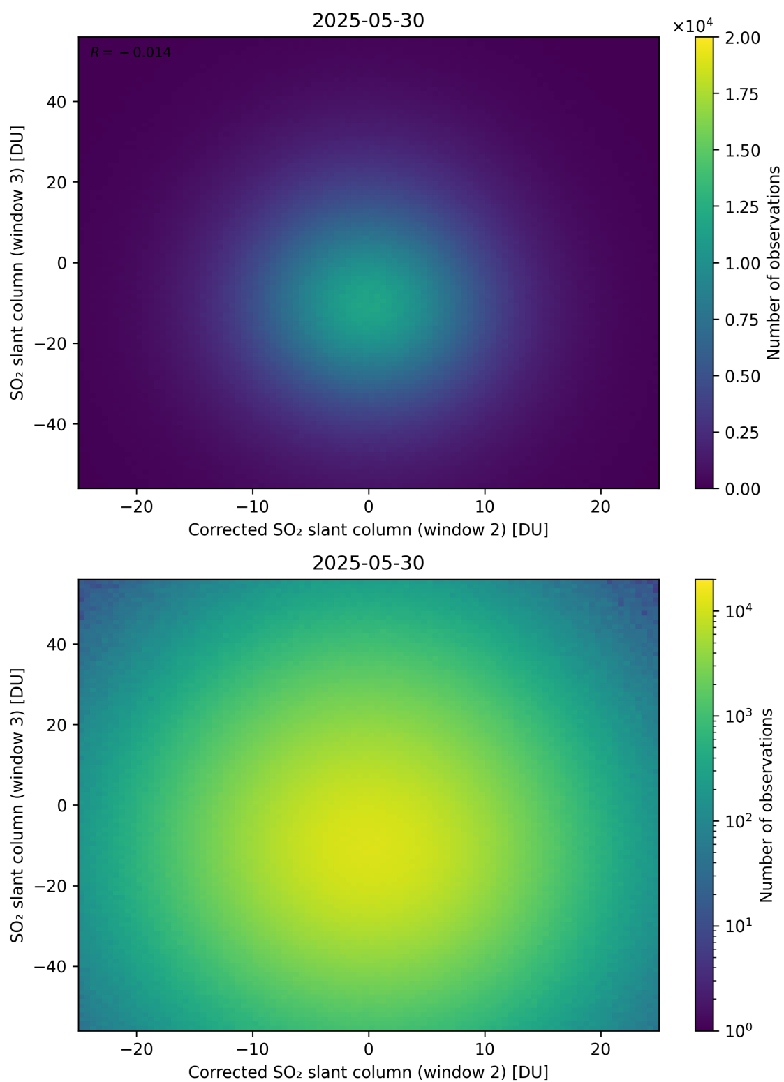
Figure 251: Scatter density plot of “Corrected SO 2 slant column (window 2)” against “SO 2 slant column (window 3)” for 2025-05-29 to 2025-05-31.
