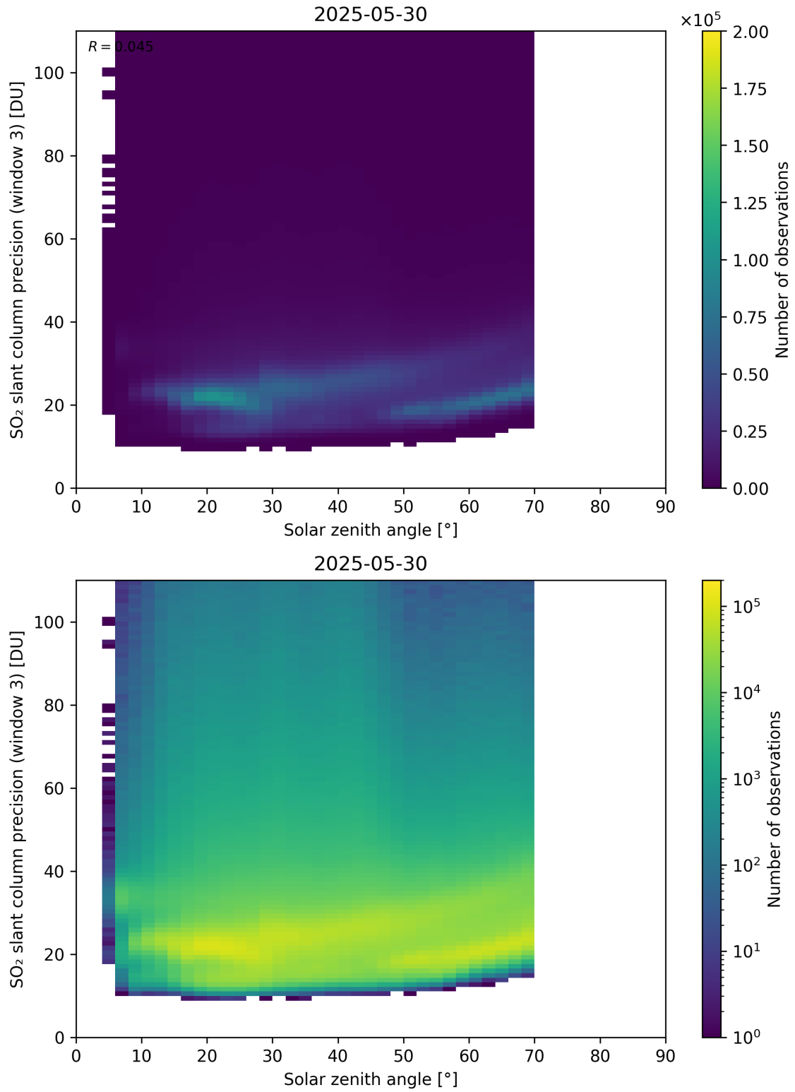
Figure 188: Scatter density plot of “Solar zenith angle” against “SO 2 slant column precision (window 3)” for 2025-05-29 to 2025-05-31.
