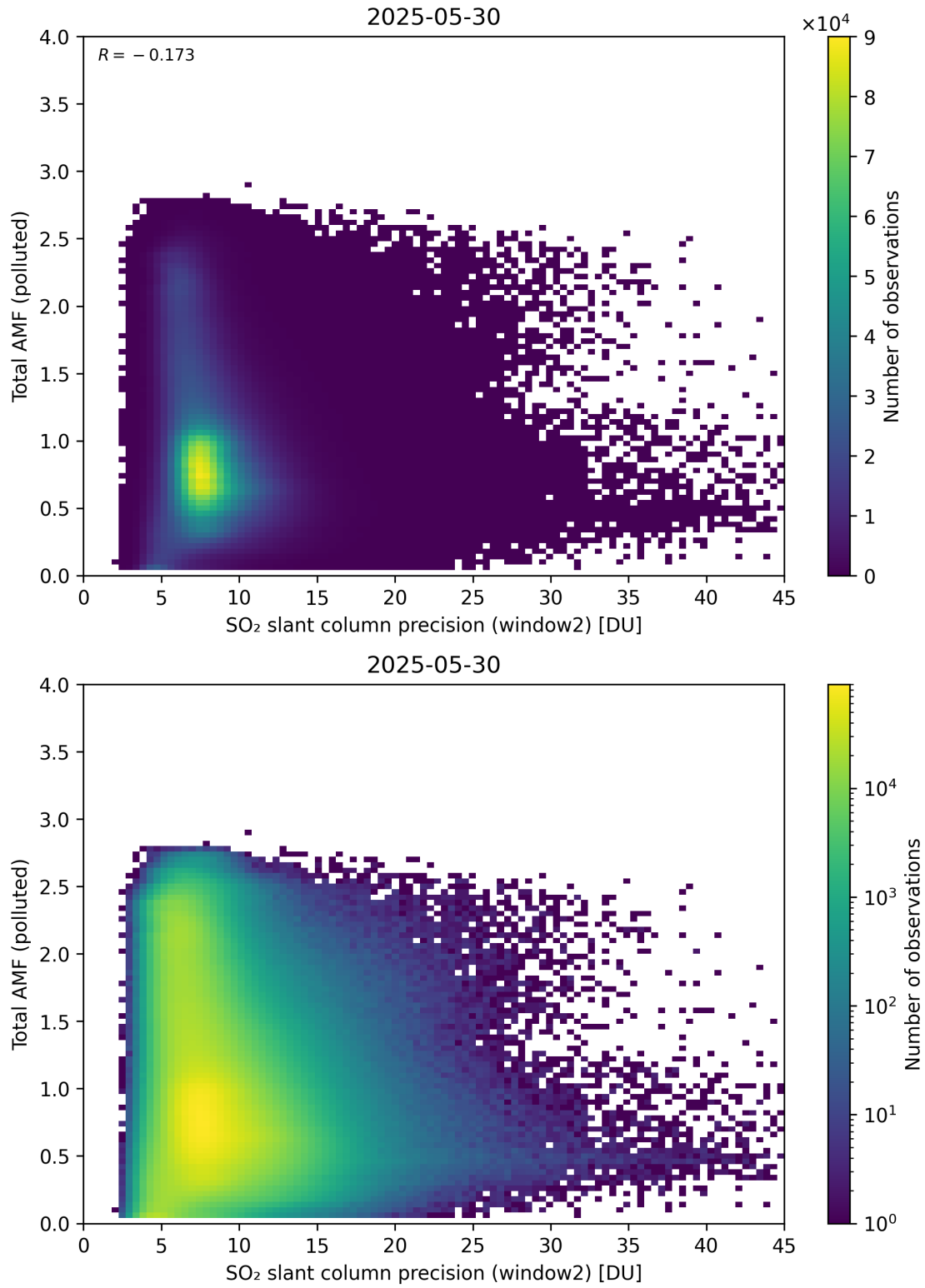
Figure 301: Scatter density plot of “SO 2 slant column precision (window2)” against “Total AMF (polluted)” for 2025-05-29 to 2025-05-31.
