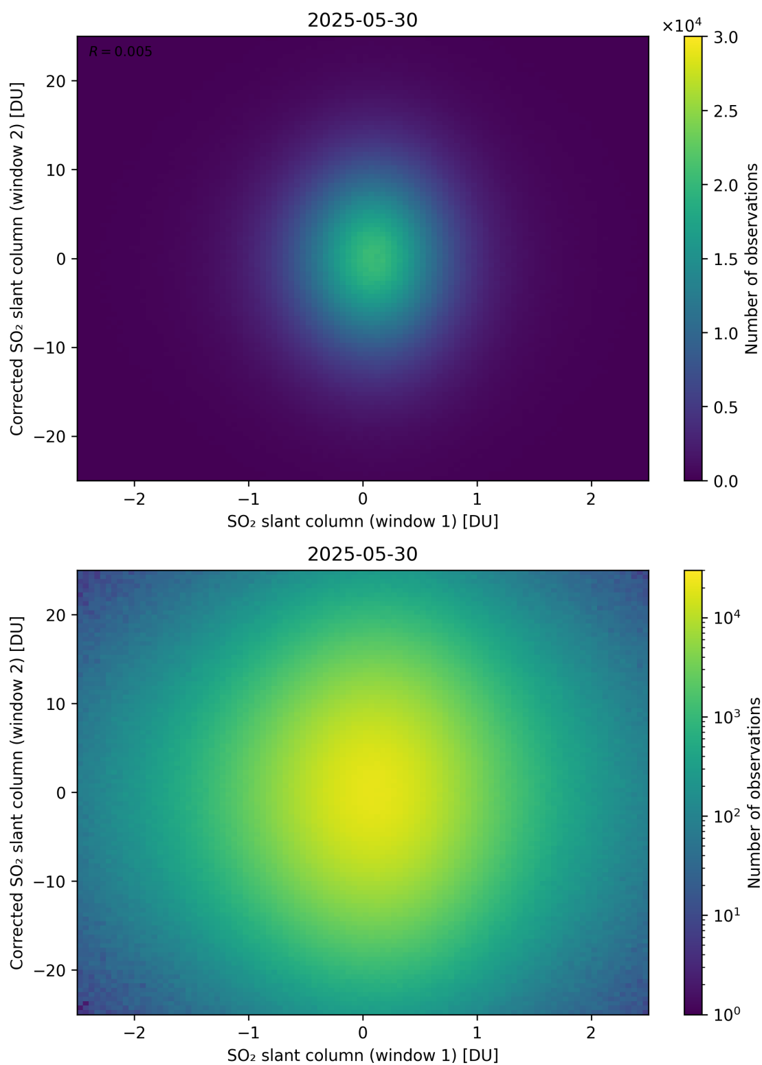
Figure 283: Scatter density plot of “SO 2 slant column (window 1)” against “Corrected SO 2 slant column (window 2)” for 2025-05-29 to 2025-05-31.
