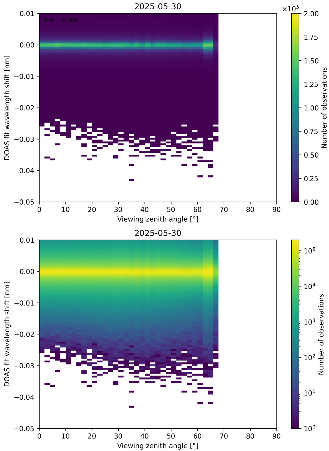
Figure 365: Scatter density plot of “Viewing zenith angle” against “DOAS fit wavelength shift” for 2025-05-29 to 2025-05-31.
