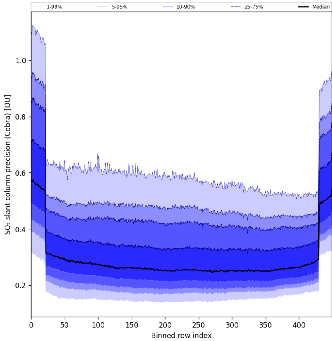
Figure 88: Along track statistics of "SO 2 slant column precision (Cobra)" for 2025-05-29 to 2025-05-31
