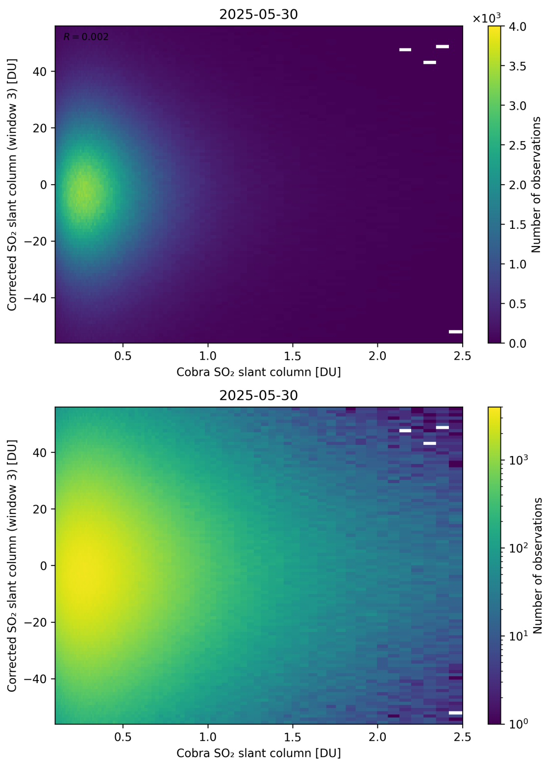
Figure 218: Scatter density plot of “Cobra SO 2 slant column” against “Corrected SO 2 slant column (window 3)” for 2025-05-29 to 2025-05-31.
