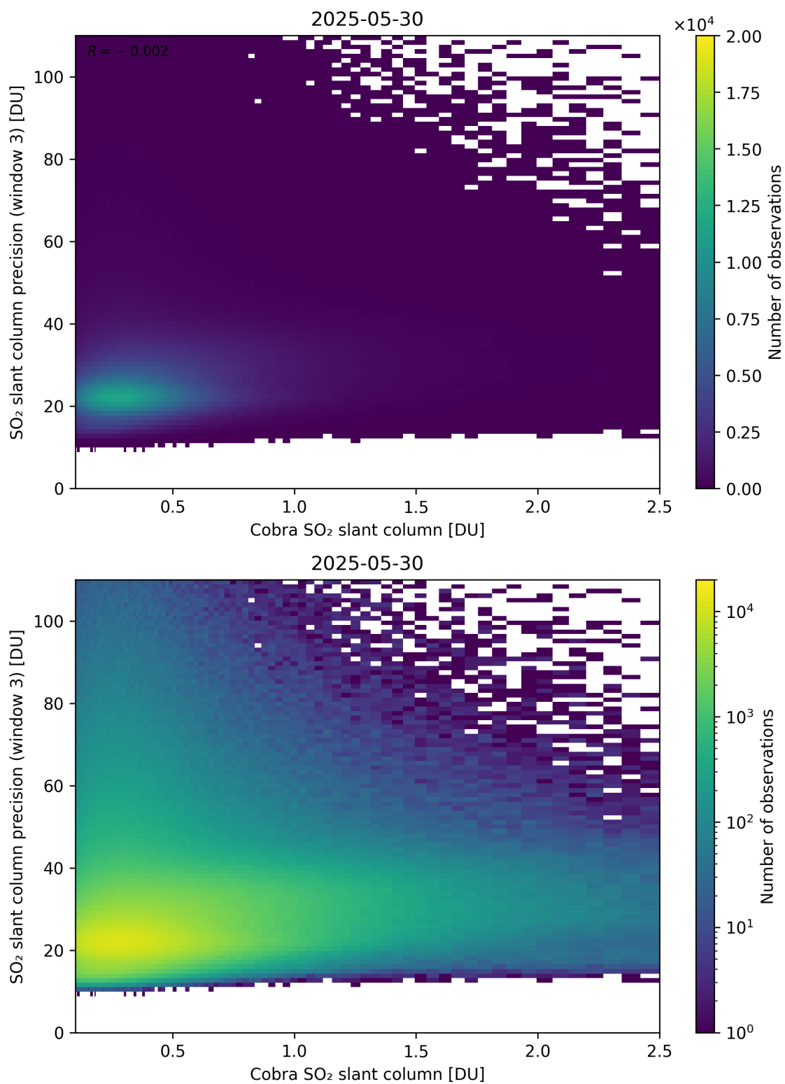
Figure 223: Scatter density plot of “Cobra SO 2 slant column” against “SO 2 slant column precision (window 3)” for 2025-05-29 to 2025-05-31.
