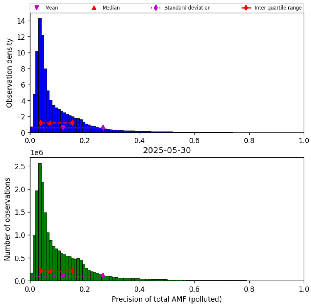
Figure 80: Histogram of “Precision of total AMF (polluted)” for 2025-05-29 to 2025-05-31
