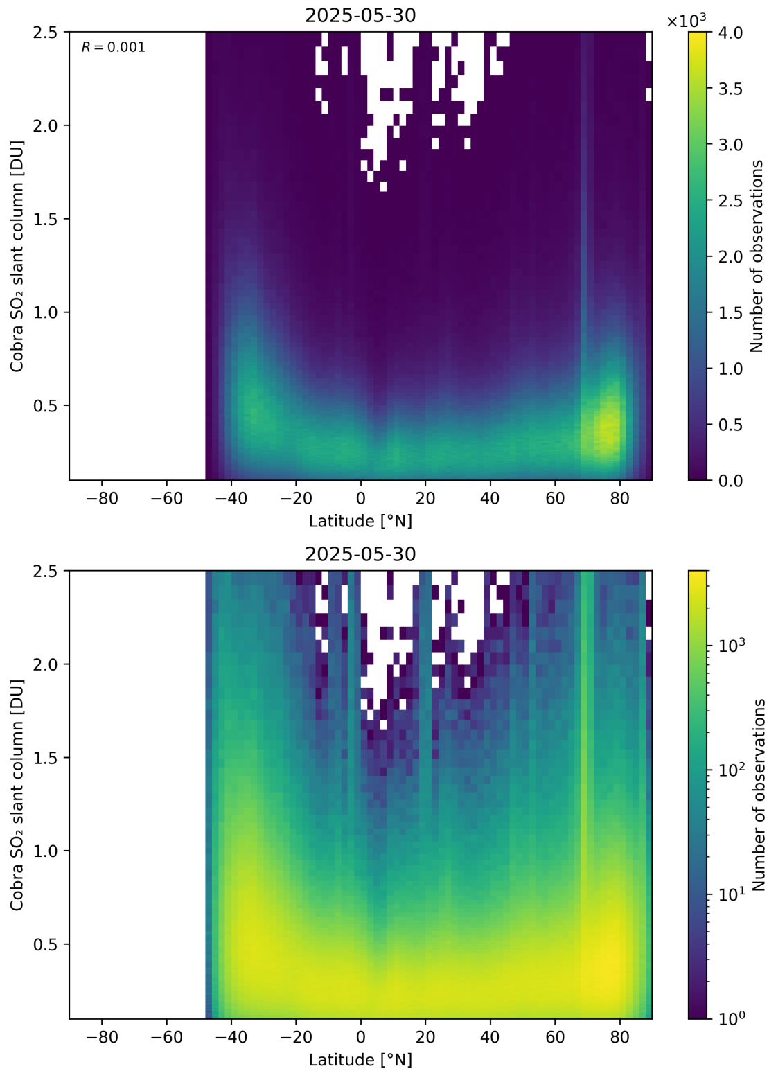
Figure 157: Scatter density plot of “Latitude” against “Cobra SO 2 slant column” for 2025-05-29 to 2025-05-31.
