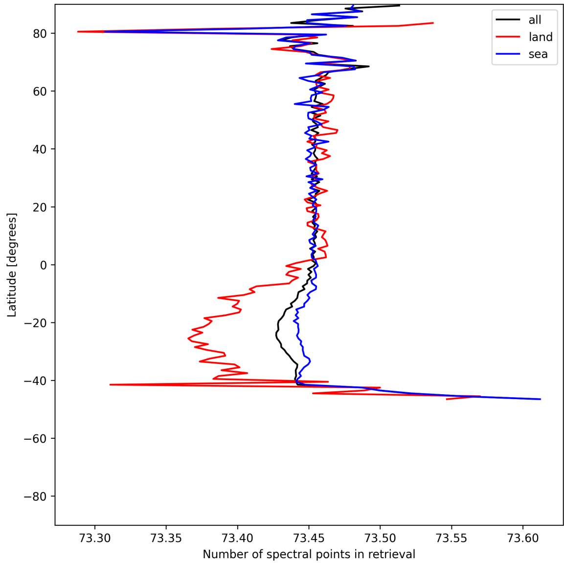
Figure 56: Zonal average of “Number of spectral points in retrieval” for 2025-05-29 to 2025-05-31.
