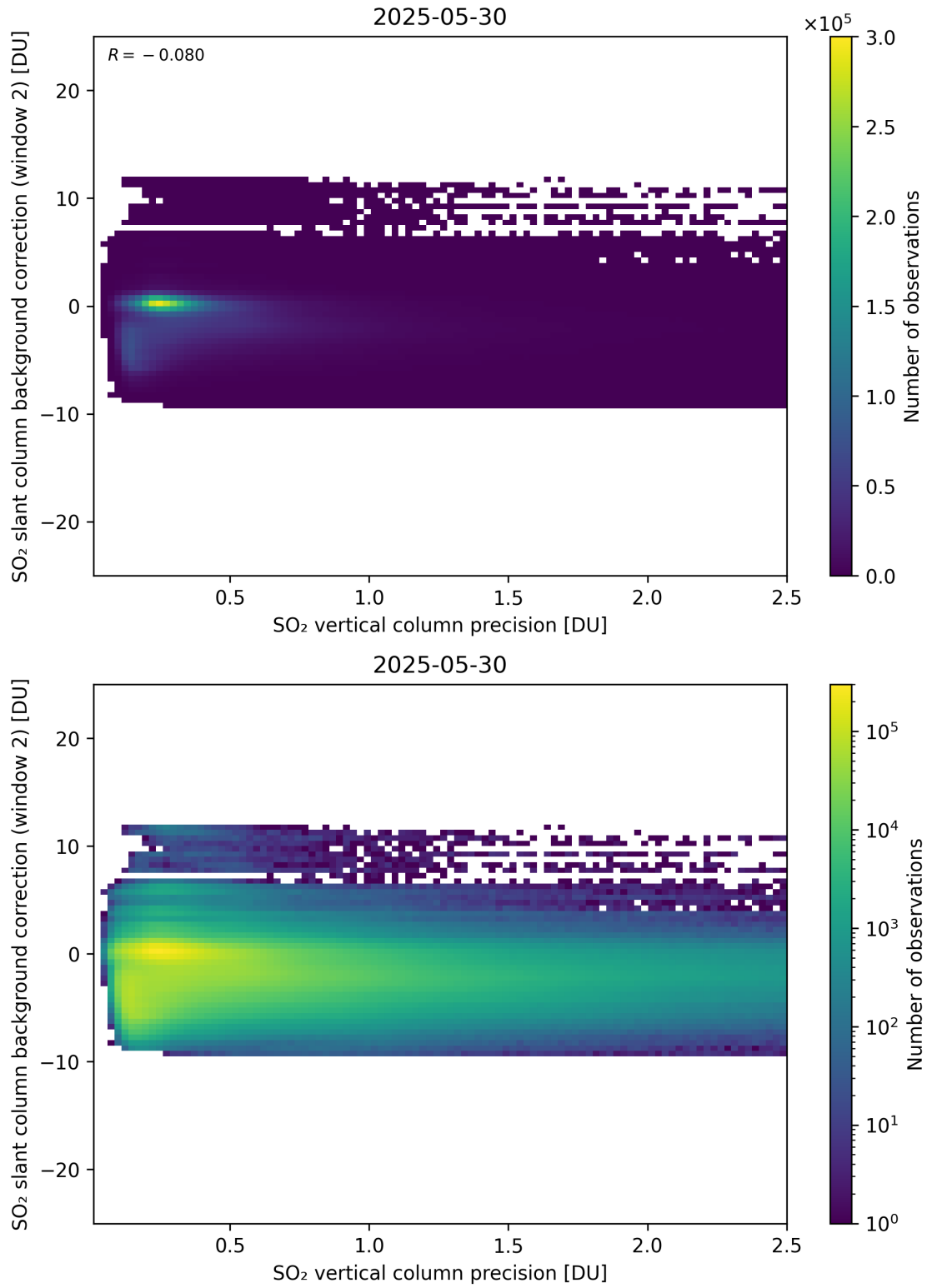
Figure 330: Scatter density plot of “SO 2 vertical column precision” against “SO 2 slant column background correction (window 2)” for 2025-05-29 to 2025-05-31.
