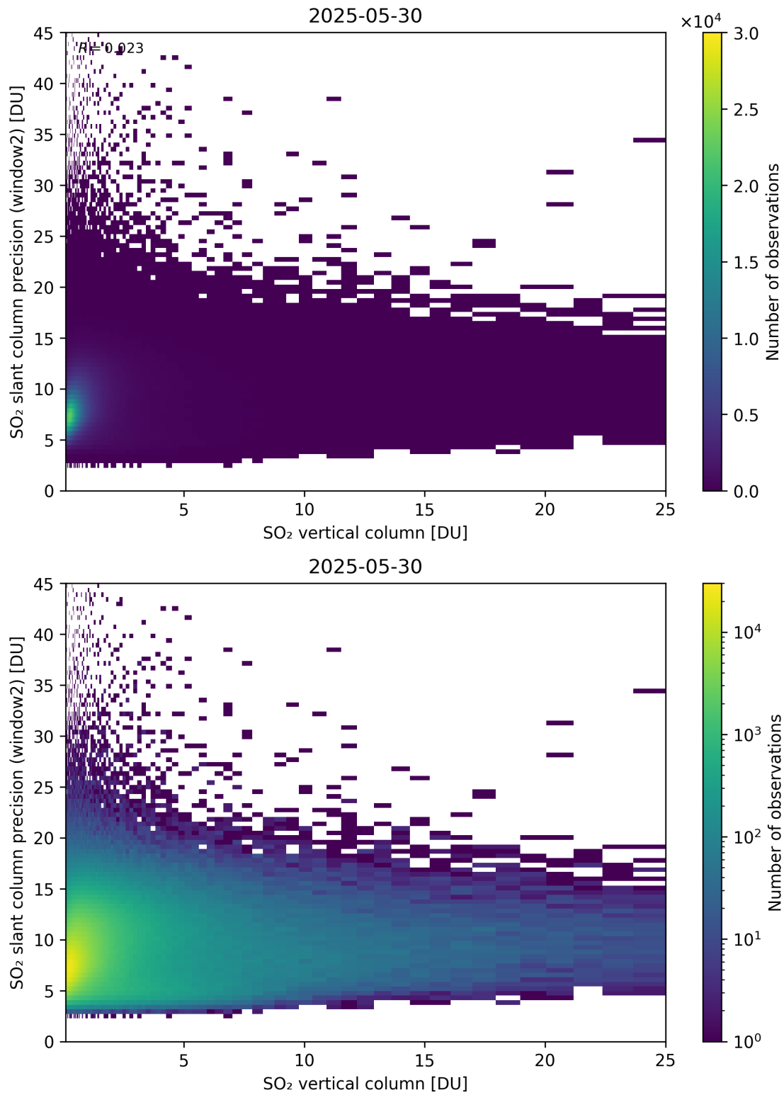
Figure 356: Scatter density plot of “SO 2 vertical column” against “SO 2 slant column precision (window2)” for 2025-05-29 to 2025-05-31.
