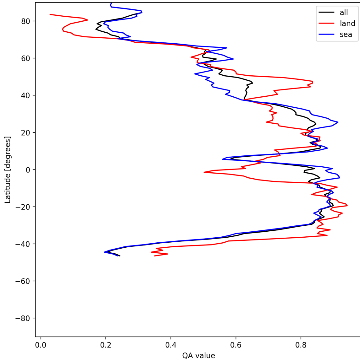
Figure 31: Zonal average of “QA value” for 2025-05-29 to 2025-05-31.
