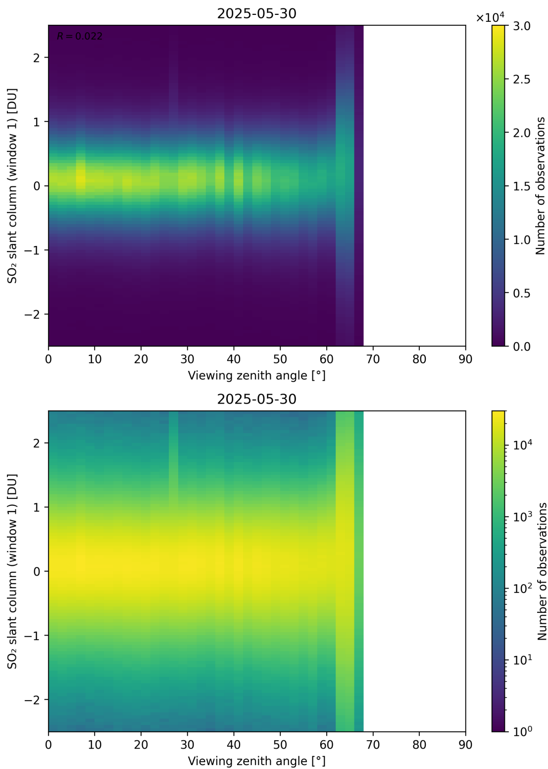
Figure 376: Scatter density plot of “Viewing zenith angle” against “SO 2 slant column (window 1)” for 2025-05-29 to 2025-05-31.
