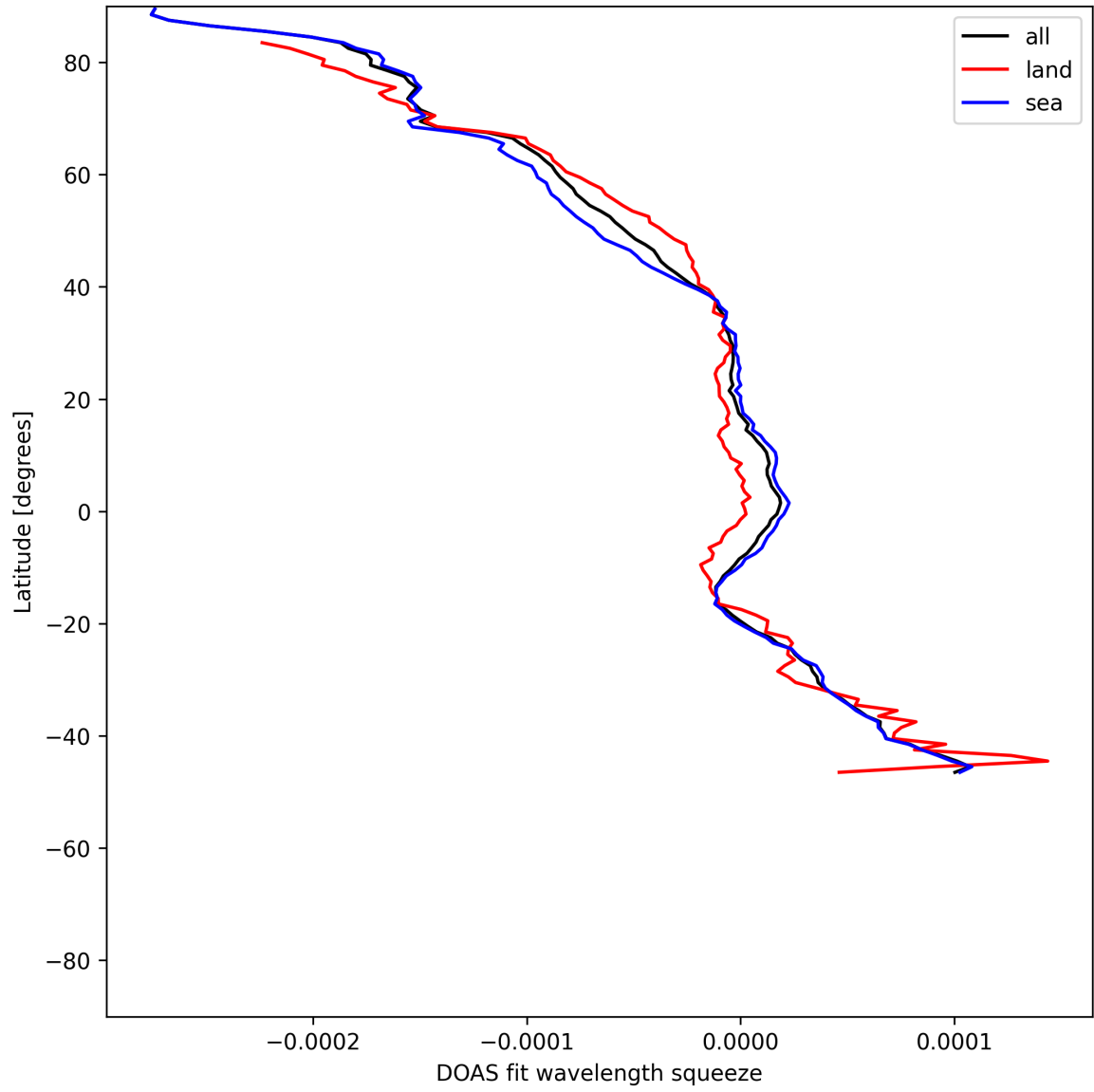
Figure 51: Zonal average of “DOAS fit wavelength squeeze” for 2025-05-29 to 2025-05-31.
