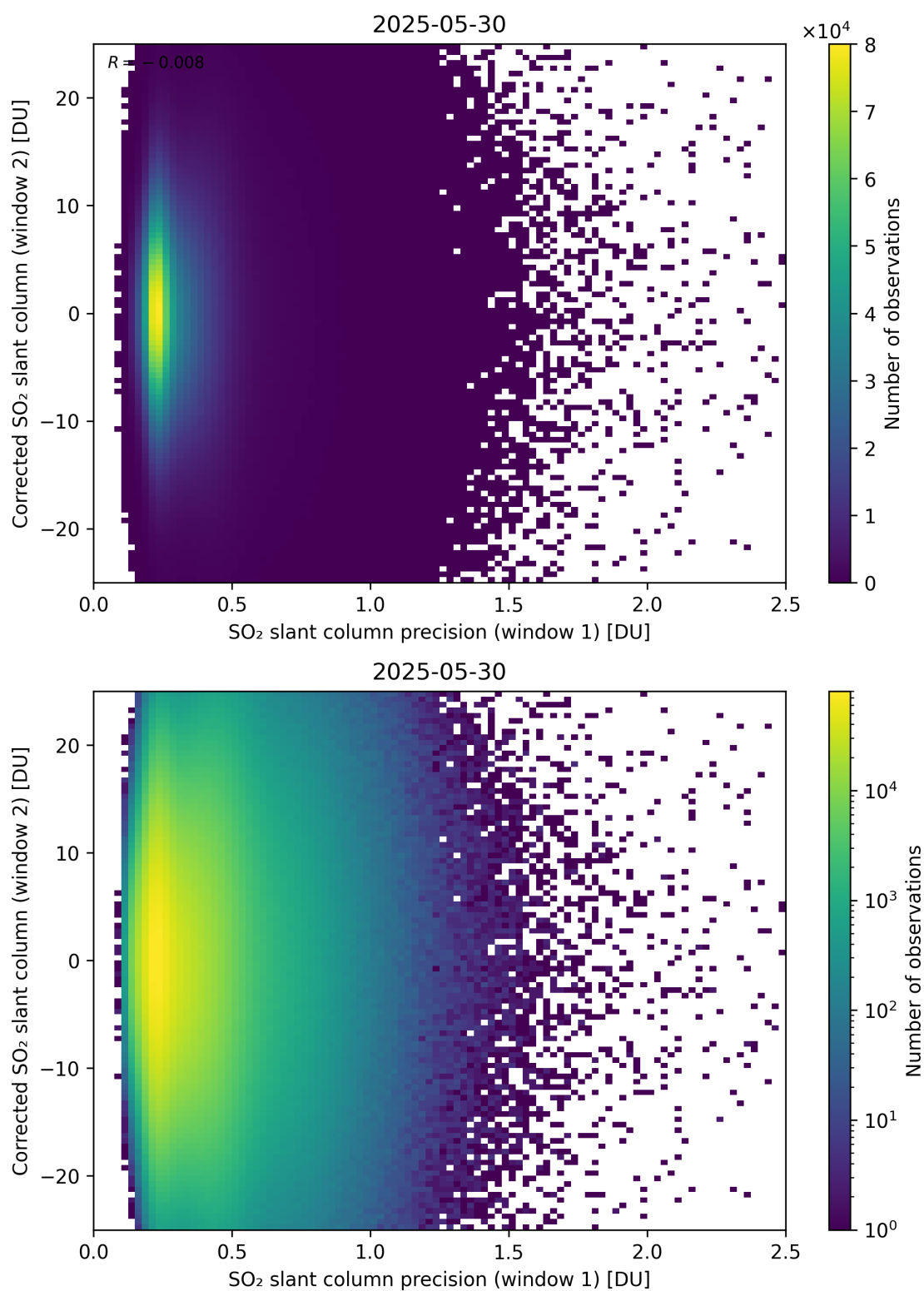
Figure 275: Scatter density plot of “SO 2 slant column precision (window 1)” against “Corrected SO 2 slant column (window 2)” for 2025-05-29 to 2025-05-31.
