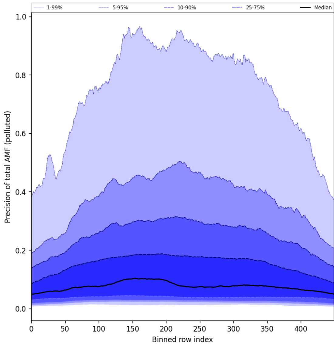
Figure 106: Along track statistics of “Precision of total AMF (polluted)” for 2025-05-29 to 2025-05-31
