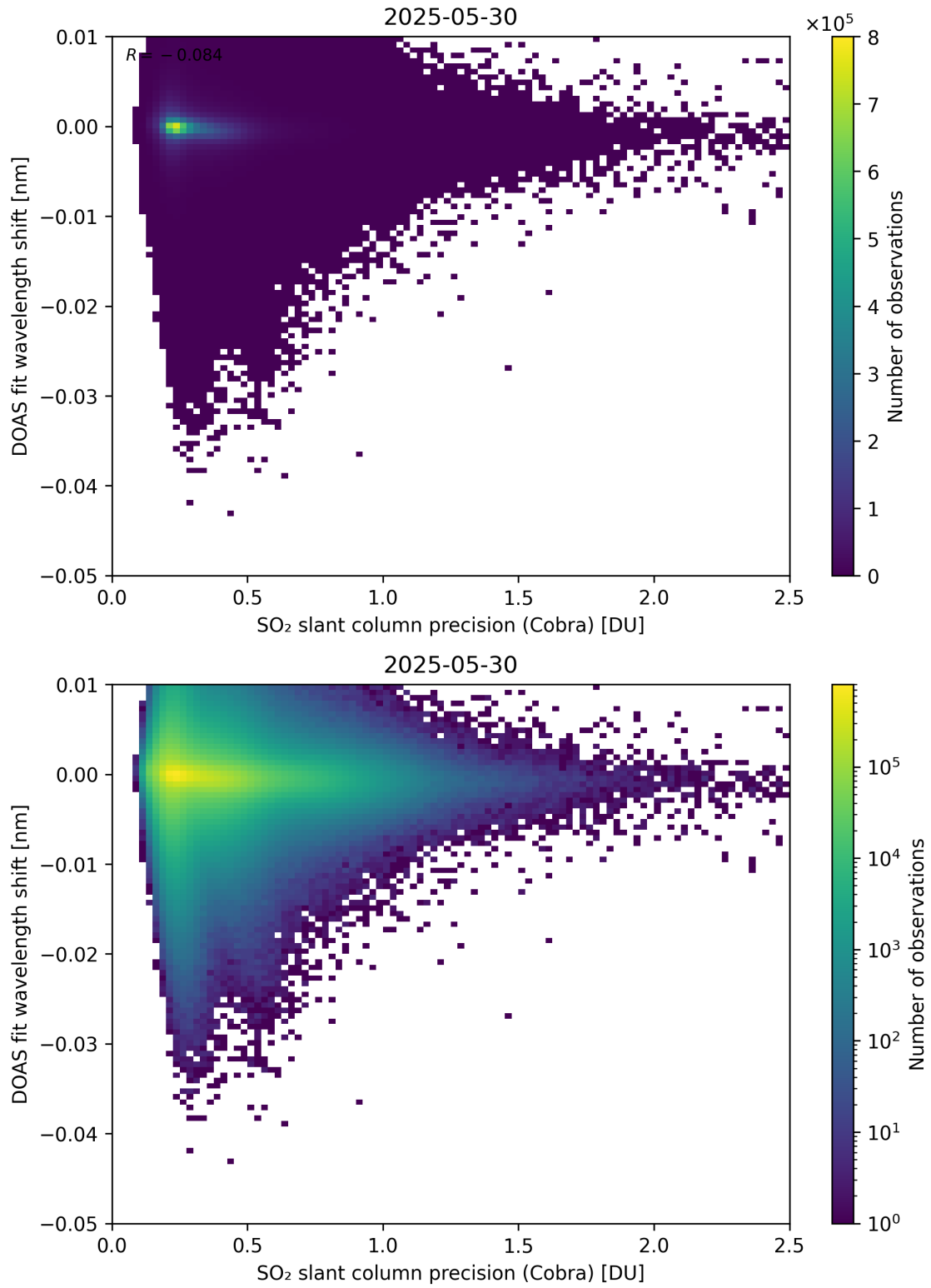
Figure 202: Scatter density plot of “SO 2 slant column precision (Cobra)” against “DOAS fit wavelength shift” for 2025-05-29 to 2025-05-31.
