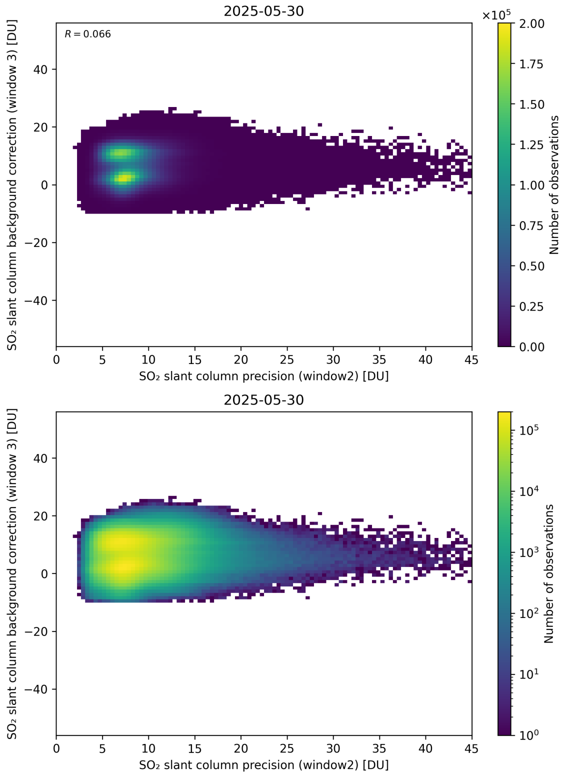
Figure 292: Scatter density plot of “SO 2 slant column precision (window2)” against “SO 2 slant column background correction (window 3)” for 2025-05-29 to 2025-05-31.
