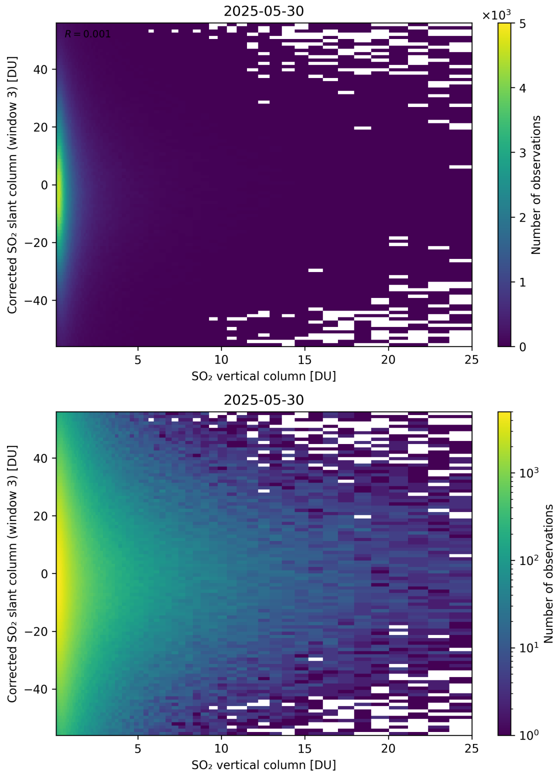
Figure 353: Scatter density plot of “SO 2 vertical column” against “Corrected SO 2 slant column (window 3)” for 2025-05-29 to 2025-05-31.
