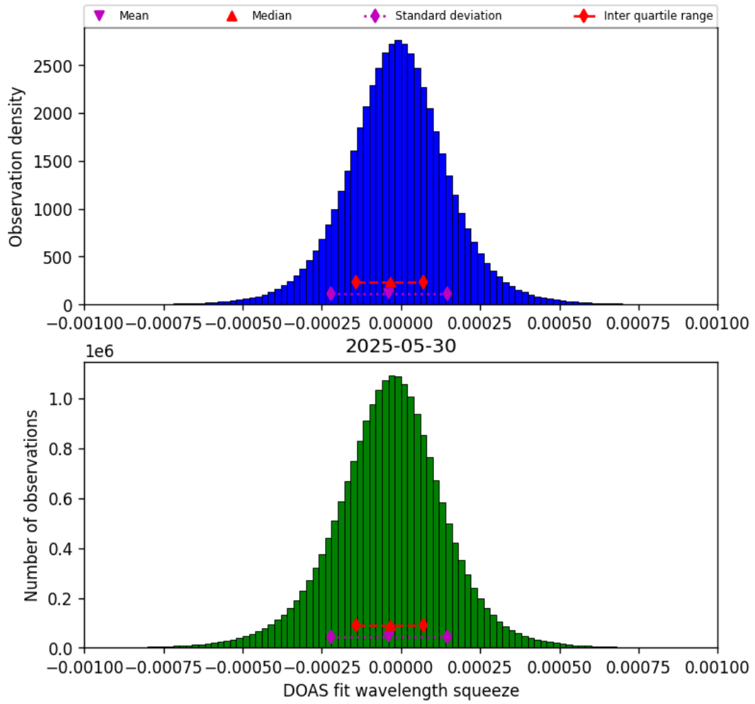
Figure 77: Histogram of “DOAS fit wavelength squeeze” for 2025-05-29 to 2025-05-31
