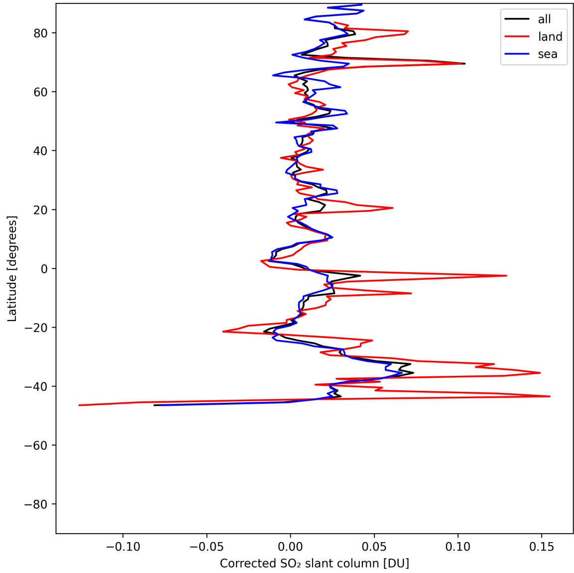
Figure 34: Zonal average of “Corrected SO 2 slant column” for 2025-05-29 to 2025-05-31.
