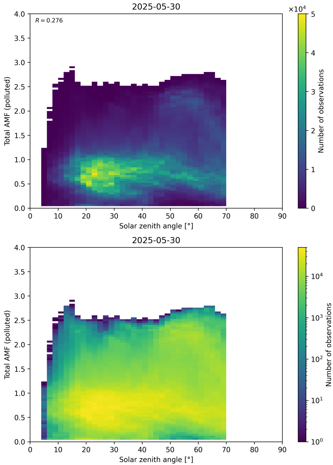
Figure 189: Scatter density plot of “Solar zenith angle” against “Total AMF (polluted)” for 2025-05-29 to 2025-05-31.
