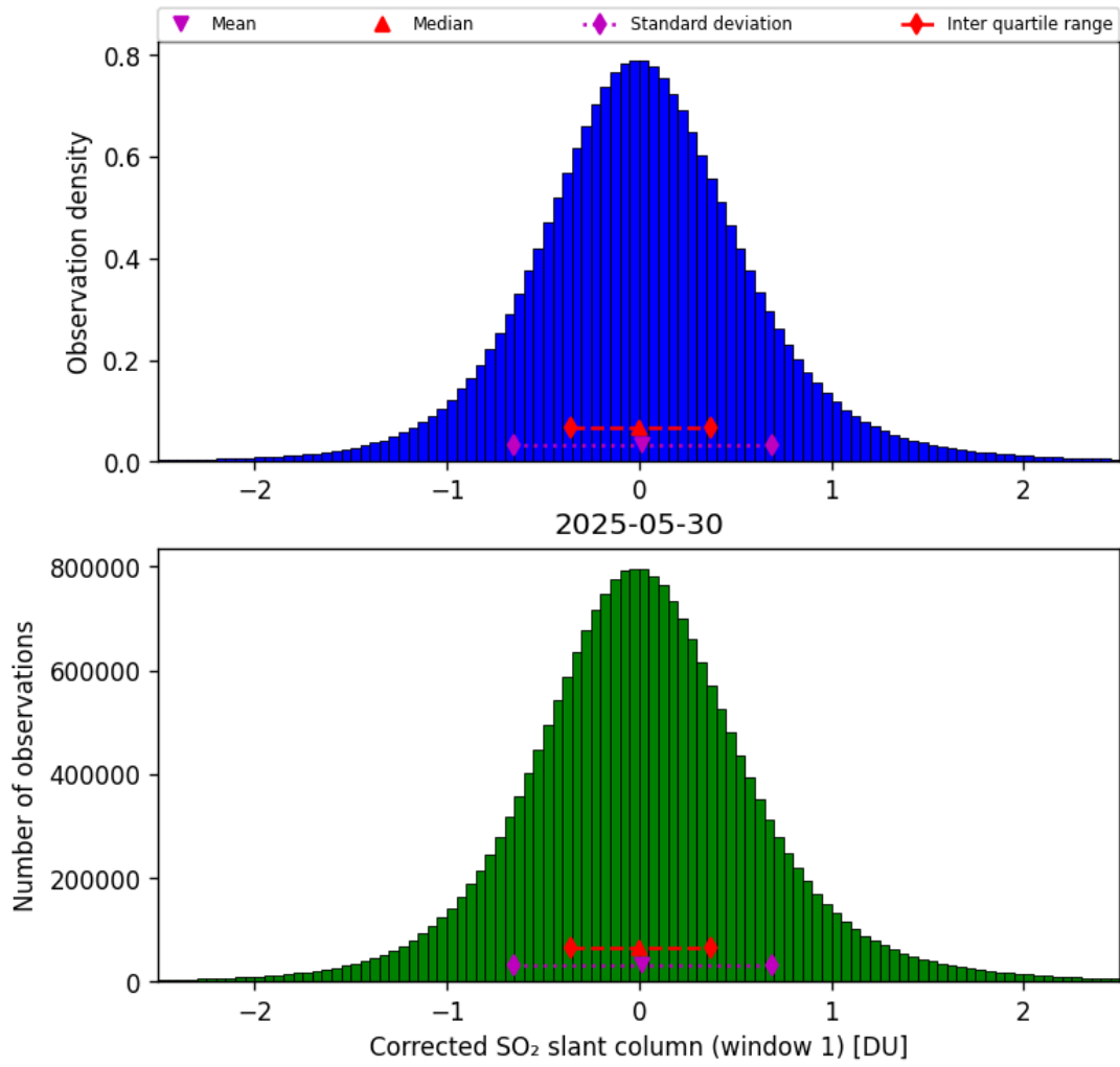
Figure 65: Histogram of “Corrected SO 2 slant column (window 1)” for 2025-05-29 to 2025-05-31
