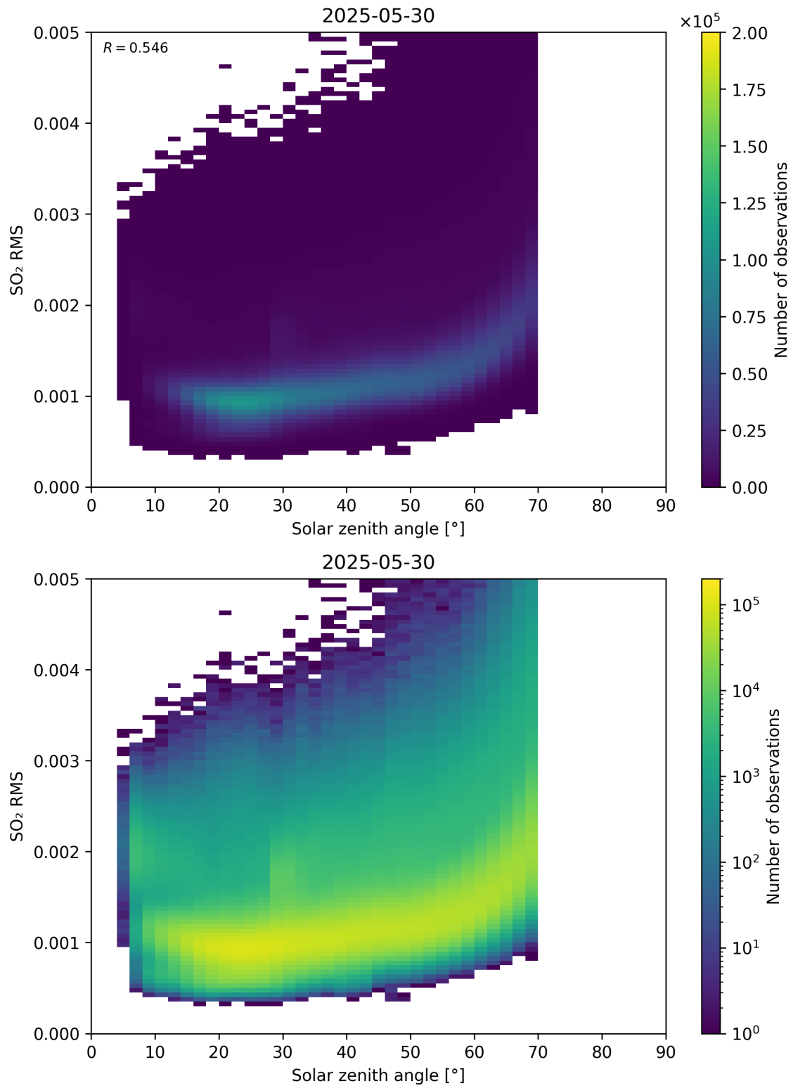
Figure 176: Scatter density plot of “Solar zenith angle” against “SO 2 RMS” for 2025-05-29 to 2025-05-31.
