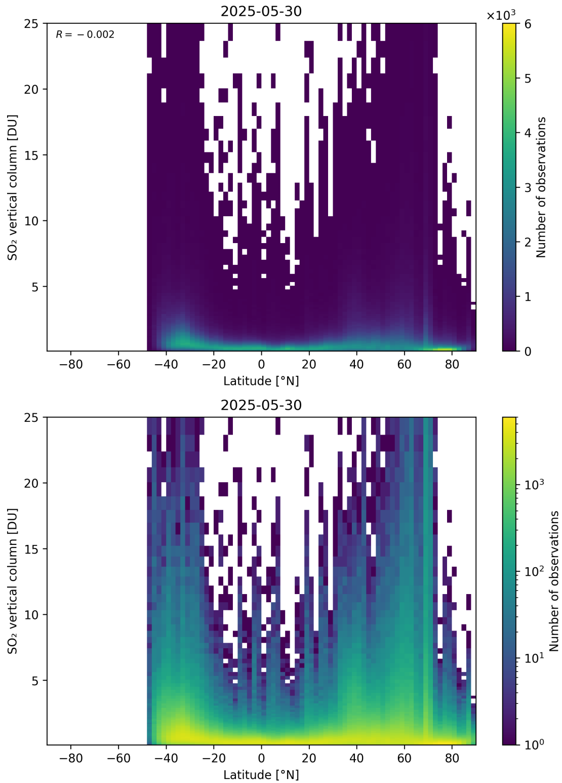
Figure 169: Scatter density plot of “Latitude” against “SO 2 vertical column” for 2025-05-29 to 2025-05-31.
