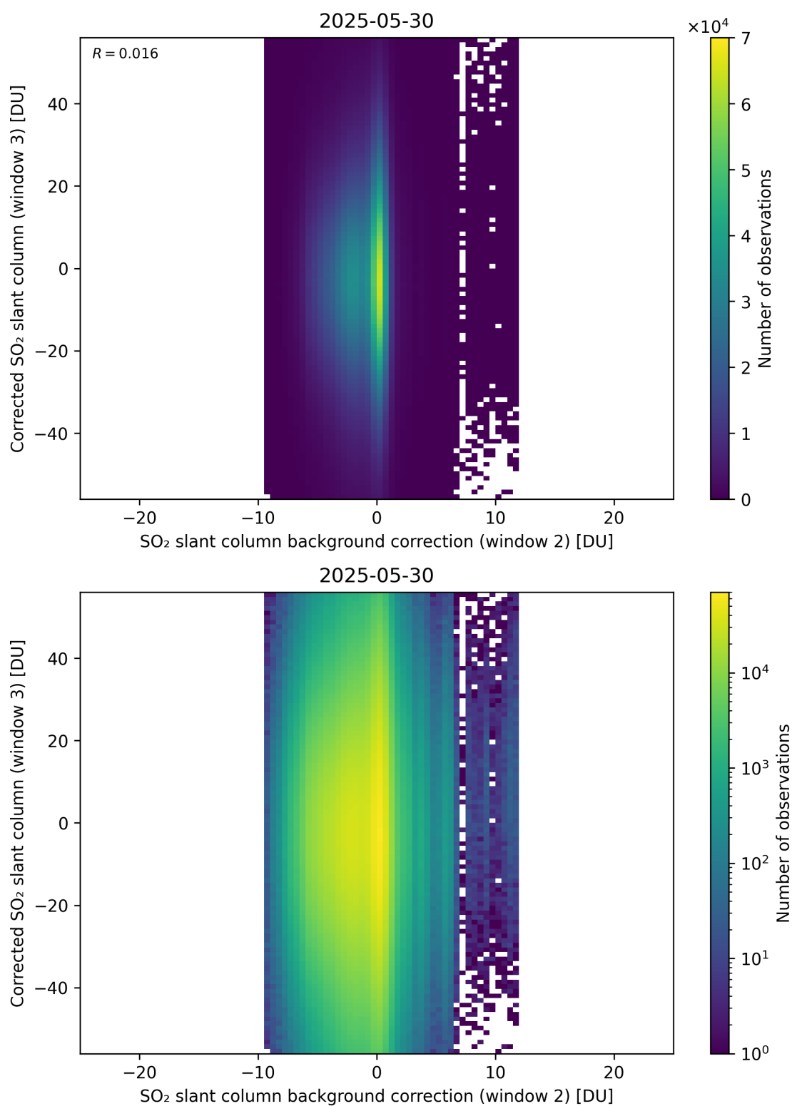
Figure 127: Scatter density plot of “SO 2 slant column background correction (window 2)” against “Corrected SO 2 slant column (window 3)” for 2025-05-29 to 2025-05-31.
