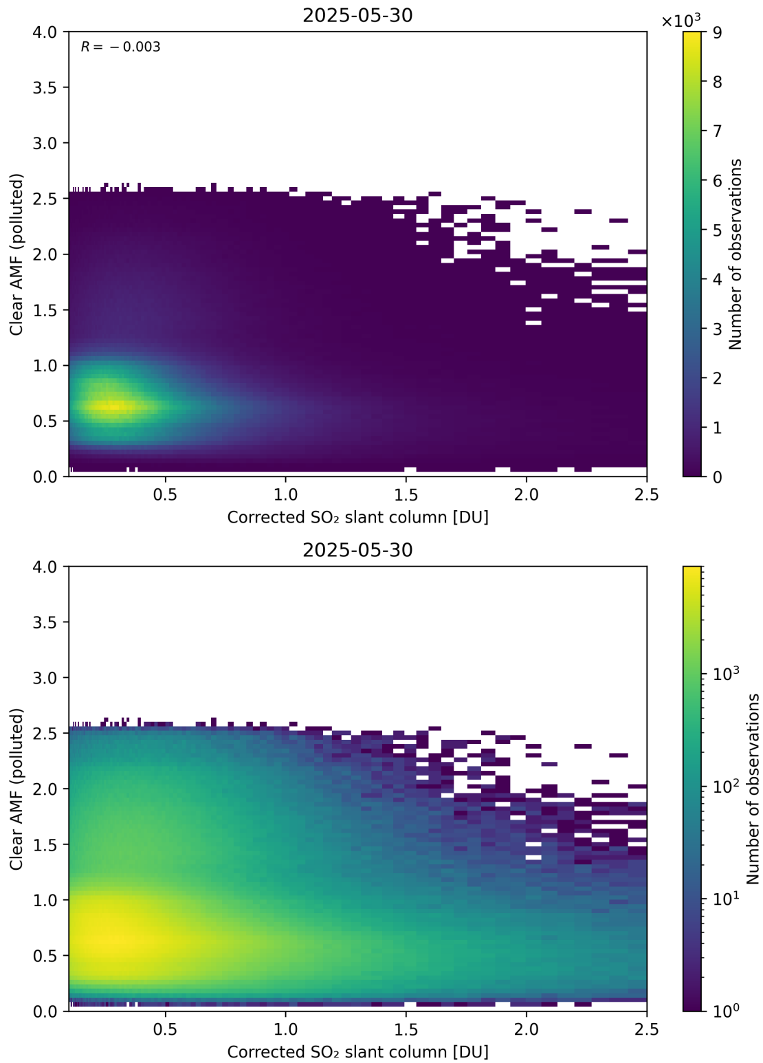
Figure 232: Scatter density plot of “Corrected SO 2 slant column” against “Clear AMF (polluted)” for 2025-05-29 to 2025-05-31.
