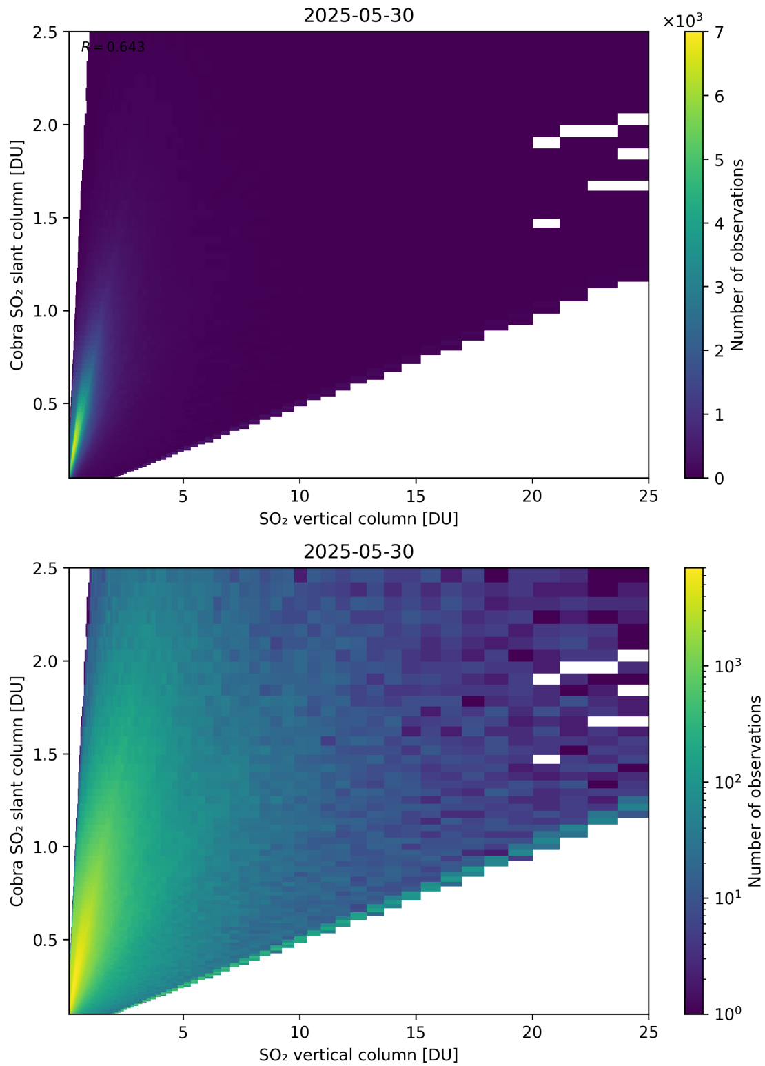
Figure 349: Scatter density plot of “SO 2 vertical column” against “Cobra SO 2 slant column” for 2025-05-29 to 2025-05-31.
