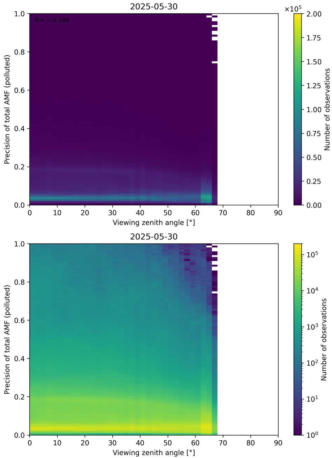
Figure 382: Scatter density plot of “Viewing zenith angle” against “Precision of total AMF (polluted)” for 2025-05-29 to 2025-05-31.
