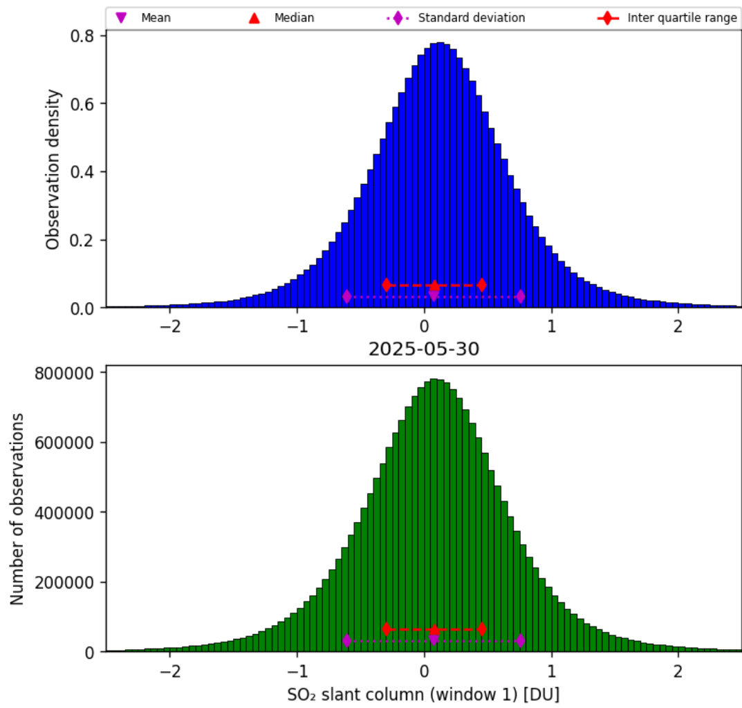
Figure 63: Histogram of “SO 2 slant column (window 1)” for 2025-05-29 to 2025-05-31
