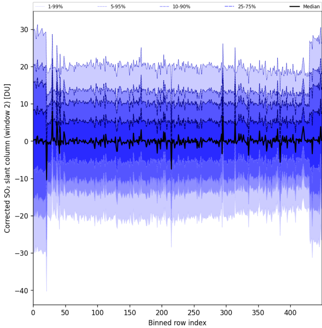
Figure 95: Along track statistics of “Corrected SO 2 slant column (window 2)” for 2025-05-29 to 2025-05-31
