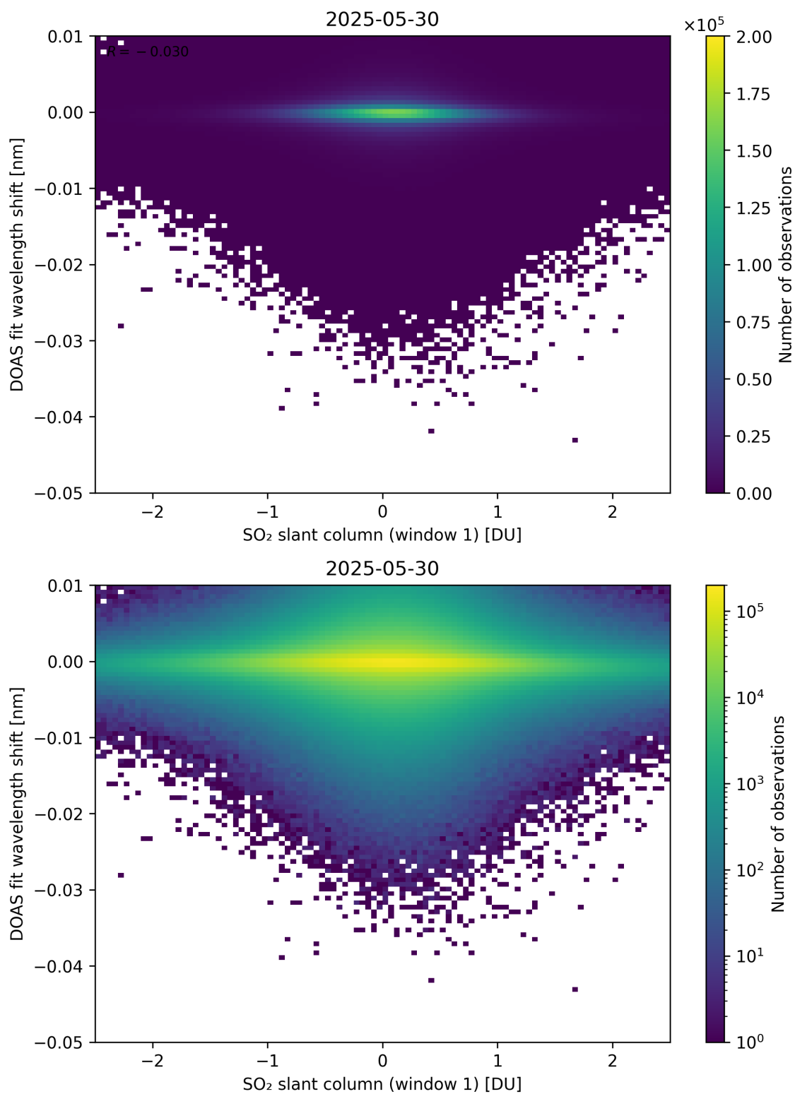
Figure 265: Scatter density plot of “SO 2 slant column (window 1)” against “DOAS fit wavelength shift” for 2025-05-29 to 2025-05-31.
