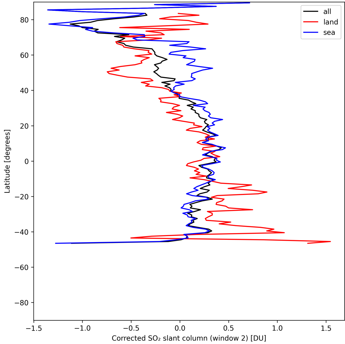
Figure 43: Zonal average of “Corrected SO 2 slant column (window 2)” for 2025-05-29 to 2025-05-31.
