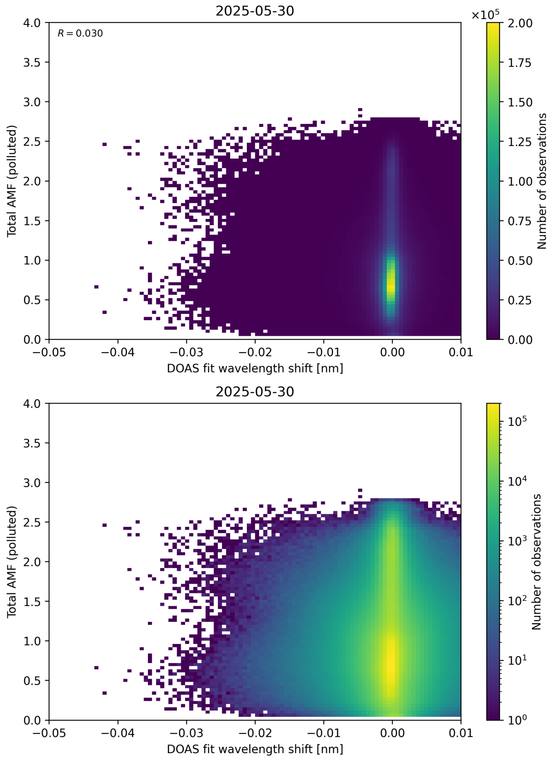
Figure 141: Scatter density plot of “DOAS fit wavelength shift” against “Total AMF (polluted)” for 2025-05-29 to 2025-05-31.
