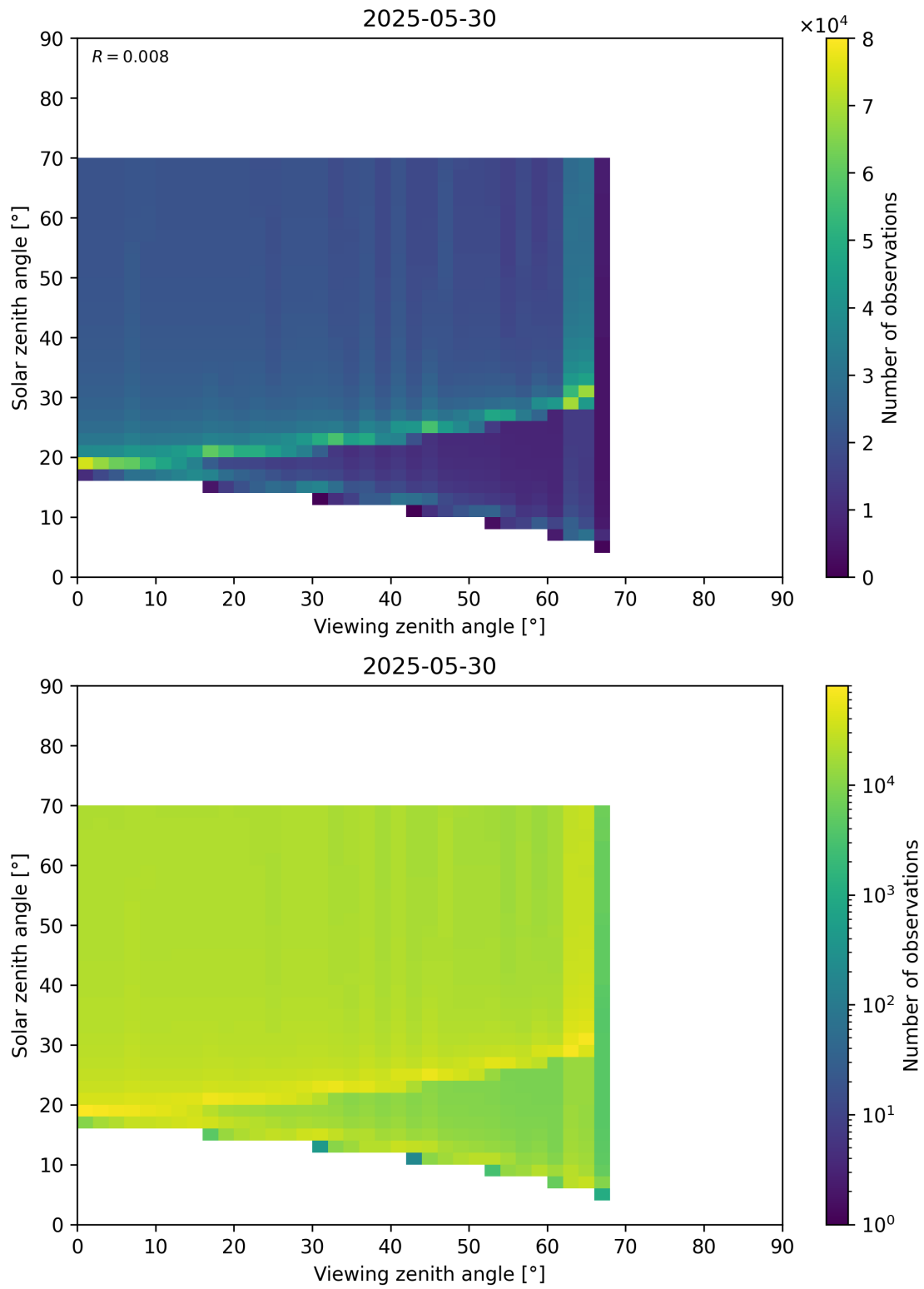
Figure 369: Scatter density plot of “Viewing zenith angle” against “Solar zenith angle” for 2025-05-29 to 2025-05-31.
