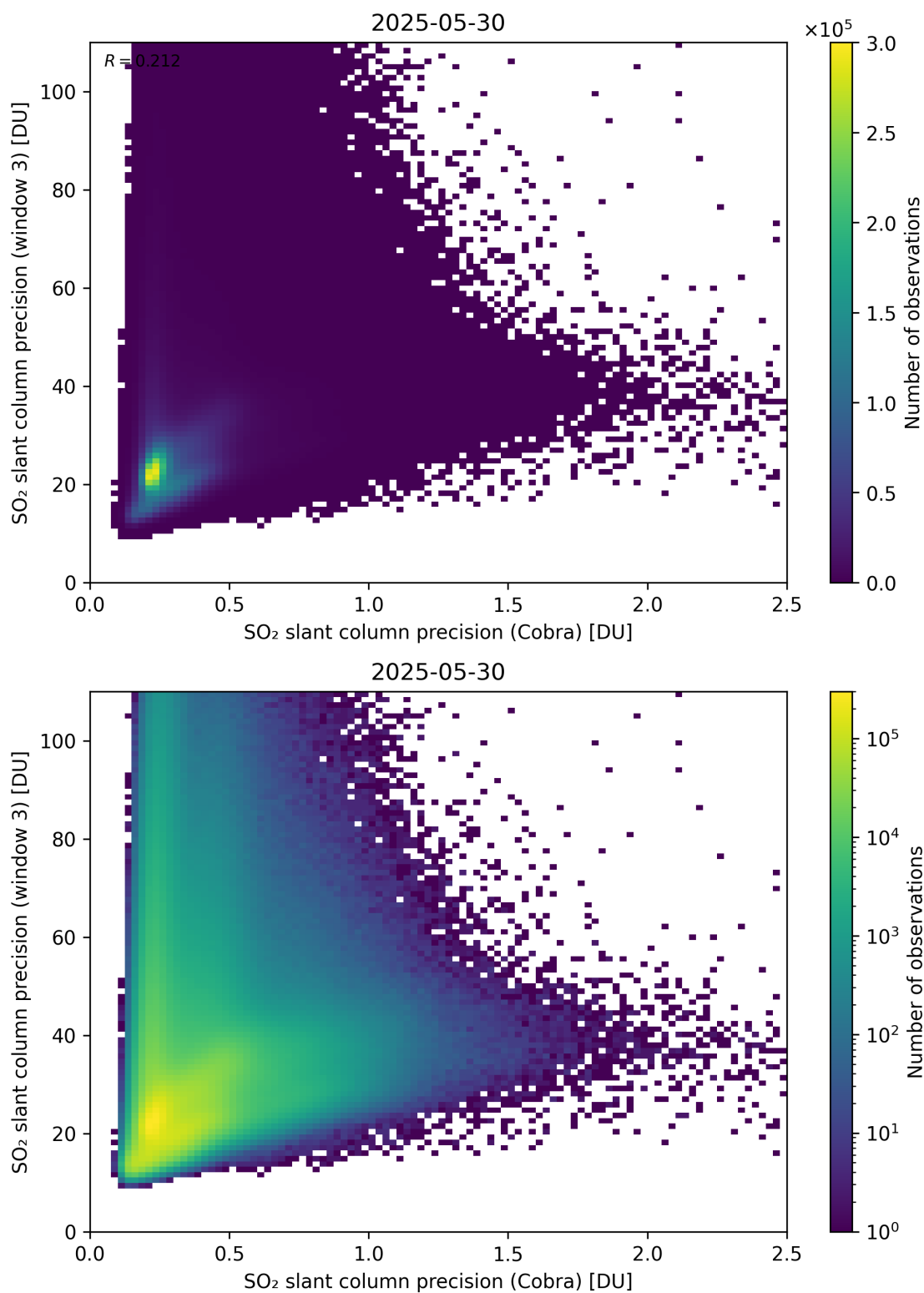
Figure 212: Scatter density plot of “SO 2 slant column precision (Cobra)” against “SO 2 slant column precision (window 3)” for 2025-05-29 to 2025-05-31.
