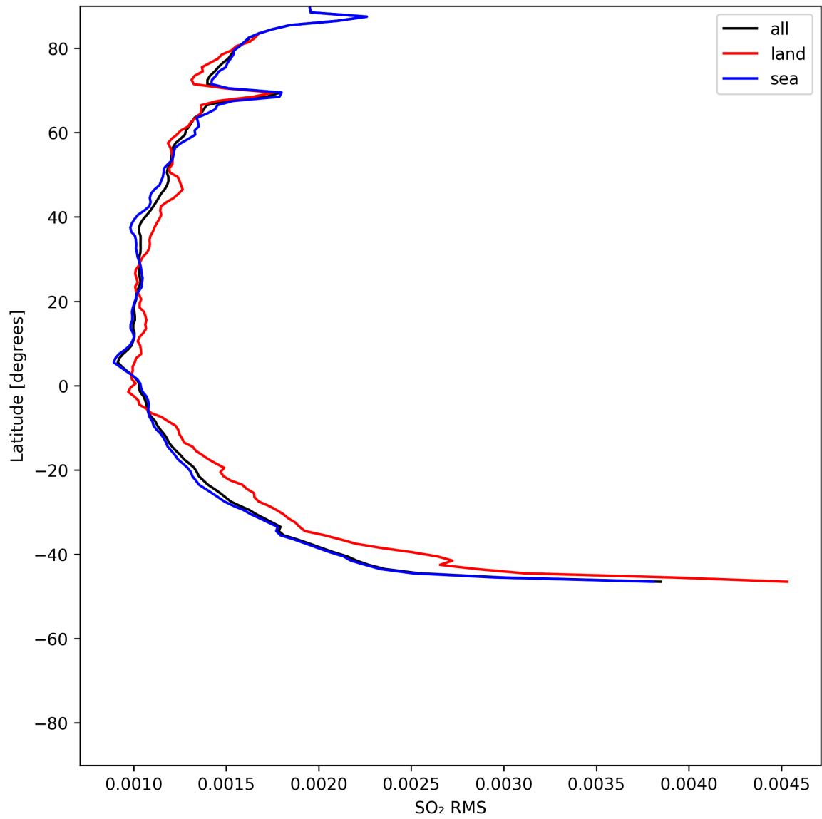
Figure 52: Zonal average of “SO 2 RMS” for 2025-05-29 to 2025-05-31.
