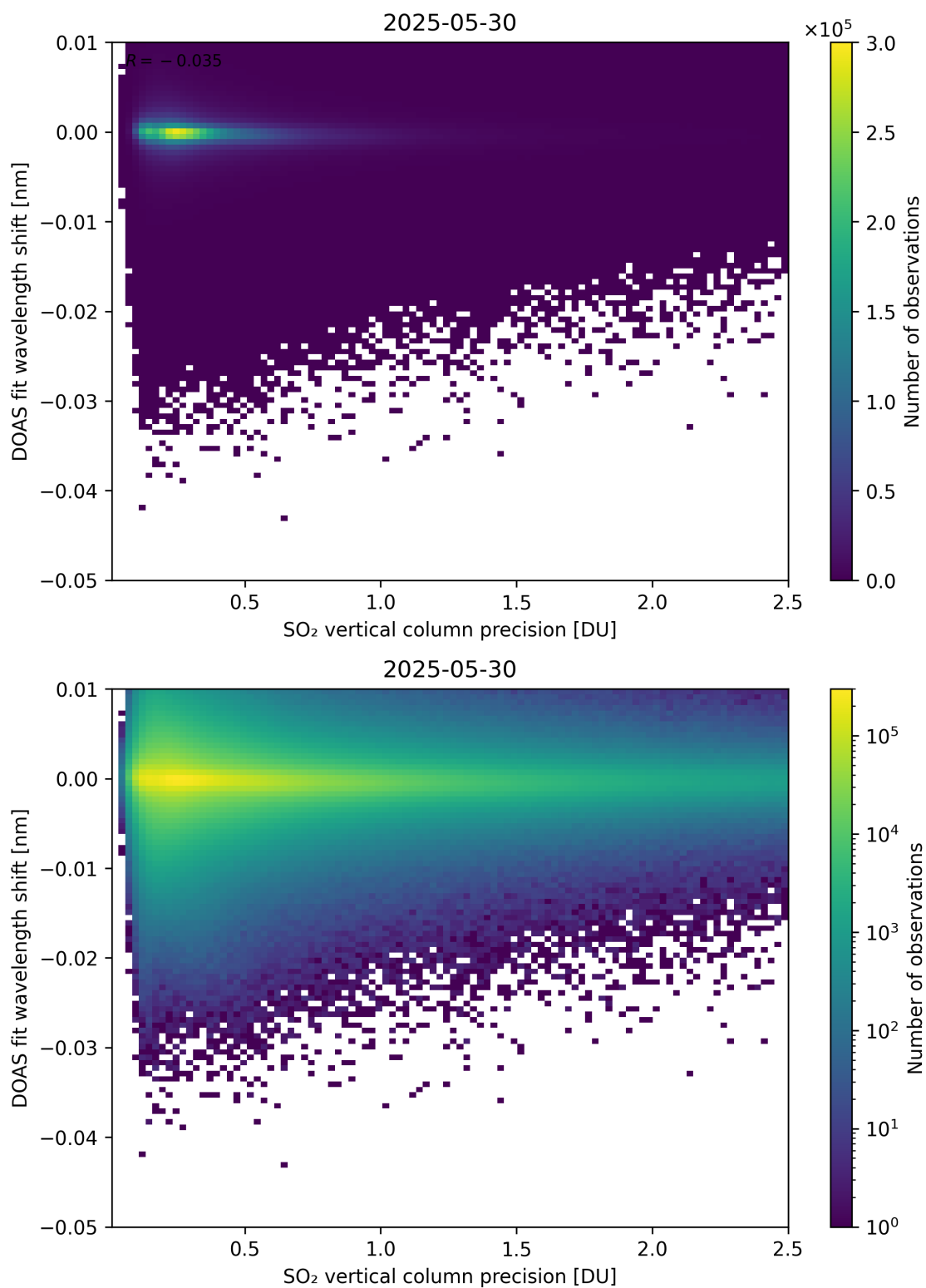
Figure 332: Scatter density plot of “SO 2 vertical column precision” against “DOAS fit wavelength shift” for 2025-05-29 to 2025-05-31.
