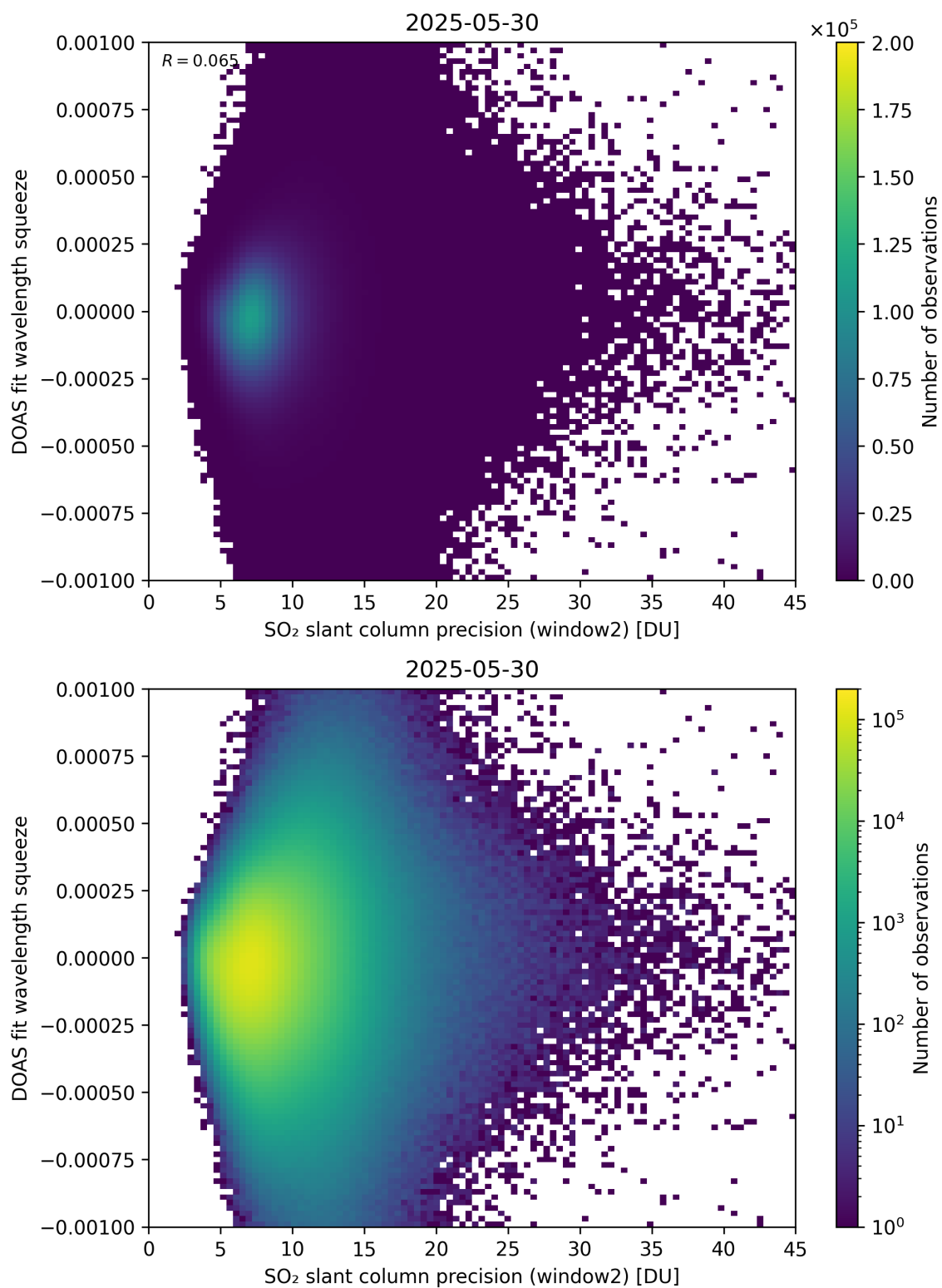
Figure 294: Scatter density plot of “SO 2 slant column precision (window2)” against “DOAS fit wavelength squeeze” for 2025-05-29 to 2025-05-31.
