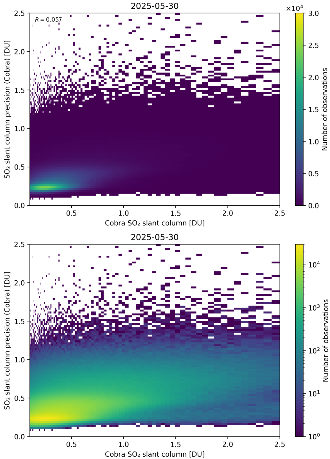
Figure 216: Scatter density plot of “Cobra SO 2 slant column” against “SO 2 slant column precision (Cobra)” for 2025-05-29 to 2025-05-31.
