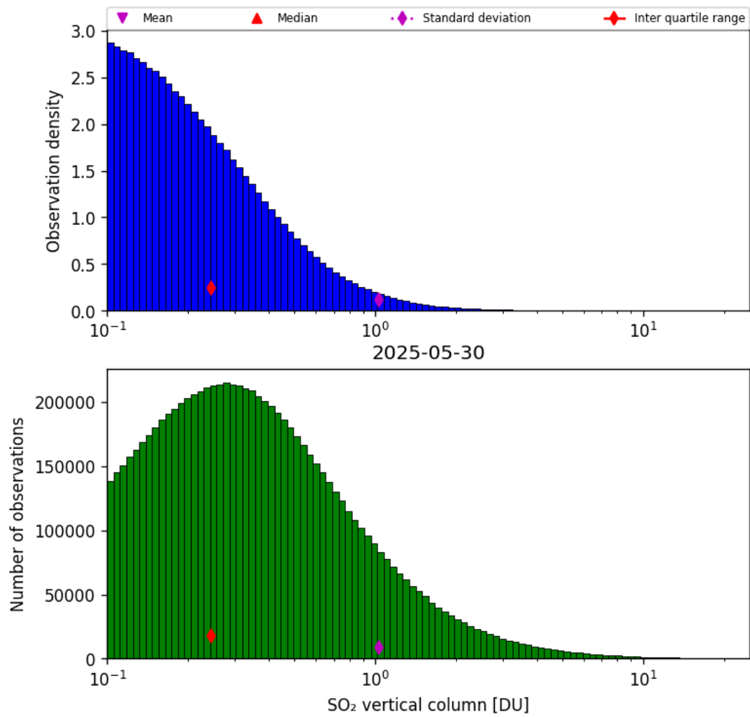
Figure 58: Histogram of “SO 2 vertical column” for 2025-05-29 to 2025-05-31
