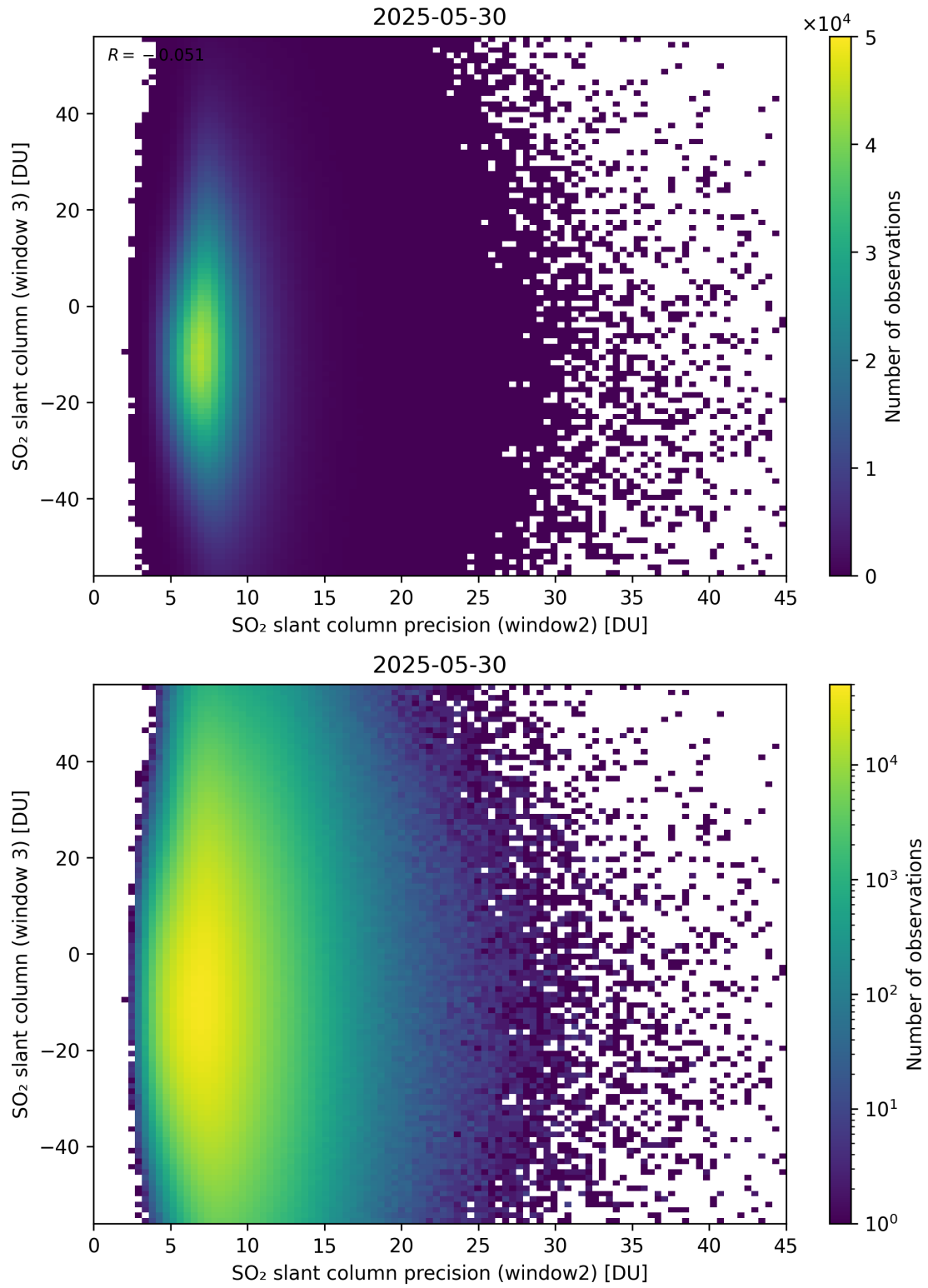
Figure 299: Scatter density plot of “SO 2 slant column precision (window2)” against “SO 2 slant column (window 3)” for 2025-05-29 to 2025-05-31.
