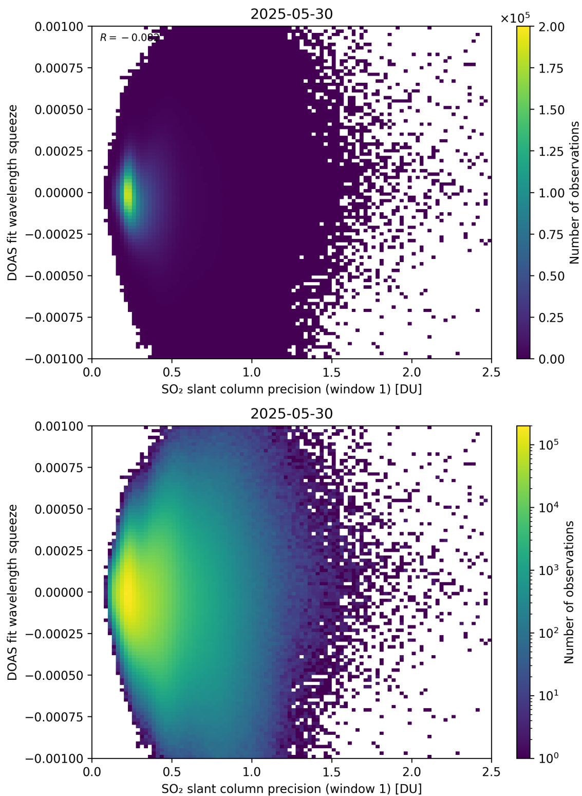
Figure 272: Scatter density plot of “SO 2 slant column precision (window 1)” against “DOAS fit wavelength squeeze” for 2025-05-29 to 2025-05-31.
