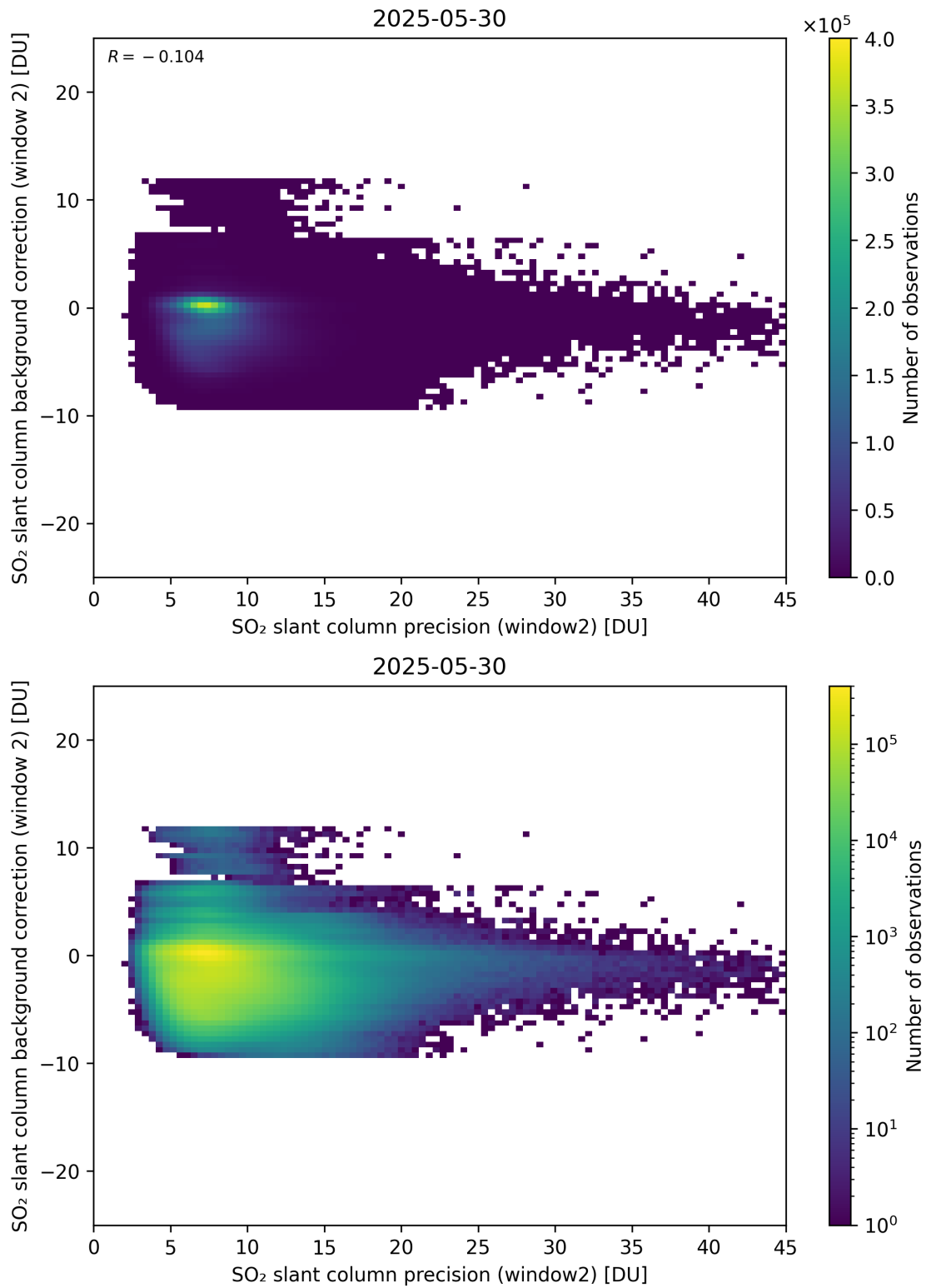
Figure 291: Scatter density plot of “SO 2 slant column precision (window2)” against “SO 2 slant column background correction (window 2)” for 2025-05-29 to 2025-05-31.
