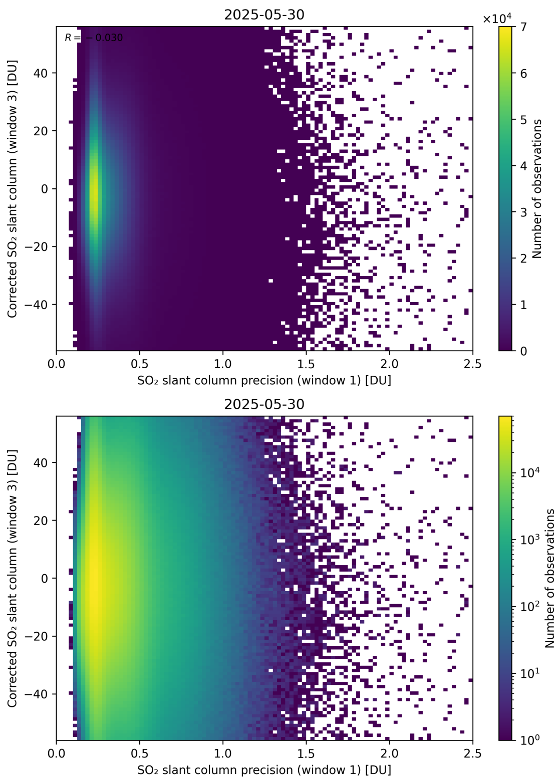
Figure 276: Scatter density plot of “SO 2 slant column precision (window 1)” against “Corrected SO 2 slant column (window 3)” for 2025-05-29 to 2025-05-31.
