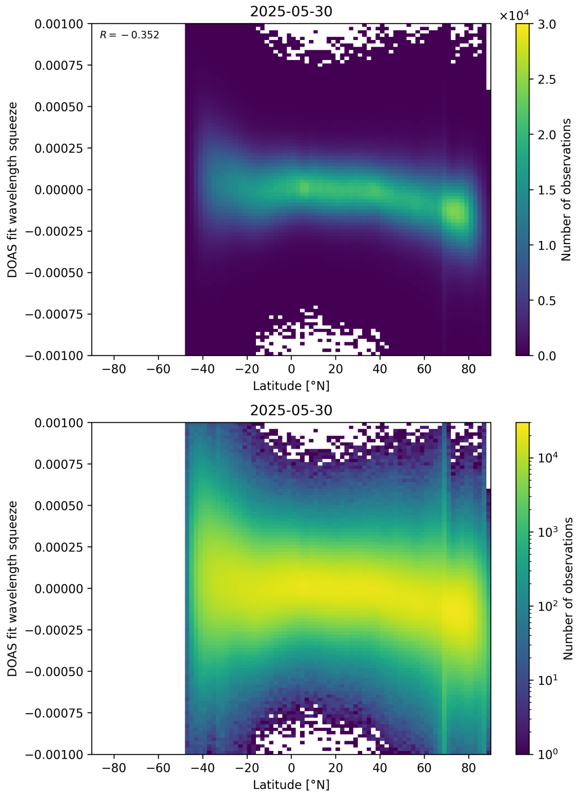
Figure 154: Scatter density plot of “Latitude” against “DOAS fit wavelength squeeze” for 2025-05-29 to 2025-05-31.
