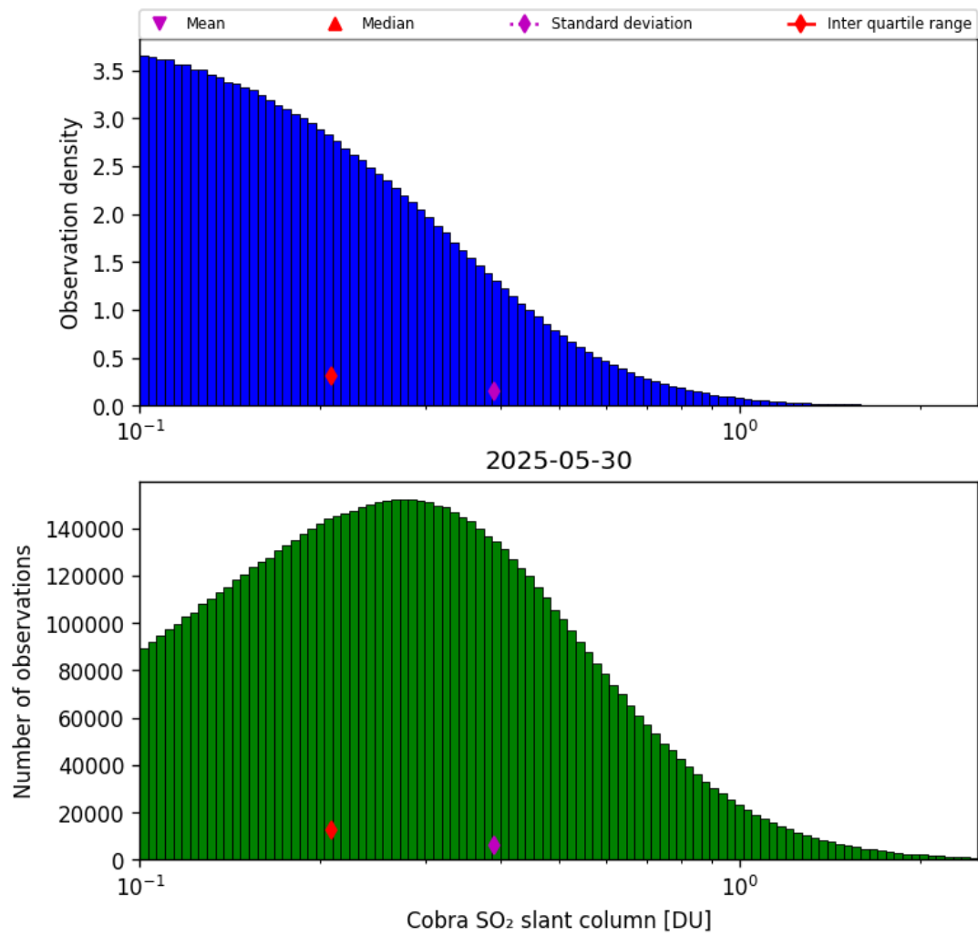
Figure 61: Histogram of “Cobra SO 2 slant column” for 2025-05-29 to 2025-05-31
