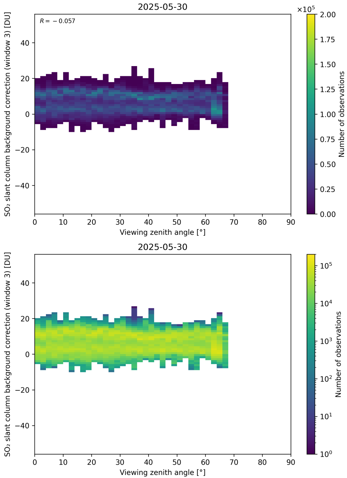
Figure 364: Scatter density plot of “Viewing zenith angle” against “SO 2 slant column background correction (window 3)” for 2025-05-29 to 2025-05-31.
