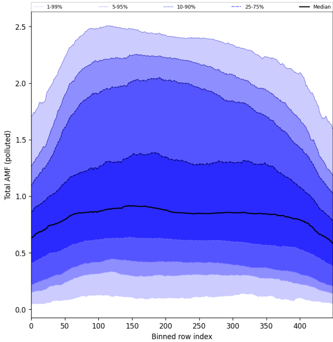
Figure 105: Along track statistics of “Total AMF (polluted)” for 2025-05-29 to 2025-05-31
