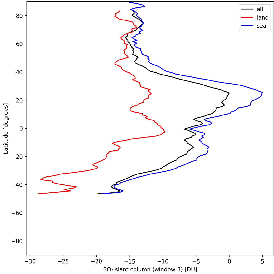
Figure 45: Zonal average of “SO 2 slant column (window 3)” for 2025-05-29 to 2025-05-31.
