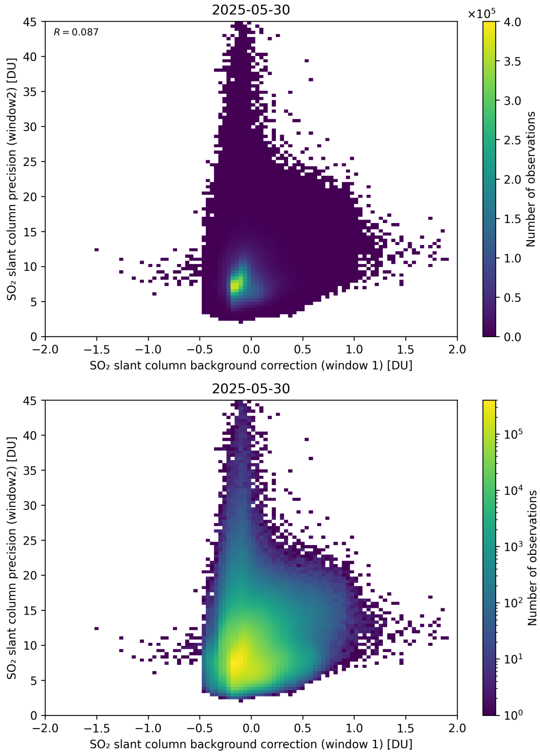
Figure 117: Scatter density plot of “SO 2 slant column background correction (window 1)” against “SO 2 slant column precision (window2)” for 2025-05-29 to 2025-05-31.
