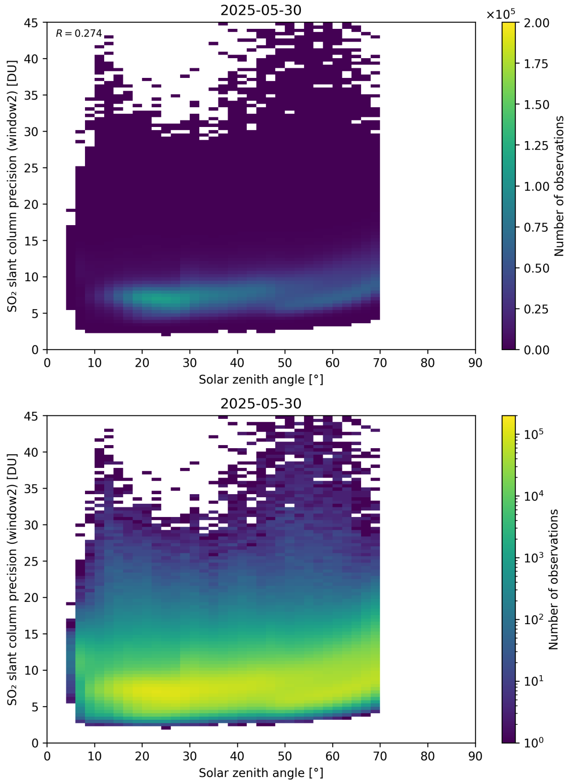
Figure 186: Scatter density plot of “Solar zenith angle” against “SO 2 slant column precision (window2)” for 2025-05-29 to 2025-05-31.
