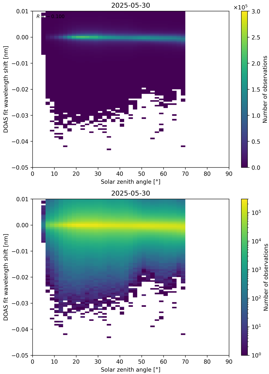
Figure 174: Scatter density plot of “Solar zenith angle” against “DOAS fit wavelength shift” for 2025-05-29 to 2025-05-31.
