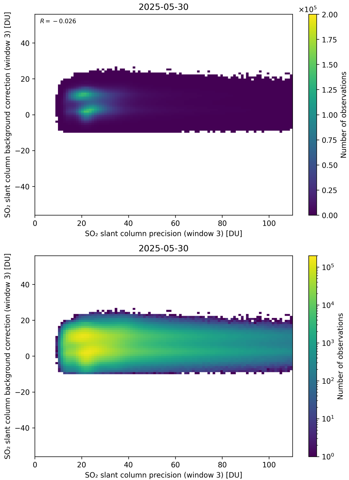
Figure 307: Scatter density plot of “SO 2 slant column precision (window 3)” against “SO 2 slant column background correction (window 3)” for 2025-05-29 to 2025-05-31.
