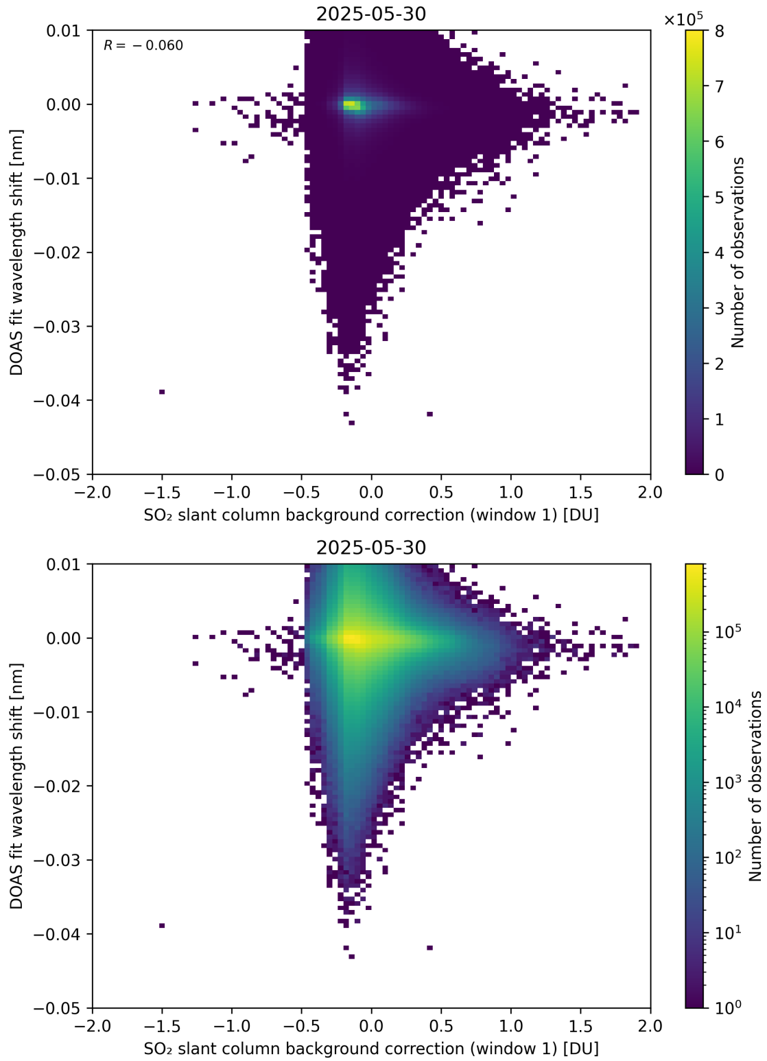
Figure 111: Scatter density plot of “SO 2 slant column background correction (window 1)” against “DOAS fit wavelength shift” for 2025-05-29 to 2025-05-31.
