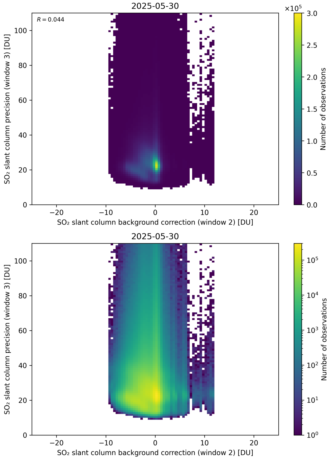
Figure 129: Scatter density plot of “SO 2 slant column background correction (window 2)” against “SO 2 slant column precision (window 3)” for 2025-05-29 to 2025-05-31.
