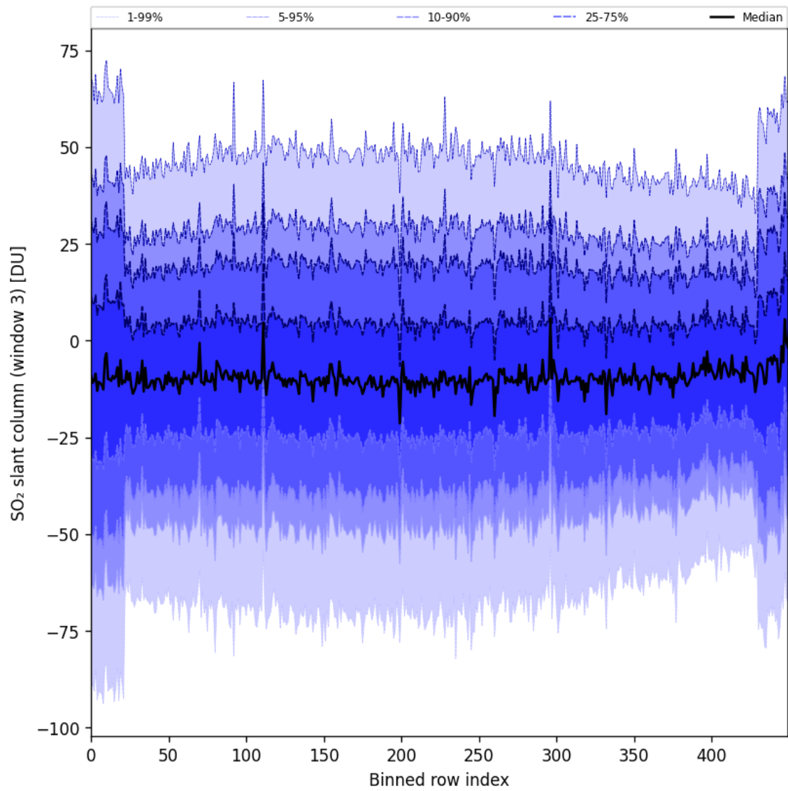
Figure 97: Along track statistics of “SO 2 slant column (window 3)” for 2025-05-29 to 2025-05-31
