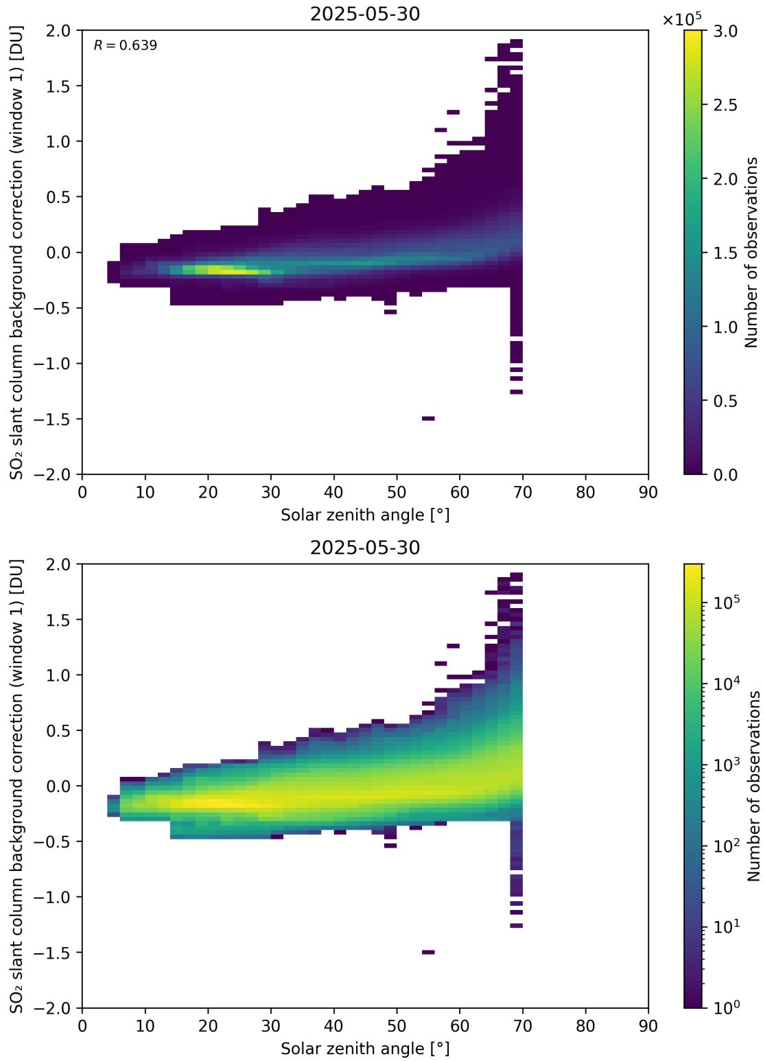
Figure 171: Scatter density plot of “Solar zenith angle” against “SO 2 slant column background correction (window 1)” for 2025-05-29 to 2025-05-31.
