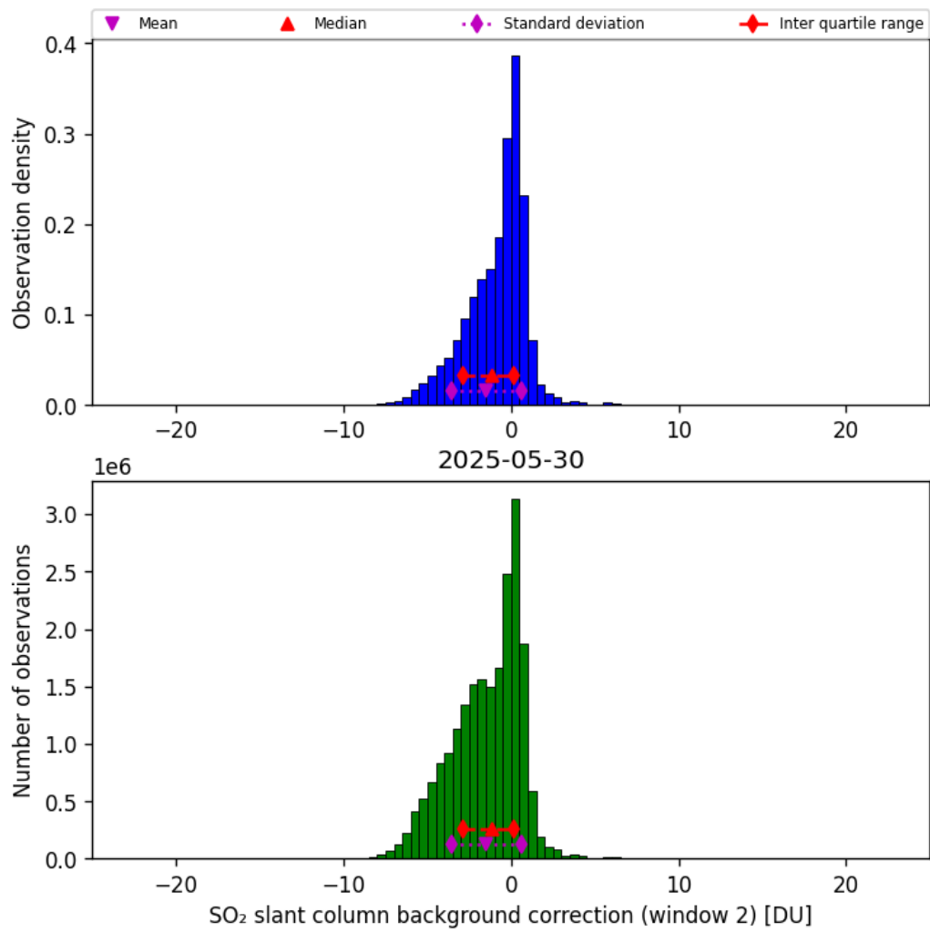
Figure 70: Histogram of “SO 2 slant column background correction (window 2)” for 2025-05-29 to 2025-05-31
