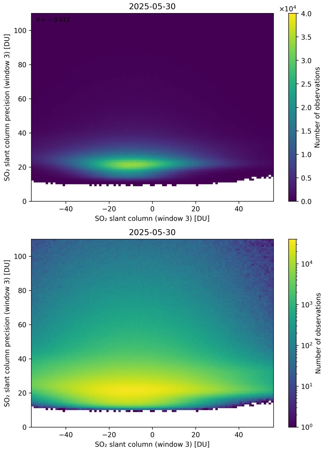
Figure 317: Scatter density plot of “SO 2 slant column (window 3)” against “SO 2 slant column precision (window 3)” for 2025-05-29 to 2025-05-31.
