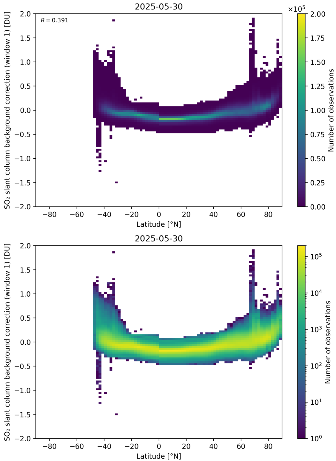
Figure 150: Scatter density plot of “Latitude” against “SO 2 slant column background correction (window 1)” for 2025-05-29 to 2025-05-31.
