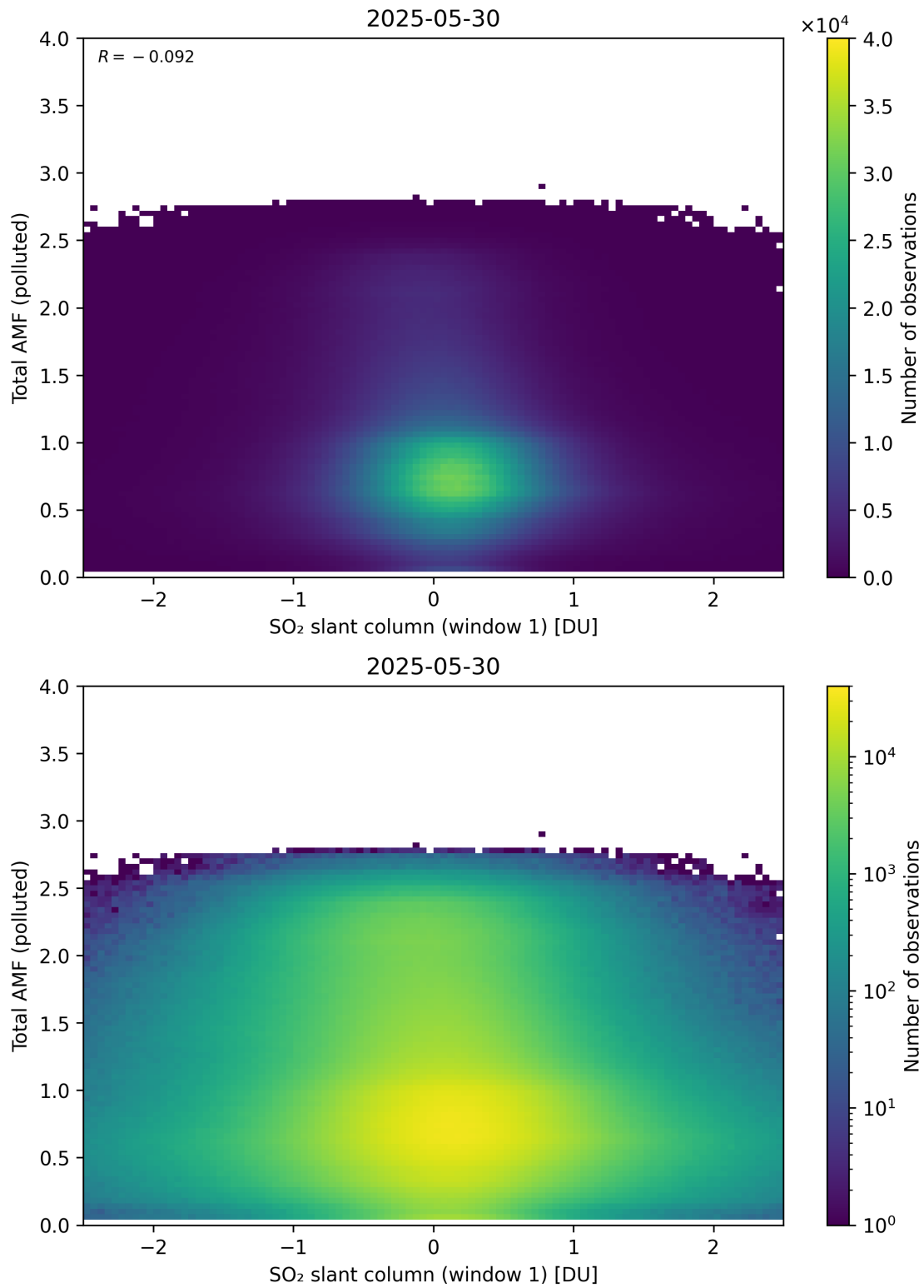
Figure 289: Scatter density plot of “SO 2 slant column (window 1)” against “Total AMF (polluted)” for 2025-05-29 to 2025-05-31.
