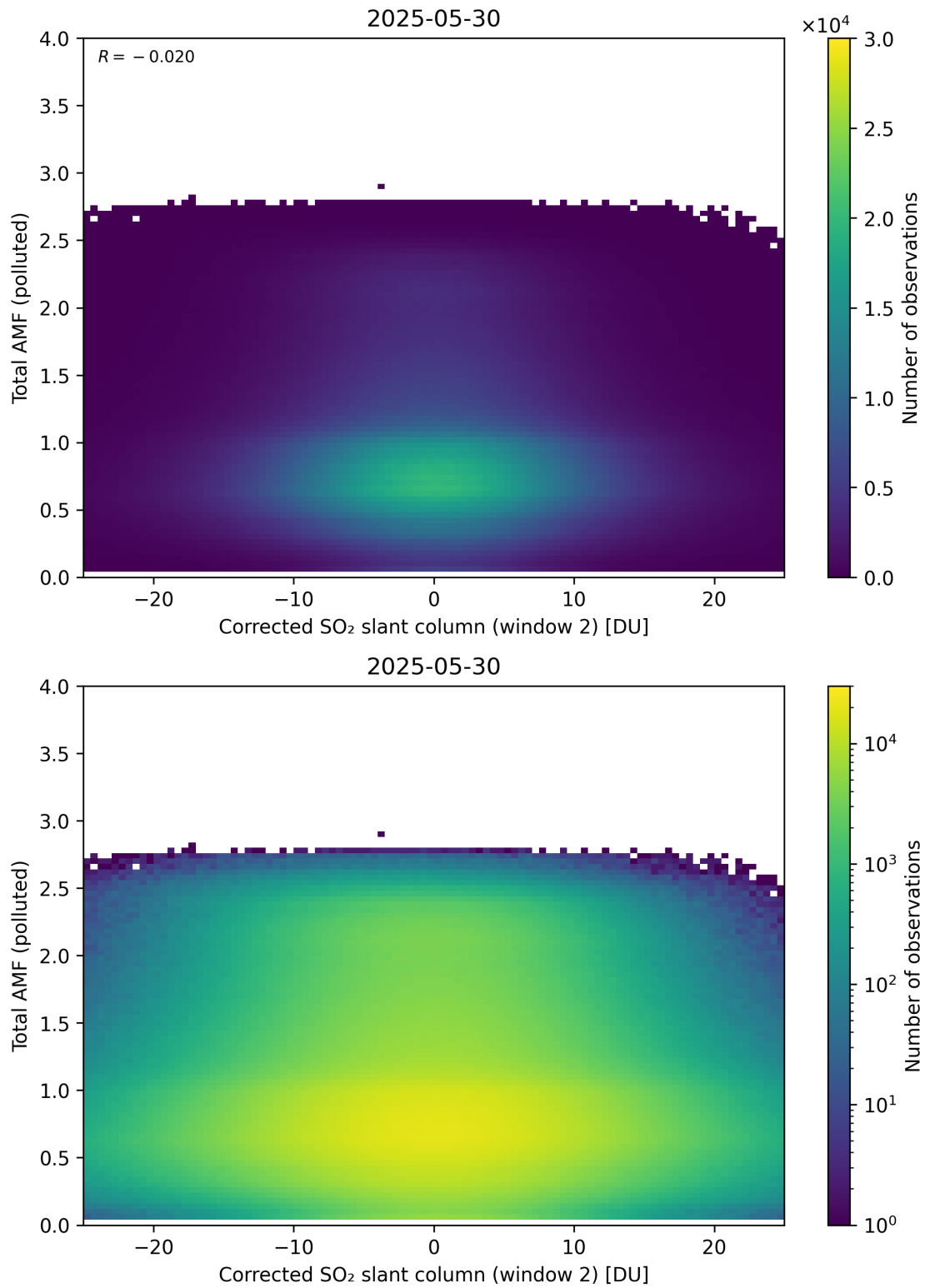
Figure 253: Scatter density plot of “Corrected SO 2 slant column (window 2)” against “Total AMF (polluted)” for 2025-05-29 to 2025-05-31.
