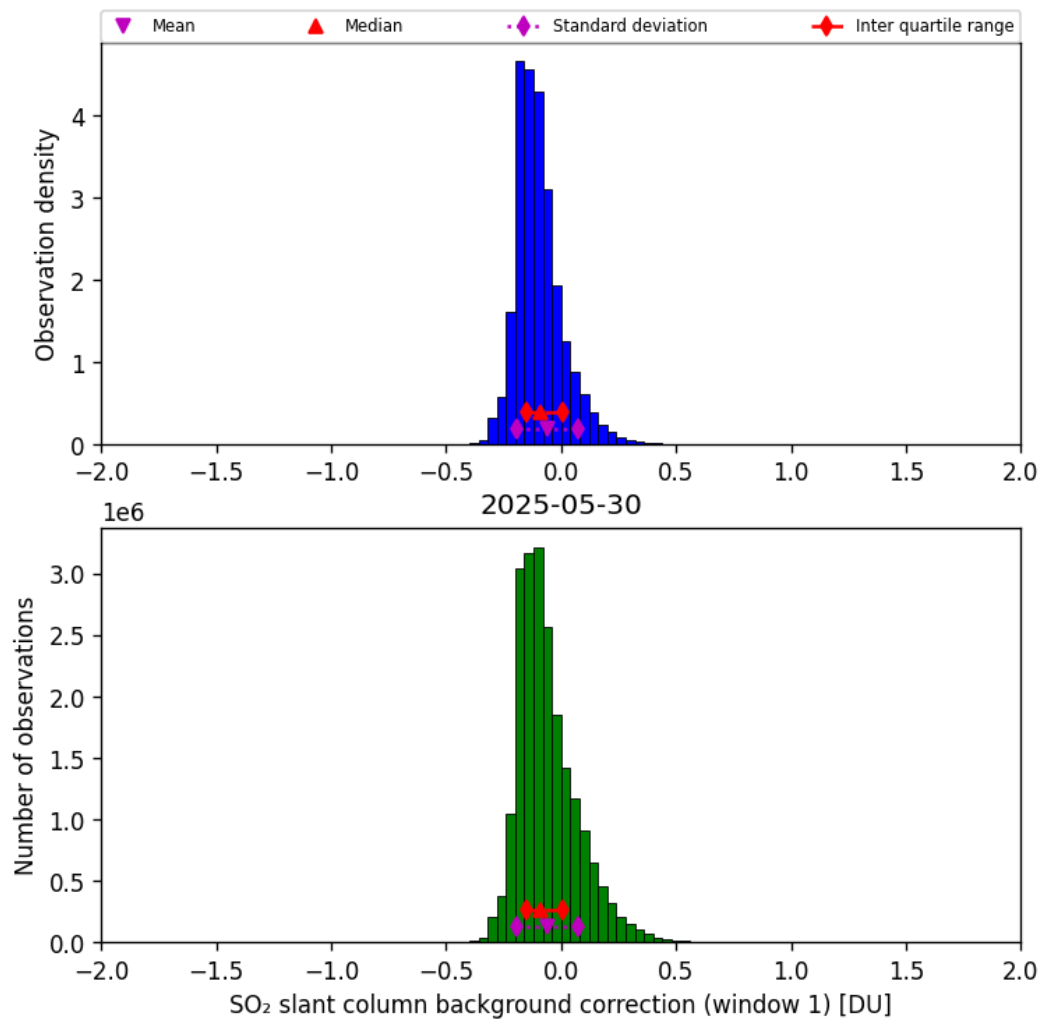
Figure 66: Histogram of “SO 2 slant column background correction (window 1)” for 2025-05-29 to 2025-05-31
