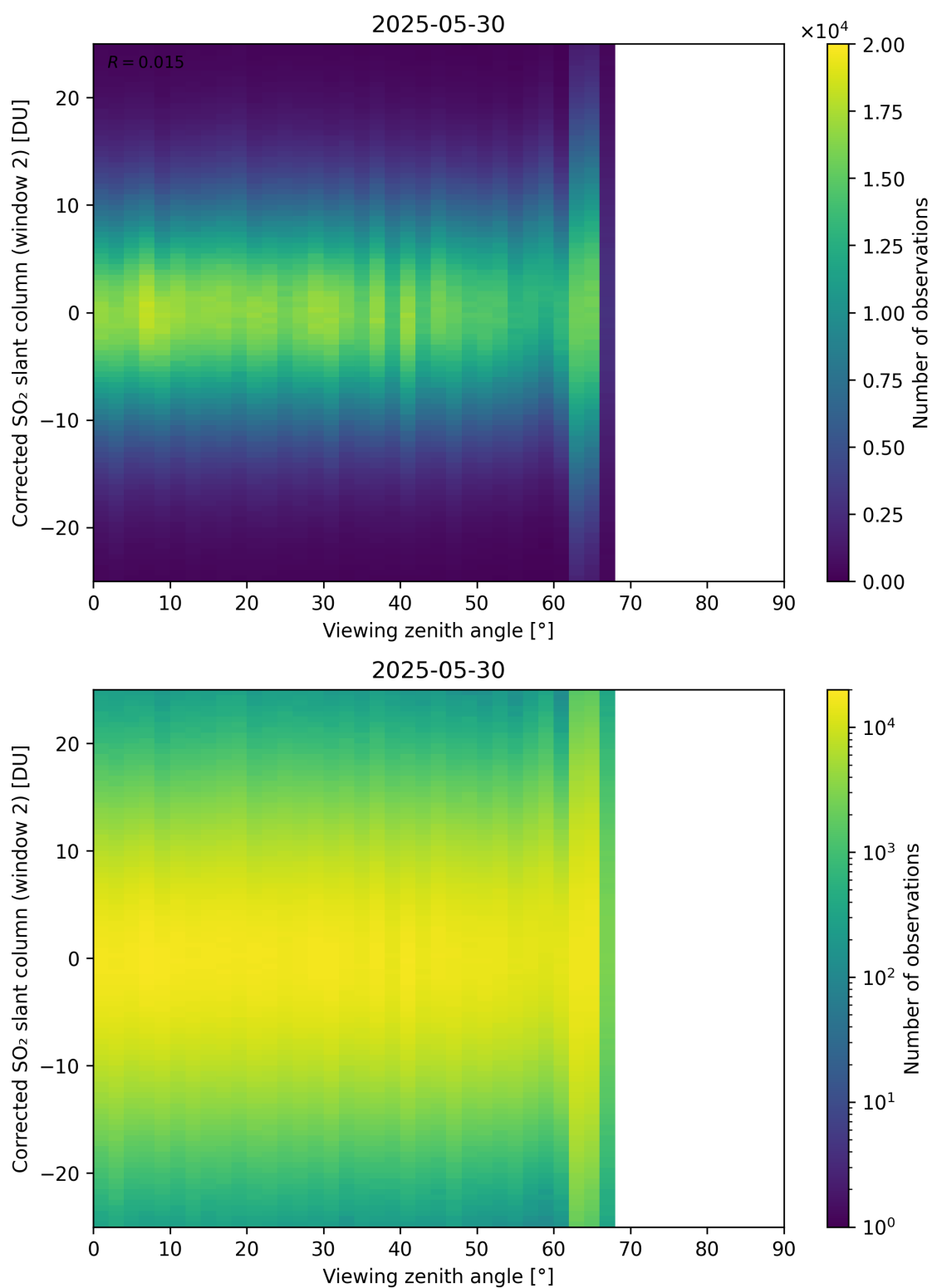
Figure 374: Scatter density plot of “Viewing zenith angle” against “Corrected SO 2 slant column (window 2)” for 2025-05-29 to 2025-05-31.
