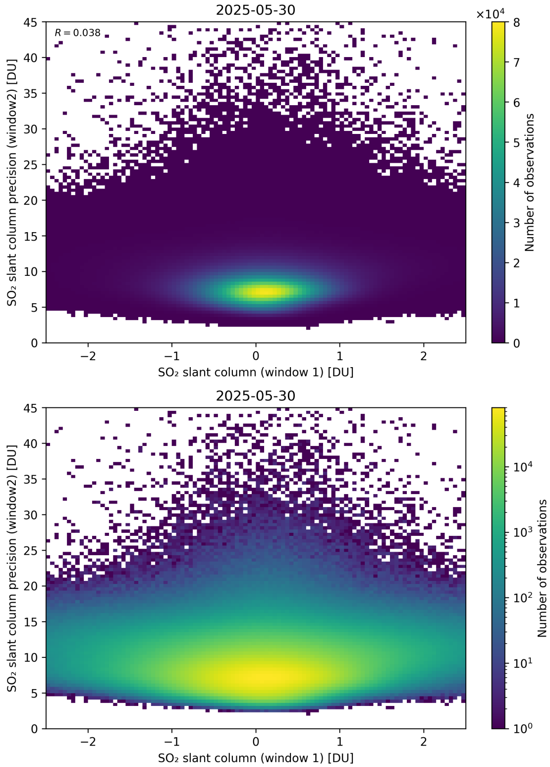
Figure 286: Scatter density plot of “SO 2 slant column (window 1)” against “SO 2 slant column precision (window2)” for 2025-05-29 to 2025-05-31.
