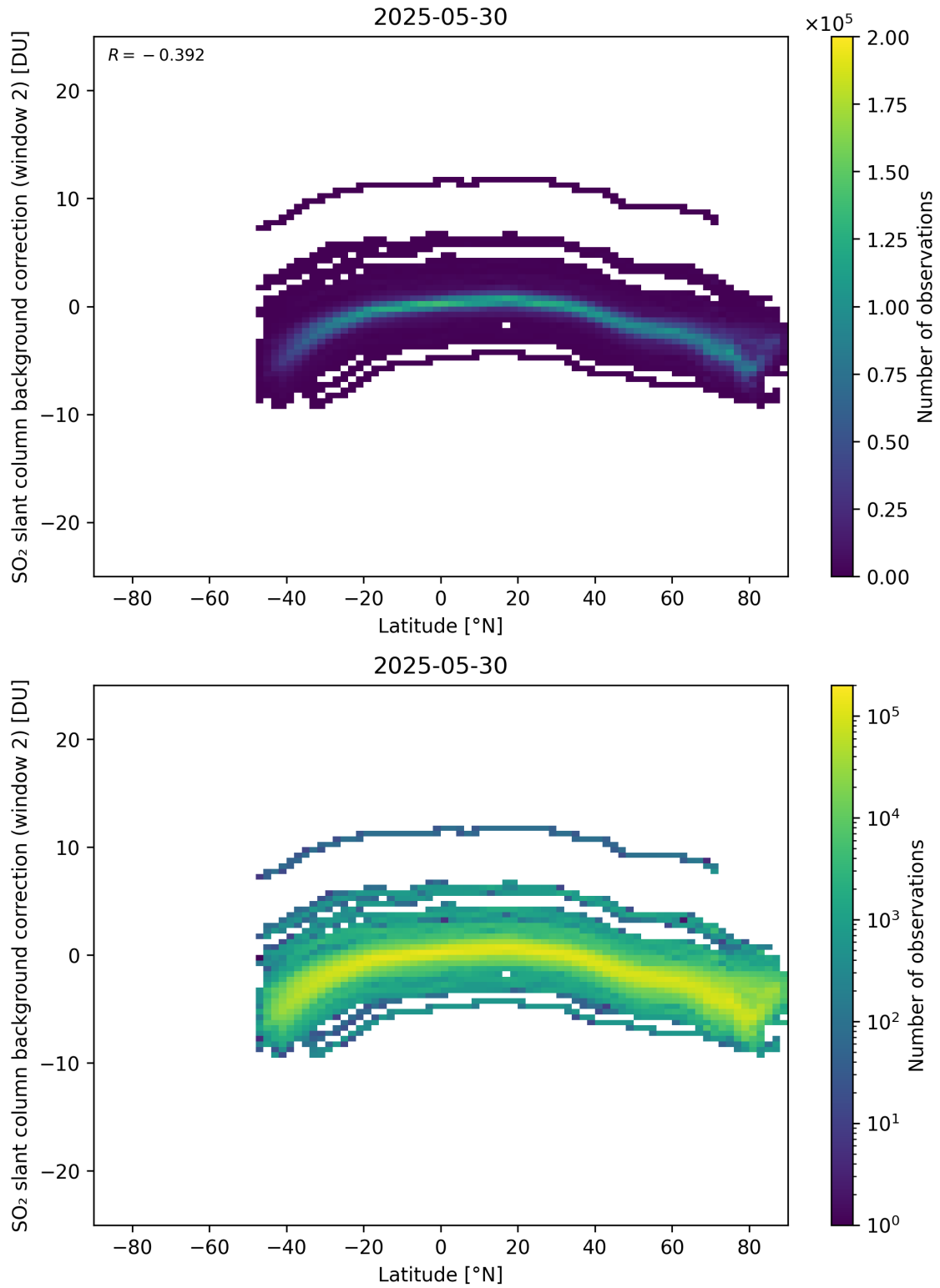
Figure 151: Scatter density plot of “Latitude” against “SO 2 slant column background correction (window 2)” for 2025-05-29 to 2025-05-31.
