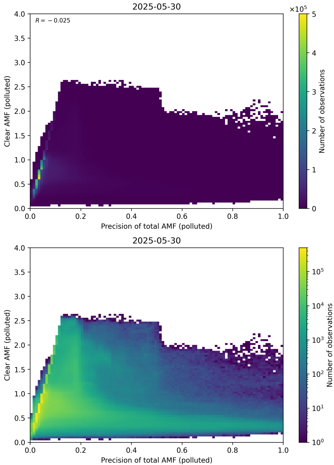
Figure 320: Scatter density plot of “Precision of total AMF (polluted)” against “Clear AMF (polluted)” for 2025-05-29 to 2025-05-31.
