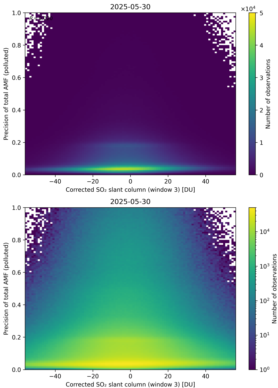
Figure 261: Scatter density plot of “Corrected SO 2 slant column (window 3)” against “Precision of total AMF (polluted)” for 2025-05-29 to 2025-05-31.
