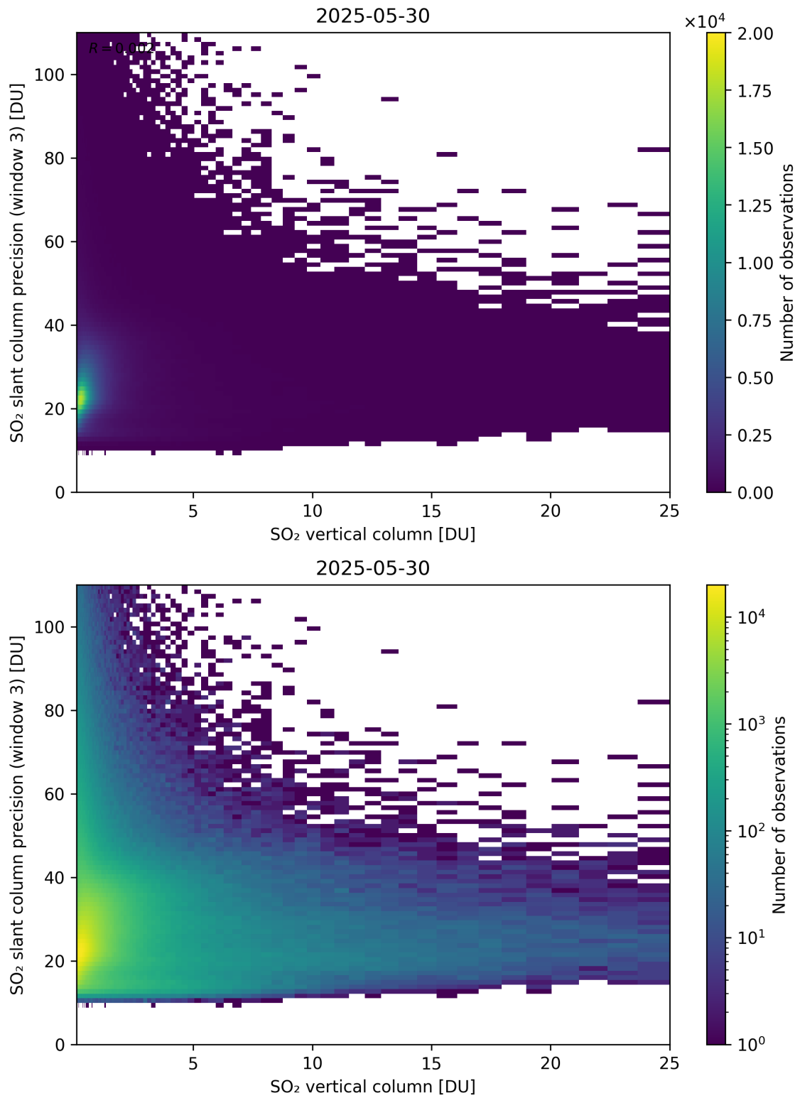
Figure 358: Scatter density plot of “SO 2 vertical column” against “SO 2 slant column precision (window 3)” for 2025-05-29 to 2025-05-31.
