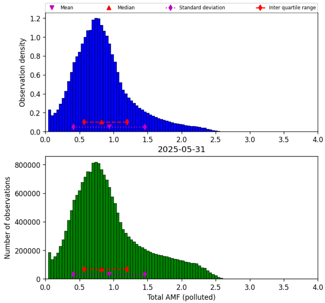
Figure 79: Histogram of “Total AMF (polluted)” for 2025-05-31 to 2025-06-01
