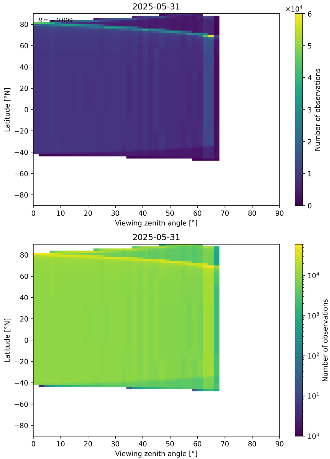
Figure 368: Scatter density plot of “Viewing zenith angle” against “Latitude” for 2025-05-31 to 2025-06-01.
