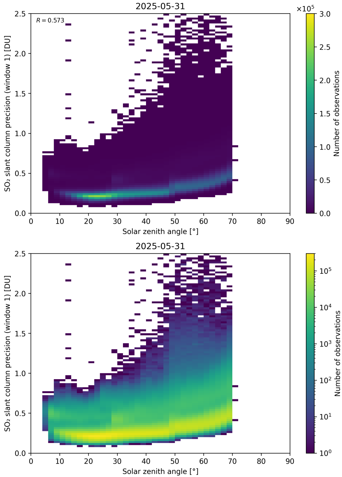
Figure 185: Scatter density plot of “Solar zenith angle” against “SO 2 slant column precision (window 1)” for 2025-05-31 to 2025-06-01.
