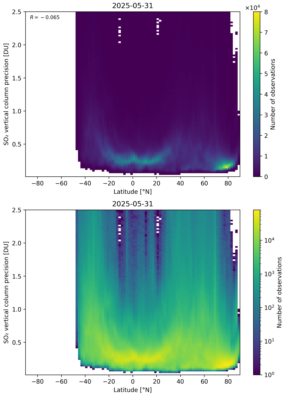
Figure 170: Scatter density plot of “Latitude” against “SO 2 vertical column precision” for 2025-05-31 to 2025-06-01.
