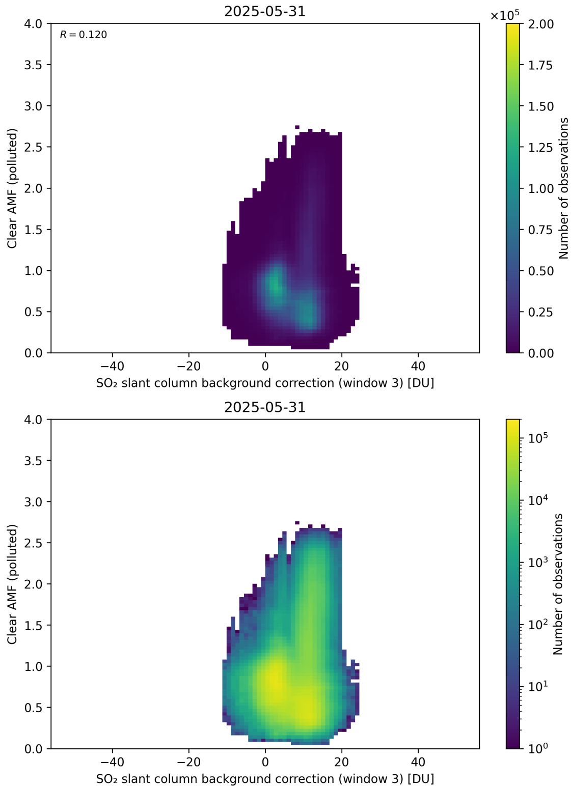
Figure 135: Scatter density plot of “SO 2 slant column background correction (window 3)” against “Clear AMF (polluted)” for 2025-05-31 to 2025-06-01.
