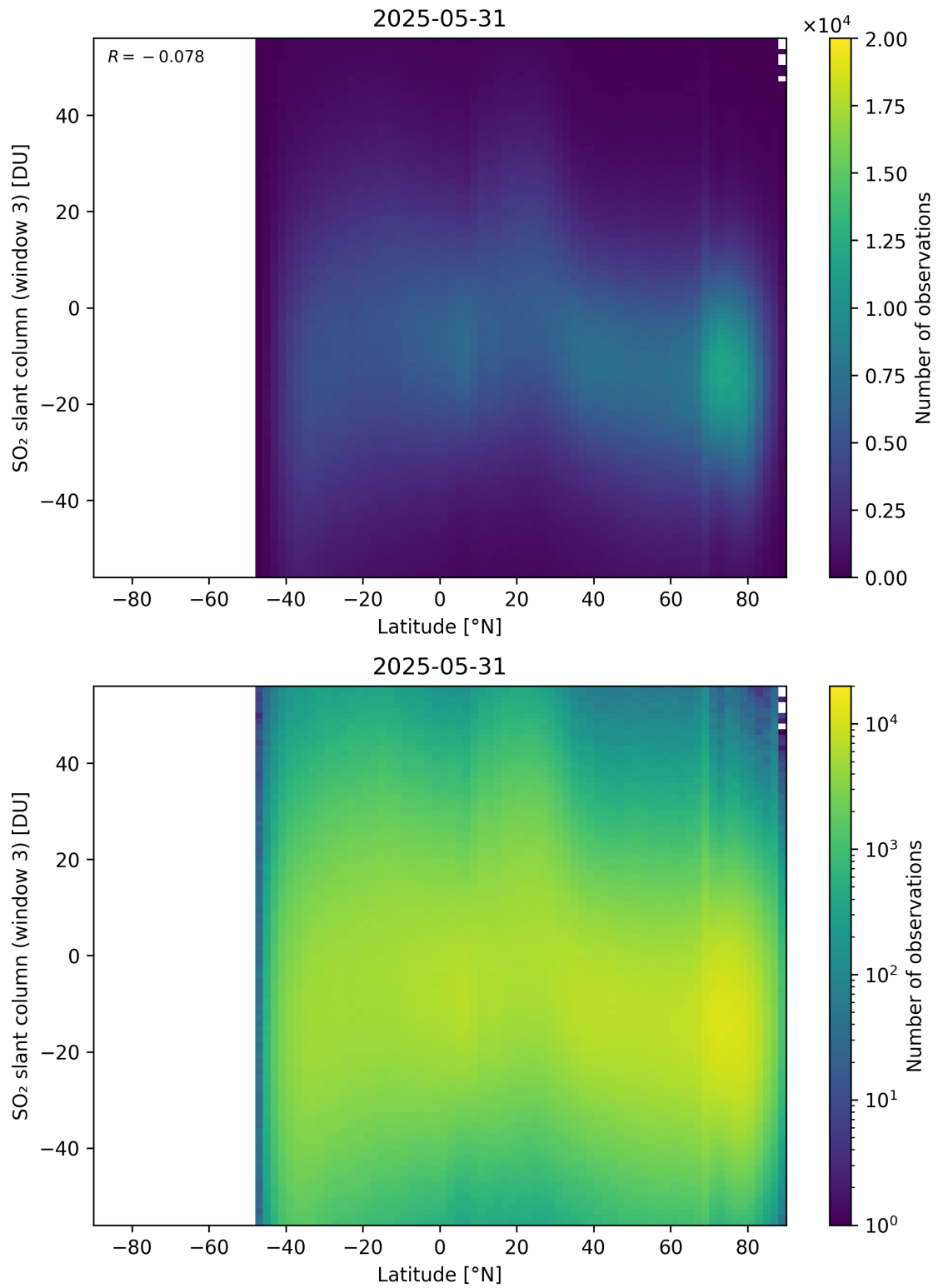
Figure 165: Scatter density plot of “Latitude” against “SO 2 slant column (window 3)” for 2025-05-31 to 2025-06-01.
