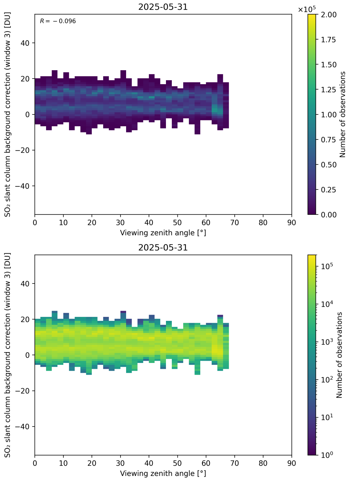
Figure 364: Scatter density plot of “Viewing zenith angle” against “SO 2 slant column background correction (window 3)” for 2025-05-31 to 2025-06-01.
