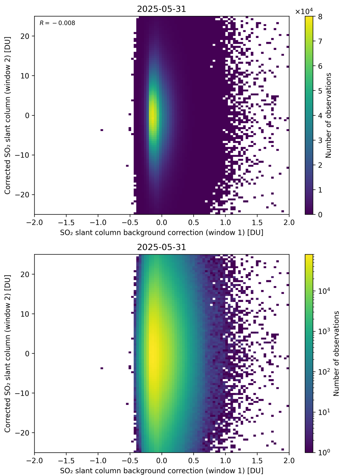
Figure 115: Scatter density plot of “SO 2 slant column background correction (window 1)” against “Corrected SO 2 slant column (window 2)” for 2025-05-31 to 2025-06-01.
