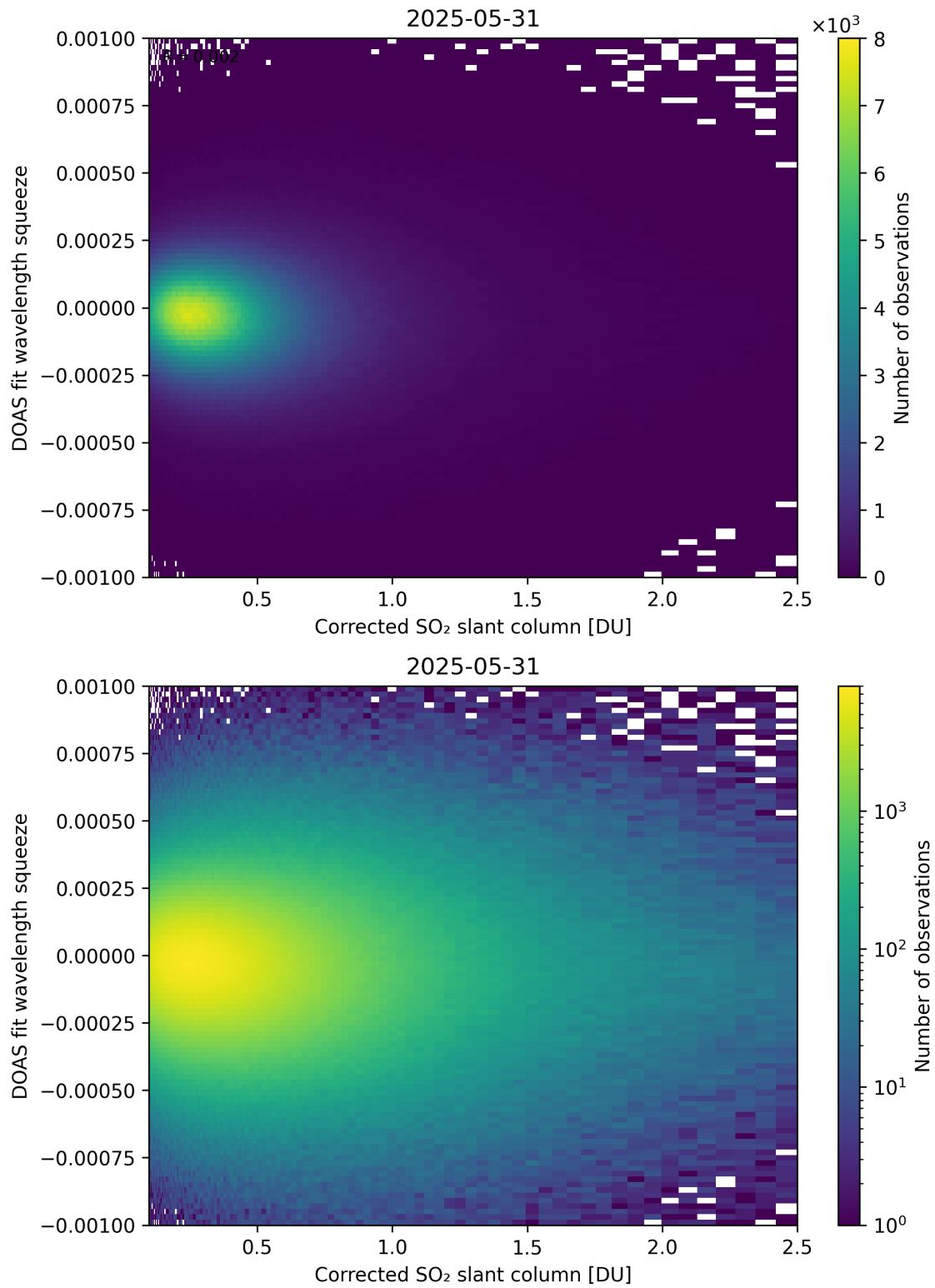
Figure 230: Scatter density plot of "Corrected SO 2 slant column" against "DOAS fit wavelength squeeze" for 2025-05-31 to 2025-06-01.
