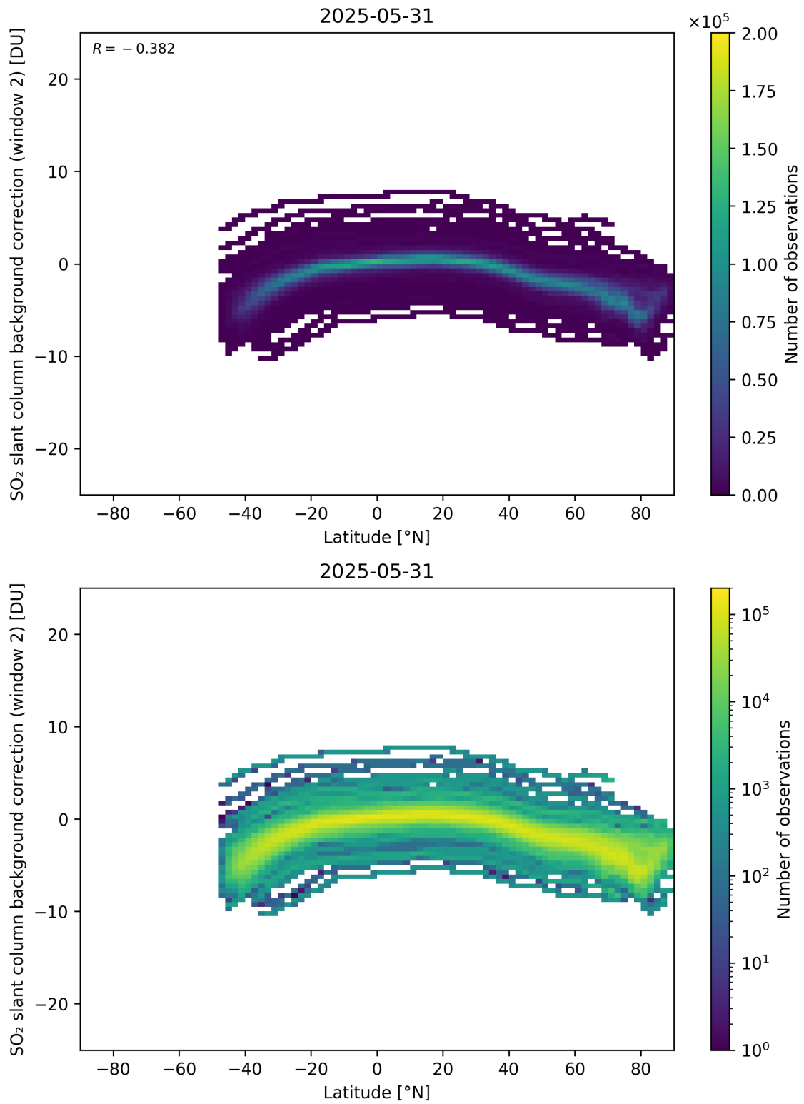
Figure 151: Scatter density plot of “Latitude” against “SO 2 slant column background correction (window 2)” for 2025-05-31 to 2025-06-01.
