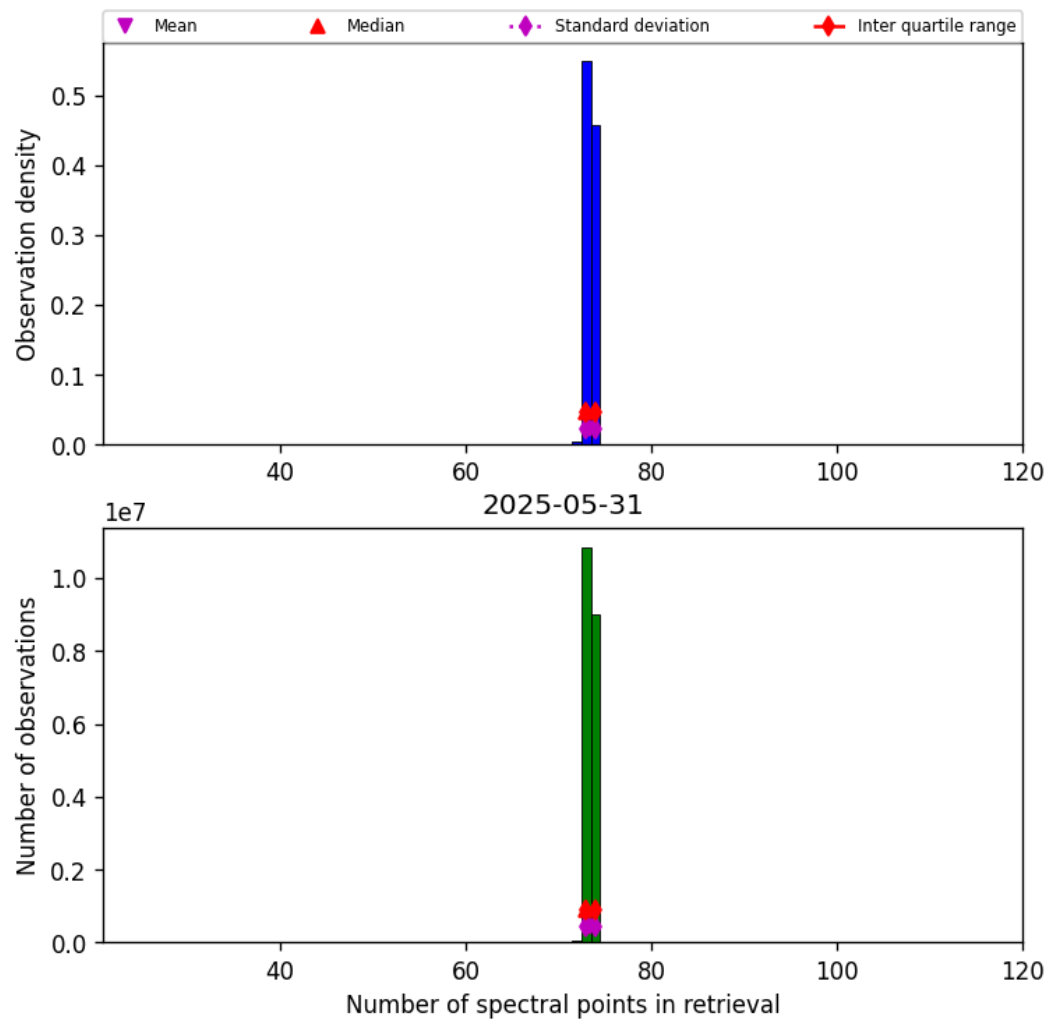
Figure 82: Histogram of “Number of spectral points in retrieval” for 2025-05-31 to 2025-06-01
