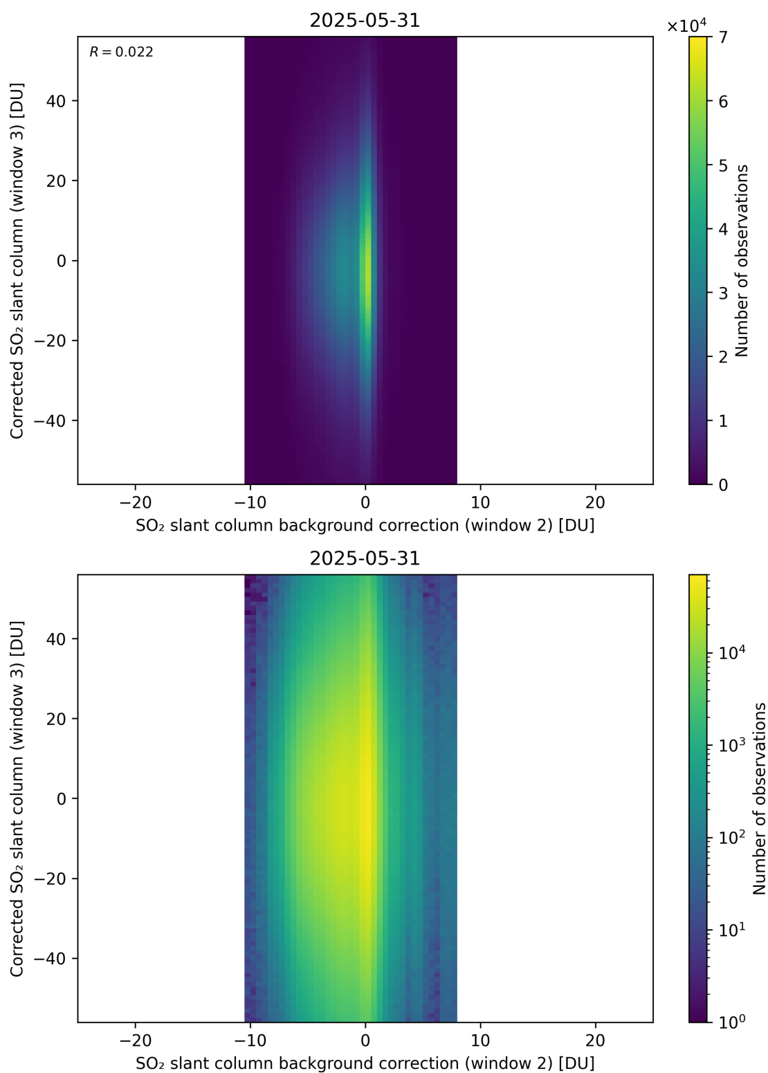
Figure 127: Scatter density plot of “SO 2 slant column background correction (window 2)” against “Corrected SO 2 slant column (window 3)” for 2025-05-31 to 2025-06-01.
