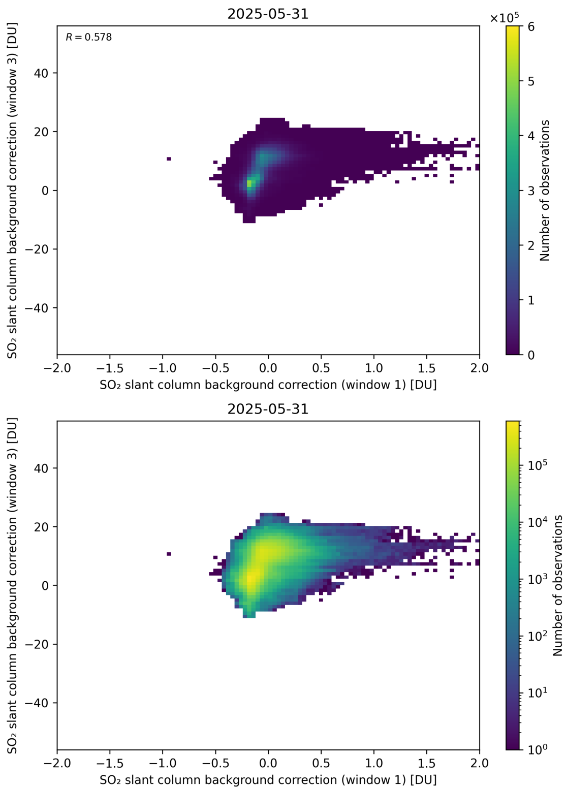
Figure 110: Scatter density plot of “SO 2 slant column background correction (window 1)” against “SO 2 slant column background correction (window 3)” for 2025-05-31 to 2025-06-01.
