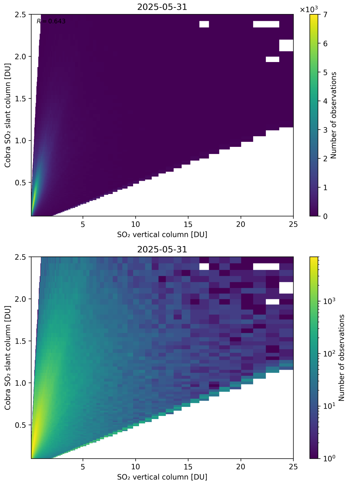
Figure 349: Scatter density plot of “SO 2 vertical column” against “Cobra SO 2 slant column” for 2025-05-31 to 2025-06-01.
