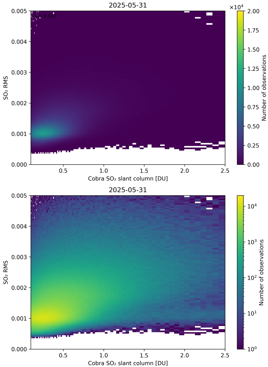
Figure 198: Scatter density plot of “Cobra SO 2 slant column” against “SO 2 RMS” for 2025-05-31 to 2025-06-01.
