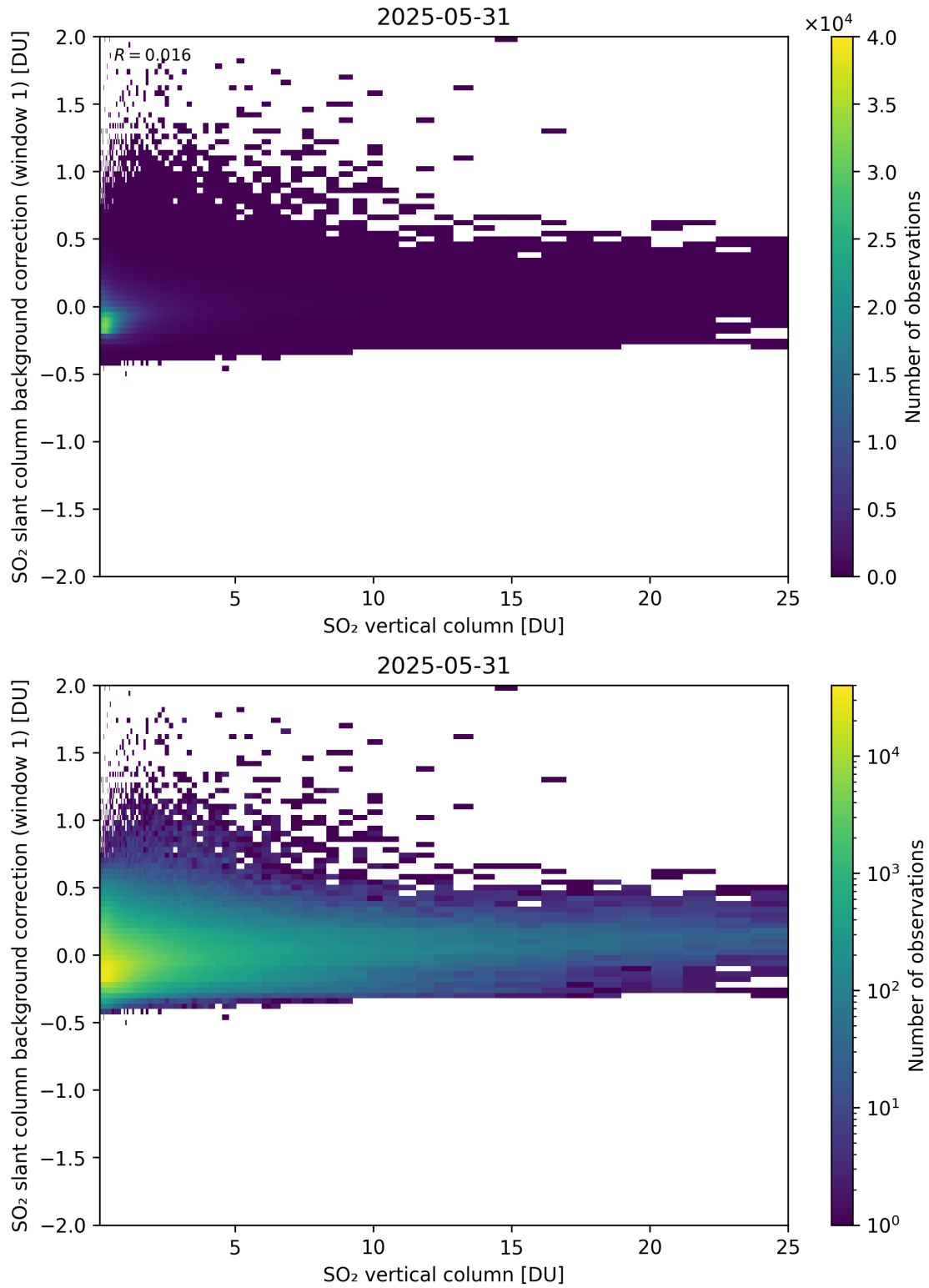
Figure 323: Scatter density plot of “SO 2 vertical column” against “SO 2 slant column background correction (window 1)” for 2025-05-31 to 2025-06-01.
