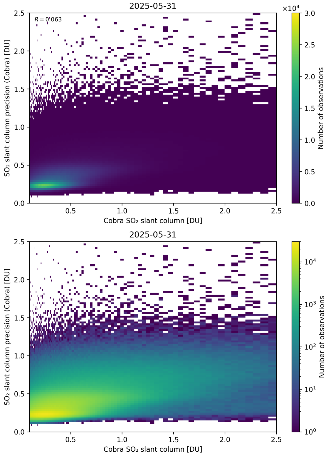
Figure 216: Scatter density plot of “Cobra SO 2 slant column” against “SO 2 slant column precision (Cobra)” for 2025-05-31 to 2025-06-01.
