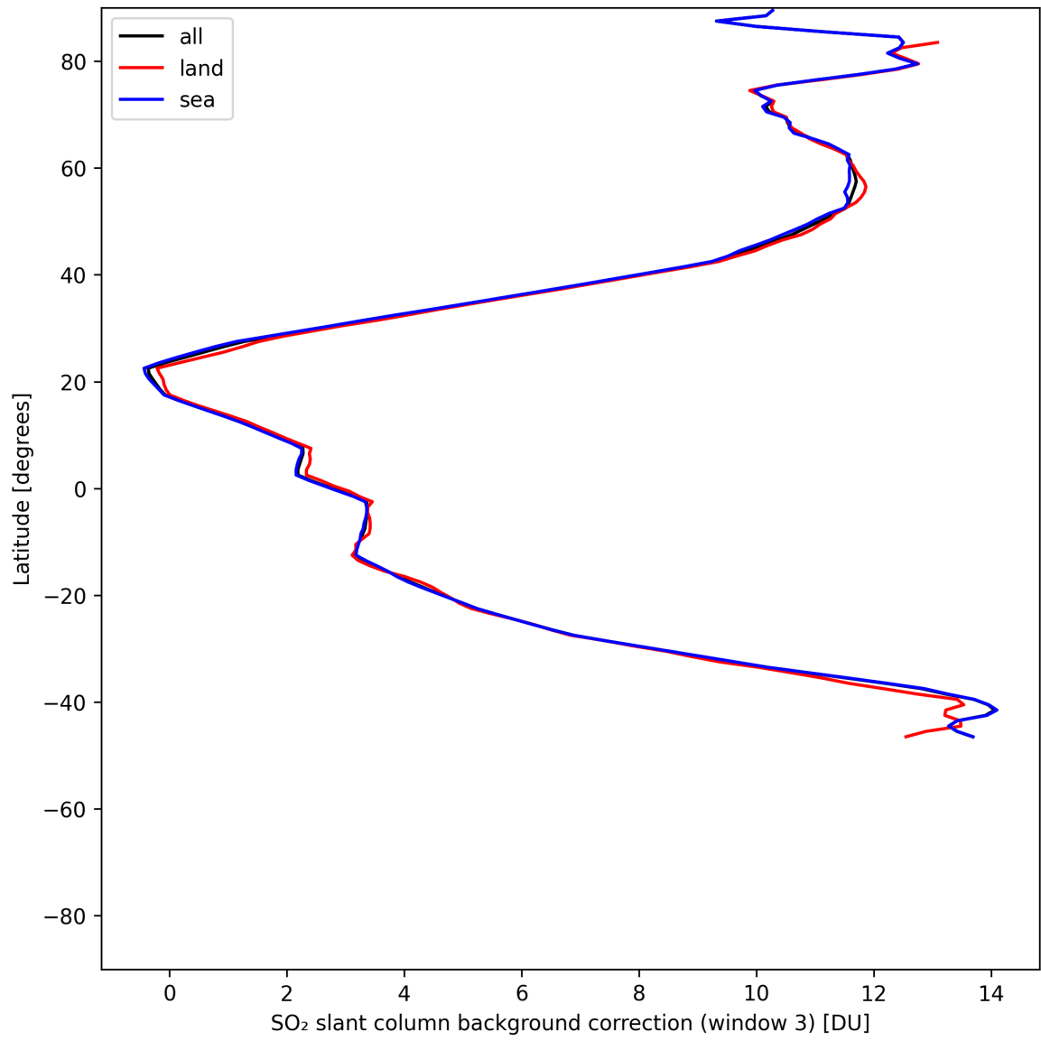
Figure 48: Zonal average of “SO 2 slant column background correction (window 3)” for 2025-05-31 to 2025-06-01.
