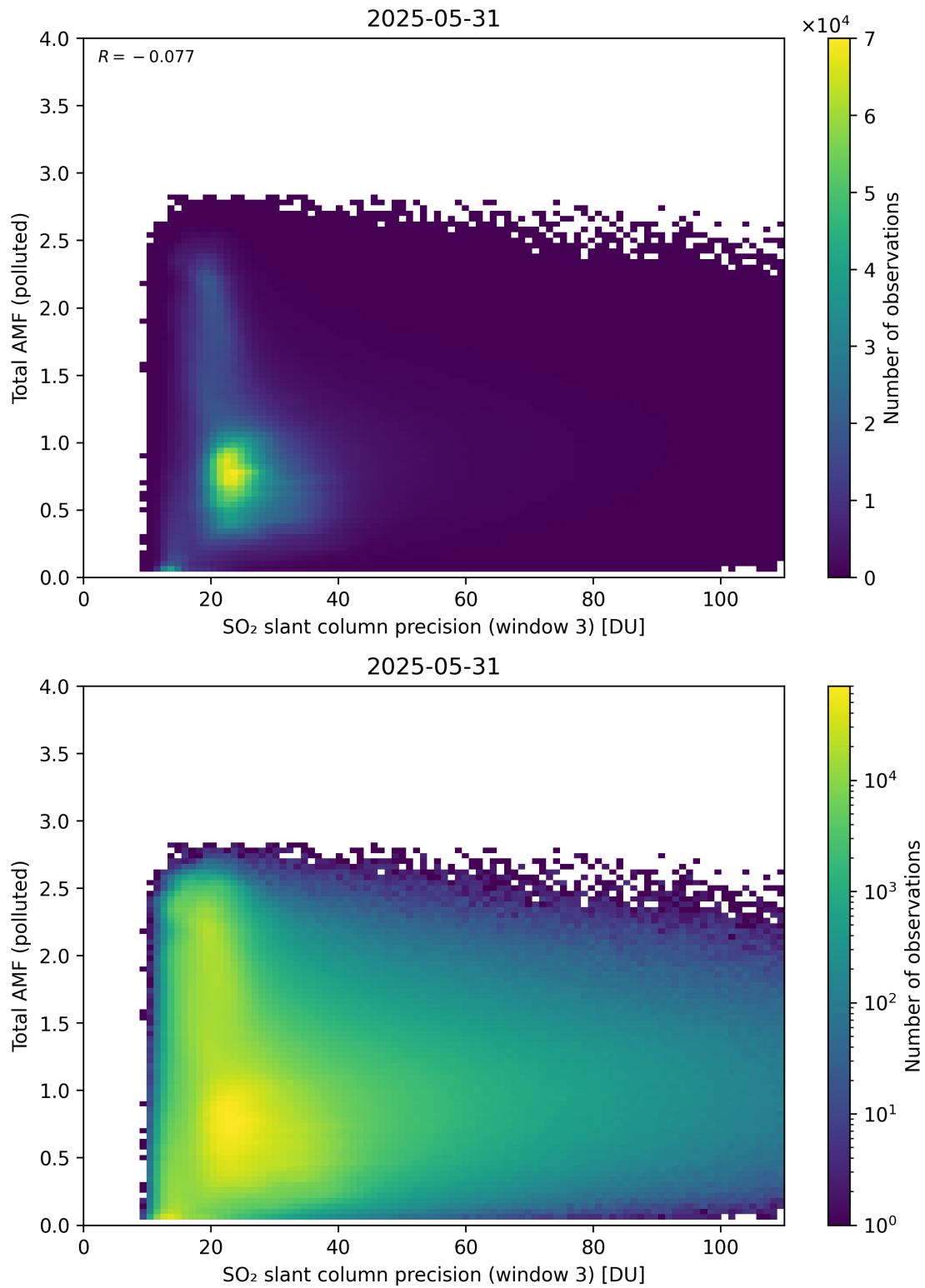
Figure 313: Scatter density plot of “SO 2 slant column precision (window 3)” against “Total AMF (polluted)” for 2025-05-31 to 2025-06-01.
