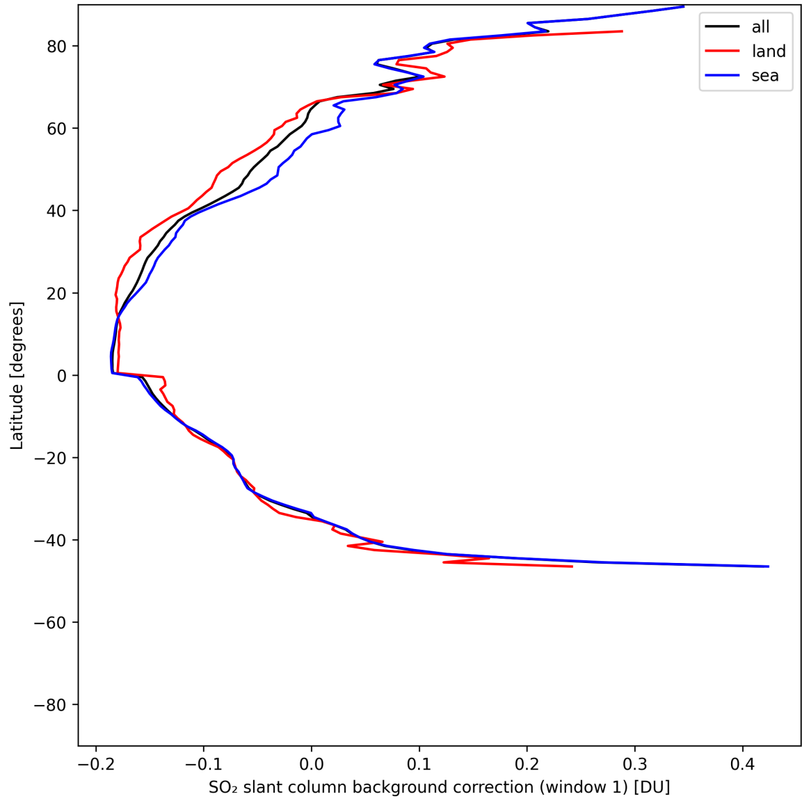
Figure 40: Zonal average of “SO 2 slant column background correction (window 1)” for 2025-05-31 to 2025-06-01.
