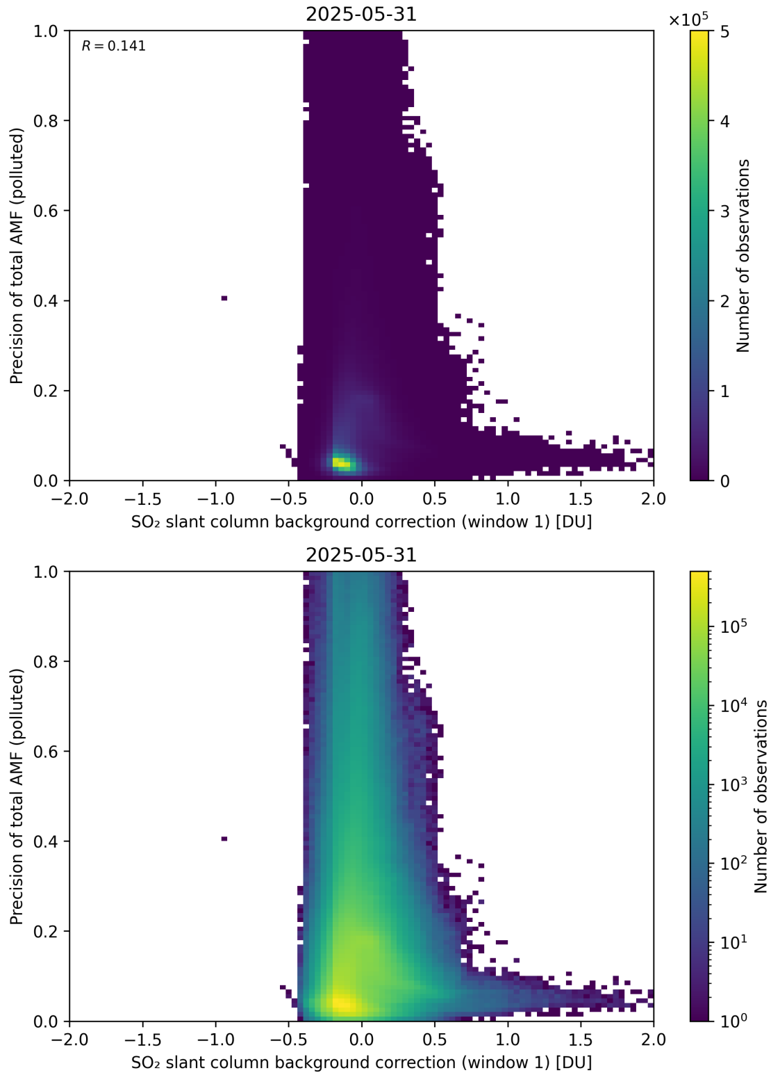
Figure 121: Scatter density plot of “SO 2 slant column background correction (window 1)” against “Precision of total AMF (polluted)” for 2025-05-31 to 2025-06-01.
