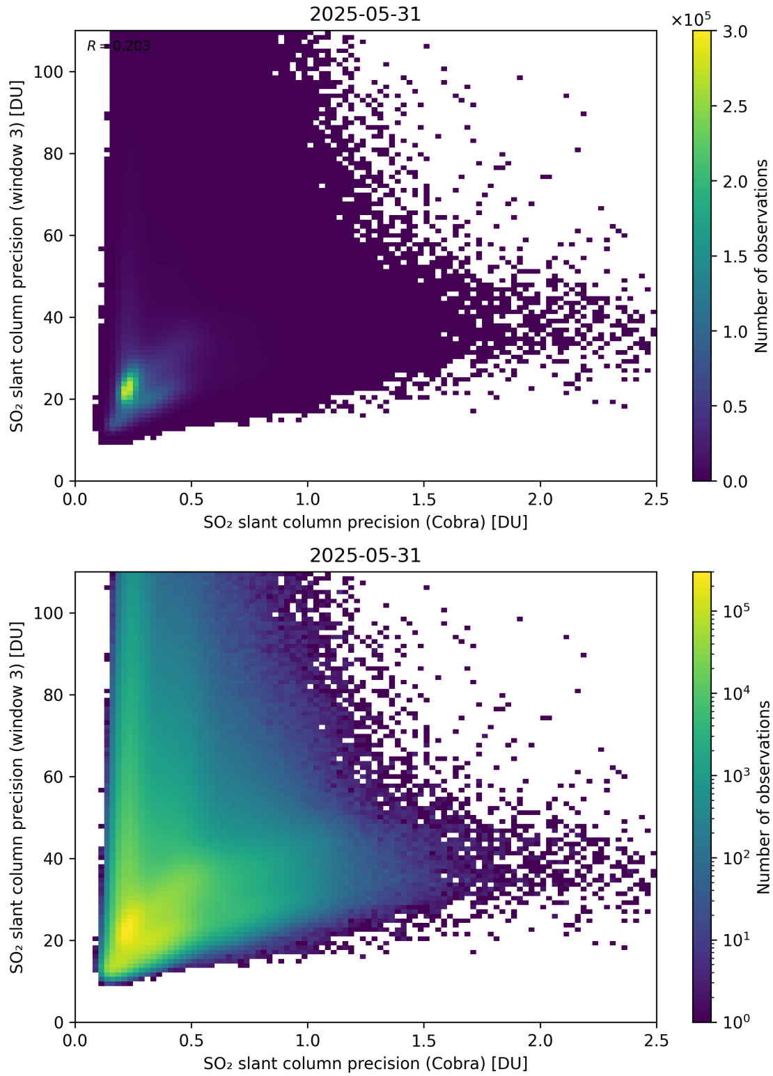
Figure 212: Scatter density plot of “SO 2 slant column precision (Cobra)” against “SO 2 slant column precision (window 3)” for 2025-05-31 to 2025-06-01.
