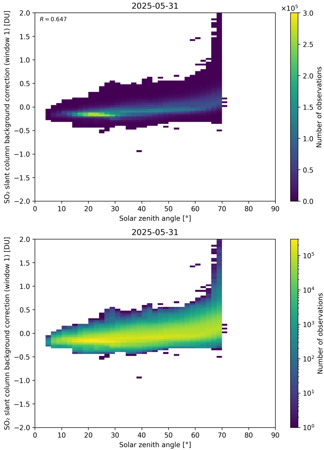
Figure 171: Scatter density plot of “Solar zenith angle” against “SO 2 slant column background correction (window 1)” for 2025-05-31 to 2025-06-01.
