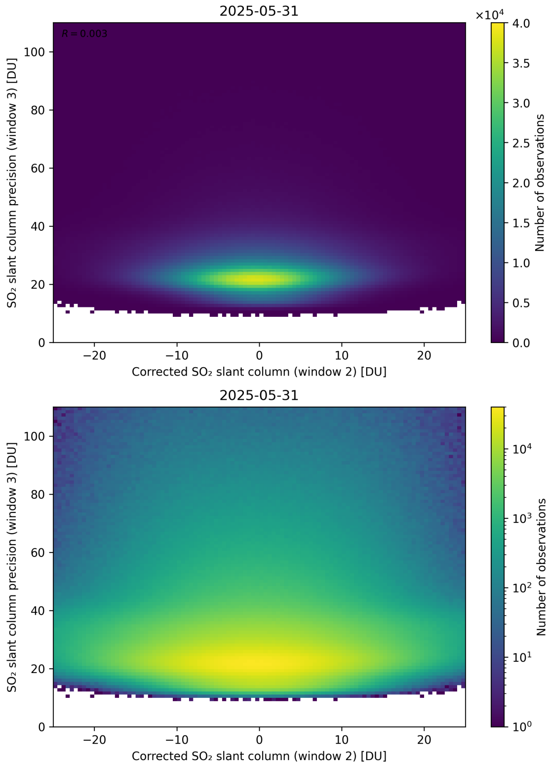
Figure 252: Scatter density plot of “Corrected SO 2 slant column (window 2)” against “SO 2 slant column precision (window 3)” for 2025-05-31 to 2025-06-01.
