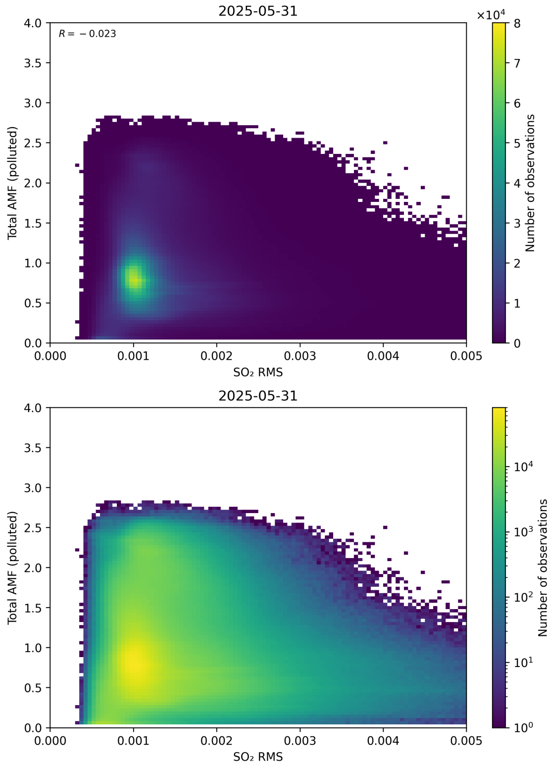
Figure 148: Scatter density plot of “SO 2 RMS” against “Total AMF (polluted)” for 2025-05-31 to 2025-06-01.
