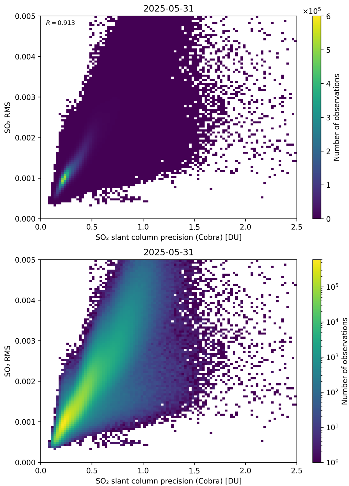
Figure 204: Scatter density plot of “SO 2 slant column precision (Cobra)” against “SO 2 RMS” for 2025-05-31 to 2025-06-01.
