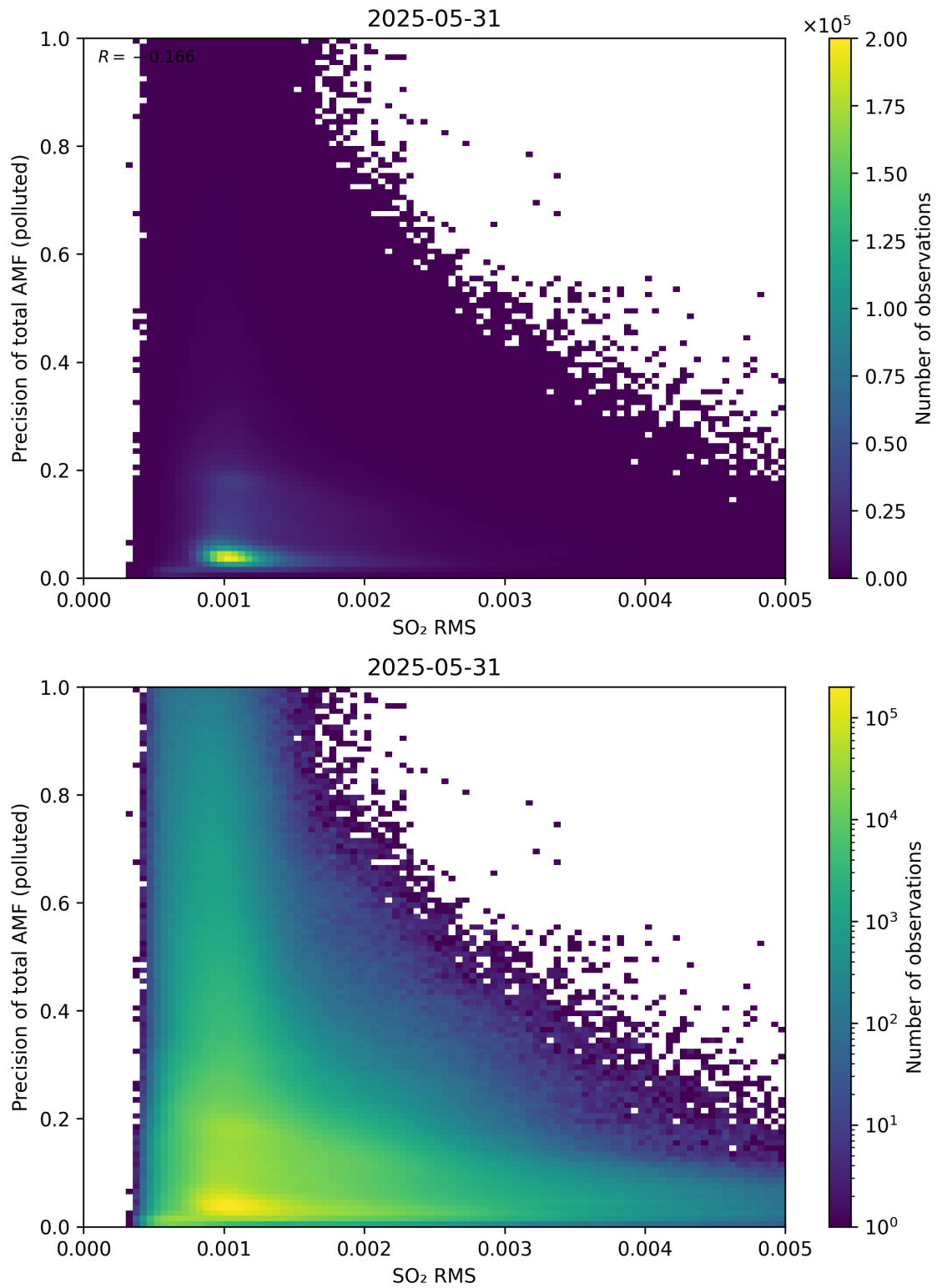
Figure 149: Scatter density plot of “SO 2 RMS” against “Precision of total AMF (polluted)” for 2025-05-31 to 2025-06-01.
