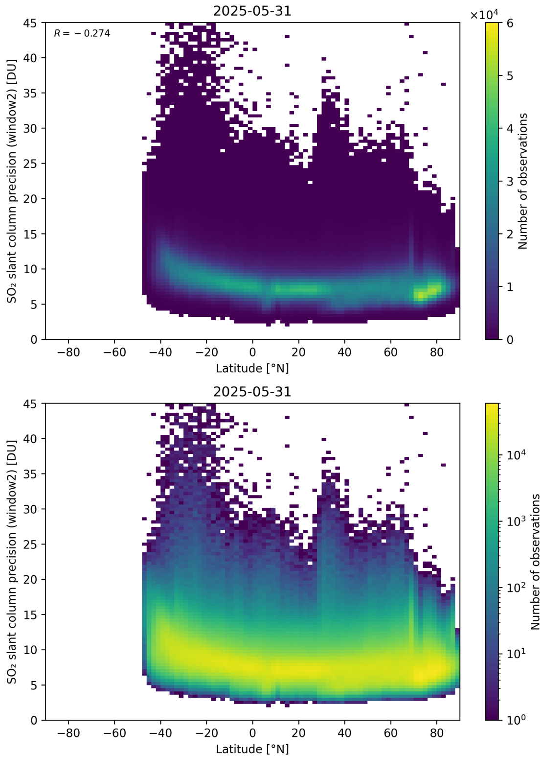
Figure 164: Scatter density plot of “Latitude” against “SO 2 slant column precision (window2)” for 2025-05-31 to 2025-06-01.
