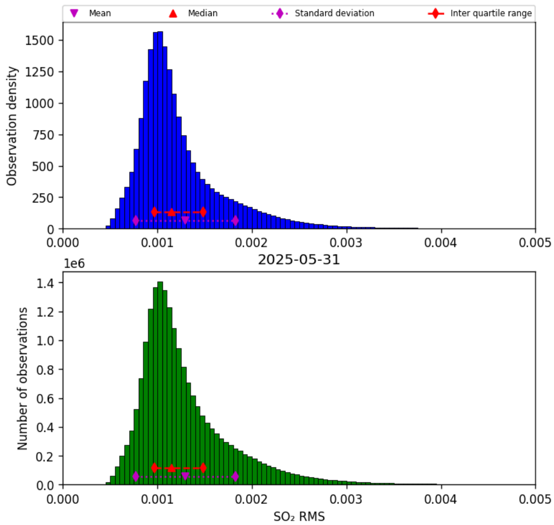
Figure 78: Histogram of “SO 2 RMS” for 2025-05-31 to 2025-06-01
