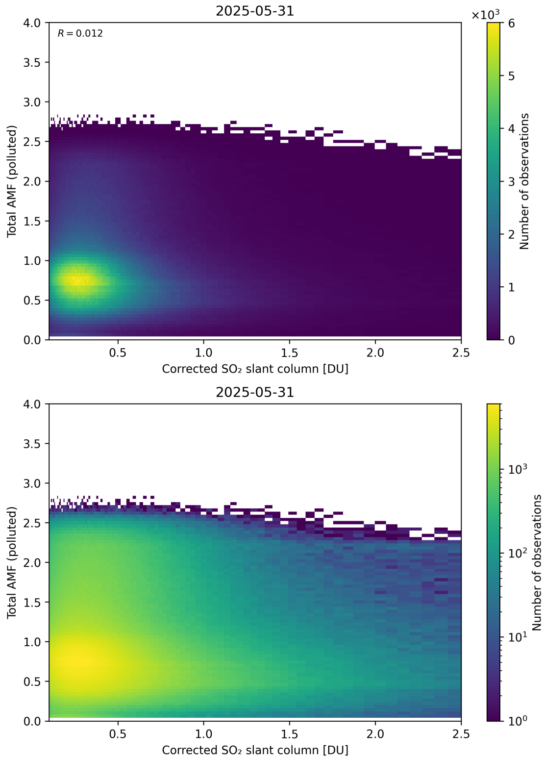
Figure 242: Scatter density plot of “Corrected SO 2 slant column” against “Total AMF (polluted)” for 2025-05-31 to 2025-06-01.
