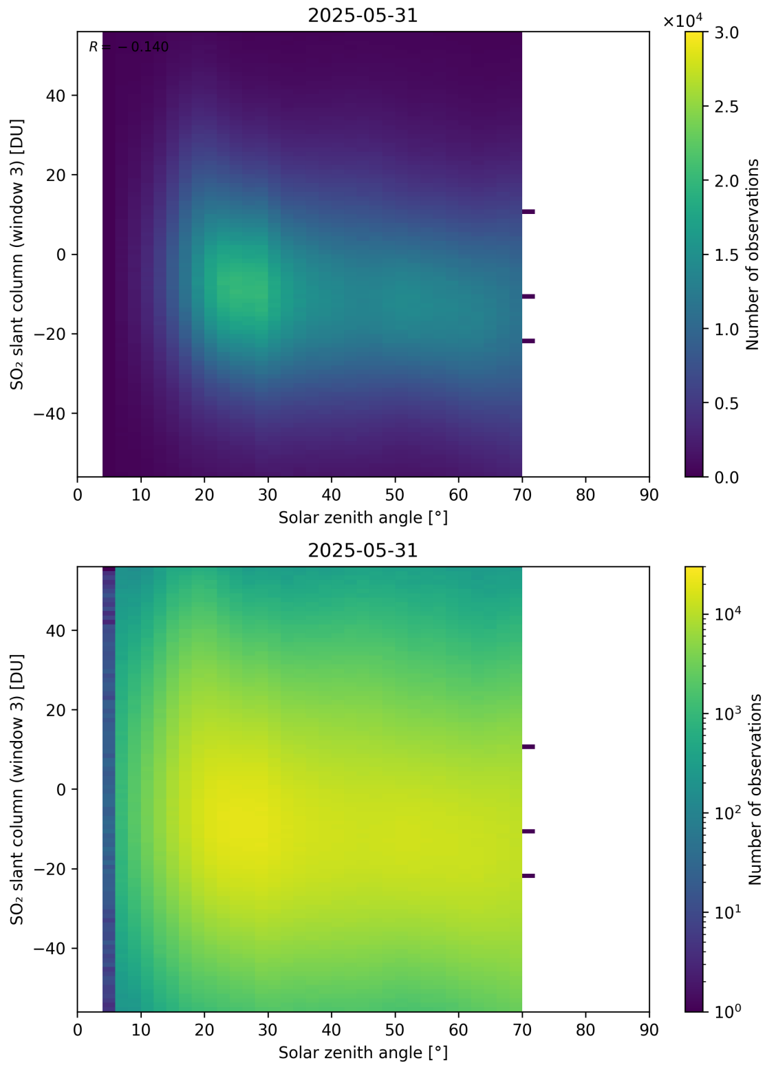
Figure 187: Scatter density plot of “Solar zenith angle” against “SO 2 slant column (window 3)” for 2025-05-31 to 2025-06-01.
