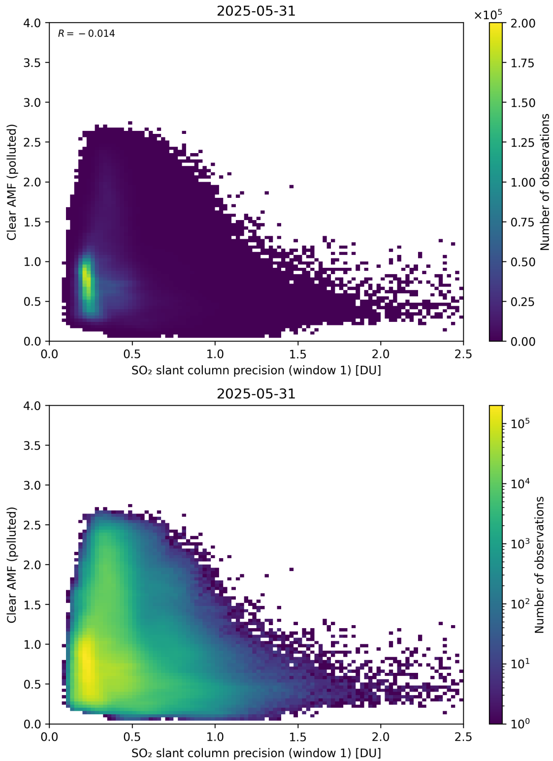
Figure 274: Scatter density plot of “SO 2 slant column precision (window 1)” against “Clear AMF (polluted)” for 2025-05-31 to 2025-06-01.
