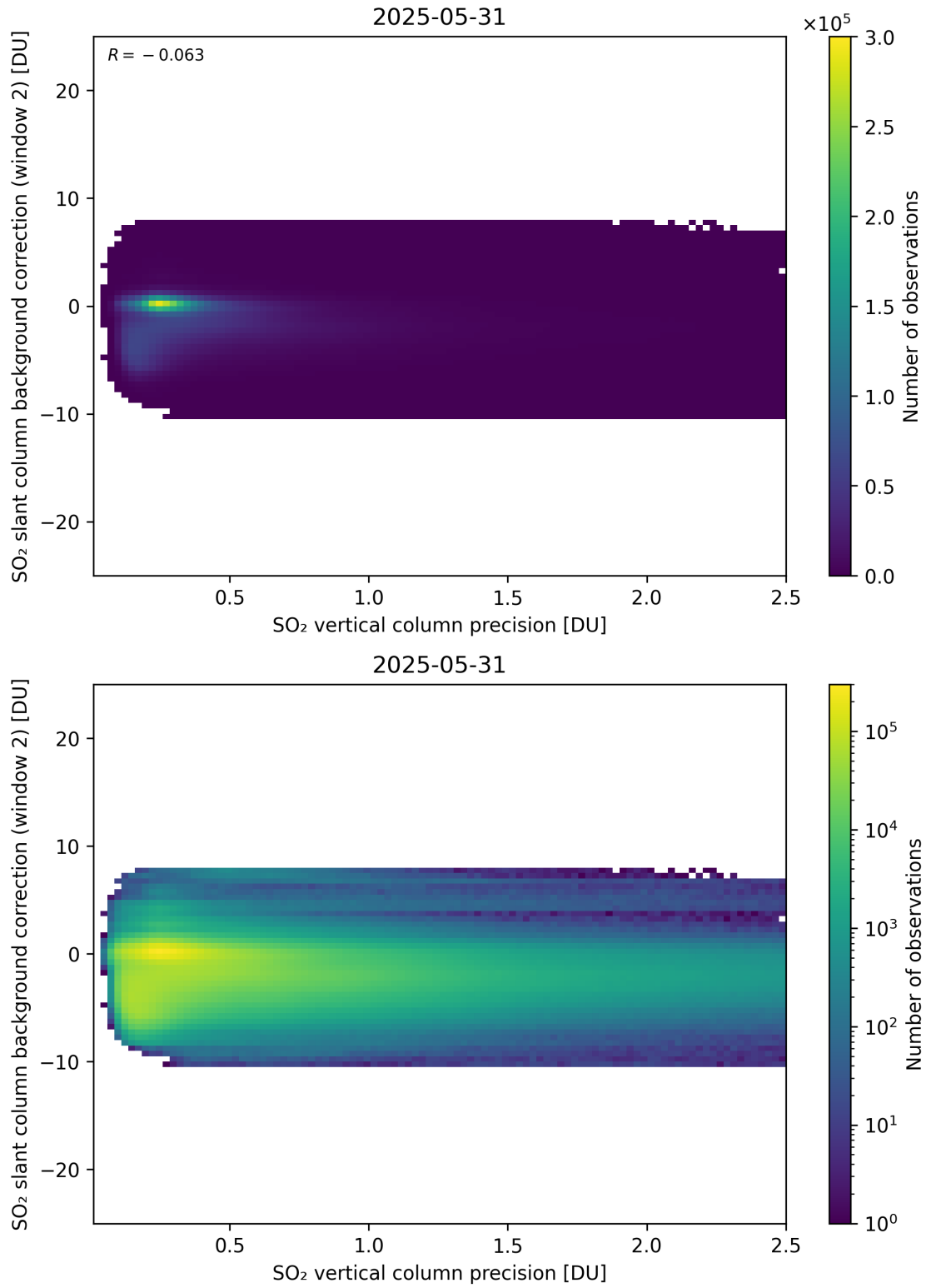
Figure 330: Scatter density plot of “SO 2 vertical column precision” against “SO 2 slant column background correction (window 2)” for 2025-05-31 to 2025-06-01.
