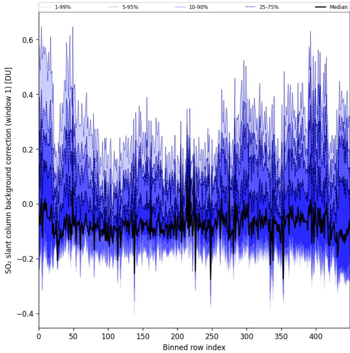
Figure 92: Along track statistics of “SO 2 slant column background correction (window 1)” for 2025-05-31 to 2025-06-01
