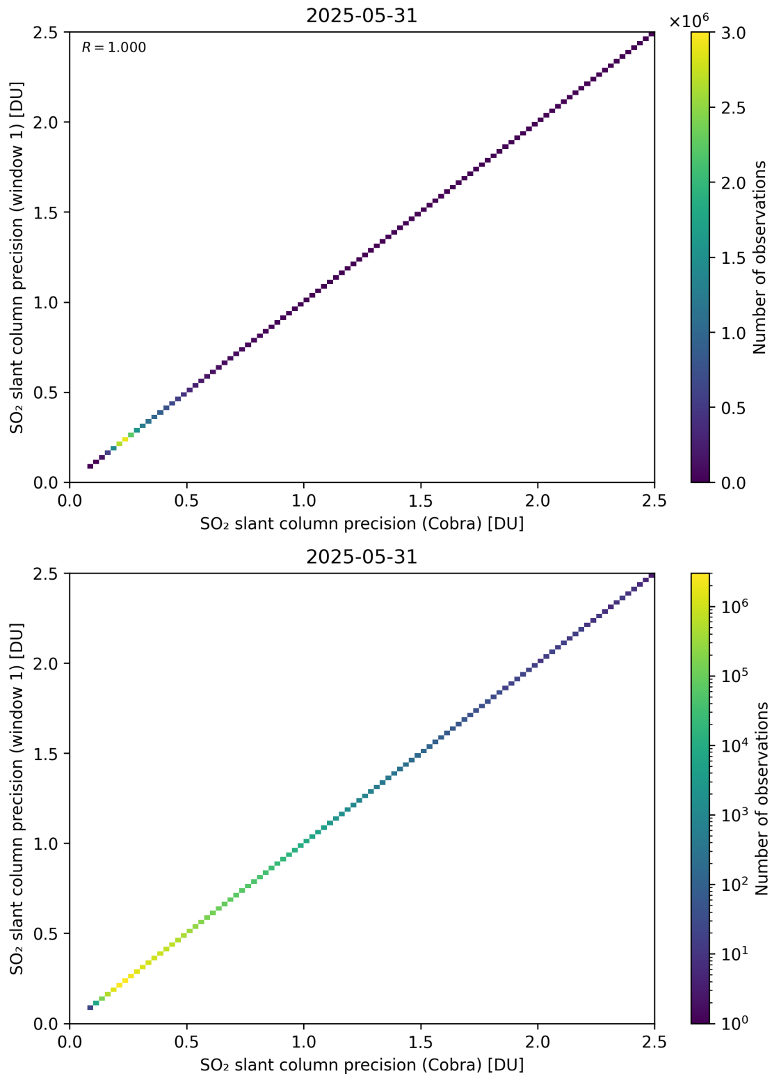
Figure 209: Scatter density plot of “SO 2 slant column precision (Cobra)” against “SO 2 slant column precision (window 1)” for 2025-05-31 to 2025-06-01.
