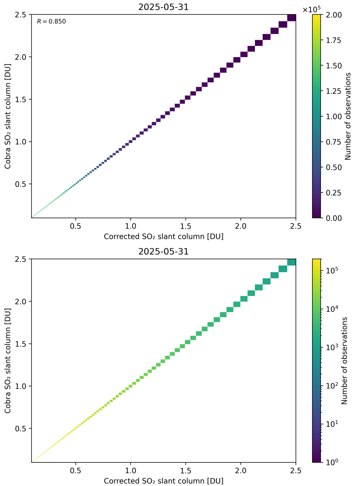
Figure 233: Scatter density plot of “Corrected SO 2 slant column” against “Cobra SO 2 slant column” for 2025-05-31 to 2025-06-01.
