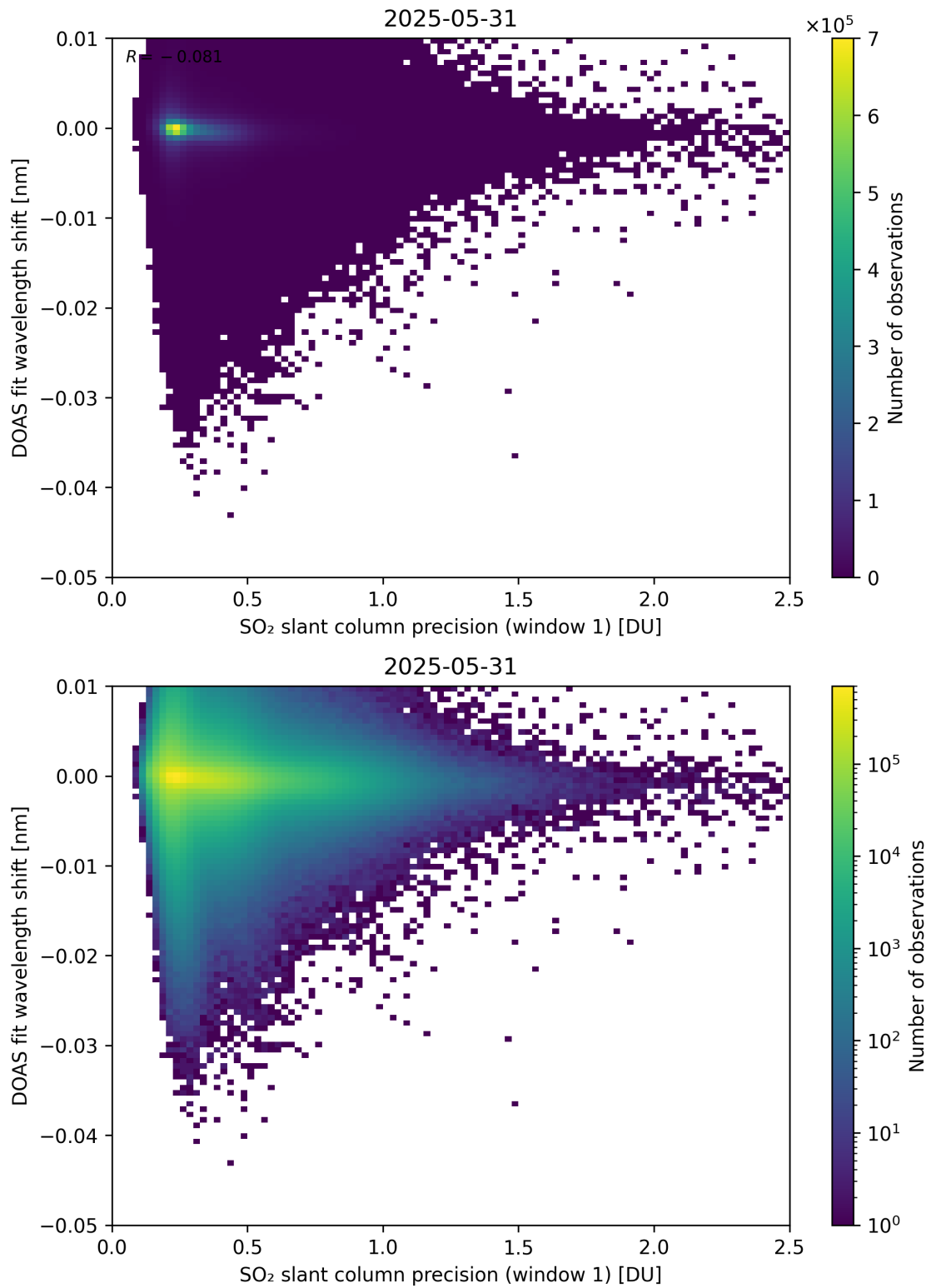
Figure 271: Scatter density plot of “SO 2 slant column precision (window 1)” against “DOAS fit wavelength shift” for 2025-05-31 to 2025-06-01.
