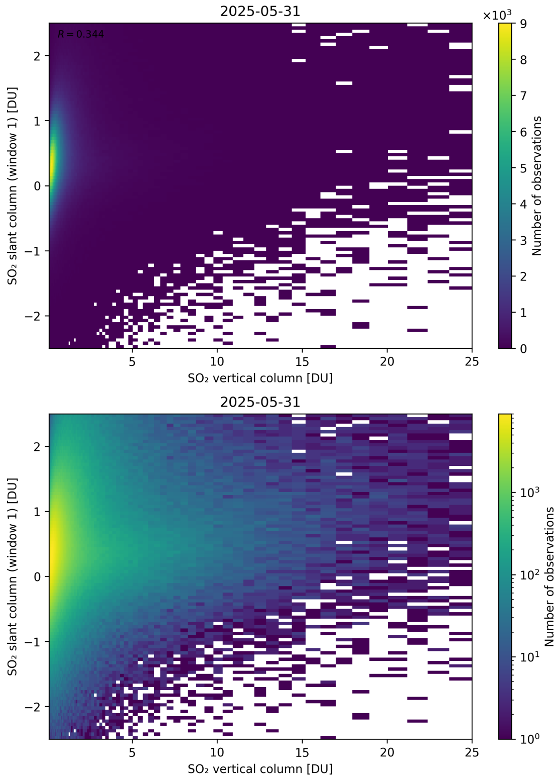
Figure 354: Scatter density plot of “SO 2 vertical column” against “SO 2 slant column (window 1)” for 2025-05-31 to 2025-06-01.
