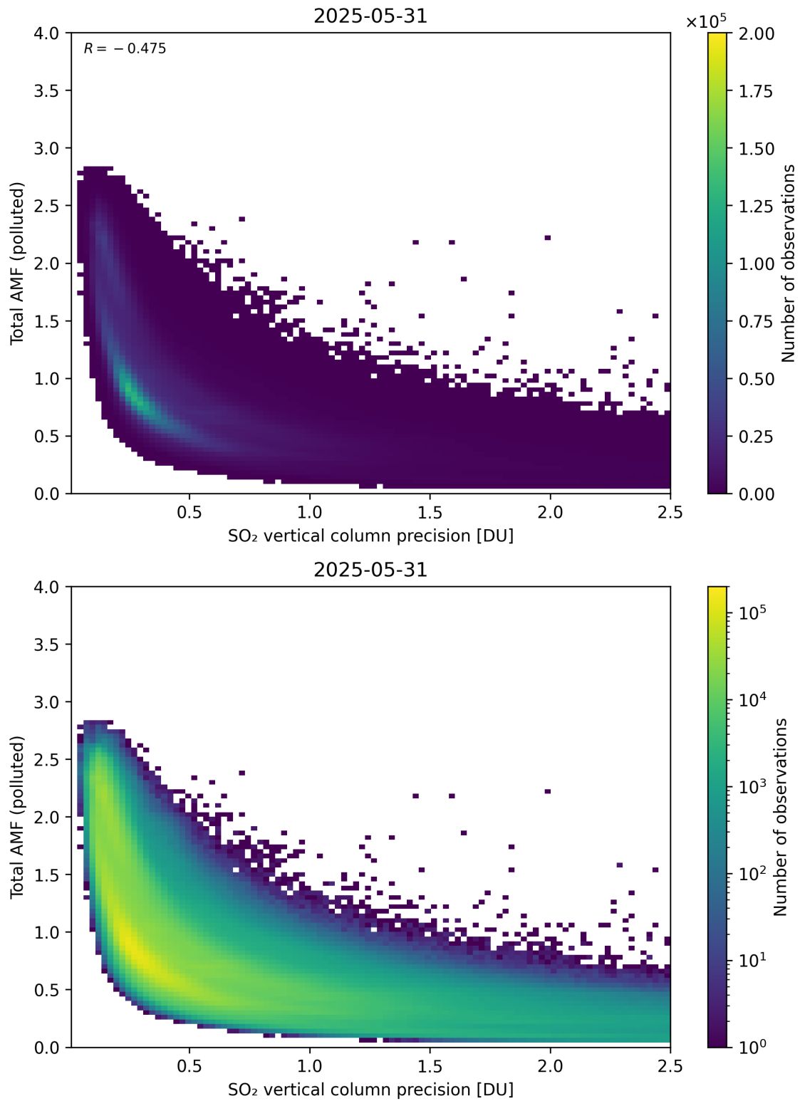
Figure 346: Scatter density plot of “SO 2 vertical column precision” against “Total AMF (polluted)” for 2025-05-31 to 2025-06-01.
