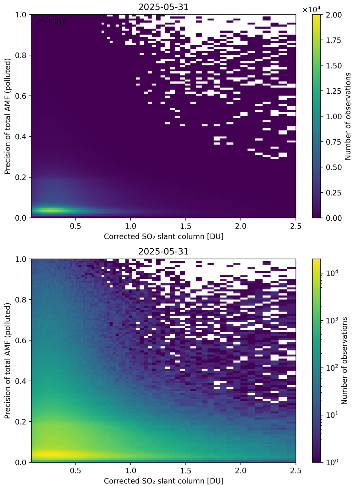
Figure 243: Scatter density plot of “Corrected SO 2 slant column” against “Precision of total AMF (polluted)” for 2025-05-31 to 2025-06-01.
