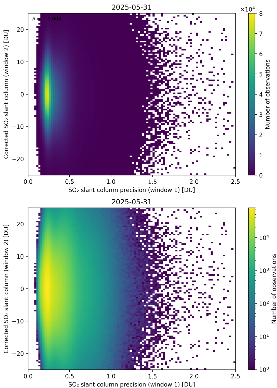
Figure 275: Scatter density plot of “SO 2 slant column precision (window 1)” against “Corrected SO 2 slant column (window 2)” for 2025-05-31 to 2025-06-01.
