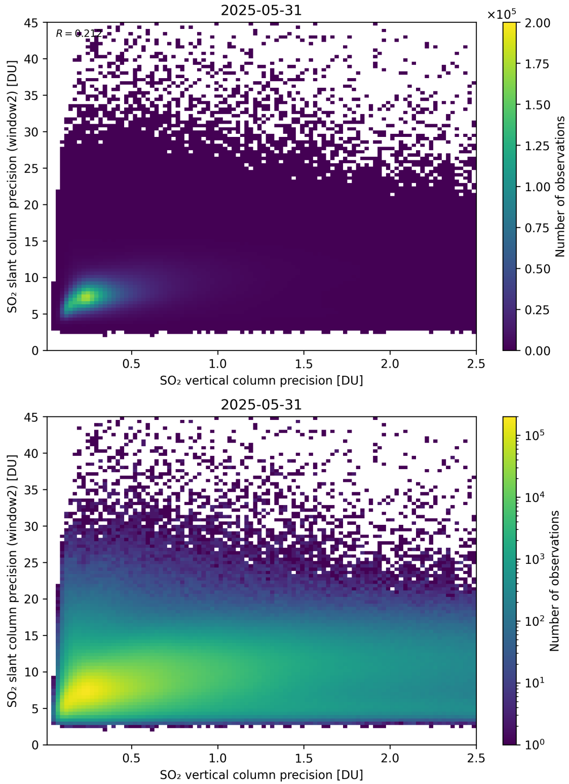
Figure 343: Scatter density plot of “SO 2 vertical column precision” against “SO 2 slant column precision (window2)” for 2025-05-31 to 2025-06-01.
