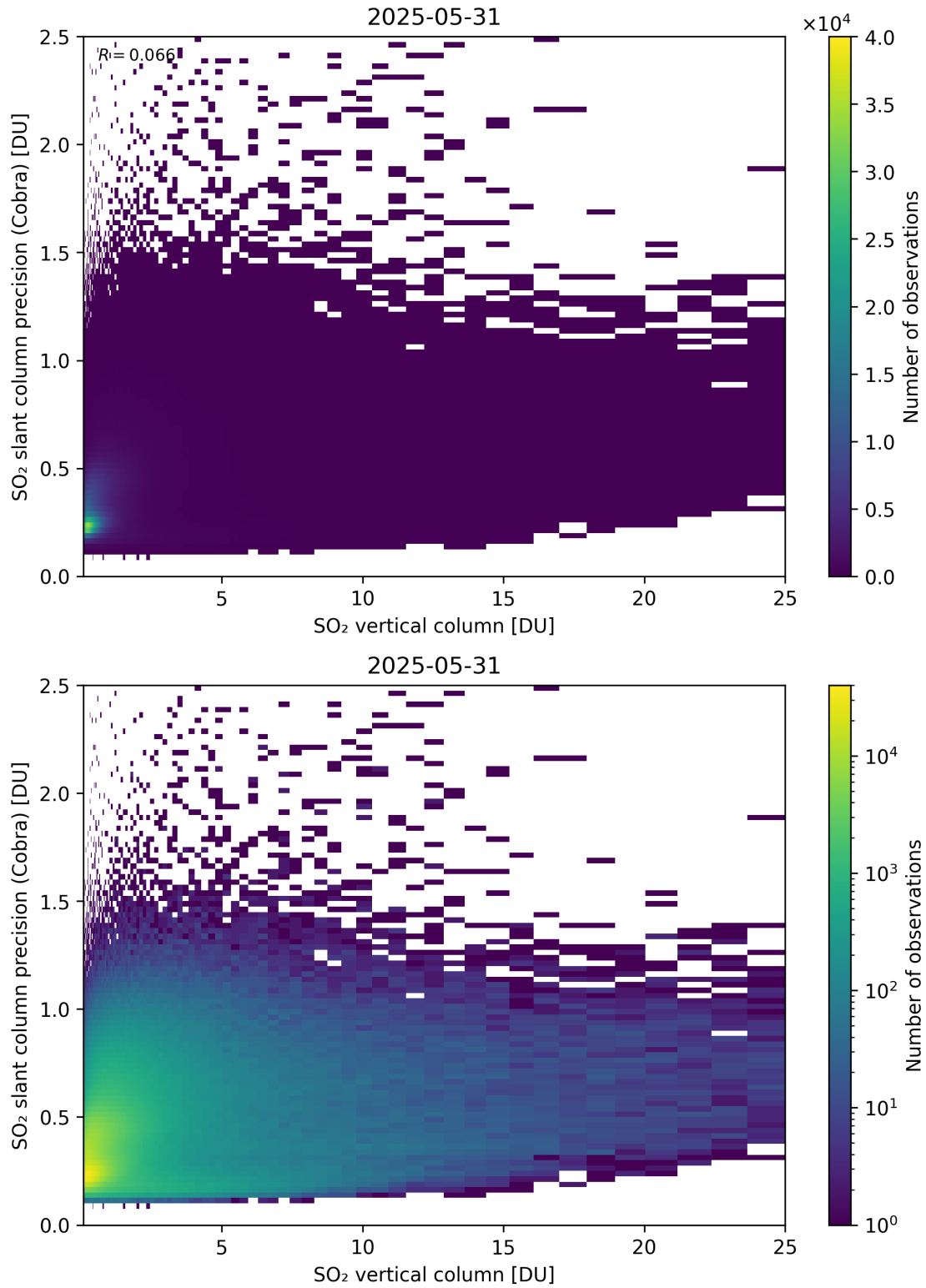
Figure 350: Scatter density plot of “SO 2 vertical column” against “SO 2 slant column precision (Cobra)” for 2025-05-31 to 2025-06-01.
