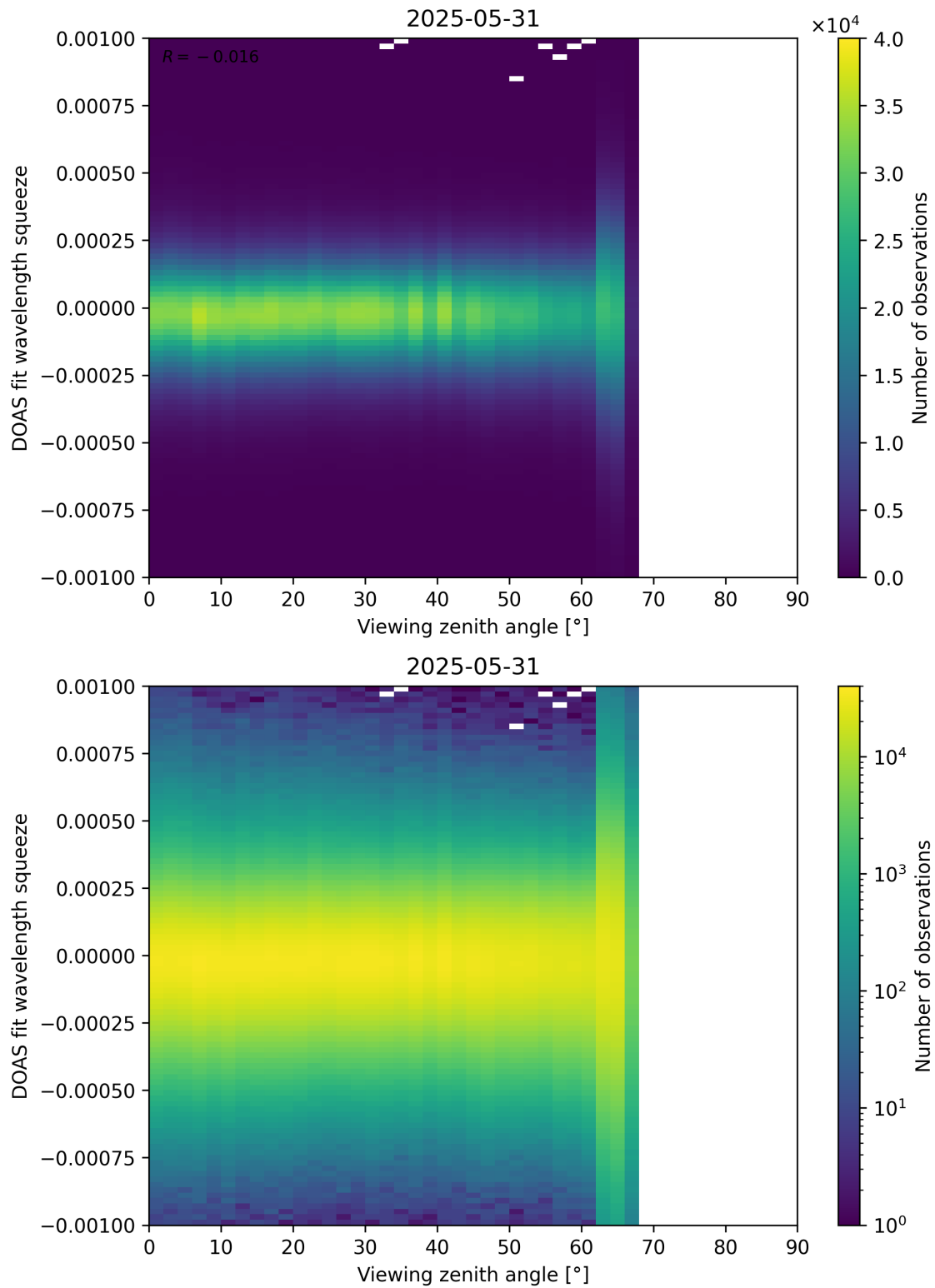
Figure 366: Scatter density plot of “Viewing zenith angle” against “DOAS fit wavelength squeeze” for 2025-05-31 to 2025-06-01.
