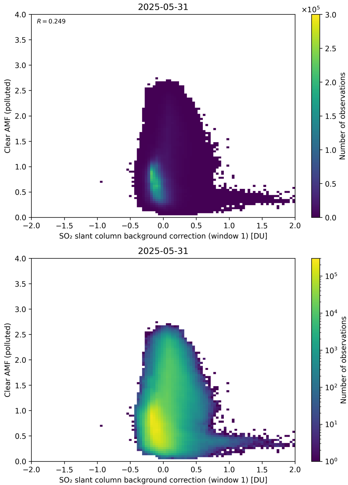
Figure 114: Scatter density plot of “SO 2 slant column background correction (window 1)” against “Clear AMF (polluted)” for 2025-05-31 to 2025-06-01.
