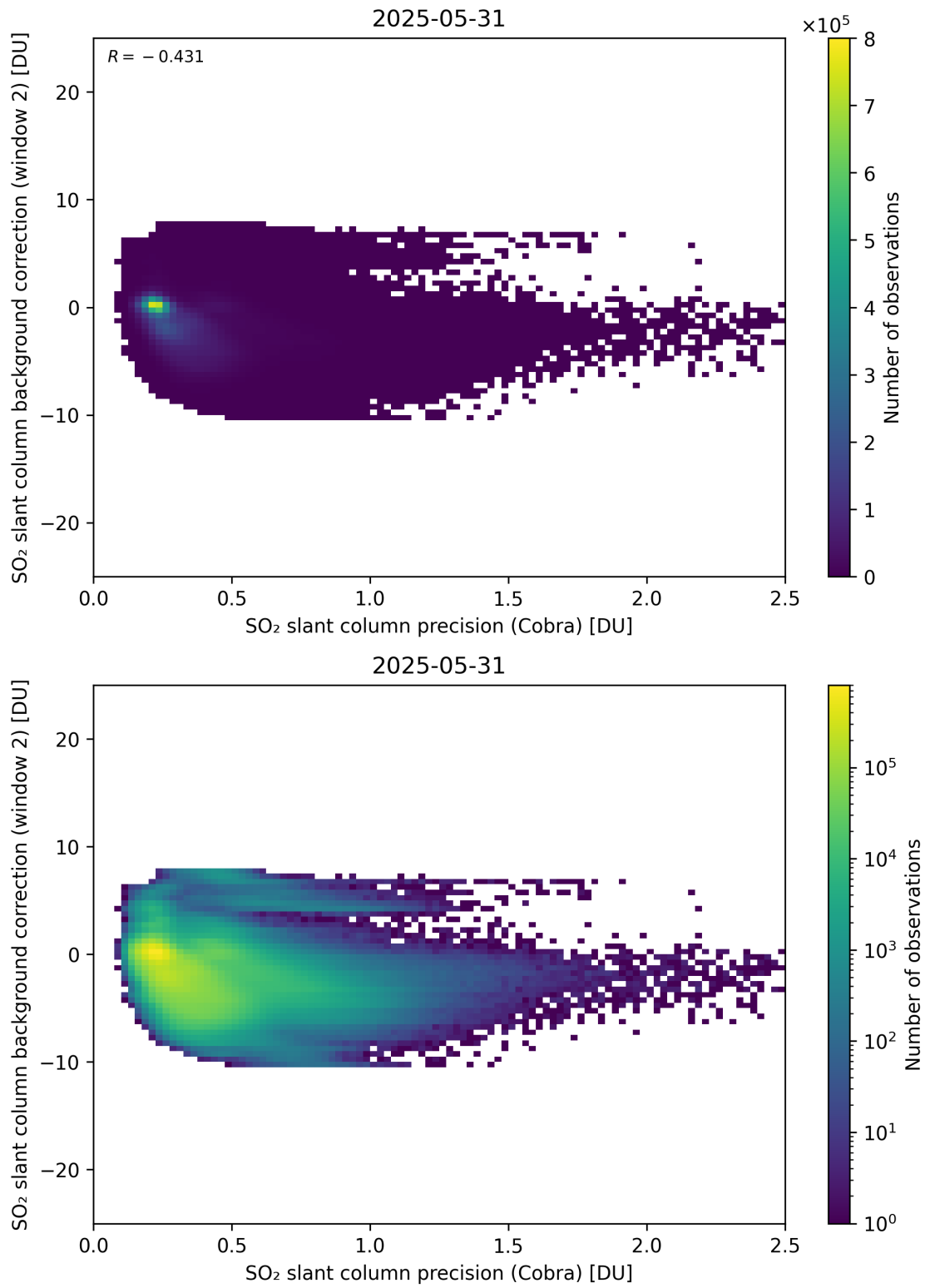
Figure 200: Scatter density plot of “SO 2 slant column precision (Cobra)” against “SO 2 slant column background correction (window 2)” for 2025-05-31 to 2025-06-01.
