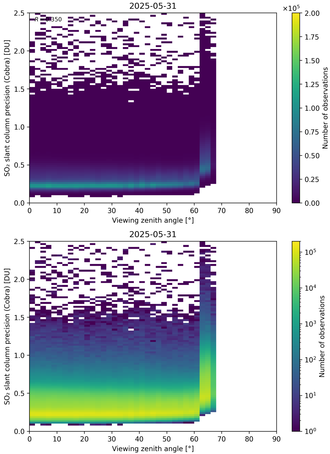
Figure 372: Scatter density plot of “Viewing zenith angle” against “SO 2 slant column precision (Cobra)” for 2025-05-31 to 2025-06-01.
