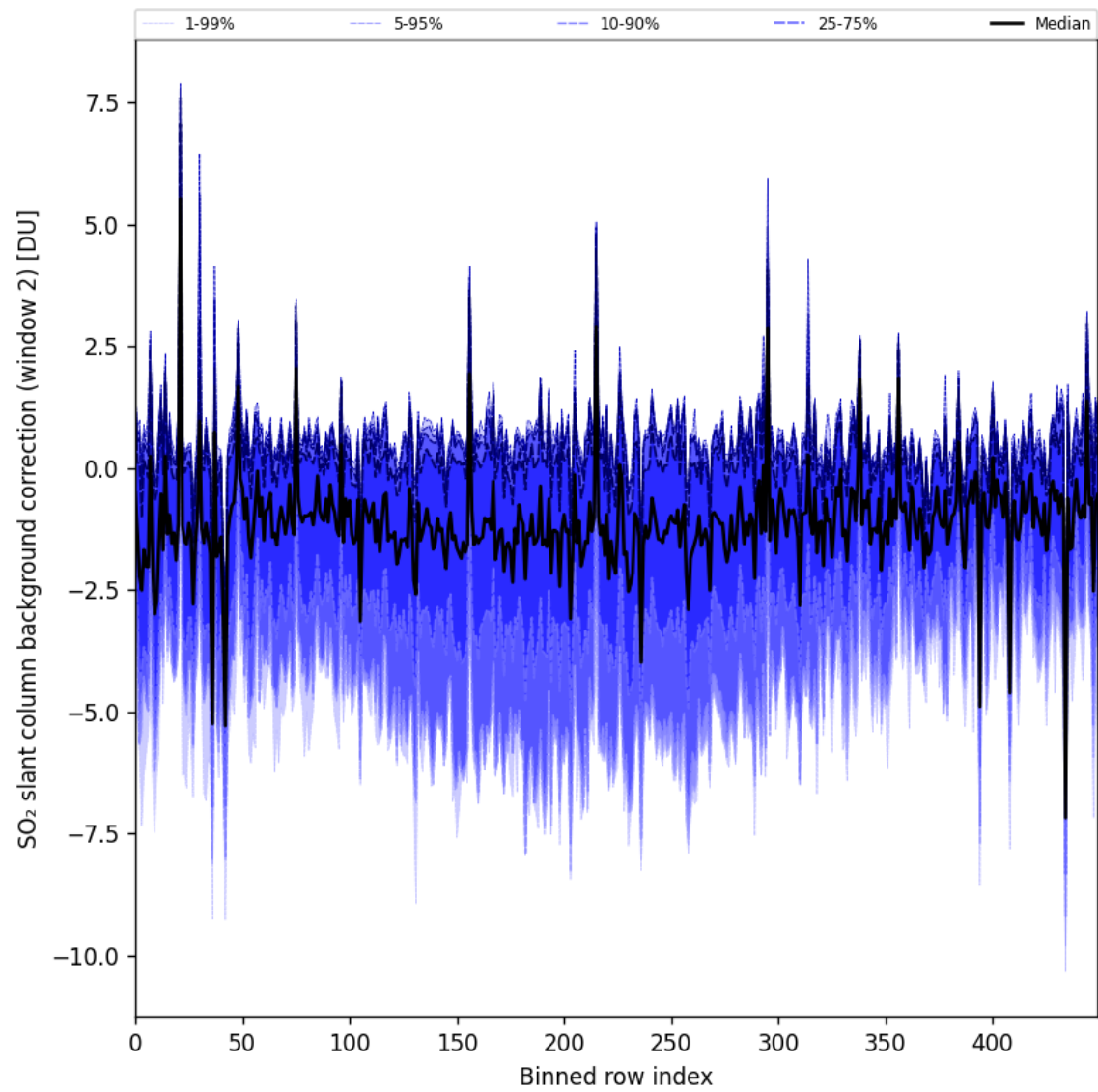
Figure 96: Along track statistics of “SO 2 slant column background correction (window 2)” for 2025-05-31 to 2025-06-01
