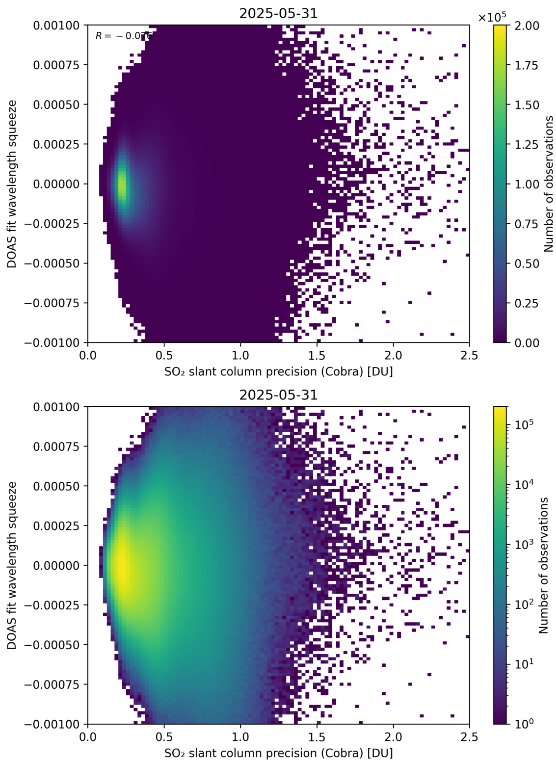
Figure 203: Scatter density plot of “SO 2 slant column precision (Cobra)” against “DOAS fit wavelength squeeze” for 2025-05-31 to 2025-06-01.
