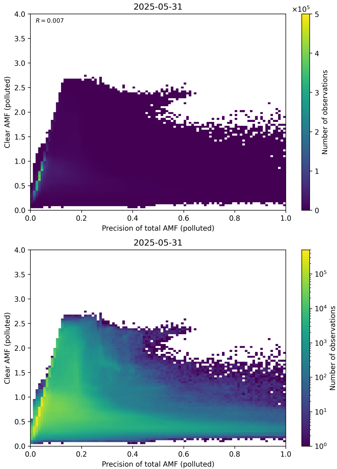
Figure 320: Scatter density plot of “Precision of total AMF (polluted)” against “Clear AMF (polluted)” for 2025-05-31 to 2025-06-01.
