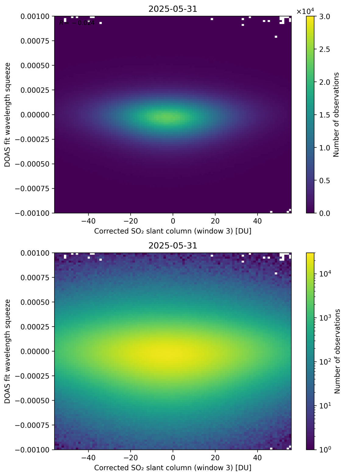
Figure 257: Scatter density plot of “Corrected SO 2 slant column (window 3)” against “DOAS fit wavelength squeeze” for 2025-05-31 to 2025-06-01.
