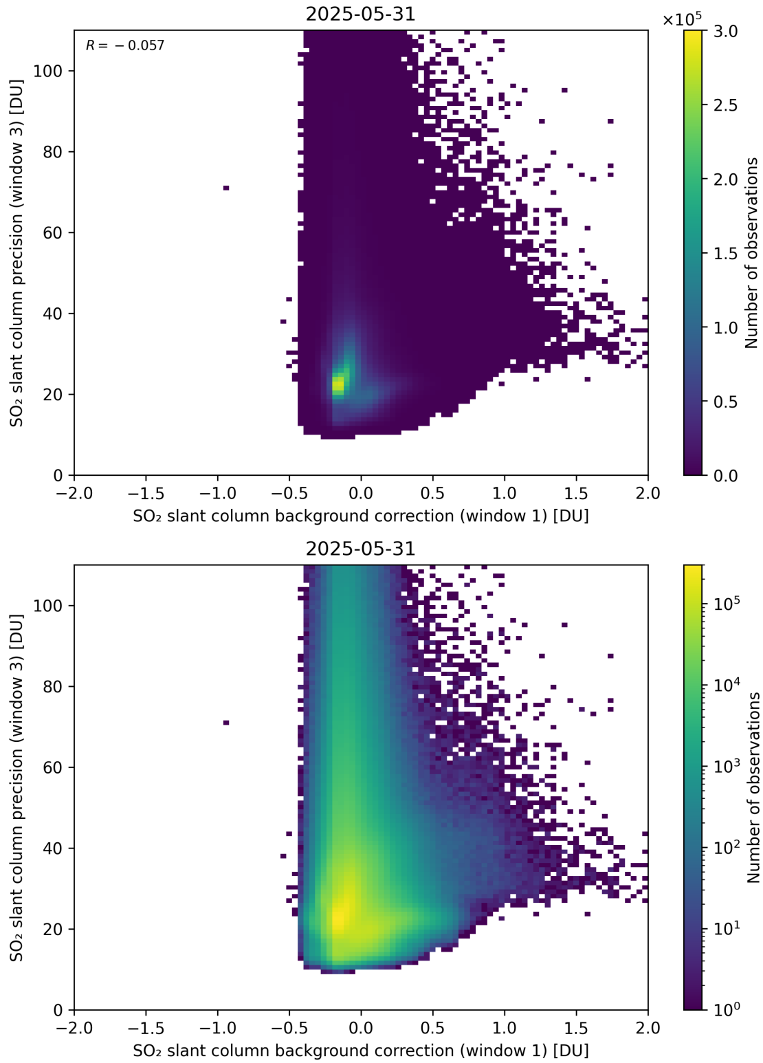
Figure 119: Scatter density plot of “SO 2 slant column background correction (window 1)” against “SO 2 slant column precision (window 3)” for 2025-05-31 to 2025-06-01.
