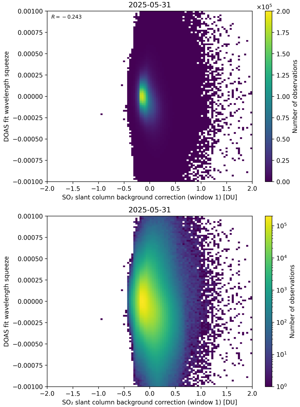
Figure 112: Scatter density plot of “SO 2 slant column background correction (window 1)” against “DOAS fit wavelength squeeze” for 2025-05-31 to 2025-06-01.
