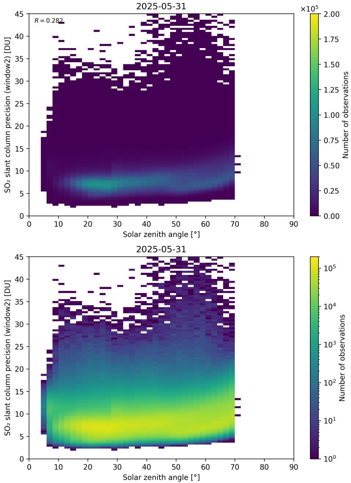
Figure 186: Scatter density plot of “Solar zenith angle” against “SO 2 slant column precision (window2)” for 2025-05-31 to 2025-06-01.
