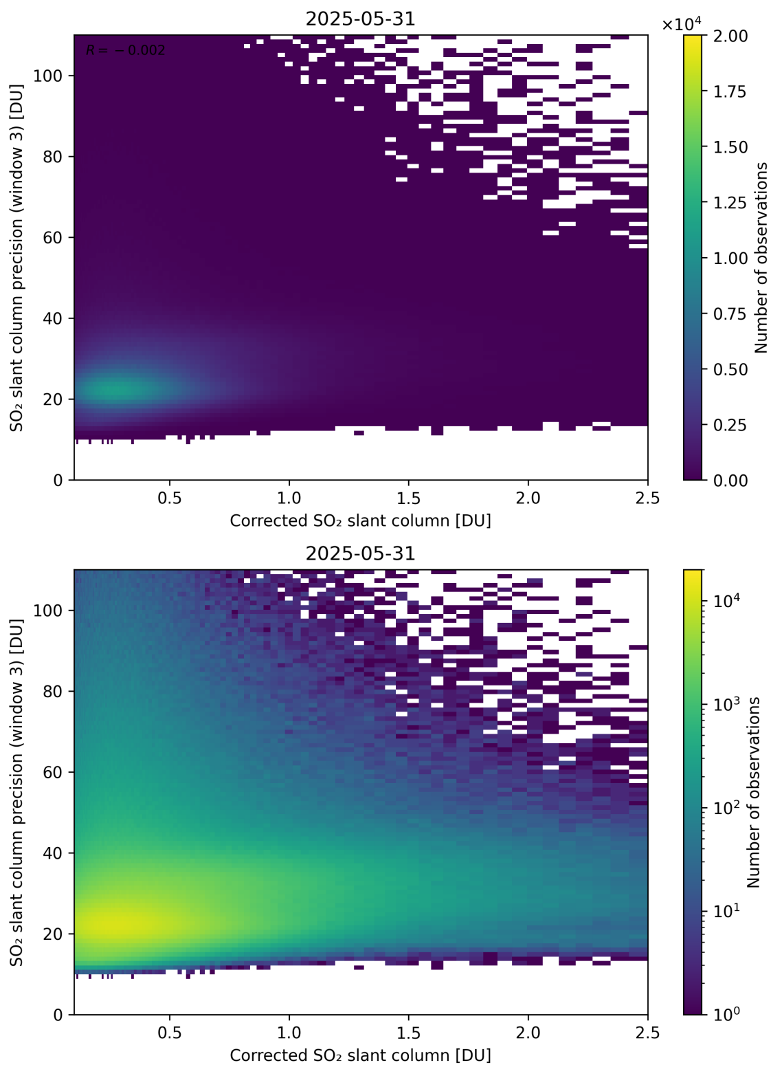
Figure 241: Scatter density plot of “Corrected SO 2 slant column” against “SO 2 slant column precision (window 3)” for 2025-05-31 to 2025-06-01.
