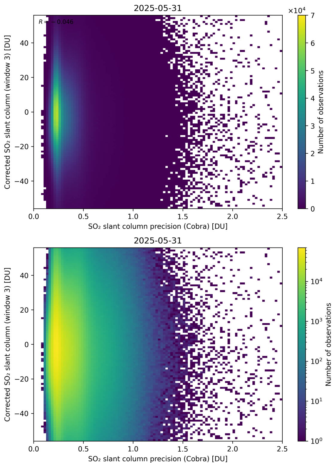
Figure 207: Scatter density plot of “SO 2 slant column precision (Cobra)” against “Corrected SO 2 slant column (window 3)” for 2025-05-31 to 2025-06-01.
