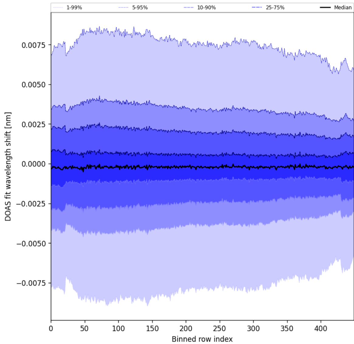
Figure 102: Along track statistics of “DOAS fit wavelength shift” for 2025-05-31 to 2025-06-01
