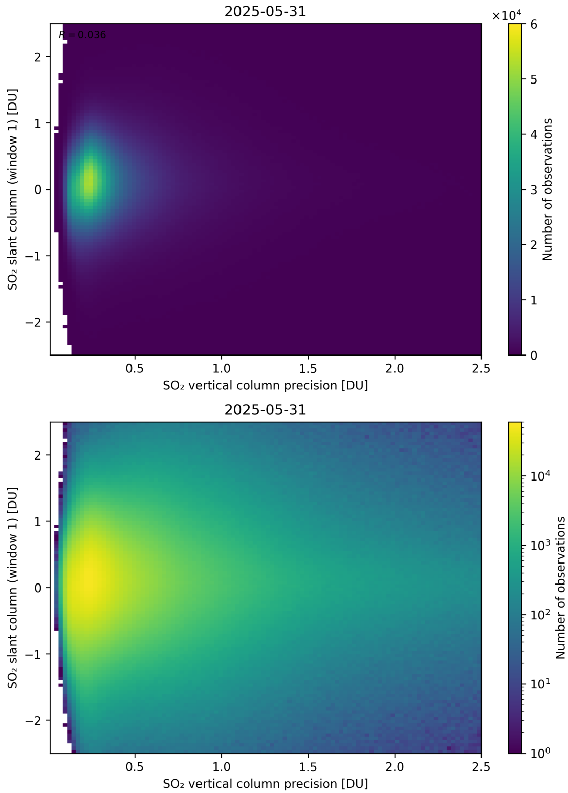
Figure 341: Scatter density plot of “SO 2 vertical column precision” against “SO 2 slant column (window 1)” for 2025-05-31 to 2025-06-01.
