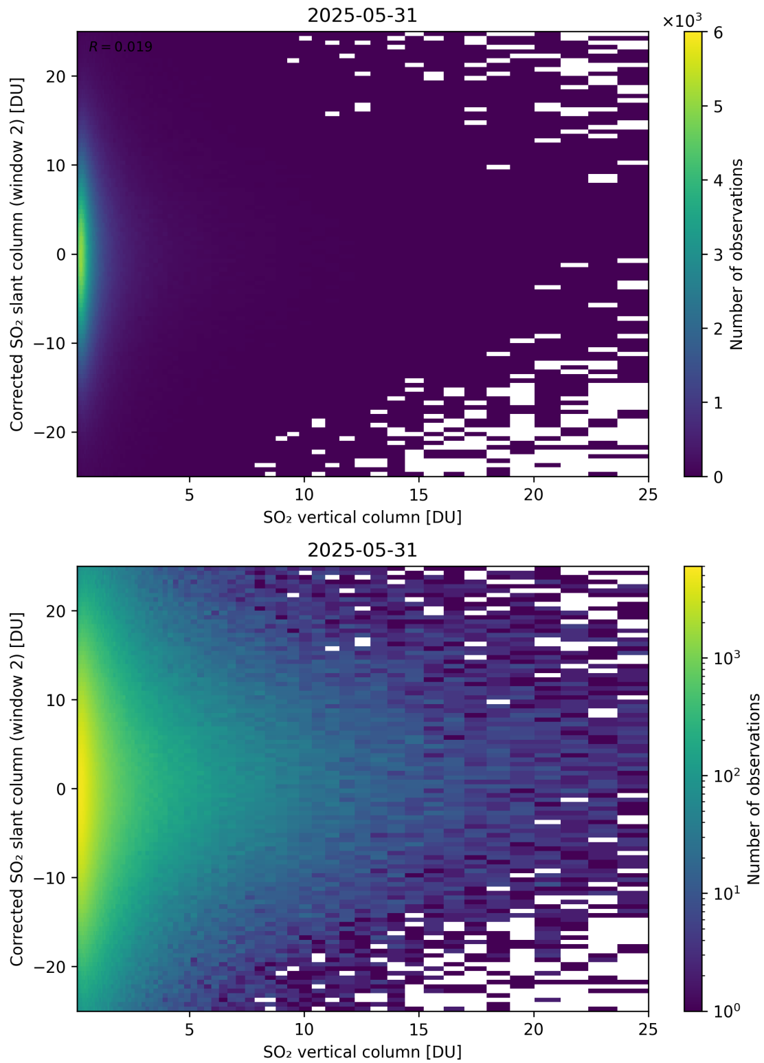
Figure 352: Scatter density plot of “SO 2 vertical column” against “Corrected SO 2 slant column (window 2)” for 2025-05-31 to 2025-06-01.
