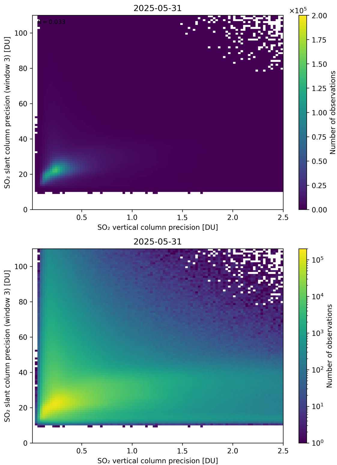
Figure 345: Scatter density plot of “SO 2 vertical column precision” against “SO 2 slant column precision (window 3)” for 2025-05-31 to 2025-06-01.
