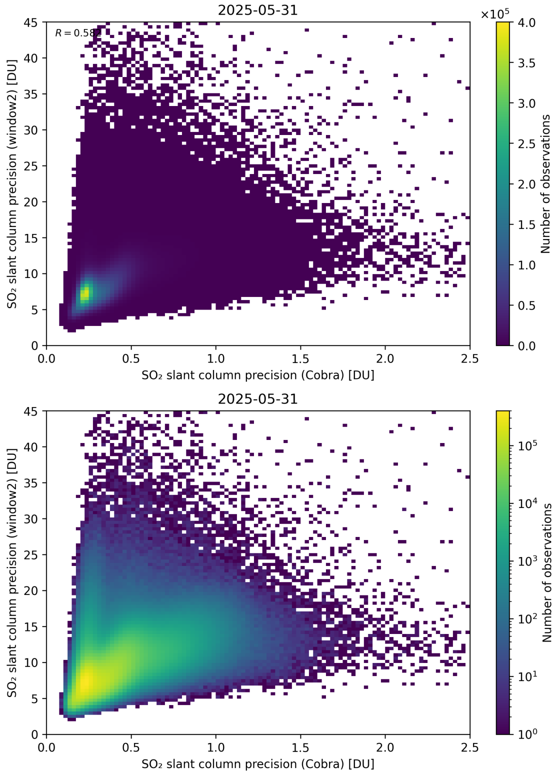
Figure 210: Scatter density plot of “SO 2 slant column precision (Cobra)” against “SO 2 slant column precision (window2)” for 2025-05-31 to 2025-06-01.
