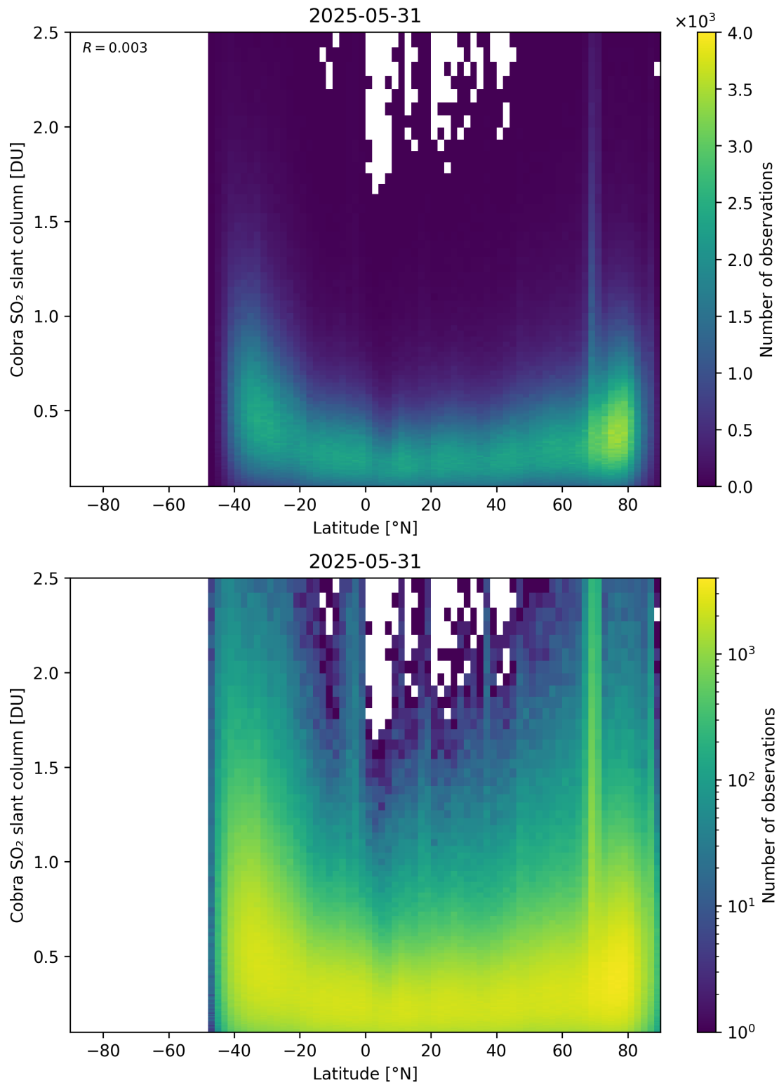
Figure 157: Scatter density plot of “Latitude” against “Cobra SO 2 slant column” for 2025-05-31 to 2025-06-01.
