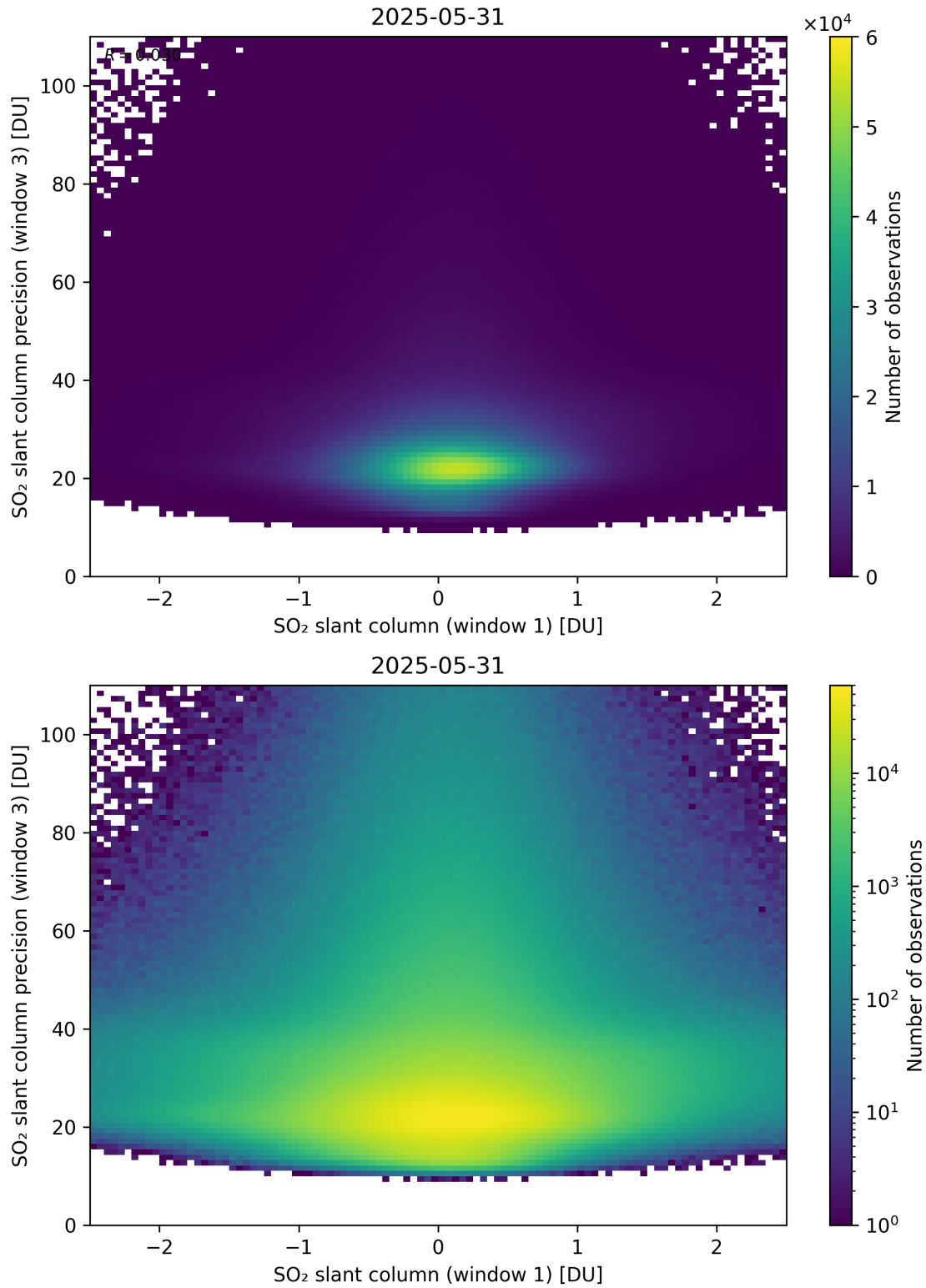
Figure 288: Scatter density plot of “SO 2 slant column (window 1)” against “SO 2 slant column precision (window 3)” for 2025-05-31 to 2025-06-01.
