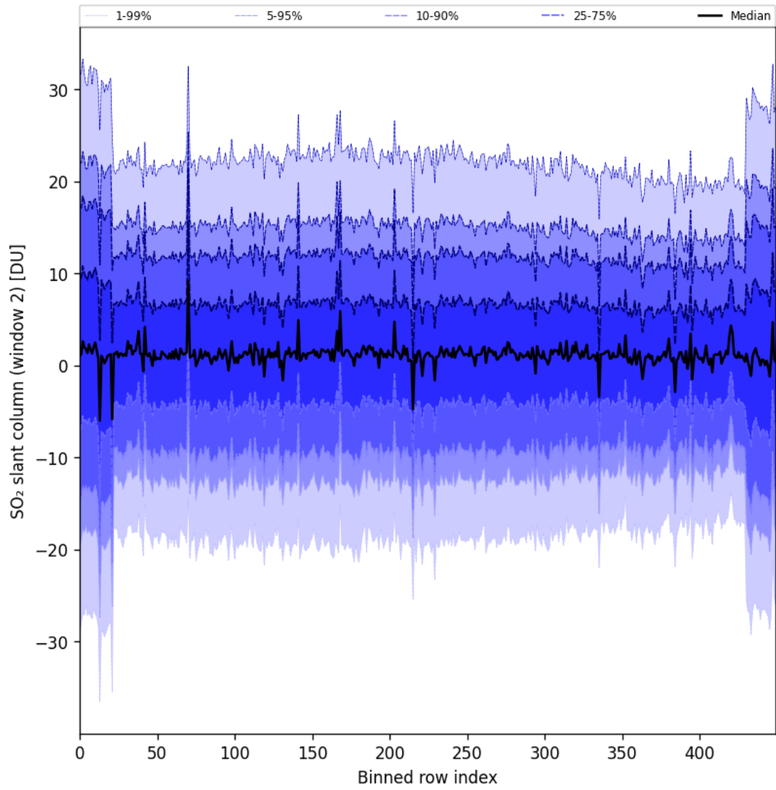
Figure 93: Along track statistics of “SO 2 slant column (window 2)” for 2025-05-31 to 2025-06-01
