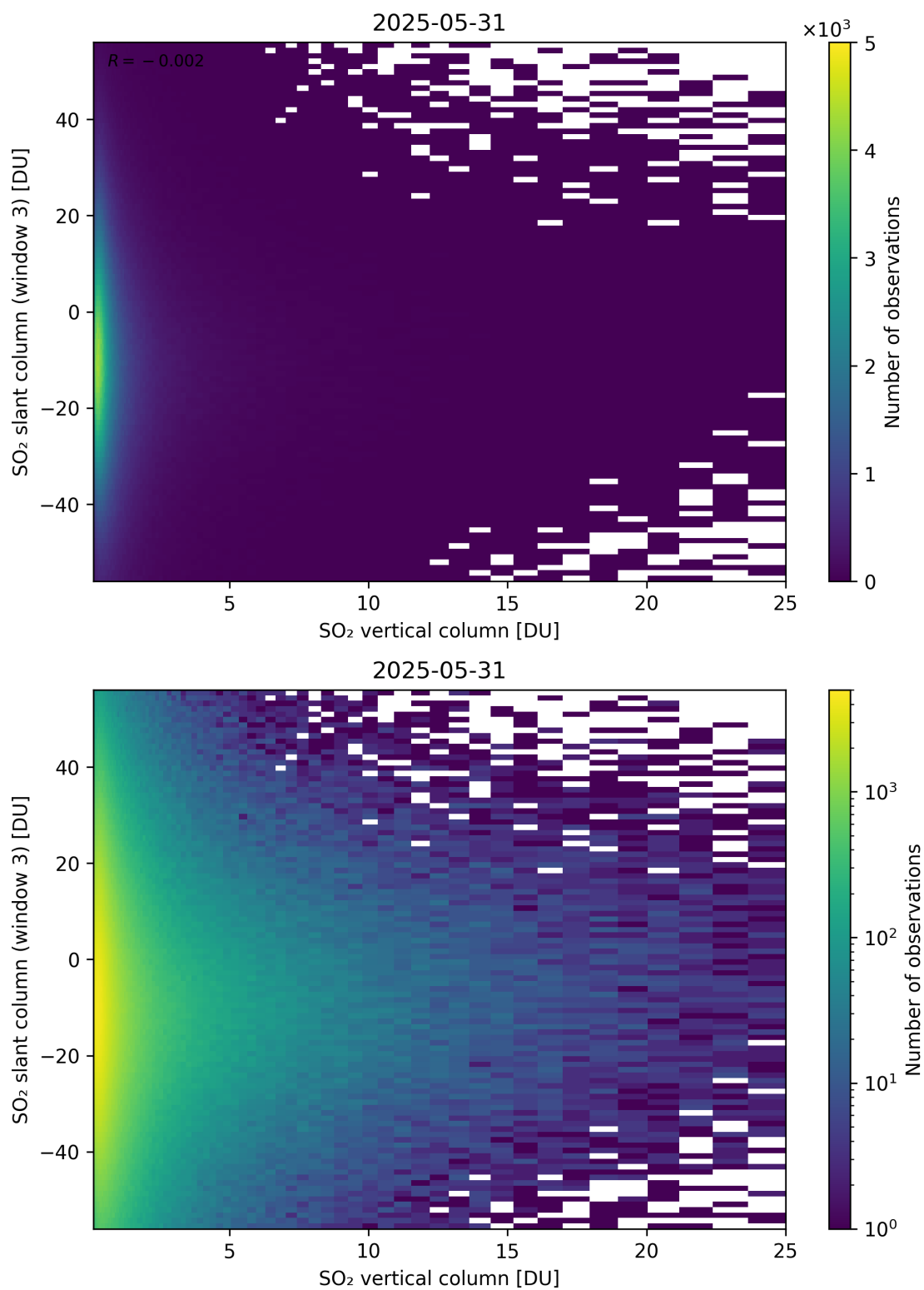
Figure 357: Scatter density plot of “SO 2 vertical column” against “SO 2 slant column (window 3)” for 2025-05-31 to 2025-06-01.
