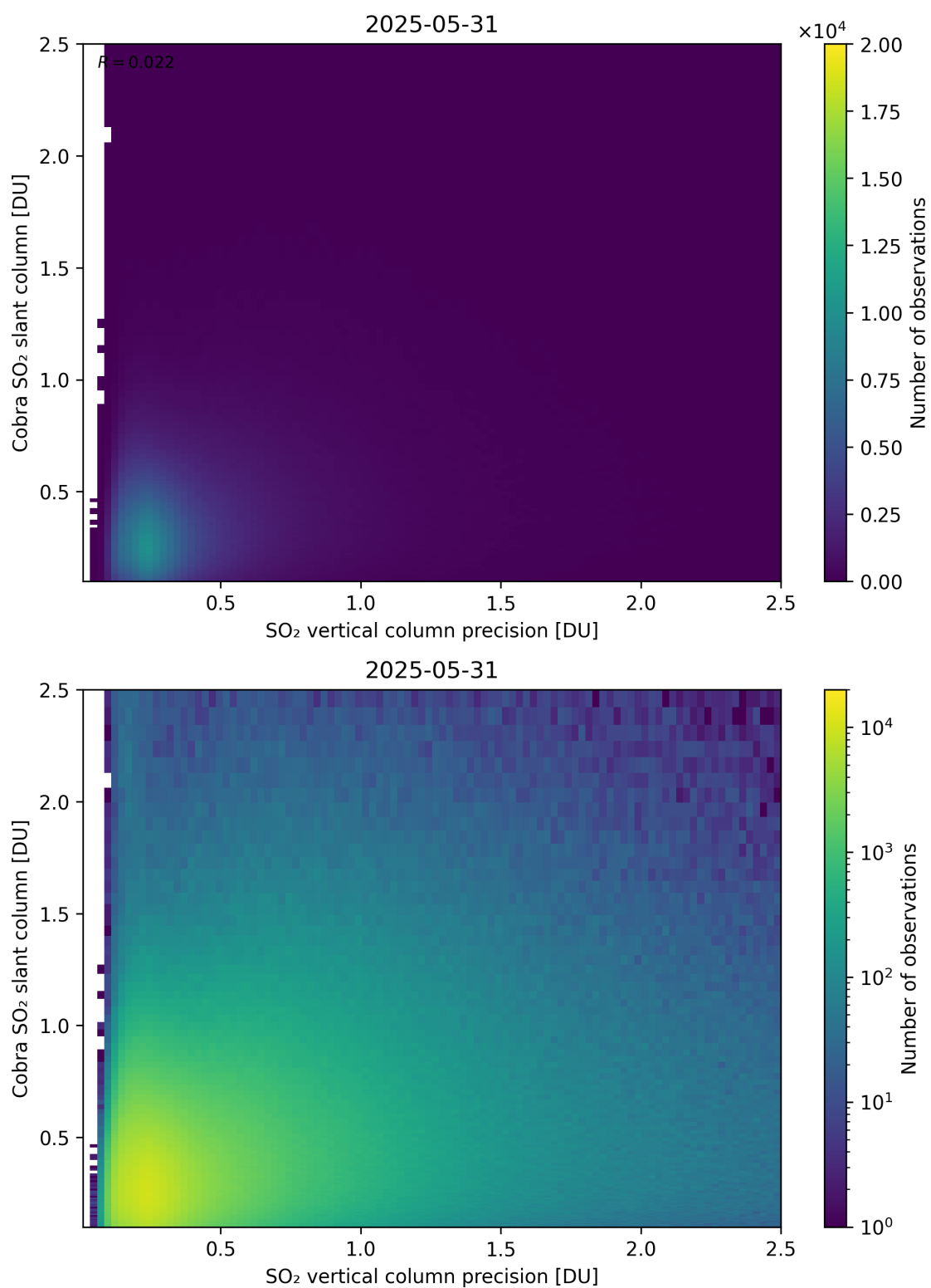
Figure 336: Scatter density plot of “SO 2 vertical column precision” against “Cobra SO 2 slant column” for 2025-05-31 to 2025-06-01.
