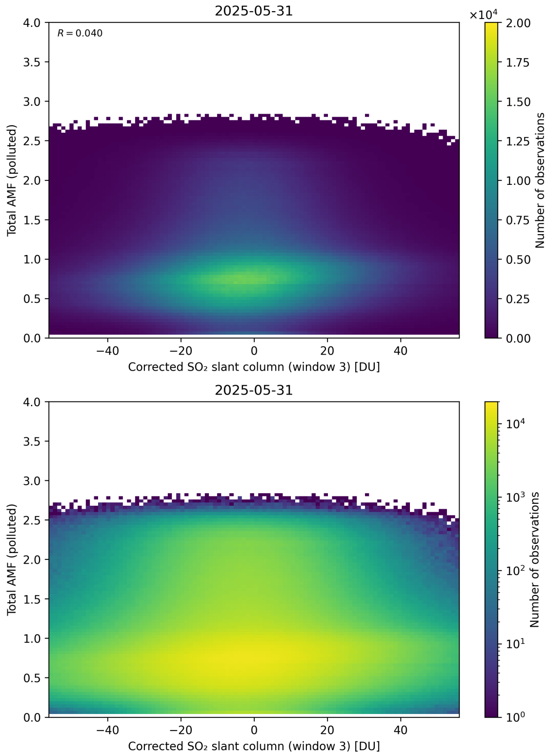
Figure 260: Scatter density plot of “Corrected SO 2 slant column (window 3)” against “Total AMF (polluted)” for 2025-05-31 to 2025-06-01.
