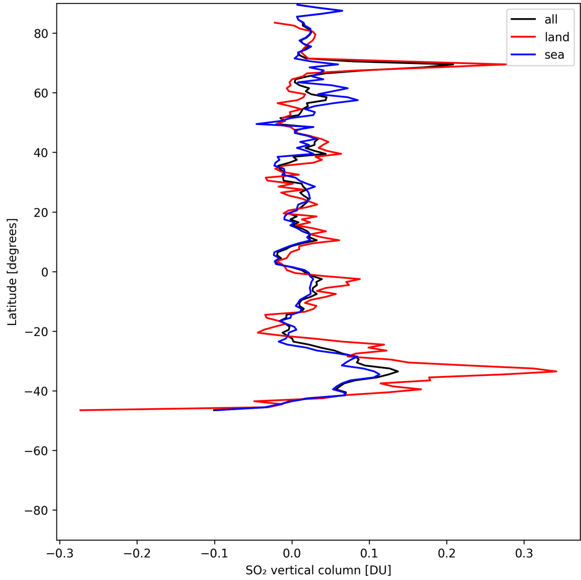
Figure 32: Zonal average of “SO 2 vertical column” for 2025-05-31 to 2025-06-01.
