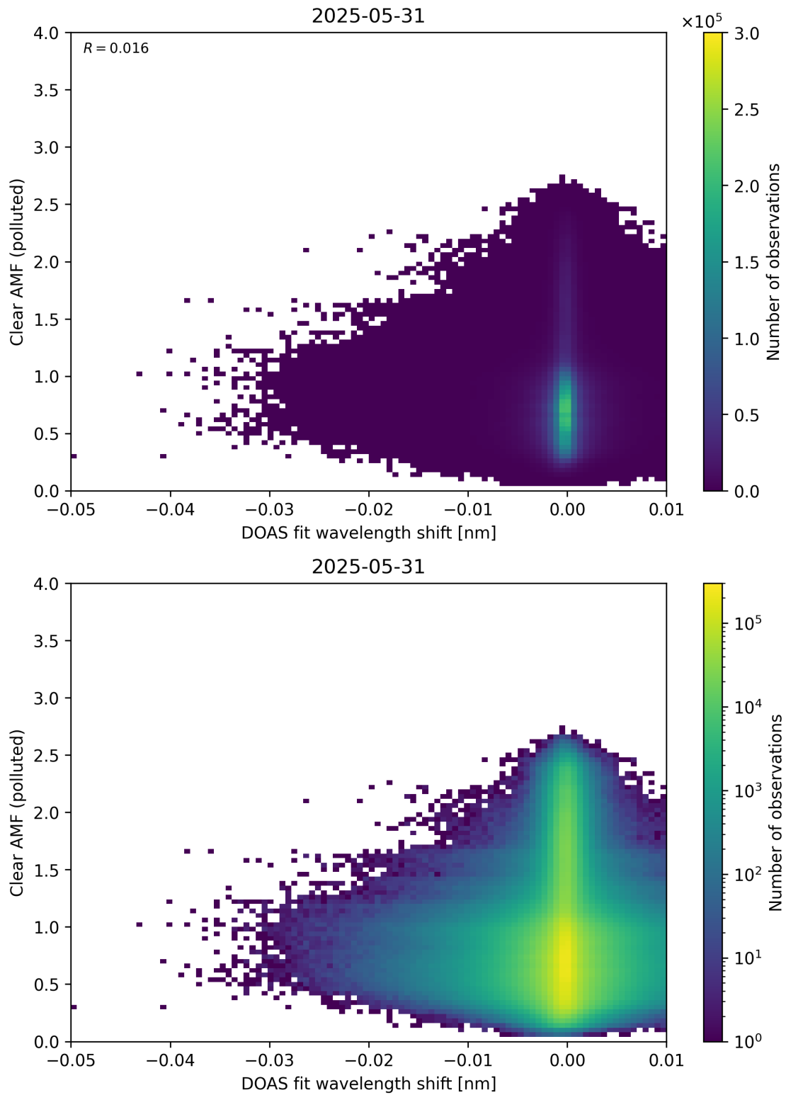
Figure 140: Scatter density plot of “DOAS fit wavelength shift” against “Clear AMF (polluted)” for 2025-05-31 to 2025-06-01.
