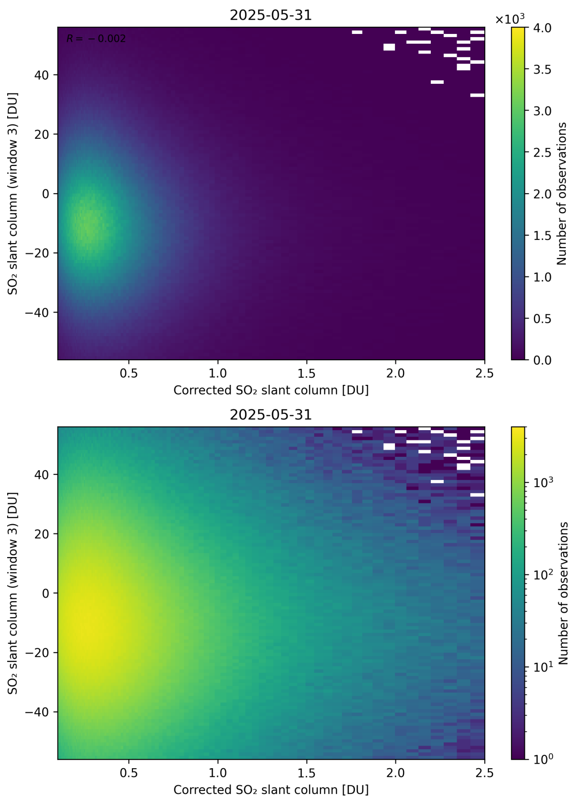
Figure 240: Scatter density plot of “Corrected SO 2 slant column” against “SO 2 slant column (window 3)” for 2025-05-31 to 2025-06-01.
