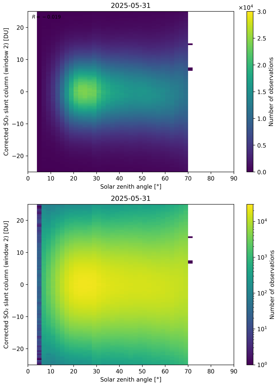
Figure 182: Scatter density plot of “Solar zenith angle” against “Corrected SO 2 slant column (window 2)” for 2025-05-31 to 2025-06-01.
