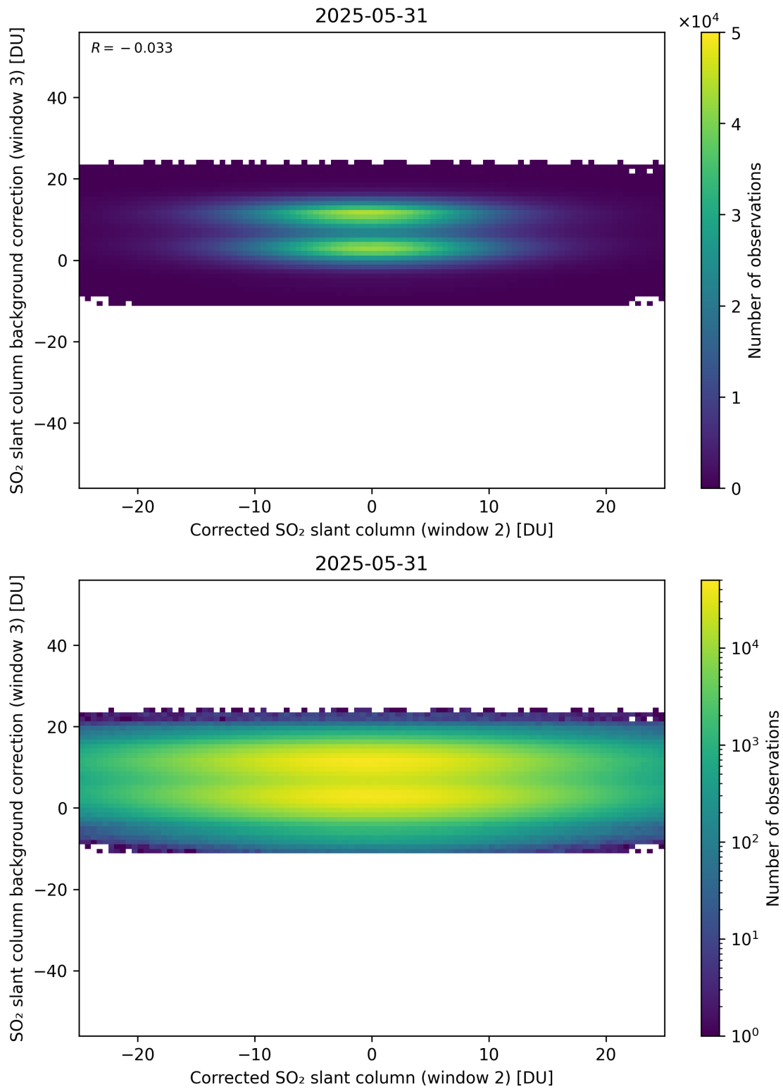
Figure 245: Scatter density plot of “Corrected SO 2 slant column (window 2)” against “SO 2 slant column background correction (window 3)” for 2025-05-31 to 2025-06-01.
