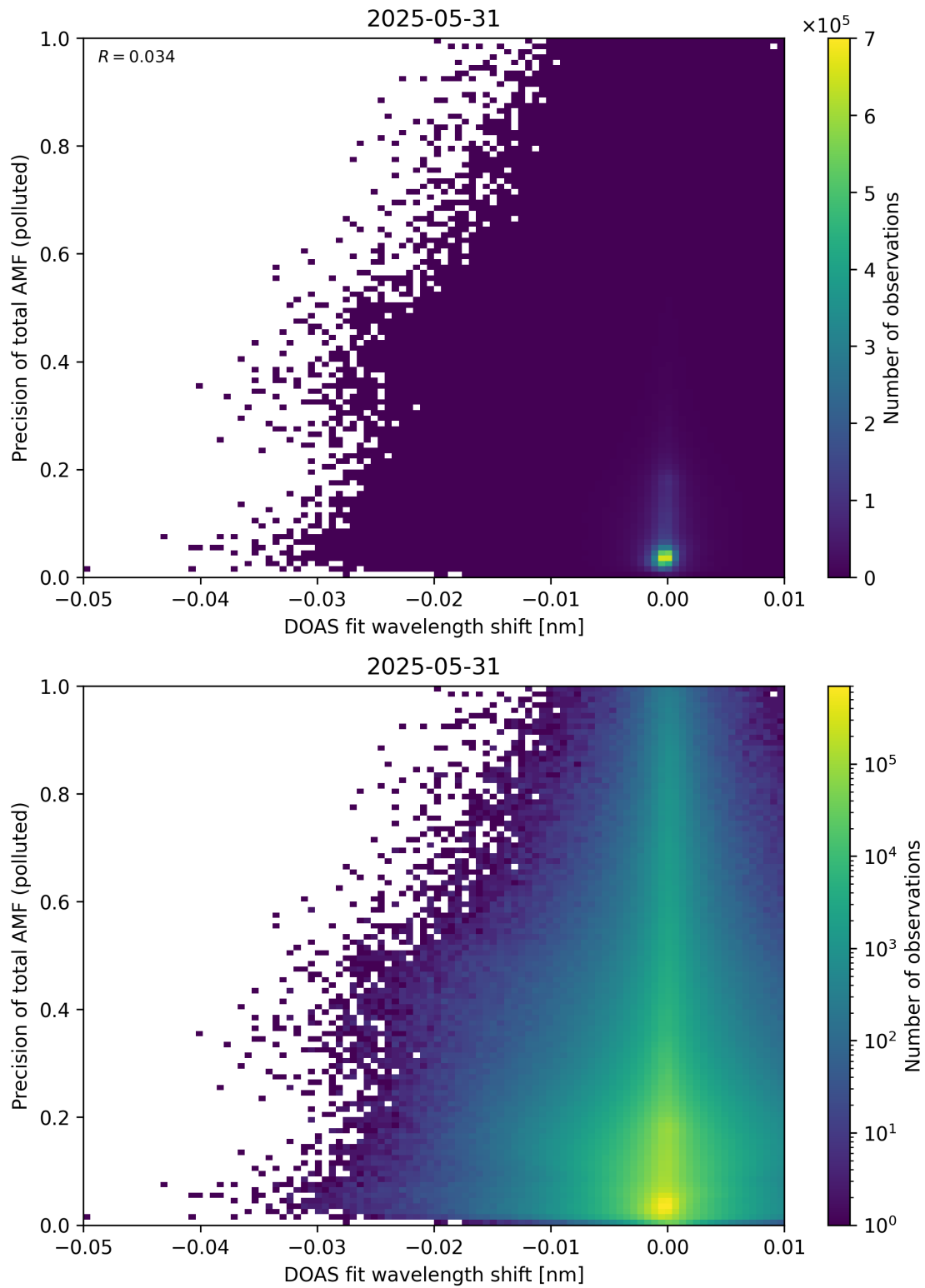
Figure 142: Scatter density plot of “DOAS fit wavelength shift” against “Precision of total AMF (polluted)” for 2025-05-31 to 2025-06-01.
