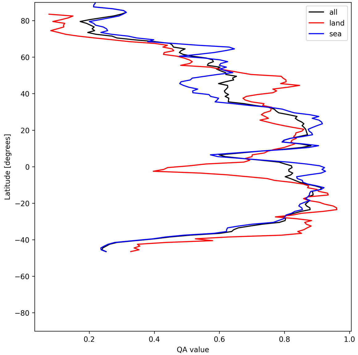
Figure 31: Zonal average of “QA value” for 2025-05-31 to 2025-06-01.
