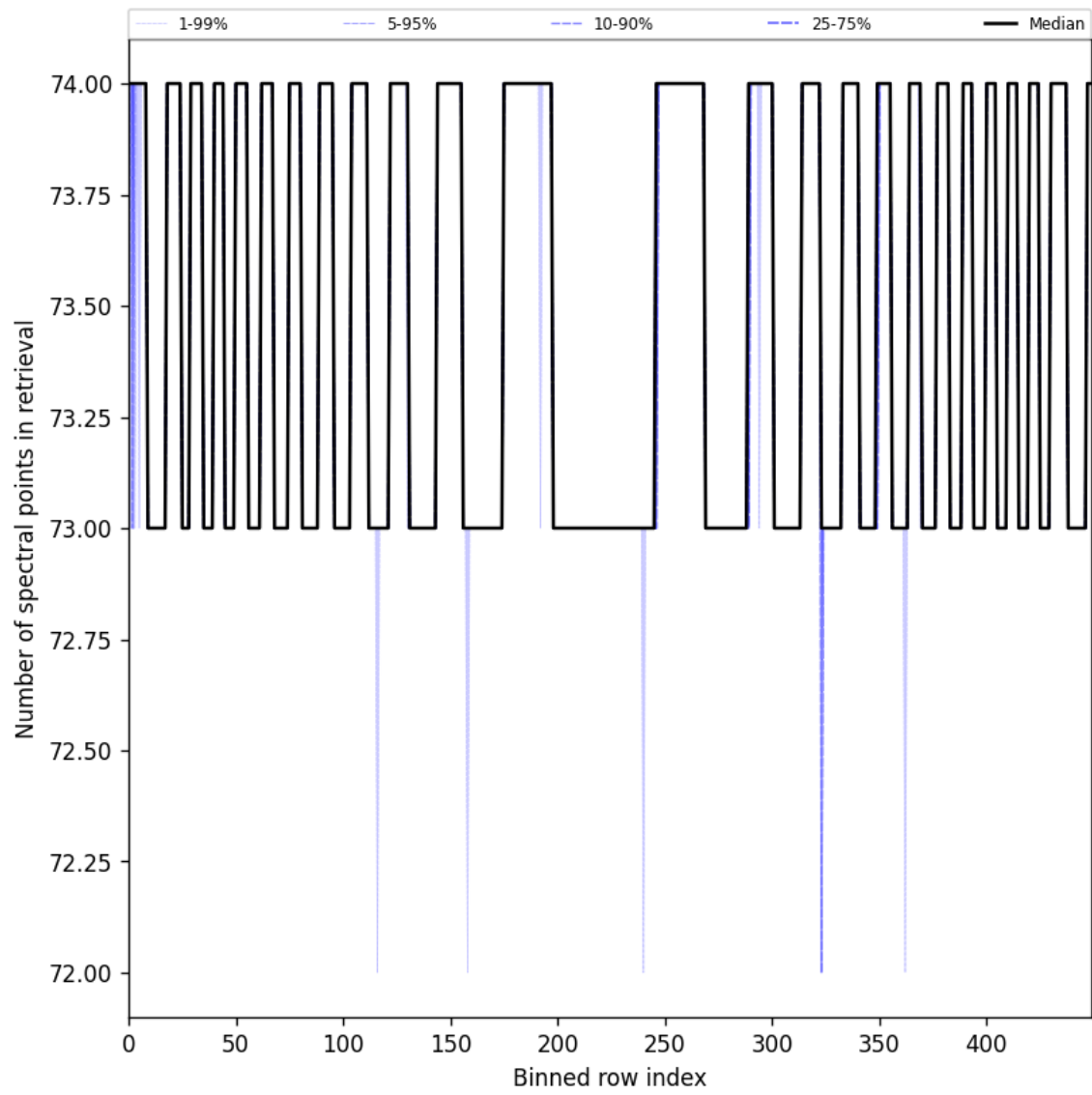
Figure 108: Along track statistics of “Number of spectral points in retrieval” for 2025-05-31 to 2025-06-01
