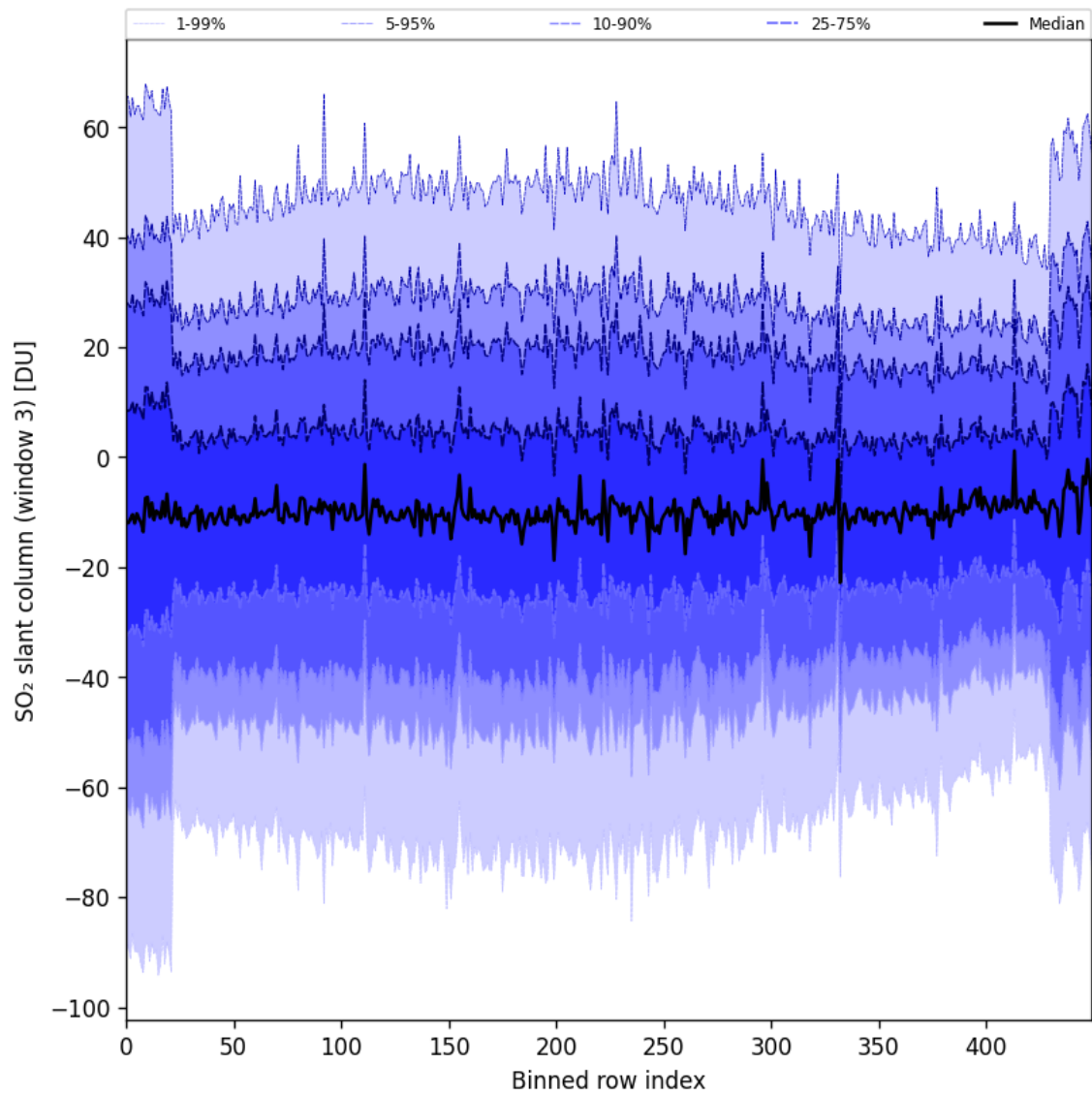
Figure 97: Along track statistics of “SO 2 slant column (window 3)” for 2025-05-31 to 2025-06-01
