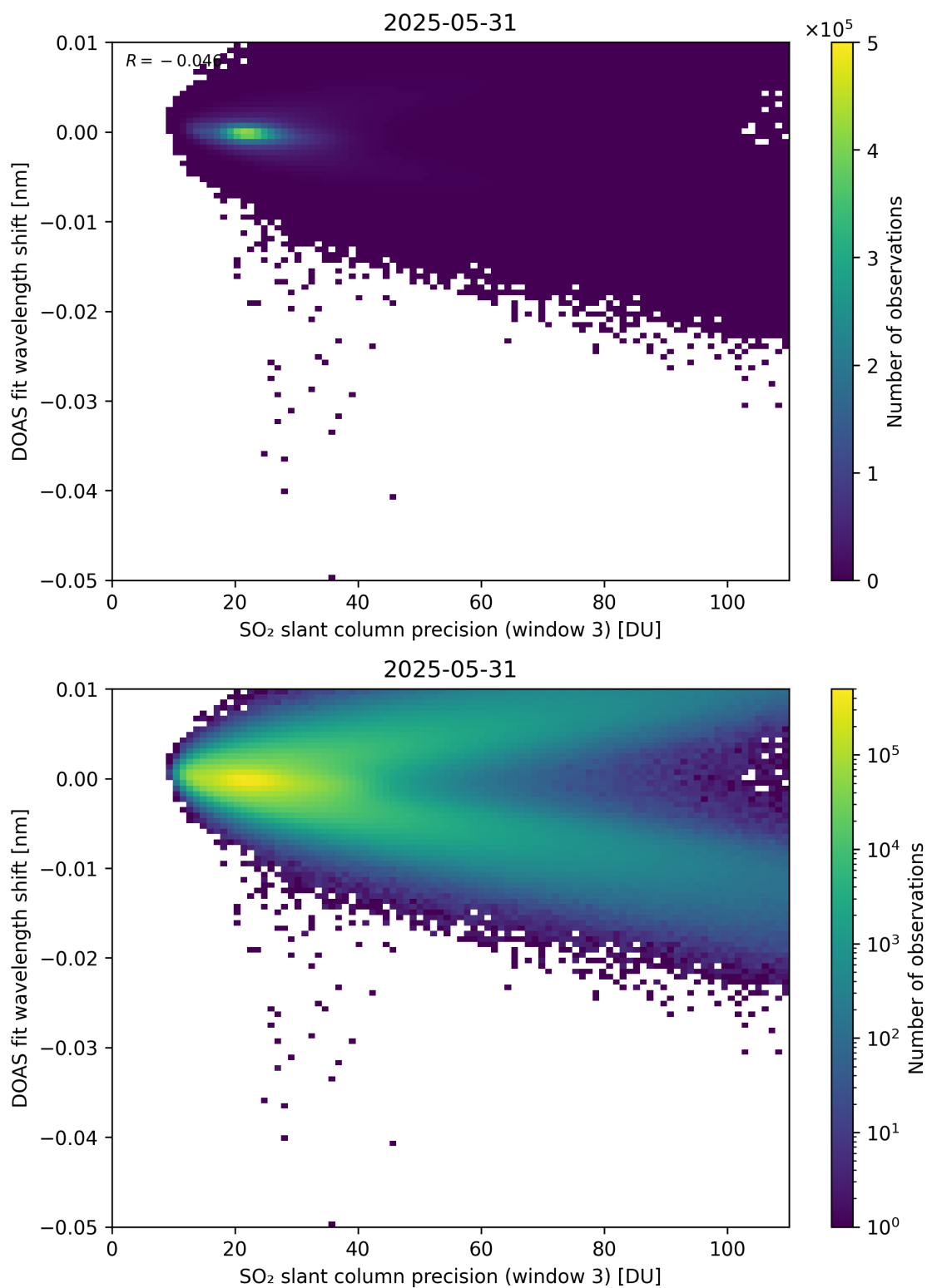
Figure 308: Scatter density plot of “SO 2 slant column precision (window 3)” against “DOAS fit wavelength shift” for 2025-05-31 to 2025-06-01.
