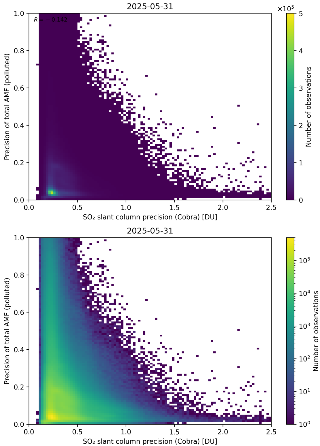
Figure 214: Scatter density plot of “SO 2 slant column precision (Cobra)” against “Precision of total AMF (polluted)” for 2025-05-31 to 2025-06-01.
