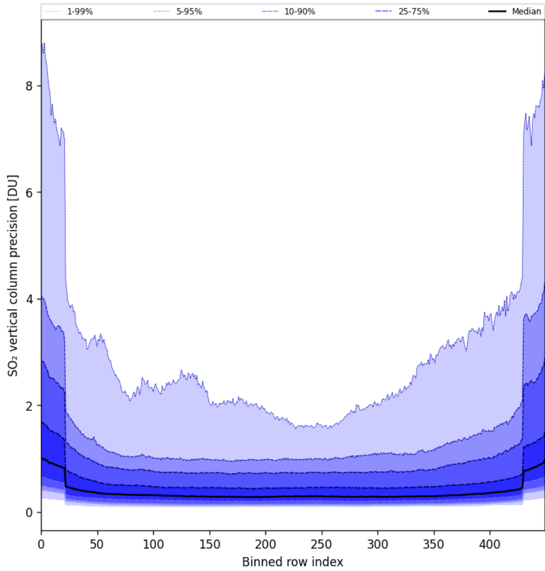
Figure 85: Along track statistics of “SO 2 vertical column precision” for 2025-05-31 to 2025-06-01
