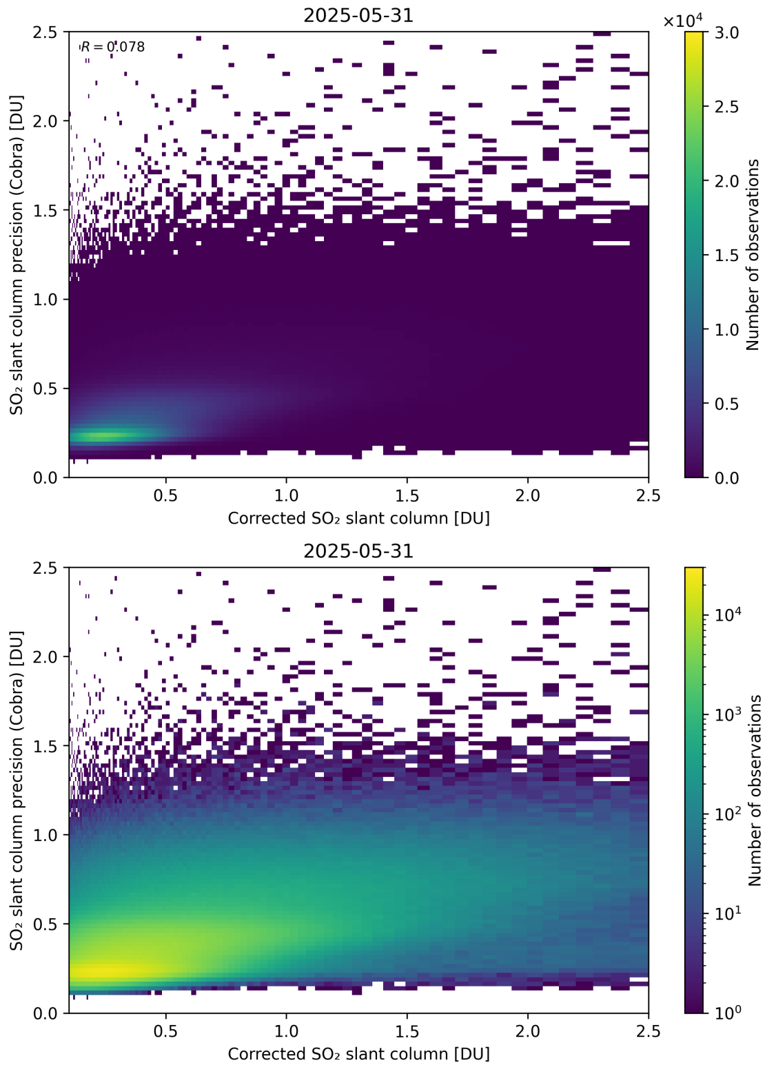
Figure 234: Scatter density plot of “Corrected SO 2 slant column” against “SO 2 slant column precision (Cobra)” for 2025-05-31 to 2025-06-01.
