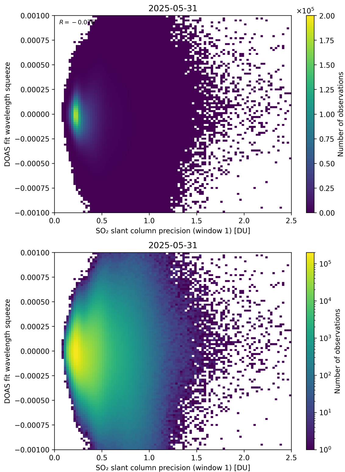
Figure 272: Scatter density plot of “SO 2 slant column precision (window 1)” against “DOAS fit wavelength squeeze” for 2025-05-31 to 2025-06-01.
