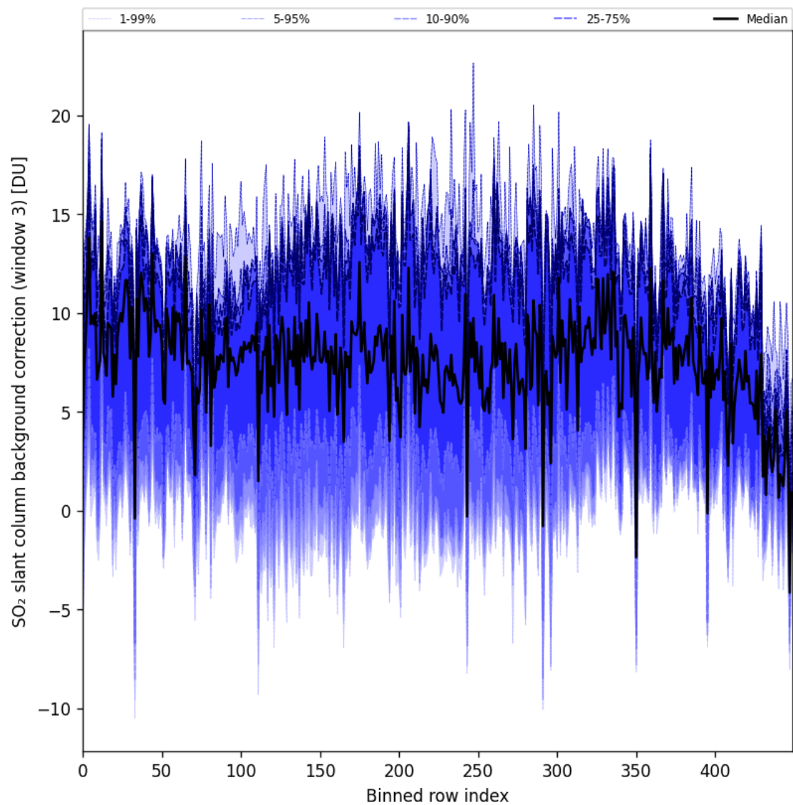
Figure 100: Along track statistics of “SO 2 slant column background correction (window 3)” for 2025-05-31 to 2025-06-01
