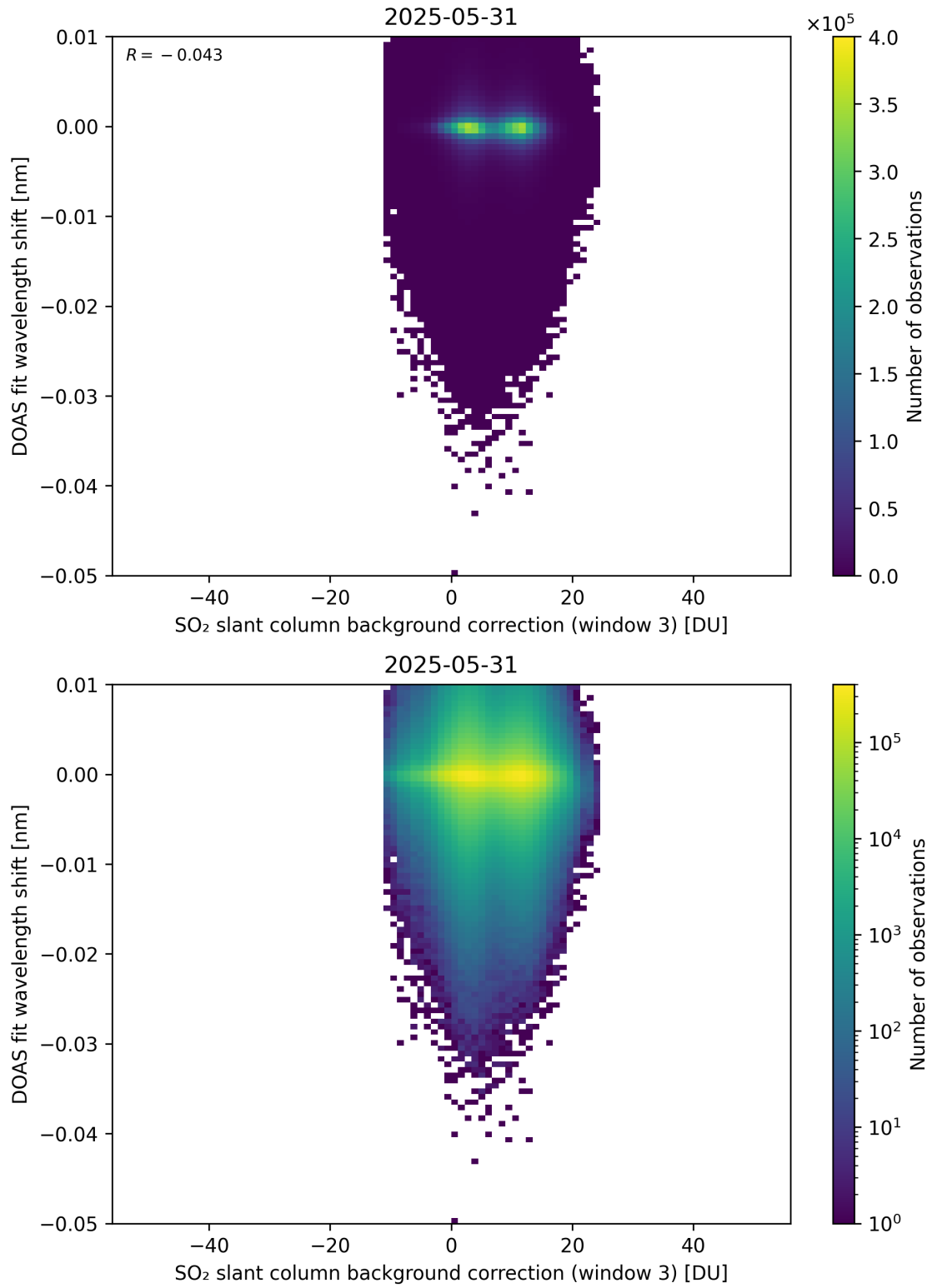
Figure 132: Scatter density plot of “SO 2 slant column background correction (window 3)” against “DOAS fit wavelength shift” for 2025-05-31 to 2025-06-01.
