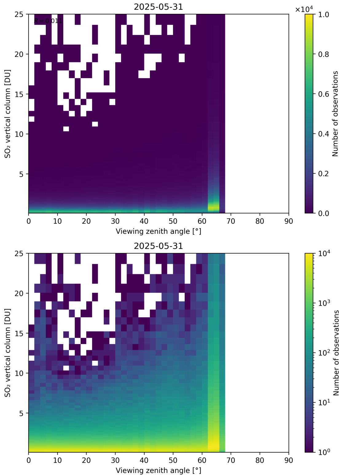
Figure 383: Scatter density plot of “Viewing zenith angle” against “SO 2 vertical column” for 2025-05-31 to 2025-06-01.
