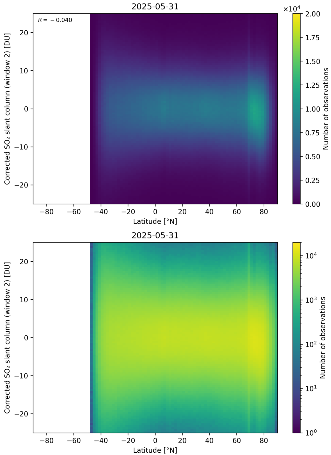
Figure 160: Scatter density plot of “Latitude” against “Corrected SO 2 slant column (window 2)” for 2025-05-31 to 2025-06-01.
