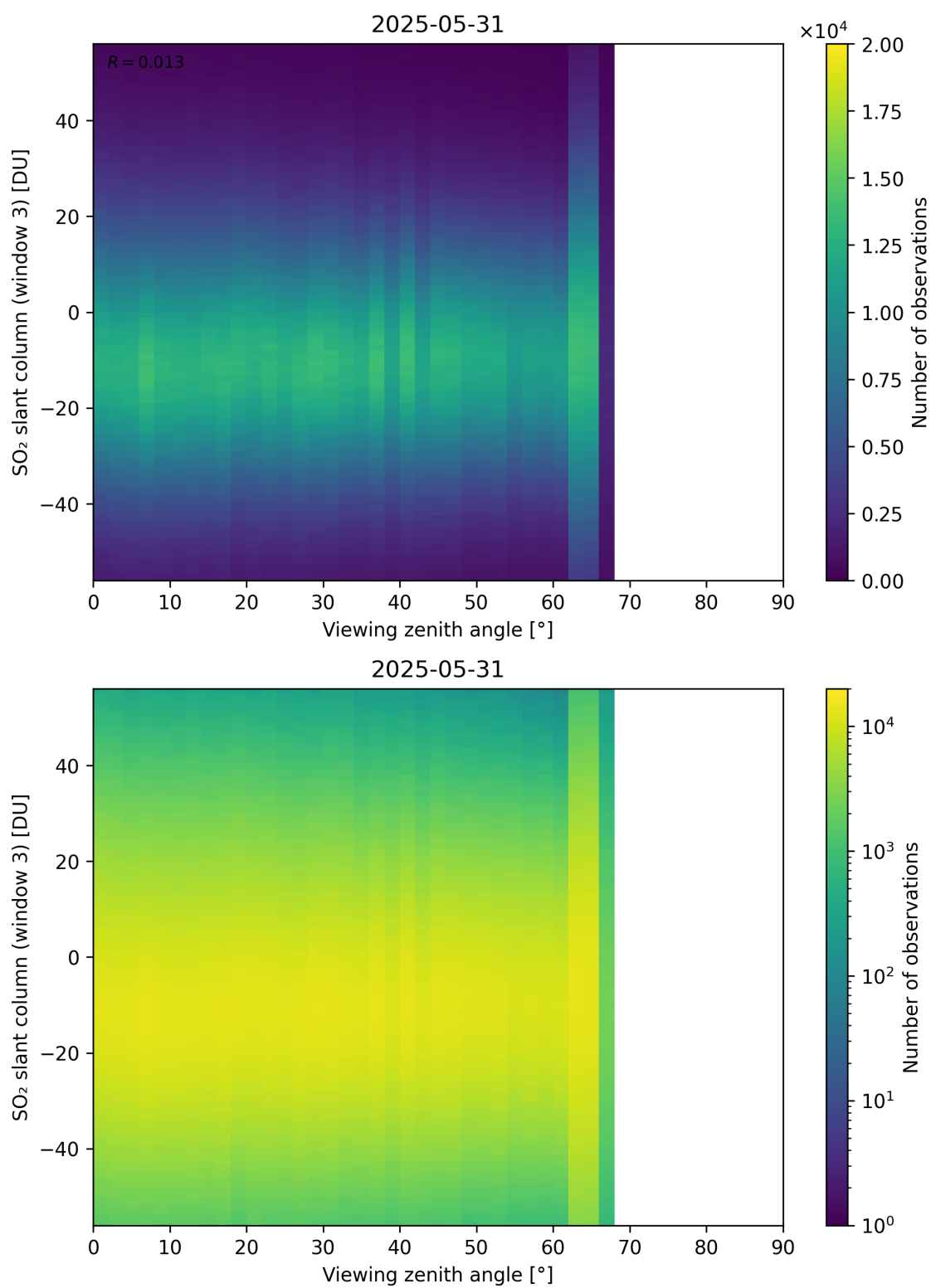
Figure 379: Scatter density plot of “Viewing zenith angle” against “SO 2 slant column (window 3)” for 2025-05-31 to 2025-06-01.
