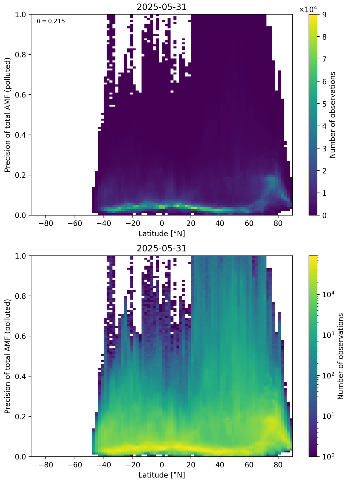
Figure 168: Scatter density plot of “Latitude” against “Precision of total AMF (polluted)” for 2025-05-31 to 2025-06-01.
