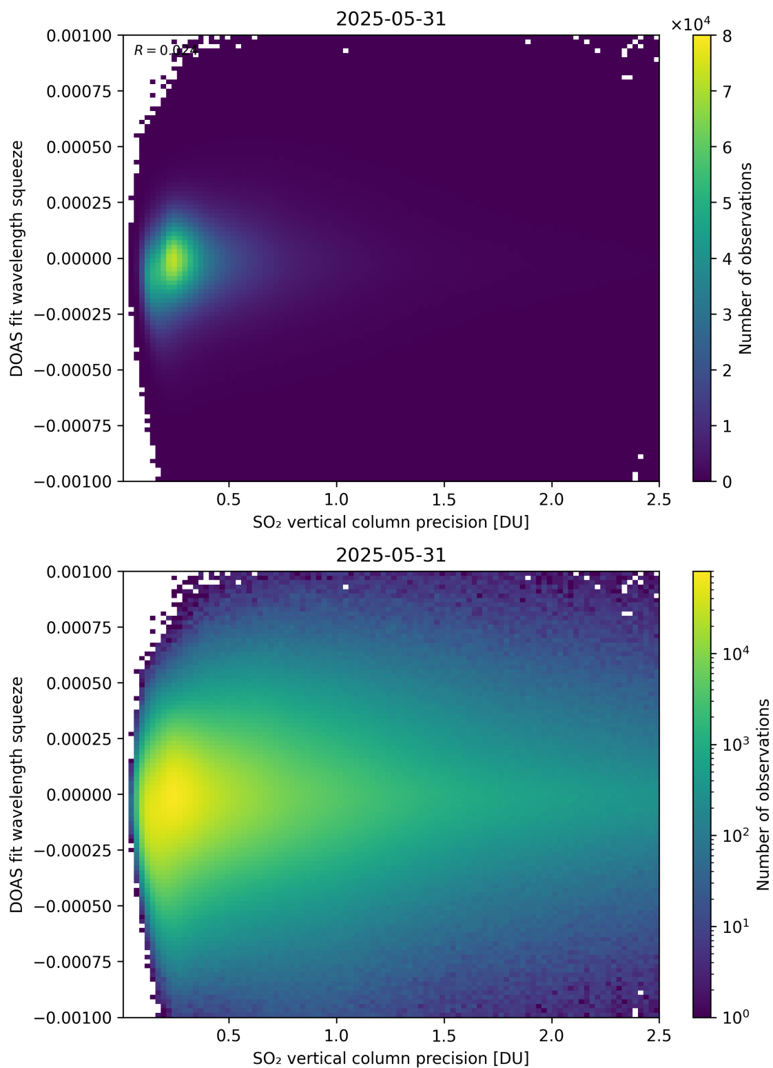
Figure 333: Scatter density plot of “SO 2 vertical column precision” against “DOAS fit wavelength squeeze” for 2025-05-31 to 2025-06-01.
