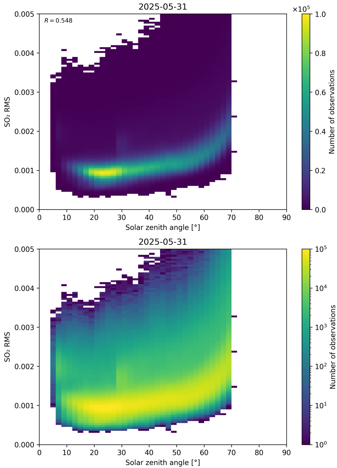
Figure 176: Scatter density plot of “Solar zenith angle” against “SO 2 RMS” for 2025-05-31 to 2025-06-01.
