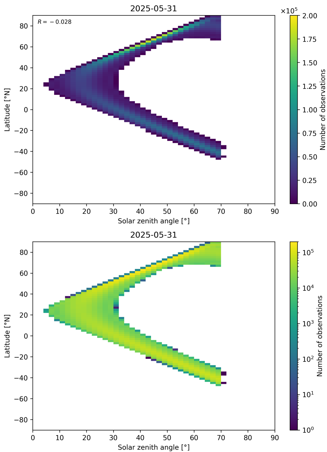
Figure 177: Scatter density plot of “Solar zenith angle” against “Latitude” for 2025-05-31 to 2025-06-01.
