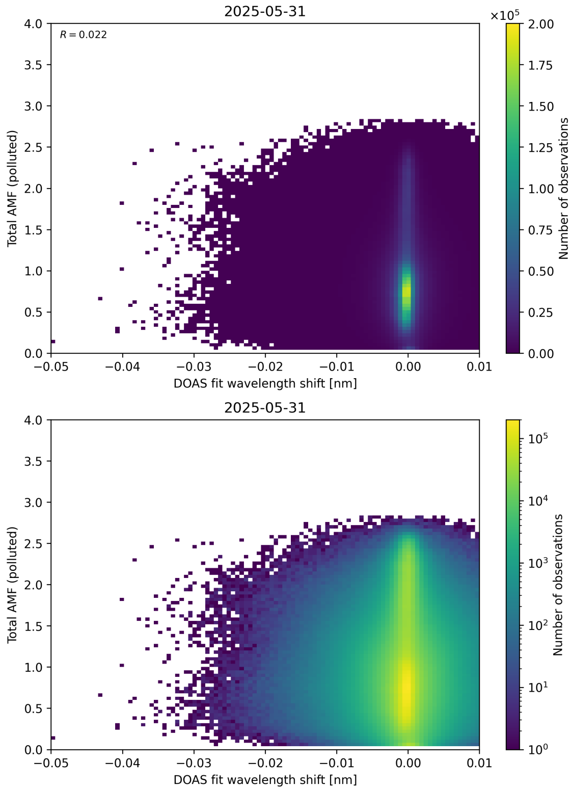
Figure 141: Scatter density plot of “DOAS fit wavelength shift” against “Total AMF (polluted)” for 2025-05-31 to 2025-06-01.
