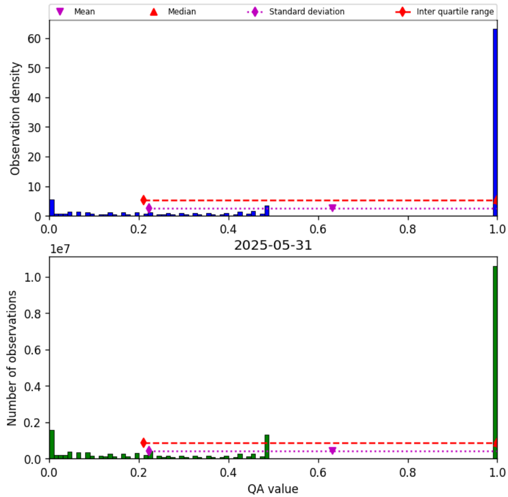
Figure 57: Histogram of “QA value” for 2025-05-31 to 2025-06-01
