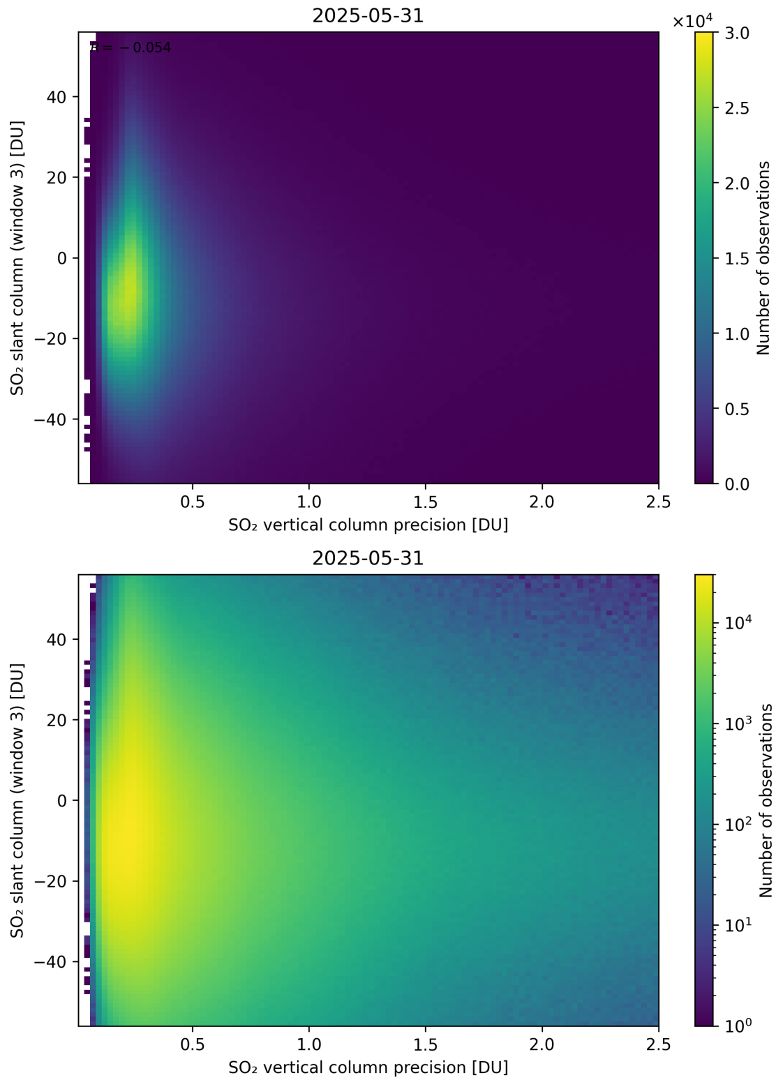
Figure 344: Scatter density plot of “SO 2 vertical column precision” against “SO 2 slant column (window 3)” for 2025-05-31 to 2025-06-01.
