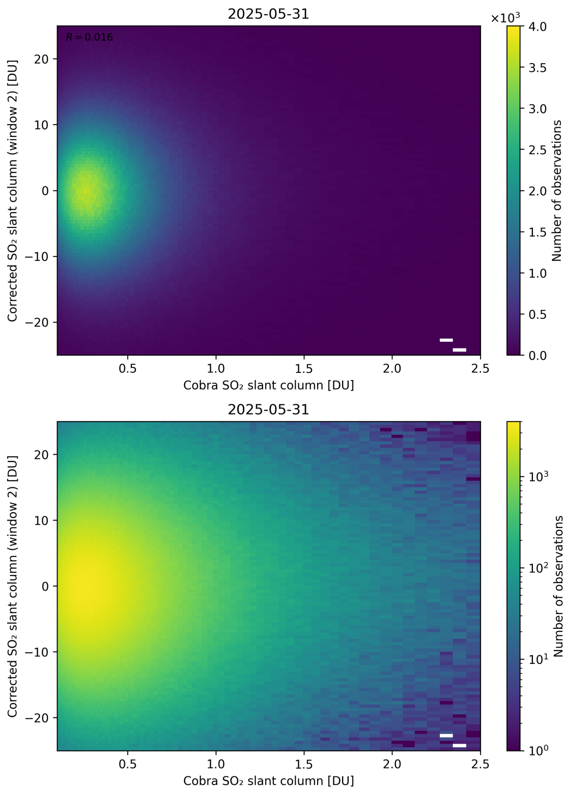
Figure 217: Scatter density plot of “Cobra SO 2 slant column” against “Corrected SO 2 slant column (window 2)” for 2025-05-31 to 2025-06-01.
