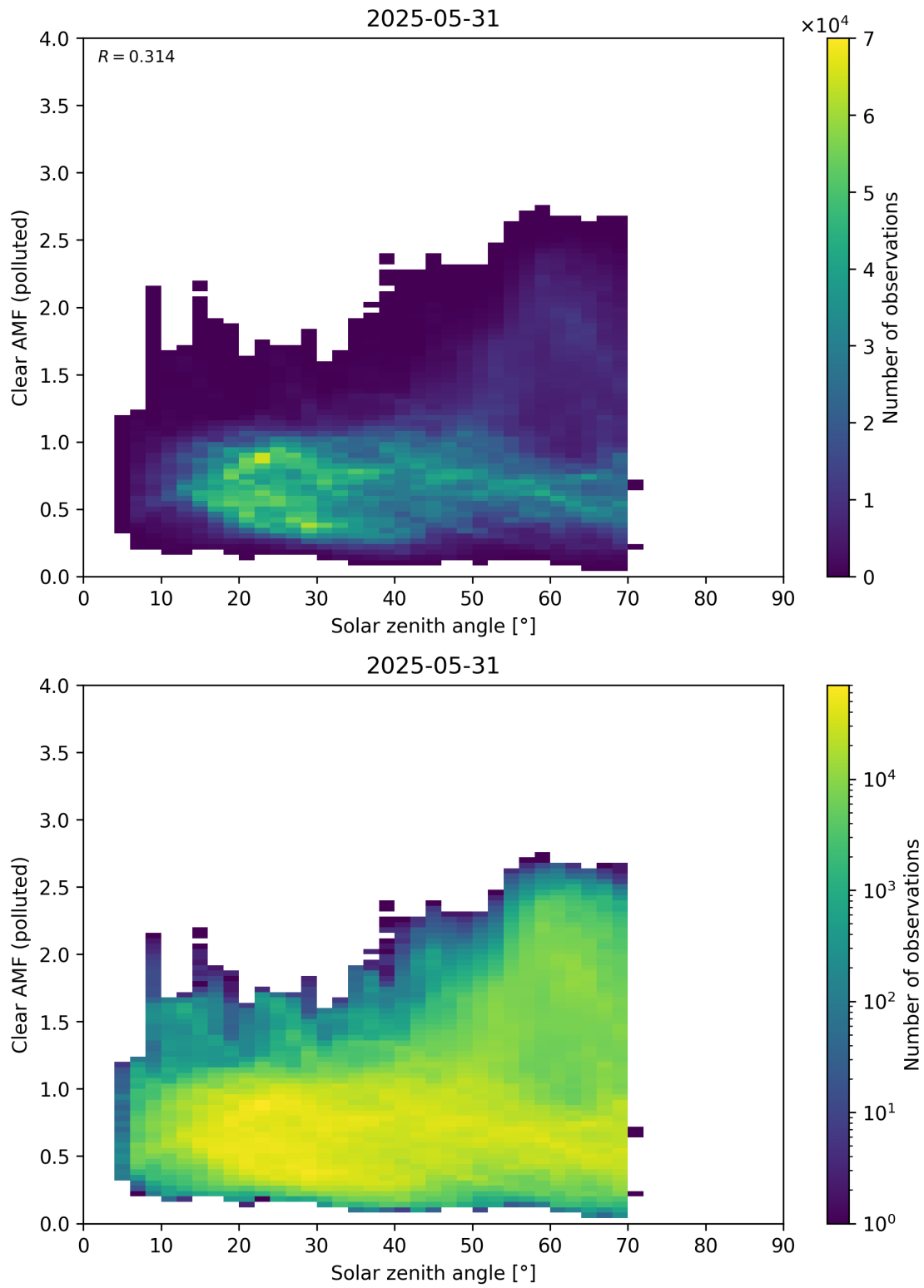
Figure 178: Scatter density plot of “Solar zenith angle” against “Clear AMF (polluted)” for 2025-05-31 to 2025-06-01.
