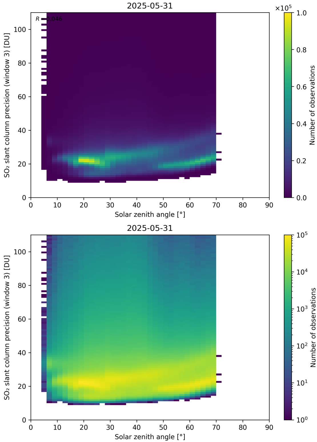
Figure 188: Scatter density plot of “Solar zenith angle” against “SO 2 slant column precision (window 3)” for 2025-05-31 to 2025-06-01.
