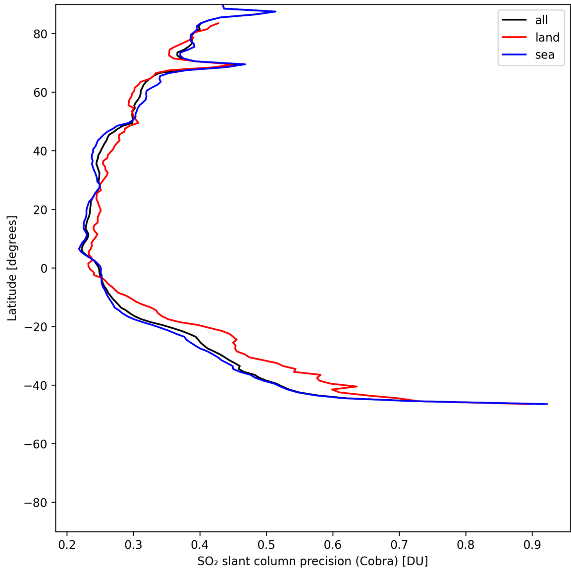
Figure 36: Zonal average of “SO 2 slant column precision (Cobra)” for 2025-05-31 to 2025-06-01.
