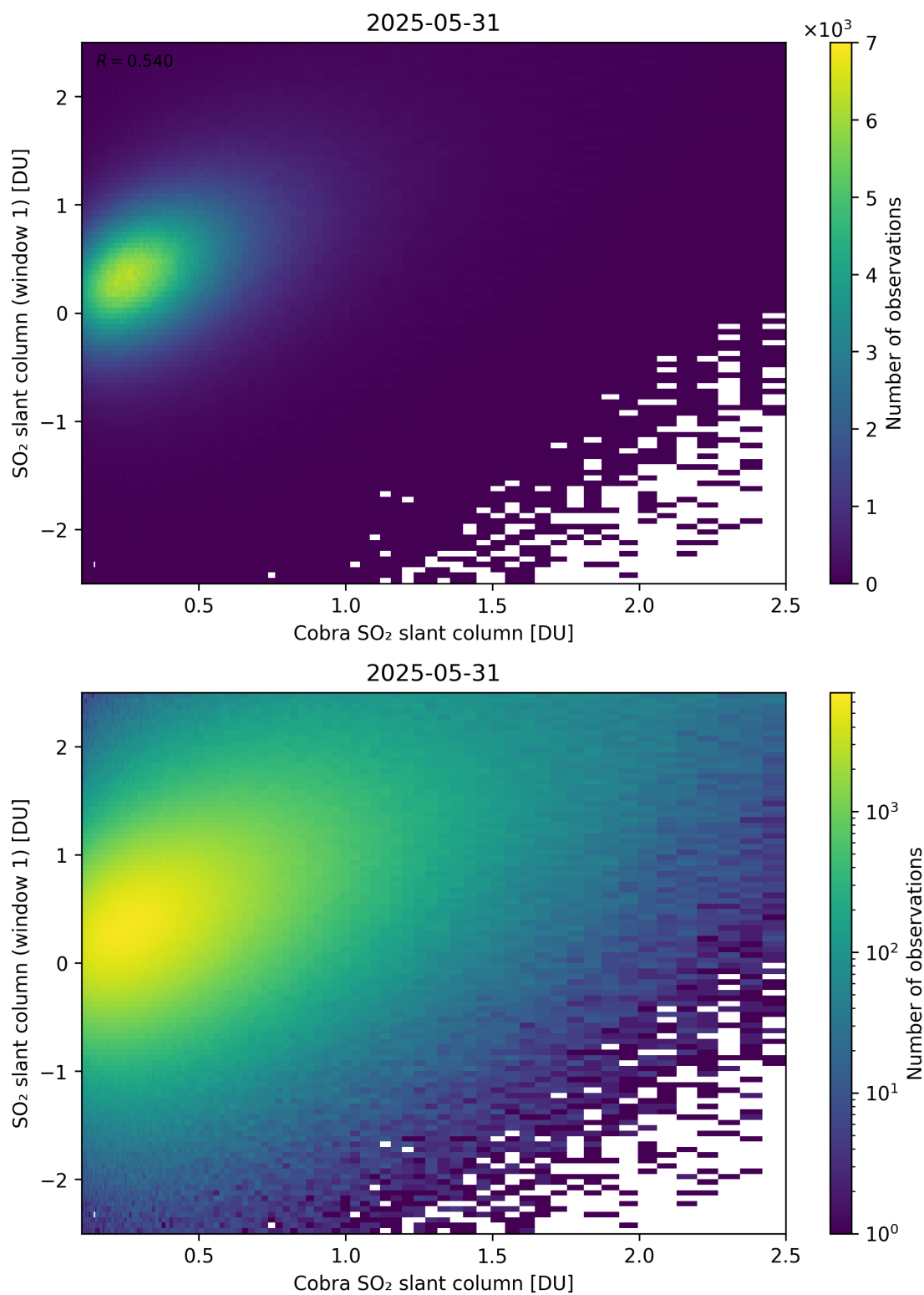
Figure 219: Scatter density plot of “Cobra SO 2 slant column” against “SO 2 slant column (window 1)” for 2025-05-31 to 2025-06-01.
