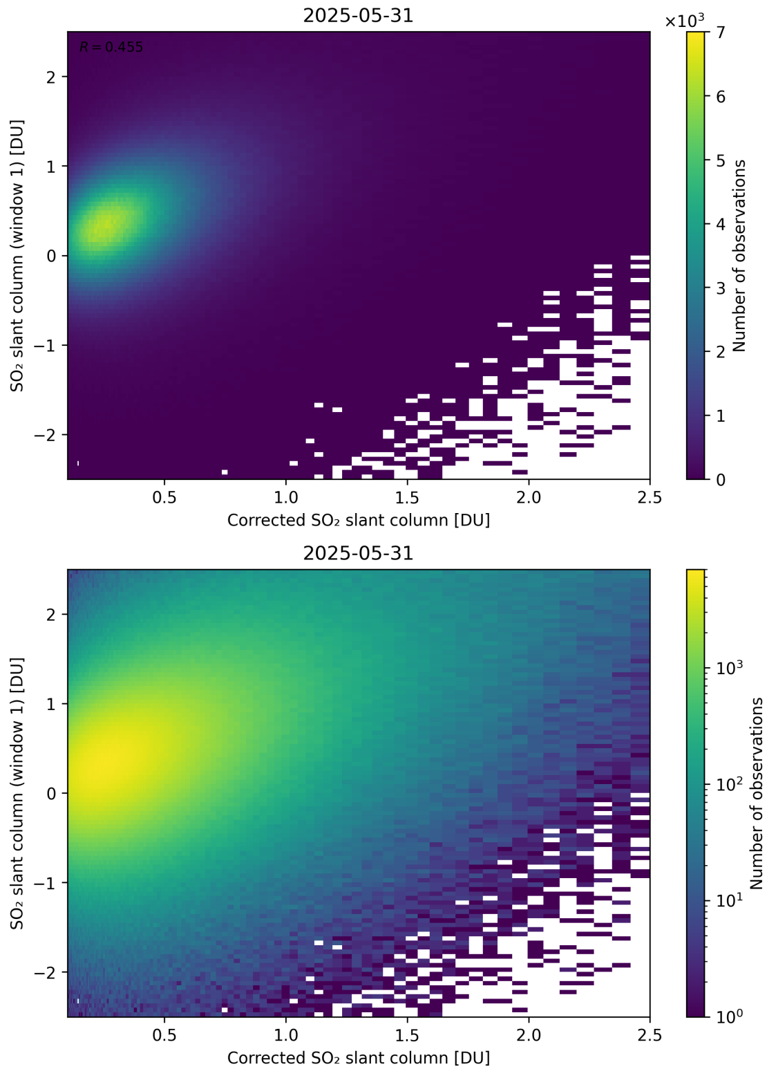
Figure 237: Scatter density plot of “Corrected SO 2 slant column” against “SO 2 slant column (window 1)” for 2025-05-31 to 2025-06-01.
