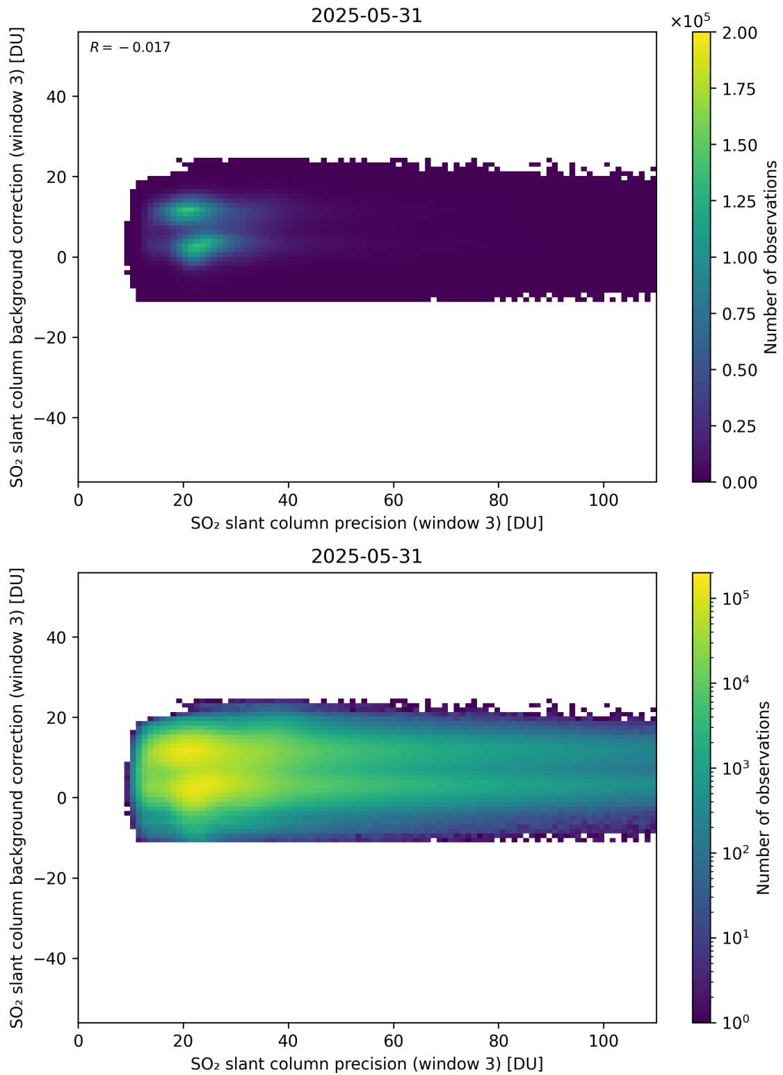
Figure 307: Scatter density plot of “SO 2 slant column precision (window 3)” against “SO 2 slant column background correction (window 3)” for 2025-05-31 to 2025-06-01.
