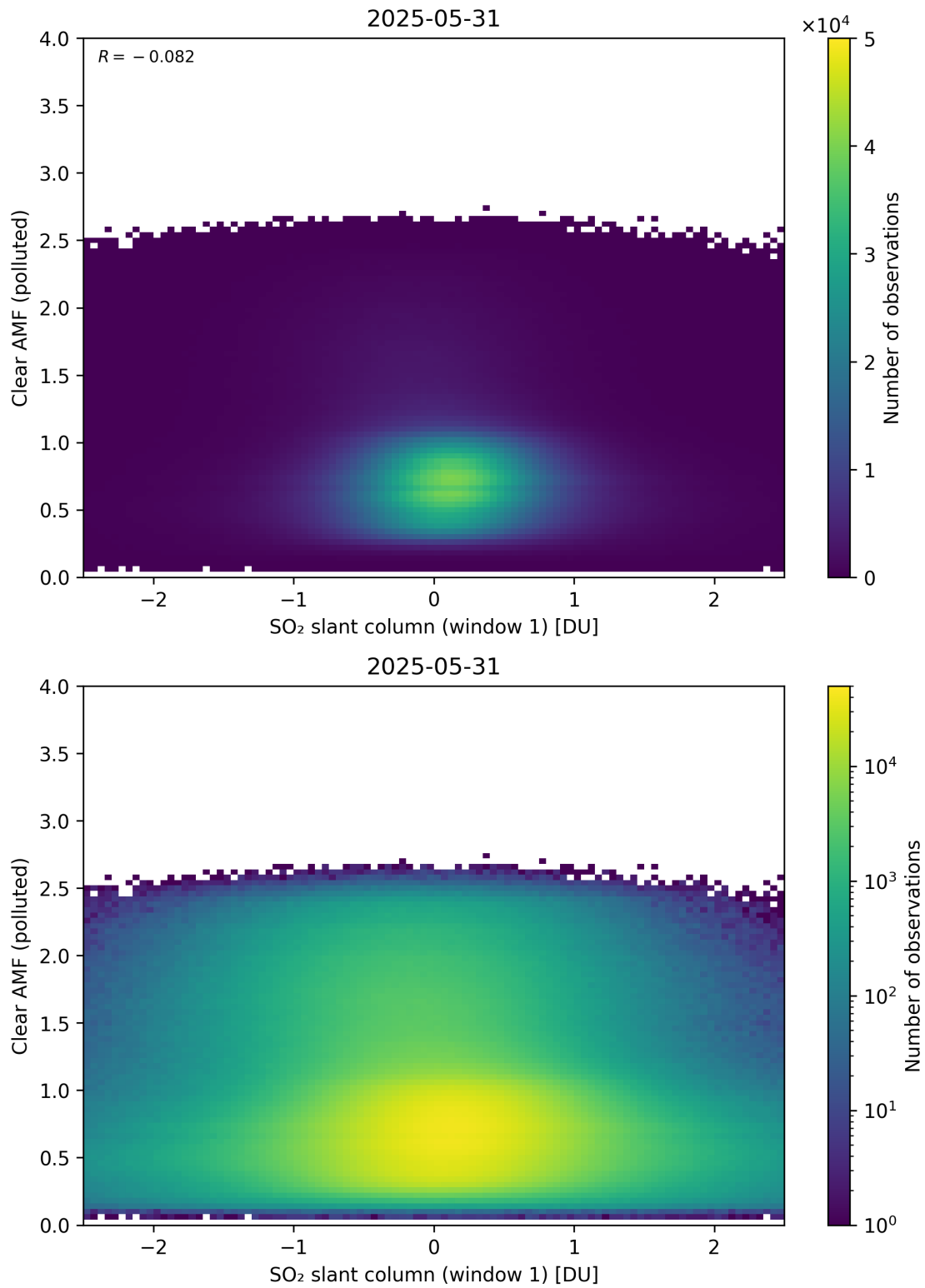
Figure 282: Scatter density plot of “SO 2 slant column (window 1)” against “Clear AMF (polluted)” for 2025-05-31 to 2025-06-01.
