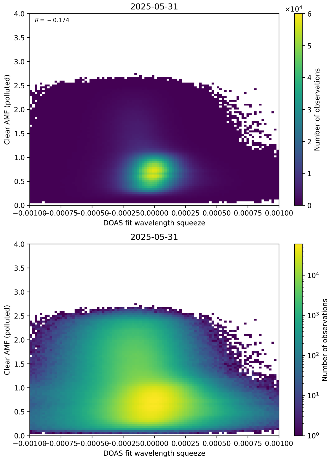
Figure 144: Scatter density plot of “DOAS fit wavelength squeeze” against “Clear AMF (polluted)” for 2025-05-31 to 2025-06-01.
