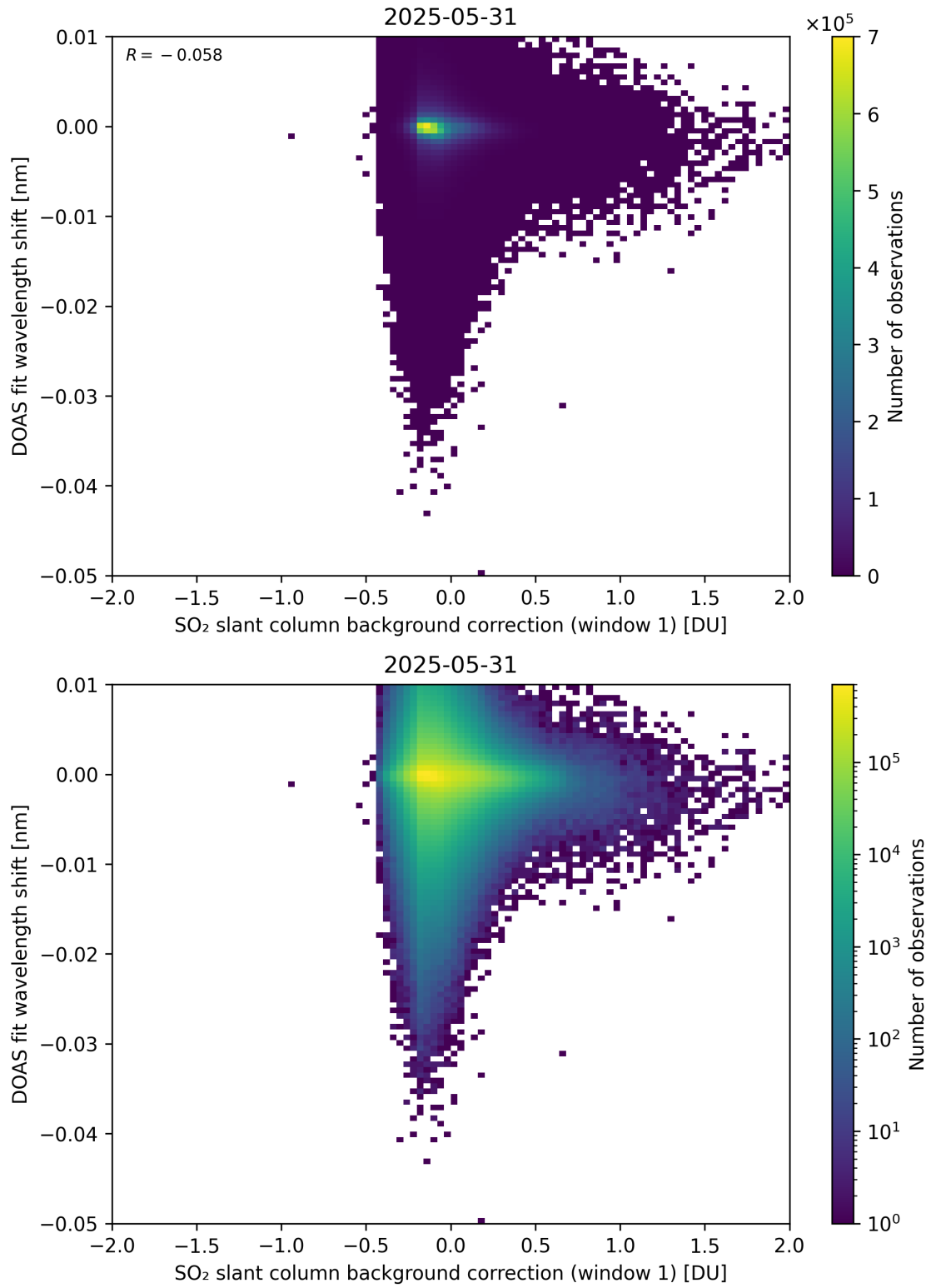
Figure 111: Scatter density plot of “SO 2 slant column background correction (window 1)” against “DOAS fit wavelength shift” for 2025-05-31 to 2025-06-01.
