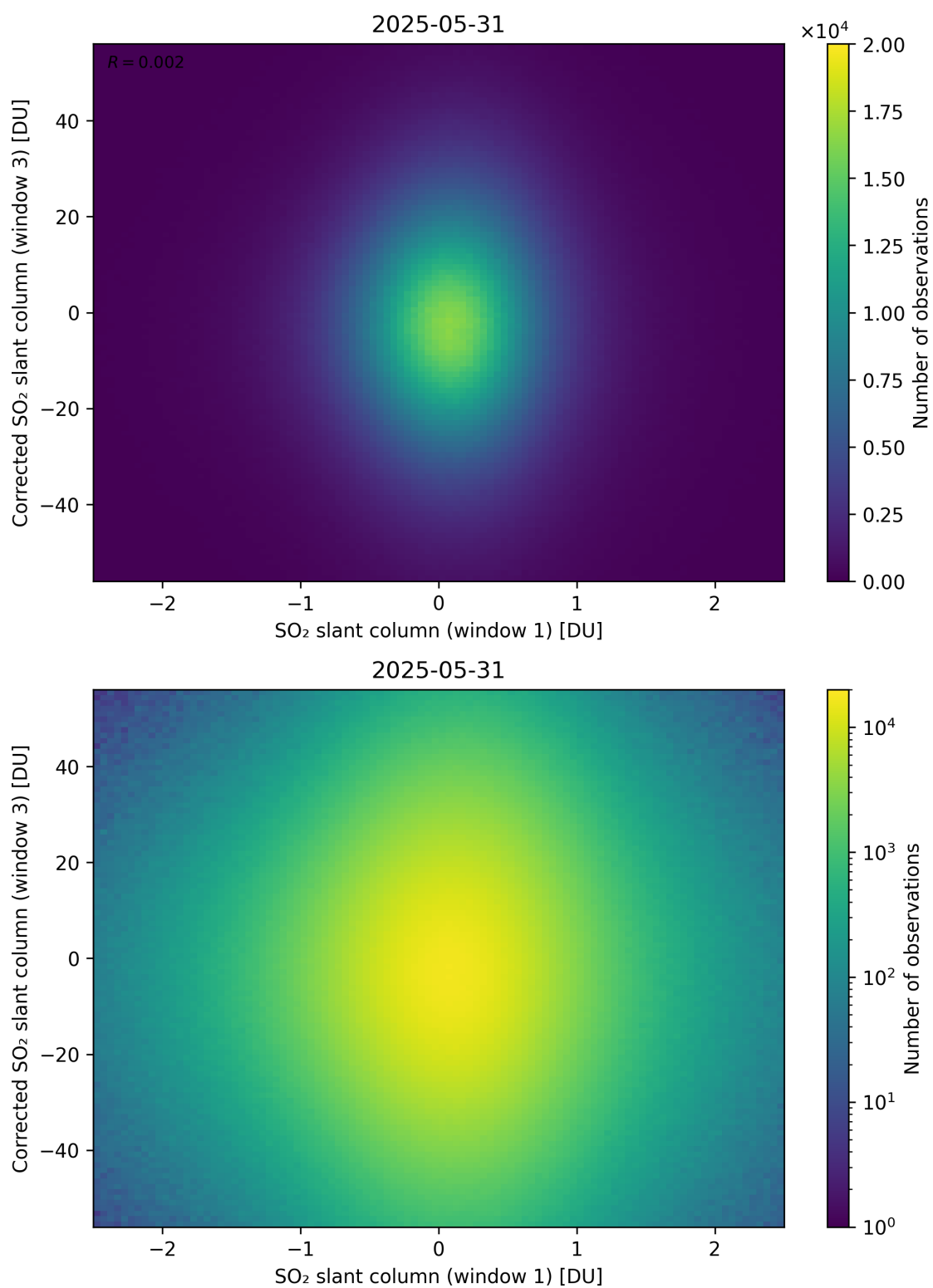
Figure 284: Scatter density plot of “SO 2 slant column (window 1)” against “Corrected SO 2 slant column (window 3)” for 2025-05-31 to 2025-06-01.
