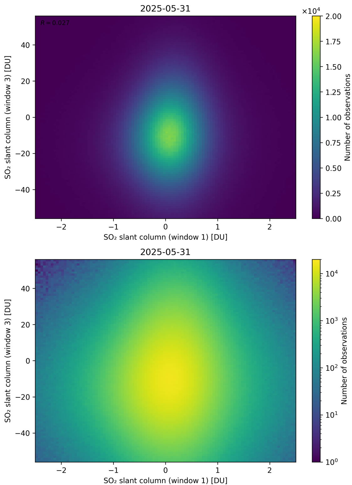
Figure 287: Scatter density plot of “SO 2 slant column (window 1)” against “SO 2 slant column (window 3)” for 2025-05-31 to 2025-06-01.
