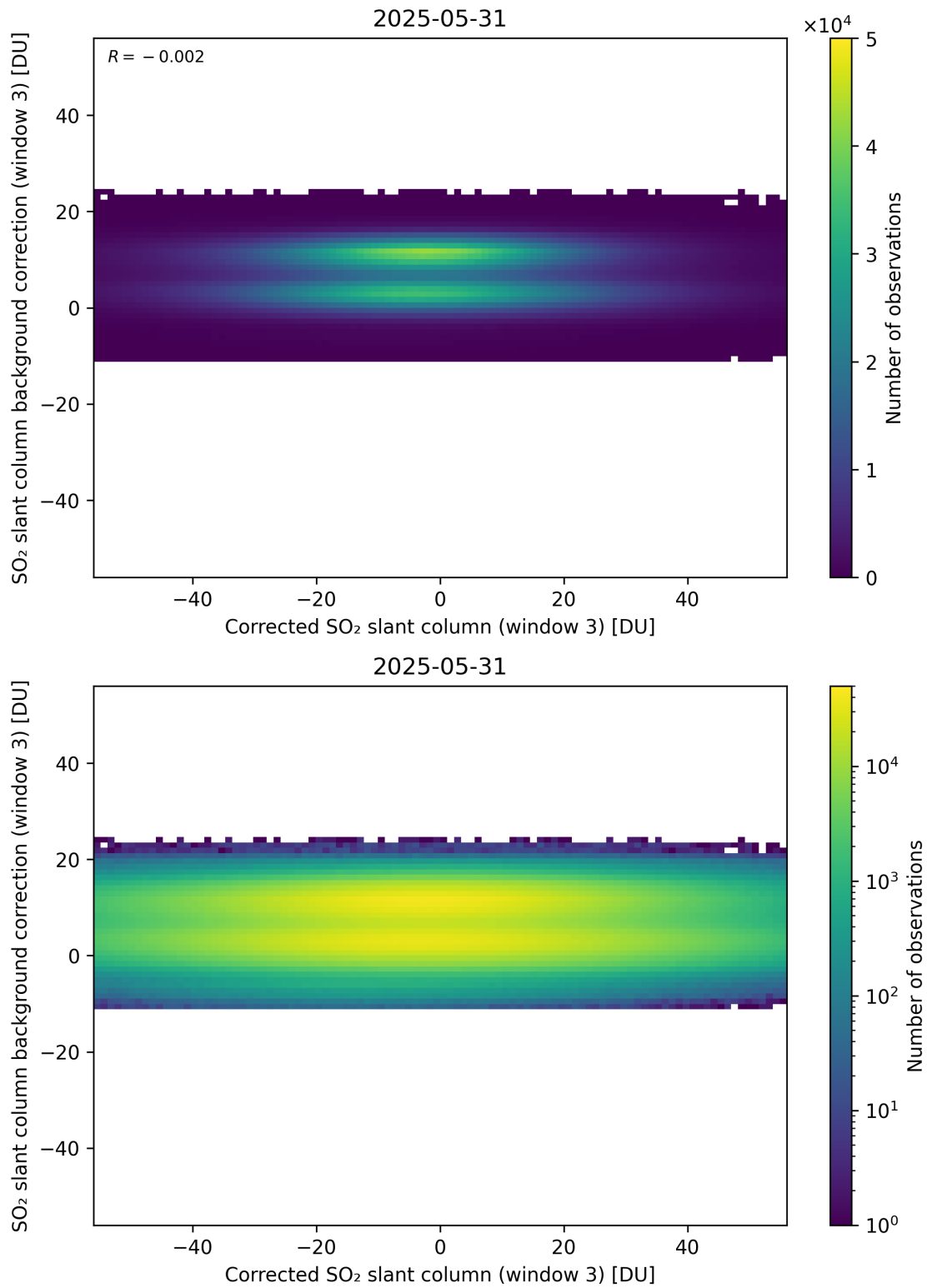
Figure 255: Scatter density plot of “Corrected SO 2 slant column (window 3)” against “SO 2 slant column background correction (window 3)” for 2025-05-31 to 2025-06-01.
