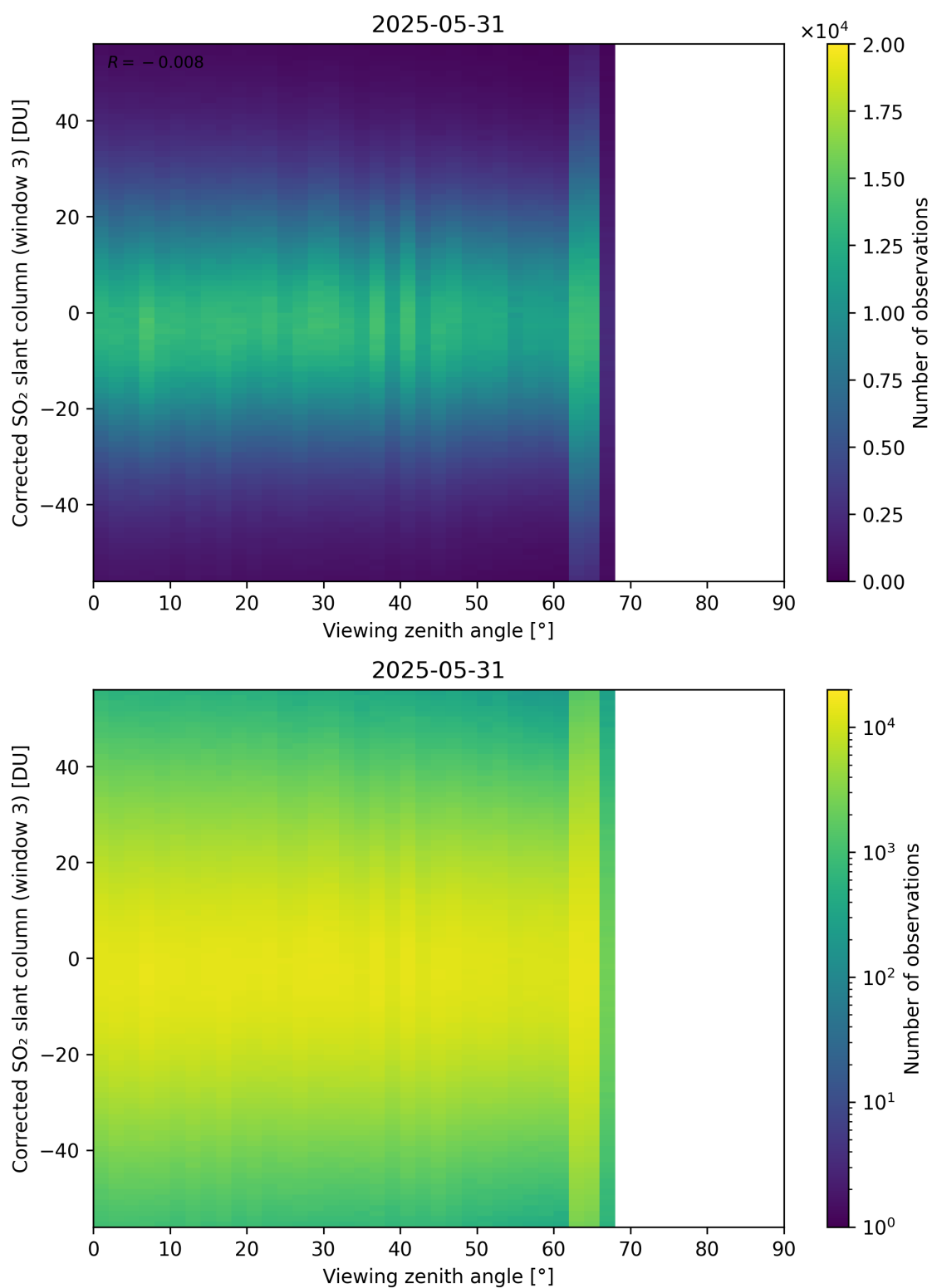
Figure 375: Scatter density plot of “Viewing zenith angle” against “Corrected SO 2 slant column (window 3)” for 2025-05-31 to 2025-06-01.
