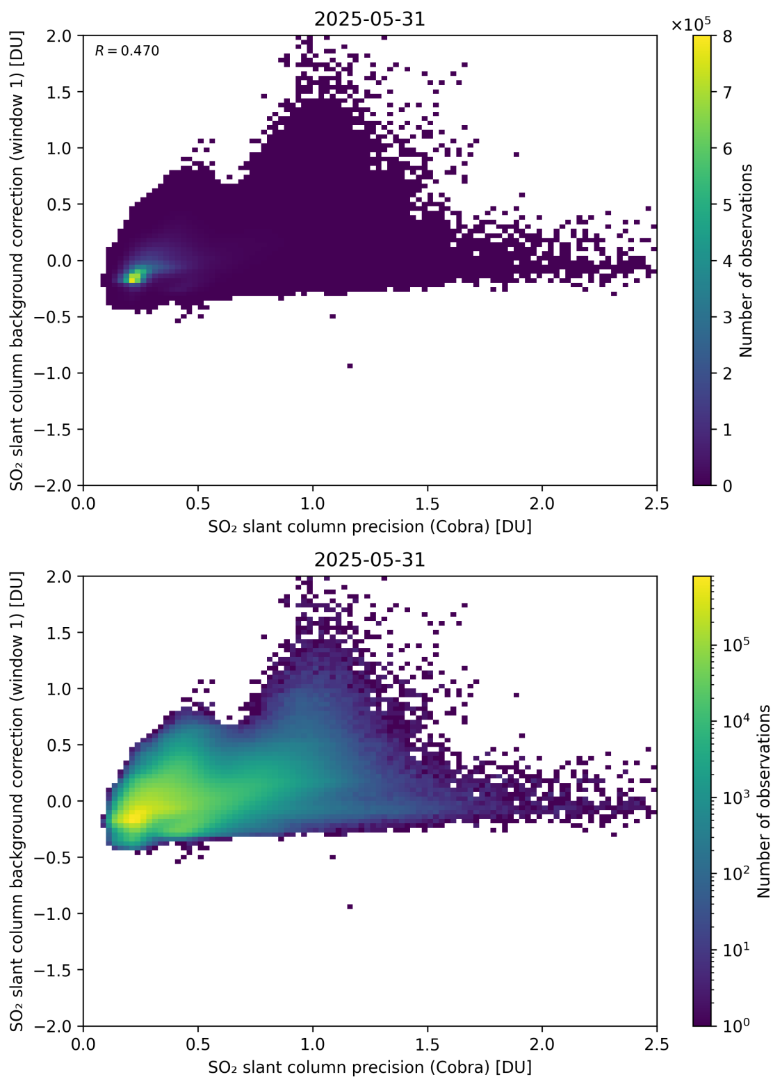
Figure 199: Scatter density plot of “SO 2 slant column precision (Cobra)” against “SO 2 slant column background correction (window 1)” for 2025-05-31 to 2025-06-01.
