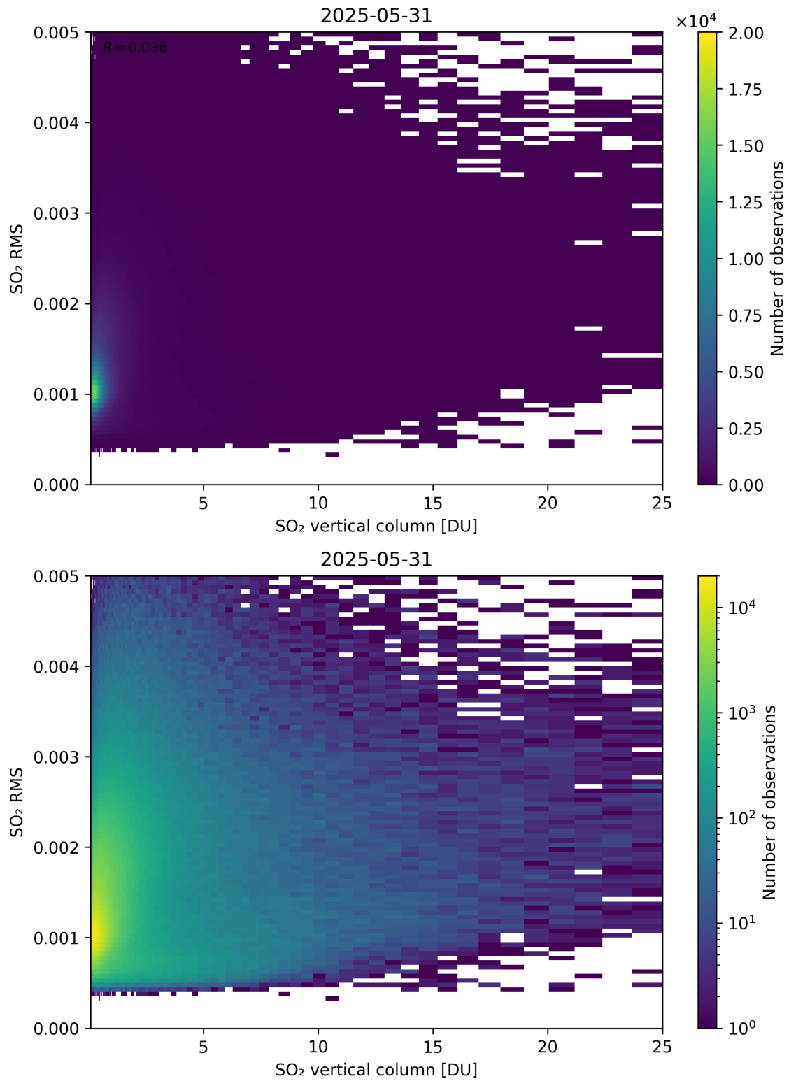
Figure 328: Scatter density plot of “SO 2 vertical column” against “SO 2 RMS” for 2025-05-31 to 2025-06-01.
