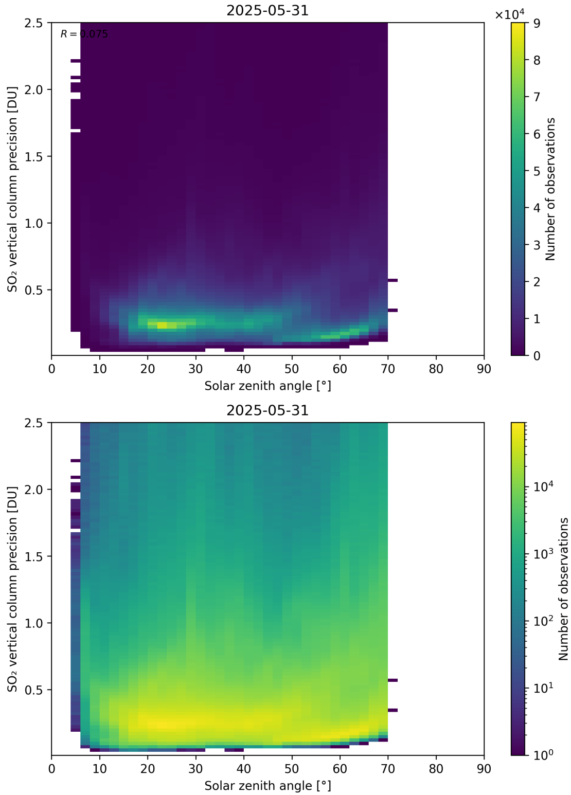
Figure 192: Scatter density plot of “Solar zenith angle” against “SO 2 vertical column precision” for 2025-05-31 to 2025-06-01.
