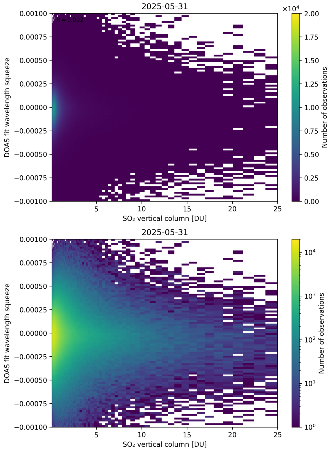
Figure 327: Scatter density plot of “SO 2 vertical column” against “DOAS fit wavelength squeeze” for 2025-05-31 to 2025-06-01.
