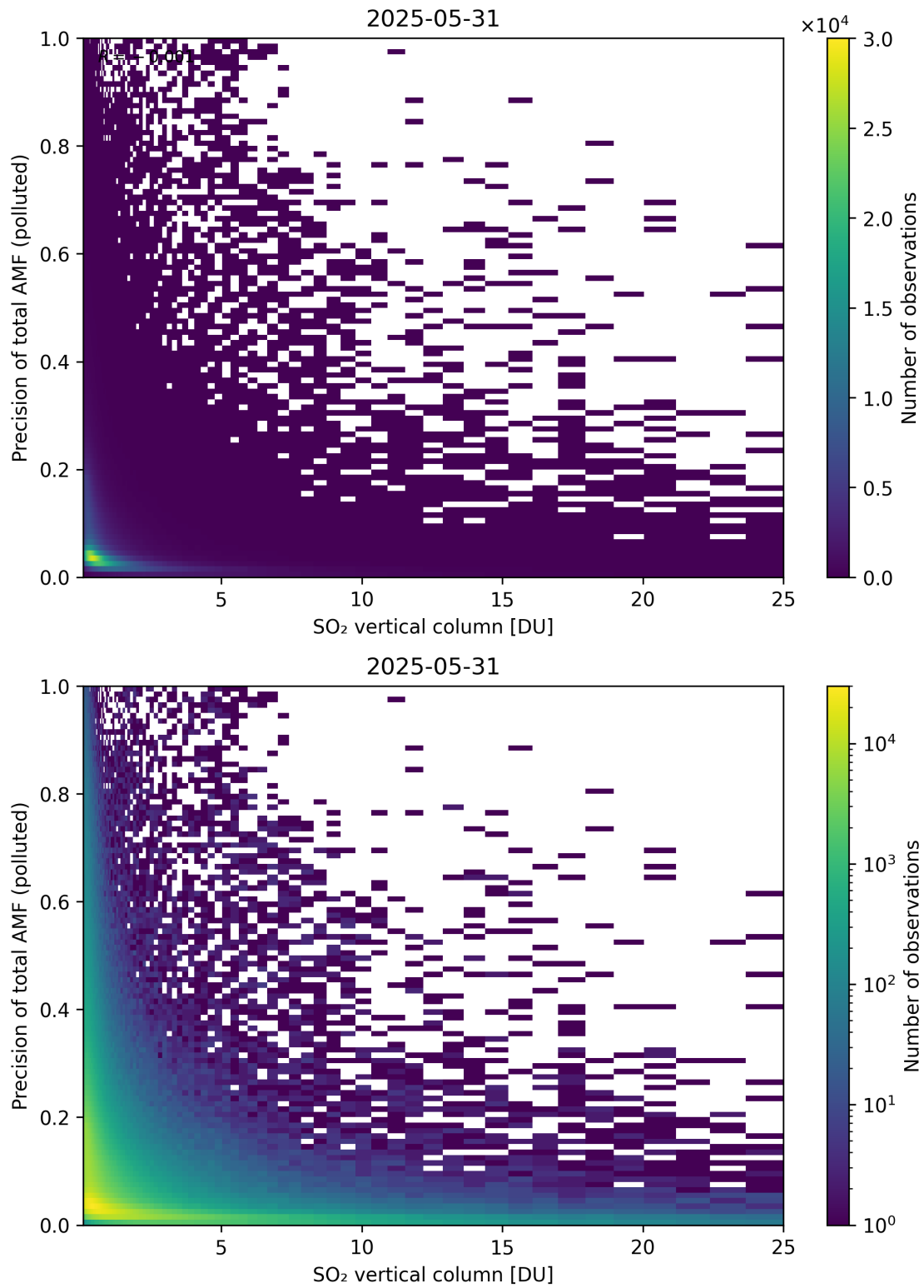
Figure 360: Scatter density plot of “SO 2 vertical column” against “Precision of total AMF (polluted)” for 2025-05-31 to 2025-06-01.
