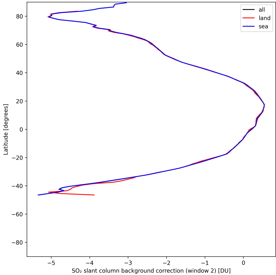
Figure 44: Zonal average of “SO 2 slant column background correction (window 2)” for 2025-05-31 to 2025-06-01.
