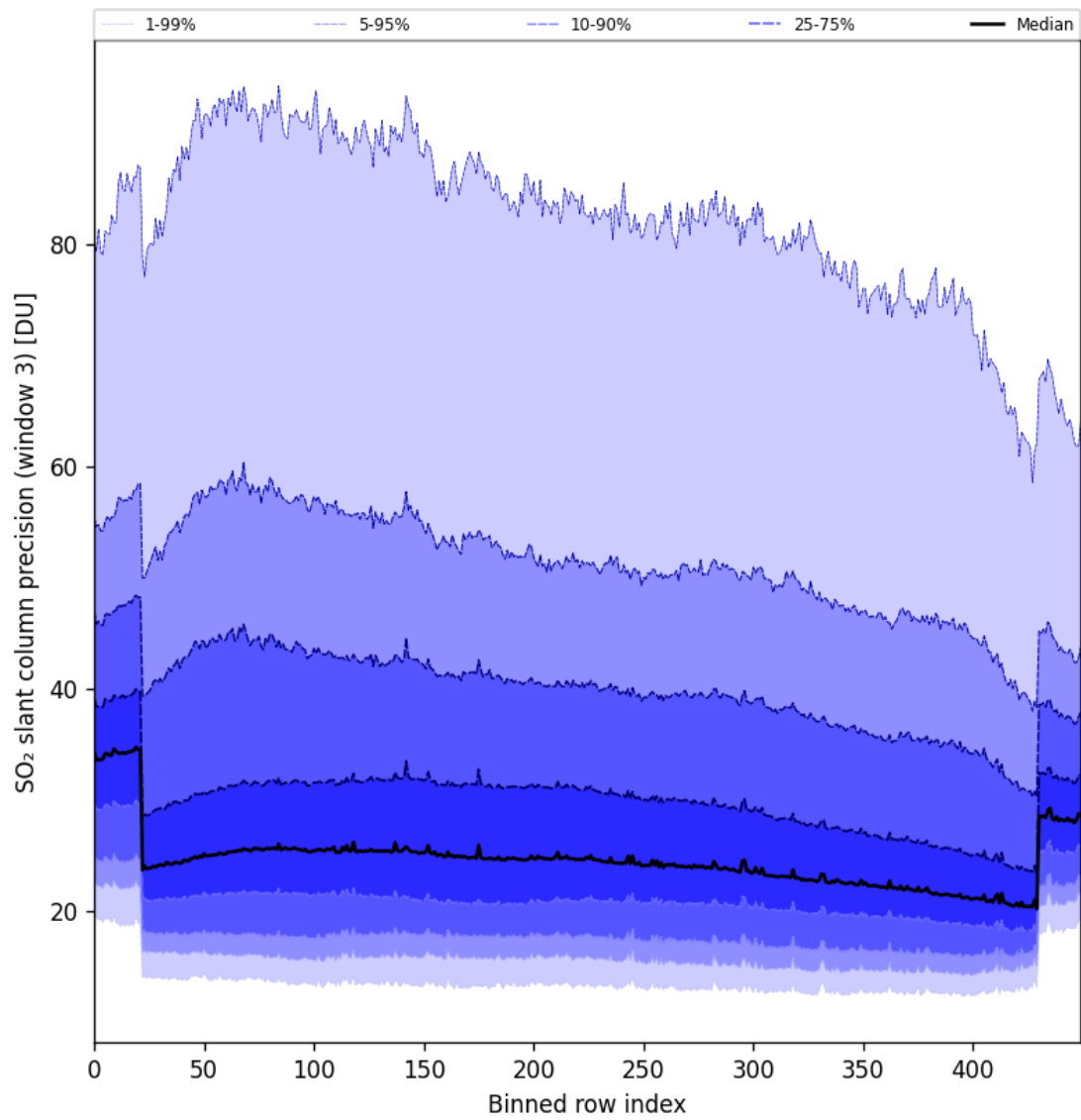
Figure 98: Along track statistics of “SO 2 slant column precision (window 3)” for 2025-05-31 to 2025-06-01
