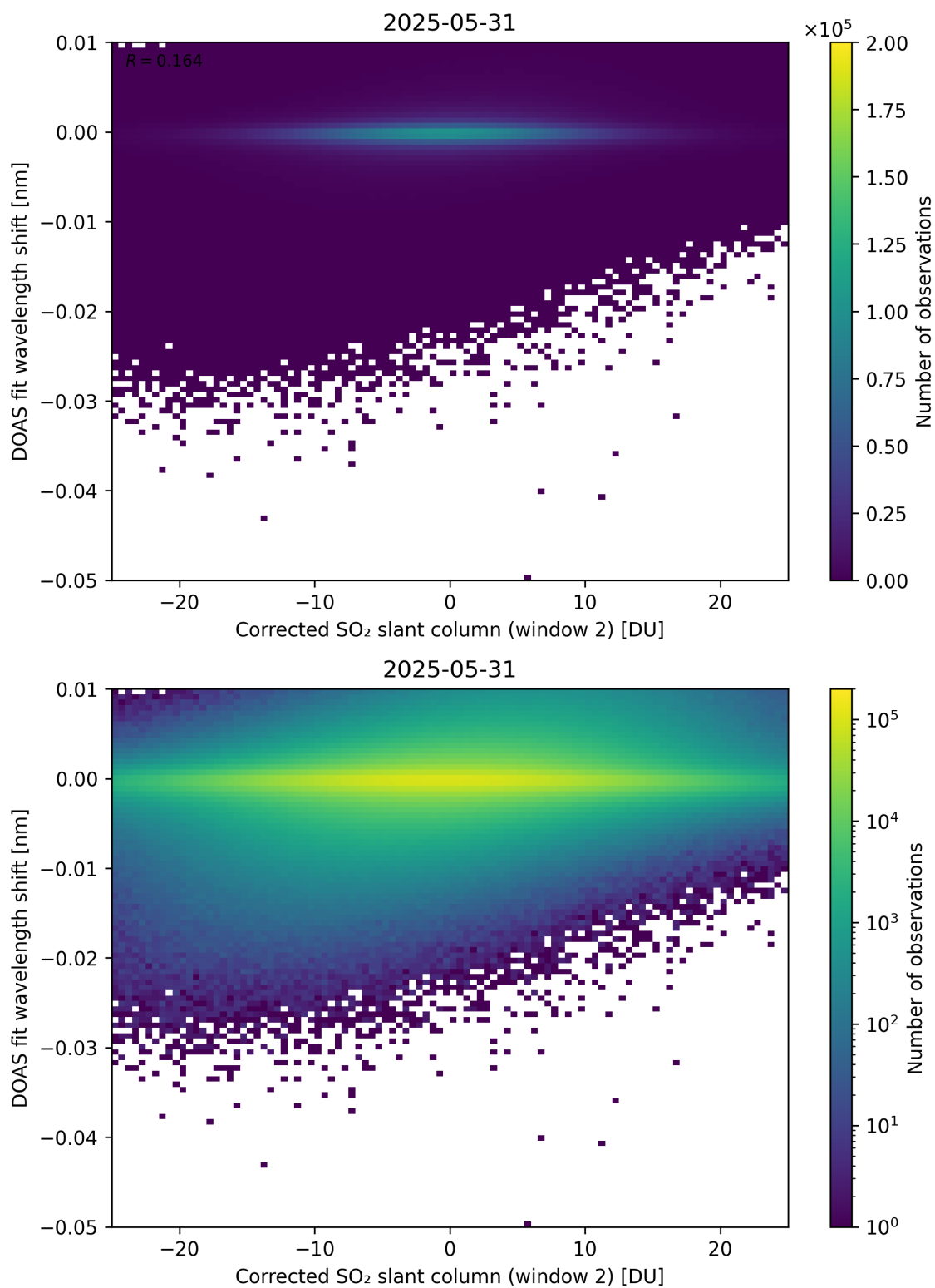
Figure 246: Scatter density plot of “Corrected SO 2 slant column (window 2)” against “DOAS fit wavelength shift” for 2025-05-31 to 2025-06-01.
