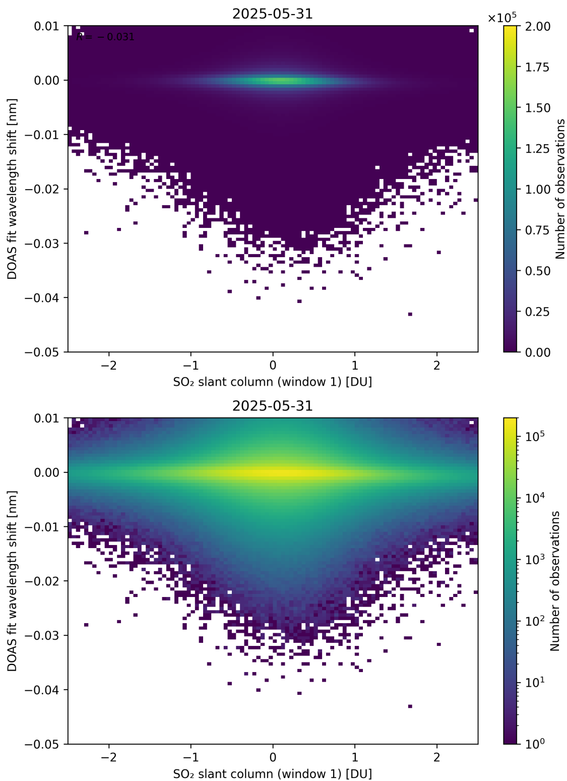
Figure 265: Scatter density plot of “SO 2 slant column (window 1)” against “DOAS fit wavelength shift” for 2025-05-31 to 2025-06-01.
