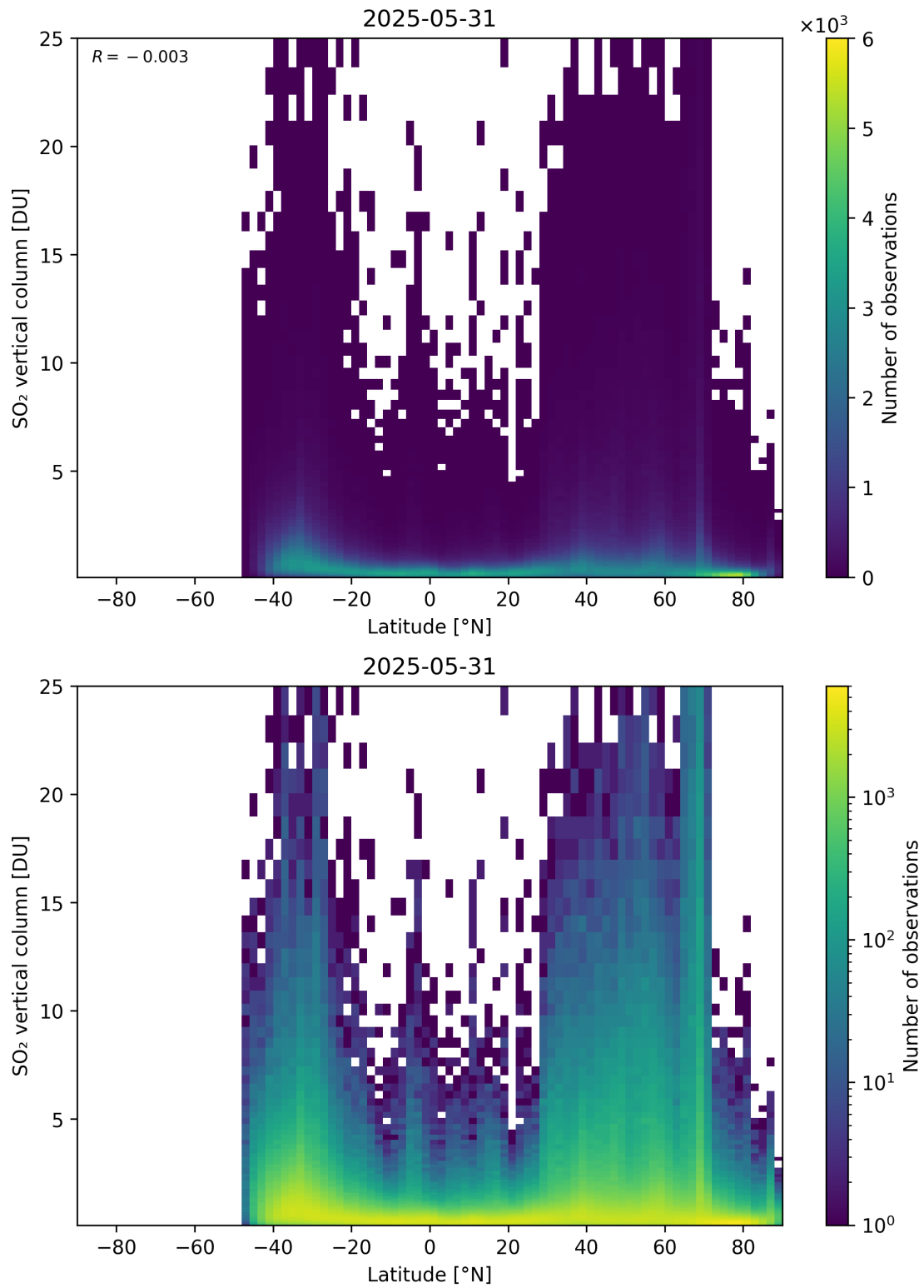
Figure 169: Scatter density plot of “Latitude” against “SO 2 vertical column” for 2025-05-31 to 2025-06-01.
