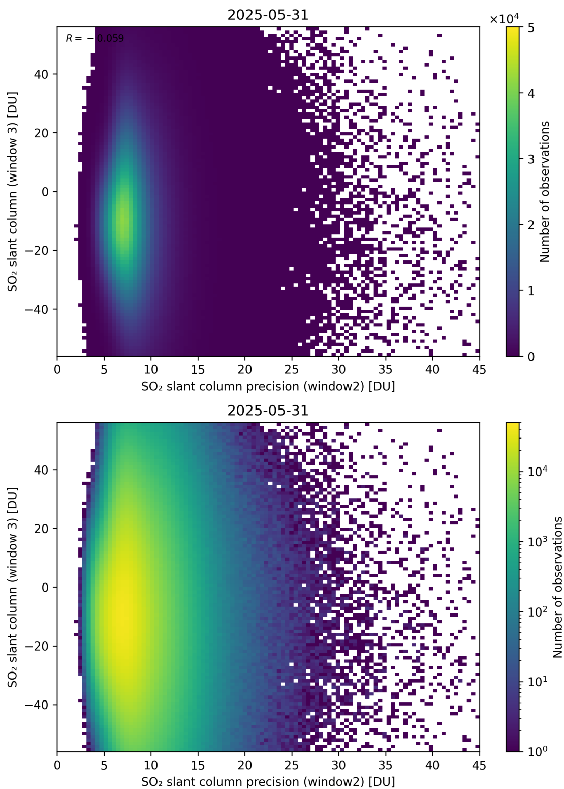
Figure 299: Scatter density plot of “SO 2 slant column precision (window2)” against “SO 2 slant column (window 3)” for 2025-05-31 to 2025-06-01.
