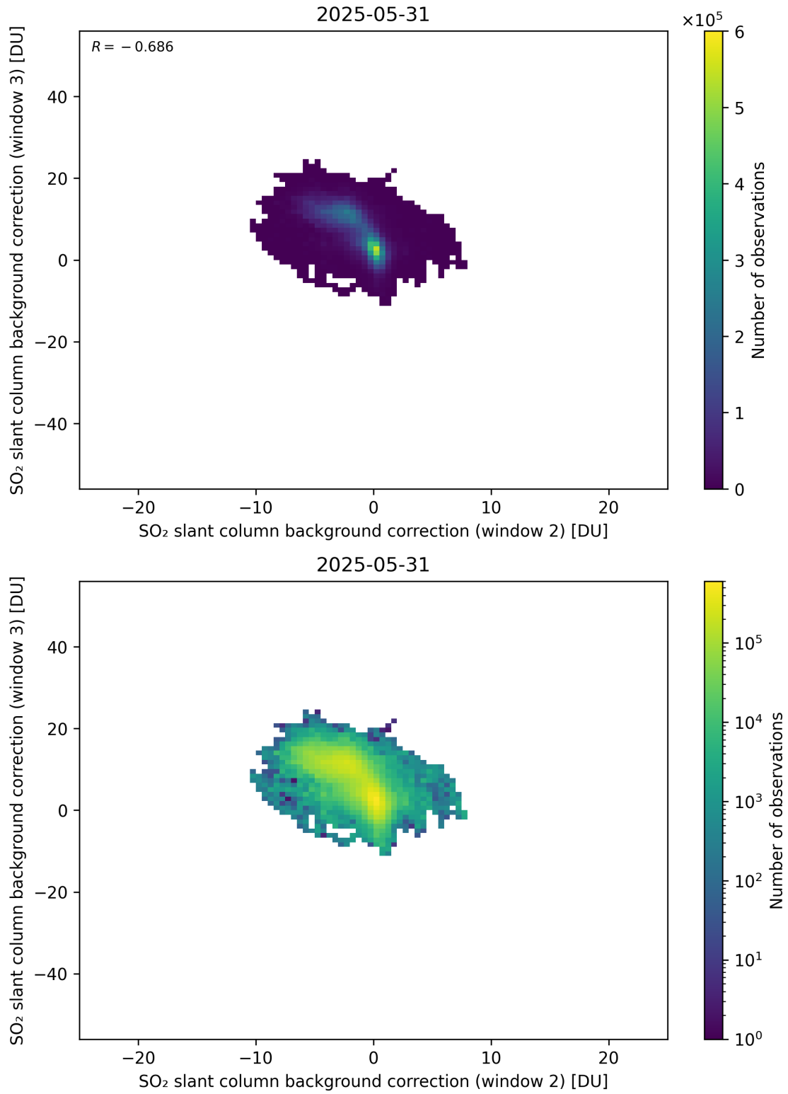
Figure 122: Scatter density plot of “SO 2 slant column background correction (window 2)” against “SO 2 slant column background correction (window 3)” for 2025-05-31 to 2025-06-01.
