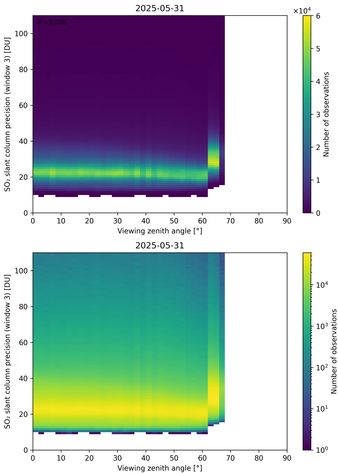
Figure 380: Scatter density plot of “Viewing zenith angle” against “SO 2 slant column precision (window 3)” for 2025-05-31 to 2025-06-01.
