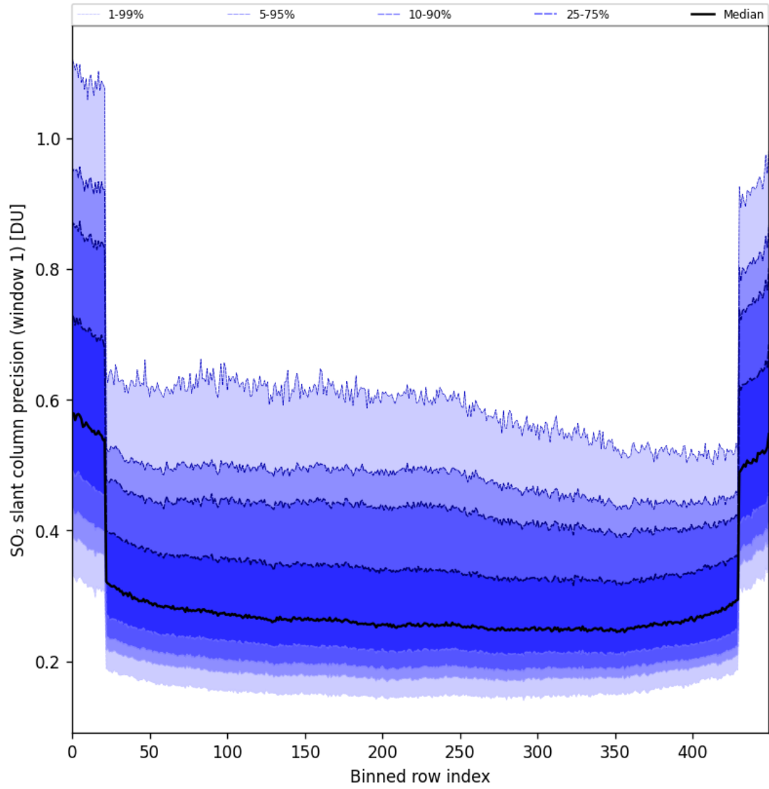
Figure 90: Along track statistics of “SO 2 slant column precision (window 1)” for 2025-05-31 to 2025-06-01
