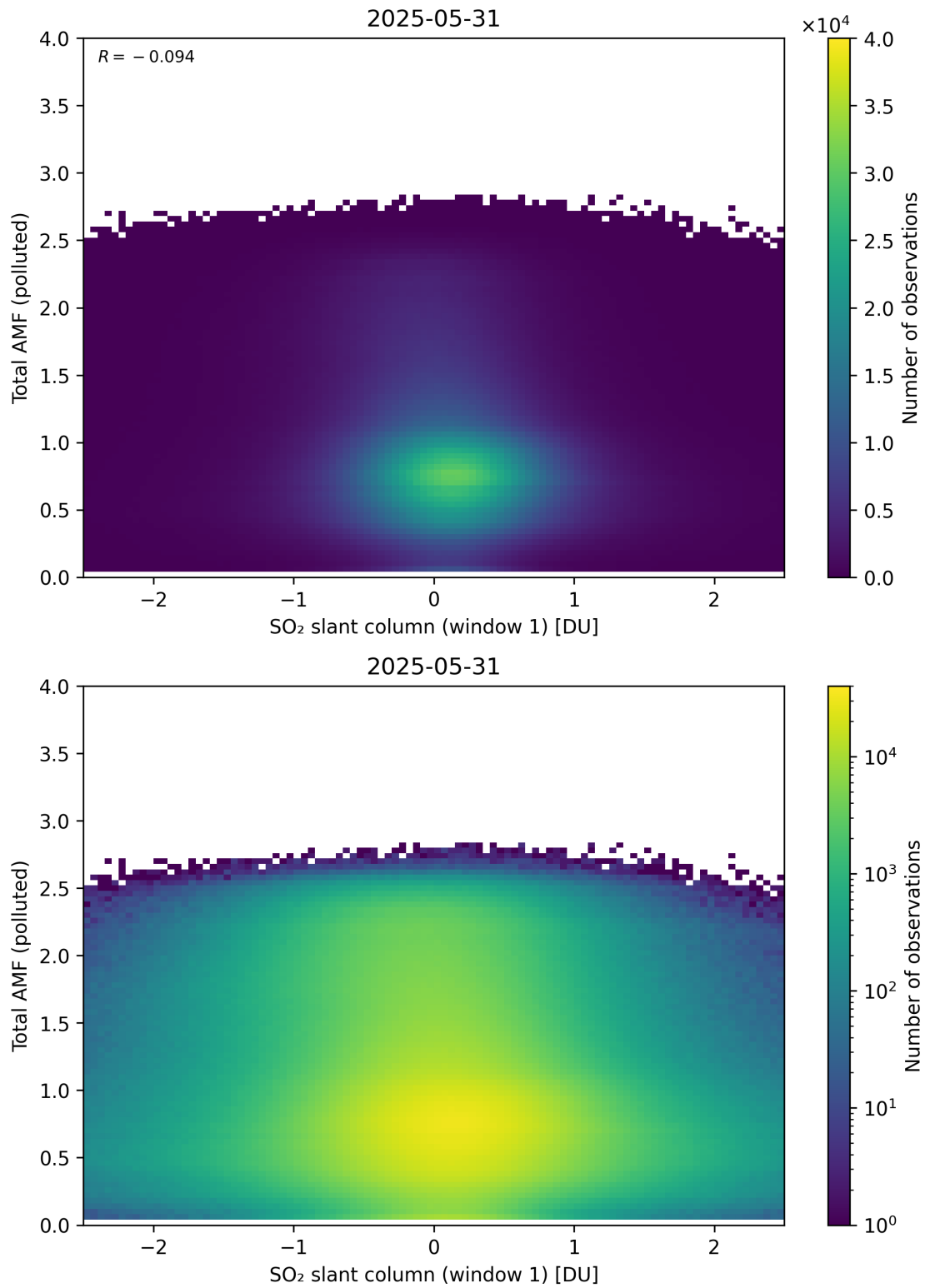
Figure 289: Scatter density plot of “SO 2 slant column (window 1)” against “Total AMF (polluted)” for 2025-05-31 to 2025-06-01.
