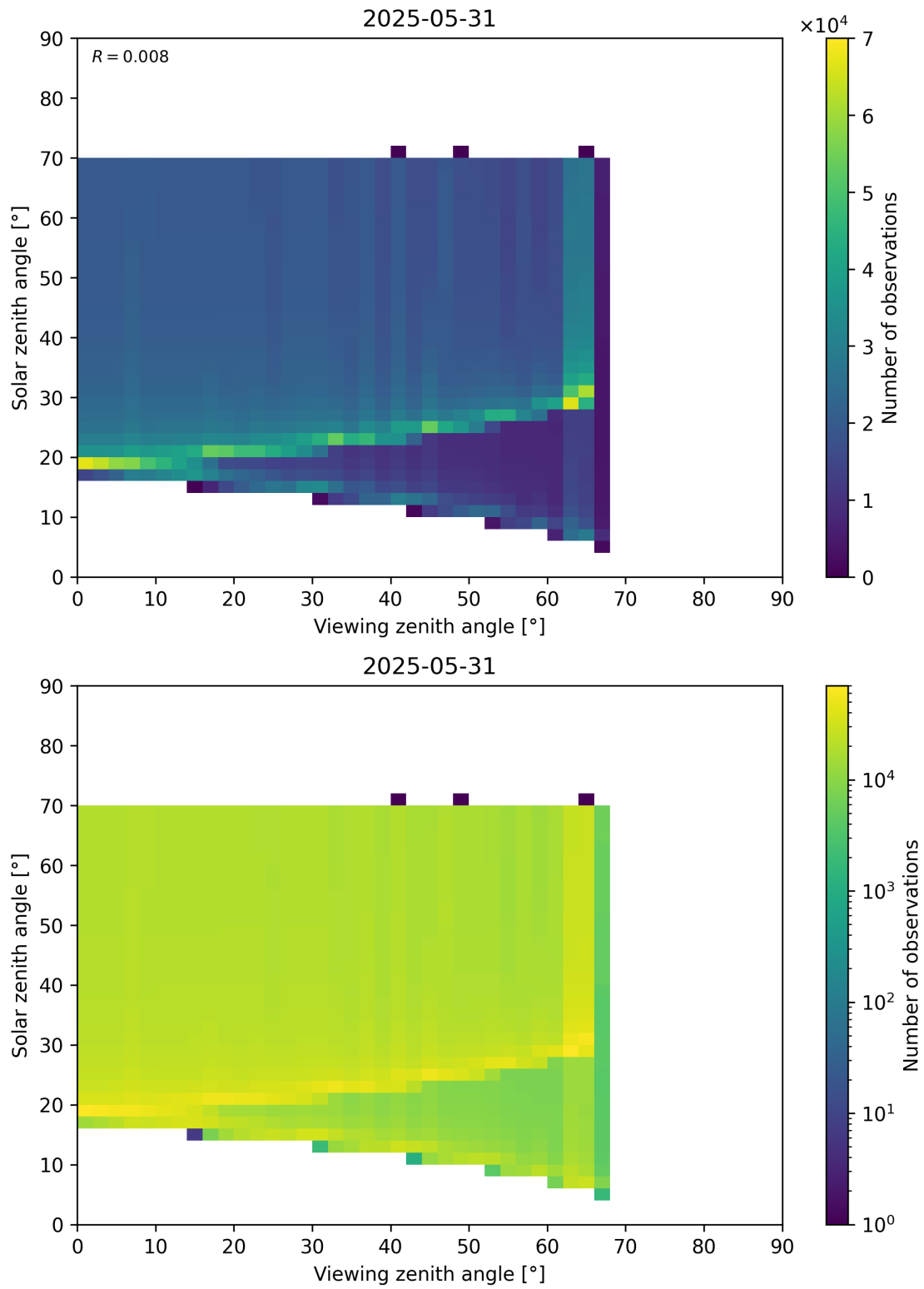
Figure 369: Scatter density plot of “Viewing zenith angle” against “Solar zenith angle” for 2025-05-31 to 2025-06-01.
