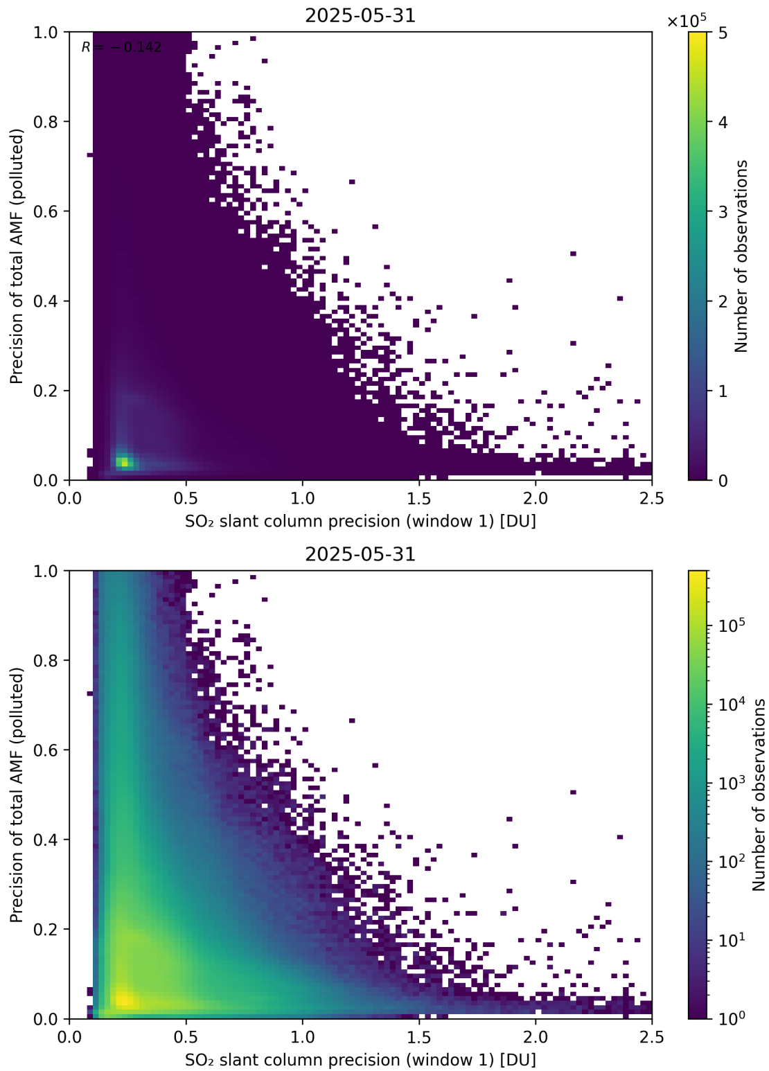
Figure 281: Scatter density plot of “SO 2 slant column precision (window 1)” against “Precision of total AMF (polluted)” for 2025-05-31 to 2025-06-01.
