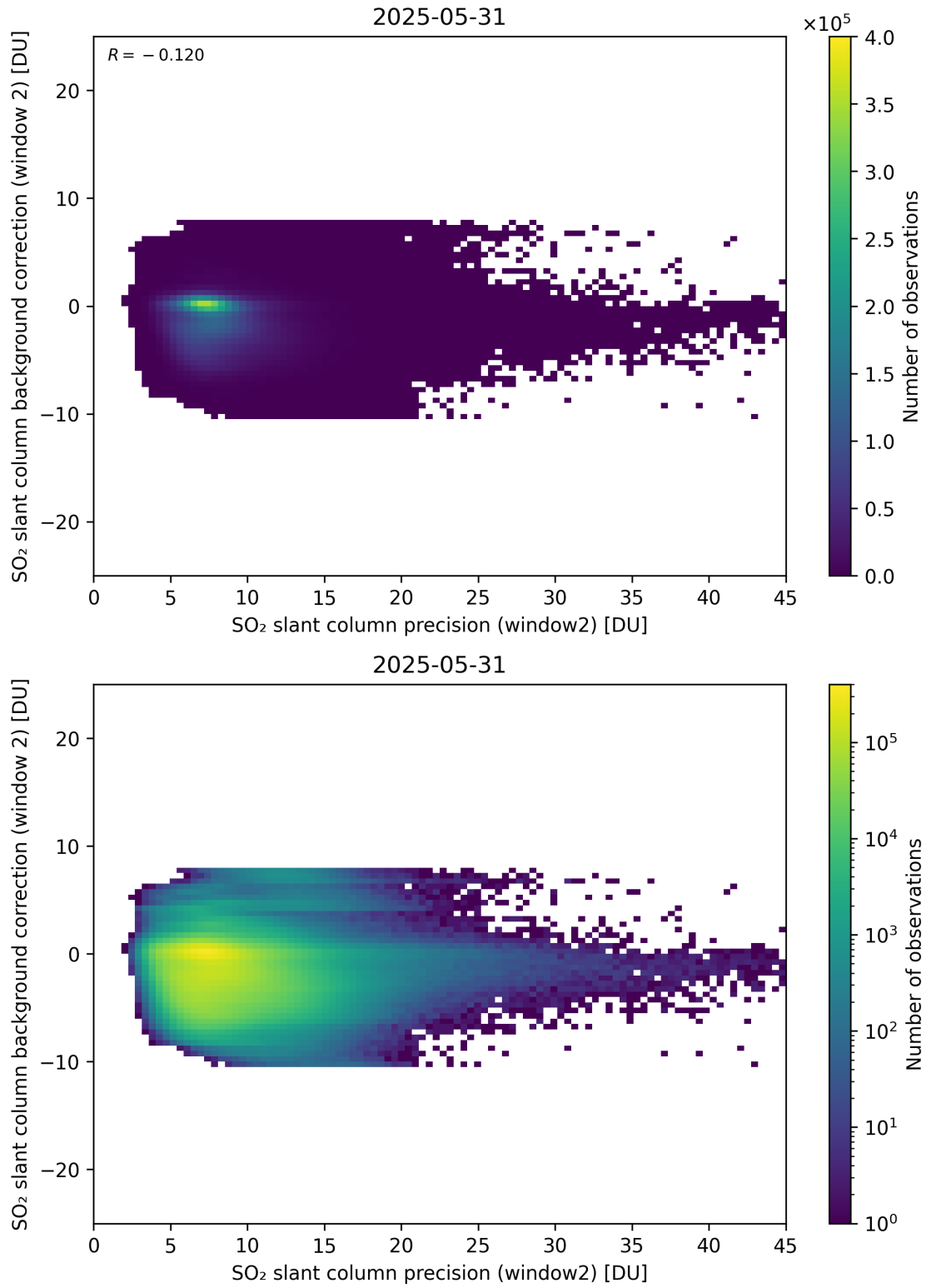
Figure 291: Scatter density plot of “SO 2 slant column precision (window2)” against “SO 2 slant column background correction (window 2)” for 2025-05-31 to 2025-06-01.
