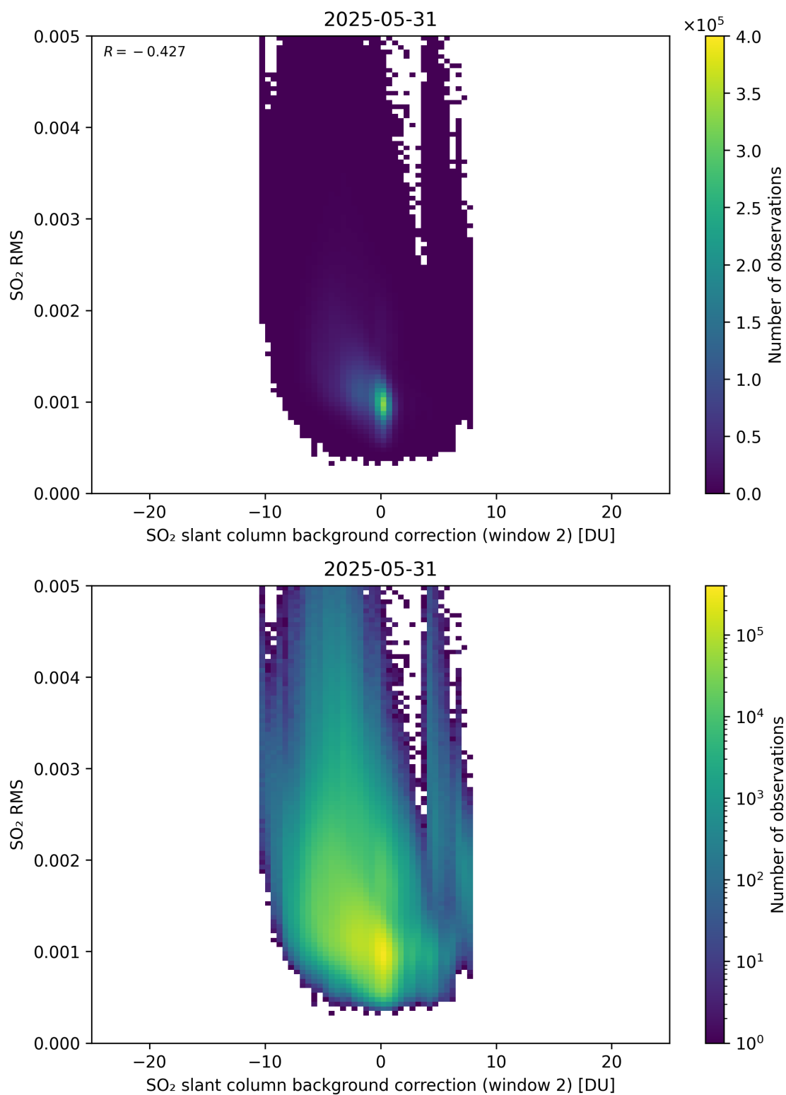
Figure 125: Scatter density plot of “SO 2 slant column background correction (window 2)” against “SO 2 RMS” for 2025-05-31 to 2025-06-01.
