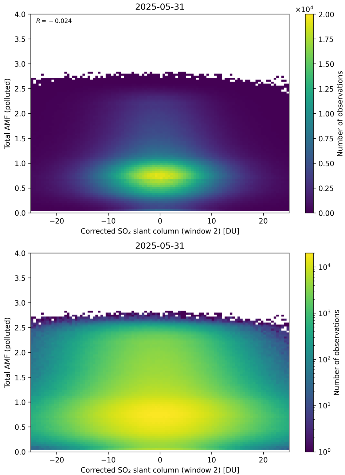
Figure 253: Scatter density plot of “Corrected SO 2 slant column (window 2)” against “Total AMF (polluted)” for 2025-05-31 to 2025-06-01.
