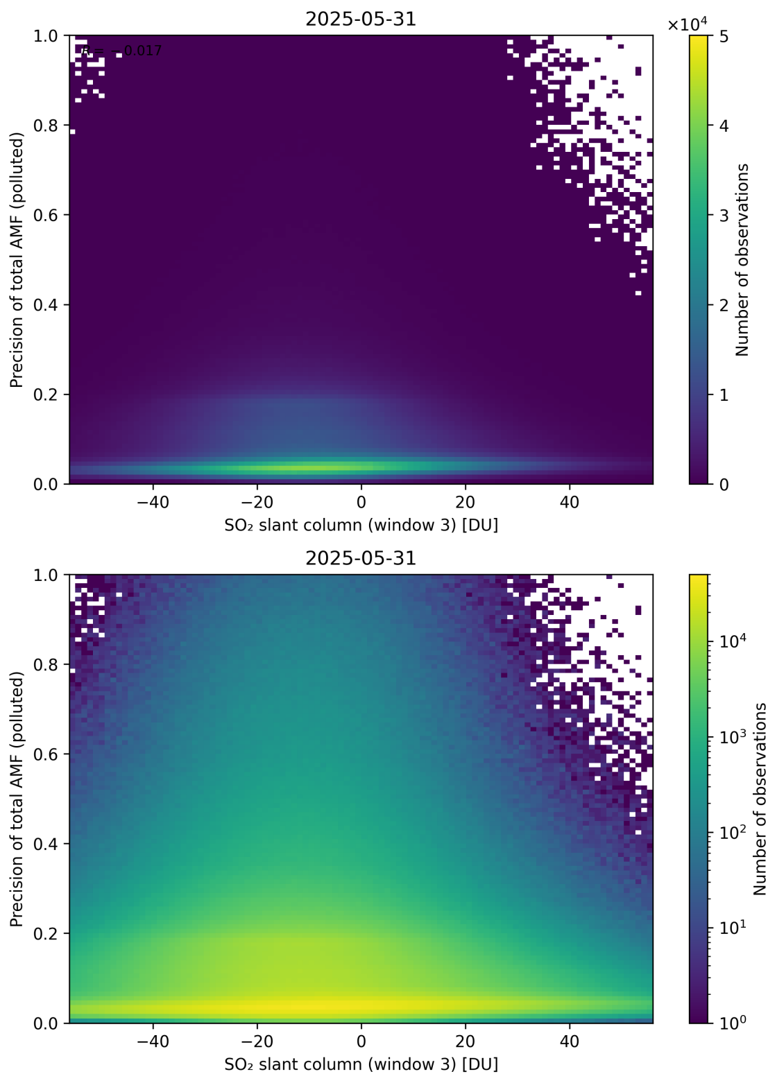
Figure 319: Scatter density plot of “SO 2 slant column (window 3)” against “Precision of total AMF (polluted)” for 2025-05-31 to 2025-06-01.
