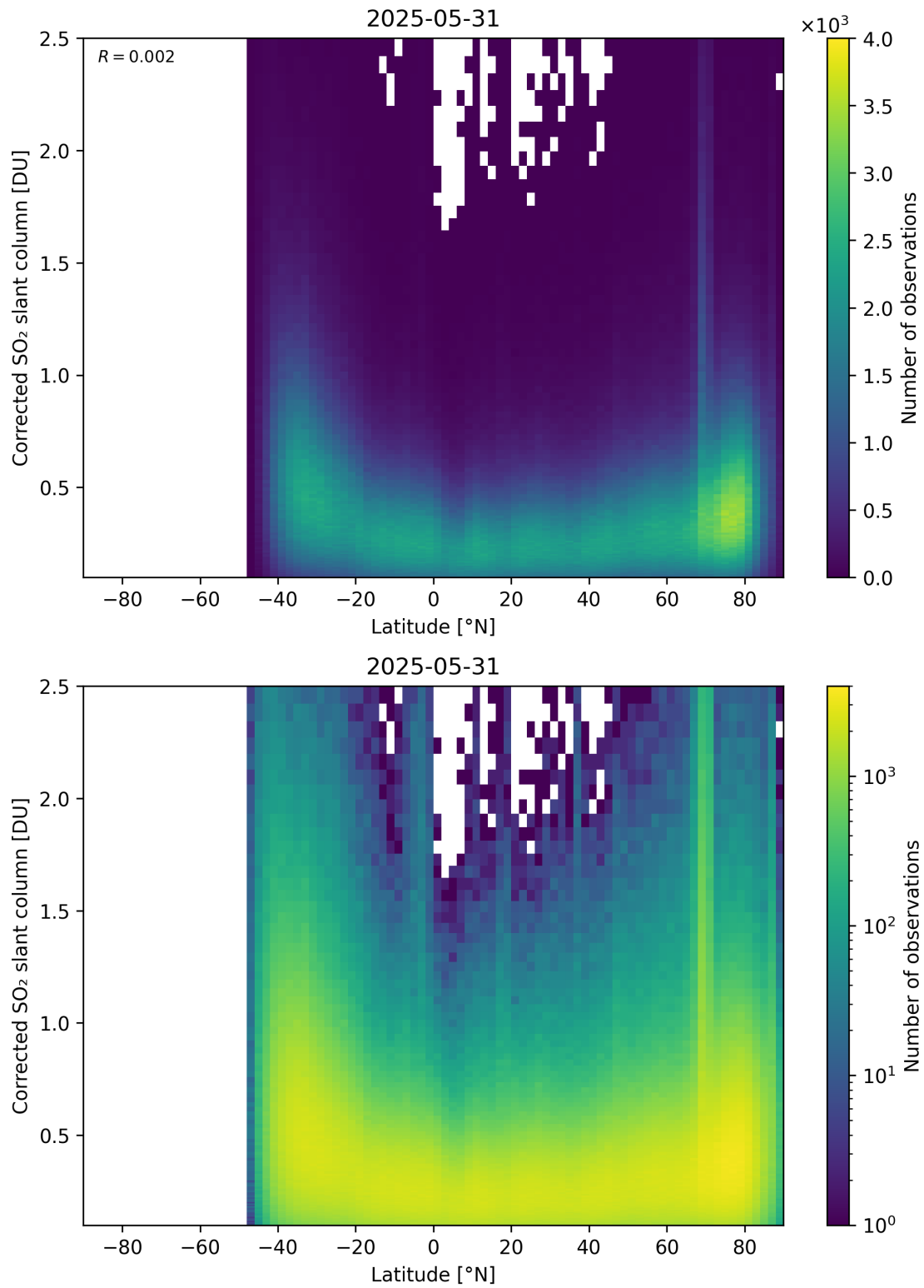
Figure 159: Scatter density plot of “Latitude” against “Corrected SO 2 slant column” for 2025-05-31 to 2025-06-01.
