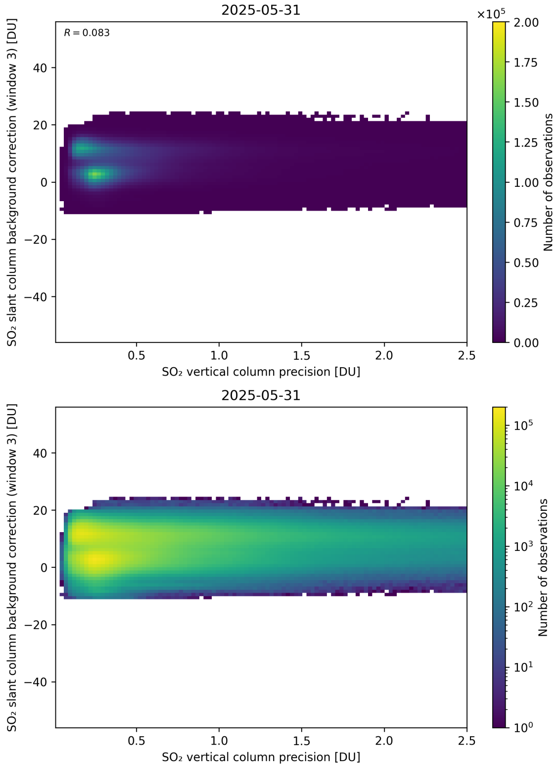
Figure 331: Scatter density plot of “SO 2 vertical column precision” against “SO 2 slant column background correction (window 3)” for 2025-05-31 to 2025-06-01.
