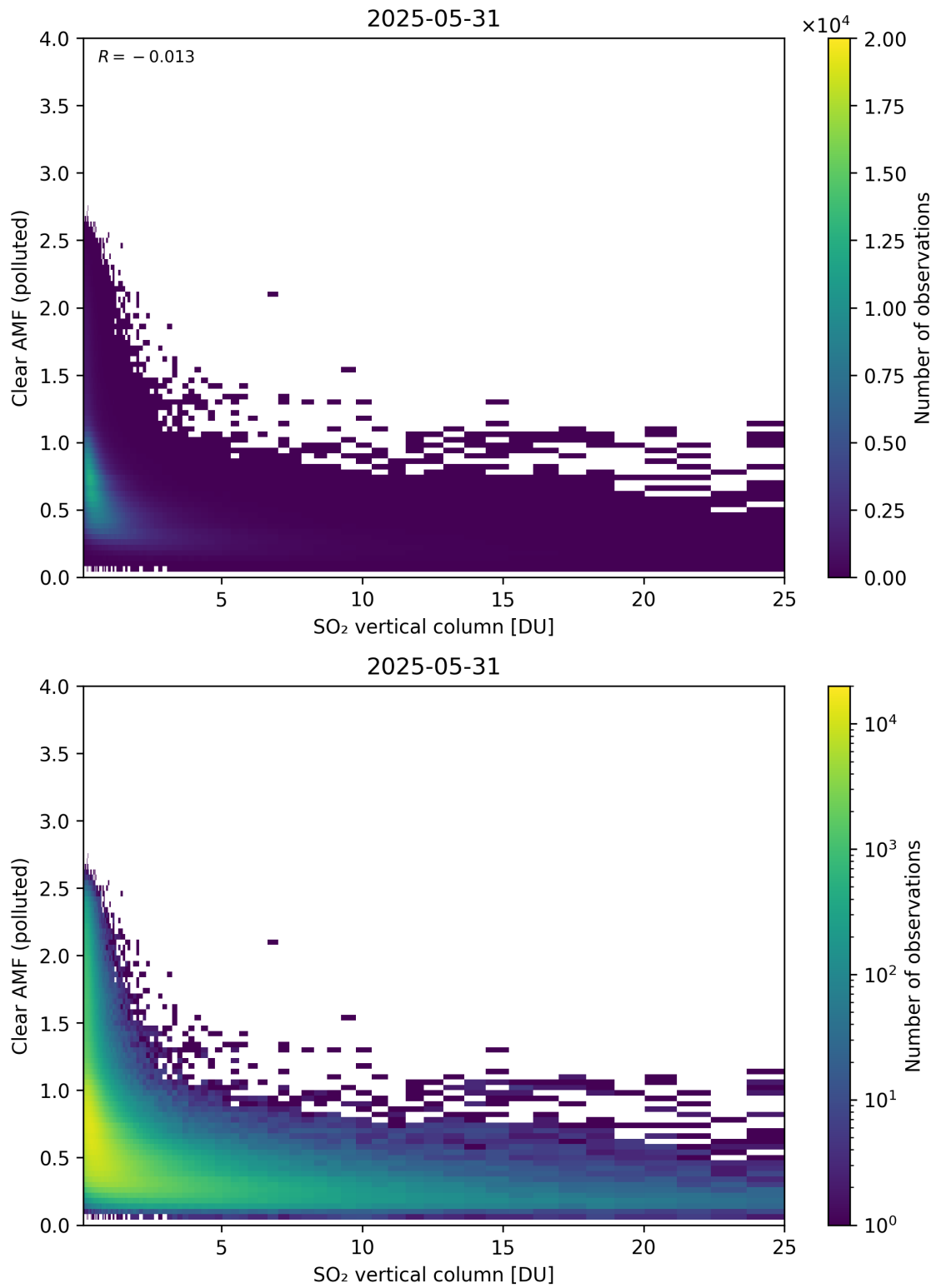
Figure 348: Scatter density plot of “SO 2 vertical column” against “Clear AMF (polluted)” for 2025-05-31 to 2025-06-01.
