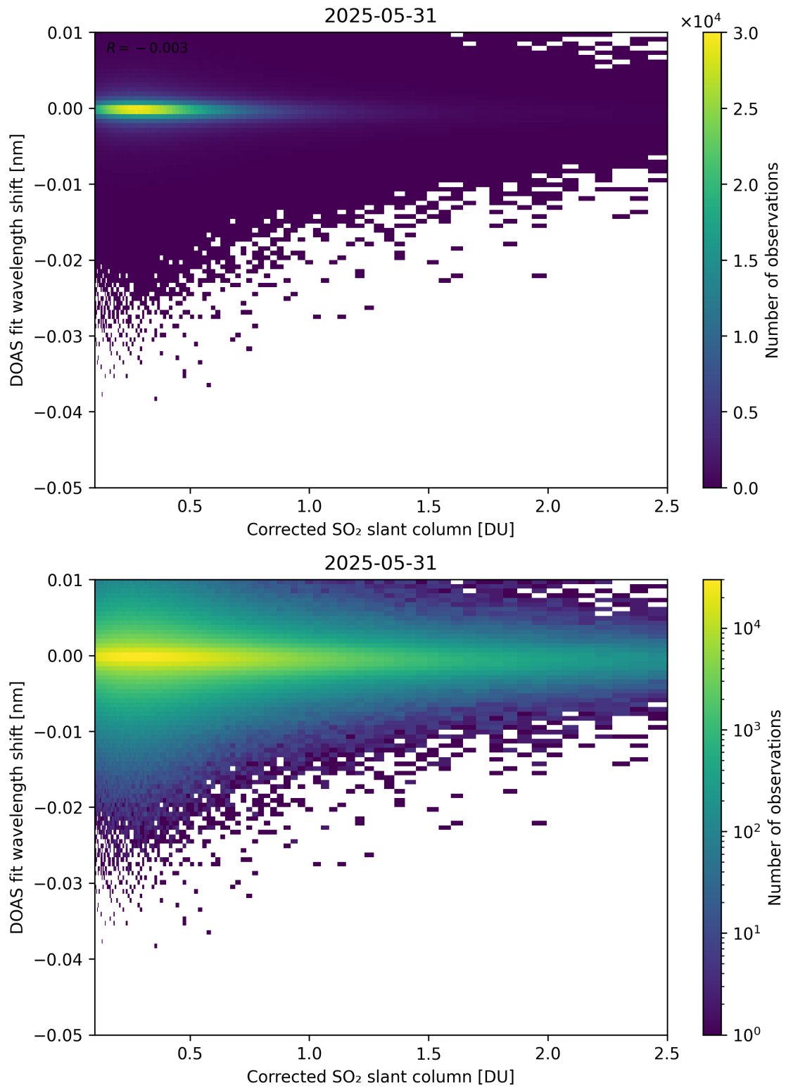
Figure 229: Scatter density plot of “Corrected SO 2 slant column” against “DOAS fit wavelength shift” for 2025-05-31 to 2025-06-01.
