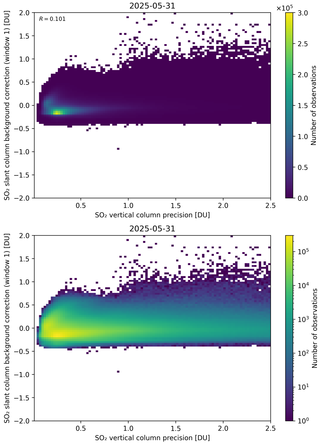
Figure 329: Scatter density plot of “SO 2 vertical column precision” against “SO 2 slant column background correction (window 1)” for 2025-05-31 to 2025-06-01.
