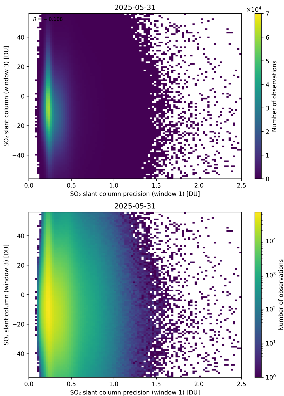
Figure 278: Scatter density plot of “SO 2 slant column precision (window 1)” against “SO 2 slant column (window 3)” for 2025-05-31 to 2025-06-01.
