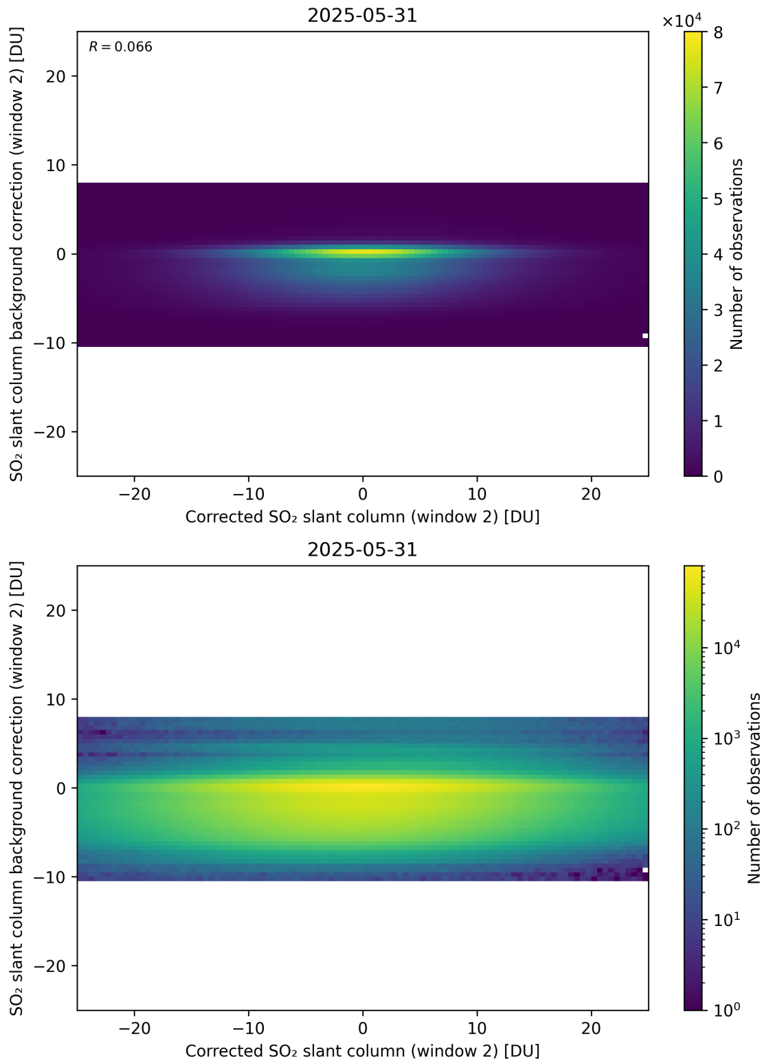
Figure 244: Scatter density plot of “Corrected SO 2 slant column (window 2)” against “SO 2 slant column background correction (window 2)” for 2025-05-31 to 2025-06-01.
