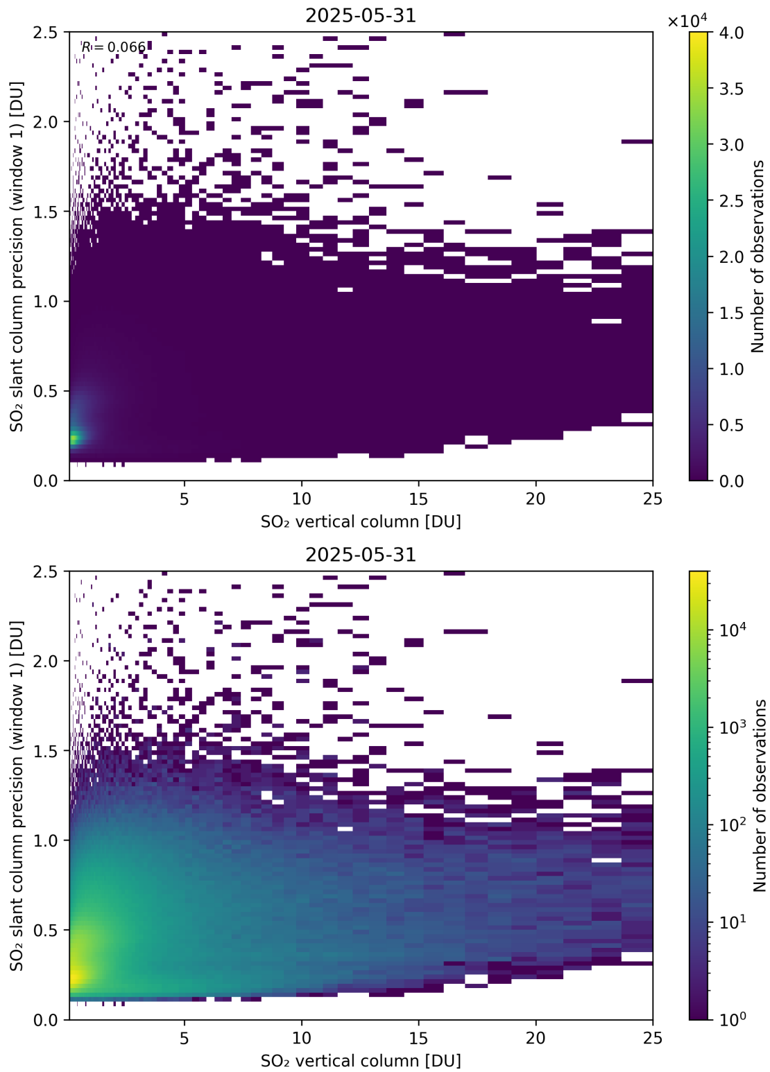
Figure 355: Scatter density plot of “SO 2 vertical column” against “SO 2 slant column precision (window 1)” for 2025-05-31 to 2025-06-01.
