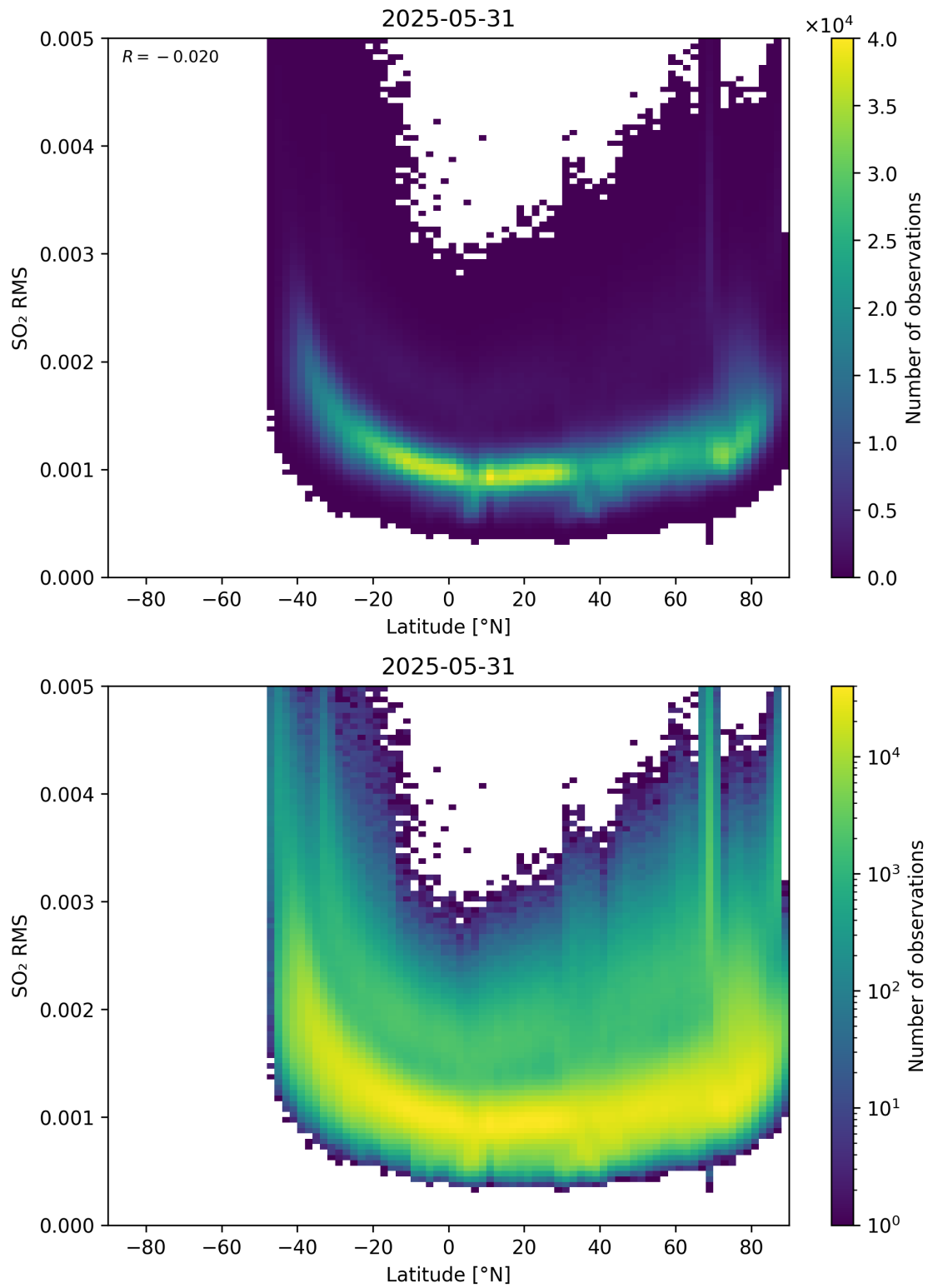
Figure 155: Scatter density plot of “Latitude” against “SO 2 RMS” for 2025-05-31 to 2025-06-01.
