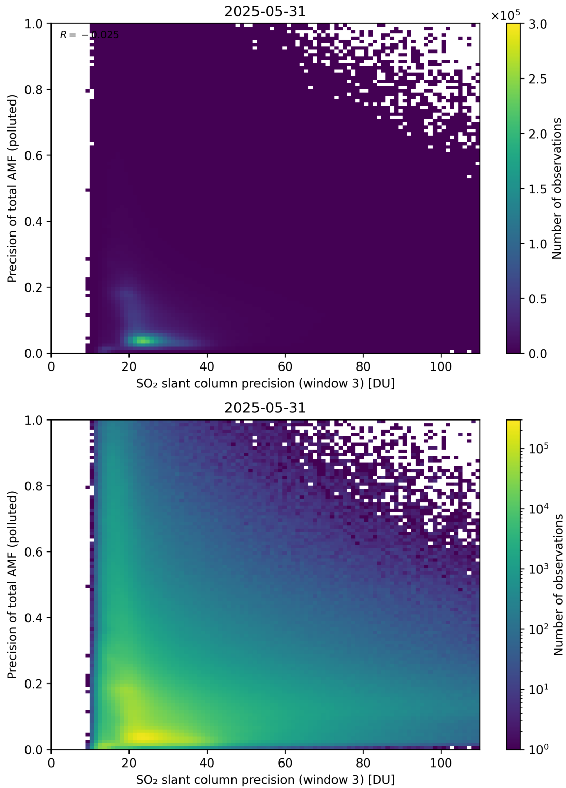
Figure 314: Scatter density plot of “SO 2 slant column precision (window 3)” against “Precision of total AMF (polluted)” for 2025-05-31 to 2025-06-01.
