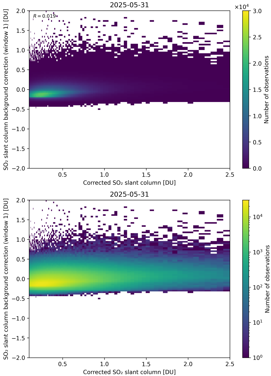
Figure 226: Scatter density plot of “Corrected SO 2 slant column” against “SO 2 slant column background correction (window 1)” for 2025-05-31 to 2025-06-01.
