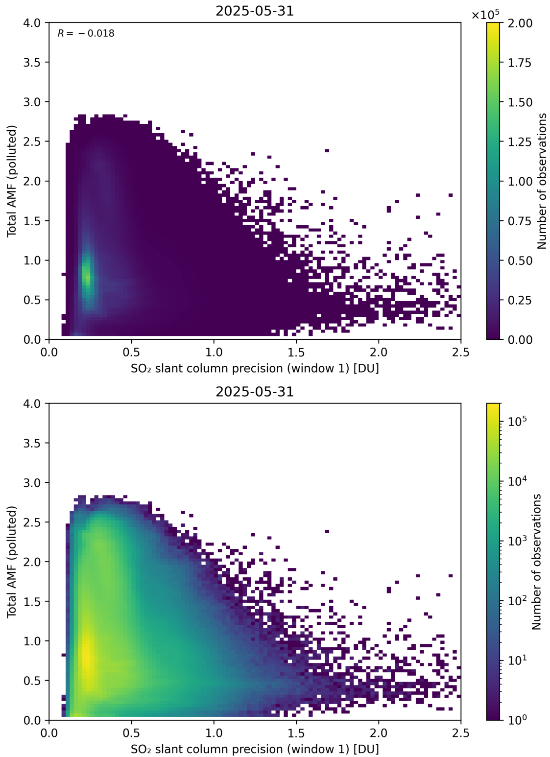
Figure 280: Scatter density plot of “SO 2 slant column precision (window 1)” against “Total AMF (polluted)” for 2025-05-31 to 2025-06-01.
