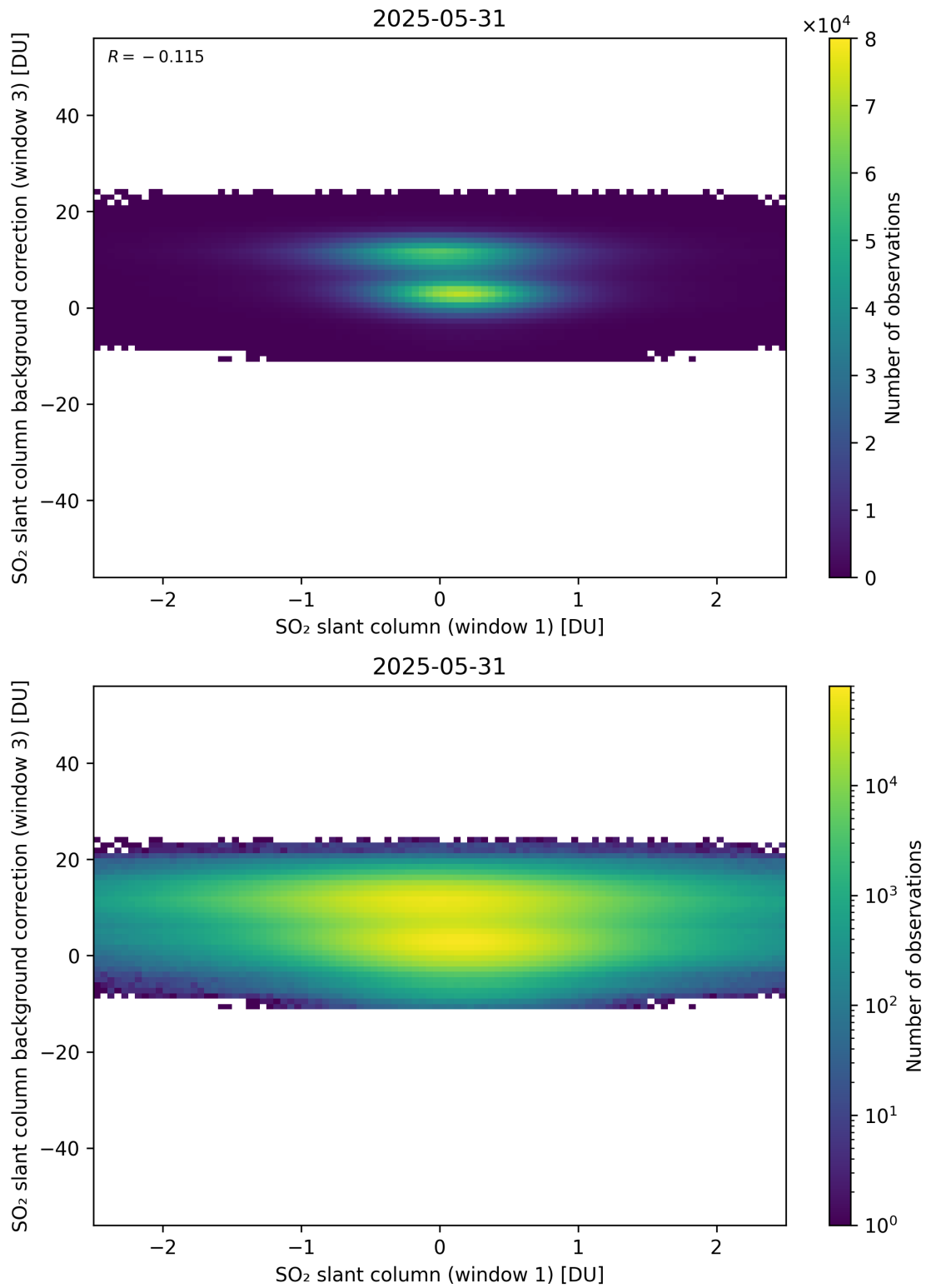
Figure 264: Scatter density plot of “SO 2 slant column (window 1)” against “SO 2 slant column background correction (window 3)” for 2025-05-31 to 2025-06-01.
