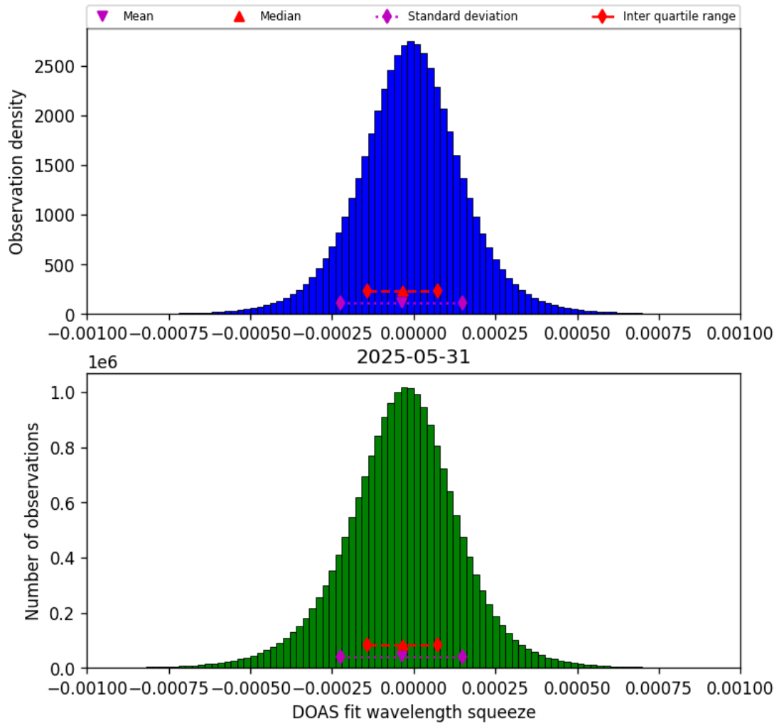
Figure 77: Histogram of “DOAS fit wavelength squeeze” for 2025-05-31 to 2025-06-01
