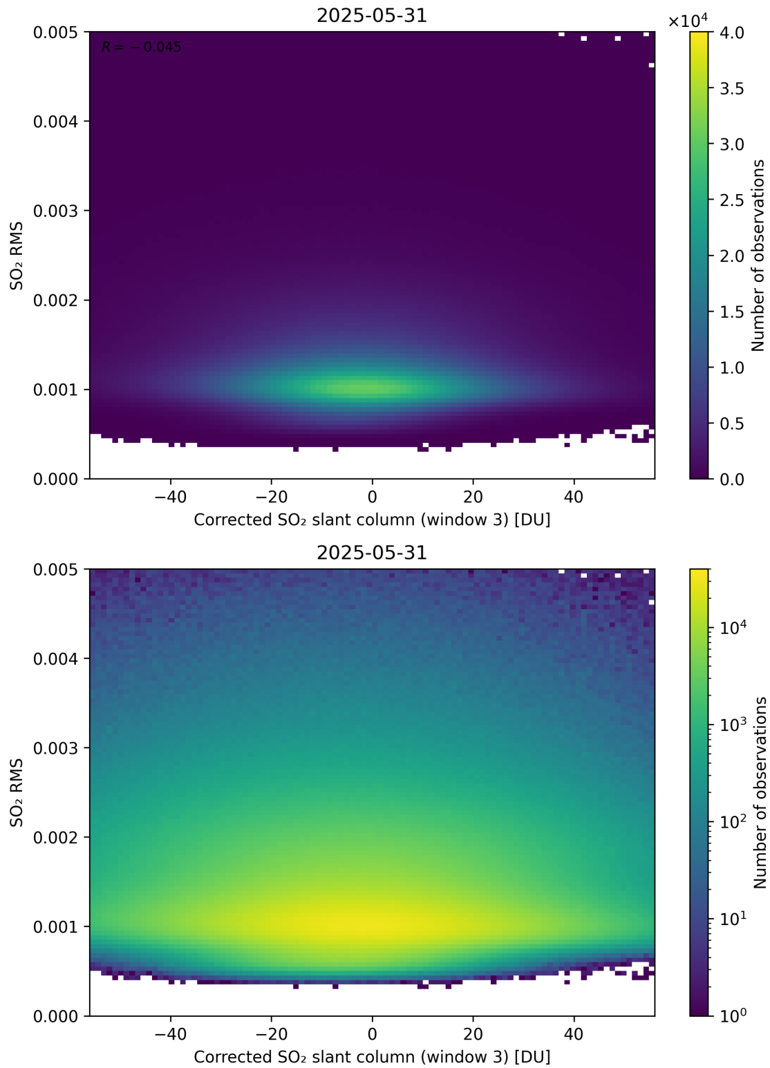
Figure 258: Scatter density plot of “Corrected SO 2 slant column (window 3)” against “SO 2 RMS” for 2025-05-31 to 2025-06-01.
