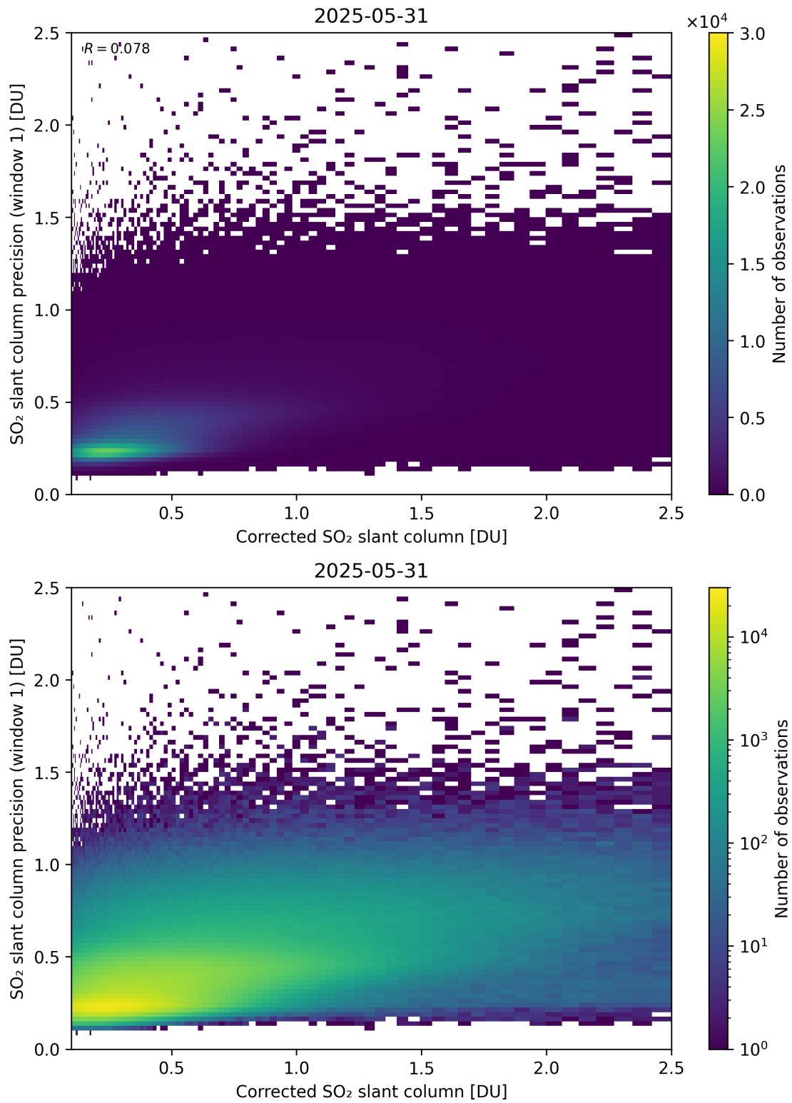
Figure 238: Scatter density plot of “Corrected SO 2 slant column” against “SO 2 slant column precision (window 1)” for 2025-05-31 to 2025-06-01.
