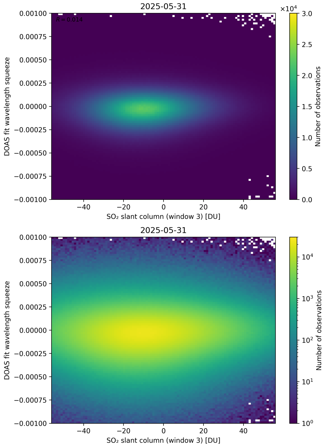
Figure 305: Scatter density plot of “SO 2 slant column (window 3)” against “DOAS fit wavelength squeeze” for 2025-05-31 to 2025-06-01.
