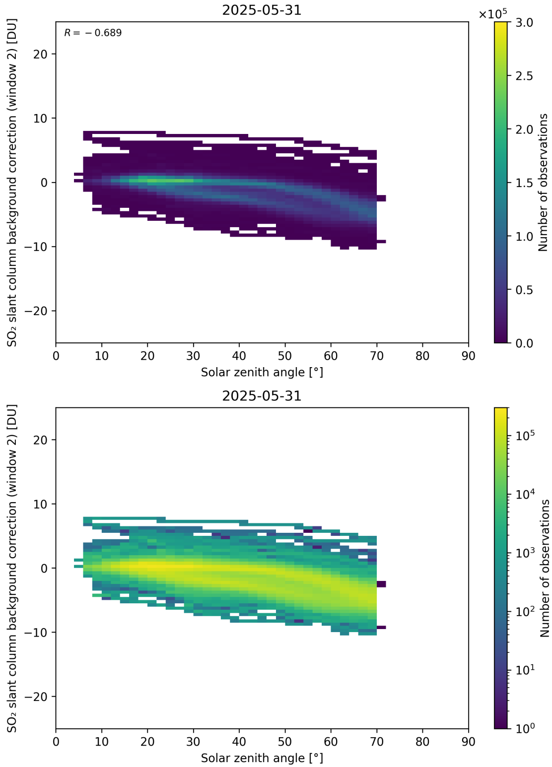
Figure 172: Scatter density plot of “Solar zenith angle” against “SO 2 slant column background correction (window 2)” for 2025-05-31 to 2025-06-01.
