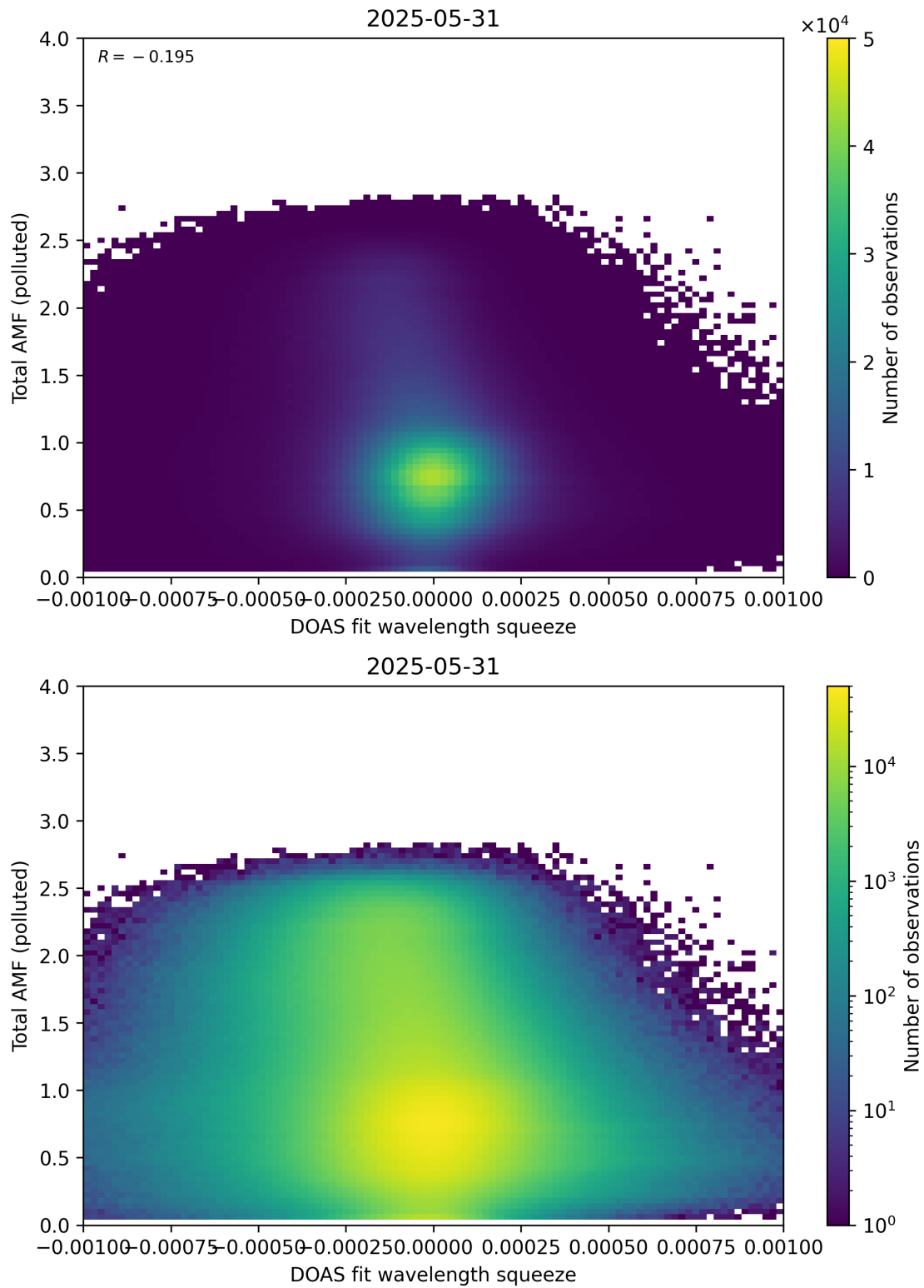
Figure 145: Scatter density plot of “DOAS fit wavelength squeeze” against “Total AMF (polluted)” for 2025-05-31 to 2025-06-01.
