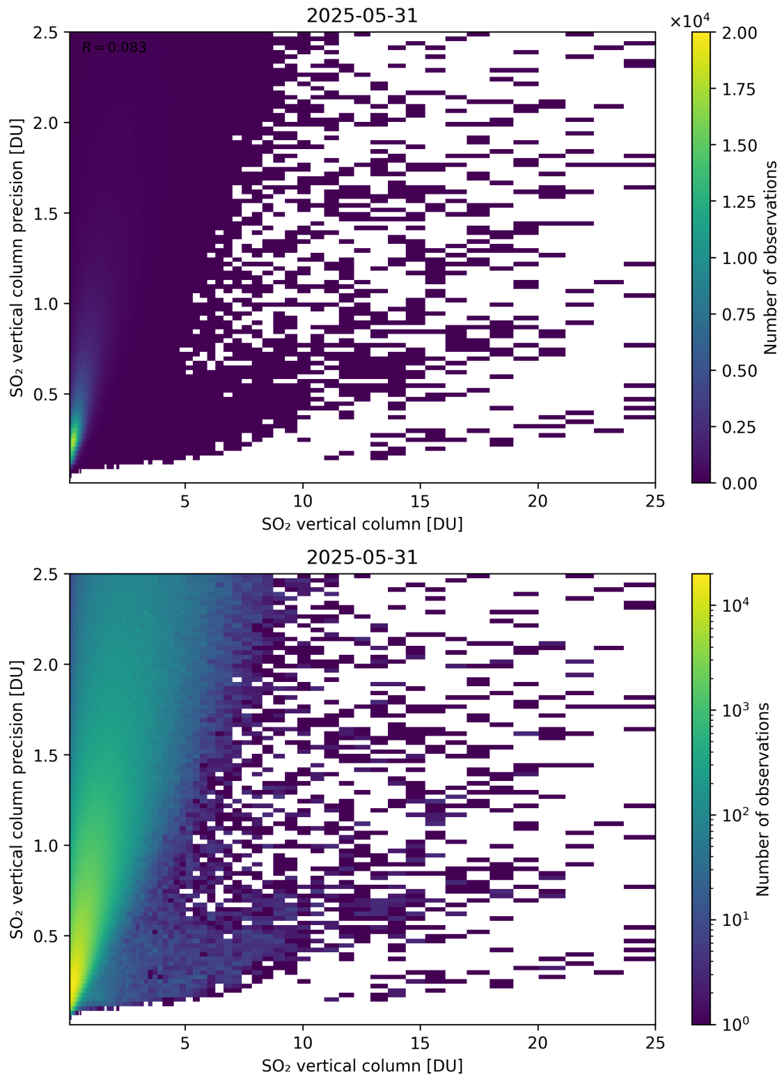
Figure 361: Scatter density plot of “SO 2 vertical column” against “SO 2 vertical column precision” for 2025-05-31 to 2025-06-01.
