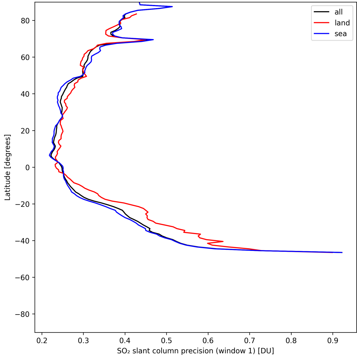
Figure 38: Zonal average of “SO 2 slant column precision (window 1)” for 2025-05-31 to 2025-06-01.
