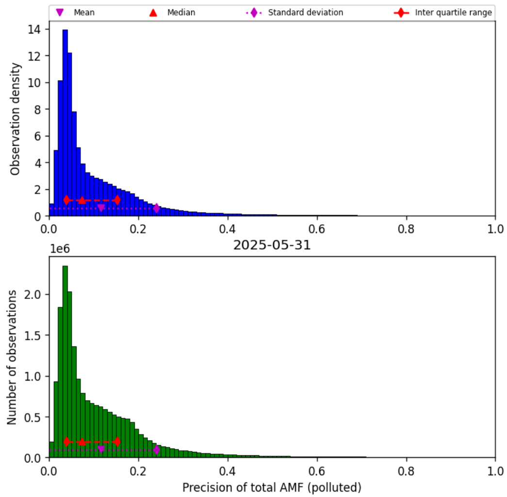
Figure 80: Histogram of “Precision of total AMF (polluted)” for 2025-05-31 to 2025-06-01
