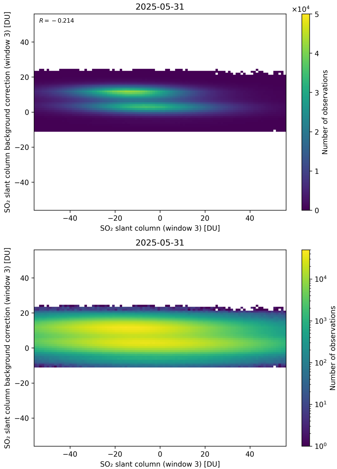
Figure 303: Scatter density plot of “SO 2 slant column (window 3)” against “SO 2 slant column background correction (window 3)” for 2025-05-31 to 2025-06-01.
