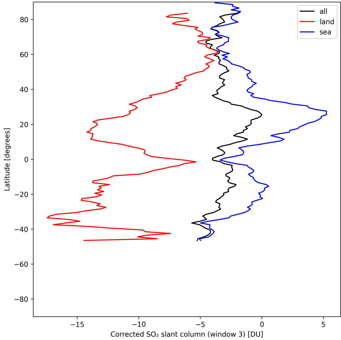
Figure 47: Zonal average of “Corrected SO 2 slant column (window 3)” for 2025-05-31 to 2025-06-01.
