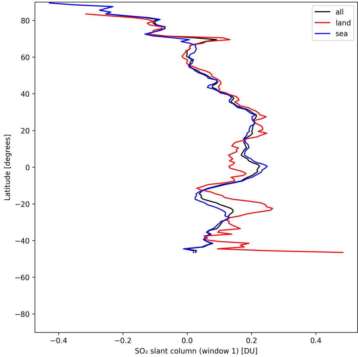
Figure 37: Zonal average of “SO 2 slant column (window 1)” for 2025-05-31 to 2025-06-01.
