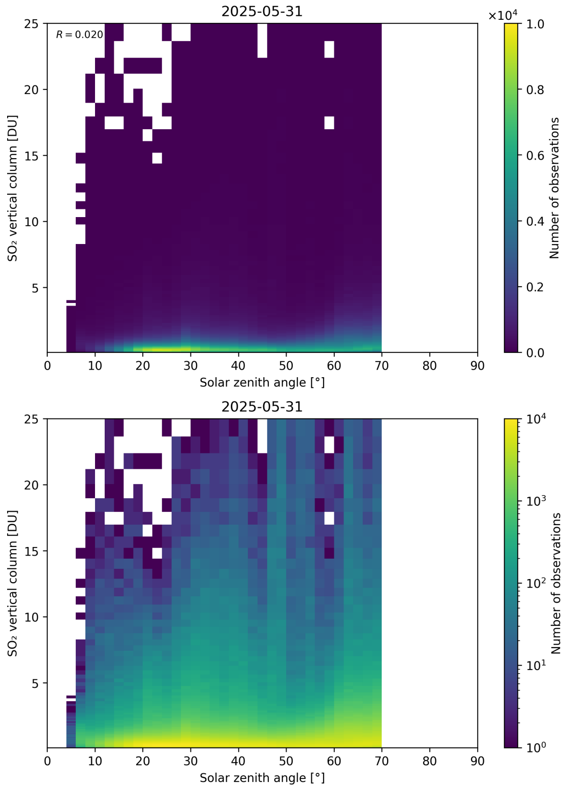
Figure 191: Scatter density plot of “Solar zenith angle” against “SO 2 vertical column” for 2025-05-31 to 2025-06-01.
