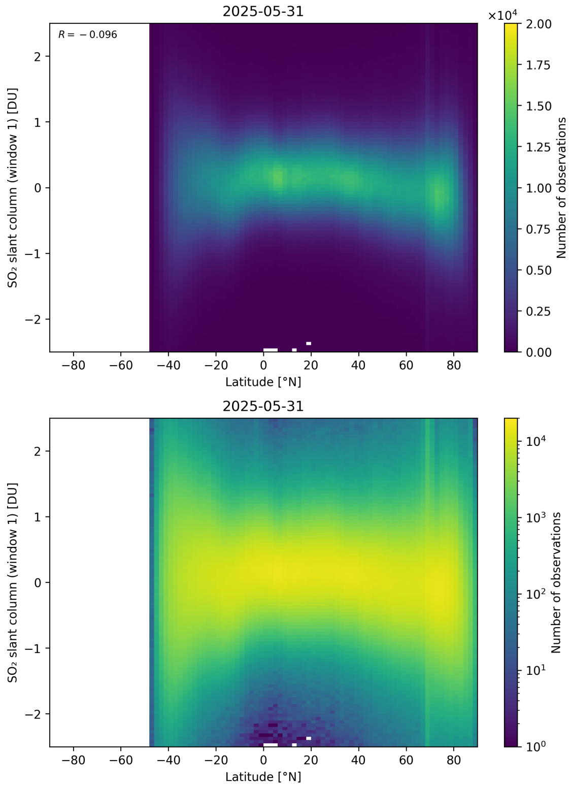
Figure 162: Scatter density plot of “Latitude” against “SO 2 slant column (window 1)” for 2025-05-31 to 2025-06-01.
