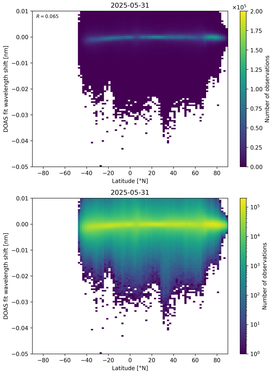
Figure 153: Scatter density plot of “Latitude” against “DOAS fit wavelength shift” for 2025-05-31 to 2025-06-01.
