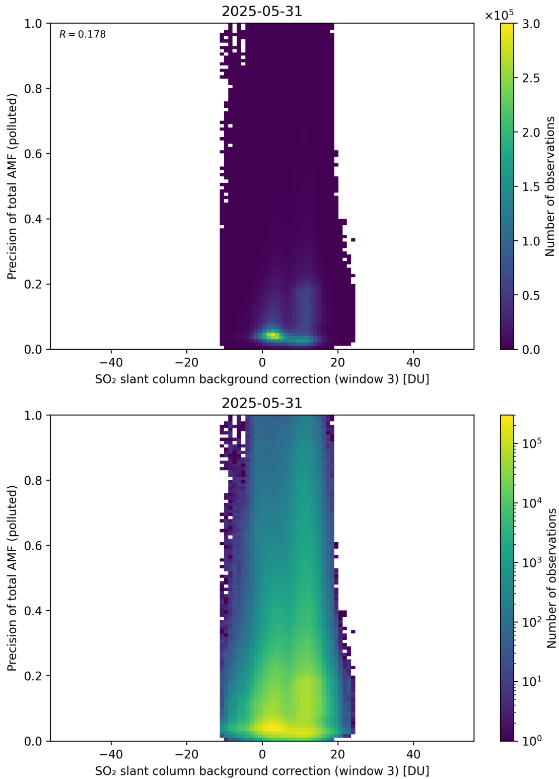
Figure 137: Scatter density plot of “SO 2 slant column background correction (window 3)” against “Precision of total AMF (polluted)” for 2025-05-31 to 2025-06-01.
