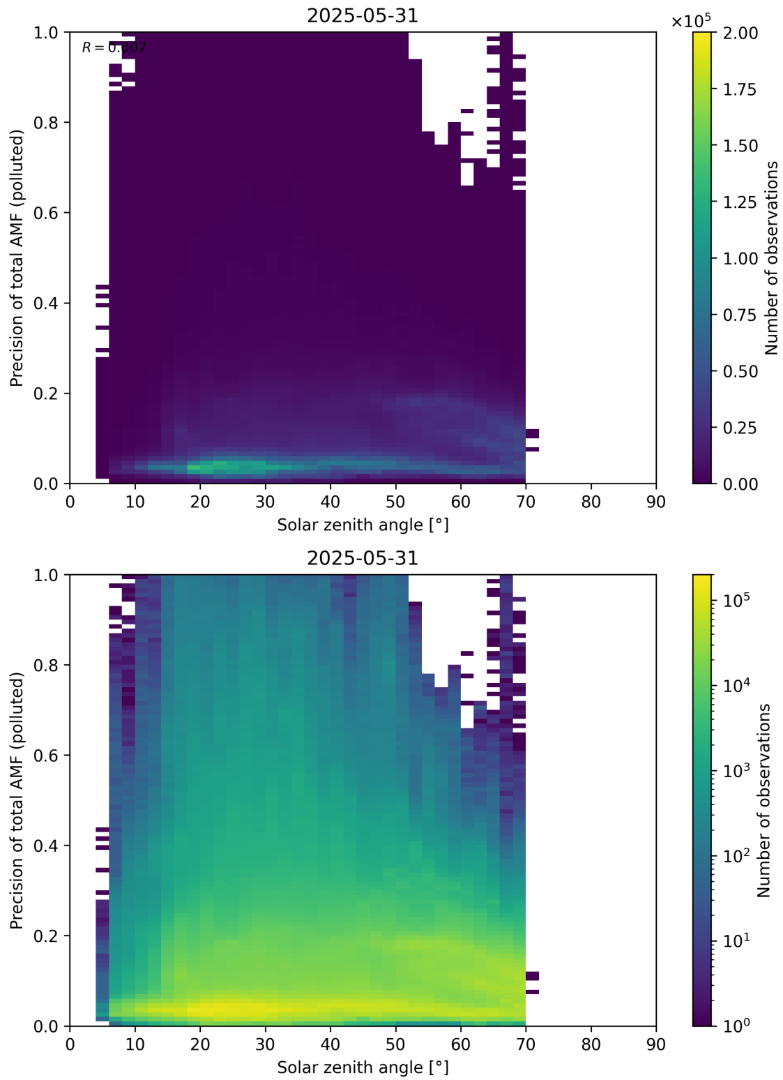
Figure 190: Scatter density plot of “Solar zenith angle” against “Precision of total AMF (polluted)” for 2025-05-31 to 2025-06-01.
