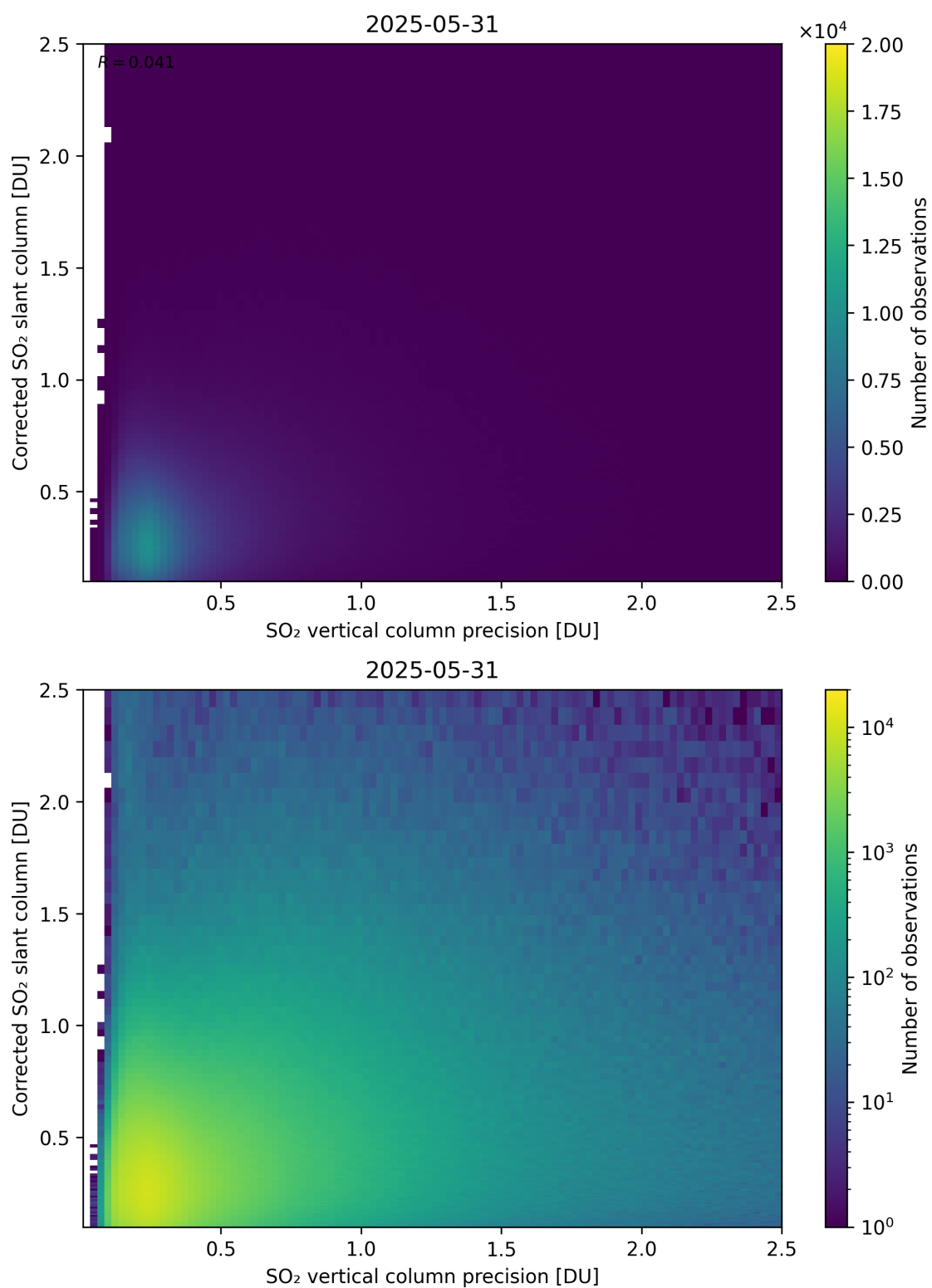
Figure 338: Scatter density plot of “SO 2 vertical column precision” against “Corrected SO 2 slant column” for 2025-05-31 to 2025-06-01.
