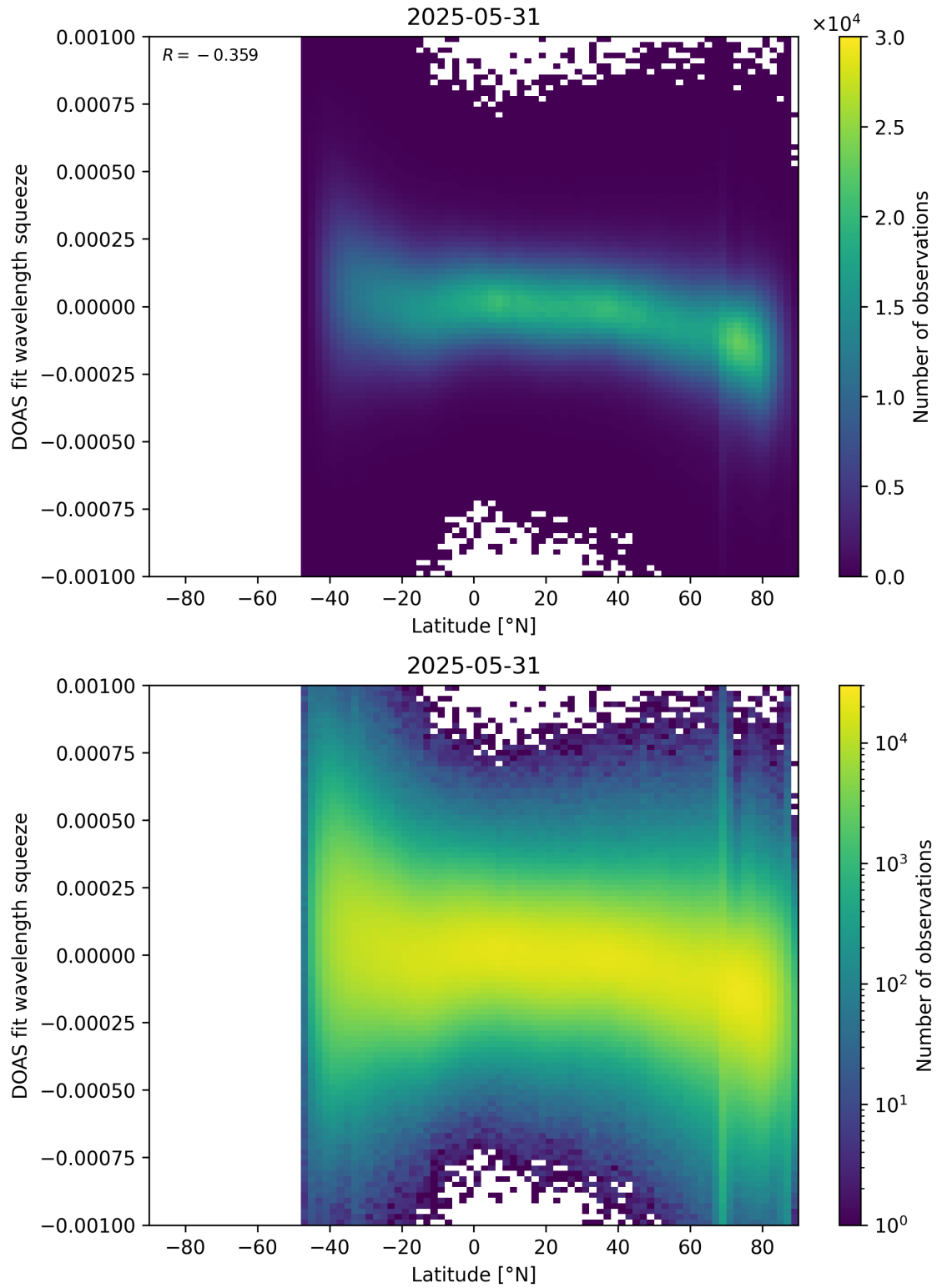
Figure 154: Scatter density plot of “Latitude” against “DOAS fit wavelength squeeze” for 2025-05-31 to 2025-06-01.
