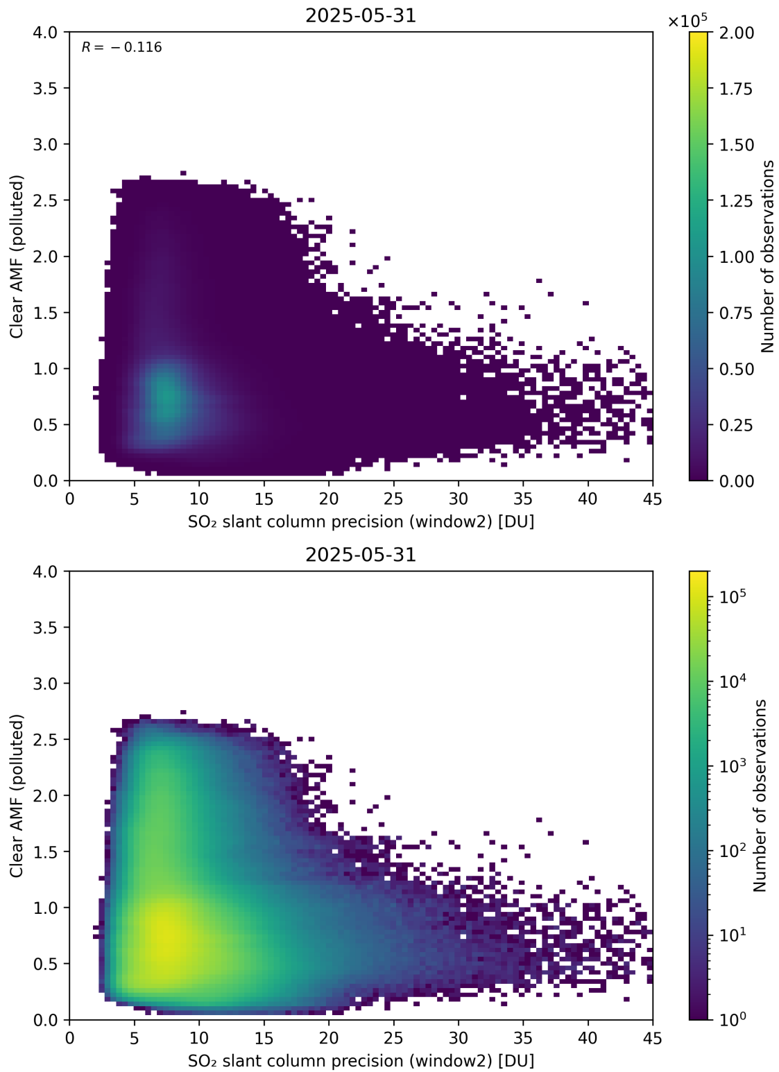
Figure 296: Scatter density plot of “SO 2 slant column precision (window2)” against “Clear AMF (polluted)” for 2025-05-31 to 2025-06-01.
