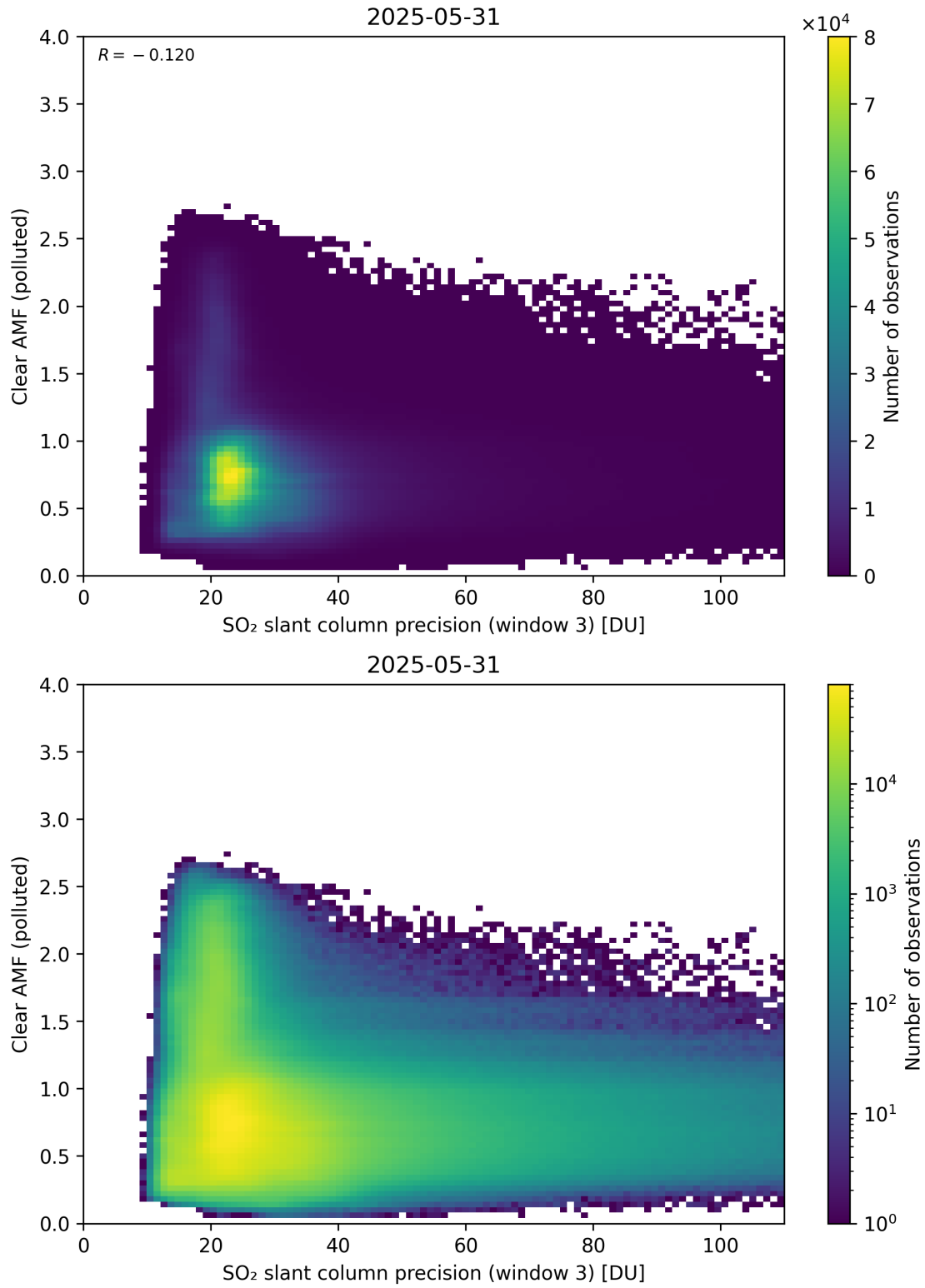
Figure 311: Scatter density plot of “SO 2 slant column precision (window 3)” against “Clear AMF (polluted)” for 2025-05-31 to 2025-06-01.
