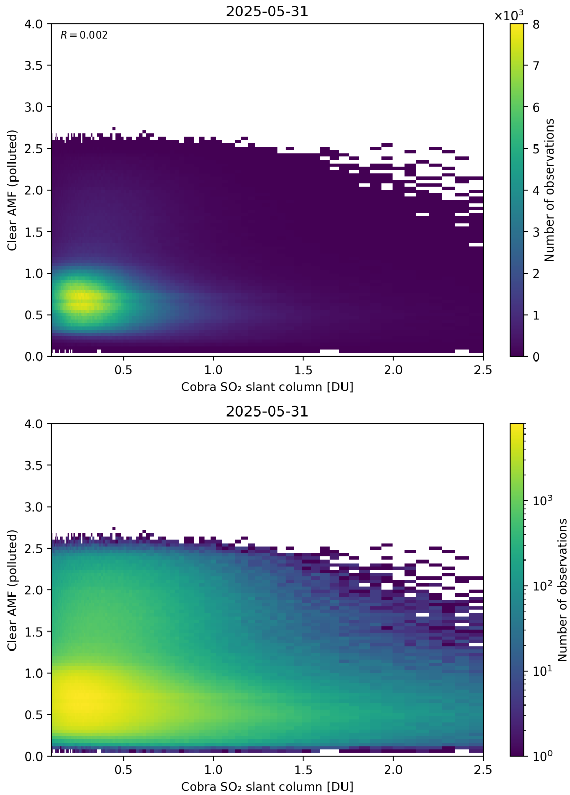
Figure 215: Scatter density plot of “Cobra SO 2 slant column” against “Clear AMF (polluted)” for 2025-05-31 to 2025-06-01.
