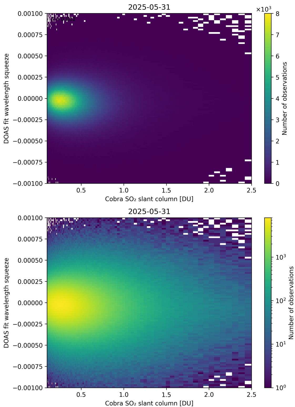
Figure 197: Scatter density plot of “Cobra SO 2 slant column” against “DOAS fit wavelength squeeze” for 2025-05-31 to 2025-06-01.
