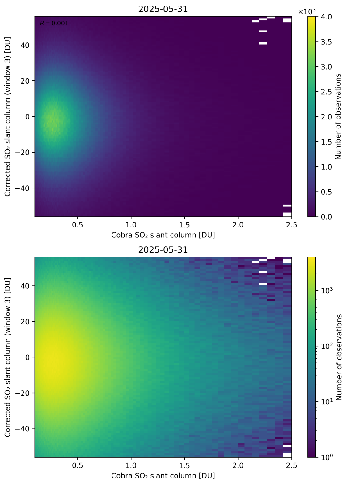
Figure 218: Scatter density plot of “Cobra SO 2 slant column” against “Corrected SO 2 slant column (window 3)” for 2025-05-31 to 2025-06-01.
