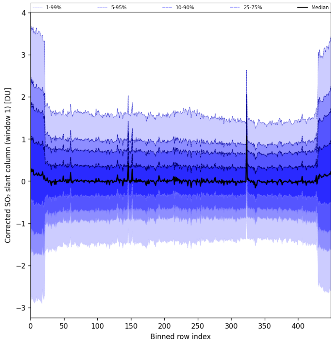
Figure 91: Along track statistics of “Corrected SO 2 slant column (window 1)” for 2025-05-31 to 2025-06-01
