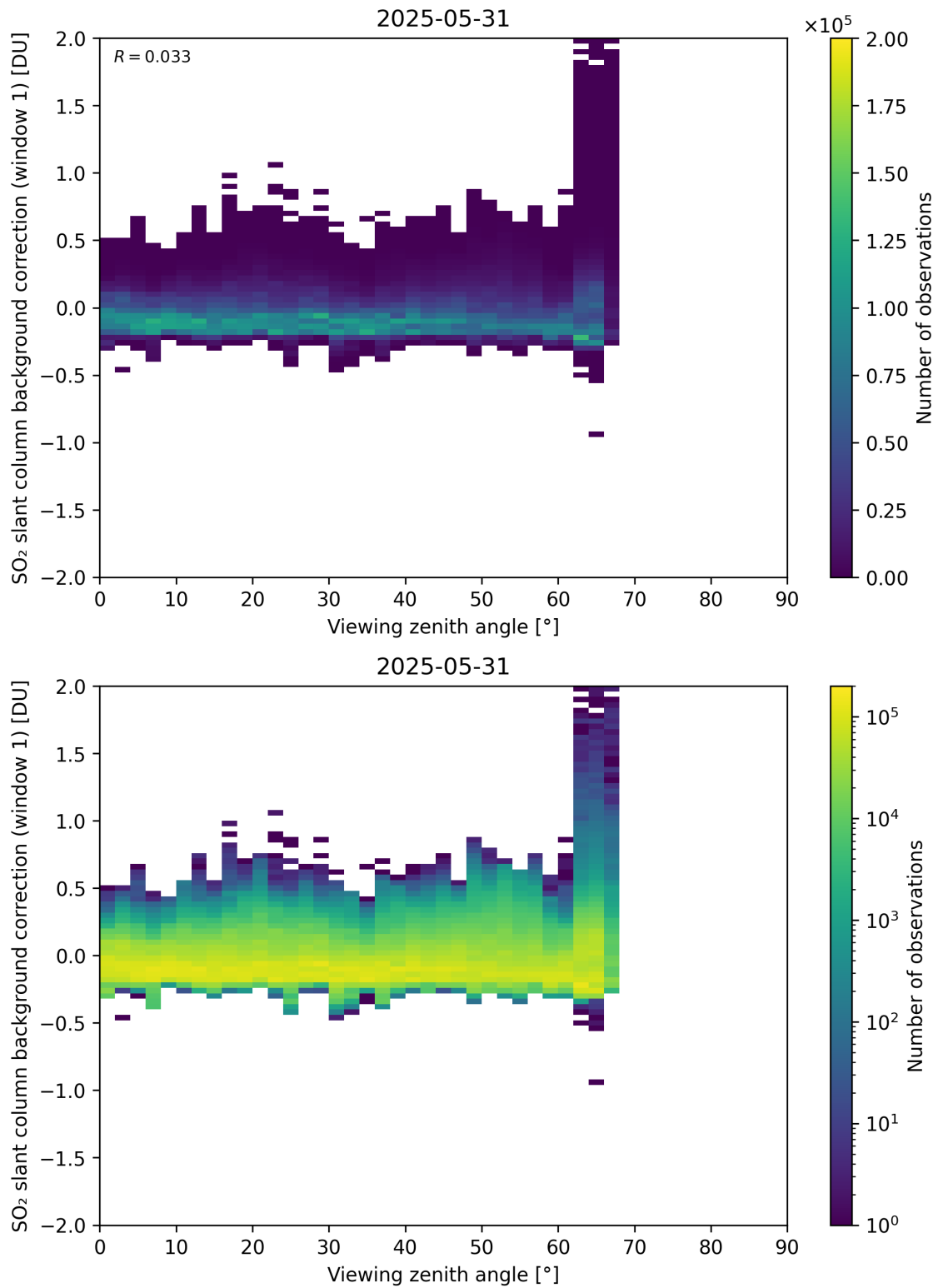
Figure 362: Scatter density plot of “Viewing zenith angle” against “SO 2 slant column background correction (window 1)” for 2025-05-31 to 2025-06-01.
