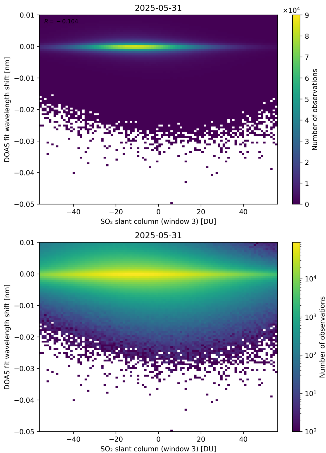
Figure 304: Scatter density plot of “SO 2 slant column (window 3)” against “DOAS fit wavelength shift” for 2025-05-31 to 2025-06-01.
