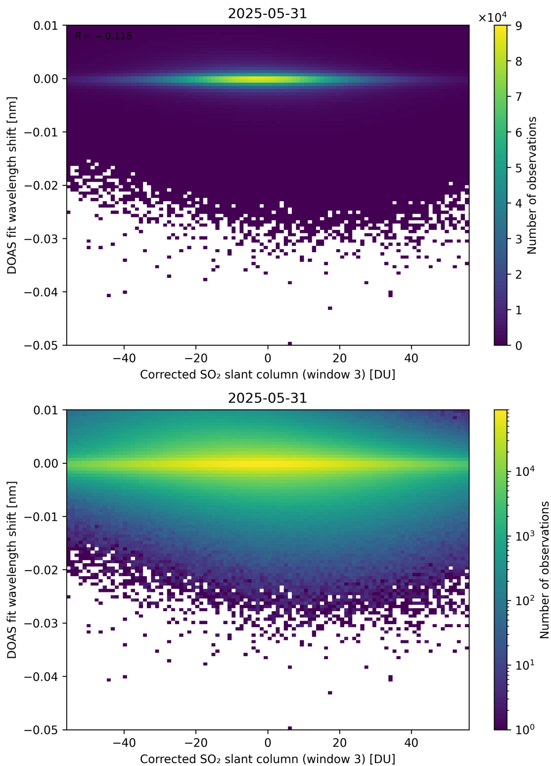
Figure 256: Scatter density plot of “Corrected SO 2 slant column (window 3)” against “DOAS fit wavelength shift” for 2025-05-31 to 2025-06-01.
