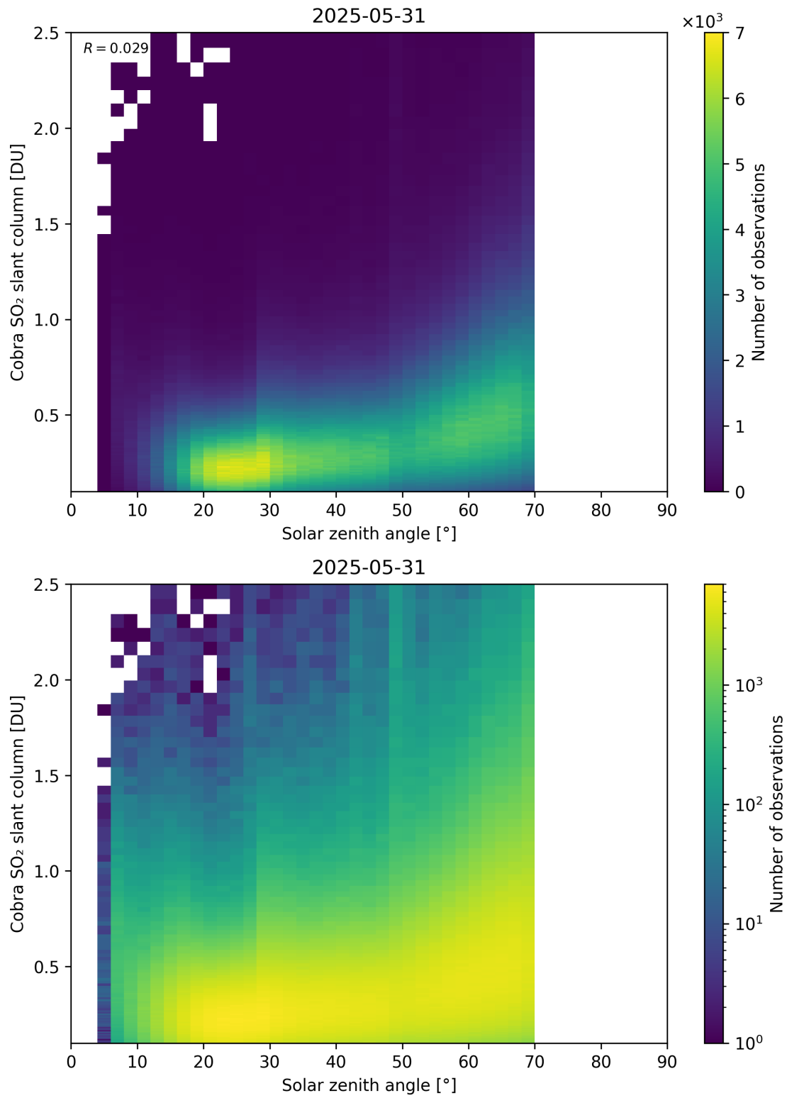
Figure 179: Scatter density plot of “Solar zenith angle” against “Cobra SO 2 slant column” for 2025-05-31 to 2025-06-01.
