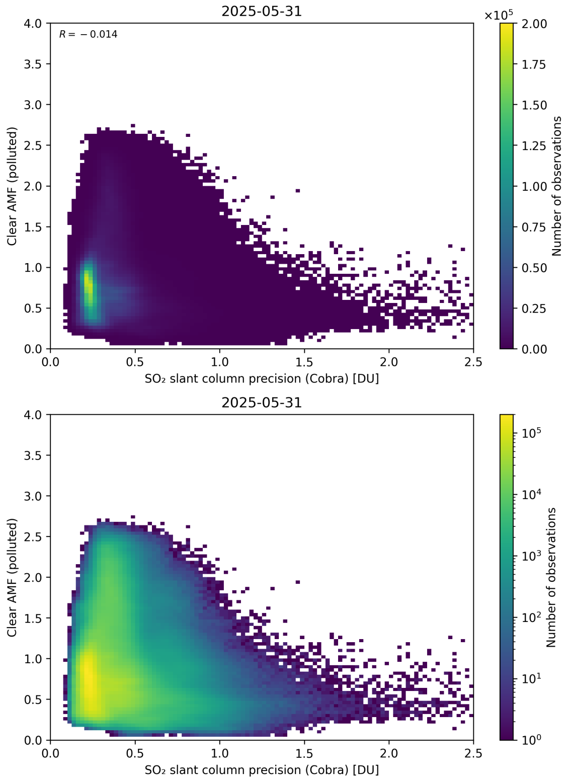
Figure 205: Scatter density plot of “SO 2 slant column precision (Cobra)” against “Clear AMF (polluted)” for 2025-05-31 to 2025-06-01.
