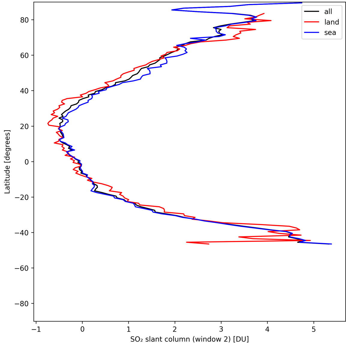
Figure 41: Zonal average of “SO 2 slant column (window 2)” for 2025-05-31 to 2025-06-01.
