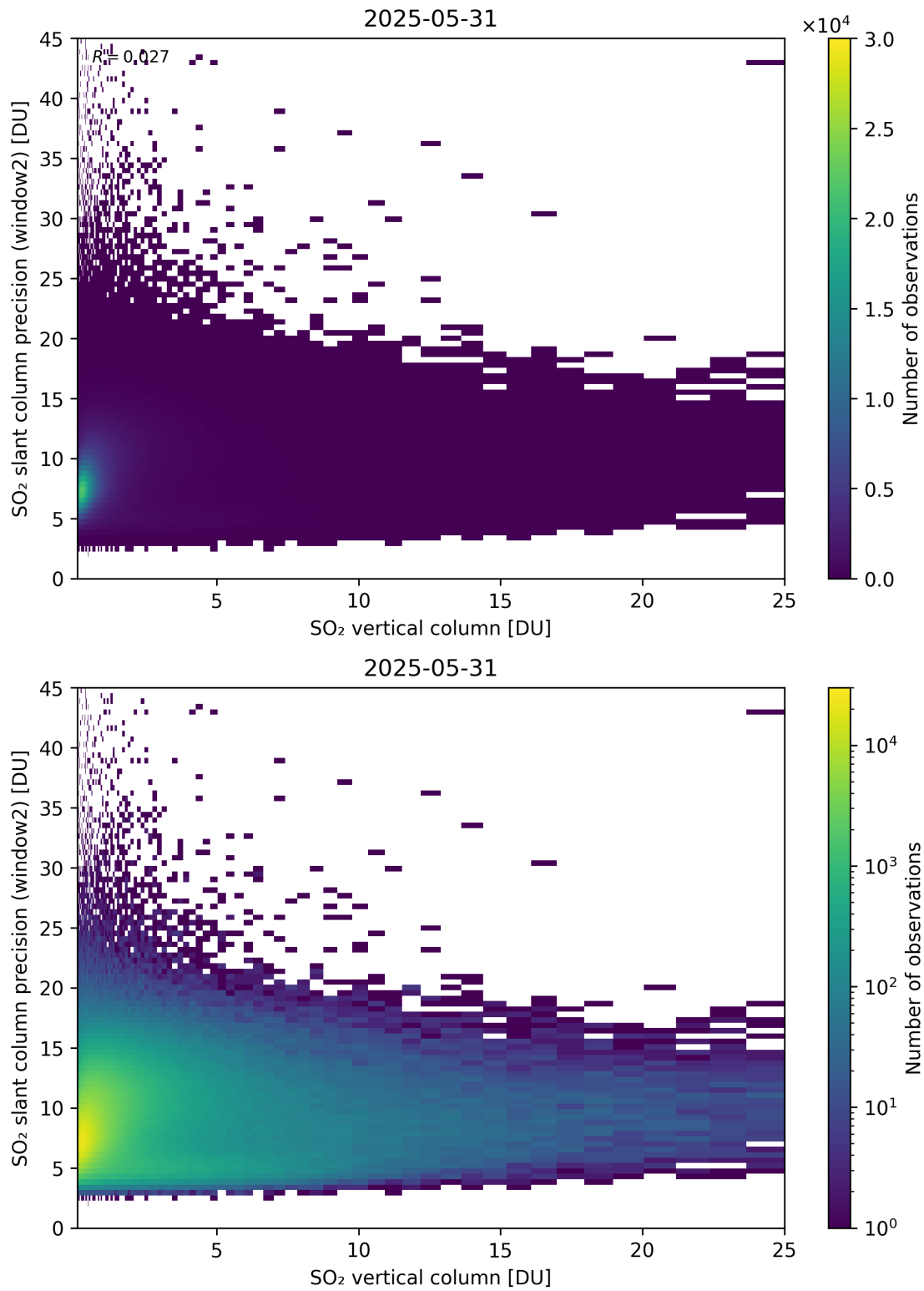
Figure 356: Scatter density plot of “SO 2 vertical column” against “SO 2 slant column precision (window2)” for 2025-05-31 to 2025-06-01.
