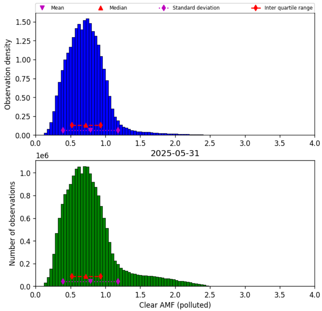
Figure 81: Histogram of “Clear AMF (polluted)” for 2025-05-31 to 2025-06-01
