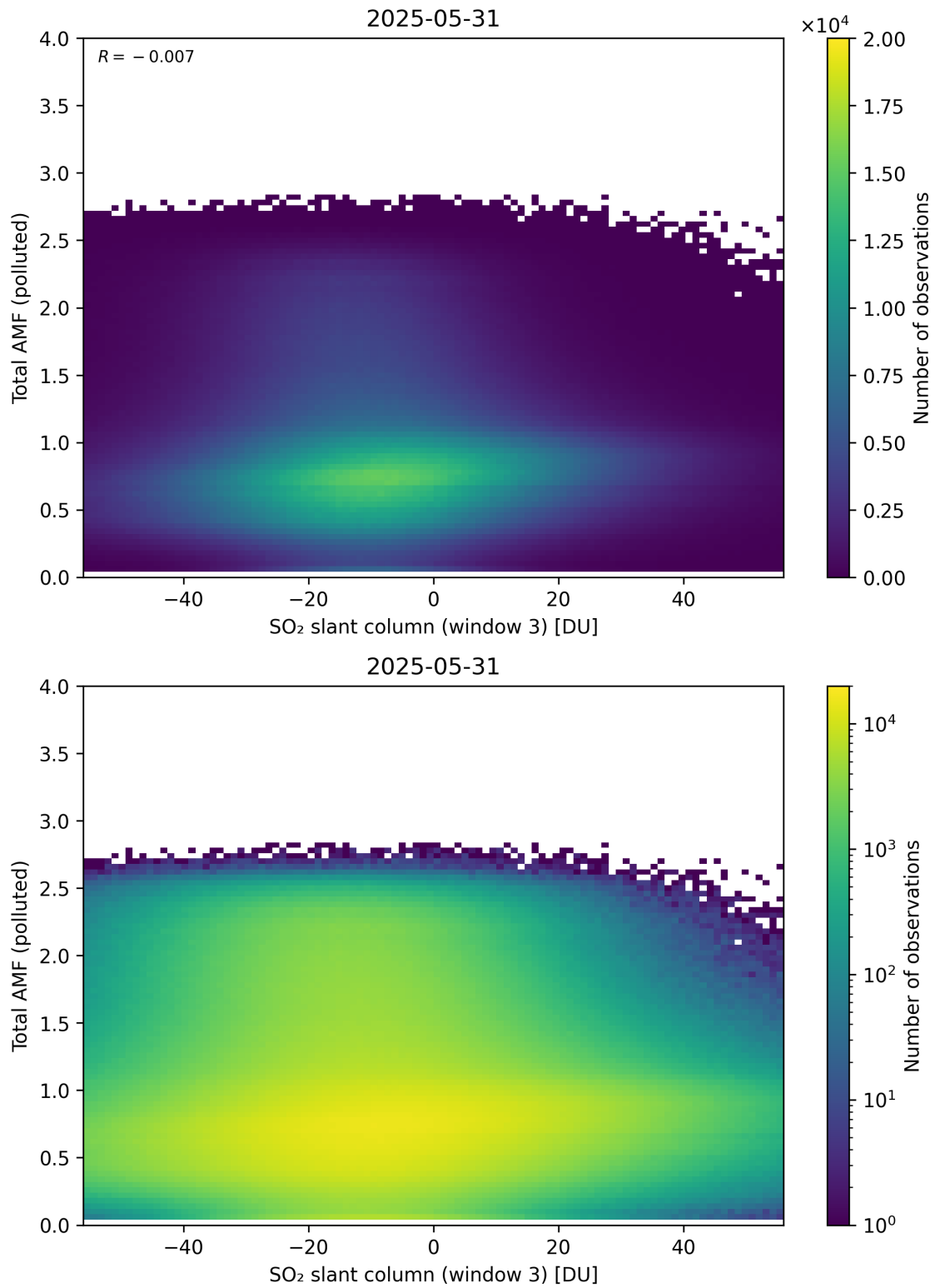
Figure 318: Scatter density plot of “SO 2 slant column (window 3)” against “Total AMF (polluted)” for 2025-05-31 to 2025-06-01.
