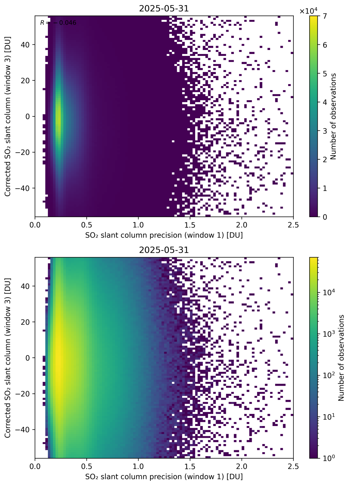
Figure 276: Scatter density plot of “SO 2 slant column precision (window 1)” against “Corrected SO 2 slant column (window 3)” for 2025-05-31 to 2025-06-01.
