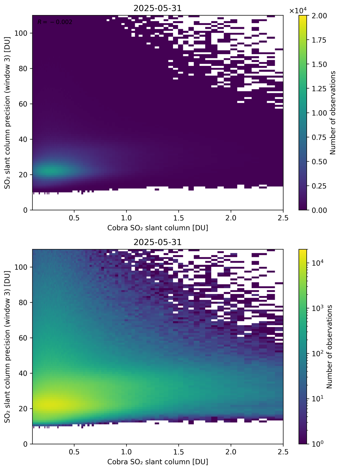
Figure 223: Scatter density plot of “Cobra SO 2 slant column” against “SO 2 slant column precision (window 3)” for 2025-05-31 to 2025-06-01.
