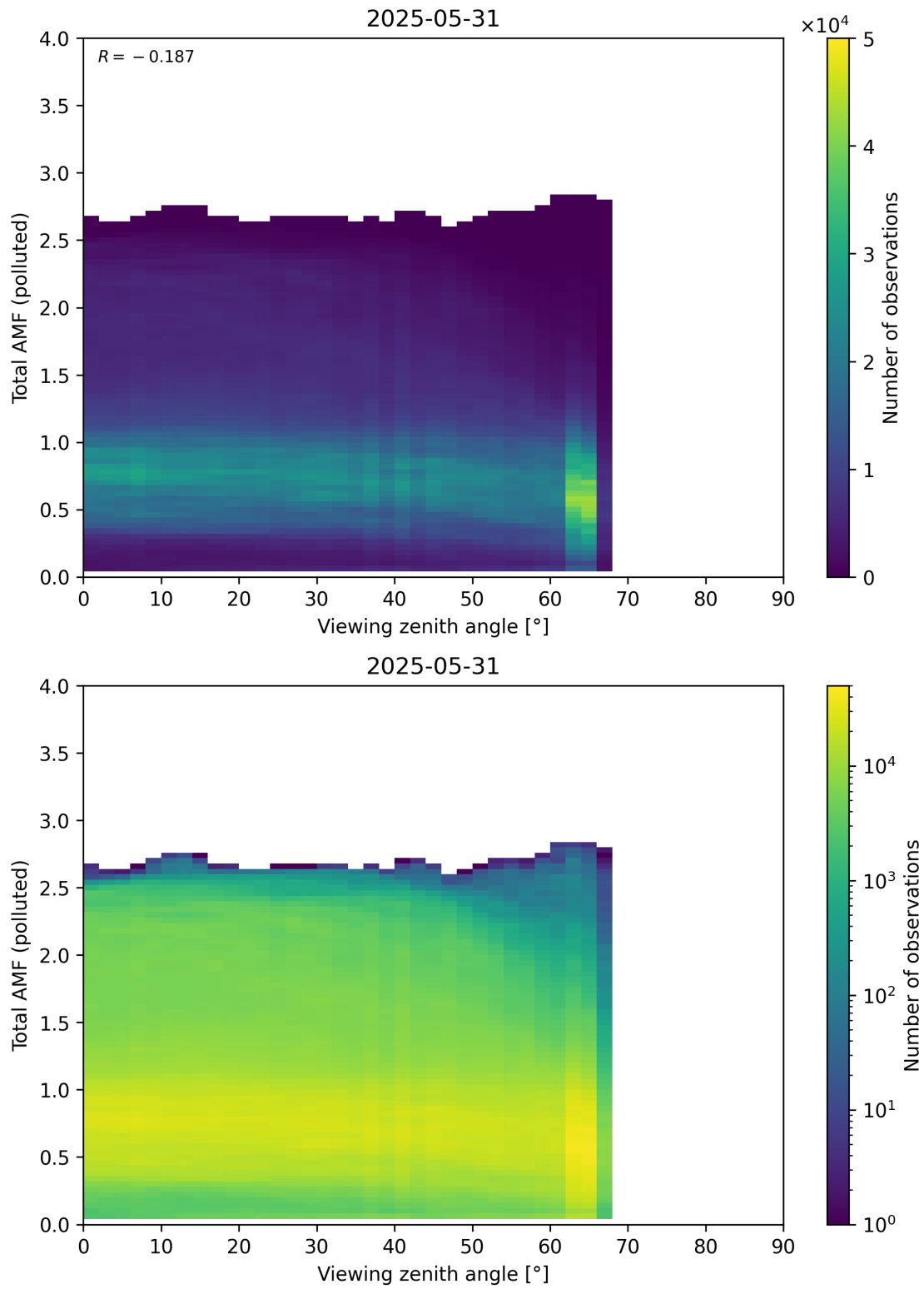
Figure 381: Scatter density plot of “Viewing zenith angle” against “Total AMF (polluted)” for 2025-05-31 to 2025-06-01.
