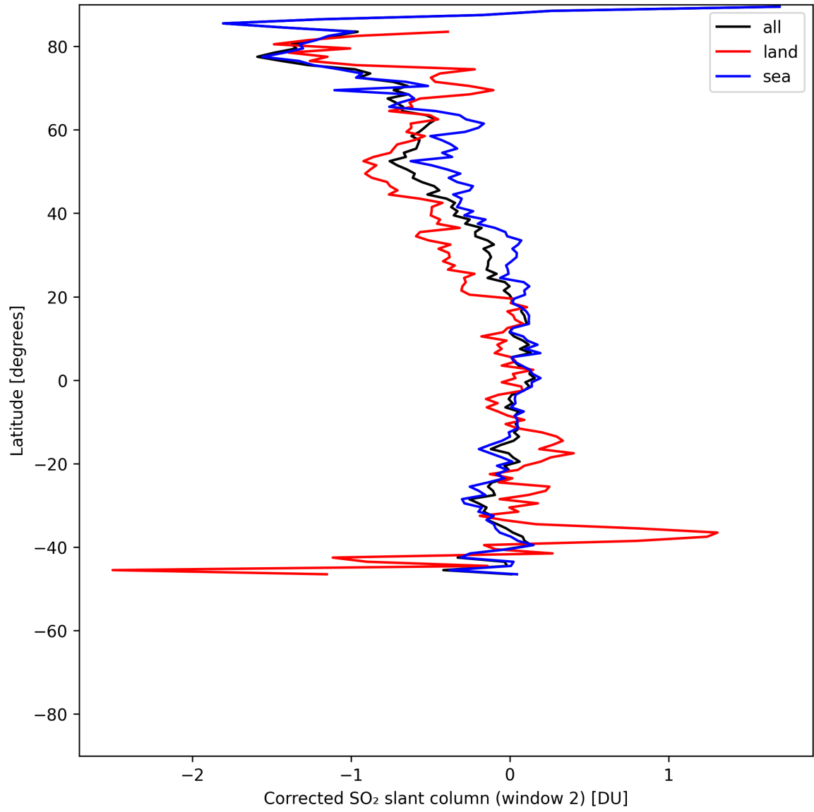
Figure 43: Zonal average of “Corrected SO 2 slant column (window 2)” for 2025-05-31 to 2025-06-01.
