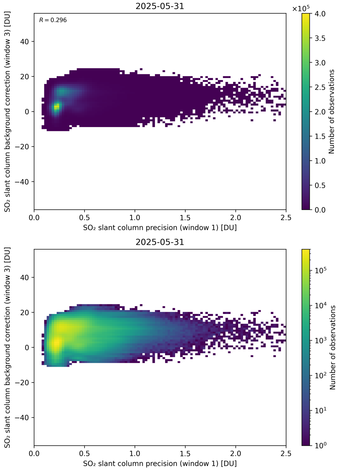
Figure 270: Scatter density plot of “SO 2 slant column precision (window 1)” against “SO 2 slant column background correction (window 3)” for 2025-05-31 to 2025-06-01.
