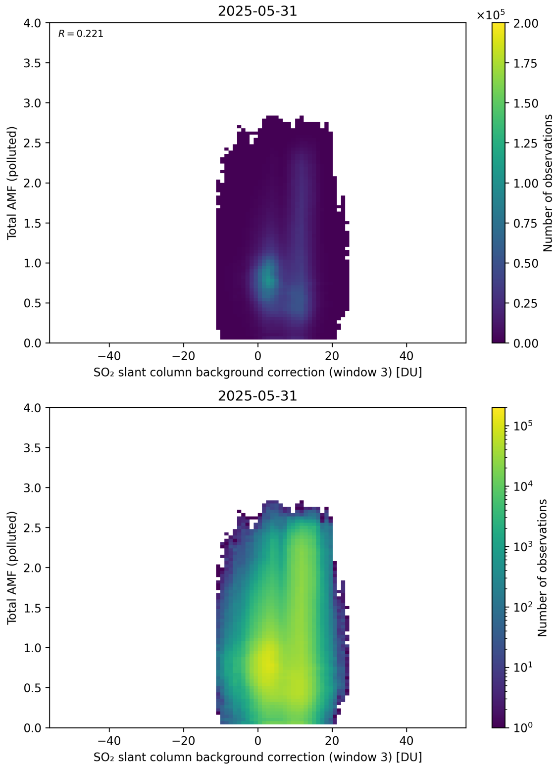
Figure 136: Scatter density plot of “SO 2 slant column background correction (window 3)” against “Total AMF (polluted)” for 2025-05-31 to 2025-06-01.
