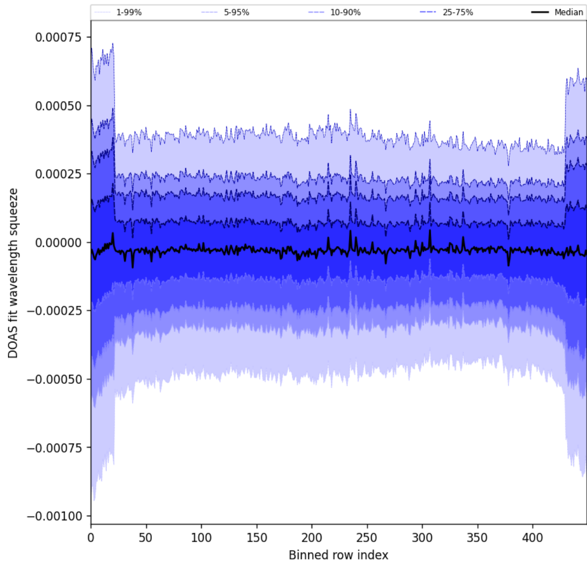
Figure 103: Along track statistics of “DOAS fit wavelength squeeze” for 2025-05-31 to 2025-06-01
