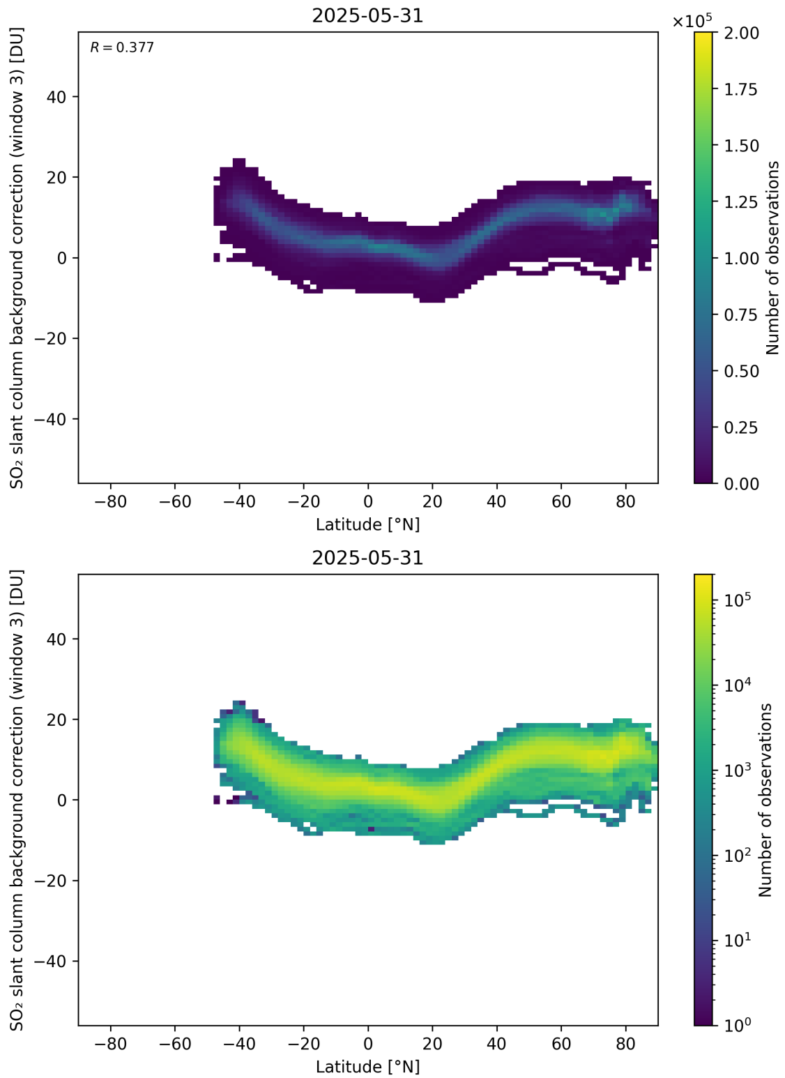
Figure 152: Scatter density plot of “Latitude” against “SO 2 slant column background correction (window 3)” for 2025-05-31 to 2025-06-01.
