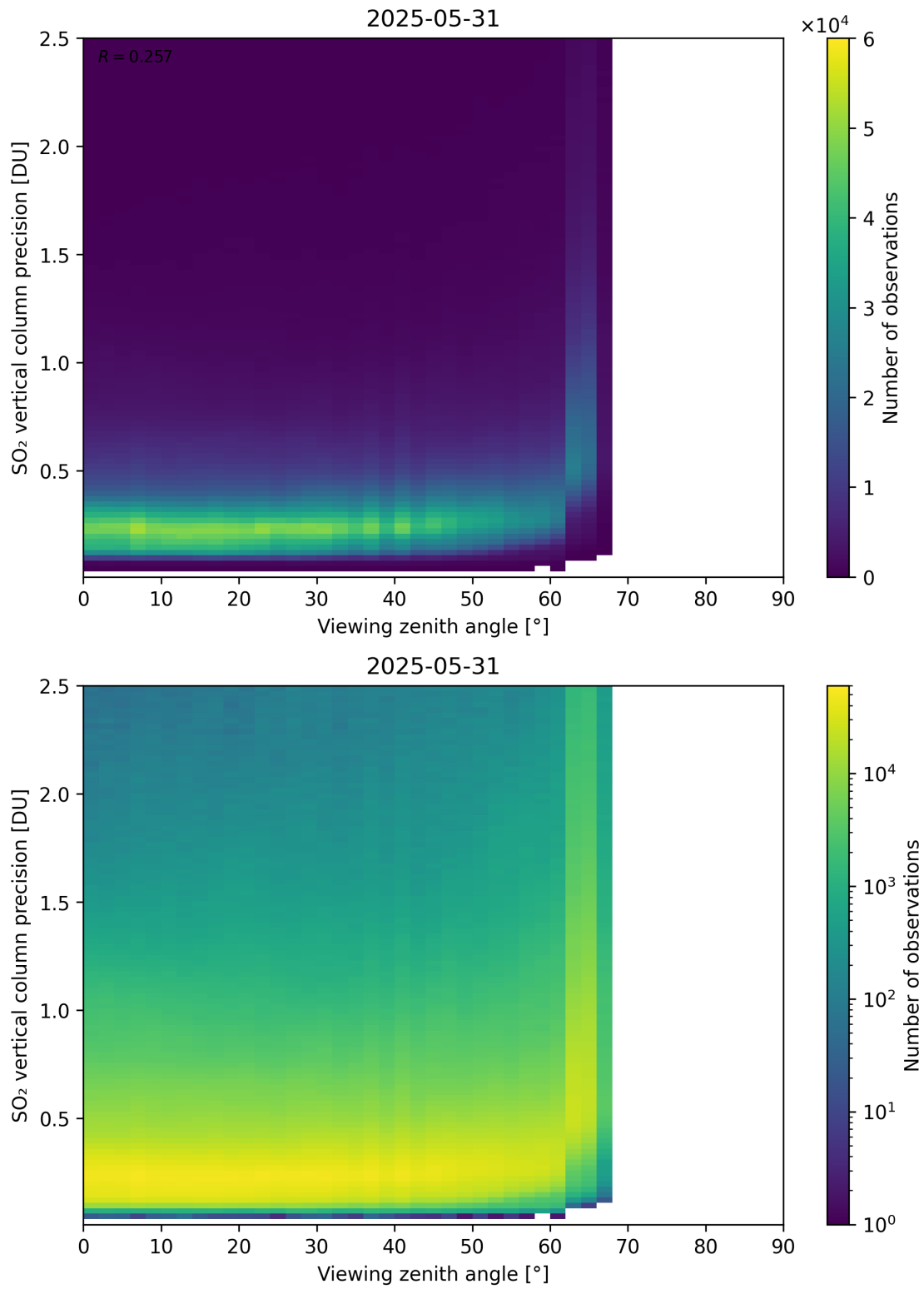
Figure 384: Scatter density plot of “Viewing zenith angle” against “SO 2 vertical column precision” for 2025-05-31 to 2025-06-01.
