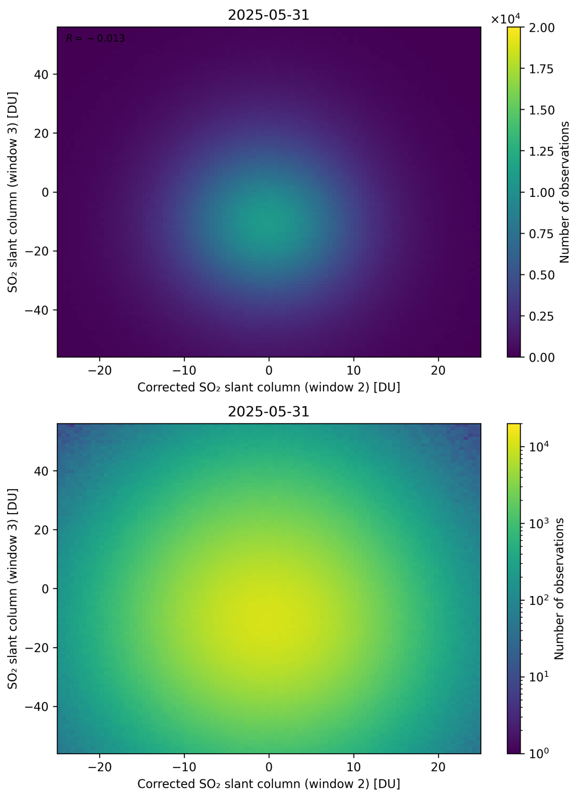
Figure 251: Scatter density plot of “Corrected SO 2 slant column (window 2)” against “SO 2 slant column (window 3)” for 2025-05-31 to 2025-06-01.
