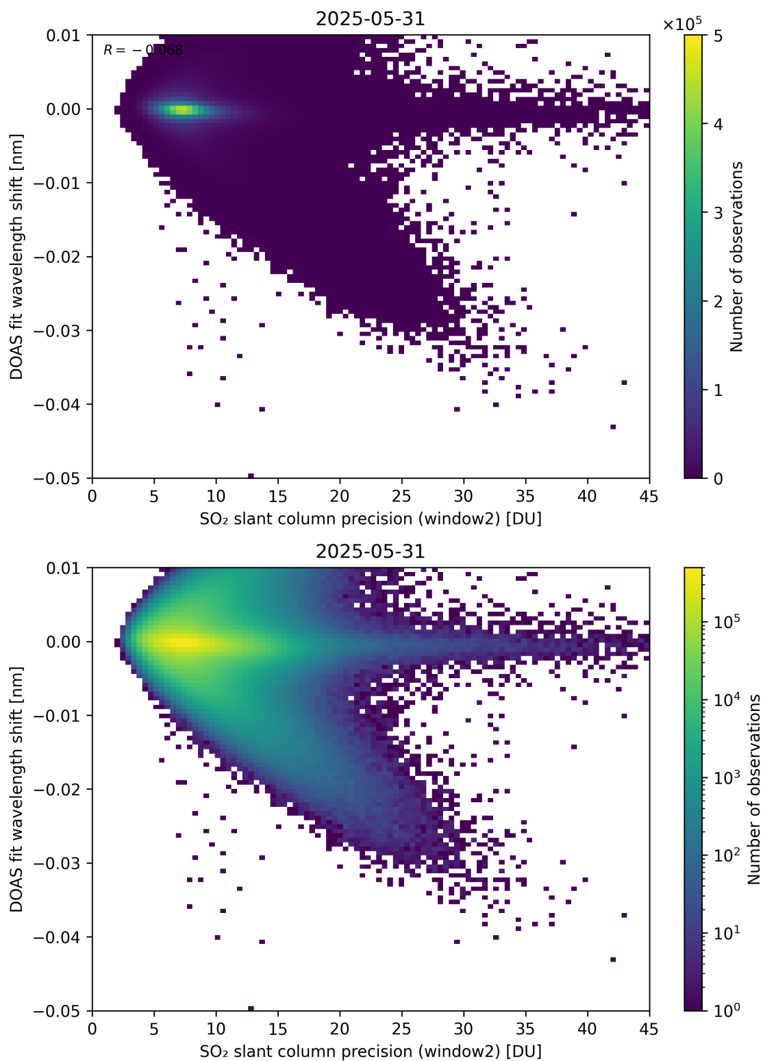
Figure 293: Scatter density plot of “SO 2 slant column precision (window2)” against “DOAS fit wavelength shift” for 2025-05-31 to 2025-06-01.
