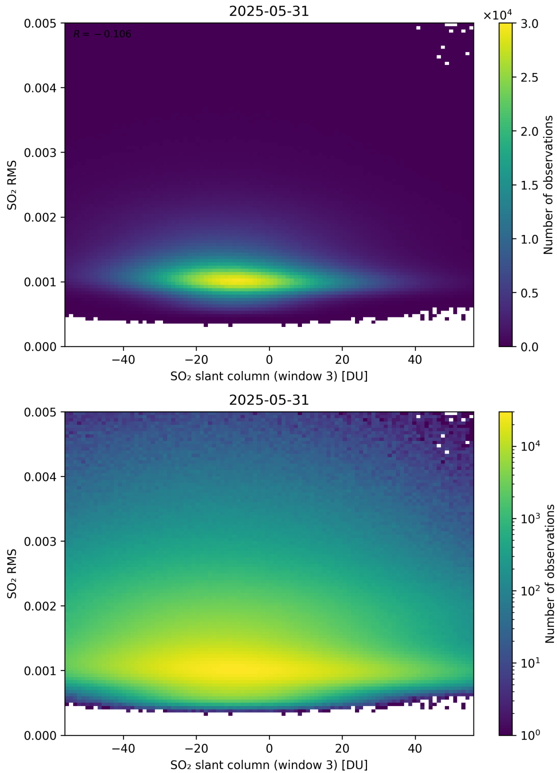
Figure 306: Scatter density plot of “SO 2 slant column (window 3)” against “SO 2 RMS” for 2025-05-31 to 2025-06-01.
