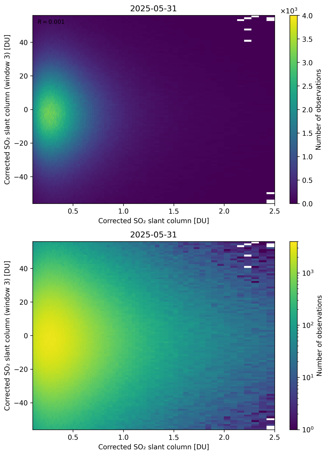
Figure 236: Scatter density plot of “Corrected SO 2 slant column” against “Corrected SO 2 slant column (window 3)” for 2025-05-31 to 2025-06-01.
