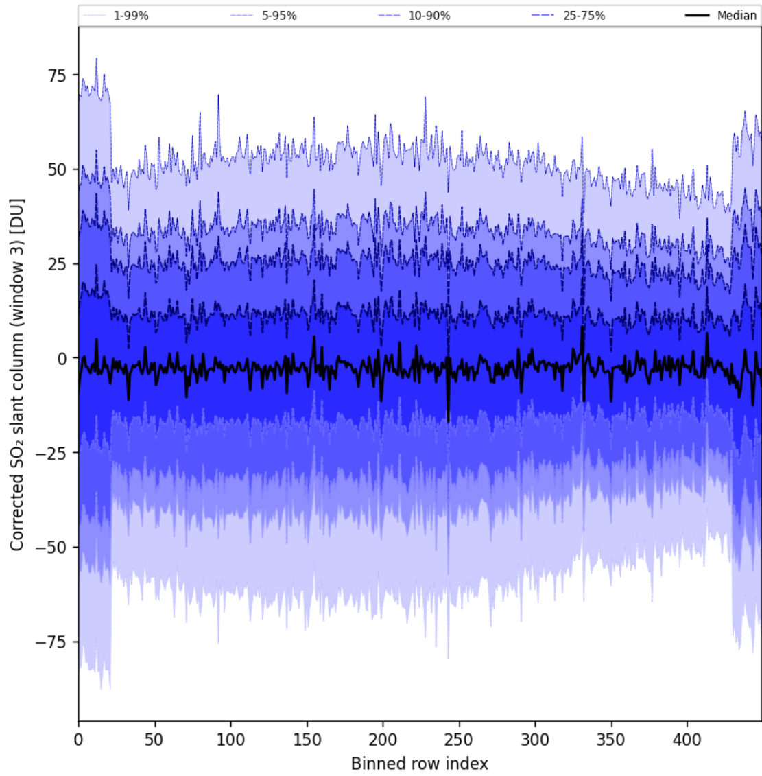
Figure 99: Along track statistics of “Corrected SO 2 slant column (window 3)” for 2025-05-31 to 2025-06-01
