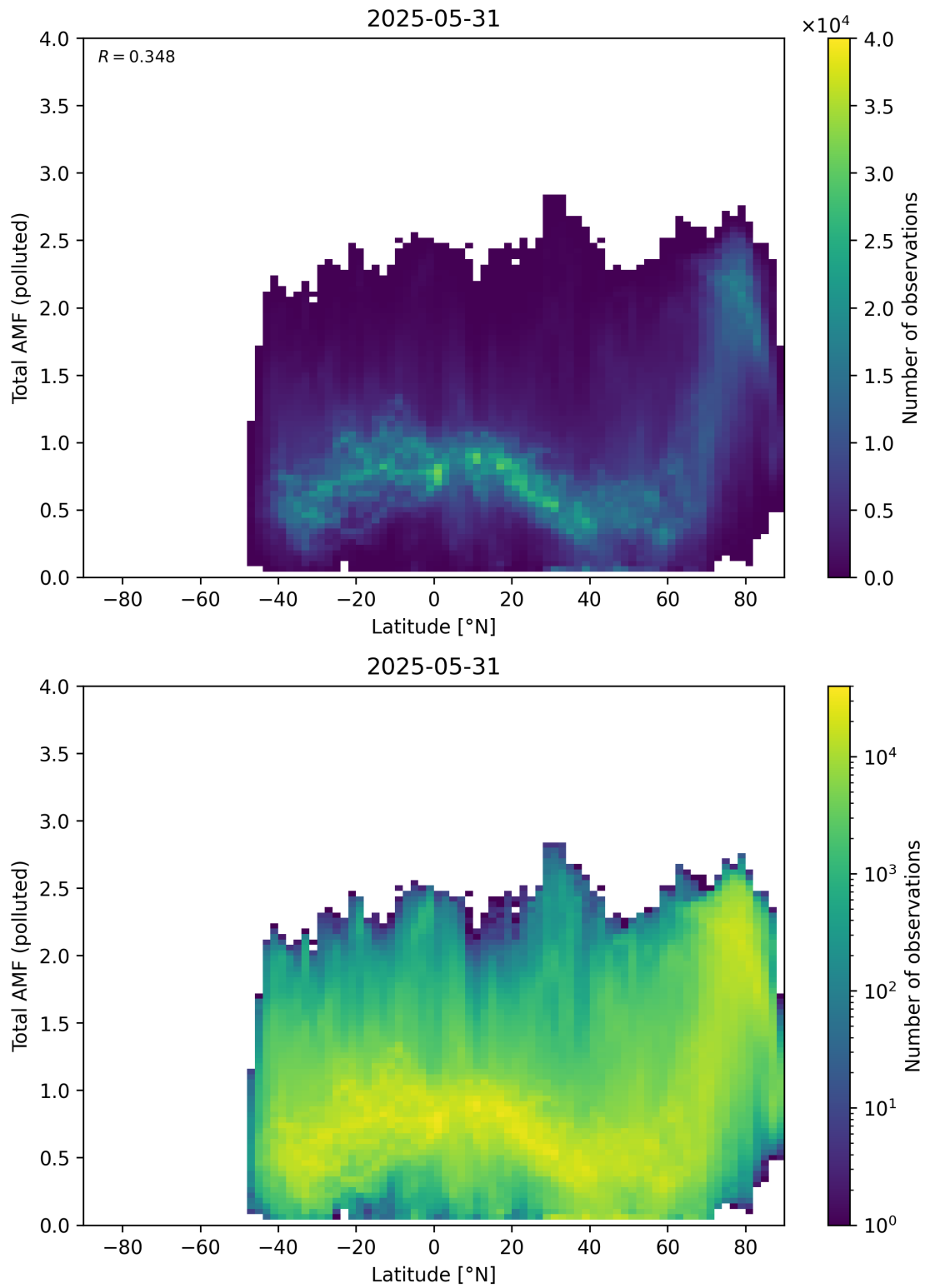
Figure 167: Scatter density plot of “Latitude” against “Total AMF (polluted)” for 2025-05-31 to 2025-06-01.
