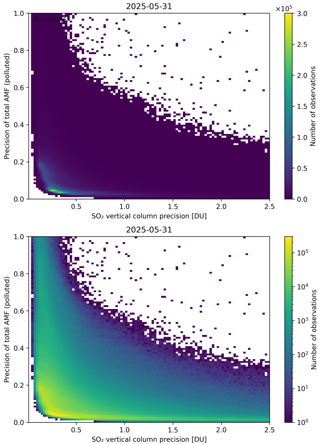
Figure 347: Scatter density plot of “SO 2 vertical column precision” against “Precision of total AMF (polluted)” for 2025-05-31 to 2025-06-01.
