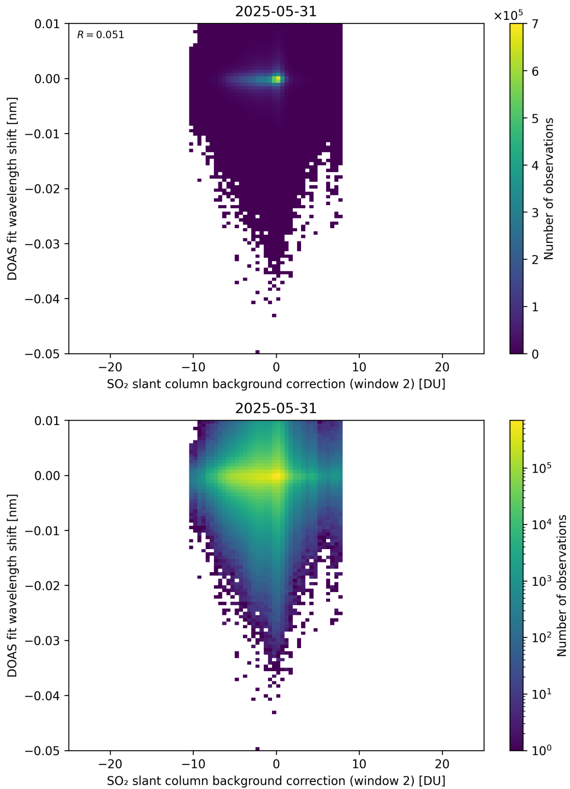
Figure 123: Scatter density plot of “SO 2 slant column background correction (window 2)” against “DOAS fit wavelength shift” for 2025-05-31 to 2025-06-01.
