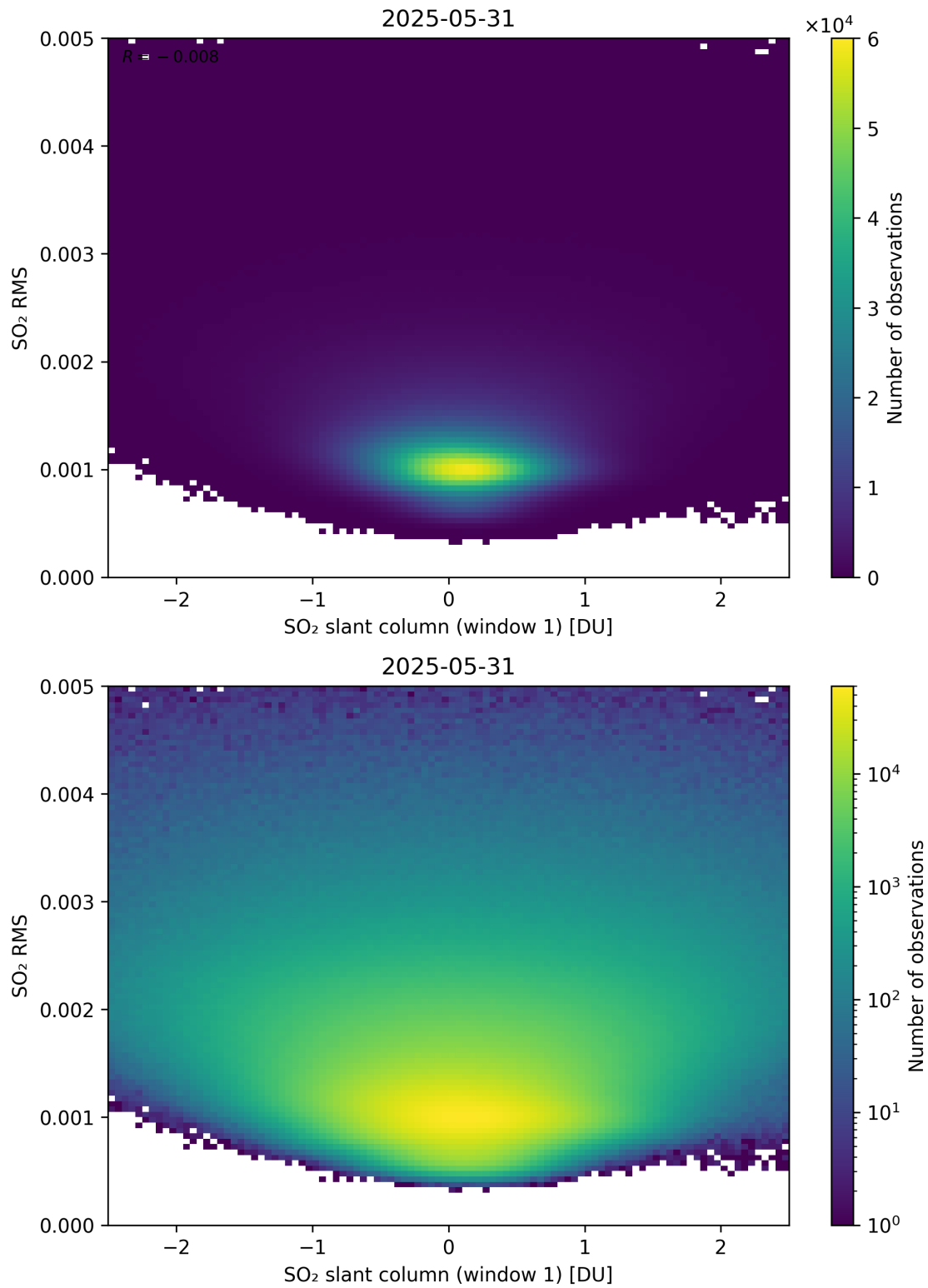
Figure 267: Scatter density plot of “SO 2 slant column (window 1)” against “SO 2 RMS” for 2025-05-31 to 2025-06-01.
