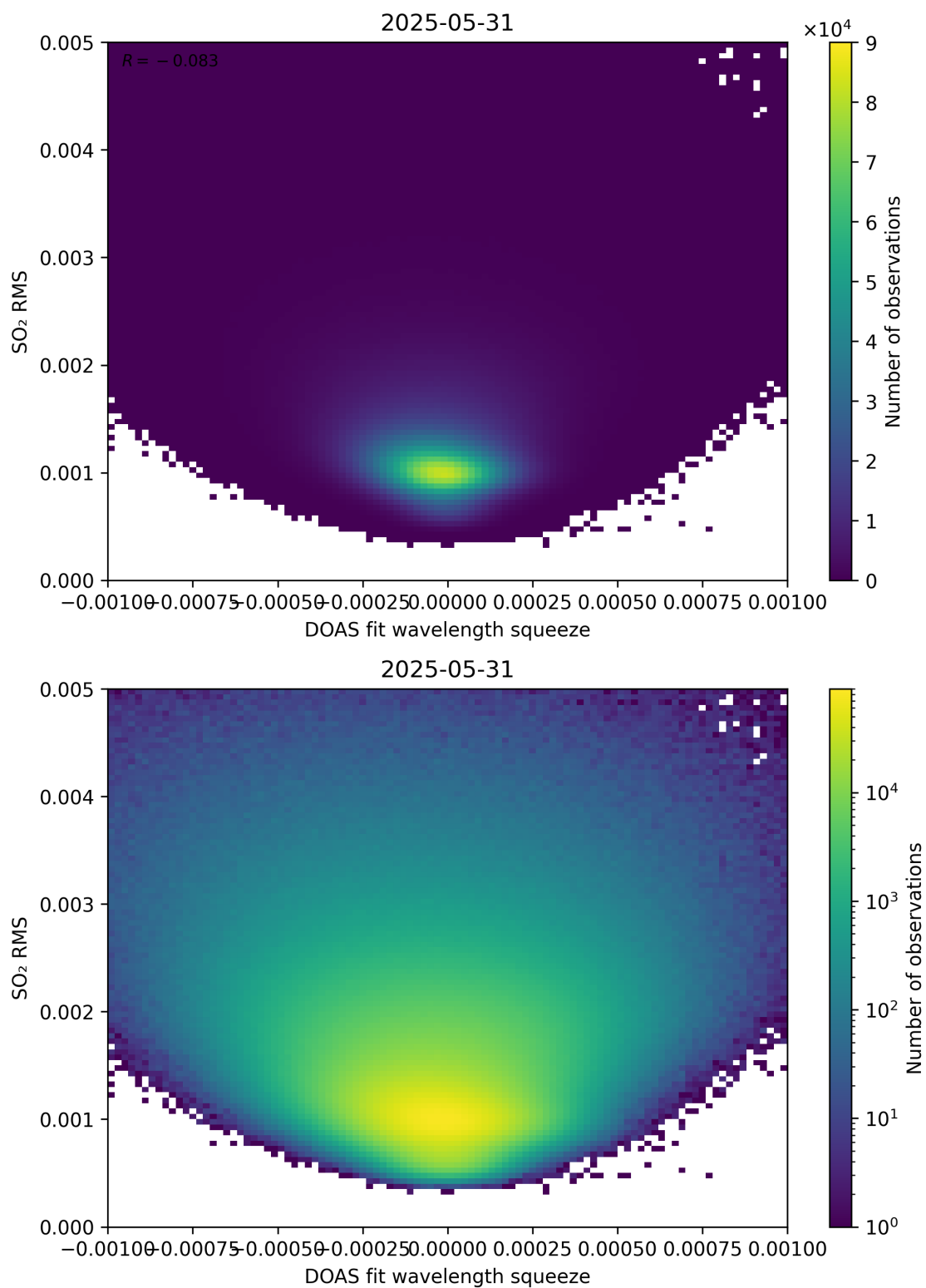
Figure 143: Scatter density plot of “DOAS fit wavelength squeeze” against “SO 2 RMS” for 2025-05-31 to 2025-06-01.
