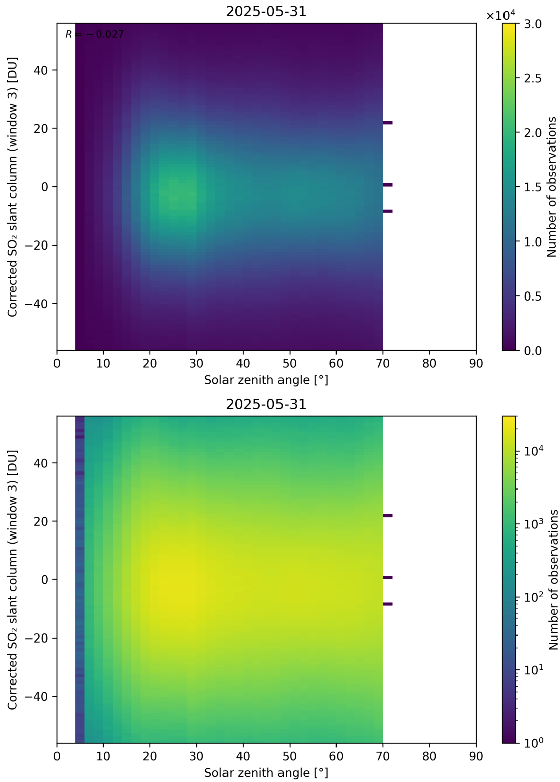
Figure 183: Scatter density plot of “Solar zenith angle” against “Corrected SO 2 slant column (window 3)” for 2025-05-31 to 2025-06-01.
