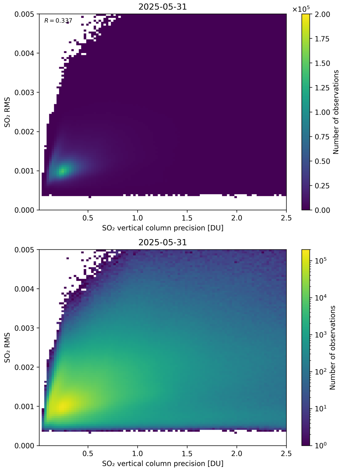
Figure 334: Scatter density plot of “SO 2 vertical column precision” against “SO 2 RMS” for 2025-05-31 to 2025-06-01.
