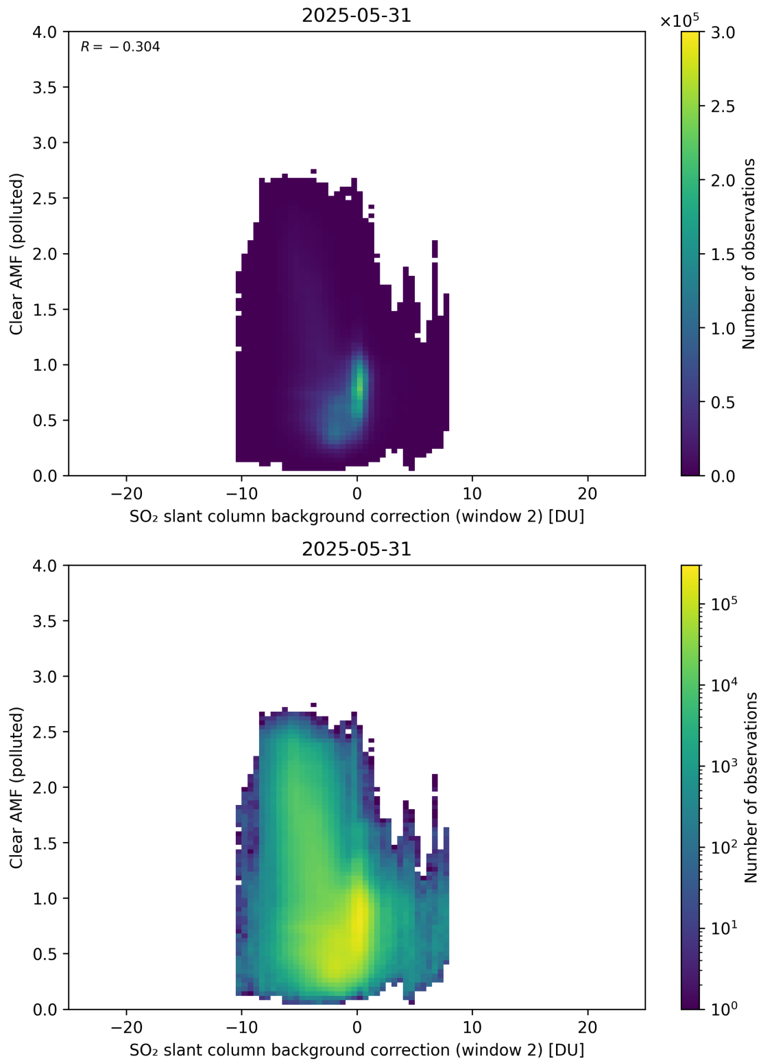
Figure 126: Scatter density plot of “SO 2 slant column background correction (window 2)” against “Clear AMF (polluted)” for 2025-05-31 to 2025-06-01.
