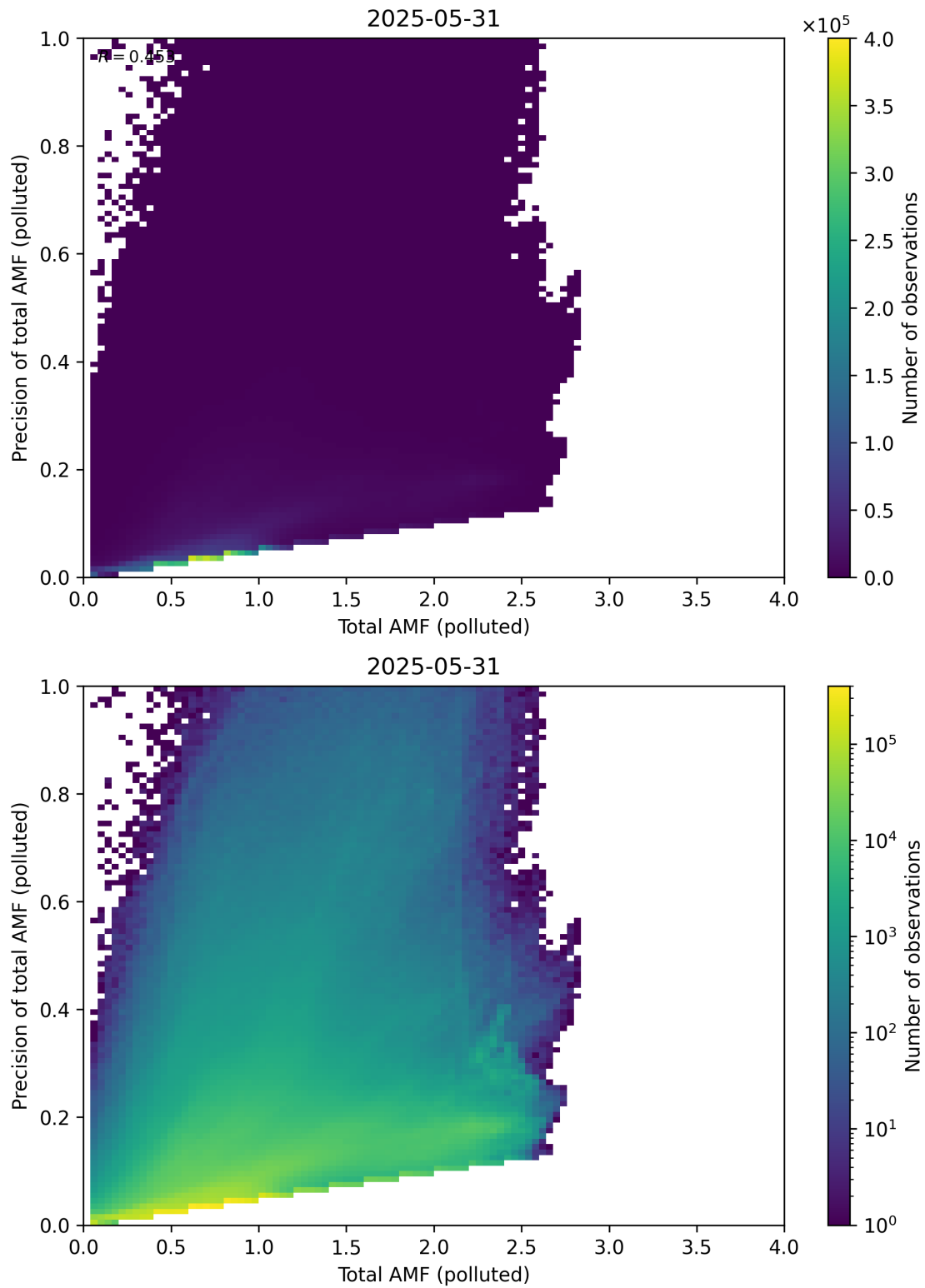
Figure 322: Scatter density plot of “Total AMF (polluted)” against “Precision of total AMF (polluted)” for 2025-05-31 to 2025-06-01.
