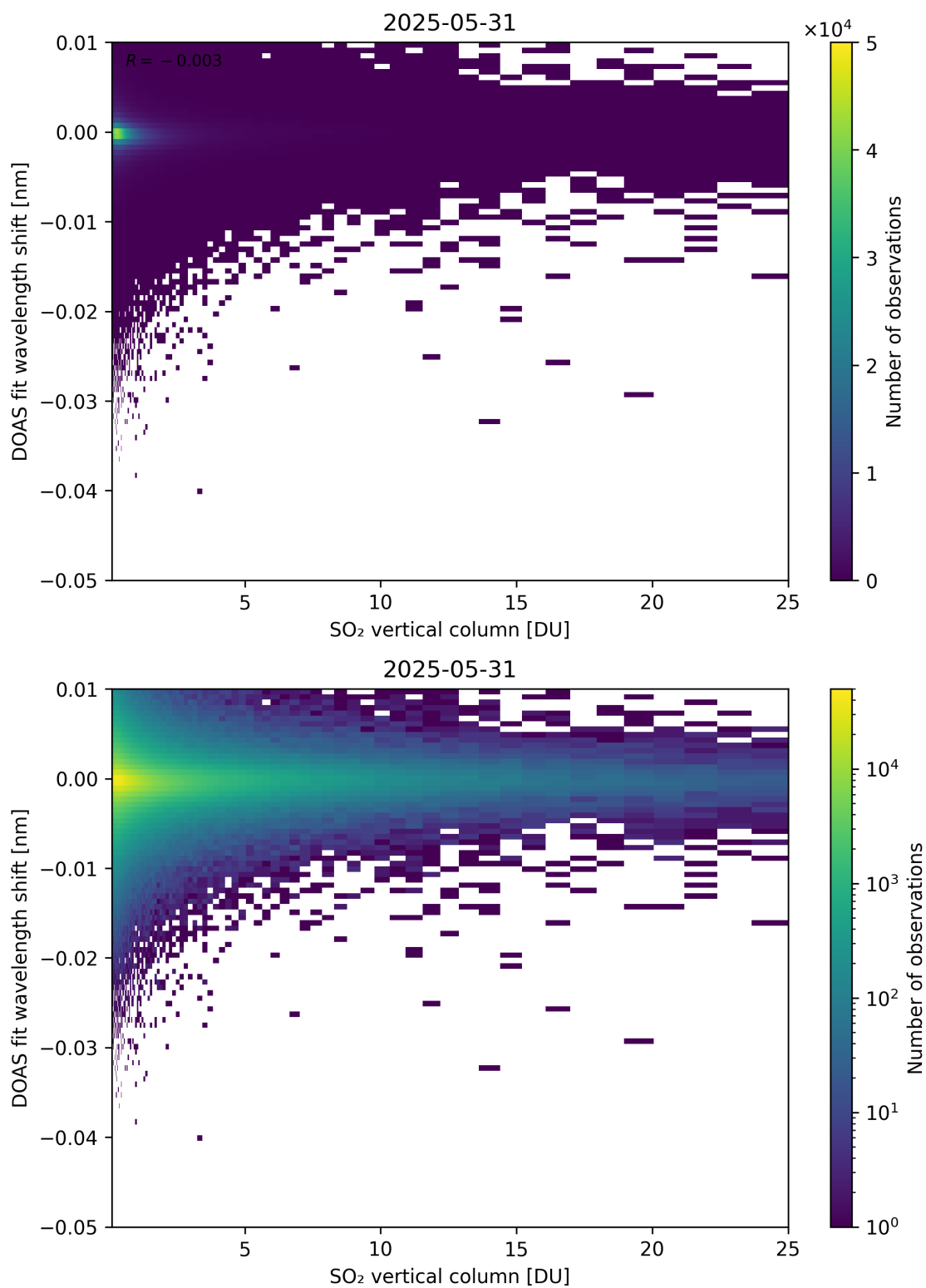
Figure 326: Scatter density plot of “SO 2 vertical column” against “DOAS fit wavelength shift” for 2025-05-31 to 2025-06-01.
