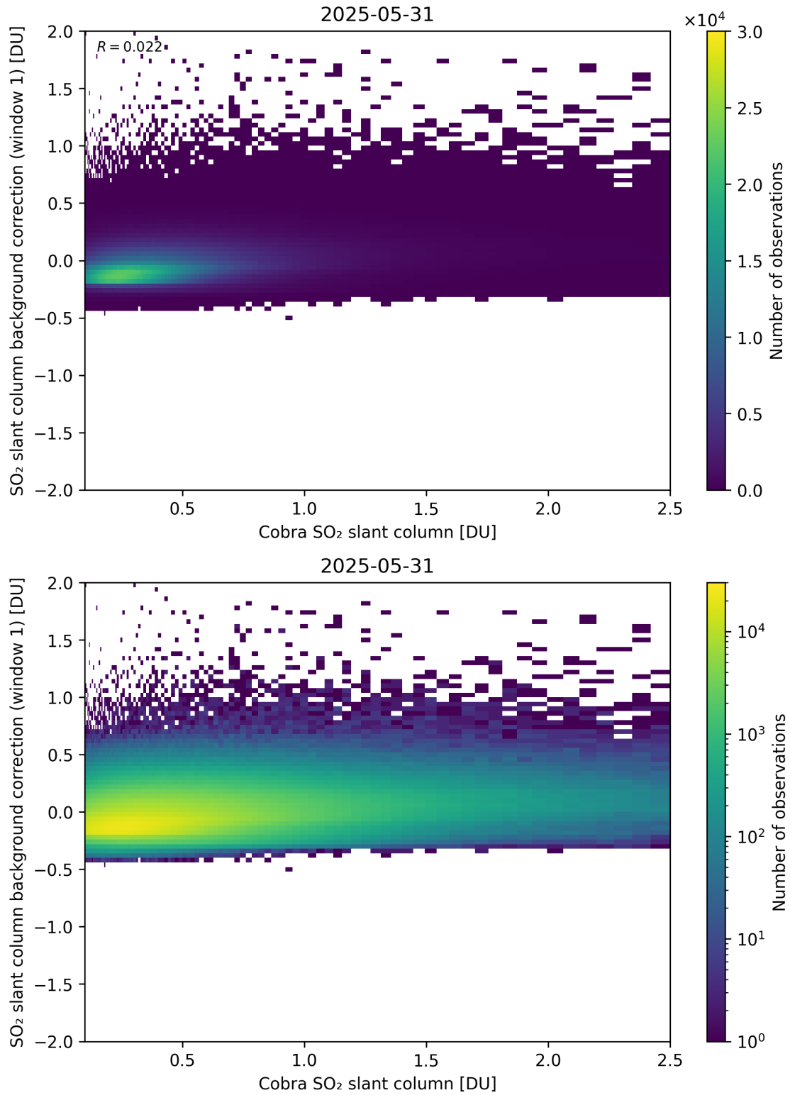
Figure 193: Scatter density plot of “Cobra SO 2 slant column” against “SO 2 slant column background correction (window 1)” for 2025-05-31 to 2025-06-01.
