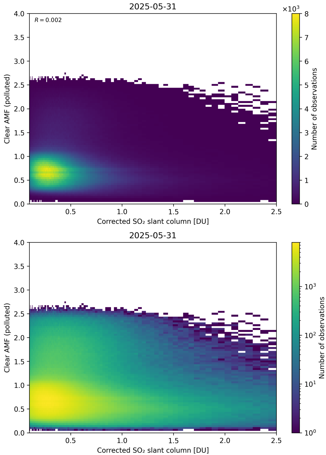
Figure 232: Scatter density plot of “Corrected SO 2 slant column” against “Clear AMF (polluted)” for 2025-05-31 to 2025-06-01.
