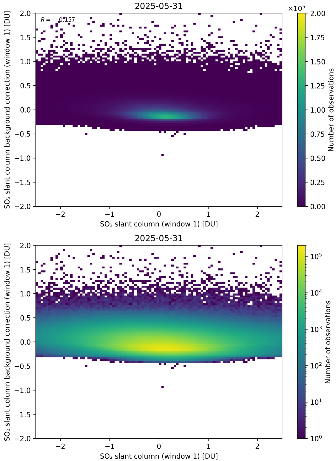
Figure 262: Scatter density plot of “SO 2 slant column (window 1)” against “SO 2 slant column background correction (window 1)” for 2025-05-31 to 2025-06-01.
