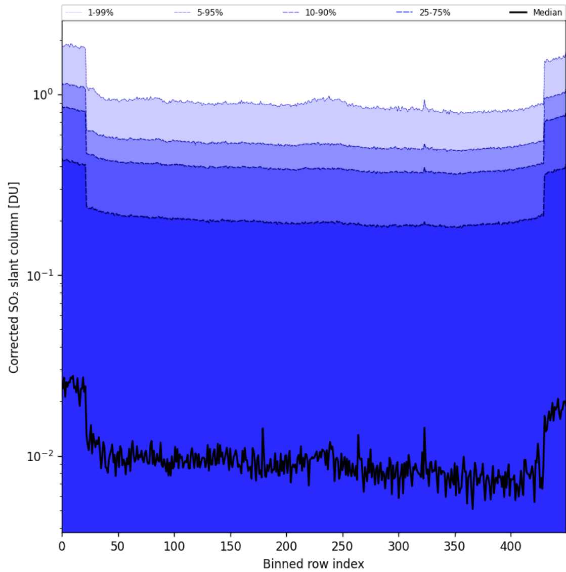
Figure 86: Along track statistics of “Corrected SO 2 slant column” for 2025-05-31 to 2025-06-01
