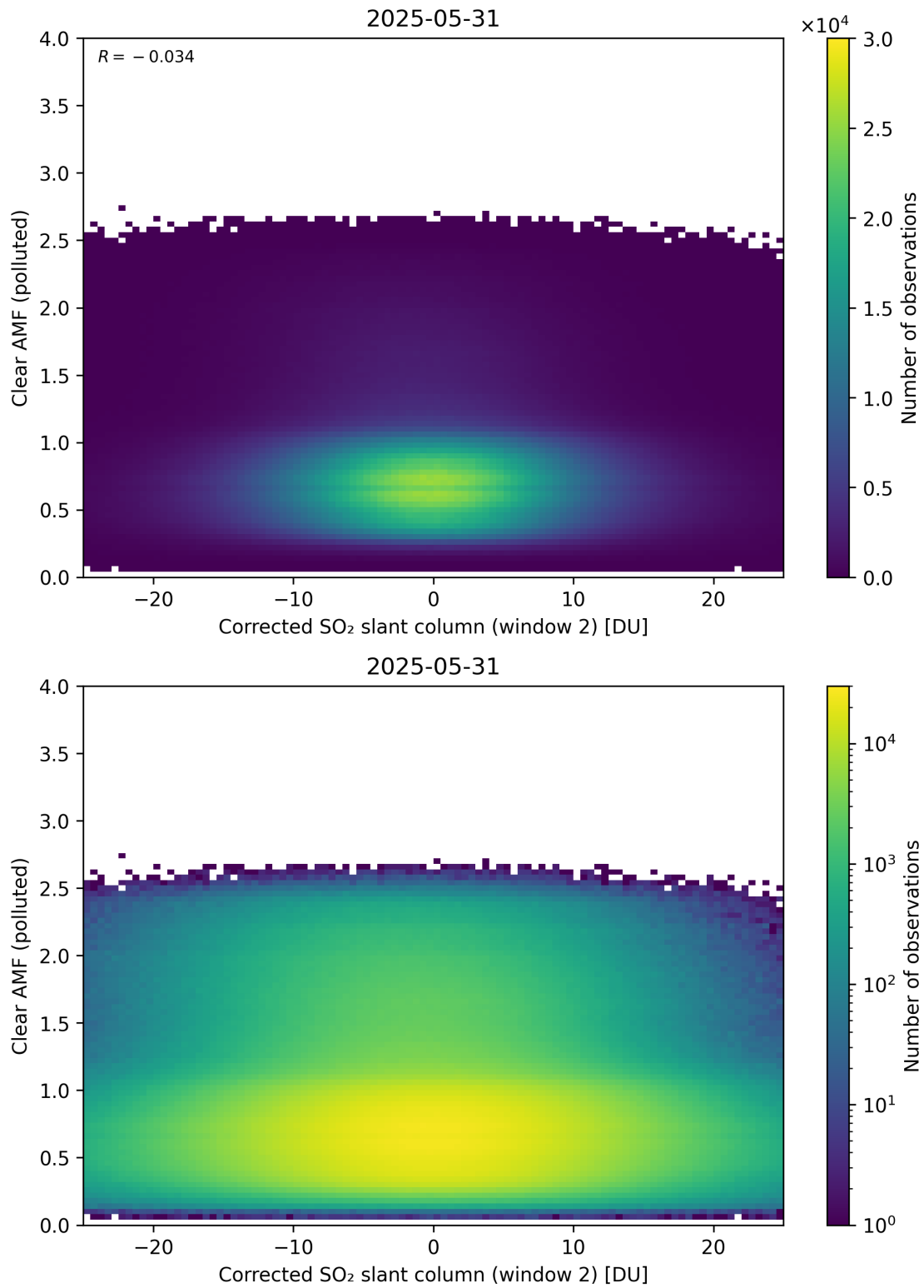
Figure 249: Scatter density plot of “Corrected SO 2 slant column (window 2)” against “Clear AMF (polluted)” for 2025-05-31 to 2025-06-01.
