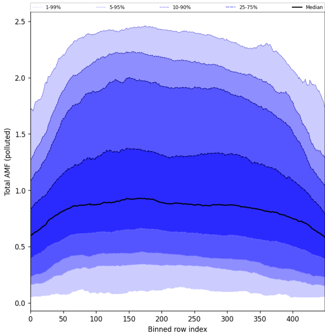
Figure 105: Along track statistics of “Total AMF (polluted)” for 2025-05-31 to 2025-06-01
