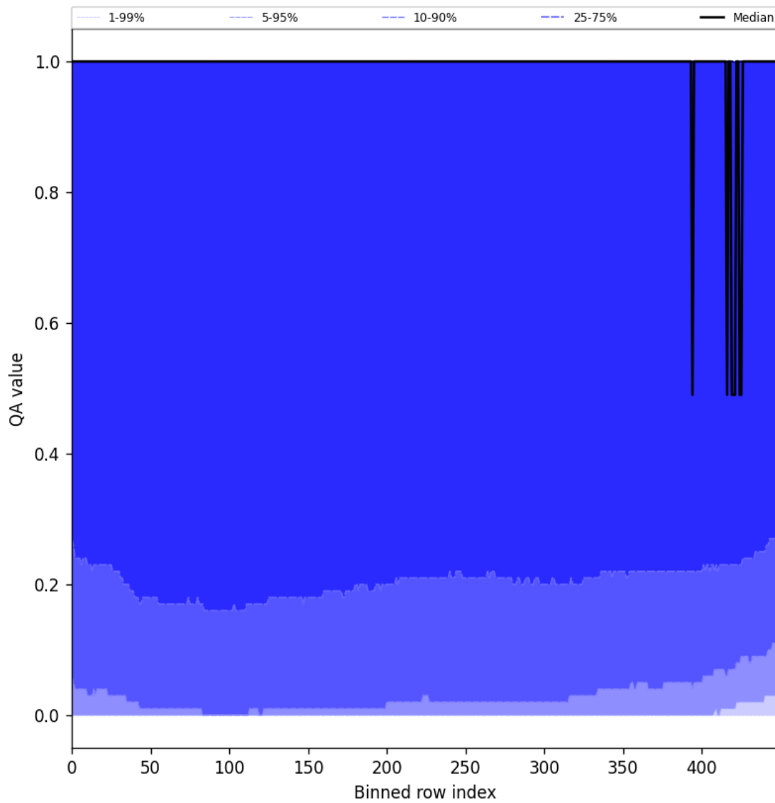
Figure 83: Along track statistics of “QA value” for 2025-05-31 to 2025-06-01
