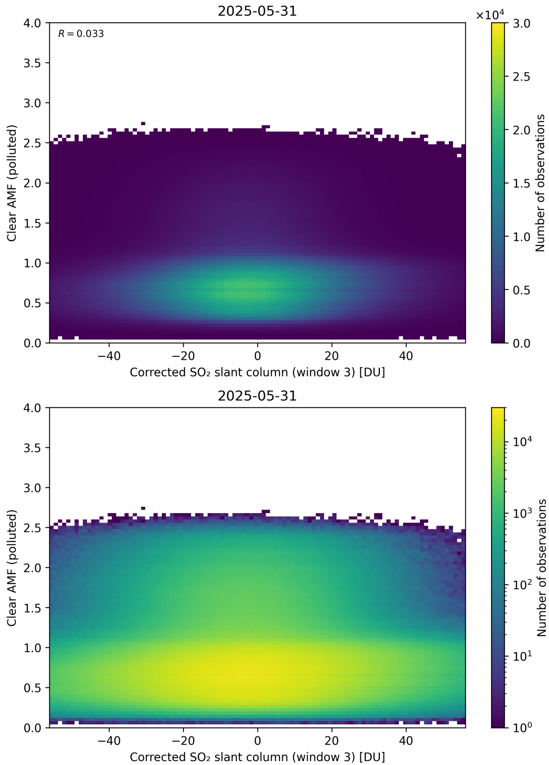
Figure 259: Scatter density plot of “Corrected SO 2 slant column (window 3)” against “Clear AMF (polluted)” for 2025-05-31 to 2025-06-01.
