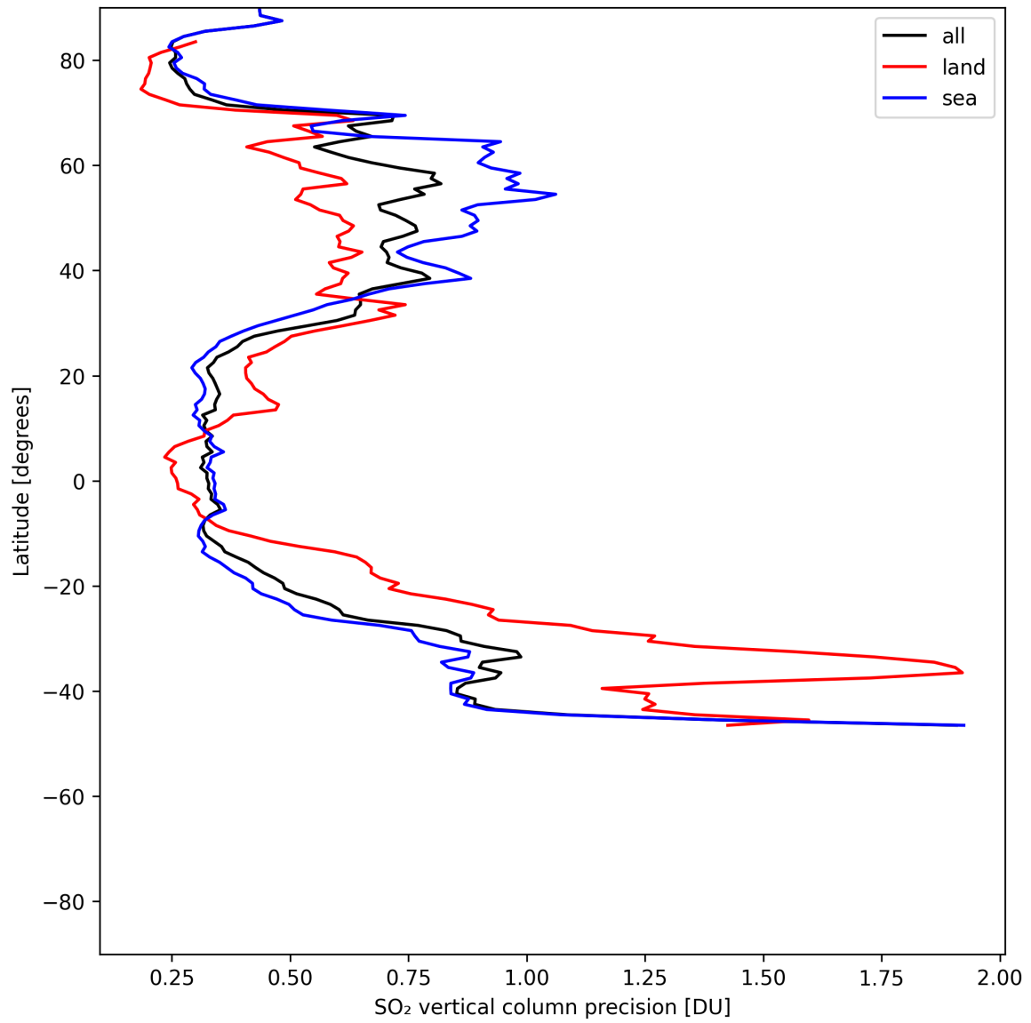
Figure 33: Zonal average of “SO 2 vertical column precision” for 2025-05-31 to 2025-06-01.
