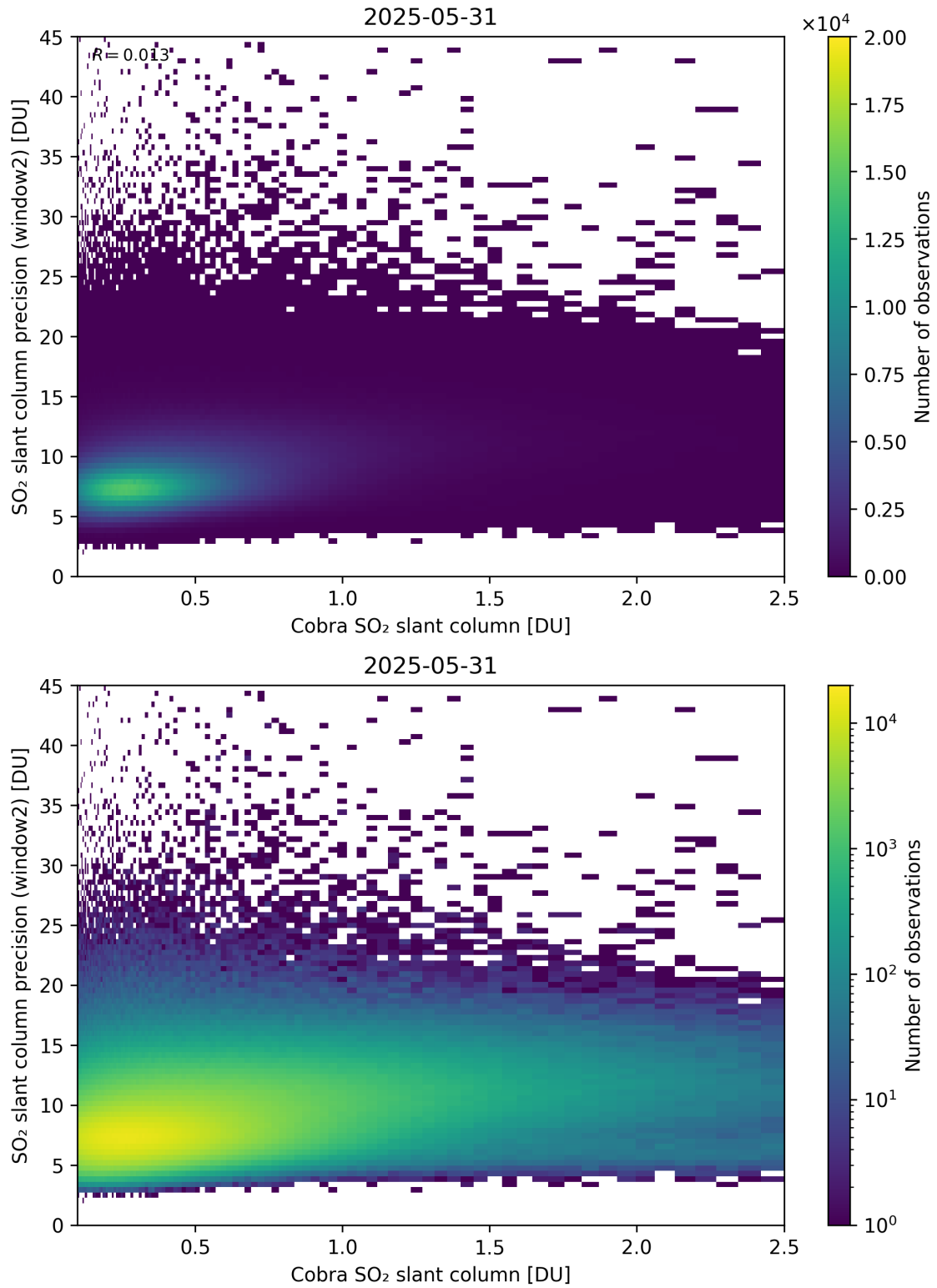
Figure 221: Scatter density plot of “Cobra SO 2 slant column” against “SO 2 slant column precision (window2)” for 2025-05-31 to 2025-06-01.
