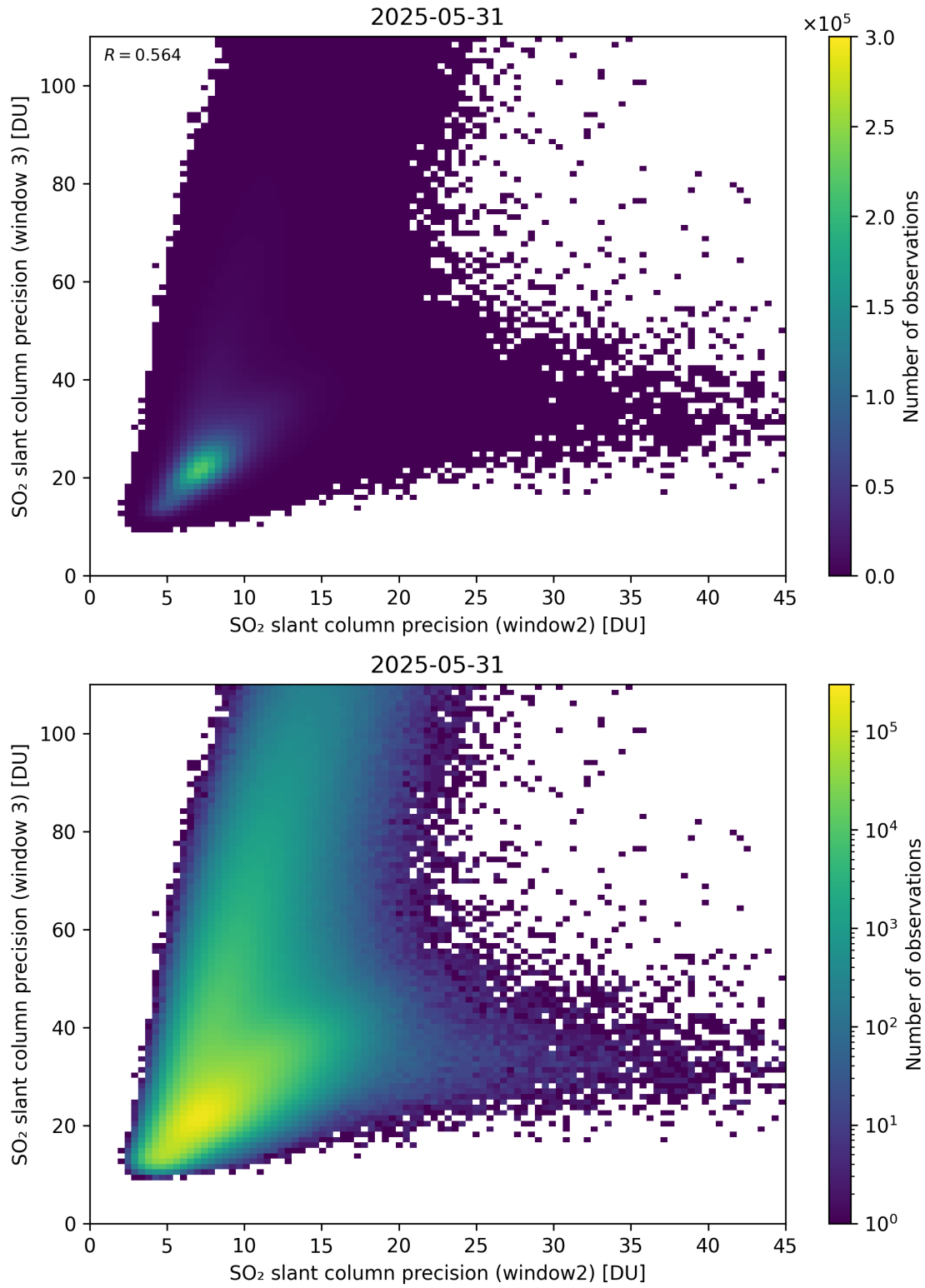
Figure 300: Scatter density plot of “SO 2 slant column precision (window2)” against “SO 2 slant column precision (window 3)” for 2025-05-31 to 2025-06-01.
