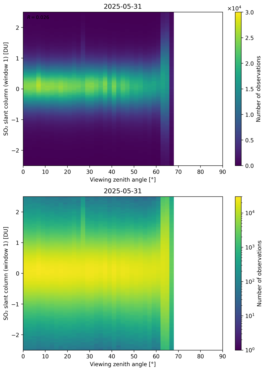
Figure 376: Scatter density plot of “Viewing zenith angle” against “SO 2 slant column (window 1)” for 2025-05-31 to 2025-06-01.
