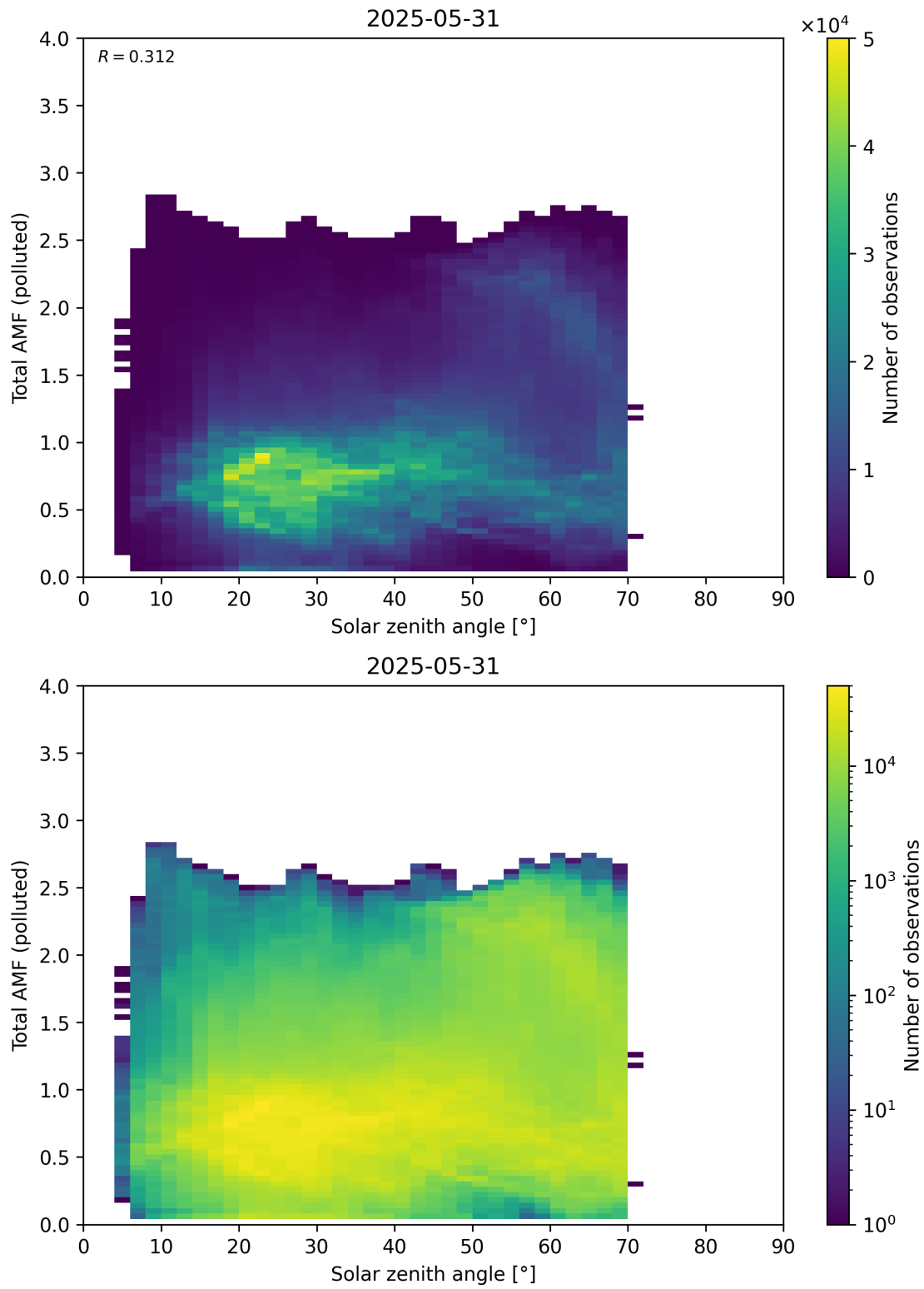
Figure 189: Scatter density plot of “Solar zenith angle” against “Total AMF (polluted)” for 2025-05-31 to 2025-06-01.
