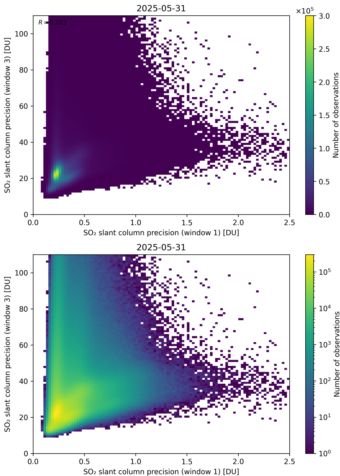
Figure 279: Scatter density plot of “SO 2 slant column precision (window 1)” against “SO 2 slant column precision (window 3)” for 2025-05-31 to 2025-06-01.
