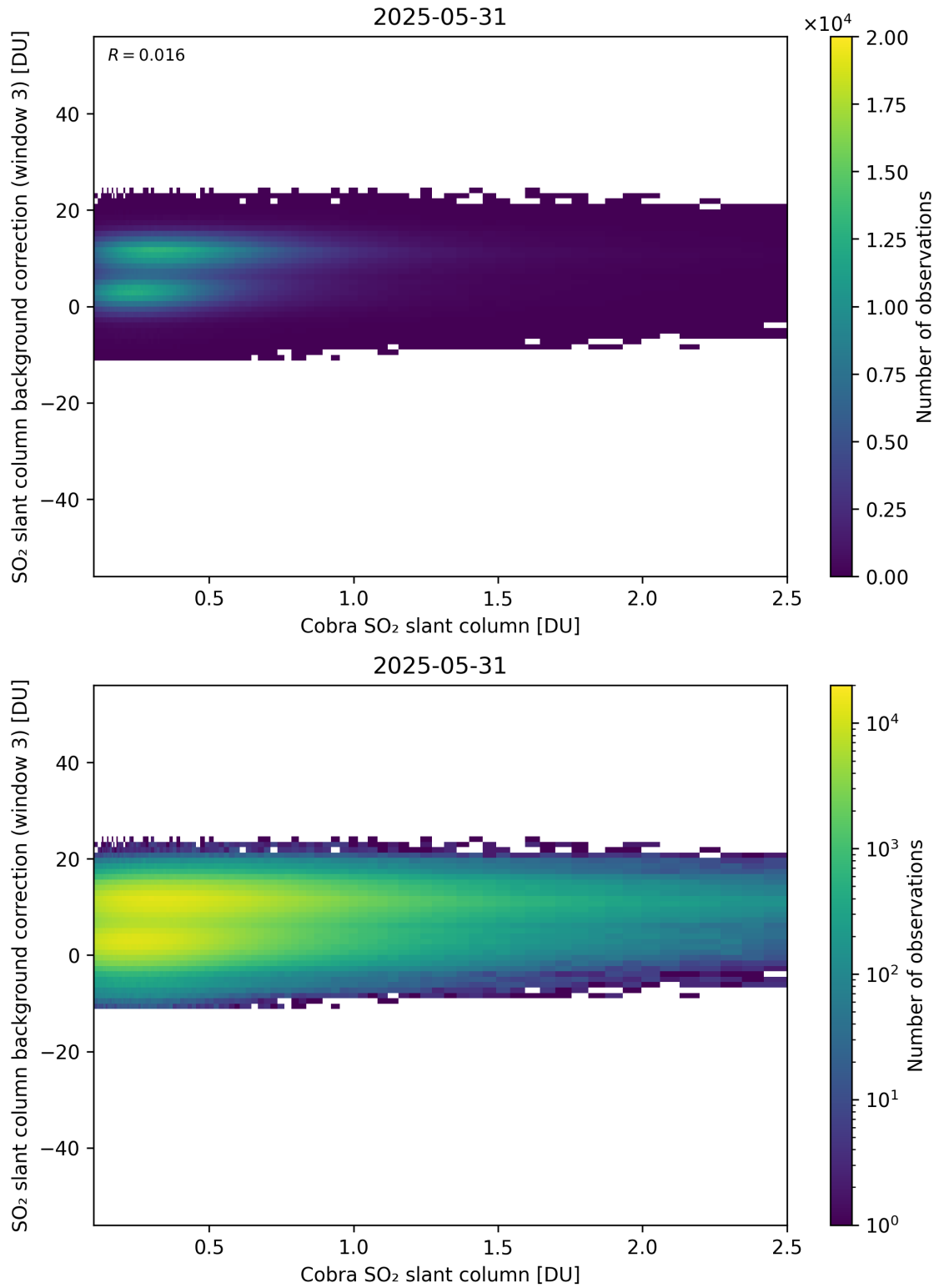
Figure 195: Scatter density plot of “Cobra SO 2 slant column” against “SO 2 slant column background correction (window 3)” for 2025-05-31 to 2025-06-01.
