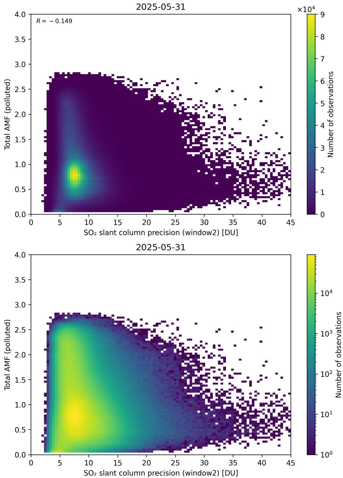
Figure 301: Scatter density plot of “SO 2 slant column precision (window2)” against “Total AMF (polluted)” for 2025-05-31 to 2025-06-01.
