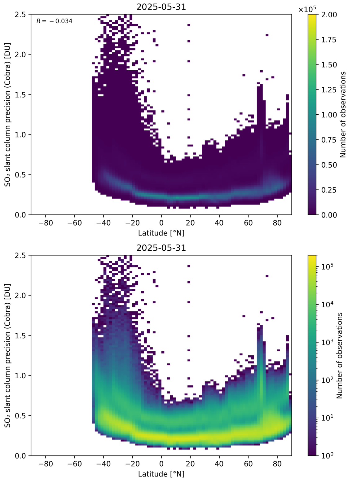
Figure 158: Scatter density plot of “Latitude” against “SO 2 slant column precision (Cobra)” for 2025-05-31 to 2025-06-01.
