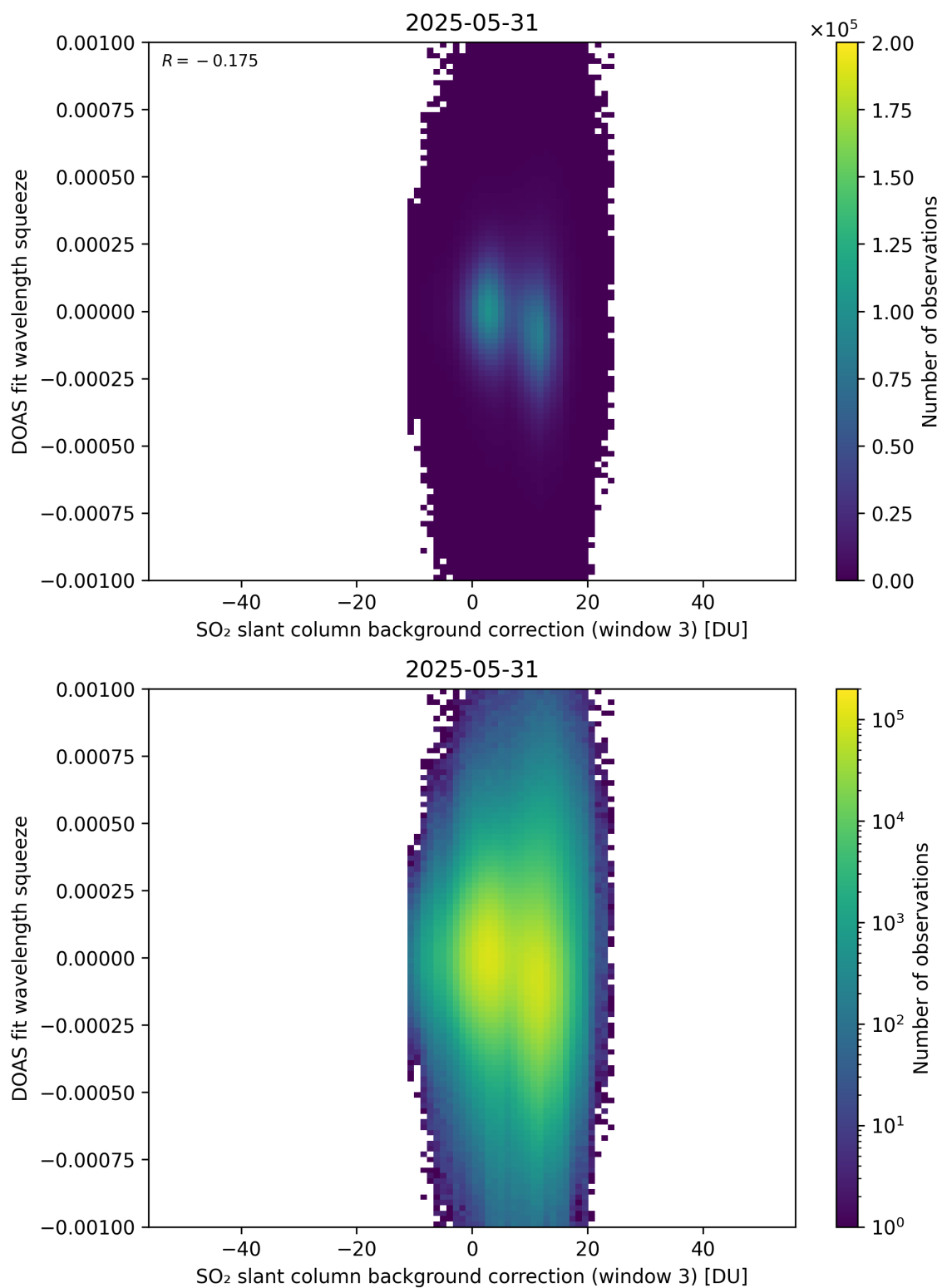
Figure 133: Scatter density plot of “SO 2 slant column background correction (window 3)” against “DOAS fit wavelength squeeze” for 2025-05-31 to 2025-06-01.
