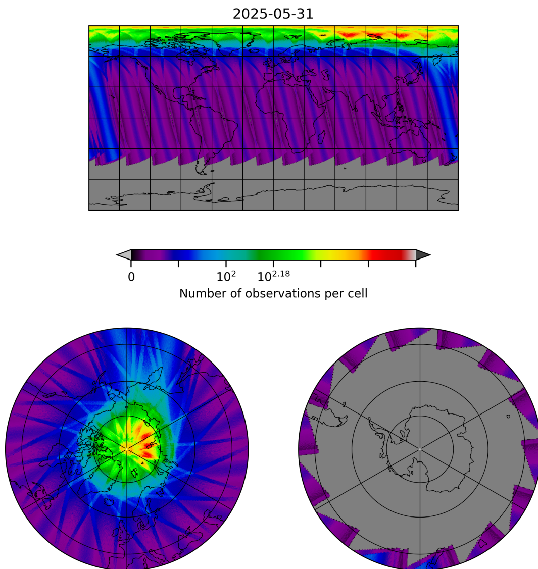
Figure 30: Map of the number of observations for 2025-05-31 to 2025-06-01
