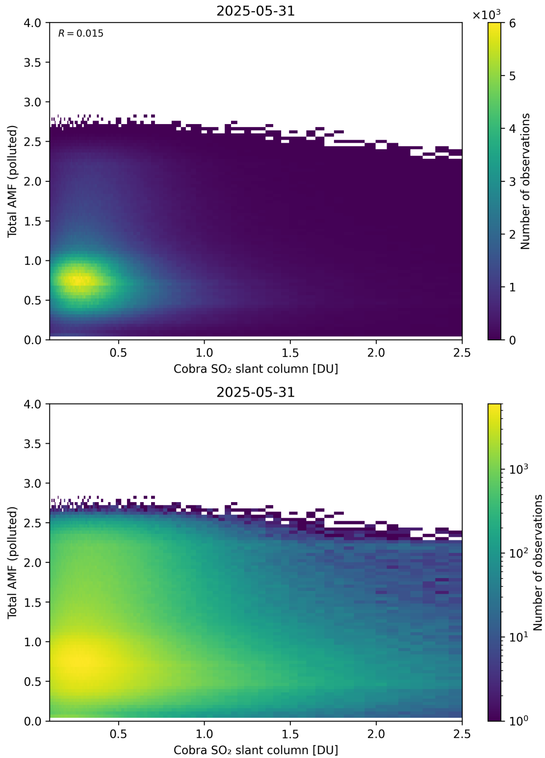
Figure 224: Scatter density plot of “Cobra SO 2 slant column” against “Total AMF (polluted)” for 2025-05-31 to 2025-06-01.
