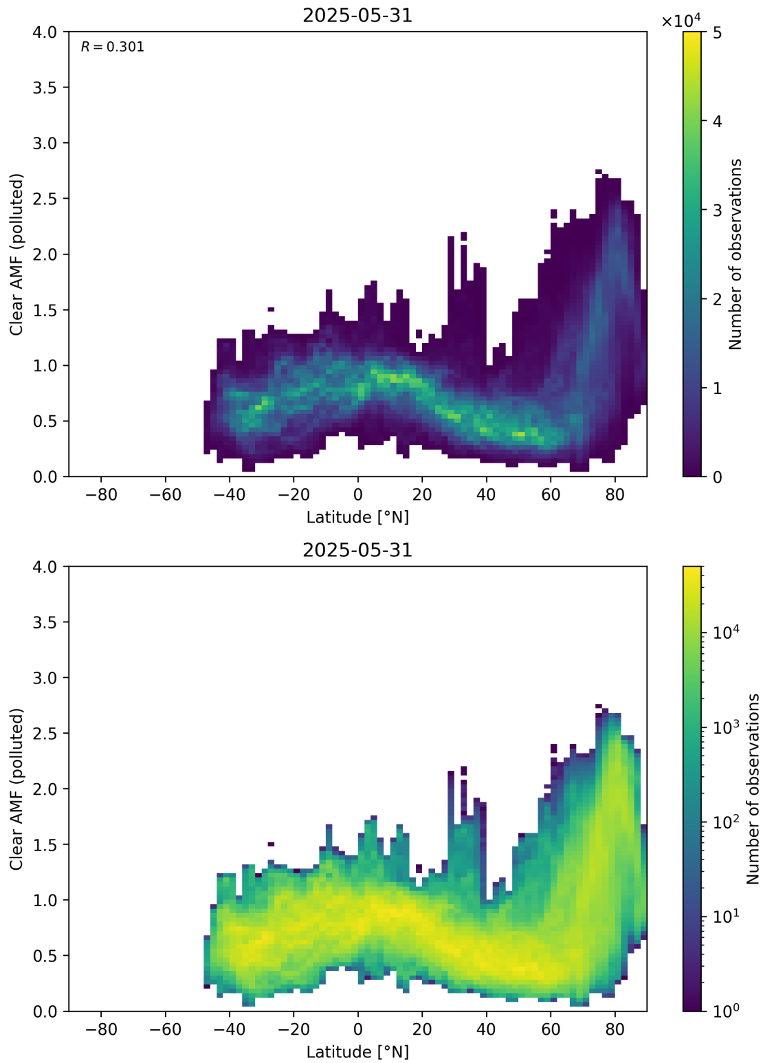
Figure 156: Scatter density plot of “Latitude” against “Clear AMF (polluted)” for 2025-05-31 to 2025-06-01.
