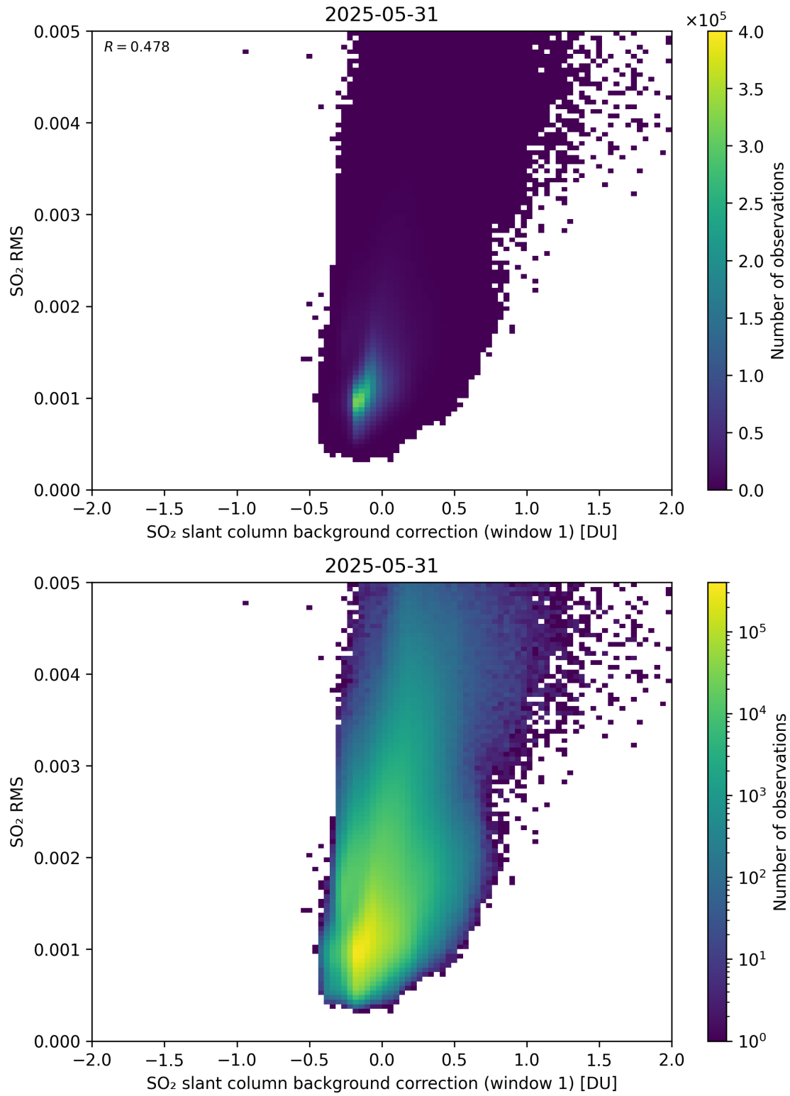
Figure 113: Scatter density plot of “SO 2 slant column background correction (window 1)” against “SO 2 RMS” for 2025-05-31 to 2025-06-01.
