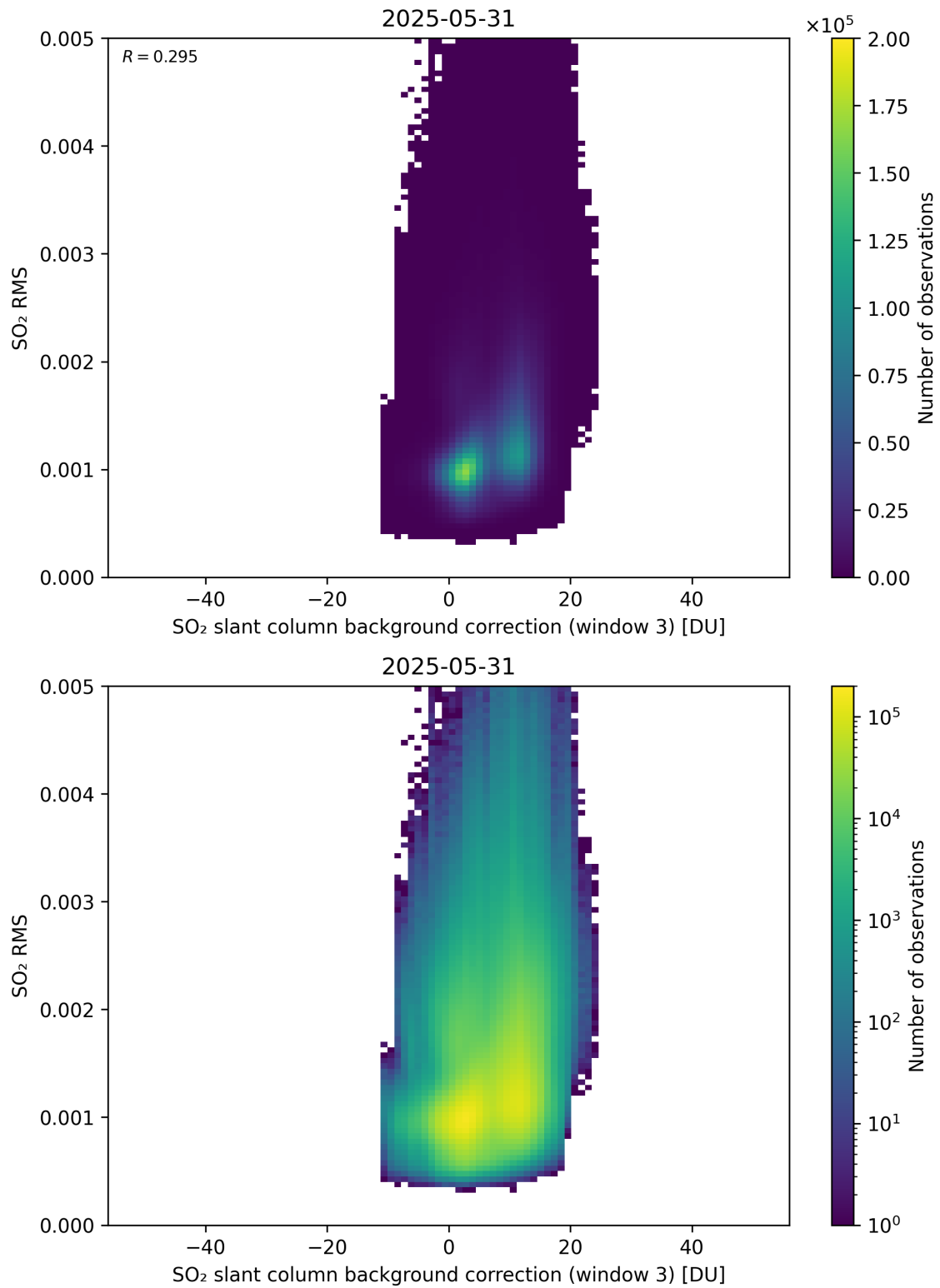
Figure 134: Scatter density plot of “SO 2 slant column background correction (window 3)” against “SO 2 RMS” for 2025-05-31 to 2025-06-01.
