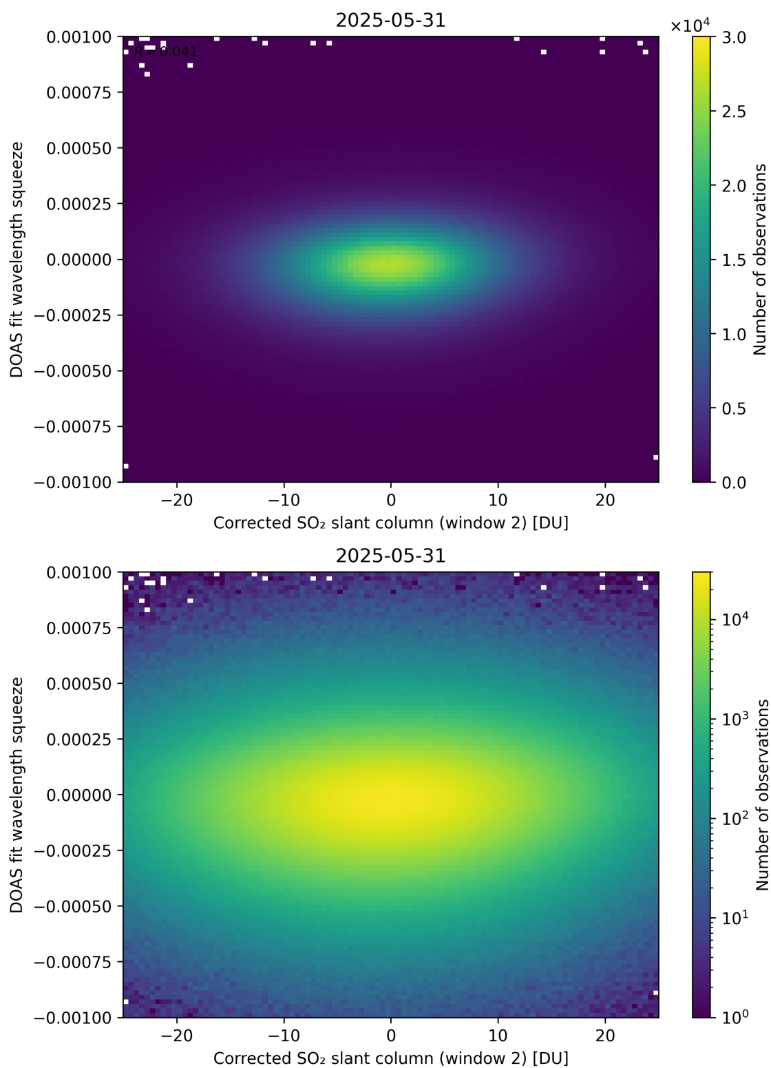
Figure 247: Scatter density plot of “Corrected SO 2 slant column (window 2)” against “DOAS fit wavelength squeeze” for 2025-05-31 to 2025-06-01.
