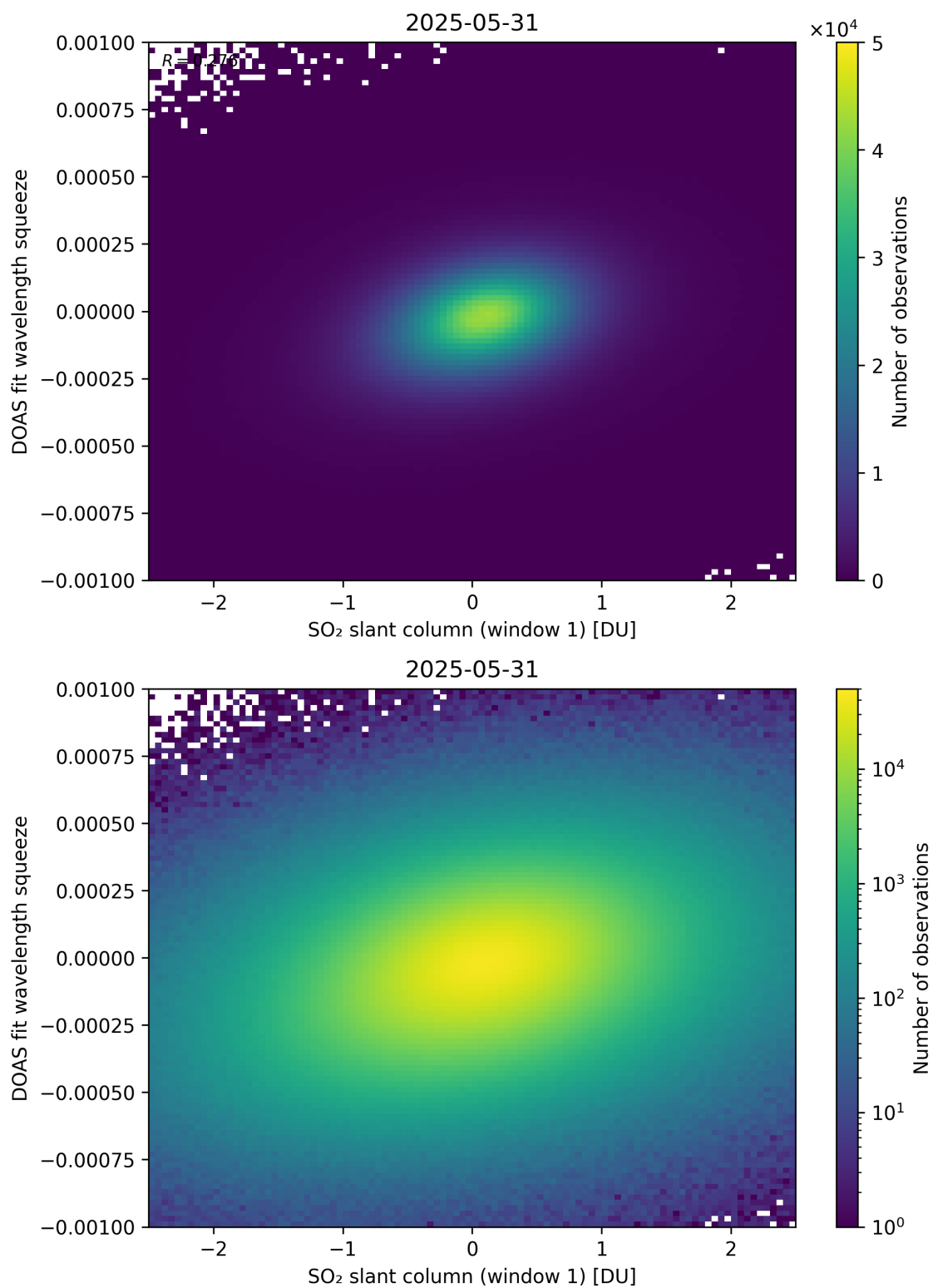
Figure 266: Scatter density plot of “SO 2 slant column (window 1)” against “DOAS fit wavelength squeeze” for 2025-05-31 to 2025-06-01.
