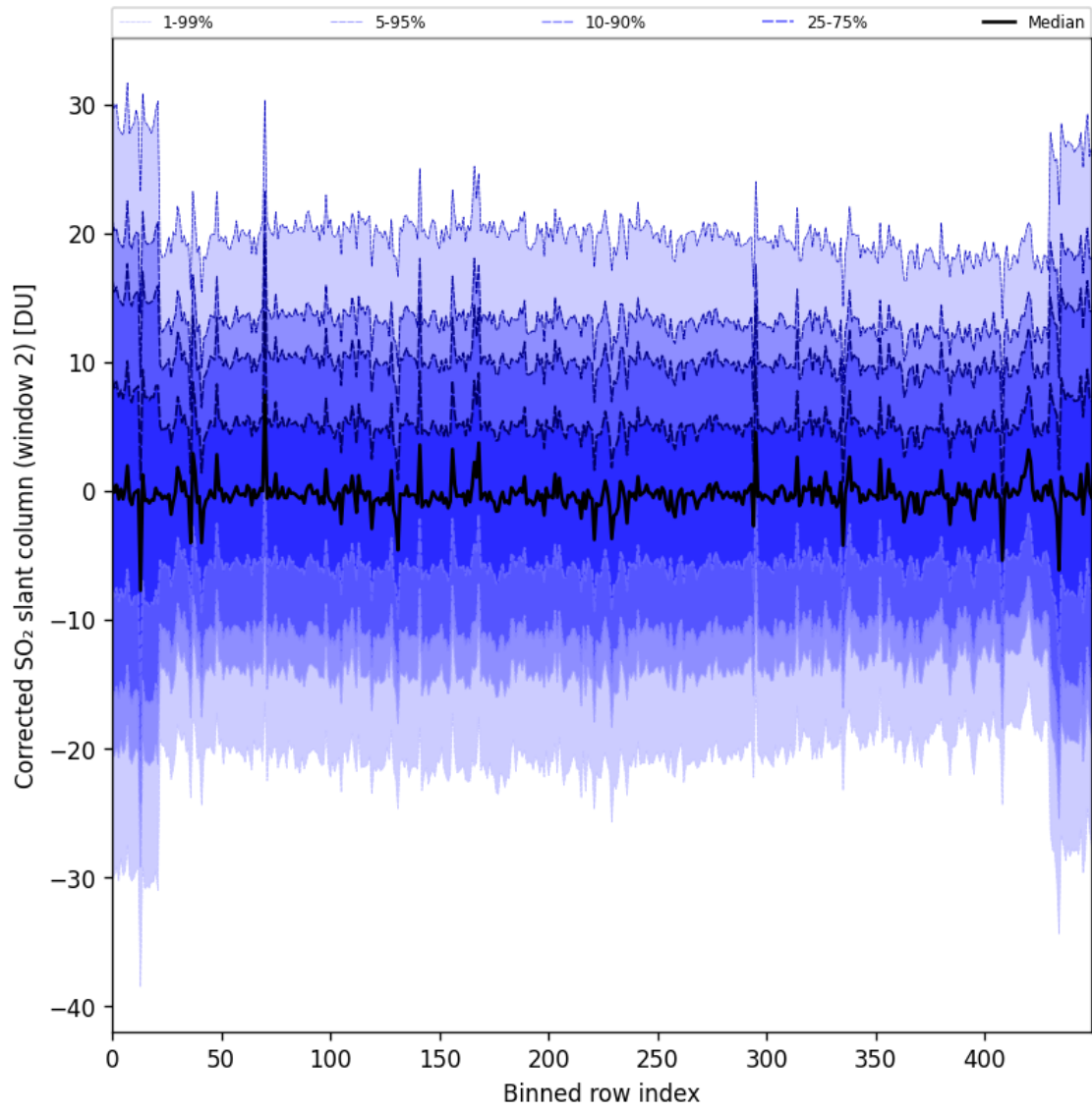
Figure 95: Along track statistics of “Corrected SO 2 slant column (window 2)” for 2025-05-31 to 2025-06-01
