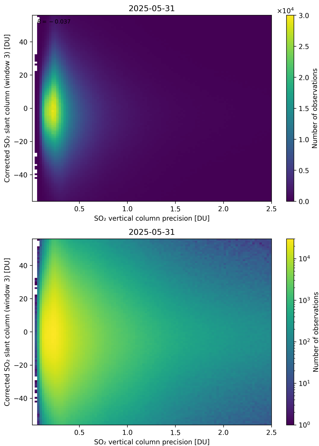
Figure 340: Scatter density plot of “SO 2 vertical column precision” against “Corrected SO 2 slant column (window 3)” for 2025-05-31 to 2025-06-01.
