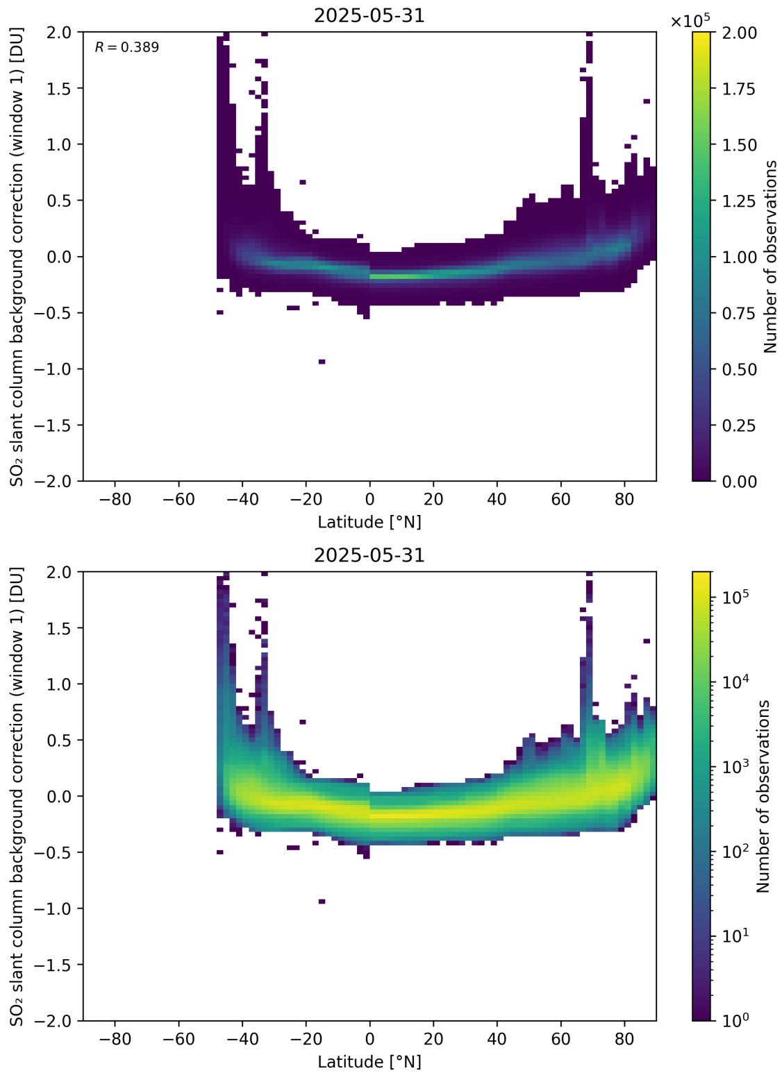
Figure 150: Scatter density plot of “Latitude” against “SO 2 slant column background correction (window 1)” for 2025-05-31 to 2025-06-01.
