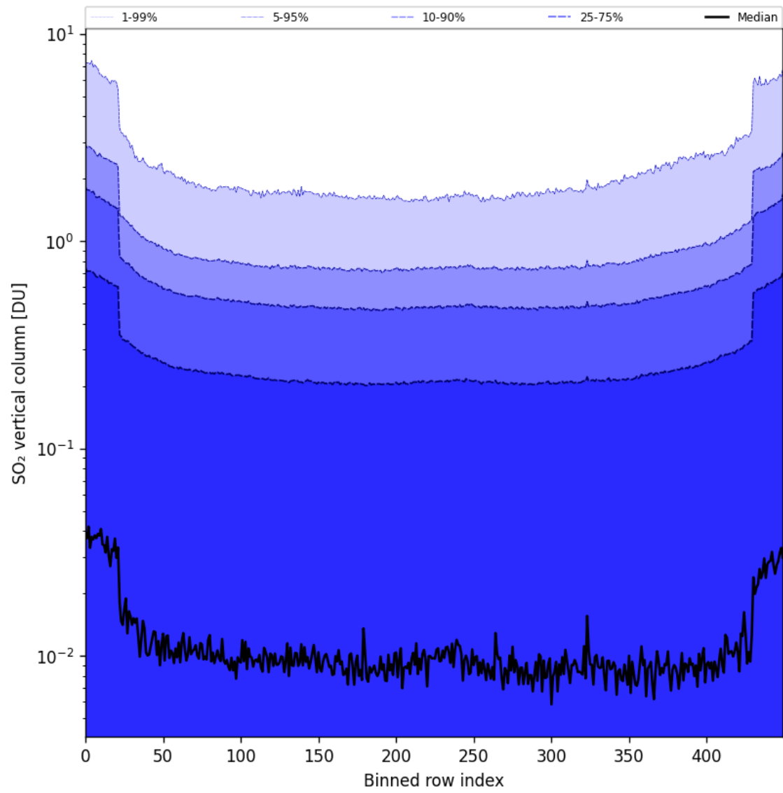
Figure 84: Along track statistics of “SO 2 vertical column” for 2025-05-31 to 2025-06-01
