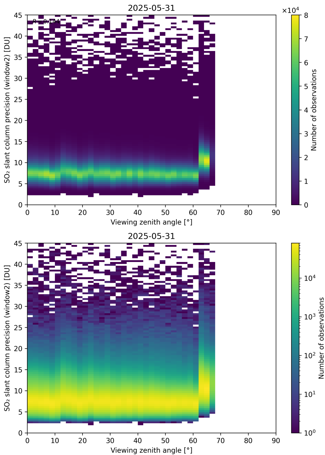
Figure 378: Scatter density plot of “Viewing zenith angle” against “SO 2 slant column precision (window2)” for 2025-05-31 to 2025-06-01.
