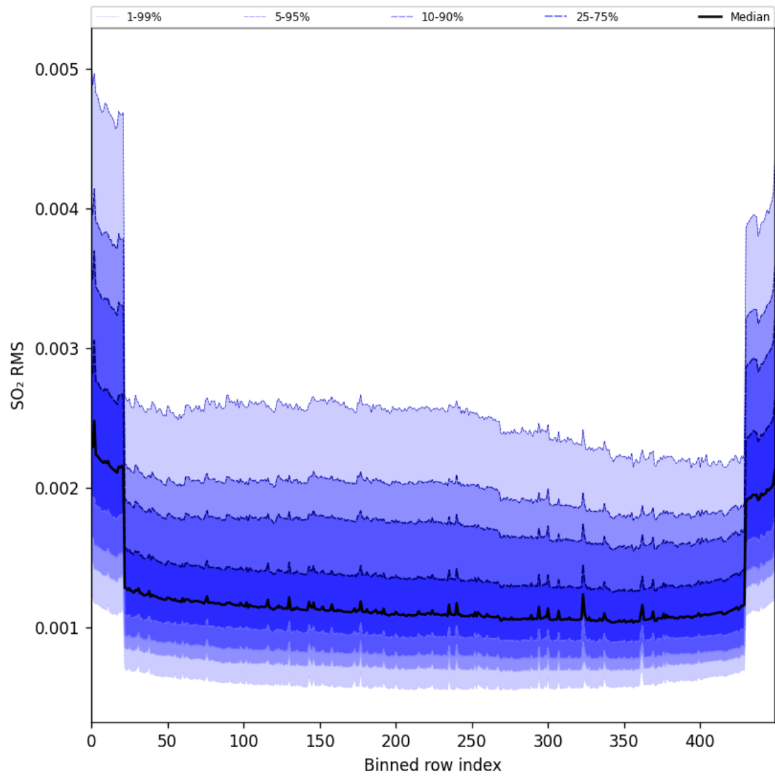
Figure 104: Along track statistics of “SO 2 RMS” for 2025-05-31 to 2025-06-01
