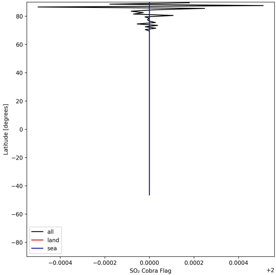
Figure 49: Zonal average of “SO 2 Cobra Flag” for 2025-05-31 to 2025-06-01.
