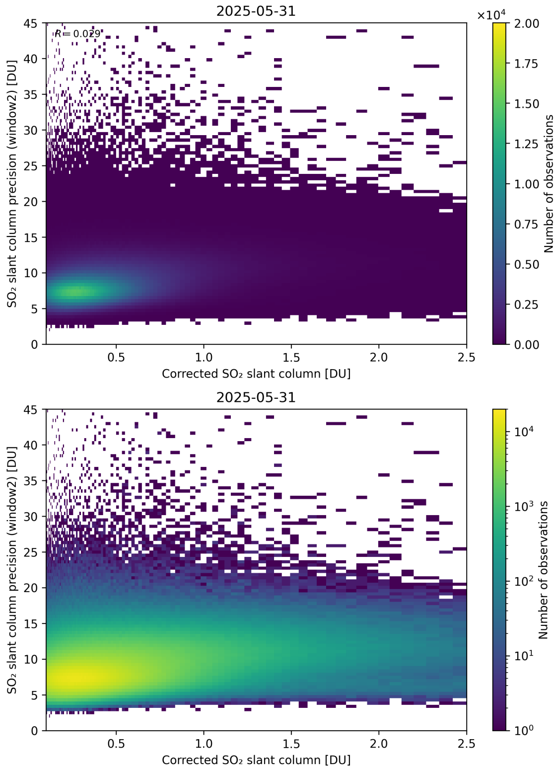
Figure 239: Scatter density plot of “Corrected SO 2 slant column” against “SO 2 slant column precision (window2)” for 2025-05-31 to 2025-06-01.
