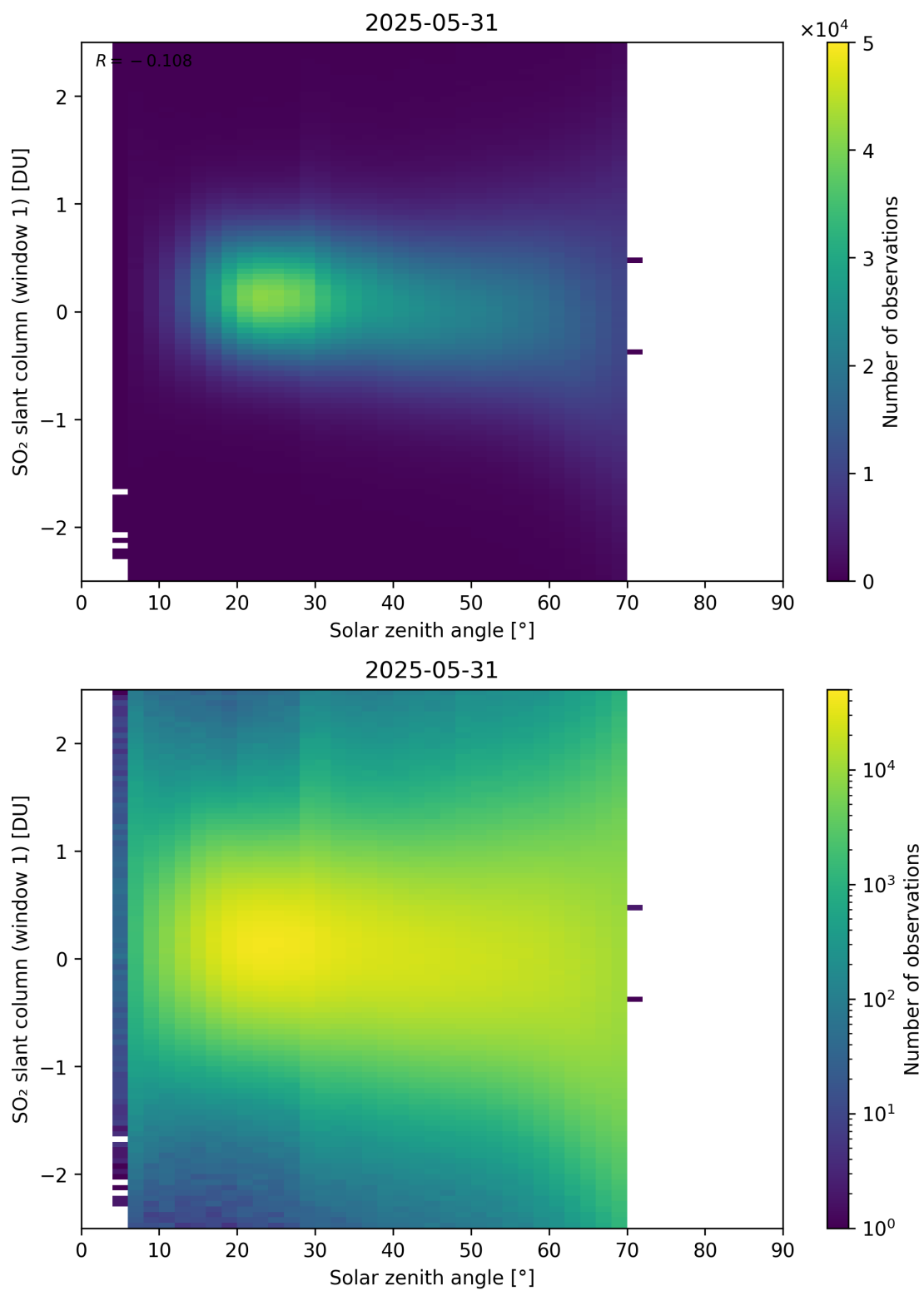
Figure 184: Scatter density plot of “Solar zenith angle” against “SO 2 slant column (window 1)” for 2025-05-31 to 2025-06-01.
