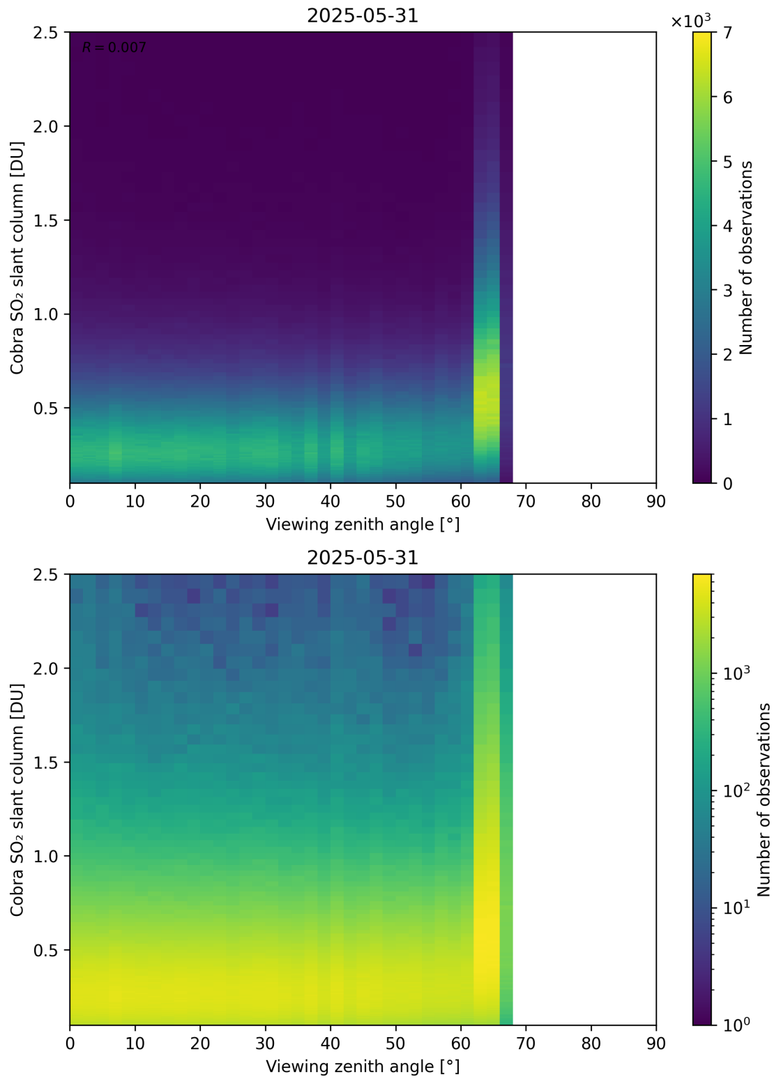
Figure 371: Scatter density plot of “Viewing zenith angle” against “Cobra SO 2 slant column” for 2025-05-31 to 2025-06-01.
