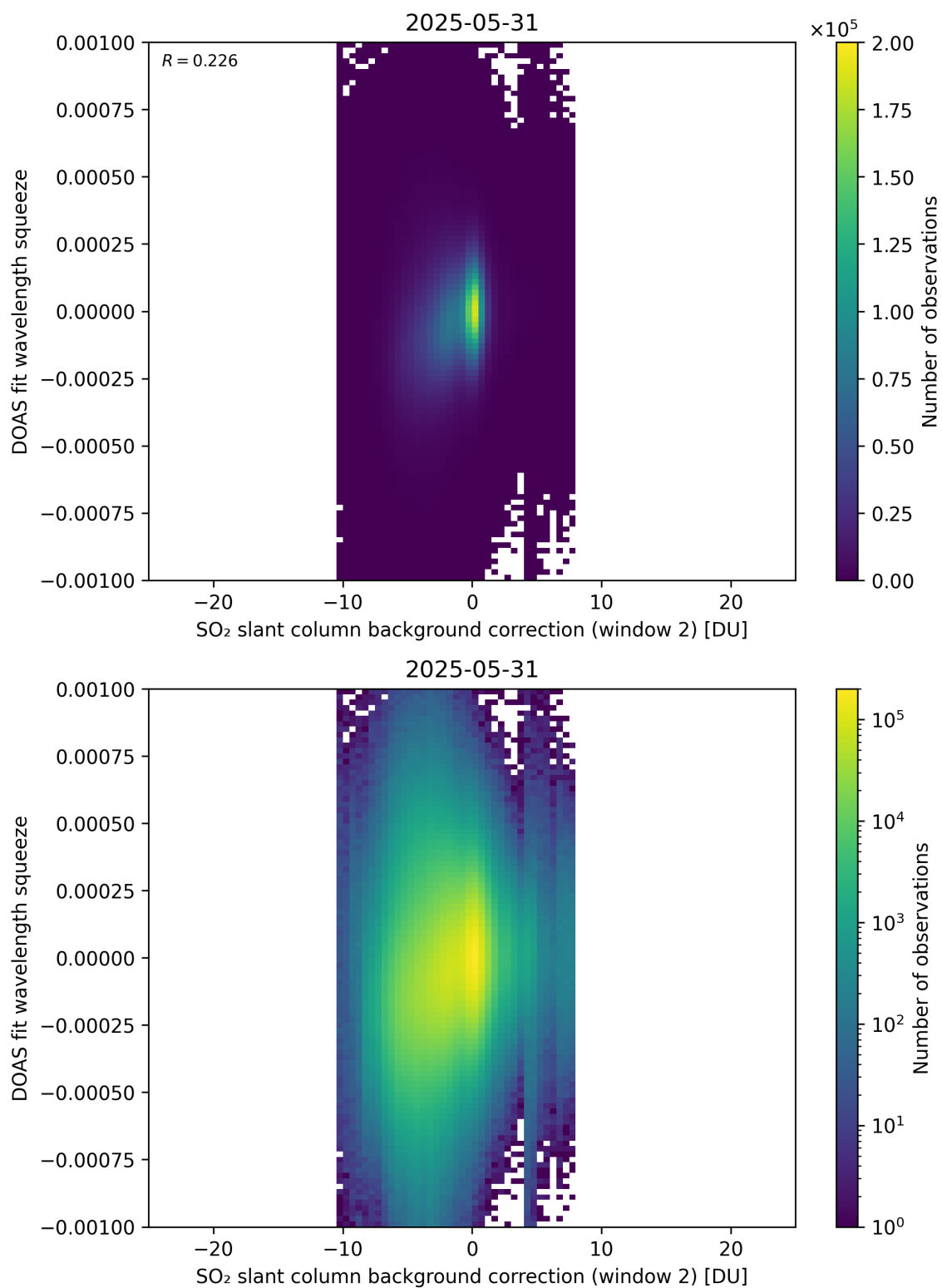
Figure 124: Scatter density plot of “SO 2 slant column background correction (window 2)” against “DOAS fit wavelength squeeze” for 2025-05-31 to 2025-06-01.
