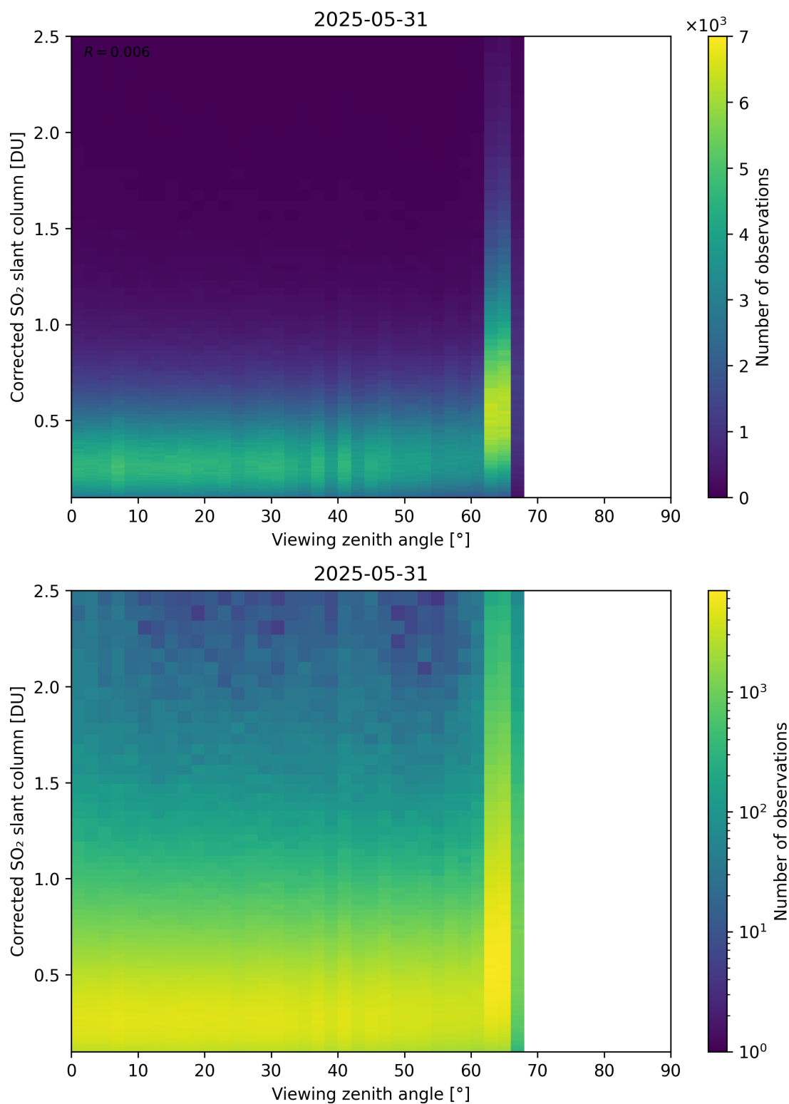
Figure 373: Scatter density plot of “Viewing zenith angle” against “Corrected SO 2 slant column” for 2025-05-31 to 2025-06-01.
