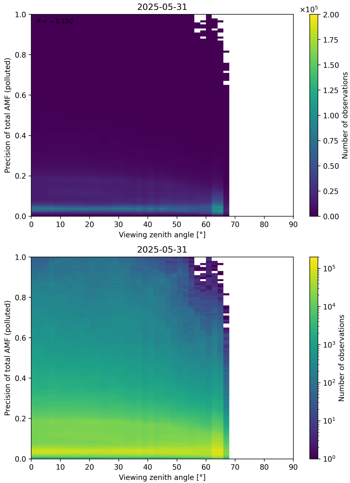
Figure 382: Scatter density plot of “Viewing zenith angle” against “Precision of total AMF (polluted)” for 2025-05-31 to 2025-06-01.
