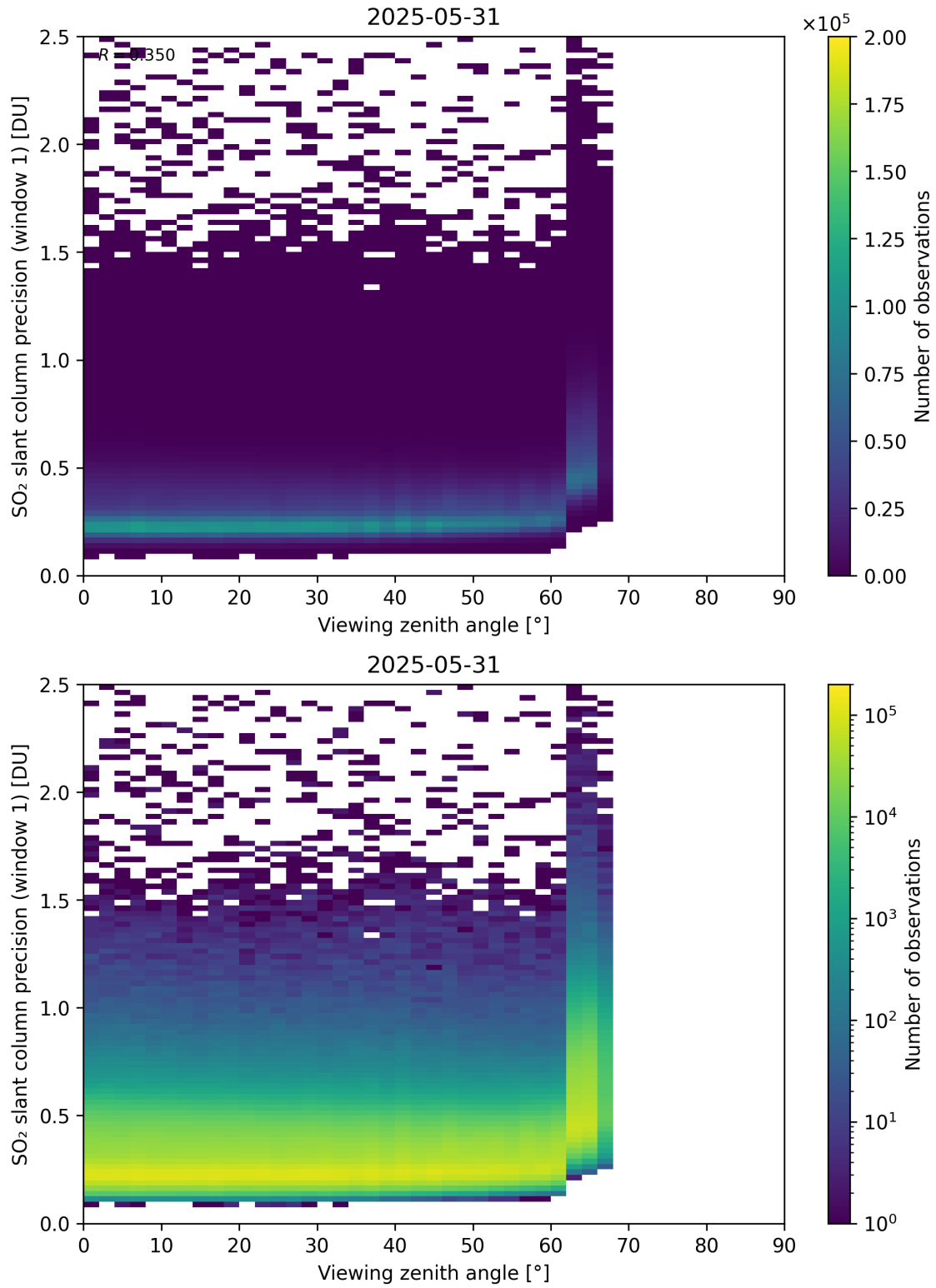
Figure 377: Scatter density plot of “Viewing zenith angle” against “SO 2 slant column precision (window 1)” for 2025-05-31 to 2025-06-01.
