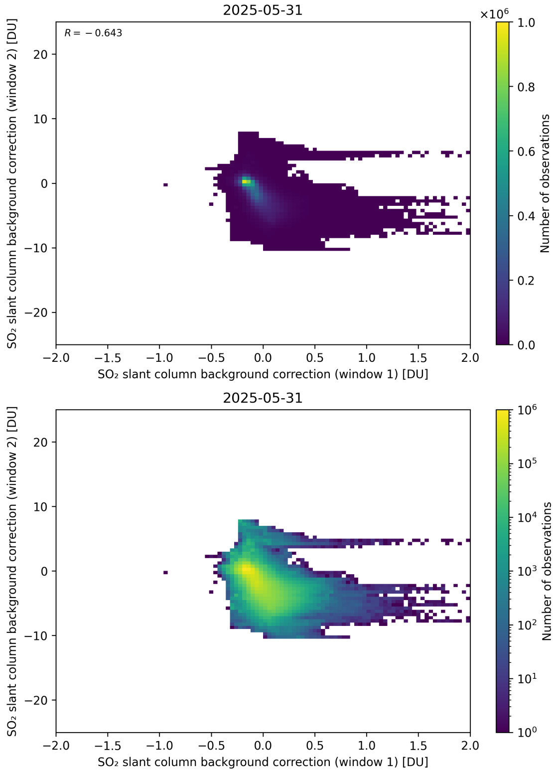
Figure 109: Scatter density plot of “SO 2 slant column background correction (window 1)” against “SO 2 slant column background correction (window 2)” for 2025-05-31 to 2025-06-01.
