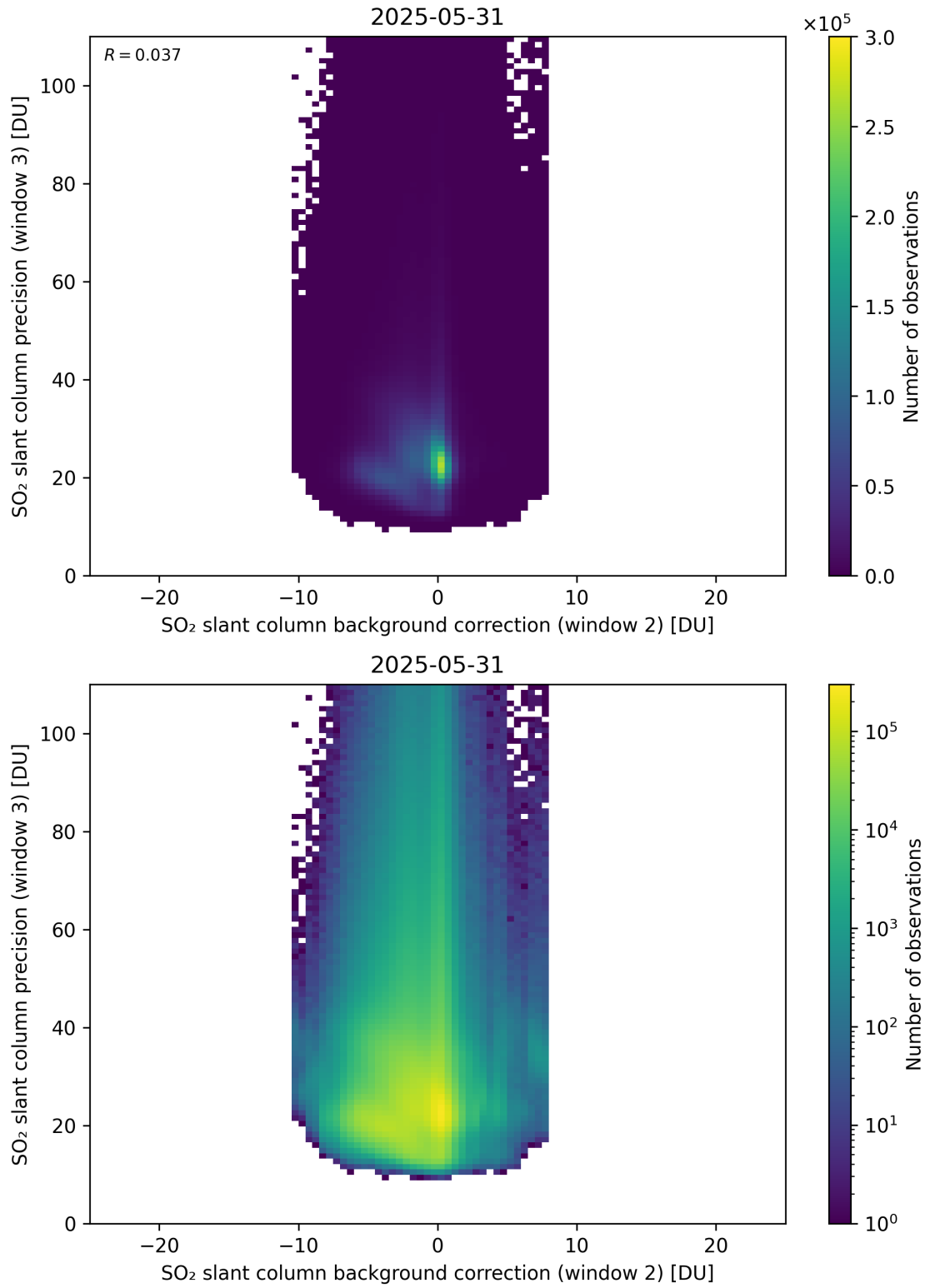
Figure 129: Scatter density plot of “SO 2 slant column background correction (window 2)” against “SO 2 slant column precision (window 3)” for 2025-05-31 to 2025-06-01.
