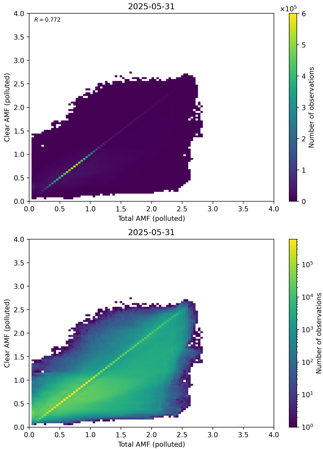
Figure 321: Scatter density plot of “Total AMF (polluted)” against “Clear AMF (polluted)” for 2025-05-31 to 2025-06-01.
