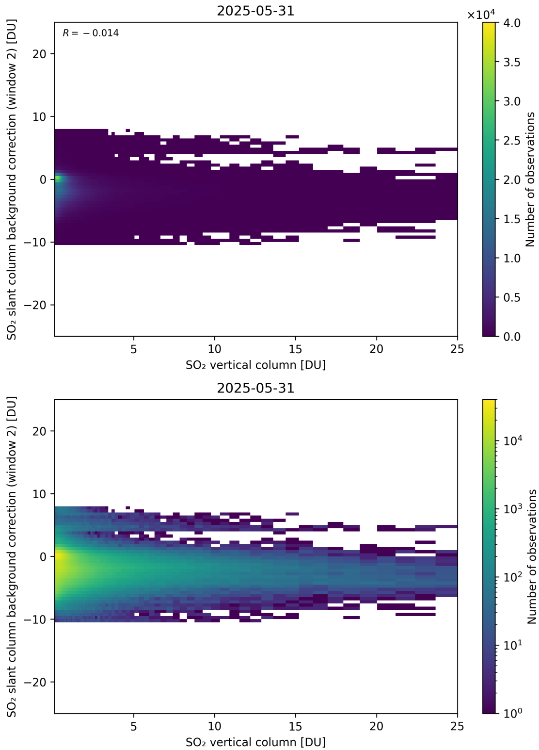
Figure 324: Scatter density plot of “SO 2 vertical column” against “SO 2 slant column background correction (window 2)” for 2025-05-31 to 2025-06-01.
