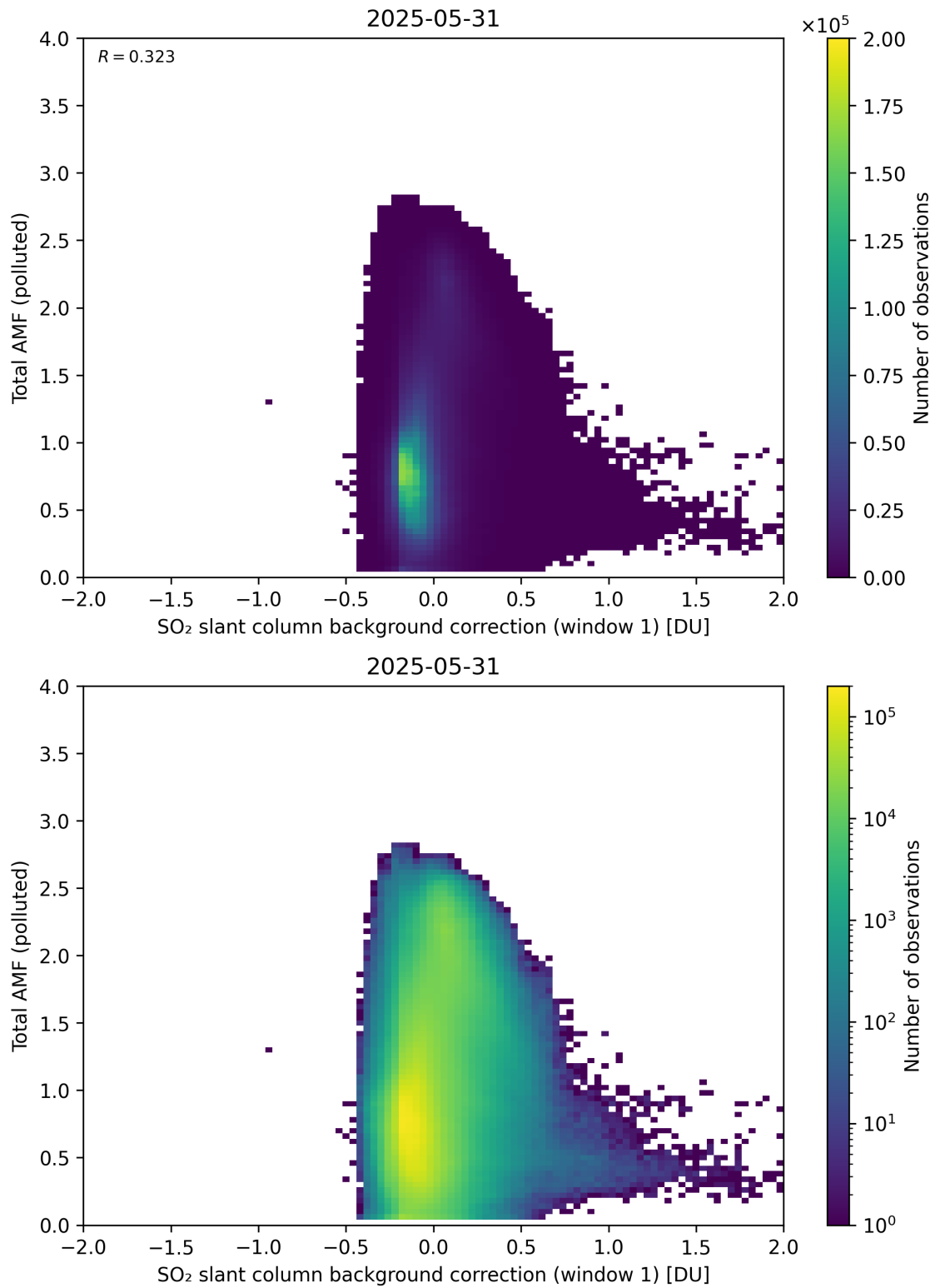
Figure 120: Scatter density plot of “SO 2 slant column background correction (window 1)” against “Total AMF (polluted)” for 2025-05-31 to 2025-06-01.
