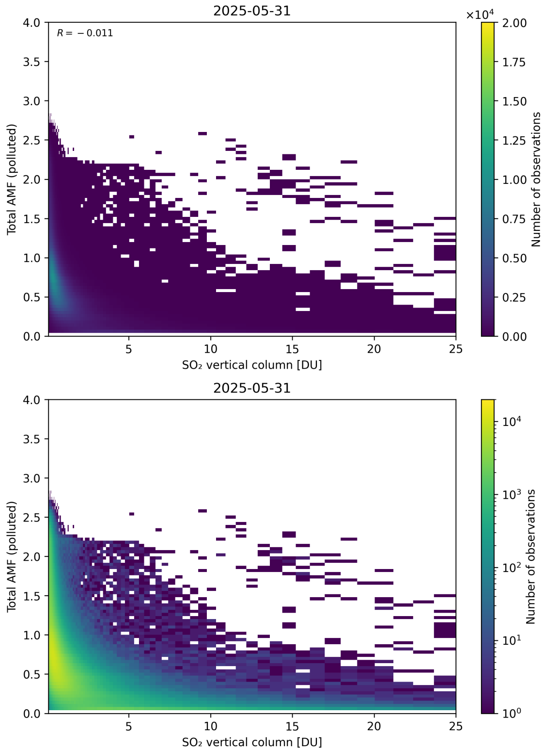
Figure 359: Scatter density plot of “SO 2 vertical column” against “Total AMF (polluted)” for 2025-05-31 to 2025-06-01.
