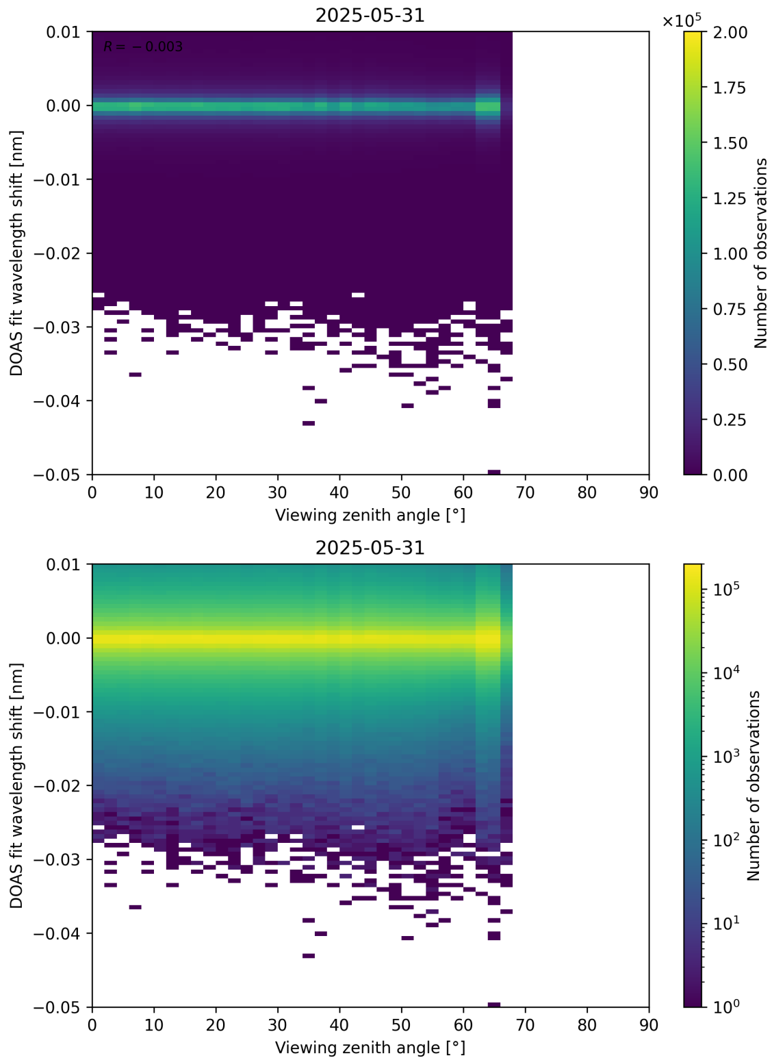
Figure 365: Scatter density plot of “Viewing zenith angle” against “DOAS fit wavelength shift” for 2025-05-31 to 2025-06-01.
