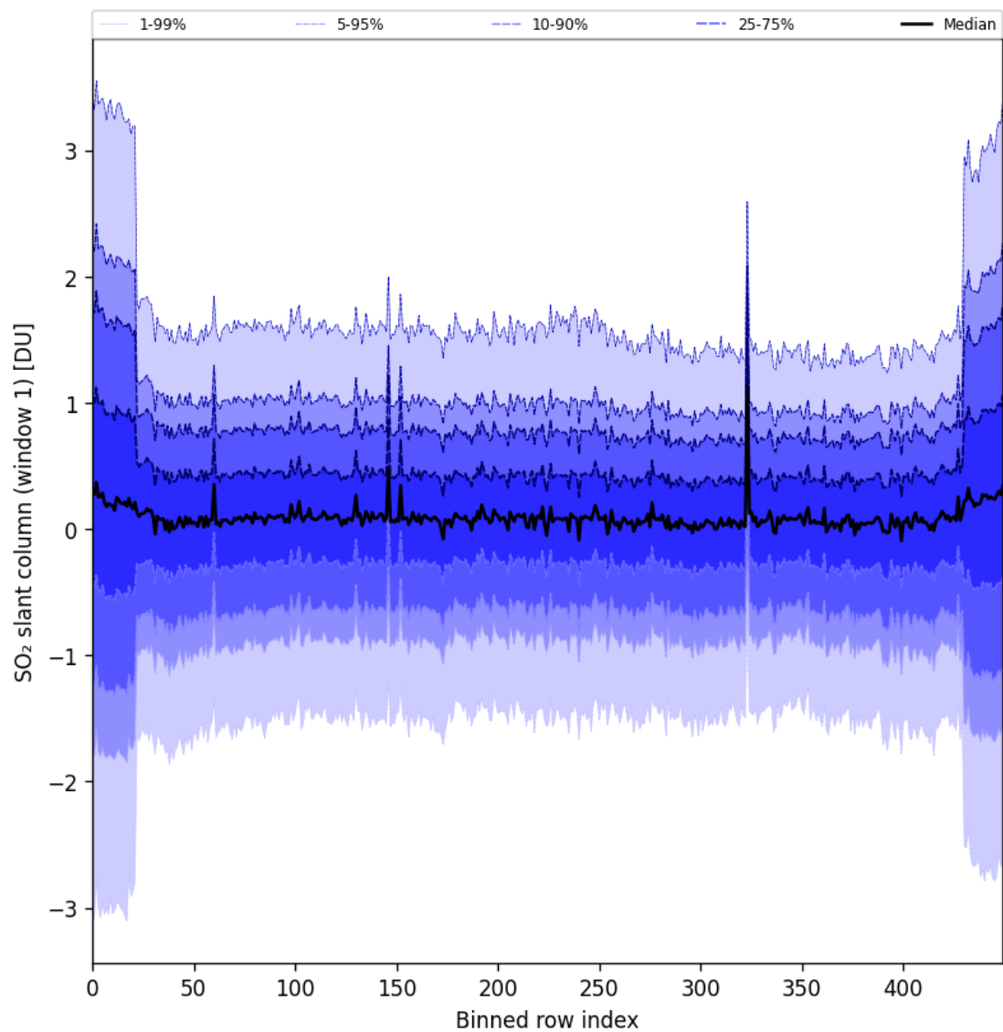
Figure 89: Along track statistics of “SO 2 slant column (window 1)” for 2025-05-31 to 2025-06-01
