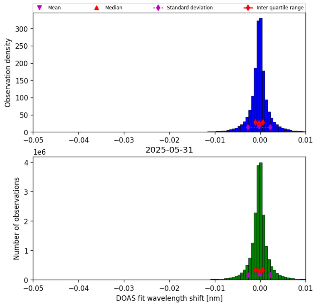
Figure 76: Histogram of “DOAS fit wavelength shift” for 2025-05-31 to 2025-06-01
