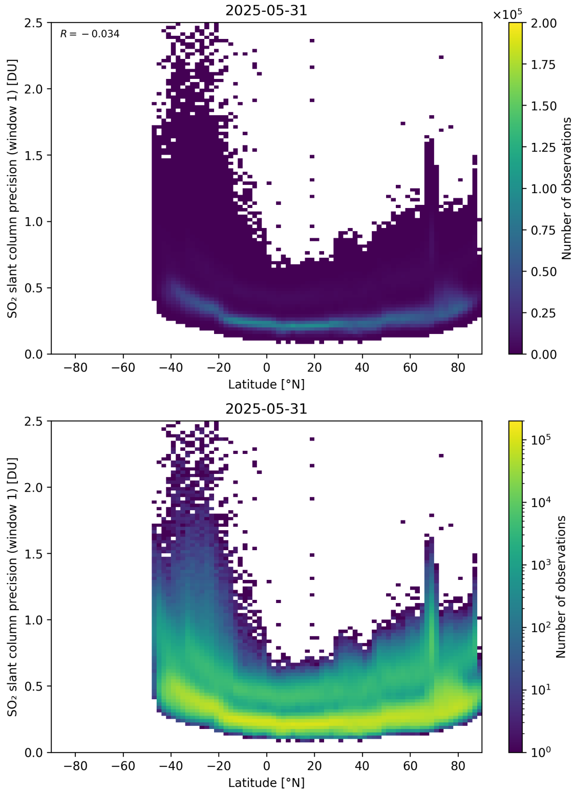
Figure 163: Scatter density plot of “Latitude” against “SO 2 slant column precision (window 1)” for 2025-05-31 to 2025-06-01.
