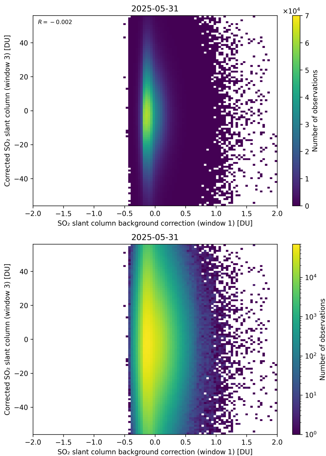
Figure 116: Scatter density plot of “SO 2 slant column background correction (window 1)” against “Corrected SO 2 slant column (window 3)” for 2025-05-31 to 2025-06-01.
