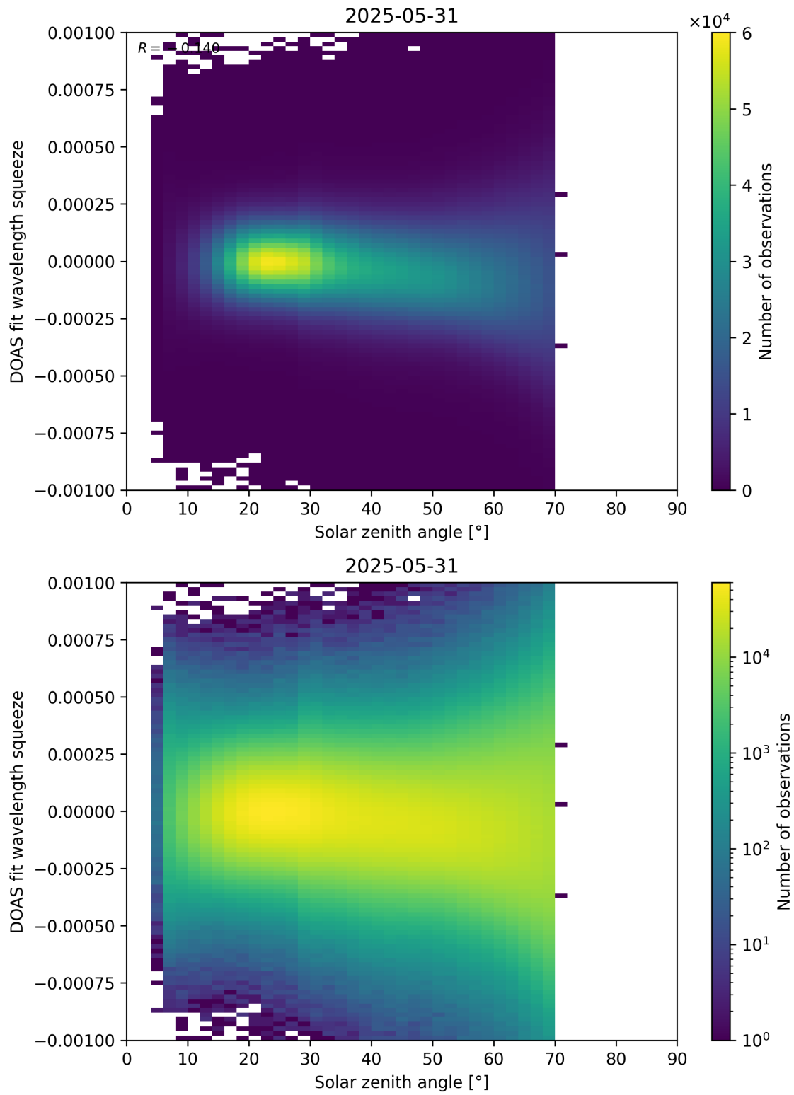
Figure 175: Scatter density plot of “Solar zenith angle” against “DOAS fit wavelength squeeze” for 2025-05-31 to 2025-06-01.
