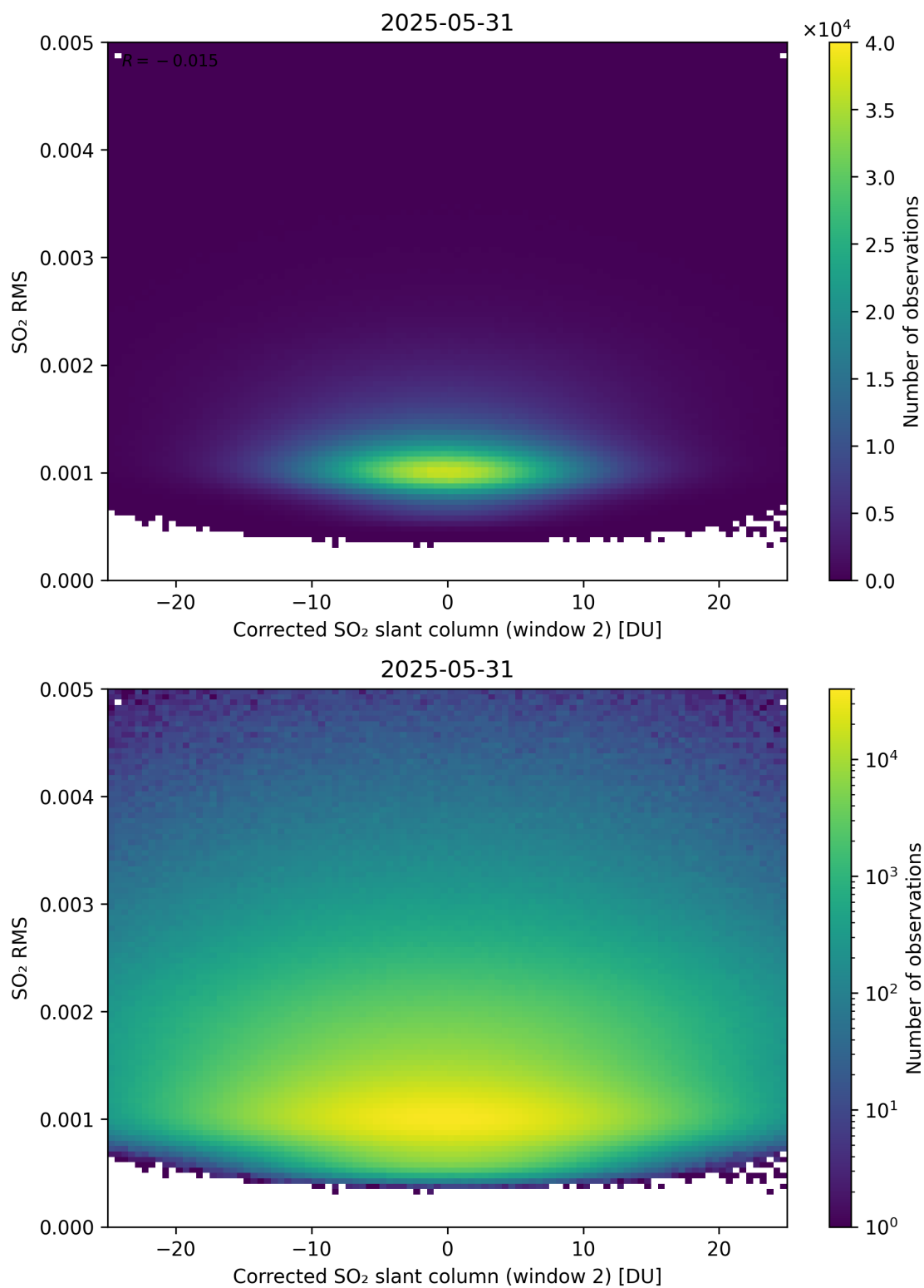
Figure 248: Scatter density plot of “Corrected SO 2 slant column (window 2)” against “SO 2 RMS” for 2025-05-31 to 2025-06-01.
