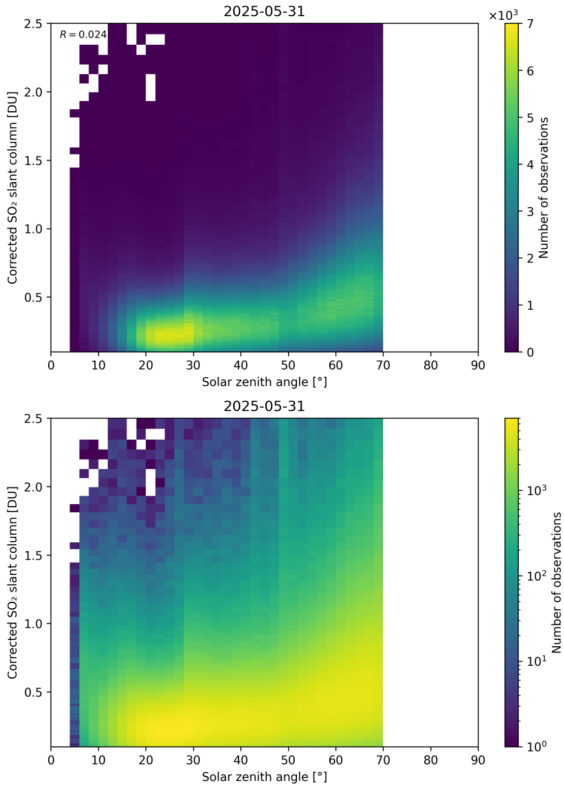
Figure 181: Scatter density plot of “Solar zenith angle” against “Corrected SO 2 slant column” for 2025-05-31 to 2025-06-01.
