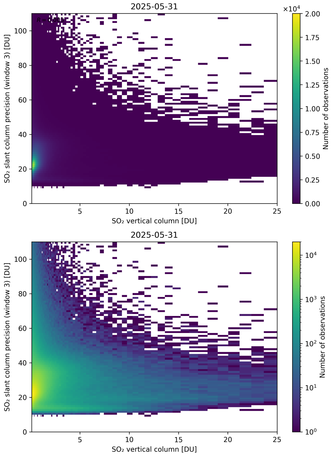
Figure 358: Scatter density plot of “SO 2 vertical column” against “SO 2 slant column precision (window 3)” for 2025-05-31 to 2025-06-01.
