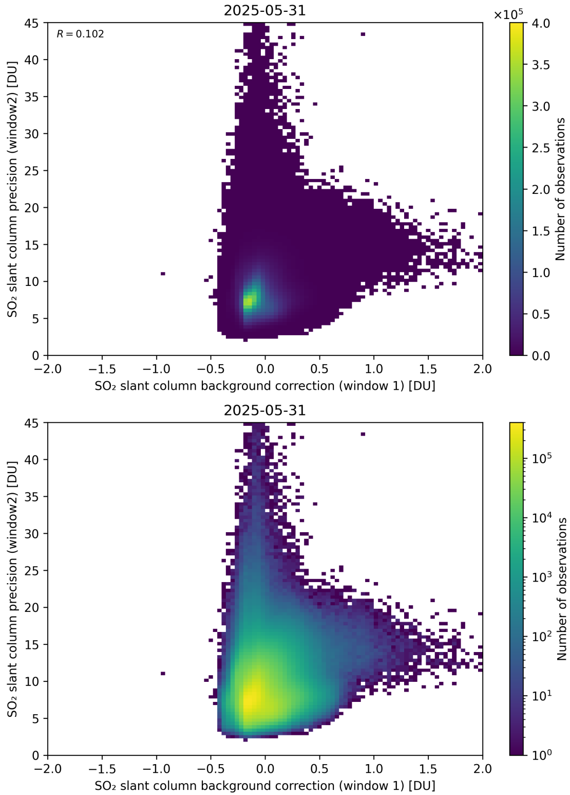
Figure 117: Scatter density plot of “SO 2 slant column background correction (window 1)” against “SO 2 slant column precision (window2)” for 2025-05-31 to 2025-06-01.
