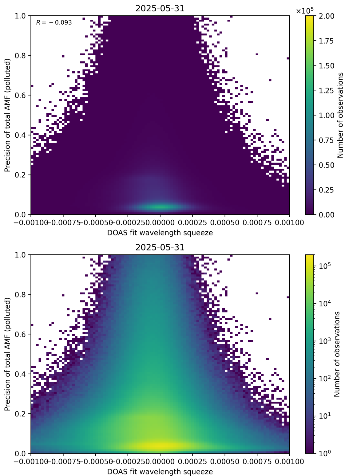
Figure 146: Scatter density plot of “DOAS fit wavelength squeeze” against “Precision of total AMF (polluted)” for 2025-05-31 to 2025-06-01.
