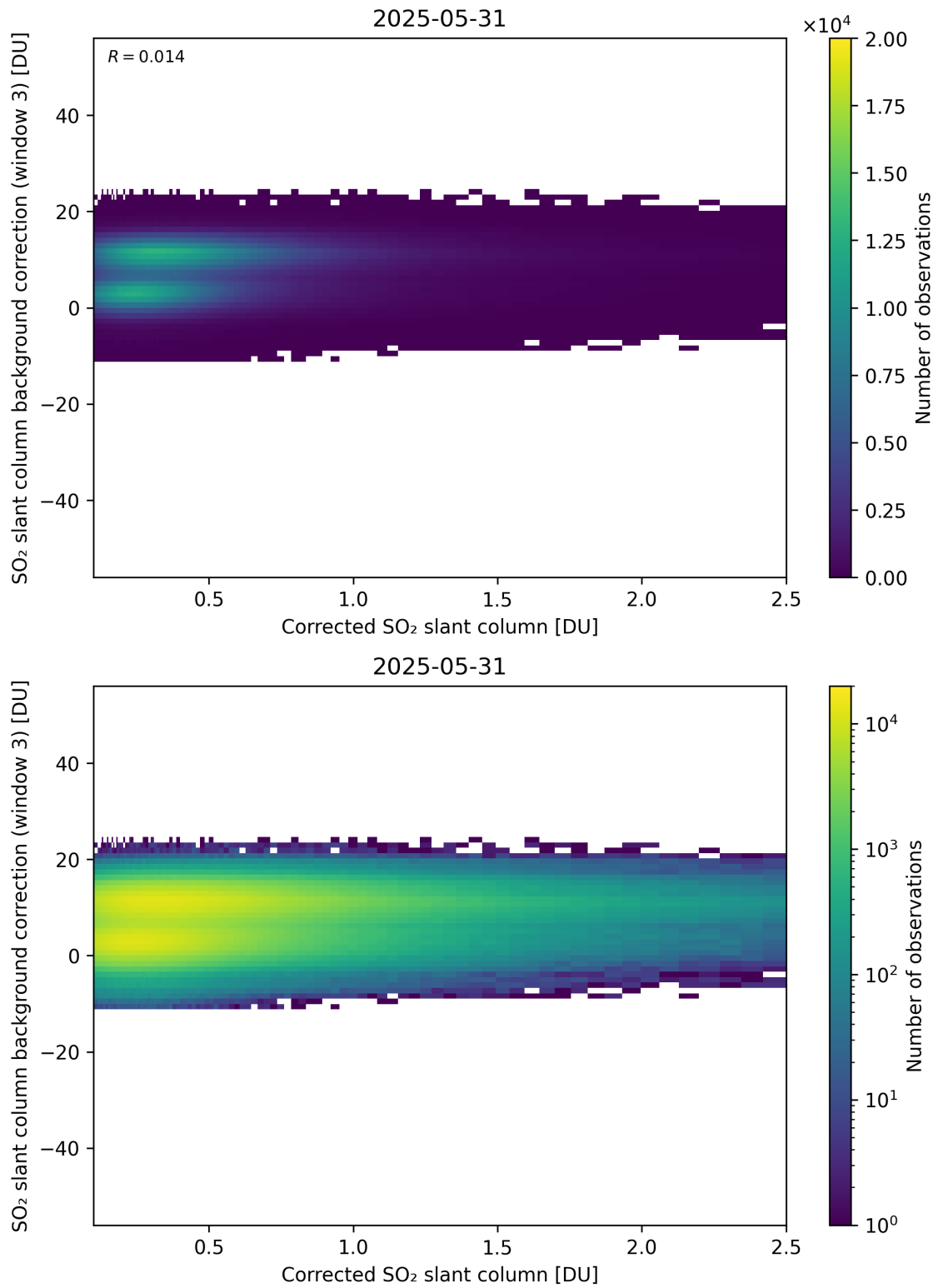
Figure 228: Scatter density plot of “Corrected SO 2 slant column” against “SO 2 slant column background correction (window 3)” for 2025-05-31 to 2025-06-01.
