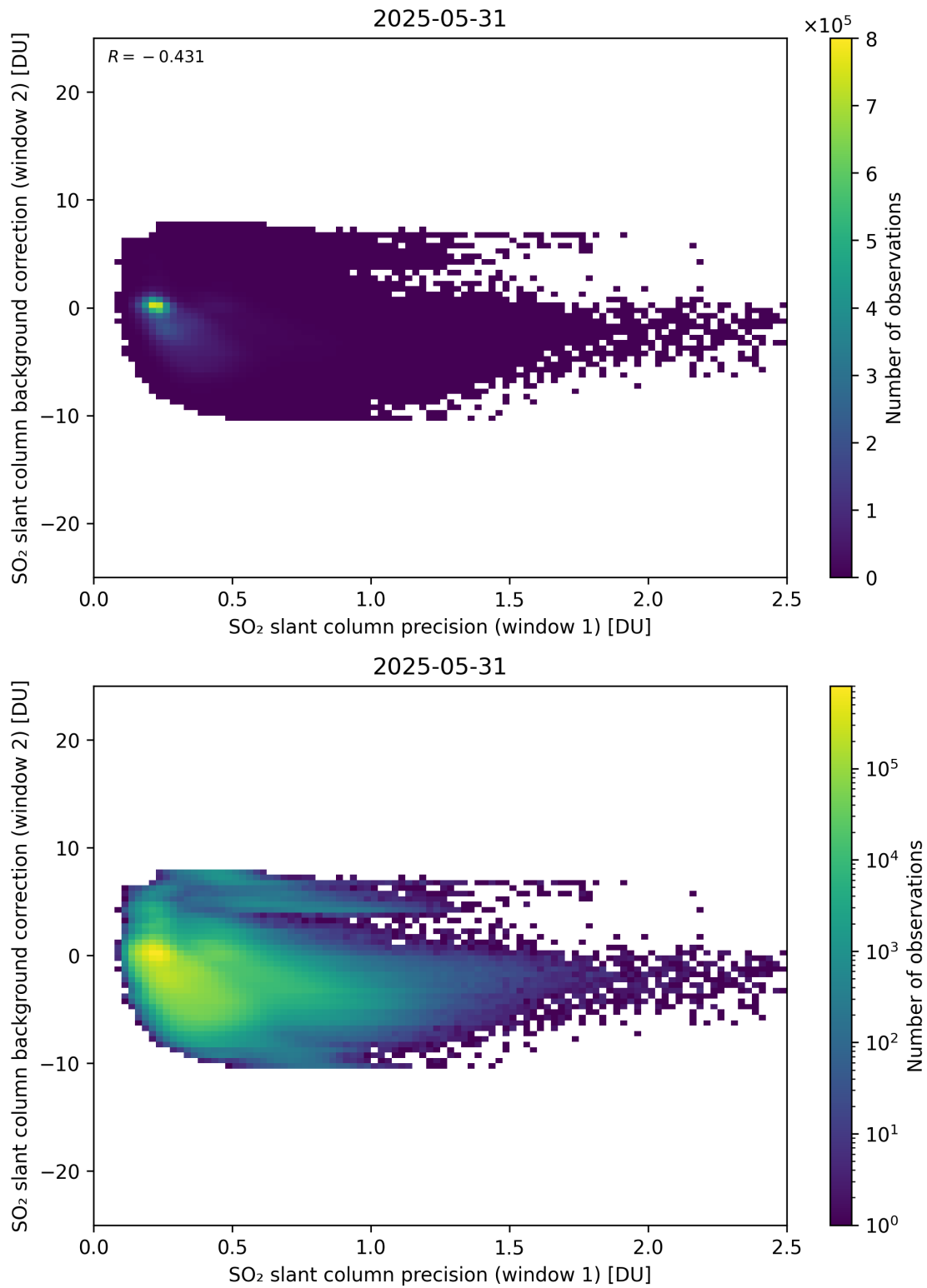
Figure 269: Scatter density plot of “SO 2 slant column precision (window 1)” against “SO 2 slant column background correction (window 2)” for 2025-05-31 to 2025-06-01.
