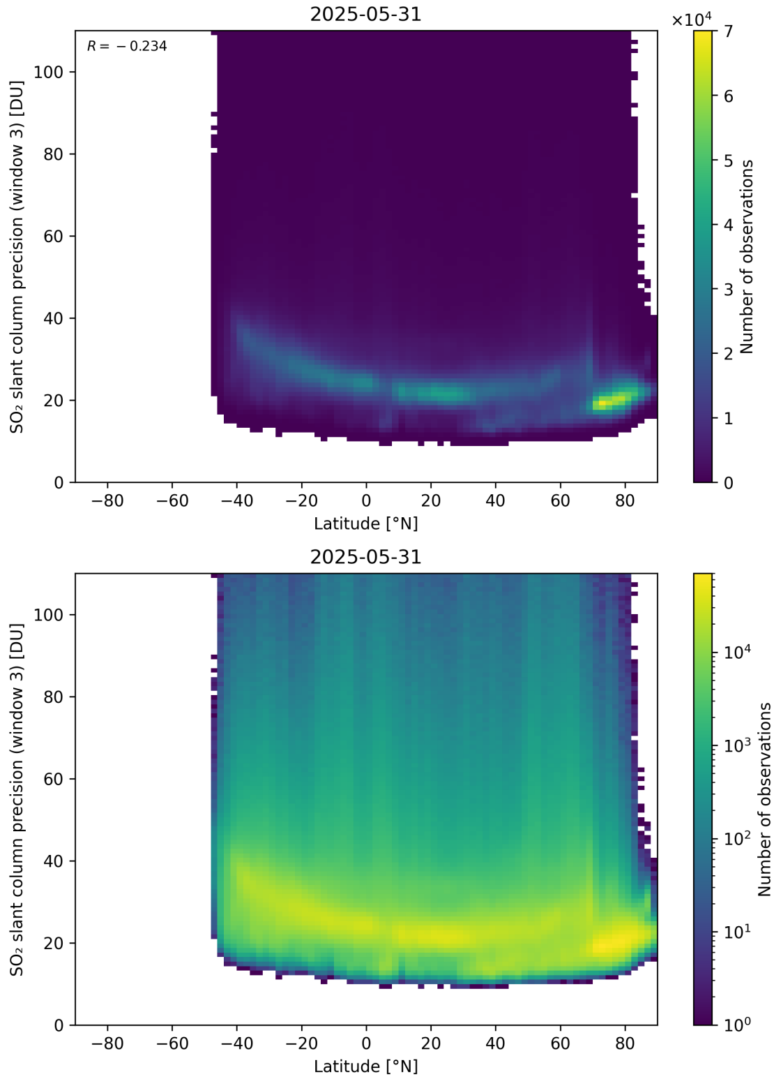
Figure 166: Scatter density plot of “Latitude” against “SO 2 slant column precision (window 3)” for 2025-05-31 to 2025-06-01.
