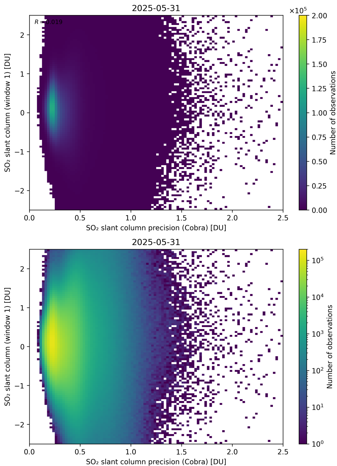
Figure 208: Scatter density plot of “SO 2 slant column precision (Cobra)” against “SO 2 slant column (window 1)” for 2025-05-31 to 2025-06-01.
