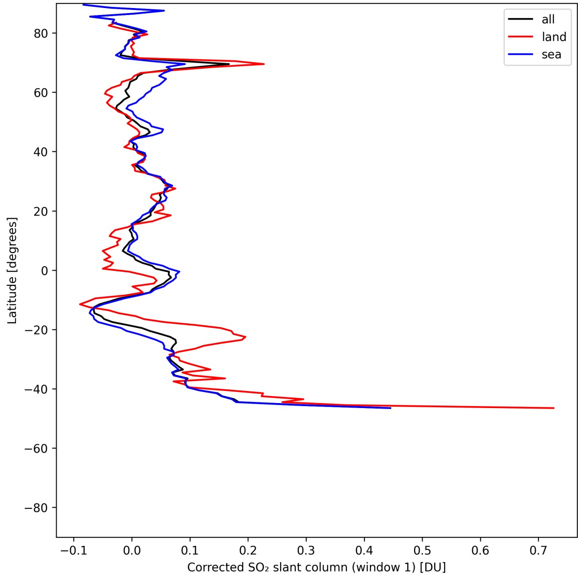
Figure 39: Zonal average of “Corrected SO 2 slant column (window 1)” for 2025-05-31 to 2025-06-01.
