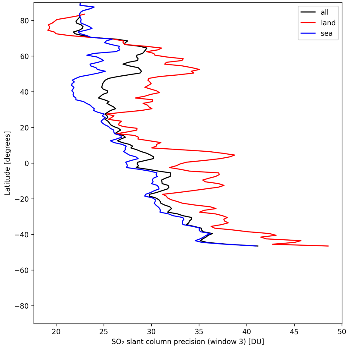
Figure 46: Zonal average of “SO 2 slant column precision (window 3)” for 2025-05-31 to 2025-06-01.
