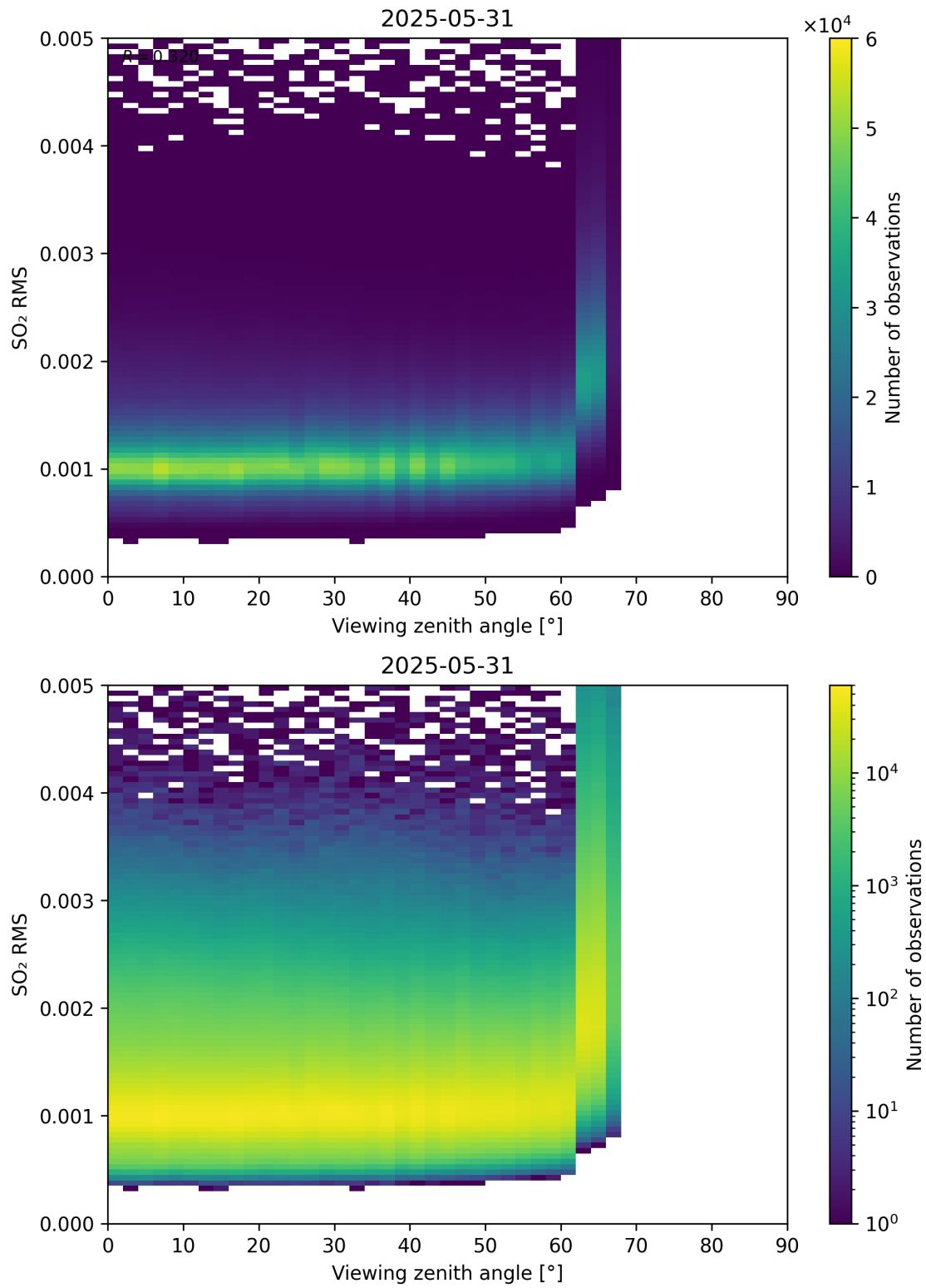
Figure 367: Scatter density plot of “Viewing zenith angle” against “SO 2 RMS” for 2025-05-31 to 2025-06-01.
