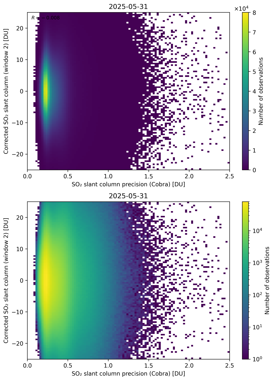
Figure 206: Scatter density plot of “SO 2 slant column precision (Cobra)” against “Corrected SO 2 slant column (window 2)” for 2025-05-31 to 2025-06-01.
