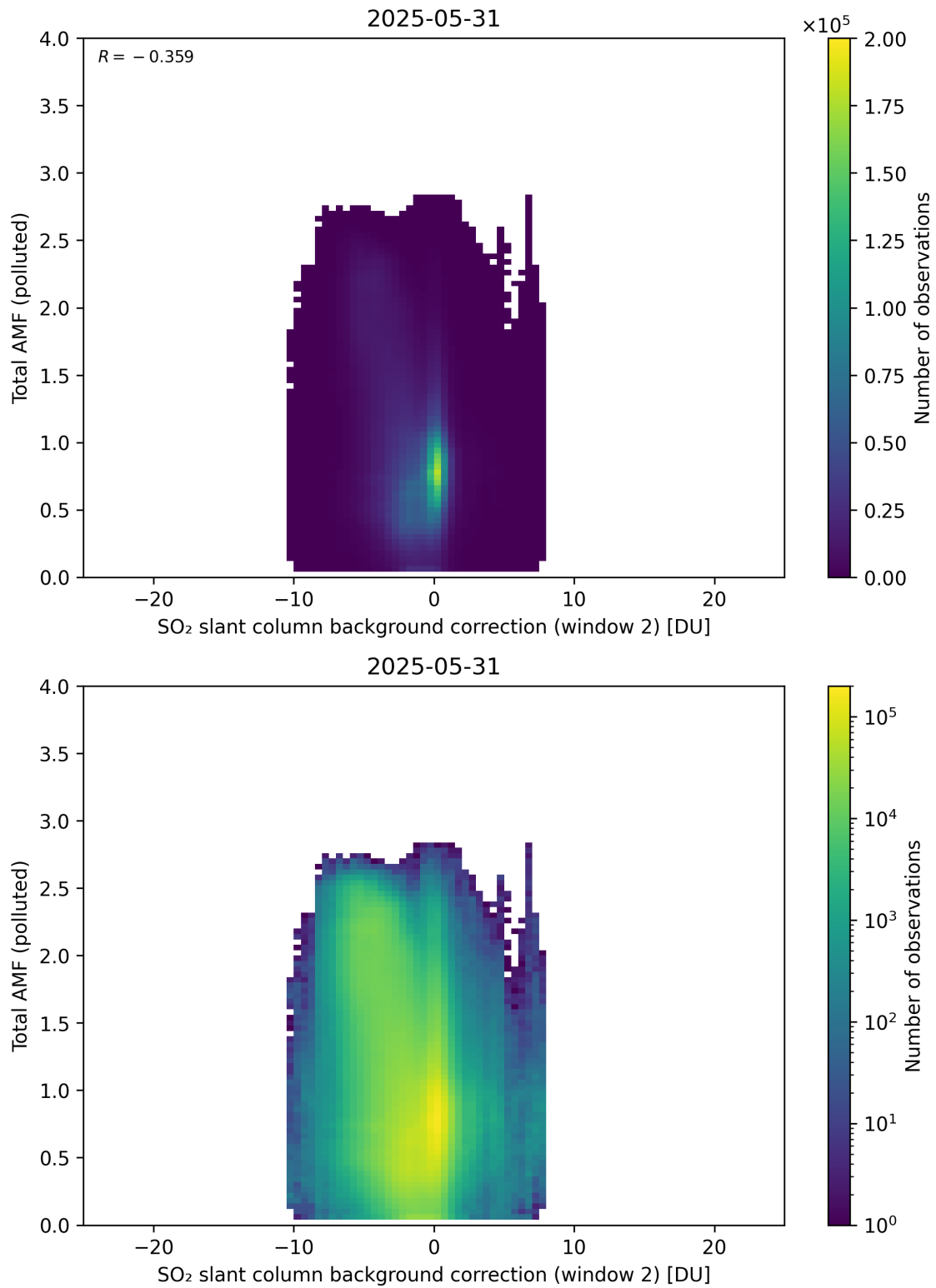
Figure 130: Scatter density plot of “SO 2 slant column background correction (window 2)” against “Total AMF (polluted)” for 2025-05-31 to 2025-06-01.
