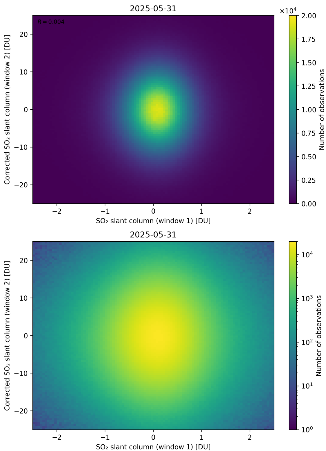
Figure 283: Scatter density plot of “SO 2 slant column (window 1)” against “Corrected SO 2 slant column (window 2)” for 2025-05-31 to 2025-06-01.
