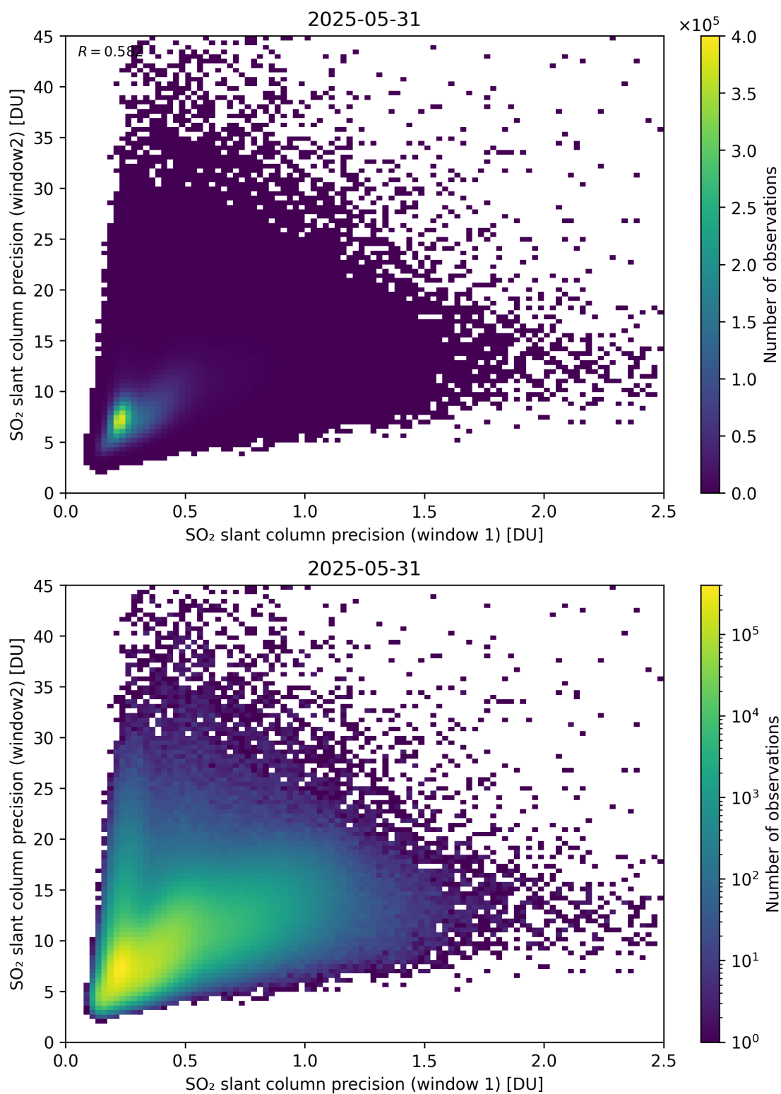
Figure 277: Scatter density plot of “SO 2 slant column precision (window 1)” against “SO 2 slant column precision (window2)” for 2025-05-31 to 2025-06-01.
