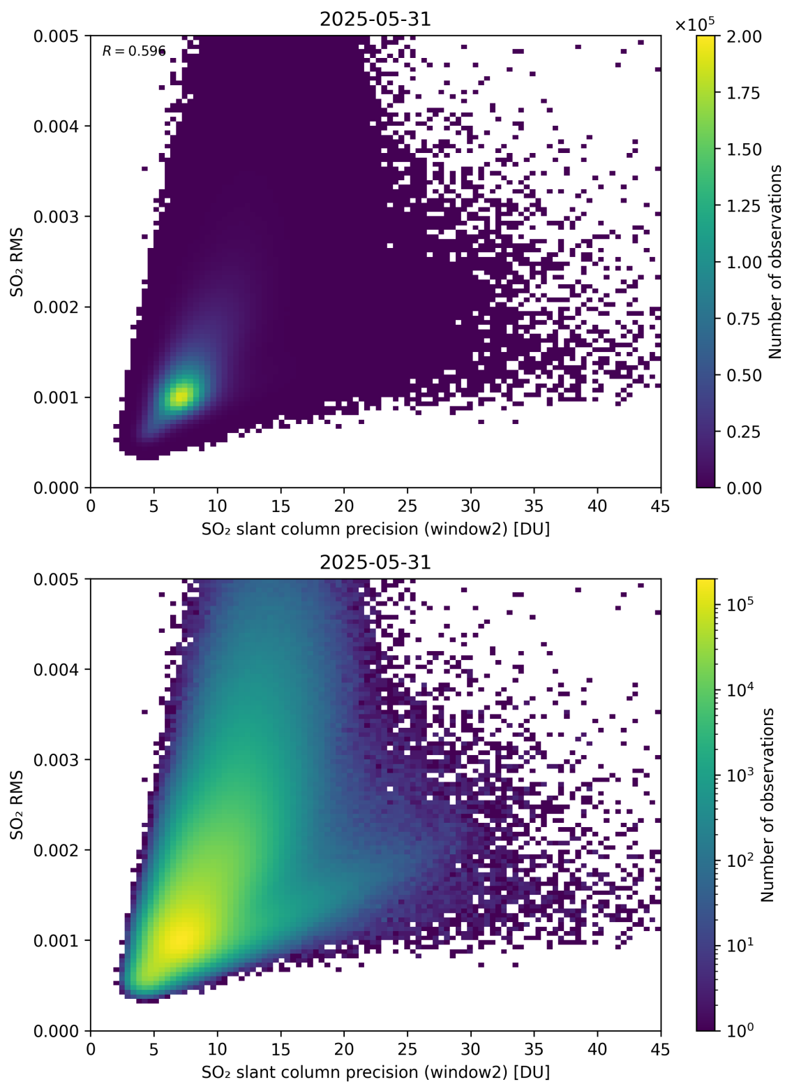
Figure 295: Scatter density plot of “SO 2 slant column precision (window2)” against “SO 2 RMS” for 2025-05-31 to 2025-06-01.
