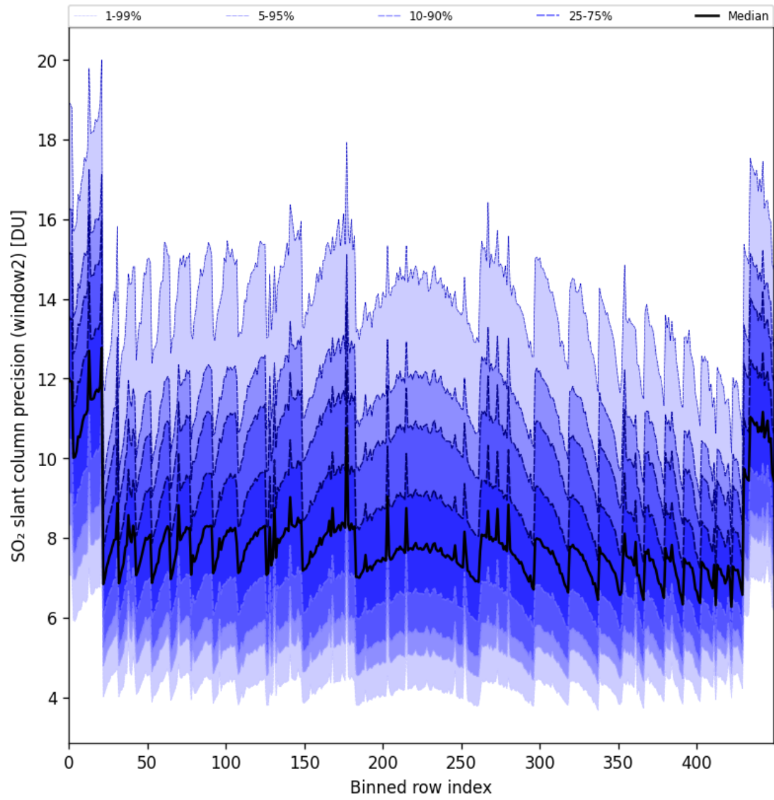
Figure 94: Along track statistics of “SO 2 slant column precision (window2)” for 2025-05-31 to 2025-06-01
