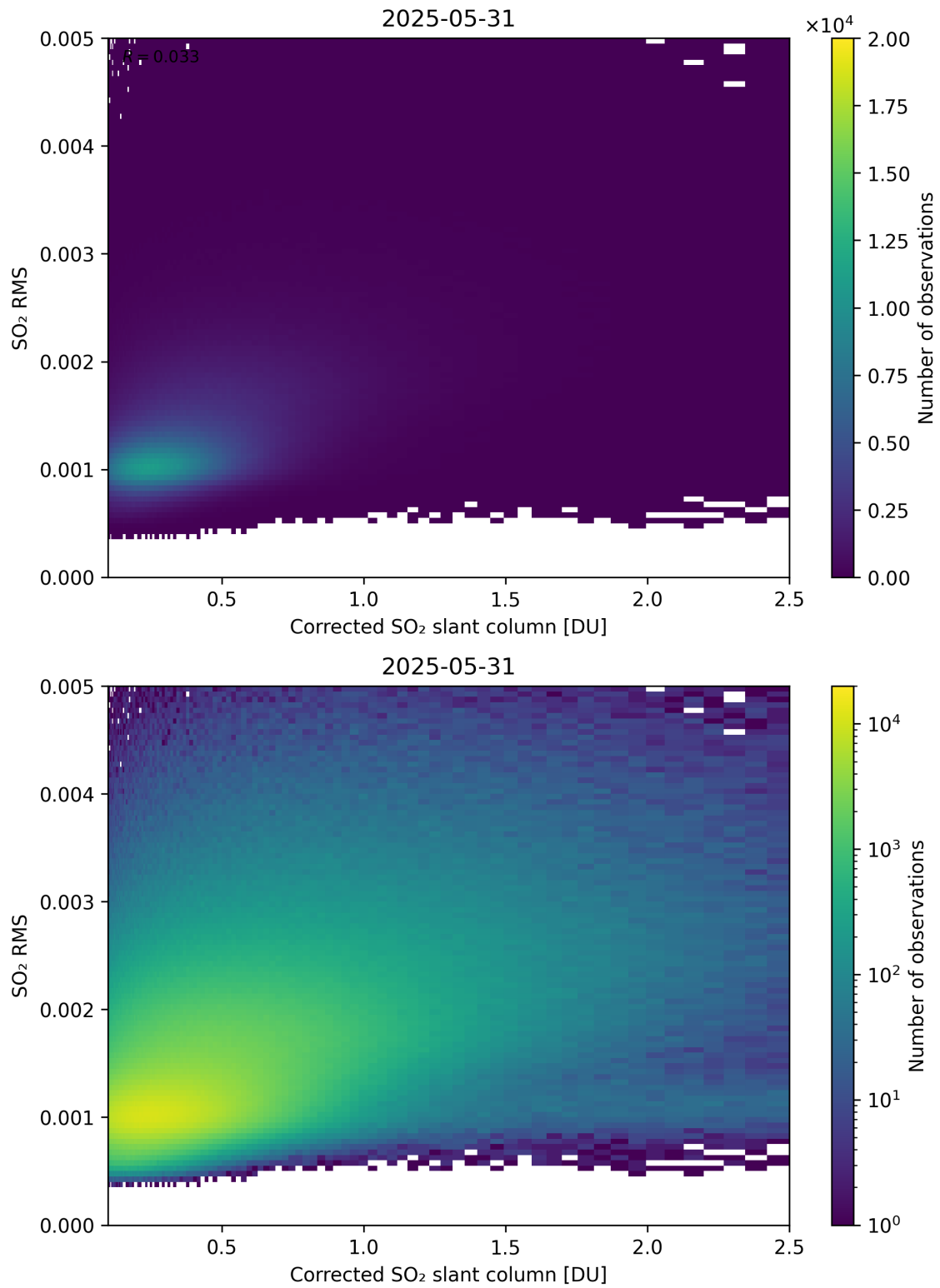
Figure 231: Scatter density plot of “Corrected SO 2 slant column” against “SO 2 RMS” for 2025-05-31 to 2025-06-01.
