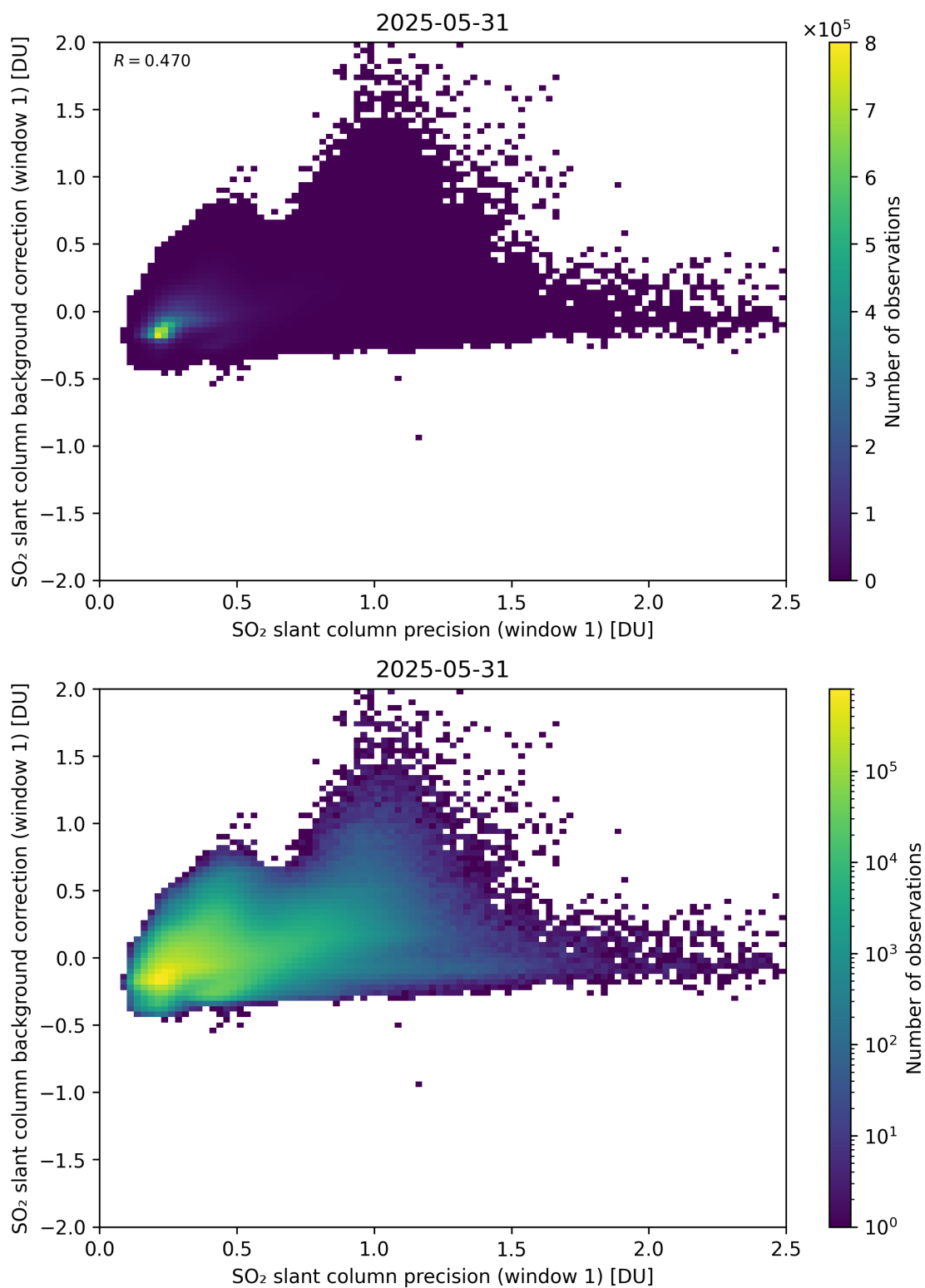
Figure 268: Scatter density plot of “SO 2 slant column precision (window 1)” against “SO 2 slant column background correction (window 1)” for 2025-05-31 to 2025-06-01.
