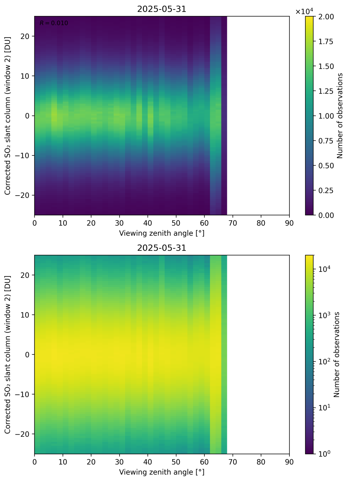
Figure 374: Scatter density plot of “Viewing zenith angle” against “Corrected SO 2 slant column (window 2)” for 2025-05-31 to 2025-06-01.
