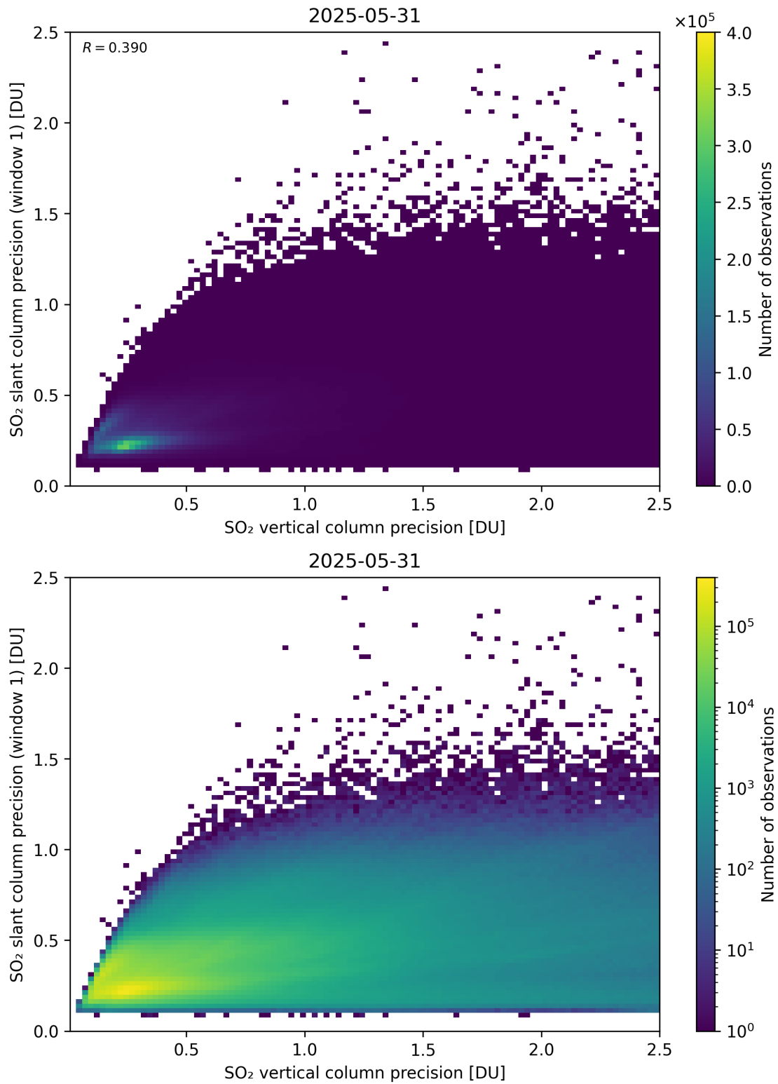
Figure 342: Scatter density plot of “SO 2 vertical column precision” against “SO 2 slant column precision (window 1)” for 2025-05-31 to 2025-06-01.
