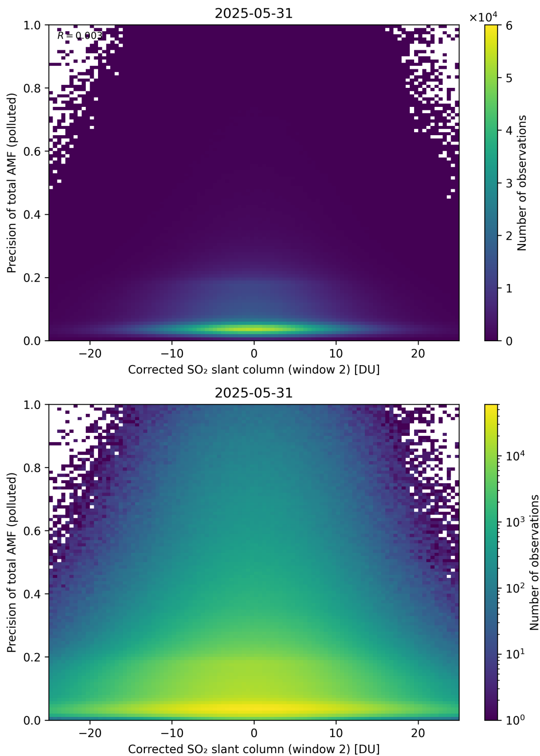
Figure 254: Scatter density plot of “Corrected SO 2 slant column (window 2)” against “Precision of total AMF (polluted)” for 2025-05-31 to 2025-06-01.
