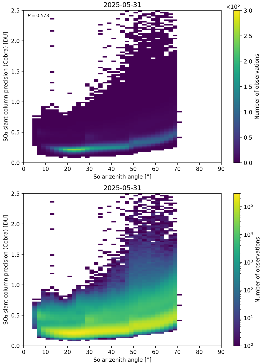
Figure 180: Scatter density plot of “Solar zenith angle” against “SO 2 slant column precision (Cobra)” for 2025-05-31 to 2025-06-01.
