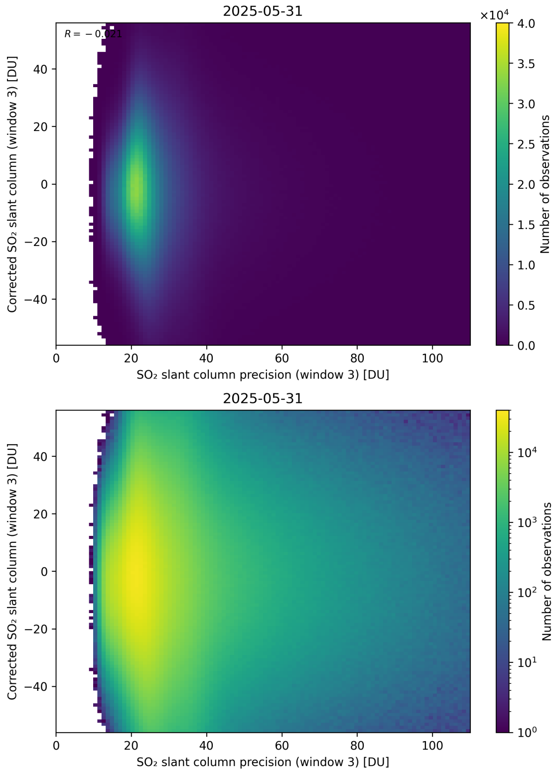
Figure 312: Scatter density plot of “SO 2 slant column precision (window 3)” against “Corrected SO 2 slant column (window 3)” for 2025-05-31 to 2025-06-01.
