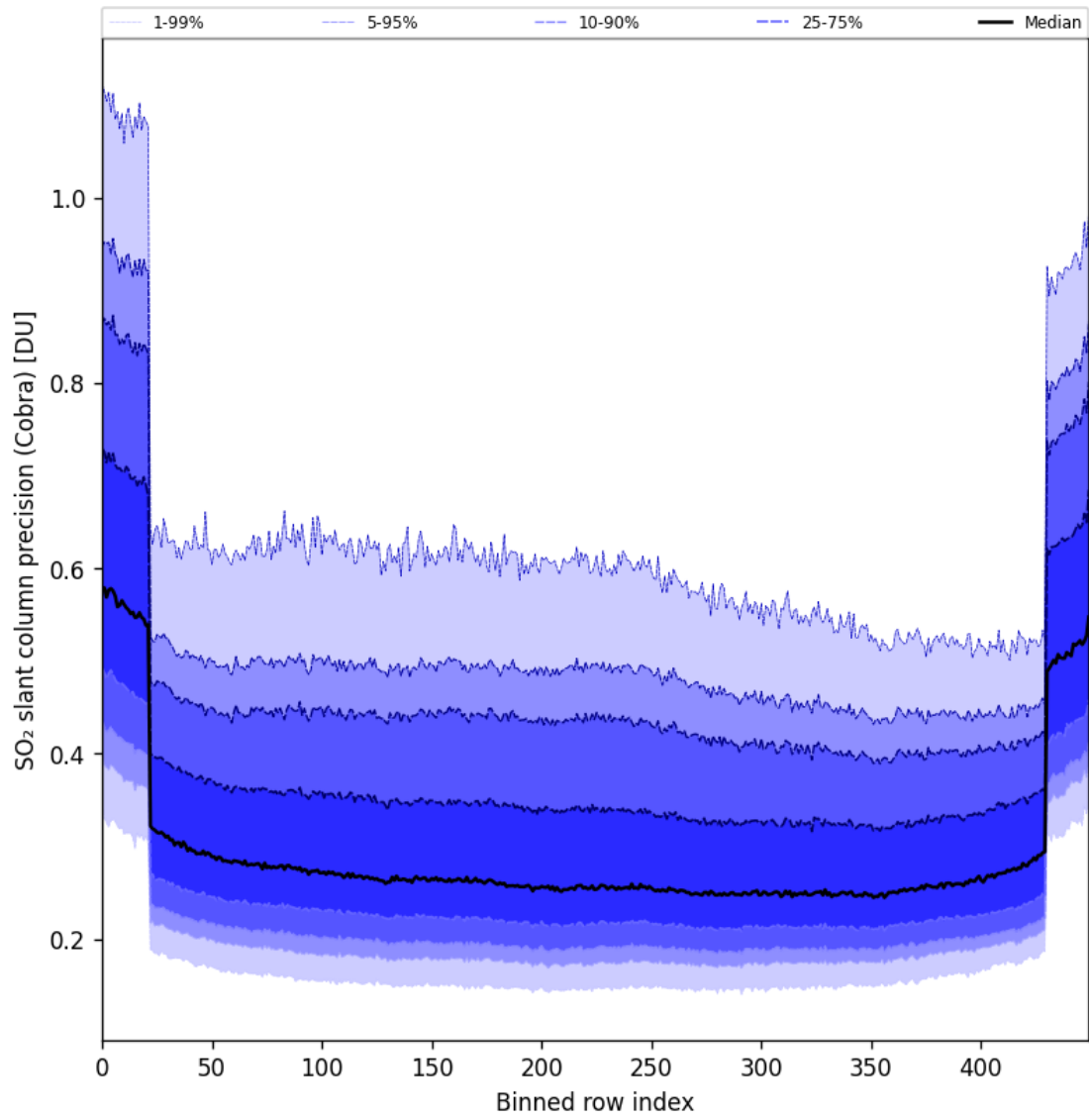
Figure 88: Along track statistics of “SO 2 slant column precision (Cobra)” for 2025-05-31 to 2025-06-01
