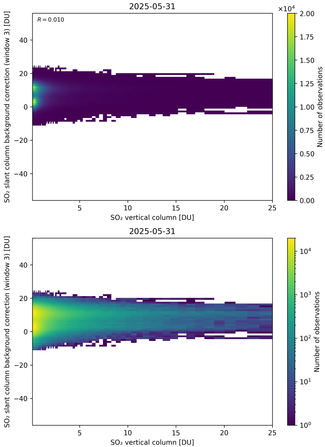
Figure 325: Scatter density plot of “SO 2 vertical column” against “SO 2 slant column background correction (window 3)” for 2025-05-31 to 2025-06-01.
