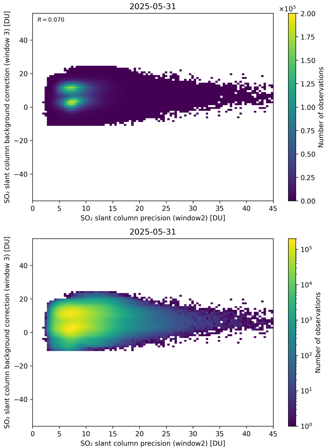
Figure 292: Scatter density plot of “SO 2 slant column precision (window2)” against “SO 2 slant column background correction (window 3)” for 2025-05-31 to 2025-06-01.
