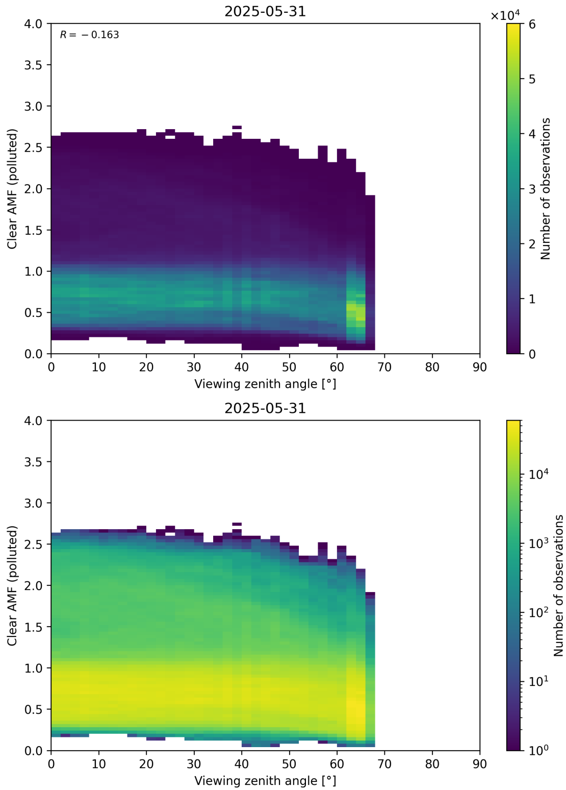
Figure 370: Scatter density plot of “Viewing zenith angle” against “Clear AMF (polluted)” for 2025-05-31 to 2025-06-01.
