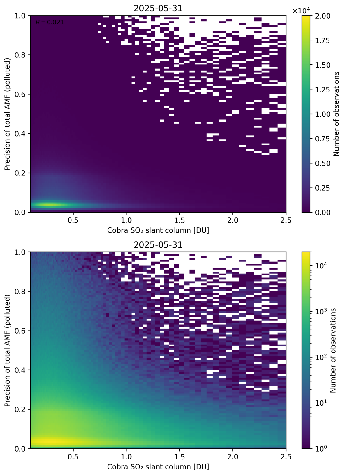
Figure 225: Scatter density plot of “Cobra SO 2 slant column” against “Precision of total AMF (polluted)” for 2025-05-31 to 2025-06-01.
