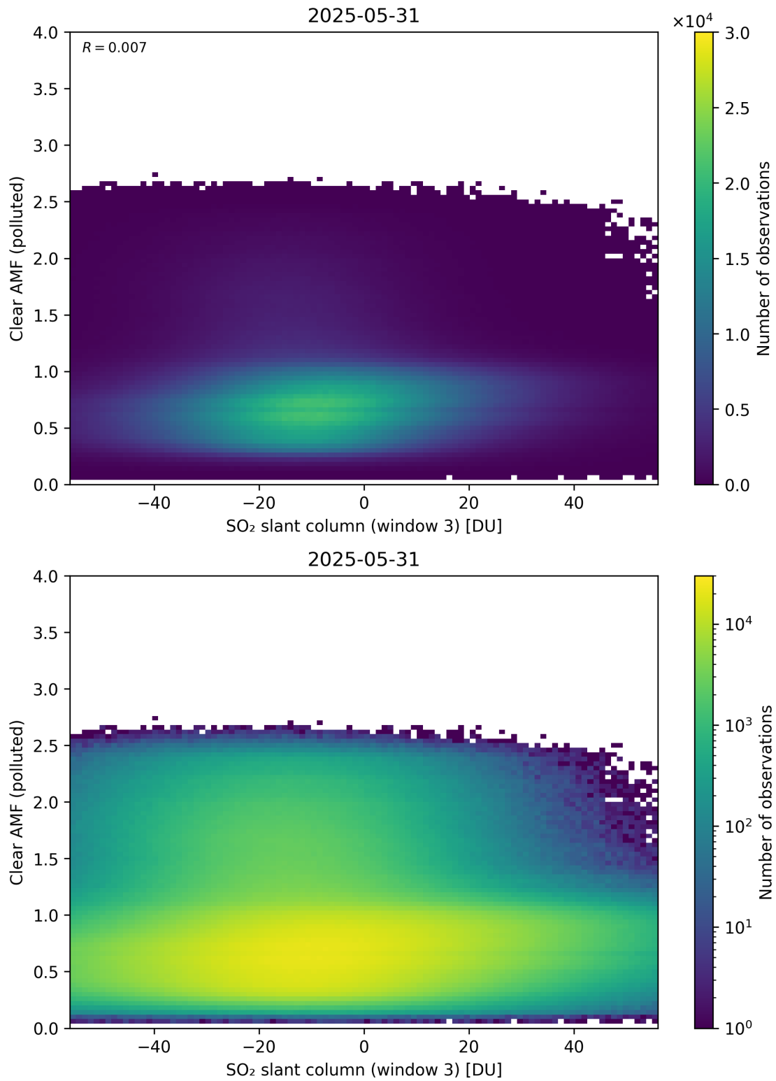
Figure 315: Scatter density plot of “SO 2 slant column (window 3)” against “Clear AMF (polluted)” for 2025-05-31 to 2025-06-01.
