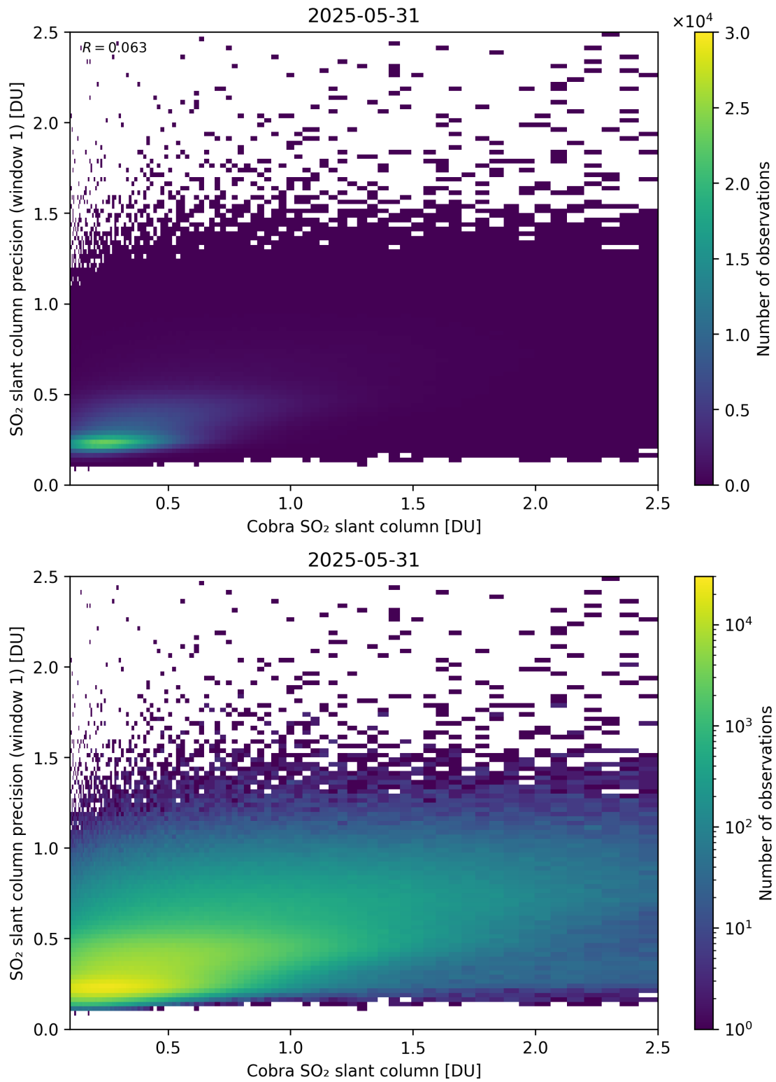
Figure 220: Scatter density plot of “Cobra SO 2 slant column” against “SO 2 slant column precision (window 1)” for 2025-05-31 to 2025-06-01.
