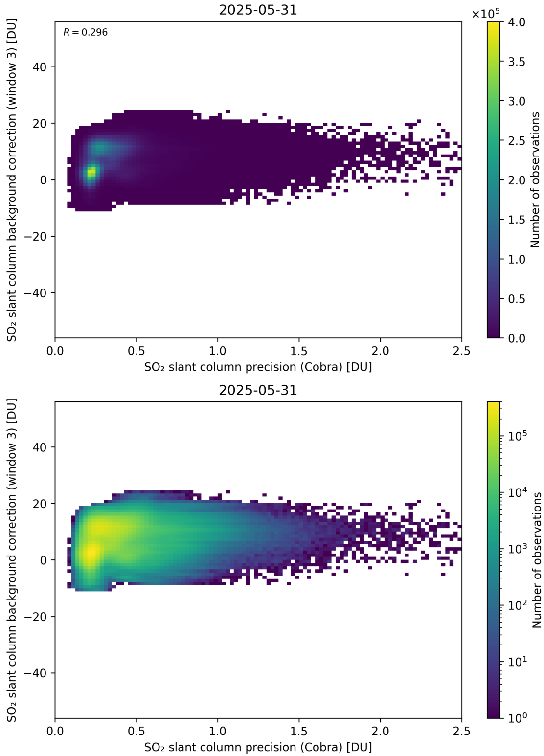
Figure 201: Scatter density plot of “SO 2 slant column precision (Cobra)” against “SO 2 slant column background correction (window 3)” for 2025-05-31 to 2025-06-01.
