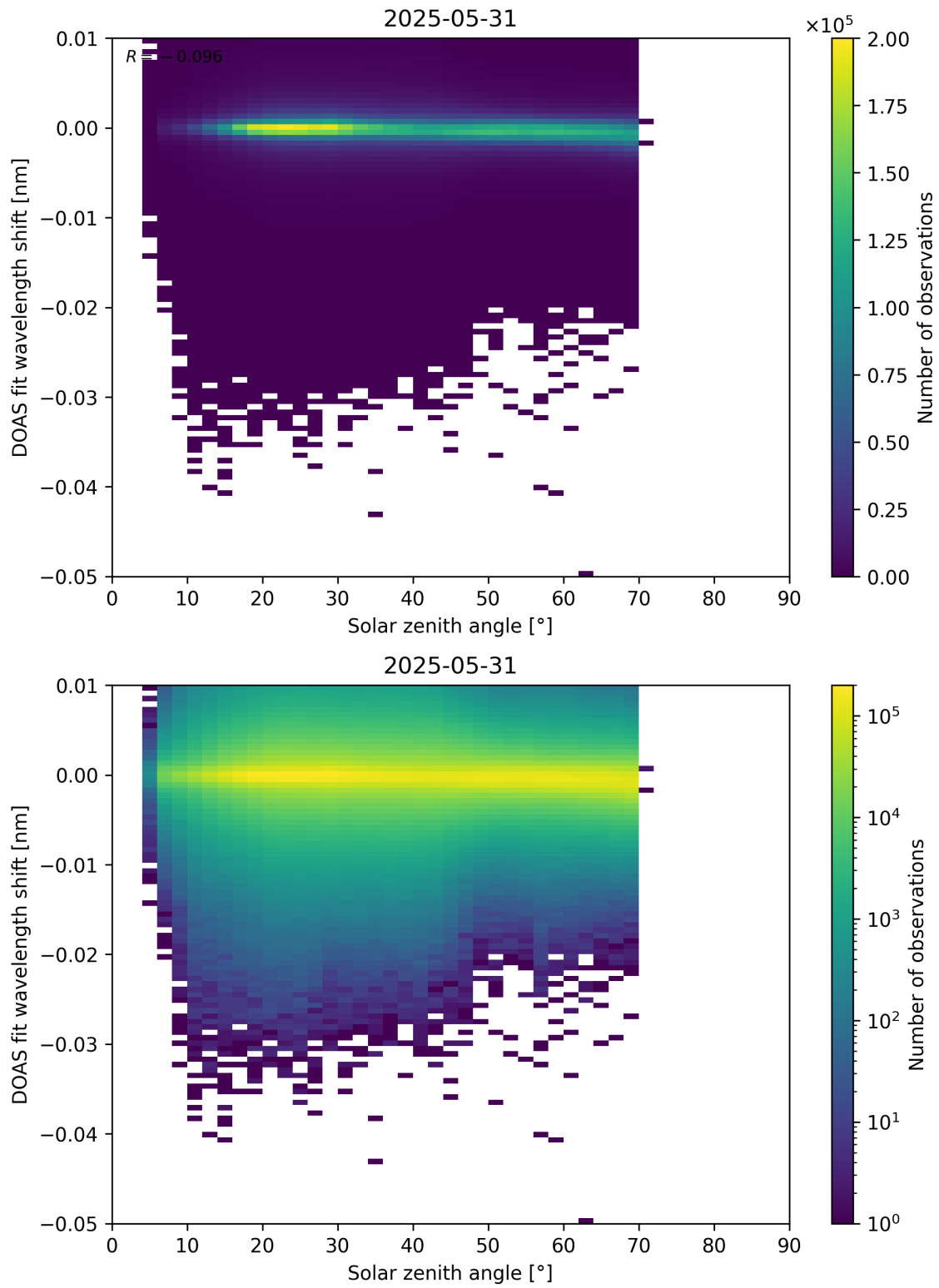
Figure 174: Scatter density plot of “Solar zenith angle” against “DOAS fit wavelength shift” for 2025-05-31 to 2025-06-01.
