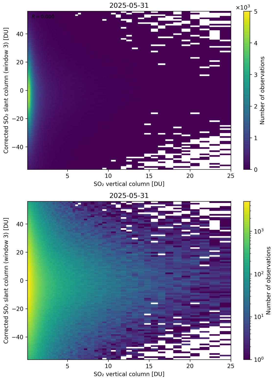
Figure 353: Scatter density plot of “SO 2 vertical column” against “Corrected SO 2 slant column (window 3)” for 2025-05-31 to 2025-06-01.
