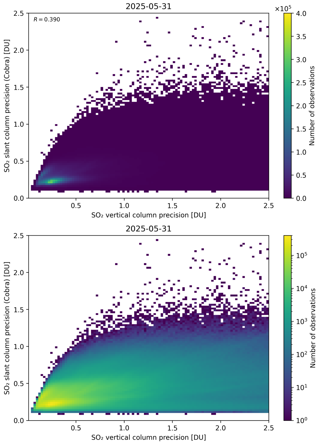
Figure 337: Scatter density plot of “SO 2 vertical column precision” against “SO 2 slant column precision (Cobra)” for 2025-05-31 to 2025-06-01.
