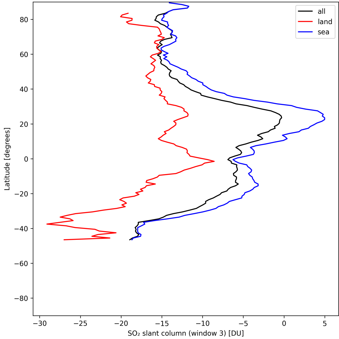
Figure 45: Zonal average of “SO 2 slant column (window 3)” for 2025-05-31 to 2025-06-01.
