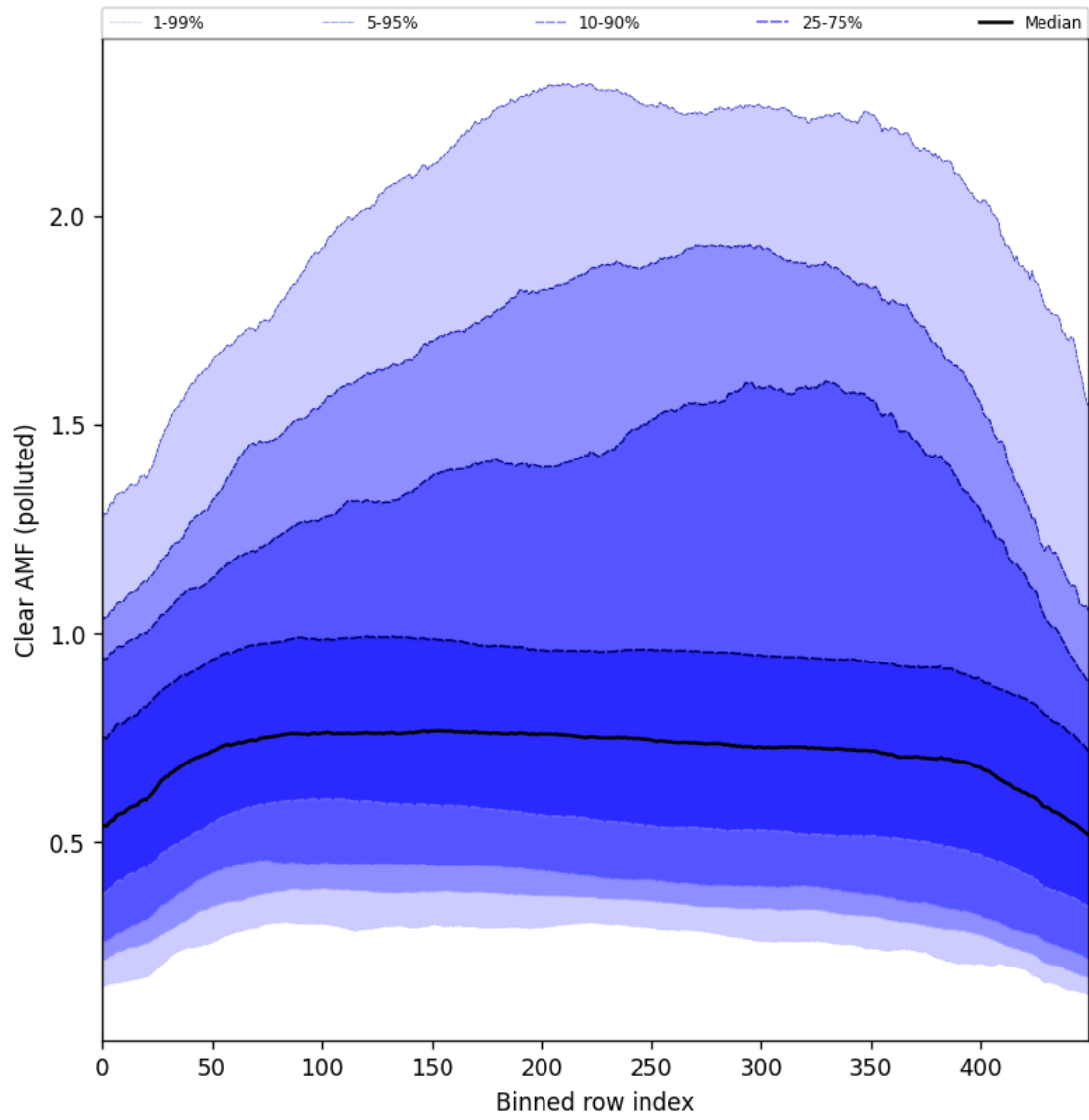
Figure 107: Along track statistics of “Clear AMF (polluted)” for 2025-05-31 to 2025-06-01
