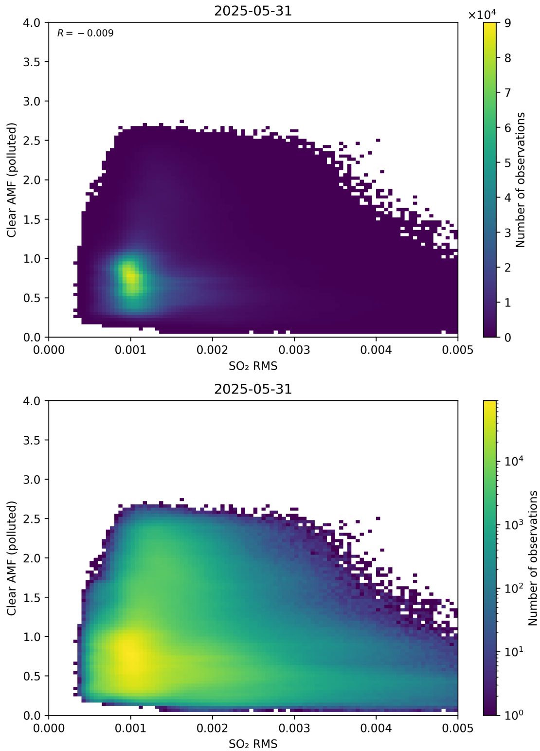
Figure 147: Scatter density plot of “SO 2 RMS” against “Clear AMF (polluted)” for 2025-05-31 to 2025-06-01.
