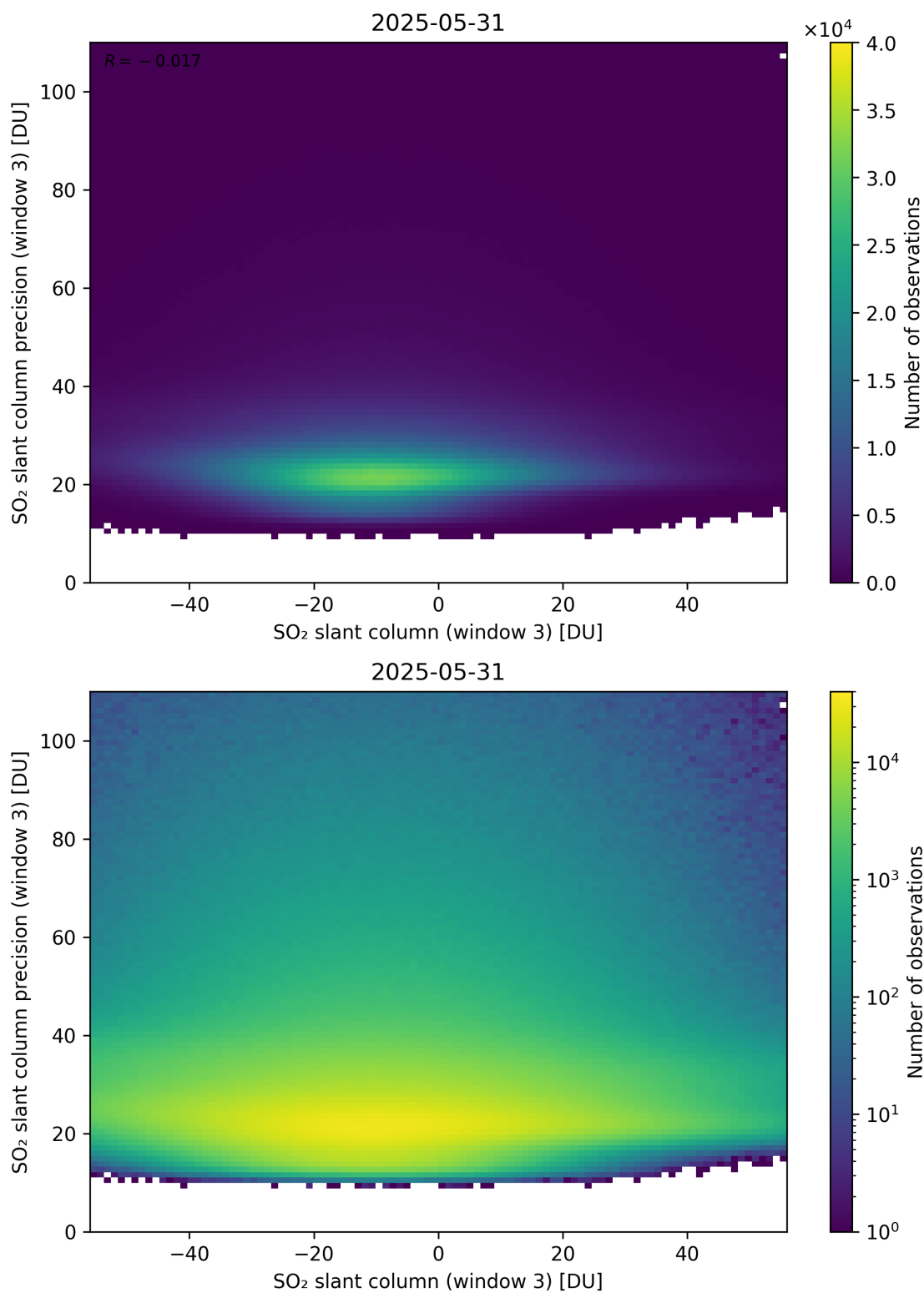
Figure 317: Scatter density plot of “SO 2 slant column (window 3)” against “SO 2 slant column precision (window 3)” for 2025-05-31 to 2025-06-01.
