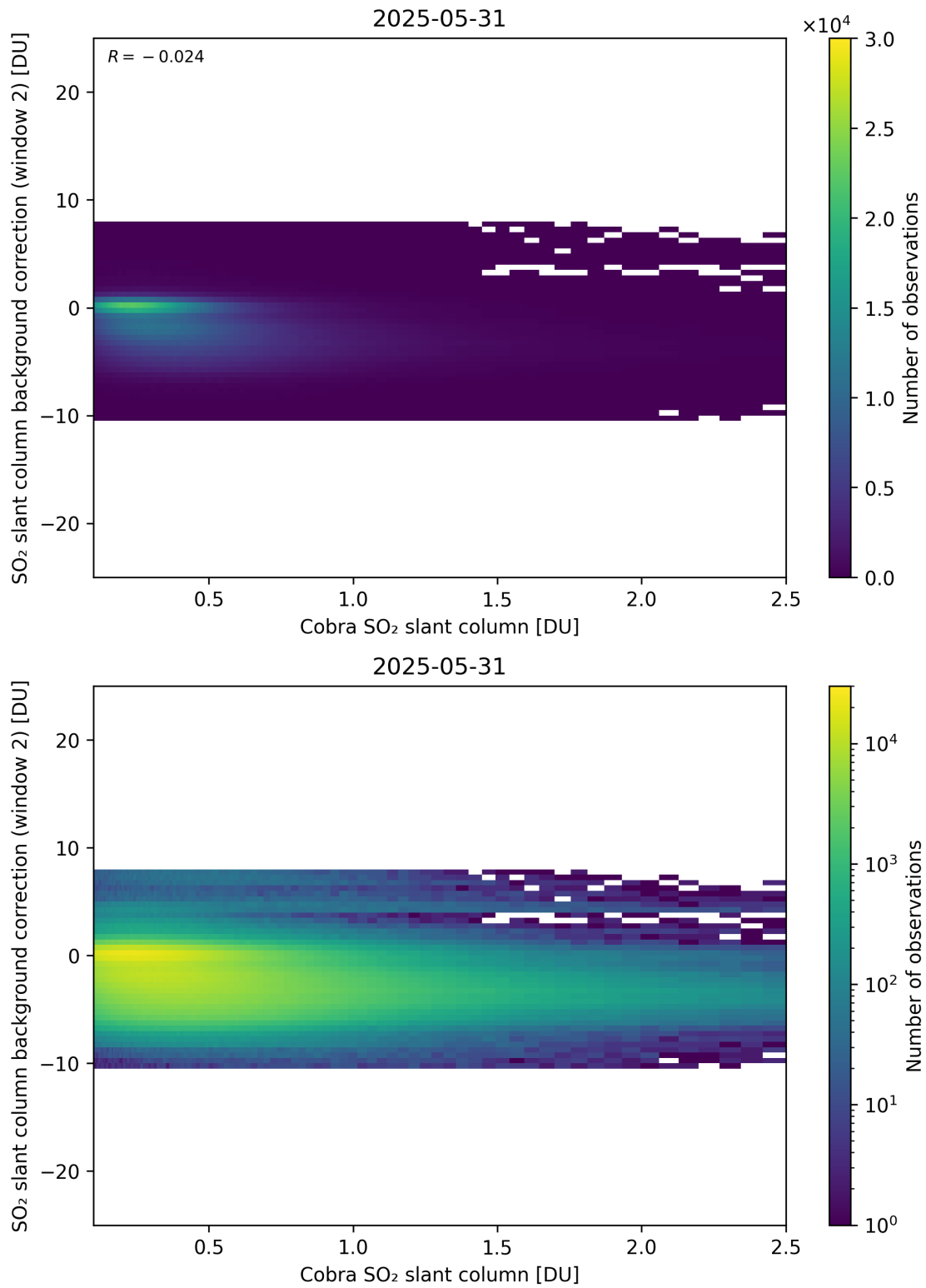
Figure 194: Scatter density plot of “Cobra SO 2 slant column” against “SO 2 slant column background correction (window 2)” for 2025-05-31 to 2025-06-01.
