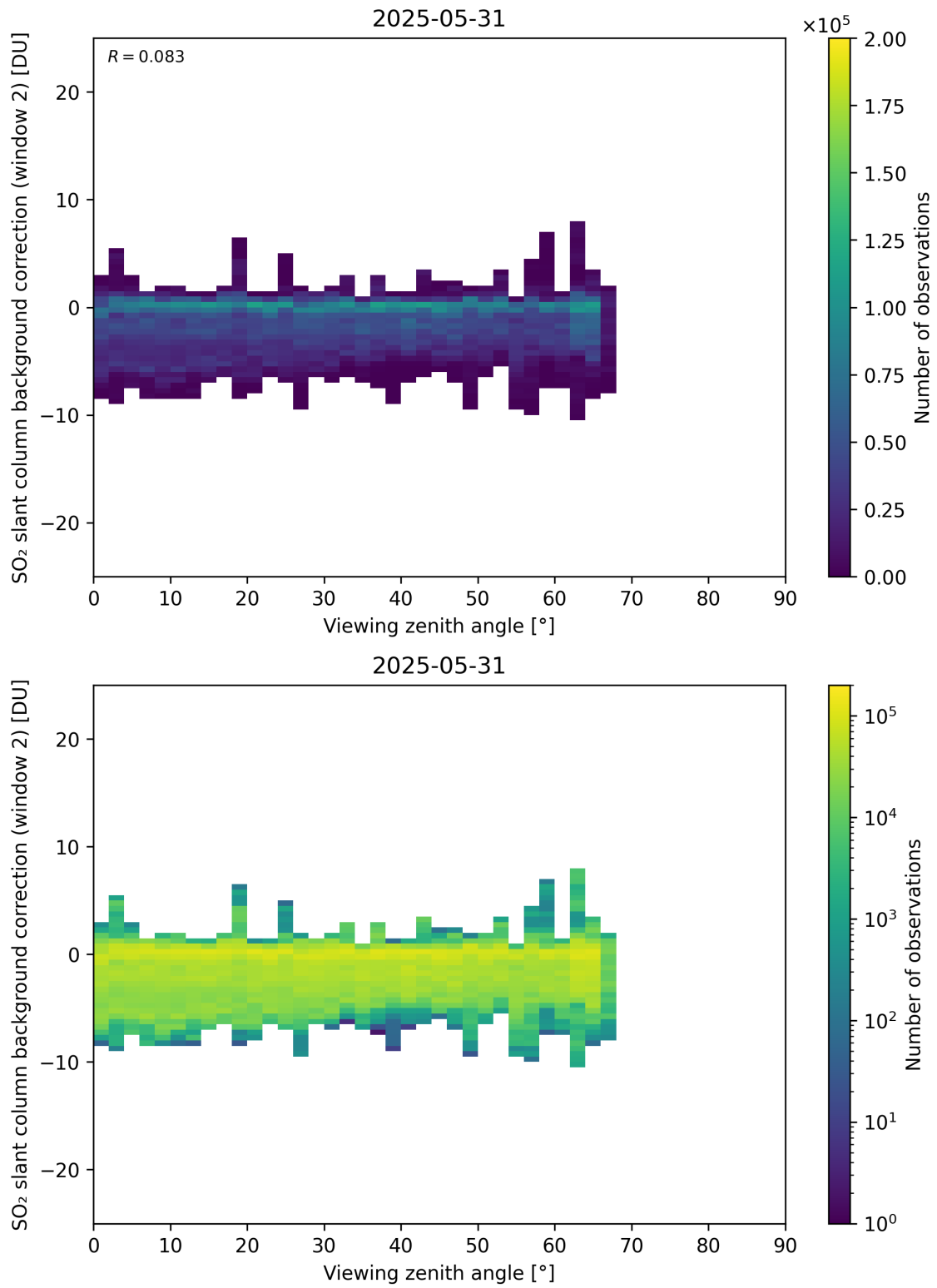
Figure 363: Scatter density plot of “Viewing zenith angle” against “SO 2 slant column background correction (window 2)” for 2025-05-31 to 2025-06-01.
