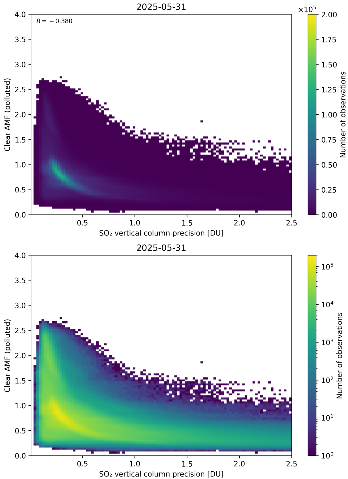
Figure 335: Scatter density plot of “SO 2 vertical column precision” against “Clear AMF (polluted)” for 2025-05-31 to 2025-06-01.
