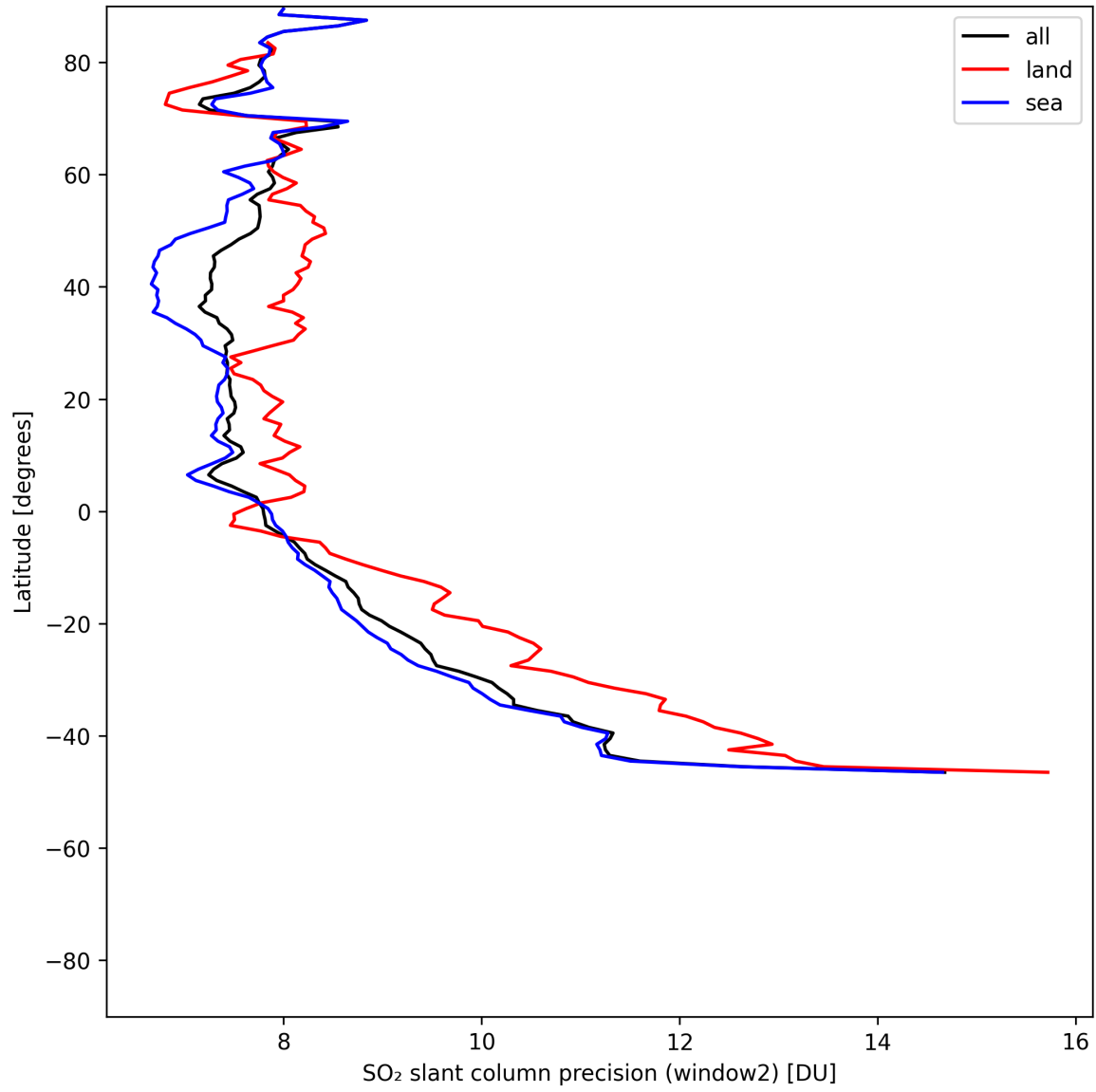
Figure 42: Zonal average of “SO 2 slant column precision (window2)” for 2025-05-31 to 2025-06-01.
