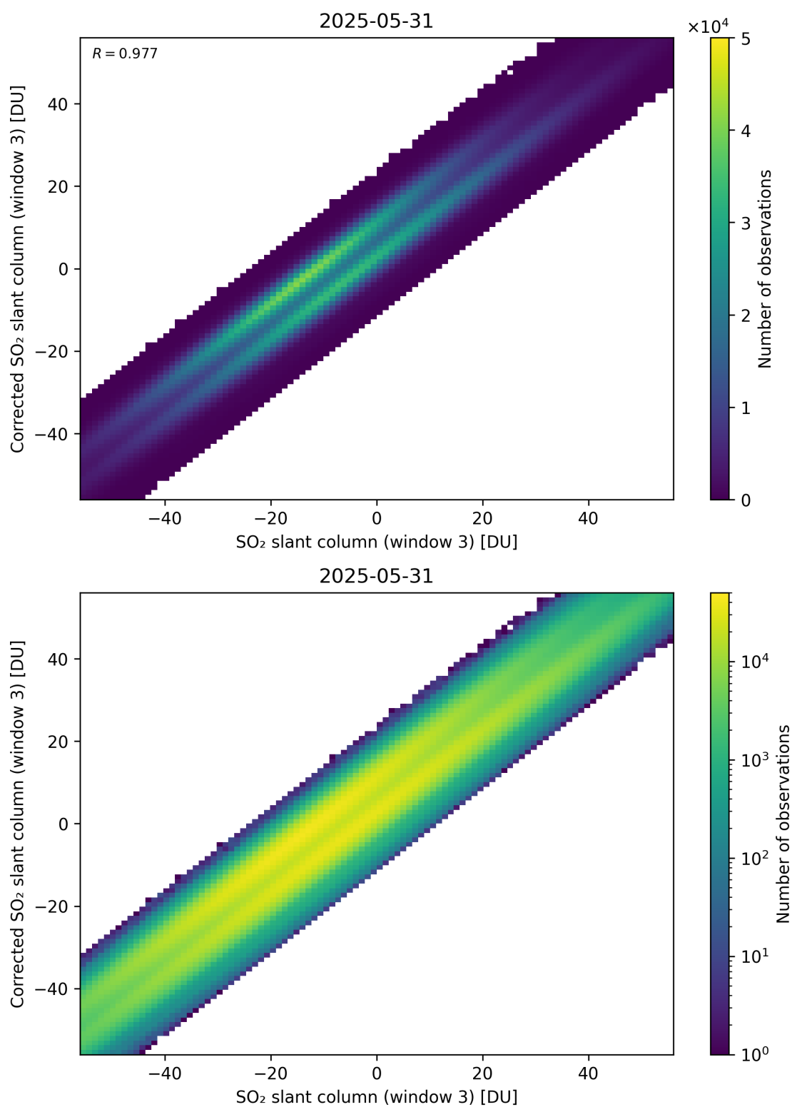
Figure 316: Scatter density plot of “SO 2 slant column (window 3)” against “Corrected SO 2 slant column (window 3)” for 2025-05-31 to 2025-06-01.
