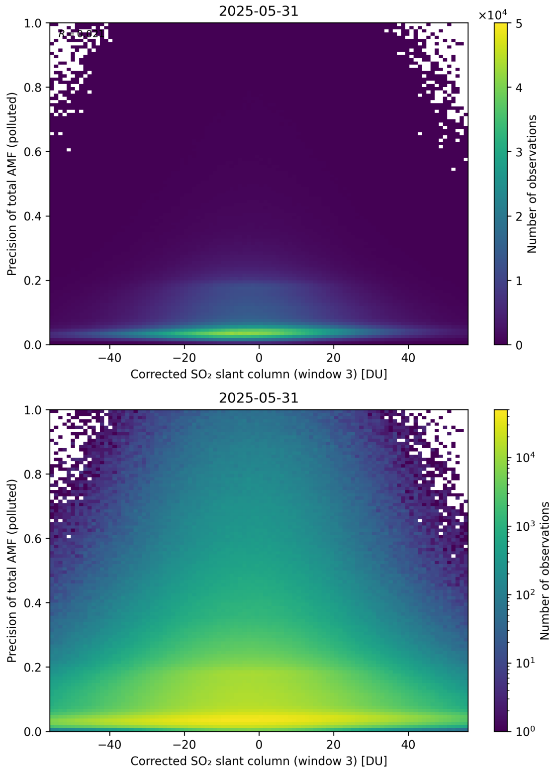
Figure 261: Scatter density plot of “Corrected SO 2 slant column (window 3)” against “Precision of total AMF (polluted)” for 2025-05-31 to 2025-06-01.
