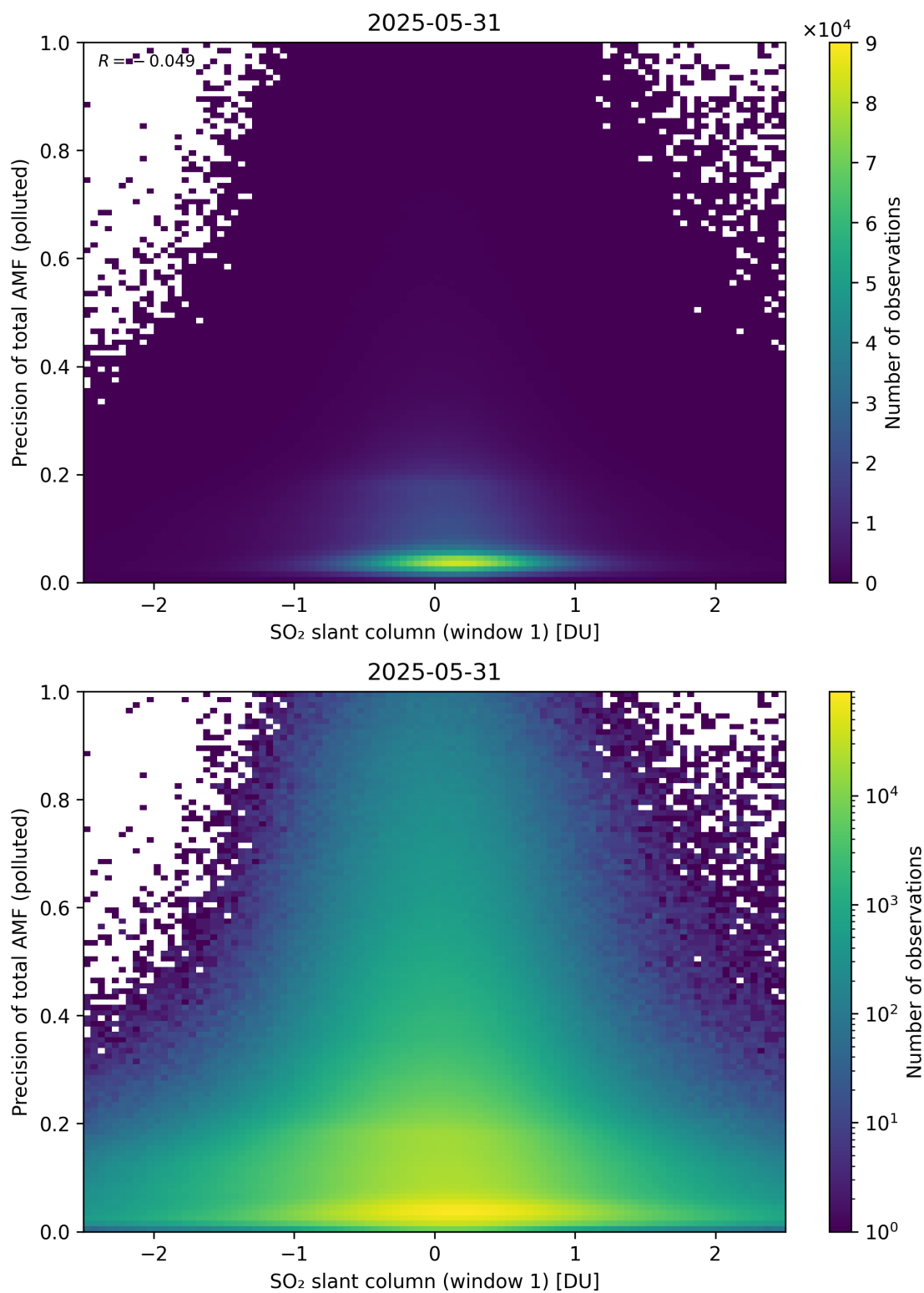
Figure 290: Scatter density plot of “SO 2 slant column (window 1)” against “Precision of total AMF (polluted)” for 2025-05-31 to 2025-06-01.
