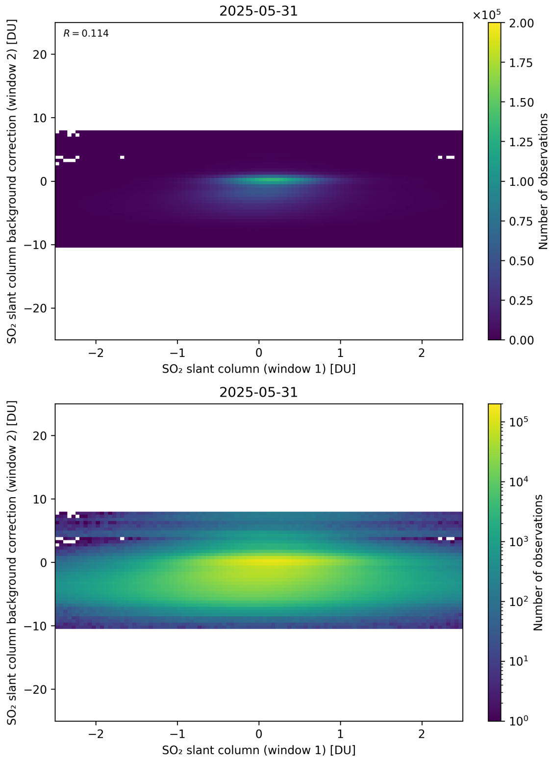
Figure 263: Scatter density plot of “SO 2 slant column (window 1)” against “SO 2 slant column background correction (window 2)” for 2025-05-31 to 2025-06-01.
