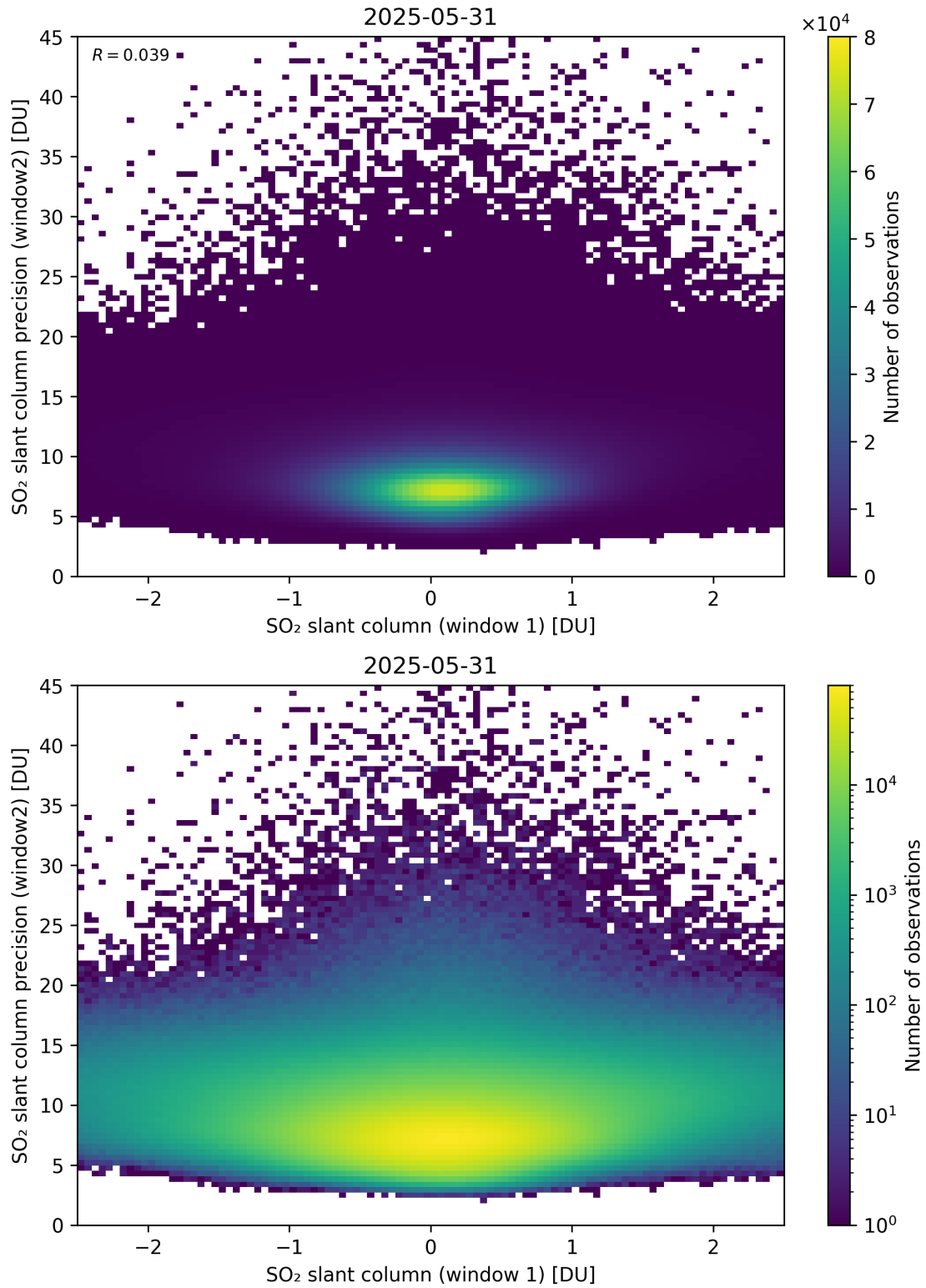
Figure 286: Scatter density plot of “SO 2 slant column (window 1)” against “SO 2 slant column precision (window2)” for 2025-05-31 to 2025-06-01.
