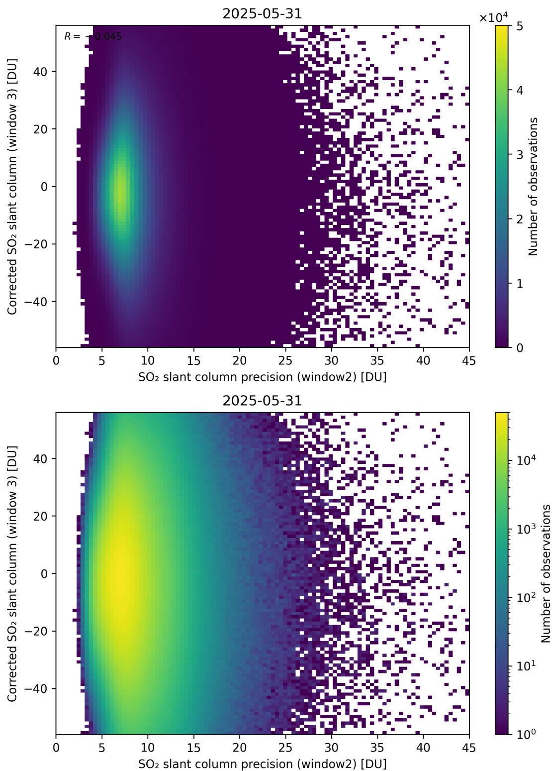
Figure 298: Scatter density plot of “SO 2 slant column precision (window2)” against “Corrected SO 2 slant column (window 3)” for 2025-05-31 to 2025-06-01.
