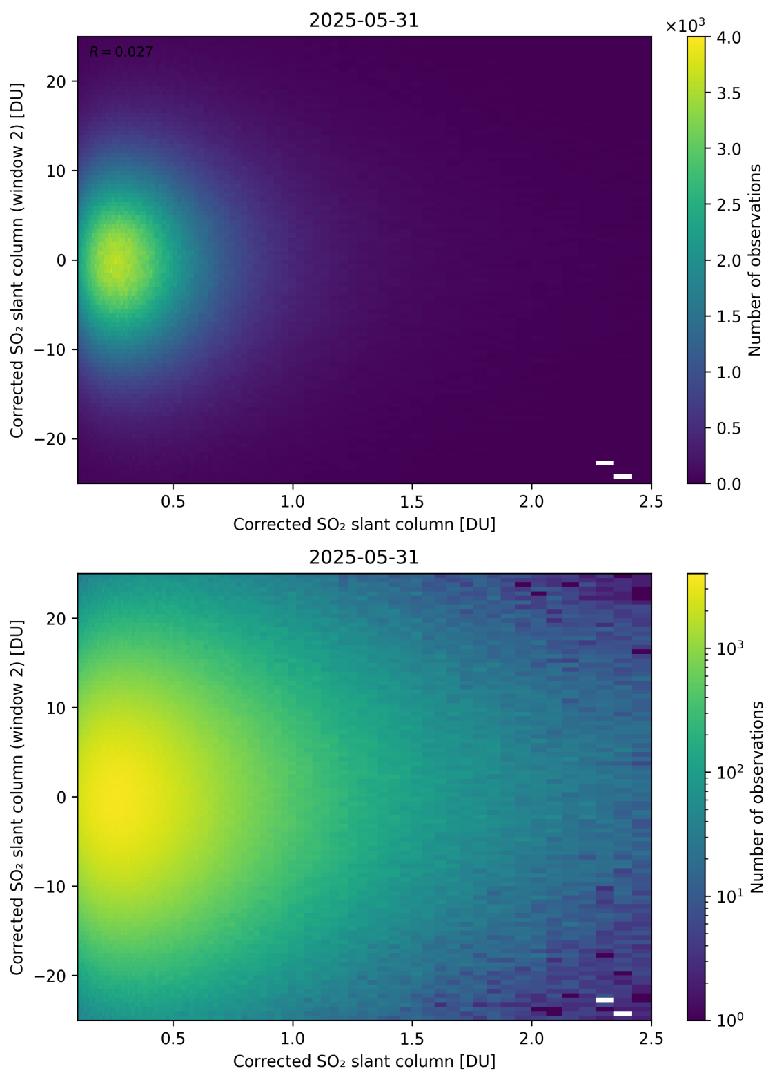
Figure 235: Scatter density plot of “Corrected SO 2 slant column” against “Corrected SO 2 slant column (window 2)” for 2025-05-31 to 2025-06-01.
