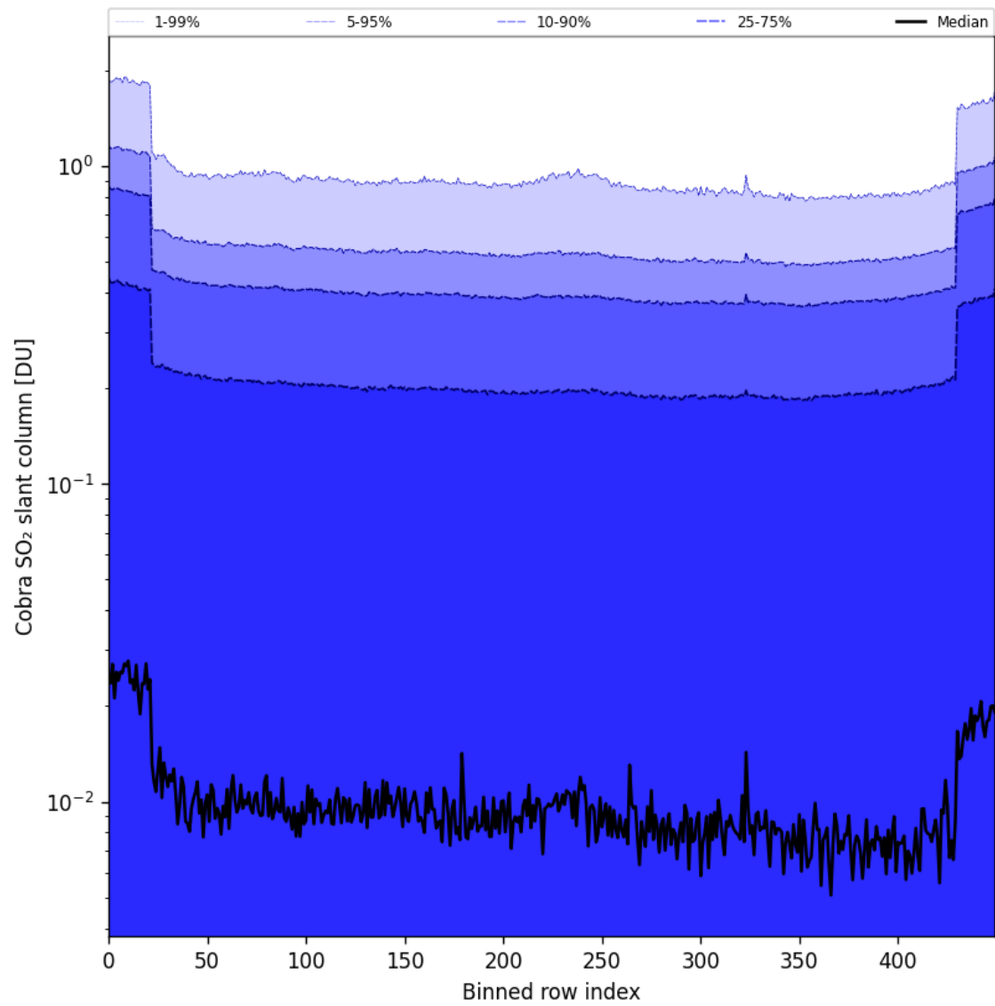
Figure 87: Along track statistics of “Cobra SO 2 slant column” for 2025-05-31 to 2025-06-01
