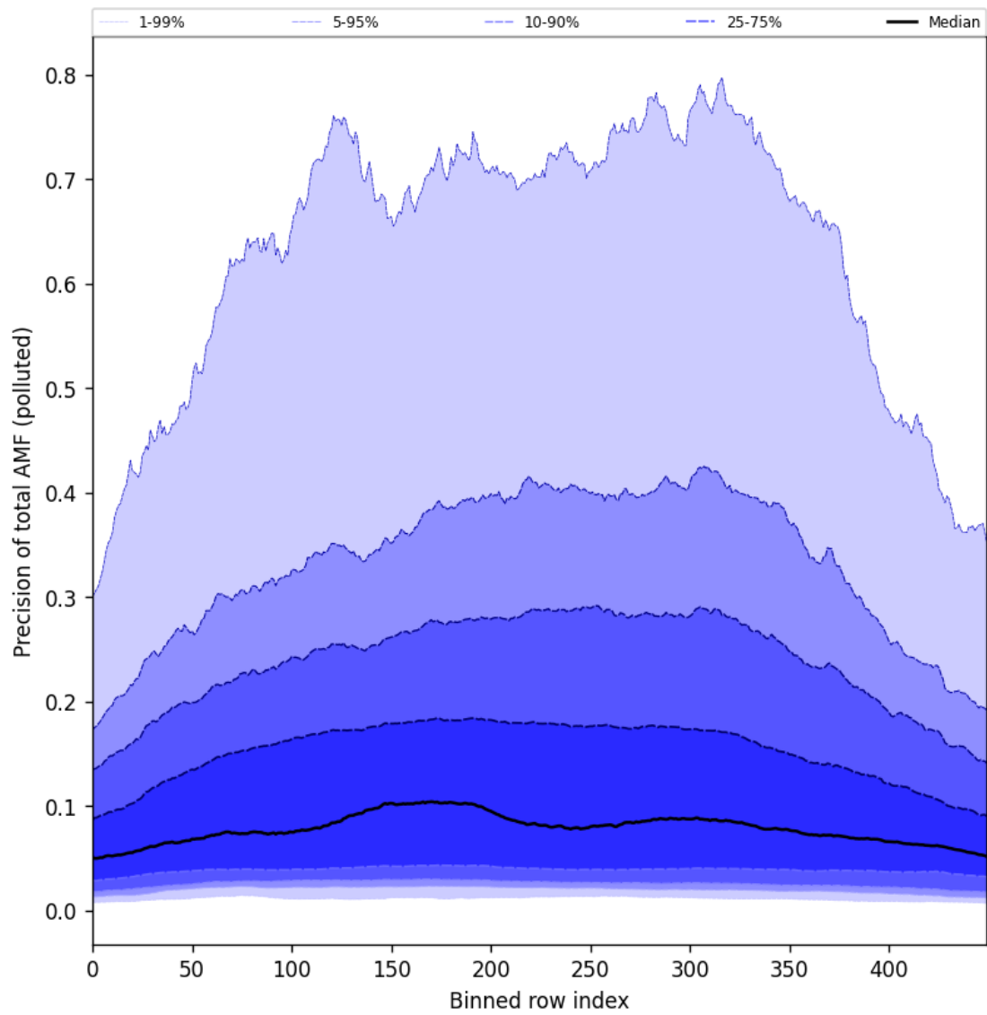
Figure 106: Along track statistics of “Precision of total AMF (polluted)” for 2025-05-31 to 2025-06-01
