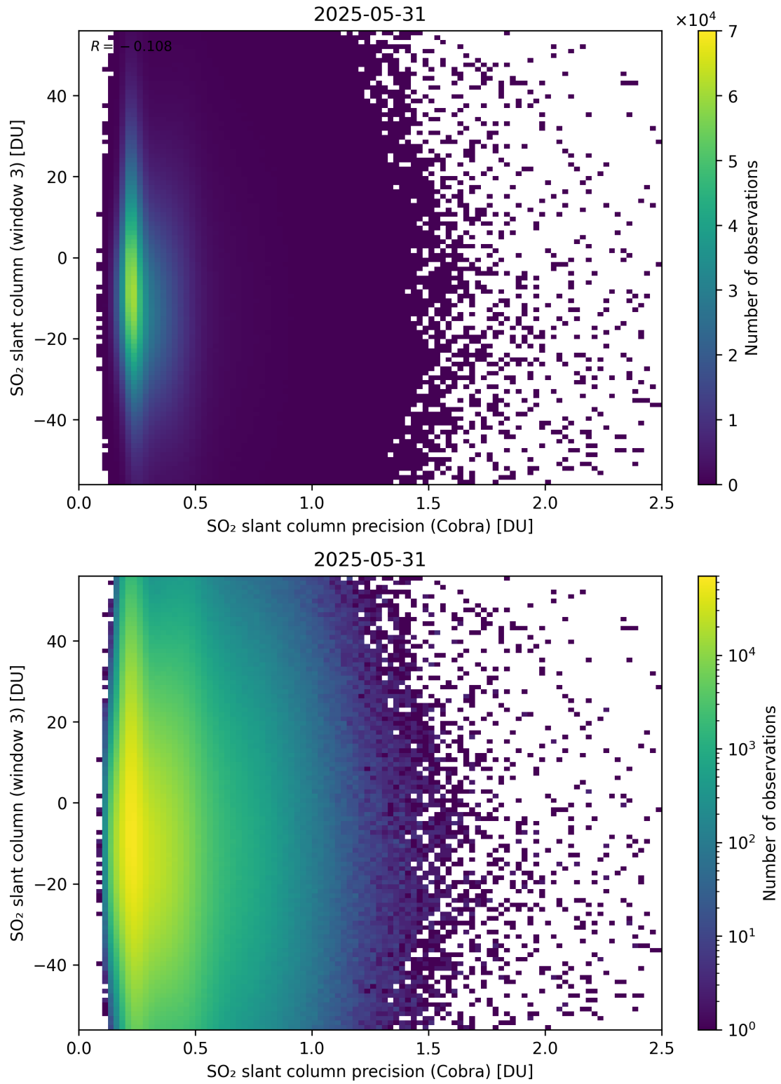
Figure 211: Scatter density plot of “SO 2 slant column precision (Cobra)” against “SO 2 slant column (window 3)” for 2025-05-31 to 2025-06-01.
