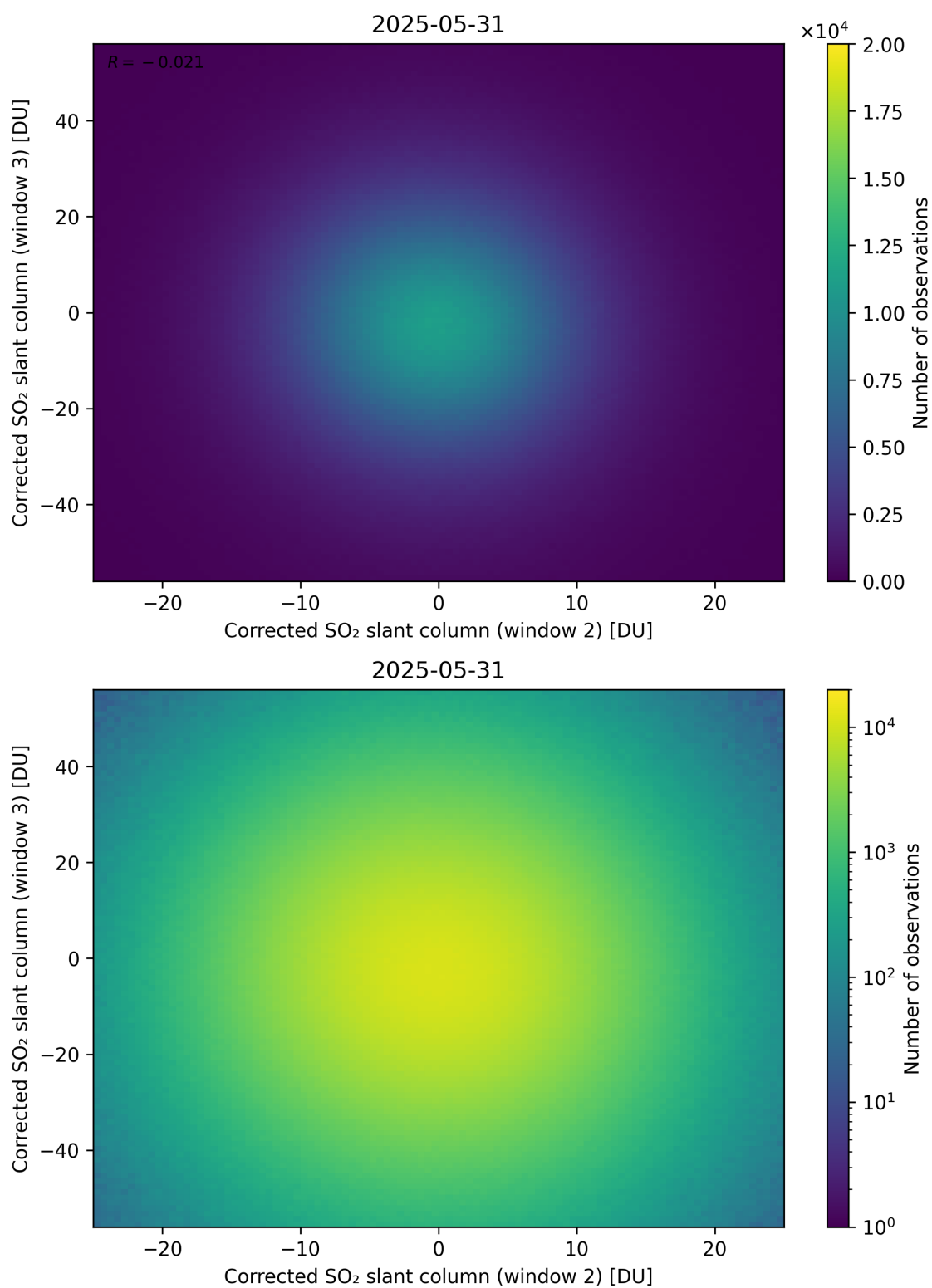
Figure 250: Scatter density plot of “Corrected SO 2 slant column (window 2)” against “Corrected SO 2 slant column (window 3)” for 2025-05-31 to 2025-06-01.
