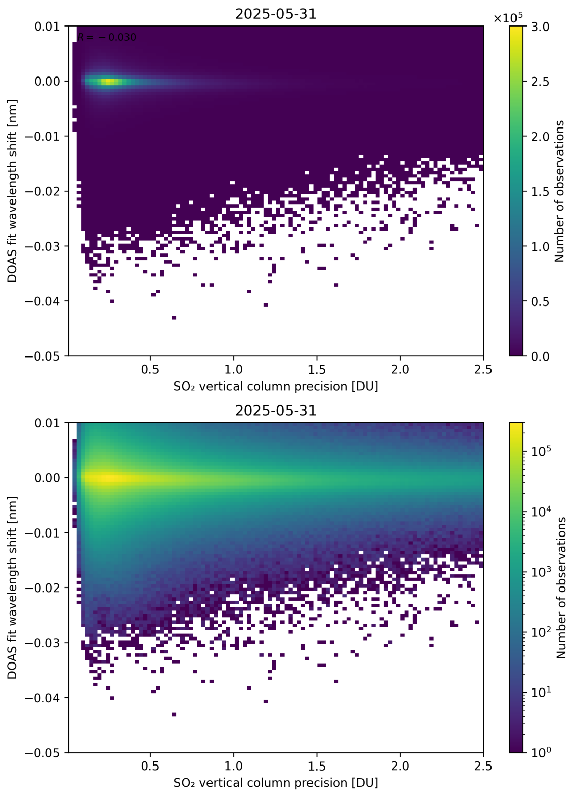
Figure 332: Scatter density plot of “SO 2 vertical column precision” against “DOAS fit wavelength shift” for 2025-05-31 to 2025-06-01.
