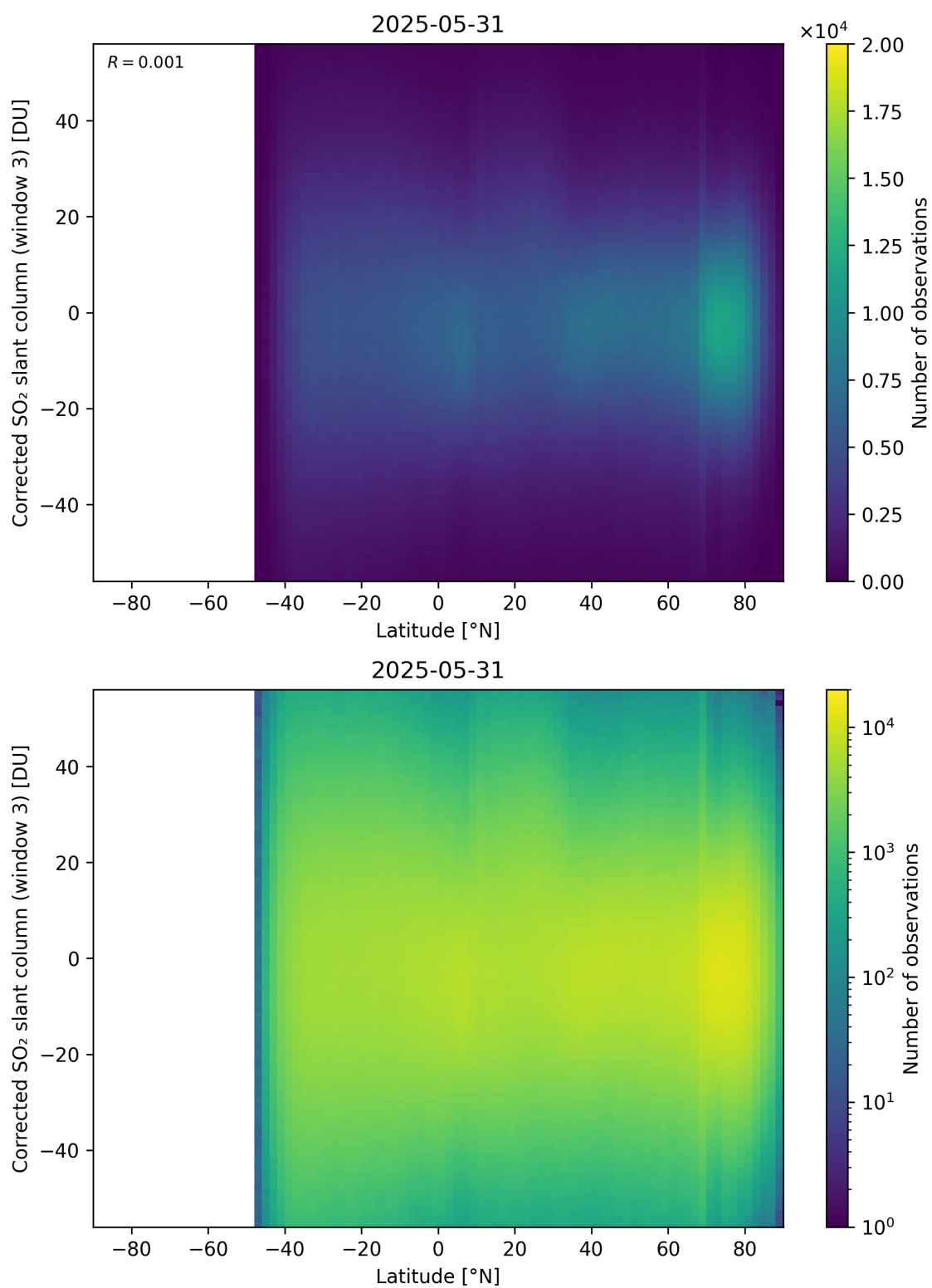
Figure 161: Scatter density plot of “Latitude” against “Corrected SO 2 slant column (window 3)” for 2025-05-31 to 2025-06-01.
