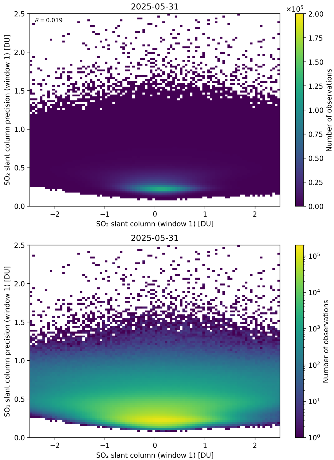
Figure 285: Scatter density plot of “SO 2 slant column (window 1)” against “SO 2 slant column precision (window 1)” for 2025-05-31 to 2025-06-01.
