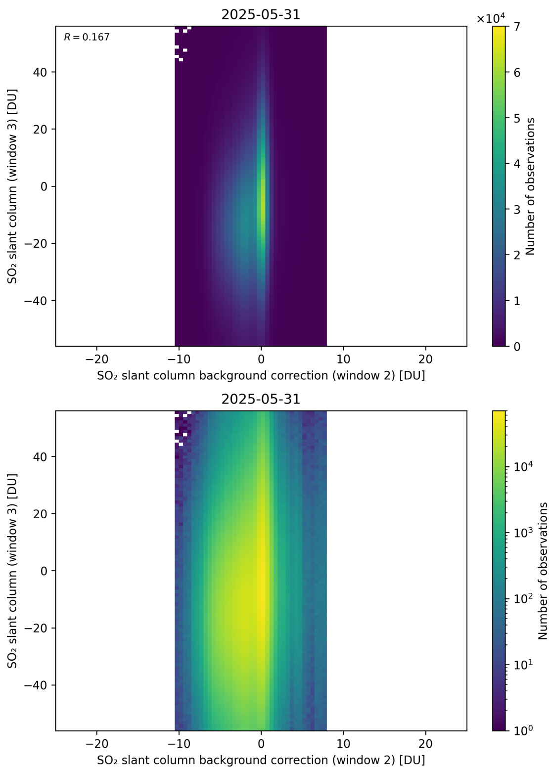
Figure 128: Scatter density plot of “SO 2 slant column background correction (window 2)” against “SO 2 slant column (window 3)” for 2025-05-31 to 2025-06-01.
