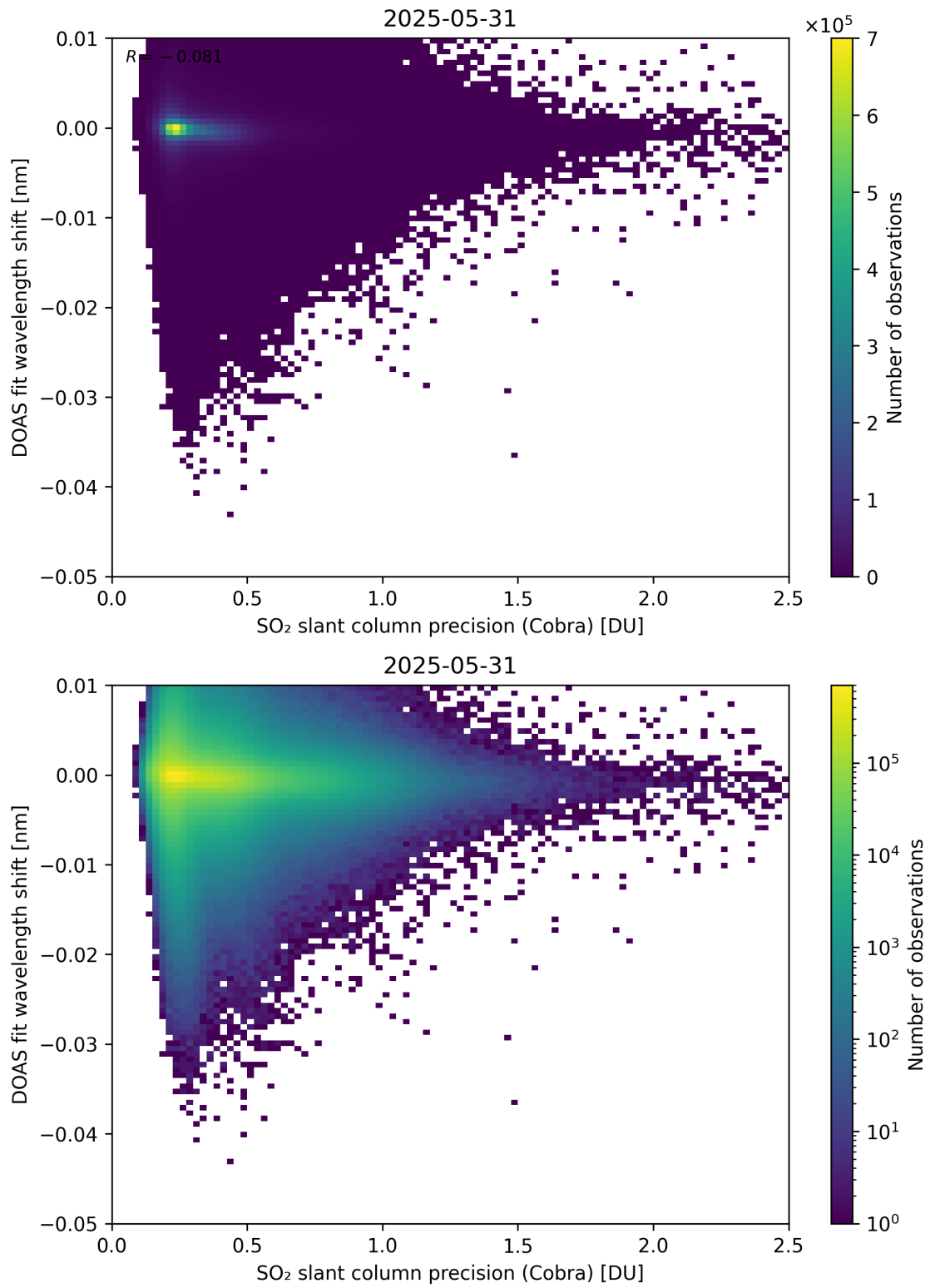
Figure 202: Scatter density plot of “SO 2 slant column precision (Cobra)” against “DOAS fit wavelength shift” for 2025-05-31 to 2025-06-01.
