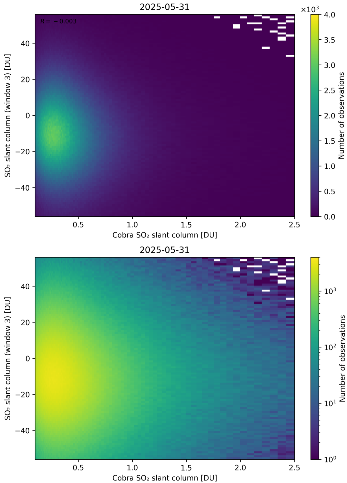
Figure 222: Scatter density plot of “Cobra SO 2 slant column” against “SO 2 slant column (window 3)” for 2025-05-31 to 2025-06-01.
