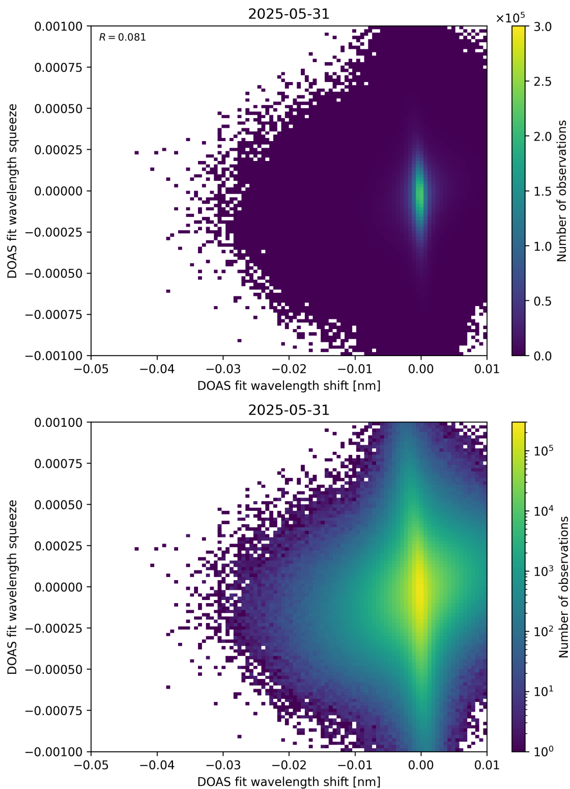
Figure 138: Scatter density plot of “DOAS fit wavelength shift” against “DOAS fit wavelength squeeze” for 2025-05-31 to 2025-06-01.
