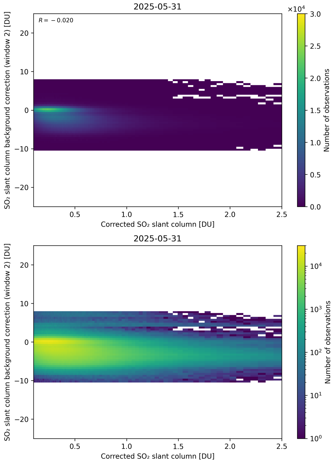
Figure 227: Scatter density plot of “Corrected SO 2 slant column” against “SO 2 slant column background correction (window 2)” for 2025-05-31 to 2025-06-01.
