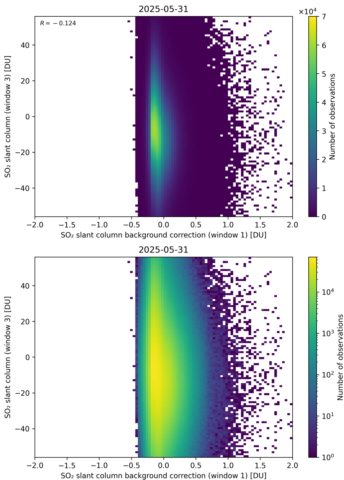
Figure 118: Scatter density plot of “SO 2 slant column background correction (window 1)” against “SO 2 slant column (window 3)” for 2025-05-31 to 2025-06-01.
