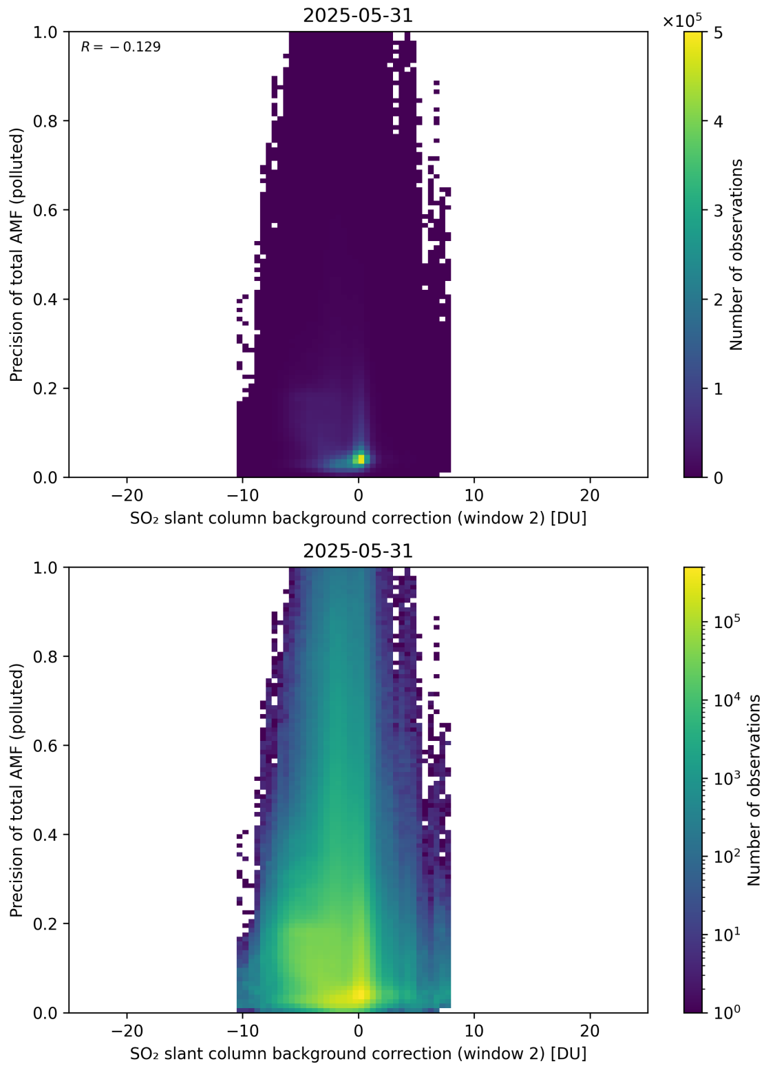
Figure 131: Scatter density plot of “SO 2 slant column background correction (window 2)” against “Precision of total AMF (polluted)” for 2025-05-31 to 2025-06-01.
