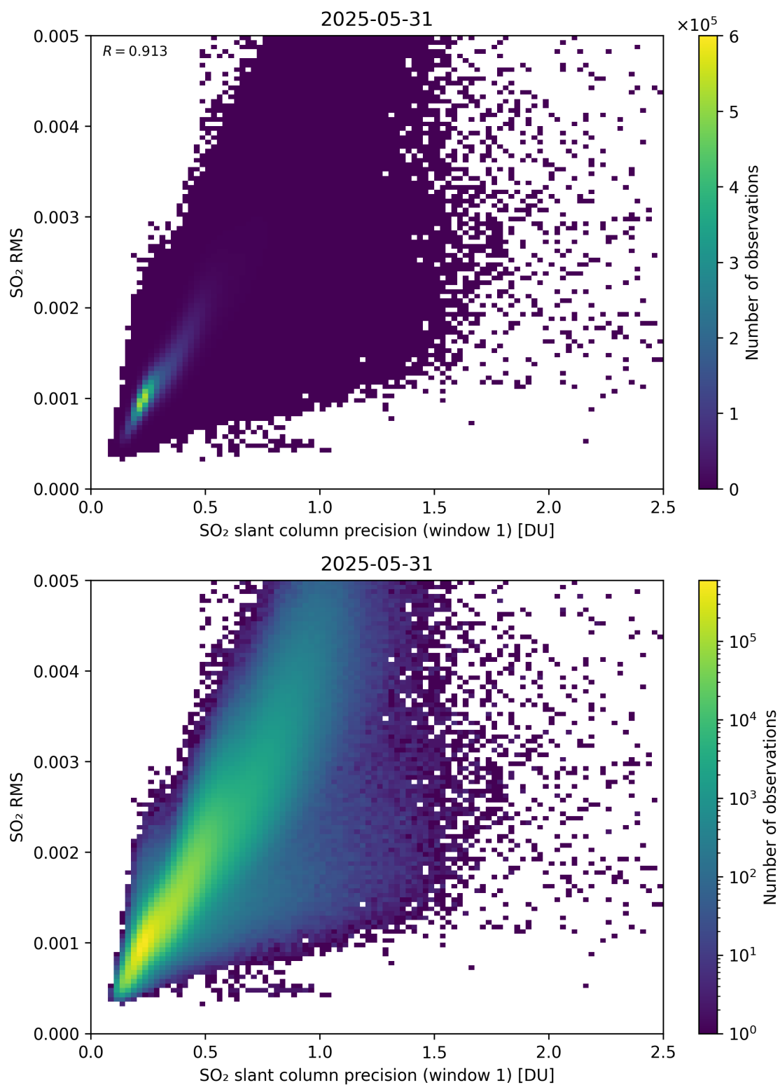
Figure 273: Scatter density plot of “SO 2 slant column precision (window 1)” against “SO 2 RMS” for 2025-05-31 to 2025-06-01.
