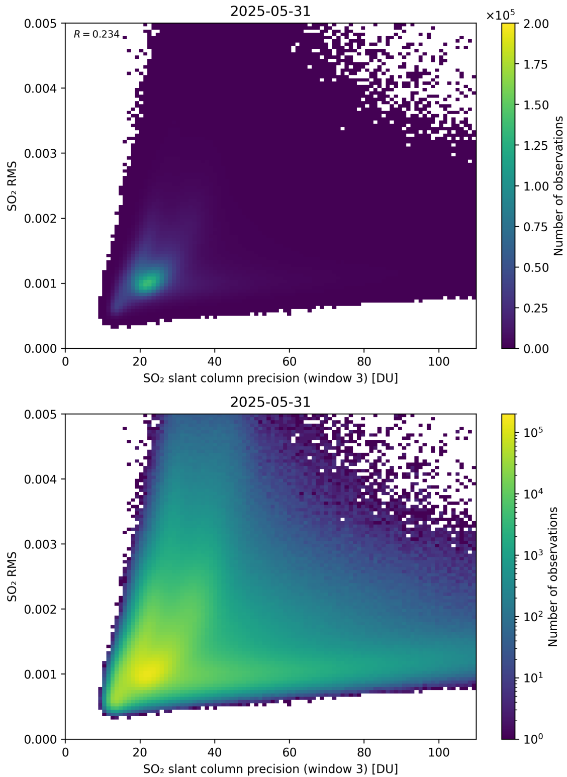
Figure 310: Scatter density plot of “SO 2 slant column precision (window 3)” against “SO 2 RMS” for 2025-05-31 to 2025-06-01.
