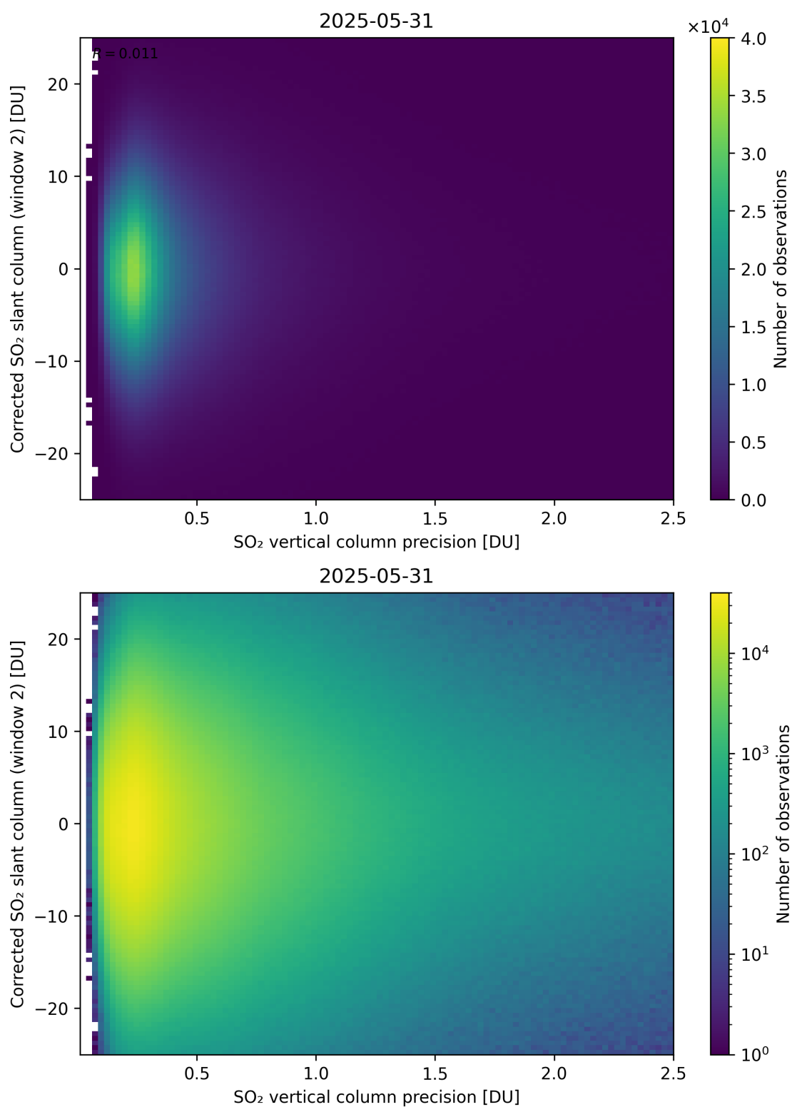
Figure 339: Scatter density plot of “SO 2 vertical column precision” against “Corrected SO 2 slant column (window 2)” for 2025-05-31 to 2025-06-01.
