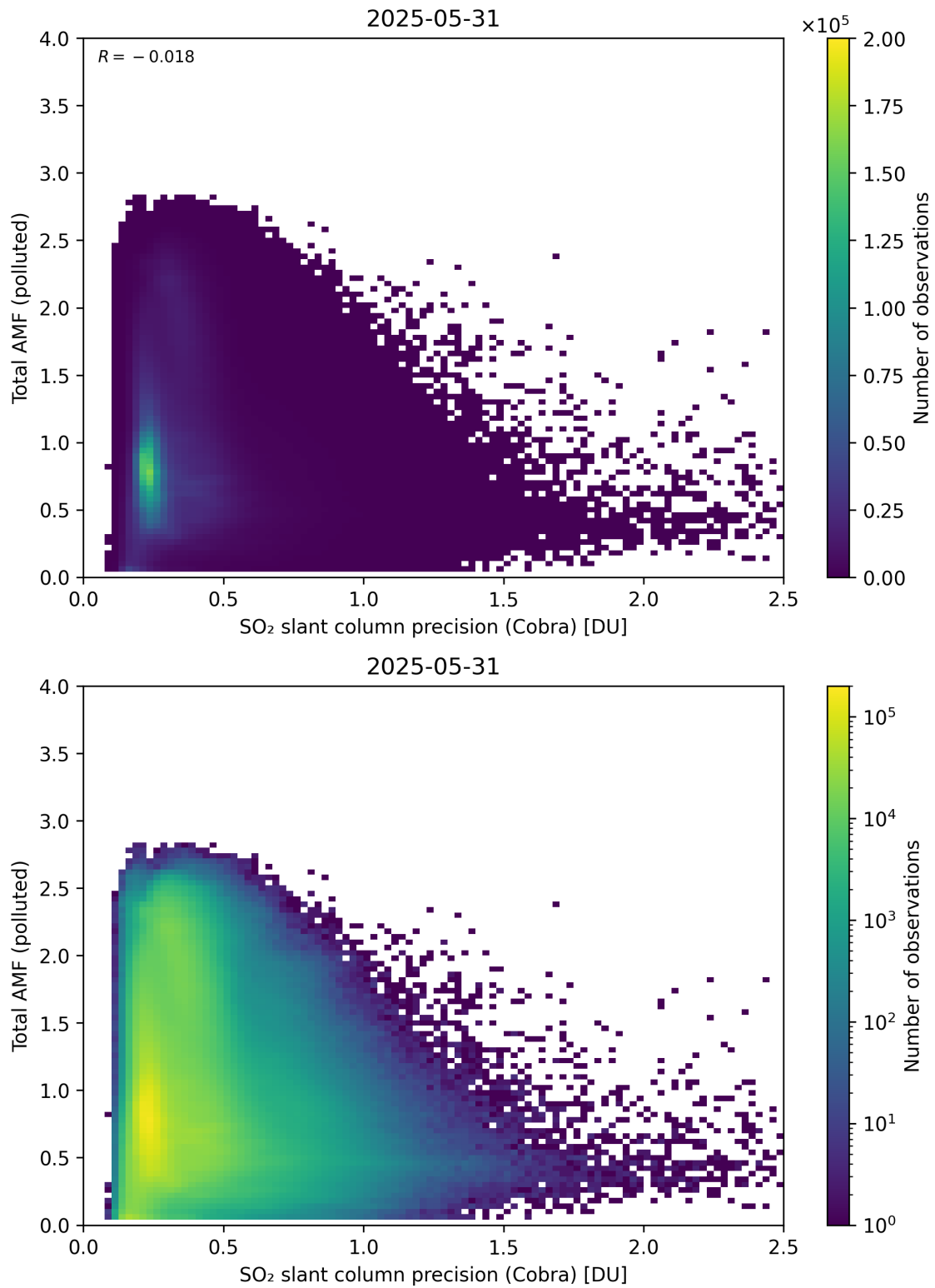
Figure 213: Scatter density plot of “SO 2 slant column precision (Cobra)” against “Total AMF (polluted)” for 2025-05-31 to 2025-06-01.
