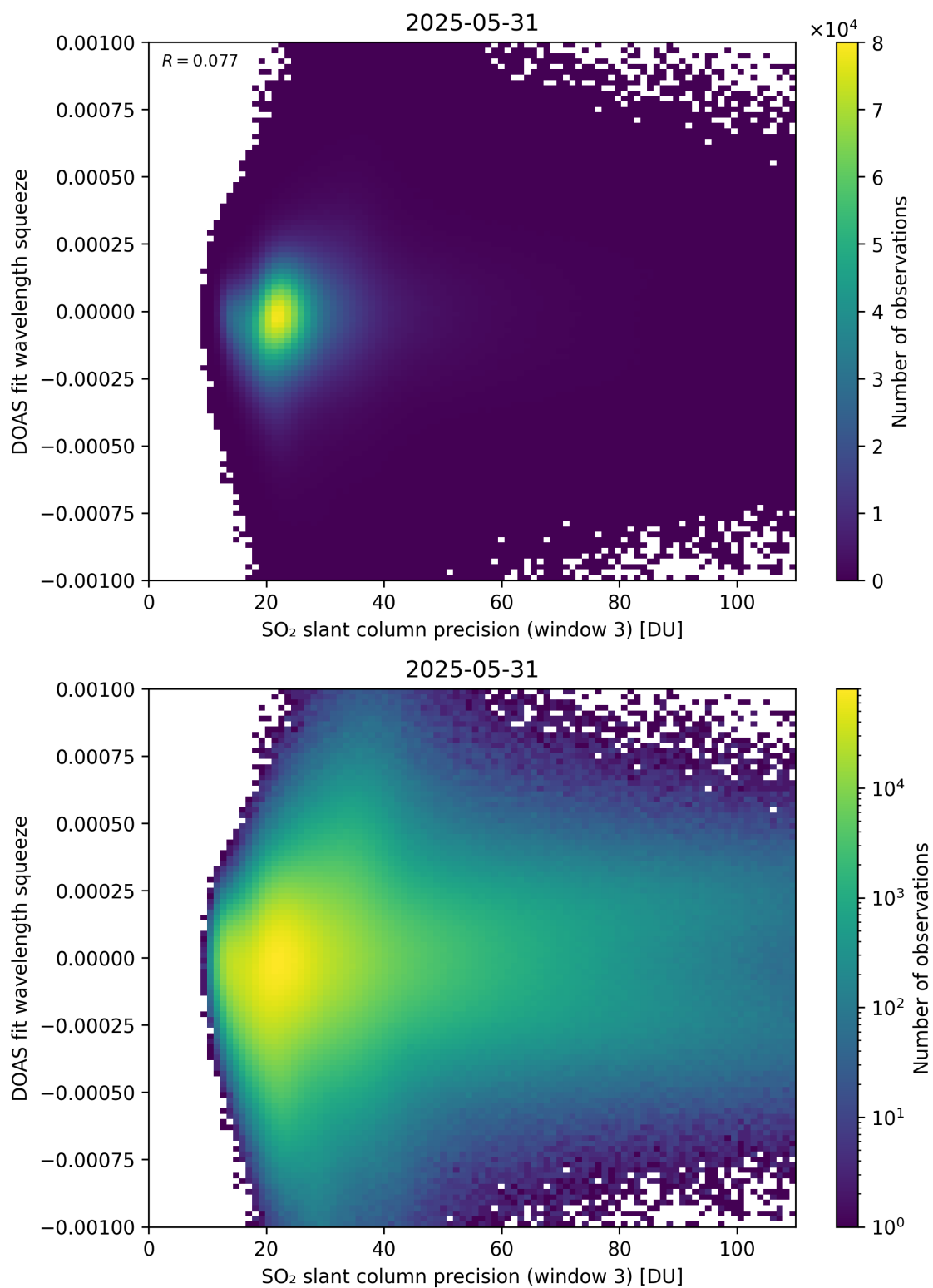
Figure 309: Scatter density plot of “SO 2 slant column precision (window 3)” against “DOAS fit wavelength squeeze” for 2025-05-31 to 2025-06-01.
