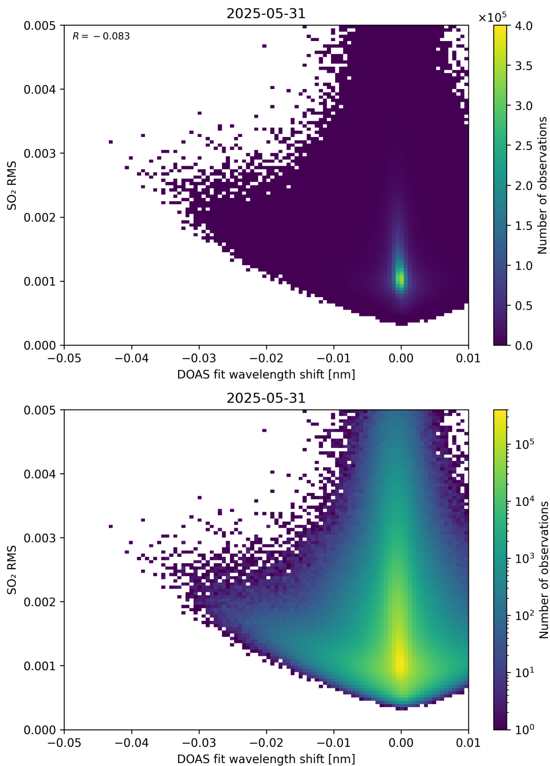
Figure 139: Scatter density plot of “DOAS fit wavelength shift” against “SO 2 RMS” for 2025-05-31 to 2025-06-01.
