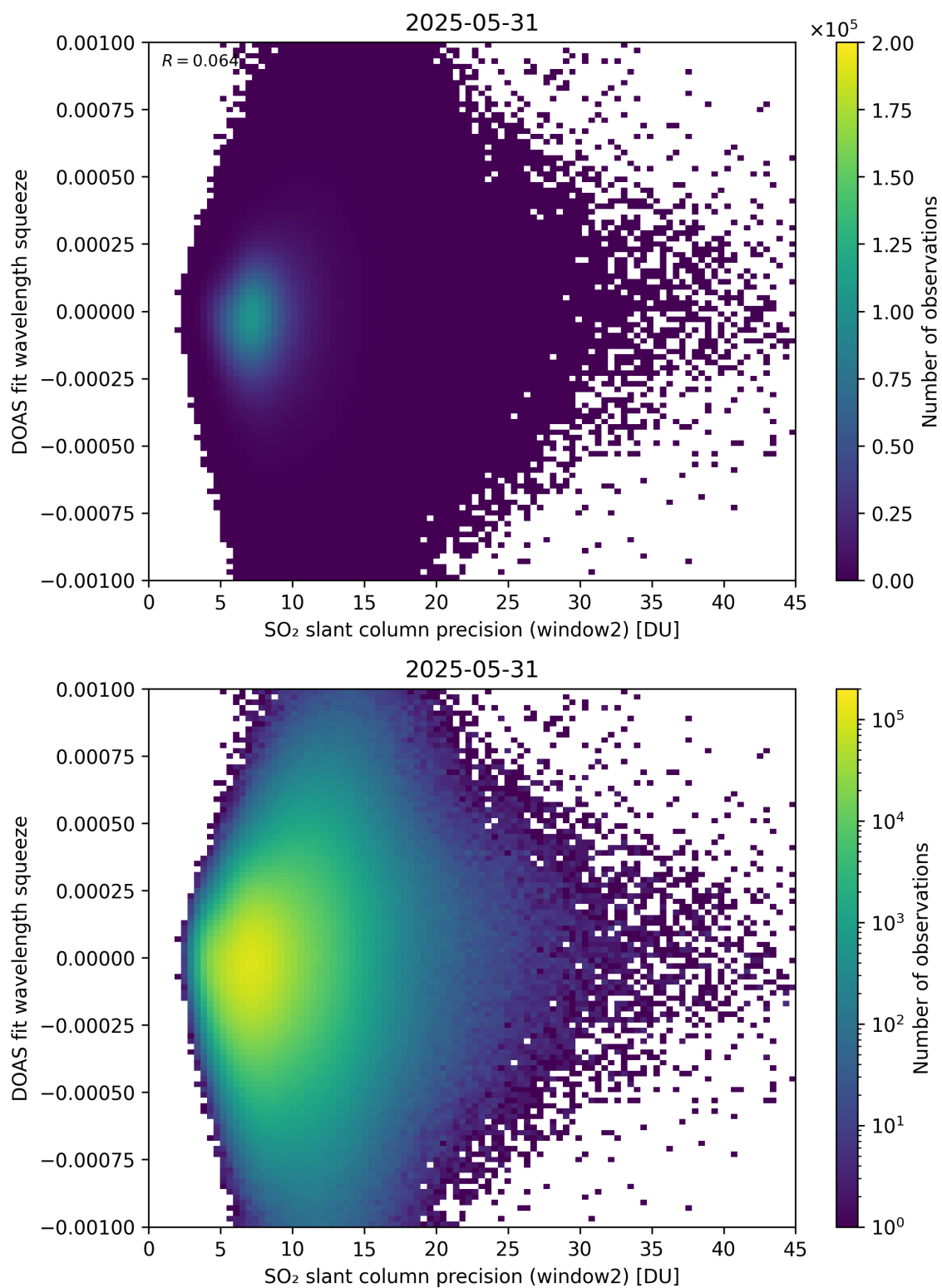
Figure 294: Scatter density plot of “SO 2 slant column precision (window2)” against “DOAS fit wavelength squeeze” for 2025-05-31 to 2025-06-01.
