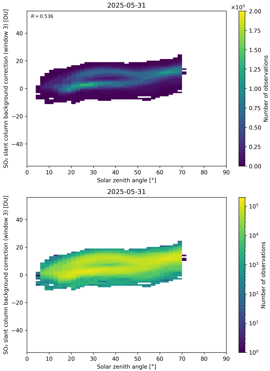
Figure 173: Scatter density plot of “Solar zenith angle” against “SO 2 slant column background correction (window 3)” for 2025-05-31 to 2025-06-01.
