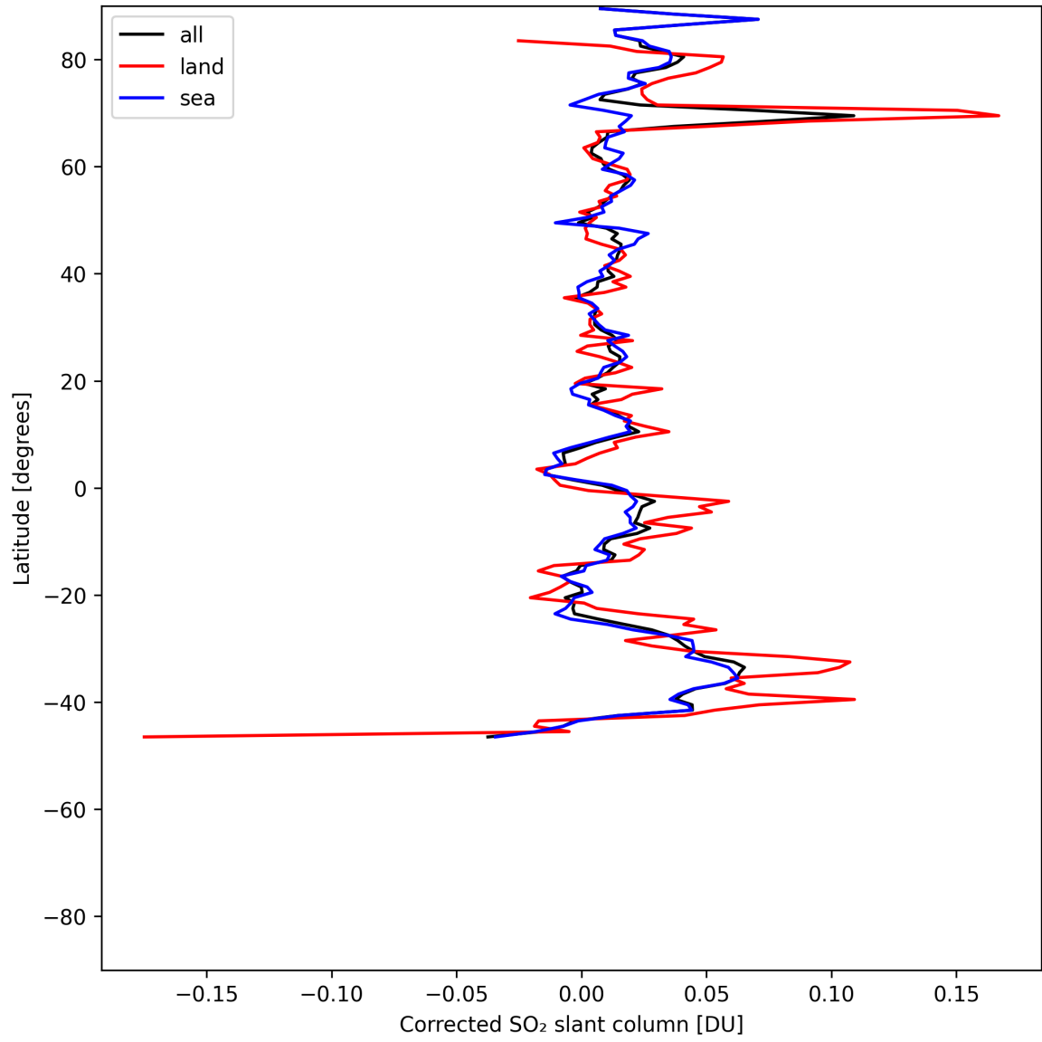
Figure 34: Zonal average of “Corrected SO 2 slant column” for 2025-05-31 to 2025-06-01.
