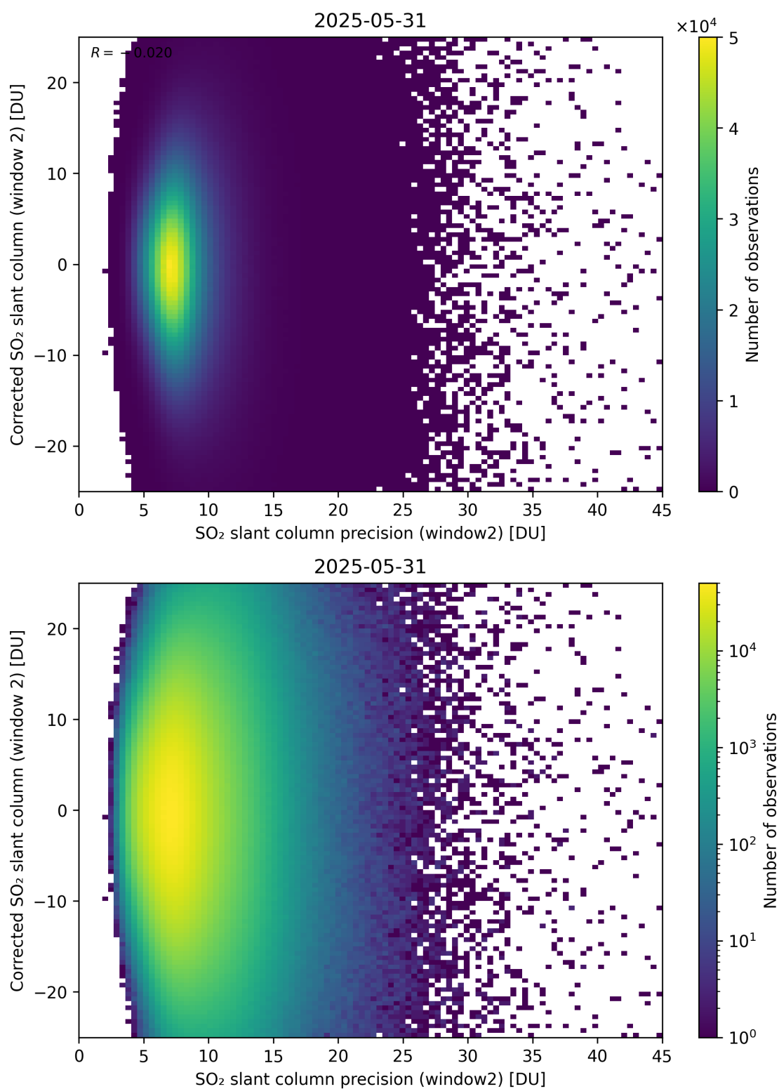
Figure 297: Scatter density plot of “SO 2 slant column precision (window2)” against “Corrected SO 2 slant column (window 2)” for 2025-05-31 to 2025-06-01.
