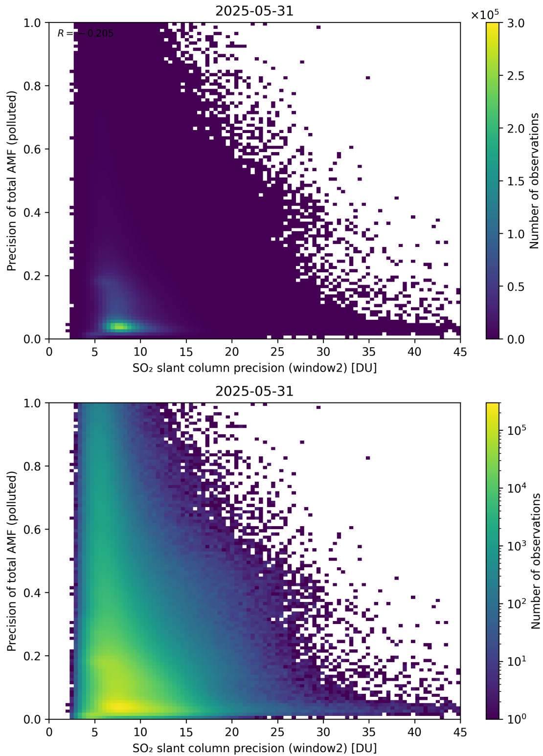
Figure 302: Scatter density plot of “SO 2 slant column precision (window2)” against “Precision of total AMF (polluted)” for 2025-05-31 to 2025-06-01.
