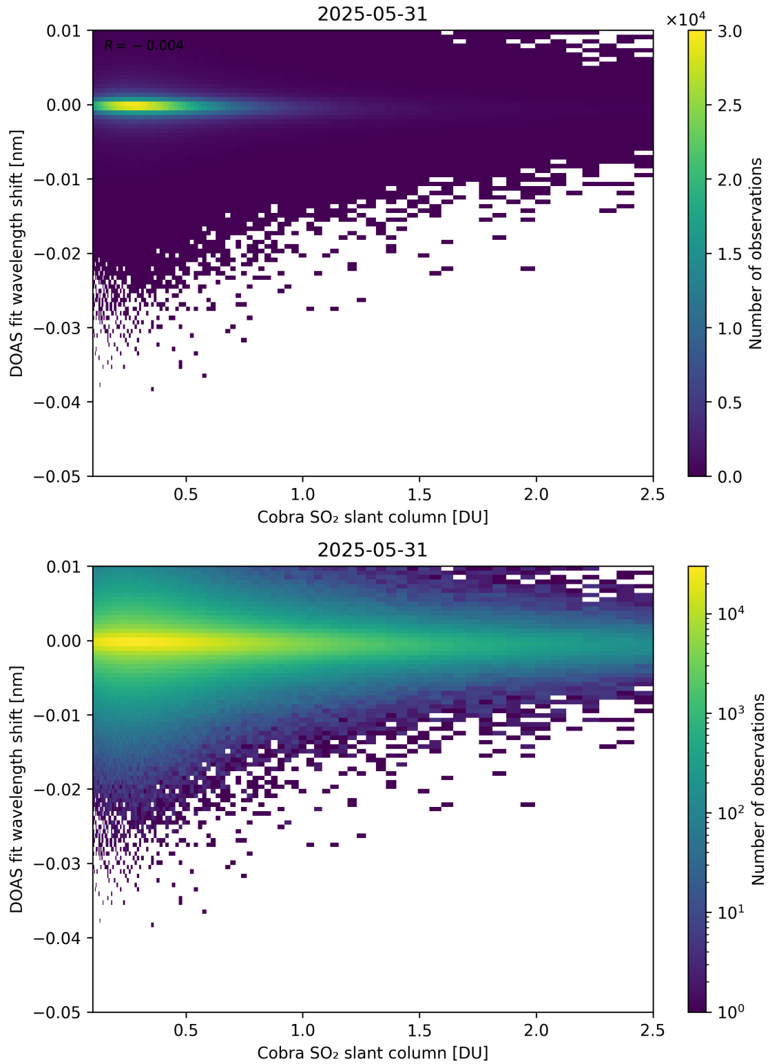
Figure 196: Scatter density plot of “Cobra SO 2 slant column” against “DOAS fit wavelength shift” for 2025-05-31 to 2025-06-01.
