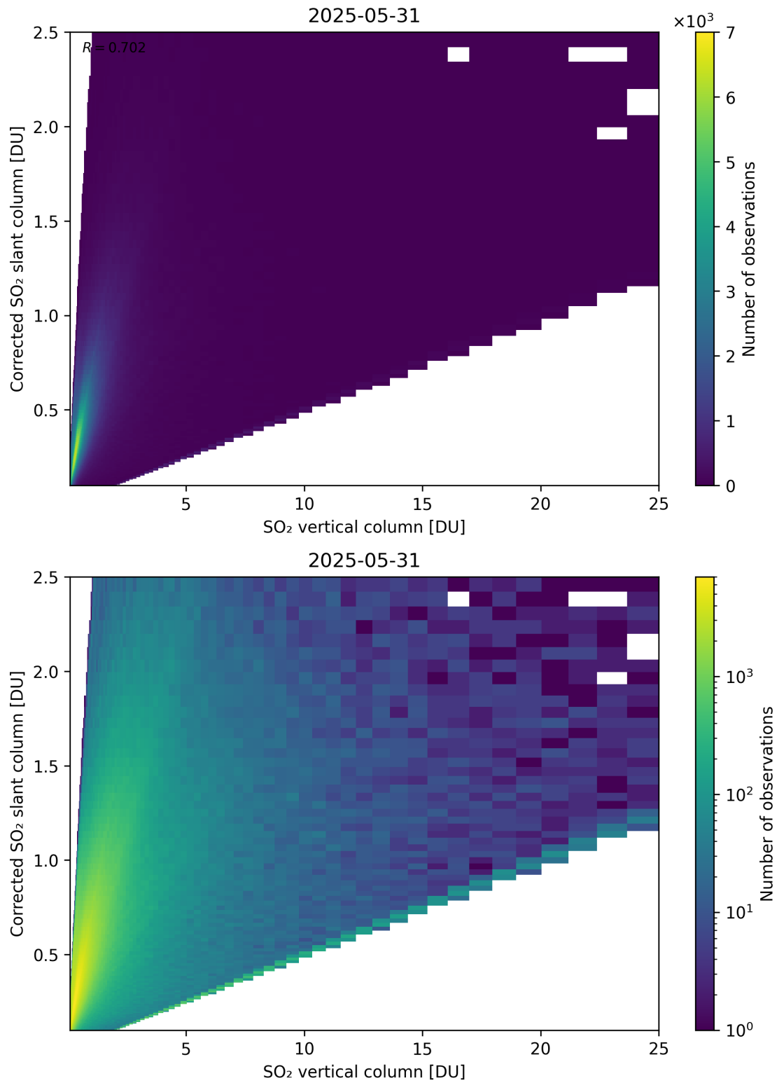
Figure 351: Scatter density plot of “SO 2 vertical column” against “Corrected SO 2 slant column” for 2025-05-31 to 2025-06-01.
