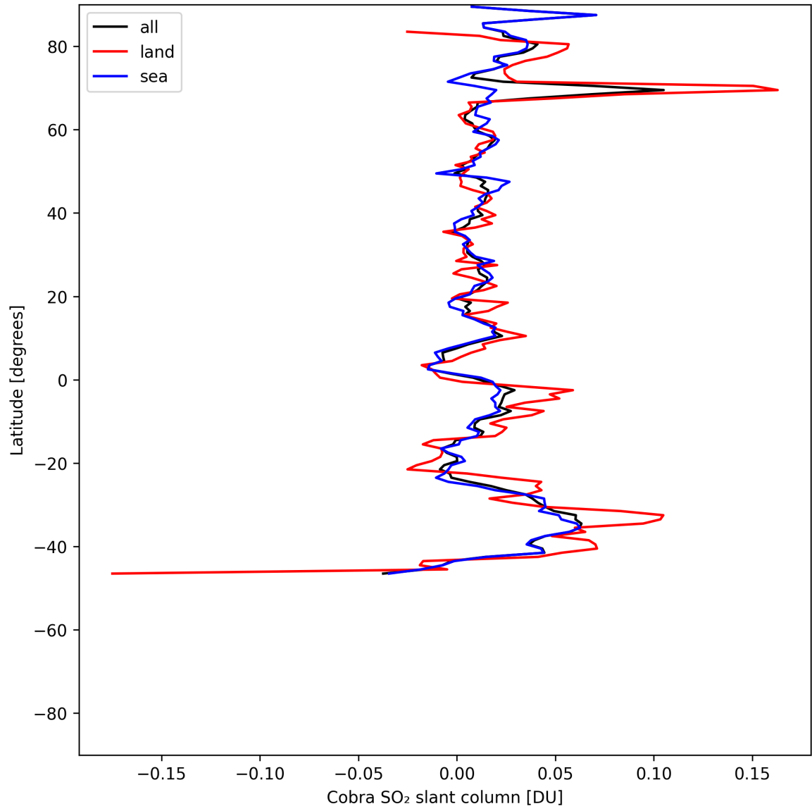
Figure 35: Zonal average of “Cobra SO 2 slant column” for 2025-05-31 to 2025-06-01.
