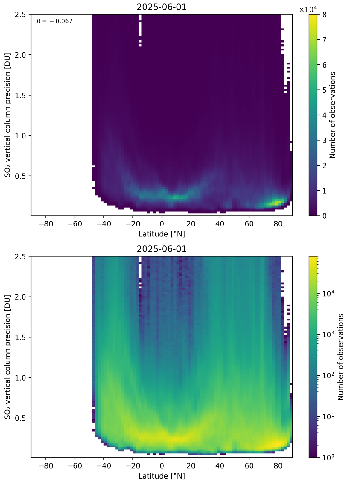
Figure 170: Scatter density plot of “Latitude” against “SO 2 vertical column precision” for 2025-06-01 to 2025-06-02.
