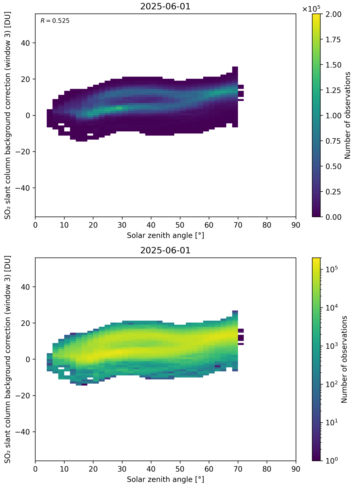
Figure 173: Scatter density plot of “Solar zenith angle” against “SO 2 slant column background correction (window 3)” for 2025-06-01 to 2025-06-02.
