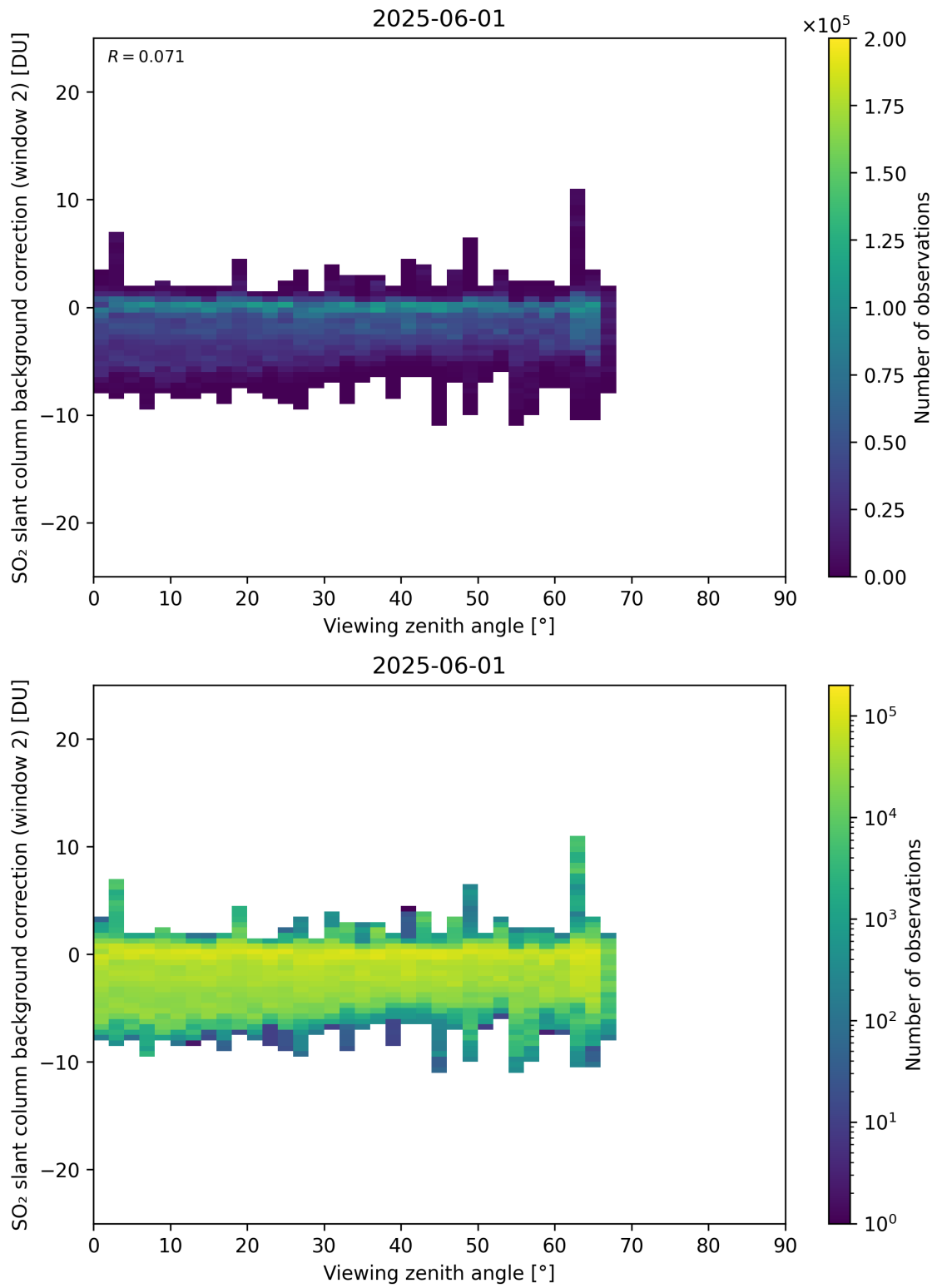
Figure 363: Scatter density plot of “Viewing zenith angle” against “SO 2 slant column background correction (window 2)” for 2025-06-01 to 2025-06-02.
