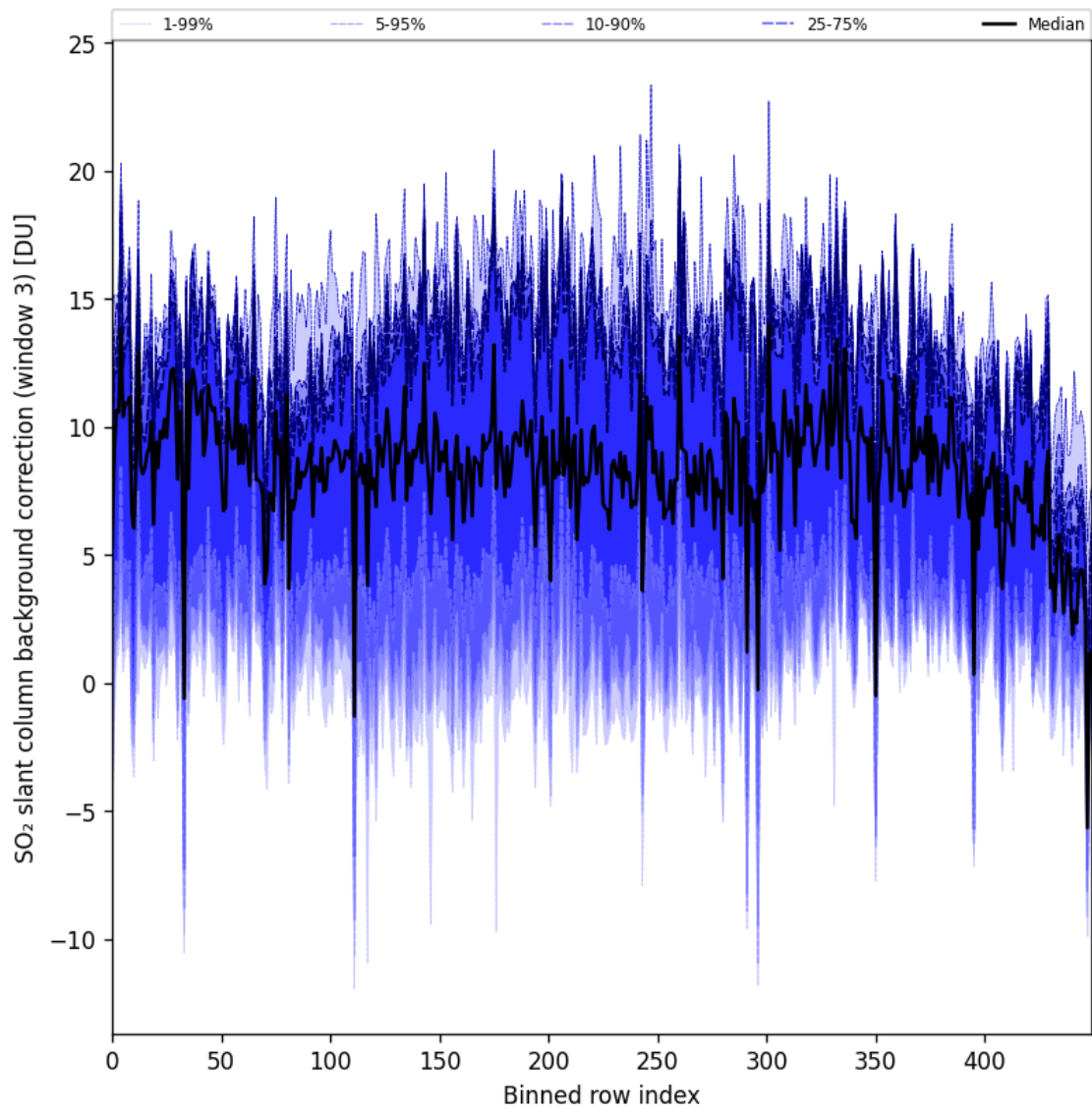
Figure 100: Along track statistics of “SO 2 slant column background correction (window 3)” for 2025-06-01 to 2025-06-02
