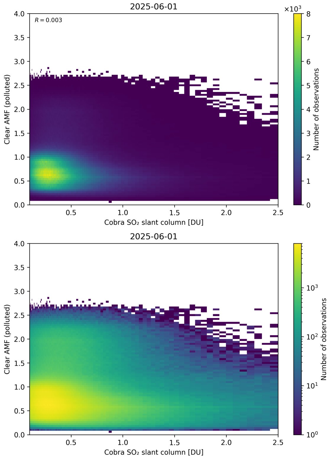
Figure 215: Scatter density plot of “Cobra SO 2 slant column” against “Clear AMF (polluted)” for 2025-06-01 to 2025-06-02.
