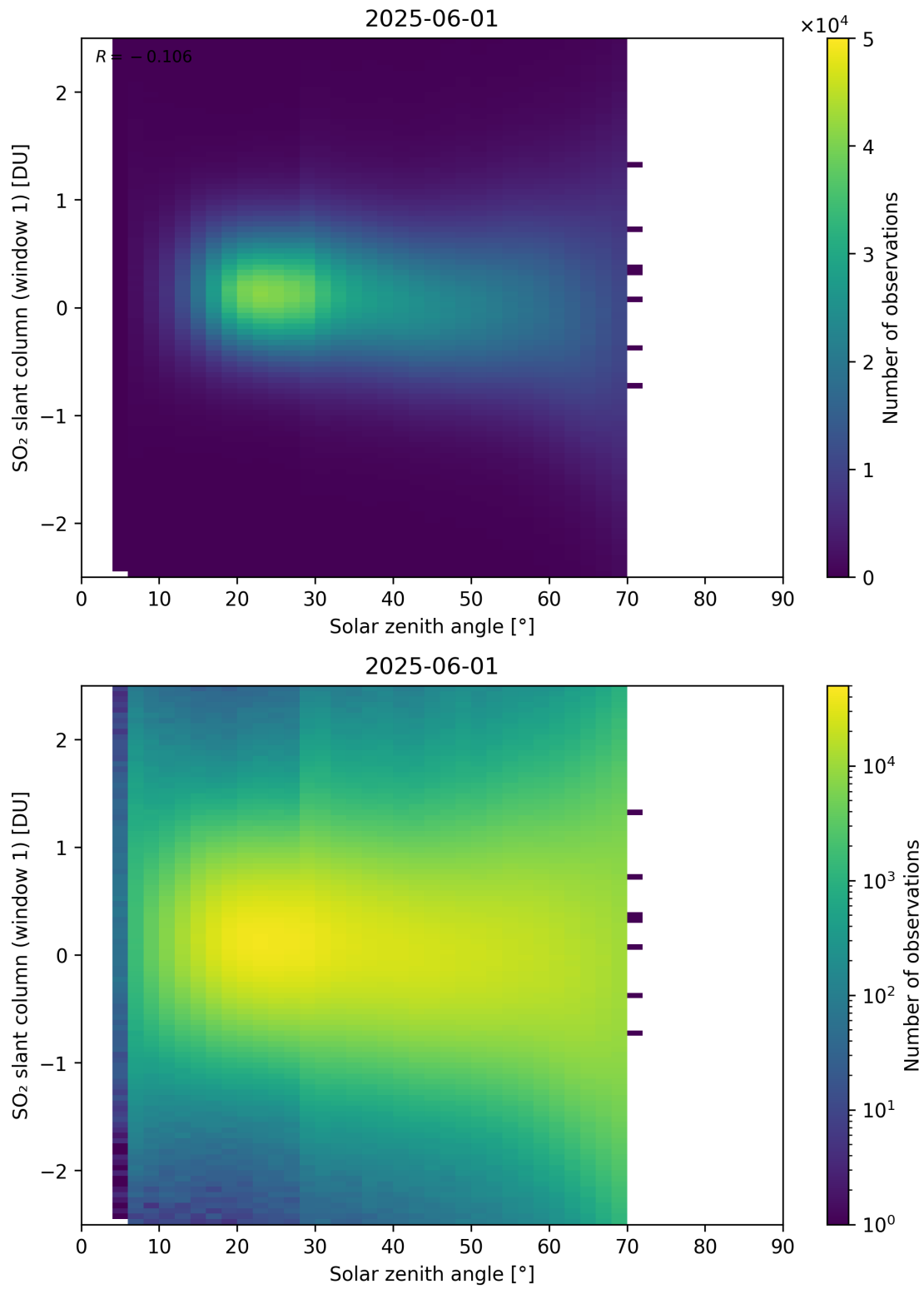
Figure 184: Scatter density plot of “Solar zenith angle” against “SO 2 slant column (window 1)” for 2025-06-01 to 2025-06-02.
