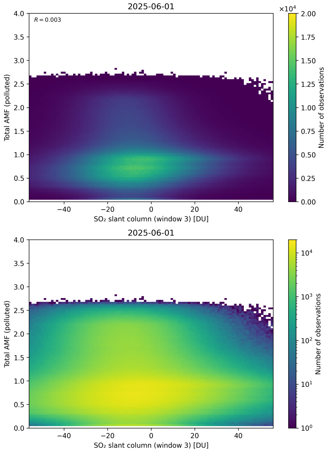
Figure 318: Scatter density plot of “SO 2 slant column (window 3)” against “Total AMF (polluted)” for 2025-06-01 to 2025-06-02.
