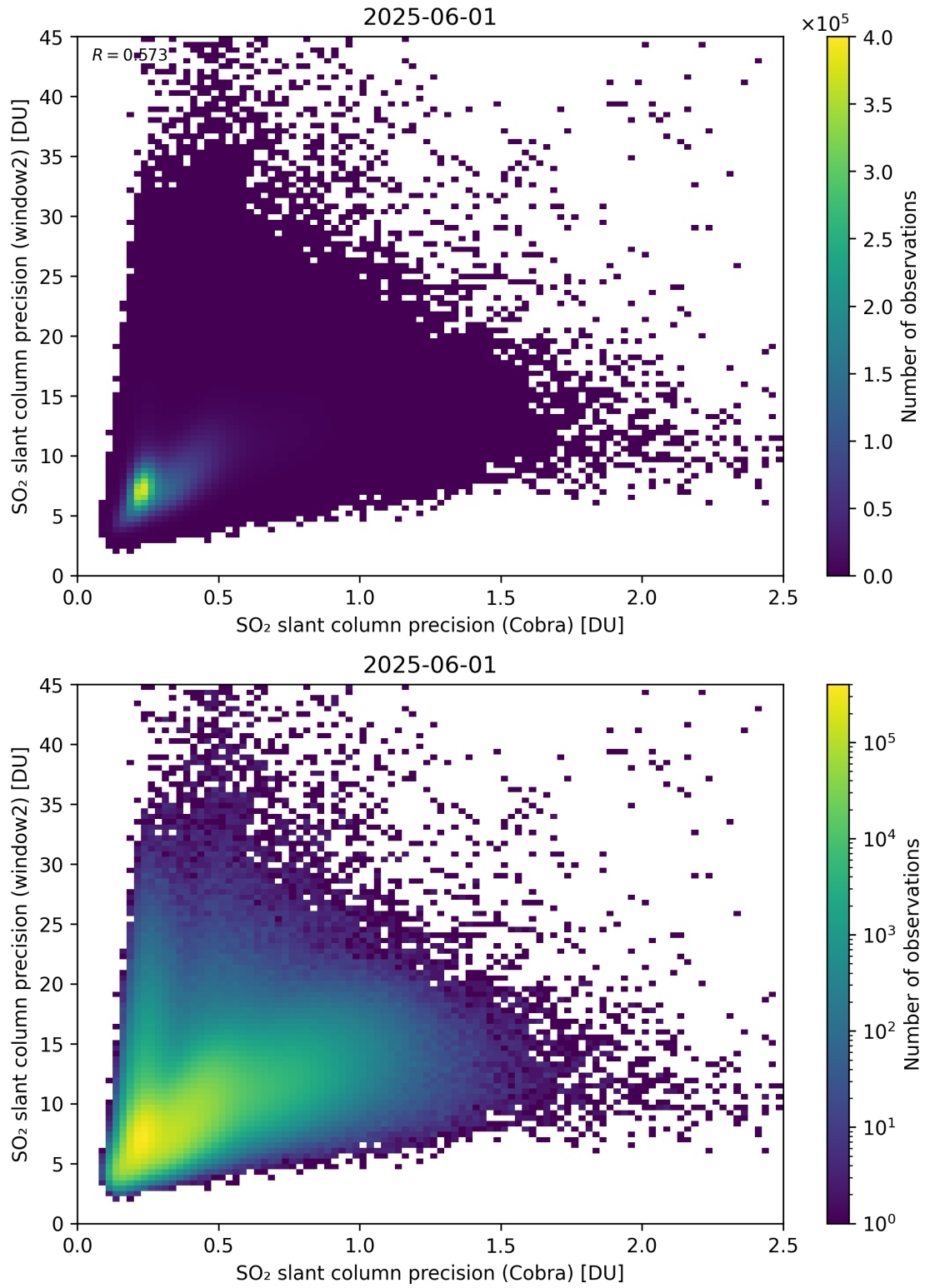
Figure 210: Scatter density plot of “SO 2 slant column precision (Cobra)” against “SO 2 slant column precision (window2)” for 2025-06-01 to 2025-06-02.
