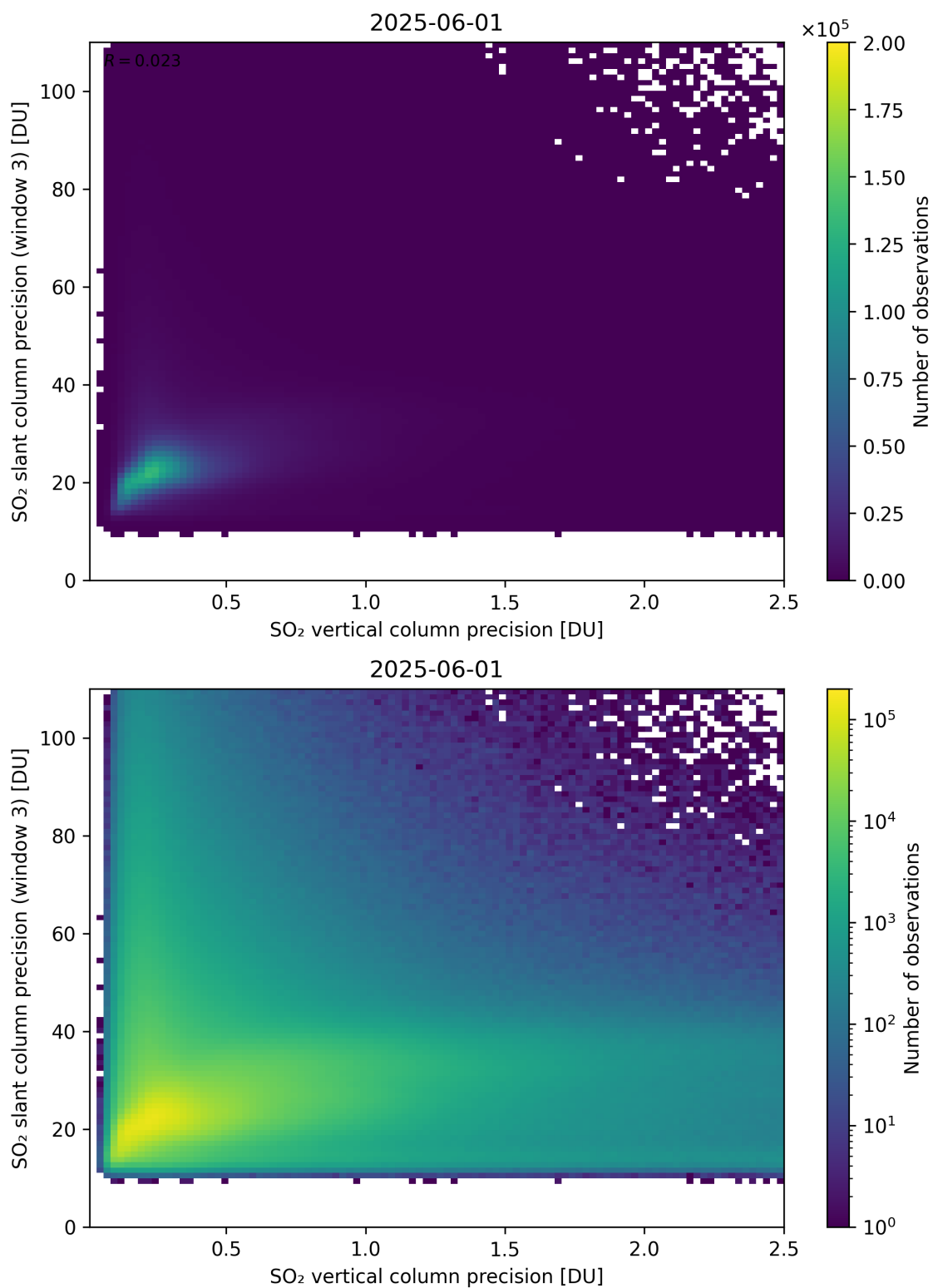
Figure 345: Scatter density plot of “SO 2 vertical column precision” against “SO 2 slant column precision (window 3)” for 2025-06-01 to 2025-06-02.
