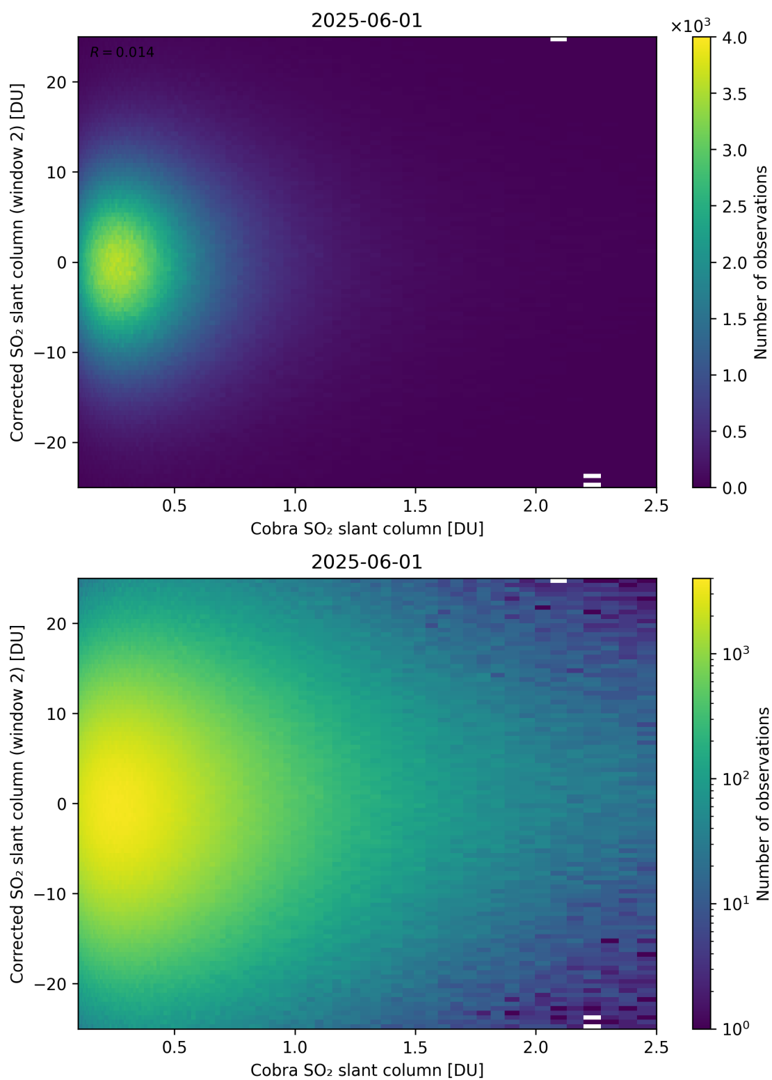
Figure 217: Scatter density plot of “Cobra SO 2 slant column” against “Corrected SO 2 slant column (window 2)” for 2025-06-01 to 2025-06-02.
