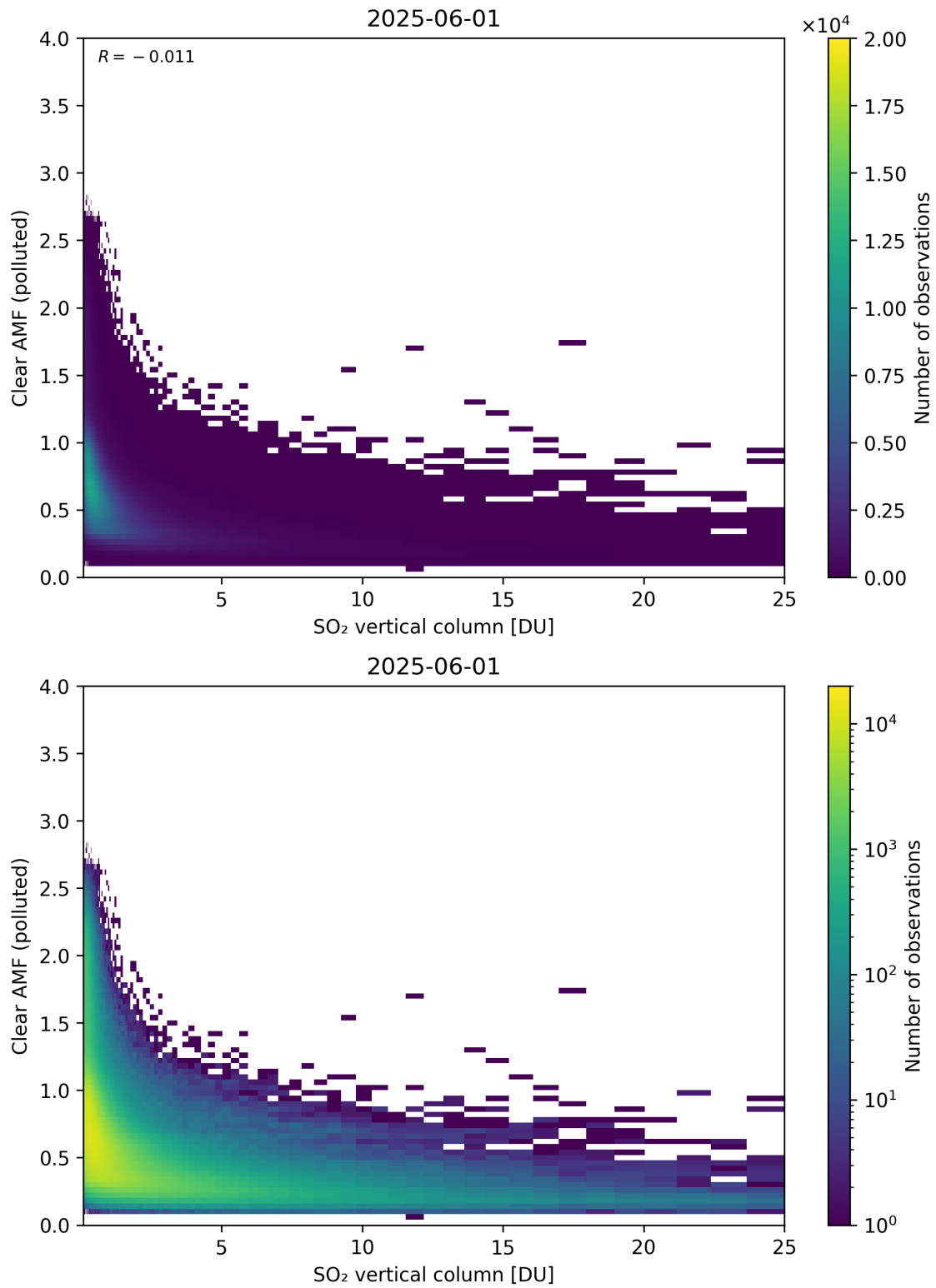
Figure 348: Scatter density plot of “SO 2 vertical column” against “Clear AMF (polluted)” for 2025-06-01 to 2025-06-02.
