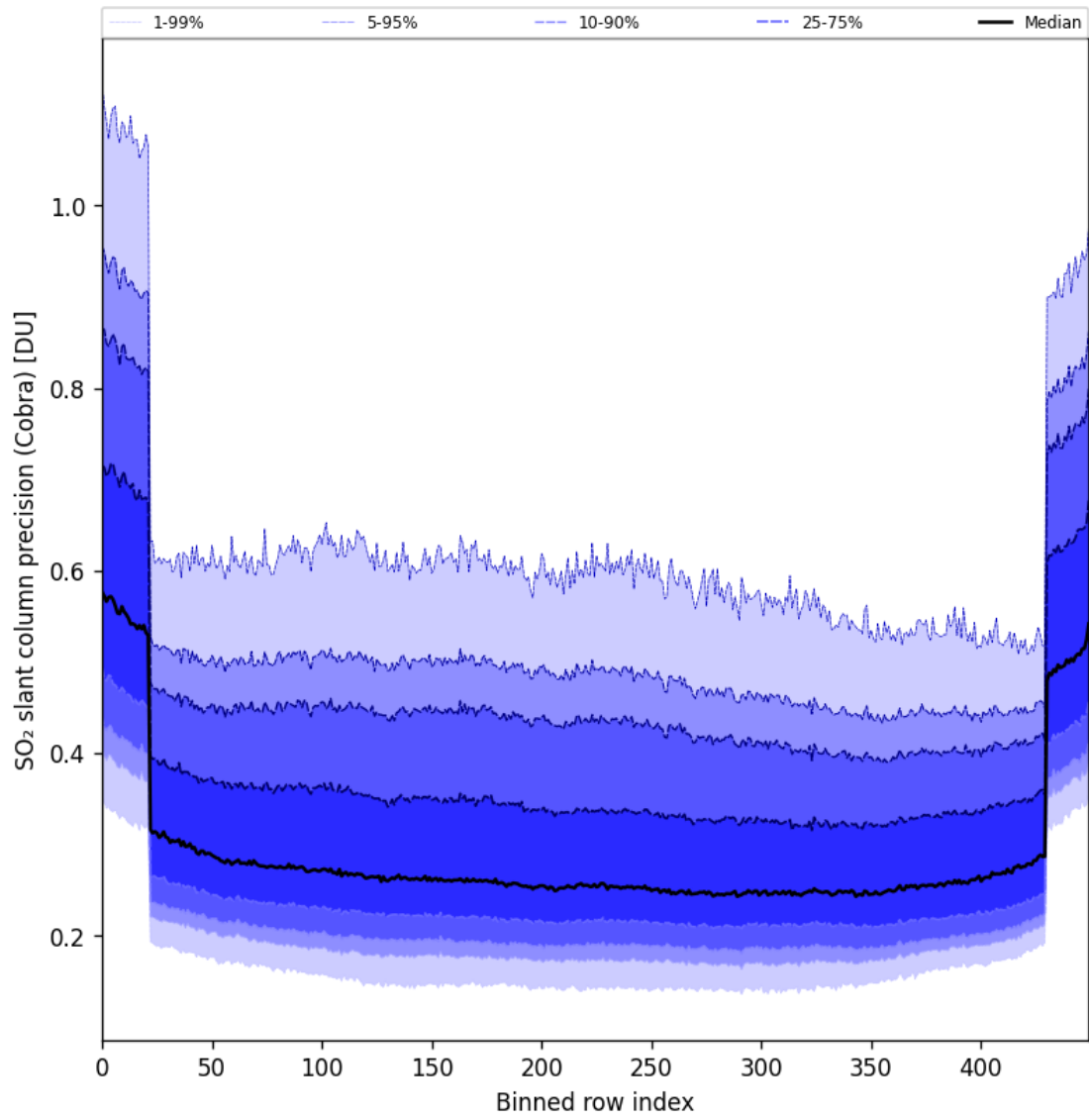
Figure 88: Along track statistics of “SO 2 slant column precision (Cobra)” for 2025-06-01 to 2025-06-02
