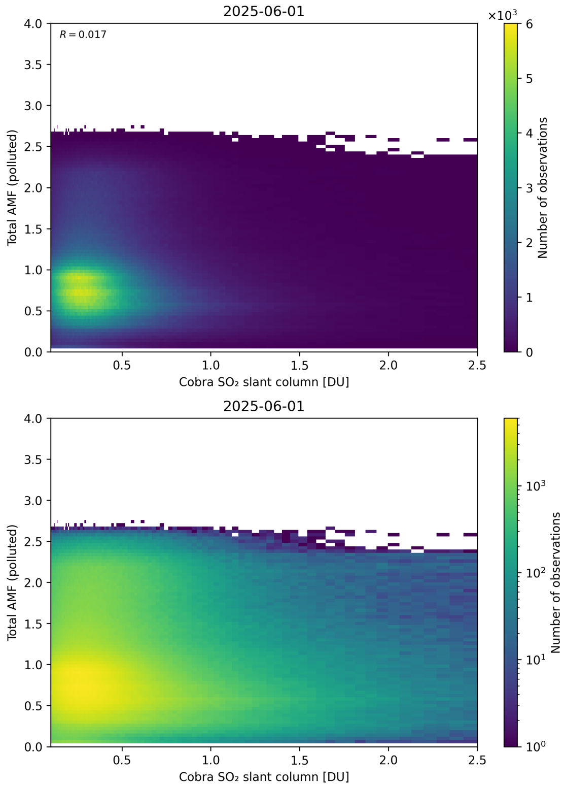
Figure 224: Scatter density plot of “Cobra SO 2 slant column” against “Total AMF (polluted)” for 2025-06-01 to 2025-06-02.
