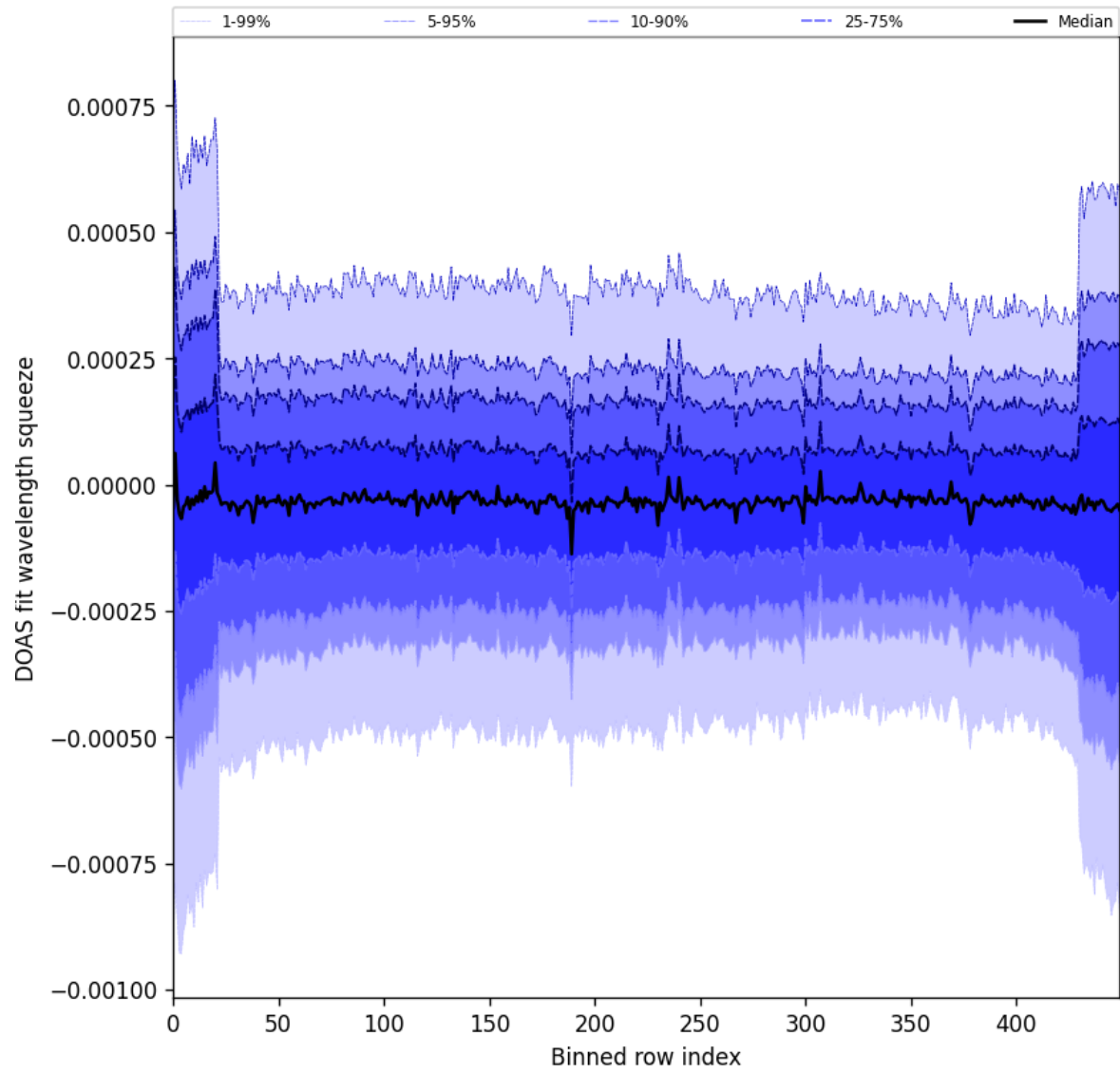
Figure 103: Along track statistics of “DOAS fit wavelength squeeze” for 2025-06-01 to 2025-06-02
