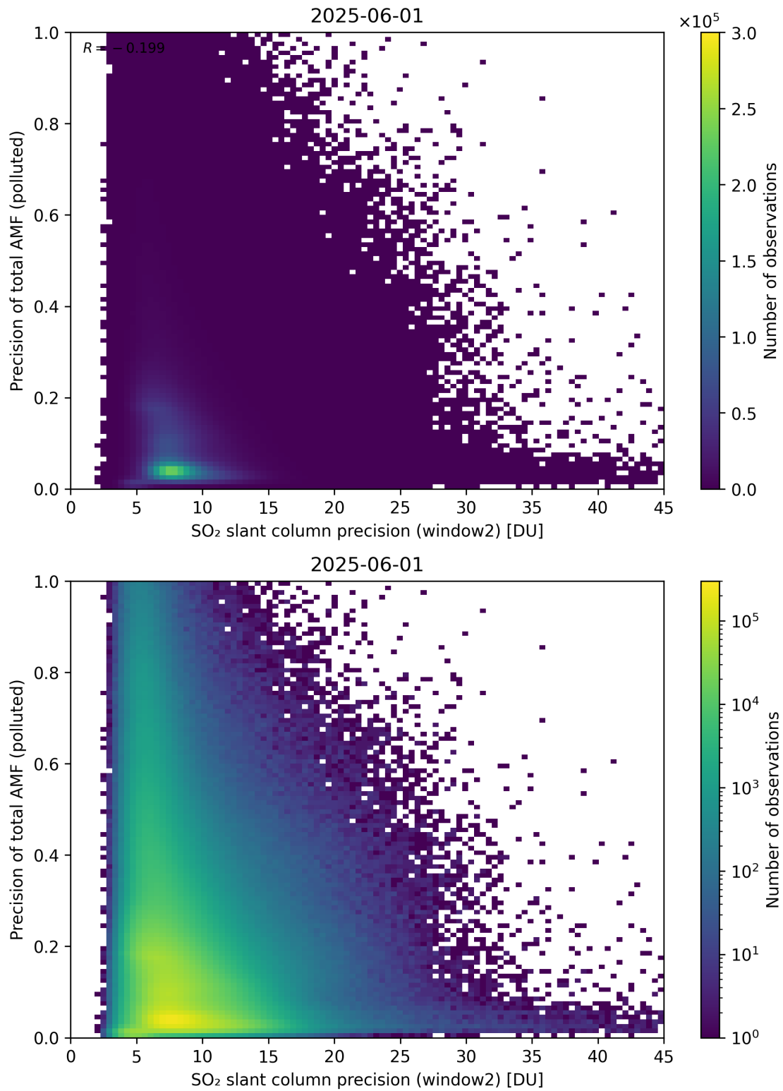
Figure 302: Scatter density plot of “SO 2 slant column precision (window2)” against “Precision of total AMF (polluted)” for 2025-06-01 to 2025-06-02.
