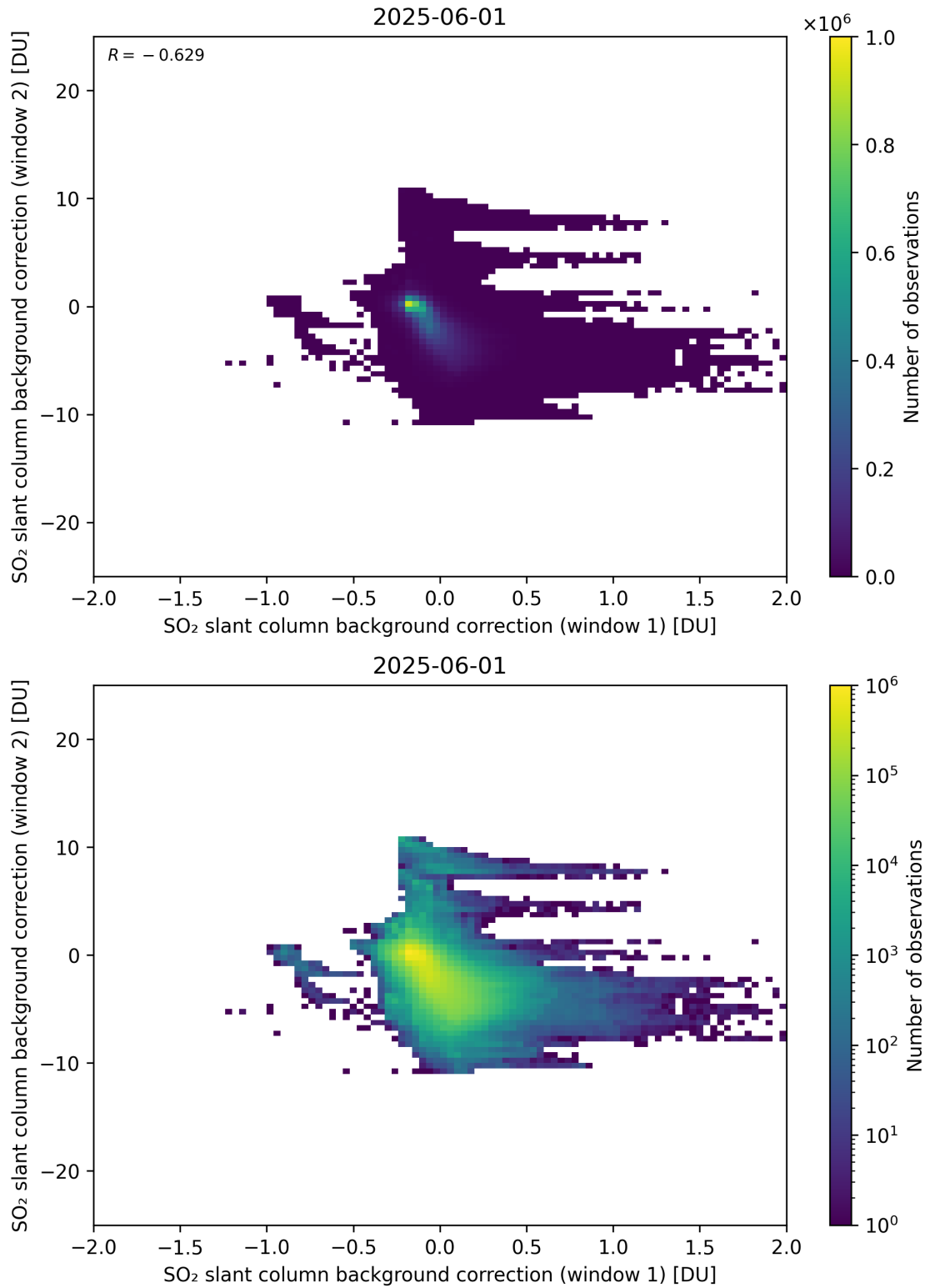
Figure 109: Scatter density plot of “SO 2 slant column background correction (window 1)” against “SO 2 slant column background correction (window 2)” for 2025-06-01 to 2025-06-02.
