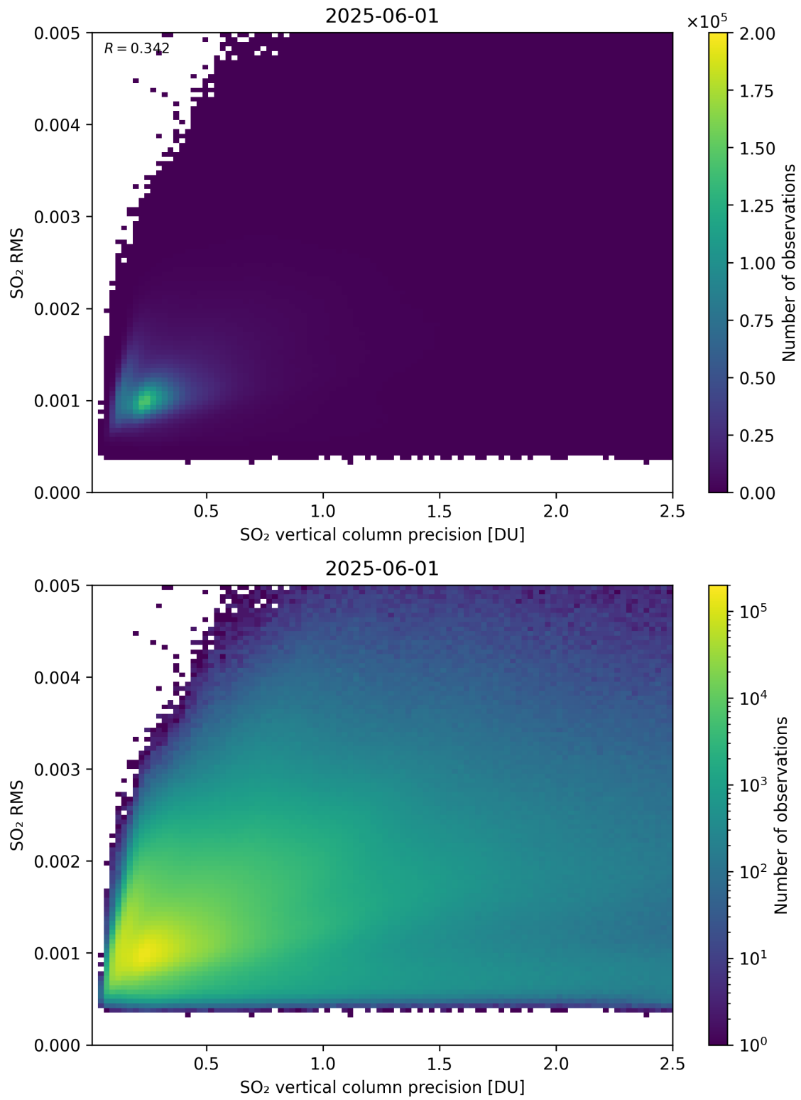
Figure 334: Scatter density plot of “SO 2 vertical column precision” against “SO 2 RMS” for 2025-06-01 to 2025-06-02.
