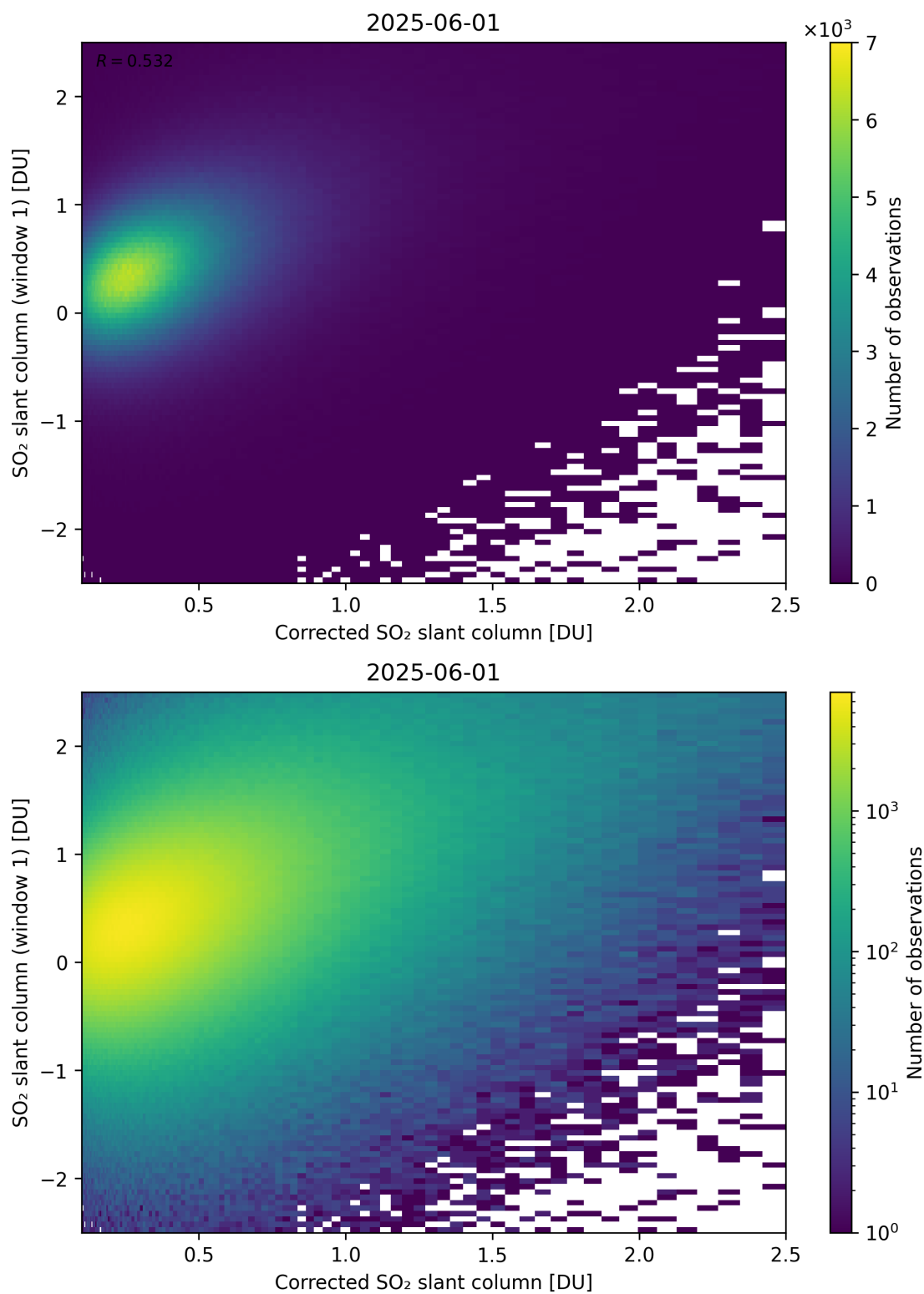
Figure 237: Scatter density plot of “Corrected SO 2 slant column” against “SO 2 slant column (window 1)” for 2025-06-01 to 2025-06-02.
