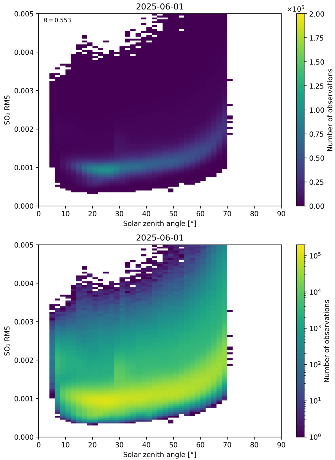
Figure 176: Scatter density plot of “Solar zenith angle” against “SO 2 RMS” for 2025-06-01 to 2025-06-02.
