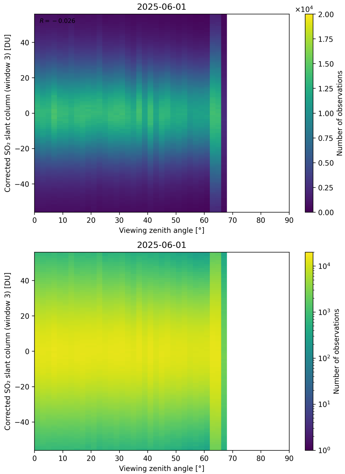
Figure 375: Scatter density plot of “Viewing zenith angle” against “Corrected SO 2 slant column (window 3)” for 2025-06-01 to 2025-06-02.
