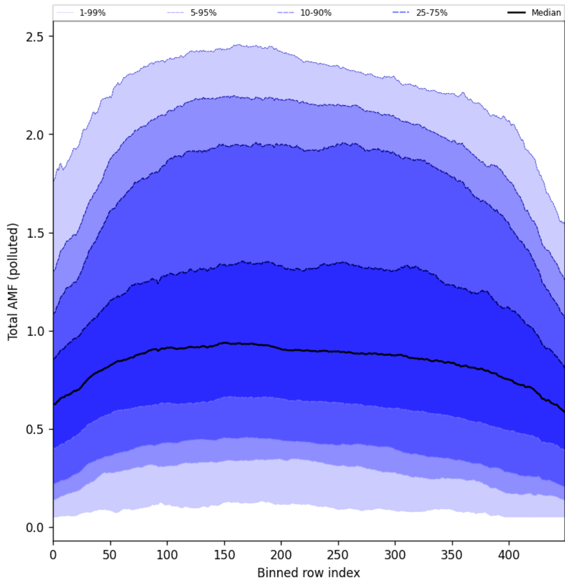
Figure 105: Along track statistics of “Total AMF (polluted)” for 2025-06-01 to 2025-06-02
