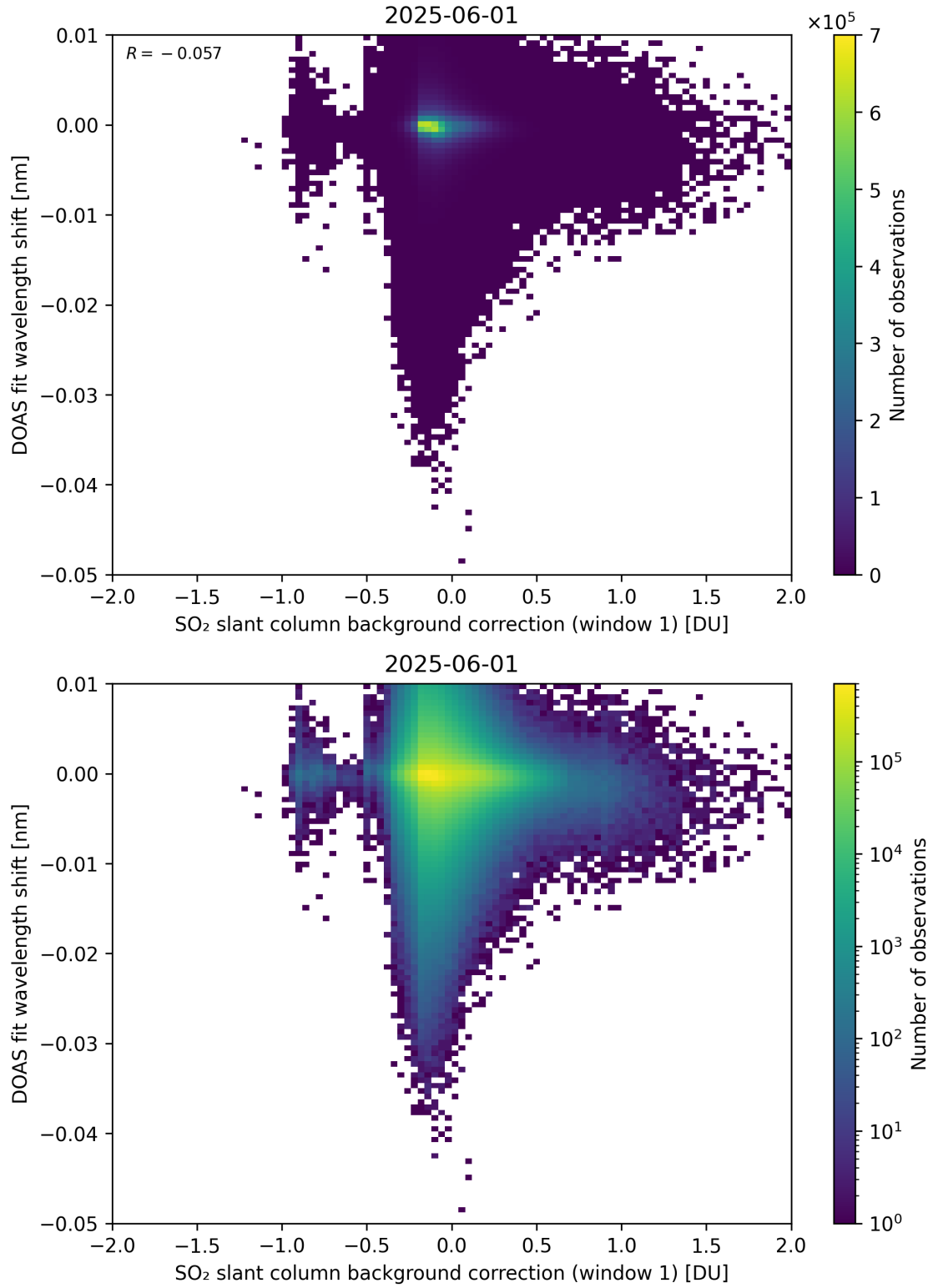
Figure 111: Scatter density plot of “SO 2 slant column background correction (window 1)” against “DOAS fit wavelength shift” for 2025-06-01 to 2025-06-02.
