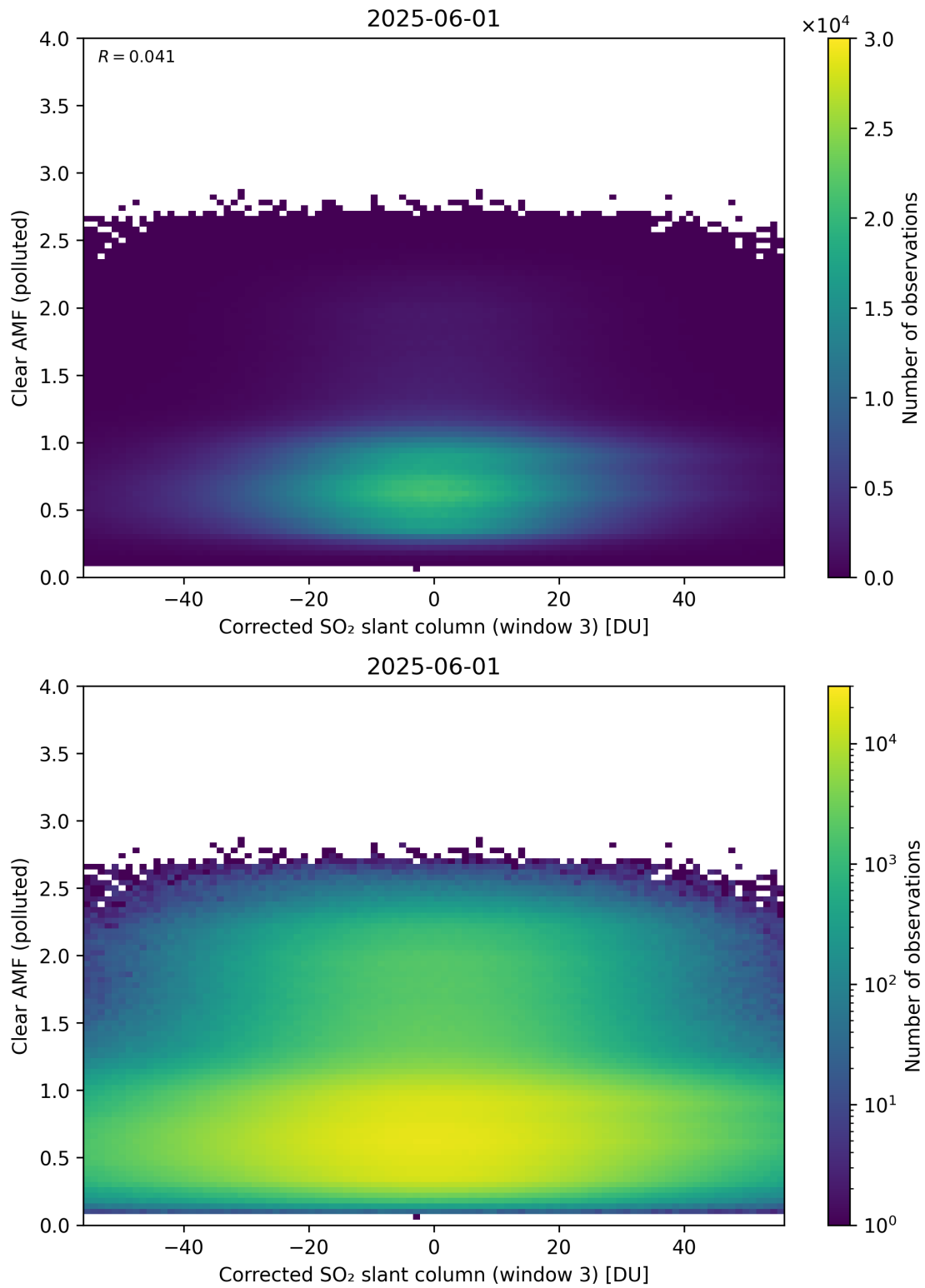
Figure 259: Scatter density plot of “Corrected SO 2 slant column (window 3)” against “Clear AMF (polluted)” for 2025-06-01 to 2025-06-02.
