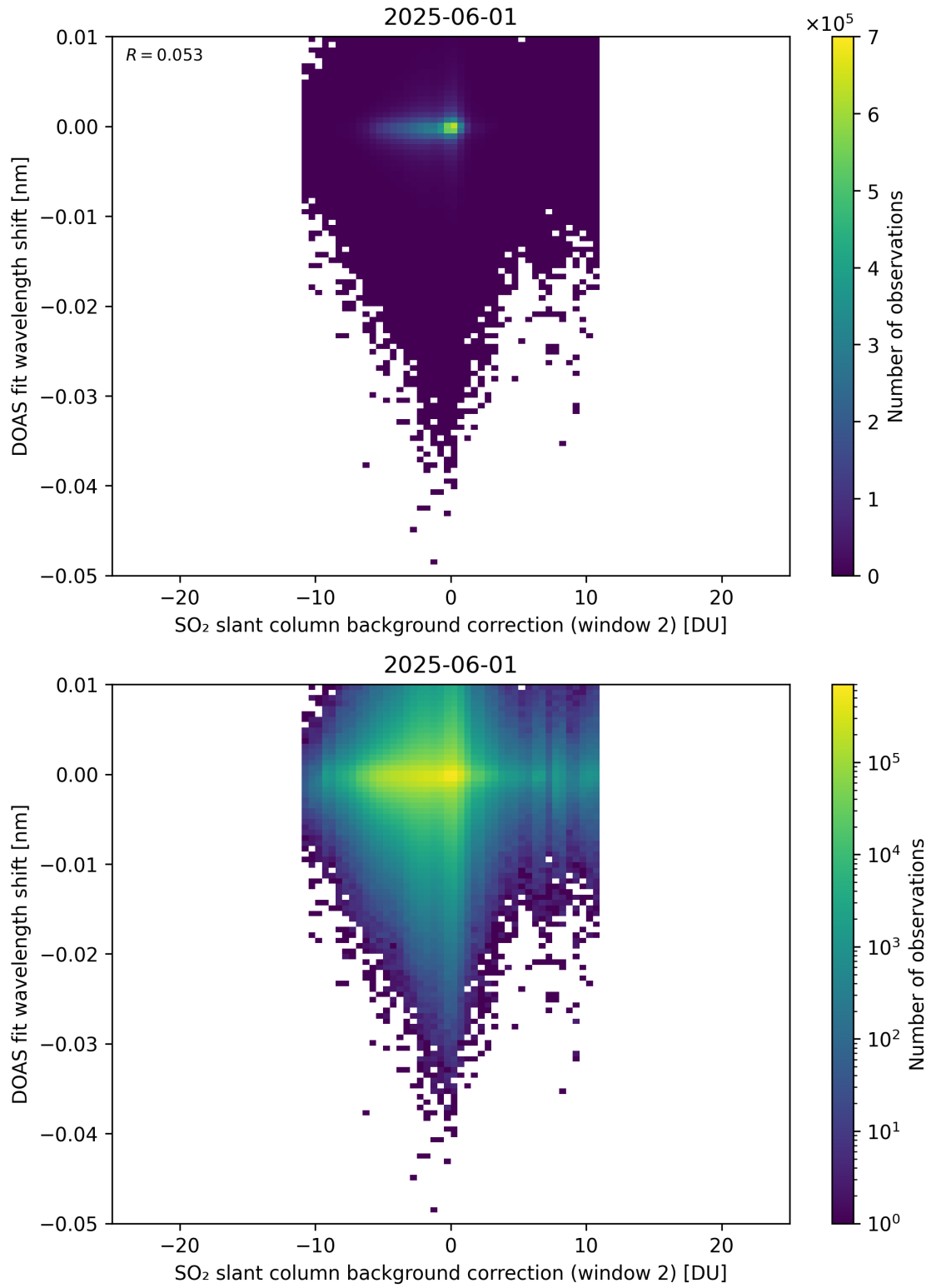
Figure 123: Scatter density plot of “SO 2 slant column background correction (window 2)” against “DOAS fit wavelength shift” for 2025-06-01 to 2025-06-02.
