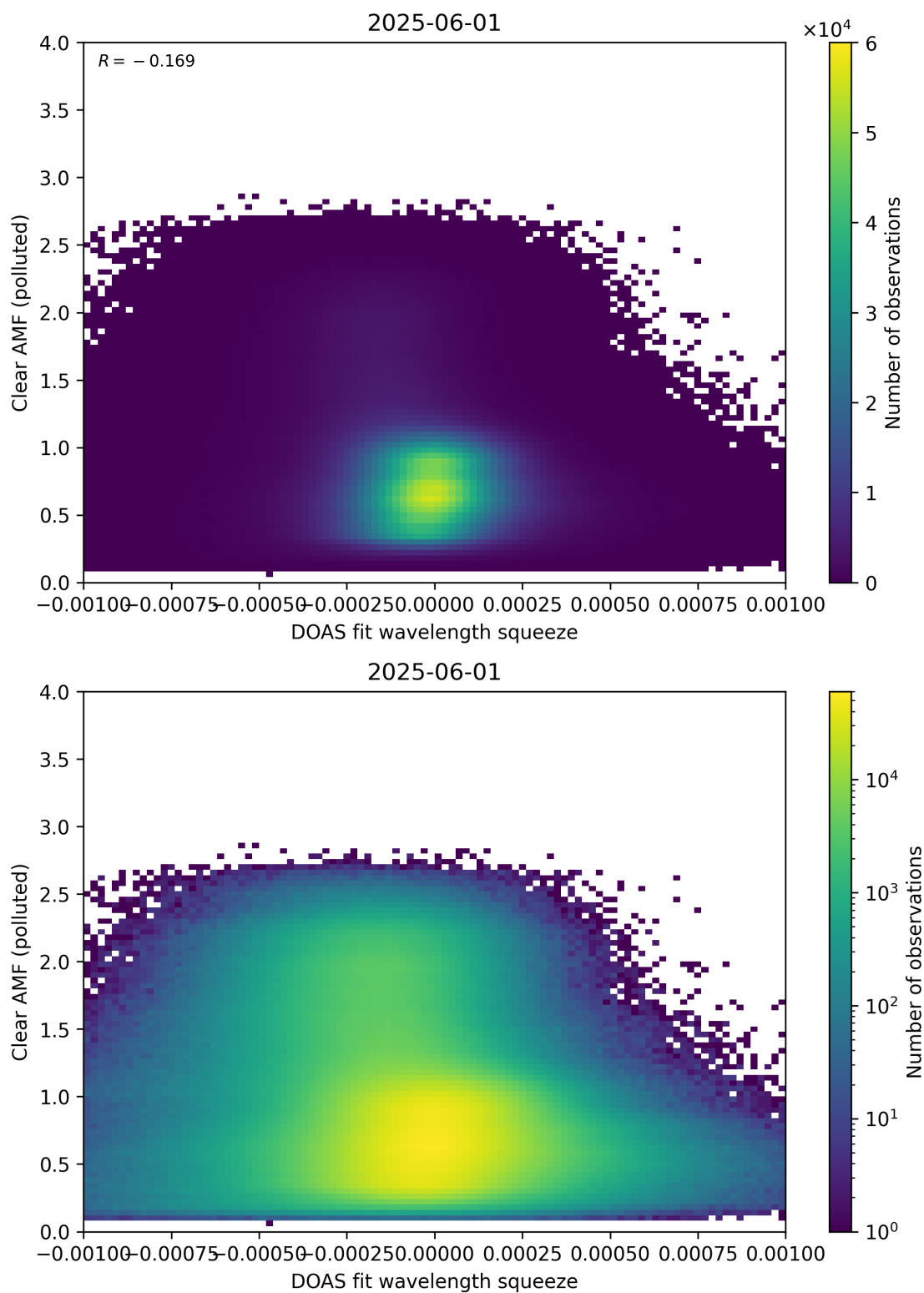
Figure 144: Scatter density plot of “DOAS fit wavelength squeeze” against “Clear AMF (polluted)” for 2025-06-01 to 2025-06-02.
