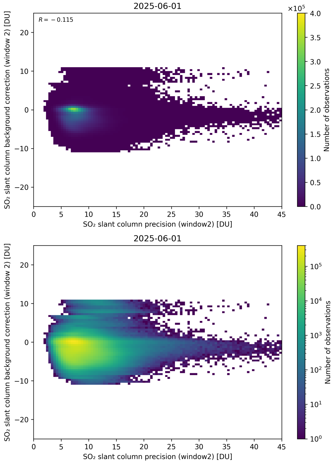
Figure 291: Scatter density plot of “SO 2 slant column precision (window2)” against “SO 2 slant column background correction (window 2)” for 2025-06-01 to 2025-06-02.
