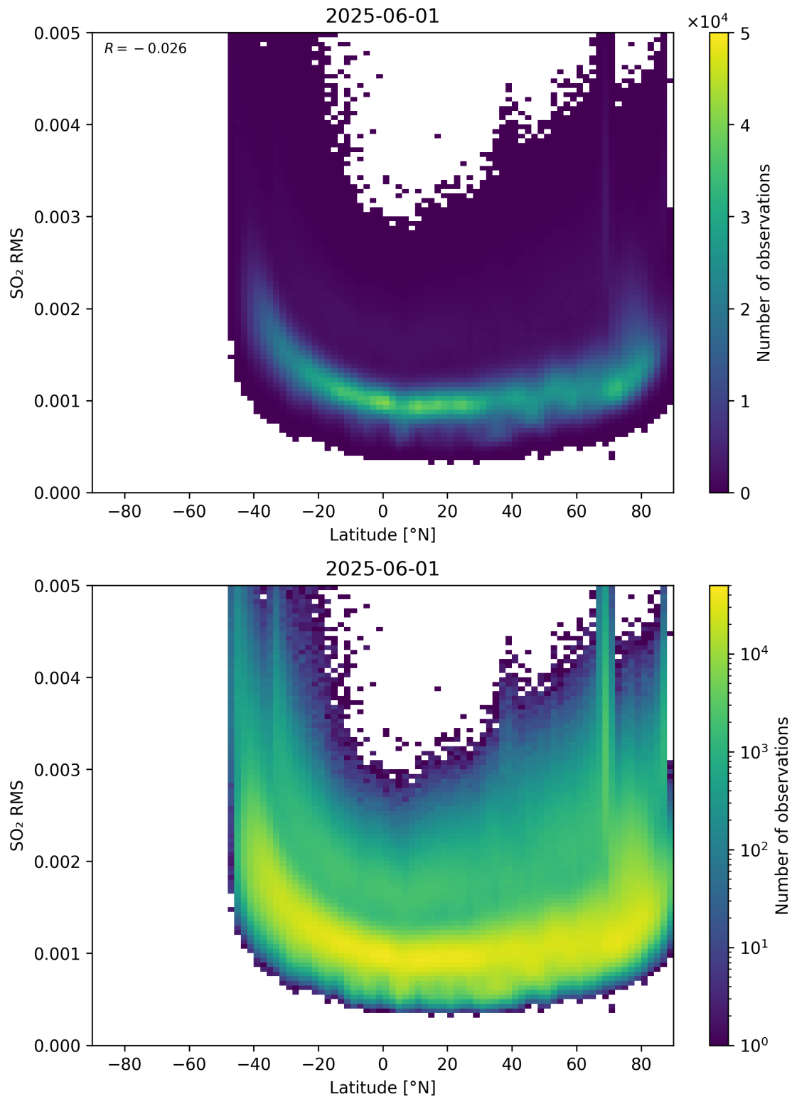
Figure 155: Scatter density plot of “Latitude” against “SO 2 RMS” for 2025-06-01 to 2025-06-02.
