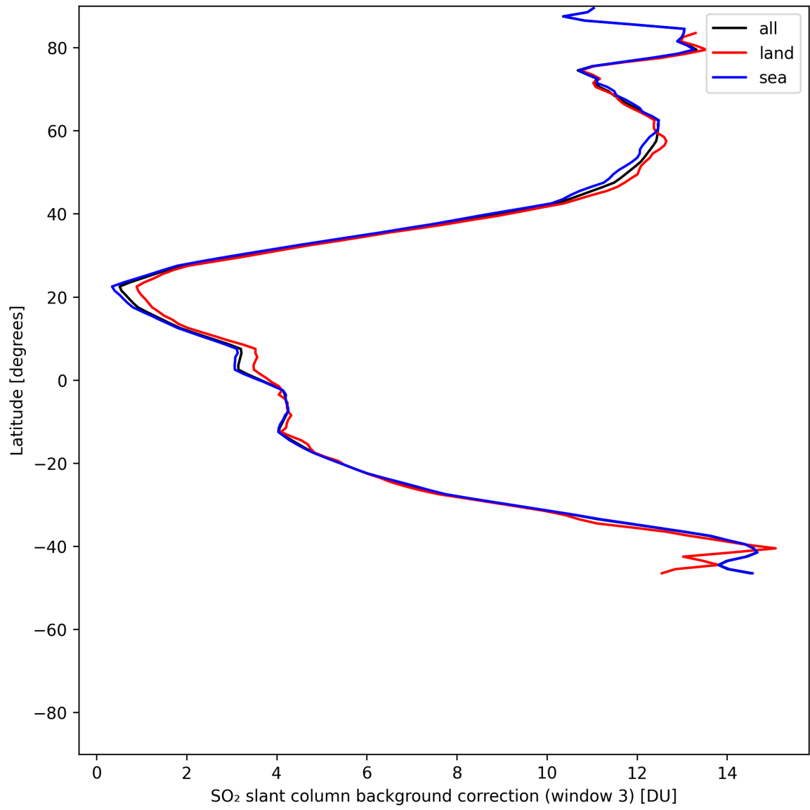
Figure 48: Zonal average of “SO 2 slant column background correction (window 3)” for 2025-06-01 to 2025-06-02.
