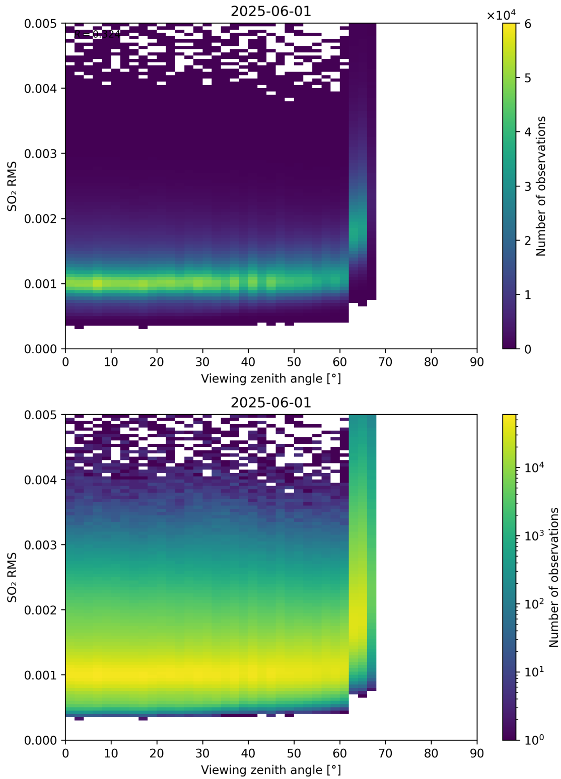
Figure 367: Scatter density plot of “Viewing zenith angle” against “SO 2 RMS” for 2025-06-01 to 2025-06-02.
