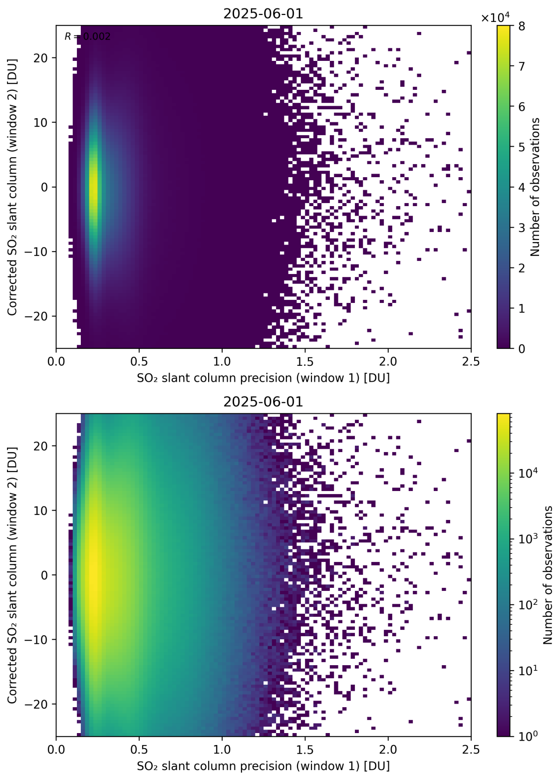
Figure 275: Scatter density plot of “SO 2 slant column precision (window 1)” against “Corrected SO 2 slant column (window 2)” for 2025-06-01 to 2025-06-02.
