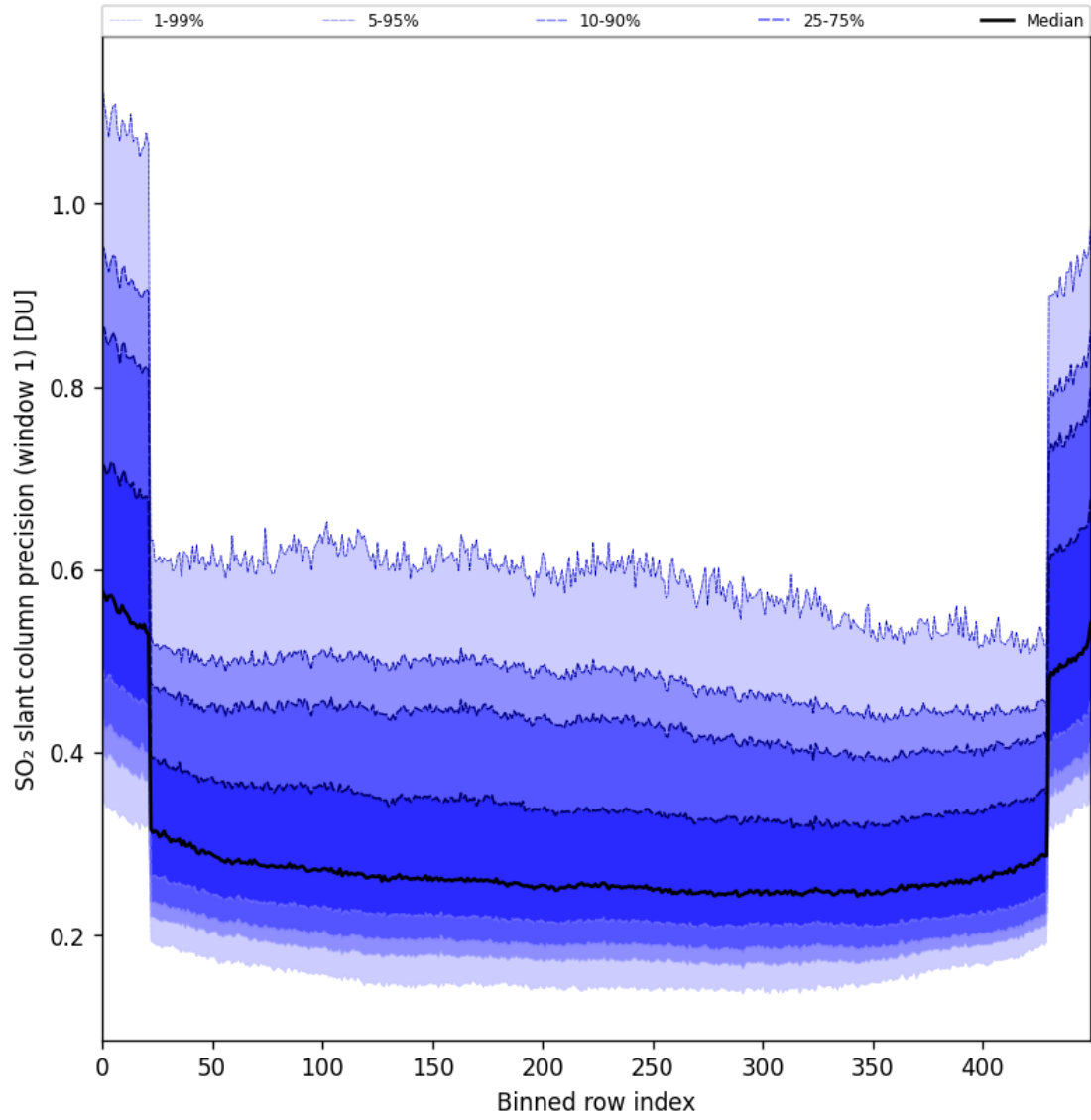
Figure 90: Along track statistics of “SO 2 slant column precision (window 1)” for 2025-06-01 to 2025-06-02
