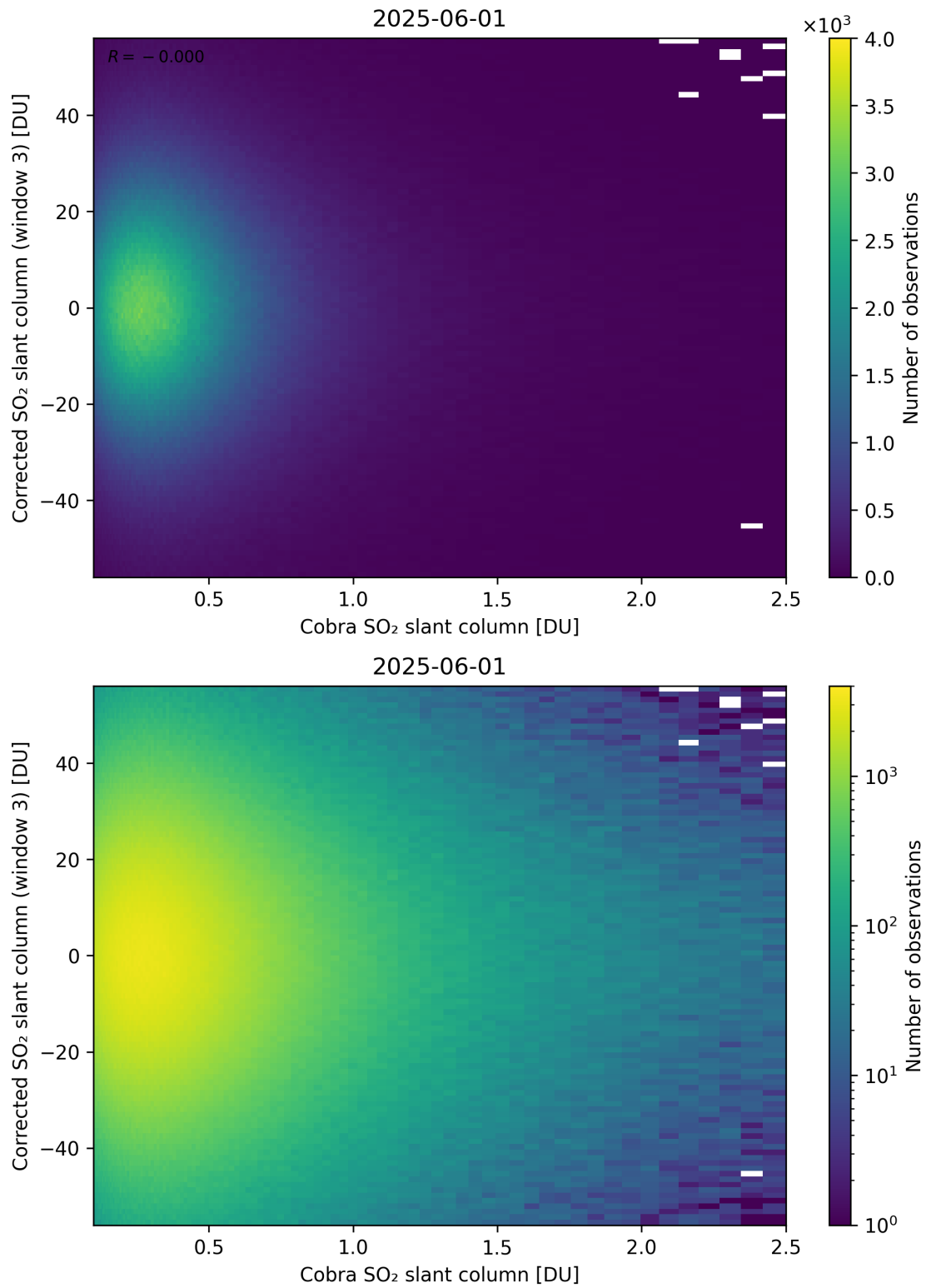
Figure 218: Scatter density plot of “Cobra SO 2 slant column” against “Corrected SO 2 slant column (window 3)” for 2025-06-01 to 2025-06-02.
