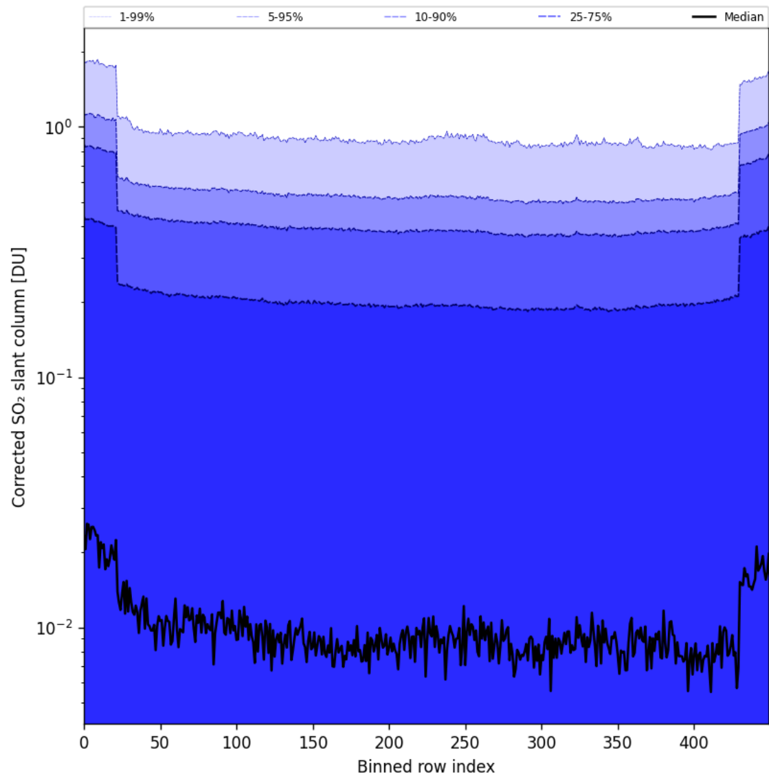
Figure 86: Along track statistics of “Corrected SO 2 slant column” for 2025-06-01 to 2025-06-02
