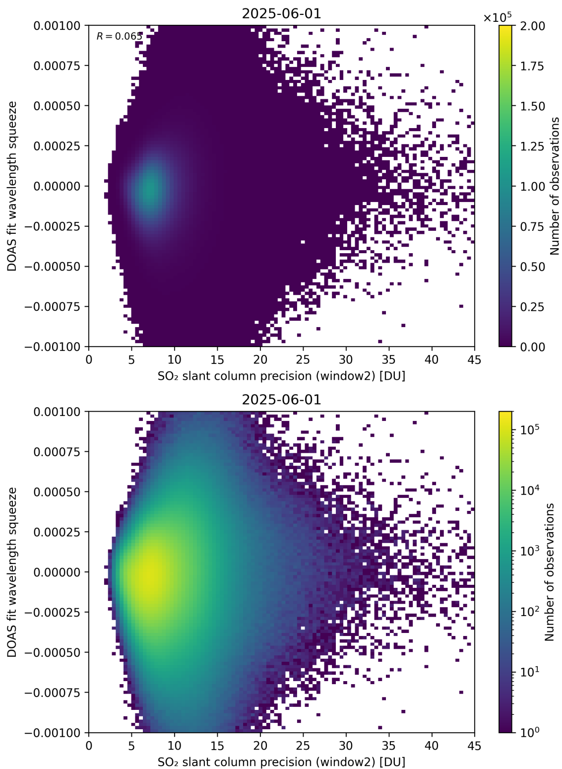
Figure 294: Scatter density plot of “SO 2 slant column precision (window2)” against “DOAS fit wavelength squeeze” for 2025-06-01 to 2025-06-02.
