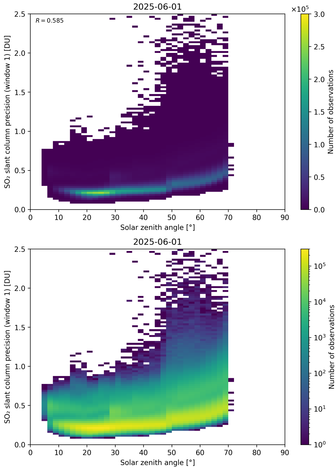
Figure 185: Scatter density plot of “Solar zenith angle” against “SO 2 slant column precision (window 1)” for 2025-06-01 to 2025-06-02.
