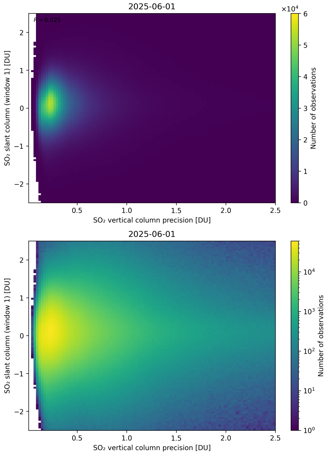
Figure 341: Scatter density plot of “SO 2 vertical column precision” against “SO 2 slant column (window 1)” for 2025-06-01 to 2025-06-02.
