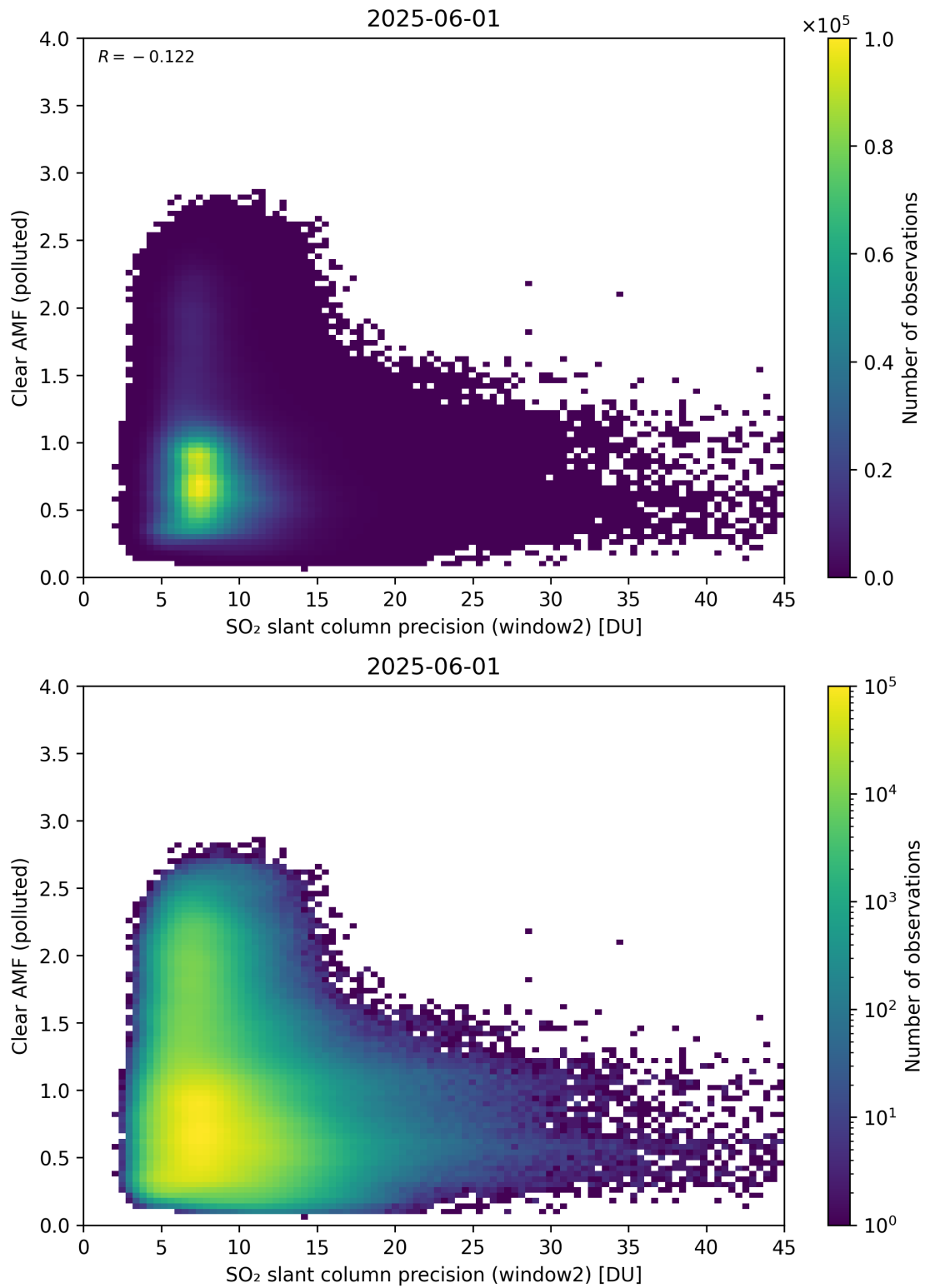
Figure 296: Scatter density plot of “SO 2 slant column precision (window2)” against “Clear AMF (polluted)” for 2025-06-01 to 2025-06-02.
