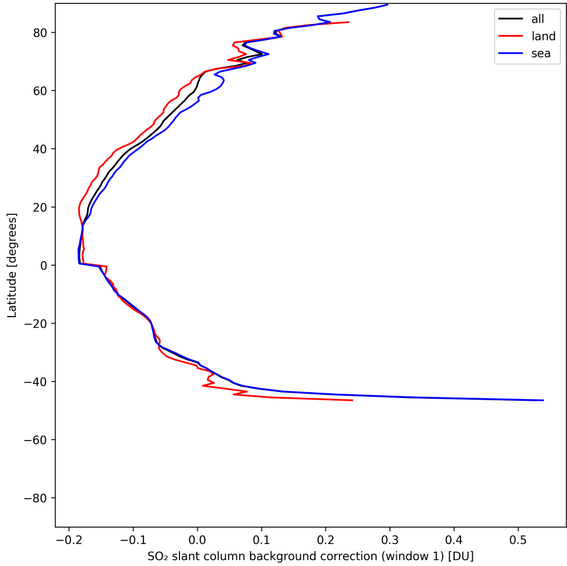
Figure 40: Zonal average of “SO 2 slant column background correction (window 1)” for 2025-06-01 to 2025-06-02.
