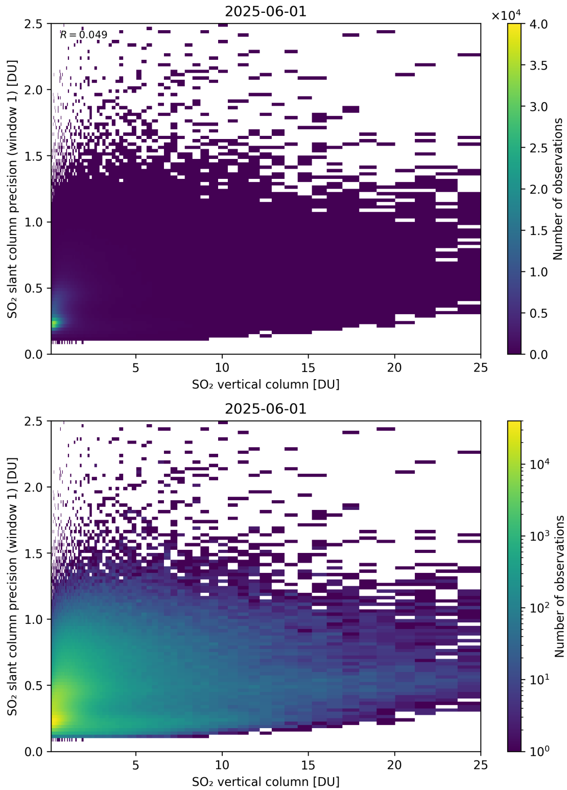
Figure 355: Scatter density plot of “SO 2 vertical column” against “SO 2 slant column precision (window 1)” for 2025-06-01 to 2025-06-02.
