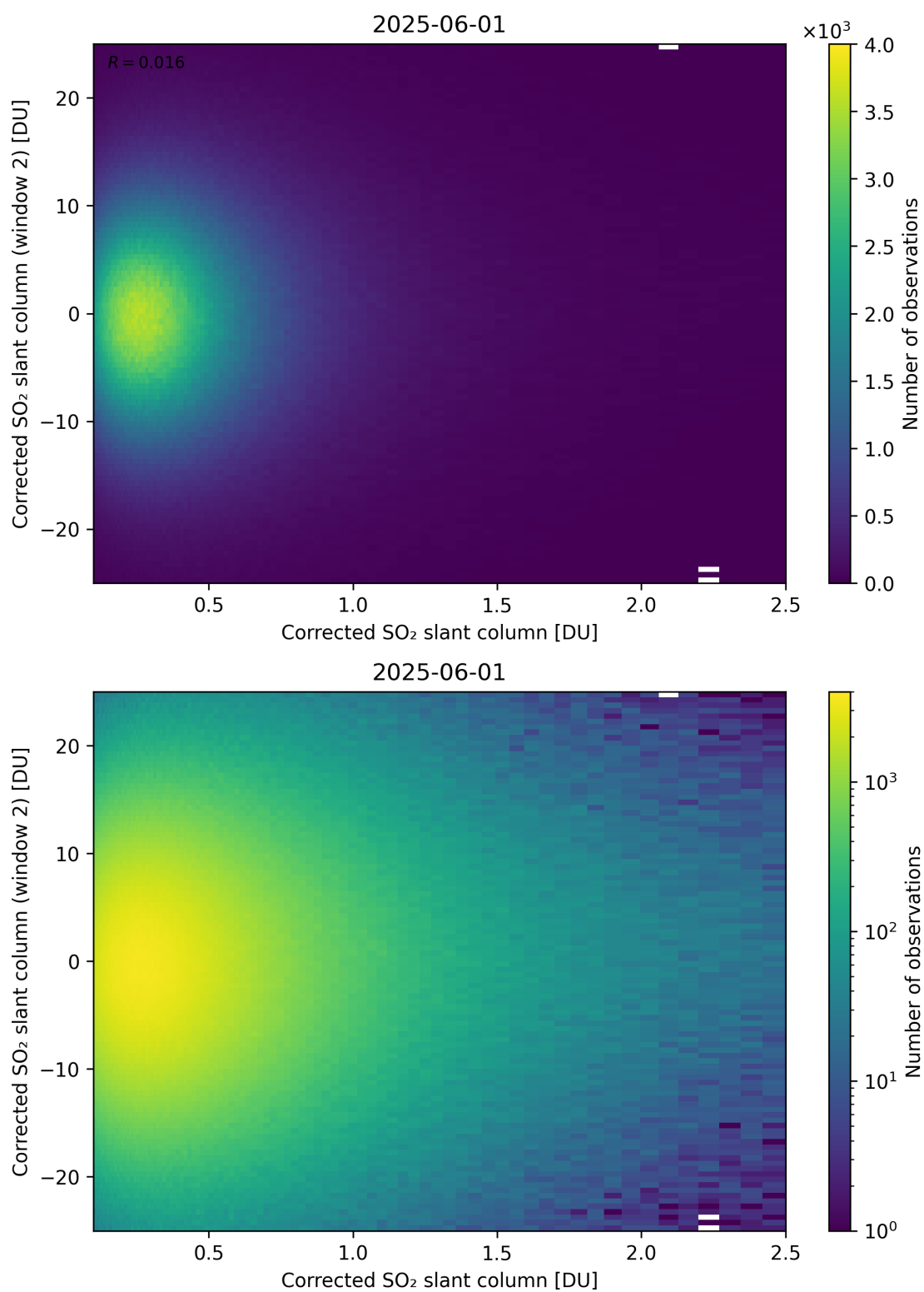
Figure 235: Scatter density plot of “Corrected SO 2 slant column” against “Corrected SO 2 slant column (window 2)” for 2025-06-01 to 2025-06-02.
