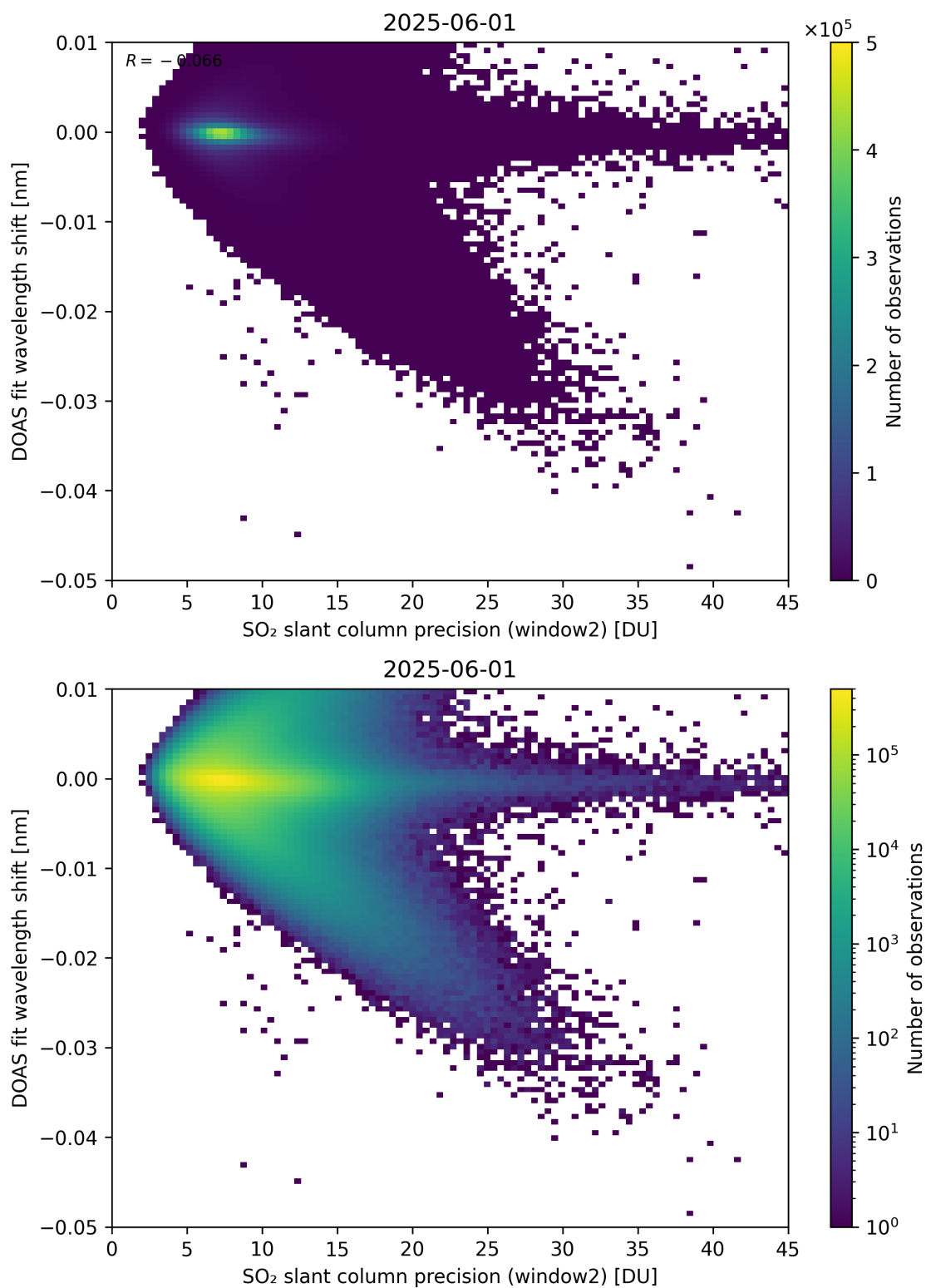
Figure 293: Scatter density plot of “SO 2 slant column precision (window2)” against “DOAS fit wavelength shift” for 2025-06-01 to 2025-06-02.
