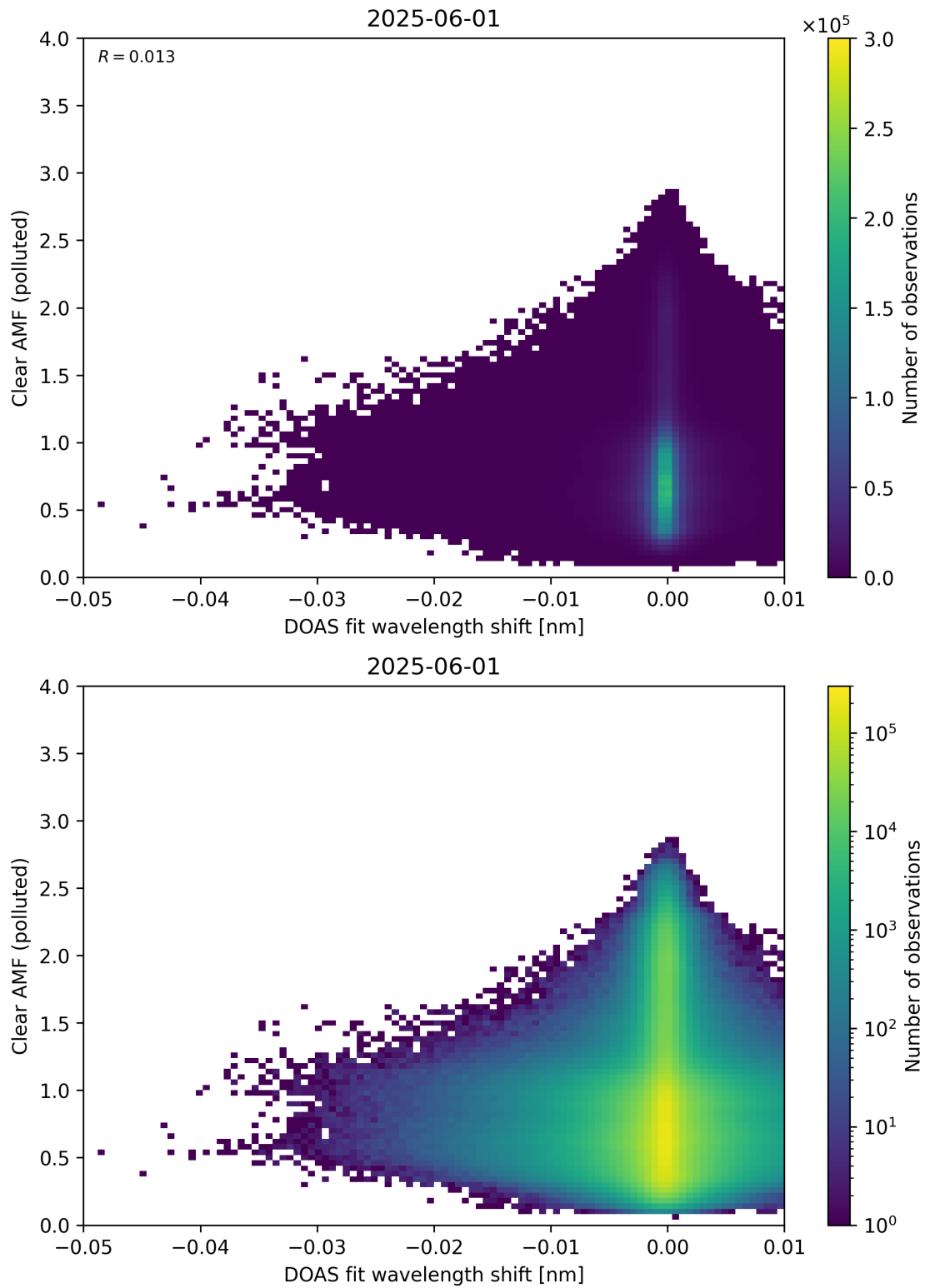
Figure 140: Scatter density plot of “DOAS fit wavelength shift” against “Clear AMF (polluted)” for 2025-06-01 to 2025-06-02.
