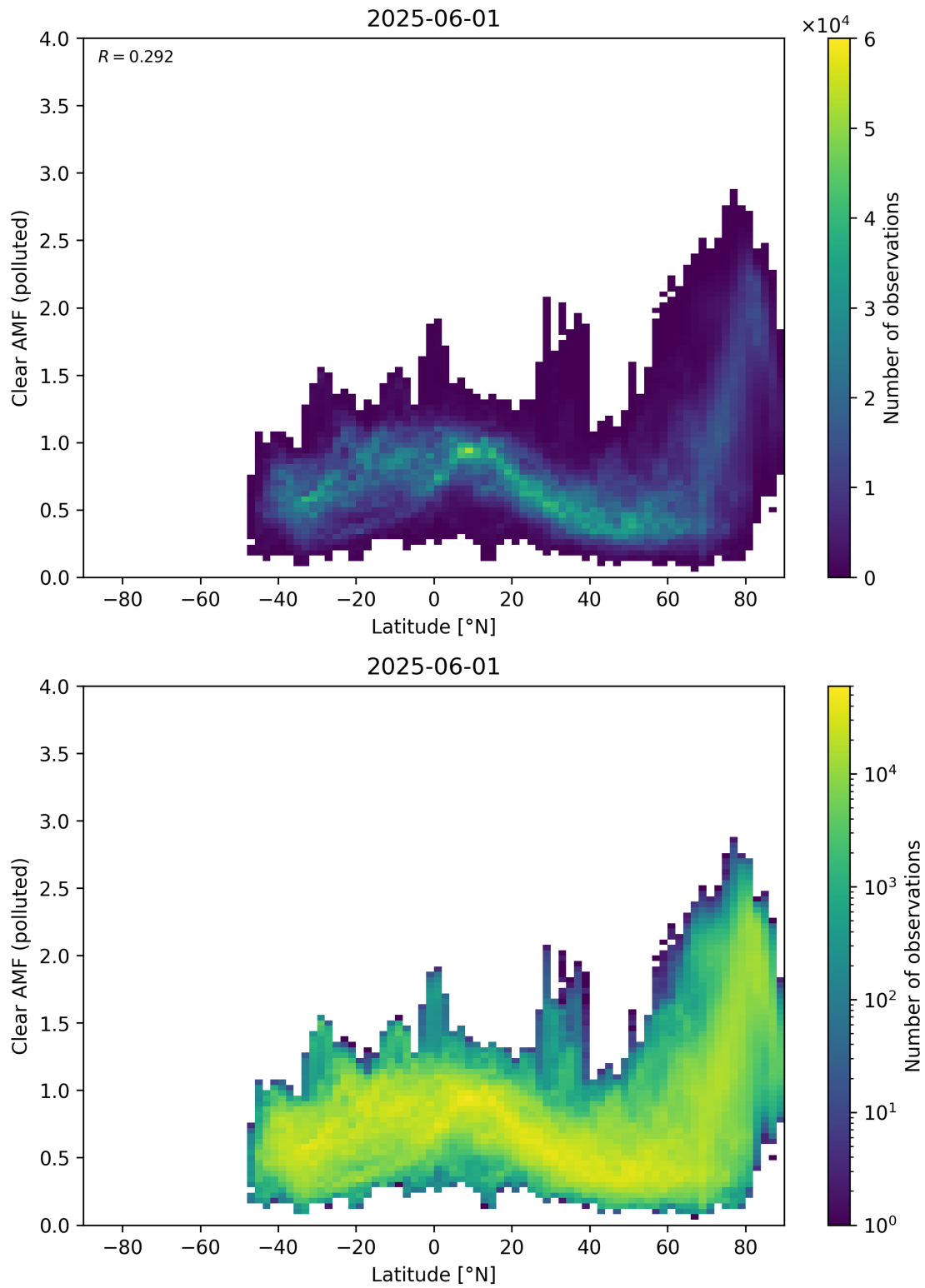
Figure 156: Scatter density plot of “Latitude” against “Clear AMF (polluted)” for 2025-06-01 to 2025-06-02.
