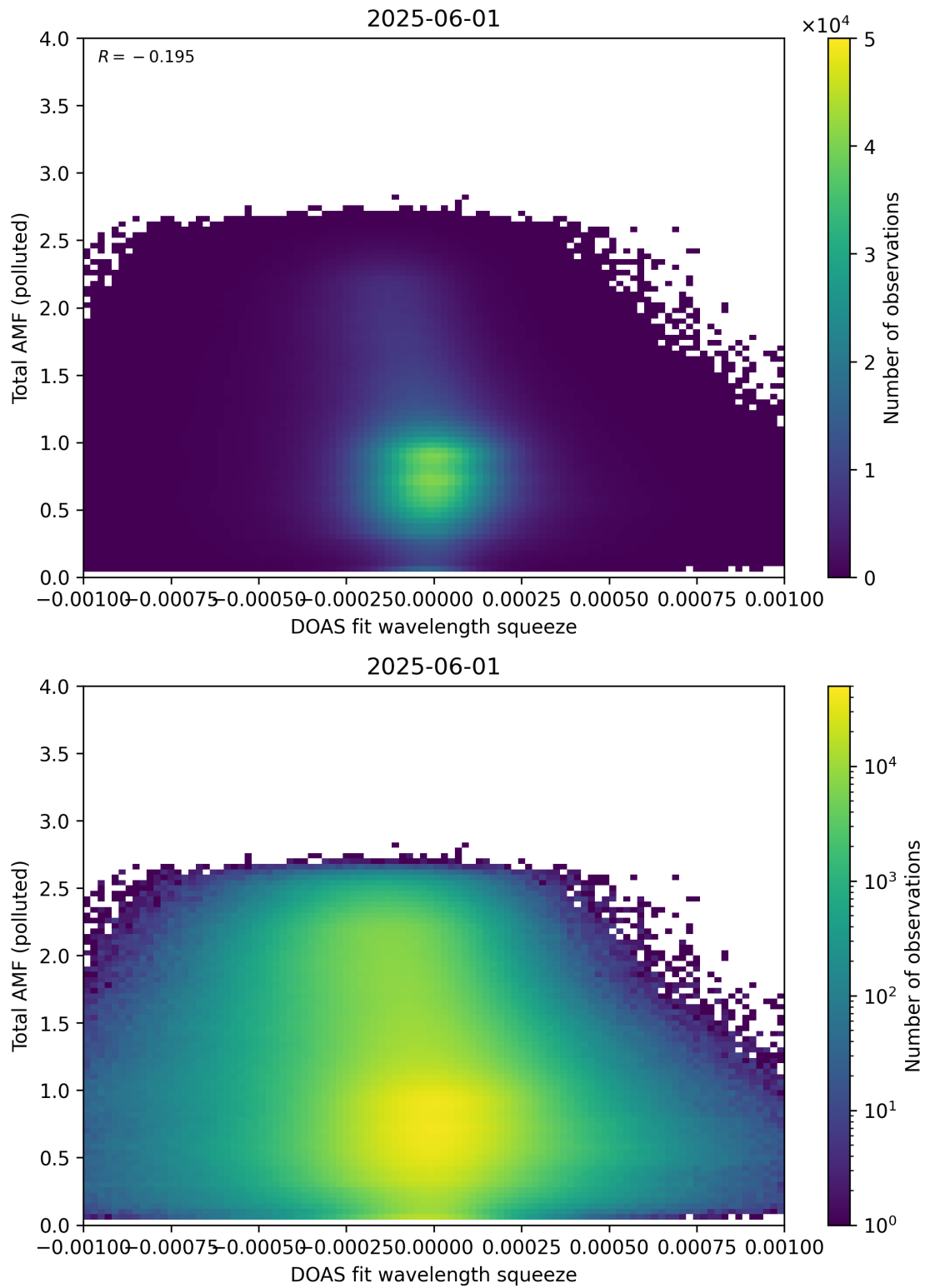
Figure 145: Scatter density plot of “DOAS fit wavelength squeeze” against “Total AMF (polluted)” for 2025-06-01 to 2025-06-02.
