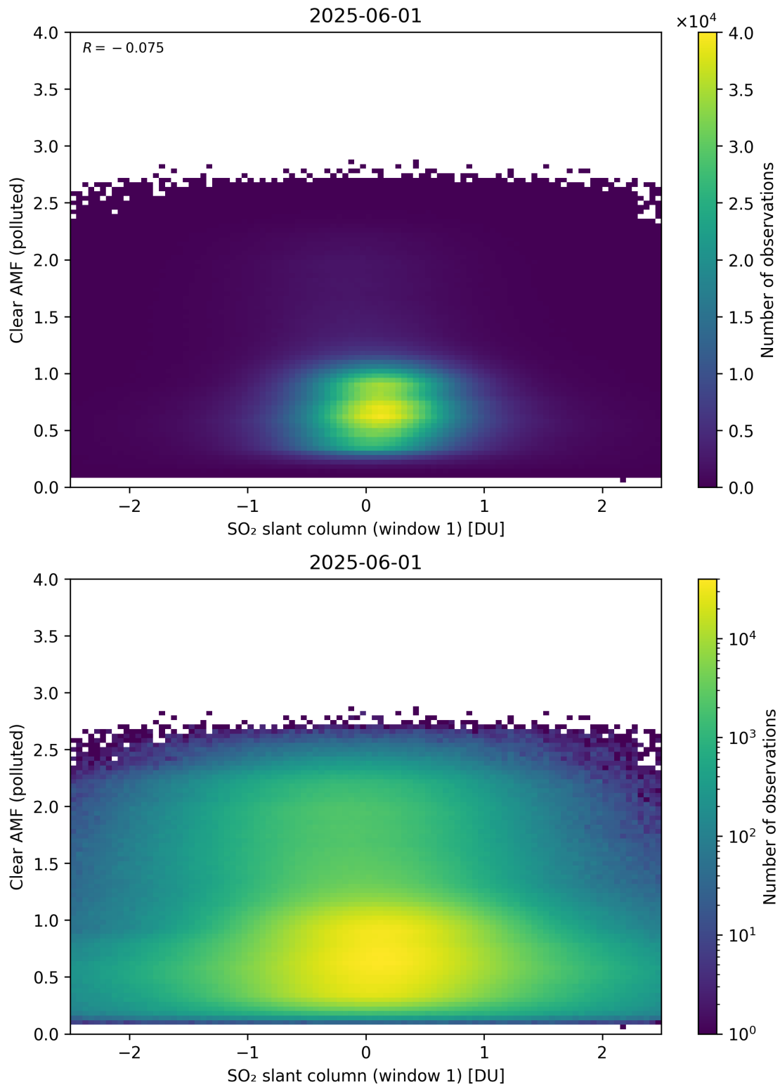
Figure 282: Scatter density plot of “SO 2 slant column (window 1)” against “Clear AMF (polluted)” for 2025-06-01 to 2025-06-02.
