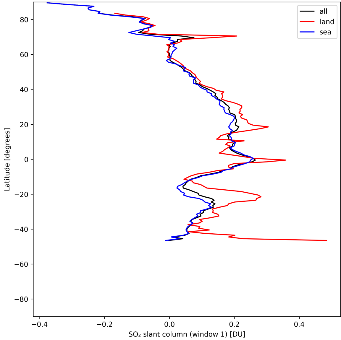
Figure 37: Zonal average of “SO 2 slant column (window 1)” for 2025-06-01 to 2025-06-02.
