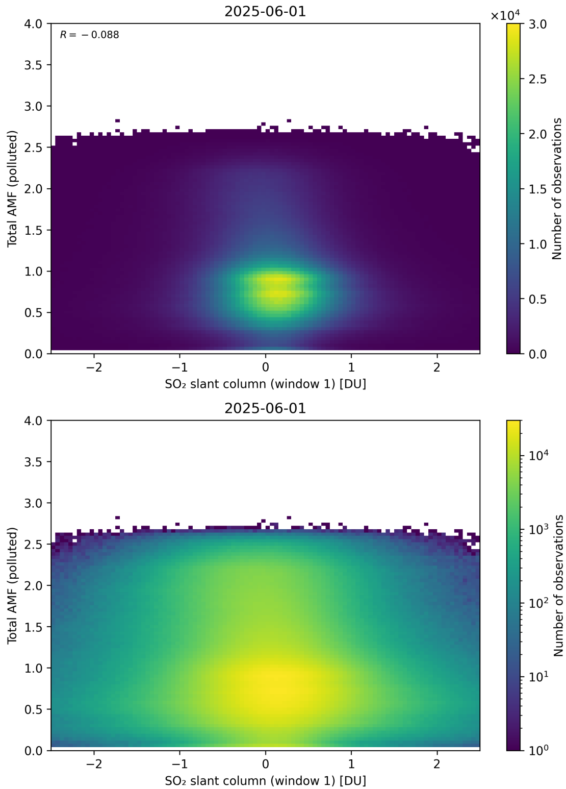
Figure 289: Scatter density plot of “SO 2 slant column (window 1)” against “Total AMF (polluted)” for 2025-06-01 to 2025-06-02.
