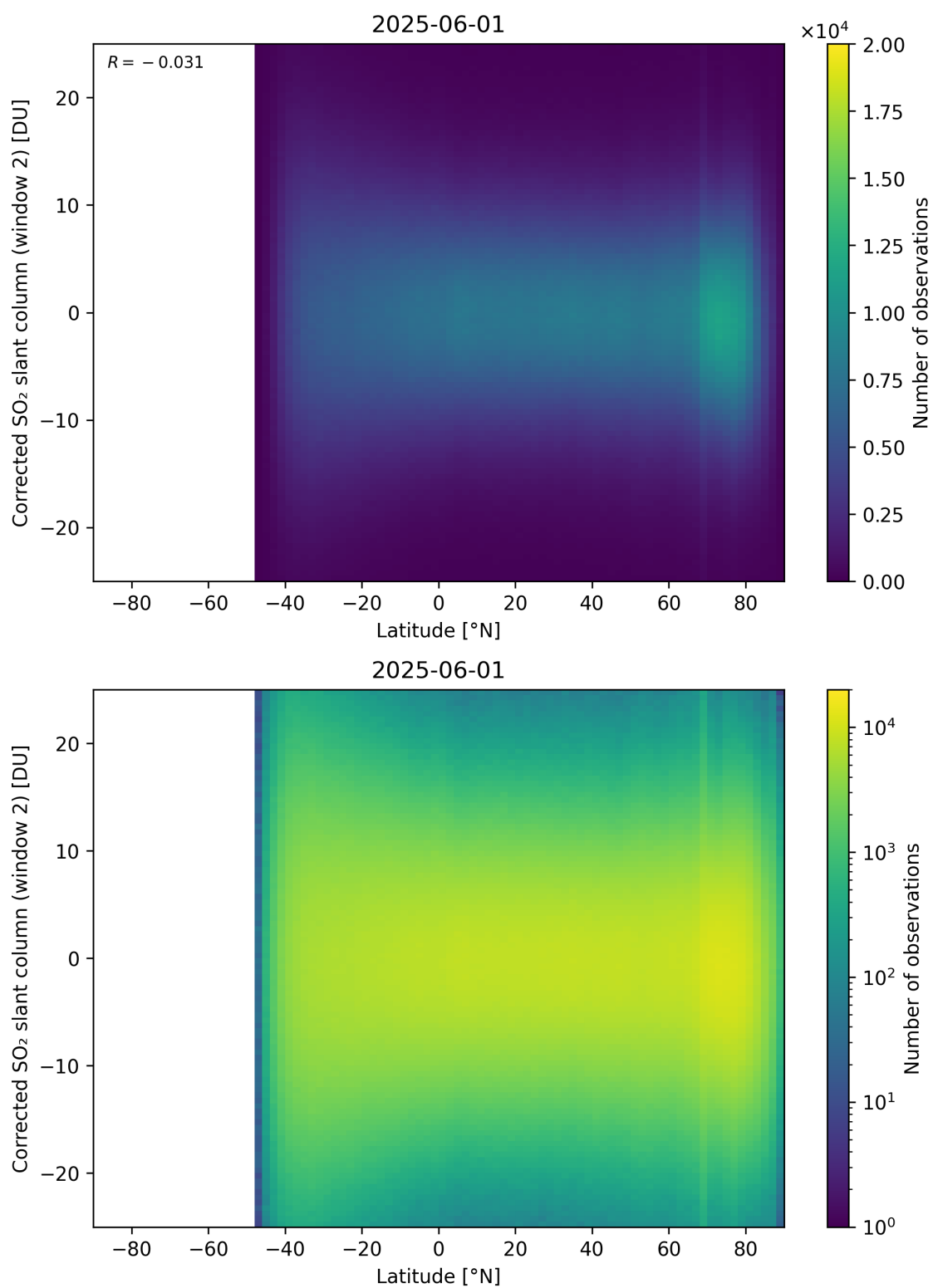
Figure 160: Scatter density plot of “Latitude” against “Corrected SO 2 slant column (window 2)” for 2025-06-01 to 2025-06-02.
