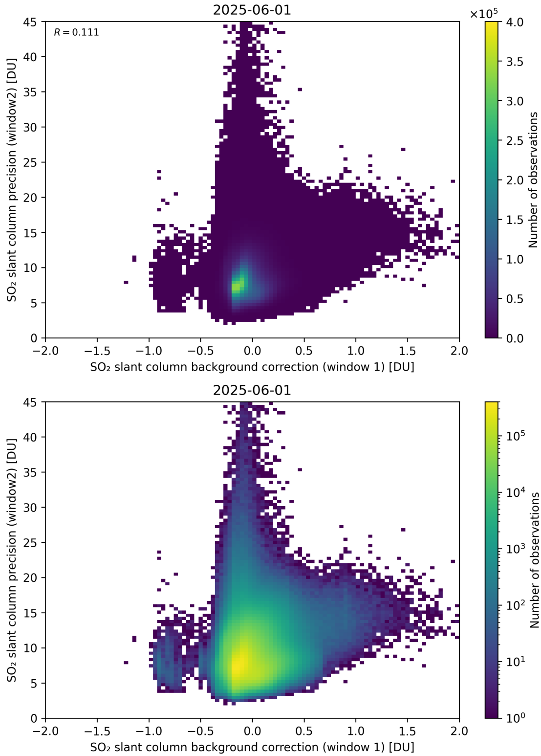
Figure 117: Scatter density plot of “SO 2 slant column background correction (window 1)” against “SO 2 slant column precision (window2)” for 2025-06-01 to 2025-06-02.
