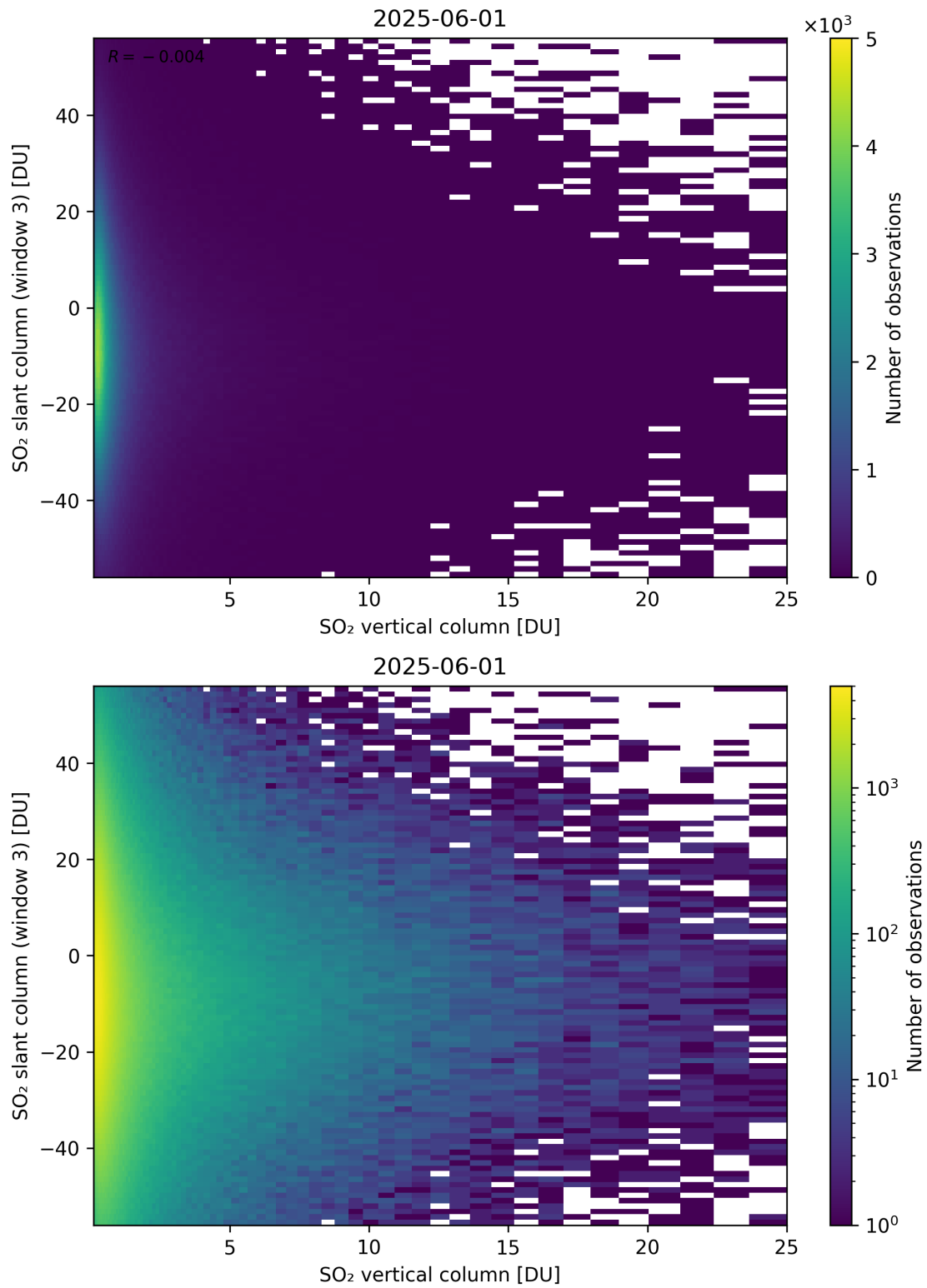
Figure 357: Scatter density plot of “SO 2 vertical column” against “SO 2 slant column (window 3)” for 2025-06-01 to 2025-06-02.
