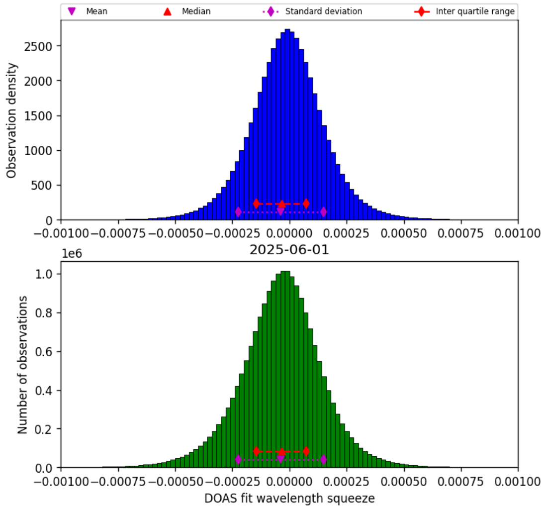
Figure 77: Histogram of “DOAS fit wavelength squeeze” for 2025-06-01 to 2025-06-02
