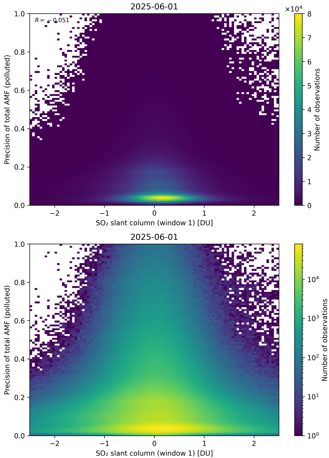
Figure 290: Scatter density plot of “SO 2 slant column (window 1)” against “Precision of total AMF (polluted)” for 2025-06-01 to 2025-06-02.
