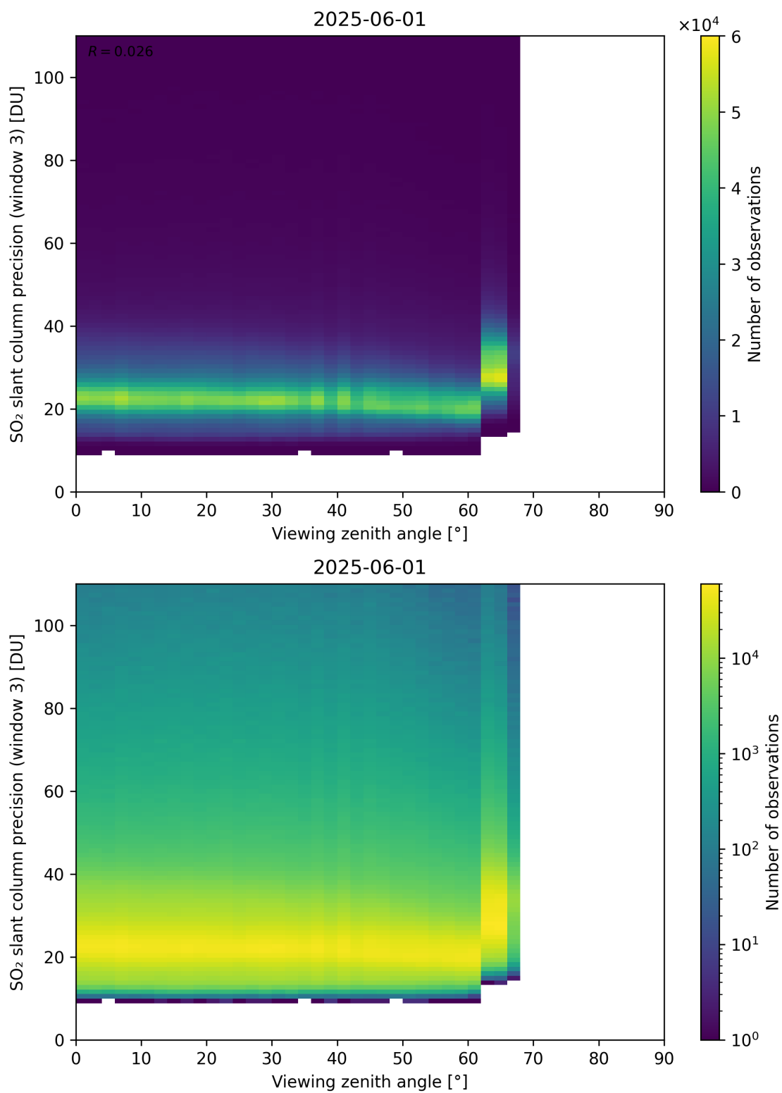
Figure 380: Scatter density plot of “Viewing zenith angle” against “SO 2 slant column precision (window 3)” for 2025-06-01 to 2025-06-02.
