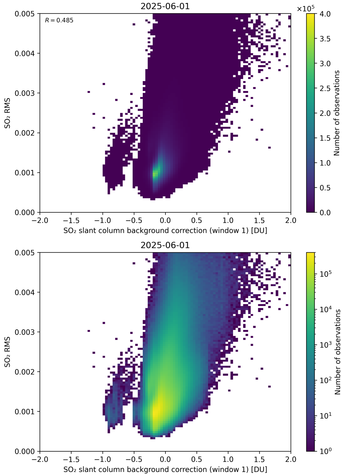
Figure 113: Scatter density plot of “SO 2 slant column background correction (window 1)” against “SO 2 RMS” for 2025-06-01 to 2025-06-02.
