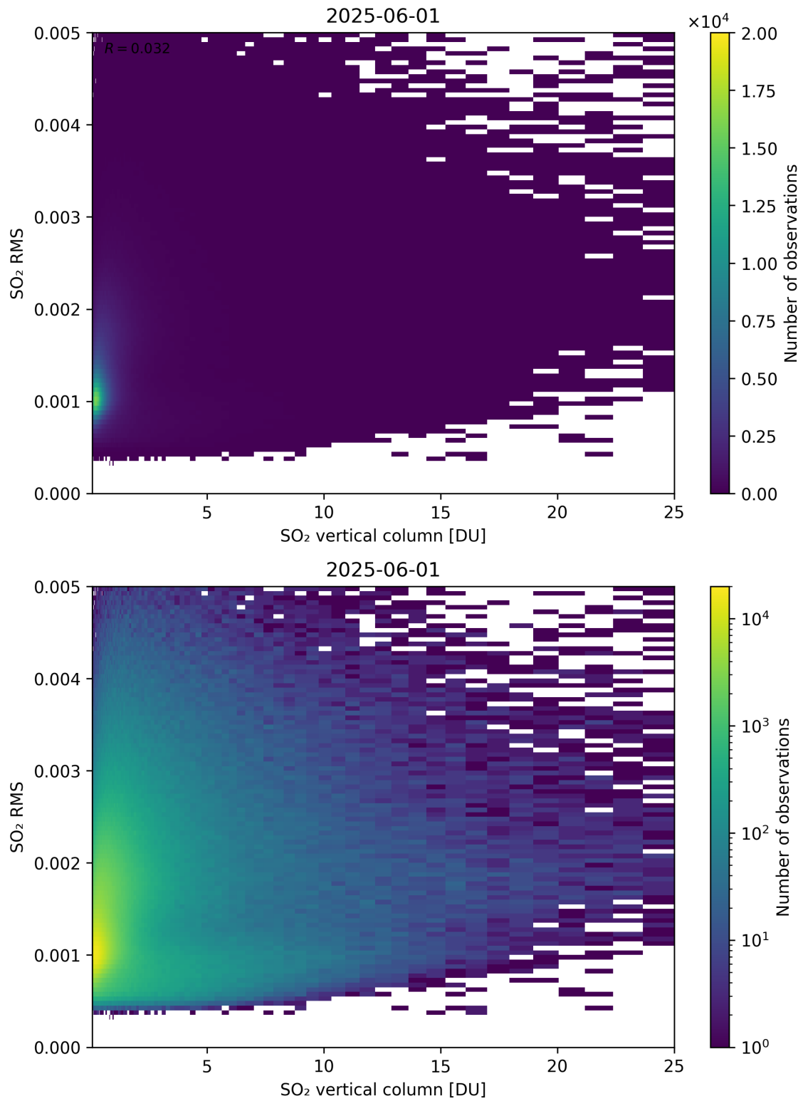
Figure 328: Scatter density plot of “SO 2 vertical column” against “SO 2 RMS” for 2025-06-01 to 2025-06-02.
