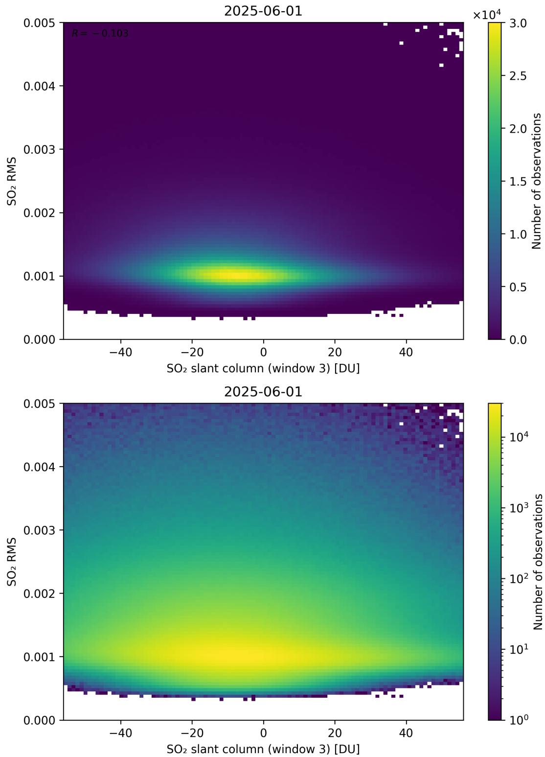
Figure 306: Scatter density plot of “SO 2 slant column (window 3)” against “SO 2 RMS” for 2025-06-01 to 2025-06-02.
