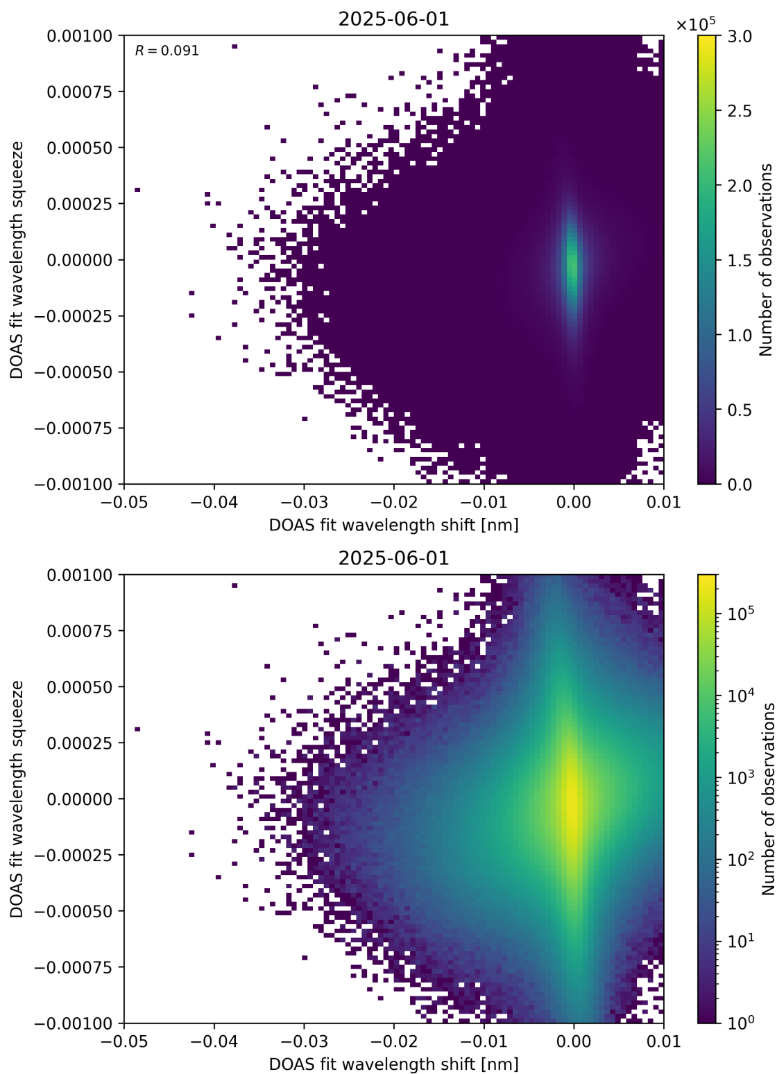
Figure 138: Scatter density plot of “DOAS fit wavelength shift” against “DOAS fit wavelength squeeze” for 2025-06-01 to 2025-06-02.
