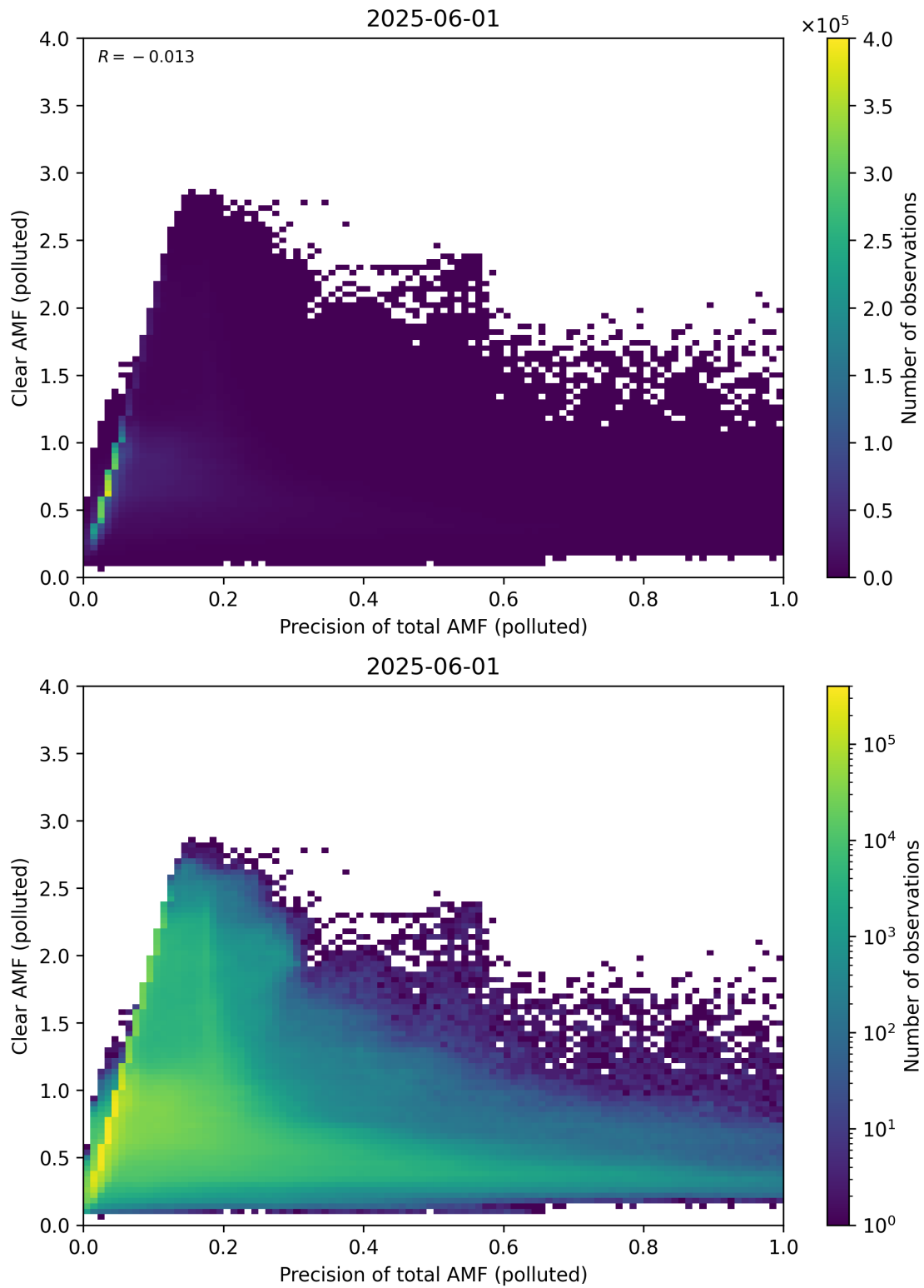
Figure 320: Scatter density plot of “Precision of total AMF (polluted)” against “Clear AMF (polluted)” for 2025-06-01 to 2025-06-02.
