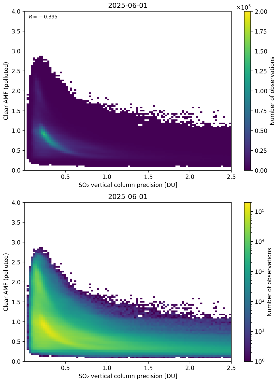
Figure 335: Scatter density plot of “SO 2 vertical column precision” against “Clear AMF (polluted)” for 2025-06-01 to 2025-06-02.
