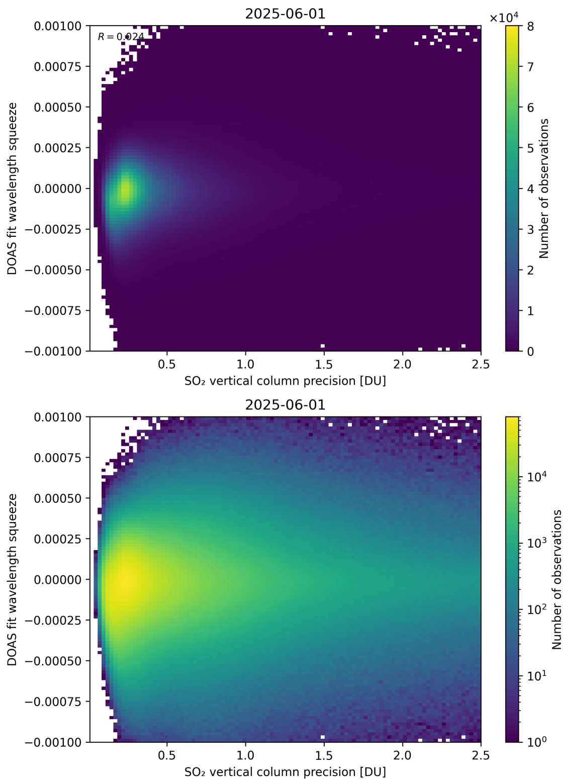
Figure 333: Scatter density plot of “SO 2 vertical column precision” against “DOAS fit wavelength squeeze” for 2025-06-01 to 2025-06-02.
