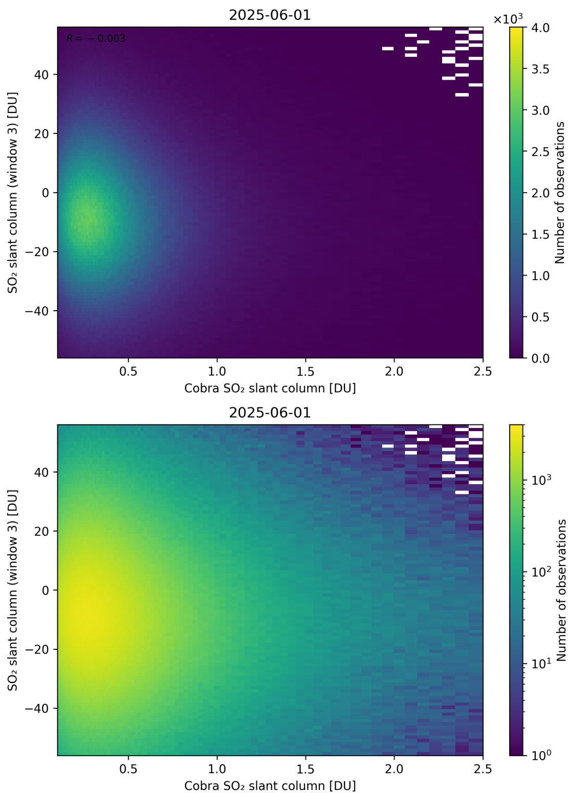
Figure 222: Scatter density plot of “Cobra SO 2 slant column” against “SO 2 slant column (window 3)” for 2025-06-01 to 2025-06-02.
