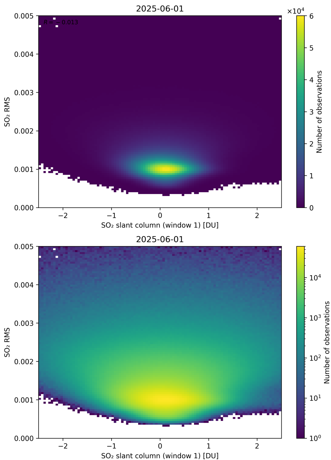
Figure 267: Scatter density plot of “SO 2 slant column (window 1)” against “SO 2 RMS” for 2025-06-01 to 2025-06-02.
