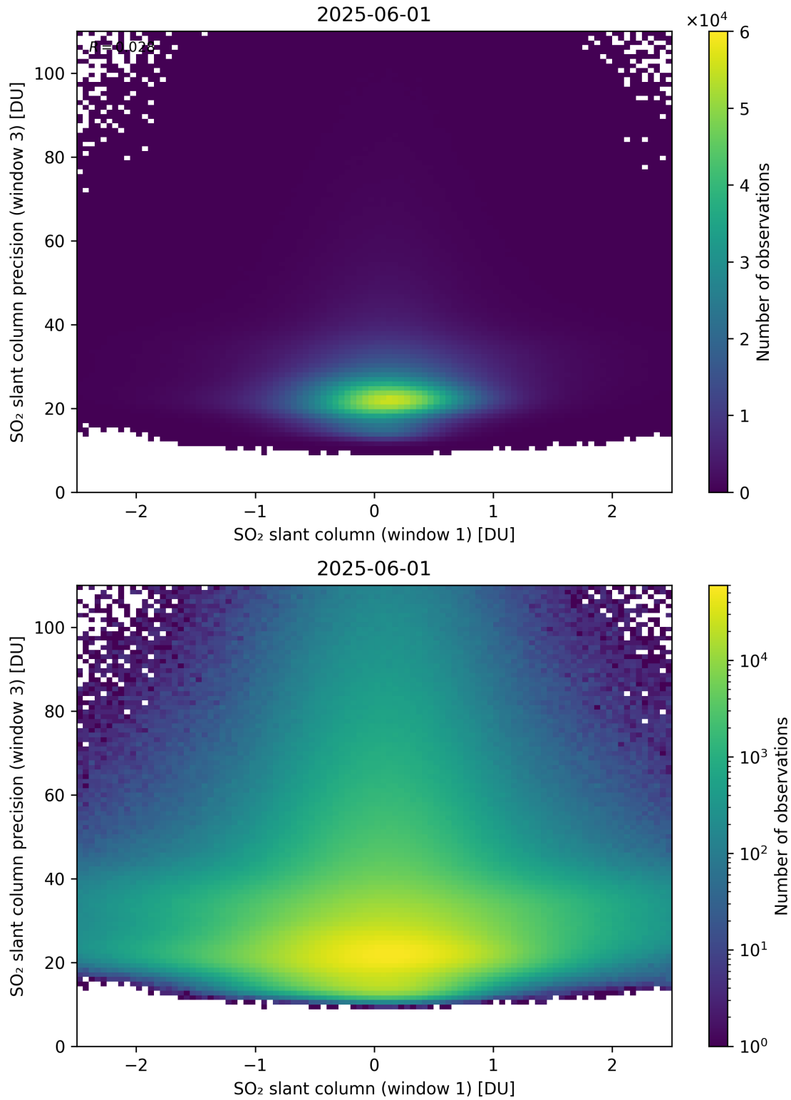
Figure 288: Scatter density plot of “SO 2 slant column (window 1)” against “SO 2 slant column precision (window 3)” for 2025-06-01 to 2025-06-02.
