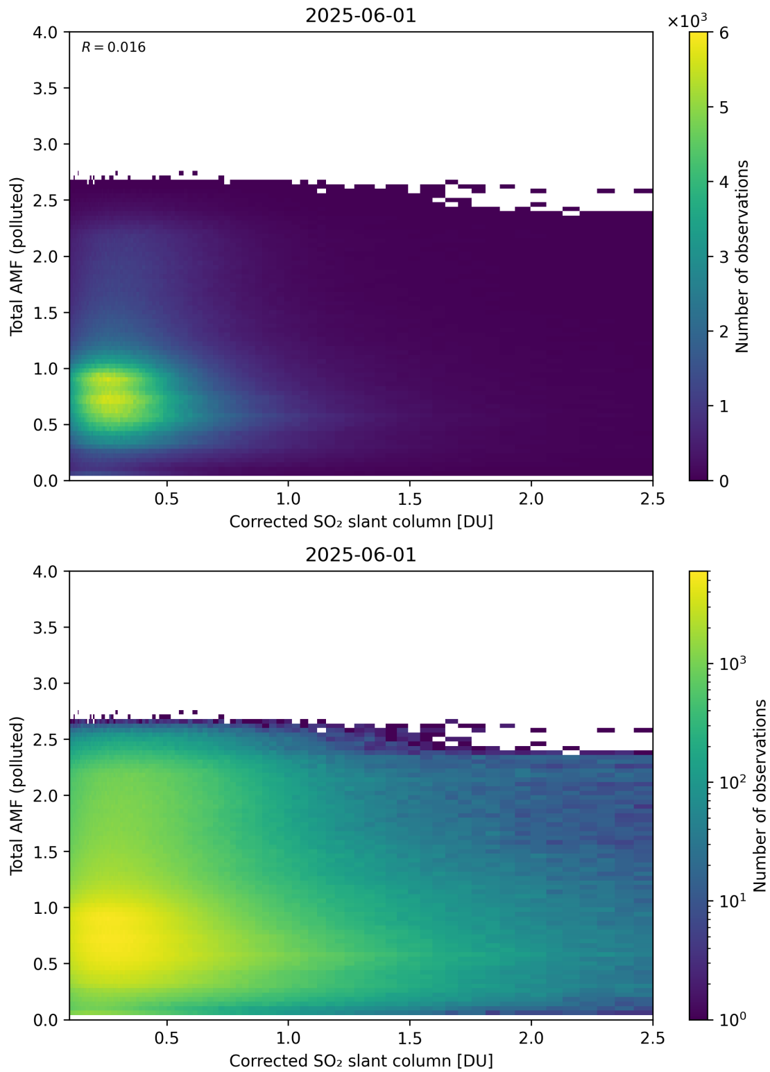
Figure 242: Scatter density plot of “Corrected SO 2 slant column” against “Total AMF (polluted)” for 2025-06-01 to 2025-06-02.
