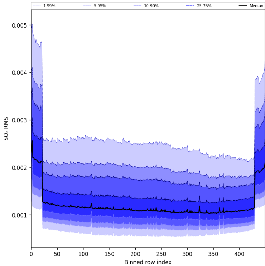
Figure 104: Along track statistics of “SO 2 RMS” for 2025-06-01 to 2025-06-02
