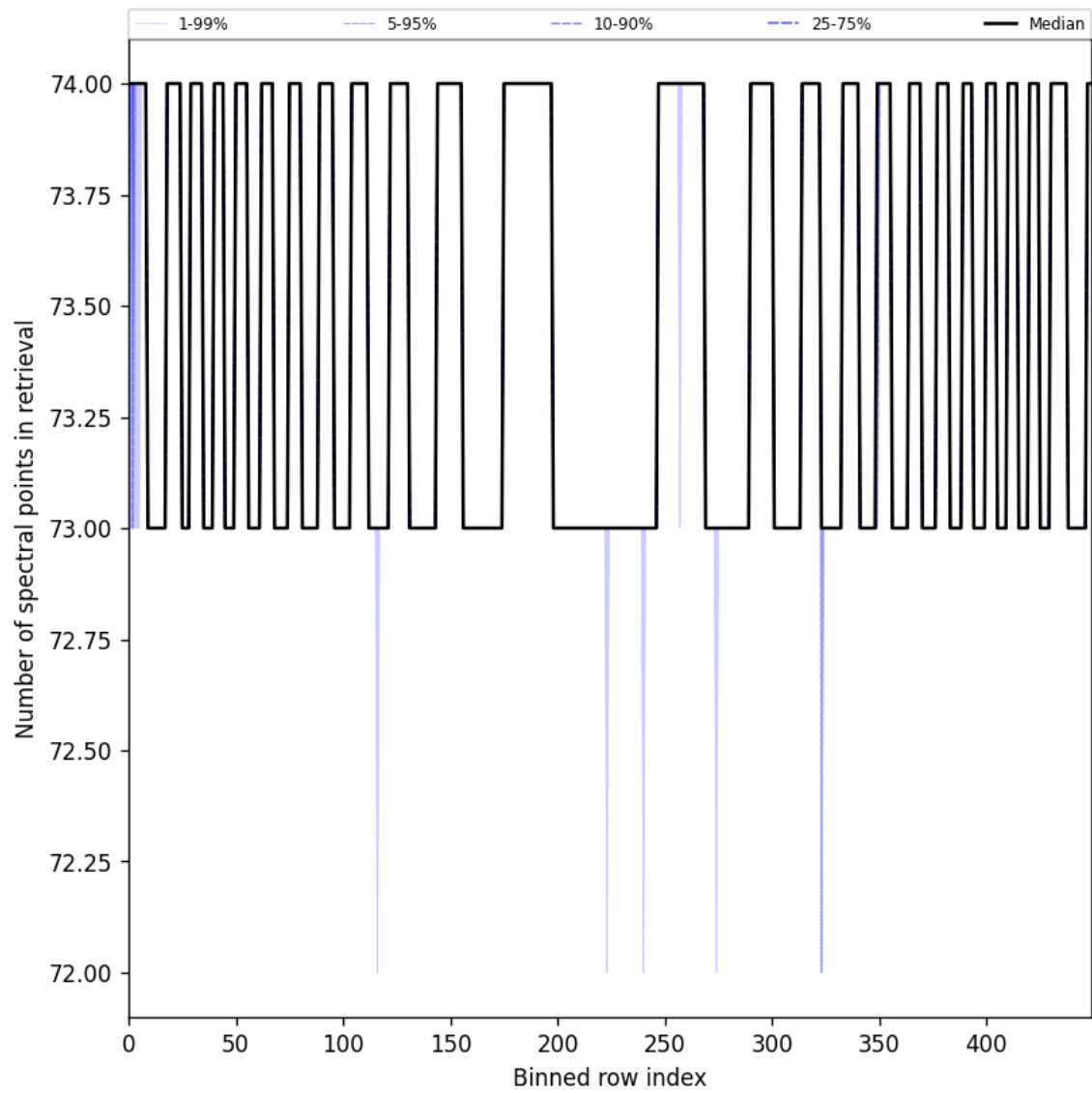
Figure 108: Along track statistics of “Number of spectral points in retrieval” for 2025-06-01 to 2025-06-02
