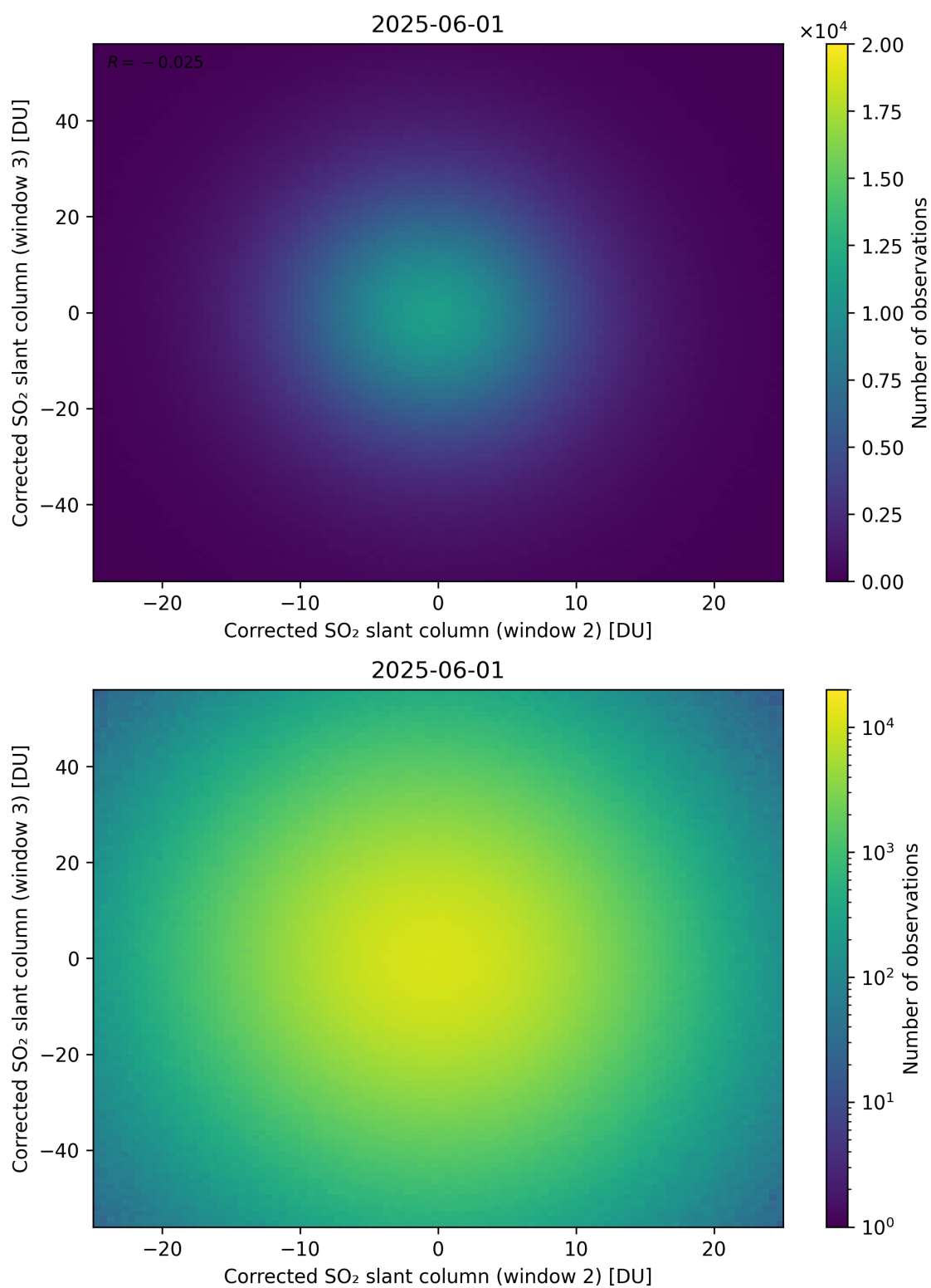
Figure 250: Scatter density plot of “Corrected SO 2 slant column (window 2)” against “Corrected SO 2 slant column (window 3)” for 2025-06-01 to 2025-06-02.
