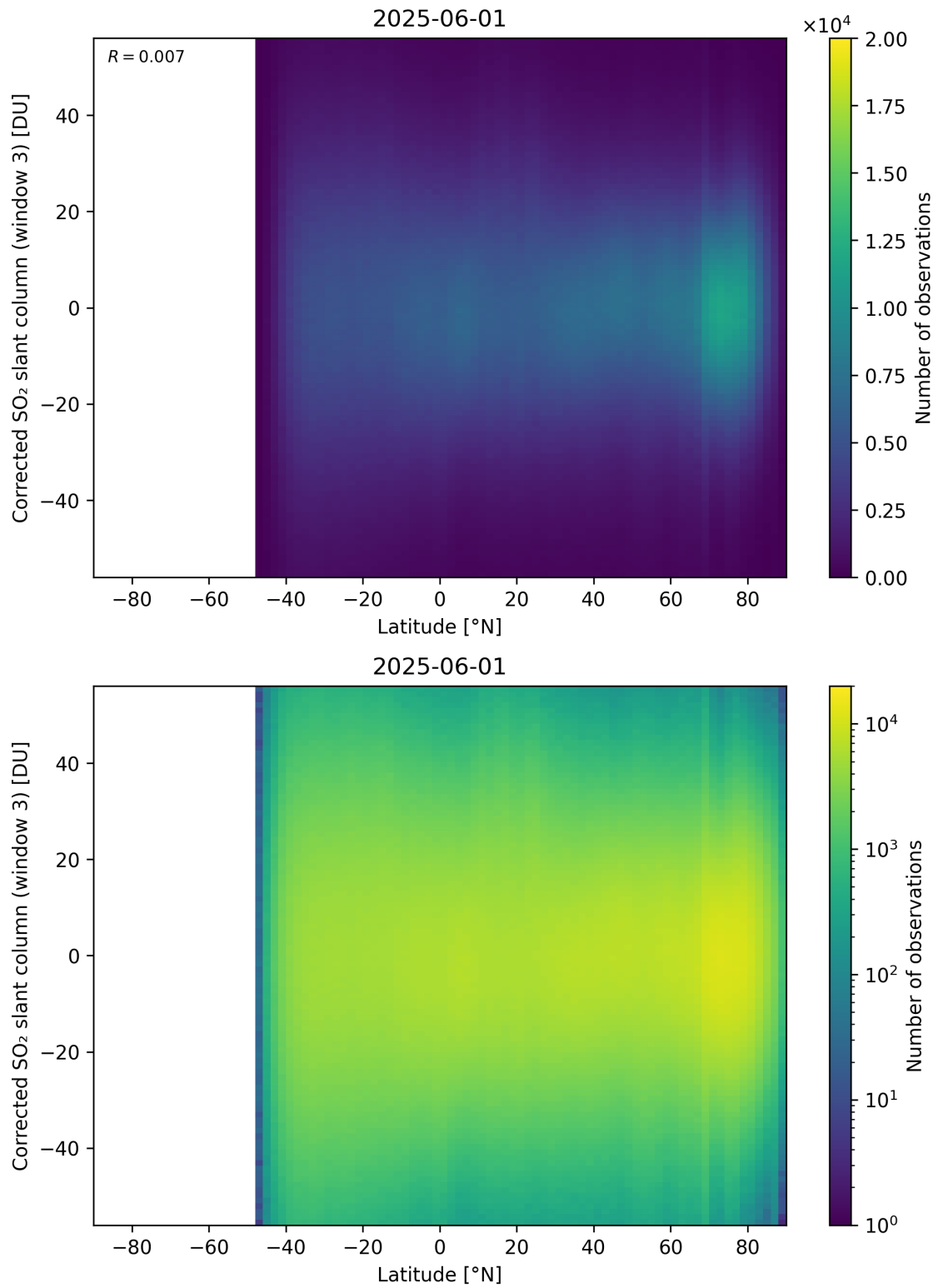
Figure 161: Scatter density plot of “Latitude” against “Corrected SO 2 slant column (window 3)” for 2025-06-01 to 2025-06-02.
