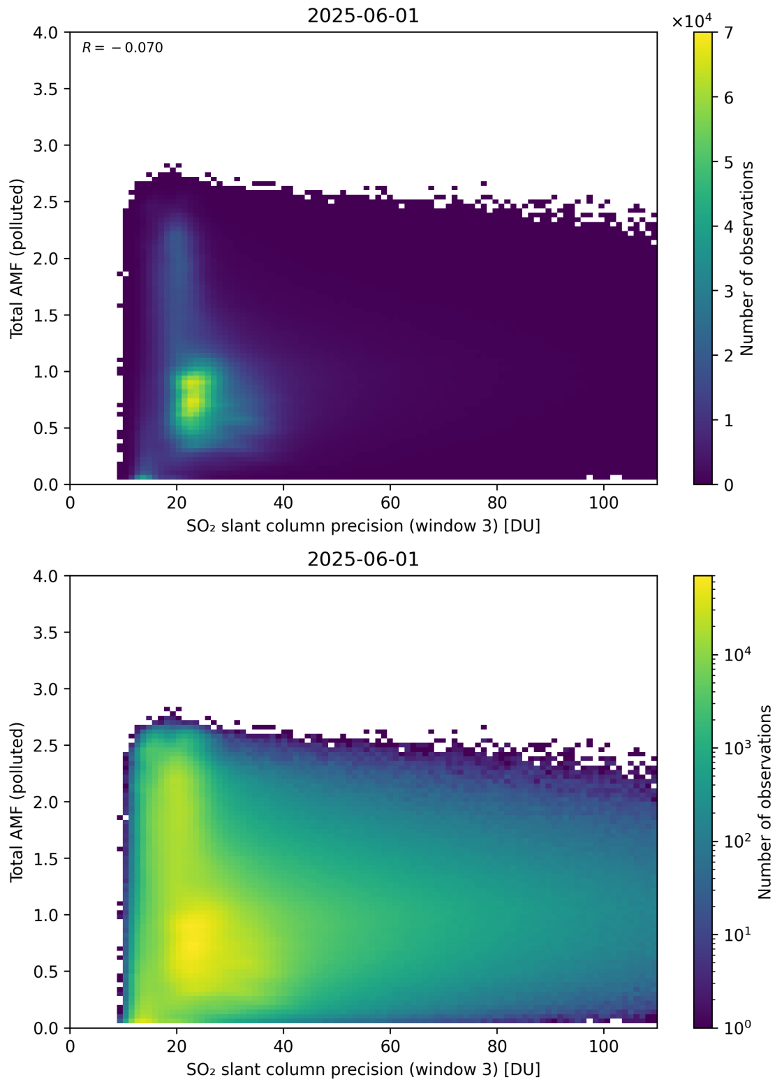
Figure 313: Scatter density plot of “SO 2 slant column precision (window 3)” against “Total AMF (polluted)” for 2025-06-01 to 2025-06-02.
