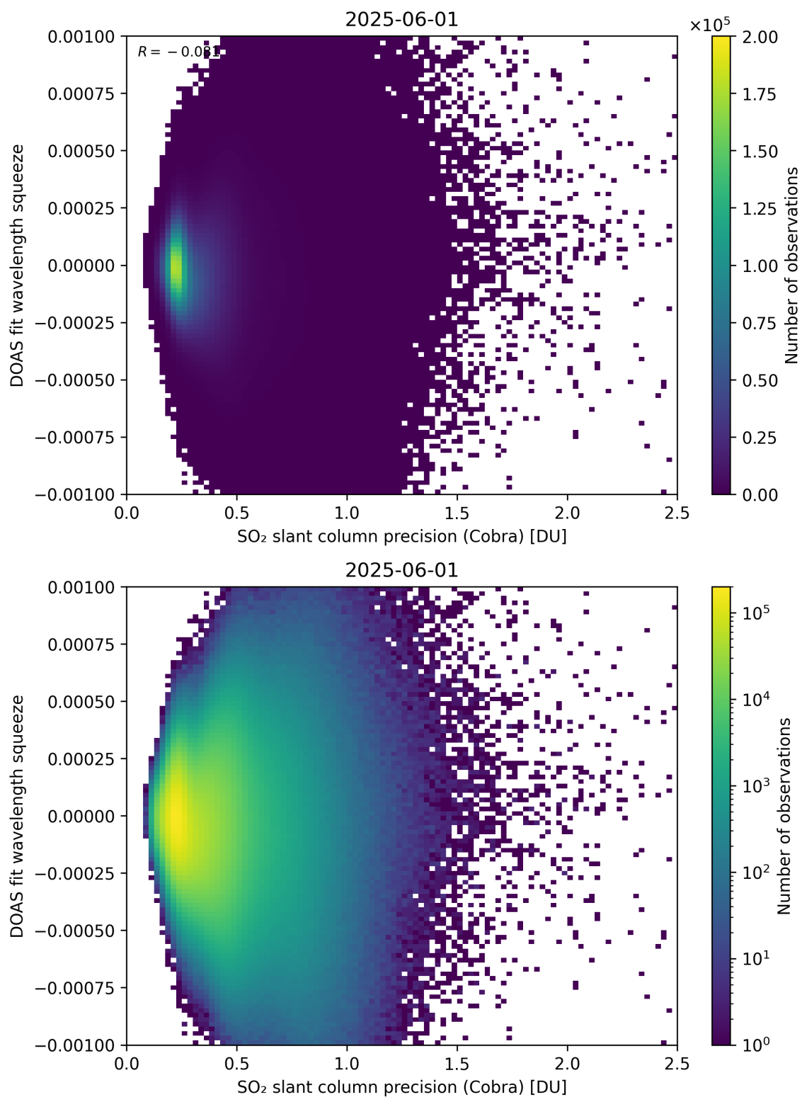
Figure 203: Scatter density plot of “SO 2 slant column precision (Cobra)” against “DOAS fit wavelength squeeze” for 2025-06-01 to 2025-06-02.
