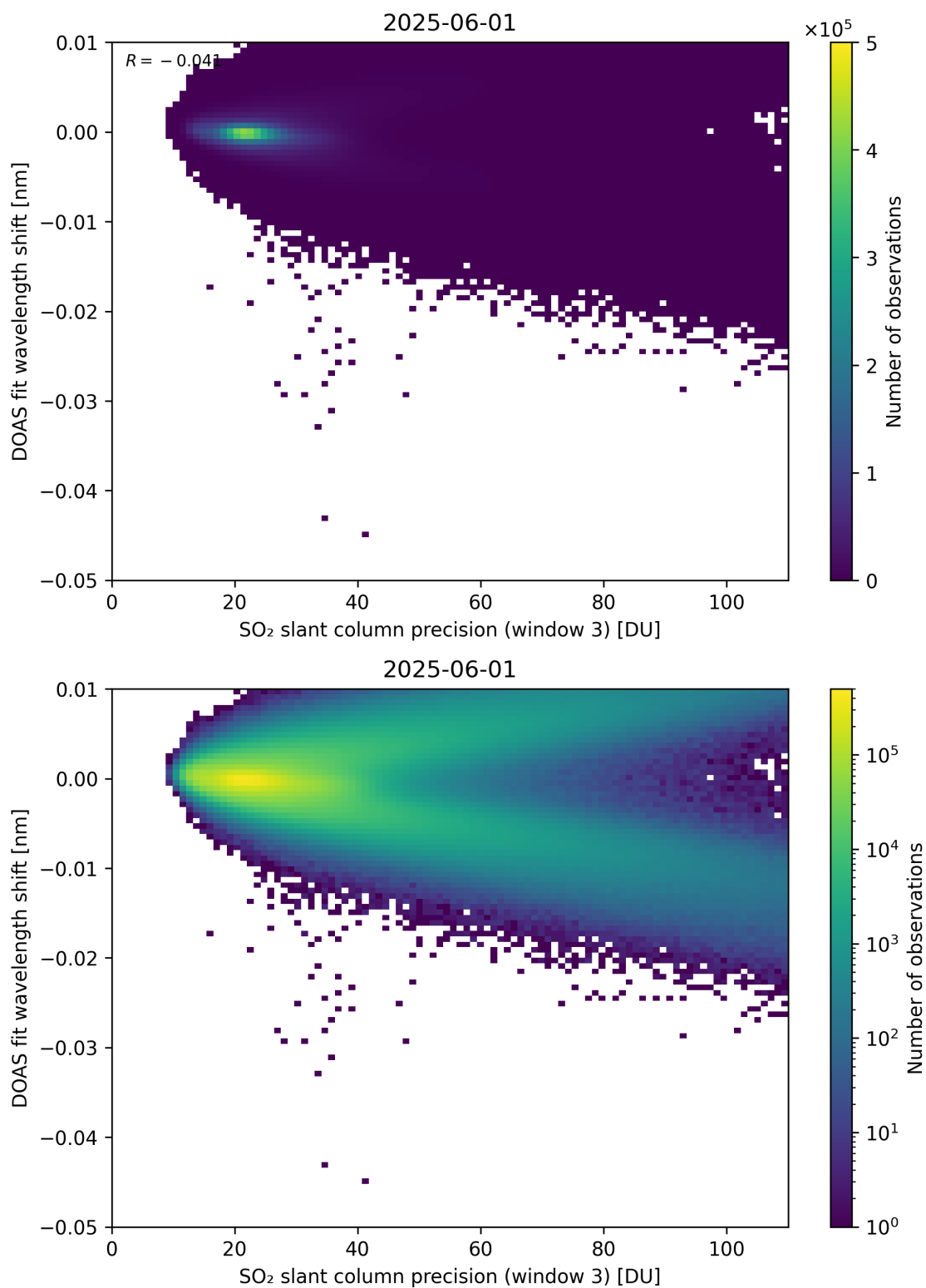
Figure 308: Scatter density plot of “SO 2 slant column precision (window 3)” against “DOAS fit wavelength shift” for 2025-06-01 to 2025-06-02.
