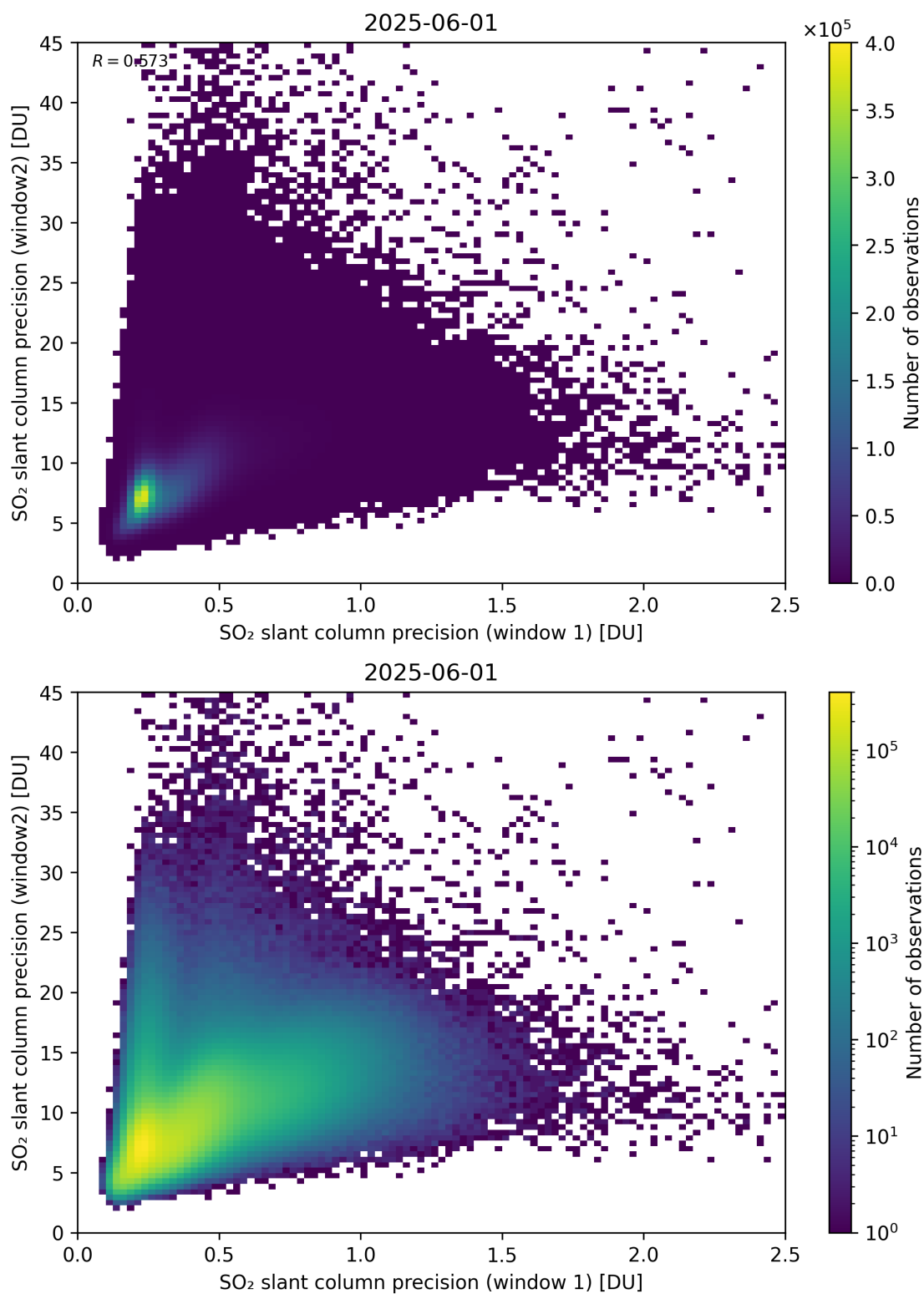
Figure 277: Scatter density plot of “SO 2 slant column precision (window 1)” against “SO 2 slant column precision (window2)” for 2025-06-01 to 2025-06-02.
