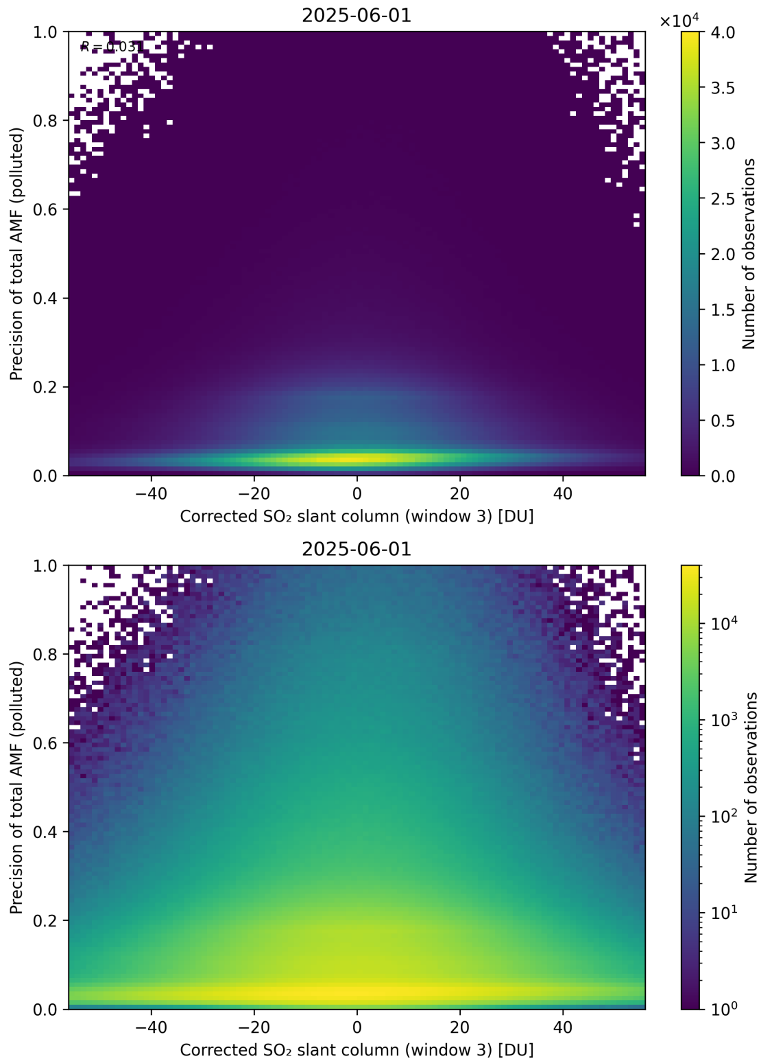
Figure 261: Scatter density plot of “Corrected SO 2 slant column (window 3)” against “Precision of total AMF (polluted)” for 2025-06-01 to 2025-06-02.
