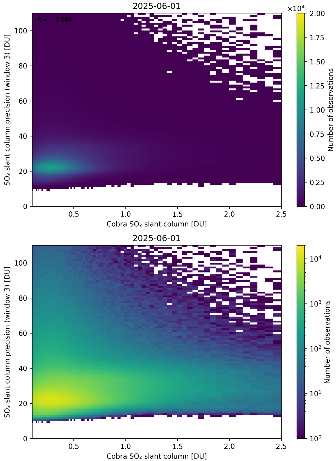
Figure 223: Scatter density plot of “Cobra SO 2 slant column” against “SO 2 slant column precision (window 3)” for 2025-06-01 to 2025-06-02.
