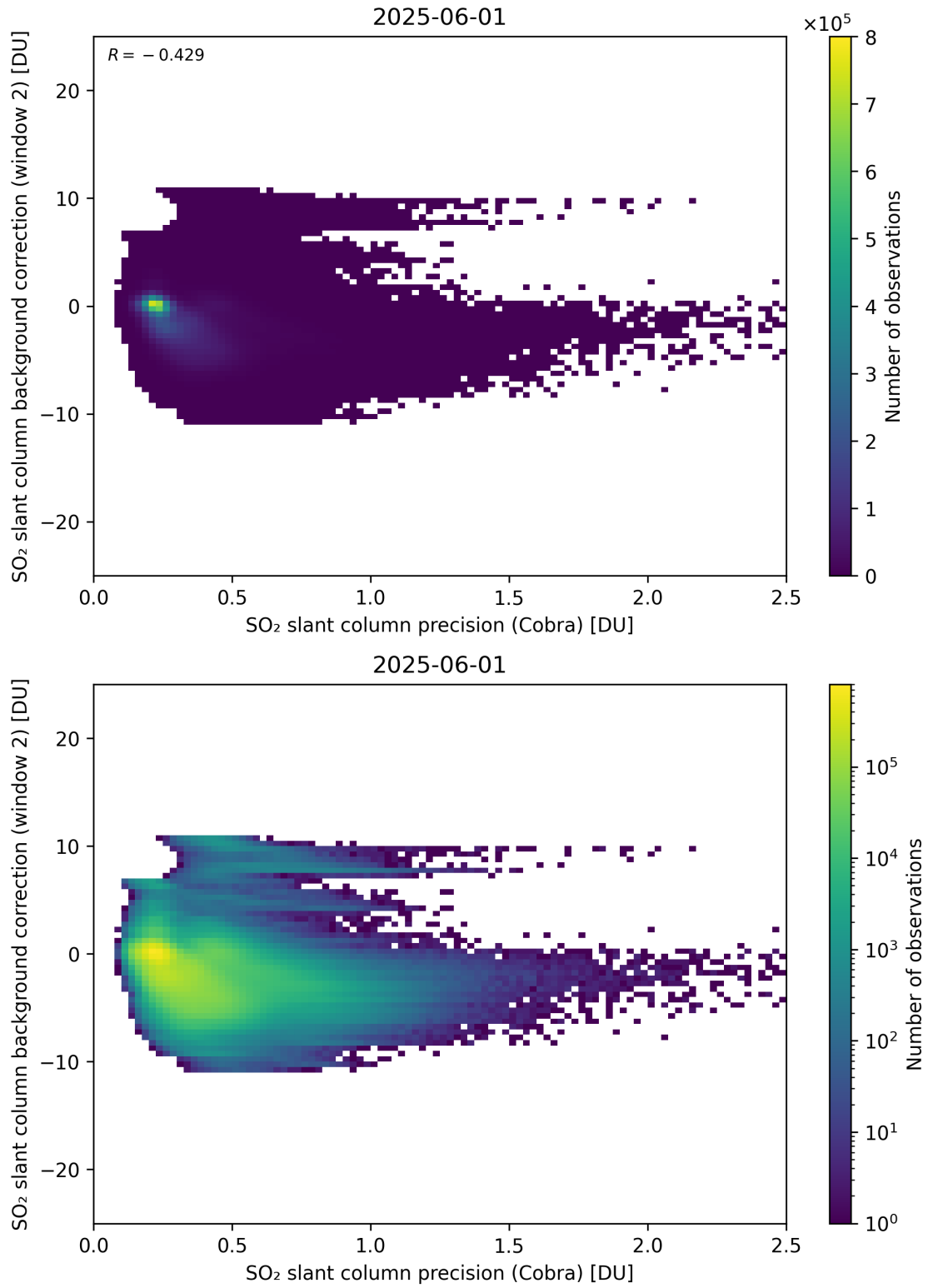
Figure 200: Scatter density plot of “SO 2 slant column precision (Cobra)” against “SO 2 slant column background correction (window 2)” for 2025-06-01 to 2025-06-02.
