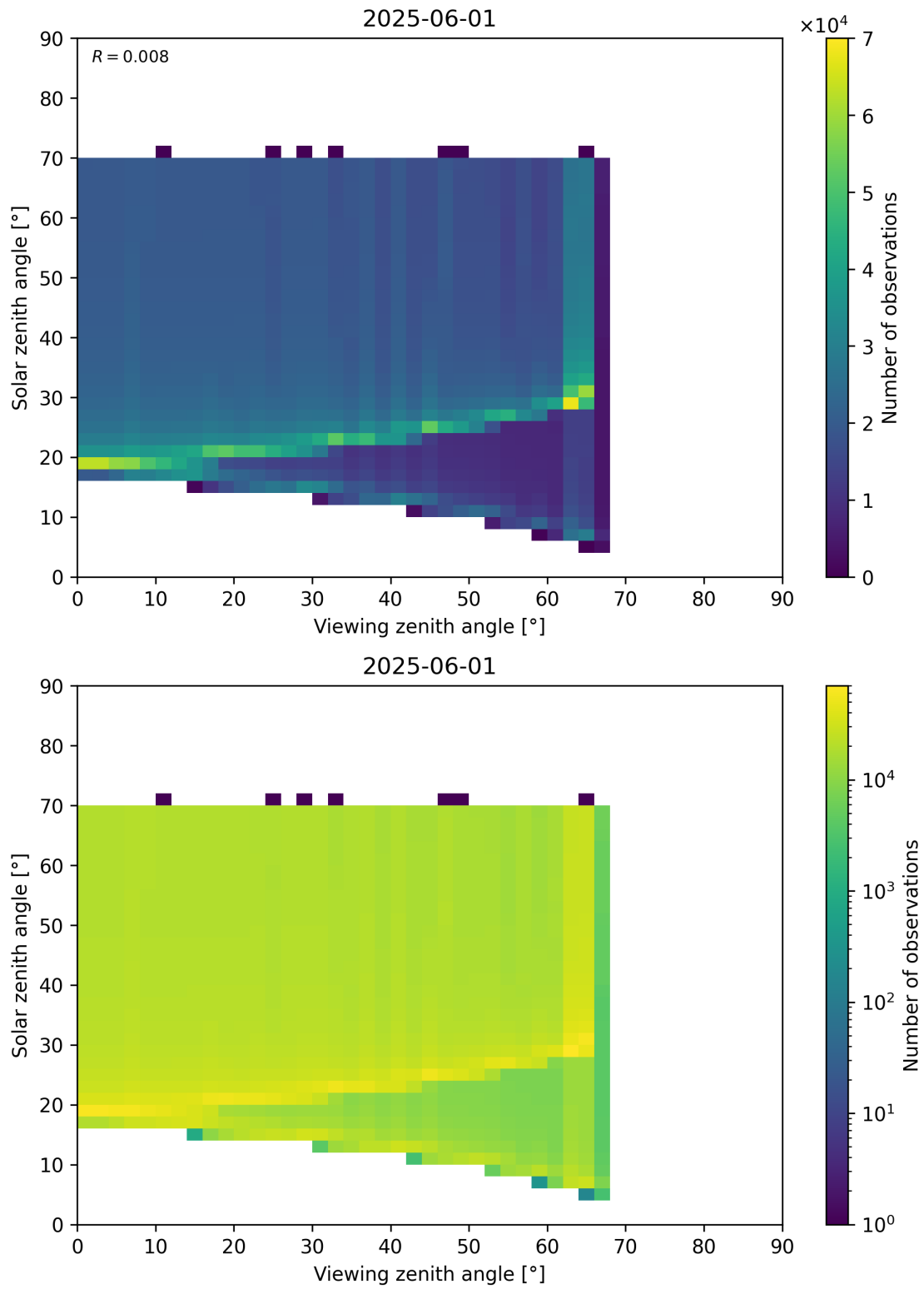
Figure 369: Scatter density plot of “Viewing zenith angle” against “Solar zenith angle” for 2025-06-01 to 2025-06-02.
