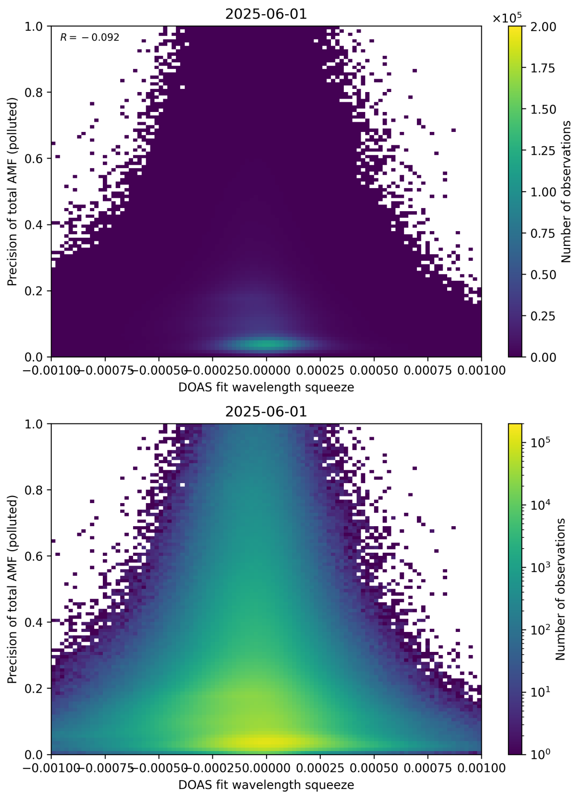
Figure 146: Scatter density plot of “DOAS fit wavelength squeeze” against “Precision of total AMF (polluted)” for 2025-06-01 to 2025-06-02.
