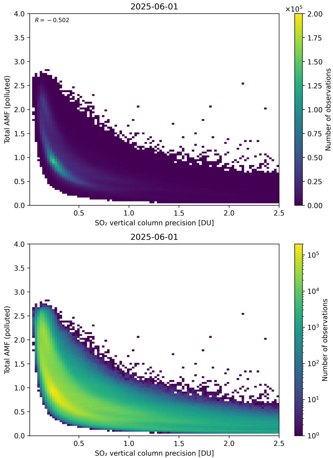
Figure 346: Scatter density plot of “SO 2 vertical column precision” against “Total AMF (polluted)” for 2025-06-01 to 2025-06-02.
