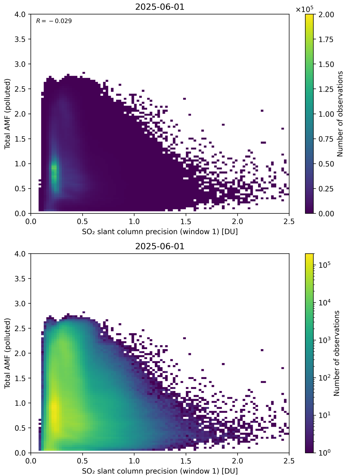
Figure 280: Scatter density plot of “SO 2 slant column precision (window 1)” against “Total AMF (polluted)” for 2025-06-01 to 2025-06-02.
