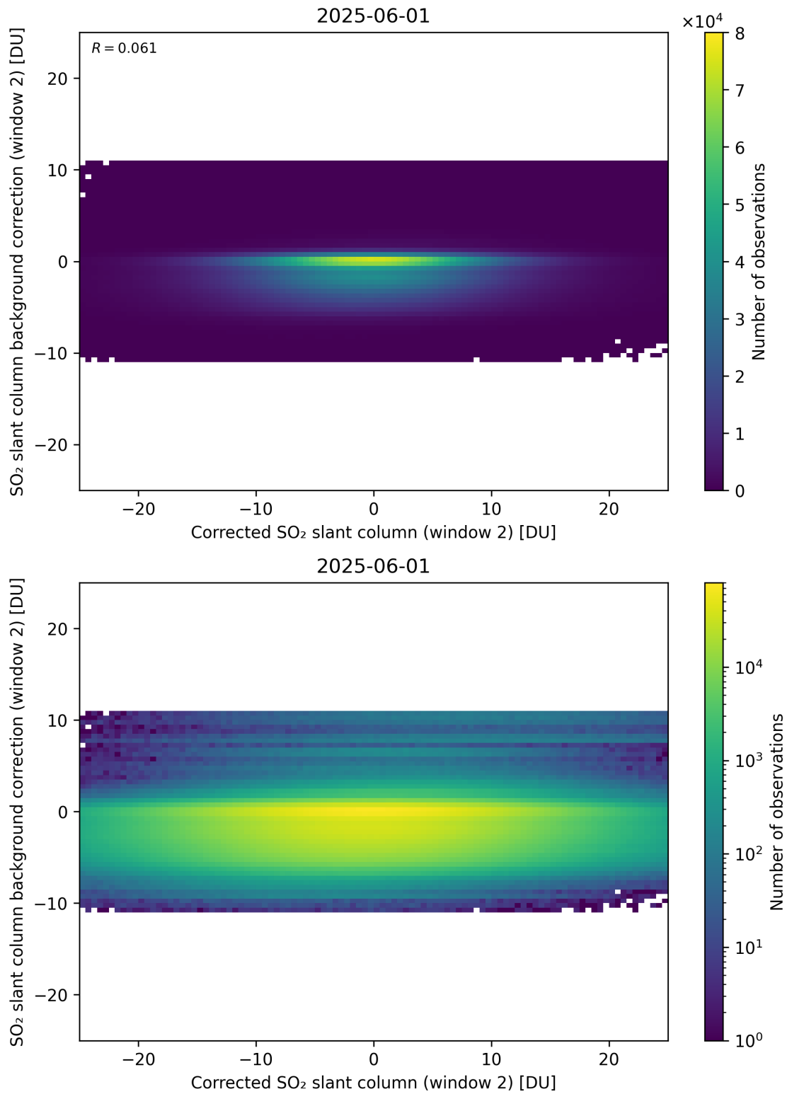
Figure 244: Scatter density plot of “Corrected SO 2 slant column (window 2)” against “SO 2 slant column background correction (window 2)” for 2025-06-01 to 2025-06-02.
