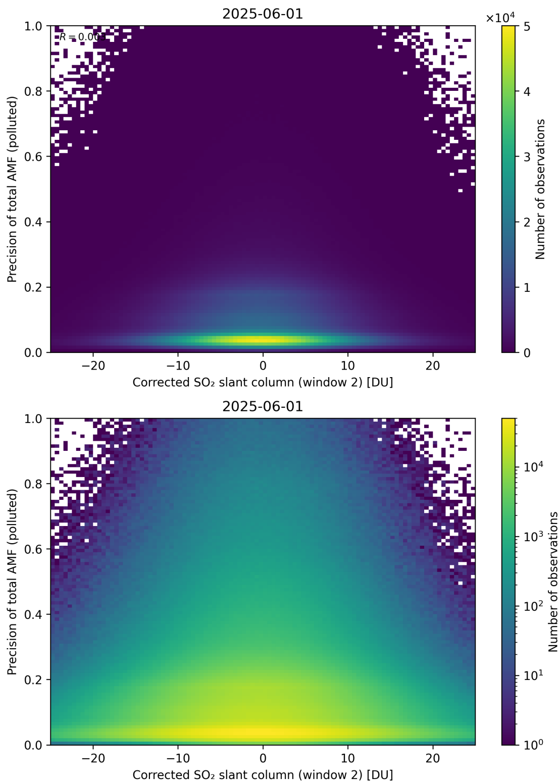
Figure 254: Scatter density plot of “Corrected SO 2 slant column (window 2)” against “Precision of total AMF (polluted)” for 2025-06-01 to 2025-06-02.
