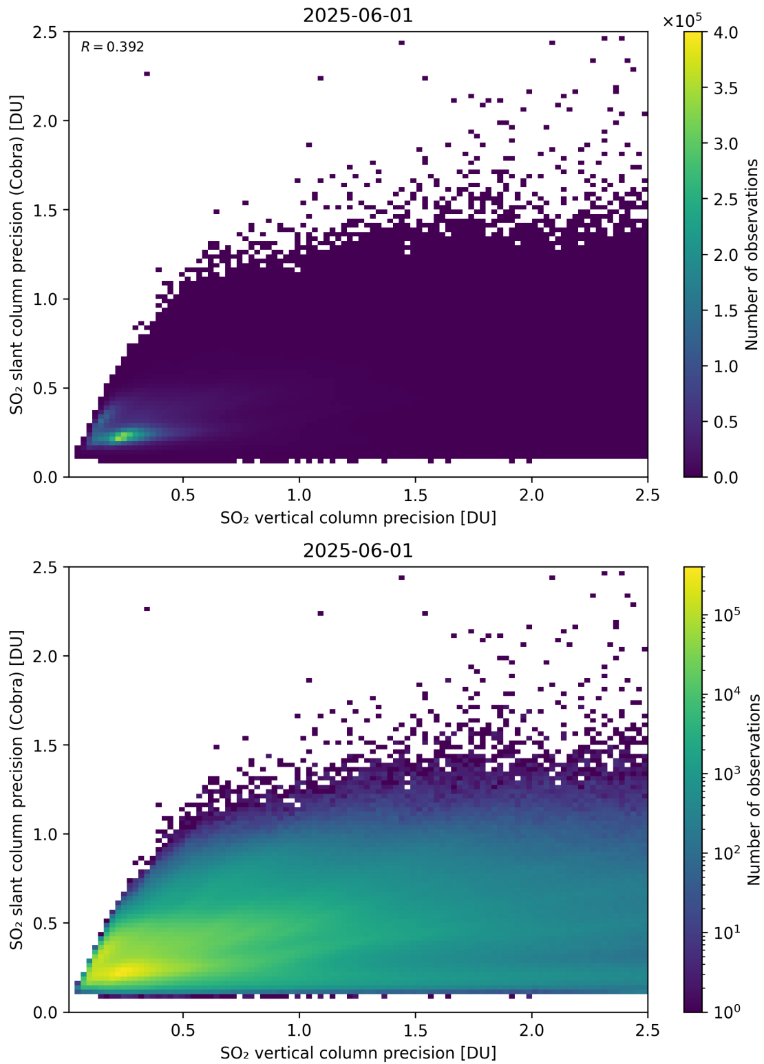
Figure 337: Scatter density plot of “SO 2 vertical column precision” against “SO 2 slant column precision (Cobra)” for 2025-06-01 to 2025-06-02.
