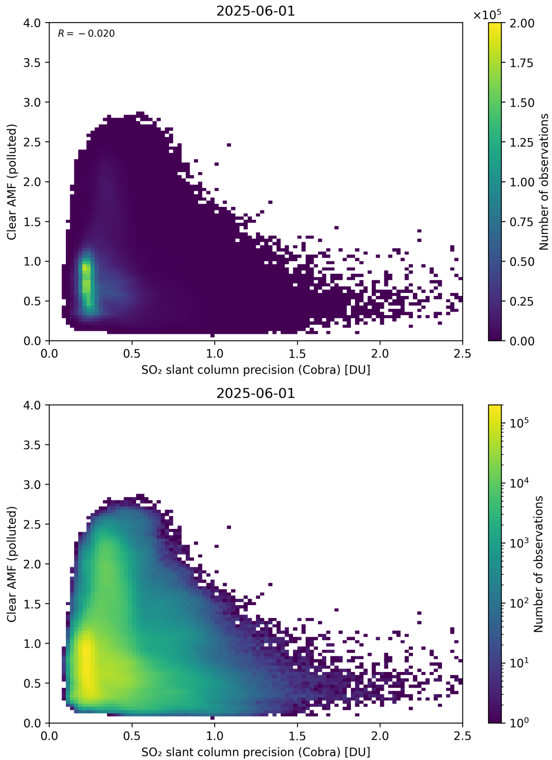
Figure 205: Scatter density plot of “SO 2 slant column precision (Cobra)” against “Clear AMF (polluted)” for 2025-06-01 to 2025-06-02.
