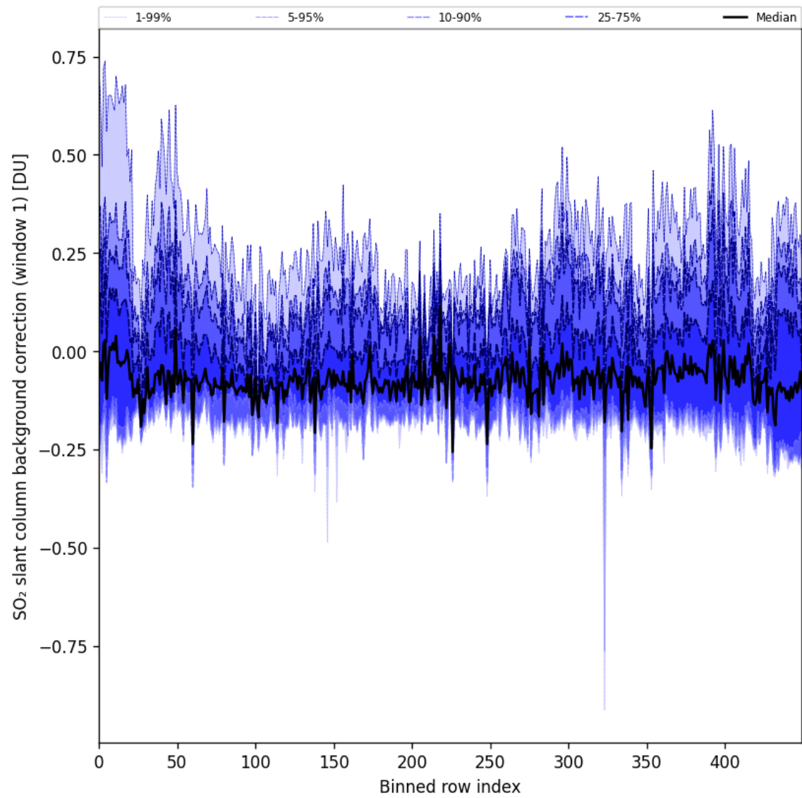
Figure 92: Along track statistics of “SO 2 slant column background correction (window 1)” for 2025-06-01 to 2025-06-02
