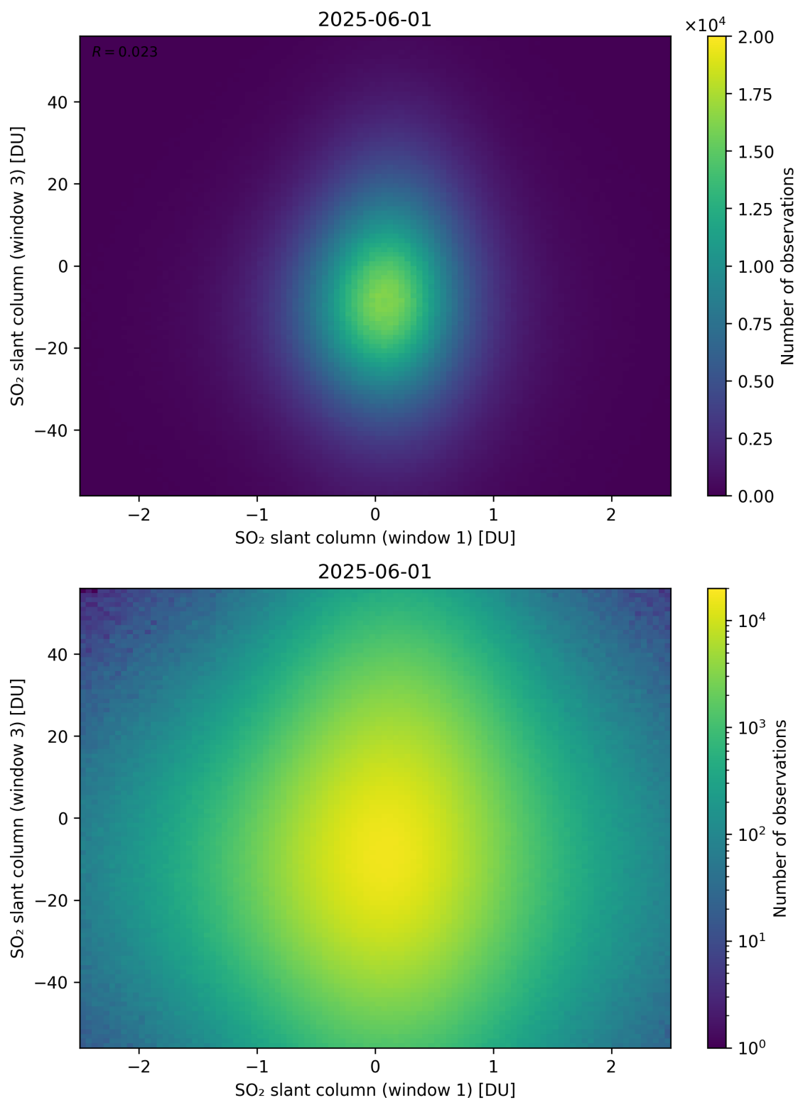
Figure 287: Scatter density plot of “SO 2 slant column (window 1)” against “SO 2 slant column (window 3)” for 2025-06-01 to 2025-06-02.
