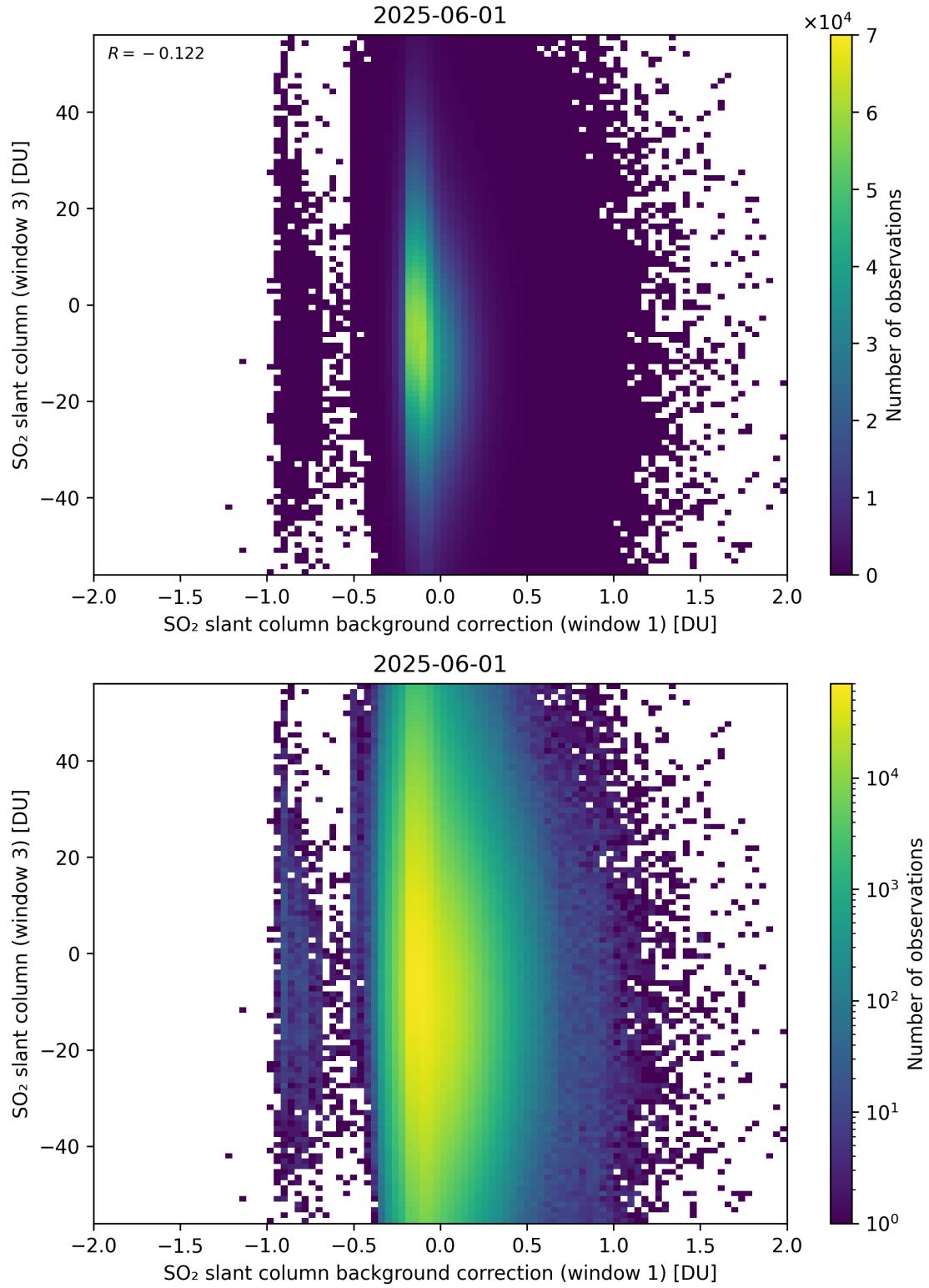
Figure 118: Scatter density plot of “SO 2 slant column background correction (window 1)” against “SO 2 slant column (window 3)” for 2025-06-01 to 2025-06-02.
