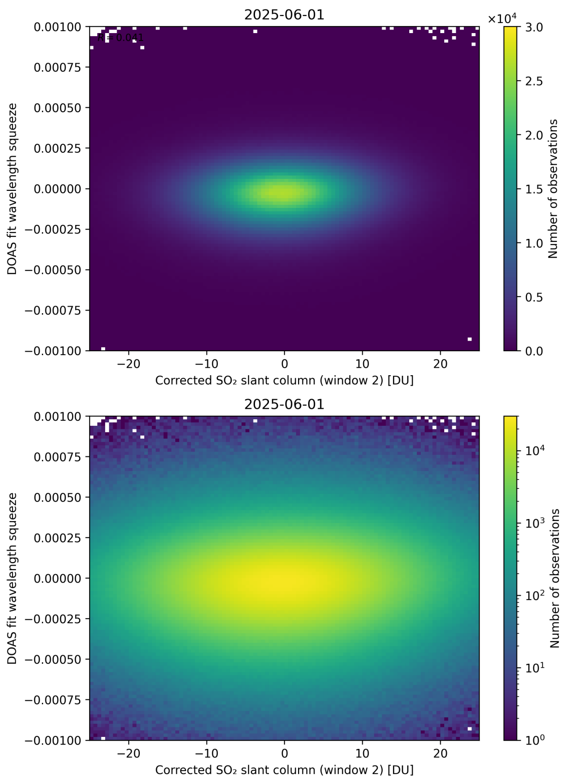
Figure 247: Scatter density plot of “Corrected SO 2 slant column (window 2)” against “DOAS fit wavelength squeeze” for 2025-06-01 to 2025-06-02.
