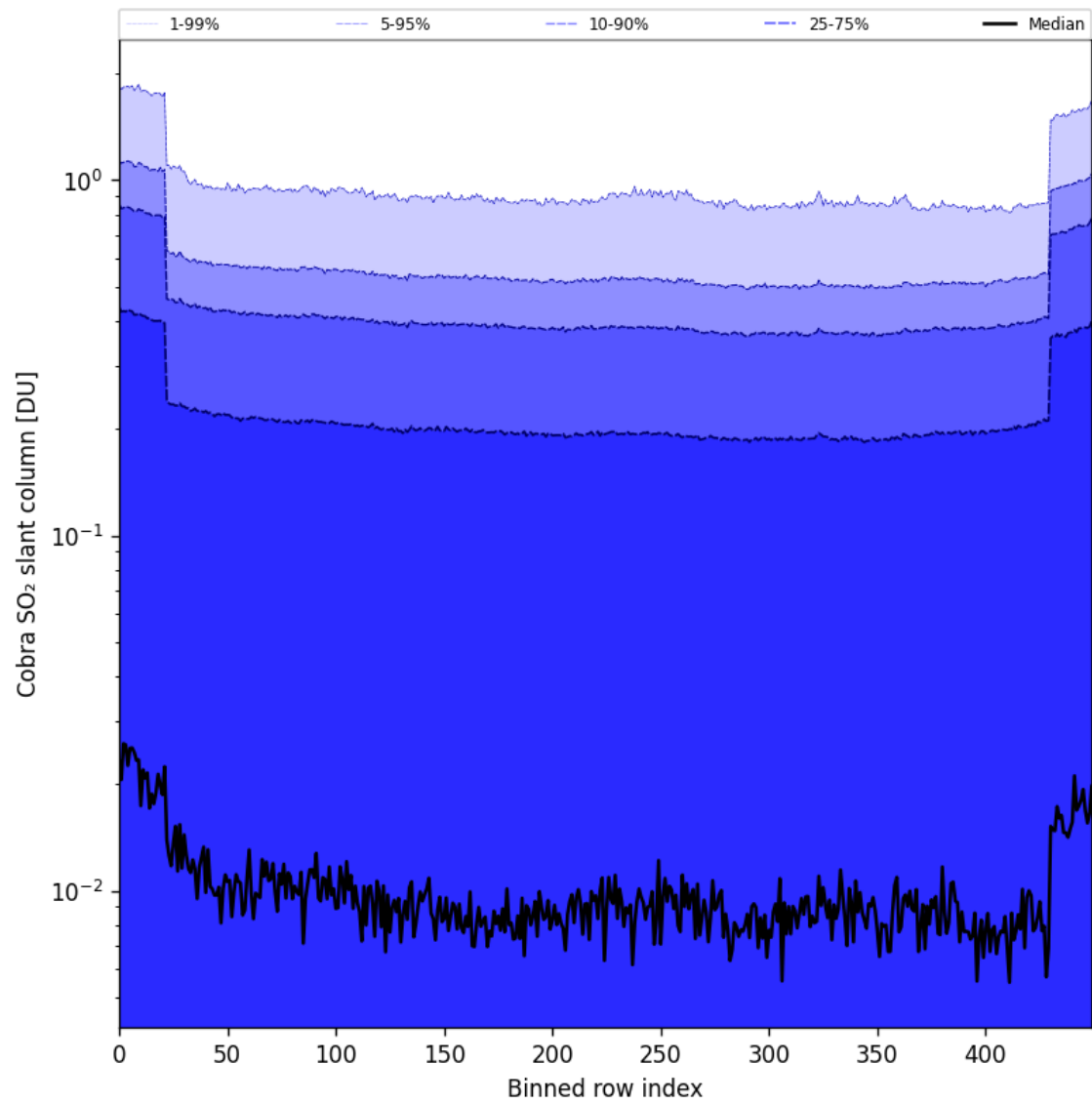
Figure 87: Along track statistics of “Cobra SO 2 slant column” for 2025-06-01 to 2025-06-02
