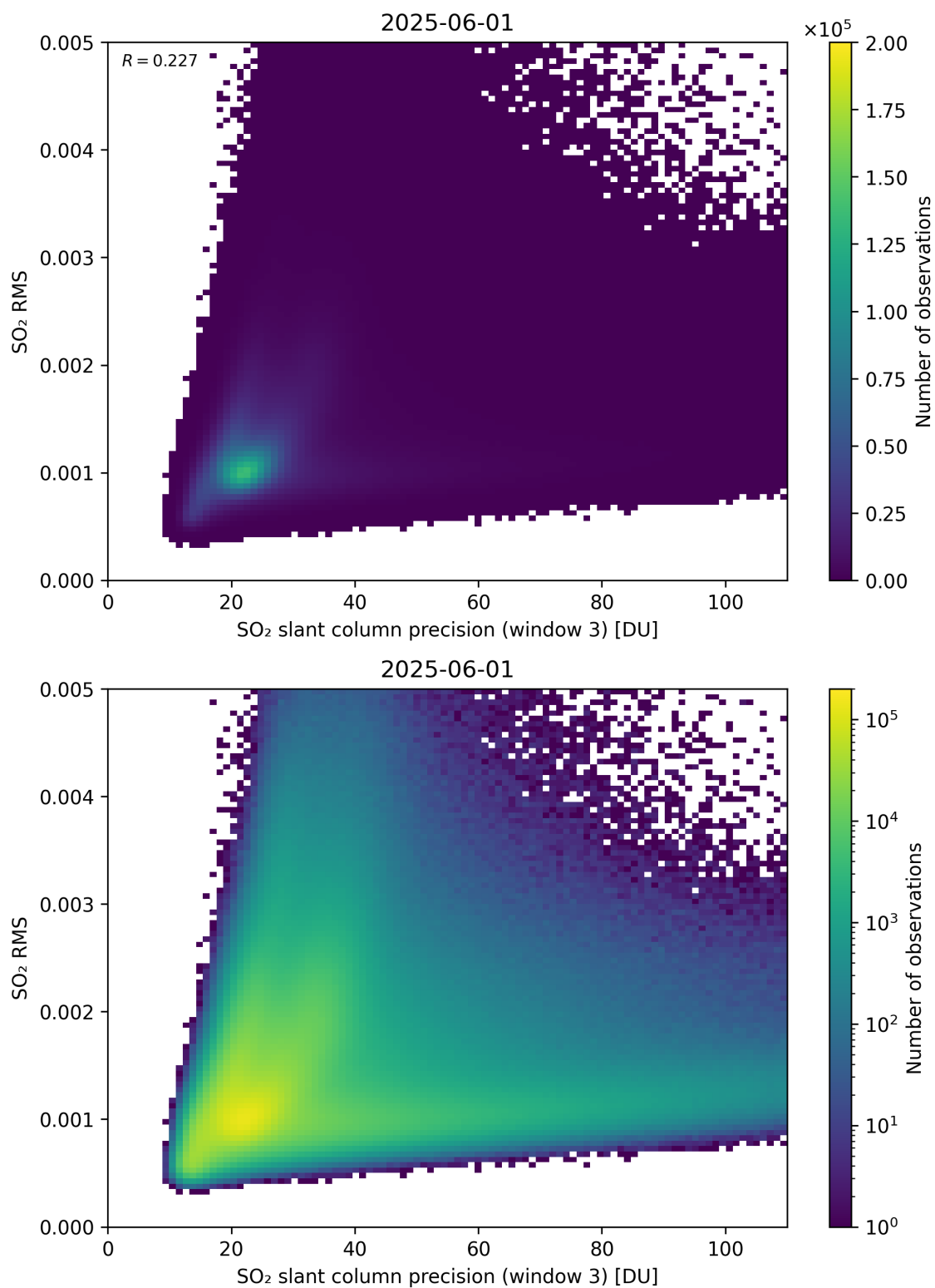
Figure 310: Scatter density plot of “SO 2 slant column precision (window 3)” against “SO 2 RMS” for 2025-06-01 to 2025-06-02.
