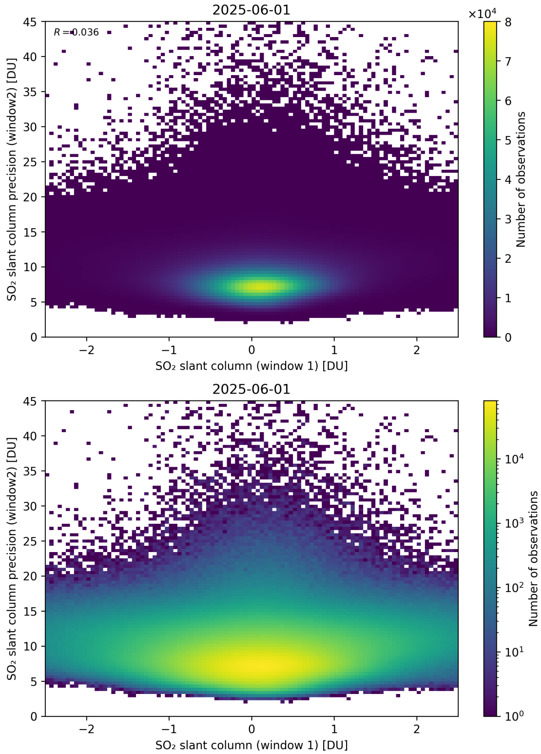
Figure 286: Scatter density plot of “SO 2 slant column (window 1)” against “SO 2 slant column precision (window2)” for 2025-06-01 to 2025-06-02.
