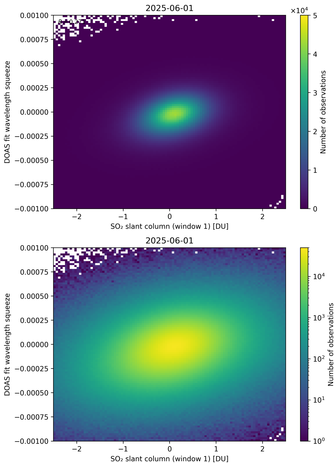
Figure 266: Scatter density plot of “SO 2 slant column (window 1)” against “DOAS fit wavelength squeeze” for 2025-06-01 to 2025-06-02.
