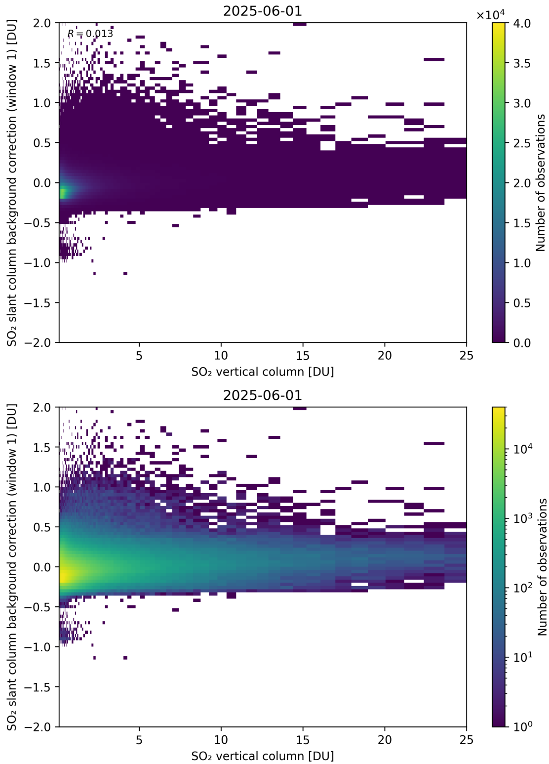
Figure 323: Scatter density plot of “SO 2 vertical column” against “SO 2 slant column background correction (window 1)” for 2025-06-01 to 2025-06-02.
