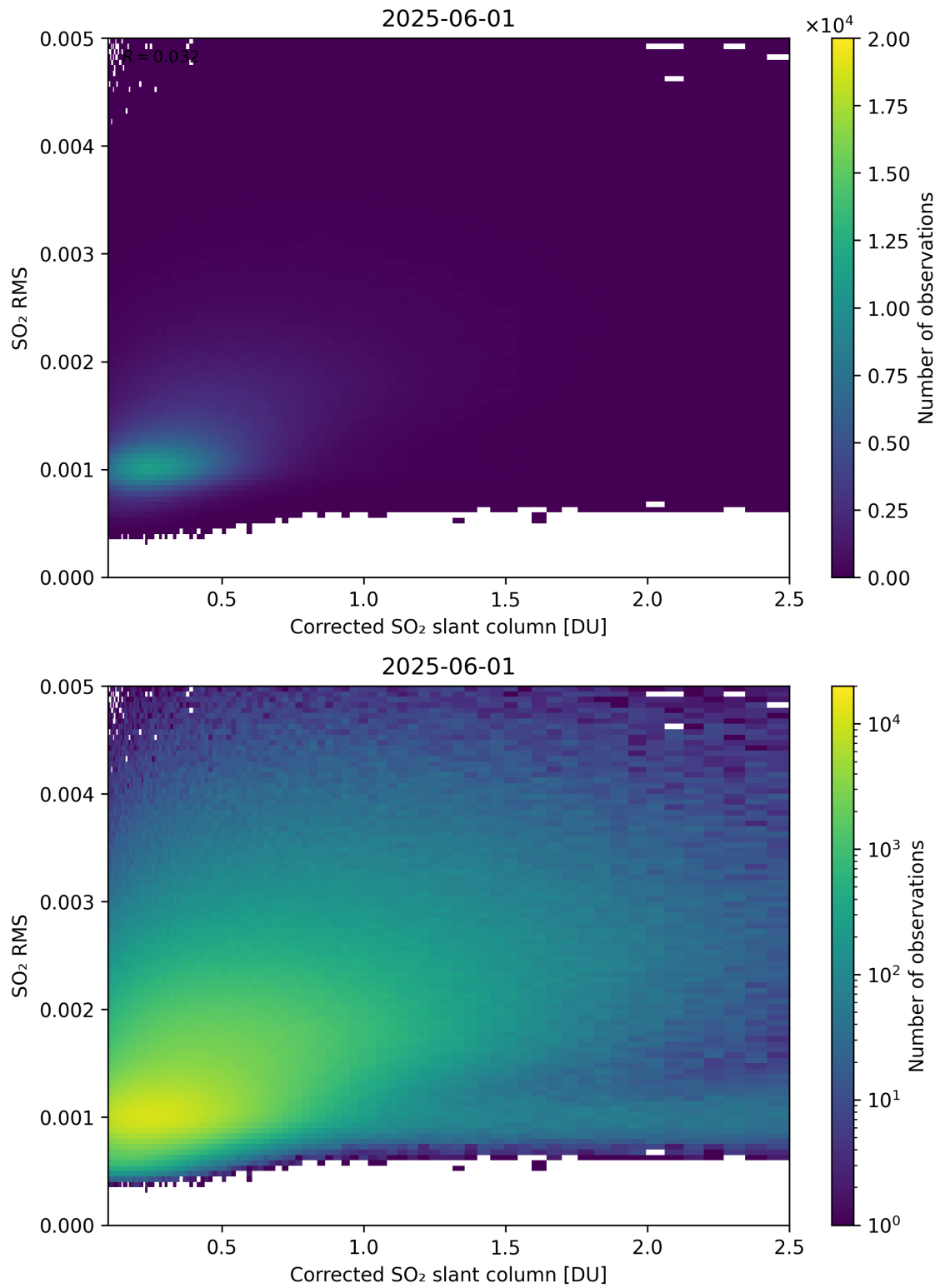
Figure 231: Scatter density plot of “Corrected SO 2 slant column” against “SO 2 RMS” for 2025-06-01 to 2025-06-02.
