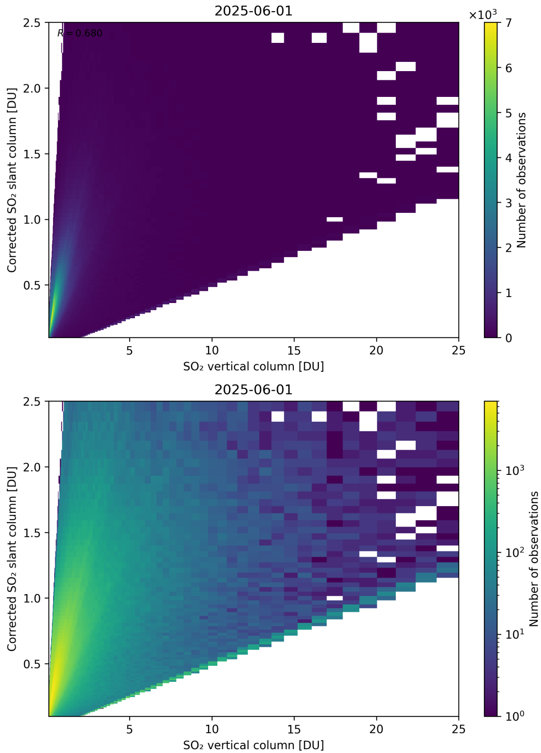
Figure 351: Scatter density plot of “SO 2 vertical column” against “Corrected SO 2 slant column” for 2025-06-01 to 2025-06-02.
