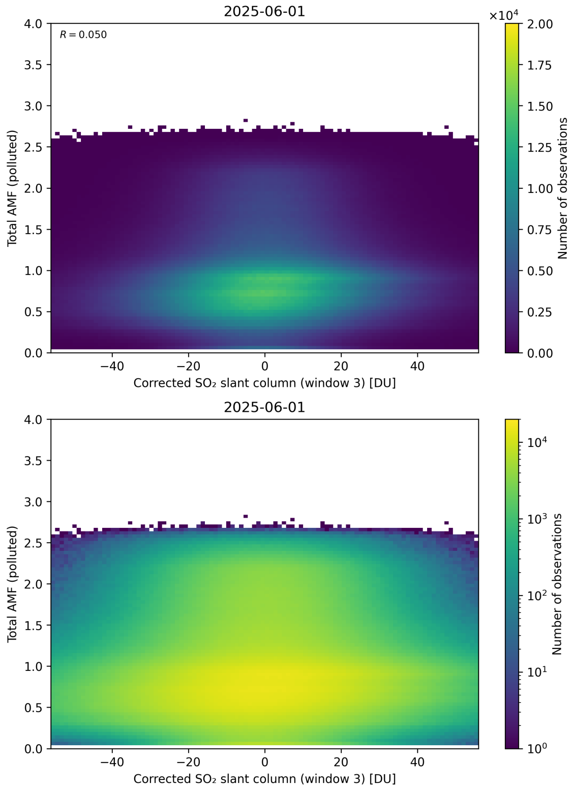
Figure 260: Scatter density plot of “Corrected SO 2 slant column (window 3)” against “Total AMF (polluted)” for 2025-06-01 to 2025-06-02.
