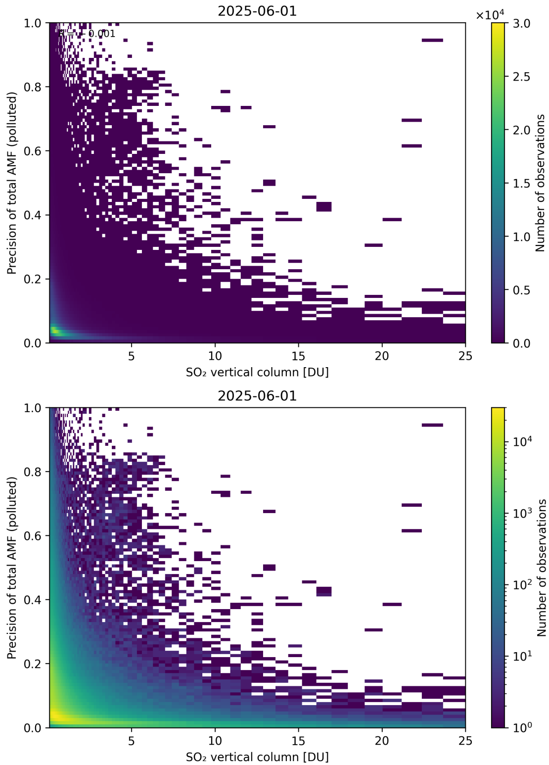
Figure 360: Scatter density plot of “SO 2 vertical column” against “Precision of total AMF (polluted)” for 2025-06-01 to 2025-06-02.
