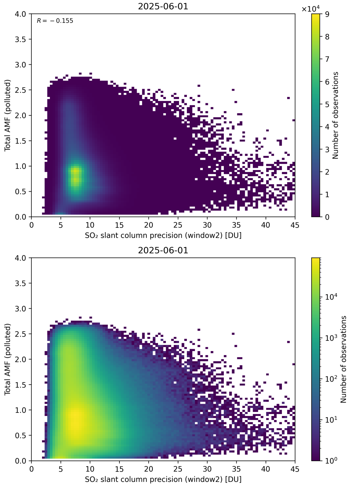
Figure 301: Scatter density plot of “SO 2 slant column precision (window2)” against “Total AMF (polluted)” for 2025-06-01 to 2025-06-02.
