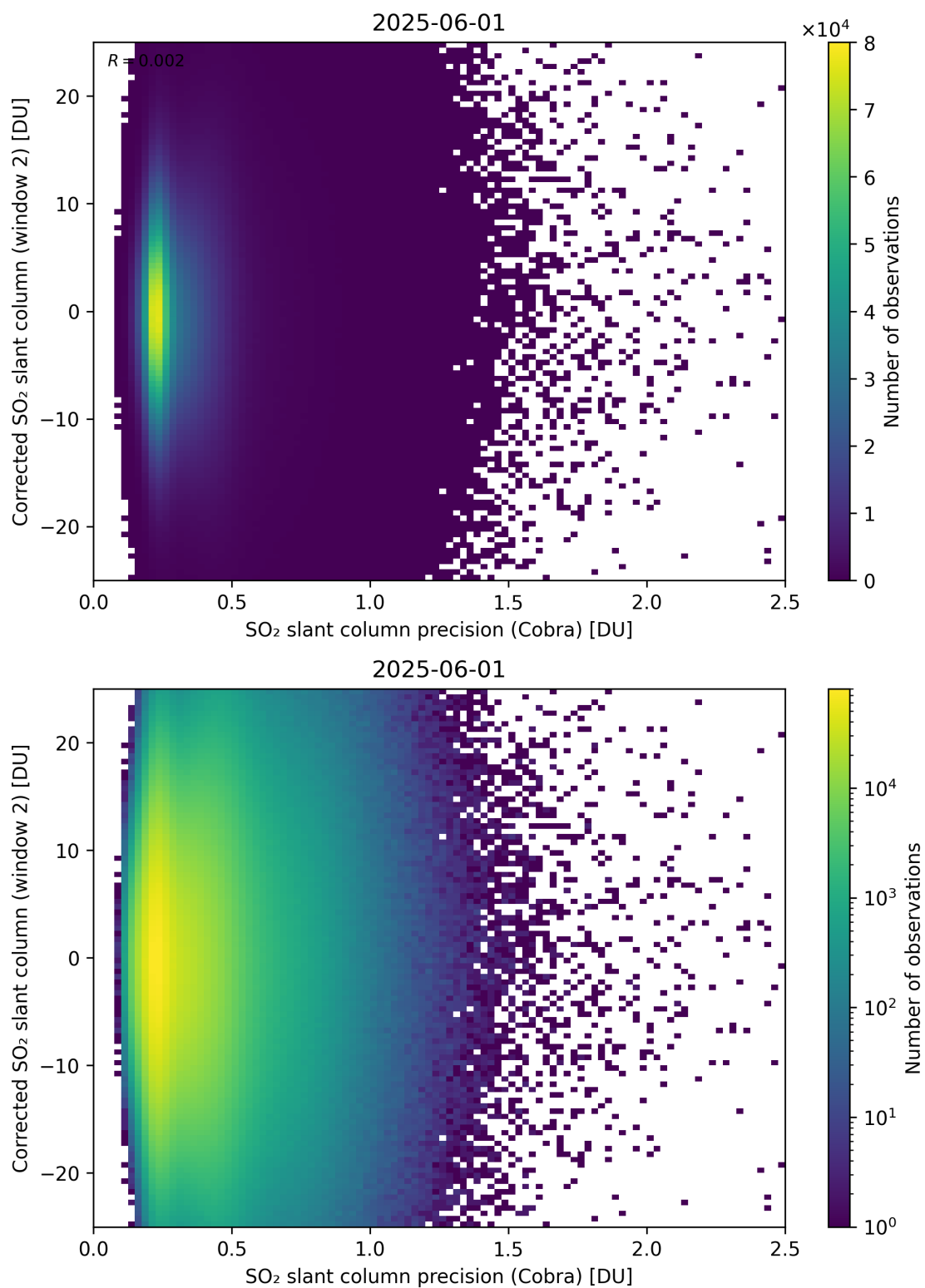
Figure 206: Scatter density plot of “SO 2 slant column precision (Cobra)” against “Corrected SO 2 slant column (window 2)” for 2025-06-01 to 2025-06-02.
