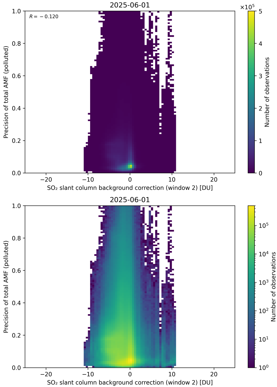
Figure 131: Scatter density plot of “SO 2 slant column background correction (window 2)” against “Precision of total AMF (polluted)” for 2025-06-01 to 2025-06-02.
