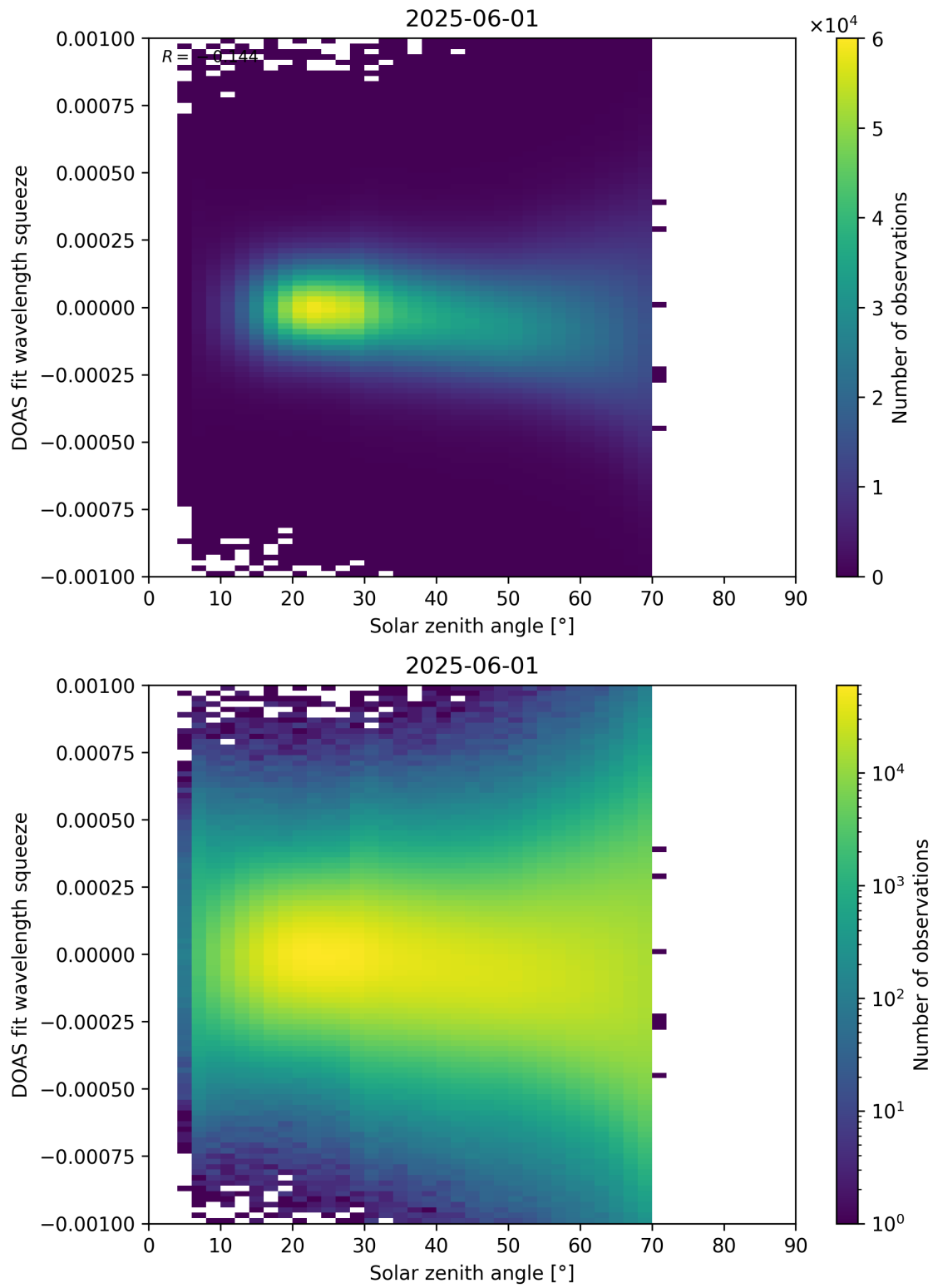
Figure 175: Scatter density plot of “Solar zenith angle” against “DOAS fit wavelength squeeze” for 2025-06-01 to 2025-06-02.
