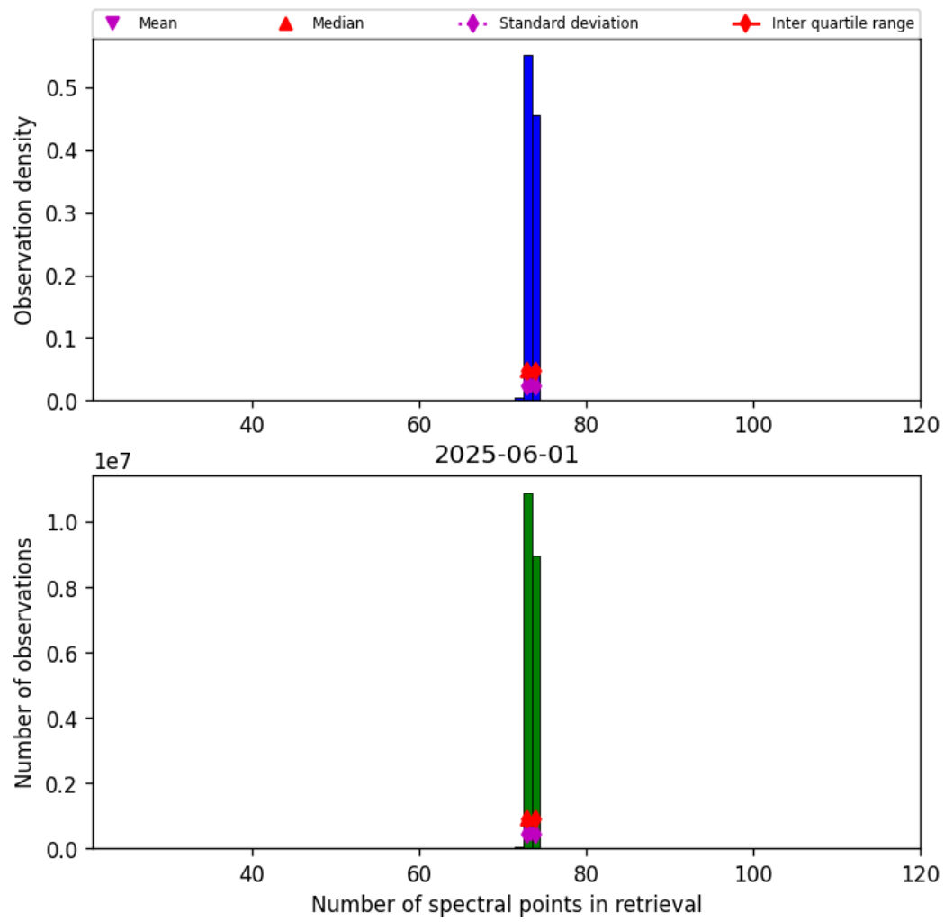
Figure 82: Histogram of “Number of spectral points in retrieval” for 2025-06-01 to 2025-06-02
