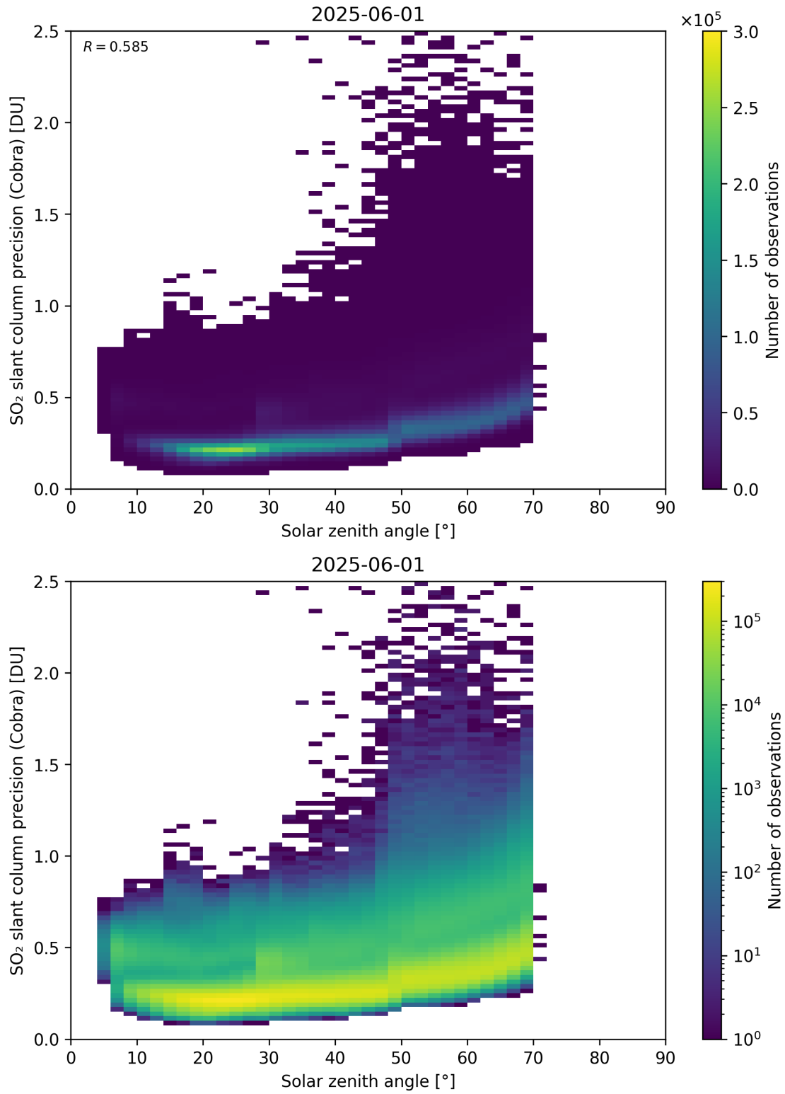
Figure 180: Scatter density plot of “Solar zenith angle” against “SO 2 slant column precision (Cobra)” for 2025-06-01 to 2025-06-02.
