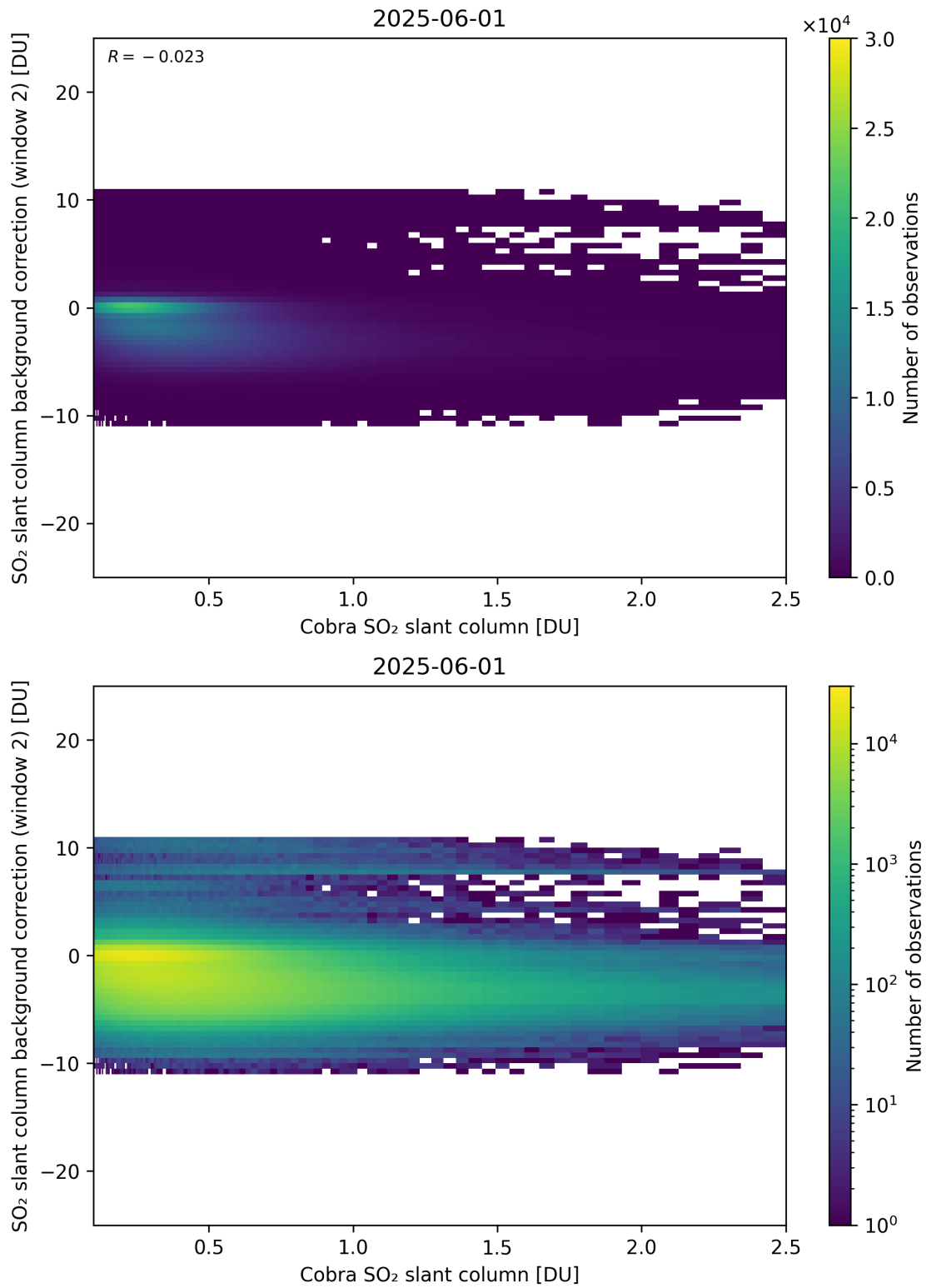
Figure 194: Scatter density plot of “Cobra SO 2 slant column” against “SO 2 slant column background correction (window 2)” for 2025-06-01 to 2025-06-02.
