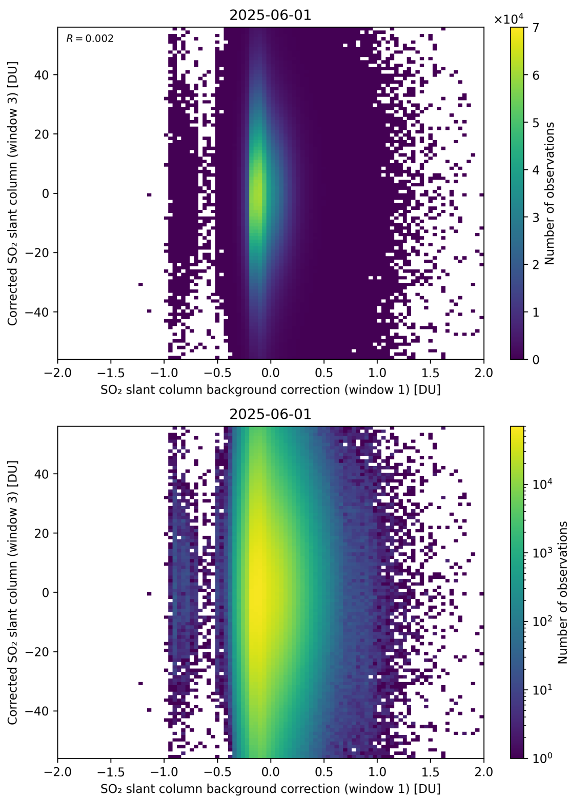
Figure 116: Scatter density plot of “SO 2 slant column background correction (window 1)” against “Corrected SO 2 slant column (window 3)” for 2025-06-01 to 2025-06-02.
