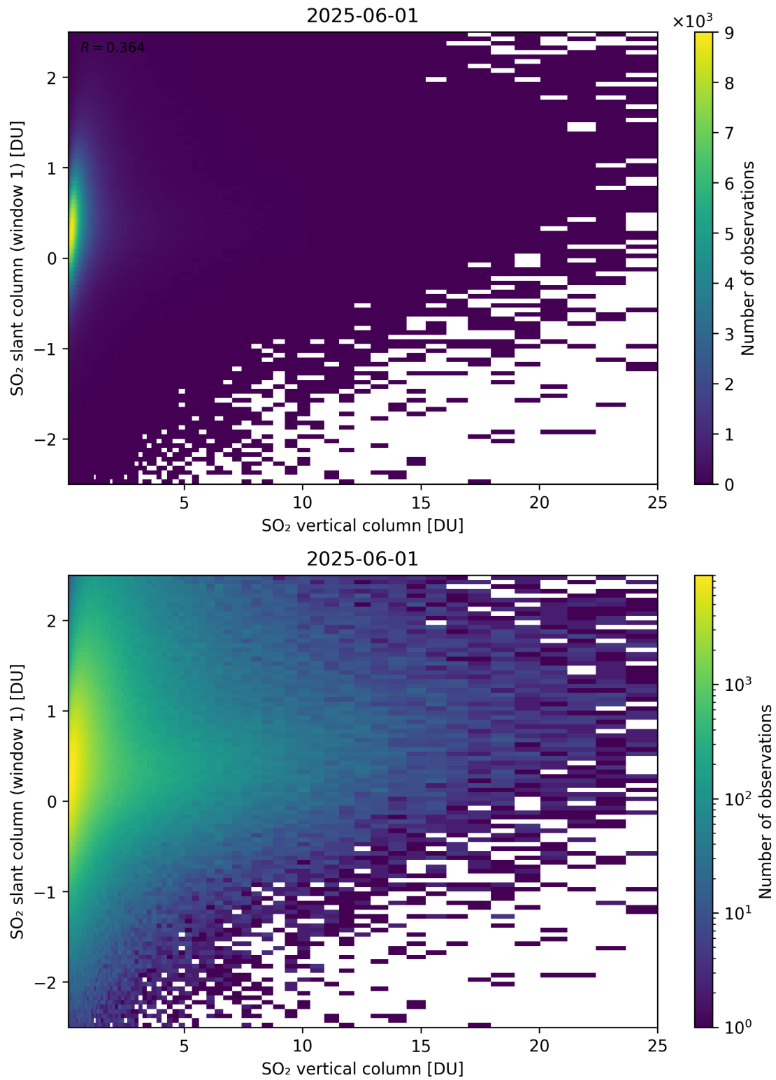
Figure 354: Scatter density plot of “SO 2 vertical column” against “SO 2 slant column (window 1)” for 2025-06-01 to 2025-06-02.
