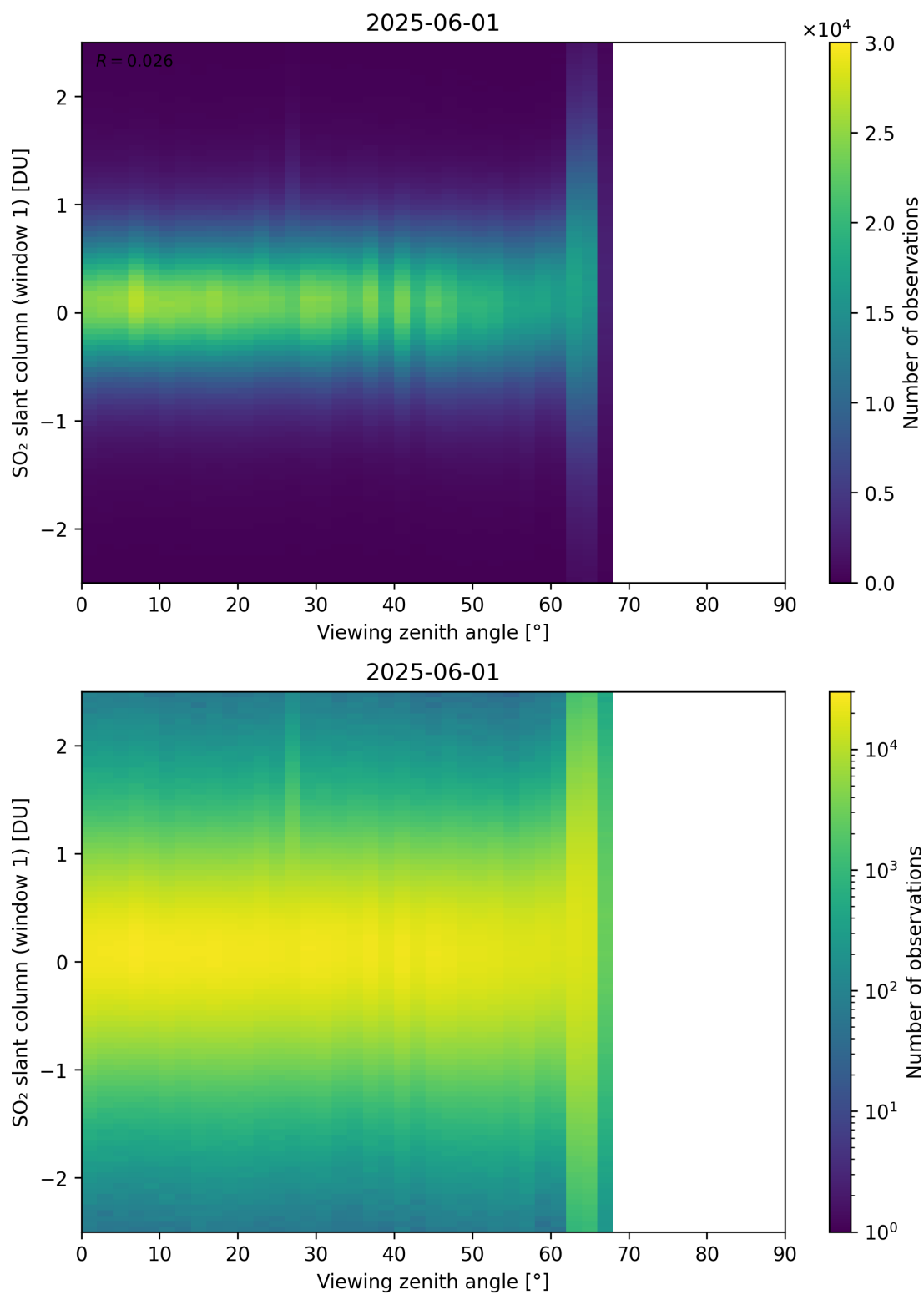
Figure 376: Scatter density plot of “Viewing zenith angle” against “SO 2 slant column (window 1)” for 2025-06-01 to 2025-06-02.
