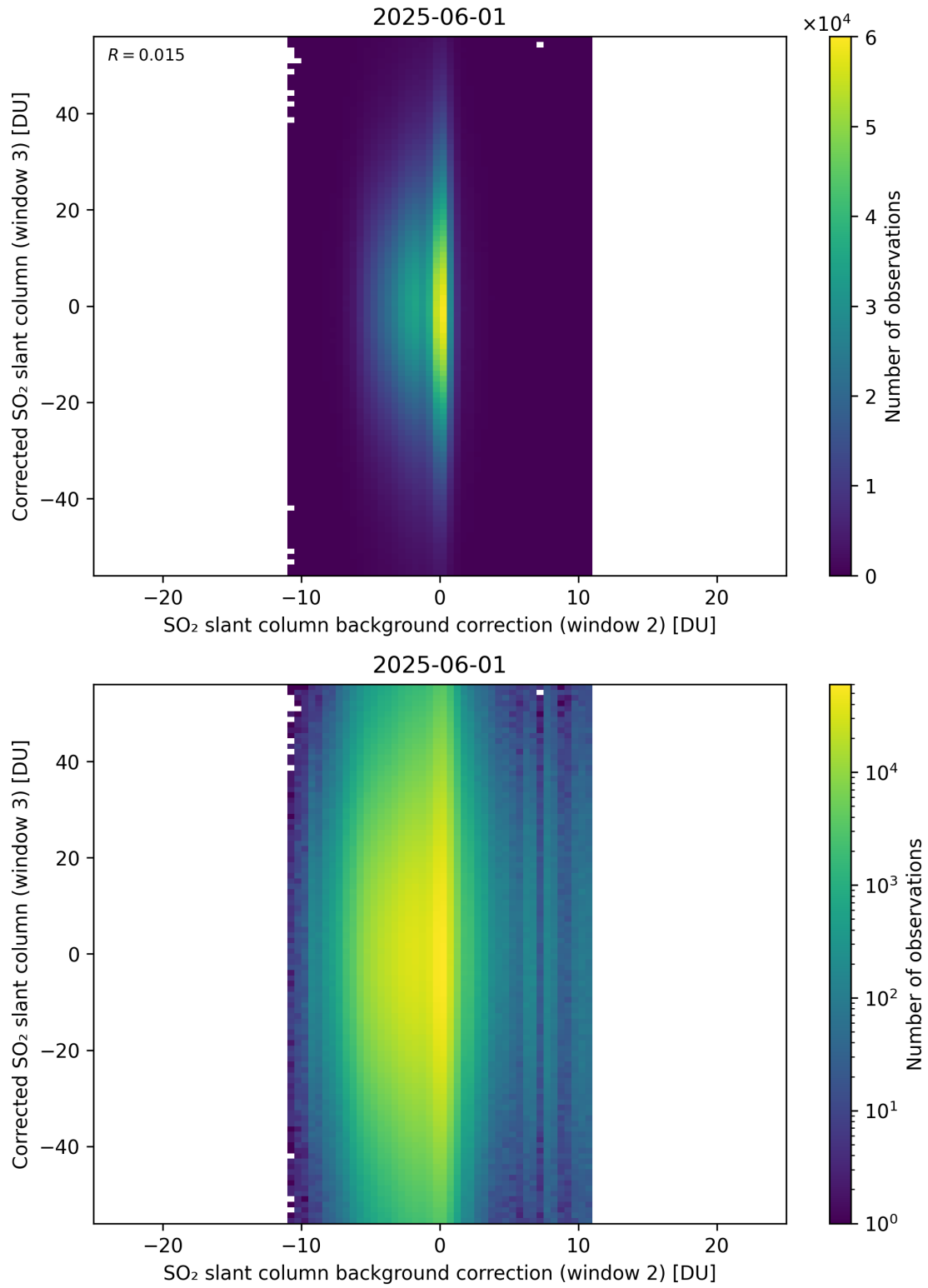
Figure 127: Scatter density plot of “SO 2 slant column background correction (window 2)” against “Corrected SO 2 slant column (window 3)” for 2025-06-01 to 2025-06-02.
