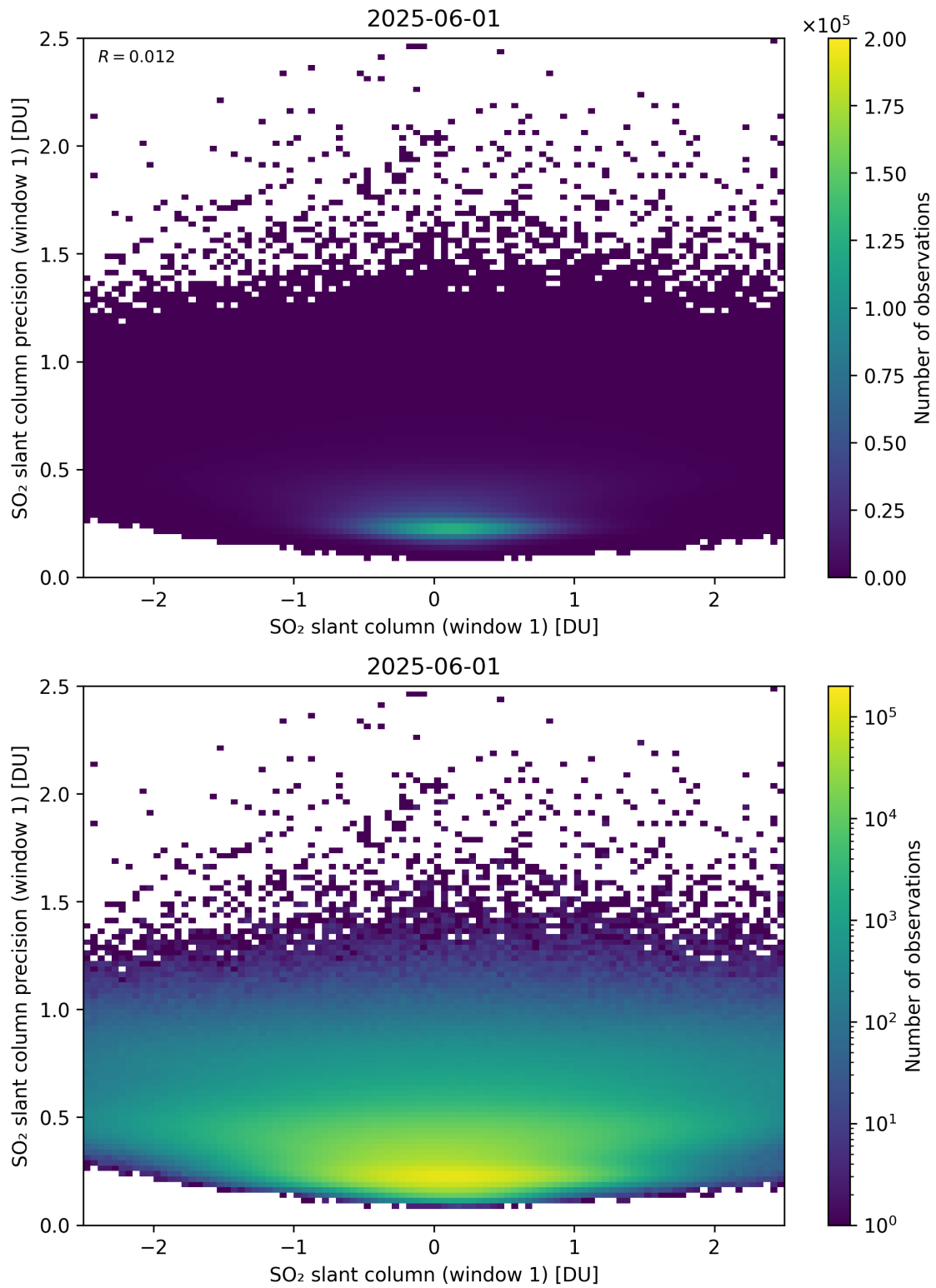
Figure 285: Scatter density plot of “SO 2 slant column (window 1)” against “SO 2 slant column precision (window 1)” for 2025-06-01 to 2025-06-02.
