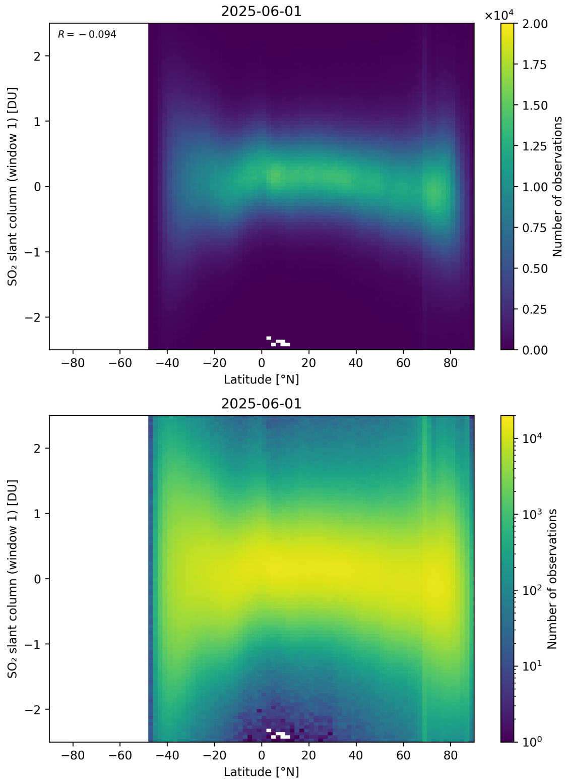
Figure 162: Scatter density plot of “Latitude” against “SO 2 slant column (window 1)” for 2025-06-01 to 2025-06-02.
