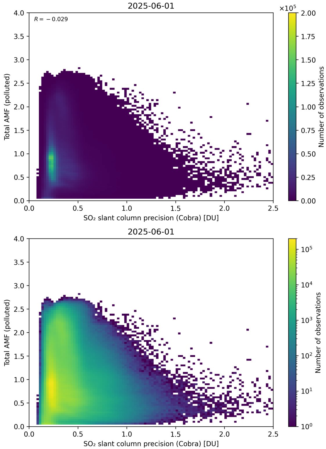
Figure 213: Scatter density plot of “SO 2 slant column precision (Cobra)” against “Total AMF (polluted)” for 2025-06-01 to 2025-06-02.
