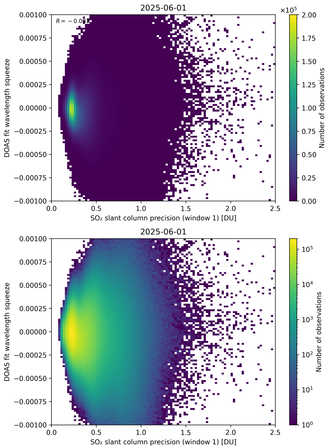
Figure 272: Scatter density plot of “SO 2 slant column precision (window 1)” against “DOAS fit wavelength squeeze” for 2025-06-01 to 2025-06-02.
