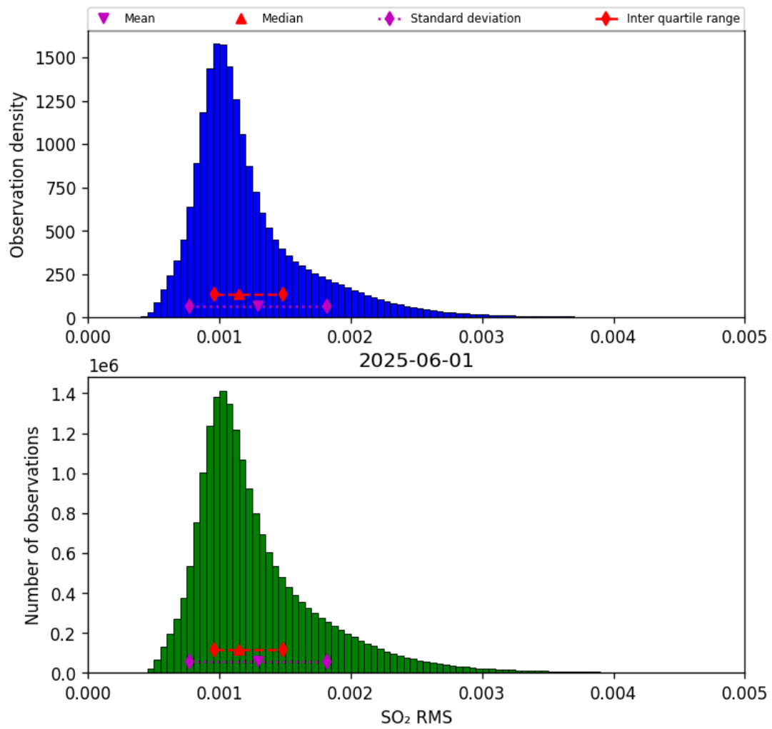
Figure 78: Histogram of “SO 2 RMS” for 2025-06-01 to 2025-06-02
