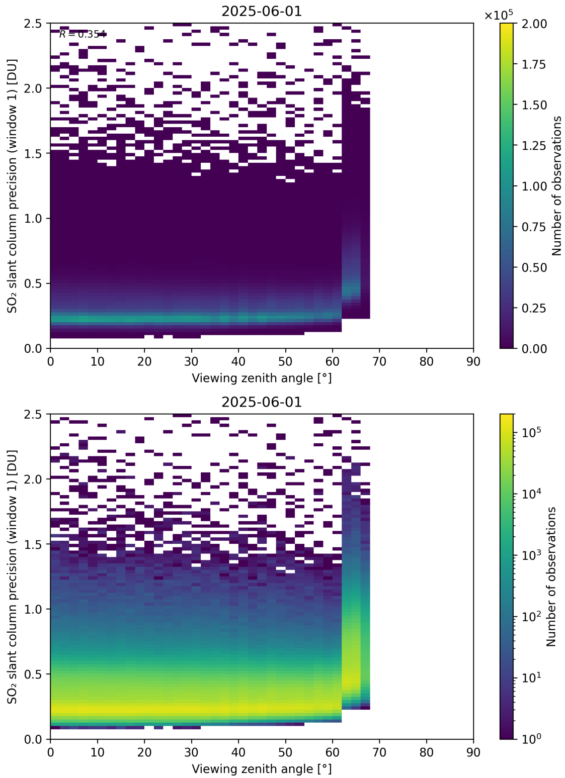
Figure 377: Scatter density plot of “Viewing zenith angle” against “SO 2 slant column precision (window 1)” for 2025-06-01 to 2025-06-02.
