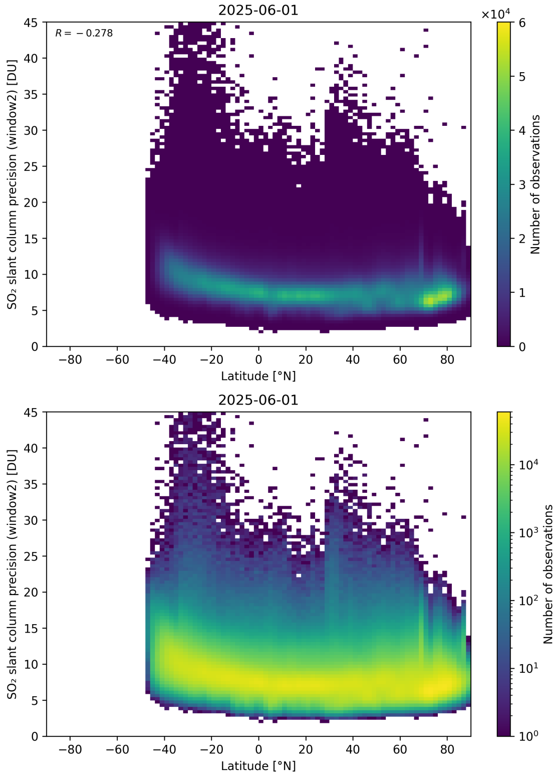
Figure 164: Scatter density plot of “Latitude” against “SO 2 slant column precision (window2)” for 2025-06-01 to 2025-06-02.
