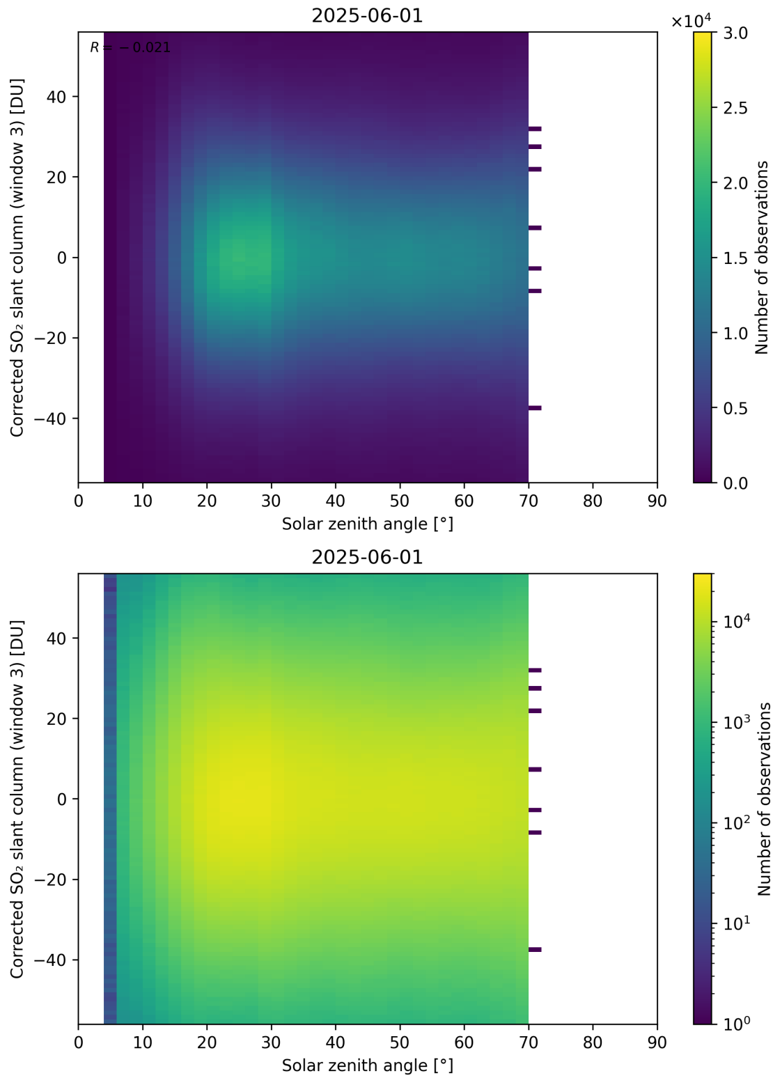
Figure 183: Scatter density plot of “Solar zenith angle” against “Corrected SO 2 slant column (window 3)” for 2025-06-01 to 2025-06-02.
