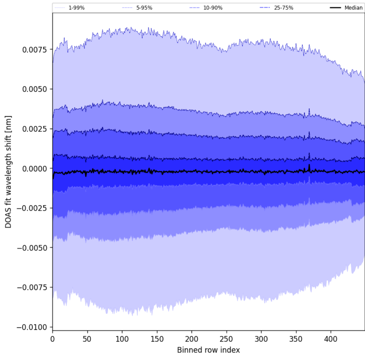
Figure 102: Along track statistics of “DOAS fit wavelength shift” for 2025-06-01 to 2025-06-02
