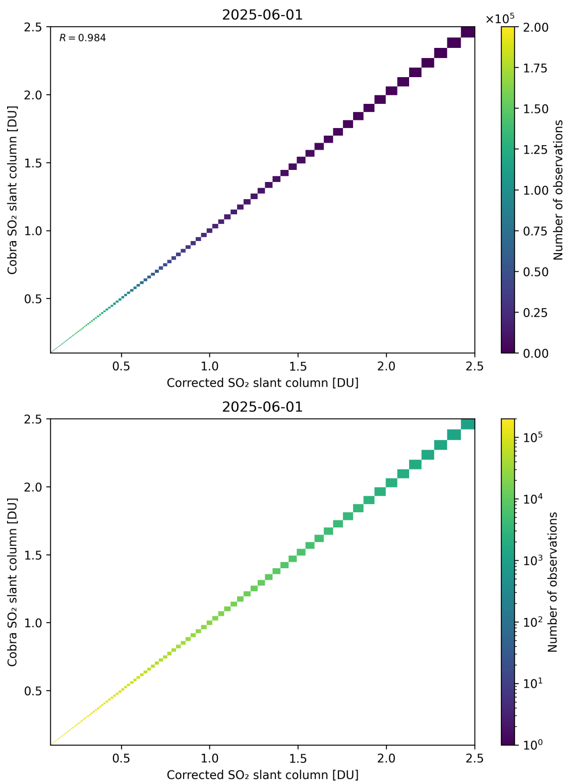
Figure 233: Scatter density plot of “Corrected SO 2 slant column” against “Cobra SO 2 slant column” for 2025-06-01 to 2025-06-02.
