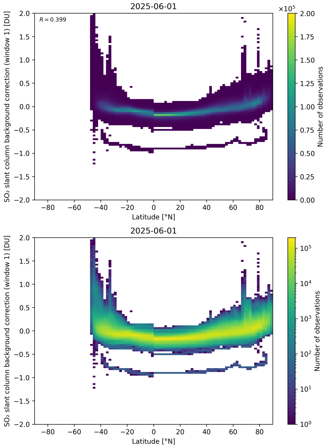
Figure 150: Scatter density plot of “Latitude” against “SO 2 slant column background correction (window 1)” for 2025-06-01 to 2025-06-02.
