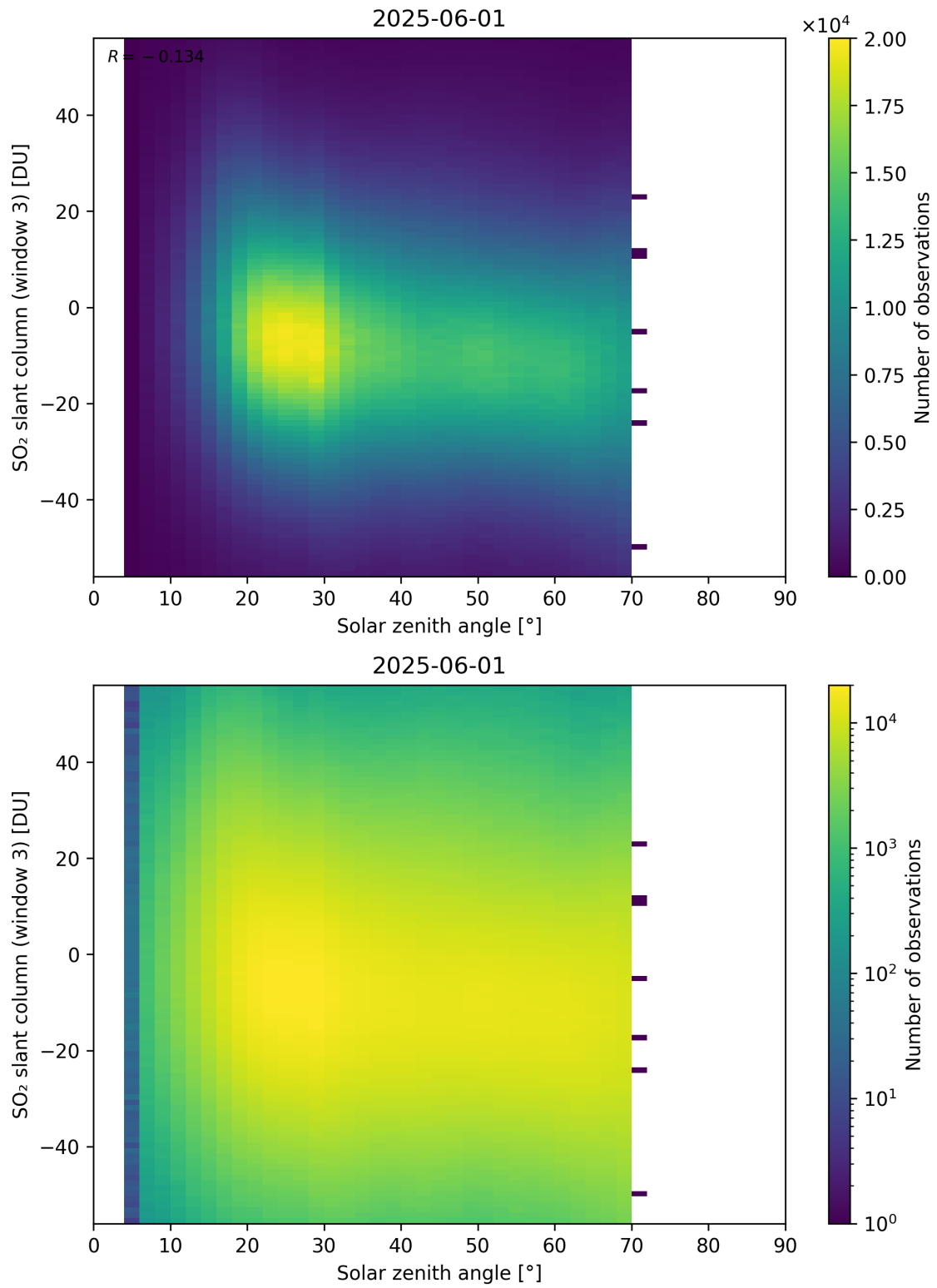
Figure 187: Scatter density plot of “Solar zenith angle” against “SO 2 slant column (window 3)” for 2025-06-01 to 2025-06-02.
