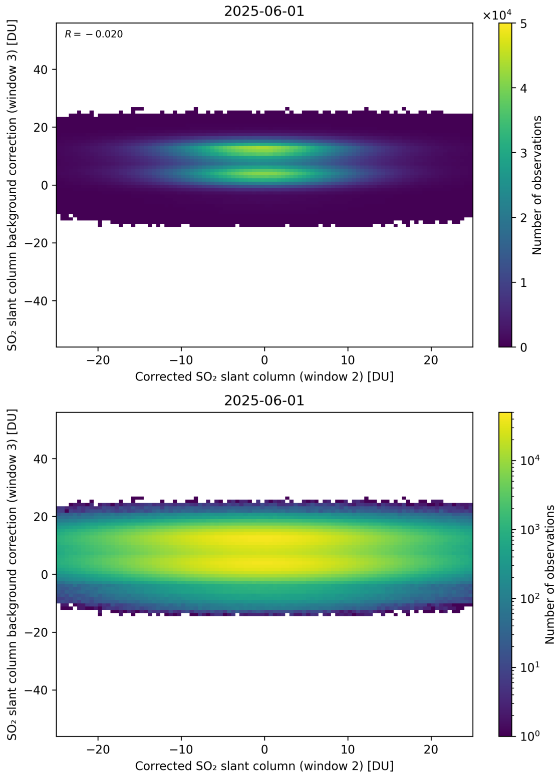
Figure 245: Scatter density plot of “Corrected SO 2 slant column (window 2)” against “SO 2 slant column background correction (window 3)” for 2025-06-01 to 2025-06-02.
