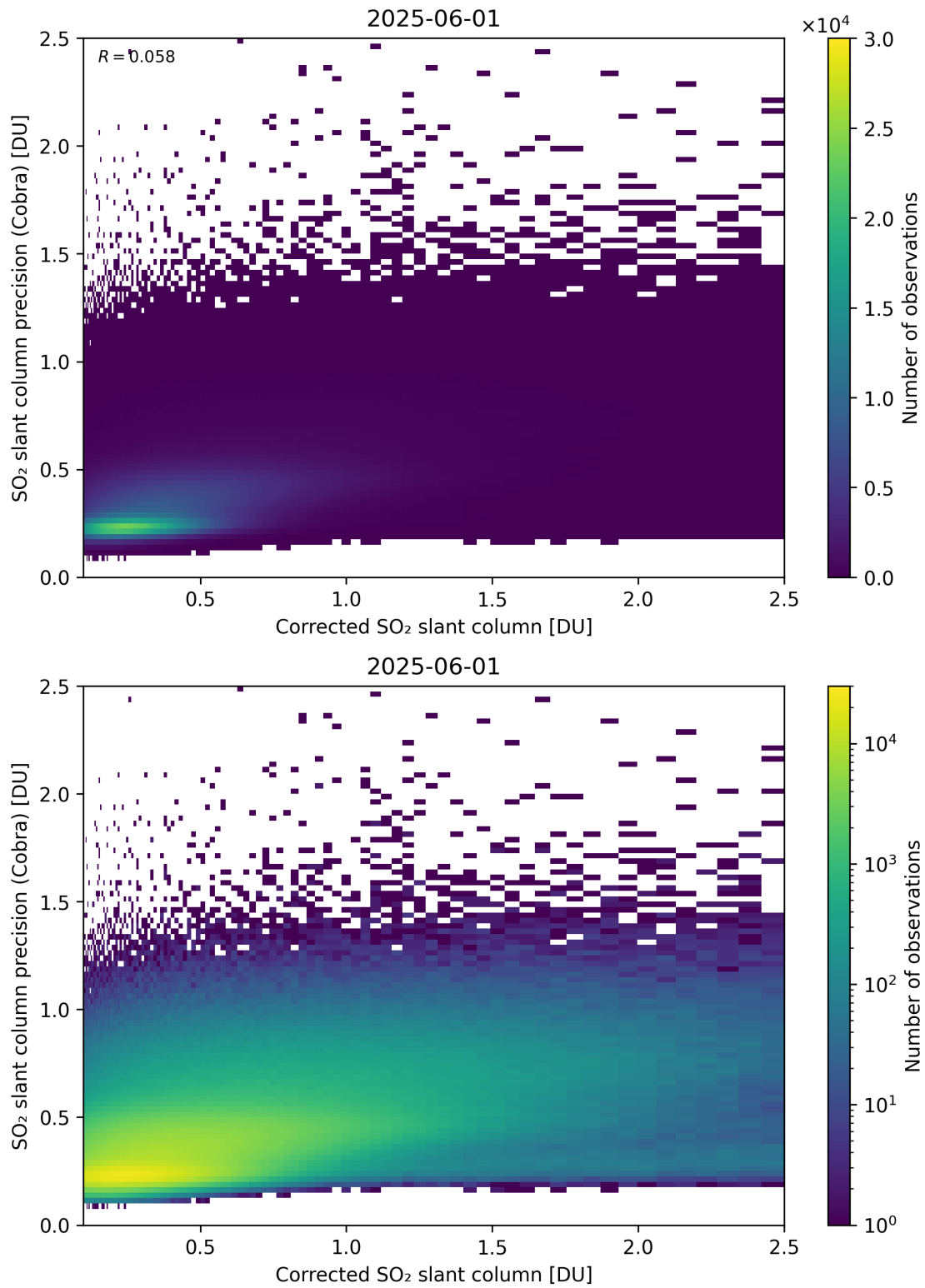
Figure 234: Scatter density plot of “Corrected SO 2 slant column” against “SO 2 slant column precision (Cobra)” for 2025-06-01 to 2025-06-02.
