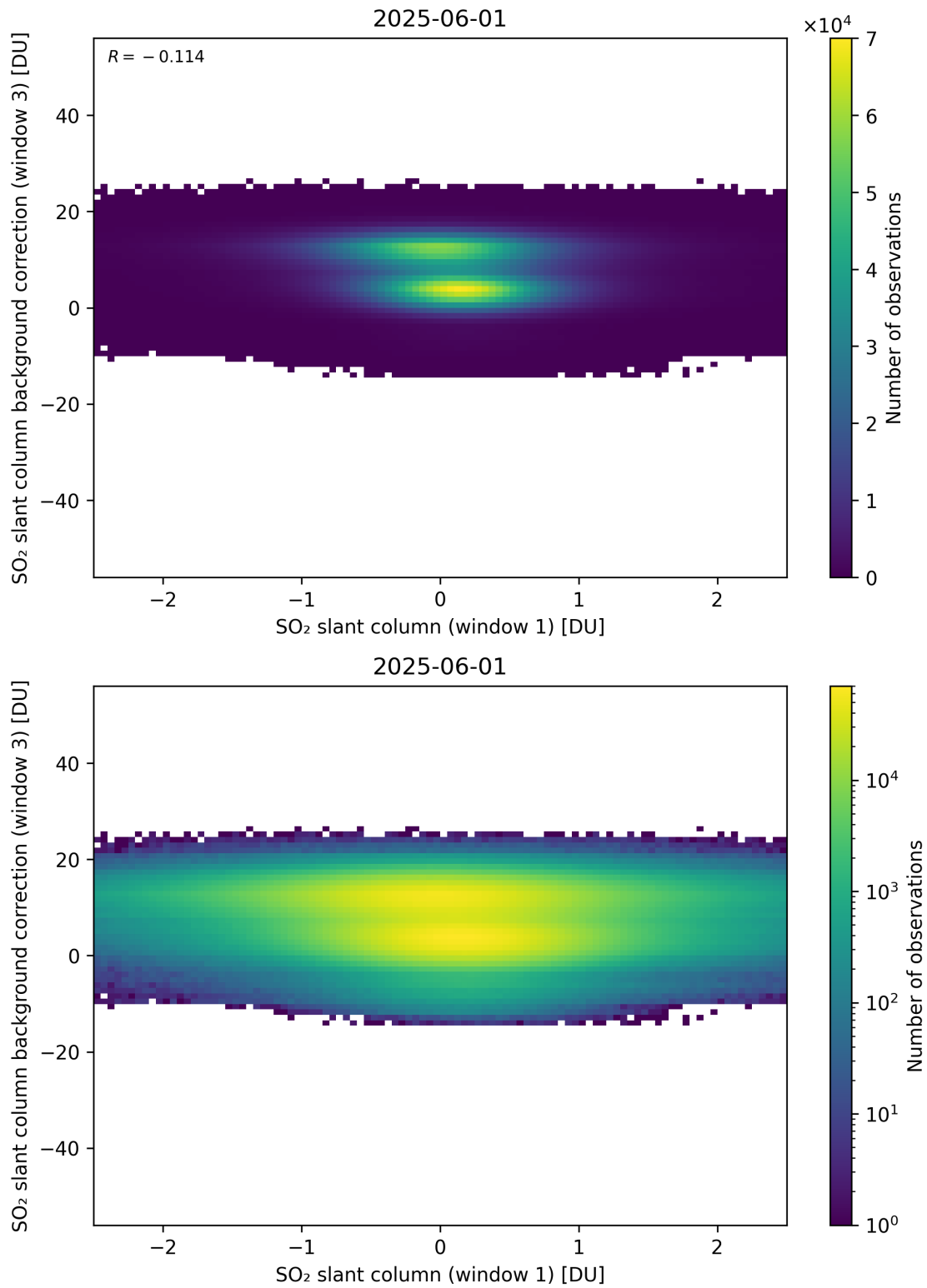
Figure 264: Scatter density plot of “SO 2 slant column (window 1)” against “SO 2 slant column background correction (window 3)” for 2025-06-01 to 2025-06-02.
