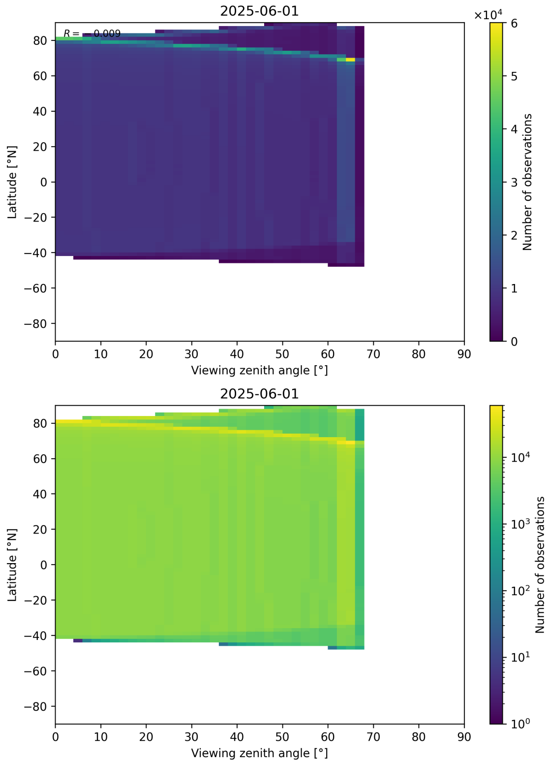
Figure 368: Scatter density plot of “Viewing zenith angle” against “Latitude” for 2025-06-01 to 2025-06-02.
