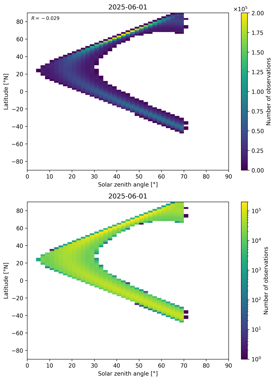
Figure 177: Scatter density plot of “Solar zenith angle” against “Latitude” for 2025-06-01 to 2025-06-02.
