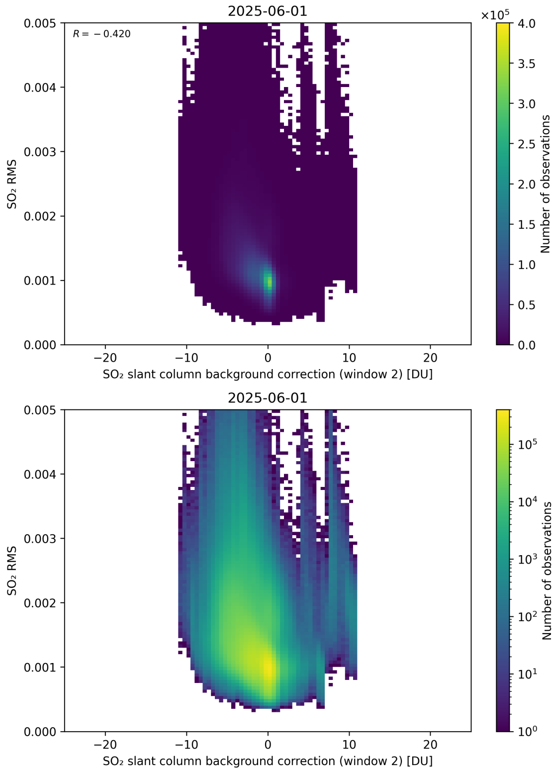
Figure 125: Scatter density plot of “SO 2 slant column background correction (window 2)” against “SO 2 RMS” for 2025-06-01 to 2025-06-02.
