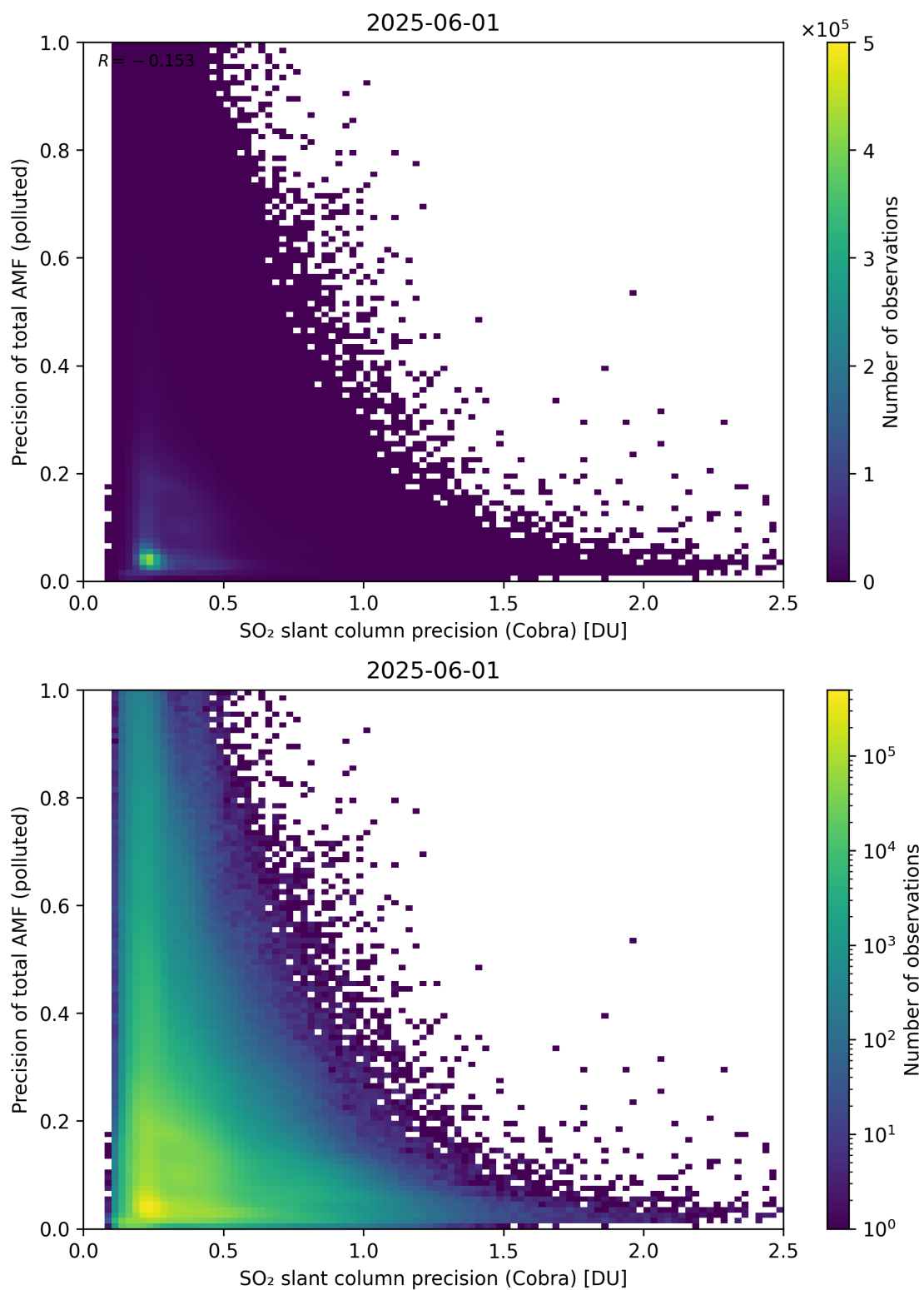
Figure 214: Scatter density plot of “SO 2 slant column precision (Cobra)” against “Precision of total AMF (polluted)” for 2025-06-01 to 2025-06-02.
