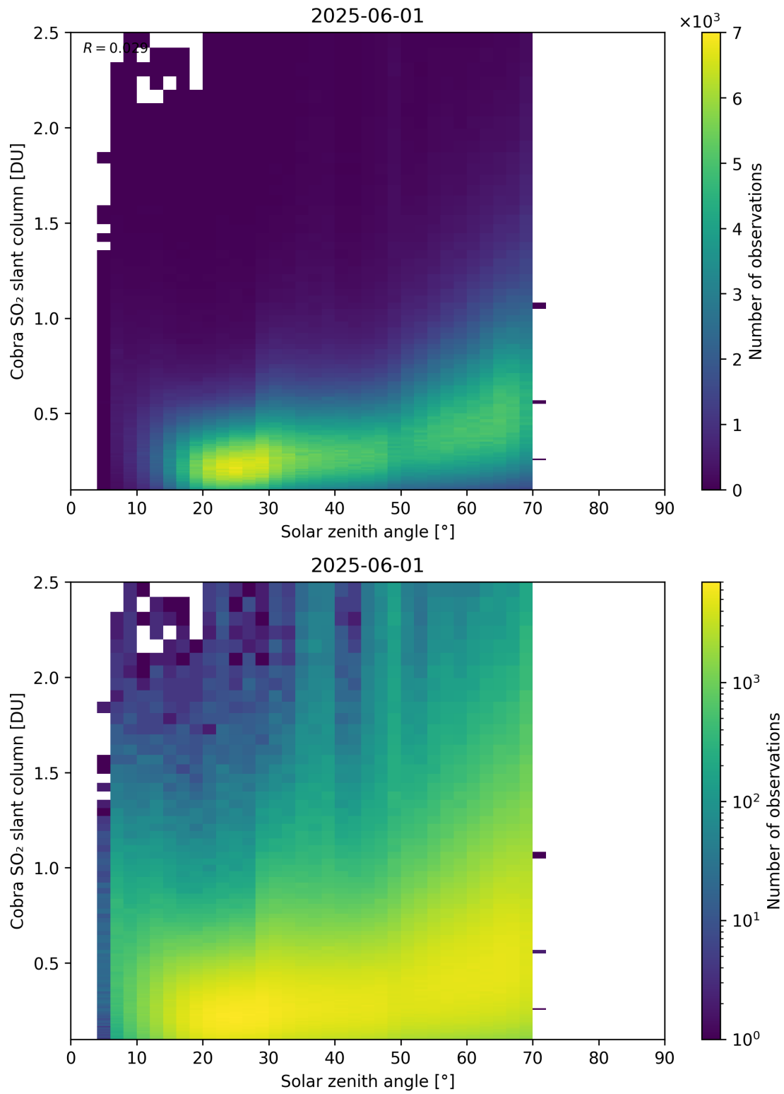
Figure 179: Scatter density plot of “Solar zenith angle” against “Cobra SO 2 slant column” for 2025-06-01 to 2025-06-02.
