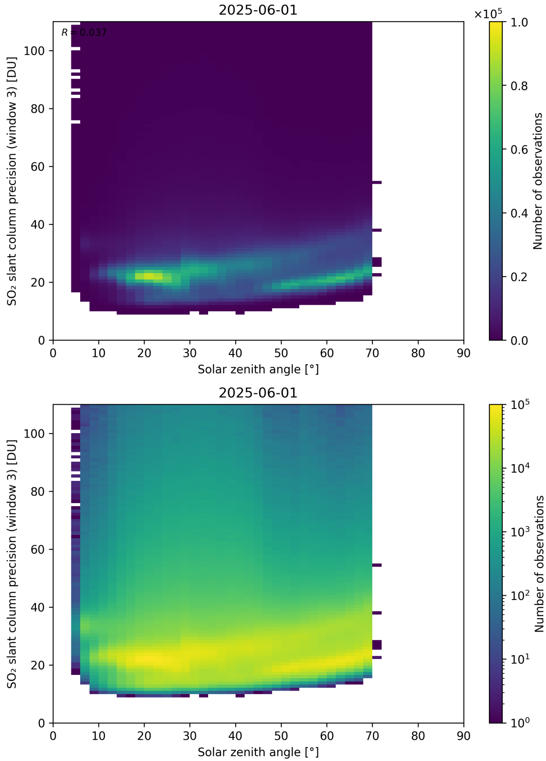
Figure 188: Scatter density plot of “Solar zenith angle” against “SO 2 slant column precision (window 3)” for 2025-06-01 to 2025-06-02.
