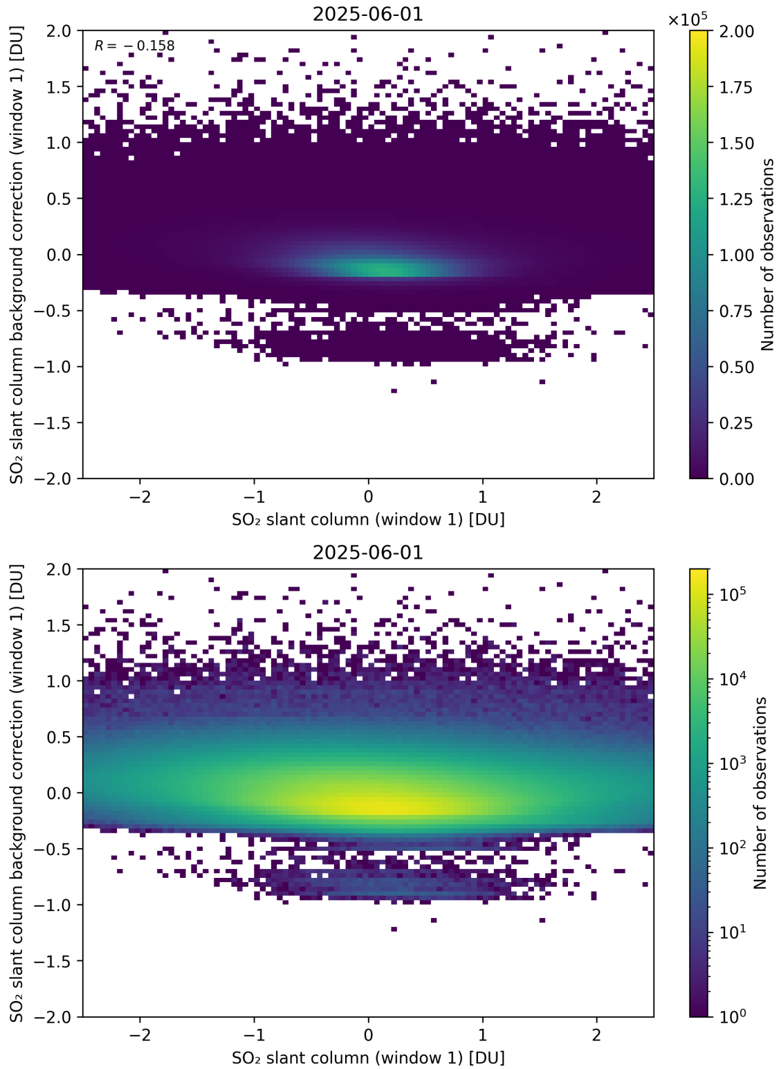
Figure 262: Scatter density plot of “SO 2 slant column (window 1)” against “SO 2 slant column background correction (window 1)” for 2025-06-01 to 2025-06-02.
