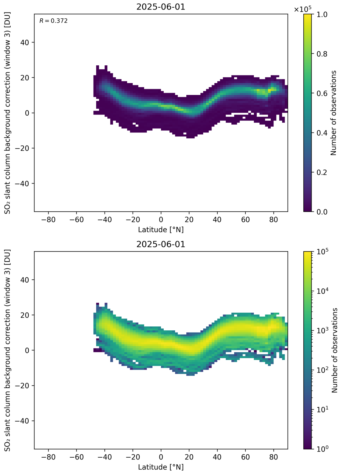
Figure 152: Scatter density plot of “Latitude” against “SO 2 slant column background correction (window 3)” for 2025-06-01 to 2025-06-02.
