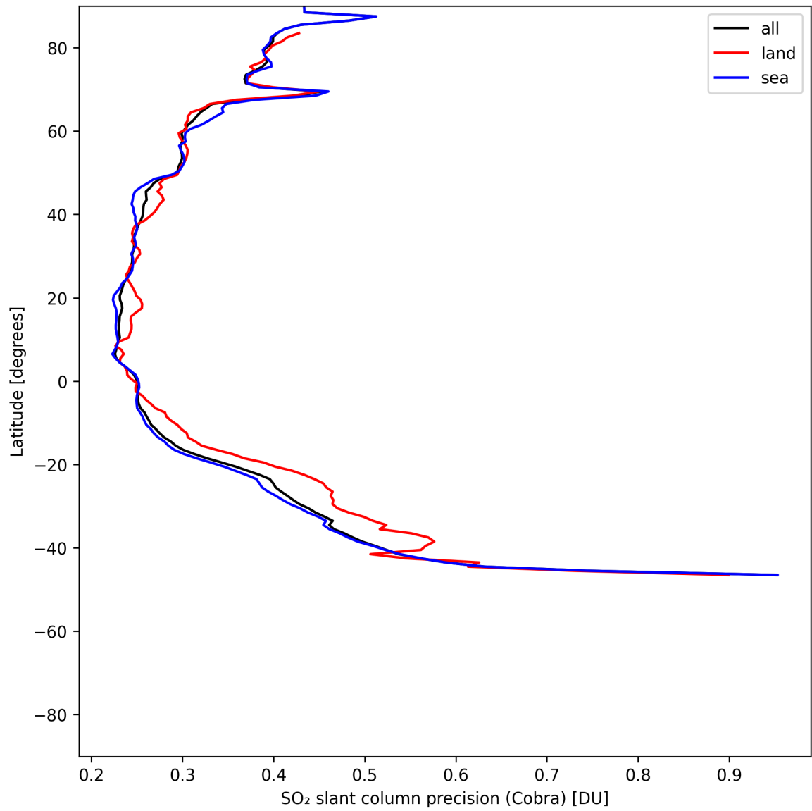
Figure 36: Zonal average of “SO 2 slant column precision (Cobra)” for 2025-06-01 to 2025-06-02.
