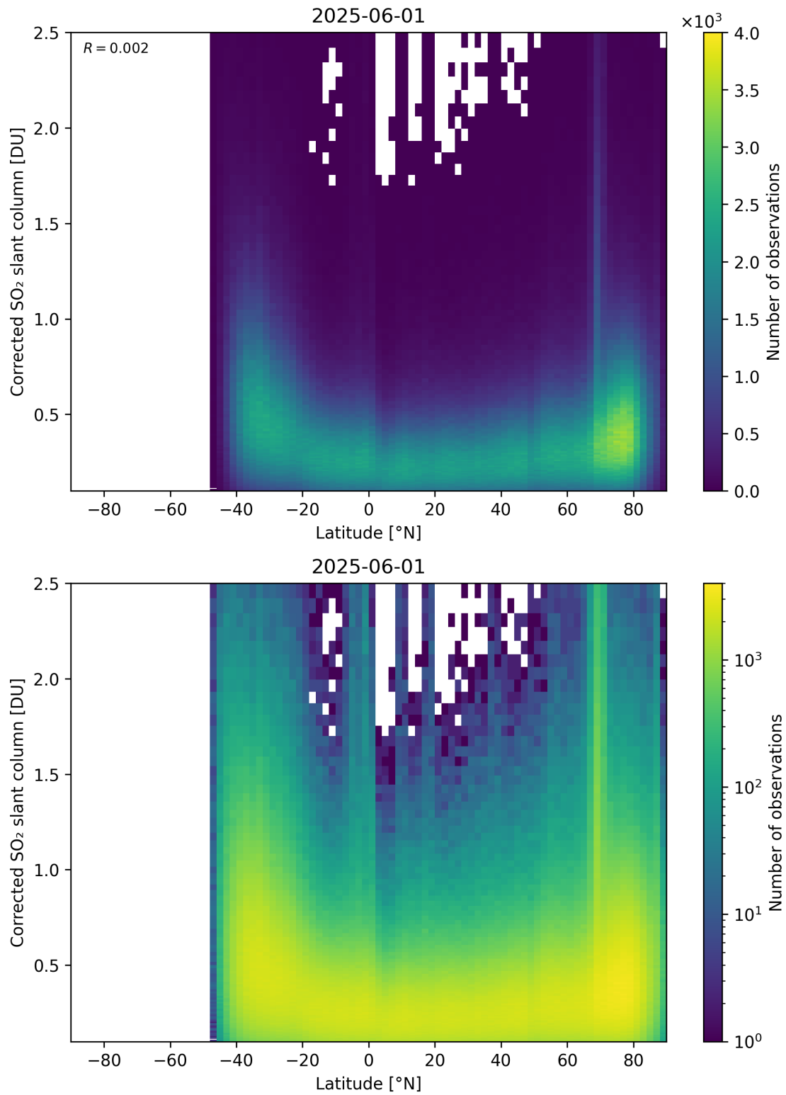
Figure 159: Scatter density plot of “Latitude” against “Corrected SO 2 slant column” for 2025-06-01 to 2025-06-02.
