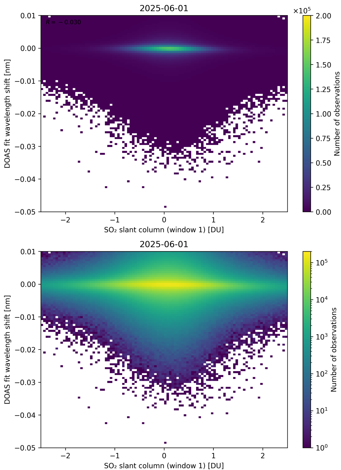
Figure 265: Scatter density plot of “SO 2 slant column (window 1)” against “DOAS fit wavelength shift” for 2025-06-01 to 2025-06-02.
