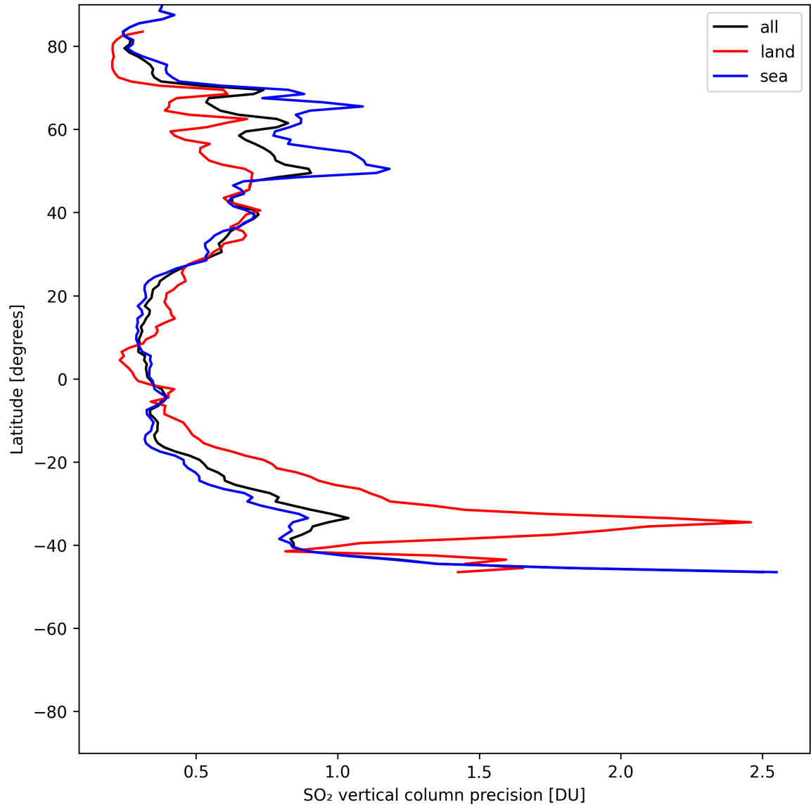
Figure 33: Zonal average of “SO 2 vertical column precision” for 2025-06-01 to 2025-06-02.
