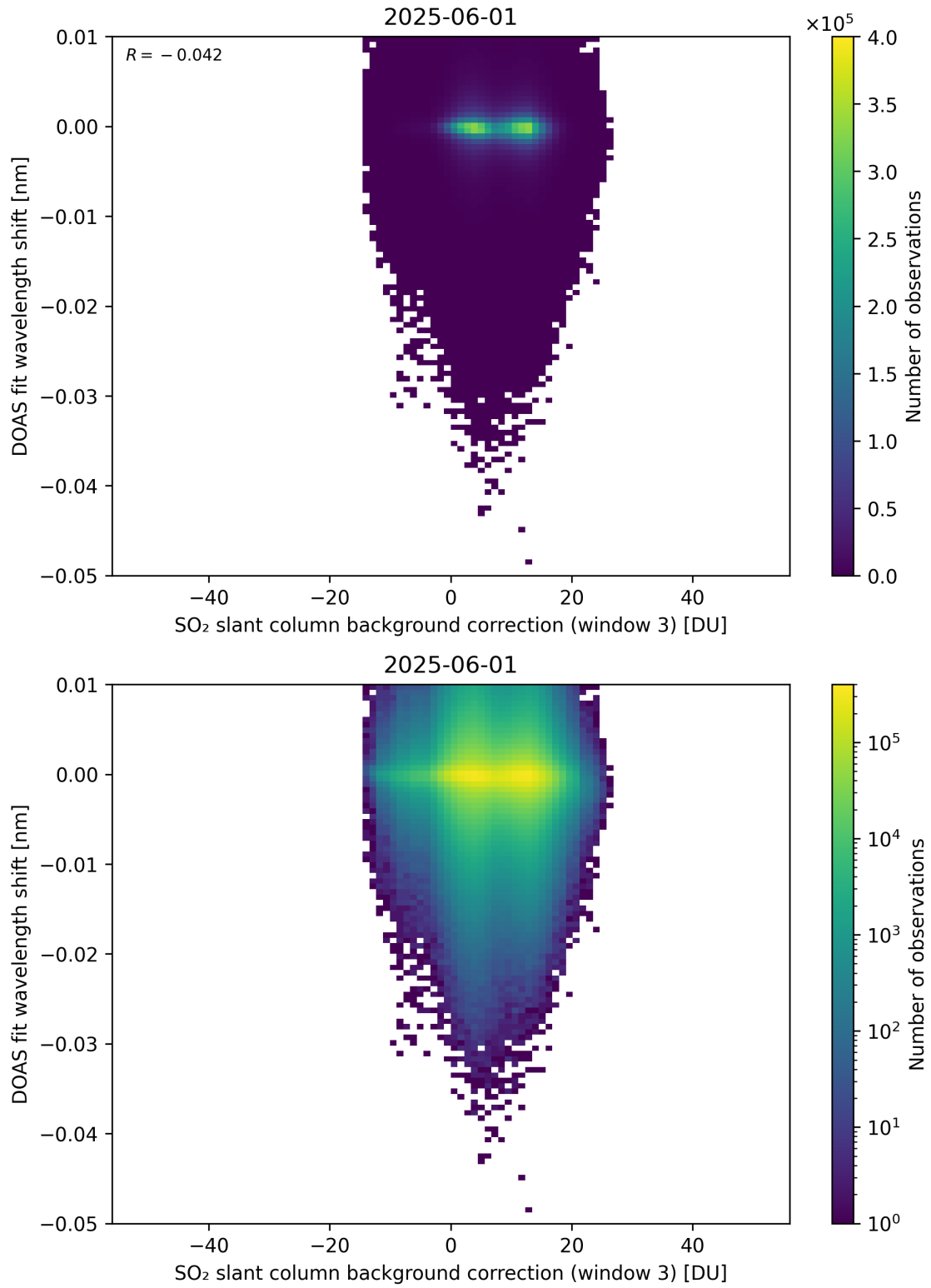
Figure 132: Scatter density plot of “SO 2 slant column background correction (window 3)” against “DOAS fit wavelength shift” for 2025-06-01 to 2025-06-02.
