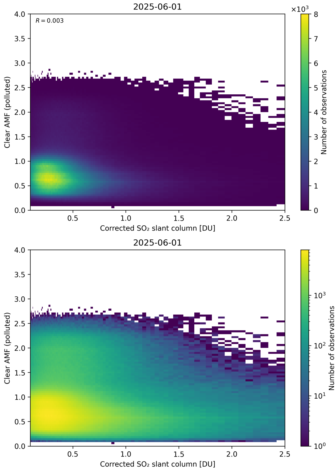
Figure 232: Scatter density plot of “Corrected SO 2 slant column” against “Clear AMF (polluted)” for 2025-06-01 to 2025-06-02.
