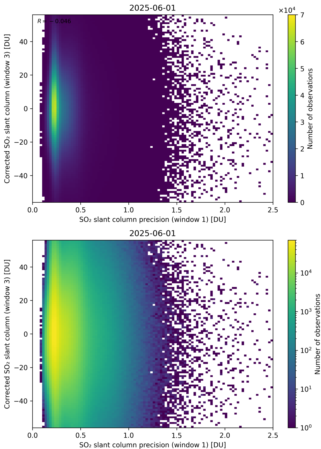
Figure 276: Scatter density plot of “SO 2 slant column precision (window 1)” against “Corrected SO 2 slant column (window 3)” for 2025-06-01 to 2025-06-02.
