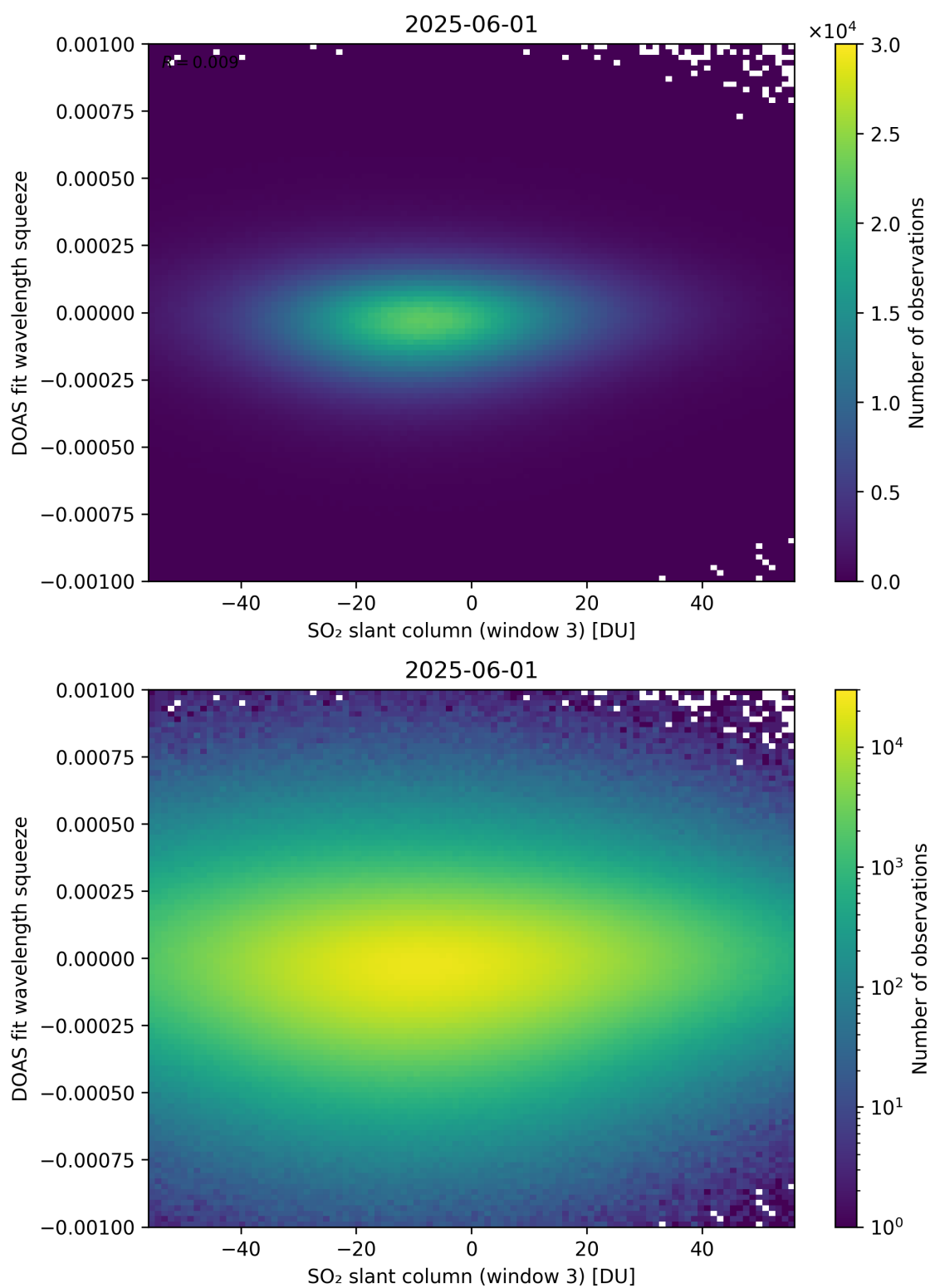
Figure 305: Scatter density plot of “SO 2 slant column (window 3)” against “DOAS fit wavelength squeeze” for 2025-06-01 to 2025-06-02.
