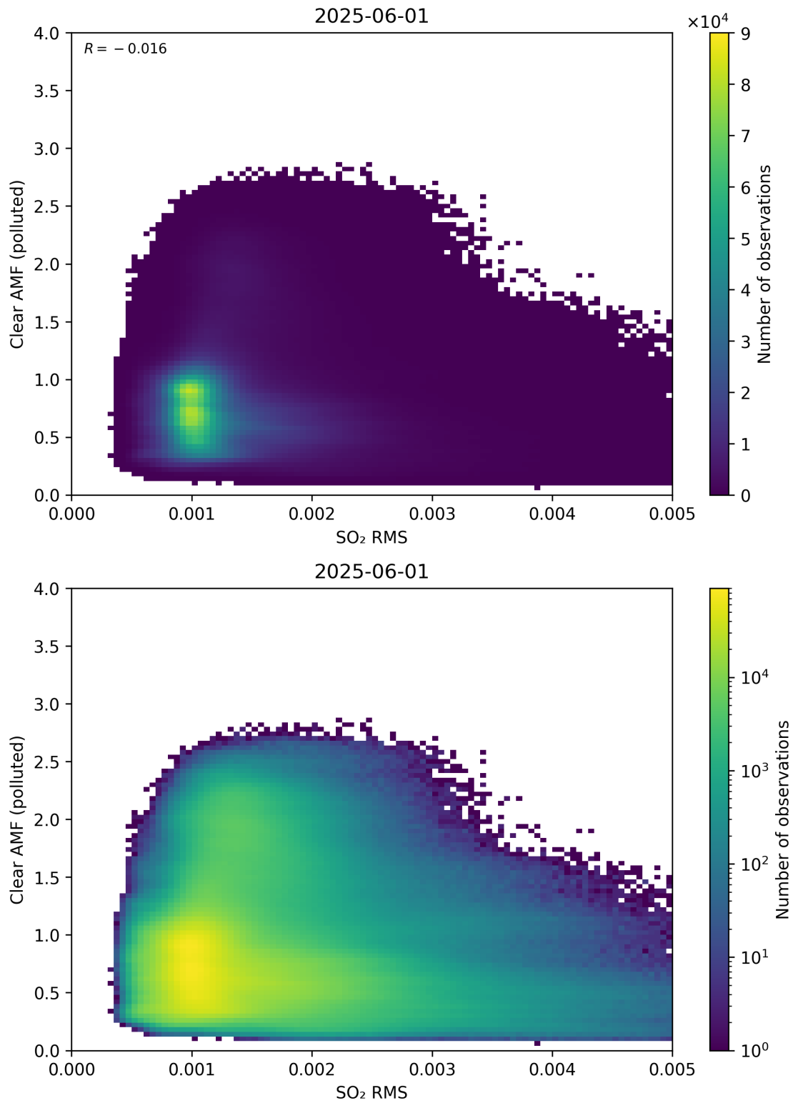
Figure 147: Scatter density plot of “SO 2 RMS” against “Clear AMF (polluted)” for 2025-06-01 to 2025-06-02.
