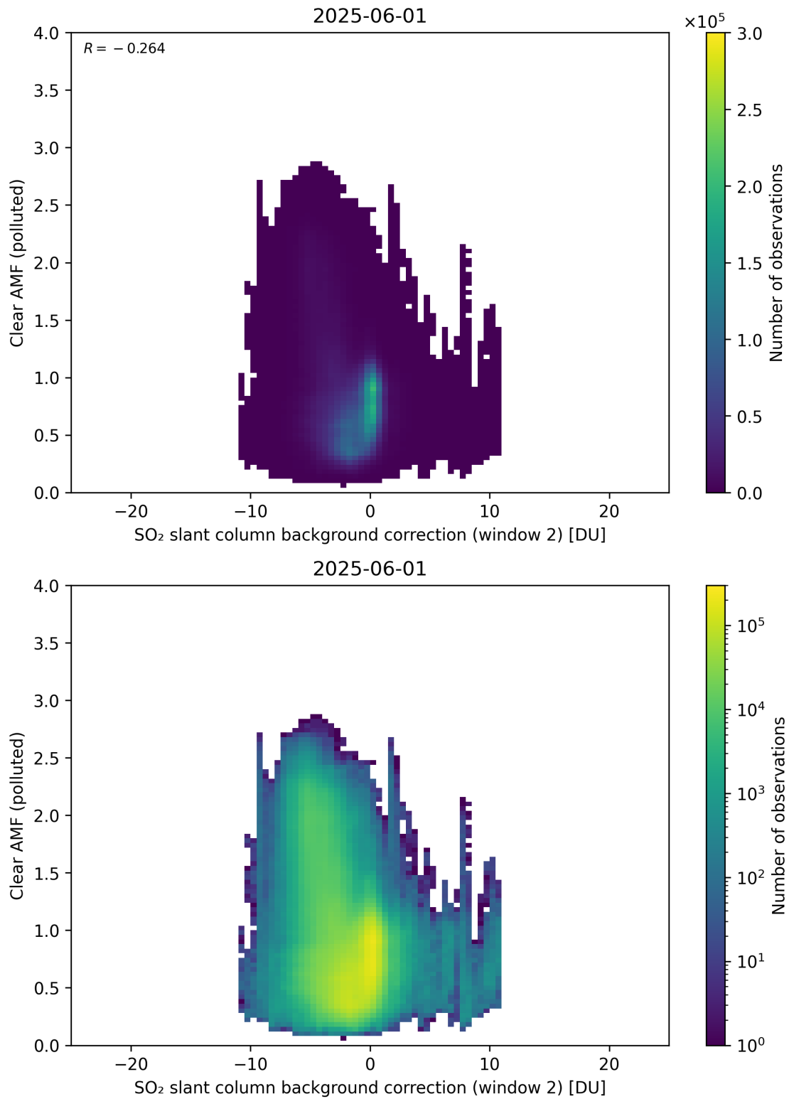
Figure 126: Scatter density plot of “SO 2 slant column background correction (window 2)” against “Clear AMF (polluted)” for 2025-06-01 to 2025-06-02.
