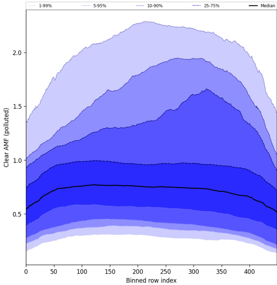
Figure 107: Along track statistics of “Clear AMF (polluted)” for 2025-06-01 to 2025-06-02
