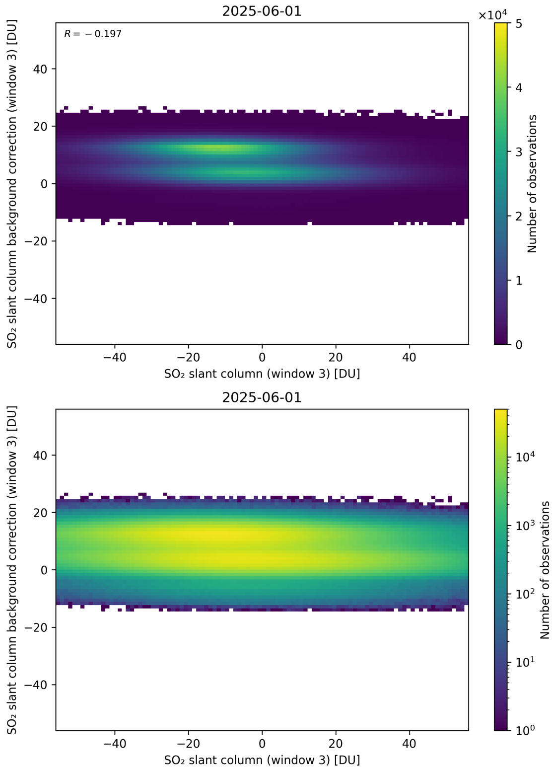
Figure 303: Scatter density plot of “SO 2 slant column (window 3)” against “SO 2 slant column background correction (window 3)” for 2025-06-01 to 2025-06-02.
