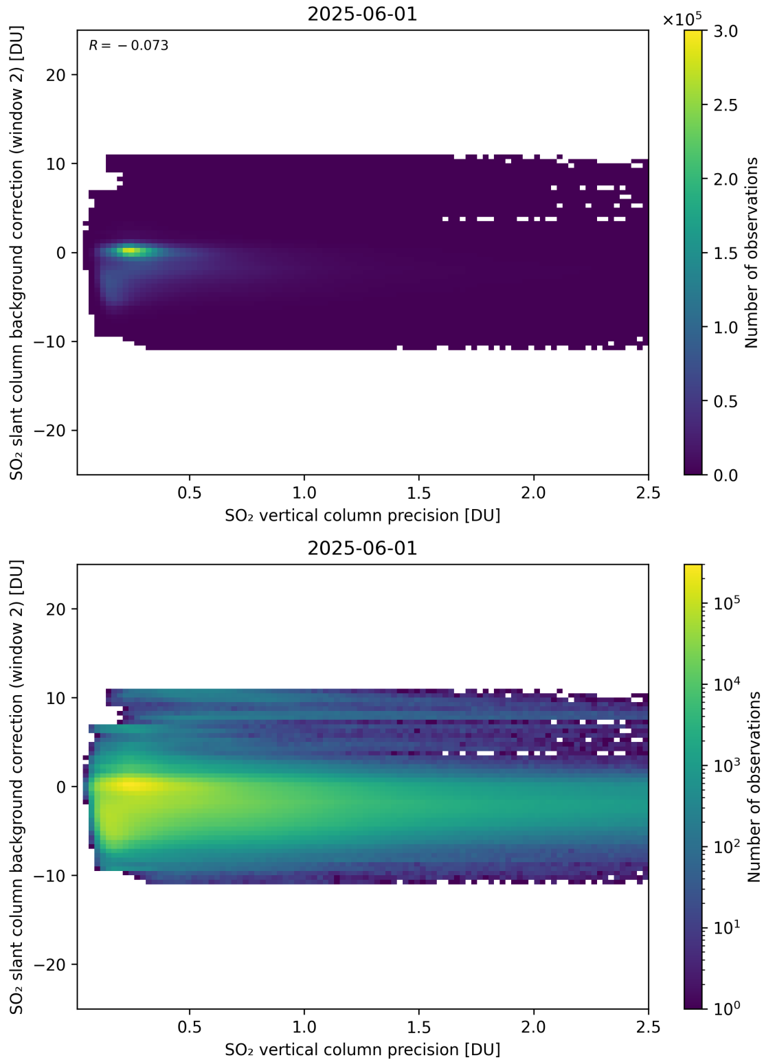
Figure 330: Scatter density plot of “SO 2 vertical column precision” against “SO 2 slant column background correction (window 2)” for 2025-06-01 to 2025-06-02.
