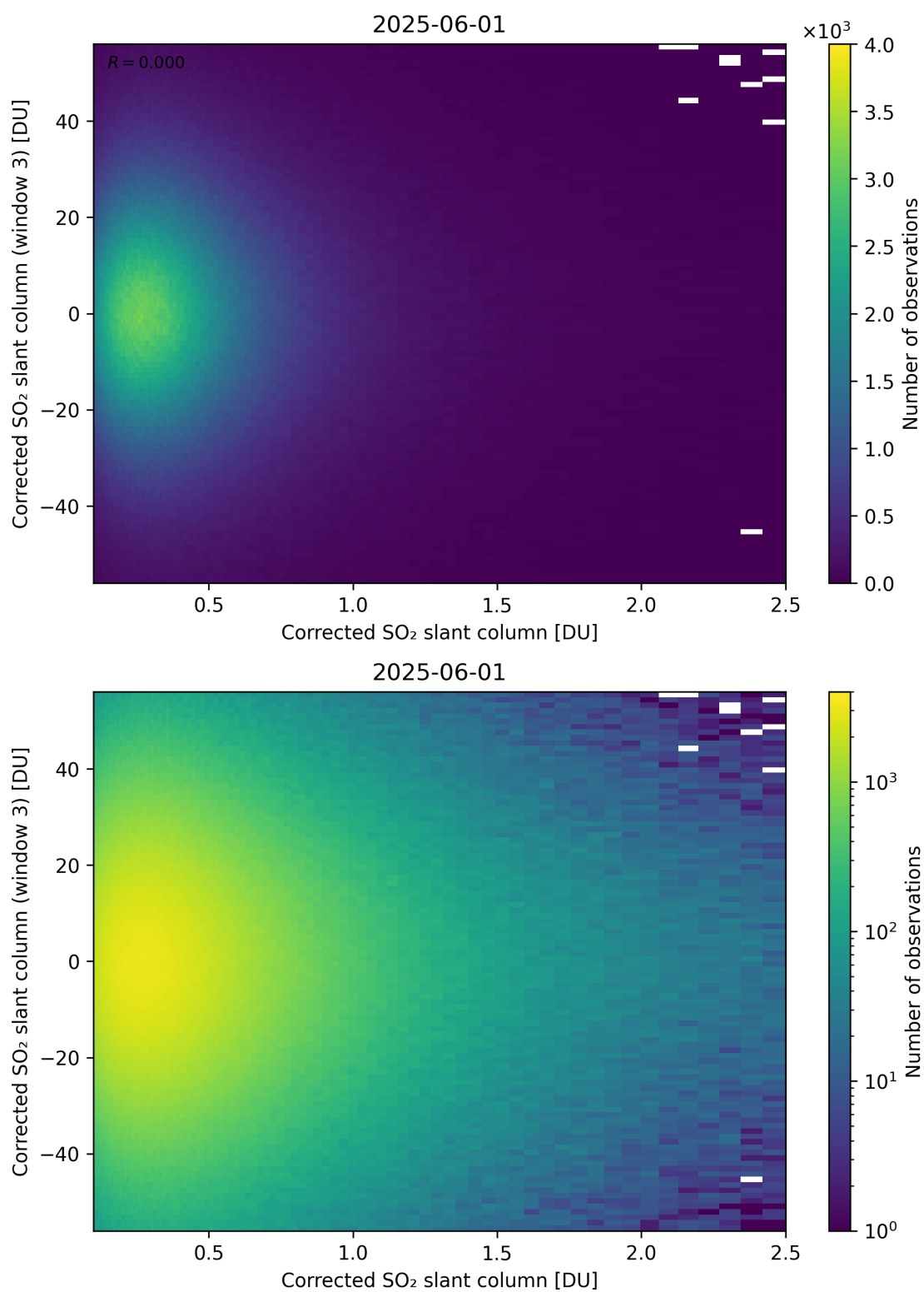
Figure 236: Scatter density plot of “Corrected SO 2 slant column” against “Corrected SO 2 slant column (window 3)” for 2025-06-01 to 2025-06-02.
