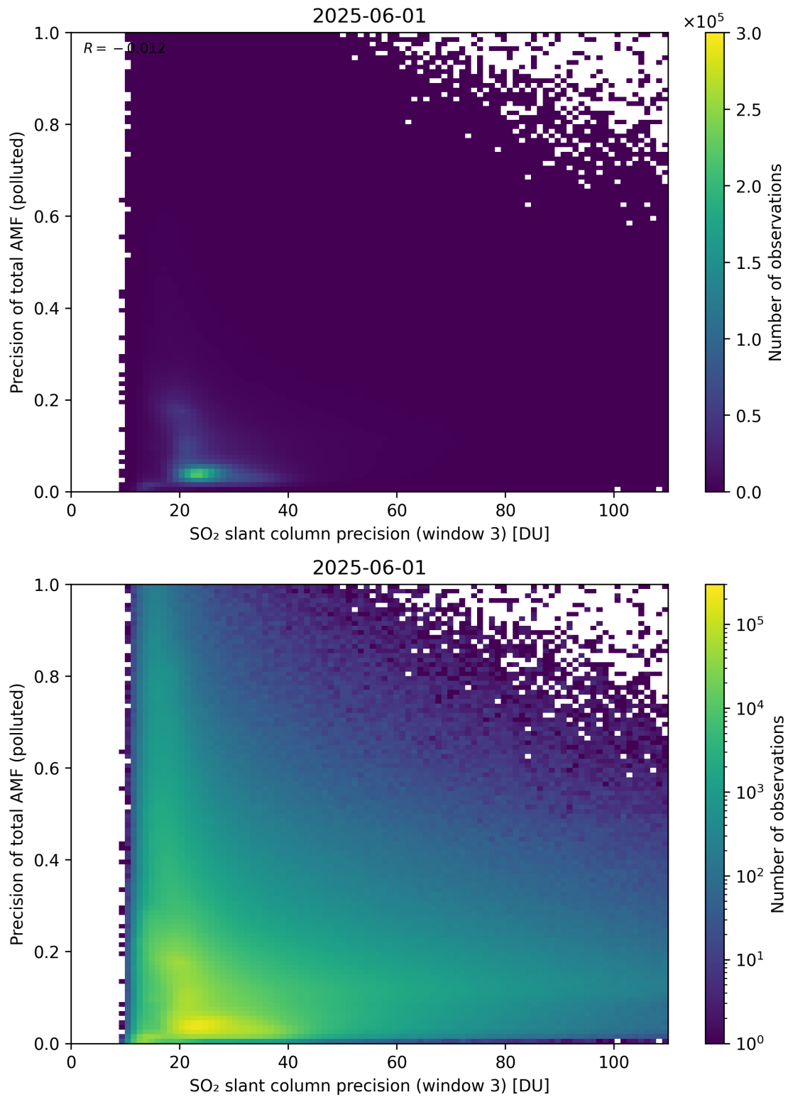
Figure 314: Scatter density plot of “SO 2 slant column precision (window 3)” against “Precision of total AMF (polluted)” for 2025-06-01 to 2025-06-02.
