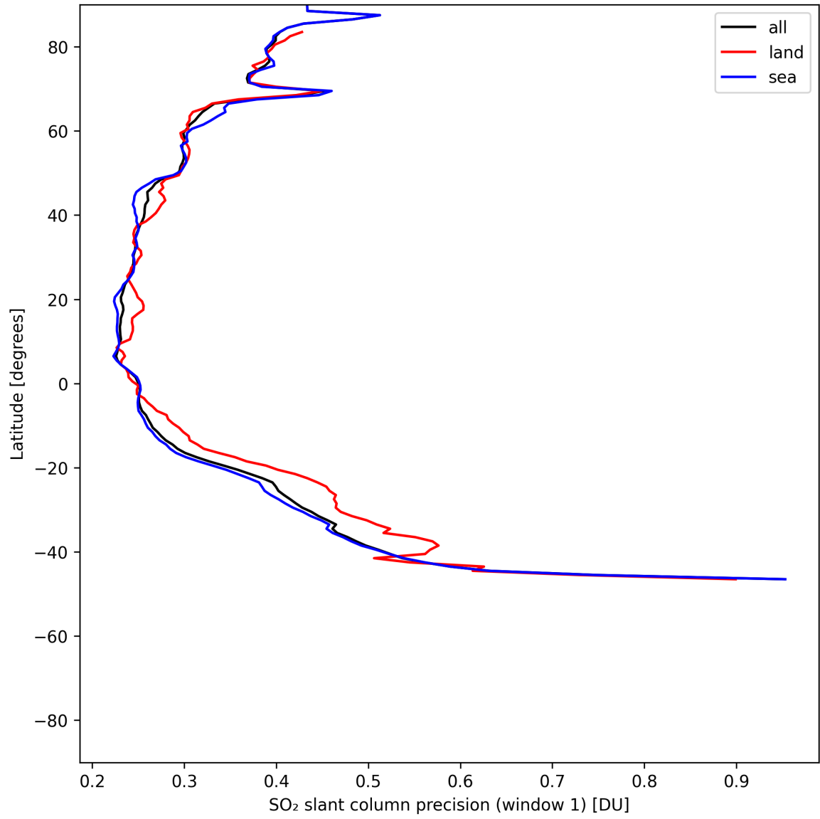
Figure 38: Zonal average of “SO 2 slant column precision (window 1)” for 2025-06-01 to 2025-06-02.
