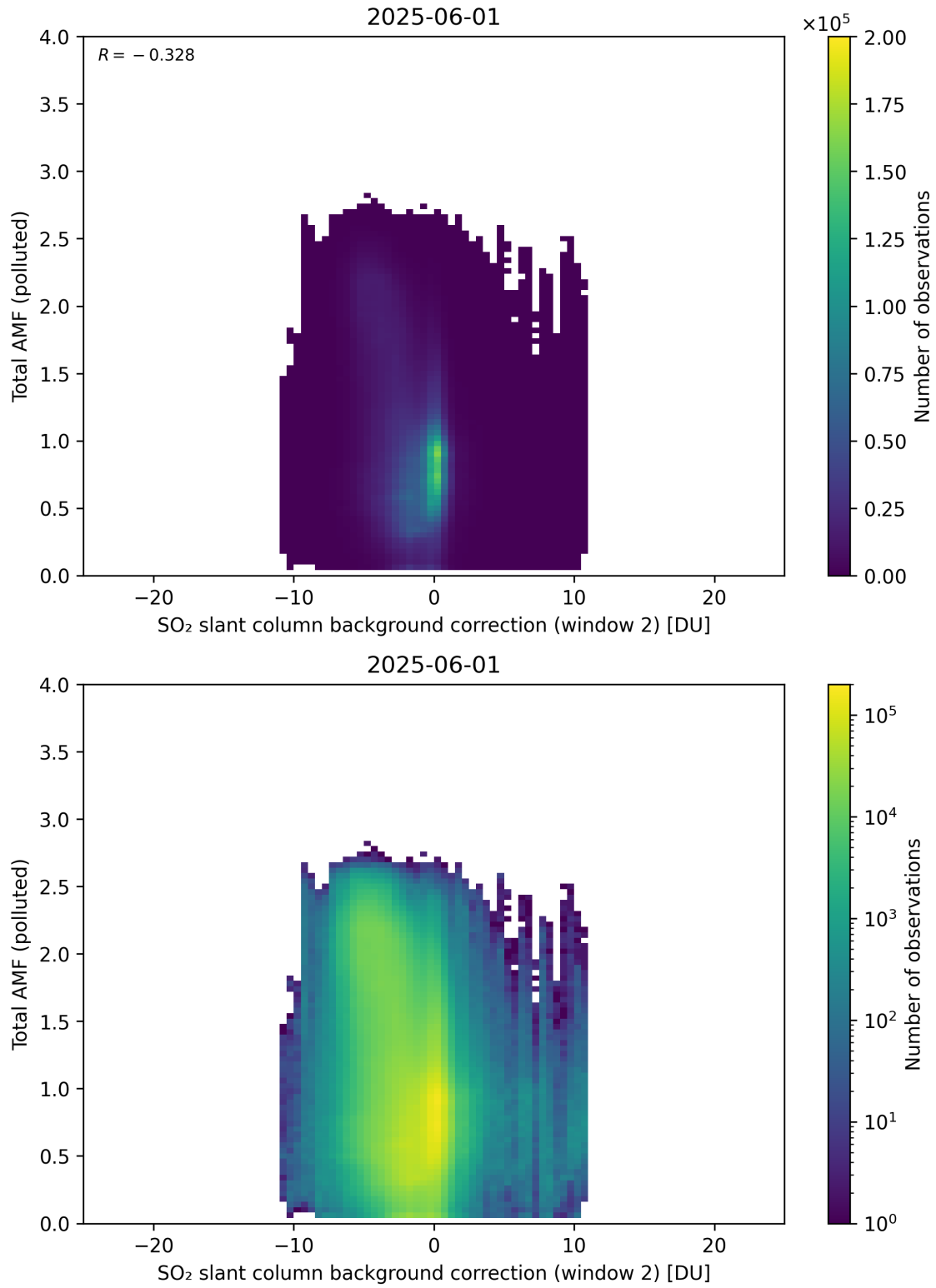
Figure 130: Scatter density plot of “SO 2 slant column background correction (window 2)” against “Total AMF (polluted)” for 2025-06-01 to 2025-06-02.
