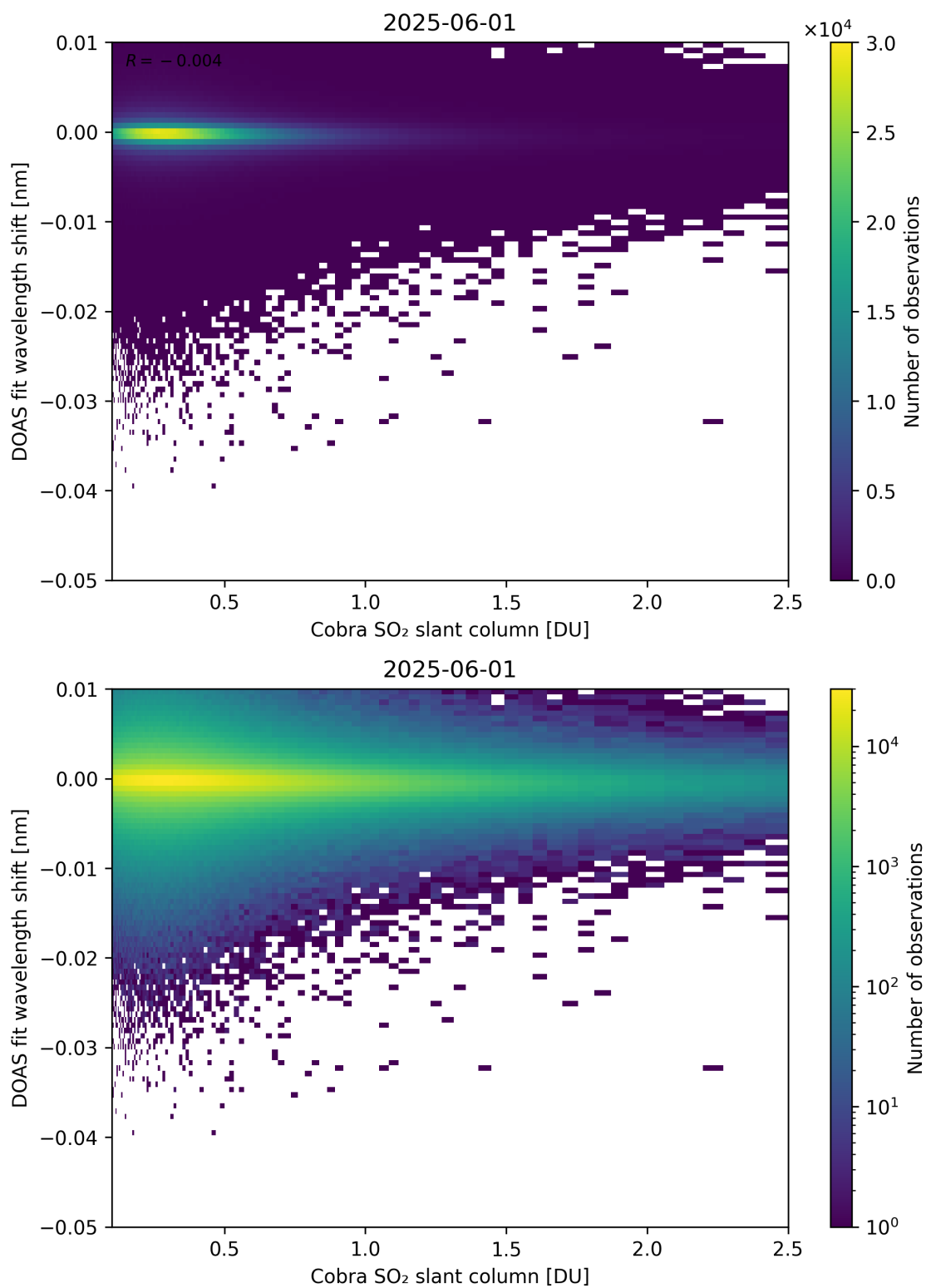
Figure 196: Scatter density plot of “Cobra SO 2 slant column” against “DOAS fit wavelength shift” for 2025-06-01 to 2025-06-02.
