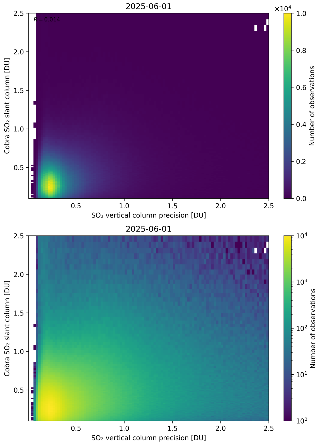
Figure 336: Scatter density plot of “SO 2 vertical column precision” against “Cobra SO 2 slant column” for 2025-06-01 to 2025-06-02.
