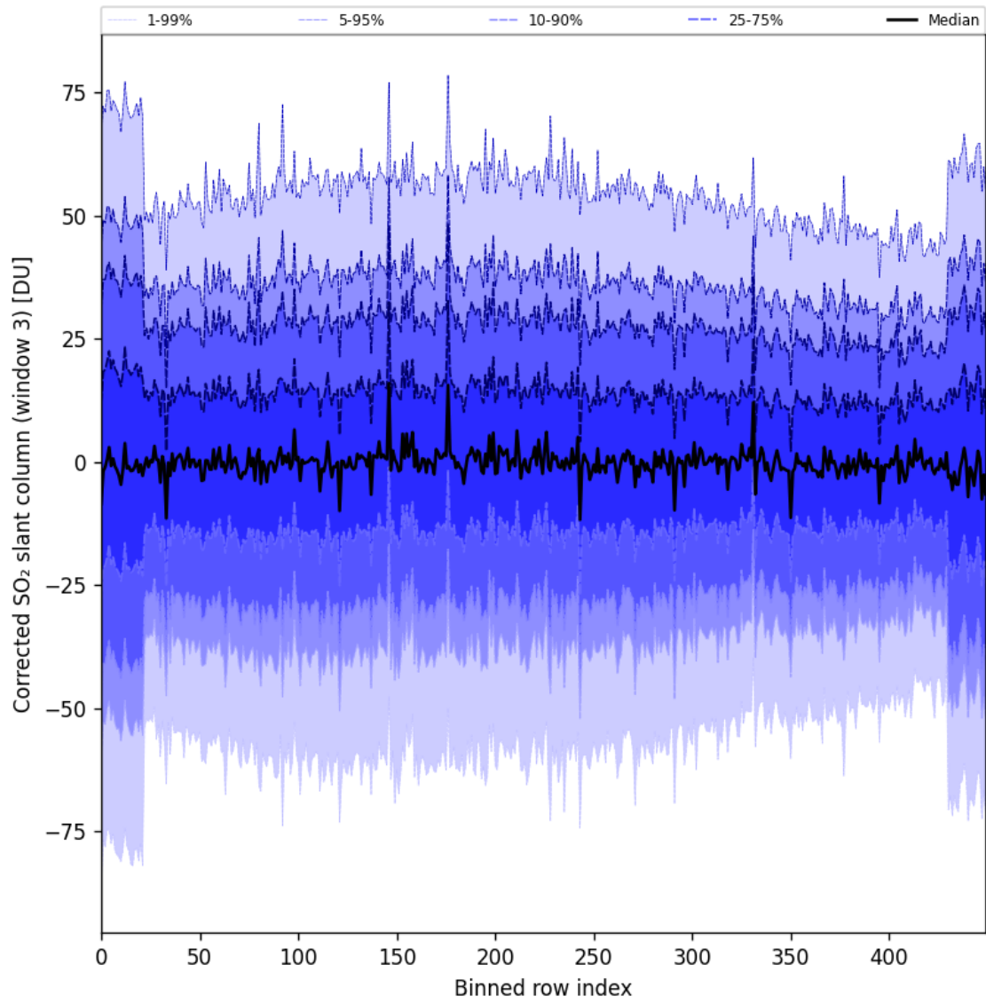
Figure 99: Along track statistics of “Corrected SO 2 slant column (window 3)” for 2025-06-01 to 2025-06-02
