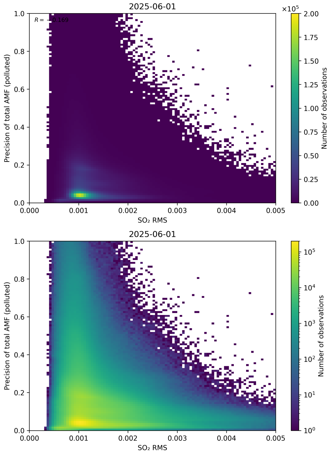
Figure 149: Scatter density plot of “SO 2 RMS” against “Precision of total AMF (polluted)” for 2025-06-01 to 2025-06-02.
