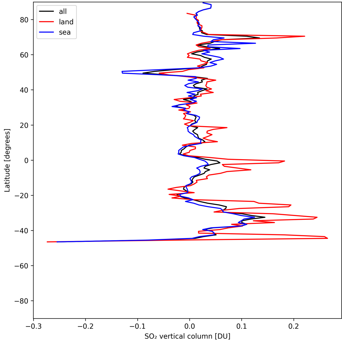
Figure 32: Zonal average of “SO 2 vertical column” for 2025-06-01 to 2025-06-02.
