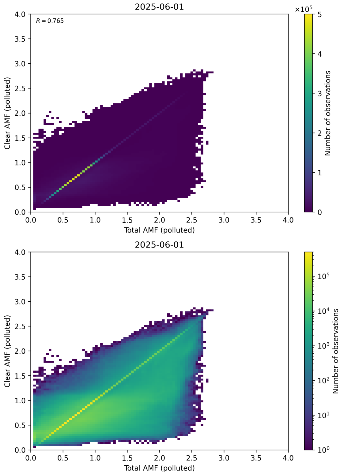
Figure 321: Scatter density plot of “Total AMF (polluted)” against “Clear AMF (polluted)” for 2025-06-01 to 2025-06-02.
