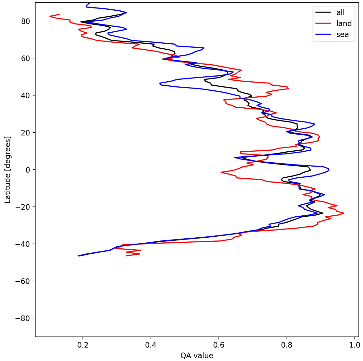
Figure 31: Zonal average of “QA value” for 2025-06-01 to 2025-06-02.
