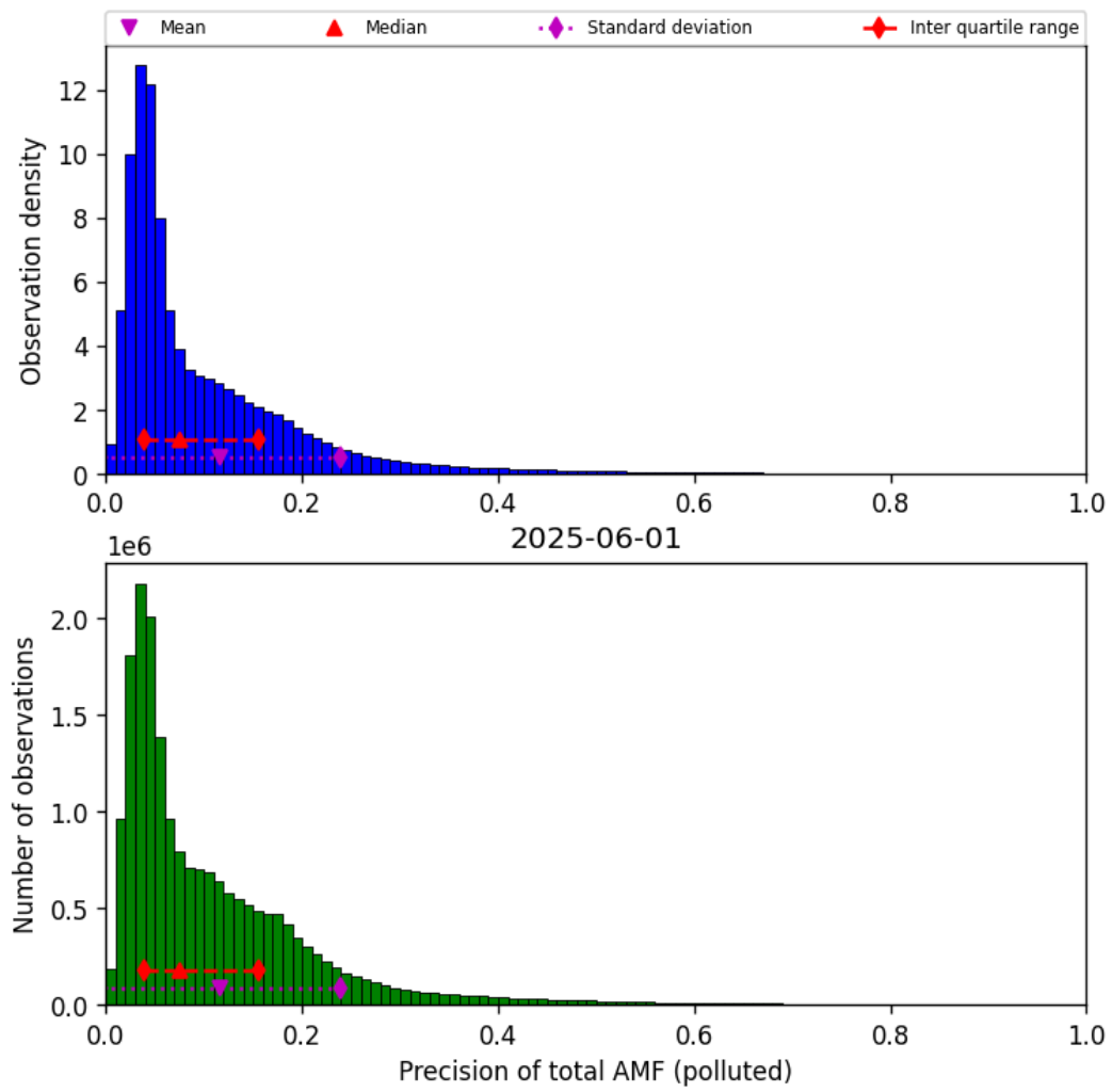
Figure 80: Histogram of “Precision of total AMF (polluted)” for 2025-06-01 to 2025-06-02
