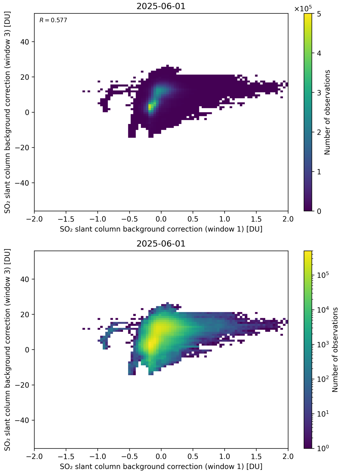
Figure 110: Scatter density plot of “SO 2 slant column background correction (window 1)” against “SO 2 slant column background correction (window 3)” for 2025-06-01 to 2025-06-02.
