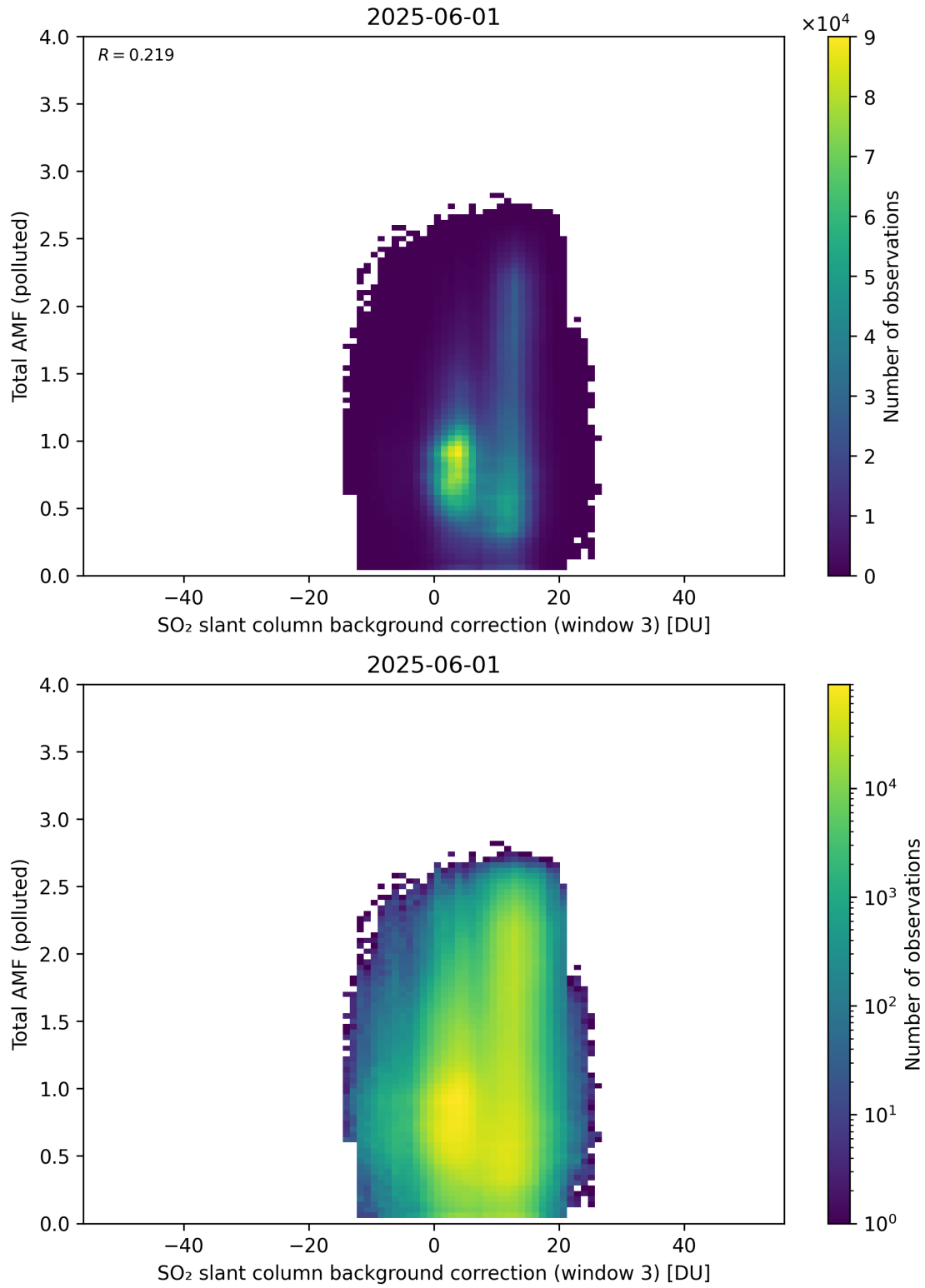
Figure 136: Scatter density plot of “SO 2 slant column background correction (window 3)” against “Total AMF (polluted)” for 2025-06-01 to 2025-06-02.
