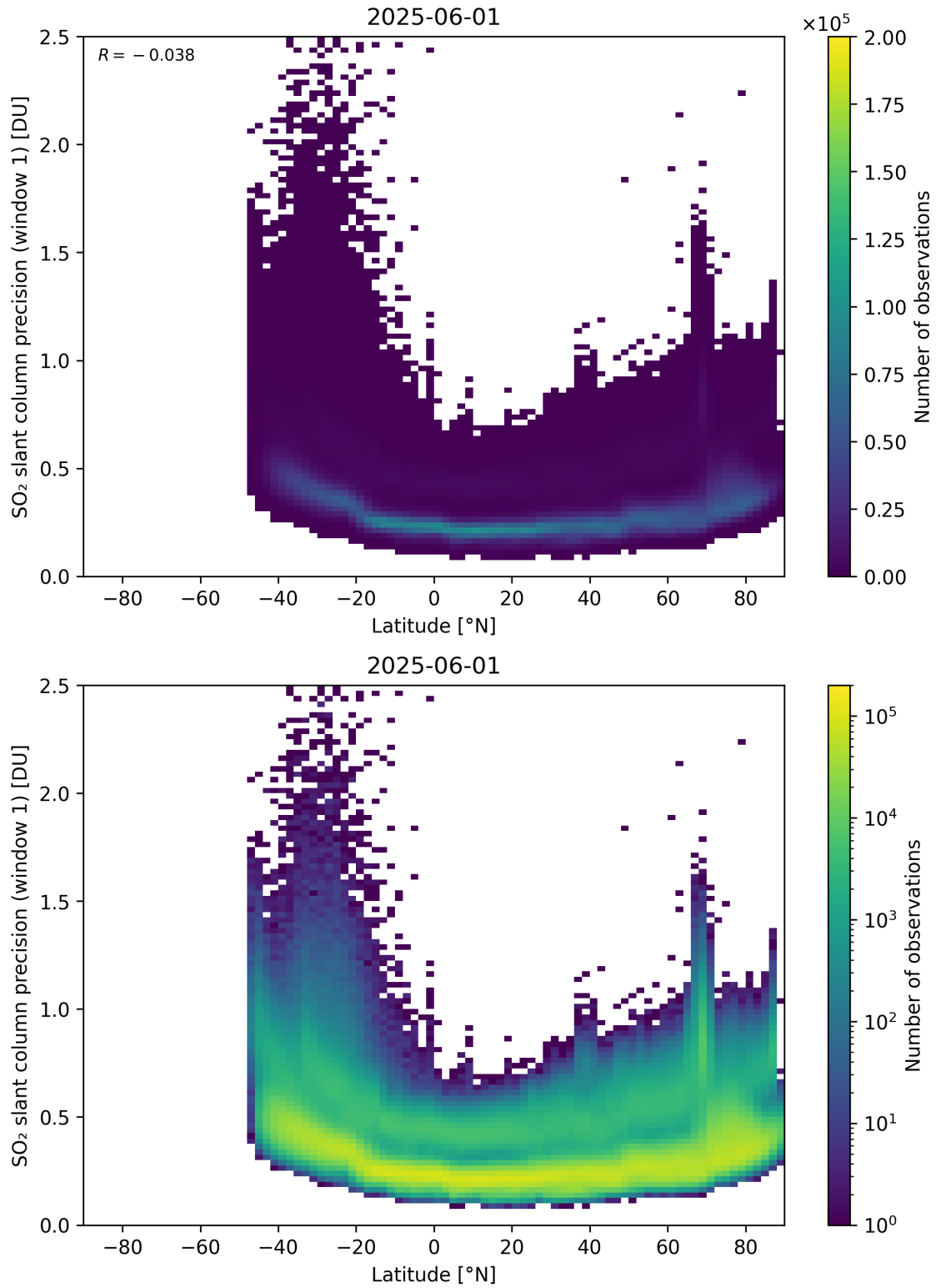
Figure 163: Scatter density plot of “Latitude” against “SO 2 slant column precision (window 1)” for 2025-06-01 to 2025-06-02.
