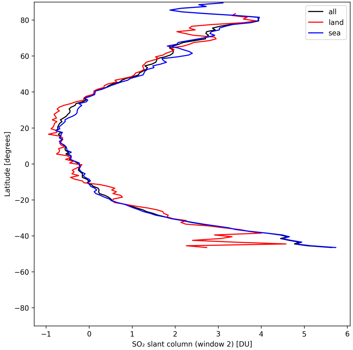
Figure 41: Zonal average of “SO 2 slant column (window 2)” for 2025-06-01 to 2025-06-02.
