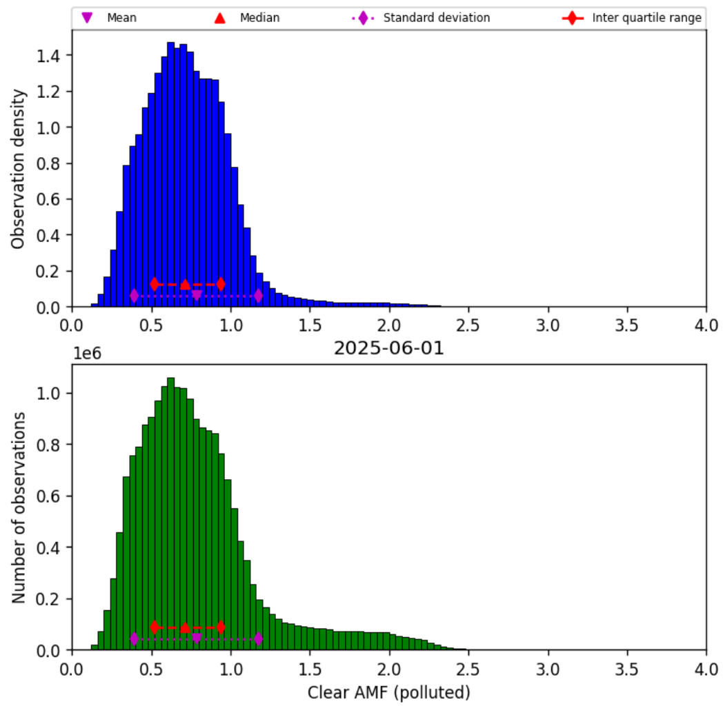
Figure 81: Histogram of “Clear AMF (polluted)” for 2025-06-01 to 2025-06-02
