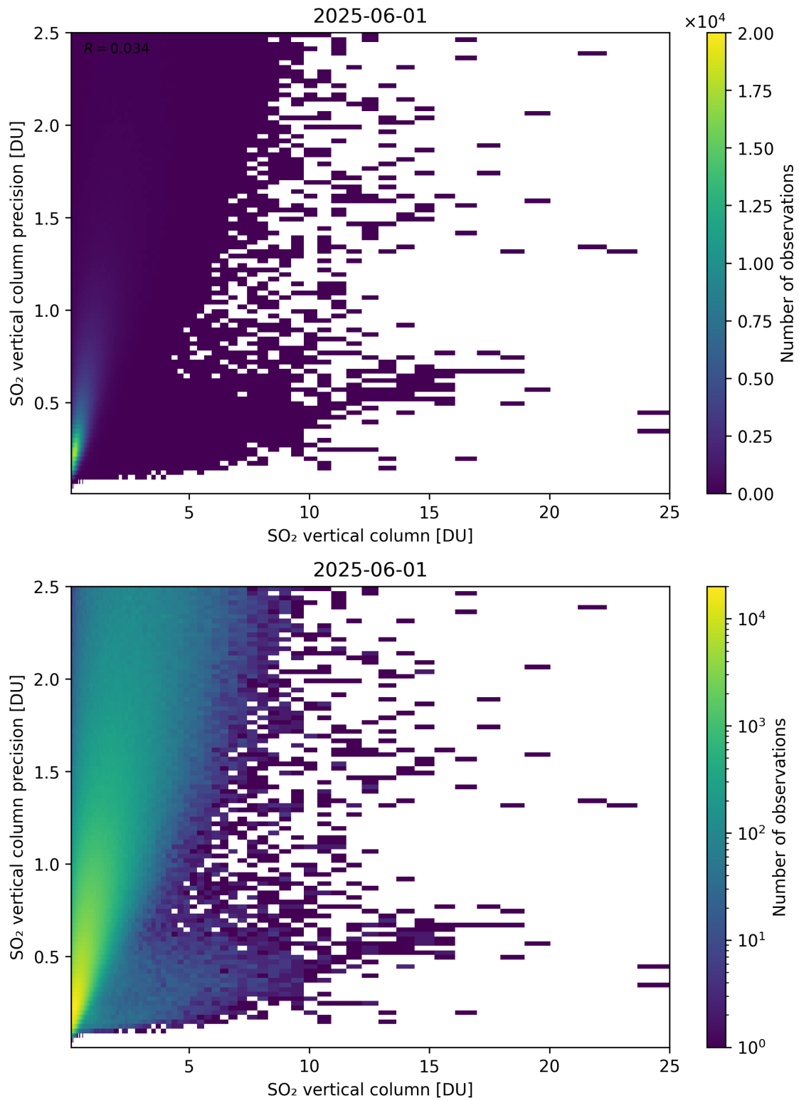
Figure 361: Scatter density plot of “SO 2 vertical column” against “SO 2 vertical column precision” for 2025-06-01 to 2025-06-02.
