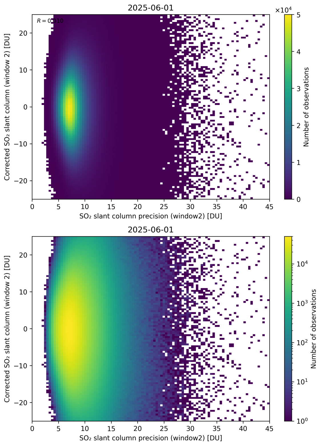
Figure 297: Scatter density plot of “SO 2 slant column precision (window2)” against “Corrected SO 2 slant column (window 2)” for 2025-06-01 to 2025-06-02.
