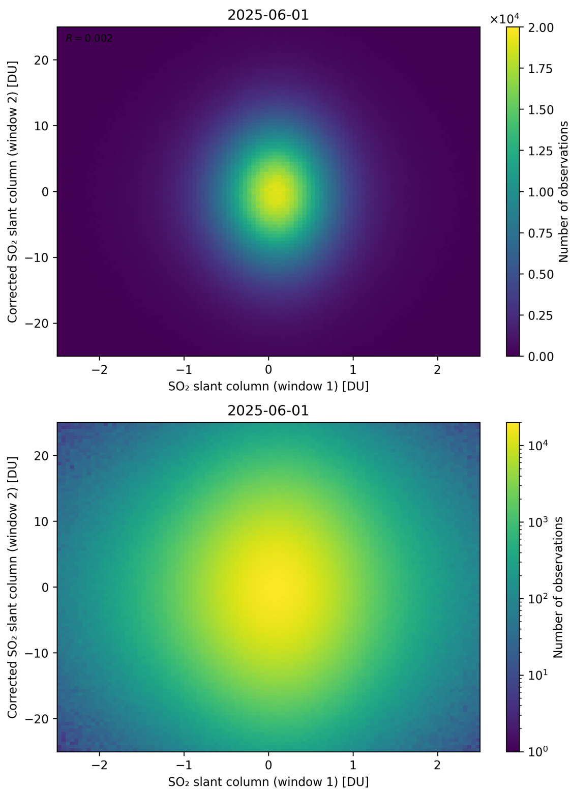
Figure 283: Scatter density plot of “SO 2 slant column (window 1)” against “Corrected SO 2 slant column (window 2)” for 2025-06-01 to 2025-06-02.
