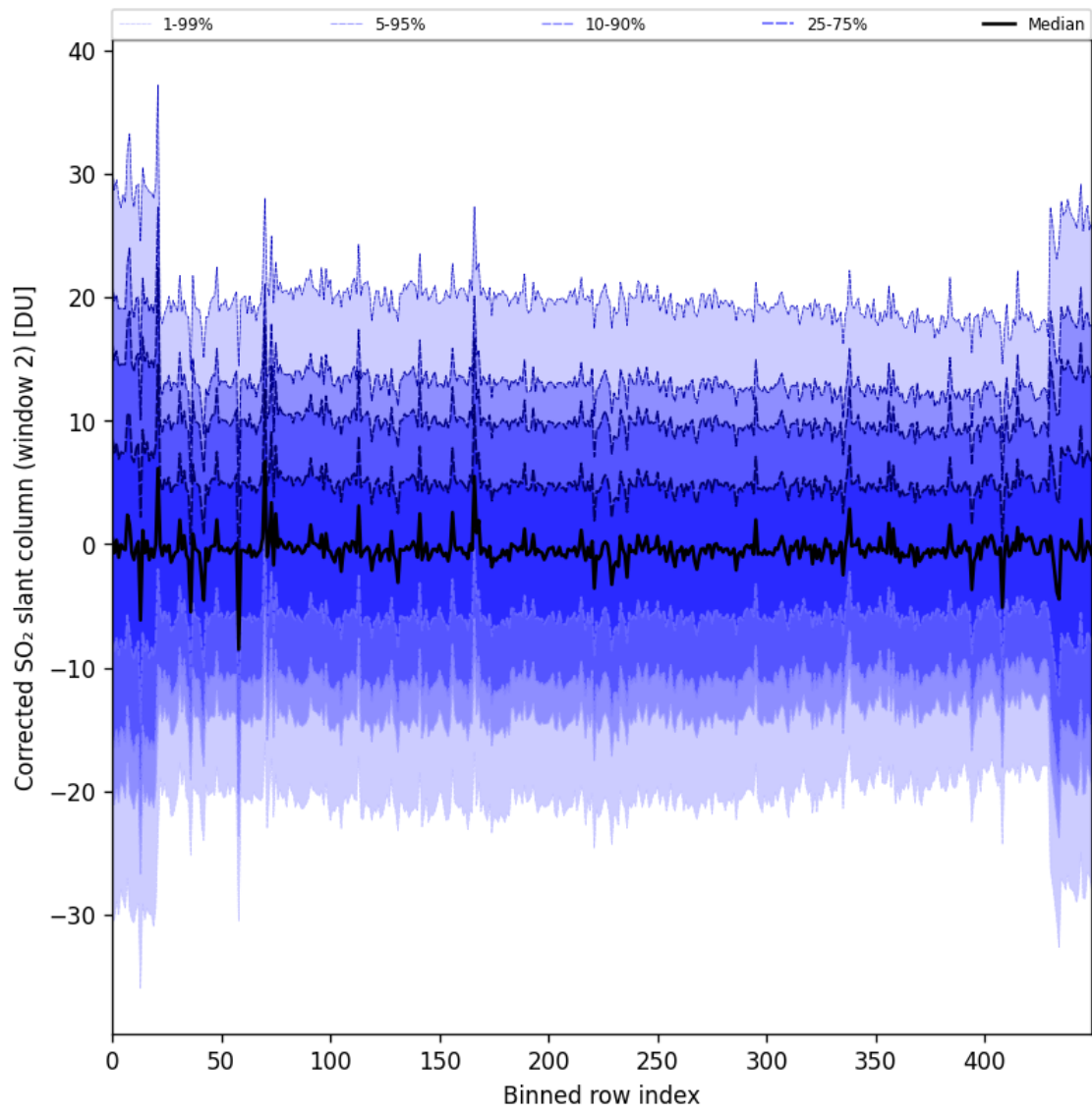
Figure 95: Along track statistics of “Corrected SO 2 slant column (window 2)” for 2025-06-01 to 2025-06-02
