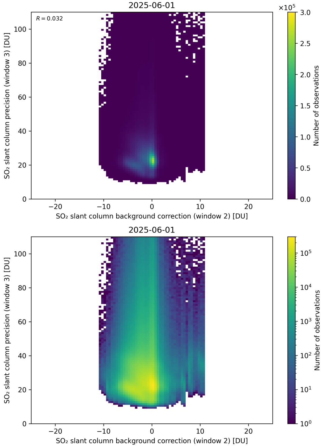
Figure 129: Scatter density plot of “SO 2 slant column background correction (window 2)” against “SO 2 slant column precision (window 3)” for 2025-06-01 to 2025-06-02.
