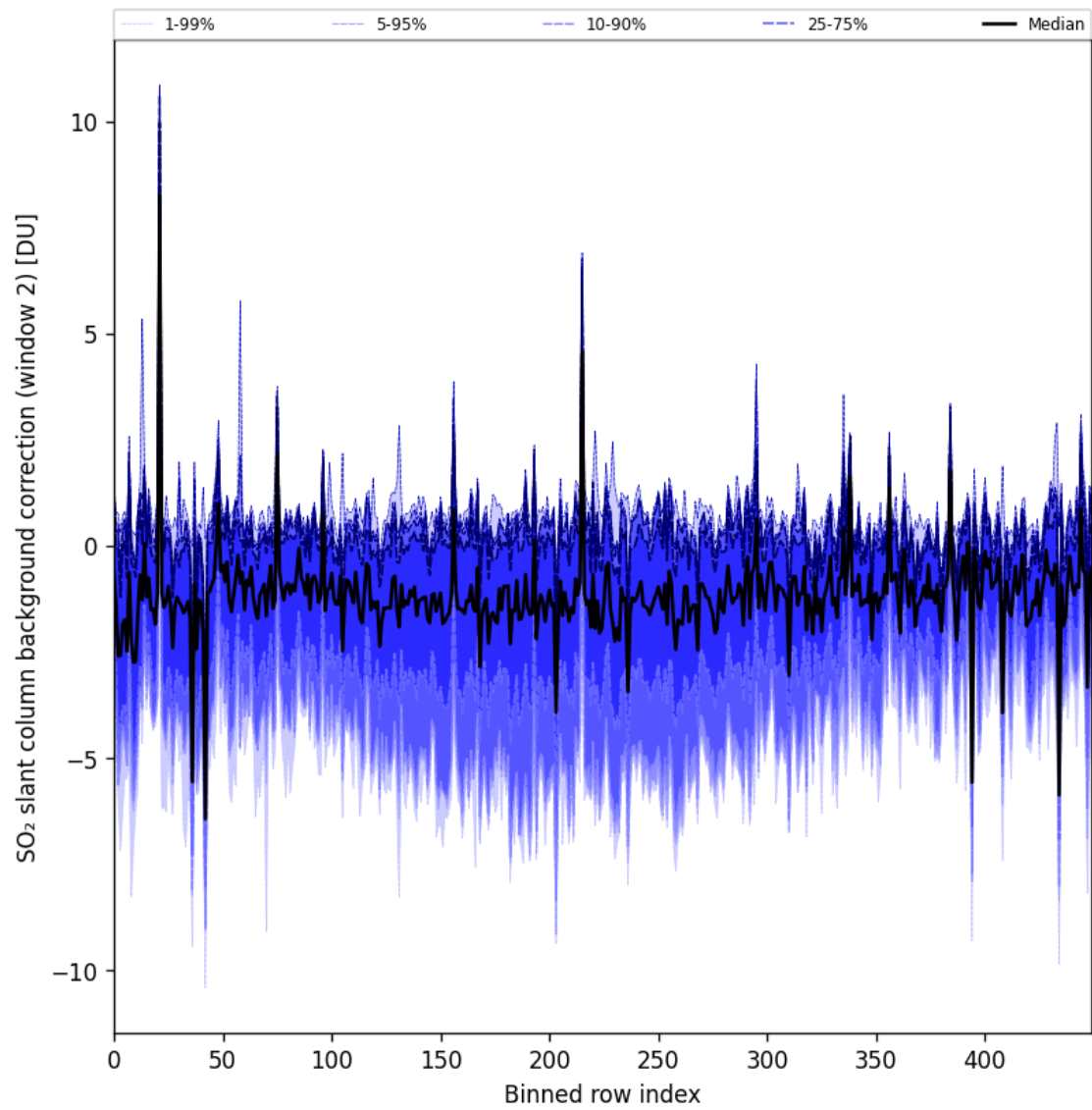
Figure 96: Along track statistics of “SO 2 slant column background correction (window 2)” for 2025-06-01 to 2025-06-02
