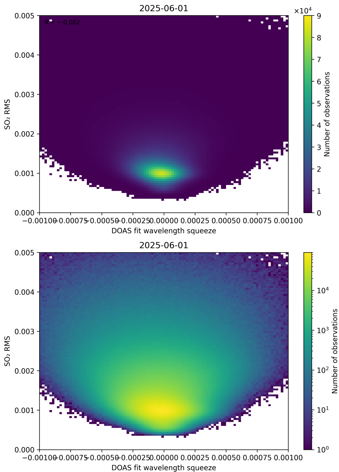
Figure 143: Scatter density plot of “DOAS fit wavelength squeeze” against “SO 2 RMS” for 2025-06-01 to 2025-06-02.
