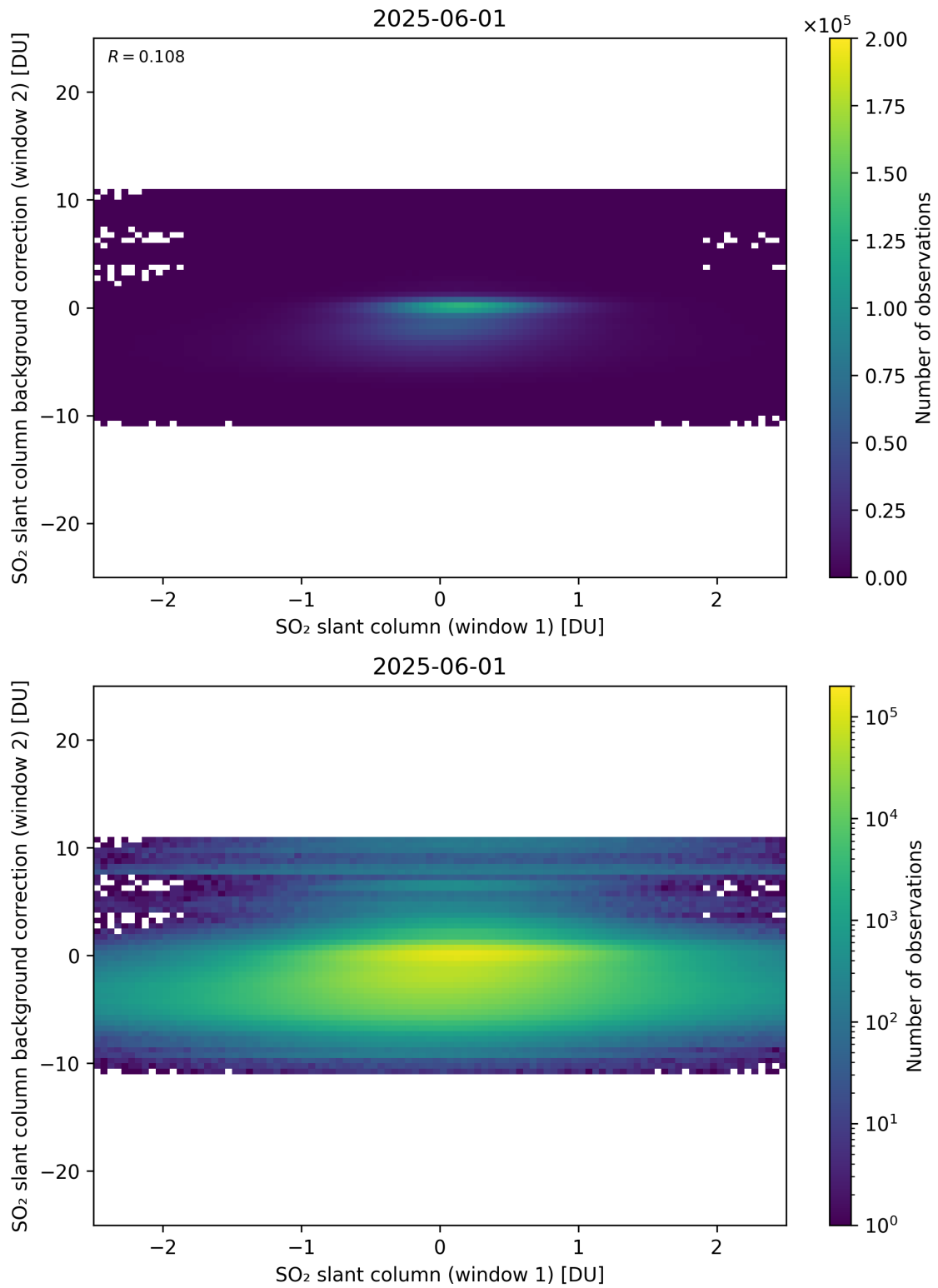
Figure 263: Scatter density plot of “SO 2 slant column (window 1)” against “SO 2 slant column background correction (window 2)” for 2025-06-01 to 2025-06-02.
