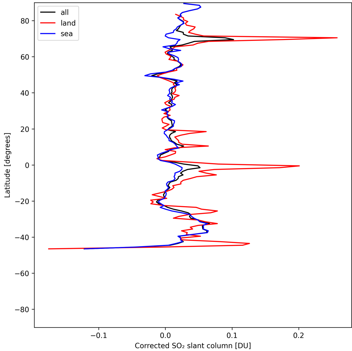
Figure 34: Zonal average of “Corrected SO 2 slant column” for 2025-06-01 to 2025-06-02.
