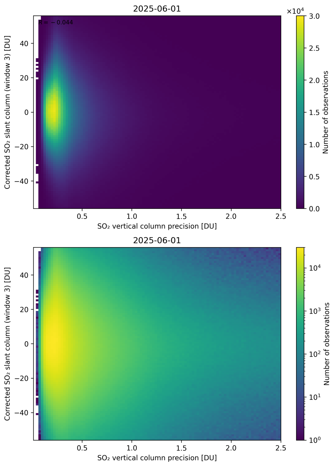
Figure 340: Scatter density plot of “SO 2 vertical column precision” against “Corrected SO 2 slant column (window 3)” for 2025-06-01 to 2025-06-02.
