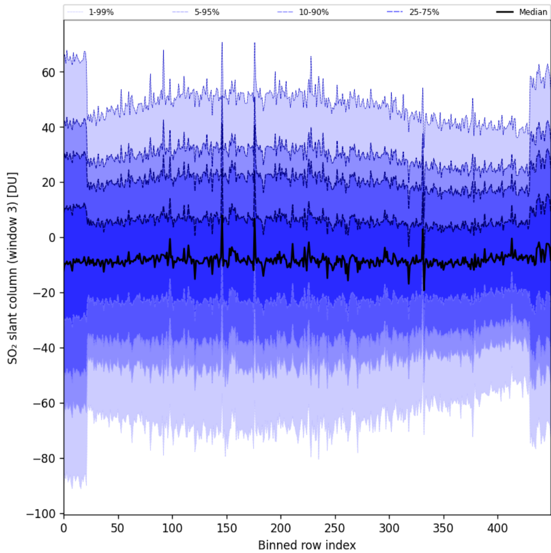
Figure 97: Along track statistics of “SO 2 slant column (window 3)” for 2025-06-01 to 2025-06-02
