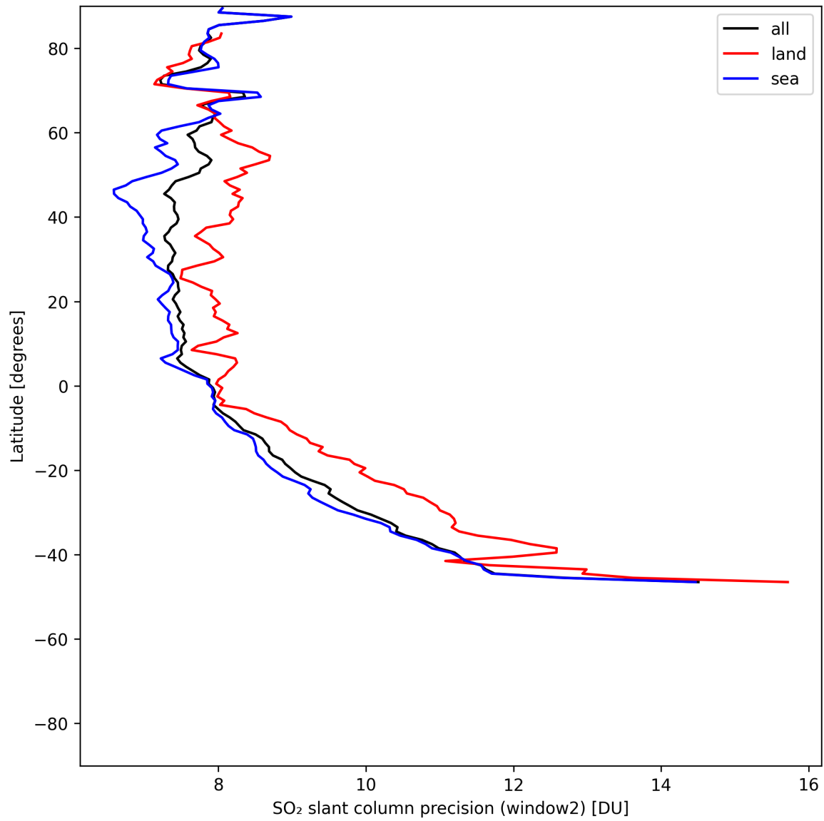
Figure 42: Zonal average of “SO 2 slant column precision (window2)” for 2025-06-01 to 2025-06-02.
