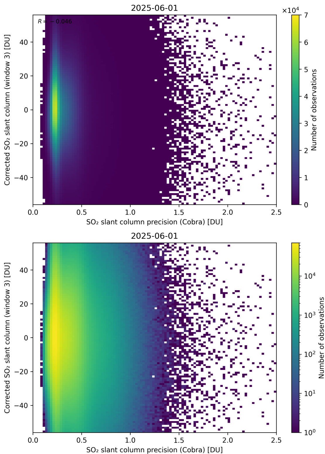
Figure 207: Scatter density plot of “SO 2 slant column precision (Cobra)” against “Corrected SO 2 slant column (window 3)” for 2025-06-01 to 2025-06-02.
