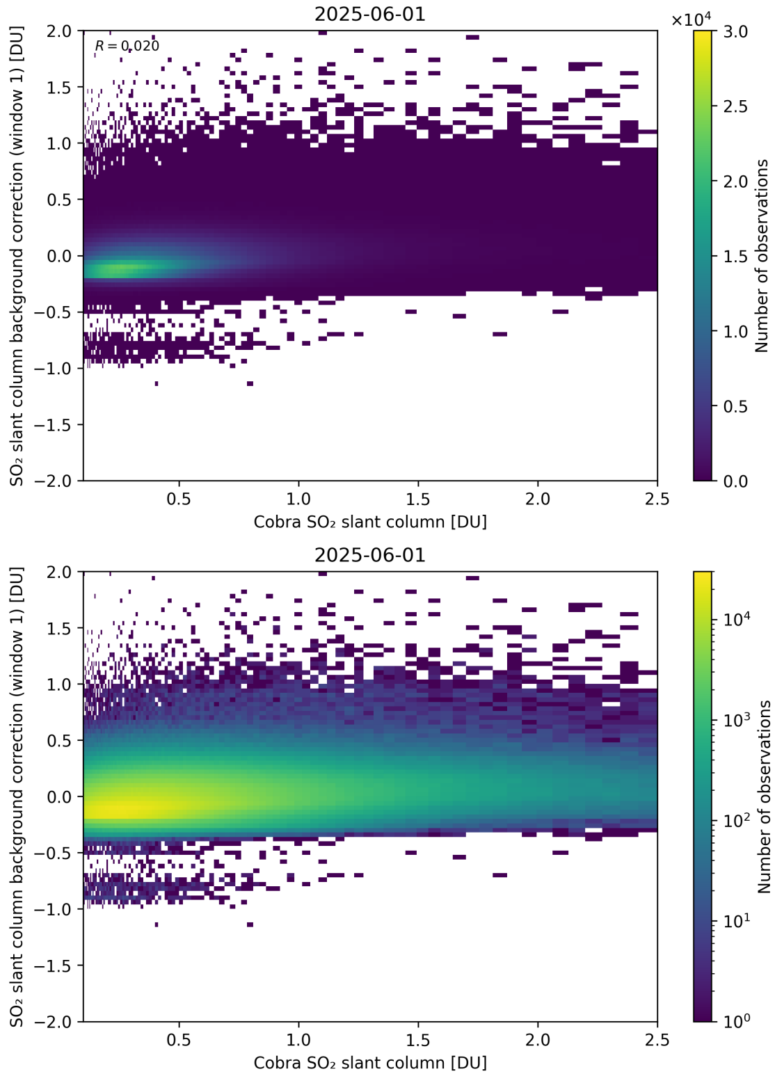
Figure 193: Scatter density plot of “Cobra SO 2 slant column” against “SO 2 slant column background correction (window 1)” for 2025-06-01 to 2025-06-02.
