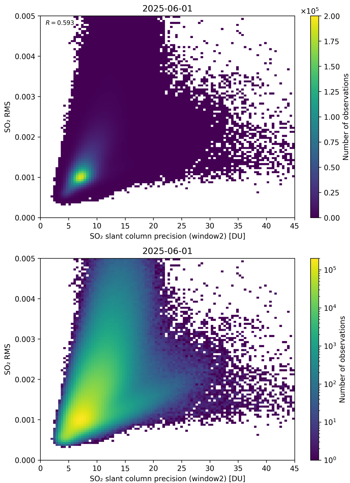
Figure 295: Scatter density plot of “SO 2 slant column precision (window2)” against “SO 2 RMS” for 2025-06-01 to 2025-06-02.
