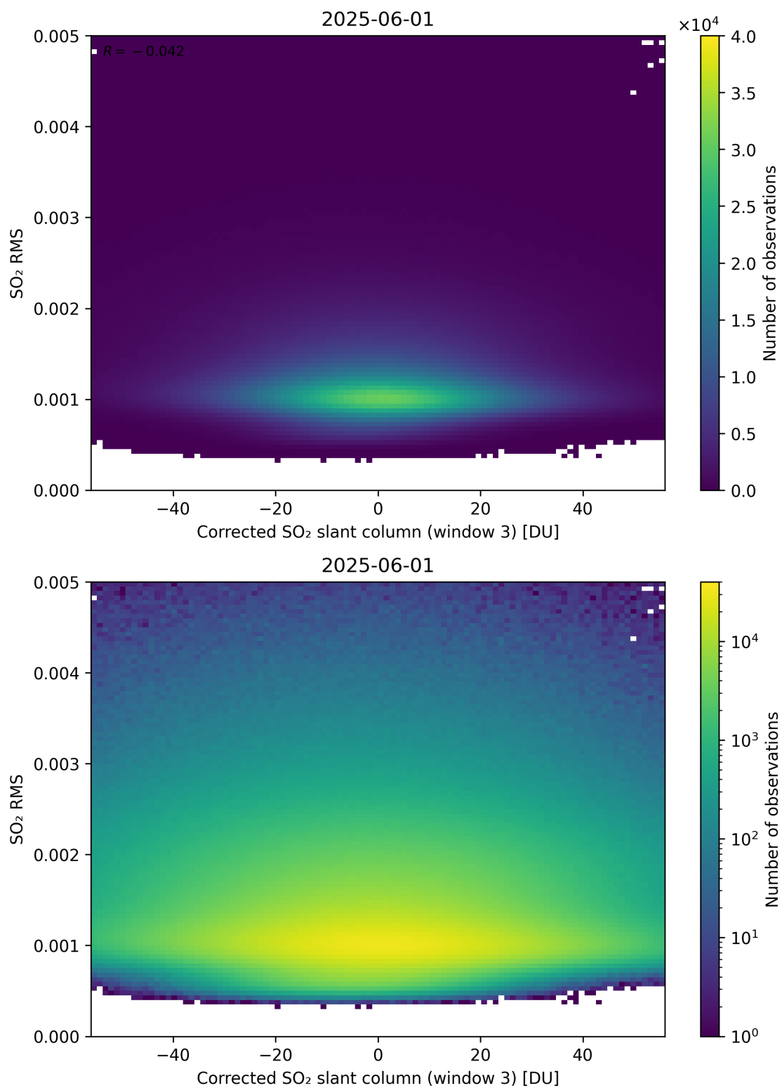
Figure 258: Scatter density plot of “Corrected SO 2 slant column (window 3)” against “SO 2 RMS” for 2025-06-01 to 2025-06-02.
