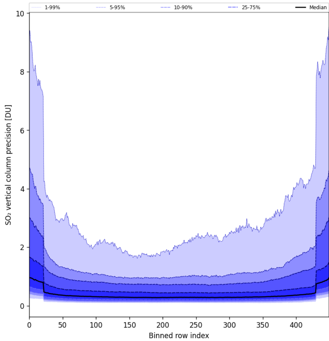
Figure 85: Along track statistics of “SO 2 vertical column precision” for 2025-06-01 to 2025-06-02
