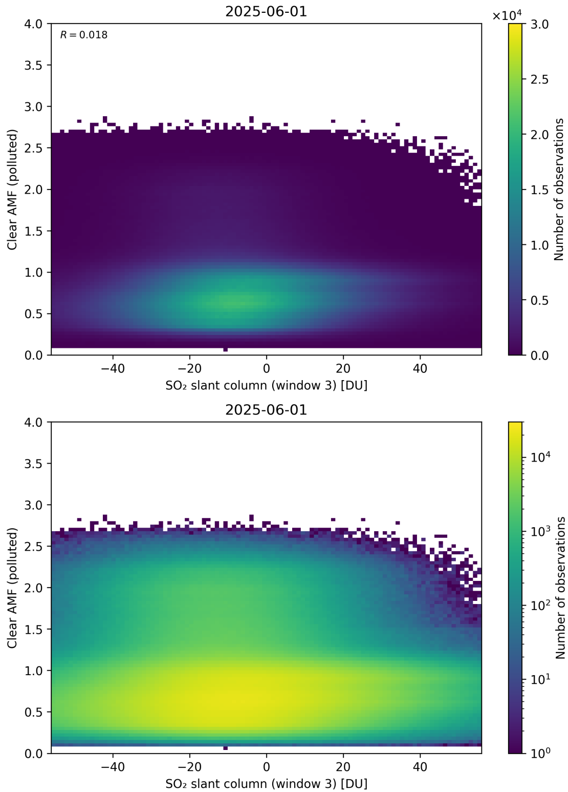
Figure 315: Scatter density plot of “SO 2 slant column (window 3)” against “Clear AMF (polluted)” for 2025-06-01 to 2025-06-02.
