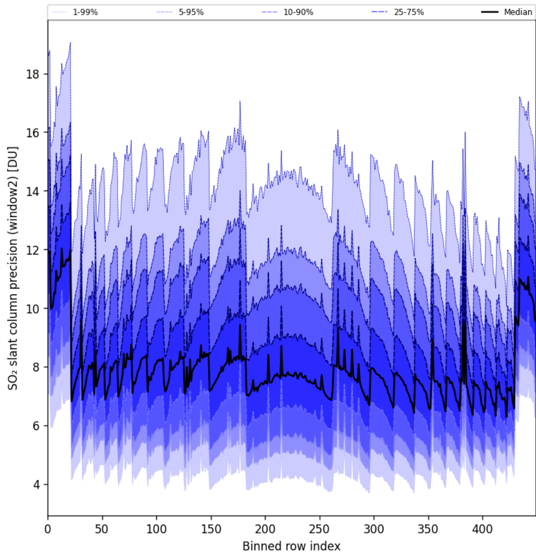
Figure 94: Along track statistics of “SO 2 slant column precision (window2)” for 2025-06-01 to 2025-06-02
