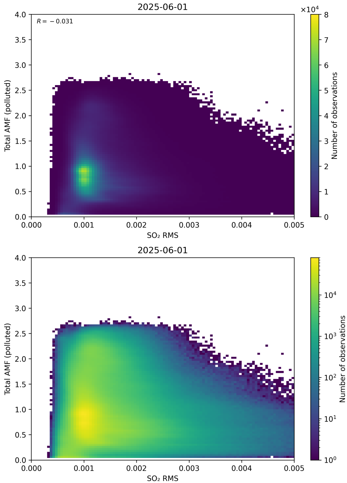
Figure 148: Scatter density plot of “SO 2 RMS” against “Total AMF (polluted)” for 2025-06-01 to 2025-06-02.
