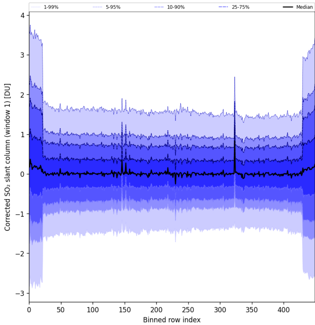
Figure 91: Along track statistics of “Corrected SO 2 slant column (window 1)” for 2025-06-01 to 2025-06-02
