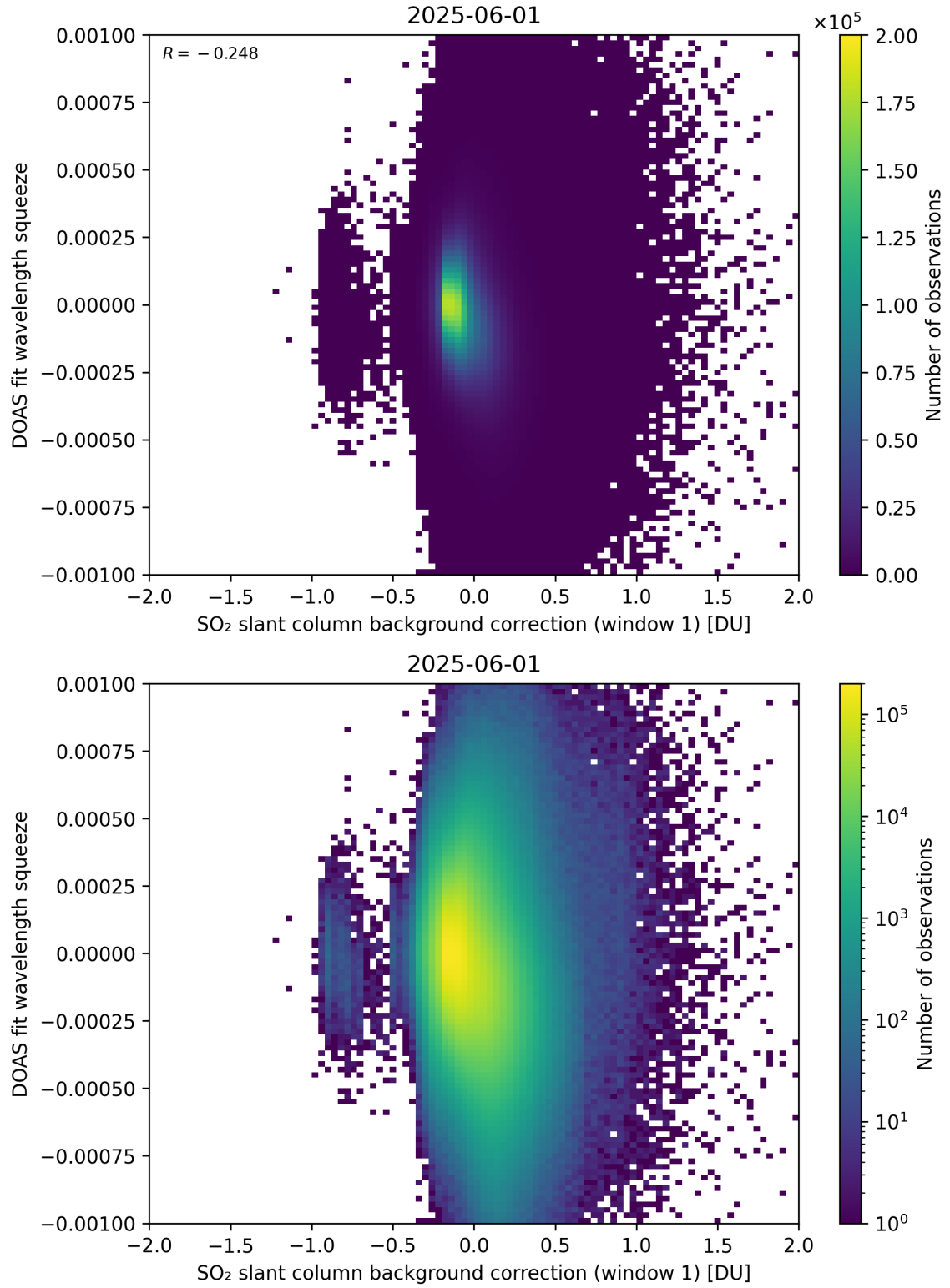
Figure 112: Scatter density plot of “SO 2 slant column background correction (window 1)” against “DOAS fit wavelength squeeze” for 2025-06-01 to 2025-06-02.
