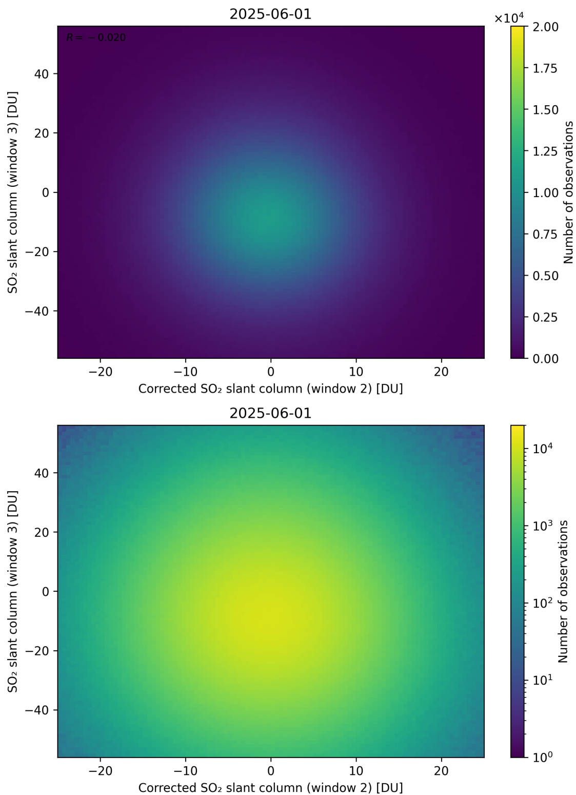
Figure 251: Scatter density plot of “Corrected SO 2 slant column (window 2)” against “SO 2 slant column (window 3)” for 2025-06-01 to 2025-06-02.
