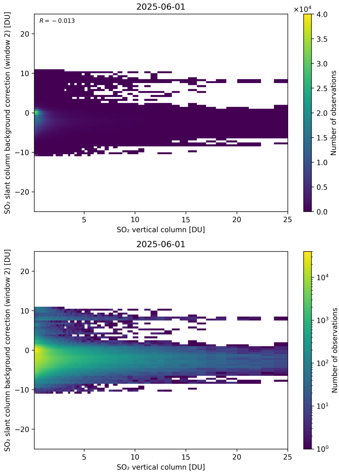
Figure 324: Scatter density plot of “SO 2 vertical column” against “SO 2 slant column background correction (window 2)” for 2025-06-01 to 2025-06-02.
