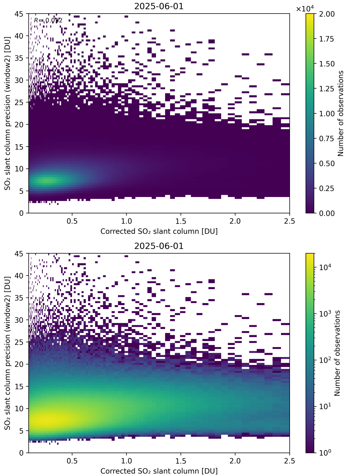
Figure 239: Scatter density plot of “Corrected SO 2 slant column” against “SO 2 slant column precision (window2)” for 2025-06-01 to 2025-06-02.
