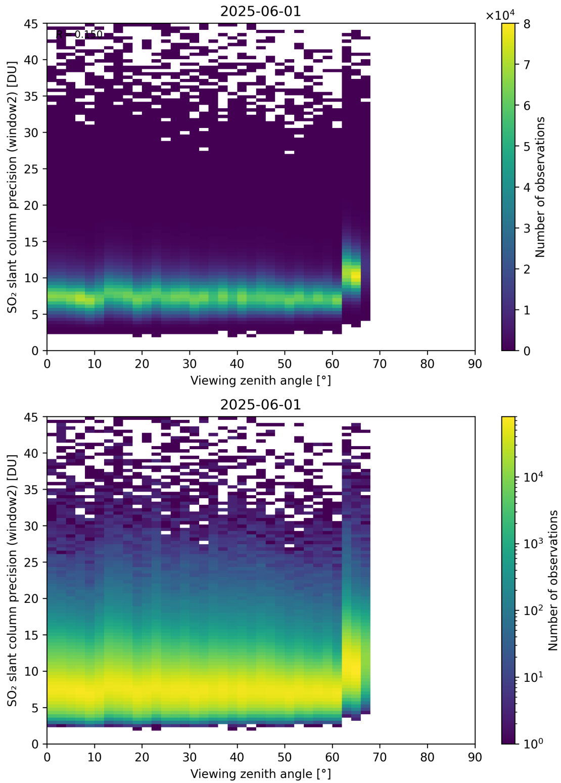
Figure 378: Scatter density plot of “Viewing zenith angle” against “SO 2 slant column precision (window2)” for 2025-06-01 to 2025-06-02.
