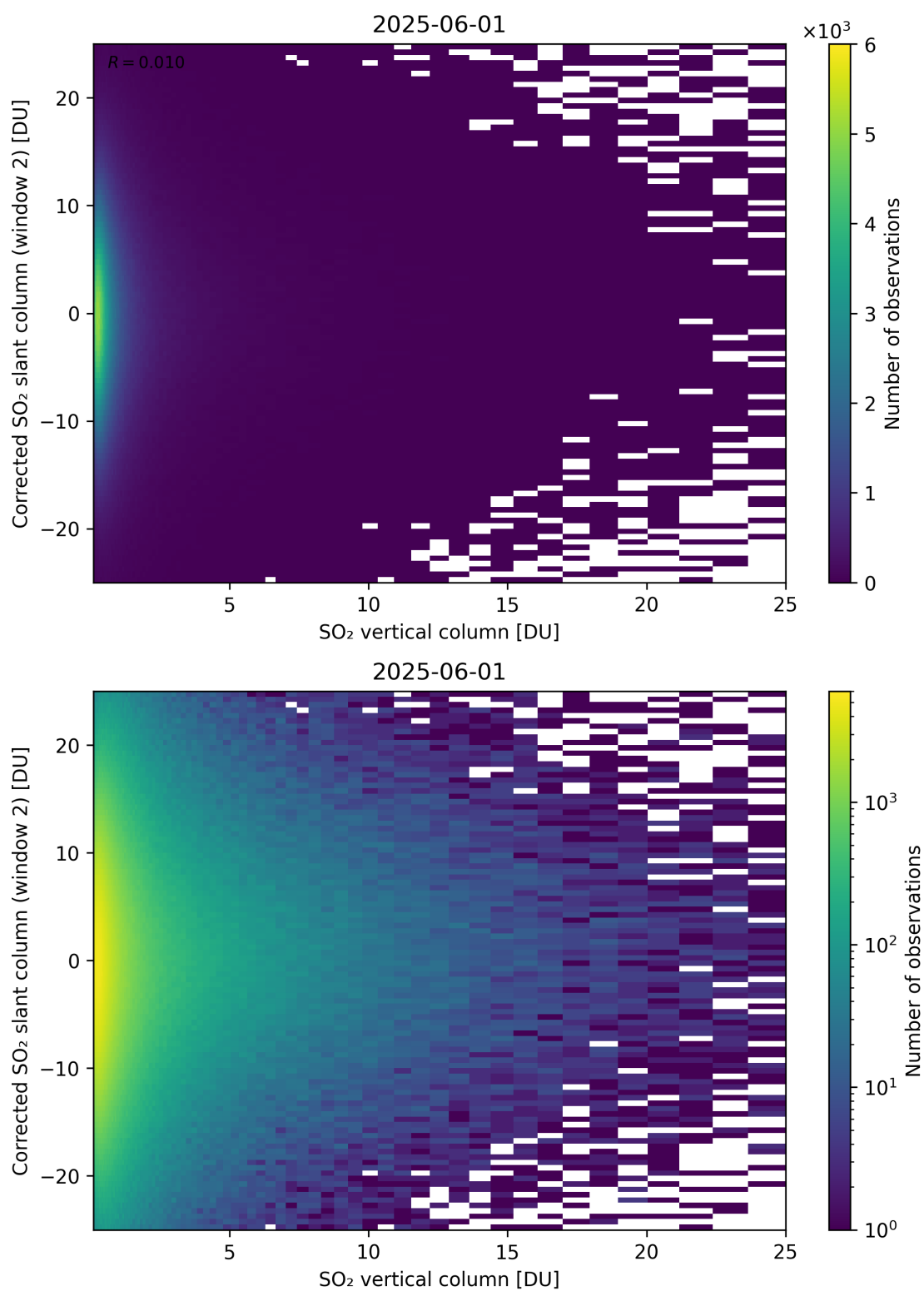
Figure 352: Scatter density plot of “SO 2 vertical column” against “Corrected SO 2 slant column (window 2)” for 2025-06-01 to 2025-06-02.
