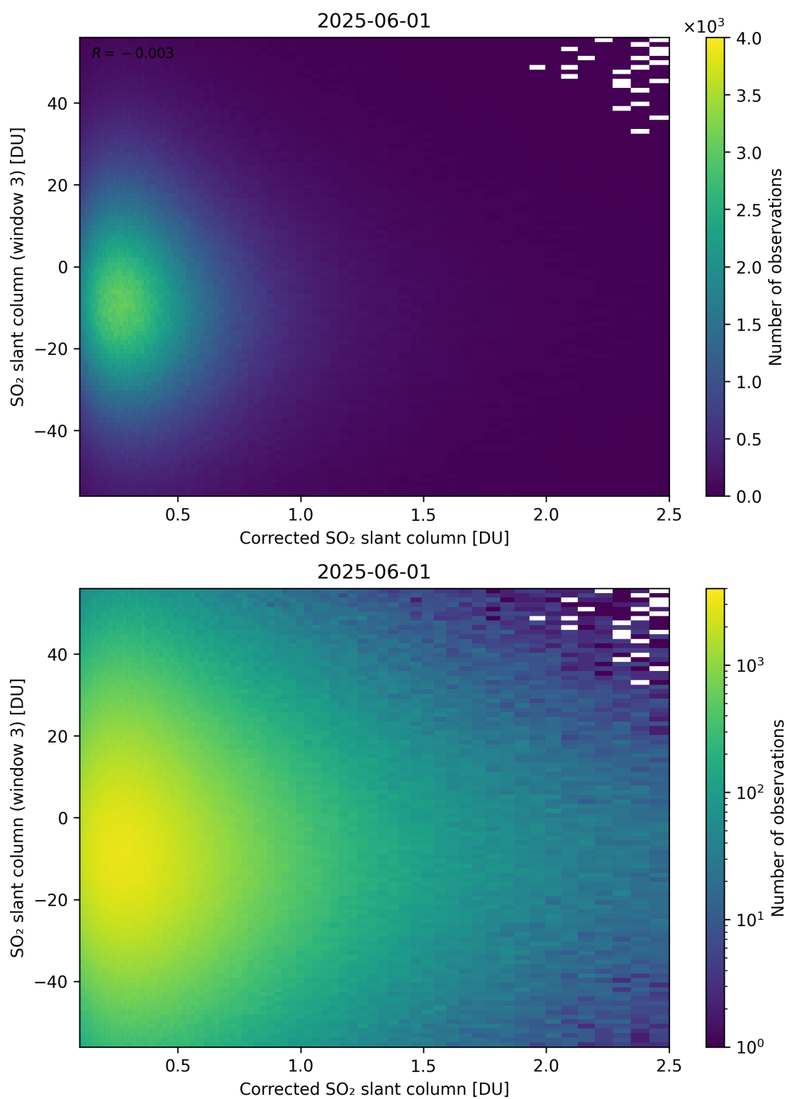
Figure 240: Scatter density plot of “Corrected SO 2 slant column” against “SO 2 slant column (window 3)” for 2025-06-01 to 2025-06-02.
