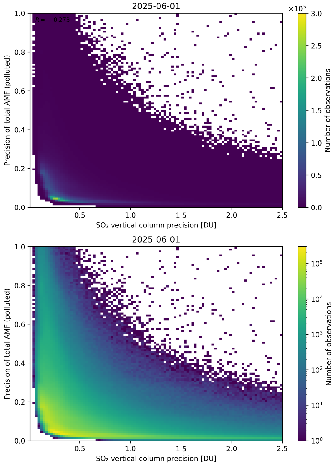
Figure 347: Scatter density plot of “SO 2 vertical column precision” against “Precision of total AMF (polluted)” for 2025-06-01 to 2025-06-02.
