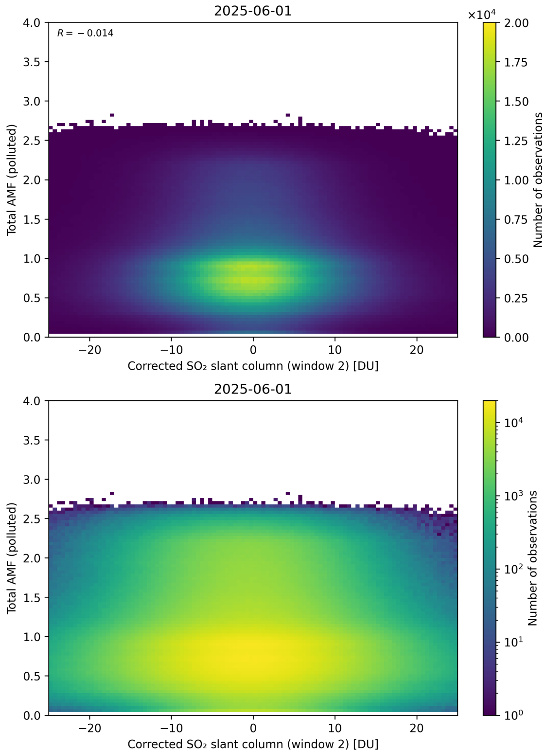
Figure 253: Scatter density plot of “Corrected SO 2 slant column (window 2)” against “Total AMF (polluted)” for 2025-06-01 to 2025-06-02.
