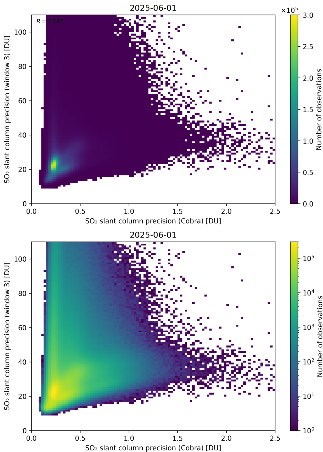
Figure 212: Scatter density plot of “SO 2 slant column precision (Cobra)” against “SO 2 slant column precision (window 3)” for 2025-06-01 to 2025-06-02.
