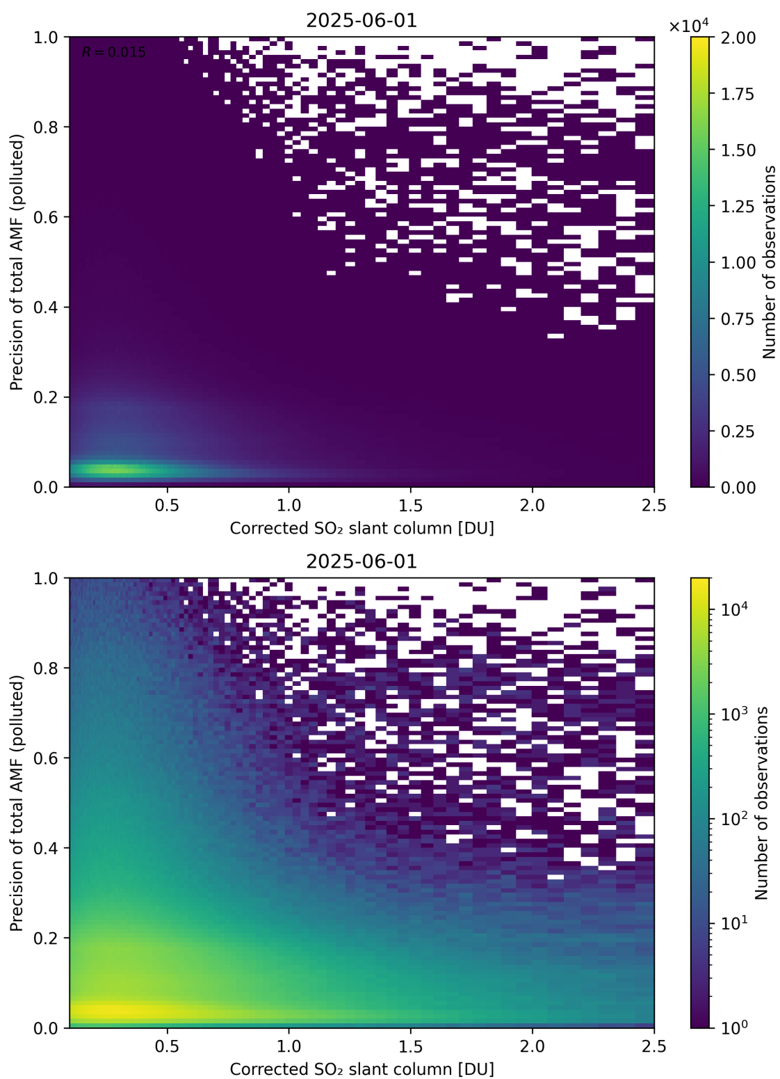
Figure 243: Scatter density plot of “Corrected SO 2 slant column” against “Precision of total AMF (polluted)” for 2025-06-01 to 2025-06-02.
