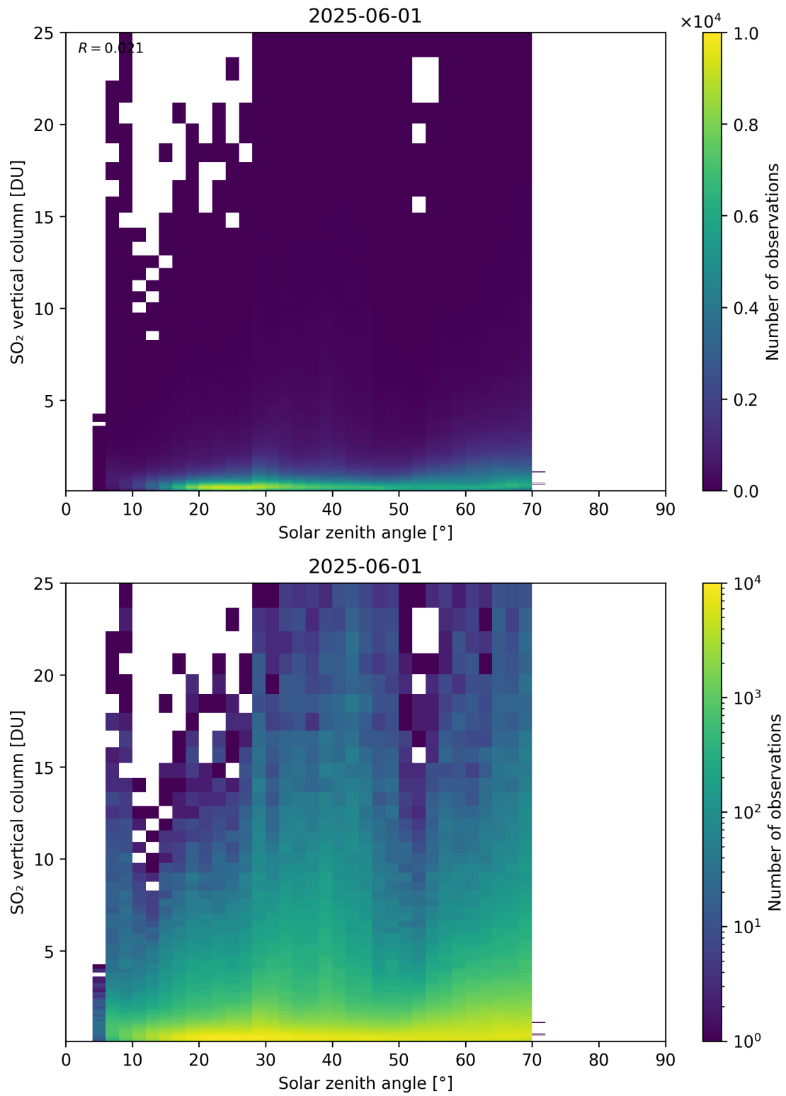
Figure 191: Scatter density plot of “Solar zenith angle” against “SO 2 vertical column” for 2025-06-01 to 2025-06-02.
