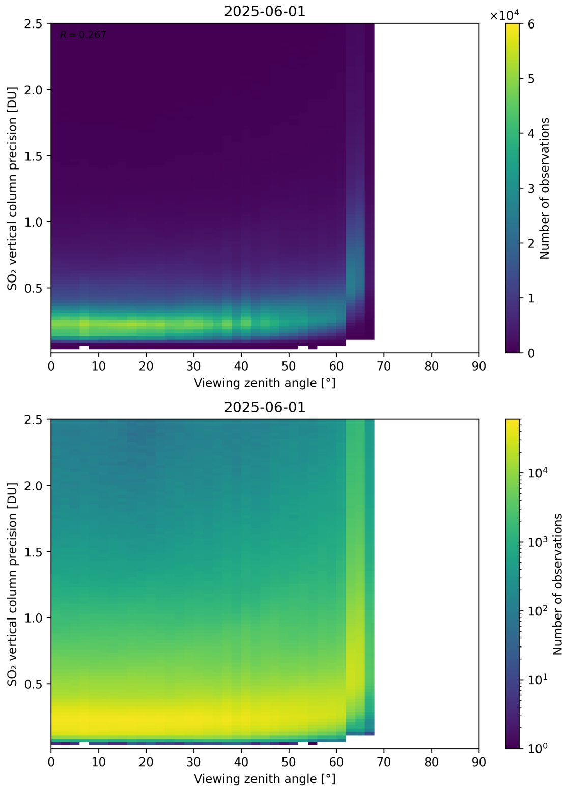
Figure 384: Scatter density plot of “Viewing zenith angle” against “SO 2 vertical column precision” for 2025-06-01 to 2025-06-02.
