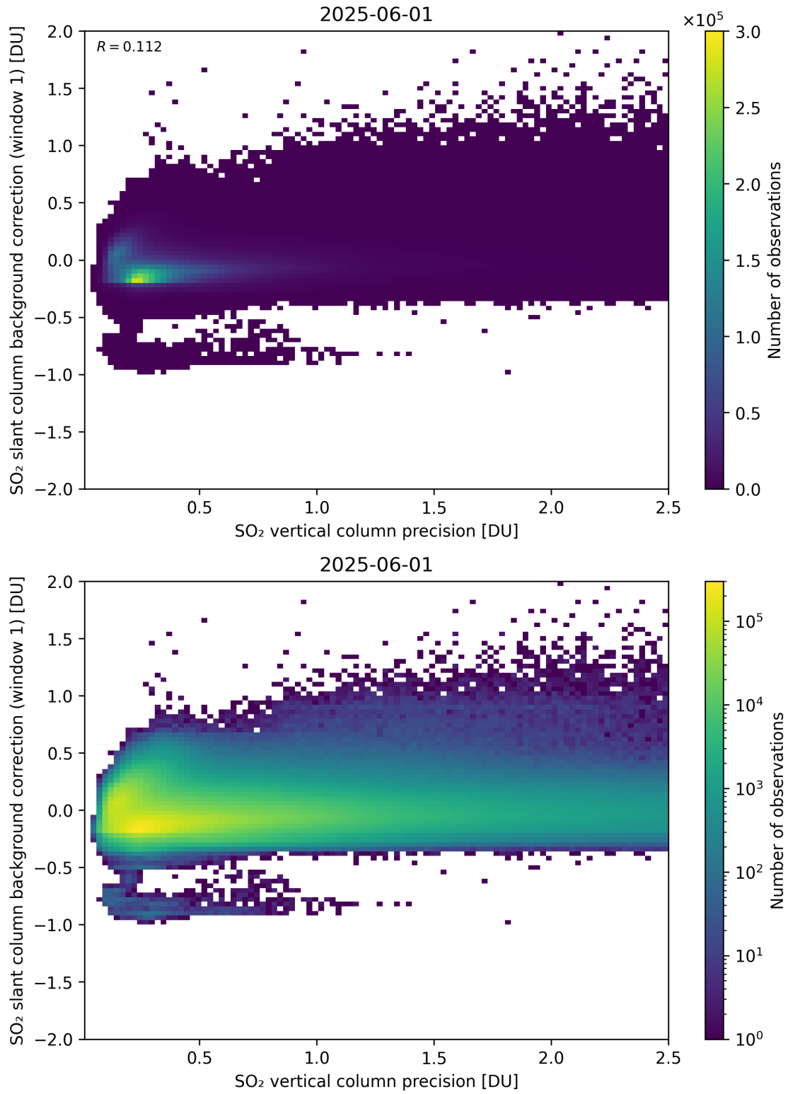
Figure 329: Scatter density plot of “SO 2 vertical column precision” against “SO 2 slant column background correction (window 1)” for 2025-06-01 to 2025-06-02.
