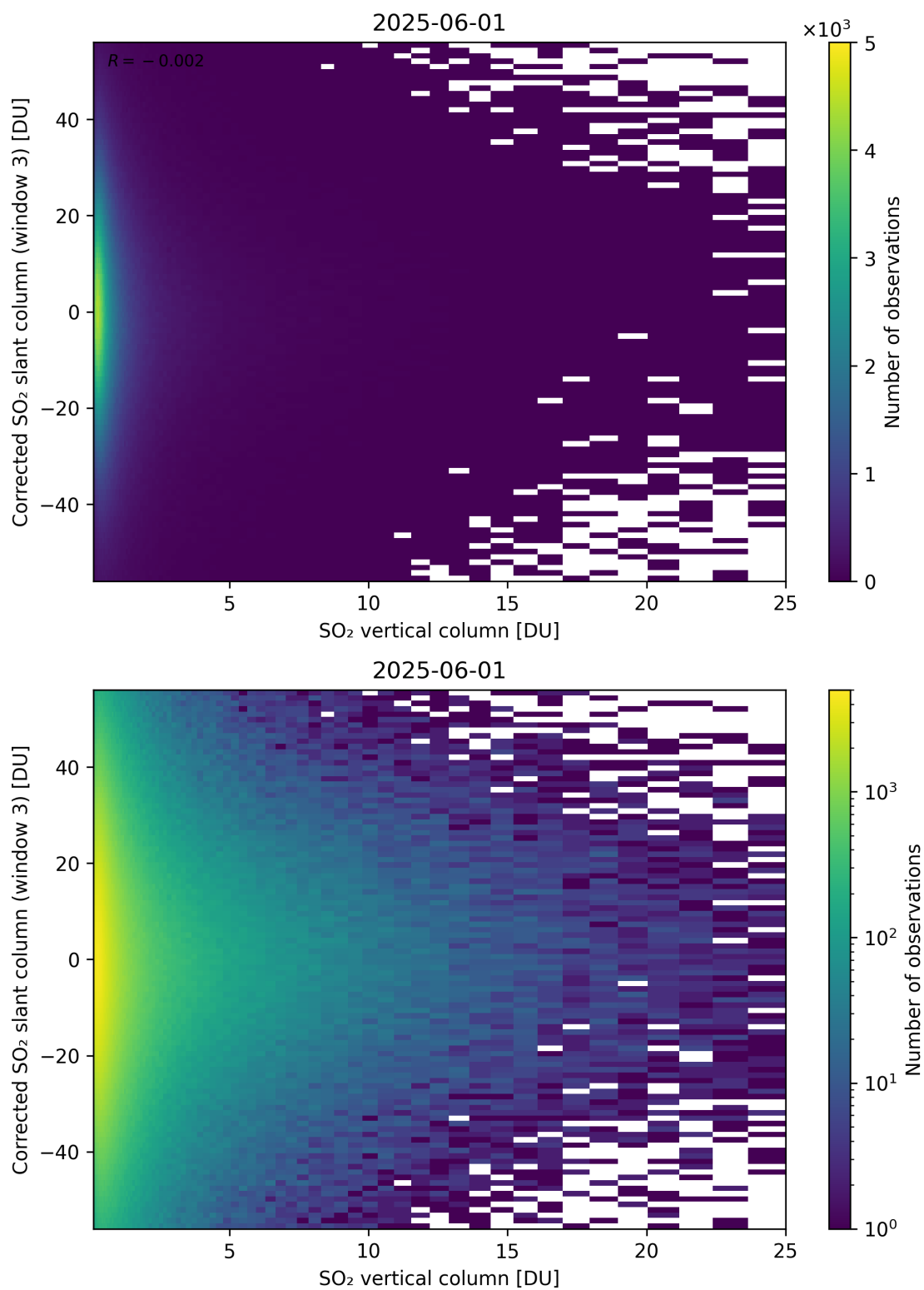
Figure 353: Scatter density plot of “SO 2 vertical column” against “Corrected SO 2 slant column (window 3)” for 2025-06-01 to 2025-06-02.
