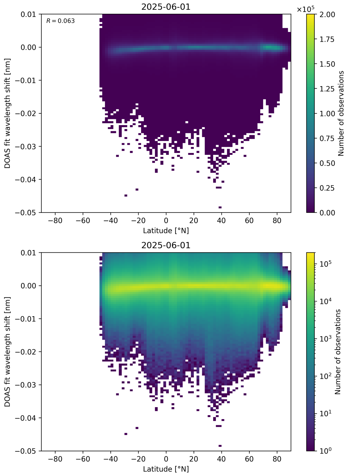
Figure 153: Scatter density plot of “Latitude” against “DOAS fit wavelength shift” for 2025-06-01 to 2025-06-02.
