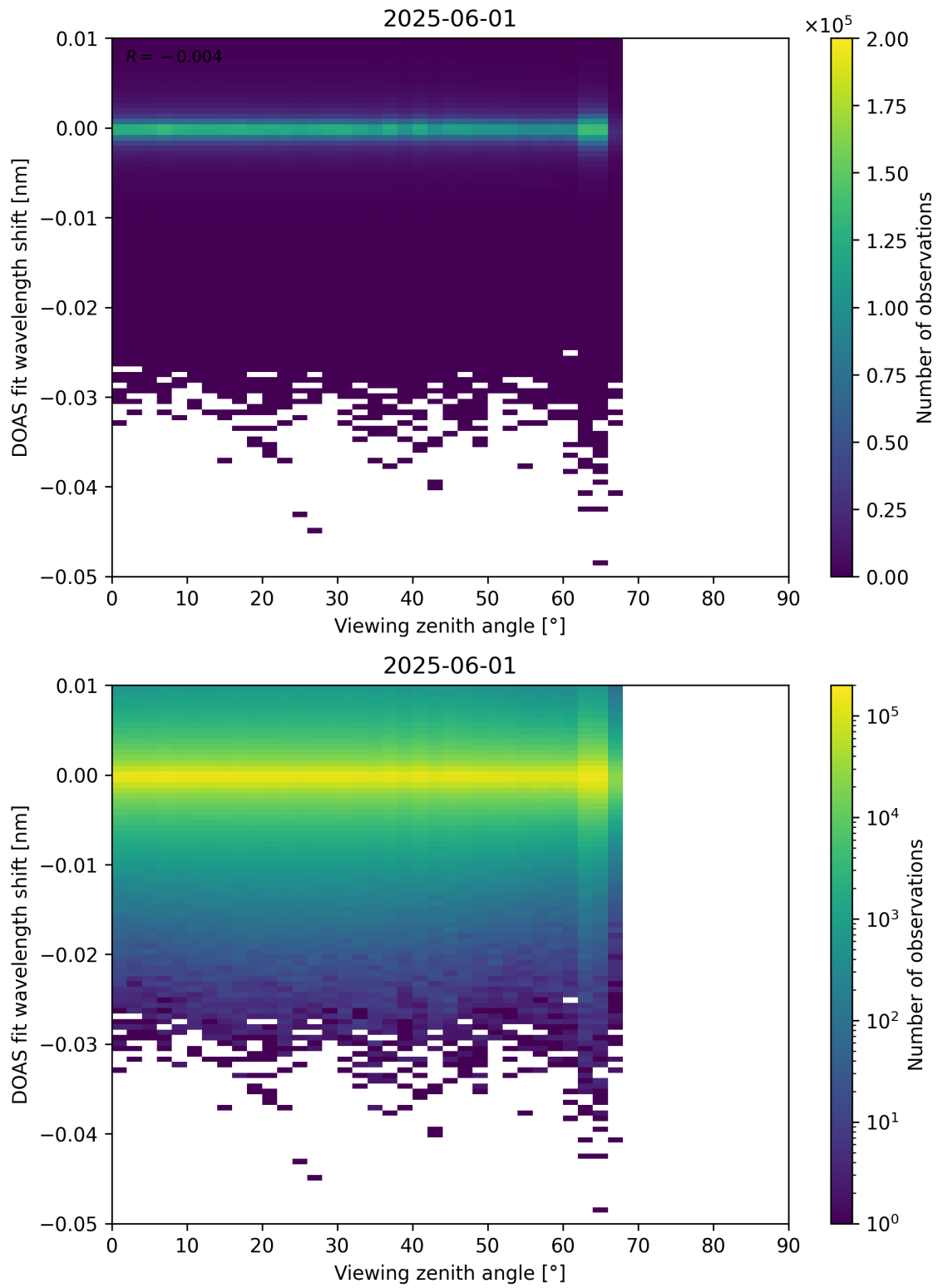
Figure 365: Scatter density plot of “Viewing zenith angle” against “DOAS fit wavelength shift” for 2025-06-01 to 2025-06-02.
