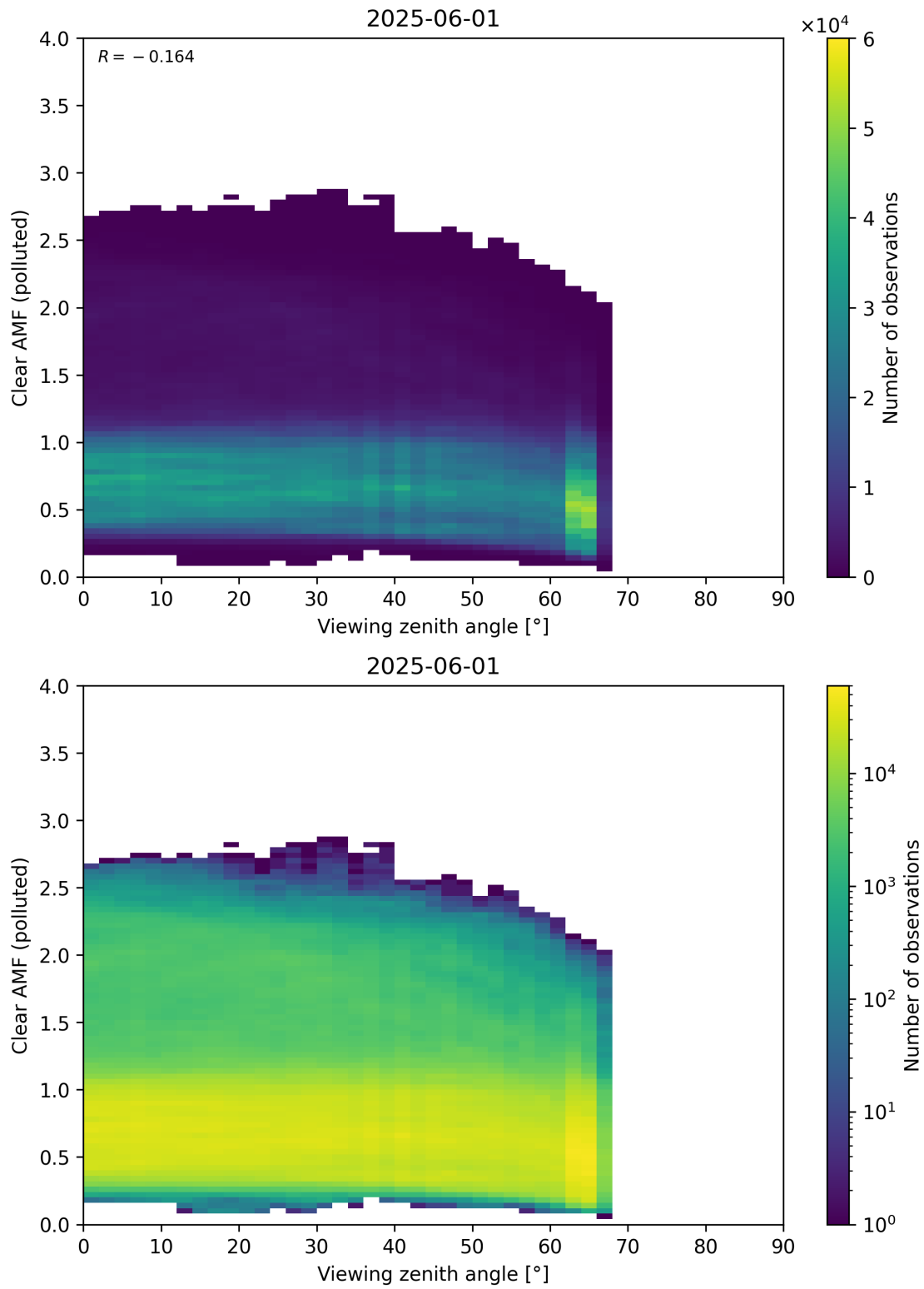
Figure 370: Scatter density plot of “Viewing zenith angle” against “Clear AMF (polluted)” for 2025-06-01 to 2025-06-02.
