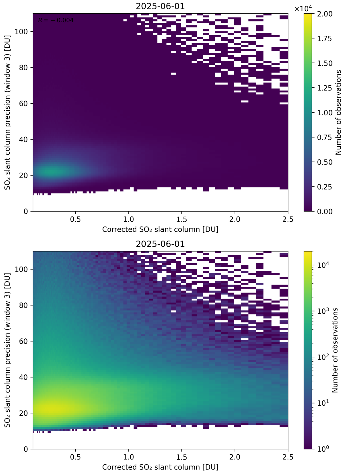
Figure 241: Scatter density plot of “Corrected SO 2 slant column” against “SO 2 slant column precision (window 3)” for 2025-06-01 to 2025-06-02.
