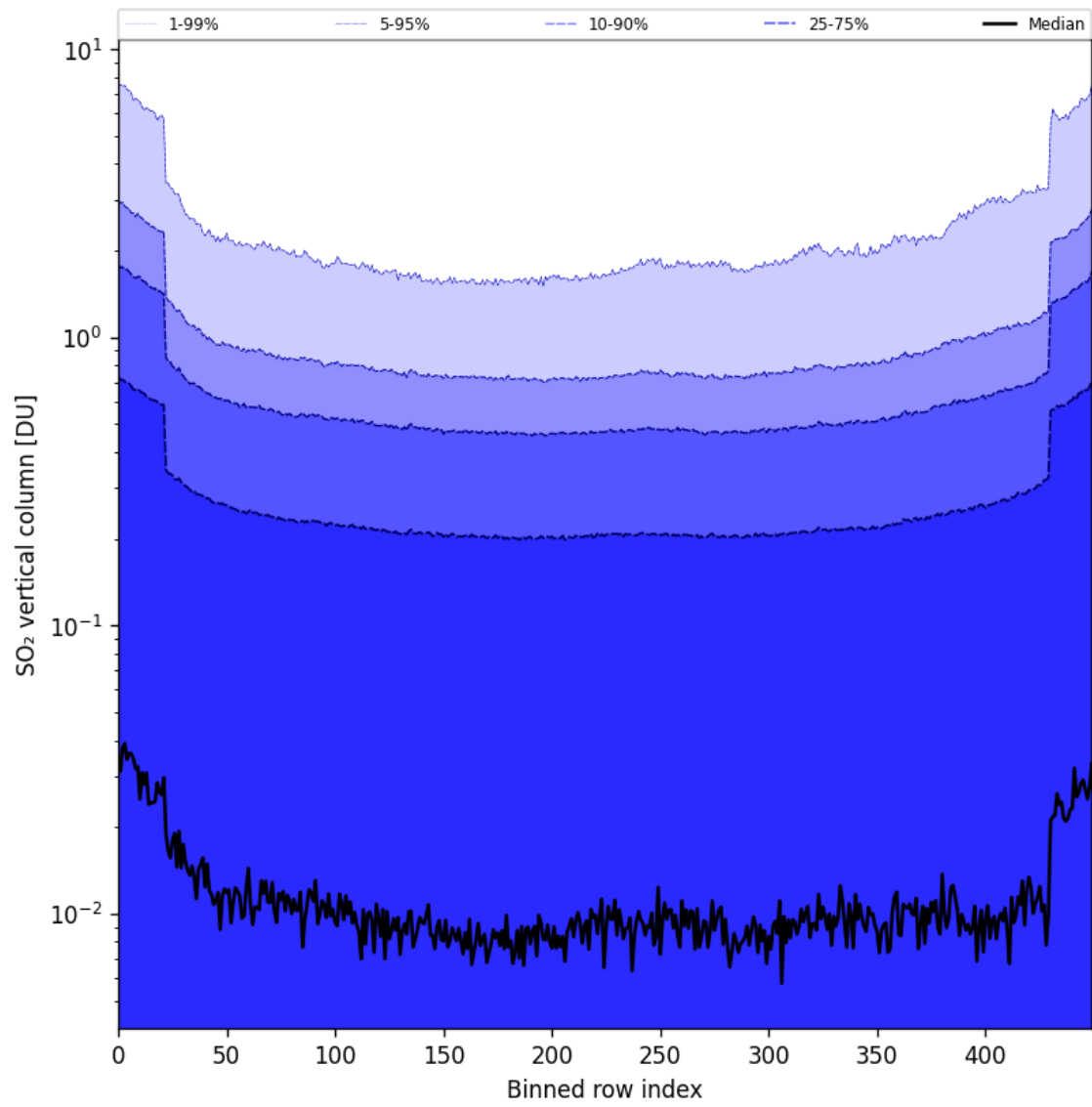
Figure 84: Along track statistics of “SO 2 vertical column” for 2025-06-01 to 2025-06-02
