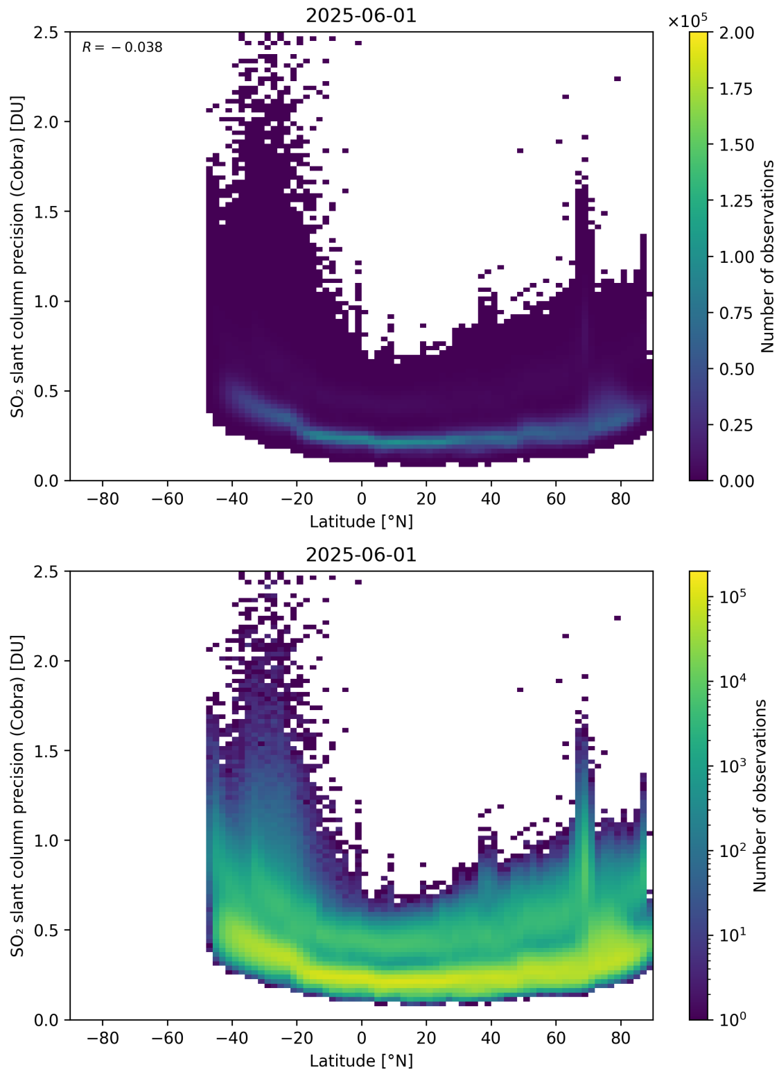
Figure 158: Scatter density plot of “Latitude” against “SO 2 slant column precision (Cobra)” for 2025-06-01 to 2025-06-02.
