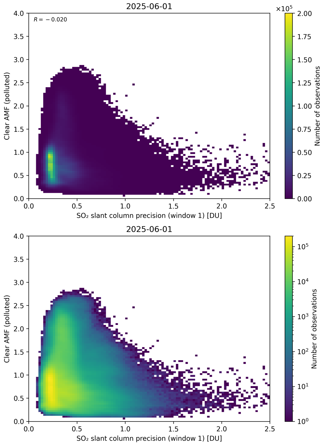
Figure 274: Scatter density plot of “SO 2 slant column precision (window 1)” against “Clear AMF (polluted)” for 2025-06-01 to 2025-06-02.
