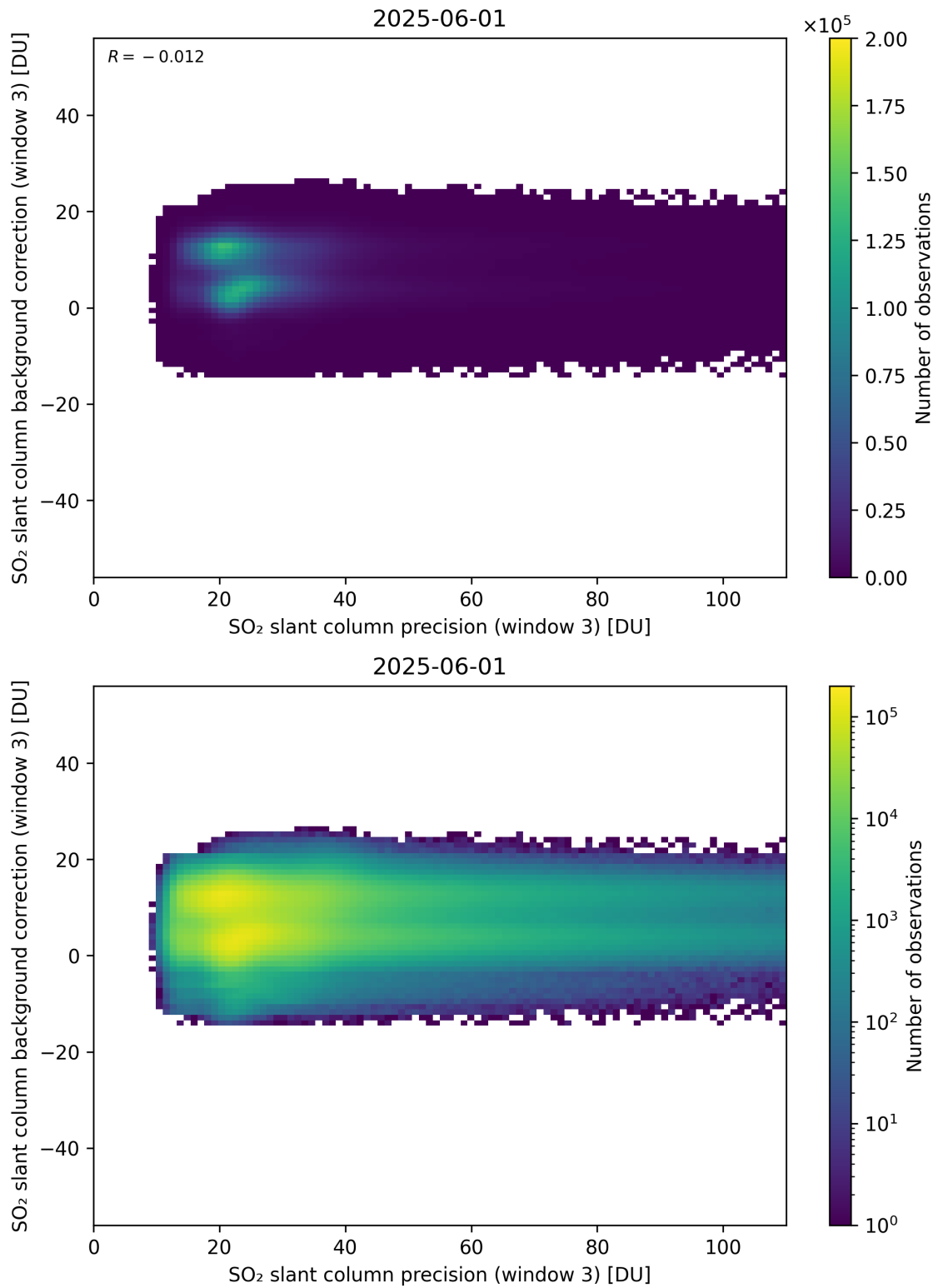
Figure 307: Scatter density plot of “SO 2 slant column precision (window 3)” against “SO 2 slant column background correction (window 3)” for 2025-06-01 to 2025-06-02.
