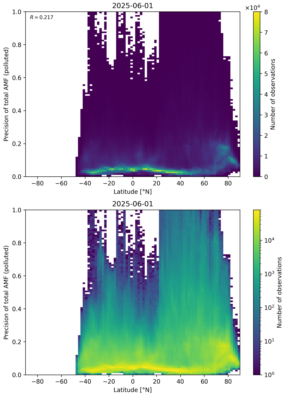
Figure 168: Scatter density plot of “Latitude” against “Precision of total AMF (polluted)” for 2025-06-01 to 2025-06-02.
