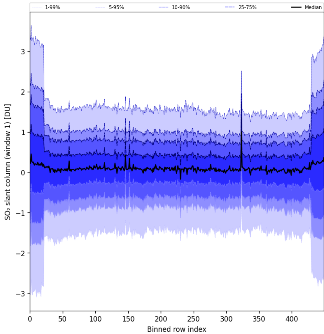
Figure 89: Along track statistics of “SO 2 slant column (window 1)” for 2025-06-01 to 2025-06-02
