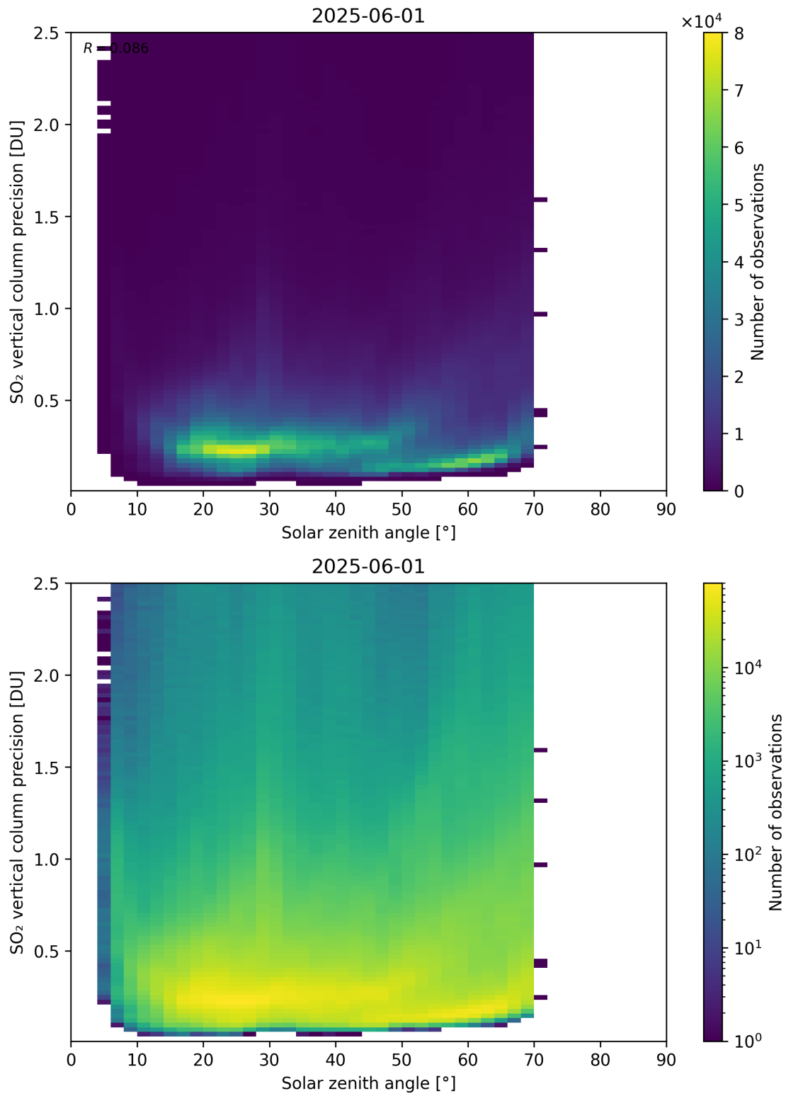
Figure 192: Scatter density plot of “Solar zenith angle” against “SO 2 vertical column precision” for 2025-06-01 to 2025-06-02.
