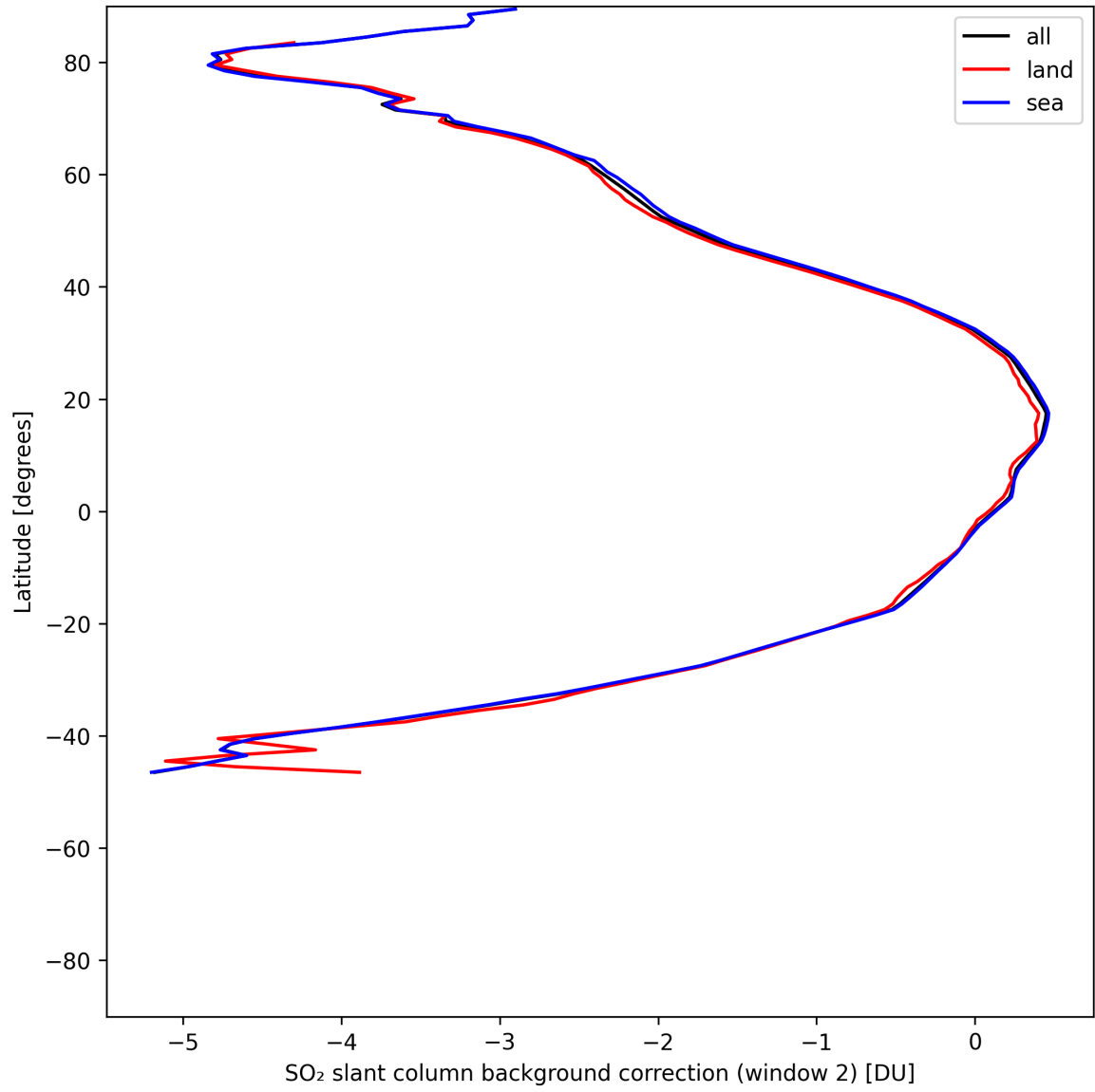
Figure 44: Zonal average of “SO 2 slant column background correction (window 2)” for 2025-06-01 to 2025-06-02.
