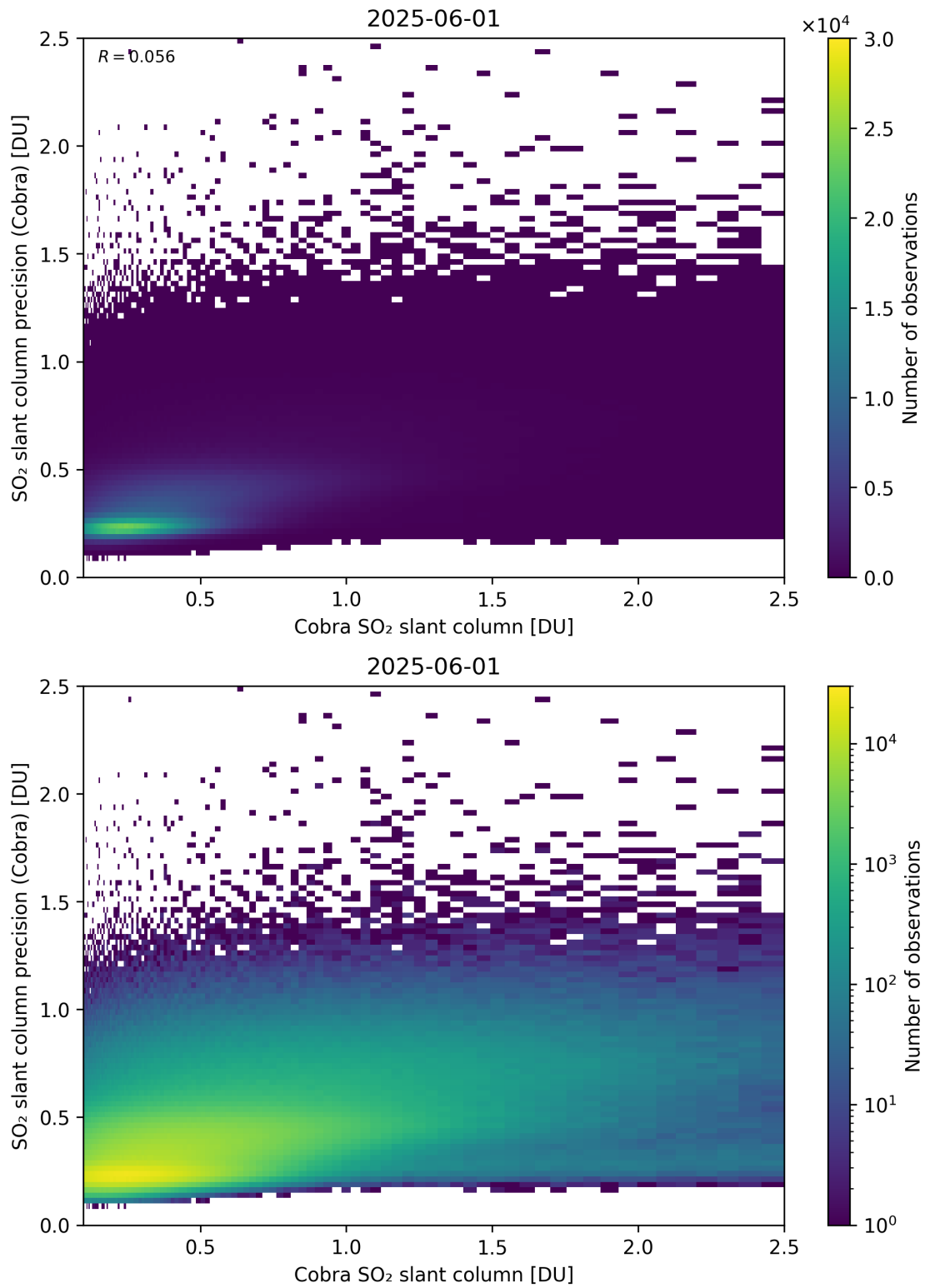
Figure 216: Scatter density plot of “Cobra SO 2 slant column” against “SO 2 slant column precision (Cobra)” for 2025-06-01 to 2025-06-02.
