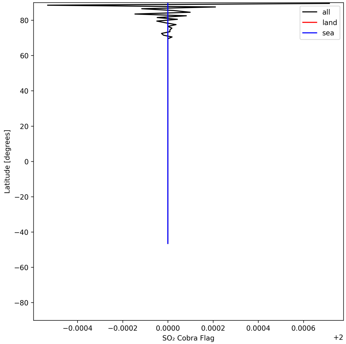
Figure 49: Zonal average of “SO 2 Cobra Flag” for 2025-06-01 to 2025-06-02.
