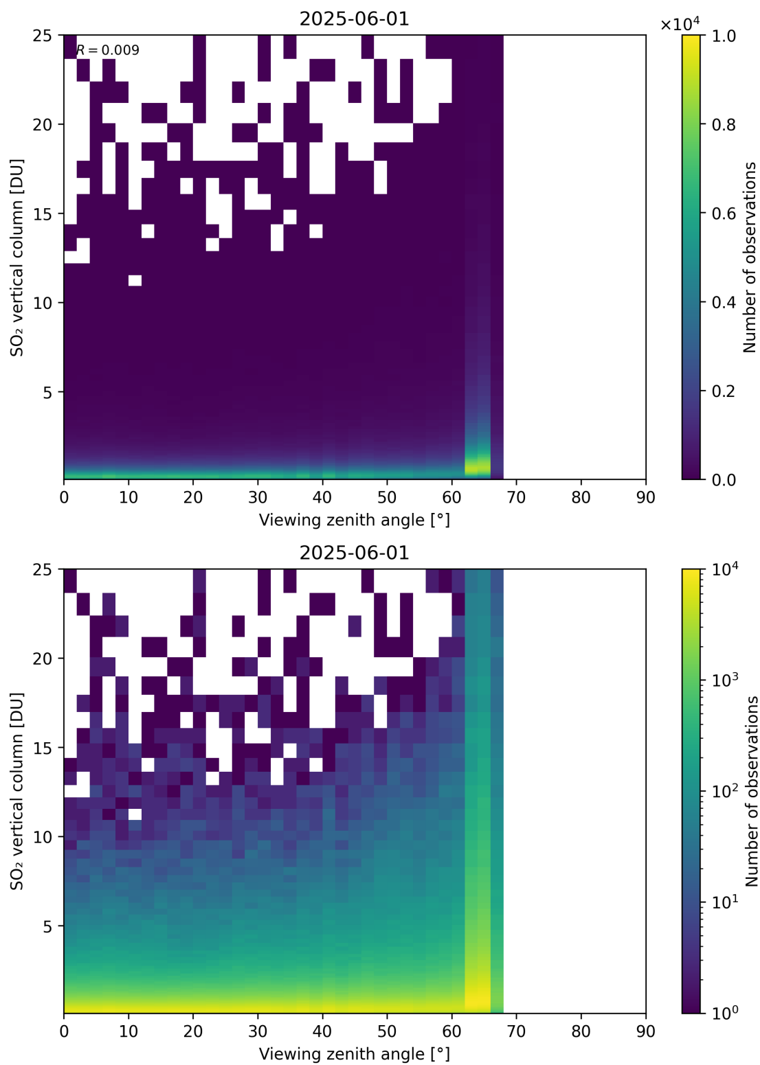
Figure 383: Scatter density plot of “Viewing zenith angle” against “SO 2 vertical column” for 2025-06-01 to 2025-06-02.
