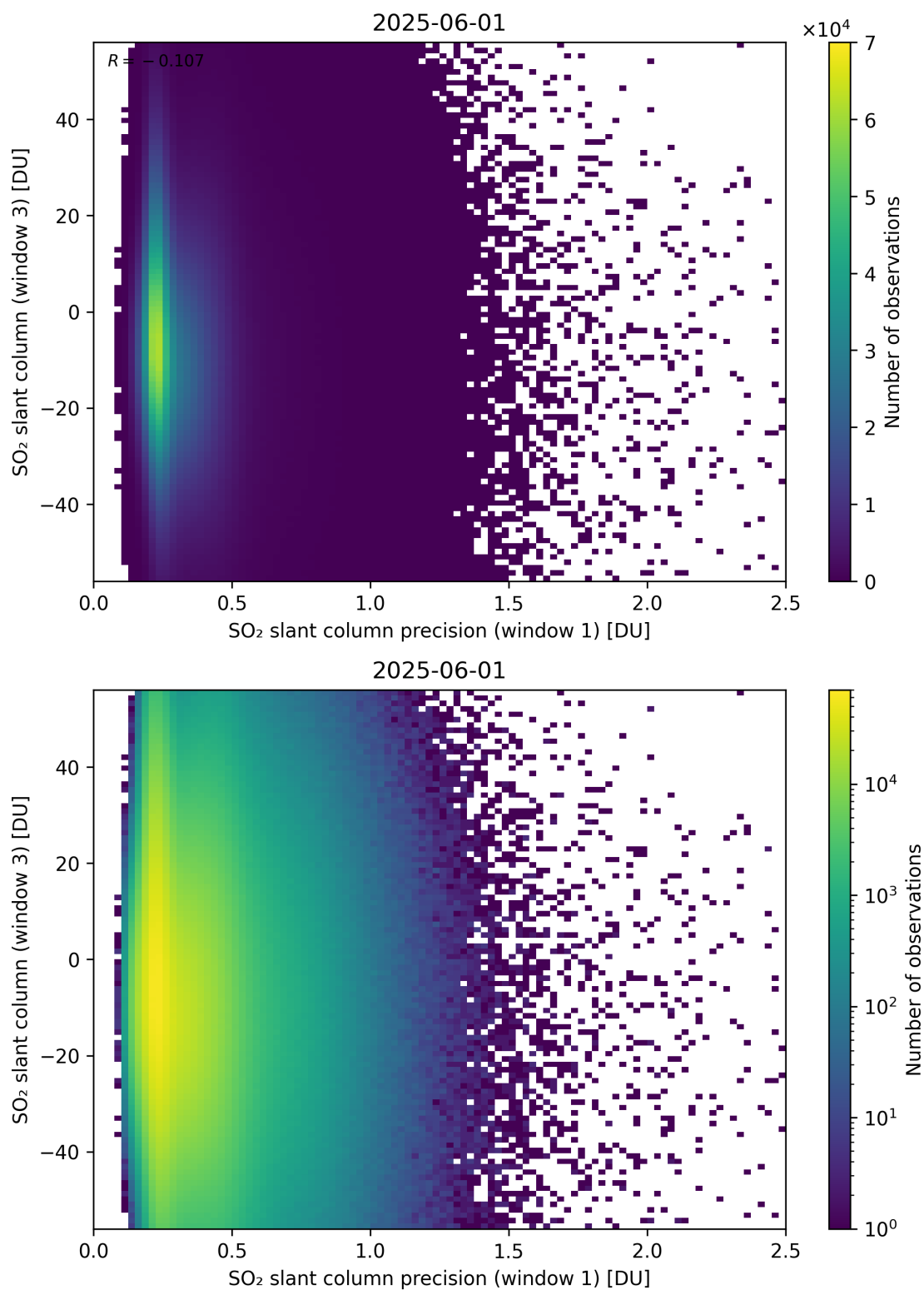
Figure 278: Scatter density plot of “SO 2 slant column precision (window 1)” against “SO 2 slant column (window 3)” for 2025-06-01 to 2025-06-02.
