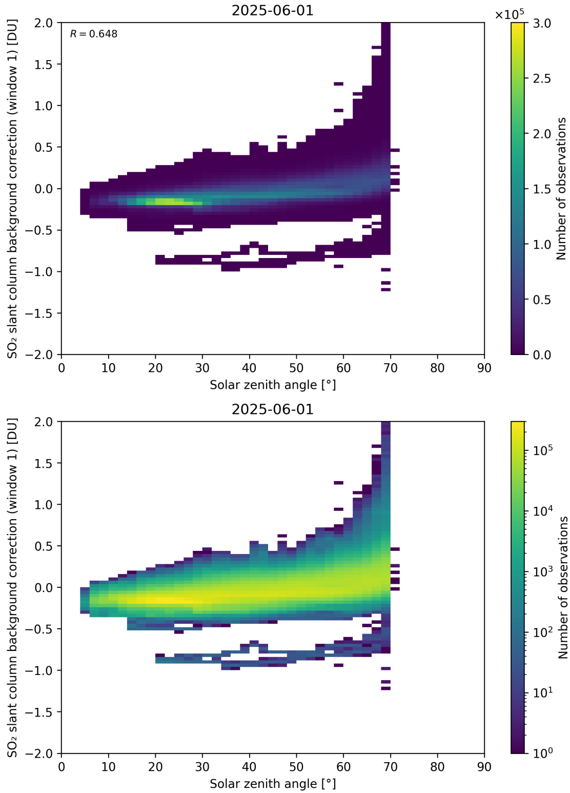
Figure 171: Scatter density plot of “Solar zenith angle” against “SO 2 slant column background correction (window 1)” for 2025-06-01 to 2025-06-02.
