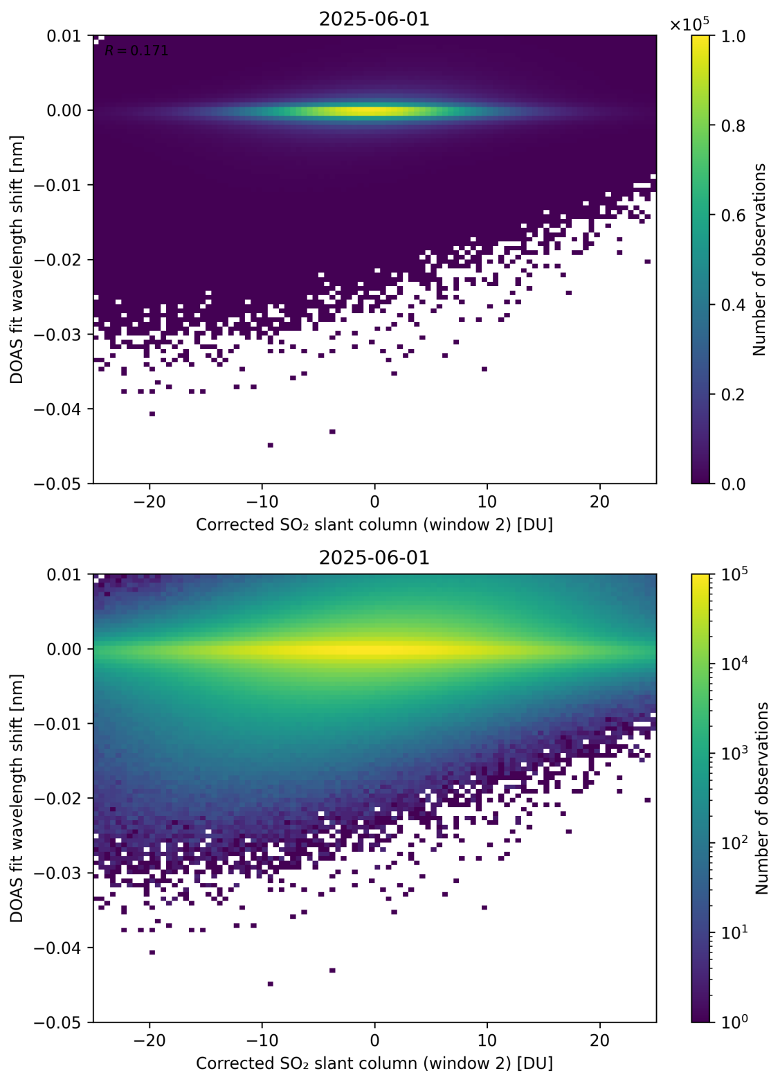
Figure 246: Scatter density plot of “Corrected SO 2 slant column (window 2)” against “DOAS fit wavelength shift” for 2025-06-01 to 2025-06-02.
