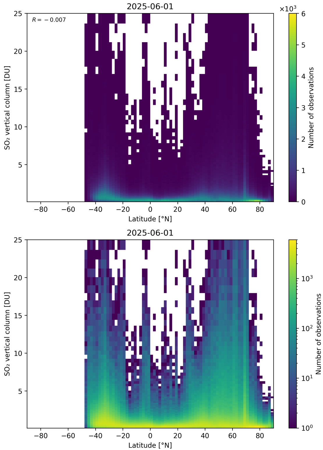
Figure 169: Scatter density plot of “Latitude” against “SO 2 vertical column” for 2025-06-01 to 2025-06-02.
