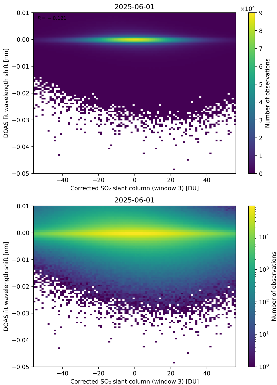
Figure 256: Scatter density plot of “Corrected SO 2 slant column (window 3)” against “DOAS fit wavelength shift” for 2025-06-01 to 2025-06-02.
