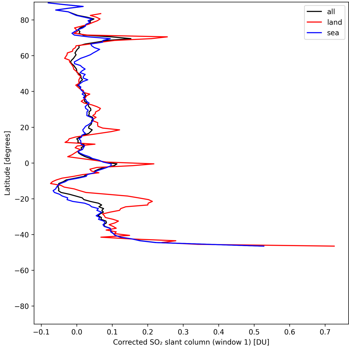
Figure 39: Zonal average of “Corrected SO 2 slant column (window 1)” for 2025-06-01 to 2025-06-02.
