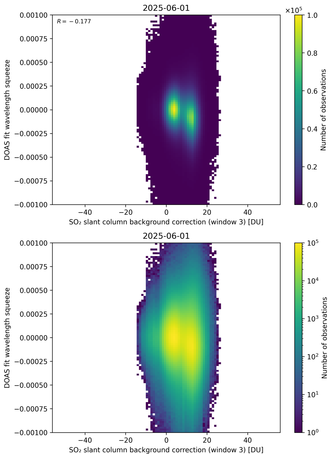
Figure 133: Scatter density plot of “SO 2 slant column background correction (window 3)” against “DOAS fit wavelength squeeze” for 2025-06-01 to 2025-06-02.
