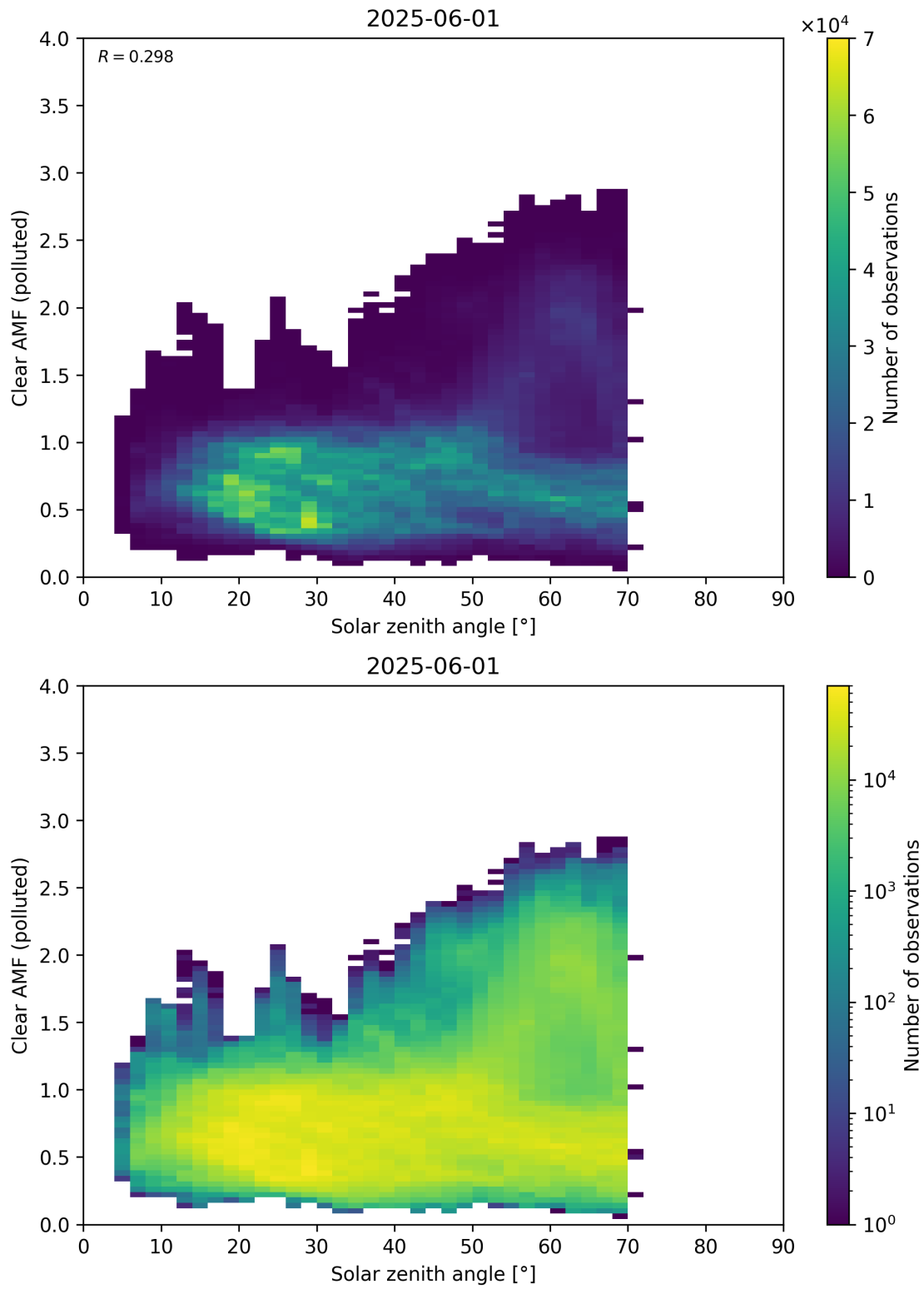
Figure 178: Scatter density plot of “Solar zenith angle” against “Clear AMF (polluted)” for 2025-06-01 to 2025-06-02.
