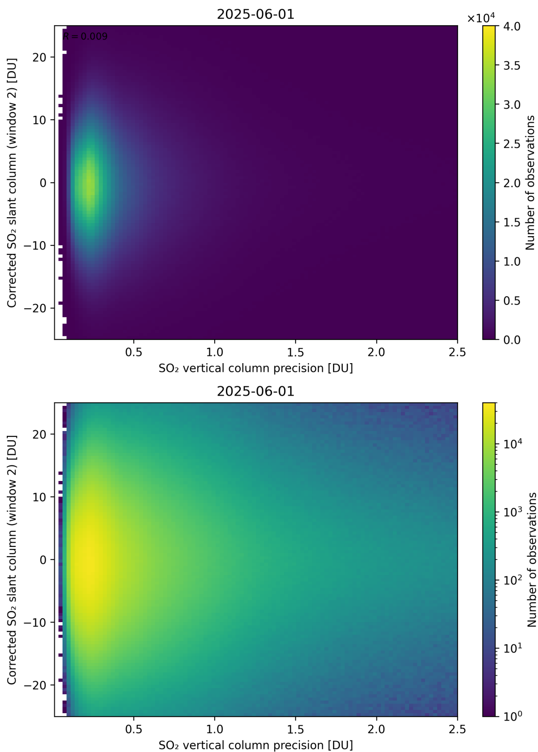
Figure 339: Scatter density plot of “SO 2 vertical column precision” against “Corrected SO 2 slant column (window 2)” for 2025-06-01 to 2025-06-02.
