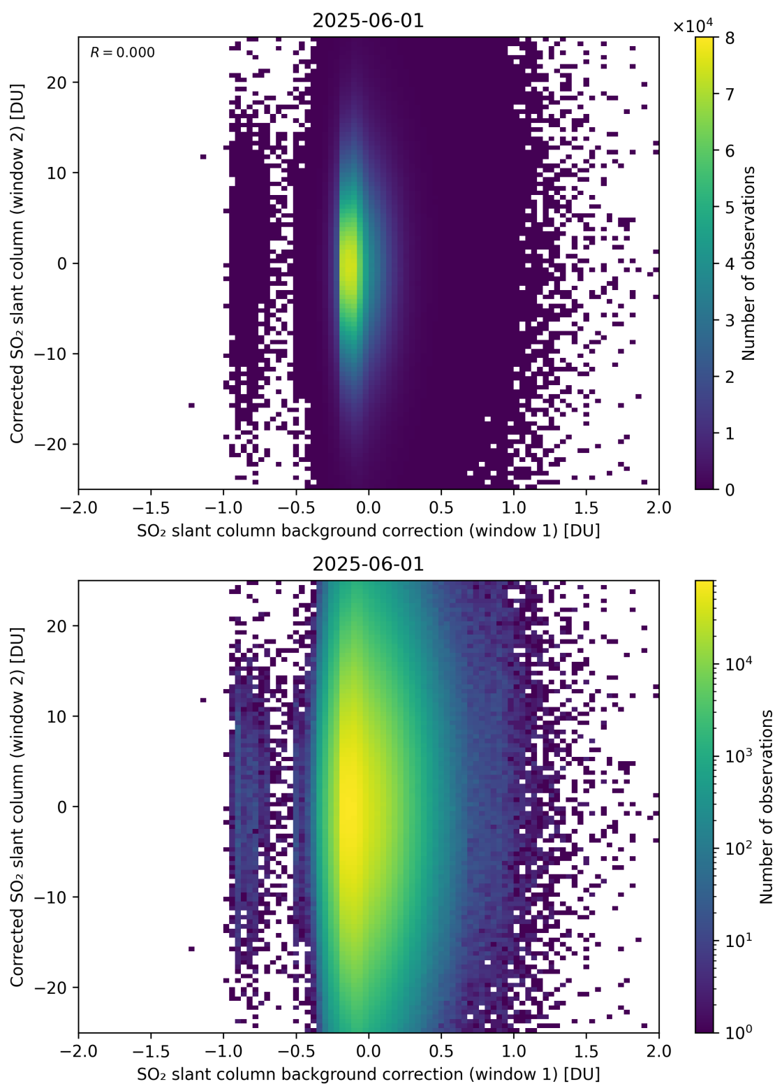
Figure 115: Scatter density plot of “SO 2 slant column background correction (window 1)” against “Corrected SO 2 slant column (window 2)” for 2025-06-01 to 2025-06-02.
