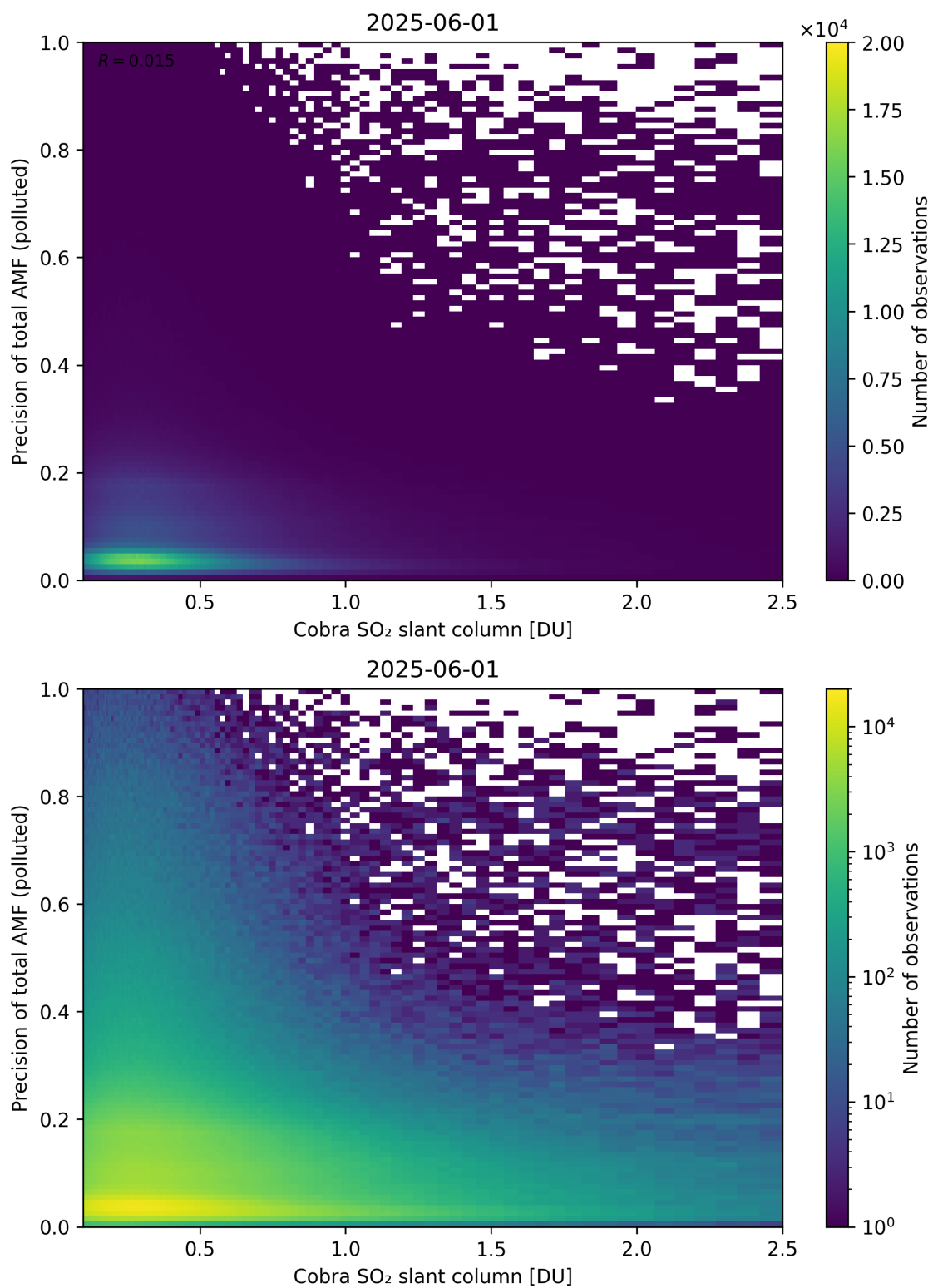
Figure 225: Scatter density plot of “Cobra SO 2 slant column” against “Precision of total AMF (polluted)” for 2025-06-01 to 2025-06-02.
