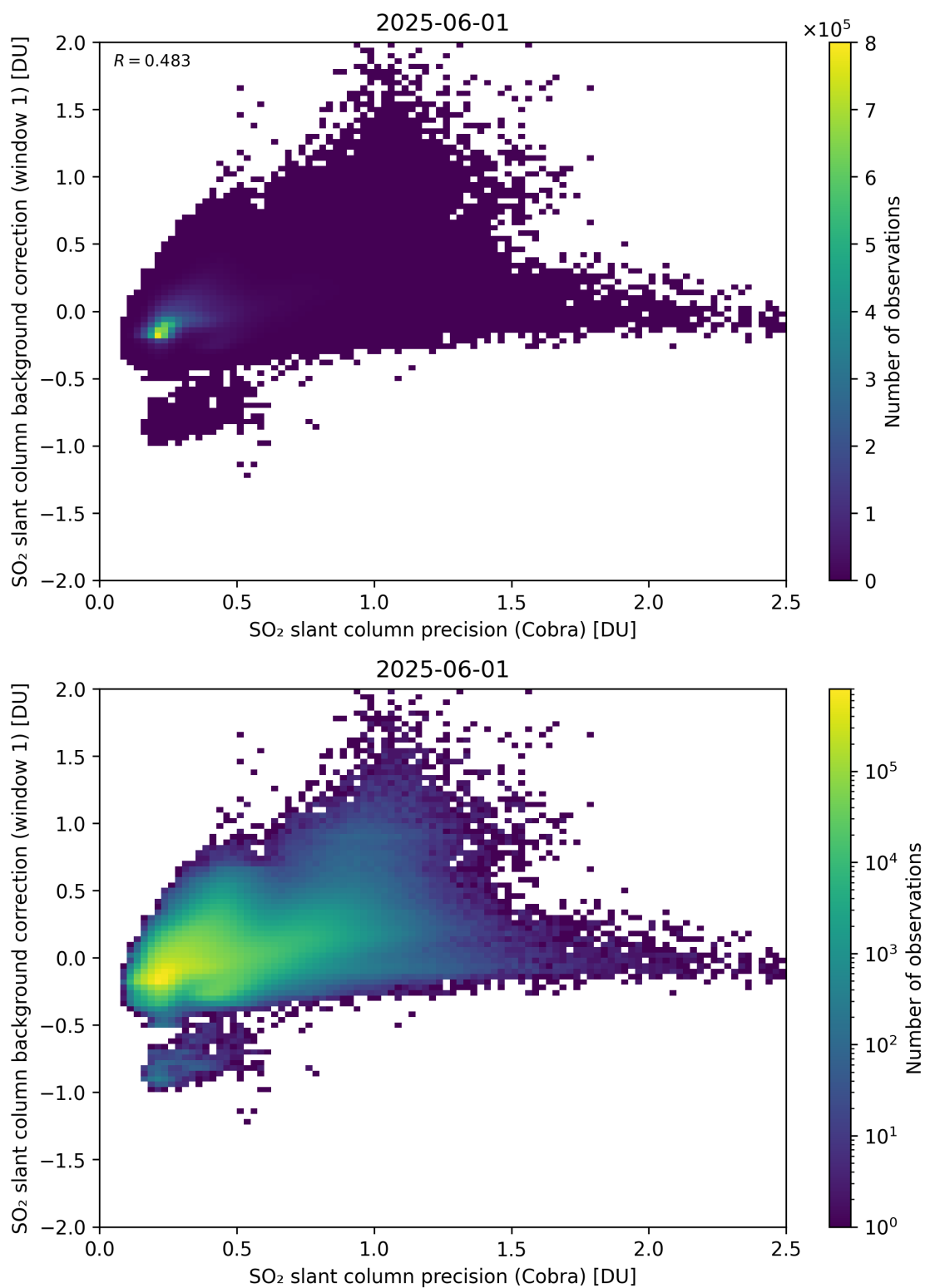
Figure 199: Scatter density plot of “SO 2 slant column precision (Cobra)” against “SO 2 slant column background correction (window 1)” for 2025-06-01 to 2025-06-02.
