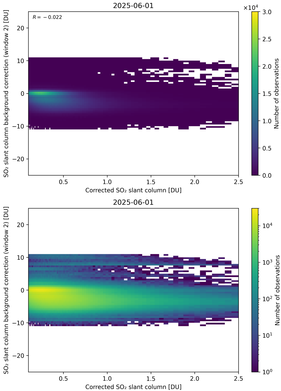
Figure 227: Scatter density plot of “Corrected SO 2 slant column” against “SO 2 slant column background correction (window 2)” for 2025-06-01 to 2025-06-02.
