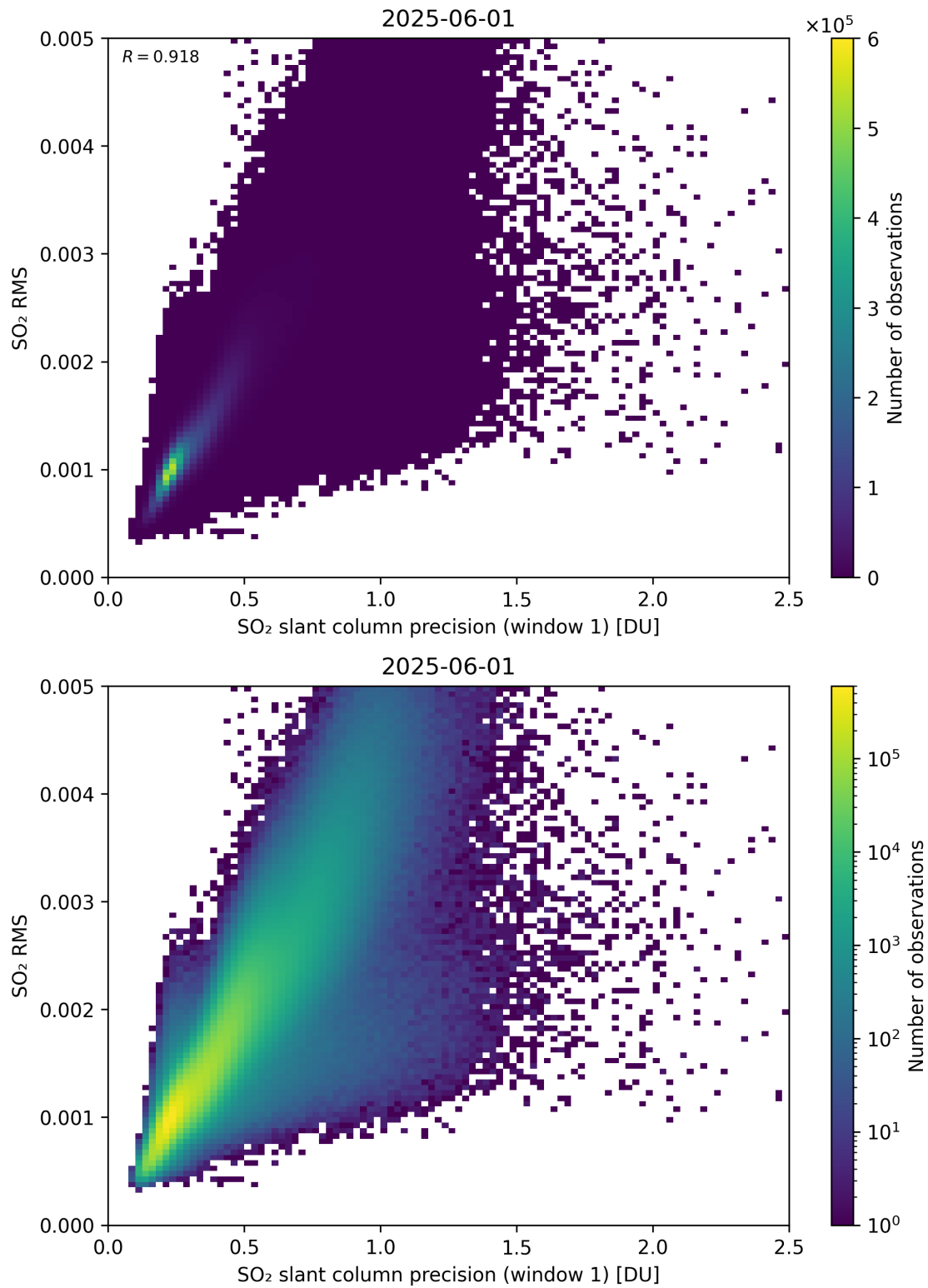
Figure 273: Scatter density plot of “SO 2 slant column precision (window 1)” against “SO 2 RMS” for 2025-06-01 to 2025-06-02.
