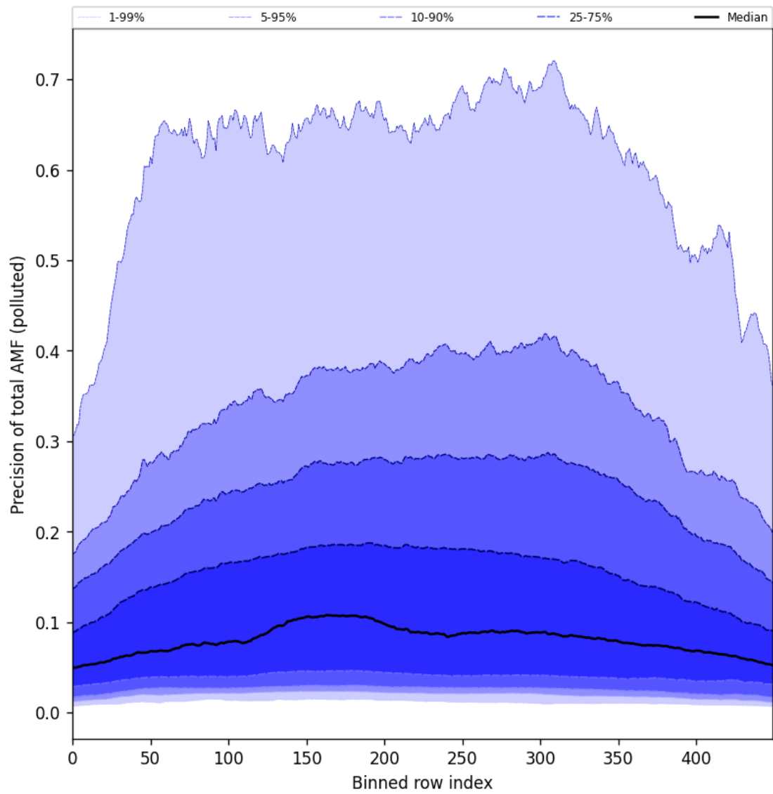
Figure 106: Along track statistics of “Precision of total AMF (polluted)” for 2025-06-01 to 2025-06-02
