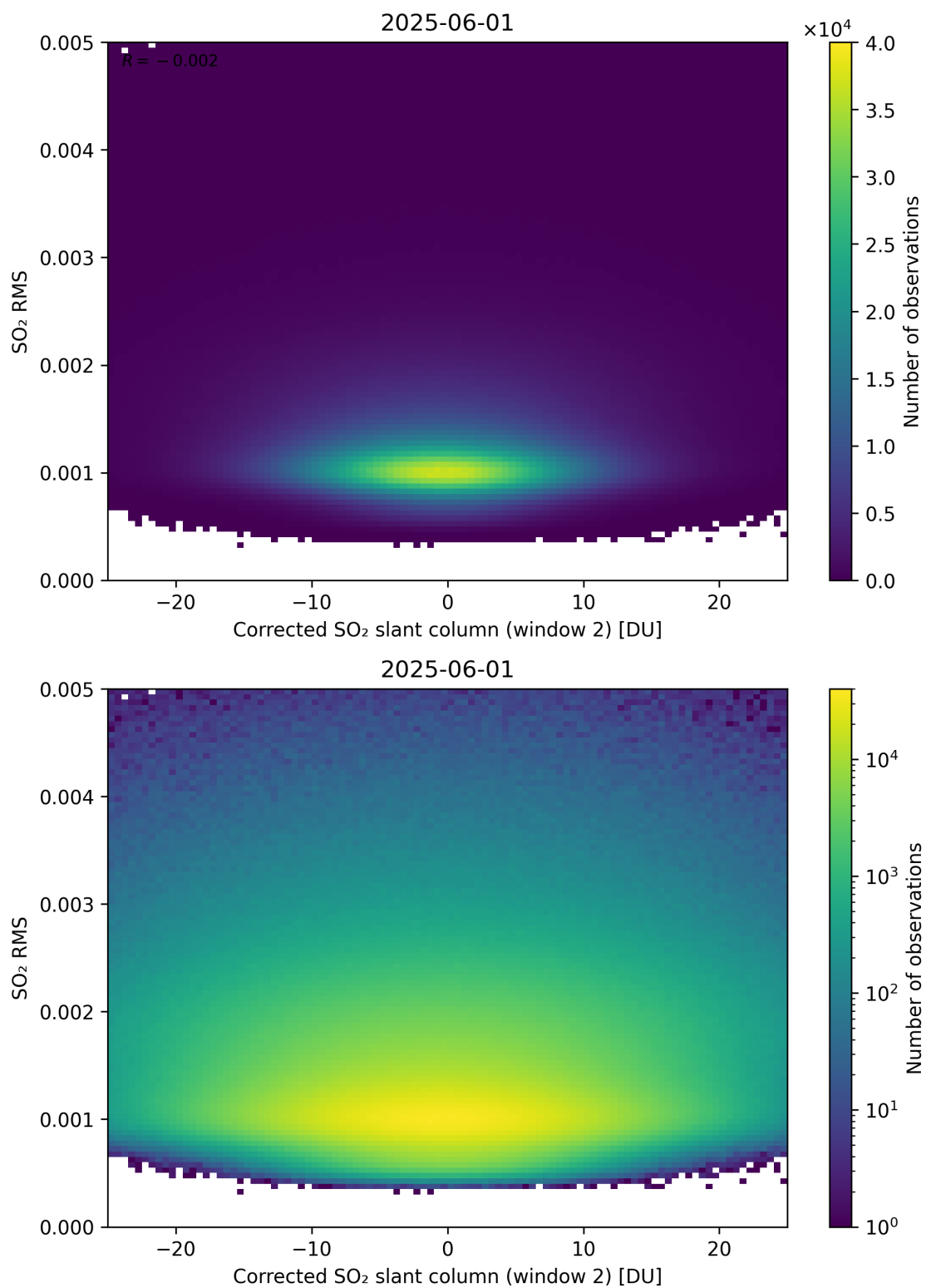
Figure 248: Scatter density plot of “Corrected SO 2 slant column (window 2)” against “SO 2 RMS” for 2025-06-01 to 2025-06-02.
