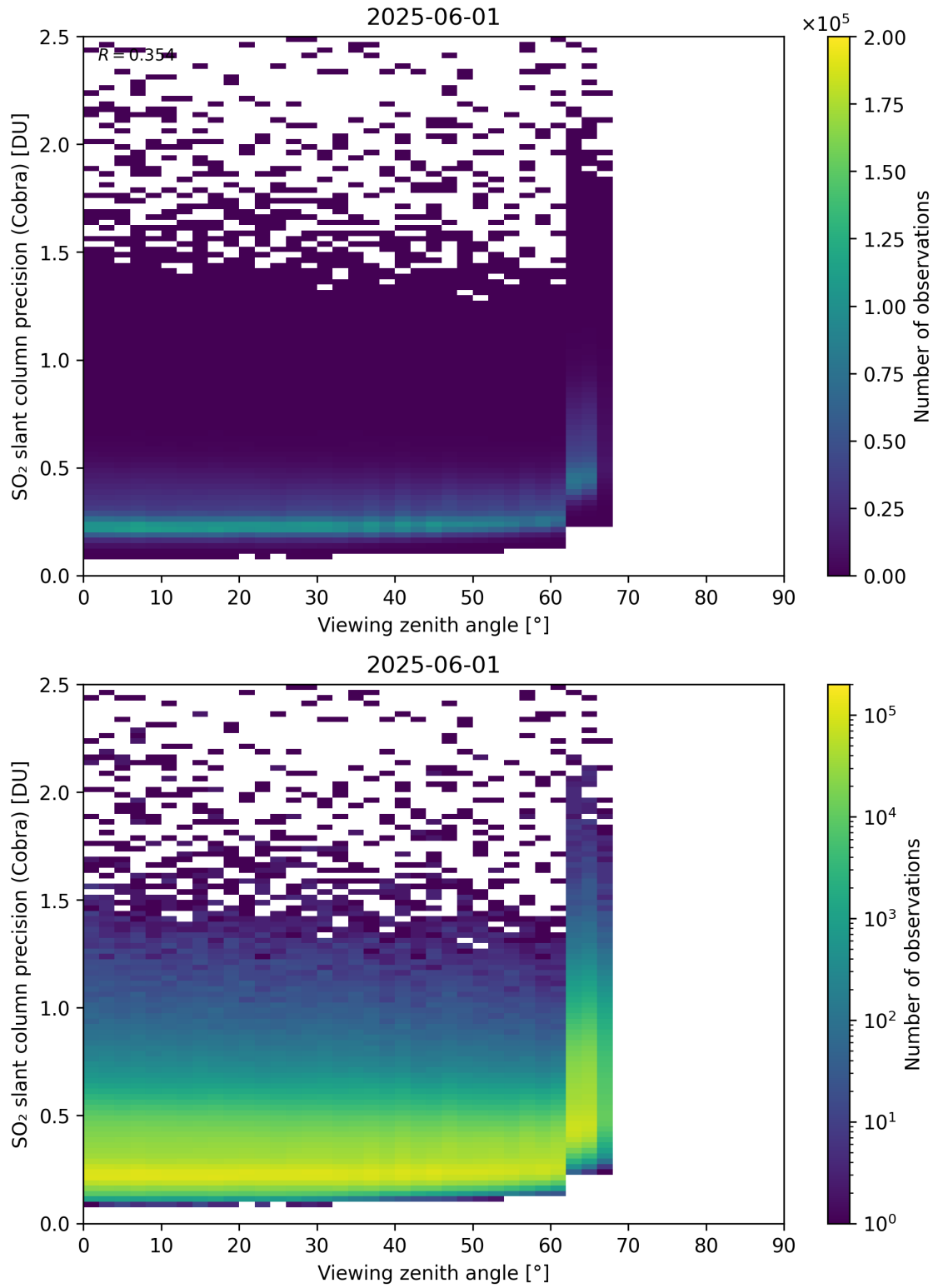
Figure 372: Scatter density plot of “Viewing zenith angle” against “SO 2 slant column precision (Cobra)” for 2025-06-01 to 2025-06-02.
