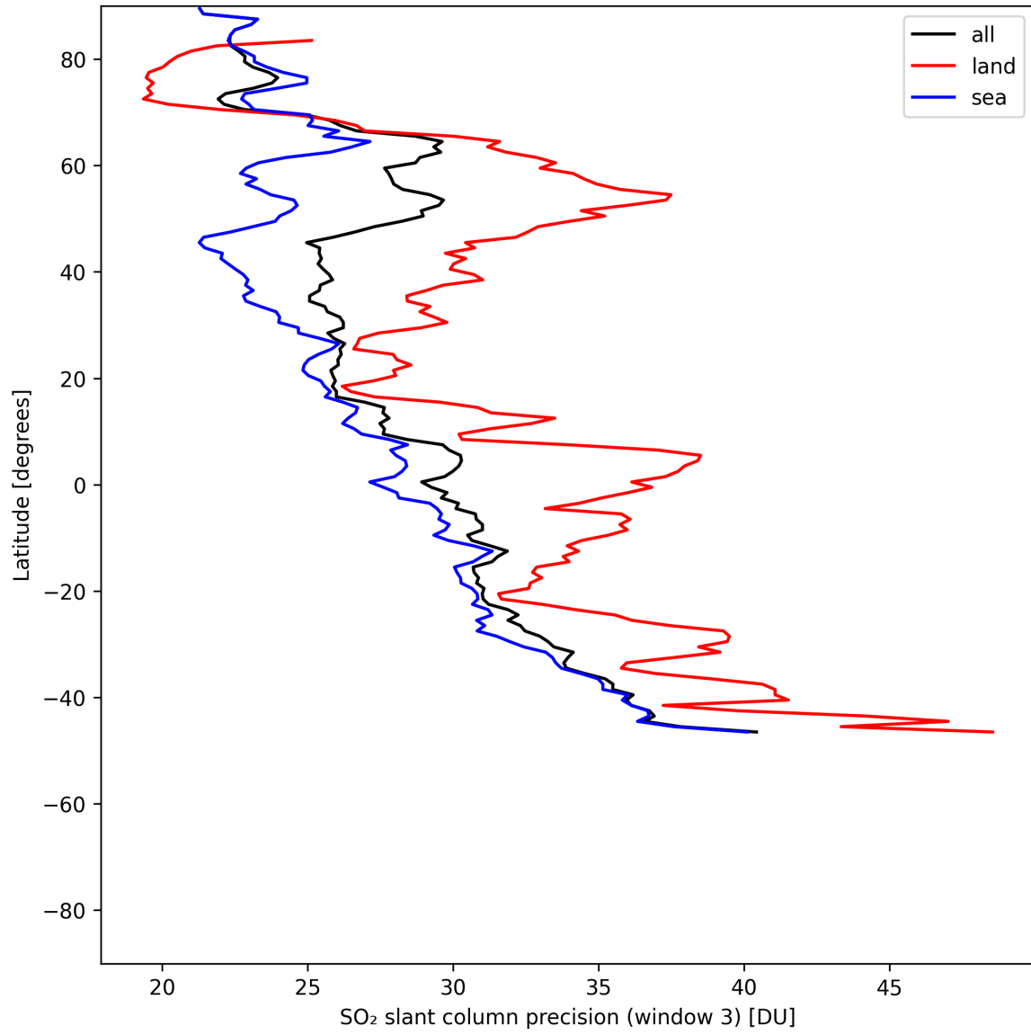
Figure 46: Zonal average of “SO 2 slant column precision (window 3)” for 2025-06-01 to 2025-06-02.
