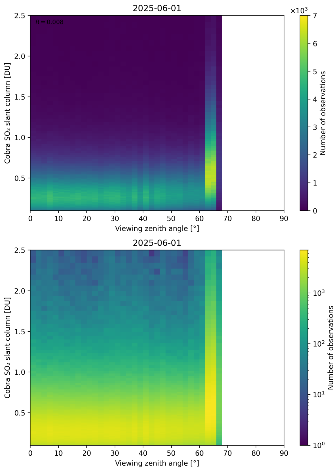
Figure 371: Scatter density plot of “Viewing zenith angle” against “Cobra SO 2 slant column” for 2025-06-01 to 2025-06-02.
