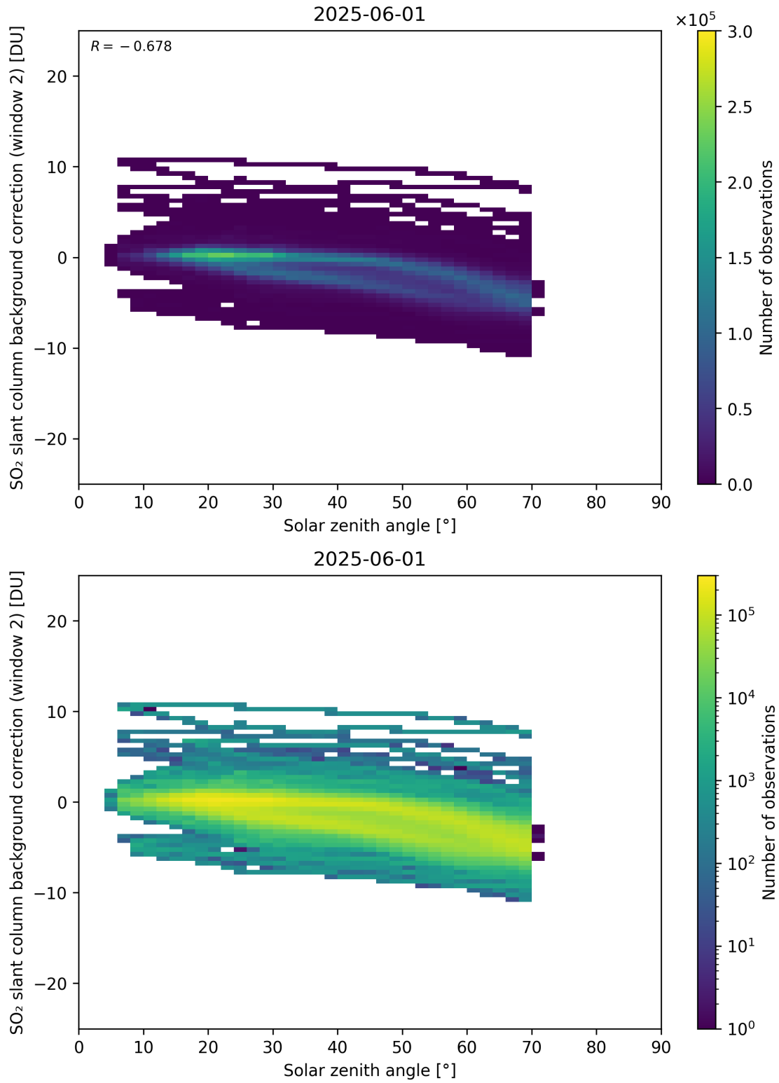
Figure 172: Scatter density plot of “Solar zenith angle” against “SO 2 slant column background correction (window 2)” for 2025-06-01 to 2025-06-02.
