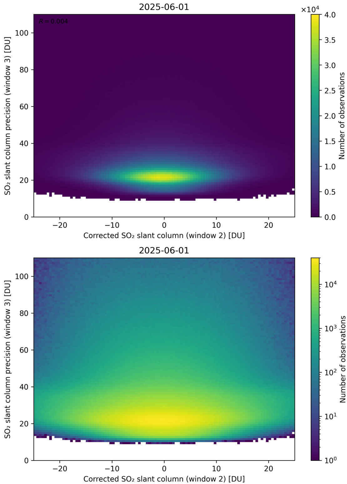
Figure 252: Scatter density plot of “Corrected SO 2 slant column (window 2)” against “SO 2 slant column precision (window 3)” for 2025-06-01 to 2025-06-02.
