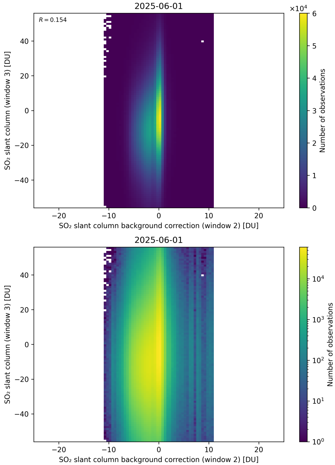
Figure 128: Scatter density plot of “SO 2 slant column background correction (window 2)” against “SO 2 slant column (window 3)” for 2025-06-01 to 2025-06-02.
