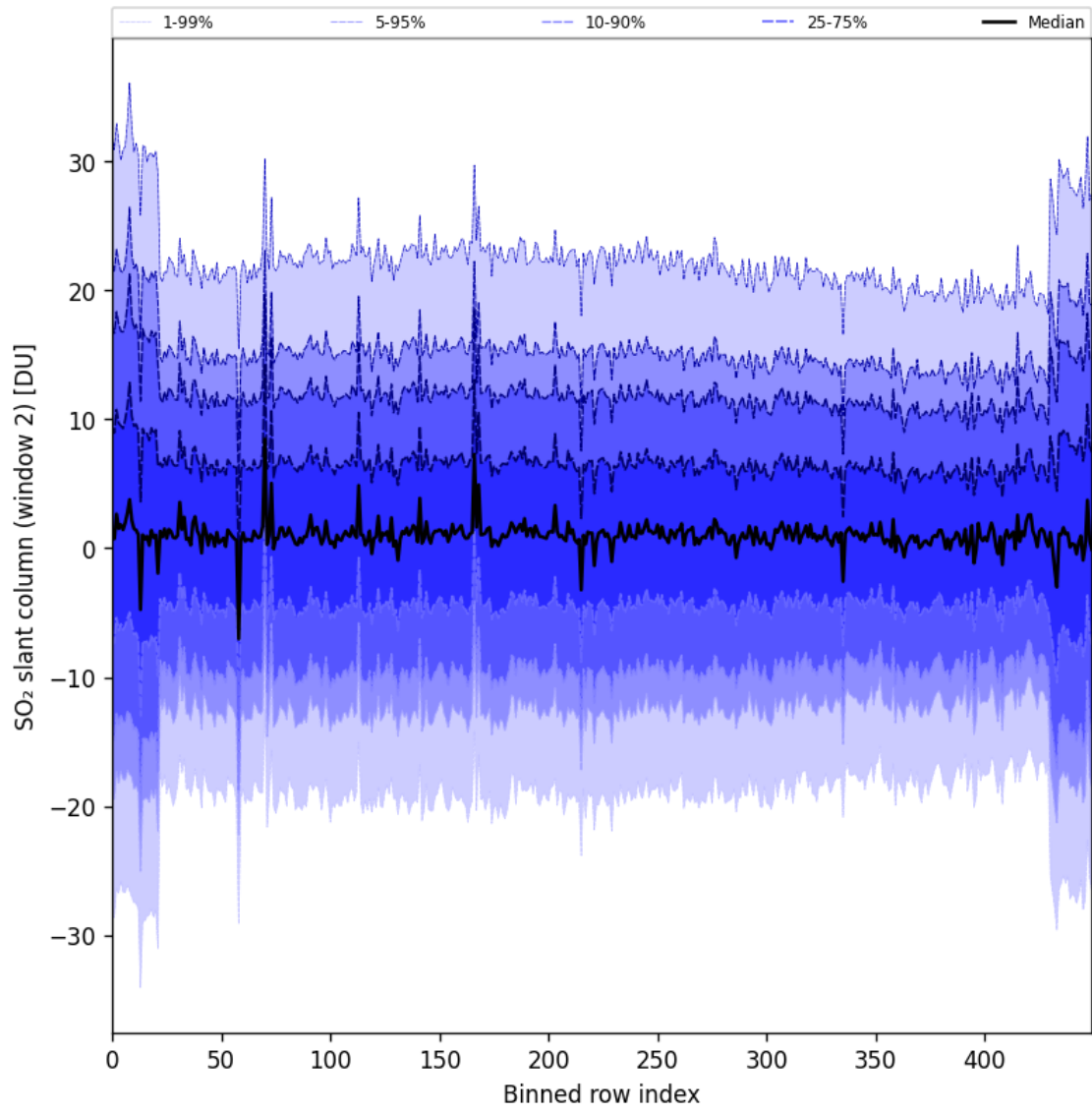
Figure 93: Along track statistics of “SO 2 slant column (window 2)” for 2025-06-01 to 2025-06-02
