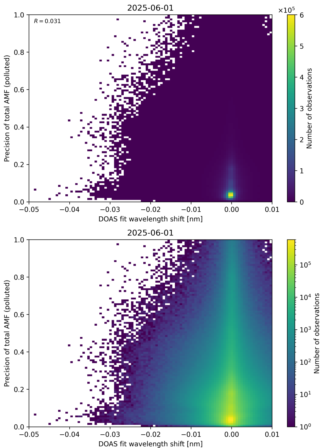
Figure 142: Scatter density plot of “DOAS fit wavelength shift” against “Precision of total AMF (polluted)” for 2025-06-01 to 2025-06-02.
