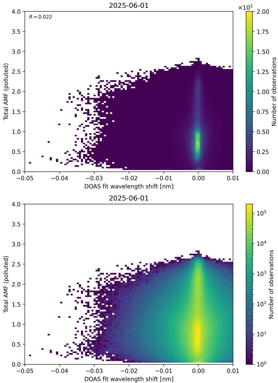
Figure 141: Scatter density plot of “DOAS fit wavelength shift” against “Total AMF (polluted)” for 2025-06-01 to 2025-06-02.
