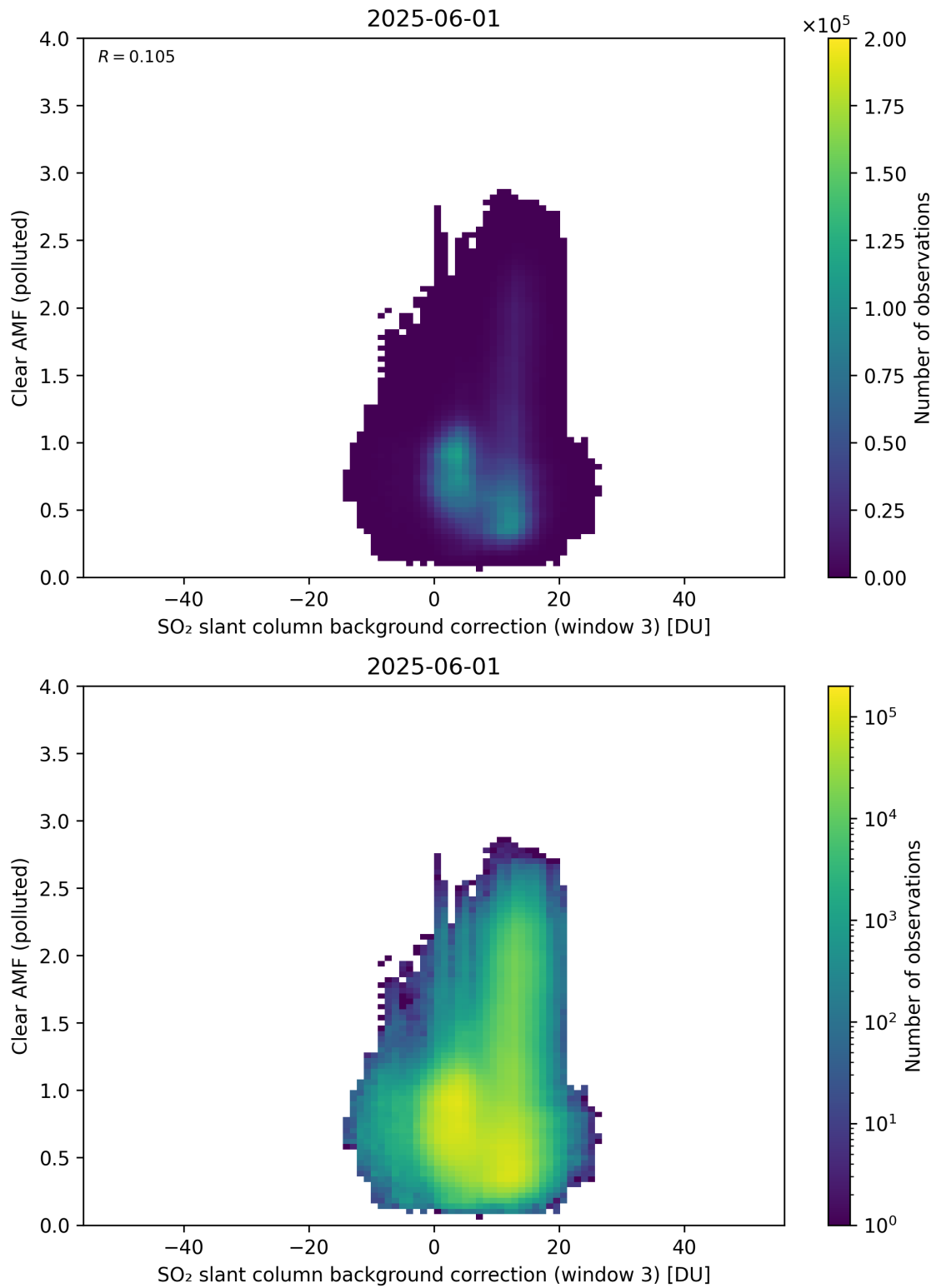
Figure 135: Scatter density plot of “SO 2 slant column background correction (window 3)” against “Clear AMF (polluted)” for 2025-06-01 to 2025-06-02.
