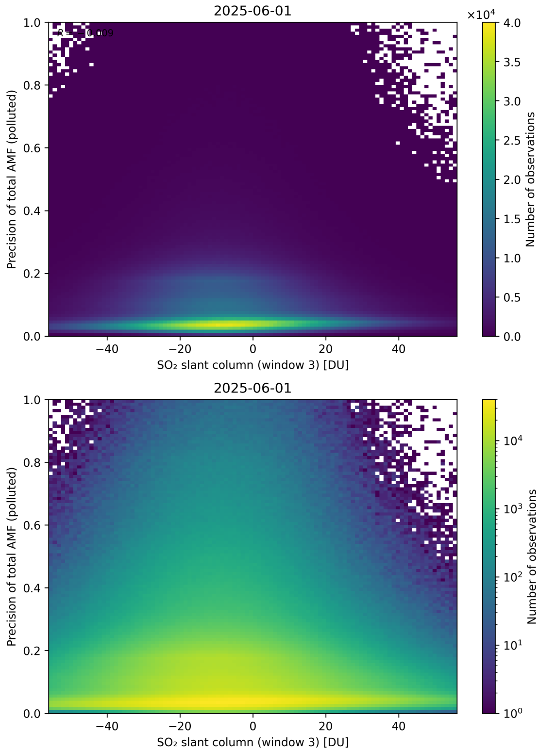
Figure 319: Scatter density plot of “SO 2 slant column (window 3)” against “Precision of total AMF (polluted)” for 2025-06-01 to 2025-06-02.
