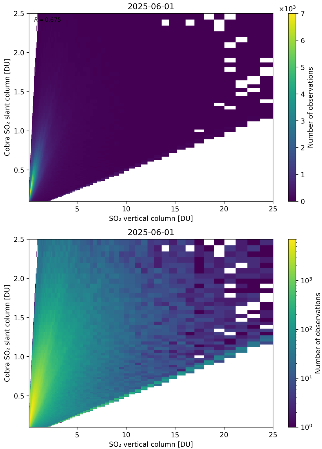
Figure 349: Scatter density plot of “SO 2 vertical column” against “Cobra SO 2 slant column” for 2025-06-01 to 2025-06-02.
