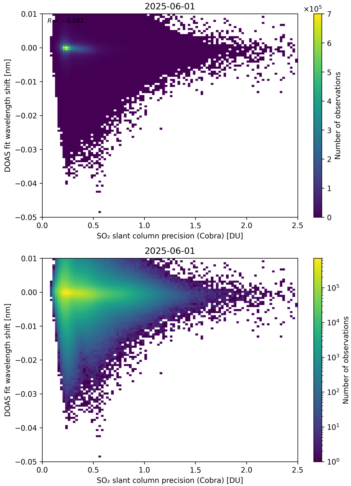
Figure 202: Scatter density plot of “SO 2 slant column precision (Cobra)” against “DOAS fit wavelength shift” for 2025-06-01 to 2025-06-02.
