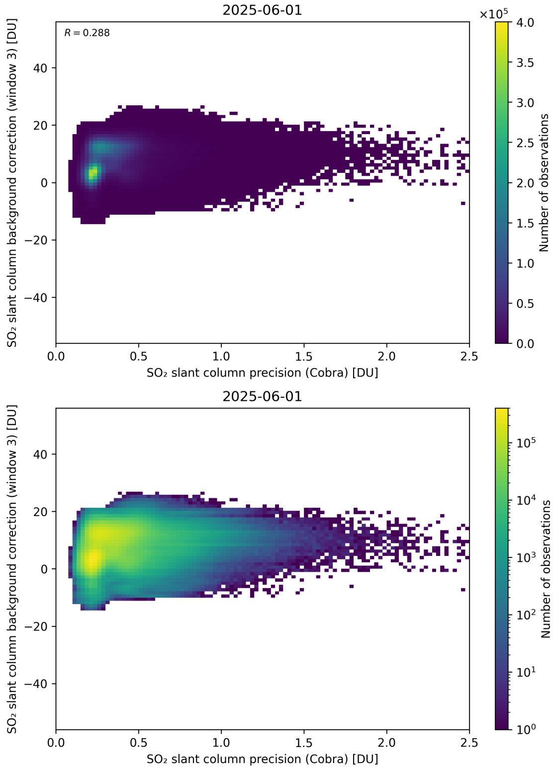
Figure 201: Scatter density plot of “SO 2 slant column precision (Cobra)” against “SO 2 slant column background correction (window 3)” for 2025-06-01 to 2025-06-02.
