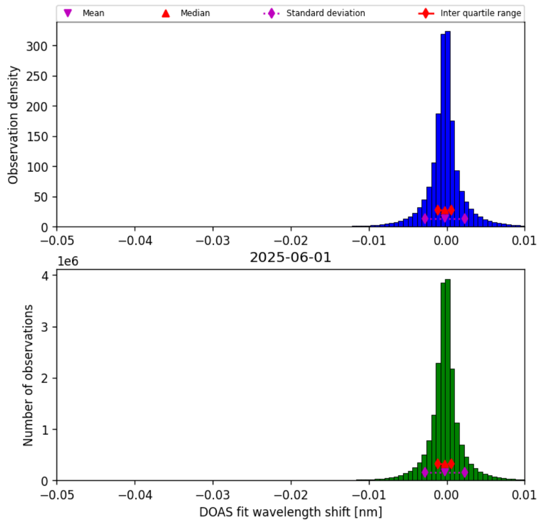
Figure 76: Histogram of “DOAS fit wavelength shift” for 2025-06-01 to 2025-06-02
