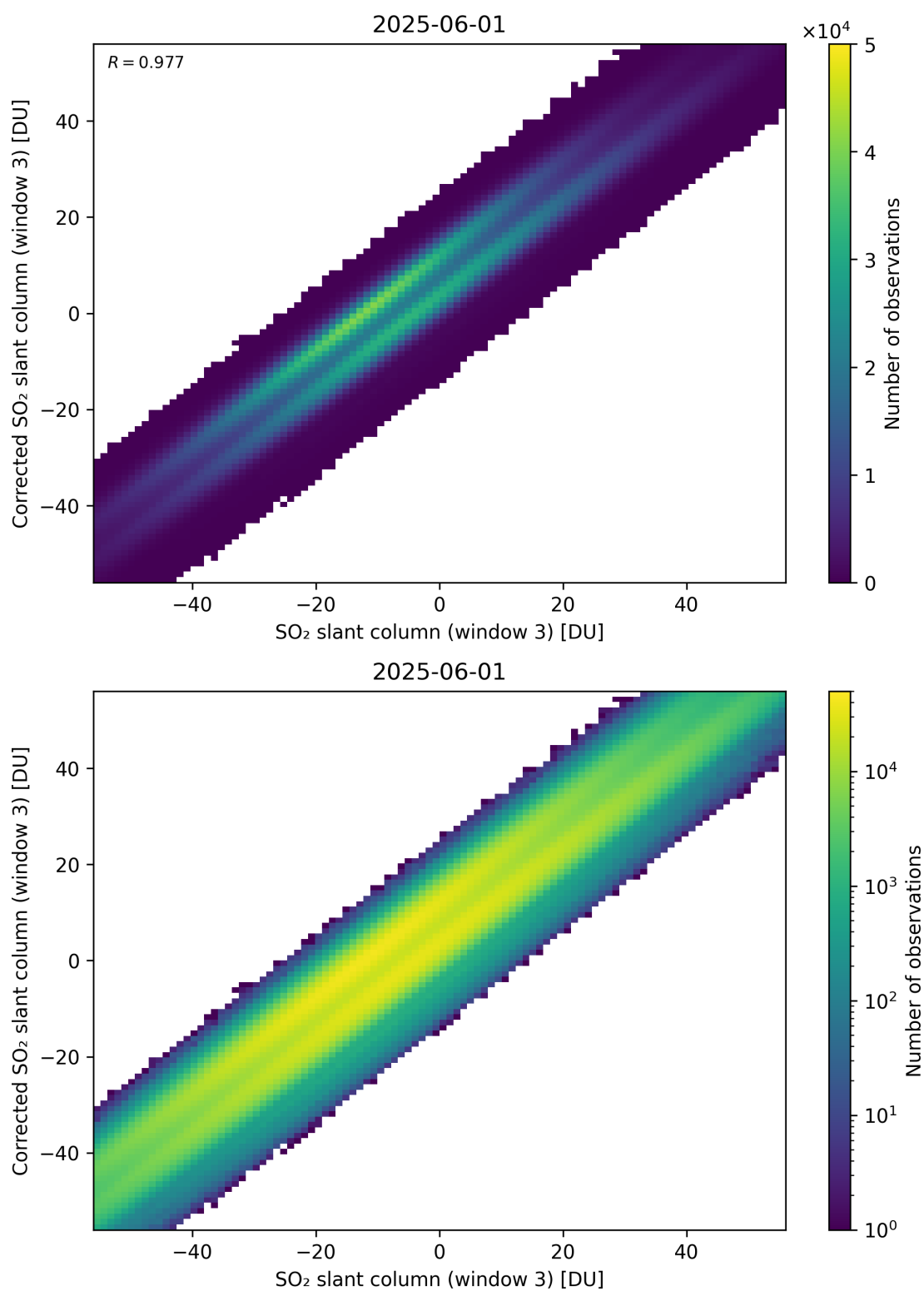
Figure 316: Scatter density plot of “SO 2 slant column (window 3)” against “Corrected SO 2 slant column (window 3)” for 2025-06-01 to 2025-06-02.
