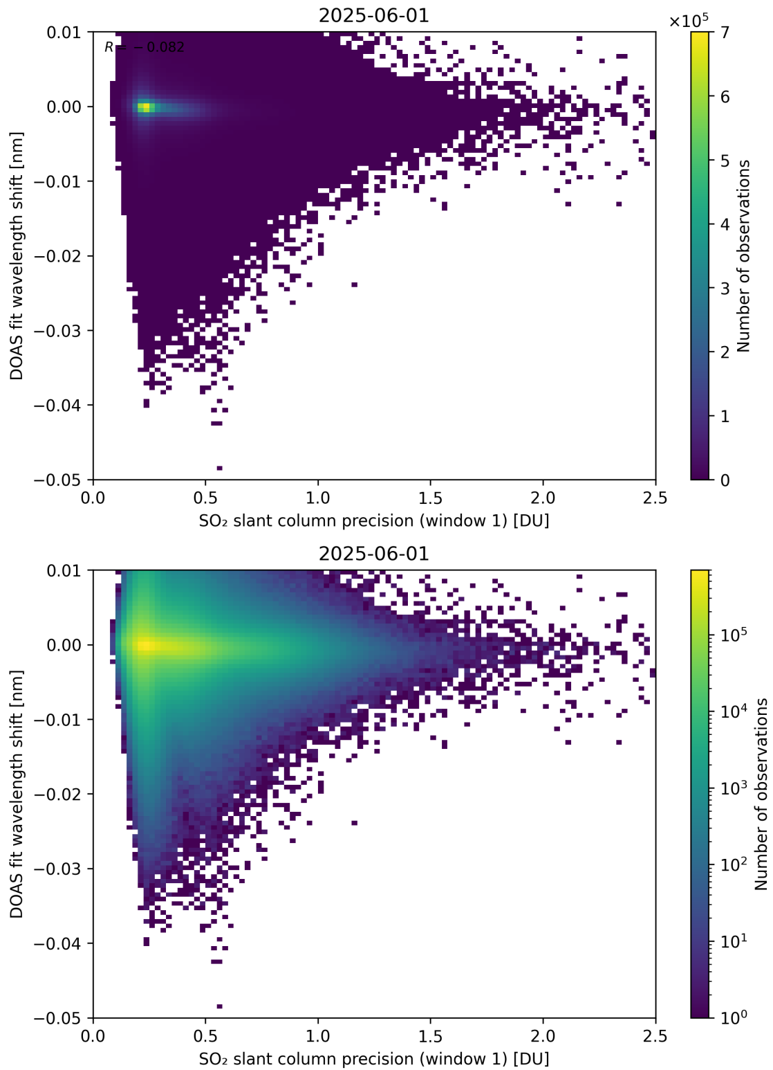
Figure 271: Scatter density plot of “SO 2 slant column precision (window 1)” against “DOAS fit wavelength shift” for 2025-06-01 to 2025-06-02.
