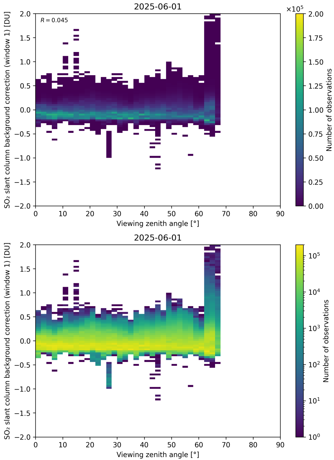
Figure 362: Scatter density plot of “Viewing zenith angle” against “SO 2 slant column background correction (window 1)” for 2025-06-01 to 2025-06-02.
