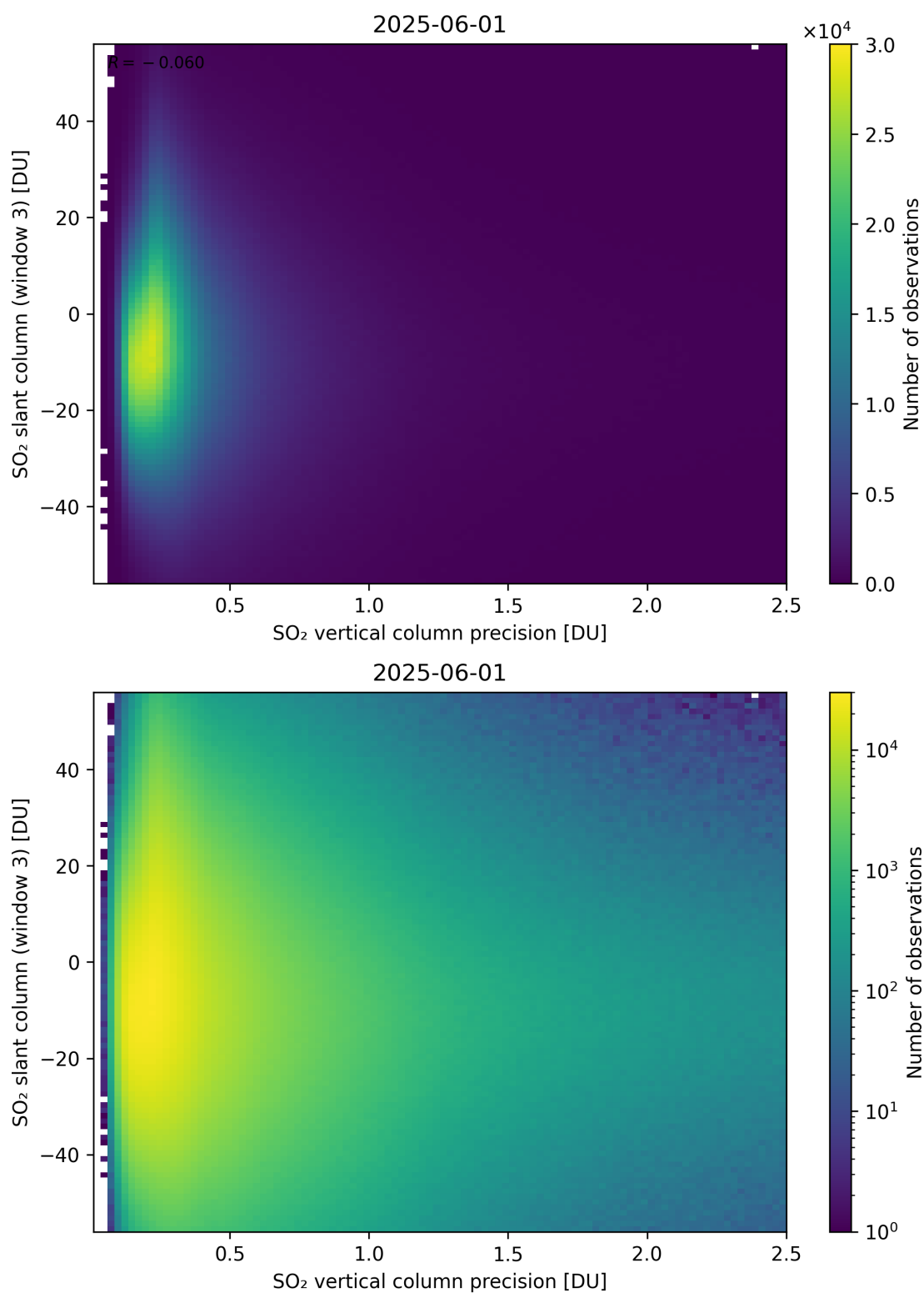
Figure 344: Scatter density plot of “SO 2 vertical column precision” against “SO 2 slant column (window 3)” for 2025-06-01 to 2025-06-02.
