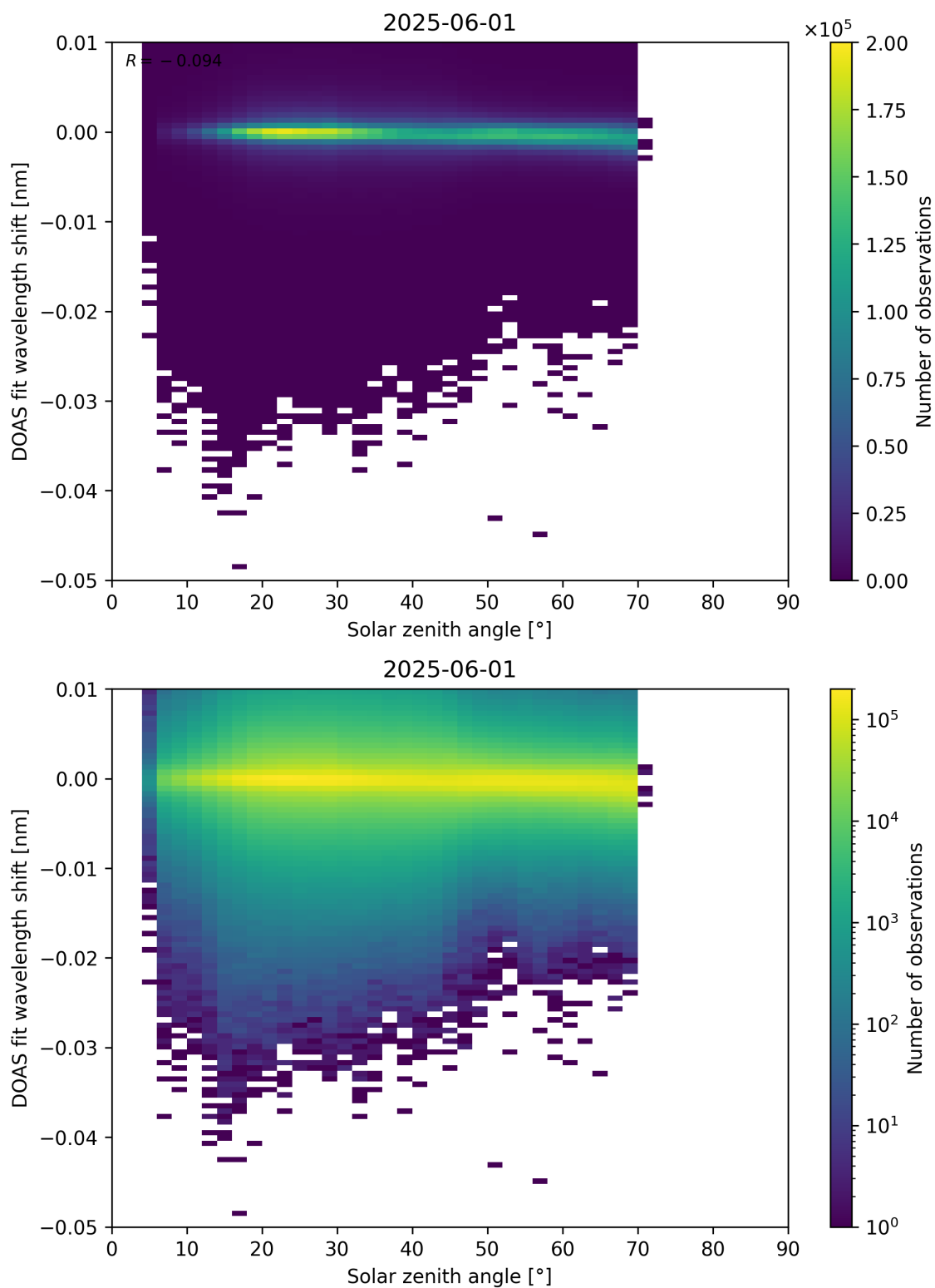
Figure 174: Scatter density plot of “Solar zenith angle” against “DOAS fit wavelength shift” for 2025-06-01 to 2025-06-02.
