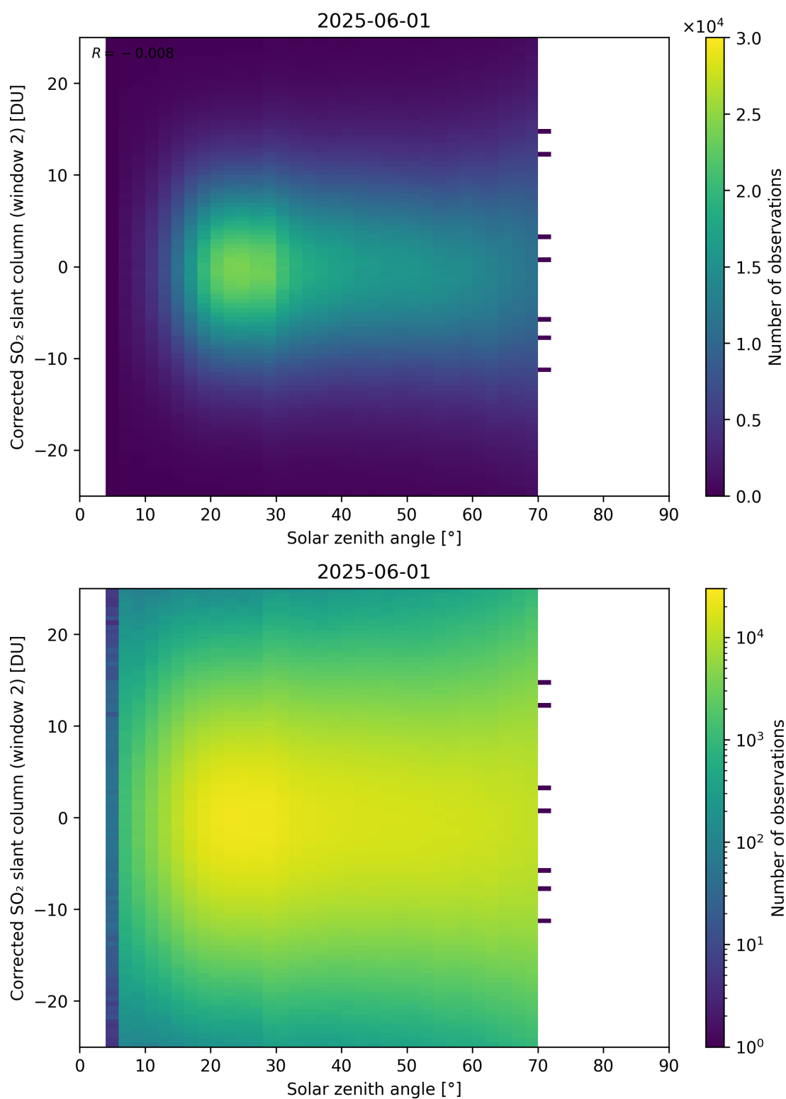
Figure 182: Scatter density plot of “Solar zenith angle” against “Corrected SO 2 slant column (window 2)” for 2025-06-01 to 2025-06-02.
