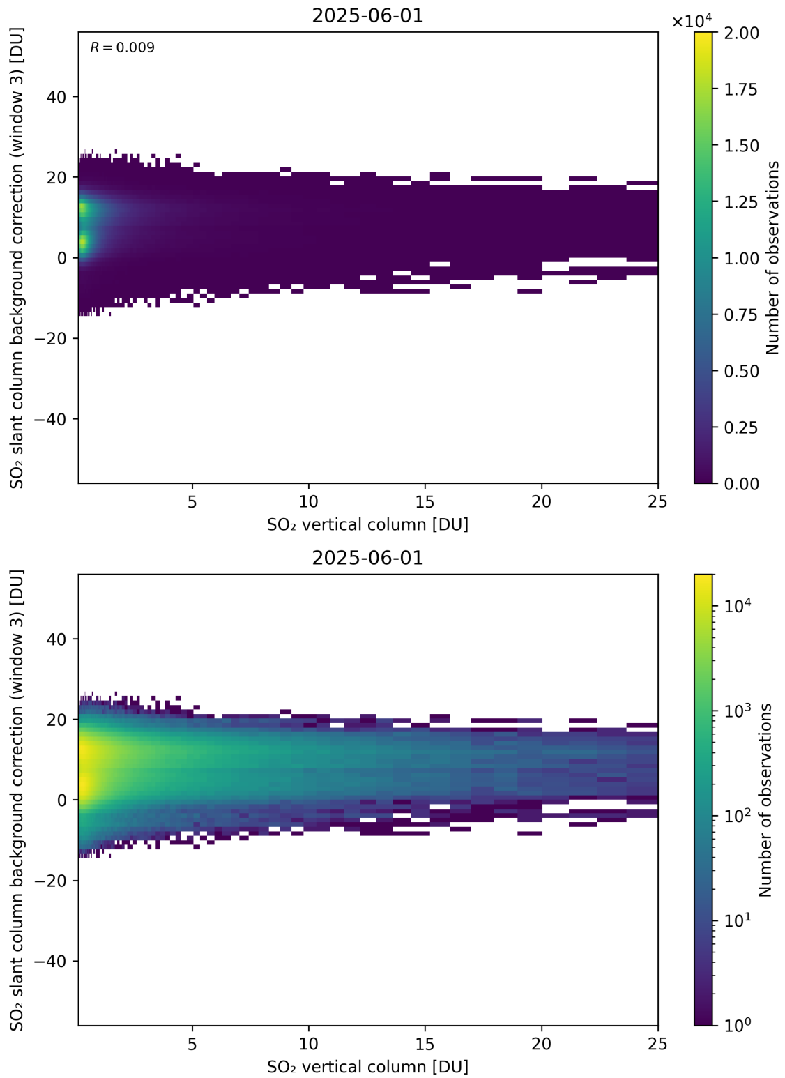
Figure 325: Scatter density plot of “SO 2 vertical column” against “SO 2 slant column background correction (window 3)” for 2025-06-01 to 2025-06-02.
