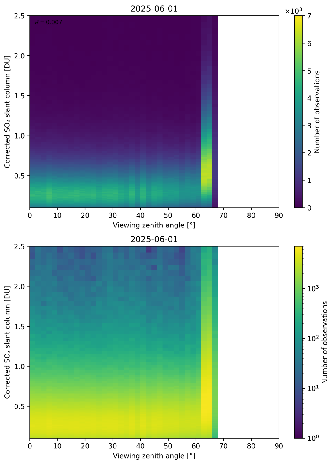
Figure 373: Scatter density plot of “Viewing zenith angle” against “Corrected SO 2 slant column” for 2025-06-01 to 2025-06-02.
