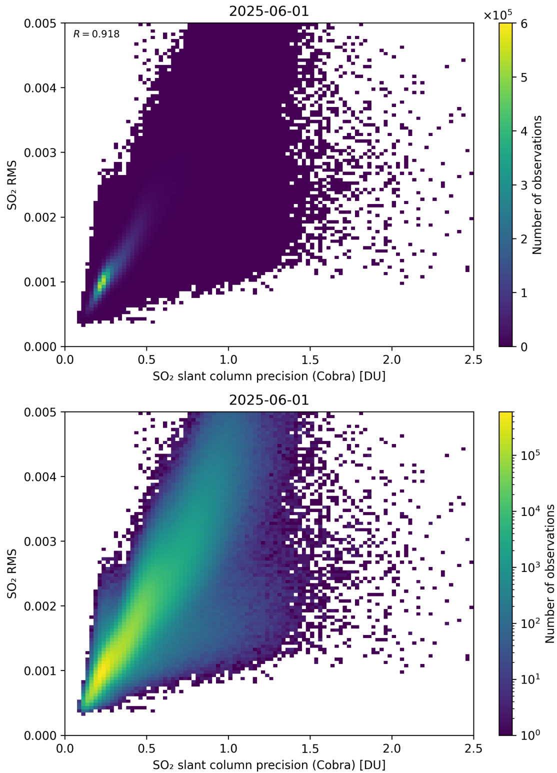
Figure 204: Scatter density plot of “SO 2 slant column precision (Cobra)” against “SO 2 RMS” for 2025-06-01 to 2025-06-02.
