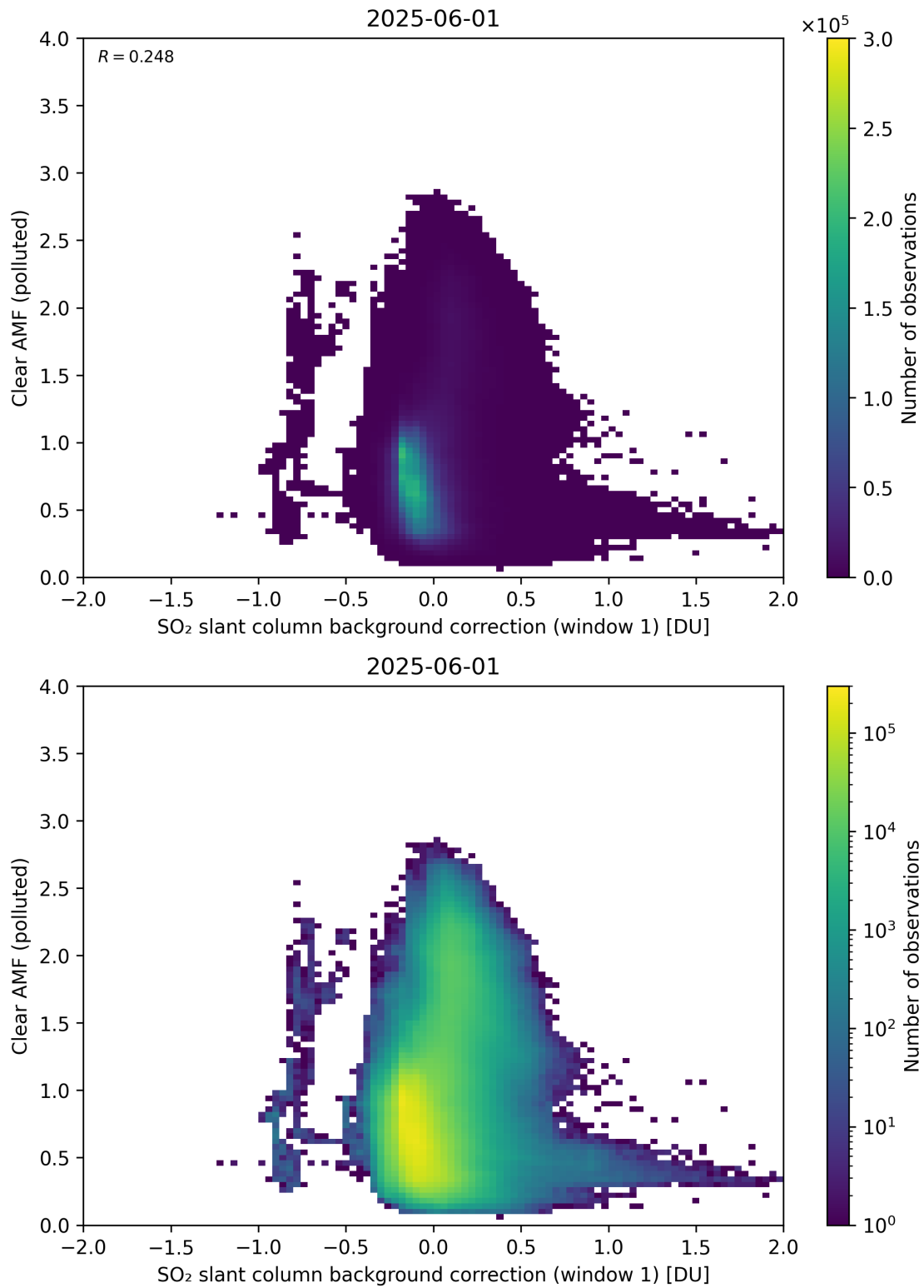
Figure 114: Scatter density plot of “SO 2 slant column background correction (window 1)” against “Clear AMF (polluted)” for 2025-06-01 to 2025-06-02.
