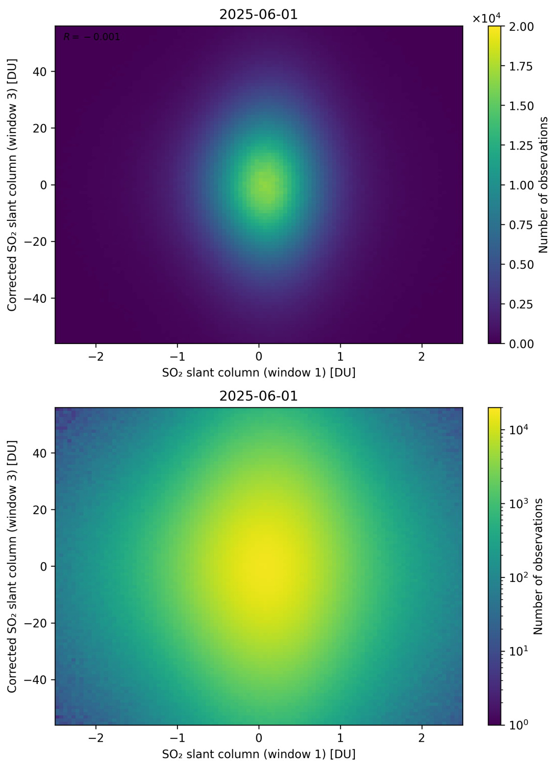
Figure 284: Scatter density plot of “SO 2 slant column (window 1)” against “Corrected SO 2 slant column (window 3)” for 2025-06-01 to 2025-06-02.
