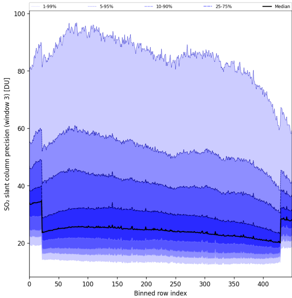
Figure 98: Along track statistics of “SO 2 slant column precision (window 3)” for 2025-06-01 to 2025-06-02
