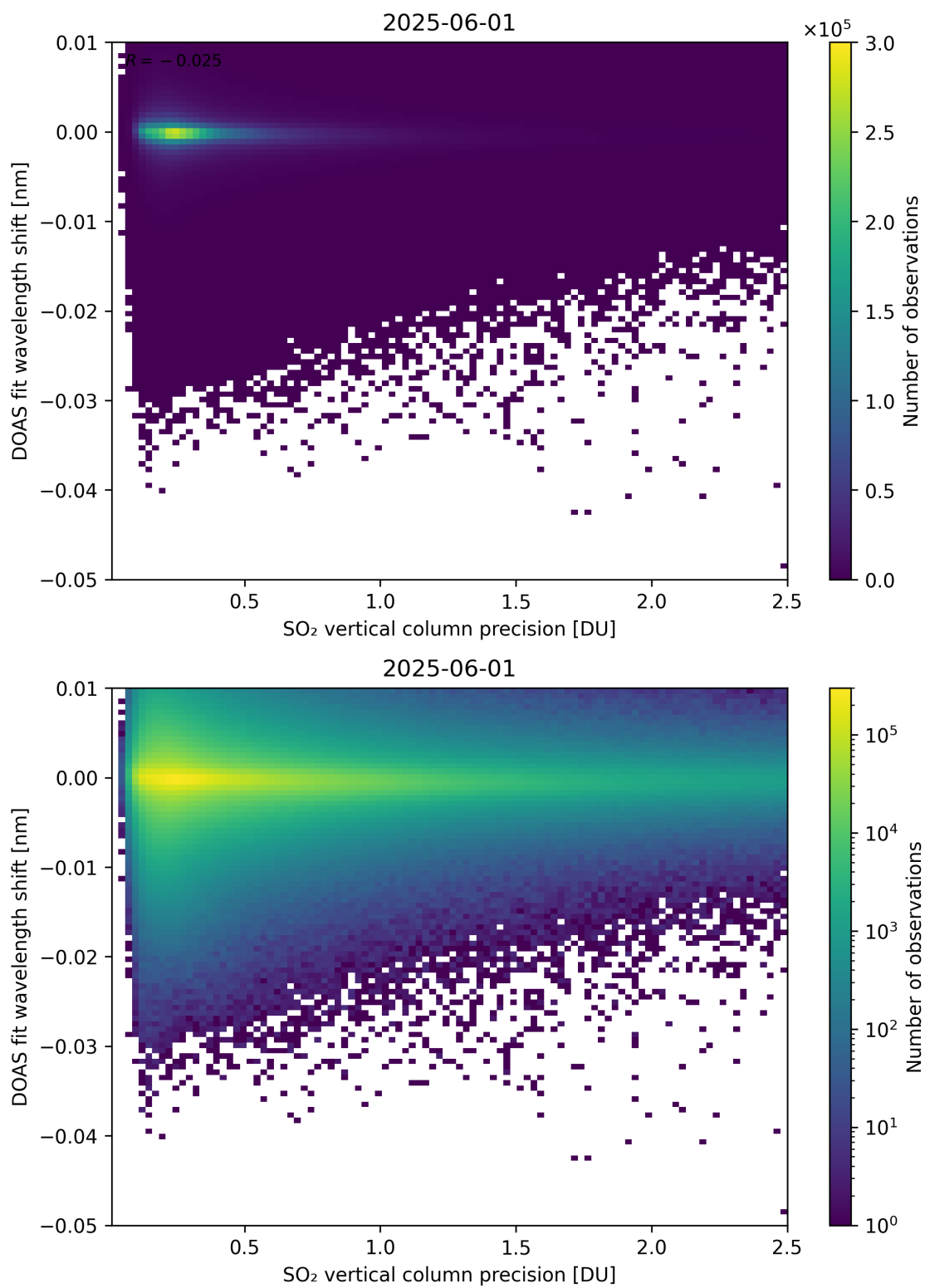
Figure 332: Scatter density plot of “SO 2 vertical column precision” against “DOAS fit wavelength shift” for 2025-06-01 to 2025-06-02.
