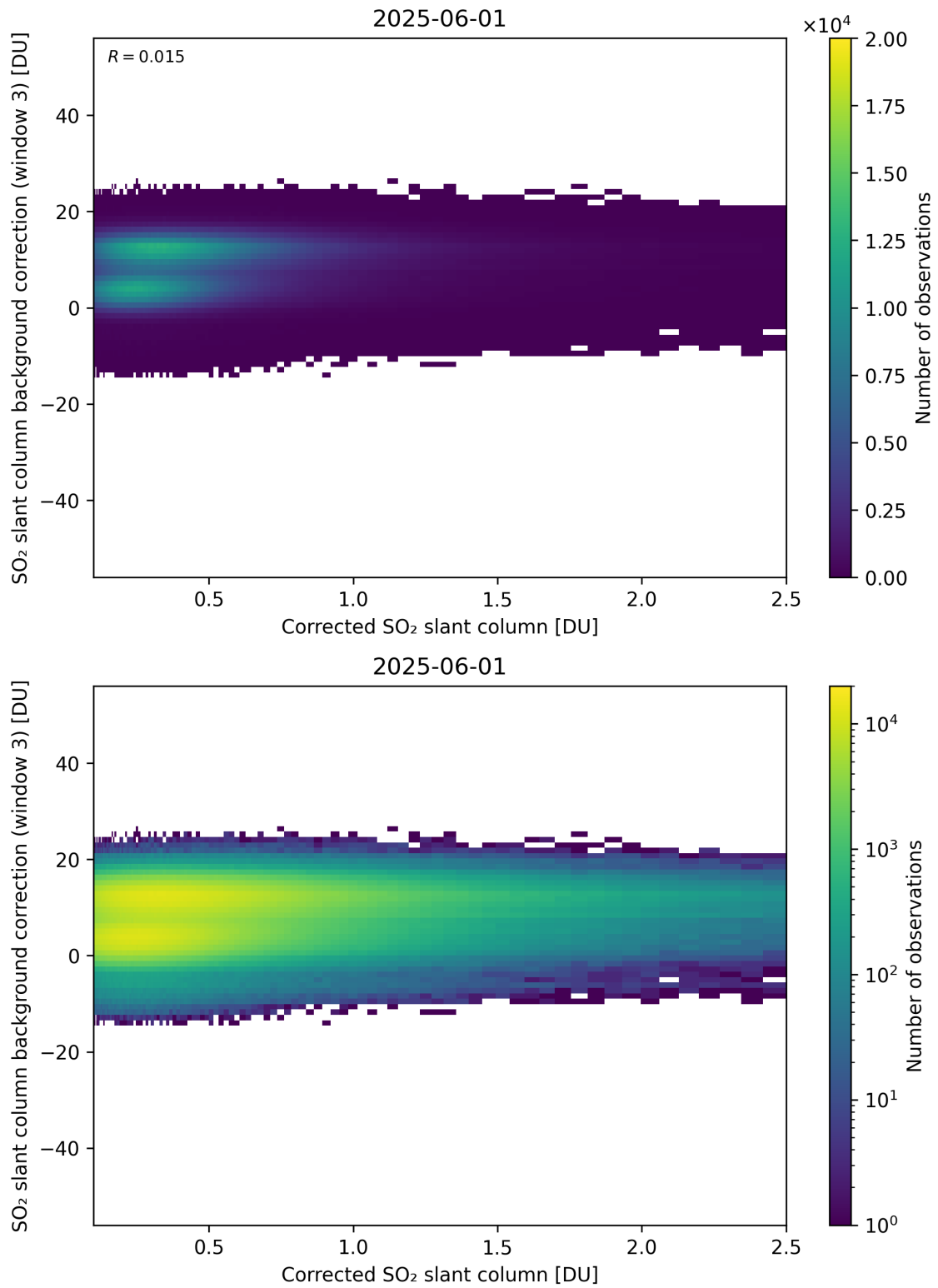
Figure 228: Scatter density plot of “Corrected SO 2 slant column” against “SO 2 slant column background correction (window 3)” for 2025-06-01 to 2025-06-02.
