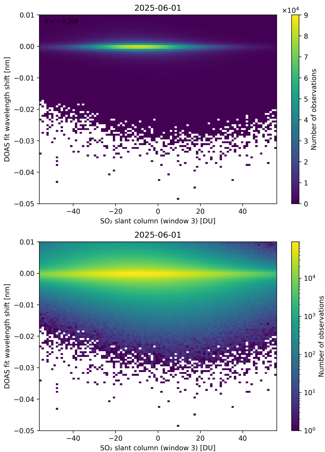
Figure 304: Scatter density plot of “SO 2 slant column (window 3)” against “DOAS fit wavelength shift” for 2025-06-01 to 2025-06-02.
