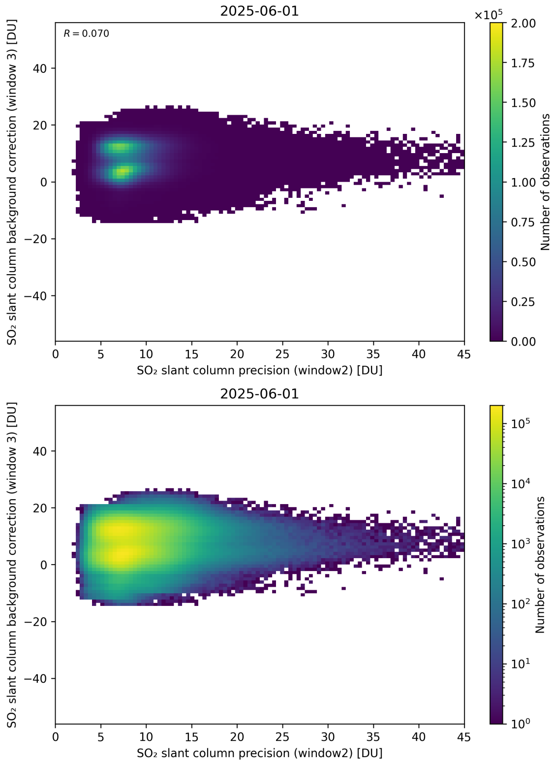
Figure 292: Scatter density plot of “SO 2 slant column precision (window2)” against “SO 2 slant column background correction (window 3)” for 2025-06-01 to 2025-06-02.
