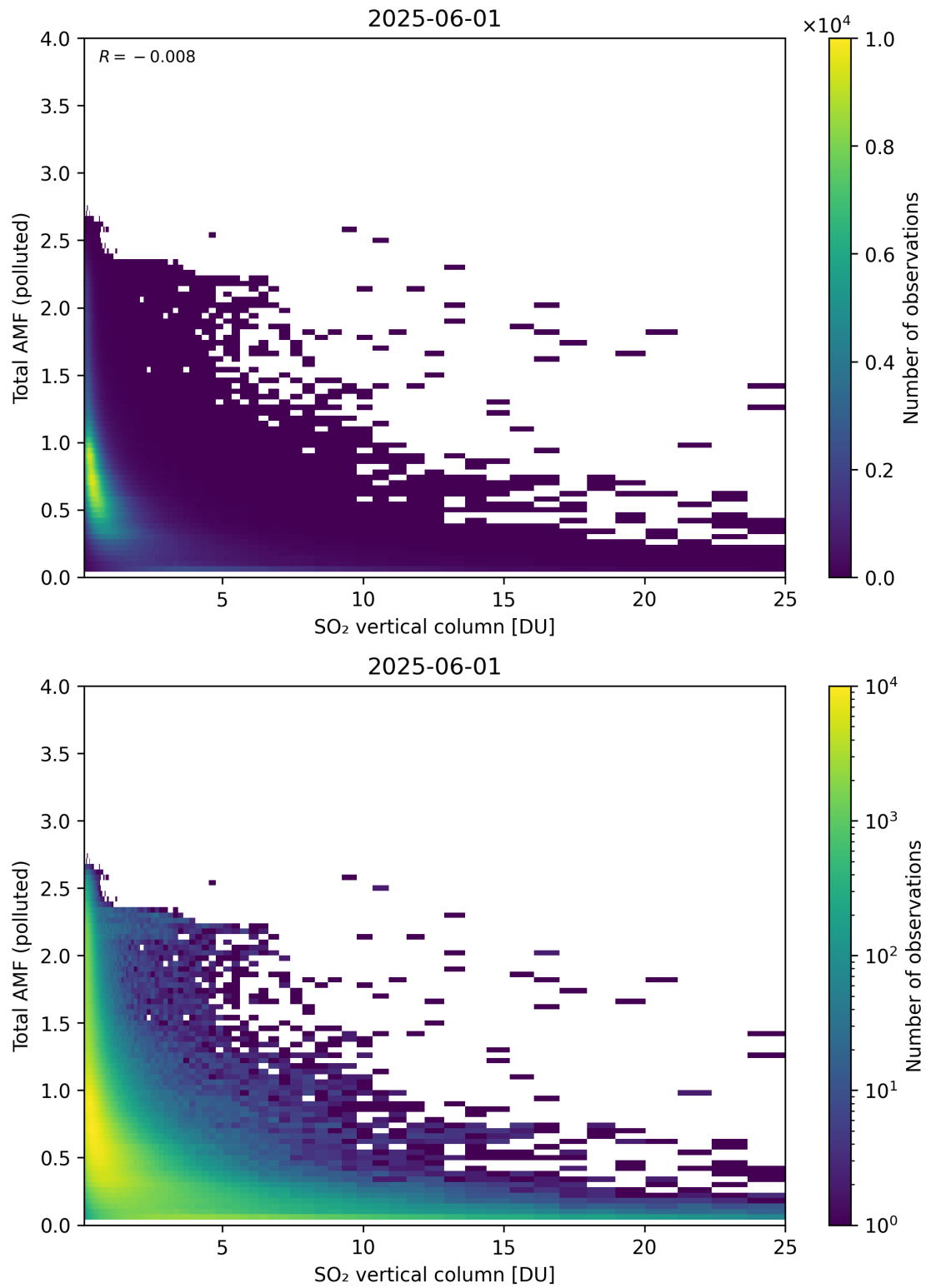
Figure 359: Scatter density plot of “SO 2 vertical column” against “Total AMF (polluted)” for 2025-06-01 to 2025-06-02.
