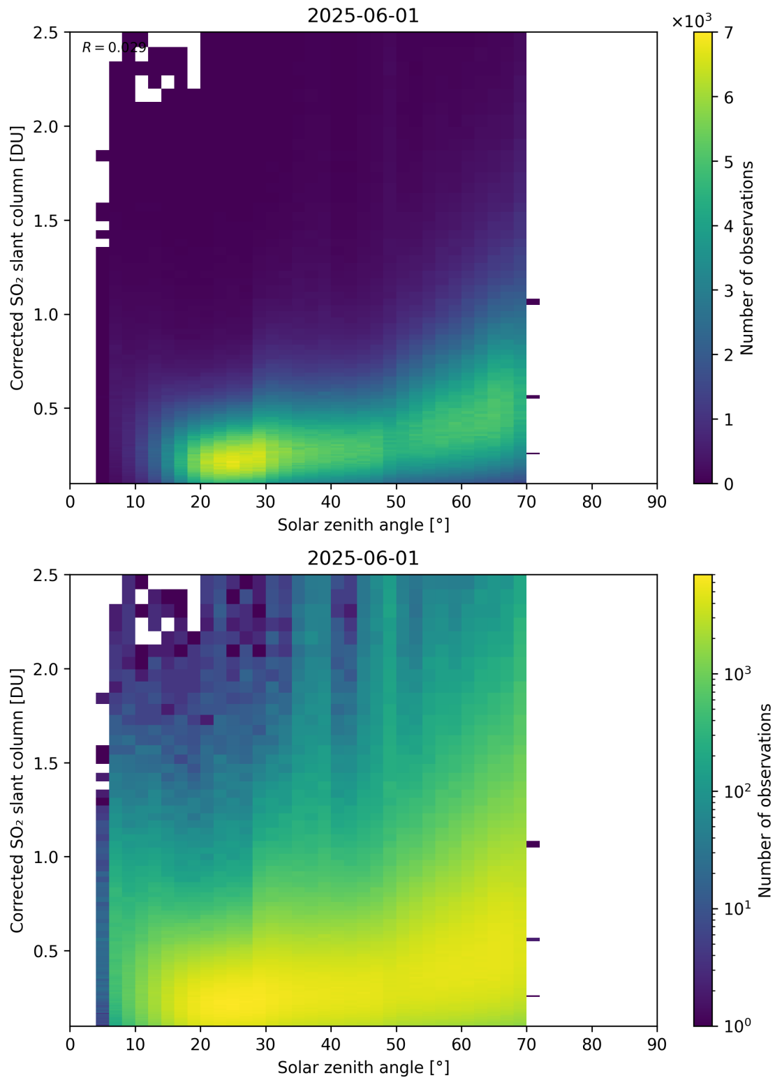
Figure 181: Scatter density plot of “Solar zenith angle” against “Corrected SO 2 slant column” for 2025-06-01 to 2025-06-02.
