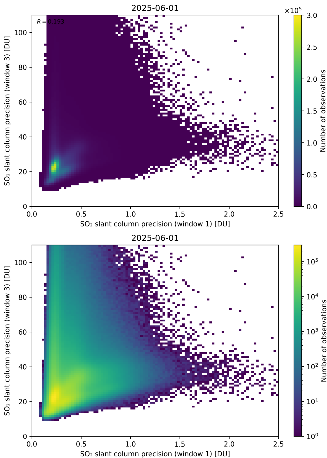
Figure 279: Scatter density plot of “SO 2 slant column precision (window 1)” against “SO 2 slant column precision (window 3)” for 2025-06-01 to 2025-06-02.
