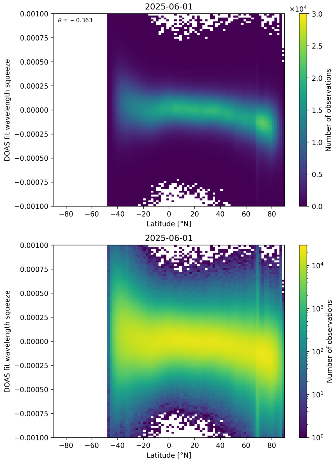
Figure 154: Scatter density plot of “Latitude” against “DOAS fit wavelength squeeze” for 2025-06-01 to 2025-06-02.
