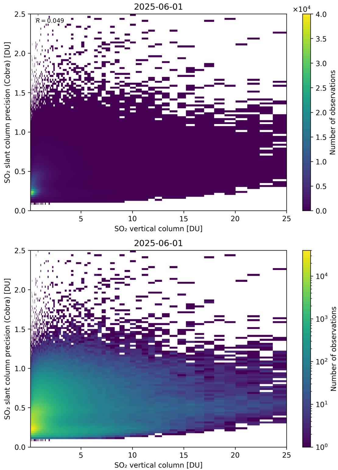
Figure 350: Scatter density plot of “SO 2 vertical column” against “SO 2 slant column precision (Cobra)” for 2025-06-01 to 2025-06-02.
