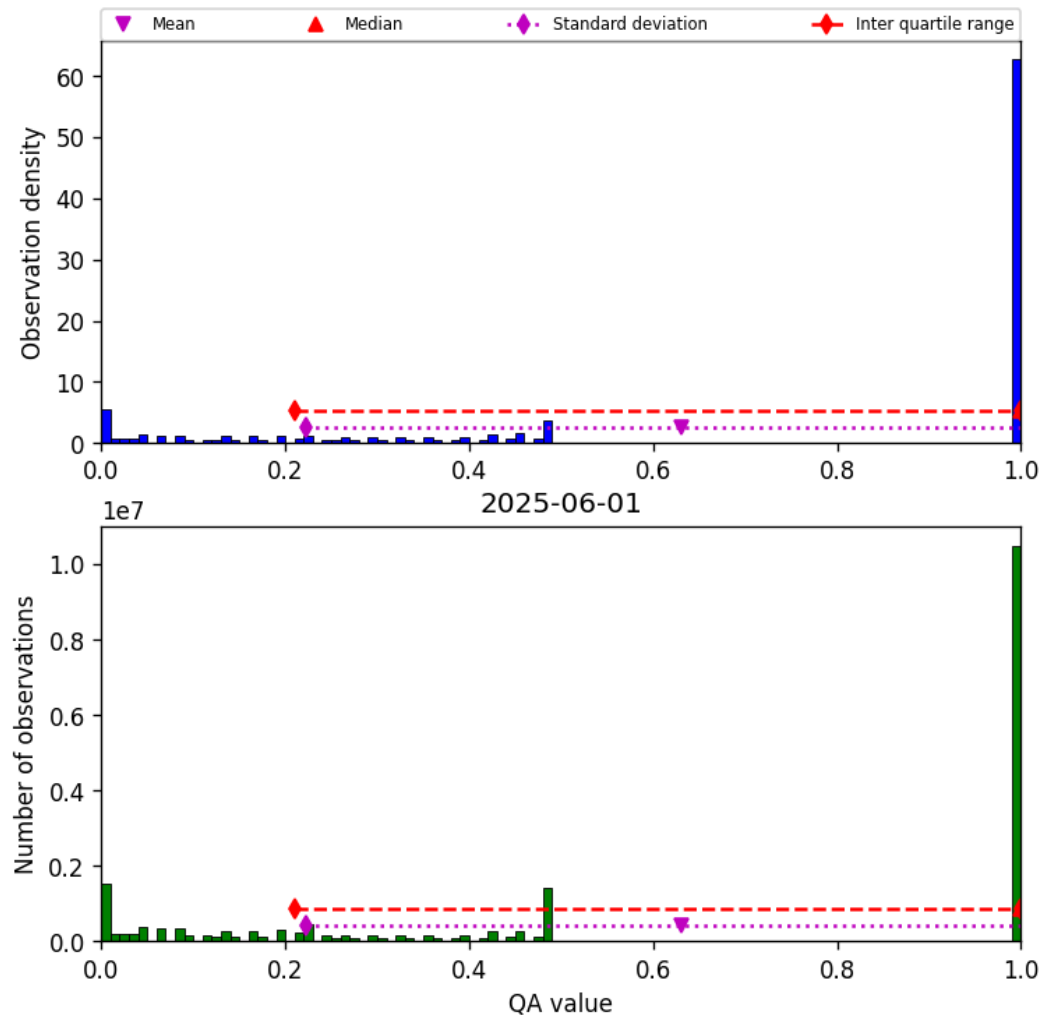
Figure 57: Histogram of “QA value” for 2025-06-01 to 2025-06-02
