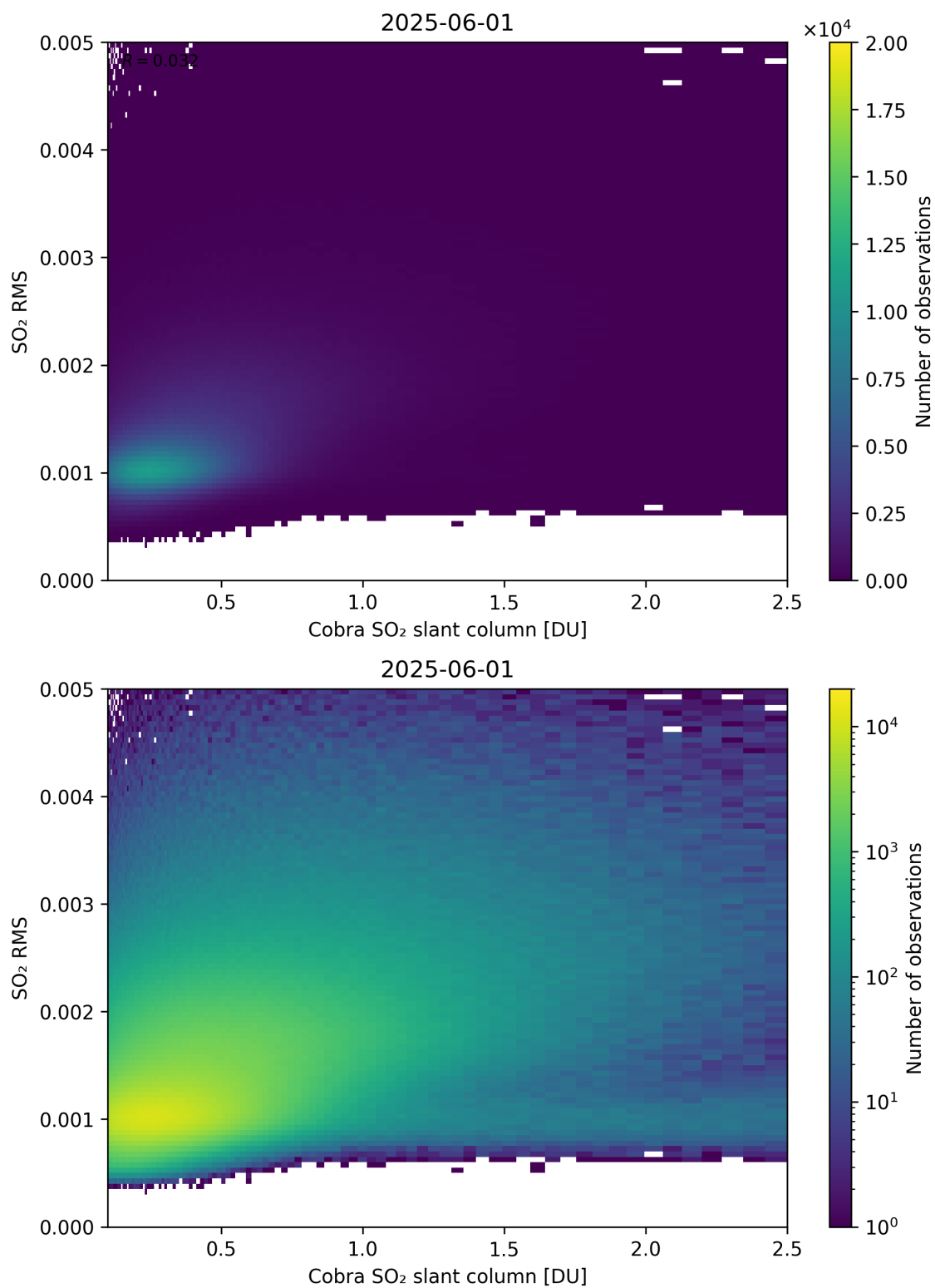
Figure 198: Scatter density plot of “Cobra SO 2 slant column” against “SO 2 RMS” for 2025-06-01 to 2025-06-02.
