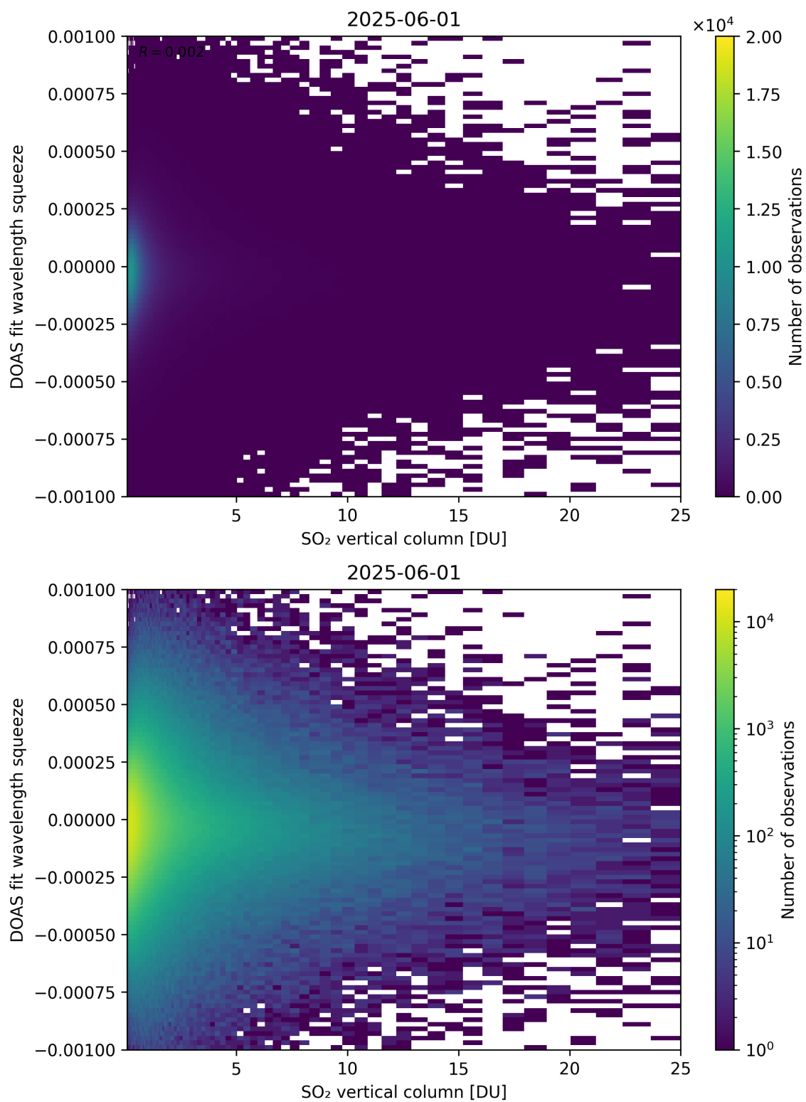
Figure 327: Scatter density plot of “SO 2 vertical column” against “DOAS fit wavelength squeeze” for 2025-06-01 to 2025-06-02.
