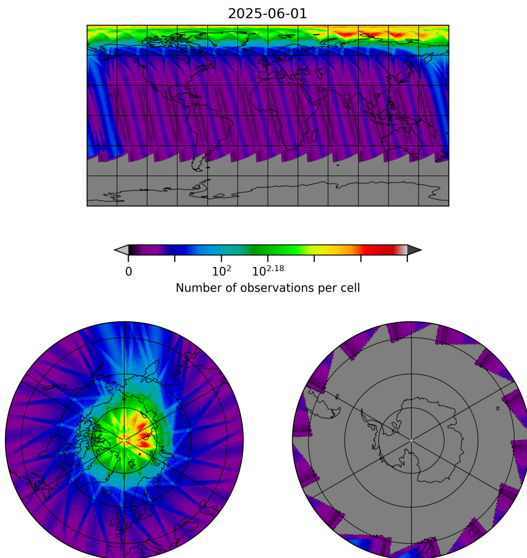
Figure 30: Map of the number of observations for 2025-06-01 to 2025-06-02
