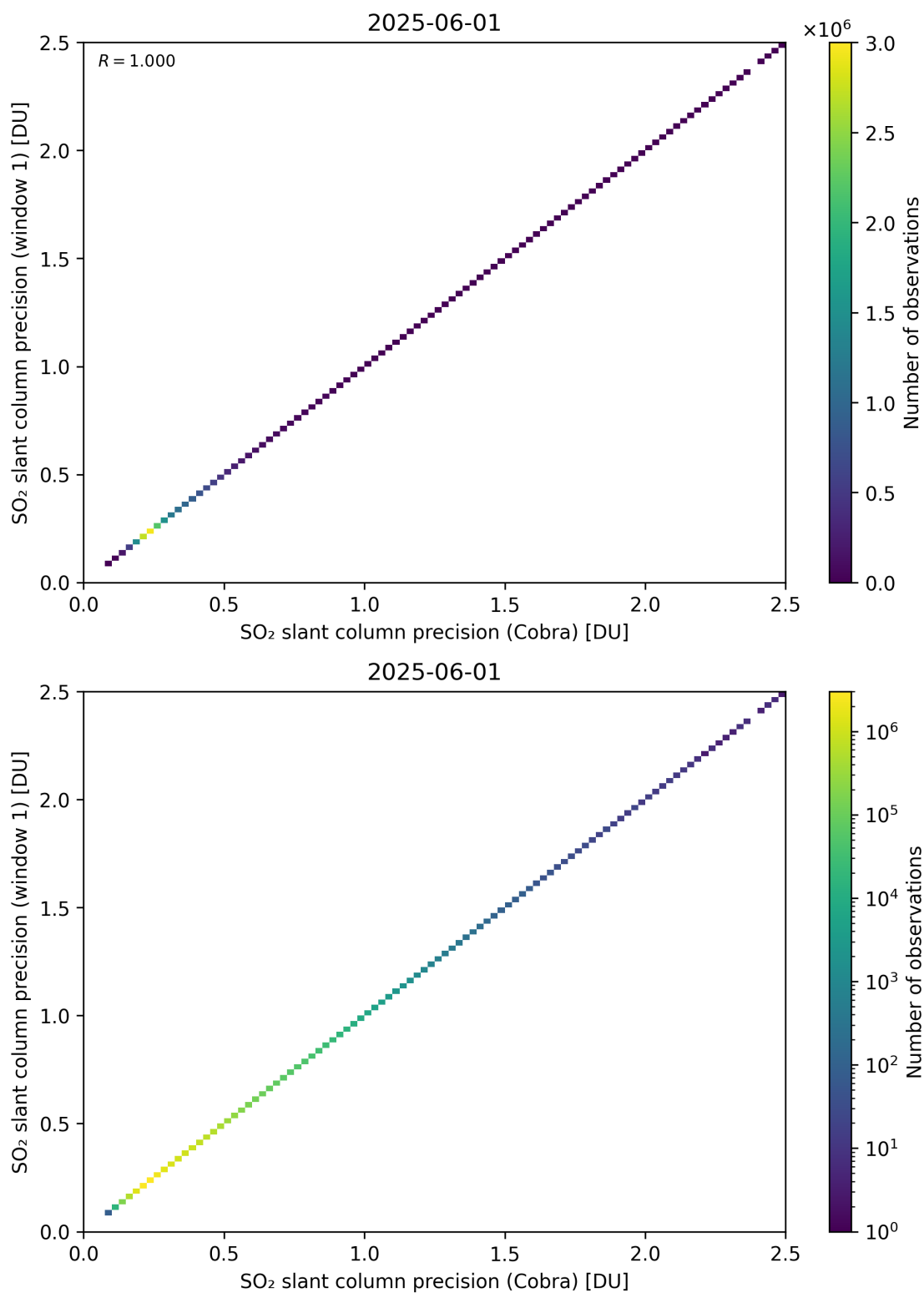
Figure 209: Scatter density plot of “SO 2 slant column precision (Cobra)” against “SO 2 slant column precision (window 1)” for 2025-06-01 to 2025-06-02.
