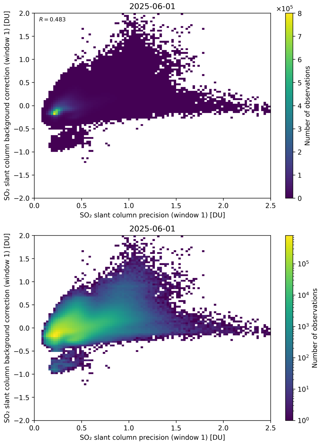
Figure 268: Scatter density plot of “SO 2 slant column precision (window 1)” against “SO 2 slant column background correction (window 1)” for 2025-06-01 to 2025-06-02.
