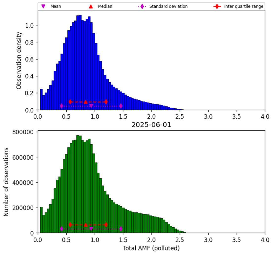
Figure 79: Histogram of “Total AMF (polluted)” for 2025-06-01 to 2025-06-02
