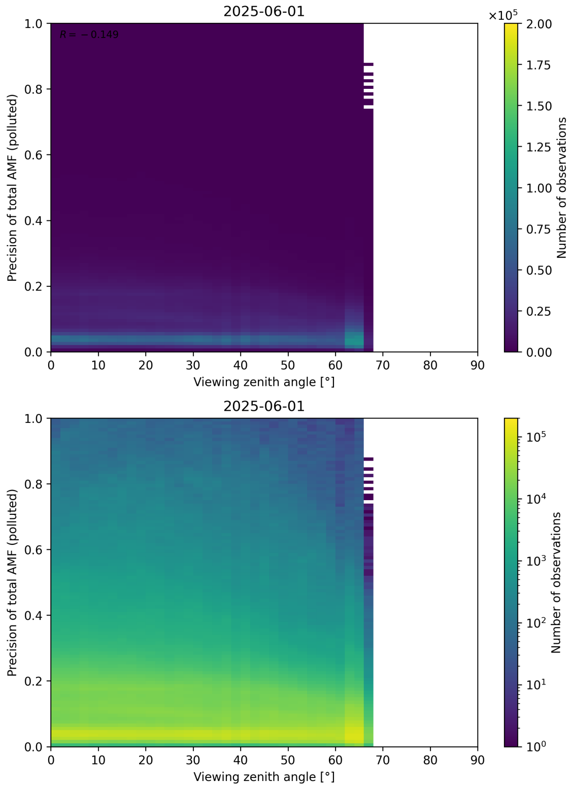
Figure 382: Scatter density plot of “Viewing zenith angle” against “Precision of total AMF (polluted)” for 2025-06-01 to 2025-06-02.
