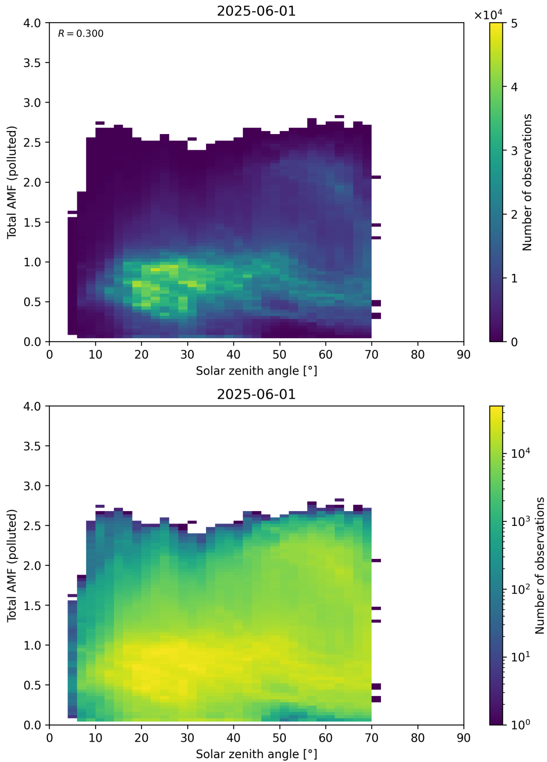
Figure 189: Scatter density plot of “Solar zenith angle” against “Total AMF (polluted)” for 2025-06-01 to 2025-06-02.
