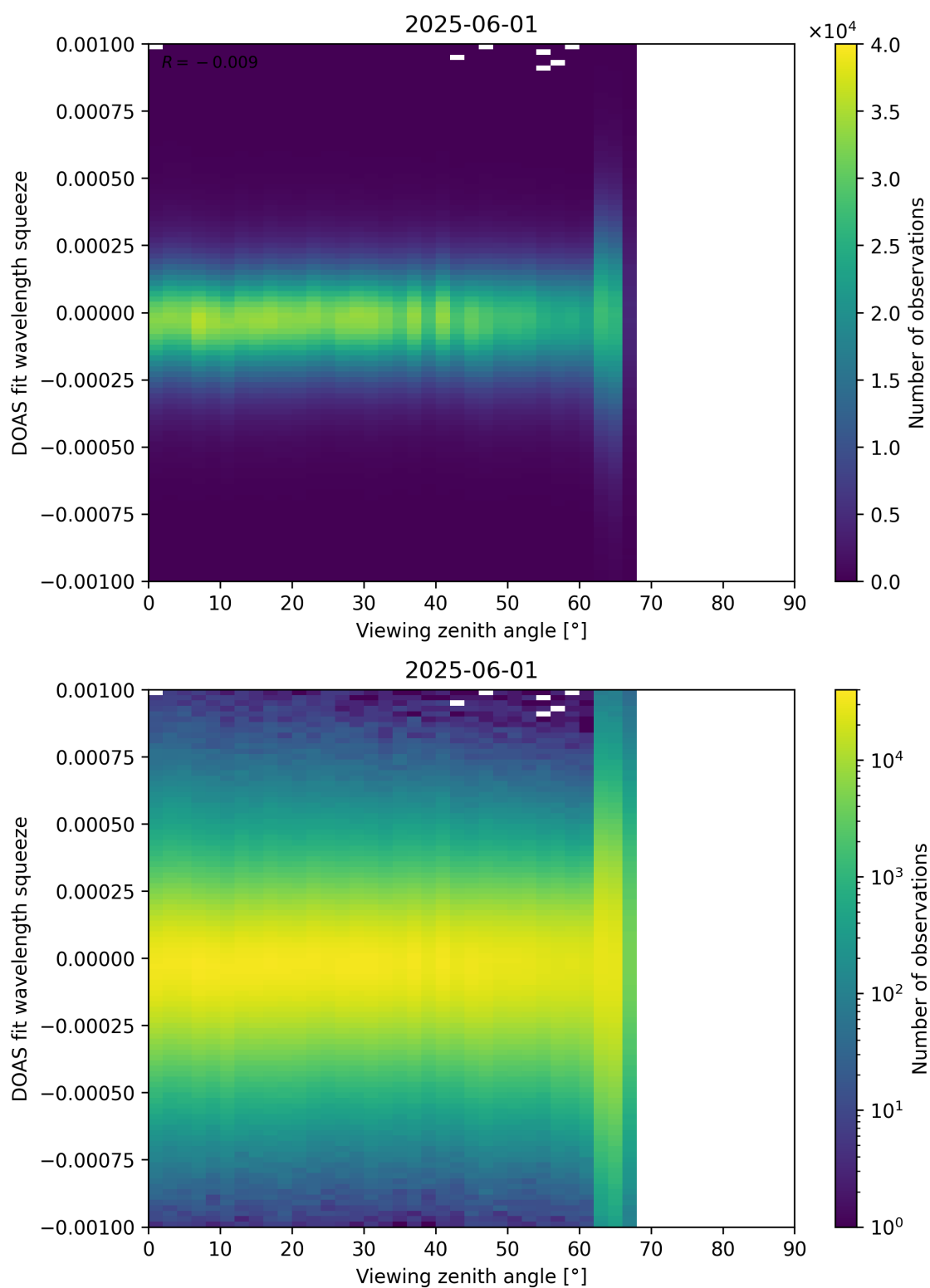
Figure 366: Scatter density plot of “Viewing zenith angle” against “DOAS fit wavelength squeeze” for 2025-06-01 to 2025-06-02.
