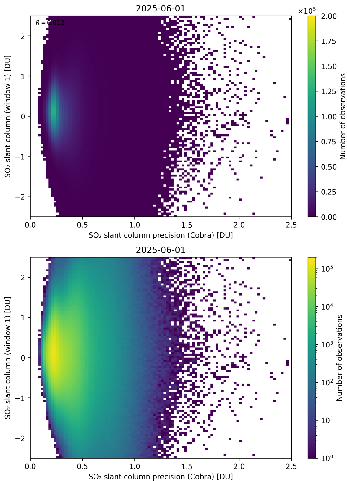
Figure 208: Scatter density plot of “SO 2 slant column precision (Cobra)” against “SO 2 slant column (window 1)” for 2025-06-01 to 2025-06-02.
