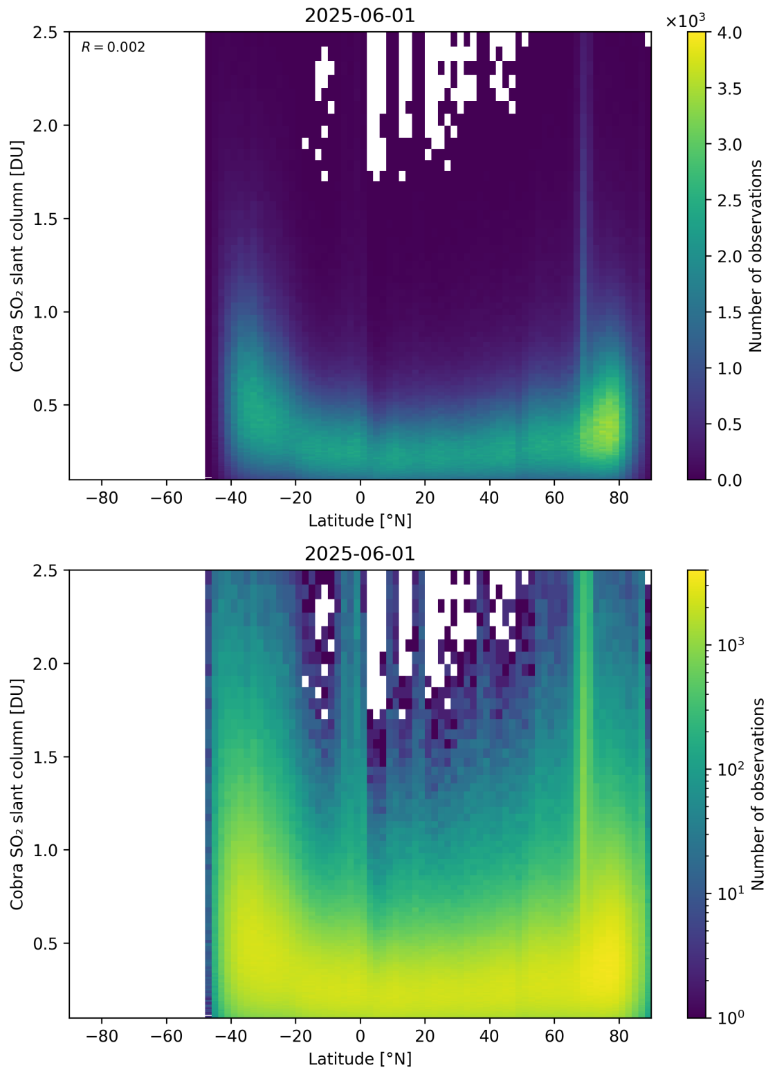
Figure 157: Scatter density plot of “Latitude” against “Cobra SO 2 slant column” for 2025-06-01 to 2025-06-02.
