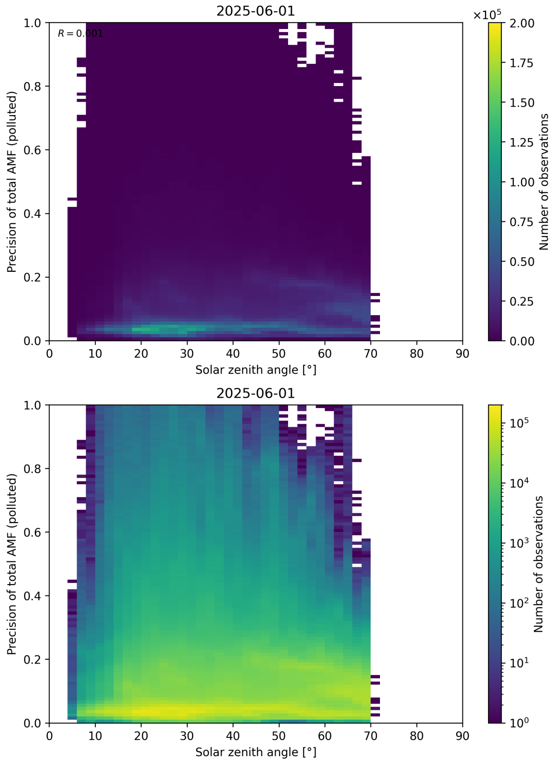
Figure 190: Scatter density plot of “Solar zenith angle” against “Precision of total AMF (polluted)” for 2025-06-01 to 2025-06-02.
