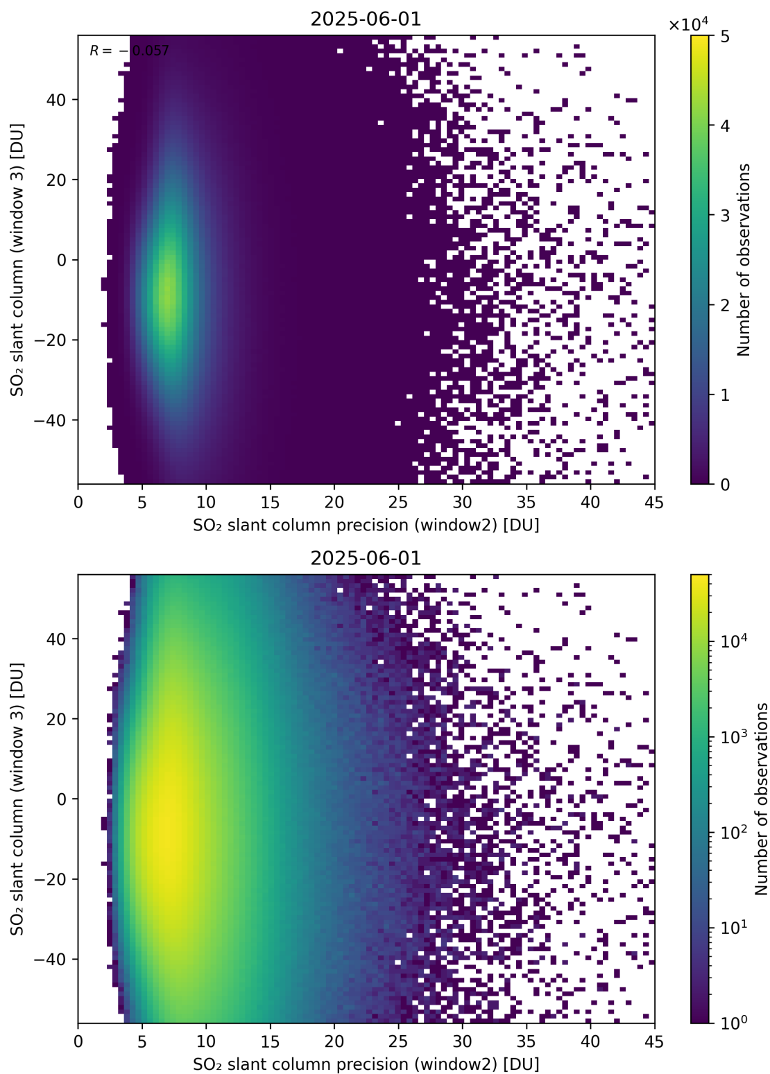
Figure 299: Scatter density plot of “SO 2 slant column precision (window2)” against “SO 2 slant column (window 3)” for 2025-06-01 to 2025-06-02.
