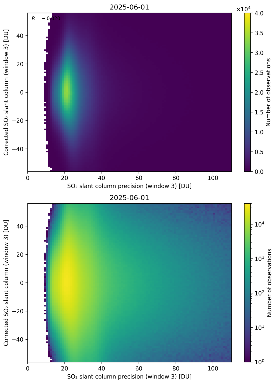
Figure 312: Scatter density plot of “SO 2 slant column precision (window 3)” against “Corrected SO 2 slant column (window 3)” for 2025-06-01 to 2025-06-02.
