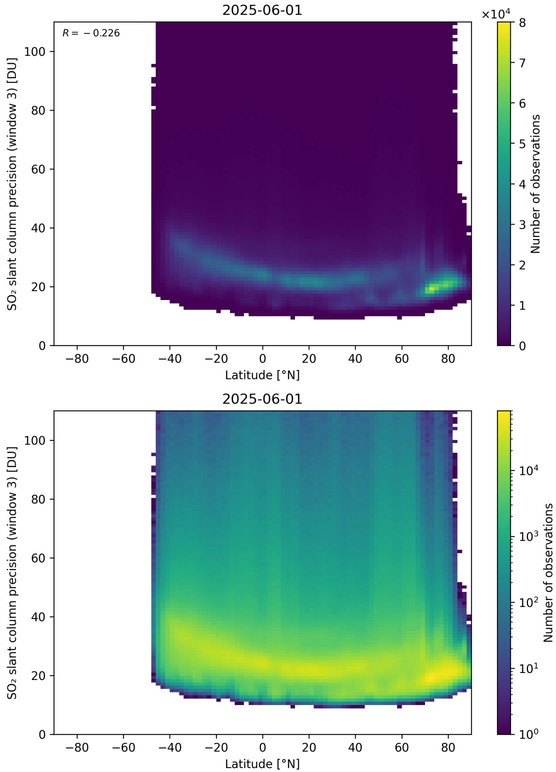
Figure 166: Scatter density plot of “Latitude” against “SO 2 slant column precision (window 3)” for 2025-06-01 to 2025-06-02.
