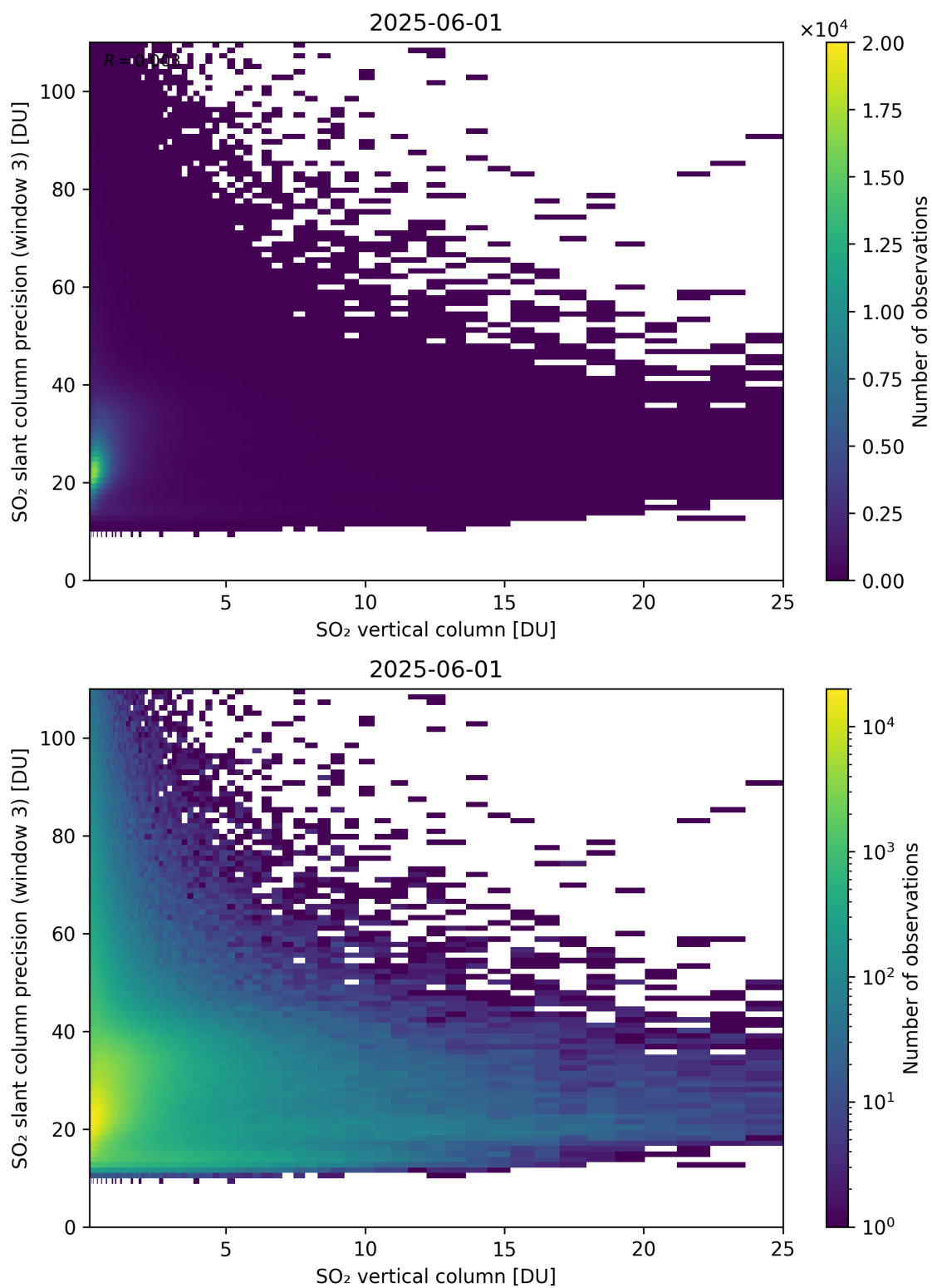
Figure 358: Scatter density plot of “SO 2 vertical column” against “SO 2 slant column precision (window 3)” for 2025-06-01 to 2025-06-02.
