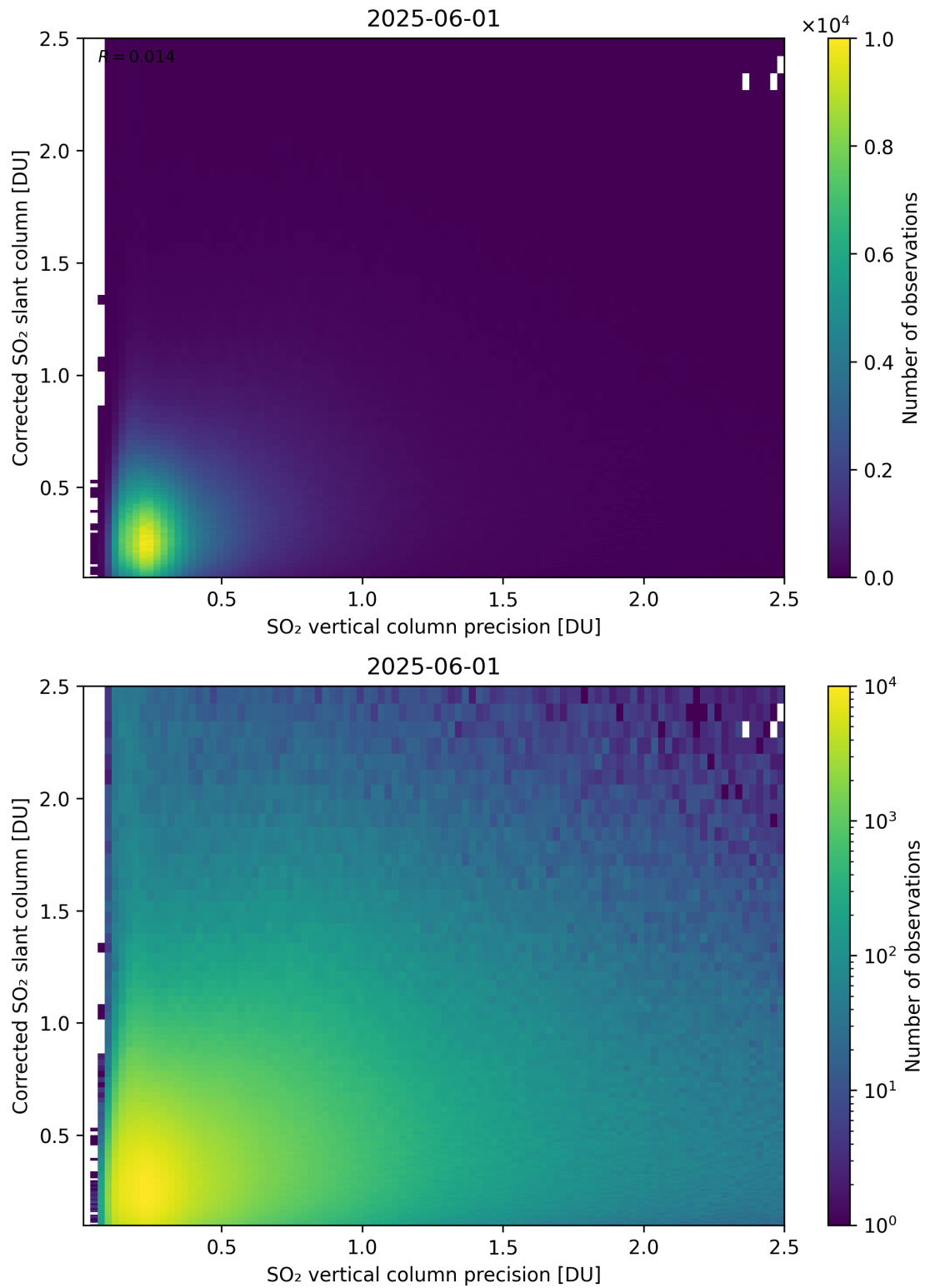
Figure 338: Scatter density plot of “SO 2 vertical column precision” against “Corrected SO 2 slant column” for 2025-06-01 to 2025-06-02.
