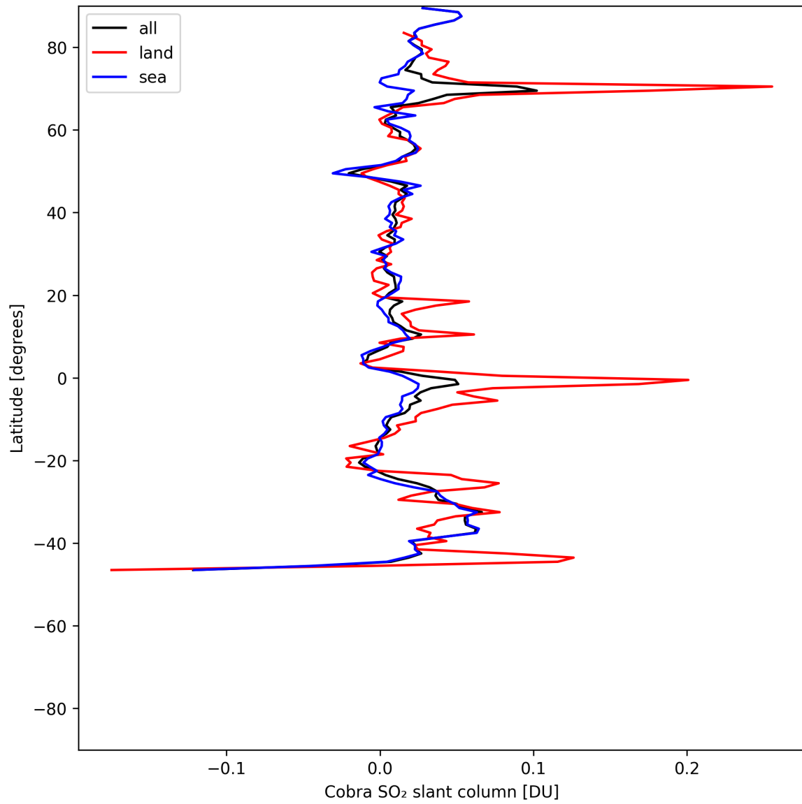
Figure 35: Zonal average of “Cobra SO 2 slant column” for 2025-06-01 to 2025-06-02.
