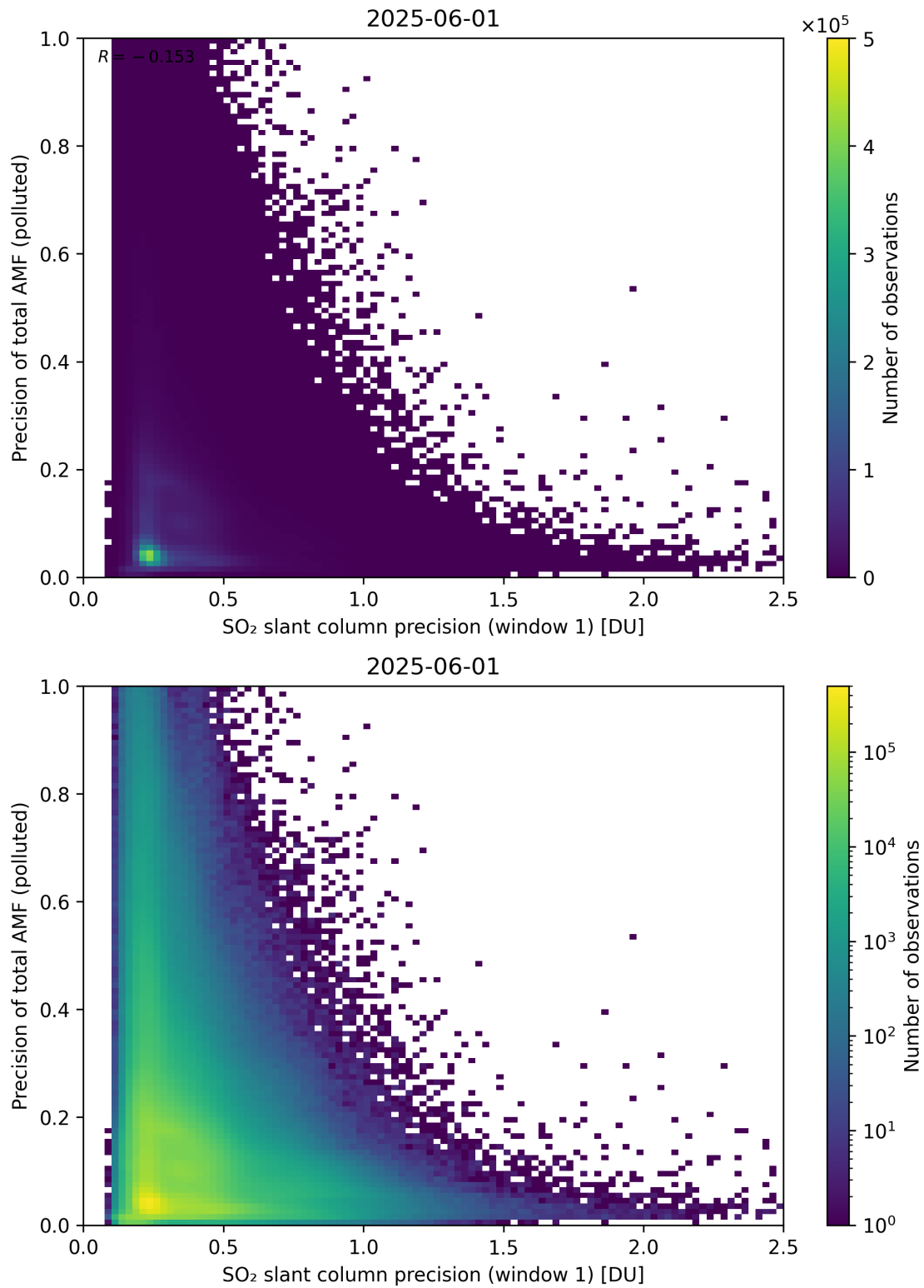
Figure 281: Scatter density plot of “SO 2 slant column precision (window 1)” against “Precision of total AMF (polluted)” for 2025-06-01 to 2025-06-02.
