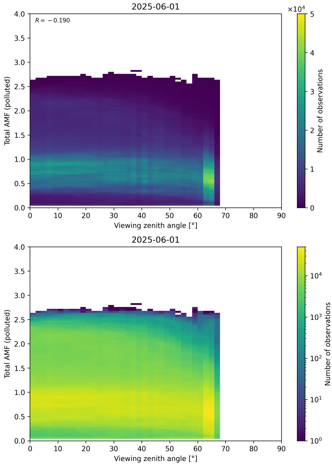
Figure 381: Scatter density plot of “Viewing zenith angle” against “Total AMF (polluted)” for 2025-06-01 to 2025-06-02.
