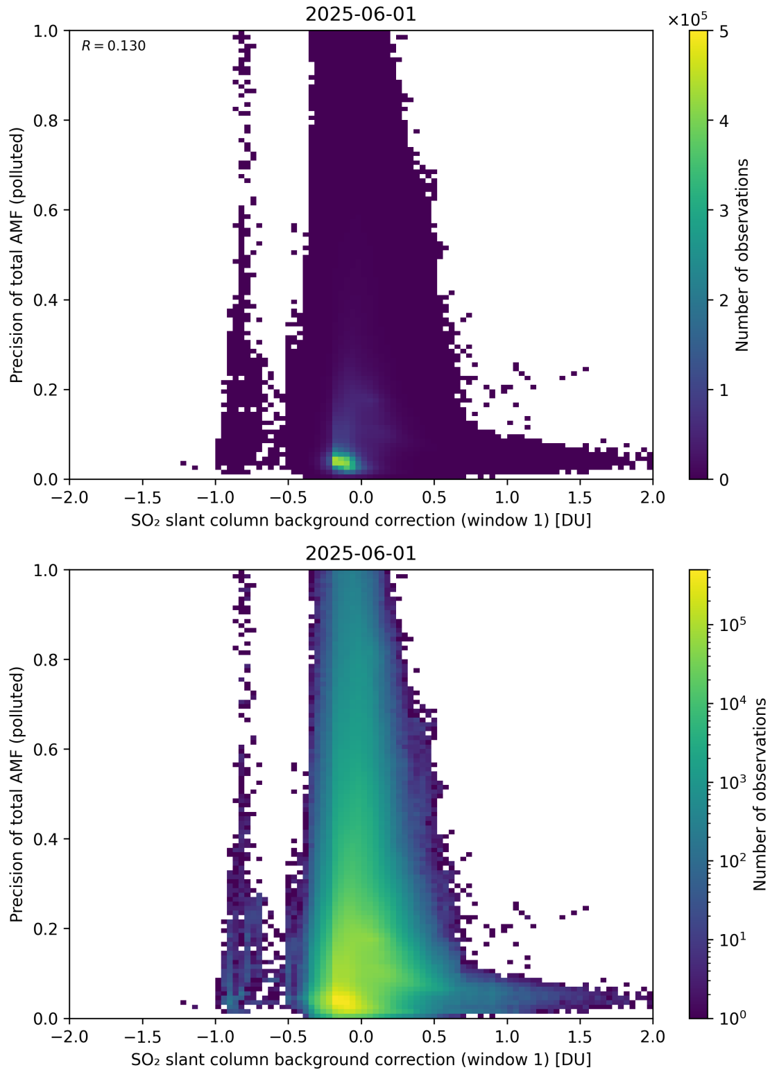
Figure 121: Scatter density plot of “SO 2 slant column background correction (window 1)” against “Precision of total AMF (polluted)” for 2025-06-01 to 2025-06-02.
