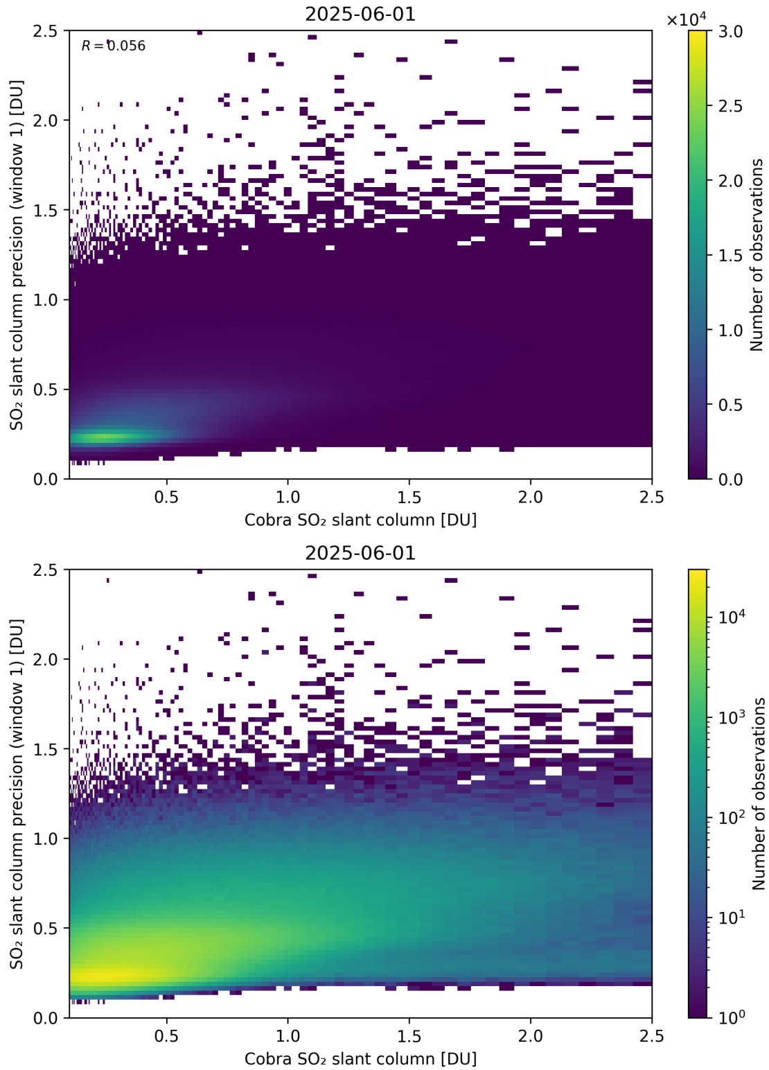
Figure 220: Scatter density plot of “Cobra SO 2 slant column” against “SO 2 slant column precision (window 1)” for 2025-06-01 to 2025-06-02.
