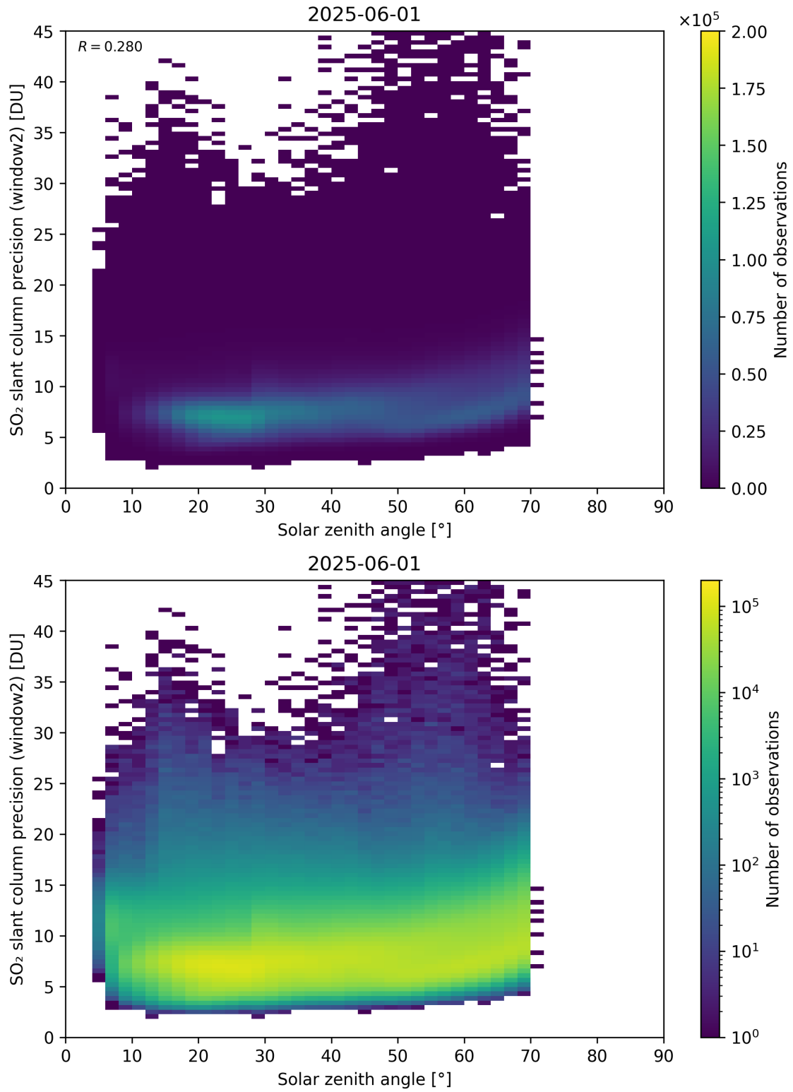
Figure 186: Scatter density plot of “Solar zenith angle” against “SO 2 slant column precision (window2)” for 2025-06-01 to 2025-06-02.
