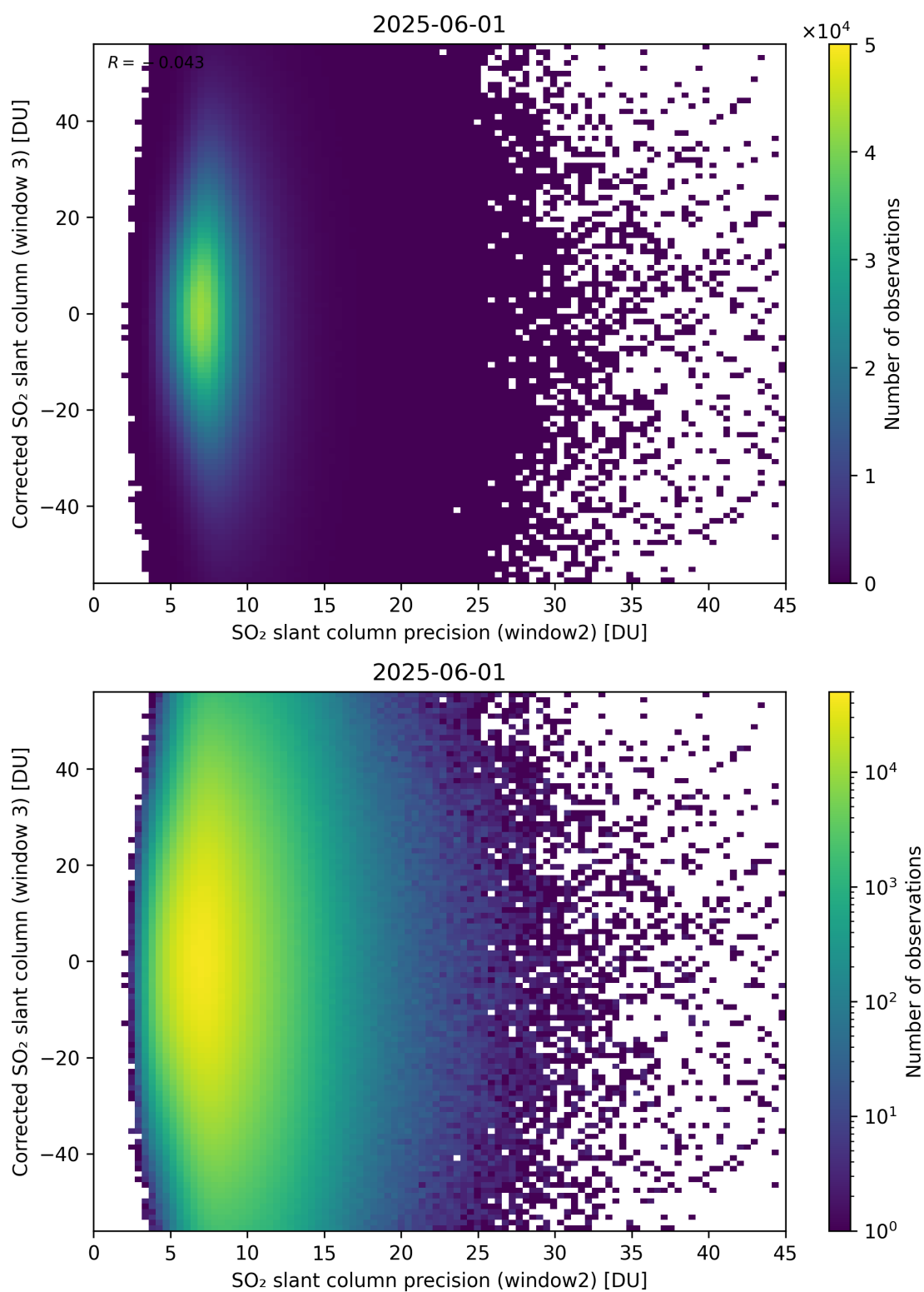
Figure 298: Scatter density plot of “SO 2 slant column precision (window2)” against “Corrected SO 2 slant column (window 3)” for 2025-06-01 to 2025-06-02.
