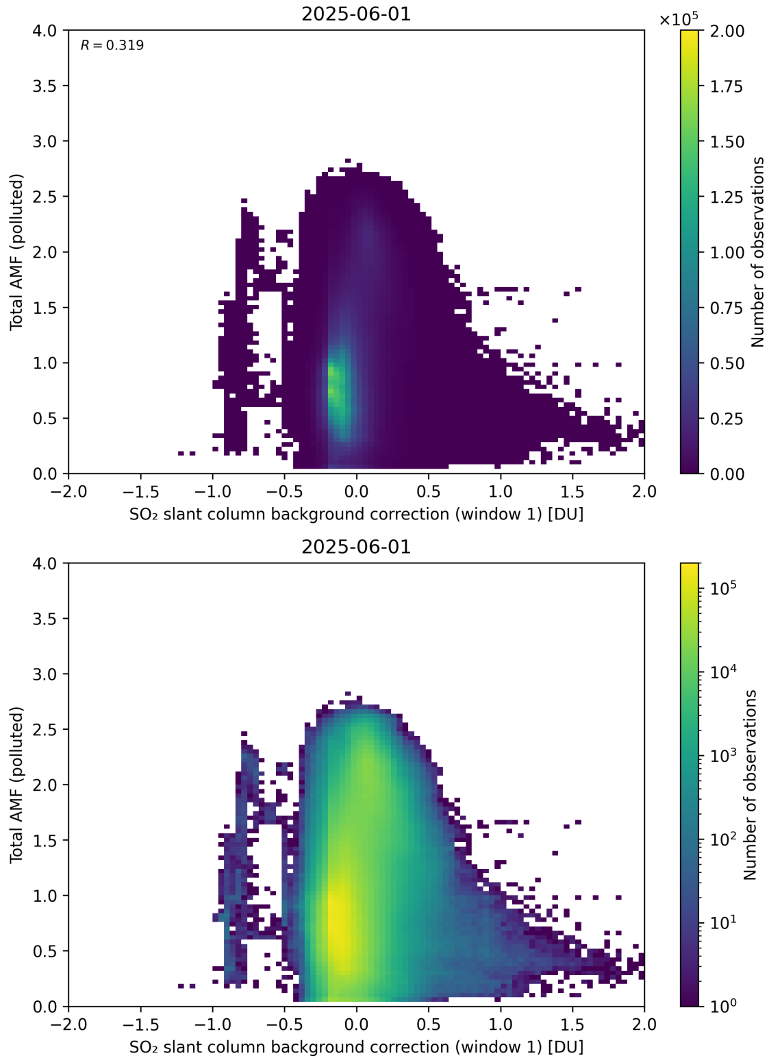
Figure 120: Scatter density plot of “SO 2 slant column background correction (window 1)” against “Total AMF (polluted)” for 2025-06-01 to 2025-06-02.
