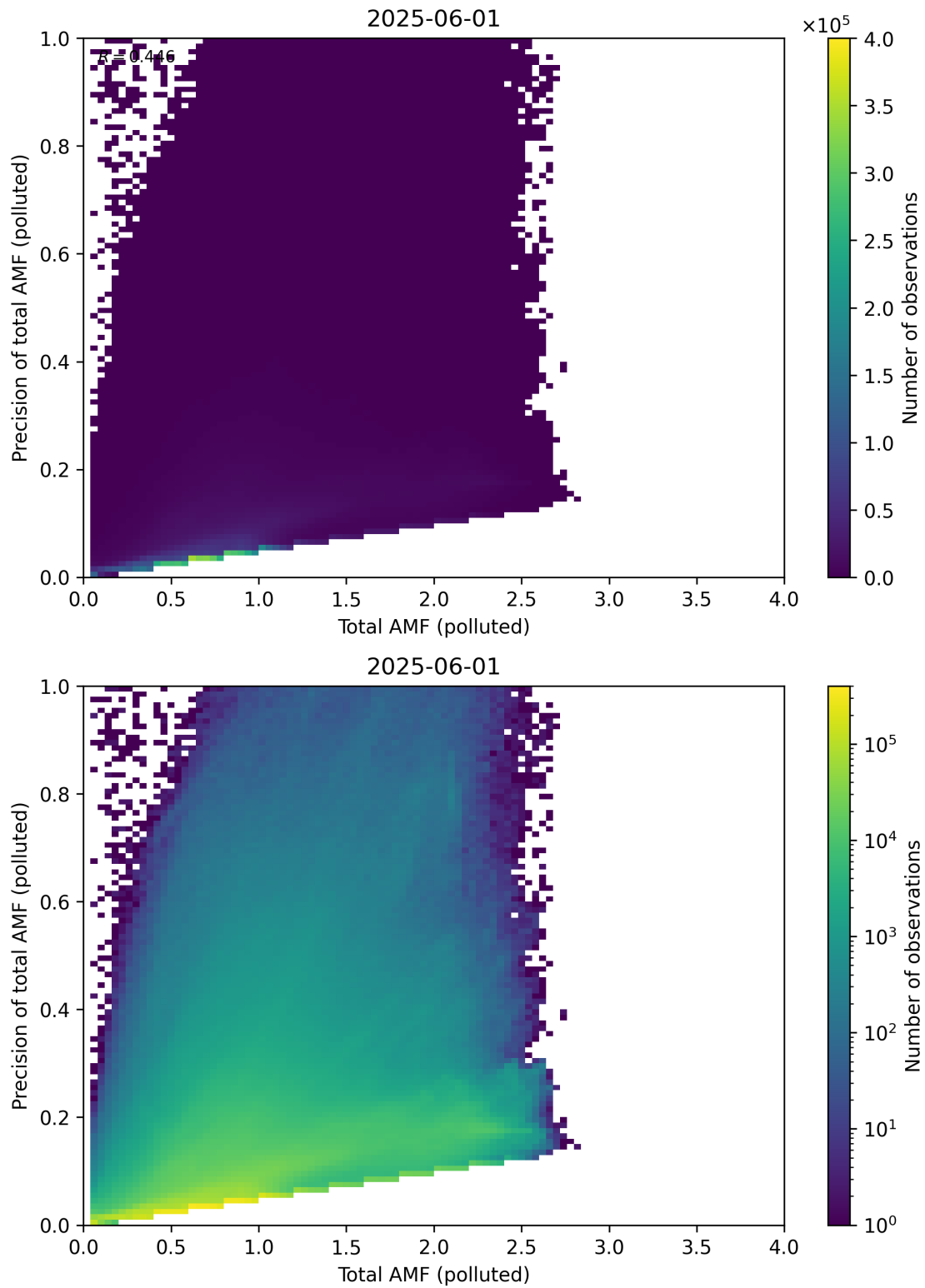
Figure 322: Scatter density plot of “Total AMF (polluted)” against “Precision of total AMF (polluted)” for 2025-06-01 to 2025-06-02.
