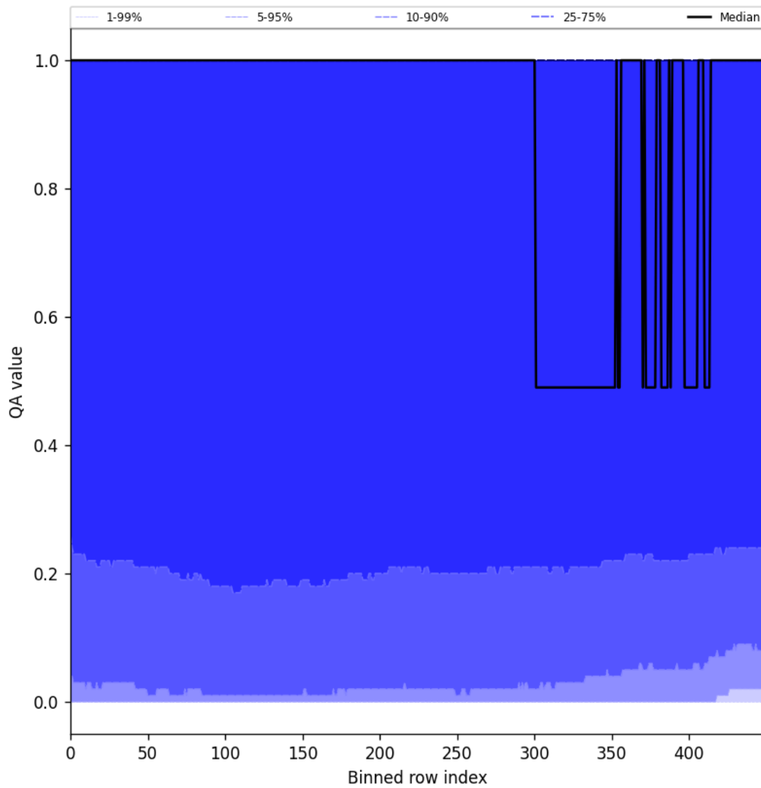
Figure 83: Along track statistics of “QA value” for 2025-06-01 to 2025-06-02
