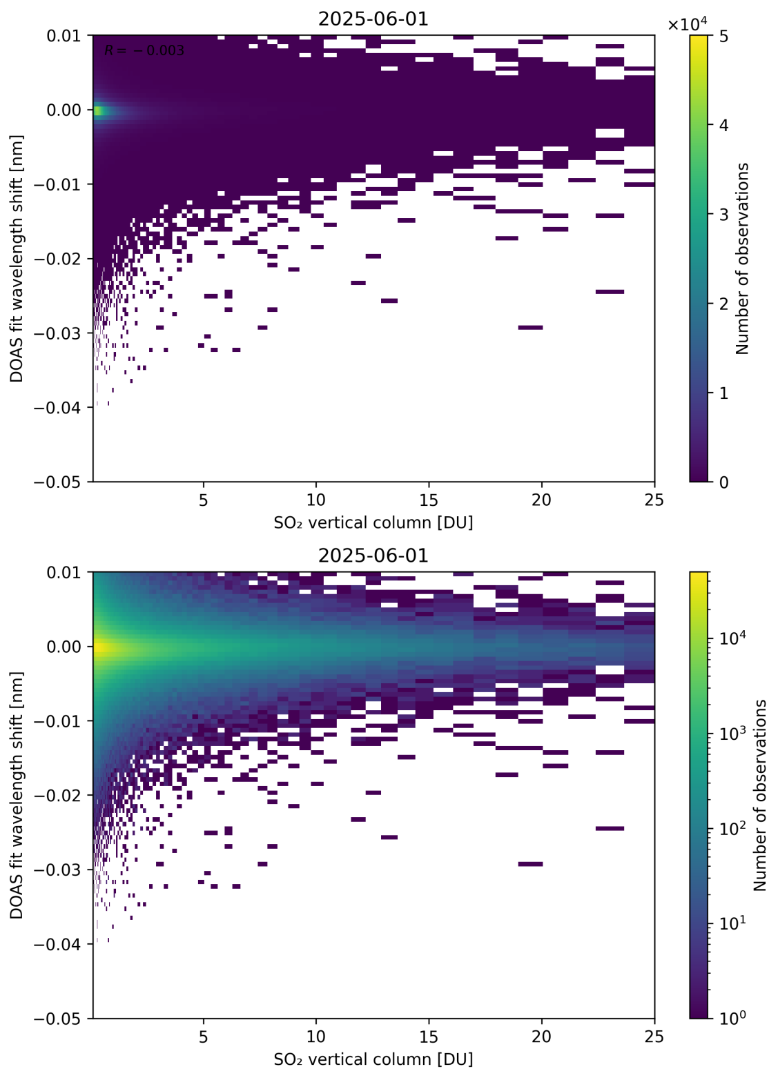
Figure 326: Scatter density plot of “SO 2 vertical column” against “DOAS fit wavelength shift” for 2025-06-01 to 2025-06-02.
