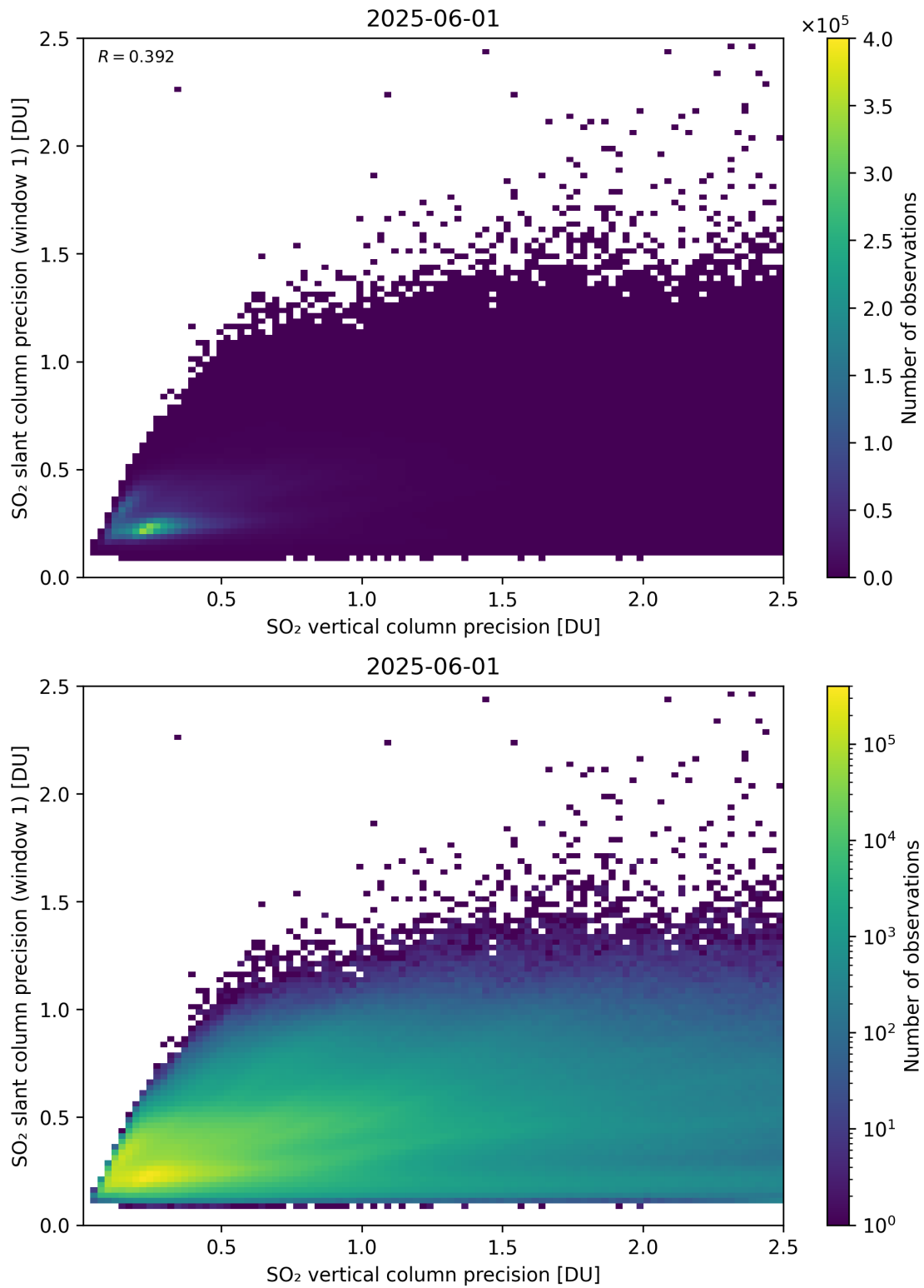
Figure 342: Scatter density plot of “SO 2 vertical column precision” against “SO 2 slant column precision (window 1)” for 2025-06-01 to 2025-06-02.
