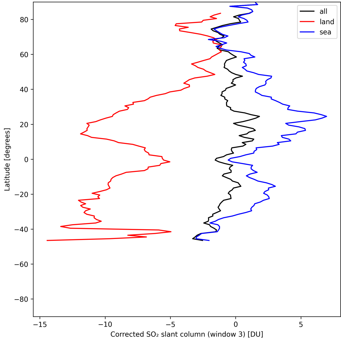
Figure 47: Zonal average of “Corrected SO 2 slant column (window 3)” for 2025-06-01 to 2025-06-02.
