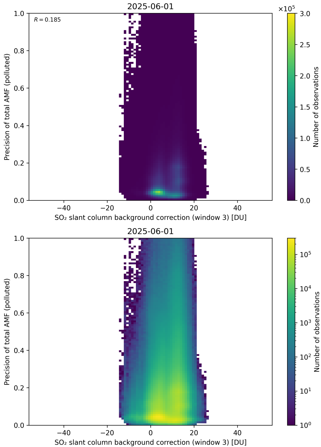
Figure 137: Scatter density plot of “SO 2 slant column background correction (window 3)” against “Precision of total AMF (polluted)” for 2025-06-01 to 2025-06-02.
