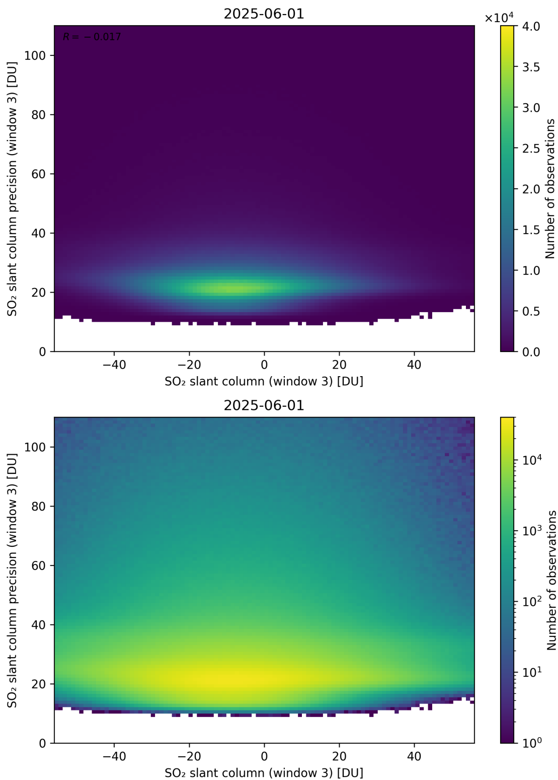
Figure 317: Scatter density plot of “SO 2 slant column (window 3)” against “SO 2 slant column precision (window 3)” for 2025-06-01 to 2025-06-02.
