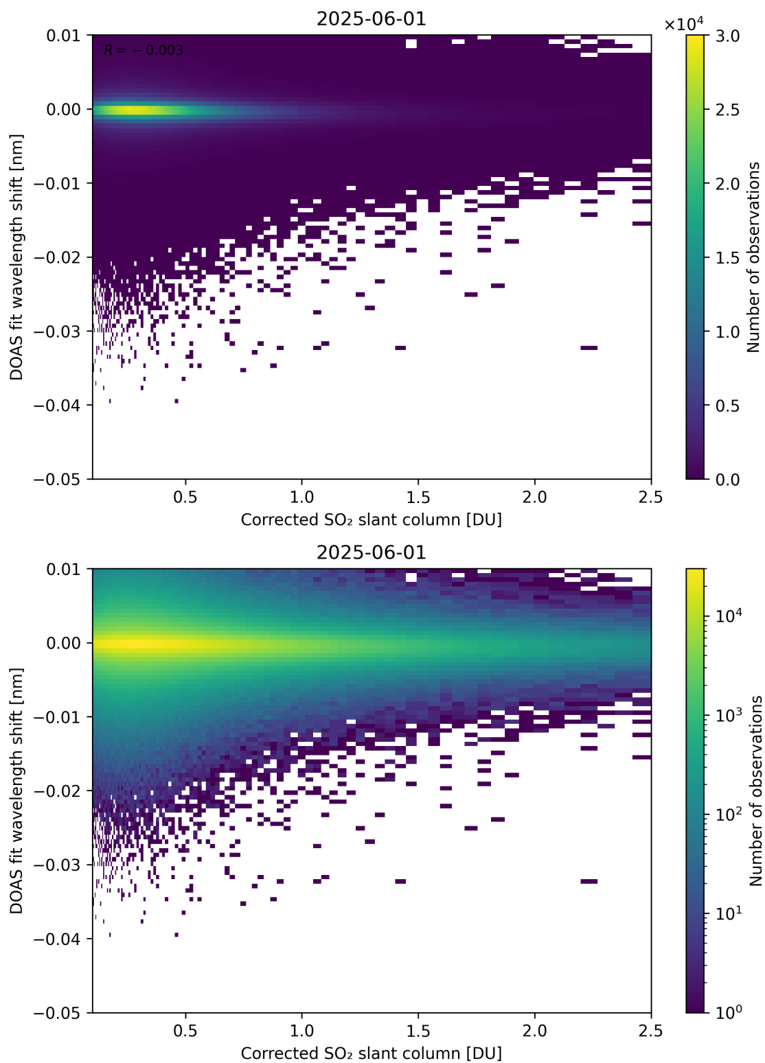
Figure 229: Scatter density plot of “Corrected SO 2 slant column” against “DOAS fit wavelength shift” for 2025-06-01 to 2025-06-02.
