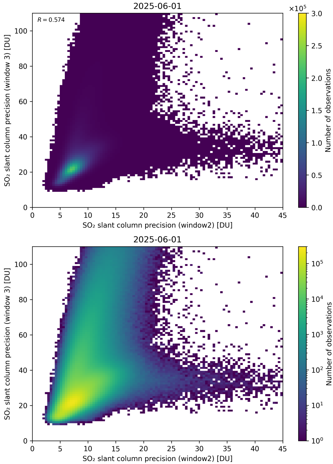
Figure 300: Scatter density plot of “SO 2 slant column precision (window2)” against “SO 2 slant column precision (window 3)” for 2025-06-01 to 2025-06-02.
