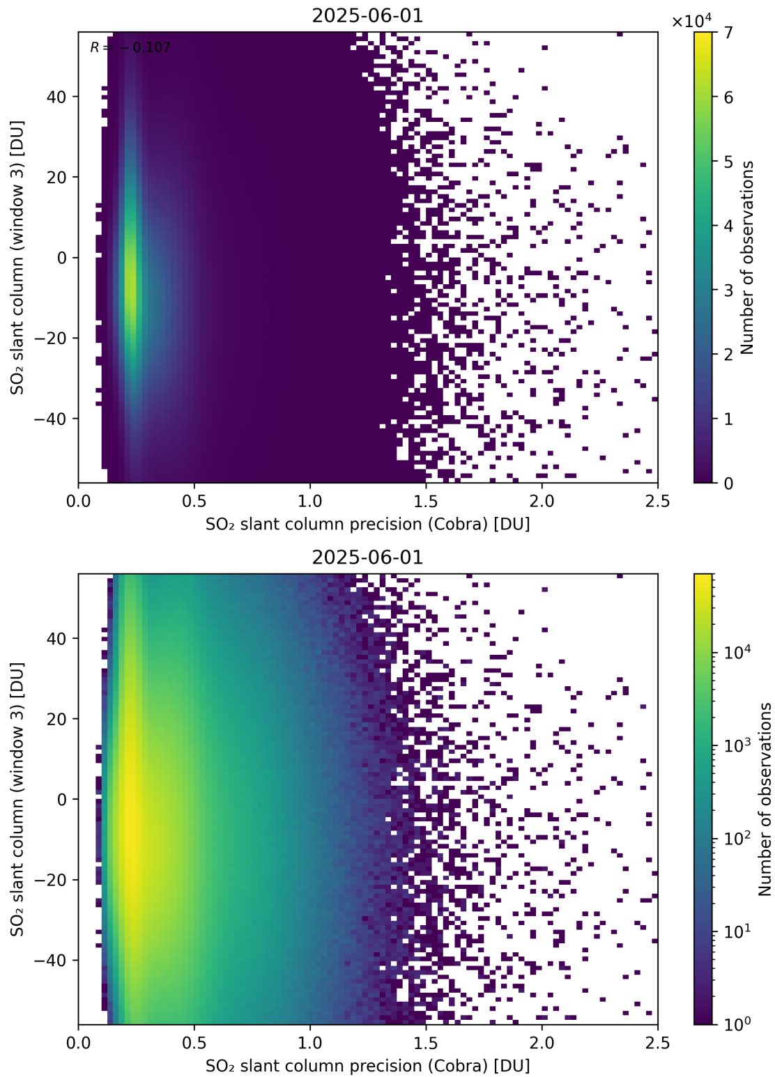
Figure 211: Scatter density plot of “SO 2 slant column precision (Cobra)” against “SO 2 slant column (window 3)” for 2025-06-01 to 2025-06-02.
