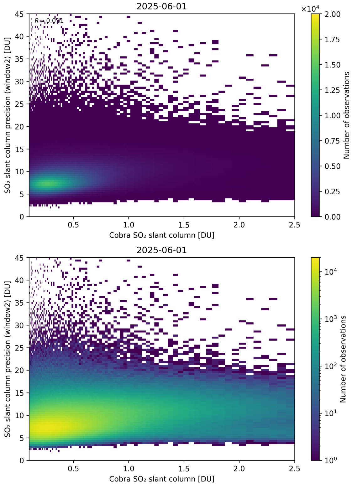
Figure 221: Scatter density plot of “Cobra SO 2 slant column” against “SO 2 slant column precision (window2)” for 2025-06-01 to 2025-06-02.
