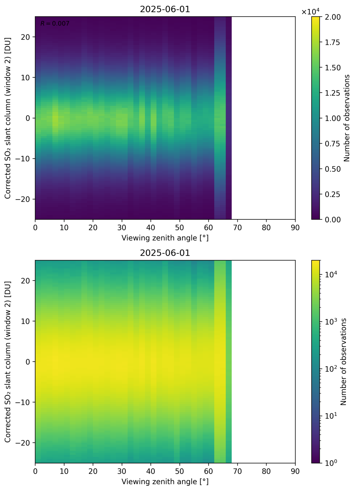
Figure 374: Scatter density plot of “Viewing zenith angle” against “Corrected SO 2 slant column (window 2)” for 2025-06-01 to 2025-06-02.
