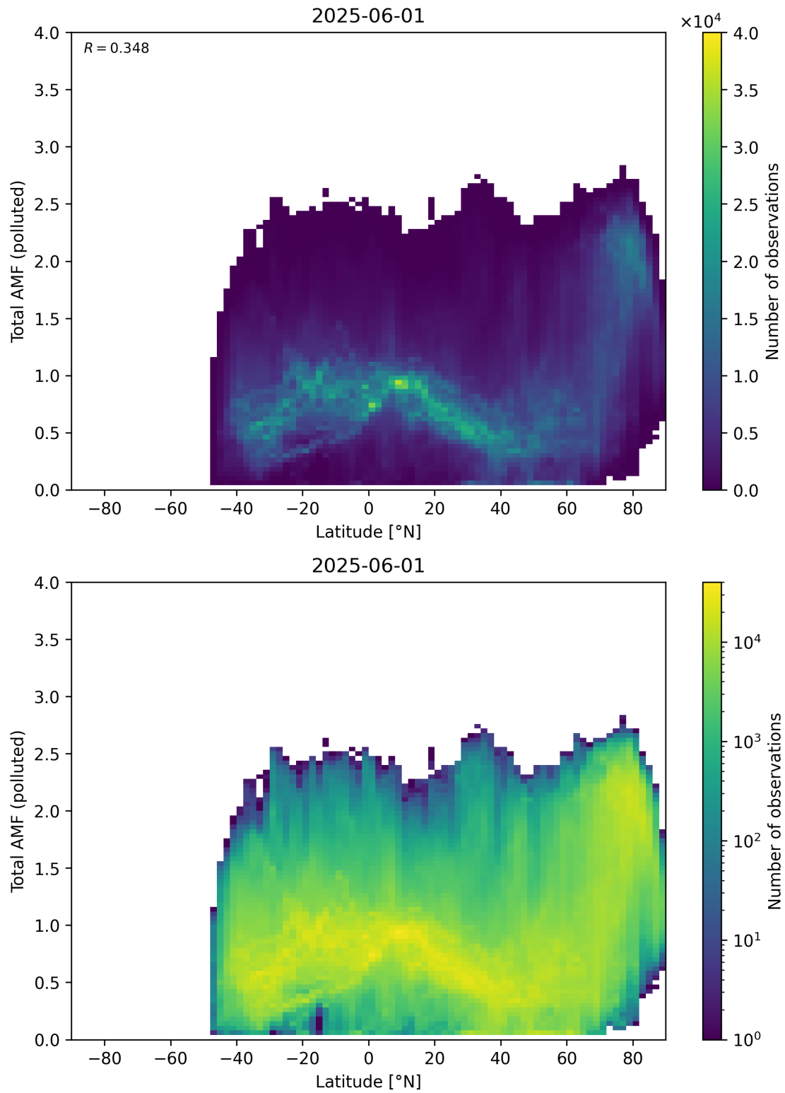
Figure 167: Scatter density plot of “Latitude” against “Total AMF (polluted)” for 2025-06-01 to 2025-06-02.
