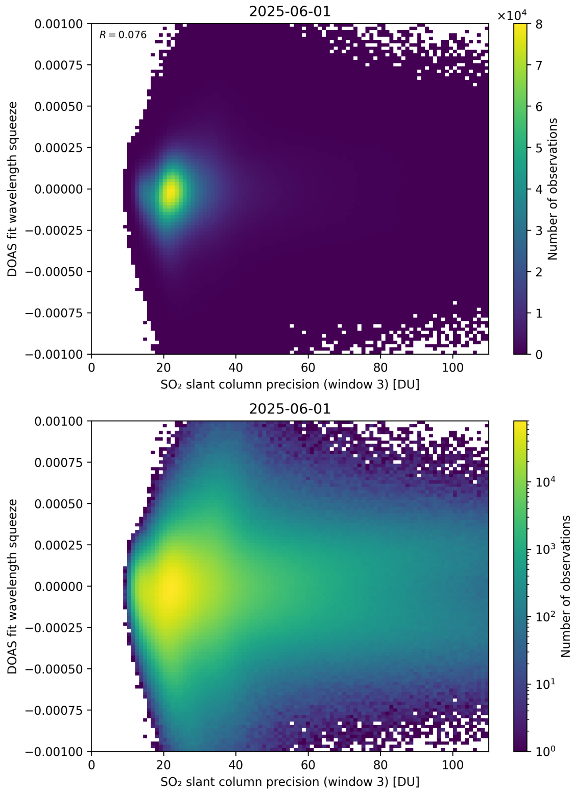
Figure 309: Scatter density plot of “SO 2 slant column precision (window 3)” against “DOAS fit wavelength squeeze” for 2025-06-01 to 2025-06-02.
