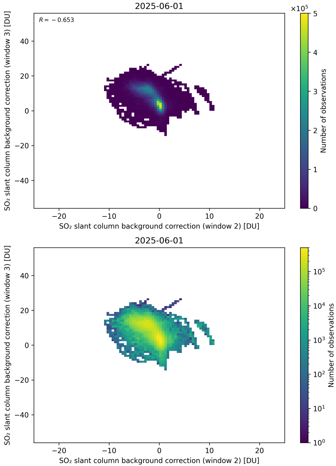
Figure 122: Scatter density plot of “SO 2 slant column background correction (window 2)” against “SO 2 slant column background correction (window 3)” for 2025-06-01 to 2025-06-02.
