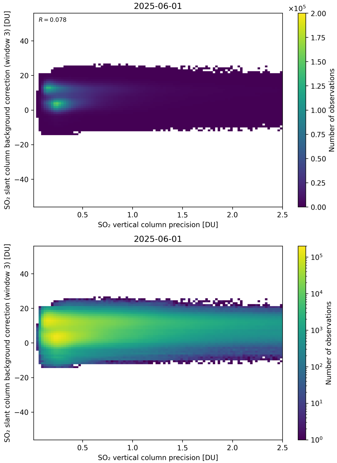
Figure 331: Scatter density plot of “SO 2 vertical column precision” against “SO 2 slant column background correction (window 3)” for 2025-06-01 to 2025-06-02.
