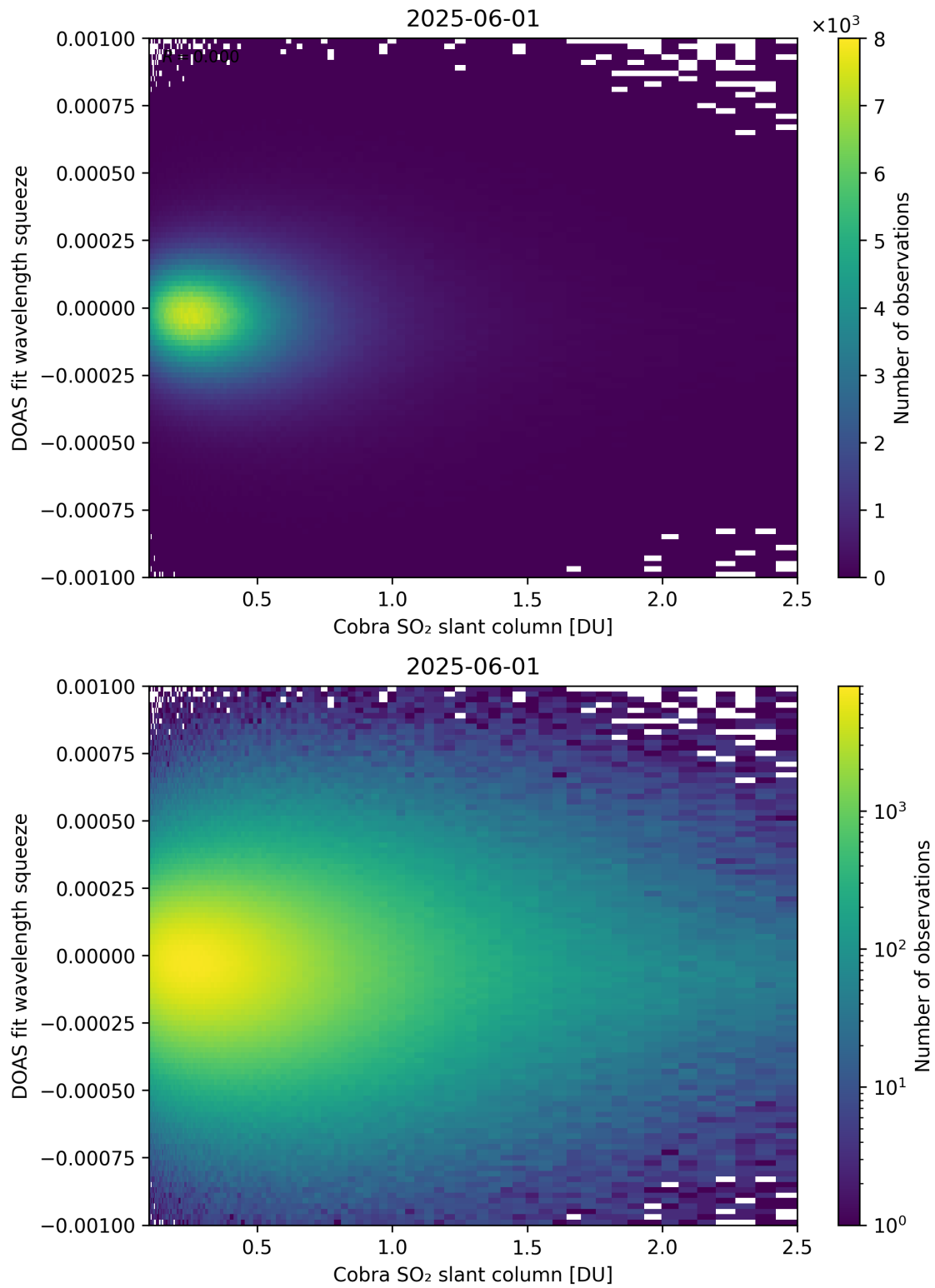
Figure 197: Scatter density plot of “Cobra SO 2 slant column” against “DOAS fit wavelength squeeze” for 2025-06-01 to 2025-06-02.
