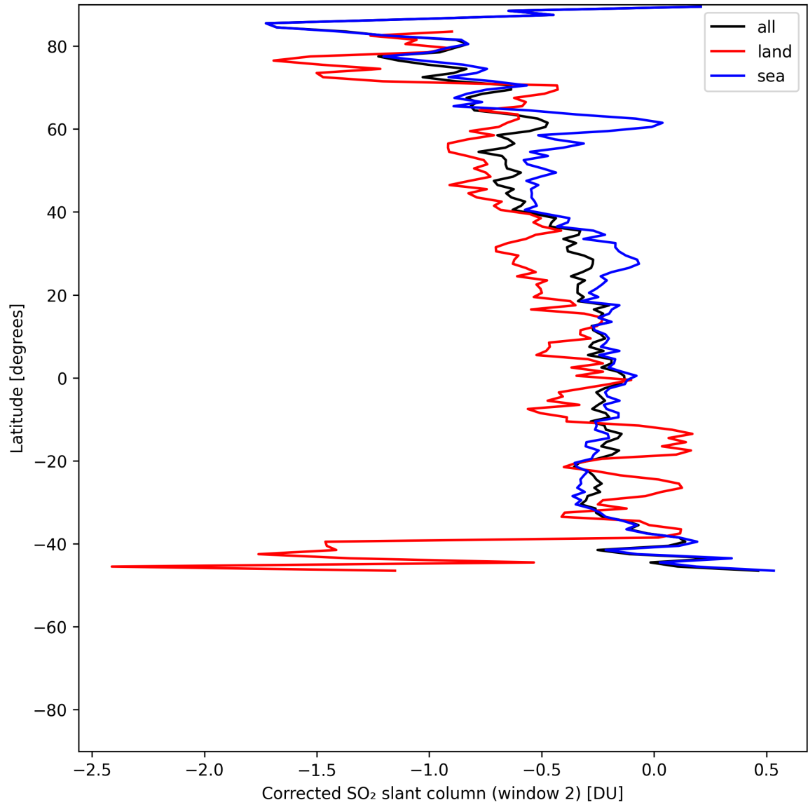
Figure 43: Zonal average of “Corrected SO 2 slant column (window 2)” for 2025-06-01 to 2025-06-02.
