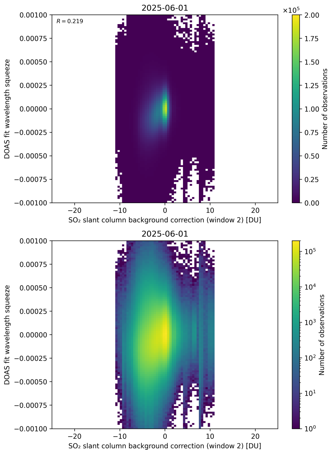
Figure 124: Scatter density plot of “SO 2 slant column background correction (window 2)” against “DOAS fit wavelength squeeze” for 2025-06-01 to 2025-06-02.
