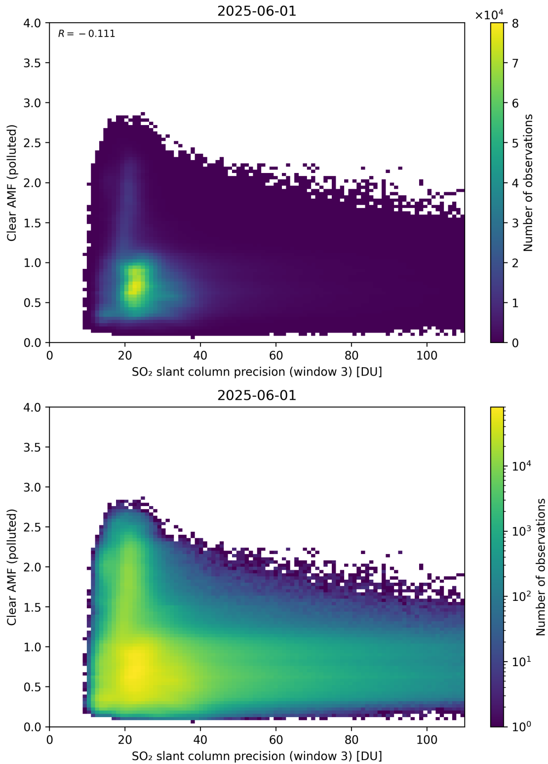
Figure 311: Scatter density plot of “SO 2 slant column precision (window 3)” against “Clear AMF (polluted)” for 2025-06-01 to 2025-06-02.
