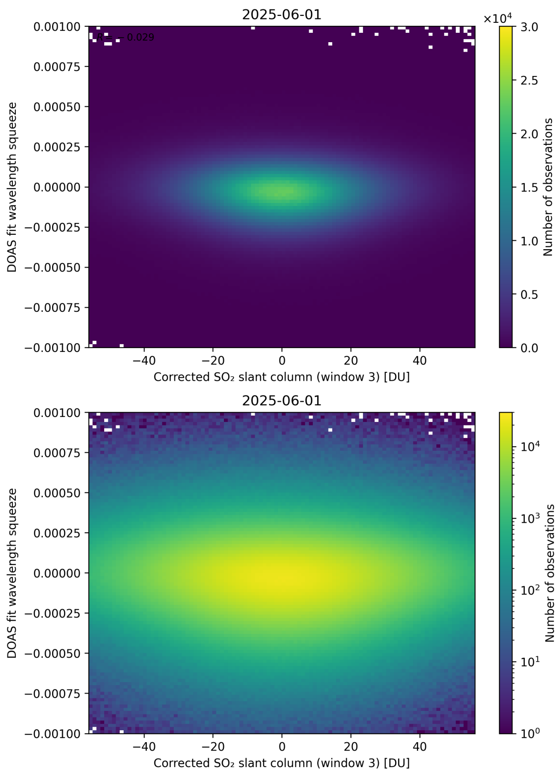
Figure 257: Scatter density plot of “Corrected SO 2 slant column (window 3)” against “DOAS fit wavelength squeeze” for 2025-06-01 to 2025-06-02.
