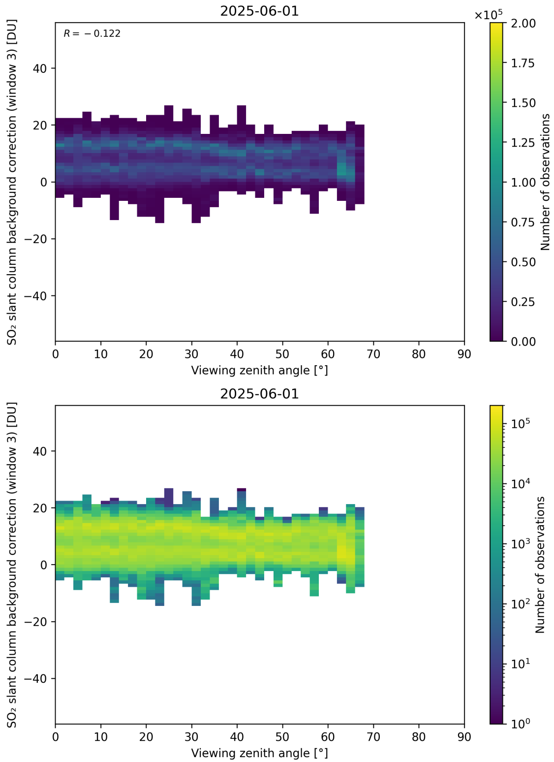
Figure 364: Scatter density plot of “Viewing zenith angle” against “SO 2 slant column background correction (window 3)” for 2025-06-01 to 2025-06-02.
