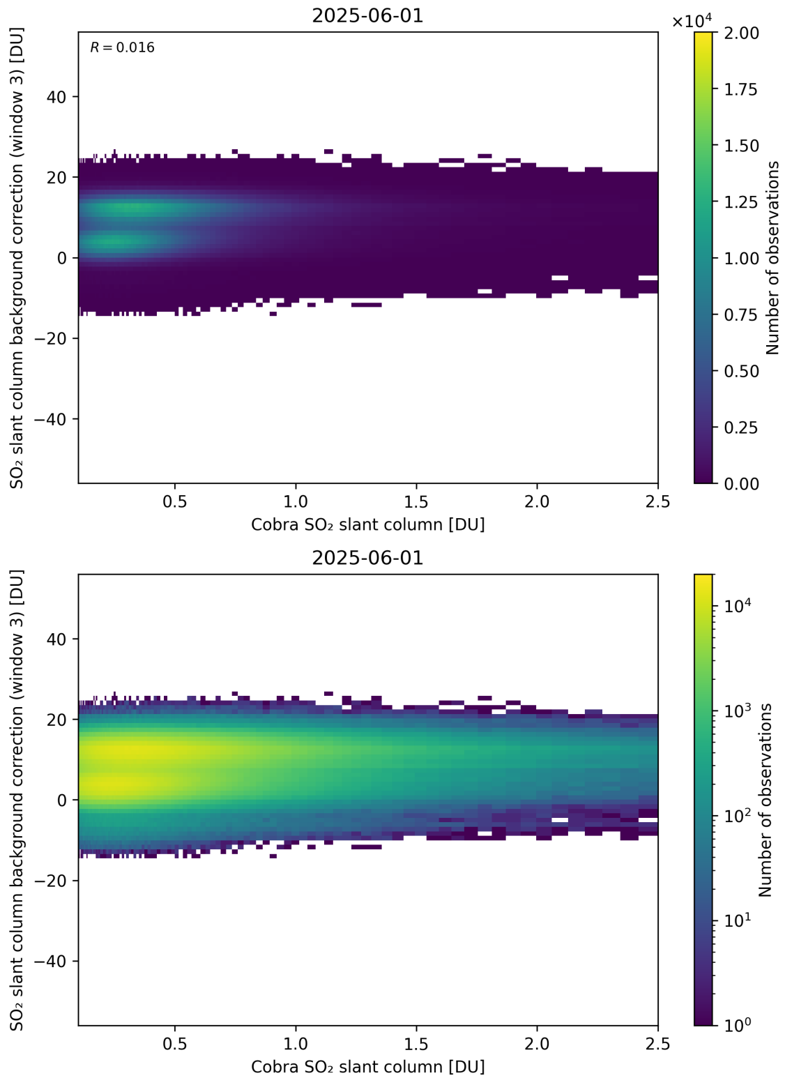
Figure 195: Scatter density plot of “Cobra SO 2 slant column” against “SO 2 slant column background correction (window 3)” for 2025-06-01 to 2025-06-02.
