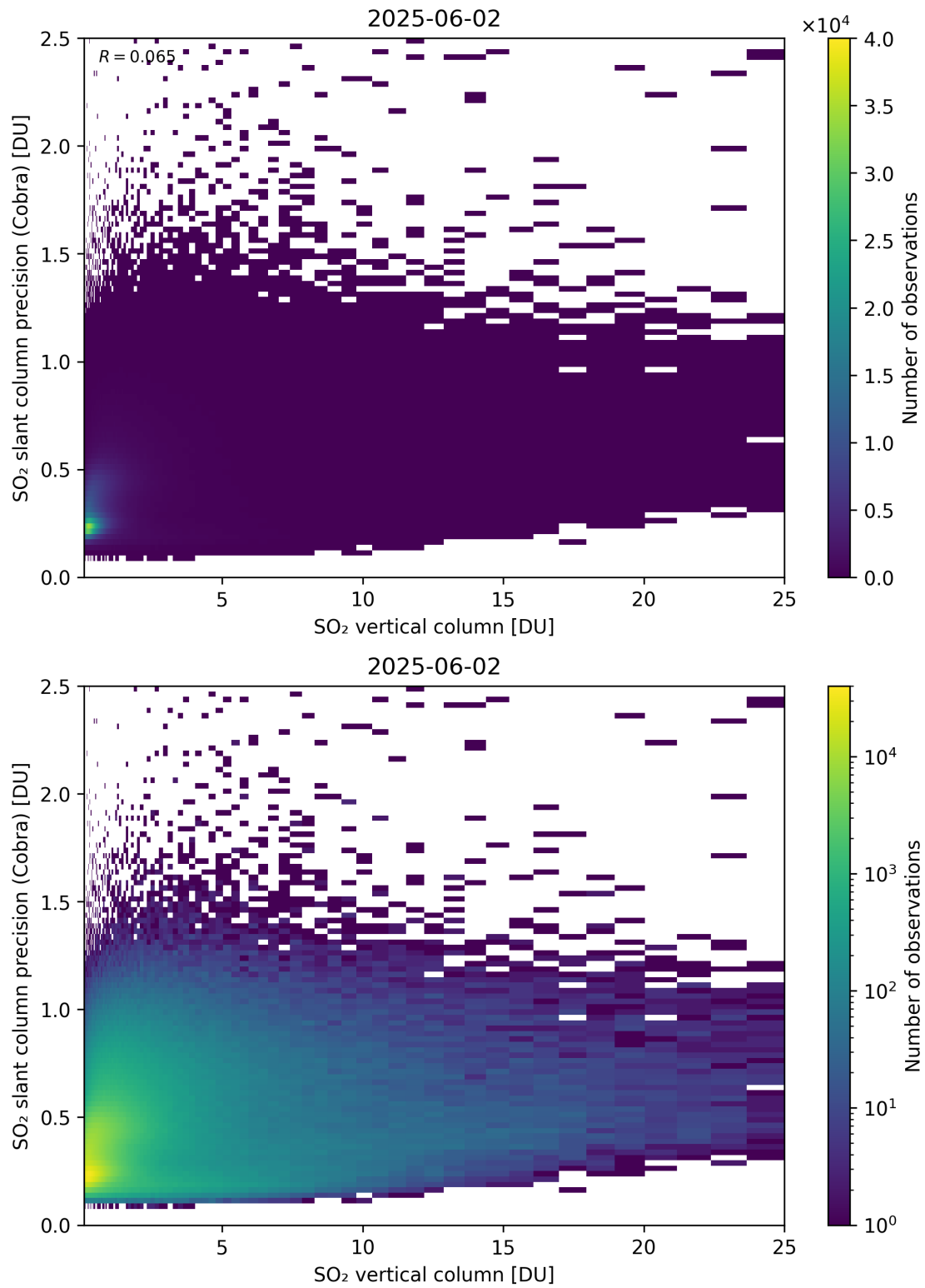
Figure 350: Scatter density plot of “SO 2 vertical column” against “SO 2 slant column precision (Cobra)” for 2025-06-01 to 2025-06-03.
