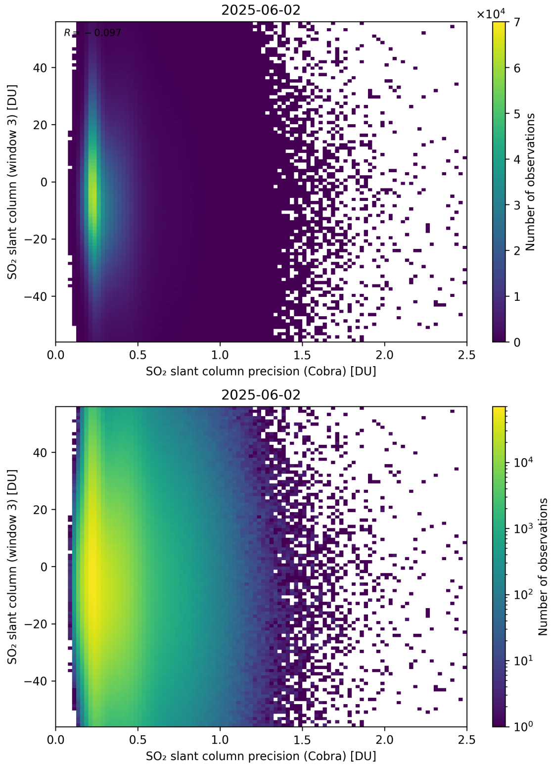
Figure 211: Scatter density plot of “SO 2 slant column precision (Cobra)” against “SO 2 slant column (window 3)” for 2025-06-01 to 2025-06-03.
