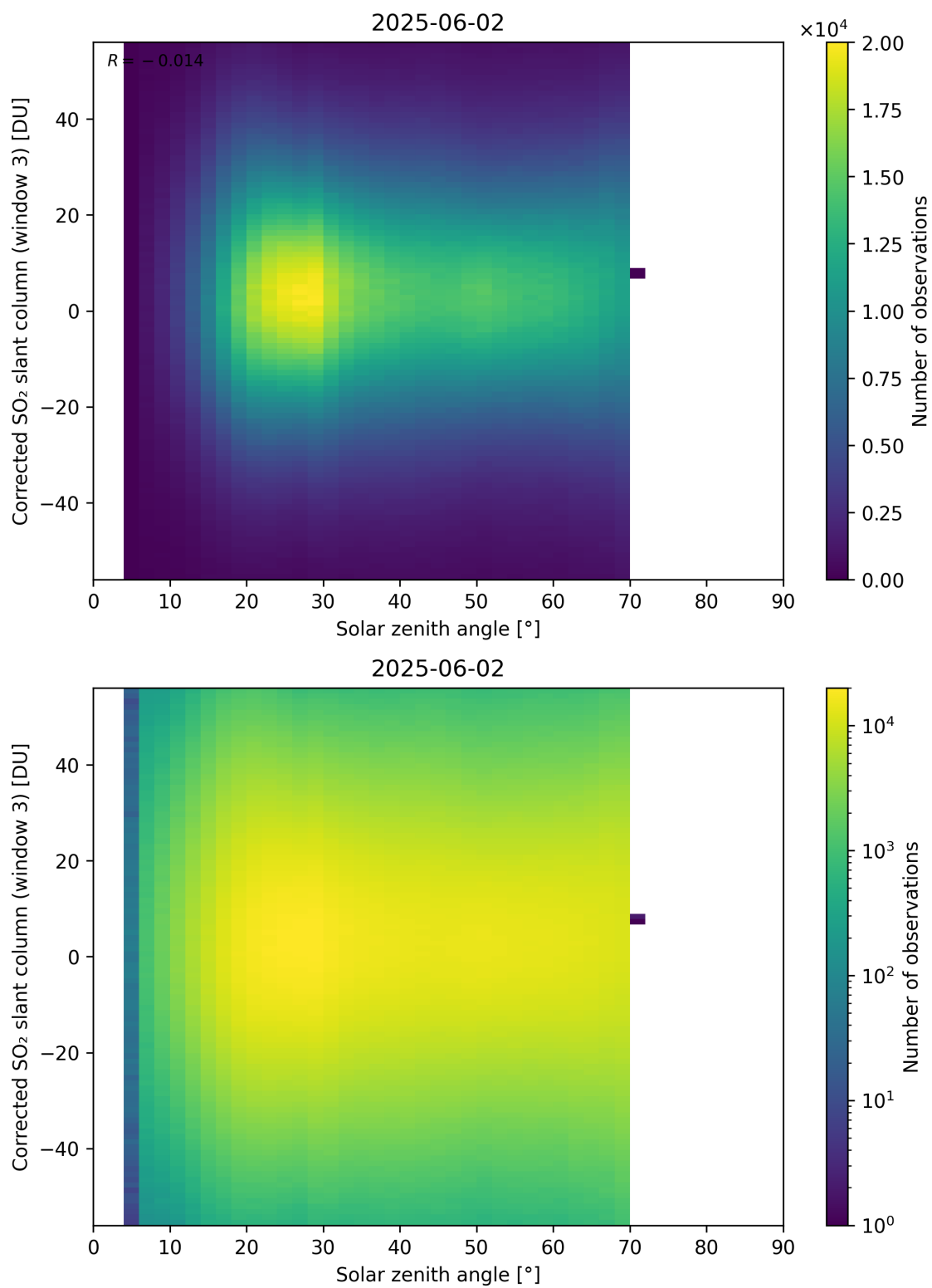
Figure 183: Scatter density plot of “Solar zenith angle” against “Corrected SO 2 slant column (window 3)” for 2025-06-01 to 2025-06-03.
