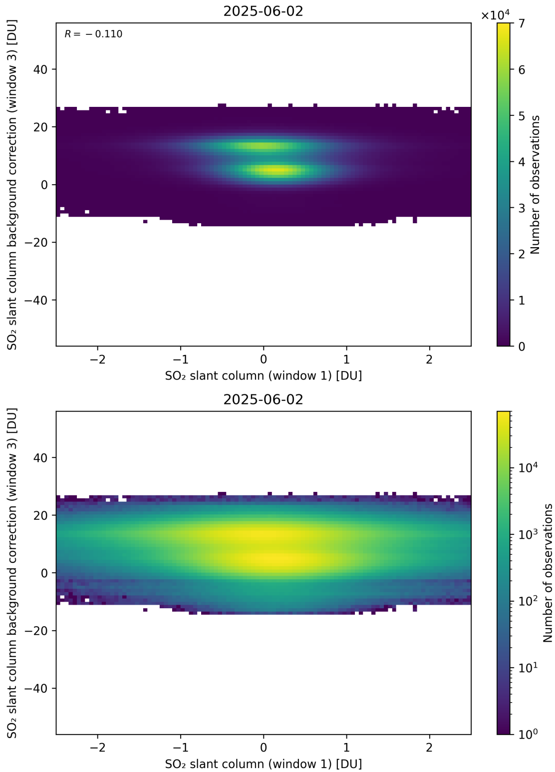
Figure 264: Scatter density plot of “SO 2 slant column (window 1)” against “SO 2 slant column background correction (window 3)” for 2025-06-01 to 2025-06-03.
