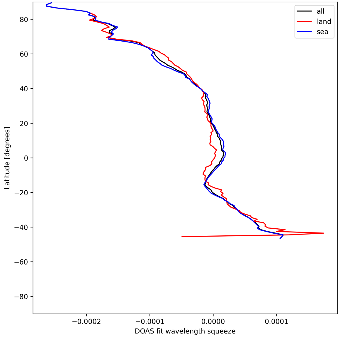
Figure 51: Zonal average of “DOAS fit wavelength squeeze” for 2025-06-01 to 2025-06-03.
