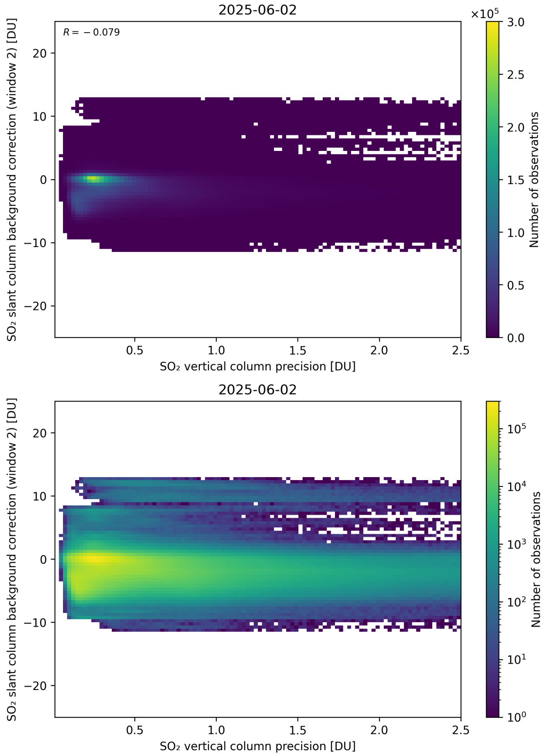
Figure 330: Scatter density plot of “SO 2 vertical column precision” against “SO 2 slant column background correction (window 2)” for 2025-06-01 to 2025-06-03.
