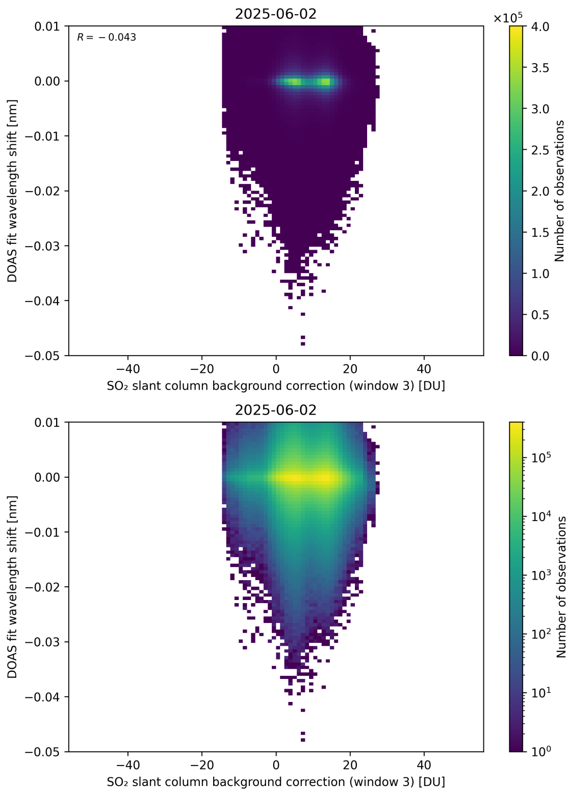
Figure 132: Scatter density plot of “SO 2 slant column background correction (window 3)” against “DOAS fit wavelength shift” for 2025-06-01 to 2025-06-03.
