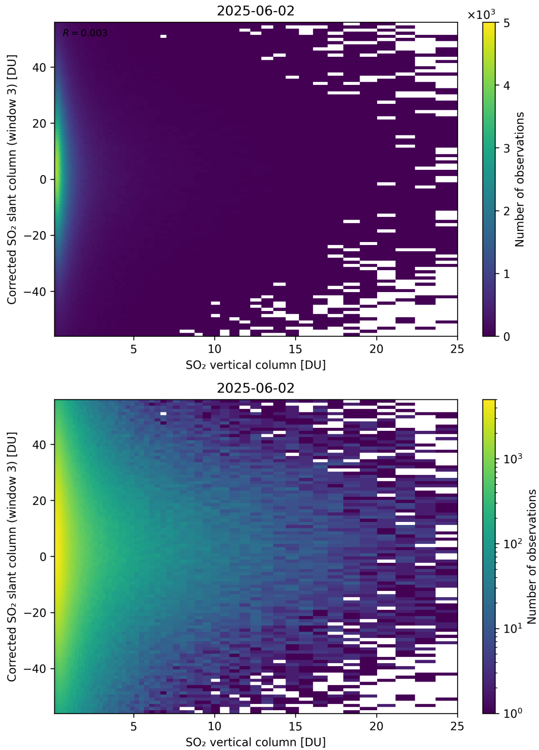
Figure 353: Scatter density plot of “SO 2 vertical column” against “Corrected SO 2 slant column (window 3)” for 2025-06-01 to 2025-06-03.
