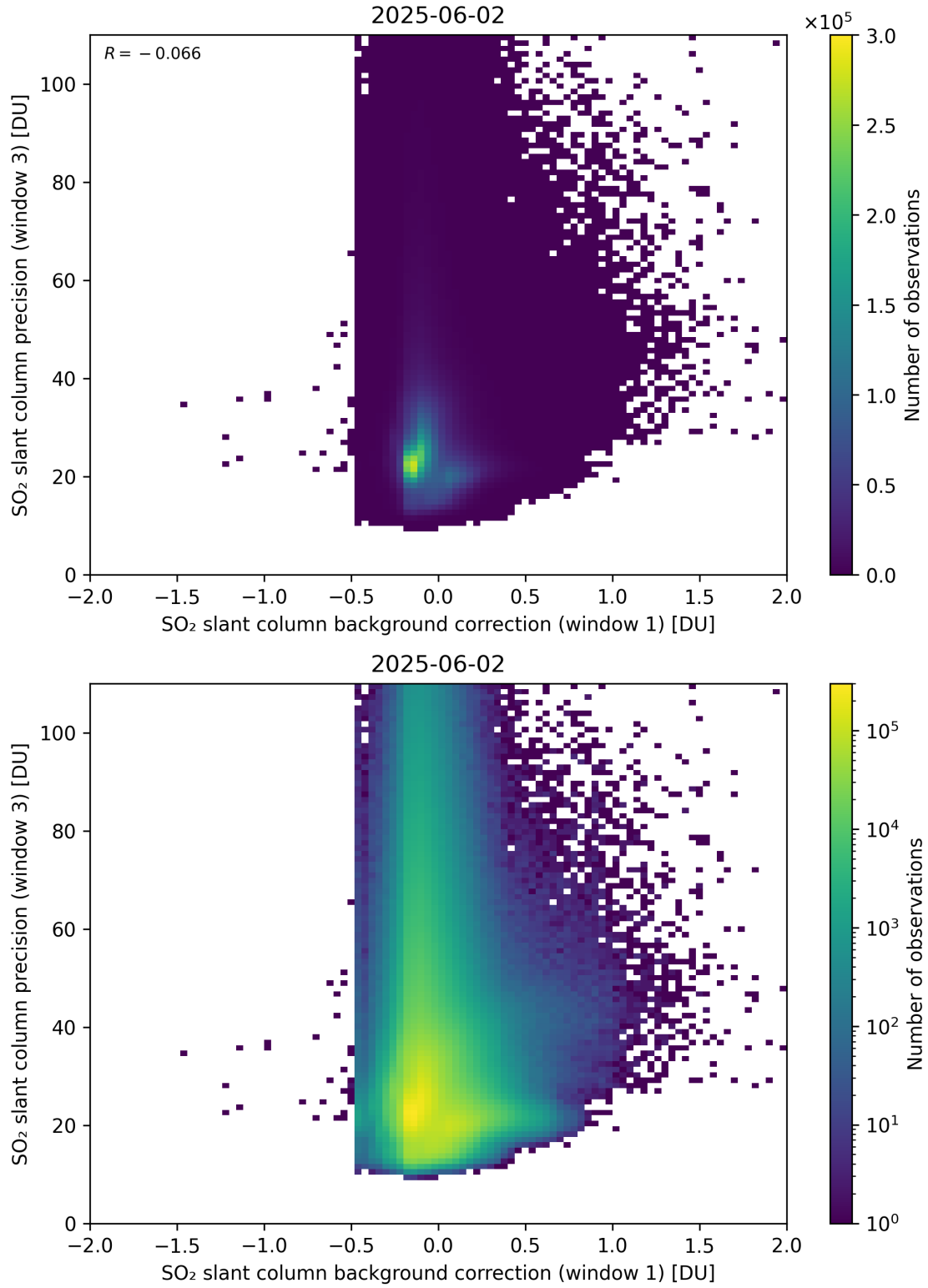
Figure 119: Scatter density plot of “SO 2 slant column background correction (window 1)” against “SO 2 slant column precision (window 3)” for 2025-06-01 to 2025-06-03.
