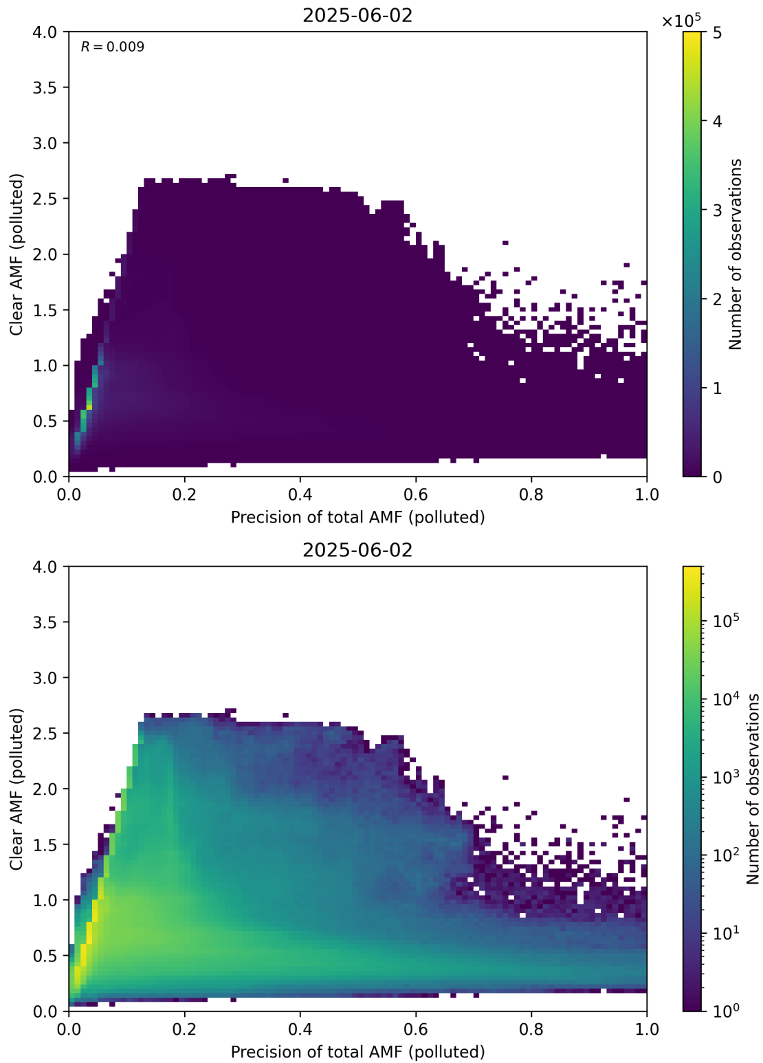
Figure 320: Scatter density plot of “Precision of total AMF (polluted)” against “Clear AMF (polluted)” for 2025-06-01 to 2025-06-03.
