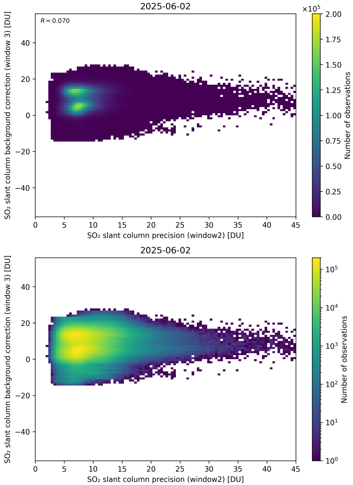
Figure 292: Scatter density plot of “SO 2 slant column precision (window2)” against “SO 2 slant column background correction (window 3)” for 2025-06-01 to 2025-06-03.
