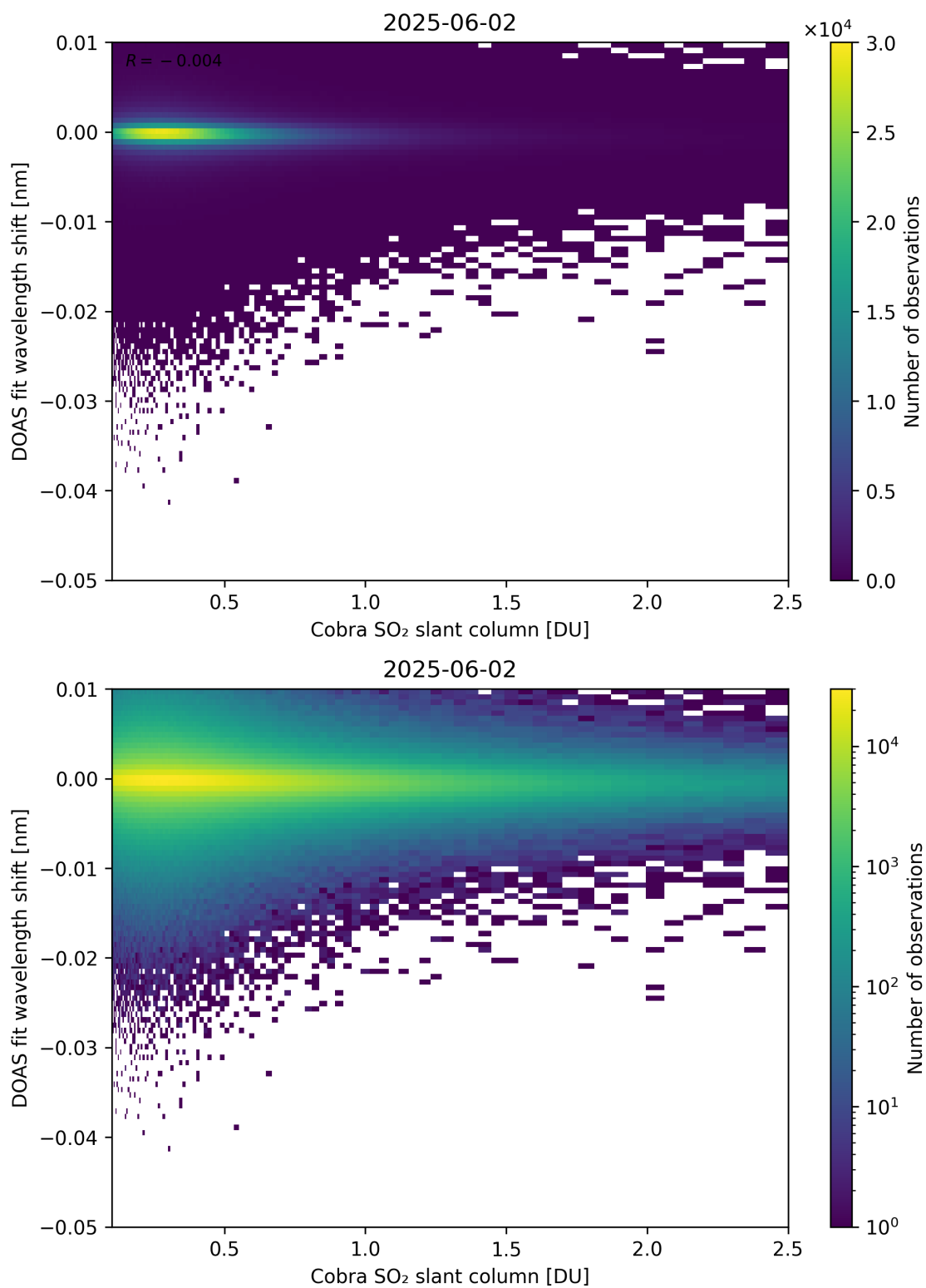
Figure 196: Scatter density plot of “Cobra SO 2 slant column” against “DOAS fit wavelength shift” for 2025-06-01 to 2025-06-03.
