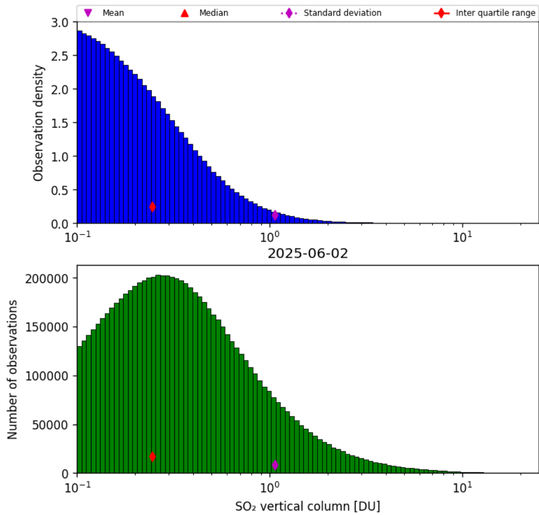
Figure 58: Histogram of “SO 2 vertical column” for 2025-06-01 to 2025-06-03
