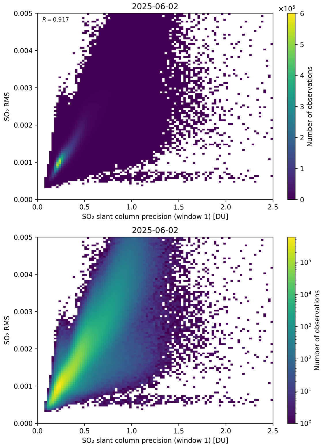
Figure 273: Scatter density plot of “SO 2 slant column precision (window 1)” against “SO 2 RMS” for 2025-06-01 to 2025-06-03.
