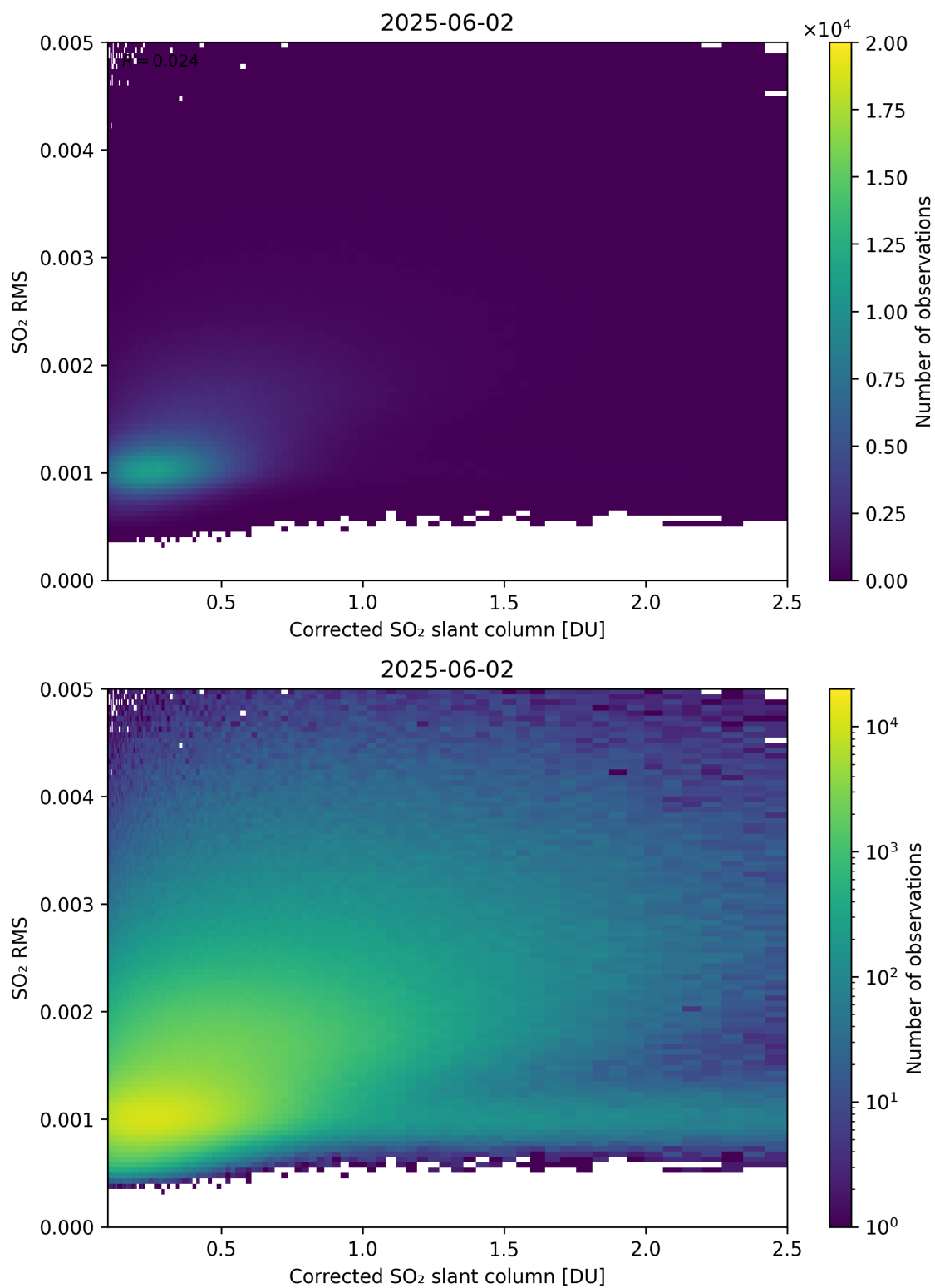
Figure 231: Scatter density plot of “Corrected SO 2 slant column” against “SO 2 RMS” for 2025-06-01 to 2025-06-03.
