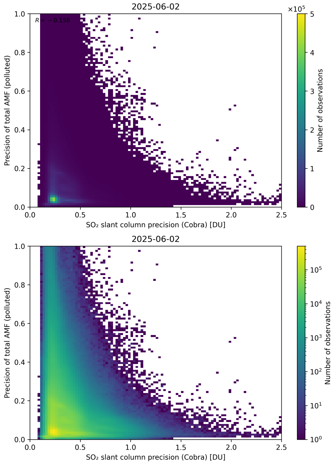
Figure 214: Scatter density plot of “SO 2 slant column precision (Cobra)” against “Precision of total AMF (polluted)” for 2025-06-01 to 2025-06-03.
