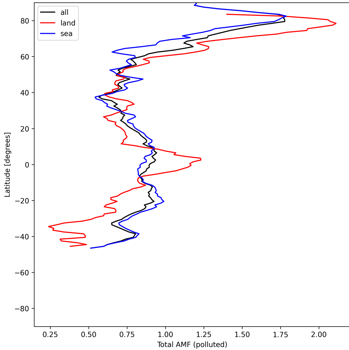
Figure 53: Zonal average of “Total AMF (polluted)” for 2025-06-01 to 2025-06-03.
