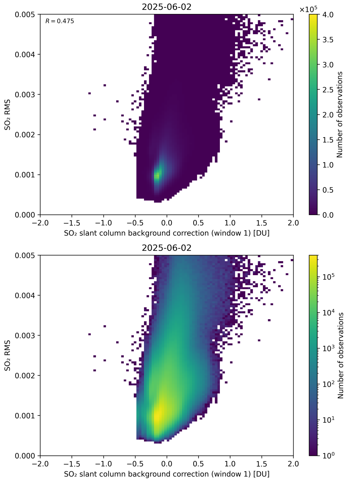
Figure 113: Scatter density plot of “SO 2 slant column background correction (window 1)” against “SO 2 RMS” for 2025-06-01 to 2025-06-03.
