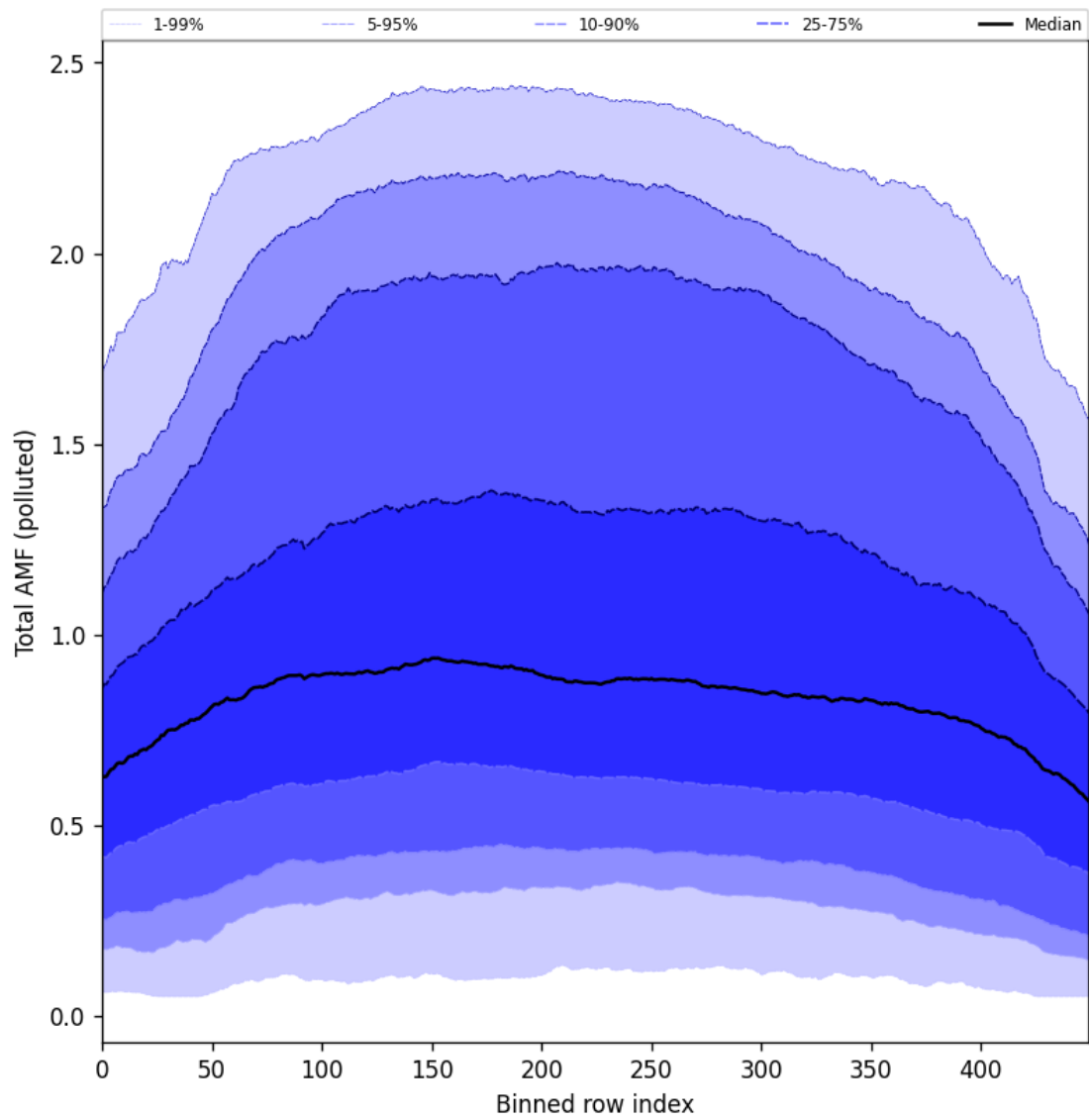
Figure 105: Along track statistics of “Total AMF (polluted)” for 2025-06-01 to 2025-06-03
