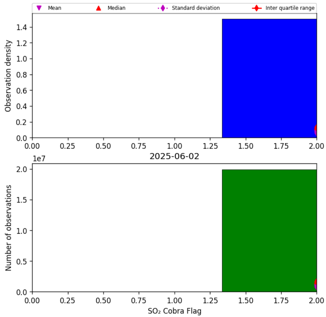
Figure 75: Histogram of “SO 2 Cobra Flag” for 2025-06-01 to 2025-06-03
