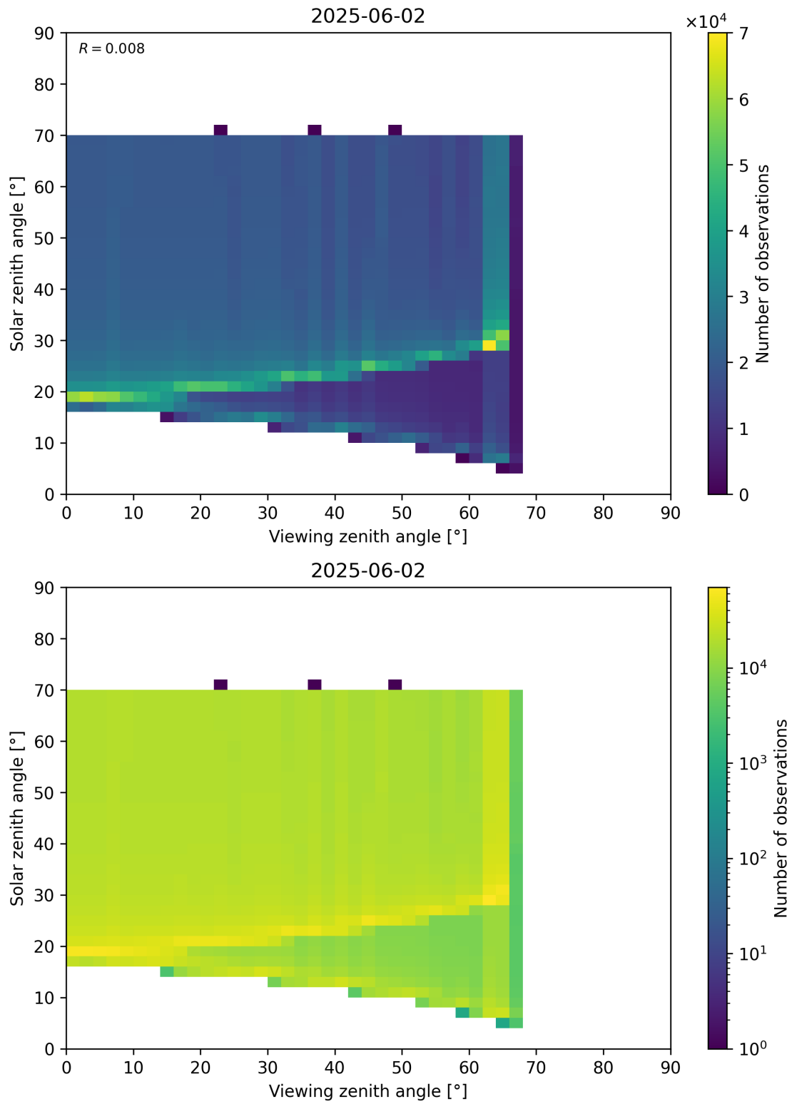
Figure 369: Scatter density plot of “Viewing zenith angle” against “Solar zenith angle” for 2025-06-01 to 2025-06-03.
