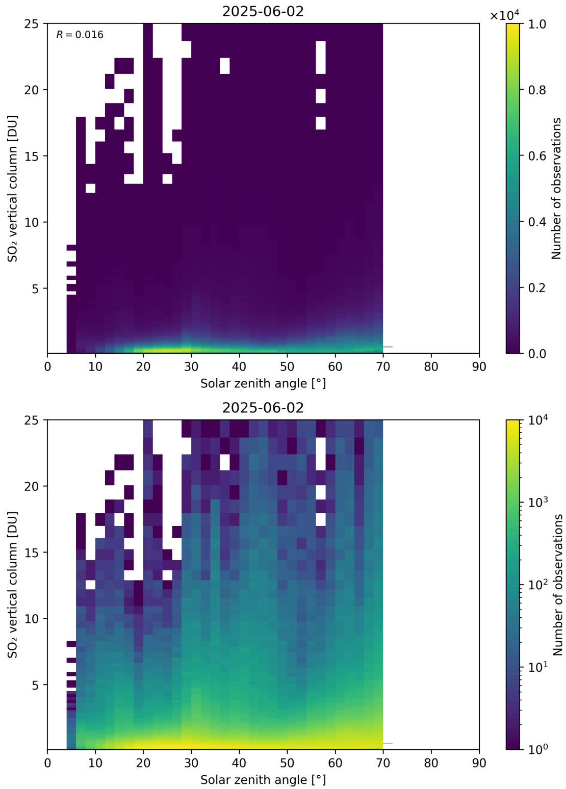
Figure 191: Scatter density plot of “Solar zenith angle” against “SO 2 vertical column” for 2025-06-01 to 2025-06-03.
