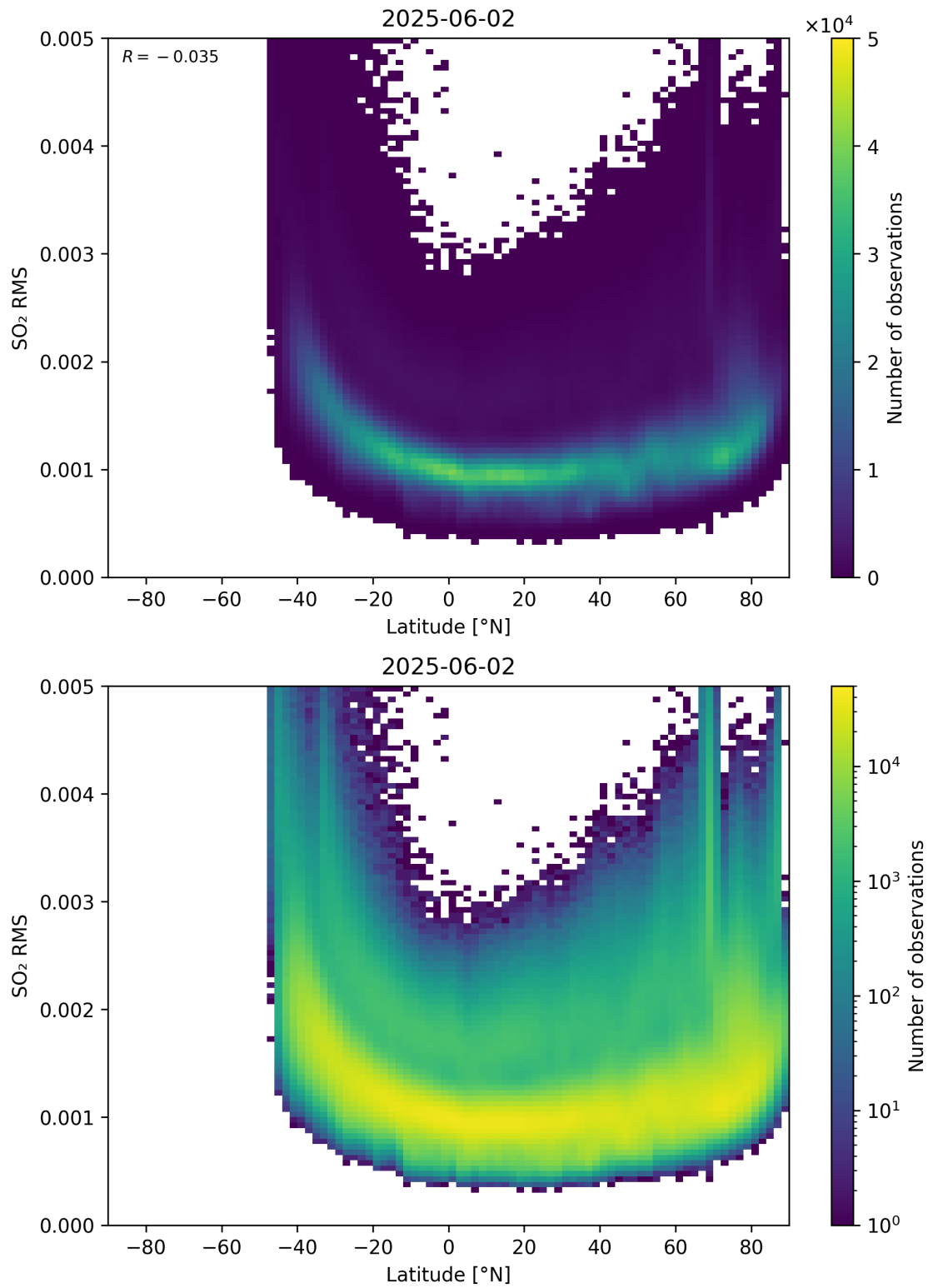
Figure 155: Scatter density plot of “Latitude” against “SO 2 RMS” for 2025-06-01 to 2025-06-03.
