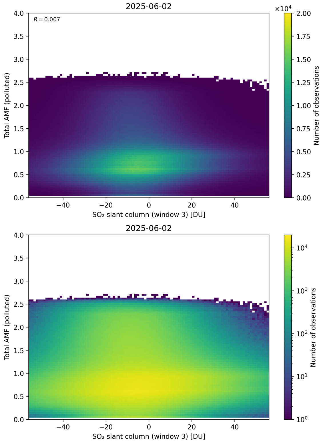
Figure 318: Scatter density plot of “SO 2 slant column (window 3)” against “Total AMF (polluted)” for 2025-06-01 to 2025-06-03.
