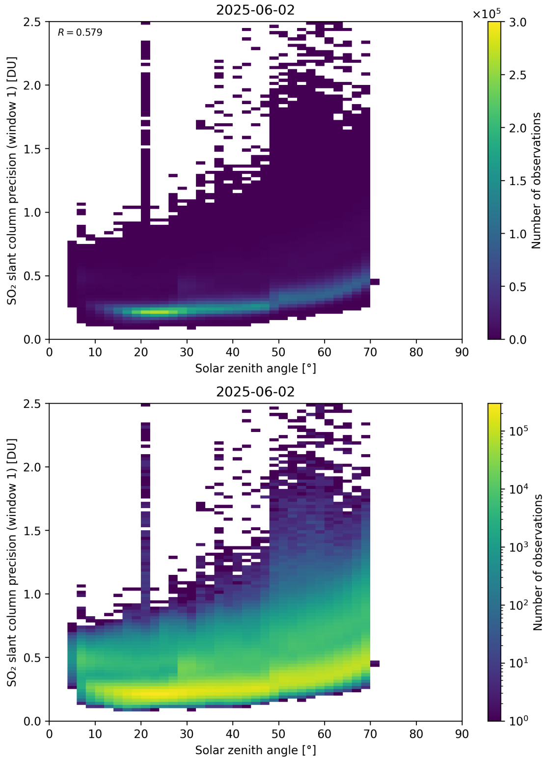
Figure 185: Scatter density plot of “Solar zenith angle” against “SO 2 slant column precision (window 1)” for 2025-06-01 to 2025-06-03.
