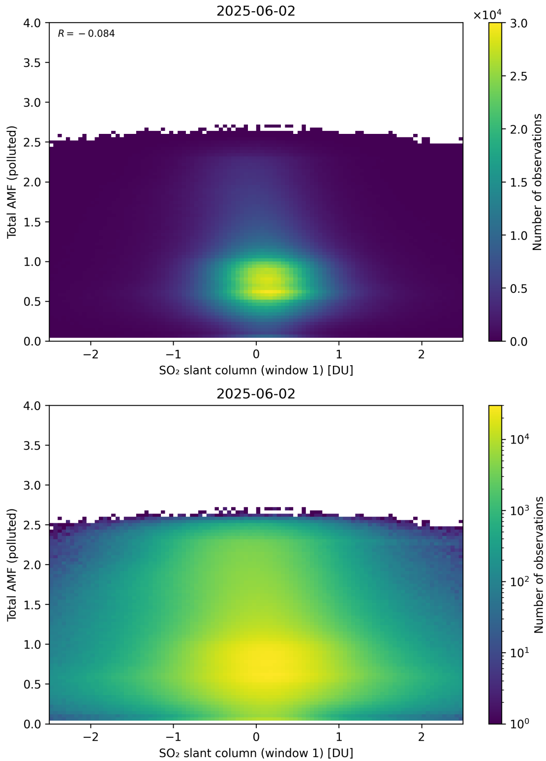
Figure 289: Scatter density plot of “SO 2 slant column (window 1)” against “Total AMF (polluted)” for 2025-06-01 to 2025-06-03.
