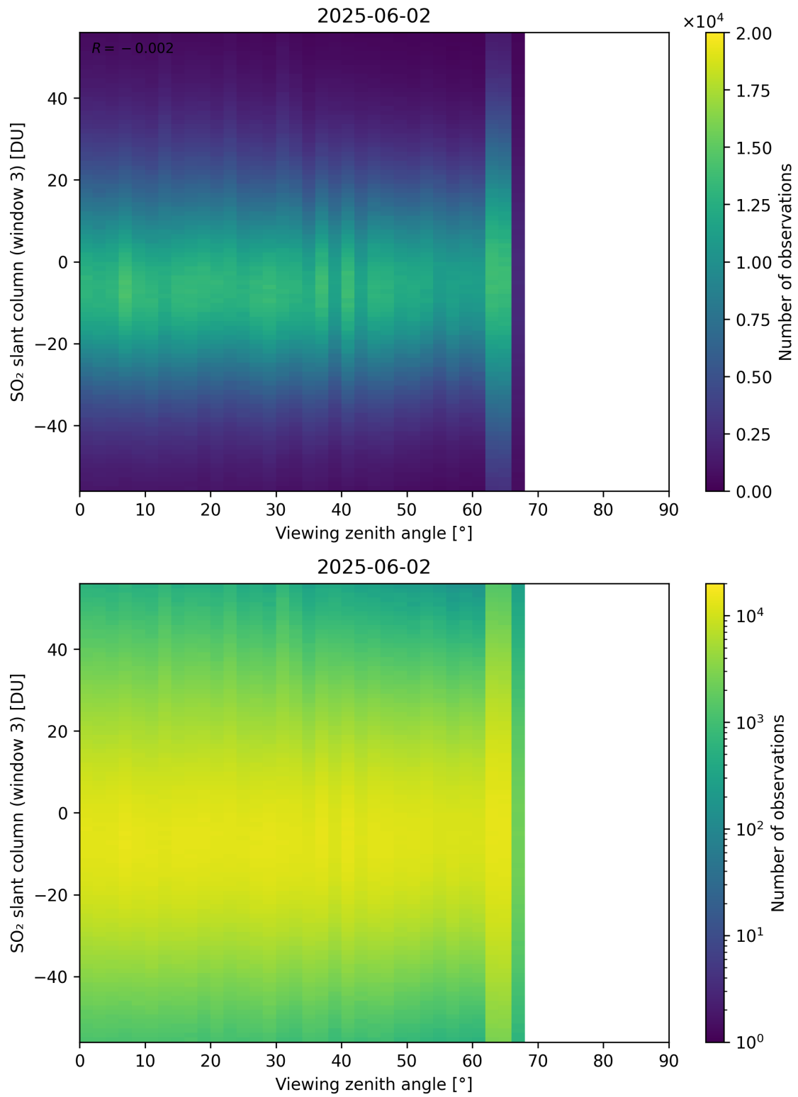
Figure 379: Scatter density plot of “Viewing zenith angle” against “SO 2 slant column (window 3)” for 2025-06-01 to 2025-06-03.
