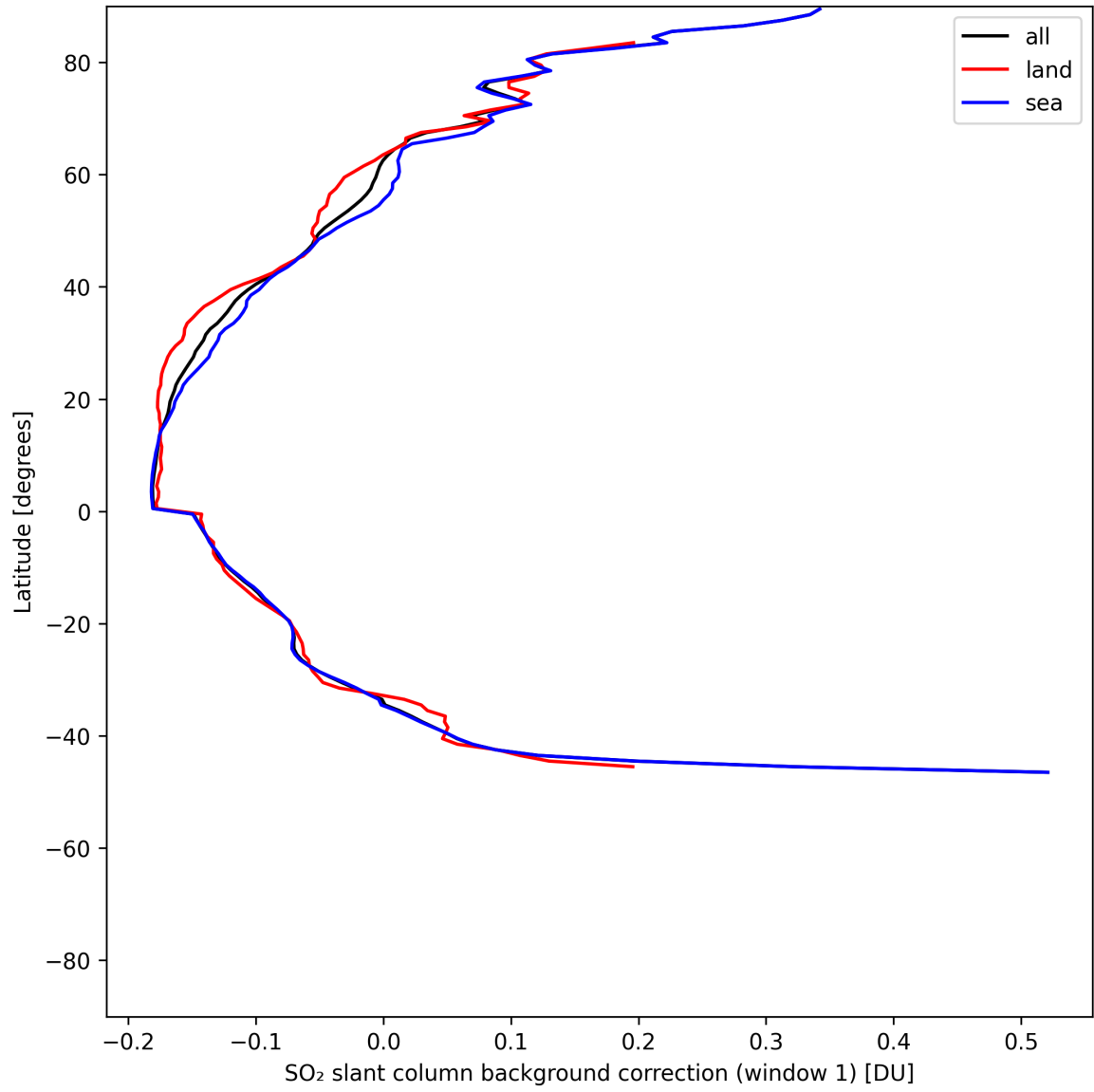
Figure 40: Zonal average of “SO 2 slant column background correction (window 1)” for 2025-06-01 to 2025-06-03.
