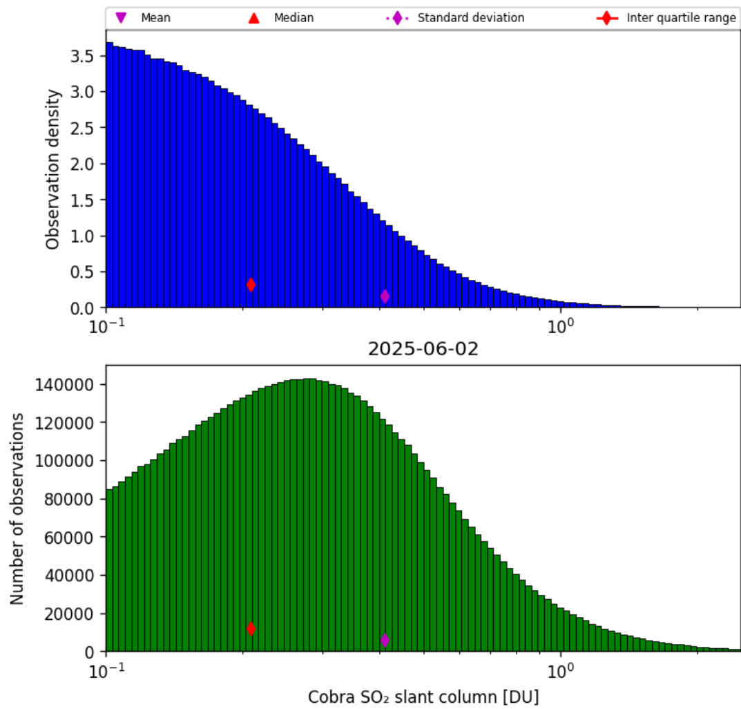
Figure 61: Histogram of “Cobra SO 2 slant column” for 2025-06-01 to 2025-06-03
