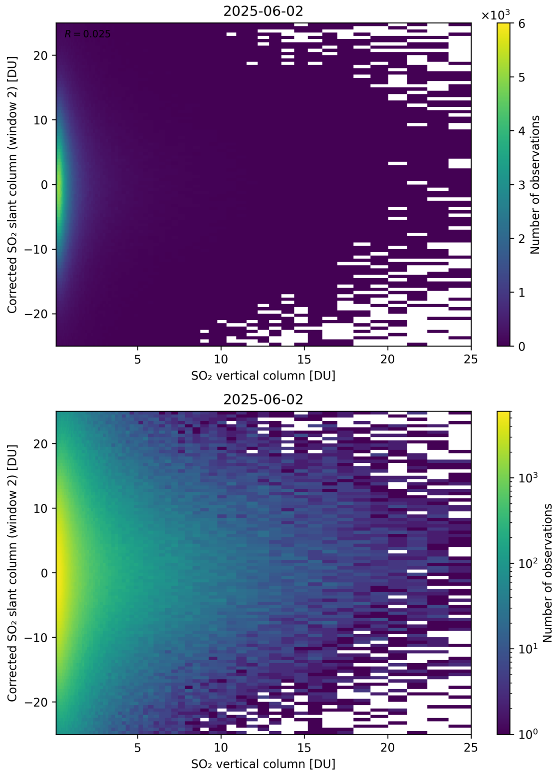
Figure 352: Scatter density plot of “SO 2 vertical column” against “Corrected SO 2 slant column (window 2)” for 2025-06-01 to 2025-06-03.
