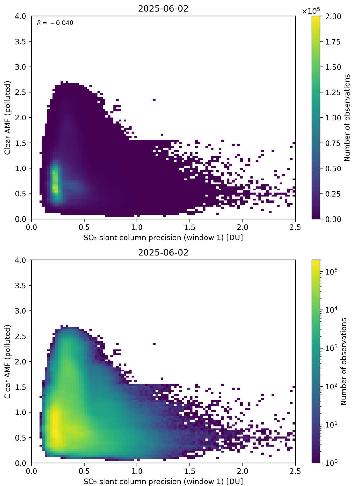
Figure 274: Scatter density plot of “SO 2 slant column precision (window 1)” against “Clear AMF (polluted)” for 2025-06-01 to 2025-06-03.
