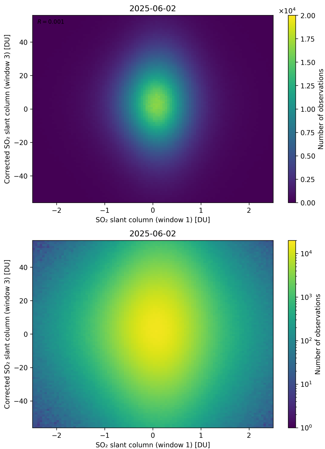
Figure 284: Scatter density plot of “SO 2 slant column (window 1)” against “Corrected SO 2 slant column (window 3)” for 2025-06-01 to 2025-06-03.
