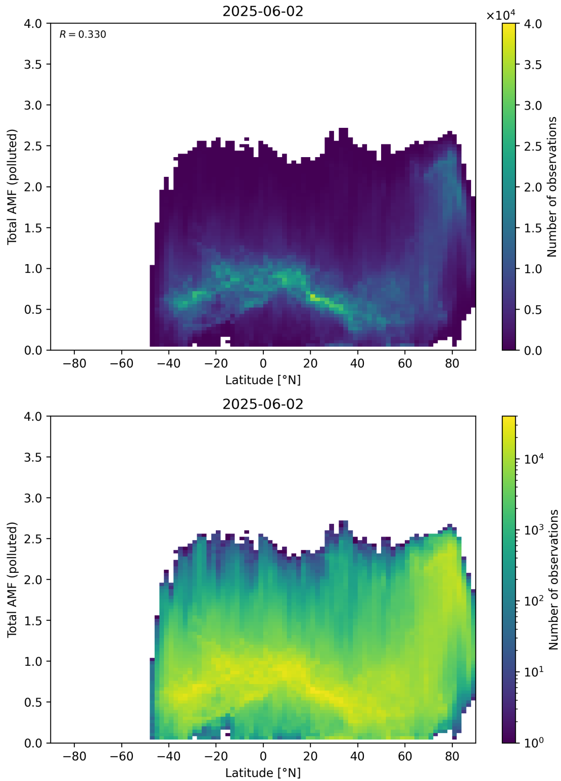
Figure 167: Scatter density plot of “Latitude” against “Total AMF (polluted)” for 2025-06-01 to 2025-06-03.
