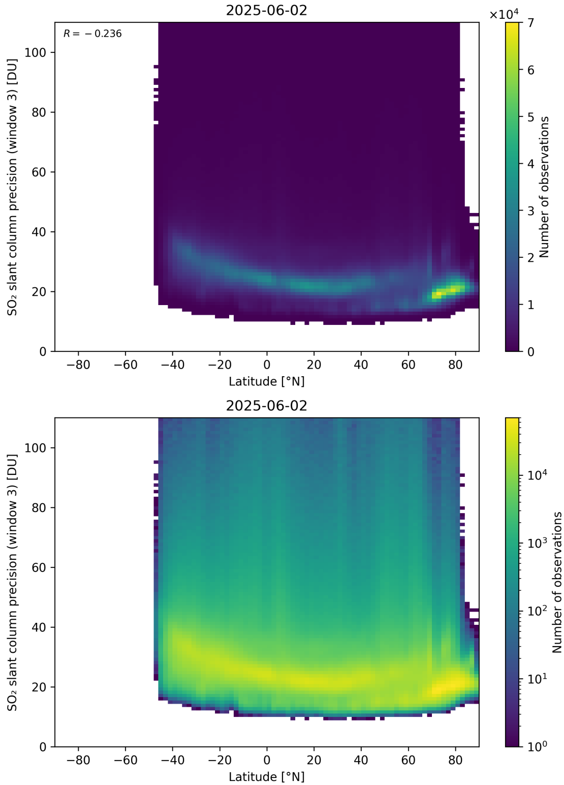
Figure 166: Scatter density plot of “Latitude” against “SO 2 slant column precision (window 3)” for 2025-06-01 to 2025-06-03.
