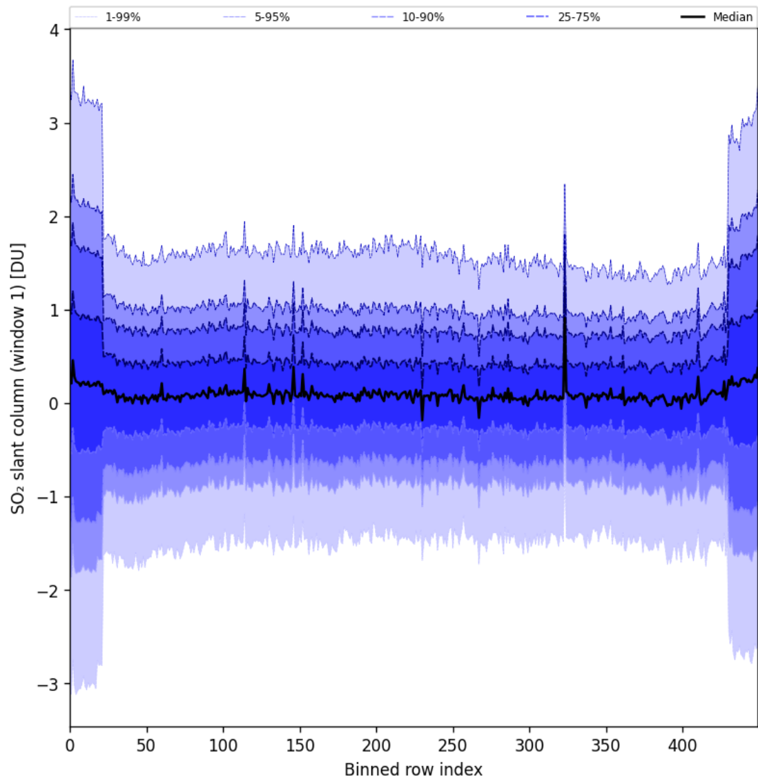
Figure 89: Along track statistics of “SO 2 slant column (window 1)” for 2025-06-01 to 2025-06-03
