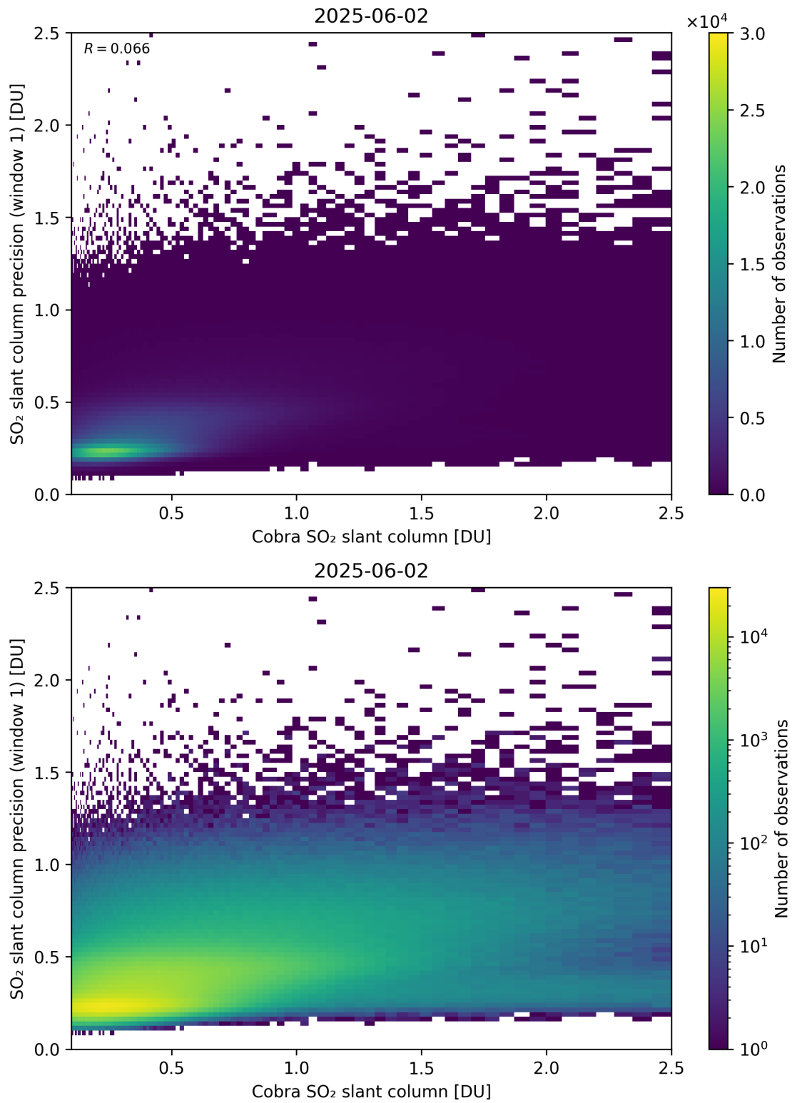
Figure 220: Scatter density plot of “Cobra SO 2 slant column” against “SO 2 slant column precision (window 1)” for 2025-06-01 to 2025-06-03.
