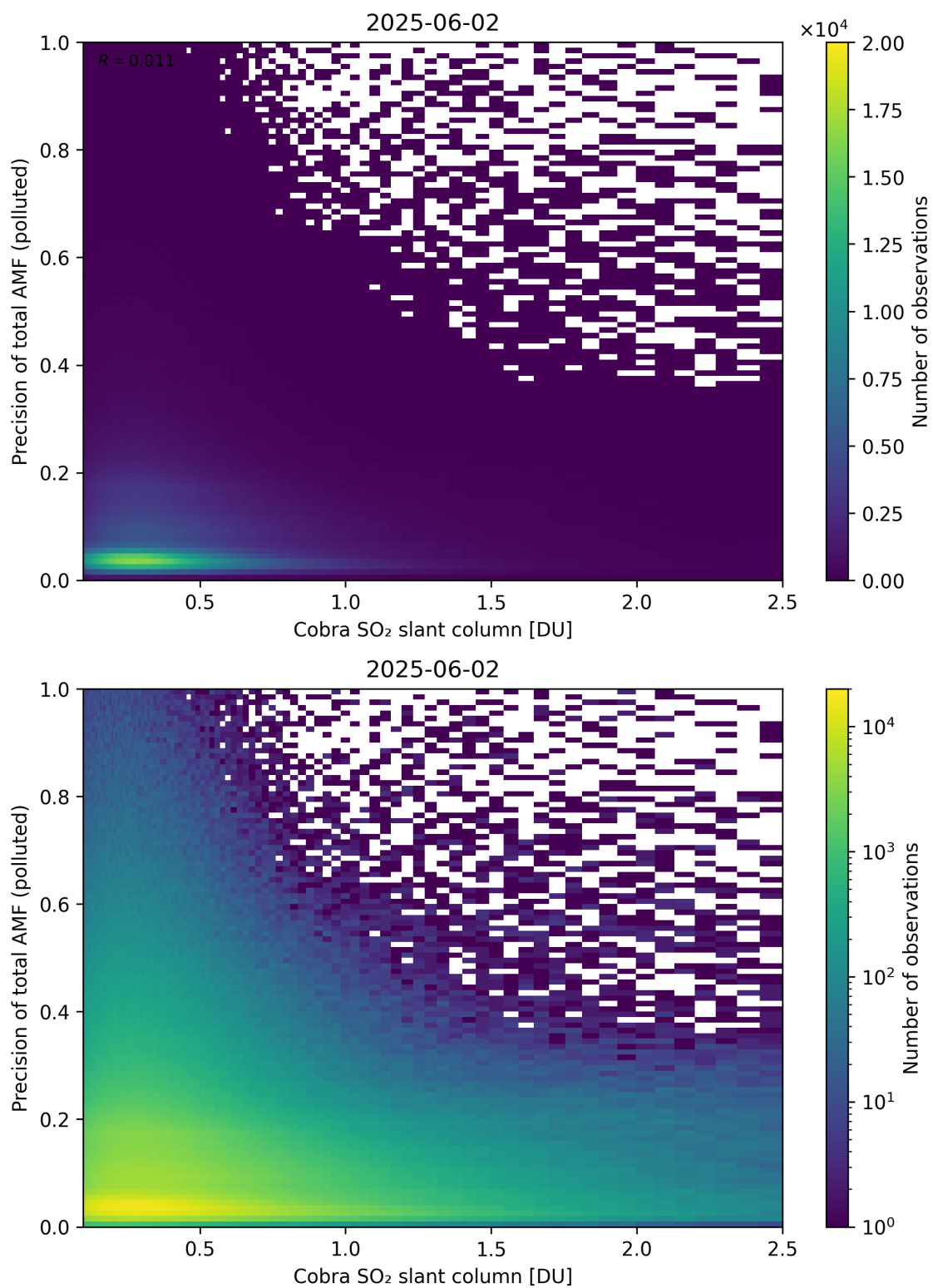
Figure 225: Scatter density plot of “Cobra SO 2 slant column” against “Precision of total AMF (polluted)” for 2025-06-01 to 2025-06-03.
