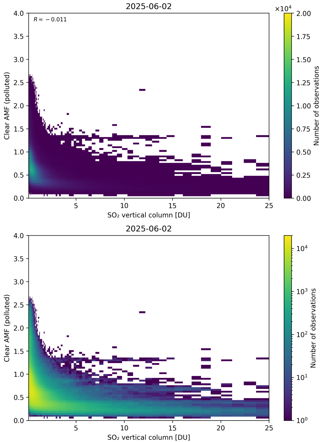
Figure 348: Scatter density plot of “SO 2 vertical column” against “Clear AMF (polluted)” for 2025-06-01 to 2025-06-03.
