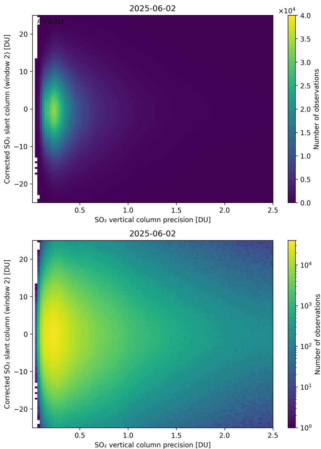
Figure 339: Scatter density plot of “SO 2 vertical column precision” against “Corrected SO 2 slant column (window 2)” for 2025-06-01 to 2025-06-03.
