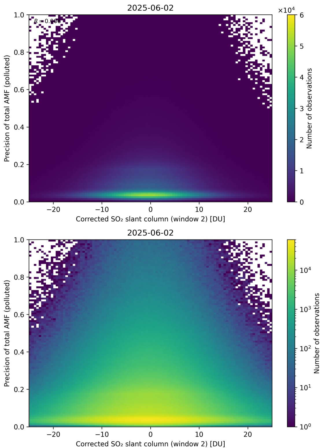
Figure 254: Scatter density plot of “Corrected SO 2 slant column (window 2)” against “Precision of total AMF (polluted)” for 2025-06-01 to 2025-06-03.
