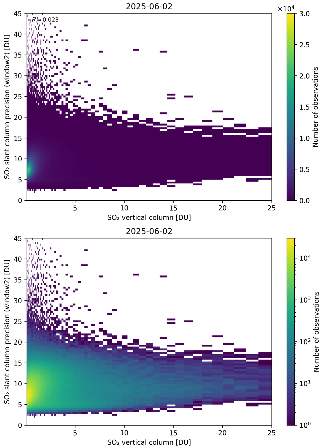
Figure 356: Scatter density plot of “SO 2 vertical column” against “SO 2 slant column precision (window2)” for 2025-06-01 to 2025-06-03.
