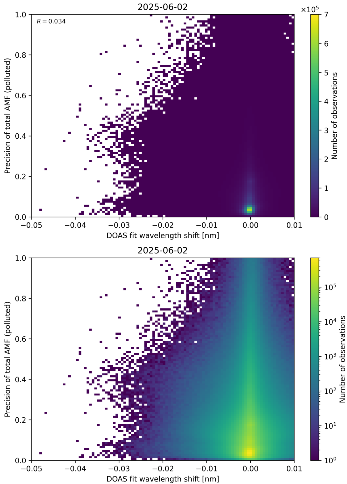
Figure 142: Scatter density plot of “DOAS fit wavelength shift” against “Precision of total AMF (polluted)” for 2025-06-01 to 2025-06-03.
