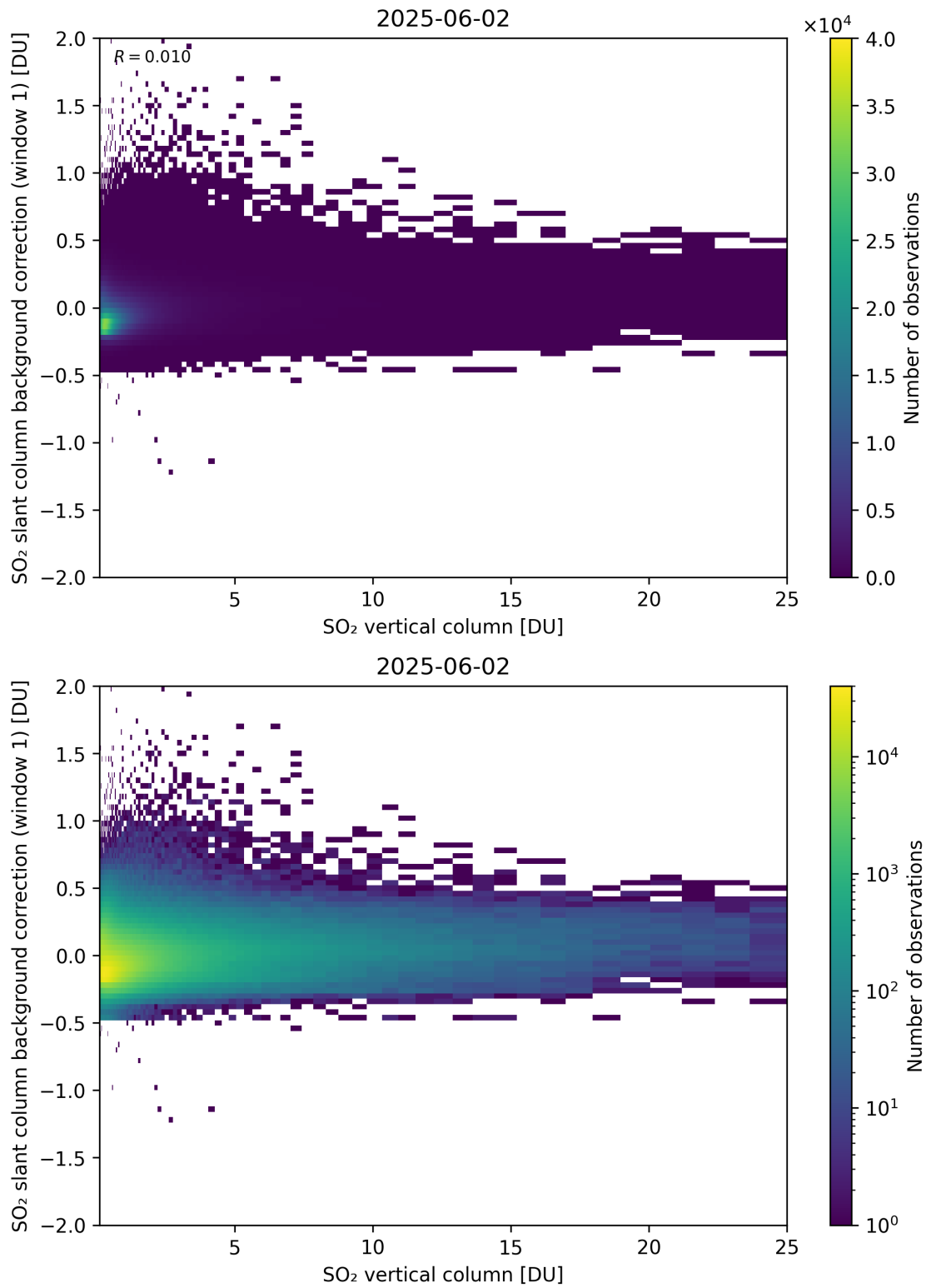
Figure 323: Scatter density plot of “SO 2 vertical column” against “SO 2 slant column background correction (window 1)” for 2025-06-01 to 2025-06-03.
