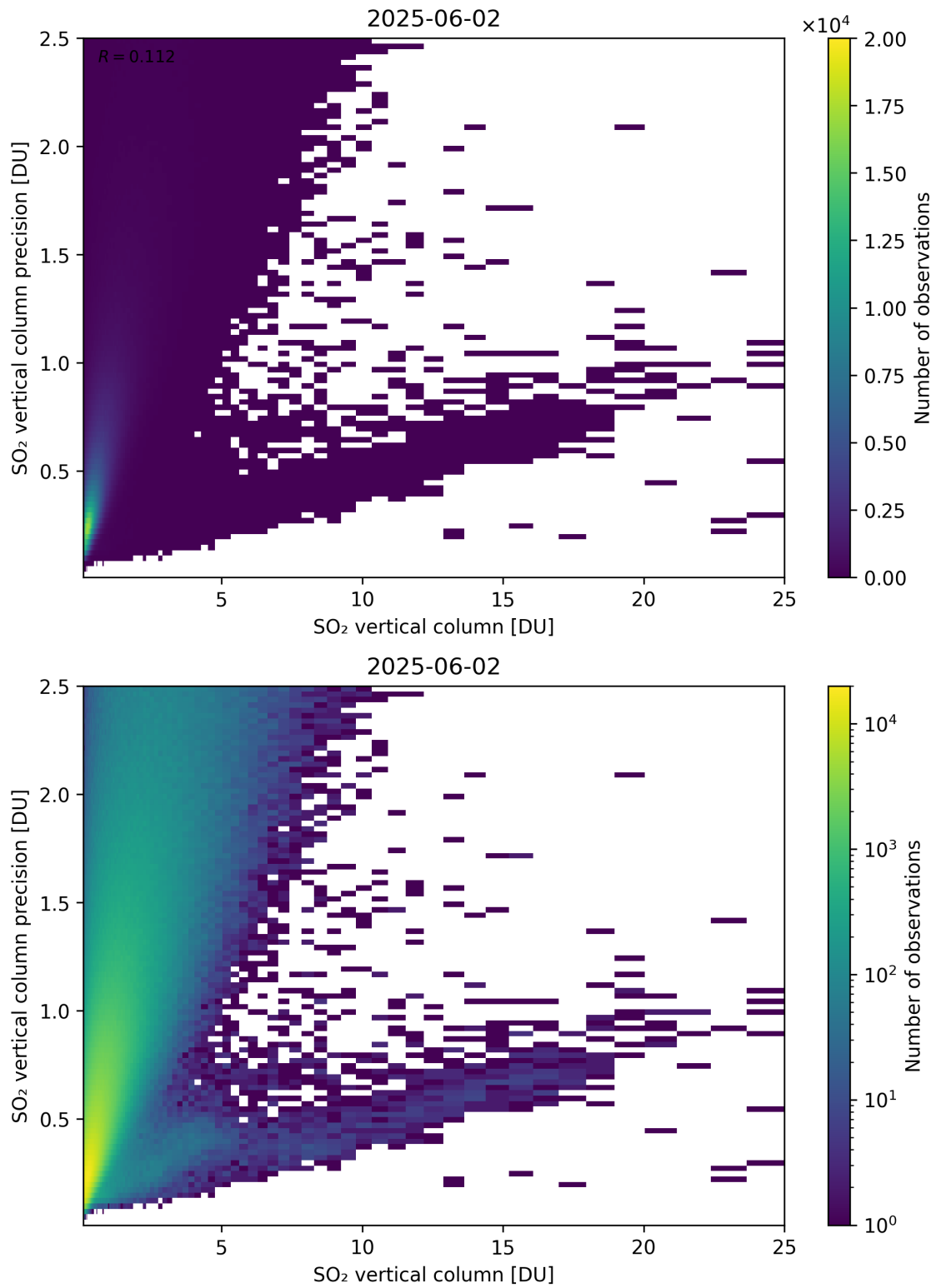
Figure 361: Scatter density plot of “SO 2 vertical column” against “SO 2 vertical column precision” for 2025-06-01 to 2025-06-03.
