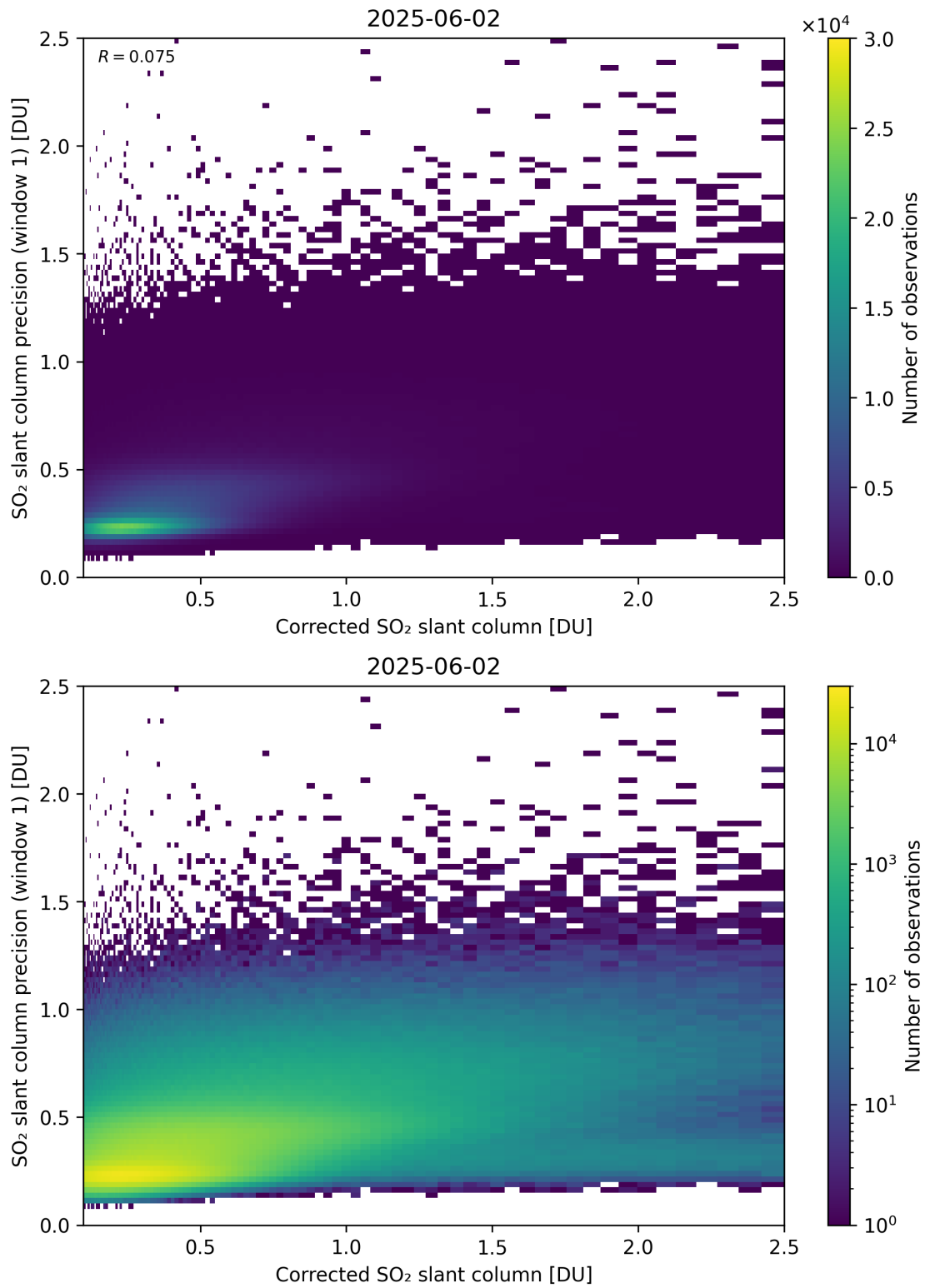
Figure 238: Scatter density plot of “Corrected SO 2 slant column” against “SO 2 slant column precision (window 1)” for 2025-06-01 to 2025-06-03.
