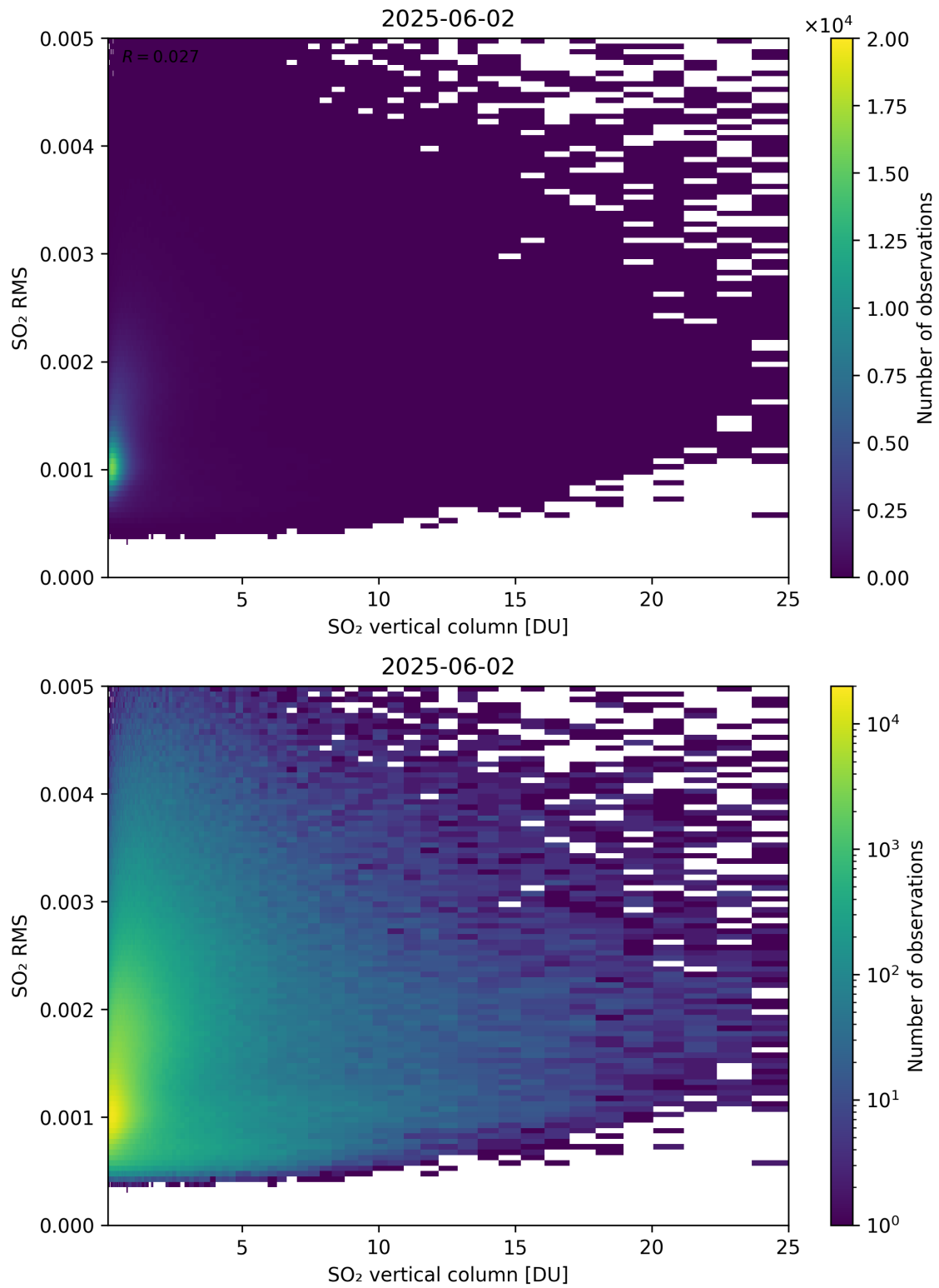
Figure 328: Scatter density plot of “SO 2 vertical column” against “SO 2 RMS” for 2025-06-01 to 2025-06-03.
