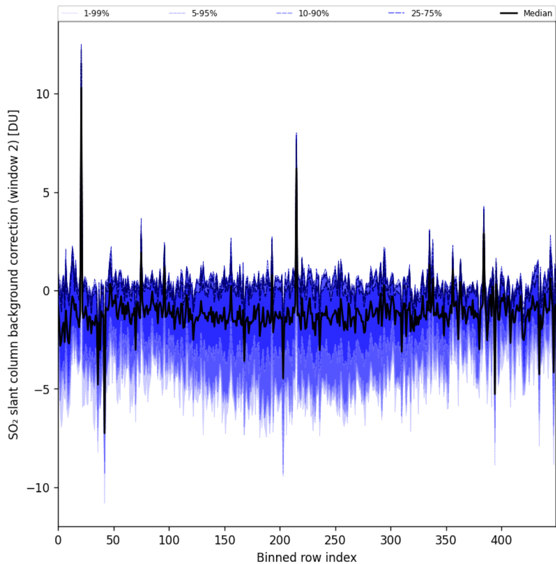
Figure 96: Along track statistics of “SO 2 slant column background correction (window 2)” for 2025-06-01 to 2025-06-03
