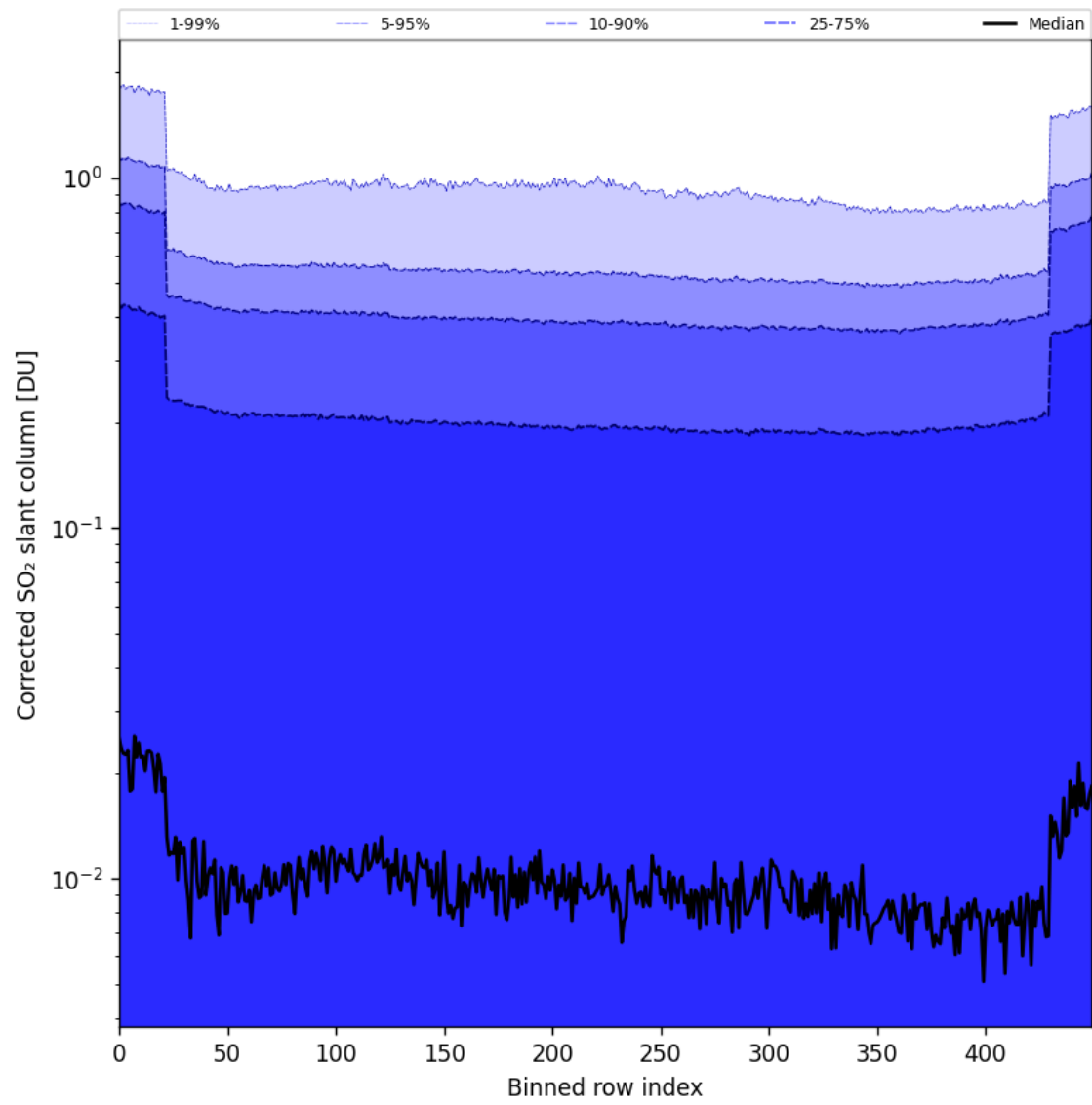
Figure 86: Along track statistics of "Corrected SO 2 slant column" for 2025-06-01 to 2025-06-03
