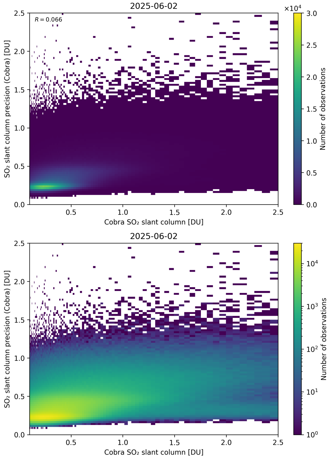
Figure 216: Scatter density plot of “Cobra SO 2 slant column” against “SO 2 slant column precision (Cobra)” for 2025-06-01 to 2025-06-03.
