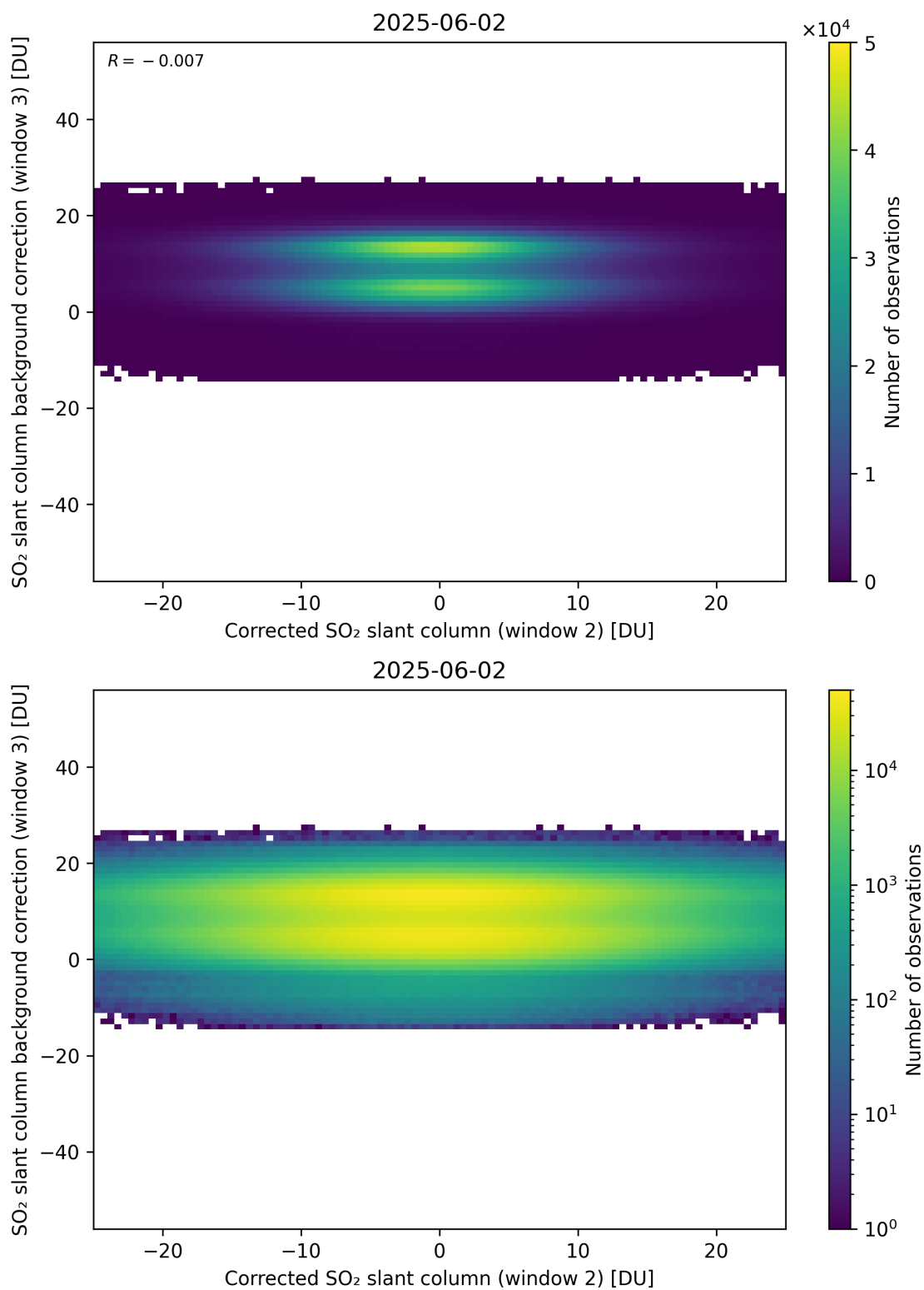
Figure 245: Scatter density plot of “Corrected SO 2 slant column (window 2)” against “SO 2 slant column background correction (window 3)” for 2025-06-01 to 2025-06-03.
