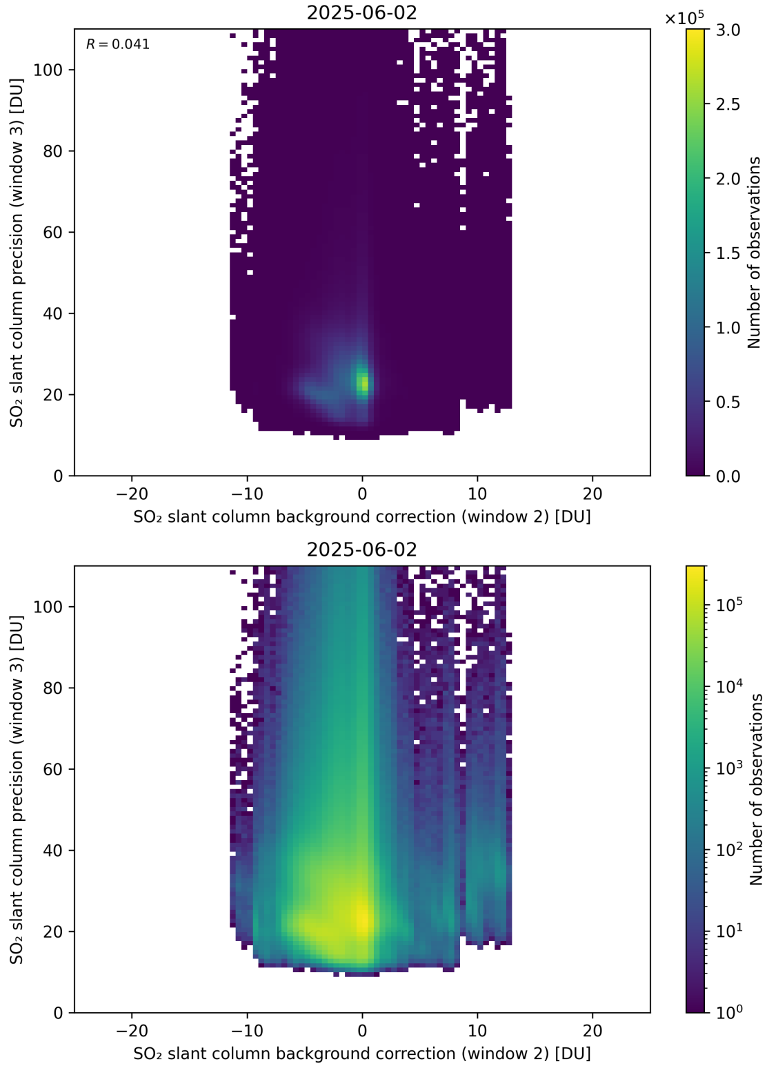
Figure 129: Scatter density plot of “SO 2 slant column background correction (window 2)” against “SO 2 slant column precision (window 3)” for 2025-06-01 to 2025-06-03.
