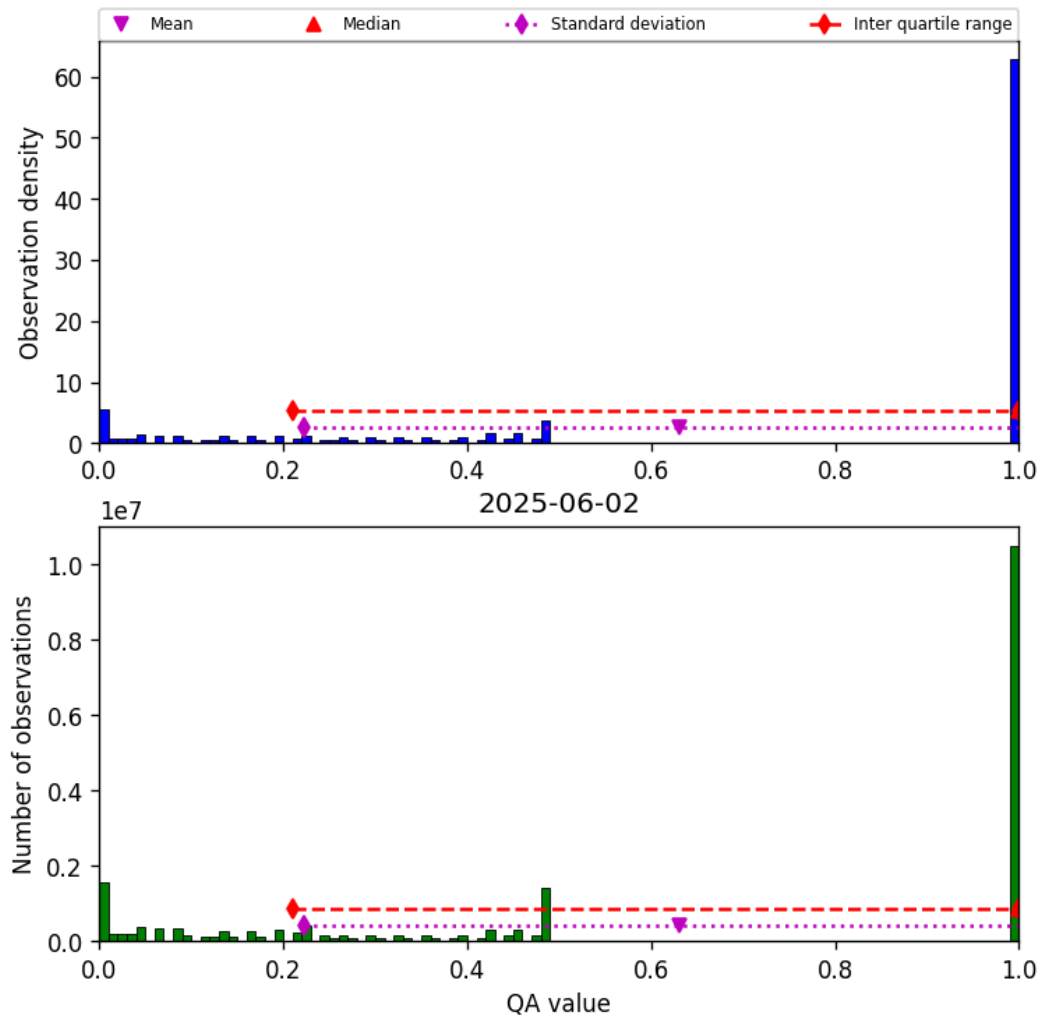
Figure 57: Histogram of “QA value” for 2025-06-01 to 2025-06-03
