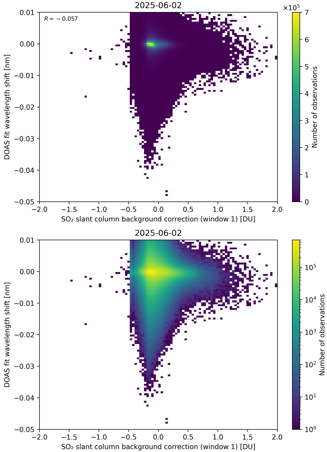
Figure 111: Scatter density plot of “SO 2 slant column background correction (window 1)” against “DOAS fit wavelength shift” for 2025-06-01 to 2025-06-03.
