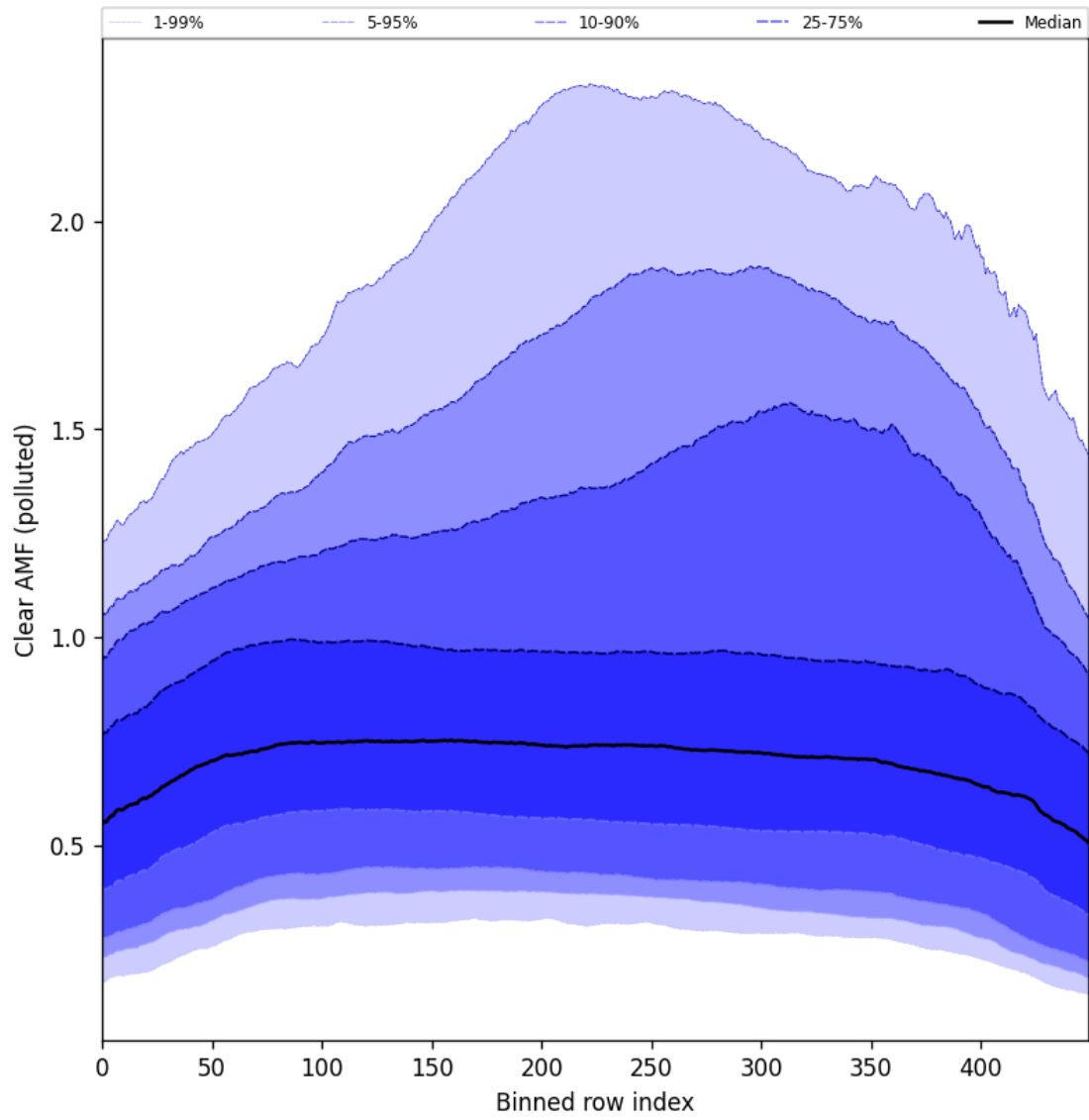
Figure 107: Along track statistics of “Clear AMF (polluted)” for 2025-06-01 to 2025-06-03
