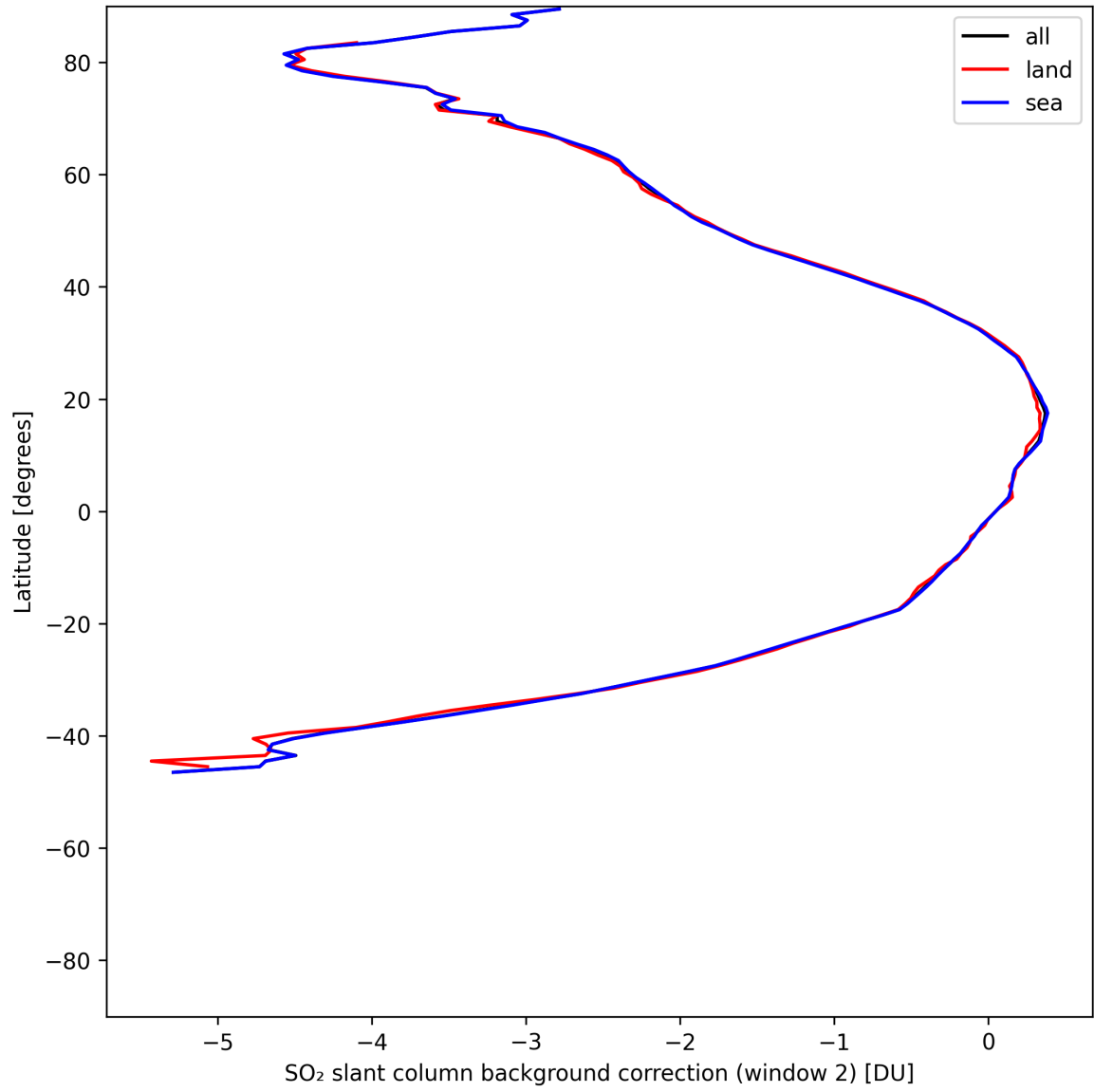
Figure 44: Zonal average of “SO 2 slant column background correction (window 2)” for 2025-06-01 to 2025-06-03.
