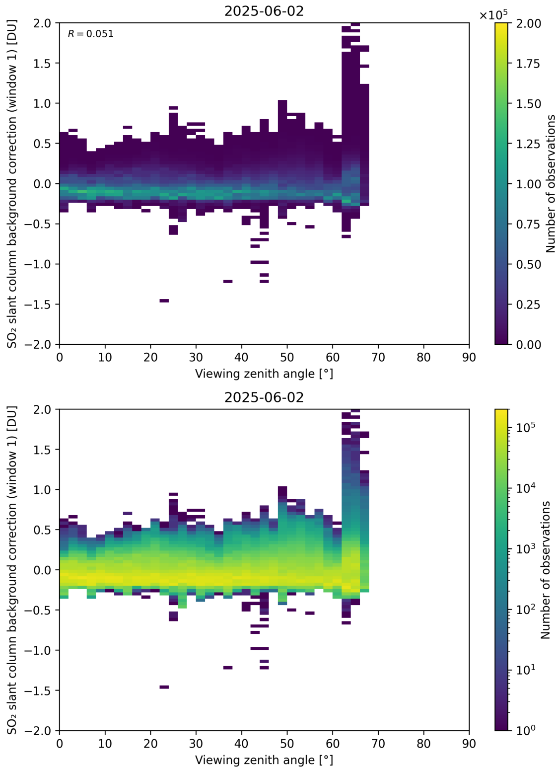
Figure 362: Scatter density plot of “Viewing zenith angle” against “SO 2 slant column background correction (window 1)” for 2025-06-01 to 2025-06-03.
