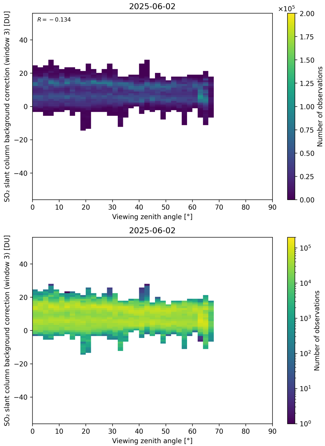
Figure 364: Scatter density plot of “Viewing zenith angle” against “SO 2 slant column background correction (window 3)” for 2025-06-01 to 2025-06-03.
