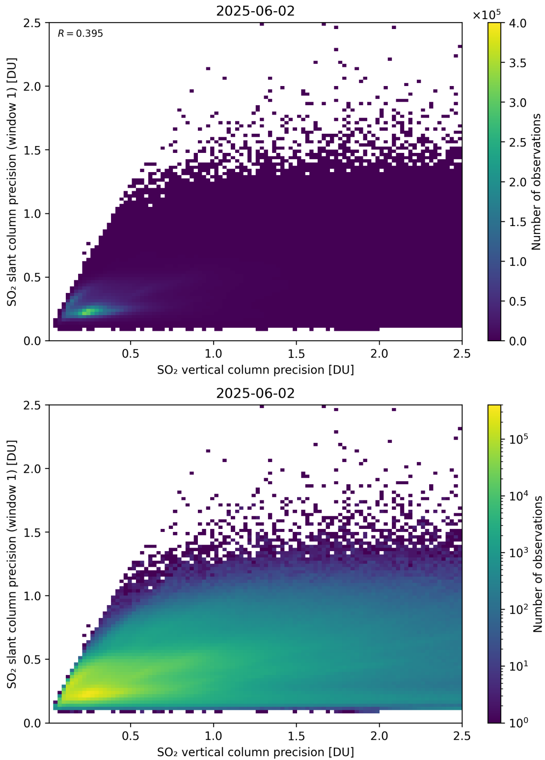
Figure 342: Scatter density plot of “SO 2 vertical column precision” against “SO 2 slant column precision (window 1)” for 2025-06-01 to 2025-06-03.
