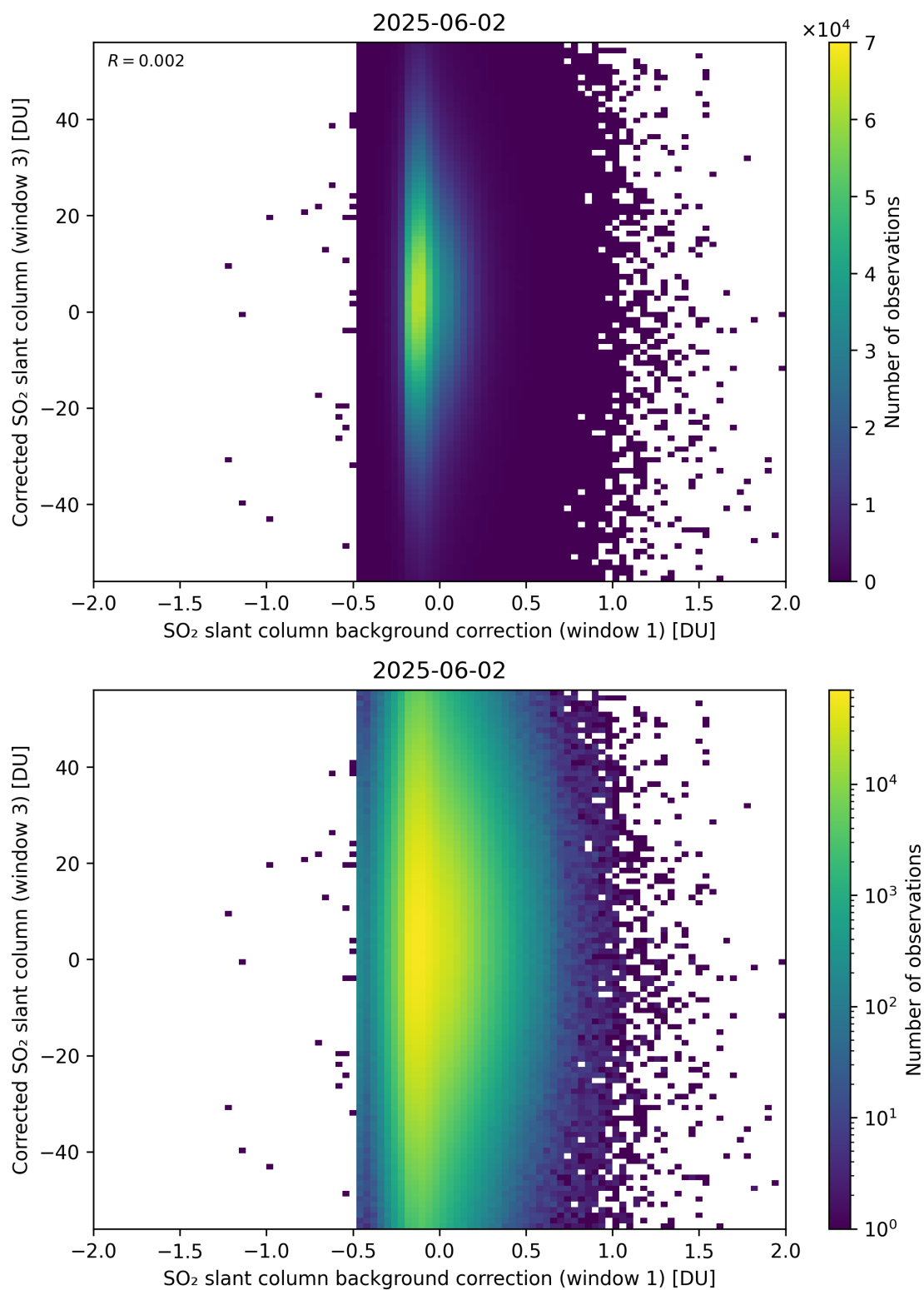
Figure 116: Scatter density plot of “SO 2 slant column background correction (window 1)” against “Corrected SO 2 slant column (window 3)” for 2025-06-01 to 2025-06-03.
