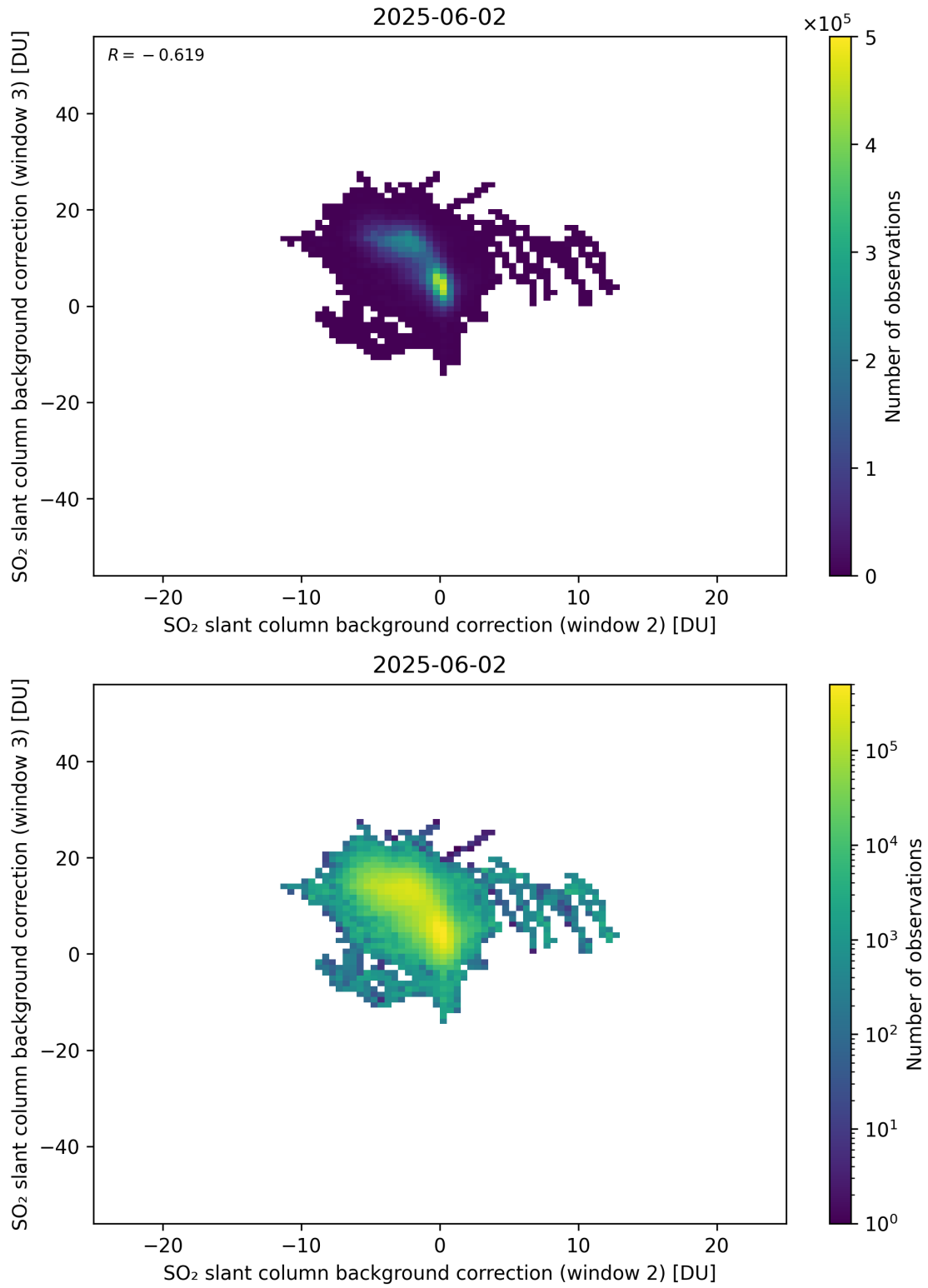
Figure 122: Scatter density plot of “SO 2 slant column background correction (window 2)” against “SO 2 slant column background correction (window 3)” for 2025-06-01 to 2025-06-03.
