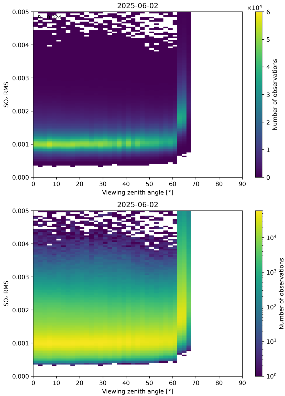
Figure 367: Scatter density plot of “Viewing zenith angle” against “SO 2 RMS” for 2025-06-01 to 2025-06-03.
