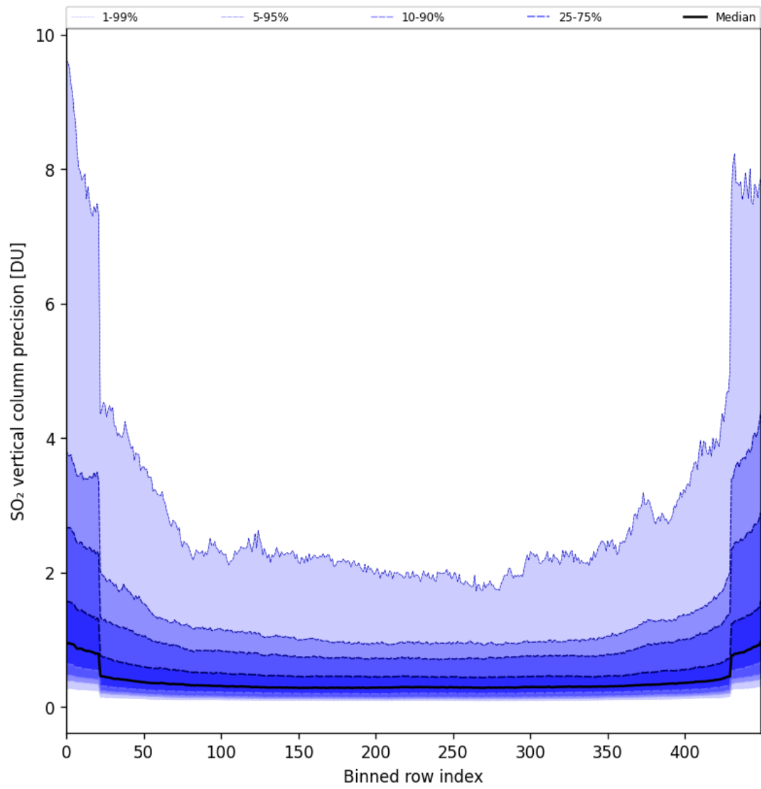
Figure 85: Along track statistics of “SO 2 vertical column precision” for 2025-06-01 to 2025-06-03
