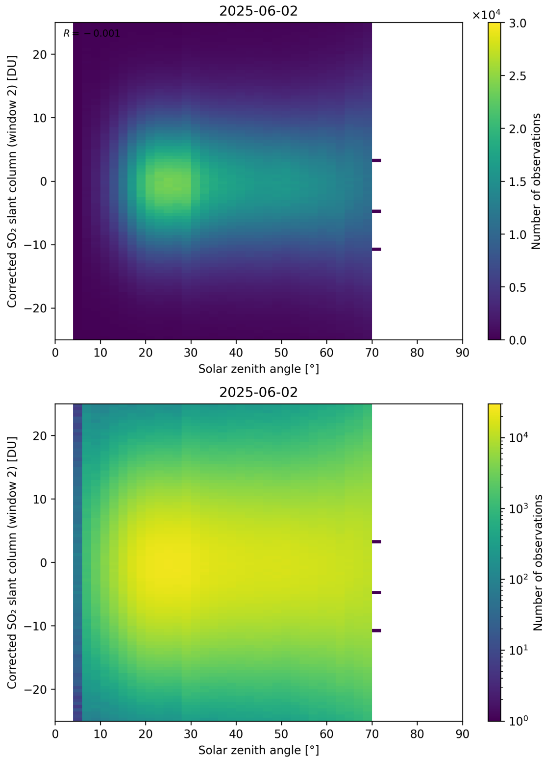
Figure 182: Scatter density plot of “Solar zenith angle” against “Corrected SO 2 slant column (window 2)” for 2025-06-01 to 2025-06-03.
