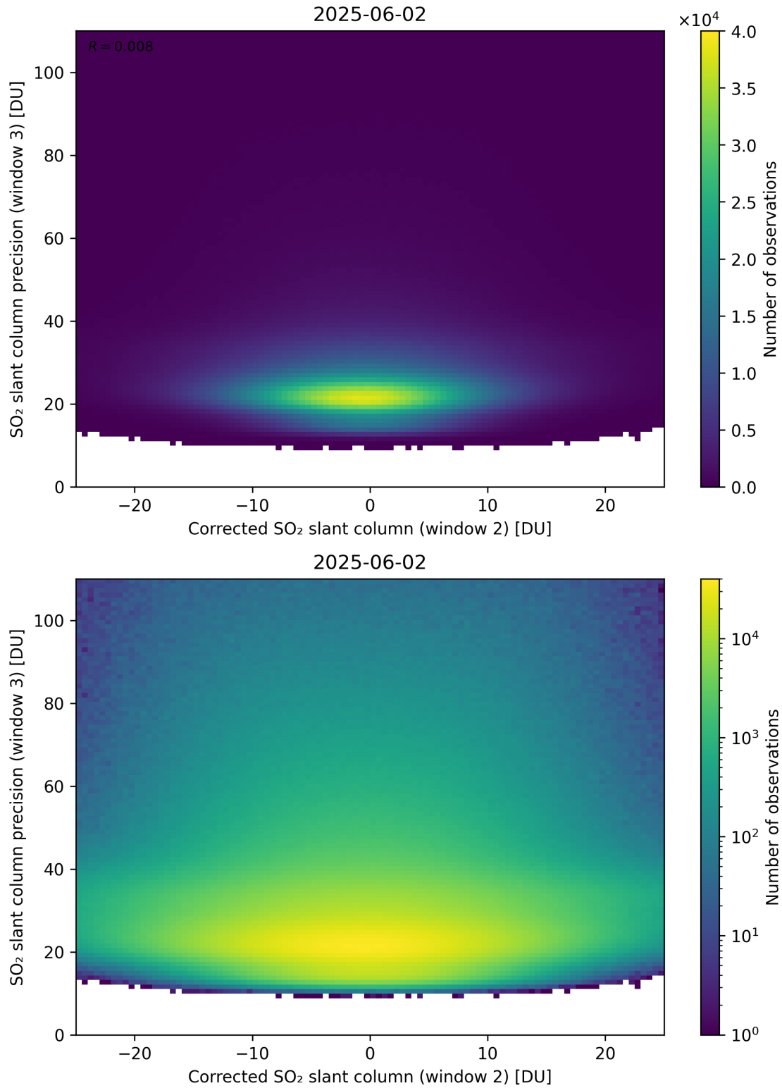
Figure 252: Scatter density plot of “Corrected SO 2 slant column (window 2)” against “SO 2 slant column precision (window 3)” for 2025-06-01 to 2025-06-03.
