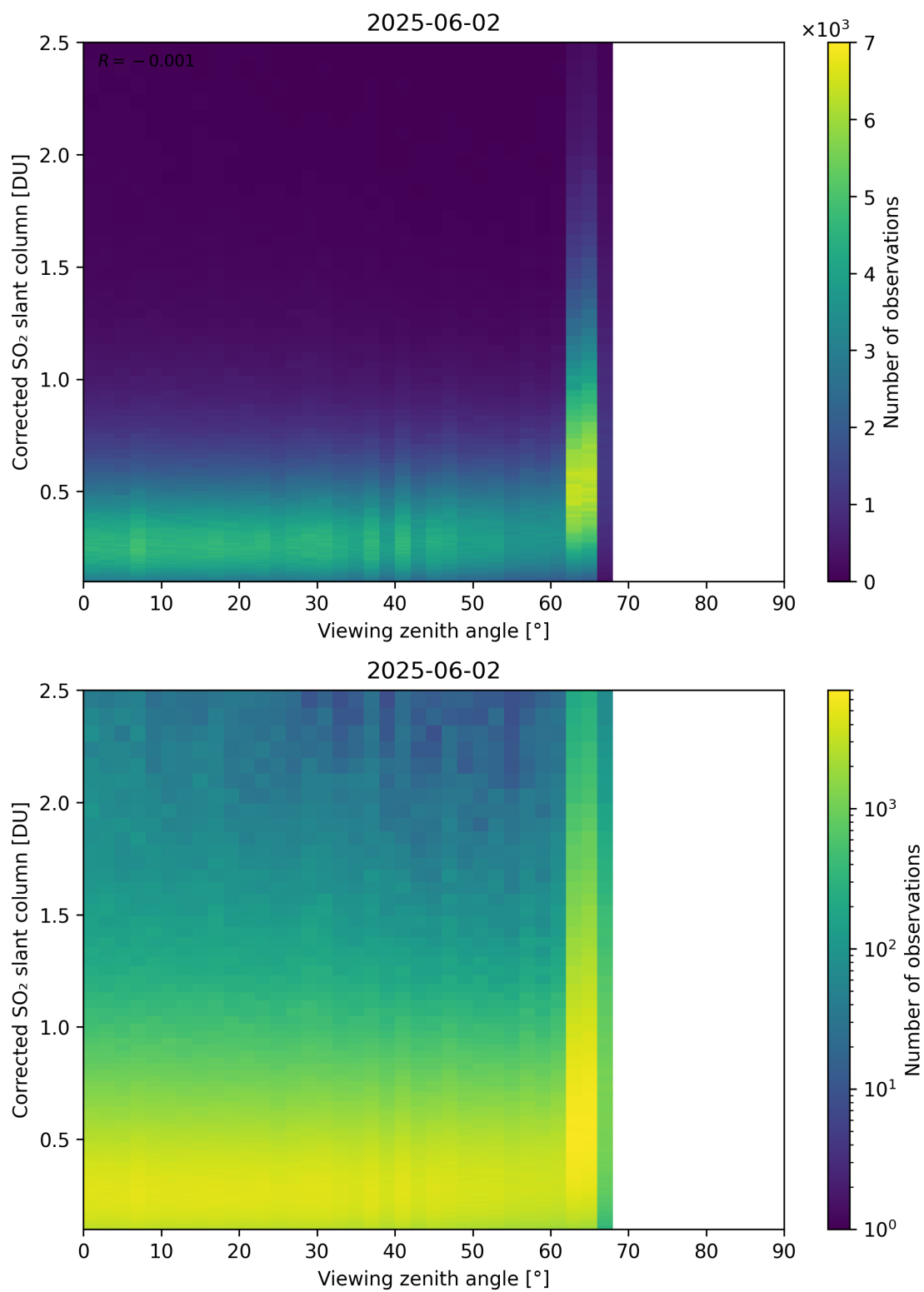
Figure 373: Scatter density plot of “Viewing zenith angle” against “Corrected SO 2 slant column” for 2025-06-01 to 2025-06-03.
