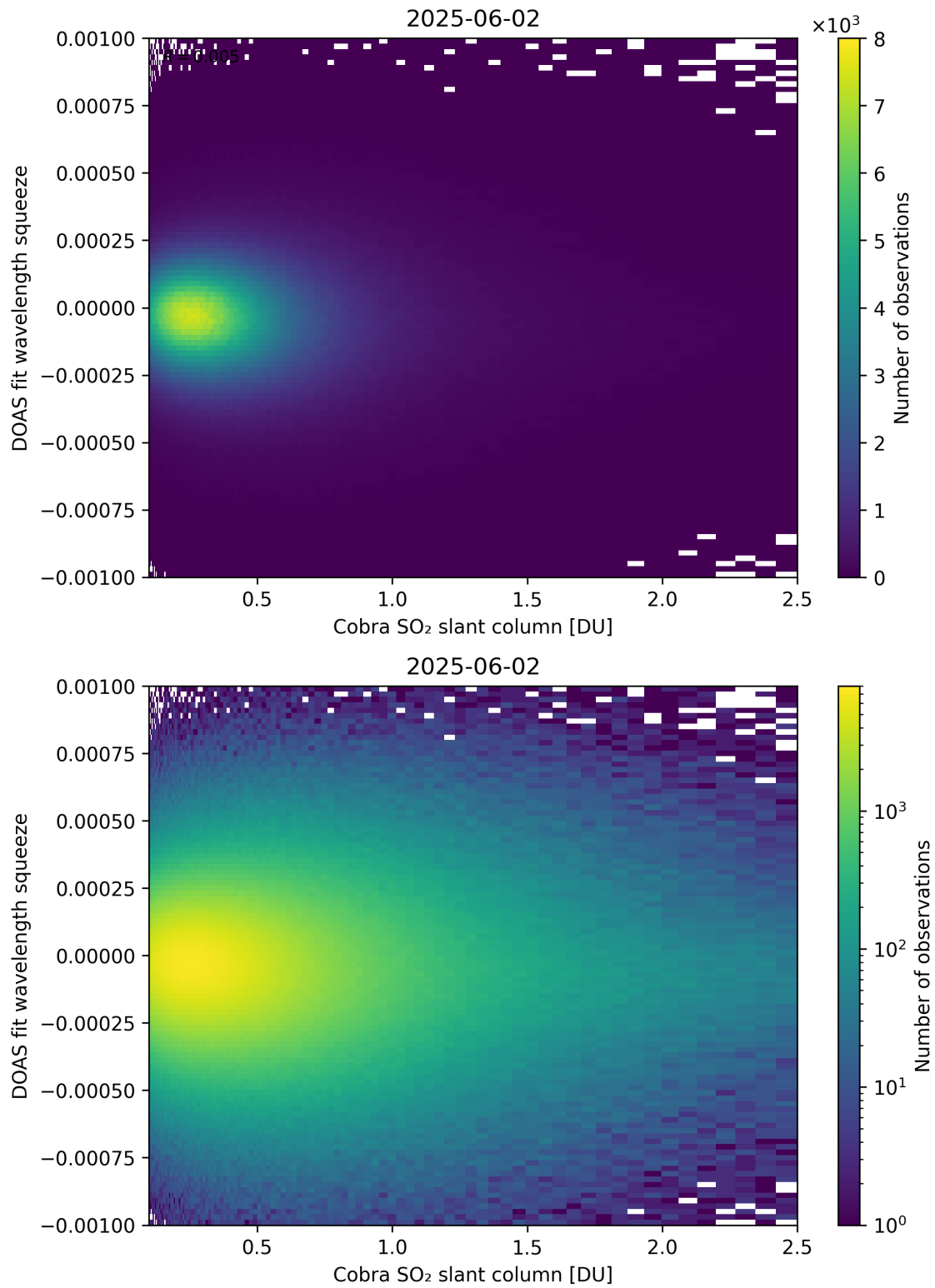
Figure 197: Scatter density plot of “Cobra SO 2 slant column” against “DOAS fit wavelength squeeze” for 2025-06-01 to 2025-06-03.
