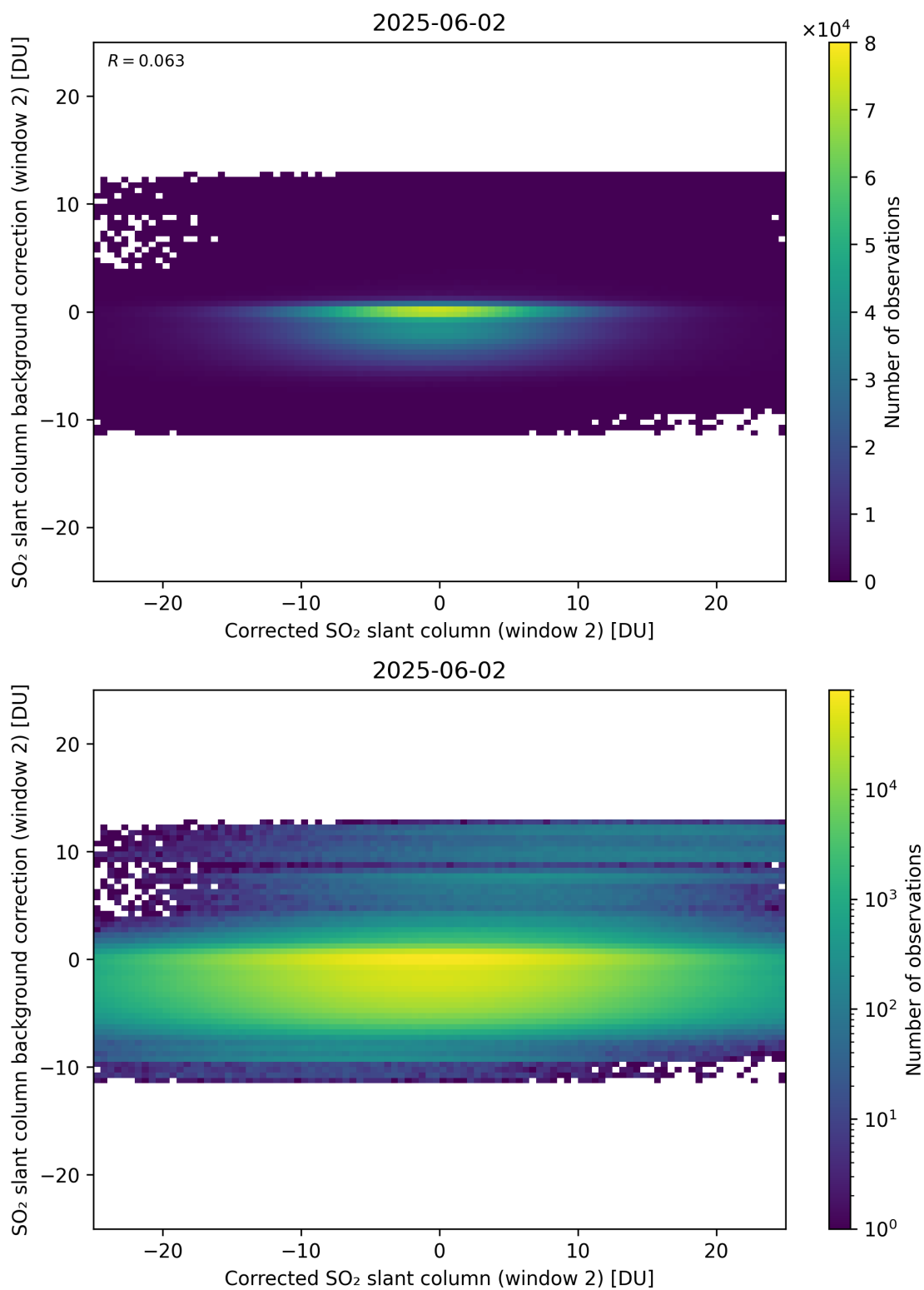
Figure 244: Scatter density plot of “Corrected SO 2 slant column (window 2)” against “SO 2 slant column background correction (window 2)” for 2025-06-01 to 2025-06-03.
