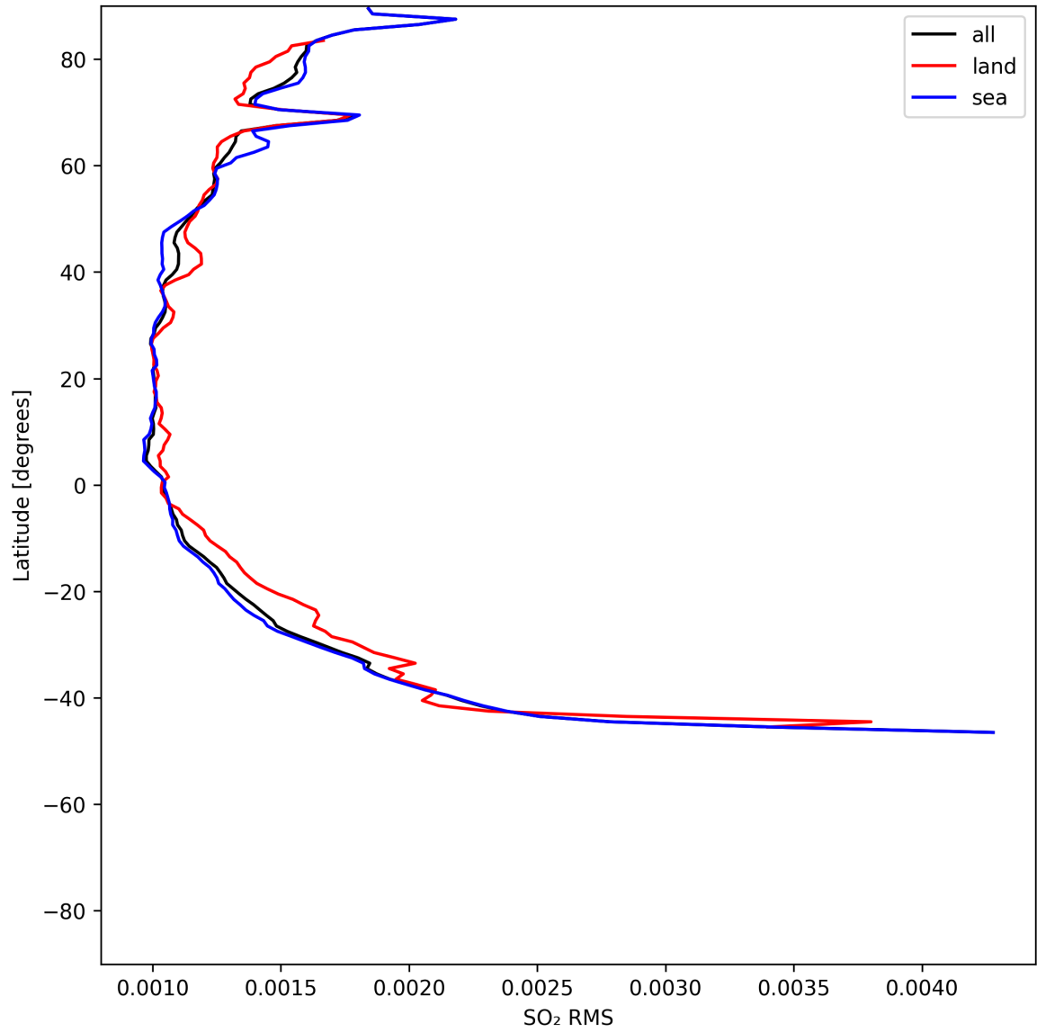
Figure 52: Zonal average of “SO 2 RMS” for 2025-06-01 to 2025-06-03.
