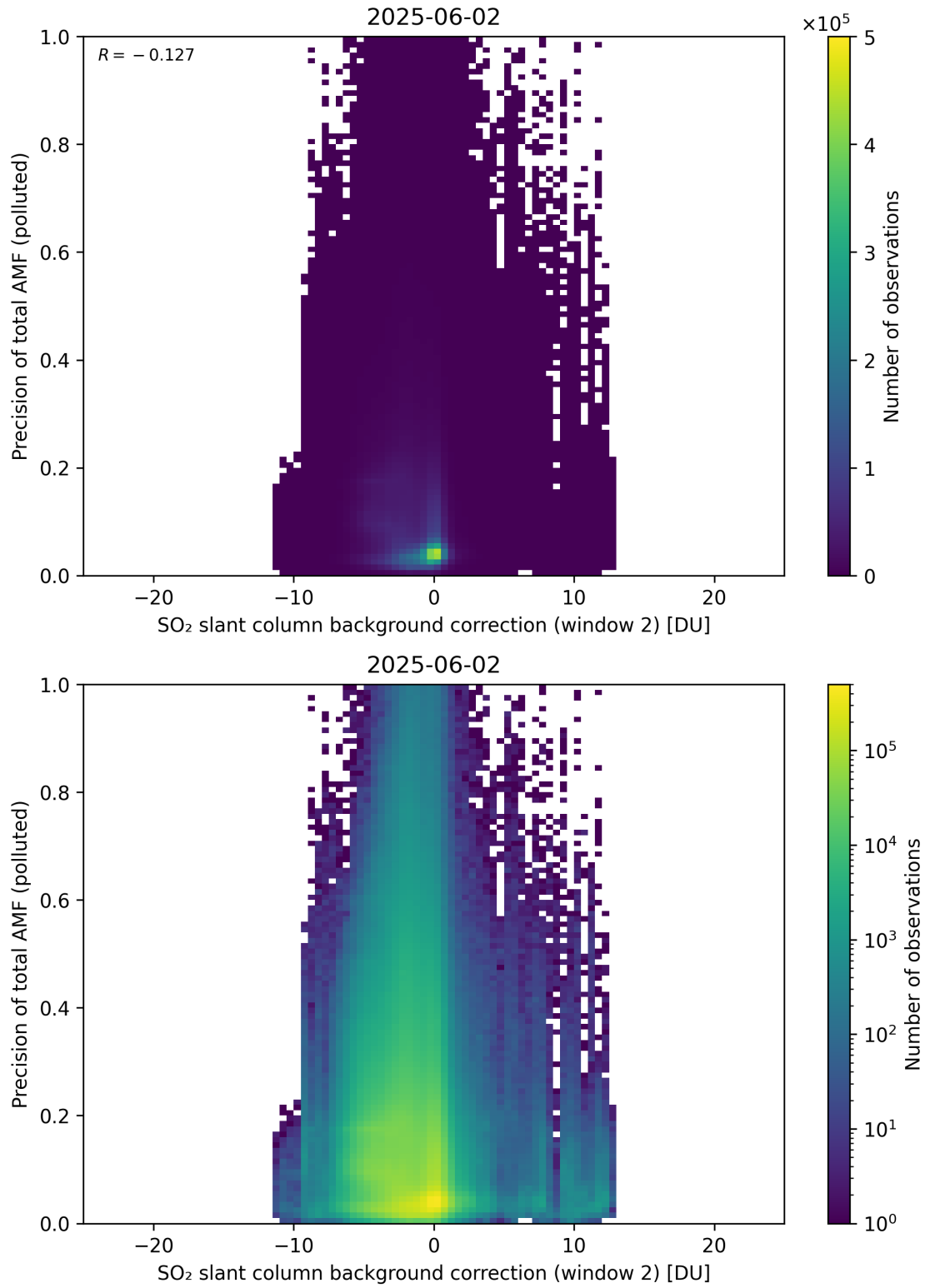
Figure 131: Scatter density plot of “SO 2 slant column background correction (window 2)” against “Precision of total AMF (polluted)” for 2025-06-01 to 2025-06-03.
