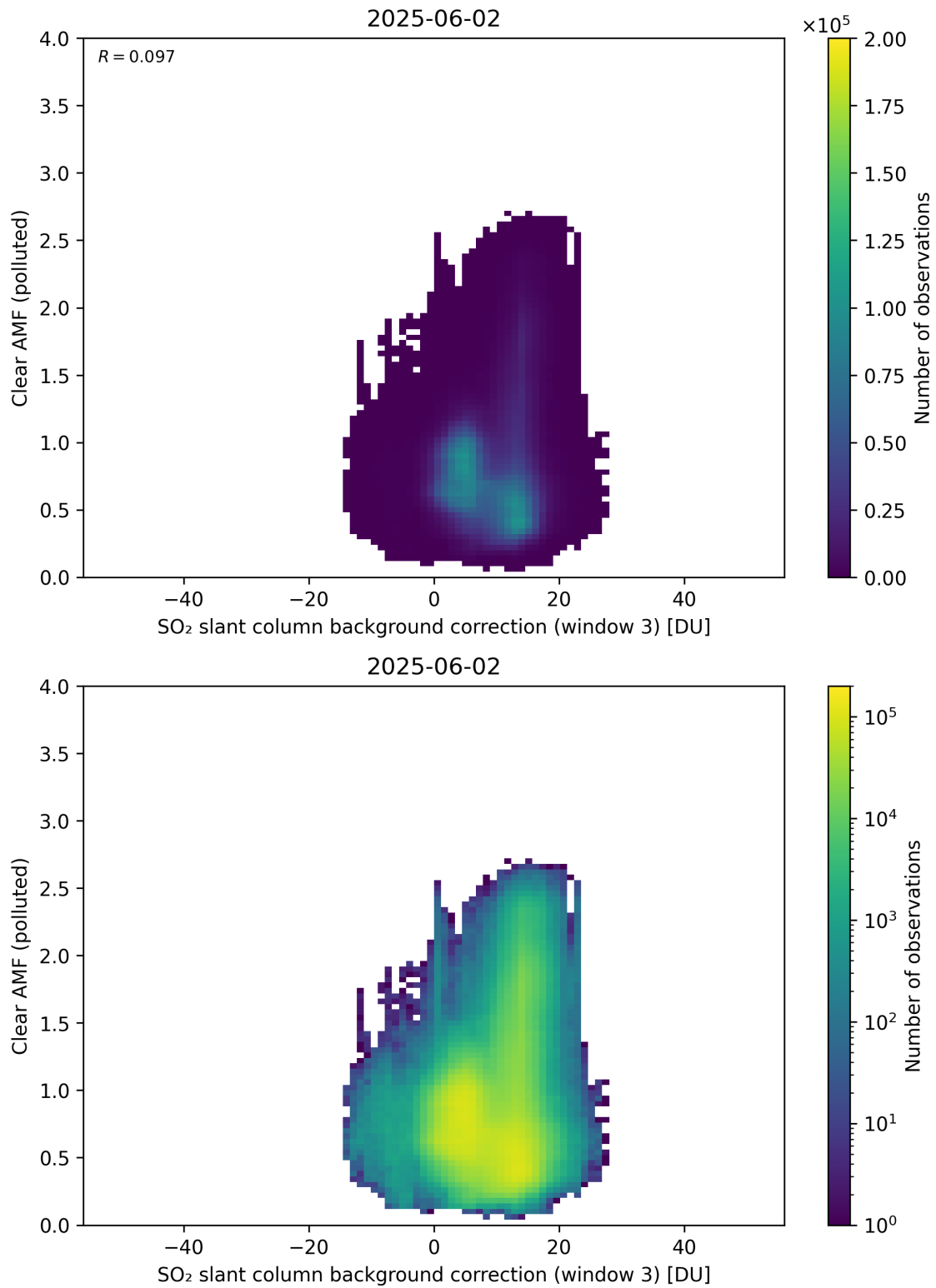
Figure 135: Scatter density plot of “SO 2 slant column background correction (window 3)” against “Clear AMF (polluted)” for 2025-06-01 to 2025-06-03.
