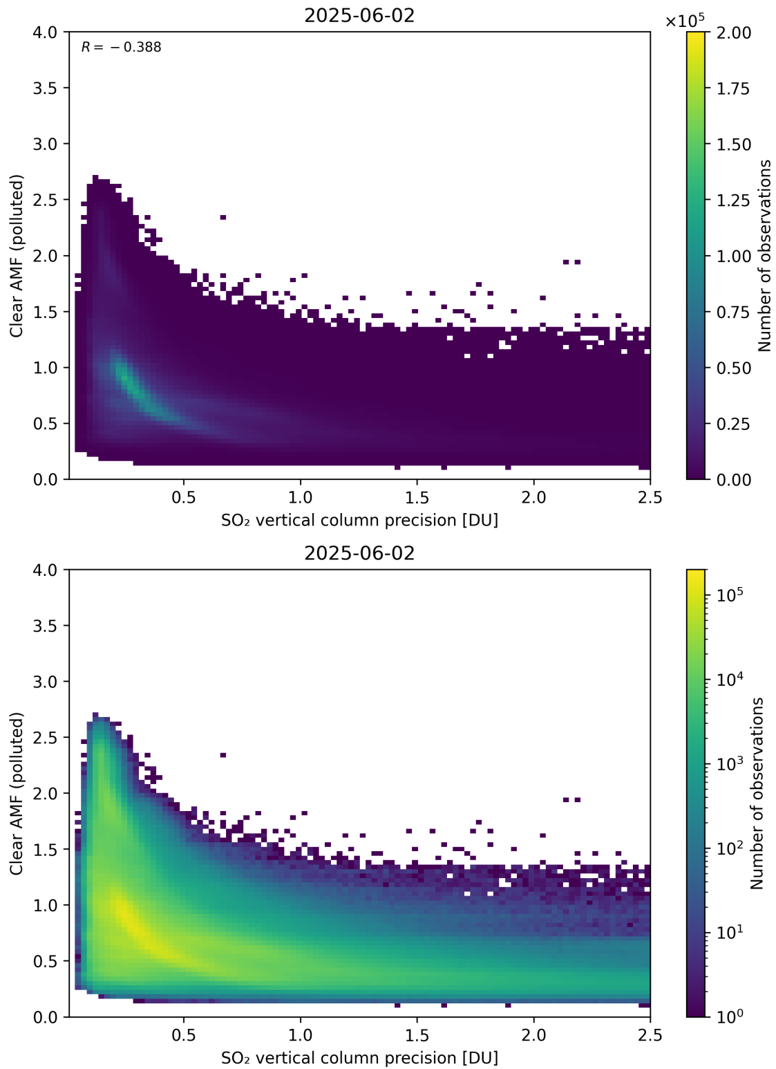
Figure 335: Scatter density plot of “SO 2 vertical column precision” against “Clear AMF (polluted)” for 2025-06-01 to 2025-06-03.
