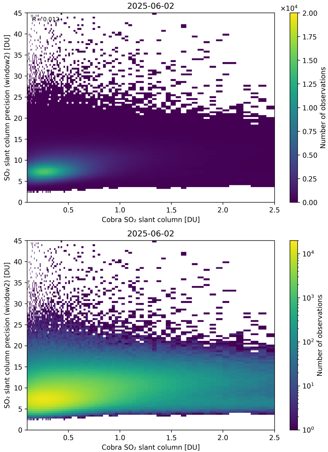
Figure 221: Scatter density plot of “Cobra SO 2 slant column” against “SO 2 slant column precision (window2)” for 2025-06-01 to 2025-06-03.
