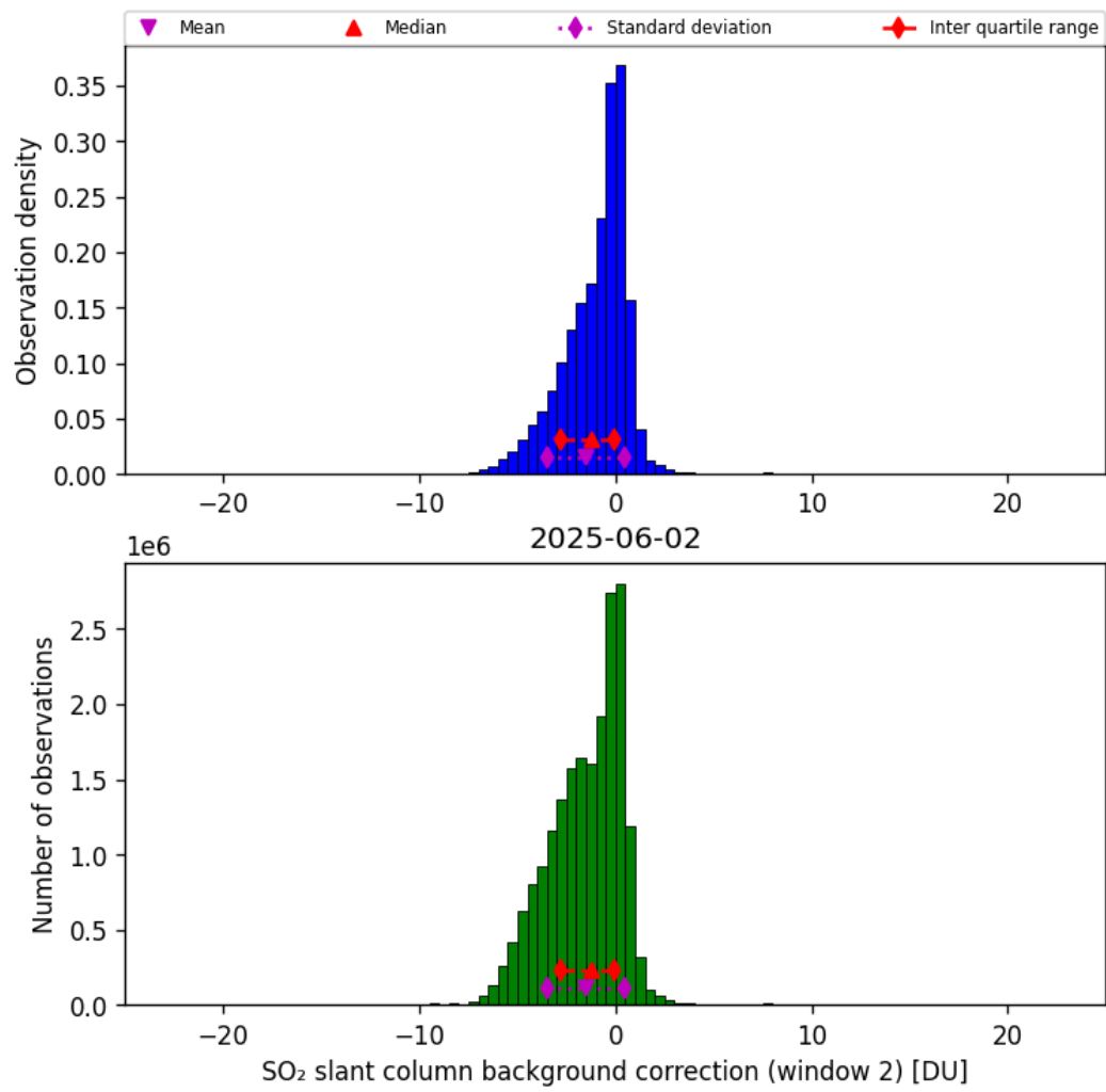
Figure 70: Histogram of “SO 2 slant column background correction (window 2)” for 2025-06-01 to 2025-06-03
