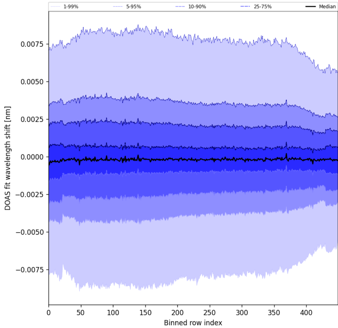
Figure 102: Along track statistics of “DOAS fit wavelength shift” for 2025-06-01 to 2025-06-03
