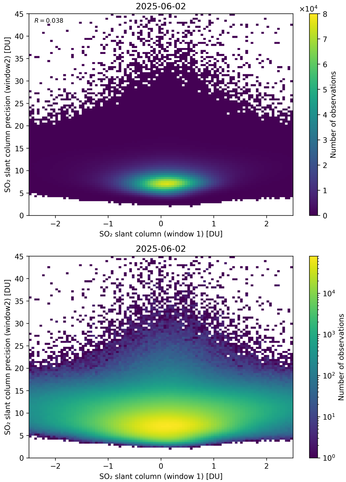
Figure 286: Scatter density plot of “SO 2 slant column (window 1)” against “SO 2 slant column precision (window2)” for 2025-06-01 to 2025-06-03.
