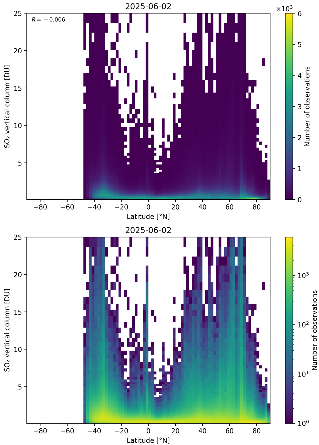
Figure 169: Scatter density plot of “Latitude” against “SO 2 vertical column” for 2025-06-01 to 2025-06-03.
