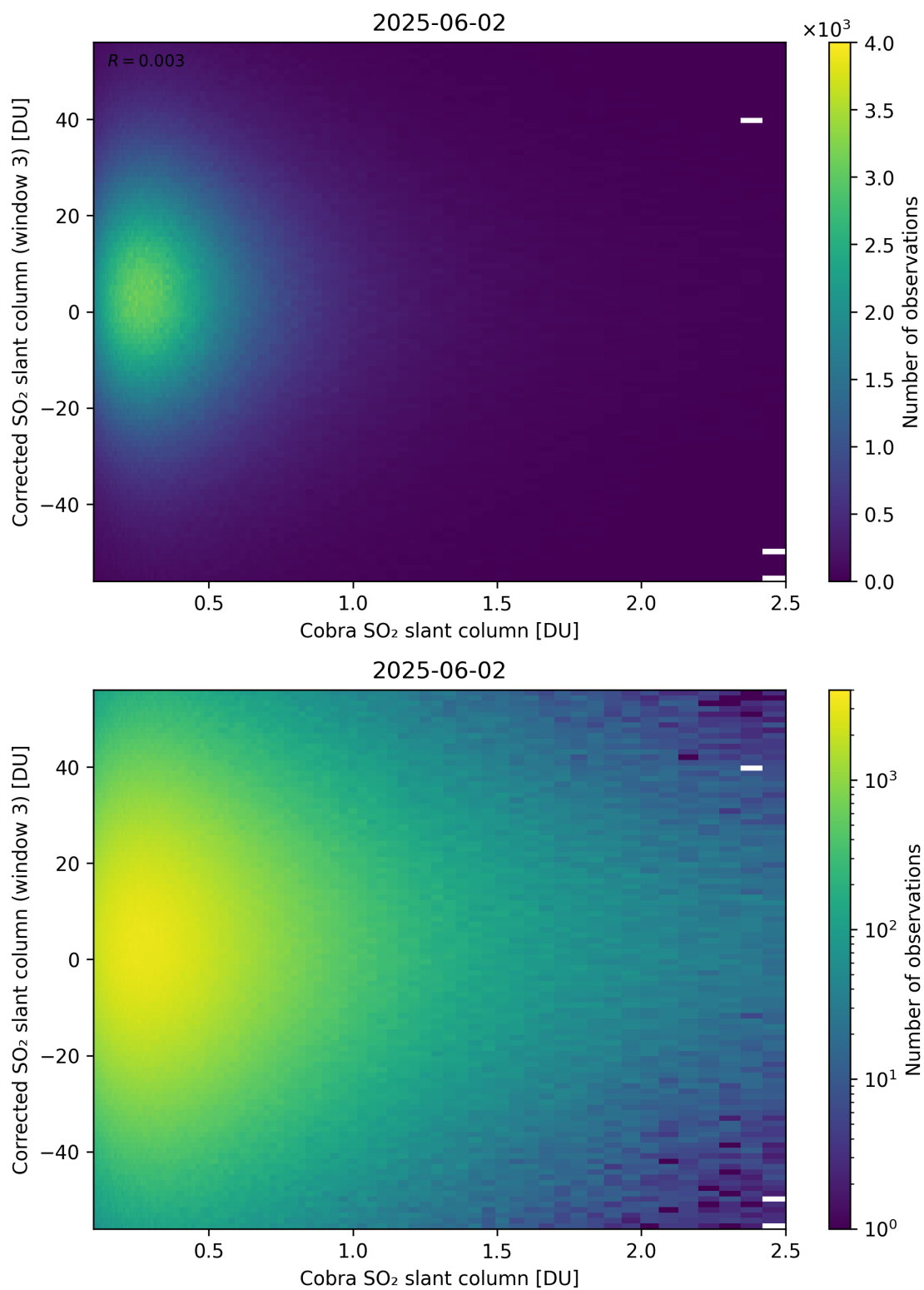
Figure 218: Scatter density plot of “Cobra SO 2 slant column” against “Corrected SO 2 slant column (window 3)” for 2025-06-01 to 2025-06-03.
