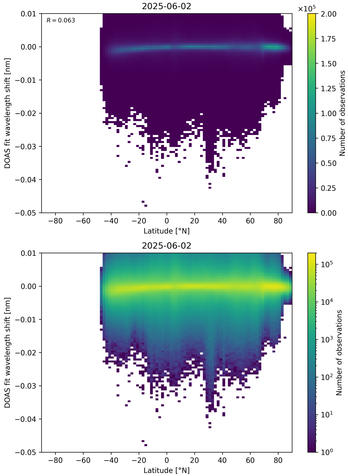
Figure 153: Scatter density plot of “Latitude” against “DOAS fit wavelength shift” for 2025-06-01 to 2025-06-03.
