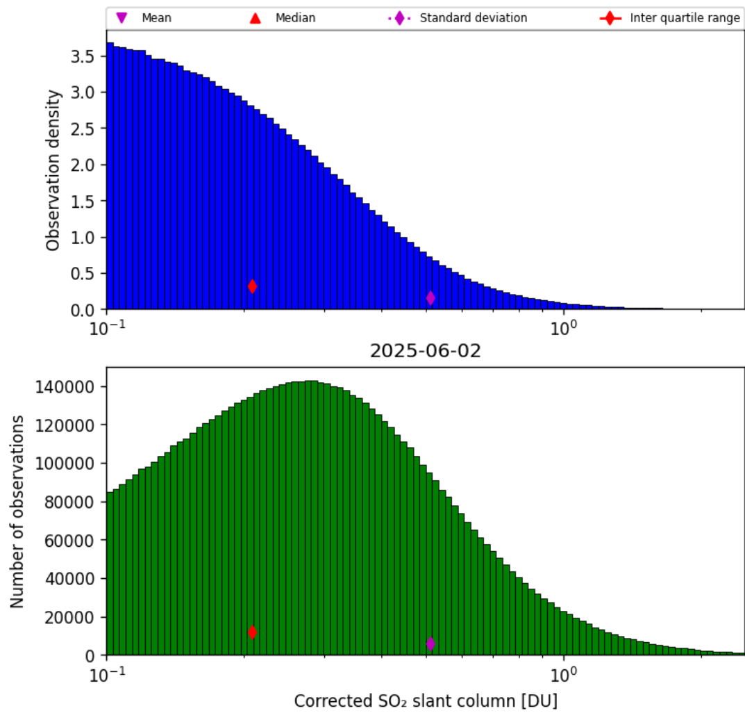
Figure 60: Histogram of “Corrected SO 2 slant column” for 2025-06-01 to 2025-06-03
