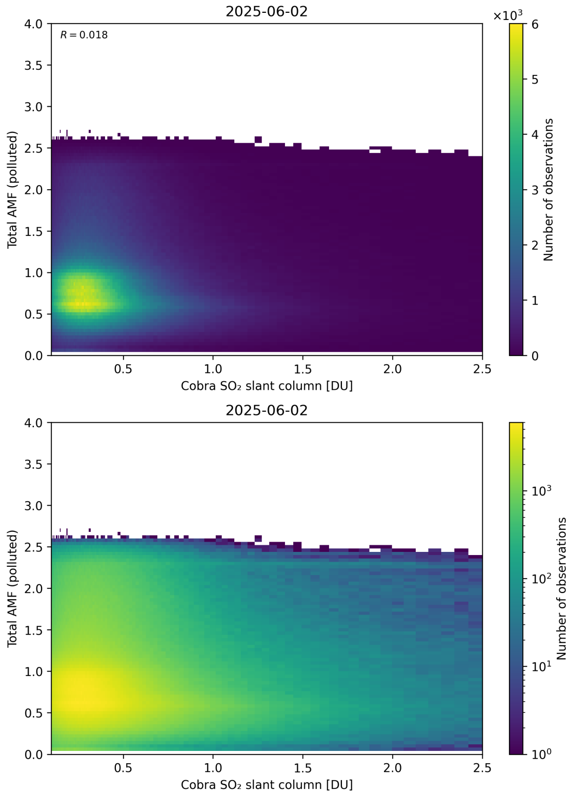
Figure 224: Scatter density plot of “Cobra SO 2 slant column” against “Total AMF (polluted)” for 2025-06-01 to 2025-06-03.
