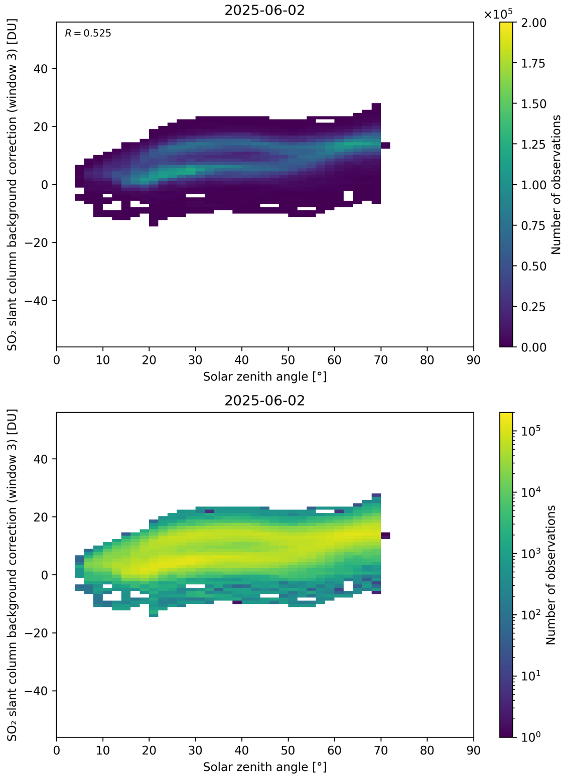
Figure 173: Scatter density plot of “Solar zenith angle” against “SO 2 slant column background correction (window 3)” for 2025-06-01 to 2025-06-03.
