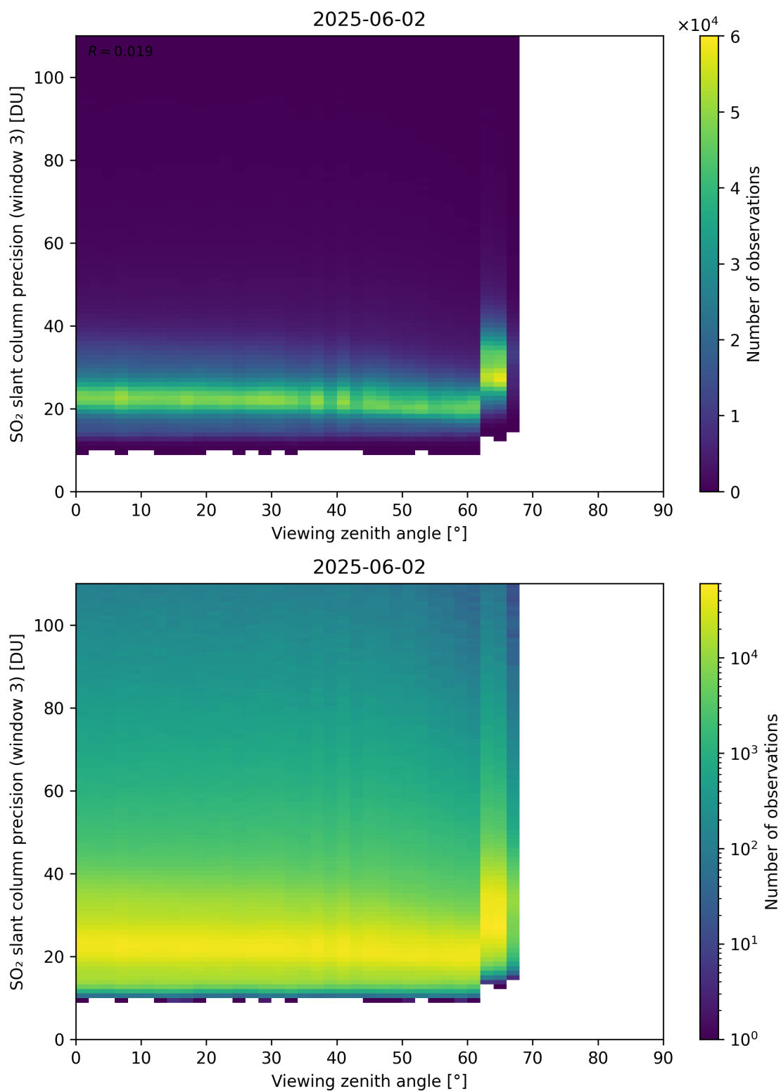
Figure 380: Scatter density plot of “Viewing zenith angle” against “SO 2 slant column precision (window 3)” for 2025-06-01 to 2025-06-03.
