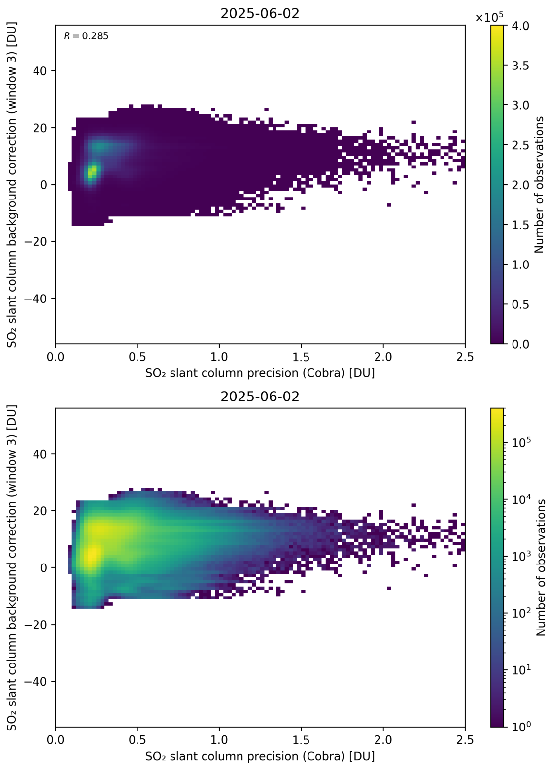
Figure 201: Scatter density plot of “SO 2 slant column precision (Cobra)” against “SO 2 slant column background correction (window 3)” for 2025-06-01 to 2025-06-03.
