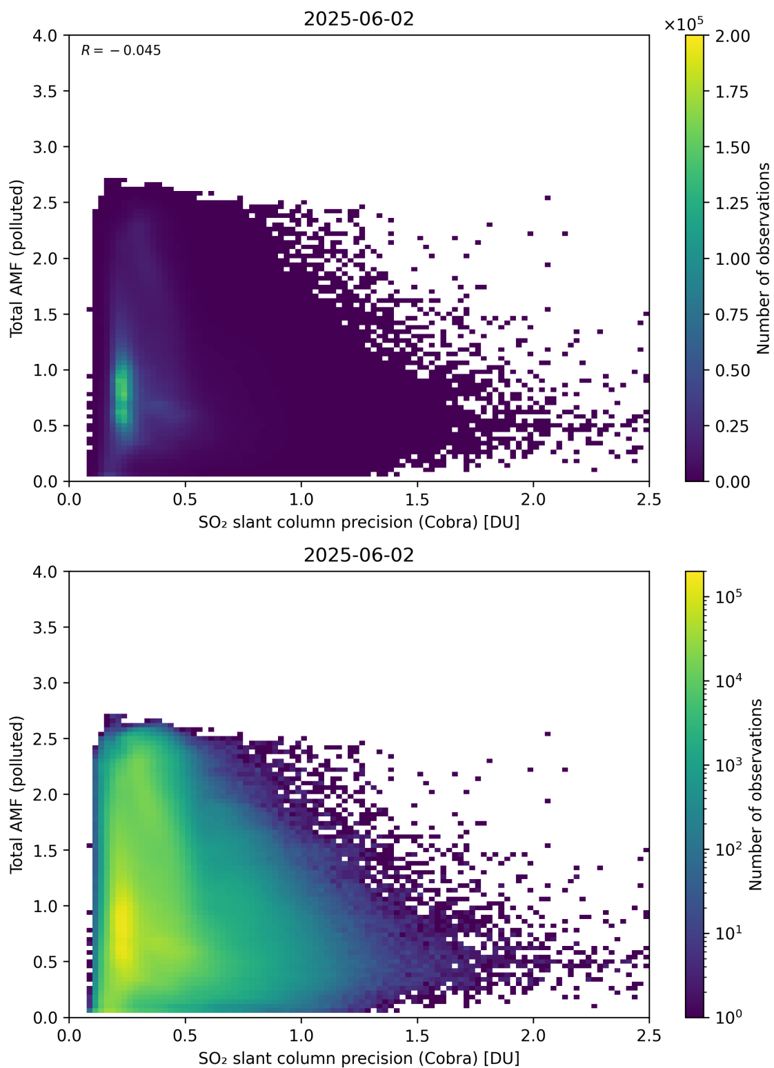
Figure 213: Scatter density plot of “SO 2 slant column precision (Cobra)” against “Total AMF (polluted)” for 2025-06-01 to 2025-06-03.
