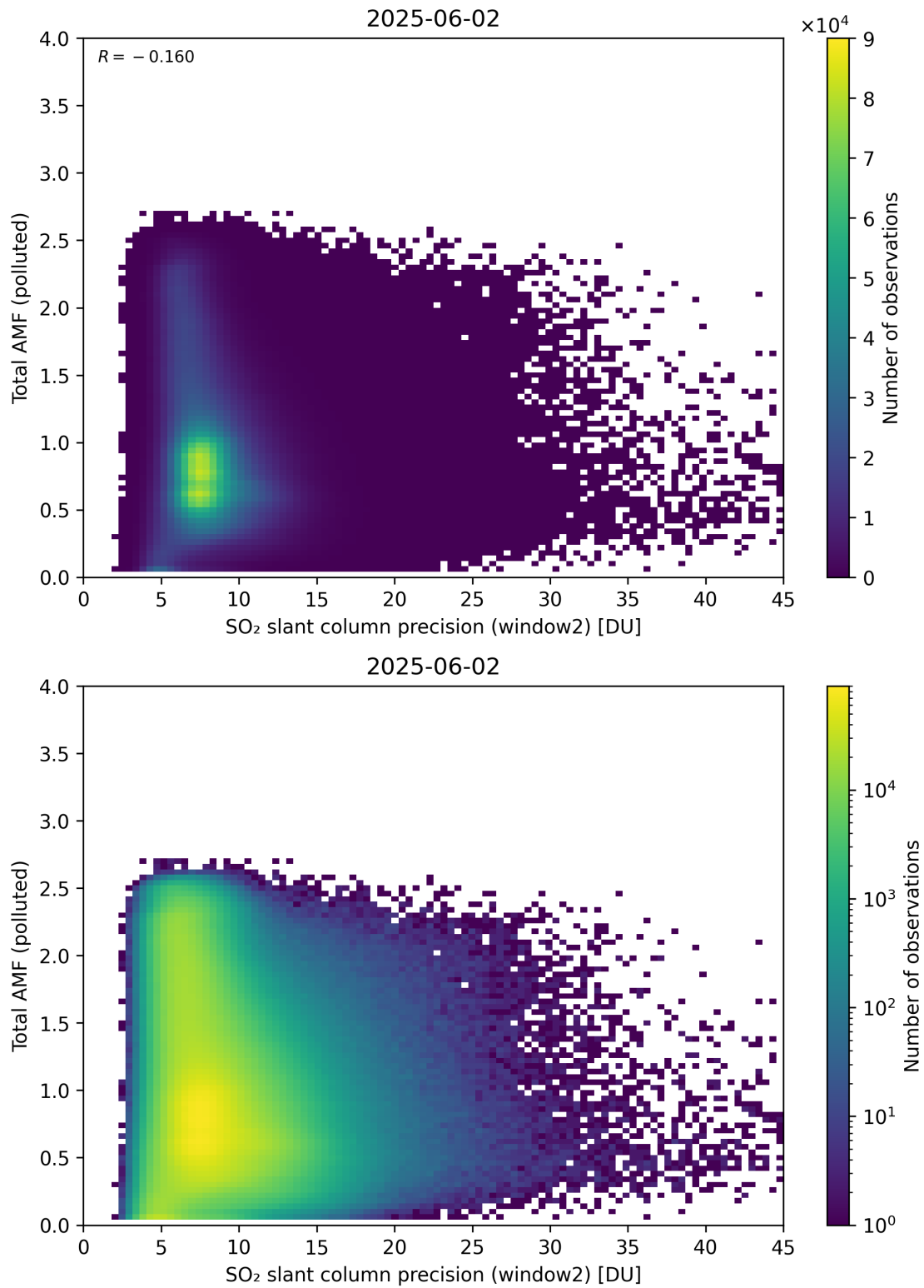
Figure 301: Scatter density plot of “SO 2 slant column precision (window2)” against “Total AMF (polluted)” for 2025-06-01 to 2025-06-03.
