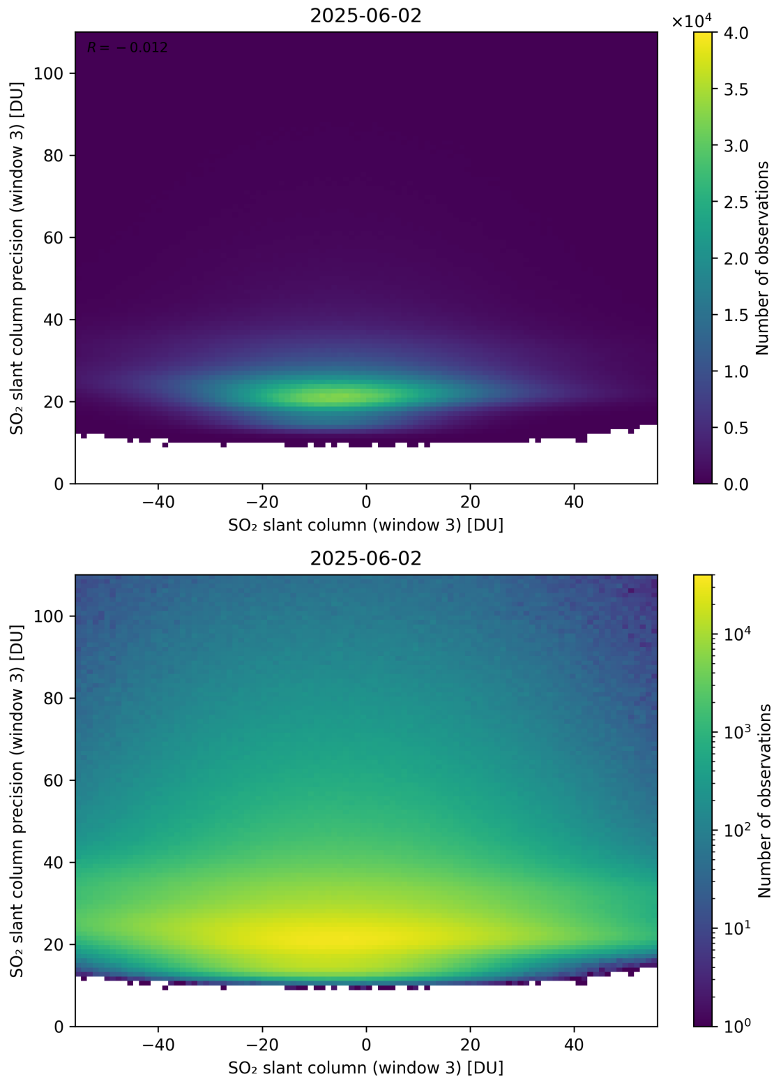
Figure 317: Scatter density plot of “SO 2 slant column (window 3)” against “SO 2 slant column precision (window 3)” for 2025-06-01 to 2025-06-03.
