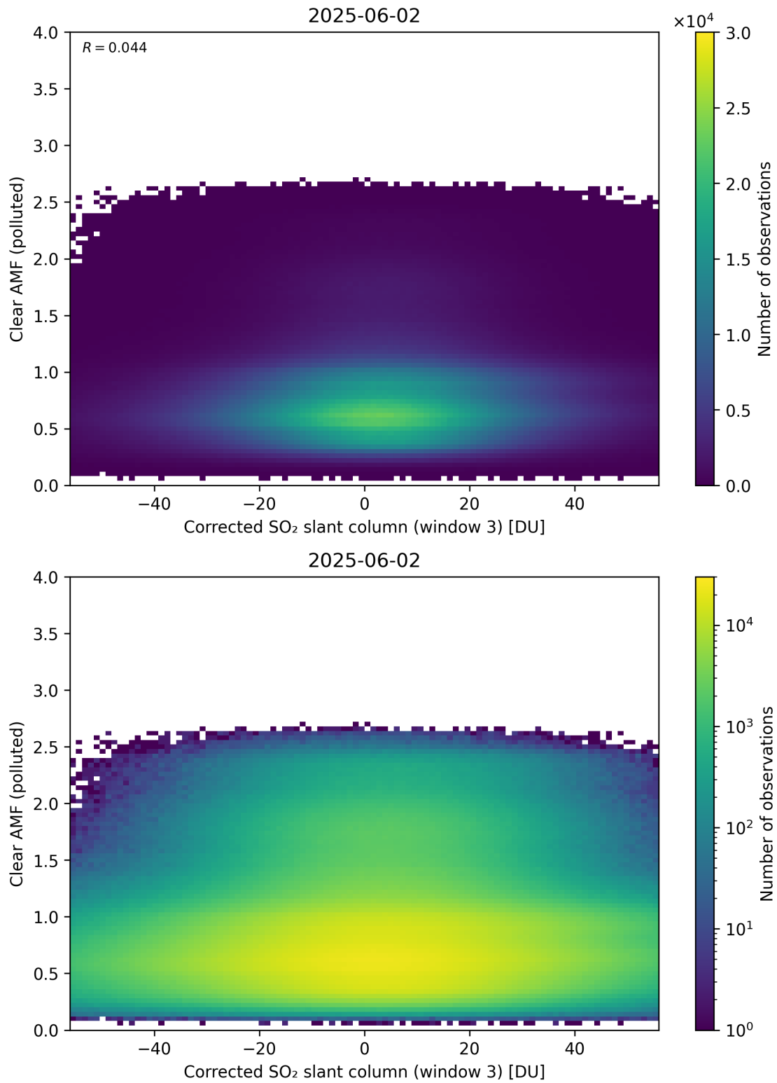
Figure 259: Scatter density plot of “Corrected SO 2 slant column (window 3)” against “Clear AMF (polluted)” for 2025-06-01 to 2025-06-03.
