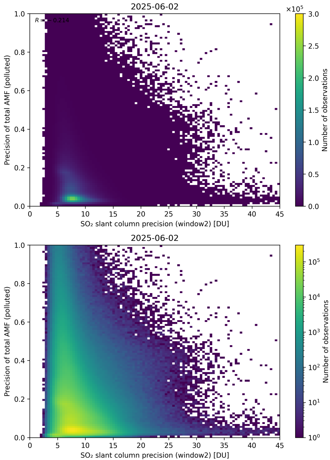
Figure 302: Scatter density plot of “SO 2 slant column precision (window2)” against “Precision of total AMF (polluted)” for 2025-06-01 to 2025-06-03.
