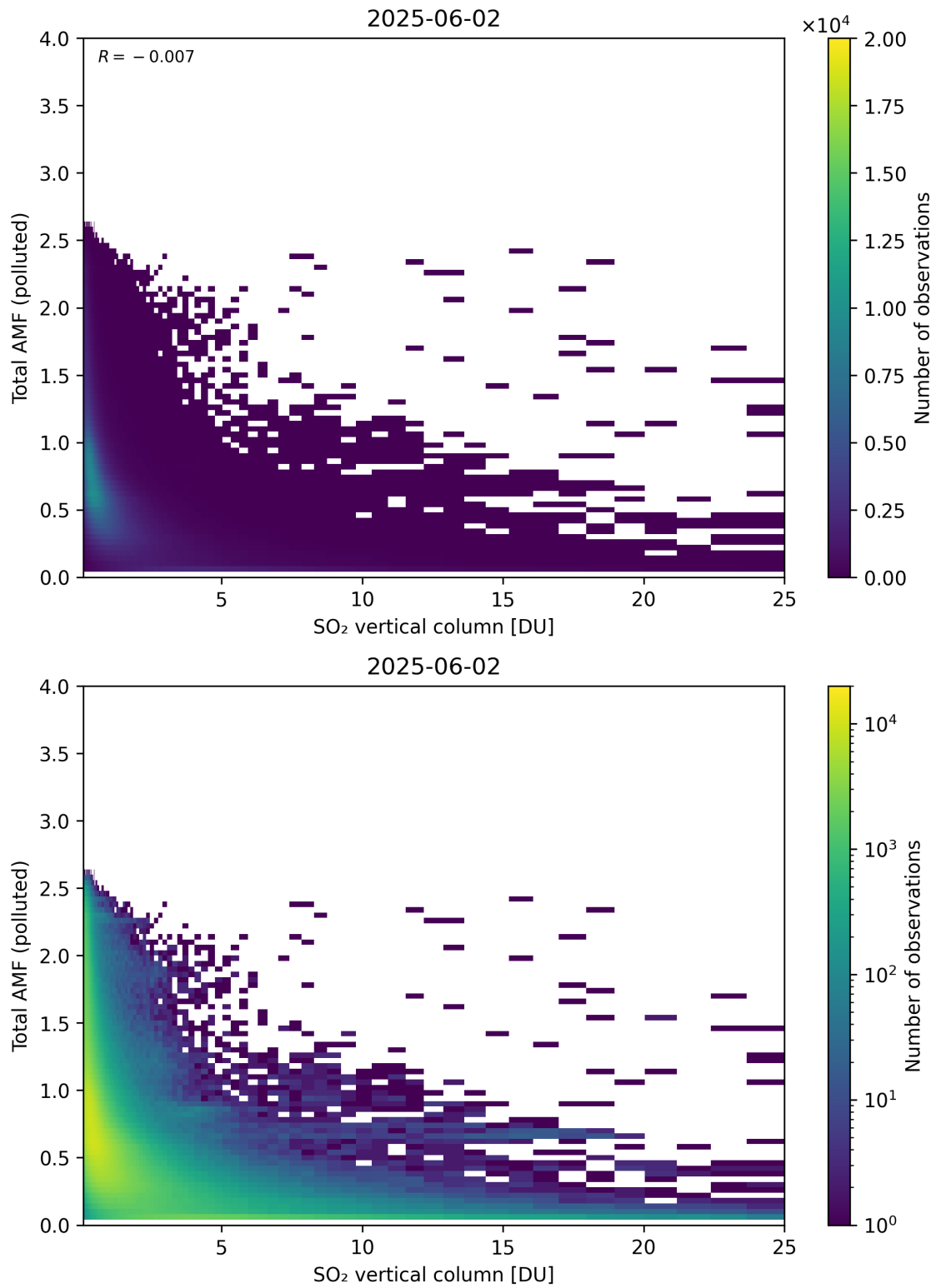
Figure 359: Scatter density plot of “SO 2 vertical column” against “Total AMF (polluted)” for 2025-06-01 to 2025-06-03.
