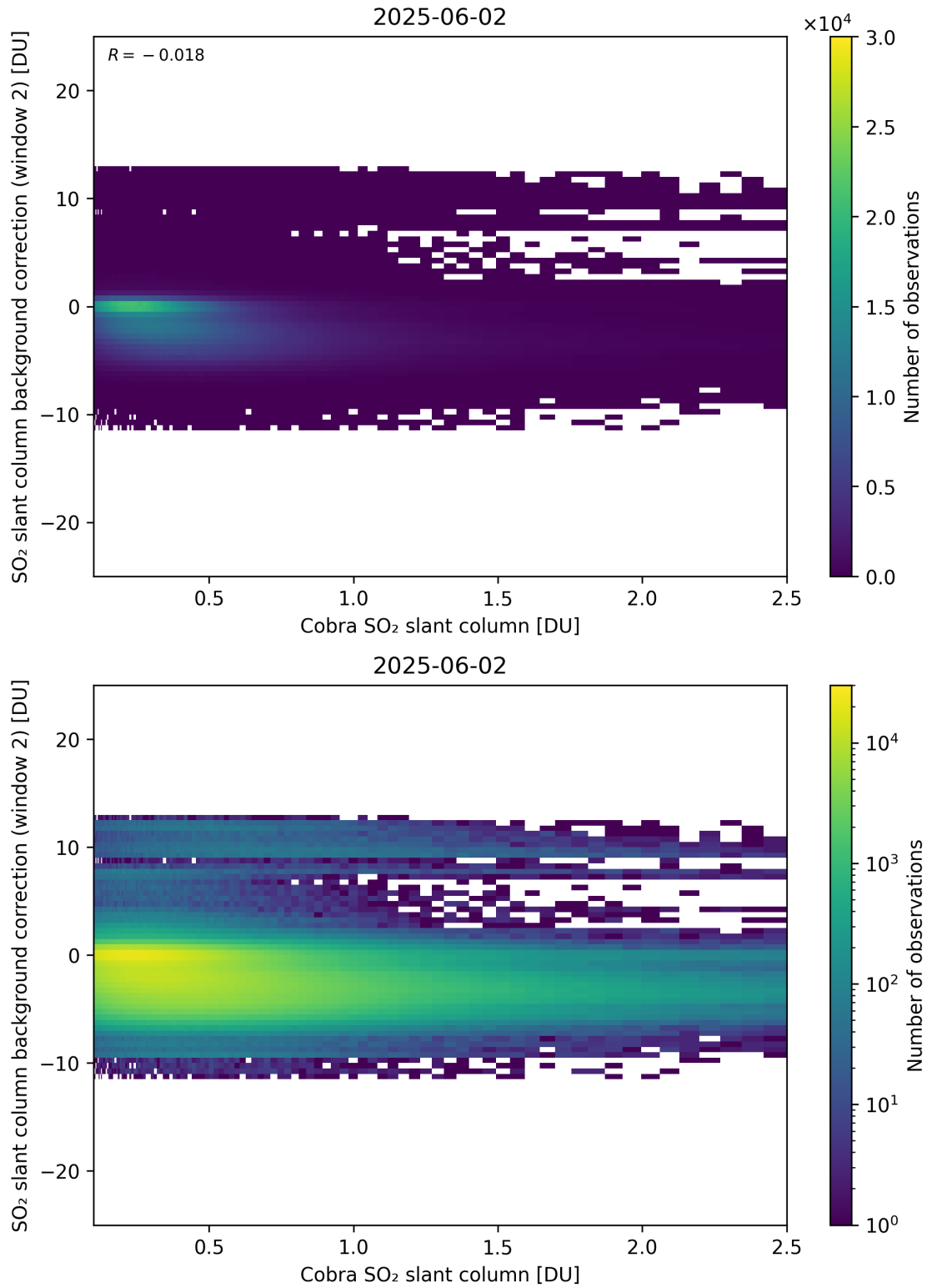
Figure 194: Scatter density plot of “Cobra SO 2 slant column” against “SO 2 slant column background correction (window 2)” for 2025-06-01 to 2025-06-03.
