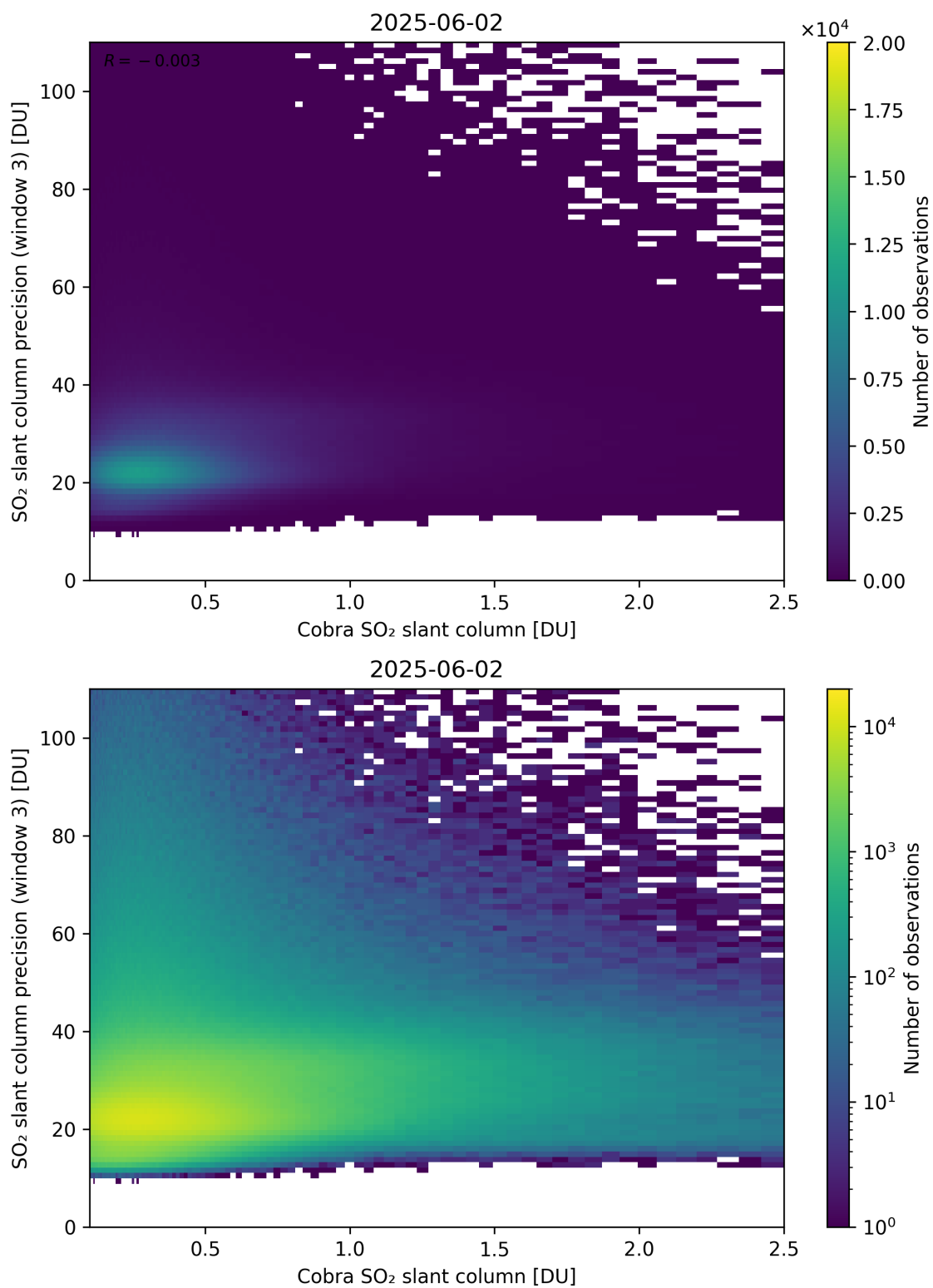
Figure 223: Scatter density plot of “Cobra SO 2 slant column” against “SO 2 slant column precision (window 3)” for 2025-06-01 to 2025-06-03.
