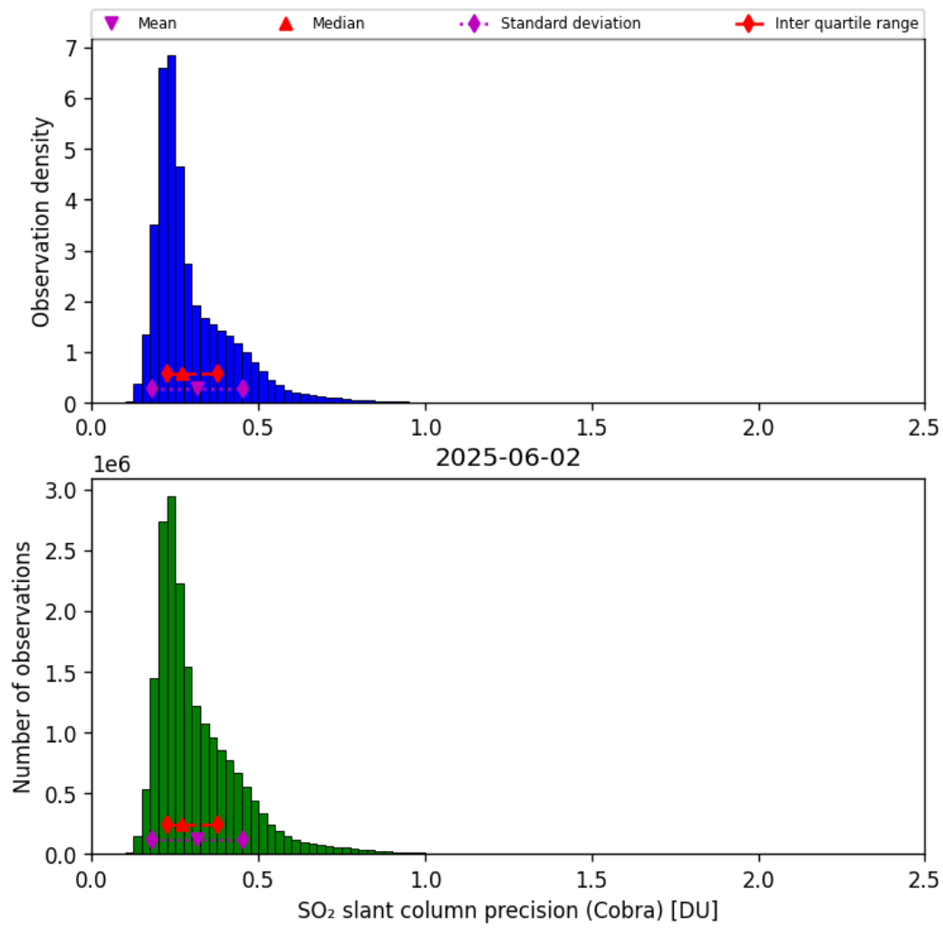
Figure 62: Histogram of “SO 2 slant column precision (Cobra)” for 2025-06-01 to 2025-06-03
