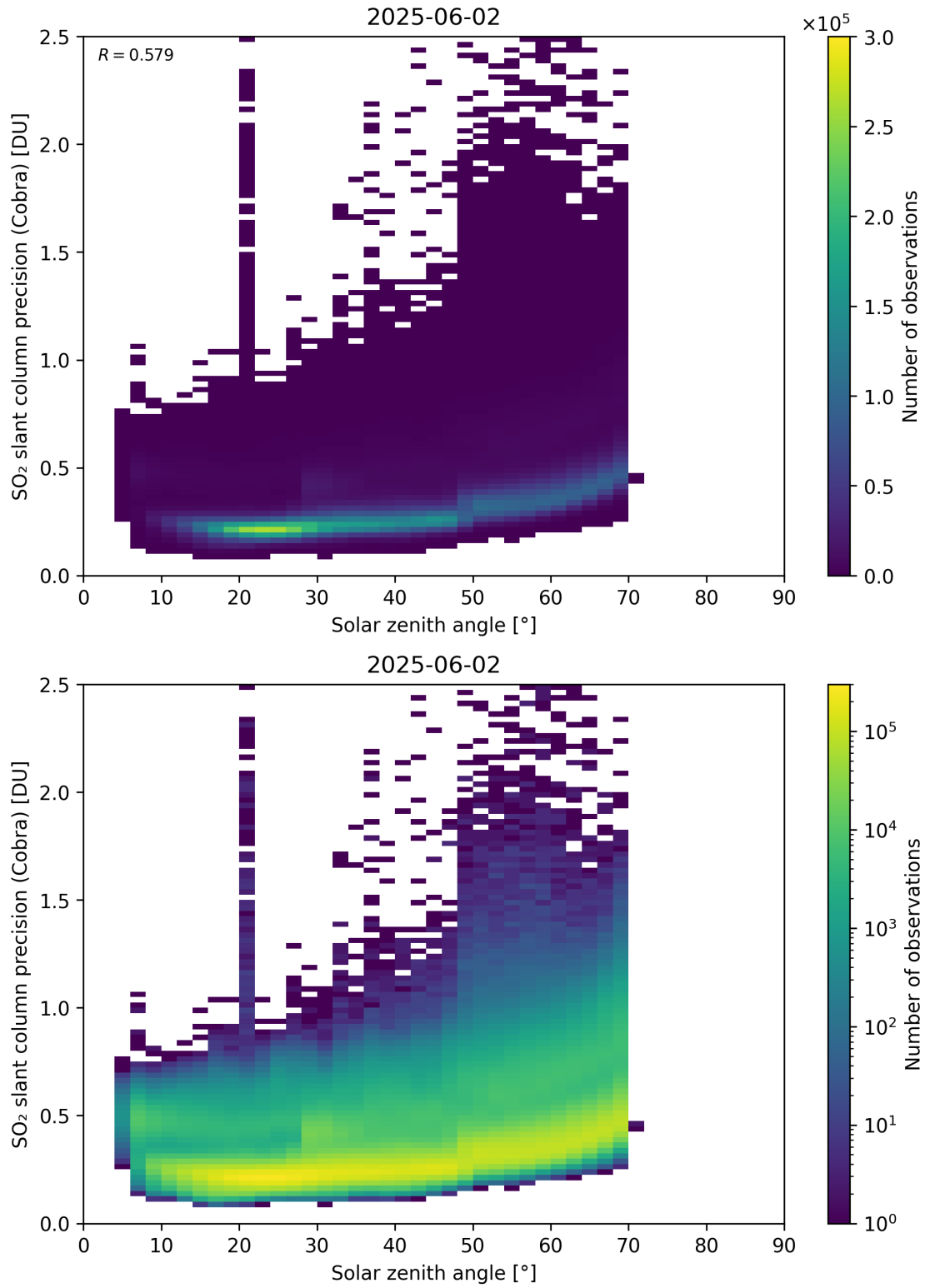
Figure 180: Scatter density plot of “Solar zenith angle” against “SO 2 slant column precision (Cobra)” for 2025-06-01 to 2025-06-03.
