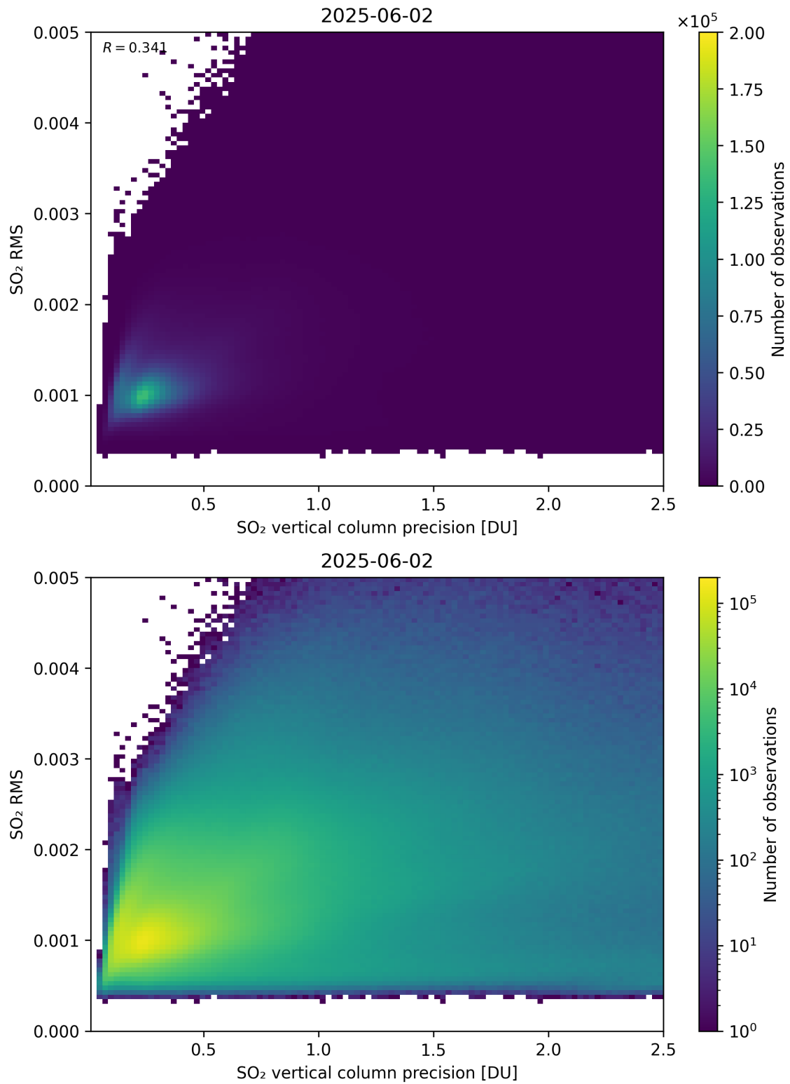
Figure 334: Scatter density plot of “SO 2 vertical column precision” against “SO 2 RMS” for 2025-06-01 to 2025-06-03.
