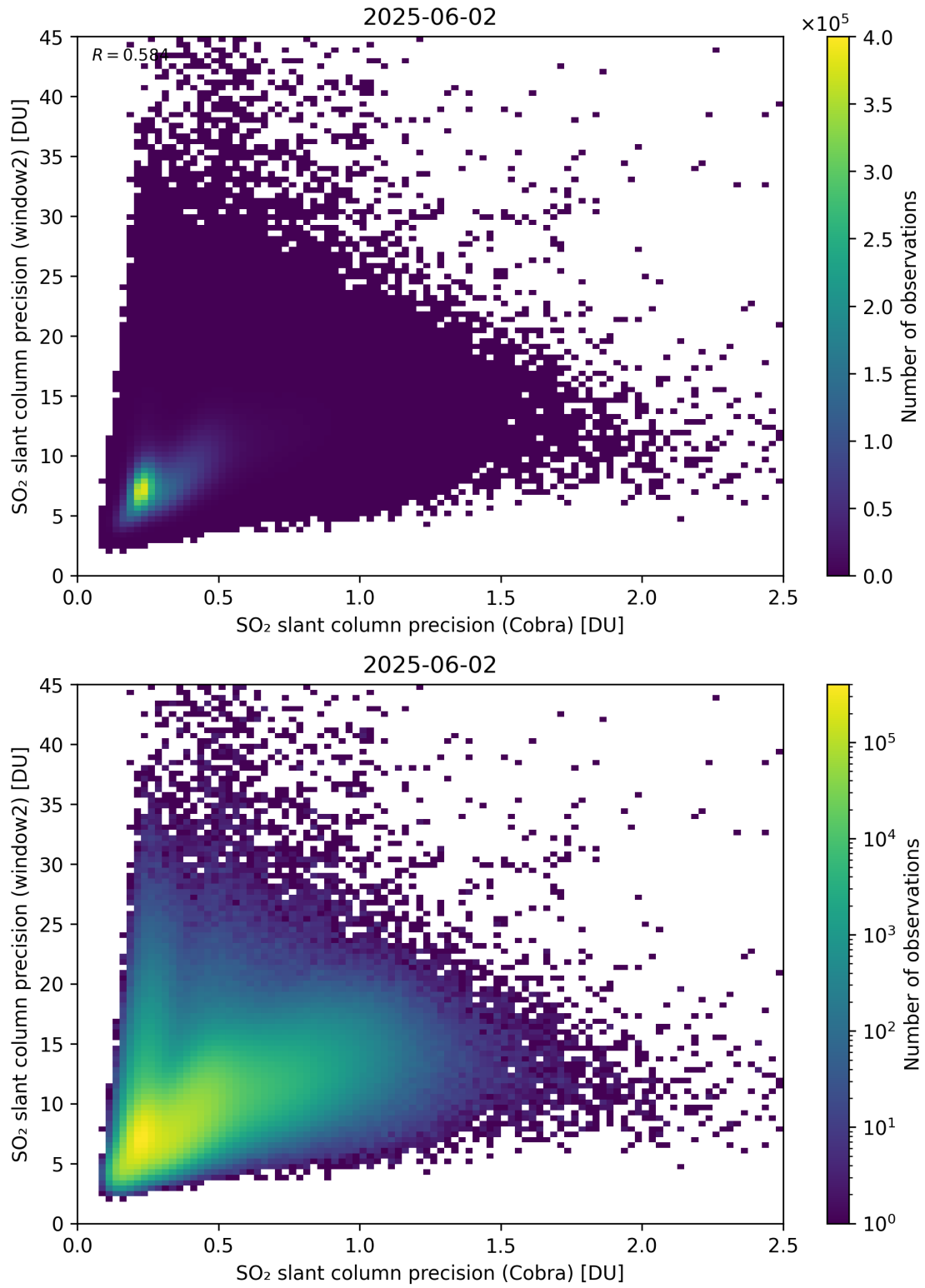
Figure 210: Scatter density plot of “SO 2 slant column precision (Cobra)” against “SO 2 slant column precision (window2)” for 2025-06-01 to 2025-06-03.
