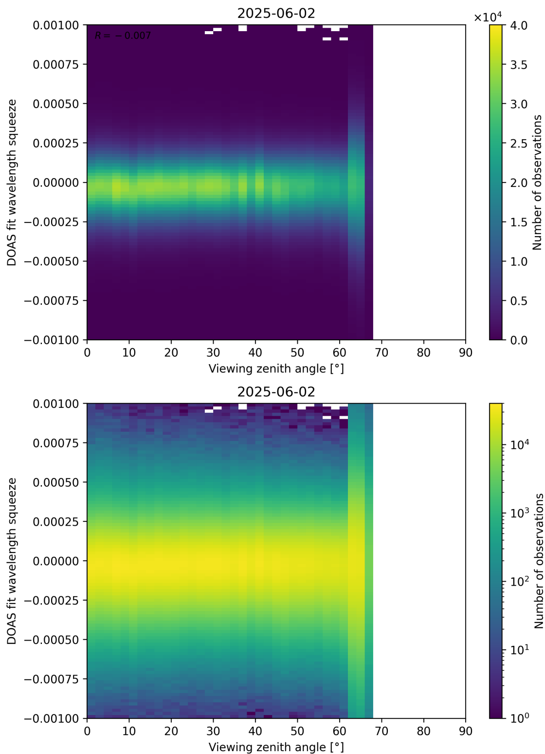
Figure 366: Scatter density plot of “Viewing zenith angle” against “DOAS fit wavelength squeeze” for 2025-06-01 to 2025-06-03.
