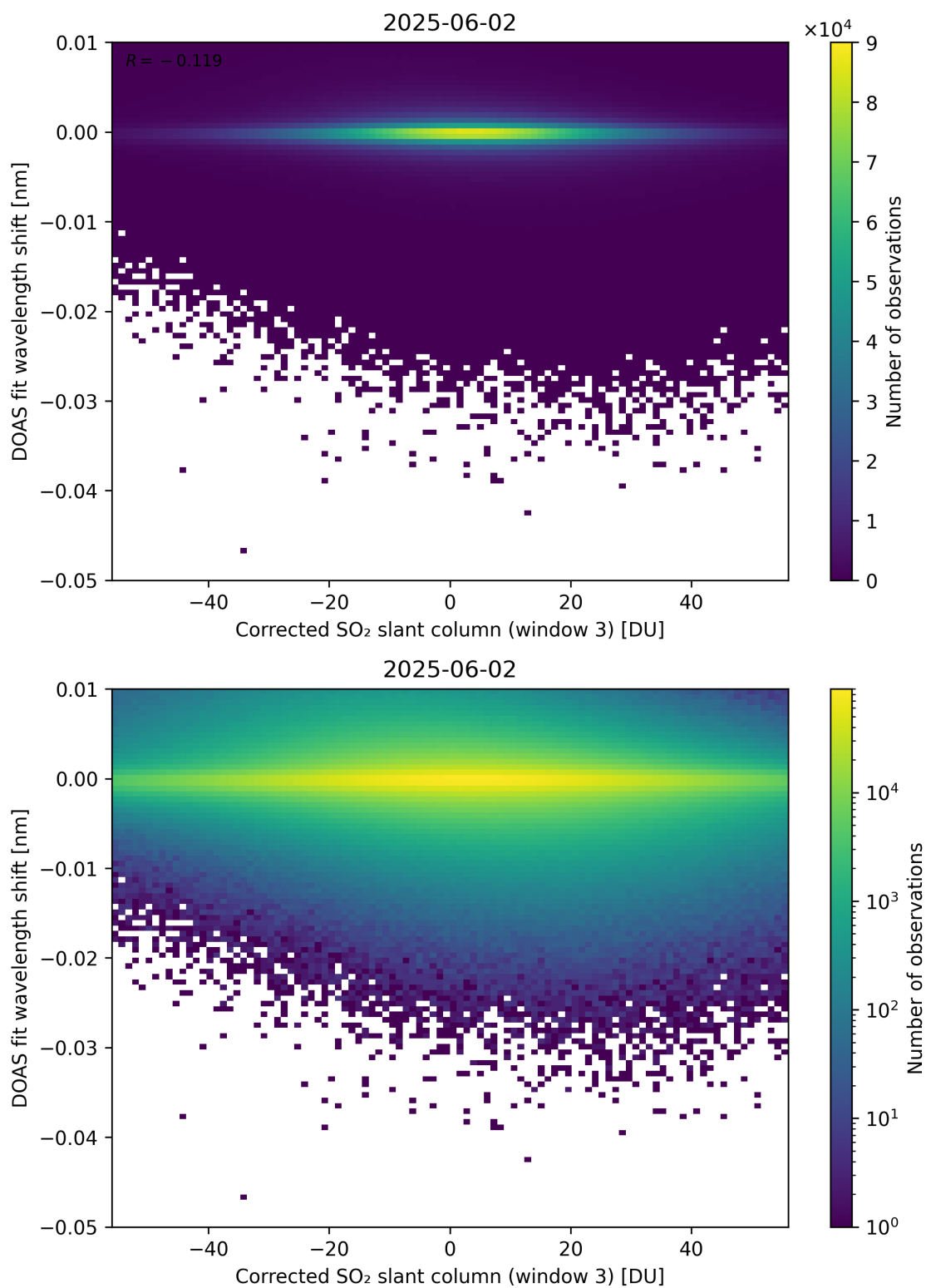
Figure 256: Scatter density plot of “Corrected SO 2 slant column (window 3)” against “DOAS fit wavelength shift” for 2025-06-01 to 2025-06-03.
