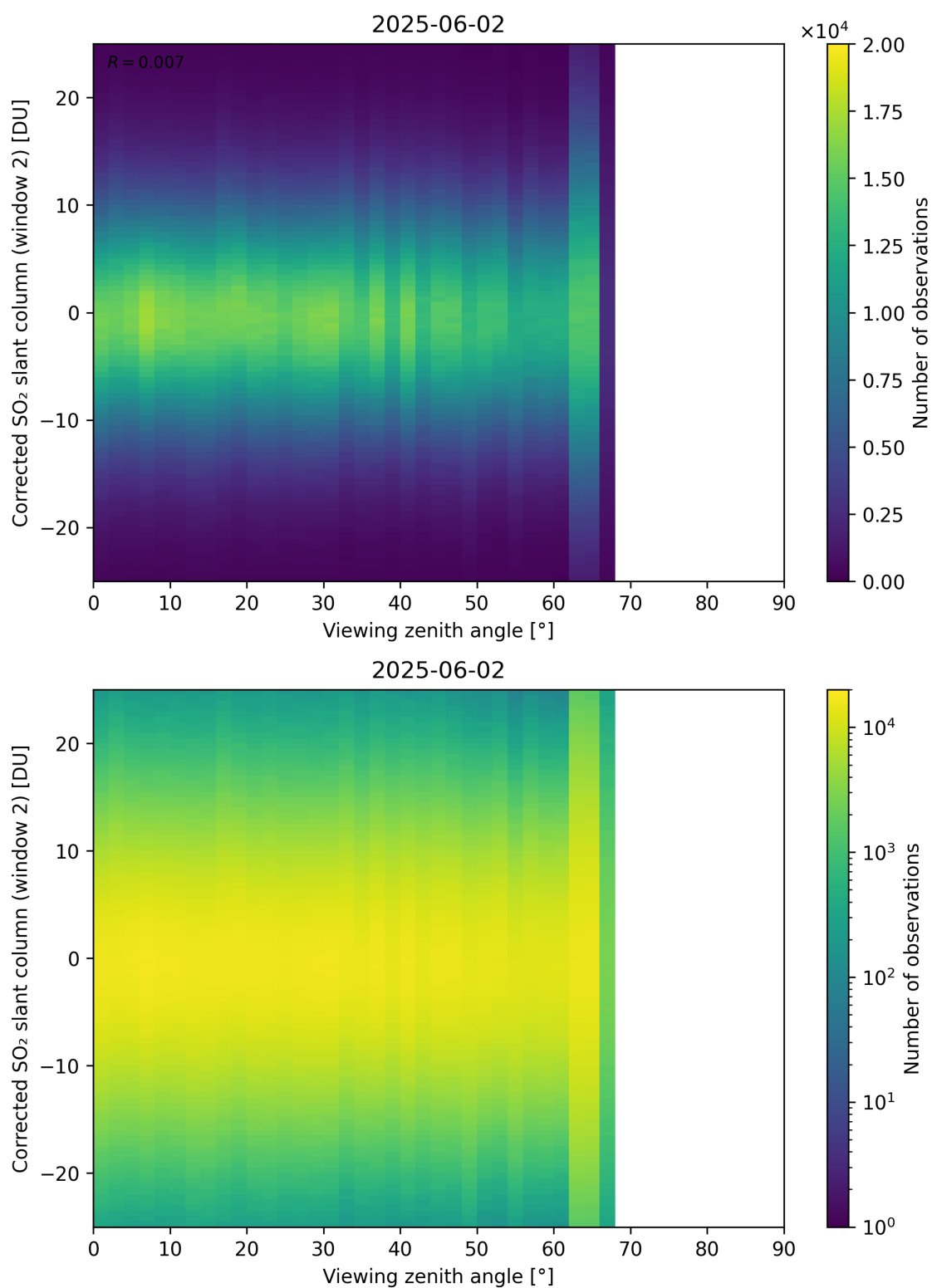
Figure 374: Scatter density plot of “Viewing zenith angle” against “Corrected SO 2 slant column (window 2)” for 2025-06-01 to 2025-06-03.
