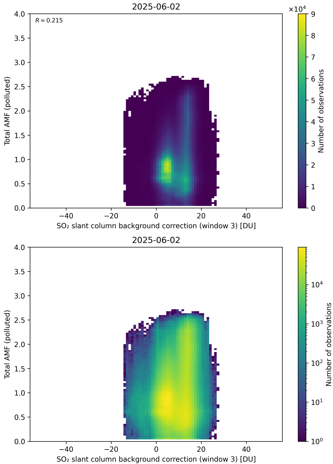
Figure 136: Scatter density plot of “SO 2 slant column background correction (window 3)” against “Total AMF (polluted)” for 2025-06-01 to 2025-06-03.
