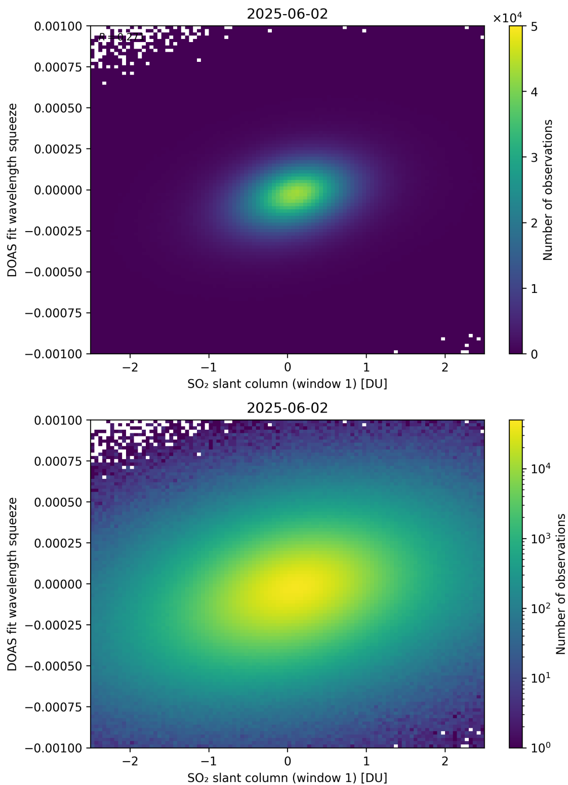
Figure 266: Scatter density plot of “SO 2 slant column (window 1)” against “DOAS fit wavelength squeeze” for 2025-06-01 to 2025-06-03.
