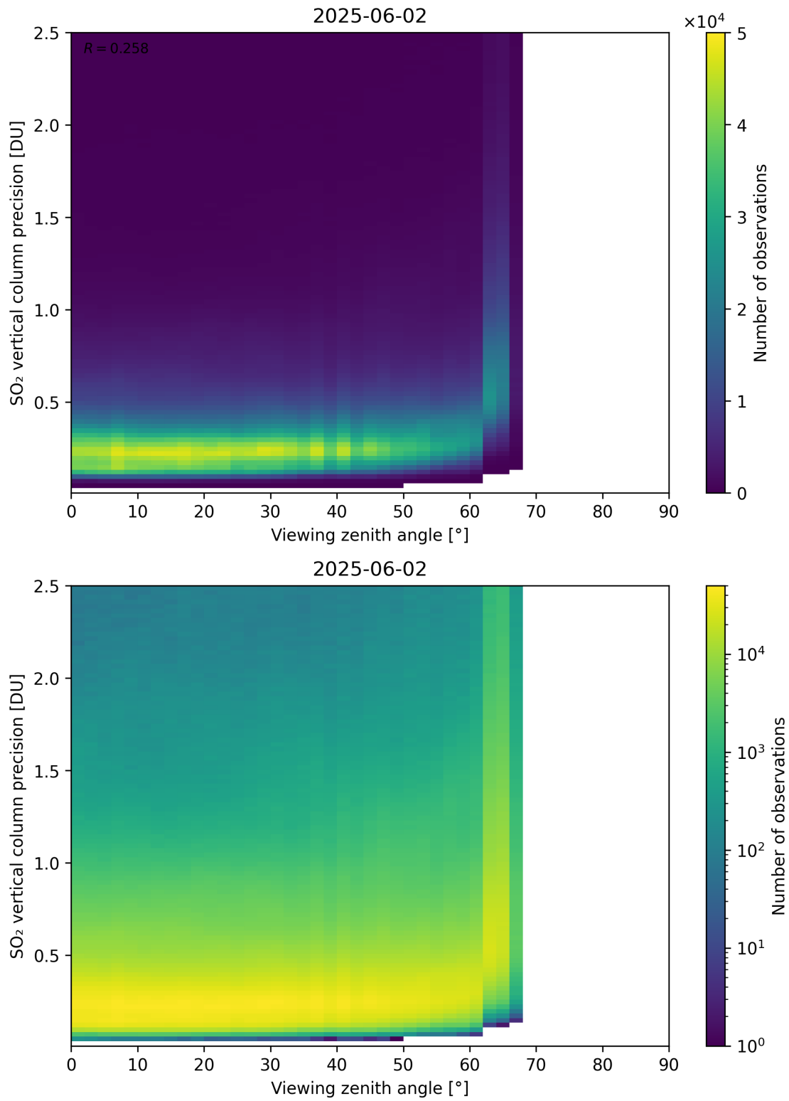
Figure 384: Scatter density plot of “Viewing zenith angle” against “SO 2 vertical column precision” for 2025-06-01 to 2025-06-03.
