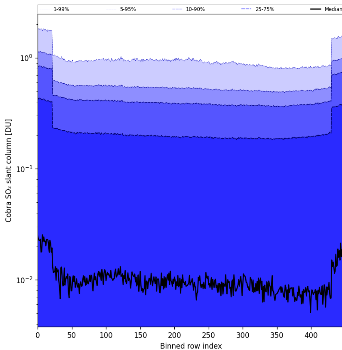
Figure 87: Along track statistics of "Cobra SO 2 slant column" for 2025-06-01 to 2025-06-03
