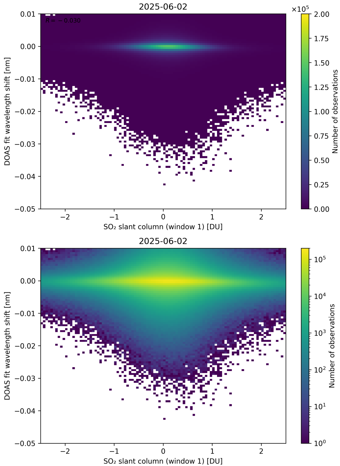
Figure 265: Scatter density plot of “SO 2 slant column (window 1)” against “DOAS fit wavelength shift” for 2025-06-01 to 2025-06-03.
