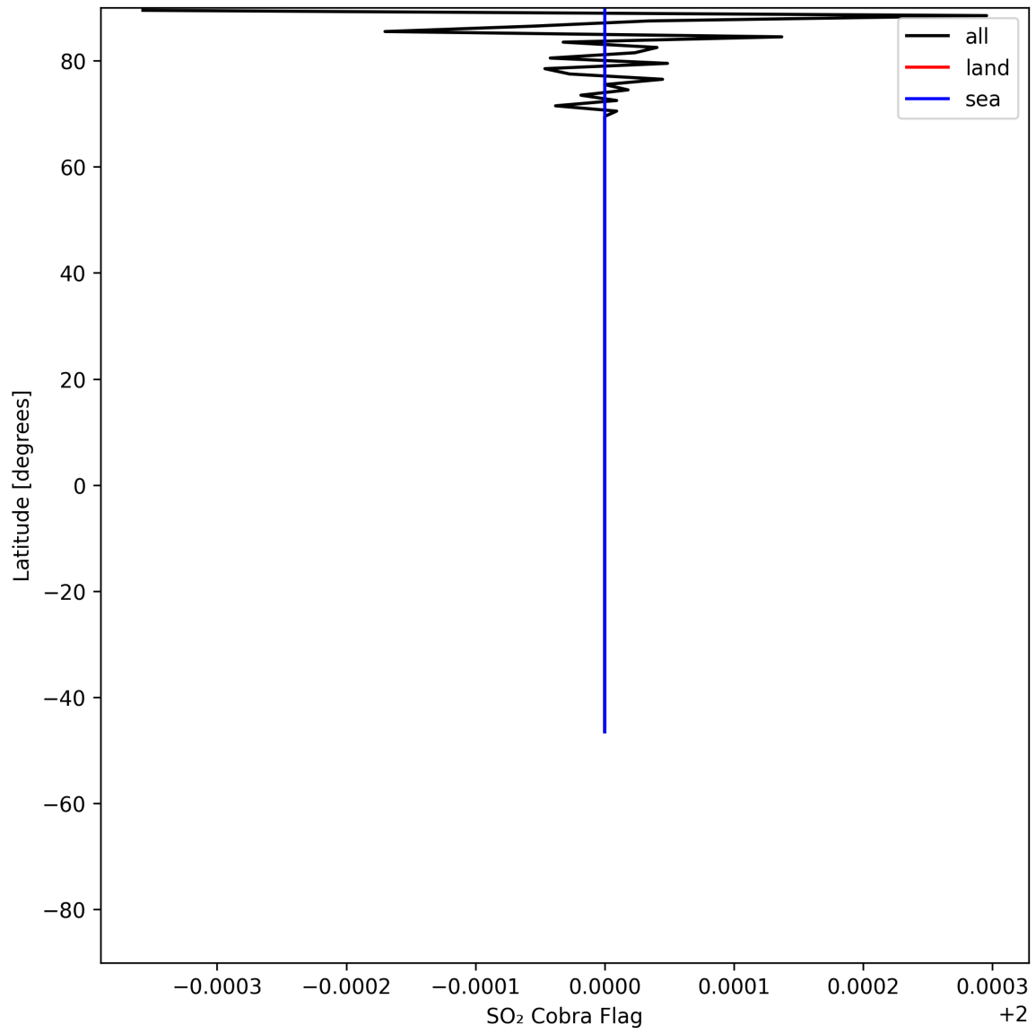
Figure 49: Zonal average of “SO 2 Cobra Flag” for 2025-06-01 to 2025-06-03.
