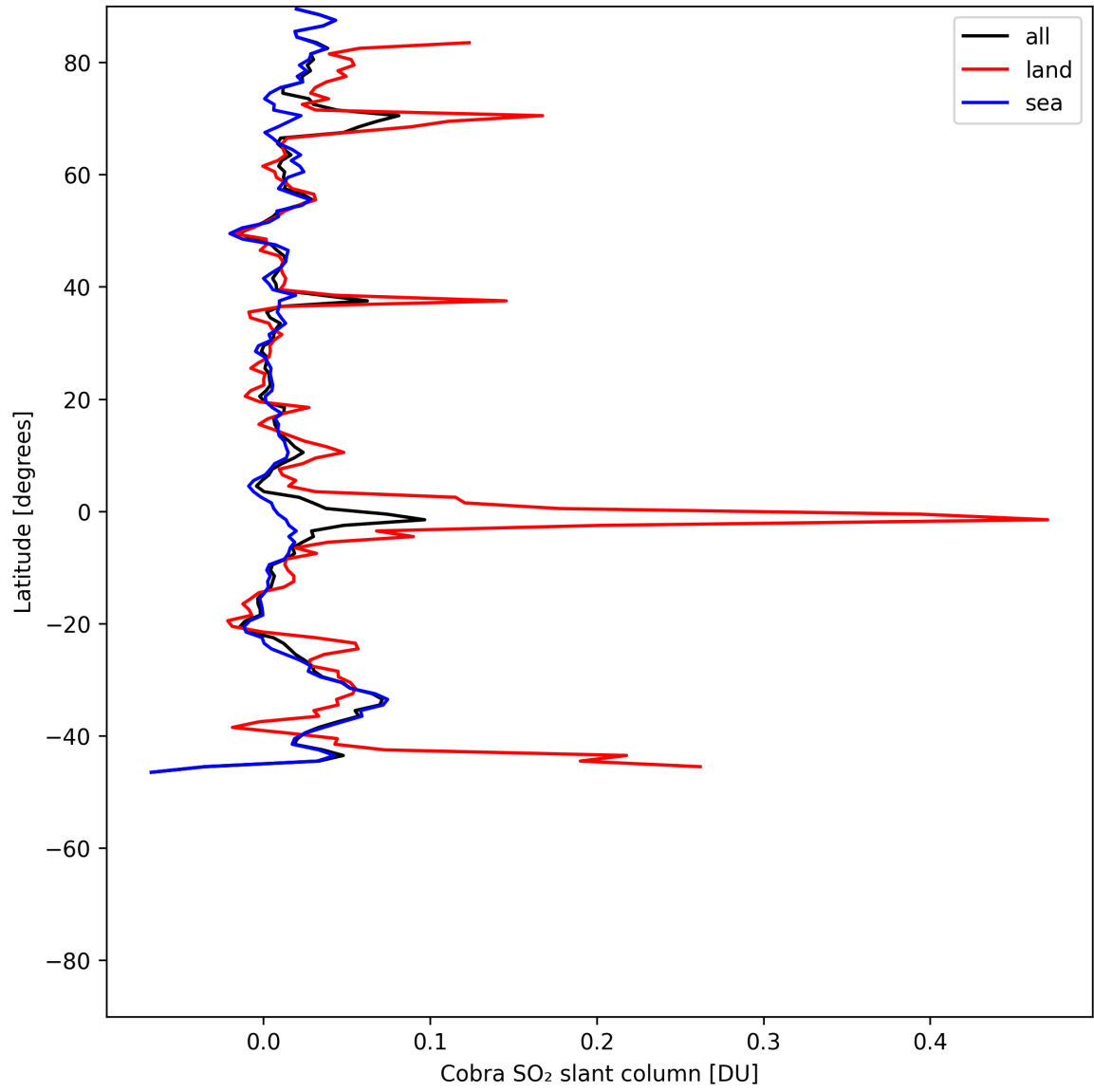
Figure 35: Zonal average of “Cobra SO 2 slant column” for 2025-06-01 to 2025-06-03.
