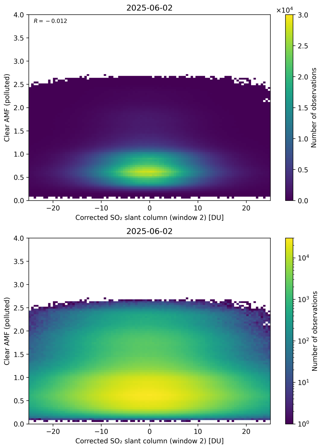
Figure 249: Scatter density plot of “Corrected SO 2 slant column (window 2)” against “Clear AMF (polluted)” for 2025-06-01 to 2025-06-03.
