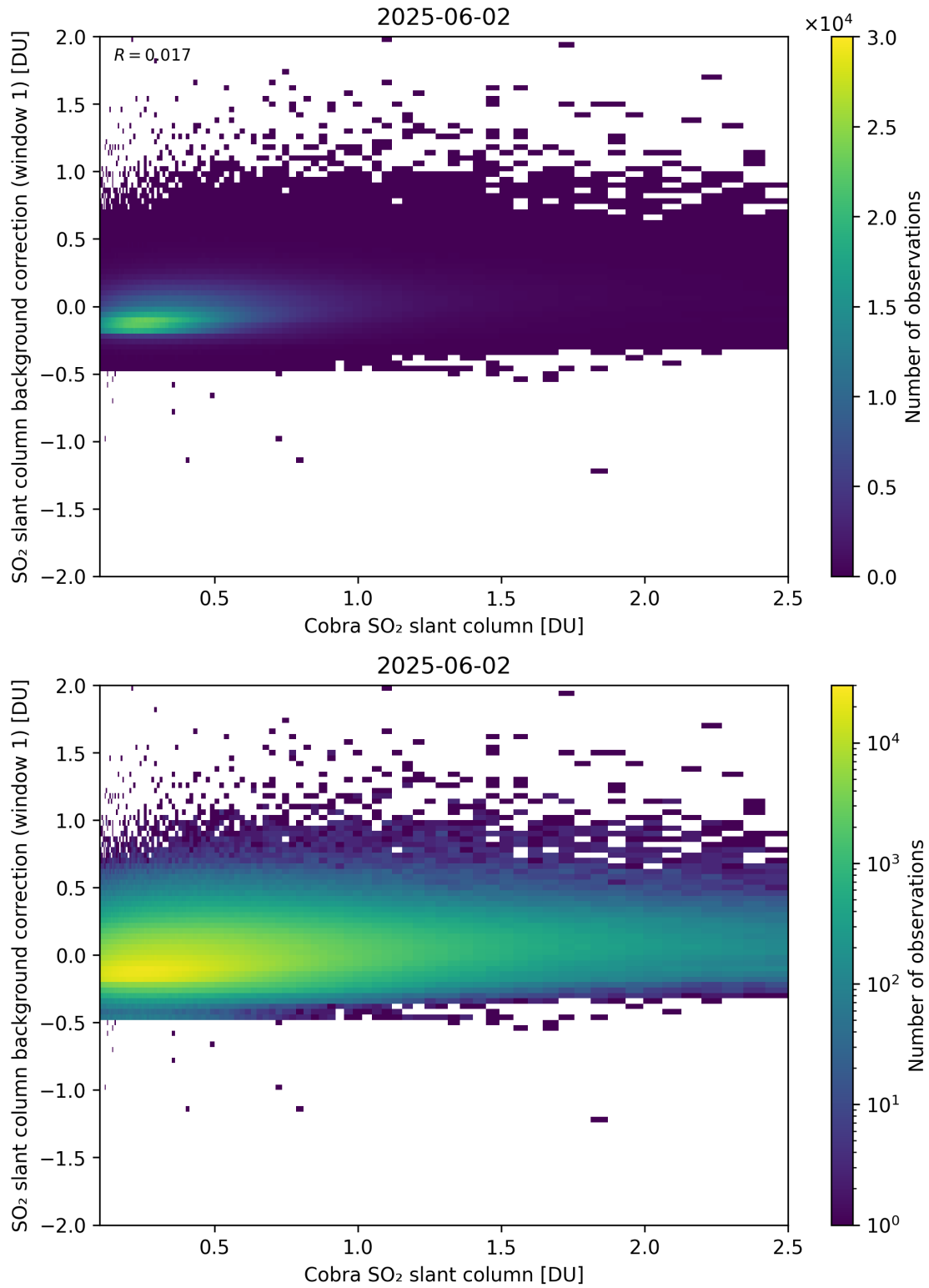
Figure 193: Scatter density plot of “Cobra SO 2 slant column” against “SO 2 slant column background correction (window 1)” for 2025-06-01 to 2025-06-03.
