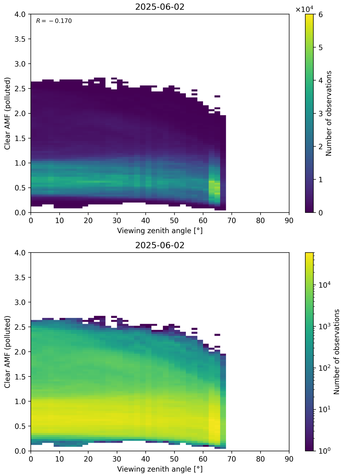
Figure 370: Scatter density plot of “Viewing zenith angle” against “Clear AMF (polluted)” for 2025-06-01 to 2025-06-03.
