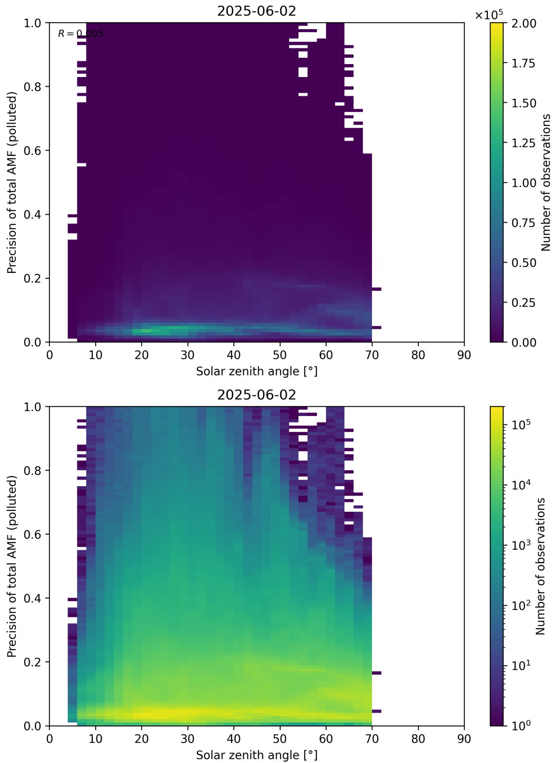
Figure 190: Scatter density plot of “Solar zenith angle” against “Precision of total AMF (polluted)” for 2025-06-01 to 2025-06-03.
