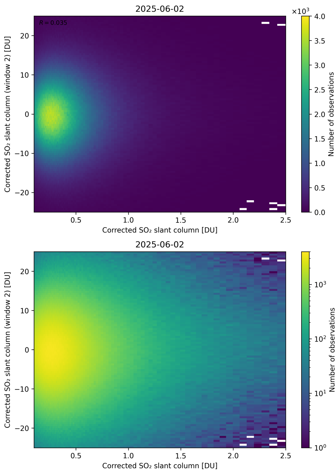
Figure 235: Scatter density plot of “Corrected SO 2 slant column” against “Corrected SO 2 slant column (window 2)” for 2025-06-01 to 2025-06-03.
