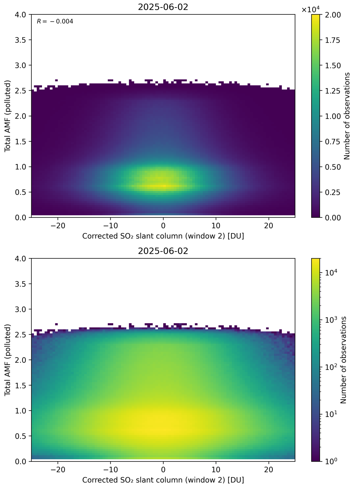
Figure 253: Scatter density plot of “Corrected SO 2 slant column (window 2)” against “Total AMF (polluted)” for 2025-06-01 to 2025-06-03.
