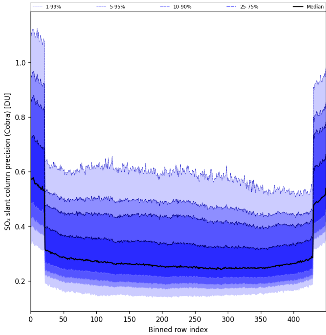
Figure 88: Along track statistics of “SO 2 slant column precision (Cobra)” for 2025-06-01 to 2025-06-03
