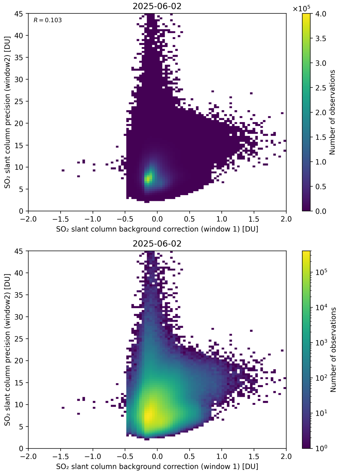
Figure 117: Scatter density plot of “SO 2 slant column background correction (window 1)” against “SO 2 slant column precision (window2)” for 2025-06-01 to 2025-06-03.
