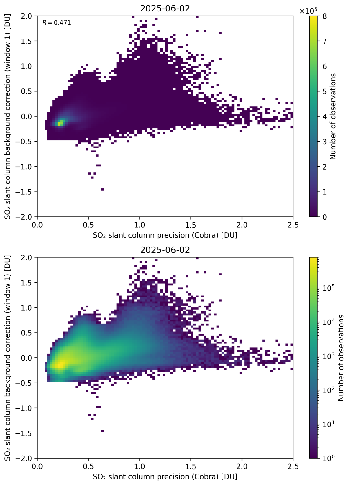
Figure 199: Scatter density plot of “SO 2 slant column precision (Cobra)” against “SO 2 slant column background correction (window 1)” for 2025-06-01 to 2025-06-03.
