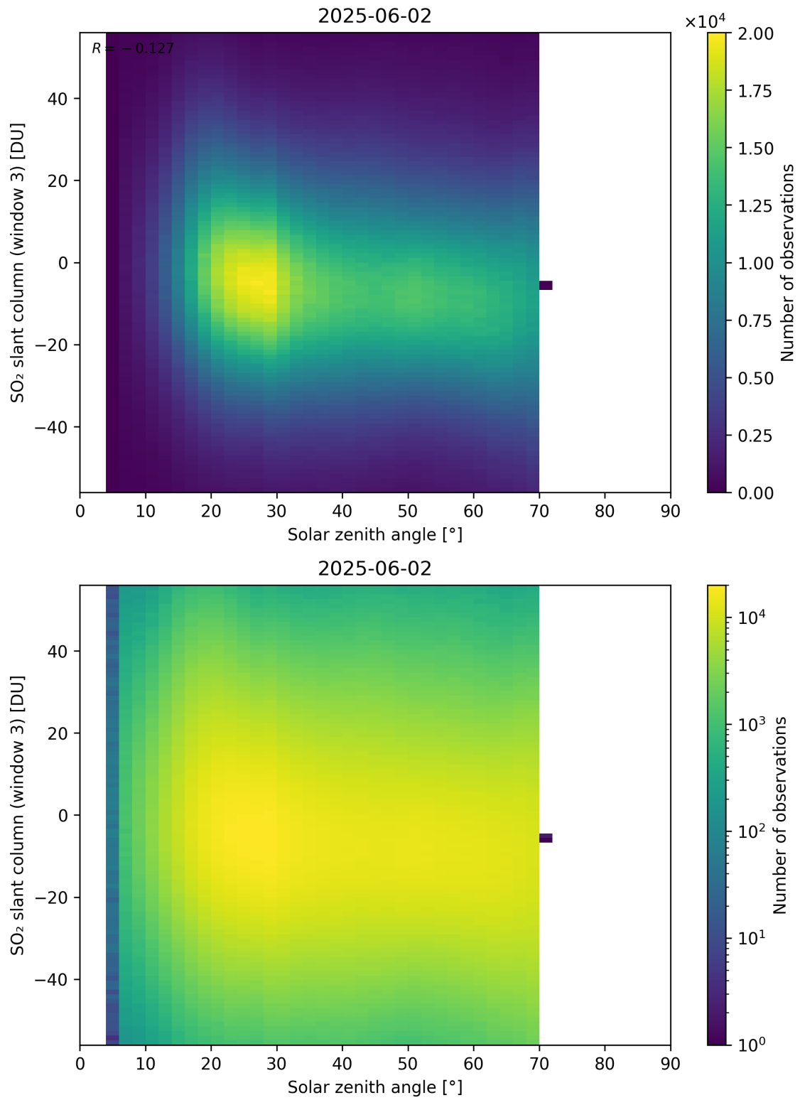
Figure 187: Scatter density plot of “Solar zenith angle” against “SO 2 slant column (window 3)” for 2025-06-01 to 2025-06-03.
