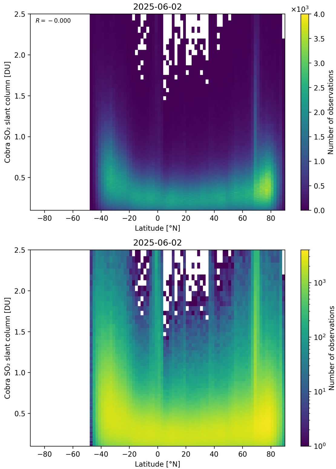
Figure 157: Scatter density plot of “Latitude” against “Cobra SO 2 slant column” for 2025-06-01 to 2025-06-03.
