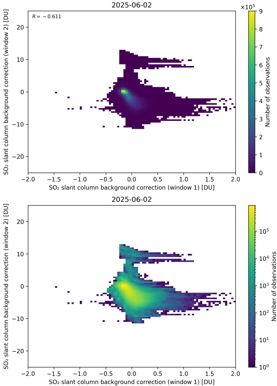
Figure 109: Scatter density plot of “SO 2 slant column background correction (window 1)” against “SO 2 slant column background correction (window 2)” for 2025-06-01 to 2025-06-03.
