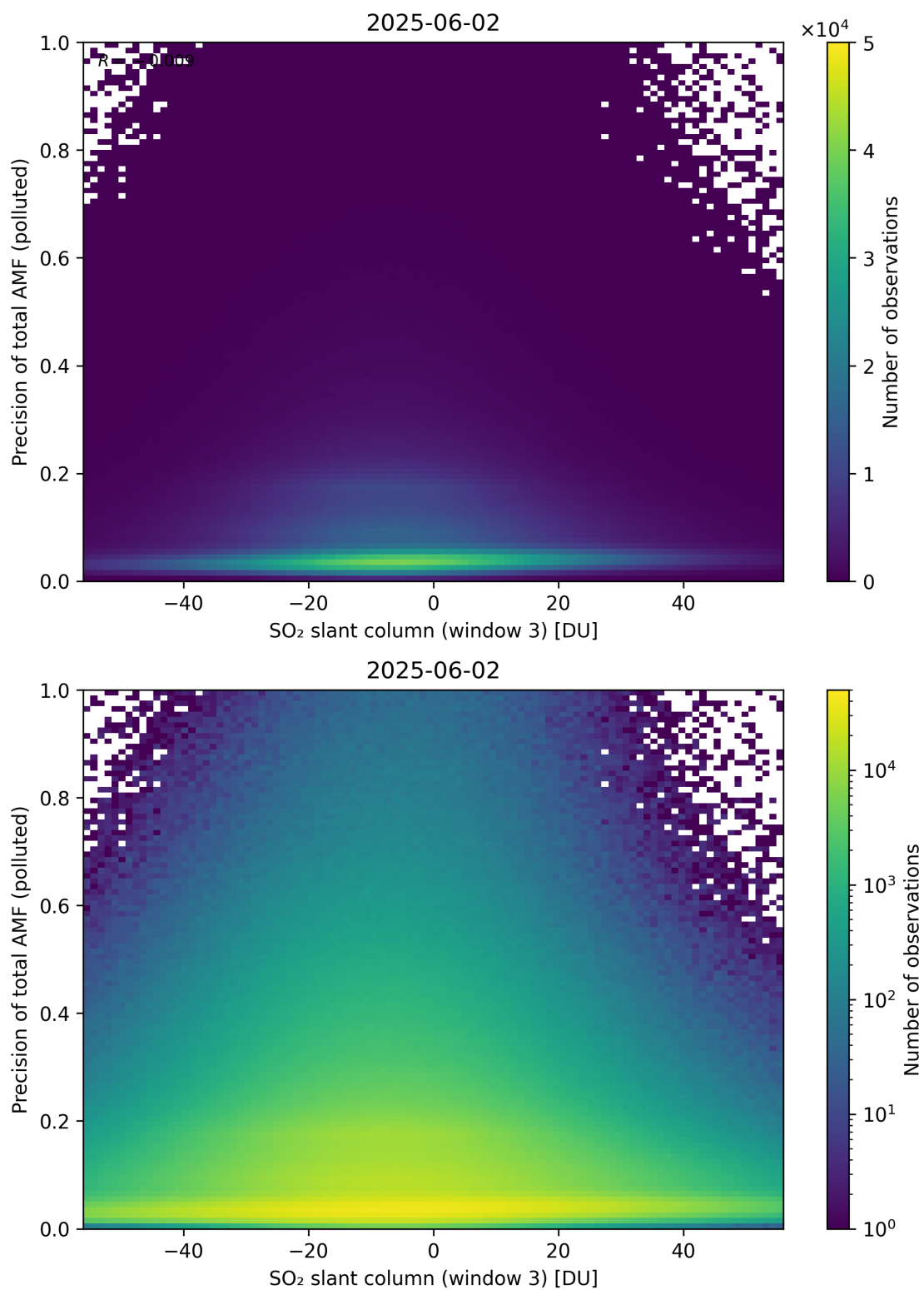
Figure 319: Scatter density plot of “SO 2 slant column (window 3)” against “Precision of total AMF (polluted)” for 2025-06-01 to 2025-06-03.
