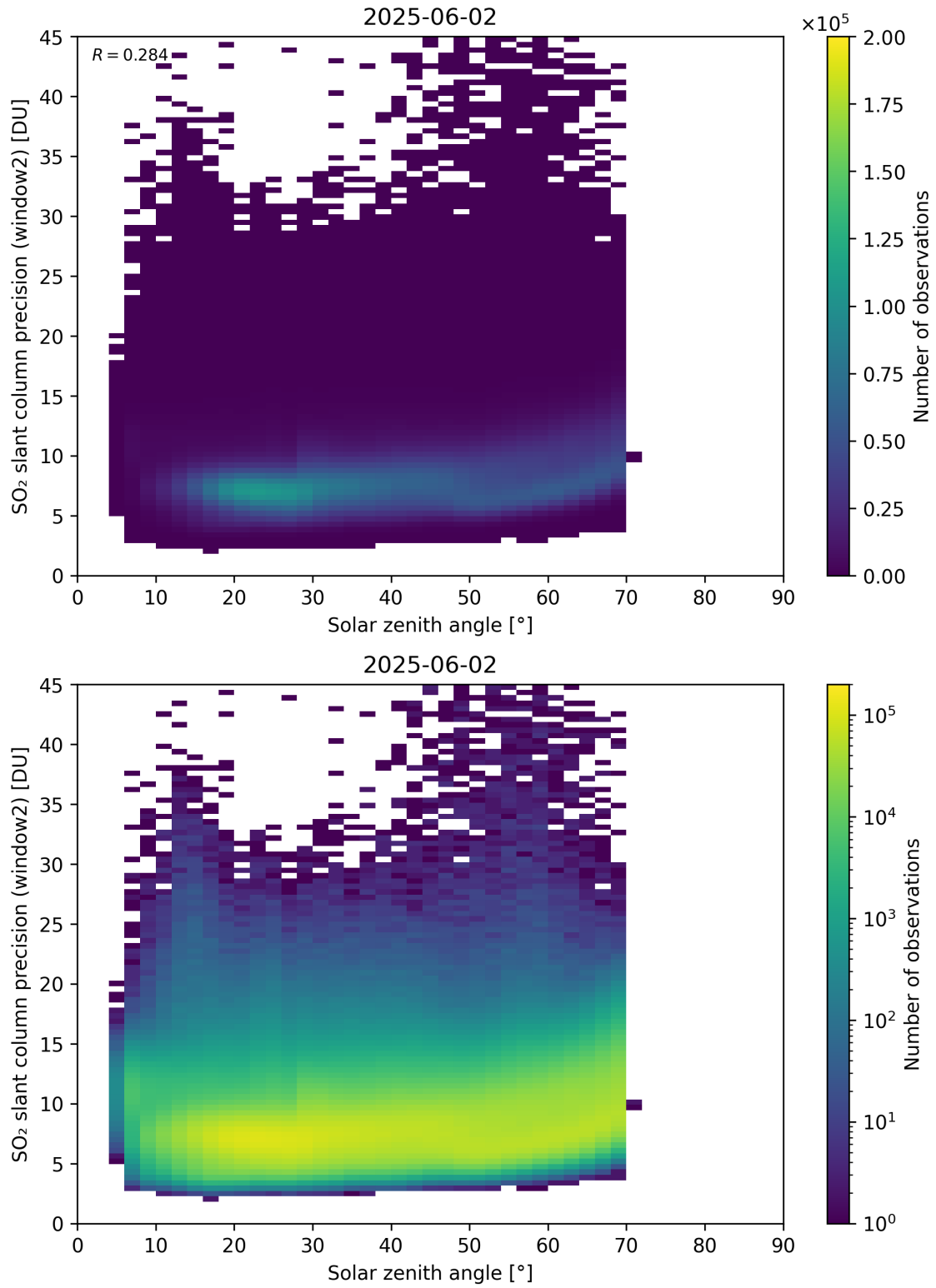
Figure 186: Scatter density plot of “Solar zenith angle” against “SO 2 slant column precision (window2)” for 2025-06-01 to 2025-06-03.
