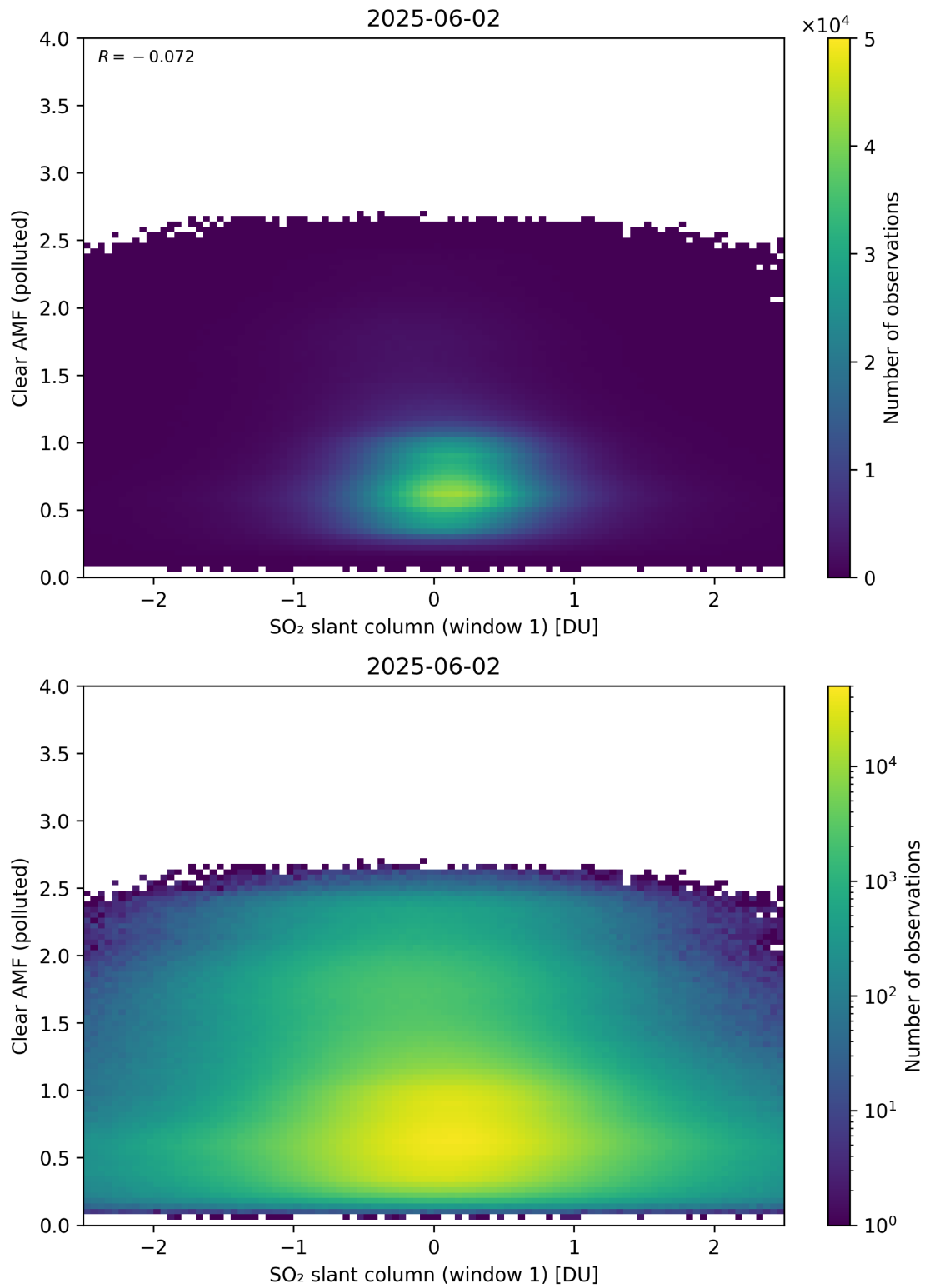
Figure 282: Scatter density plot of “SO 2 slant column (window 1)” against “Clear AMF (polluted)” for 2025-06-01 to 2025-06-03.
