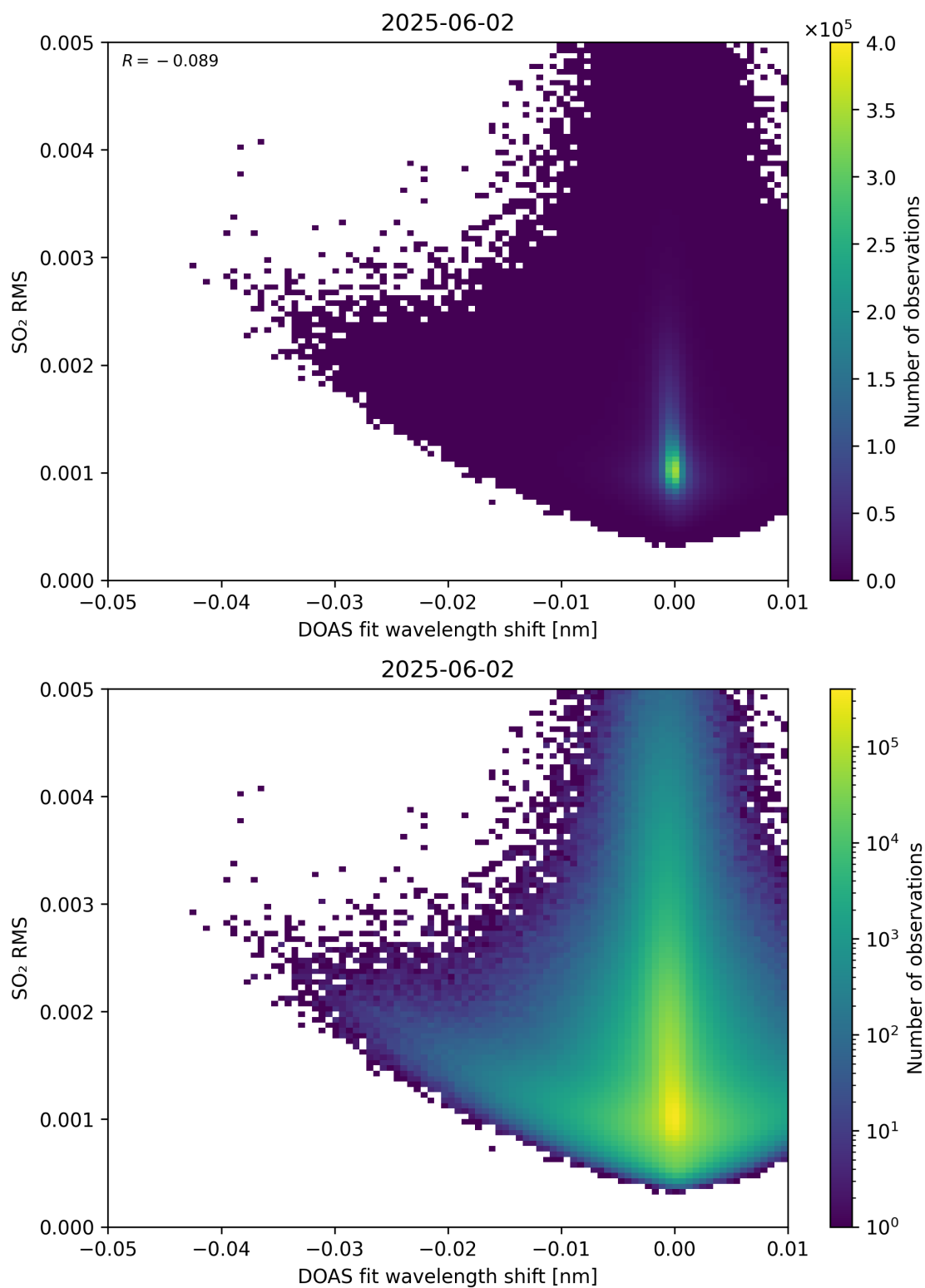
Figure 139: Scatter density plot of “DOAS fit wavelength shift” against “SO 2 RMS” for 2025-06-01 to 2025-06-03.
