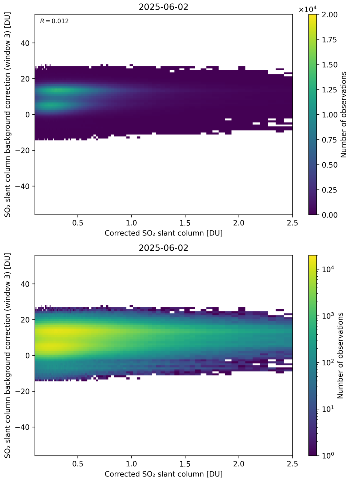
Figure 228: Scatter density plot of “Corrected SO 2 slant column” against “SO 2 slant column background correction (window 3)” for 2025-06-01 to 2025-06-03.
