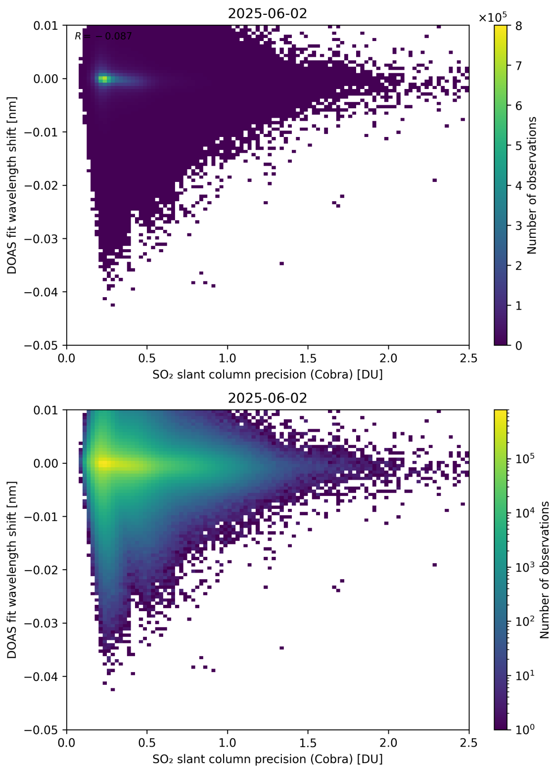
Figure 202: Scatter density plot of “SO 2 slant column precision (Cobra)” against “DOAS fit wavelength shift” for 2025-06-01 to 2025-06-03.
