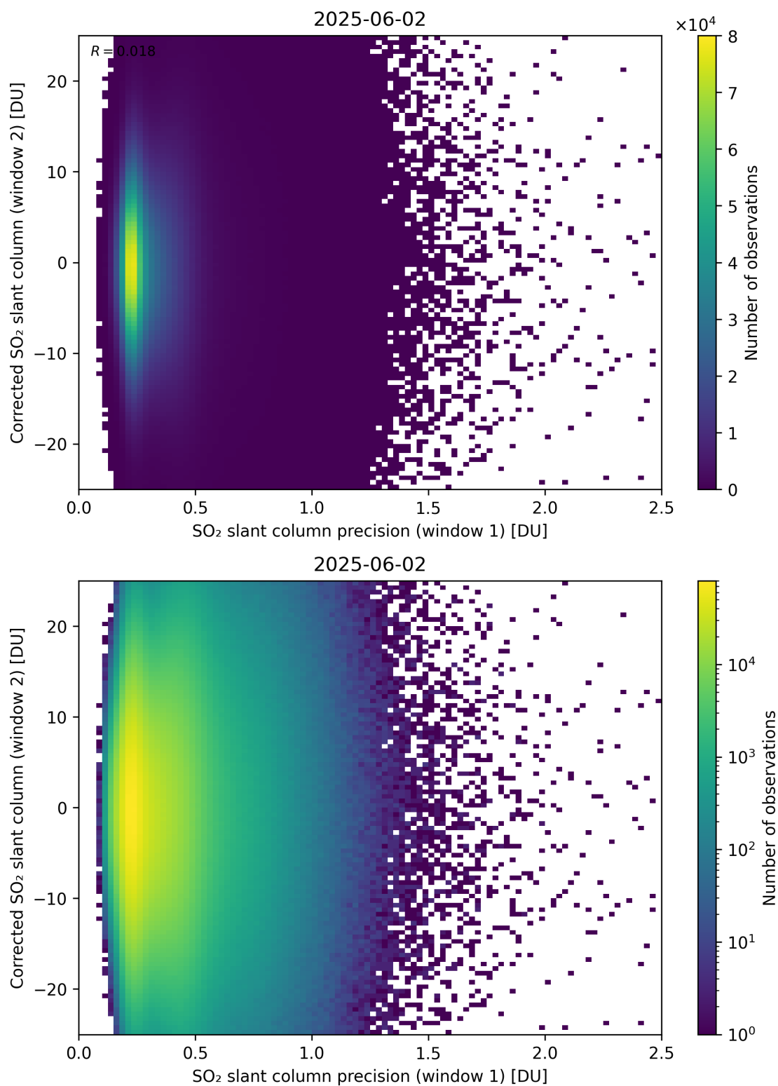
Figure 275: Scatter density plot of “SO 2 slant column precision (window 1)” against “Corrected SO 2 slant column (window 2)” for 2025-06-01 to 2025-06-03.
