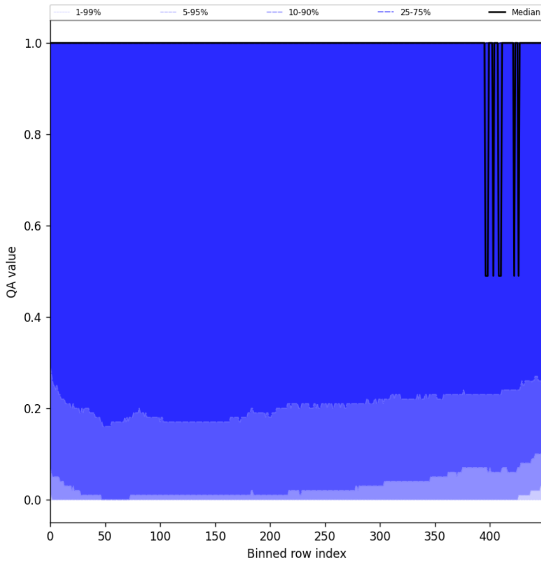
Figure 83: Along track statistics of “QA value” for 2025-06-01 to 2025-06-03
