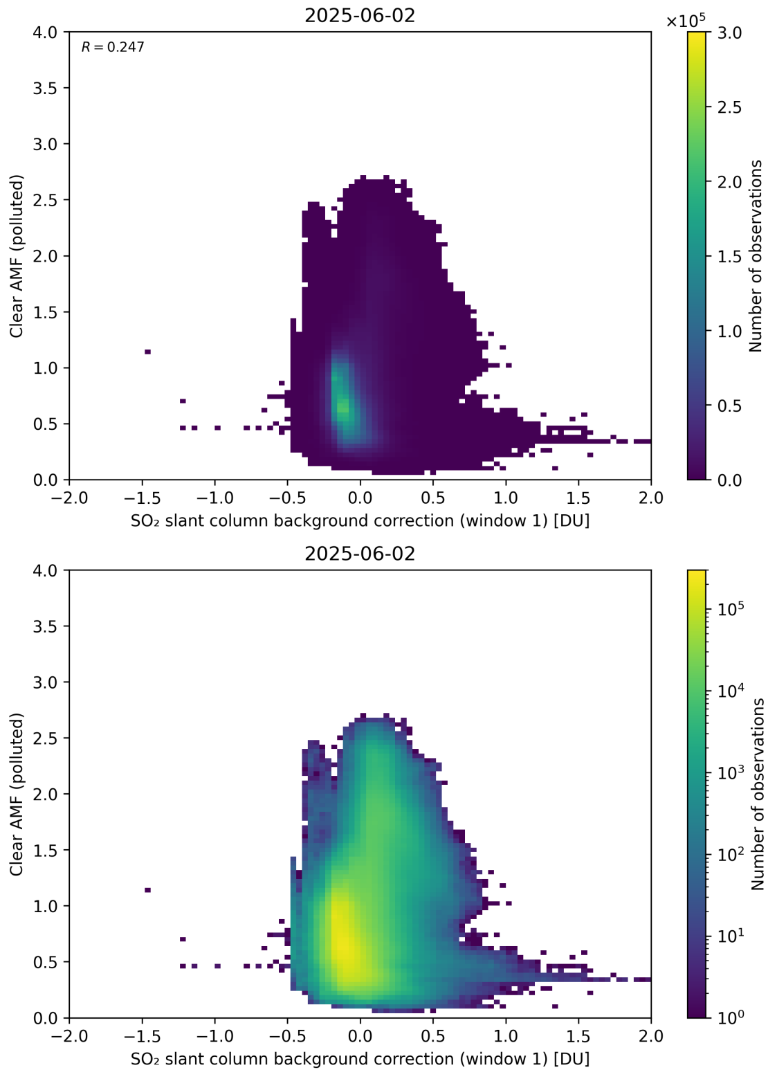
Figure 114: Scatter density plot of “SO 2 slant column background correction (window 1)” against “Clear AMF (polluted)” for 2025-06-01 to 2025-06-03.
