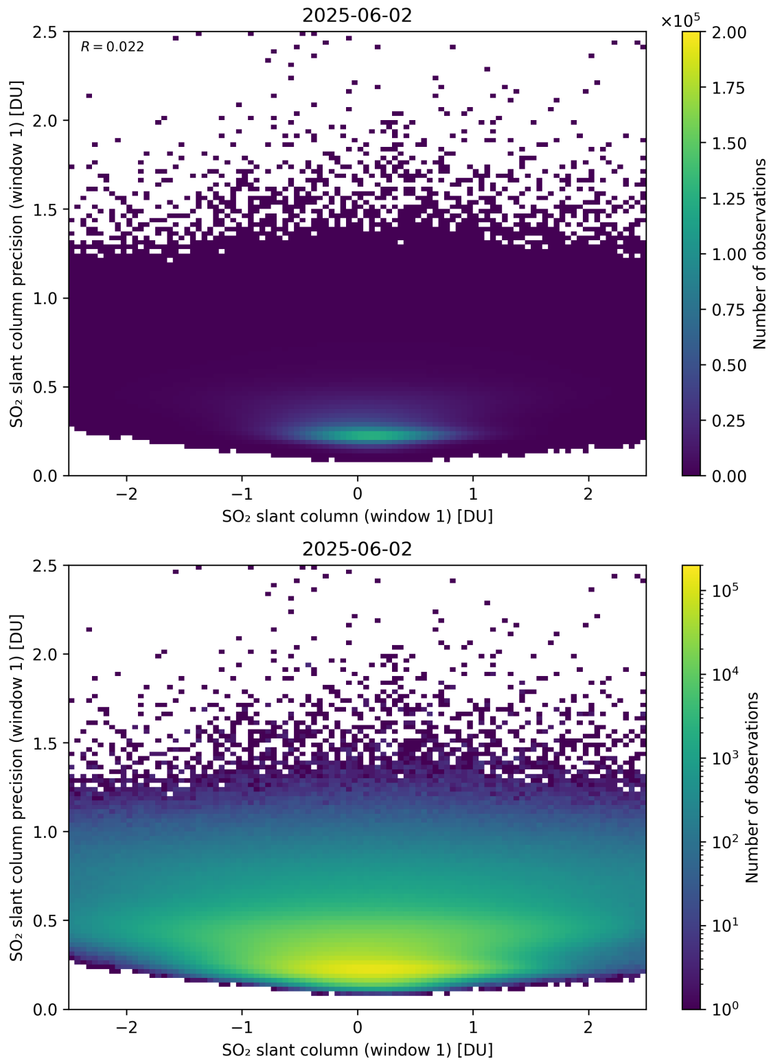
Figure 285: Scatter density plot of “SO 2 slant column (window 1)” against “SO 2 slant column precision (window 1)” for 2025-06-01 to 2025-06-03.
