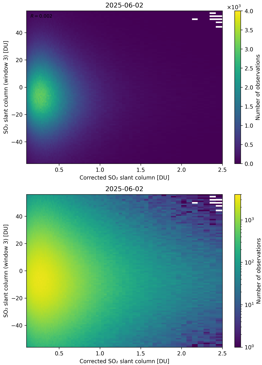
Figure 240: Scatter density plot of “Corrected SO 2 slant column” against “SO 2 slant column (window 3)” for 2025-06-01 to 2025-06-03.
