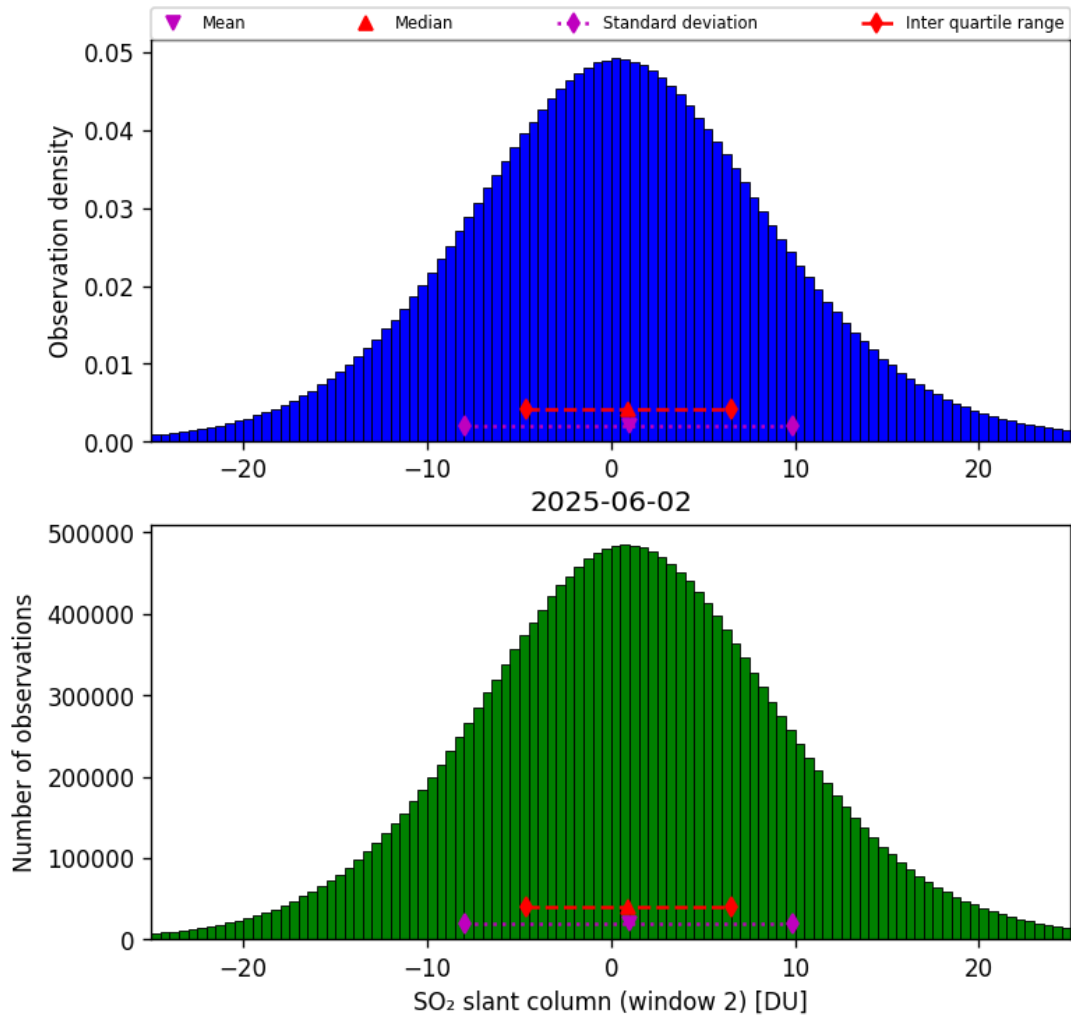
Figure 67: Histogram of “SO 2 slant column (window 2)” for 2025-06-01 to 2025-06-03
