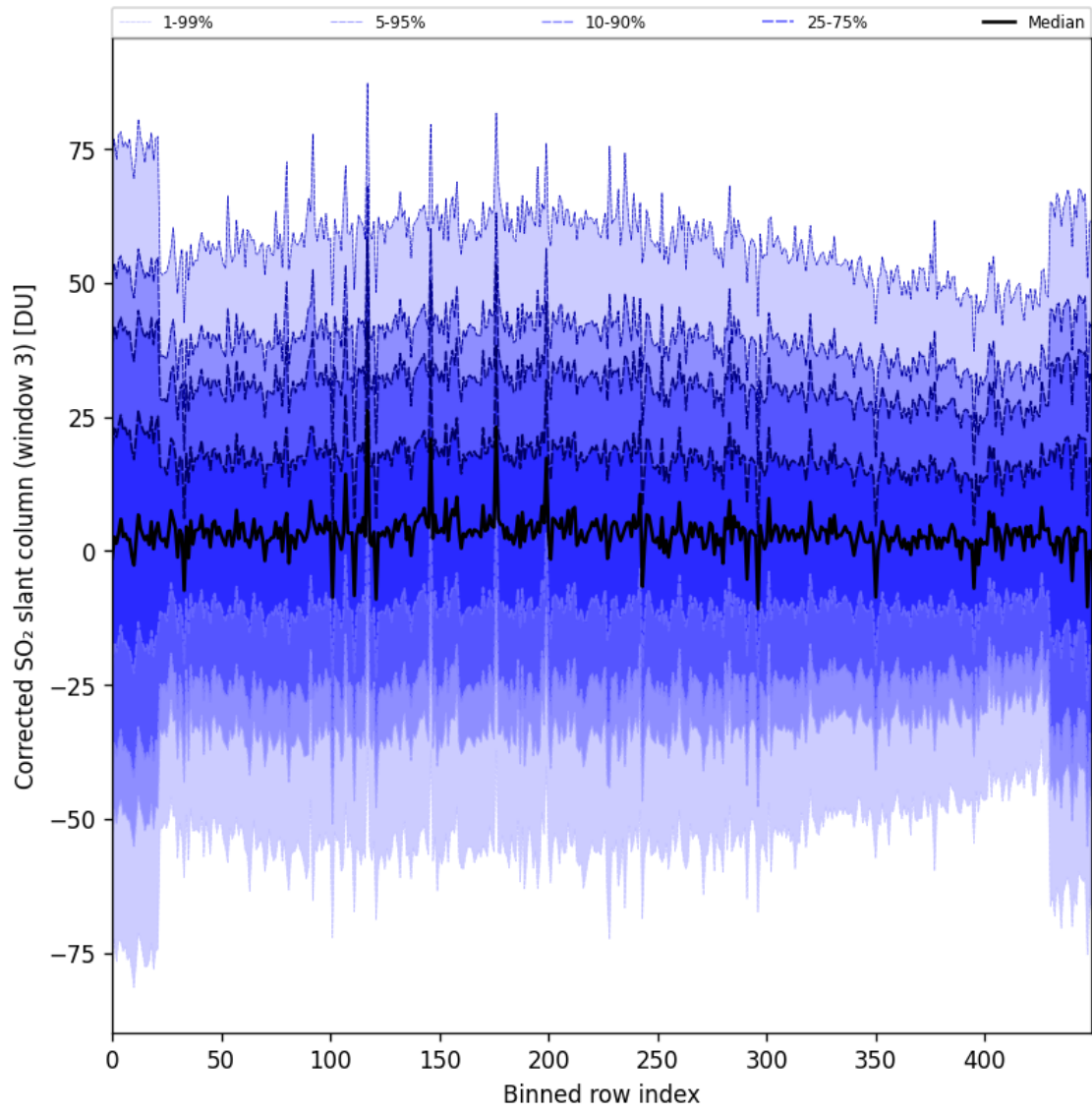
Figure 99: Along track statistics of “Corrected SO 2 slant column (window 3)” for 2025-06-01 to 2025-06-03
