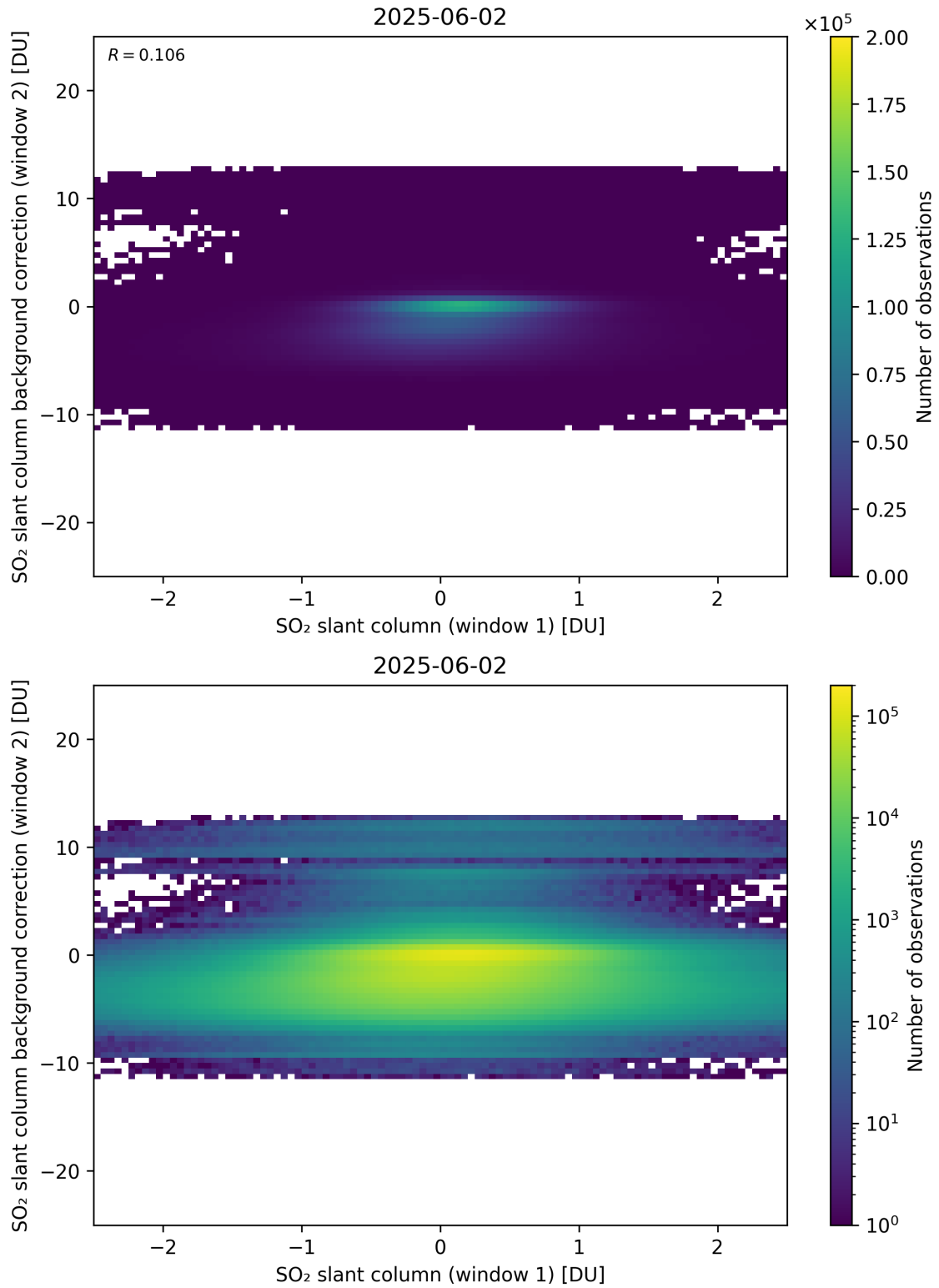
Figure 263: Scatter density plot of “SO 2 slant column (window 1)” against “SO 2 slant column background correction (window 2)” for 2025-06-01 to 2025-06-03.
