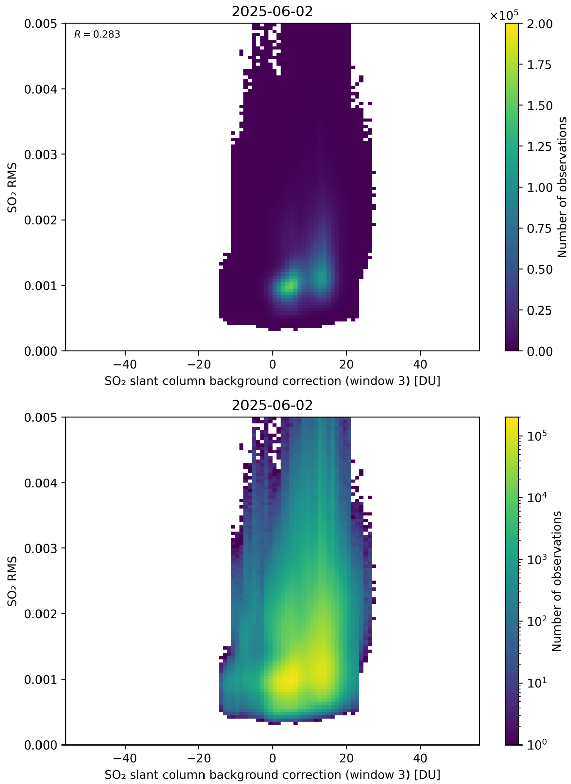
Figure 134: Scatter density plot of “SO 2 slant column background correction (window 3)” against “SO 2 RMS” for 2025-06-01 to 2025-06-03.
