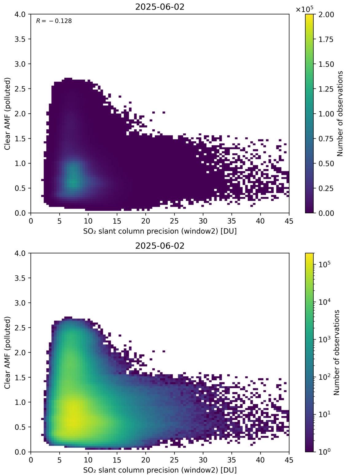
Figure 296: Scatter density plot of “SO 2 slant column precision (window2)” against “Clear AMF (polluted)” for 2025-06-01 to 2025-06-03.
