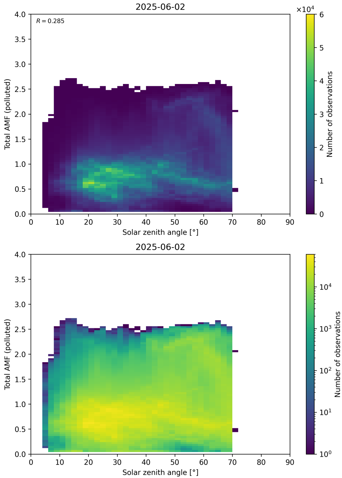
Figure 189: Scatter density plot of “Solar zenith angle” against “Total AMF (polluted)” for 2025-06-01 to 2025-06-03.
