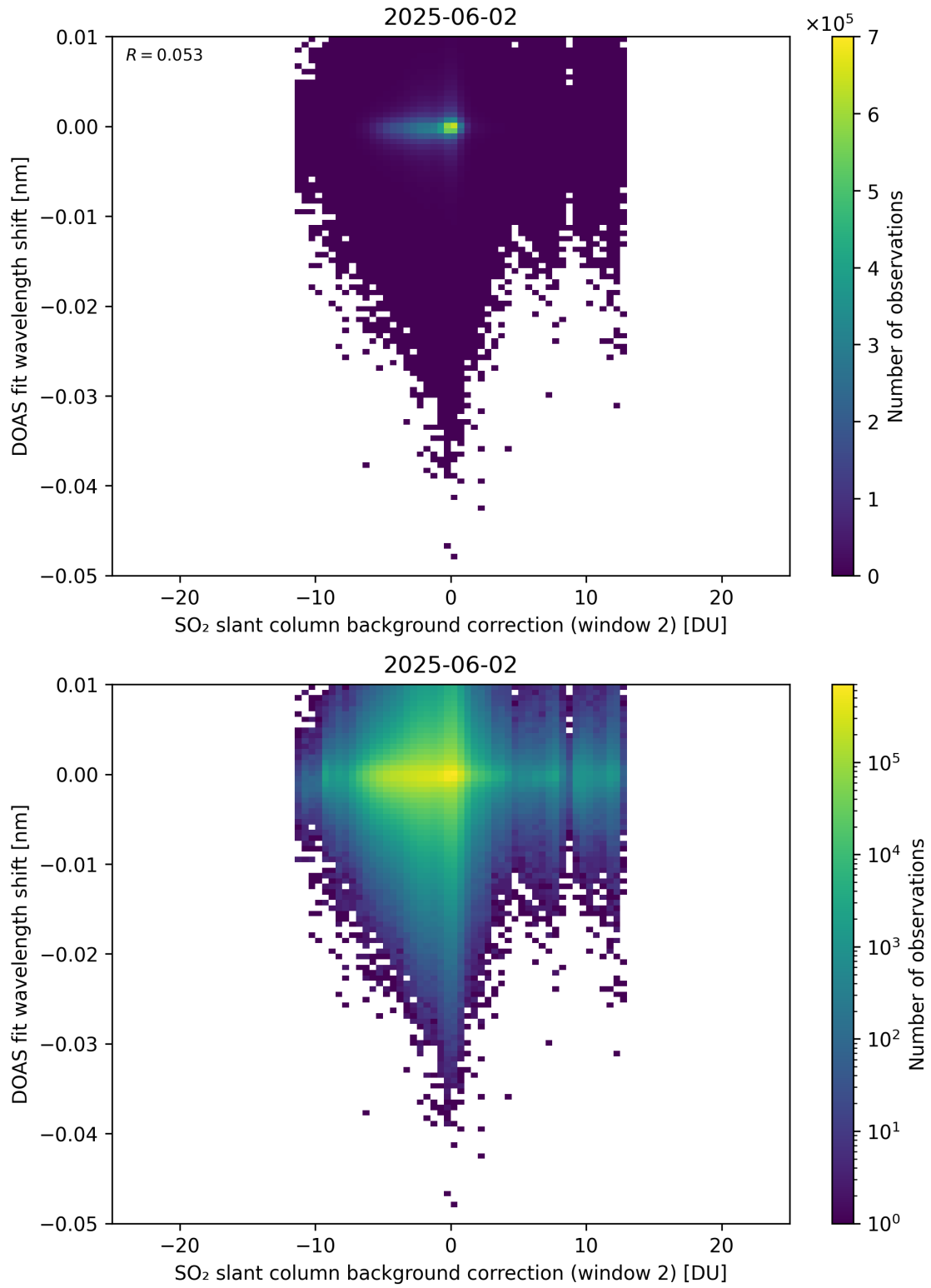
Figure 123: Scatter density plot of “SO 2 slant column background correction (window 2)” against “DOAS fit wavelength shift” for 2025-06-01 to 2025-06-03.
