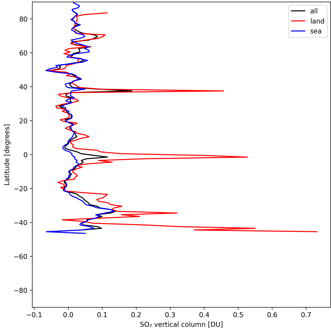
Figure 32: Zonal average of “SO 2 vertical column” for 2025-06-01 to 2025-06-03.
