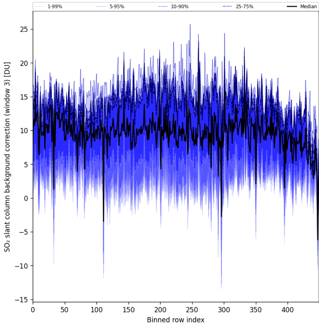
Figure 100: Along track statistics of “SO 2 slant column background correction (window 3)” for 2025-06-01 to 2025-06-03
