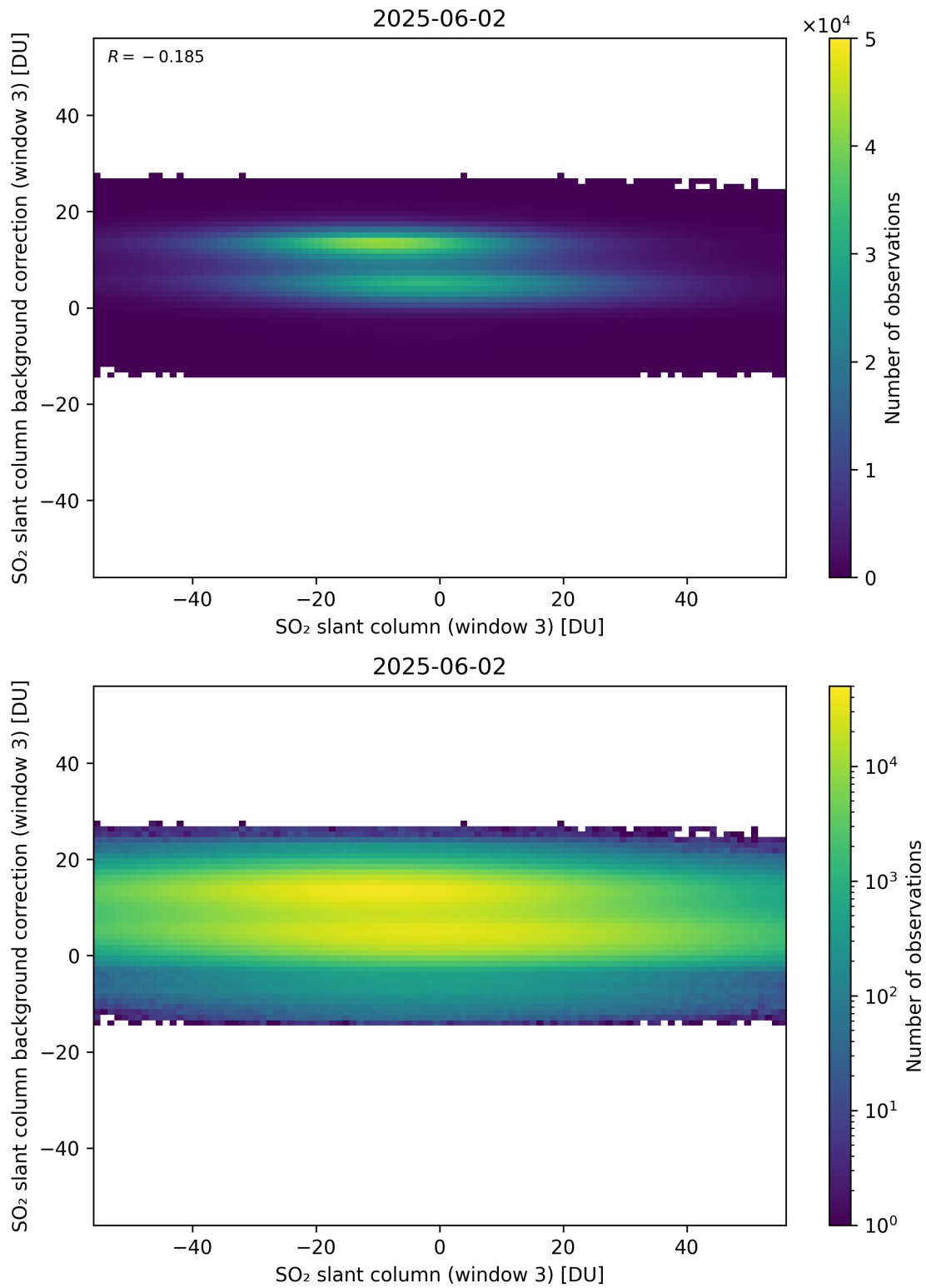
Figure 303: Scatter density plot of “SO 2 slant column (window 3)” against “SO 2 slant column background correction (window 3)” for 2025-06-01 to 2025-06-03.
