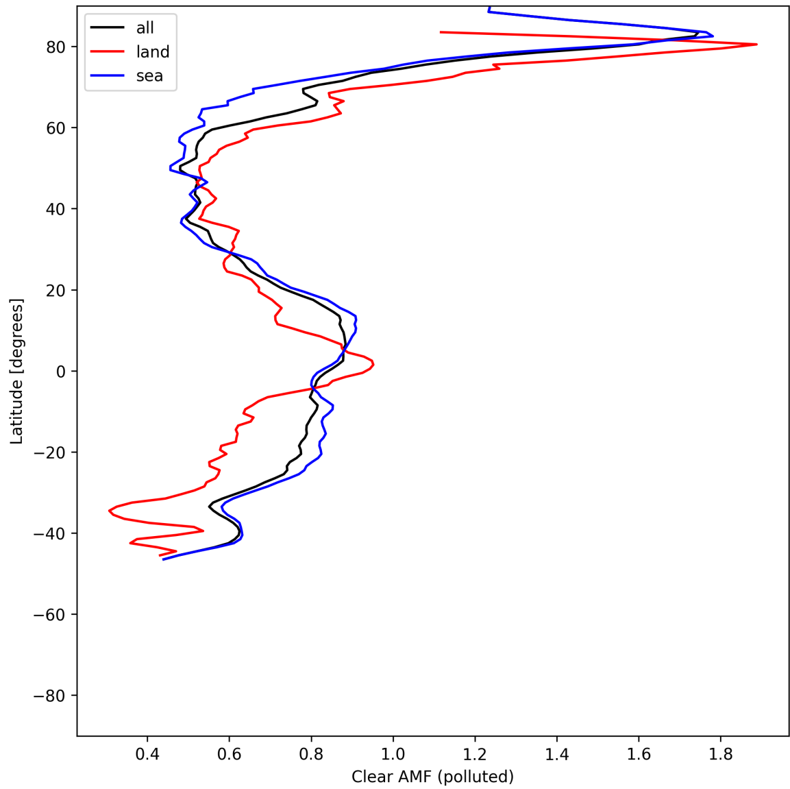
Figure 55: Zonal average of “Clear AMF (polluted)” for 2025-06-01 to 2025-06-03.
