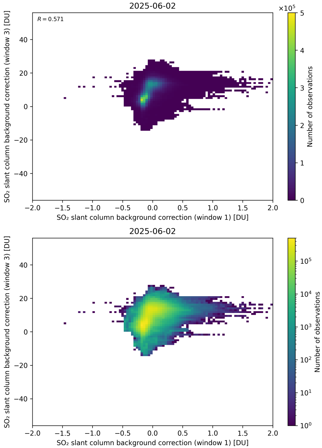
Figure 110: Scatter density plot of “SO 2 slant column background correction (window 1)” against “SO 2 slant column background correction (window 3)” for 2025-06-01 to 2025-06-03.
