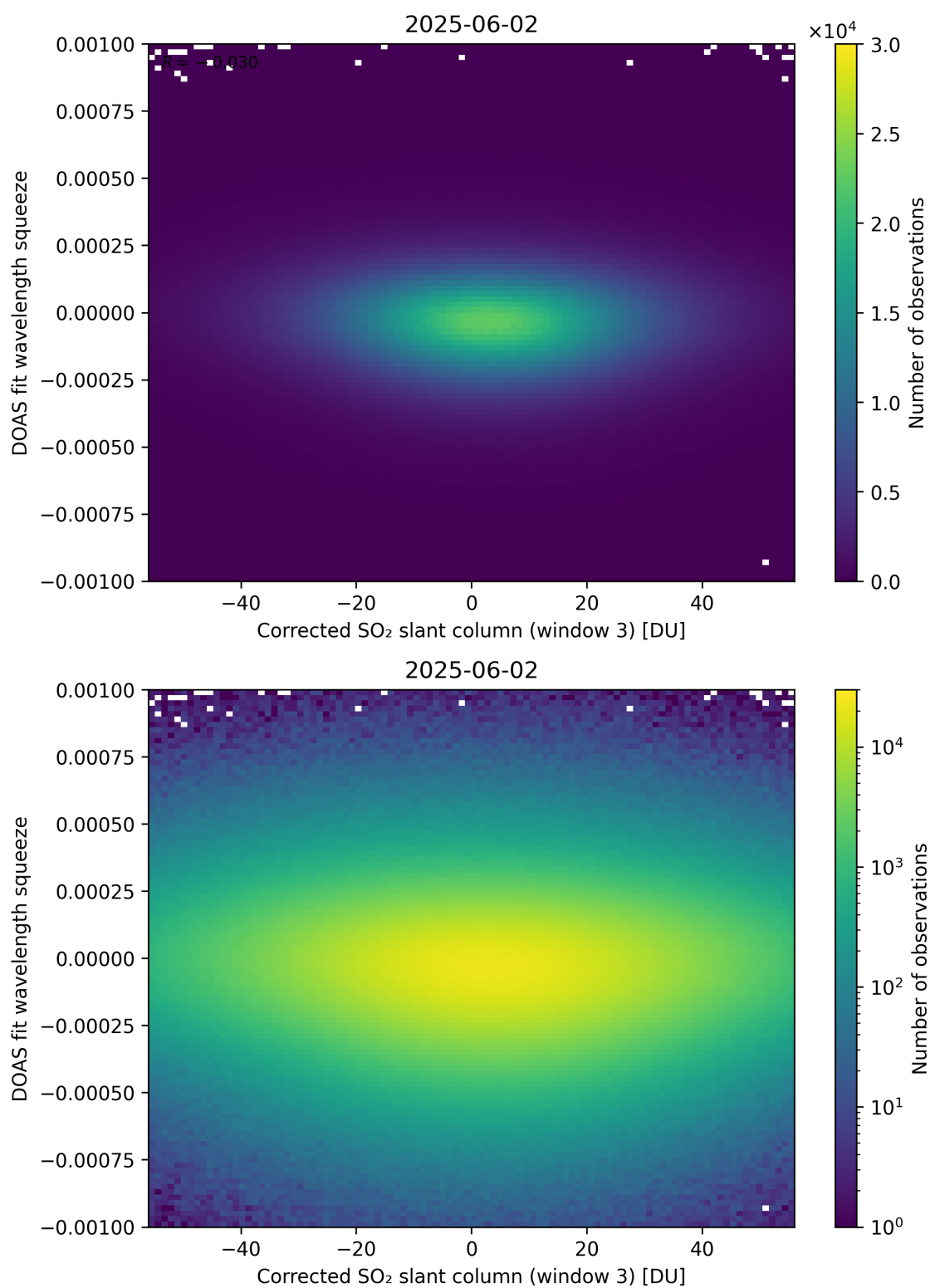
Figure 257: Scatter density plot of “Corrected SO 2 slant column (window 3)” against “DOAS fit wavelength squeeze” for 2025-06-01 to 2025-06-03.
