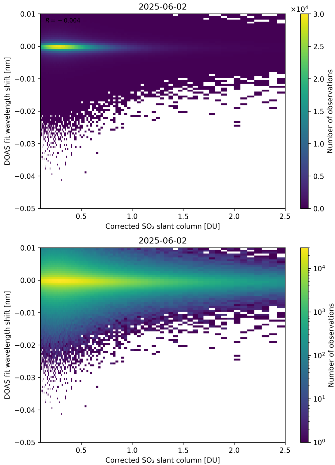
Figure 229: Scatter density plot of “Corrected SO 2 slant column” against “DOAS fit wavelength shift” for 2025-06-01 to 2025-06-03.
