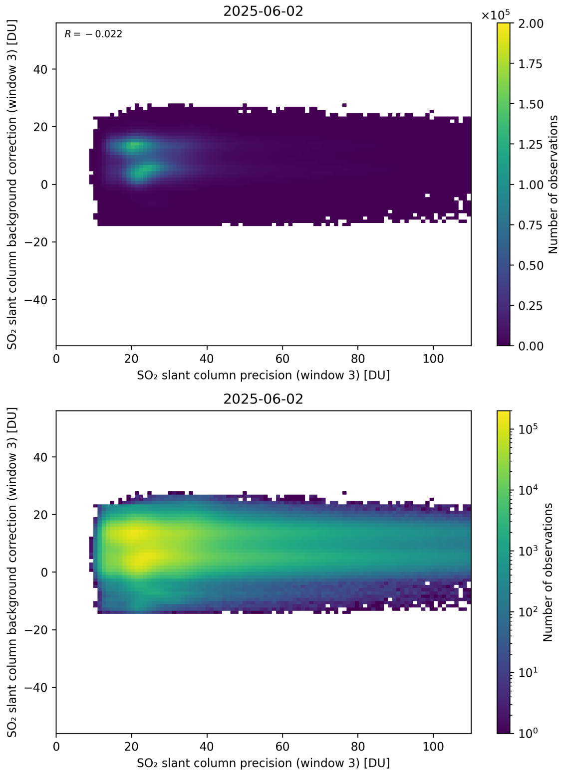
Figure 307: Scatter density plot of “SO 2 slant column precision (window 3)” against “SO 2 slant column background correction (window 3)” for 2025-06-01 to 2025-06-03.
