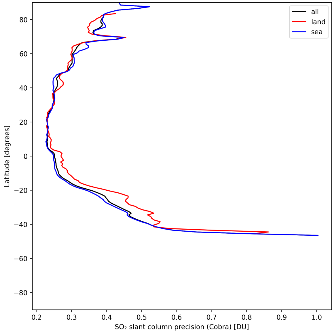
Figure 36: Zonal average of “SO 2 slant column precision (Cobra)” for 2025-06-01 to 2025-06-03.
