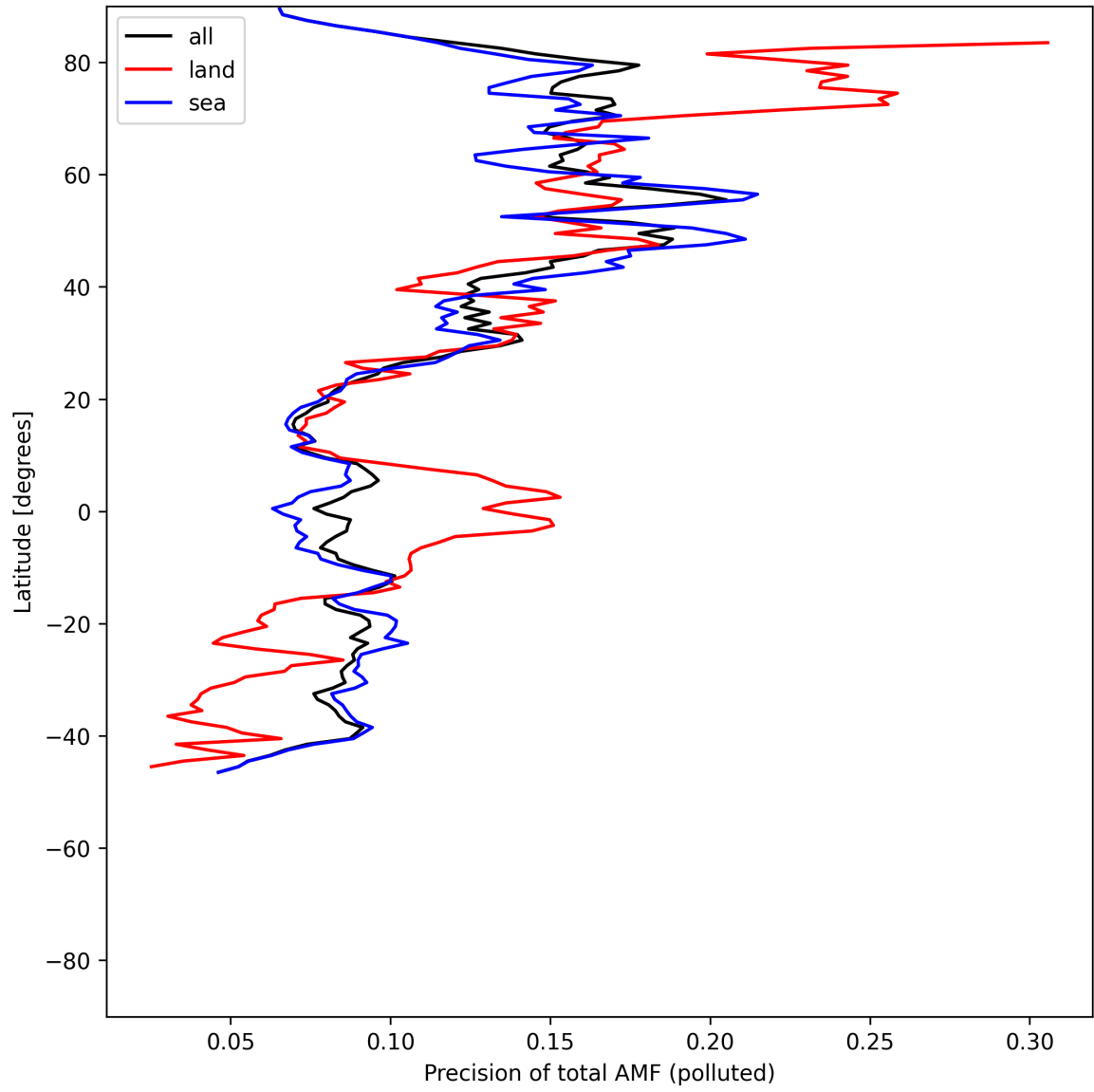
Figure 54: Zonal average of “Precision of total AMF (polluted)” for 2025-06-01 to 2025-06-03.
