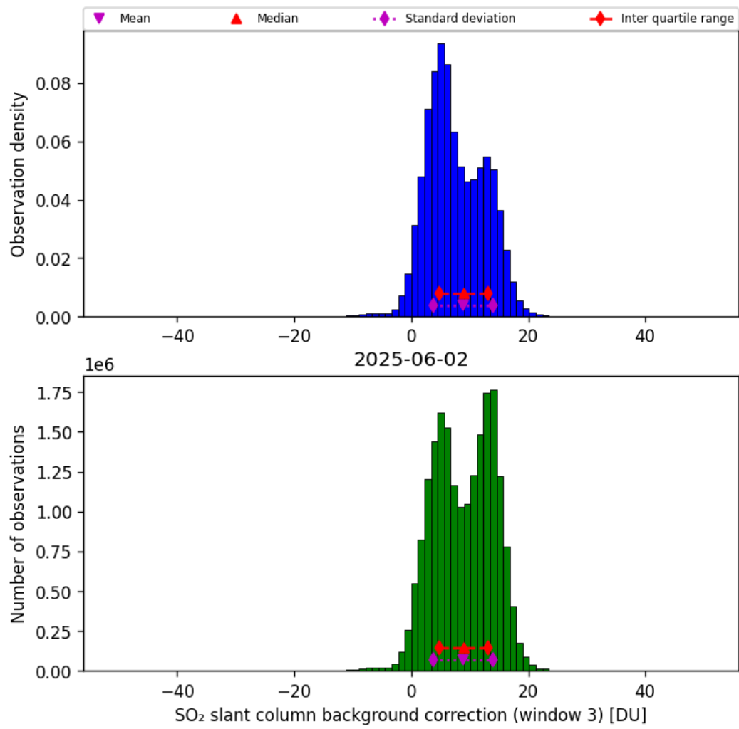
Figure 74: Histogram of “SO 2 slant column background correction (window 3)” for 2025-06-01 to 2025-06-03
