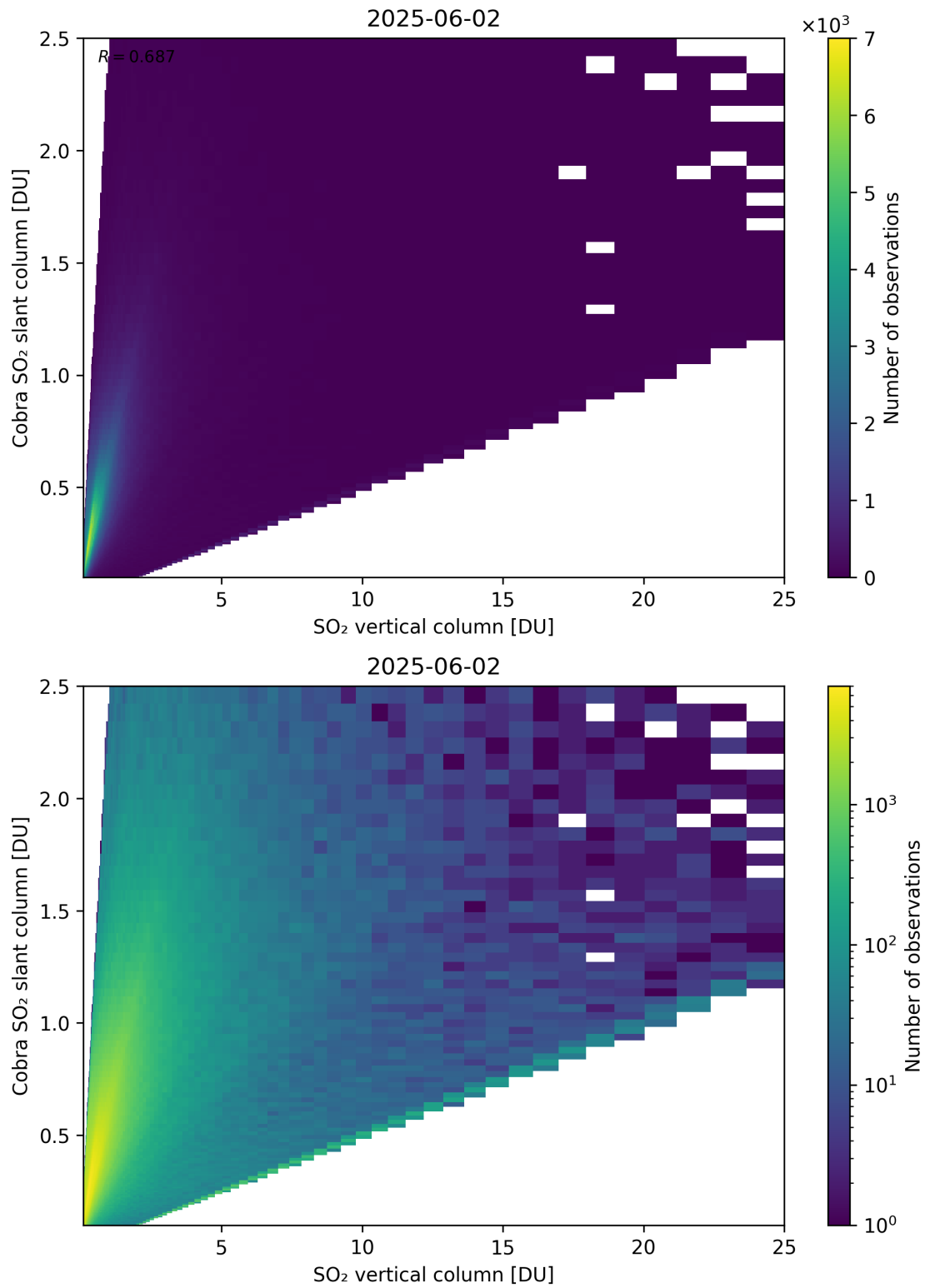
Figure 349: Scatter density plot of “SO 2 vertical column” against “Cobra SO 2 slant column” for 2025-06-01 to 2025-06-03.
