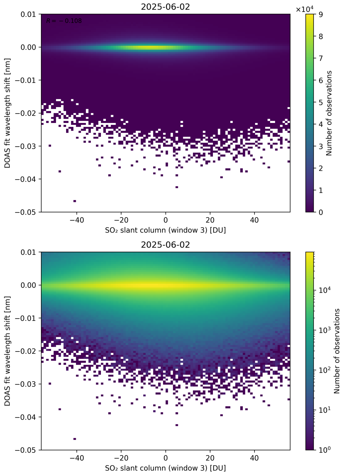
Figure 304: Scatter density plot of “SO 2 slant column (window 3)” against “DOAS fit wavelength shift” for 2025-06-01 to 2025-06-03.
