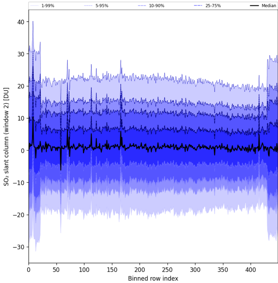
Figure 93: Along track statistics of “SO 2 slant column (window 2)” for 2025-06-01 to 2025-06-03
