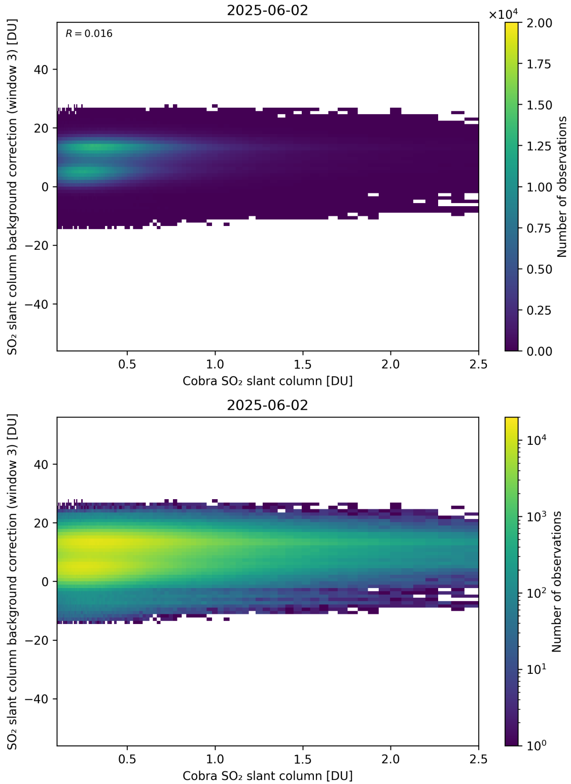
Figure 195: Scatter density plot of “Cobra SO 2 slant column” against “SO 2 slant column background correction (window 3)” for 2025-06-01 to 2025-06-03.
