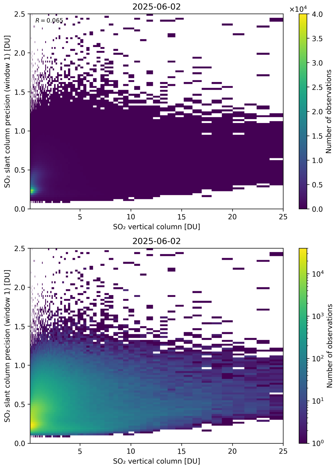
Figure 355: Scatter density plot of “SO 2 vertical column” against “SO 2 slant column precision (window 1)” for 2025-06-01 to 2025-06-03.
