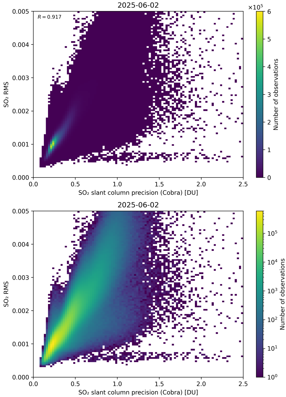
Figure 204: Scatter density plot of “SO 2 slant column precision (Cobra)” against “SO 2 RMS” for 2025-06-01 to 2025-06-03.
