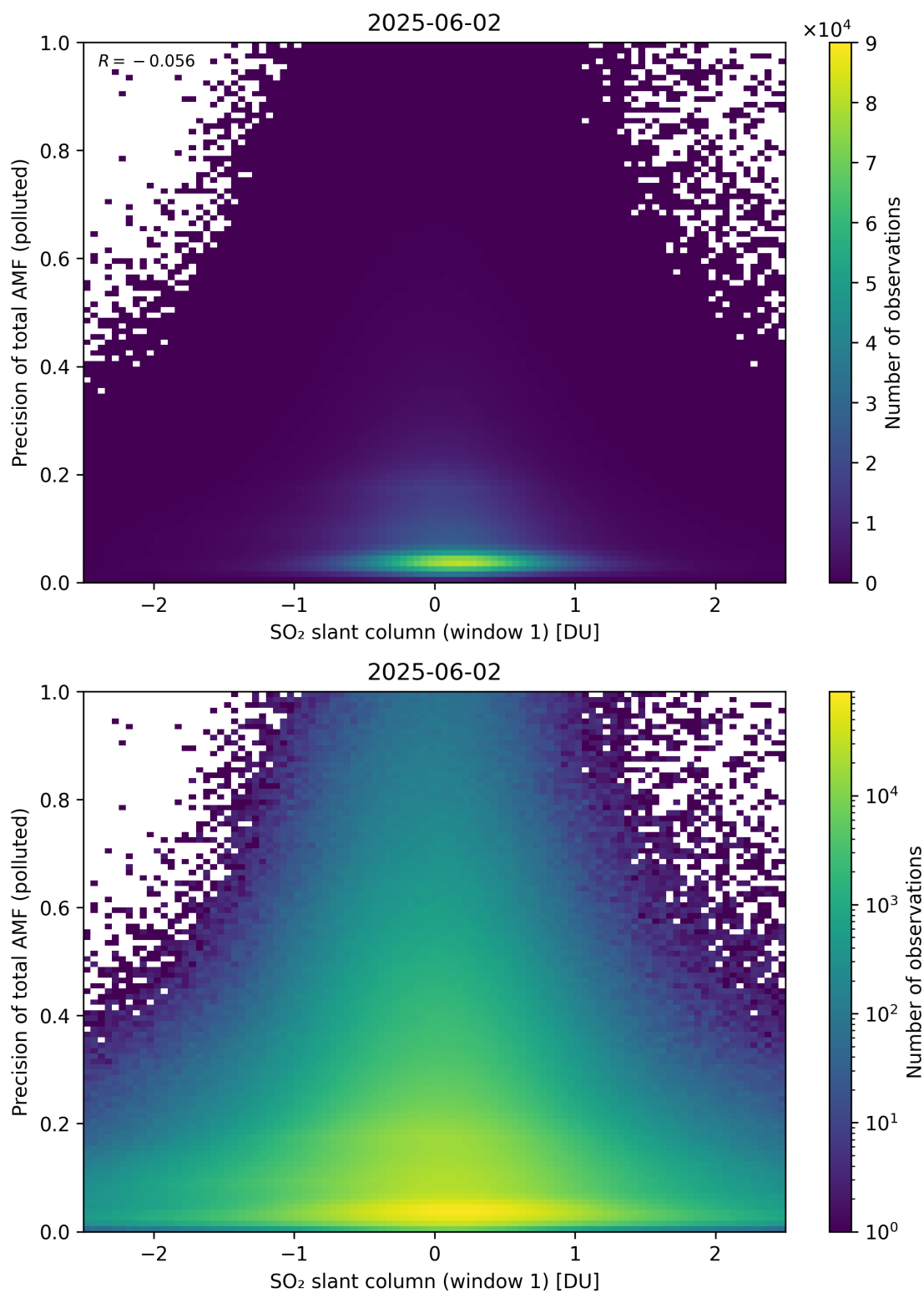
Figure 290: Scatter density plot of “SO 2 slant column (window 1)” against “Precision of total AMF (polluted)” for 2025-06-01 to 2025-06-03.
