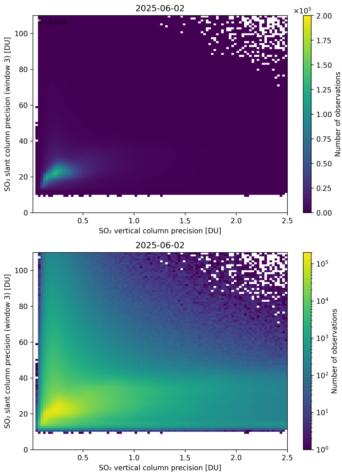
Figure 345: Scatter density plot of “SO 2 vertical column precision” against “SO 2 slant column precision (window 3)” for 2025-06-01 to 2025-06-03.
