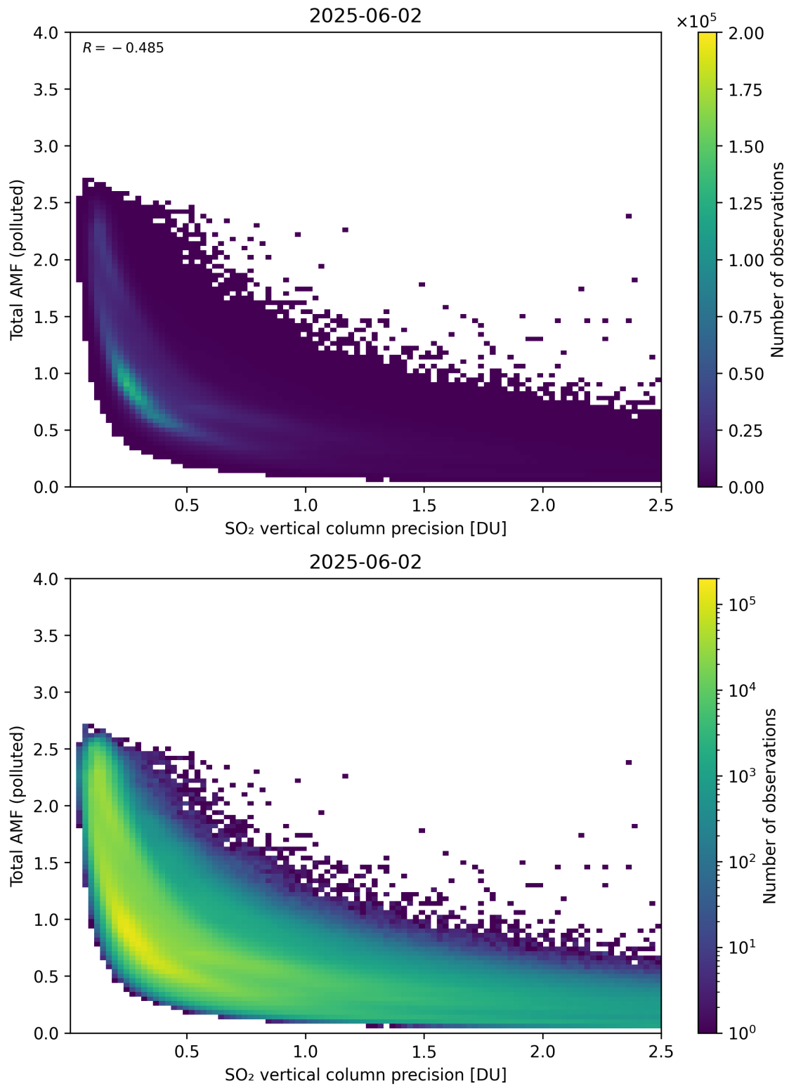
Figure 346: Scatter density plot of “SO 2 vertical column precision” against “Total AMF (polluted)” for 2025-06-01 to 2025-06-03.
