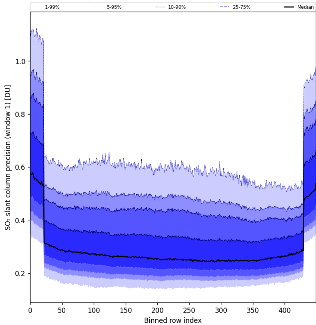
Figure 90: Along track statistics of “SO 2 slant column precision (window 1)” for 2025-06-01 to 2025-06-03
