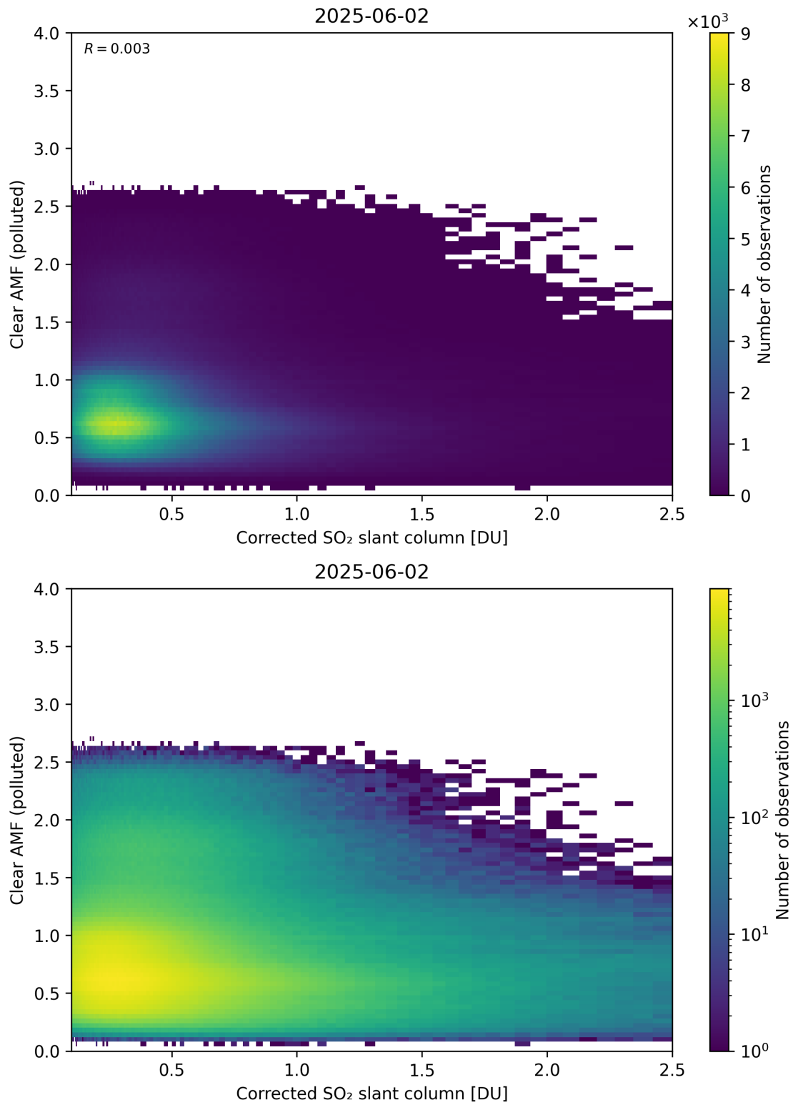
Figure 232: Scatter density plot of “Corrected SO 2 slant column” against “Clear AMF (polluted)” for 2025-06-01 to 2025-06-03.
