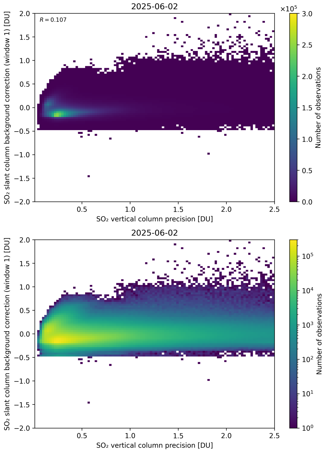
Figure 329: Scatter density plot of “SO 2 vertical column precision” against “SO 2 slant column background correction (window 1)” for 2025-06-01 to 2025-06-03.
