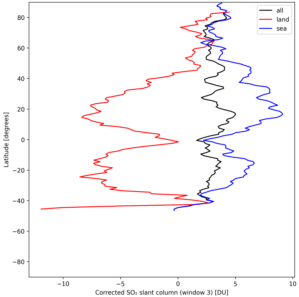
Figure 47: Zonal average of “Corrected SO 2 slant column (window 3)” for 2025-06-01 to 2025-06-03.
