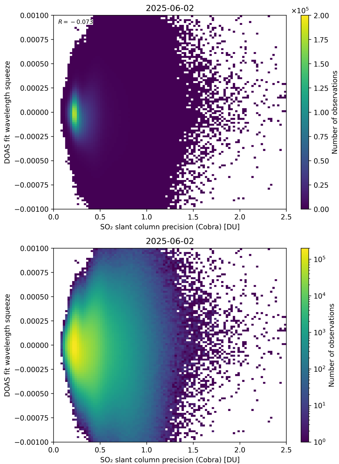
Figure 203: Scatter density plot of “SO 2 slant column precision (Cobra)” against “DOAS fit wavelength squeeze” for 2025-06-01 to 2025-06-03.
