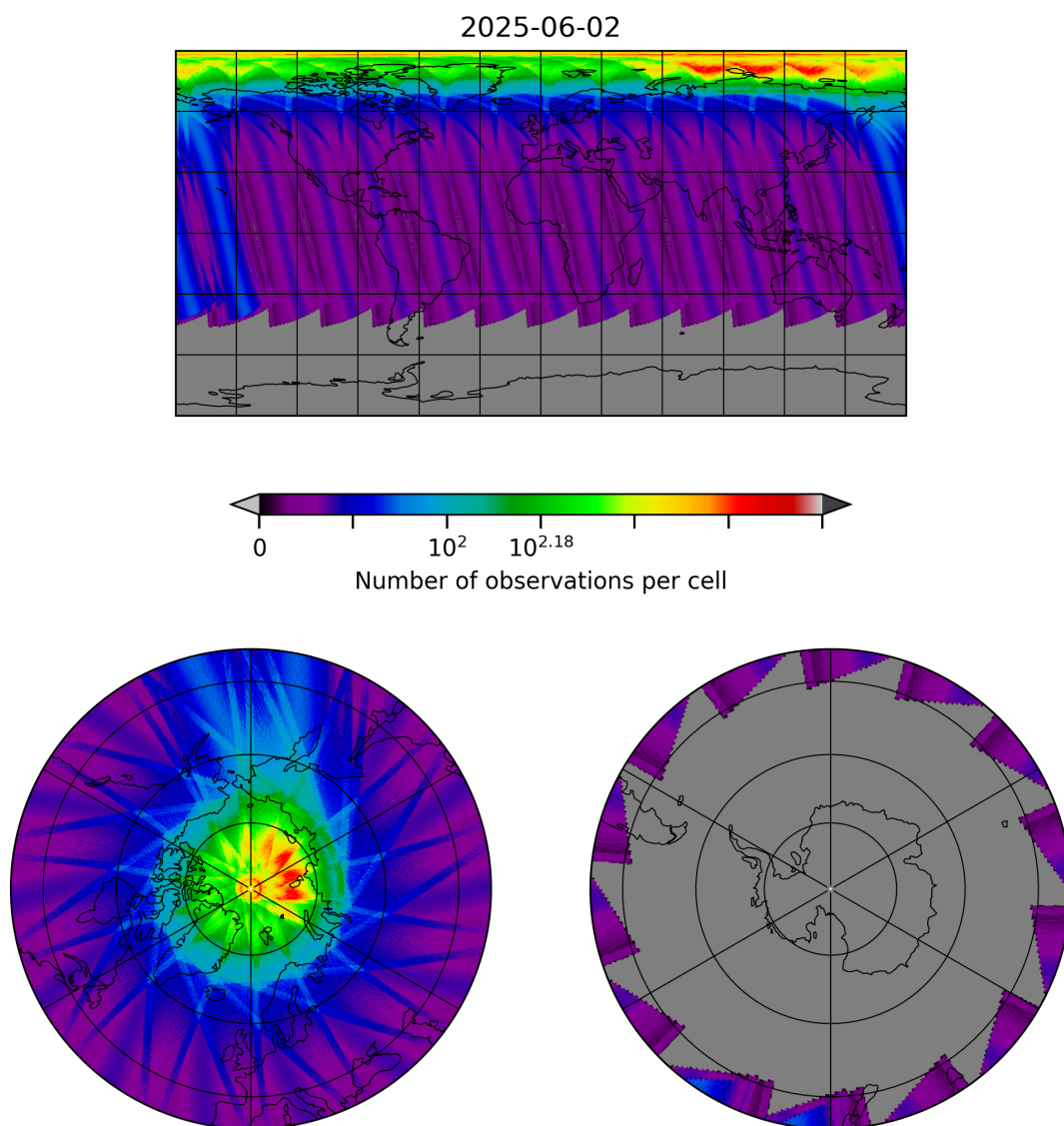
Figure 30: Map of the number of observations for 2025-06-01 to 2025-06-03
