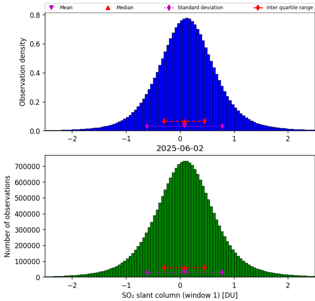
Figure 63: Histogram of “SO 2 slant column (window 1)” for 2025-06-01 to 2025-06-03
