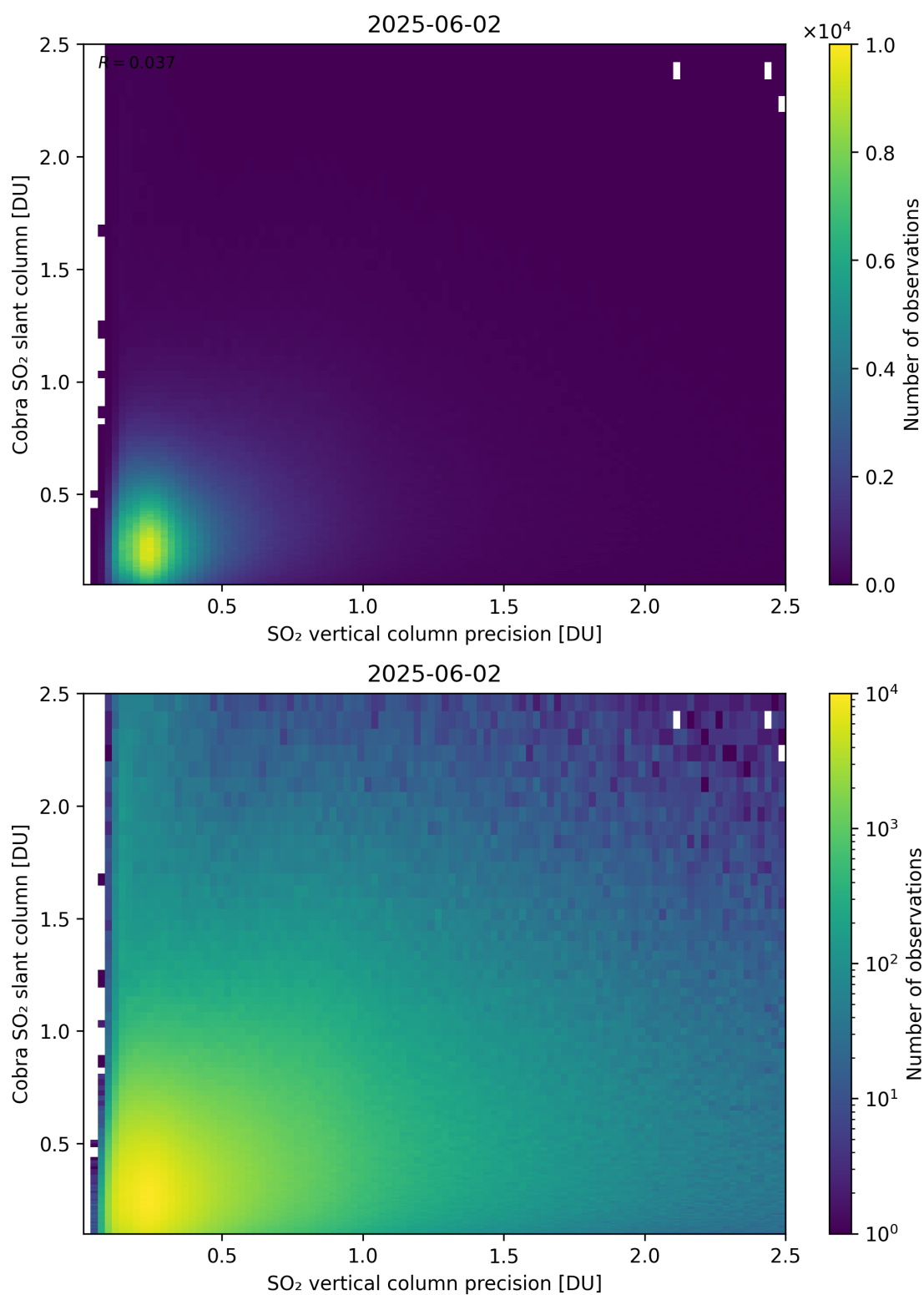
Figure 336: Scatter density plot of “SO 2 vertical column precision” against “Cobra SO 2 slant column” for 2025-06-01 to 2025-06-03.
