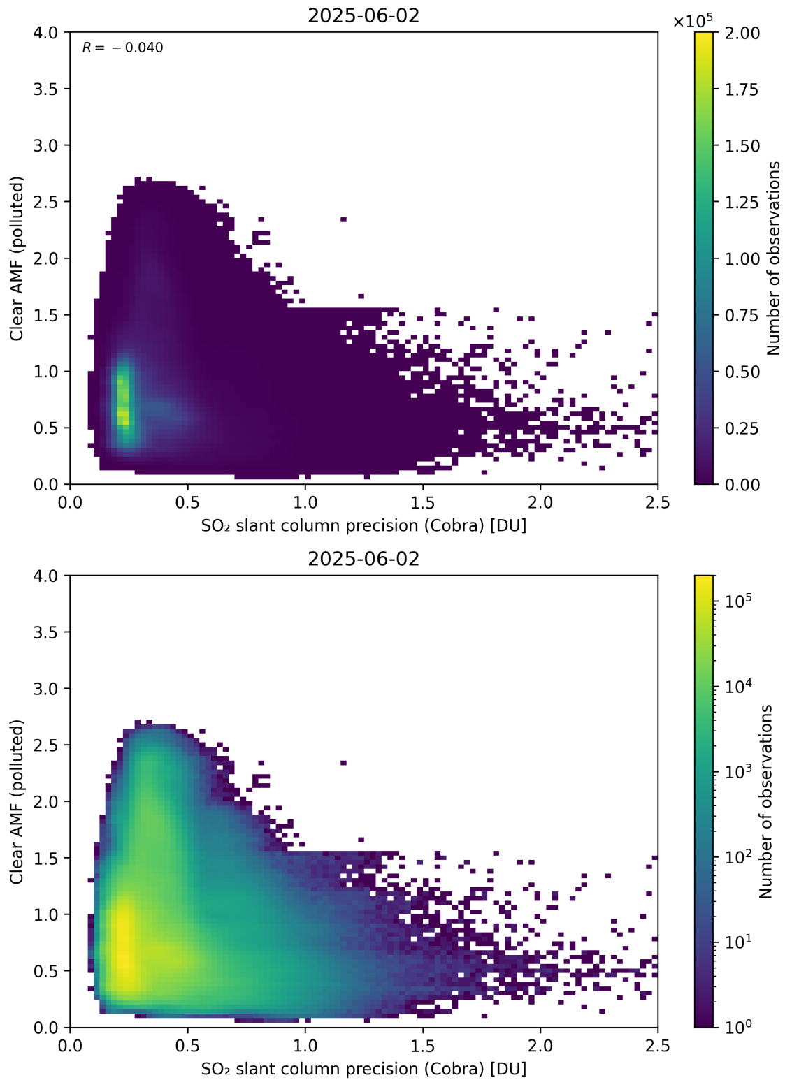
Figure 205: Scatter density plot of “SO 2 slant column precision (Cobra)” against “Clear AMF (polluted)” for 2025-06-01 to 2025-06-03.
