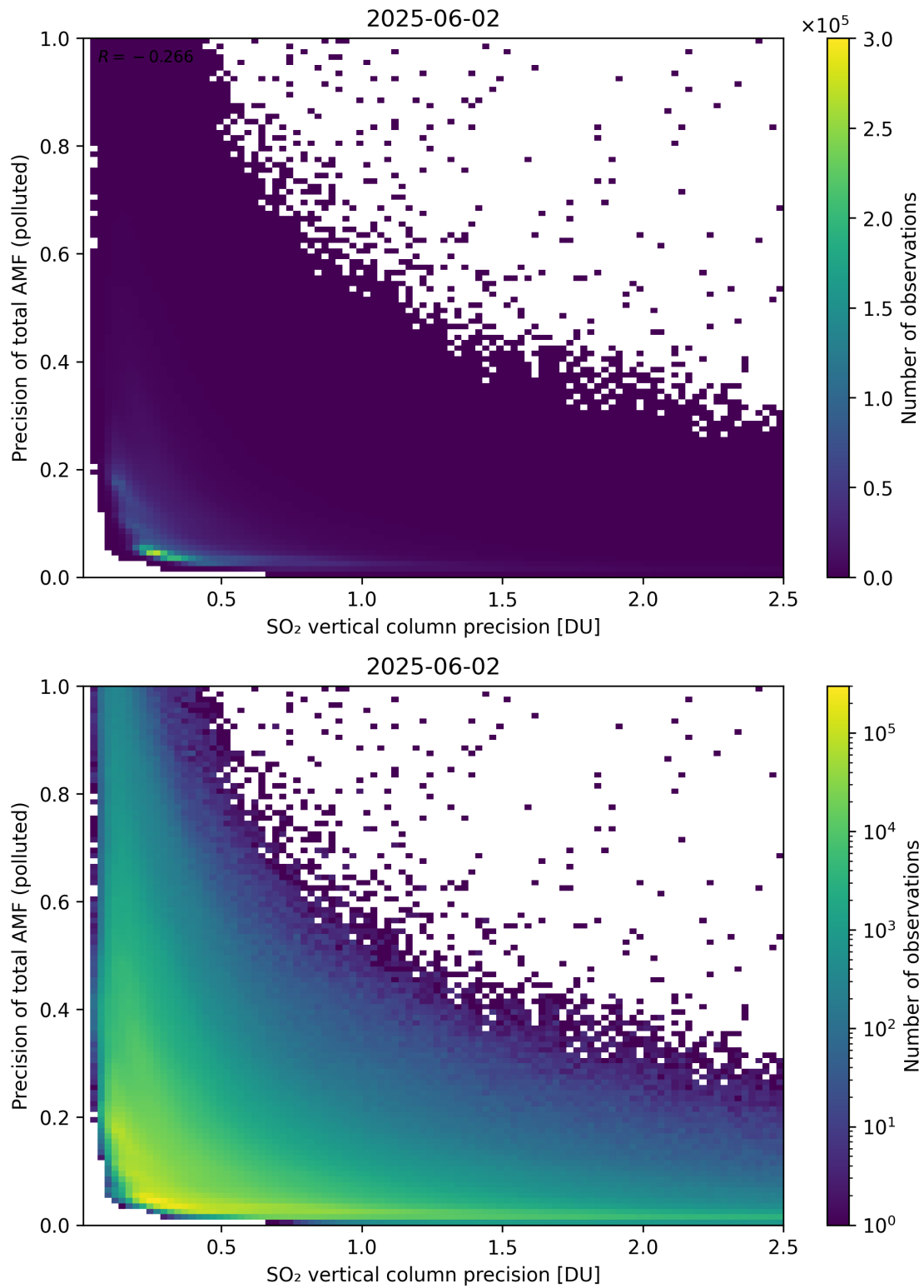
Figure 347: Scatter density plot of “SO 2 vertical column precision” against “Precision of total AMF (polluted)” for 2025-06-01 to 2025-06-03.
