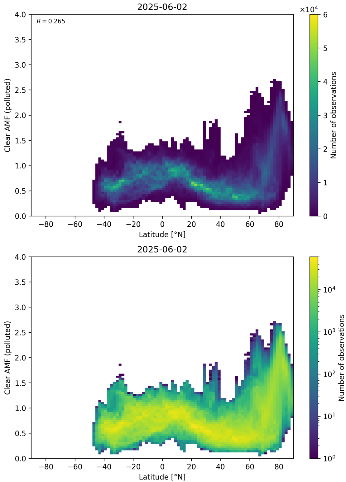
Figure 156: Scatter density plot of “Latitude” against “Clear AMF (polluted)” for 2025-06-01 to 2025-06-03.
