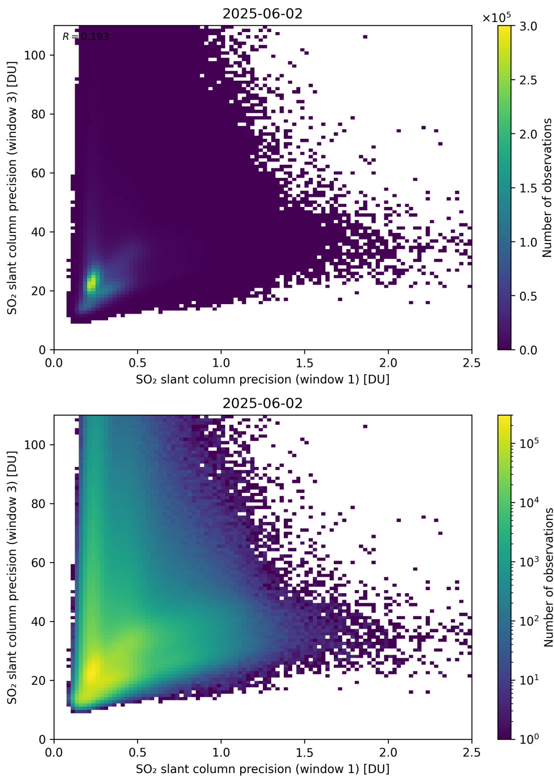
Figure 279: Scatter density plot of “SO 2 slant column precision (window 1)” against “SO 2 slant column precision (window 3)” for 2025-06-01 to 2025-06-03.
