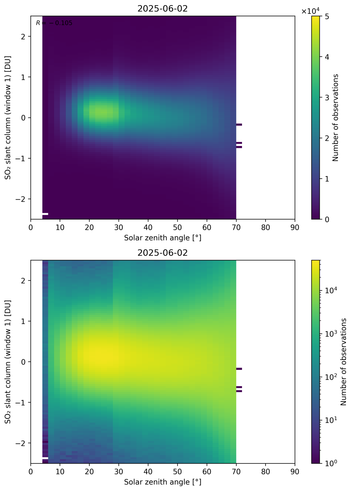
Figure 184: Scatter density plot of “Solar zenith angle” against “SO 2 slant column (window 1)” for 2025-06-01 to 2025-06-03.
