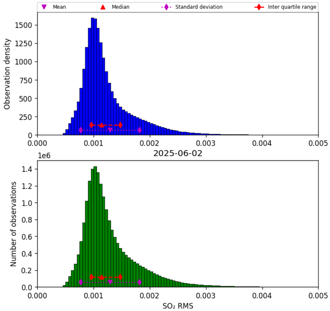
Figure 78: Histogram of “SO 2 RMS” for 2025-06-01 to 2025-06-03
