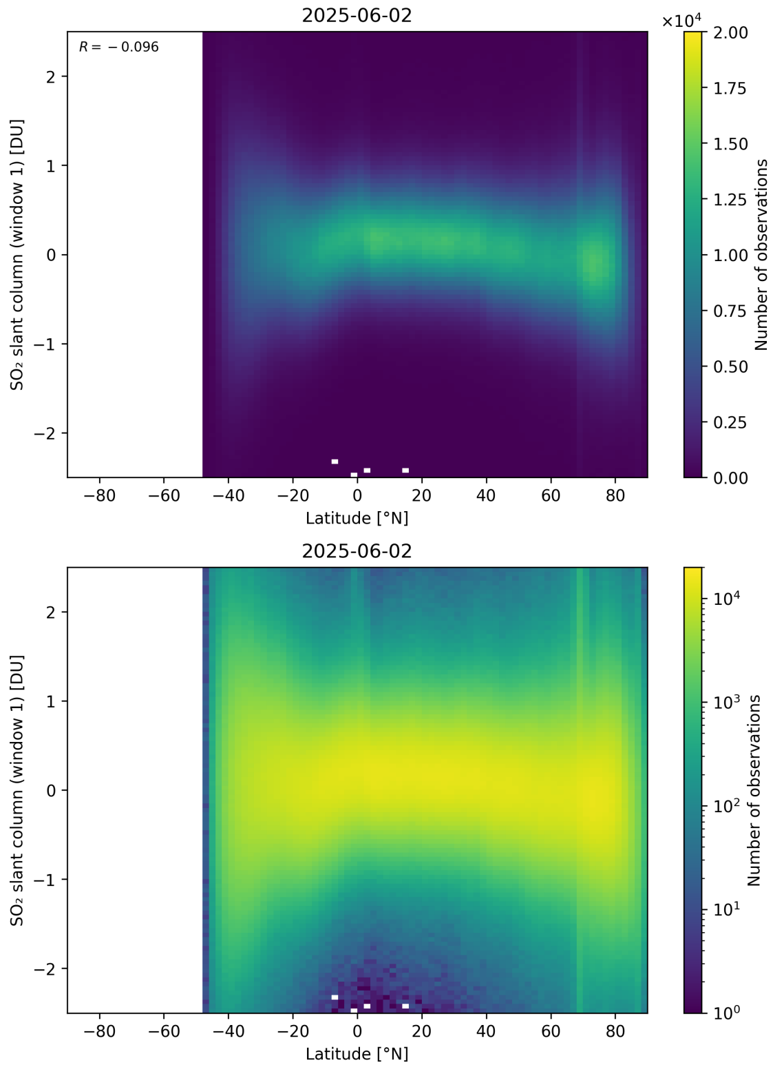
Figure 162: Scatter density plot of “Latitude” against “SO 2 slant column (window 1)” for 2025-06-01 to 2025-06-03.
