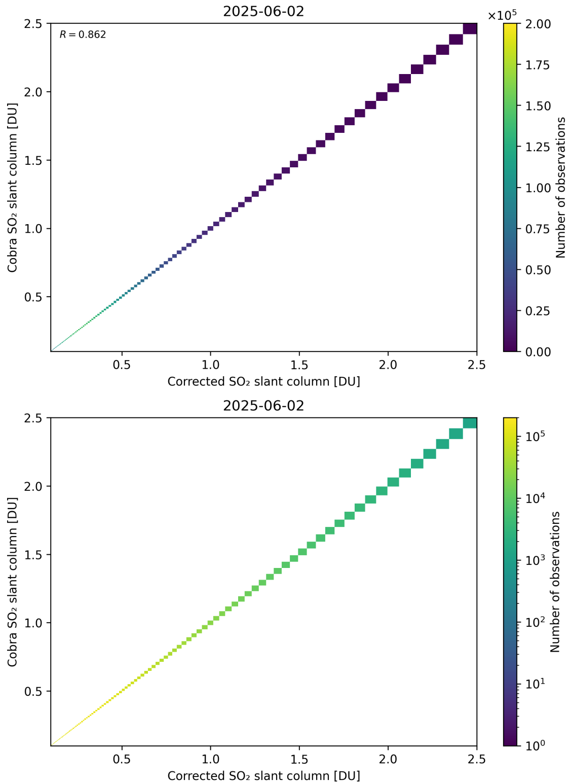
Figure 233: Scatter density plot of “Corrected SO 2 slant column” against “Cobra SO 2 slant column” for 2025-06-01 to 2025-06-03.
