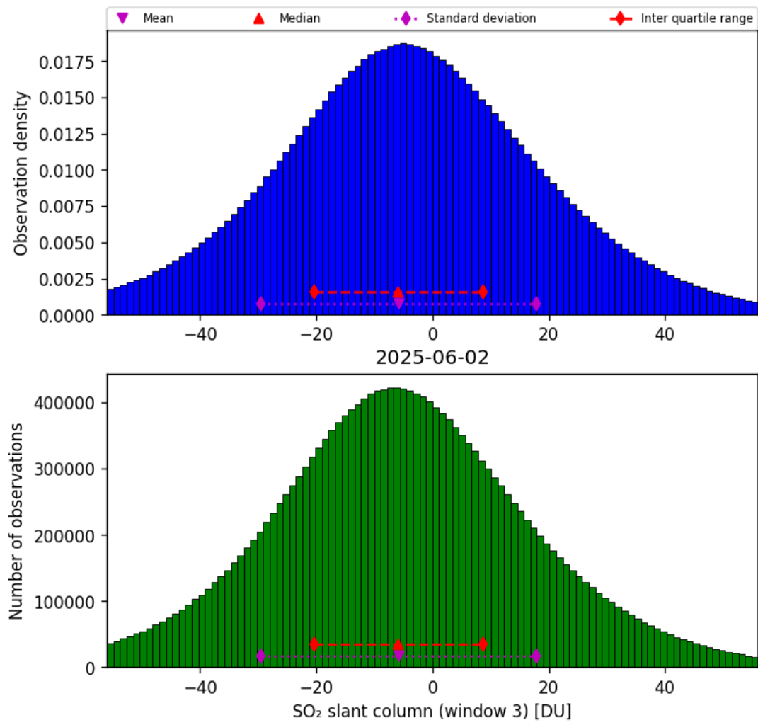
Figure 71: Histogram of “SO 2 slant column (window 3)” for 2025-06-01 to 2025-06-03
