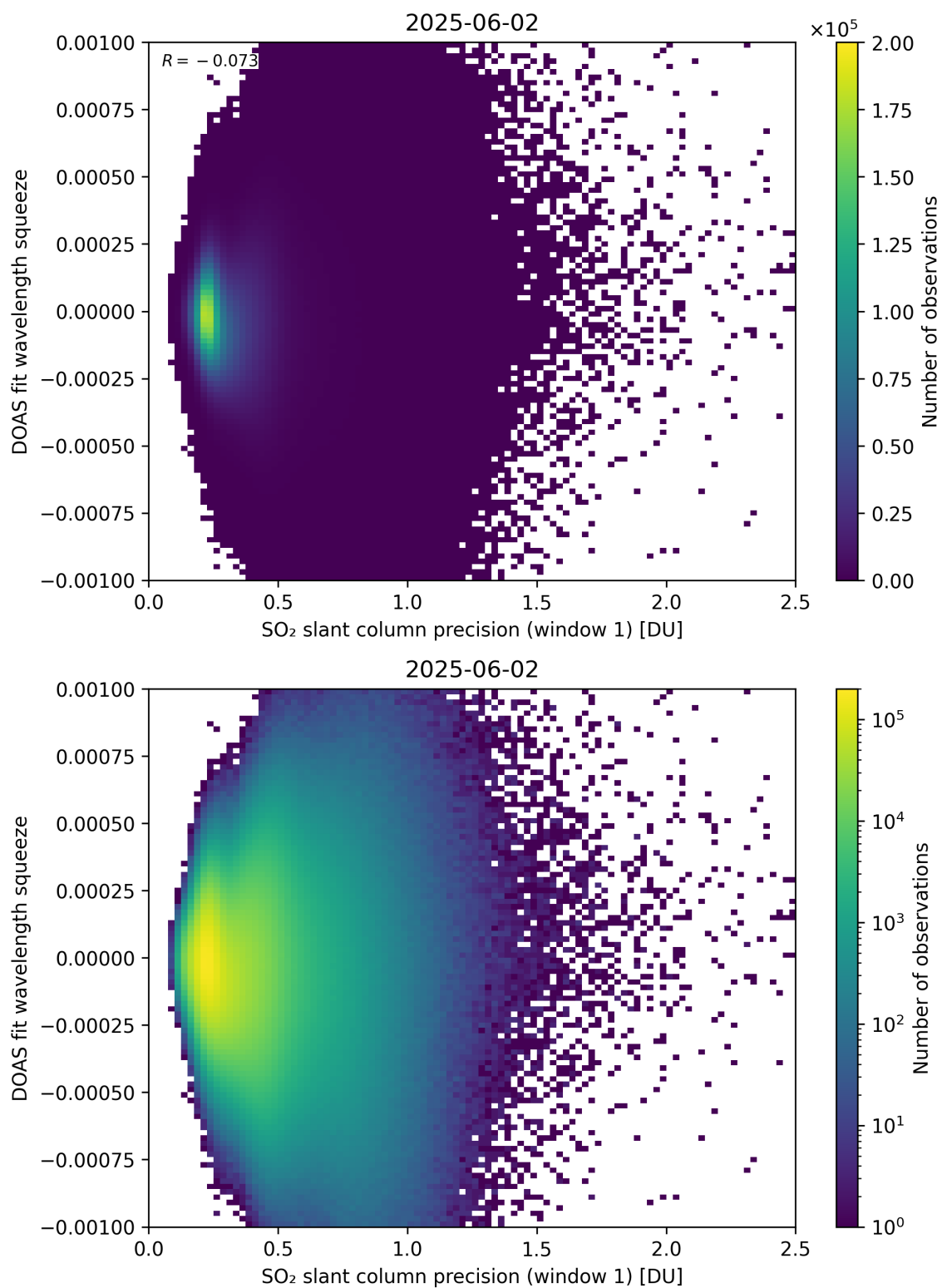
Figure 272: Scatter density plot of “SO 2 slant column precision (window 1)” against “DOAS fit wavelength squeeze” for 2025-06-01 to 2025-06-03.
