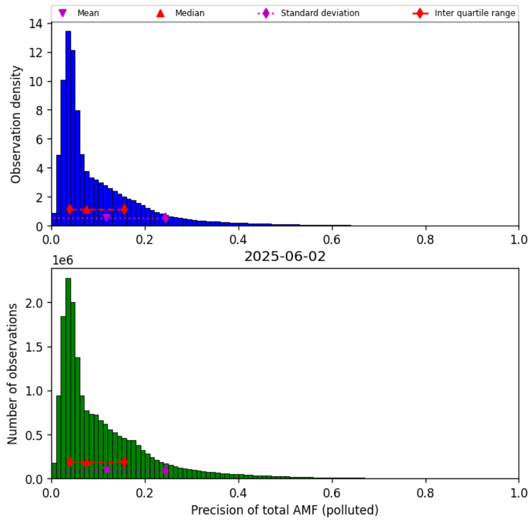
Figure 80: Histogram of “Precision of total AMF (polluted)” for 2025-06-01 to 2025-06-03
