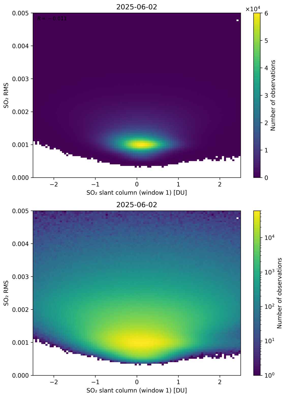
Figure 267: Scatter density plot of “SO 2 slant column (window 1)” against “SO 2 RMS” for 2025-06-01 to 2025-06-03.
