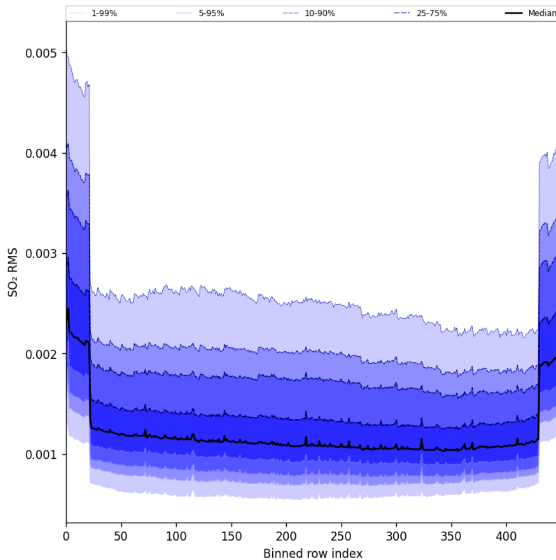
Figure 104: Along track statistics of “SO 2 RMS” for 2025-06-01 to 2025-06-03
