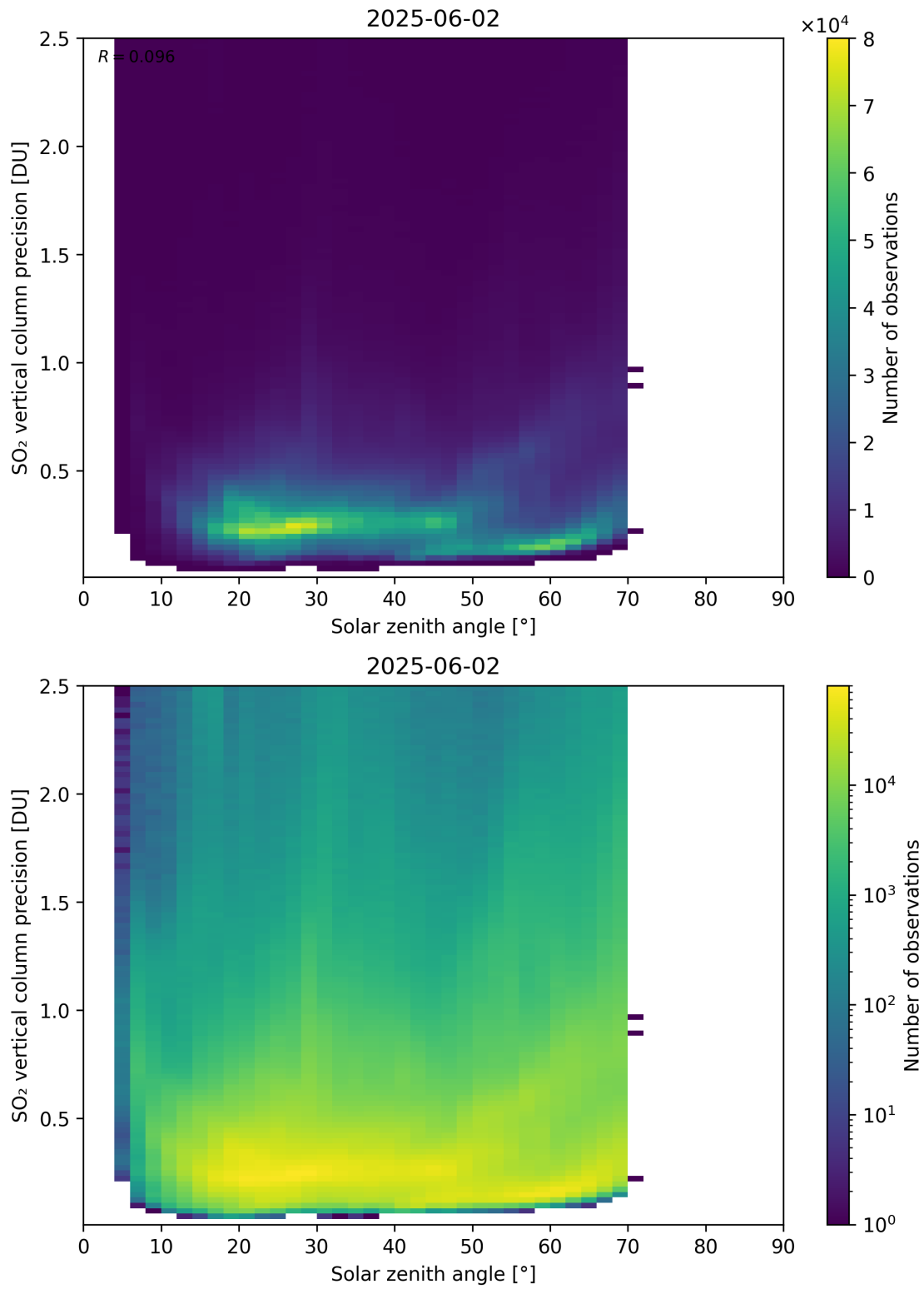
Figure 192: Scatter density plot of “Solar zenith angle” against “SO 2 vertical column precision” for 2025-06-01 to 2025-06-03.
