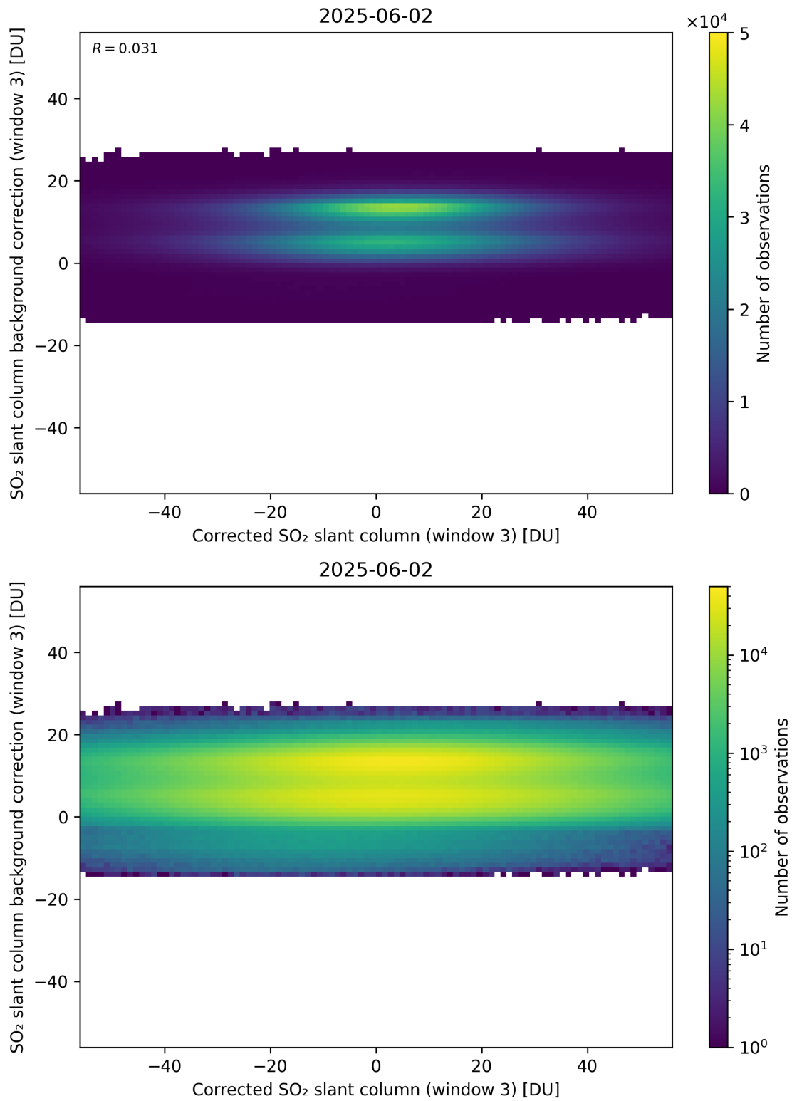
Figure 255: Scatter density plot of “Corrected SO 2 slant column (window 3)” against “SO 2 slant column background correction (window 3)” for 2025-06-01 to 2025-06-03.
