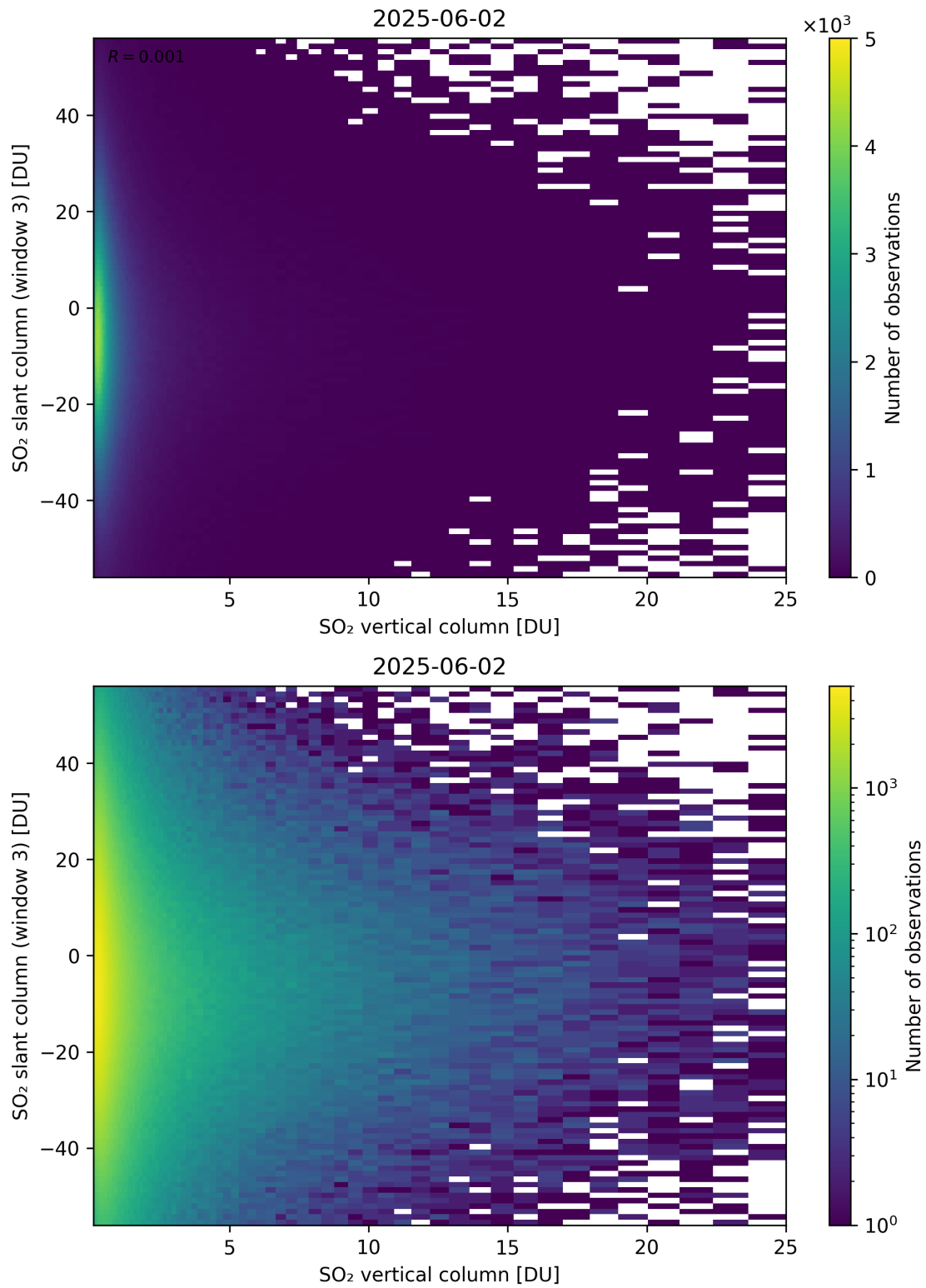
Figure 357: Scatter density plot of “SO 2 vertical column” against “SO 2 slant column (window 3)” for 2025-06-01 to 2025-06-03.
