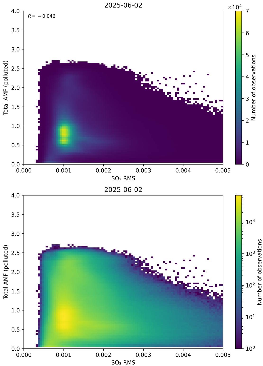
Figure 148: Scatter density plot of “SO 2 RMS” against “Total AMF (polluted)” for 2025-06-01 to 2025-06-03.
