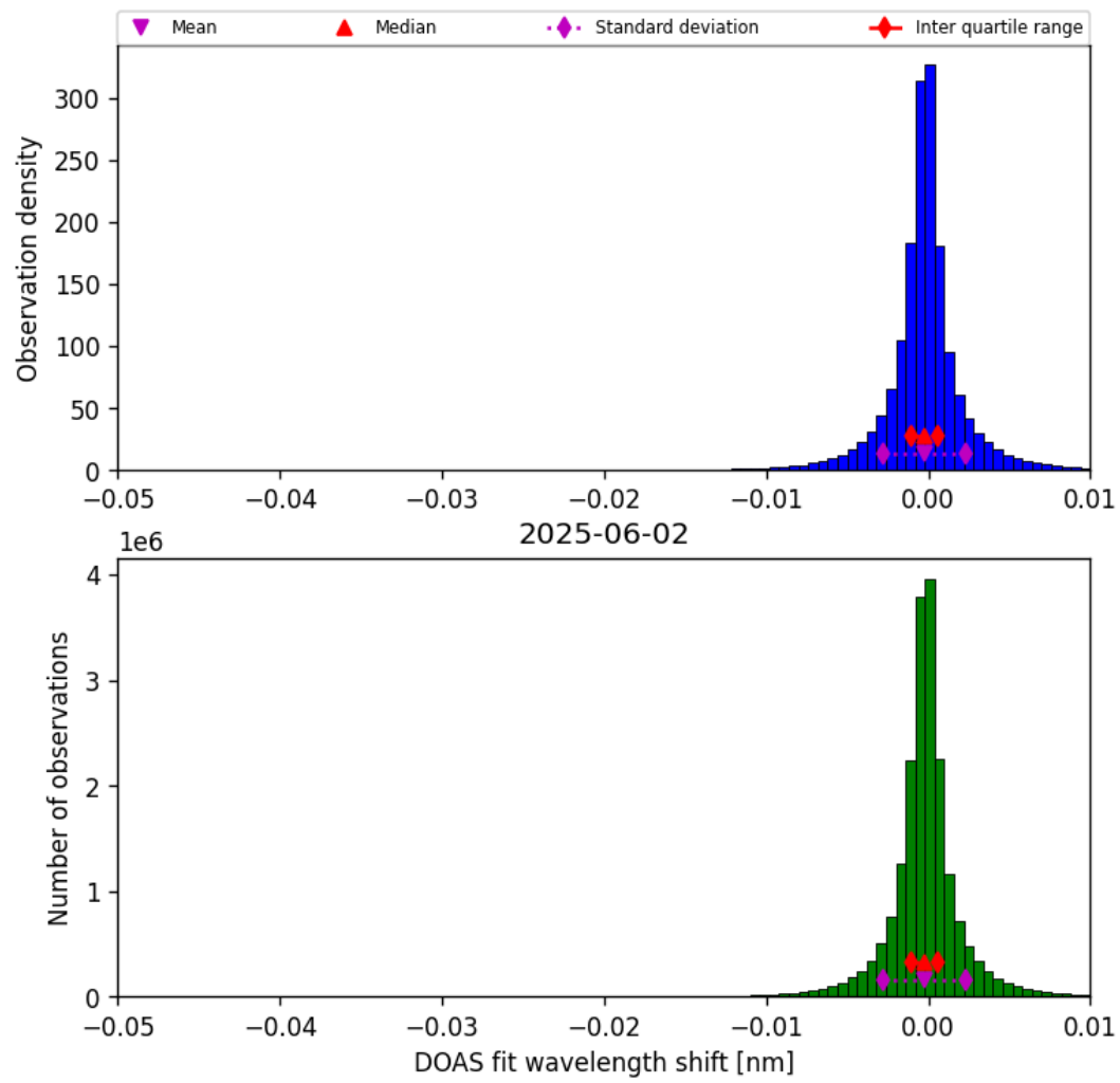
Figure 76: Histogram of “DOAS fit wavelength shift” for 2025-06-01 to 2025-06-03
