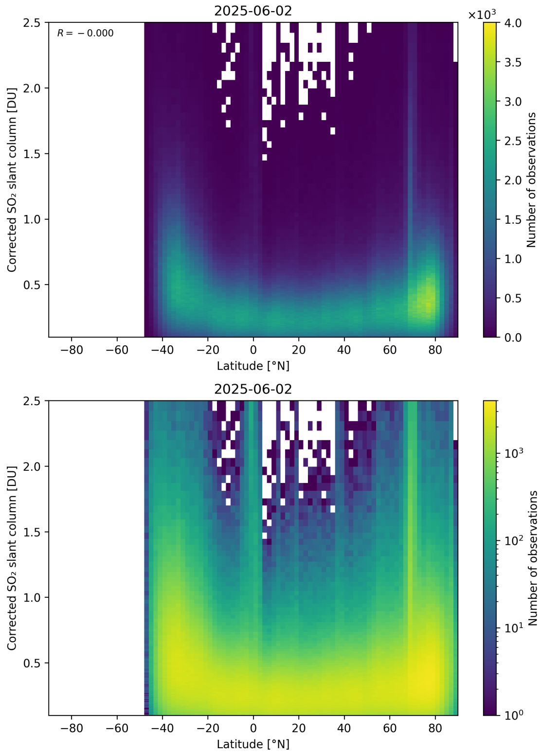
Figure 159: Scatter density plot of “Latitude” against “Corrected SO 2 slant column” for 2025-06-01 to 2025-06-03.
