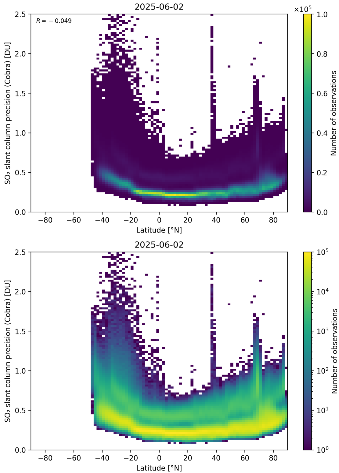
Figure 158: Scatter density plot of “Latitude” against “SO 2 slant column precision (Cobra)” for 2025-06-01 to 2025-06-03.
