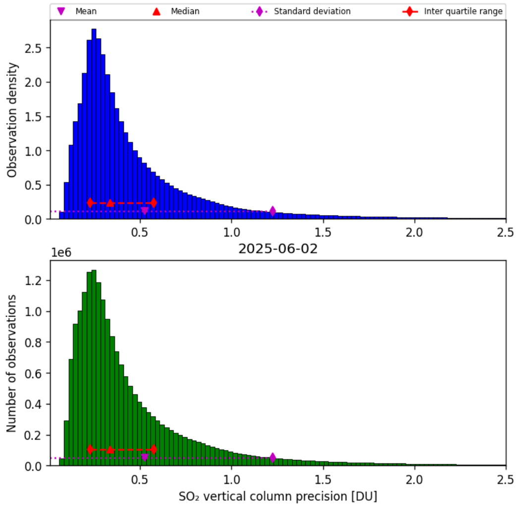
Figure 59: Histogram of “SO 2 vertical column precision” for 2025-06-01 to 2025-06-03
