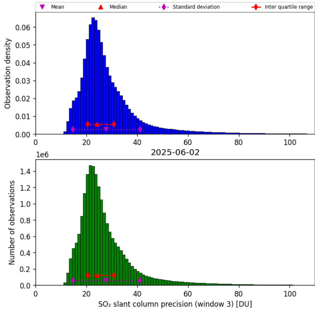
Figure 72: Histogram of “SO 2 slant column precision (window 3)” for 2025-06-01 to 2025-06-03
