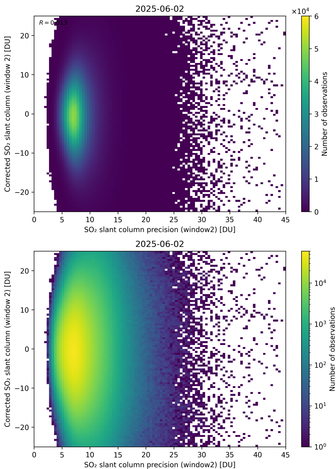
Figure 297: Scatter density plot of “SO 2 slant column precision (window2)” against “Corrected SO 2 slant column (window 2)” for 2025-06-01 to 2025-06-03.
