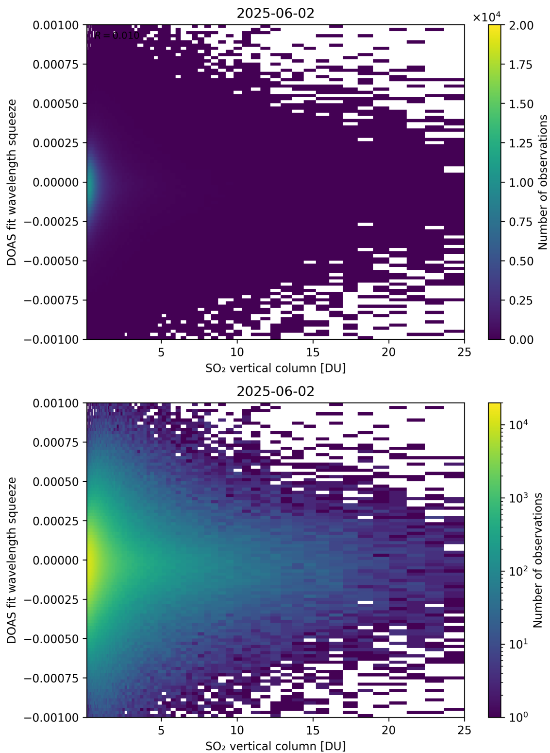
Figure 327: Scatter density plot of “SO 2 vertical column” against “DOAS fit wavelength squeeze” for 2025-06-01 to 2025-06-03.
