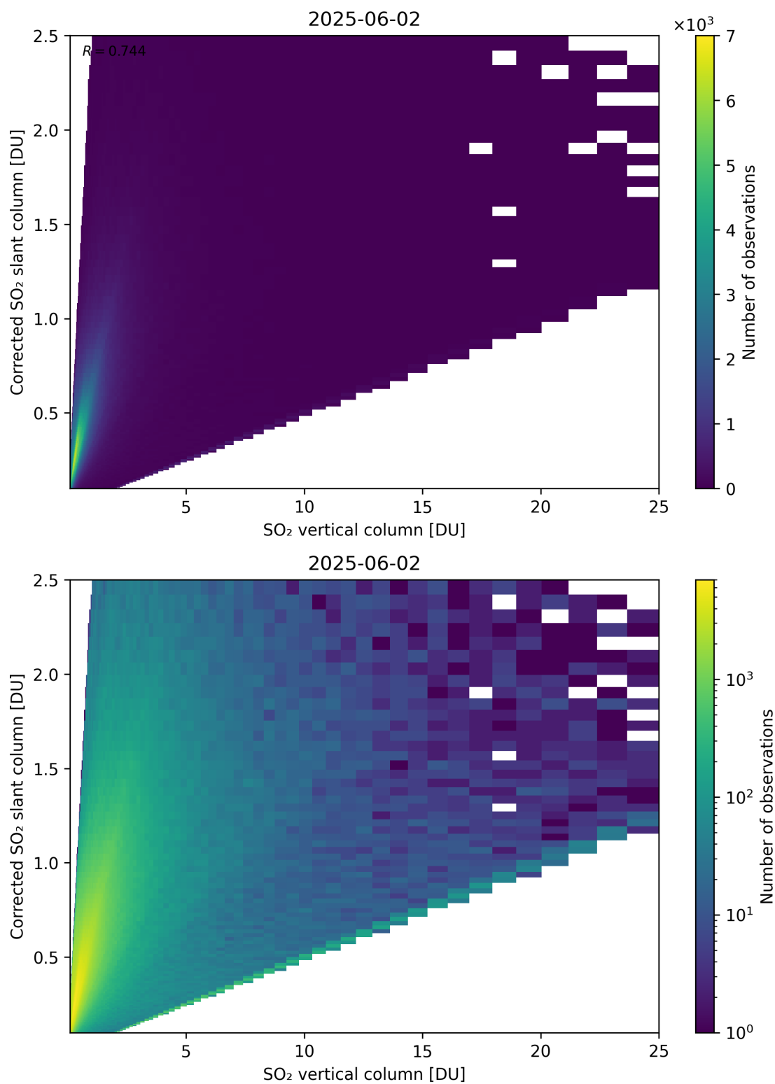
Figure 351: Scatter density plot of “SO 2 vertical column” against “Corrected SO 2 slant column” for 2025-06-01 to 2025-06-03.
