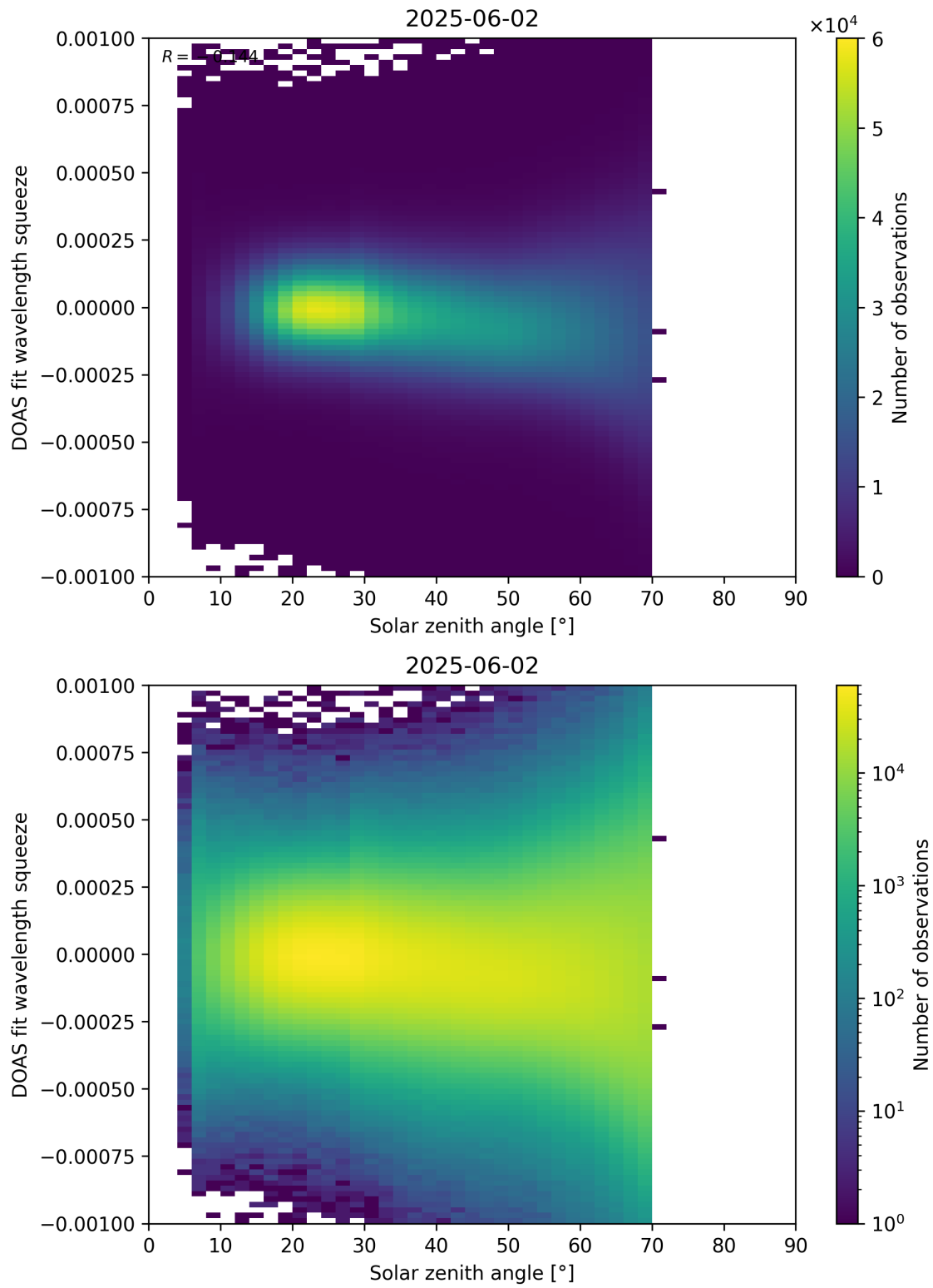
Figure 175: Scatter density plot of “Solar zenith angle” against “DOAS fit wavelength squeeze” for 2025-06-01 to 2025-06-03.
