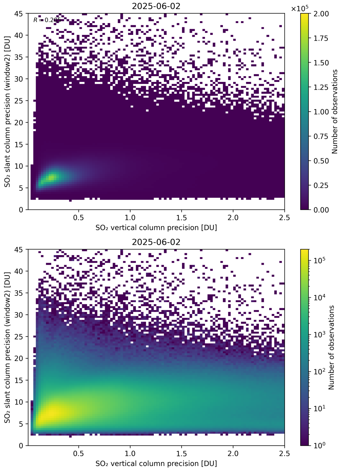
Figure 343: Scatter density plot of “SO 2 vertical column precision” against “SO 2 slant column precision (window2)” for 2025-06-01 to 2025-06-03.
