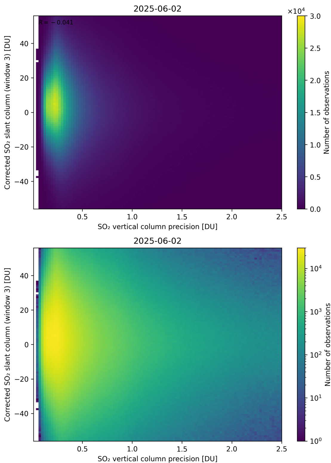
Figure 340: Scatter density plot of “SO 2 vertical column precision” against “Corrected SO 2 slant column (window 3)” for 2025-06-01 to 2025-06-03.
