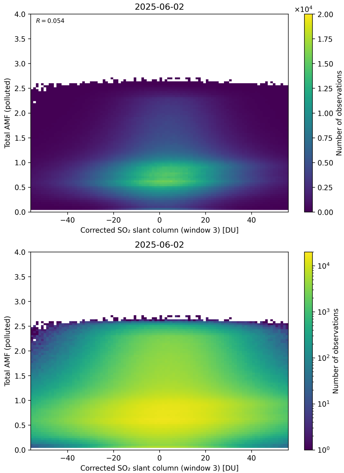
Figure 260: Scatter density plot of “Corrected SO 2 slant column (window 3)” against “Total AMF (polluted)” for 2025-06-01 to 2025-06-03.
