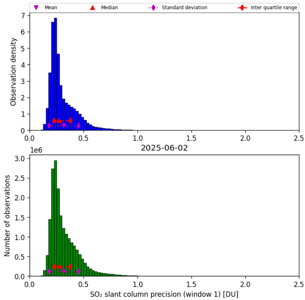
Figure 64: Histogram of “SO 2 slant column precision (window 1)” for 2025-06-01 to 2025-06-03
