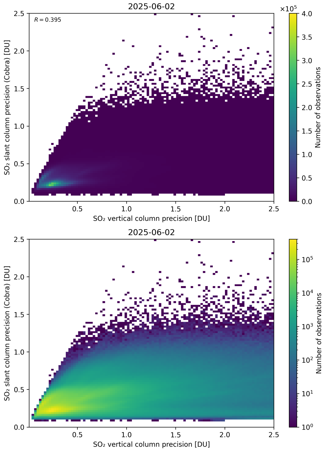
Figure 337: Scatter density plot of “SO 2 vertical column precision” against “SO 2 slant column precision (Cobra)” for 2025-06-01 to 2025-06-03.
