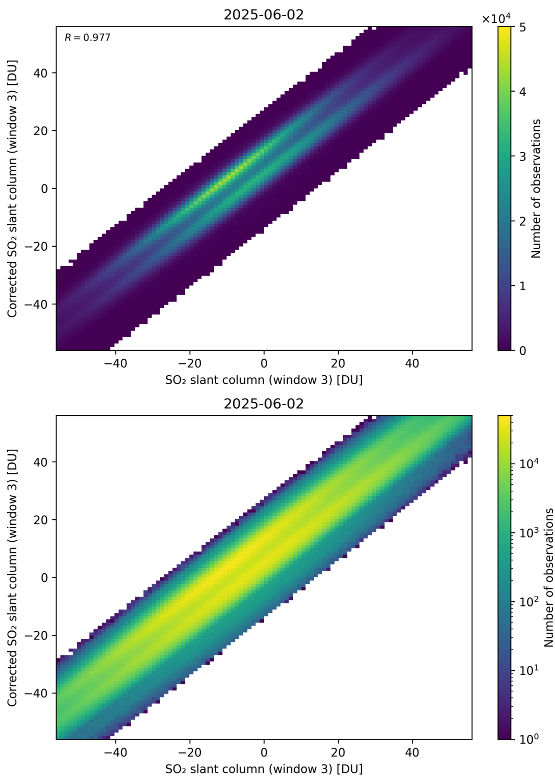
Figure 316: Scatter density plot of “SO 2 slant column (window 3)” against “Corrected SO 2 slant column (window 3)” for 2025-06-01 to 2025-06-03.
