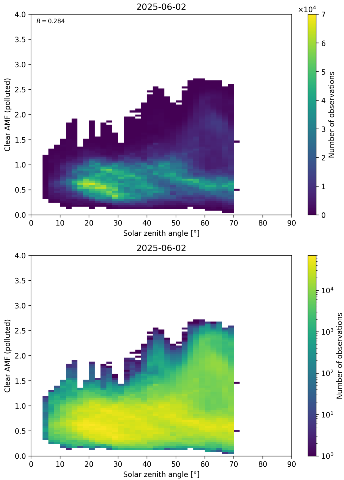
Figure 178: Scatter density plot of “Solar zenith angle” against “Clear AMF (polluted)” for 2025-06-01 to 2025-06-03.
