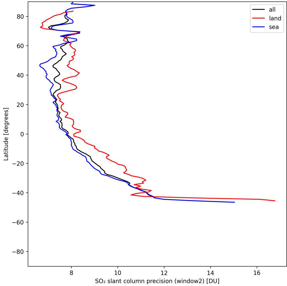
Figure 42: Zonal average of “SO 2 slant column precision (window2)” for 2025-06-01 to 2025-06-03.
