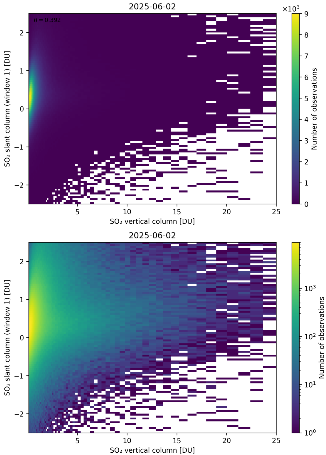
Figure 354: Scatter density plot of “SO 2 vertical column” against “SO 2 slant column (window 1)” for 2025-06-01 to 2025-06-03.
