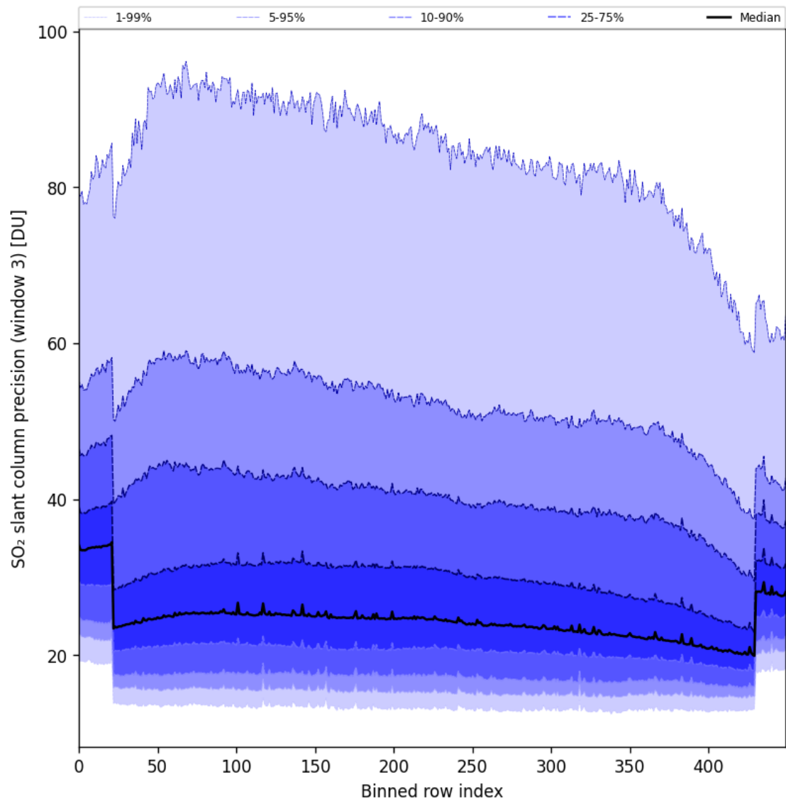
Figure 98: Along track statistics of “SO 2 slant column precision (window 3)” for 2025-06-01 to 2025-06-03
