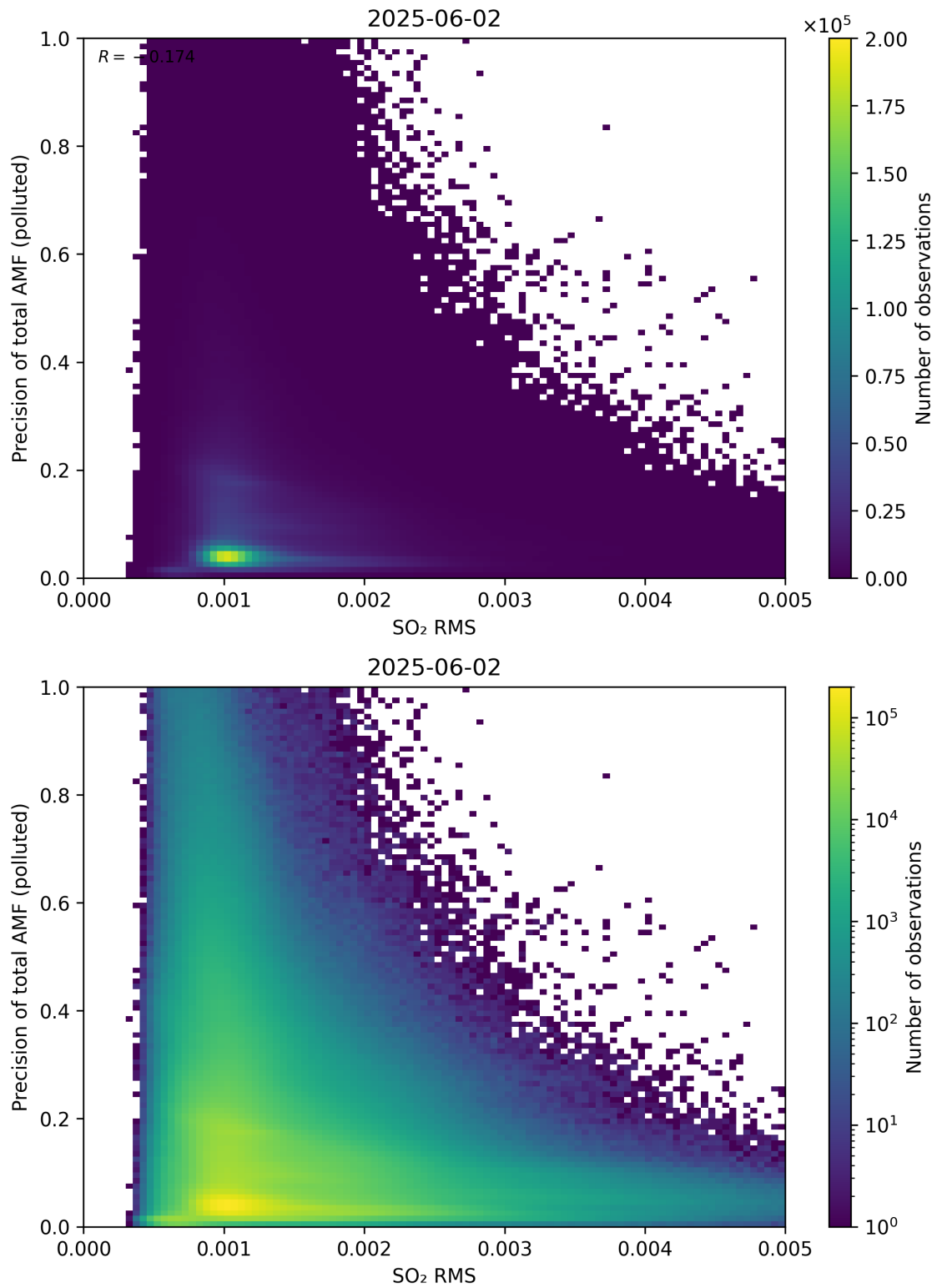
Figure 149: Scatter density plot of “SO 2 RMS” against “Precision of total AMF (polluted)” for 2025-06-01 to 2025-06-03.
