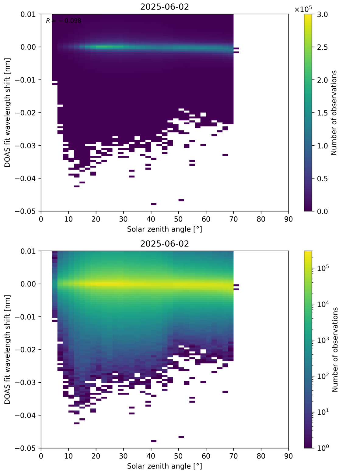
Figure 174: Scatter density plot of “Solar zenith angle” against “DOAS fit wavelength shift” for 2025-06-01 to 2025-06-03.
