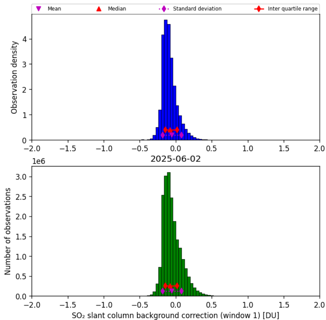
Figure 66: Histogram of “SO 2 slant column background correction (window 1)” for 2025-06-01 to 2025-06-03
