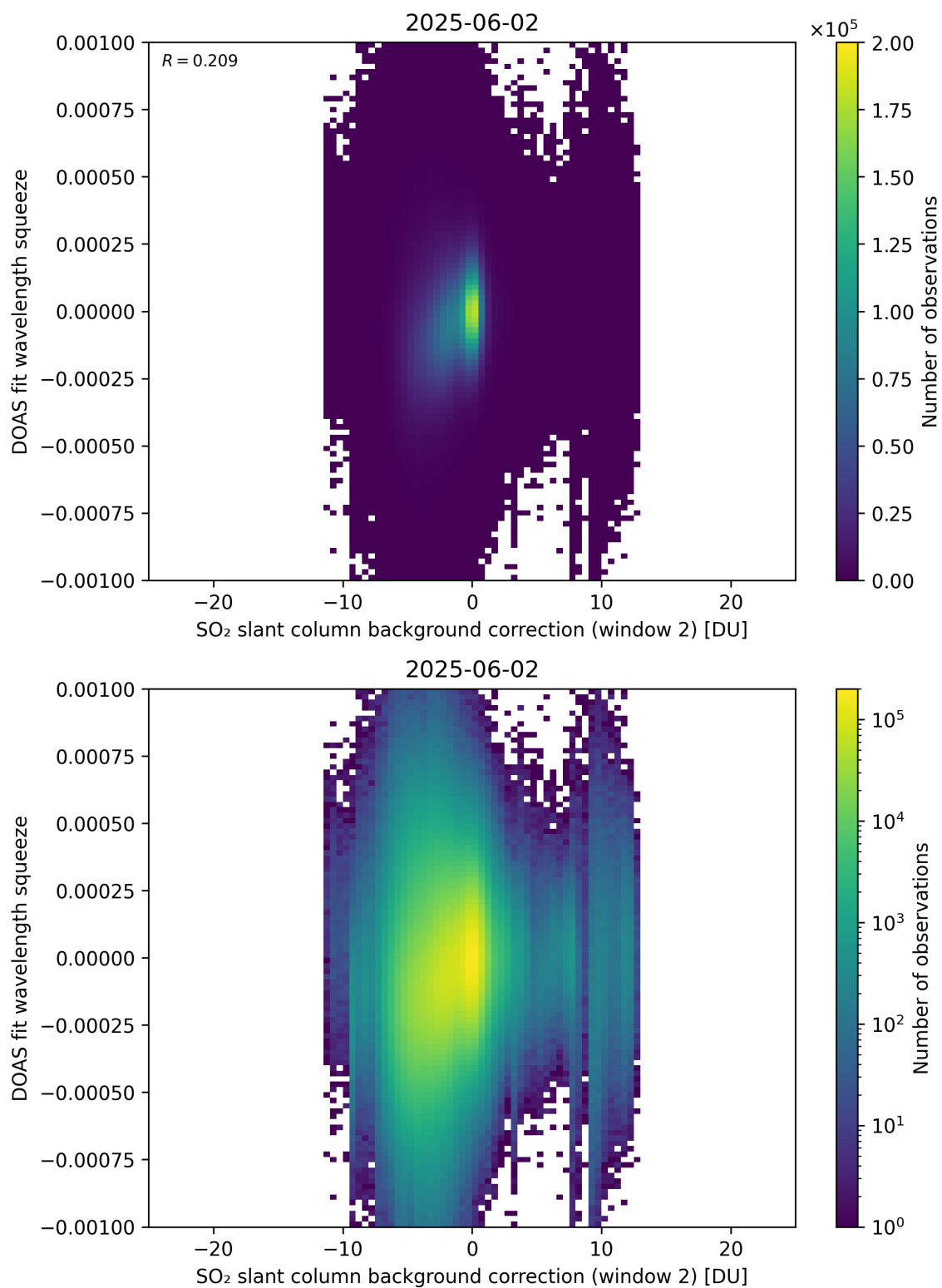
Figure 124: Scatter density plot of “SO 2 slant column background correction (window 2)” against “DOAS fit wavelength squeeze” for 2025-06-01 to 2025-06-03.
