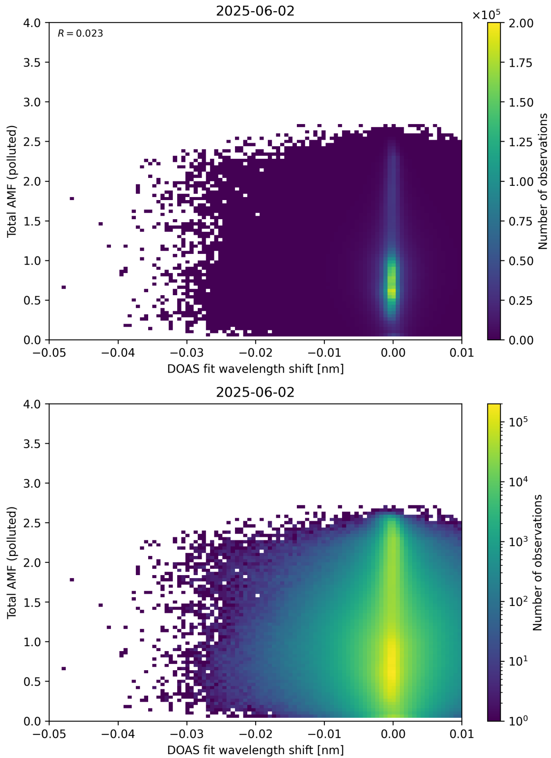
Figure 141: Scatter density plot of “DOAS fit wavelength shift” against “Total AMF (polluted)” for 2025-06-01 to 2025-06-03.
