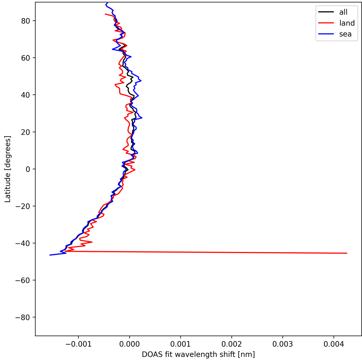
Figure 50: Zonal average of “DOAS fit wavelength shift” for 2025-06-01 to 2025-06-03.
