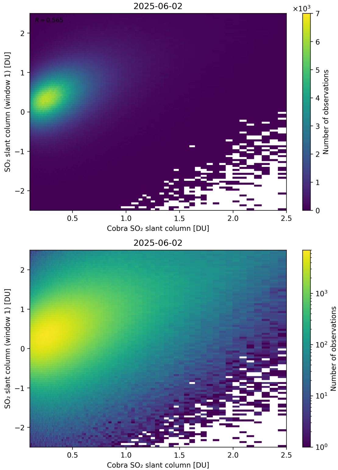
Figure 219: Scatter density plot of “Cobra SO 2 slant column” against “SO 2 slant column (window 1)” for 2025-06-01 to 2025-06-03.
