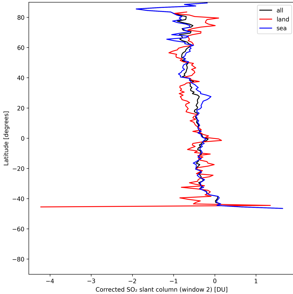
Figure 43: Zonal average of “Corrected SO 2 slant column (window 2)” for 2025-06-01 to 2025-06-03.
