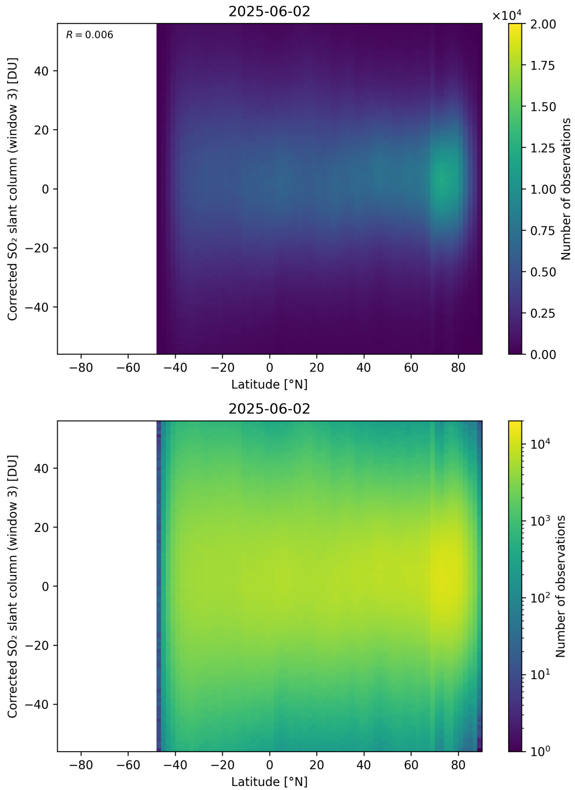
Figure 161: Scatter density plot of “Latitude” against “Corrected SO 2 slant column (window 3)” for 2025-06-01 to 2025-06-03.
