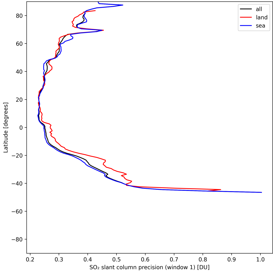
Figure 38: Zonal average of “SO 2 slant column precision (window 1)” for 2025-06-01 to 2025-06-03.
