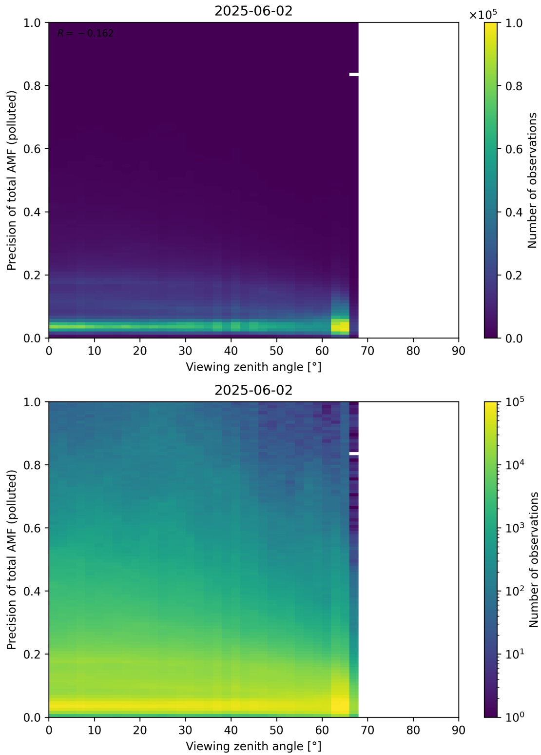
Figure 382: Scatter density plot of “Viewing zenith angle” against “Precision of total AMF (polluted)” for 2025-06-01 to 2025-06-03.
