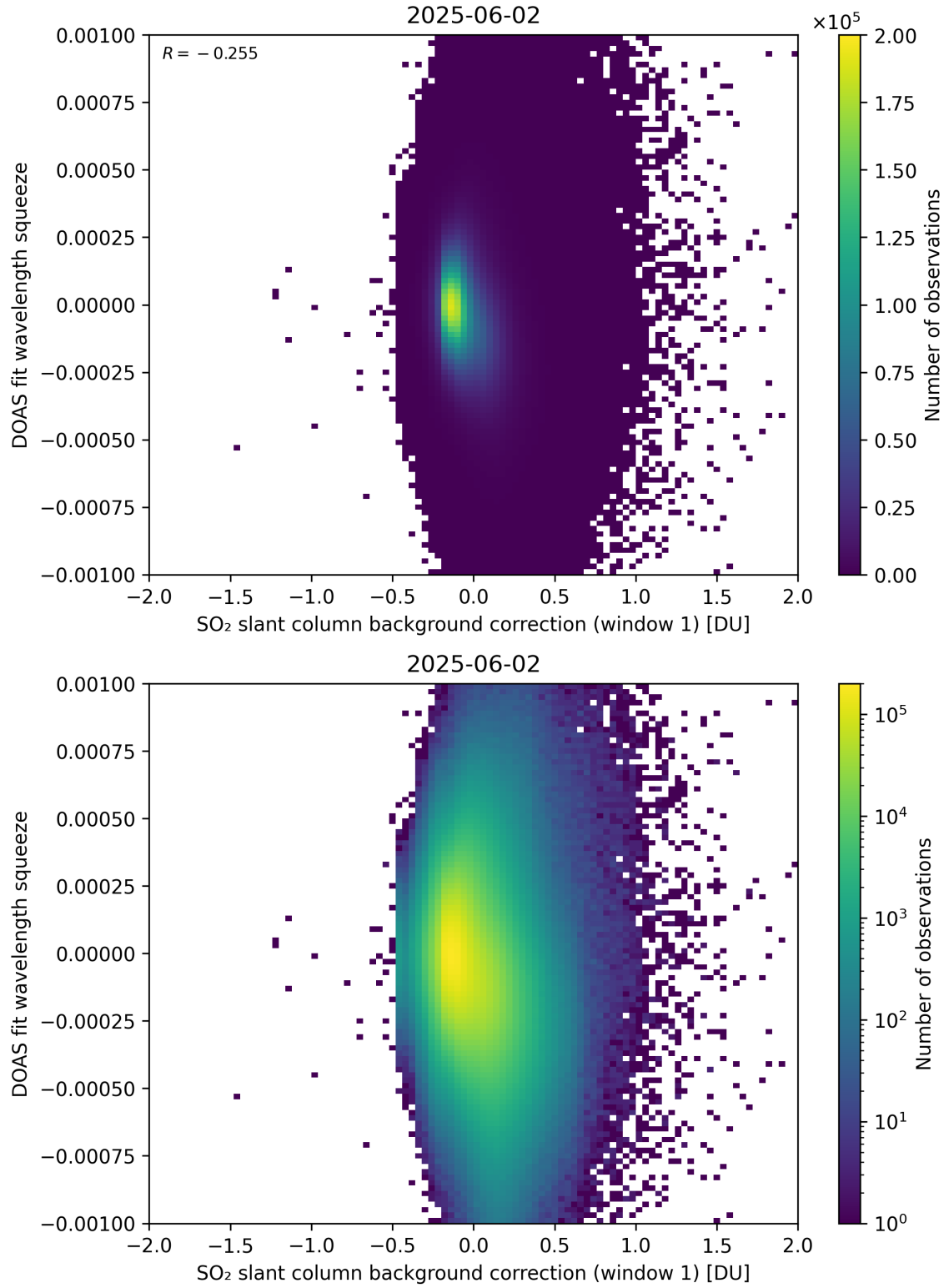
Figure 112: Scatter density plot of “SO 2 slant column background correction (window 1)” against “DOAS fit wavelength squeeze” for 2025-06-01 to 2025-06-03.
