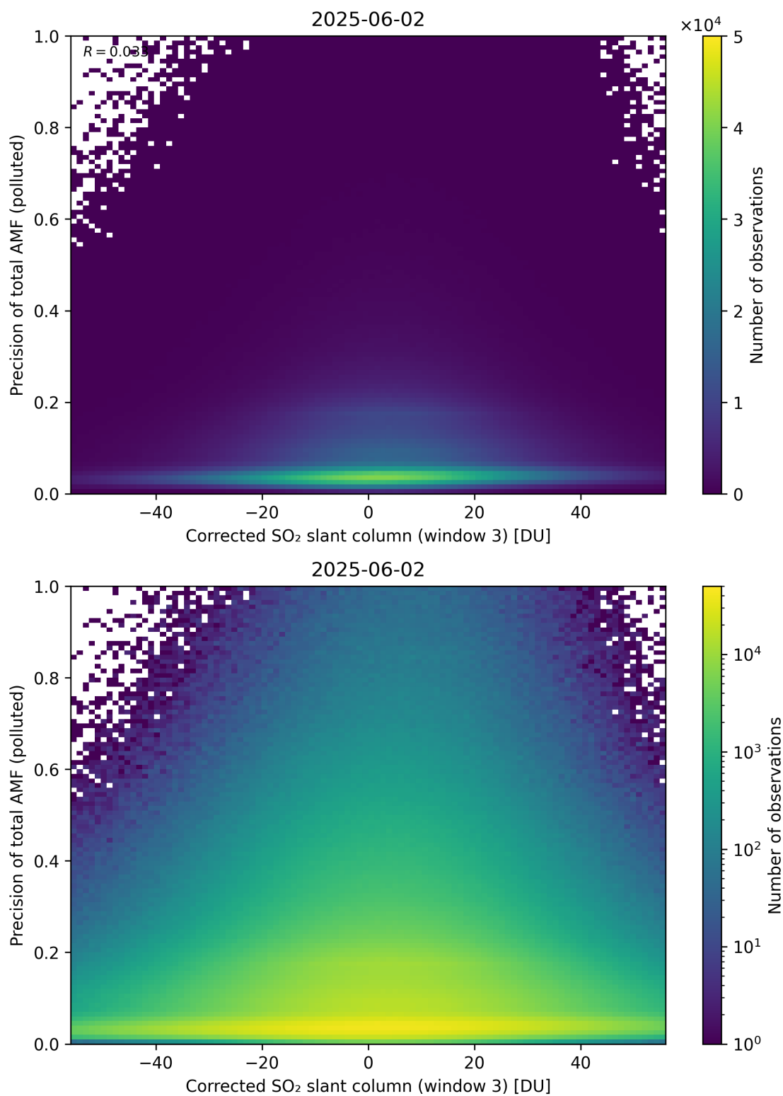
Figure 261: Scatter density plot of “Corrected SO 2 slant column (window 3)” against “Precision of total AMF (polluted)” for 2025-06-01 to 2025-06-03.
