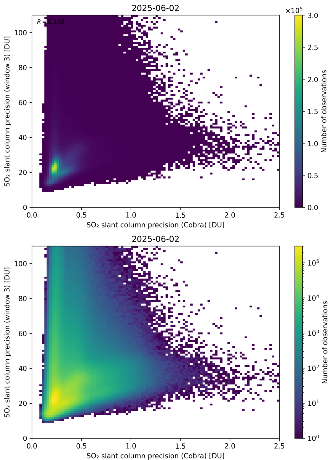
Figure 212: Scatter density plot of “SO 2 slant column precision (Cobra)” against “SO 2 slant column precision (window 3)” for 2025-06-01 to 2025-06-03.
