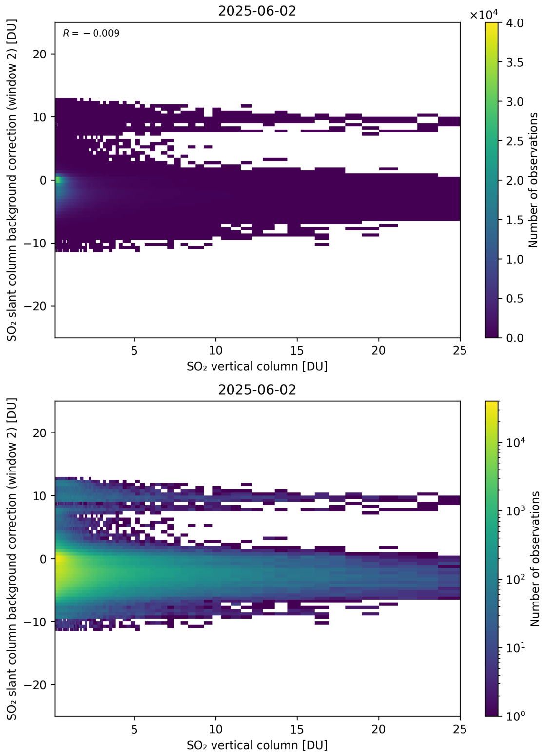
Figure 324: Scatter density plot of “SO 2 vertical column” against “SO 2 slant column background correction (window 2)” for 2025-06-01 to 2025-06-03.
