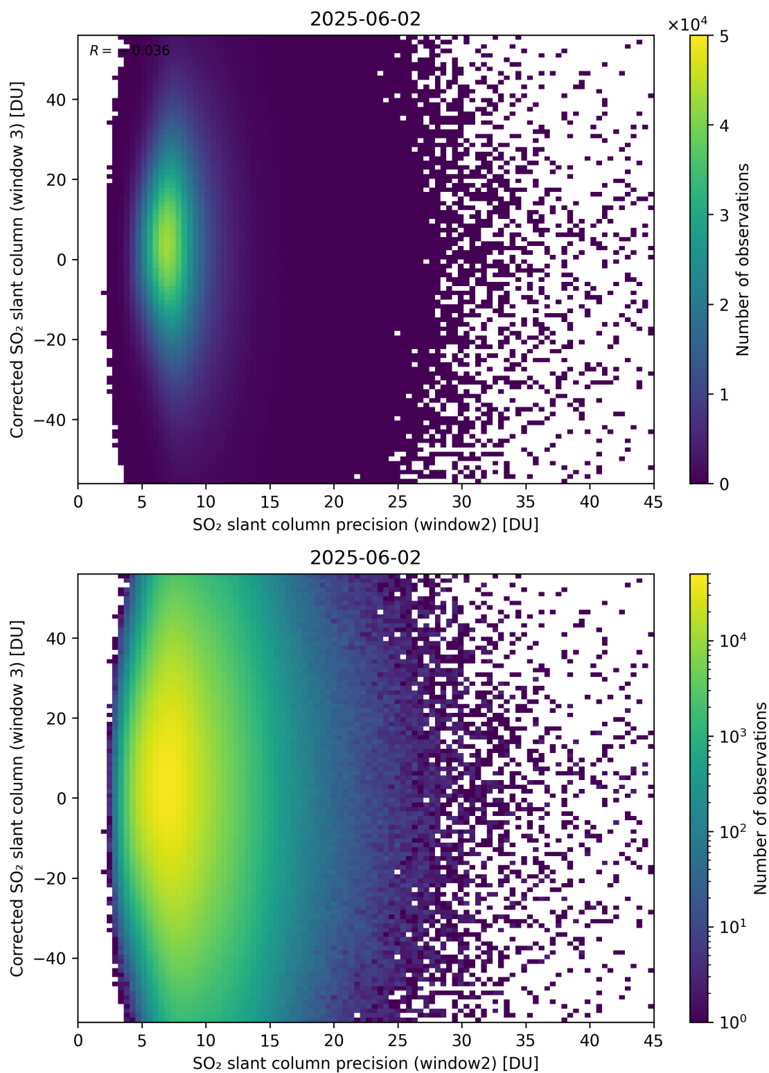
Figure 298: Scatter density plot of “SO 2 slant column precision (window2)” against “Corrected SO 2 slant column (window 3)” for 2025-06-01 to 2025-06-03.
