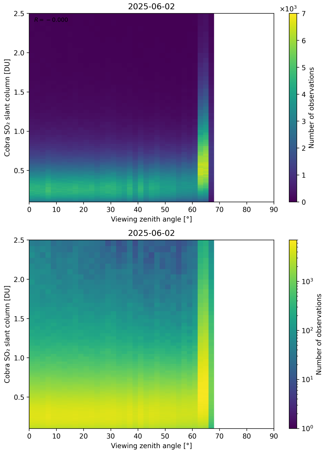
Figure 371: Scatter density plot of “Viewing zenith angle” against “Cobra SO 2 slant column” for 2025-06-01 to 2025-06-03.
