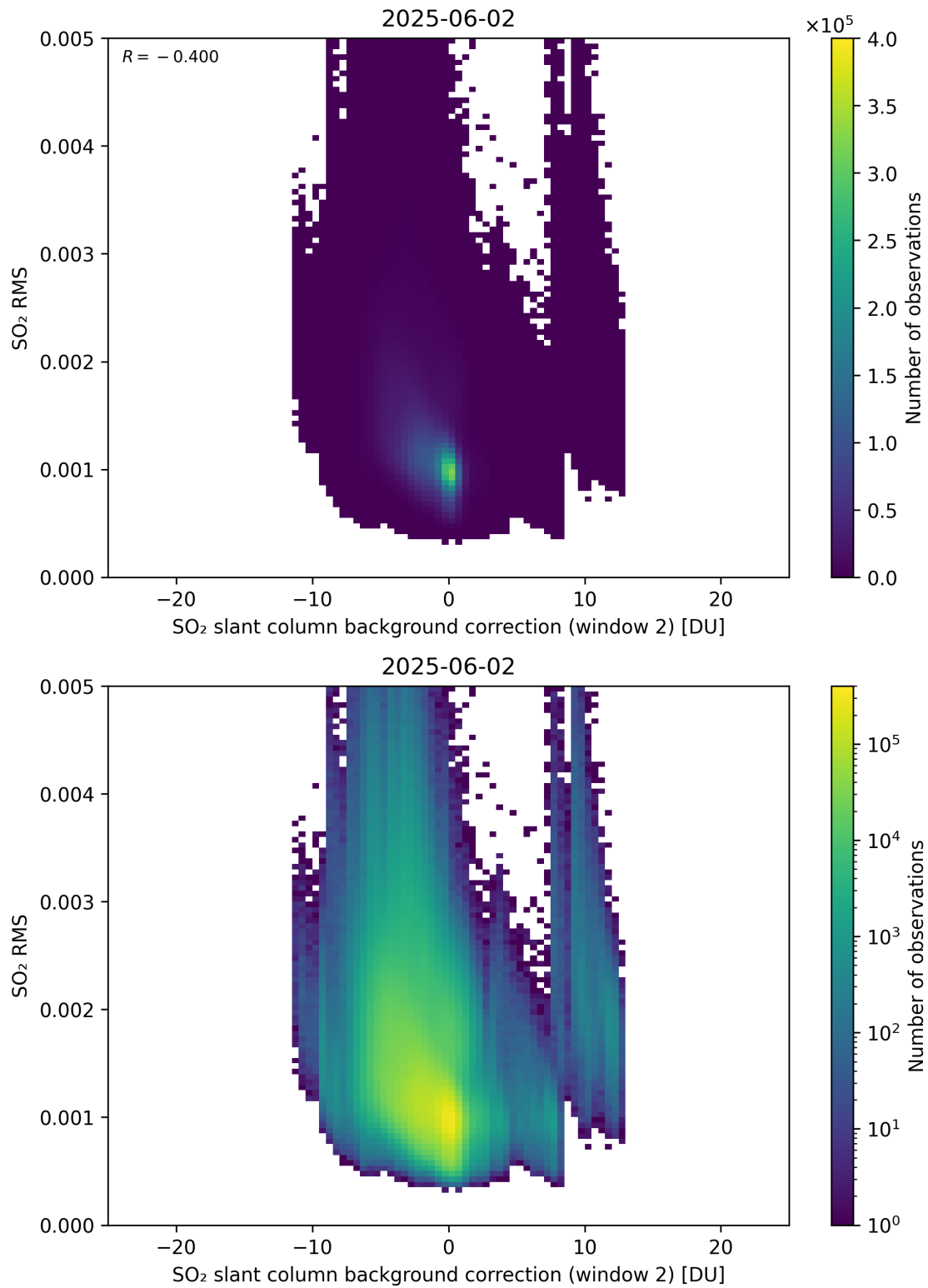
Figure 125: Scatter density plot of “SO 2 slant column background correction (window 2)” against “SO 2 RMS” for 2025-06-01 to 2025-06-03.
