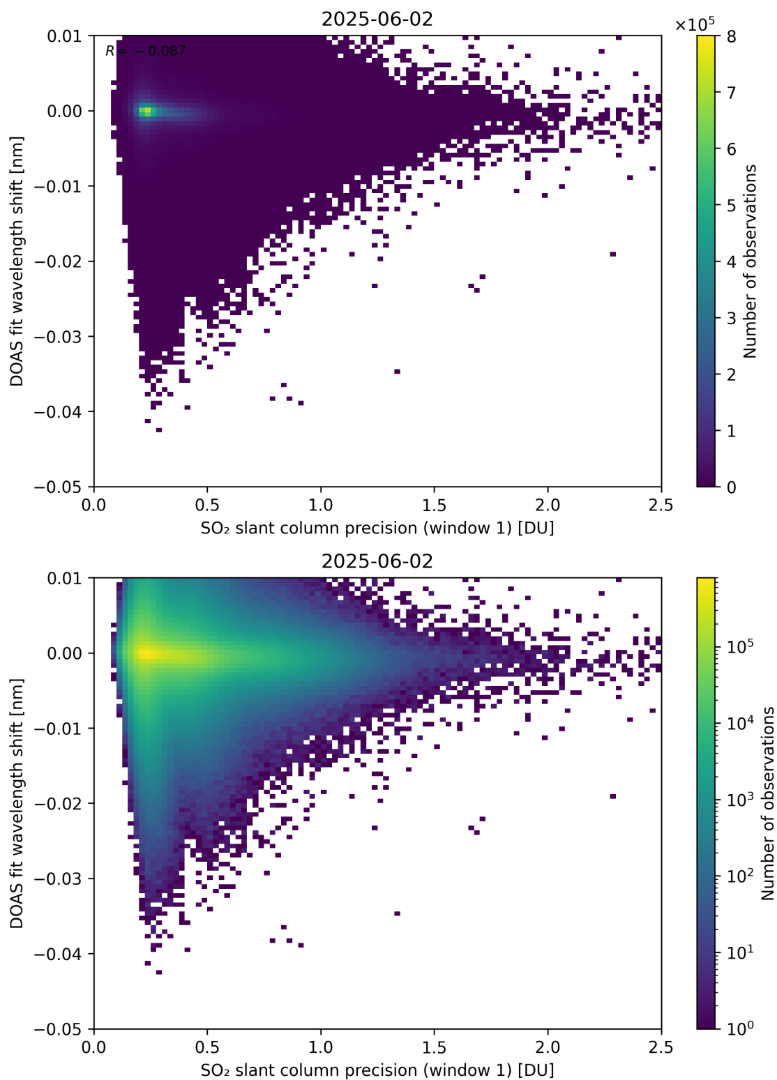
Figure 271: Scatter density plot of “SO 2 slant column precision (window 1)” against “DOAS fit wavelength shift” for 2025-06-01 to 2025-06-03.
