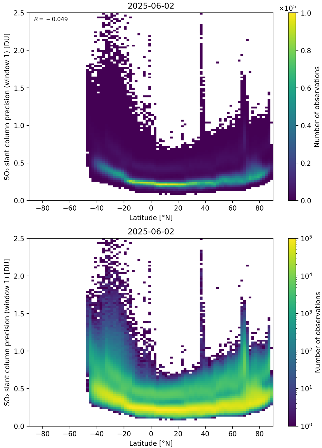
Figure 163: Scatter density plot of “Latitude” against “SO 2 slant column precision (window 1)” for 2025-06-01 to 2025-06-03.
