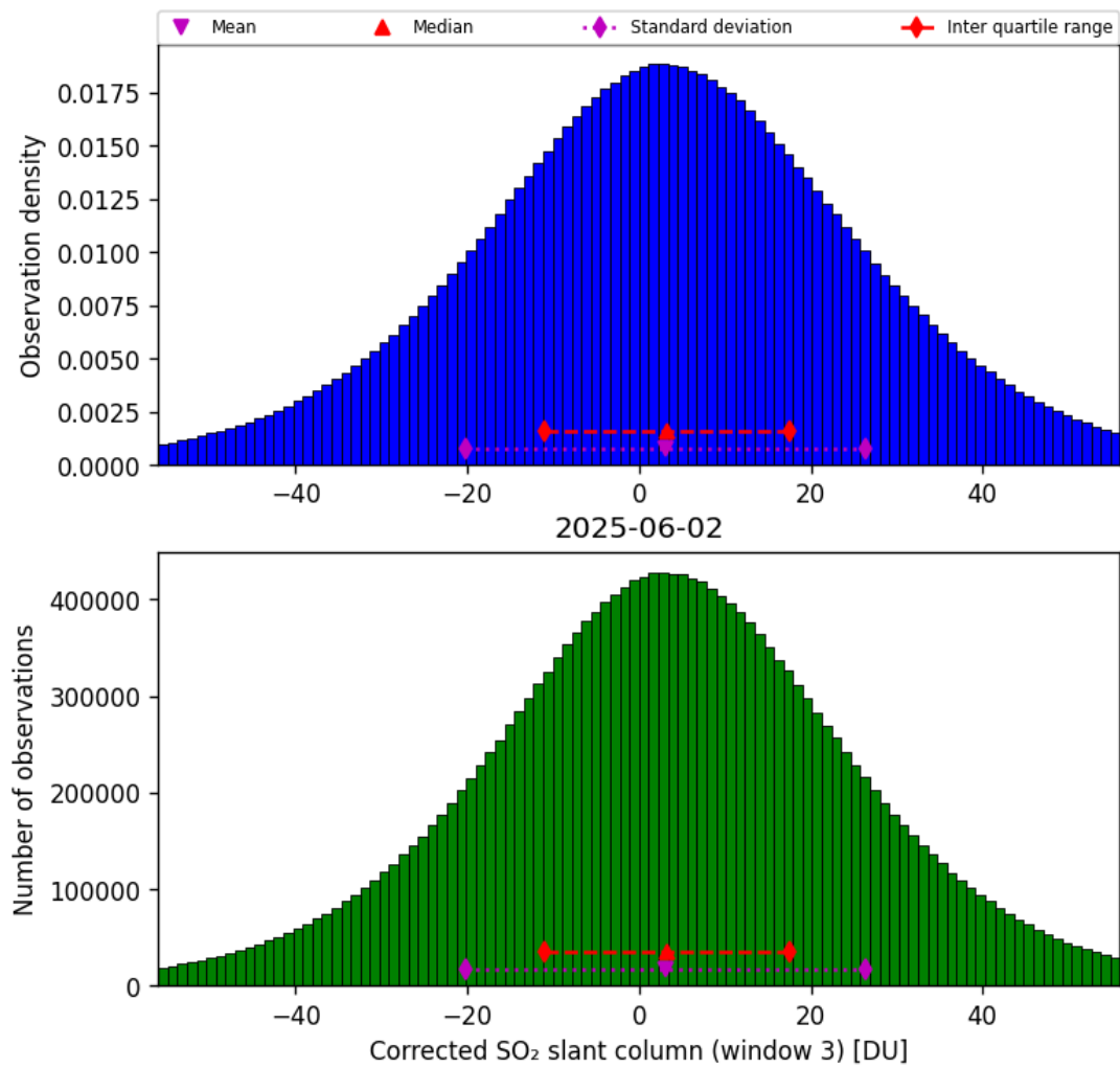
Figure 73: Histogram of “Corrected SO 2 slant column (window 3)” for 2025-06-01 to 2025-06-03
