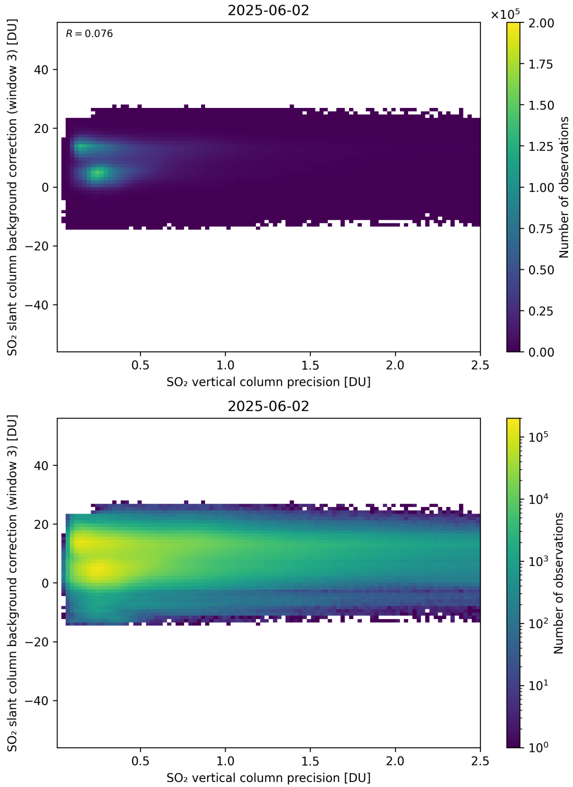
Figure 331: Scatter density plot of “SO 2 vertical column precision” against “SO 2 slant column background correction (window 3)” for 2025-06-01 to 2025-06-03.
