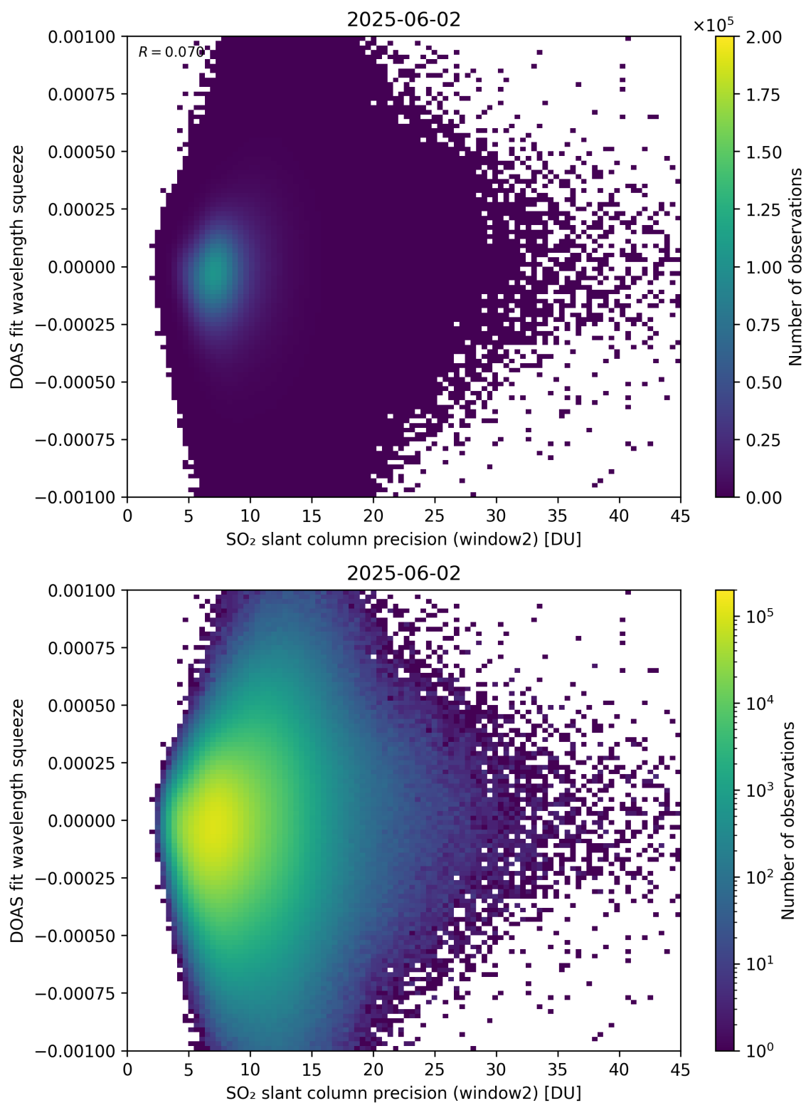
Figure 294: Scatter density plot of “SO 2 slant column precision (window2)” against “DOAS fit wavelength squeeze” for 2025-06-01 to 2025-06-03.
