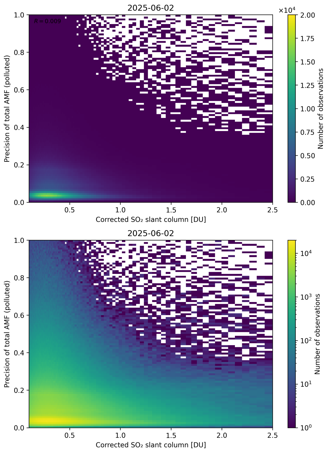
Figure 243: Scatter density plot of “Corrected SO 2 slant column” against “Precision of total AMF (polluted)” for 2025-06-01 to 2025-06-03.
