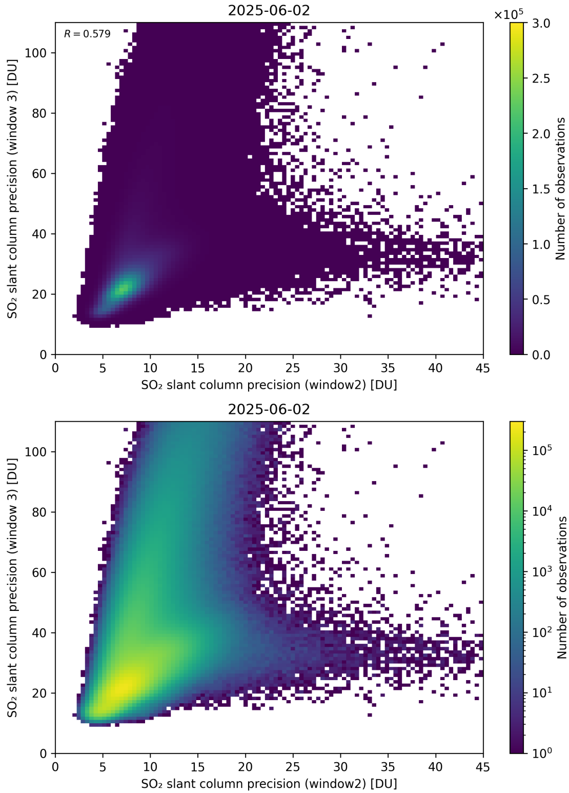
Figure 300: Scatter density plot of “SO 2 slant column precision (window2)” against “SO 2 slant column precision (window 3)” for 2025-06-01 to 2025-06-03.
