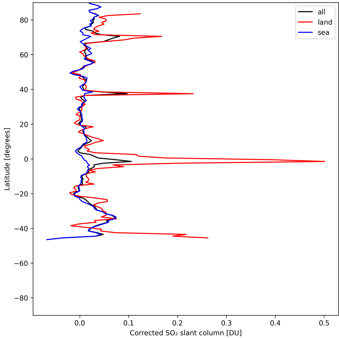
Figure 34: Zonal average of “Corrected SO 2 slant column” for 2025-06-01 to 2025-06-03.
