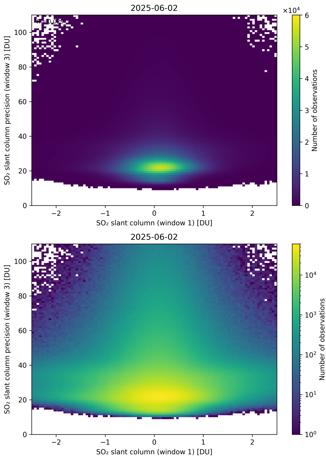
Figure 288: Scatter density plot of “SO 2 slant column (window 1)” against “SO 2 slant column precision (window 3)” for 2025-06-01 to 2025-06-03.
