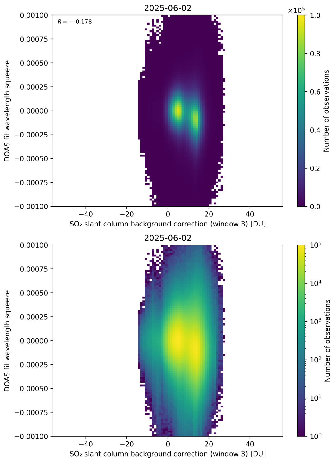
Figure 133: Scatter density plot of “SO 2 slant column background correction (window 3)” against “DOAS fit wavelength squeeze” for 2025-06-01 to 2025-06-03.
