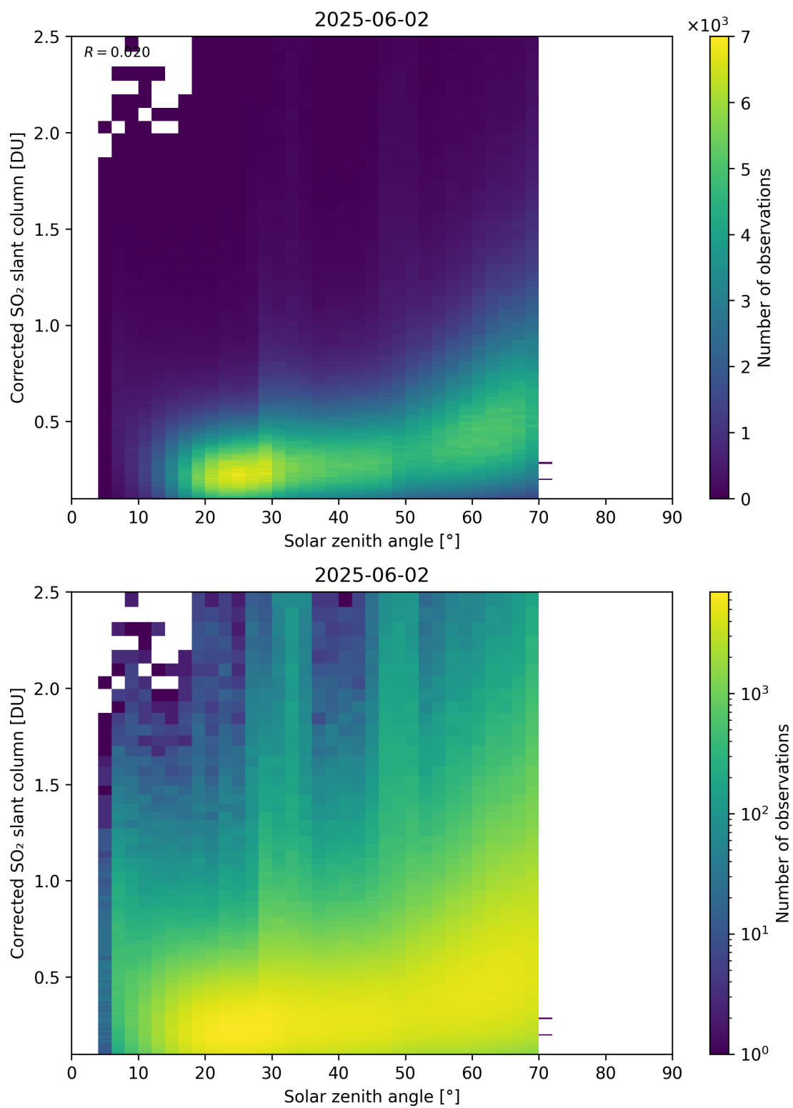
Figure 181: Scatter density plot of “Solar zenith angle” against “Corrected SO 2 slant column” for 2025-06-01 to 2025-06-03.
