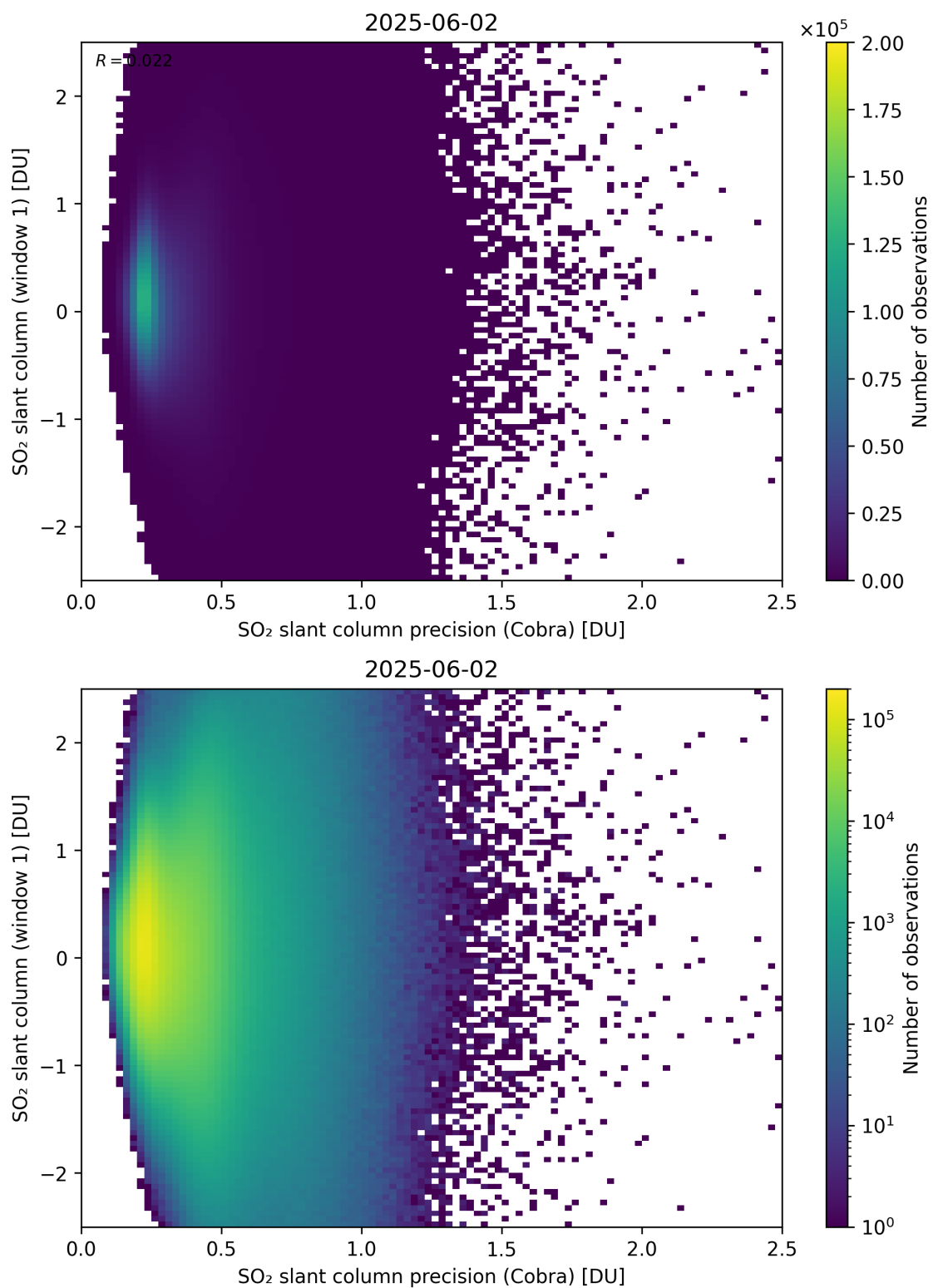
Figure 208: Scatter density plot of “SO 2 slant column precision (Cobra)” against “SO 2 slant column (window 1)” for 2025-06-01 to 2025-06-03.
