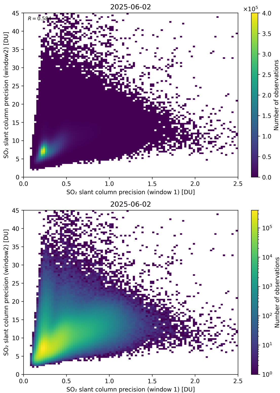
Figure 277: Scatter density plot of “SO 2 slant column precision (window 1)” against “SO 2 slant column precision (window2)” for 2025-06-01 to 2025-06-03.
