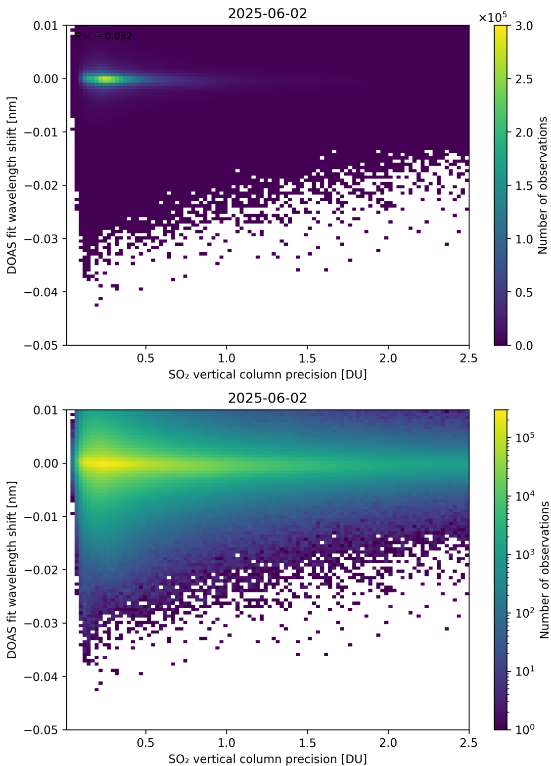
Figure 332: Scatter density plot of “SO 2 vertical column precision” against “DOAS fit wavelength shift” for 2025-06-01 to 2025-06-03.
