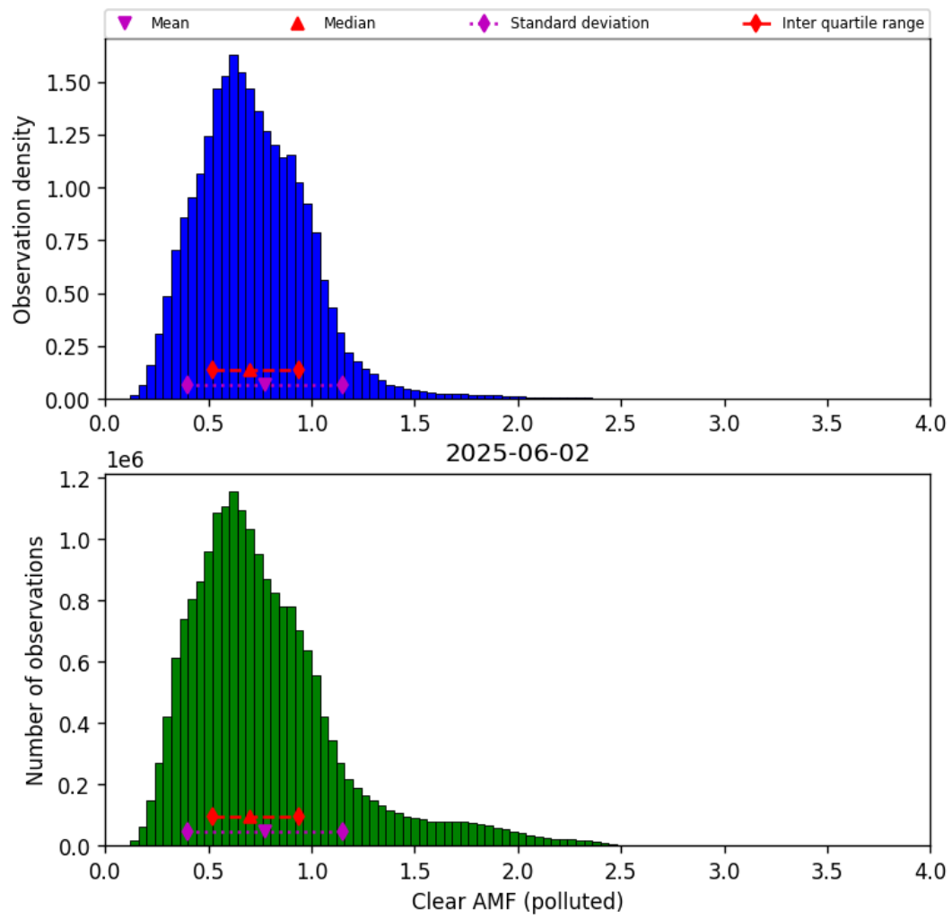
Figure 81: Histogram of “Clear AMF (polluted)” for 2025-06-01 to 2025-06-03
