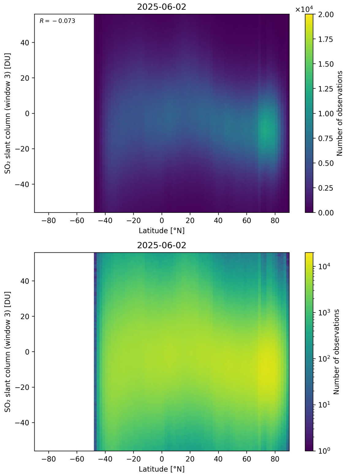
Figure 165: Scatter density plot of “Latitude” against “SO 2 slant column (window 3)” for 2025-06-01 to 2025-06-03.
