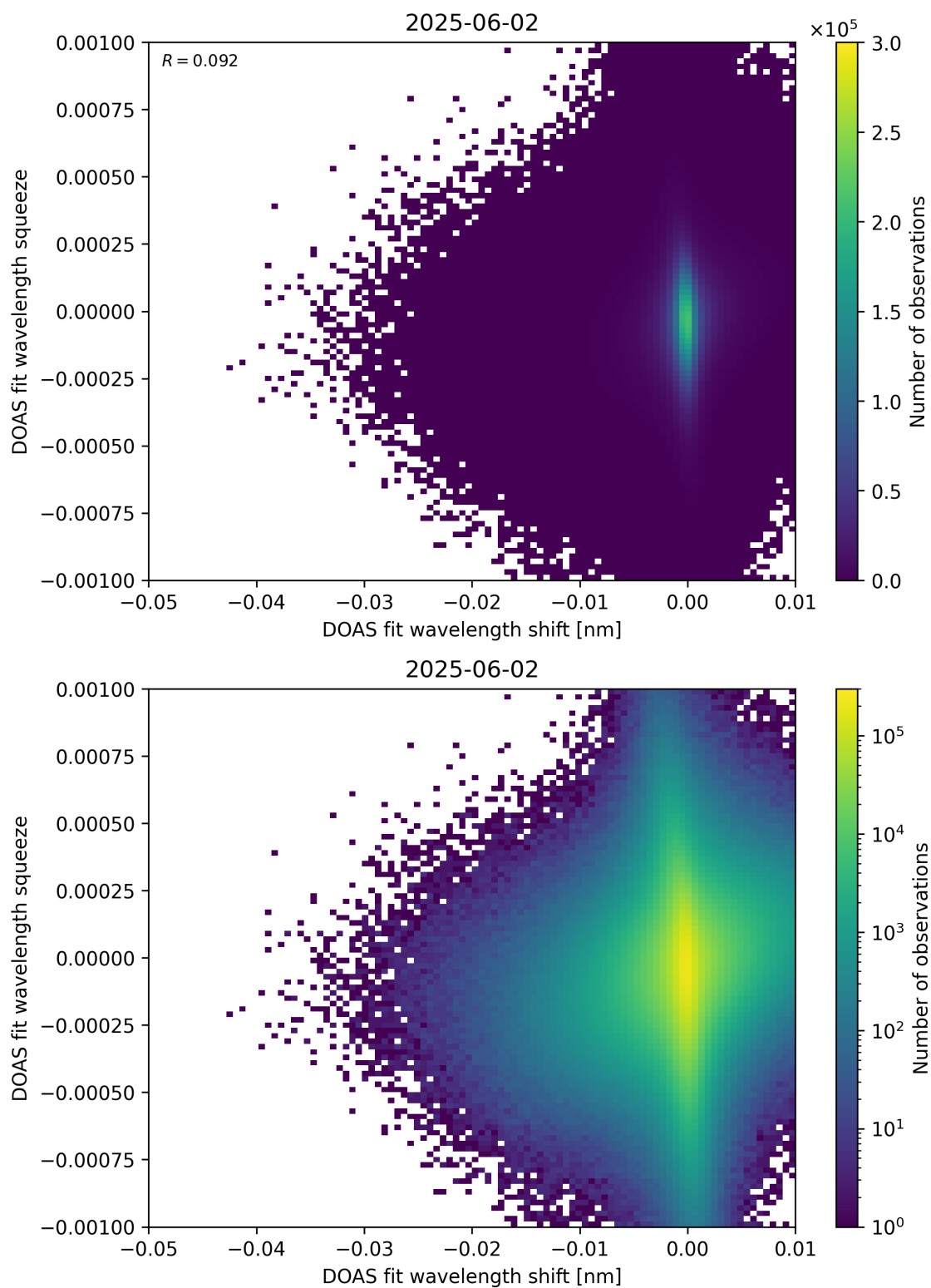
Figure 138: Scatter density plot of “DOAS fit wavelength shift” against “DOAS fit wavelength squeeze” for 2025-06-01 to 2025-06-03.
