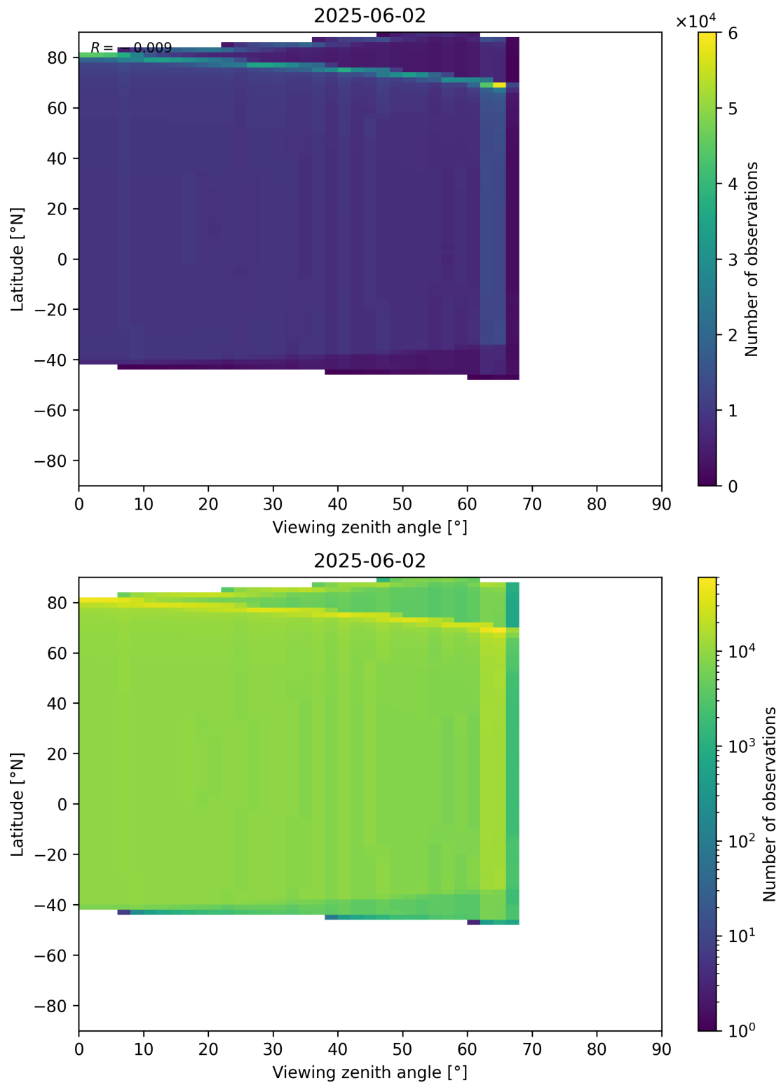
Figure 368: Scatter density plot of “Viewing zenith angle” against “Latitude” for 2025-06-01 to 2025-06-03.
