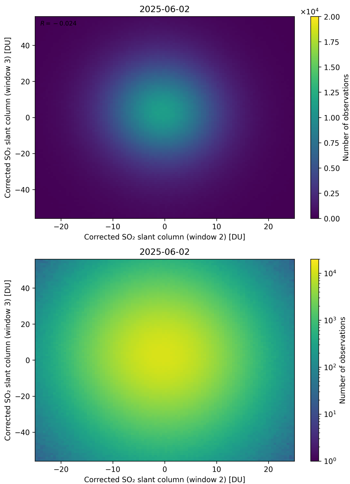
Figure 250: Scatter density plot of “Corrected SO 2 slant column (window 2)” against “Corrected SO 2 slant column (window 3)” for 2025-06-01 to 2025-06-03.
