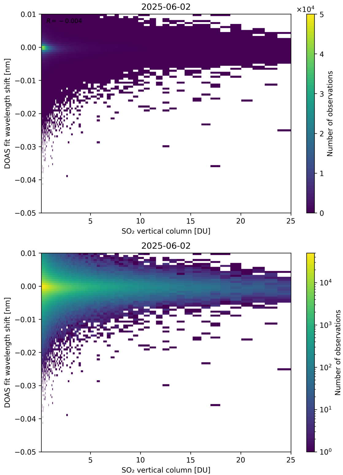
Figure 326: Scatter density plot of “SO 2 vertical column” against “DOAS fit wavelength shift” for 2025-06-01 to 2025-06-03.
