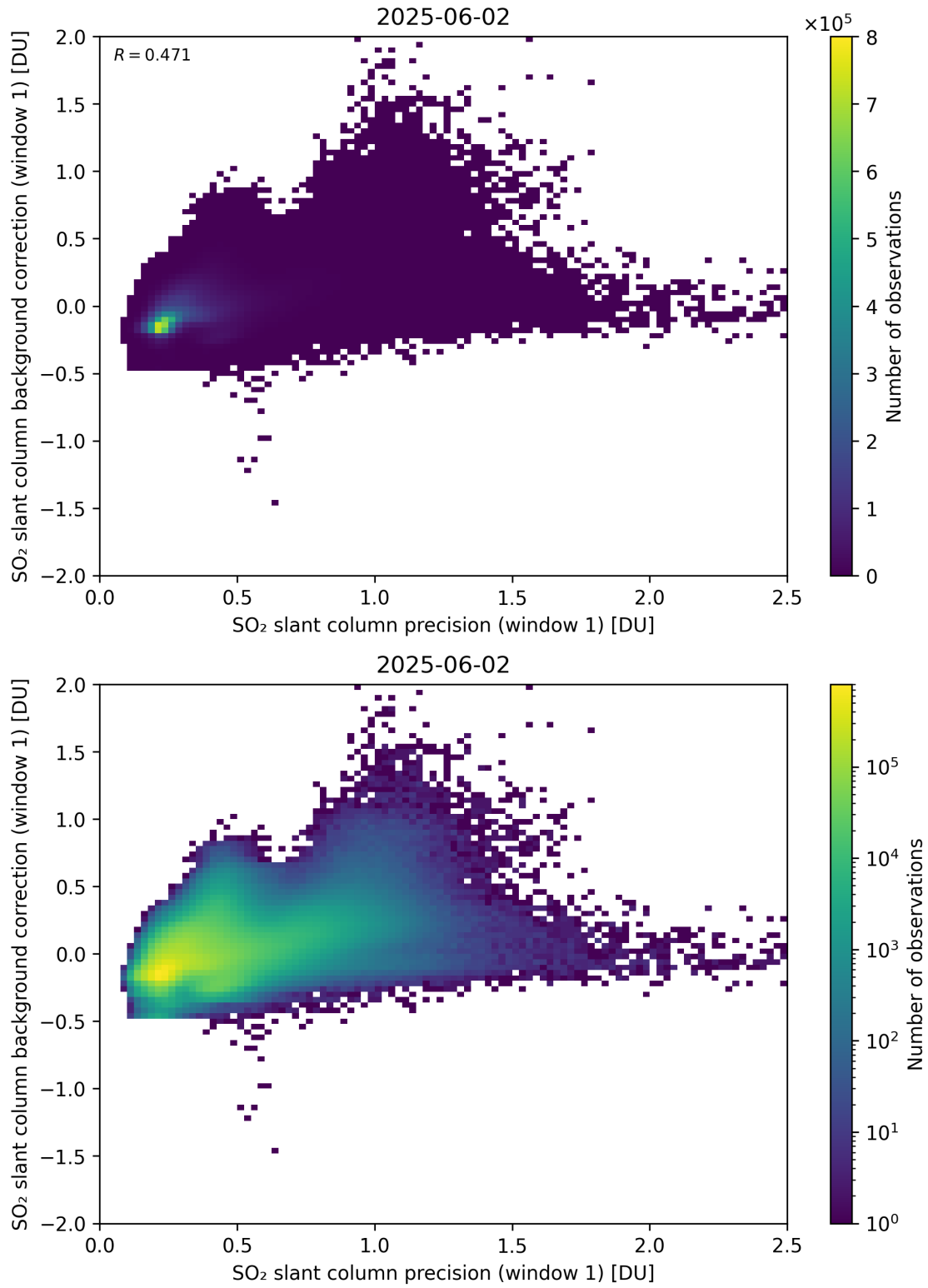
Figure 268: Scatter density plot of “SO 2 slant column precision (window 1)” against “SO 2 slant column background correction (window 1)” for 2025-06-01 to 2025-06-03.
