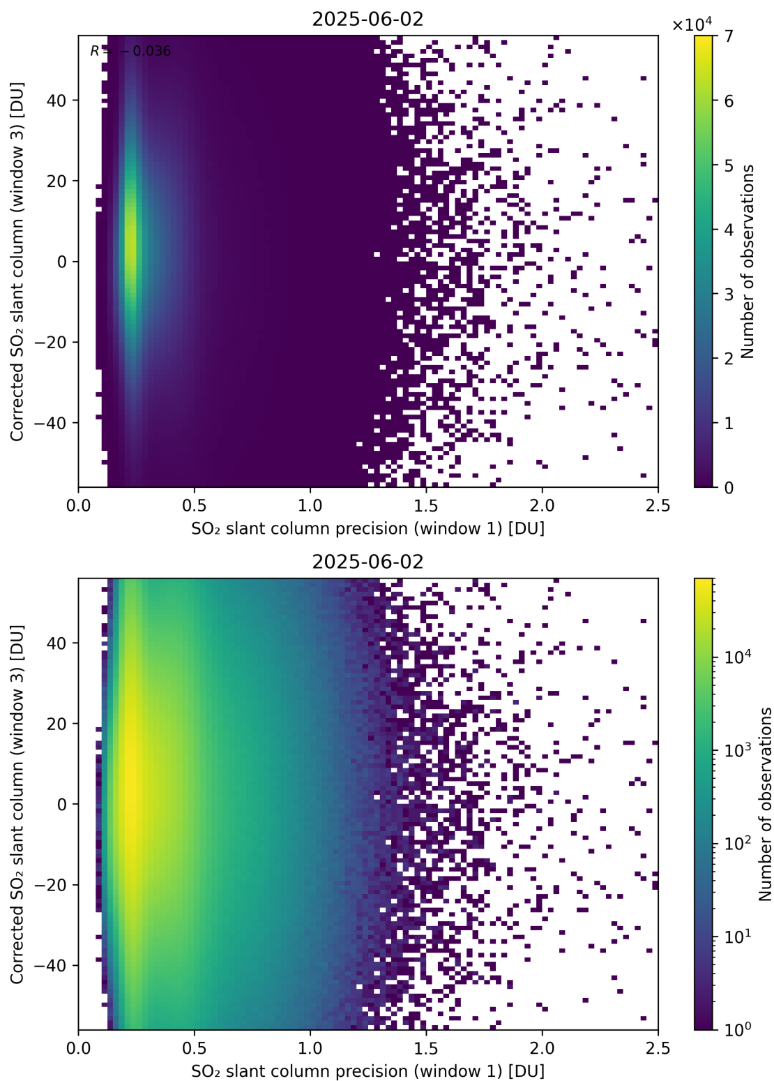
Figure 276: Scatter density plot of “SO 2 slant column precision (window 1)” against “Corrected SO 2 slant column (window 3)” for 2025-06-01 to 2025-06-03.
