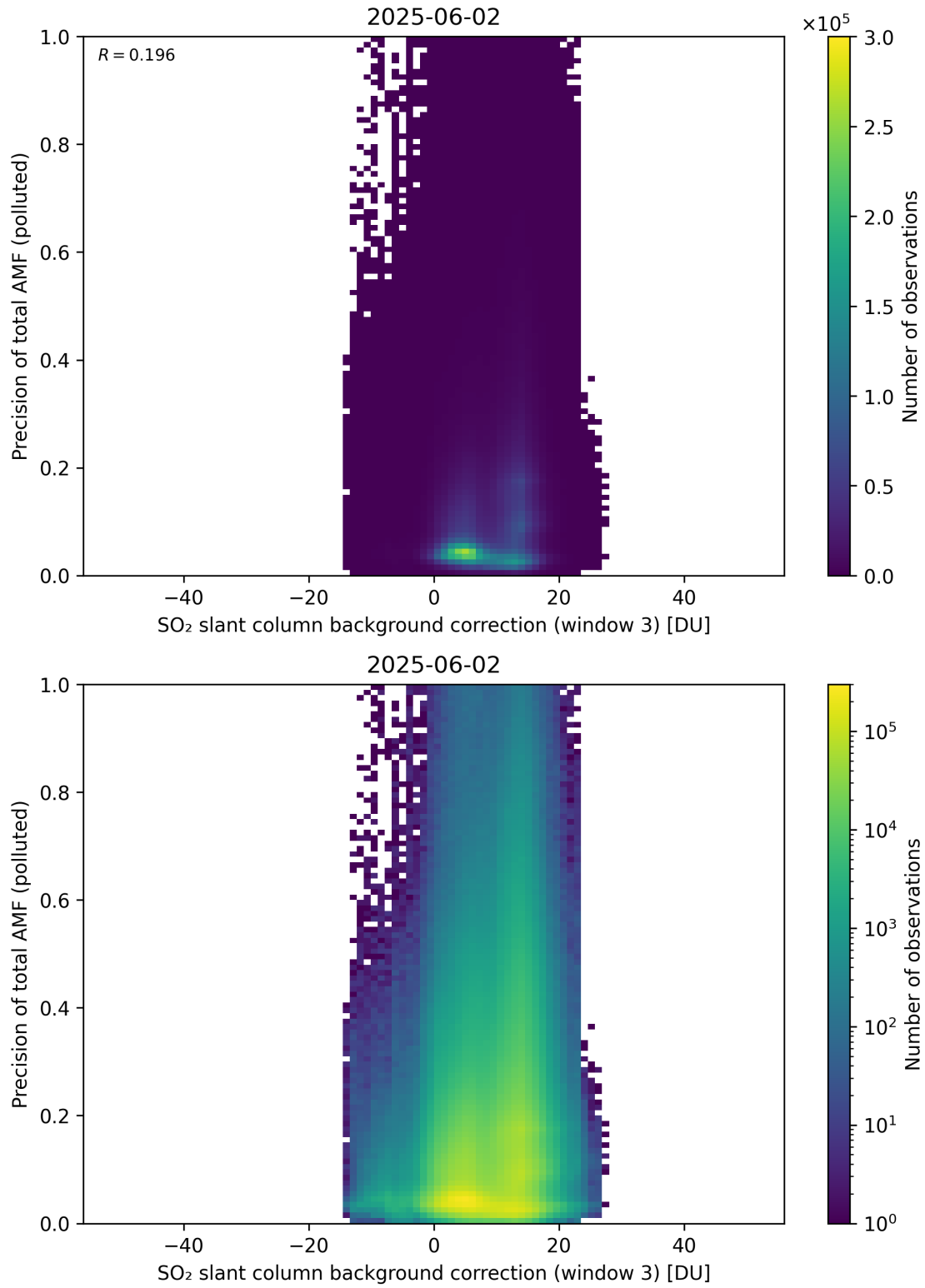
Figure 137: Scatter density plot of “SO 2 slant column background correction (window 3)” against “Precision of total AMF (polluted)” for 2025-06-01 to 2025-06-03.
