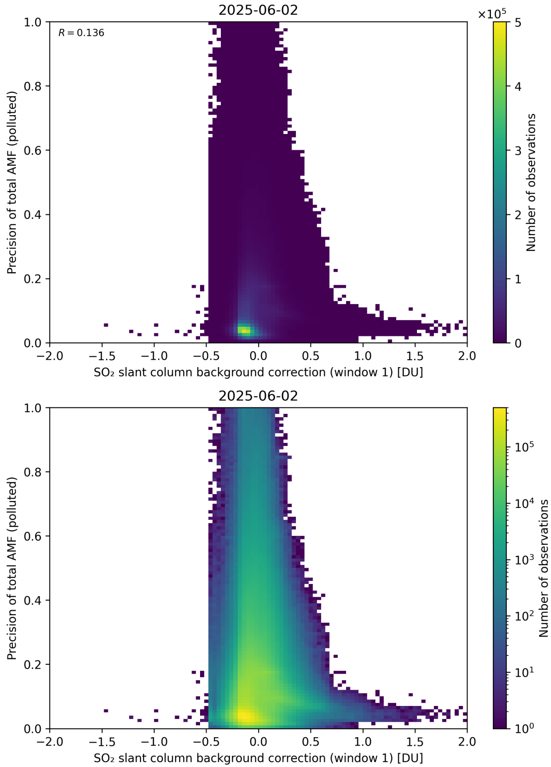
Figure 121: Scatter density plot of “SO 2 slant column background correction (window 1)” against “Precision of total AMF (polluted)” for 2025-06-01 to 2025-06-03.
