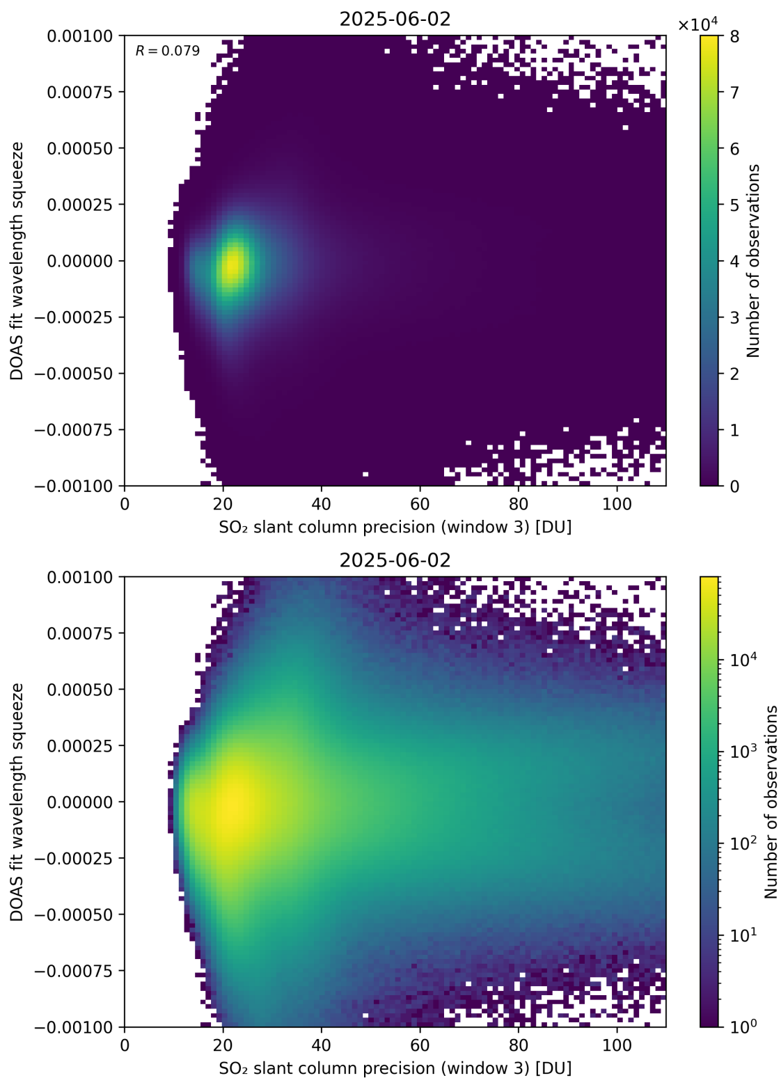
Figure 309: Scatter density plot of “SO 2 slant column precision (window 3)” against “DOAS fit wavelength squeeze” for 2025-06-01 to 2025-06-03.
