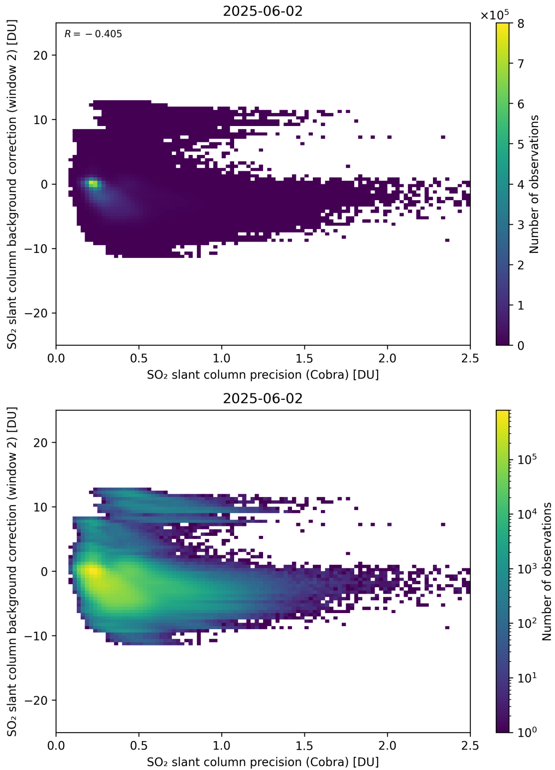
Figure 200: Scatter density plot of “SO 2 slant column precision (Cobra)” against “SO 2 slant column background correction (window 2)” for 2025-06-01 to 2025-06-03.
