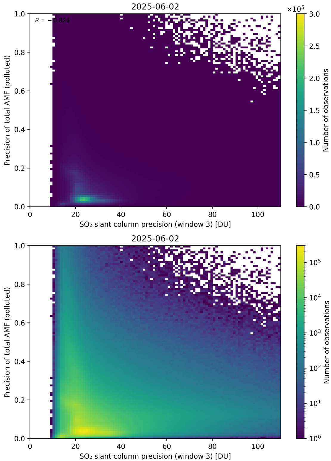
Figure 314: Scatter density plot of “SO 2 slant column precision (window 3)” against “Precision of total AMF (polluted)” for 2025-06-01 to 2025-06-03.
