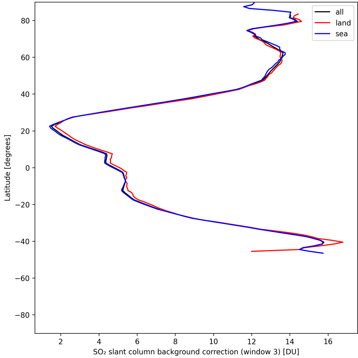
Figure 48: Zonal average of “SO 2 slant column background correction (window 3)” for 2025-06-01 to 2025-06-03.
