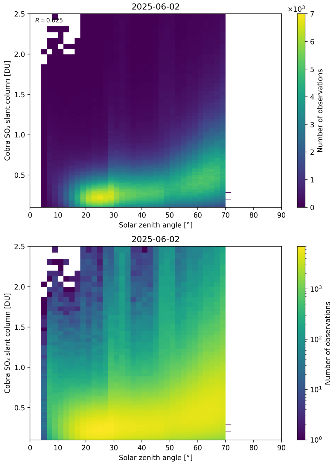
Figure 179: Scatter density plot of “Solar zenith angle” against “Cobra SO 2 slant column” for 2025-06-01 to 2025-06-03.
