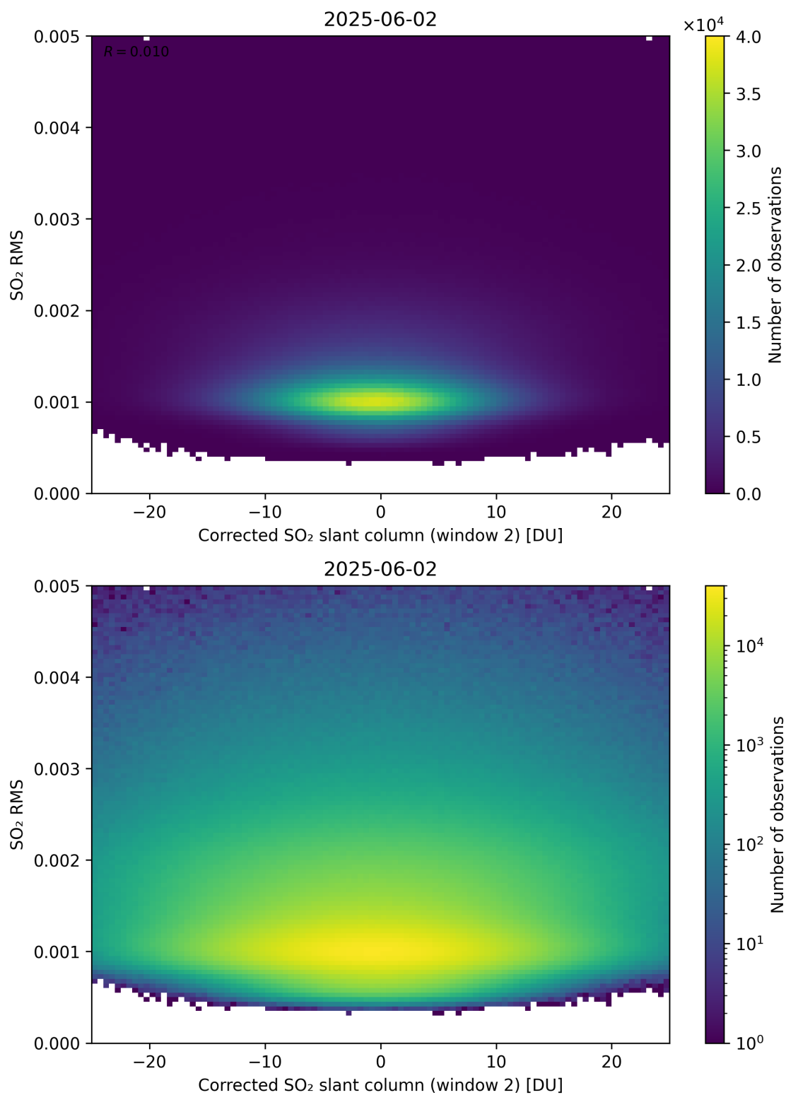
Figure 248: Scatter density plot of “Corrected SO 2 slant column (window 2)” against “SO 2 RMS” for 2025-06-01 to 2025-06-03.
