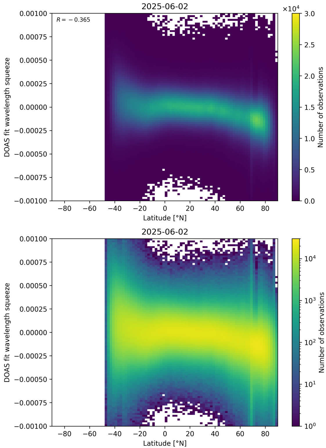
Figure 154: Scatter density plot of “Latitude” against “DOAS fit wavelength squeeze” for 2025-06-01 to 2025-06-03.
