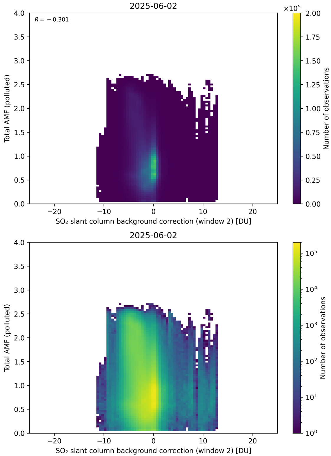
Figure 130: Scatter density plot of “SO 2 slant column background correction (window 2)” against “Total AMF (polluted)” for 2025-06-01 to 2025-06-03.
