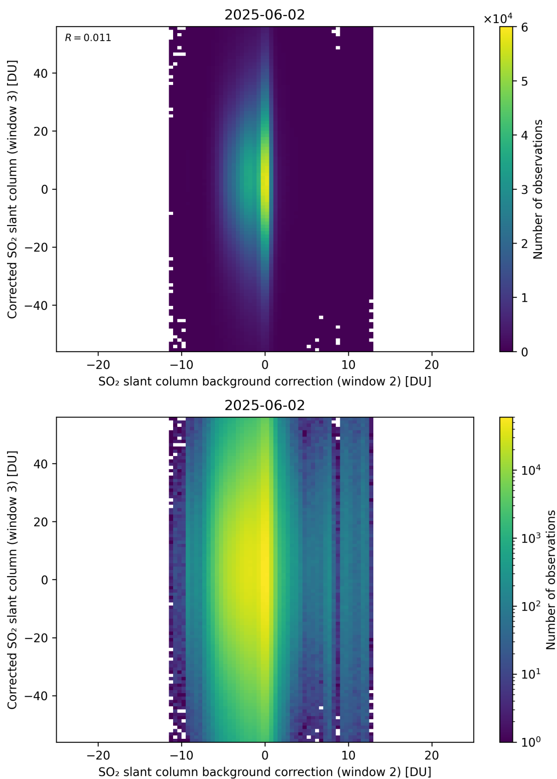
Figure 127: Scatter density plot of “SO 2 slant column background correction (window 2)” against “Corrected SO 2 slant column (window 3)” for 2025-06-01 to 2025-06-03.
