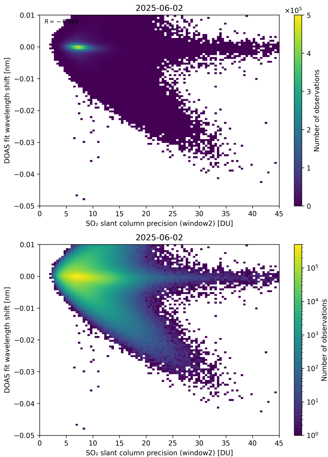
Figure 293: Scatter density plot of “SO 2 slant column precision (window2)” against “DOAS fit wavelength shift” for 2025-06-01 to 2025-06-03.
