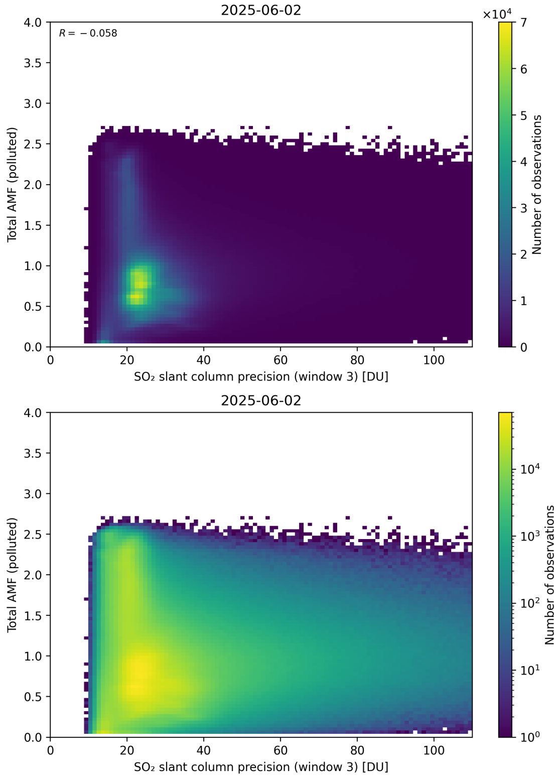
Figure 313: Scatter density plot of “SO 2 slant column precision (window 3)” against “Total AMF (polluted)” for 2025-06-01 to 2025-06-03.
