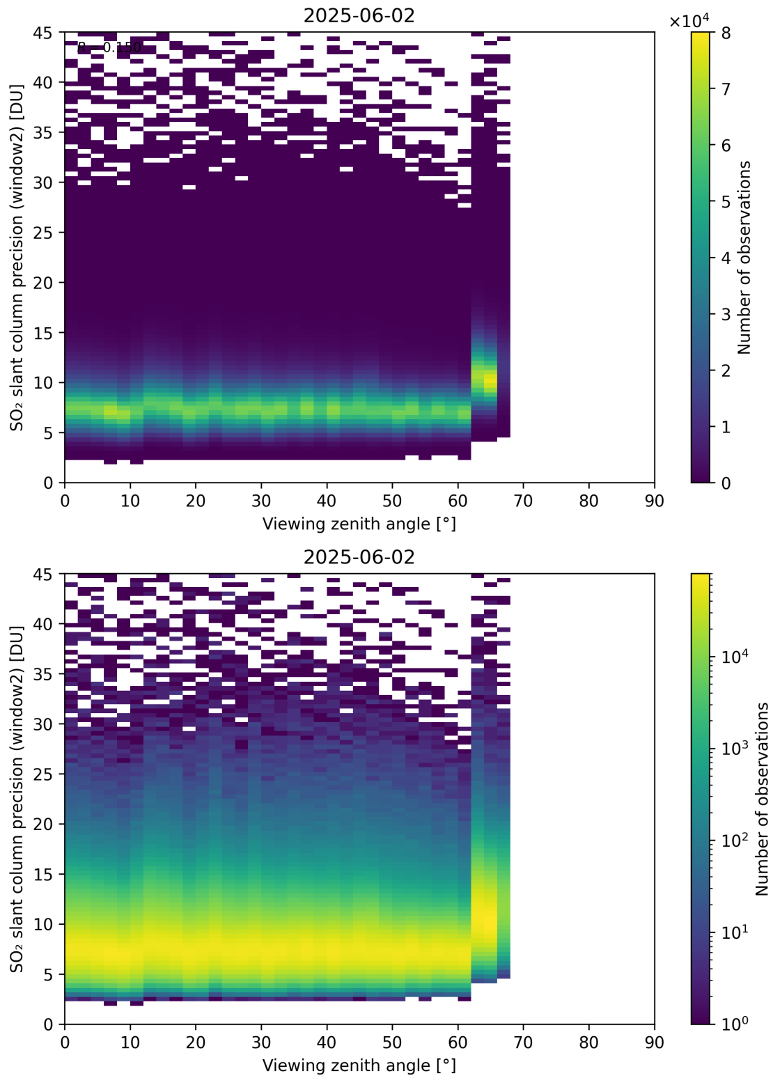
Figure 378: Scatter density plot of “Viewing zenith angle” against “SO 2 slant column precision (window2)” for 2025-06-01 to 2025-06-03.
