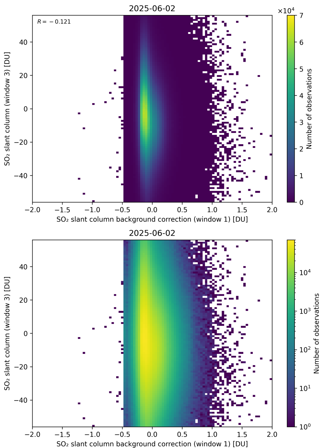
Figure 118: Scatter density plot of “SO 2 slant column background correction (window 1)” against “SO 2 slant column (window 3)” for 2025-06-01 to 2025-06-03.
