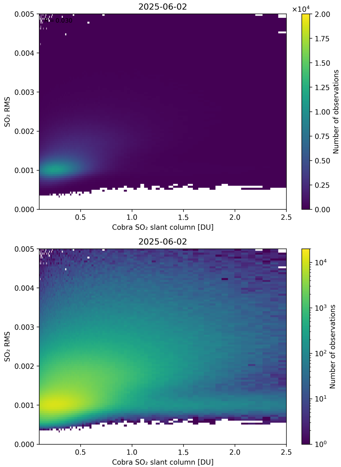
Figure 198: Scatter density plot of “Cobra SO 2 slant column” against “SO 2 RMS” for 2025-06-01 to 2025-06-03.
