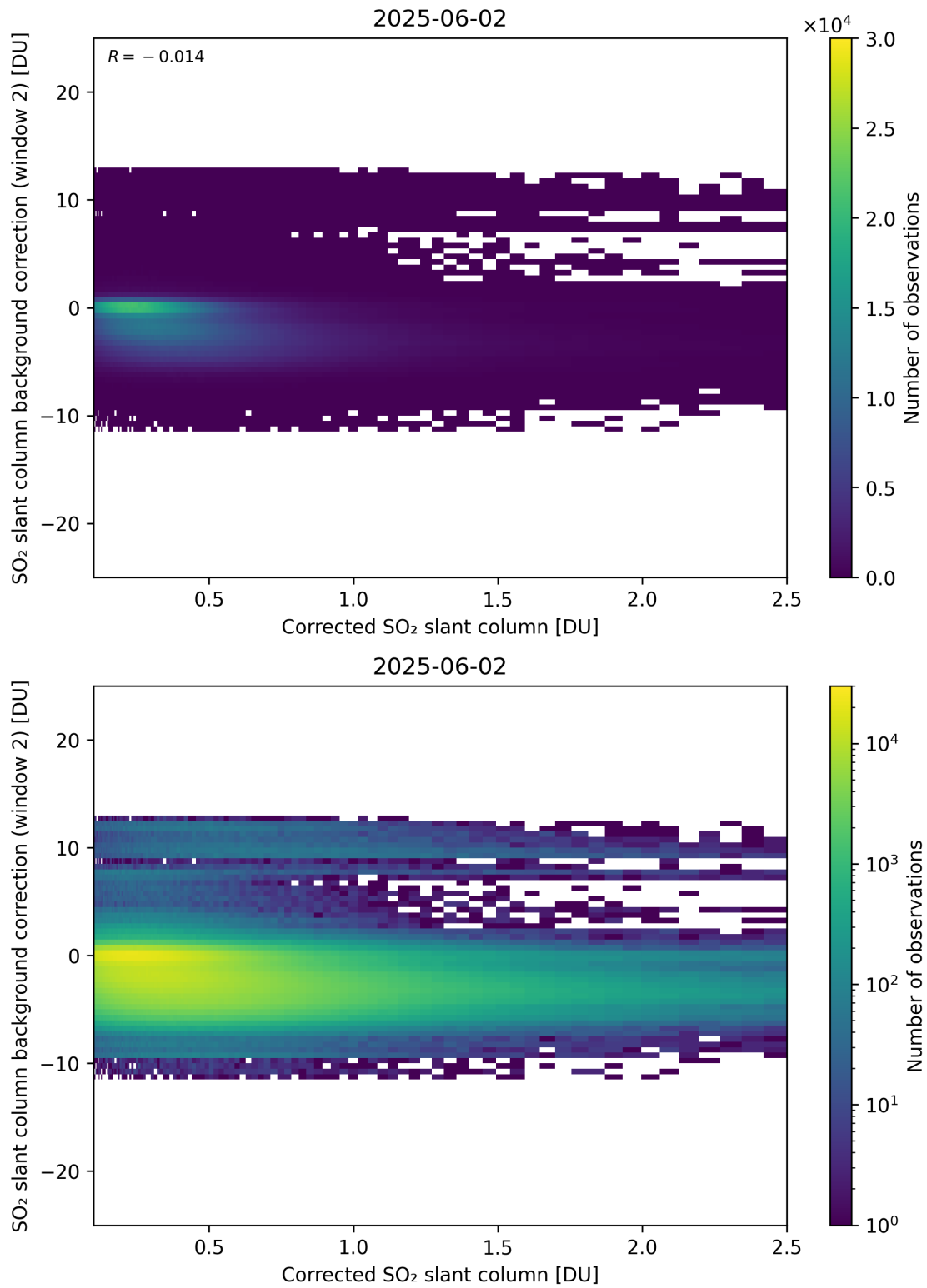
Figure 227: Scatter density plot of “Corrected SO 2 slant column” against “SO 2 slant column background correction (window 2)” for 2025-06-01 to 2025-06-03.
