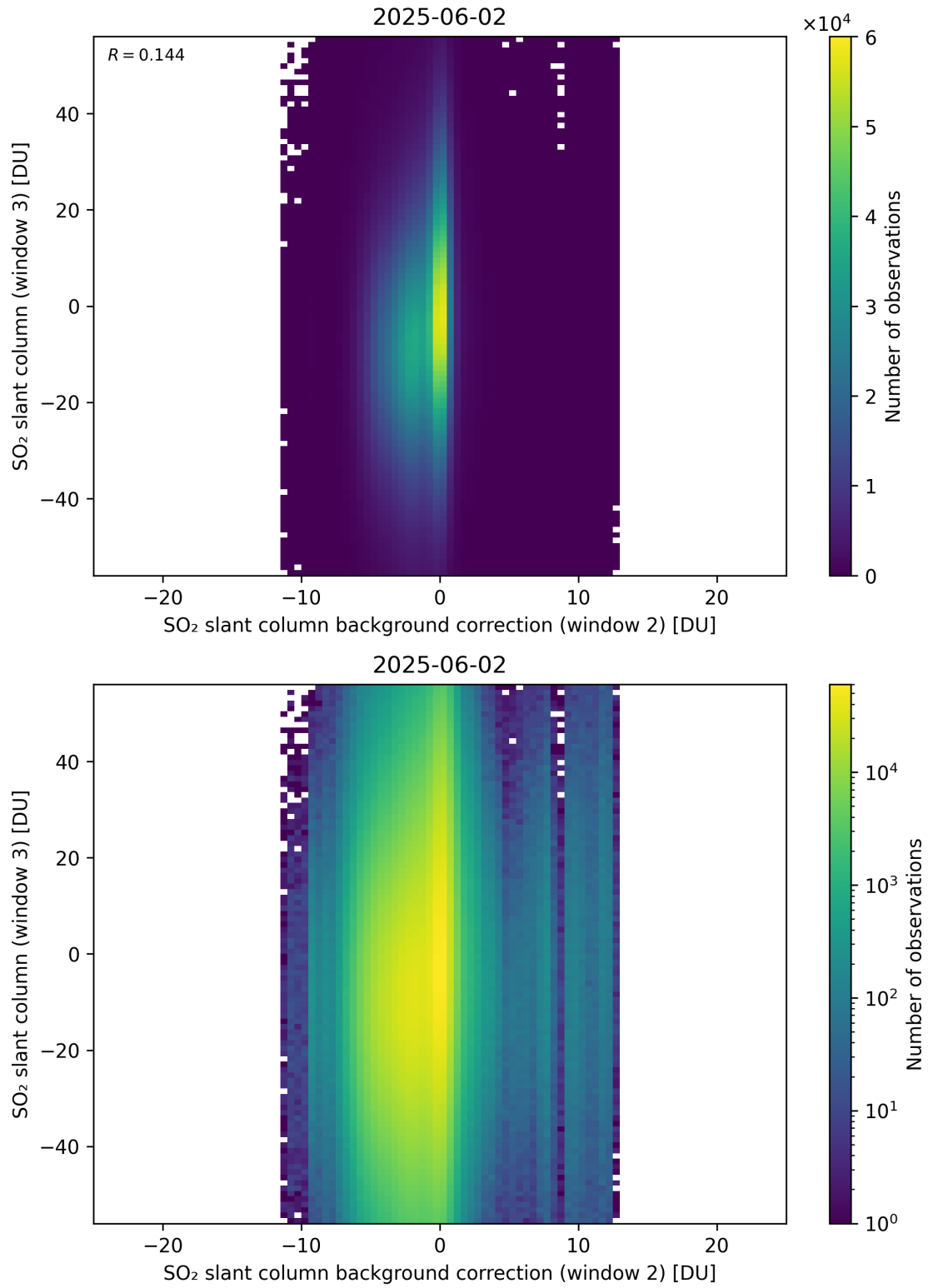
Figure 128: Scatter density plot of “SO 2 slant column background correction (window 2)” against “SO 2 slant column (window 3)” for 2025-06-01 to 2025-06-03.
