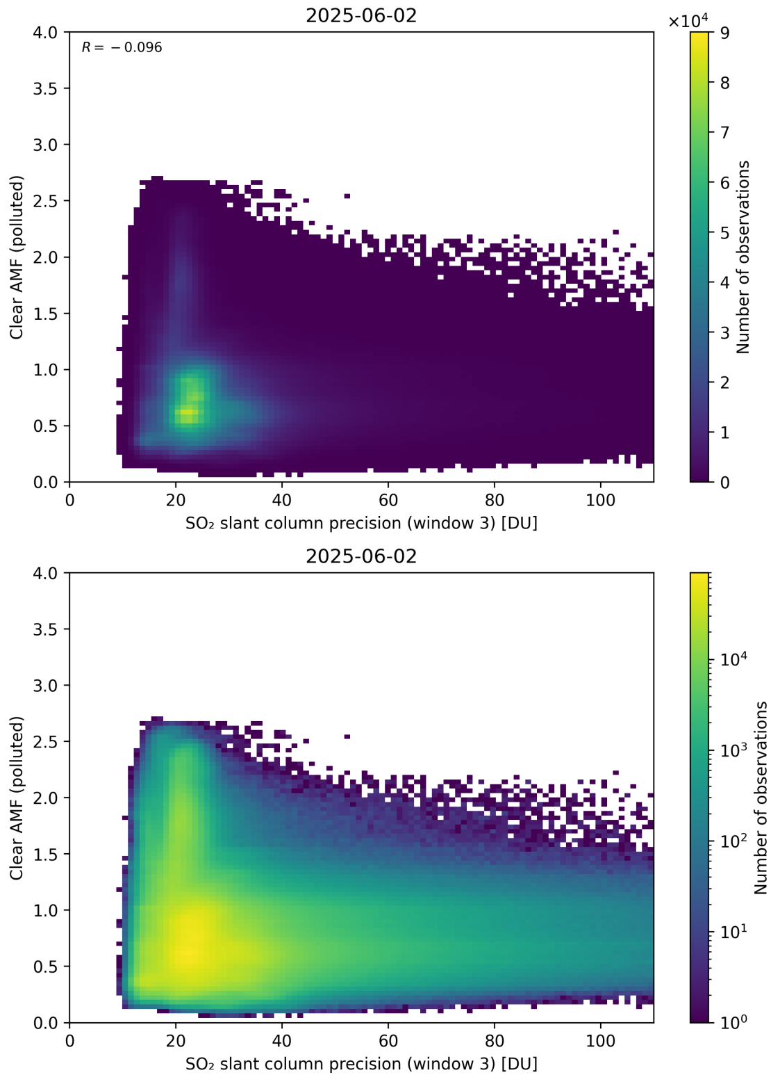
Figure 311: Scatter density plot of “SO 2 slant column precision (window 3)” against “Clear AMF (polluted)” for 2025-06-01 to 2025-06-03.
