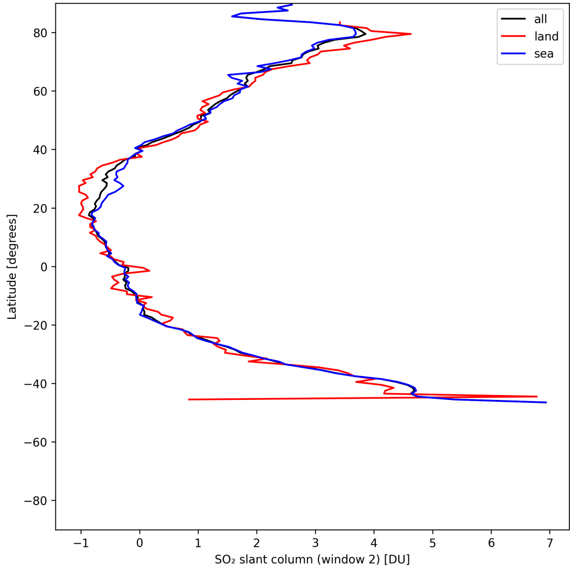
Figure 41: Zonal average of “SO 2 slant column (window 2)” for 2025-06-01 to 2025-06-03.
