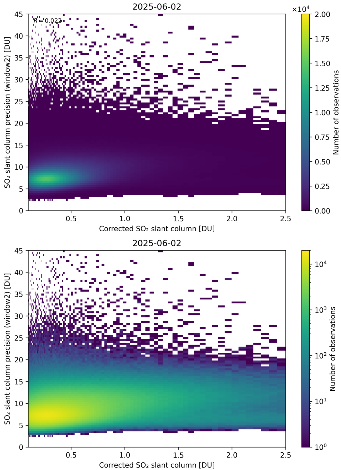
Figure 239: Scatter density plot of “Corrected SO 2 slant column” against “SO 2 slant column precision (window2)” for 2025-06-01 to 2025-06-03.
