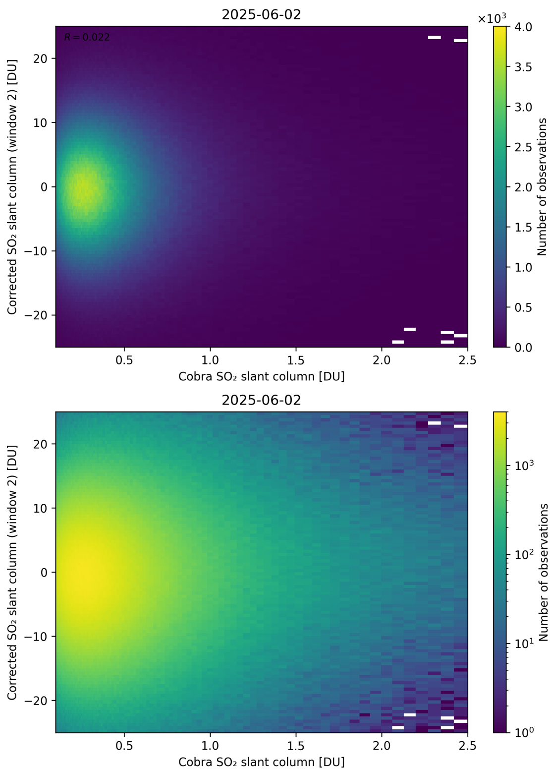
Figure 217: Scatter density plot of “Cobra SO 2 slant column” against “Corrected SO 2 slant column (window 2)” for 2025-06-01 to 2025-06-03.
