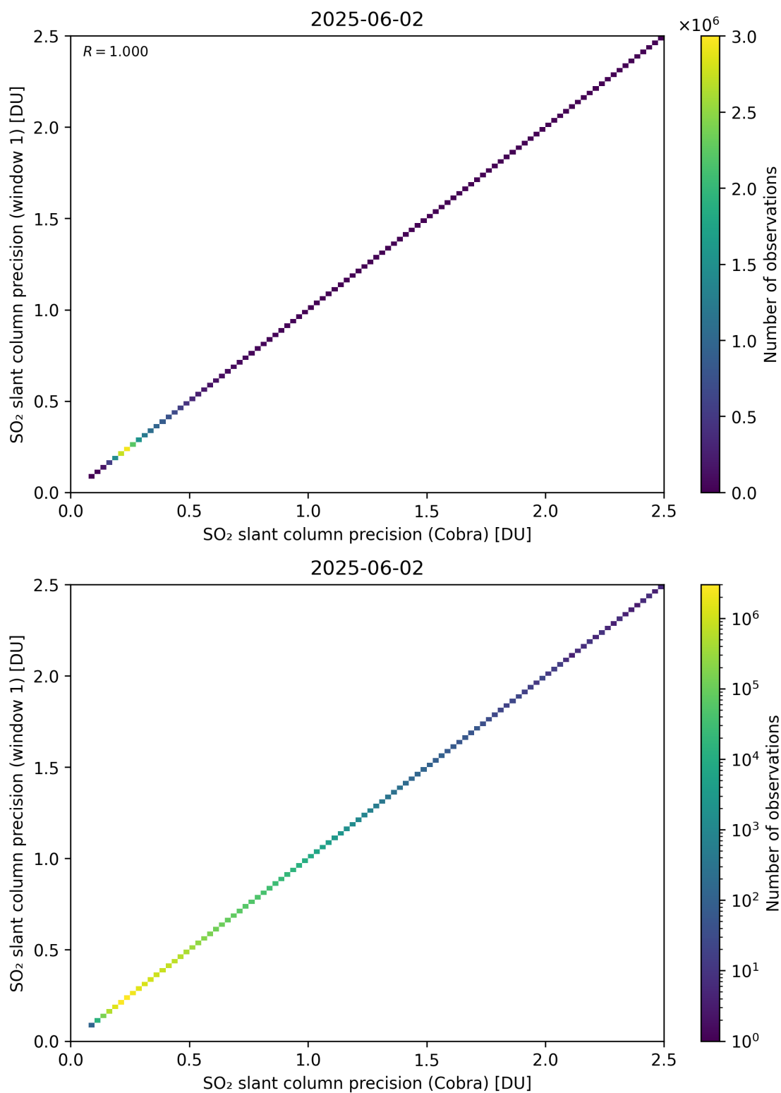
Figure 209: Scatter density plot of “SO 2 slant column precision (Cobra)” against “SO 2 slant column precision (window 1)” for 2025-06-01 to 2025-06-03.
