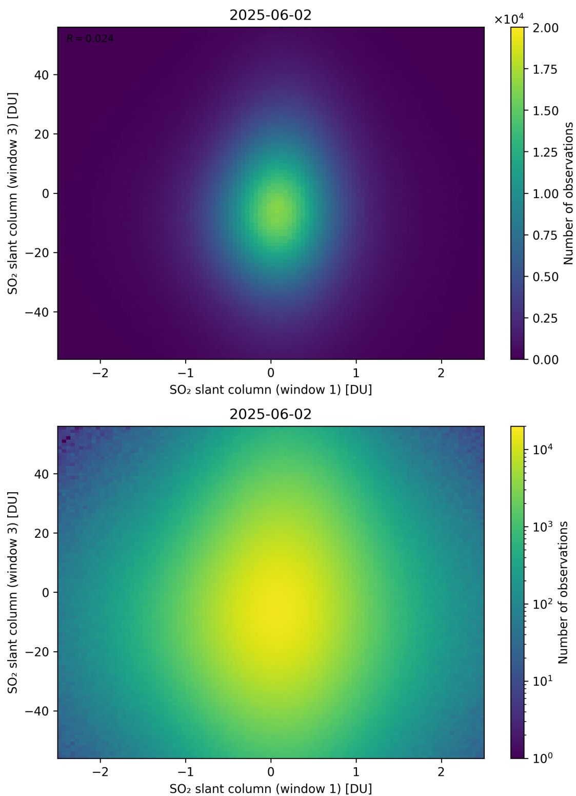
Figure 287: Scatter density plot of “SO 2 slant column (window 1)” against “SO 2 slant column (window 3)” for 2025-06-01 to 2025-06-03.
