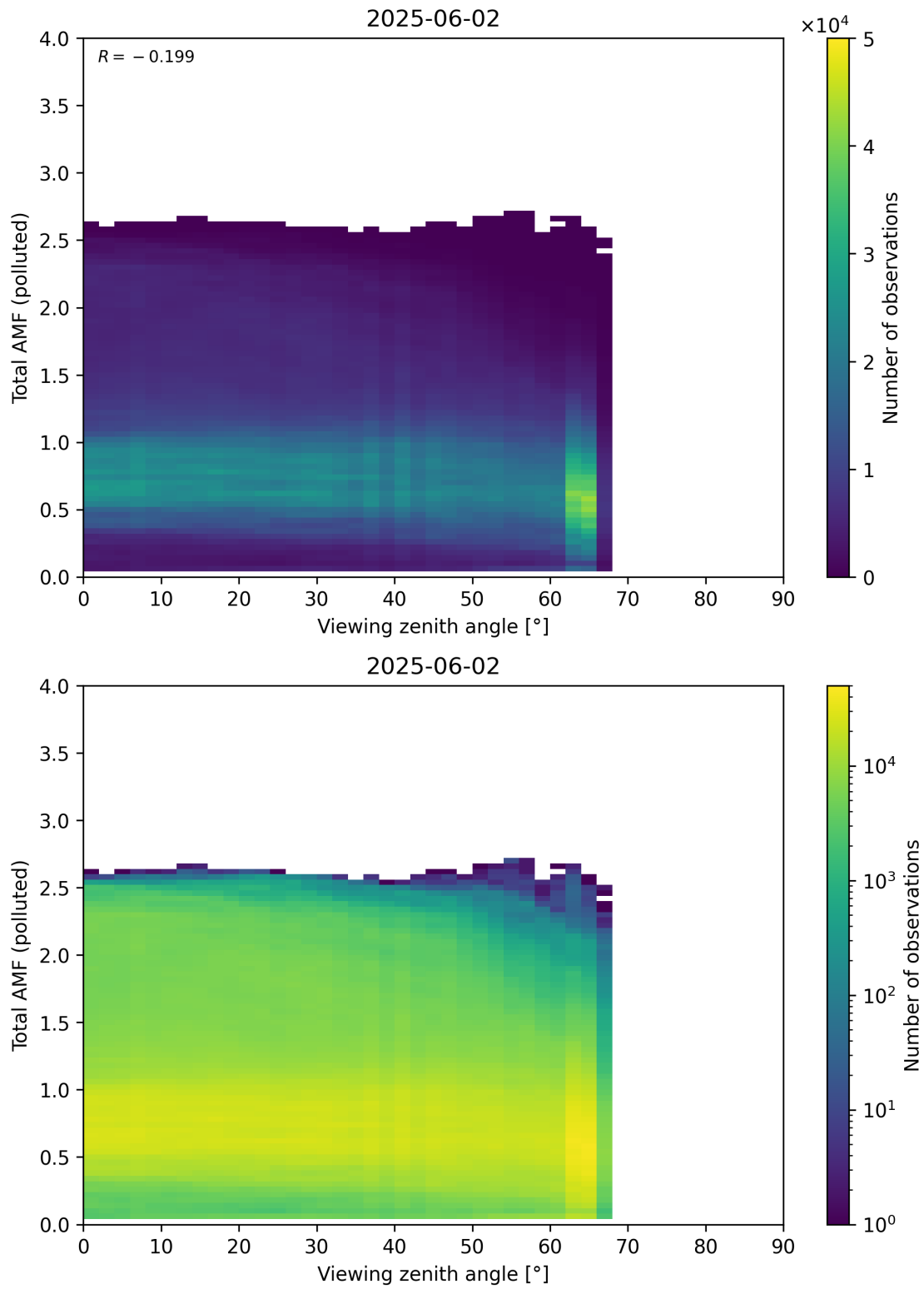
Figure 381: Scatter density plot of “Viewing zenith angle” against “Total AMF (polluted)” for 2025-06-01 to 2025-06-03.
