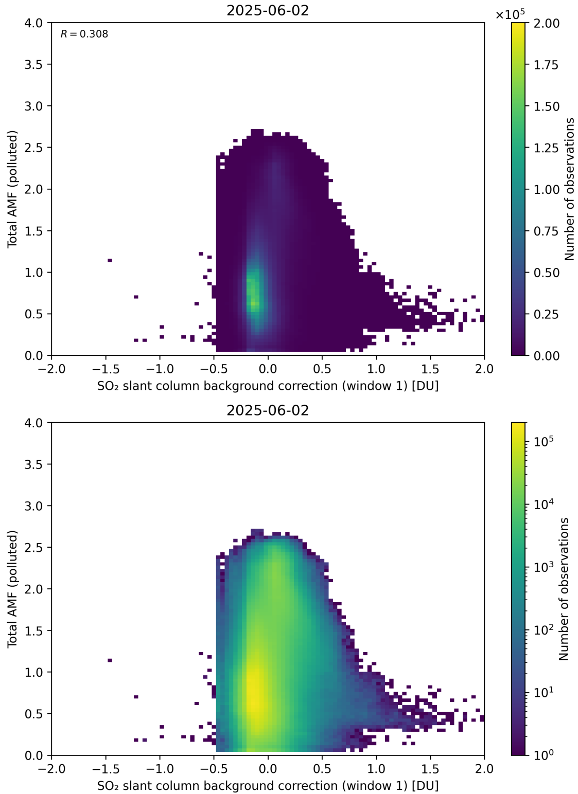
Figure 120: Scatter density plot of “SO 2 slant column background correction (window 1)” against “Total AMF (polluted)” for 2025-06-01 to 2025-06-03.
