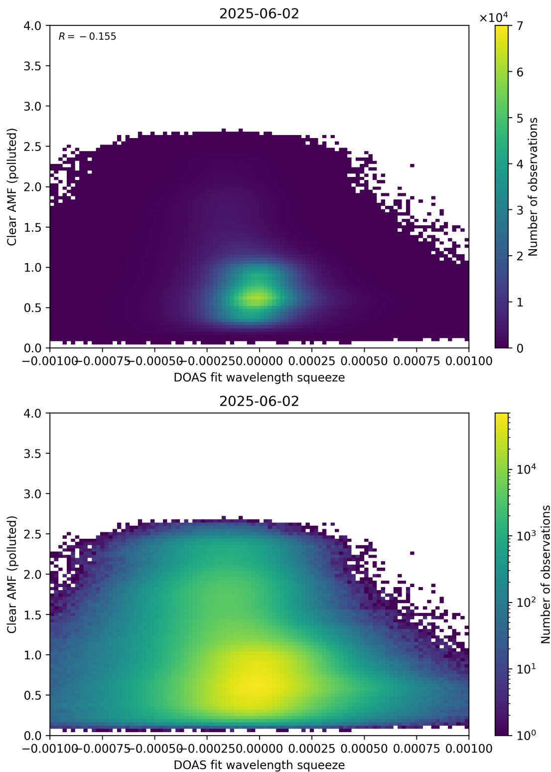
Figure 144: Scatter density plot of “DOAS fit wavelength squeeze” against “Clear AMF (polluted)” for 2025-06-01 to 2025-06-03.
