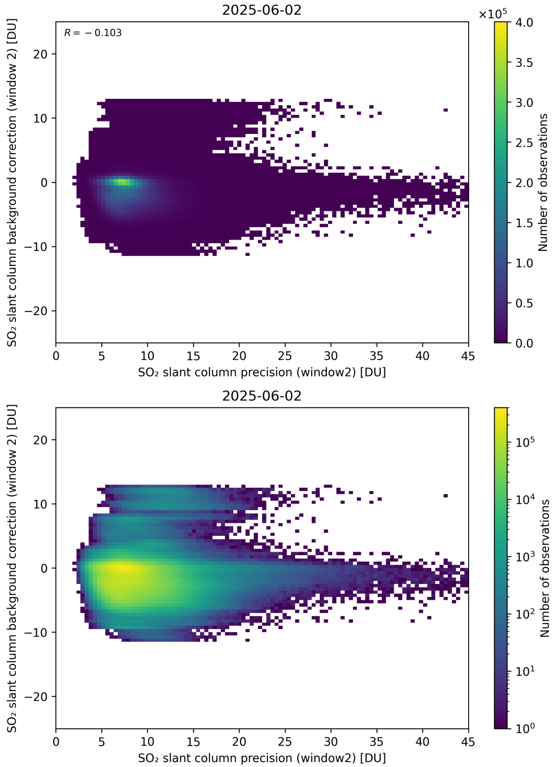
Figure 291: Scatter density plot of “SO 2 slant column precision (window2)” against “SO 2 slant column background correction (window 2)” for 2025-06-01 to 2025-06-03.
