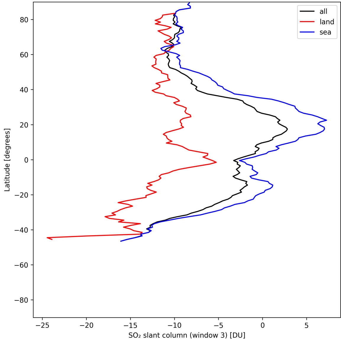
Figure 45: Zonal average of “SO 2 slant column (window 3)” for 2025-06-01 to 2025-06-03.
