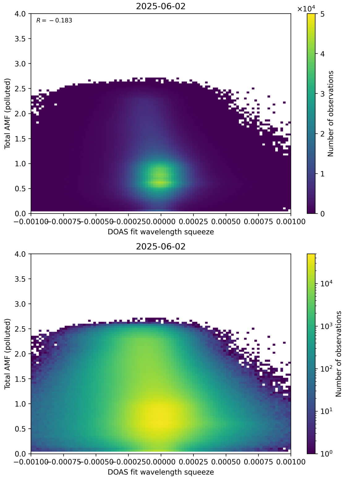
Figure 145: Scatter density plot of “DOAS fit wavelength squeeze” against “Total AMF (polluted)” for 2025-06-01 to 2025-06-03.
