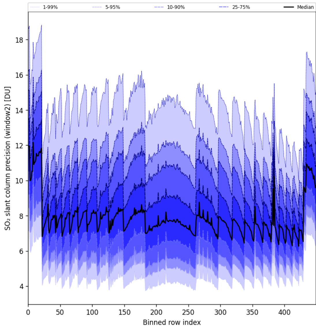
Figure 94: Along track statistics of “SO 2 slant column precision (window2)” for 2025-06-01 to 2025-06-03
