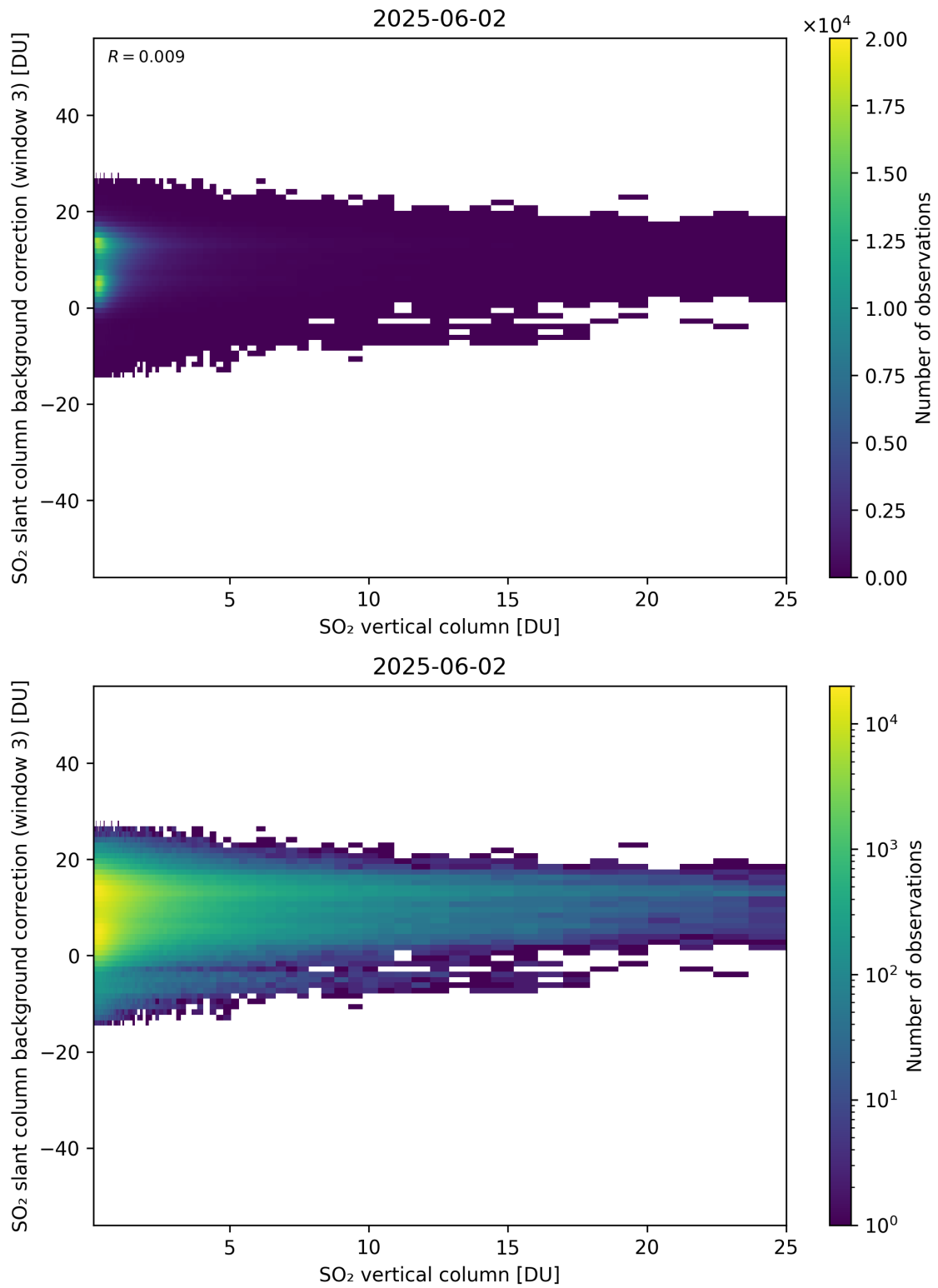
Figure 325: Scatter density plot of “SO 2 vertical column” against “SO 2 slant column background correction (window 3)” for 2025-06-01 to 2025-06-03.
