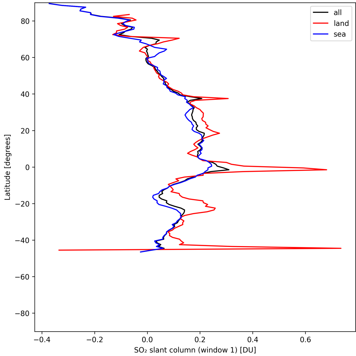
Figure 37: Zonal average of “SO 2 slant column (window 1)” for 2025-06-01 to 2025-06-03.
