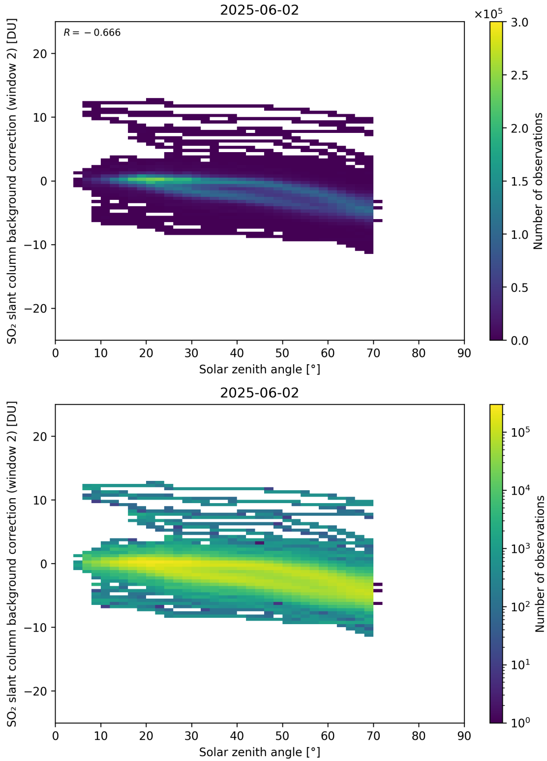
Figure 172: Scatter density plot of “Solar zenith angle” against “SO 2 slant column background correction (window 2)” for 2025-06-01 to 2025-06-03.
