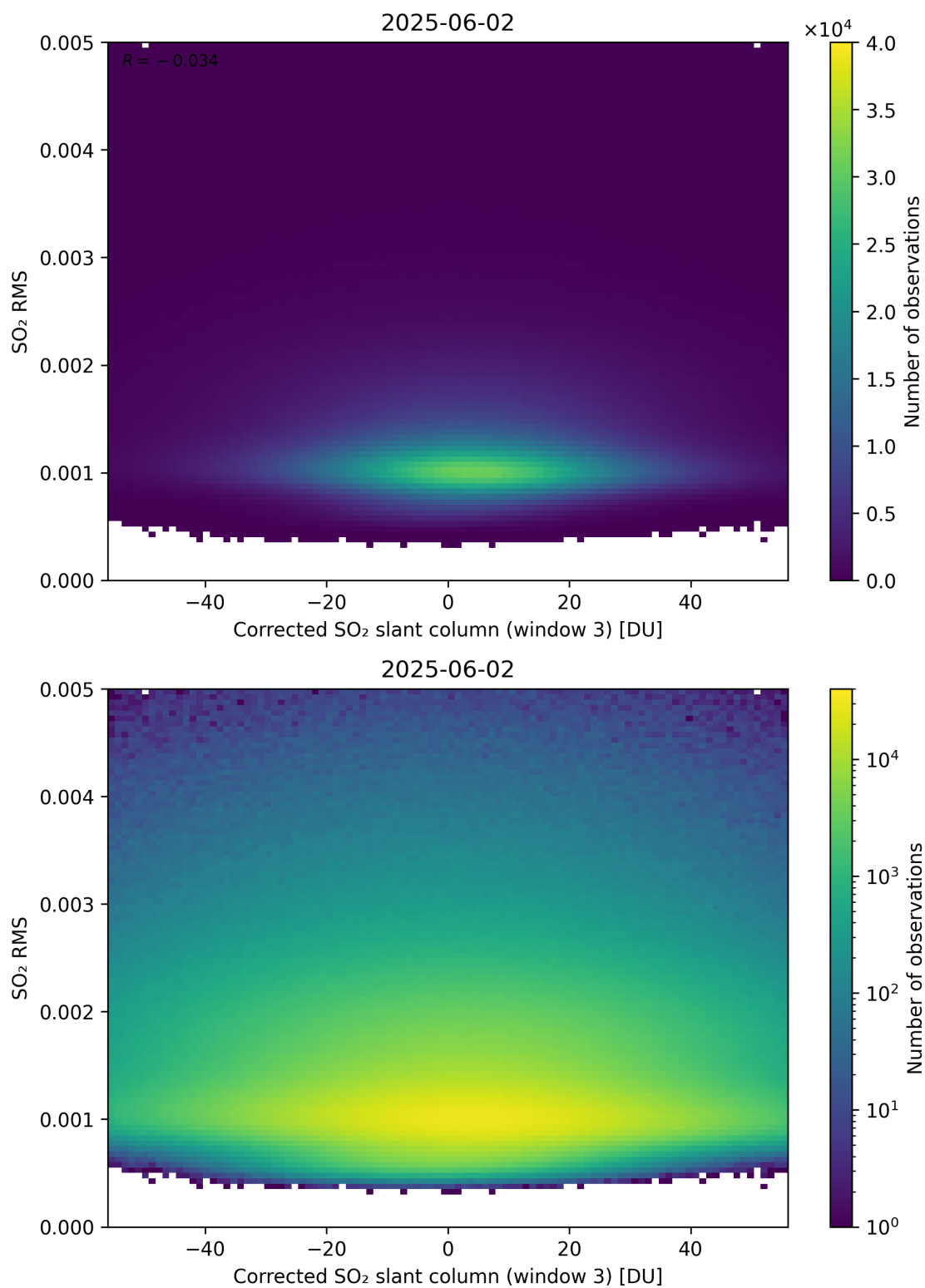
Figure 258: Scatter density plot of “Corrected SO 2 slant column (window 3)” against “SO 2 RMS” for 2025-06-01 to 2025-06-03.
