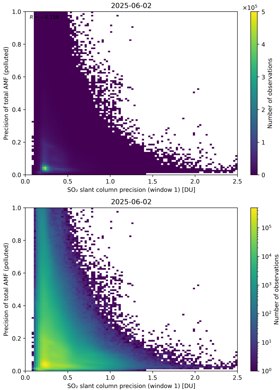
Figure 281: Scatter density plot of “SO 2 slant column precision (window 1)” against “Precision of total AMF (polluted)” for 2025-06-01 to 2025-06-03.
