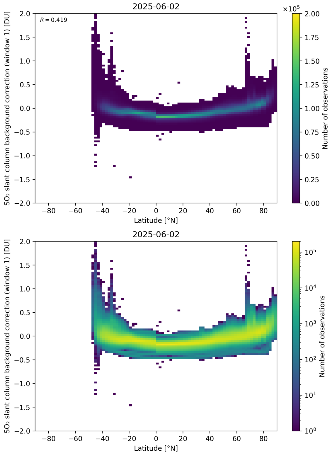
Figure 150: Scatter density plot of “Latitude” against “SO 2 slant column background correction (window 1)” for 2025-06-01 to 2025-06-03.
