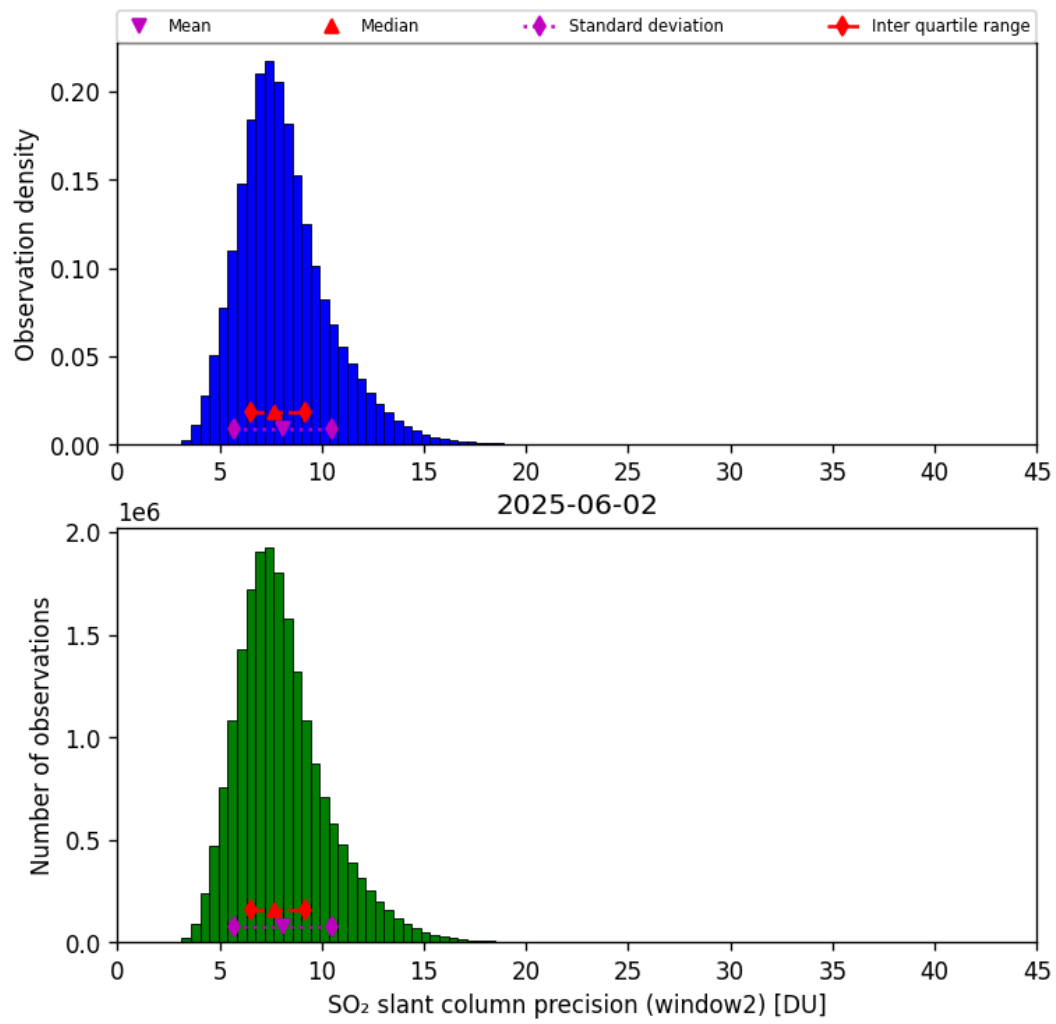
Figure 68: Histogram of “SO 2 slant column precision (window2)” for 2025-06-01 to 2025-06-03
