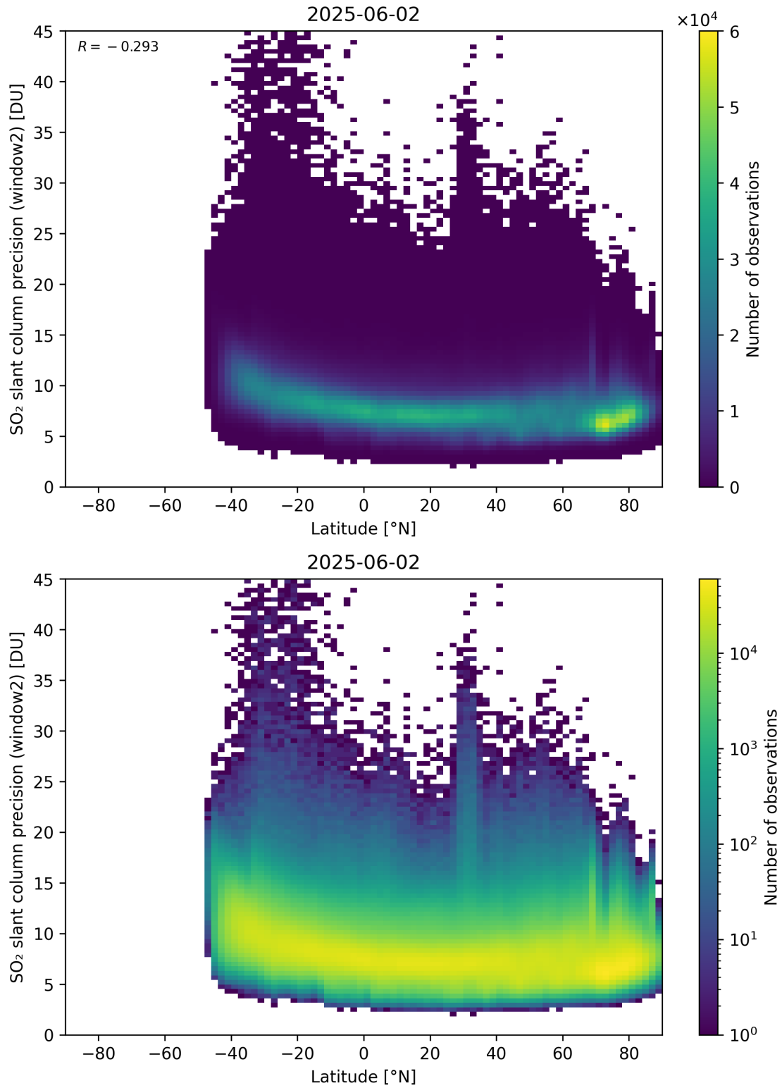
Figure 164: Scatter density plot of “Latitude” against “SO 2 slant column precision (window2)” for 2025-06-01 to 2025-06-03.
