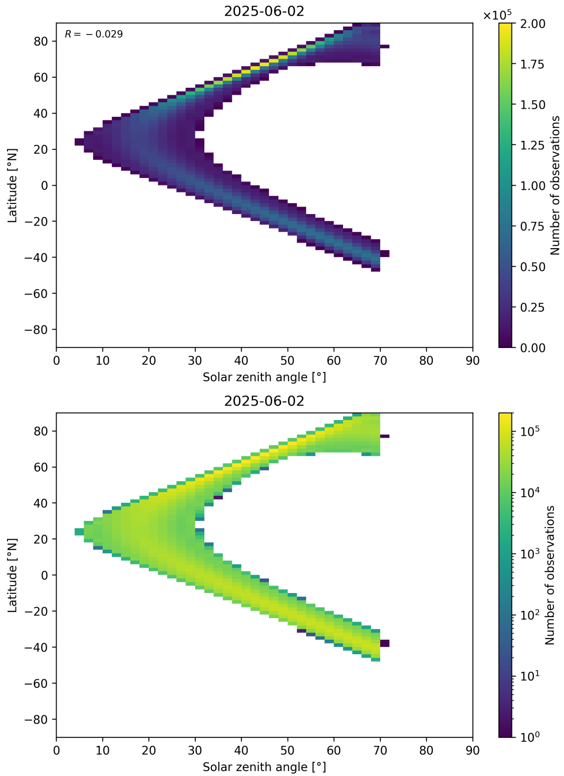
Figure 177: Scatter density plot of “Solar zenith angle” against “Latitude” for 2025-06-01 to 2025-06-03.
