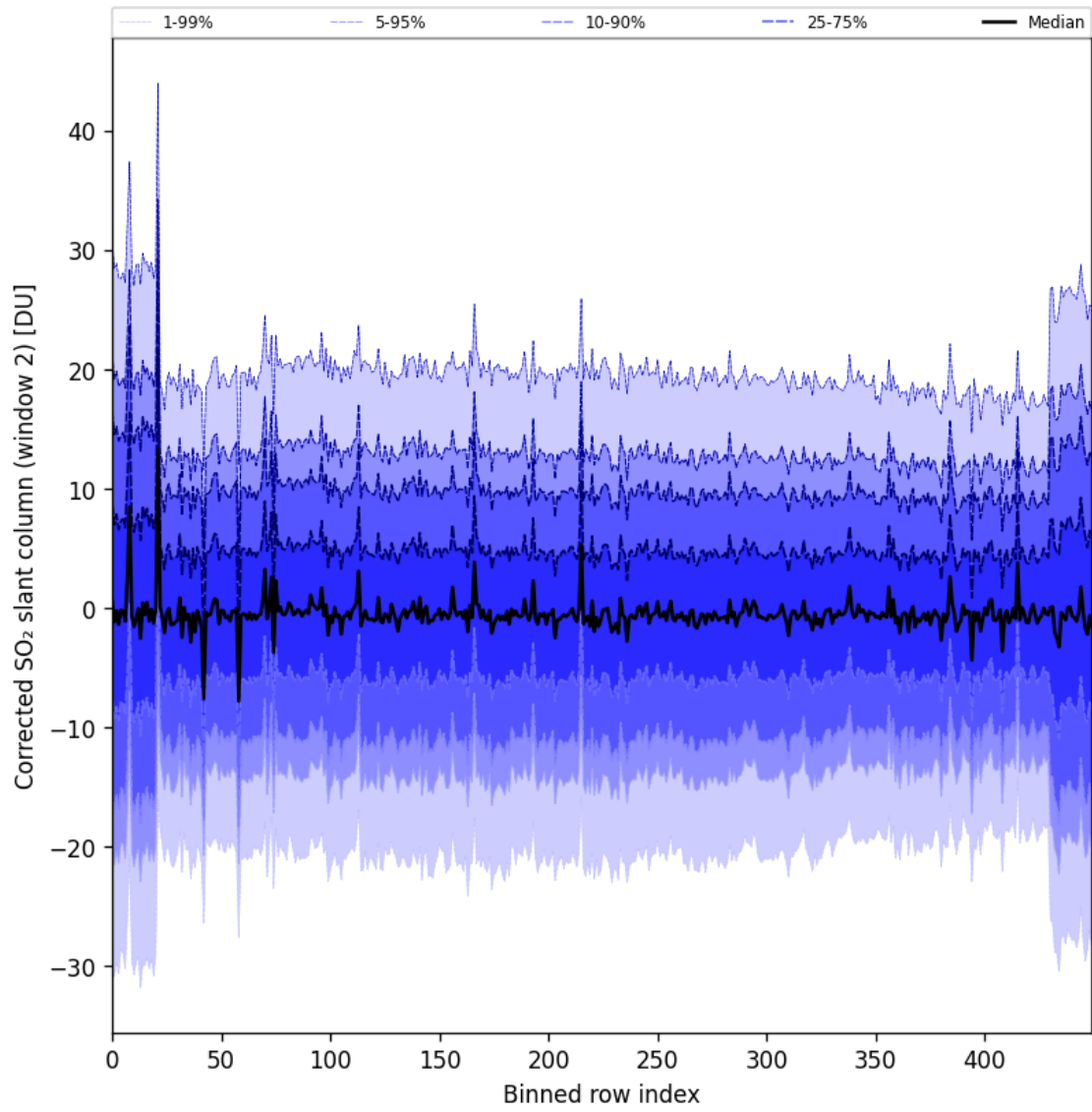
Figure 95: Along track statistics of “Corrected SO 2 slant column (window 2)” for 2025-06-01 to 2025-06-03
