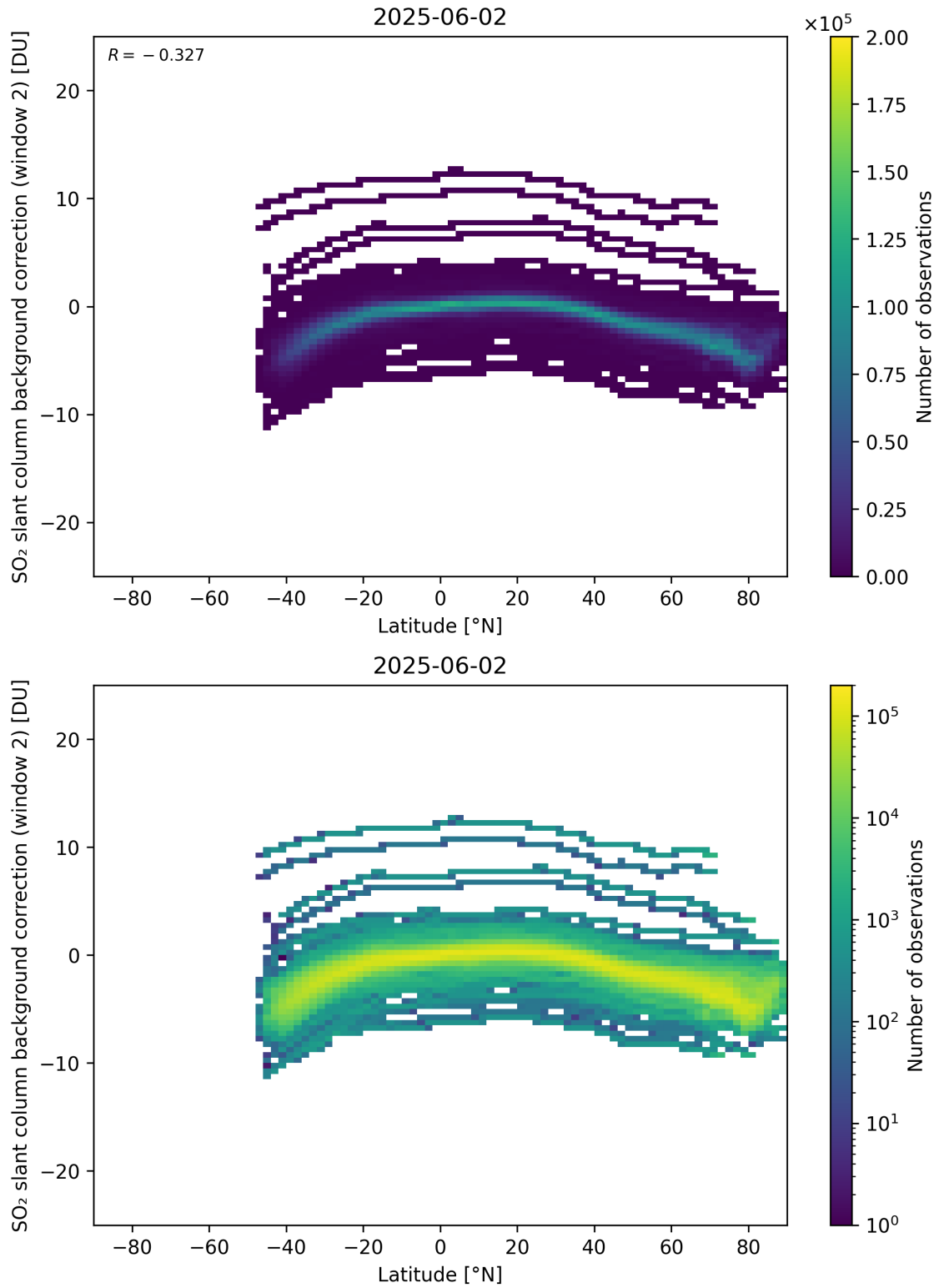
Figure 151: Scatter density plot of “Latitude” against “SO 2 slant column background correction (window 2)” for 2025-06-01 to 2025-06-03.
