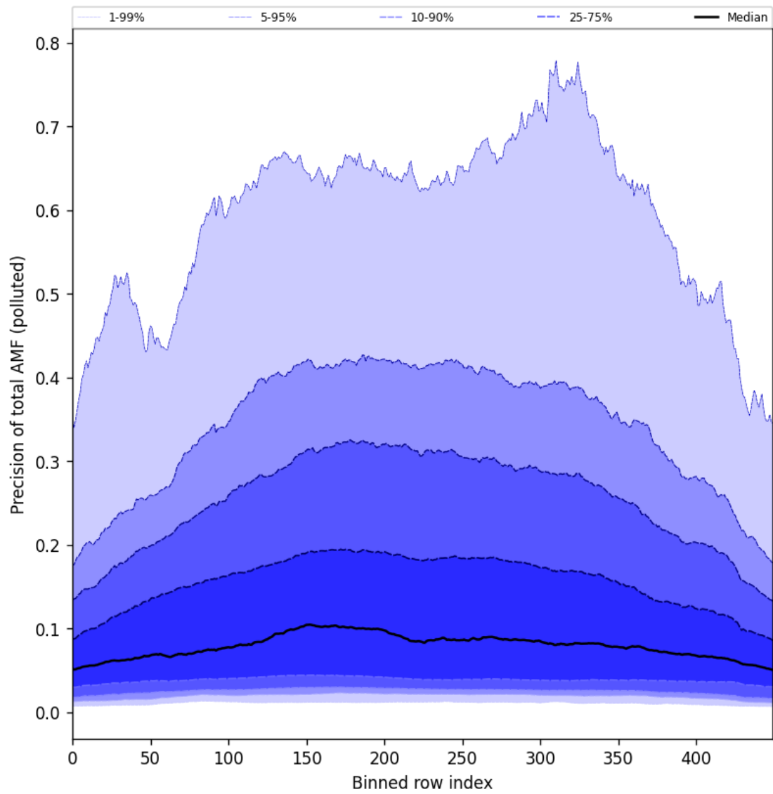
Figure 106: Along track statistics of “Precision of total AMF (polluted)” for 2025-06-01 to 2025-06-03
