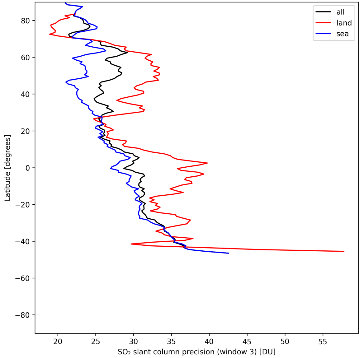
Figure 46: Zonal average of “SO 2 slant column precision (window 3)” for 2025-06-01 to 2025-06-03.
