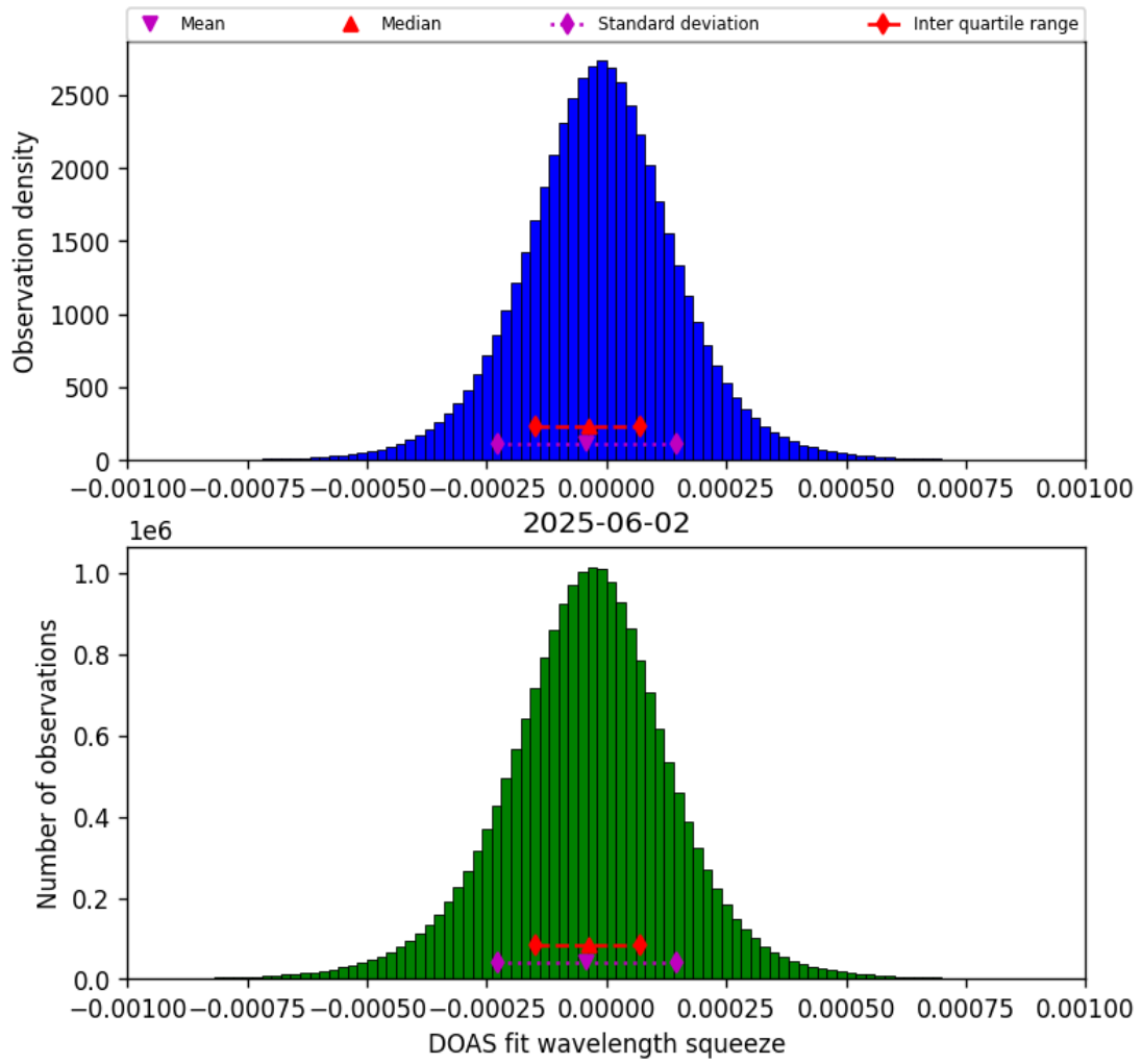
Figure 77: Histogram of “DOAS fit wavelength squeeze” for 2025-06-01 to 2025-06-03
