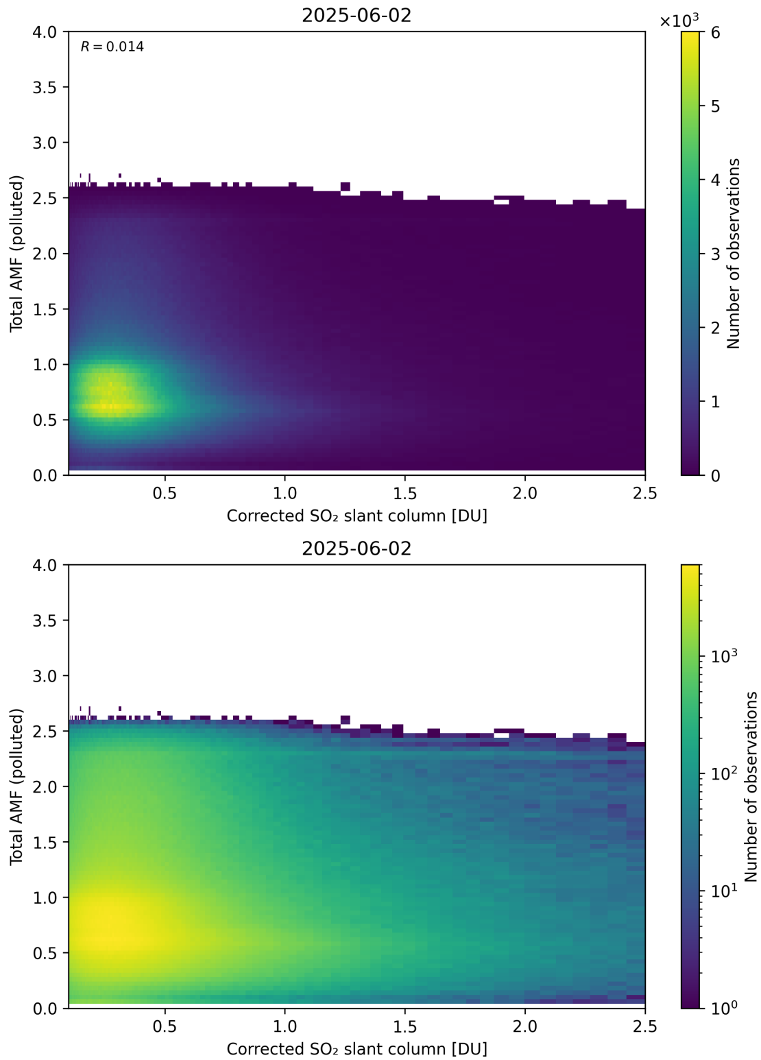
Figure 242: Scatter density plot of “Corrected SO 2 slant column” against “Total AMF (polluted)” for 2025-06-01 to 2025-06-03.
