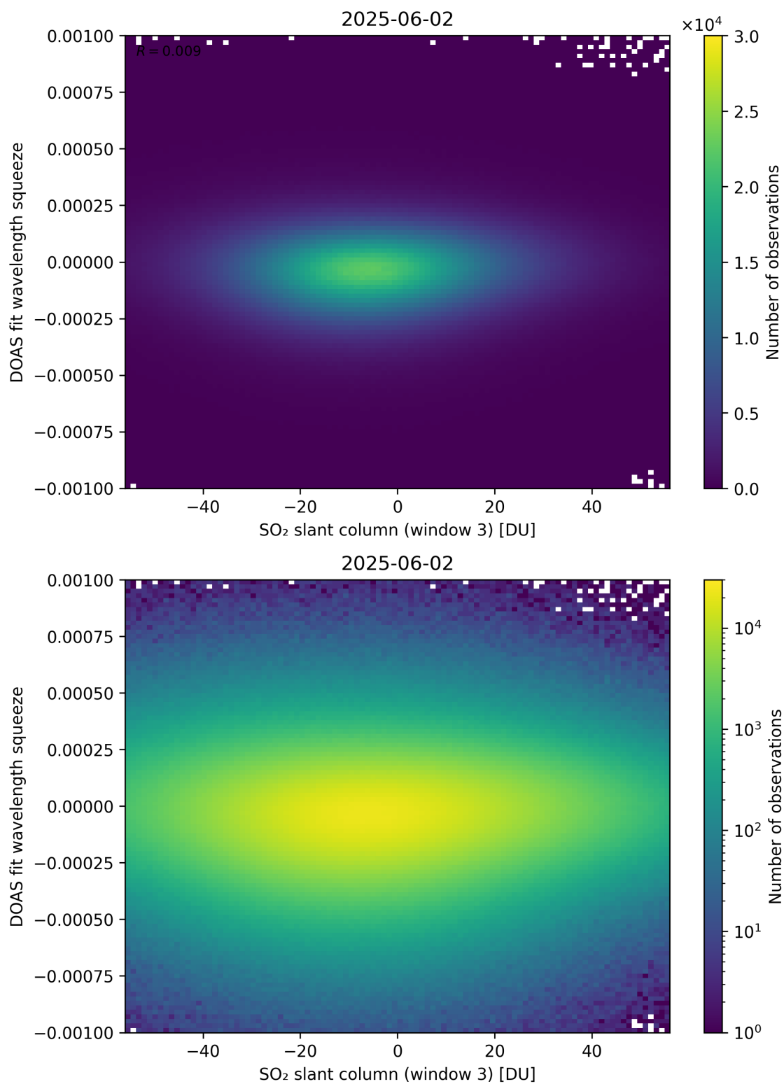
Figure 305: Scatter density plot of “SO 2 slant column (window 3)” against “DOAS fit wavelength squeeze” for 2025-06-01 to 2025-06-03.
