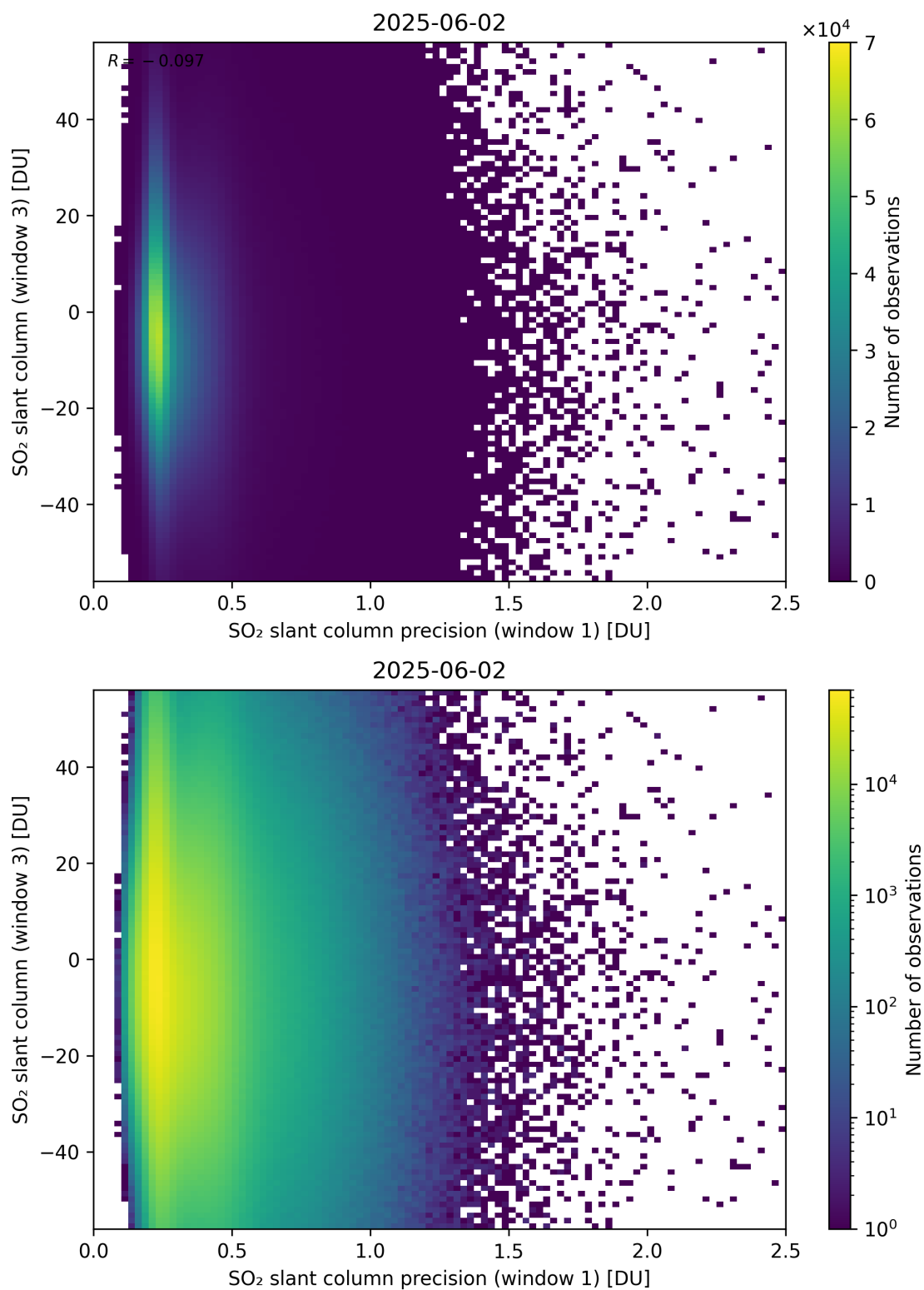
Figure 278: Scatter density plot of “SO 2 slant column precision (window 1)” against “SO 2 slant column (window 3)” for 2025-06-01 to 2025-06-03.
