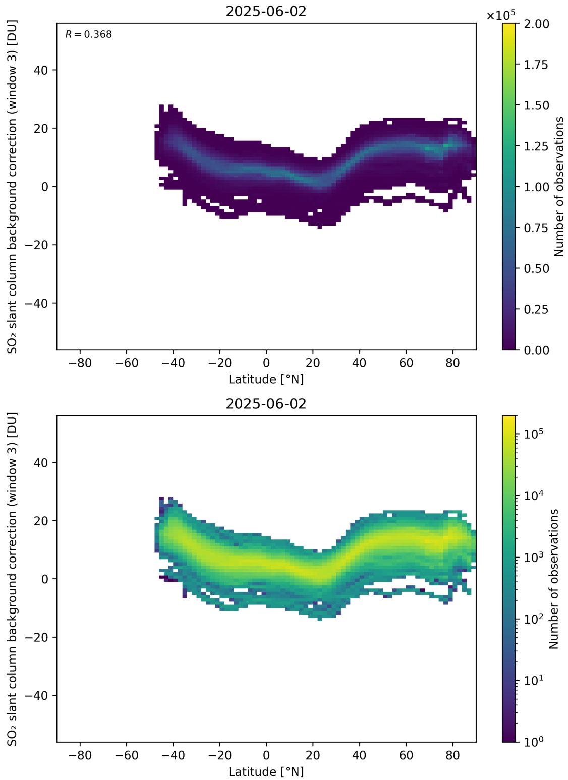
Figure 152: Scatter density plot of “Latitude” against “SO 2 slant column background correction (window 3)” for 2025-06-01 to 2025-06-03.
