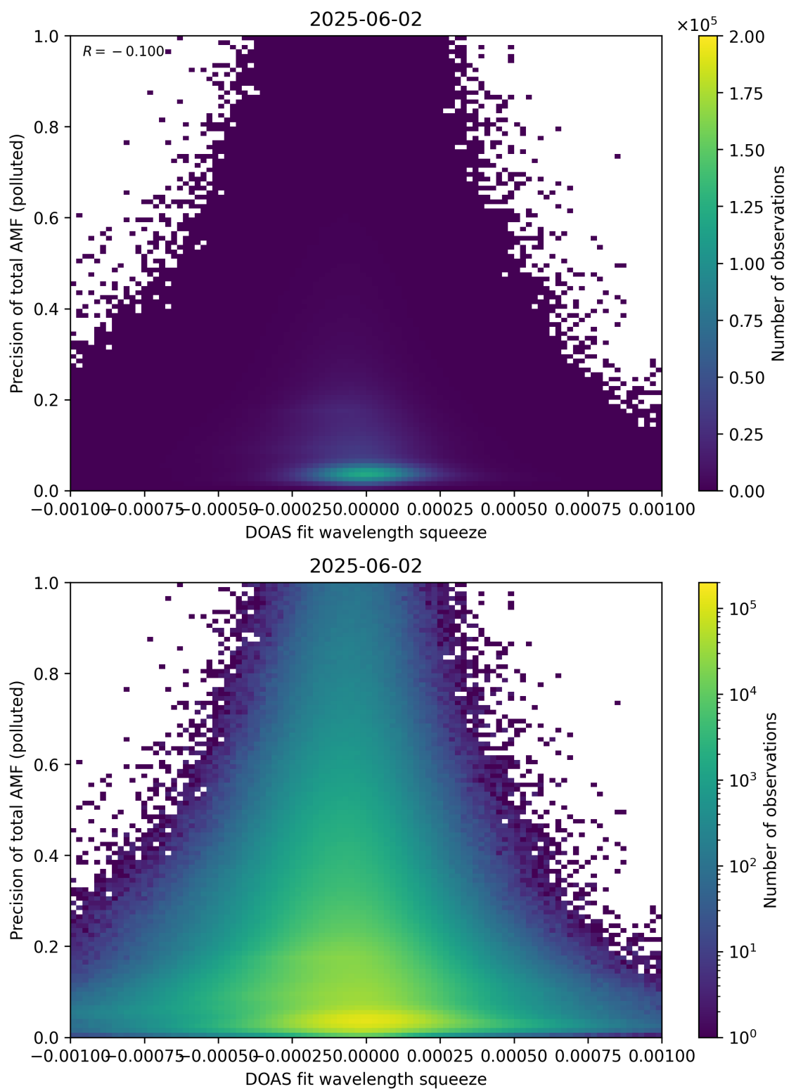
Figure 146: Scatter density plot of “DOAS fit wavelength squeeze” against “Precision of total AMF (polluted)” for 2025-06-01 to 2025-06-03.
