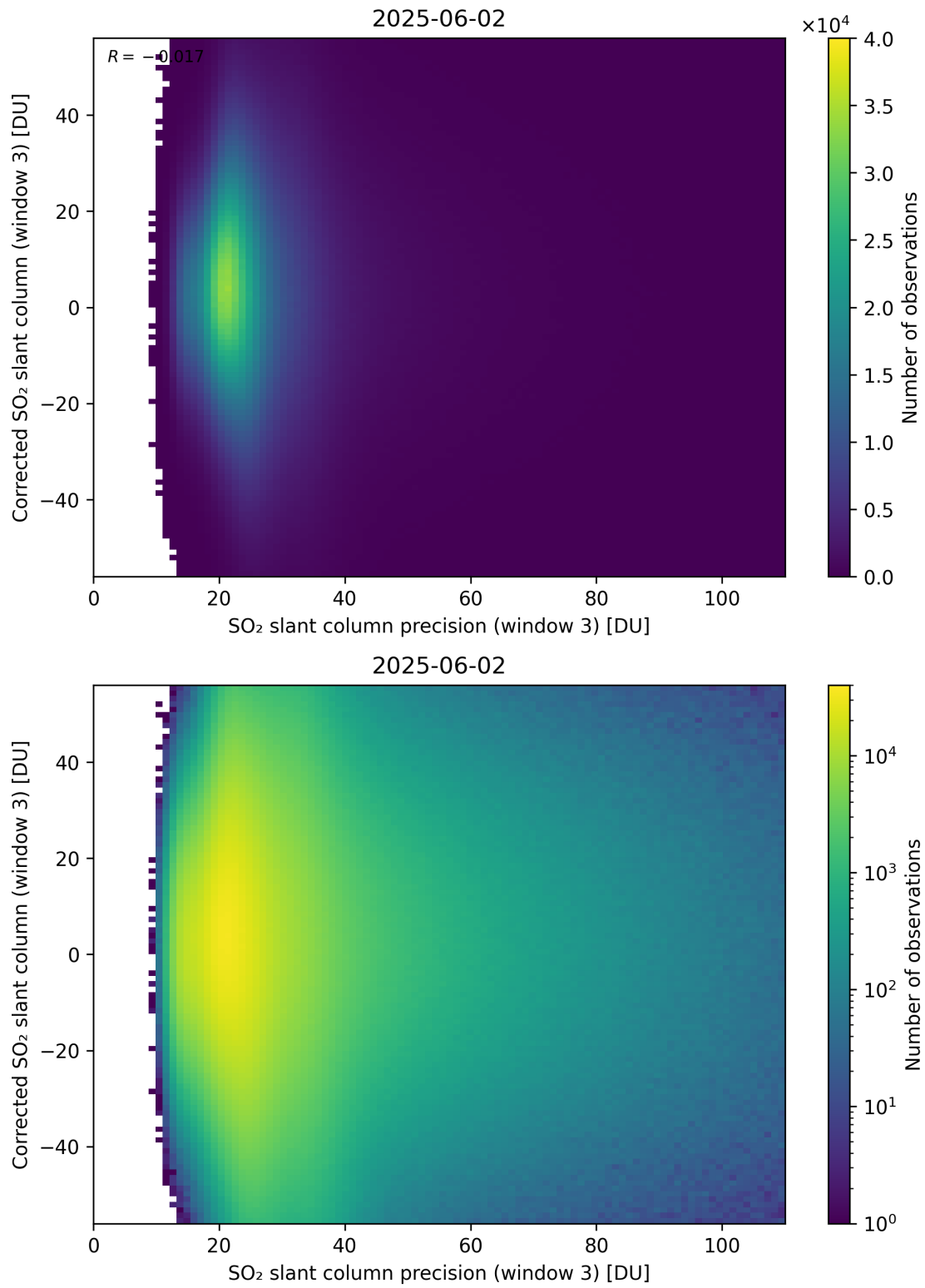
Figure 312: Scatter density plot of “SO 2 slant column precision (window 3)” against “Corrected SO 2 slant column (window 3)” for 2025-06-01 to 2025-06-03.
