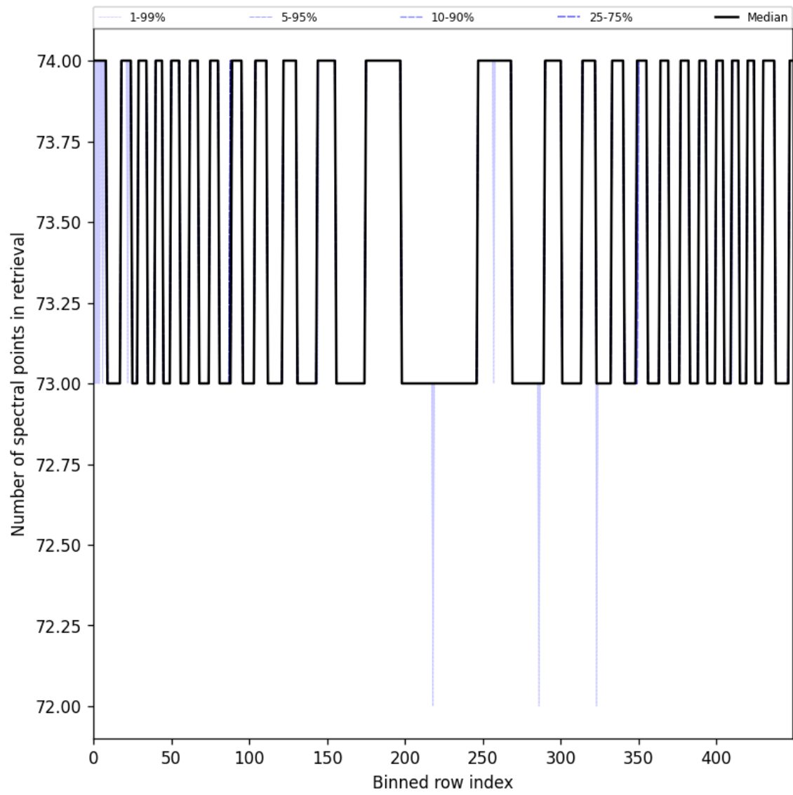
Figure 108: Along track statistics of “Number of spectral points in retrieval” for 2025-06-01 to 2025-06-03
