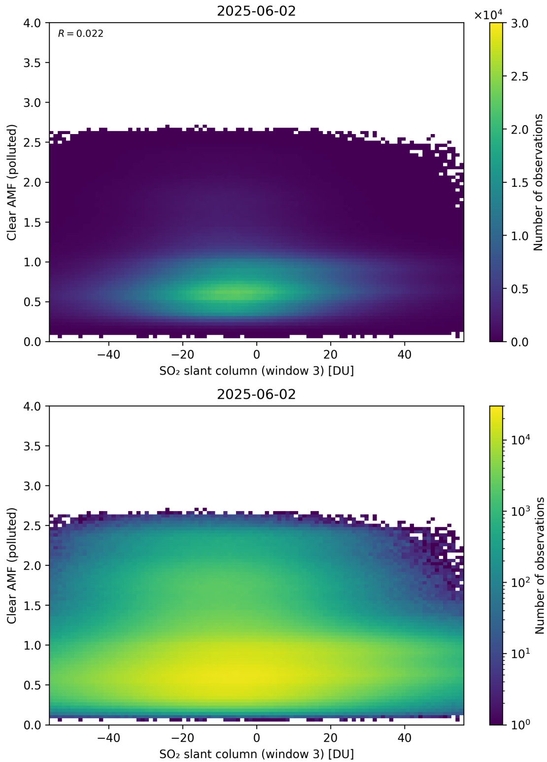
Figure 315: Scatter density plot of “SO 2 slant column (window 3)” against “Clear AMF (polluted)” for 2025-06-01 to 2025-06-03.
