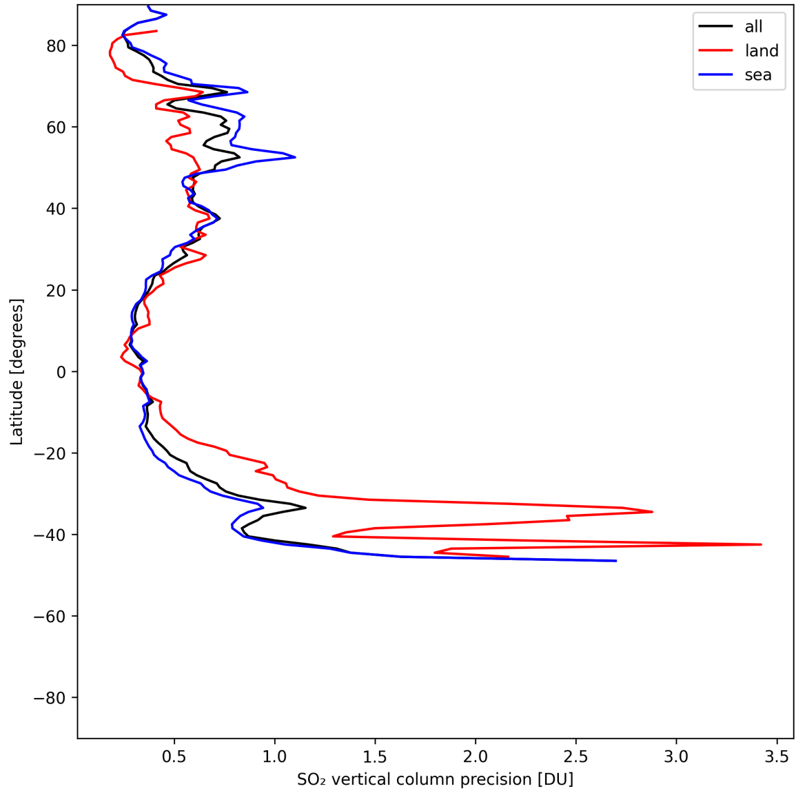
Figure 33: Zonal average of “SO 2 vertical column precision” for 2025-06-01 to 2025-06-03.
