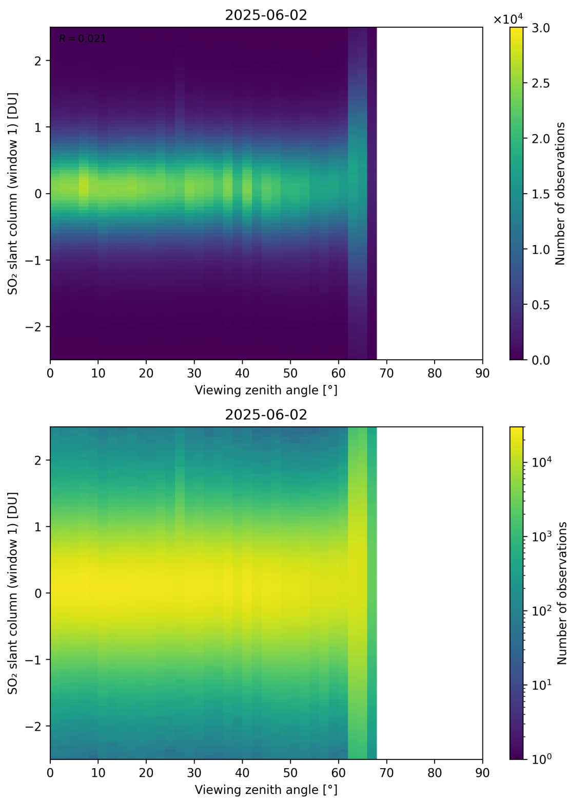
Figure 376: Scatter density plot of “Viewing zenith angle” against “SO 2 slant column (window 1)” for 2025-06-01 to 2025-06-03.
