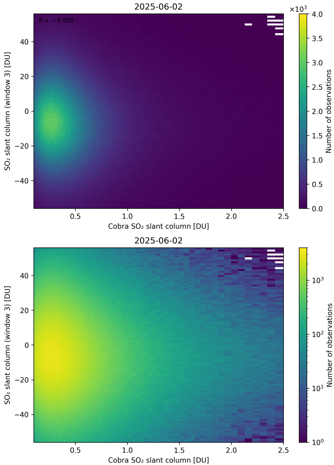
Figure 222: Scatter density plot of “Cobra SO 2 slant column” against “SO 2 slant column (window 3)” for 2025-06-01 to 2025-06-03.
