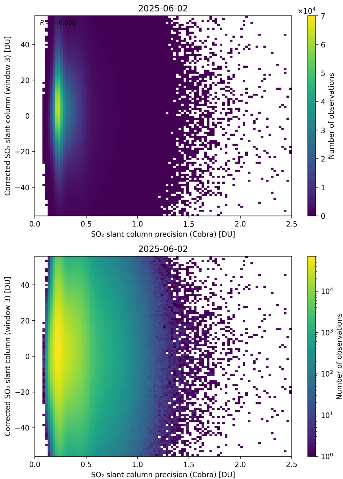
Figure 207: Scatter density plot of “SO 2 slant column precision (Cobra)” against “Corrected SO 2 slant column (window 3)” for 2025-06-01 to 2025-06-03.
