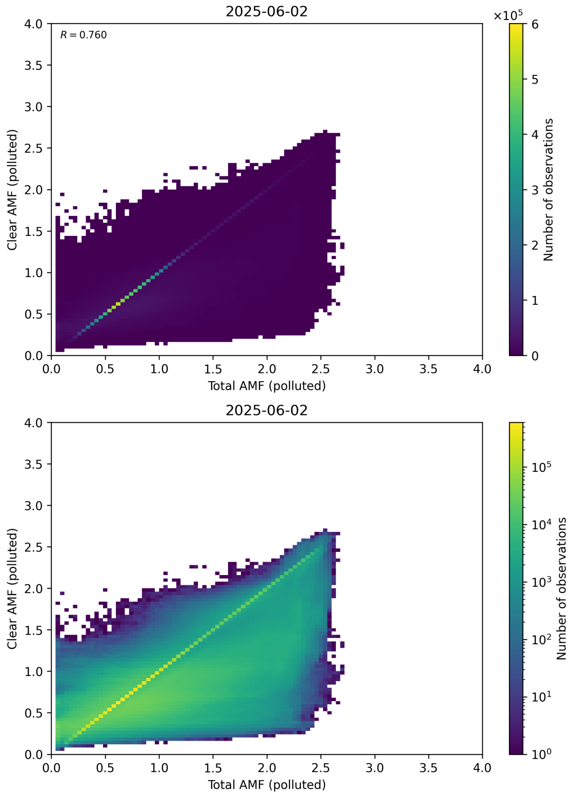
Figure 321: Scatter density plot of “Total AMF (polluted)” against “Clear AMF (polluted)” for 2025-06-01 to 2025-06-03.
