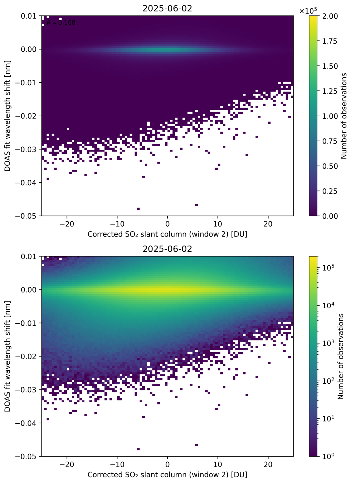
Figure 246: Scatter density plot of “Corrected SO 2 slant column (window 2)” against “DOAS fit wavelength shift” for 2025-06-01 to 2025-06-03.
