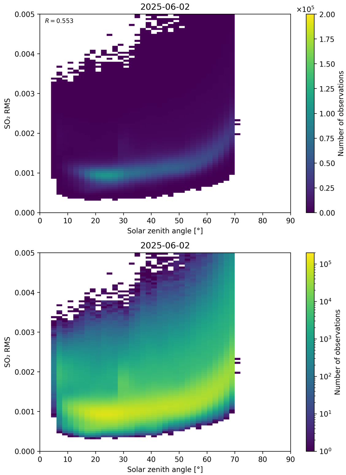
Figure 176: Scatter density plot of “Solar zenith angle” against “SO 2 RMS” for 2025-06-01 to 2025-06-03.
