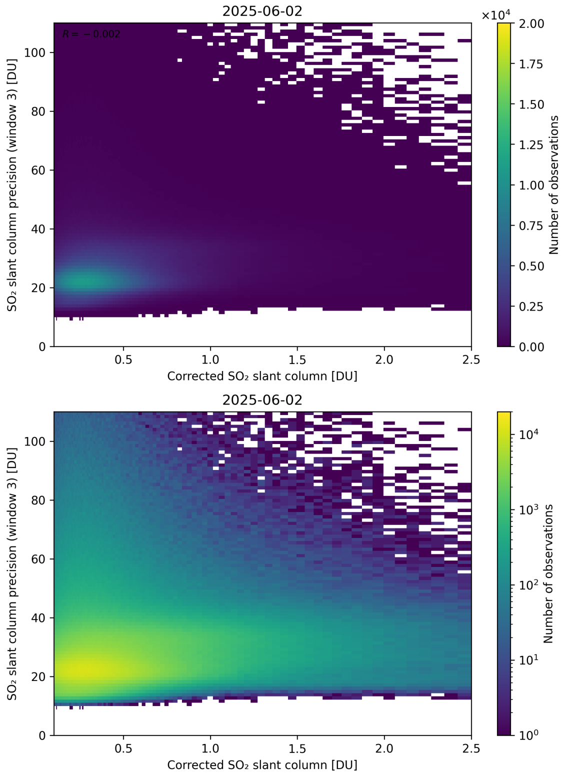
Figure 241: Scatter density plot of “Corrected SO 2 slant column” against “SO 2 slant column precision (window 3)” for 2025-06-01 to 2025-06-03.
