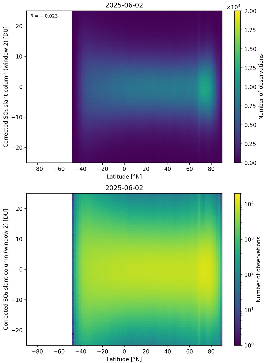
Figure 160: Scatter density plot of “Latitude” against “Corrected SO 2 slant column (window 2)” for 2025-06-01 to 2025-06-03.
