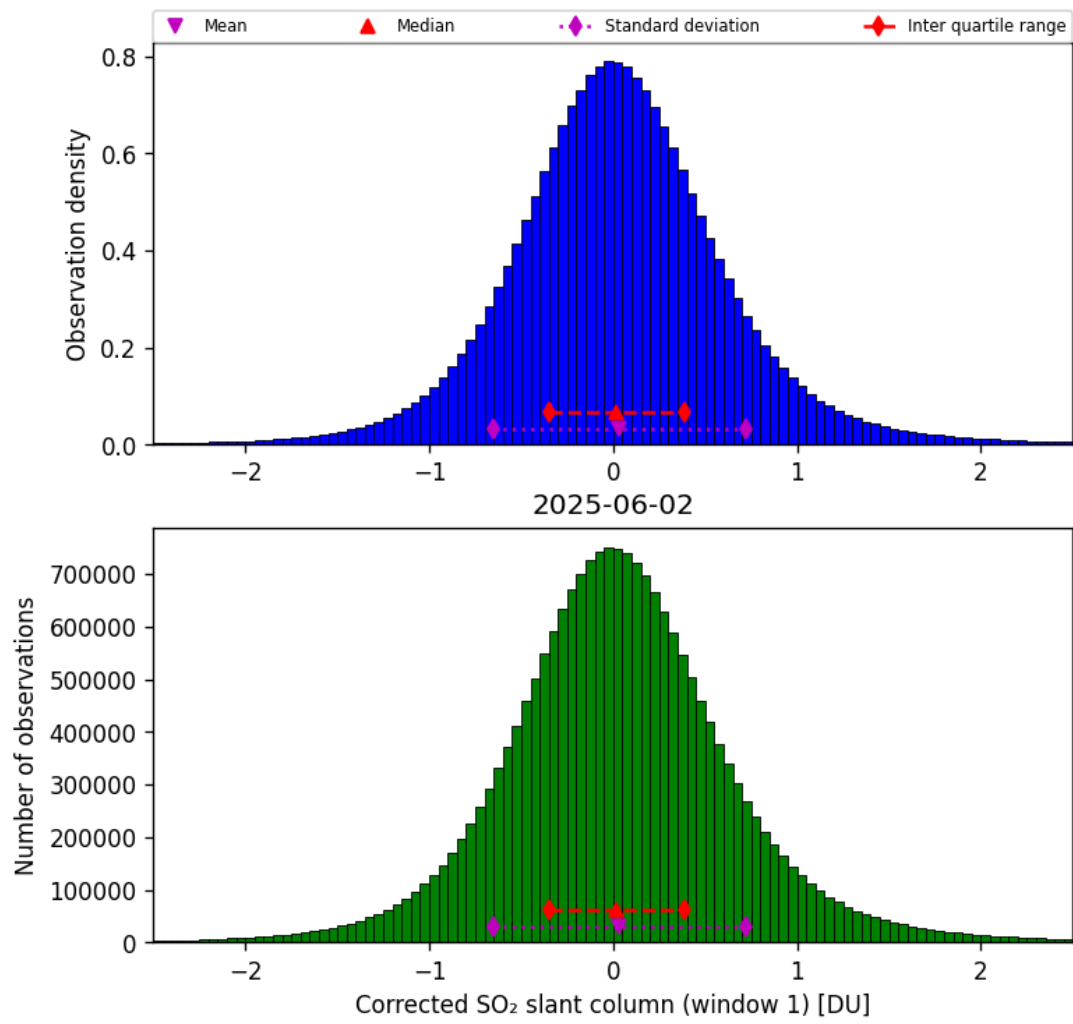
Figure 65: Histogram of “Corrected SO 2 slant column (window 1)” for 2025-06-01 to 2025-06-03
