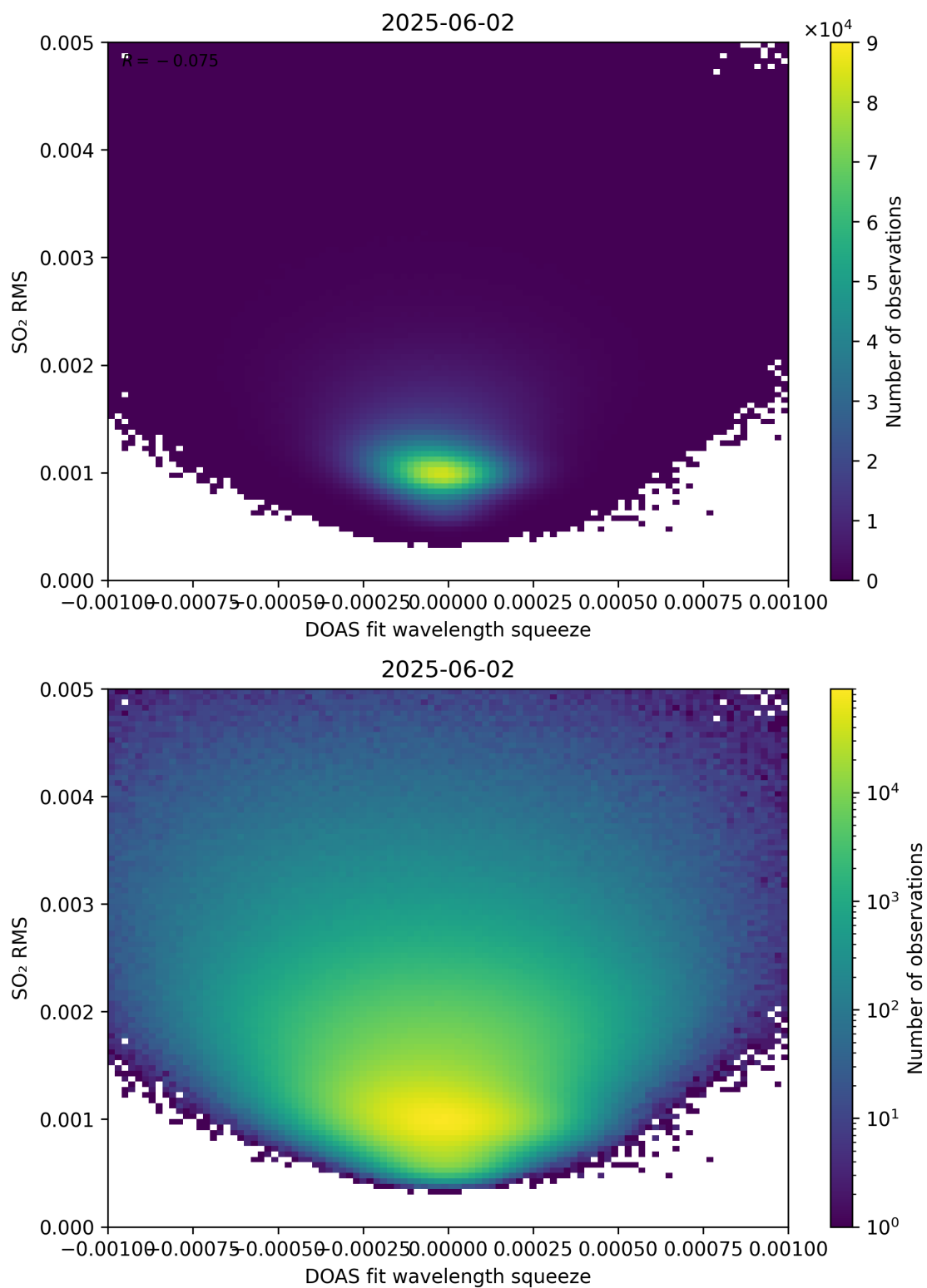
Figure 143: Scatter density plot of “DOAS fit wavelength squeeze” against “SO 2 RMS” for 2025-06-01 to 2025-06-03.
