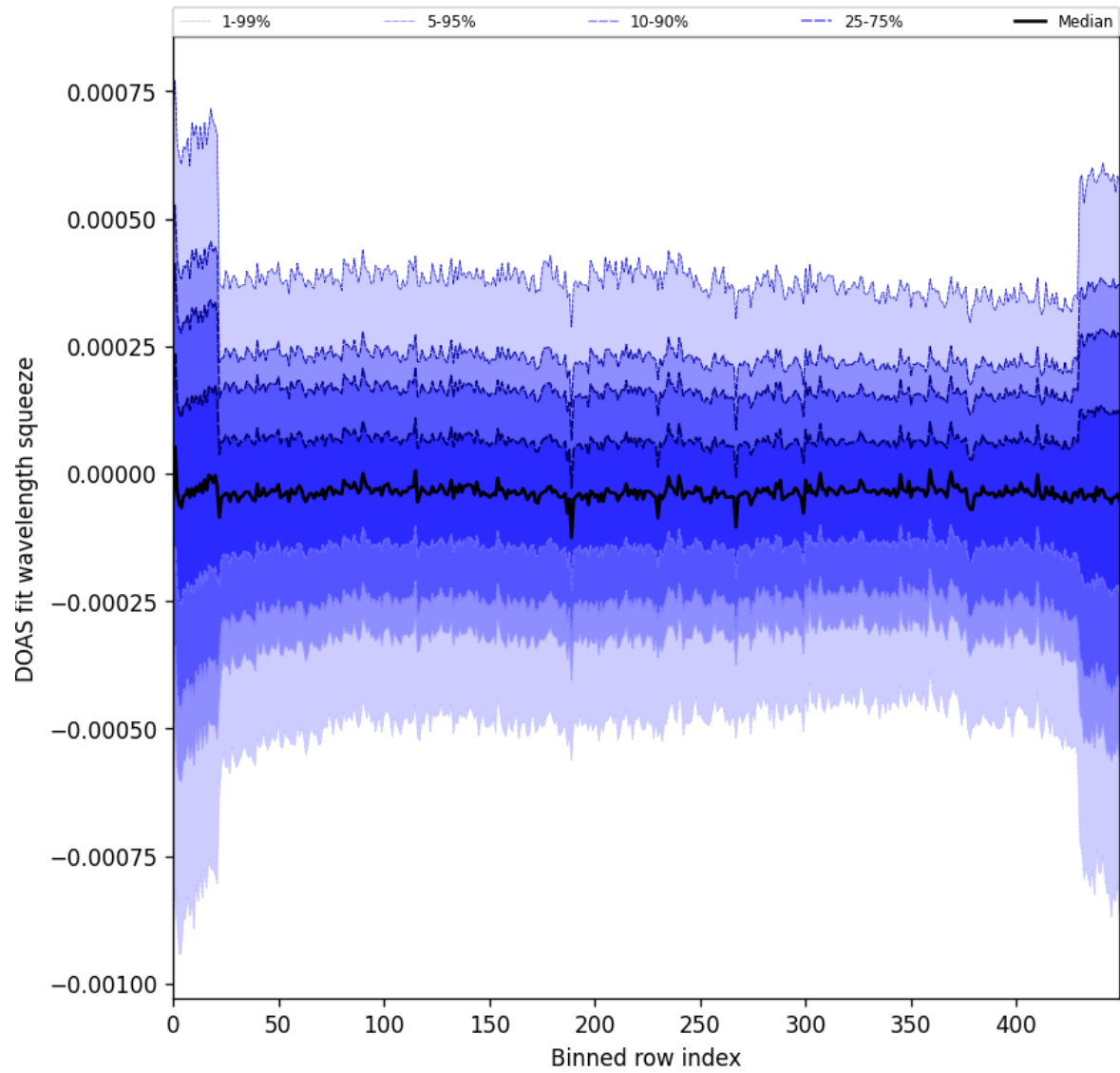
Figure 103: Along track statistics of “DOAS fit wavelength squeeze” for 2025-06-01 to 2025-06-03
