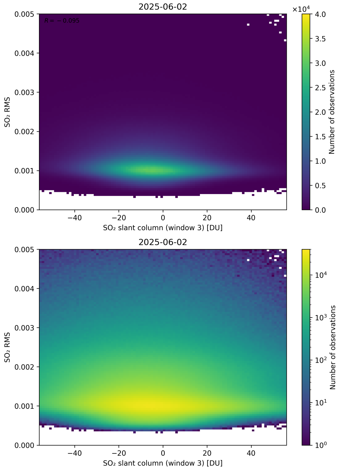
Figure 306: Scatter density plot of “SO 2 slant column (window 3)” against “SO 2 RMS” for 2025-06-01 to 2025-06-03.
