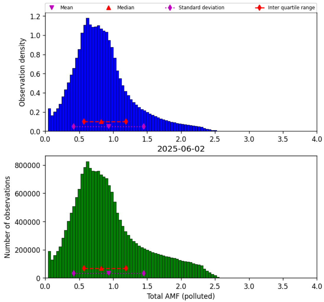
Figure 79: Histogram of “Total AMF (polluted)” for 2025-06-01 to 2025-06-03
