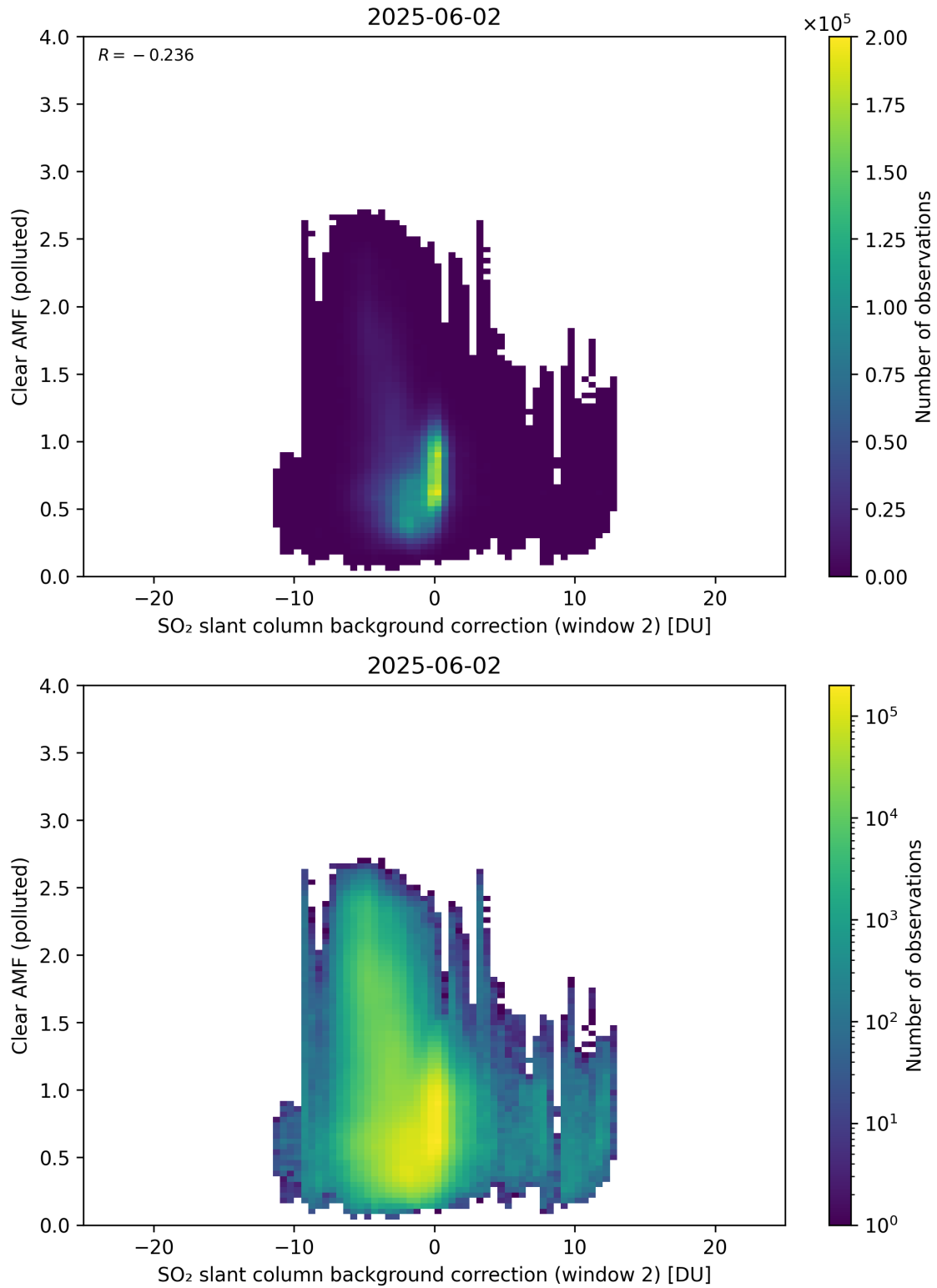
Figure 126: Scatter density plot of “SO 2 slant column background correction (window 2)” against “Clear AMF (polluted)” for 2025-06-01 to 2025-06-03.
