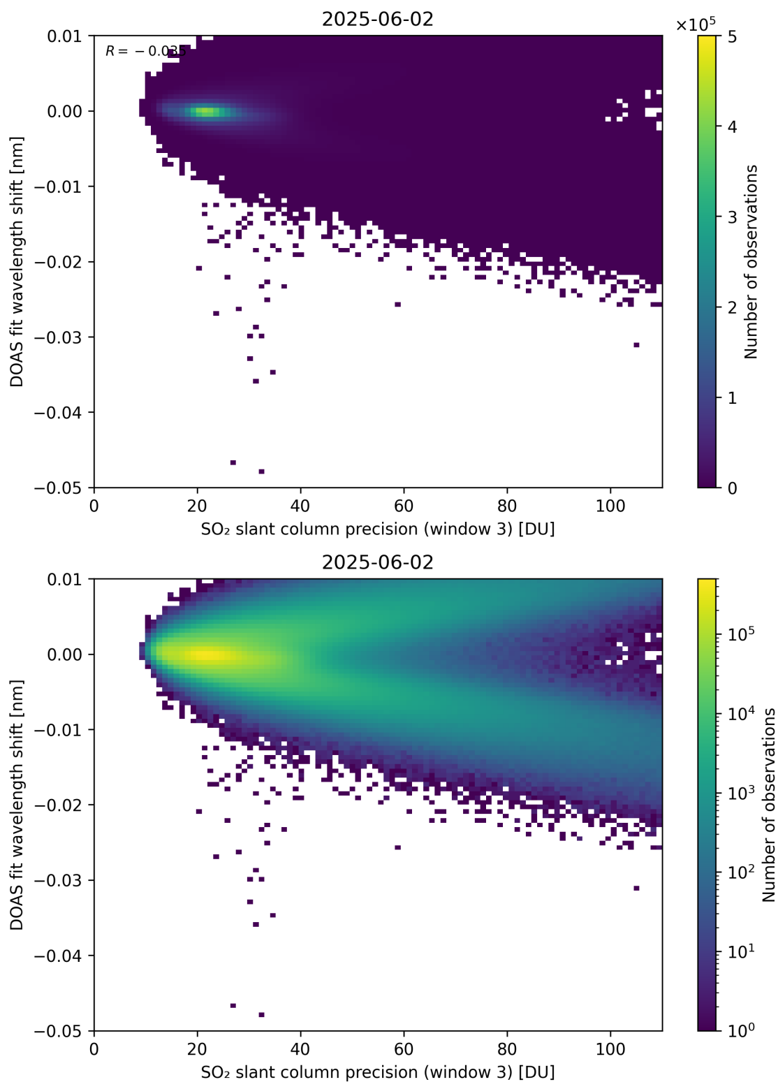
Figure 308: Scatter density plot of “SO 2 slant column precision (window 3)” against “DOAS fit wavelength shift” for 2025-06-01 to 2025-06-03.
