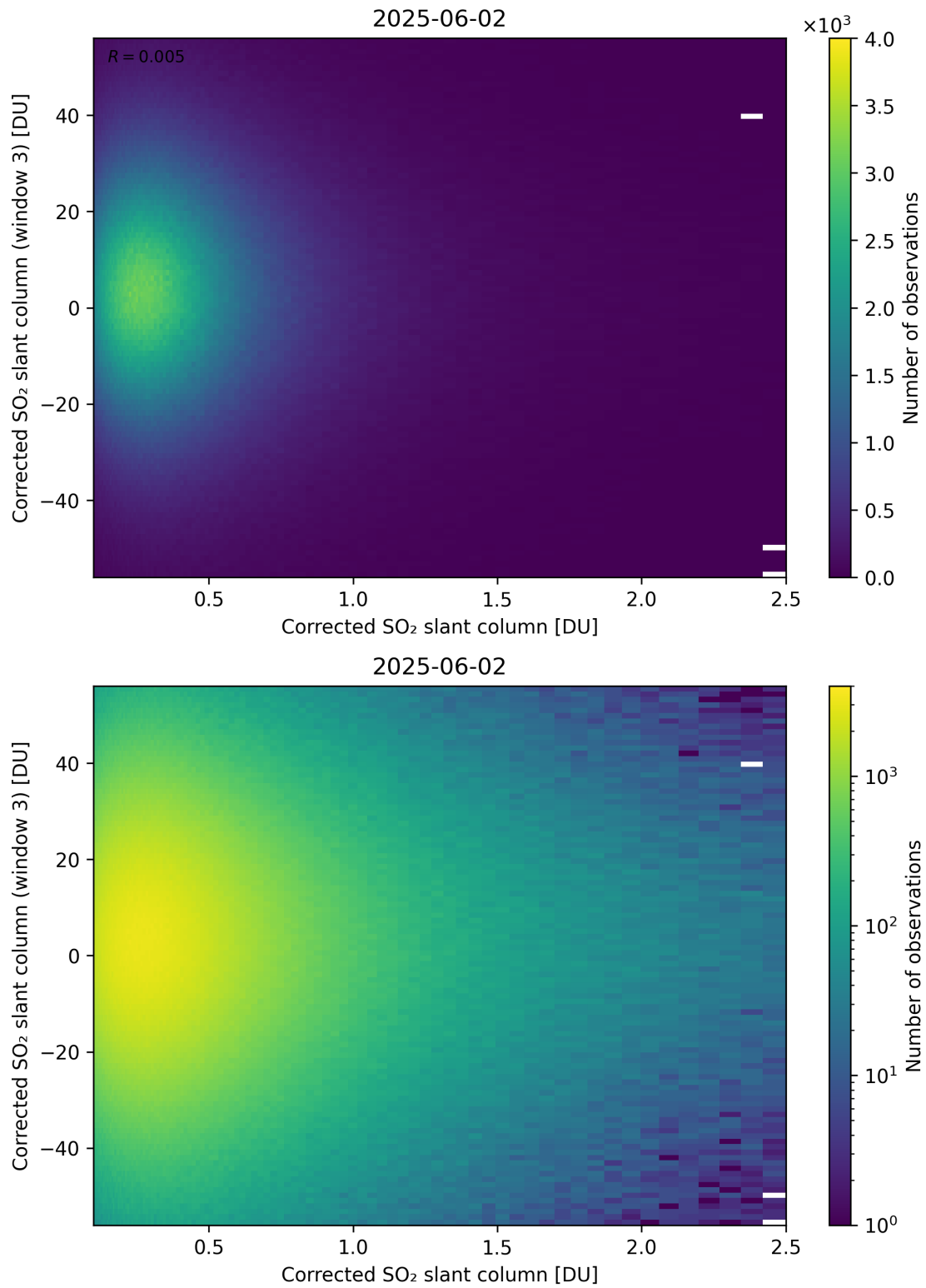
Figure 236: Scatter density plot of “Corrected SO 2 slant column” against “Corrected SO 2 slant column (window 3)” for 2025-06-01 to 2025-06-03.
