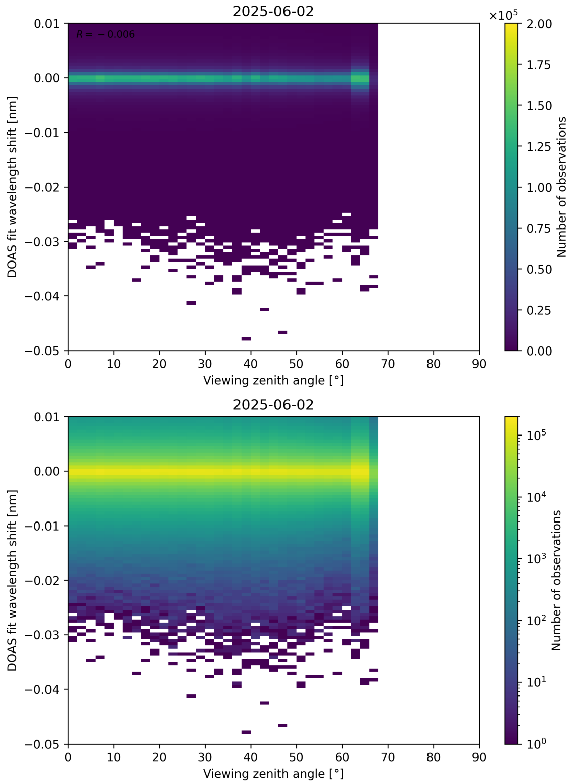
Figure 365: Scatter density plot of “Viewing zenith angle” against “DOAS fit wavelength shift” for 2025-06-01 to 2025-06-03.
