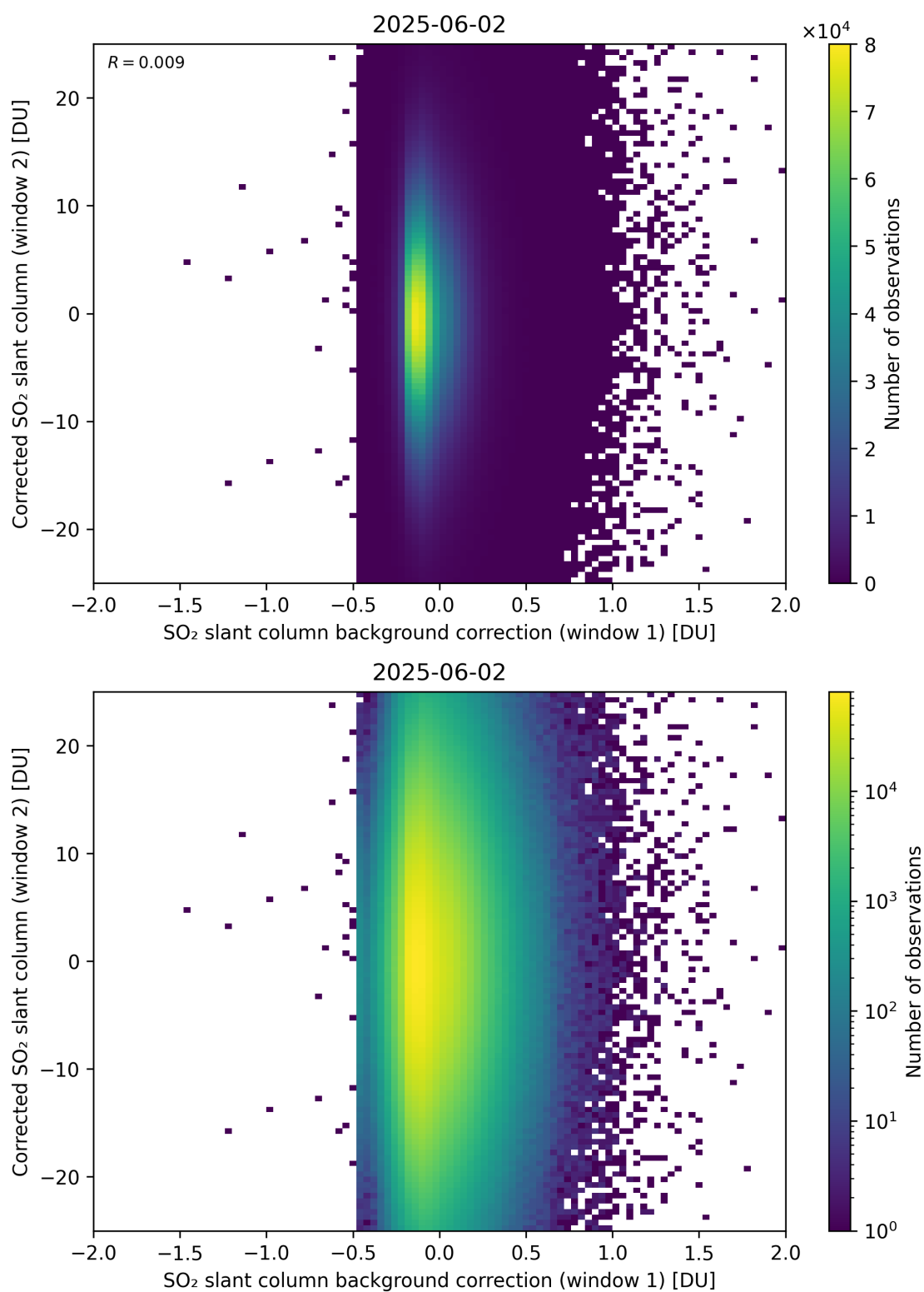
Figure 115: Scatter density plot of “SO 2 slant column background correction (window 1)” against “Corrected SO 2 slant column (window 2)” for 2025-06-01 to 2025-06-03.
