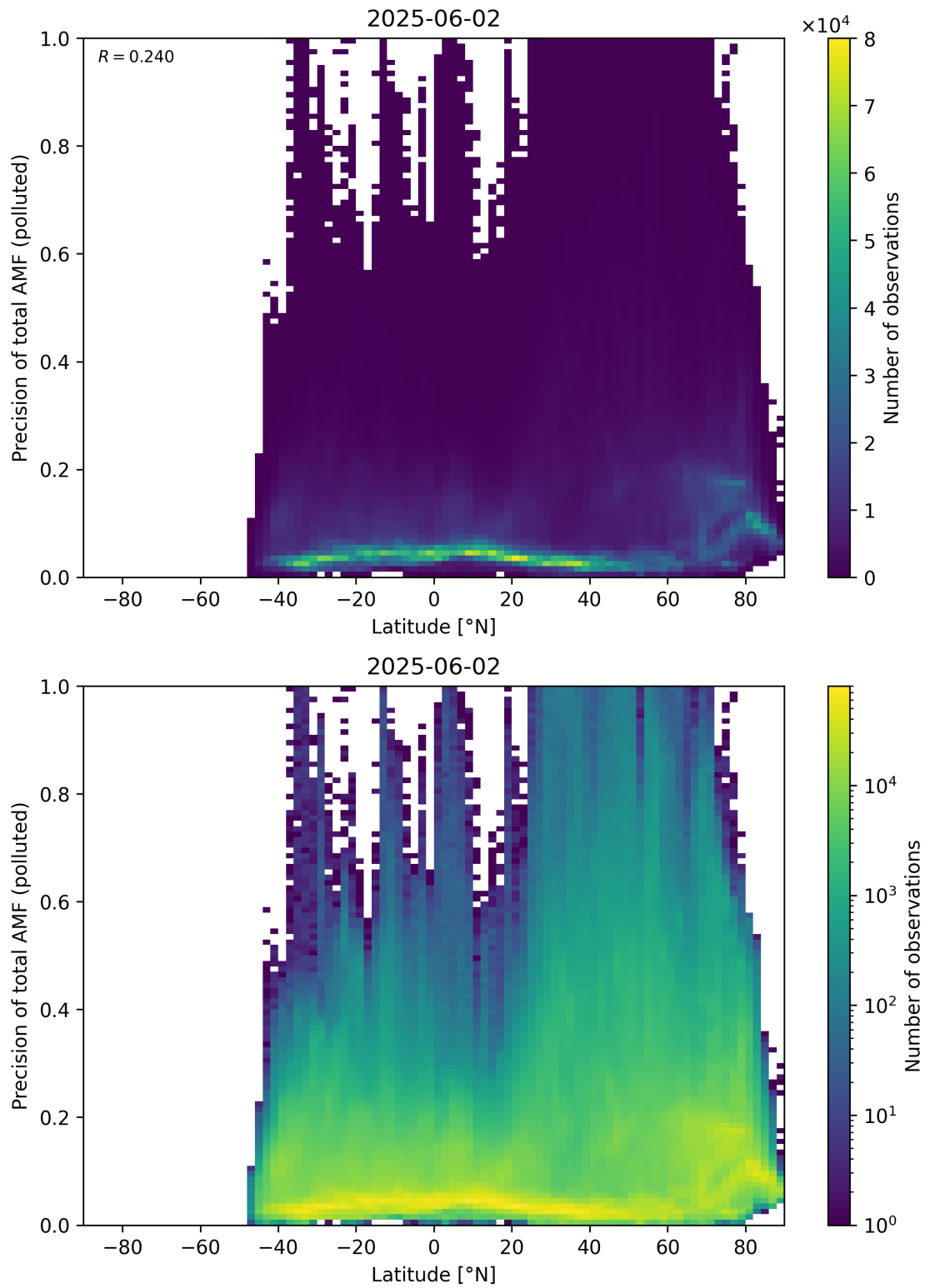
Figure 168: Scatter density plot of “Latitude” against “Precision of total AMF (polluted)” for 2025-06-01 to 2025-06-03.
