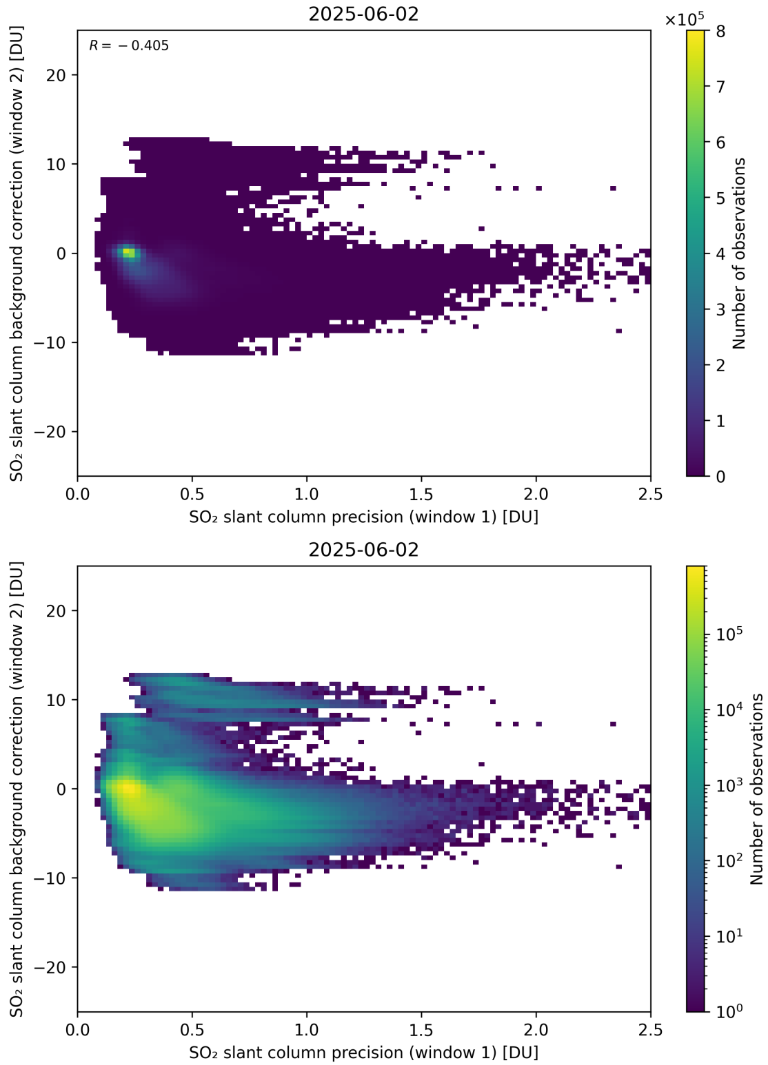
Figure 269: Scatter density plot of “SO 2 slant column precision (window 1)” against “SO 2 slant column background correction (window 2)” for 2025-06-01 to 2025-06-03.
