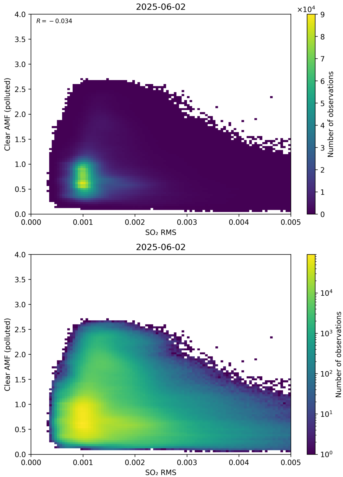
Figure 147: Scatter density plot of “SO 2 RMS” against “Clear AMF (polluted)” for 2025-06-01 to 2025-06-03.
