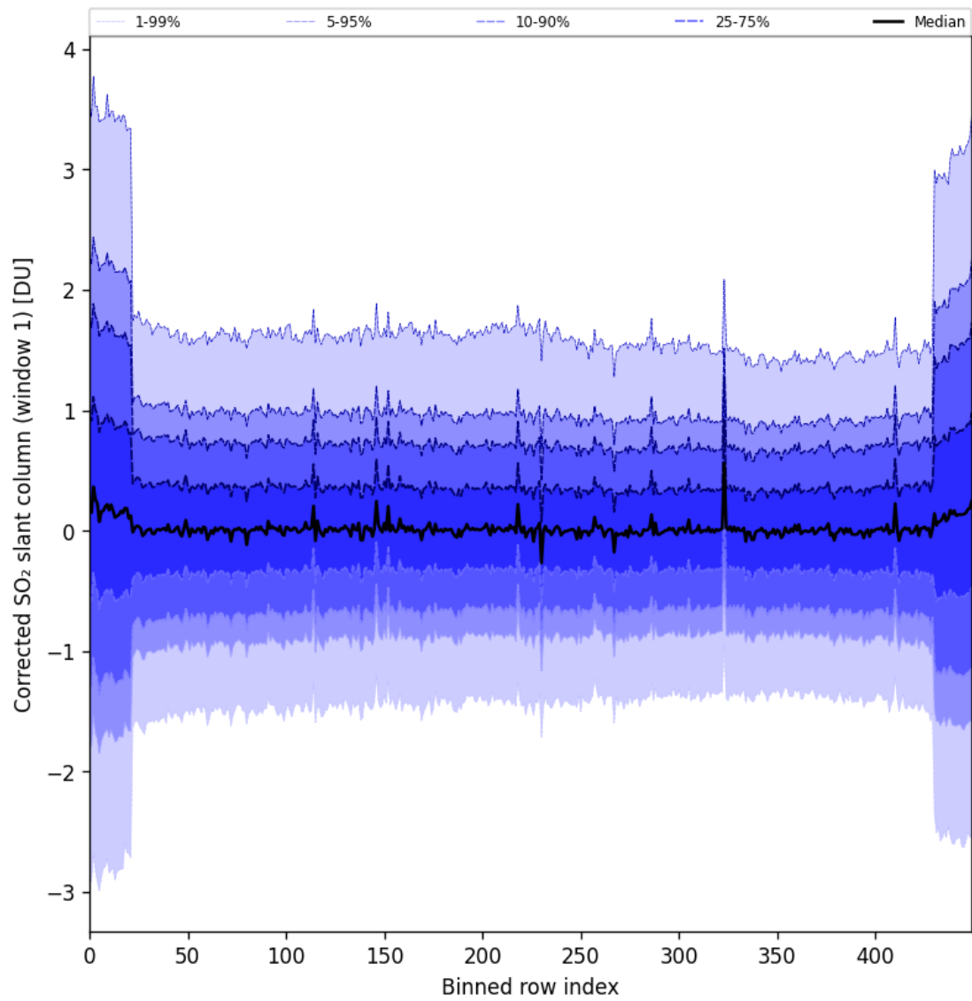
Figure 91: Along track statistics of “Corrected SO 2 slant column (window 1)” for 2025-06-01 to 2025-06-03
