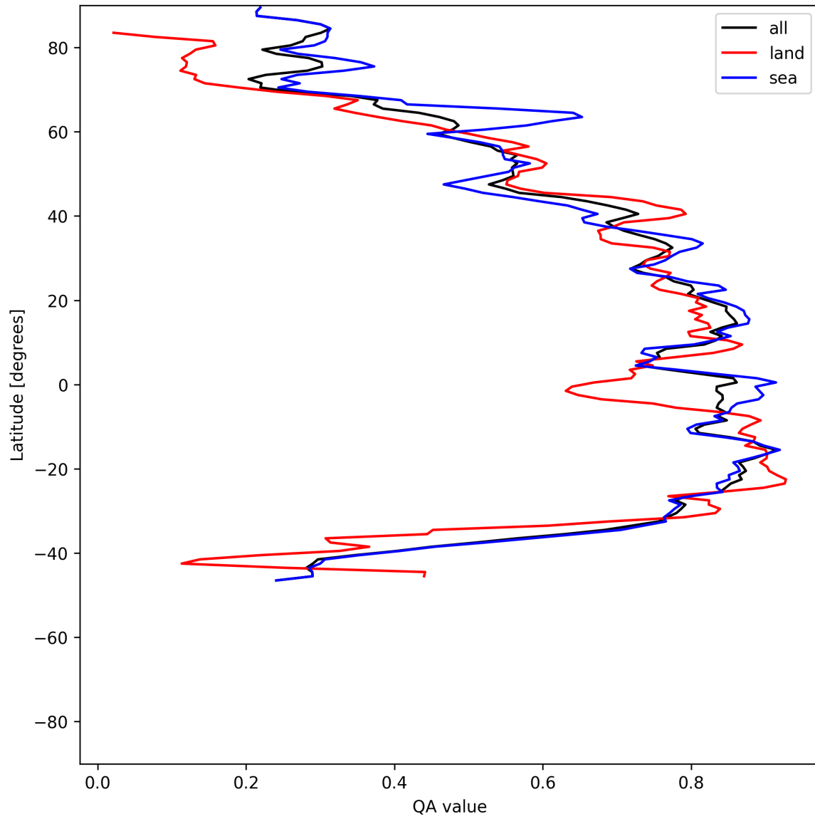
Figure 31: Zonal average of “QA value” for 2025-06-01 to 2025-06-03.
