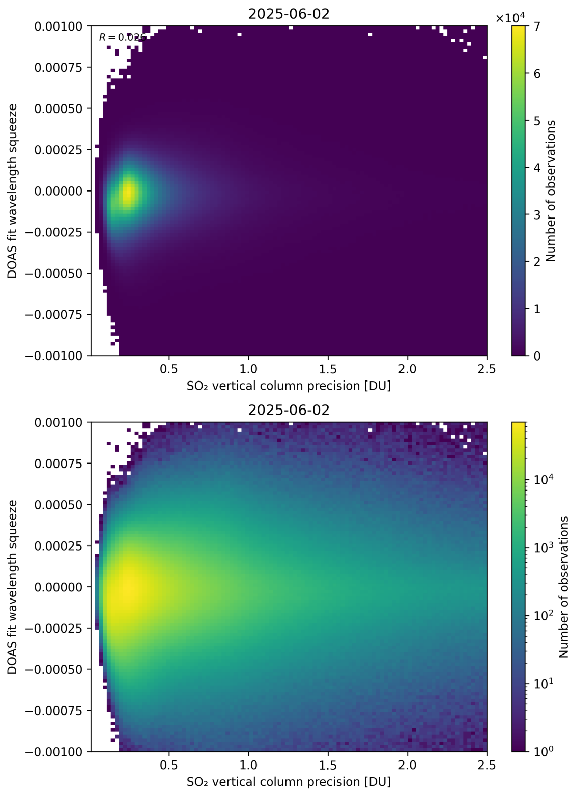
Figure 333: Scatter density plot of “SO 2 vertical column precision” against “DOAS fit wavelength squeeze” for 2025-06-01 to 2025-06-03.
