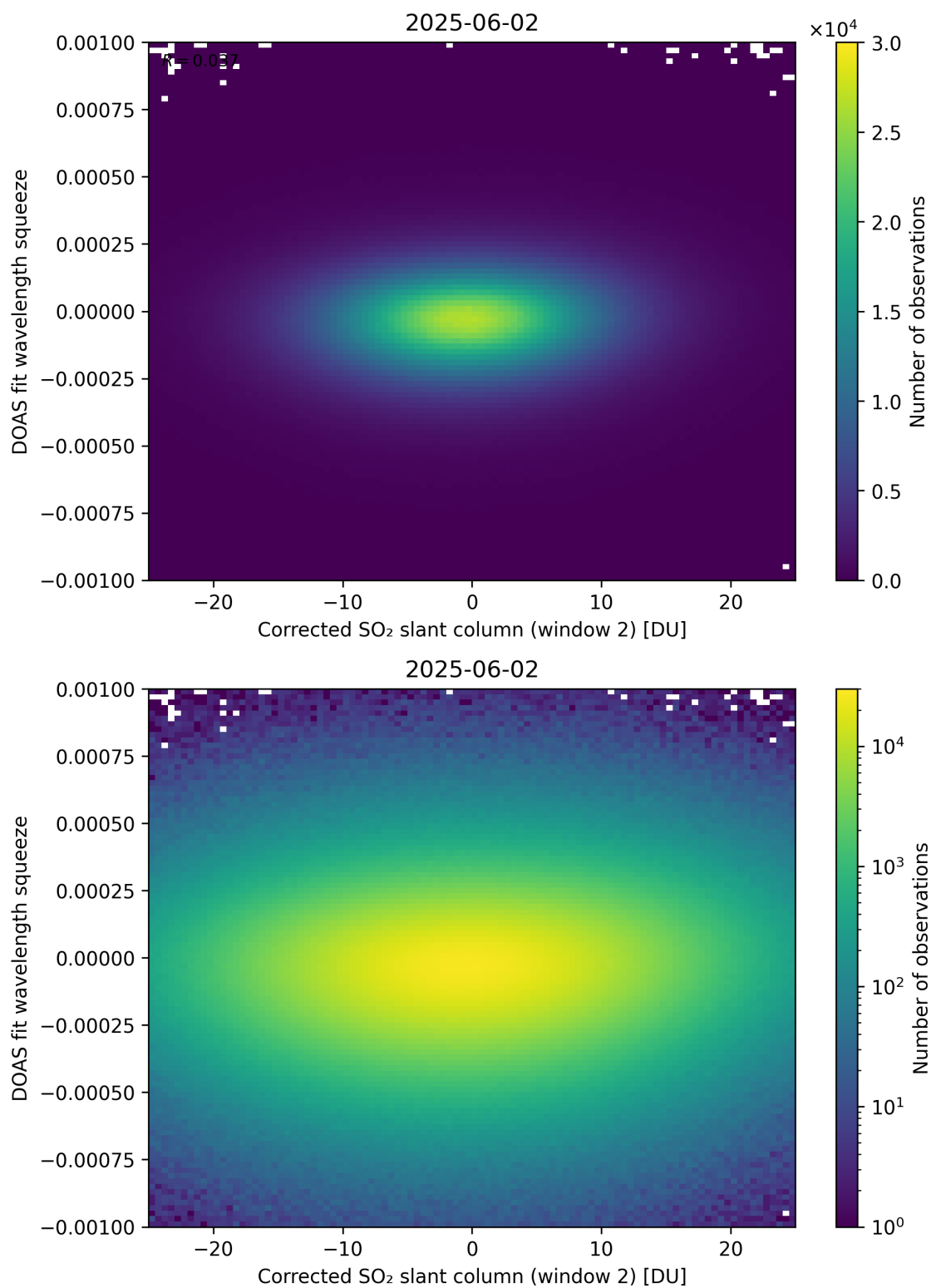
Figure 247: Scatter density plot of “Corrected SO 2 slant column (window 2)” against “DOAS fit wavelength squeeze” for 2025-06-01 to 2025-06-03.
