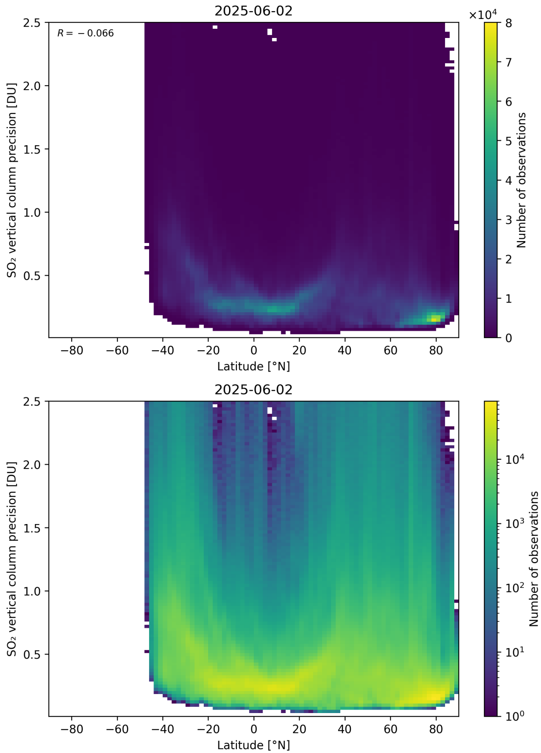
Figure 170: Scatter density plot of “Latitude” against “SO 2 vertical column precision” for 2025-06-01 to 2025-06-03.
