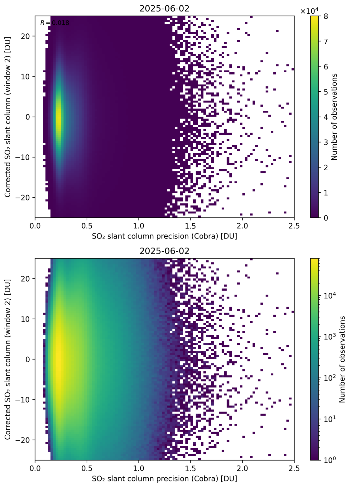
Figure 206: Scatter density plot of “SO 2 slant column precision (Cobra)” against “Corrected SO 2 slant column (window 2)” for 2025-06-01 to 2025-06-03.
