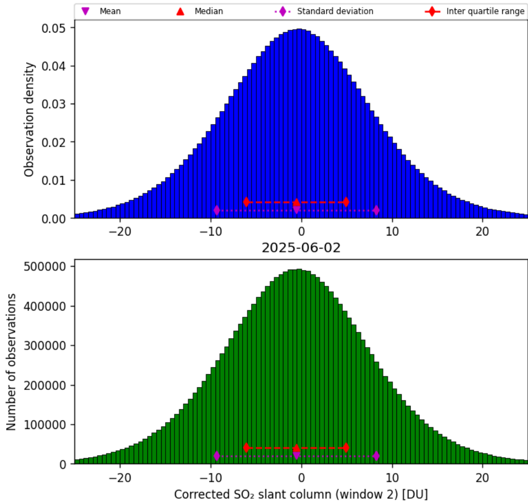
Figure 69: Histogram of “Corrected SO 2 slant column (window 2)” for 2025-06-01 to 2025-06-03
