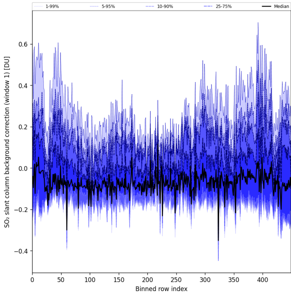
Figure 92: Along track statistics of “SO 2 slant column background correction (window 1)” for 2025-06-01 to 2025-06-03
