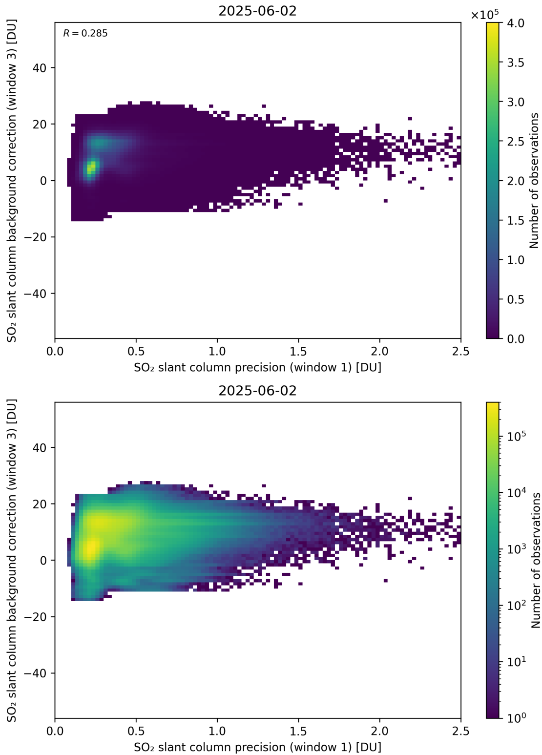
Figure 270: Scatter density plot of “SO 2 slant column precision (window 1)” against “SO 2 slant column background correction (window 3)” for 2025-06-01 to 2025-06-03.
