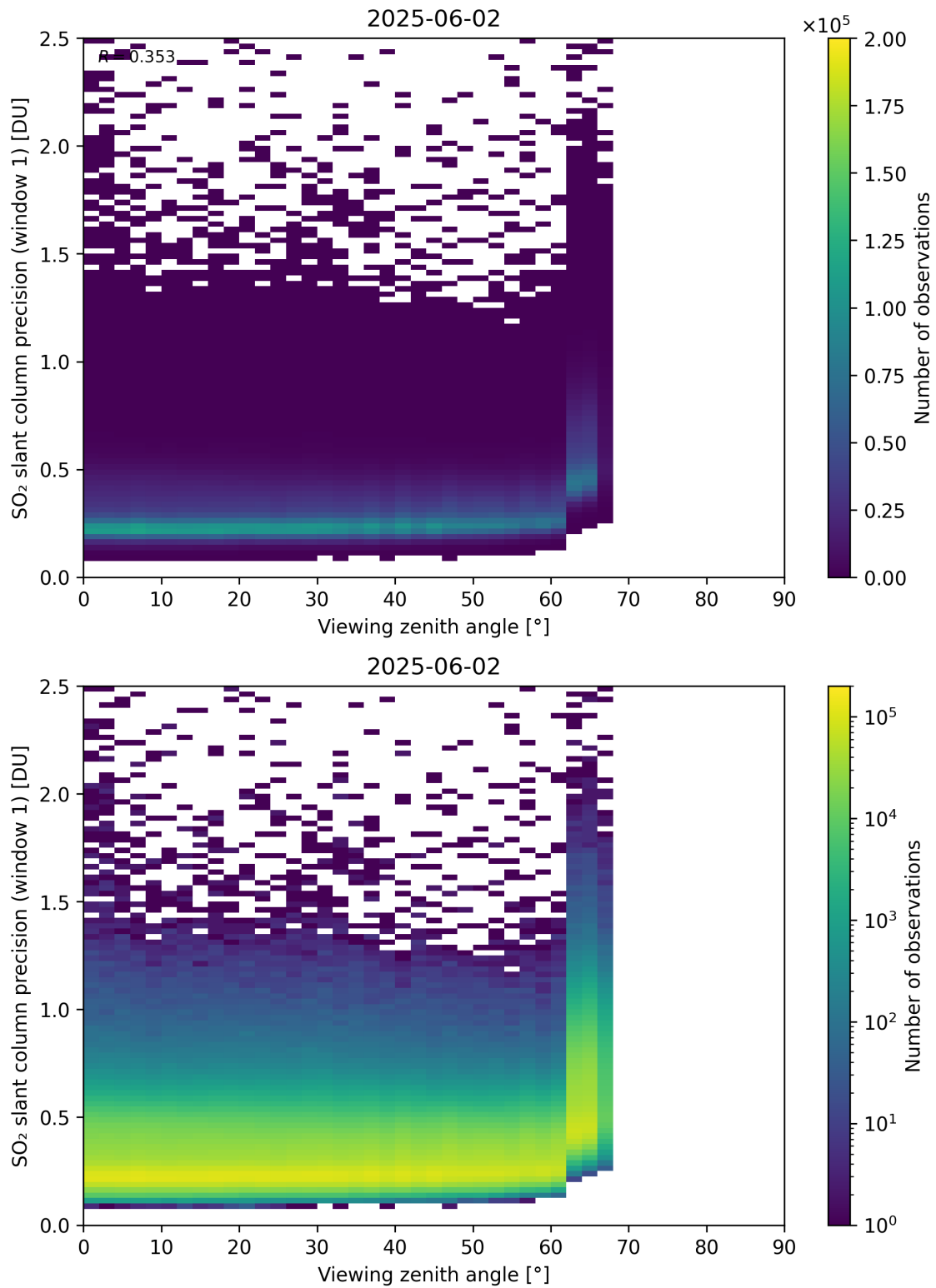
Figure 377: Scatter density plot of “Viewing zenith angle” against “SO 2 slant column precision (window 1)” for 2025-06-01 to 2025-06-03.
