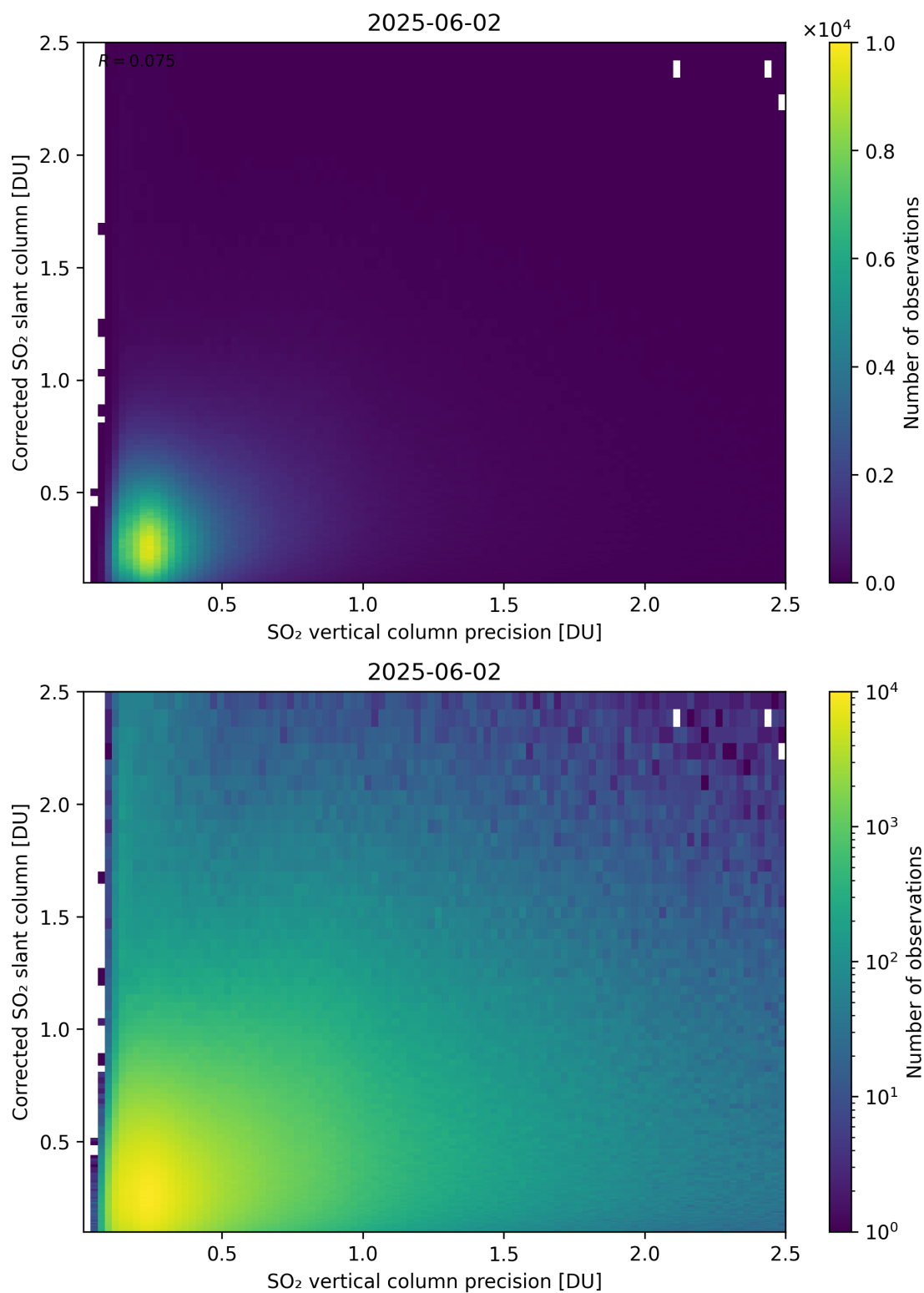
Figure 338: Scatter density plot of “SO 2 vertical column precision” against “Corrected SO 2 slant column” for 2025-06-01 to 2025-06-03.
