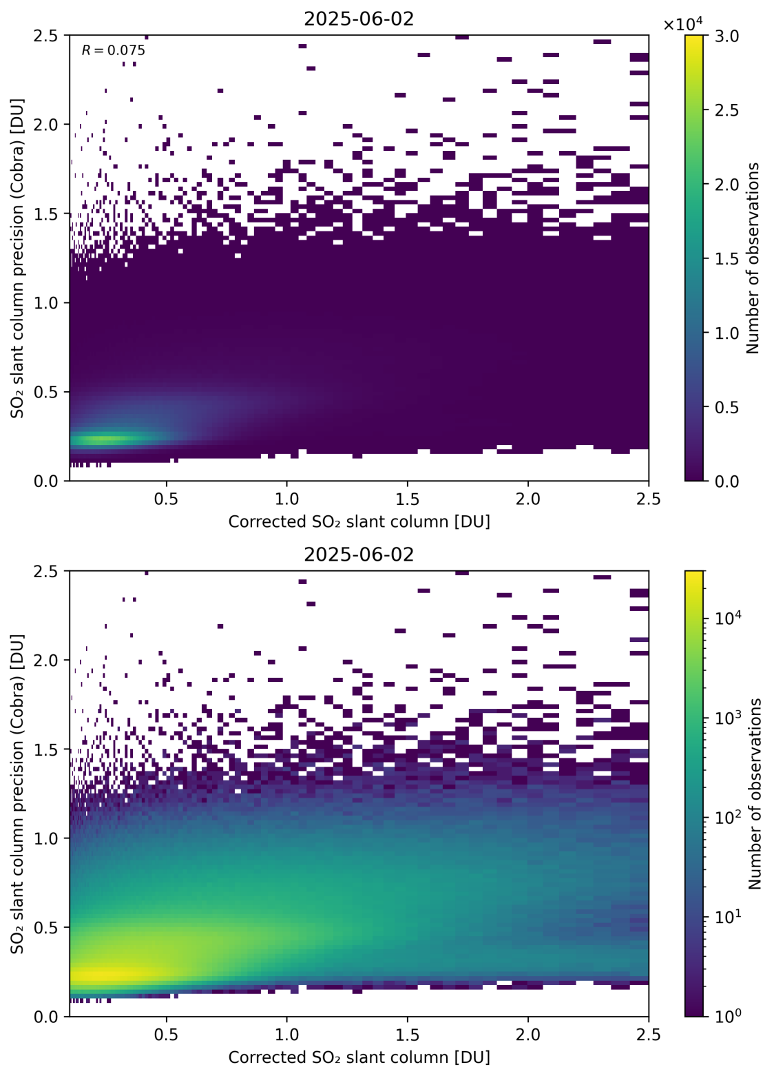
Figure 234: Scatter density plot of “Corrected SO 2 slant column” against “SO 2 slant column precision (Cobra)” for 2025-06-01 to 2025-06-03.
