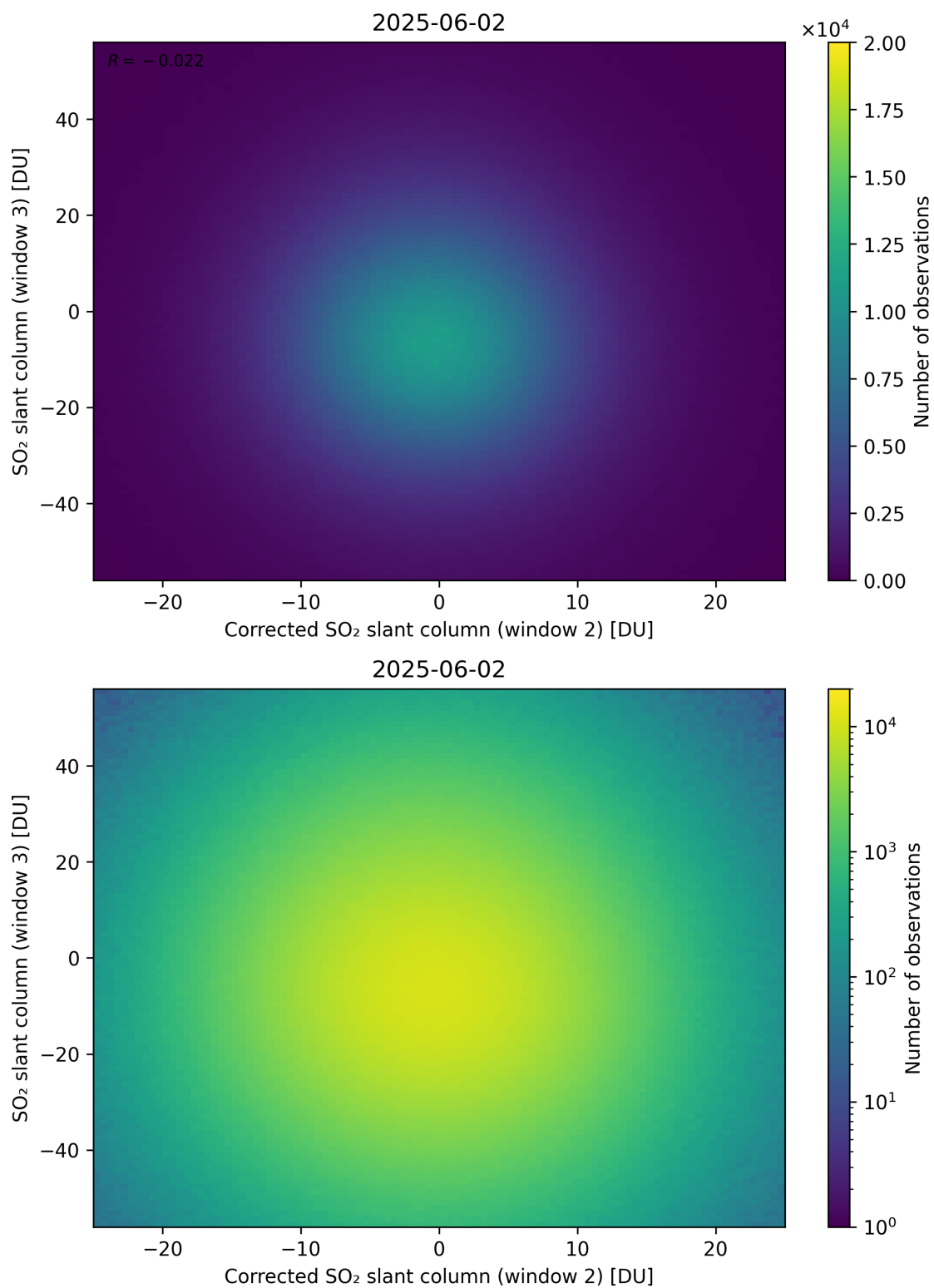
Figure 251: Scatter density plot of “Corrected SO 2 slant column (window 2)” against “SO 2 slant column (window 3)” for 2025-06-01 to 2025-06-03.
