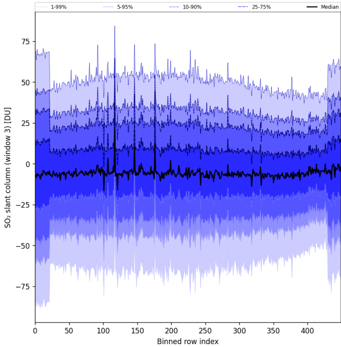
Figure 97: Along track statistics of “SO 2 slant column (window 3)” for 2025-06-01 to 2025-06-03
