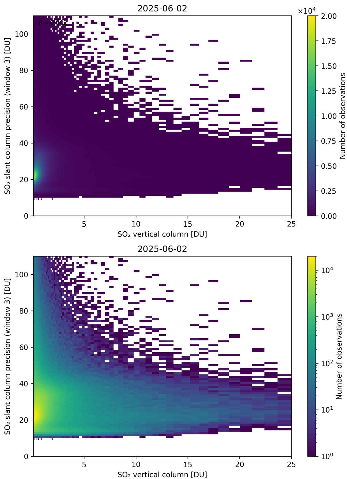
Figure 358: Scatter density plot of “SO 2 vertical column” against “SO 2 slant column precision (window 3)” for 2025-06-01 to 2025-06-03.
