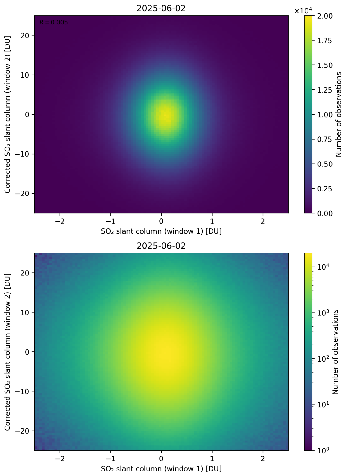
Figure 283: Scatter density plot of “SO 2 slant column (window 1)” against “Corrected SO 2 slant column (window 2)” for 2025-06-01 to 2025-06-03.
