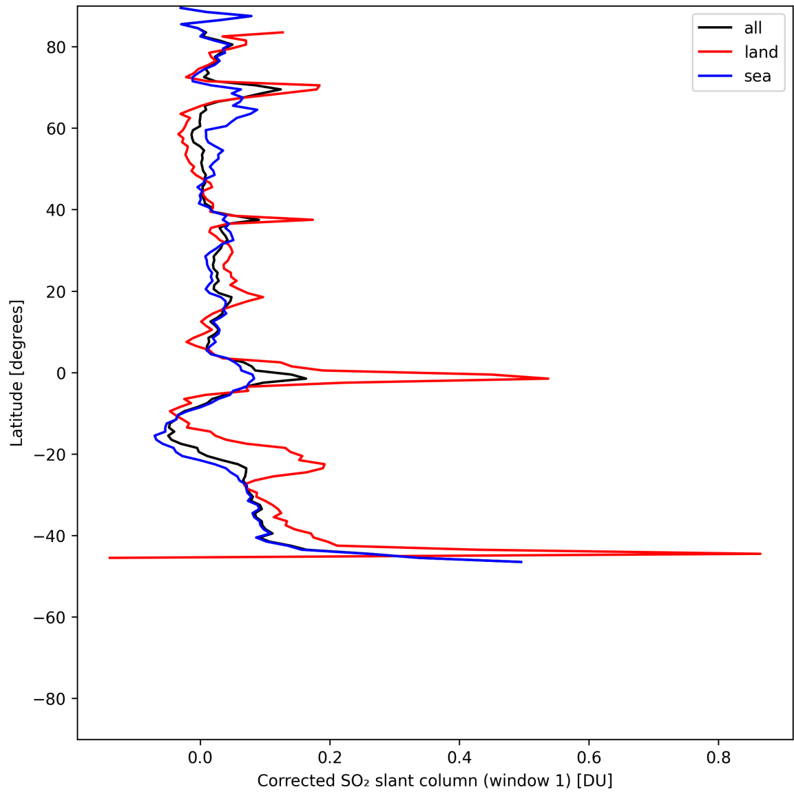
Figure 39: Zonal average of “Corrected SO 2 slant column (window 1)” for 2025-06-01 to 2025-06-03.
