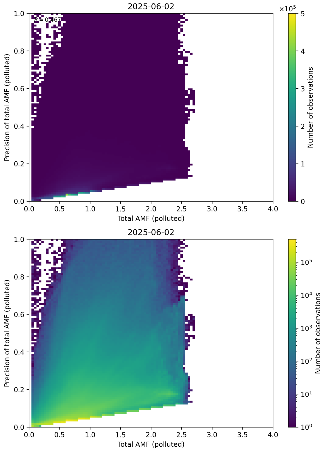
Figure 322: Scatter density plot of “Total AMF (polluted)” against “Precision of total AMF (polluted)” for 2025-06-01 to 2025-06-03.
