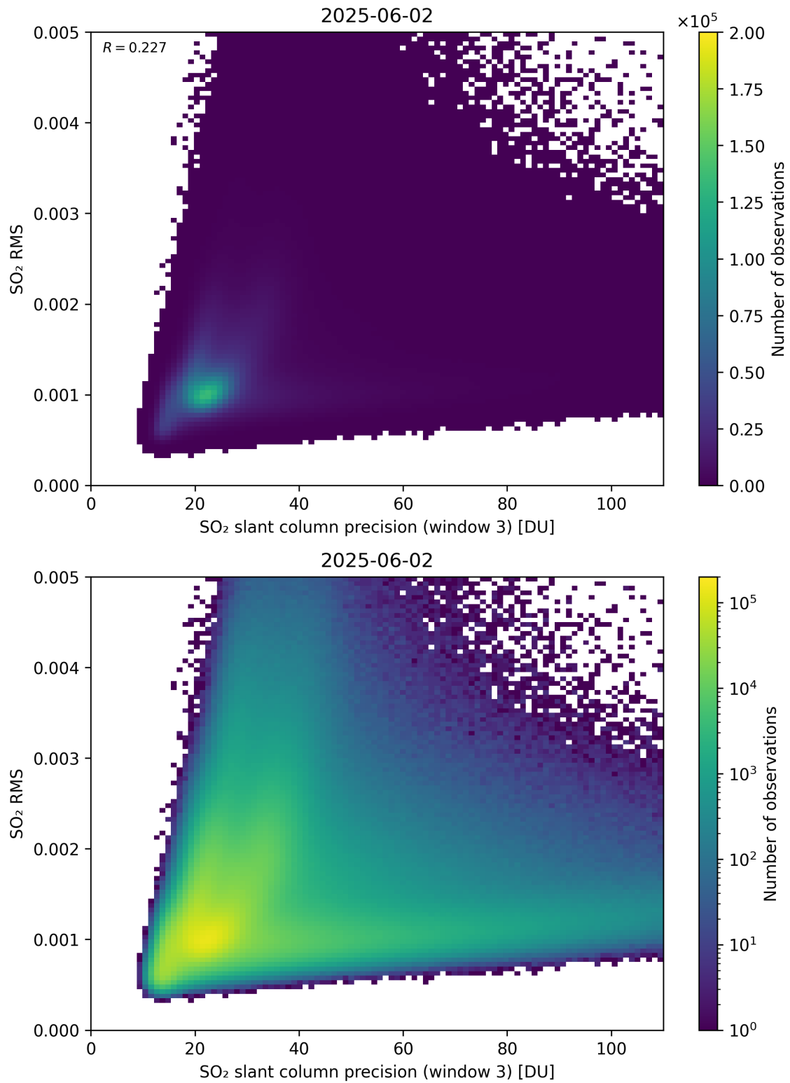
Figure 310: Scatter density plot of “SO 2 slant column precision (window 3)” against “SO 2 RMS” for 2025-06-01 to 2025-06-03.
