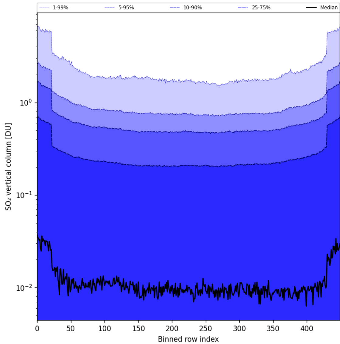
Figure 84: Along track statistics of “SO 2 vertical column” for 2025-06-01 to 2025-06-03
