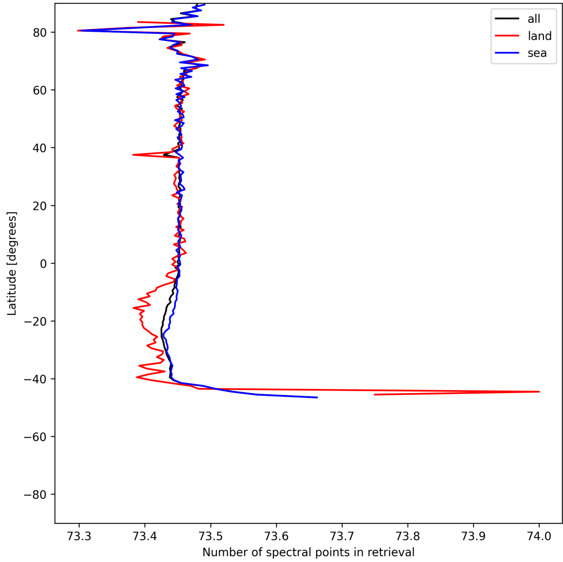
Figure 56: Zonal average of “Number of spectral points in retrieval” for 2025-06-01 to 2025-06-03.
