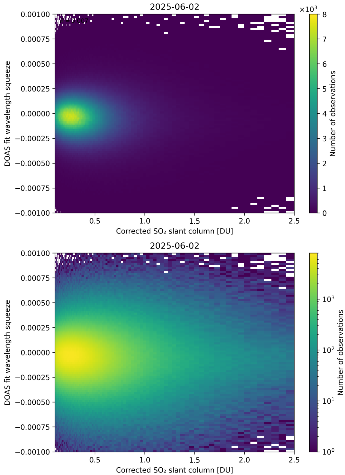
Figure 230: Scatter density plot of "Corrected SO 2 slant column" against "DOAS fit wavelength squeeze" for 2025-06-01 to 2025-06-03.
