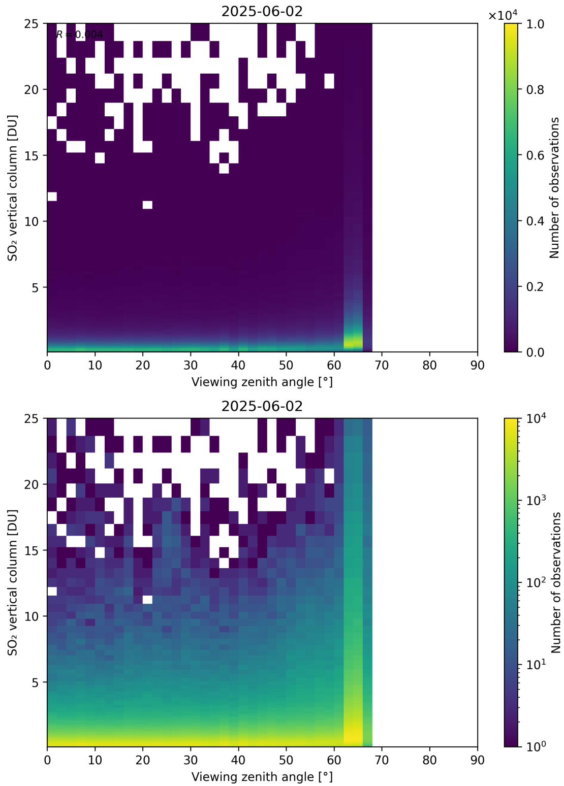
Figure 383: Scatter density plot of “Viewing zenith angle” against “SO 2 vertical column” for 2025-06-01 to 2025-06-03.
