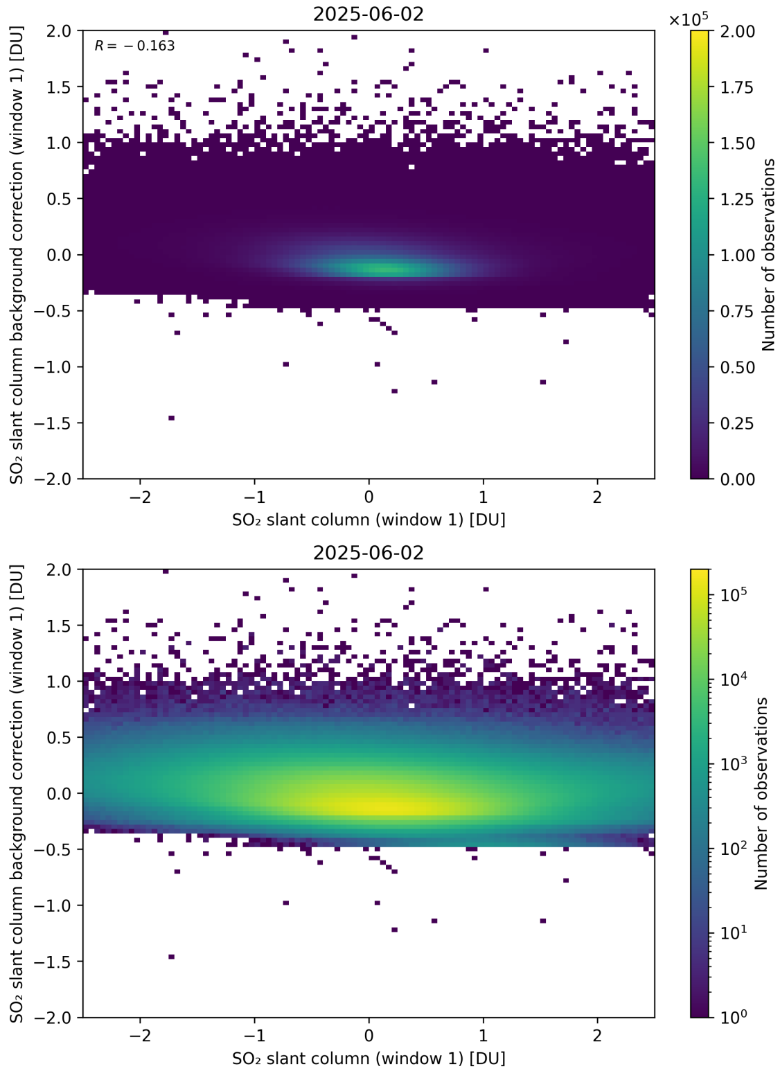
Figure 262: Scatter density plot of “SO 2 slant column (window 1)” against “SO 2 slant column background correction (window 1)” for 2025-06-01 to 2025-06-03.
