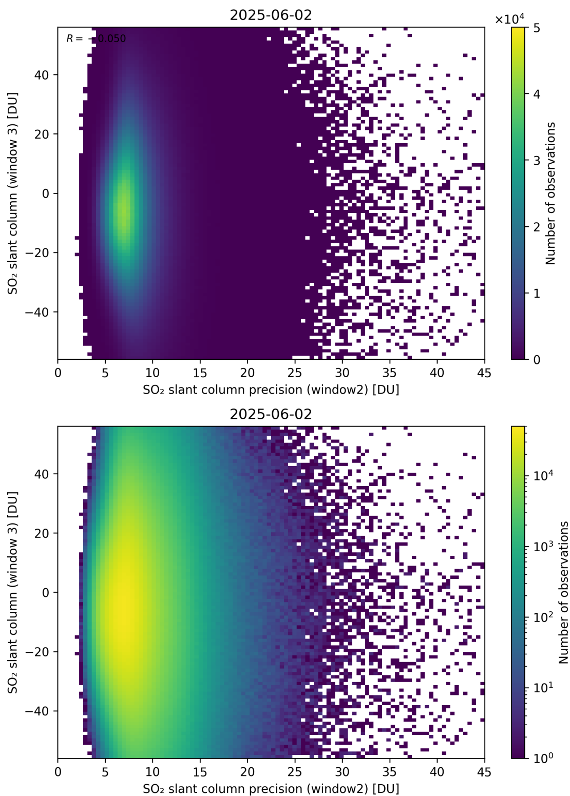
Figure 299: Scatter density plot of “SO 2 slant column precision (window2)” against “SO 2 slant column (window 3)” for 2025-06-01 to 2025-06-03.
