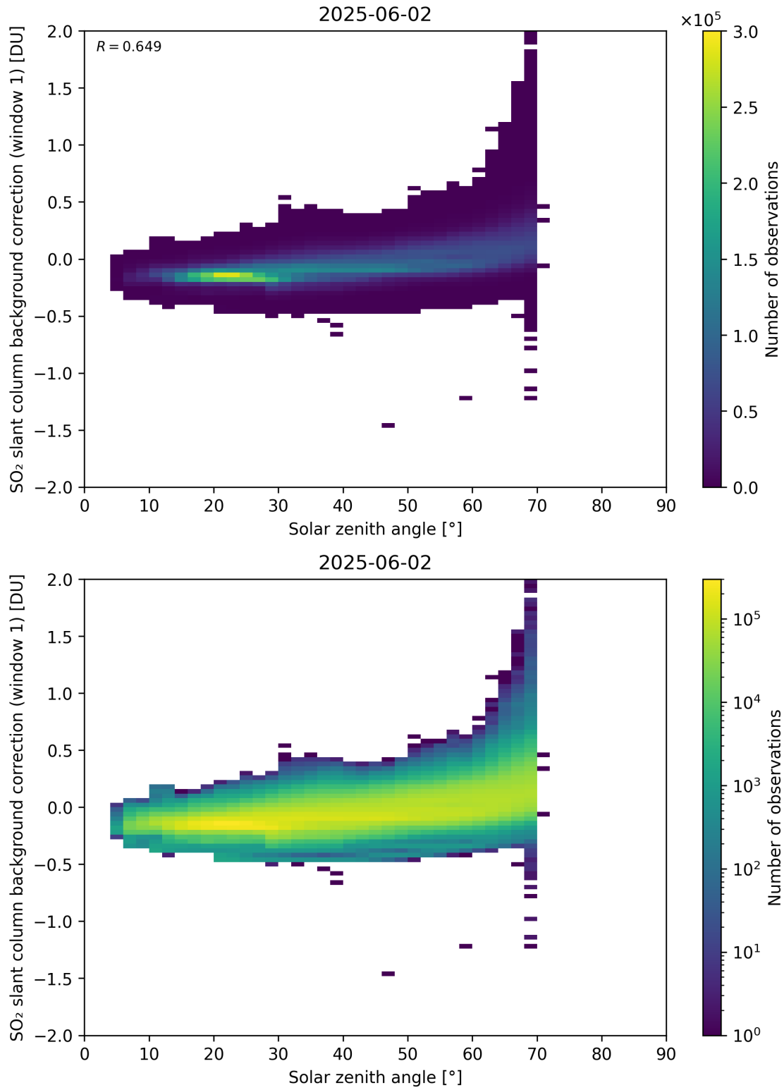
Figure 171: Scatter density plot of “Solar zenith angle” against “SO 2 slant column background correction (window 1)” for 2025-06-01 to 2025-06-03.
