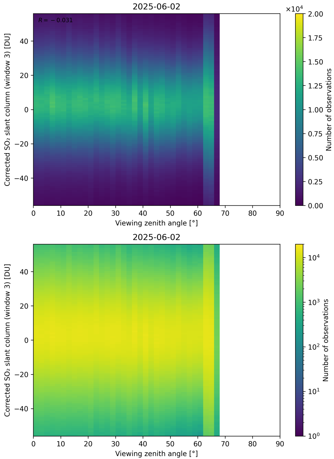
Figure 375: Scatter density plot of “Viewing zenith angle” against “Corrected SO 2 slant column (window 3)” for 2025-06-01 to 2025-06-03.
