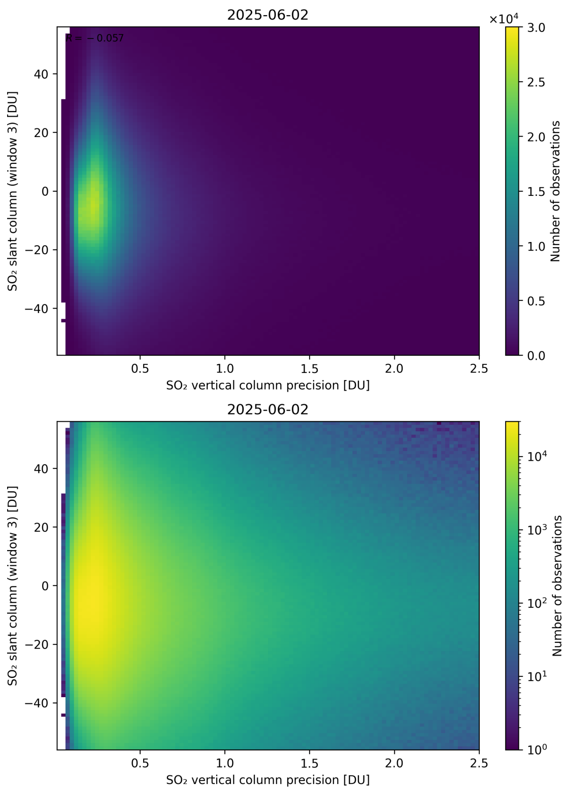
Figure 344: Scatter density plot of “SO 2 vertical column precision” against “SO 2 slant column (window 3)” for 2025-06-01 to 2025-06-03.
