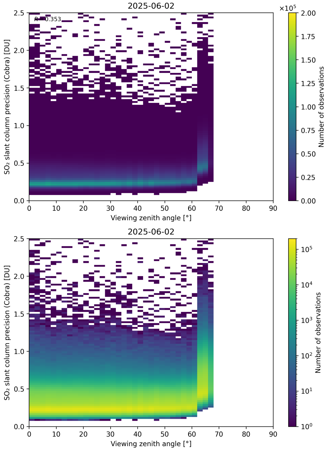
Figure 372: Scatter density plot of “Viewing zenith angle” against “SO 2 slant column precision (Cobra)” for 2025-06-01 to 2025-06-03.
