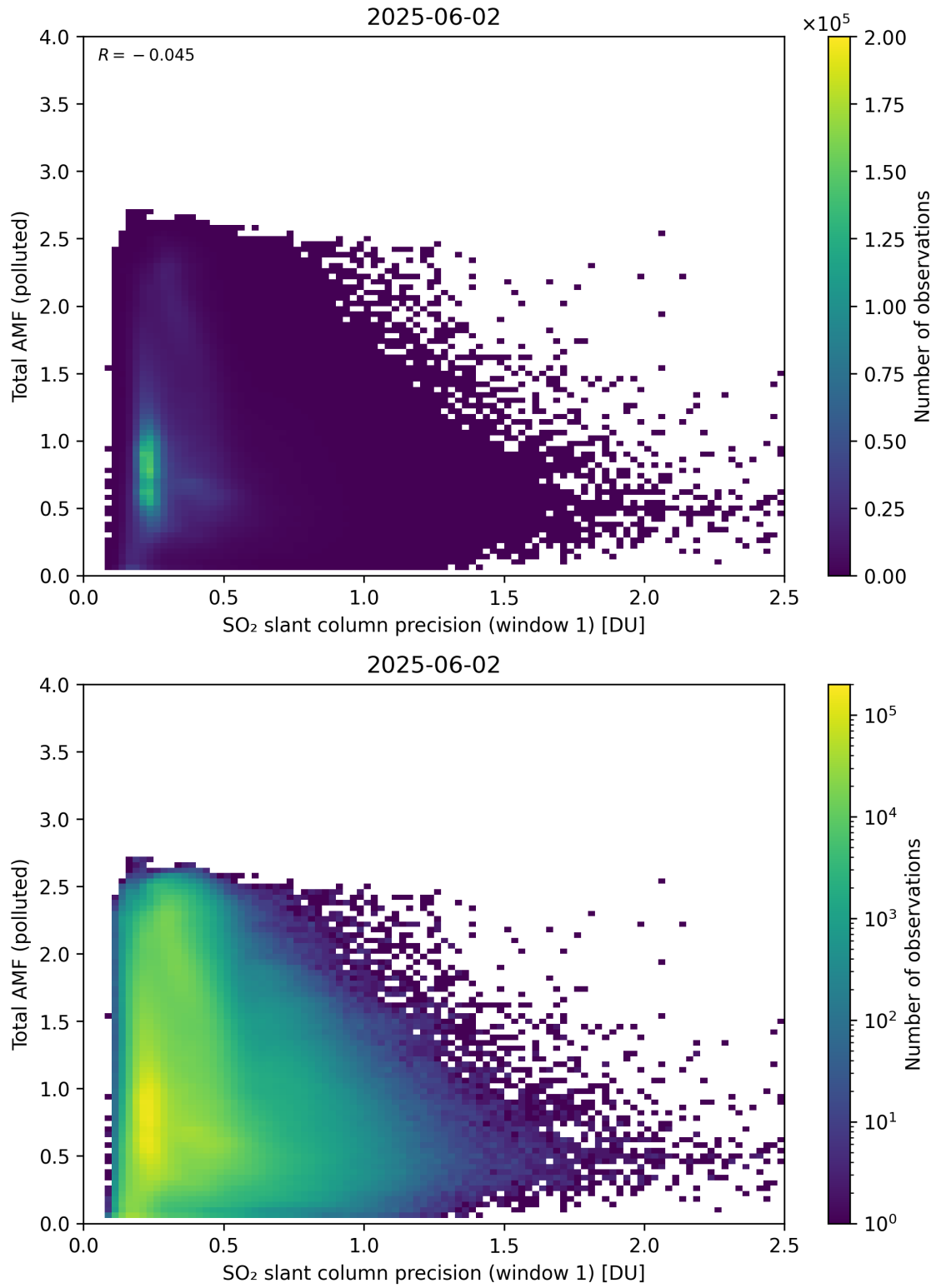
Figure 280: Scatter density plot of “SO 2 slant column precision (window 1)” against “Total AMF (polluted)” for 2025-06-01 to 2025-06-03.
