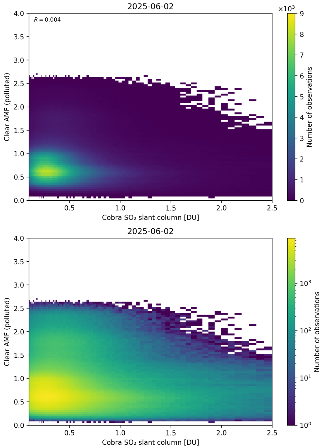
Figure 215: Scatter density plot of “Cobra SO 2 slant column” against “Clear AMF (polluted)” for 2025-06-01 to 2025-06-03.
