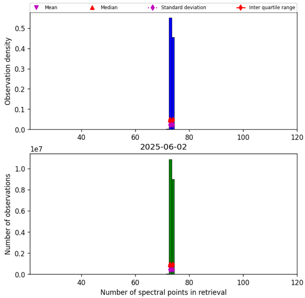
Figure 82: Histogram of “Number of spectral points in retrieval” for 2025-06-01 to 2025-06-03
