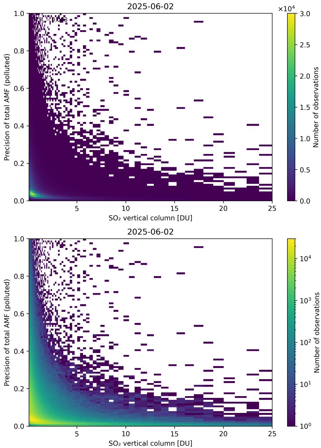
Figure 360: Scatter density plot of “SO 2 vertical column” against “Precision of total AMF (polluted)” for 2025-06-01 to 2025-06-03.
