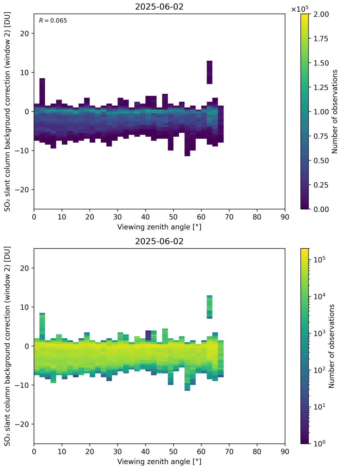
Figure 363: Scatter density plot of “Viewing zenith angle” against “SO 2 slant column background correction (window 2)” for 2025-06-01 to 2025-06-03.
