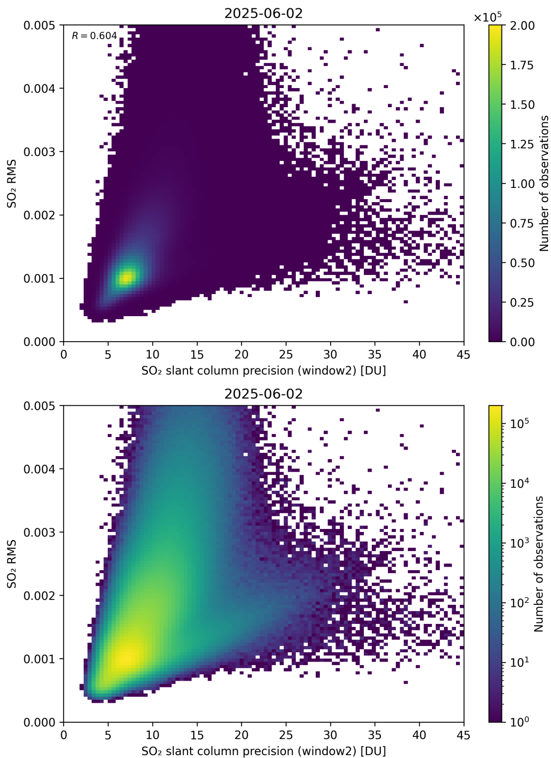
Figure 295: Scatter density plot of “SO 2 slant column precision (window2)” against “SO 2 RMS” for 2025-06-01 to 2025-06-03.
