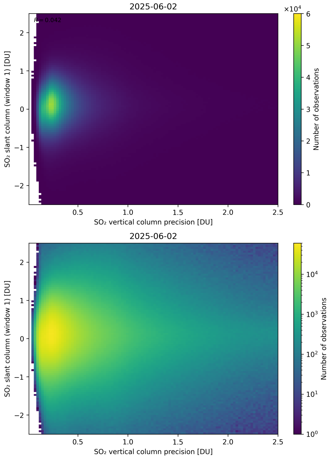
Figure 341: Scatter density plot of “SO 2 vertical column precision” against “SO 2 slant column (window 1)” for 2025-06-01 to 2025-06-03.
