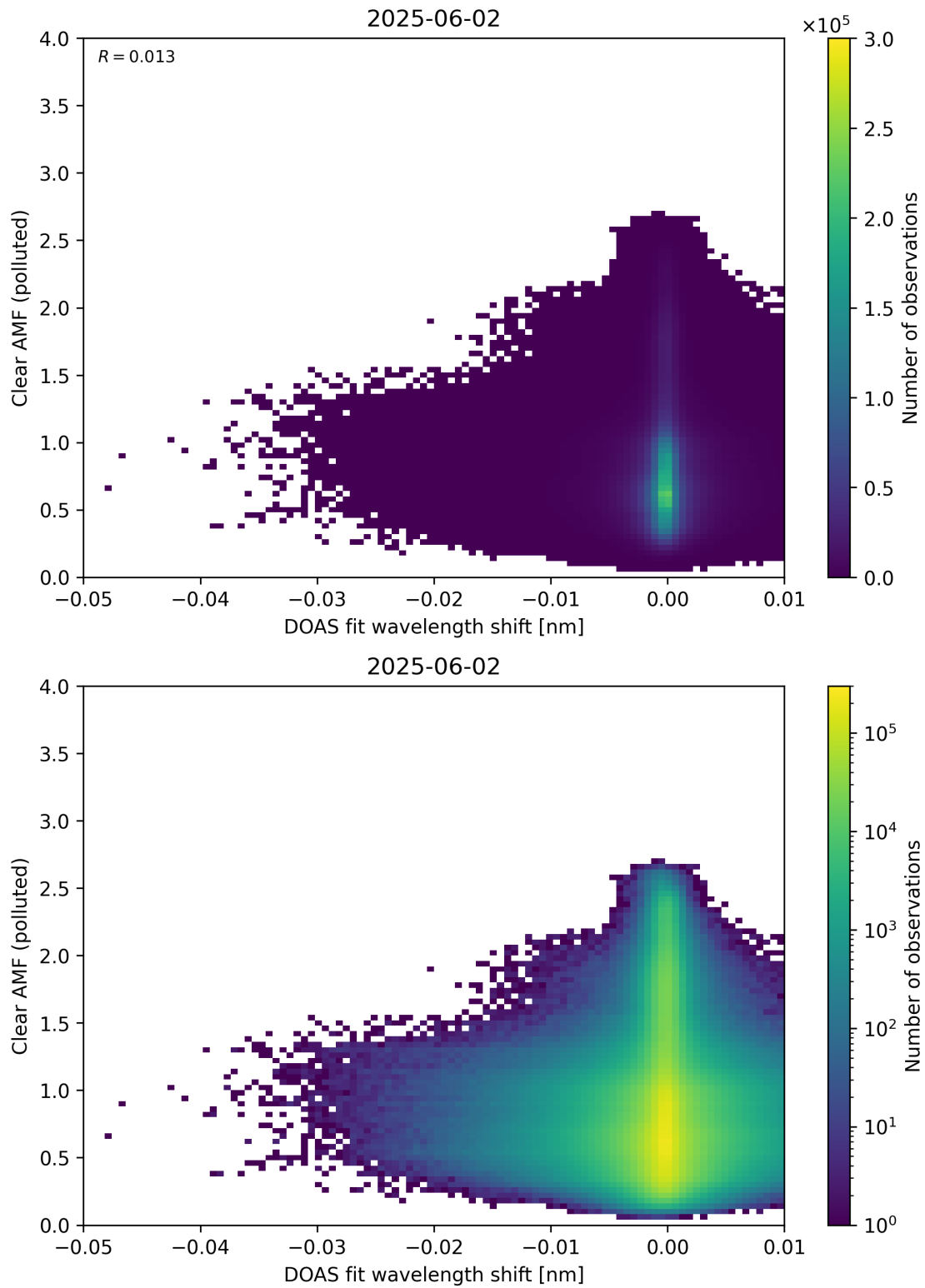
Figure 140: Scatter density plot of “DOAS fit wavelength shift” against “Clear AMF (polluted)” for 2025-06-01 to 2025-06-03.
