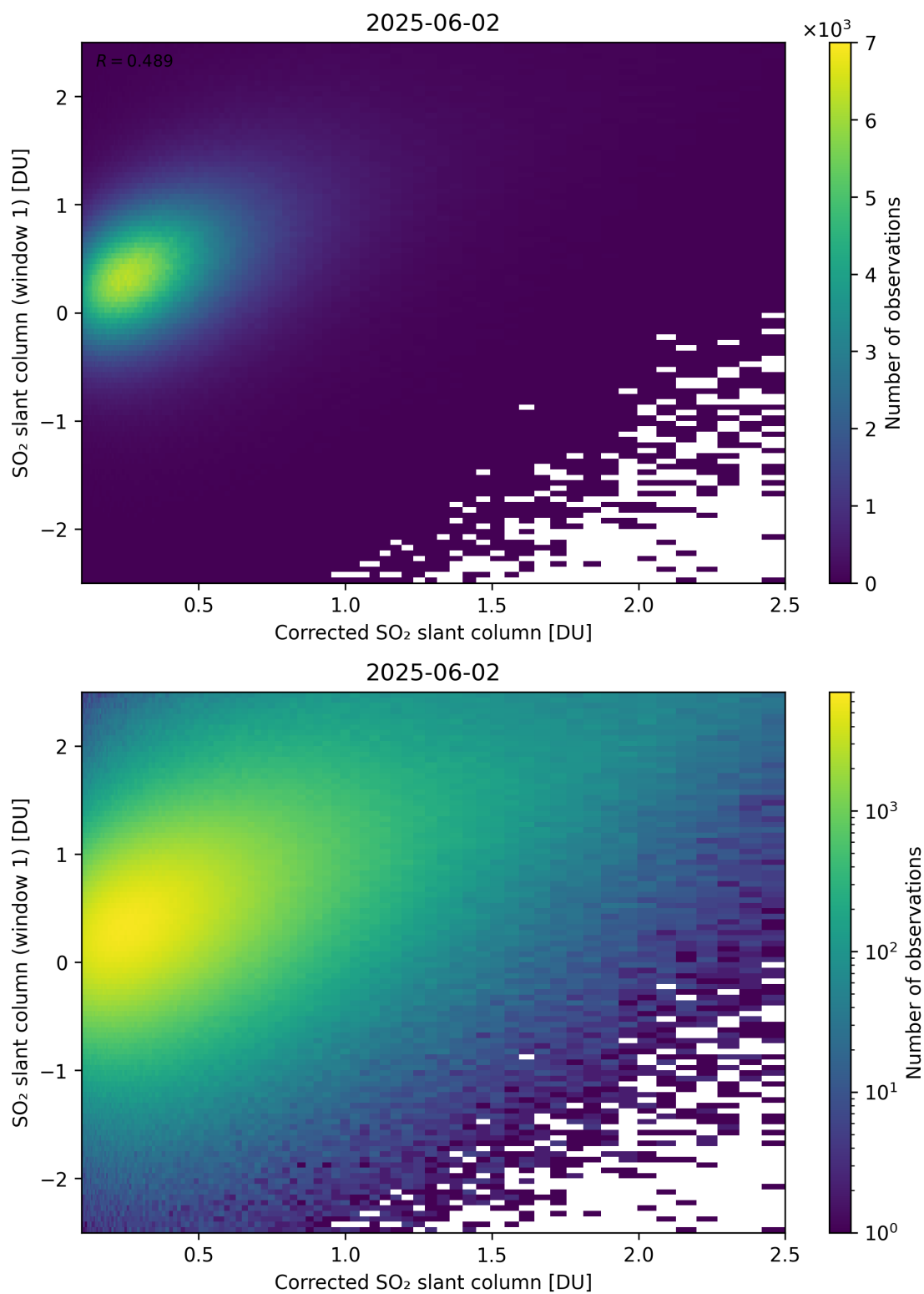
Figure 237: Scatter density plot of “Corrected SO 2 slant column” against “SO 2 slant column (window 1)” for 2025-06-01 to 2025-06-03.
