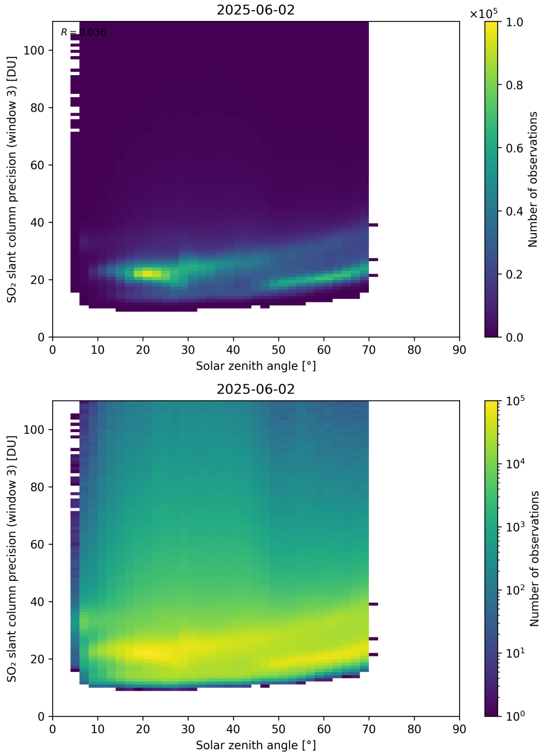
Figure 188: Scatter density plot of “Solar zenith angle” against “SO 2 slant column precision (window 3)” for 2025-06-01 to 2025-06-03.
