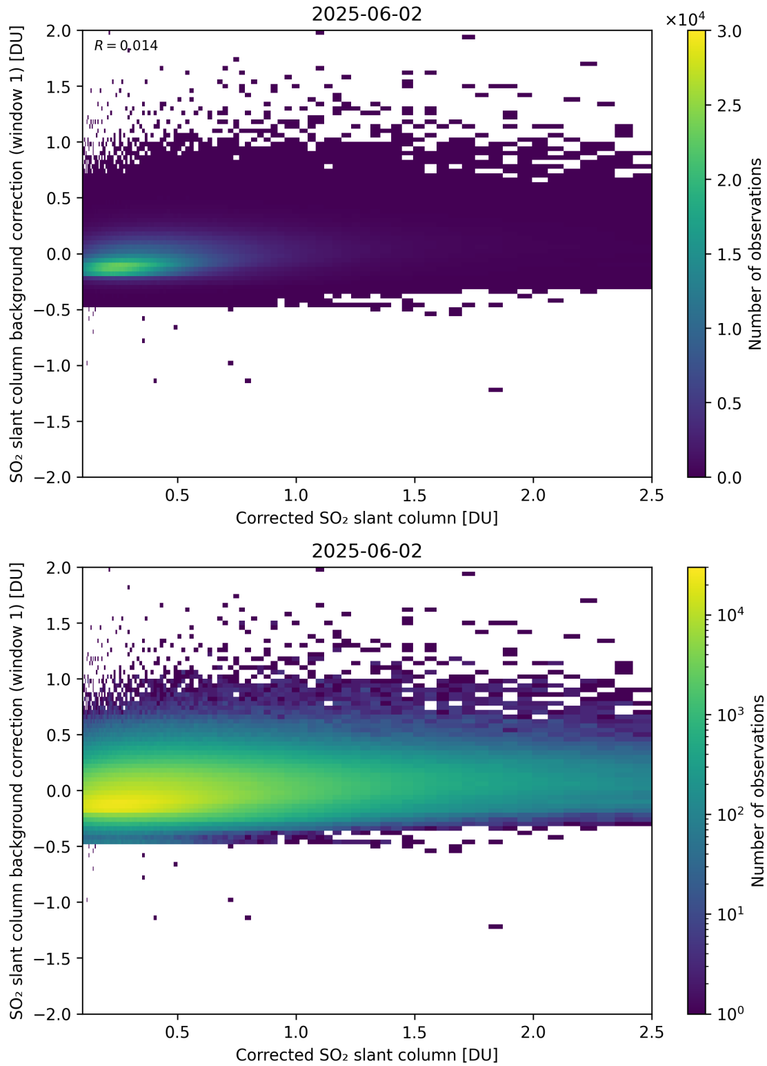
Figure 226: Scatter density plot of “Corrected SO 2 slant column” against “SO 2 slant column background correction (window 1)” for 2025-06-01 to 2025-06-03.
