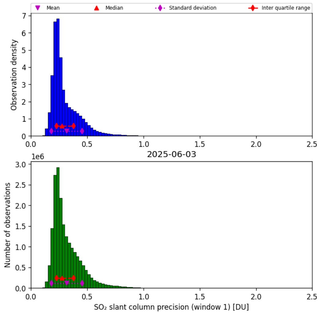
Figure 64: Histogram of “SO 2 slant column precision (window 1)” for 2025-06-02 to 2025-06-04
