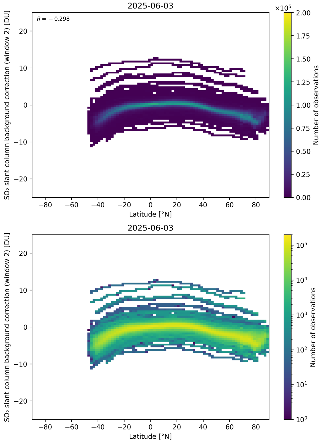
Figure 151: Scatter density plot of “Latitude” against “SO 2 slant column background correction (window 2)” for 2025-06-02 to 2025-06-04.
