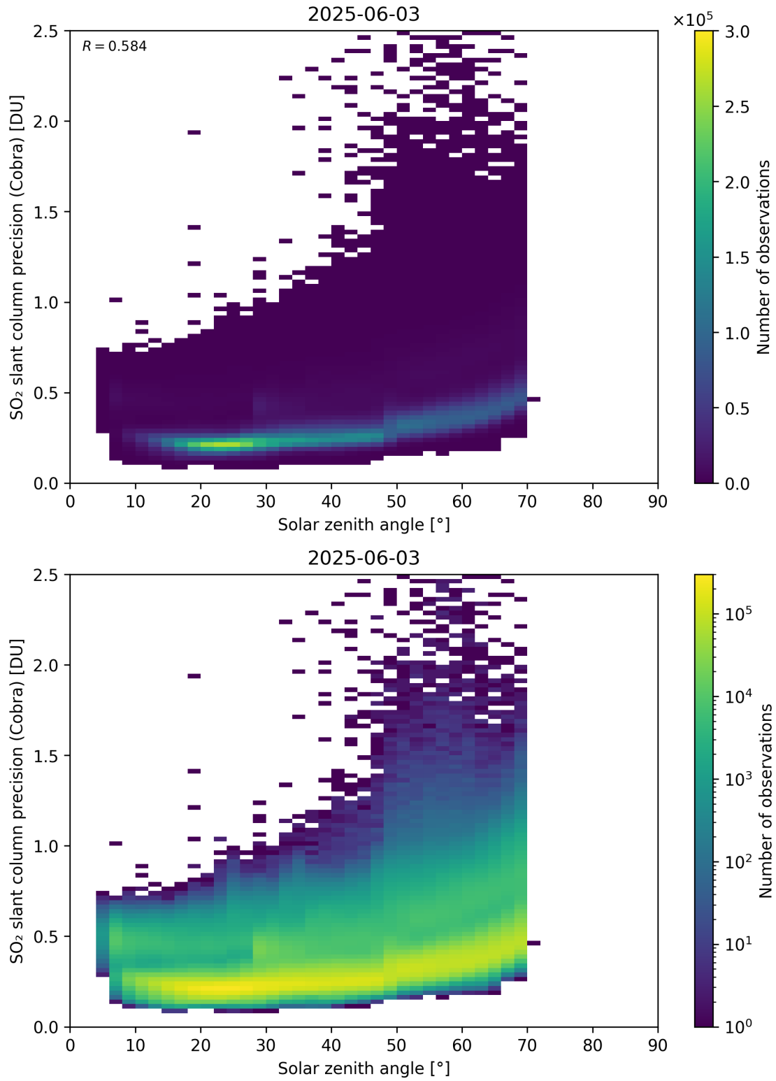
Figure 180: Scatter density plot of “Solar zenith angle” against “SO 2 slant column precision (Cobra)” for 2025-06-02 to 2025-06-04.
