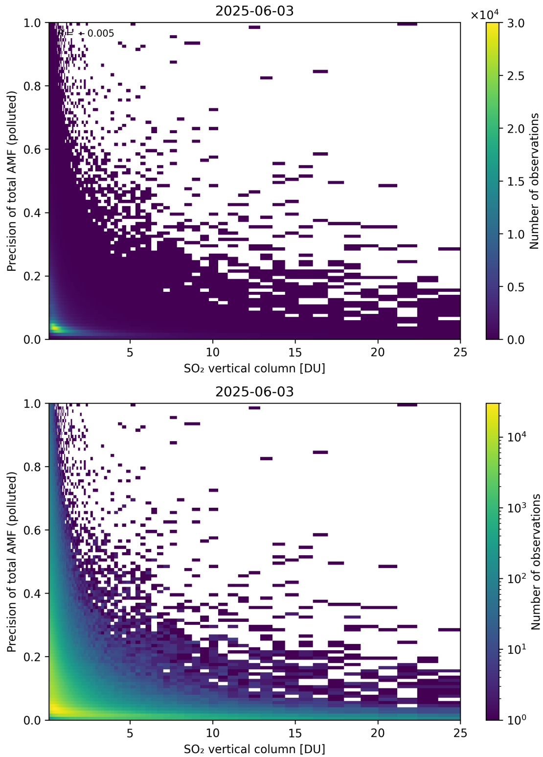
Figure 360: Scatter density plot of “SO 2 vertical column” against “Precision of total AMF (polluted)” for 2025-06-02 to 2025-06-04.
