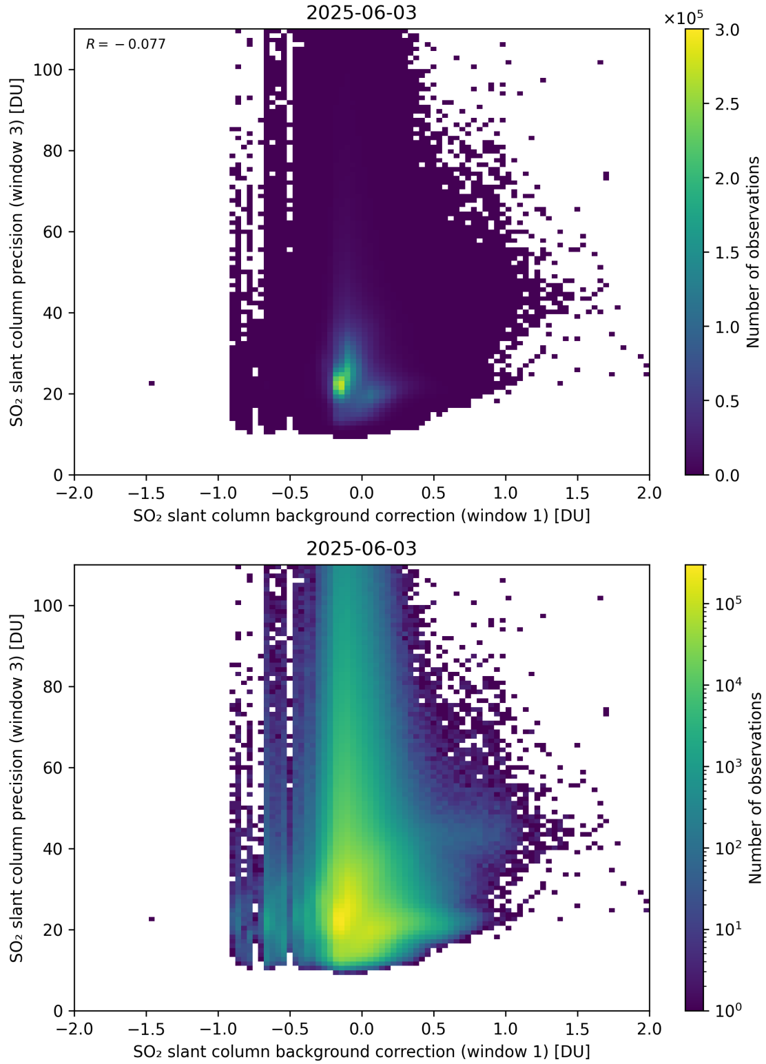
Figure 119: Scatter density plot of “SO 2 slant column background correction (window 1)” against “SO 2 slant column precision (window 3)” for 2025-06-02 to 2025-06-04.
