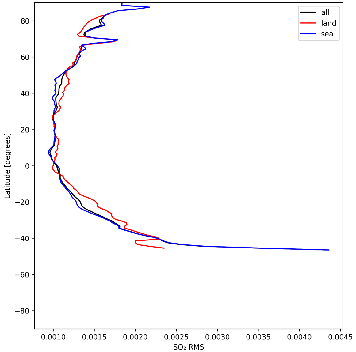
Figure 52: Zonal average of “SO 2 RMS” for 2025-06-02 to 2025-06-04.
