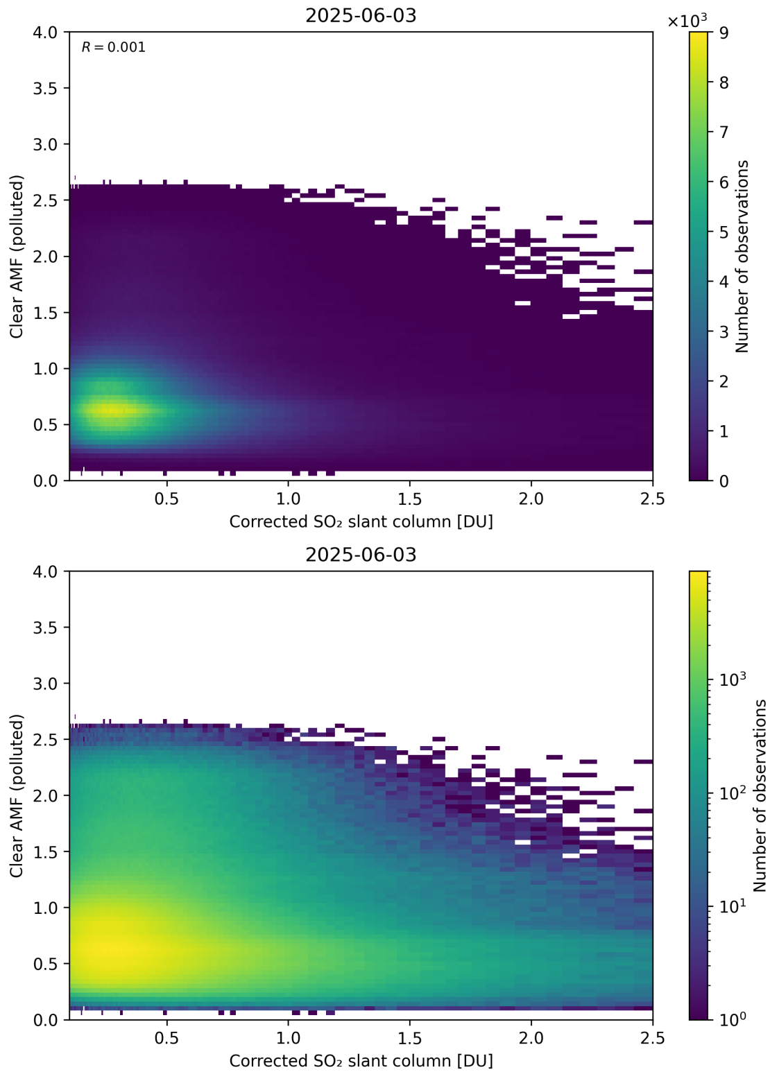
Figure 232: Scatter density plot of “Corrected SO 2 slant column” against “Clear AMF (polluted)” for 2025-06-02 to 2025-06-04.
