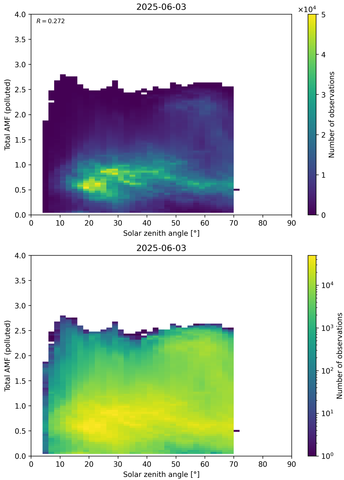
Figure 189: Scatter density plot of “Solar zenith angle” against “Total AMF (polluted)” for 2025-06-02 to 2025-06-04.
