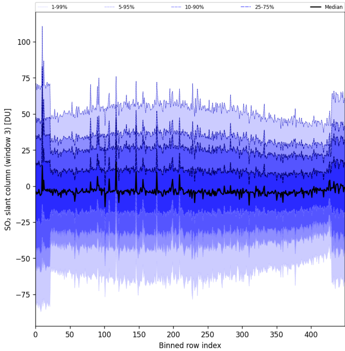
Figure 97: Along track statistics of “SO 2 slant column (window 3)” for 2025-06-02 to 2025-06-04
