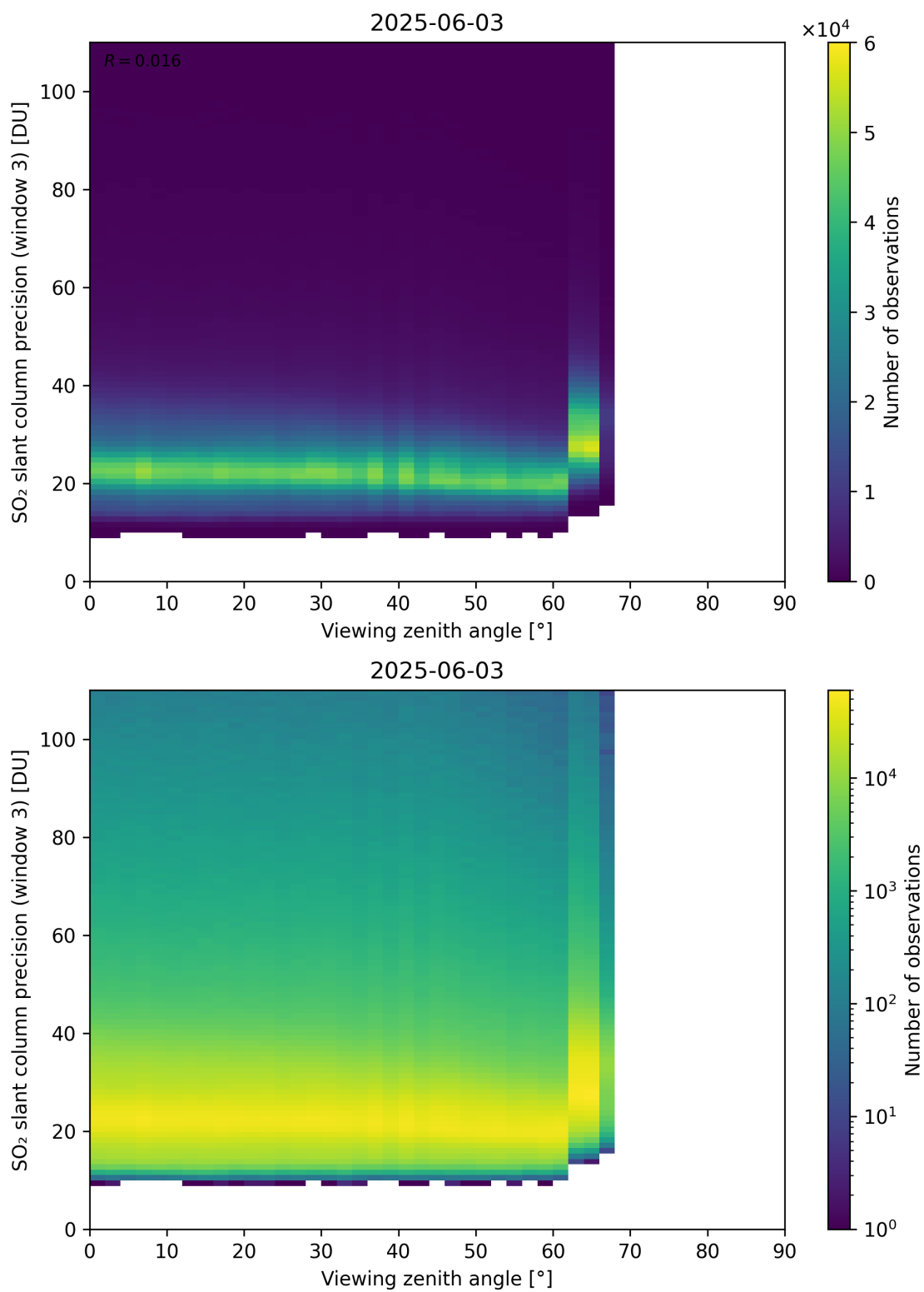
Figure 380: Scatter density plot of “Viewing zenith angle” against “SO 2 slant column precision (window 3)” for 2025-06-02 to 2025-06-04.
