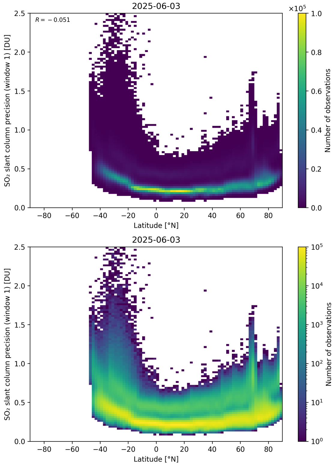
Figure 163: Scatter density plot of “Latitude” against “SO 2 slant column precision (window 1)” for 2025-06-02 to 2025-06-04.
