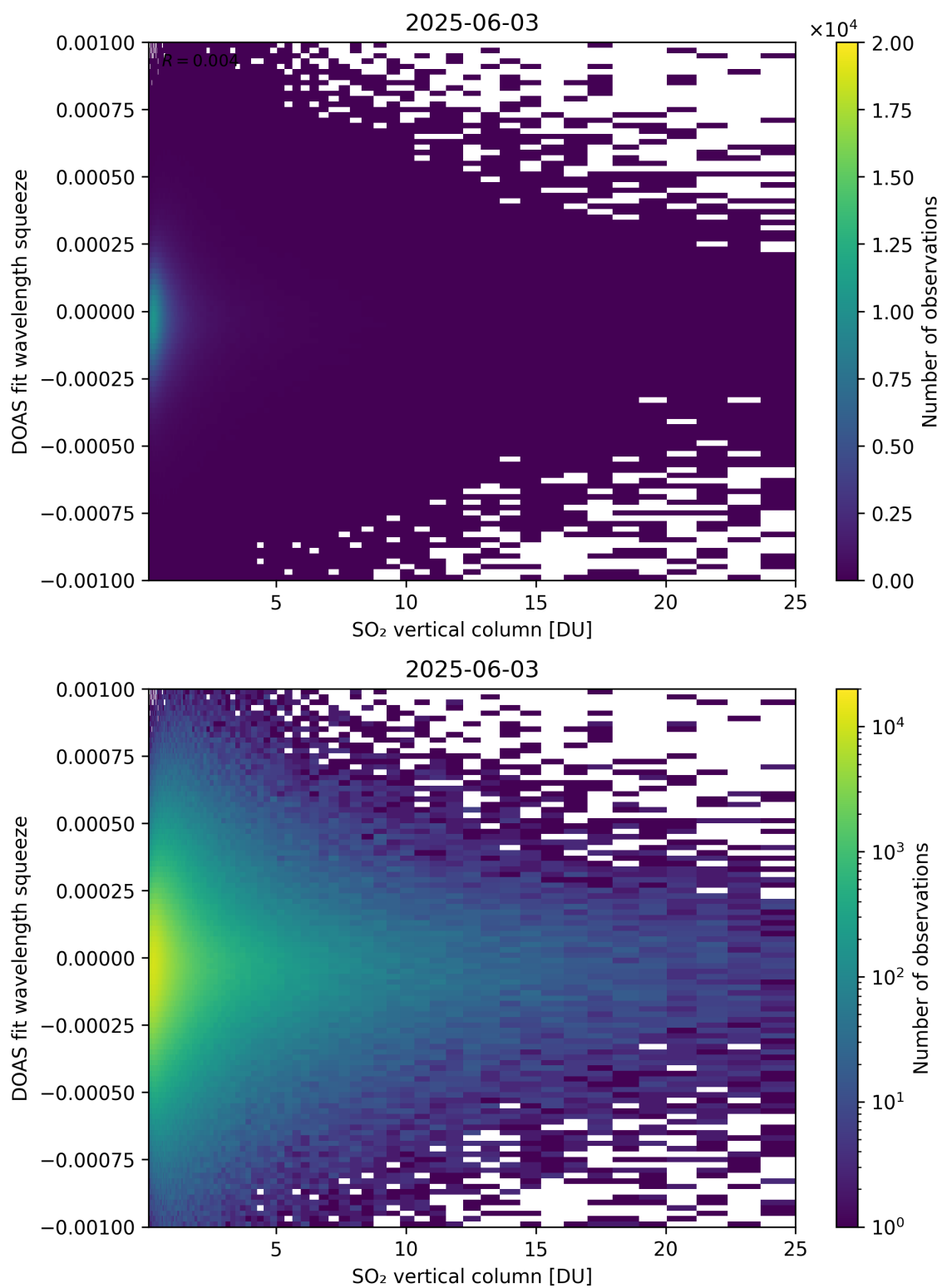
Figure 327: Scatter density plot of “SO 2 vertical column” against “DOAS fit wavelength squeeze” for 2025-06-02 to 2025-06-04.
