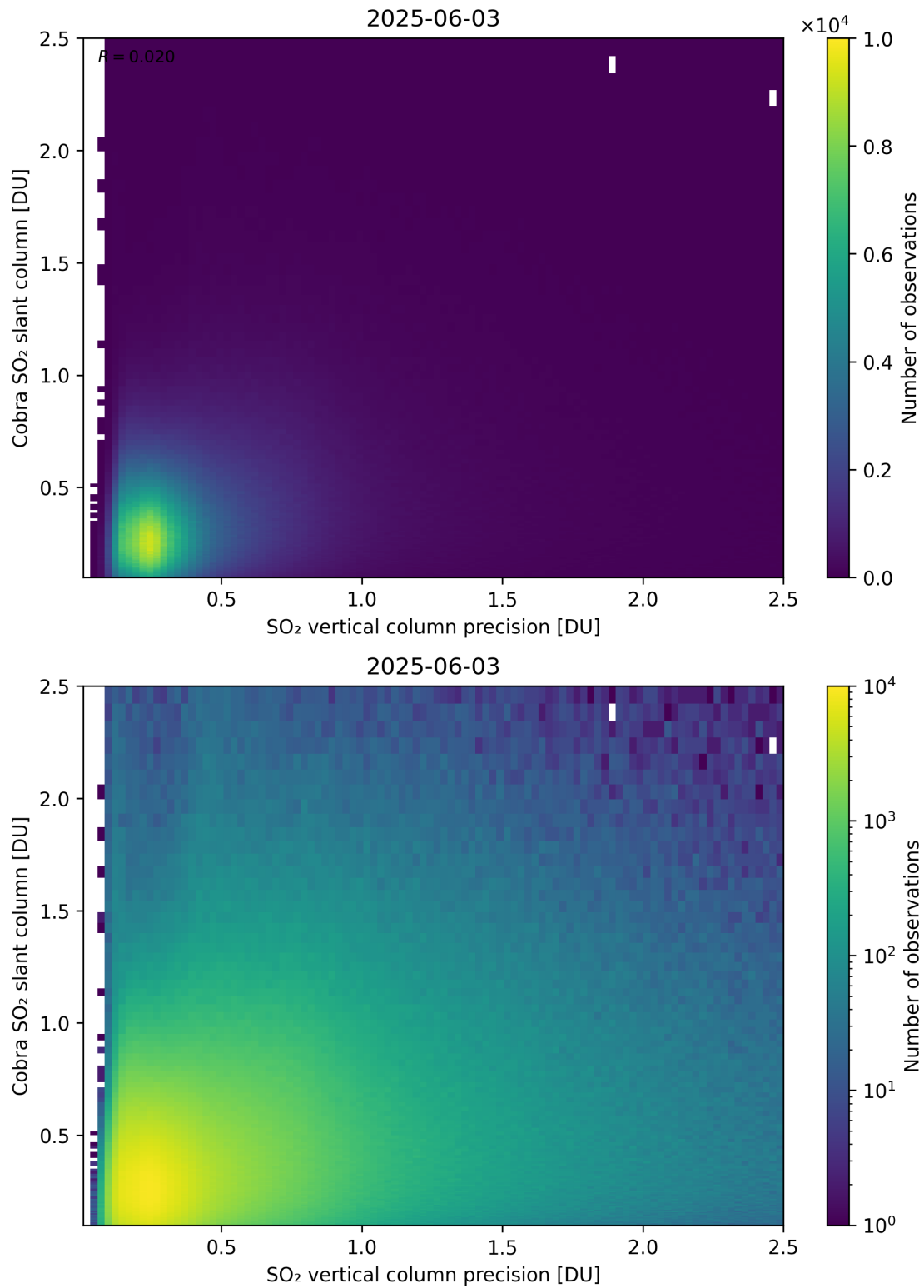
Figure 336: Scatter density plot of “SO 2 vertical column precision” against “Cobra SO 2 slant column” for 2025-06-02 to 2025-06-04.
