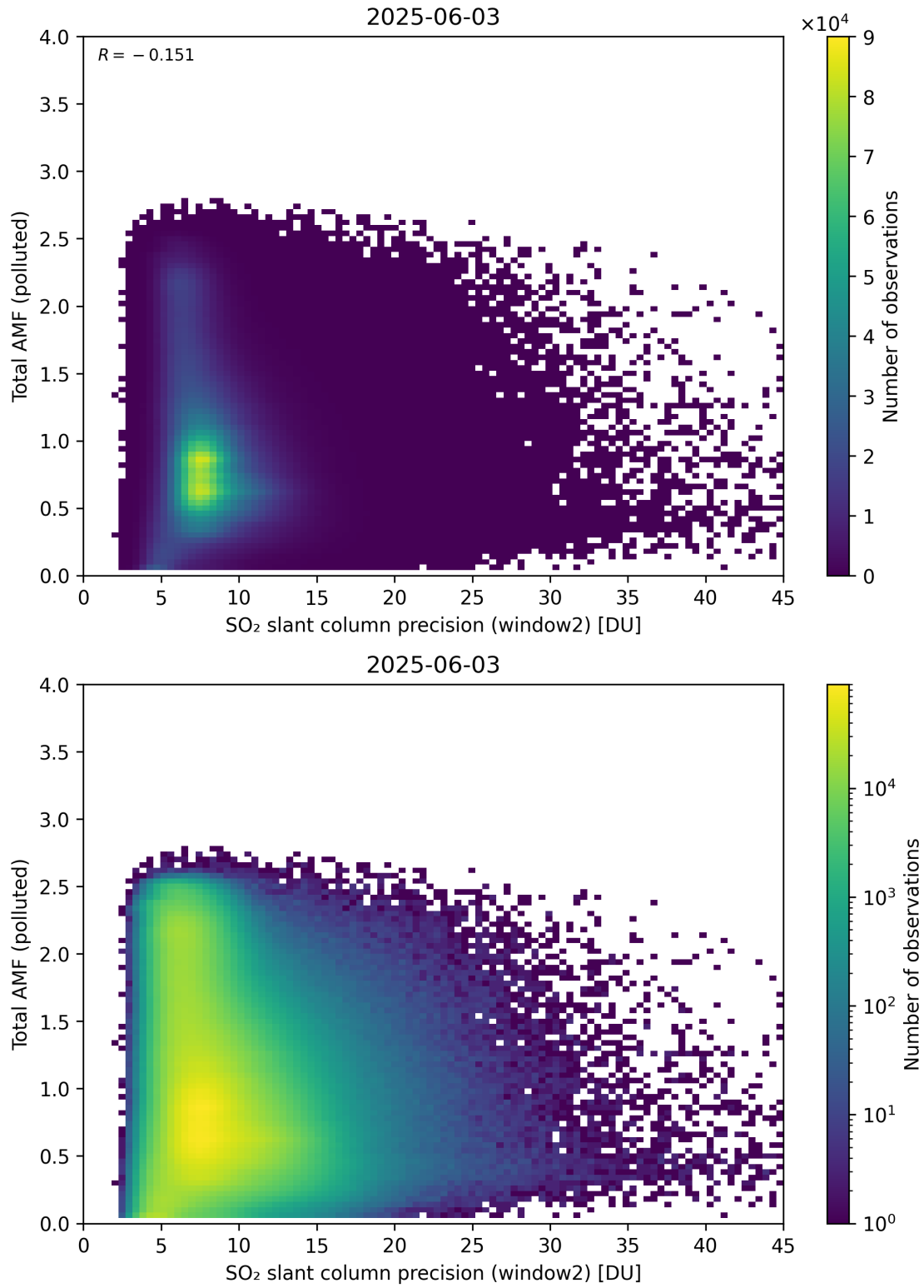
Figure 301: Scatter density plot of “SO 2 slant column precision (window2)” against “Total AMF (polluted)” for 2025-06-02 to 2025-06-04.
