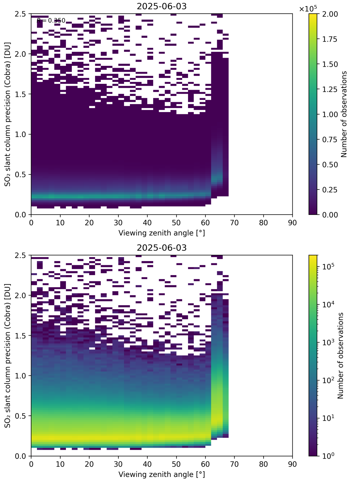
Figure 372: Scatter density plot of “Viewing zenith angle” against “SO 2 slant column precision (Cobra)” for 2025-06-02 to 2025-06-04.
