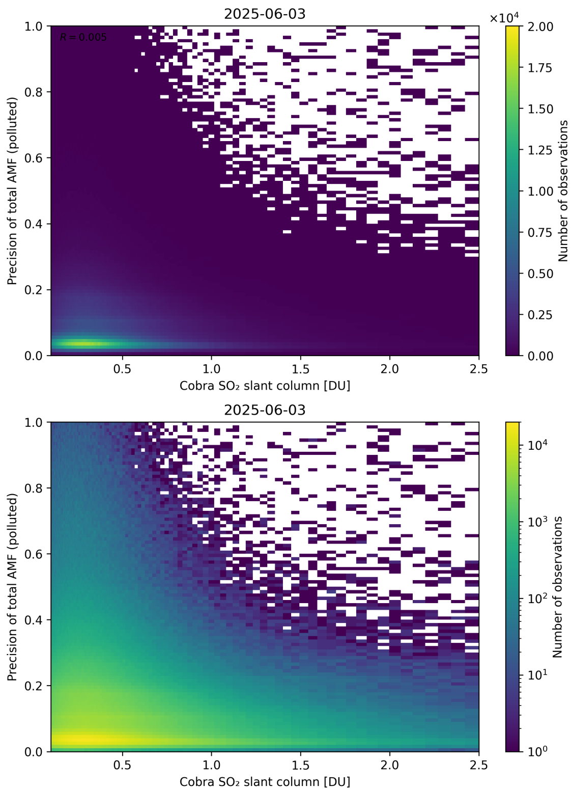
Figure 225: Scatter density plot of “Cobra SO 2 slant column” against “Precision of total AMF (polluted)” for 2025-06-02 to 2025-06-04.
