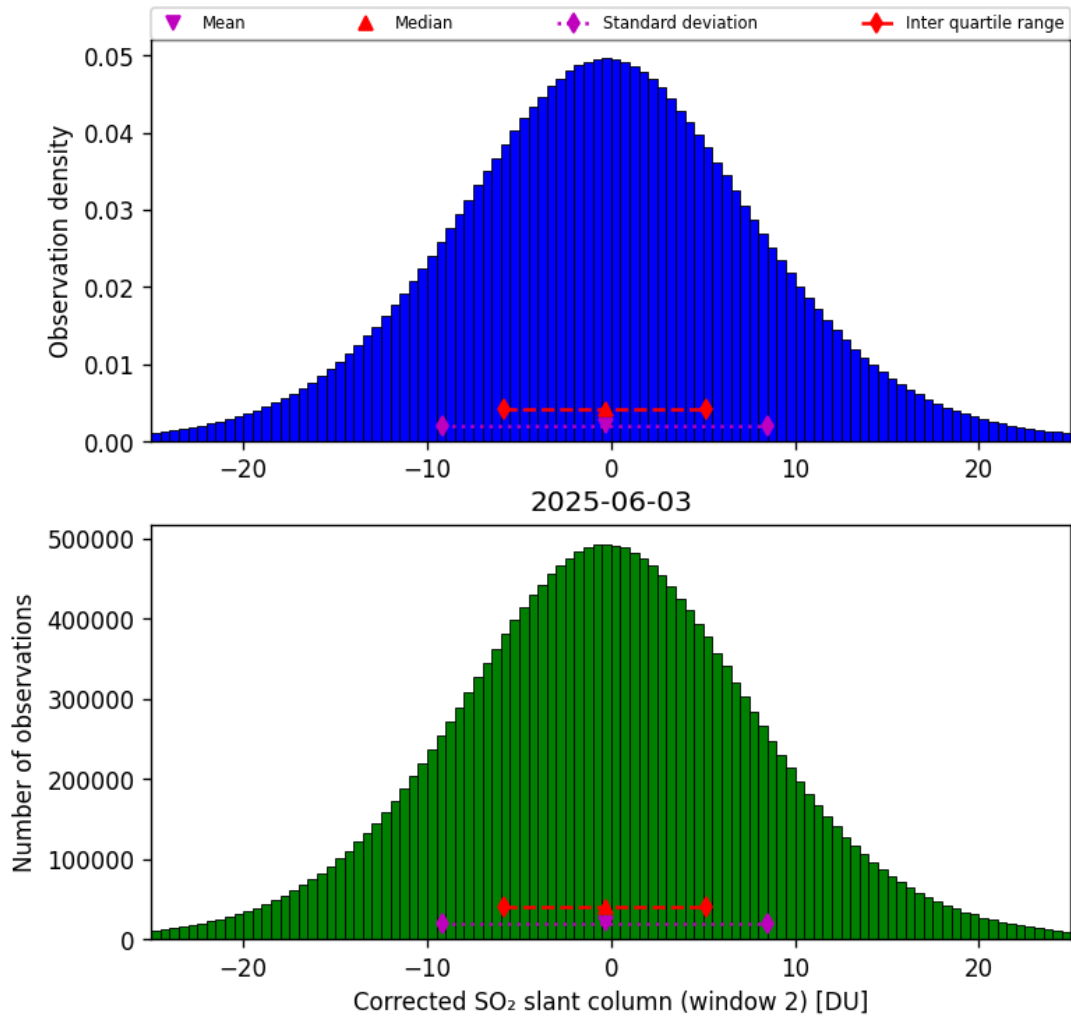
Figure 69: Histogram of “Corrected SO 2 slant column (window 2)” for 2025-06-02 to 2025-06-04
