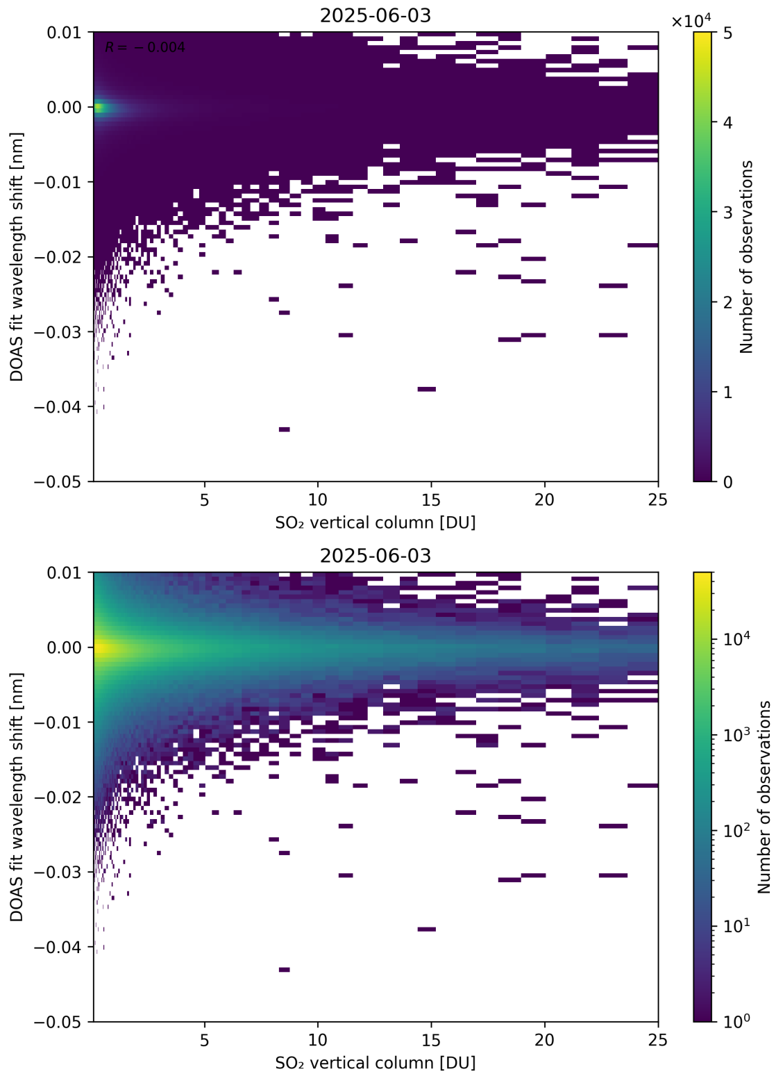
Figure 326: Scatter density plot of “SO 2 vertical column” against “DOAS fit wavelength shift” for 2025-06-02 to 2025-06-04.
