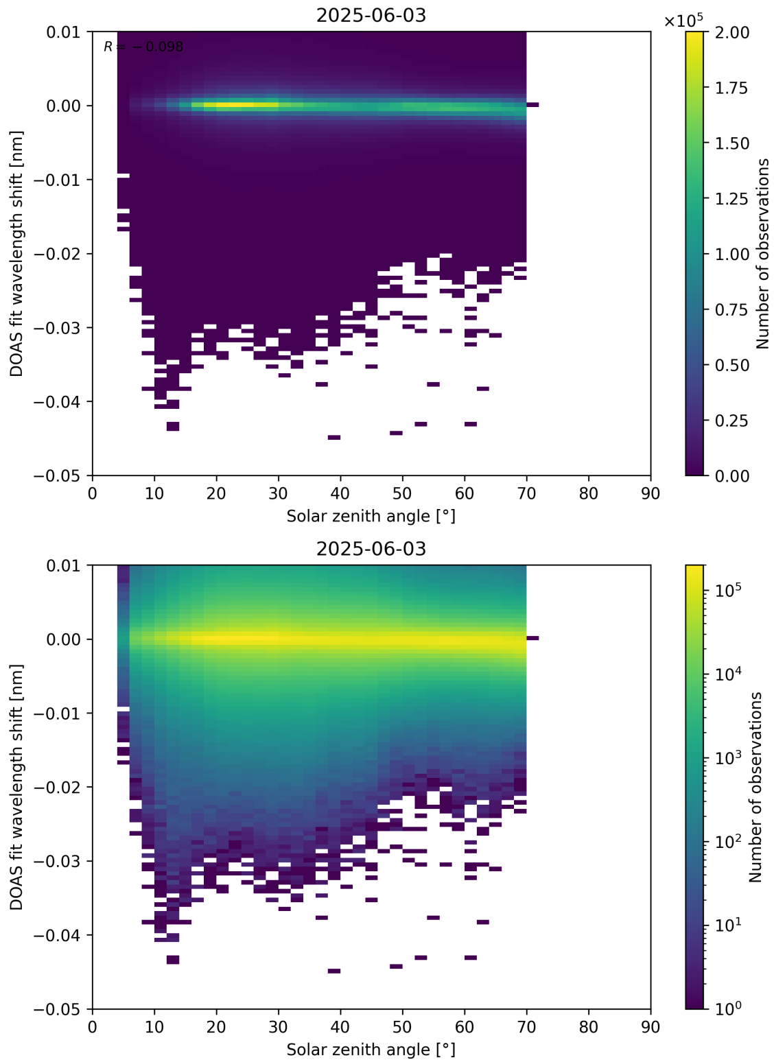
Figure 174: Scatter density plot of “Solar zenith angle” against “DOAS fit wavelength shift” for 2025-06-02 to 2025-06-04.
