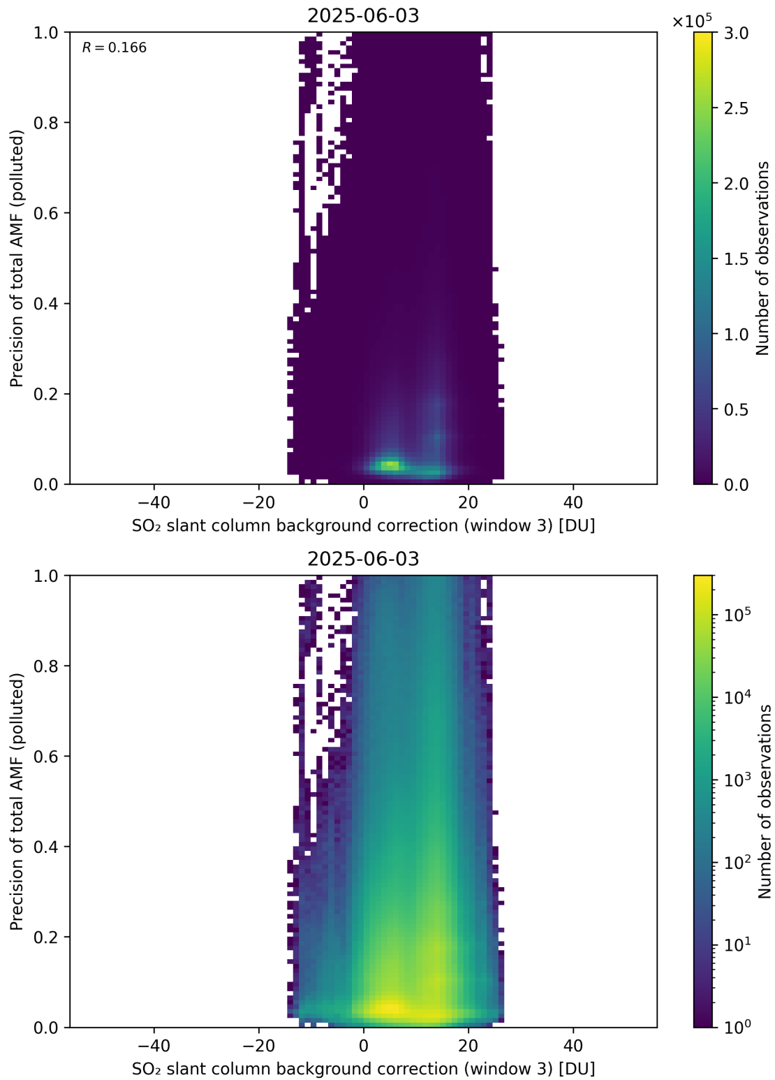
Figure 137: Scatter density plot of “SO 2 slant column background correction (window 3)” against “Precision of total AMF (polluted)” for 2025-06-02 to 2025-06-04.
