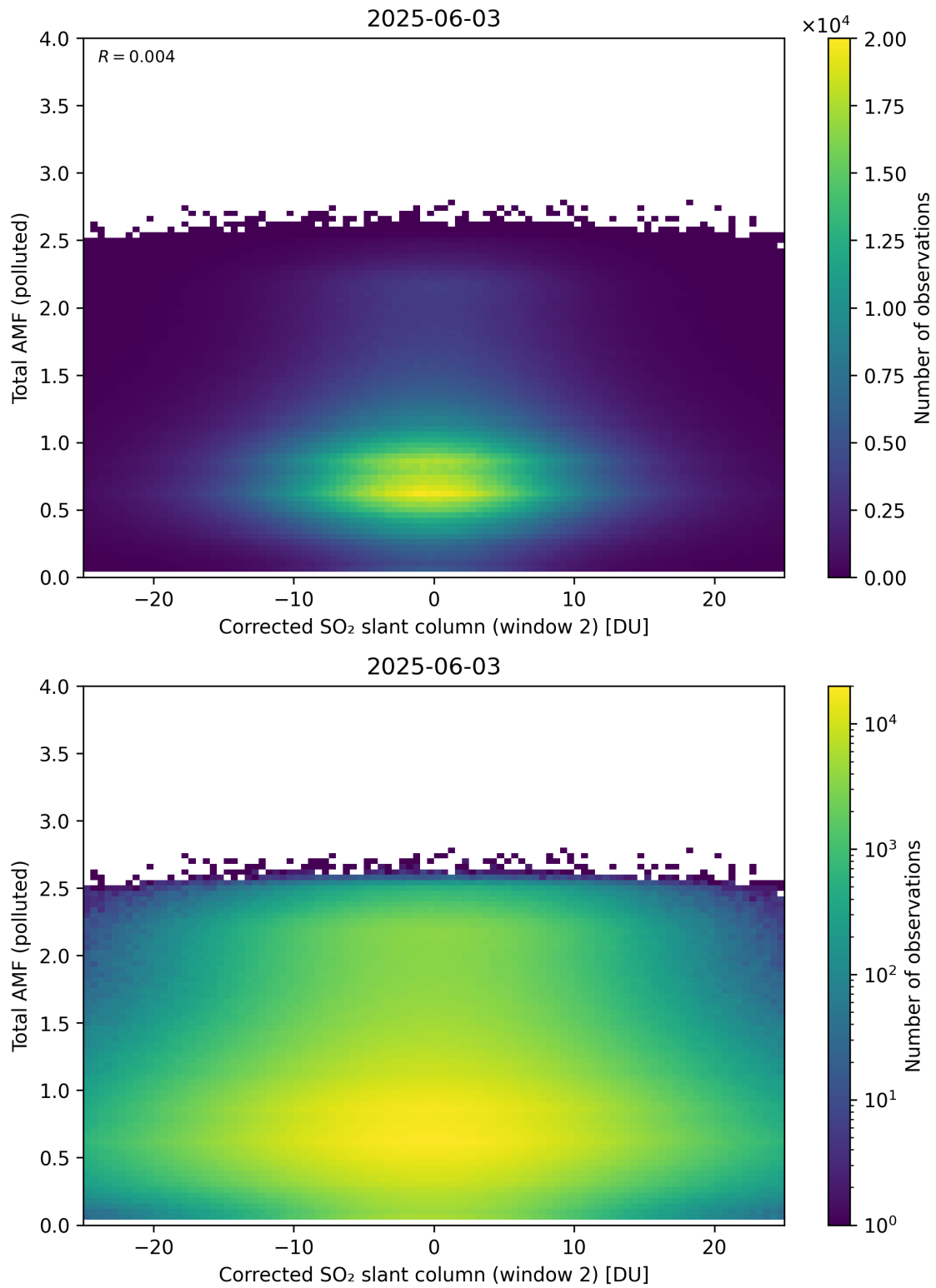
Figure 253: Scatter density plot of “Corrected SO 2 slant column (window 2)” against “Total AMF (polluted)” for 2025-06-02 to 2025-06-04.
