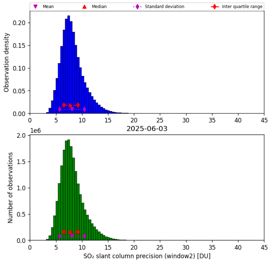
Figure 68: Histogram of “SO 2 slant column precision (window2)” for 2025-06-02 to 2025-06-04
