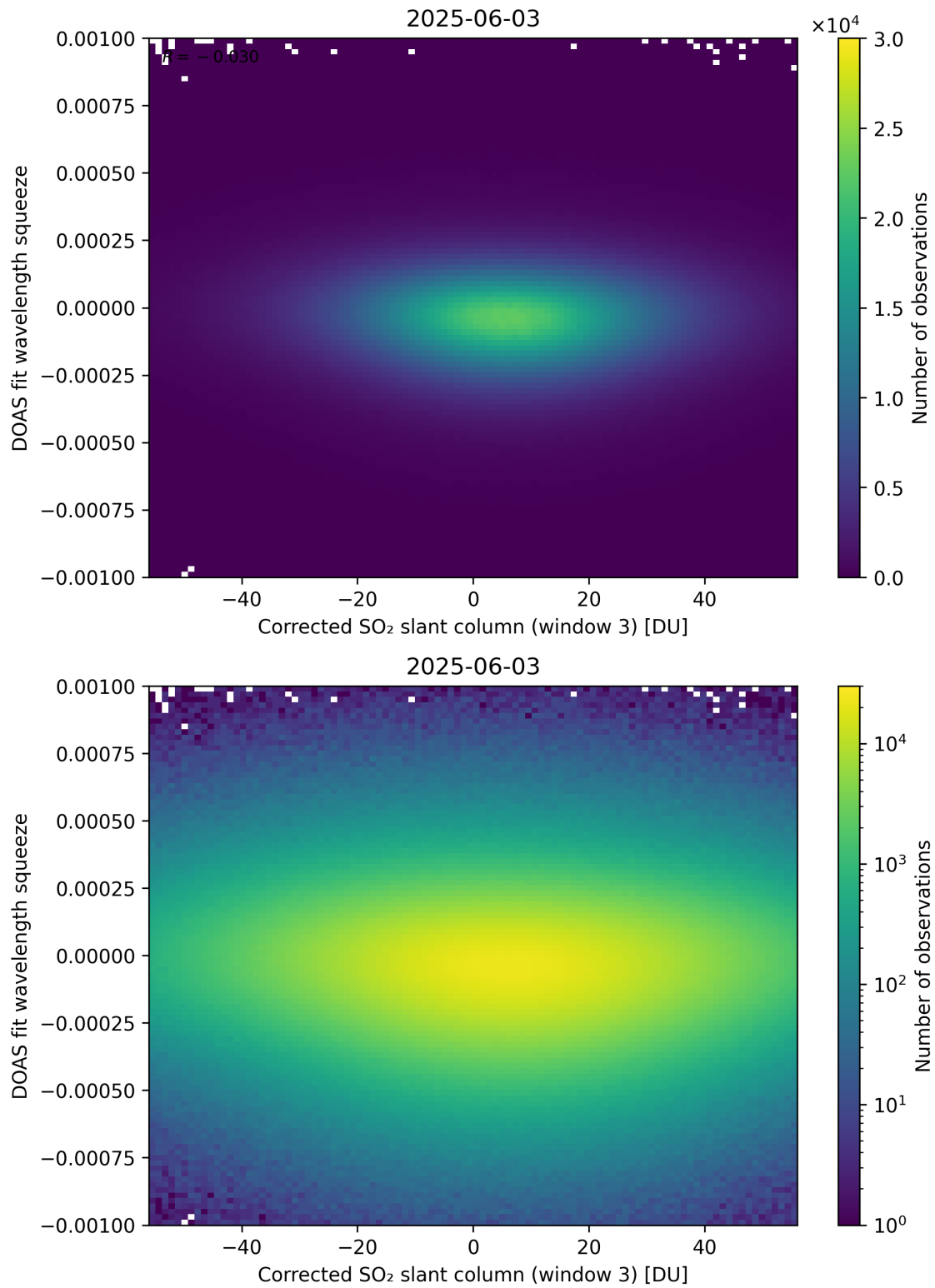
Figure 257: Scatter density plot of “Corrected SO 2 slant column (window 3)” against “DOAS fit wavelength squeeze” for 2025-06-02 to 2025-06-04.
