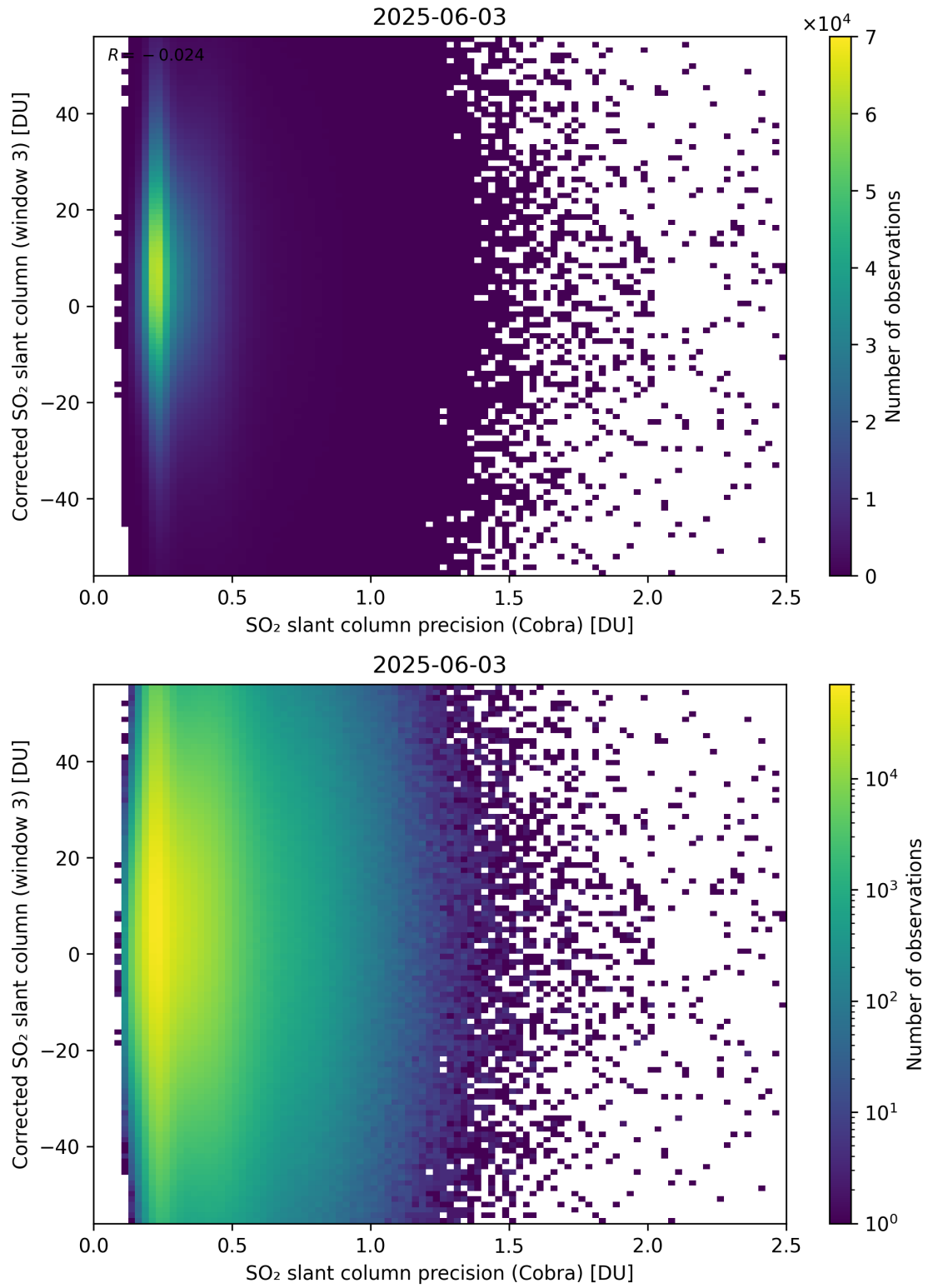
Figure 207: Scatter density plot of “SO 2 slant column precision (Cobra)” against “Corrected SO 2 slant column (window 3)” for 2025-06-02 to 2025-06-04.
