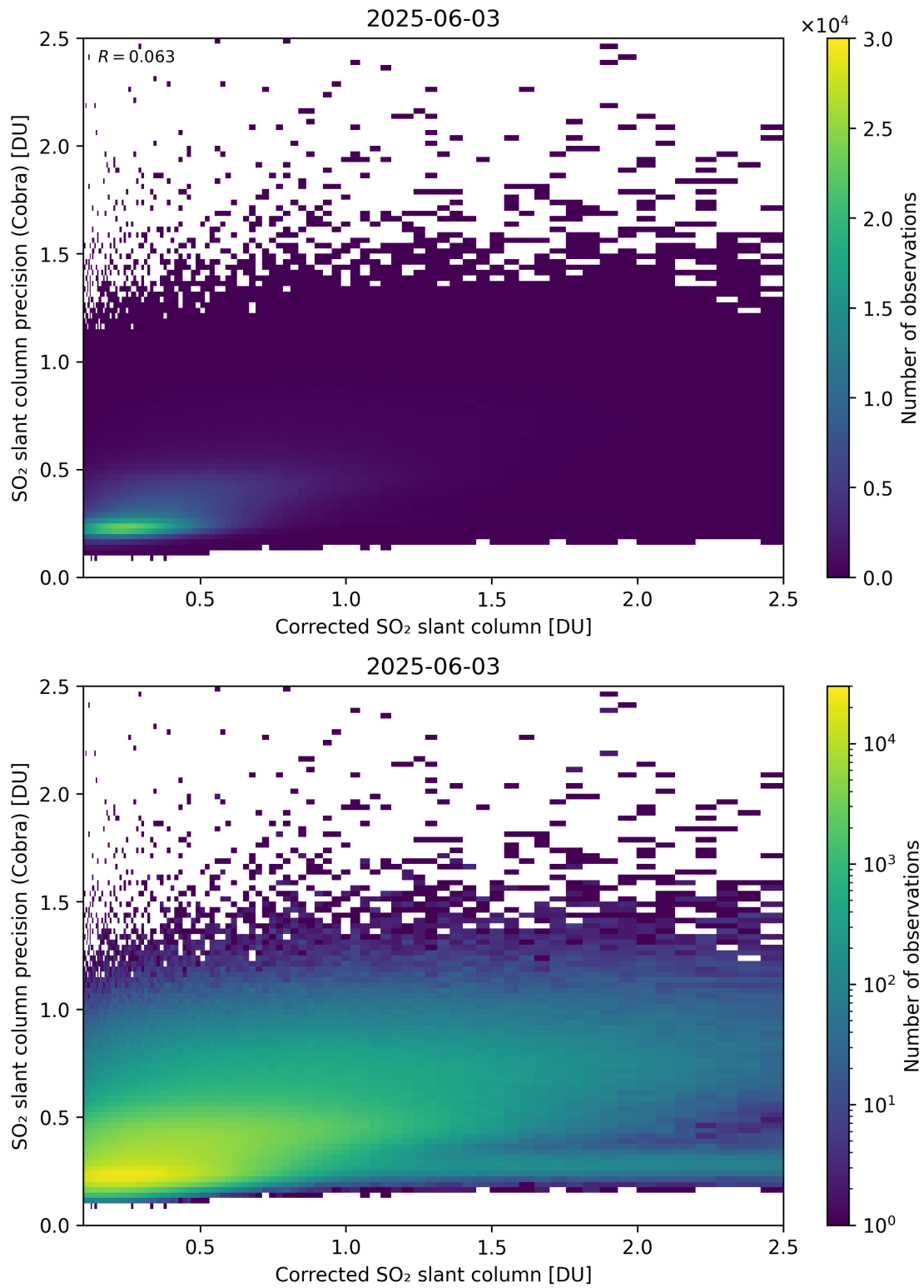
Figure 234: Scatter density plot of “Corrected SO 2 slant column” against “SO 2 slant column precision (Cobra)” for 2025-06-02 to 2025-06-04.
