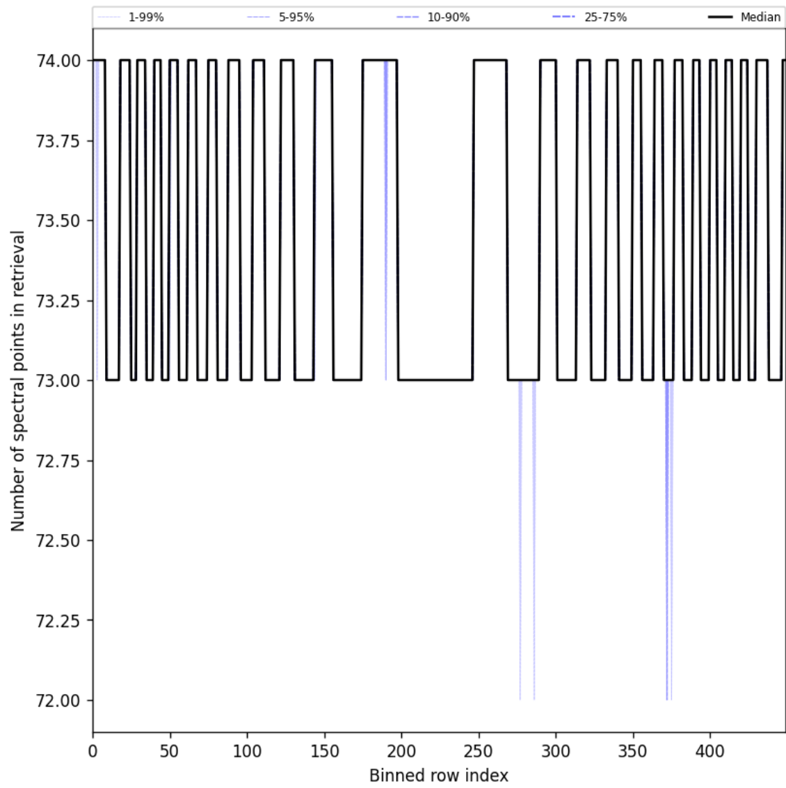
Figure 108: Along track statistics of “Number of spectral points in retrieval” for 2025-06-02 to 2025-06-04
