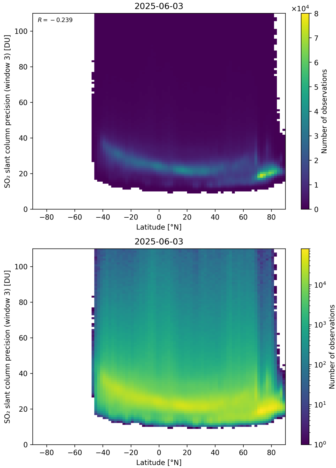
Figure 166: Scatter density plot of “Latitude” against “SO 2 slant column precision (window 3)” for 2025-06-02 to 2025-06-04.
