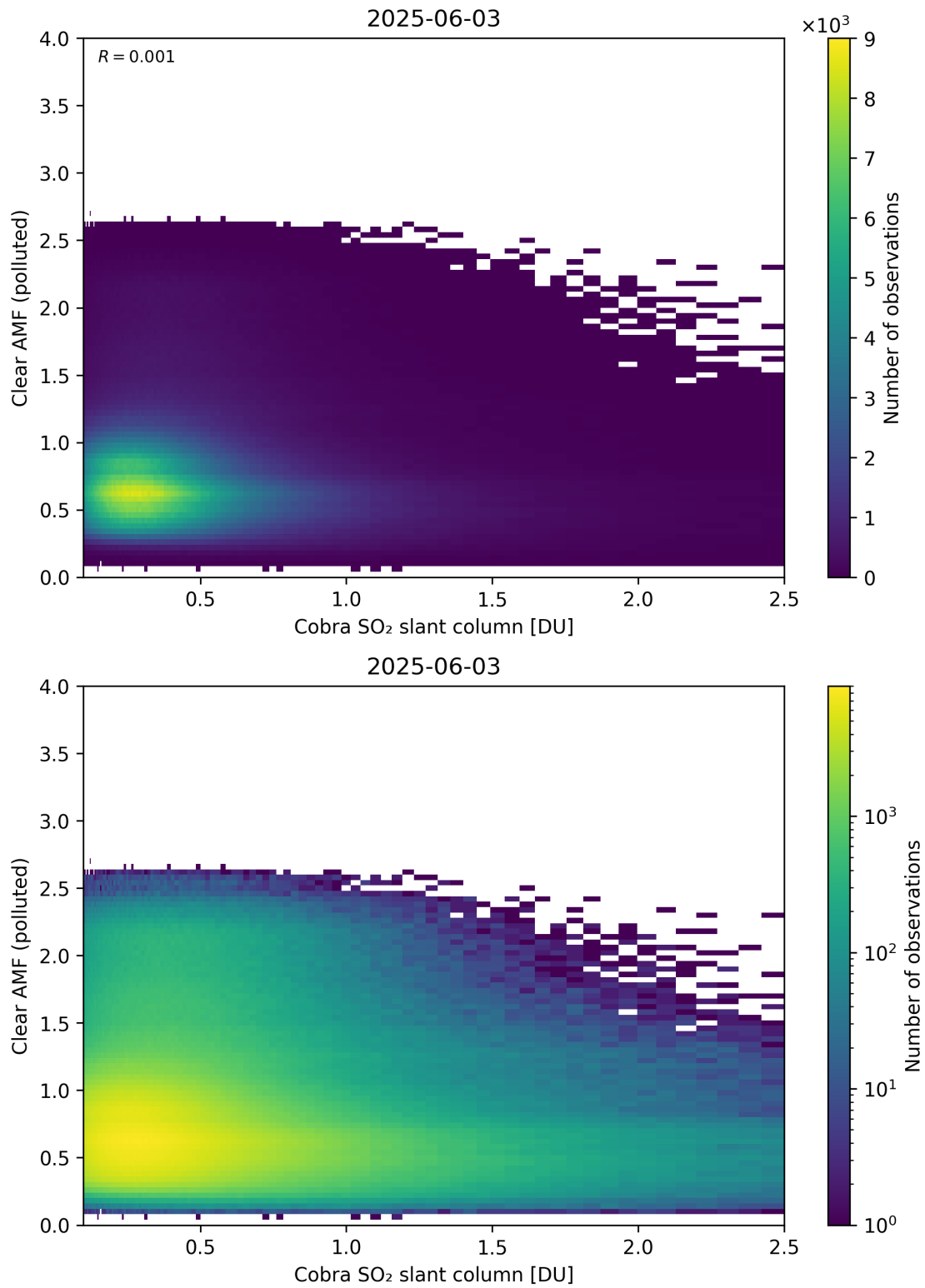
Figure 215: Scatter density plot of “Cobra SO 2 slant column” against “Clear AMF (polluted)” for 2025-06-02 to 2025-06-04.
