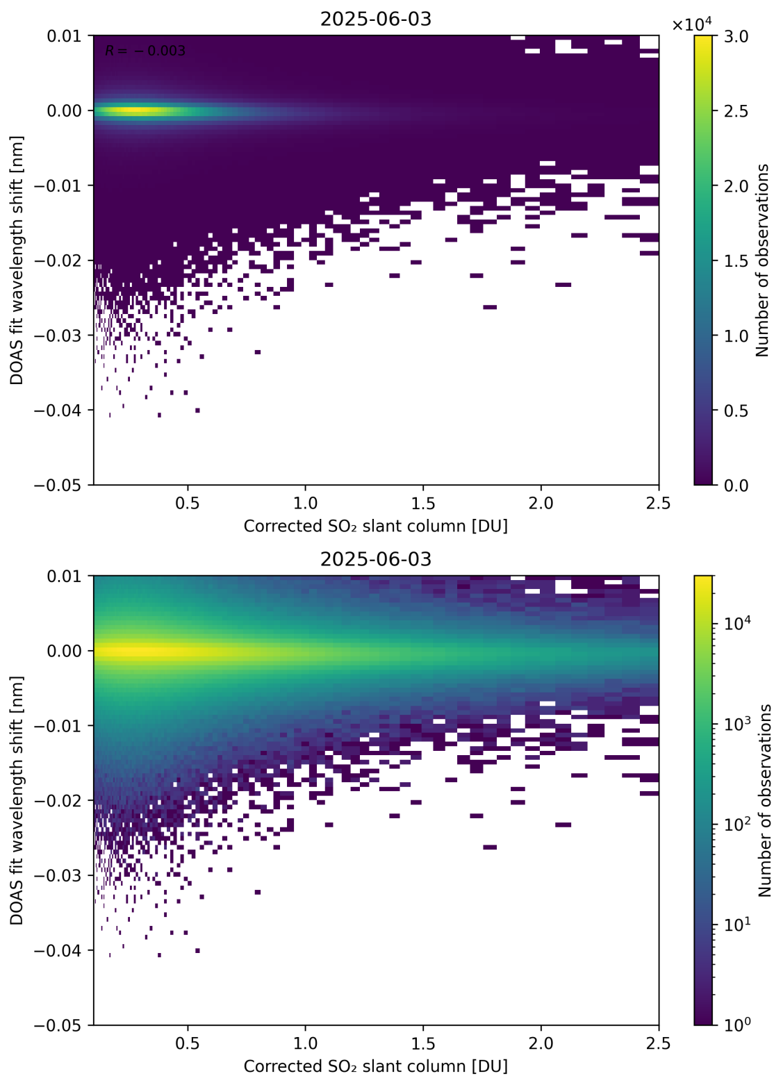
Figure 229: Scatter density plot of “Corrected SO 2 slant column” against “DOAS fit wavelength shift” for 2025-06-02 to 2025-06-04.
