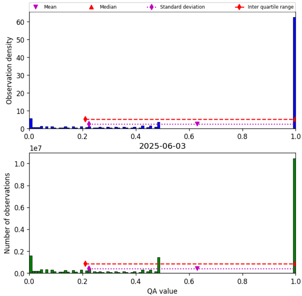
Figure 57: Histogram of “QA value” for 2025-06-02 to 2025-06-04
