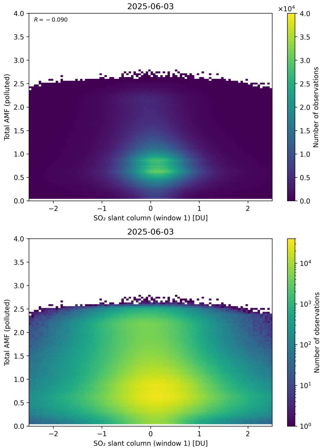
Figure 289: Scatter density plot of “SO 2 slant column (window 1)” against “Total AMF (polluted)” for 2025-06-02 to 2025-06-04.
