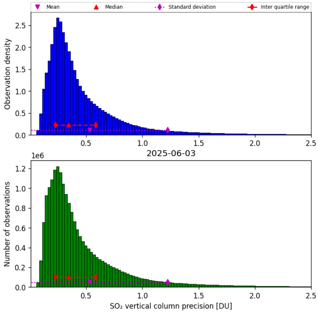
Figure 59: Histogram of “SO 2 vertical column precision” for 2025-06-02 to 2025-06-04
