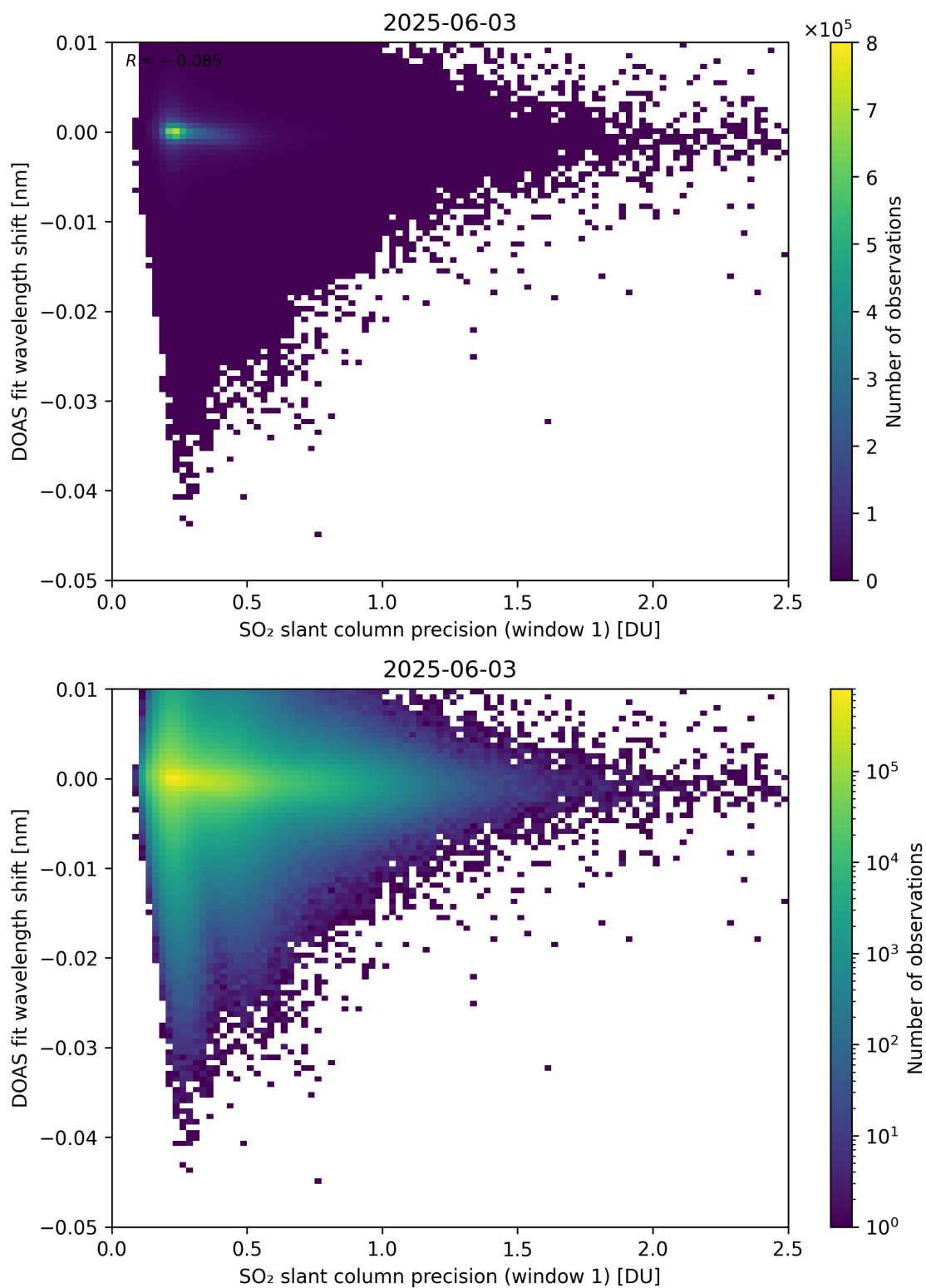
Figure 271: Scatter density plot of “SO 2 slant column precision (window 1)” against “DOAS fit wavelength shift” for 2025-06-02 to 2025-06-04.
