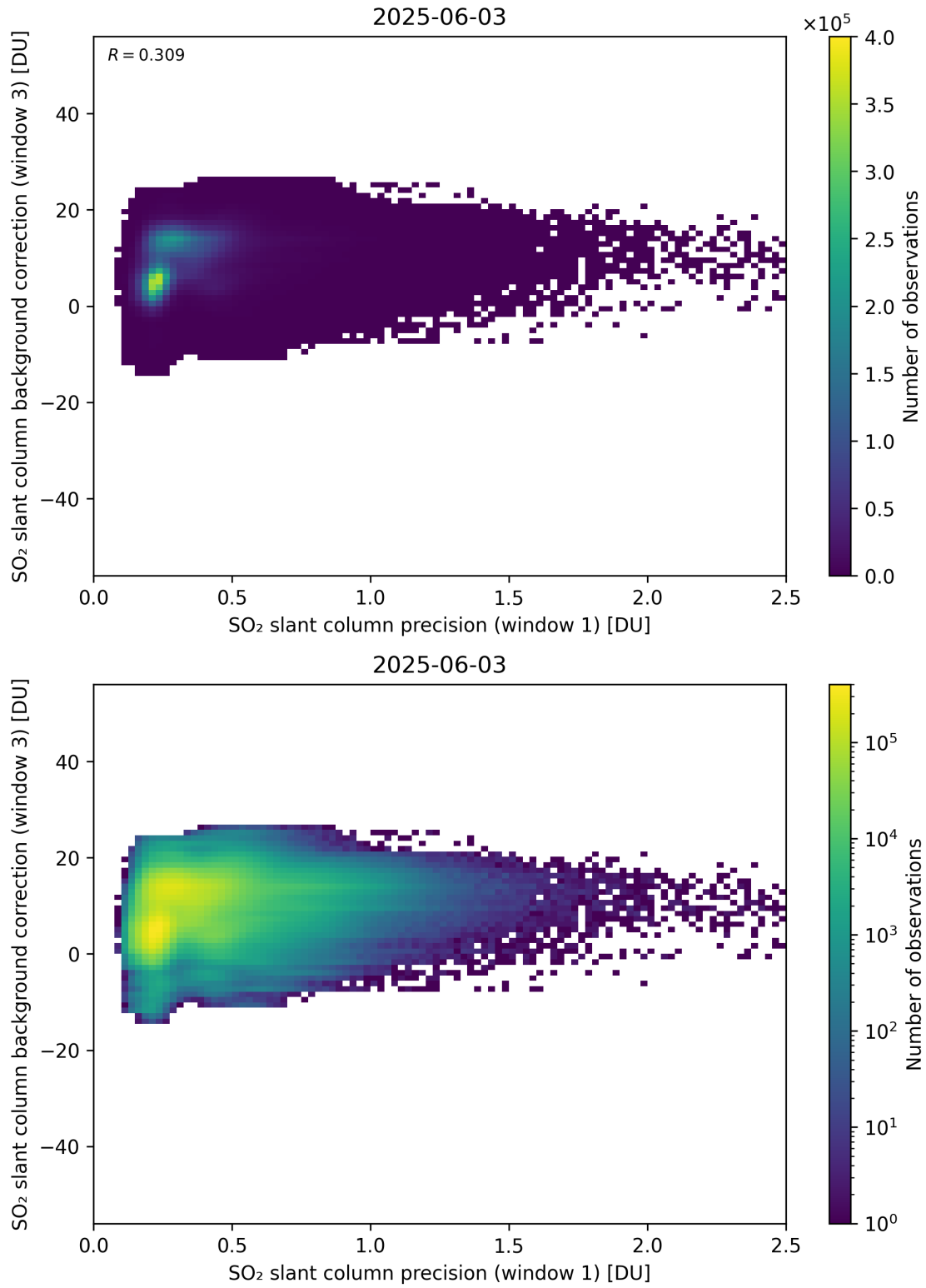
Figure 270: Scatter density plot of “SO 2 slant column precision (window 1)” against “SO 2 slant column background correction (window 3)” for 2025-06-02 to 2025-06-04.
