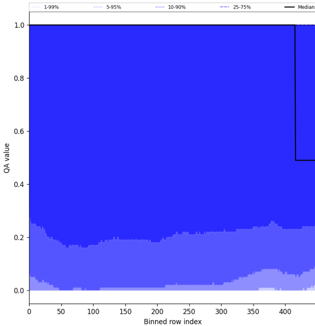
Figure 83: Along track statistics of “QA value” for 2025-06-02 to 2025-06-04
