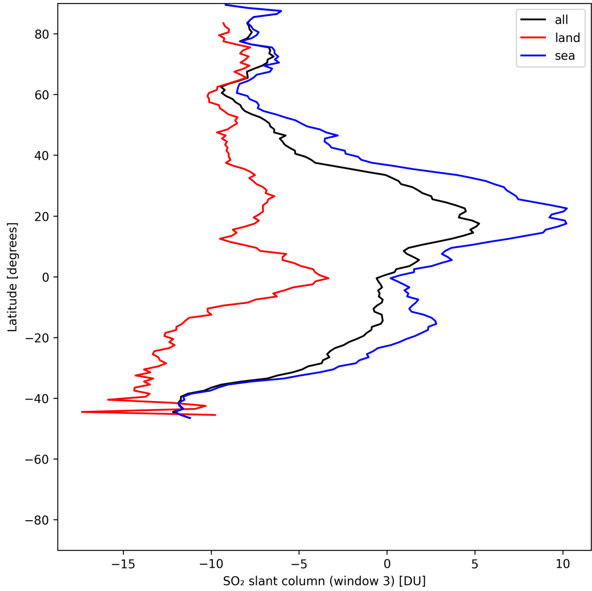
Figure 45: Zonal average of “SO 2 slant column (window 3)” for 2025-06-02 to 2025-06-04.
