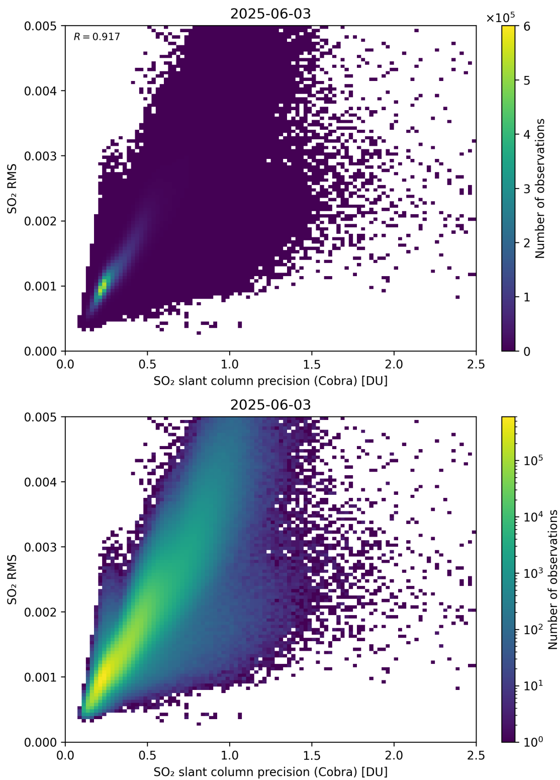
Figure 204: Scatter density plot of “SO 2 slant column precision (Cobra)” against “SO 2 RMS” for 2025-06-02 to 2025-06-04.
