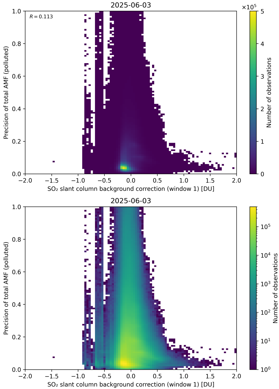
Figure 121: Scatter density plot of “SO 2 slant column background correction (window 1)” against “Precision of total AMF (polluted)” for 2025-06-02 to 2025-06-04.
