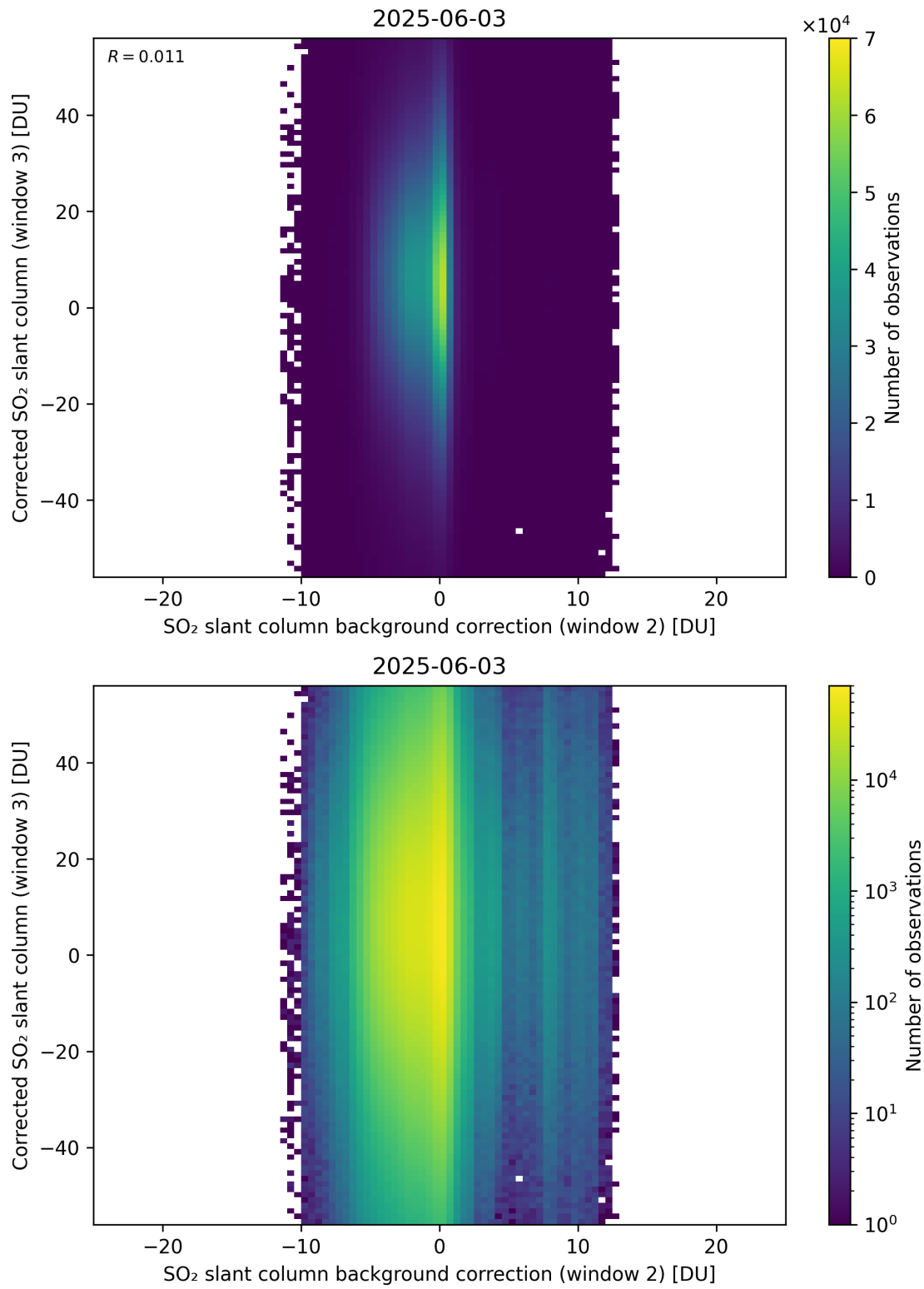
Figure 127: Scatter density plot of “SO 2 slant column background correction (window 2)” against “Corrected SO 2 slant column (window 3)” for 2025-06-02 to 2025-06-04.
