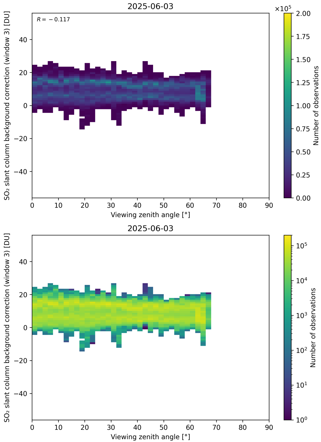
Figure 364: Scatter density plot of “Viewing zenith angle” against “SO 2 slant column background correction (window 3)” for 2025-06-02 to 2025-06-04.
