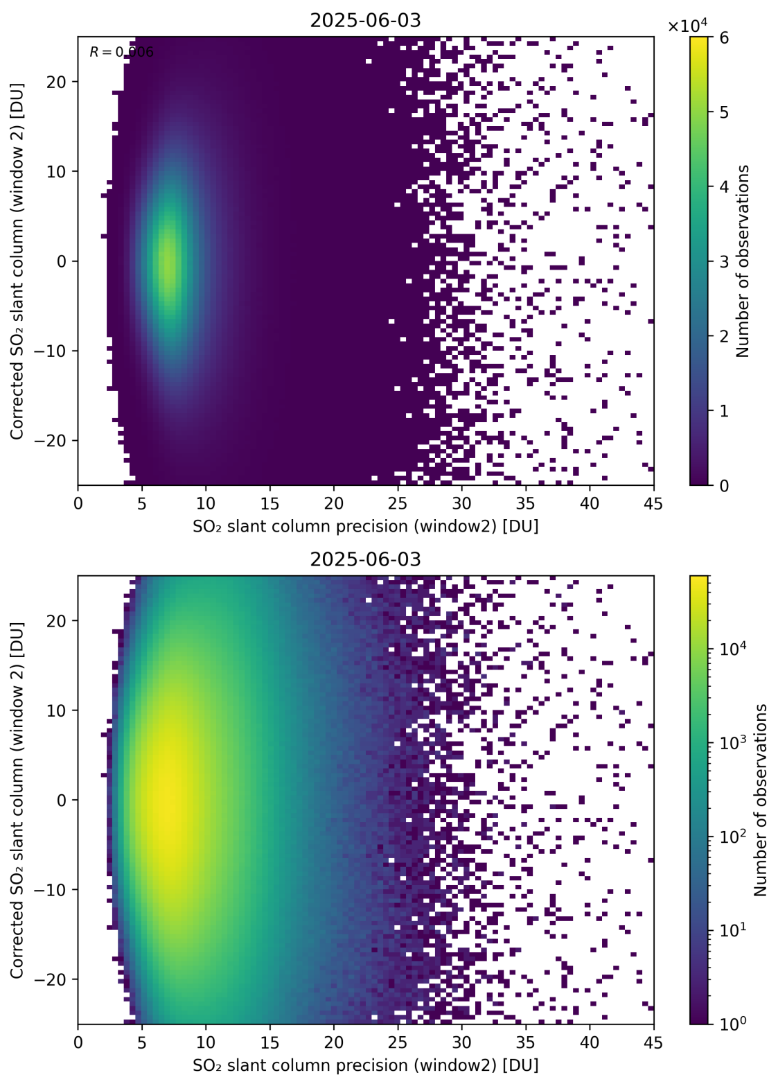
Figure 297: Scatter density plot of “SO 2 slant column precision (window2)” against “Corrected SO 2 slant column (window 2)” for 2025-06-02 to 2025-06-04.
