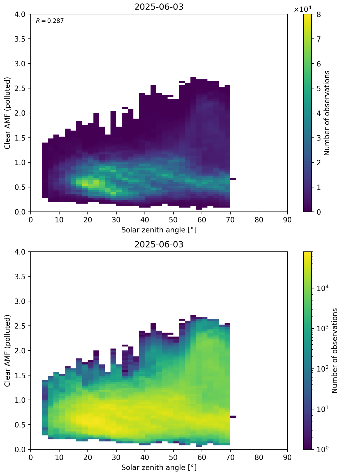
Figure 178: Scatter density plot of “Solar zenith angle” against “Clear AMF (polluted)” for 2025-06-02 to 2025-06-04.
