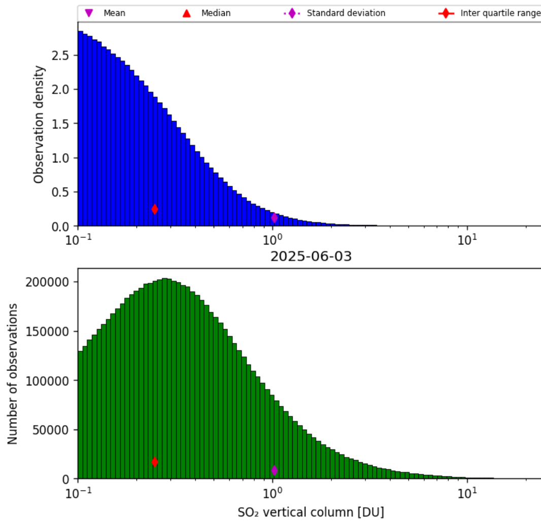
Figure 58: Histogram of “SO 2 vertical column” for 2025-06-02 to 2025-06-04
