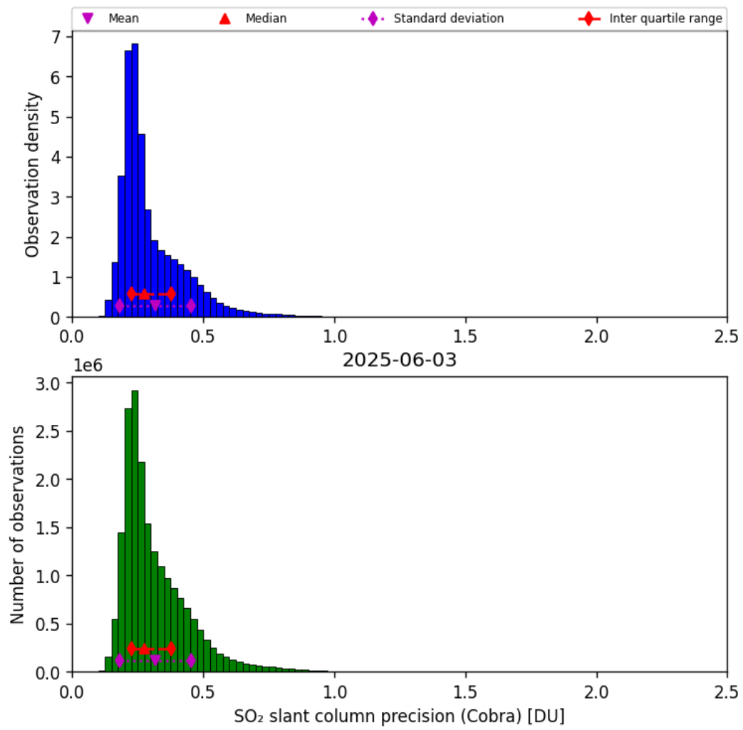
Figure 62: Histogram of “SO 2 slant column precision (Cobra)” for 2025-06-02 to 2025-06-04
