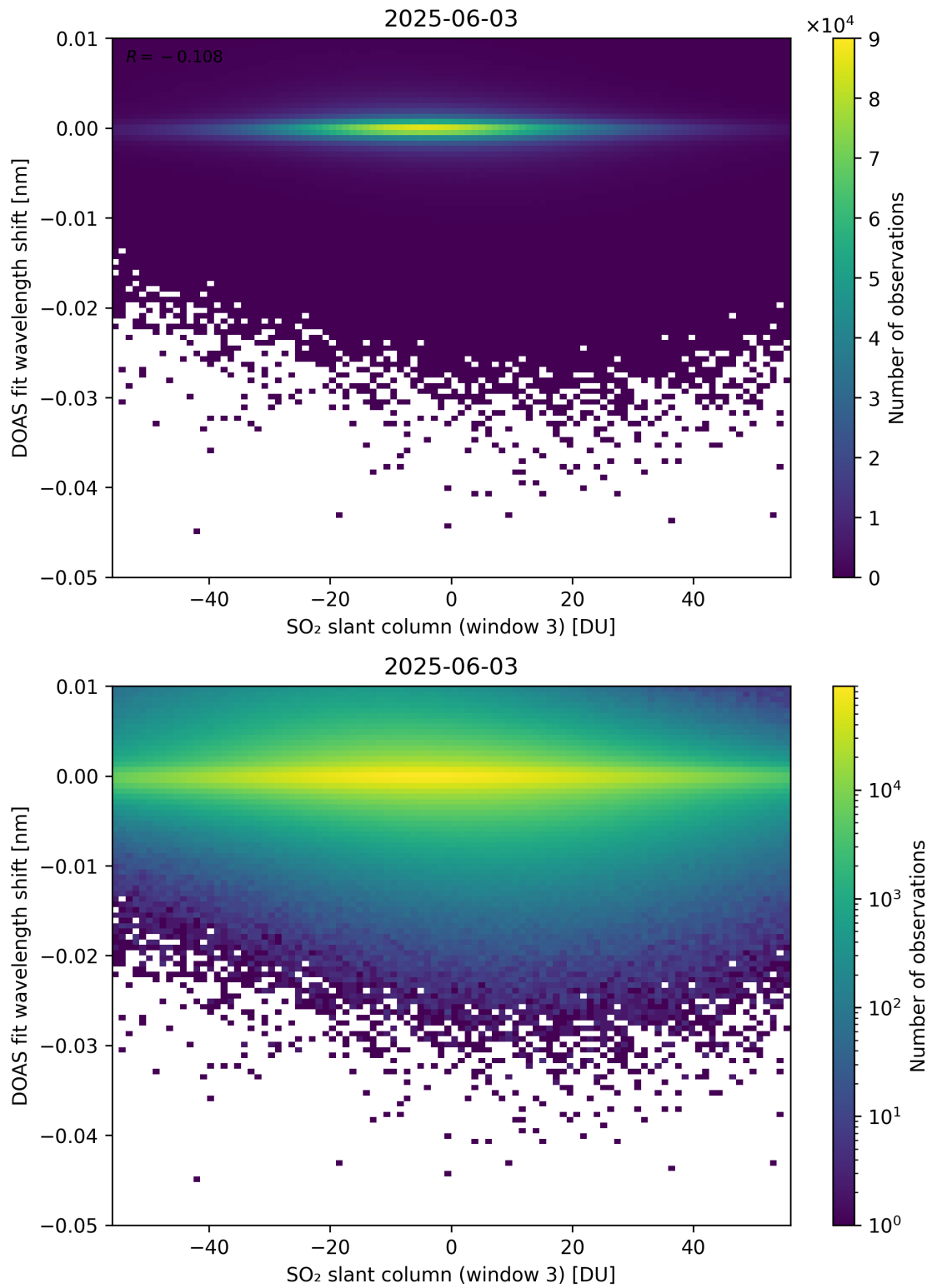
Figure 304: Scatter density plot of “SO 2 slant column (window 3)” against “DOAS fit wavelength shift” for 2025-06-02 to 2025-06-04.
