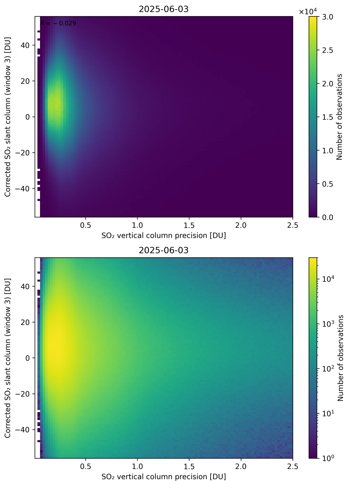
Figure 340: Scatter density plot of “SO 2 vertical column precision” against “Corrected SO 2 slant column (window 3)” for 2025-06-02 to 2025-06-04.
