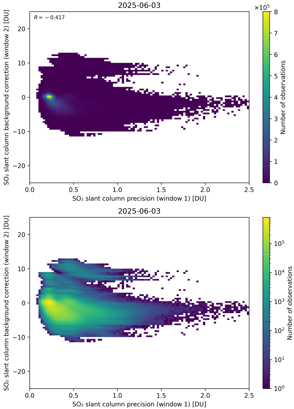
Figure 269: Scatter density plot of “SO 2 slant column precision (window 1)” against “SO 2 slant column background correction (window 2)” for 2025-06-02 to 2025-06-04.
