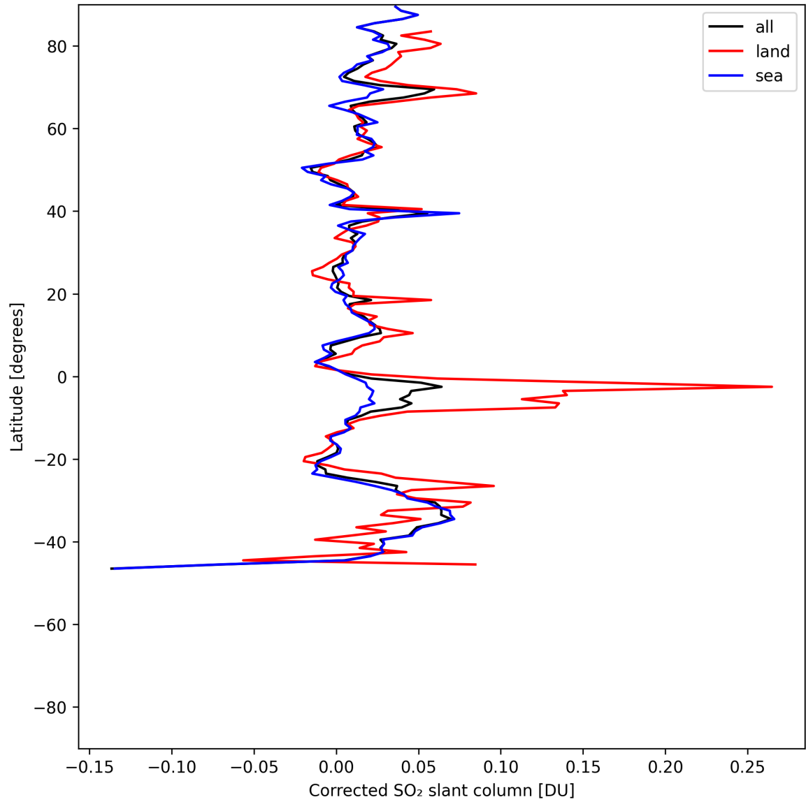
Figure 34: Zonal average of “Corrected SO 2 slant column” for 2025-06-02 to 2025-06-04.
