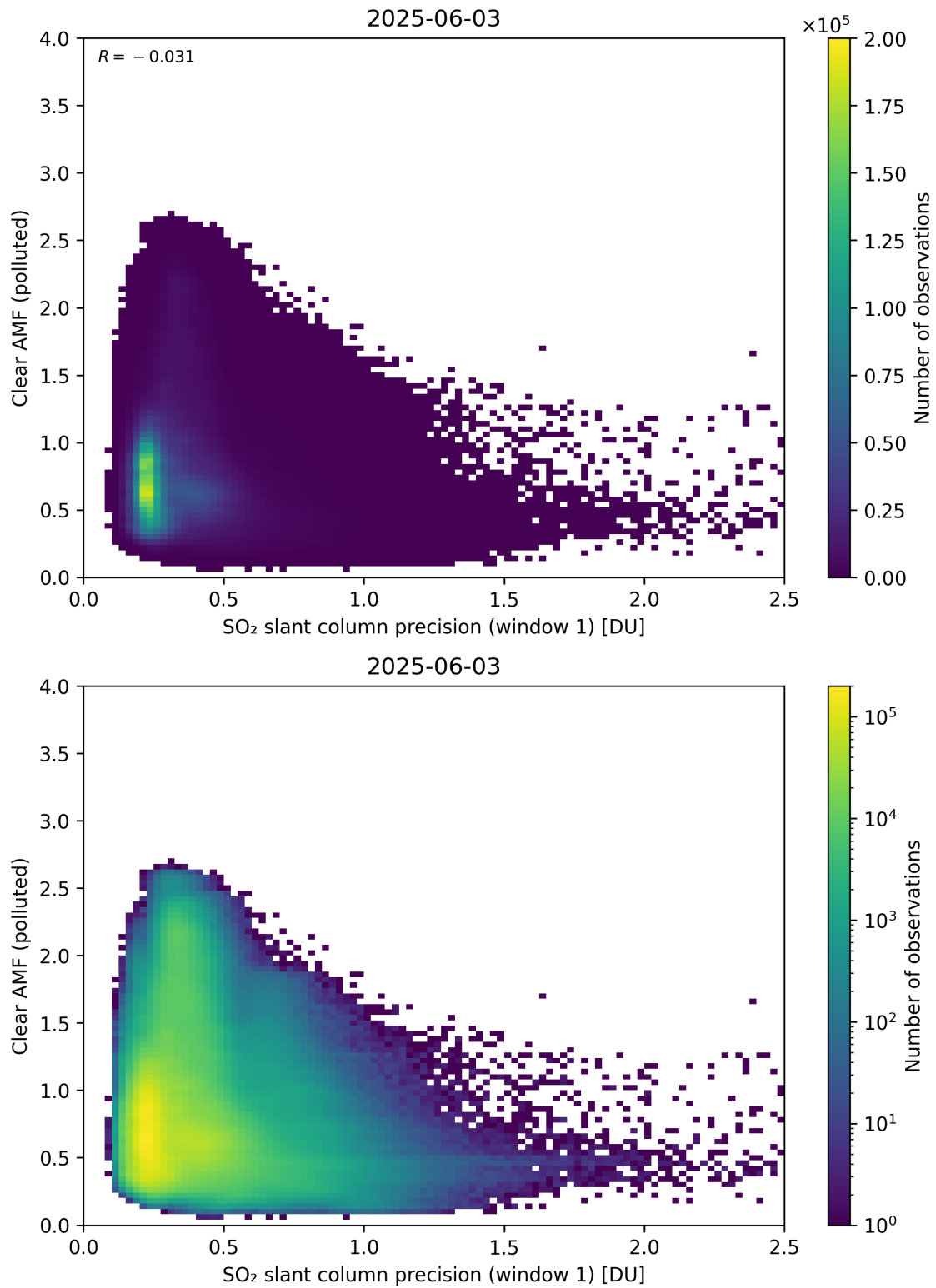
Figure 274: Scatter density plot of “SO 2 slant column precision (window 1)” against “Clear AMF (polluted)” for 2025-06-02 to 2025-06-04.
