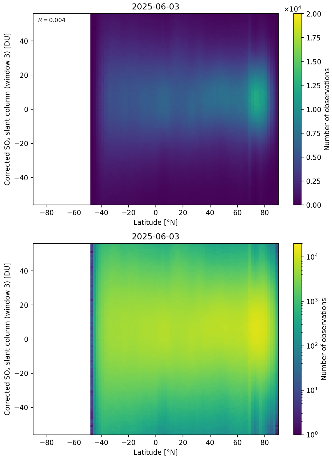
Figure 161: Scatter density plot of “Latitude” against “Corrected SO 2 slant column (window 3)” for 2025-06-02 to 2025-06-04.
