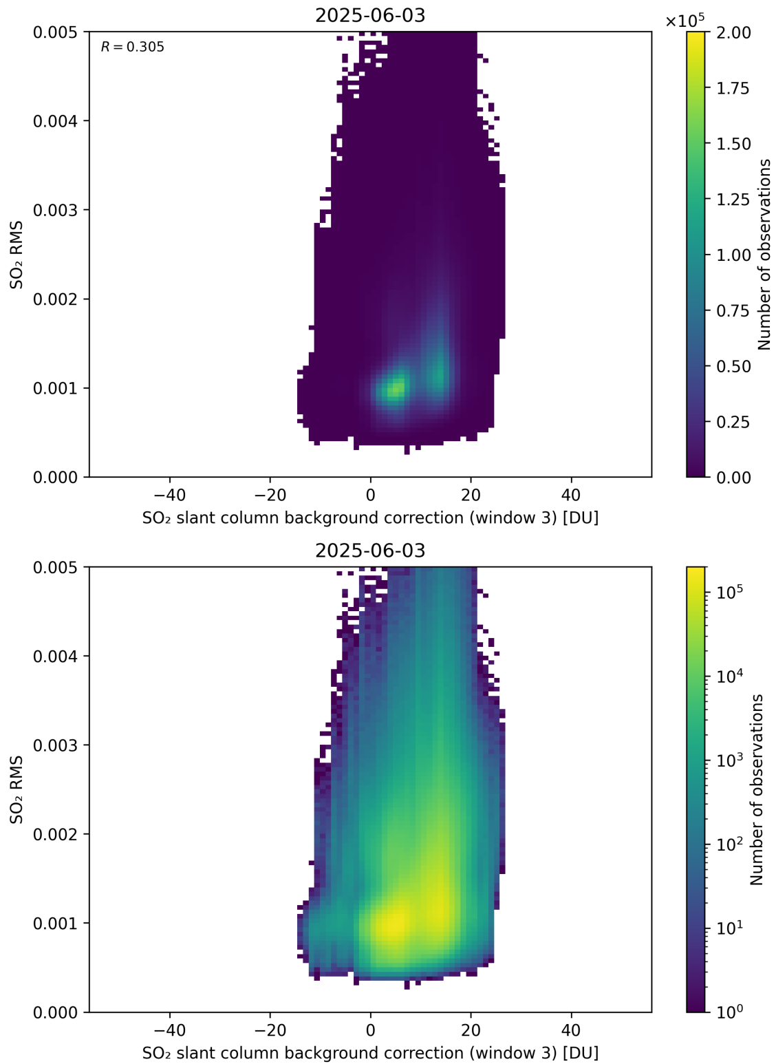
Figure 134: Scatter density plot of “SO 2 slant column background correction (window 3)” against “SO 2 RMS” for 2025-06-02 to 2025-06-04.
