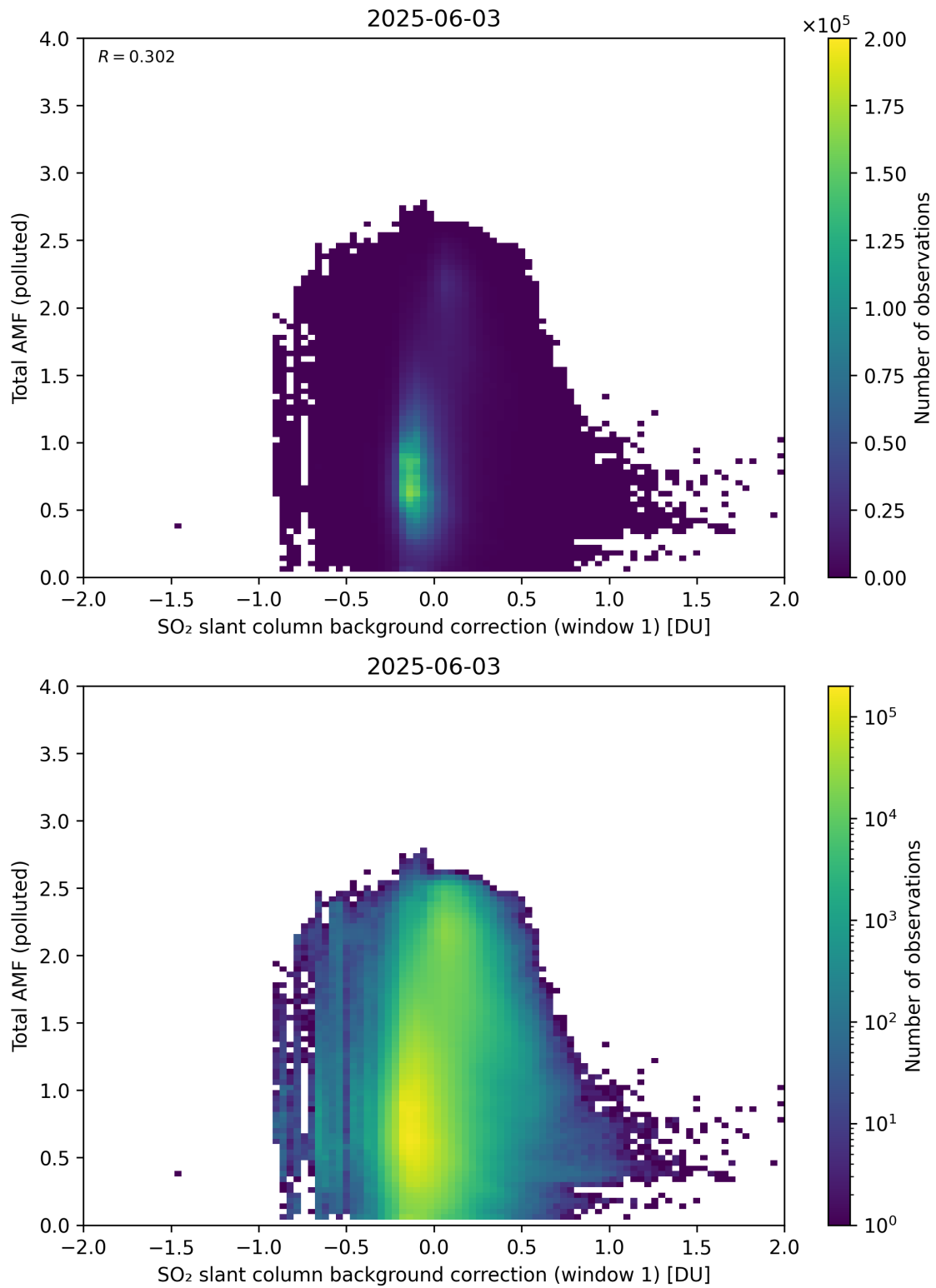
Figure 120: Scatter density plot of “SO 2 slant column background correction (window 1)” against “Total AMF (polluted)” for 2025-06-02 to 2025-06-04.
