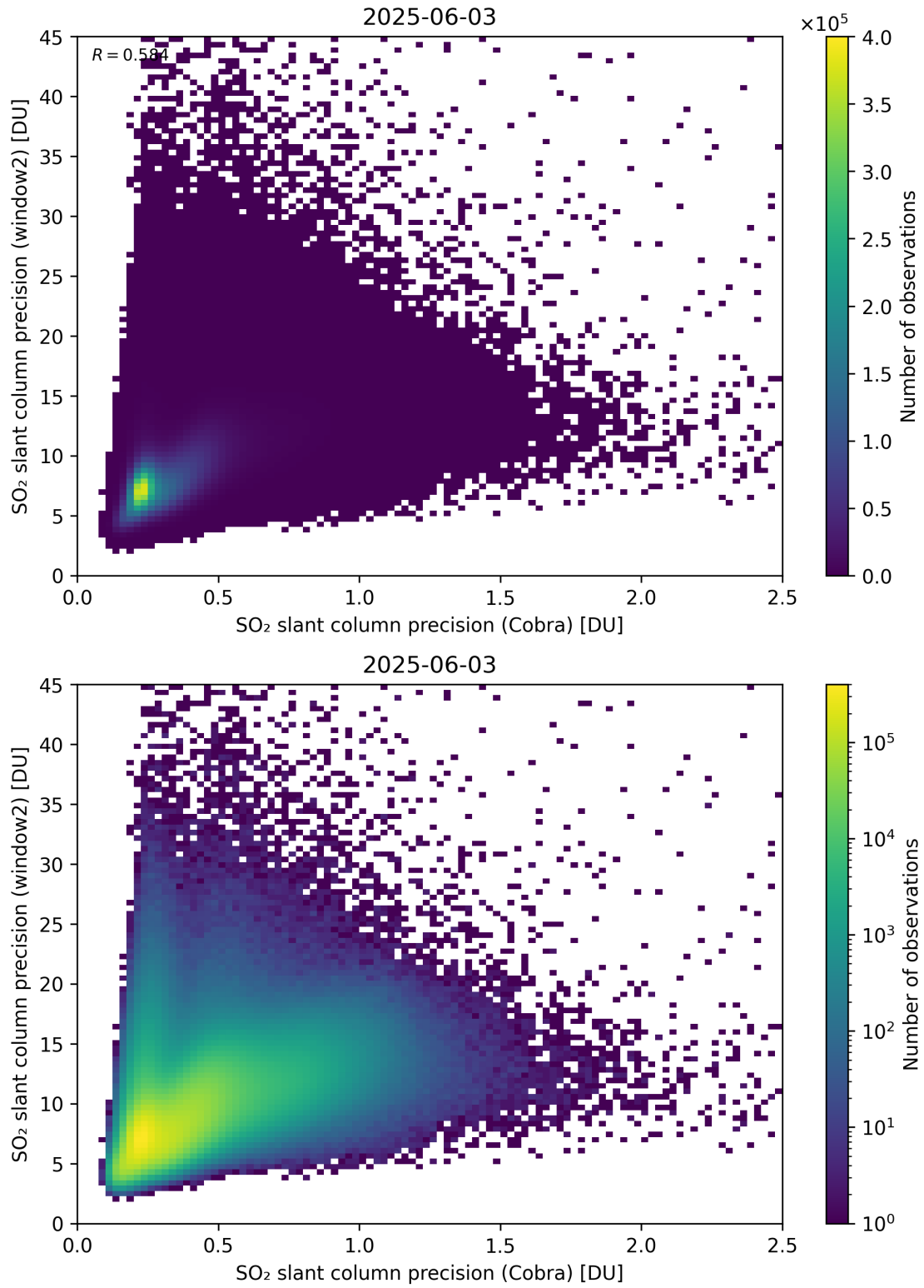
Figure 210: Scatter density plot of “SO 2 slant column precision (Cobra)” against “SO 2 slant column precision (window2)” for 2025-06-02 to 2025-06-04.
