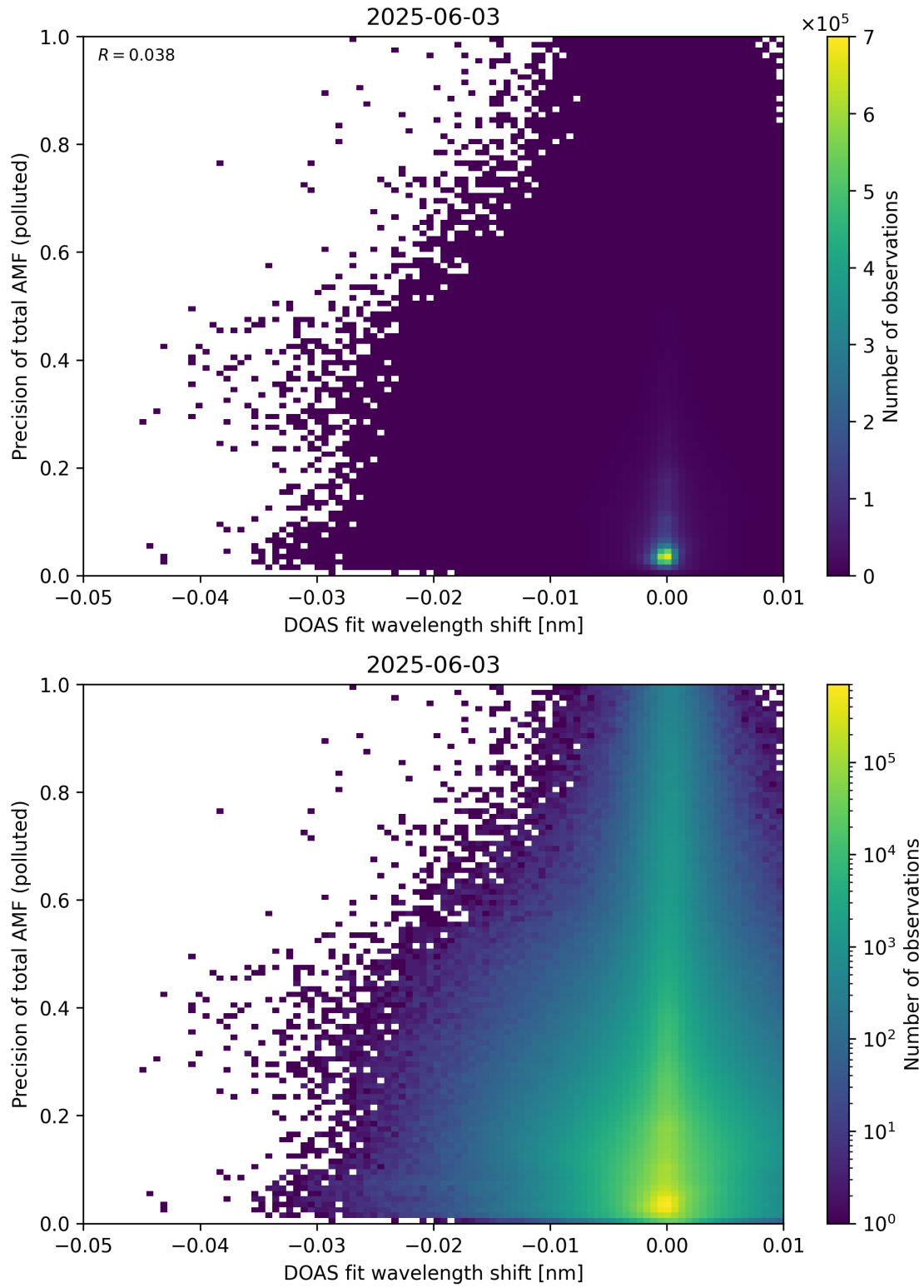
Figure 142: Scatter density plot of “DOAS fit wavelength shift” against “Precision of total AMF (polluted)” for 2025-06-02 to 2025-06-04.
