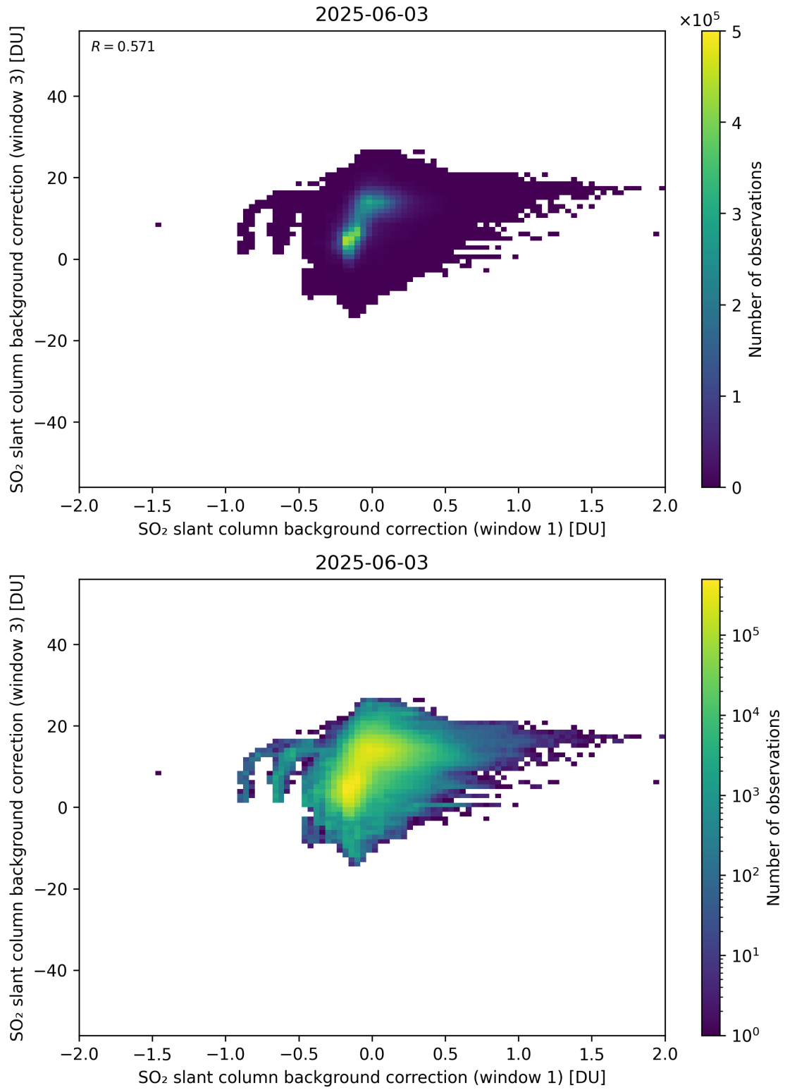
Figure 110: Scatter density plot of “SO 2 slant column background correction (window 1)” against “SO 2 slant column background correction (window 3)” for 2025-06-02 to 2025-06-04.
