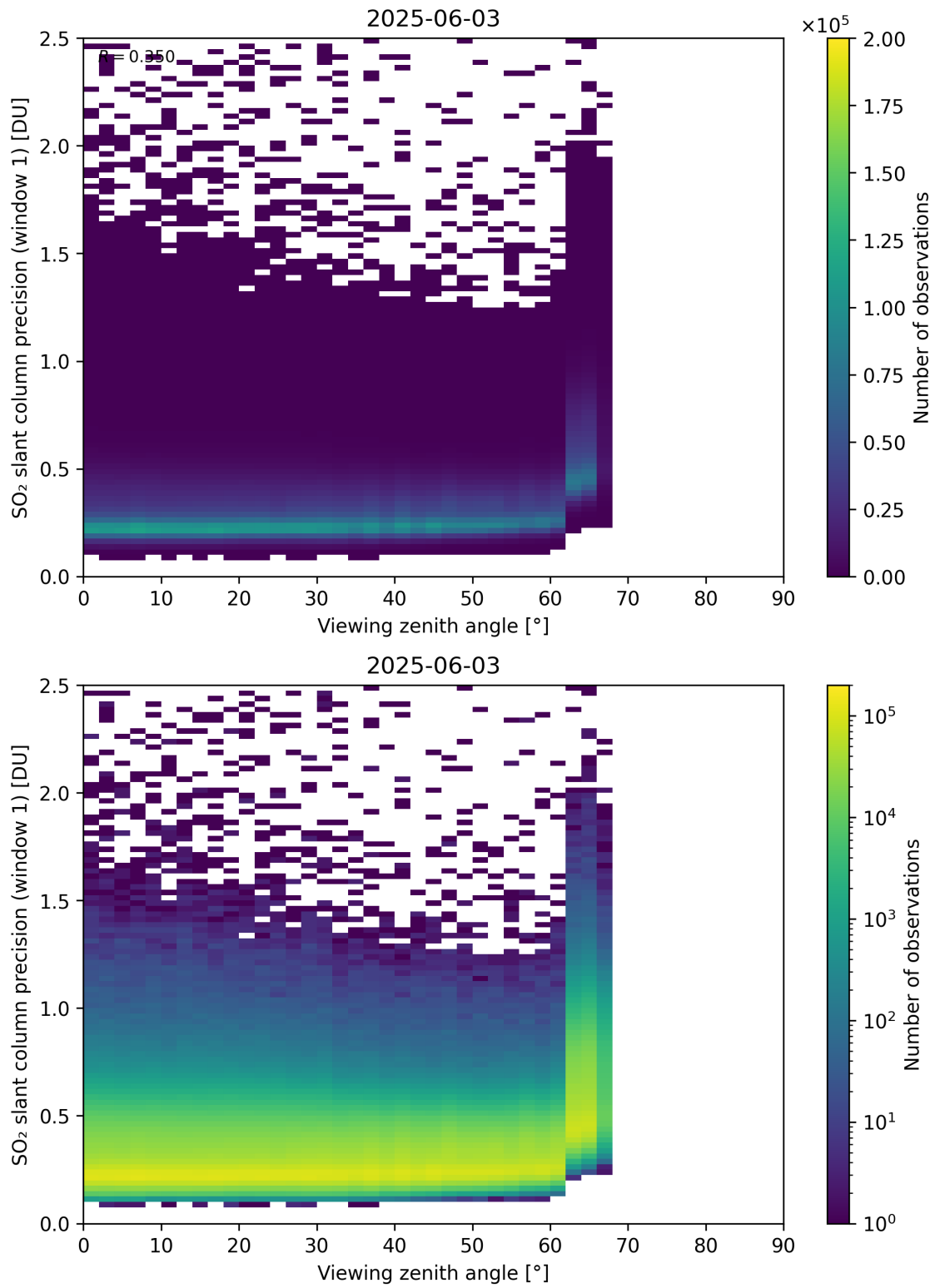
Figure 377: Scatter density plot of “Viewing zenith angle” against “SO 2 slant column precision (window 1)” for 2025-06-02 to 2025-06-04.
