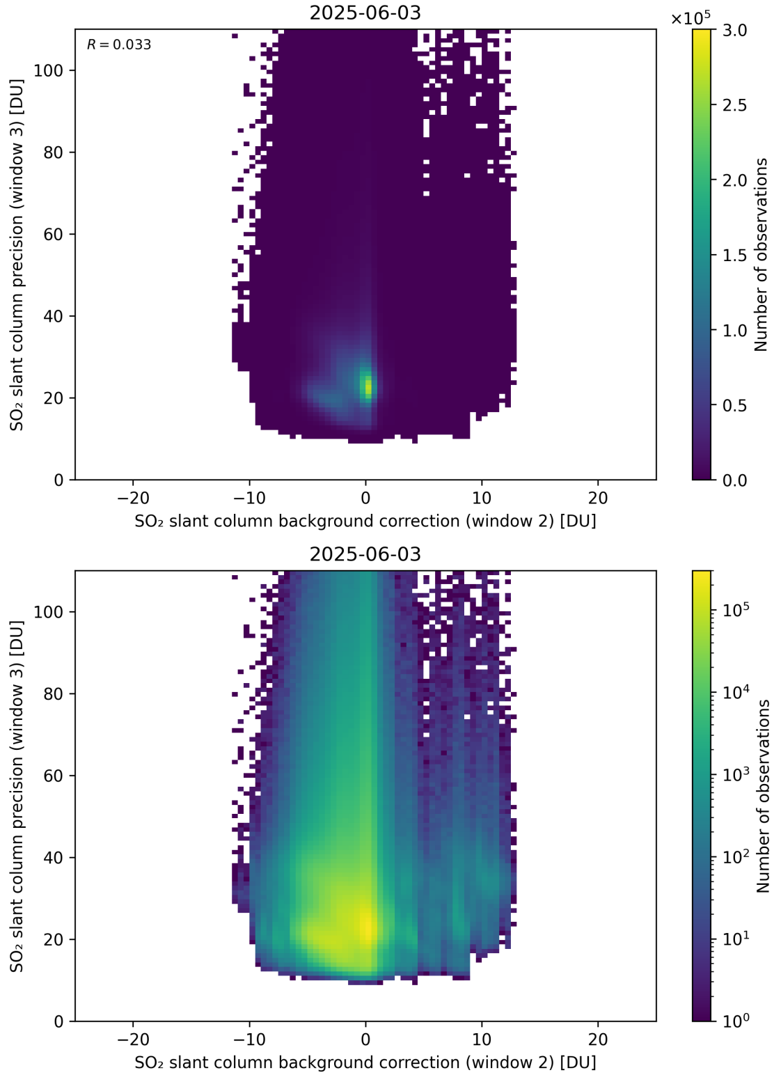
Figure 129: Scatter density plot of “SO 2 slant column background correction (window 2)” against “SO 2 slant column precision (window 3)” for 2025-06-02 to 2025-06-04.
