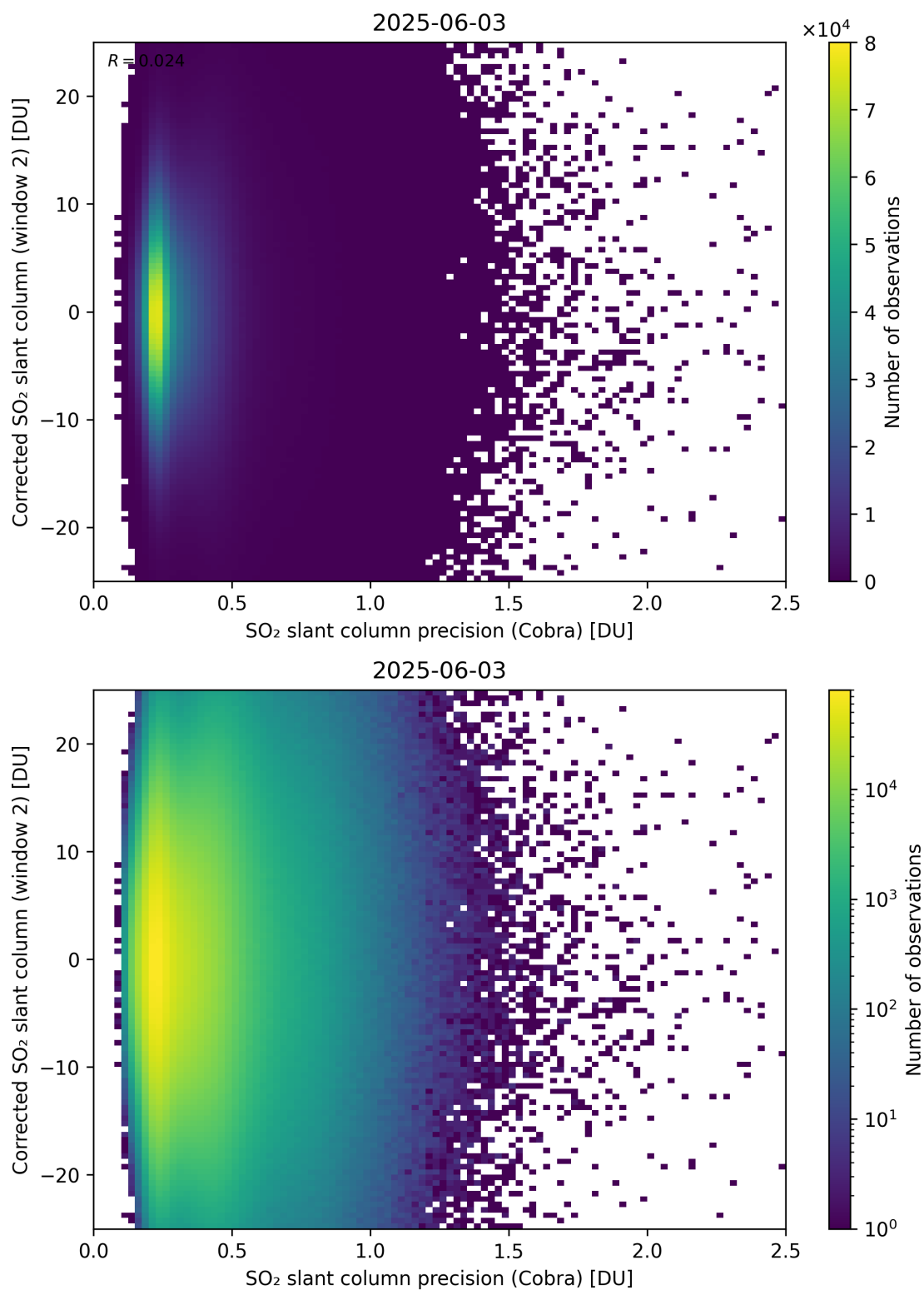
Figure 206: Scatter density plot of “SO 2 slant column precision (Cobra)” against “Corrected SO 2 slant column (window 2)” for 2025-06-02 to 2025-06-04.
