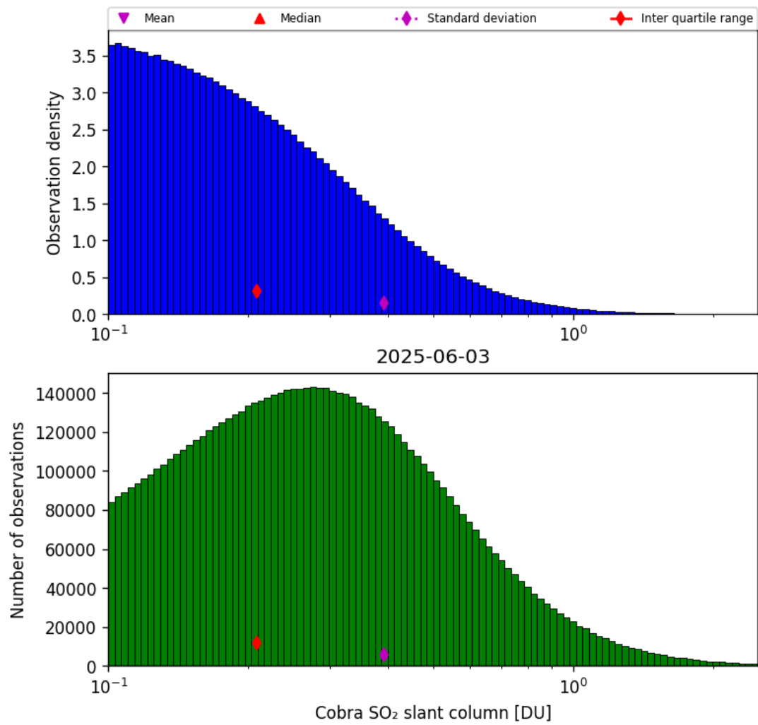
Figure 61: Histogram of “Cobra SO 2 slant column” for 2025-06-02 to 2025-06-04
