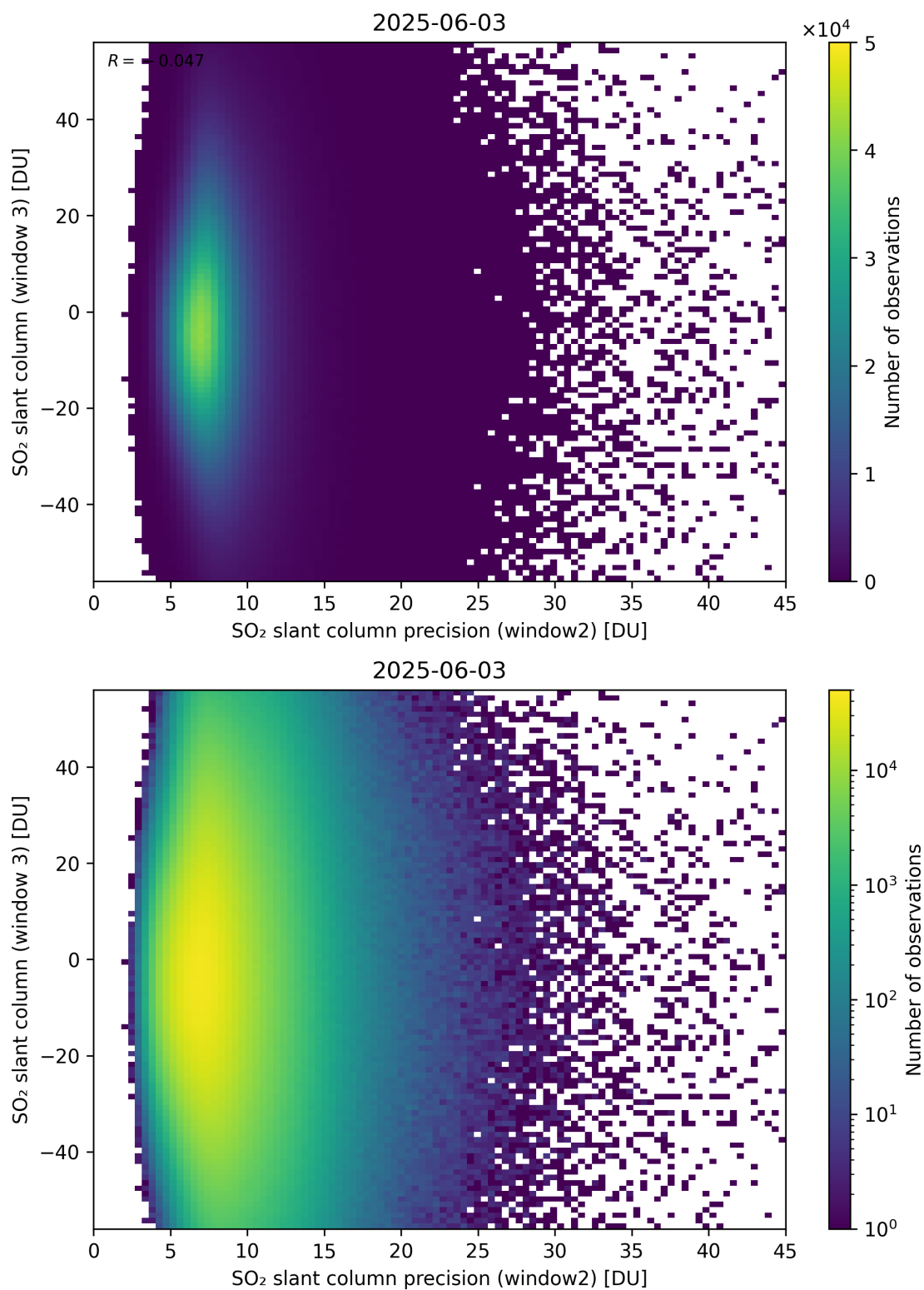
Figure 299: Scatter density plot of “SO 2 slant column precision (window2)” against “SO 2 slant column (window 3)” for 2025-06-02 to 2025-06-04.
