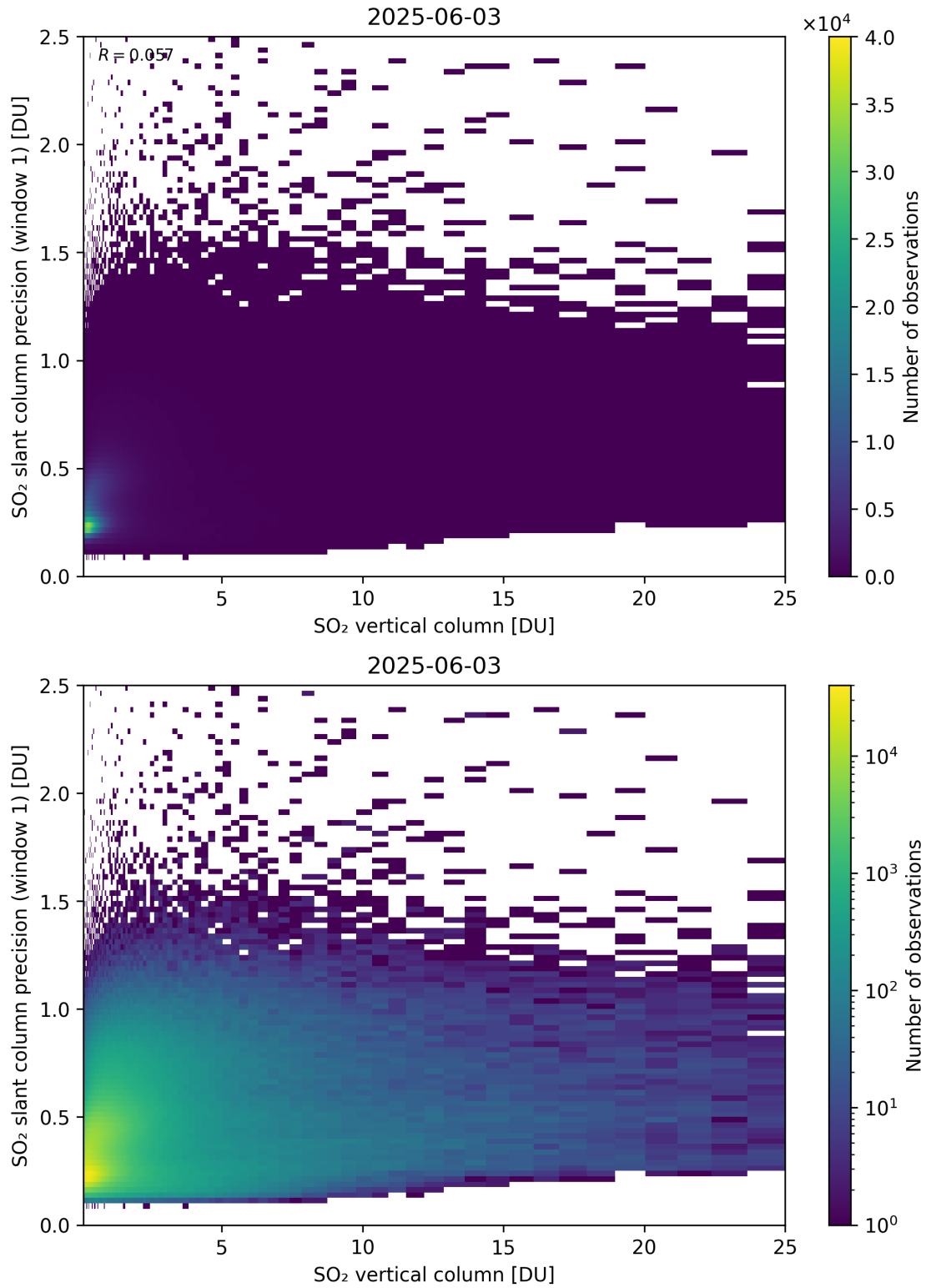
Figure 355: Scatter density plot of “SO 2 vertical column” against “SO 2 slant column precision (window 1)” for 2025-06-02 to 2025-06-04.
