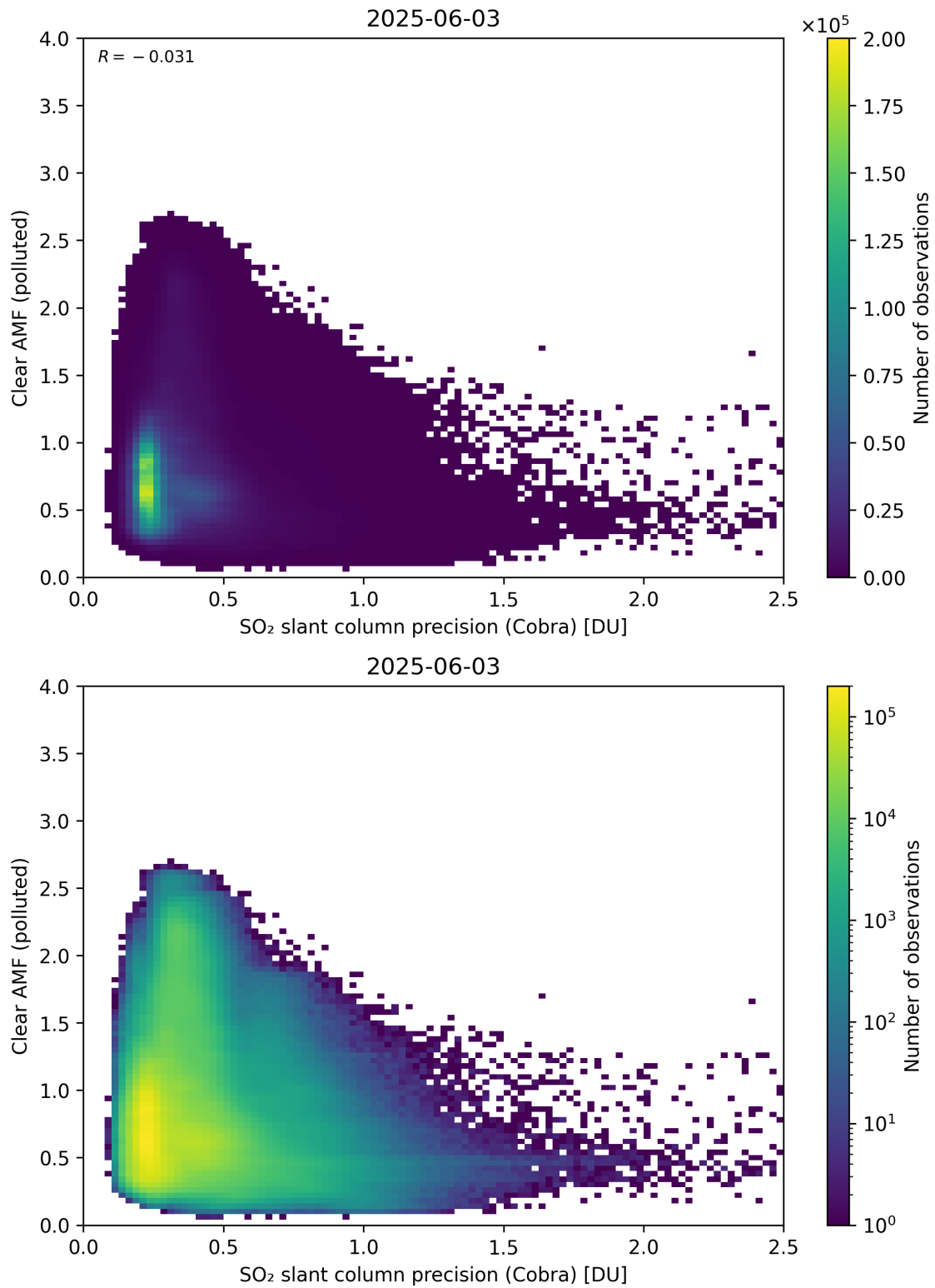
Figure 205: Scatter density plot of “SO 2 slant column precision (Cobra)” against “Clear AMF (polluted)” for 2025-06-02 to 2025-06-04.
