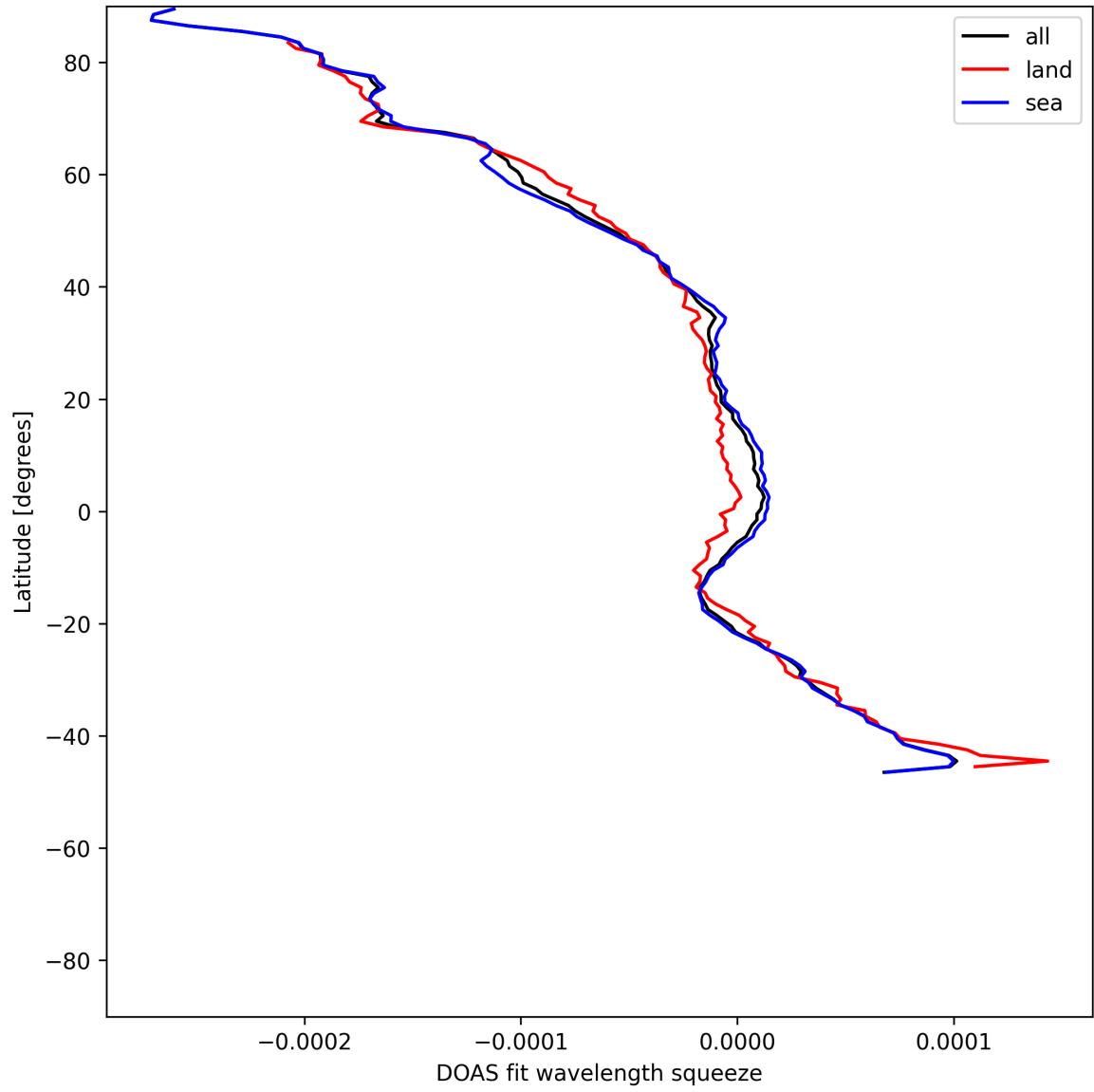
Figure 51: Zonal average of “DOAS fit wavelength squeeze” for 2025-06-02 to 2025-06-04.
