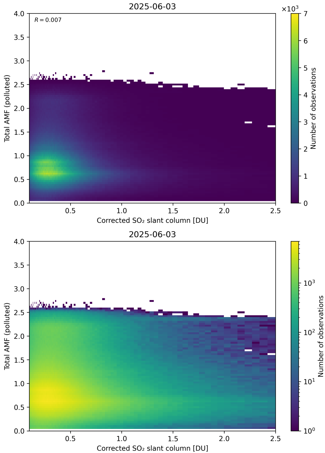
Figure 242: Scatter density plot of “Corrected SO 2 slant column” against “Total AMF (polluted)” for 2025-06-02 to 2025-06-04.
