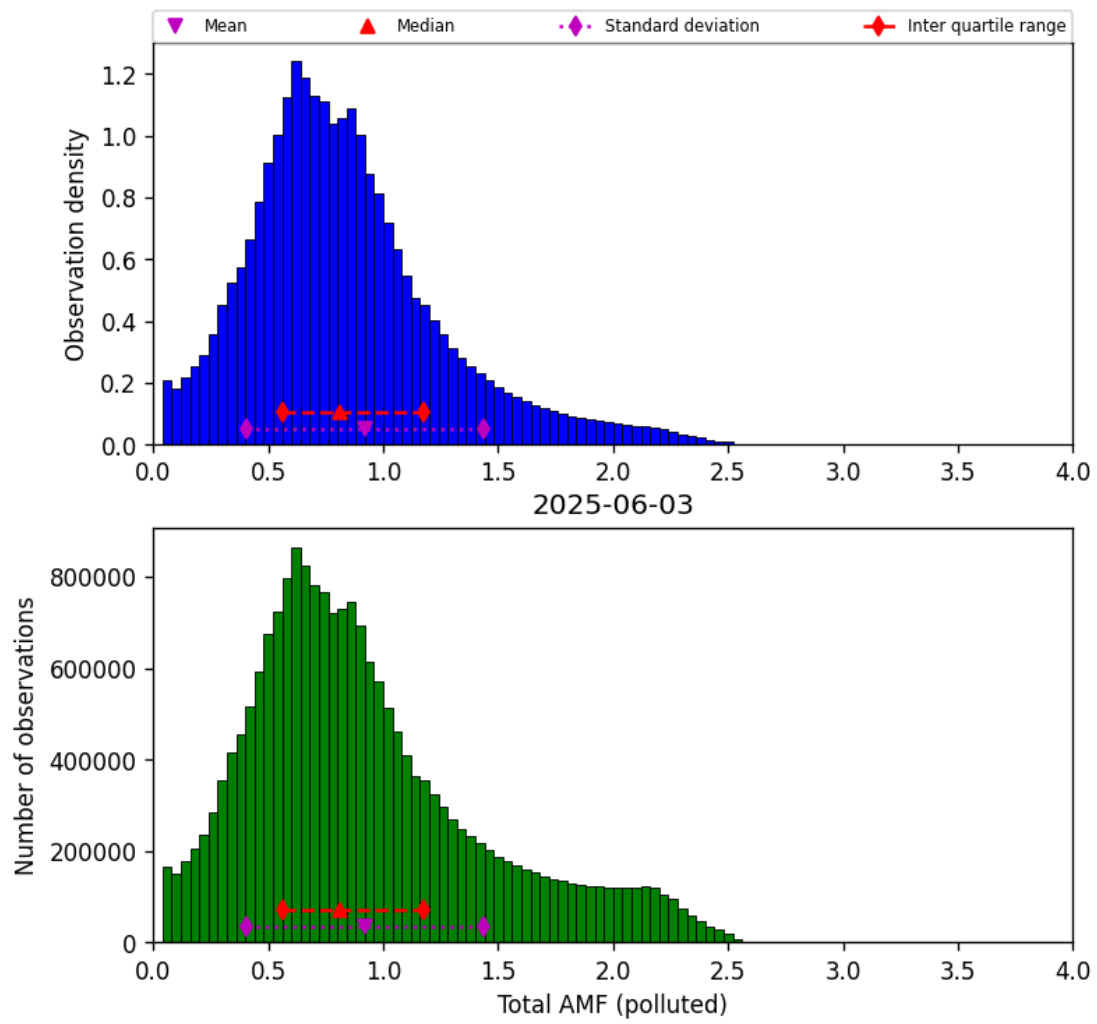
Figure 79: Histogram of “Total AMF (polluted)” for 2025-06-02 to 2025-06-04
