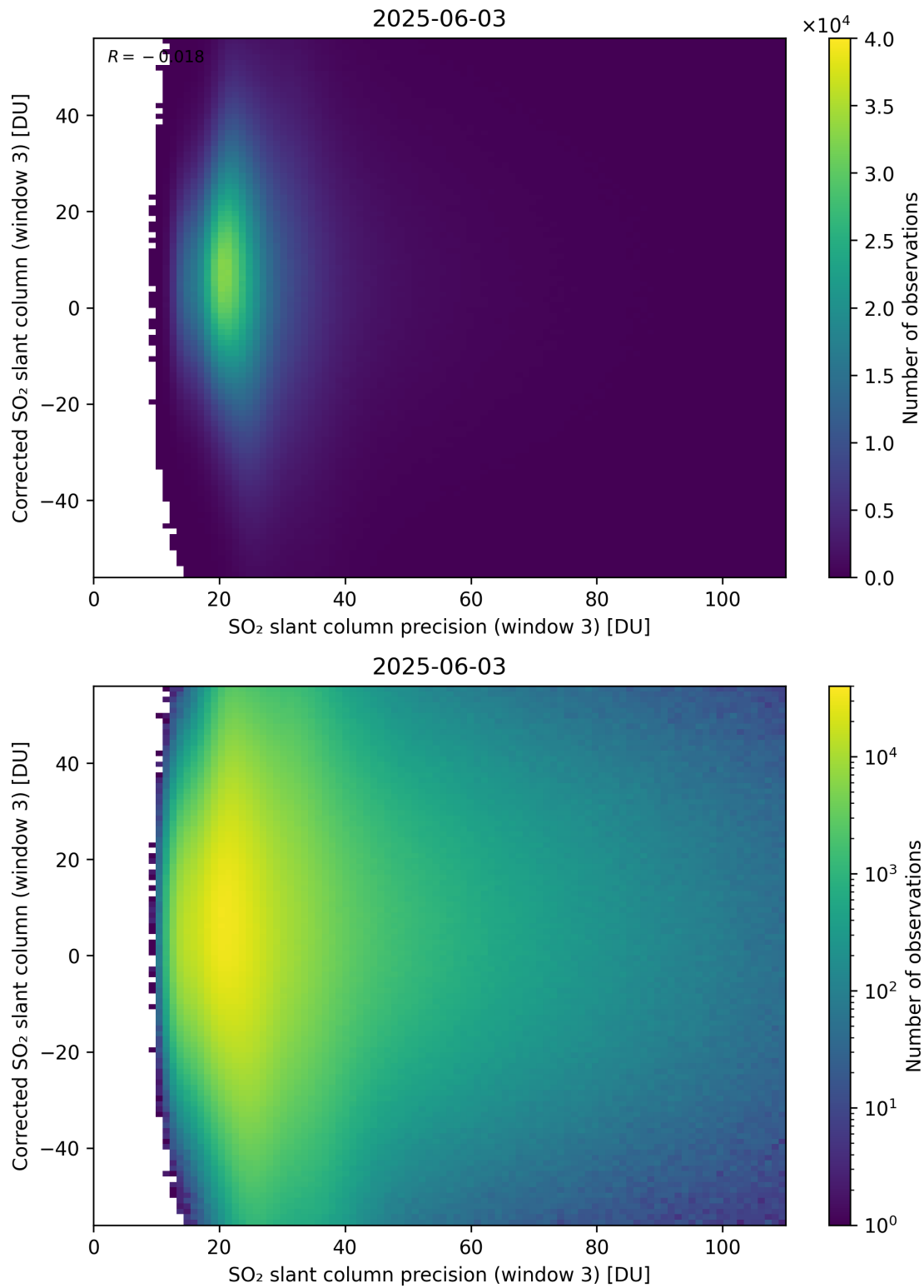
Figure 312: Scatter density plot of “SO 2 slant column precision (window 3)” against “Corrected SO 2 slant column (window 3)” for 2025-06-02 to 2025-06-04.
