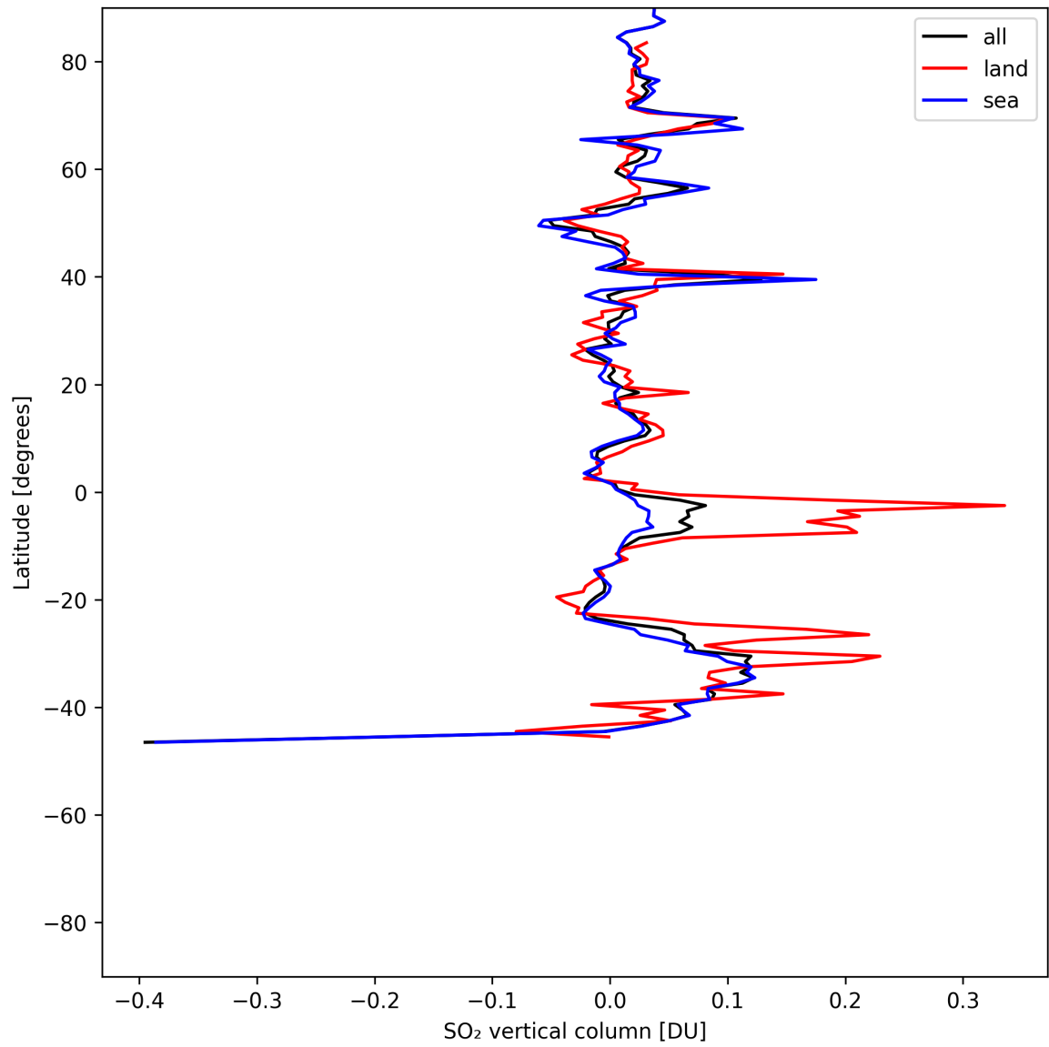
Figure 32: Zonal average of “SO 2 vertical column” for 2025-06-02 to 2025-06-04.
