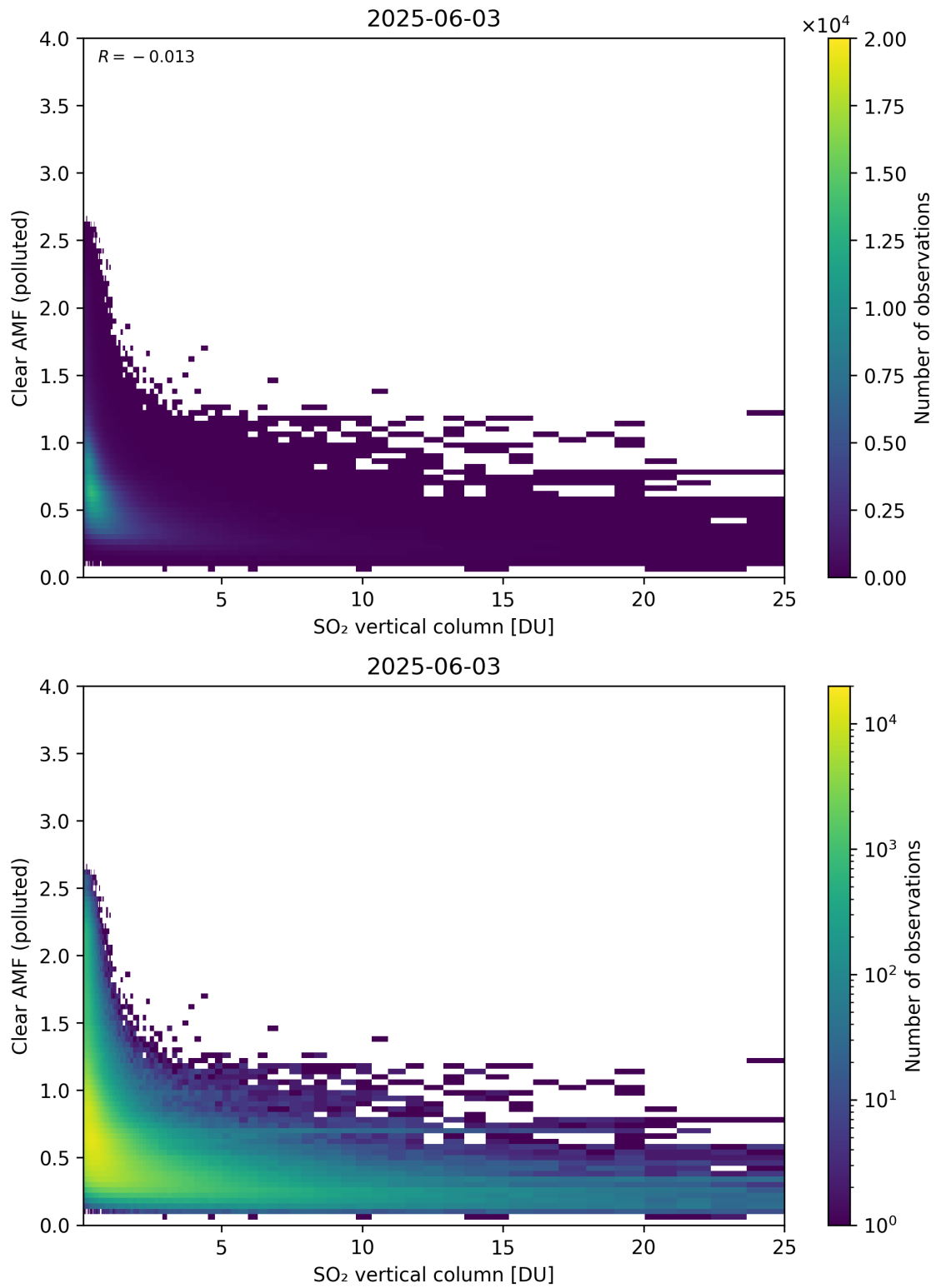
Figure 348: Scatter density plot of “SO 2 vertical column” against “Clear AMF (polluted)” for 2025-06-02 to 2025-06-04.
