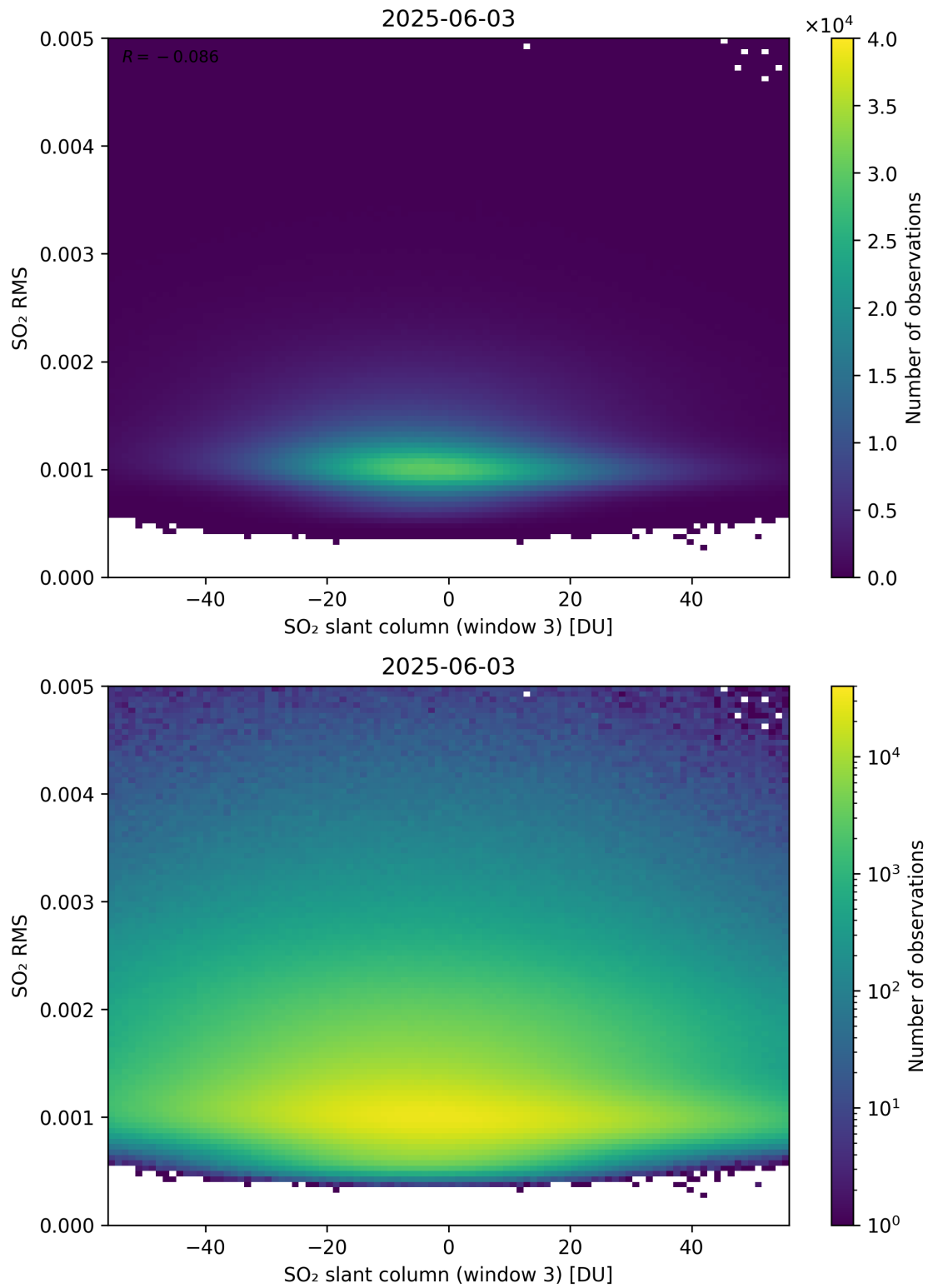
Figure 306: Scatter density plot of “SO 2 slant column (window 3)” against “SO 2 RMS” for 2025-06-02 to 2025-06-04.
