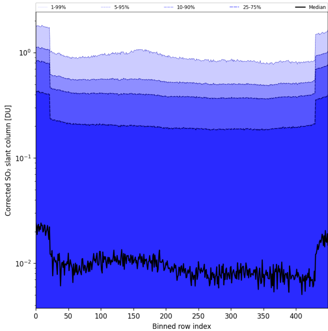
Figure 86: Along track statistics of “Corrected SO 2 slant column” for 2025-06-02 to 2025-06-04
