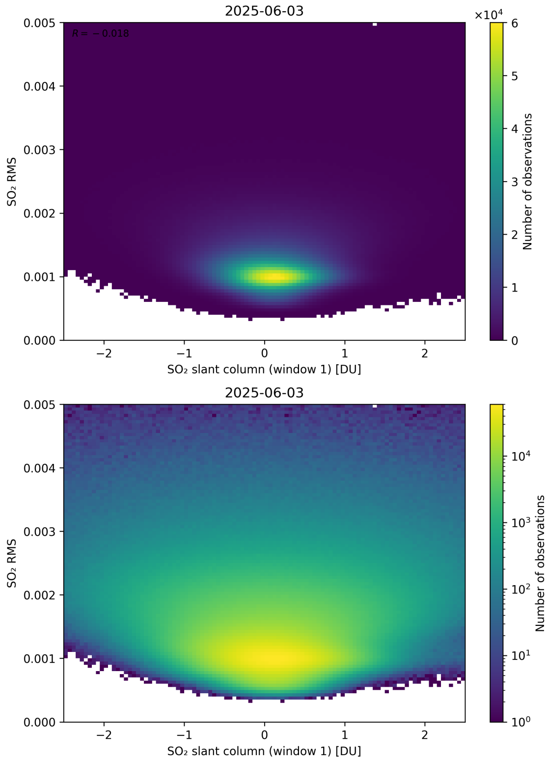
Figure 267: Scatter density plot of “SO 2 slant column (window 1)” against “SO 2 RMS” for 2025-06-02 to 2025-06-04.
