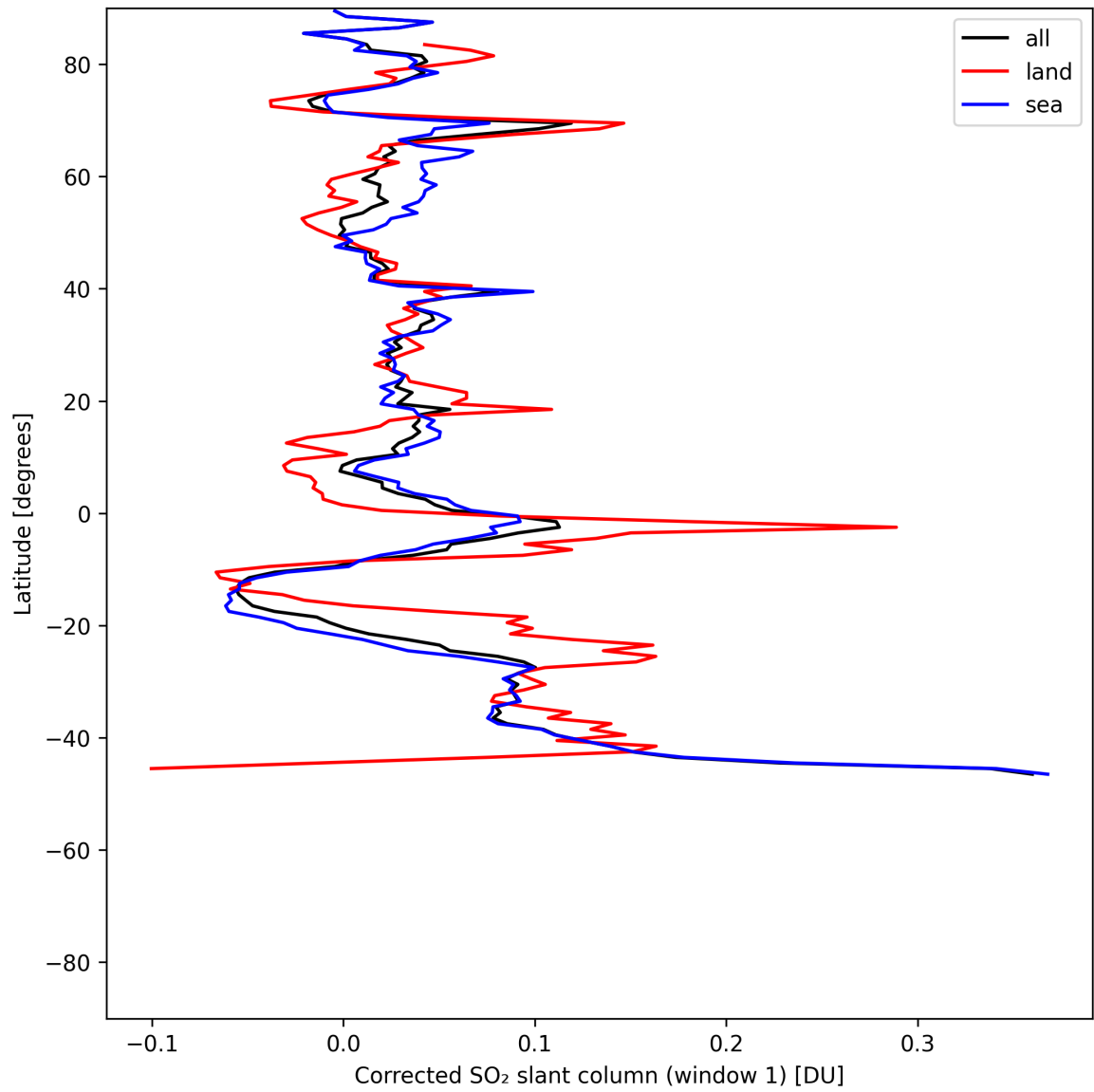
Figure 39: Zonal average of “Corrected SO 2 slant column (window 1)” for 2025-06-02 to 2025-06-04.
