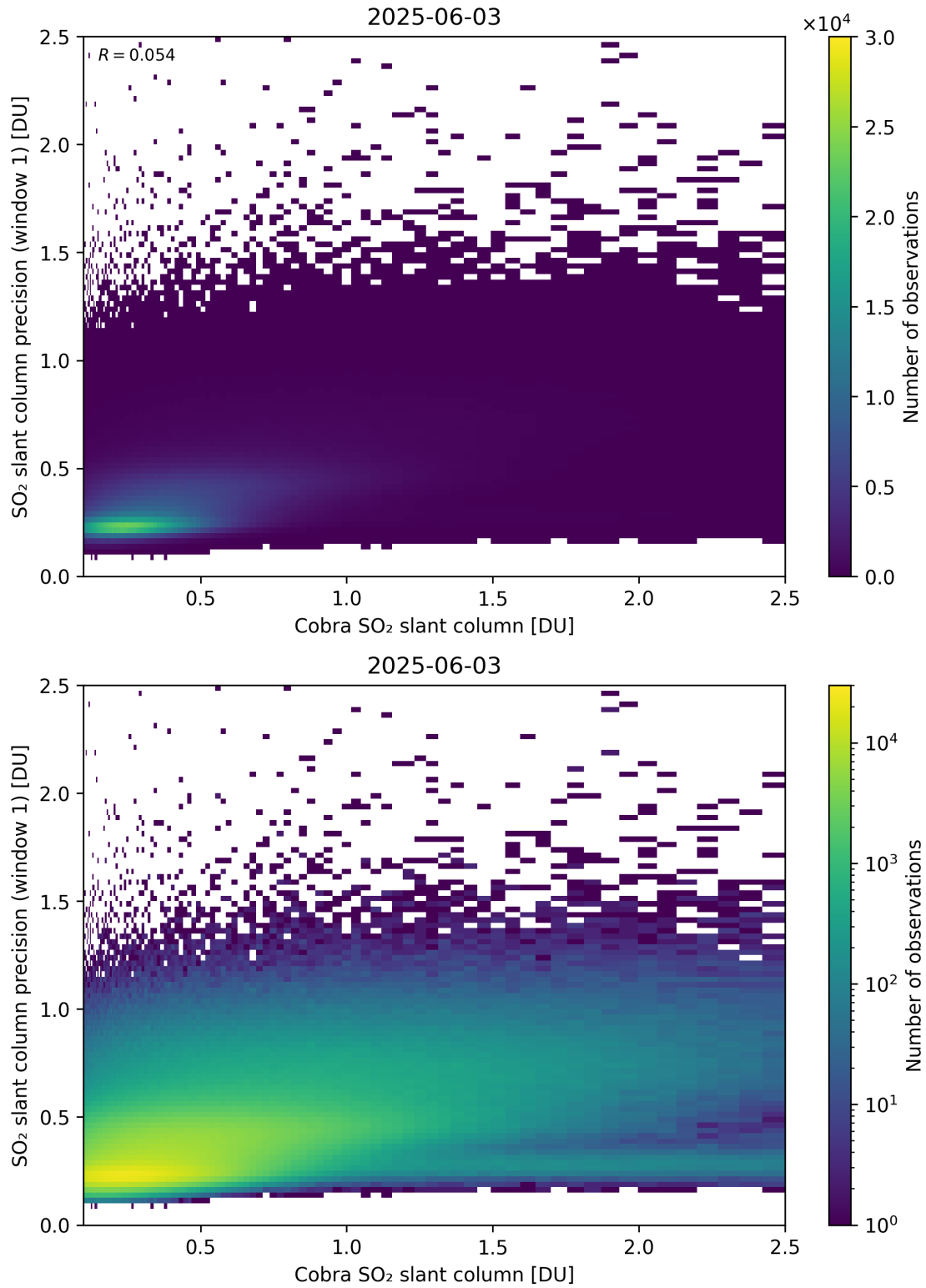
Figure 220: Scatter density plot of “Cobra SO 2 slant column” against “SO 2 slant column precision (window 1)” for 2025-06-02 to 2025-06-04.
