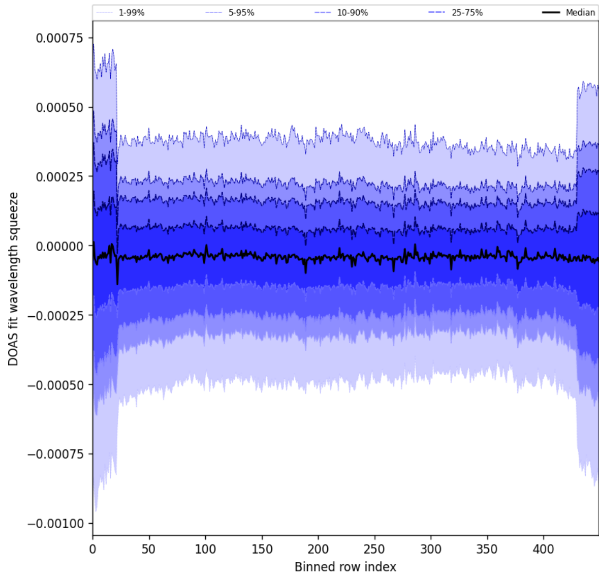
Figure 103: Along track statistics of “DOAS fit wavelength squeeze” for 2025-06-02 to 2025-06-04
