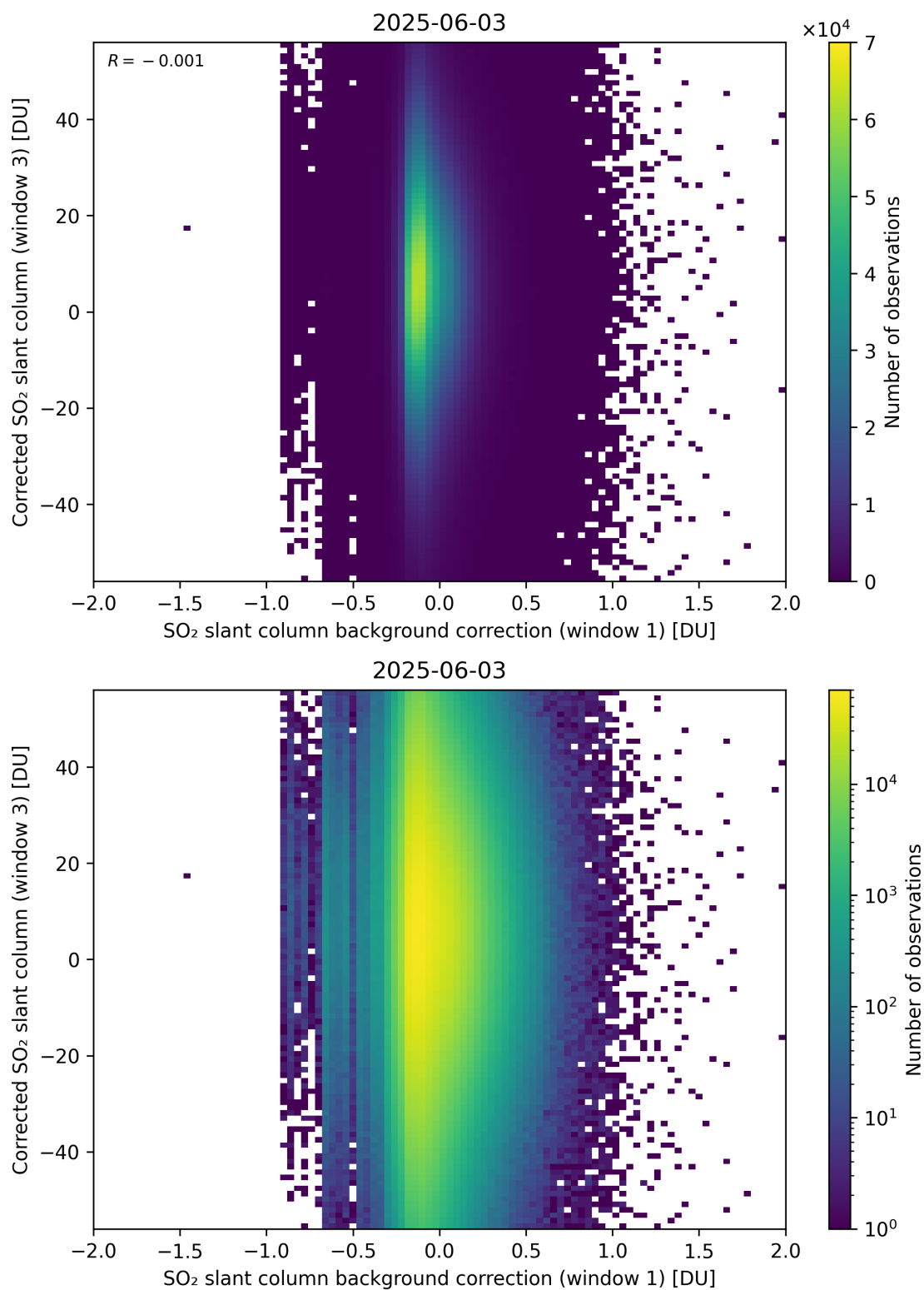
Figure 116: Scatter density plot of “SO 2 slant column background correction (window 1)” against “Corrected SO 2 slant column (window 3)” for 2025-06-02 to 2025-06-04.
