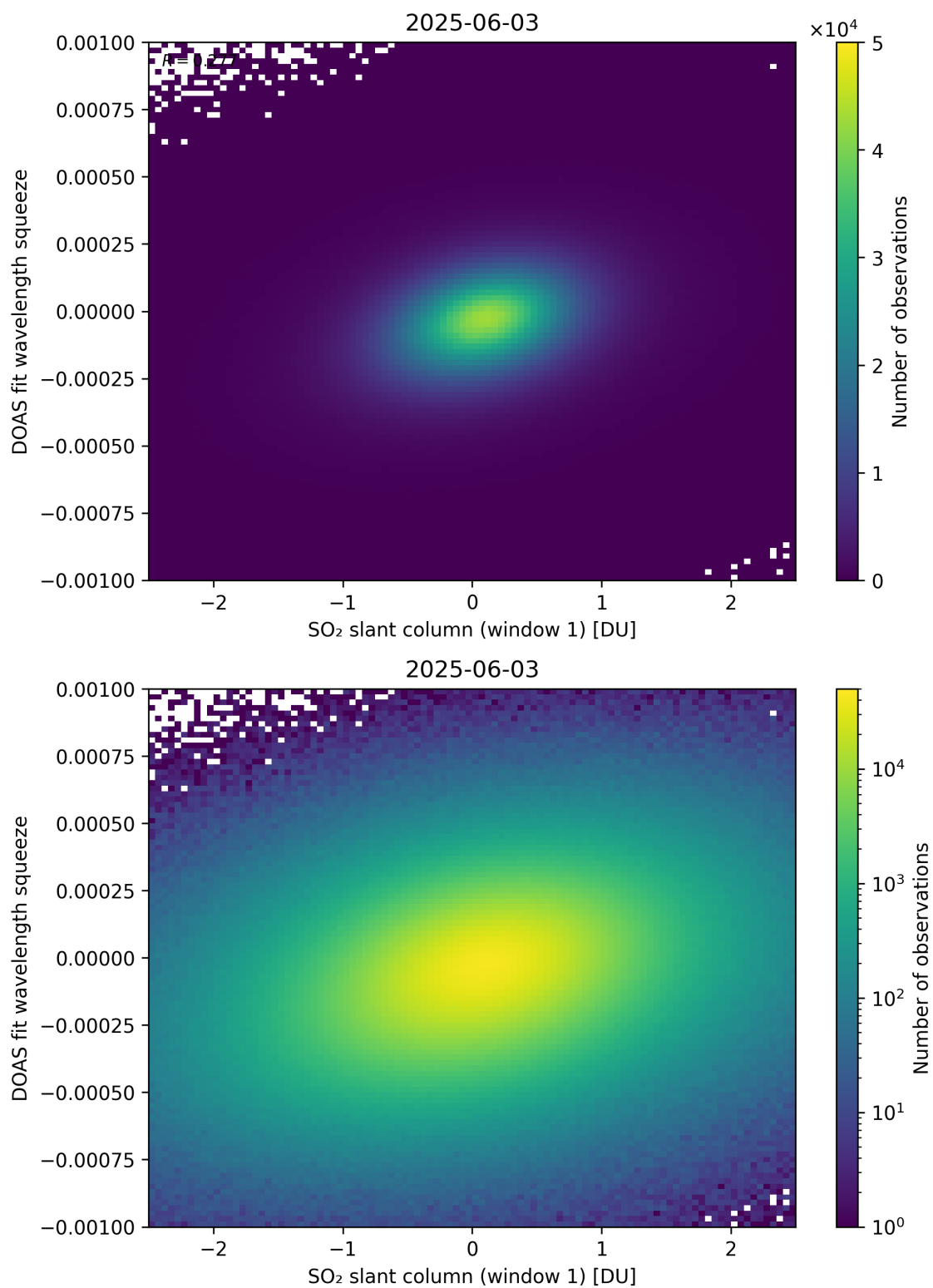
Figure 266: Scatter density plot of “SO 2 slant column (window 1)” against “DOAS fit wavelength squeeze” for 2025-06-02 to 2025-06-04.
