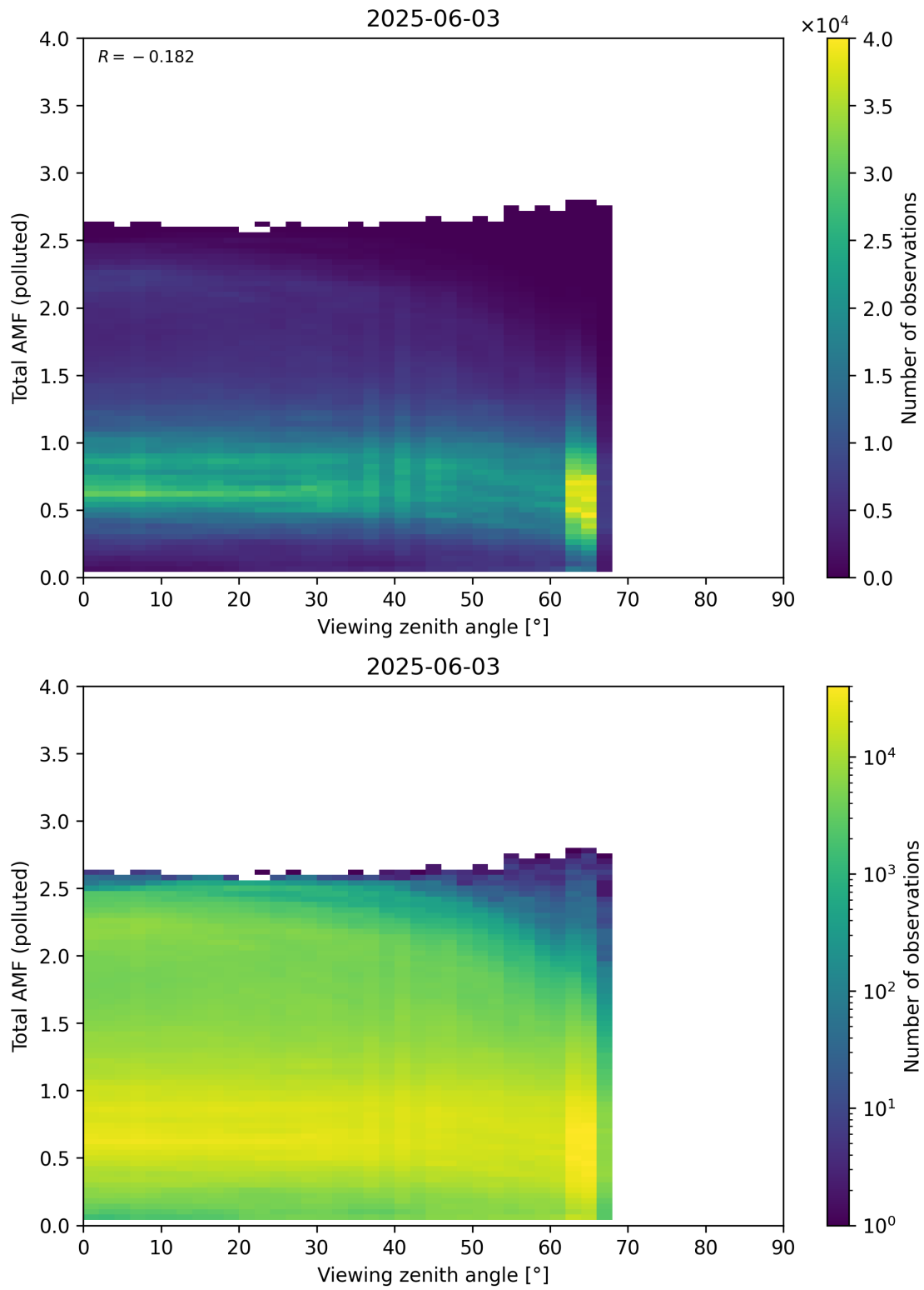
Figure 381: Scatter density plot of “Viewing zenith angle” against “Total AMF (polluted)” for 2025-06-02 to 2025-06-04.
