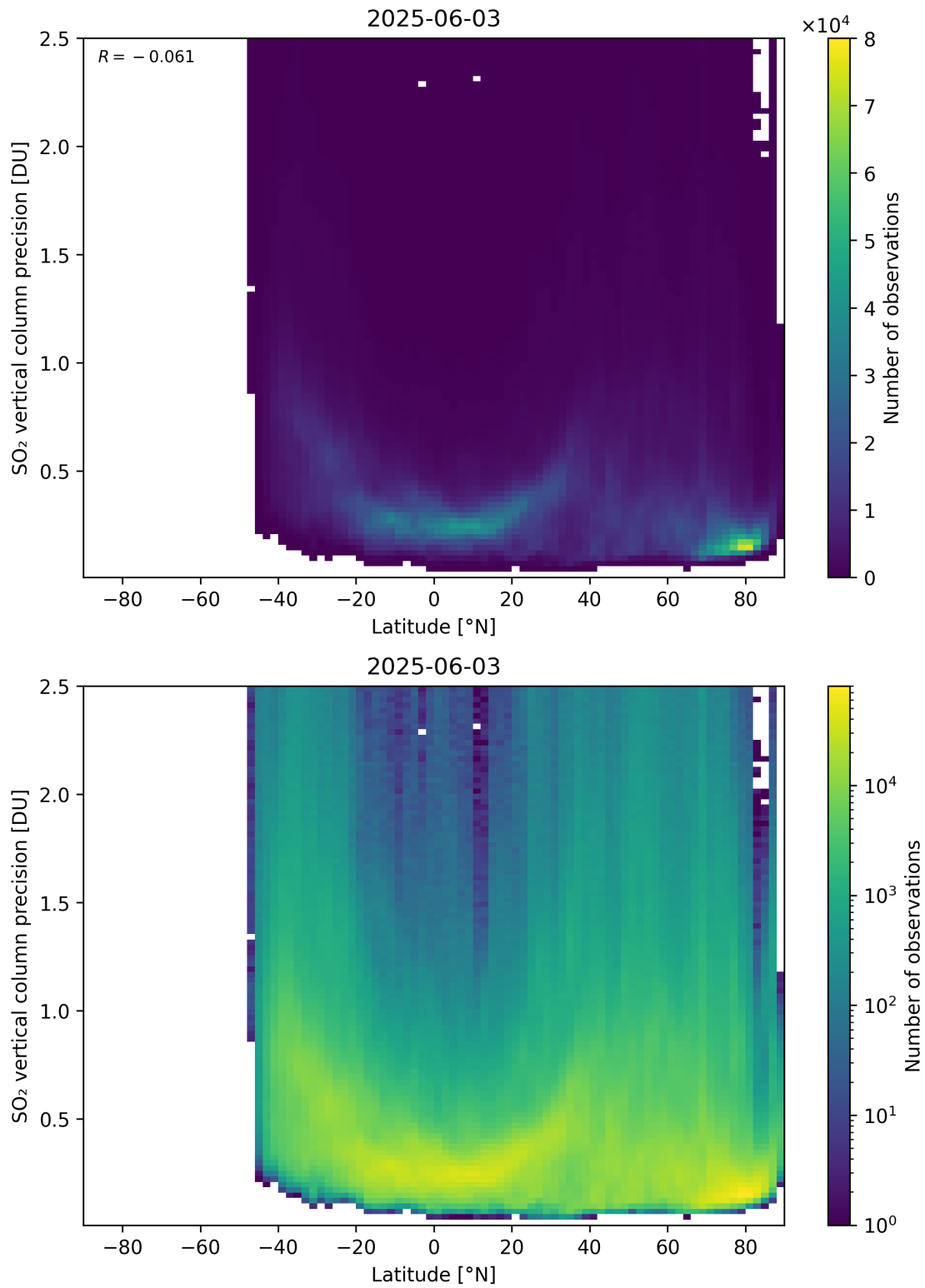
Figure 170: Scatter density plot of “Latitude” against “SO 2 vertical column precision” for 2025-06-02 to 2025-06-04.
