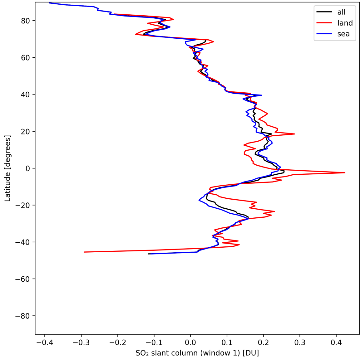
Figure 37: Zonal average of “SO 2 slant column (window 1)” for 2025-06-02 to 2025-06-04.
