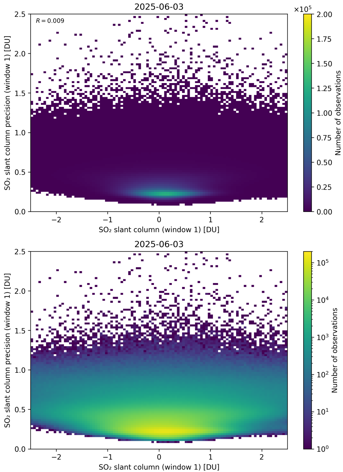
Figure 285: Scatter density plot of “SO 2 slant column (window 1)” against “SO 2 slant column precision (window 1)” for 2025-06-02 to 2025-06-04.
