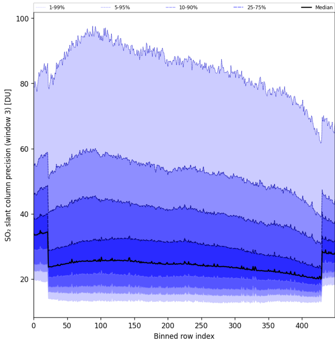
Figure 98: Along track statistics of “SO 2 slant column precision (window 3)” for 2025-06-02 to 2025-06-04
