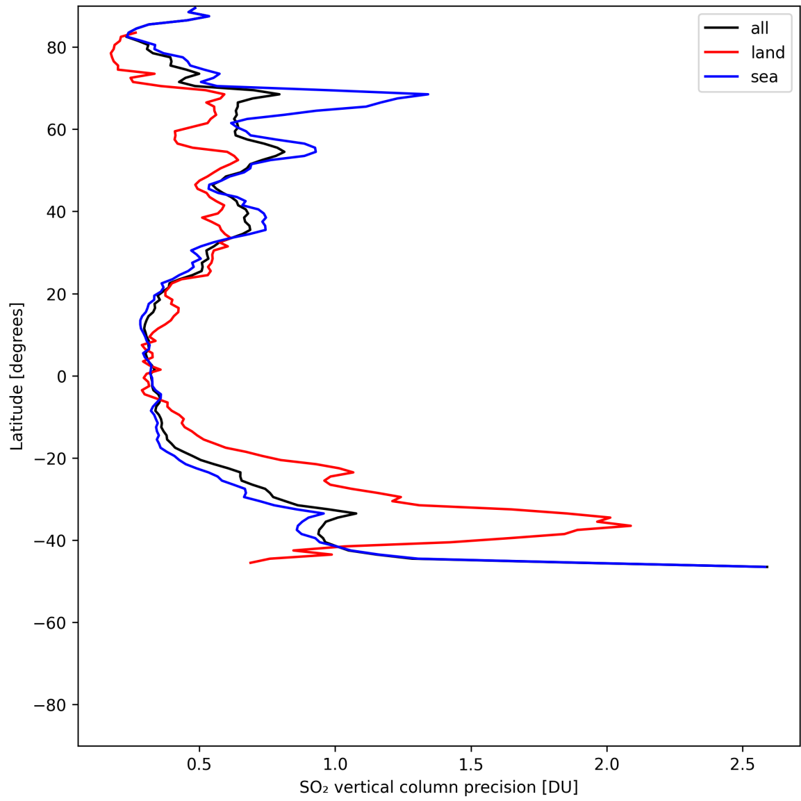
Figure 33: Zonal average of “SO 2 vertical column precision” for 2025-06-02 to 2025-06-04.
