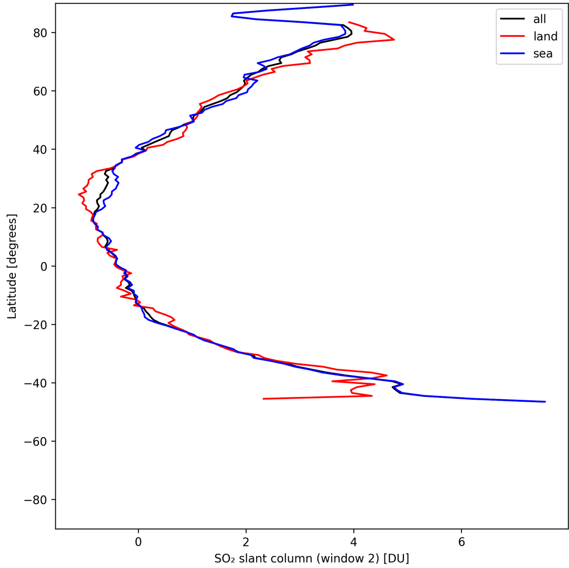
Figure 41: Zonal average of “SO 2 slant column (window 2)” for 2025-06-02 to 2025-06-04.
