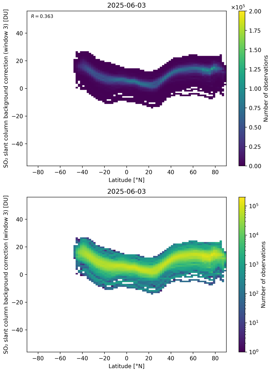
Figure 152: Scatter density plot of “Latitude” against “SO 2 slant column background correction (window 3)” for 2025-06-02 to 2025-06-04.
