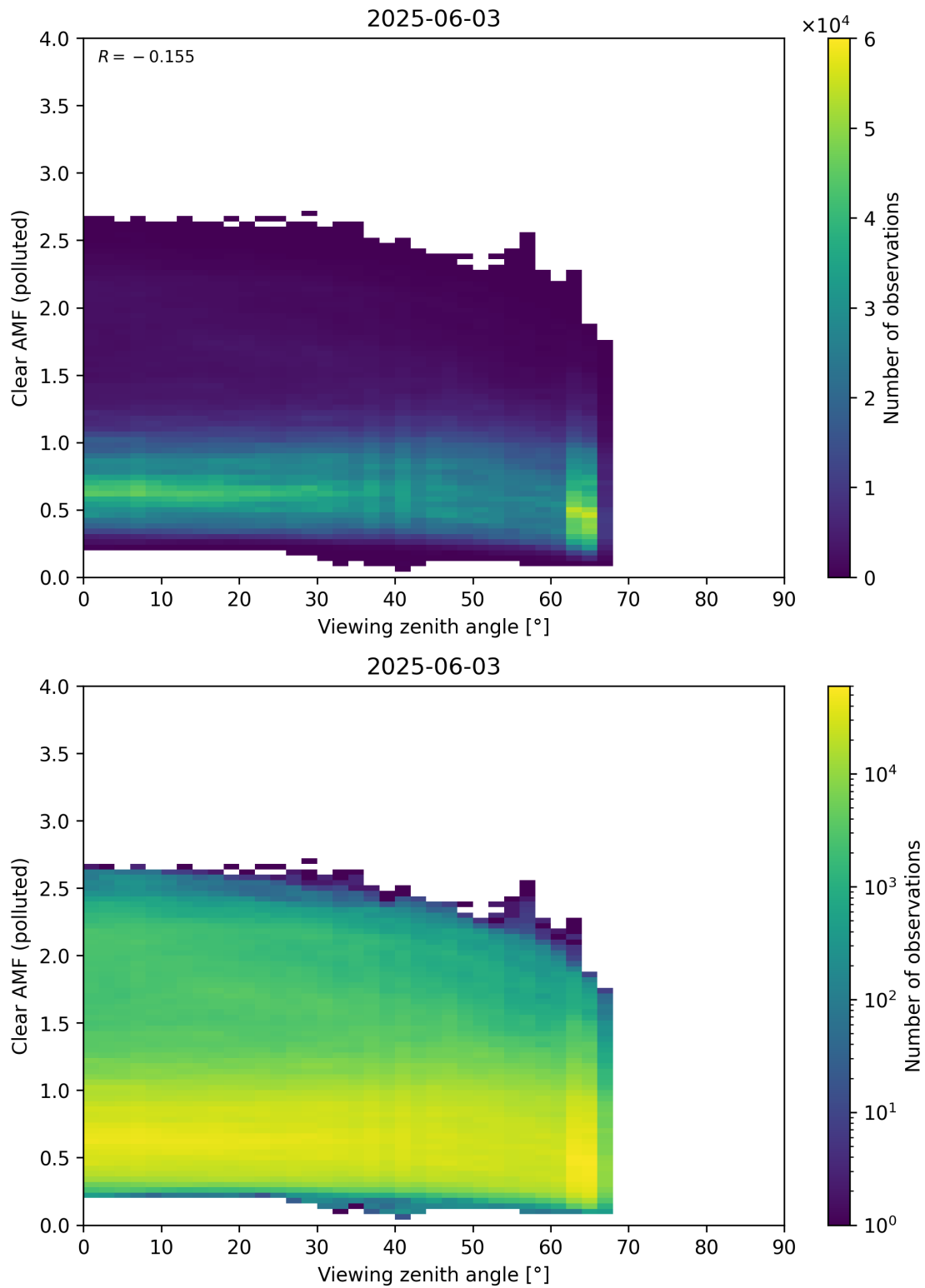
Figure 370: Scatter density plot of “Viewing zenith angle” against “Clear AMF (polluted)” for 2025-06-02 to 2025-06-04.
