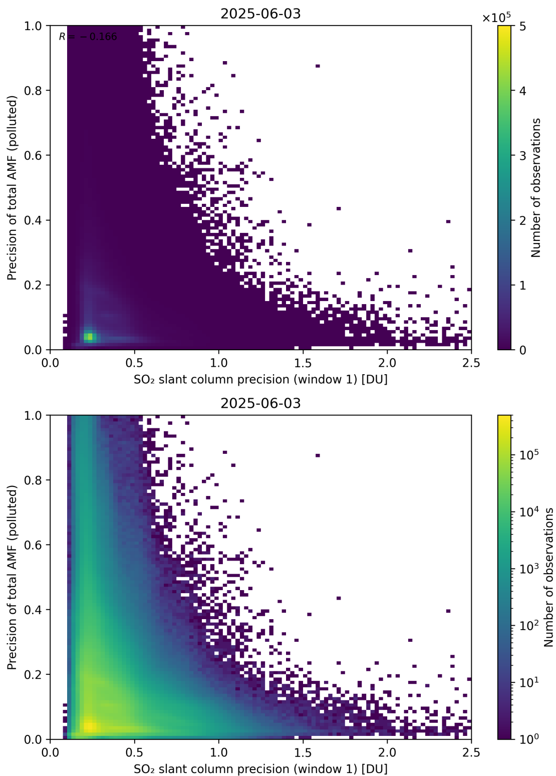
Figure 281: Scatter density plot of “SO 2 slant column precision (window 1)” against “Precision of total AMF (polluted)” for 2025-06-02 to 2025-06-04.
