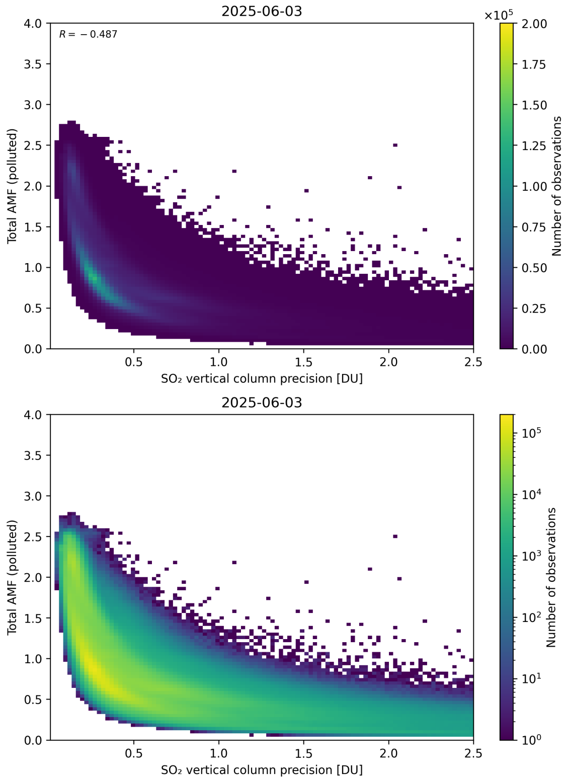
Figure 346: Scatter density plot of “SO 2 vertical column precision” against “Total AMF (polluted)” for 2025-06-02 to 2025-06-04.
