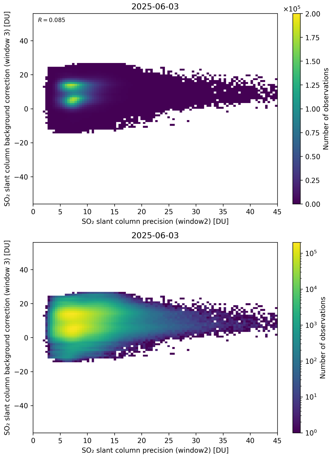
Figure 292: Scatter density plot of “SO 2 slant column precision (window2)” against “SO 2 slant column background correction (window 3)” for 2025-06-02 to 2025-06-04.
