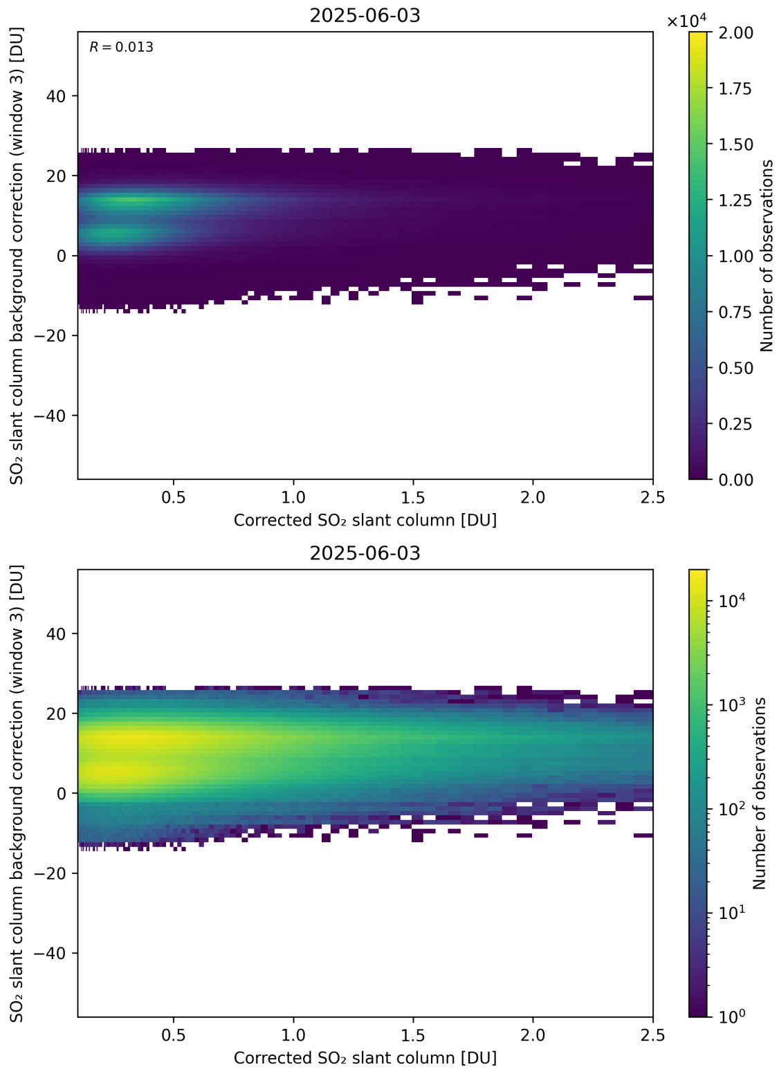
Figure 228: Scatter density plot of “Corrected SO 2 slant column” against “SO 2 slant column background correction (window 3)” for 2025-06-02 to 2025-06-04.
