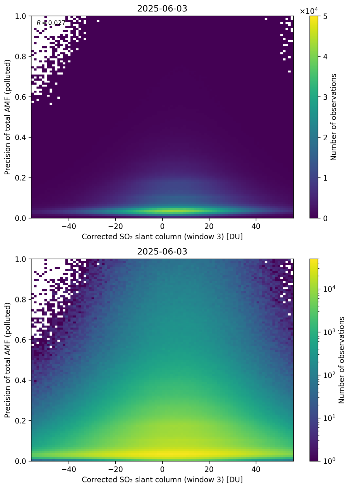
Figure 261: Scatter density plot of “Corrected SO 2 slant column (window 3)” against “Precision of total AMF (polluted)” for 2025-06-02 to 2025-06-04.
