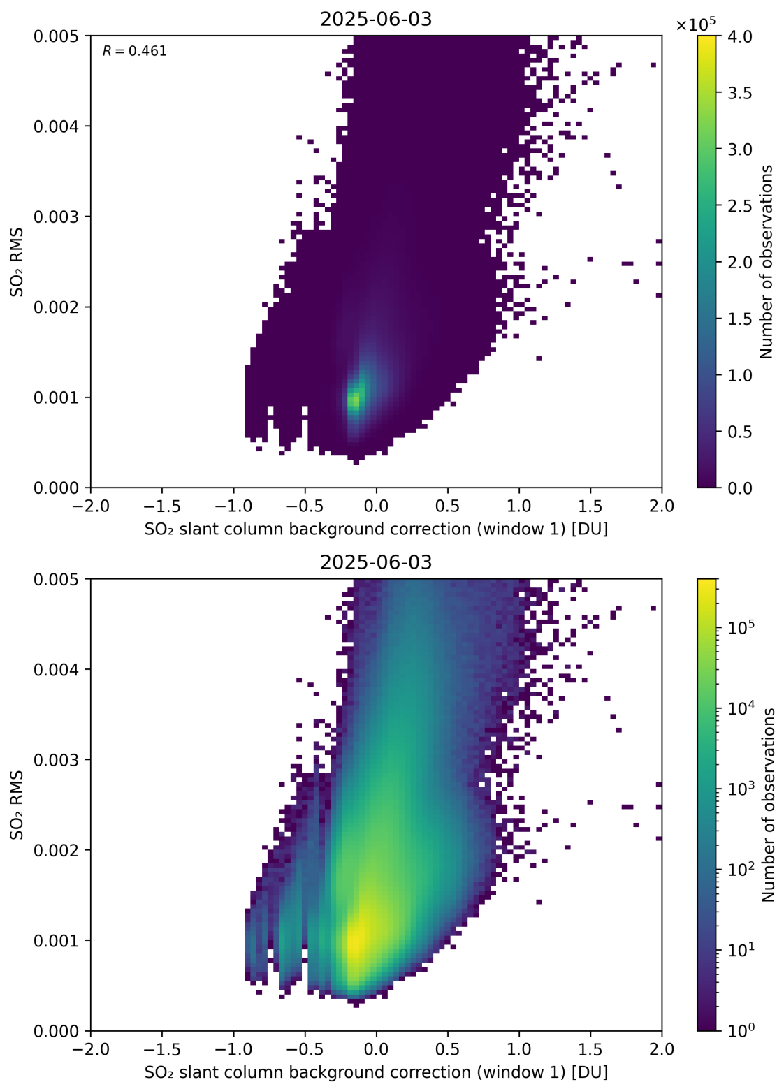
Figure 113: Scatter density plot of “SO 2 slant column background correction (window 1)” against “SO 2 RMS” for 2025-06-02 to 2025-06-04.
