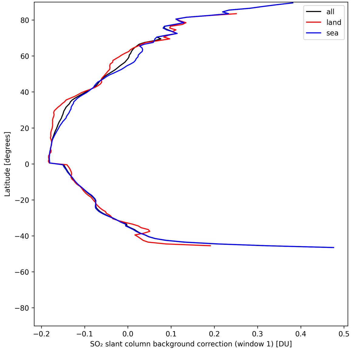
Figure 40: Zonal average of "SO 2 slant column background correction (window 1)" for 2025-06-02 to 2025-06-04.
