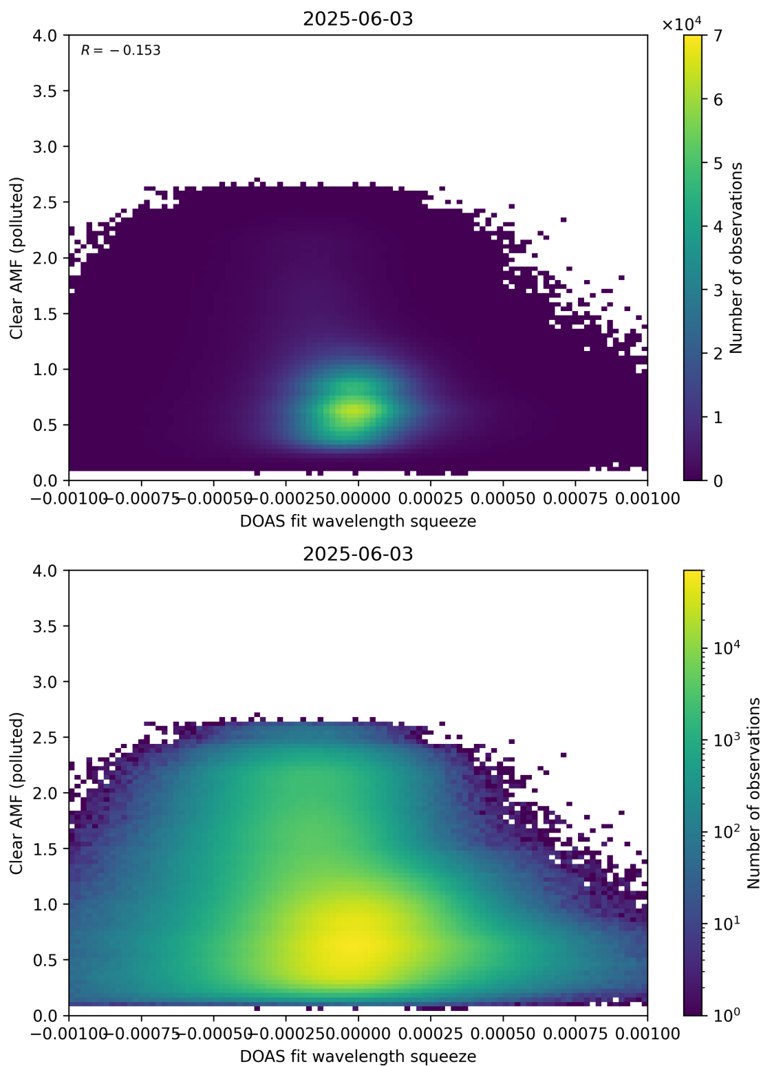
Figure 144: Scatter density plot of “DOAS fit wavelength squeeze” against “Clear AMF (polluted)” for 2025-06-02 to 2025-06-04.
