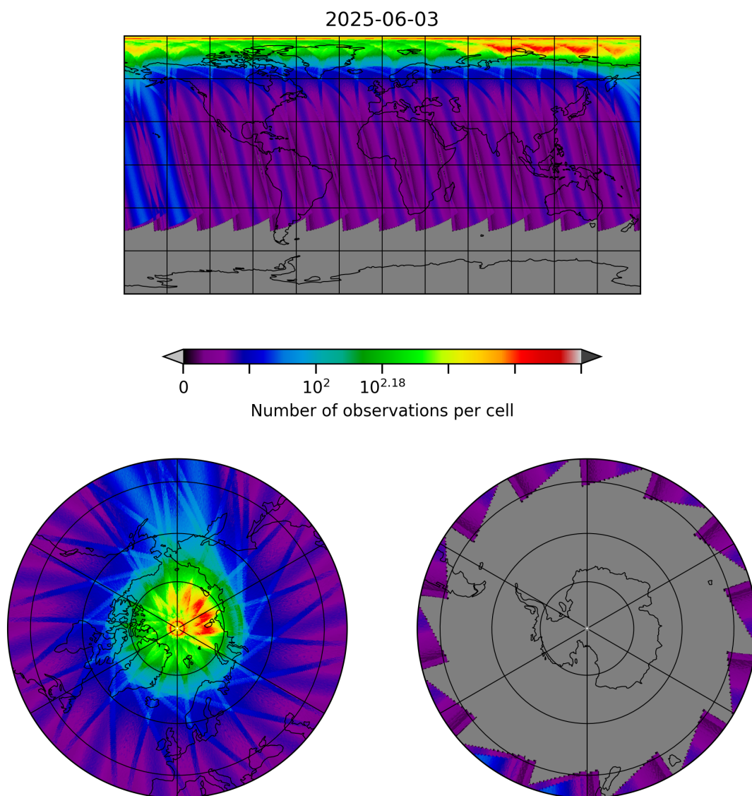
Figure 30: Map of the number of observations for 2025-06-02 to 2025-06-04
