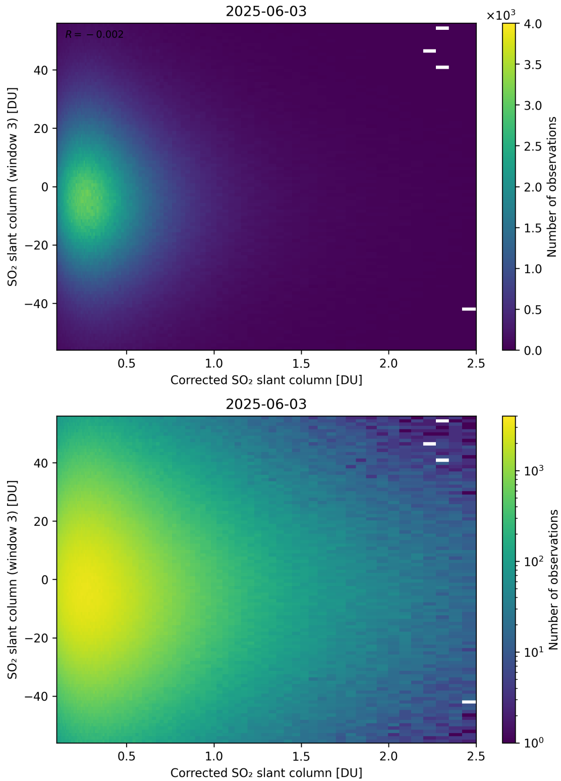
Figure 240: Scatter density plot of “Corrected SO 2 slant column” against “SO 2 slant column (window 3)” for 2025-06-02 to 2025-06-04.
