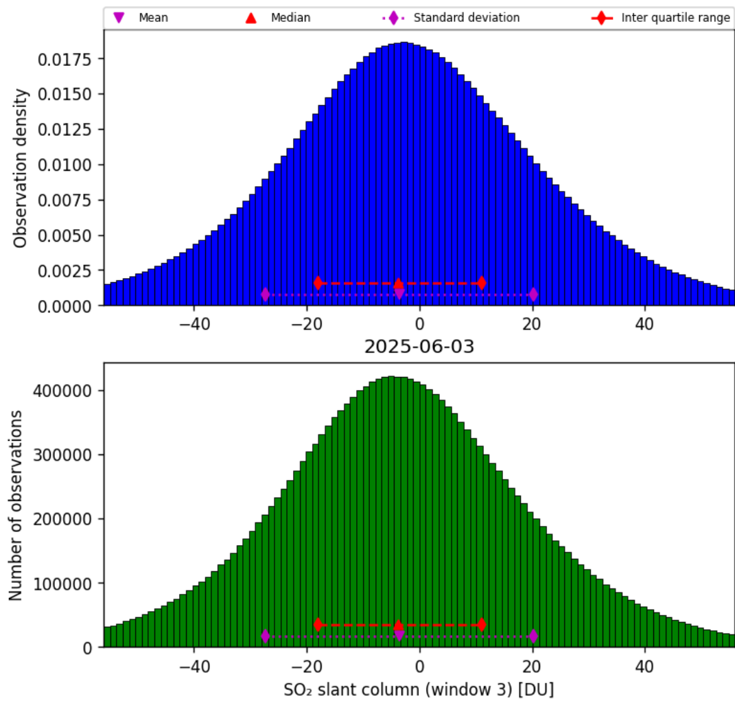
Figure 71: Histogram of “SO 2 slant column (window 3)” for 2025-06-02 to 2025-06-04
