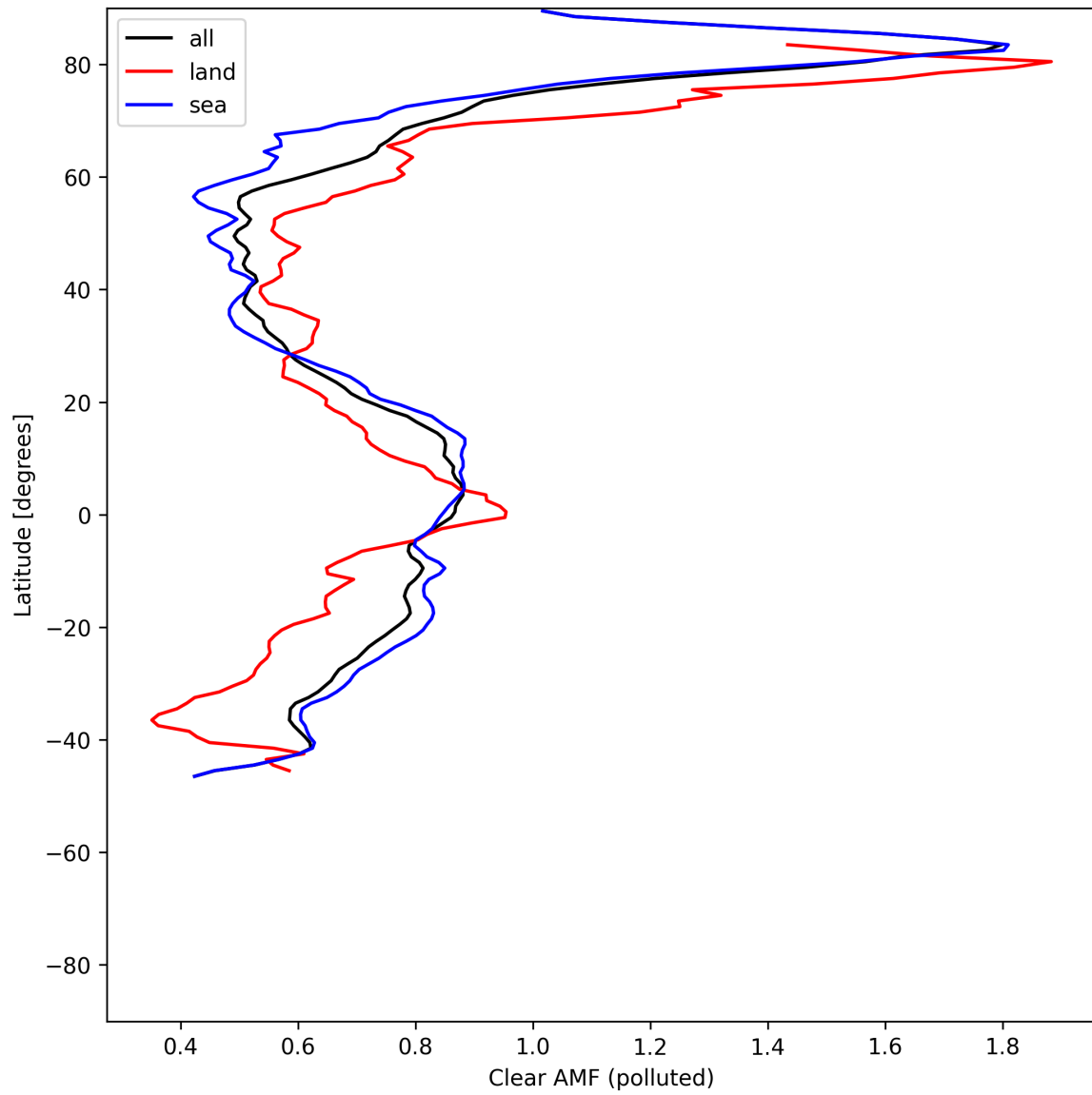
Figure 55: Zonal average of “Clear AMF (polluted)” for 2025-06-02 to 2025-06-04.
