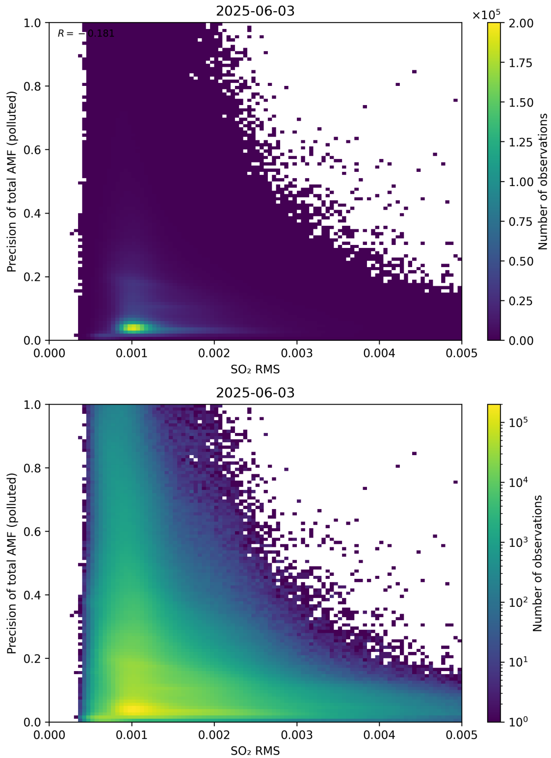
Figure 149: Scatter density plot of “SO 2 RMS” against “Precision of total AMF (polluted)” for 2025-06-02 to 2025-06-04.
