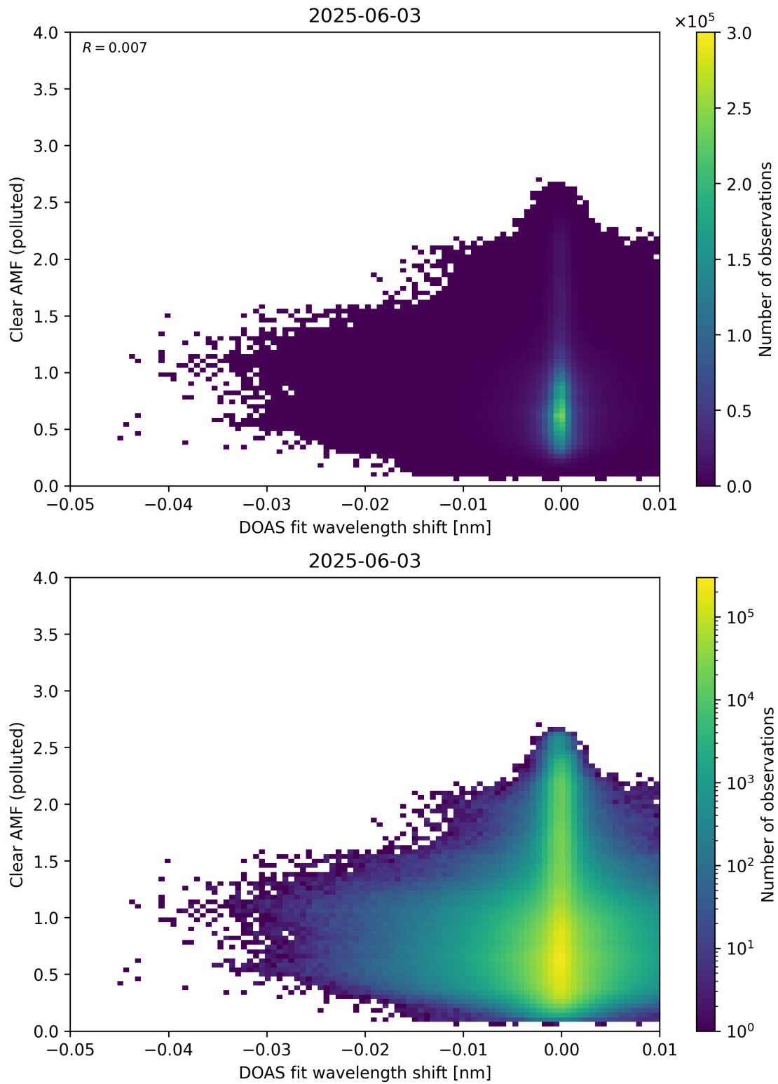
Figure 140: Scatter density plot of “DOAS fit wavelength shift” against “Clear AMF (polluted)” for 2025-06-02 to 2025-06-04.
