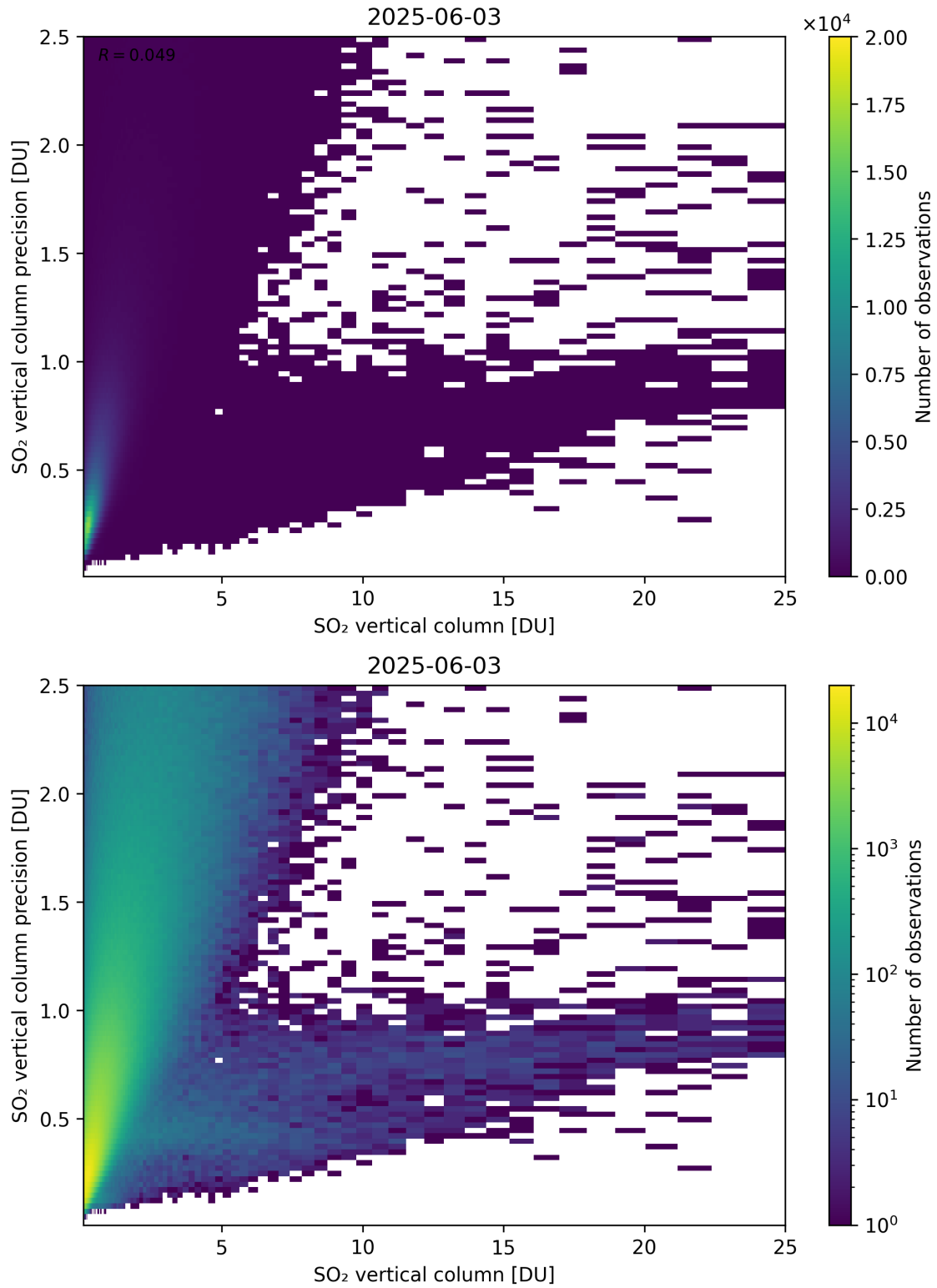
Figure 361: Scatter density plot of “SO 2 vertical column” against “SO 2 vertical column precision” for 2025-06-02 to 2025-06-04.
