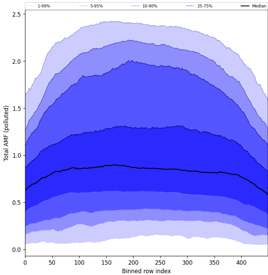
Figure 105: Along track statistics of “Total AMF (polluted)” for 2025-06-02 to 2025-06-04
