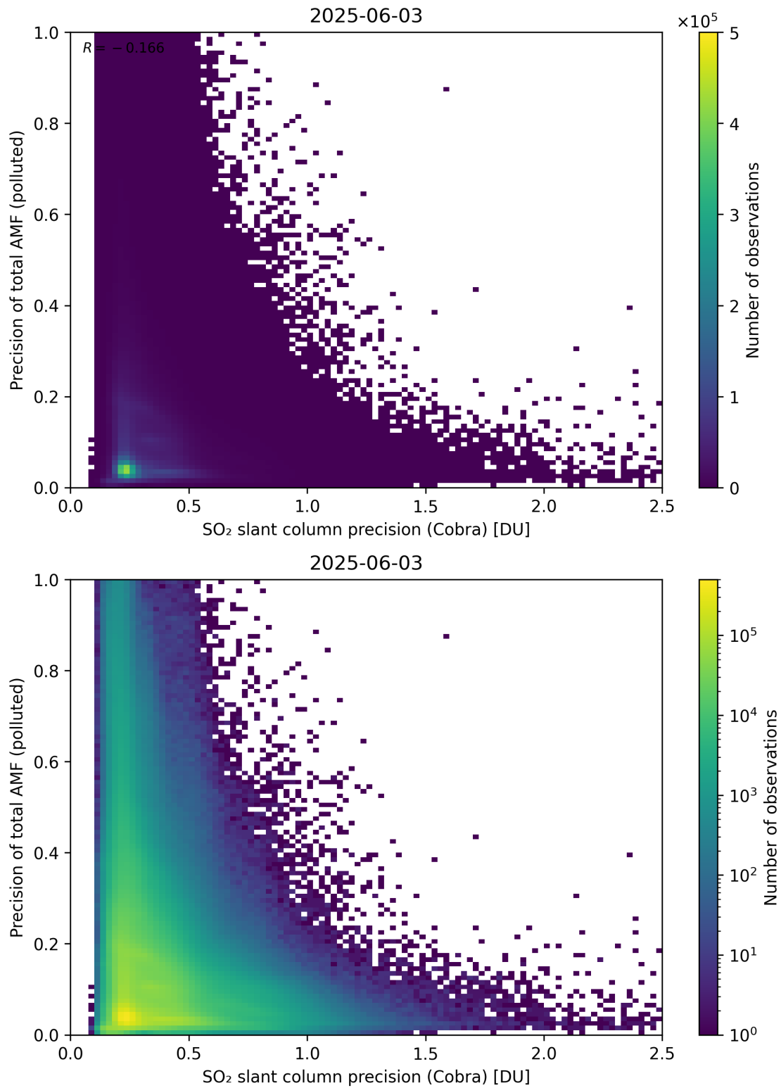
Figure 214: Scatter density plot of “SO 2 slant column precision (Cobra)” against “Precision of total AMF (polluted)” for 2025-06-02 to 2025-06-04.
