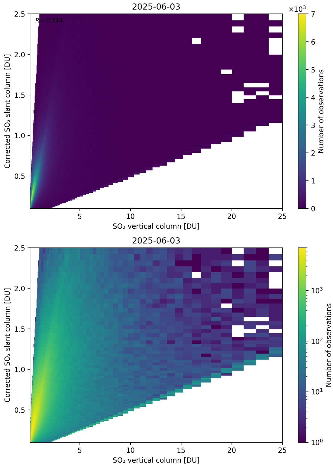
Figure 351: Scatter density plot of “SO 2 vertical column” against “Corrected SO 2 slant column” for 2025-06-02 to 2025-06-04.
