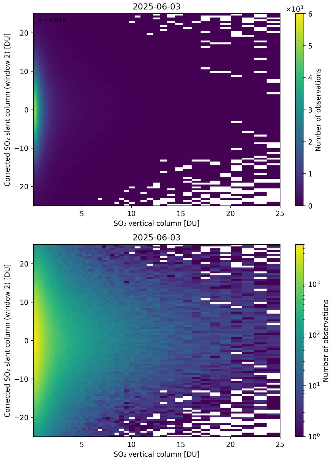
Figure 352: Scatter density plot of “SO 2 vertical column” against “Corrected SO 2 slant column (window 2)” for 2025-06-02 to 2025-06-04.
