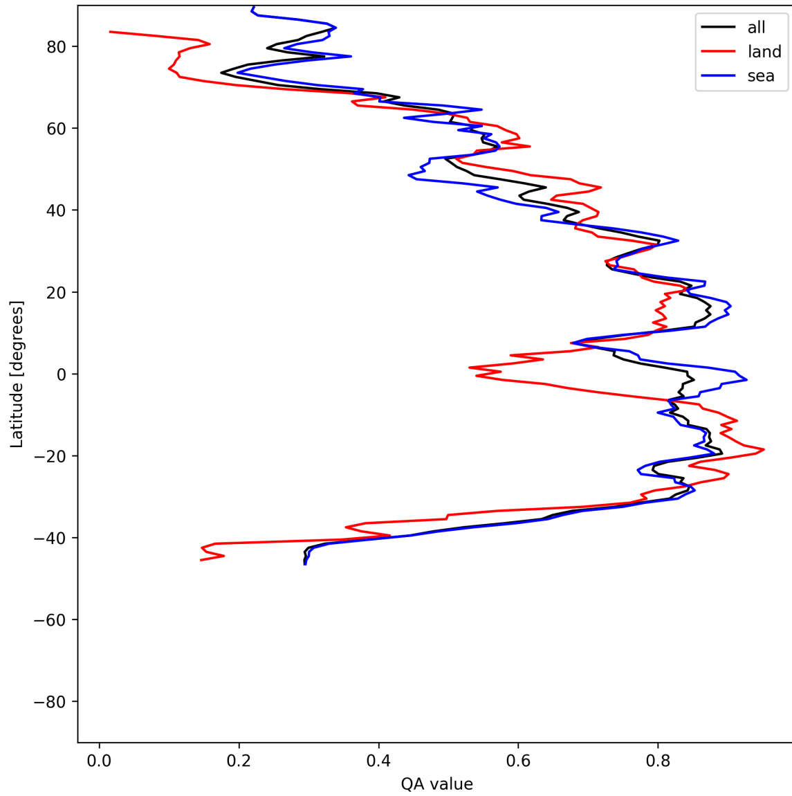
Figure 31: Zonal average of “QA value” for 2025-06-02 to 2025-06-04.
