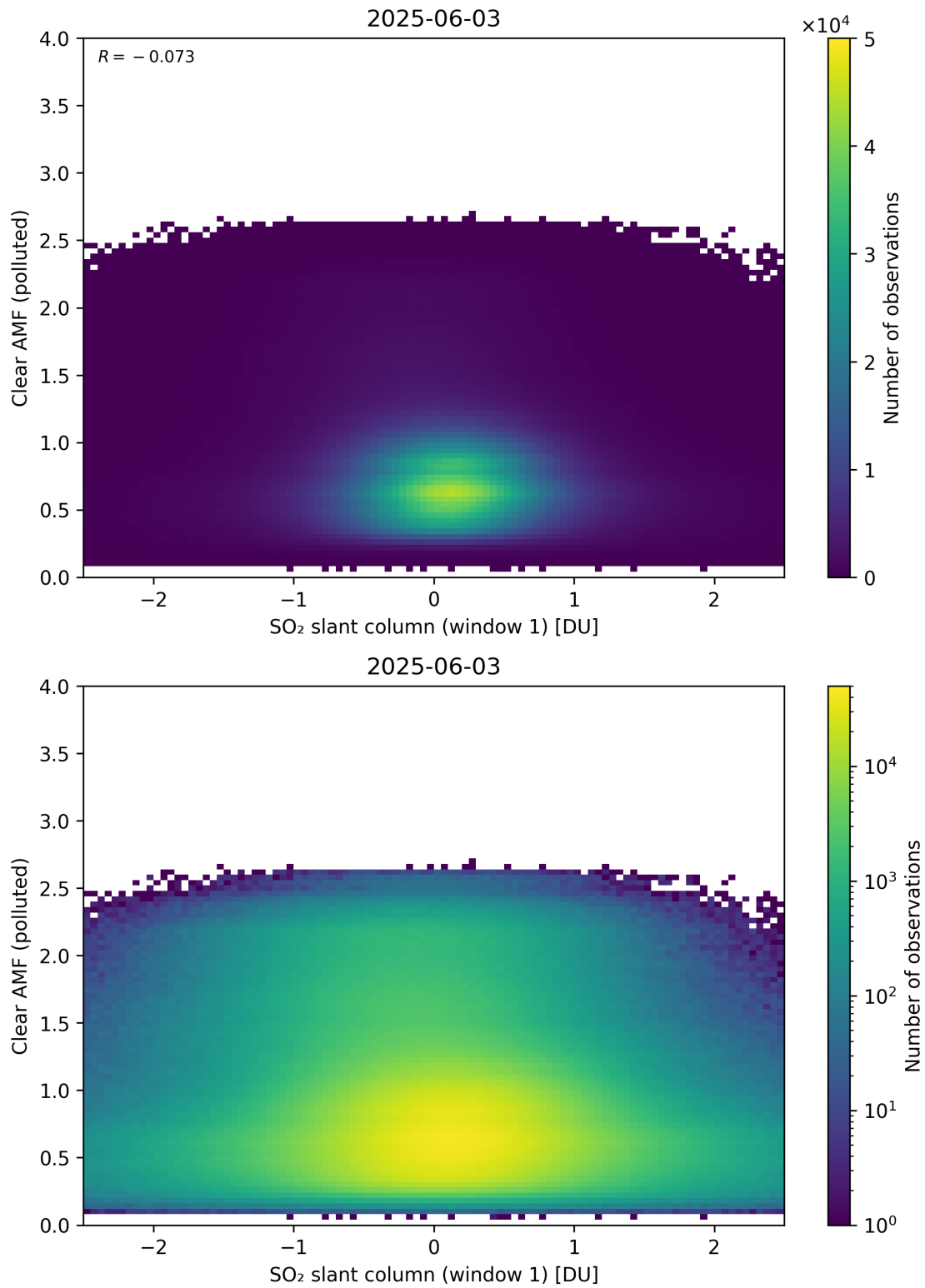
Figure 282: Scatter density plot of “SO 2 slant column (window 1)” against “Clear AMF (polluted)” for 2025-06-02 to 2025-06-04.
