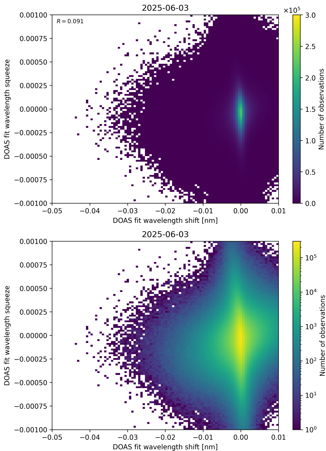
Figure 138: Scatter density plot of “DOAS fit wavelength shift” against “DOAS fit wavelength squeeze” for 2025-06-02 to 2025-06-04.
