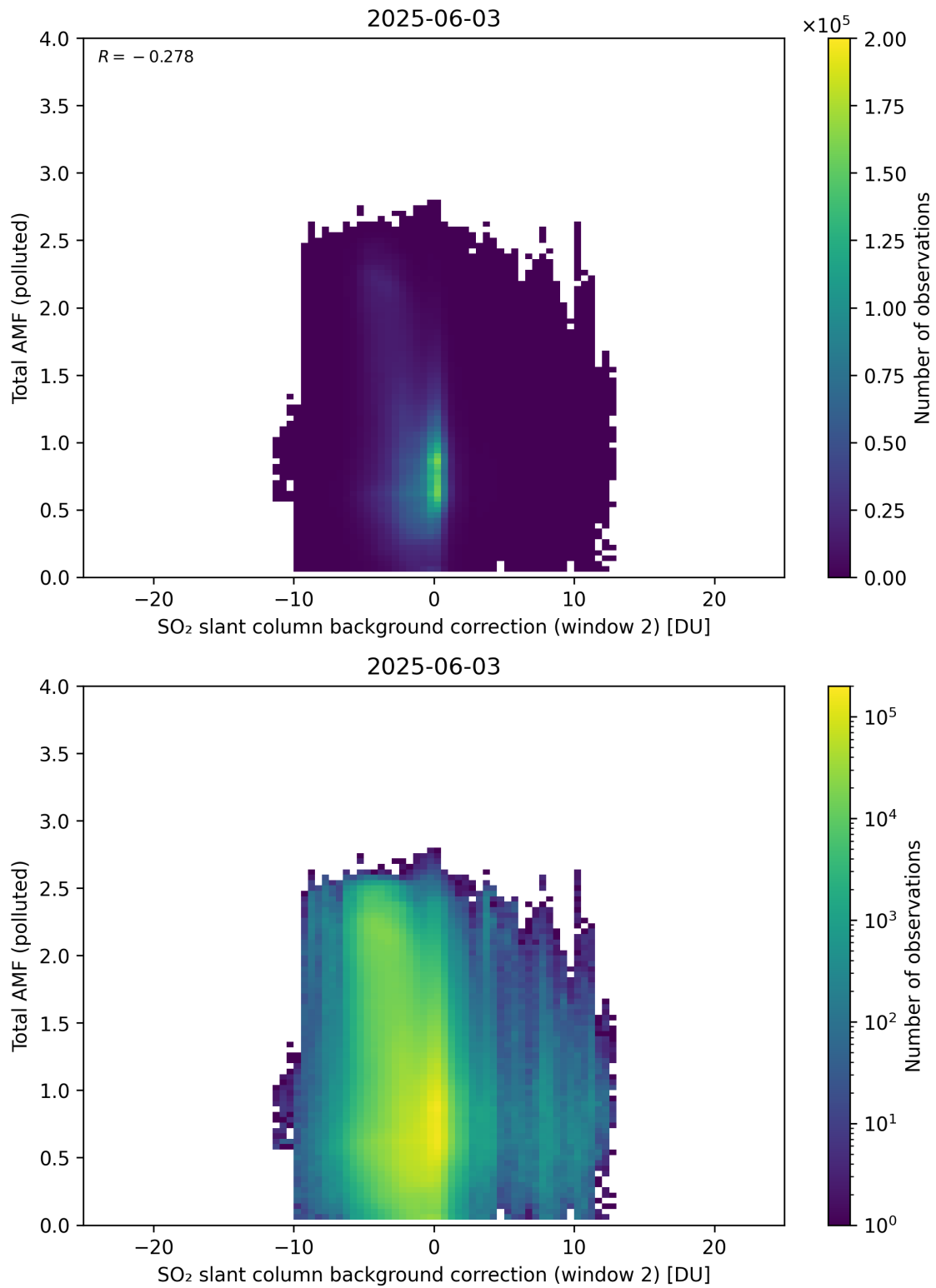
Figure 130: Scatter density plot of “SO 2 slant column background correction (window 2)” against “Total AMF (polluted)” for 2025-06-02 to 2025-06-04.
