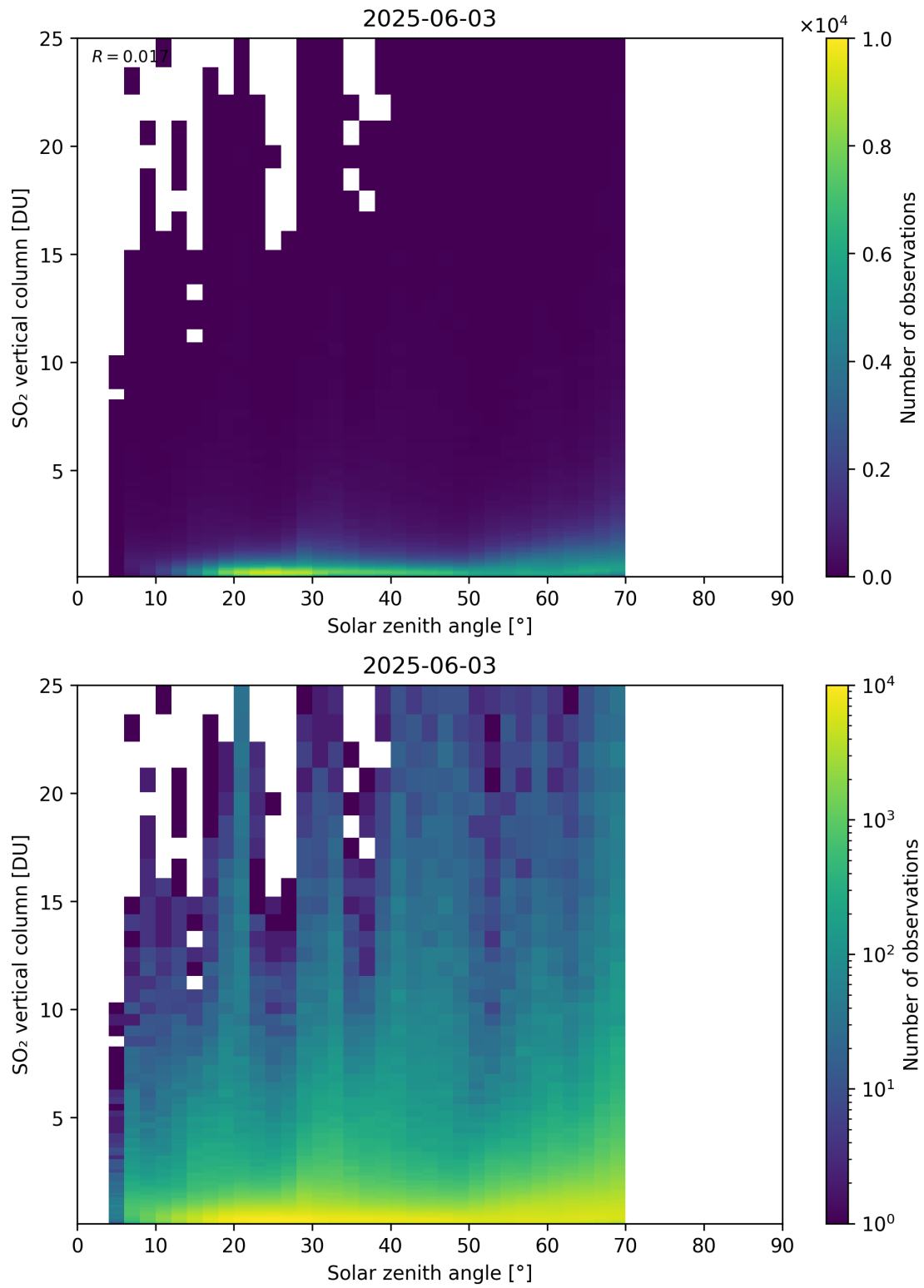
Figure 191: Scatter density plot of “Solar zenith angle” against “SO 2 vertical column” for 2025-06-02 to 2025-06-04.
