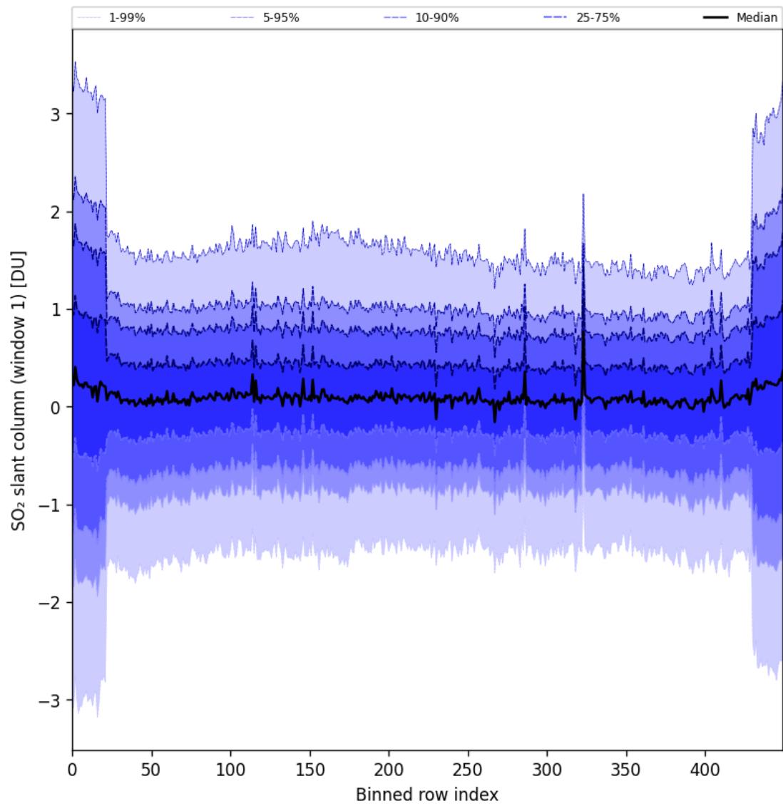
Figure 89: Along track statistics of “SO 2 slant column (window 1)” for 2025-06-02 to 2025-06-04
