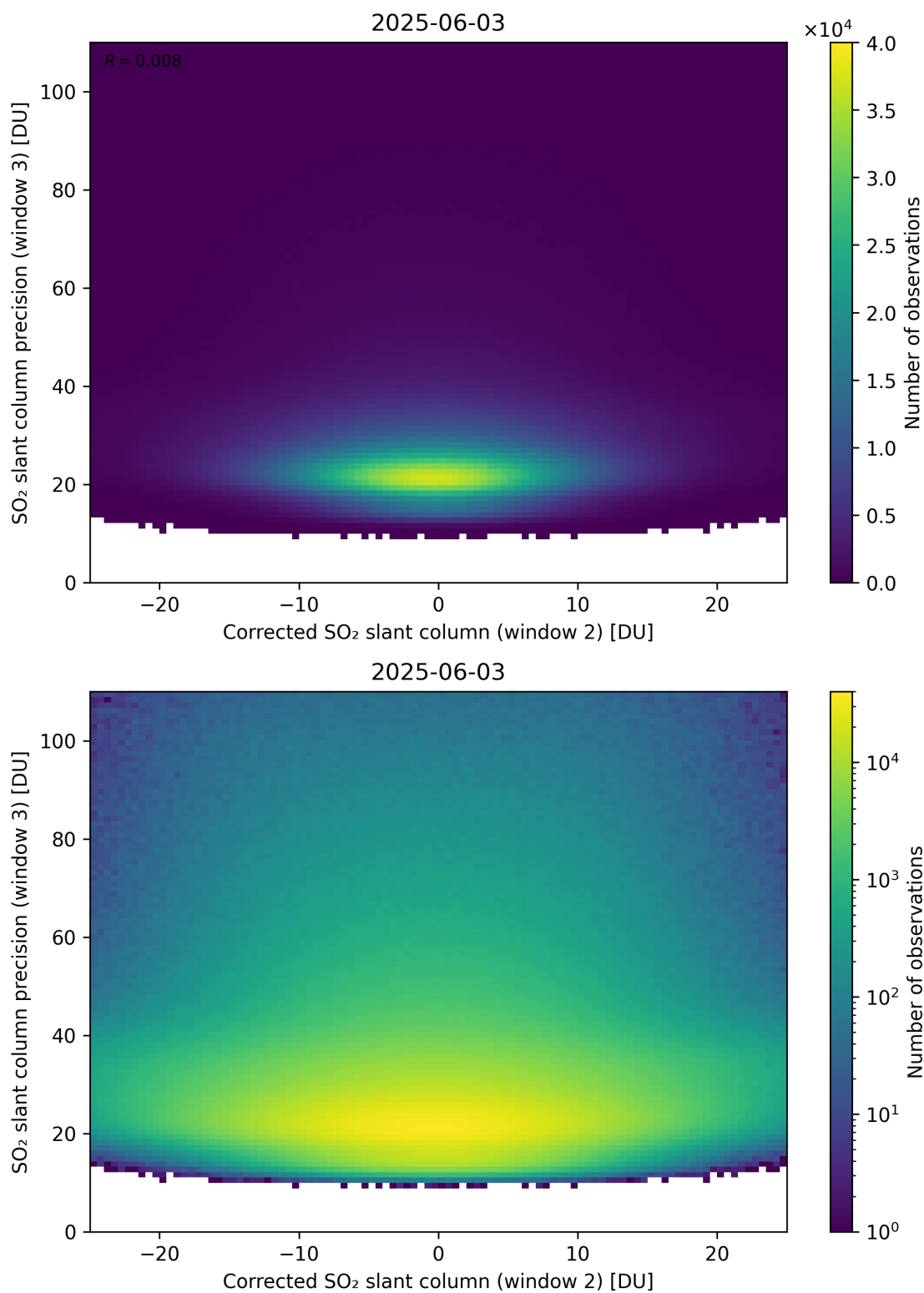
Figure 252: Scatter density plot of “Corrected SO 2 slant column (window 2)” against “SO 2 slant column precision (window 3)” for 2025-06-02 to 2025-06-04.
