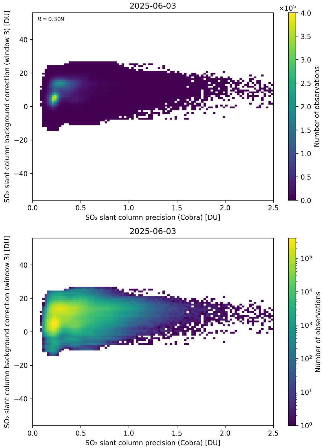
Figure 201: Scatter density plot of “SO 2 slant column precision (Cobra)” against “SO 2 slant column background correction (window 3)” for 2025-06-02 to 2025-06-04.
