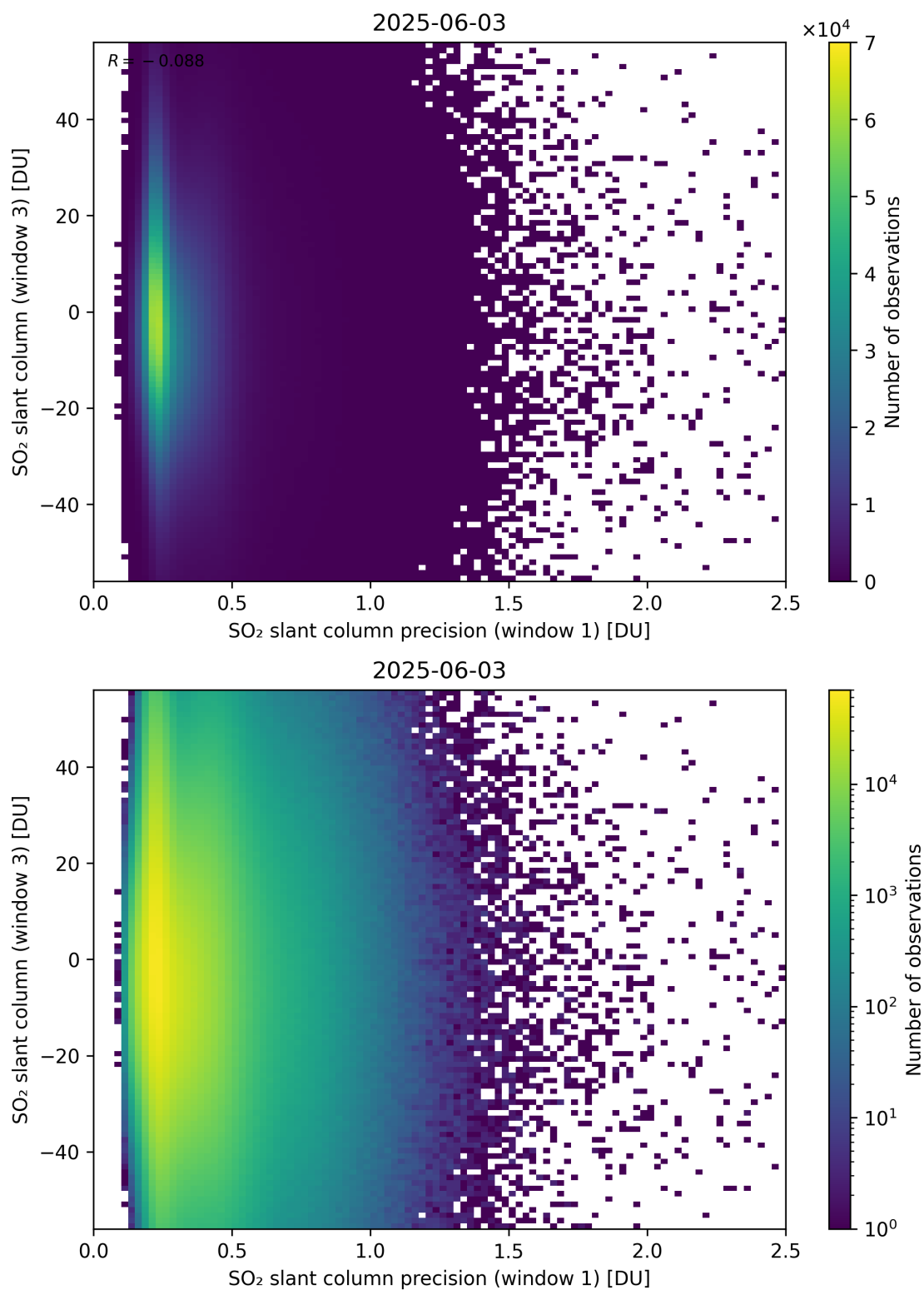
Figure 278: Scatter density plot of “SO 2 slant column precision (window 1)” against “SO 2 slant column (window 3)” for 2025-06-02 to 2025-06-04.
