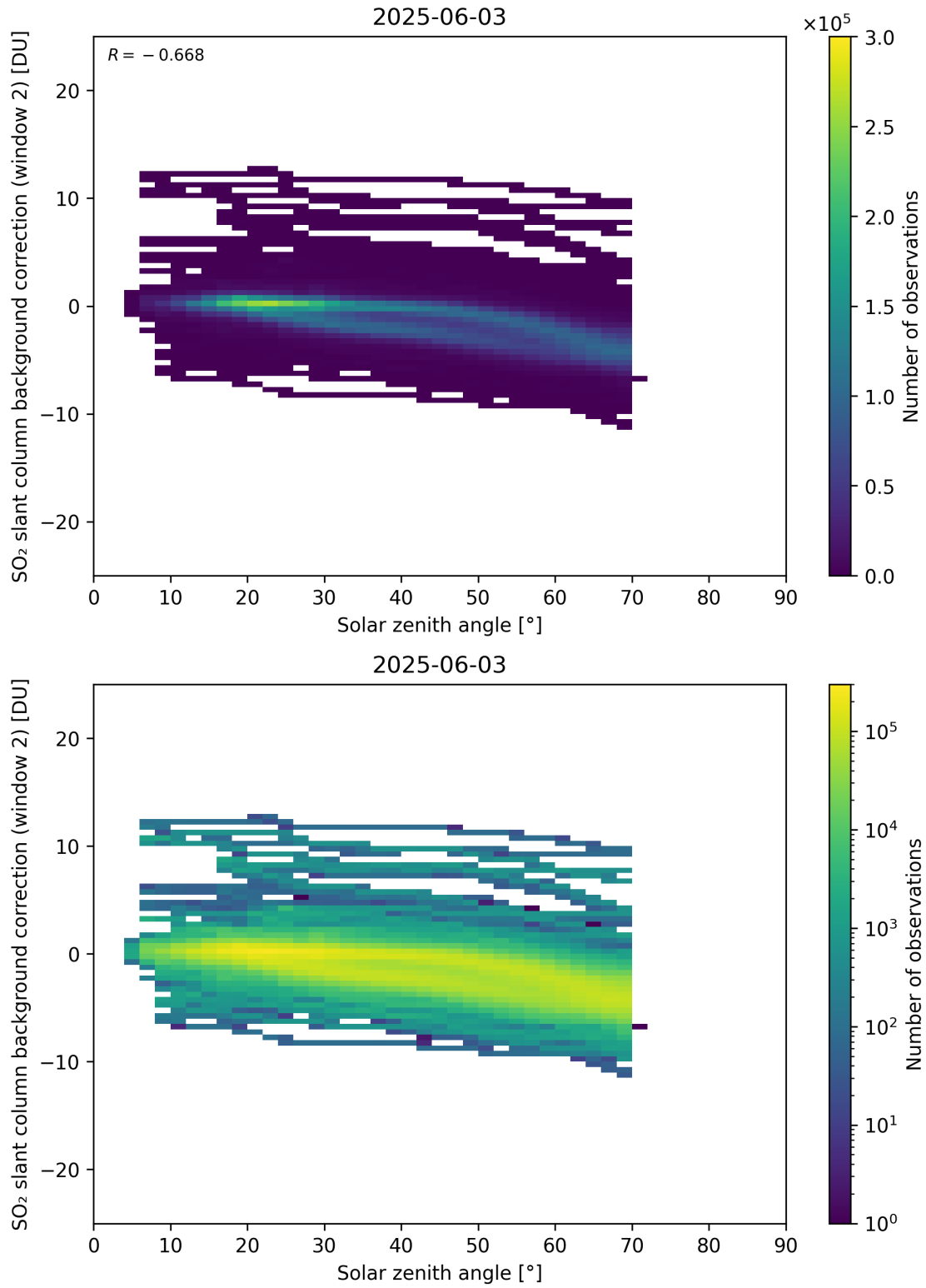
Figure 172: Scatter density plot of “Solar zenith angle” against “SO 2 slant column background correction (window 2)” for 2025-06-02 to 2025-06-04.
