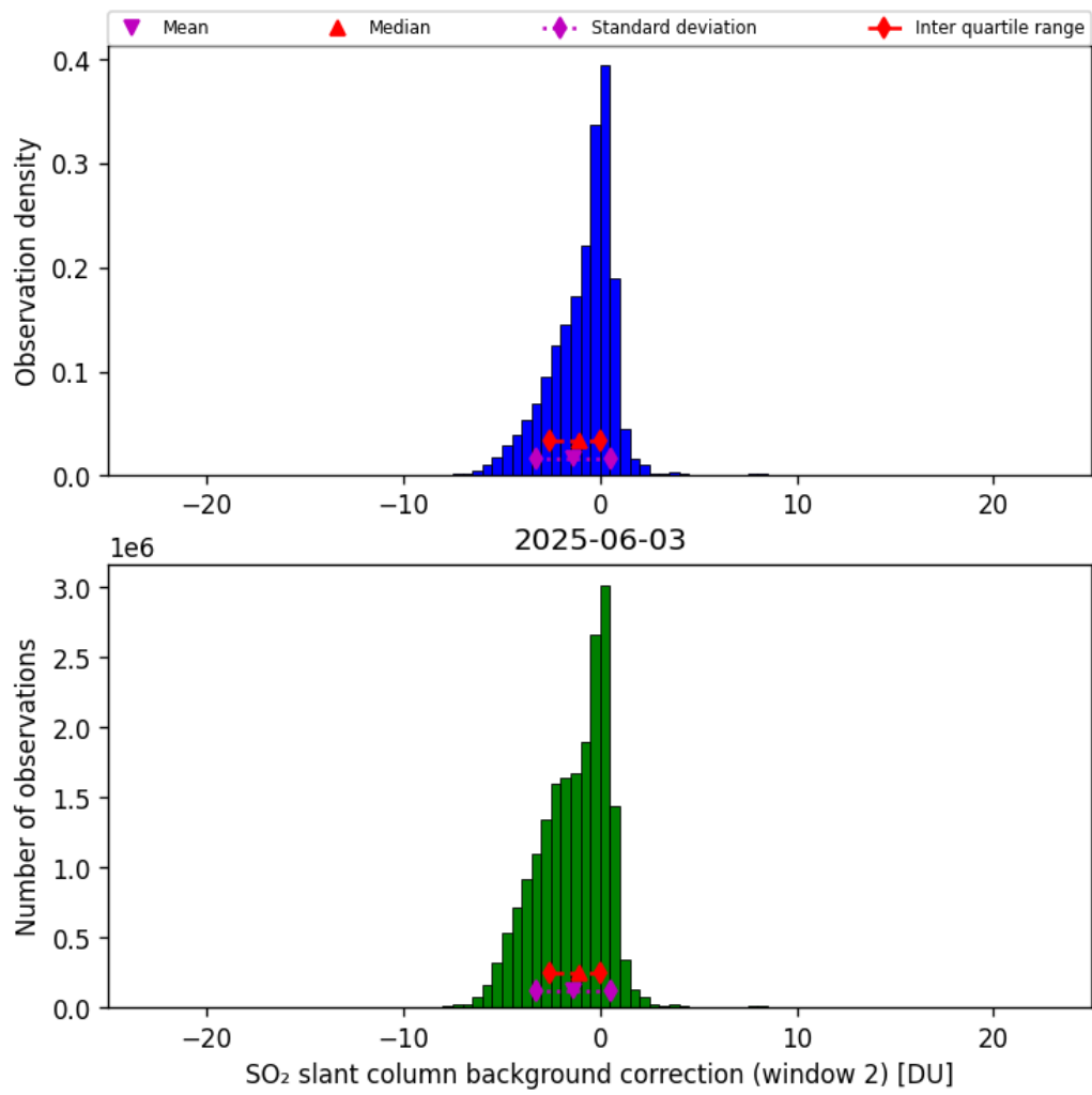
Figure 70: Histogram of “SO 2 slant column background correction (window 2)” for 2025-06-02 to 2025-06-04
