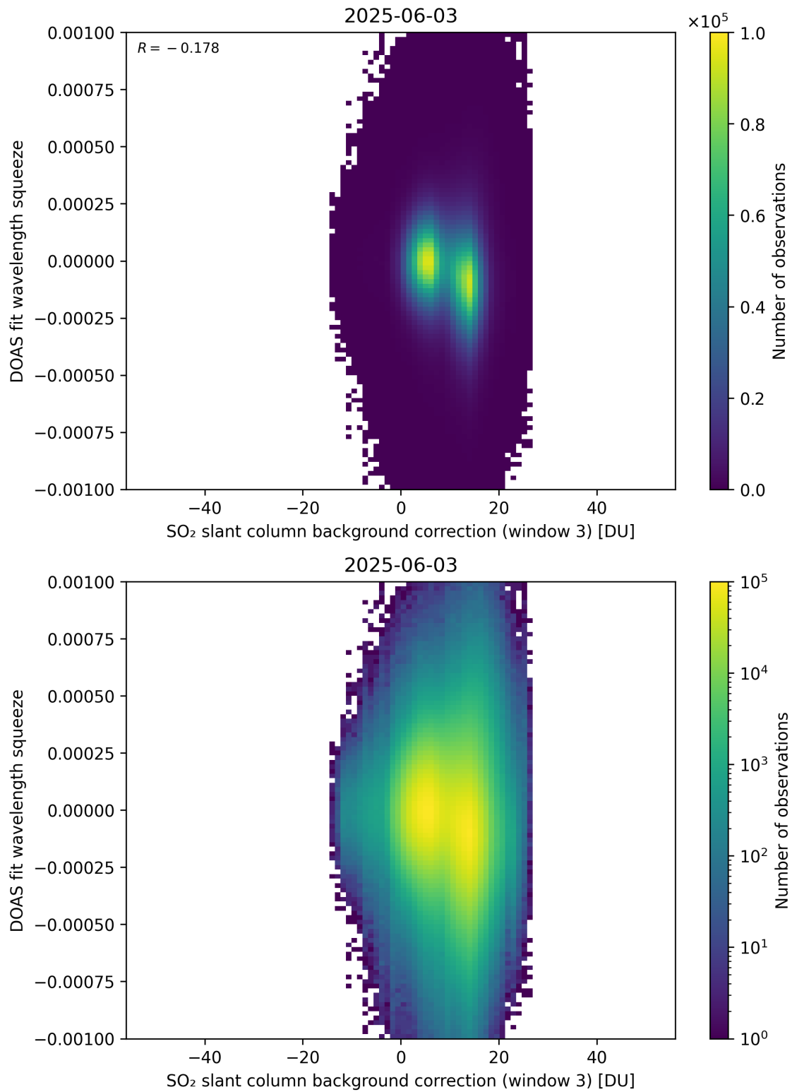
Figure 133: Scatter density plot of “SO 2 slant column background correction (window 3)” against “DOAS fit wavelength squeeze” for 2025-06-02 to 2025-06-04.
