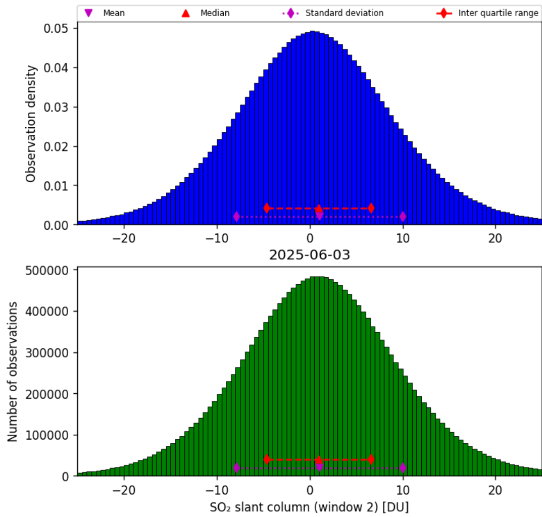
Figure 67: Histogram of “SO 2 slant column (window 2)” for 2025-06-02 to 2025-06-04
