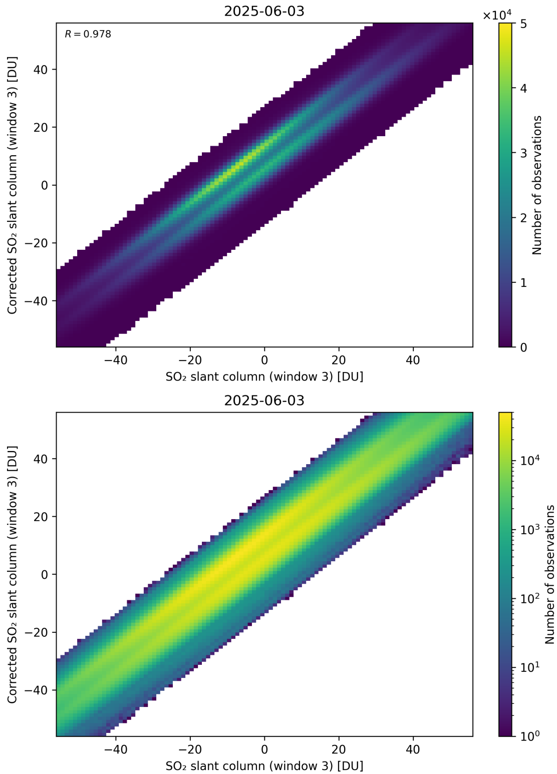
Figure 316: Scatter density plot of “SO 2 slant column (window 3)” against “Corrected SO 2 slant column (window 3)” for 2025-06-02 to 2025-06-04.
