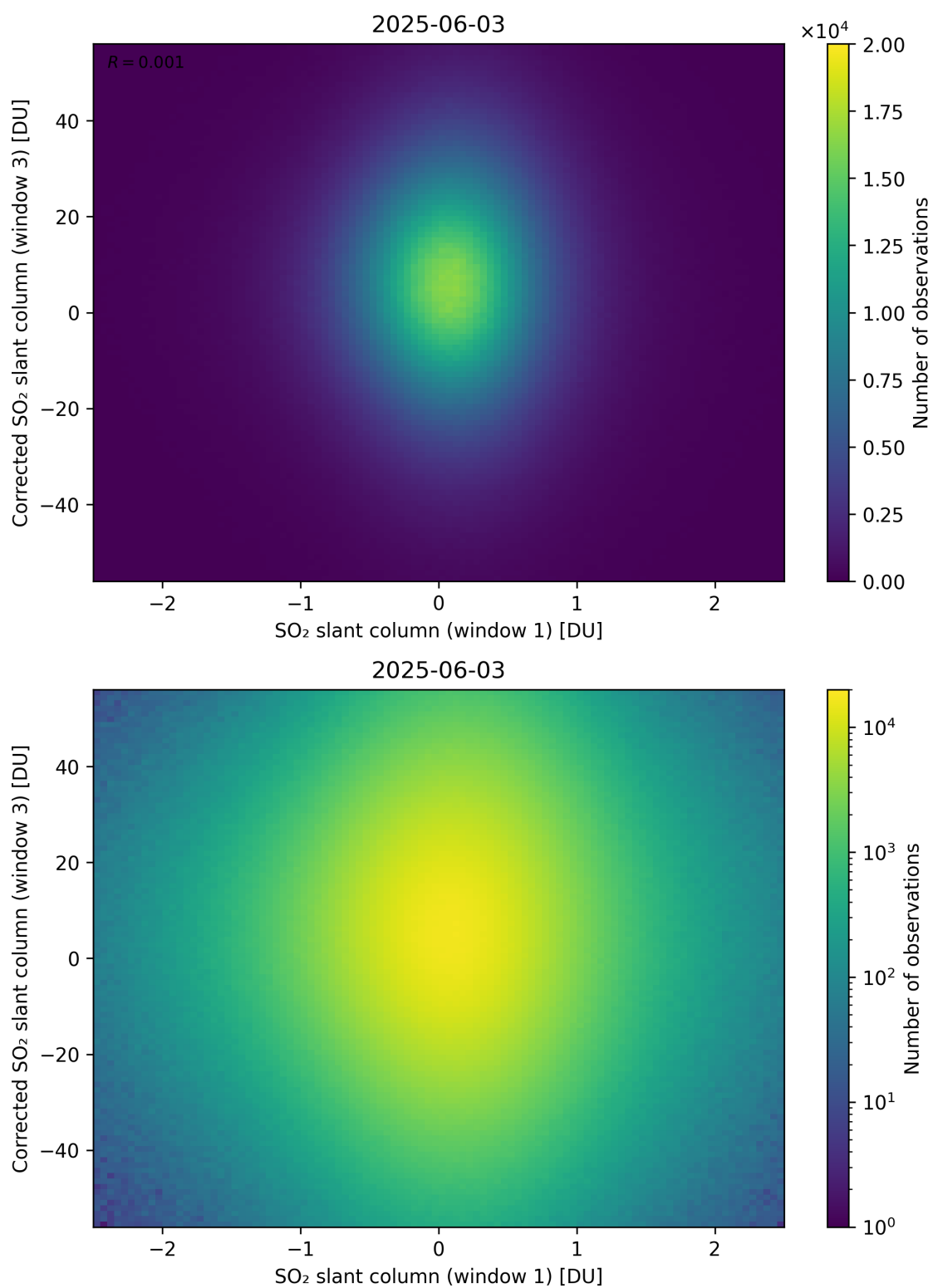
Figure 284: Scatter density plot of “SO 2 slant column (window 1)” against “Corrected SO 2 slant column (window 3)” for 2025-06-02 to 2025-06-04.
