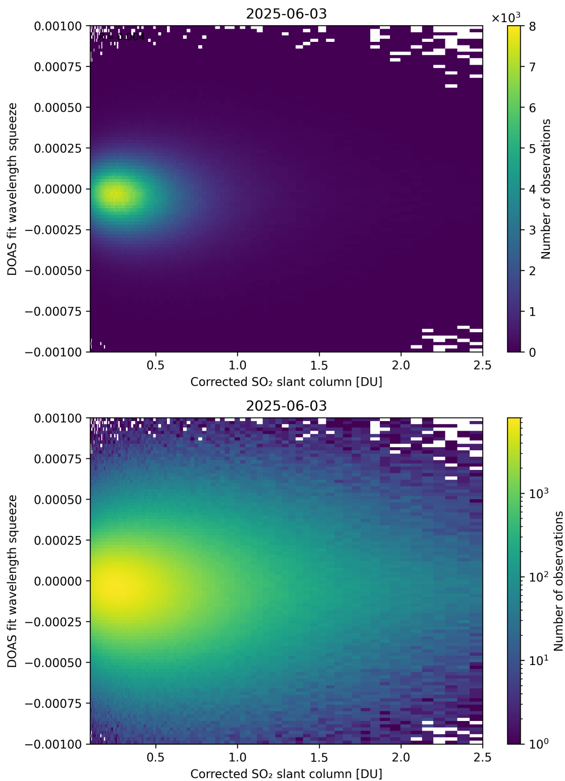
Figure 230: Scatter density plot of “Corrected SO 2 slant column” against “DOAS fit wavelength squeeze” for 2025-06-02 to 2025-06-04.
