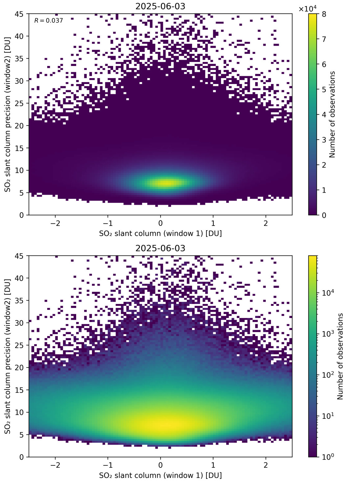
Figure 286: Scatter density plot of “SO 2 slant column (window 1)” against “SO 2 slant column precision (window2)” for 2025-06-02 to 2025-06-04.
