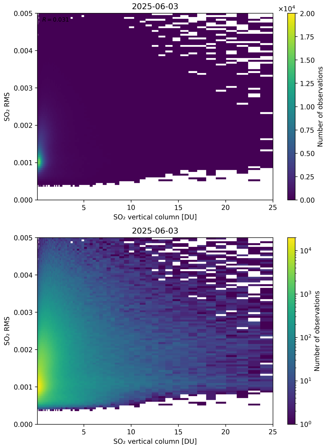
Figure 328: Scatter density plot of “SO 2 vertical column” against “SO 2 RMS” for 2025-06-02 to 2025-06-04.
