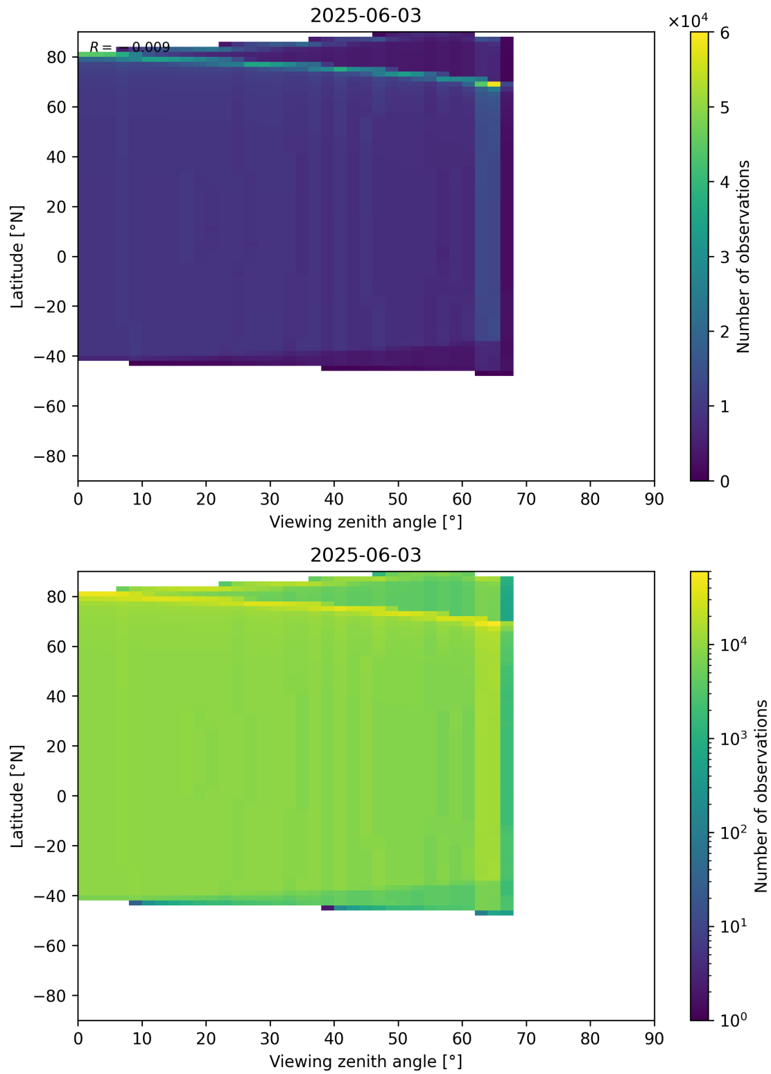
Figure 368: Scatter density plot of “Viewing zenith angle” against “Latitude” for 2025-06-02 to 2025-06-04.
