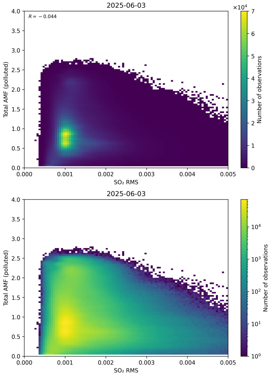
Figure 148: Scatter density plot of “SO 2 RMS” against “Total AMF (polluted)” for 2025-06-02 to 2025-06-04.
