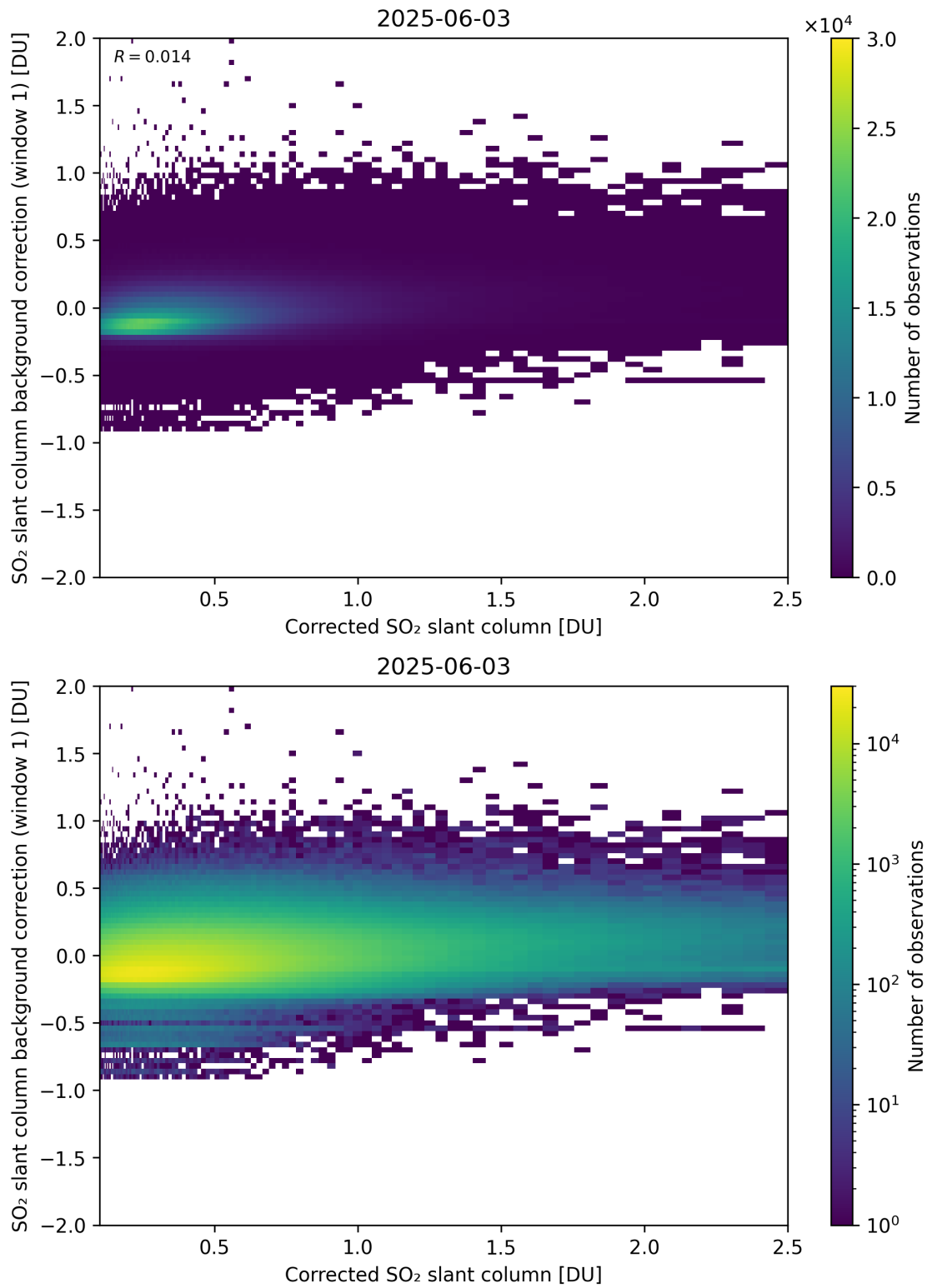
Figure 226: Scatter density plot of “Corrected SO 2 slant column” against “SO 2 slant column background correction (window 1)” for 2025-06-02 to 2025-06-04.
