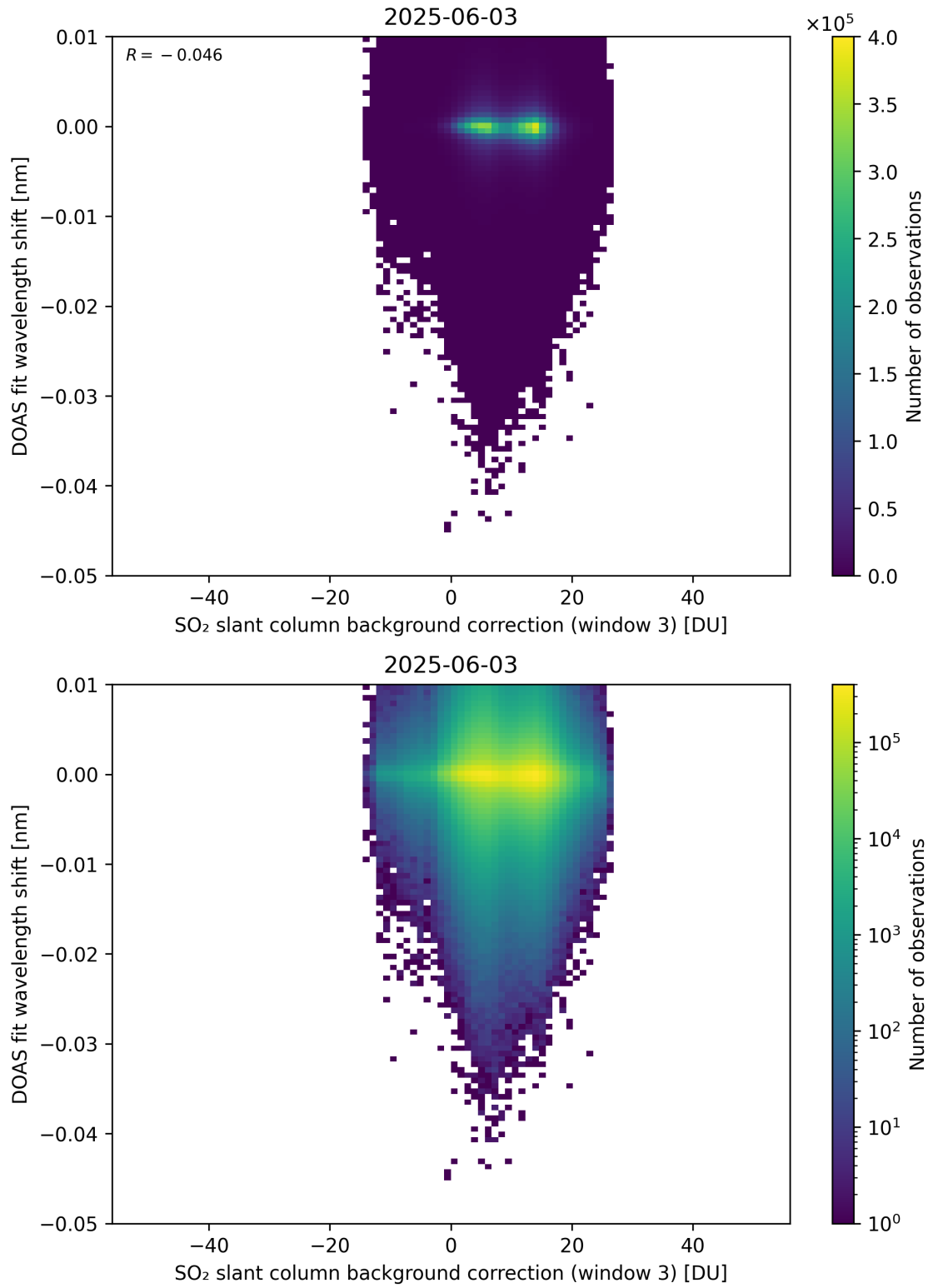
Figure 132: Scatter density plot of “SO 2 slant column background correction (window 3)” against “DOAS fit wavelength shift” for 2025-06-02 to 2025-06-04.
