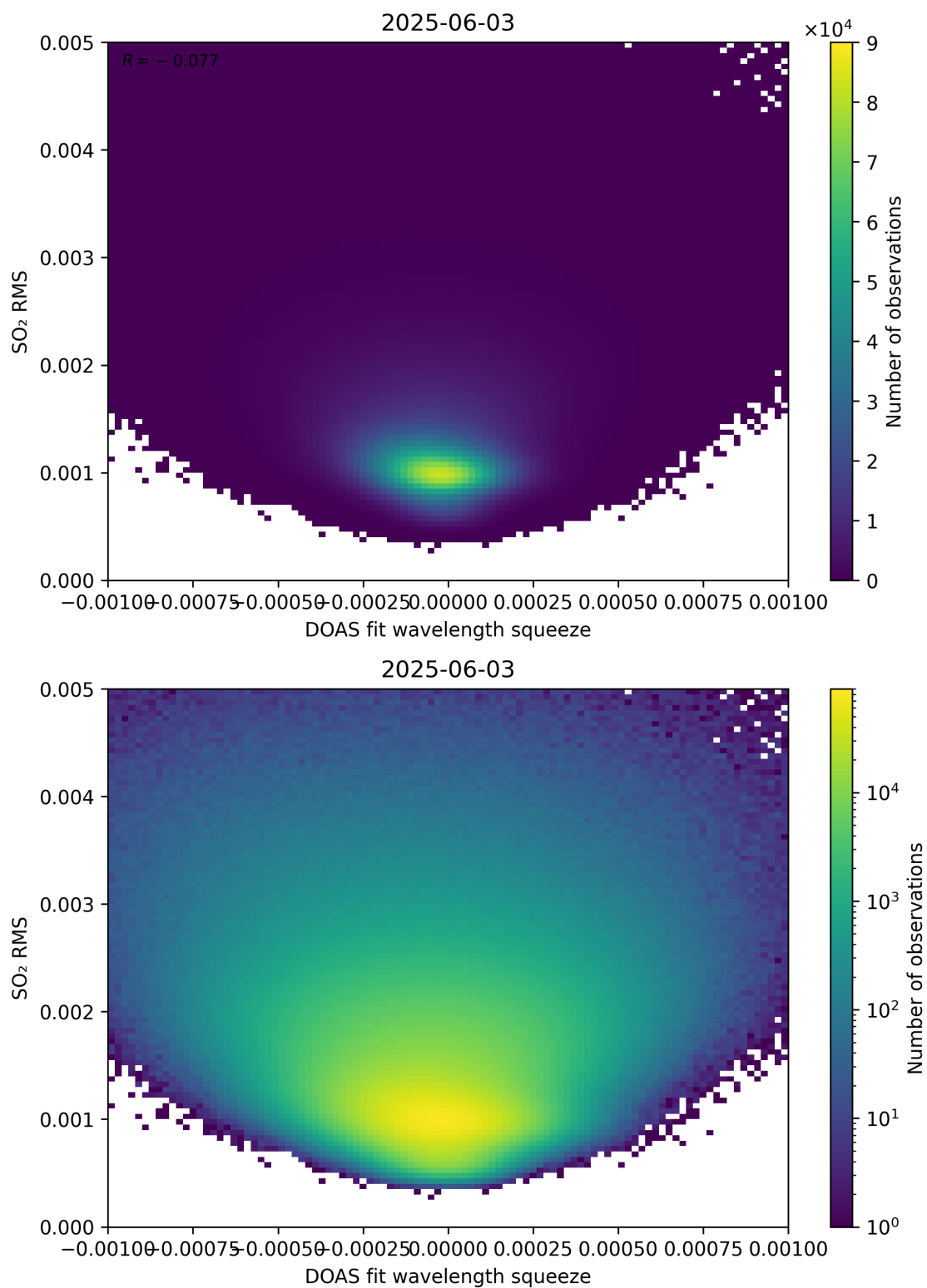
Figure 143: Scatter density plot of “DOAS fit wavelength squeeze” against “SO 2 RMS” for 2025-06-02 to 2025-06-04.
