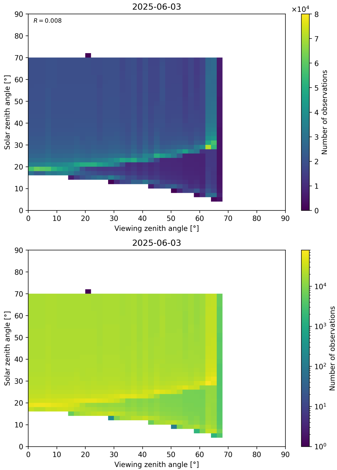
Figure 369: Scatter density plot of “Viewing zenith angle” against “Solar zenith angle” for 2025-06-02 to 2025-06-04.
