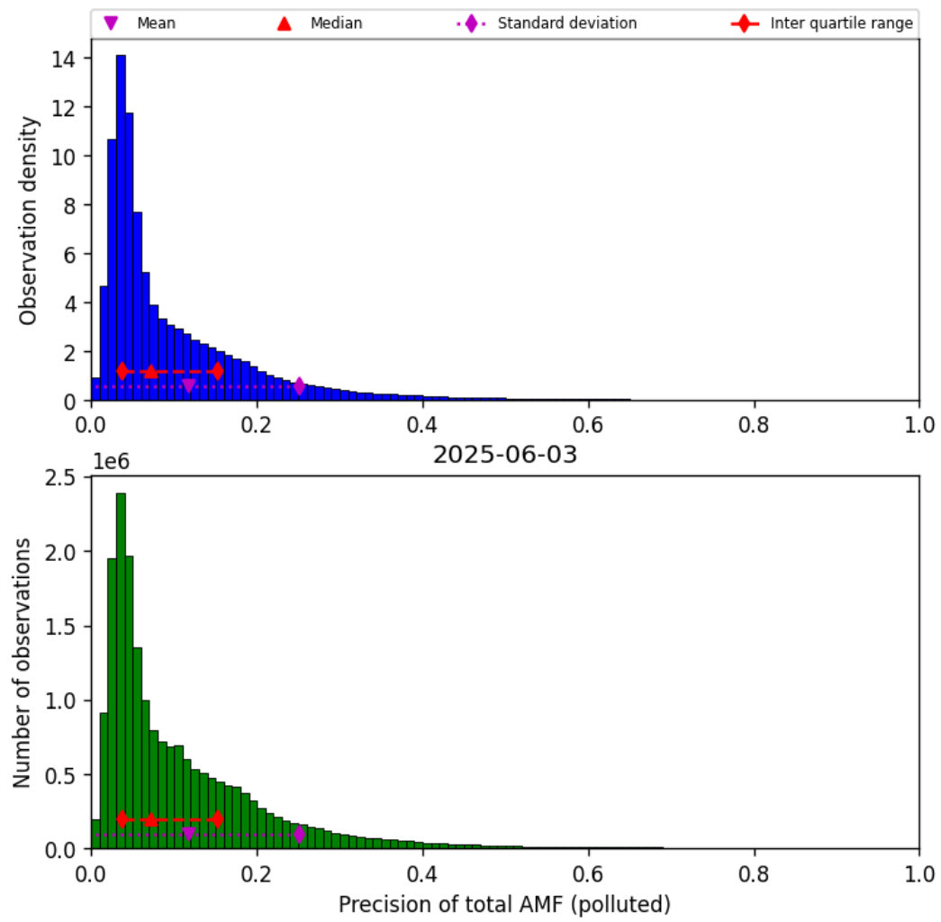
Figure 80: Histogram of “Precision of total AMF (polluted)” for 2025-06-02 to 2025-06-04
