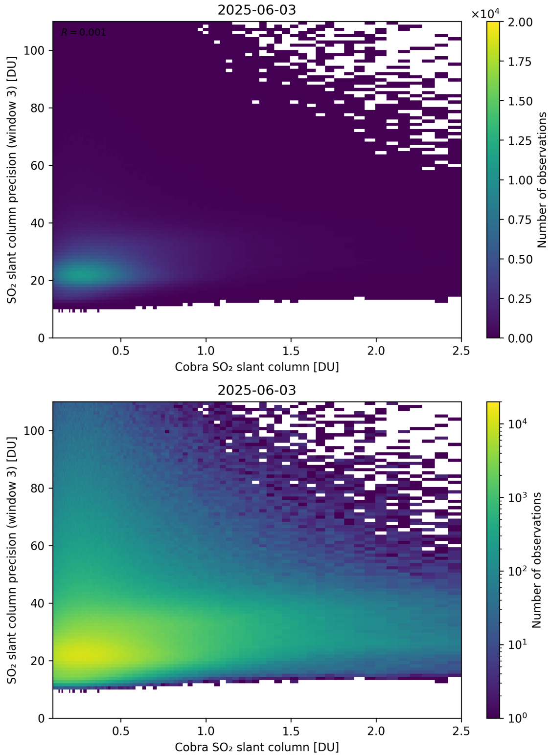
Figure 223: Scatter density plot of “Cobra SO 2 slant column” against “SO 2 slant column precision (window 3)” for 2025-06-02 to 2025-06-04.
