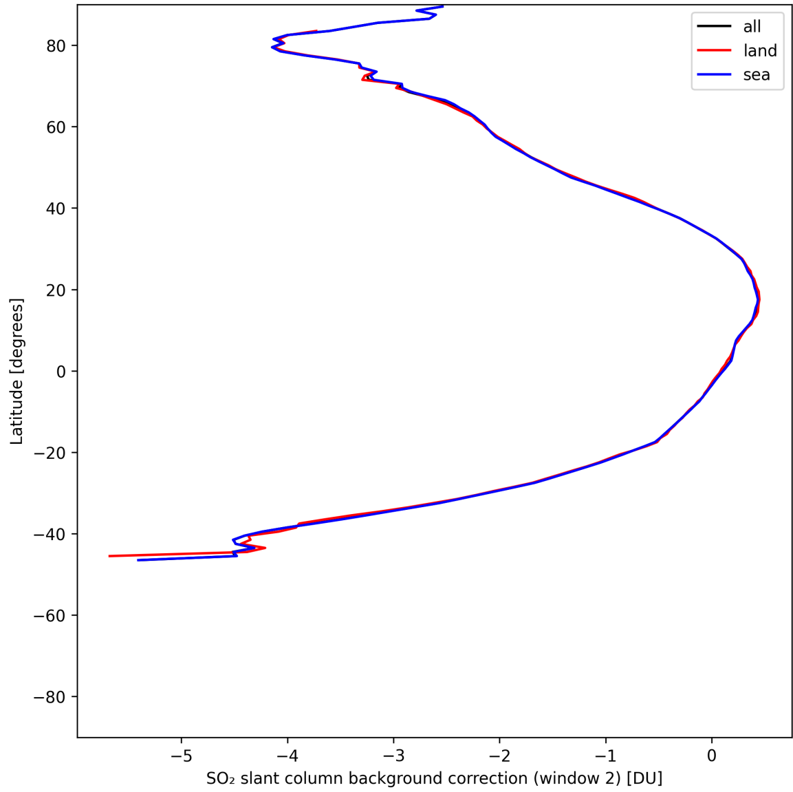
Figure 44: Zonal average of "SO 2 slant column background correction (window 2)" for 2025-06-02 to 2025-06-04.
