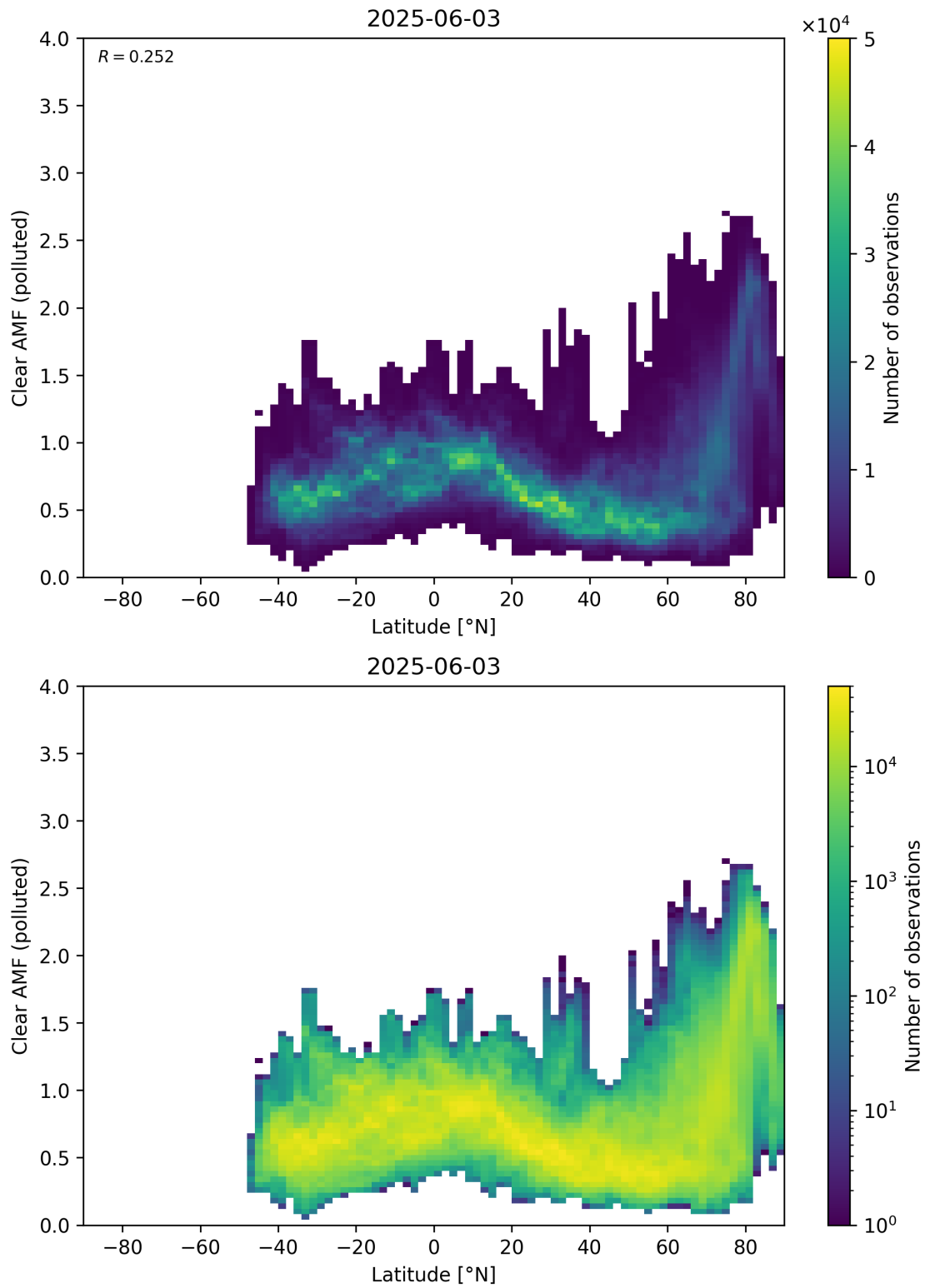
Figure 156: Scatter density plot of “Latitude” against “Clear AMF (polluted)” for 2025-06-02 to 2025-06-04.
