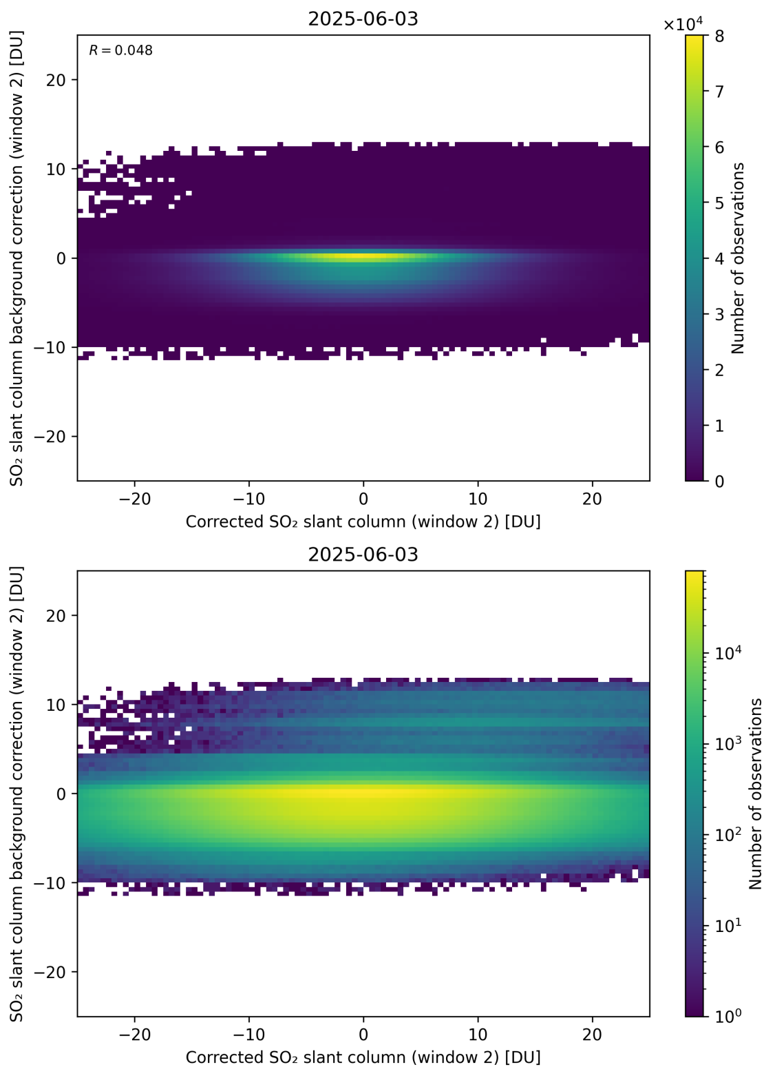
Figure 244: Scatter density plot of “Corrected SO 2 slant column (window 2)” against “SO 2 slant column background correction (window 2)” for 2025-06-02 to 2025-06-04.
