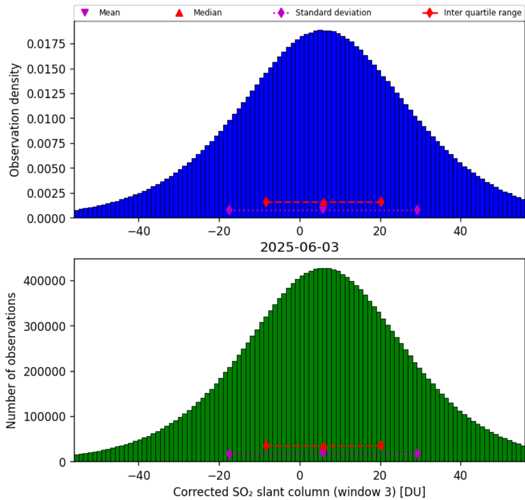
Figure 73: Histogram of “Corrected SO 2 slant column (window 3)” for 2025-06-02 to 2025-06-04
