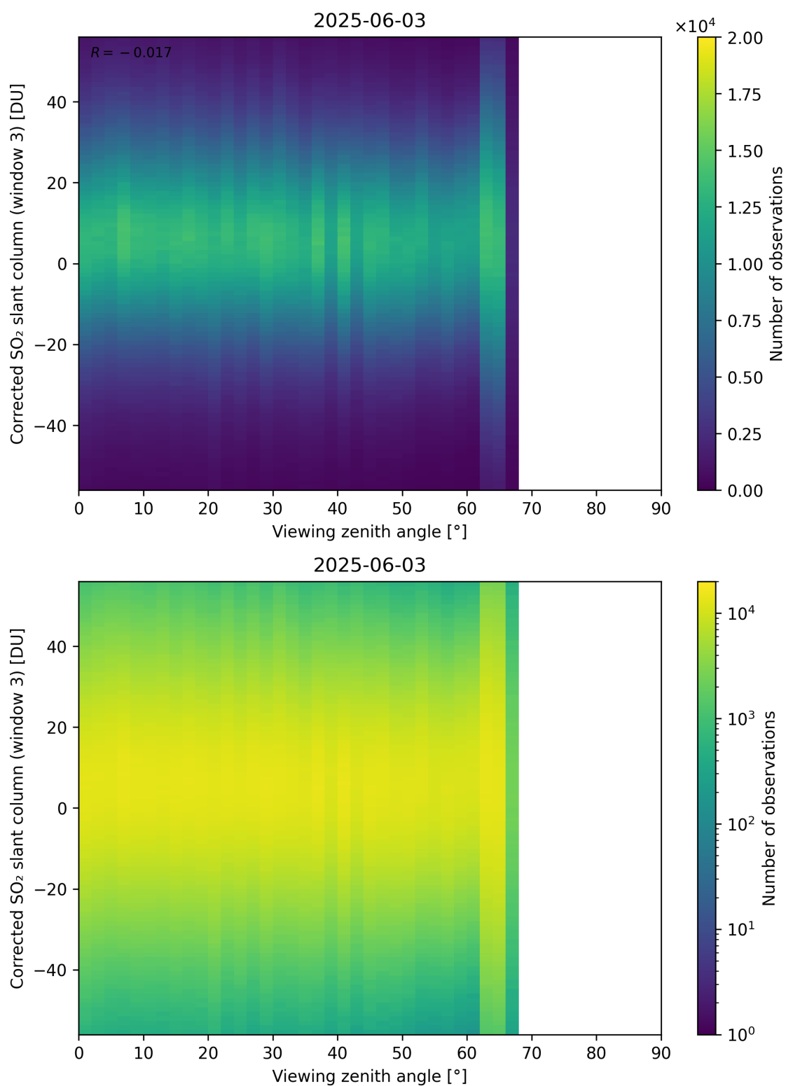
Figure 375: Scatter density plot of “Viewing zenith angle” against “Corrected SO 2 slant column (window 3)” for 2025-06-02 to 2025-06-04.
