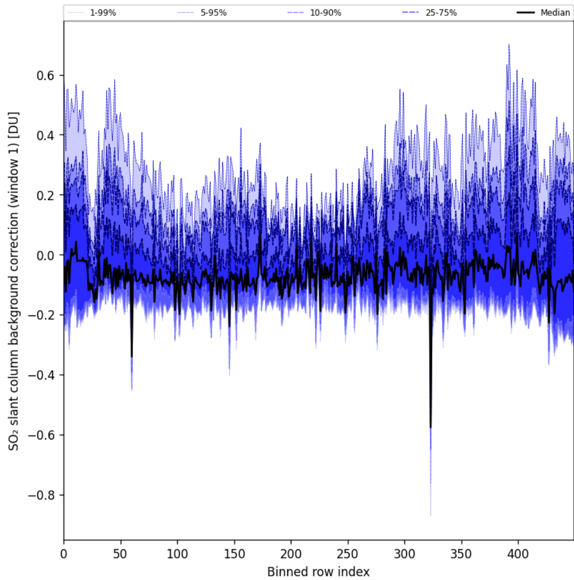
Figure 92: Along track statistics of “SO 2 slant column background correction (window 1)” for 2025-06-02 to 2025-06-04
