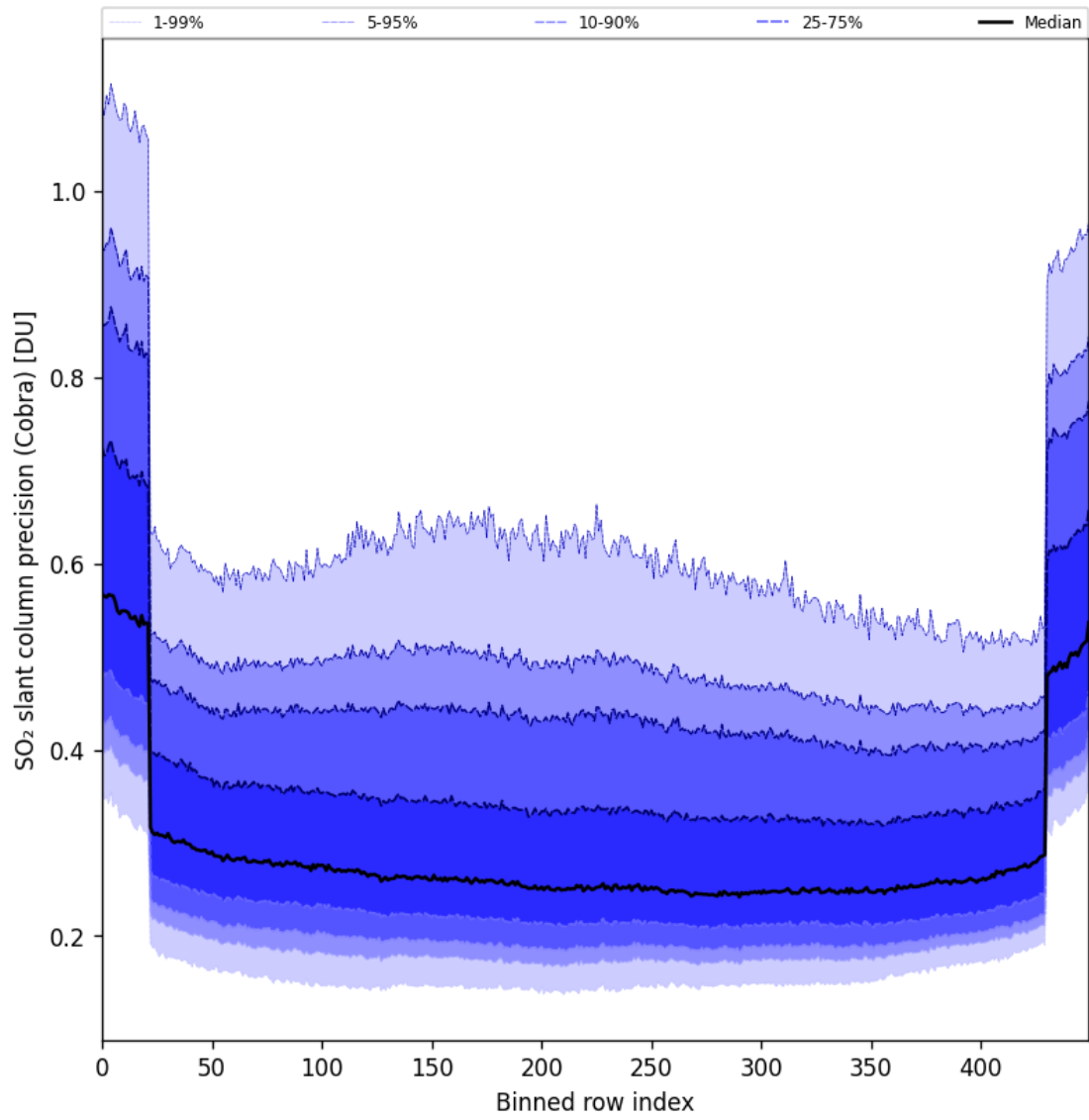
Figure 88: Along track statistics of “SO 2 slant column precision (Cobra)” for 2025-06-02 to 2025-06-04
