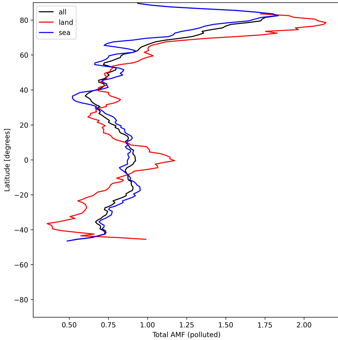
Figure 53: Zonal average of “Total AMF (polluted)” for 2025-06-02 to 2025-06-04.
