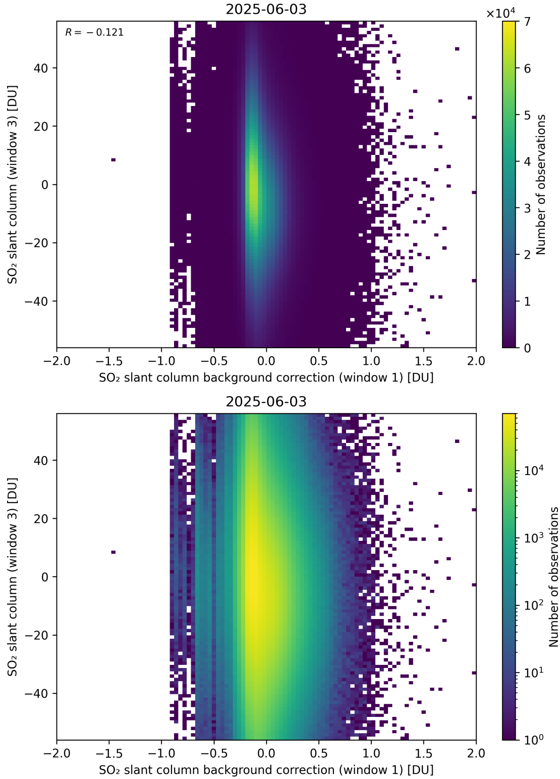
Figure 118: Scatter density plot of “SO 2 slant column background correction (window 1)” against “SO 2 slant column (window 3)” for 2025-06-02 to 2025-06-04.
