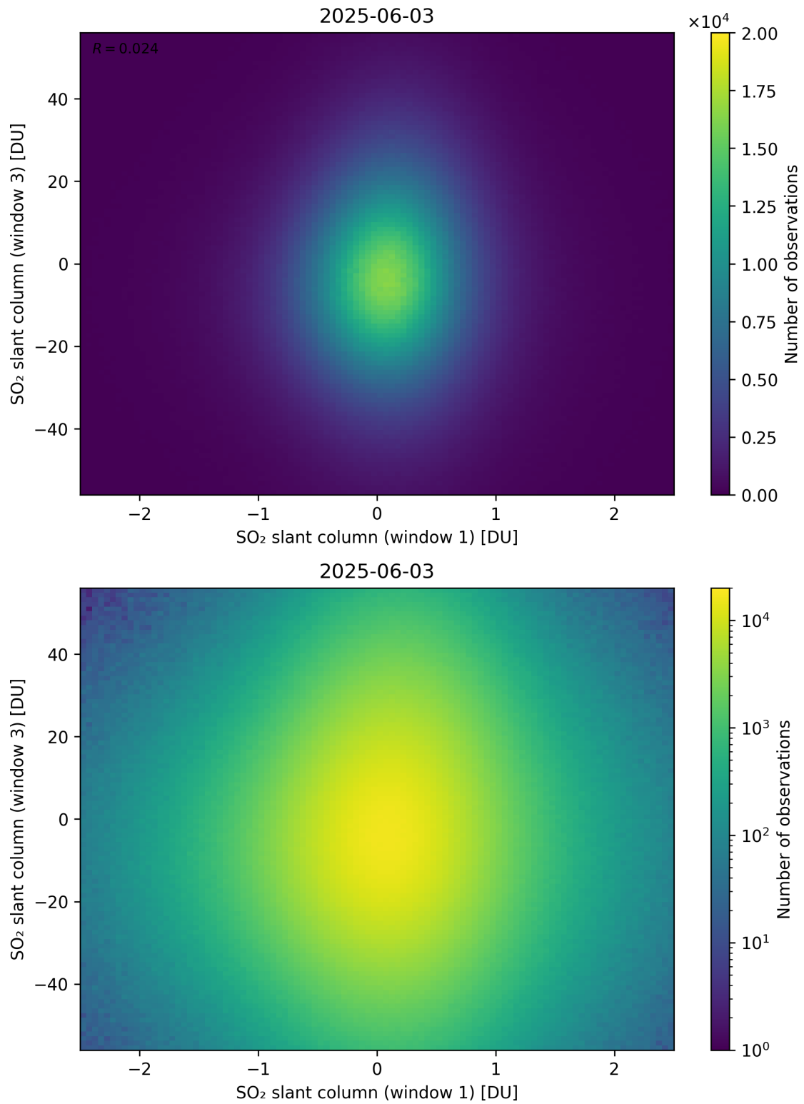
Figure 287: Scatter density plot of “SO 2 slant column (window 1)” against “SO 2 slant column (window 3)” for 2025-06-02 to 2025-06-04.
