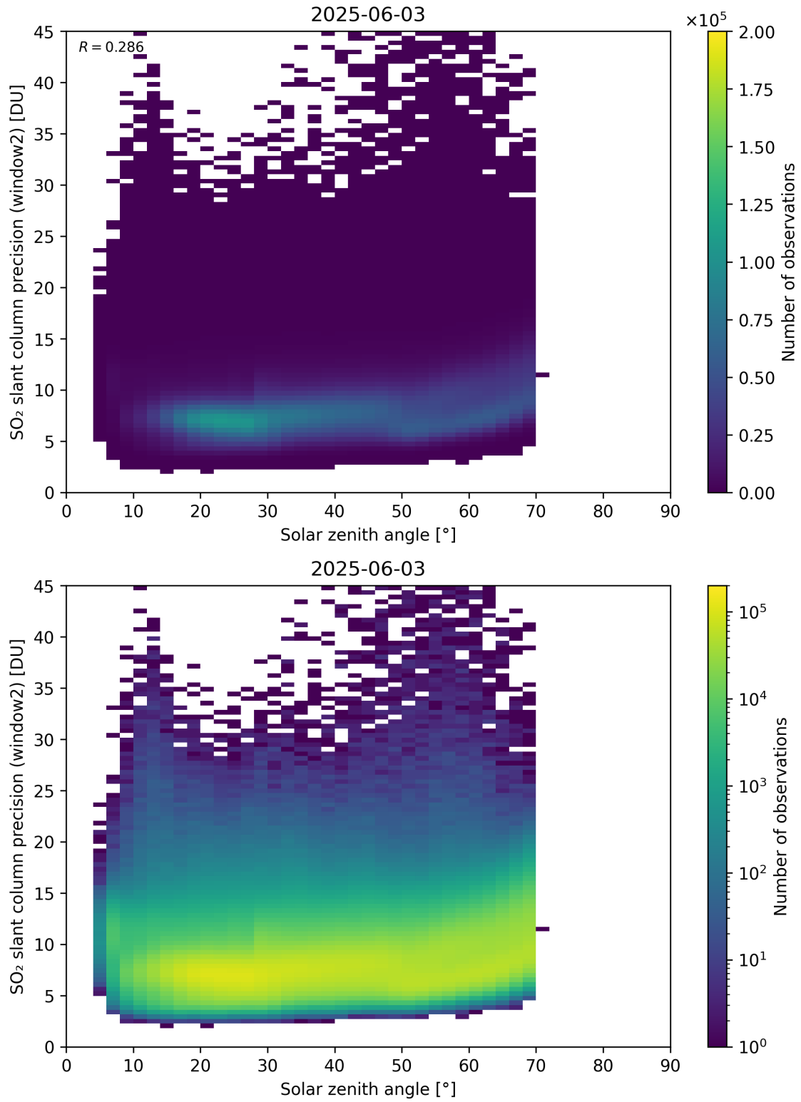
Figure 186: Scatter density plot of “Solar zenith angle” against “SO 2 slant column precision (window2)” for 2025-06-02 to 2025-06-04.
