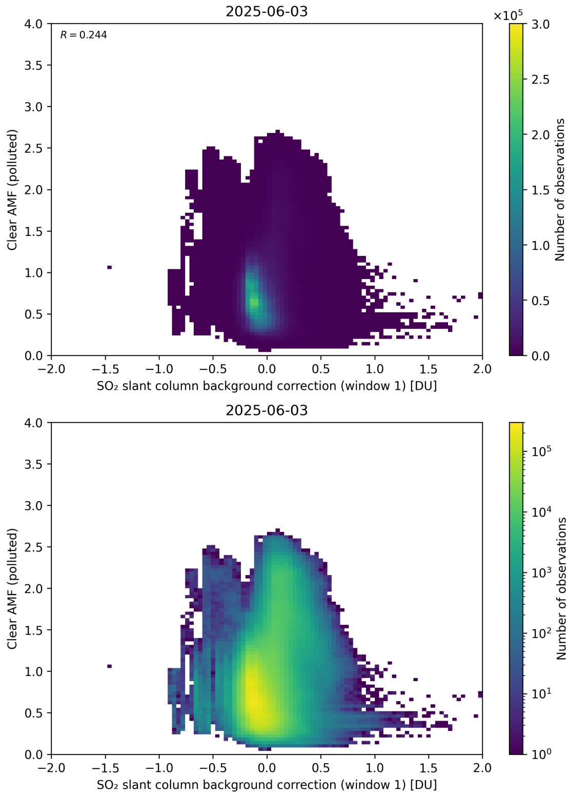
Figure 114: Scatter density plot of “SO 2 slant column background correction (window 1)” against “Clear AMF (polluted)” for 2025-06-02 to 2025-06-04.
