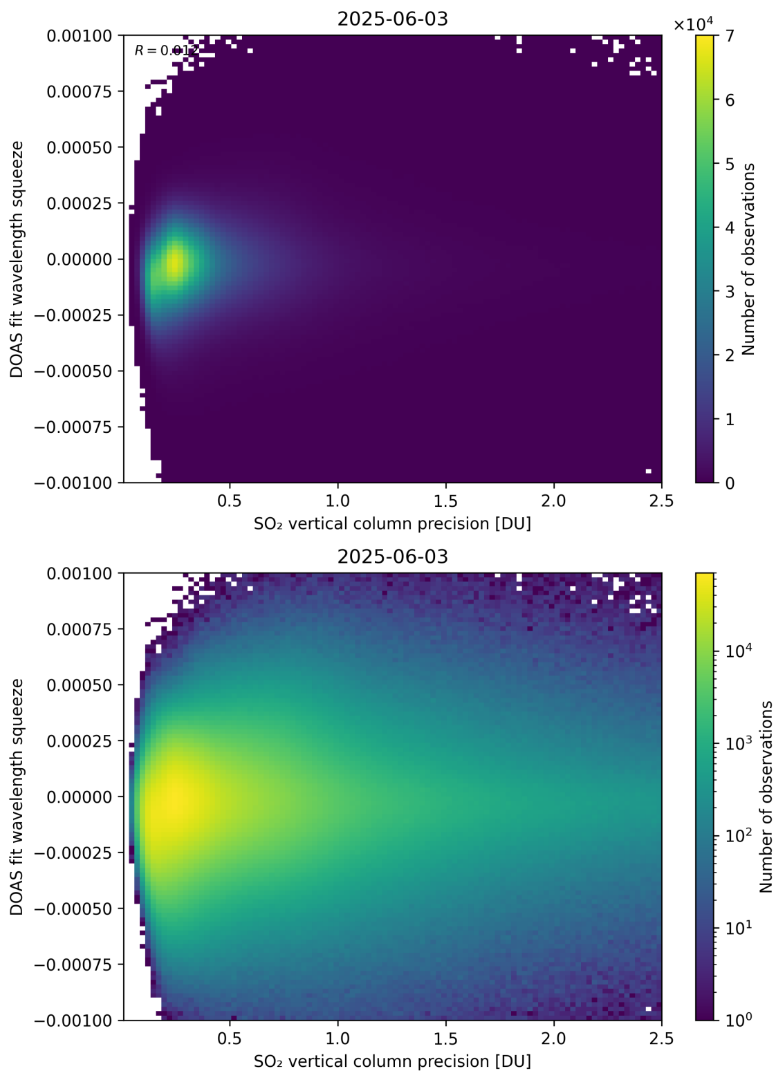
Figure 333: Scatter density plot of “SO 2 vertical column precision” against “DOAS fit wavelength squeeze” for 2025-06-02 to 2025-06-04.
