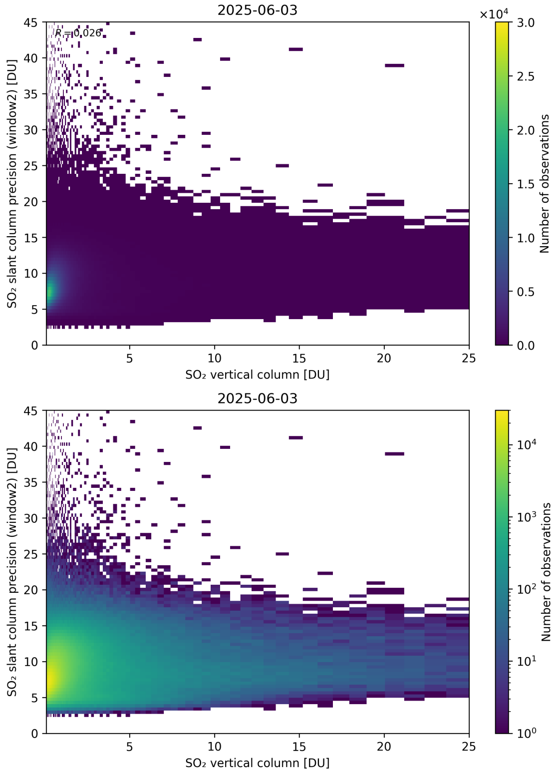
Figure 356: Scatter density plot of “SO 2 vertical column” against “SO 2 slant column precision (window2)” for 2025-06-02 to 2025-06-04.
