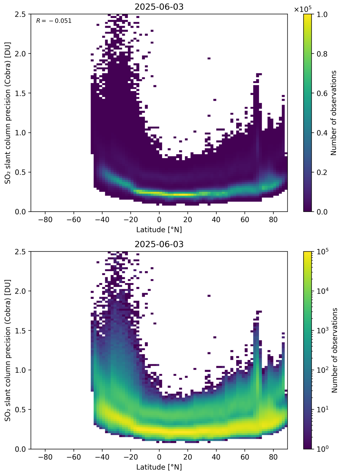
Figure 158: Scatter density plot of “Latitude” against “SO 2 slant column precision (Cobra)” for 2025-06-02 to 2025-06-04.
