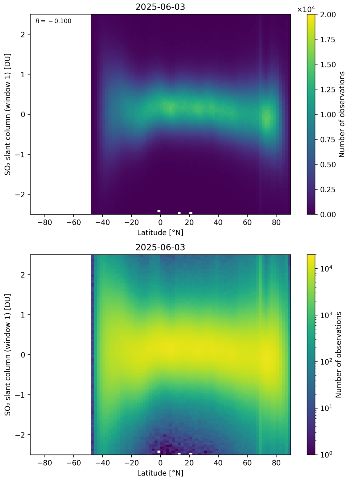
Figure 162: Scatter density plot of “Latitude” against “SO 2 slant column (window 1)” for 2025-06-02 to 2025-06-04.
