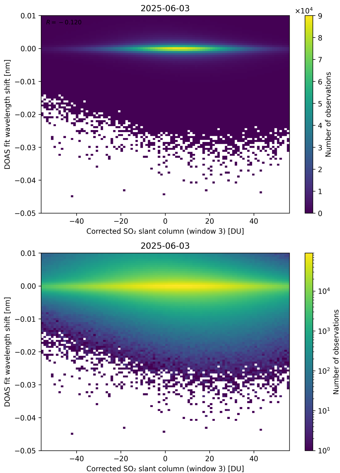
Figure 256: Scatter density plot of “Corrected SO 2 slant column (window 3)” against “DOAS fit wavelength shift” for 2025-06-02 to 2025-06-04.
