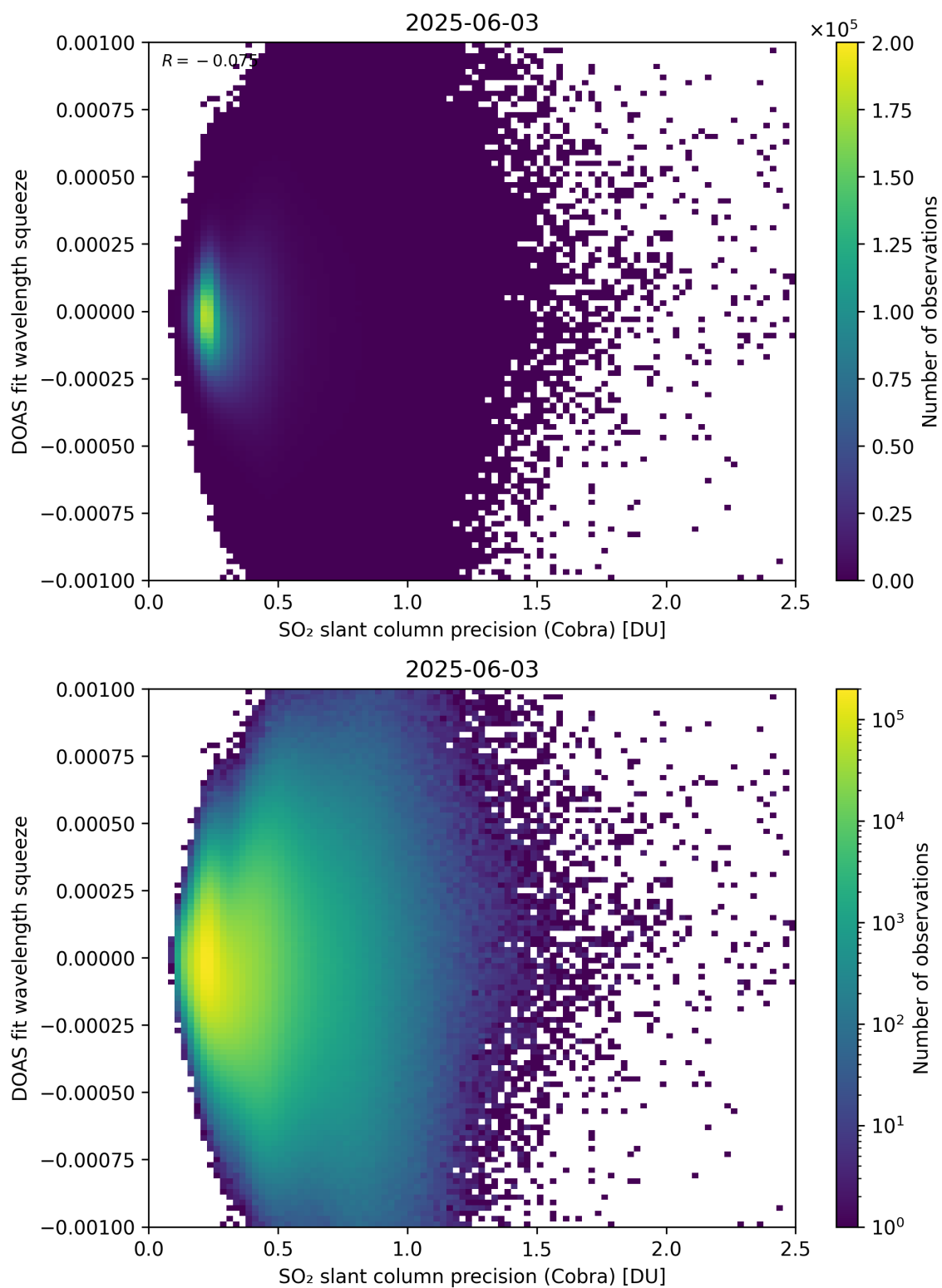
Figure 203: Scatter density plot of “SO 2 slant column precision (Cobra)” against “DOAS fit wavelength squeeze” for 2025-06-02 to 2025-06-04.
