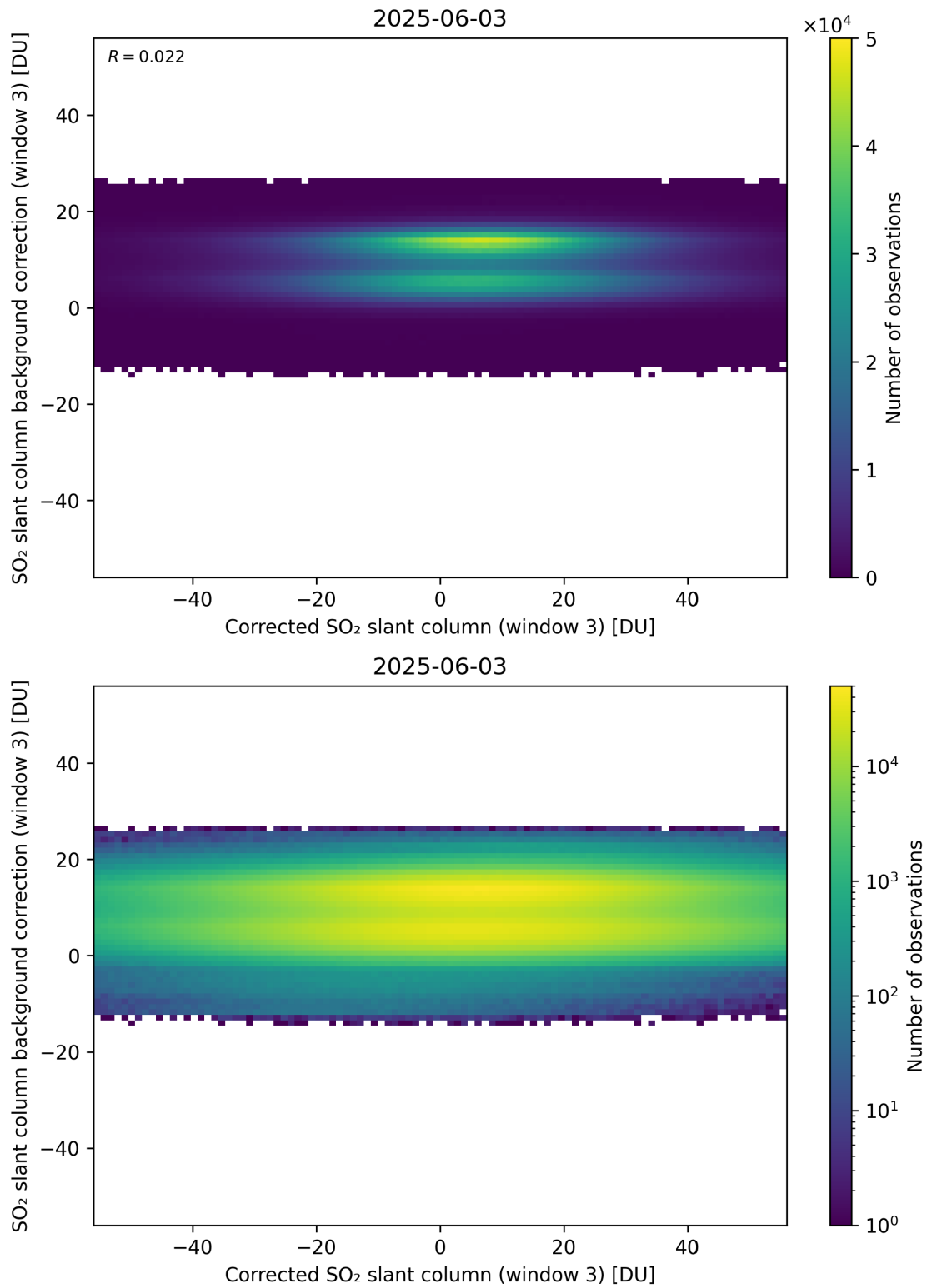
Figure 255: Scatter density plot of “Corrected SO 2 slant column (window 3)” against “SO 2 slant column background correction (window 3)” for 2025-06-02 to 2025-06-04.
