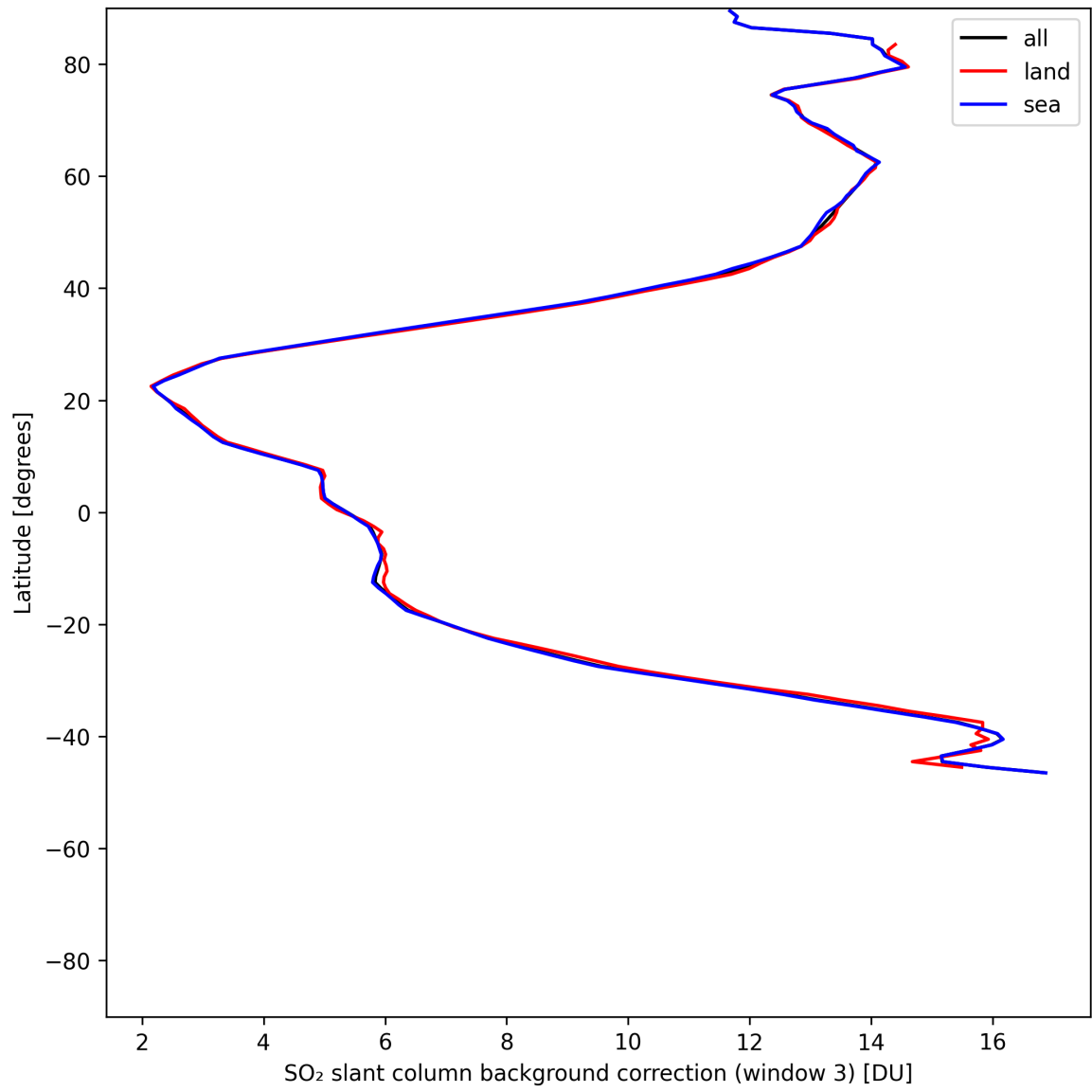
Figure 48: Zonal average of “SO 2 slant column background correction (window 3)” for 2025-06-02 to 2025-06-04.
