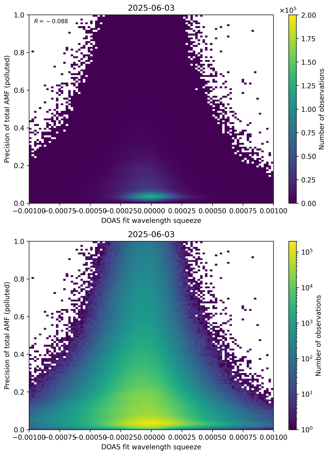
Figure 146: Scatter density plot of “DOAS fit wavelength squeeze” against “Precision of total AMF (polluted)” for 2025-06-02 to 2025-06-04.
