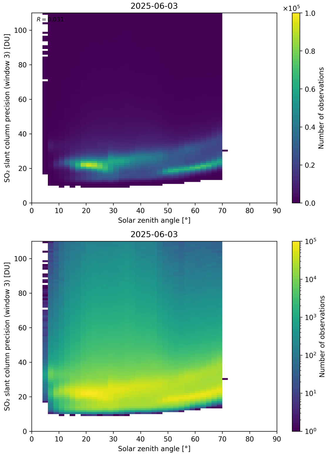
Figure 188: Scatter density plot of “Solar zenith angle” against “SO 2 slant column precision (window 3)” for 2025-06-02 to 2025-06-04.
