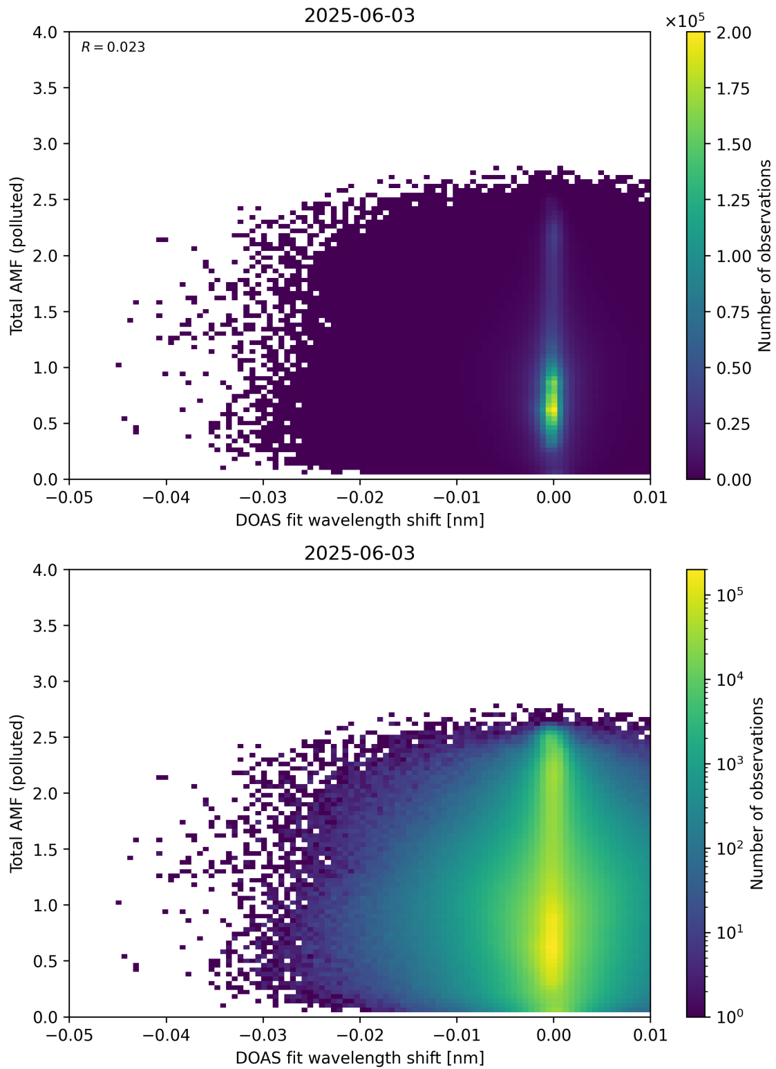
Figure 141: Scatter density plot of “DOAS fit wavelength shift” against “Total AMF (polluted)” for 2025-06-02 to 2025-06-04.
