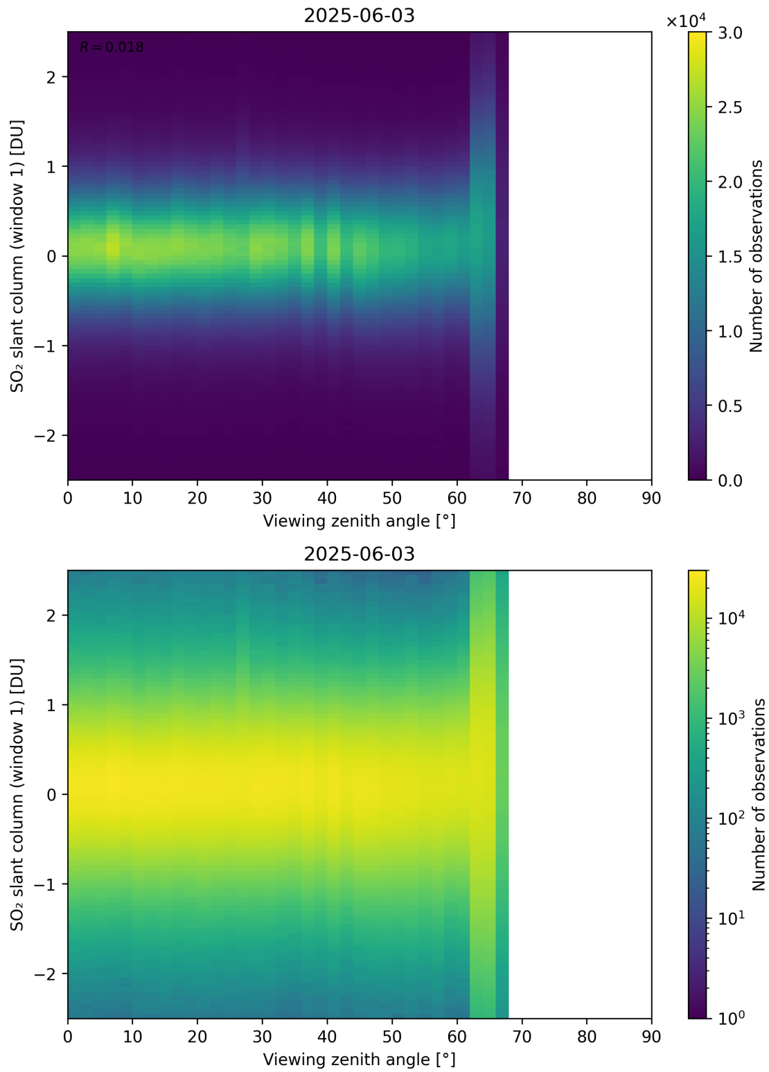
Figure 376: Scatter density plot of “Viewing zenith angle” against “SO 2 slant column (window 1)” for 2025-06-02 to 2025-06-04.
