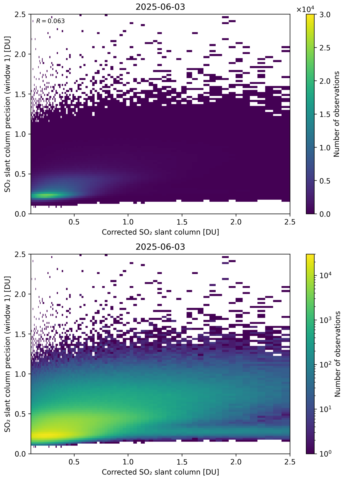
Figure 238: Scatter density plot of “Corrected SO 2 slant column” against “SO 2 slant column precision (window 1)” for 2025-06-02 to 2025-06-04.
