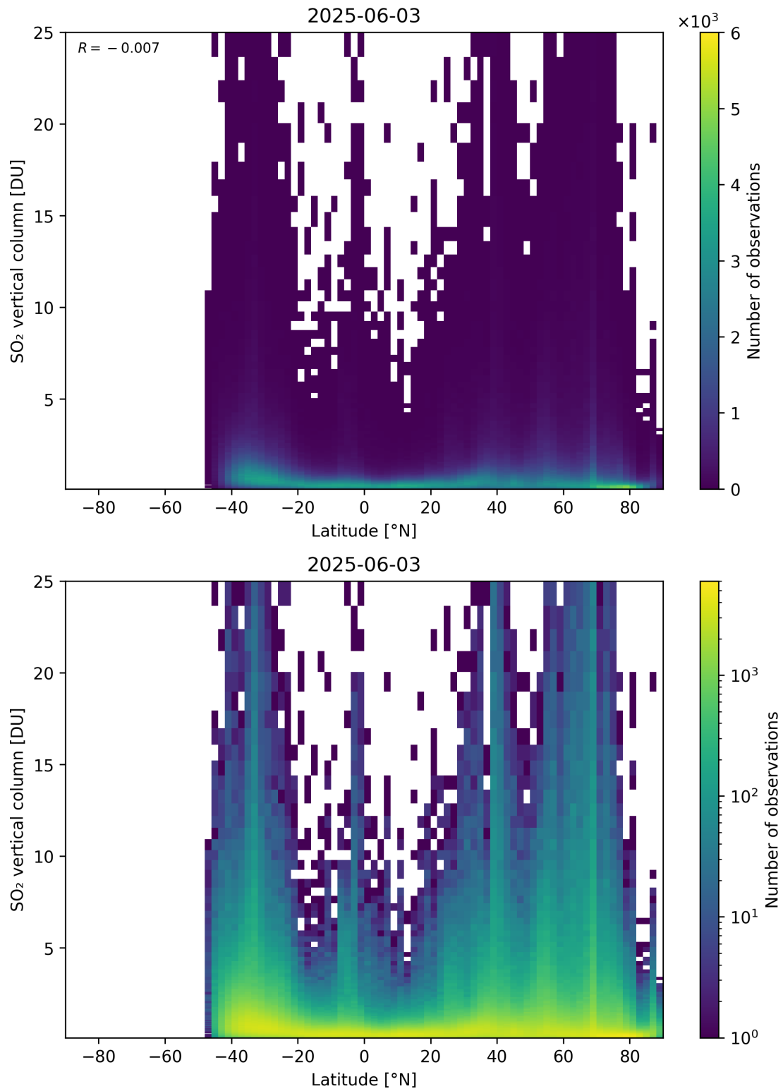
Figure 169: Scatter density plot of “Latitude” against “SO 2 vertical column” for 2025-06-02 to 2025-06-04.
