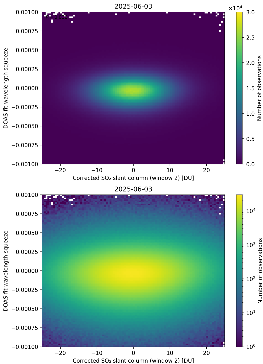
Figure 247: Scatter density plot of “Corrected SO 2 slant column (window 2)” against “DOAS fit wavelength squeeze” for 2025-06-02 to 2025-06-04.
