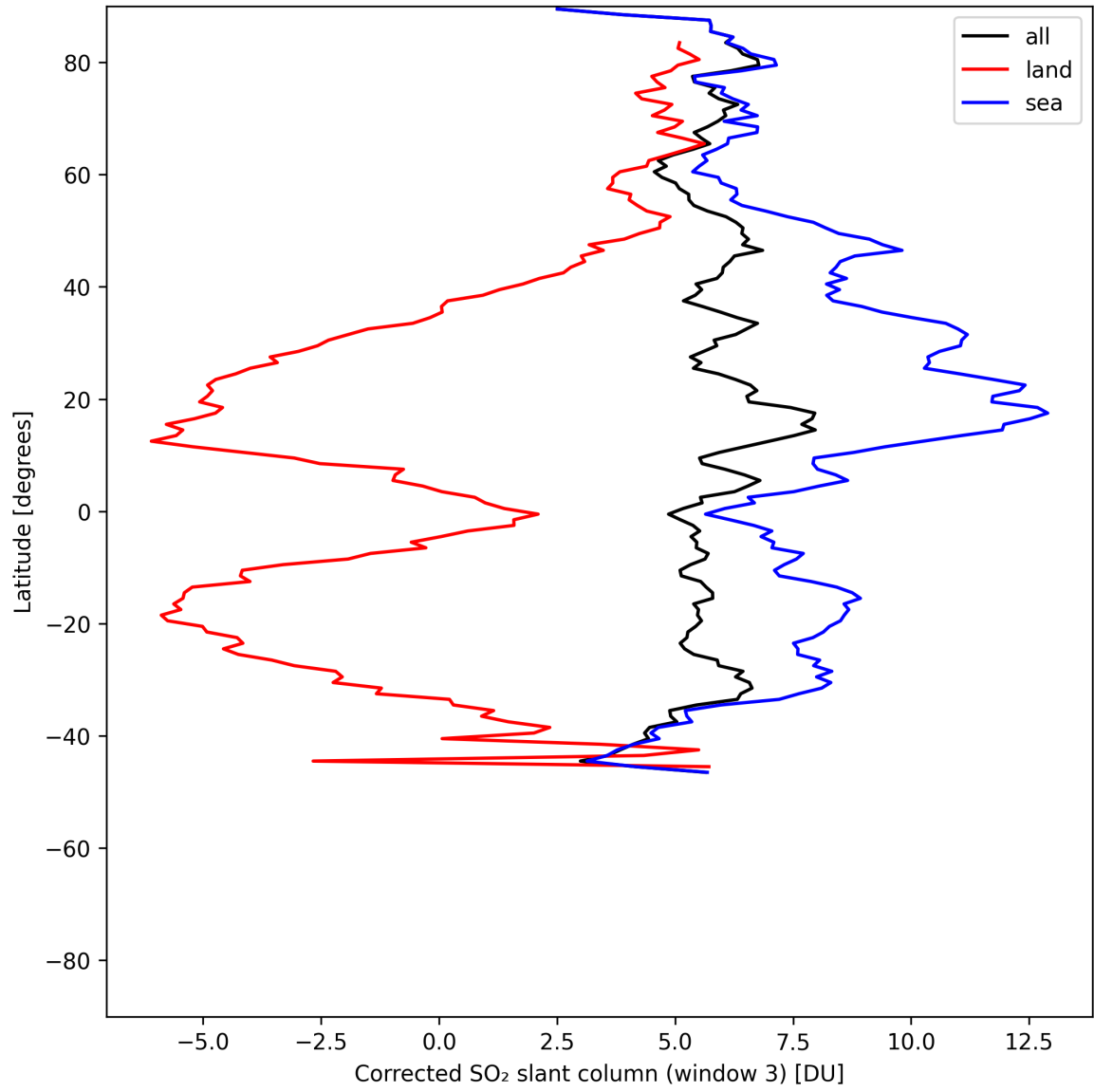
Figure 47: Zonal average of “Corrected SO 2 slant column (window 3)” for 2025-06-02 to 2025-06-04.
