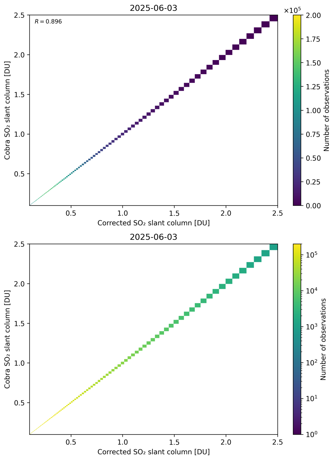
Figure 233: Scatter density plot of “Corrected SO 2 slant column” against “Cobra SO 2 slant column” for 2025-06-02 to 2025-06-04.
