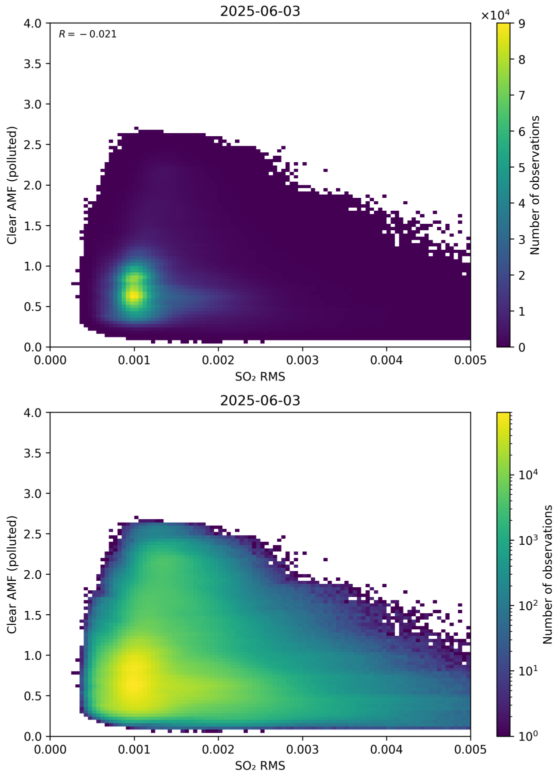
Figure 147: Scatter density plot of “SO 2 RMS” against “Clear AMF (polluted)” for 2025-06-02 to 2025-06-04.
