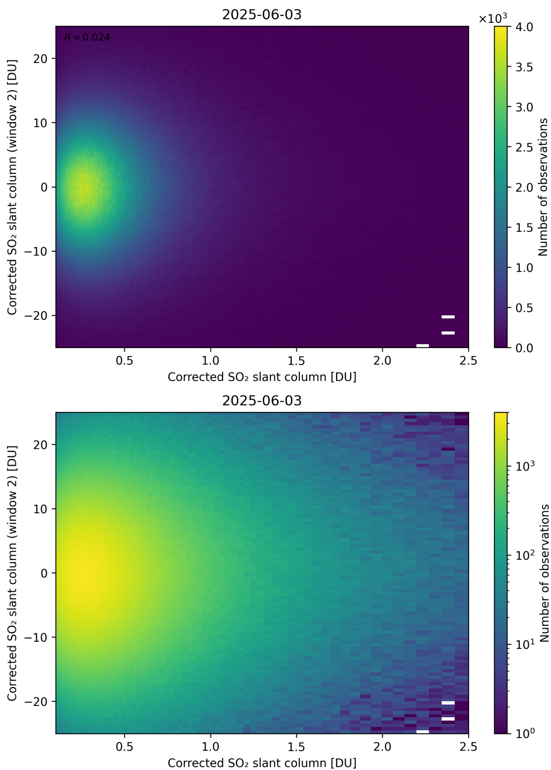
Figure 235: Scatter density plot of “Corrected SO 2 slant column” against “Corrected SO 2 slant column (window 2)” for 2025-06-02 to 2025-06-04.
