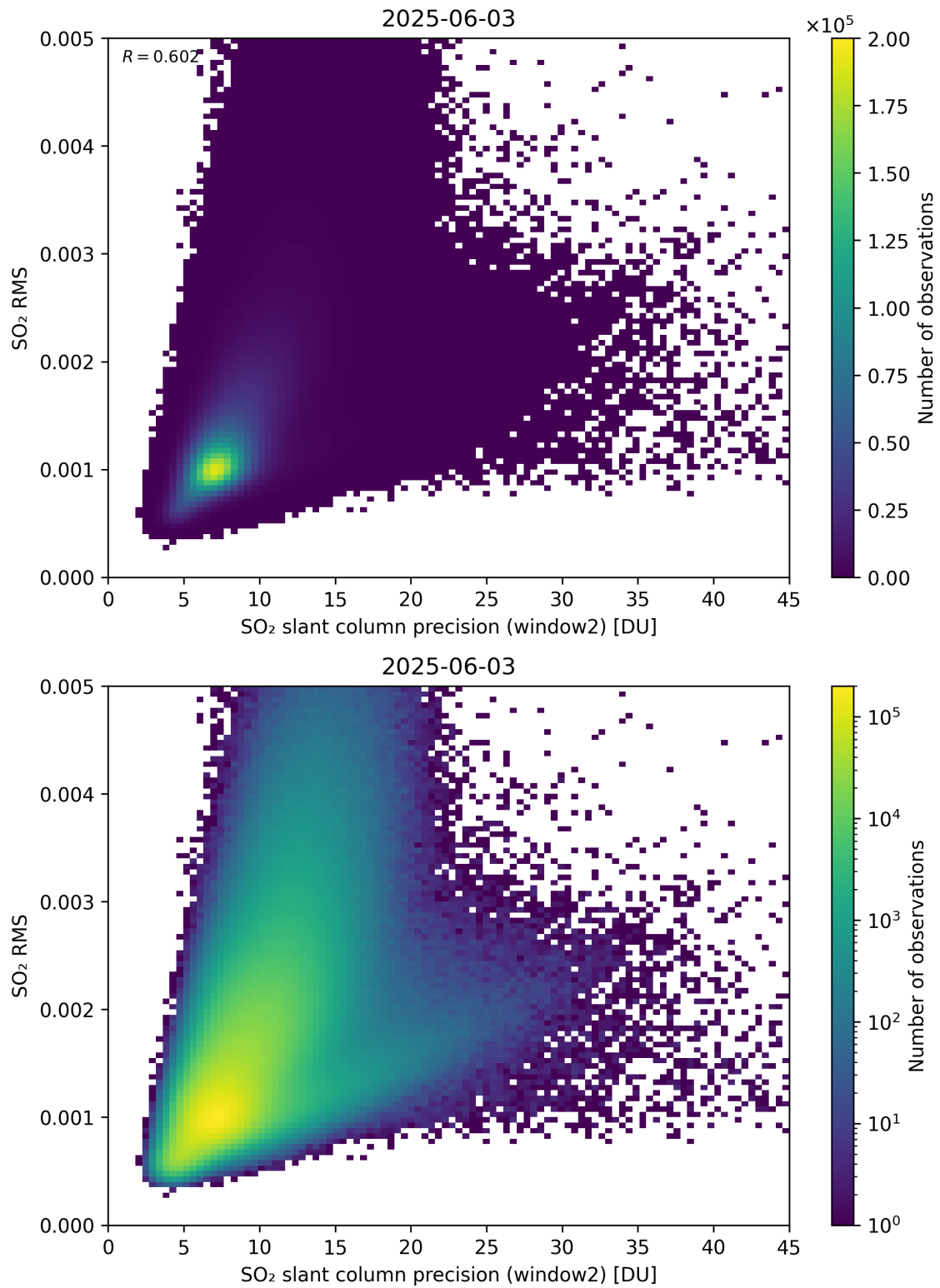
Figure 295: Scatter density plot of “SO 2 slant column precision (window2)” against “SO 2 RMS” for 2025-06-02 to 2025-06-04.
