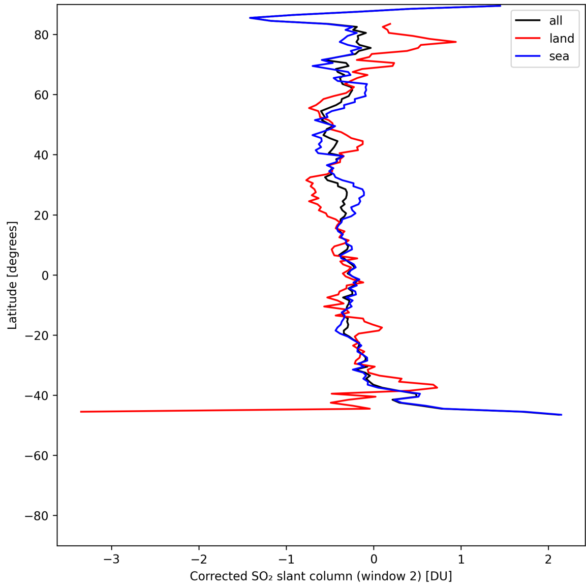
Figure 43: Zonal average of “Corrected SO 2 slant column (window 2)” for 2025-06-02 to 2025-06-04.
