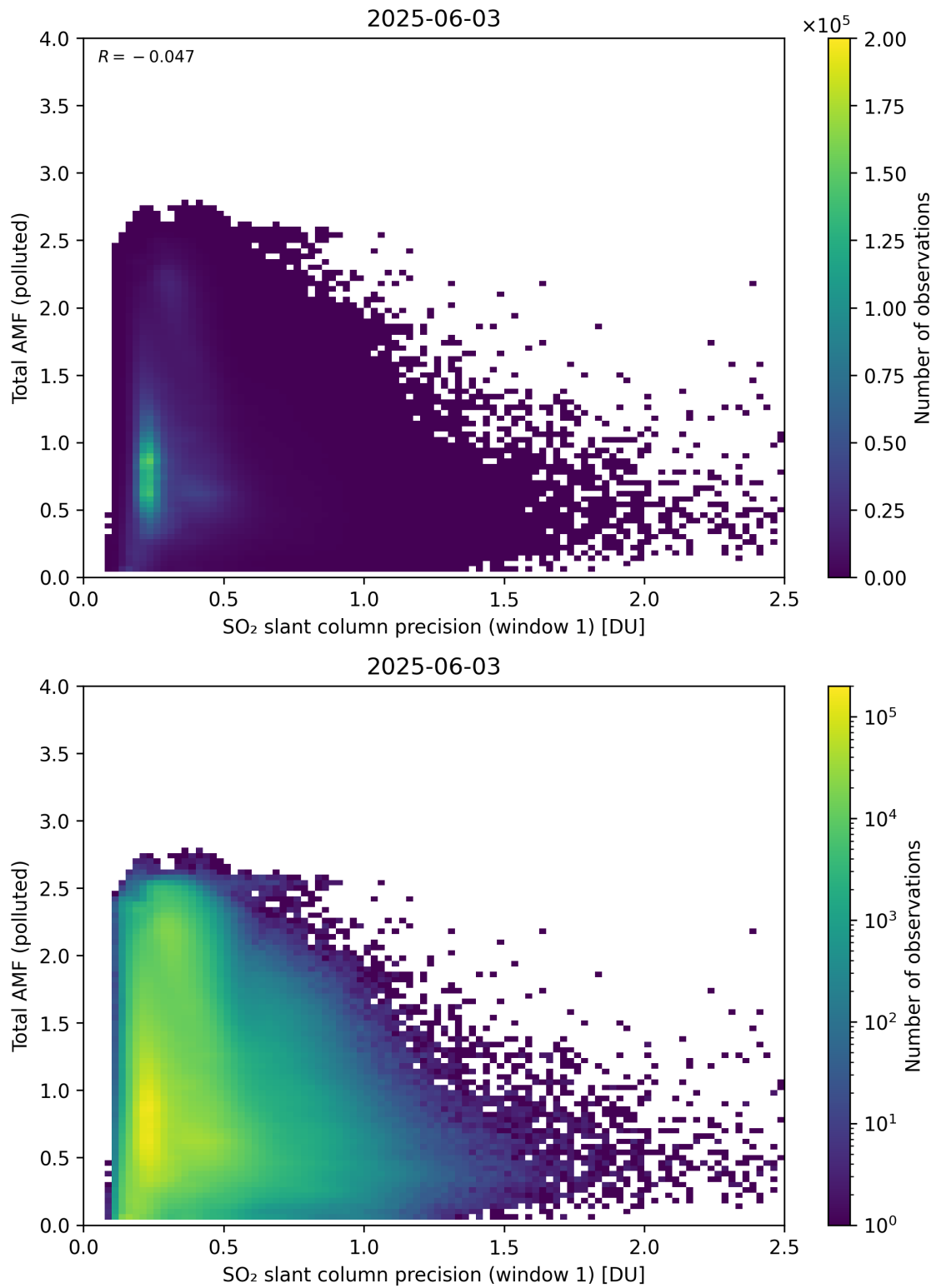
Figure 280: Scatter density plot of “SO 2 slant column precision (window 1)” against “Total AMF (polluted)” for 2025-06-02 to 2025-06-04.
