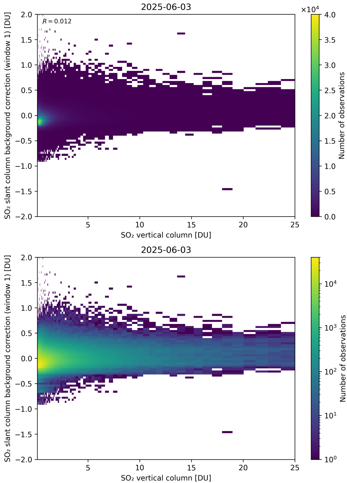
Figure 323: Scatter density plot of “SO 2 vertical column” against “SO 2 slant column background correction (window 1)” for 2025-06-02 to 2025-06-04.
