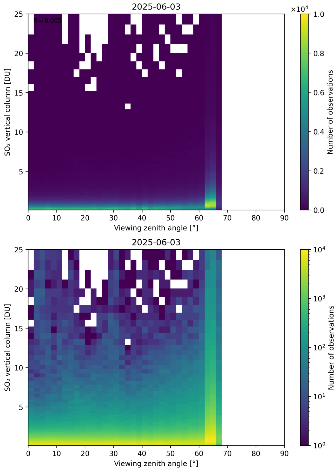
Figure 383: Scatter density plot of “Viewing zenith angle” against “SO 2 vertical column” for 2025-06-02 to 2025-06-04.
