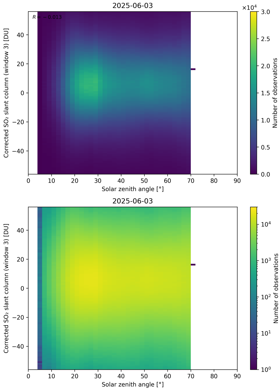
Figure 183: Scatter density plot of “Solar zenith angle” against “Corrected SO 2 slant column (window 3)” for 2025-06-02 to 2025-06-04.
