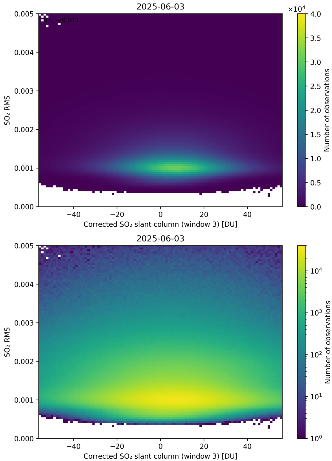
Figure 258: Scatter density plot of “Corrected SO 2 slant column (window 3)” against “SO 2 RMS” for 2025-06-02 to 2025-06-04.
