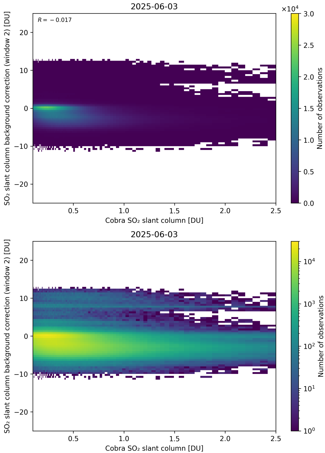
Figure 194: Scatter density plot of “Cobra SO 2 slant column” against “SO 2 slant column background correction (window 2)” for 2025-06-02 to 2025-06-04.
