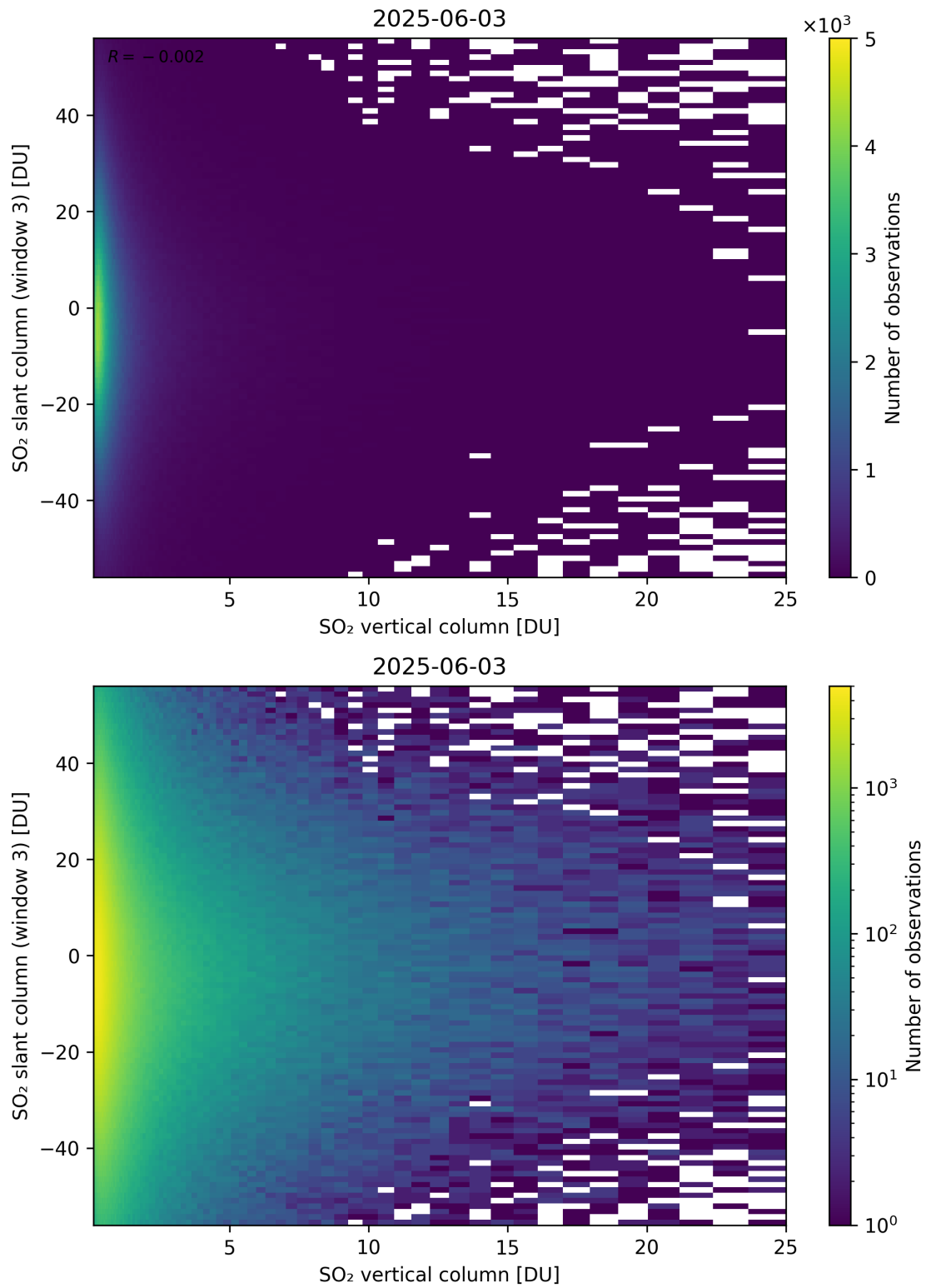
Figure 357: Scatter density plot of “SO 2 vertical column” against “SO 2 slant column (window 3)” for 2025-06-02 to 2025-06-04.
