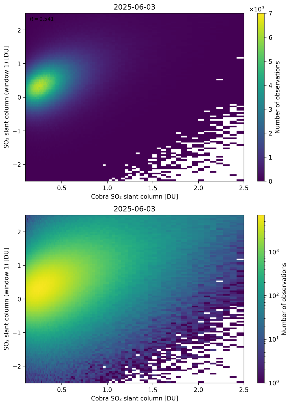
Figure 219: Scatter density plot of “Cobra SO 2 slant column” against “SO 2 slant column (window 1)” for 2025-06-02 to 2025-06-04.
