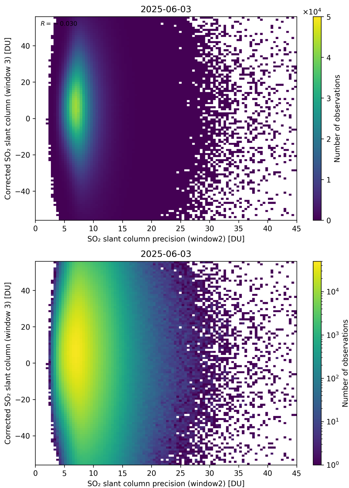
Figure 298: Scatter density plot of “SO 2 slant column precision (window2)” against “Corrected SO 2 slant column (window 3)” for 2025-06-02 to 2025-06-04.
