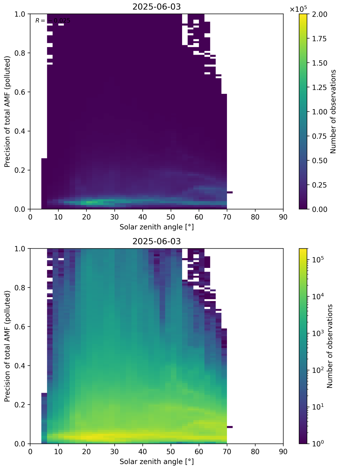
Figure 190: Scatter density plot of “Solar zenith angle” against “Precision of total AMF (polluted)” for 2025-06-02 to 2025-06-04.
