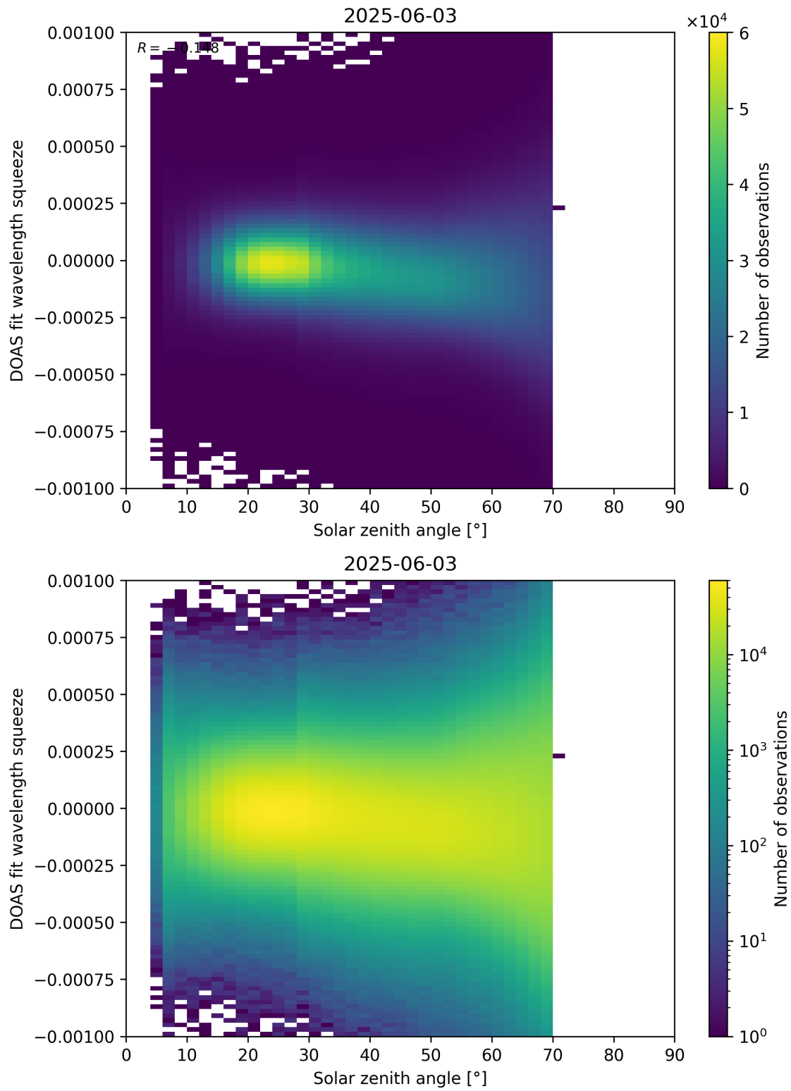
Figure 175: Scatter density plot of “Solar zenith angle” against “DOAS fit wavelength squeeze” for 2025-06-02 to 2025-06-04.
