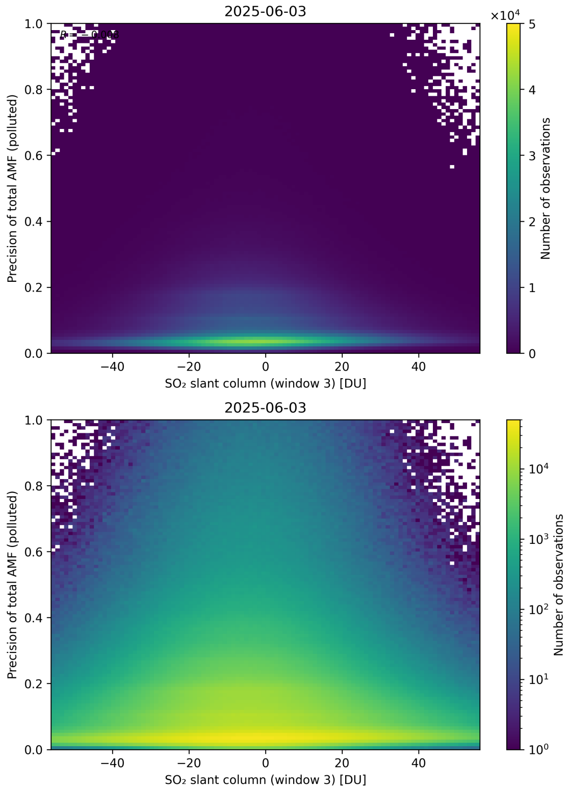
Figure 319: Scatter density plot of “SO 2 slant column (window 3)” against “Precision of total AMF (polluted)” for 2025-06-02 to 2025-06-04.
