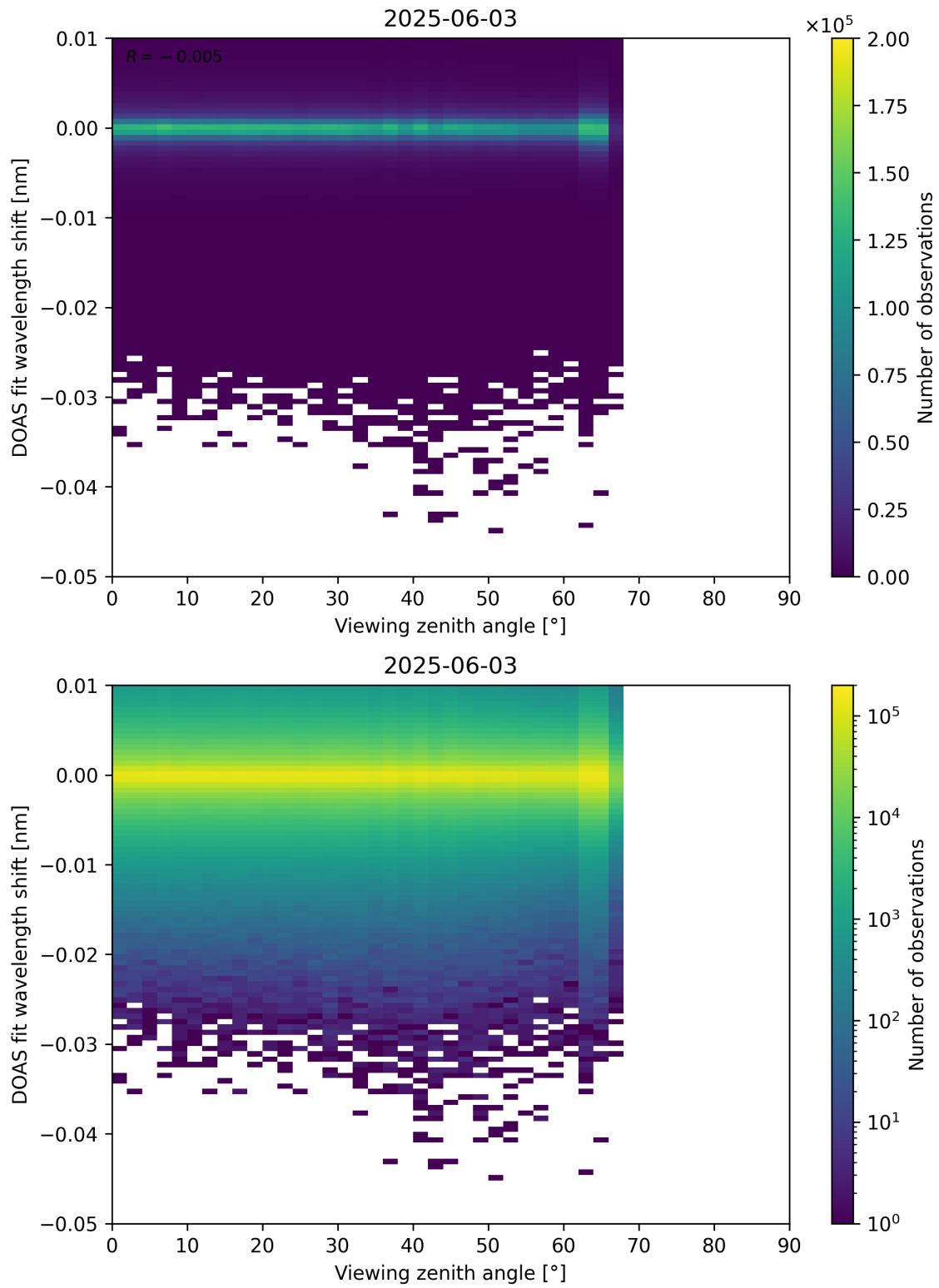
Figure 365: Scatter density plot of “Viewing zenith angle” against “DOAS fit wavelength shift” for 2025-06-02 to 2025-06-04.
