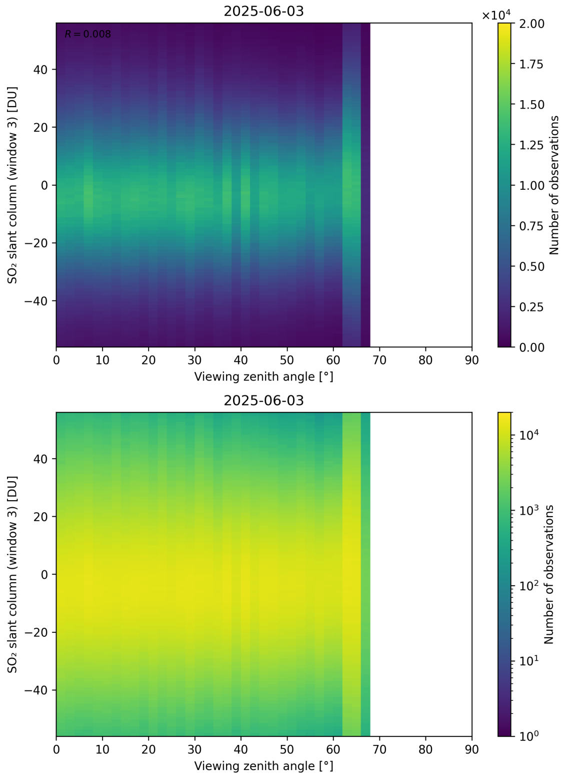
Figure 379: Scatter density plot of “Viewing zenith angle” against “SO 2 slant column (window 3)” for 2025-06-02 to 2025-06-04.
