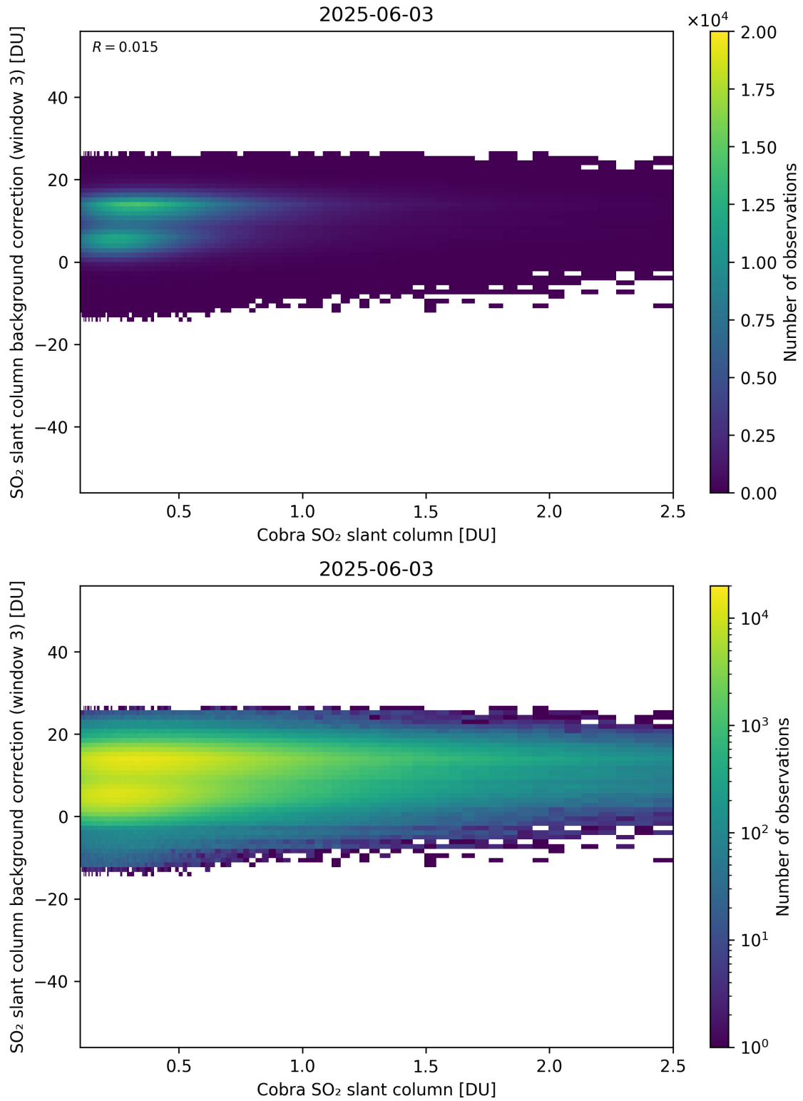
Figure 195: Scatter density plot of “Cobra SO 2 slant column” against “SO 2 slant column background correction (window 3)” for 2025-06-02 to 2025-06-04.
