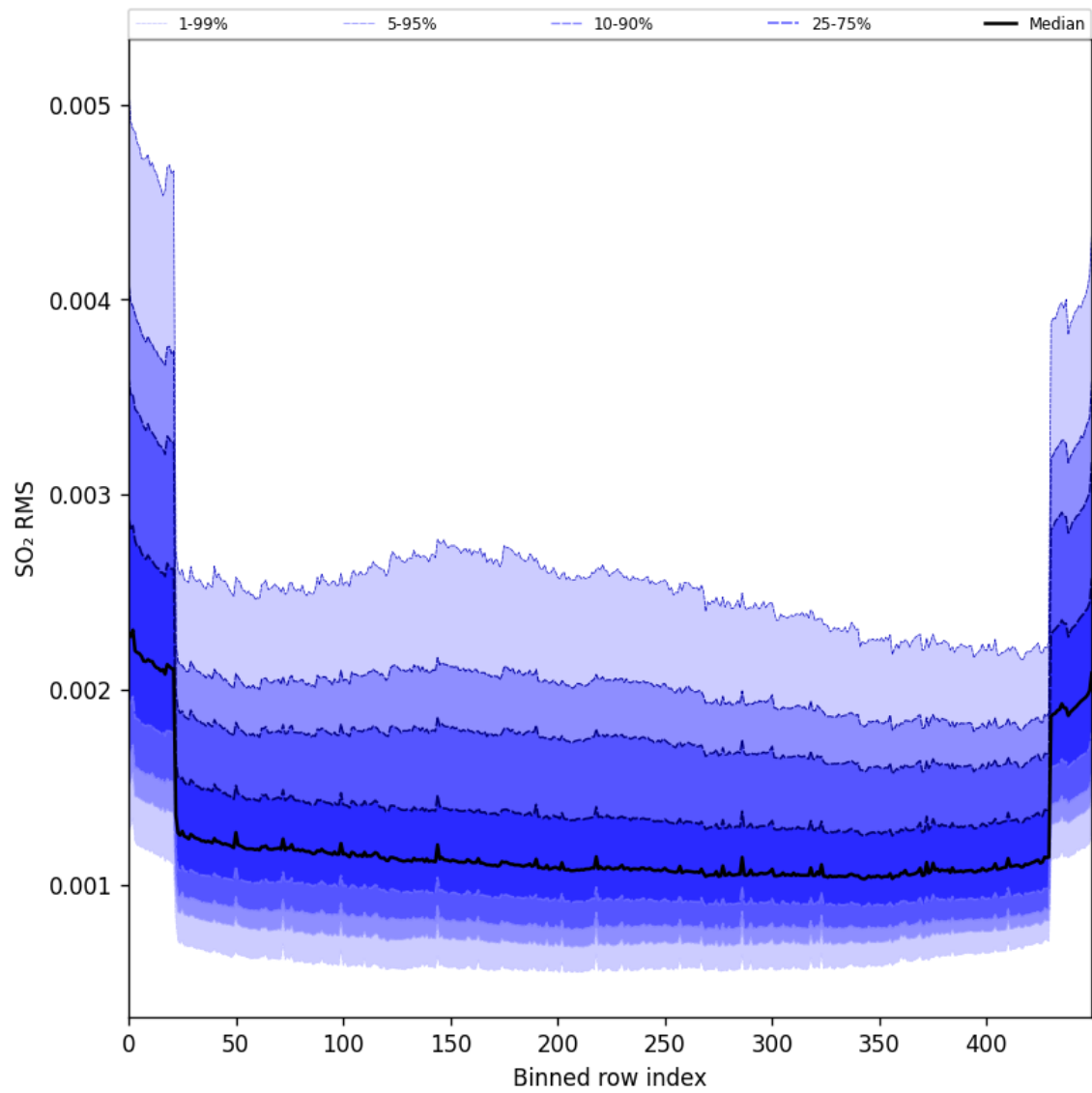
Figure 104: Along track statistics of “SO 2 RMS” for 2025-06-02 to 2025-06-04
