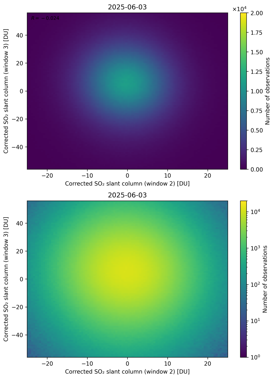
Figure 250: Scatter density plot of “Corrected SO 2 slant column (window 2)” against “Corrected SO 2 slant column (window 3)” for 2025-06-02 to 2025-06-04.
