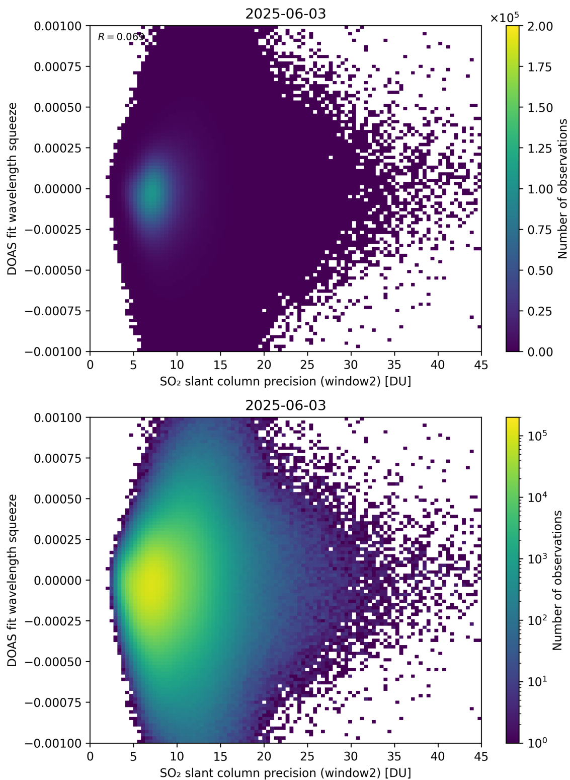
Figure 294: Scatter density plot of “SO 2 slant column precision (window2)” against “DOAS fit wavelength squeeze” for 2025-06-02 to 2025-06-04.
