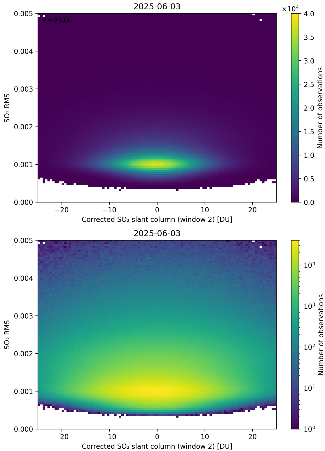
Figure 248: Scatter density plot of “Corrected SO 2 slant column (window 2)” against “SO 2 RMS” for 2025-06-02 to 2025-06-04.
