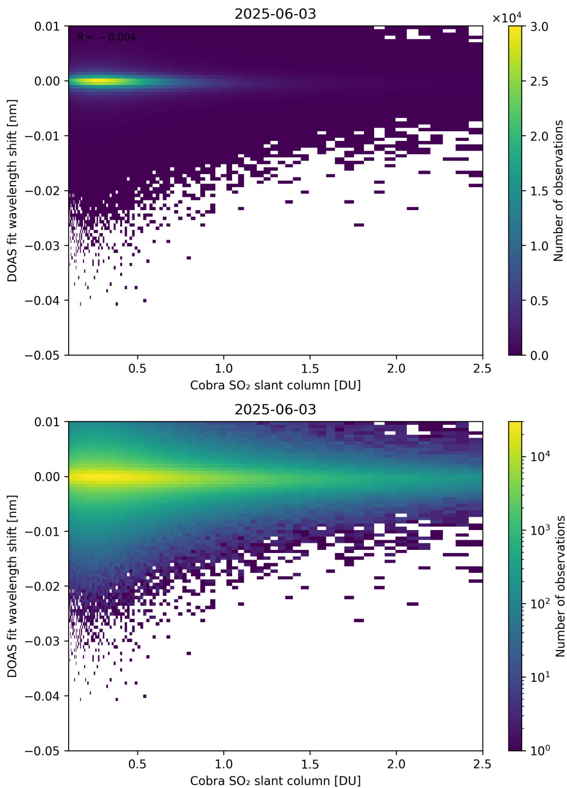
Figure 196: Scatter density plot of “Cobra SO 2 slant column” against “DOAS fit wavelength shift” for 2025-06-02 to 2025-06-04.
