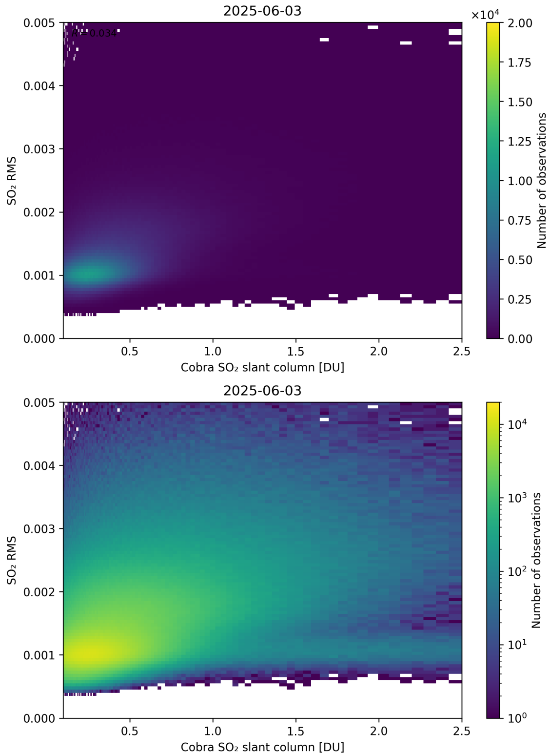
Figure 198: Scatter density plot of “Cobra SO 2 slant column” against “SO 2 RMS” for 2025-06-02 to 2025-06-04.
