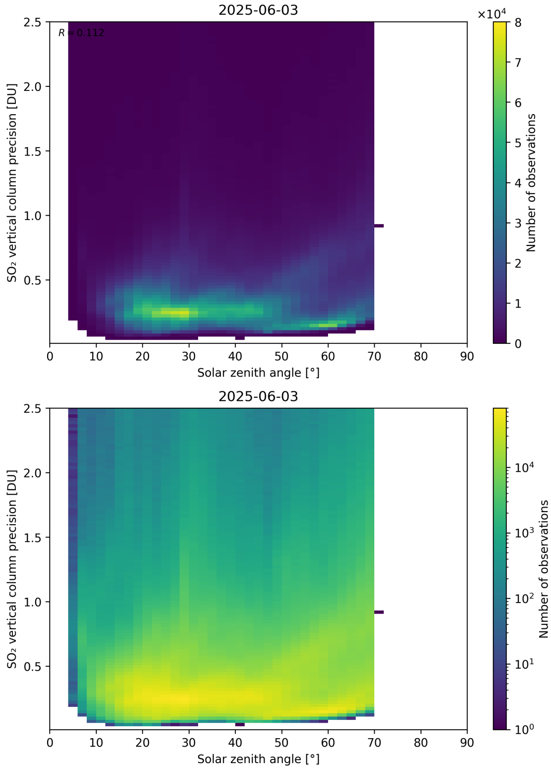
Figure 192: Scatter density plot of “Solar zenith angle” against “SO 2 vertical column precision” for 2025-06-02 to 2025-06-04.
