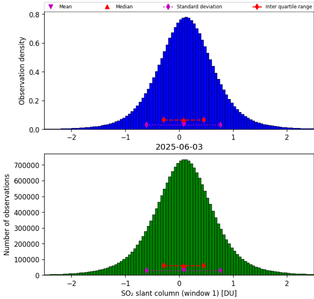
Figure 63: Histogram of “SO 2 slant column (window 1)” for 2025-06-02 to 2025-06-04
