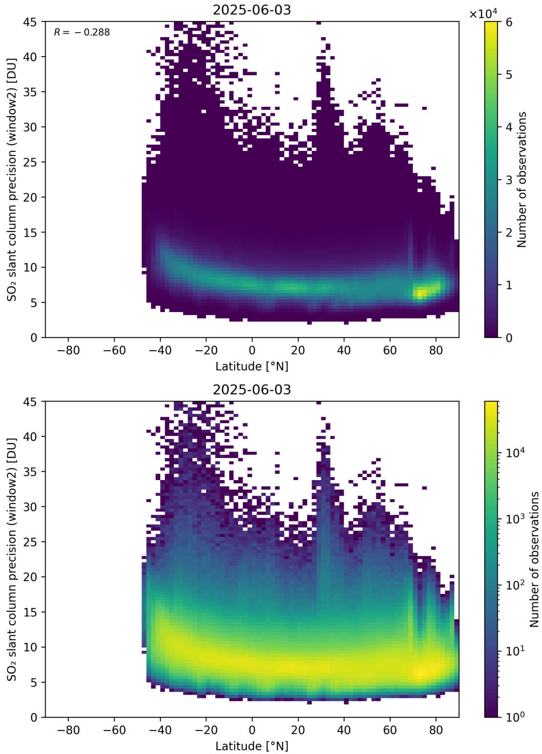
Figure 164: Scatter density plot of “Latitude” against “SO 2 slant column precision (window2)” for 2025-06-02 to 2025-06-04.
