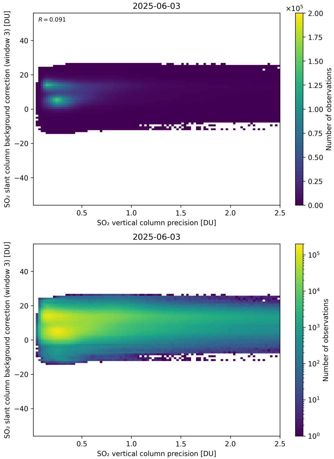
Figure 331: Scatter density plot of “SO 2 vertical column precision” against “SO 2 slant column background correction (window 3)” for 2025-06-02 to 2025-06-04.
