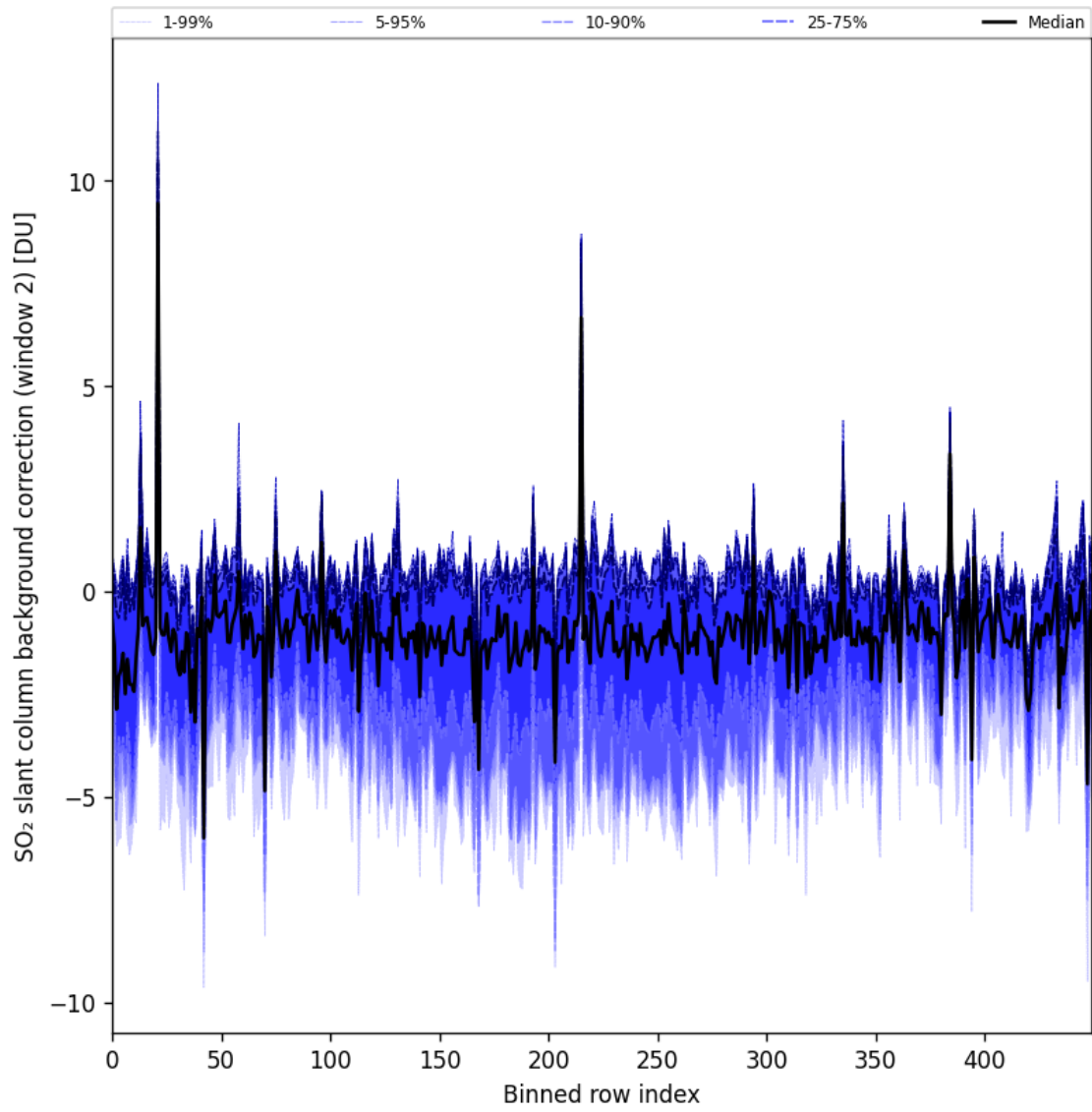
Figure 96: Along track statistics of “SO 2 slant column background correction (window 2)” for 2025-06-02 to 2025-06-04
