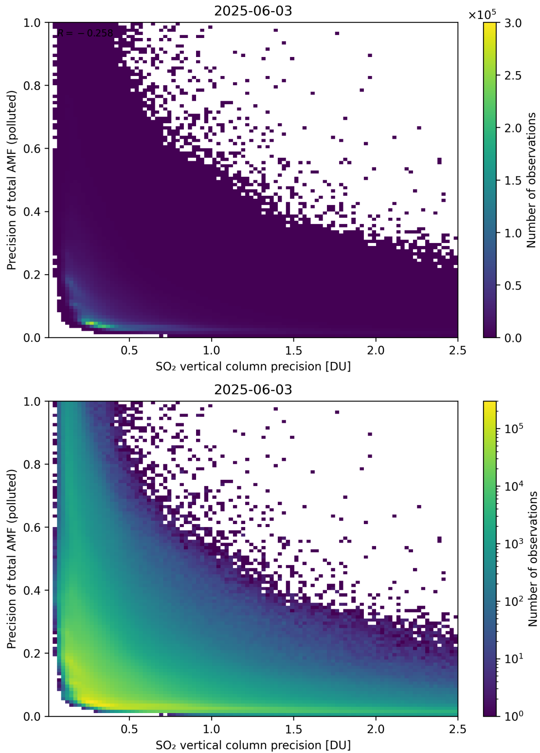
Figure 347: Scatter density plot of “SO 2 vertical column precision” against “Precision of total AMF (polluted)” for 2025-06-02 to 2025-06-04.
