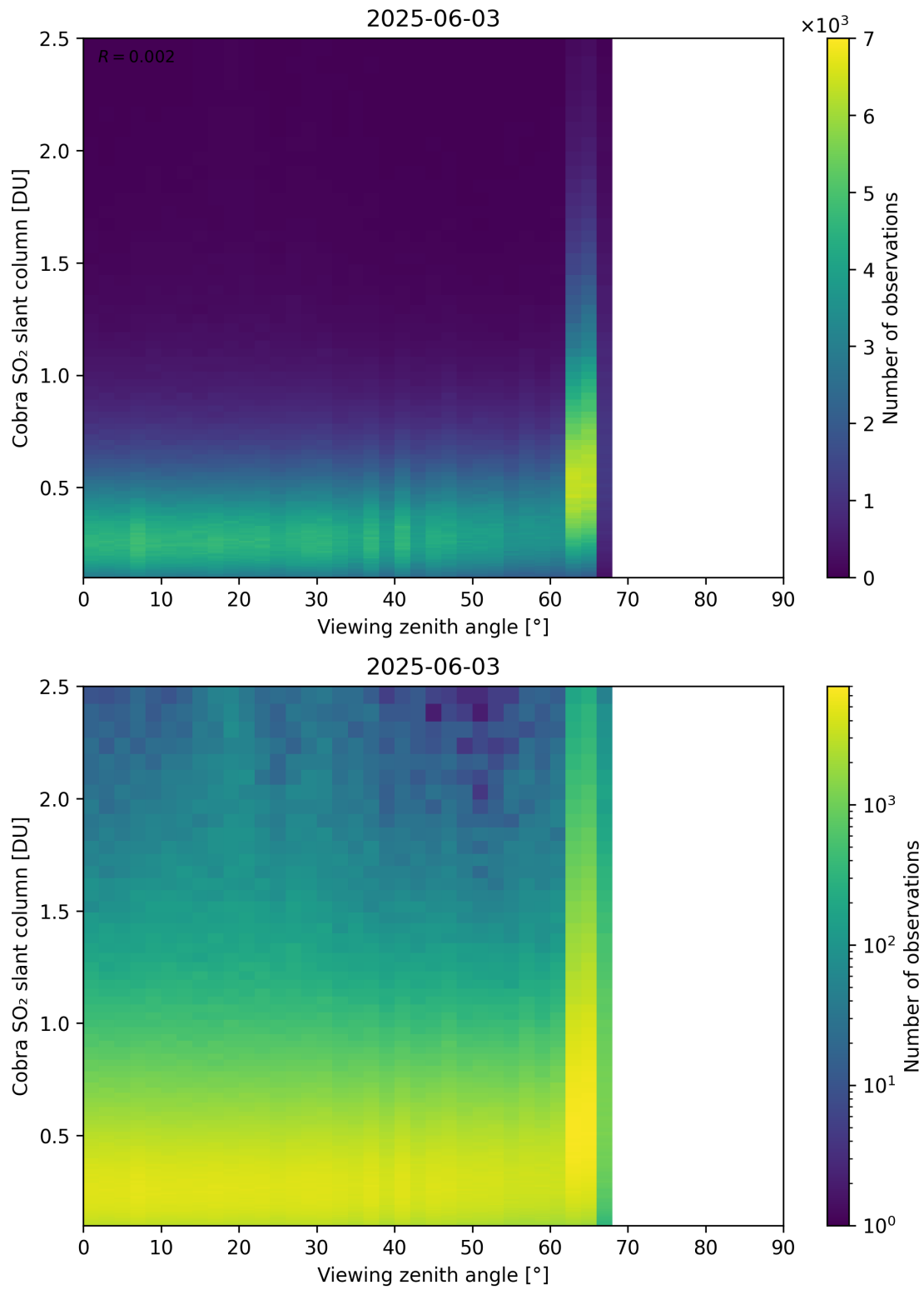
Figure 371: Scatter density plot of “Viewing zenith angle” against “Cobra SO 2 slant column” for 2025-06-02 to 2025-06-04.
