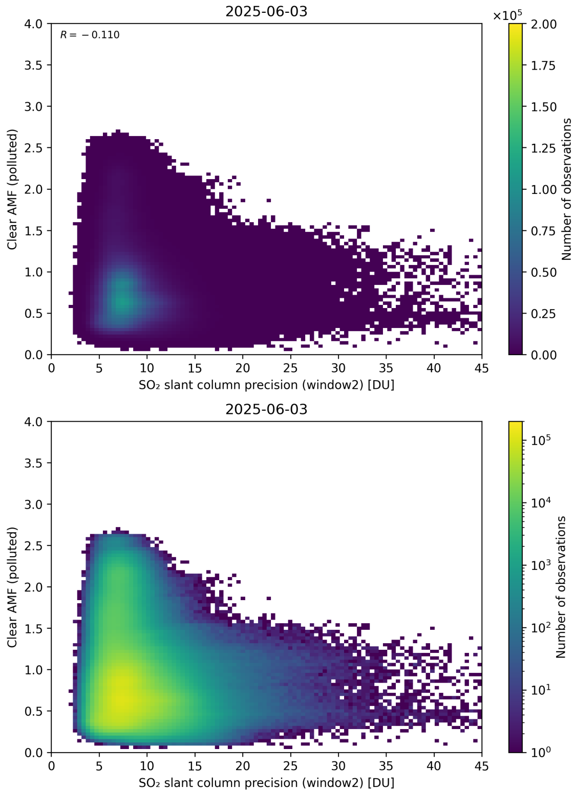
Figure 296: Scatter density plot of “SO 2 slant column precision (window2)” against “Clear AMF (polluted)” for 2025-06-02 to 2025-06-04.
