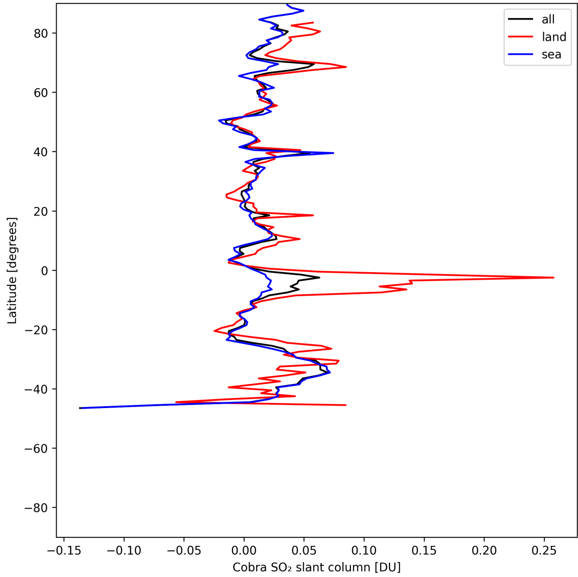
Figure 35: Zonal average of “Cobra SO 2 slant column” for 2025-06-02 to 2025-06-04.
