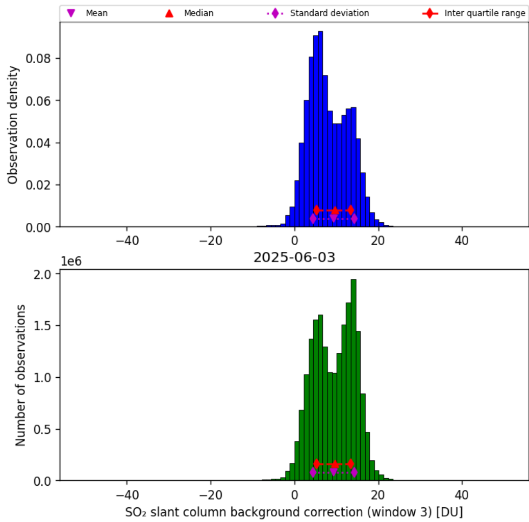
Figure 74: Histogram of “SO 2 slant column background correction (window 3)” for 2025-06-02 to 2025-06-04
