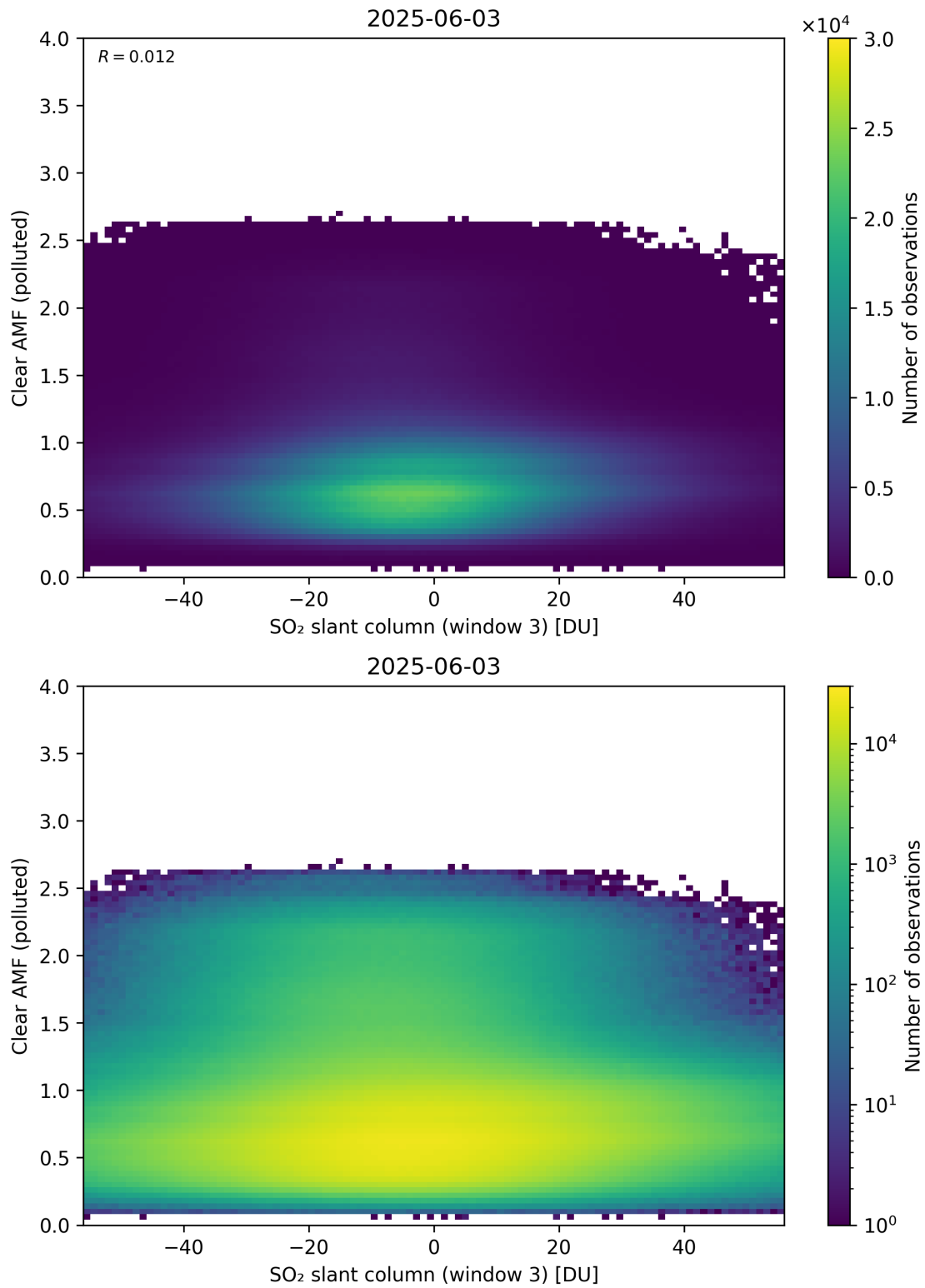
Figure 315: Scatter density plot of “SO 2 slant column (window 3)” against “Clear AMF (polluted)” for 2025-06-02 to 2025-06-04.
