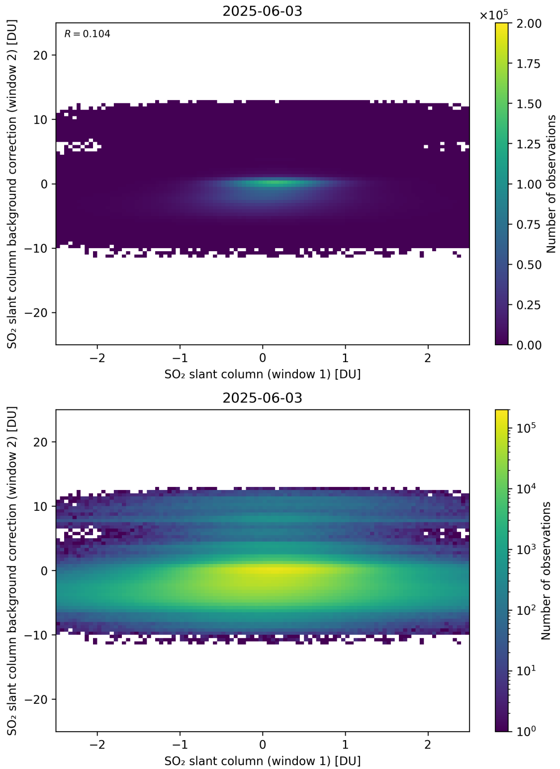
Figure 263: Scatter density plot of “SO 2 slant column (window 1)” against “SO 2 slant column background correction (window 2)” for 2025-06-02 to 2025-06-04.
