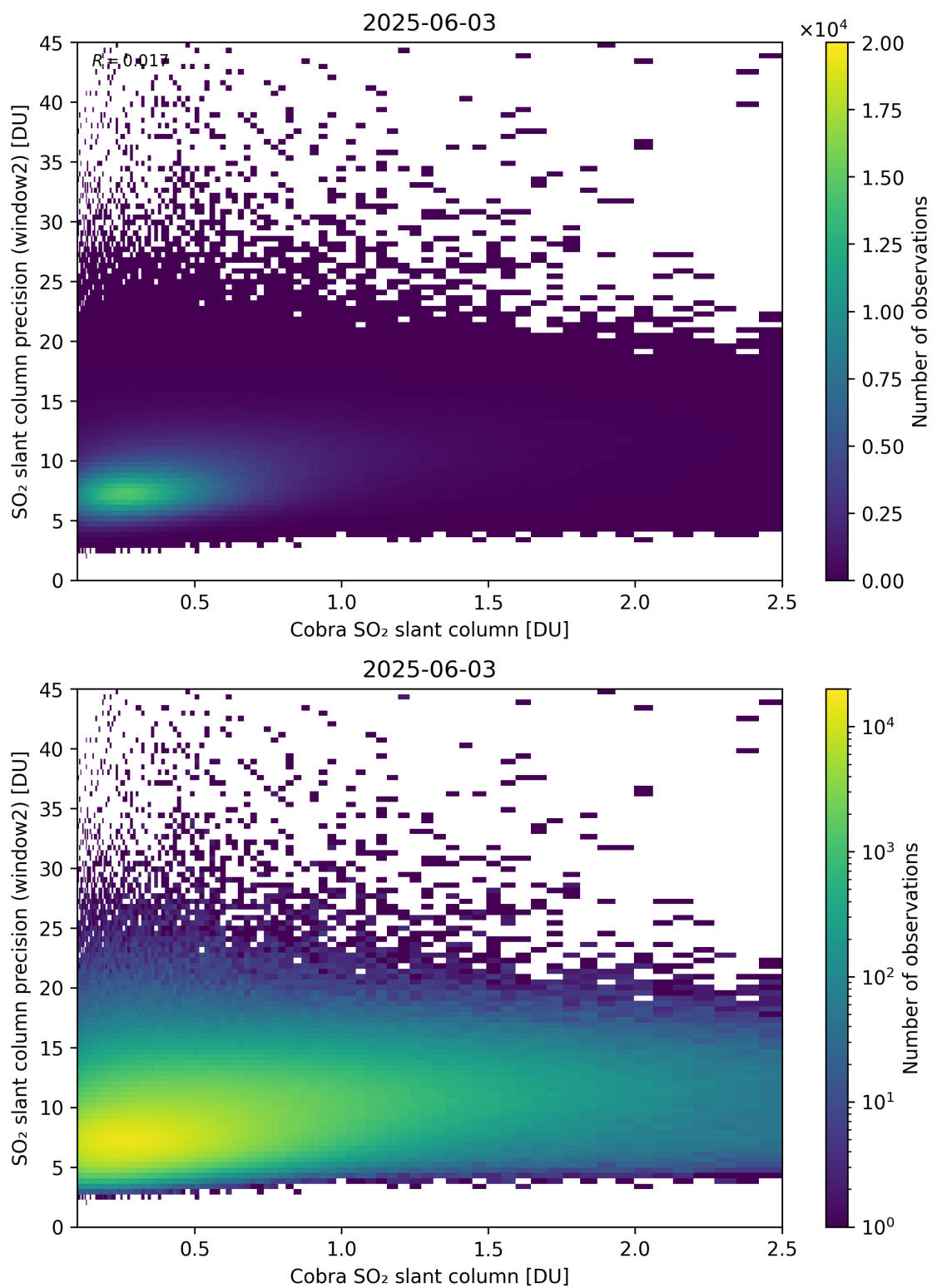
Figure 221: Scatter density plot of “Cobra SO 2 slant column” against “SO 2 slant column precision (window2)” for 2025-06-02 to 2025-06-04.
