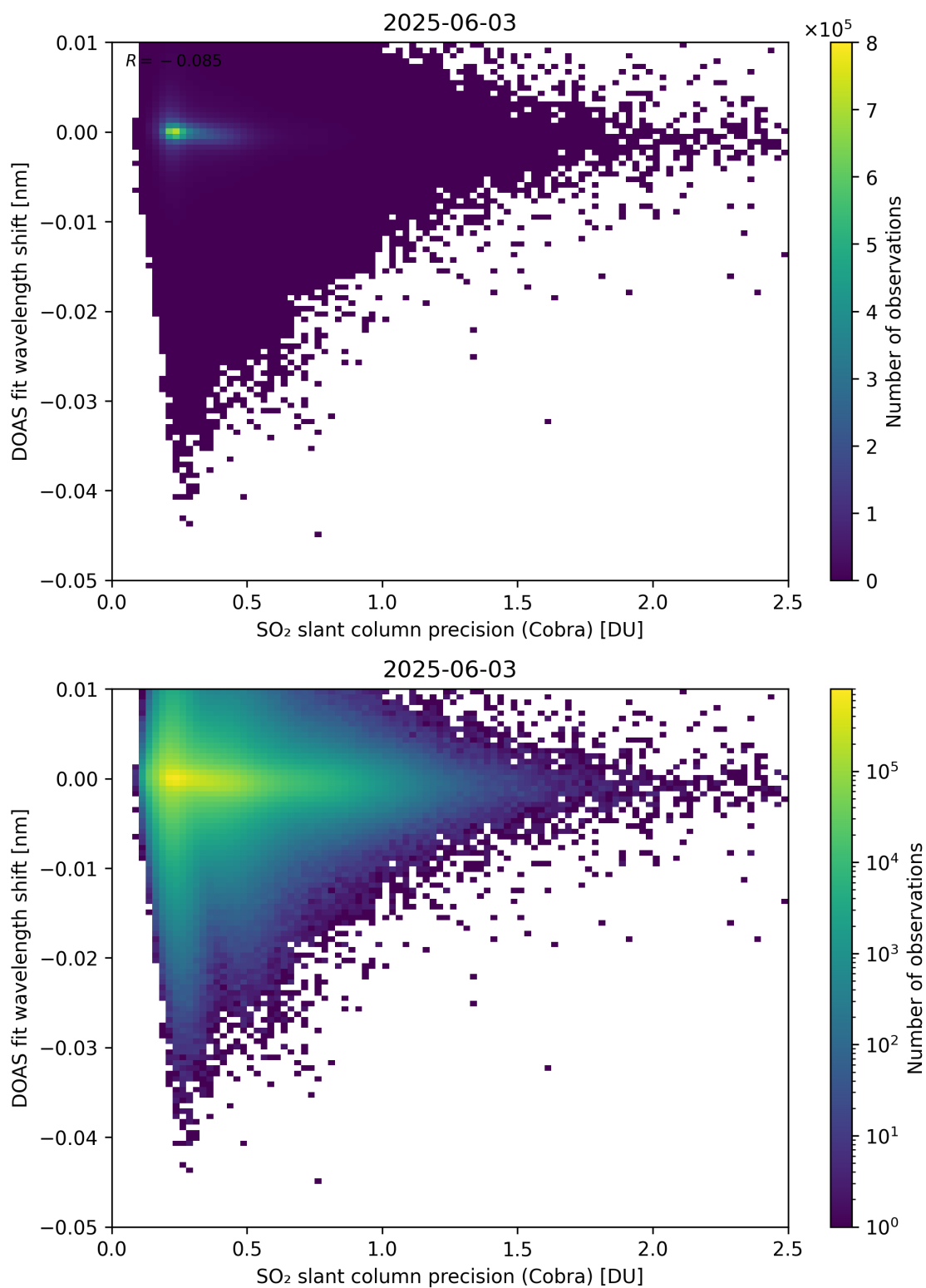
Figure 202: Scatter density plot of “SO 2 slant column precision (Cobra)” against “DOAS fit wavelength shift” for 2025-06-02 to 2025-06-04.
