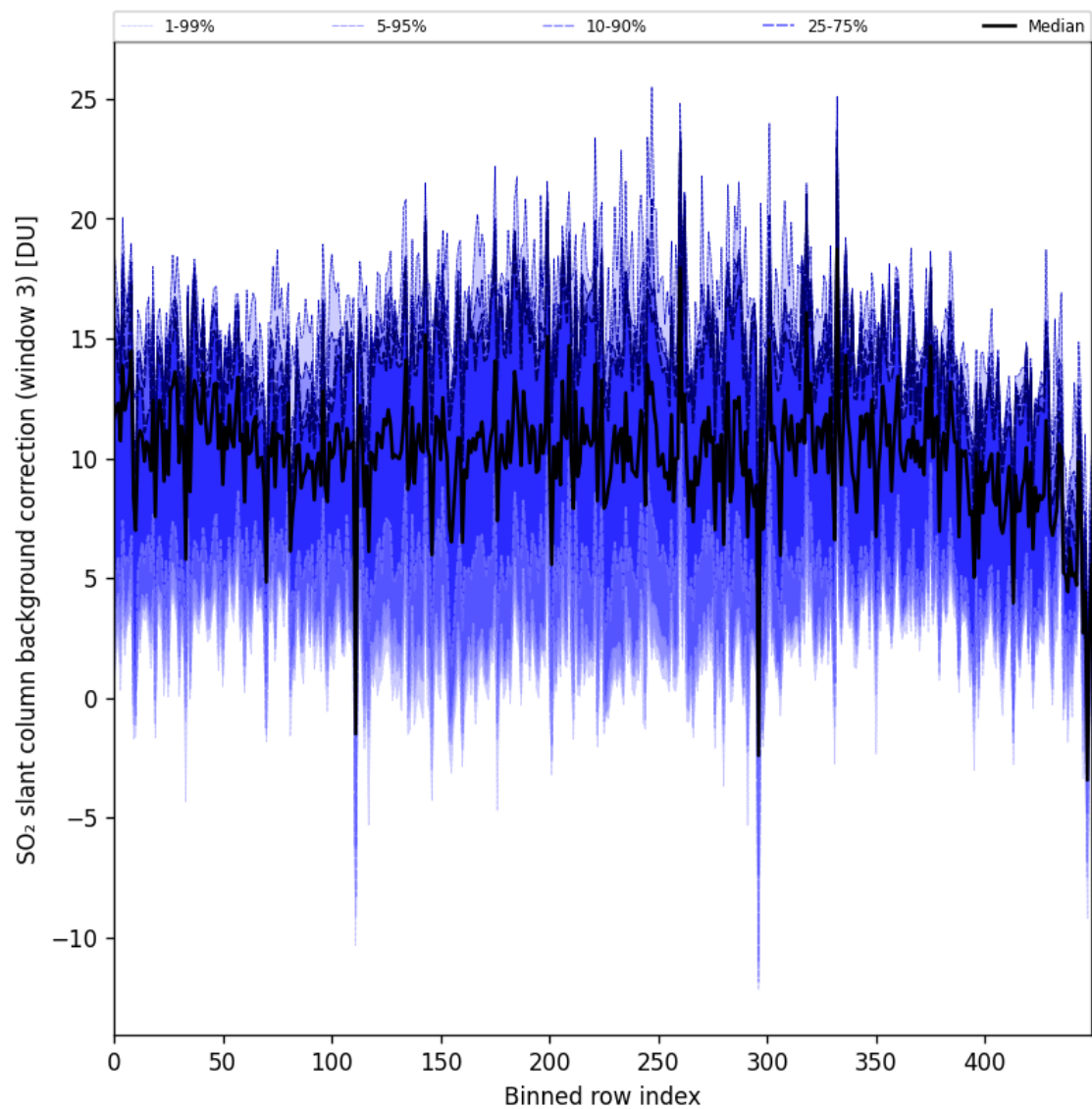
Figure 100: Along track statistics of “SO 2 slant column background correction (window 3)” for 2025-06-02 to 2025-06-04
