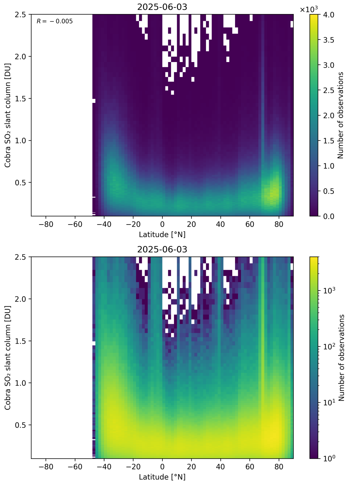
Figure 157: Scatter density plot of “Latitude” against “Cobra SO 2 slant column” for 2025-06-02 to 2025-06-04.
