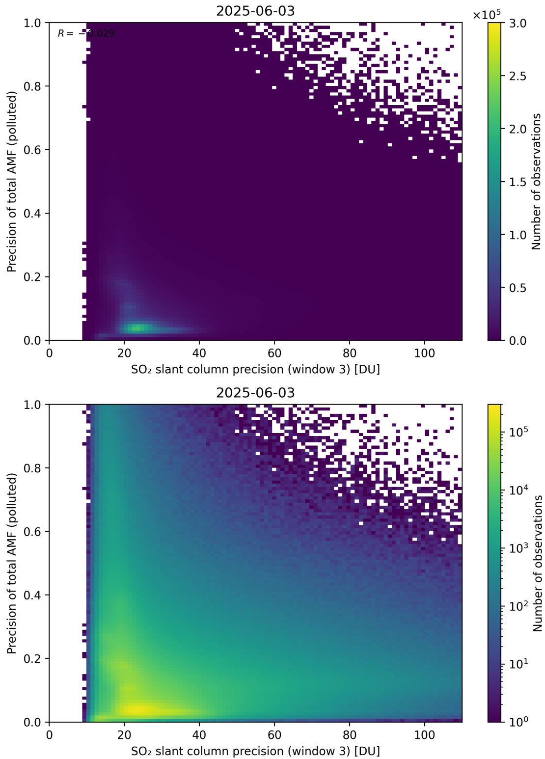
Figure 314: Scatter density plot of “SO 2 slant column precision (window 3)” against “Precision of total AMF (polluted)” for 2025-06-02 to 2025-06-04.
