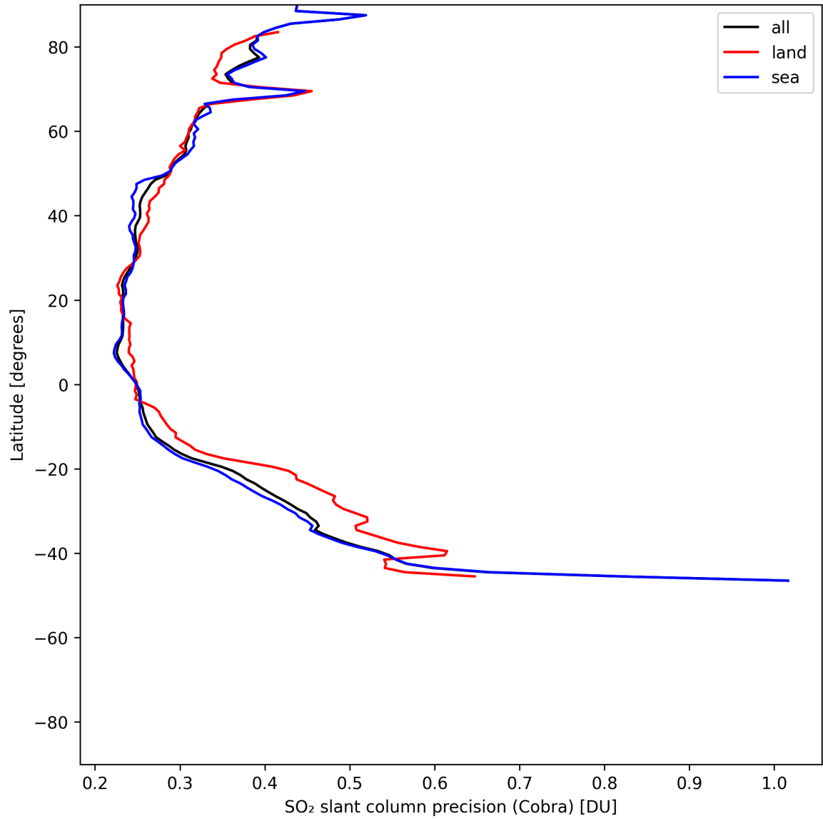
Figure 36: Zonal average of “SO 2 slant column precision (Cobra)” for 2025-06-02 to 2025-06-04.
