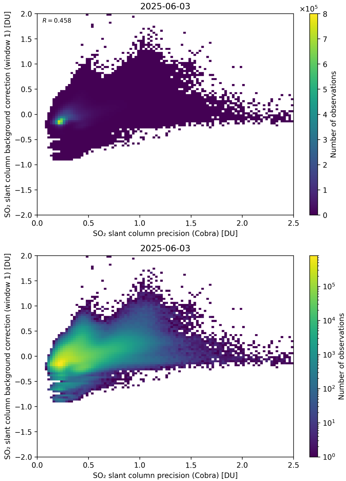
Figure 199: Scatter density plot of “SO 2 slant column precision (Cobra)” against “SO 2 slant column background correction (window 1)” for 2025-06-02 to 2025-06-04.
