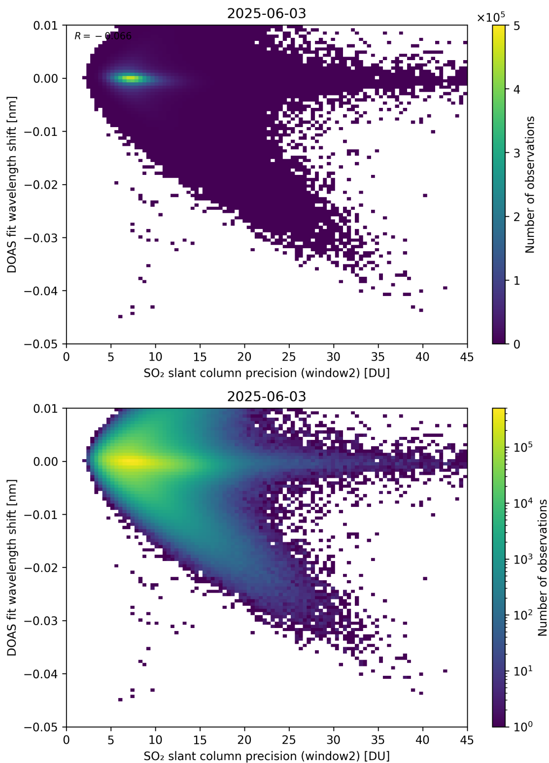
Figure 293: Scatter density plot of “SO 2 slant column precision (window2)” against “DOAS fit wavelength shift” for 2025-06-02 to 2025-06-04.
