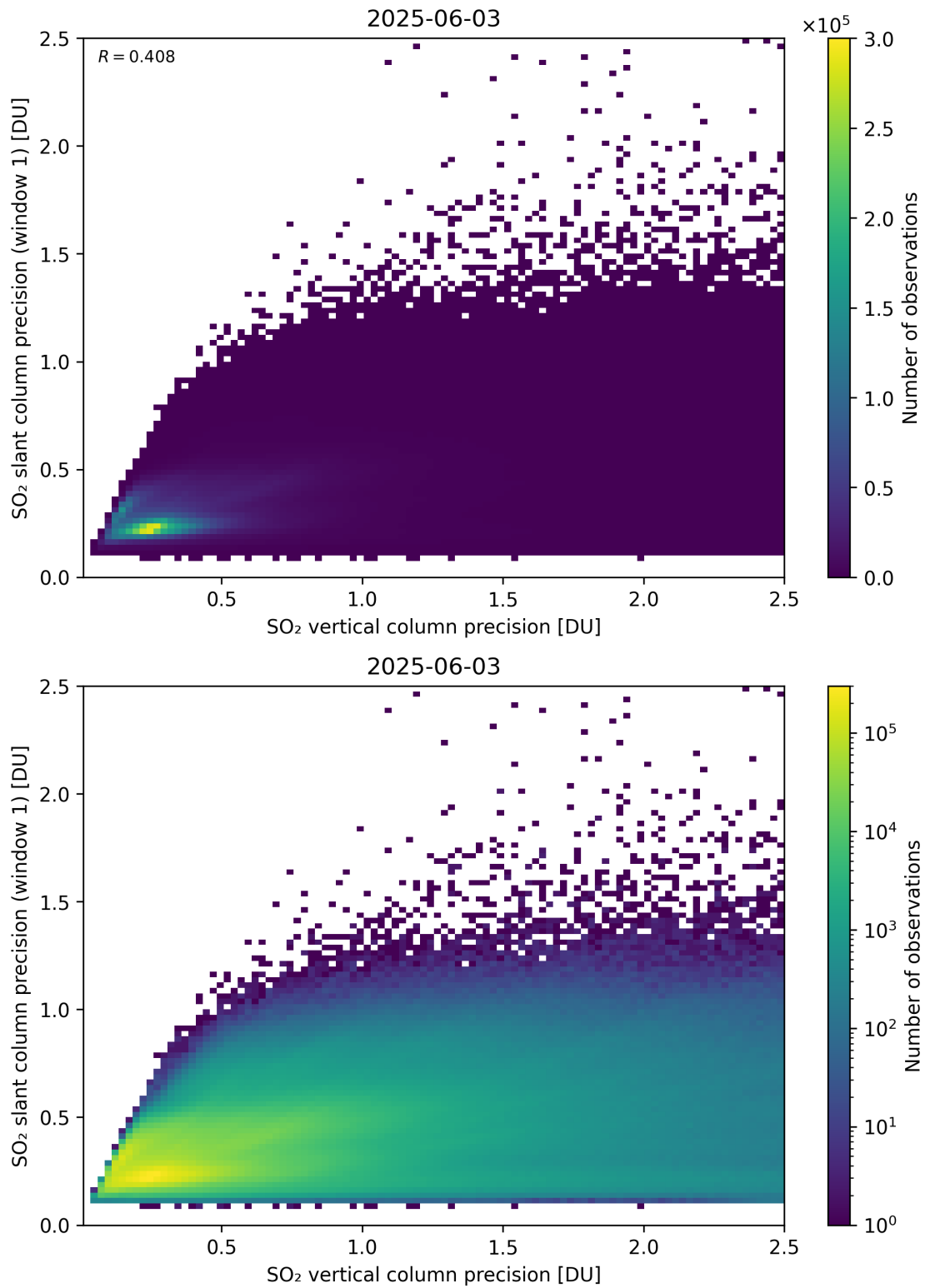
Figure 342: Scatter density plot of “SO 2 vertical column precision” against “SO 2 slant column precision (window 1)” for 2025-06-02 to 2025-06-04.
