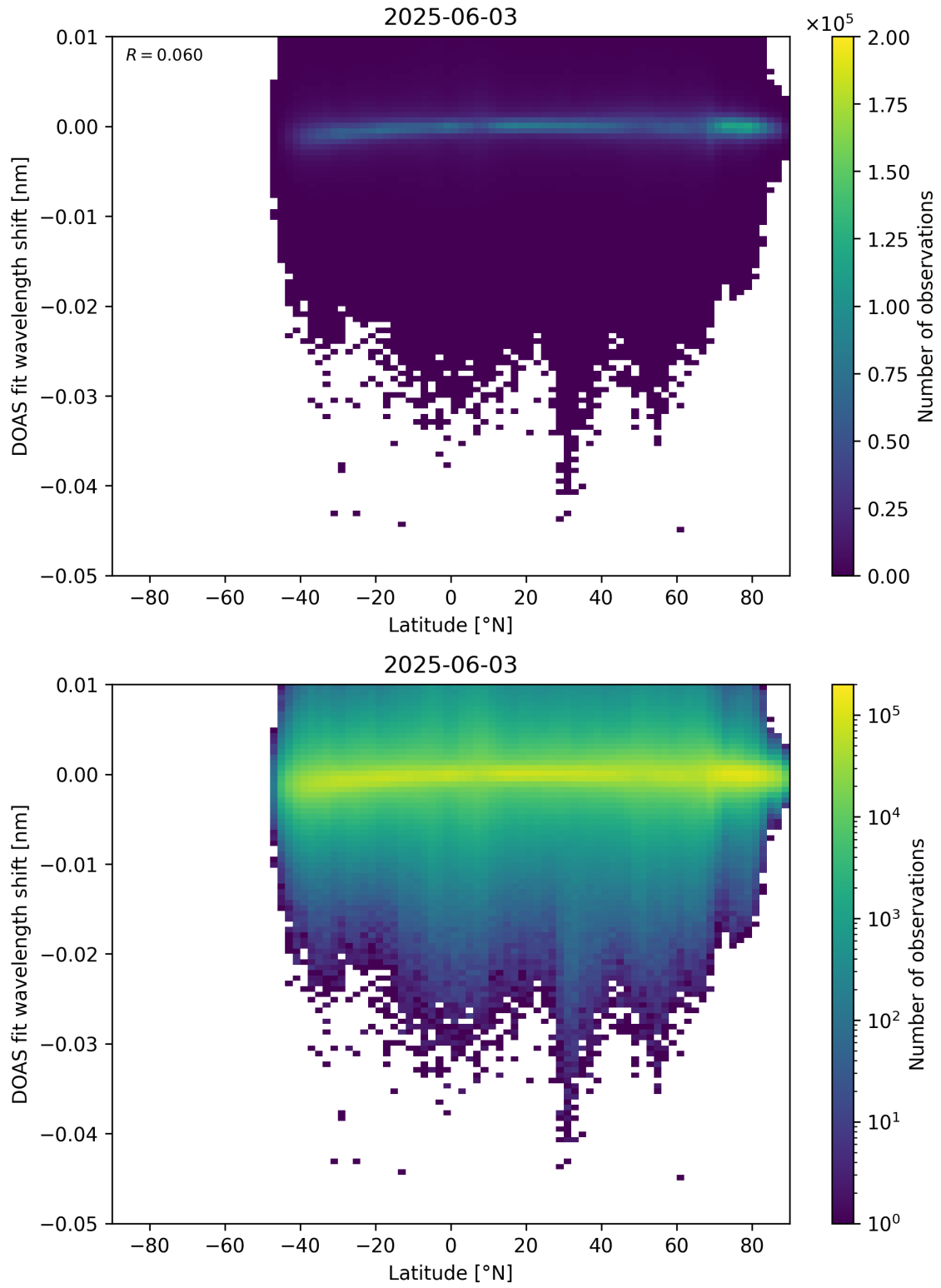
Figure 153: Scatter density plot of “Latitude” against “DOAS fit wavelength shift” for 2025-06-02 to 2025-06-04.
