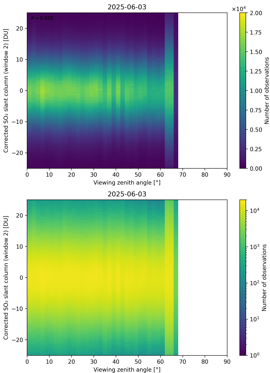
Figure 374: Scatter density plot of “Viewing zenith angle” against “Corrected SO 2 slant column (window 2)” for 2025-06-02 to 2025-06-04.
