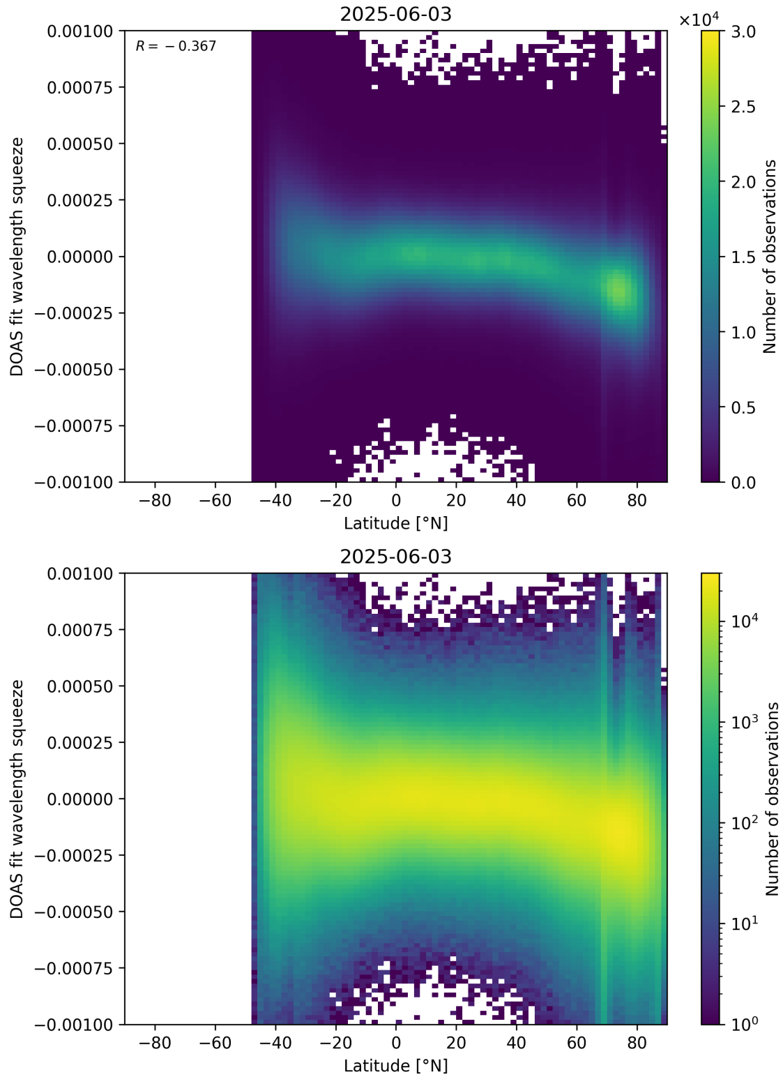
Figure 154: Scatter density plot of “Latitude” against “DOAS fit wavelength squeeze” for 2025-06-02 to 2025-06-04.
