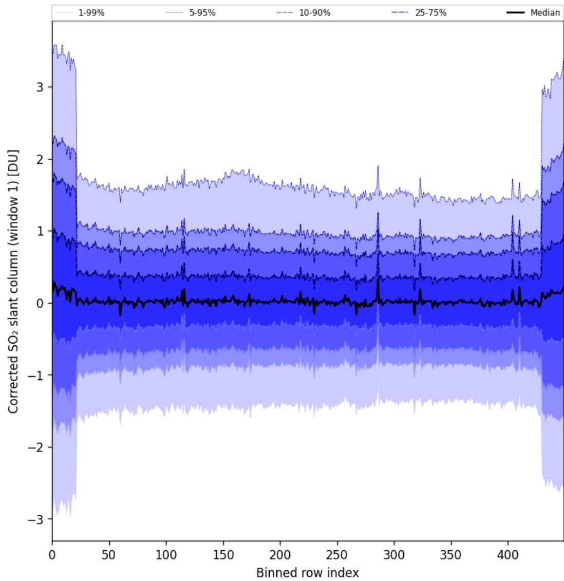
Figure 91: Along track statistics of “Corrected SO 2 slant column (window 1)” for 2025-06-02 to 2025-06-04
