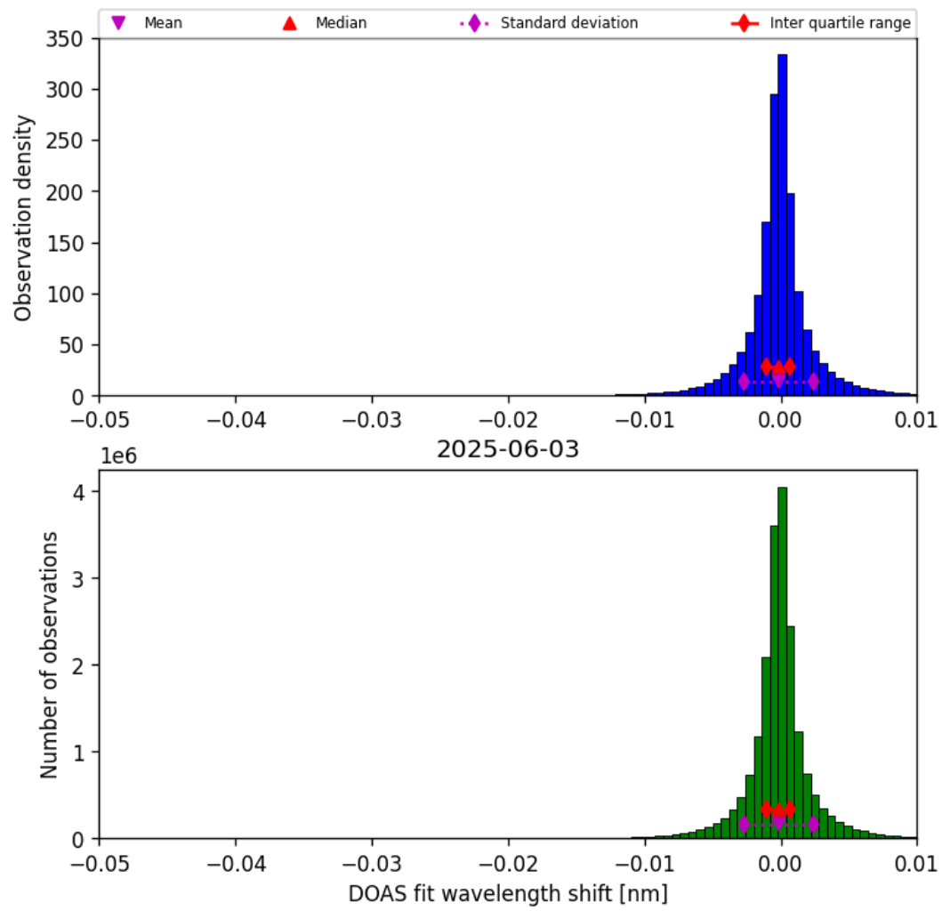
Figure 76: Histogram of “DOAS fit wavelength shift” for 2025-06-02 to 2025-06-04
