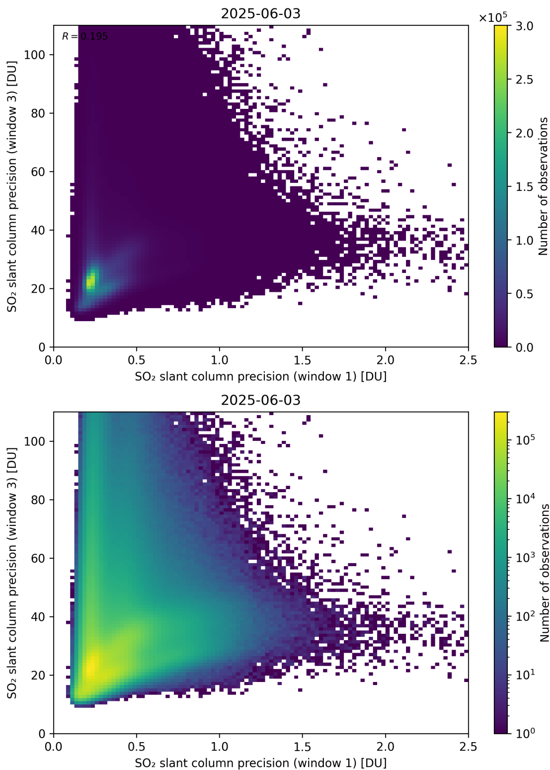
Figure 279: Scatter density plot of “SO 2 slant column precision (window 1)” against “SO 2 slant column precision (window 3)” for 2025-06-02 to 2025-06-04.
