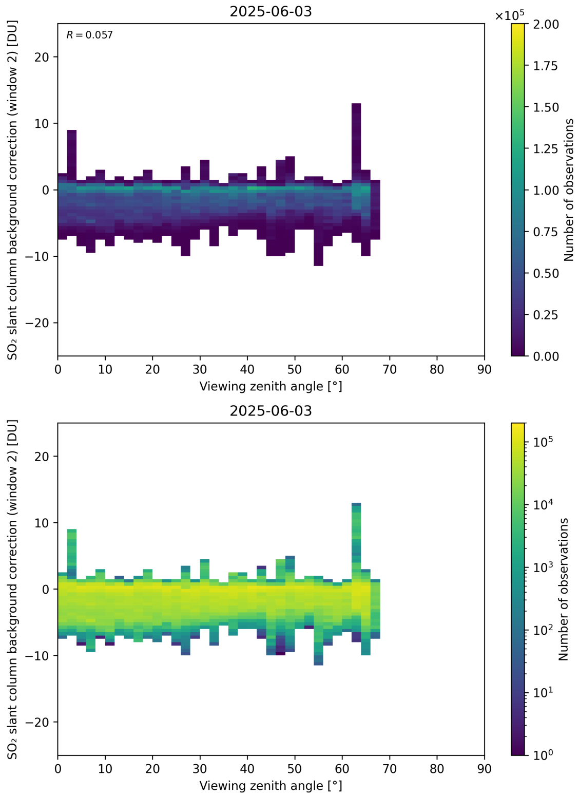
Figure 363: Scatter density plot of “Viewing zenith angle” against “SO 2 slant column background correction (window 2)” for 2025-06-02 to 2025-06-04.
