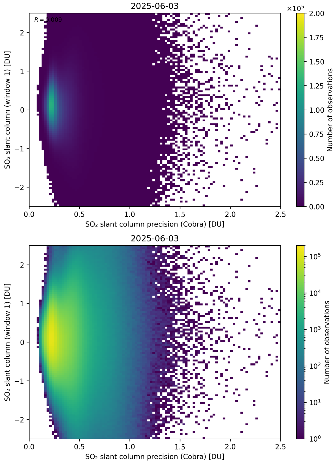
Figure 208: Scatter density plot of “SO 2 slant column precision (Cobra)” against “SO 2 slant column (window 1)” for 2025-06-02 to 2025-06-04.
