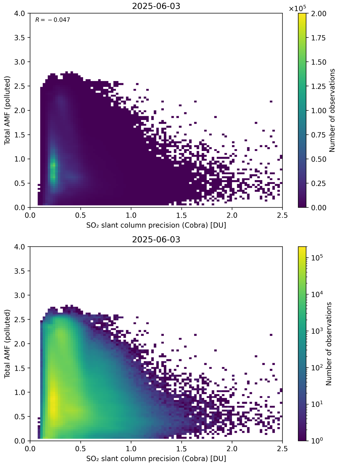
Figure 213: Scatter density plot of “SO 2 slant column precision (Cobra)” against “Total AMF (polluted)” for 2025-06-02 to 2025-06-04.
