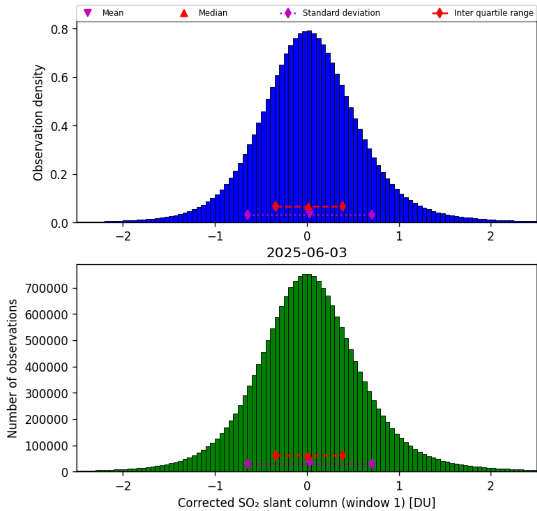
Figure 65: Histogram of "Corrected SO 2 slant column (window 1)" for 2025-06-02 to 2025-06-04
