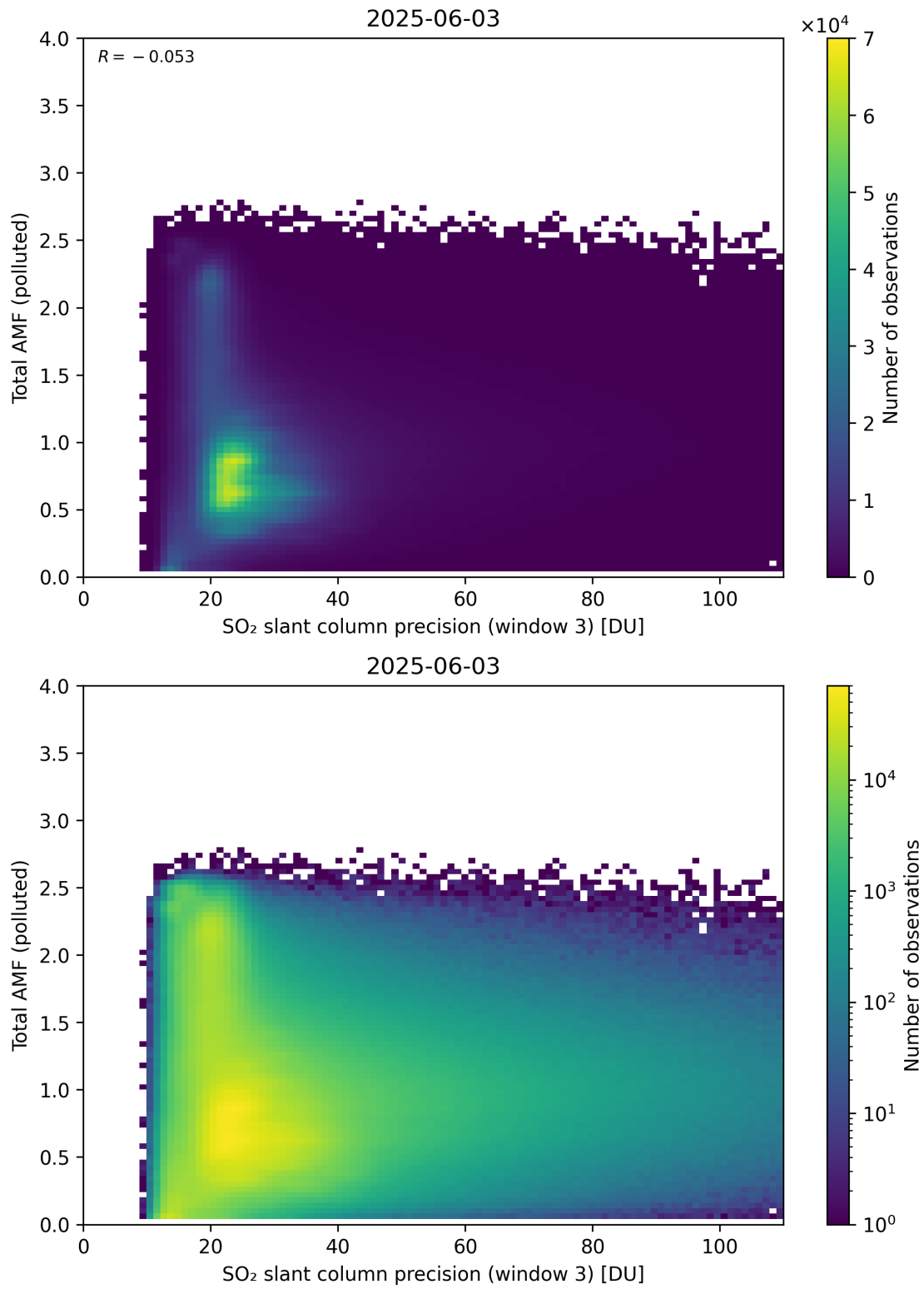
Figure 313: Scatter density plot of “SO 2 slant column precision (window 3)” against “Total AMF (polluted)” for 2025-06-02 to 2025-06-04.
