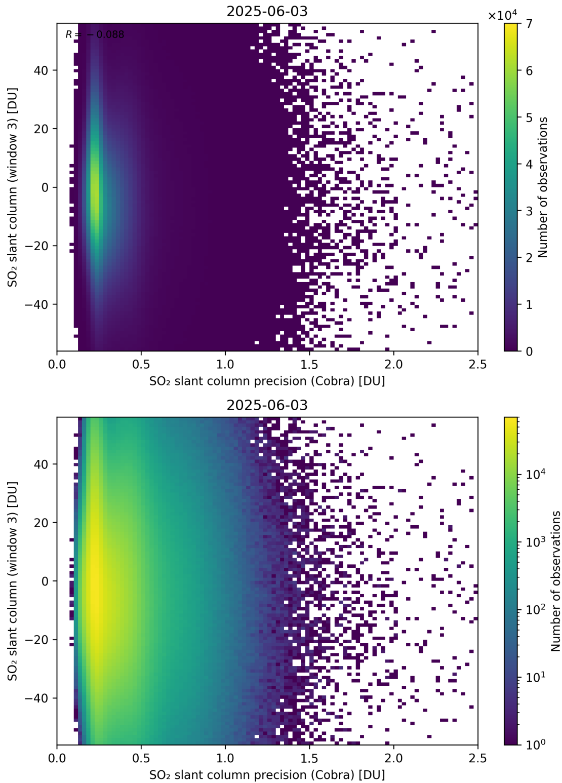
Figure 211: Scatter density plot of “SO 2 slant column precision (Cobra)” against “SO 2 slant column (window 3)” for 2025-06-02 to 2025-06-04.
