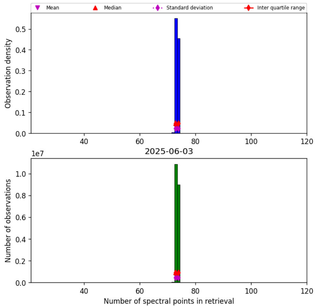
Figure 82: Histogram of “Number of spectral points in retrieval” for 2025-06-02 to 2025-06-04
