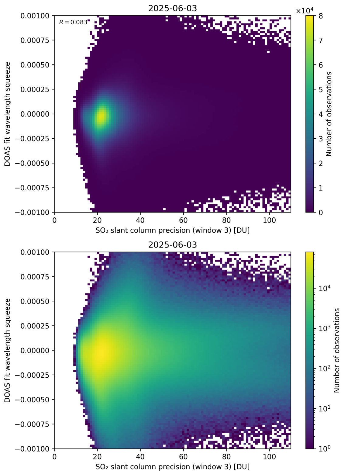
Figure 309: Scatter density plot of “SO 2 slant column precision (window 3)” against “DOAS fit wavelength squeeze” for 2025-06-02 to 2025-06-04.
