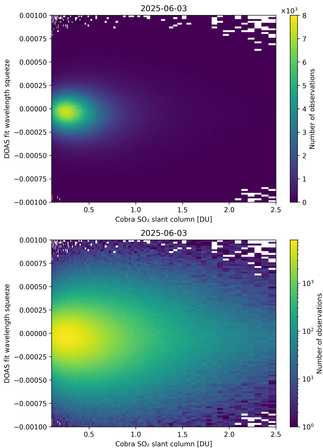
Figure 197: Scatter density plot of “Cobra SO 2 slant column” against “DOAS fit wavelength squeeze” for 2025-06-02 to 2025-06-04.
