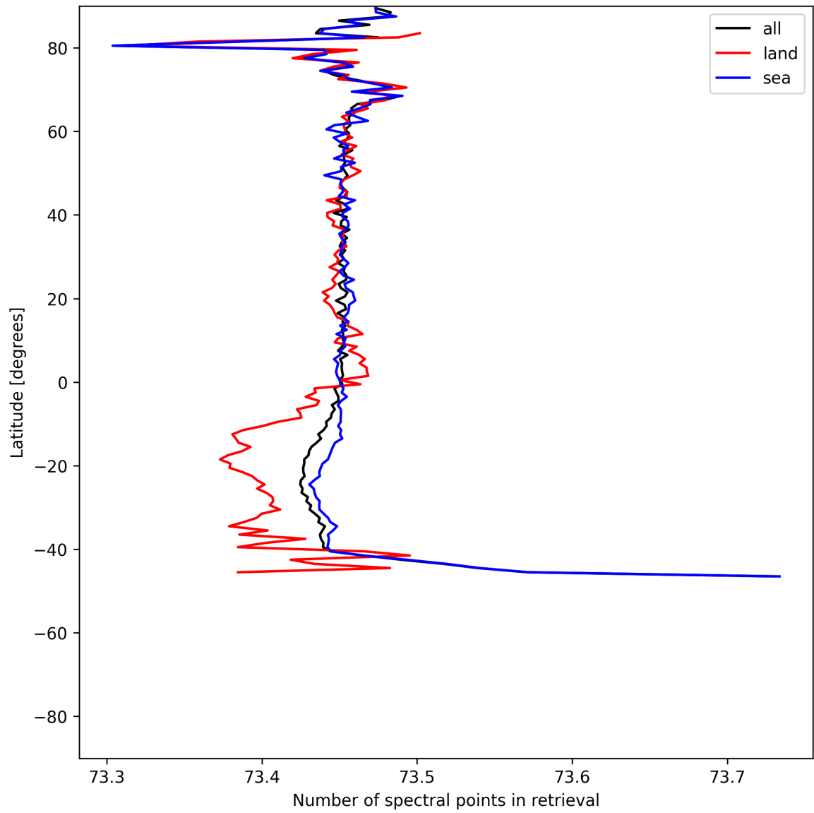
Figure 56: Zonal average of “Number of spectral points in retrieval” for 2025-06-02 to 2025-06-04.
