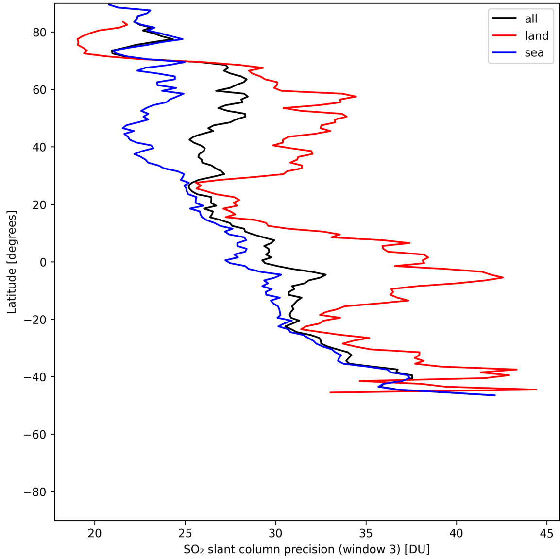
Figure 46: Zonal average of “SO 2 slant column precision (window 3)” for 2025-06-02 to 2025-06-04.
