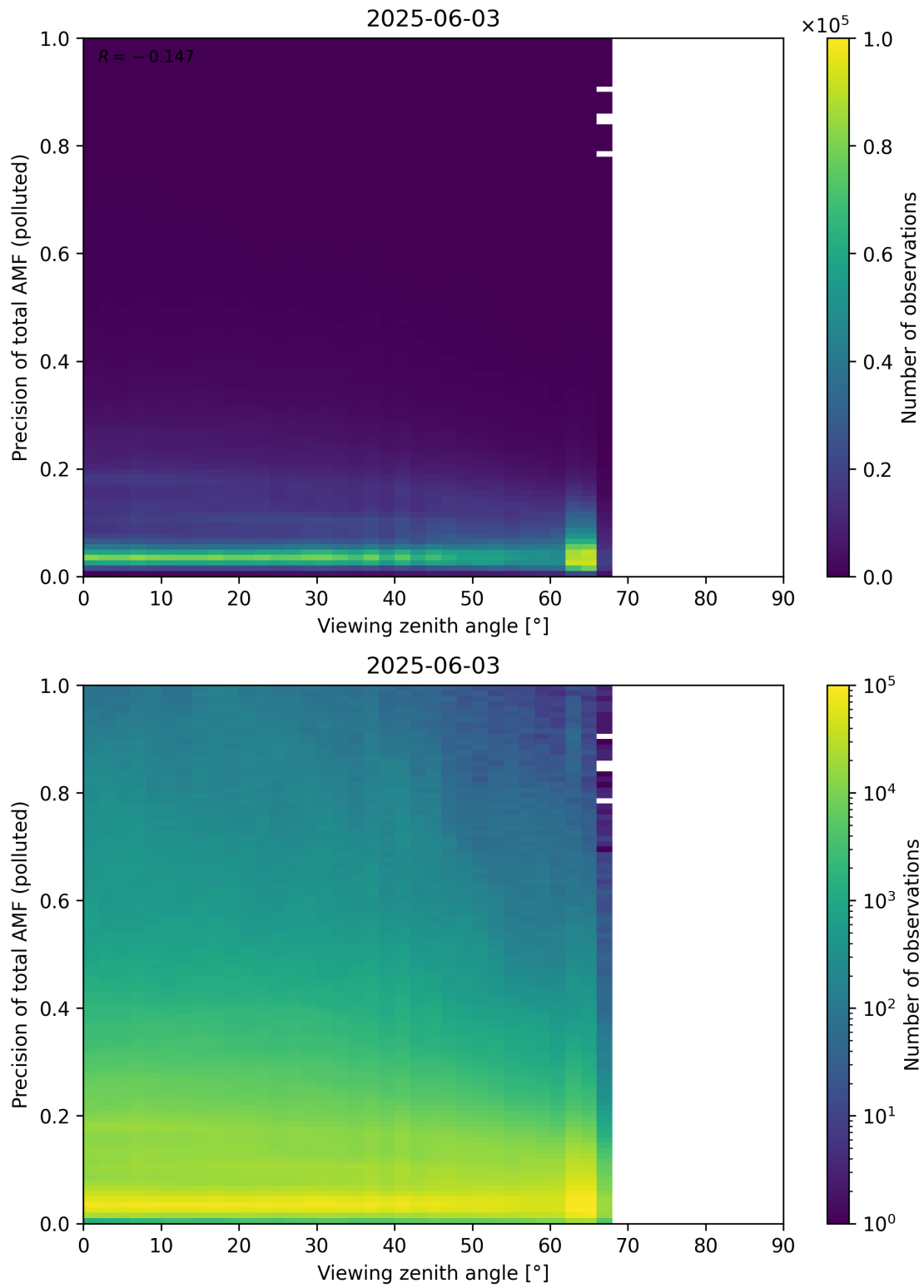
Figure 382: Scatter density plot of “Viewing zenith angle” against “Precision of total AMF (polluted)” for 2025-06-02 to 2025-06-04.
