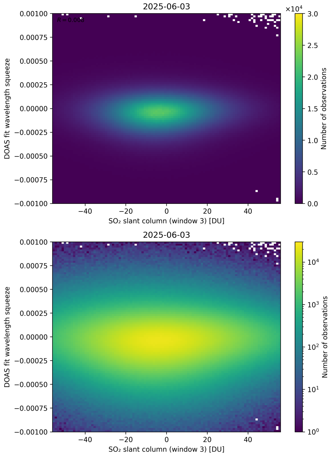
Figure 305: Scatter density plot of “SO 2 slant column (window 3)” against “DOAS fit wavelength squeeze” for 2025-06-02 to 2025-06-04.
