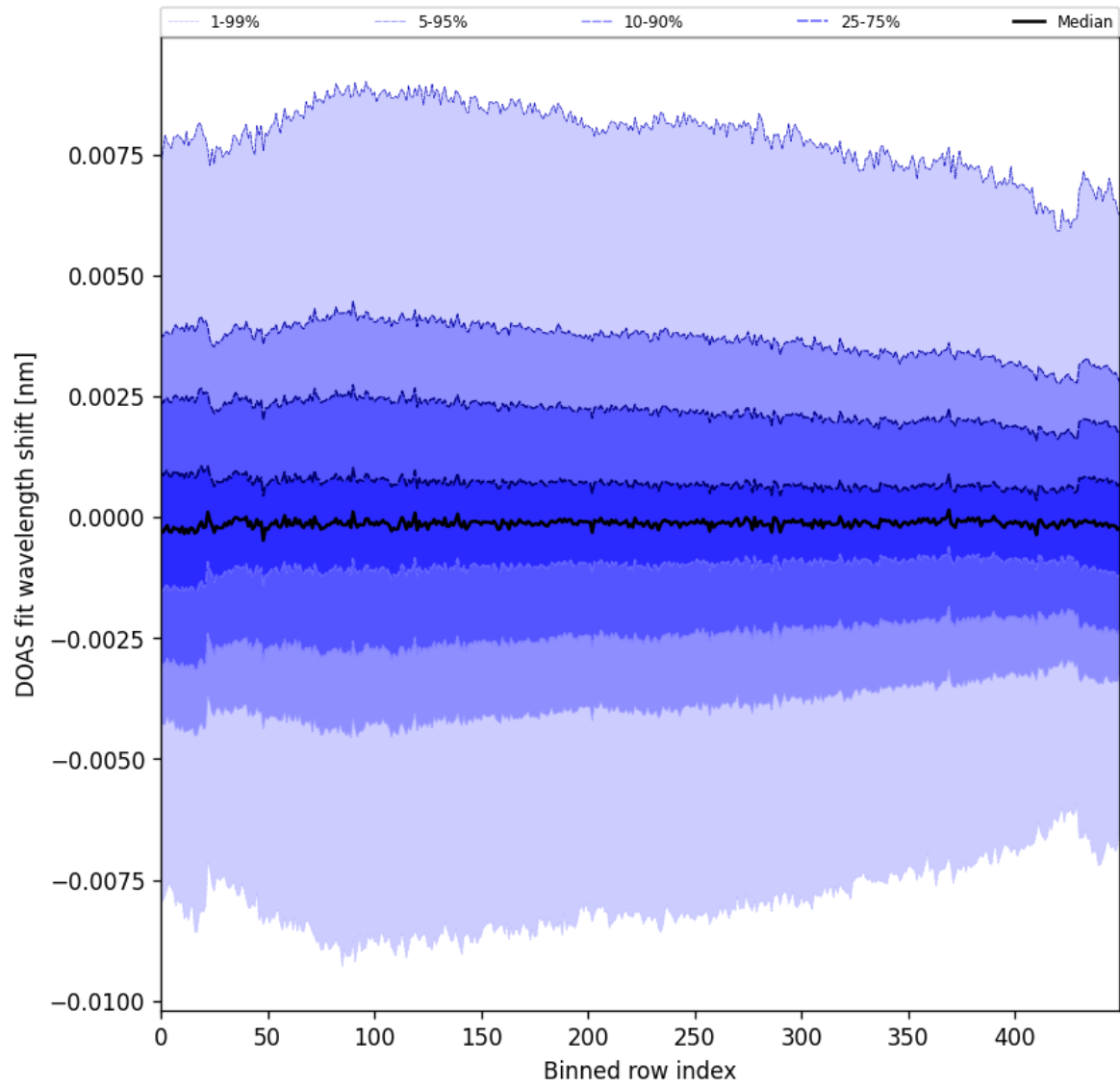
Figure 102: Along track statistics of “DOAS fit wavelength shift” for 2025-06-02 to 2025-06-04
