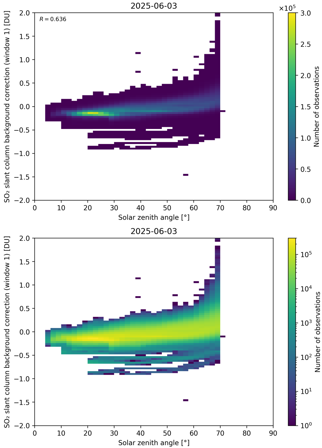
Figure 171: Scatter density plot of “Solar zenith angle” against “SO 2 slant column background correction (window 1)” for 2025-06-02 to 2025-06-04.
