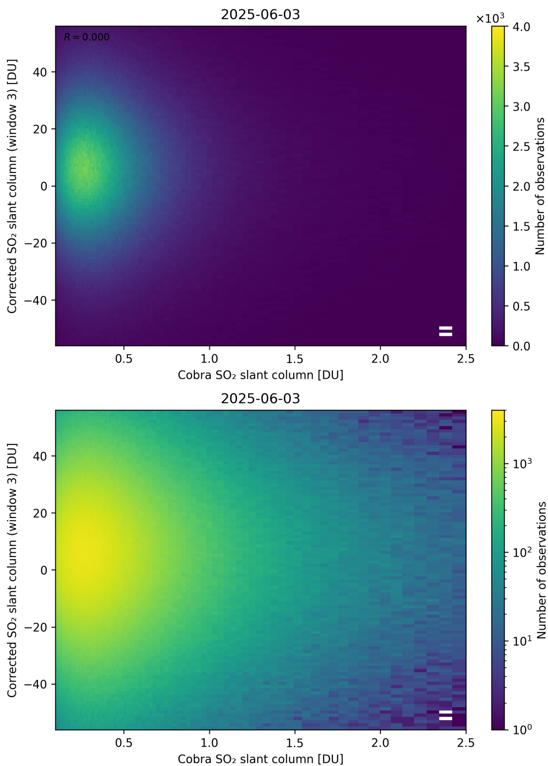
Figure 218: Scatter density plot of “Cobra SO 2 slant column” against “Corrected SO 2 slant column (window 3)” for 2025-06-02 to 2025-06-04.
