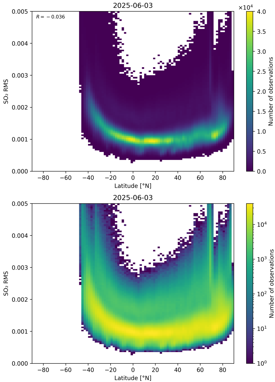
Figure 155: Scatter density plot of “Latitude” against “SO 2 RMS” for 2025-06-02 to 2025-06-04.
