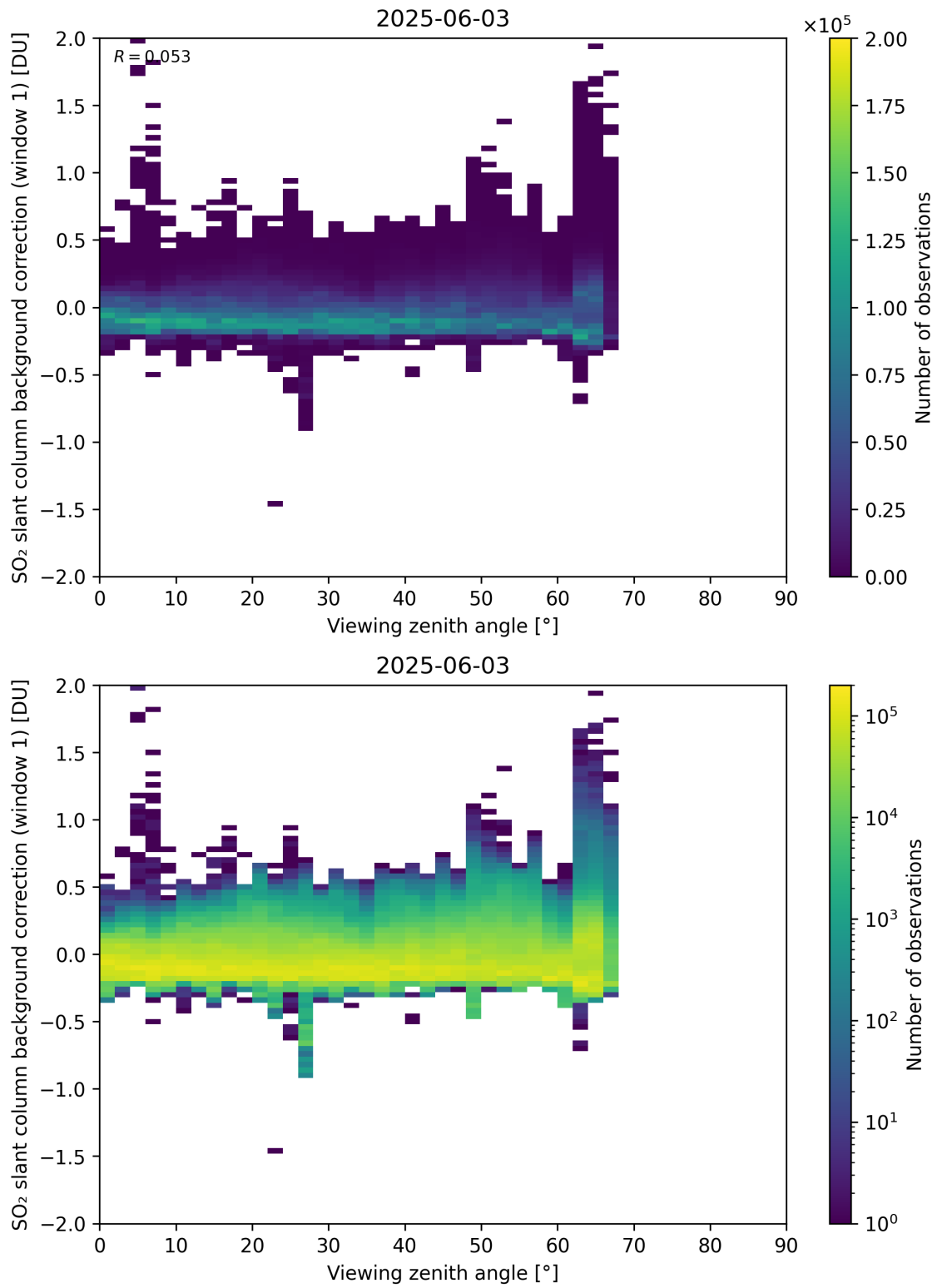
Figure 362: Scatter density plot of “Viewing zenith angle” against “SO 2 slant column background correction (window 1)” for 2025-06-02 to 2025-06-04.
