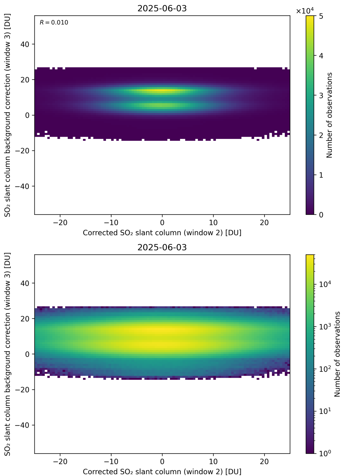
Figure 245: Scatter density plot of “Corrected SO 2 slant column (window 2)” against “SO 2 slant column background correction (window 3)” for 2025-06-02 to 2025-06-04.
