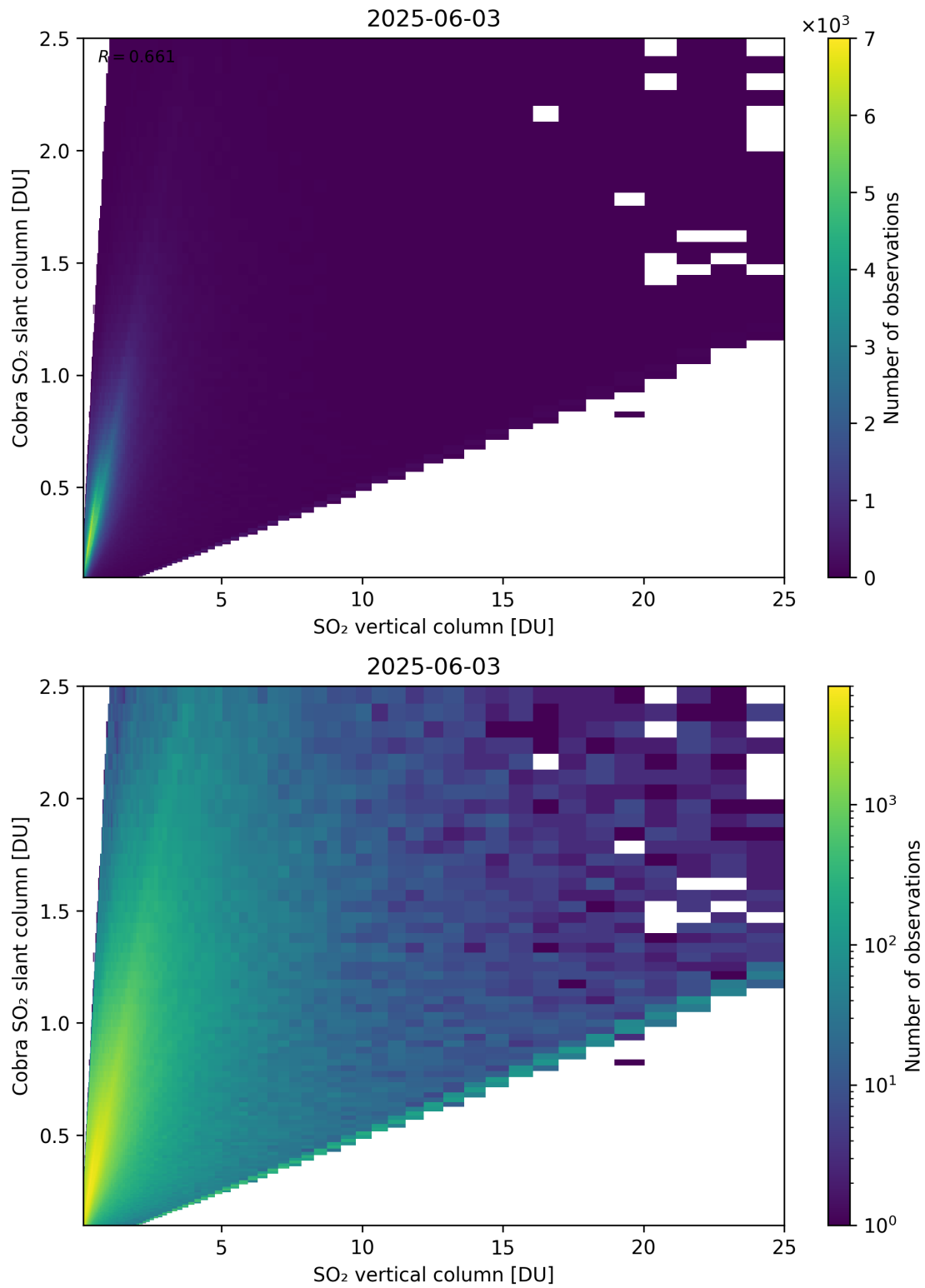
Figure 349: Scatter density plot of “SO 2 vertical column” against “Cobra SO 2 slant column” for 2025-06-02 to 2025-06-04.
