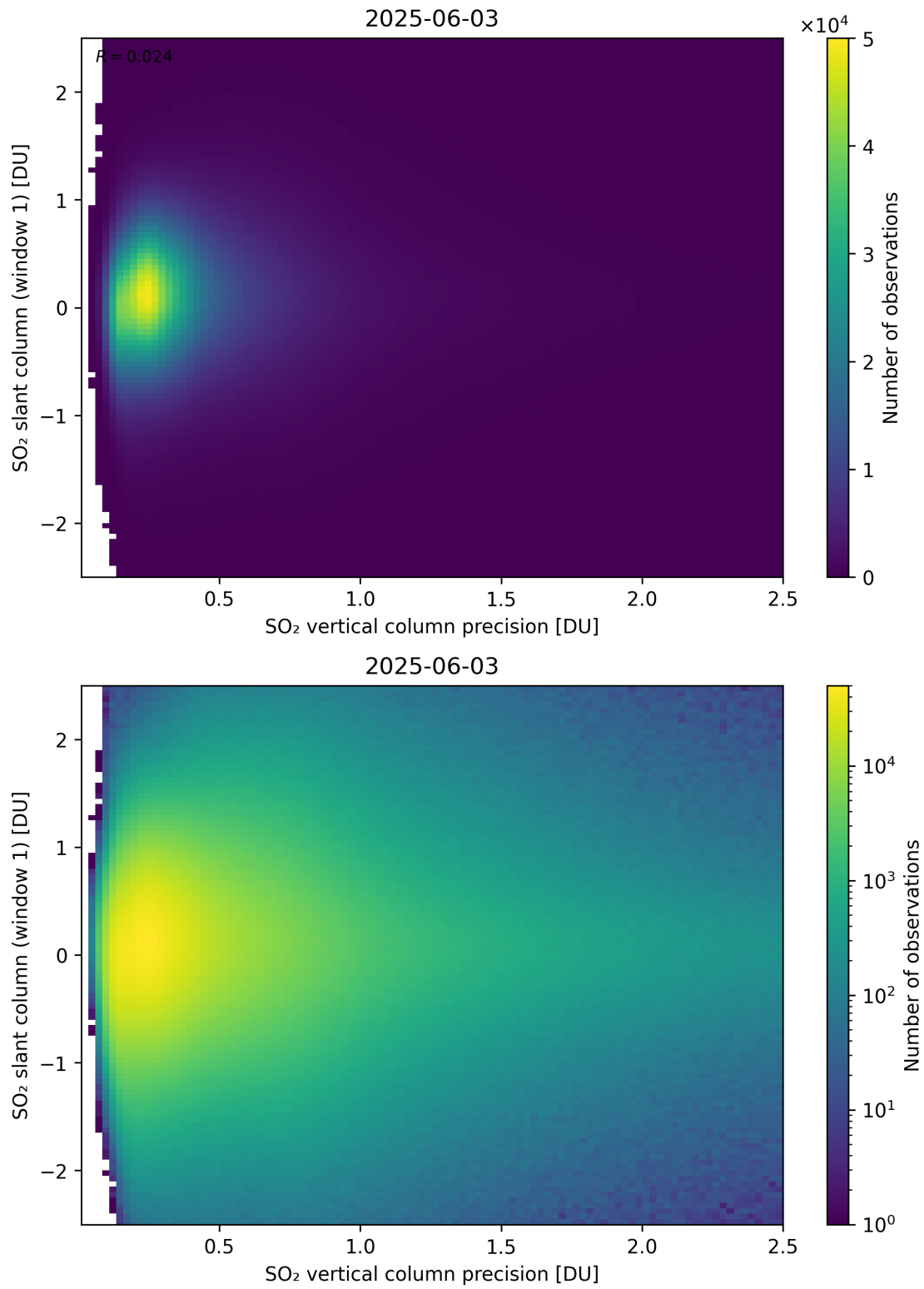
Figure 341: Scatter density plot of “SO 2 vertical column precision” against “SO 2 slant column (window 1)” for 2025-06-02 to 2025-06-04.
