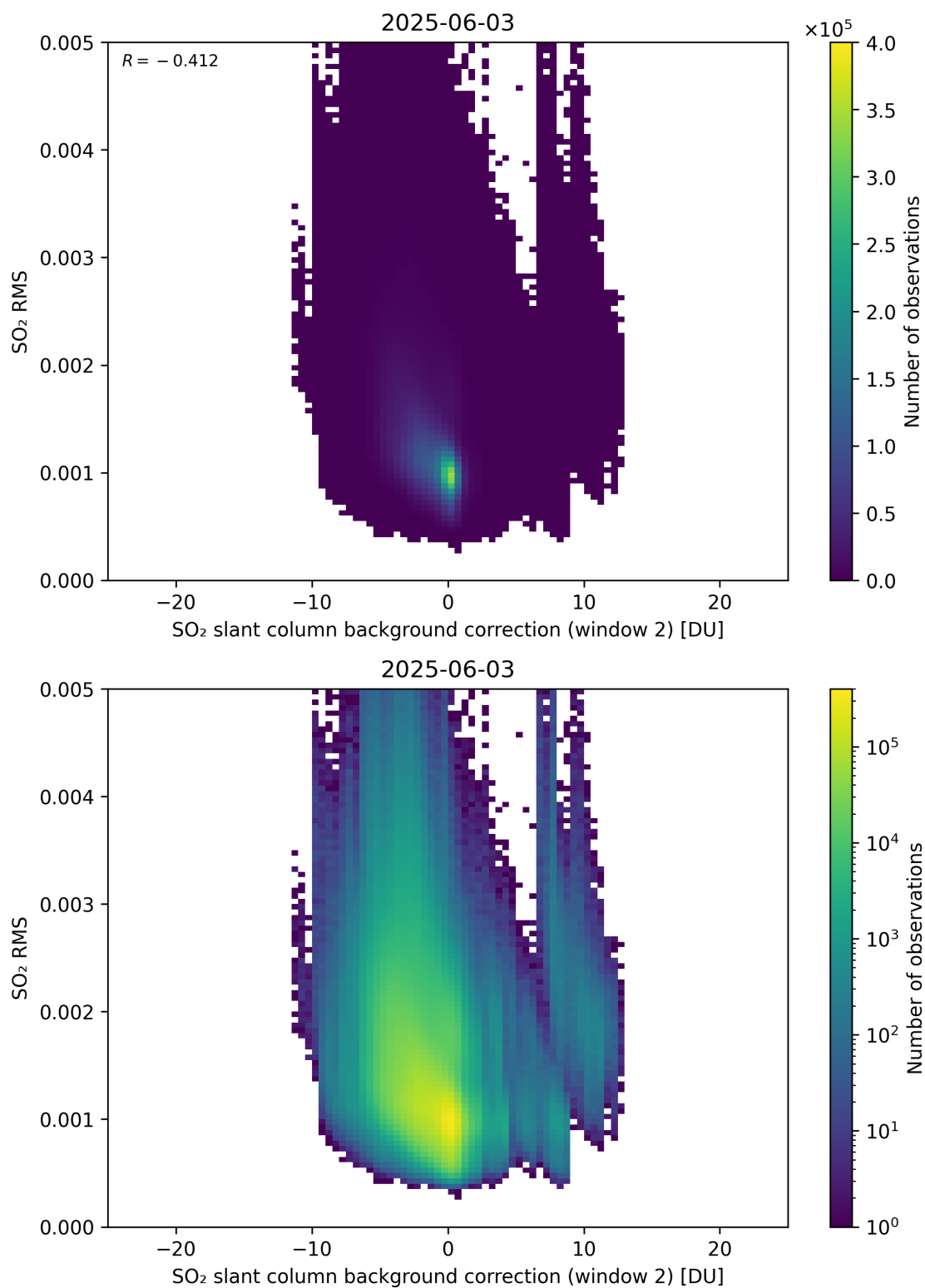
Figure 125: Scatter density plot of “SO 2 slant column background correction (window 2)” against “SO 2 RMS” for 2025-06-02 to 2025-06-04.
