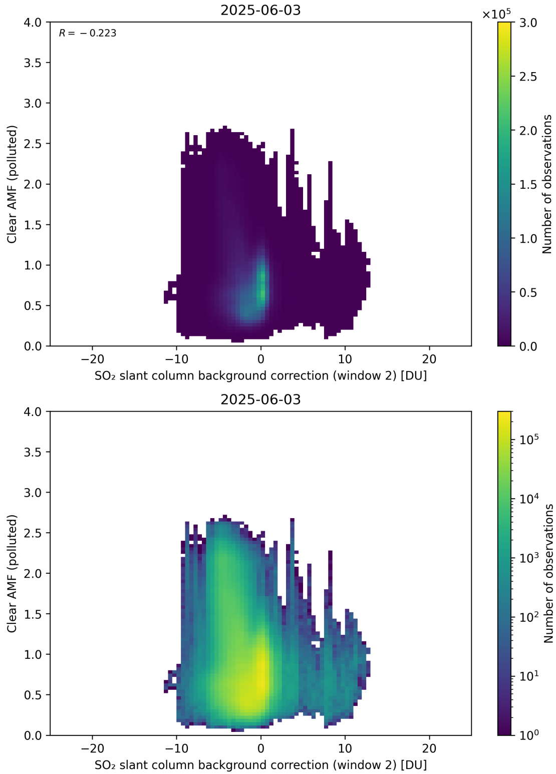
Figure 126: Scatter density plot of “SO 2 slant column background correction (window 2)” against “Clear AMF (polluted)” for 2025-06-02 to 2025-06-04.
