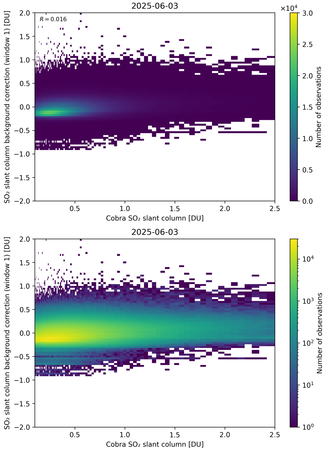
Figure 193: Scatter density plot of “Cobra SO 2 slant column” against “SO 2 slant column background correction (window 1)” for 2025-06-02 to 2025-06-04.
