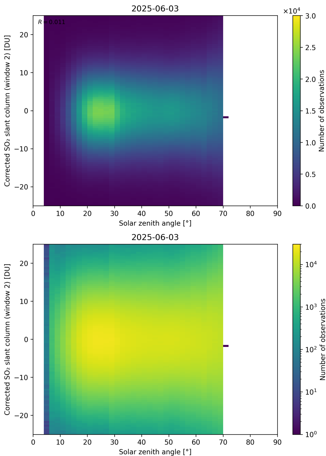
Figure 182: Scatter density plot of “Solar zenith angle” against “Corrected SO 2 slant column (window 2)” for 2025-06-02 to 2025-06-04.
