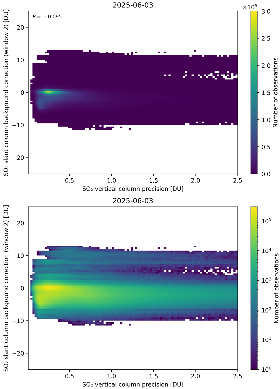
Figure 330: Scatter density plot of “SO 2 vertical column precision” against “SO 2 slant column background correction (window 2)” for 2025-06-02 to 2025-06-04.
