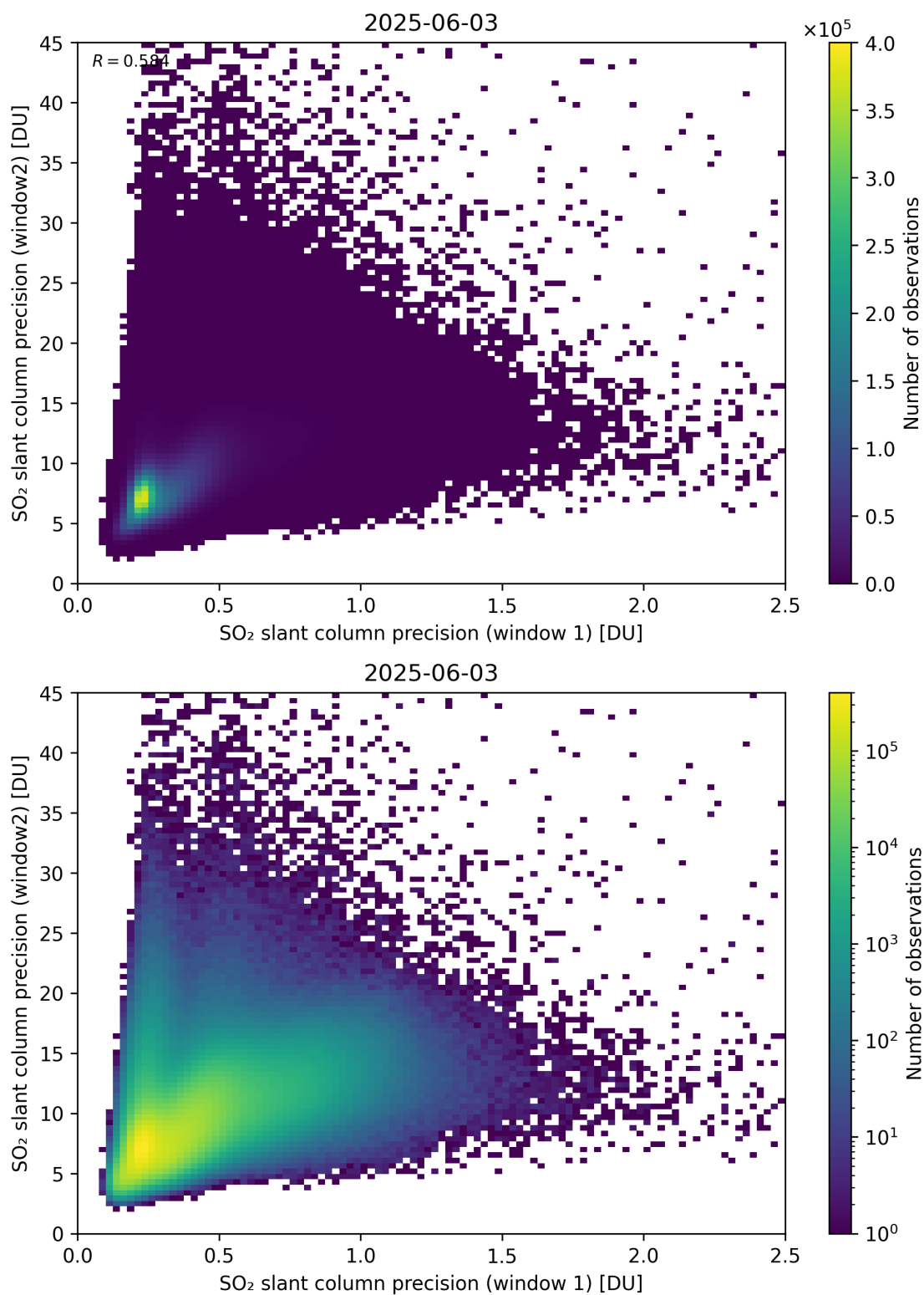
Figure 277: Scatter density plot of “SO 2 slant column precision (window 1)” against “SO 2 slant column precision (window2)” for 2025-06-02 to 2025-06-04.
