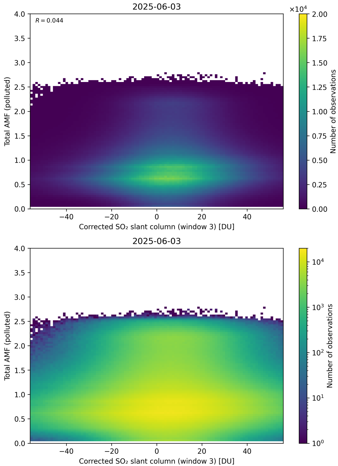
Figure 260: Scatter density plot of “Corrected SO 2 slant column (window 3)” against “Total AMF (polluted)” for 2025-06-02 to 2025-06-04.
