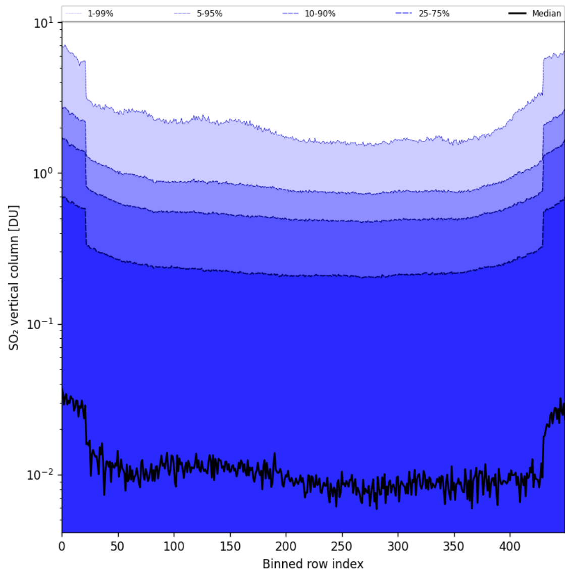
Figure 84: Along track statistics of “SO 2 vertical column” for 2025-06-02 to 2025-06-04
