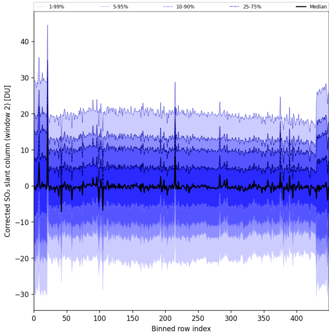
Figure 95: Along track statistics of “Corrected SO 2 slant column (window 2)” for 2025-06-02 to 2025-06-04
