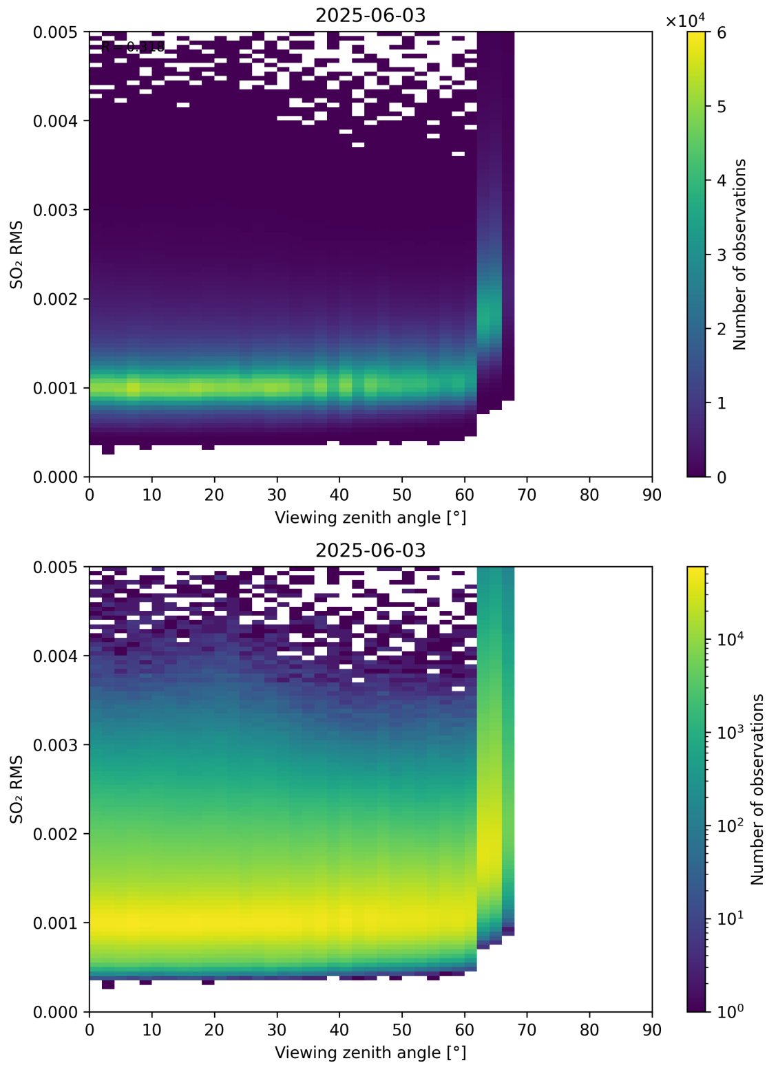
Figure 367: Scatter density plot of “Viewing zenith angle” against “SO 2 RMS” for 2025-06-02 to 2025-06-04.
