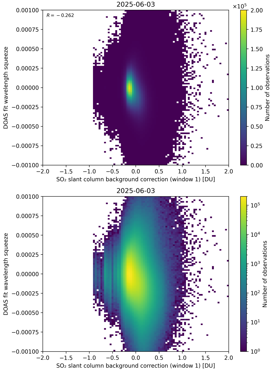
Figure 112: Scatter density plot of “SO 2 slant column background correction (window 1)” against “DOAS fit wavelength squeeze” for 2025-06-02 to 2025-06-04.
