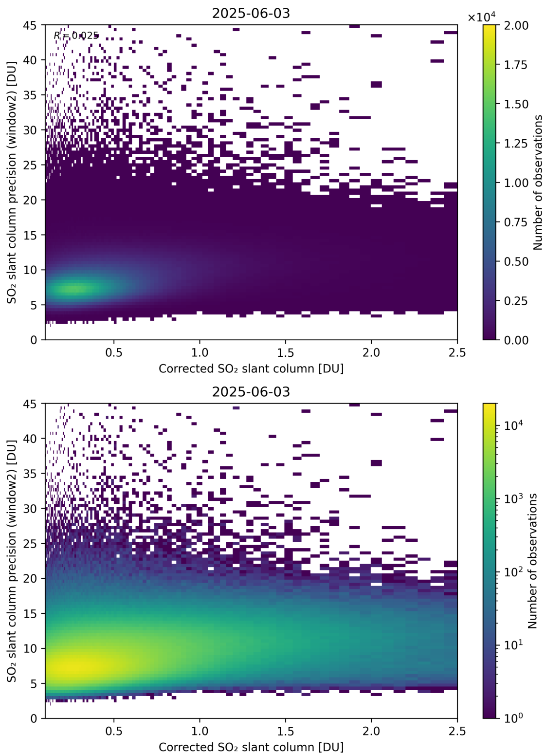
Figure 239: Scatter density plot of “Corrected SO 2 slant column” against “SO 2 slant column precision (window2)” for 2025-06-02 to 2025-06-04.
