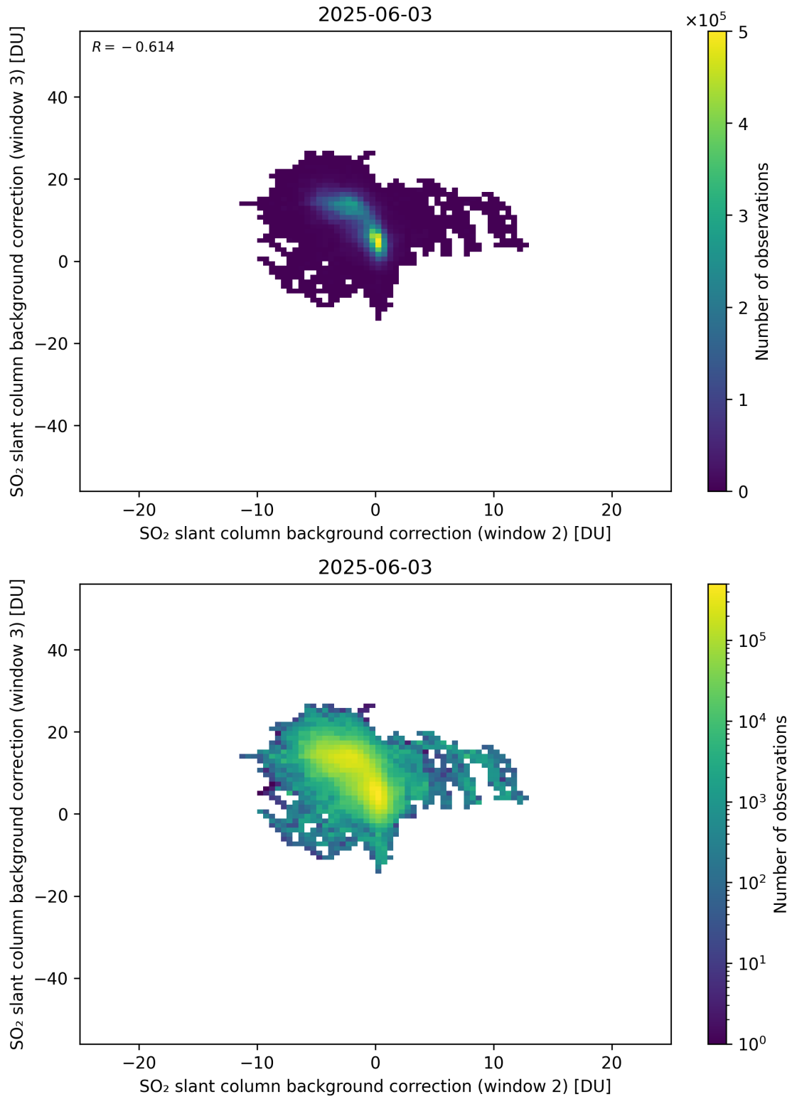
Figure 122: Scatter density plot of “SO 2 slant column background correction (window 2)” against “SO 2 slant column background correction (window 3)” for 2025-06-02 to 2025-06-04.
