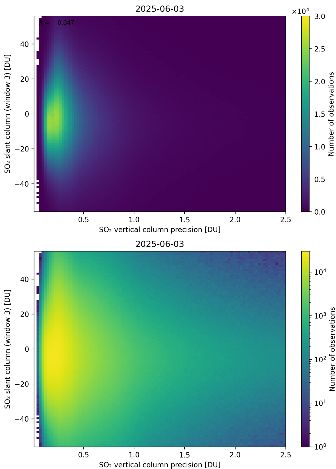
Figure 344: Scatter density plot of “SO 2 vertical column precision” against “SO 2 slant column (window 3)” for 2025-06-02 to 2025-06-04.
