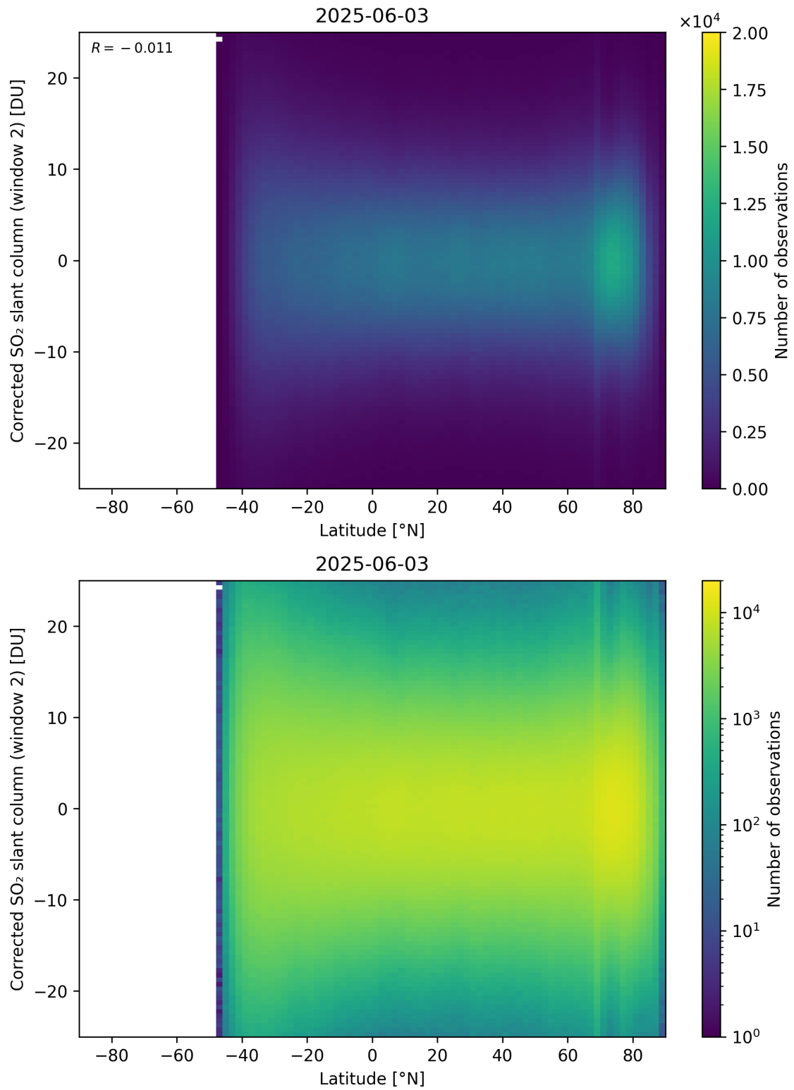
Figure 160: Scatter density plot of “Latitude” against “Corrected SO 2 slant column (window 2)” for 2025-06-02 to 2025-06-04.
