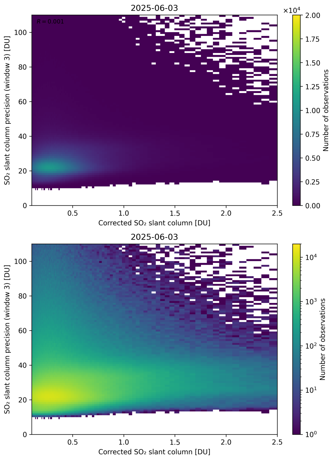
Figure 241: Scatter density plot of “Corrected SO 2 slant column” against “SO 2 slant column precision (window 3)” for 2025-06-02 to 2025-06-04.
