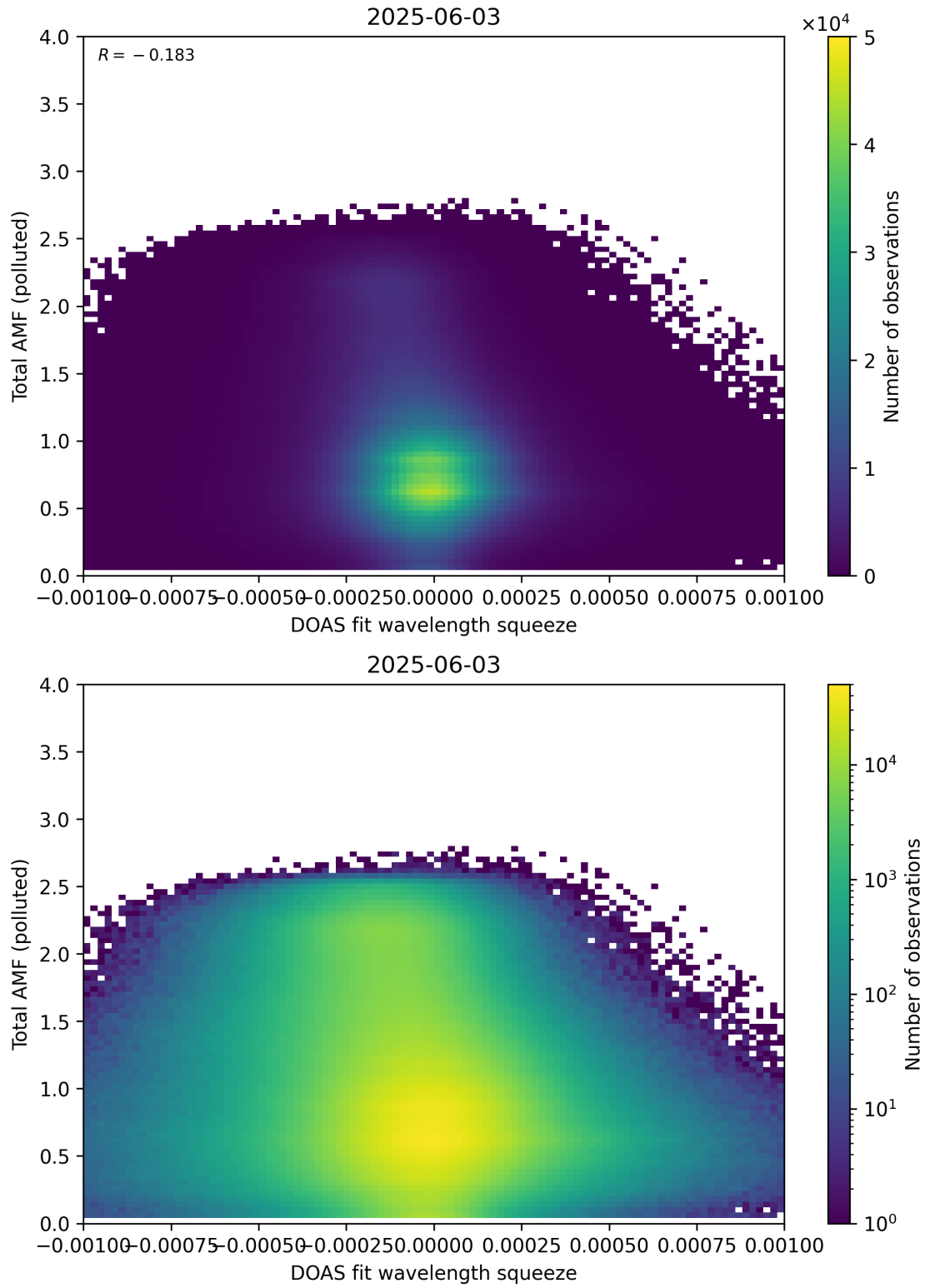
Figure 145: Scatter density plot of “DOAS fit wavelength squeeze” against “Total AMF (polluted)” for 2025-06-02 to 2025-06-04.
