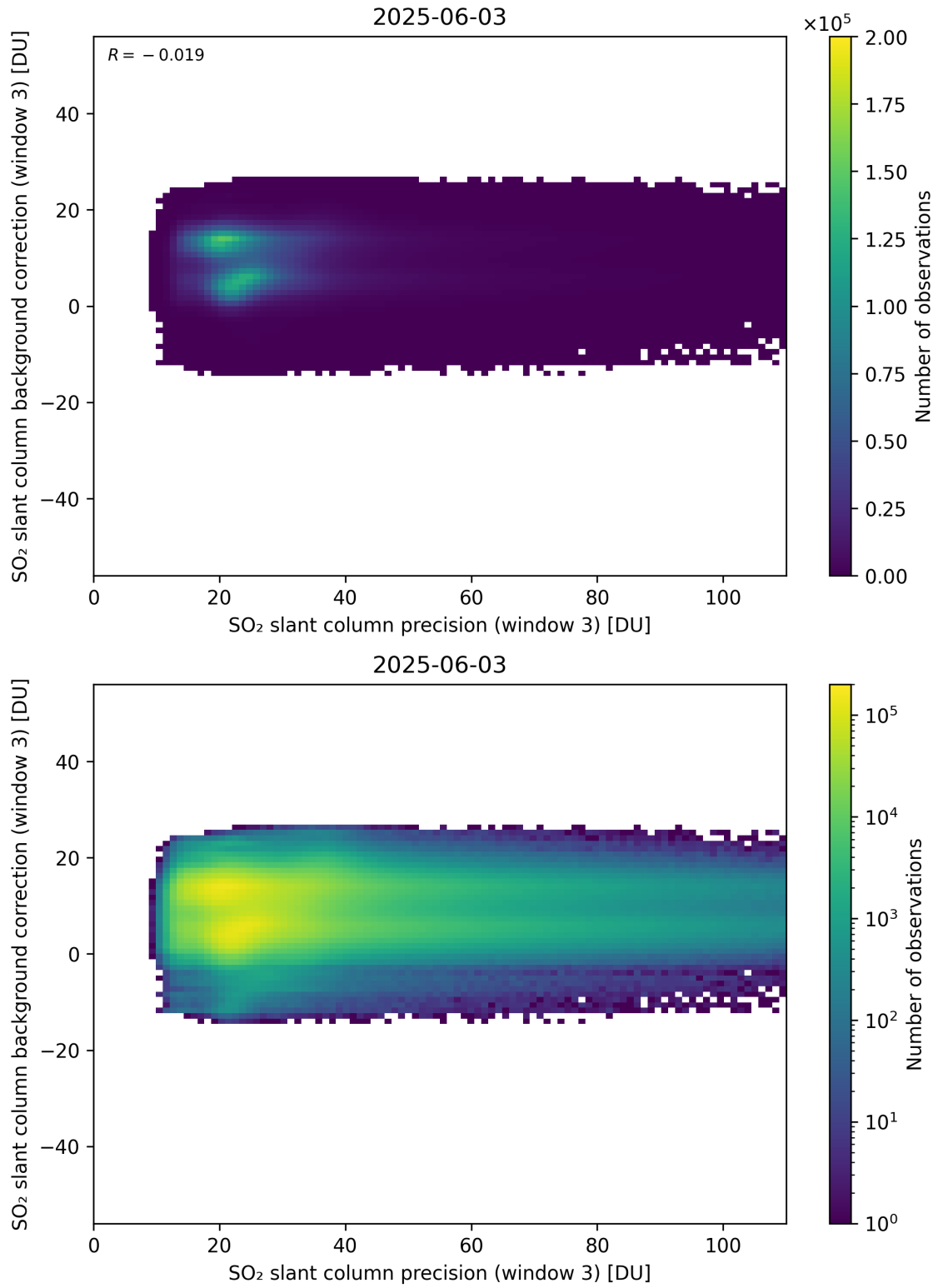
Figure 307: Scatter density plot of “SO 2 slant column precision (window 3)” against “SO 2 slant column background correction (window 3)” for 2025-06-02 to 2025-06-04.
