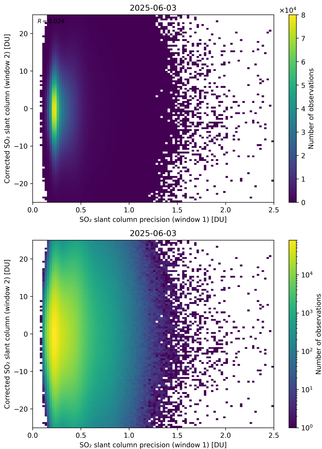
Figure 275: Scatter density plot of “SO 2 slant column precision (window 1)” against “Corrected SO 2 slant column (window 2)” for 2025-06-02 to 2025-06-04.
