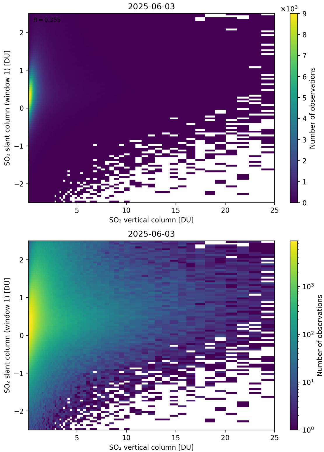
Figure 354: Scatter density plot of “SO 2 vertical column” against “SO 2 slant column (window 1)” for 2025-06-02 to 2025-06-04.
