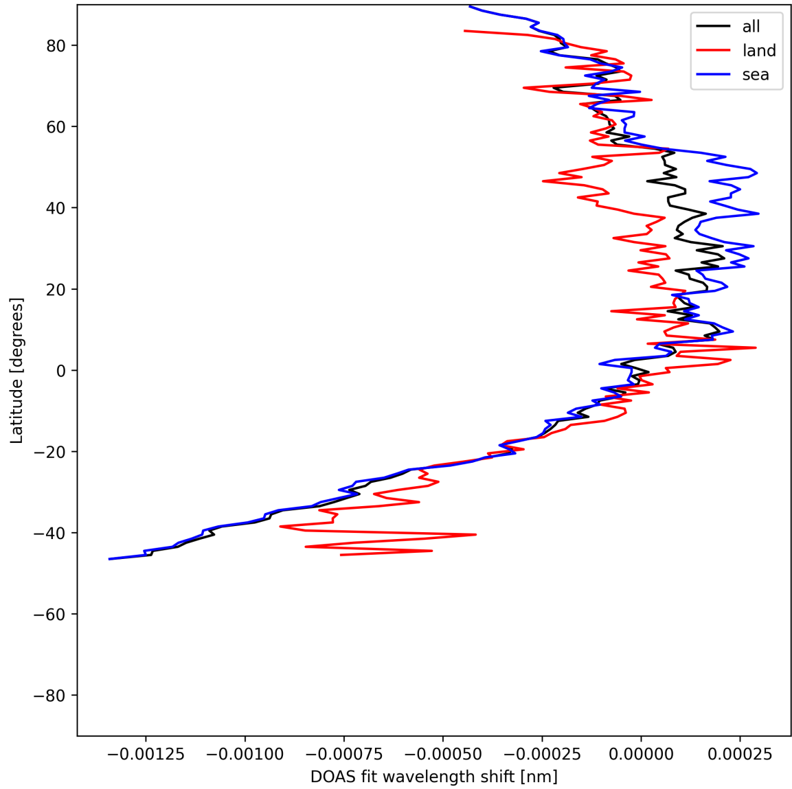
Figure 50: Zonal average of "DOAS fit wavelength shift" for 2025-06-02 to 2025-06-04.
