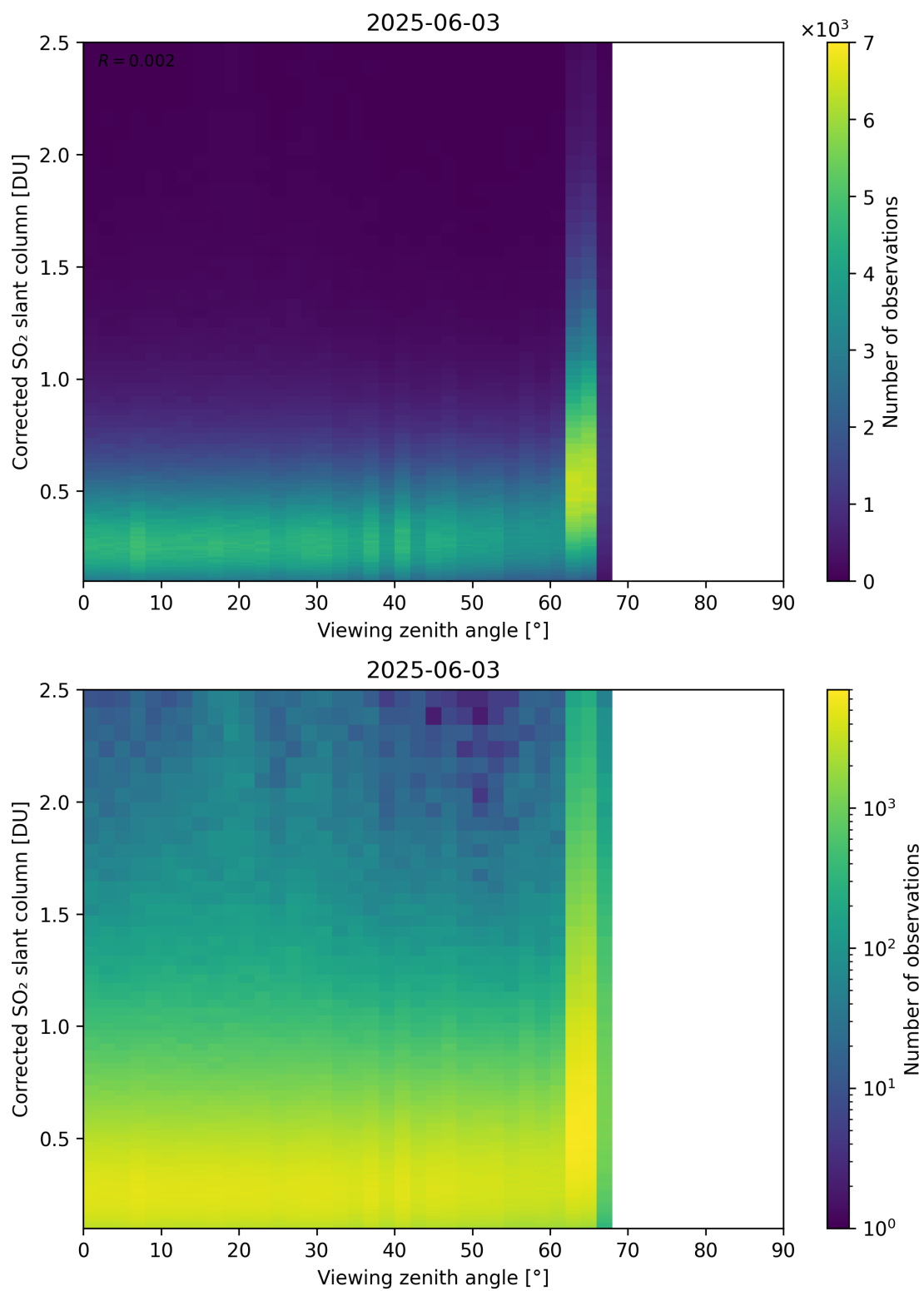
Figure 373: Scatter density plot of “Viewing zenith angle” against “Corrected SO 2 slant column” for 2025-06-02 to 2025-06-04.
