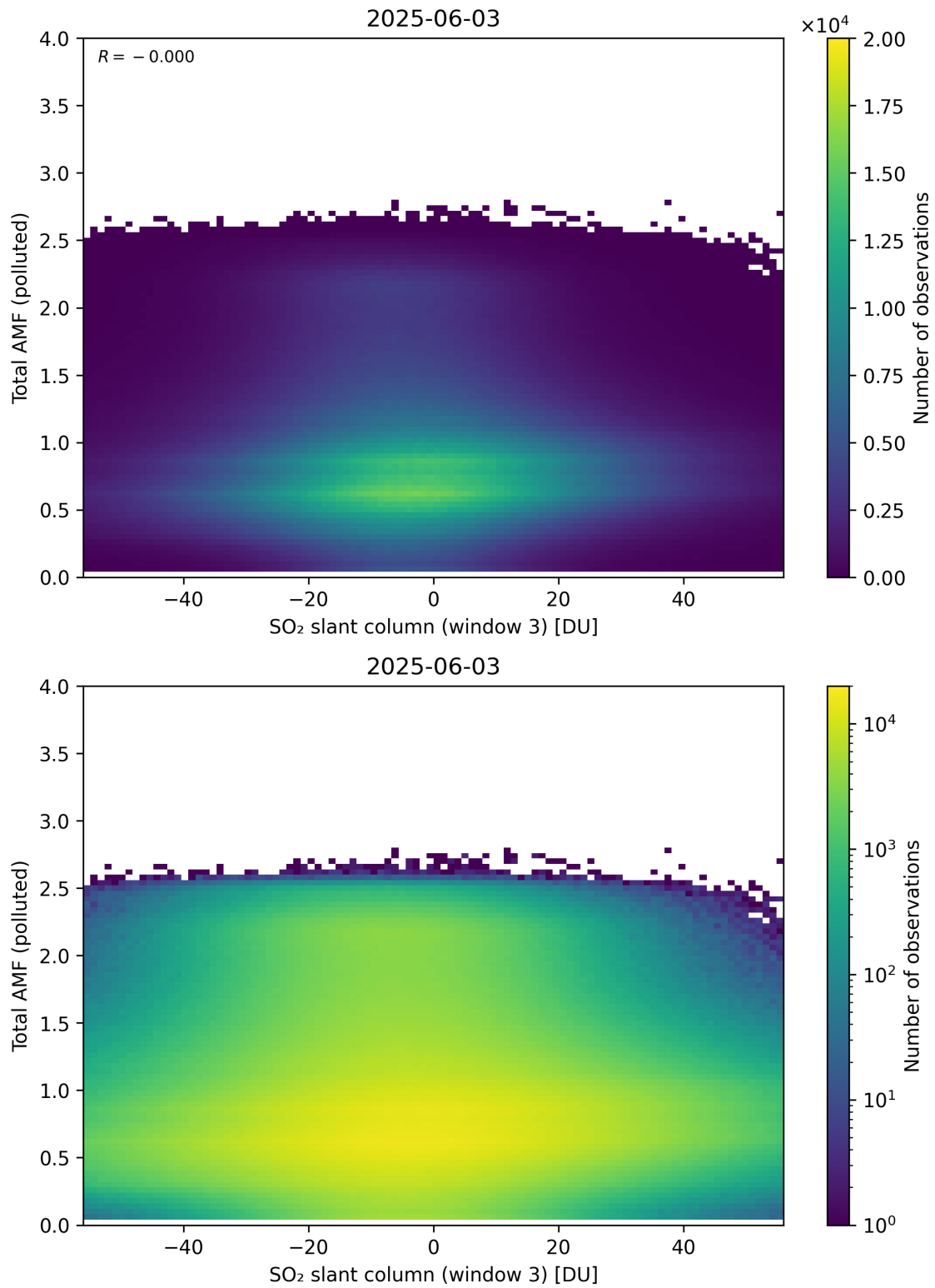
Figure 318: Scatter density plot of “SO 2 slant column (window 3)” against “Total AMF (polluted)” for 2025-06-02 to 2025-06-04.
