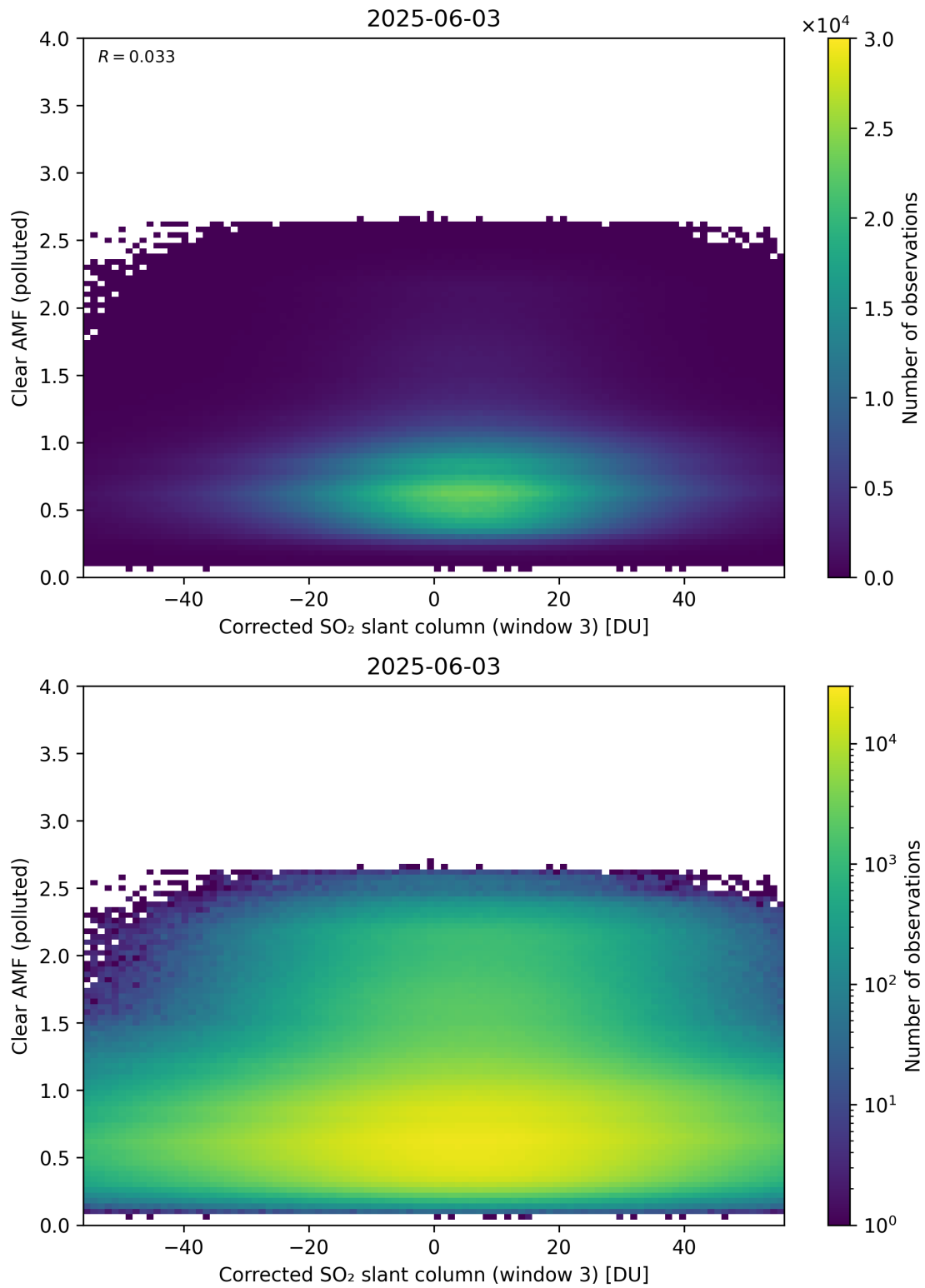
Figure 259: Scatter density plot of “Corrected SO 2 slant column (window 3)” against “Clear AMF (polluted)” for 2025-06-02 to 2025-06-04.
