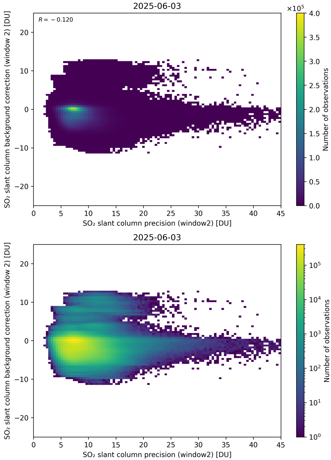
Figure 291: Scatter density plot of “SO 2 slant column precision (window2)” against “SO 2 slant column background correction (window 2)” for 2025-06-02 to 2025-06-04.
