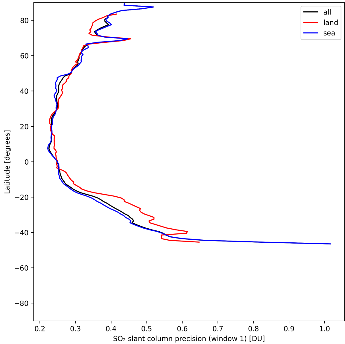
Figure 38: Zonal average of “SO 2 slant column precision (window 1)” for 2025-06-02 to 2025-06-04.
