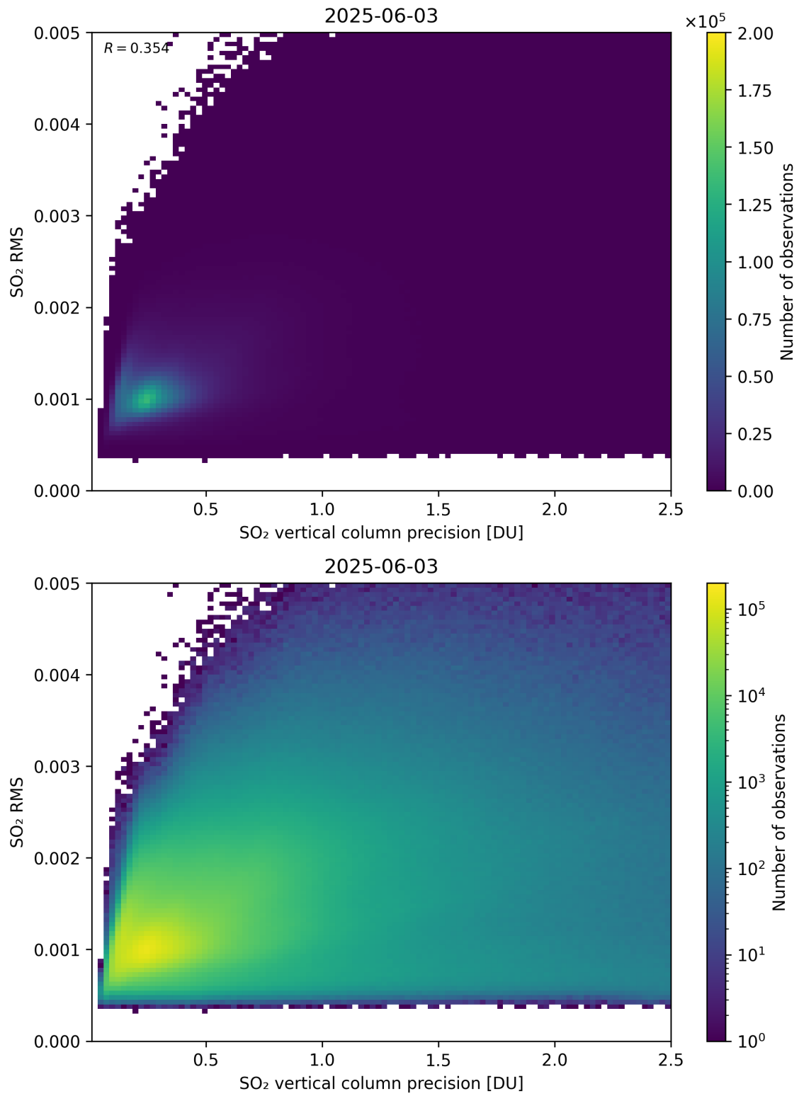
Figure 334: Scatter density plot of “SO 2 vertical column precision” against “SO 2 RMS” for 2025-06-02 to 2025-06-04.
