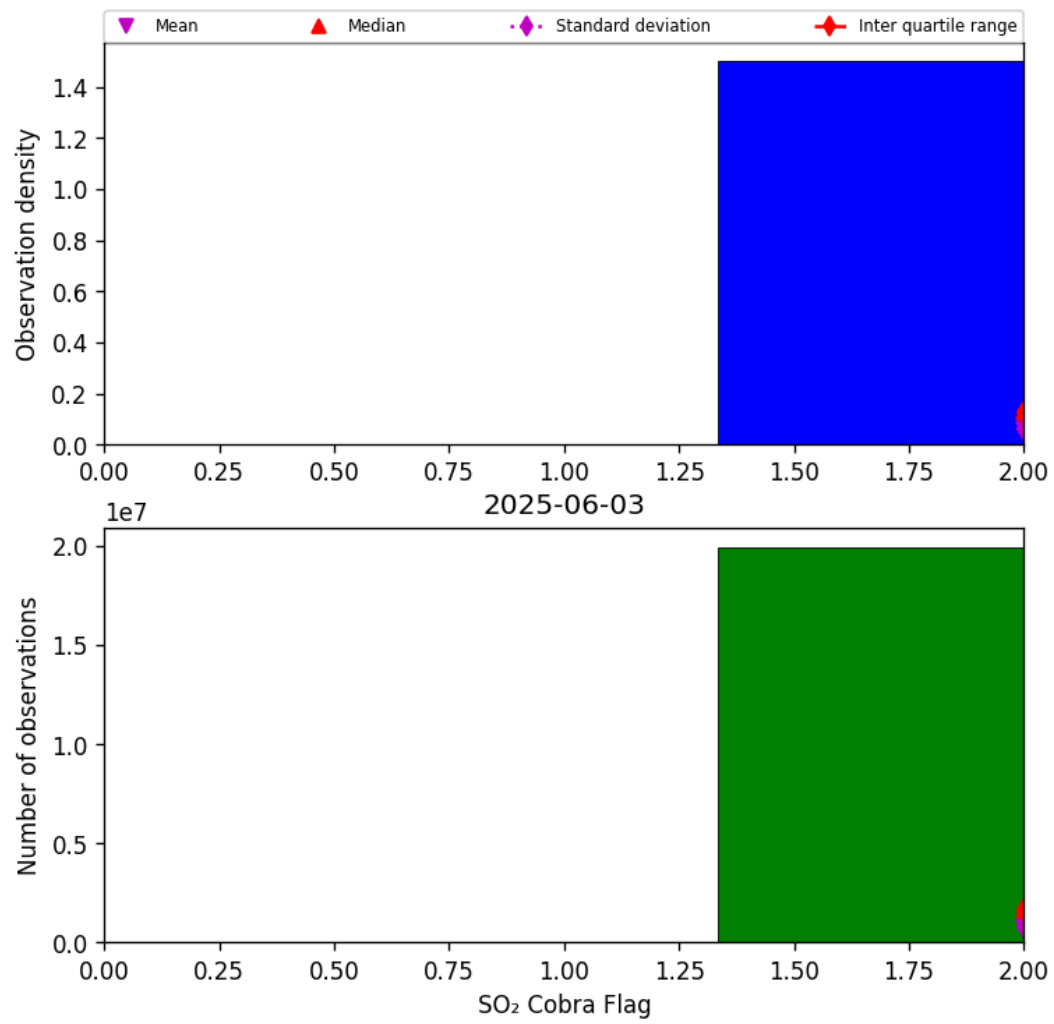
Figure 75: Histogram of “SO 2 Cobra Flag” for 2025-06-02 to 2025-06-04
