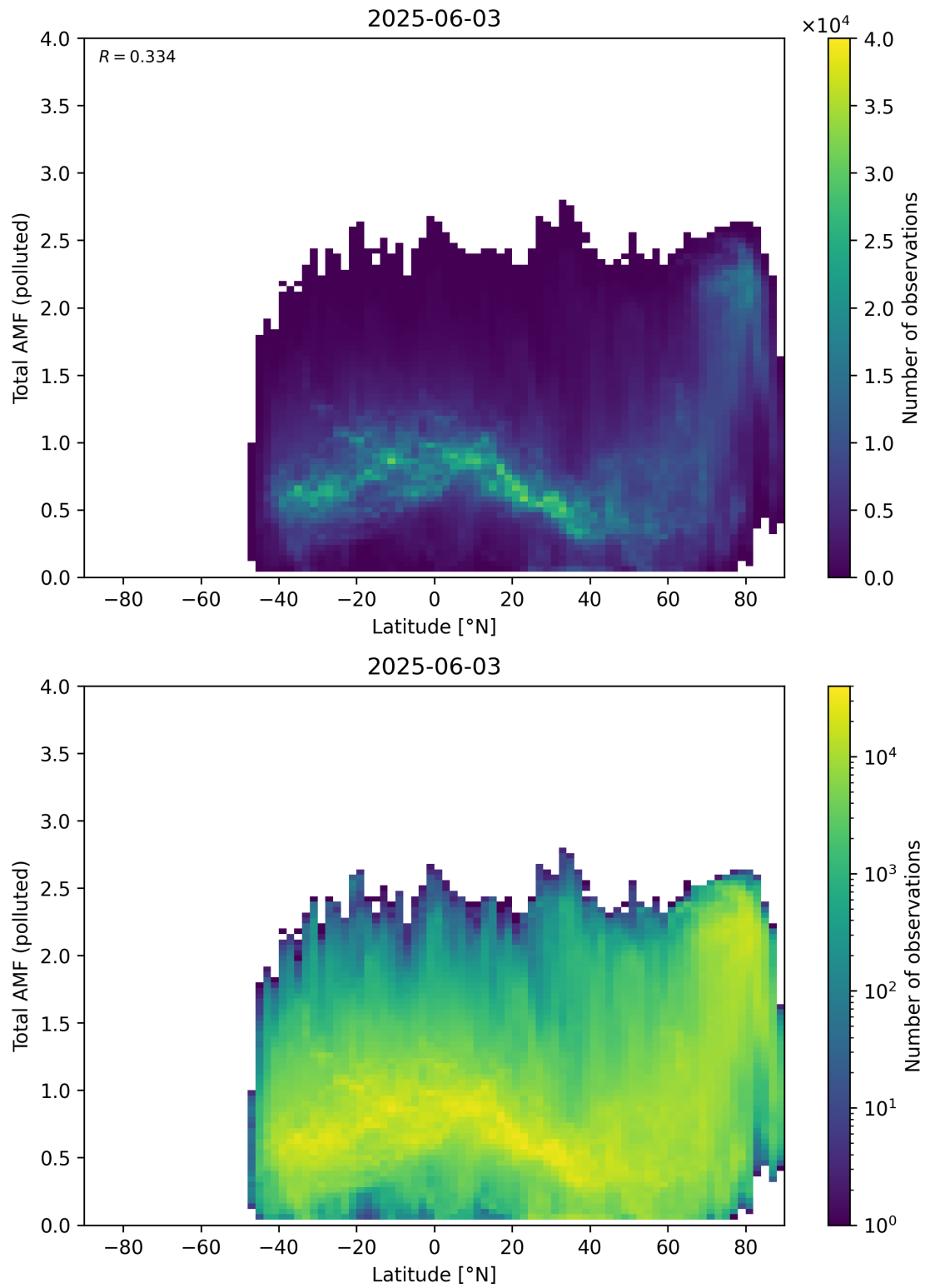
Figure 167: Scatter density plot of “Latitude” against “Total AMF (polluted)” for 2025-06-02 to 2025-06-04.
