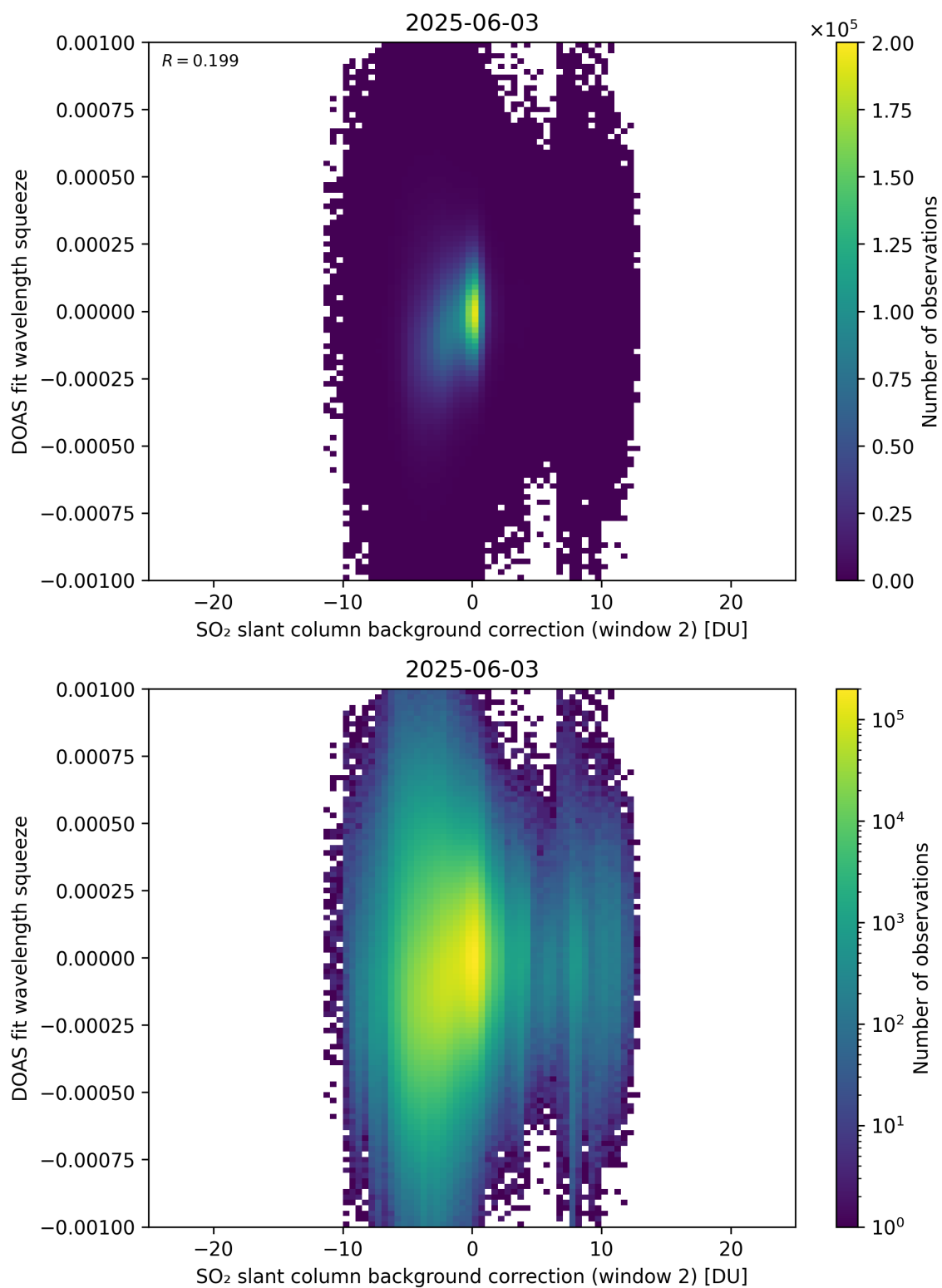
Figure 124: Scatter density plot of “SO 2 slant column background correction (window 2)” against “DOAS fit wavelength squeeze” for 2025-06-02 to 2025-06-04.
