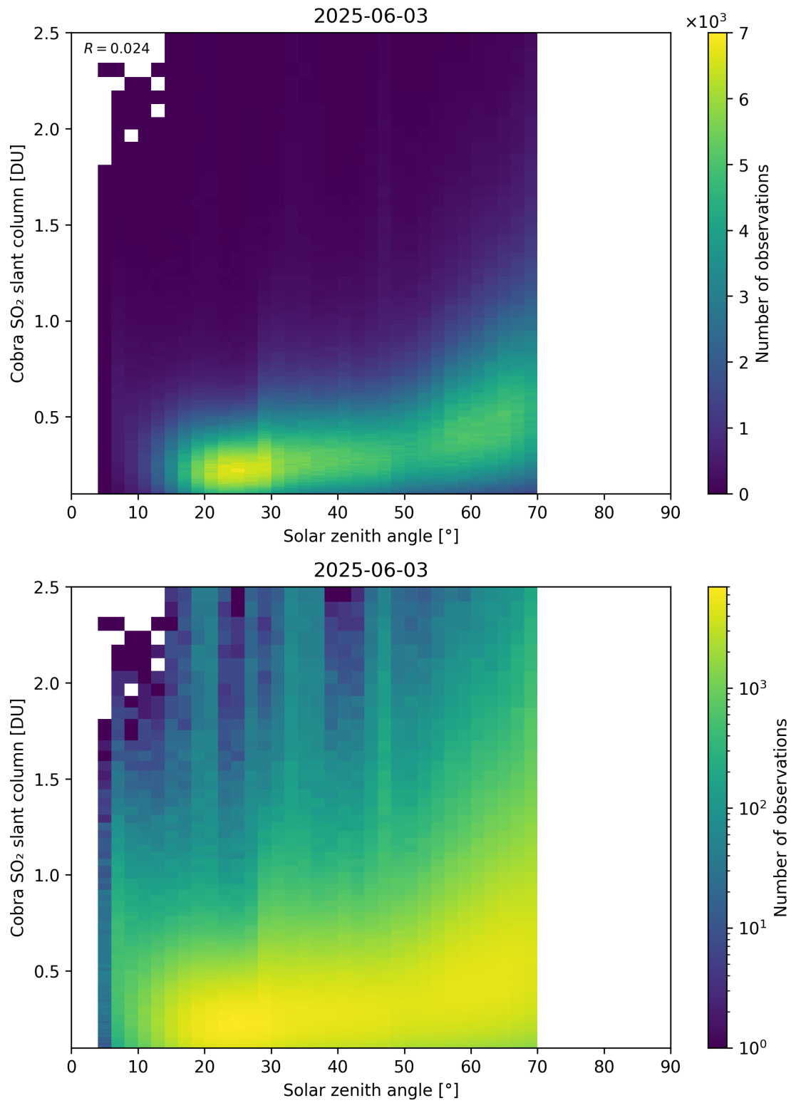
Figure 179: Scatter density plot of “Solar zenith angle” against “Cobra SO 2 slant column” for 2025-06-02 to 2025-06-04.
