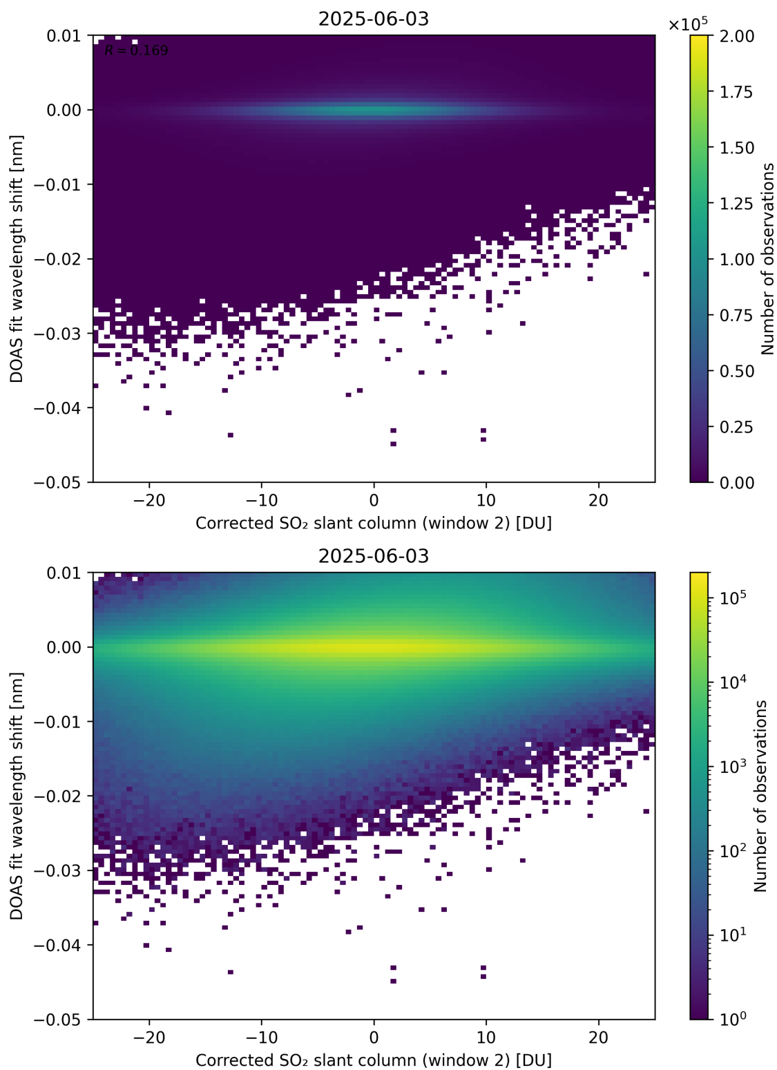
Figure 246: Scatter density plot of “Corrected SO 2 slant column (window 2)” against “DOAS fit wavelength shift” for 2025-06-02 to 2025-06-04.
