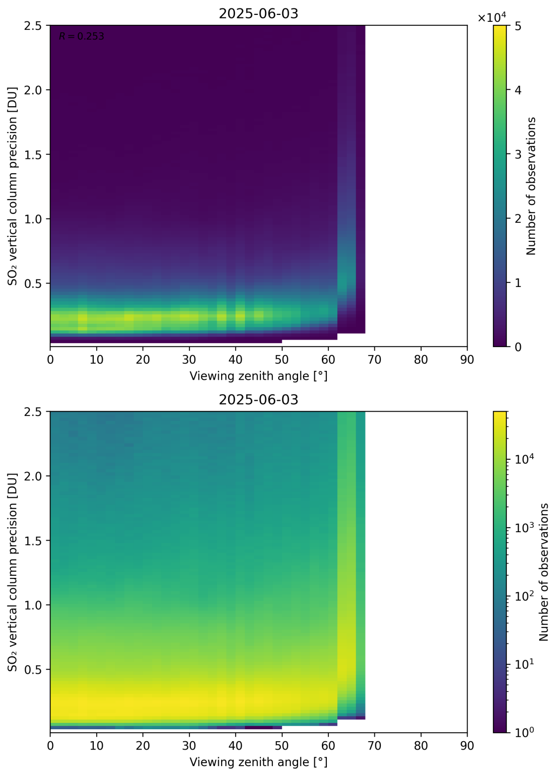
Figure 384: Scatter density plot of “Viewing zenith angle” against “SO 2 vertical column precision” for 2025-06-02 to 2025-06-04.
