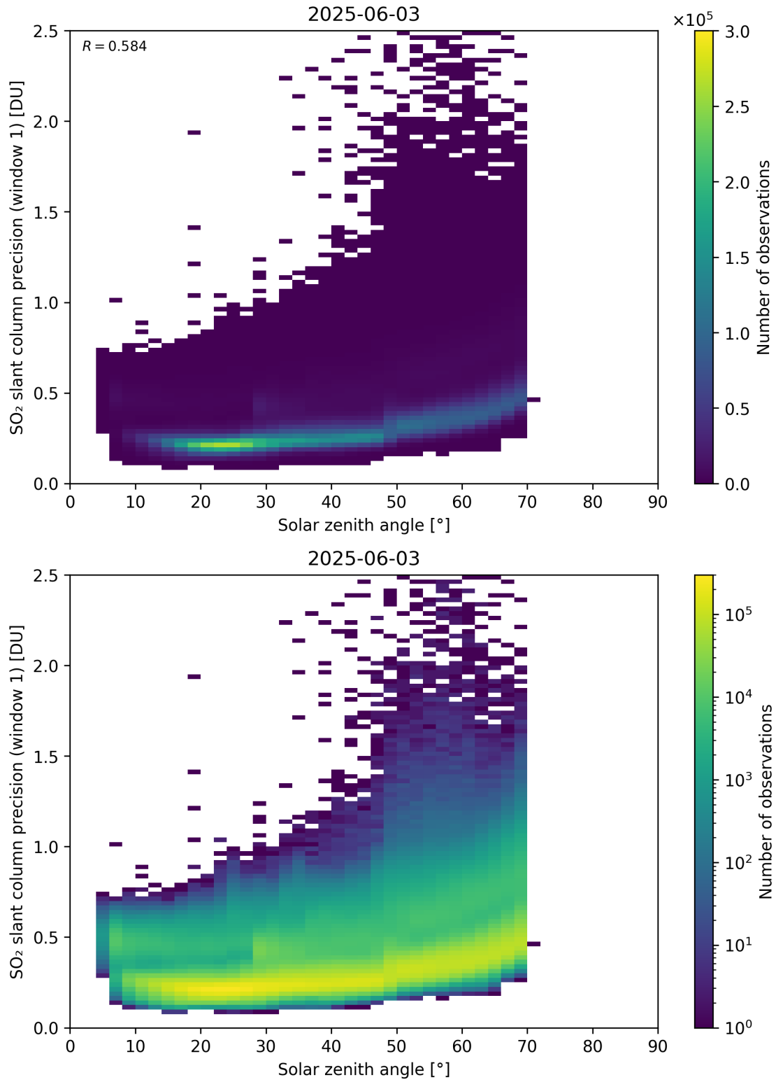
Figure 185: Scatter density plot of “Solar zenith angle” against “SO 2 slant column precision (window 1)” for 2025-06-02 to 2025-06-04.
