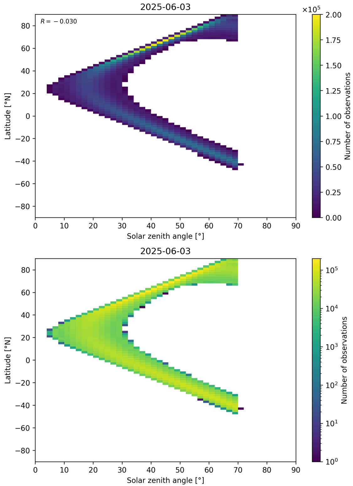
Figure 177: Scatter density plot of “Solar zenith angle” against “Latitude” for 2025-06-02 to 2025-06-04.
