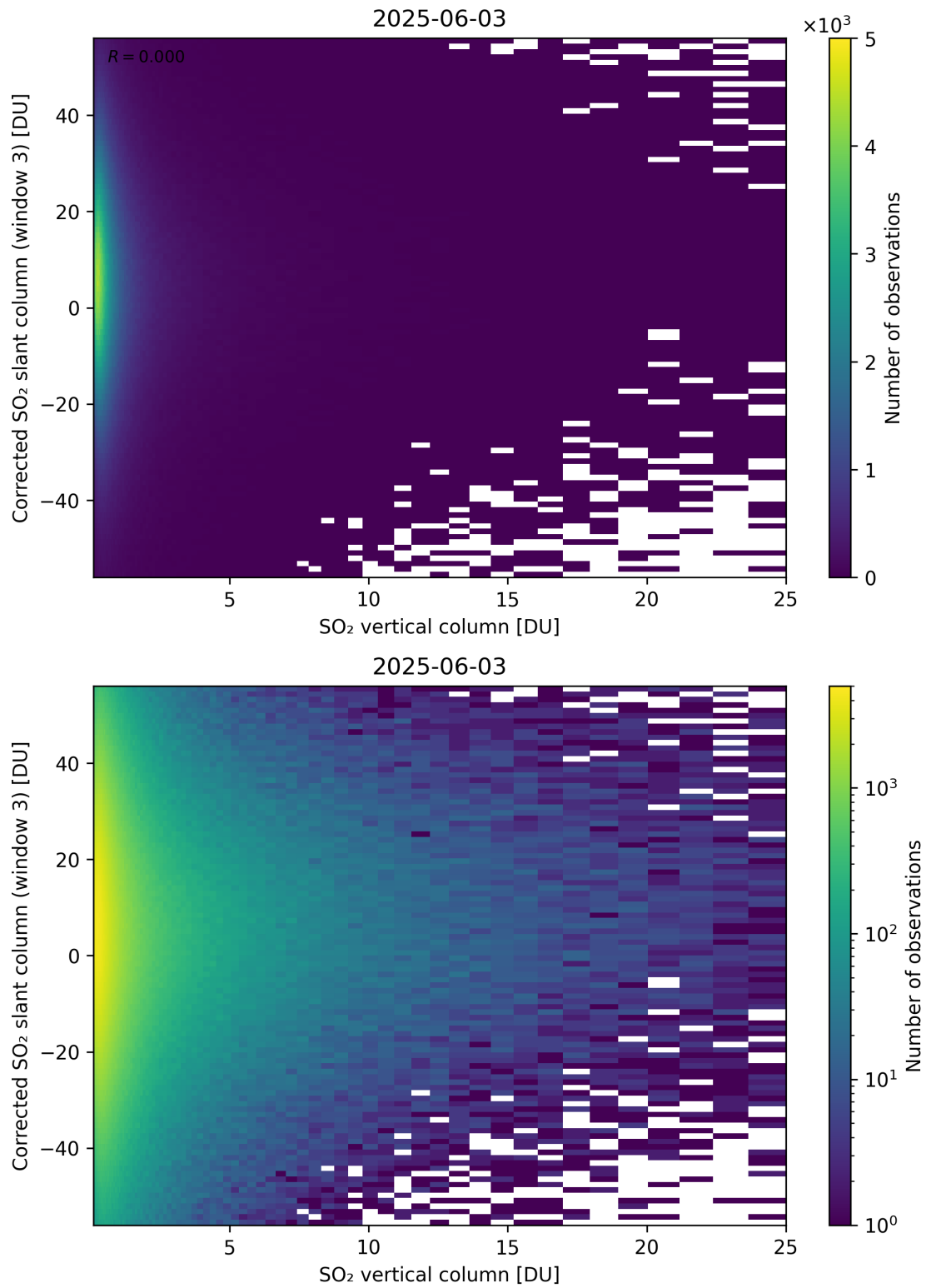
Figure 353: Scatter density plot of “SO 2 vertical column” against “Corrected SO 2 slant column (window 3)” for 2025-06-02 to 2025-06-04.
