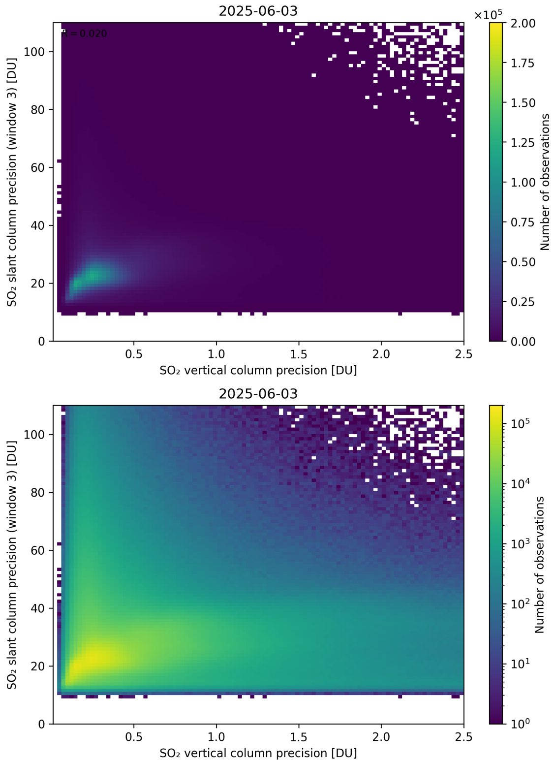
Figure 345: Scatter density plot of “SO 2 vertical column precision” against “SO 2 slant column precision (window 3)” for 2025-06-02 to 2025-06-04.
