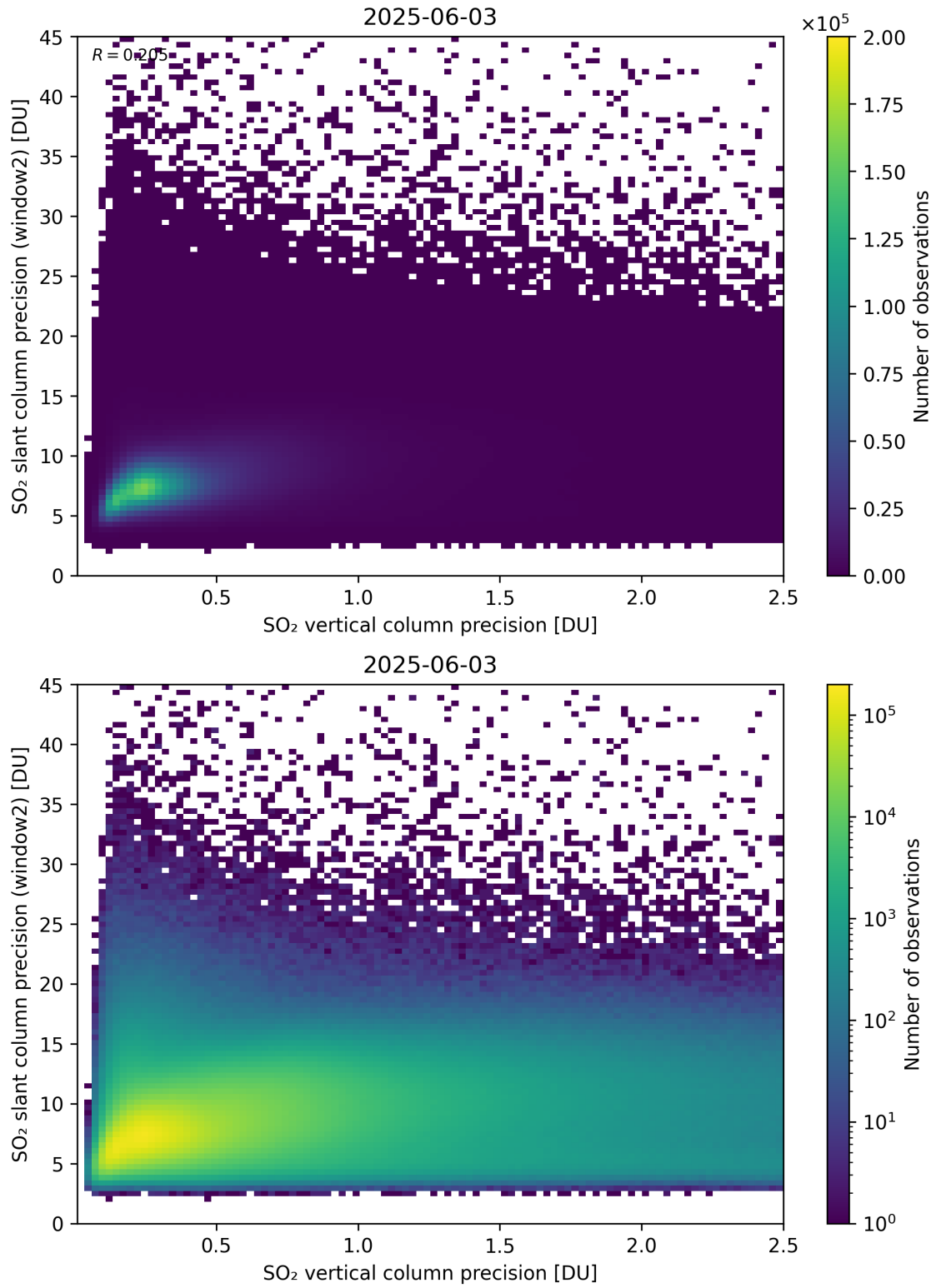
Figure 343: Scatter density plot of “SO 2 vertical column precision” against “SO 2 slant column precision (window2)” for 2025-06-02 to 2025-06-04.
