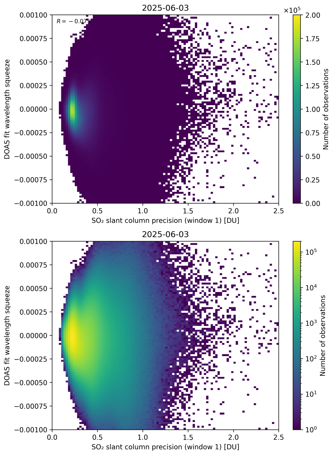
Figure 272: Scatter density plot of “SO 2 slant column precision (window 1)” against “DOAS fit wavelength squeeze” for 2025-06-02 to 2025-06-04.
