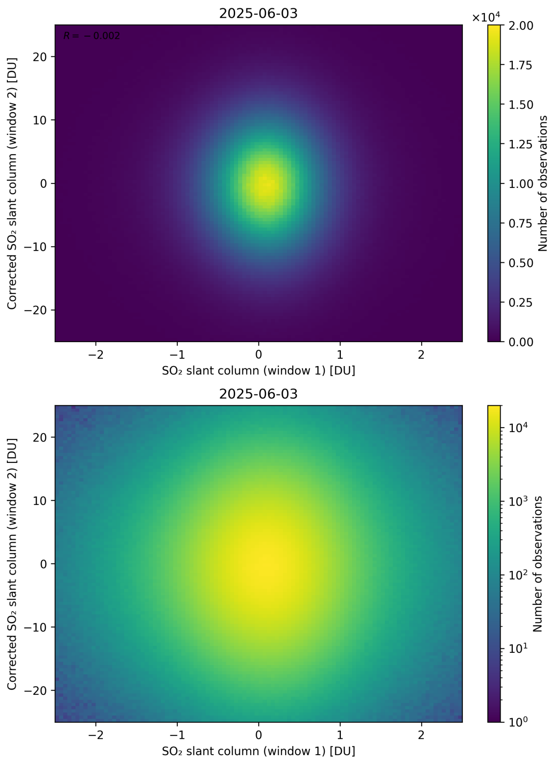
Figure 283: Scatter density plot of “SO 2 slant column (window 1)” against “Corrected SO 2 slant column (window 2)” for 2025-06-02 to 2025-06-04.
