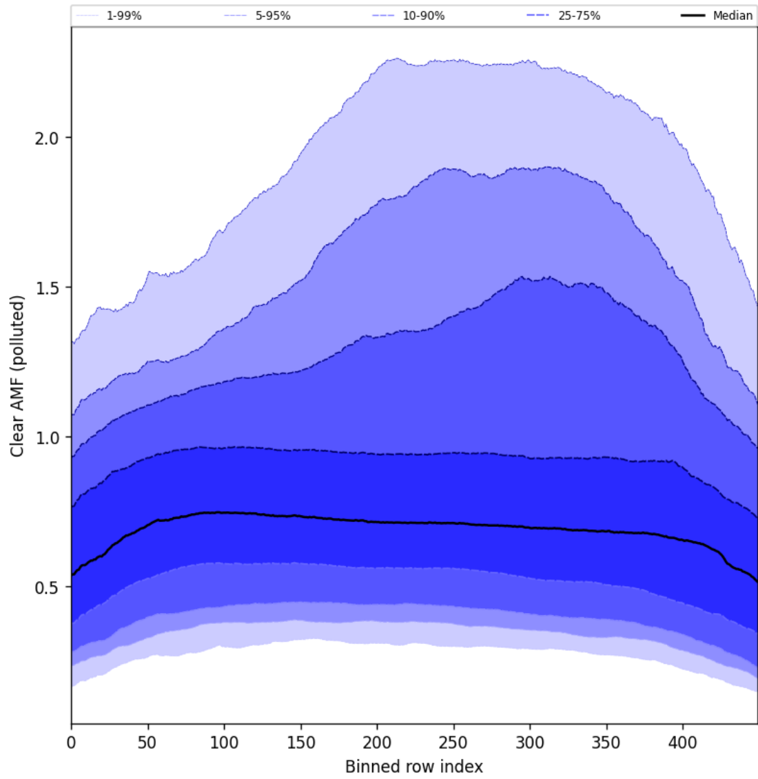
Figure 107: Along track statistics of “Clear AMF (polluted)” for 2025-06-02 to 2025-06-04
