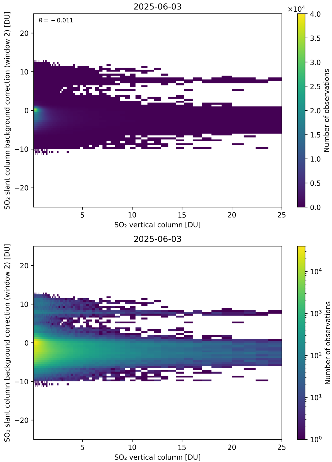
Figure 324: Scatter density plot of “SO 2 vertical column” against “SO 2 slant column background correction (window 2)” for 2025-06-02 to 2025-06-04.
