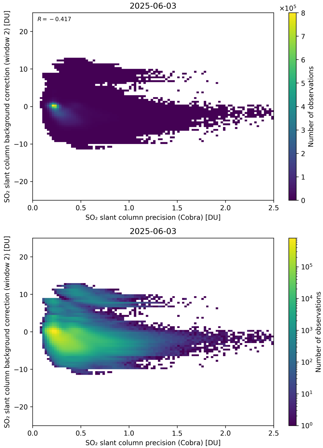
Figure 200: Scatter density plot of “SO 2 slant column precision (Cobra)” against “SO 2 slant column background correction (window 2)” for 2025-06-02 to 2025-06-04.
