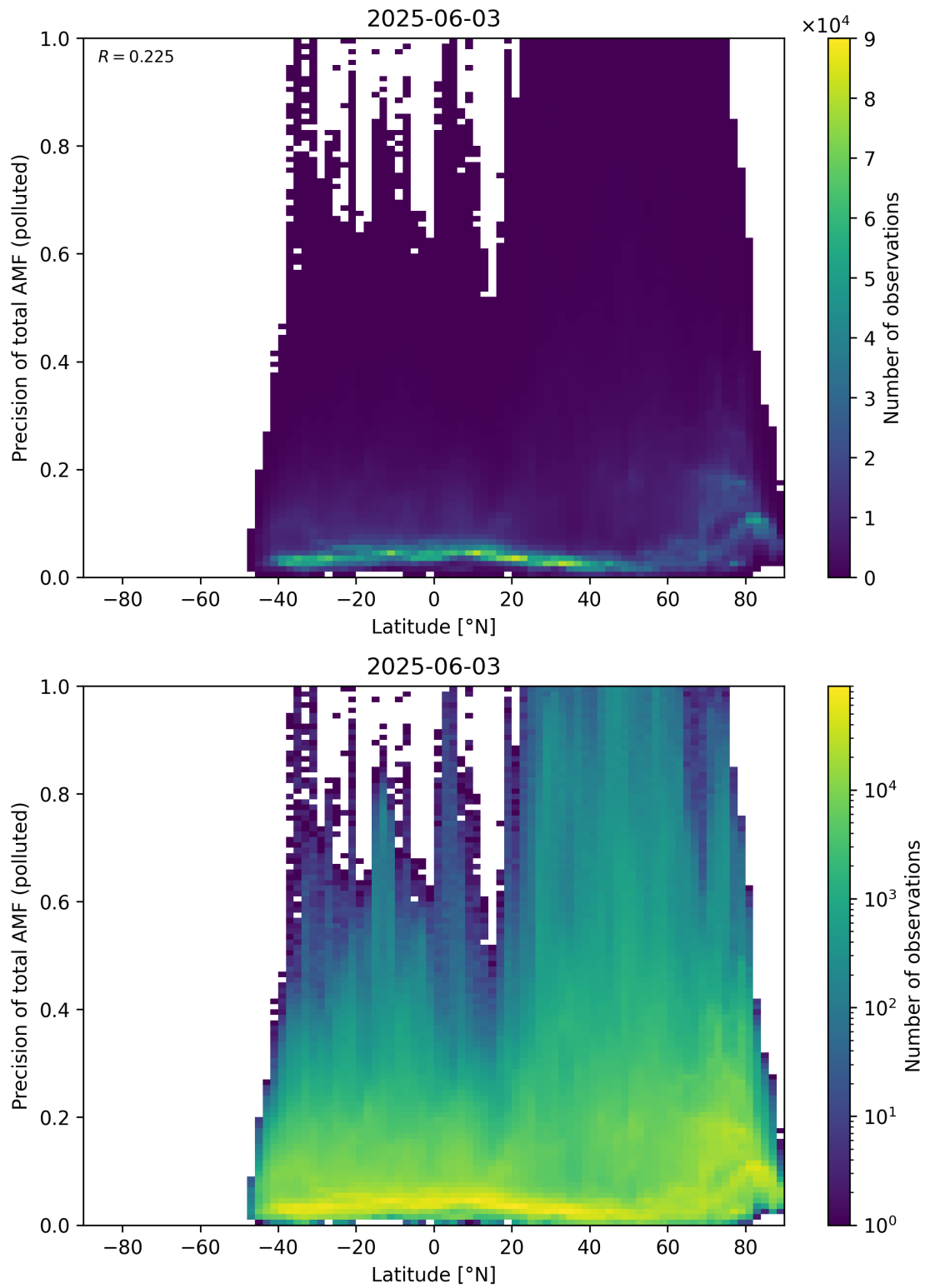
Figure 168: Scatter density plot of “Latitude” against “Precision of total AMF (polluted)” for 2025-06-02 to 2025-06-04.
