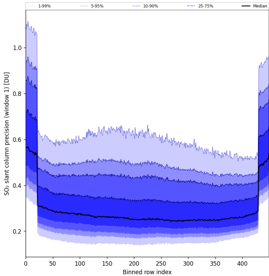
Figure 90: Along track statistics of “SO 2 slant column precision (window 1)” for 2025-06-02 to 2025-06-04
