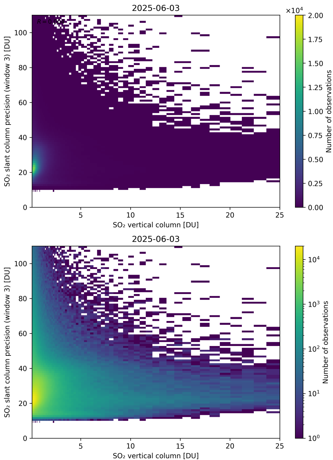
Figure 358: Scatter density plot of “SO 2 vertical column” against “SO 2 slant column precision (window 3)” for 2025-06-02 to 2025-06-04.
