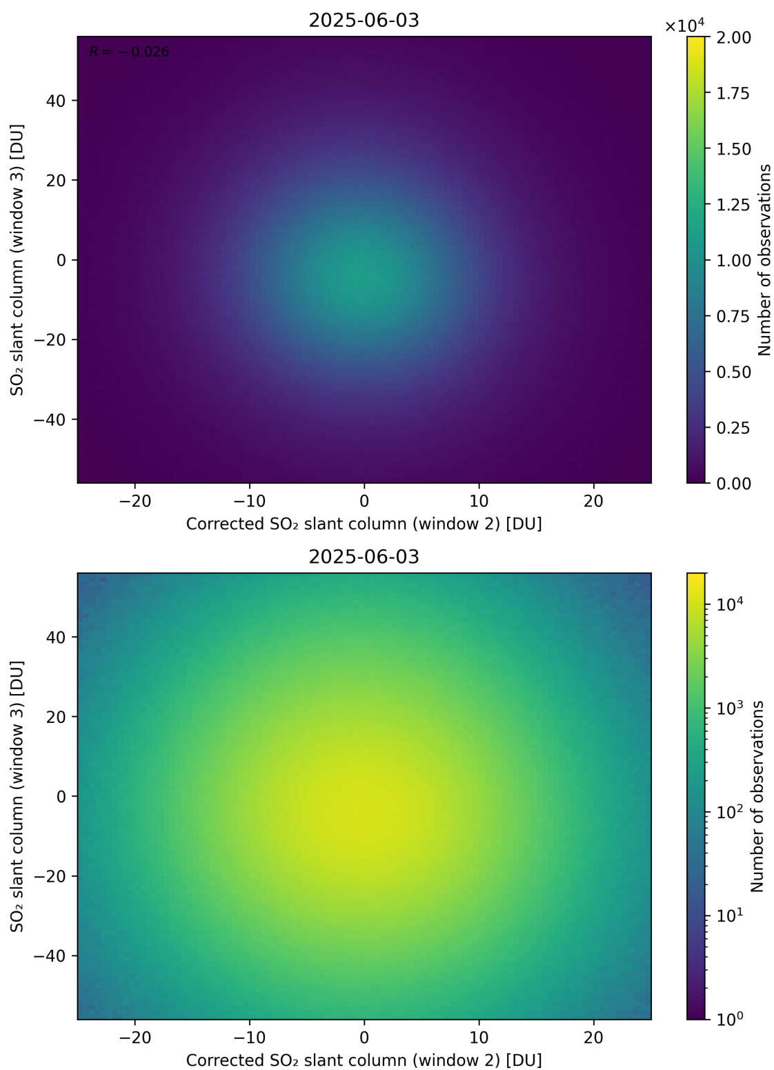
Figure 251: Scatter density plot of “Corrected SO 2 slant column (window 2)” against “SO 2 slant column (window 3)” for 2025-06-02 to 2025-06-04.
