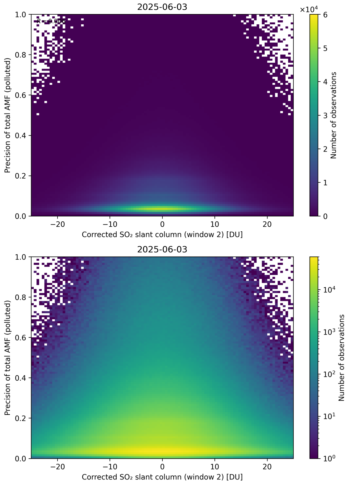
Figure 254: Scatter density plot of “Corrected SO 2 slant column (window 2)” against “Precision of total AMF (polluted)” for 2025-06-02 to 2025-06-04.
