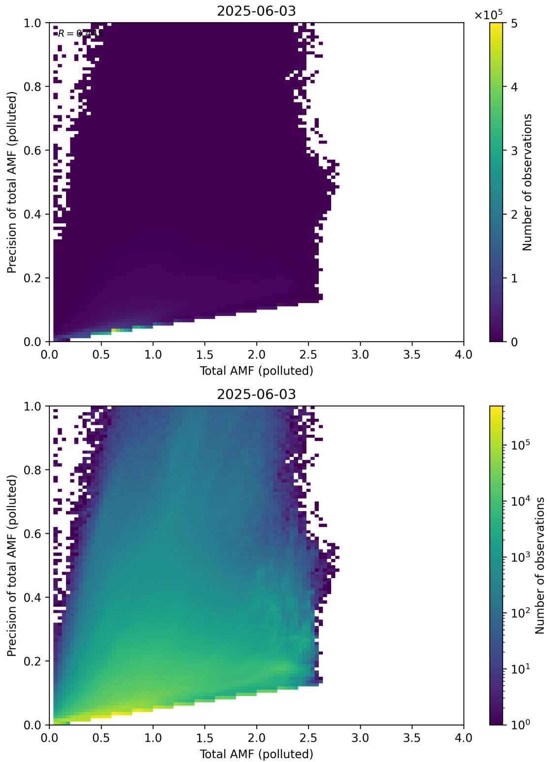
Figure 322: Scatter density plot of “Total AMF (polluted)” against “Precision of total AMF (polluted)” for 2025-06-02 to 2025-06-04.
