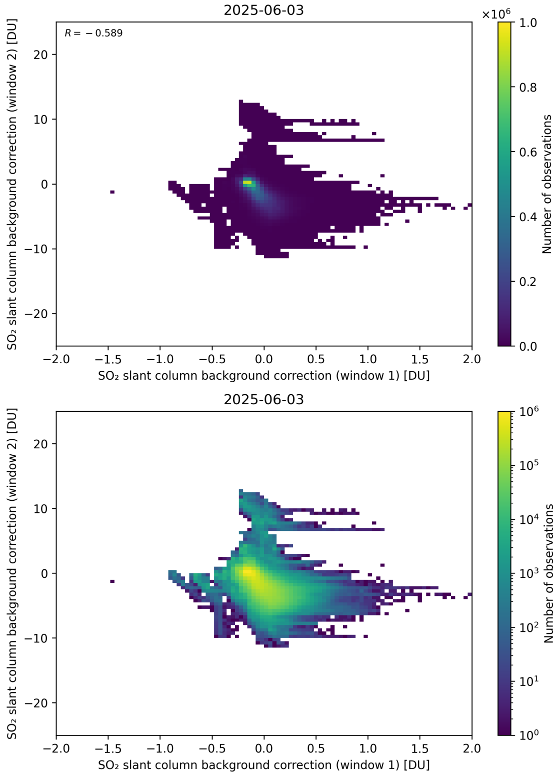
Figure 109: Scatter density plot of “SO 2 slant column background correction (window 1)” against “SO 2 slant column background correction (window 2)” for 2025-06-02 to 2025-06-04.
