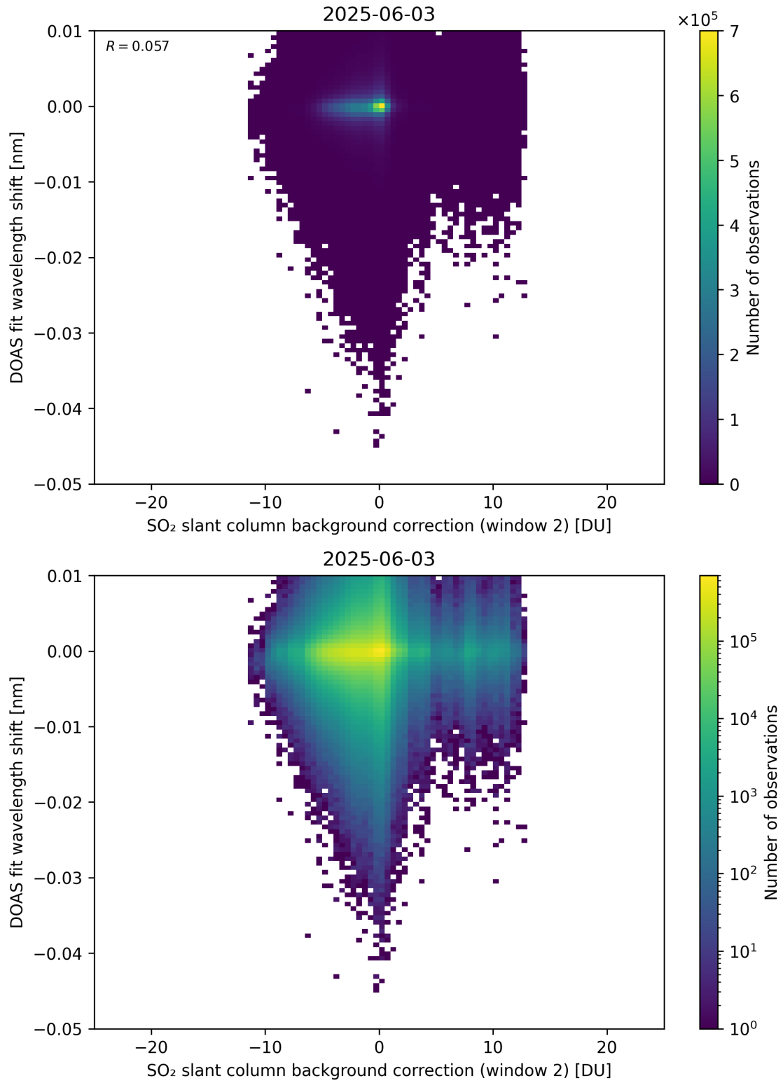
Figure 123: Scatter density plot of “SO 2 slant column background correction (window 2)” against “DOAS fit wavelength shift” for 2025-06-02 to 2025-06-04.
