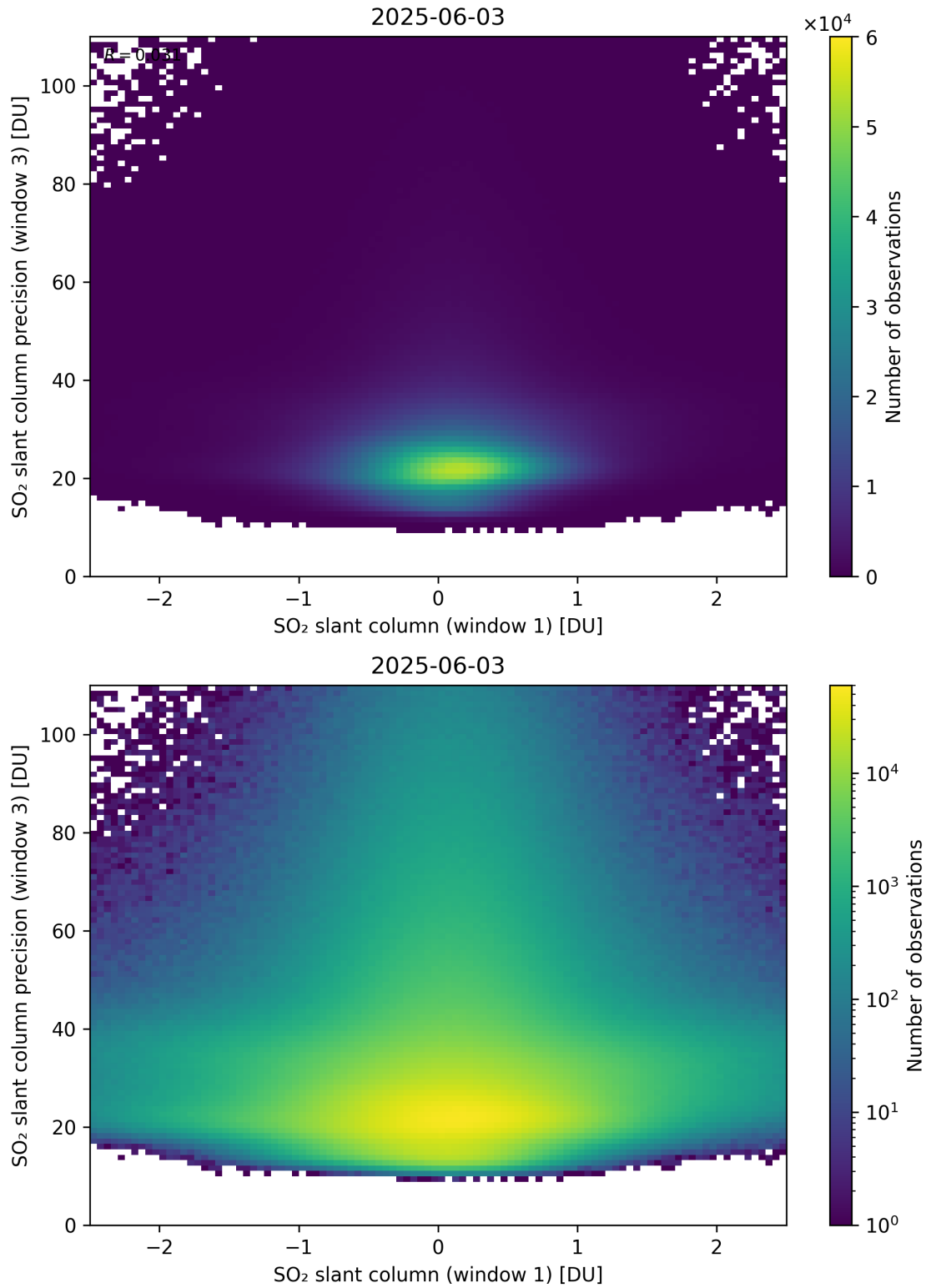
Figure 288: Scatter density plot of “SO 2 slant column (window 1)” against “SO 2 slant column precision (window 3)” for 2025-06-02 to 2025-06-04.
