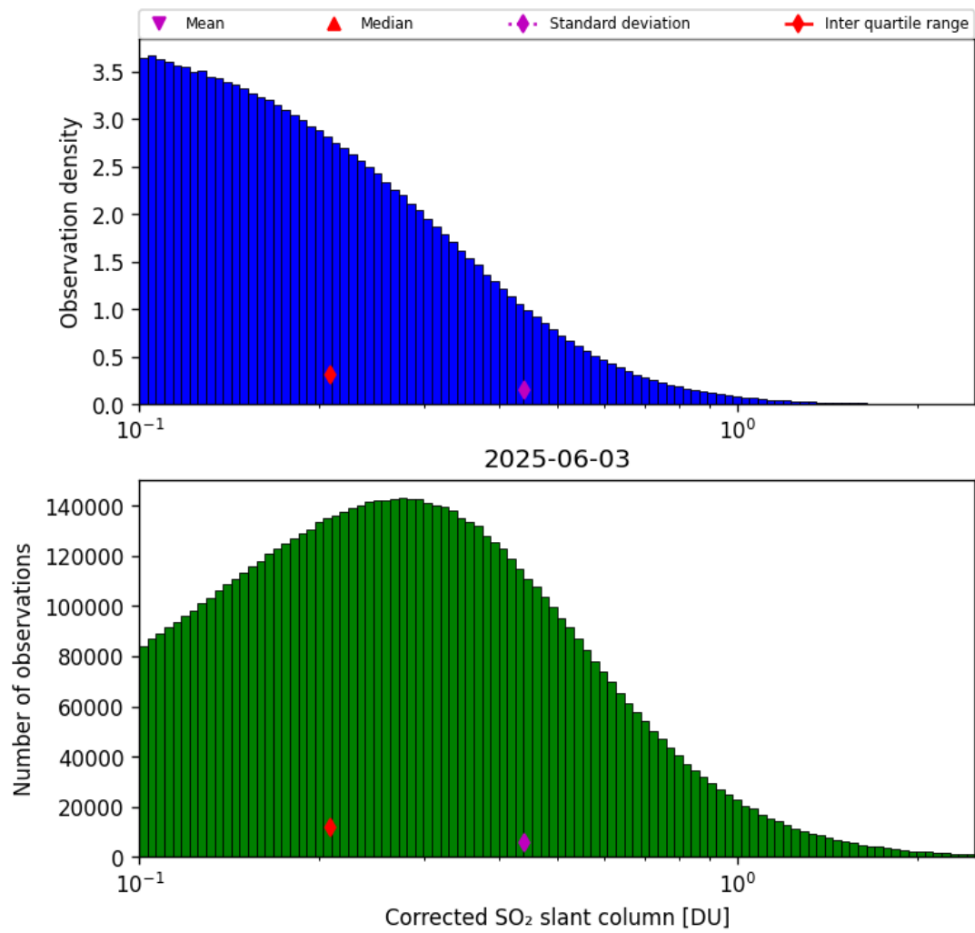
Figure 60: Histogram of "Corrected SO 2 slant column" for 2025-06-02 to 2025-06-04
