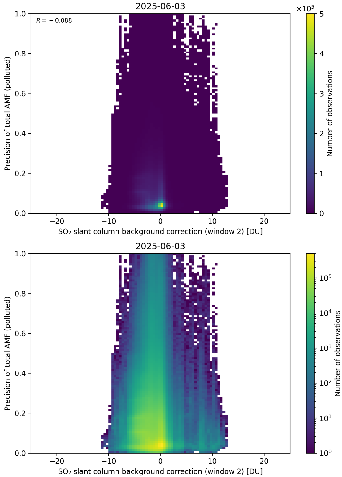
Figure 131: Scatter density plot of “SO 2 slant column background correction (window 2)” against “Precision of total AMF (polluted)” for 2025-06-02 to 2025-06-04.
