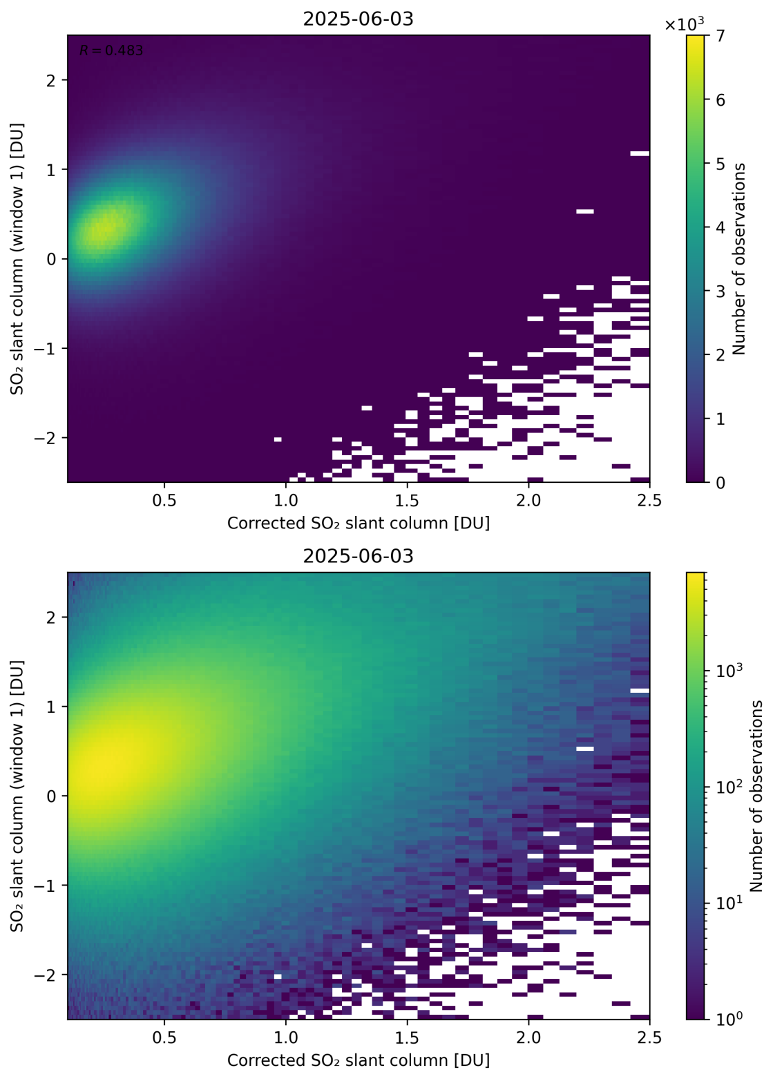
Figure 237: Scatter density plot of “Corrected SO 2 slant column” against “SO 2 slant column (window 1)” for 2025-06-02 to 2025-06-04.
