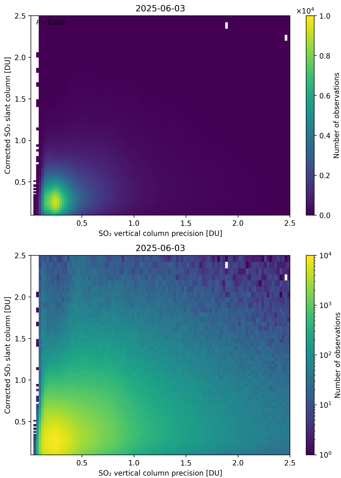
Figure 338: Scatter density plot of “SO 2 vertical column precision” against “Corrected SO 2 slant column” for 2025-06-02 to 2025-06-04.
