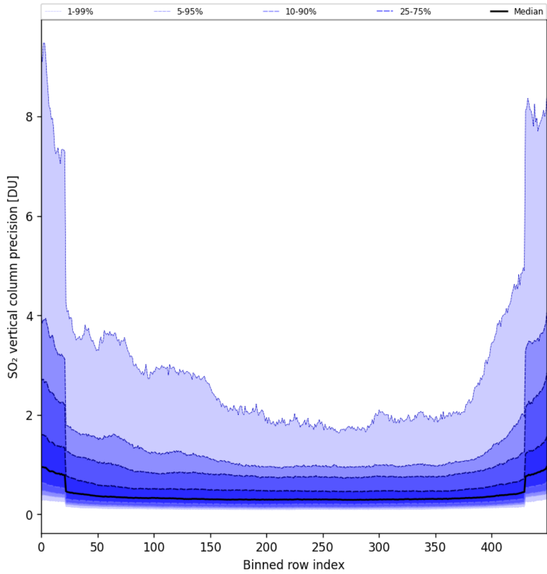
Figure 85: Along track statistics of “SO 2 vertical column precision” for 2025-06-02 to 2025-06-04
