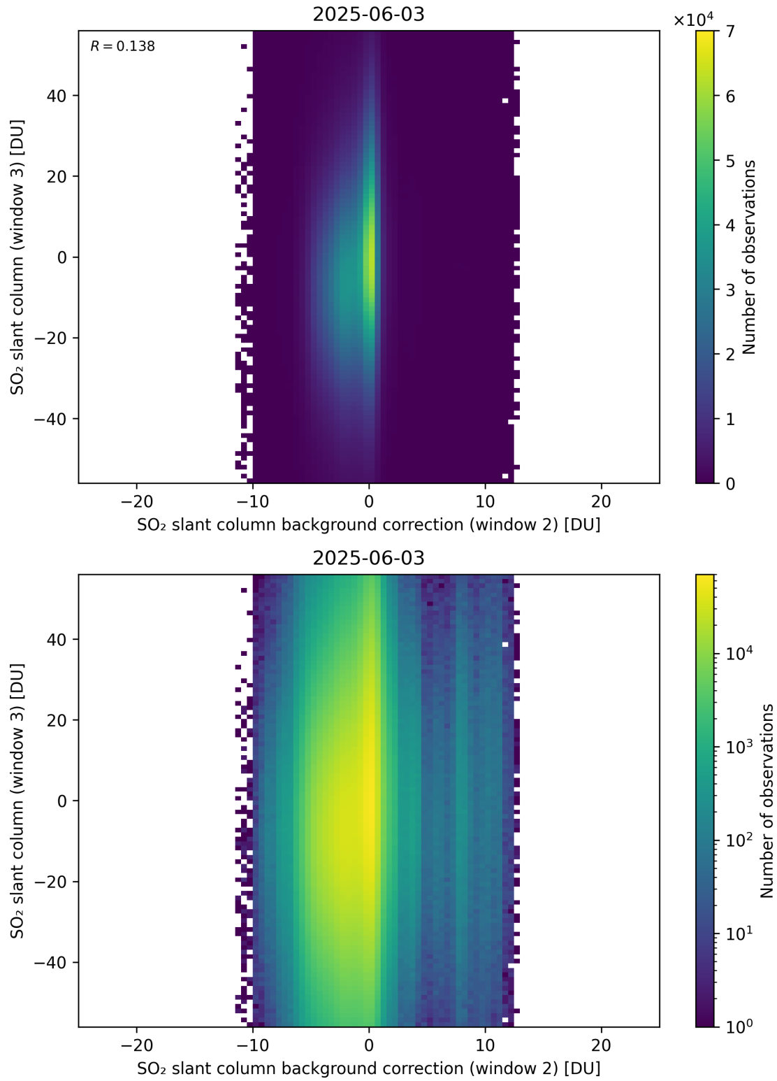
Figure 128: Scatter density plot of “SO 2 slant column background correction (window 2)” against “SO 2 slant column (window 3)” for 2025-06-02 to 2025-06-04.
