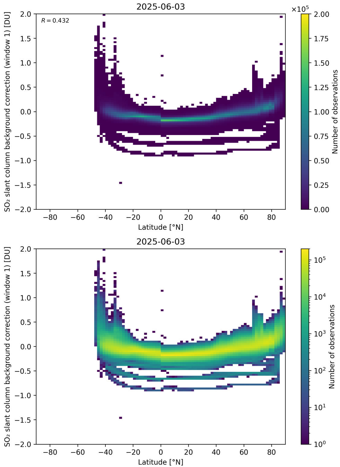
Figure 150: Scatter density plot of “Latitude” against “SO 2 slant column background correction (window 1)” for 2025-06-02 to 2025-06-04.
