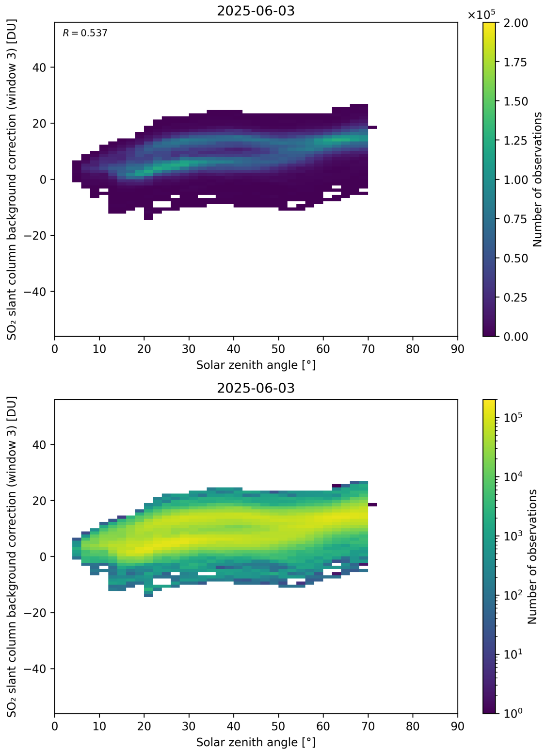
Figure 173: Scatter density plot of “Solar zenith angle” against “SO 2 slant column background correction (window 3)” for 2025-06-02 to 2025-06-04.
