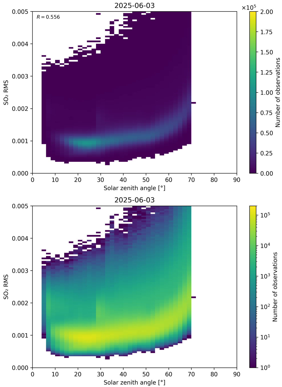
Figure 176: Scatter density plot of “Solar zenith angle” against “SO 2 RMS” for 2025-06-02 to 2025-06-04.
