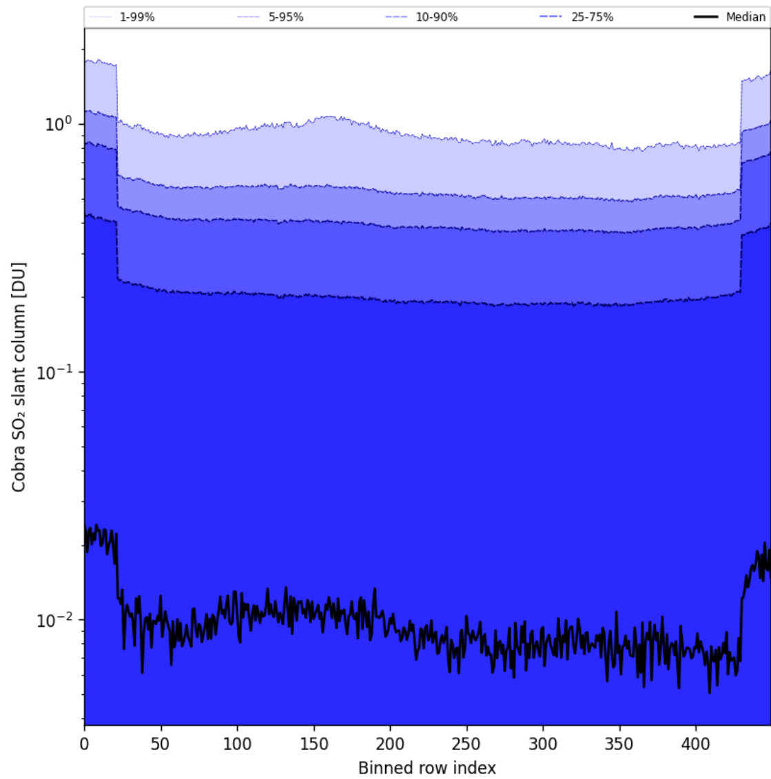
Figure 87: Along track statistics of "Cobra SO 2 slant column" for 2025-06-02 to 2025-06-04
