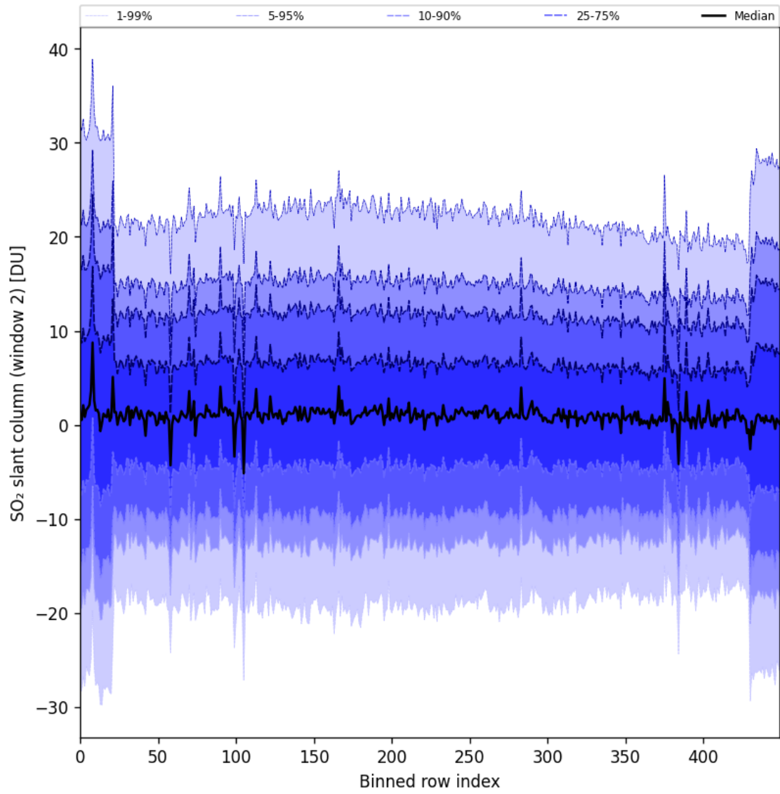
Figure 93: Along track statistics of “SO 2 slant column (window 2)” for 2025-06-02 to 2025-06-04
