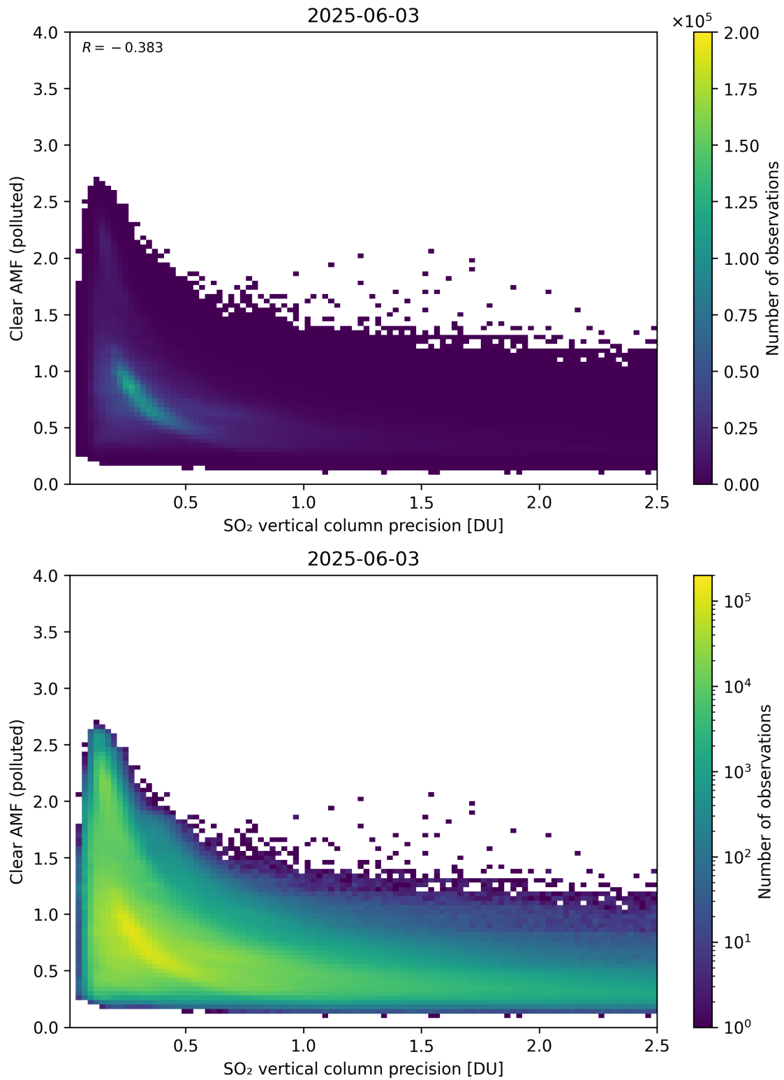
Figure 335: Scatter density plot of “SO 2 vertical column precision” against “Clear AMF (polluted)” for 2025-06-02 to 2025-06-04.
