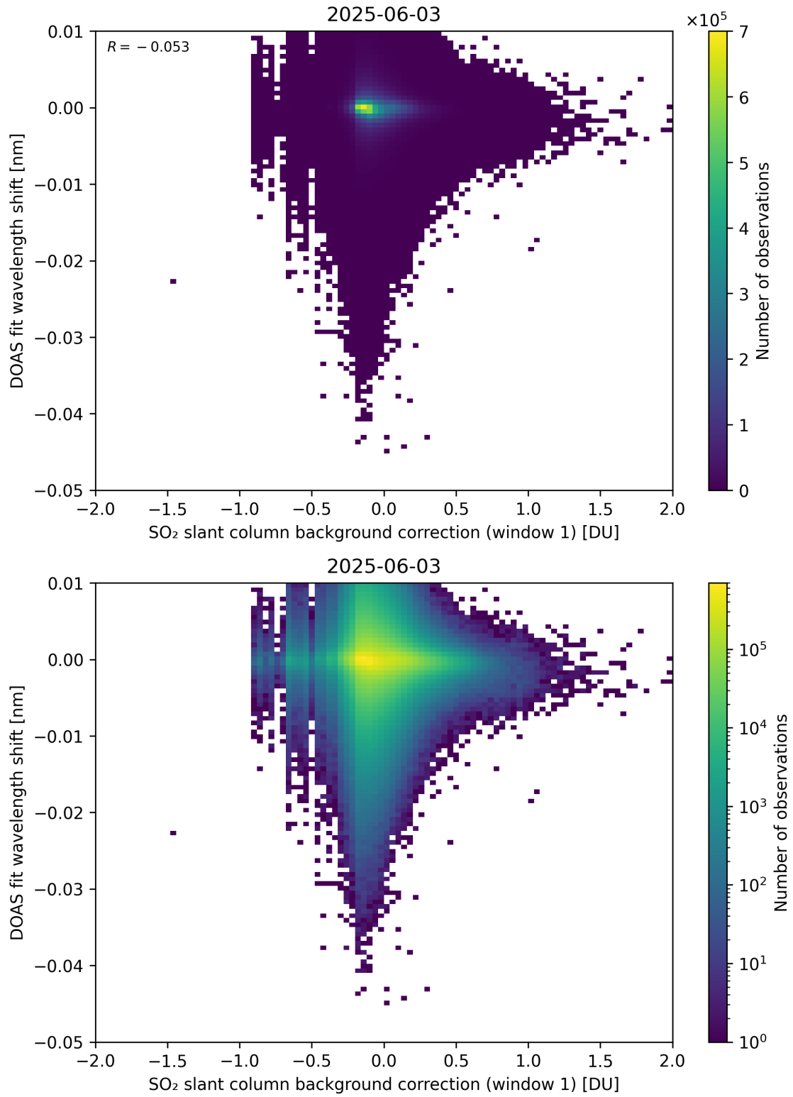
Figure 111: Scatter density plot of “SO 2 slant column background correction (window 1)” against “DOAS fit wavelength shift” for 2025-06-02 to 2025-06-04.
