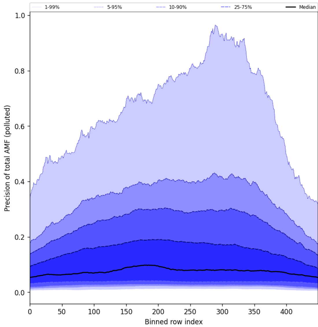
Figure 106: Along track statistics of “Precision of total AMF (polluted)” for 2025-06-02 to 2025-06-04
