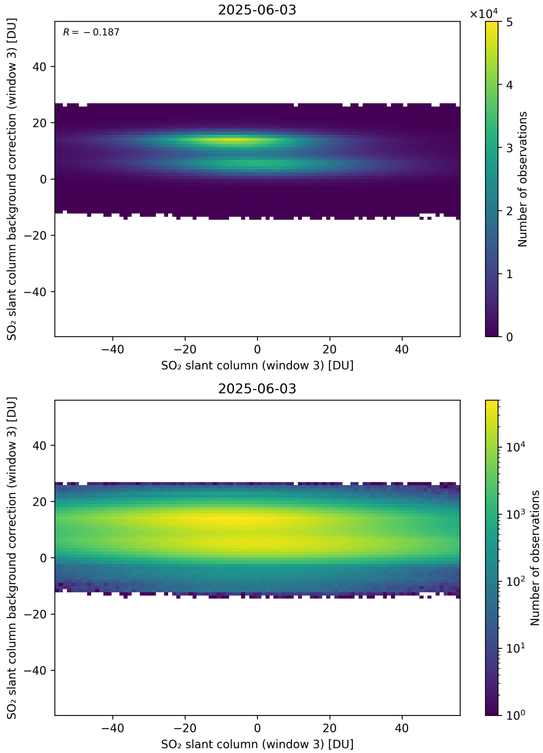
Figure 303: Scatter density plot of “SO 2 slant column (window 3)” against “SO 2 slant column background correction (window 3)” for 2025-06-02 to 2025-06-04.
