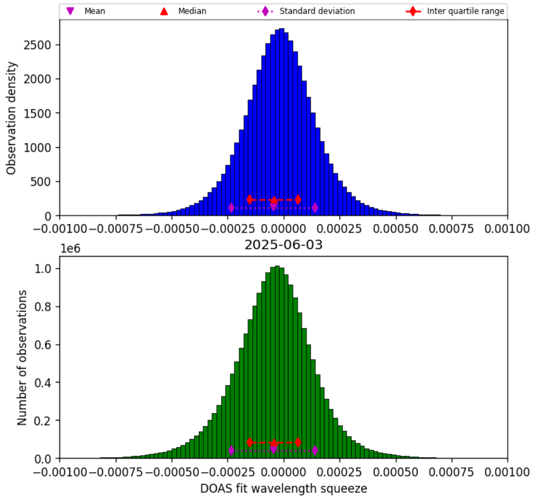
Figure 77: Histogram of “DOAS fit wavelength squeeze” for 2025-06-02 to 2025-06-04
