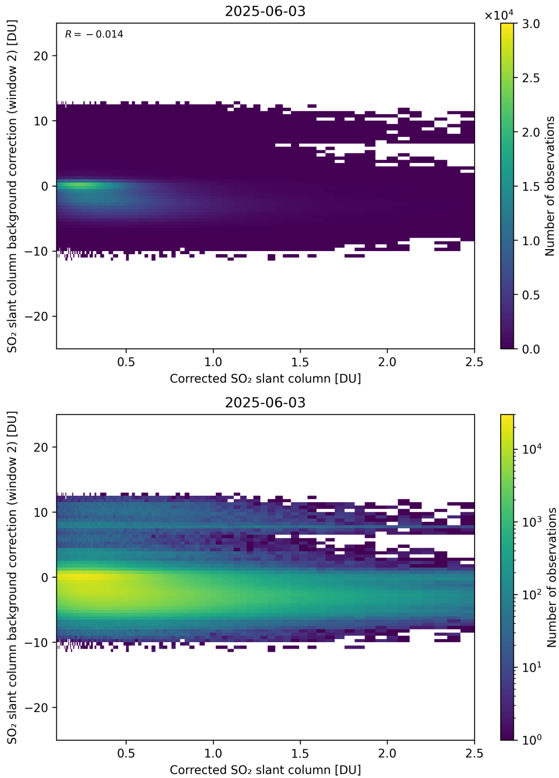
Figure 227: Scatter density plot of “Corrected SO 2 slant column” against “SO 2 slant column background correction (window 2)” for 2025-06-02 to 2025-06-04.
