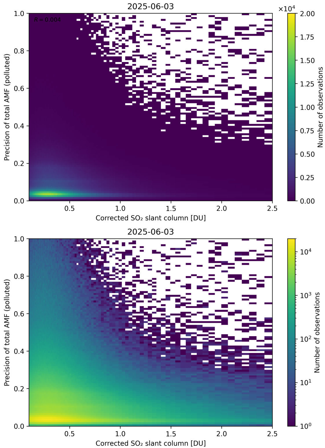
Figure 243: Scatter density plot of “Corrected SO 2 slant column” against “Precision of total AMF (polluted)” for 2025-06-02 to 2025-06-04.
