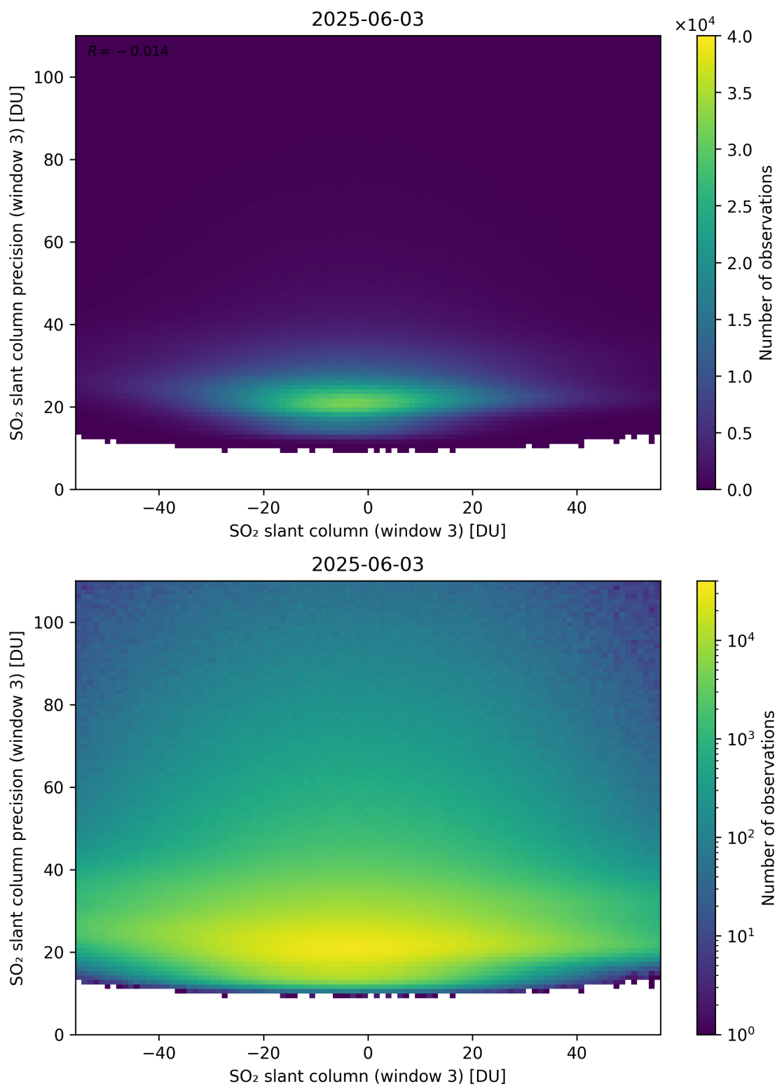
Figure 317: Scatter density plot of “SO 2 slant column (window 3)” against “SO 2 slant column precision (window 3)” for 2025-06-02 to 2025-06-04.
