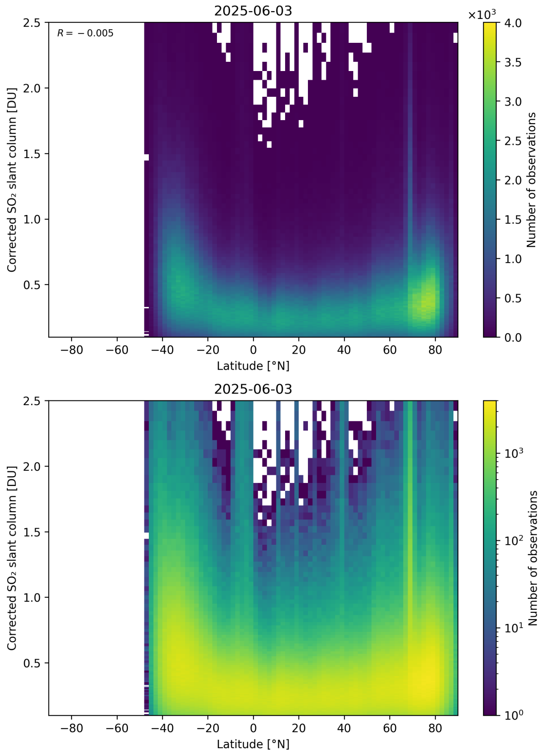
Figure 159: Scatter density plot of “Latitude” against “Corrected SO 2 slant column” for 2025-06-02 to 2025-06-04.
