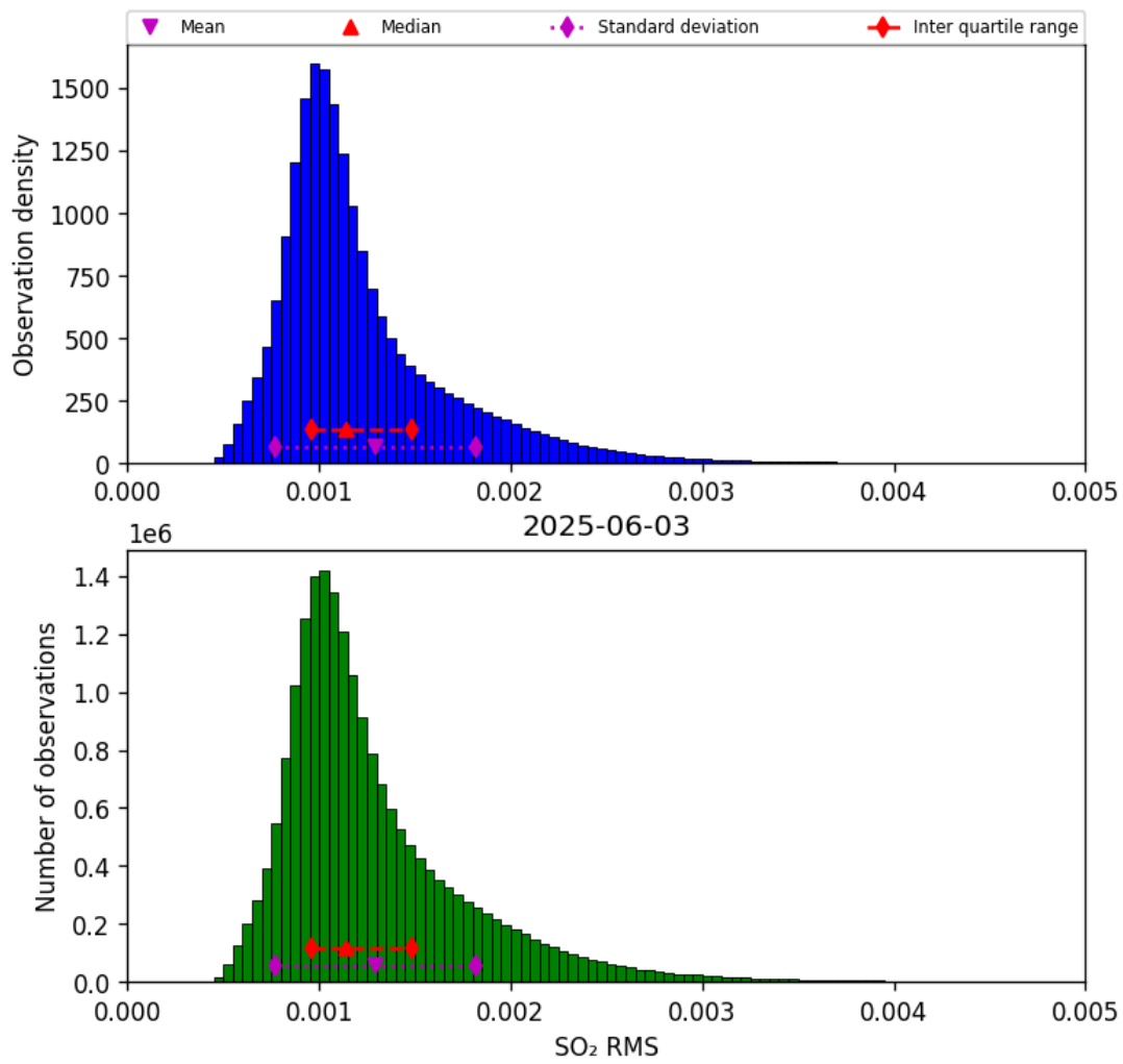
Figure 78: Histogram of “SO 2 RMS” for 2025-06-02 to 2025-06-04
