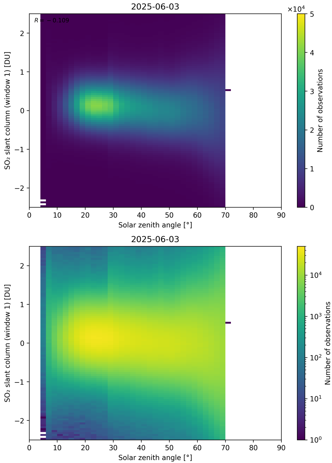
Figure 184: Scatter density plot of “Solar zenith angle” against “SO 2 slant column (window 1)” for 2025-06-02 to 2025-06-04.
