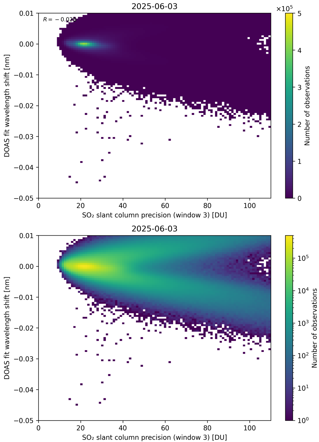
Figure 308: Scatter density plot of “SO 2 slant column precision (window 3)” against “DOAS fit wavelength shift” for 2025-06-02 to 2025-06-04.
