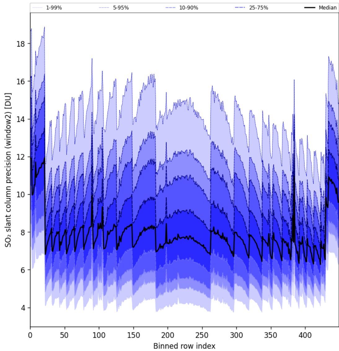
Figure 94: Along track statistics of “SO 2 slant column precision (window2)” for 2025-06-02 to 2025-06-04
