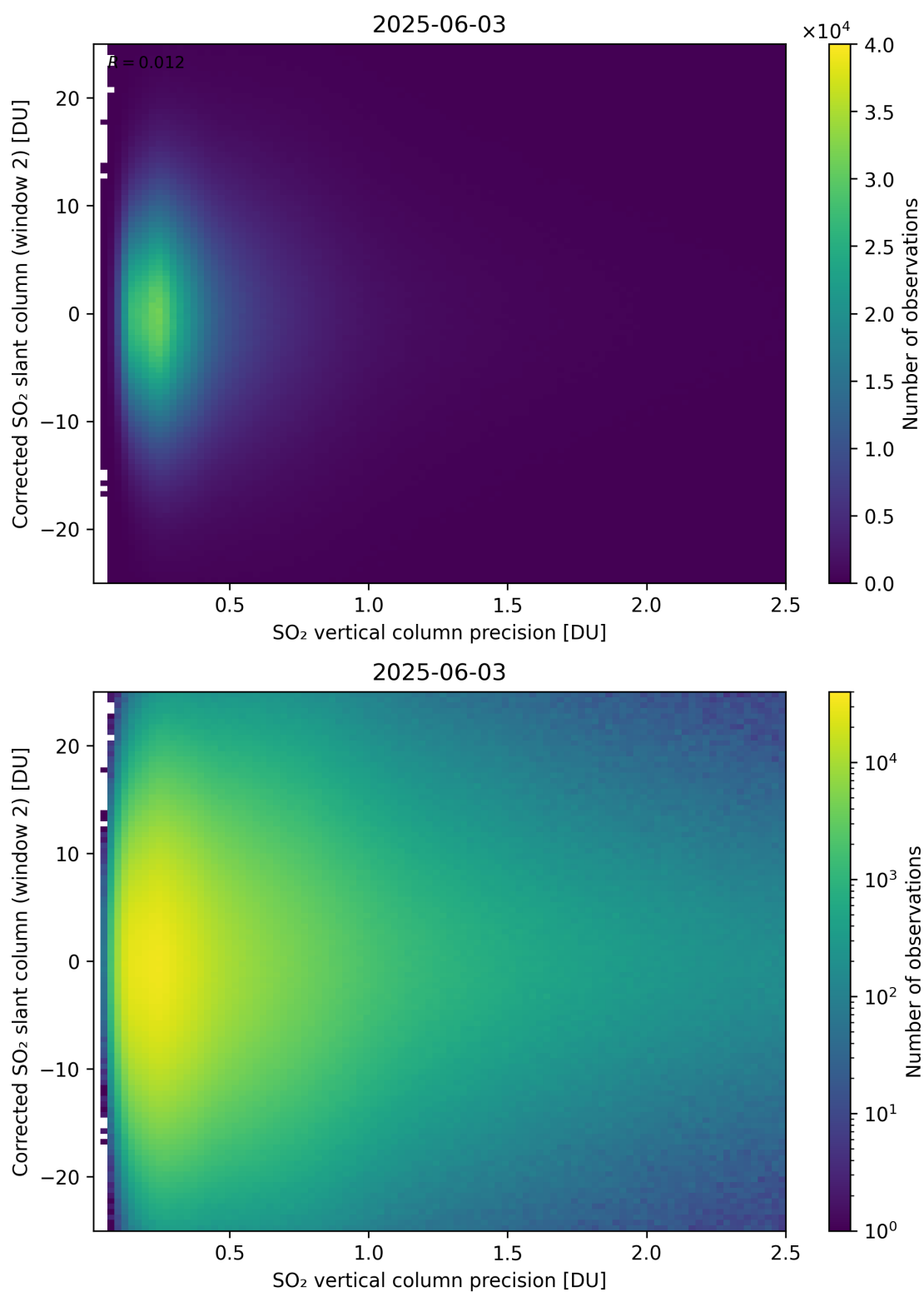
Figure 339: Scatter density plot of “SO 2 vertical column precision” against “Corrected SO 2 slant column (window 2)” for 2025-06-02 to 2025-06-04.
