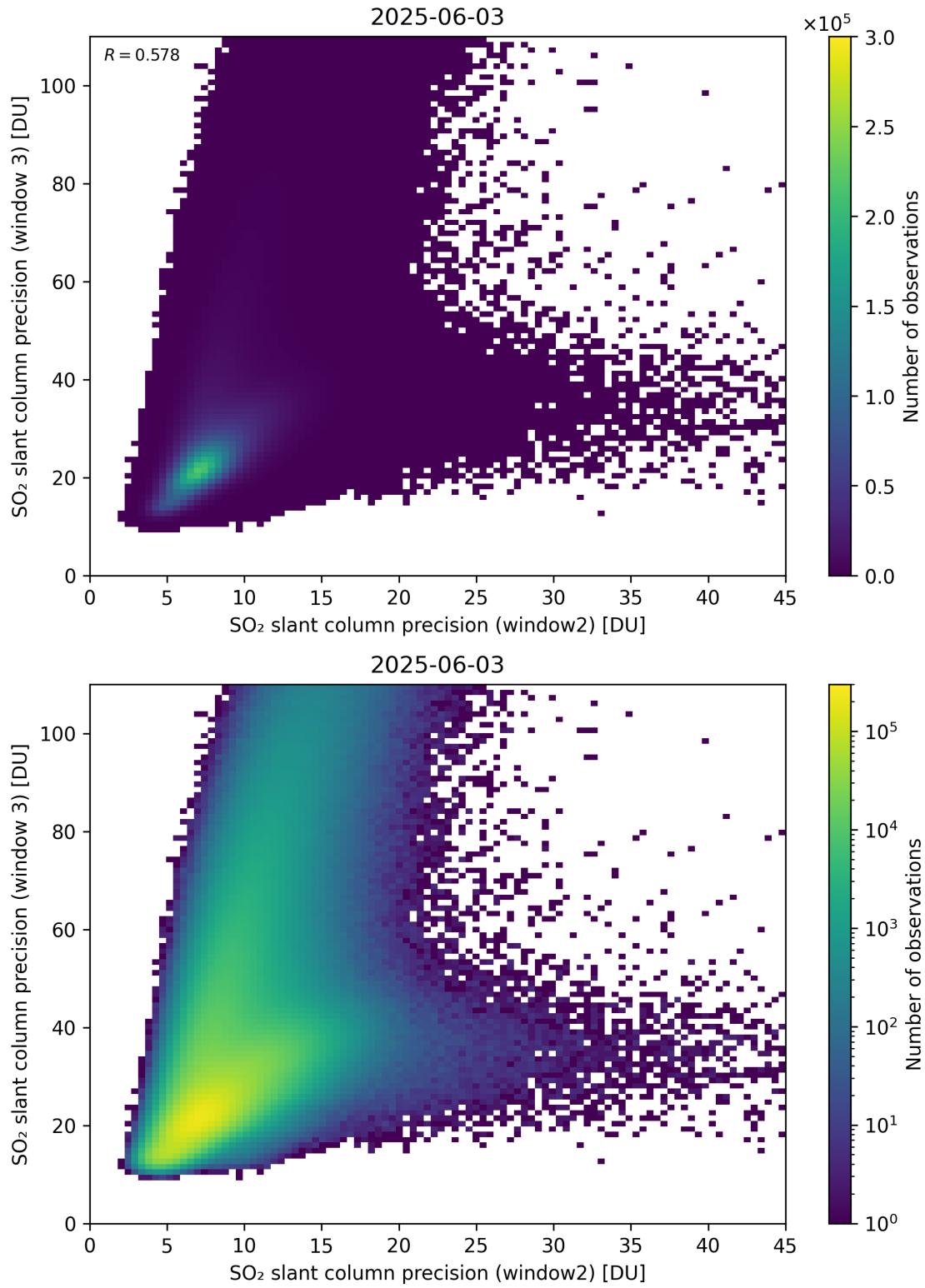
Figure 300: Scatter density plot of “SO 2 slant column precision (window2)” against “SO 2 slant column precision (window 3)” for 2025-06-02 to 2025-06-04.
