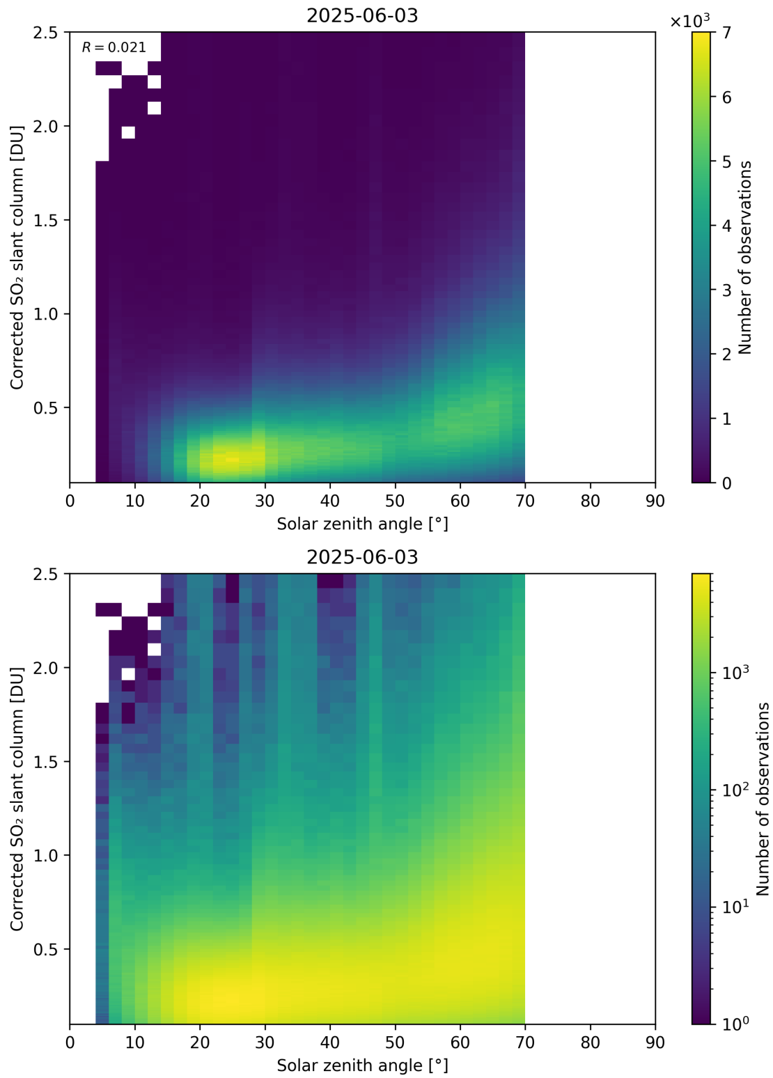
Figure 181: Scatter density plot of “Solar zenith angle” against “Corrected SO 2 slant column” for 2025-06-02 to 2025-06-04.
