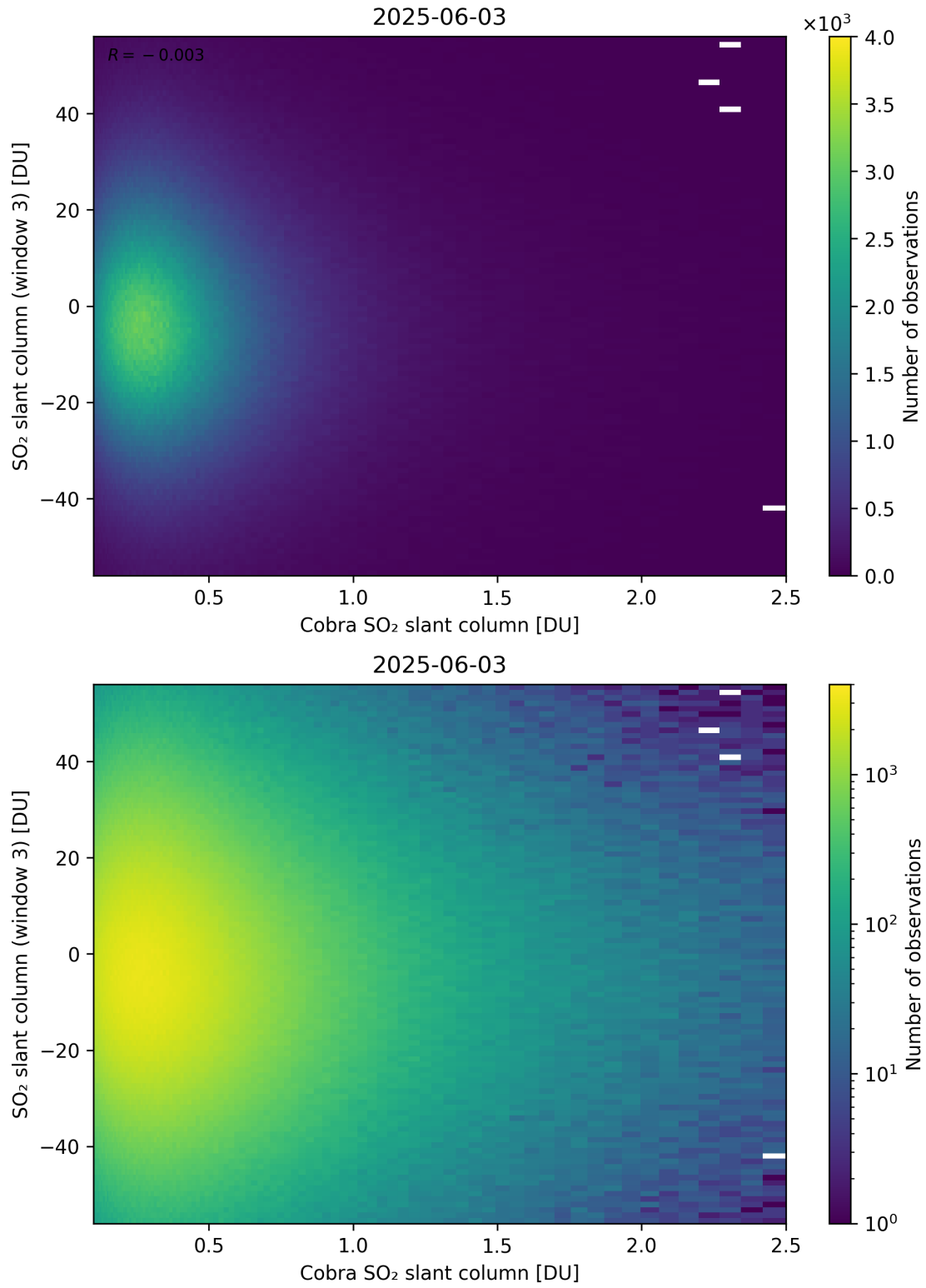
Figure 222: Scatter density plot of “Cobra SO 2 slant column” against “SO 2 slant column (window 3)” for 2025-06-02 to 2025-06-04.
