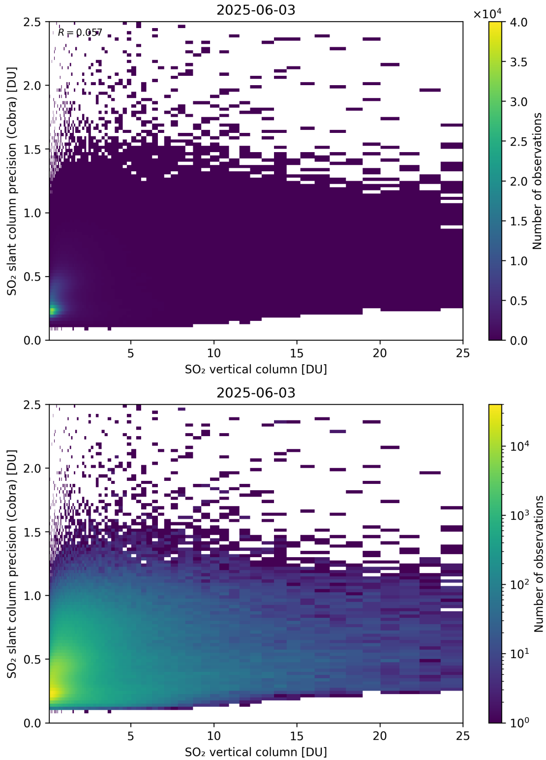
Figure 350: Scatter density plot of “SO 2 vertical column” against “SO 2 slant column precision (Cobra)” for 2025-06-02 to 2025-06-04.
