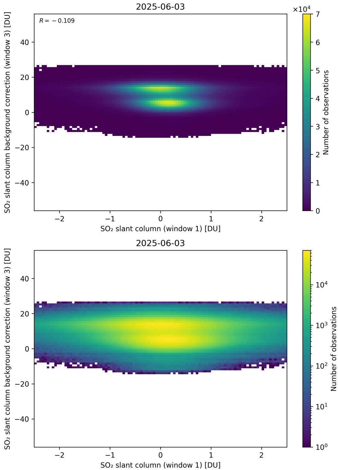
Figure 264: Scatter density plot of “SO 2 slant column (window 1)” against “SO 2 slant column background correction (window 3)” for 2025-06-02 to 2025-06-04.
