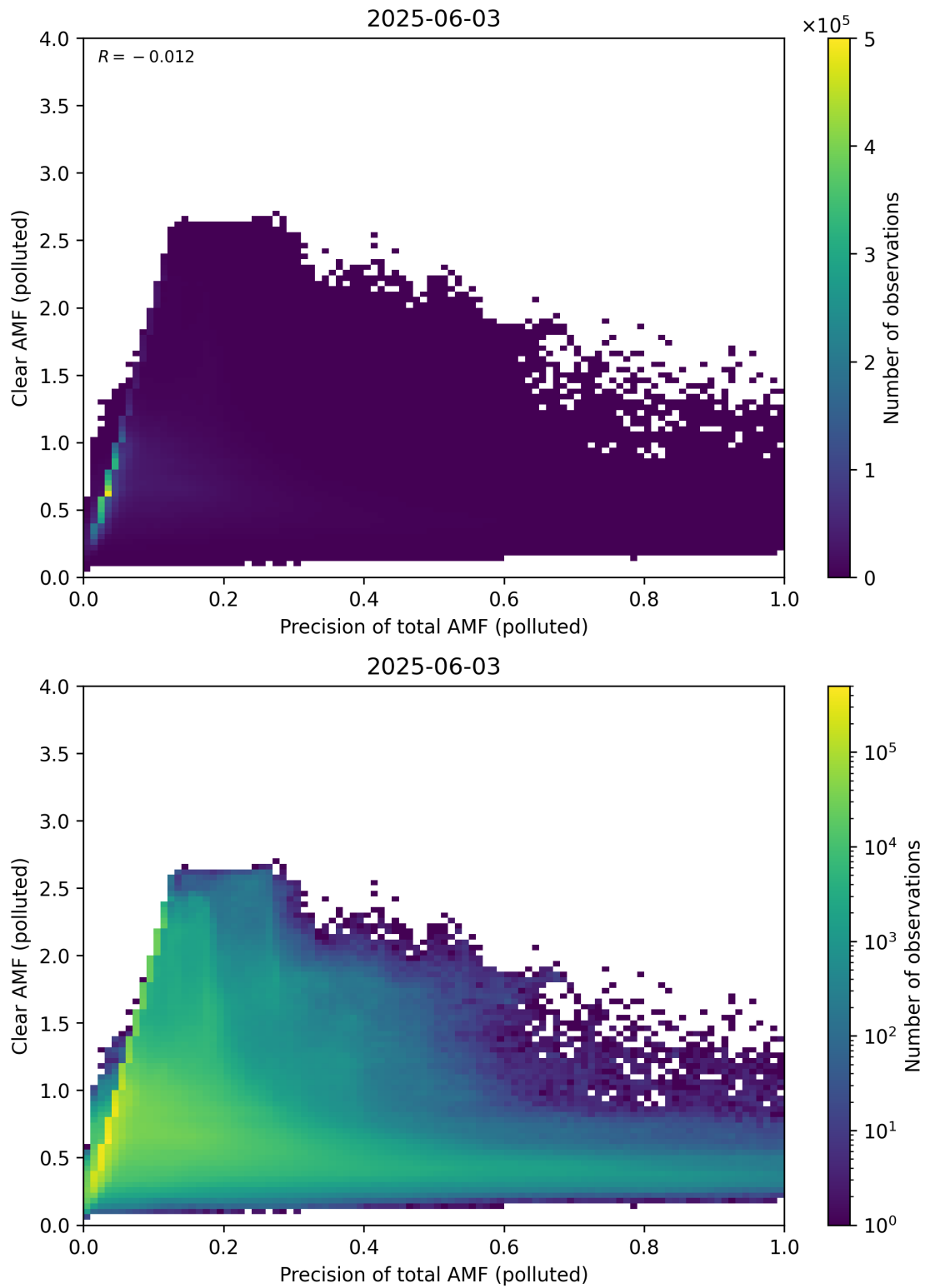
Figure 320: Scatter density plot of “Precision of total AMF (polluted)” against “Clear AMF (polluted)” for 2025-06-02 to 2025-06-04.
