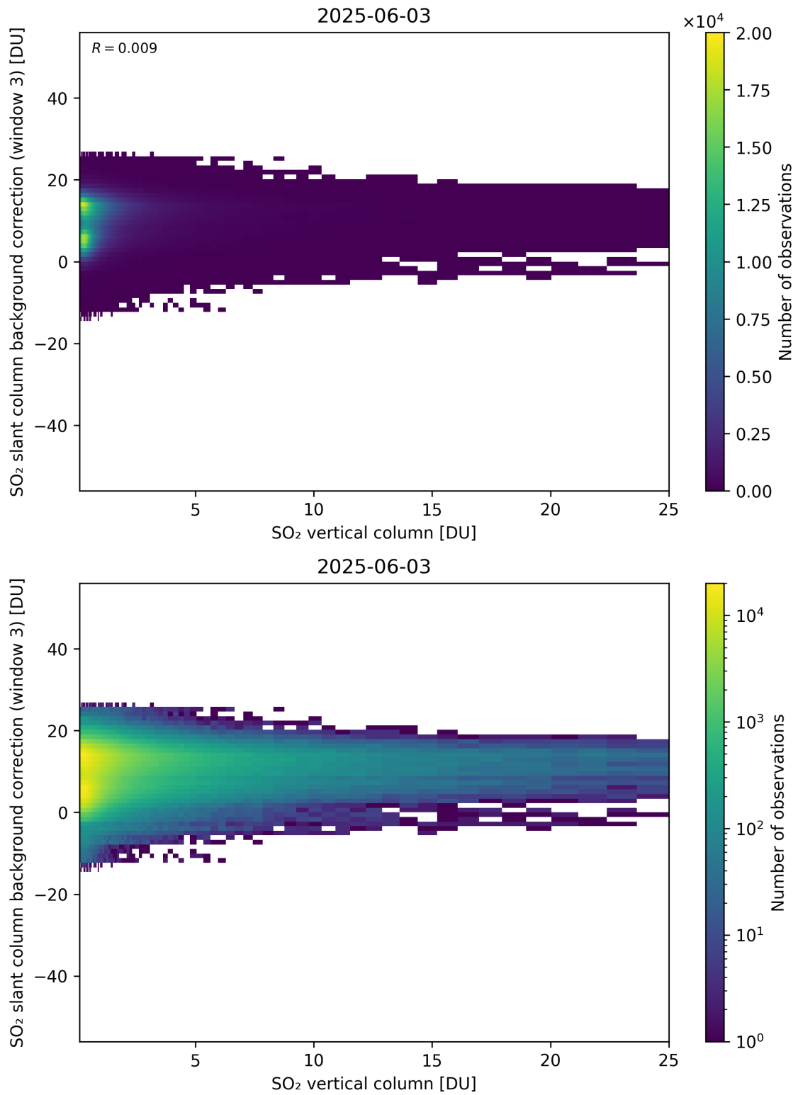
Figure 325: Scatter density plot of “SO 2 vertical column” against “SO 2 slant column background correction (window 3)” for 2025-06-02 to 2025-06-04.
