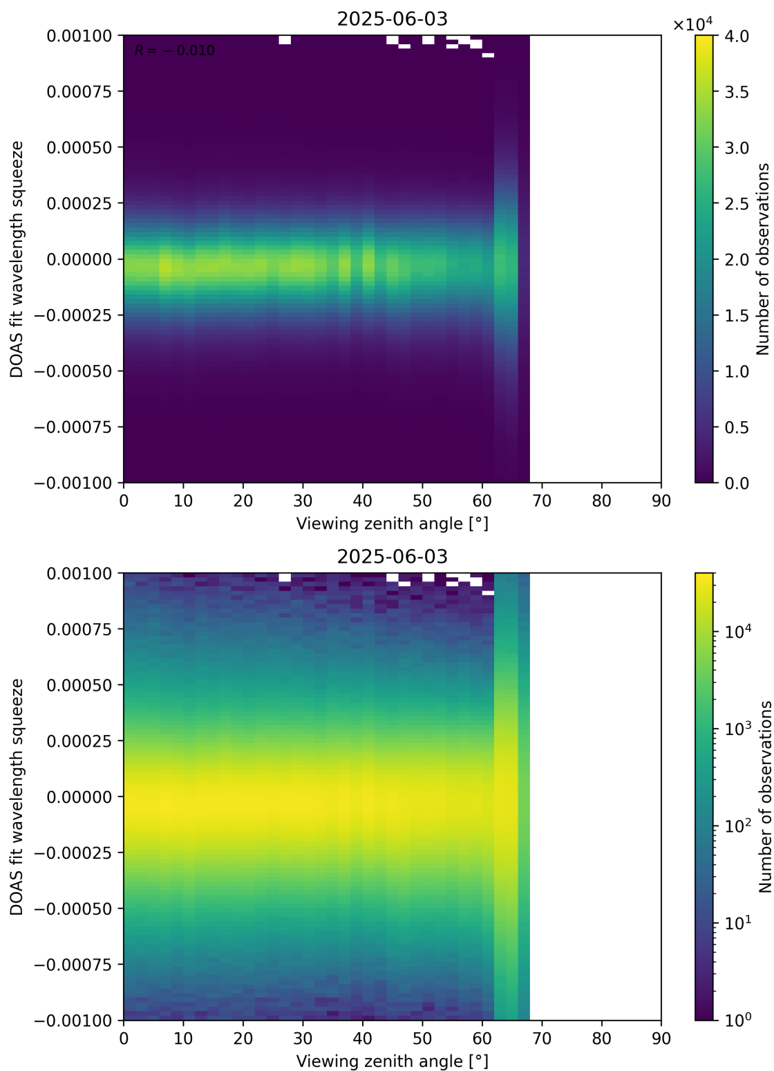
Figure 366: Scatter density plot of “Viewing zenith angle” against “DOAS fit wavelength squeeze” for 2025-06-02 to 2025-06-04.
