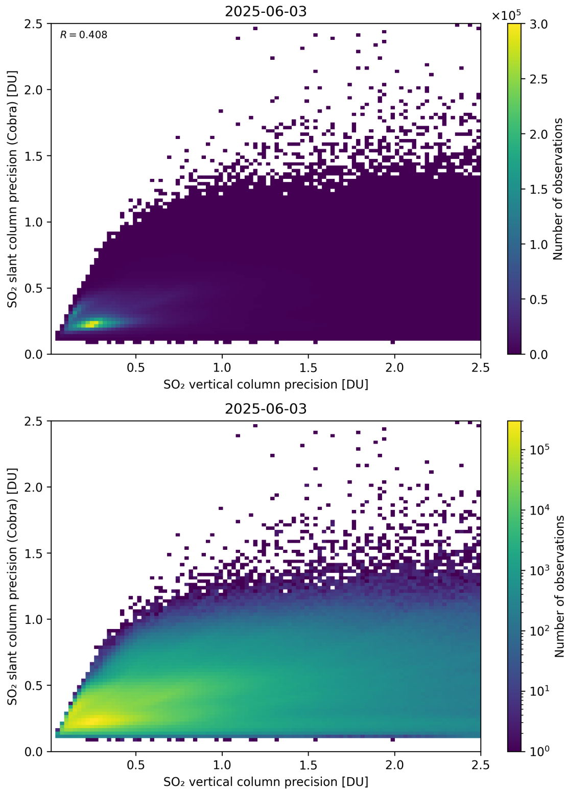
Figure 337: Scatter density plot of “SO 2 vertical column precision” against “SO 2 slant column precision (Cobra)” for 2025-06-02 to 2025-06-04.
