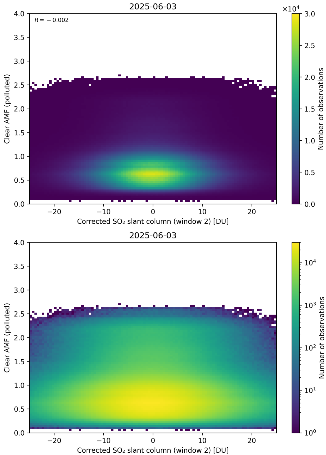
Figure 249: Scatter density plot of “Corrected SO 2 slant column (window 2)” against “Clear AMF (polluted)” for 2025-06-02 to 2025-06-04.
