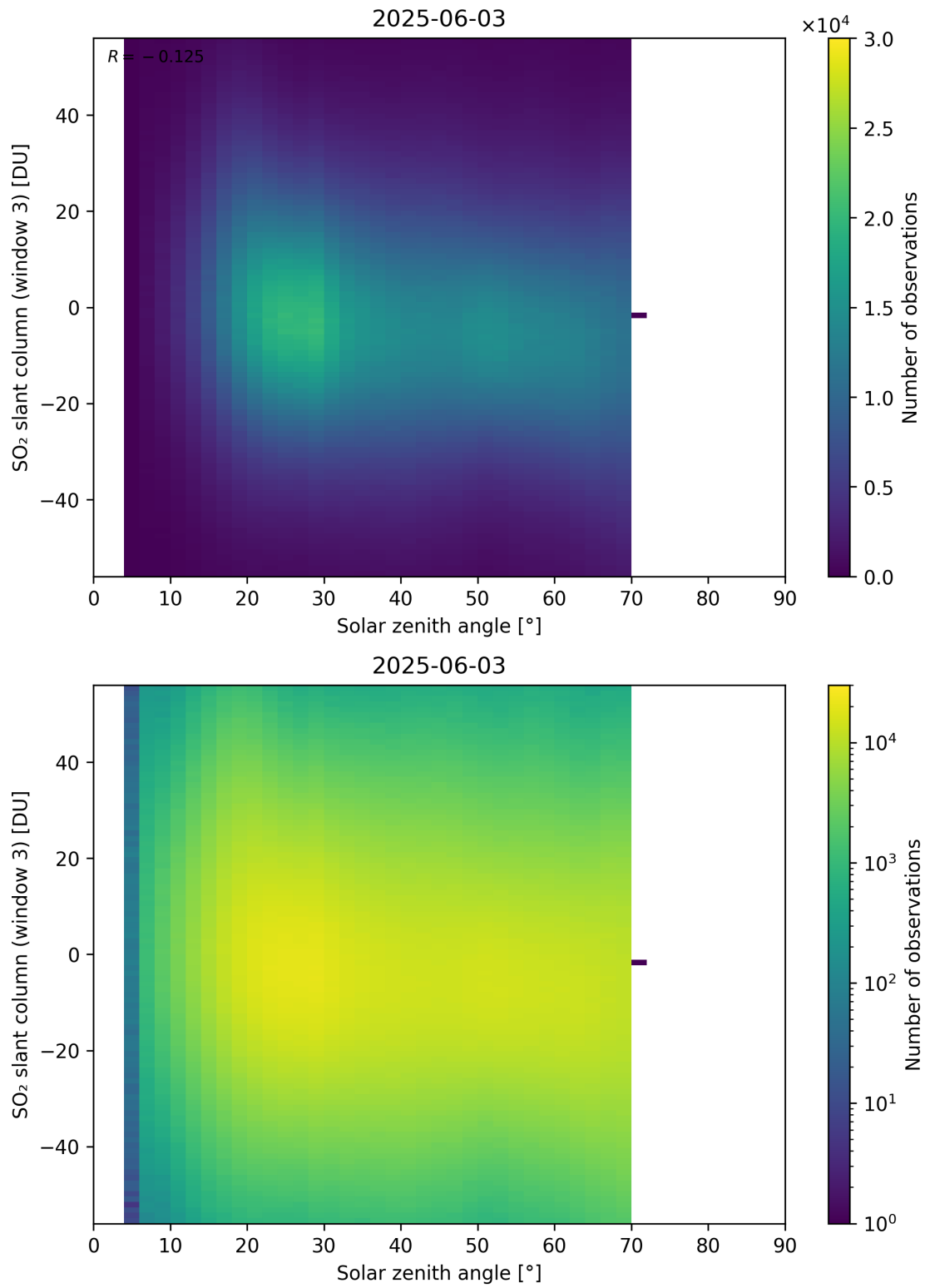
Figure 187: Scatter density plot of “Solar zenith angle” against “SO 2 slant column (window 3)” for 2025-06-02 to 2025-06-04.
