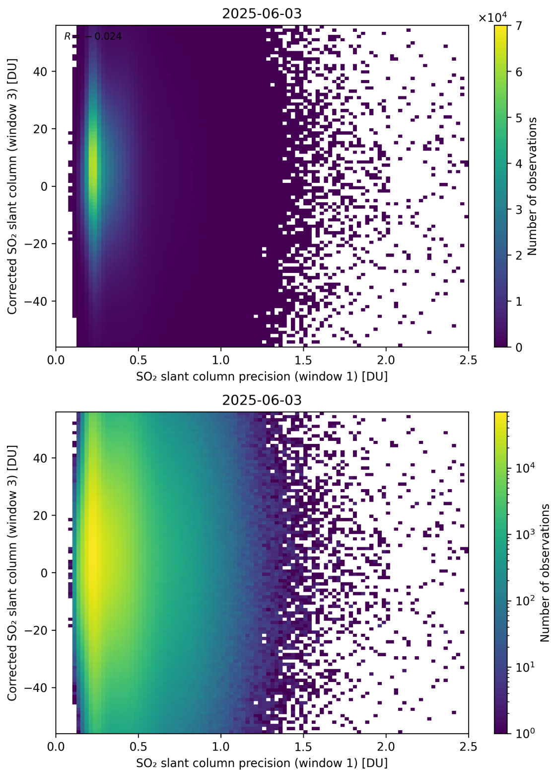
Figure 276: Scatter density plot of “SO 2 slant column precision (window 1)” against “Corrected SO 2 slant column (window 3)” for 2025-06-02 to 2025-06-04.
