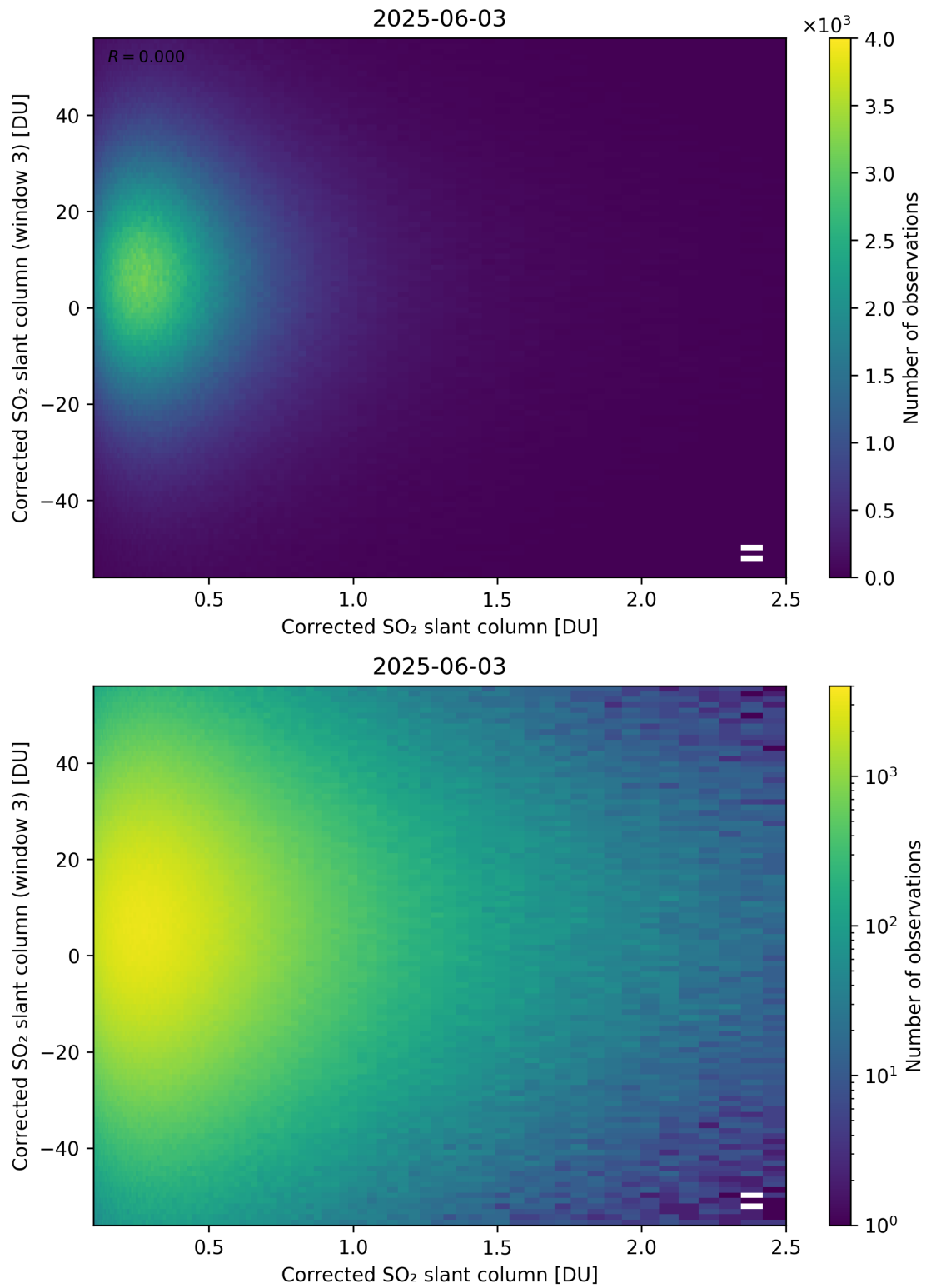
Figure 236: Scatter density plot of “Corrected SO 2 slant column” against “Corrected SO 2 slant column (window 3)” for 2025-06-02 to 2025-06-04.
