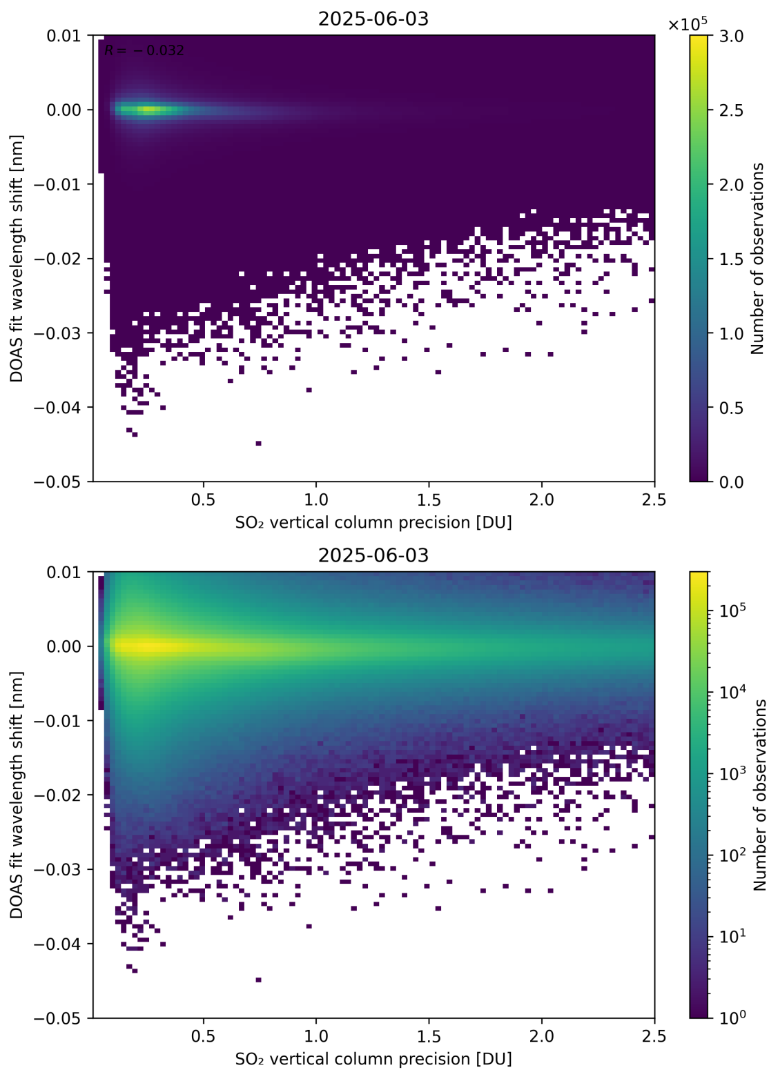
Figure 332: Scatter density plot of “SO 2 vertical column precision” against “DOAS fit wavelength shift” for 2025-06-02 to 2025-06-04.
