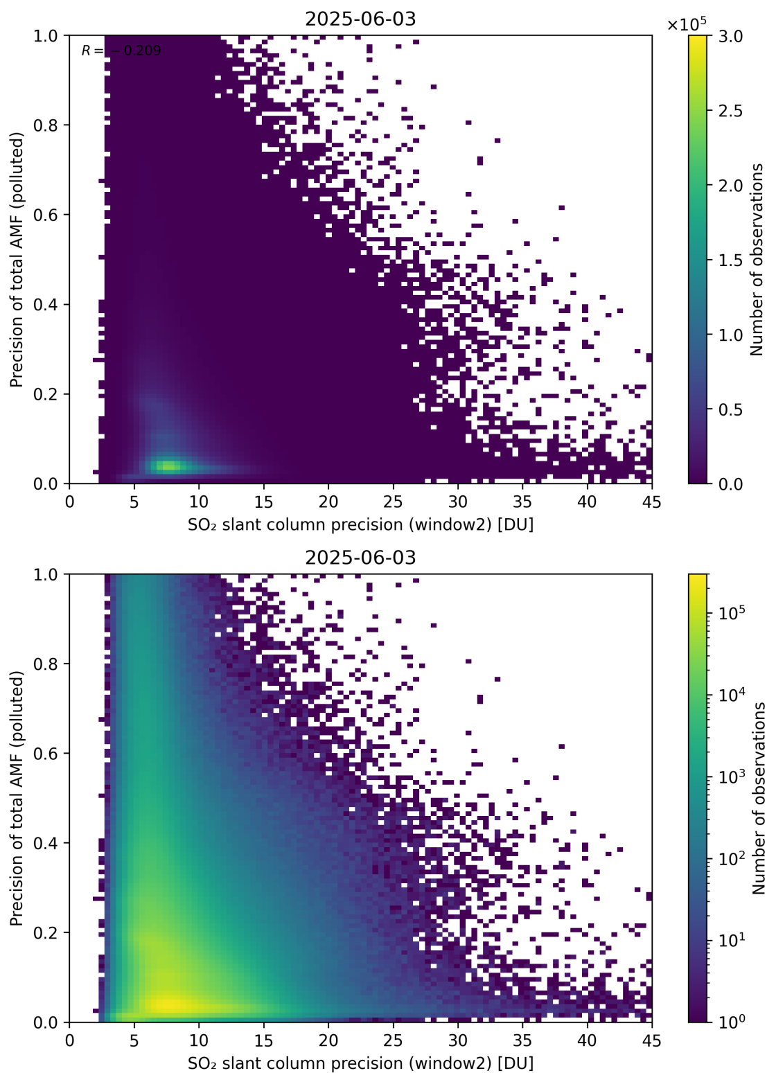
Figure 302: Scatter density plot of “SO 2 slant column precision (window2)” against “Precision of total AMF (polluted)” for 2025-06-02 to 2025-06-04.
