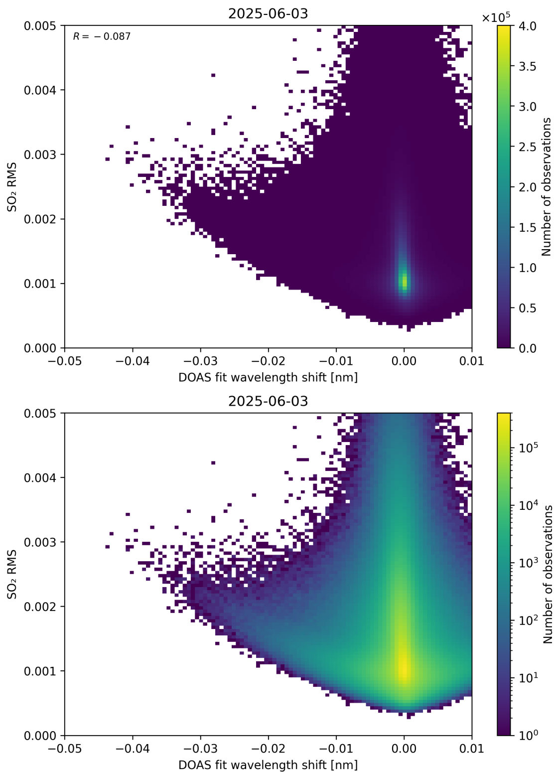
Figure 139: Scatter density plot of “DOAS fit wavelength shift” against “SO 2 RMS” for 2025-06-02 to 2025-06-04.
