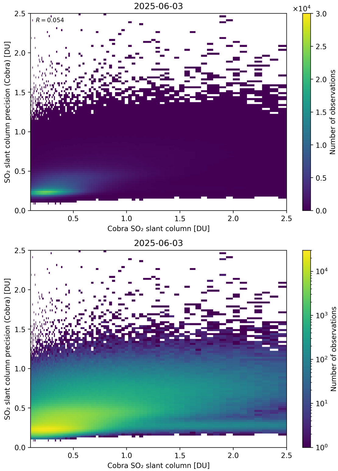
Figure 216: Scatter density plot of “Cobra SO 2 slant column” against “SO 2 slant column precision (Cobra)” for 2025-06-02 to 2025-06-04.
