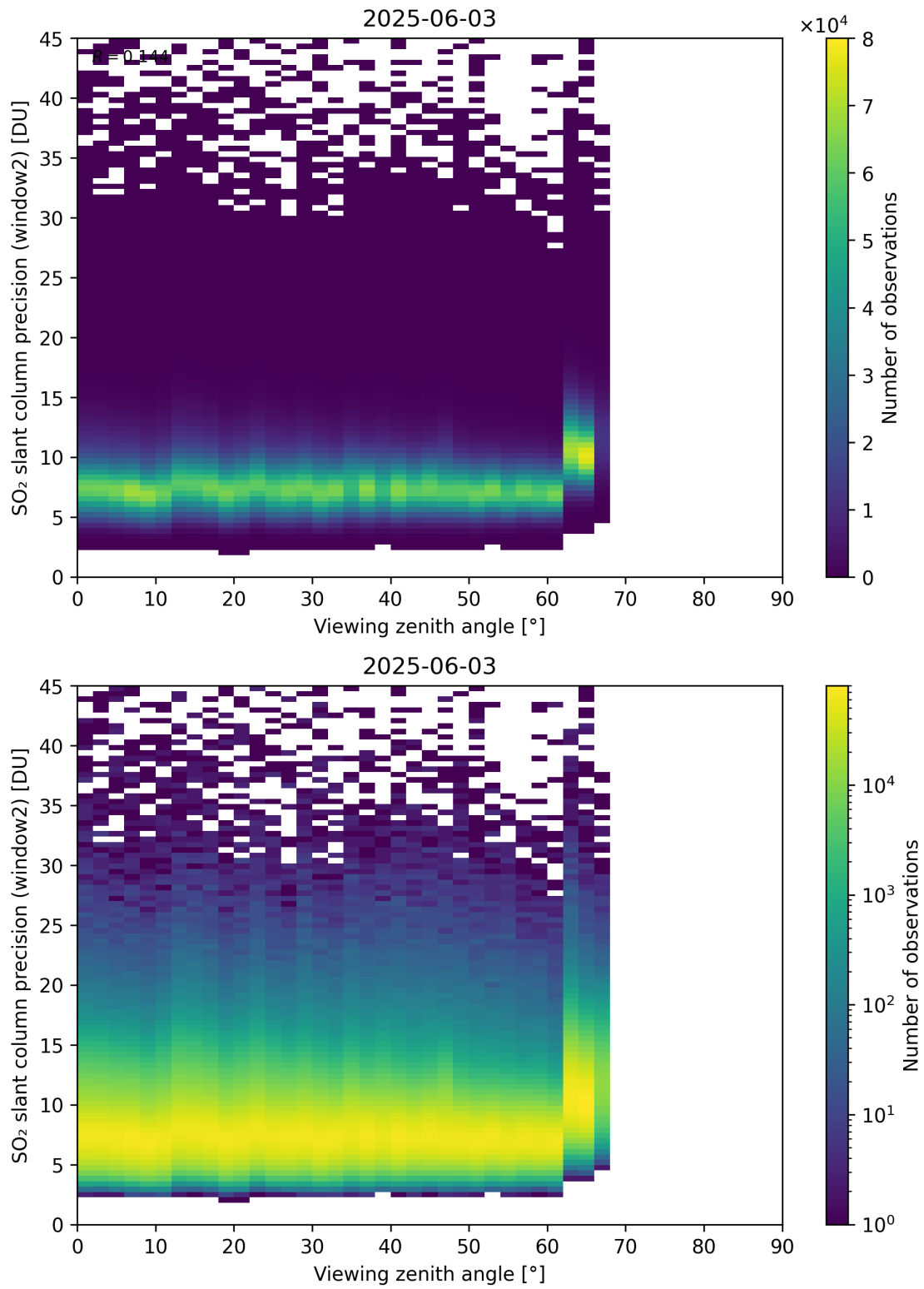
Figure 378: Scatter density plot of “Viewing zenith angle” against “SO 2 slant column precision (window2)” for 2025-06-02 to 2025-06-04.
