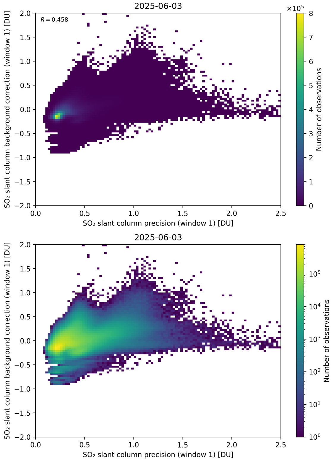
Figure 268: Scatter density plot of “SO 2 slant column precision (window 1)” against “SO 2 slant column background correction (window 1)” for 2025-06-02 to 2025-06-04.
