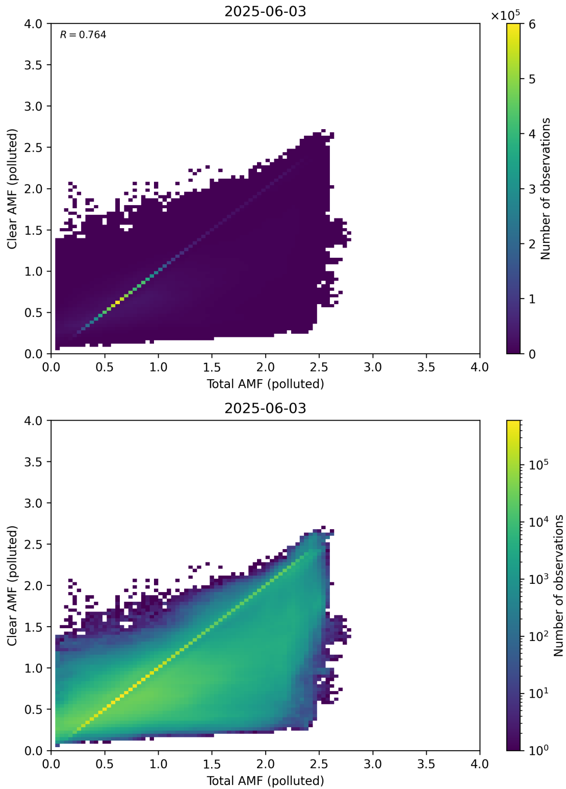
Figure 321: Scatter density plot of “Total AMF (polluted)” against “Clear AMF (polluted)” for 2025-06-02 to 2025-06-04.
