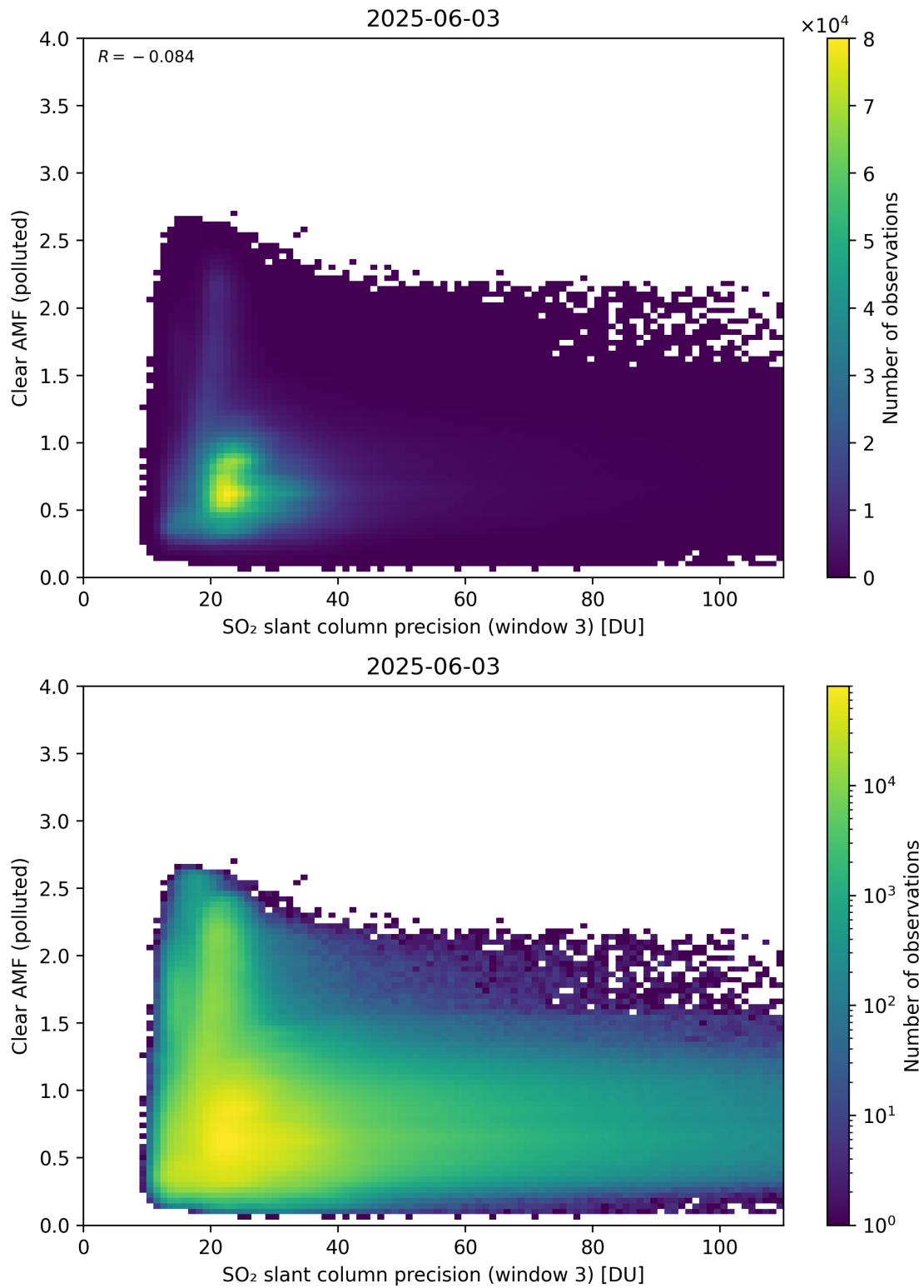
Figure 311: Scatter density plot of “SO 2 slant column precision (window 3)” against “Clear AMF (polluted)” for 2025-06-02 to 2025-06-04.
