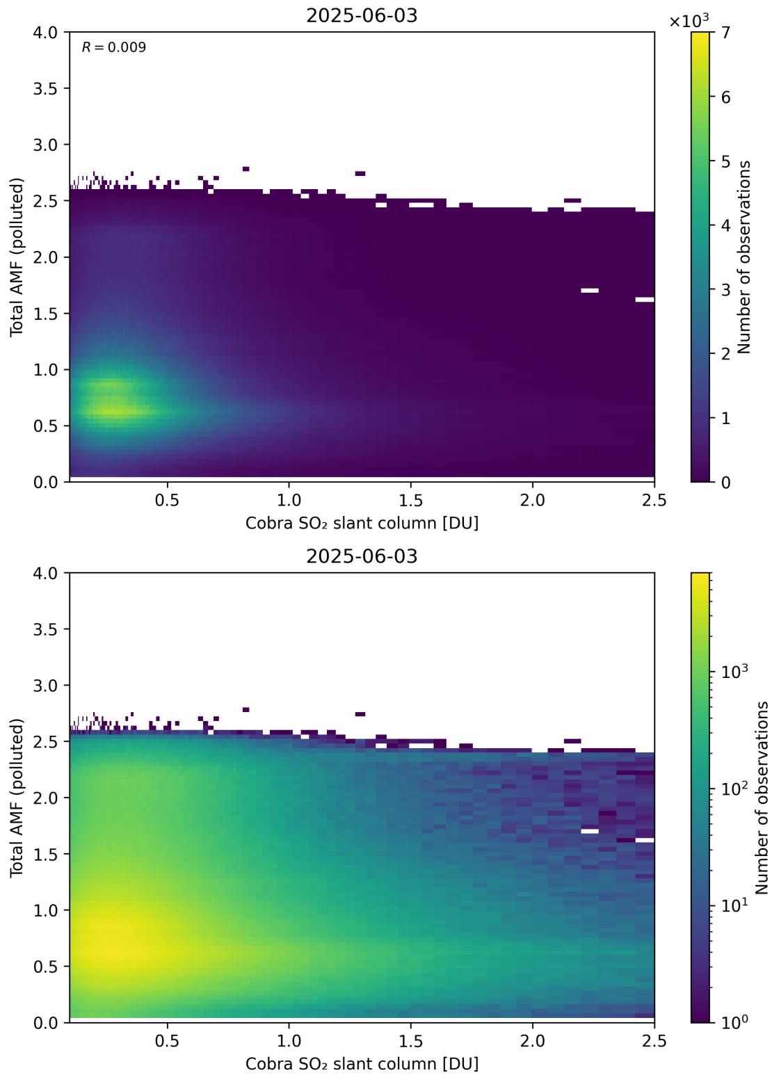
Figure 224: Scatter density plot of “Cobra SO 2 slant column” against “Total AMF (polluted)” for 2025-06-02 to 2025-06-04.
