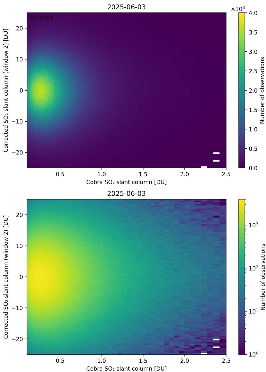
Figure 217: Scatter density plot of “Cobra SO 2 slant column” against “Corrected SO 2 slant column (window 2)” for 2025-06-02 to 2025-06-04.
