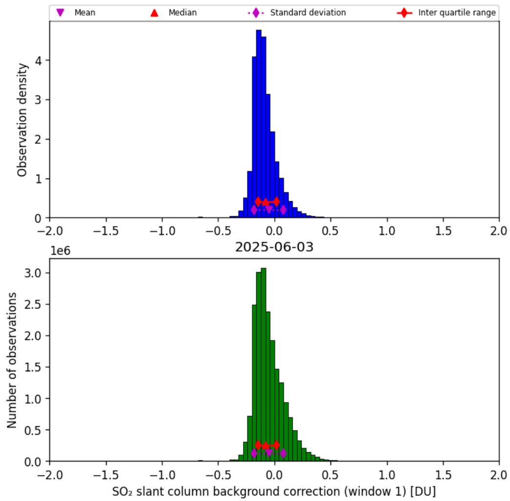
Figure 66: Histogram of “SO 2 slant column background correction (window 1)” for 2025-06-02 to 2025-06-04
