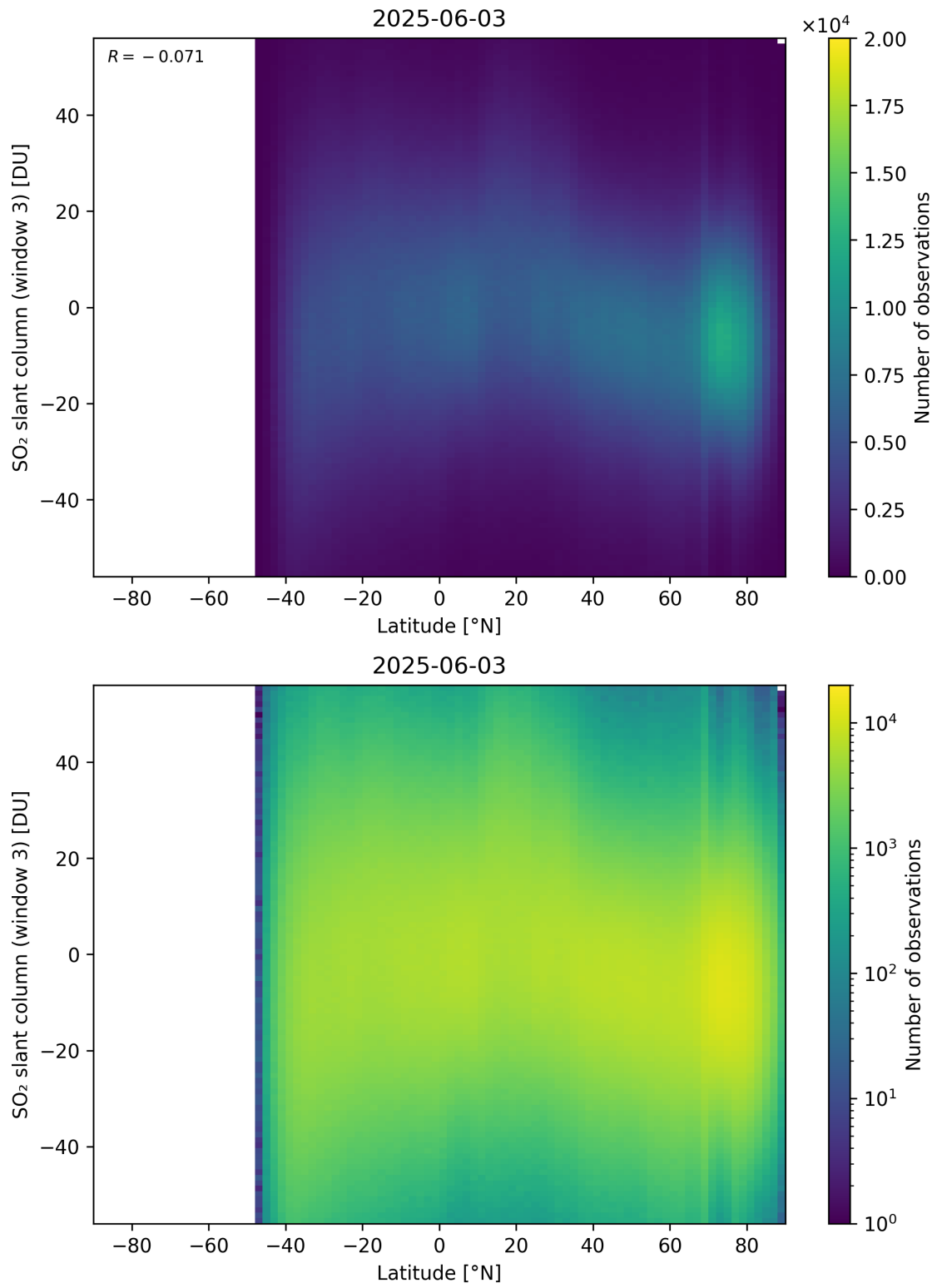
Figure 165: Scatter density plot of “Latitude” against “SO 2 slant column (window 3)” for 2025-06-02 to 2025-06-04.
