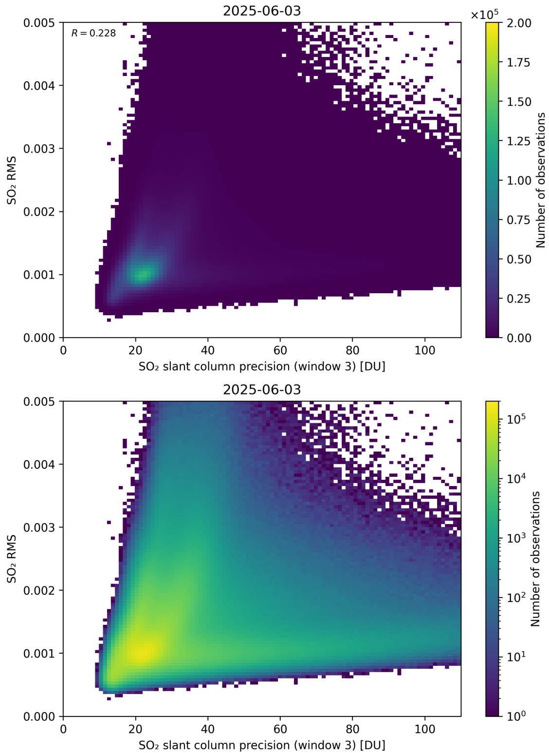
Figure 310: Scatter density plot of “SO 2 slant column precision (window 3)” against “SO 2 RMS” for 2025-06-02 to 2025-06-04.
