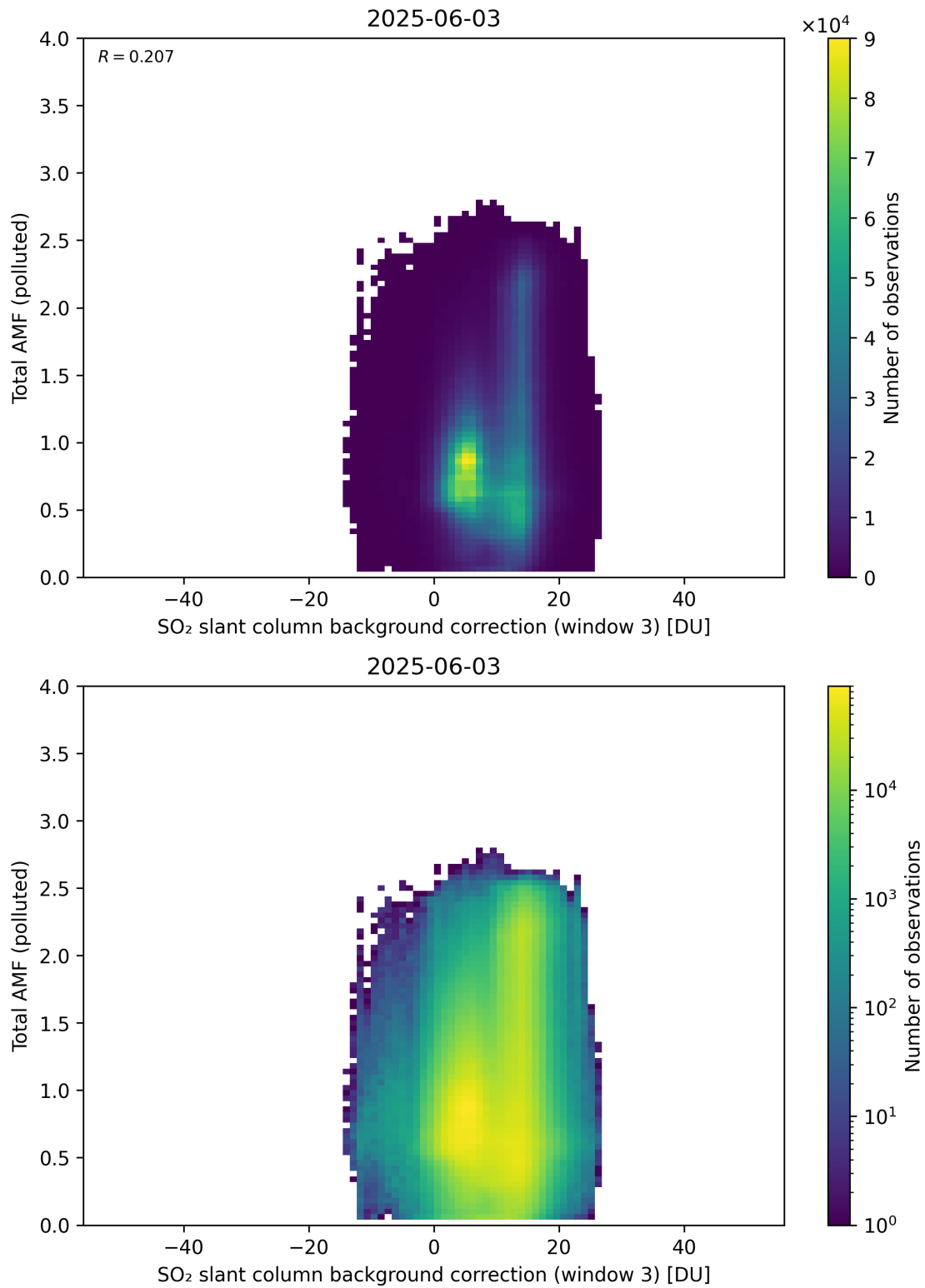
Figure 136: Scatter density plot of “SO 2 slant column background correction (window 3)” against “Total AMF (polluted)” for 2025-06-02 to 2025-06-04.
