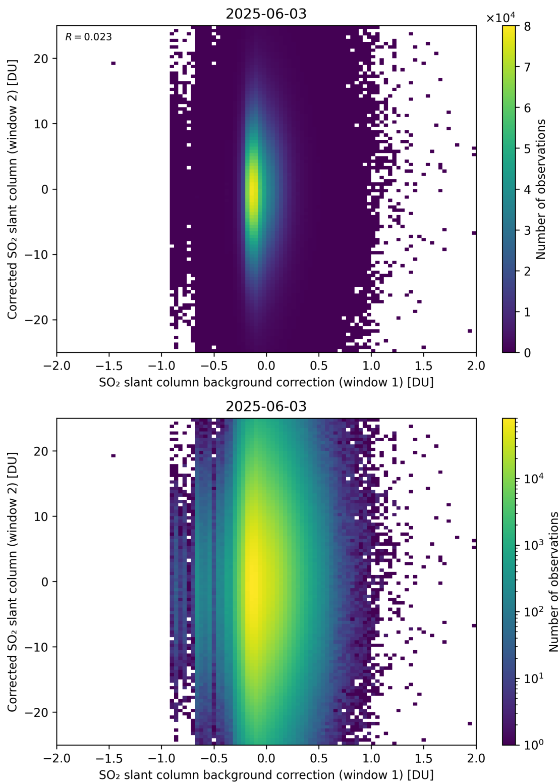
Figure 115: Scatter density plot of “SO 2 slant column background correction (window 1)” against “Corrected SO 2 slant column (window 2)” for 2025-06-02 to 2025-06-04.
