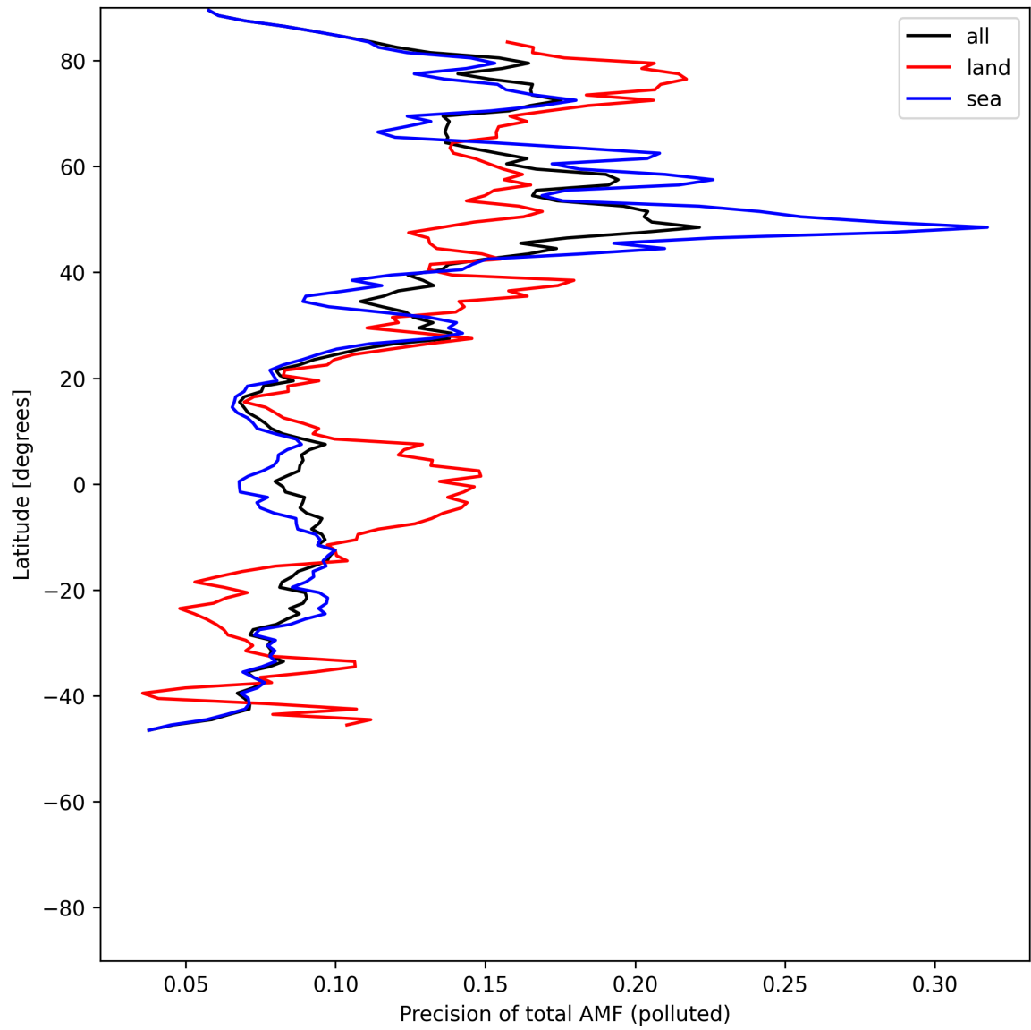
Figure 54: Zonal average of “Precision of total AMF (polluted)” for 2025-06-02 to 2025-06-04.
