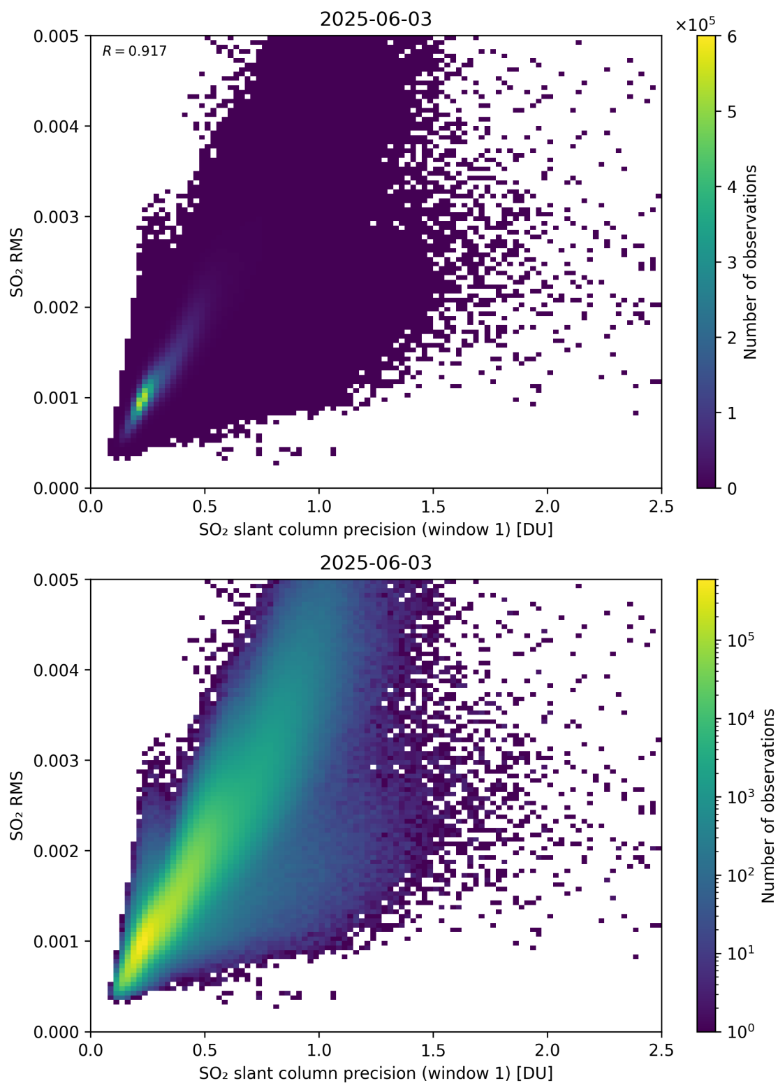
Figure 273: Scatter density plot of “SO 2 slant column precision (window 1)” against “SO 2 RMS” for 2025-06-02 to 2025-06-04.
