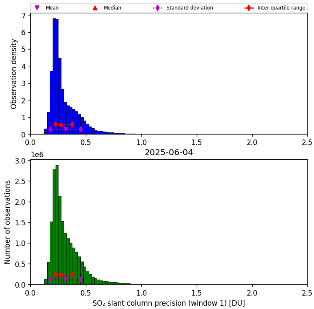
Figure 64: Histogram of “SO 2 slant column precision (window 1)” for 2025-06-03 to 2025-06-05
