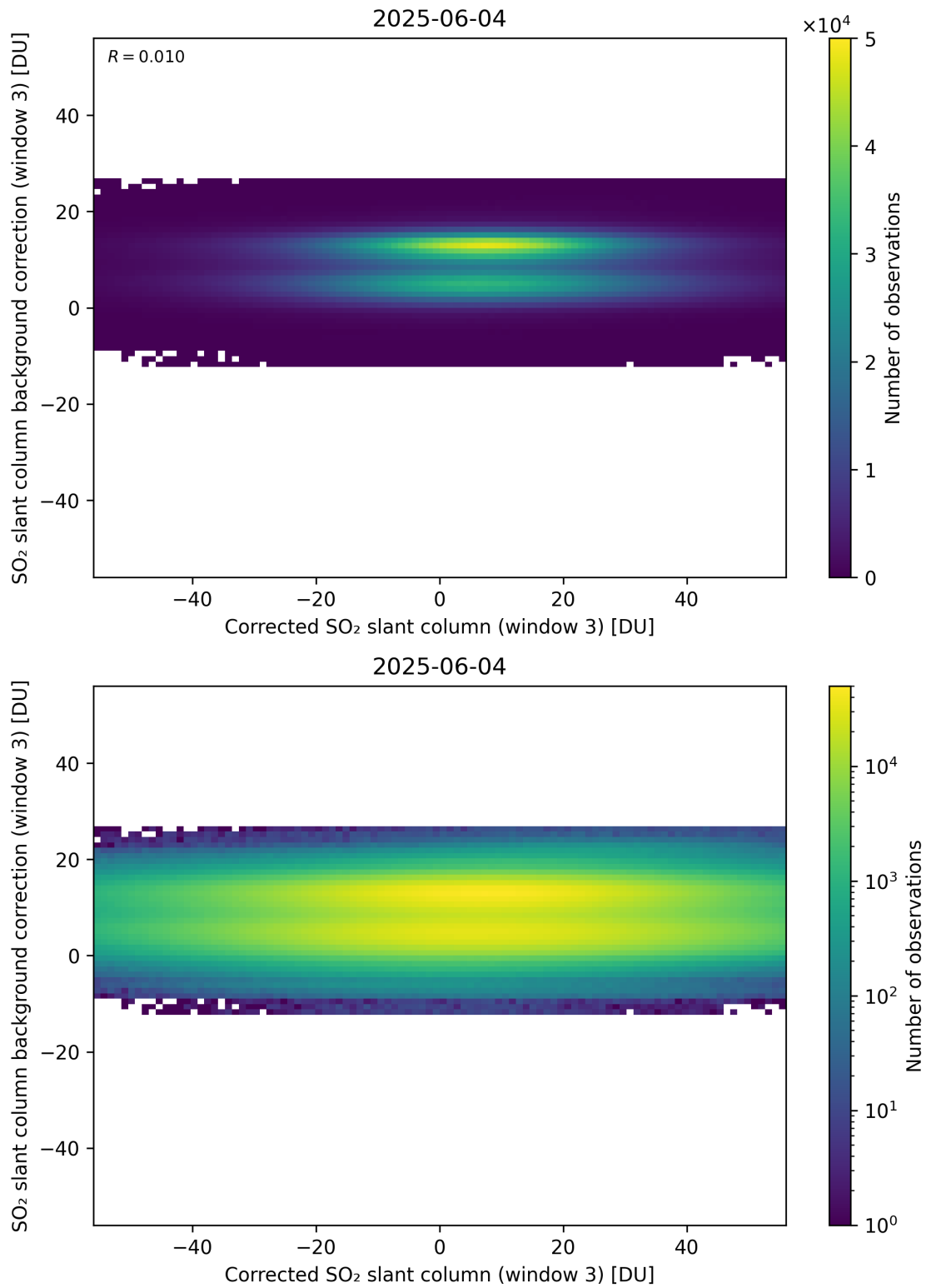
Figure 255: Scatter density plot of “Corrected SO 2 slant column (window 3)” against “SO 2 slant column background correction (window 3)” for 2025-06-03 to 2025-06-05.
