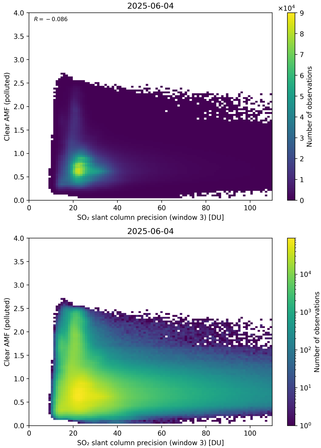
Figure 311: Scatter density plot of “SO 2 slant column precision (window 3)” against “Clear AMF (polluted)” for 2025-06-03 to 2025-06-05.
