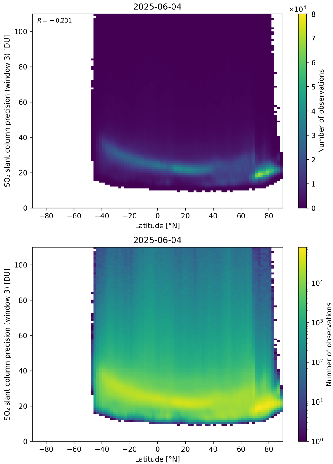
Figure 166: Scatter density plot of “Latitude” against “SO 2 slant column precision (window 3)” for 2025-06-03 to 2025-06-05.
