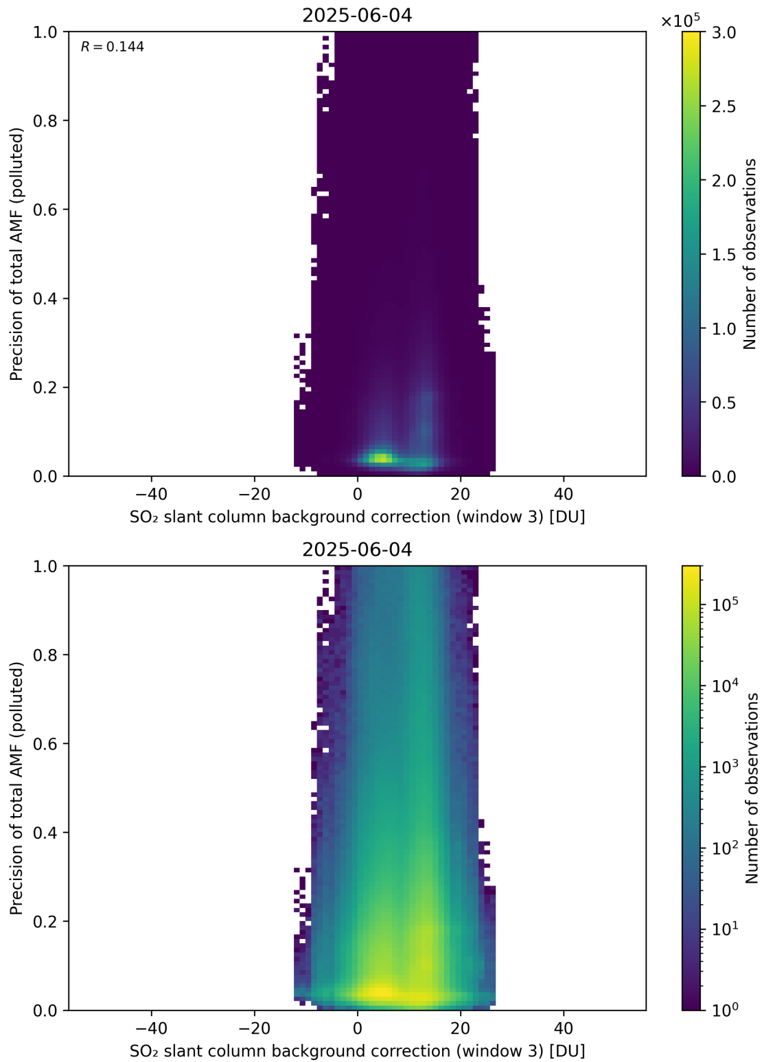
Figure 137: Scatter density plot of “SO 2 slant column background correction (window 3)” against “Precision of total AMF (polluted)” for 2025-06-03 to 2025-06-05.
