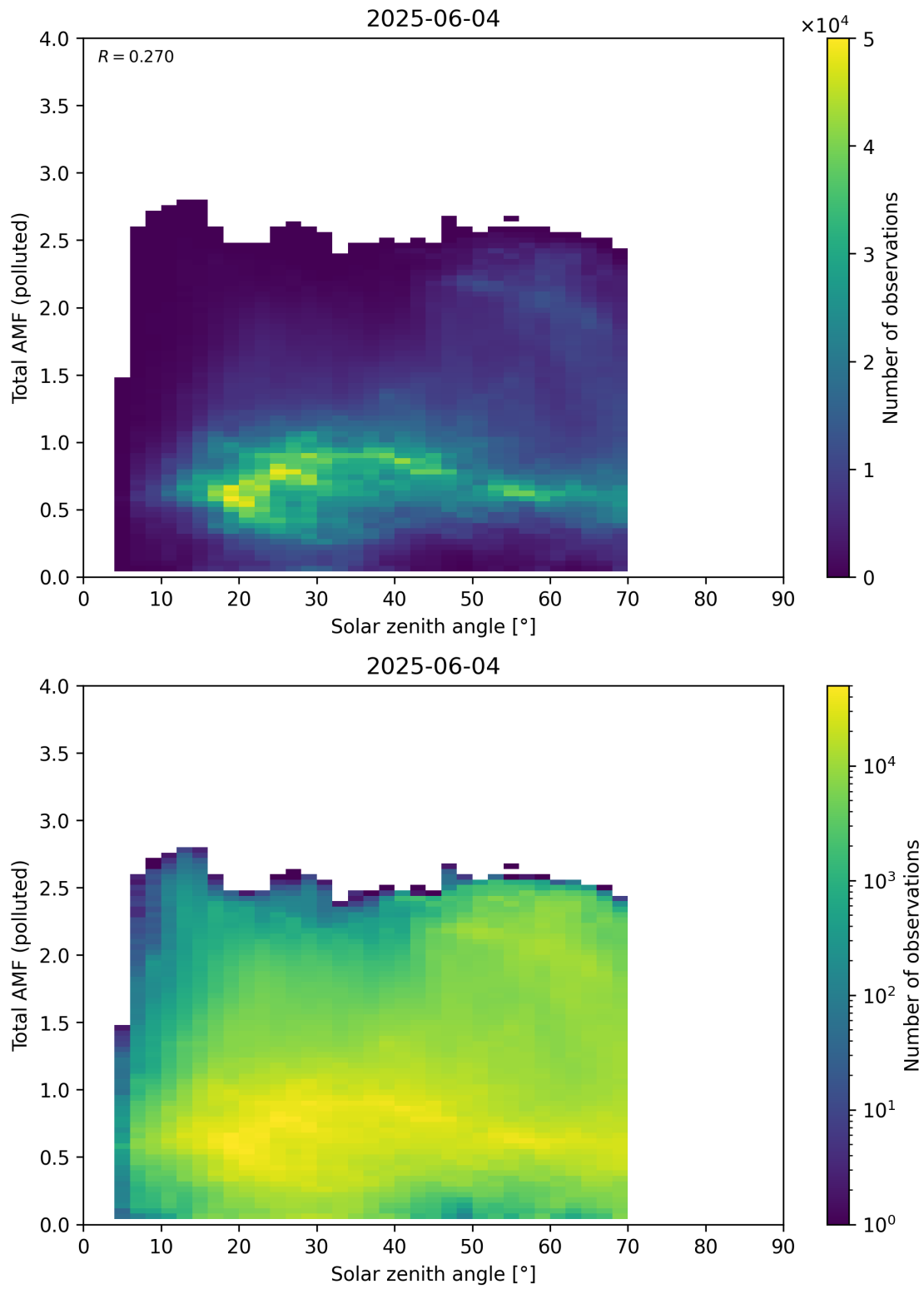
Figure 189: Scatter density plot of “Solar zenith angle” against “Total AMF (polluted)” for 2025-06-03 to 2025-06-05.
