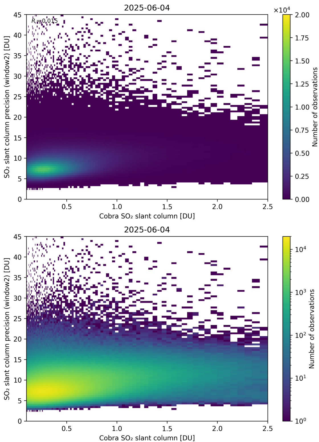
Figure 221: Scatter density plot of “Cobra SO 2 slant column” against “SO 2 slant column precision (window2)” for 2025-06-03 to 2025-06-05.
