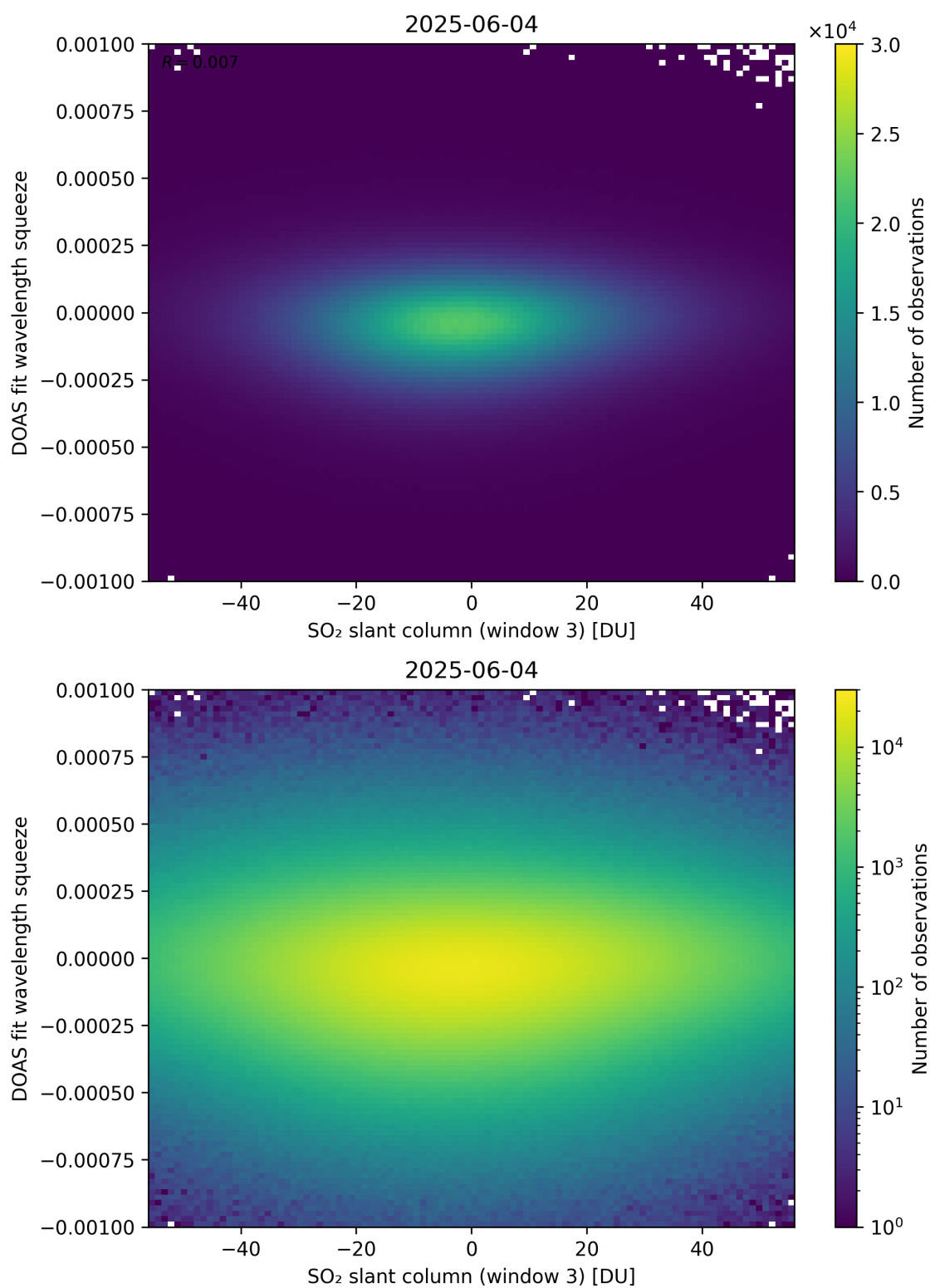
Figure 305: Scatter density plot of “SO 2 slant column (window 3)” against “DOAS fit wavelength squeeze” for 2025-06-03 to 2025-06-05.
