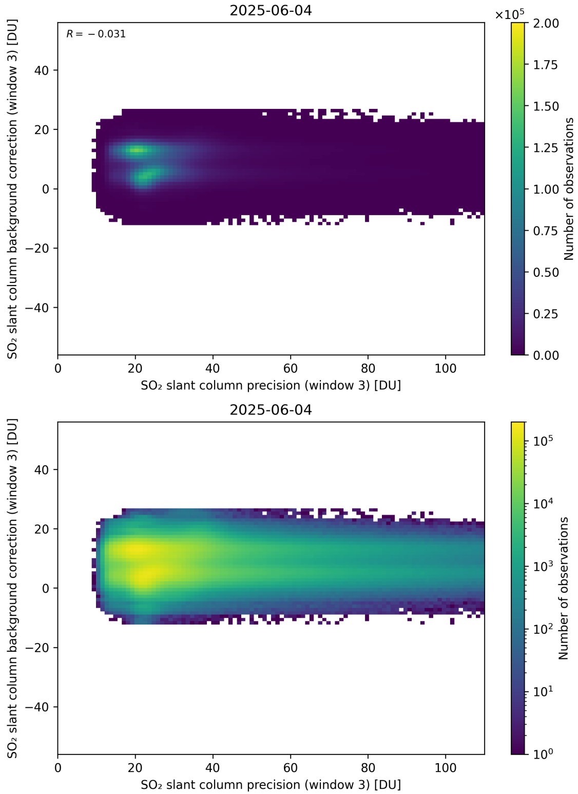
Figure 307: Scatter density plot of “SO 2 slant column precision (window 3)” against “SO 2 slant column background correction (window 3)” for 2025-06-03 to 2025-06-05.
