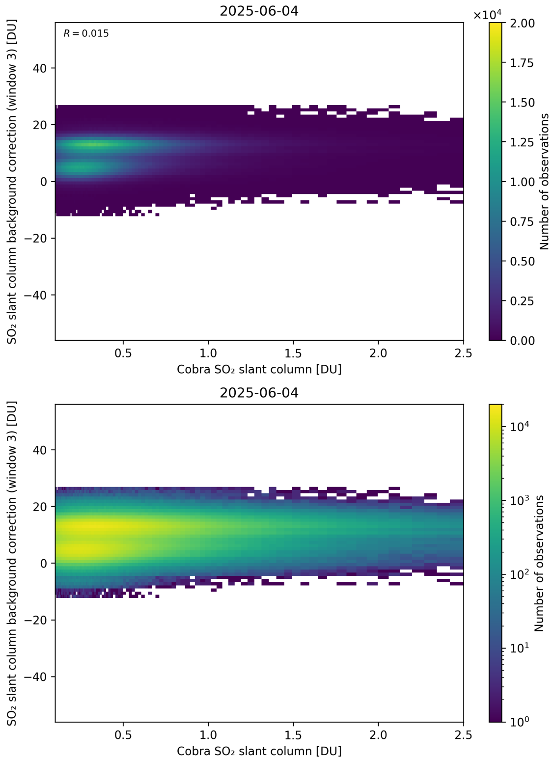
Figure 195: Scatter density plot of “Cobra SO 2 slant column” against “SO 2 slant column background correction (window 3)” for 2025-06-03 to 2025-06-05.
