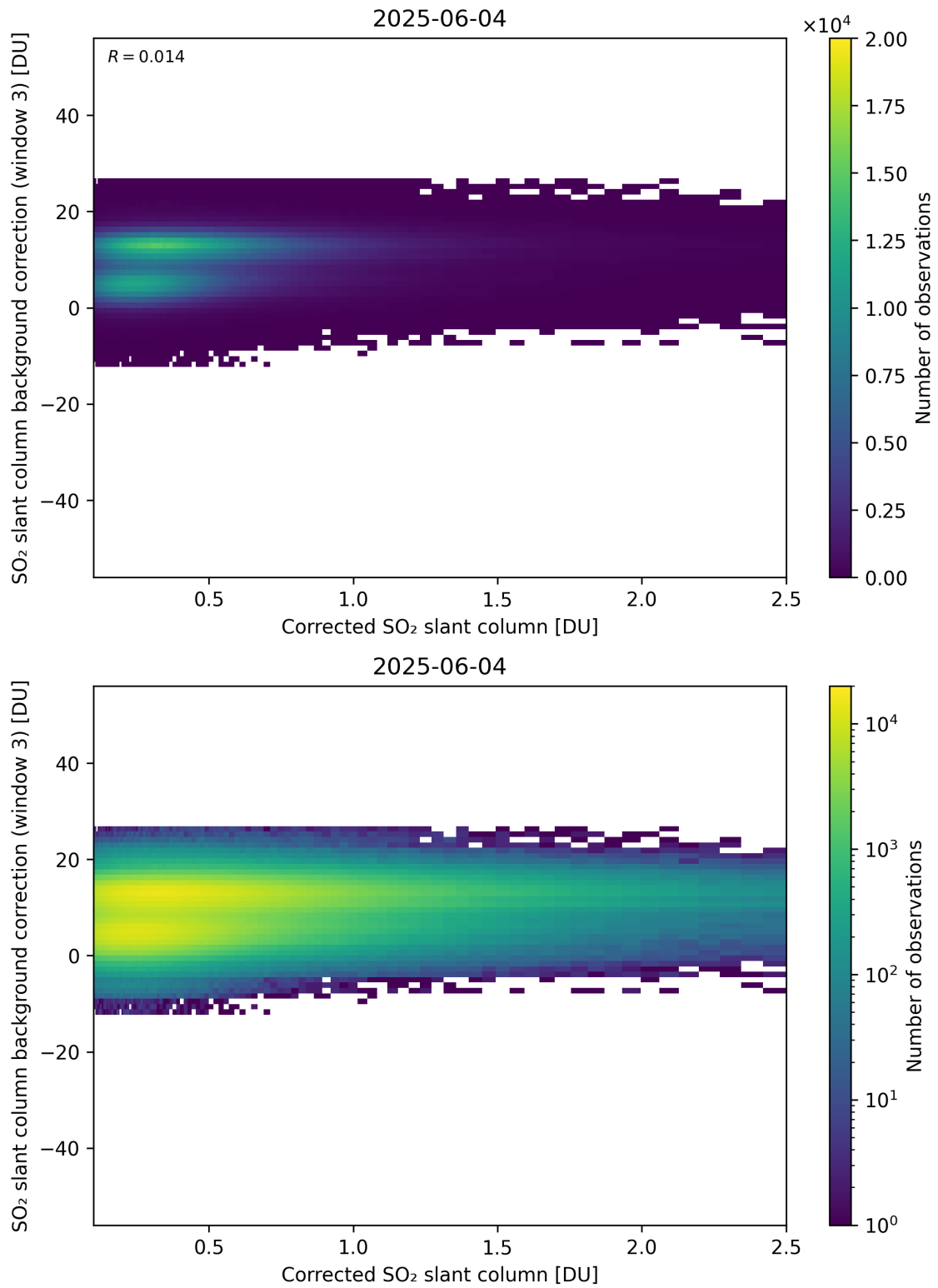
Figure 228: Scatter density plot of “Corrected SO 2 slant column” against “SO 2 slant column background correction (window 3)” for 2025-06-03 to 2025-06-05.
