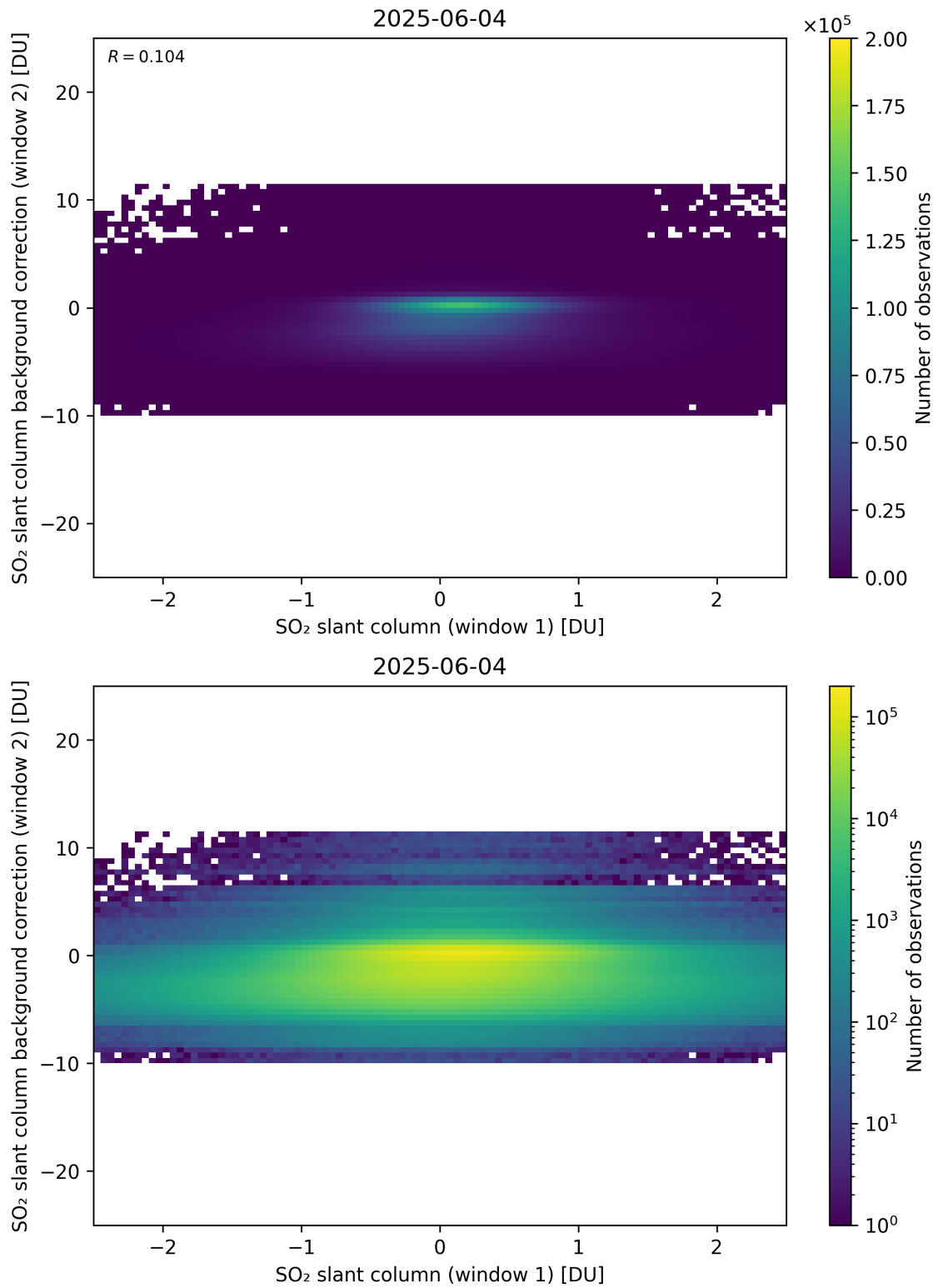
Figure 263: Scatter density plot of “SO 2 slant column (window 1)” against “SO 2 slant column background correction (window 2)” for 2025-06-03 to 2025-06-05.
