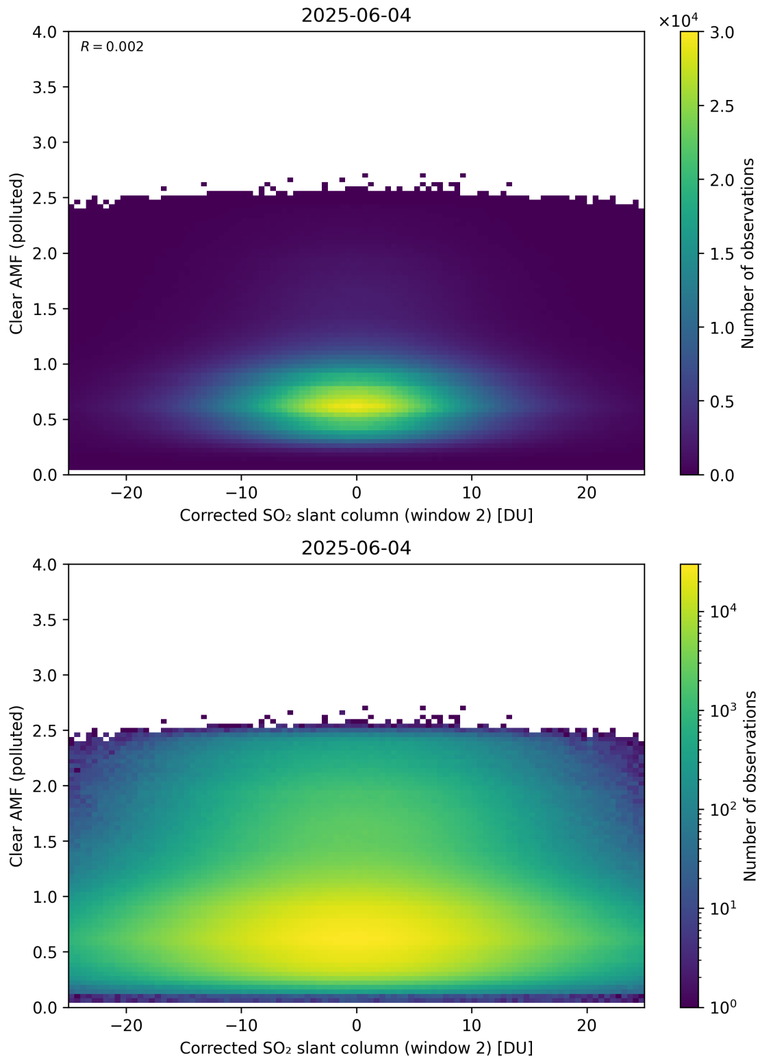
Figure 249: Scatter density plot of “Corrected SO 2 slant column (window 2)” against “Clear AMF (polluted)” for 2025-06-03 to 2025-06-05.
