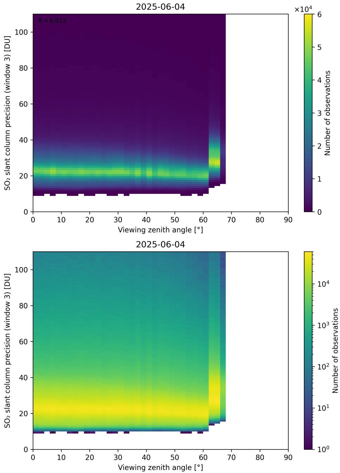
Figure 380: Scatter density plot of “Viewing zenith angle” against “SO 2 slant column precision (window 3)” for 2025-06-03 to 2025-06-05.
