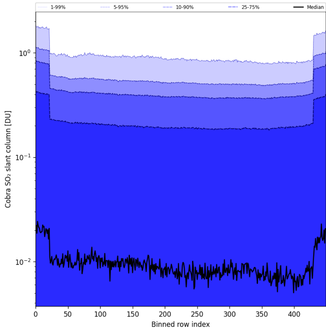
Figure 87: Along track statistics of “Cobra SO 2 slant column” for 2025-06-03 to 2025-06-05
