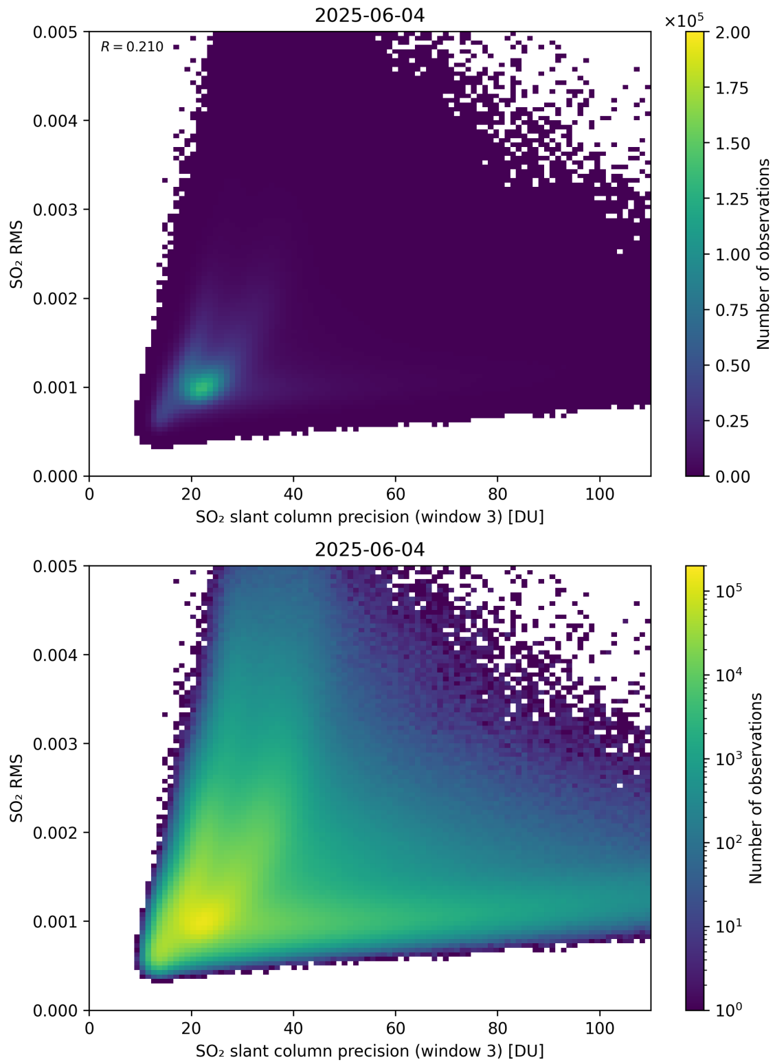
Figure 310: Scatter density plot of “SO 2 slant column precision (window 3)” against “SO 2 RMS” for 2025-06-03 to 2025-06-05.
