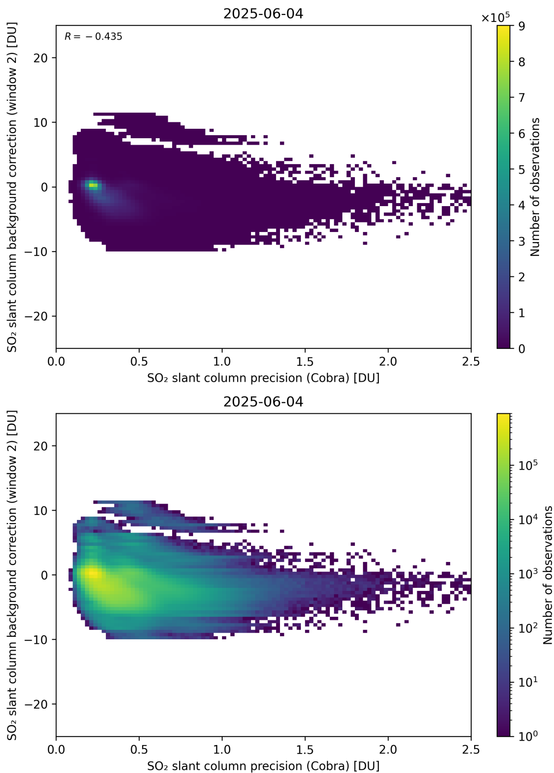
Figure 200: Scatter density plot of “SO 2 slant column precision (Cobra)” against “SO 2 slant column background correction (window 2)” for 2025-06-03 to 2025-06-05.
