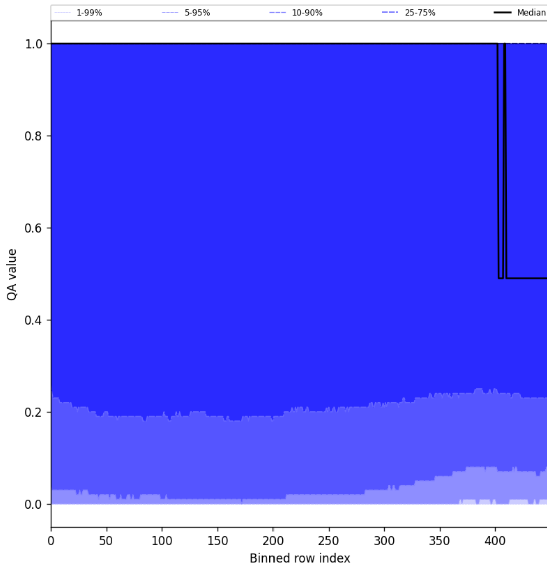
Figure 83: Along track statistics of “QA value” for 2025-06-03 to 2025-06-05
