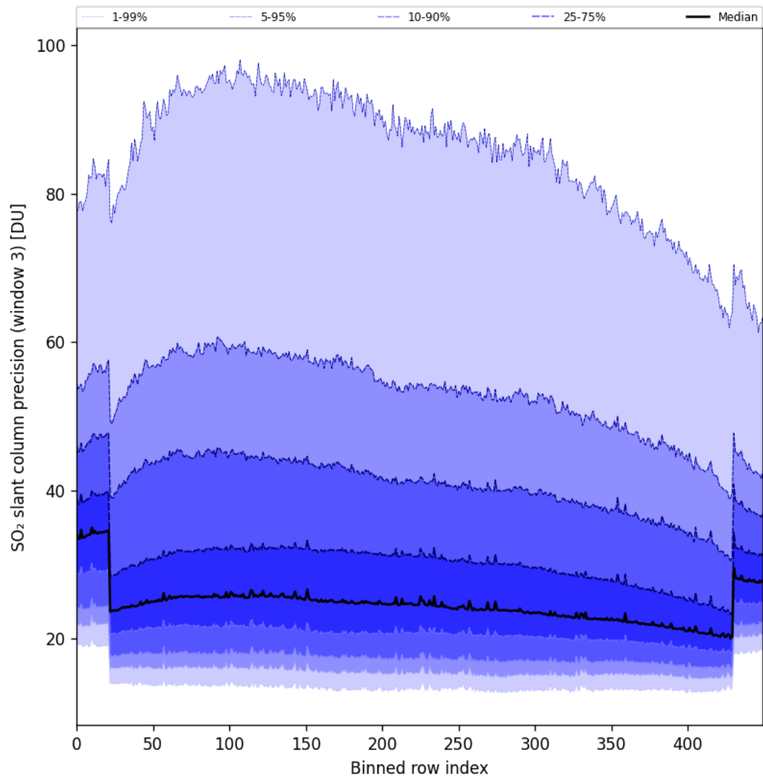
Figure 98: Along track statistics of “SO 2 slant column precision (window 3)” for 2025-06-03 to 2025-06-05
