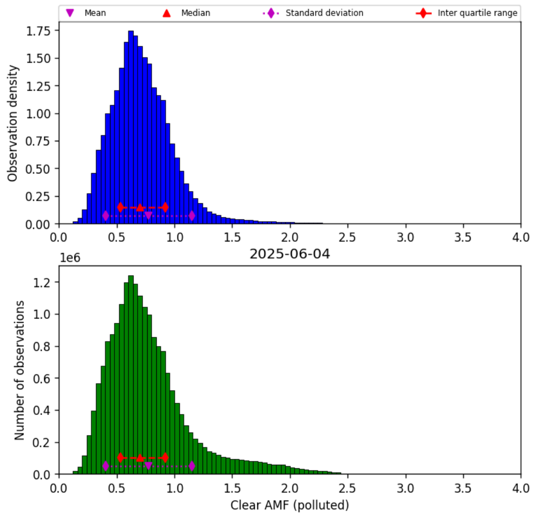
Figure 81: Histogram of “Clear AMF (polluted)” for 2025-06-03 to 2025-06-05
