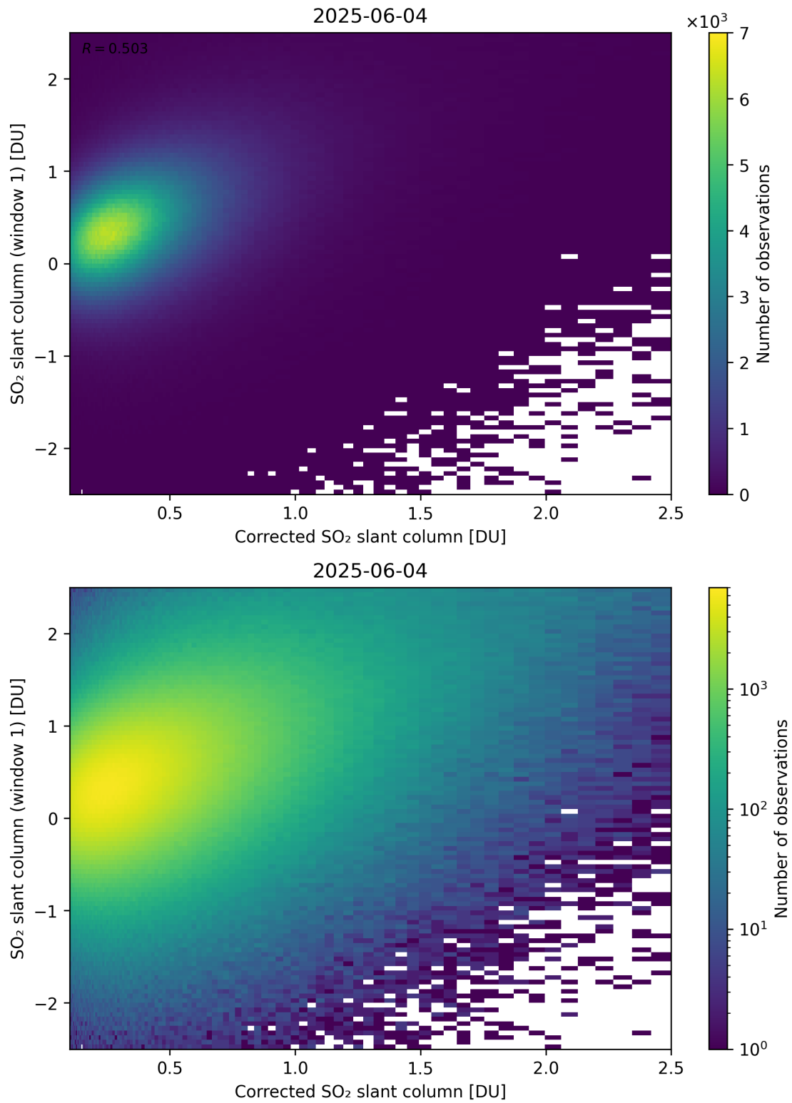
Figure 237: Scatter density plot of “Corrected SO 2 slant column” against “SO 2 slant column (window 1)” for 2025-06-03 to 2025-06-05.
