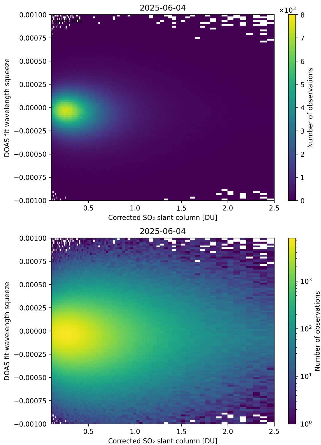
Figure 230: Scatter density plot of “Corrected SO 2 slant column” against “DOAS fit wavelength squeeze” for 2025-06-03 to 2025-06-05.
