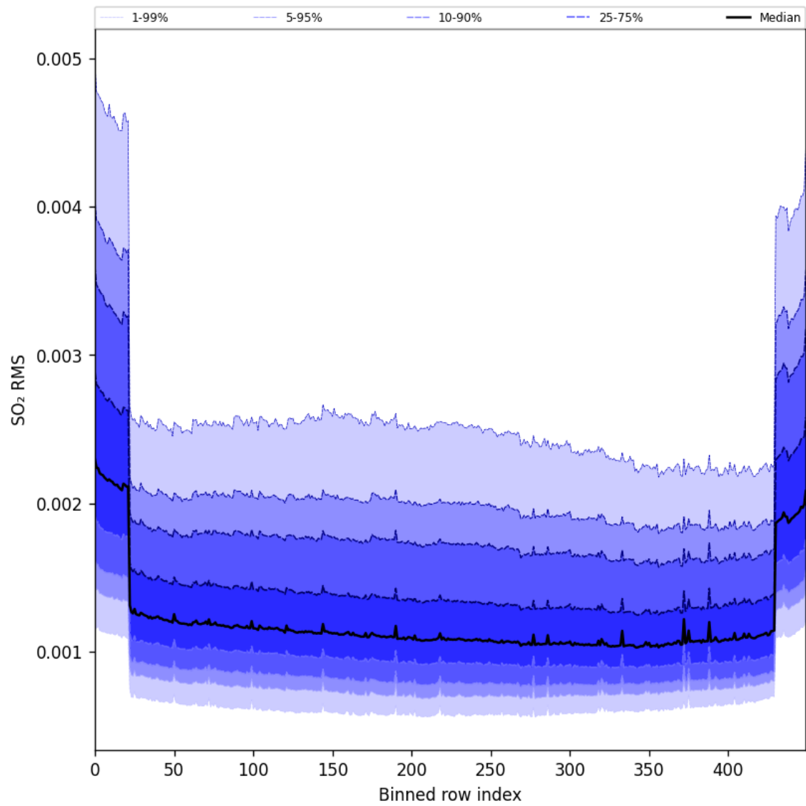
Figure 104: Along track statistics of “SO 2 RMS” for 2025-06-03 to 2025-06-05
