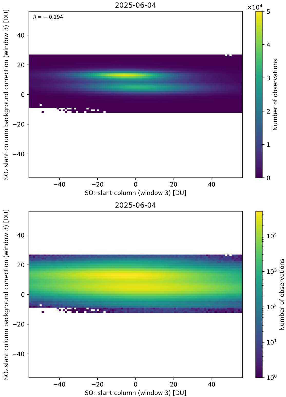
Figure 303: Scatter density plot of “SO 2 slant column (window 3)” against “SO 2 slant column background correction (window 3)” for 2025-06-03 to 2025-06-05.
