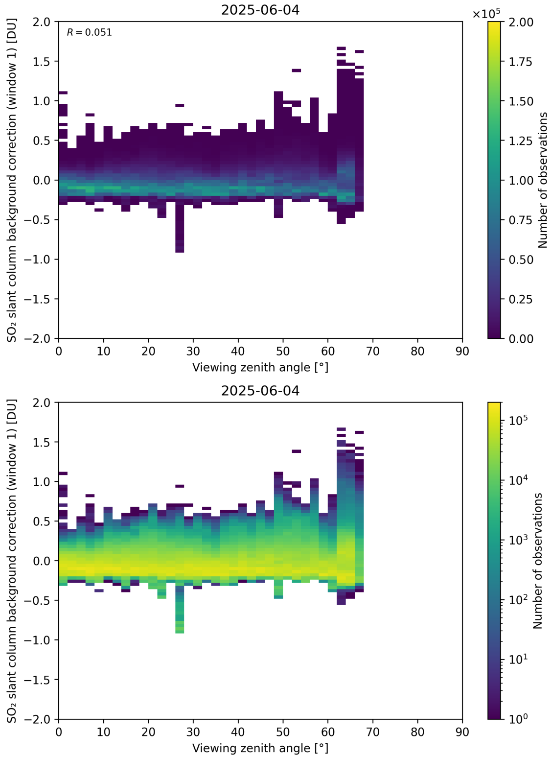
Figure 362: Scatter density plot of “Viewing zenith angle” against “SO 2 slant column background correction (window 1)” for 2025-06-03 to 2025-06-05.
