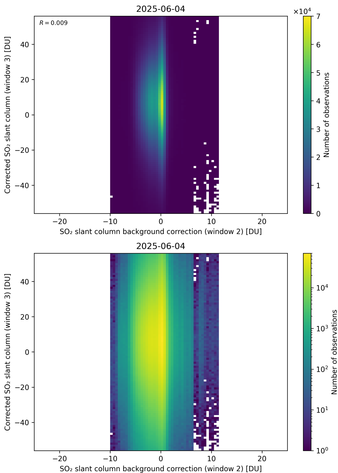
Figure 127: Scatter density plot of “SO 2 slant column background correction (window 2)” against “Corrected SO 2 slant column (window 3)” for 2025-06-03 to 2025-06-05.
