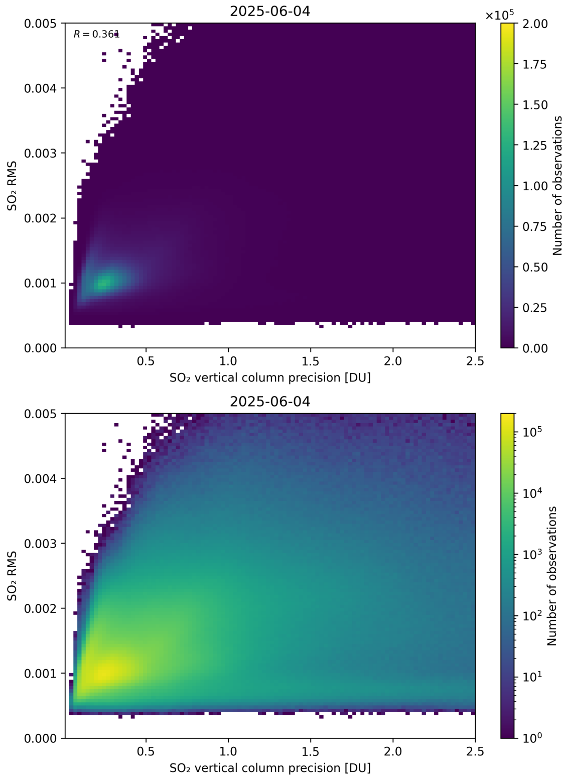
Figure 334: Scatter density plot of “SO 2 vertical column precision” against “SO 2 RMS” for 2025-06-03 to 2025-06-05.
