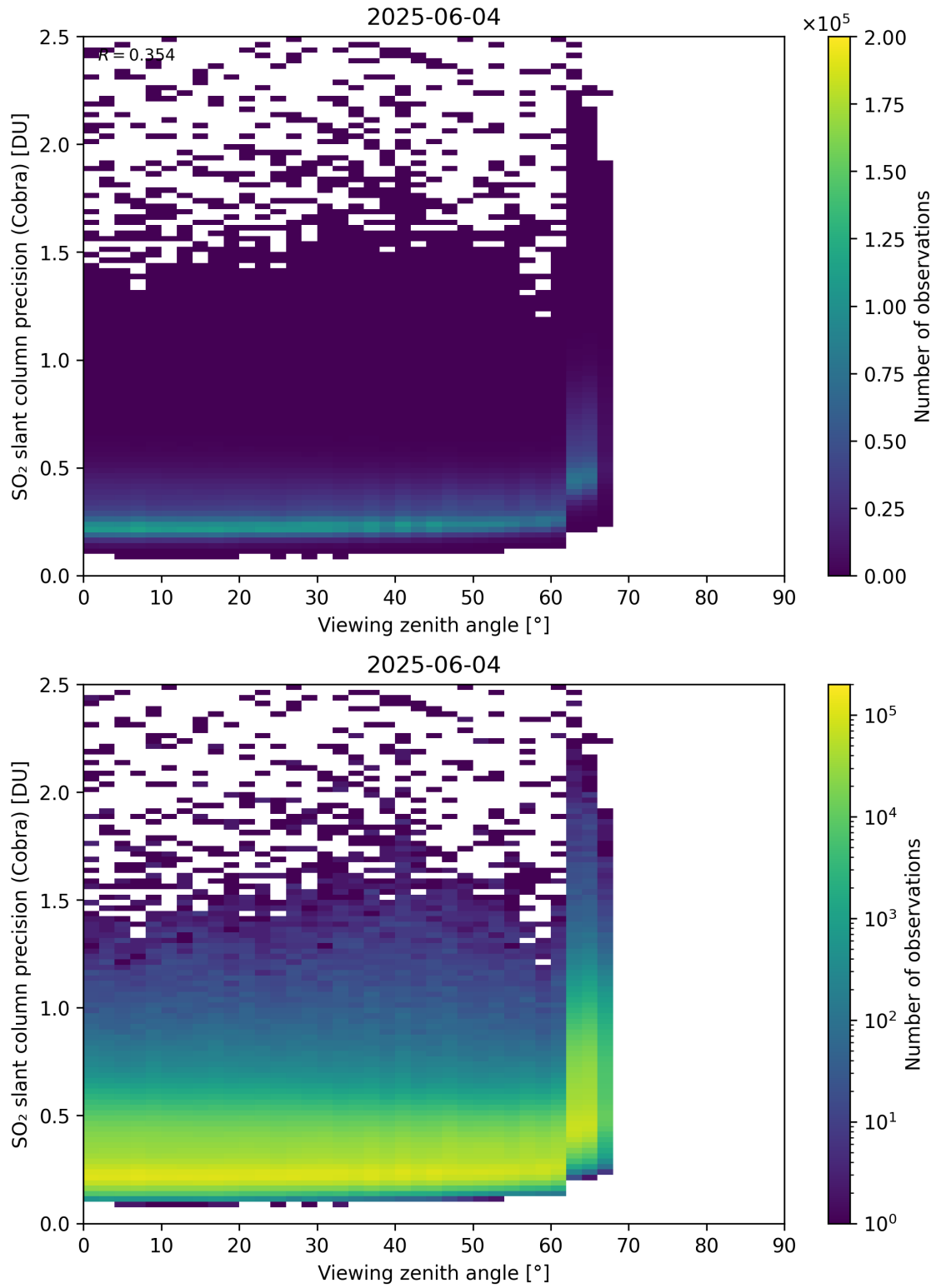
Figure 372: Scatter density plot of “Viewing zenith angle” against “SO 2 slant column precision (Cobra)” for 2025-06-03 to 2025-06-05.
