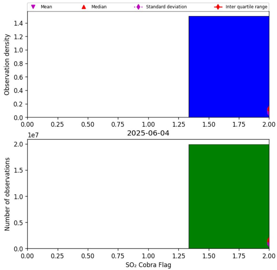
Figure 75: Histogram of “SO 2 Cobra Flag” for 2025-06-03 to 2025-06-05
