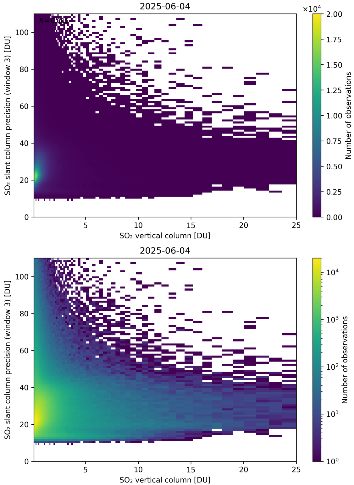
Figure 358: Scatter density plot of “SO 2 vertical column” against “SO 2 slant column precision (window 3)” for 2025-06-03 to 2025-06-05.
