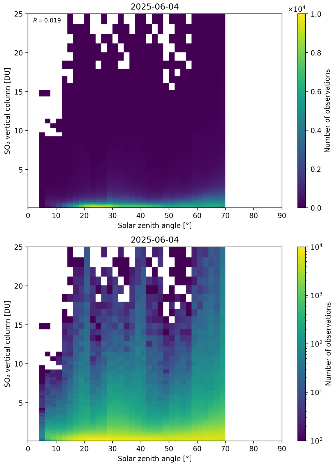
Figure 191: Scatter density plot of “Solar zenith angle” against “SO 2 vertical column” for 2025-06-03 to 2025-06-05.
