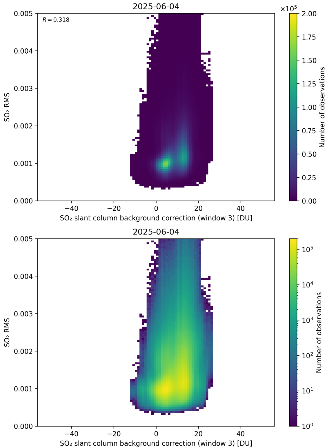
Figure 134: Scatter density plot of “SO 2 slant column background correction (window 3)” against “SO 2 RMS” for 2025-06-03 to 2025-06-05.
