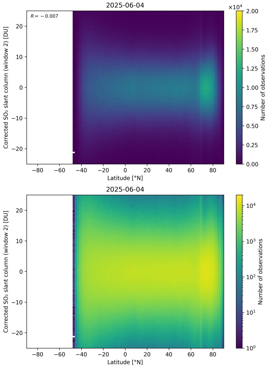
Figure 160: Scatter density plot of “Latitude” against “Corrected SO 2 slant column (window 2)” for 2025-06-03 to 2025-06-05.
