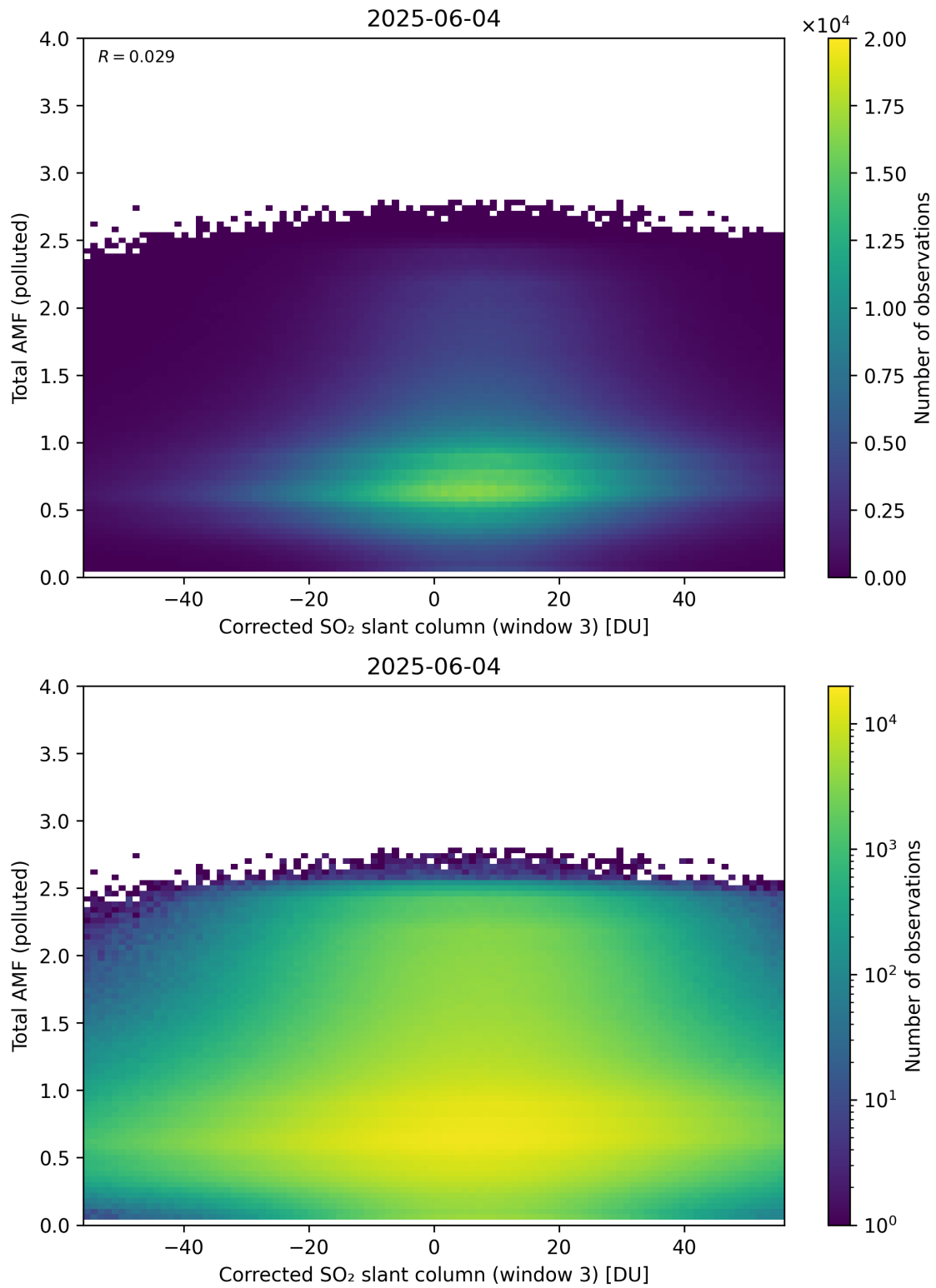
Figure 260: Scatter density plot of “Corrected SO 2 slant column (window 3)” against “Total AMF (polluted)” for 2025-06-03 to 2025-06-05.
