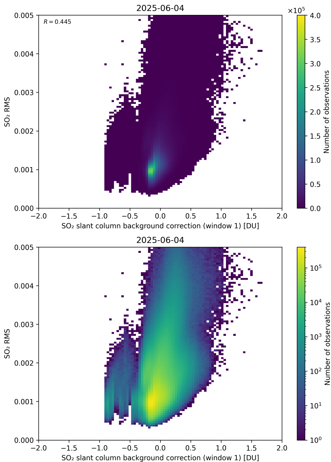
Figure 113: Scatter density plot of “SO 2 slant column background correction (window 1)” against “SO 2 RMS” for 2025-06-03 to 2025-06-05.
