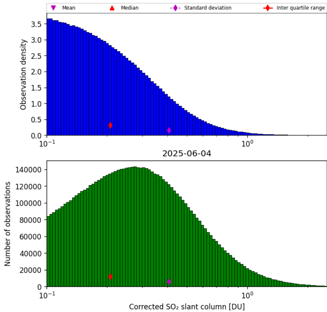
Figure 60: Histogram of "Corrected SO 2 slant column" for 2025-06-03 to 2025-06-05
