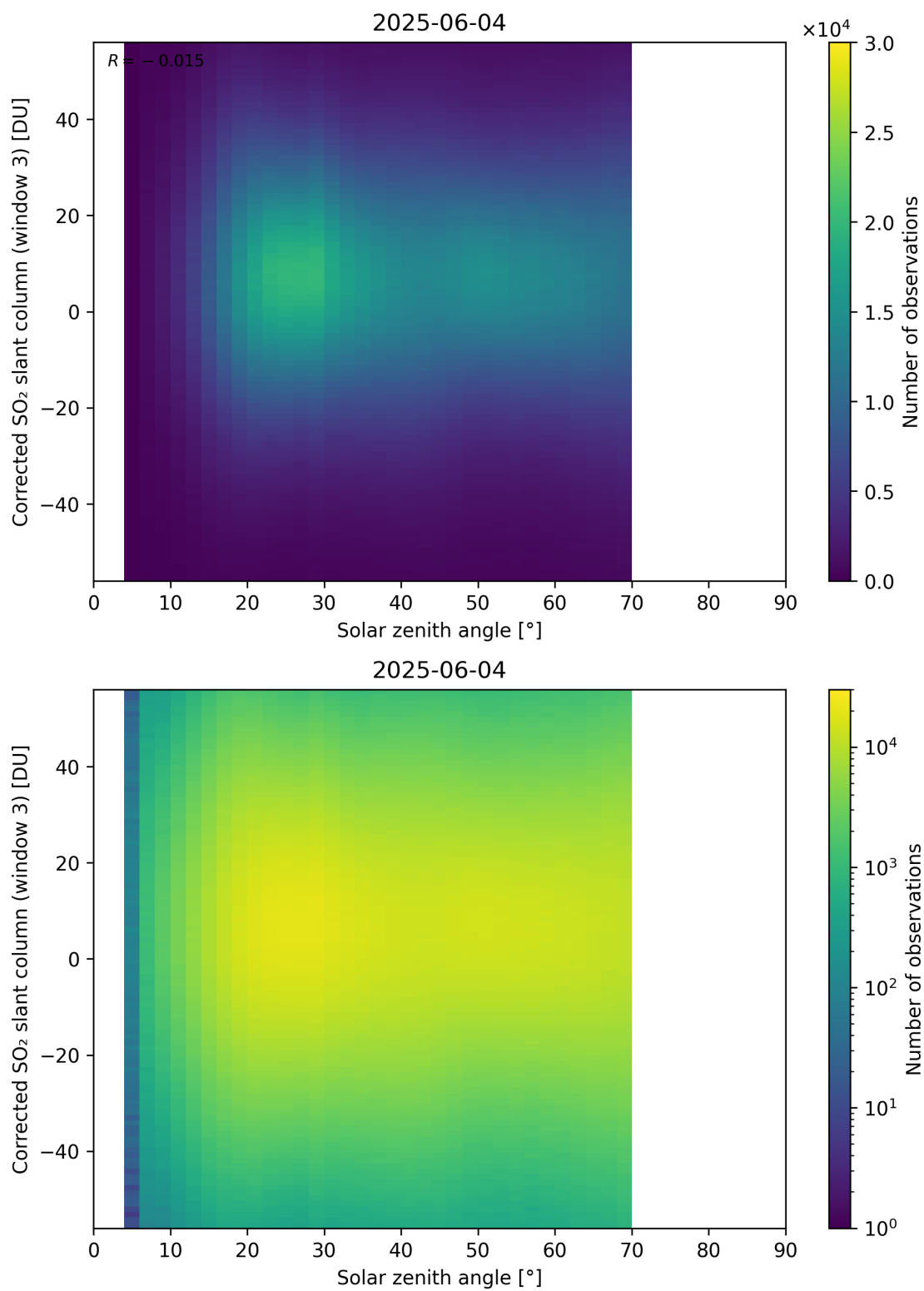
Figure 183: Scatter density plot of “Solar zenith angle” against “Corrected SO 2 slant column (window 3)” for 2025-06-03 to 2025-06-05.
