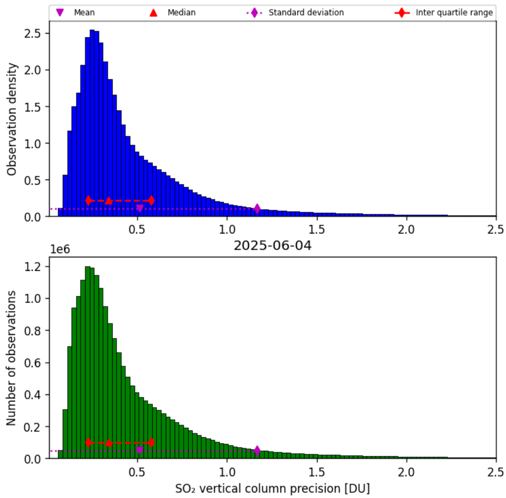
Figure 59: Histogram of “SO 2 vertical column precision” for 2025-06-03 to 2025-06-05
