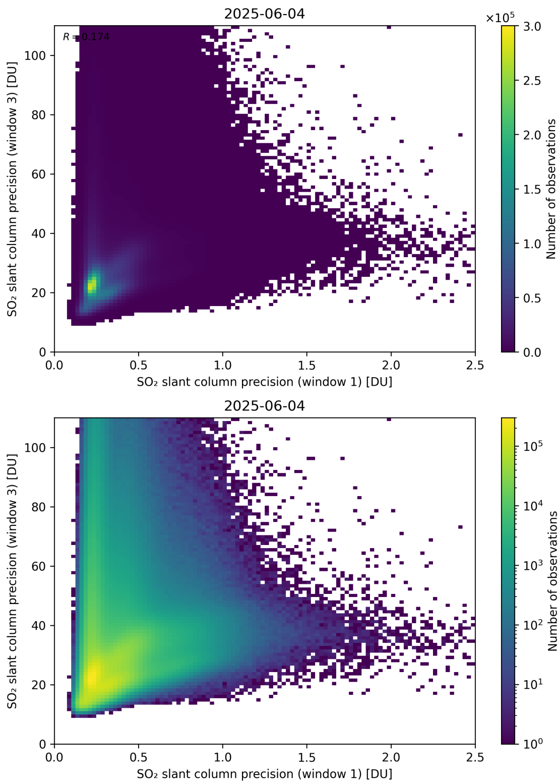
Figure 279: Scatter density plot of “SO 2 slant column precision (window 1)” against “SO 2 slant column precision (window 3)” for 2025-06-03 to 2025-06-05.
