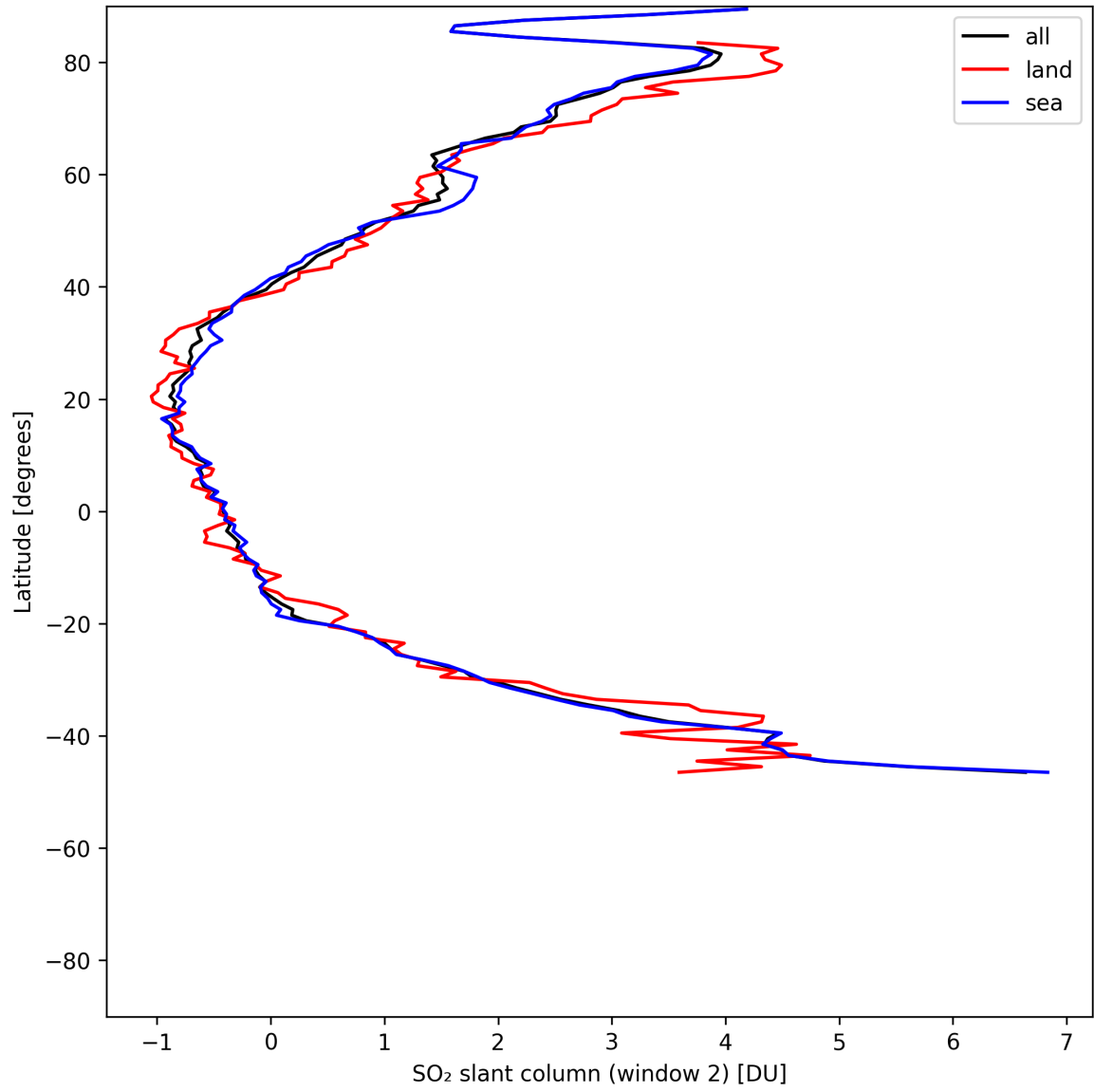
Figure 41: Zonal average of “SO 2 slant column (window 2)” for 2025-06-03 to 2025-06-05.
