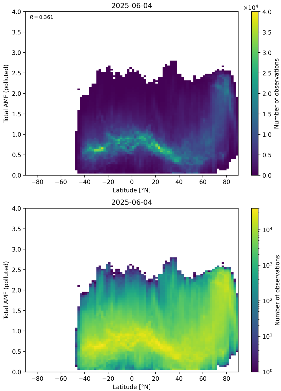
Figure 167: Scatter density plot of “Latitude” against “Total AMF (polluted)” for 2025-06-03 to 2025-06-05.
