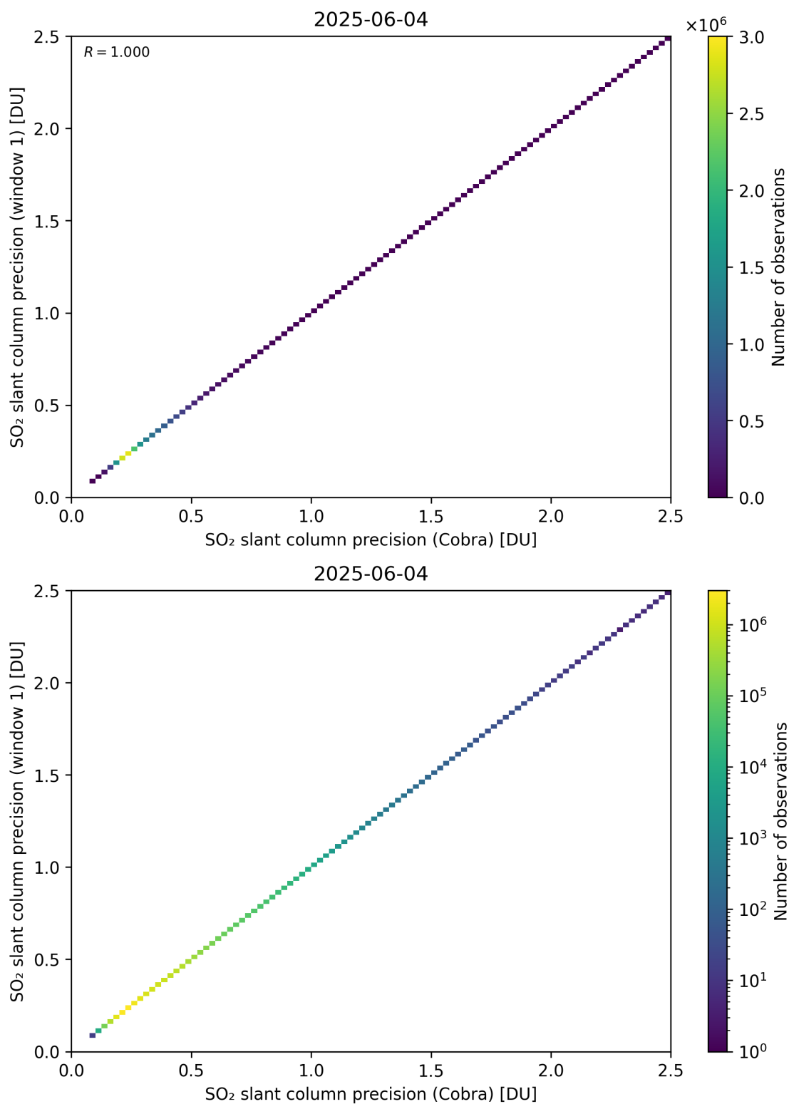
Figure 209: Scatter density plot of “SO 2 slant column precision (Cobra)” against “SO 2 slant column precision (window 1)” for 2025-06-03 to 2025-06-05.
