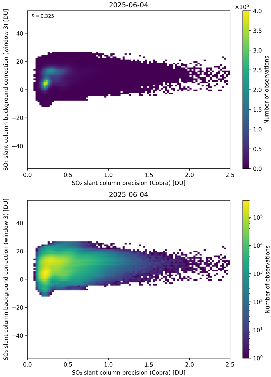
Figure 201: Scatter density plot of “SO 2 slant column precision (Cobra)” against “SO 2 slant column background correction (window 3)” for 2025-06-03 to 2025-06-05.
