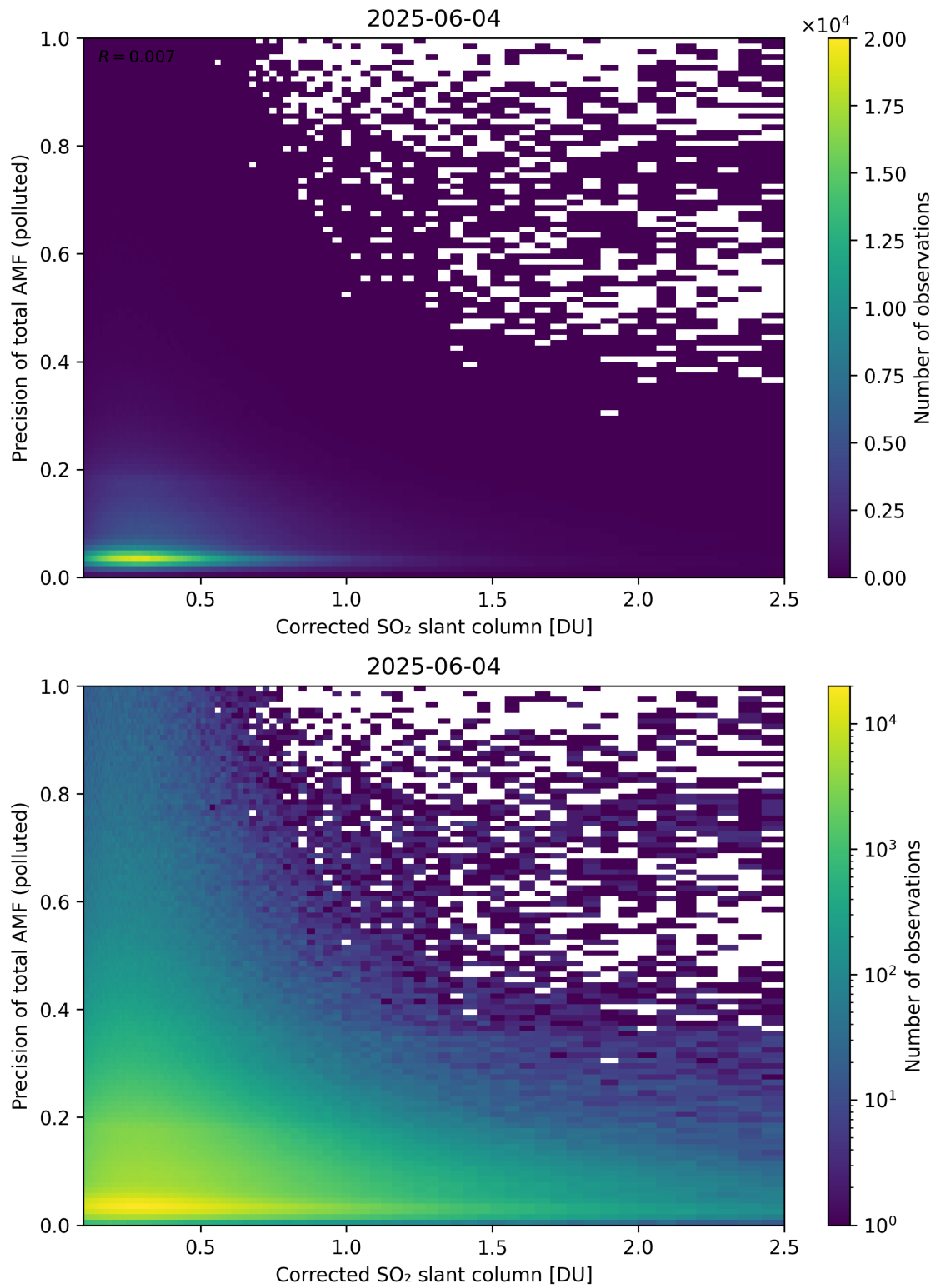
Figure 243: Scatter density plot of “Corrected SO 2 slant column” against “Precision of total AMF (polluted)” for 2025-06-03 to 2025-06-05.
