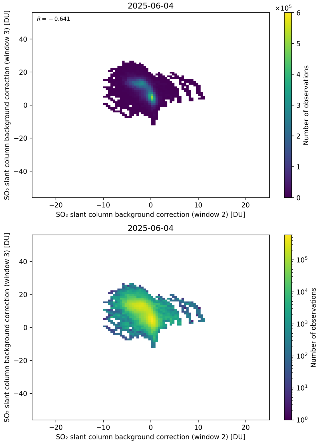
Figure 122: Scatter density plot of “SO 2 slant column background correction (window 2)” against “SO 2 slant column background correction (window 3)” for 2025-06-03 to 2025-06-05.
