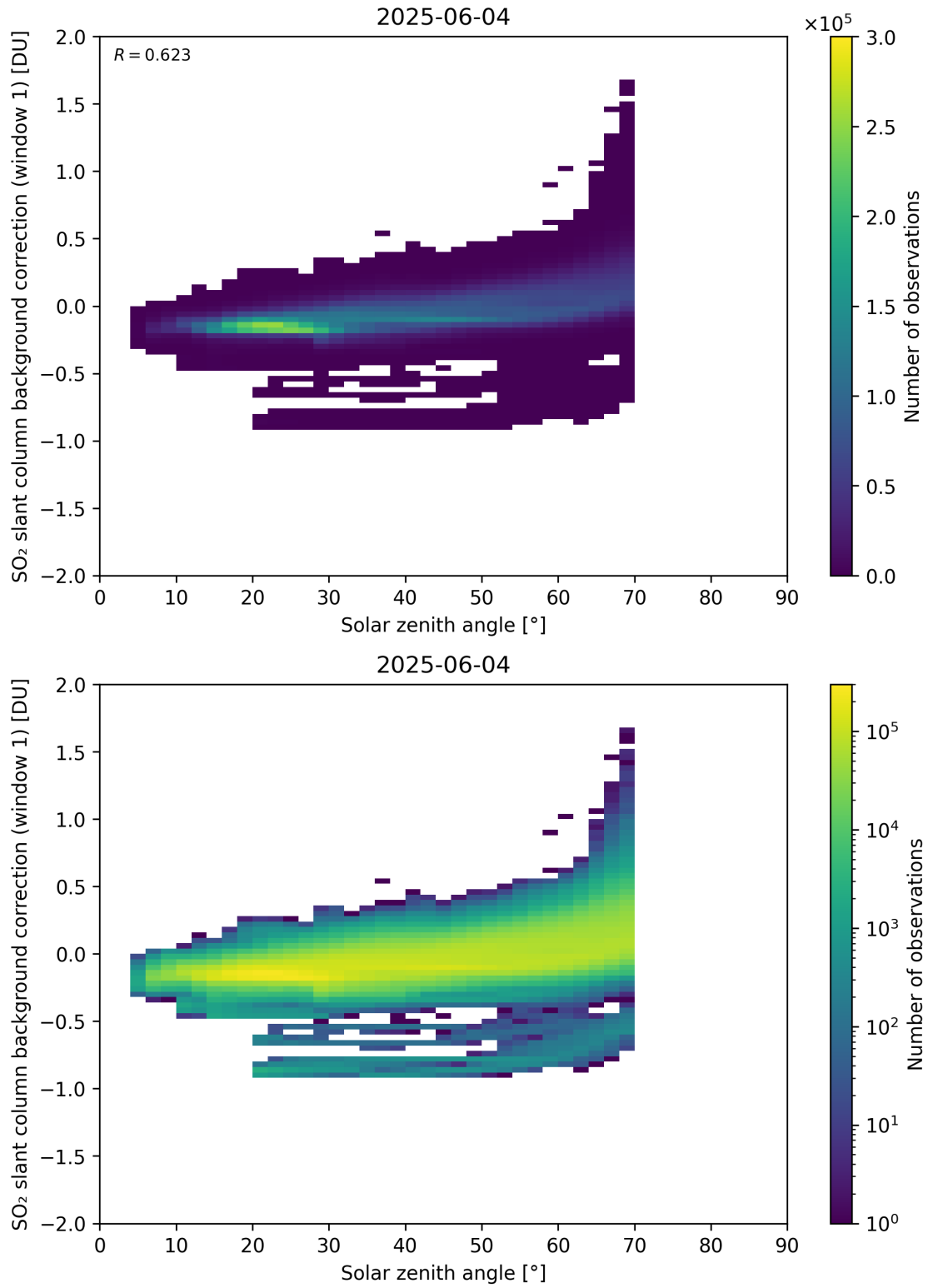
Figure 171: Scatter density plot of “Solar zenith angle” against “SO 2 slant column background correction (window 1)” for 2025-06-03 to 2025-06-05.
