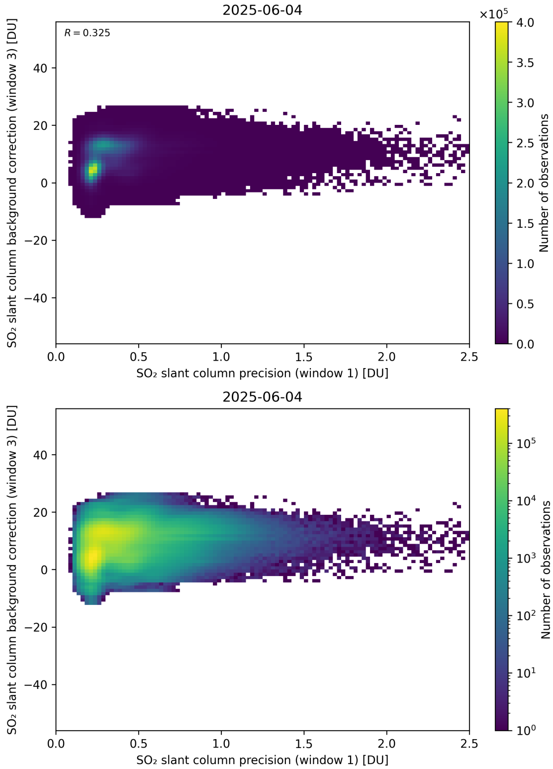
Figure 270: Scatter density plot of “SO 2 slant column precision (window 1)” against “SO 2 slant column background correction (window 3)” for 2025-06-03 to 2025-06-05.
