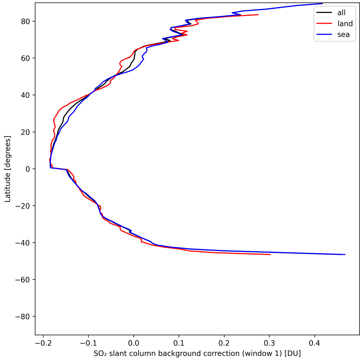
Figure 40: Zonal average of “SO 2 slant column background correction (window 1)” for 2025-06-03 to 2025-06-05.
