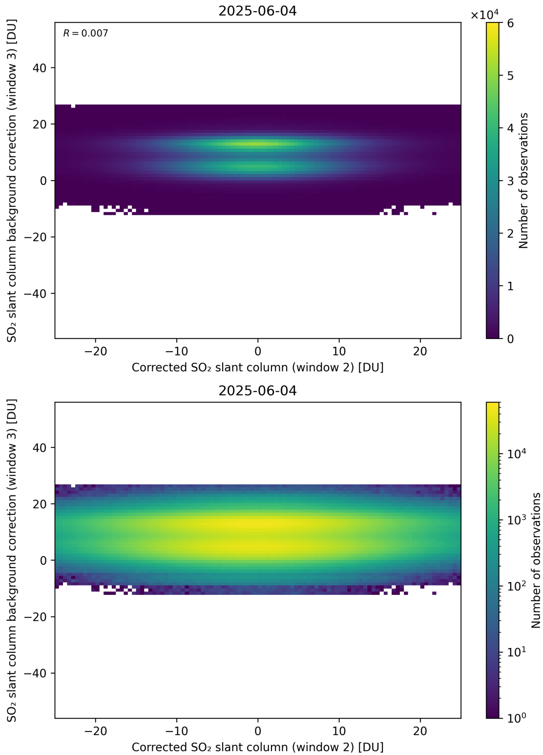
Figure 245: Scatter density plot of “Corrected SO 2 slant column (window 2)” against “SO 2 slant column background correction (window 3)” for 2025-06-03 to 2025-06-05.
