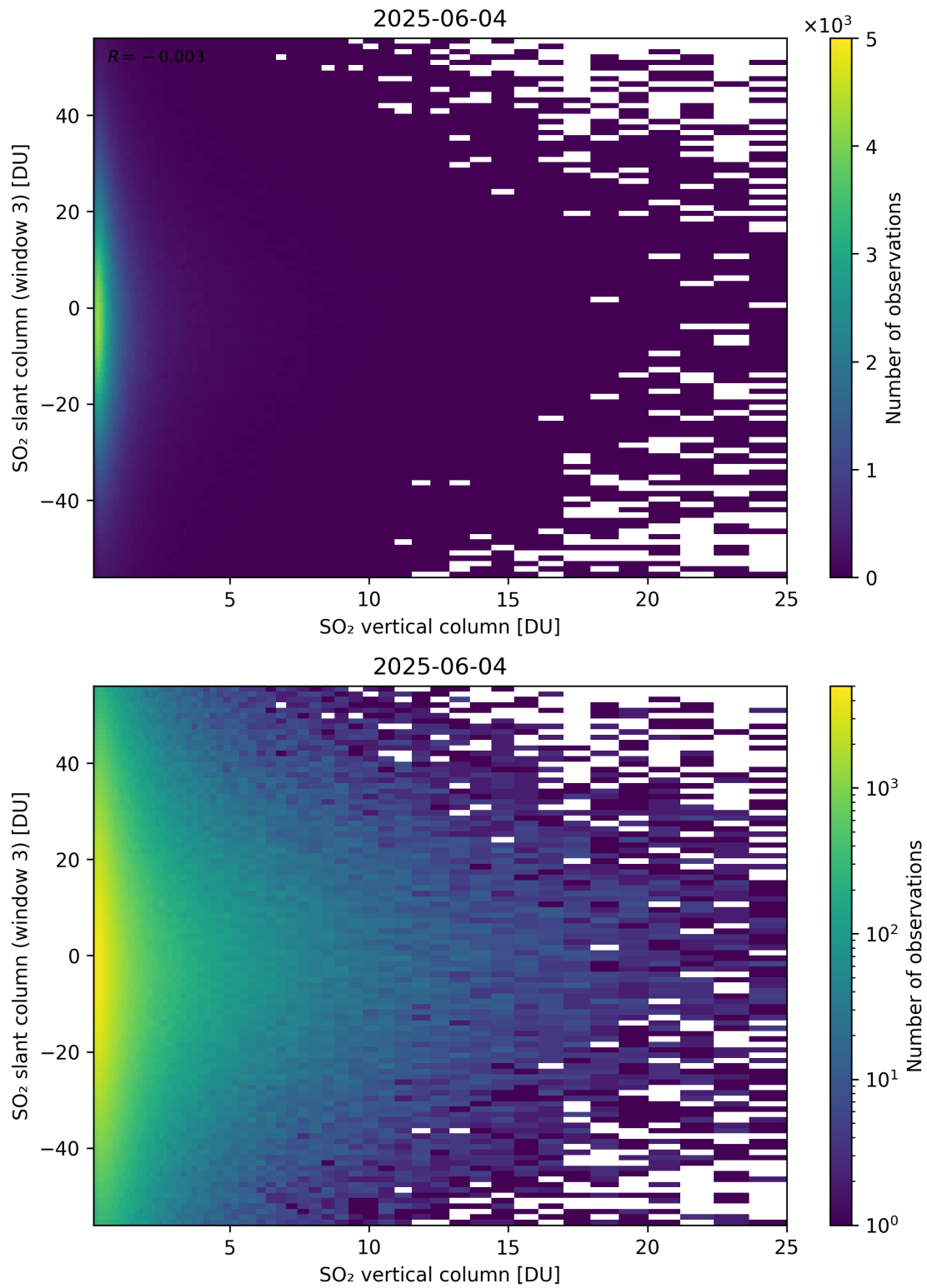
Figure 357: Scatter density plot of “SO 2 vertical column” against “SO 2 slant column (window 3)” for 2025-06-03 to 2025-06-05.
