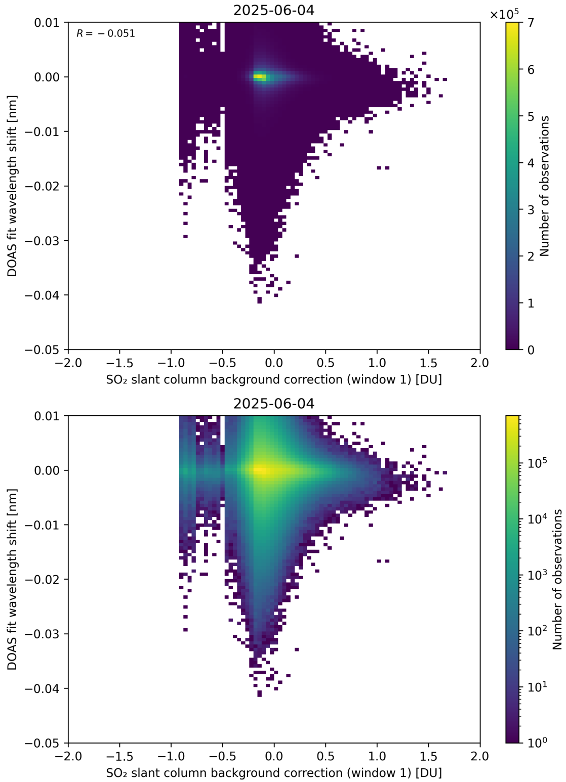
Figure 111: Scatter density plot of “SO 2 slant column background correction (window 1)” against “DOAS fit wavelength shift” for 2025-06-03 to 2025-06-05.
