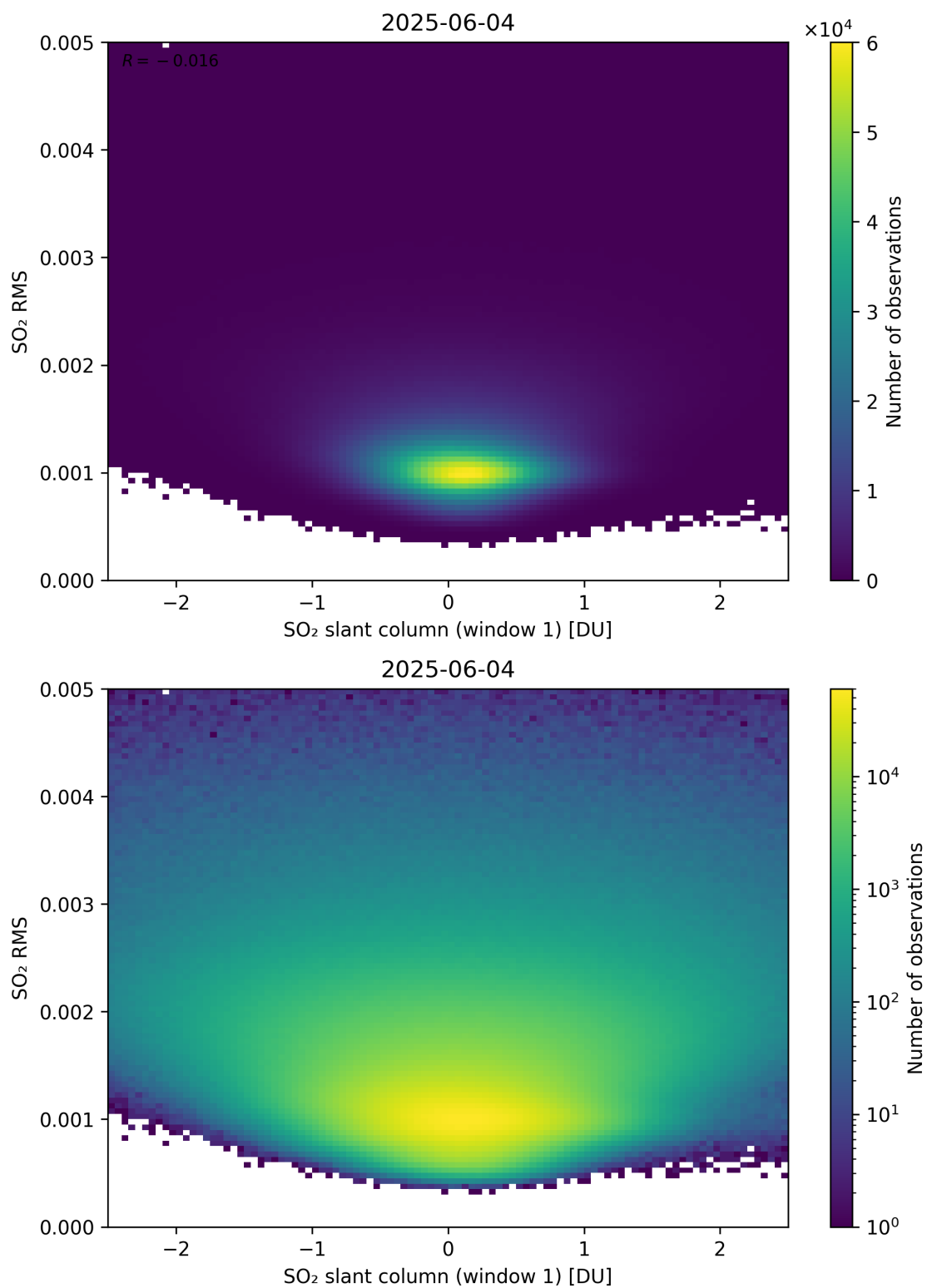
Figure 267: Scatter density plot of “SO 2 slant column (window 1)” against “SO 2 RMS” for 2025-06-03 to 2025-06-05.
