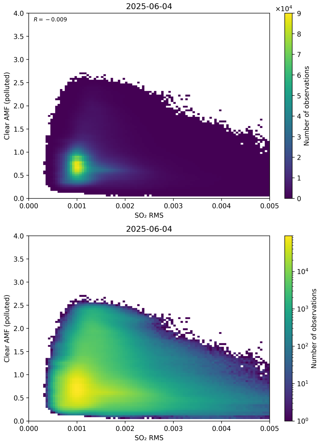
Figure 147: Scatter density plot of “SO 2 RMS” against “Clear AMF (polluted)” for 2025-06-03 to 2025-06-05.
