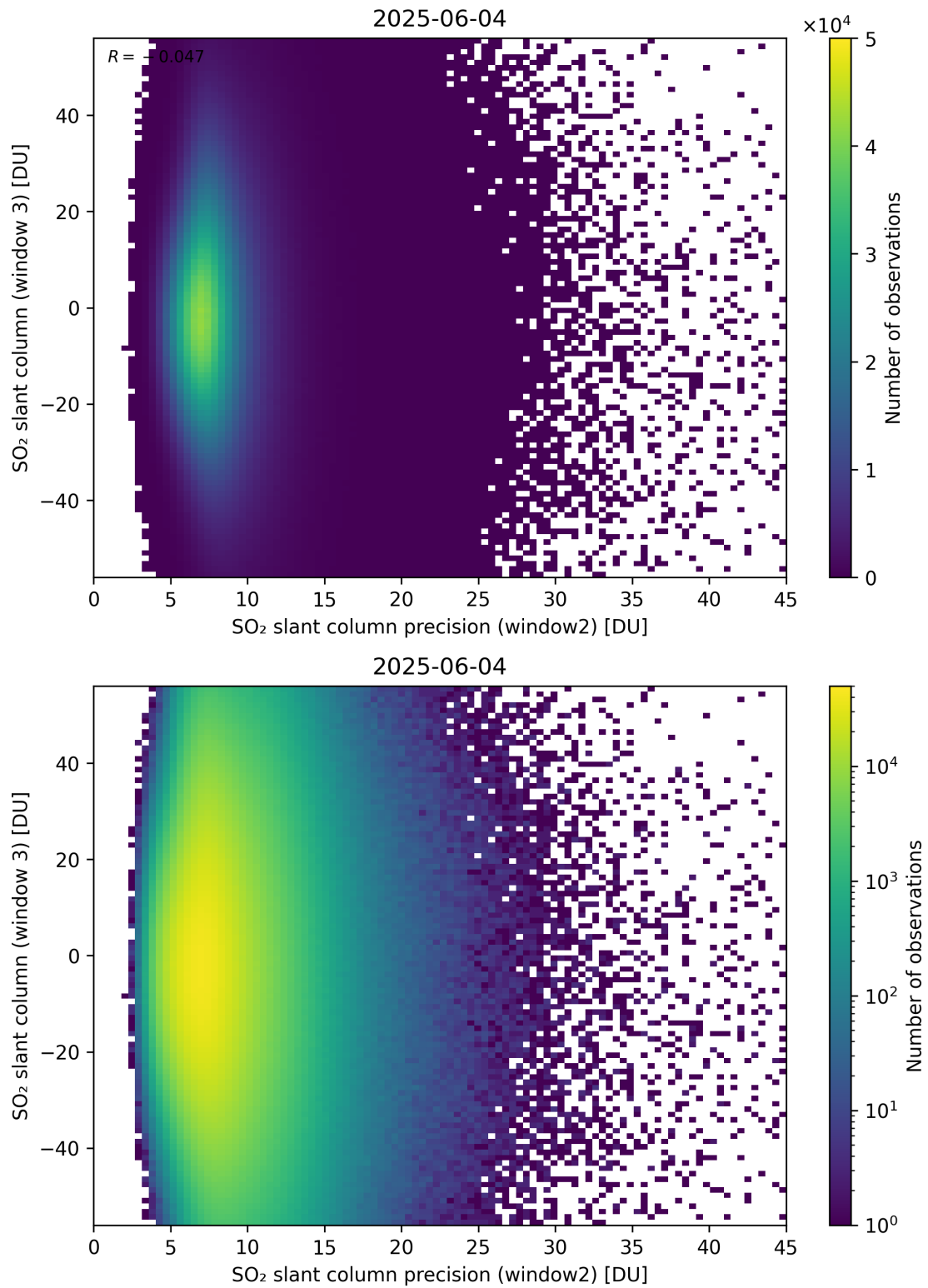
Figure 299: Scatter density plot of “SO 2 slant column precision (window2)” against “SO 2 slant column (window 3)” for 2025-06-03 to 2025-06-05.
