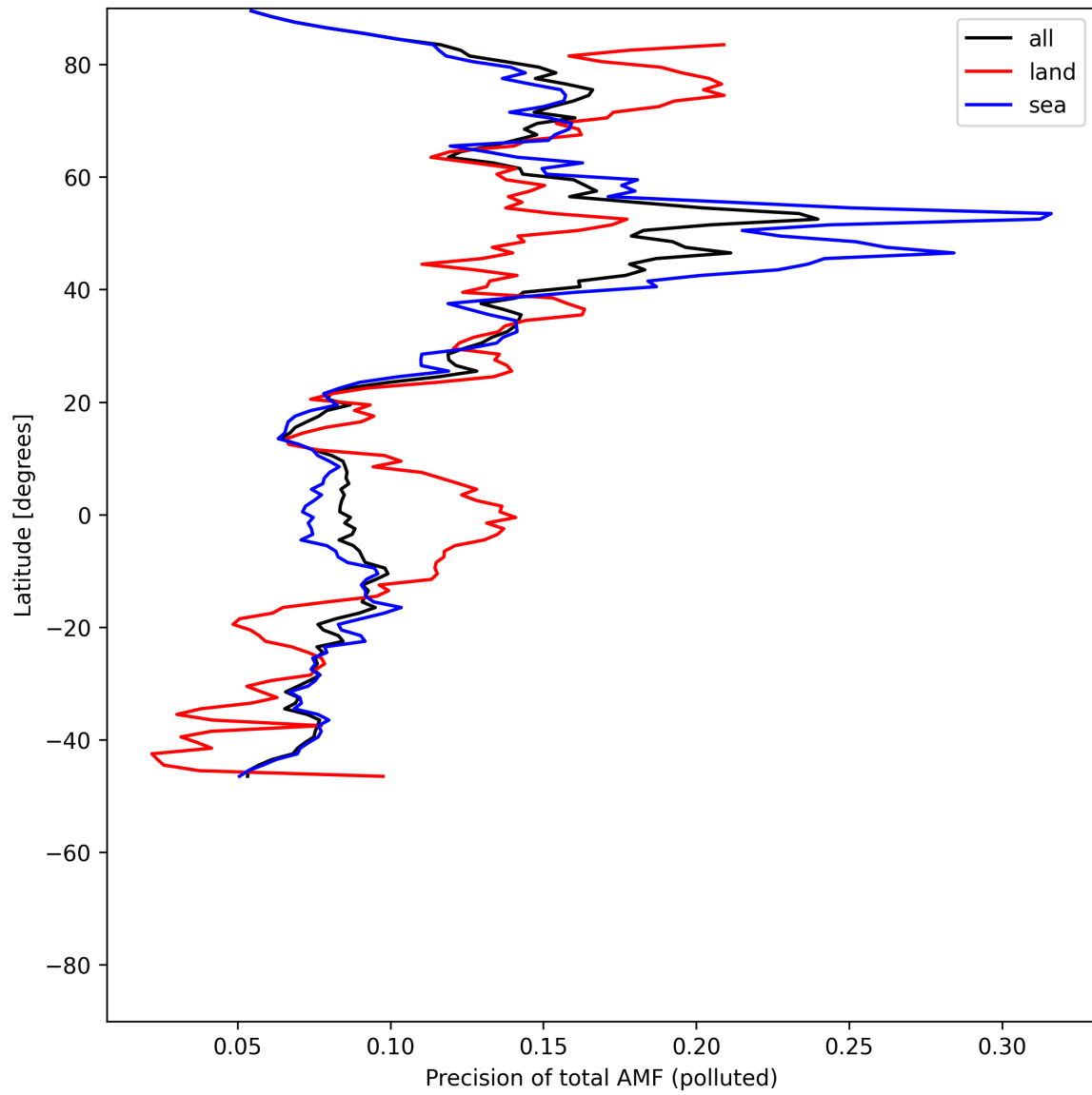
Figure 54: Zonal average of “Precision of total AMF (polluted)” for 2025-06-03 to 2025-06-05.
