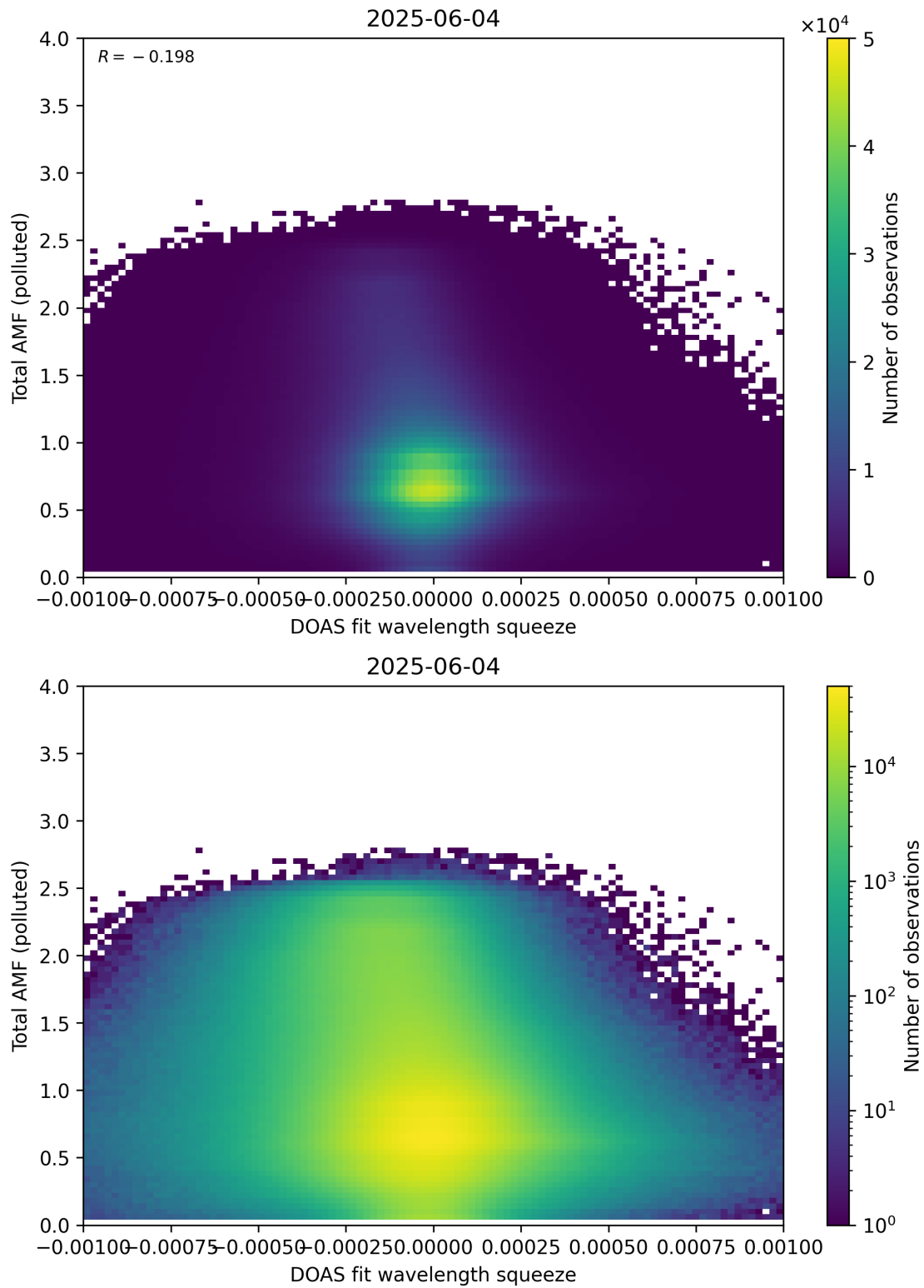
Figure 145: Scatter density plot of “DOAS fit wavelength squeeze” against “Total AMF (polluted)” for 2025-06-03 to 2025-06-05.
