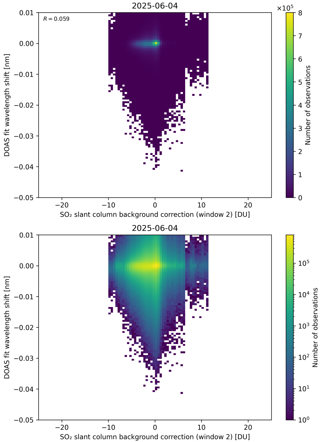
Figure 123: Scatter density plot of “SO 2 slant column background correction (window 2)” against “DOAS fit wavelength shift” for 2025-06-03 to 2025-06-05.
