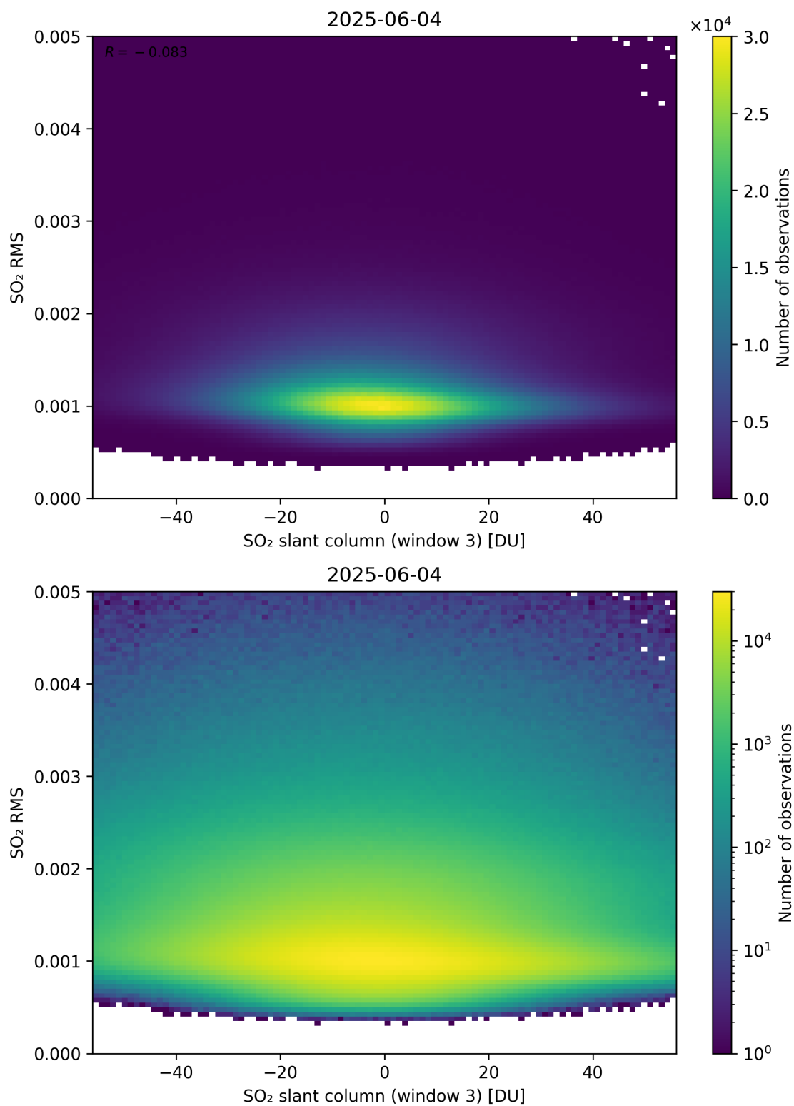
Figure 306: Scatter density plot of “SO 2 slant column (window 3)” against “SO 2 RMS” for 2025-06-03 to 2025-06-05.
