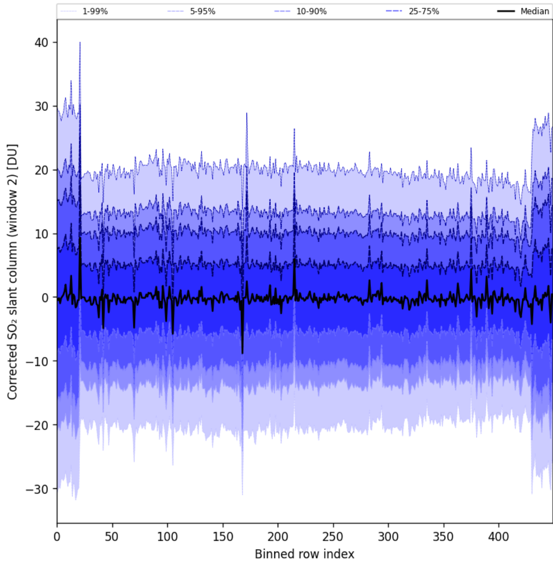
Figure 95: Along track statistics of “Corrected SO 2 slant column (window 2)” for 2025-06-03 to 2025-06-05
