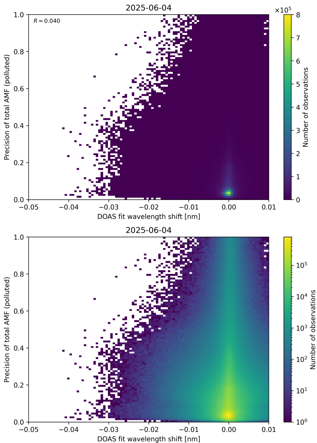
Figure 142: Scatter density plot of “DOAS fit wavelength shift” against “Precision of total AMF (polluted)” for 2025-06-03 to 2025-06-05.
