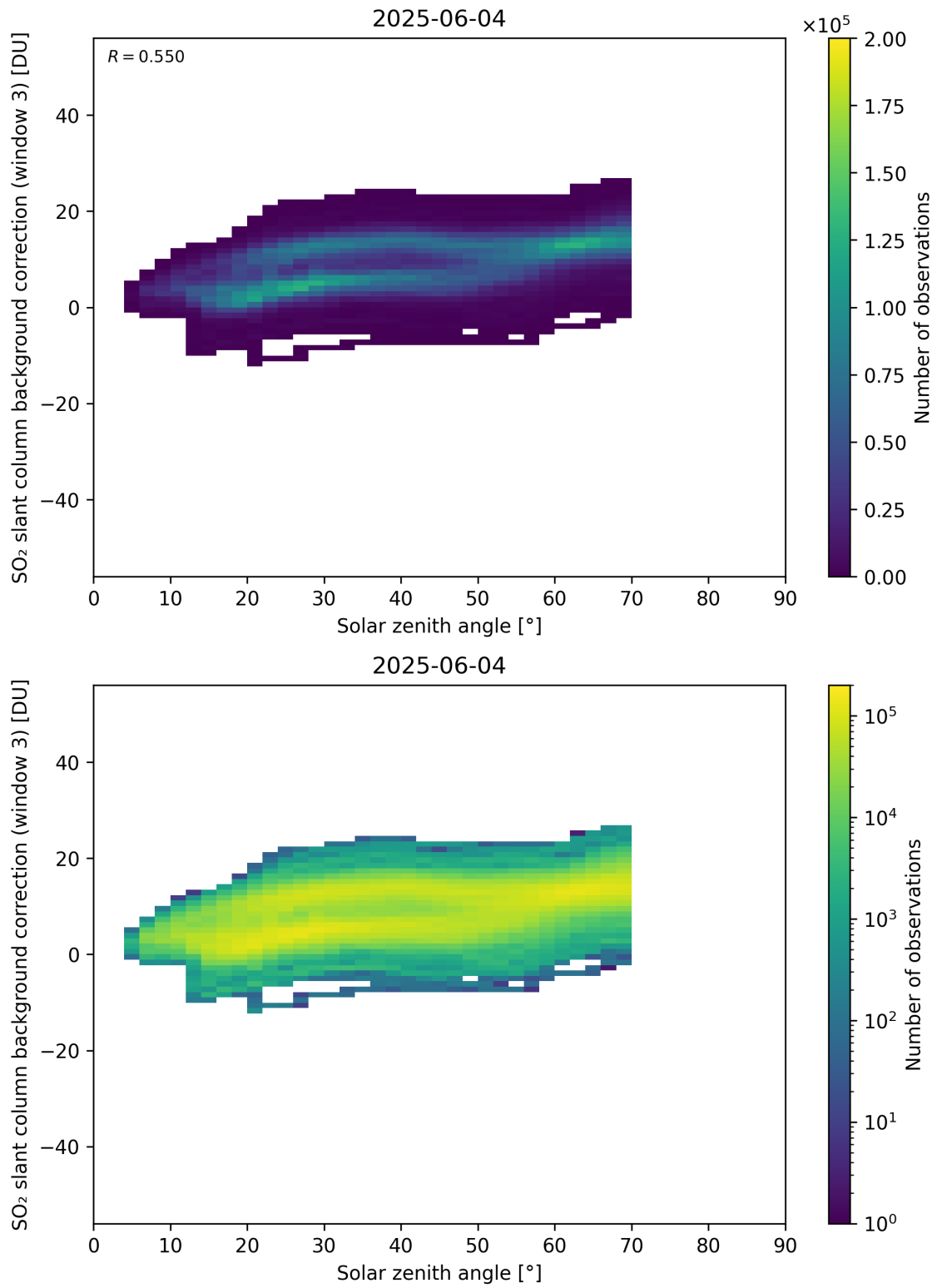
Figure 173: Scatter density plot of “Solar zenith angle” against “SO 2 slant column background correction (window 3)” for 2025-06-03 to 2025-06-05.
