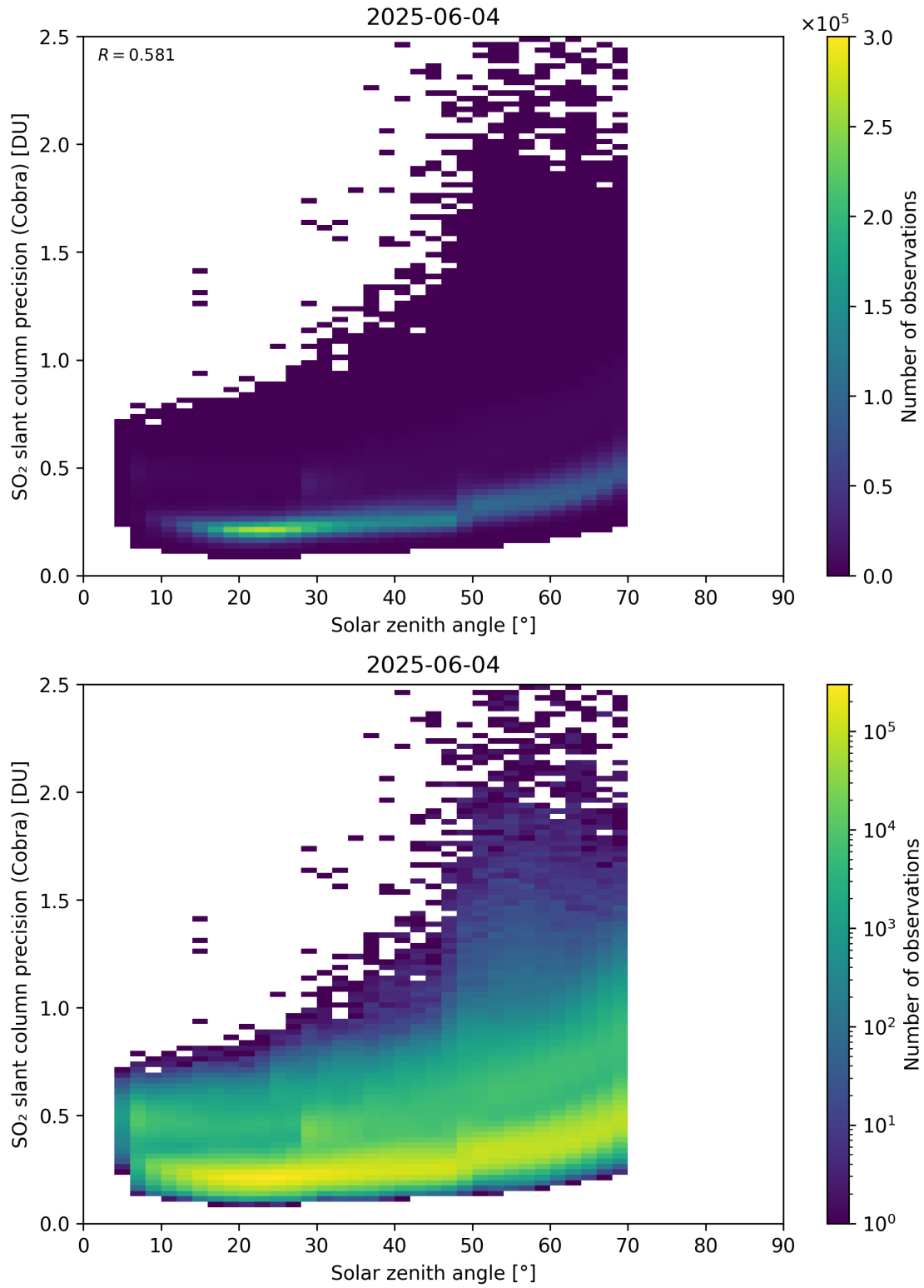
Figure 180: Scatter density plot of “Solar zenith angle” against “SO 2 slant column precision (Cobra)” for 2025-06-03 to 2025-06-05.
