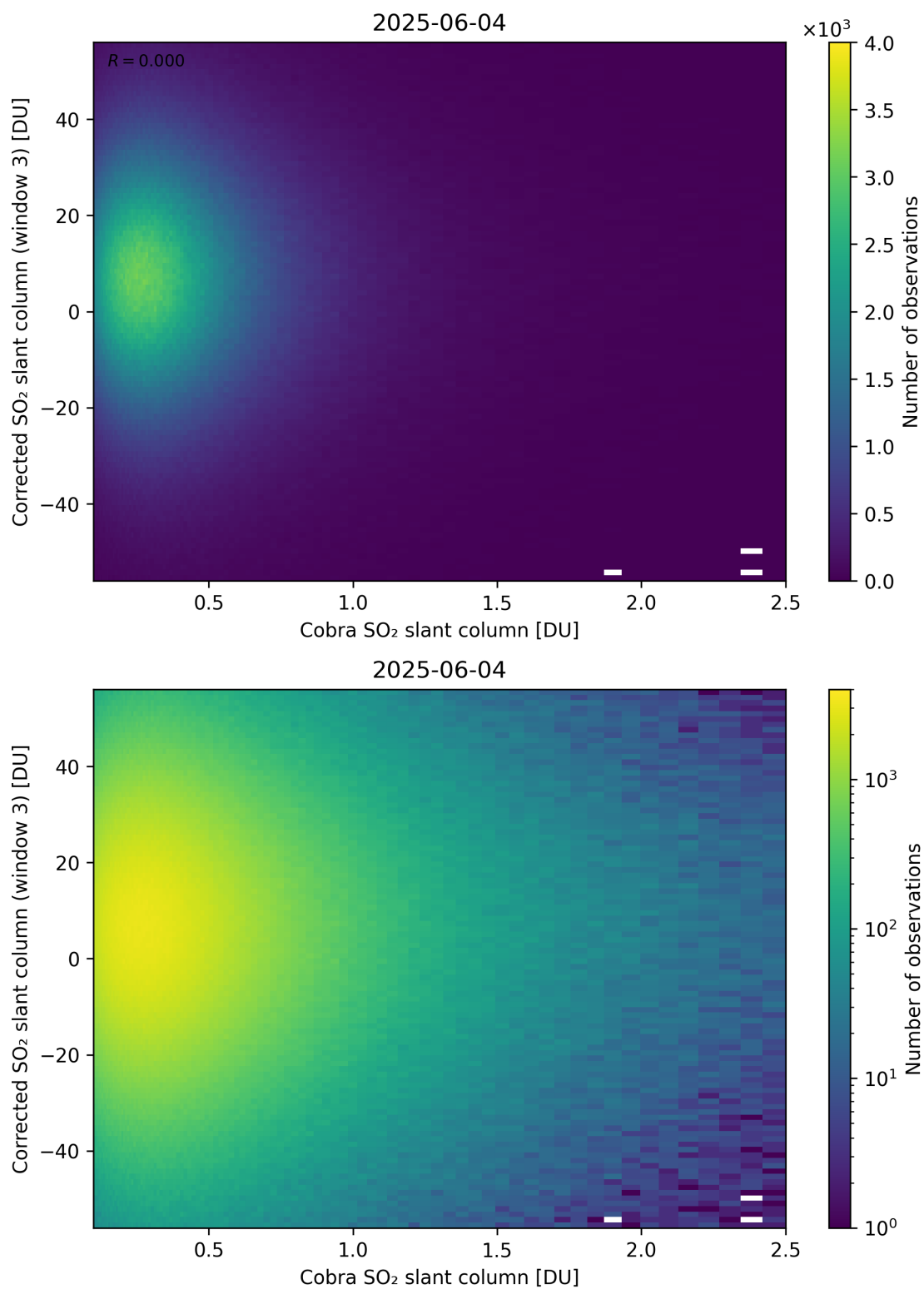
Figure 218: Scatter density plot of “Cobra SO 2 slant column” against “Corrected SO 2 slant column (window 3)” for 2025-06-03 to 2025-06-05.
