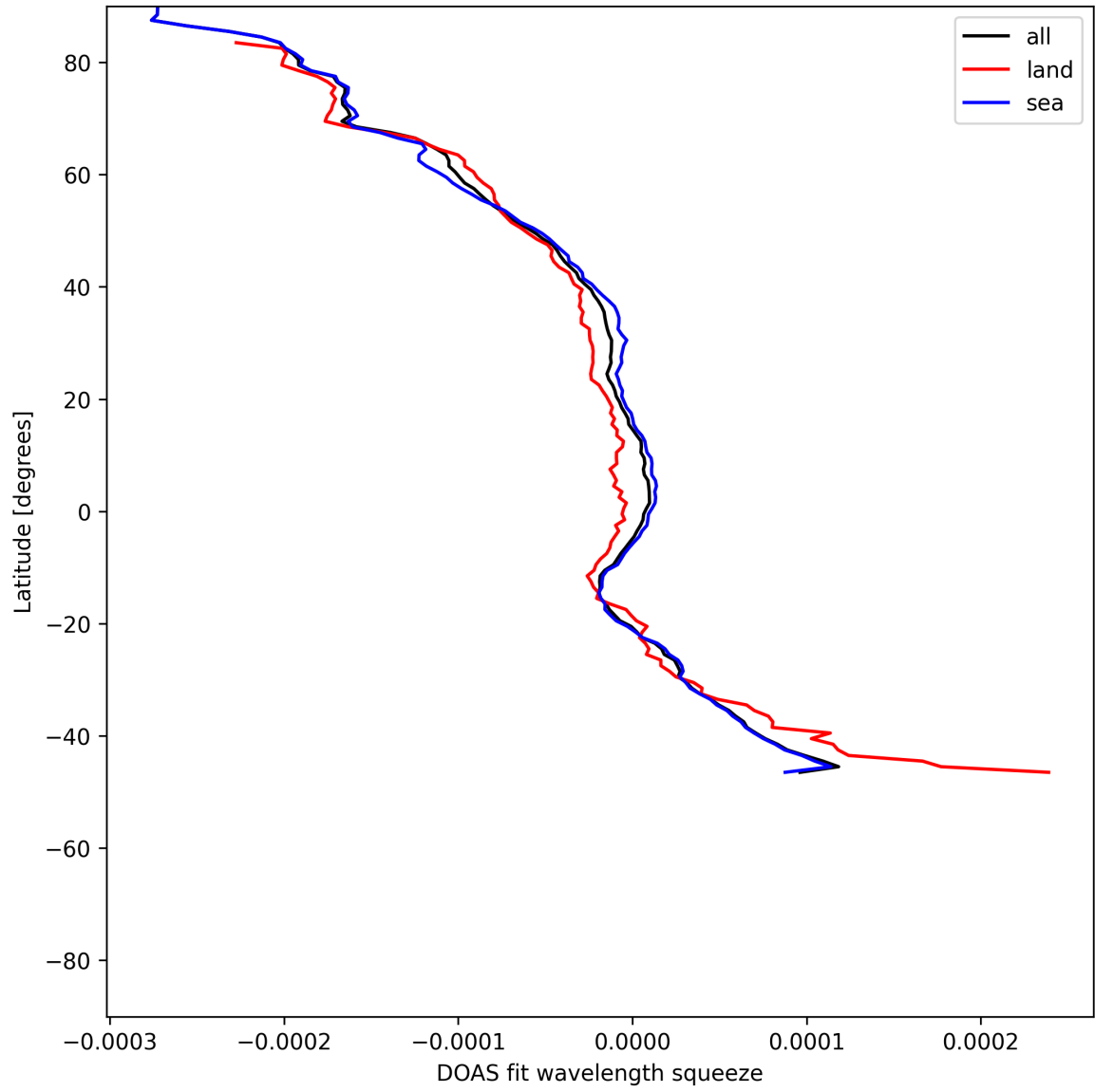
Figure 51: Zonal average of “DOAS fit wavelength squeeze” for 2025-06-03 to 2025-06-05.
