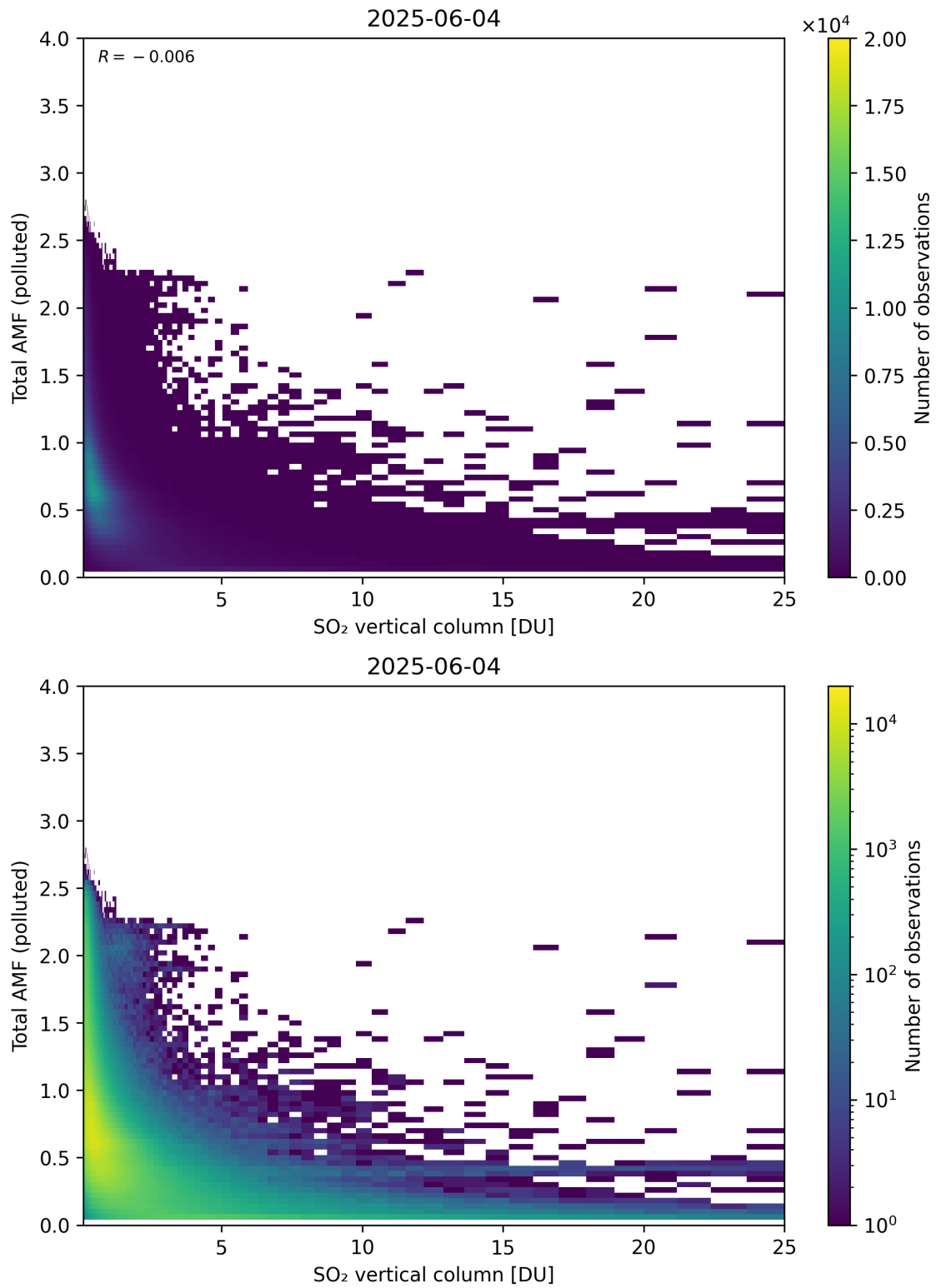
Figure 359: Scatter density plot of “SO 2 vertical column” against “Total AMF (polluted)” for 2025-06-03 to 2025-06-05.
