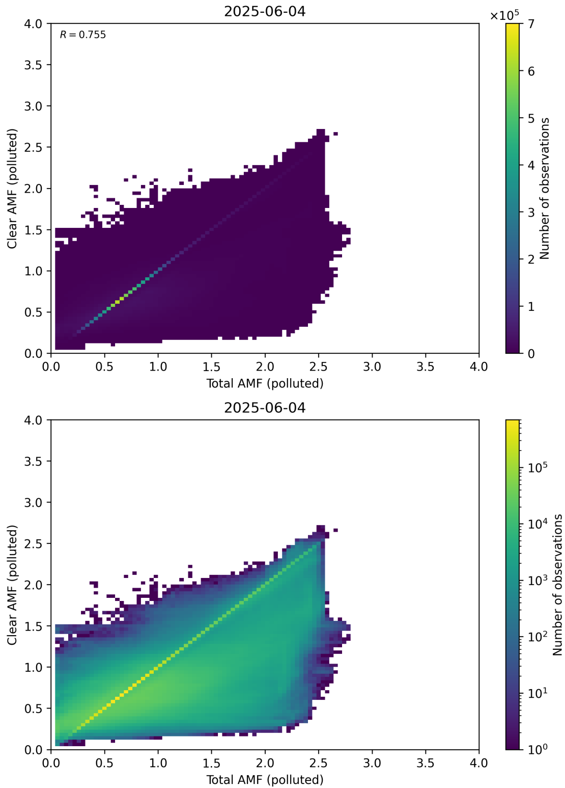
Figure 321: Scatter density plot of “Total AMF (polluted)” against “Clear AMF (polluted)” for 2025-06-03 to 2025-06-05.
