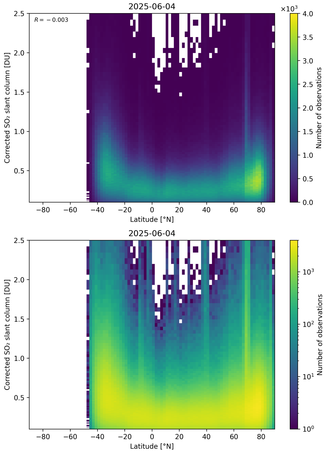
Figure 159: Scatter density plot of “Latitude” against “Corrected SO 2 slant column” for 2025-06-03 to 2025-06-05.
