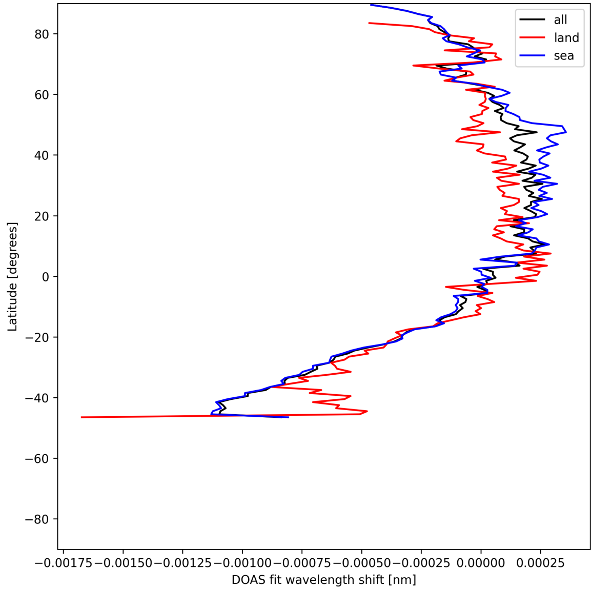
Figure 50: Zonal average of “DOAS fit wavelength shift” for 2025-06-03 to 2025-06-05.
