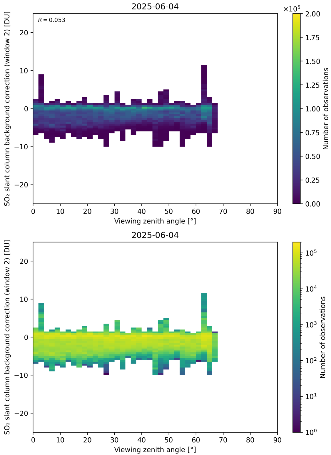
Figure 363: Scatter density plot of “Viewing zenith angle” against “SO 2 slant column background correction (window 2)” for 2025-06-03 to 2025-06-05.
