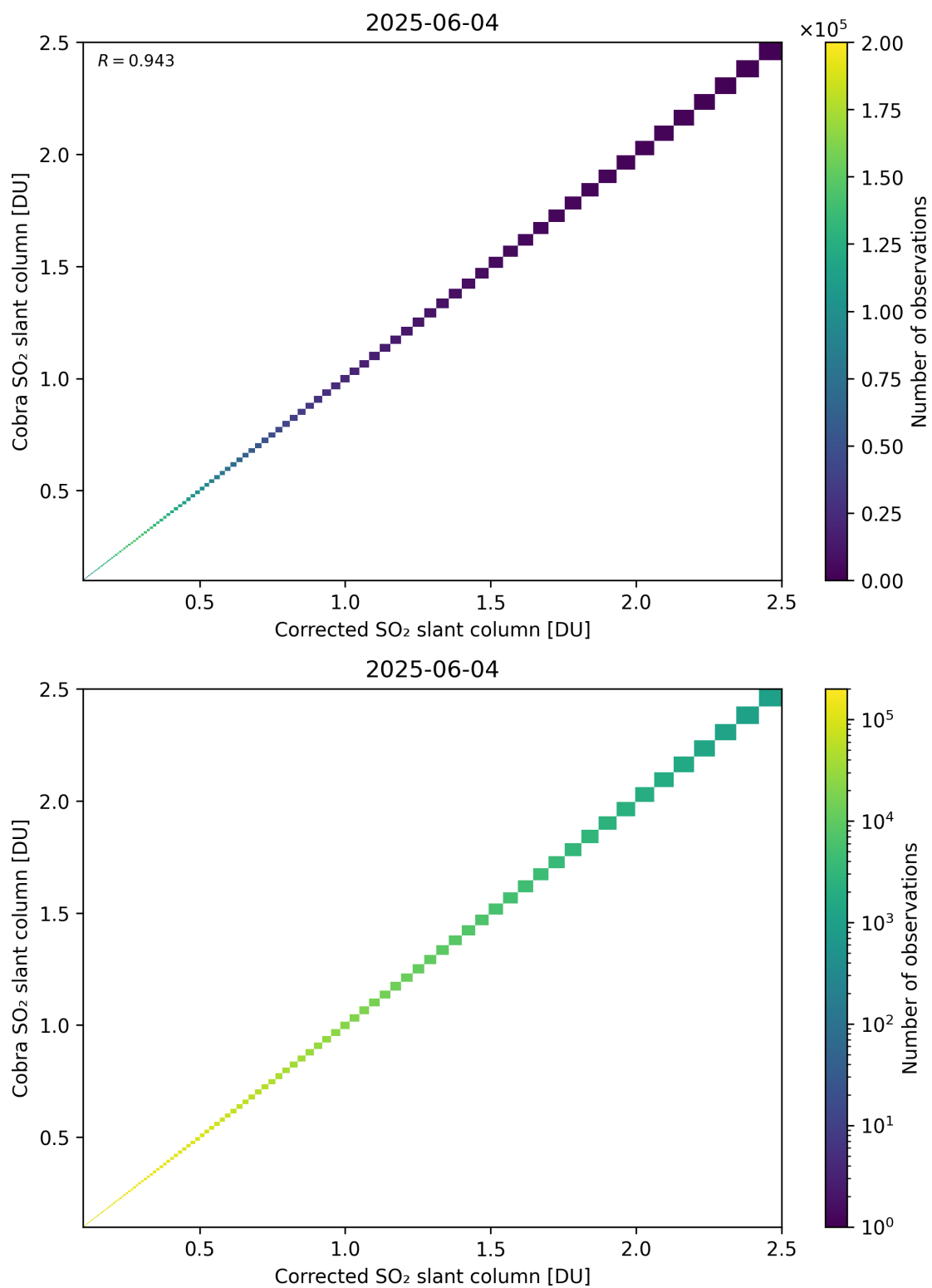
Figure 233: Scatter density plot of “Corrected SO 2 slant column” against “Cobra SO 2 slant column” for 2025-06-03 to 2025-06-05.
