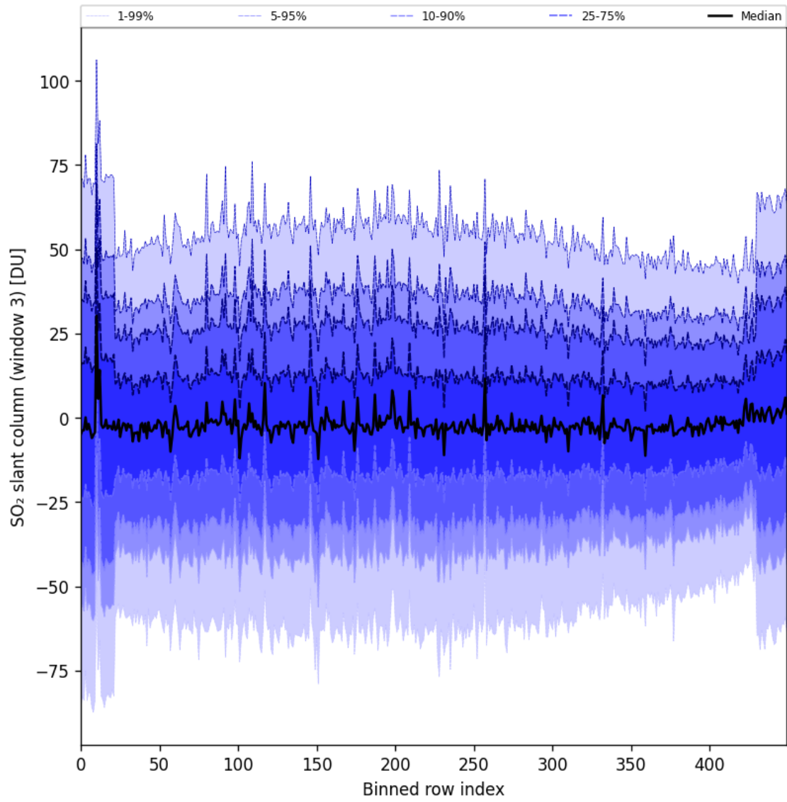
Figure 97: Along track statistics of “SO 2 slant column (window 3)” for 2025-06-03 to 2025-06-05
