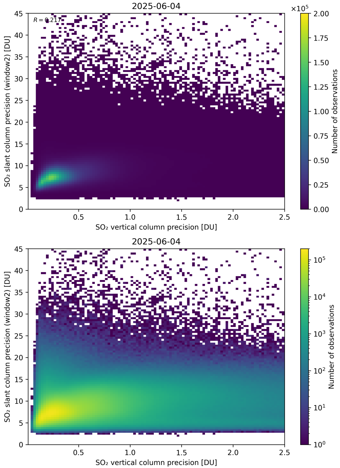
Figure 343: Scatter density plot of “SO 2 vertical column precision” against “SO 2 slant column precision (window2)” for 2025-06-03 to 2025-06-05.
