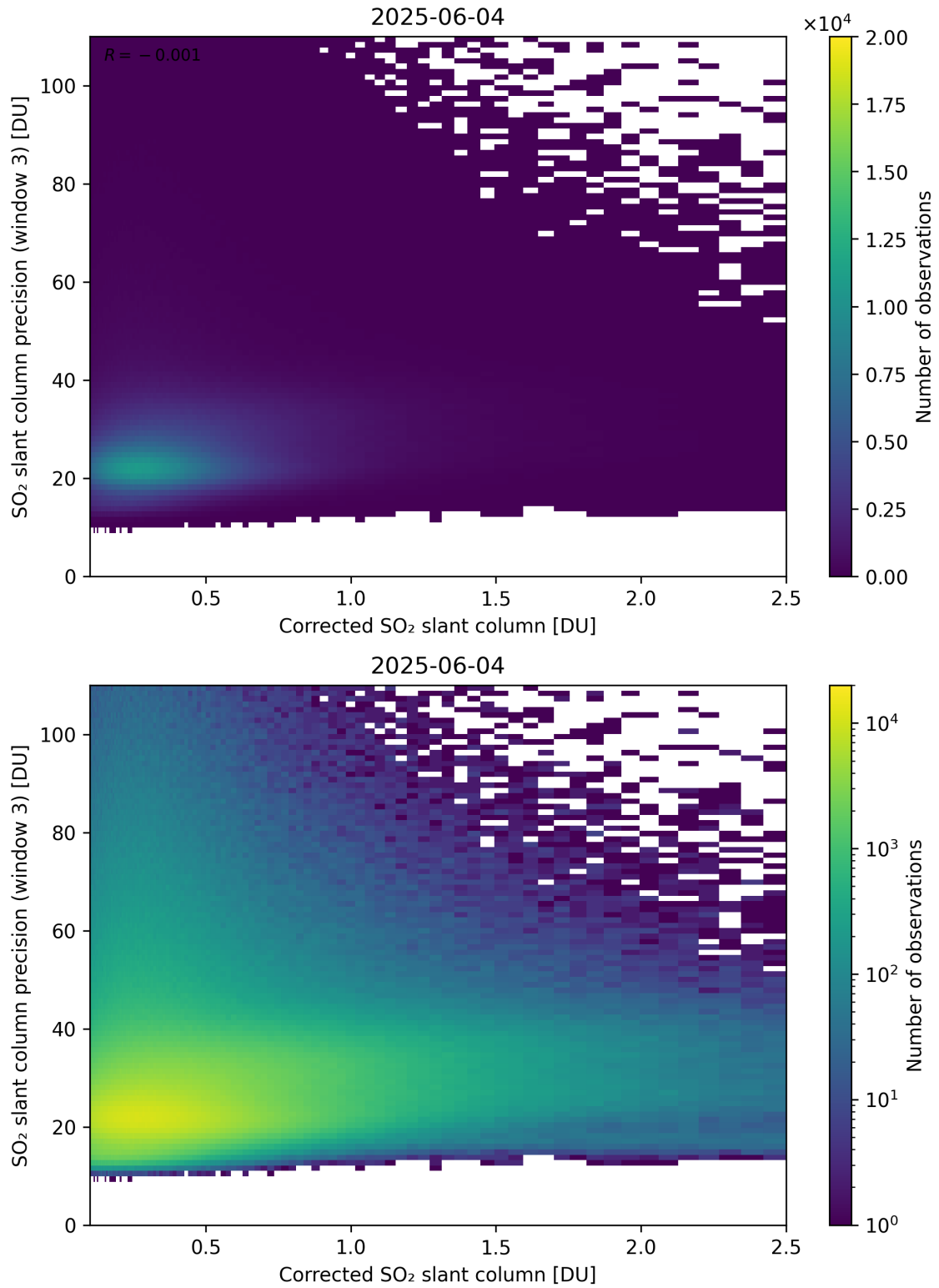
Figure 241: Scatter density plot of “Corrected SO 2 slant column” against “SO 2 slant column precision (window 3)” for 2025-06-03 to 2025-06-05.
