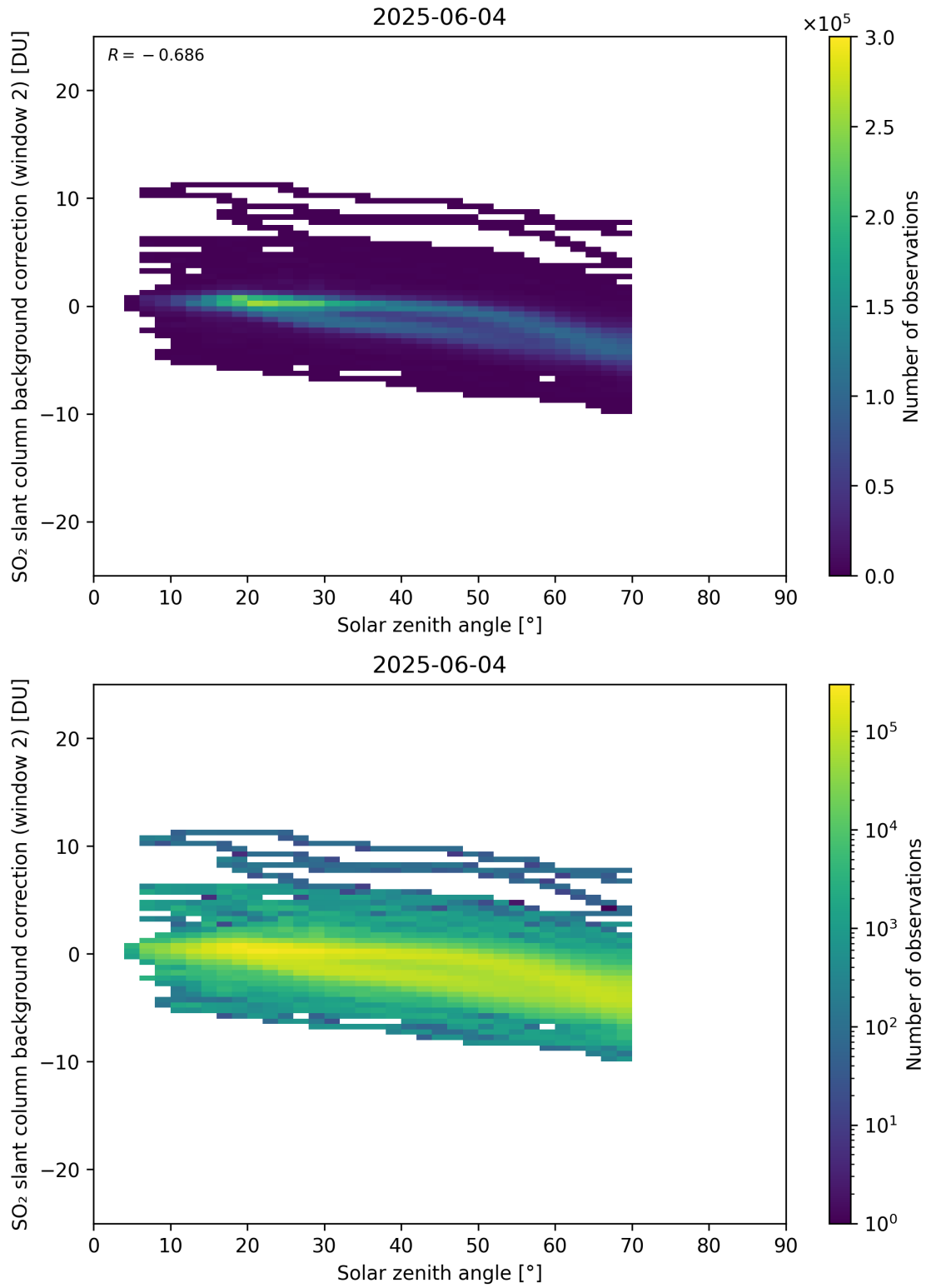
Figure 172: Scatter density plot of “Solar zenith angle” against “SO 2 slant column background correction (window 2)” for 2025-06-03 to 2025-06-05.
