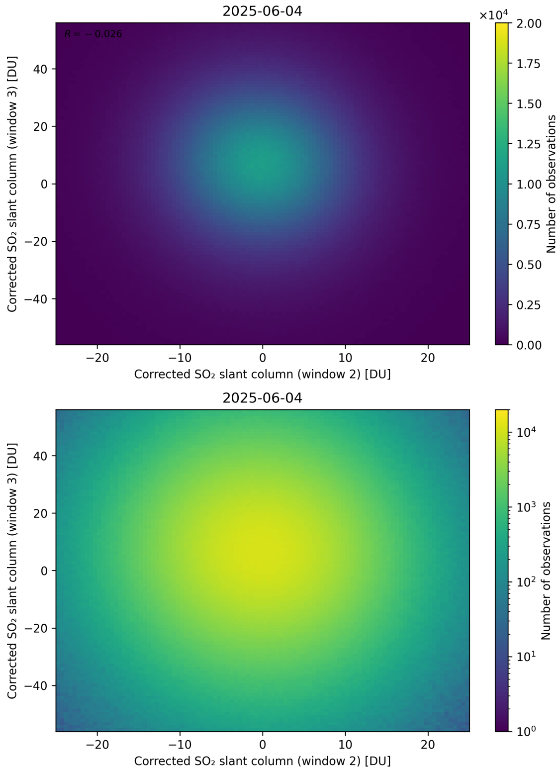
Figure 250: Scatter density plot of “Corrected SO 2 slant column (window 2)” against “Corrected SO 2 slant column (window 3)” for 2025-06-03 to 2025-06-05.
