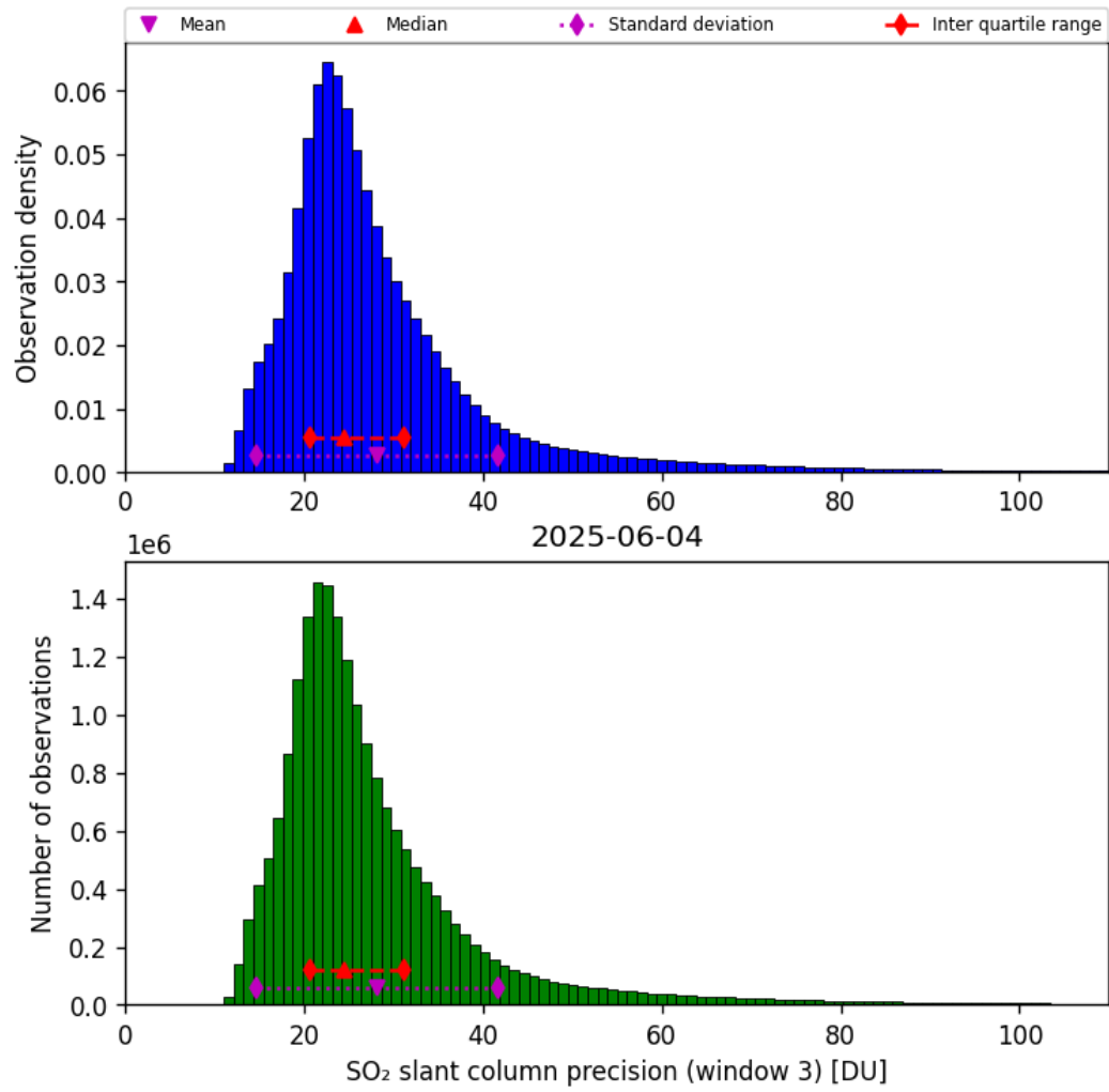
Figure 72: Histogram of “SO 2 slant column precision (window 3)” for 2025-06-03 to 2025-06-05
