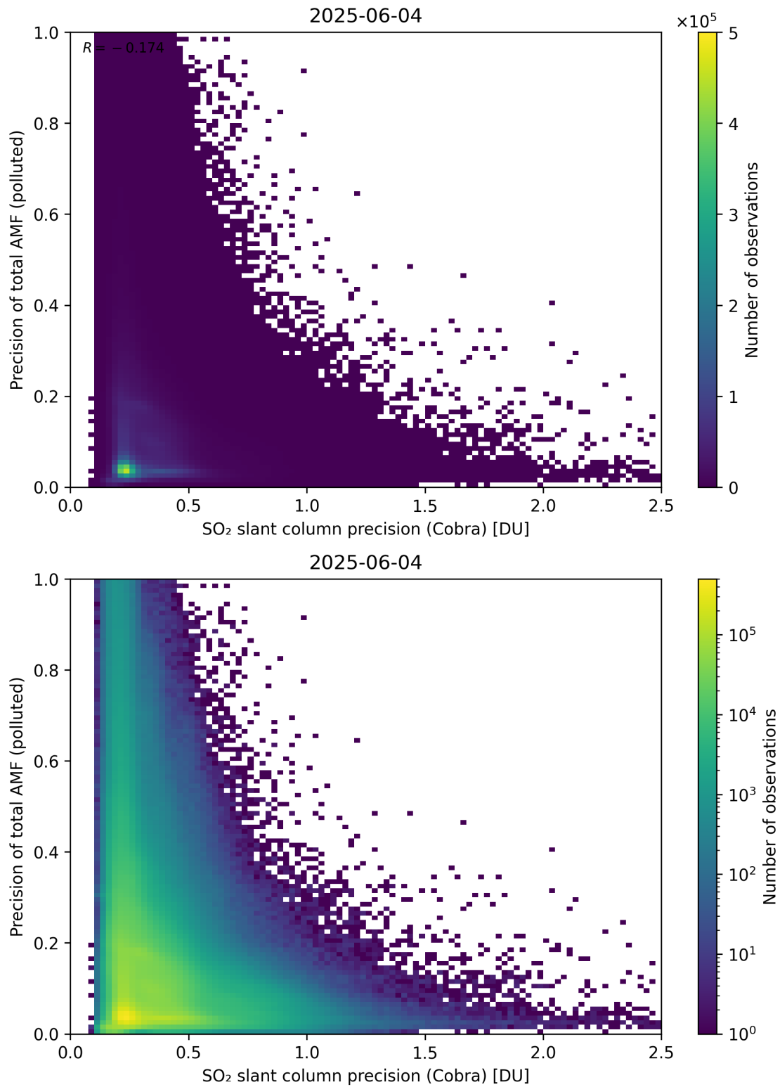
Figure 214: Scatter density plot of “SO 2 slant column precision (Cobra)” against “Precision of total AMF (polluted)” for 2025-06-03 to 2025-06-05.
