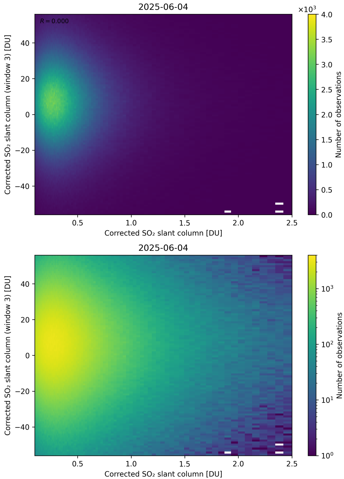
Figure 236: Scatter density plot of “Corrected SO 2 slant column” against “Corrected SO 2 slant column (window 3)” for 2025-06-03 to 2025-06-05.
