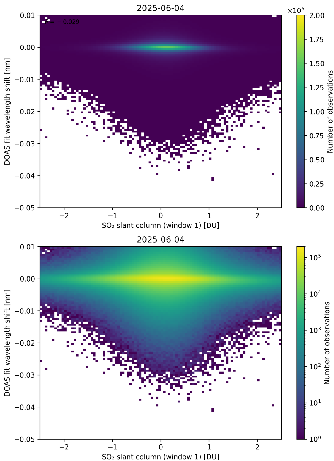
Figure 265: Scatter density plot of “SO 2 slant column (window 1)” against “DOAS fit wavelength shift” for 2025-06-03 to 2025-06-05.
