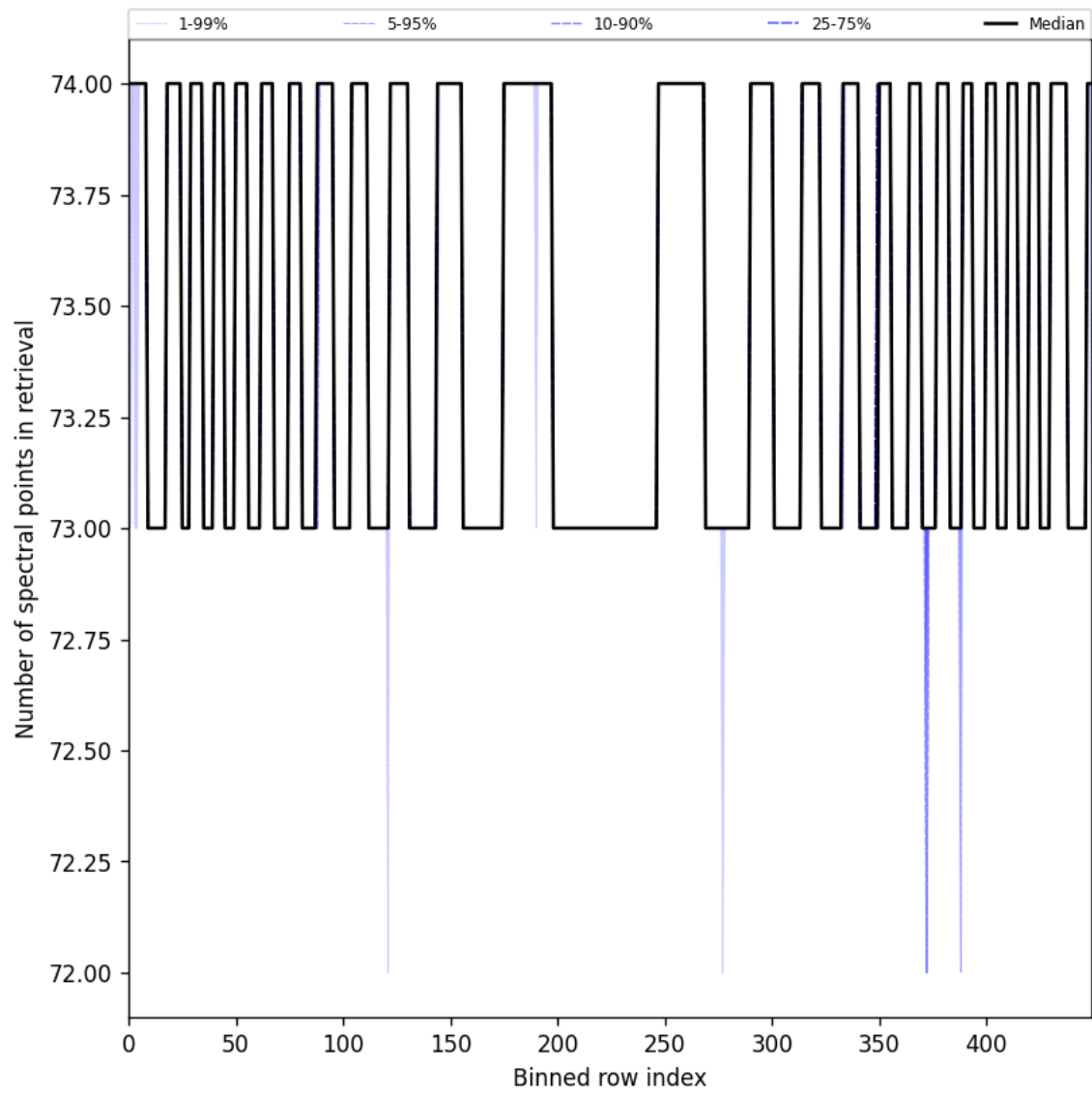
Figure 108: Along track statistics of “Number of spectral points in retrieval” for 2025-06-03 to 2025-06-05
