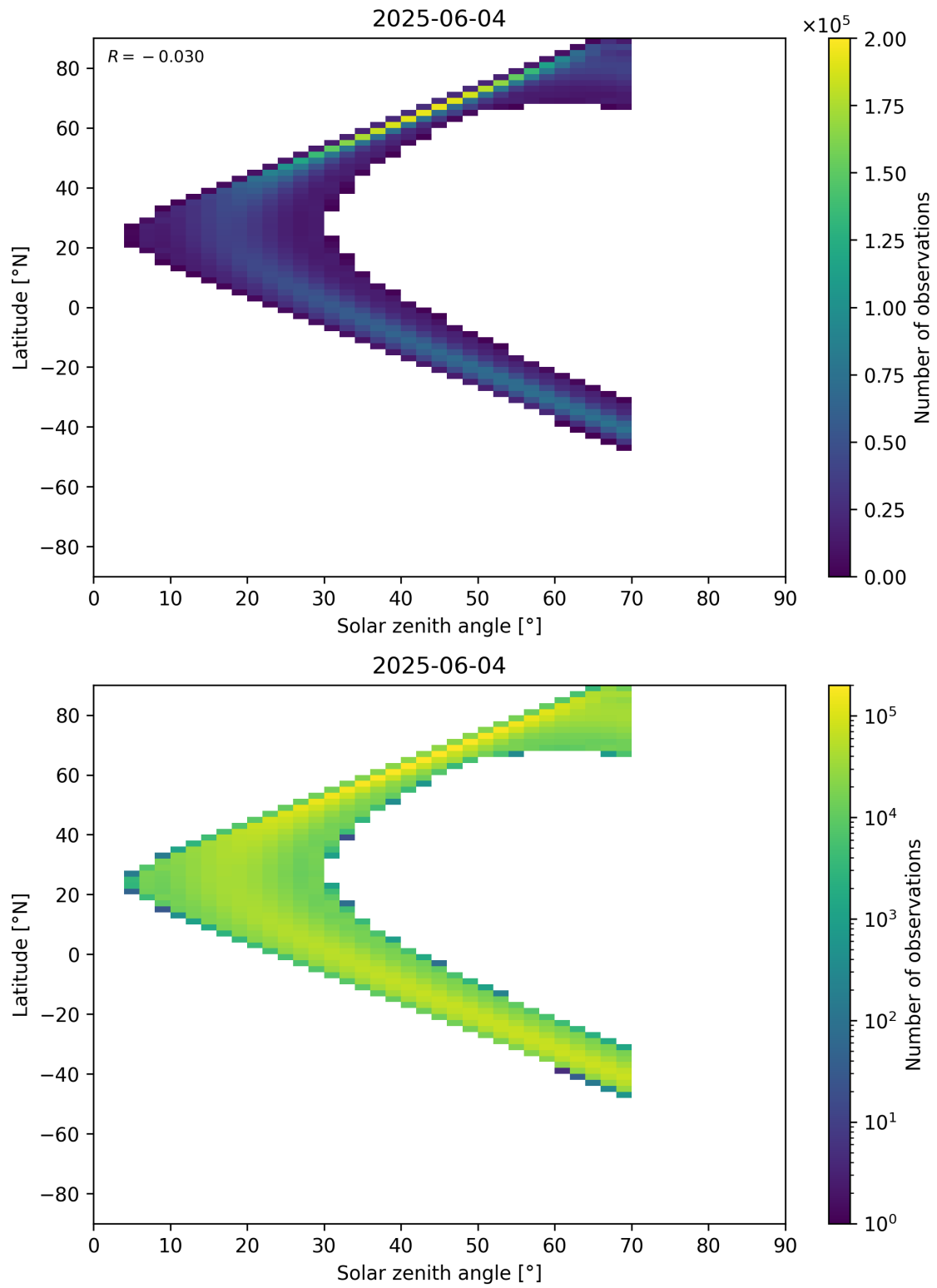
Figure 177: Scatter density plot of “Solar zenith angle” against “Latitude” for 2025-06-03 to 2025-06-05.
