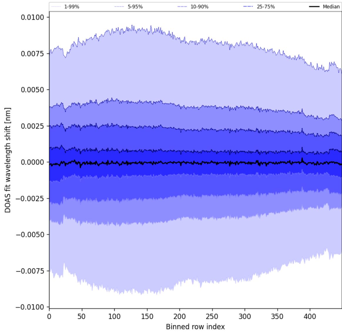
Figure 102: Along track statistics of “DOAS fit wavelength shift” for 2025-06-03 to 2025-06-05
