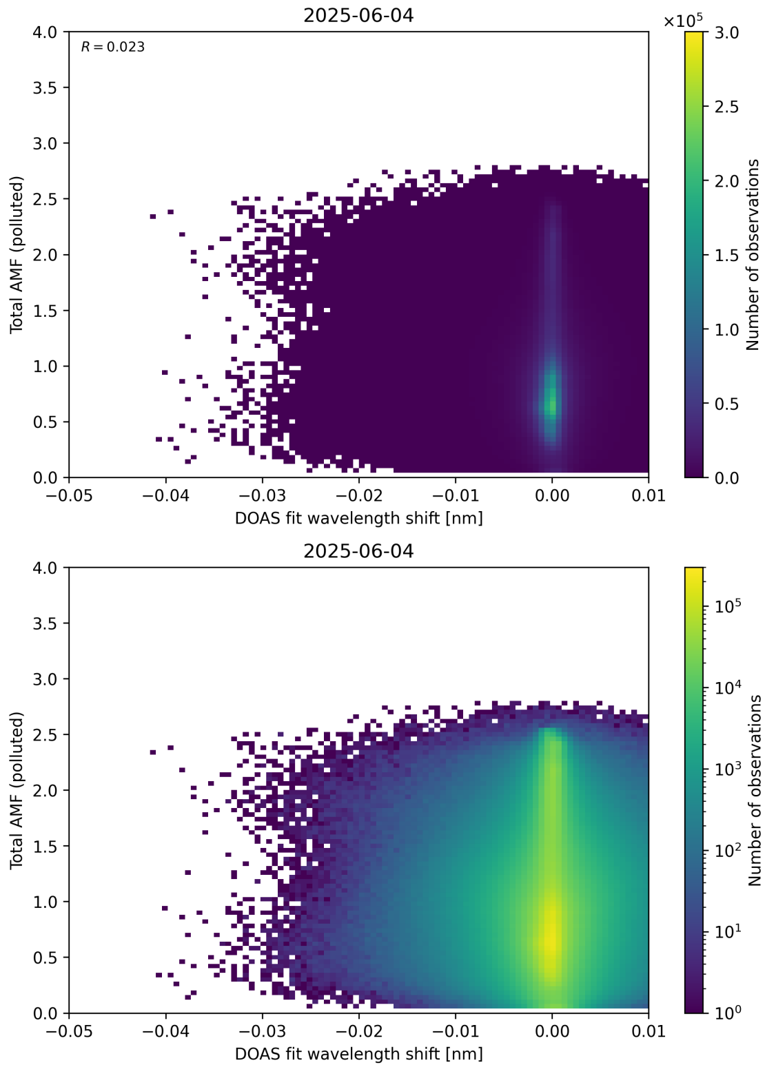
Figure 141: Scatter density plot of “DOAS fit wavelength shift” against “Total AMF (polluted)” for 2025-06-03 to 2025-06-05.
