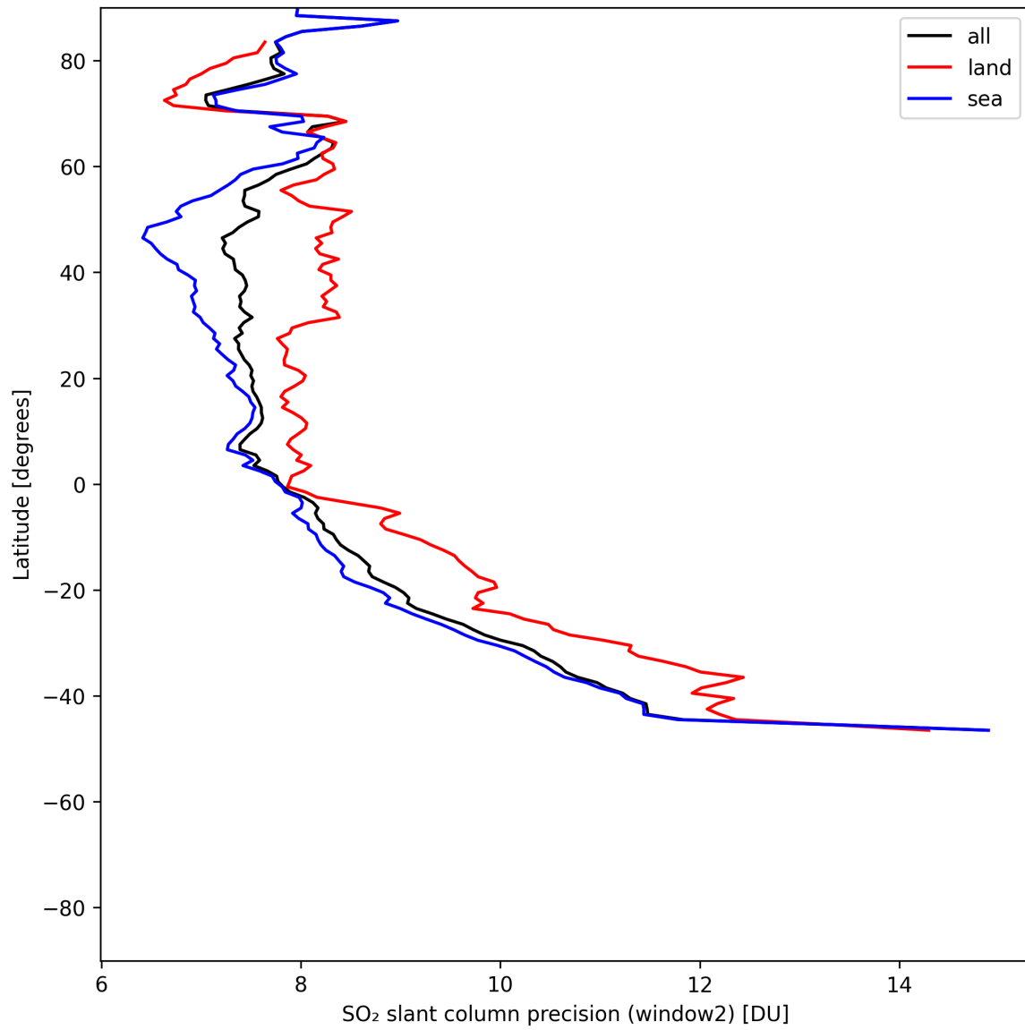
Figure 42: Zonal average of “SO 2 slant column precision (window2)” for 2025-06-03 to 2025-06-05.
