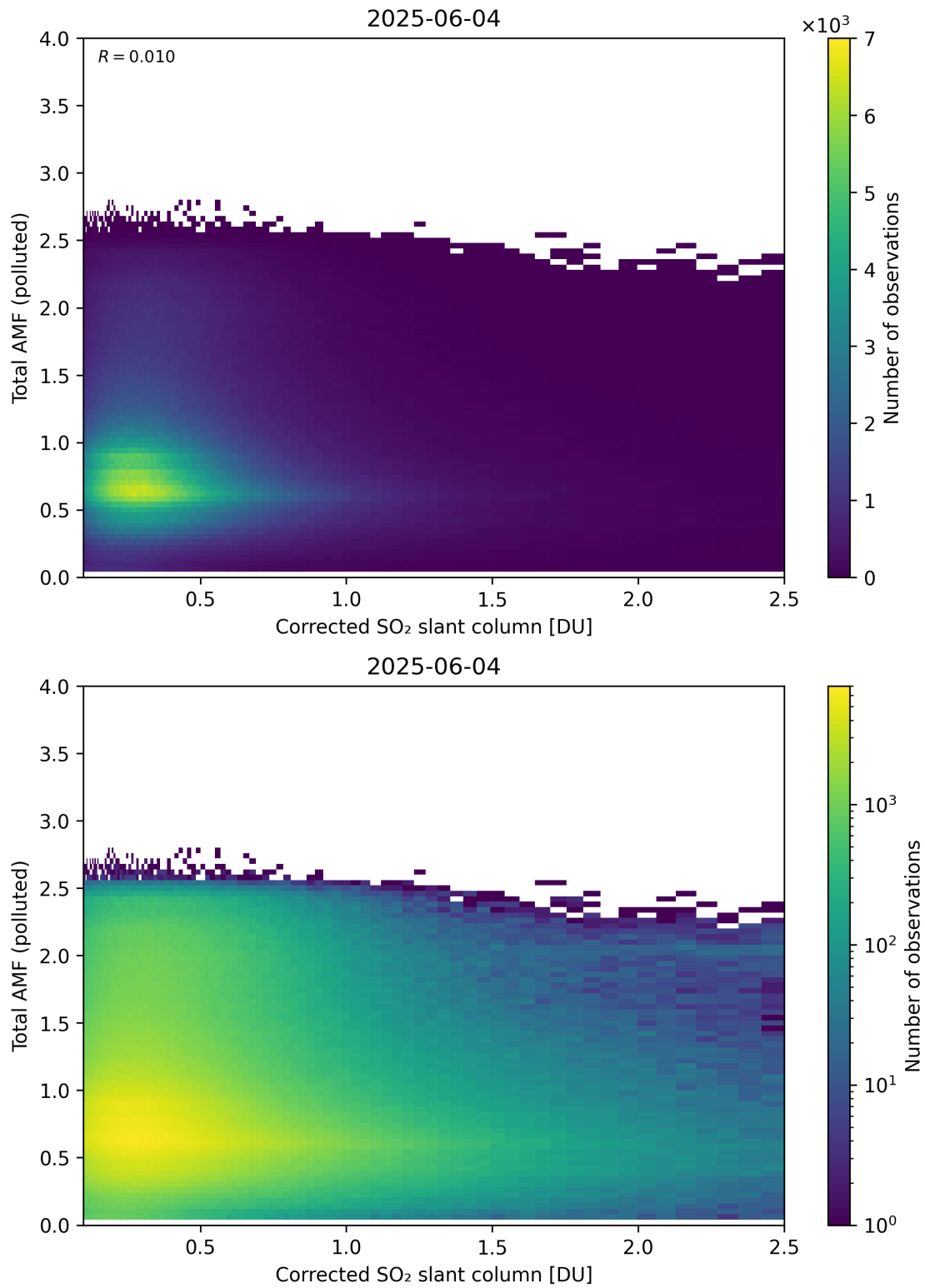
Figure 242: Scatter density plot of “Corrected SO 2 slant column” against “Total AMF (polluted)” for 2025-06-03 to 2025-06-05.
