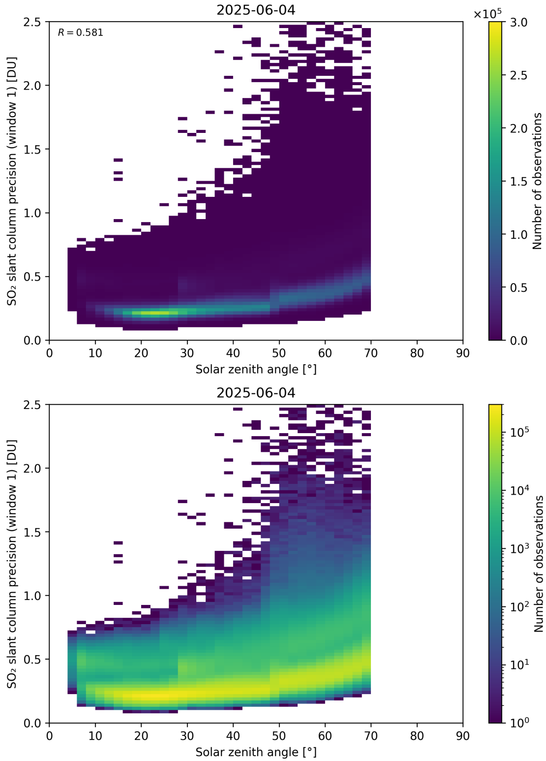
Figure 185: Scatter density plot of “Solar zenith angle” against “SO 2 slant column precision (window 1)” for 2025-06-03 to 2025-06-05.
