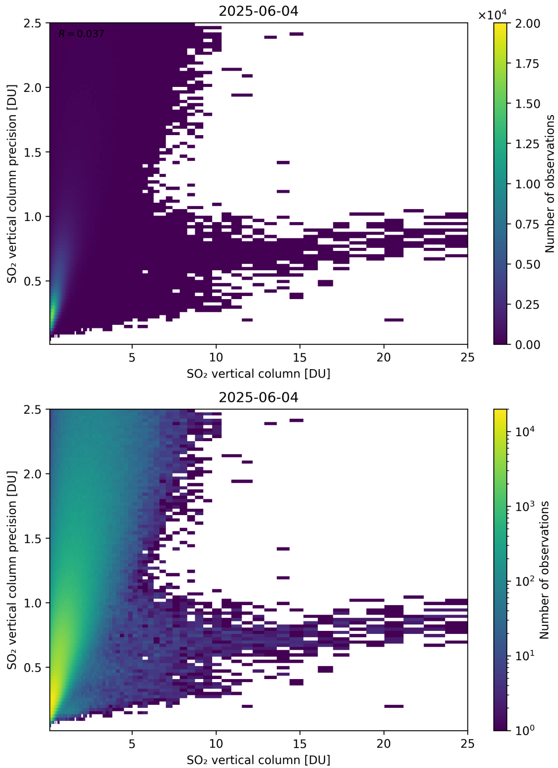
Figure 361: Scatter density plot of “SO 2 vertical column” against “SO 2 vertical column precision” for 2025-06-03 to 2025-06-05.
