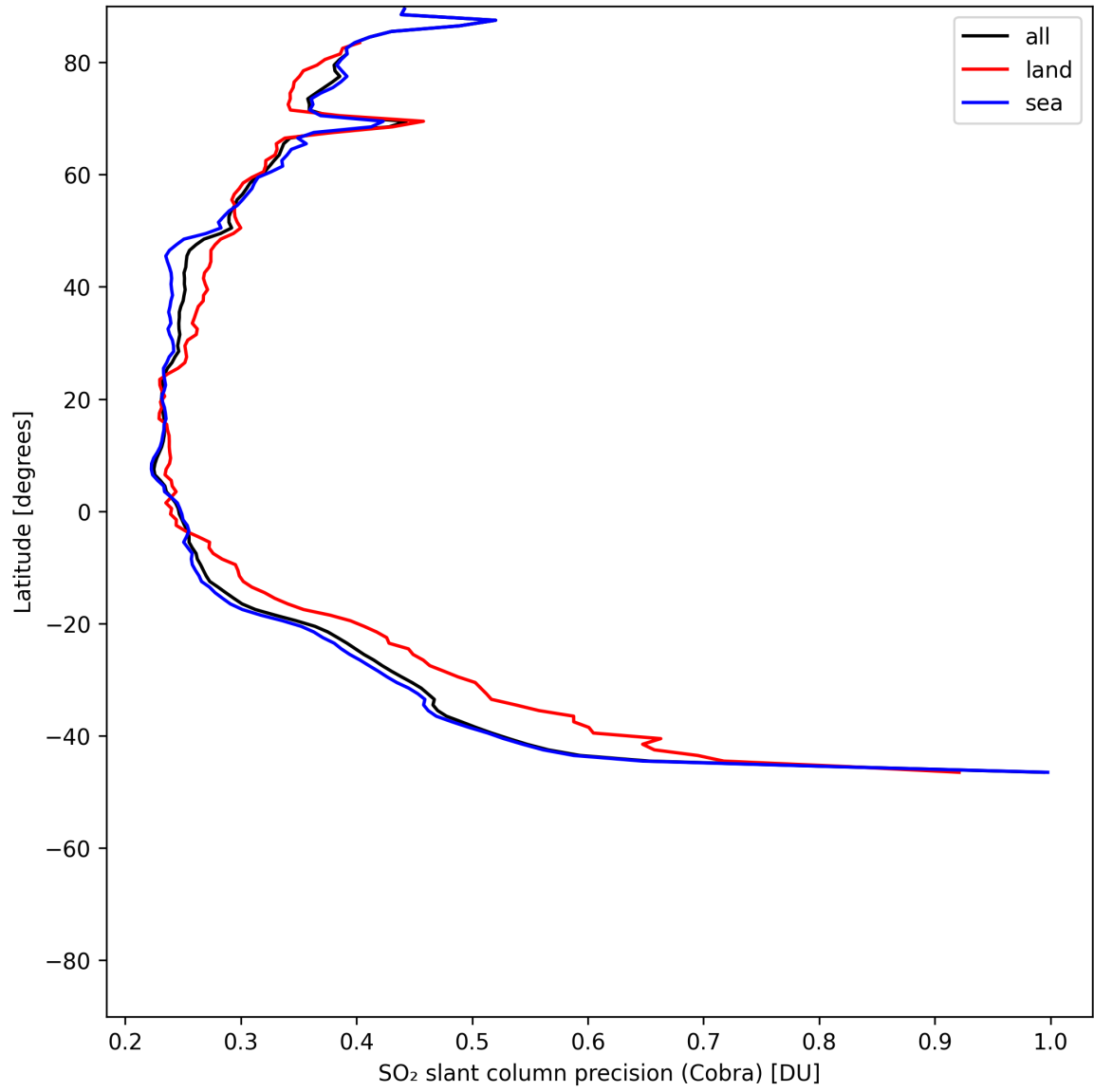
Figure 36: Zonal average of “SO 2 slant column precision (Cobra)” for 2025-06-03 to 2025-06-05.
