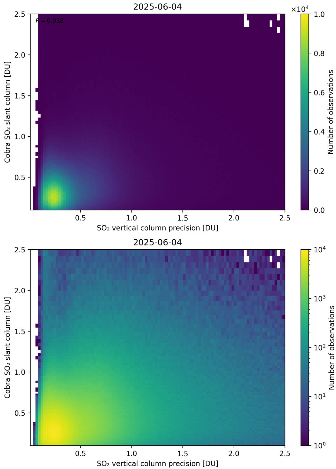
Figure 336: Scatter density plot of “SO 2 vertical column precision” against “Cobra SO 2 slant column” for 2025-06-03 to 2025-06-05.
