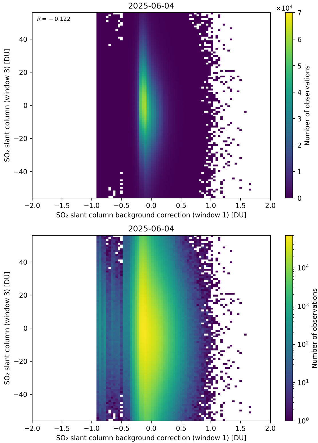
Figure 118: Scatter density plot of “SO 2 slant column background correction (window 1)” against “SO 2 slant column (window 3)” for 2025-06-03 to 2025-06-05.
