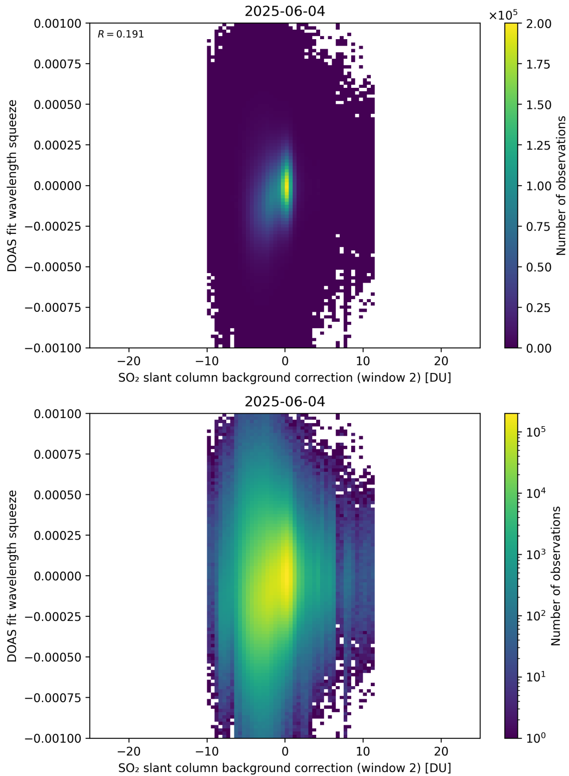
Figure 124: Scatter density plot of “SO 2 slant column background correction (window 2)” against “DOAS fit wavelength squeeze” for 2025-06-03 to 2025-06-05.
