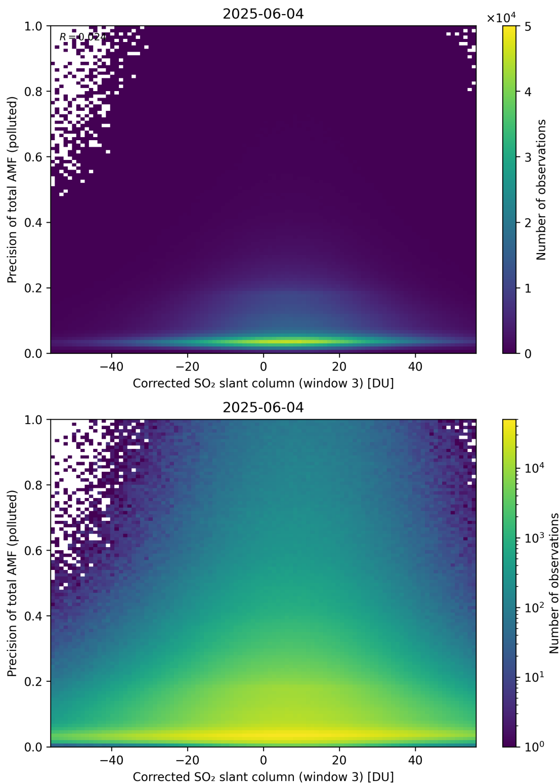
Figure 261: Scatter density plot of “Corrected SO 2 slant column (window 3)” against “Precision of total AMF (polluted)” for 2025-06-03 to 2025-06-05.
