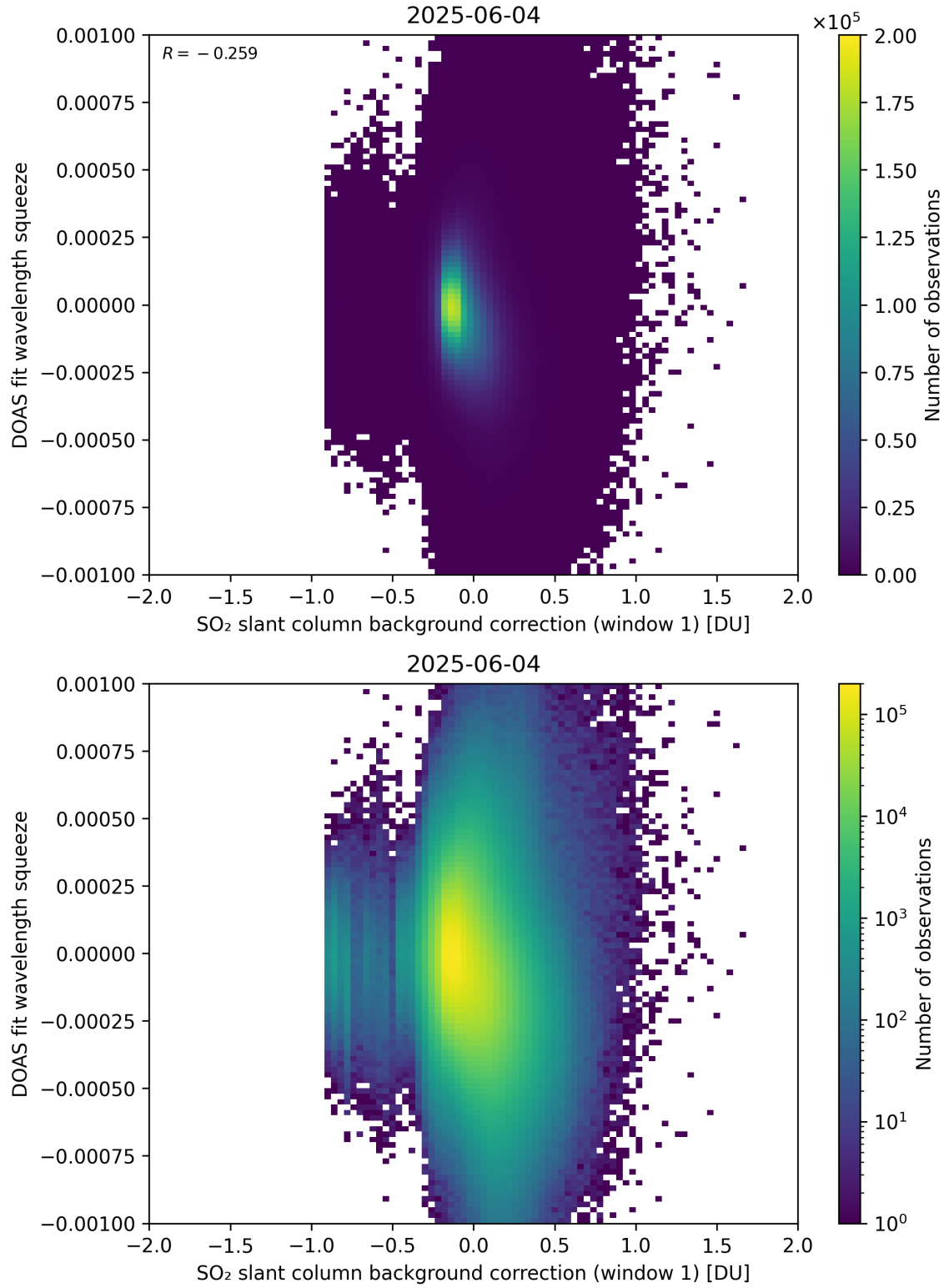
Figure 112: Scatter density plot of “SO 2 slant column background correction (window 1)” against “DOAS fit wavelength squeeze” for 2025-06-03 to 2025-06-05.
