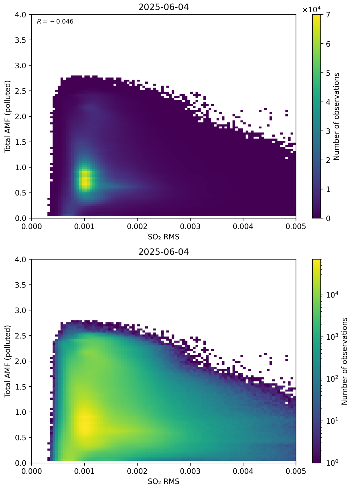
Figure 148: Scatter density plot of “SO 2 RMS” against “Total AMF (polluted)” for 2025-06-03 to 2025-06-05.
