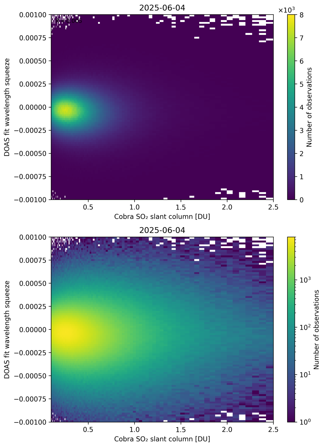
Figure 197: Scatter density plot of “Cobra SO 2 slant column” against “DOAS fit wavelength squeeze” for 2025-06-03 to 2025-06-05.
