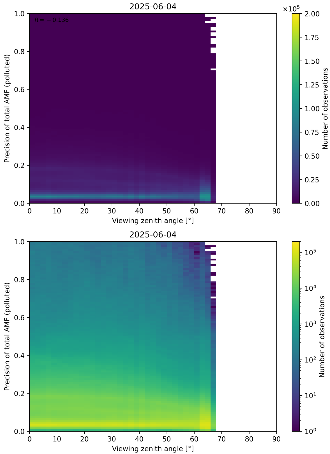
Figure 382: Scatter density plot of “Viewing zenith angle” against “Precision of total AMF (polluted)” for 2025-06-03 to 2025-06-05.
