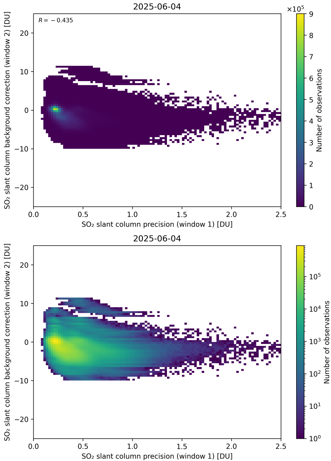
Figure 269: Scatter density plot of “SO 2 slant column precision (window 1)” against “SO 2 slant column background correction (window 2)” for 2025-06-03 to 2025-06-05.
