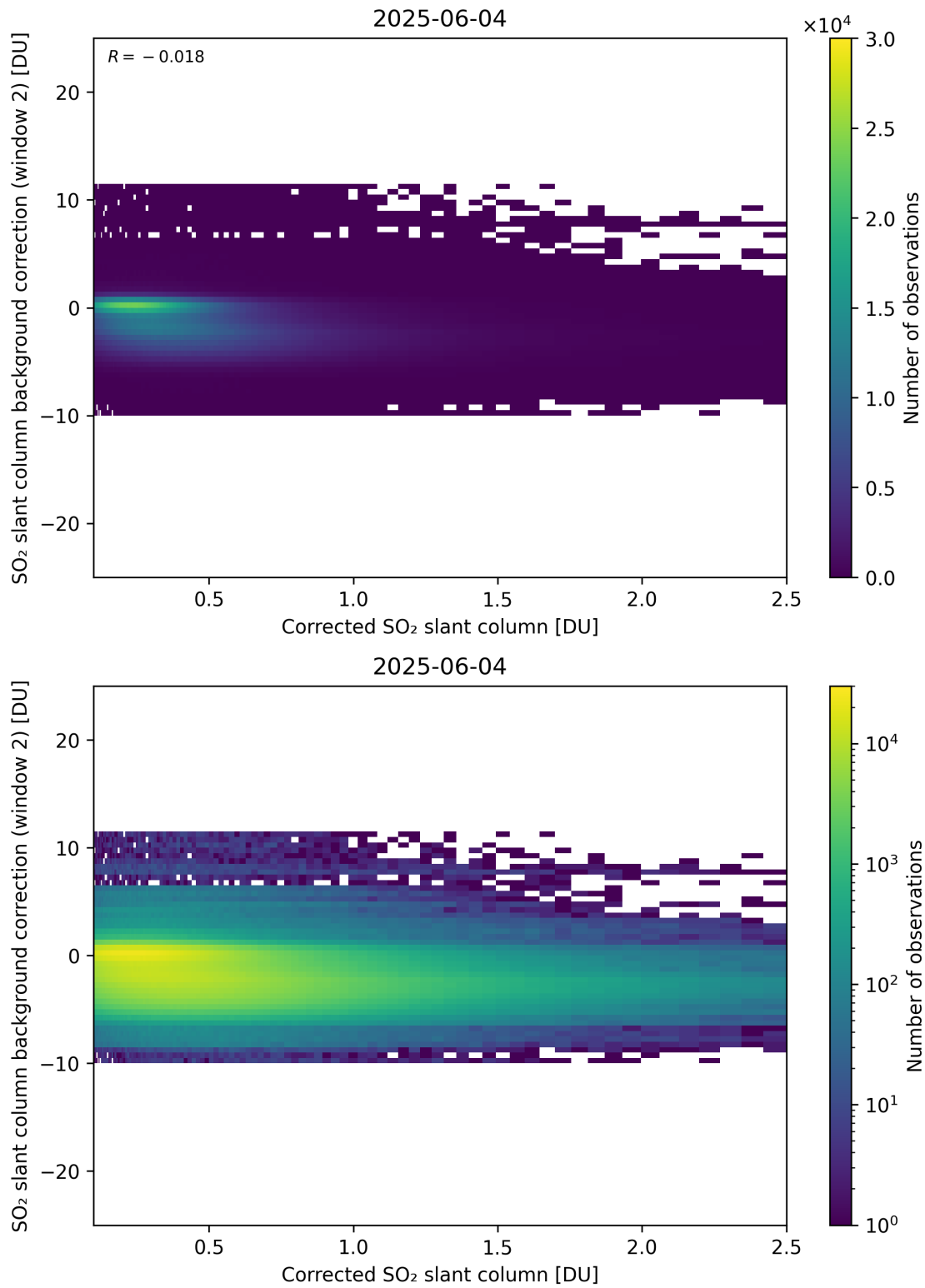
Figure 227: Scatter density plot of “Corrected SO 2 slant column” against “SO 2 slant column background correction (window 2)” for 2025-06-03 to 2025-06-05.
