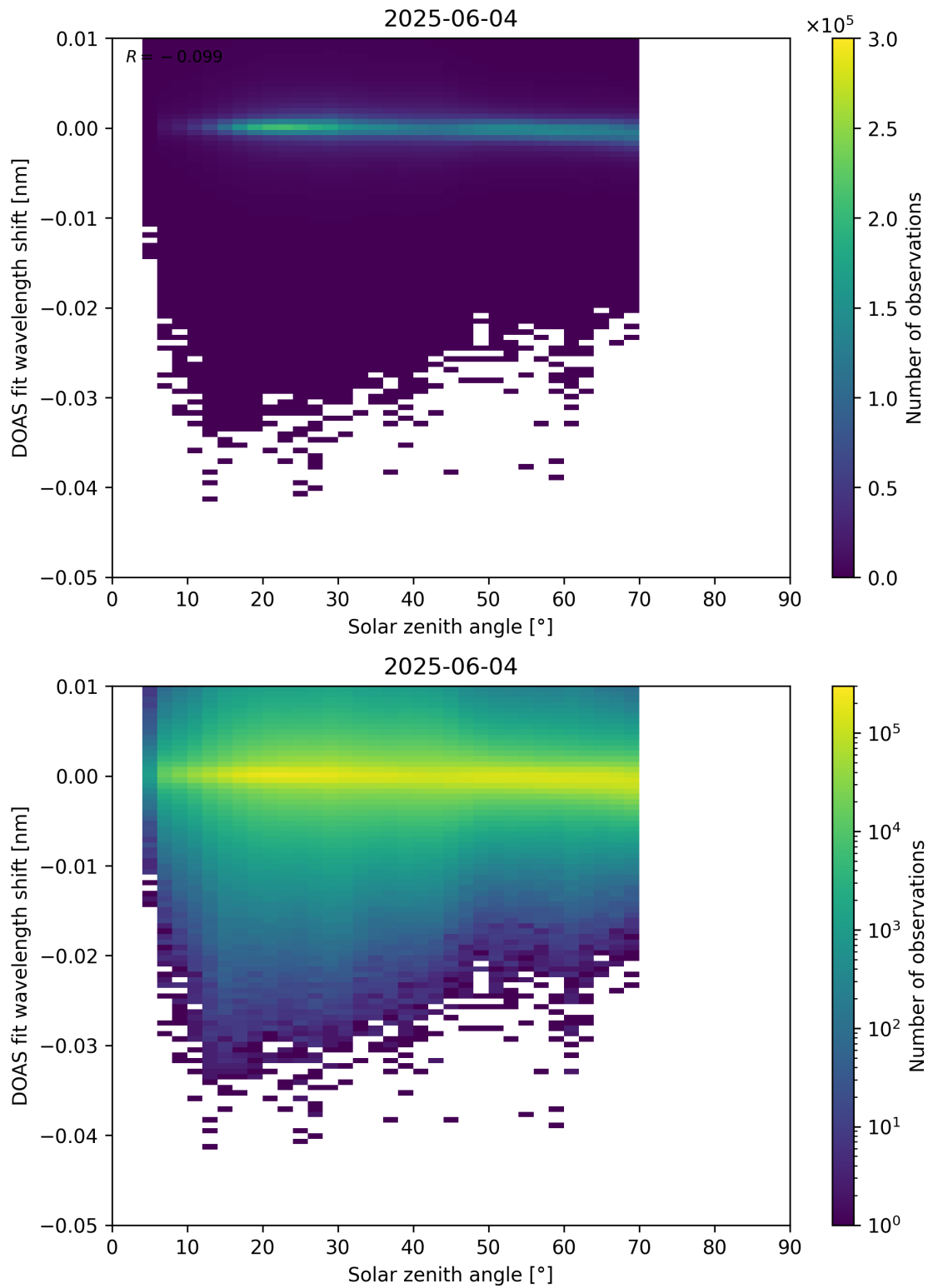
Figure 174: Scatter density plot of “Solar zenith angle” against “DOAS fit wavelength shift” for 2025-06-03 to 2025-06-05.
