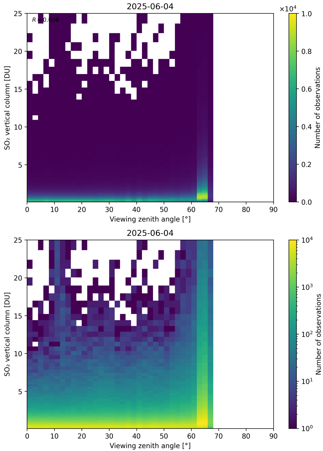
Figure 383: Scatter density plot of “Viewing zenith angle” against “SO 2 vertical column” for 2025-06-03 to 2025-06-05.
