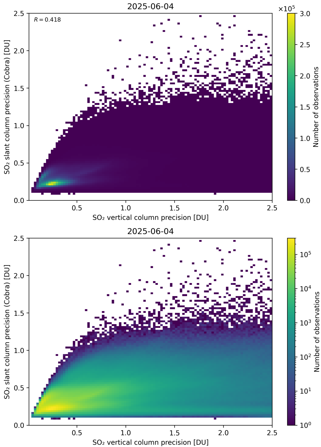
Figure 337: Scatter density plot of “SO 2 vertical column precision” against “SO 2 slant column precision (Cobra)” for 2025-06-03 to 2025-06-05.
