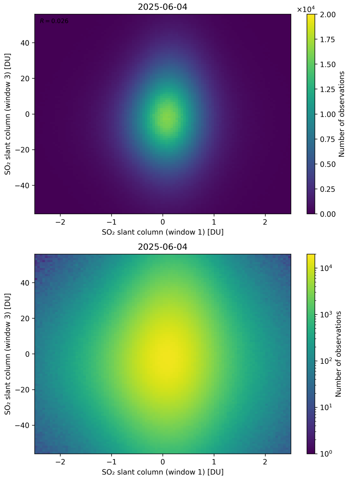
Figure 287: Scatter density plot of “SO 2 slant column (window 1)” against “SO 2 slant column (window 3)” for 2025-06-03 to 2025-06-05.
