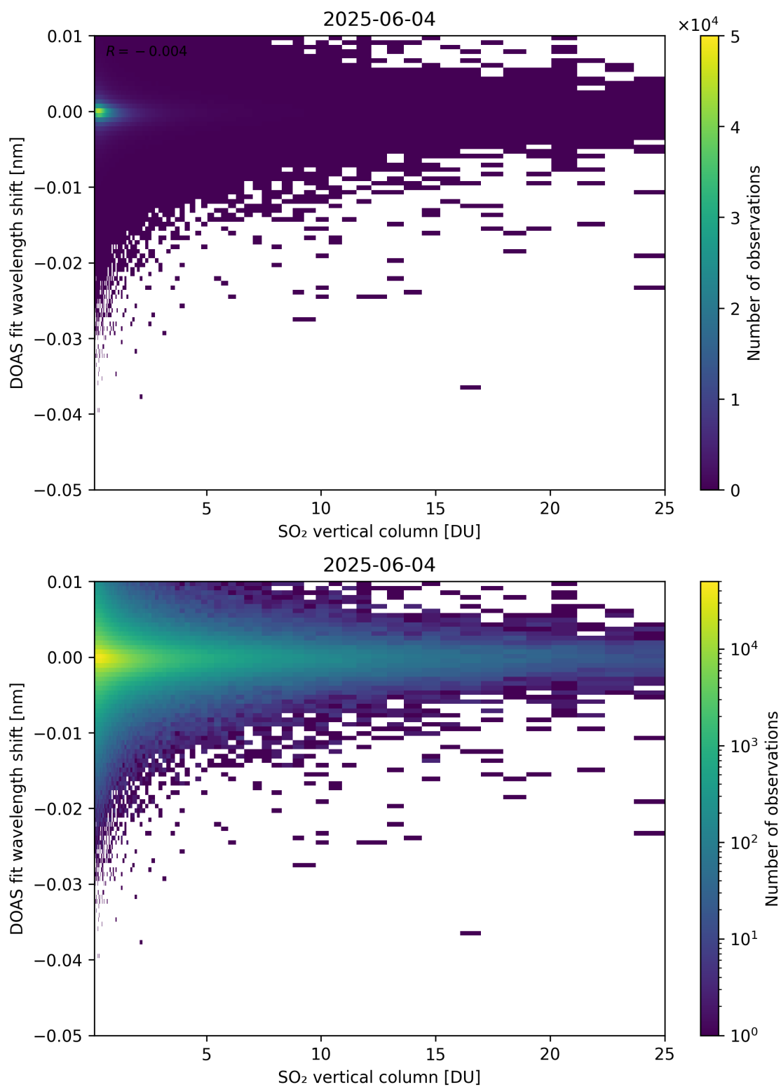
Figure 326: Scatter density plot of “SO 2 vertical column” against “DOAS fit wavelength shift” for 2025-06-03 to 2025-06-05.
