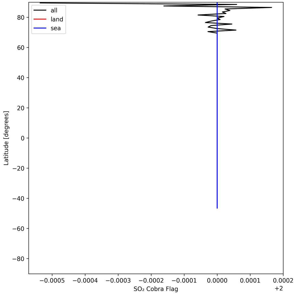
Figure 49: Zonal average of “SO 2 Cobra Flag” for 2025-06-03 to 2025-06-05.
