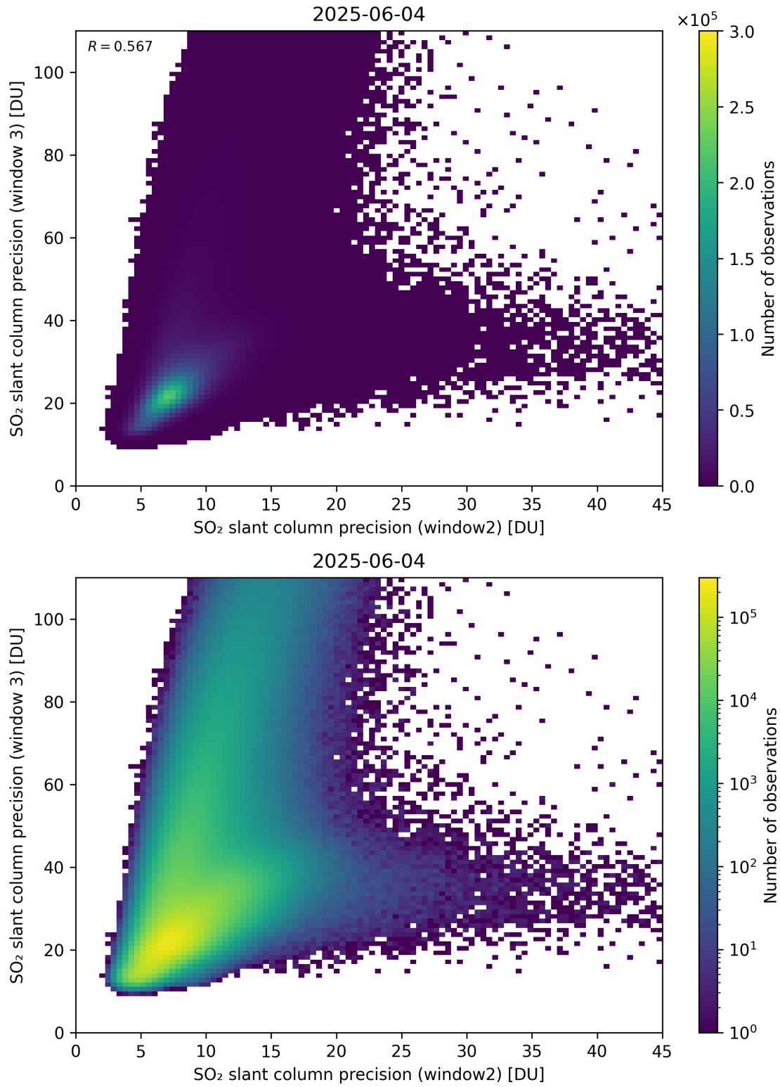
Figure 300: Scatter density plot of “SO 2 slant column precision (window2)” against “SO 2 slant column precision (window 3)” for 2025-06-03 to 2025-06-05.
