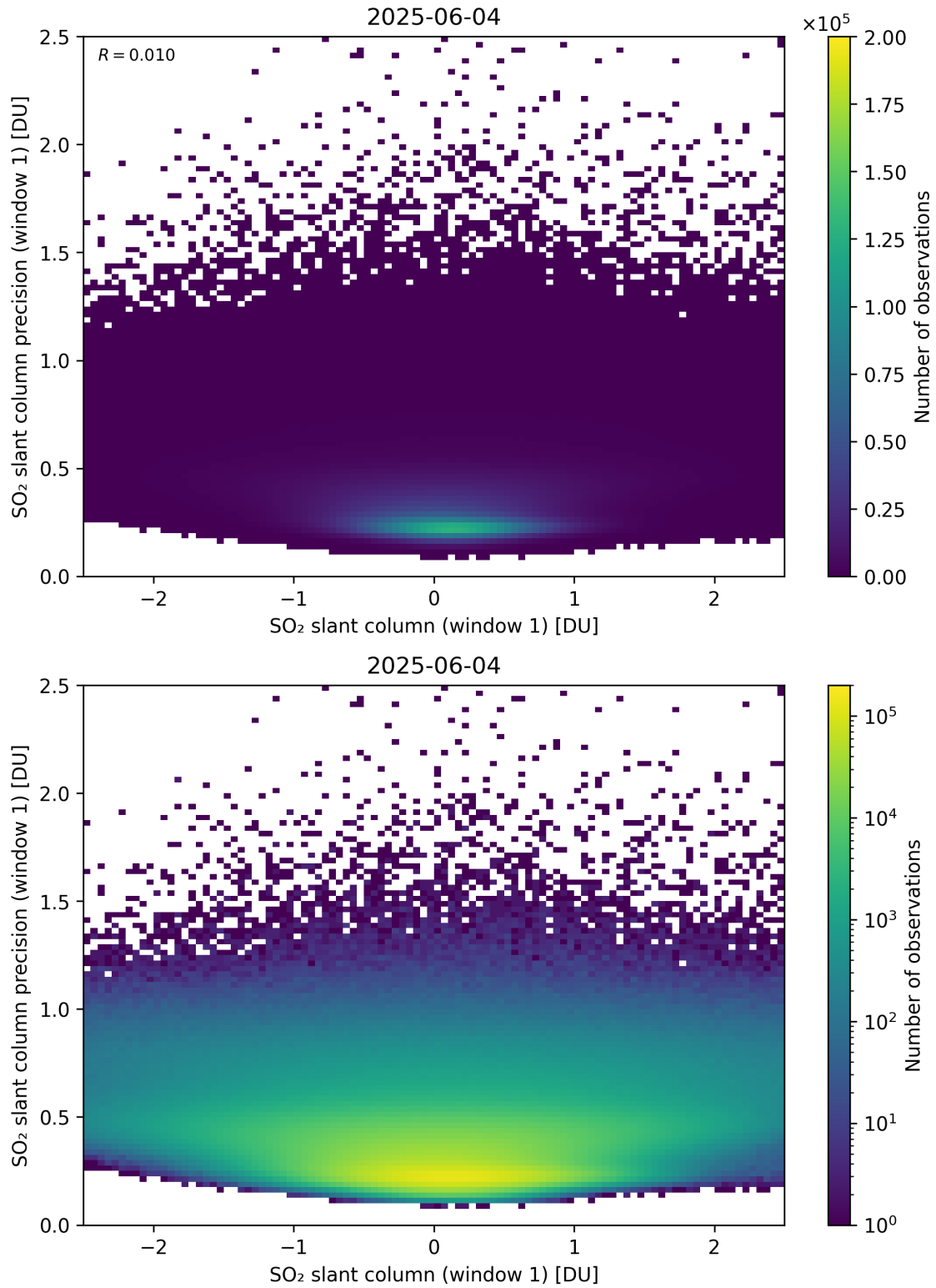
Figure 285: Scatter density plot of “SO 2 slant column (window 1)” against “SO 2 slant column precision (window 1)” for 2025-06-03 to 2025-06-05.
