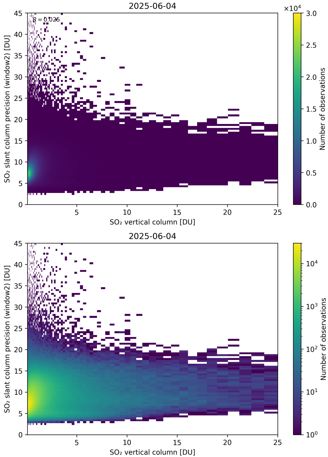
Figure 356: Scatter density plot of “SO 2 vertical column” against “SO 2 slant column precision (window2)” for 2025-06-03 to 2025-06-05.
