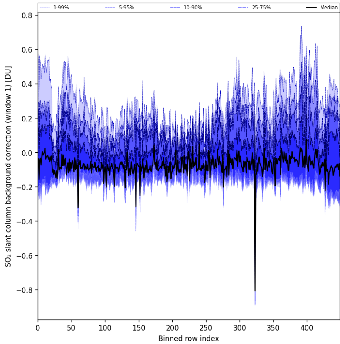
Figure 92: Along track statistics of “SO 2 slant column background correction (window 1)” for 2025-06-03 to 2025-06-05
