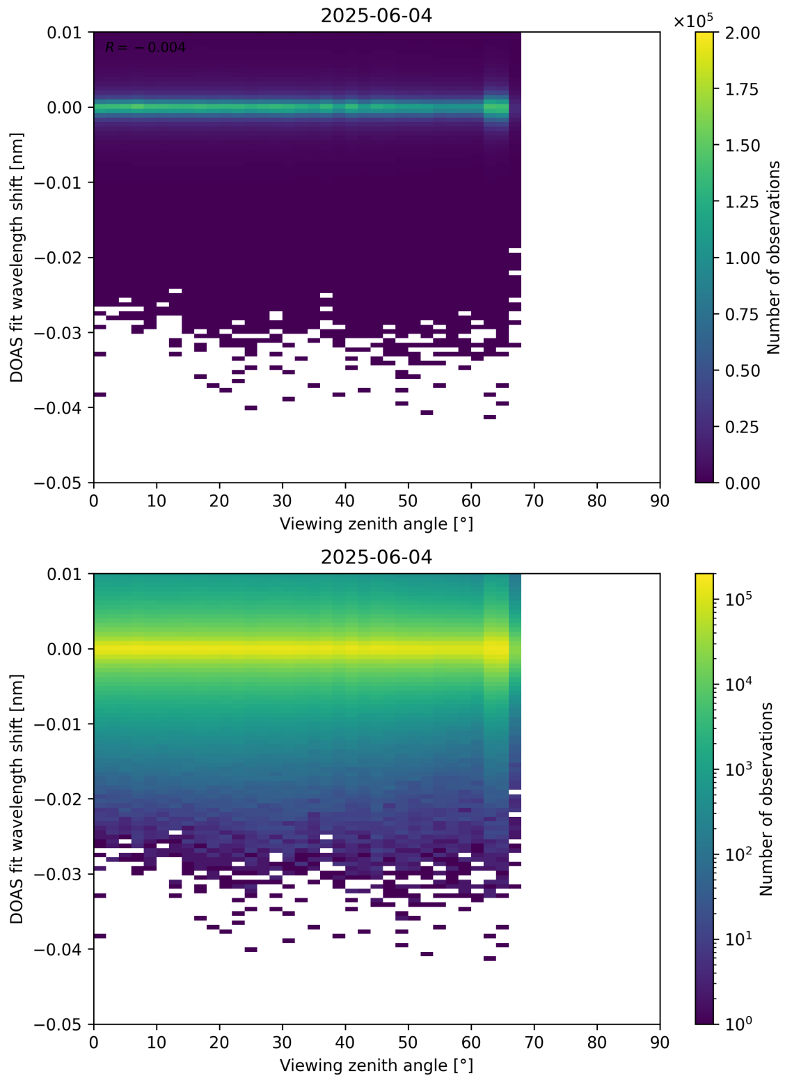
Figure 365: Scatter density plot of “Viewing zenith angle” against “DOAS fit wavelength shift” for 2025-06-03 to 2025-06-05.
