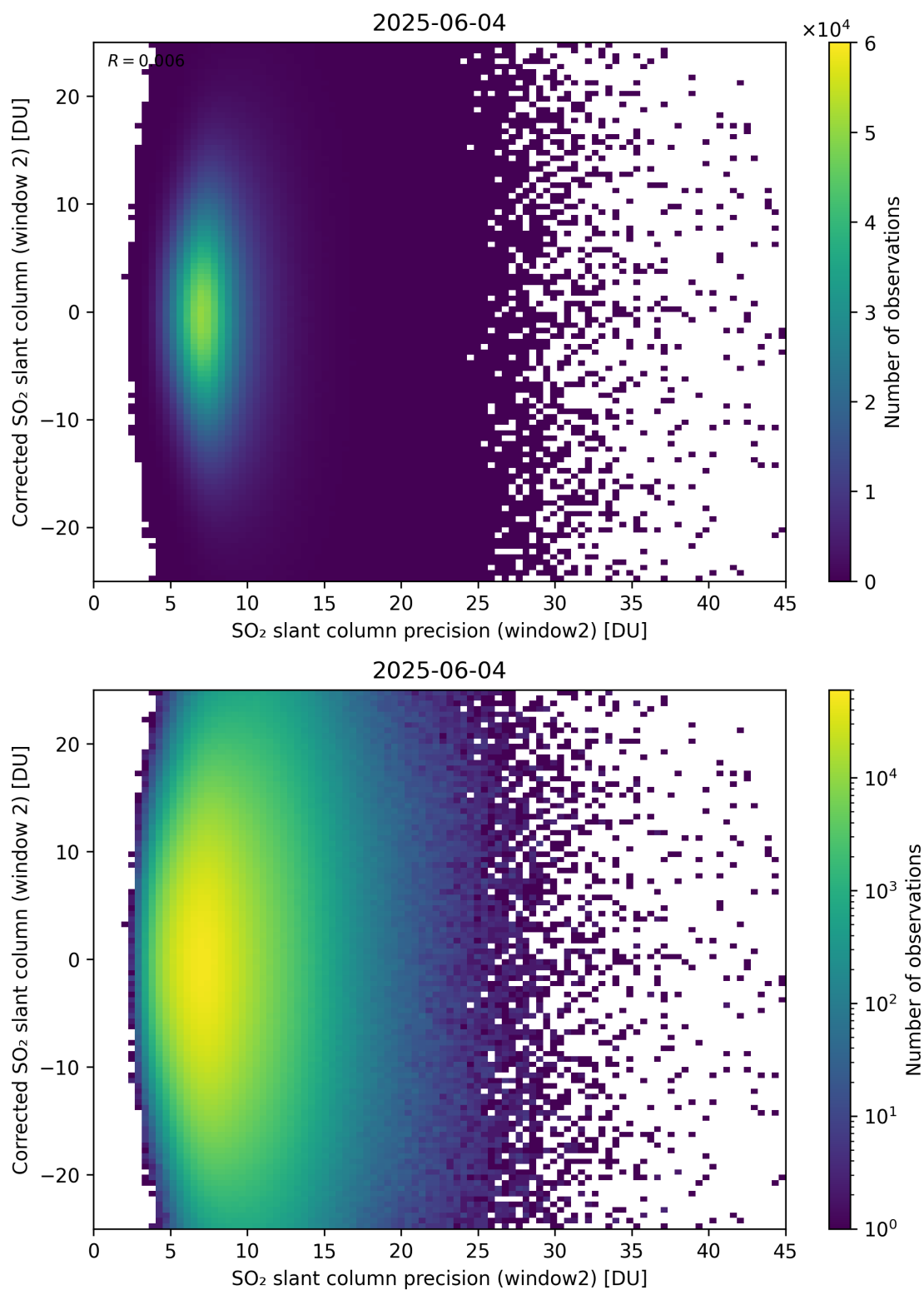
Figure 297: Scatter density plot of “SO 2 slant column precision (window2)” against “Corrected SO 2 slant column (window 2)” for 2025-06-03 to 2025-06-05.
