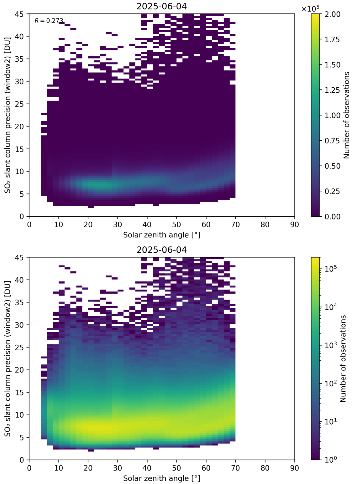
Figure 186: Scatter density plot of “Solar zenith angle” against “SO 2 slant column precision (window2)” for 2025-06-03 to 2025-06-05.
