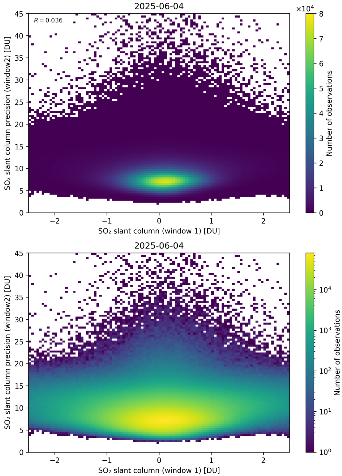
Figure 286: Scatter density plot of “SO 2 slant column (window 1)” against “SO 2 slant column precision (window2)” for 2025-06-03 to 2025-06-05.
