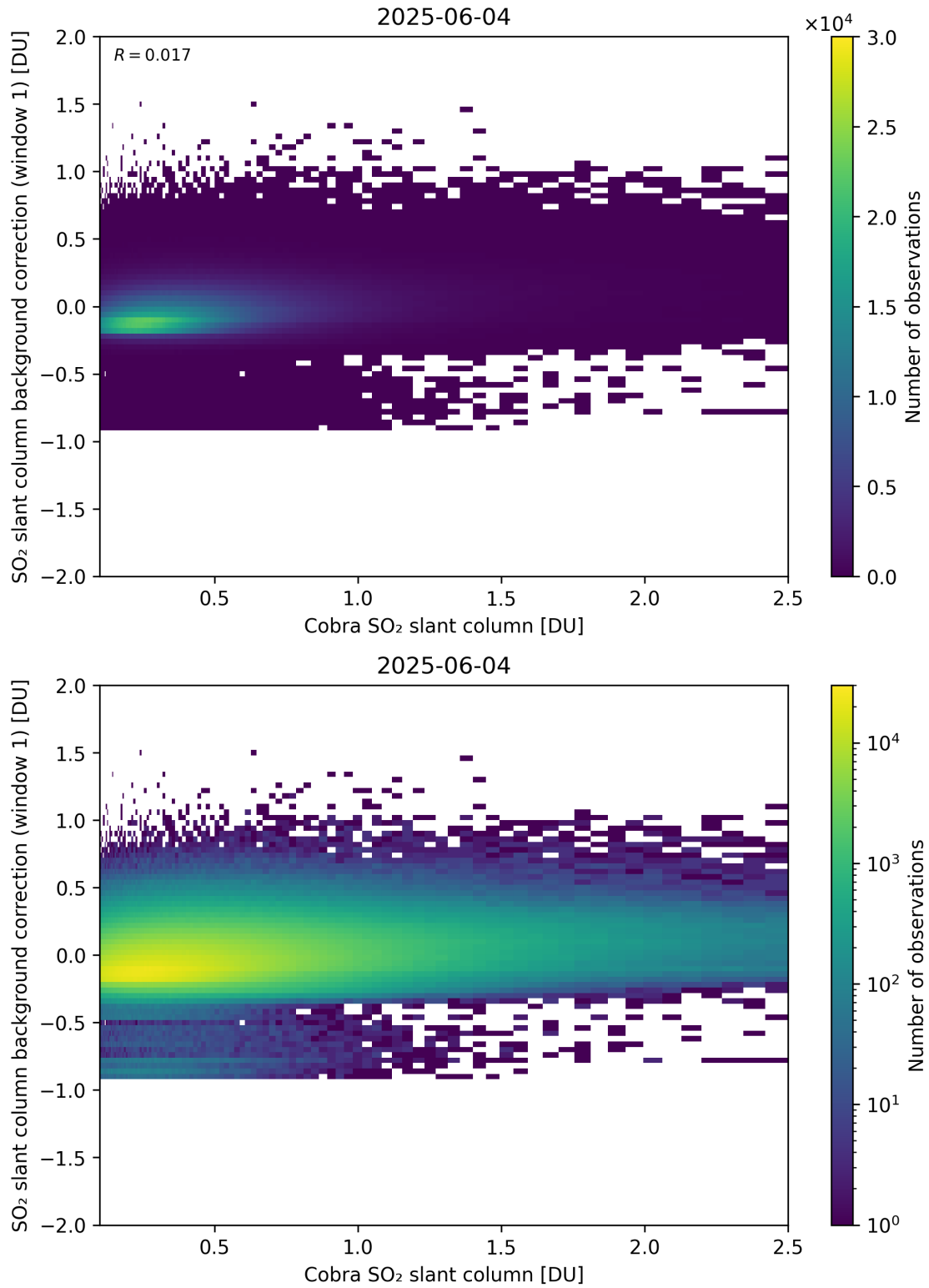
Figure 193: Scatter density plot of “Cobra SO 2 slant column” against “SO 2 slant column background correction (window 1)” for 2025-06-03 to 2025-06-05.
