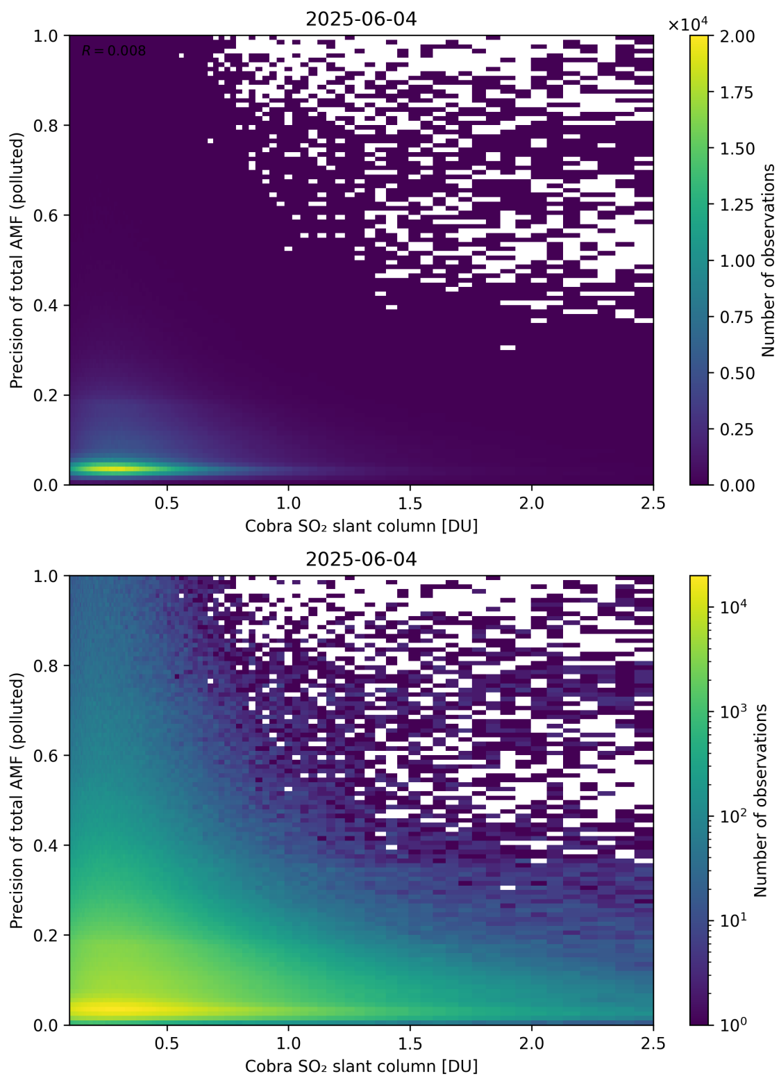
Figure 225: Scatter density plot of “Cobra SO 2 slant column” against “Precision of total AMF (polluted)” for 2025-06-03 to 2025-06-05.
