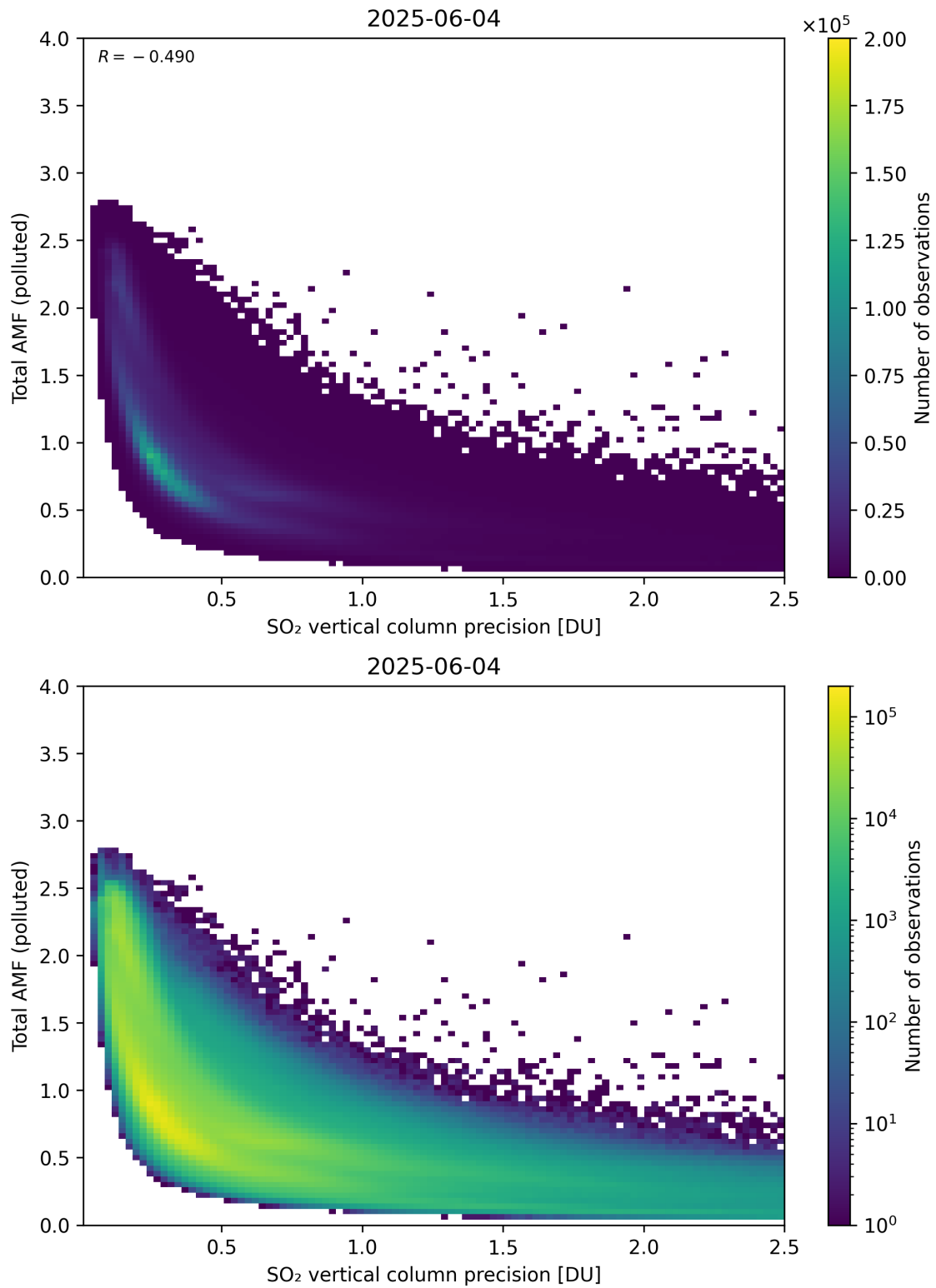
Figure 346: Scatter density plot of “SO 2 vertical column precision” against “Total AMF (polluted)” for 2025-06-03 to 2025-06-05.
