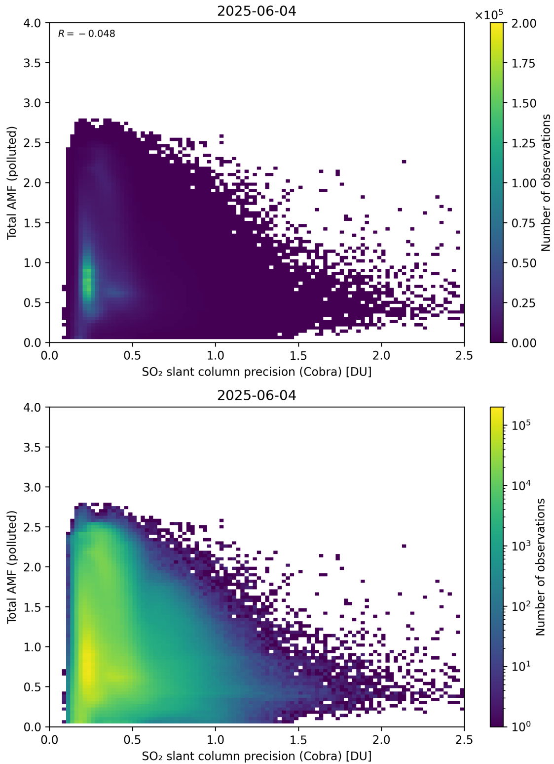
Figure 213: Scatter density plot of “SO 2 slant column precision (Cobra)” against “Total AMF (polluted)” for 2025-06-03 to 2025-06-05.
