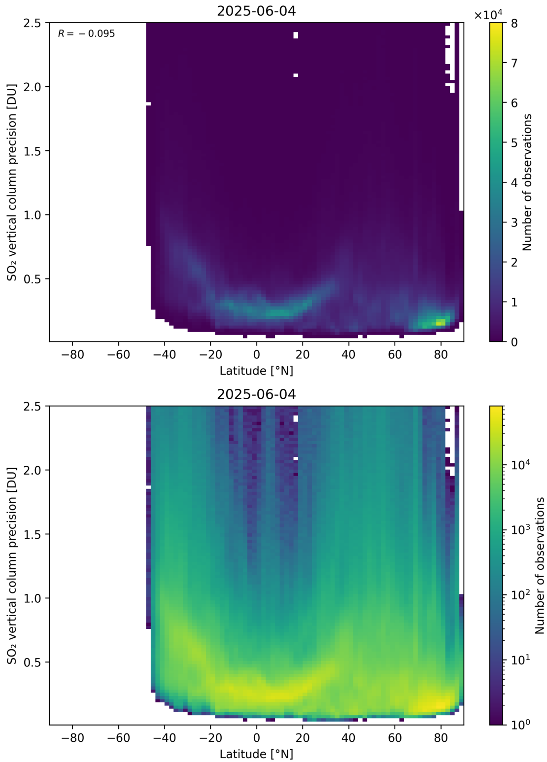
Figure 170: Scatter density plot of “Latitude” against “SO 2 vertical column precision” for 2025-06-03 to 2025-06-05.
