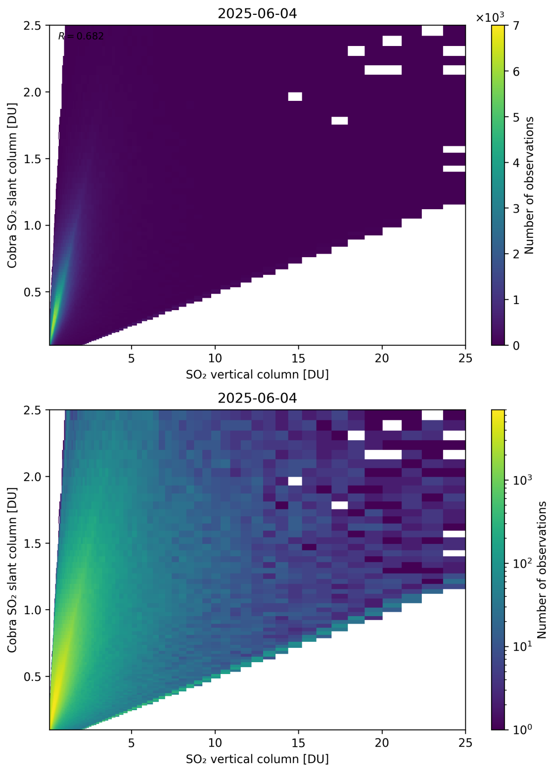
Figure 349: Scatter density plot of “SO 2 vertical column” against “Cobra SO 2 slant column” for 2025-06-03 to 2025-06-05.
