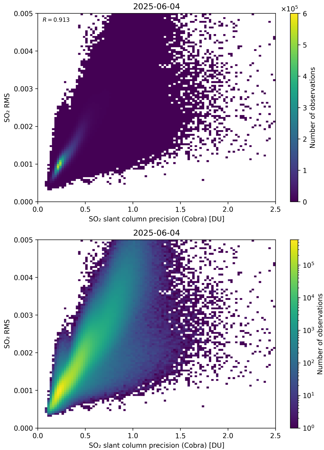
Figure 204: Scatter density plot of “SO 2 slant column precision (Cobra)” against “SO 2 RMS” for 2025-06-03 to 2025-06-05.
