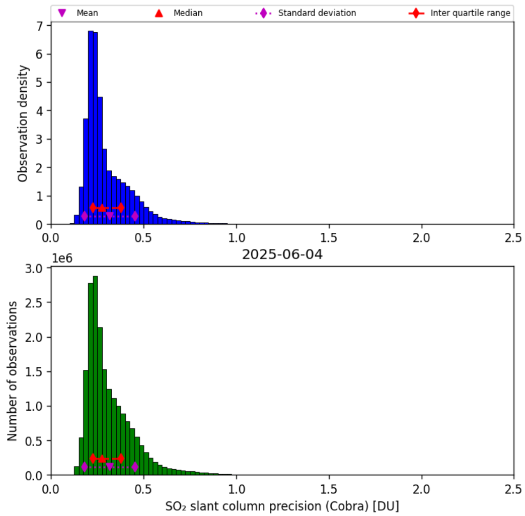
Figure 62: Histogram of “SO 2 slant column precision (Cobra)” for 2025-06-03 to 2025-06-05
