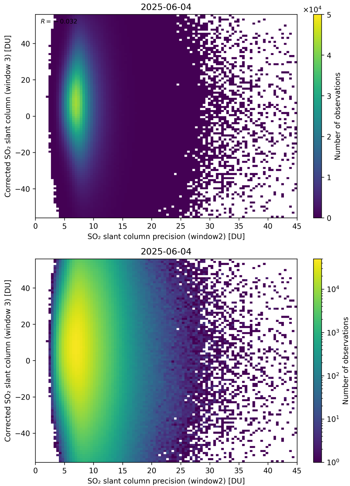
Figure 298: Scatter density plot of “SO 2 slant column precision (window2)” against “Corrected SO 2 slant column (window 3)” for 2025-06-03 to 2025-06-05.
