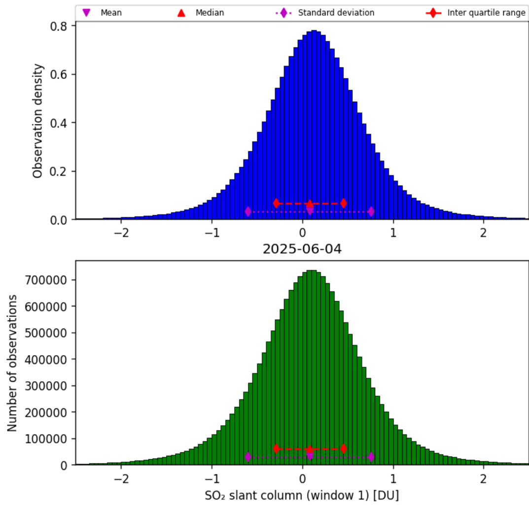
Figure 63: Histogram of “SO 2 slant column (window 1)” for 2025-06-03 to 2025-06-05
