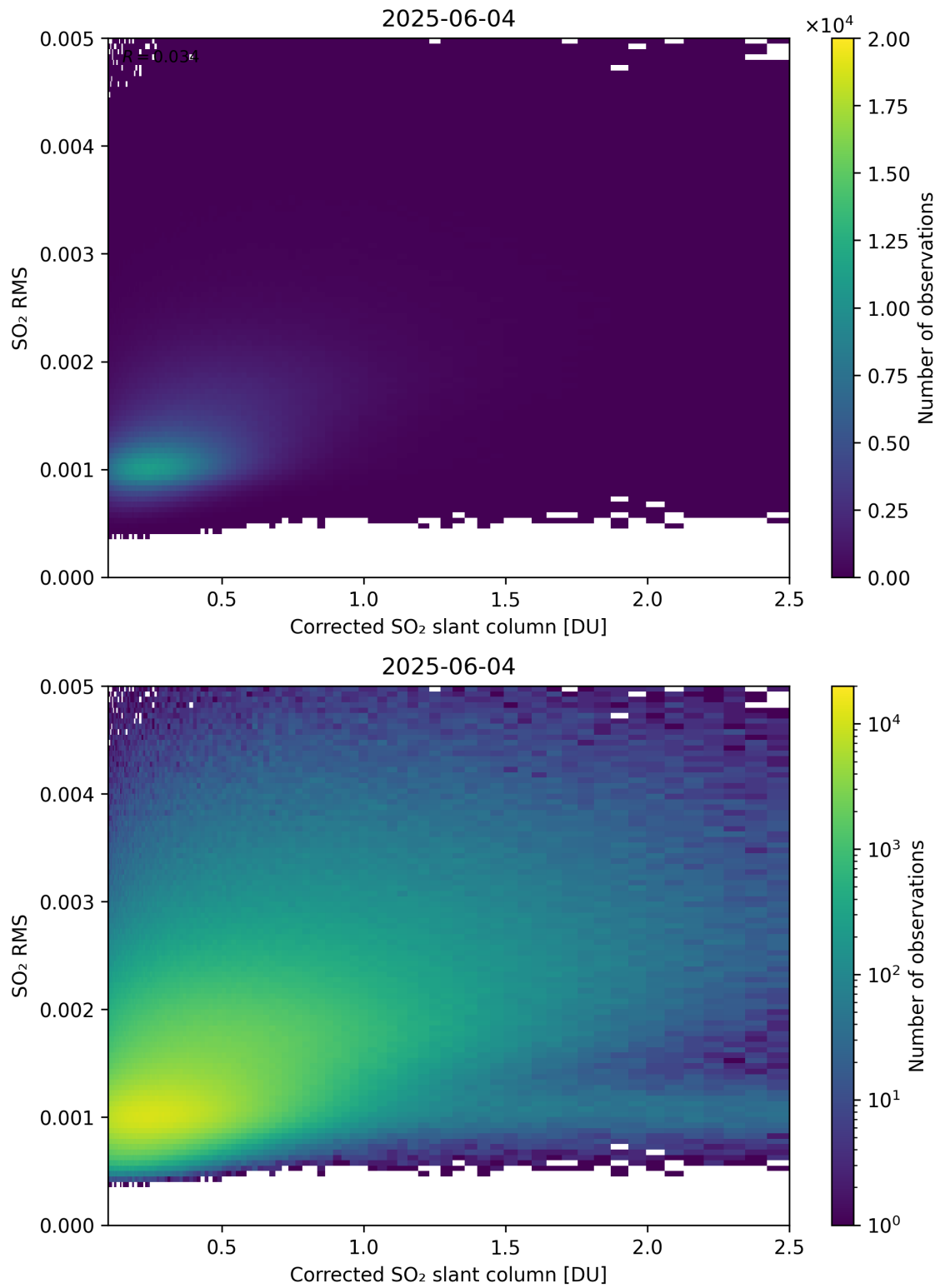
Figure 231: Scatter density plot of “Corrected SO 2 slant column” against “SO 2 RMS” for 2025-06-03 to 2025-06-05.
