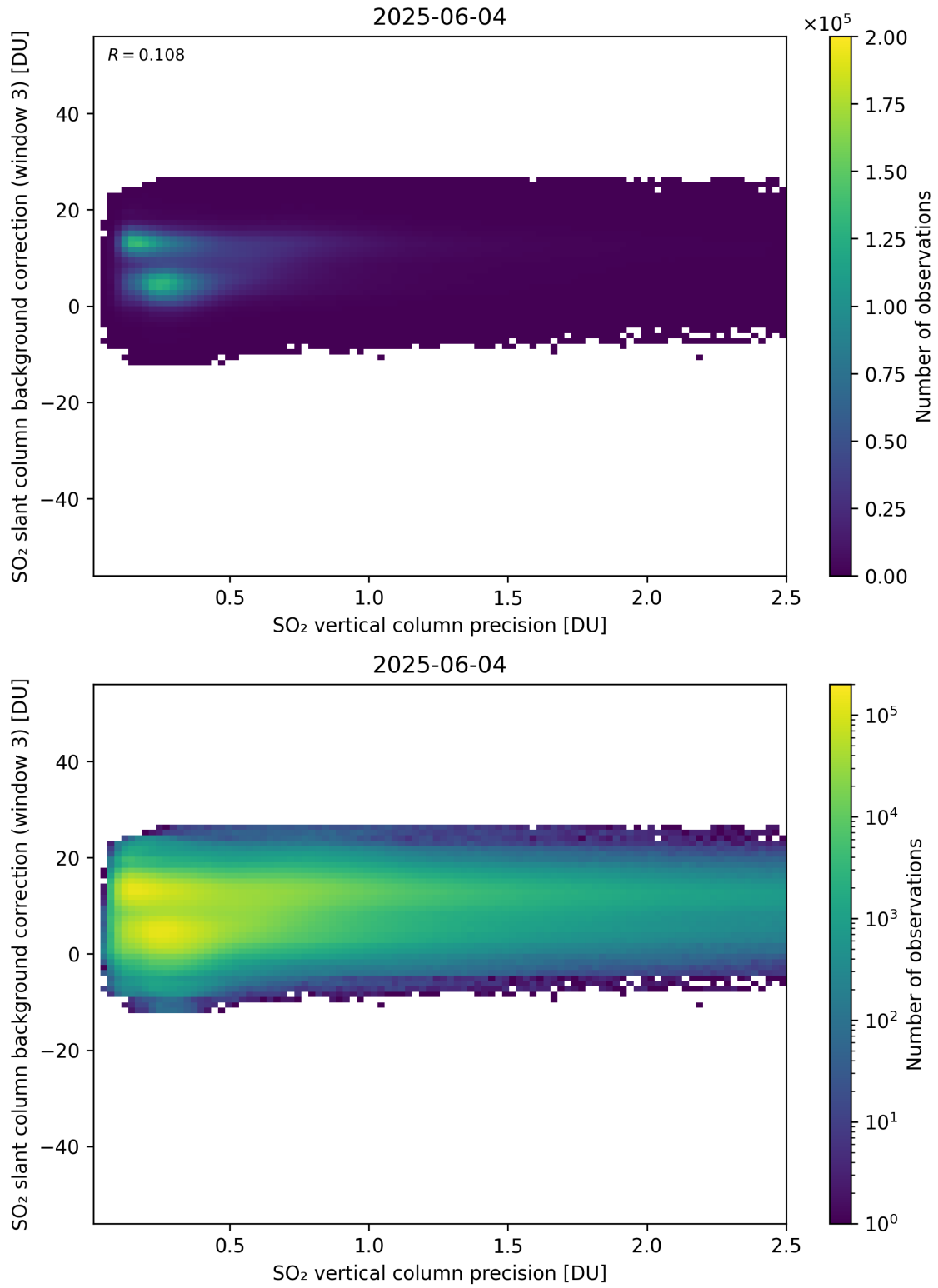
Figure 331: Scatter density plot of “SO 2 vertical column precision” against “SO 2 slant column background correction (window 3)” for 2025-06-03 to 2025-06-05.
