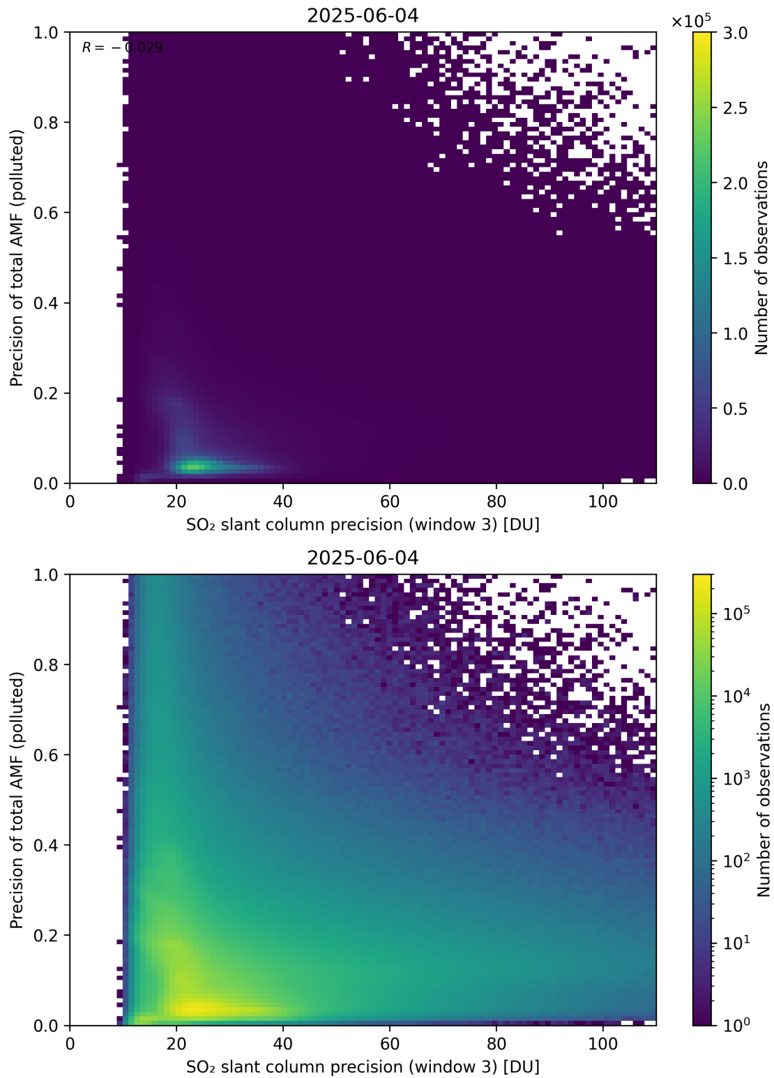
Figure 314: Scatter density plot of “SO 2 slant column precision (window 3)” against “Precision of total AMF (polluted)” for 2025-06-03 to 2025-06-05.
