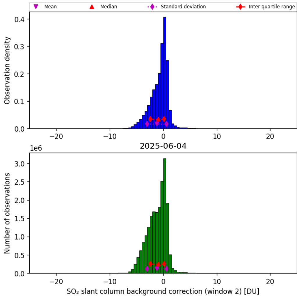
Figure 70: Histogram of “SO 2 slant column background correction (window 2)” for 2025-06-03 to 2025-06-05
