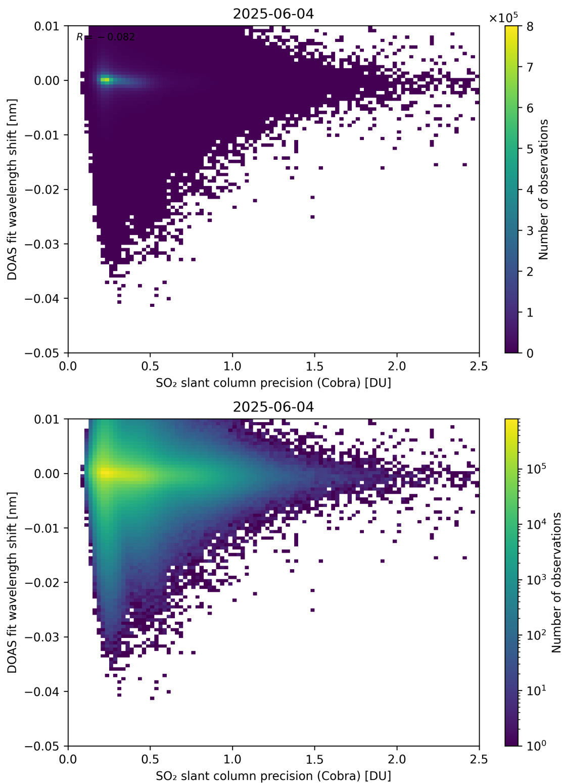
Figure 202: Scatter density plot of “SO 2 slant column precision (Cobra)” against “DOAS fit wavelength shift” for 2025-06-03 to 2025-06-05.
