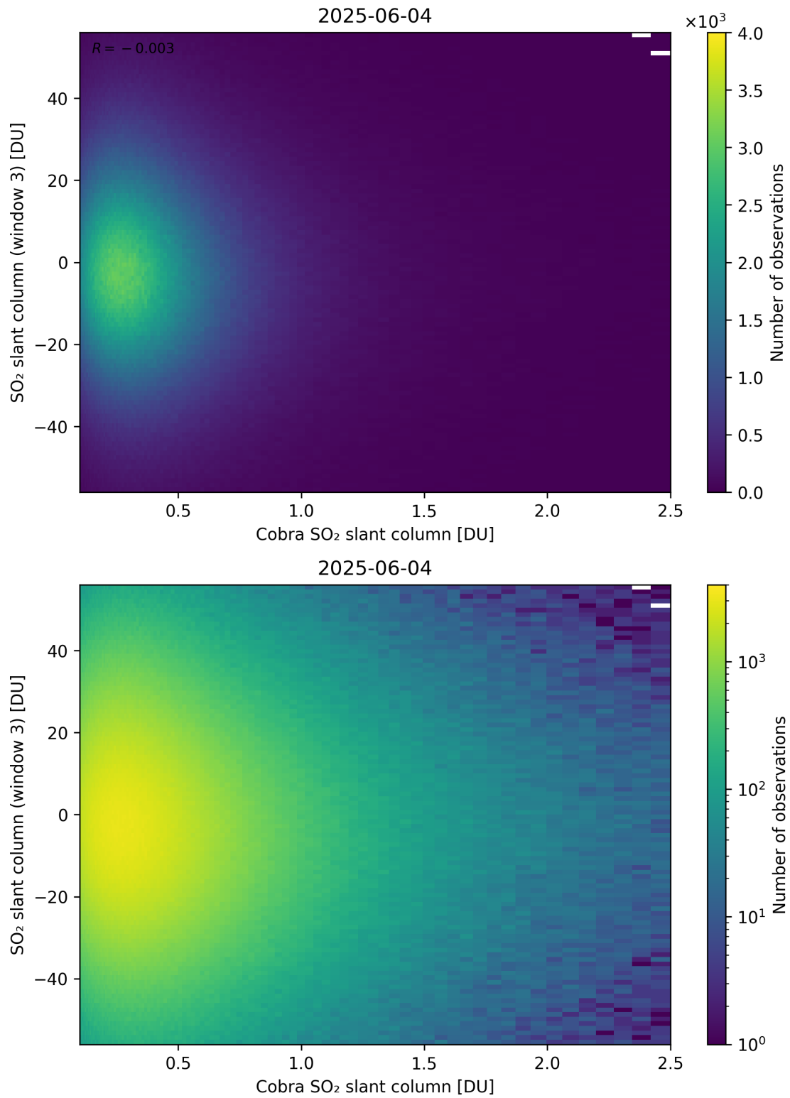
Figure 222: Scatter density plot of “Cobra SO 2 slant column” against “SO 2 slant column (window 3)” for 2025-06-03 to 2025-06-05.
