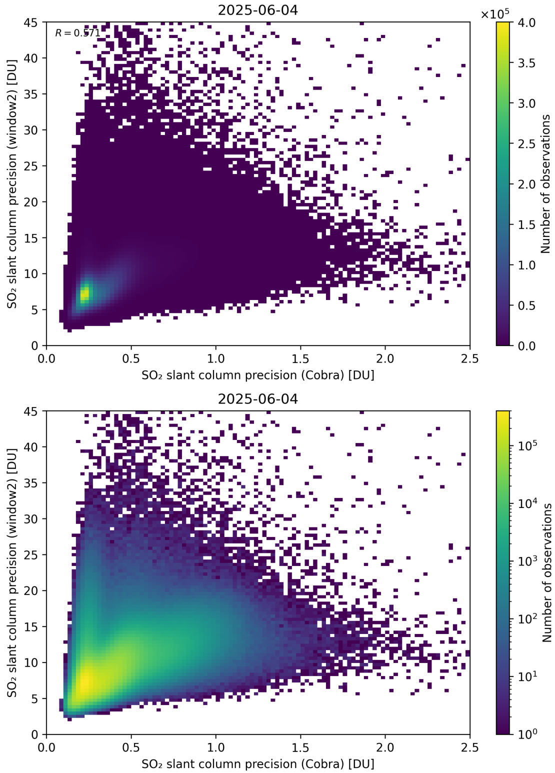
Figure 210: Scatter density plot of “SO 2 slant column precision (Cobra)” against “SO 2 slant column precision (window2)” for 2025-06-03 to 2025-06-05.
