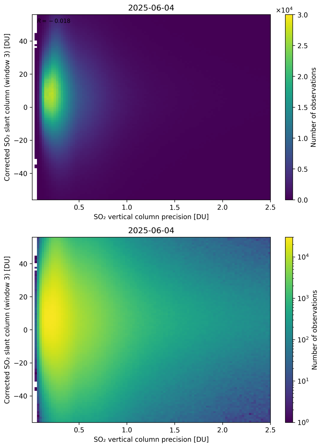
Figure 340: Scatter density plot of “SO 2 vertical column precision” against “Corrected SO 2 slant column (window 3)” for 2025-06-03 to 2025-06-05.
