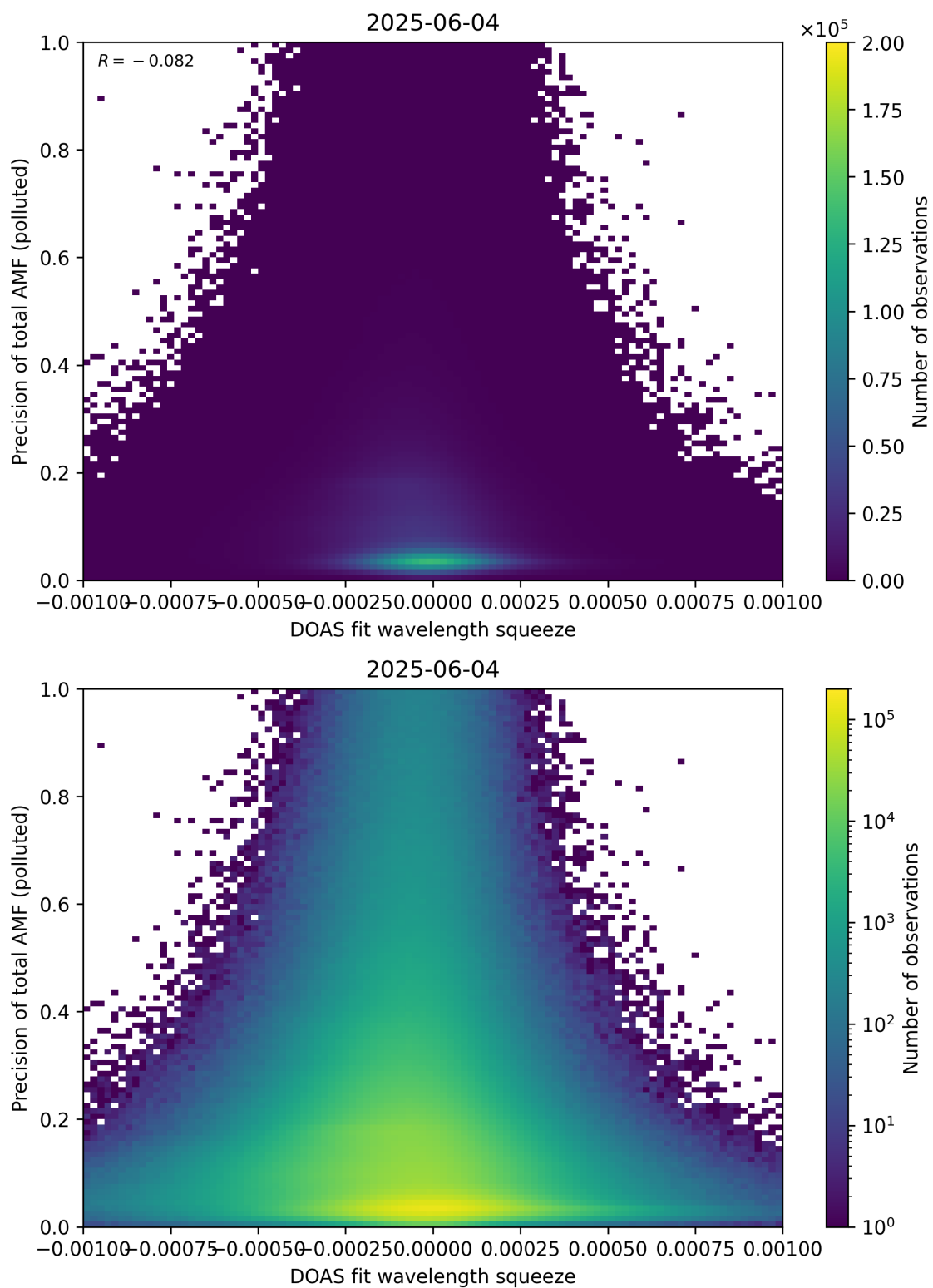
Figure 146: Scatter density plot of “DOAS fit wavelength squeeze” against “Precision of total AMF (polluted)” for 2025-06-03 to 2025-06-05.
