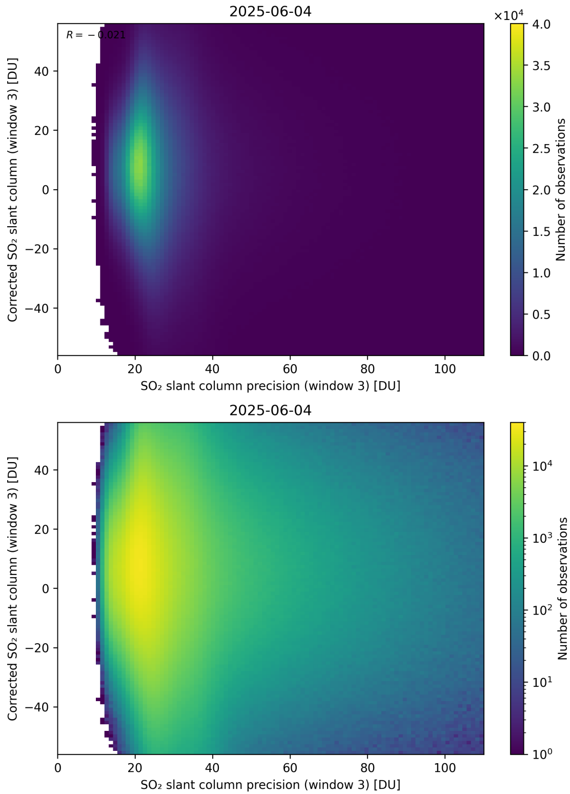
Figure 312: Scatter density plot of “SO 2 slant column precision (window 3)” against “Corrected SO 2 slant column (window 3)” for 2025-06-03 to 2025-06-05.
