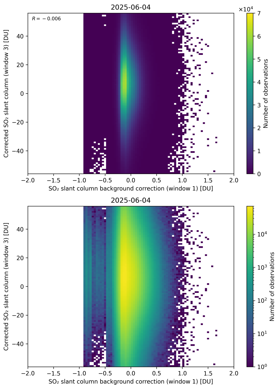
Figure 116: Scatter density plot of “SO 2 slant column background correction (window 1)” against “Corrected SO 2 slant column (window 3)” for 2025-06-03 to 2025-06-05.
