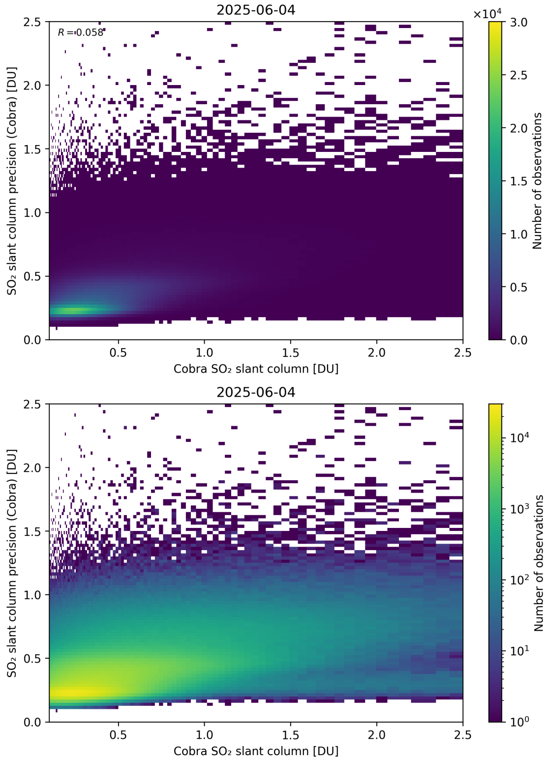
Figure 216: Scatter density plot of “Cobra SO 2 slant column” against “SO 2 slant column precision (Cobra)” for 2025-06-03 to 2025-06-05.
