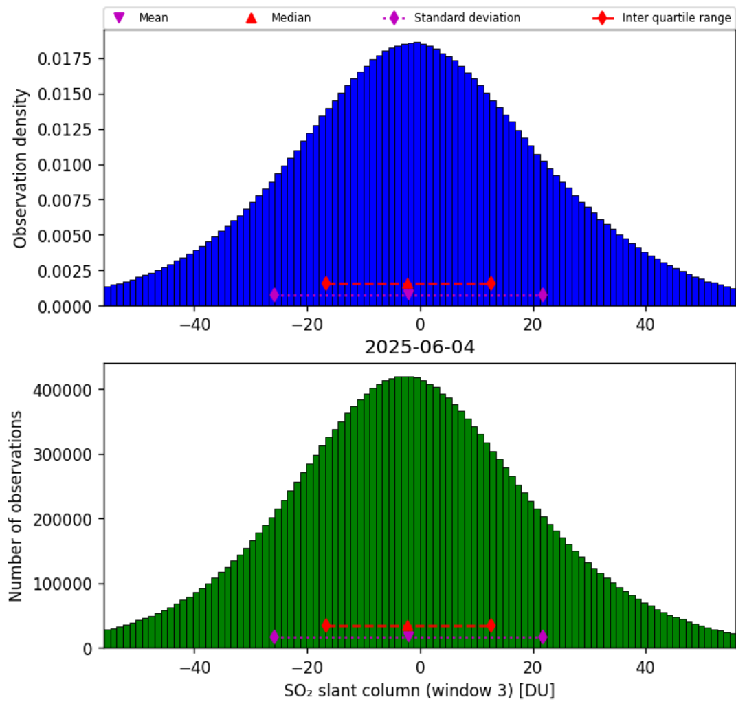
Figure 71: Histogram of “SO 2 slant column (window 3)” for 2025-06-03 to 2025-06-05
