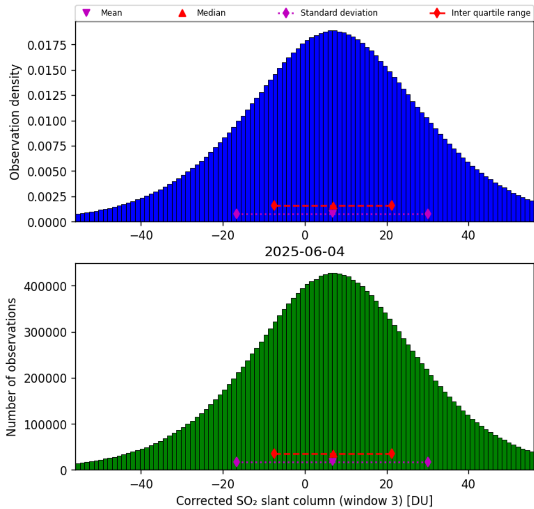
Figure 73: Histogram of “Corrected SO 2 slant column (window 3)” for 2025-06-03 to 2025-06-05
