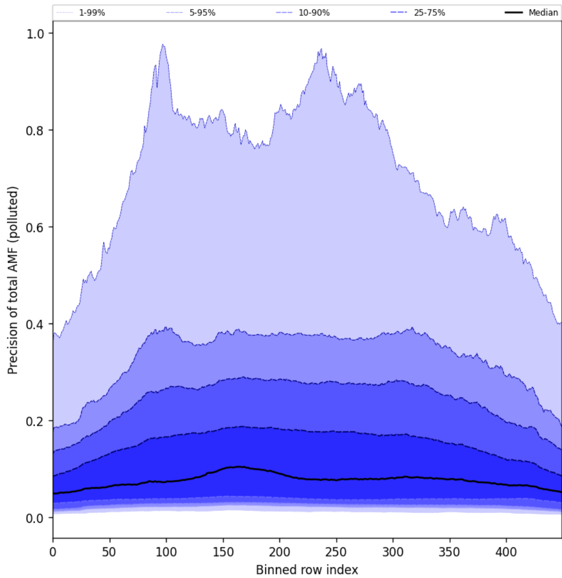
Figure 106: Along track statistics of “Precision of total AMF (polluted)” for 2025-06-03 to 2025-06-05
