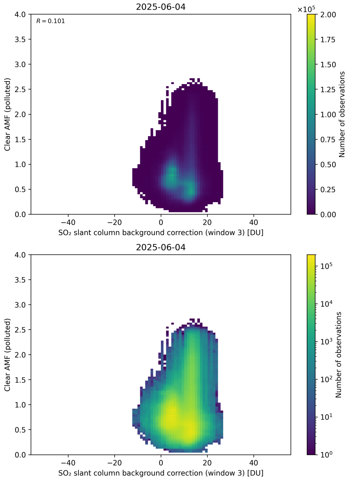
Figure 135: Scatter density plot of “SO 2 slant column background correction (window 3)” against “Clear AMF (polluted)” for 2025-06-03 to 2025-06-05.
