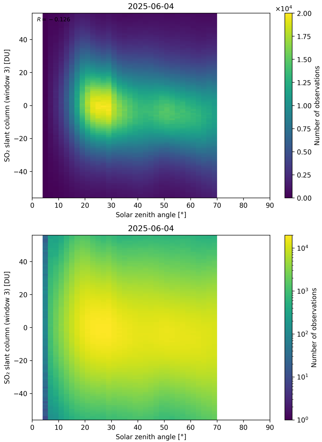
Figure 187: Scatter density plot of “Solar zenith angle” against “SO 2 slant column (window 3)” for 2025-06-03 to 2025-06-05.
