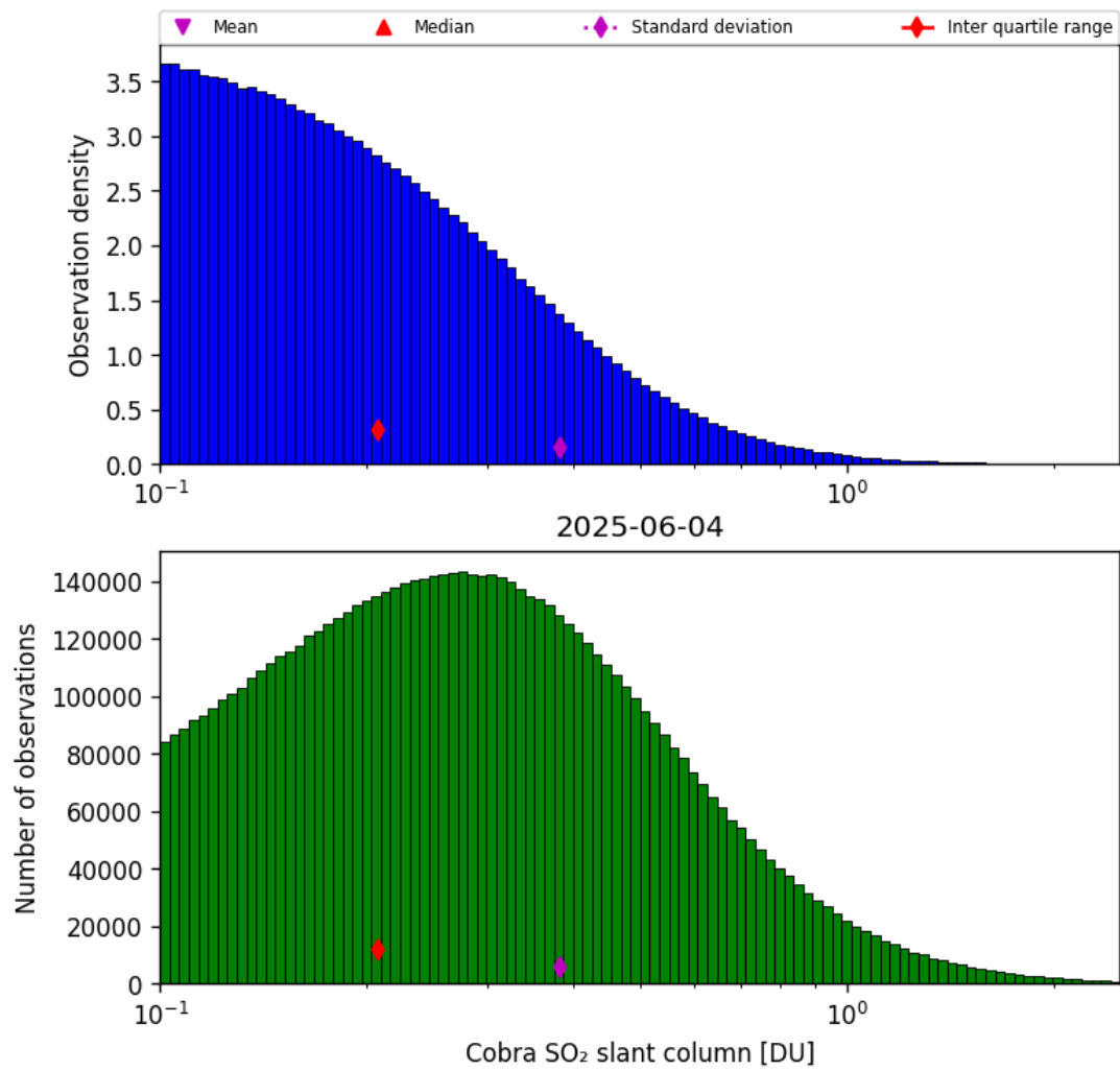
Figure 61: Histogram of “Cobra SO 2 slant column” for 2025-06-03 to 2025-06-05
