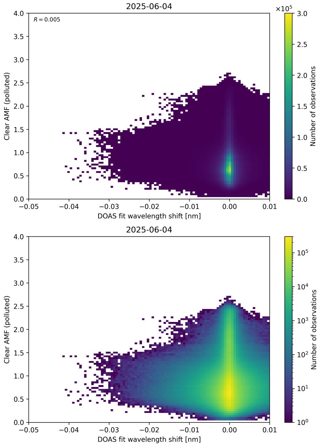
Figure 140: Scatter density plot of “DOAS fit wavelength shift” against “Clear AMF (polluted)” for 2025-06-03 to 2025-06-05.
