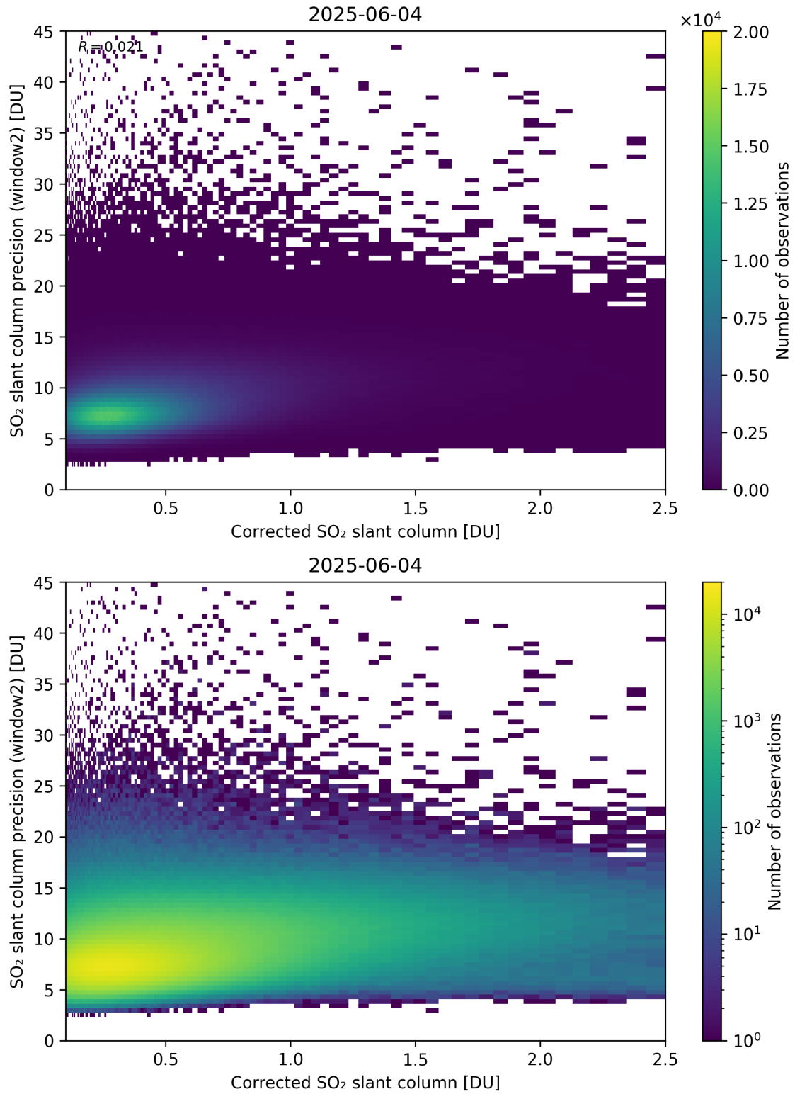
Figure 239: Scatter density plot of “Corrected SO 2 slant column” against “SO 2 slant column precision (window2)” for 2025-06-03 to 2025-06-05.
