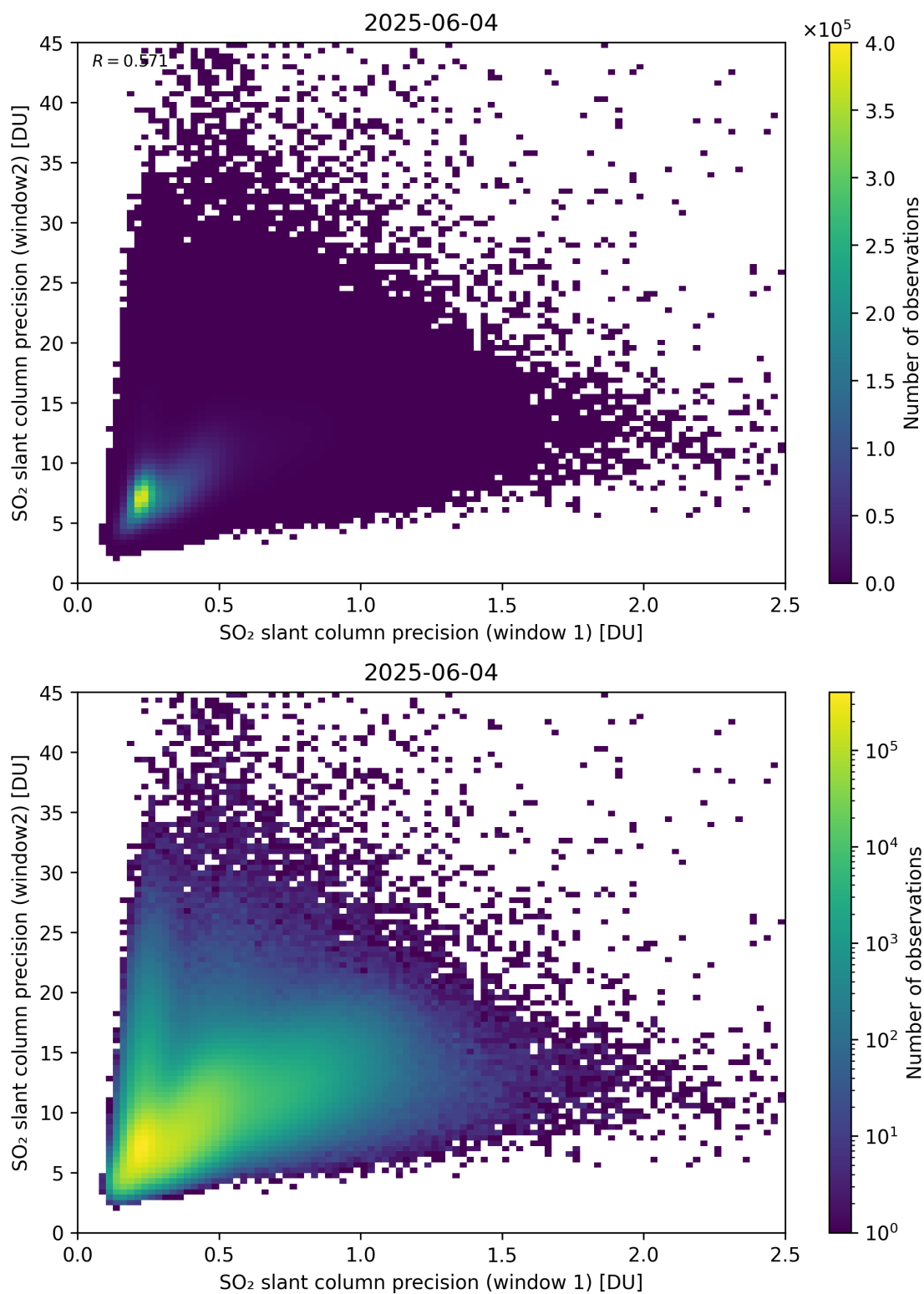
Figure 277: Scatter density plot of “SO 2 slant column precision (window 1)” against “SO 2 slant column precision (window2)” for 2025-06-03 to 2025-06-05.
