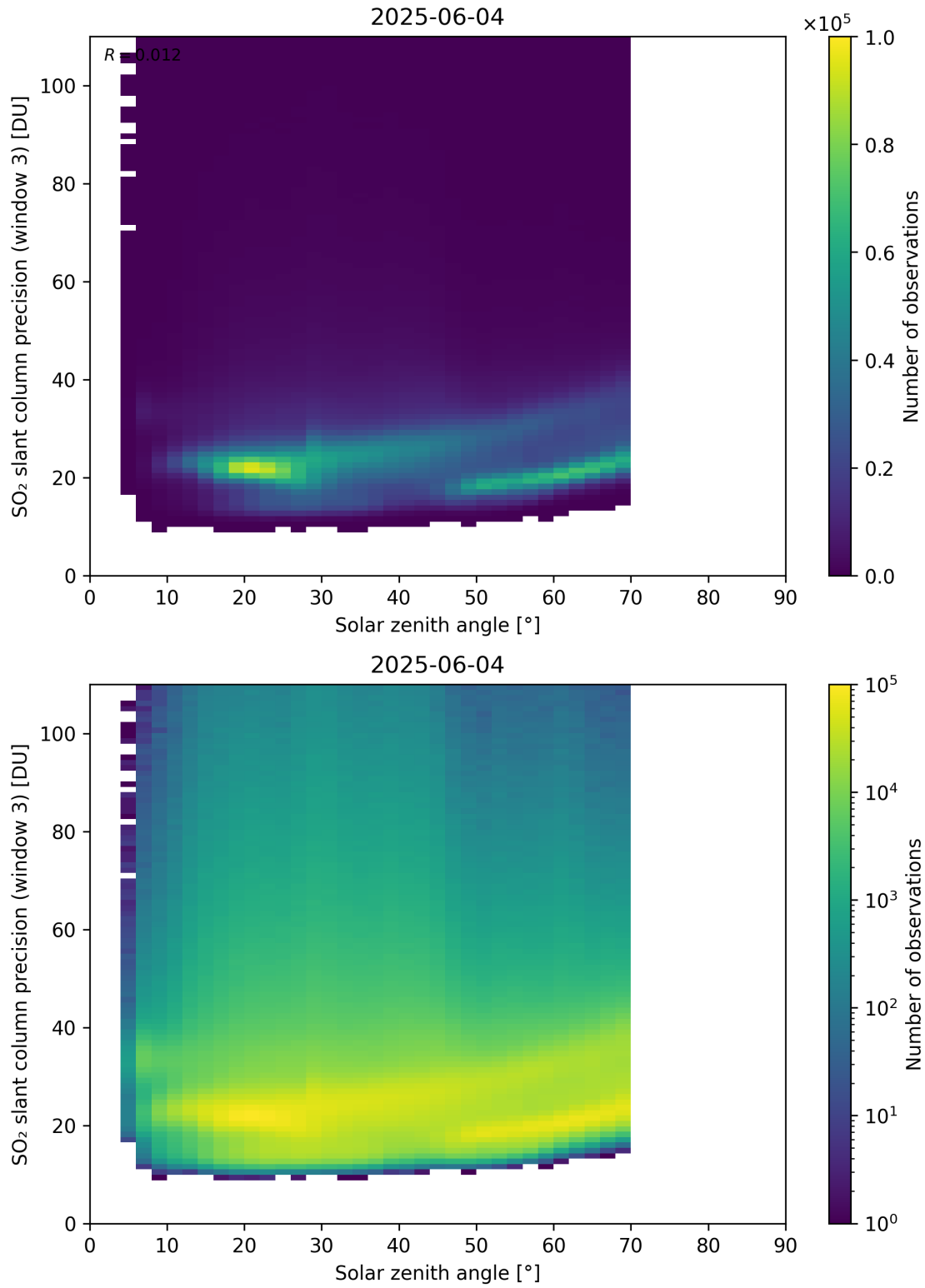
Figure 188: Scatter density plot of “Solar zenith angle” against “SO 2 slant column precision (window 3)” for 2025-06-03 to 2025-06-05.
