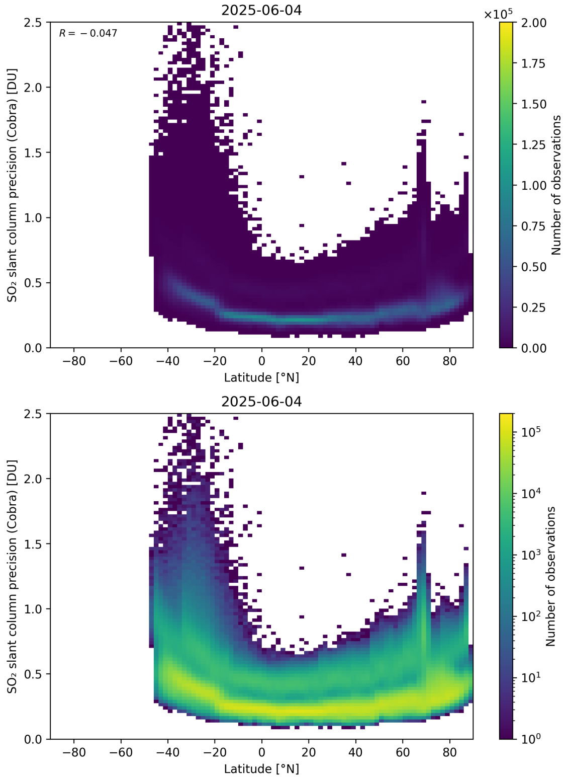
Figure 158: Scatter density plot of “Latitude” against “SO 2 slant column precision (Cobra)” for 2025-06-03 to 2025-06-05.
