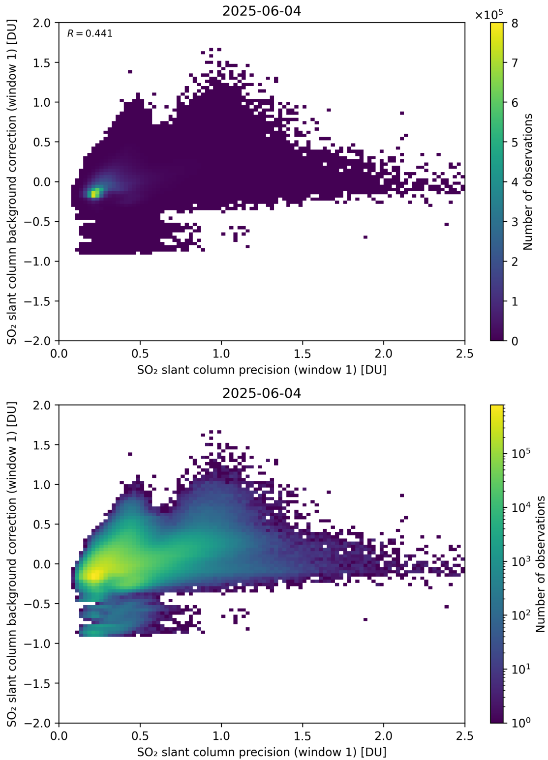
Figure 268: Scatter density plot of “SO 2 slant column precision (window 1)” against “SO 2 slant column background correction (window 1)” for 2025-06-03 to 2025-06-05.
