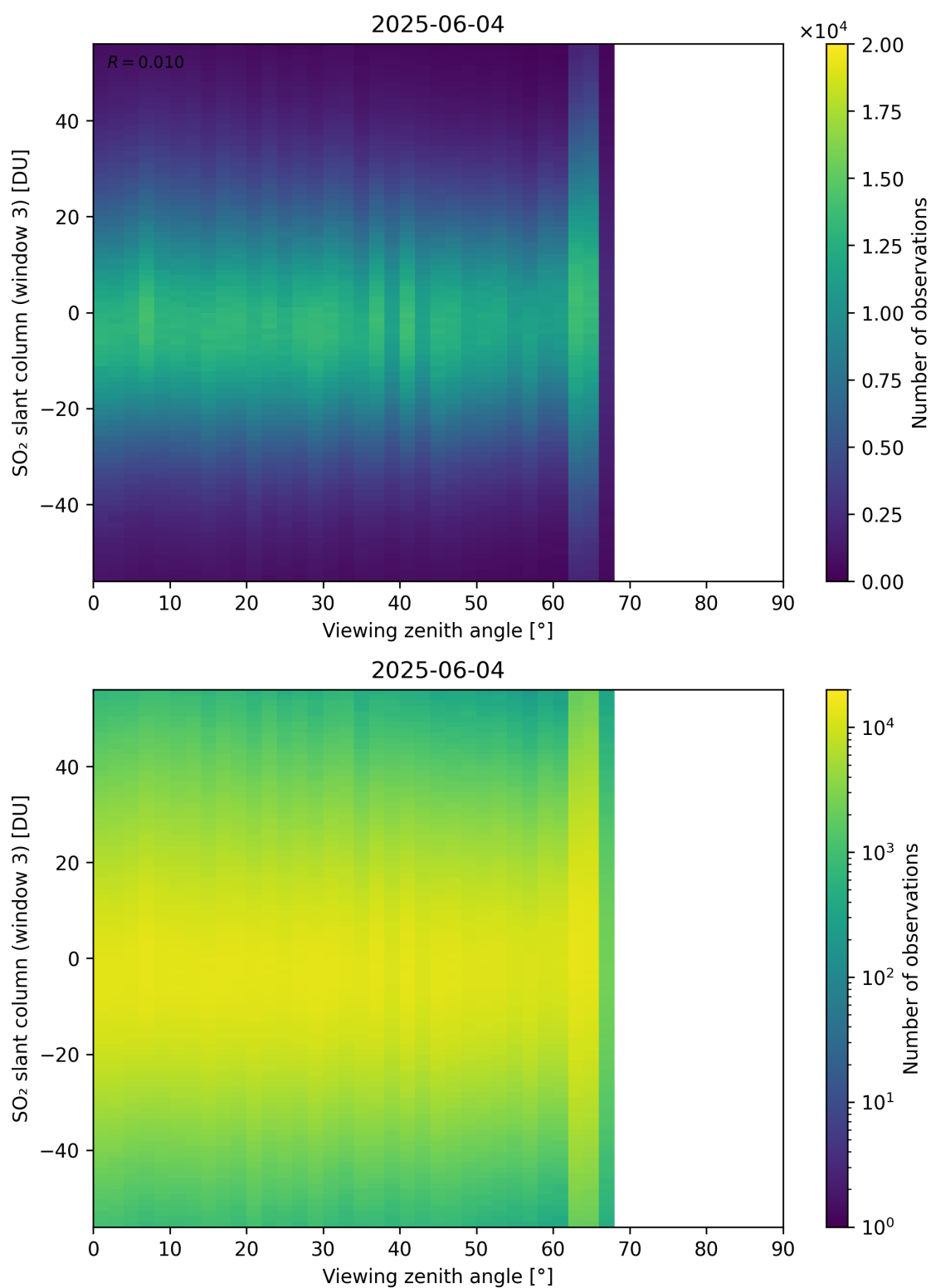
Figure 379: Scatter density plot of “Viewing zenith angle” against “SO 2 slant column (window 3)” for 2025-06-03 to 2025-06-05.
