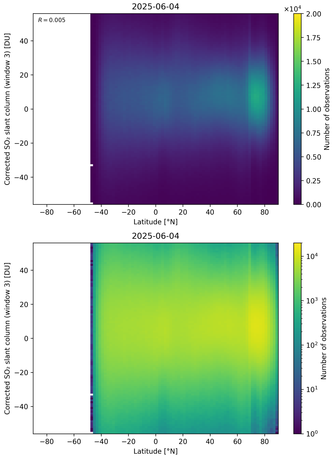
Figure 161: Scatter density plot of “Latitude” against “Corrected SO 2 slant column (window 3)” for 2025-06-03 to 2025-06-05.
