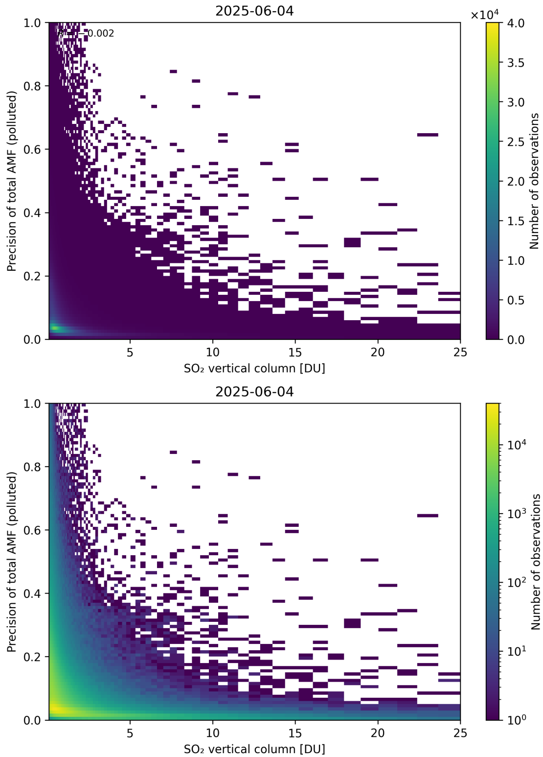
Figure 360: Scatter density plot of “SO 2 vertical column” against “Precision of total AMF (polluted)” for 2025-06-03 to 2025-06-05.
