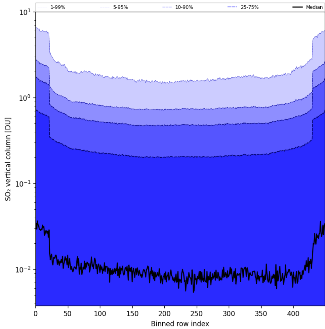
Figure 84: Along track statistics of “SO 2 vertical column” for 2025-06-03 to 2025-06-05
