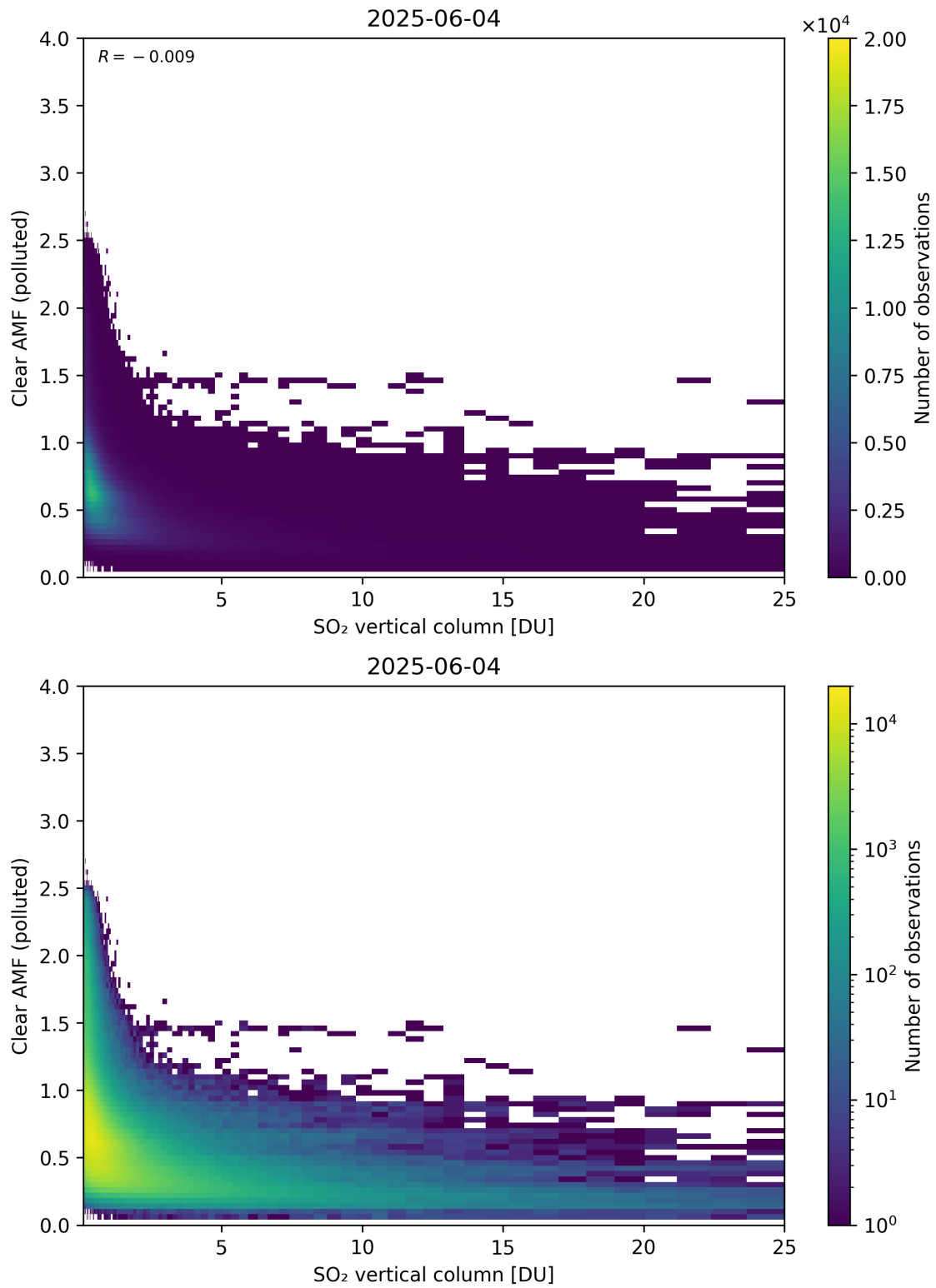
Figure 348: Scatter density plot of “SO 2 vertical column” against “Clear AMF (polluted)” for 2025-06-03 to 2025-06-05.
