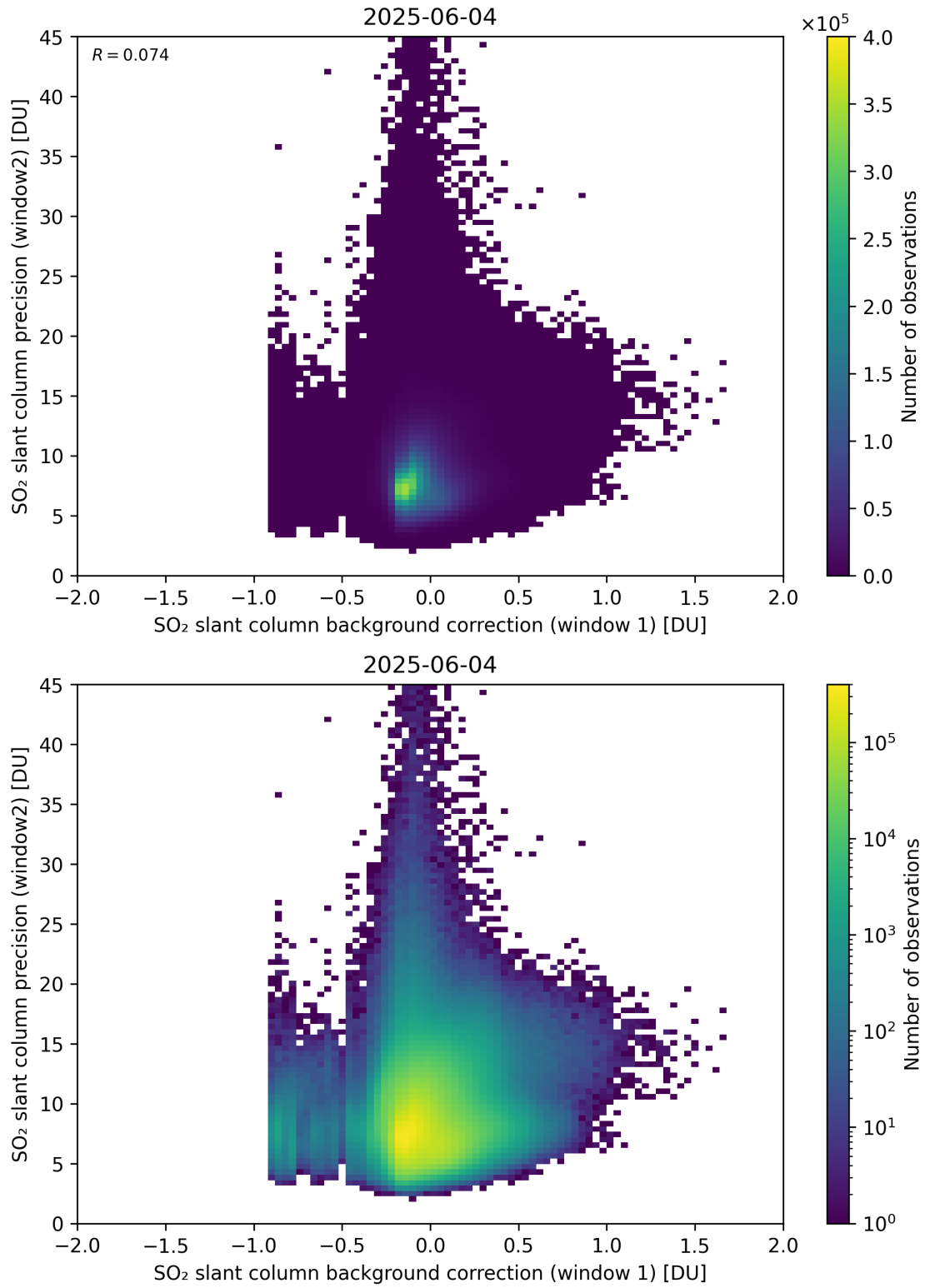
Figure 117: Scatter density plot of “SO 2 slant column background correction (window 1)” against “SO 2 slant column precision (window2)” for 2025-06-03 to 2025-06-05.
