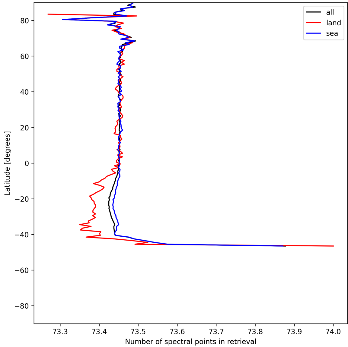
Figure 56: Zonal average of “Number of spectral points in retrieval” for 2025-06-03 to 2025-06-05.
