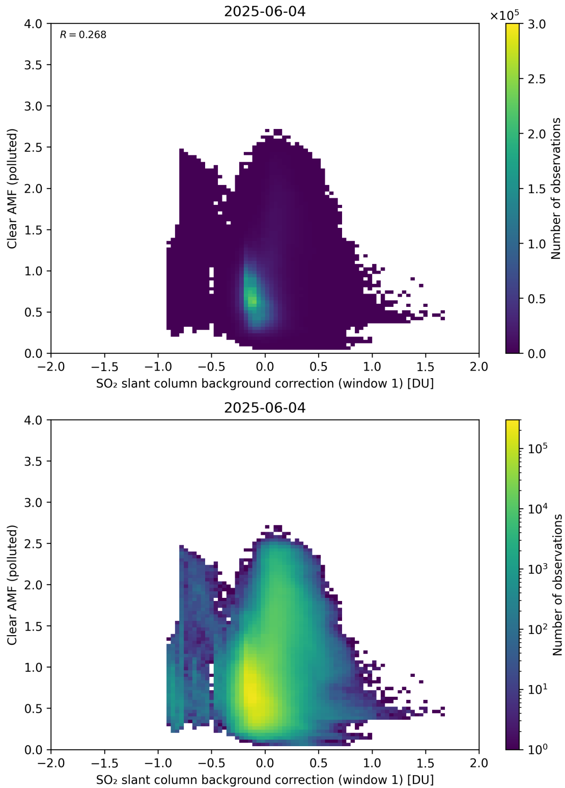
Figure 114: Scatter density plot of “SO 2 slant column background correction (window 1)” against “Clear AMF (polluted)” for 2025-06-03 to 2025-06-05.
