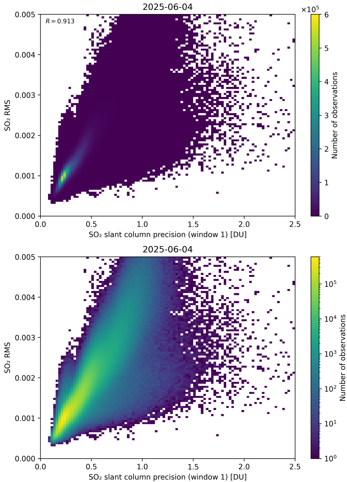
Figure 273: Scatter density plot of “SO 2 slant column precision (window 1)” against “SO 2 RMS” for 2025-06-03 to 2025-06-05.
