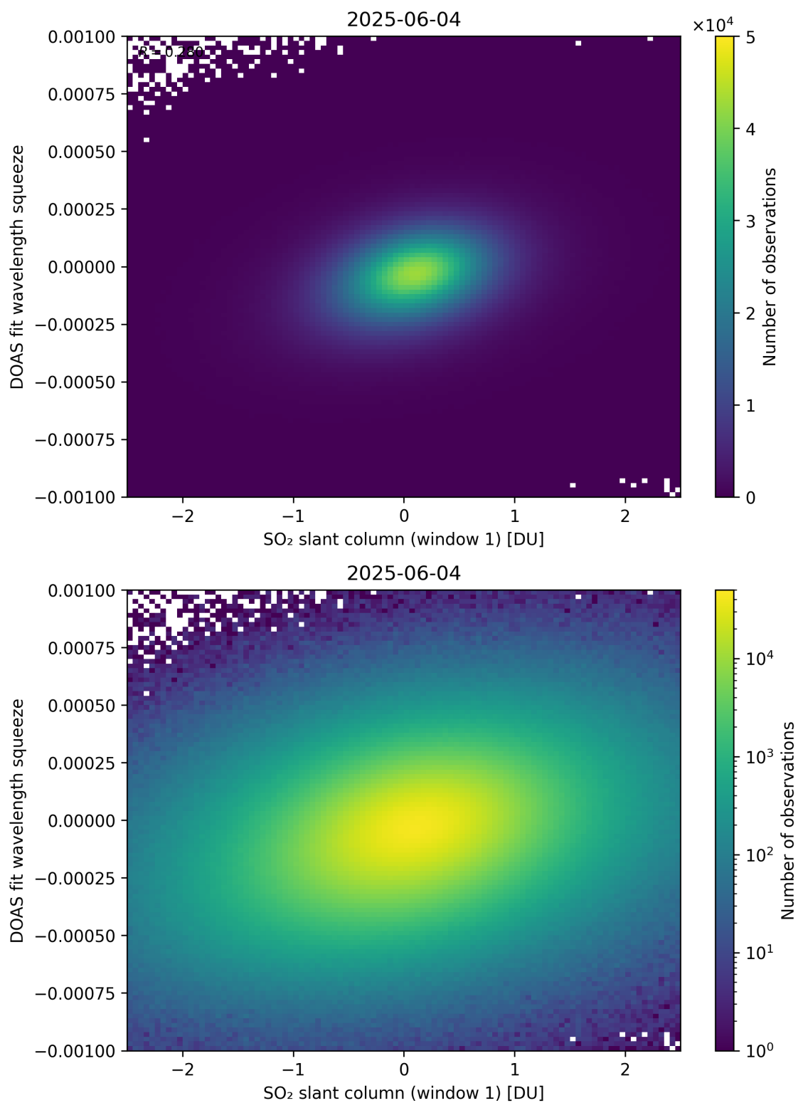
Figure 266: Scatter density plot of “SO 2 slant column (window 1)” against “DOAS fit wavelength squeeze” for 2025-06-03 to 2025-06-05.
