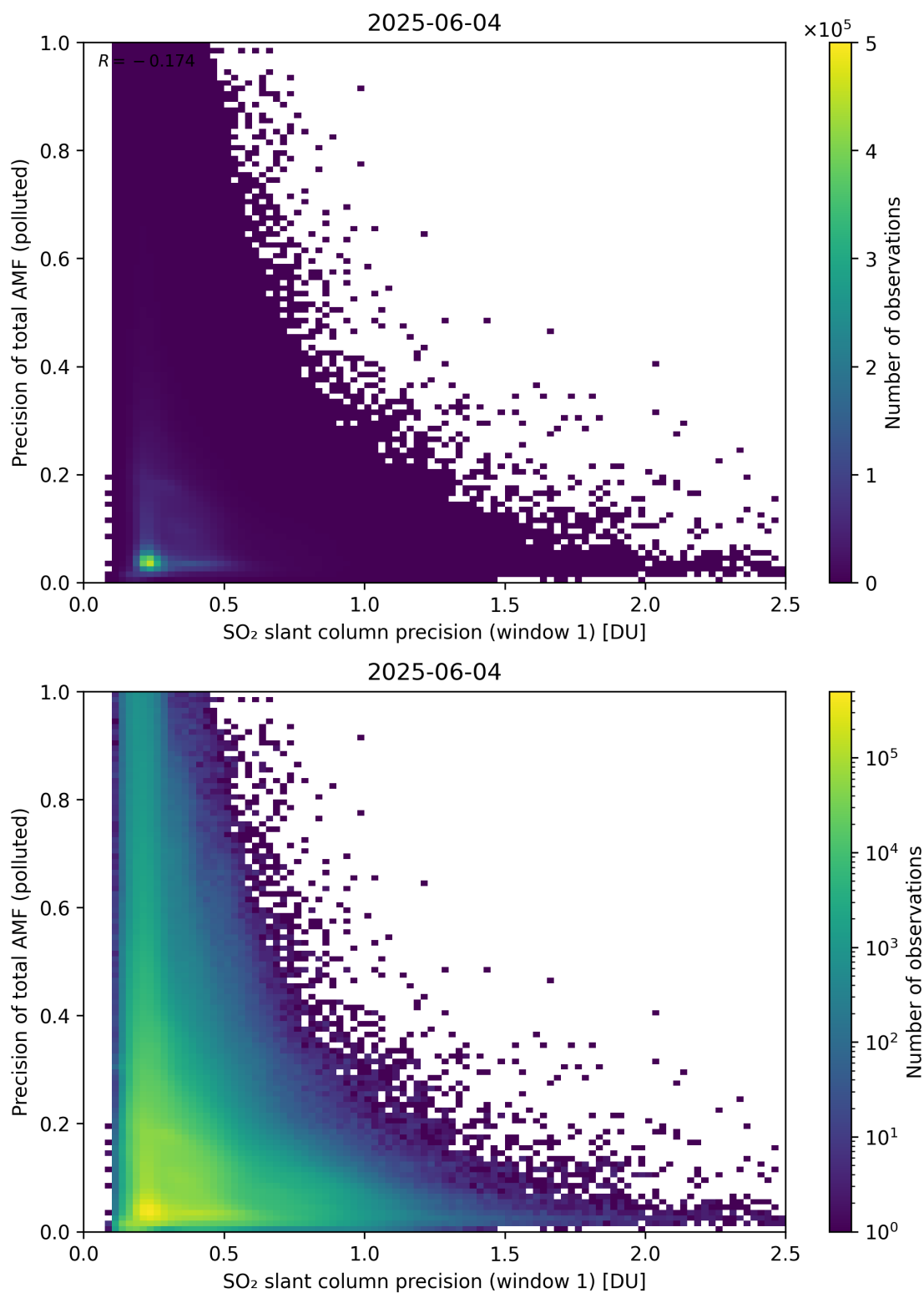
Figure 281: Scatter density plot of “SO 2 slant column precision (window 1)” against “Precision of total AMF (polluted)” for 2025-06-03 to 2025-06-05.
