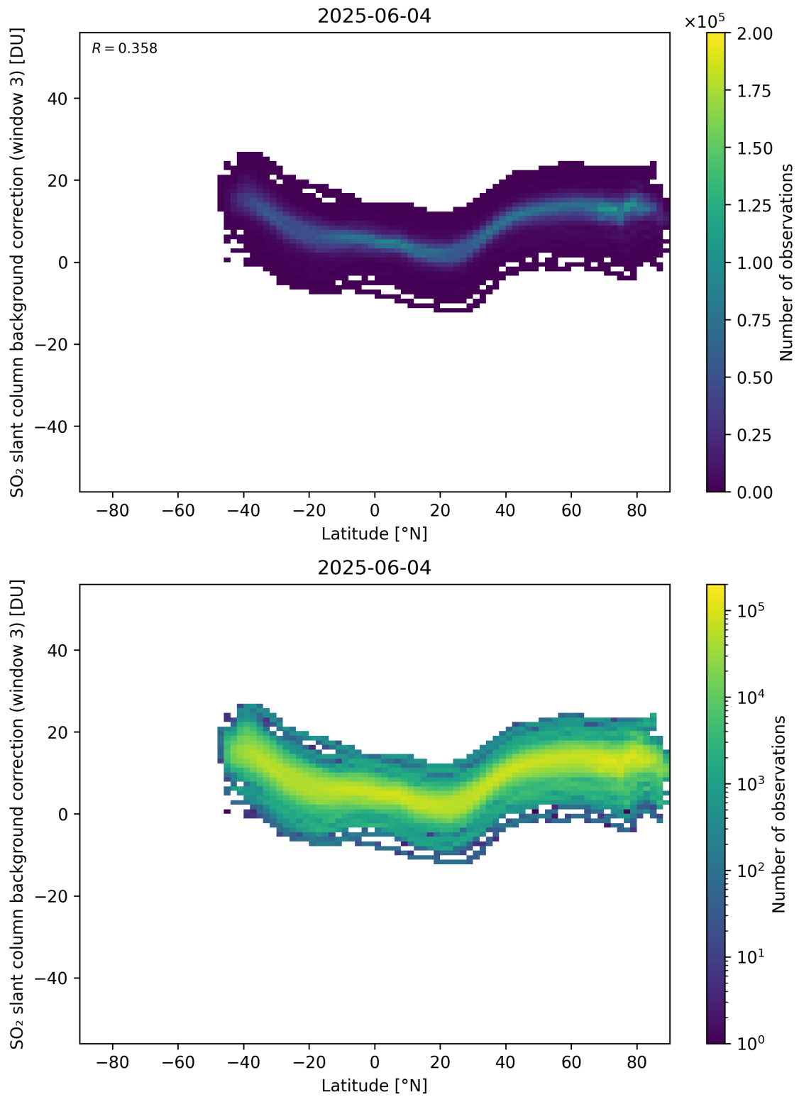
Figure 152: Scatter density plot of “Latitude” against “SO 2 slant column background correction (window 3)” for 2025-06-03 to 2025-06-05.
