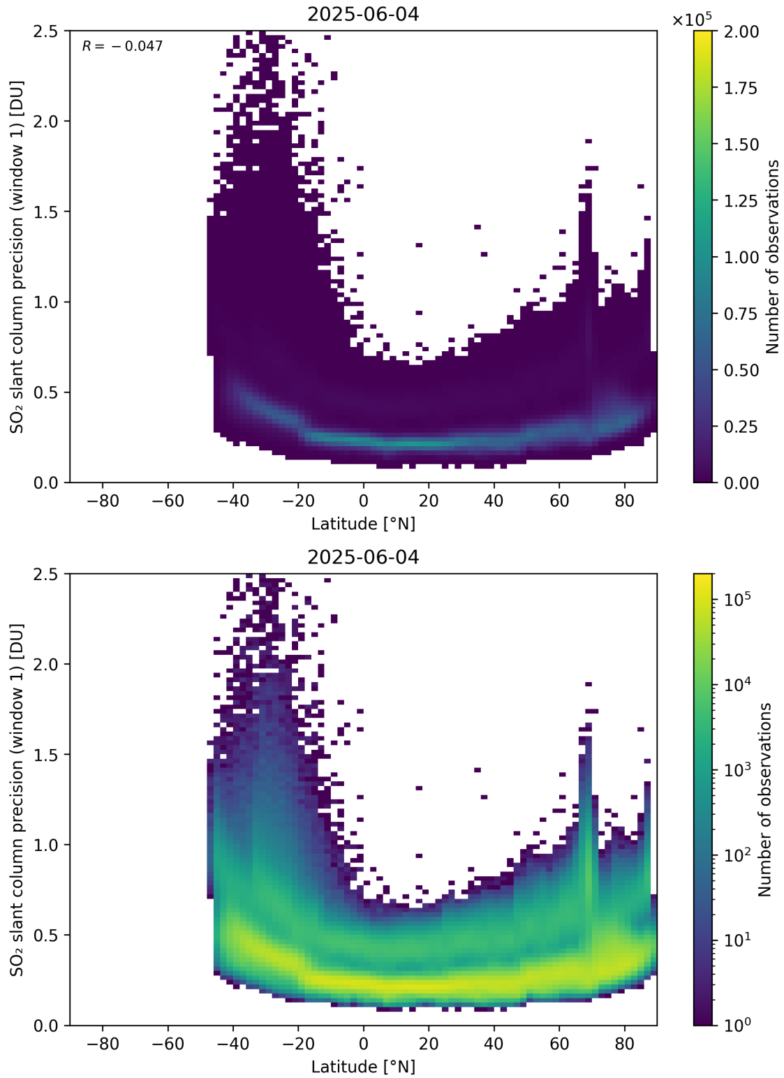
Figure 163: Scatter density plot of “Latitude” against “SO 2 slant column precision (window 1)” for 2025-06-03 to 2025-06-05.
