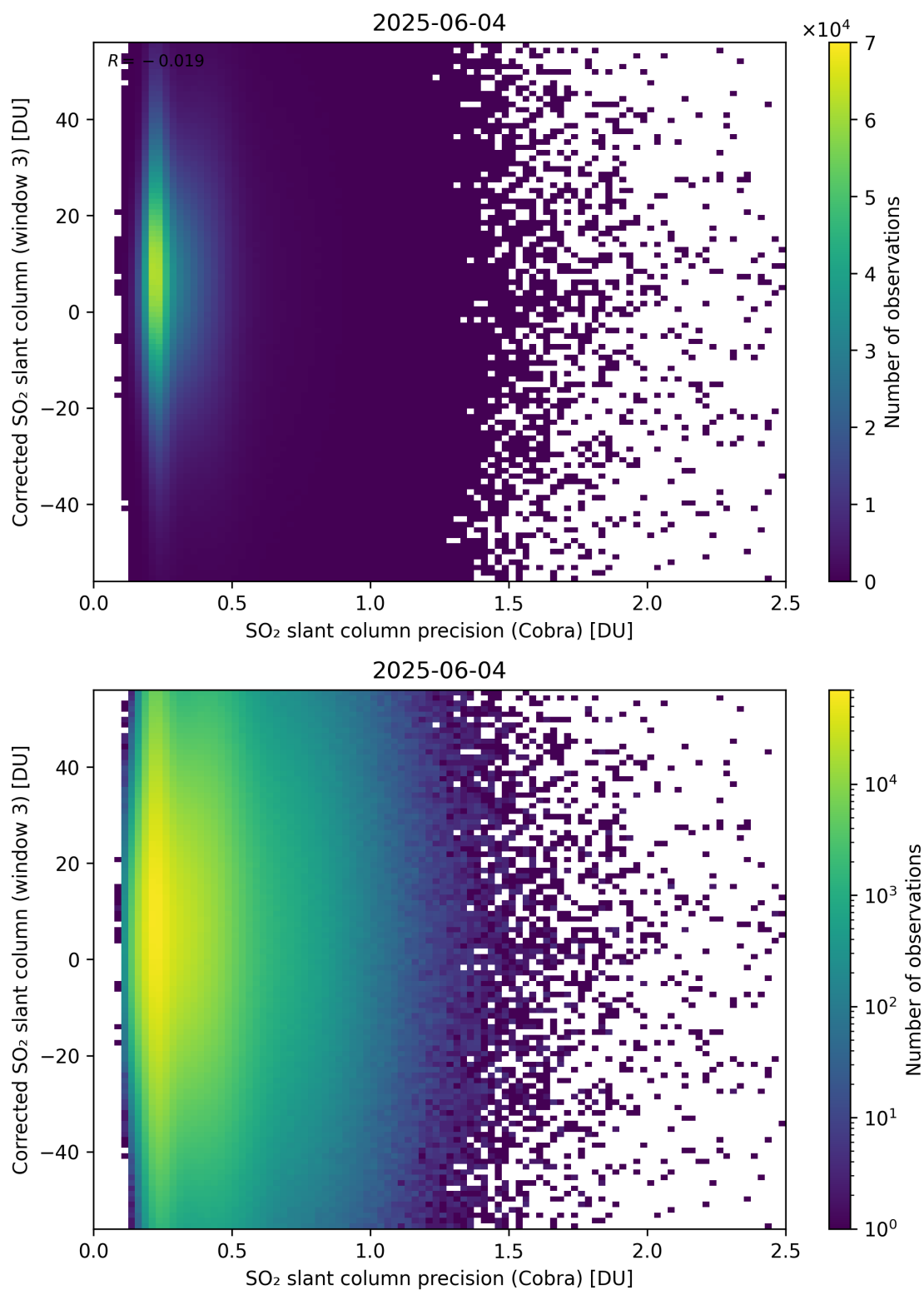
Figure 207: Scatter density plot of “SO 2 slant column precision (Cobra)” against “Corrected SO 2 slant column (window 3)” for 2025-06-03 to 2025-06-05.
