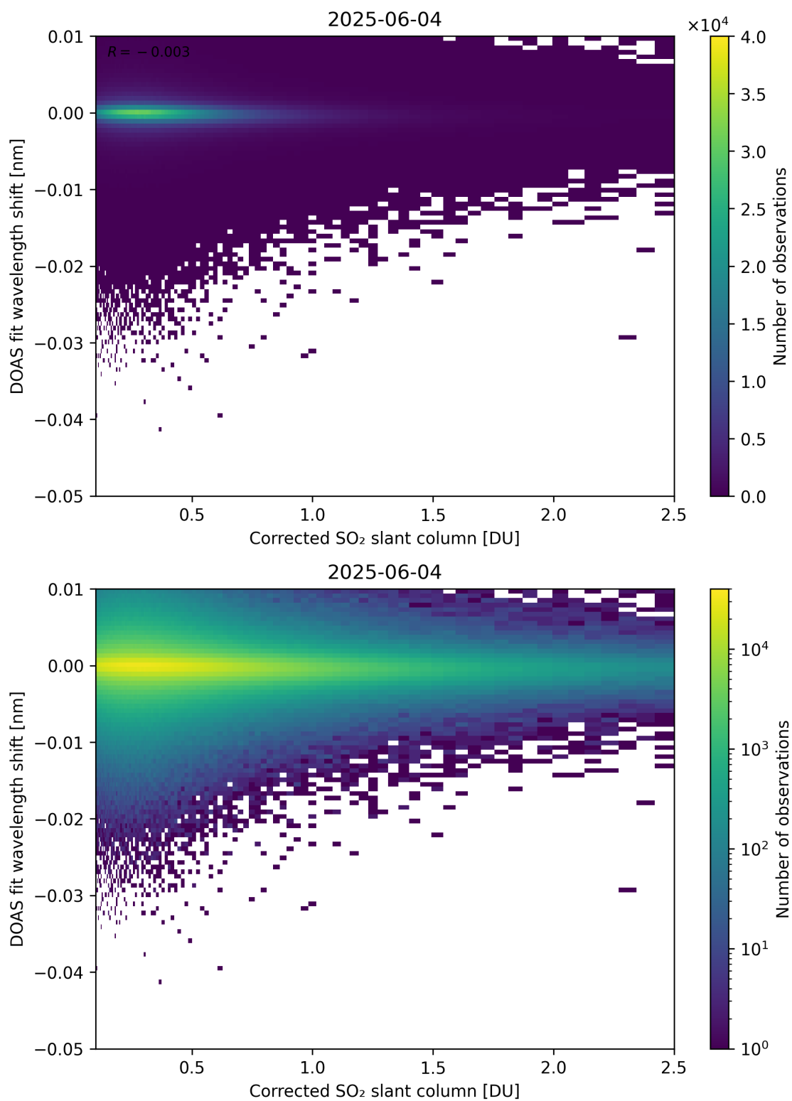
Figure 229: Scatter density plot of “Corrected SO 2 slant column” against “DOAS fit wavelength shift” for 2025-06-03 to 2025-06-05.
