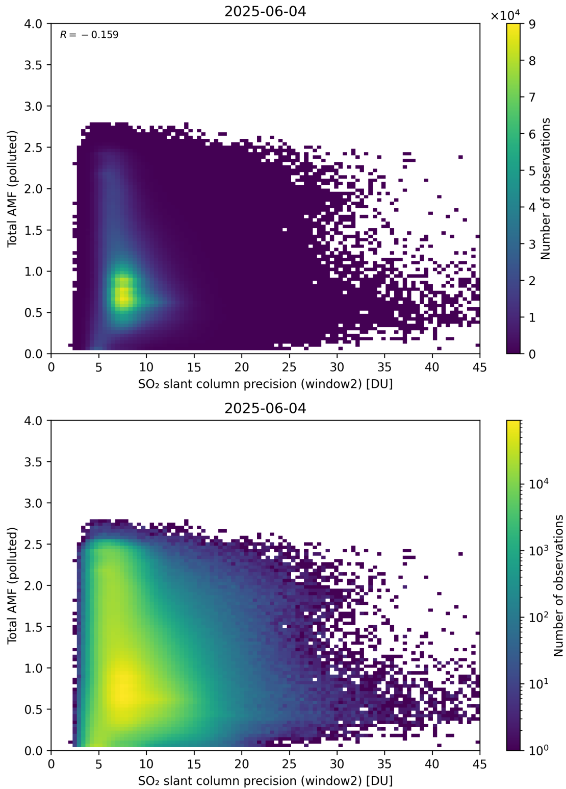
Figure 301: Scatter density plot of “SO 2 slant column precision (window2)” against “Total AMF (polluted)” for 2025-06-03 to 2025-06-05.
