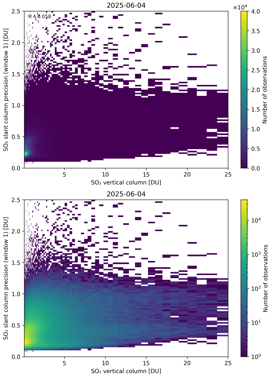
Figure 355: Scatter density plot of “SO 2 vertical column” against “SO 2 slant column precision (window 1)” for 2025-06-03 to 2025-06-05.
