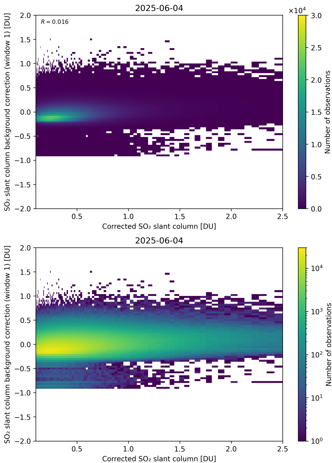
Figure 226: Scatter density plot of “Corrected SO 2 slant column” against “SO 2 slant column background correction (window 1)” for 2025-06-03 to 2025-06-05.
