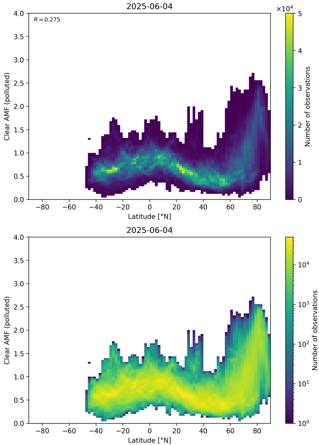
Figure 156: Scatter density plot of “Latitude” against “Clear AMF (polluted)” for 2025-06-03 to 2025-06-05.
