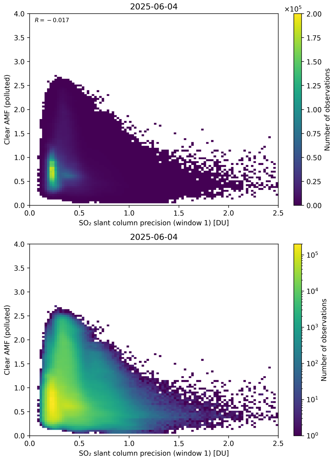
Figure 274: Scatter density plot of “SO 2 slant column precision (window 1)” against “Clear AMF (polluted)” for 2025-06-03 to 2025-06-05.
