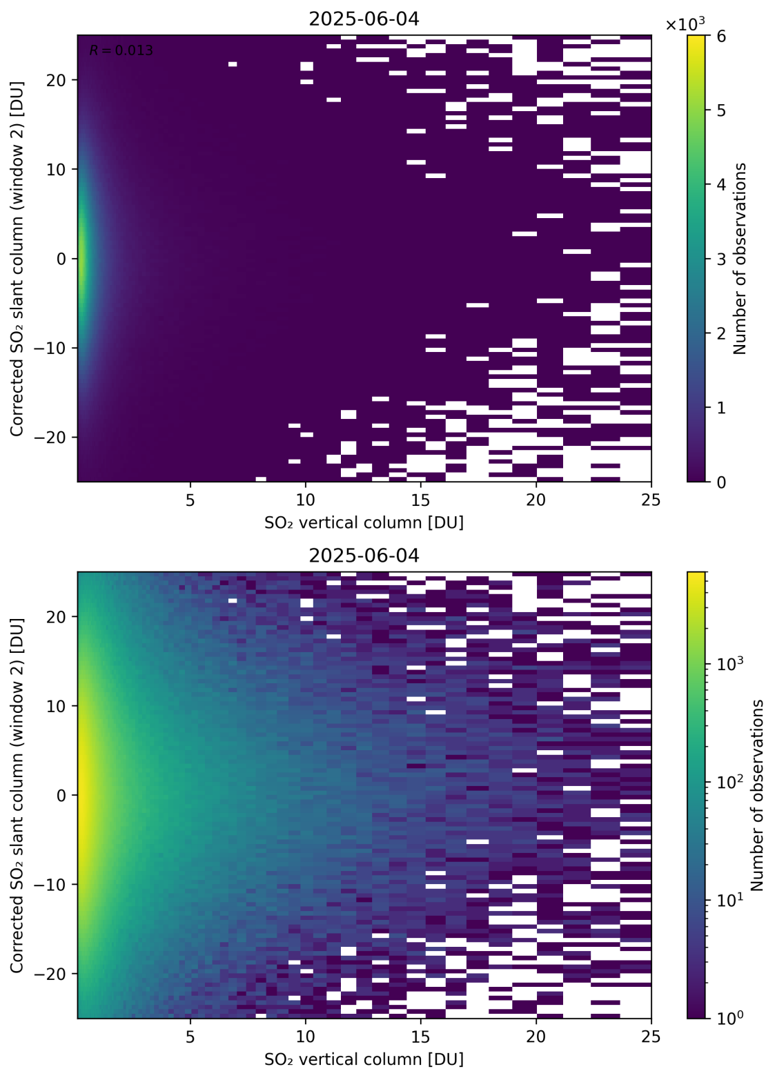
Figure 352: Scatter density plot of “SO 2 vertical column” against “Corrected SO 2 slant column (window 2)” for 2025-06-03 to 2025-06-05.
