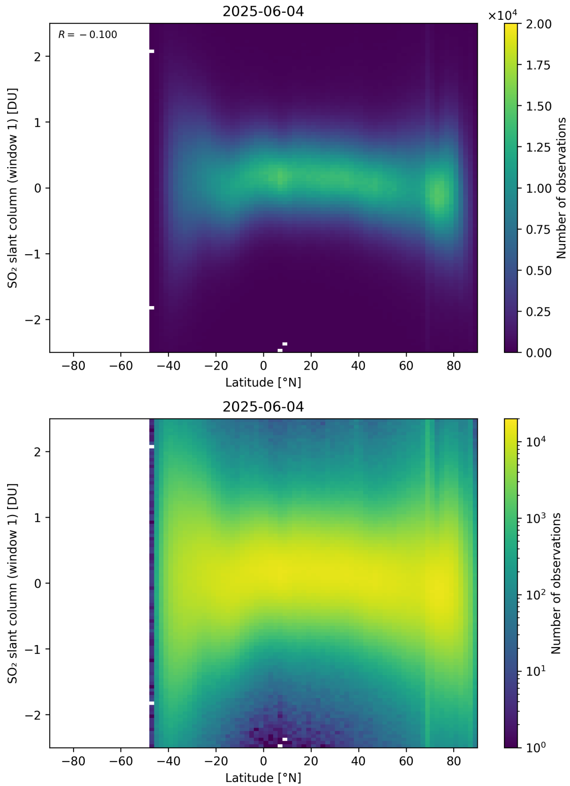
Figure 162: Scatter density plot of “Latitude” against “SO 2 slant column (window 1)” for 2025-06-03 to 2025-06-05.
