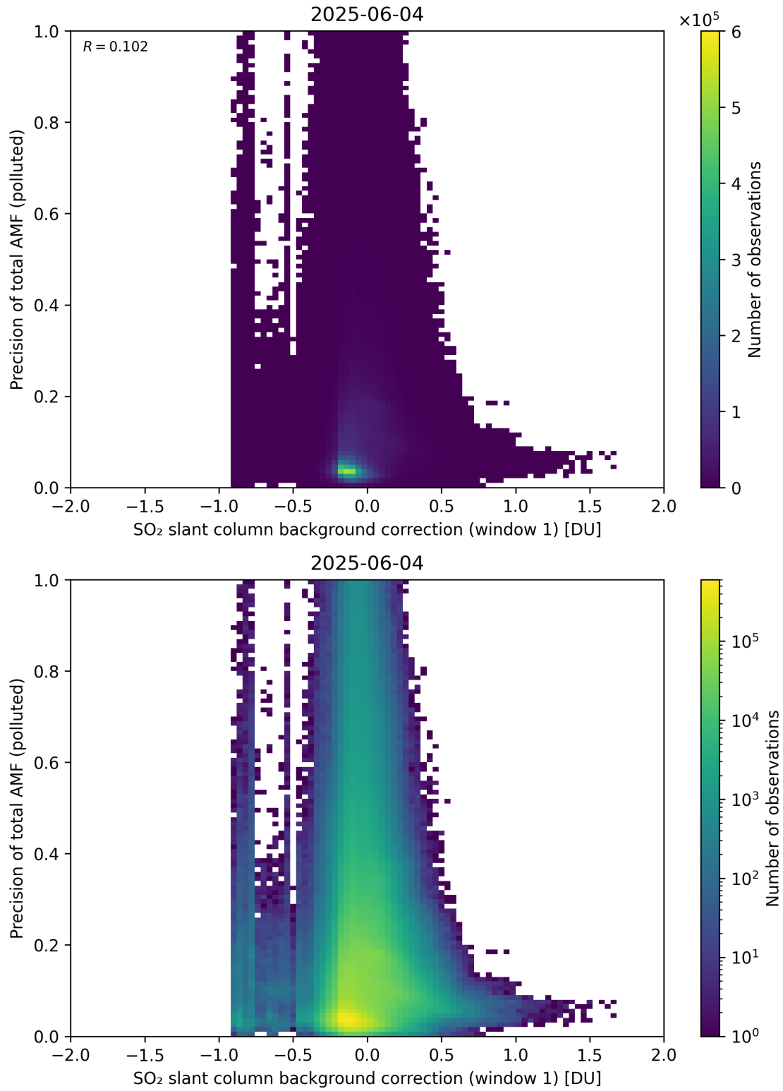
Figure 121: Scatter density plot of “SO 2 slant column background correction (window 1)” against “Precision of total AMF (polluted)” for 2025-06-03 to 2025-06-05.
