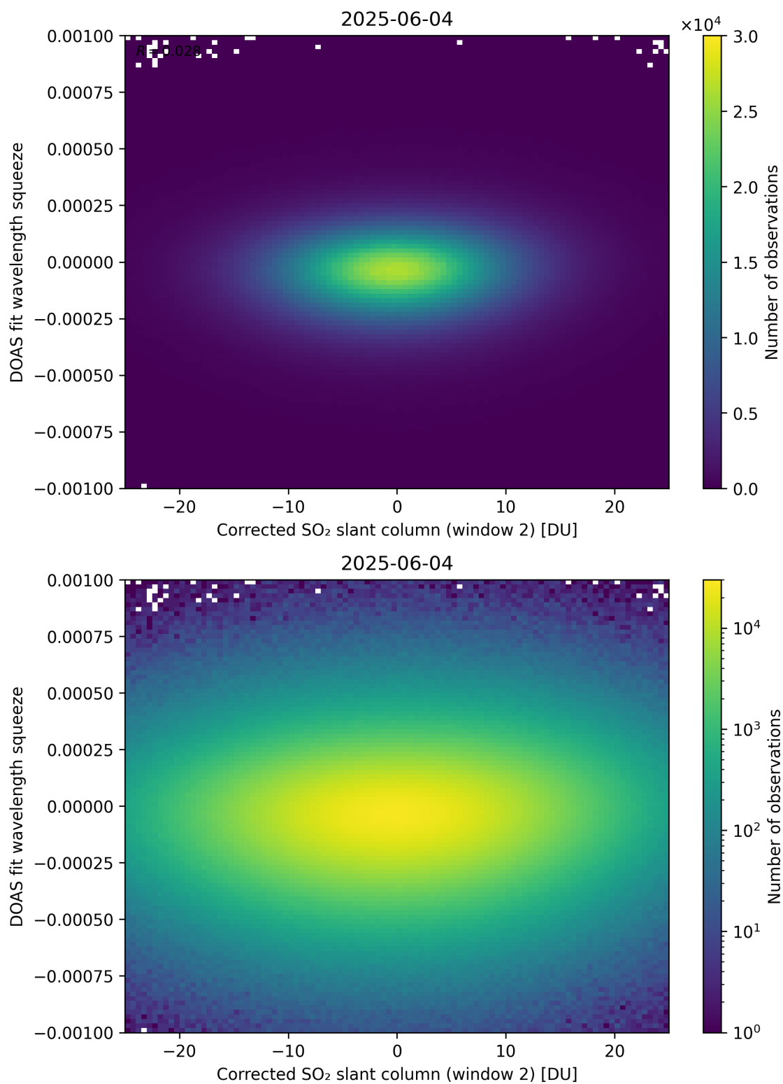
Figure 247: Scatter density plot of “Corrected SO 2 slant column (window 2)” against “DOAS fit wavelength squeeze” for 2025-06-03 to 2025-06-05.
