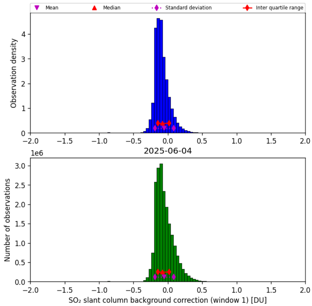
Figure 66: Histogram of “SO 2 slant column background correction (window 1)” for 2025-06-03 to 2025-06-05
