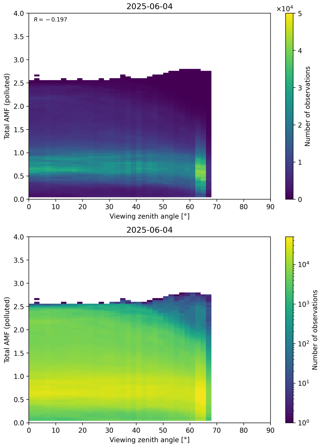
Figure 381: Scatter density plot of “Viewing zenith angle” against “Total AMF (polluted)” for 2025-06-03 to 2025-06-05.
