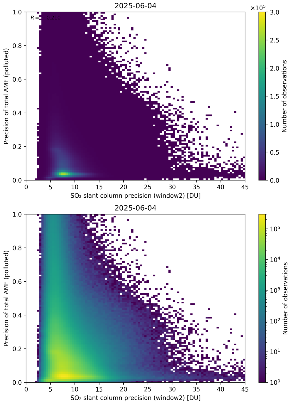
Figure 302: Scatter density plot of “SO 2 slant column precision (window2)” against “Precision of total AMF (polluted)” for 2025-06-03 to 2025-06-05.
