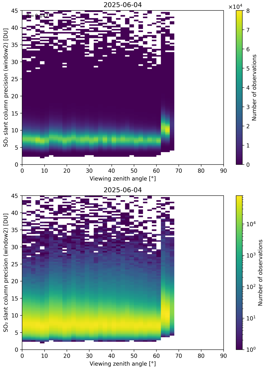
Figure 378: Scatter density plot of “Viewing zenith angle” against “SO 2 slant column precision (window2)” for 2025-06-03 to 2025-06-05.
