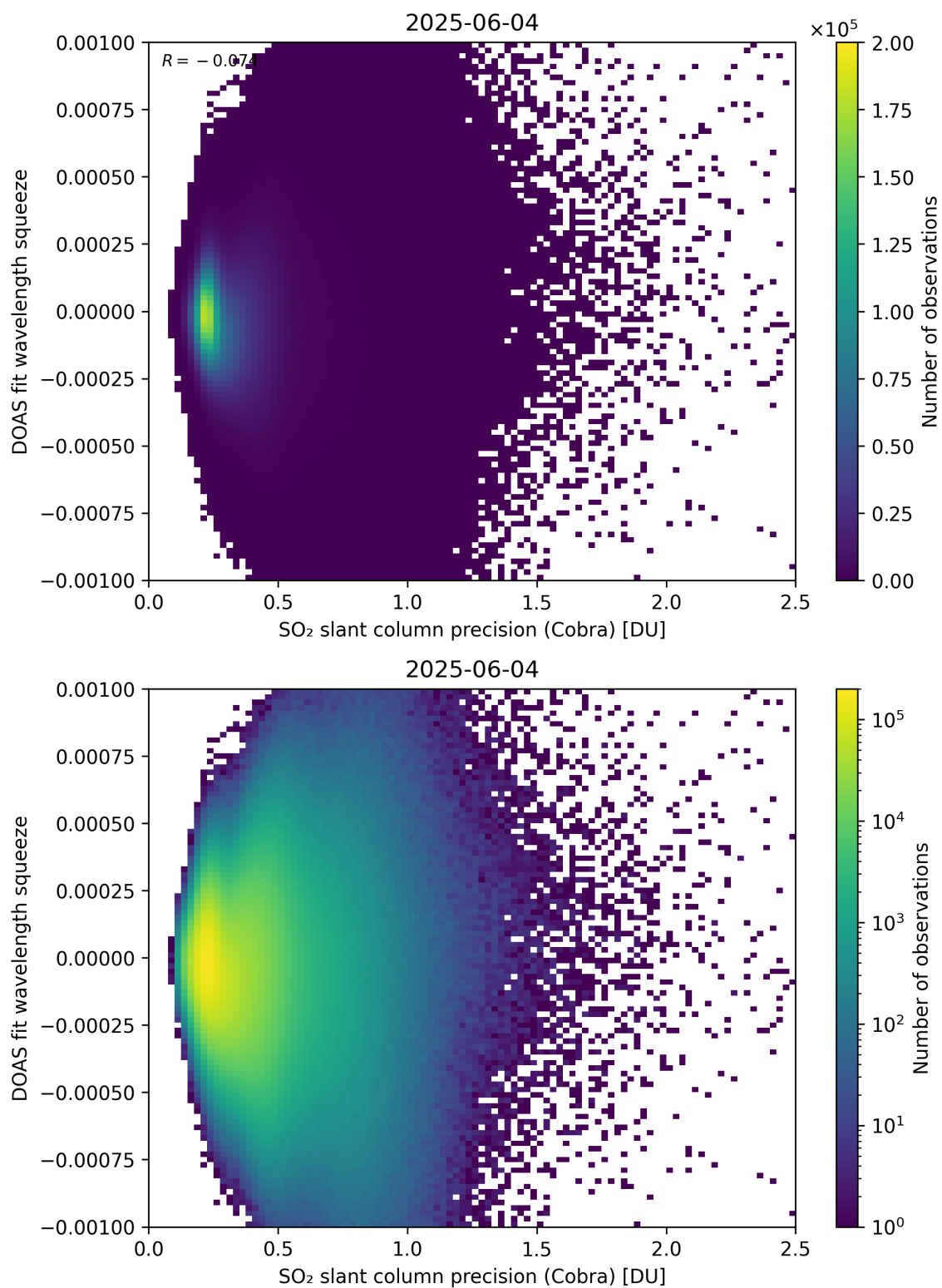
Figure 203: Scatter density plot of “SO 2 slant column precision (Cobra)” against “DOAS fit wavelength squeeze” for 2025-06-03 to 2025-06-05.
