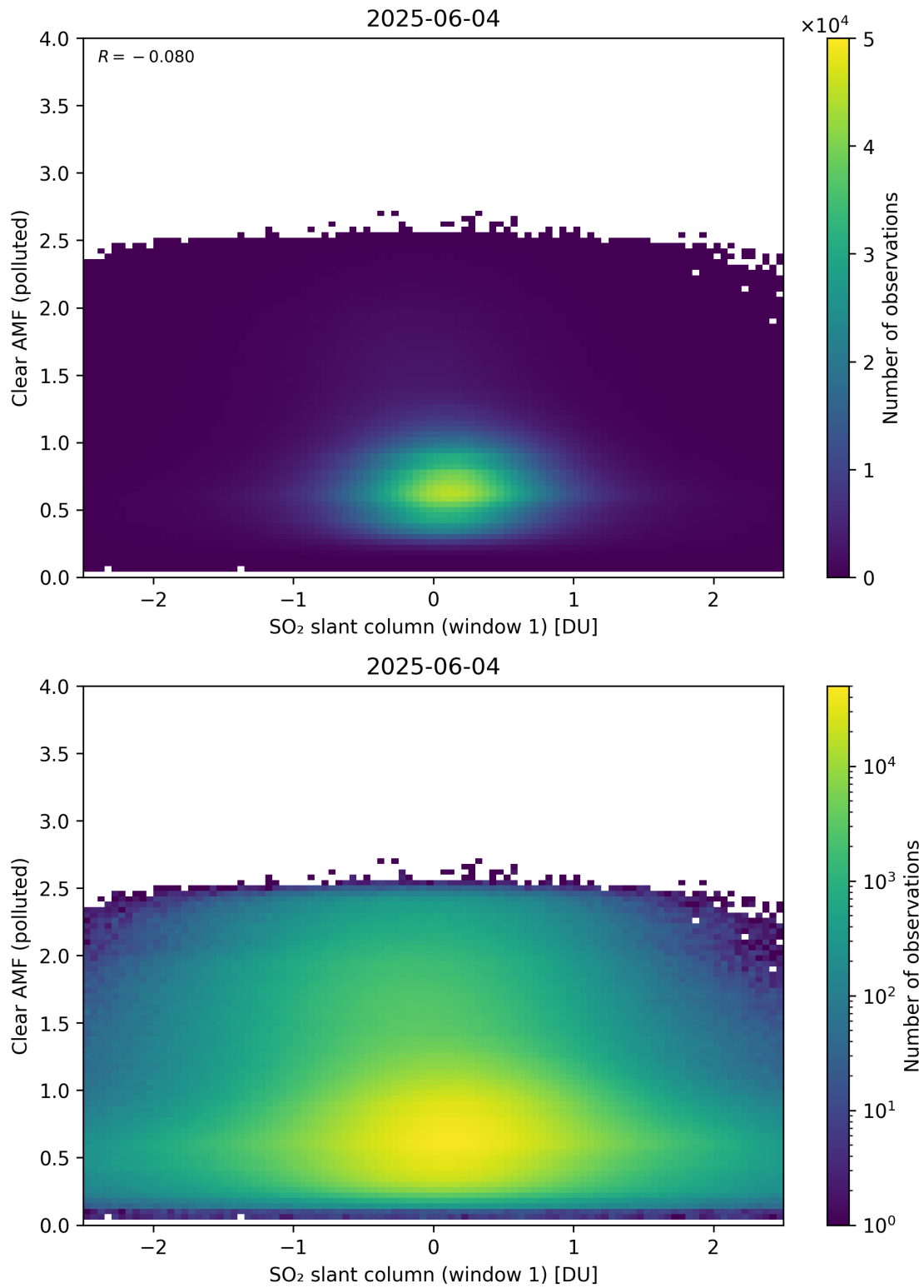
Figure 282: Scatter density plot of “SO 2 slant column (window 1)” against “Clear AMF (polluted)” for 2025-06-03 to 2025-06-05.
