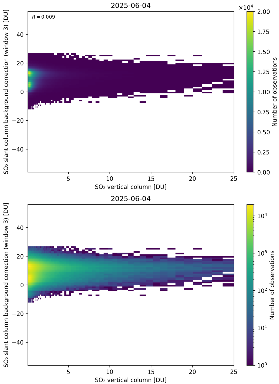
Figure 325: Scatter density plot of “SO 2 vertical column” against “SO 2 slant column background correction (window 3)” for 2025-06-03 to 2025-06-05.
