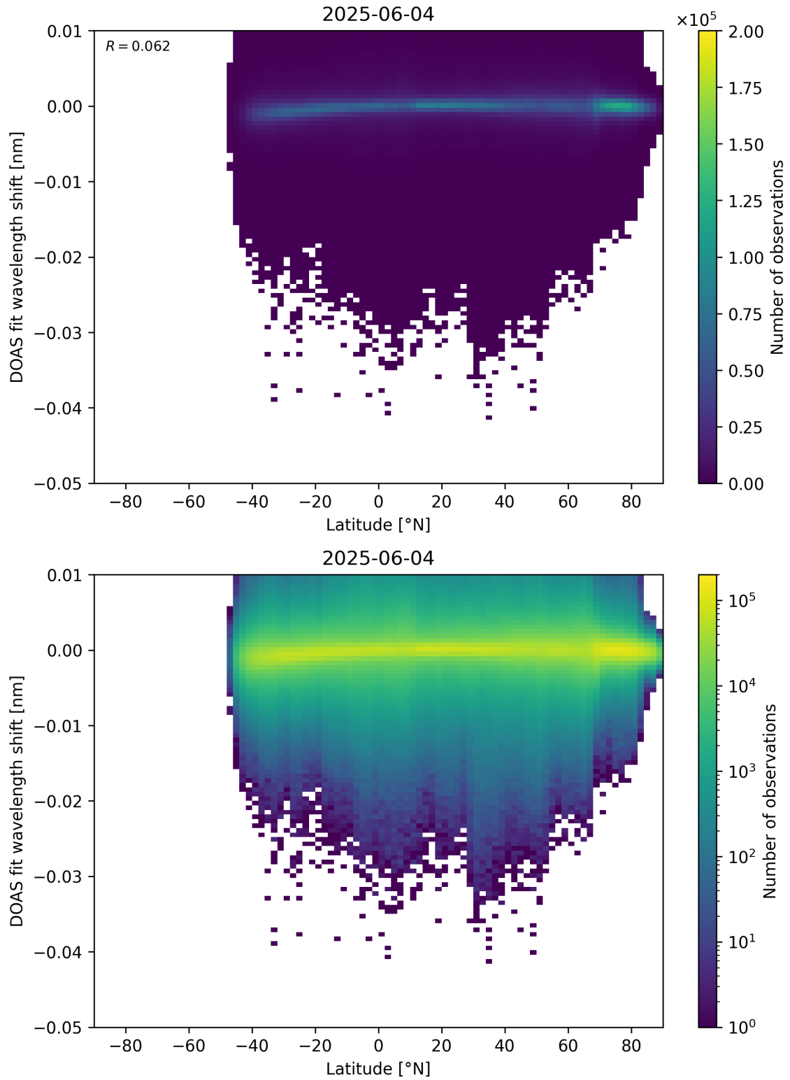
Figure 153: Scatter density plot of “Latitude” against “DOAS fit wavelength shift” for 2025-06-03 to 2025-06-05.
