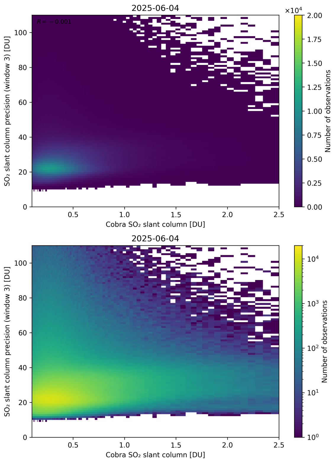
Figure 223: Scatter density plot of “Cobra SO 2 slant column” against “SO 2 slant column precision (window 3)” for 2025-06-03 to 2025-06-05.
