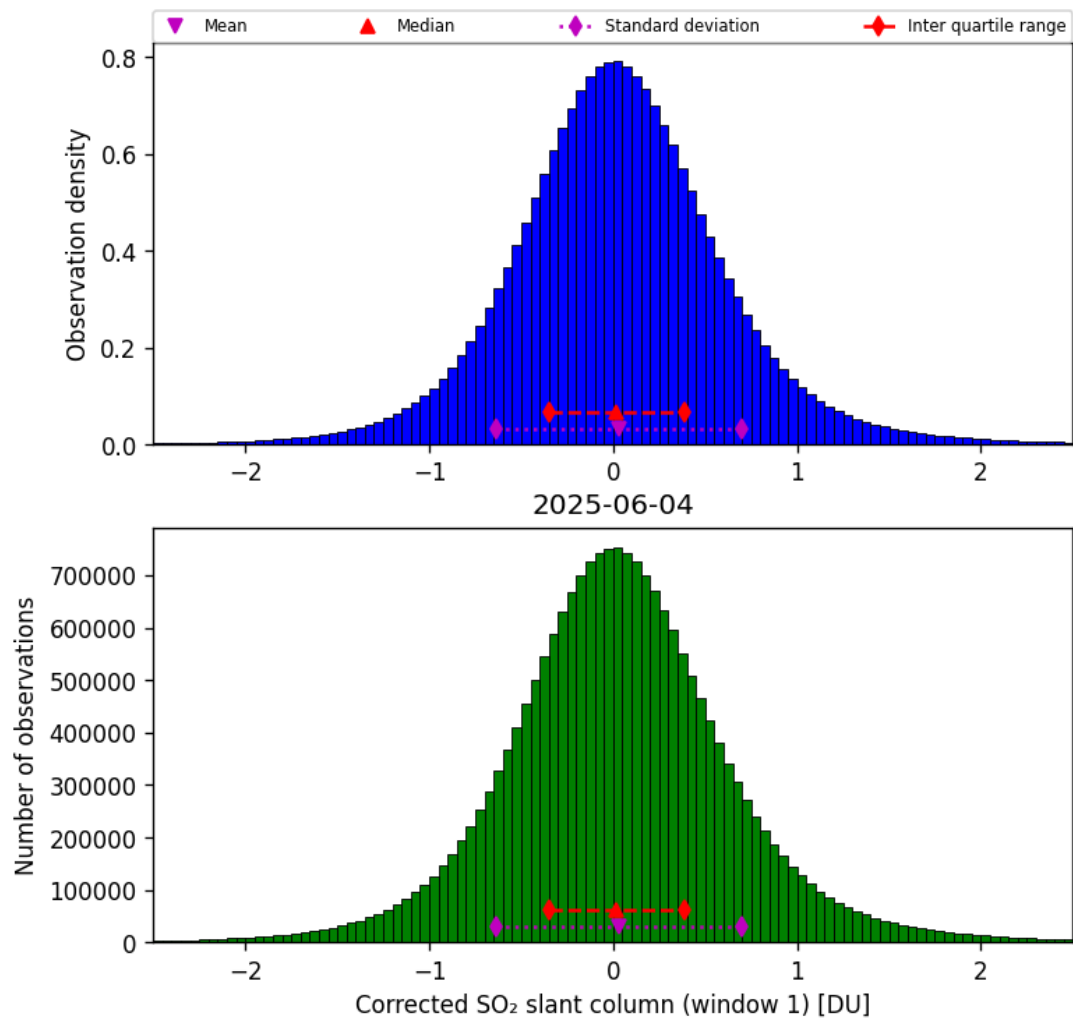
Figure 65: Histogram of “Corrected SO 2 slant column (window 1)” for 2025-06-03 to 2025-06-05
