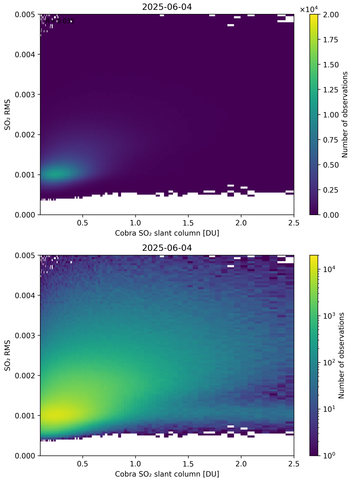
Figure 198: Scatter density plot of “Cobra SO 2 slant column” against “SO 2 RMS” for 2025-06-03 to 2025-06-05.
