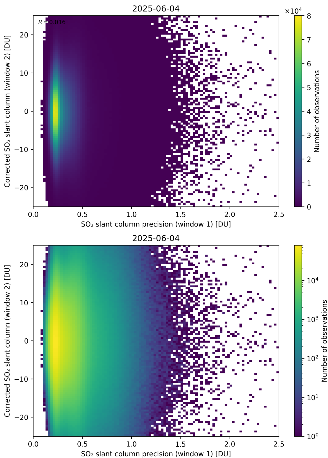
Figure 275: Scatter density plot of “SO 2 slant column precision (window 1)” against “Corrected SO 2 slant column (window 2)” for 2025-06-03 to 2025-06-05.
