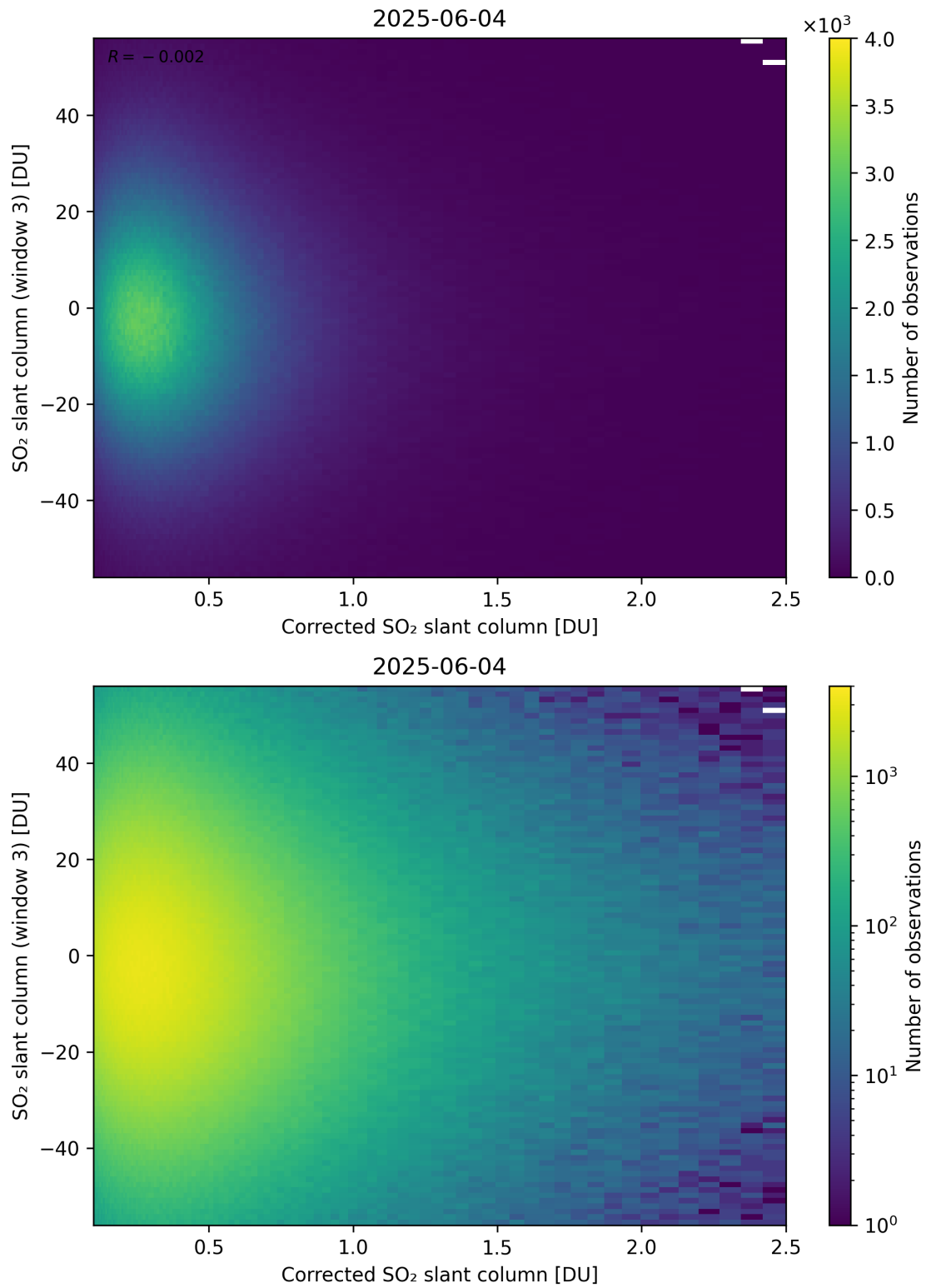
Figure 240: Scatter density plot of “Corrected SO 2 slant column” against “SO 2 slant column (window 3)” for 2025-06-03 to 2025-06-05.
