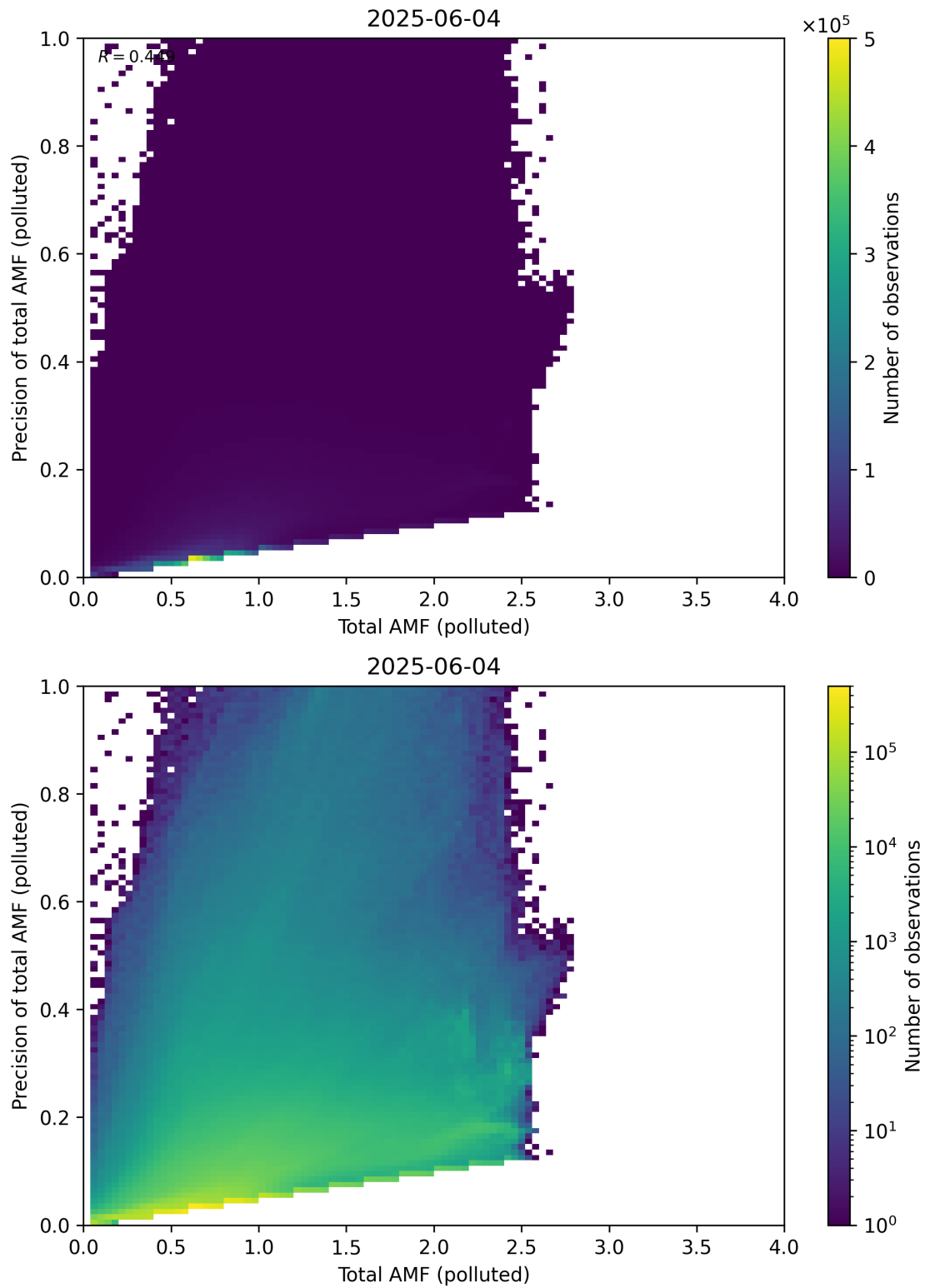
Figure 322: Scatter density plot of “Total AMF (polluted)” against “Precision of total AMF (polluted)” for 2025-06-03 to 2025-06-05.
