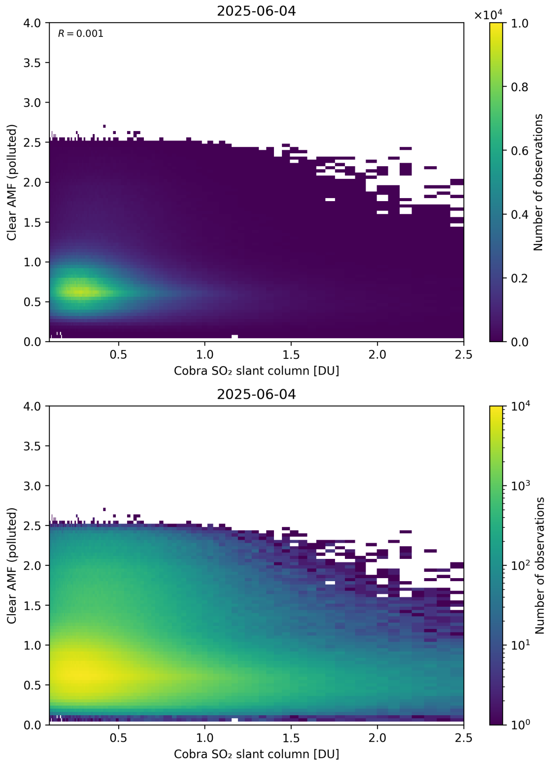
Figure 215: Scatter density plot of “Cobra SO 2 slant column” against “Clear AMF (polluted)” for 2025-06-03 to 2025-06-05.
