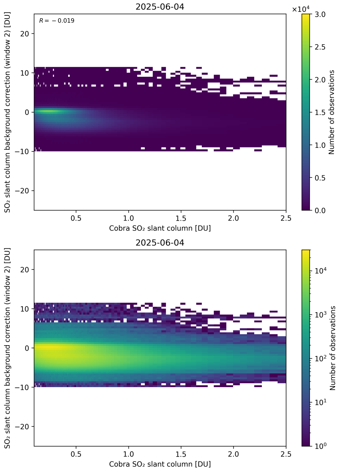
Figure 194: Scatter density plot of “Cobra SO 2 slant column” against “SO 2 slant column background correction (window 2)” for 2025-06-03 to 2025-06-05.
