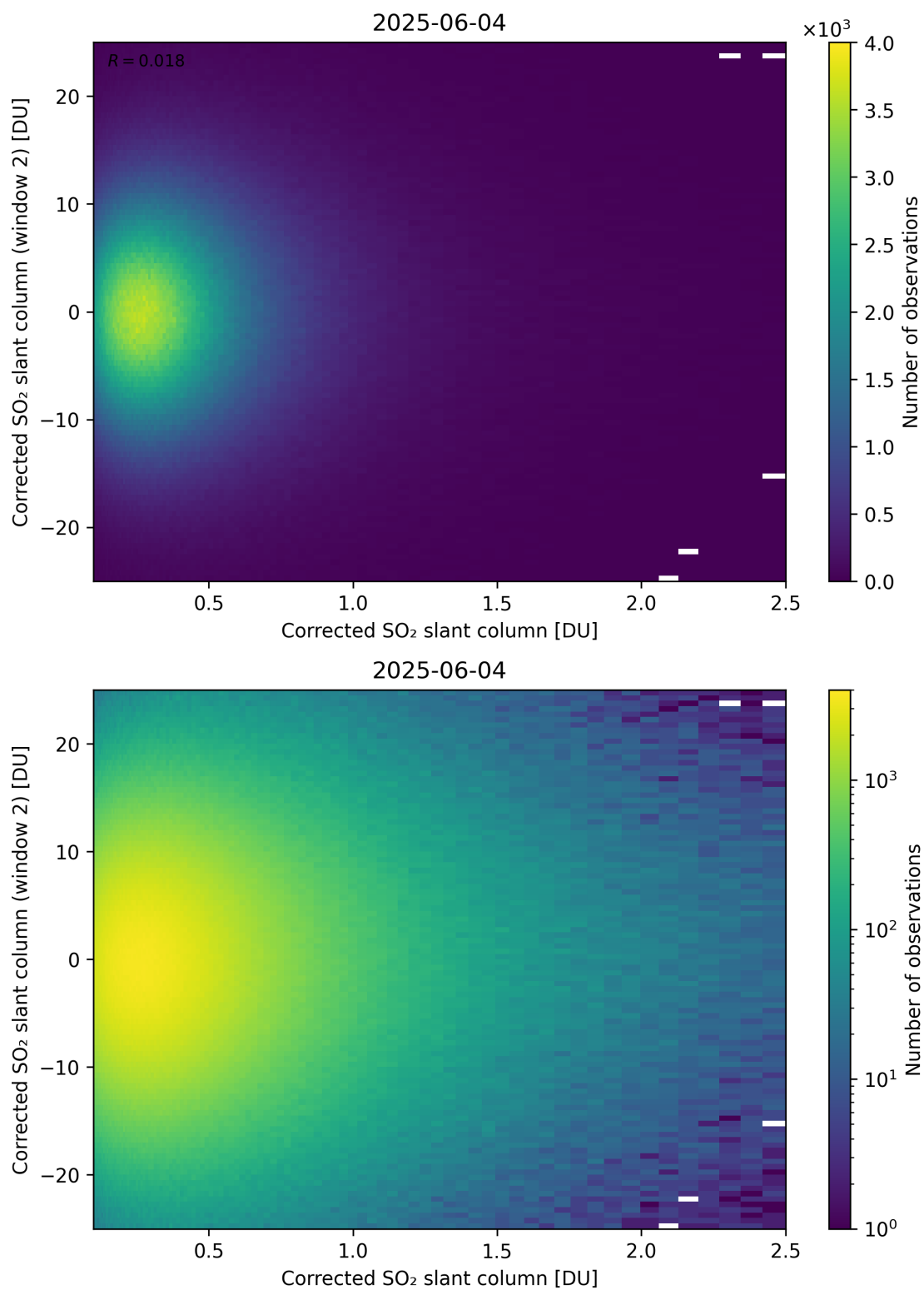
Figure 235: Scatter density plot of “Corrected SO 2 slant column” against “Corrected SO 2 slant column (window 2)” for 2025-06-03 to 2025-06-05.
