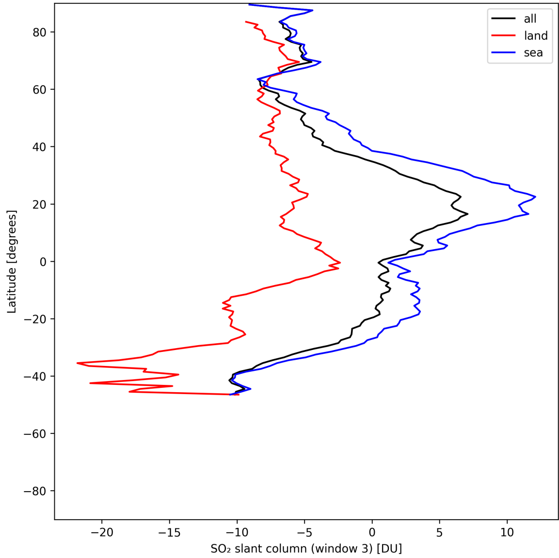
Figure 45: Zonal average of “SO 2 slant column (window 3)” for 2025-06-03 to 2025-06-05.
