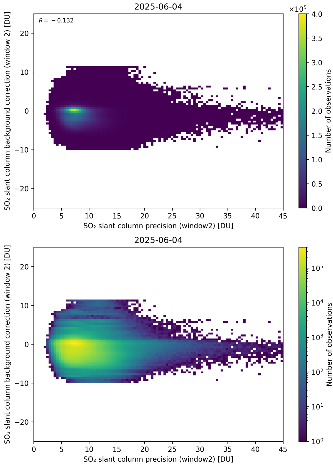
Figure 291: Scatter density plot of “SO 2 slant column precision (window2)” against “SO 2 slant column background correction (window 2)” for 2025-06-03 to 2025-06-05.
