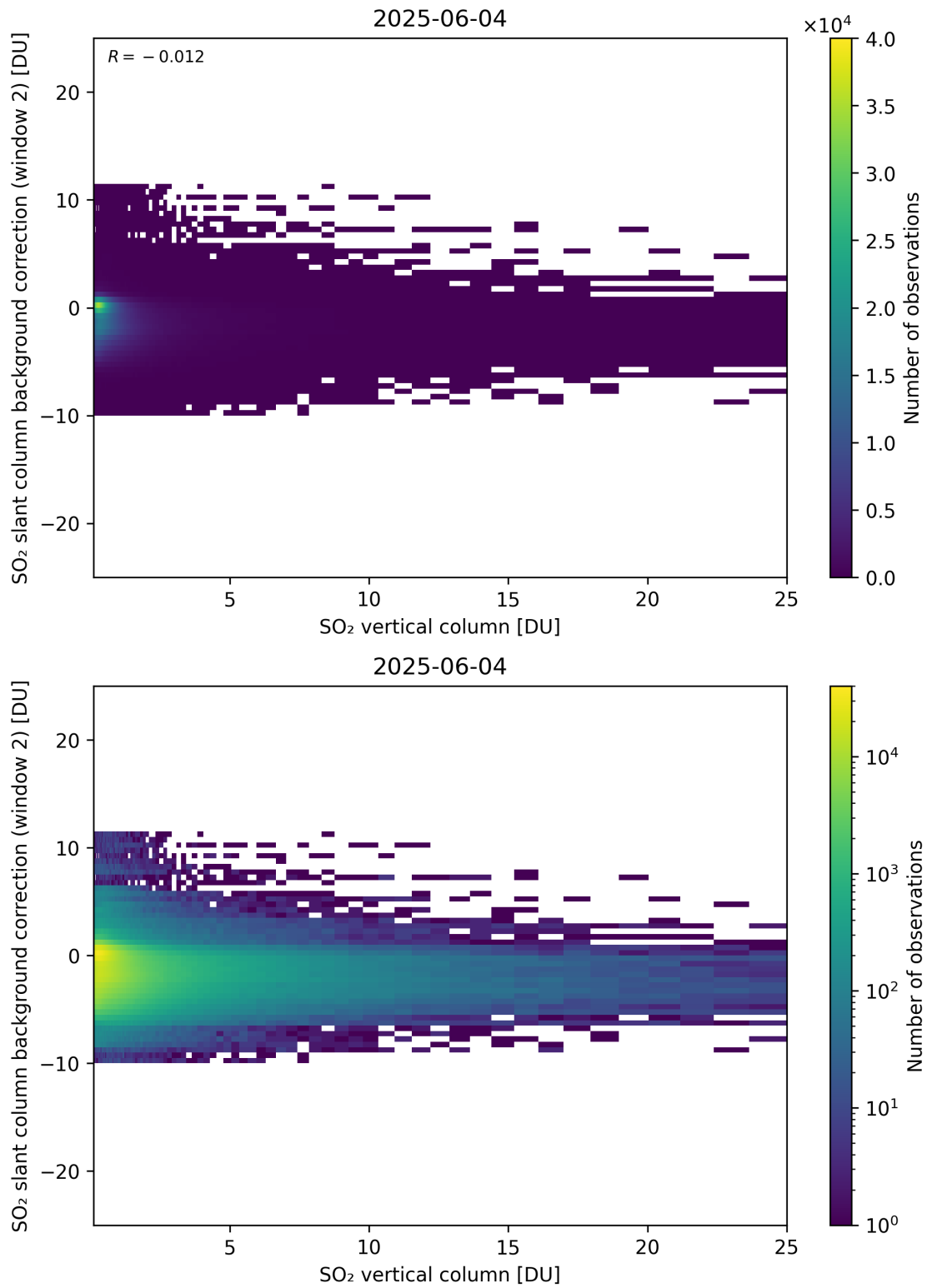
Figure 324: Scatter density plot of “SO 2 vertical column” against “SO 2 slant column background correction (window 2)” for 2025-06-03 to 2025-06-05.
