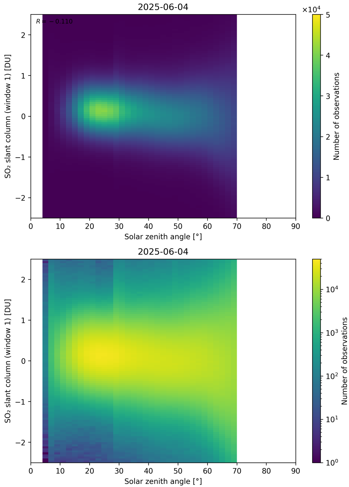
Figure 184: Scatter density plot of “Solar zenith angle” against “SO 2 slant column (window 1)” for 2025-06-03 to 2025-06-05.
