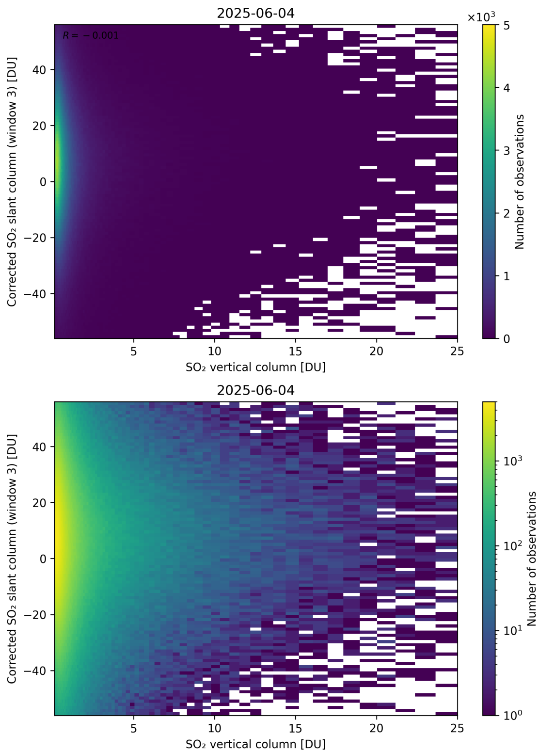
Figure 353: Scatter density plot of “SO 2 vertical column” against “Corrected SO 2 slant column (window 3)” for 2025-06-03 to 2025-06-05.
