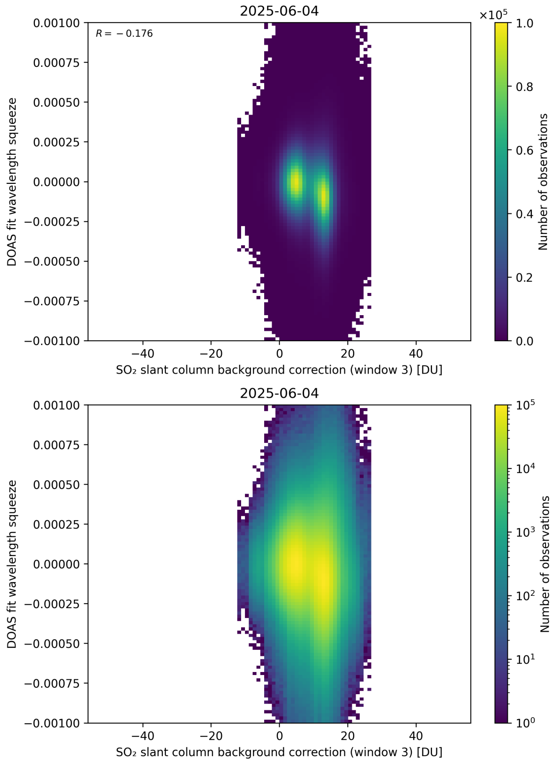
Figure 133: Scatter density plot of “SO 2 slant column background correction (window 3)” against “DOAS fit wavelength squeeze” for 2025-06-03 to 2025-06-05.
