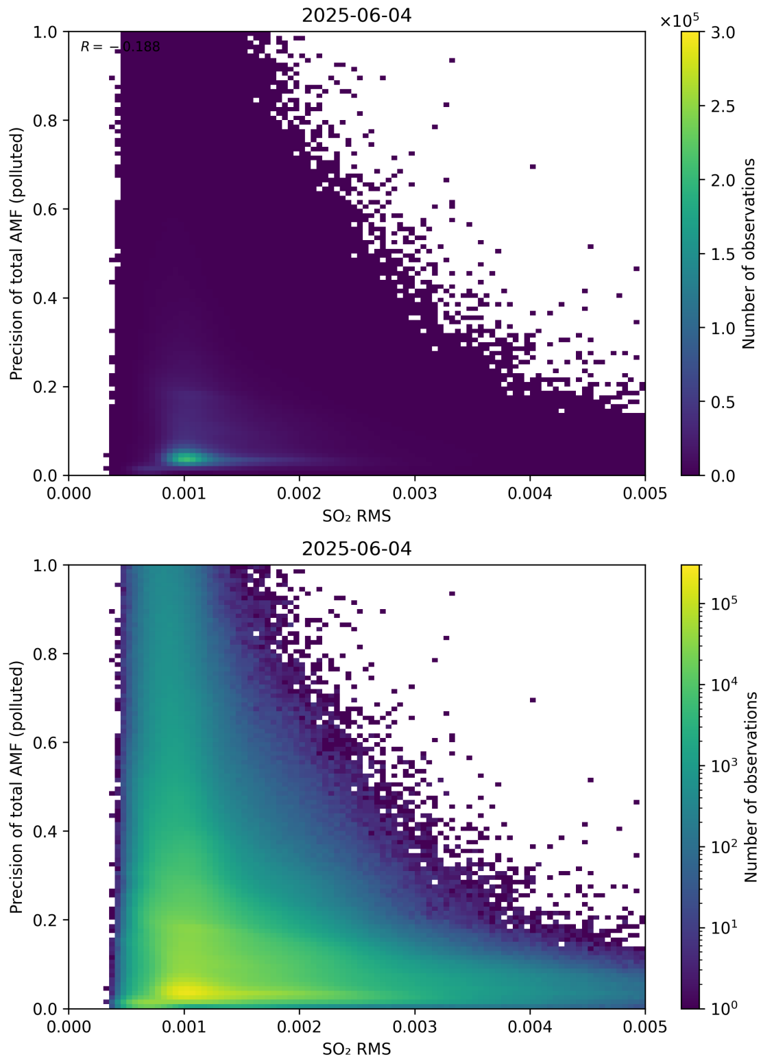
Figure 149: Scatter density plot of “SO 2 RMS” against “Precision of total AMF (polluted)” for 2025-06-03 to 2025-06-05.
