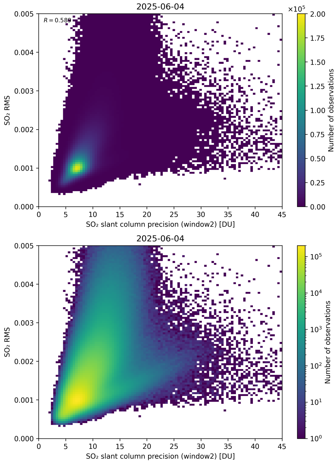
Figure 295: Scatter density plot of “SO 2 slant column precision (window2)” against “SO 2 RMS” for 2025-06-03 to 2025-06-05.
