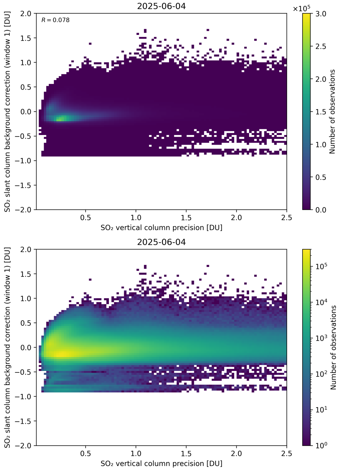
Figure 329: Scatter density plot of “SO 2 vertical column precision” against “SO 2 slant column background correction (window 1)” for 2025-06-03 to 2025-06-05.
