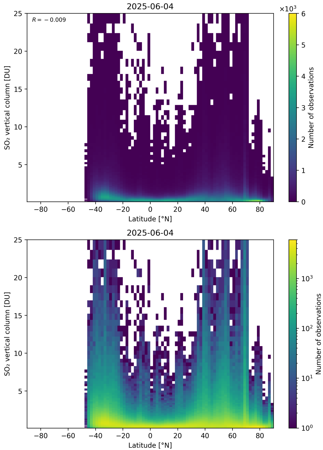
Figure 169: Scatter density plot of “Latitude” against “SO 2 vertical column” for 2025-06-03 to 2025-06-05.
