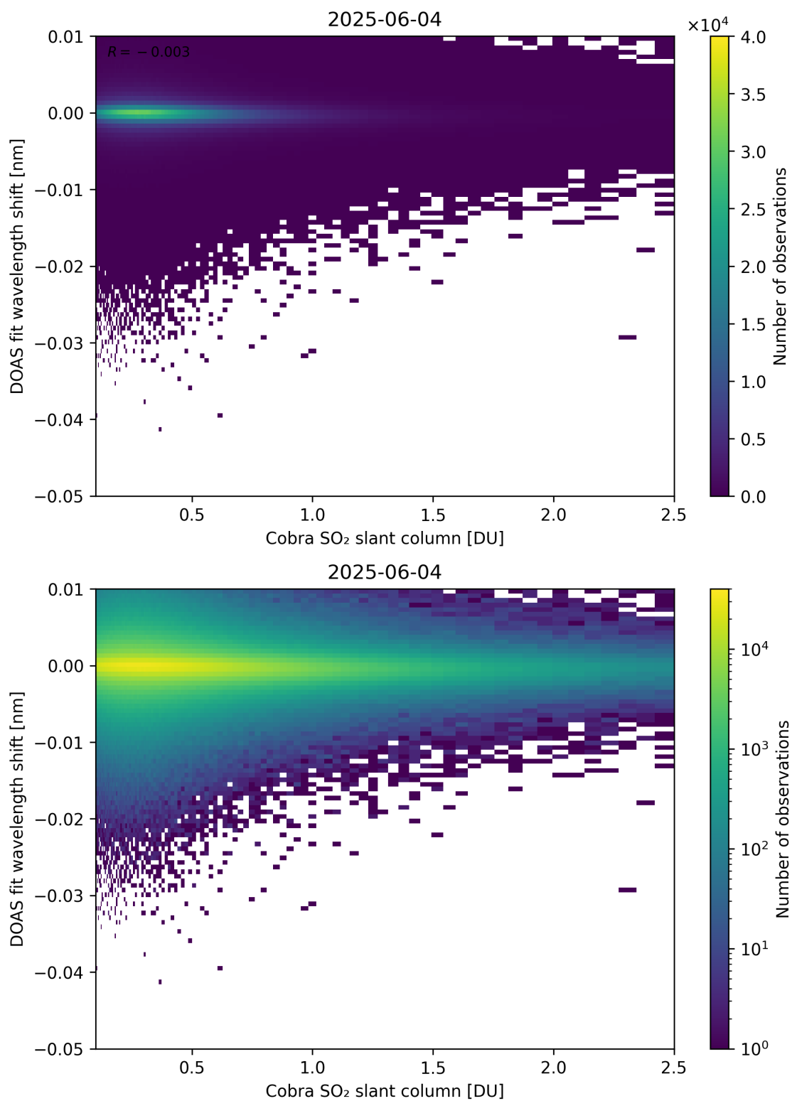
Figure 196: Scatter density plot of “Cobra SO 2 slant column” against “DOAS fit wavelength shift” for 2025-06-03 to 2025-06-05.
