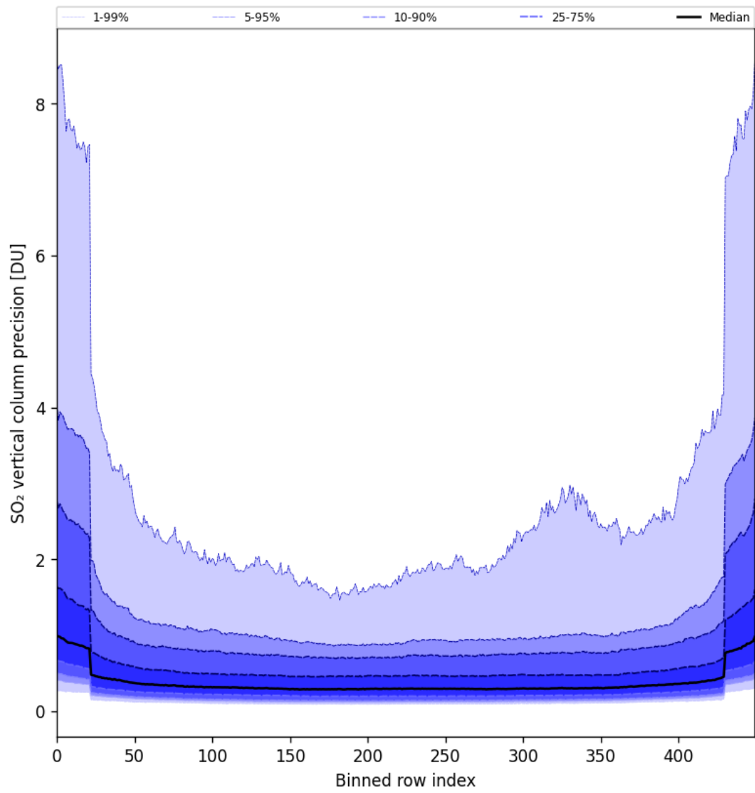
Figure 85: Along track statistics of “SO 2 vertical column precision” for 2025-06-03 to 2025-06-05
