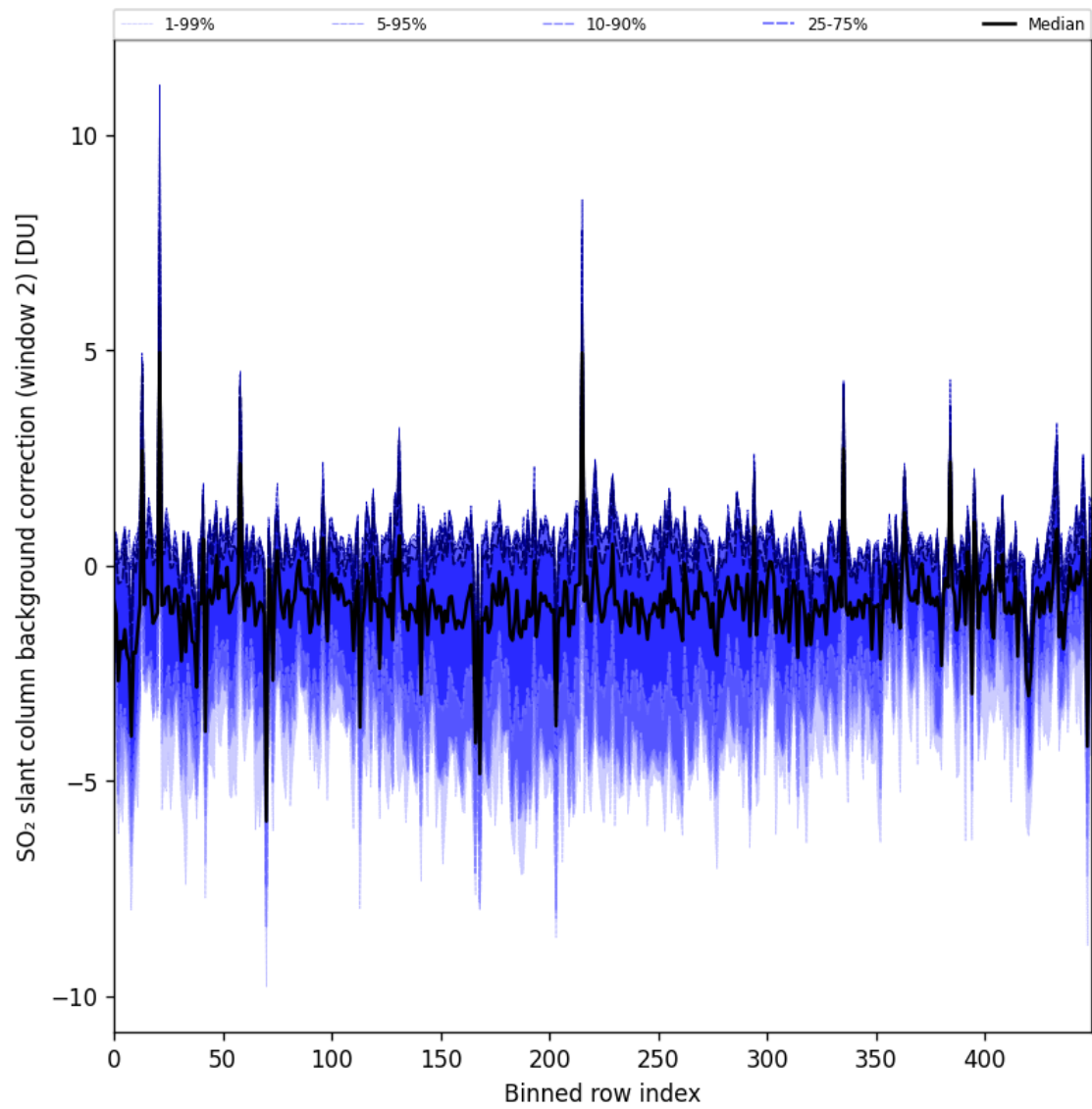
Figure 96: Along track statistics of “SO 2 slant column background correction (window 2)” for 2025-06-03 to 2025-06-05
