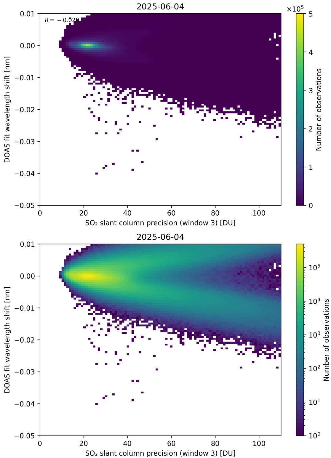
Figure 308: Scatter density plot of “SO 2 slant column precision (window 3)” against “DOAS fit wavelength shift” for 2025-06-03 to 2025-06-05.
