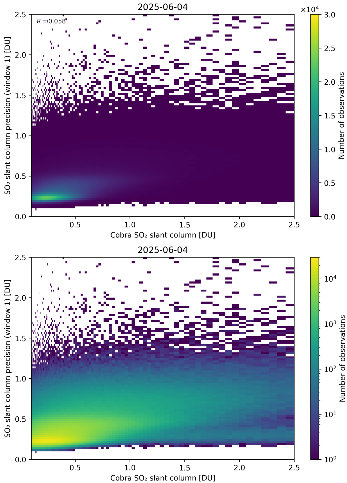
Figure 220: Scatter density plot of “Cobra SO 2 slant column” against “SO 2 slant column precision (window 1)” for 2025-06-03 to 2025-06-05.
