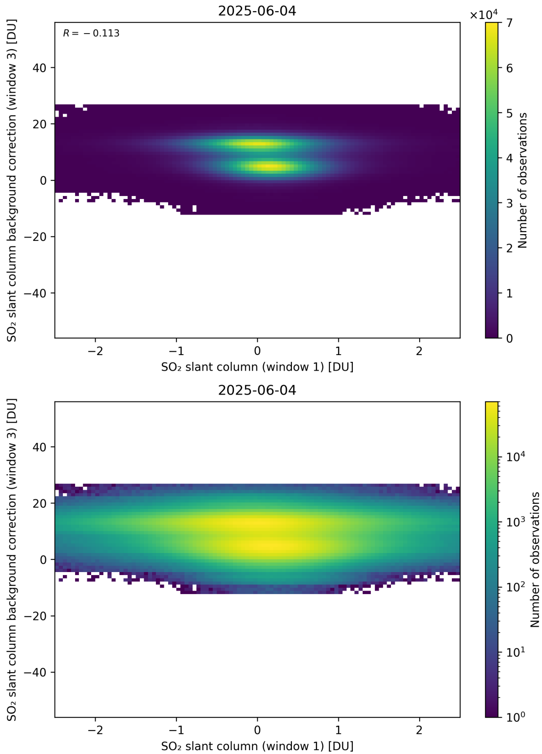
Figure 264: Scatter density plot of “SO 2 slant column (window 1)” against “SO 2 slant column background correction (window 3)” for 2025-06-03 to 2025-06-05.
