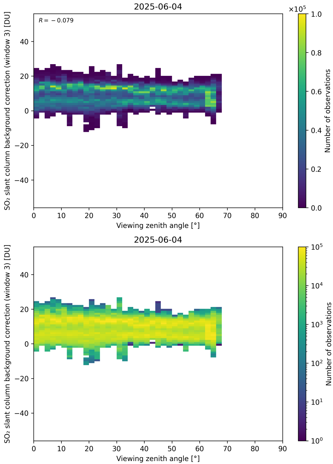
Figure 364: Scatter density plot of “Viewing zenith angle” against “SO 2 slant column background correction (window 3)” for 2025-06-03 to 2025-06-05.
