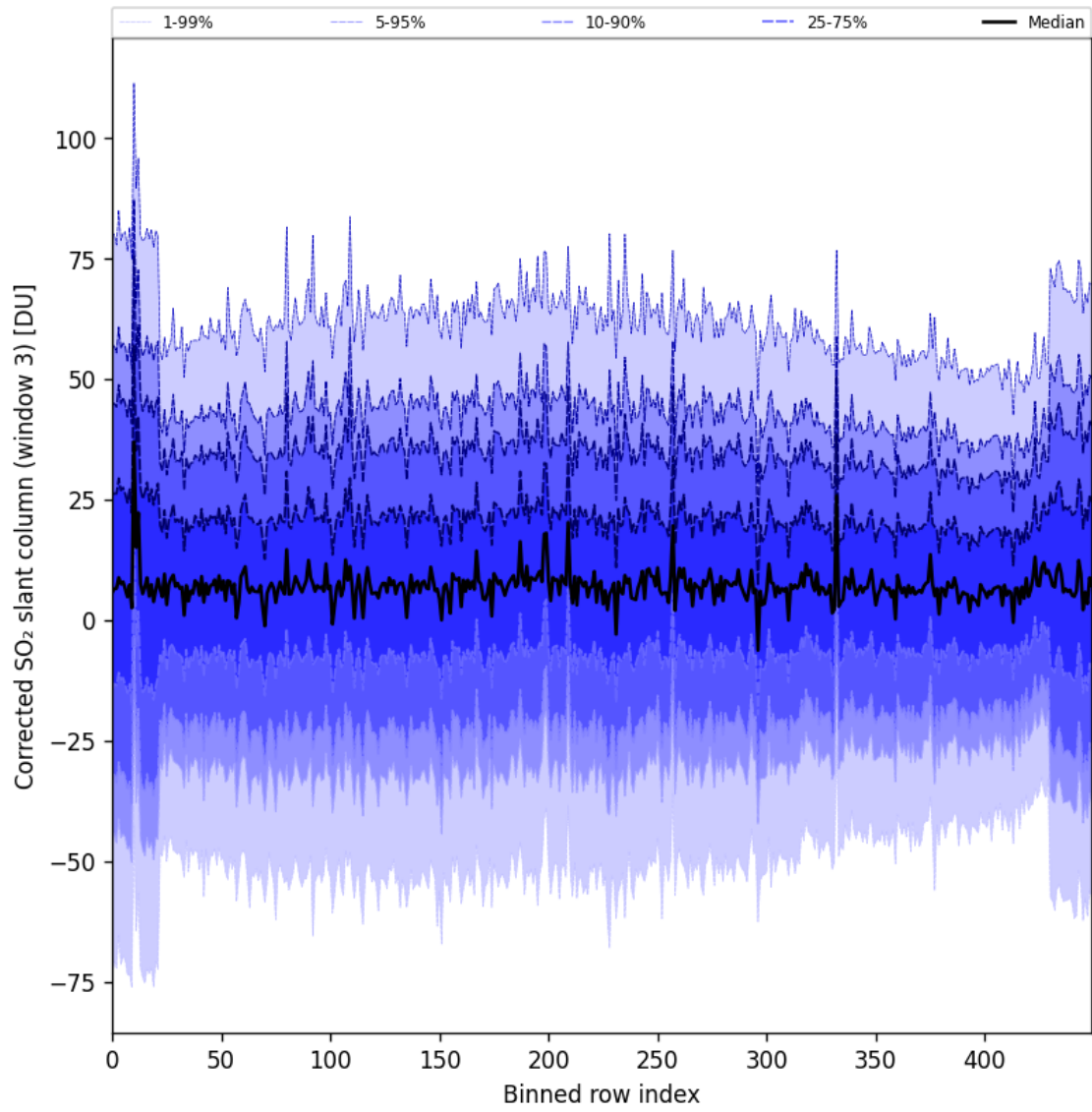
Figure 99: Along track statistics of “Corrected SO 2 slant column (window 3)” for 2025-06-03 to 2025-06-05
