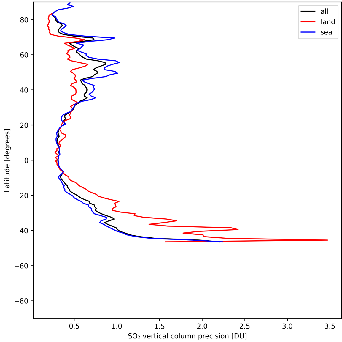
Figure 33: Zonal average of “SO 2 vertical column precision” for 2025-06-03 to 2025-06-05.
