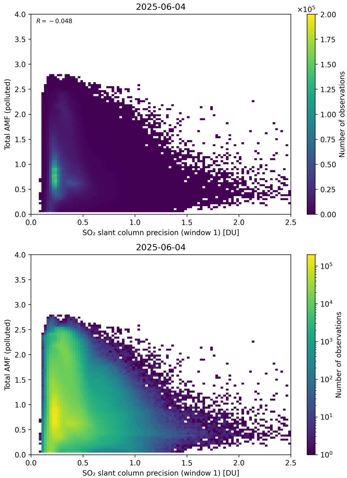
Figure 280: Scatter density plot of “SO 2 slant column precision (window 1)” against “Total AMF (polluted)” for 2025-06-03 to 2025-06-05.
