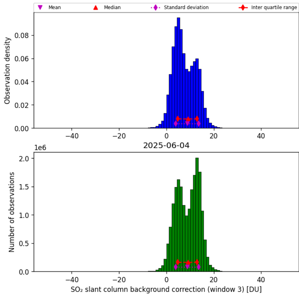
Figure 74: Histogram of “SO 2 slant column background correction (window 3)” for 2025-06-03 to 2025-06-05
