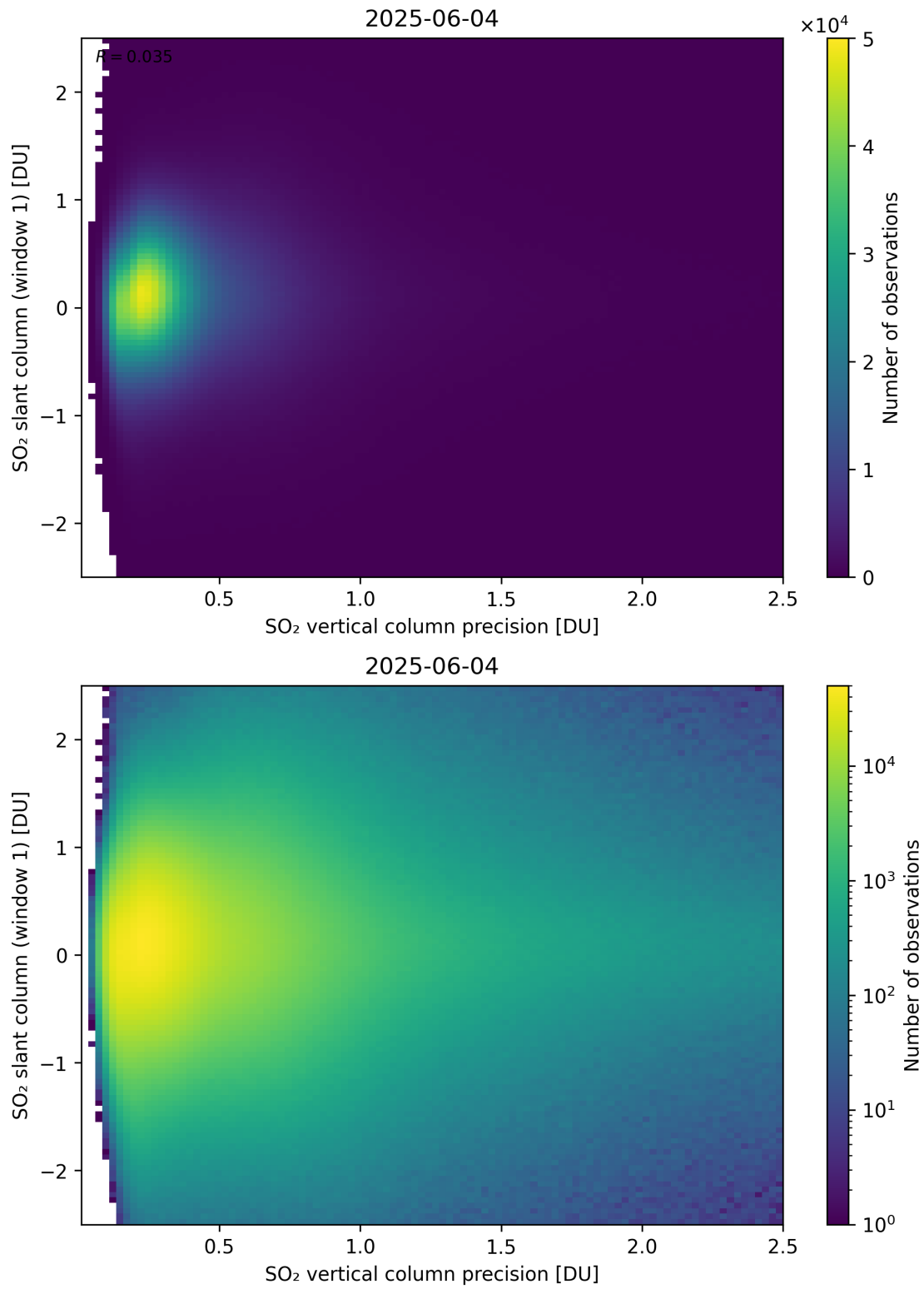
Figure 341: Scatter density plot of “SO 2 vertical column precision” against “SO 2 slant column (window 1)” for 2025-06-03 to 2025-06-05.
