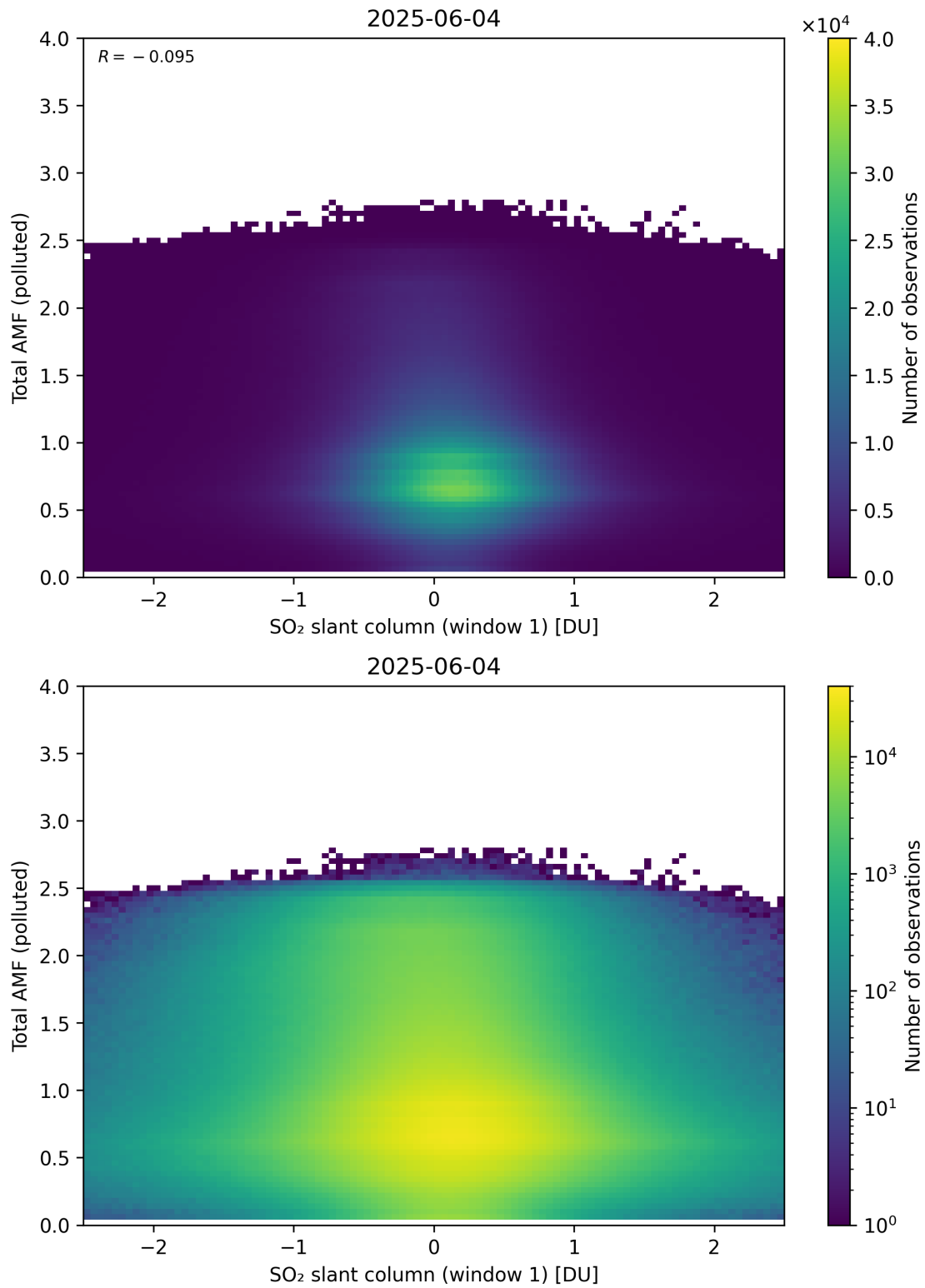
Figure 289: Scatter density plot of “SO 2 slant column (window 1)” against “Total AMF (polluted)” for 2025-06-03 to 2025-06-05.
