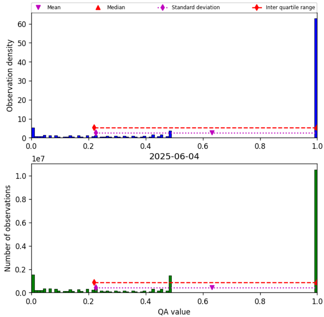
Figure 57: Histogram of “QA value” for 2025-06-03 to 2025-06-05
