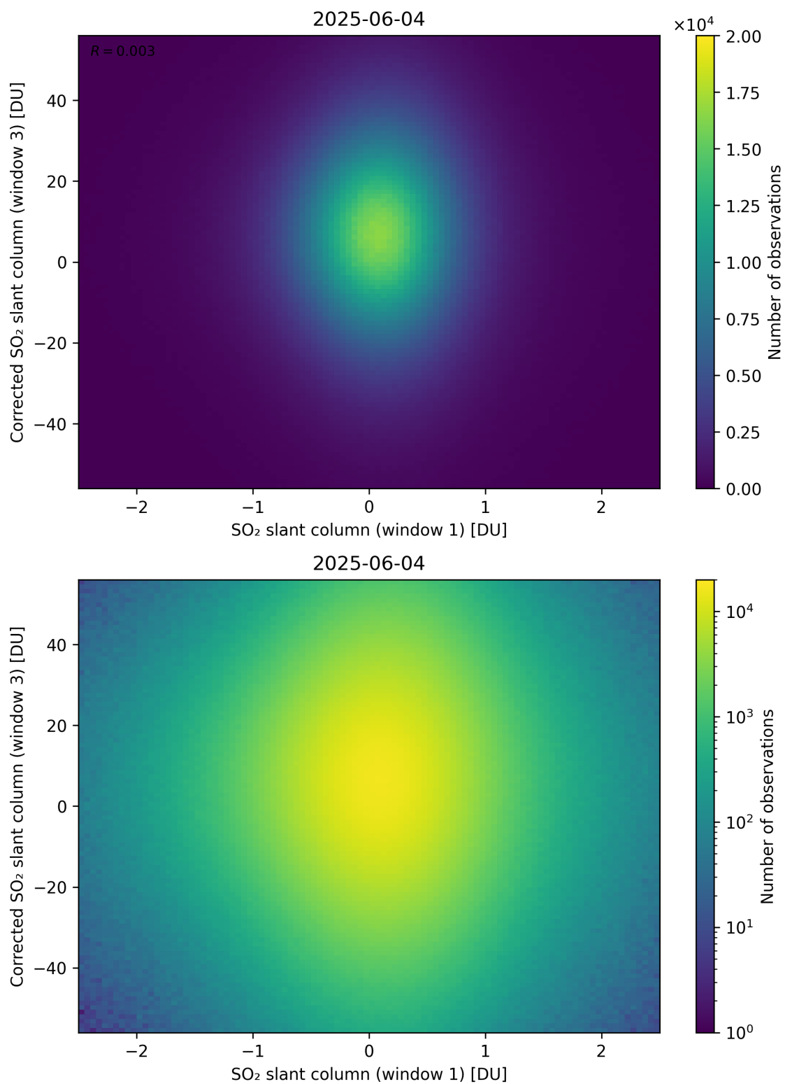
Figure 284: Scatter density plot of “SO 2 slant column (window 1)” against “Corrected SO 2 slant column (window 3)” for 2025-06-03 to 2025-06-05.
