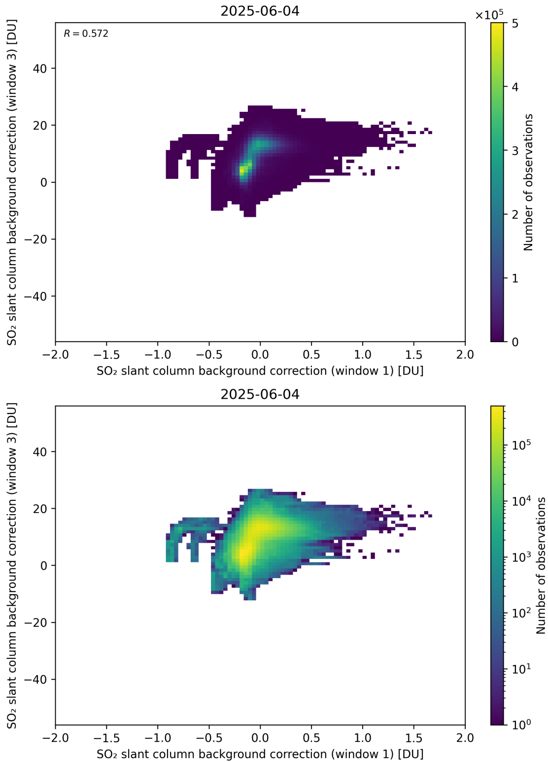
Figure 110: Scatter density plot of “SO 2 slant column background correction (window 1)” against “SO 2 slant column background correction (window 3)” for 2025-06-03 to 2025-06-05.
