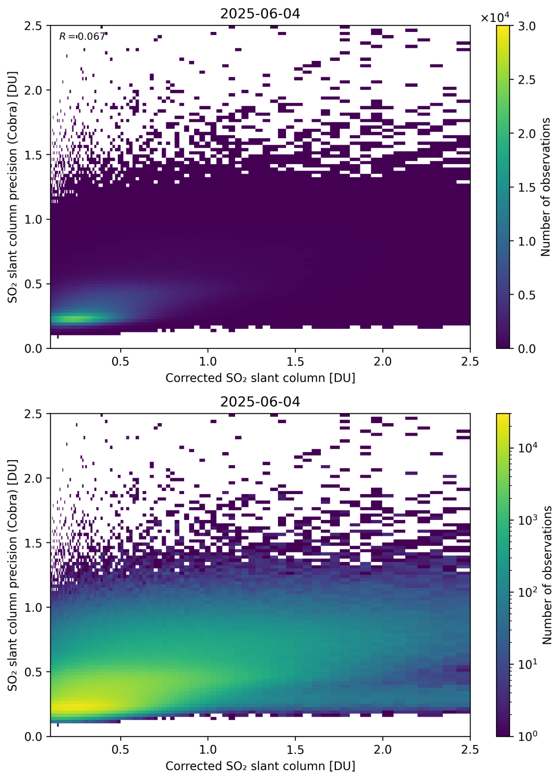
Figure 234: Scatter density plot of “Corrected SO 2 slant column” against “SO 2 slant column precision (Cobra)” for 2025-06-03 to 2025-06-05.
