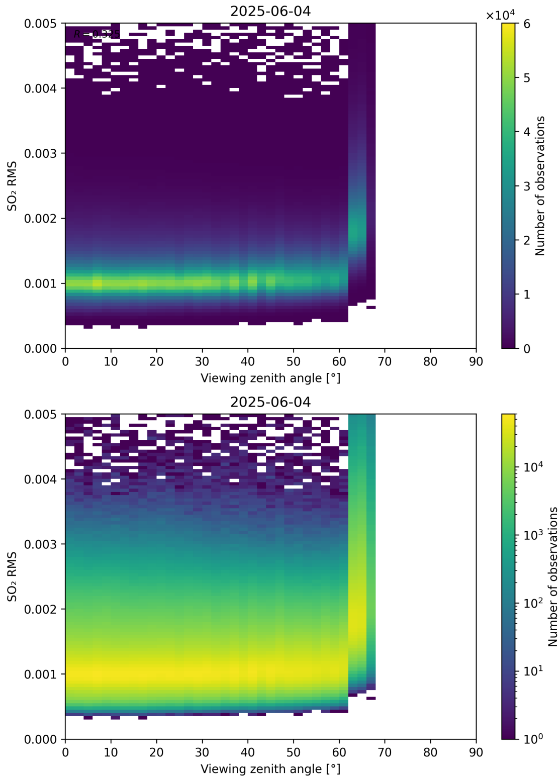
Figure 367: Scatter density plot of “Viewing zenith angle” against “SO 2 RMS” for 2025-06-03 to 2025-06-05.
