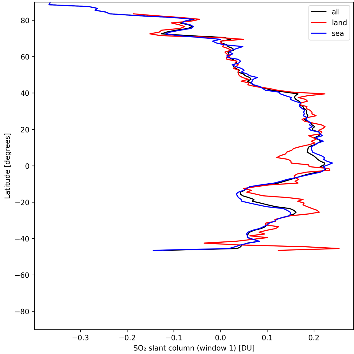
Figure 37: Zonal average of “SO 2 slant column (window 1)” for 2025-06-03 to 2025-06-05.
