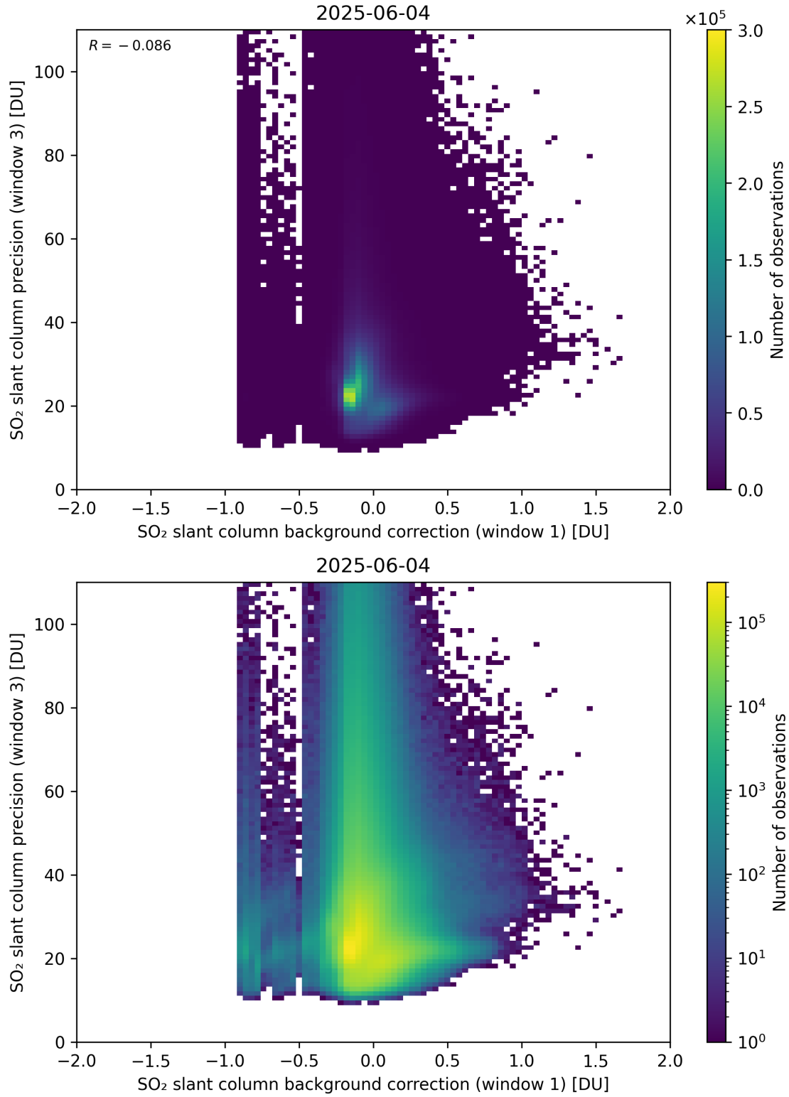
Figure 119: Scatter density plot of “SO 2 slant column background correction (window 1)” against “SO 2 slant column precision (window 3)” for 2025-06-03 to 2025-06-05.
