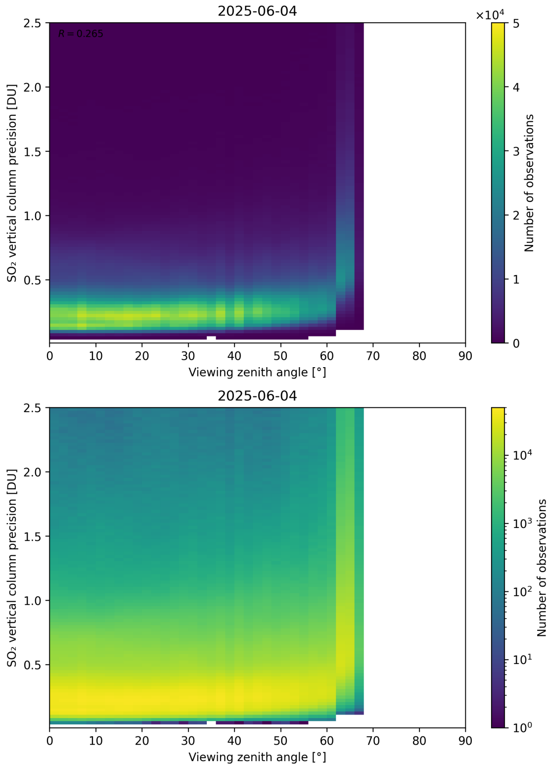
Figure 384: Scatter density plot of “Viewing zenith angle” against “SO 2 vertical column precision” for 2025-06-03 to 2025-06-05.
