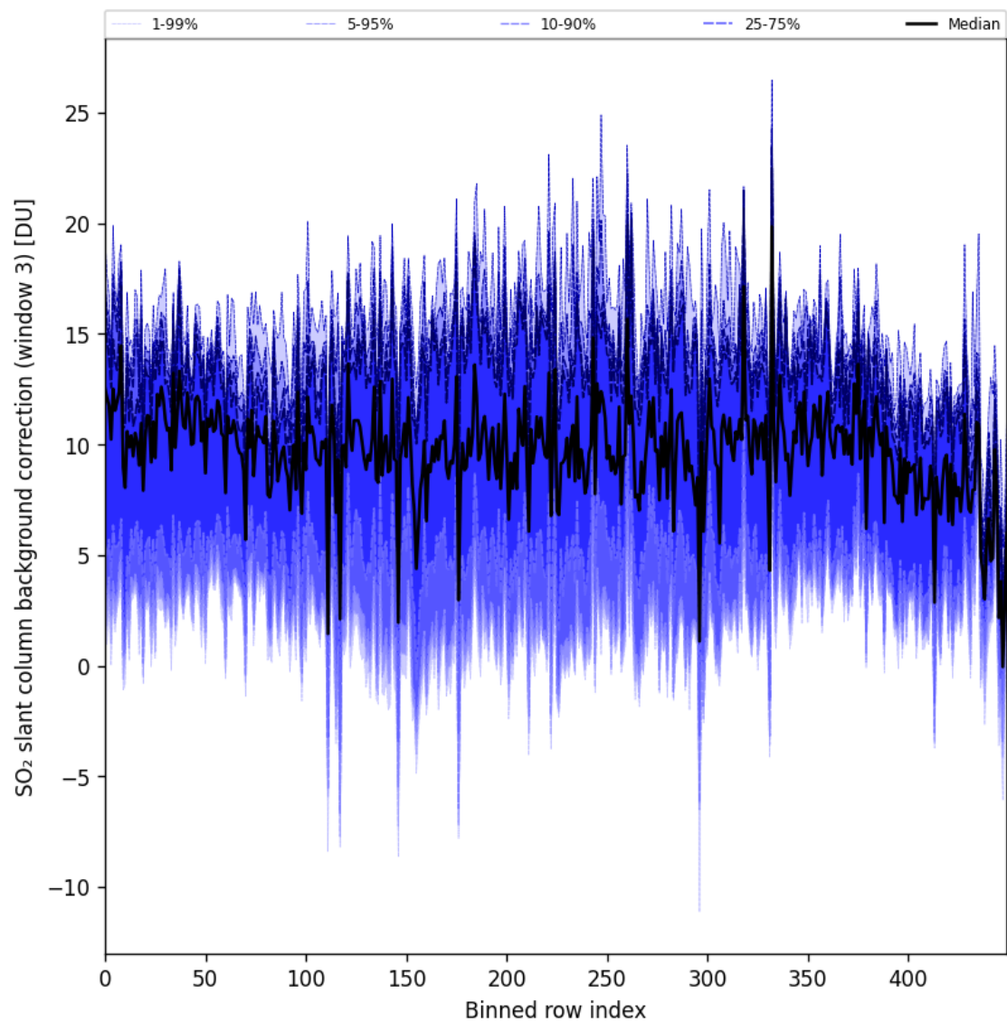
Figure 100: Along track statistics of “SO 2 slant column background correction (window 3)” for 2025-06-03 to 2025-06-05
