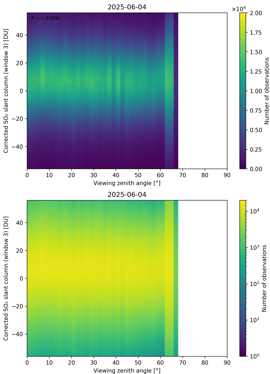
Figure 375: Scatter density plot of “Viewing zenith angle” against “Corrected SO 2 slant column (window 3)” for 2025-06-03 to 2025-06-05.
