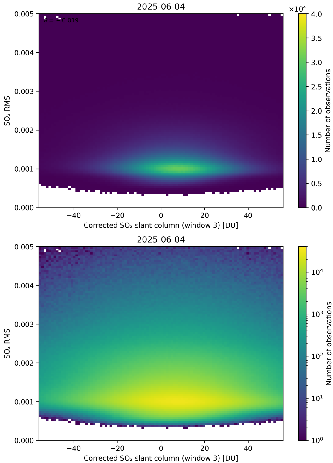
Figure 258: Scatter density plot of “Corrected SO 2 slant column (window 3)” against “SO 2 RMS” for 2025-06-03 to 2025-06-05.
