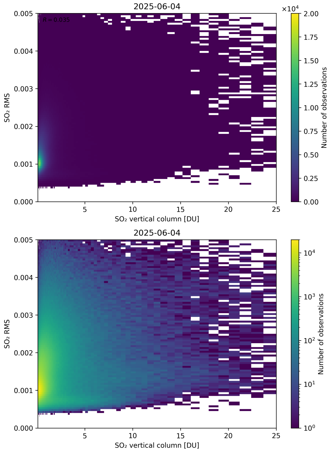
Figure 328: Scatter density plot of “SO 2 vertical column” against “SO 2 RMS” for 2025-06-03 to 2025-06-05.
