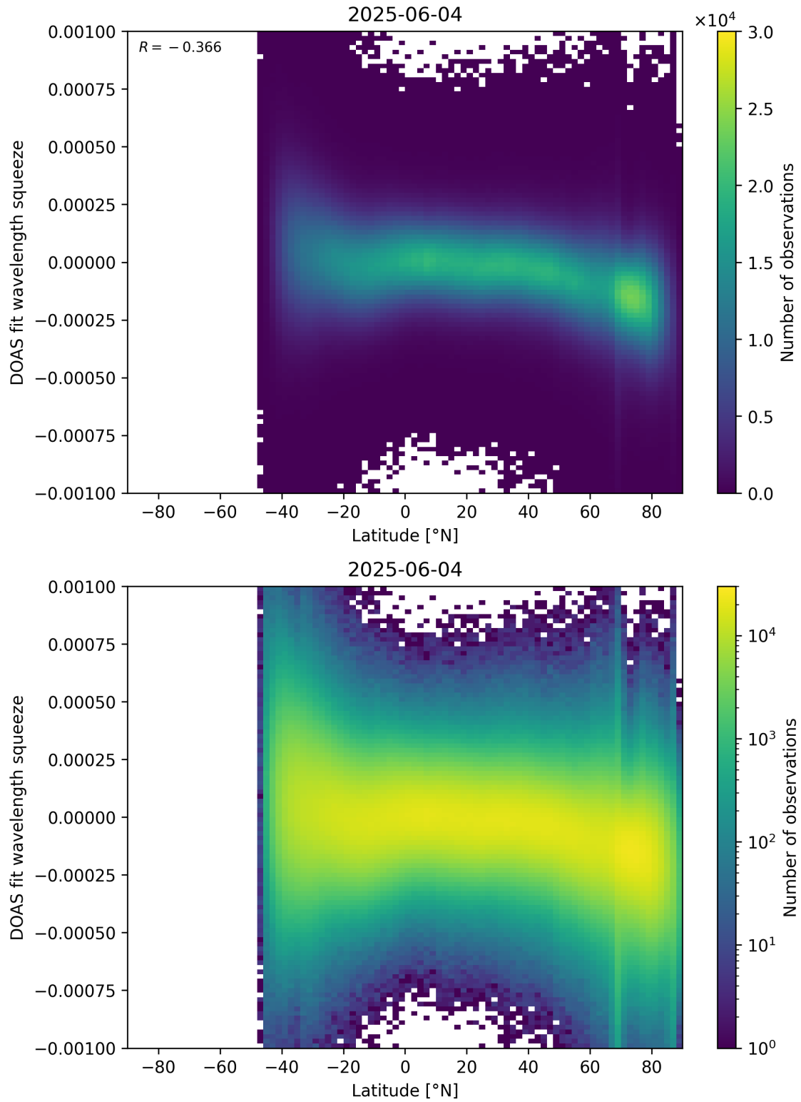
Figure 154: Scatter density plot of “Latitude” against “DOAS fit wavelength squeeze” for 2025-06-03 to 2025-06-05.
