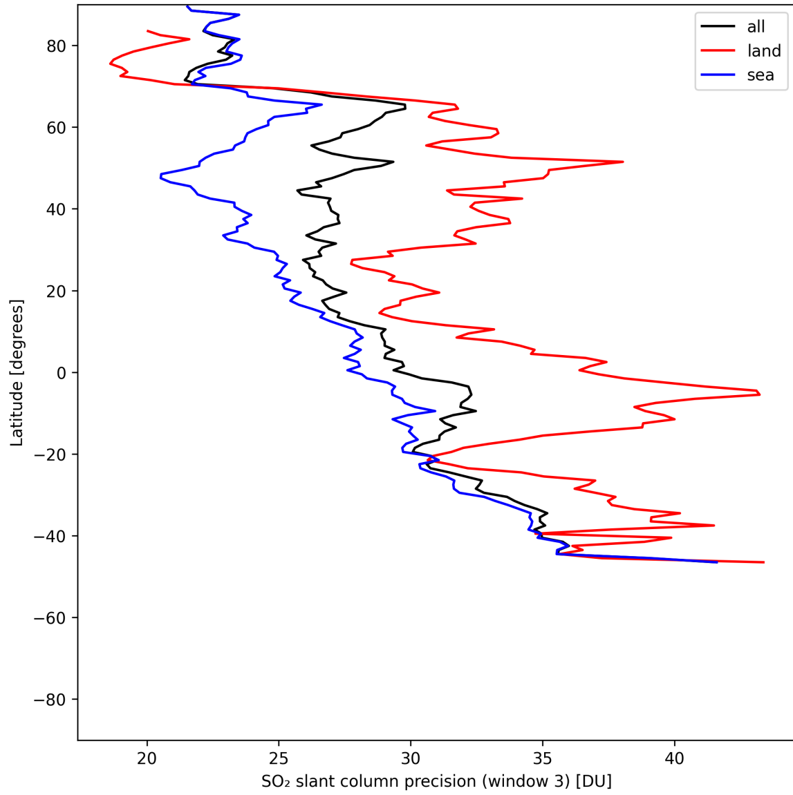
Figure 46: Zonal average of “SO 2 slant column precision (window 3)” for 2025-06-03 to 2025-06-05.
