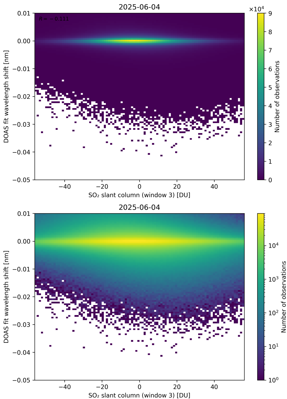
Figure 304: Scatter density plot of “SO 2 slant column (window 3)” against “DOAS fit wavelength shift” for 2025-06-03 to 2025-06-05.
