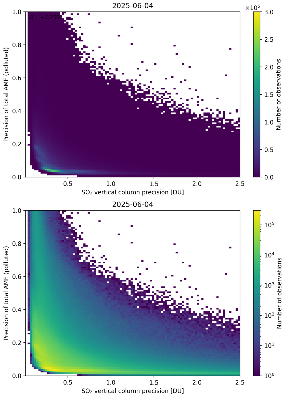
Figure 347: Scatter density plot of “SO 2 vertical column precision” against “Precision of total AMF (polluted)” for 2025-06-03 to 2025-06-05.
