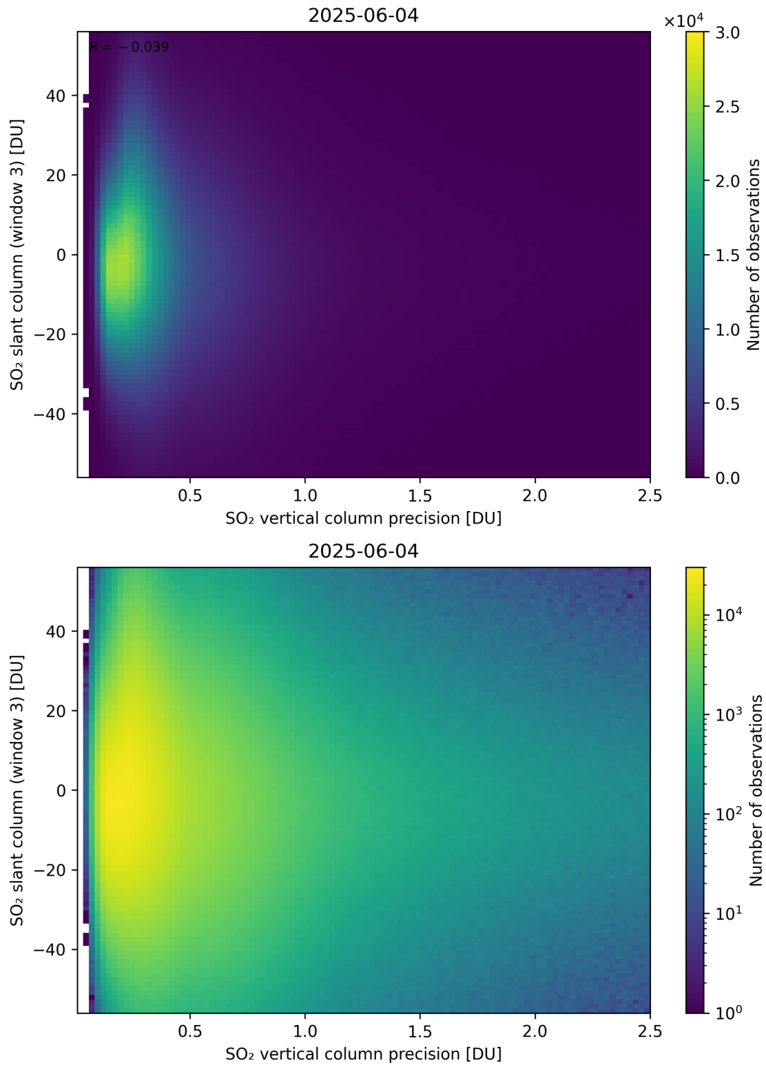
Figure 344: Scatter density plot of “SO 2 vertical column precision” against “SO 2 slant column (window 3)” for 2025-06-03 to 2025-06-05.
