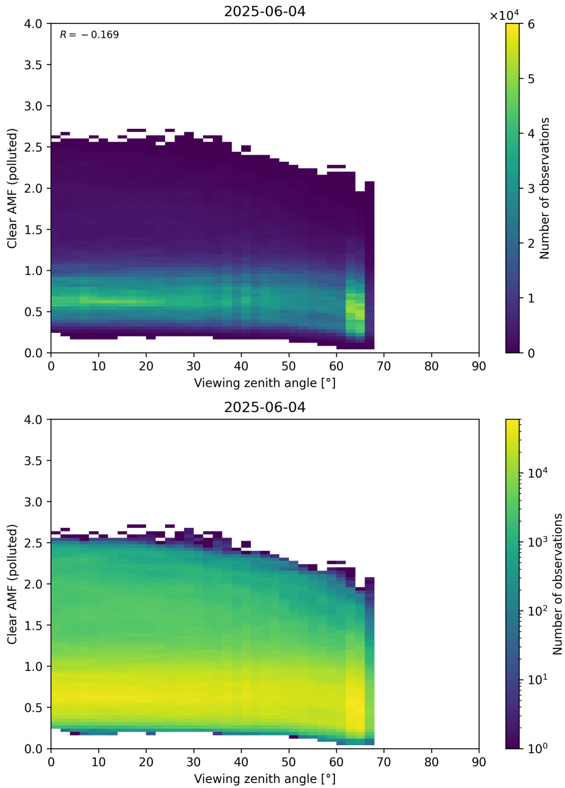
Figure 370: Scatter density plot of “Viewing zenith angle” against “Clear AMF (polluted)” for 2025-06-03 to 2025-06-05.
