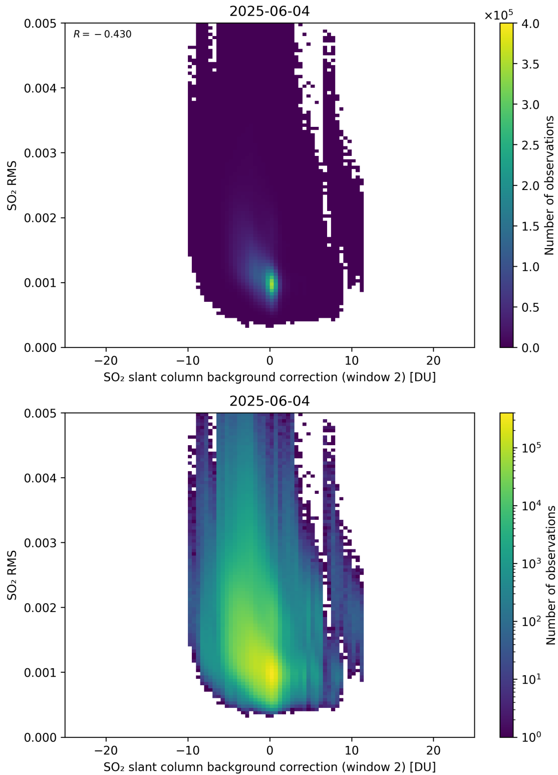
Figure 125: Scatter density plot of “SO 2 slant column background correction (window 2)” against “SO 2 RMS” for 2025-06-03 to 2025-06-05.
