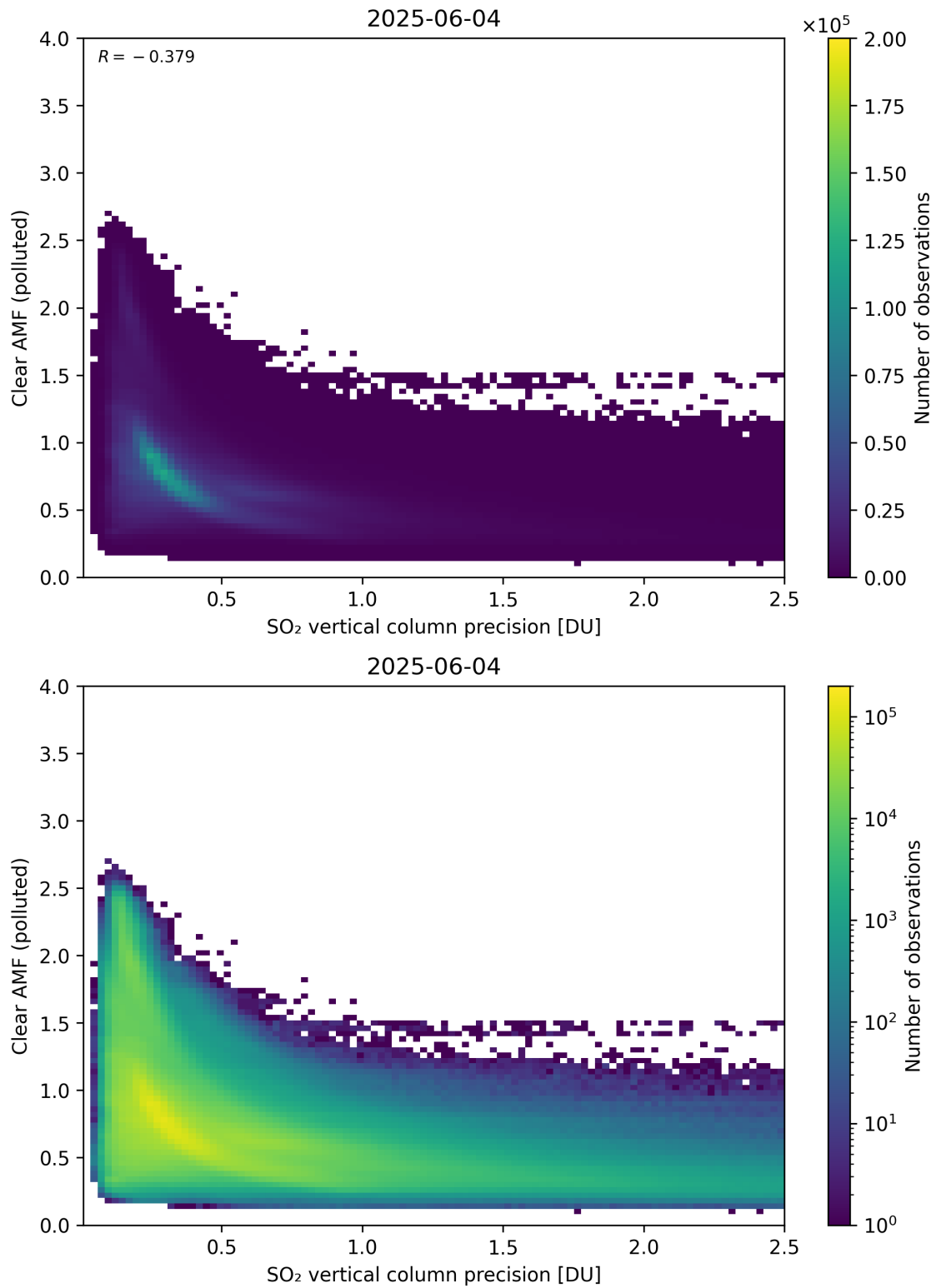
Figure 335: Scatter density plot of “SO 2 vertical column precision” against “Clear AMF (polluted)” for 2025-06-03 to 2025-06-05.
