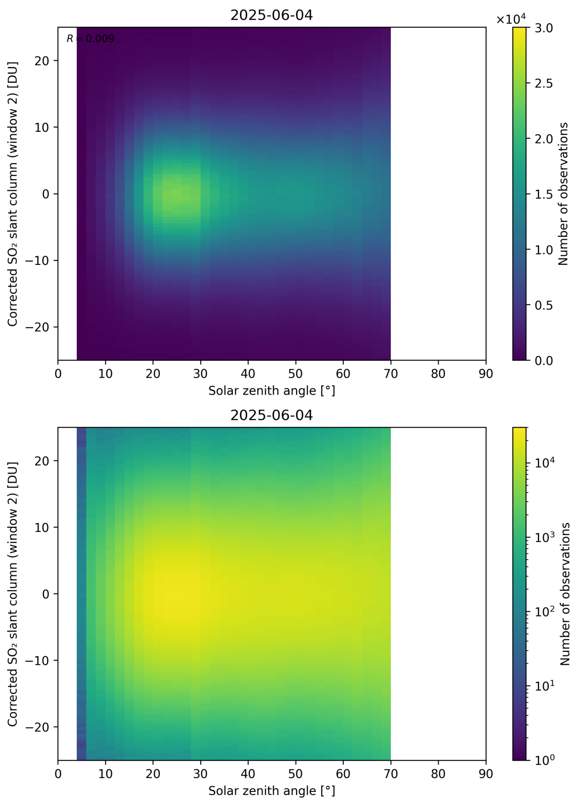
Figure 182: Scatter density plot of “Solar zenith angle” against “Corrected SO 2 slant column (window 2)” for 2025-06-03 to 2025-06-05.
