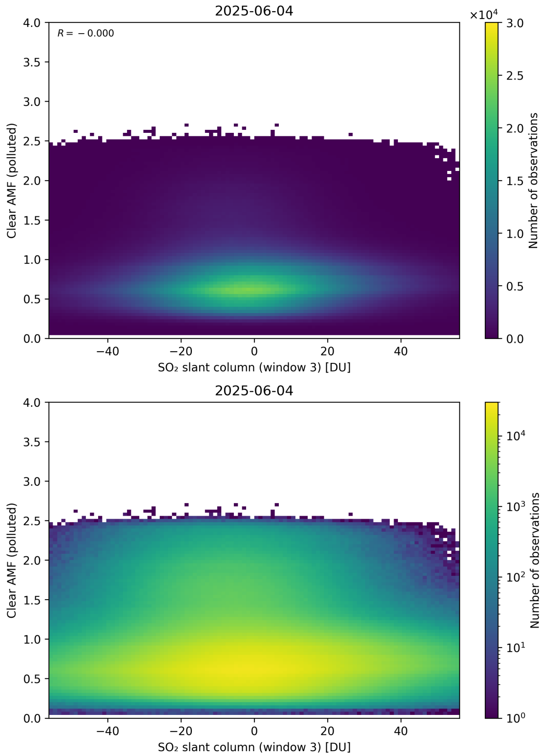
Figure 315: Scatter density plot of “SO 2 slant column (window 3)” against “Clear AMF (polluted)” for 2025-06-03 to 2025-06-05.
