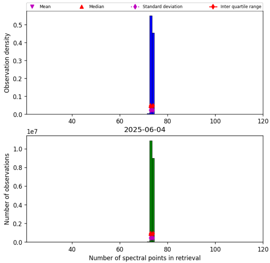
Figure 82: Histogram of “Number of spectral points in retrieval” for 2025-06-03 to 2025-06-05
