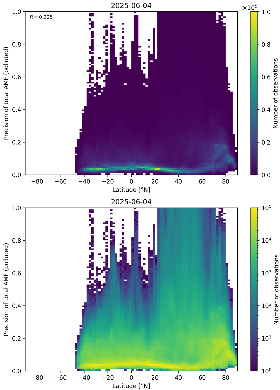
Figure 168: Scatter density plot of “Latitude” against “Precision of total AMF (polluted)” for 2025-06-03 to 2025-06-05.
