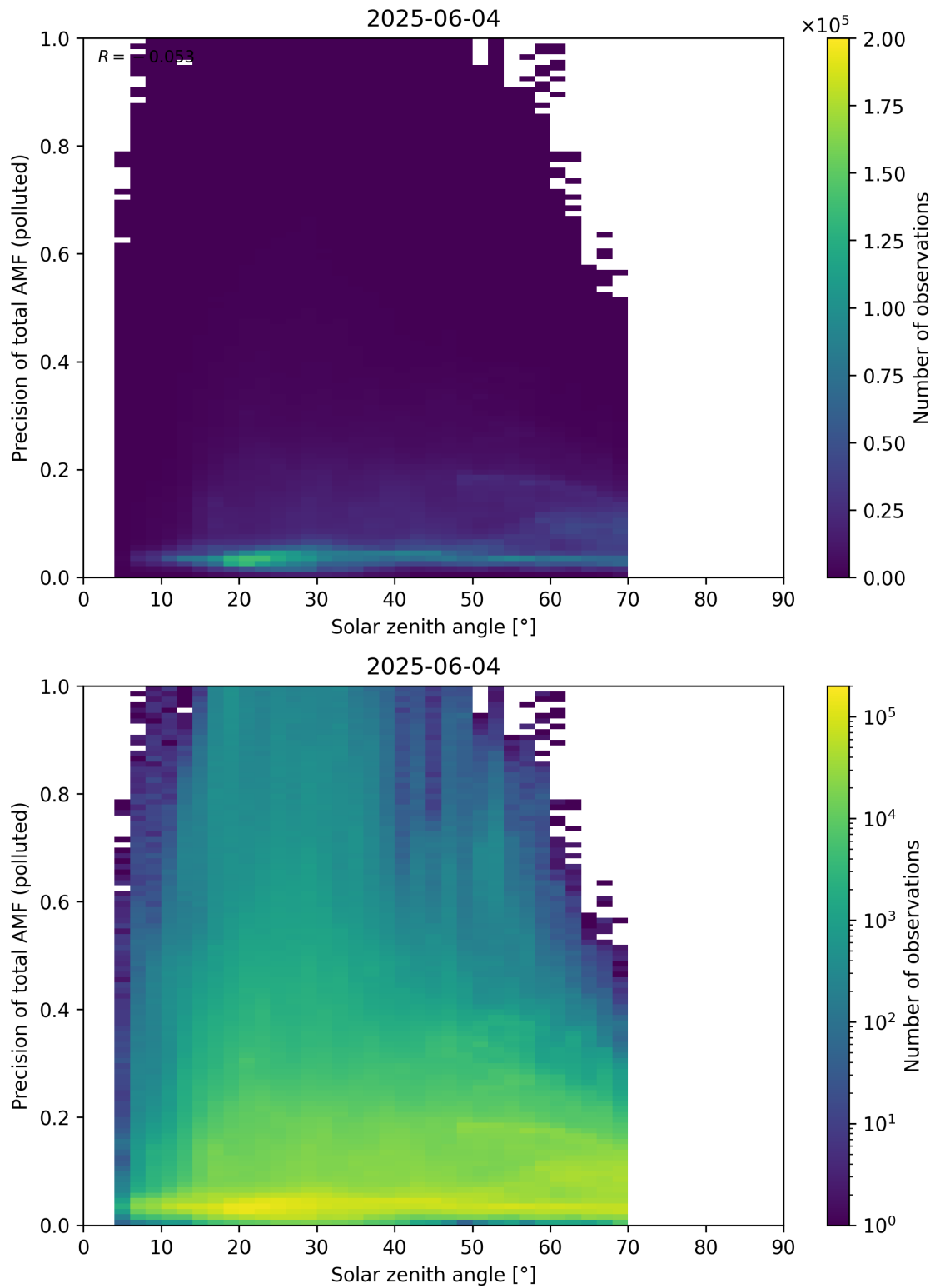
Figure 190: Scatter density plot of “Solar zenith angle” against “Precision of total AMF (polluted)” for 2025-06-03 to 2025-06-05.
