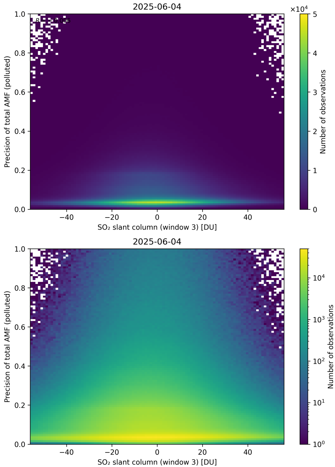
Figure 319: Scatter density plot of “SO 2 slant column (window 3)” against “Precision of total AMF (polluted)” for 2025-06-03 to 2025-06-05.
