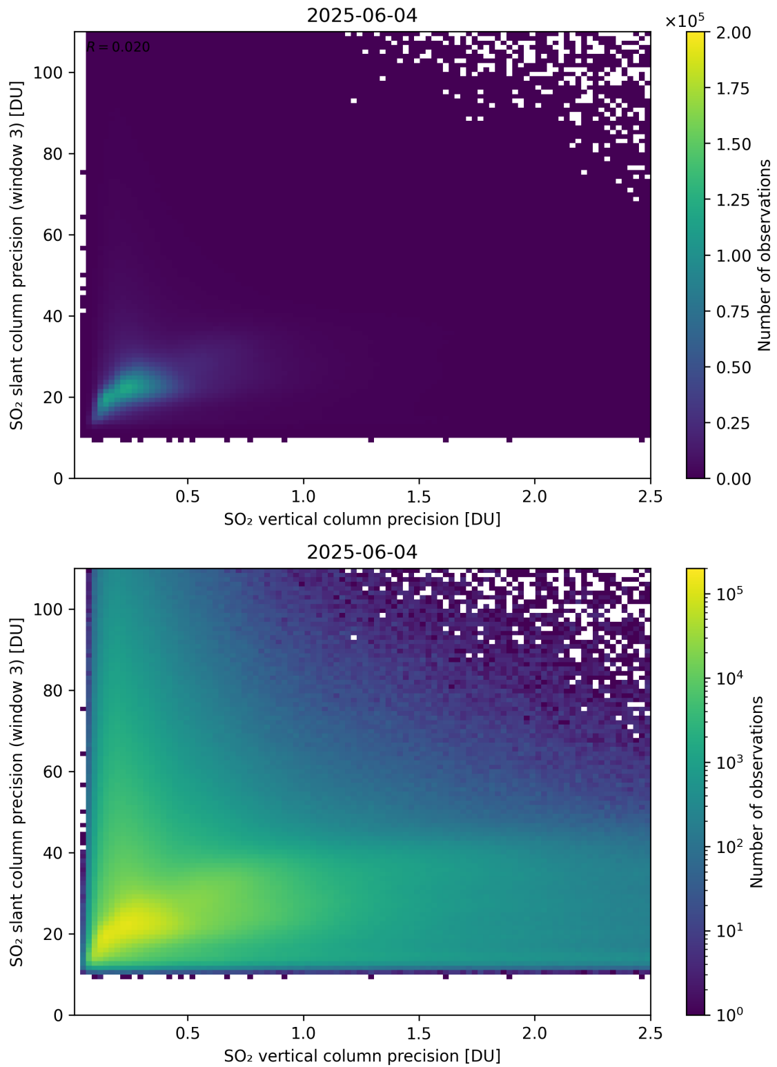
Figure 345: Scatter density plot of “SO 2 vertical column precision” against “SO 2 slant column precision (window 3)” for 2025-06-03 to 2025-06-05.
