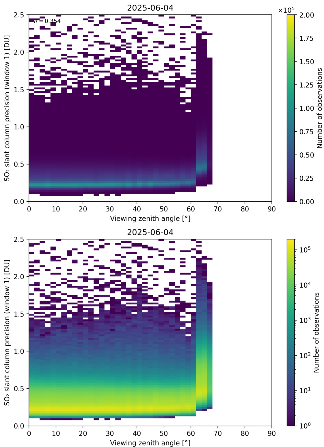
Figure 377: Scatter density plot of “Viewing zenith angle” against “SO 2 slant column precision (window 1)” for 2025-06-03 to 2025-06-05.
