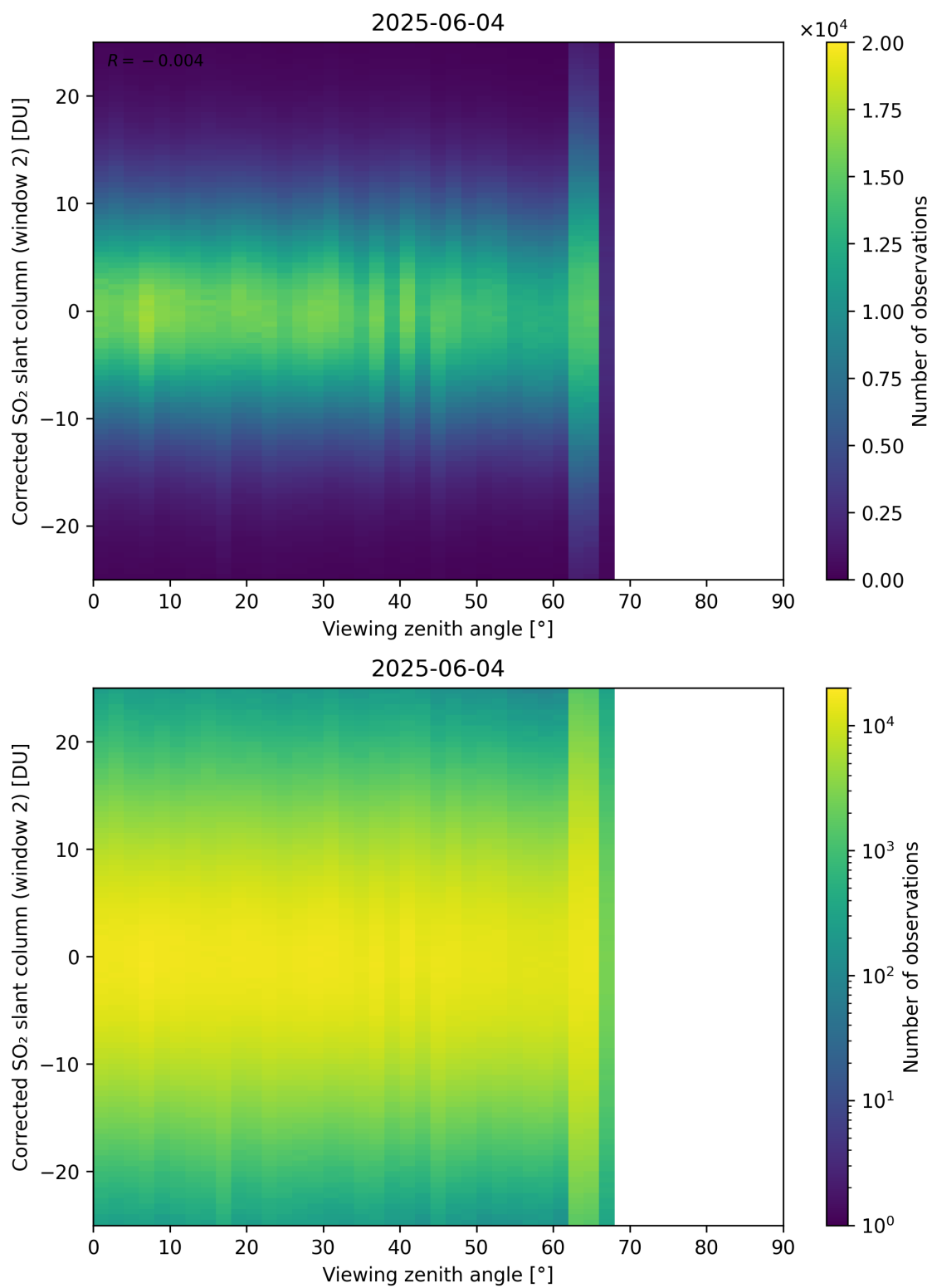
Figure 374: Scatter density plot of “Viewing zenith angle” against “Corrected SO 2 slant column (window 2)” for 2025-06-03 to 2025-06-05.
