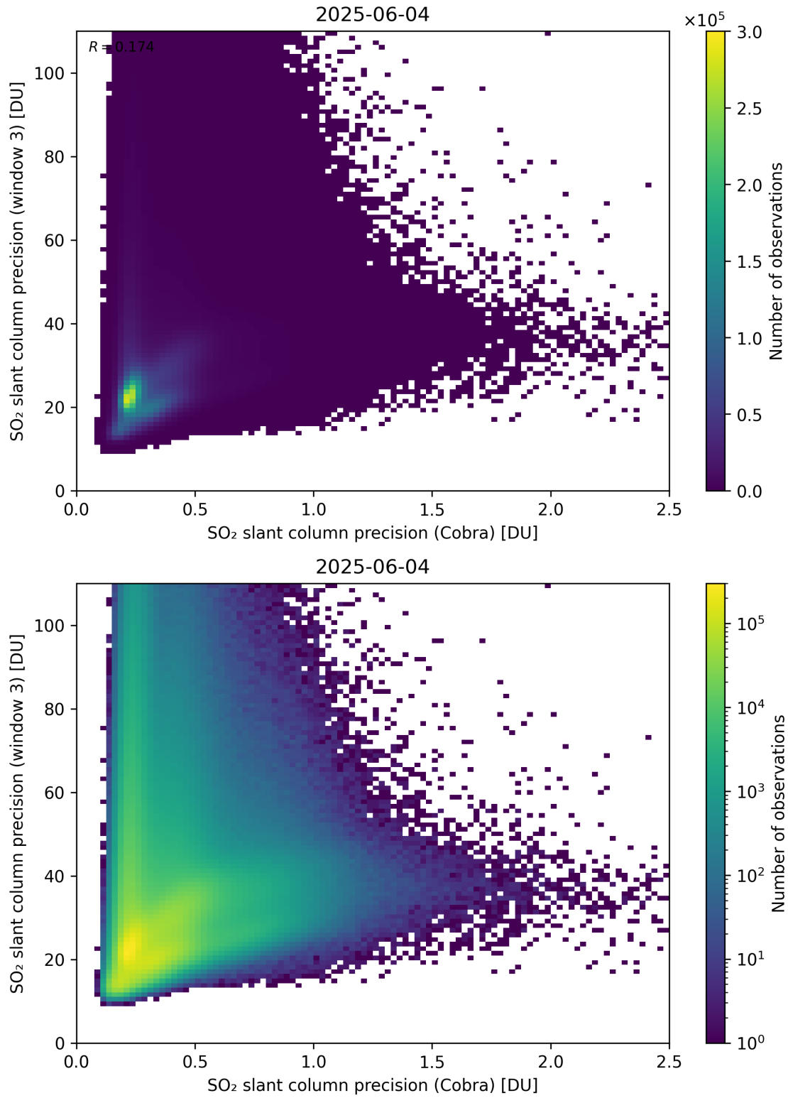
Figure 212: Scatter density plot of “SO 2 slant column precision (Cobra)” against “SO 2 slant column precision (window 3)” for 2025-06-03 to 2025-06-05.
