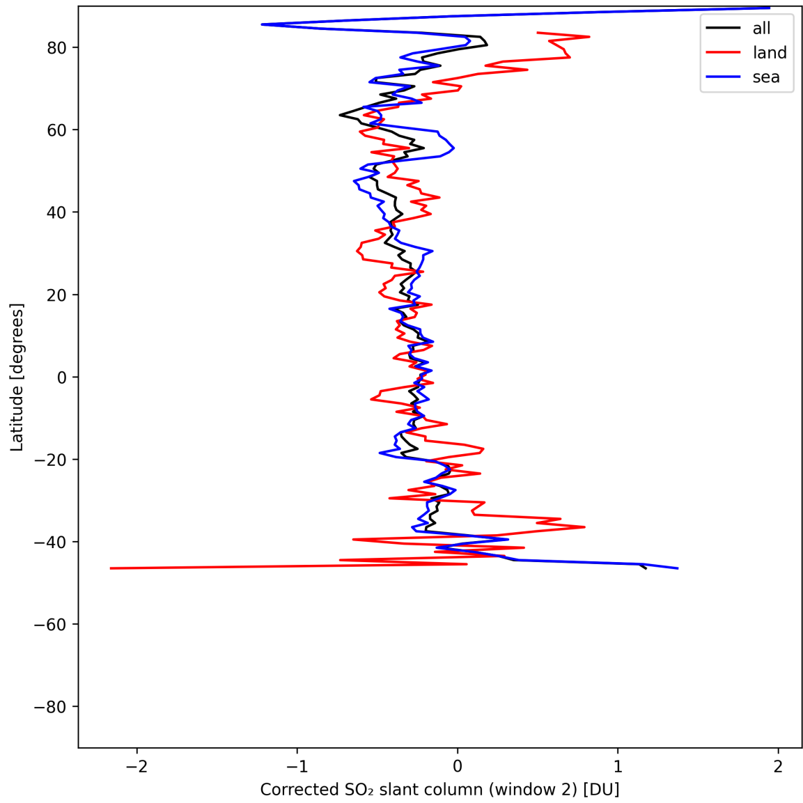
Figure 43: Zonal average of “Corrected SO 2 slant column (window 2)” for 2025-06-03 to 2025-06-05.
