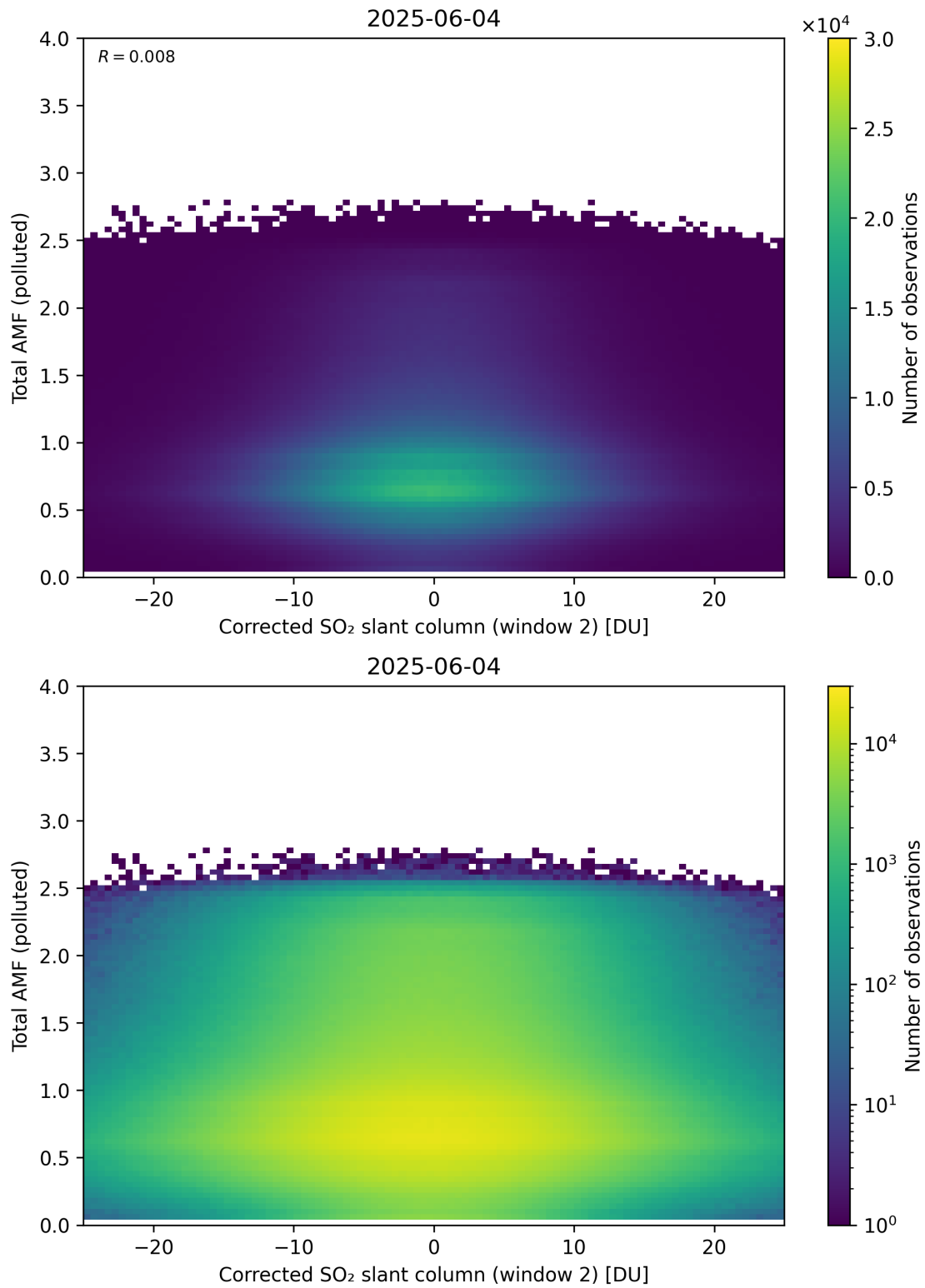
Figure 253: Scatter density plot of “Corrected SO 2 slant column (window 2)” against “Total AMF (polluted)” for 2025-06-03 to 2025-06-05.
