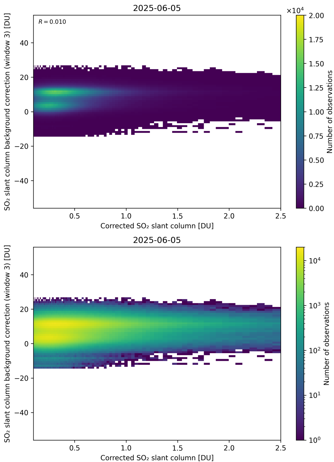
Figure 228: Scatter density plot of “Corrected SO 2 slant column” against “SO 2 slant column background correction (window 3)” for 2025-06-04 to 2025-06-06.
