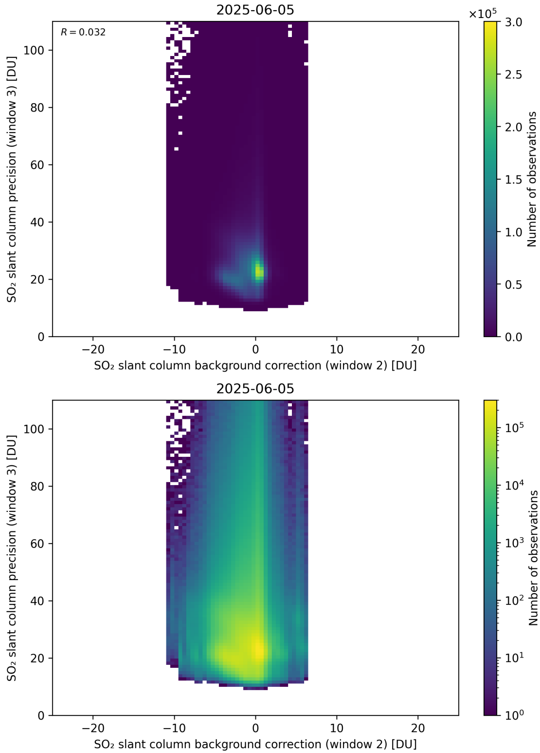
Figure 129: Scatter density plot of “SO 2 slant column background correction (window 2)” against “SO 2 slant column precision (window 3)” for 2025-06-04 to 2025-06-06.
