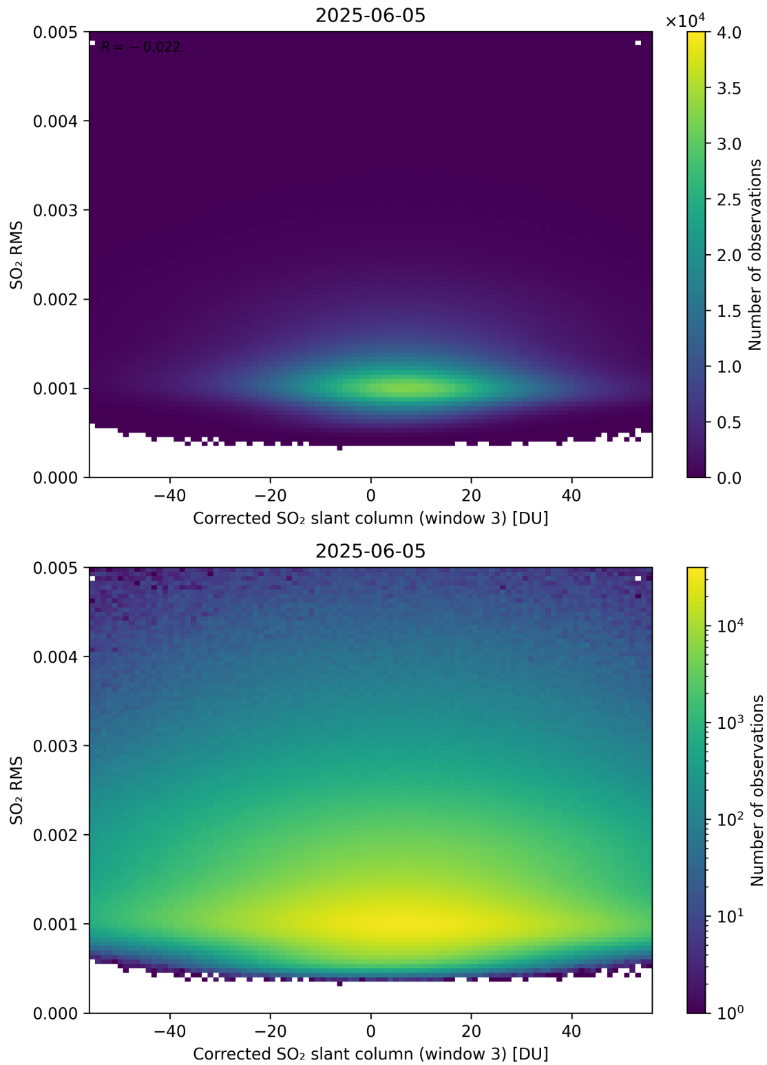
Figure 258: Scatter density plot of “Corrected SO 2 slant column (window 3)” against “SO 2 RMS” for 2025-06-04 to 2025-06-06.
