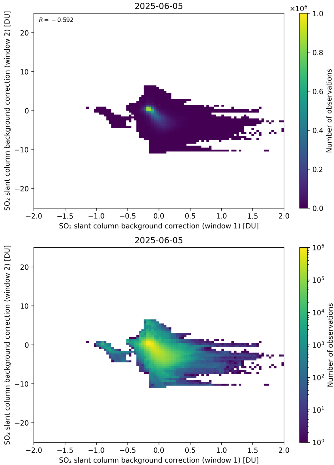
Figure 109: Scatter density plot of “SO 2 slant column background correction (window 1)” against “SO 2 slant column background correction (window 2)” for 2025-06-04 to 2025-06-06.
