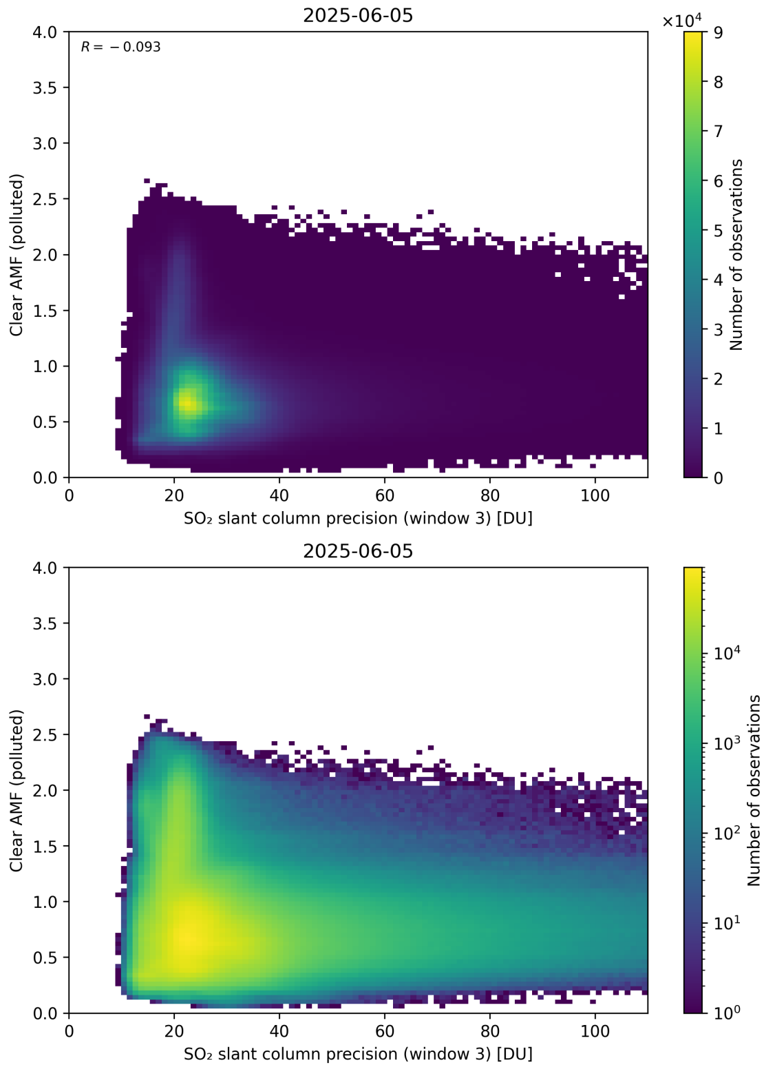
Figure 311: Scatter density plot of “SO 2 slant column precision (window 3)” against “Clear AMF (polluted)” for 2025-06-04 to 2025-06-06.
