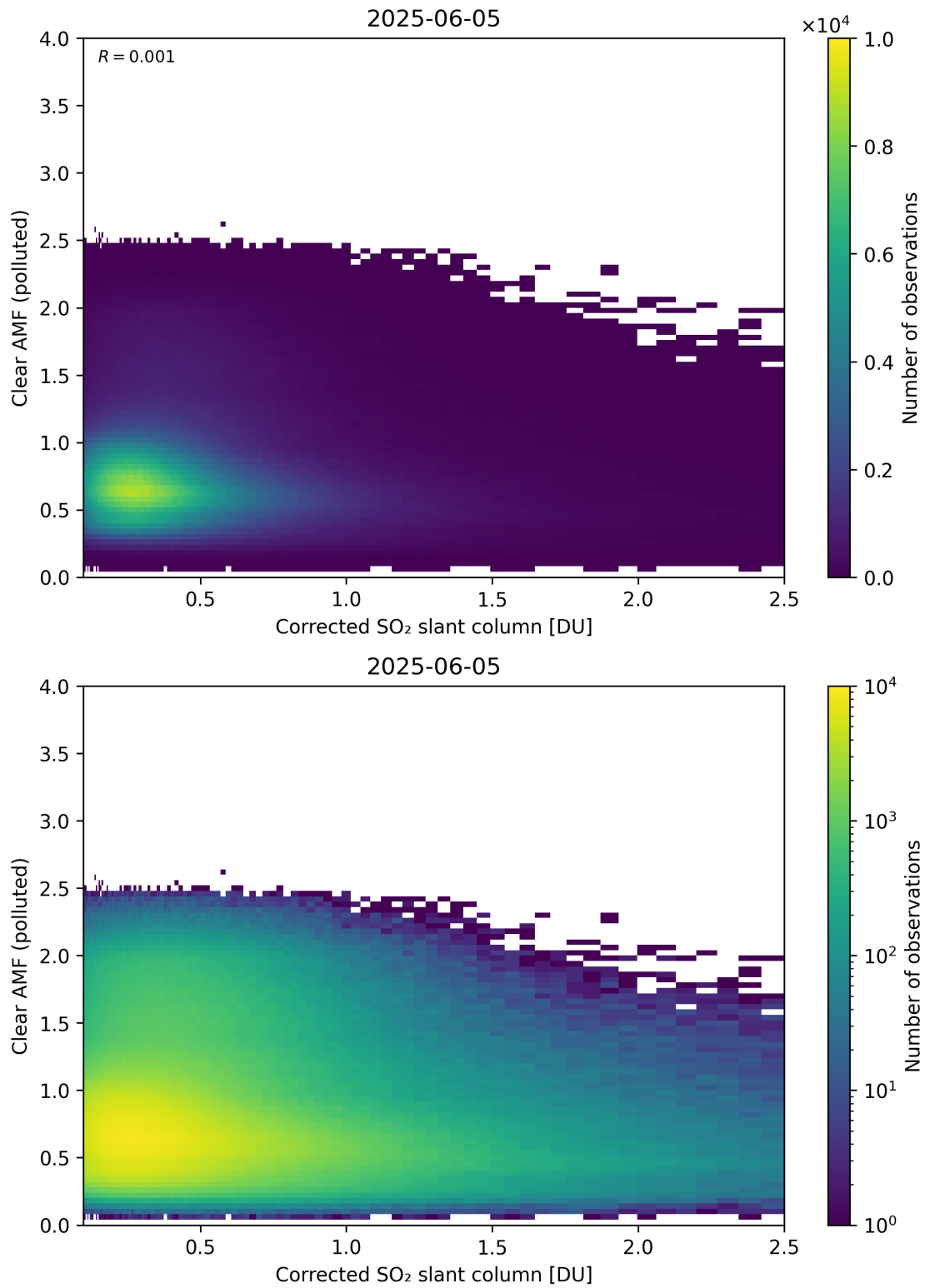
Figure 232: Scatter density plot of “Corrected SO 2 slant column” against “Clear AMF (polluted)” for 2025-06-04 to 2025-06-06.
