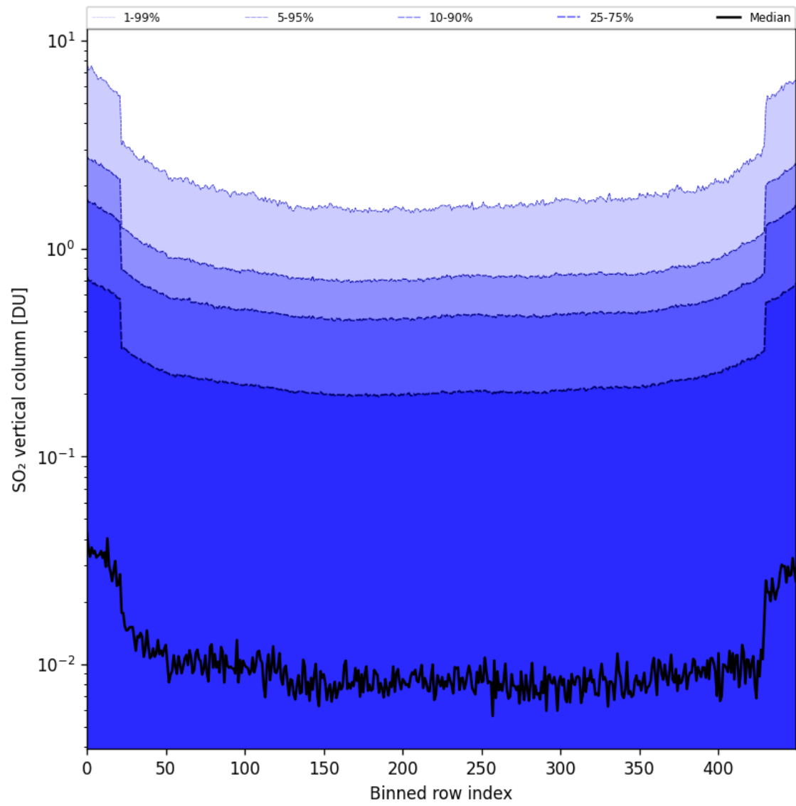
Figure 84: Along track statistics of “SO 2 vertical column” for 2025-06-04 to 2025-06-06
