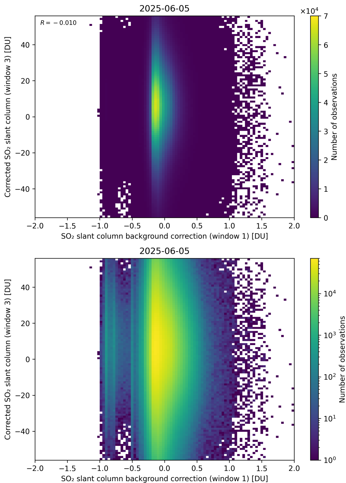
Figure 116: Scatter density plot of “SO 2 slant column background correction (window 1)” against “Corrected SO 2 slant column (window 3)” for 2025-06-04 to 2025-06-06.
