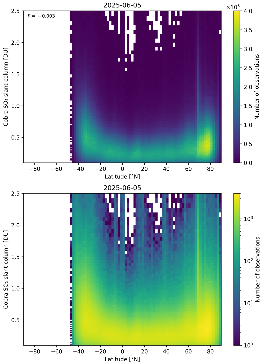
Figure 157: Scatter density plot of “Latitude” against “Cobra SO 2 slant column” for 2025-06-04 to 2025-06-06.
