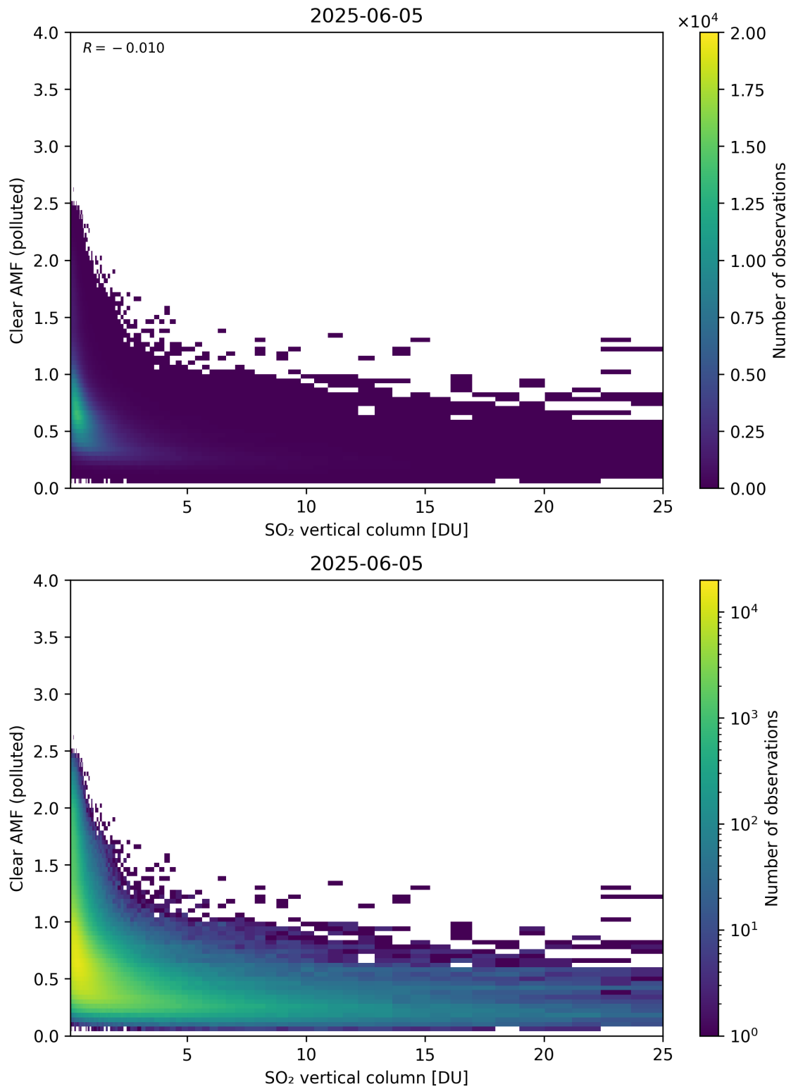
Figure 348: Scatter density plot of “SO 2 vertical column” against “Clear AMF (polluted)” for 2025-06-04 to 2025-06-06.
