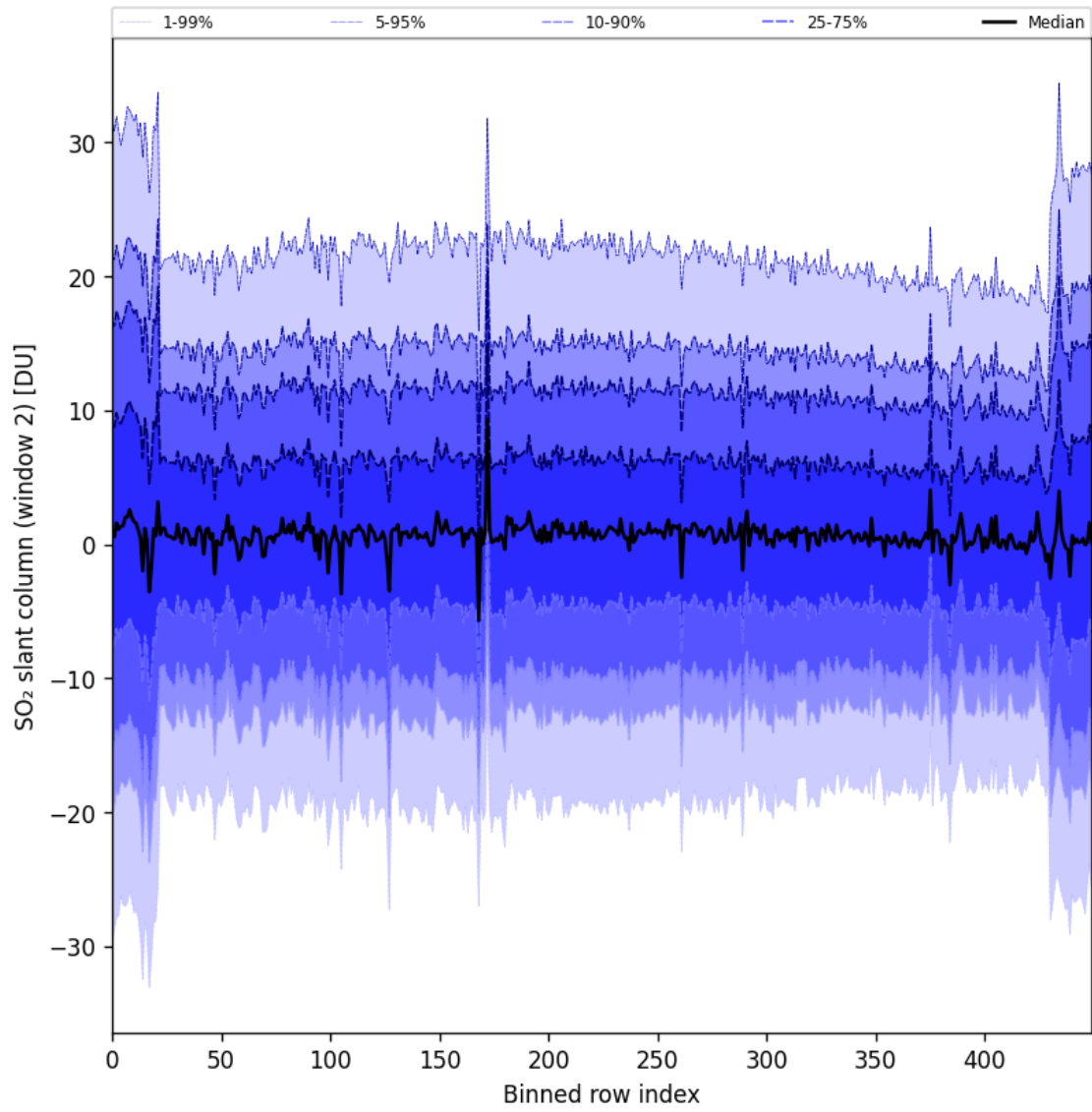
Figure 93: Along track statistics of “SO 2 slant column (window 2)” for 2025-06-04 to 2025-06-06
