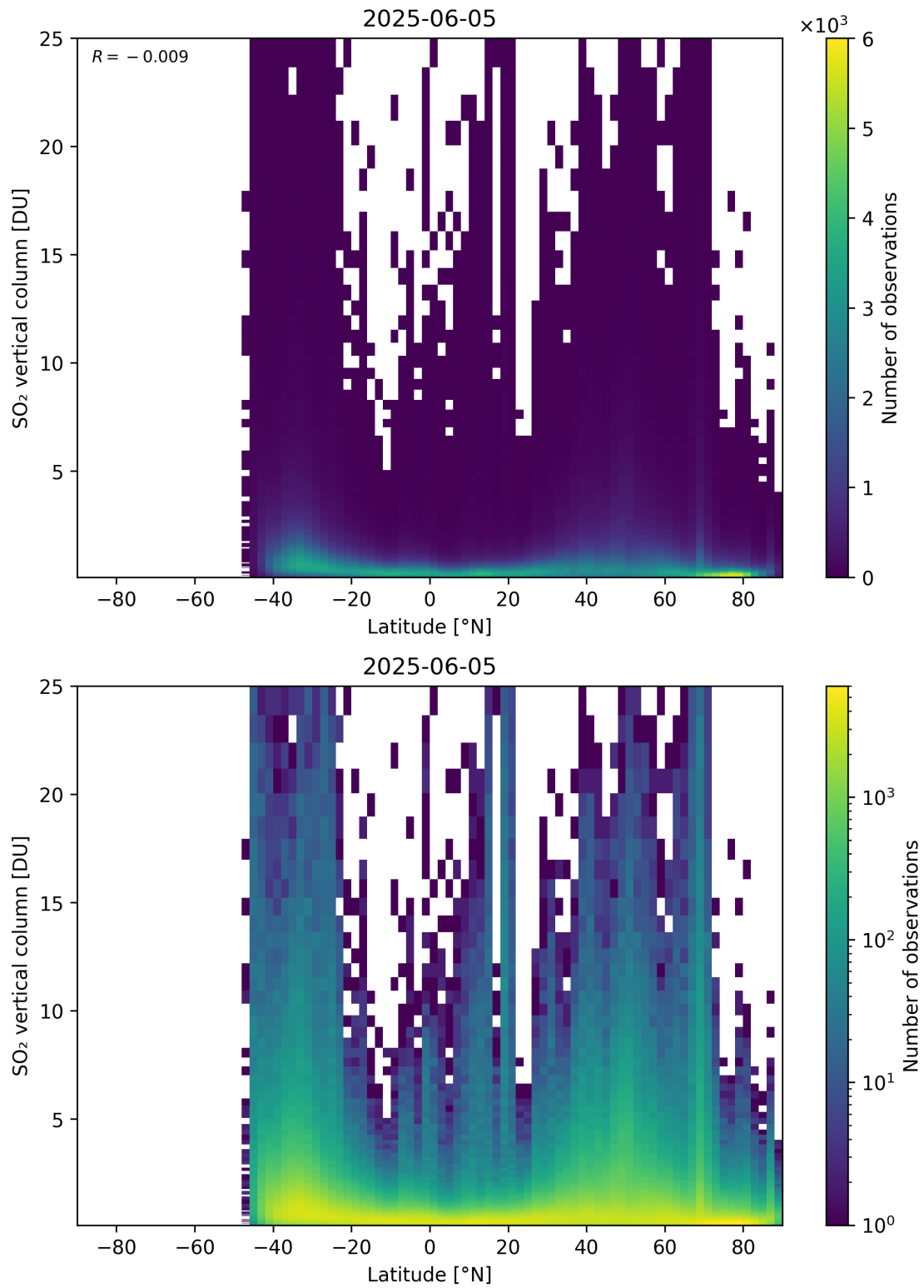
Figure 169: Scatter density plot of “Latitude” against “SO 2 vertical column” for 2025-06-04 to 2025-06-06.
