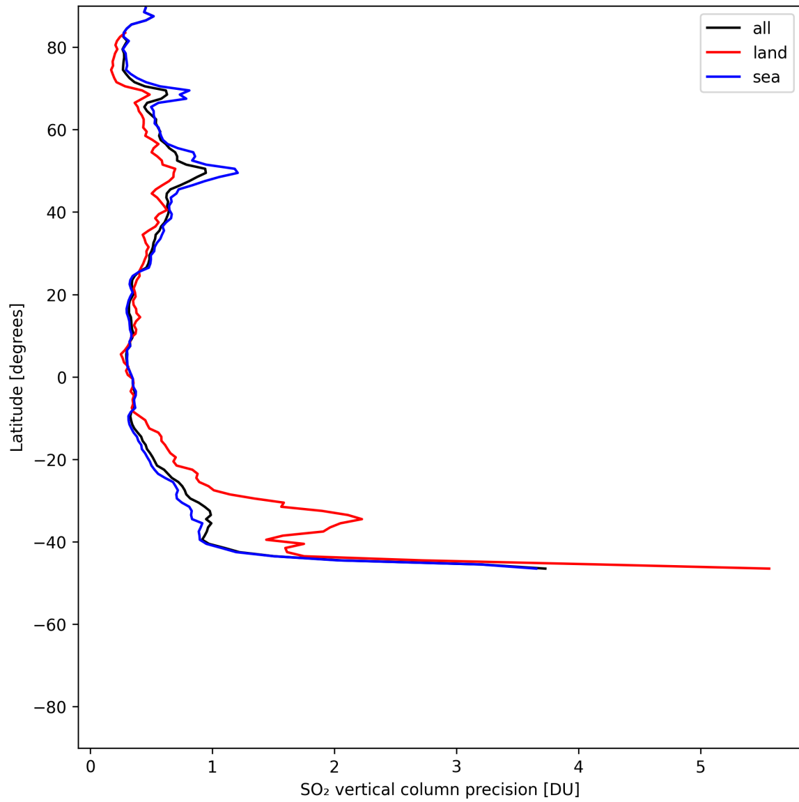
Figure 33: Zonal average of “SO 2 vertical column precision” for 2025-06-04 to 2025-06-06.
