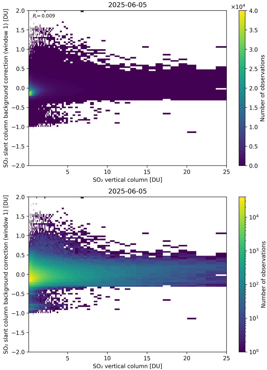
Figure 323: Scatter density plot of “SO 2 vertical column” against “SO 2 slant column background correction (window 1)” for 2025-06-04 to 2025-06-06.
