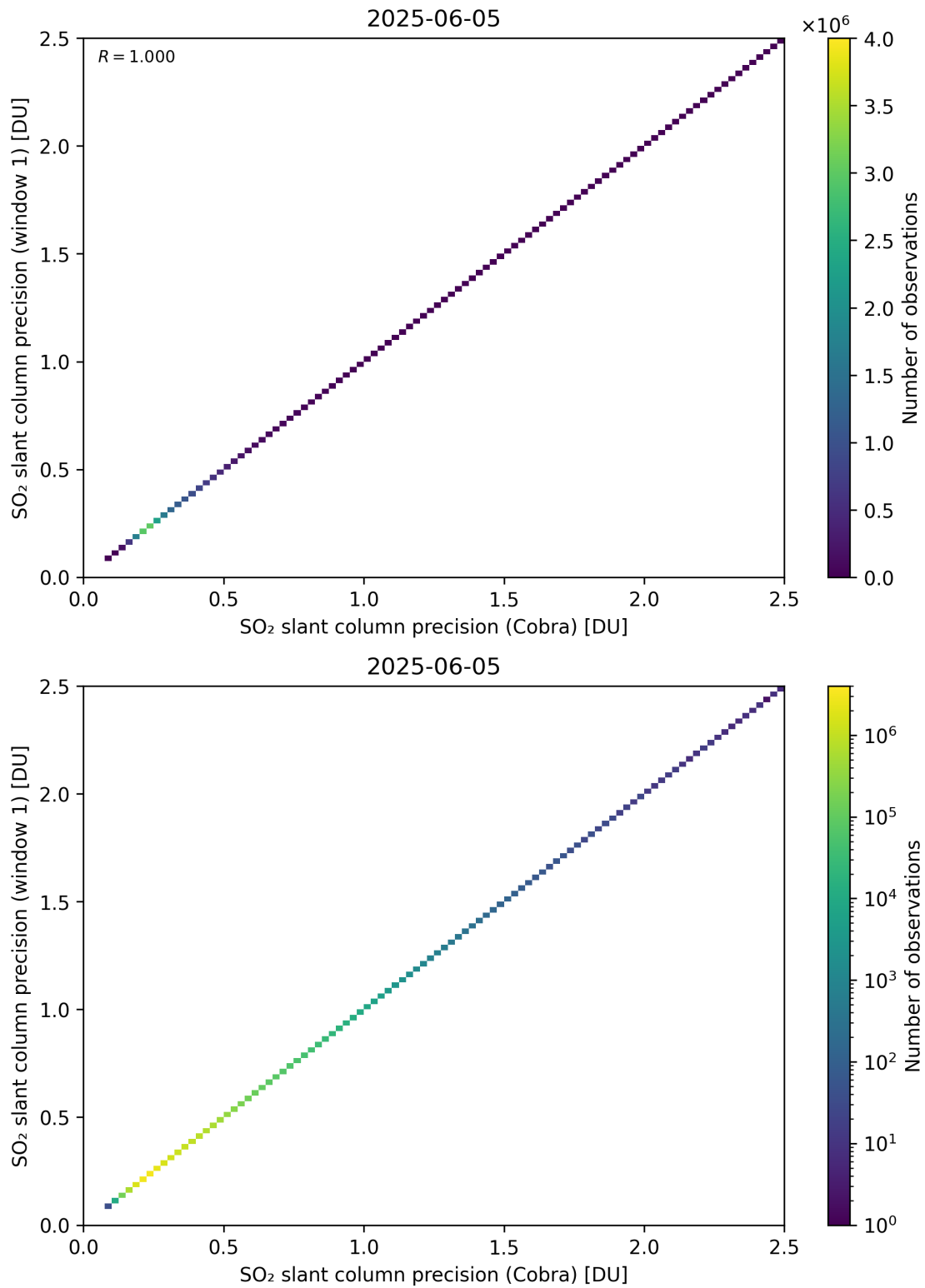
Figure 209: Scatter density plot of “SO 2 slant column precision (Cobra)” against “SO 2 slant column precision (window 1)” for 2025-06-04 to 2025-06-06.
