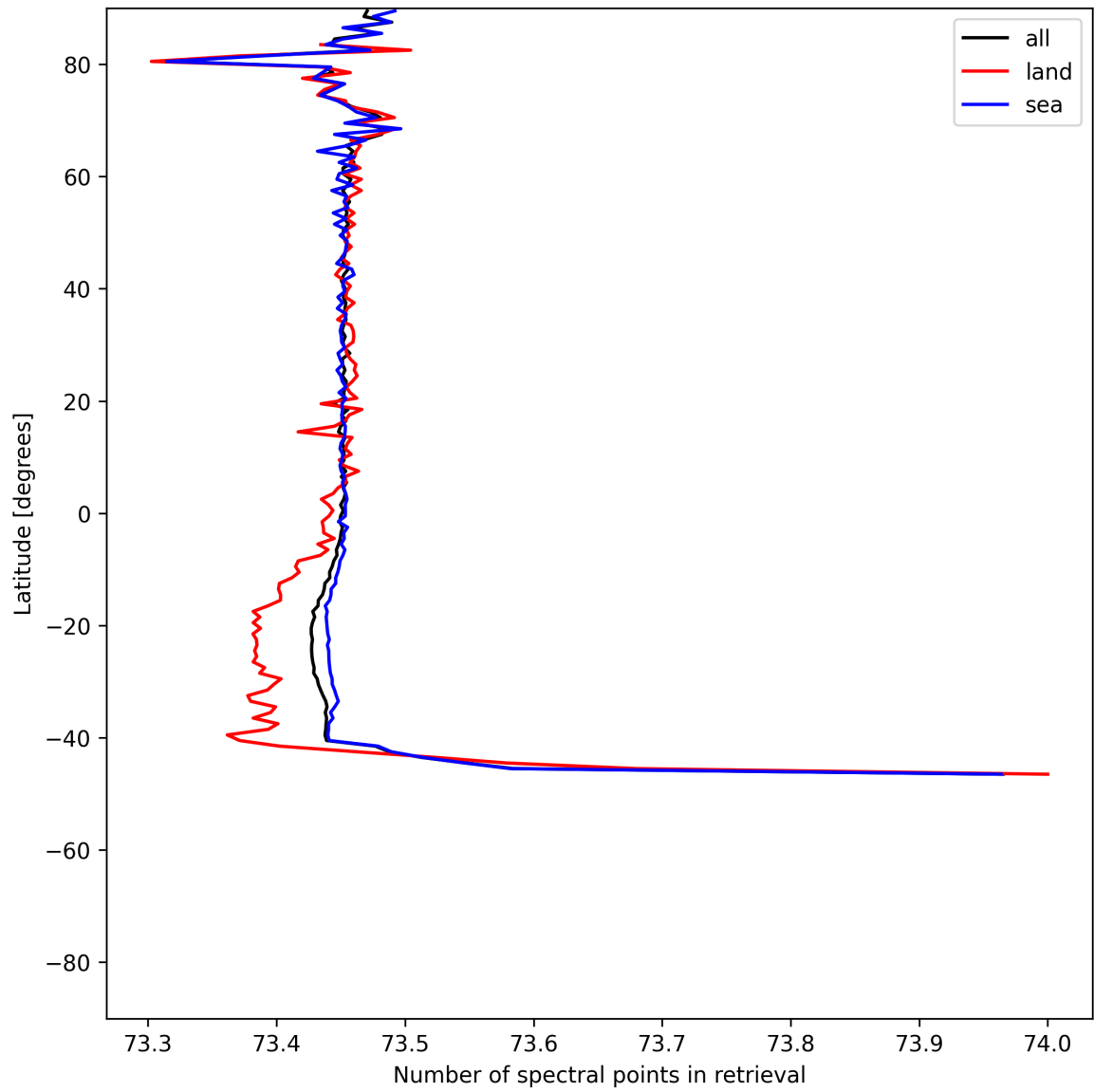
Figure 56: Zonal average of “Number of spectral points in retrieval” for 2025-06-04 to 2025-06-06.
