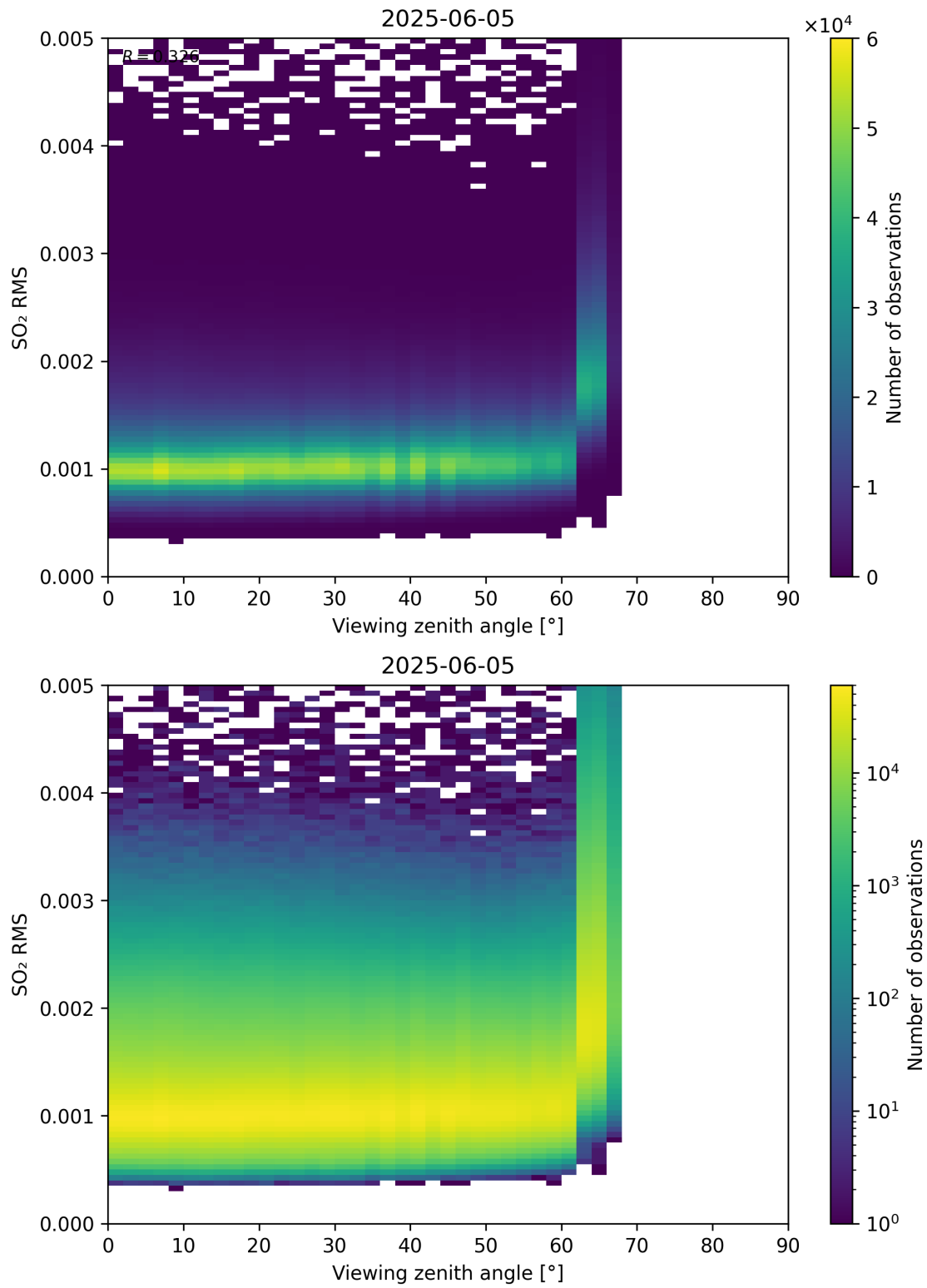
Figure 367: Scatter density plot of “Viewing zenith angle” against “SO 2 RMS” for 2025-06-04 to 2025-06-06.
