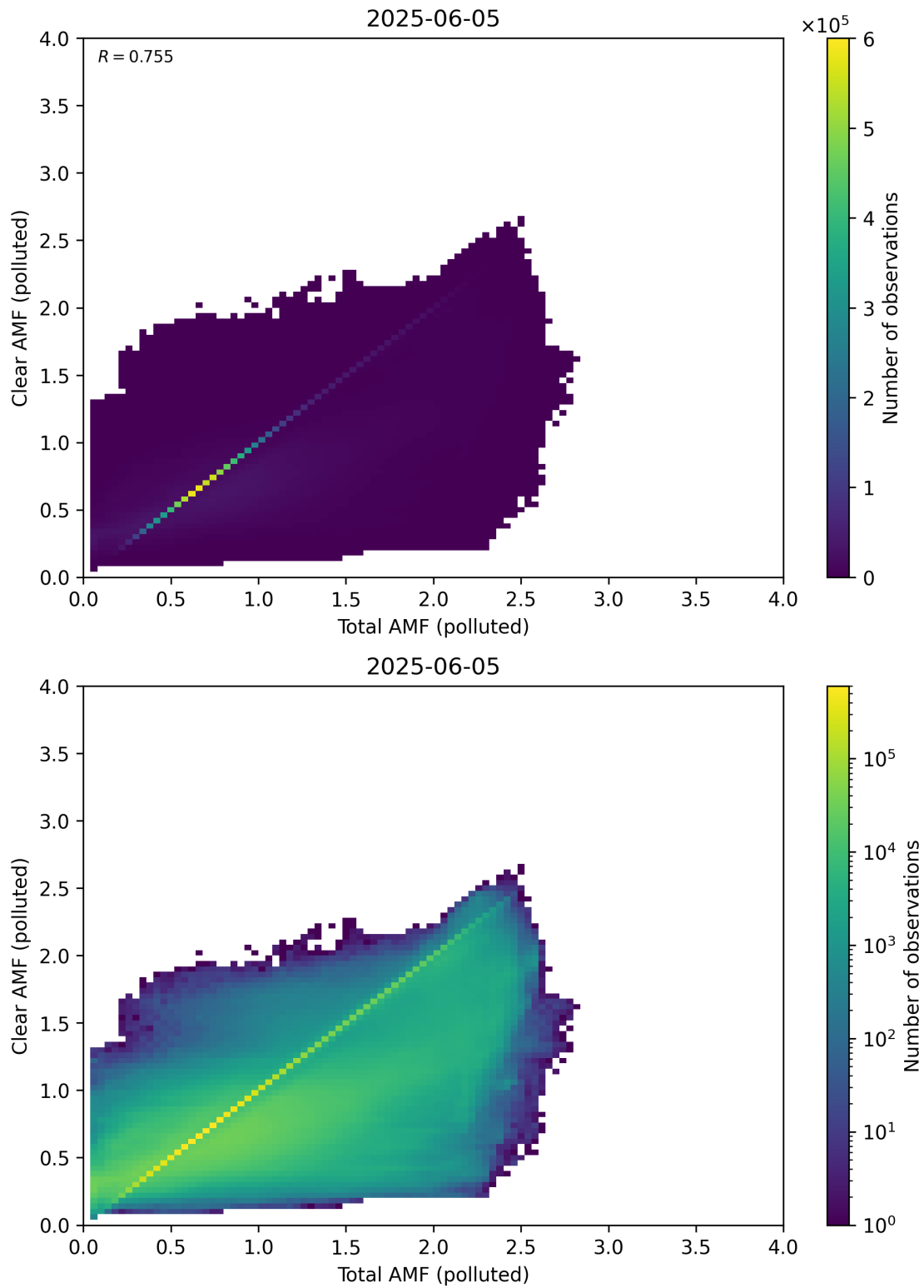
Figure 321: Scatter density plot of “Total AMF (polluted)” against “Clear AMF (polluted)” for 2025-06-04 to 2025-06-06.
