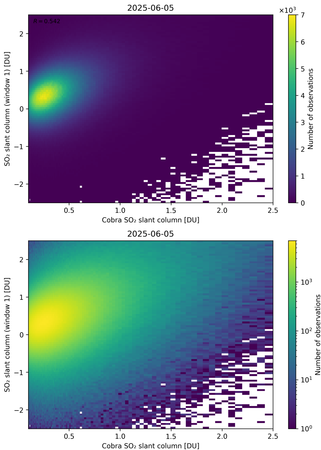
Figure 219: Scatter density plot of “Cobra SO 2 slant column” against “SO 2 slant column (window 1)” for 2025-06-04 to 2025-06-06.
