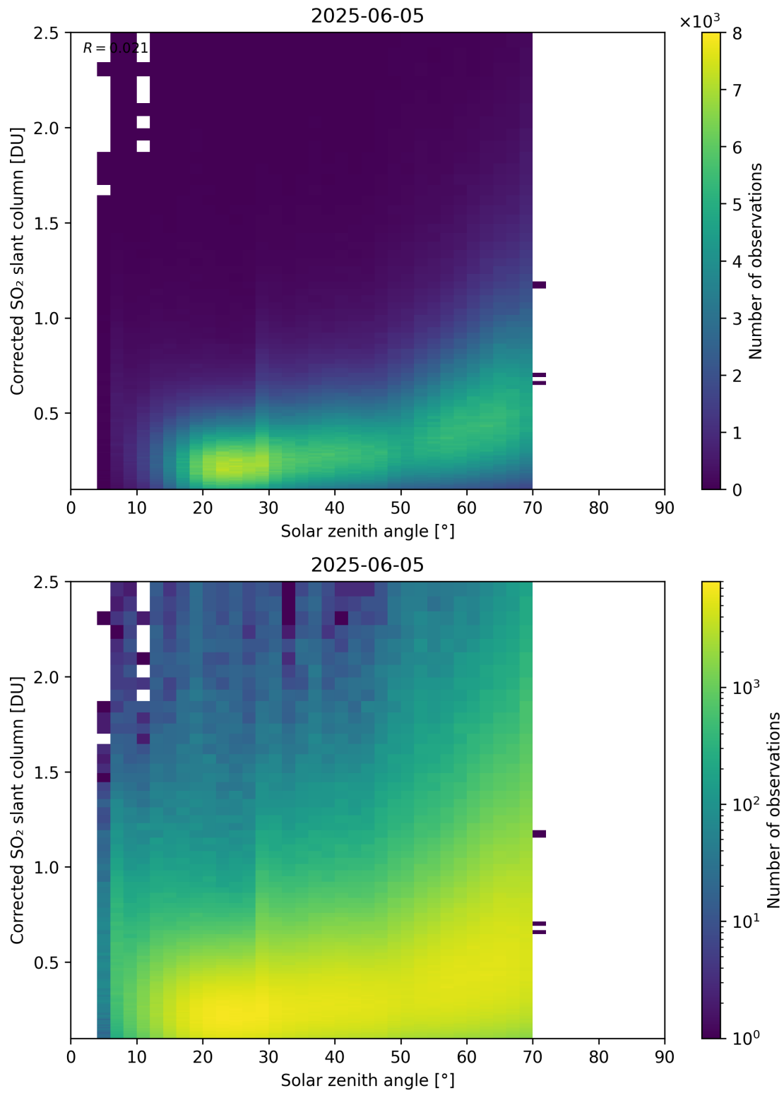
Figure 181: Scatter density plot of “Solar zenith angle” against “Corrected SO 2 slant column” for 2025-06-04 to 2025-06-06.
