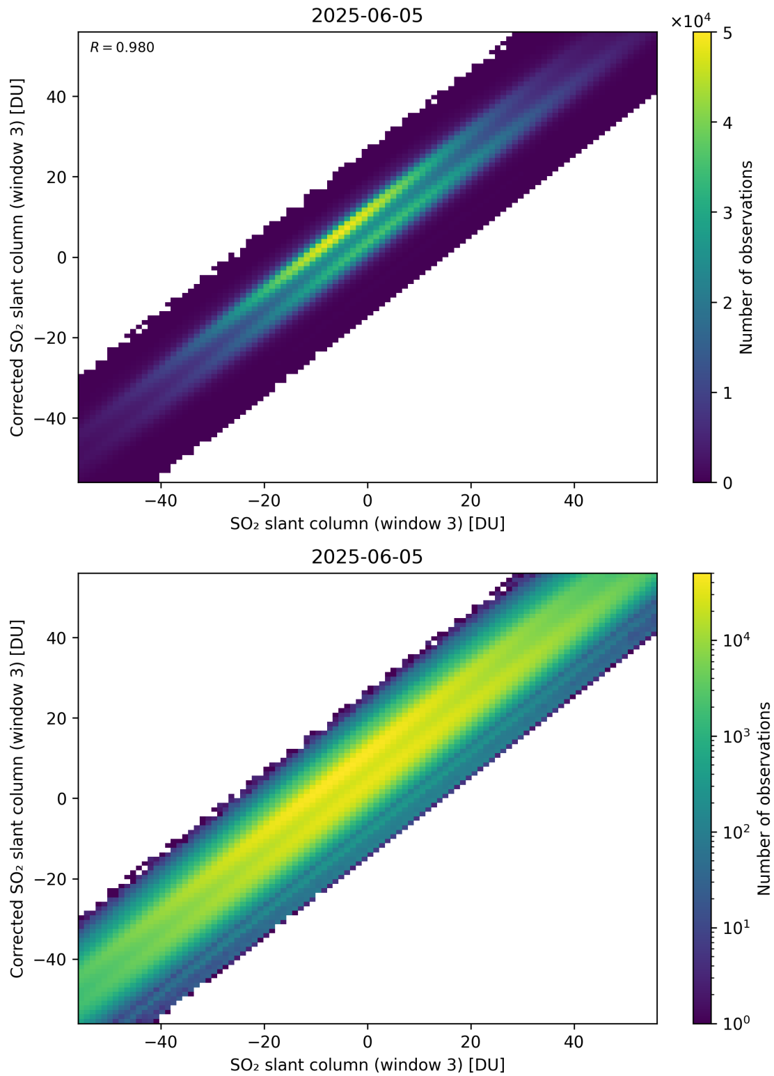
Figure 316: Scatter density plot of “SO 2 slant column (window 3)” against “Corrected SO 2 slant column (window 3)” for 2025-06-04 to 2025-06-06.
