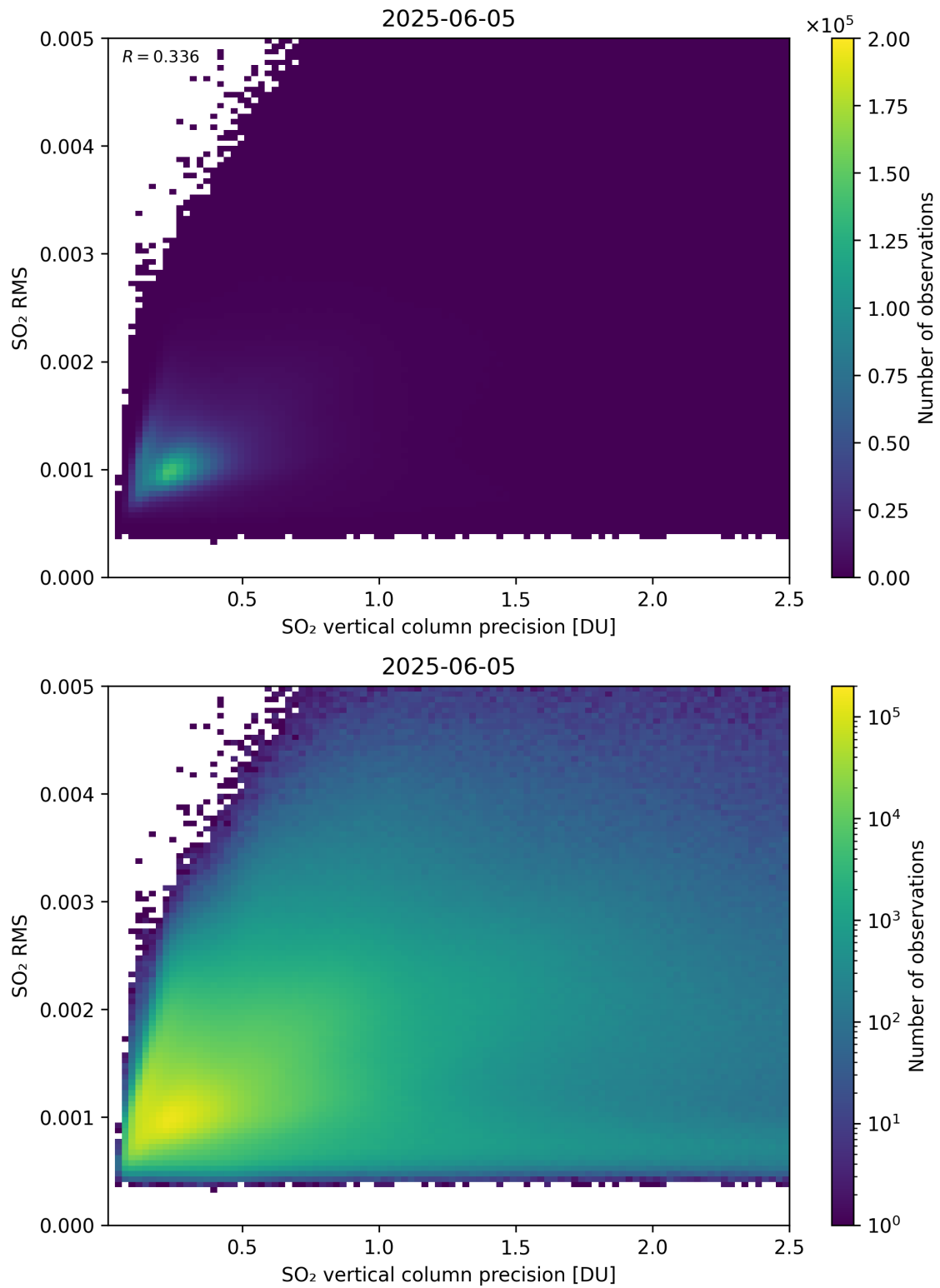
Figure 334: Scatter density plot of “SO 2 vertical column precision” against “SO 2 RMS” for 2025-06-04 to 2025-06-06.
