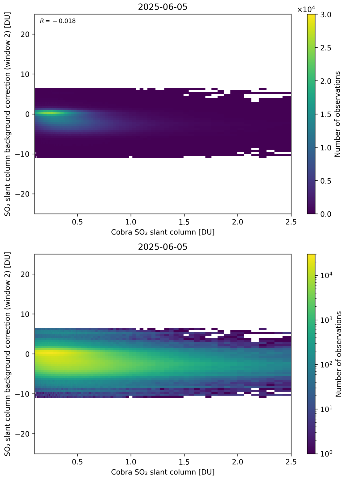
Figure 194: Scatter density plot of “Cobra SO 2 slant column” against “SO 2 slant column background correction (window 2)” for 2025-06-04 to 2025-06-06.
