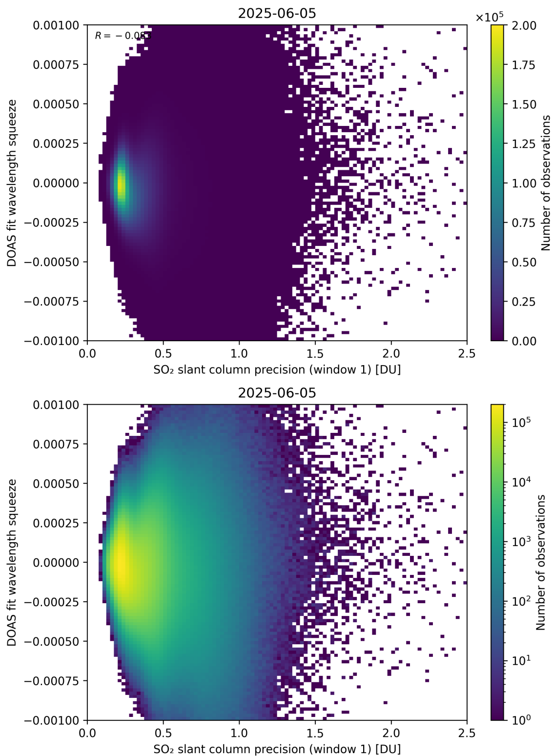
Figure 272: Scatter density plot of “SO 2 slant column precision (window 1)” against “DOAS fit wavelength squeeze” for 2025-06-04 to 2025-06-06.
