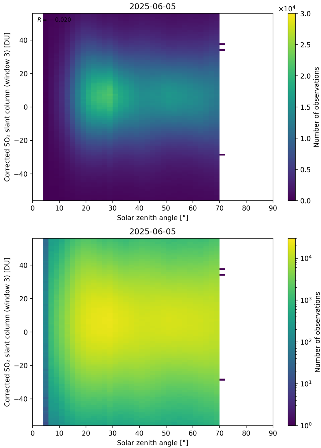
Figure 183: Scatter density plot of “Solar zenith angle” against “Corrected SO 2 slant column (window 3)” for 2025-06-04 to 2025-06-06.
