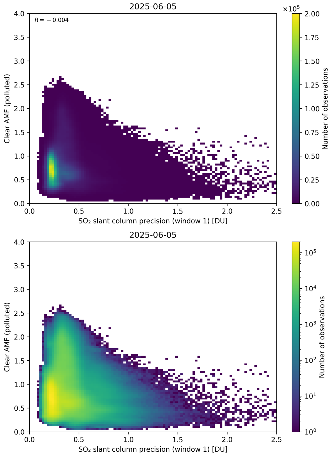
Figure 274: Scatter density plot of “SO 2 slant column precision (window 1)” against “Clear AMF (polluted)” for 2025-06-04 to 2025-06-06.
