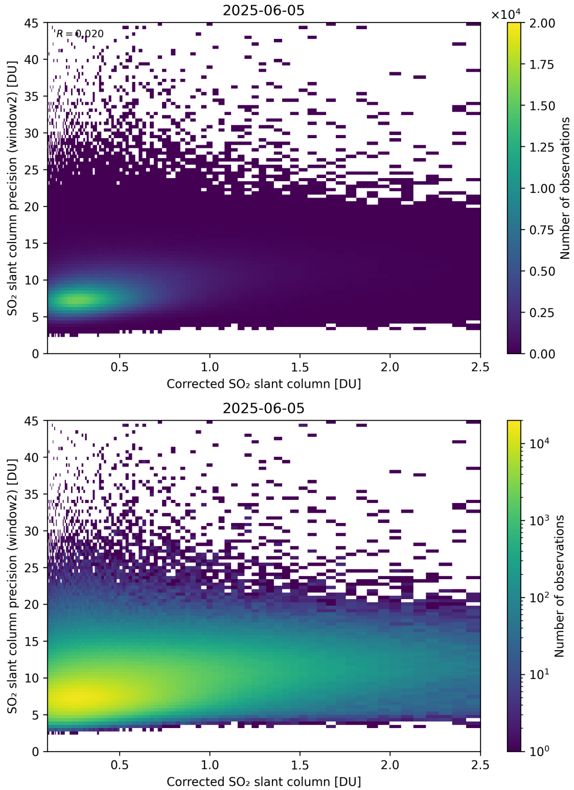
Figure 239: Scatter density plot of “Corrected SO 2 slant column” against “SO 2 slant column precision (window2)” for 2025-06-04 to 2025-06-06.
