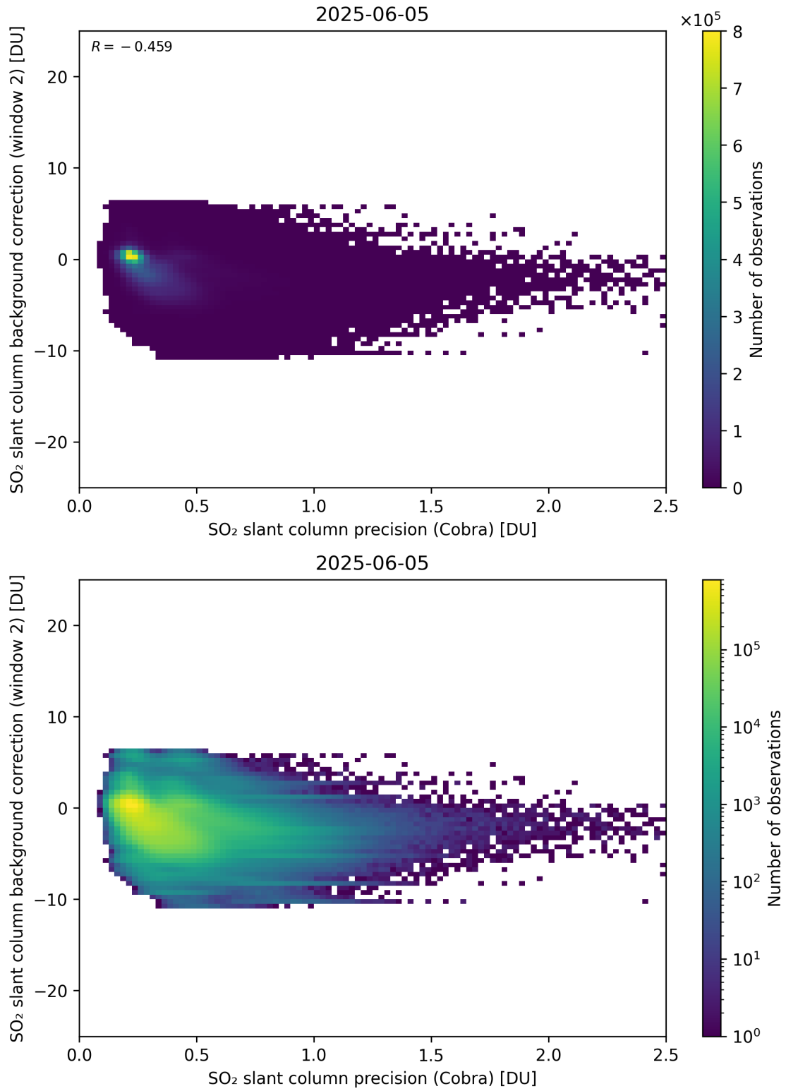
Figure 200: Scatter density plot of “SO 2 slant column precision (Cobra)” against “SO 2 slant column background correction (window 2)” for 2025-06-04 to 2025-06-06.
