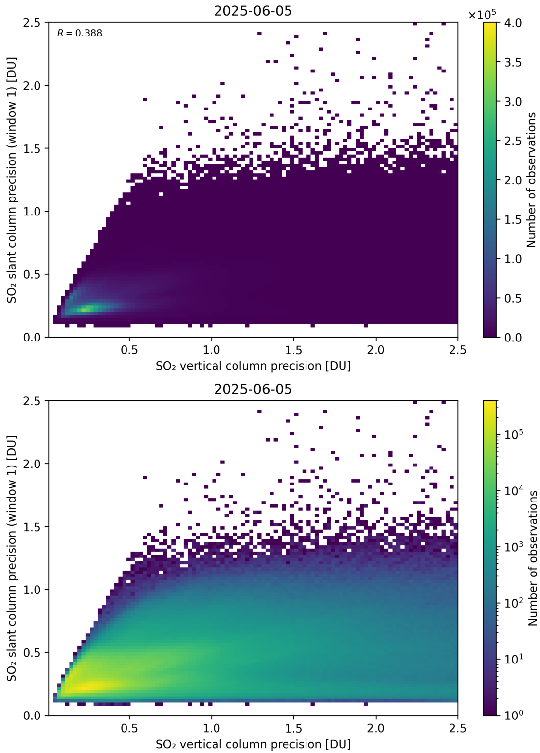
Figure 342: Scatter density plot of “SO 2 vertical column precision” against “SO 2 slant column precision (window 1)” for 2025-06-04 to 2025-06-06.
