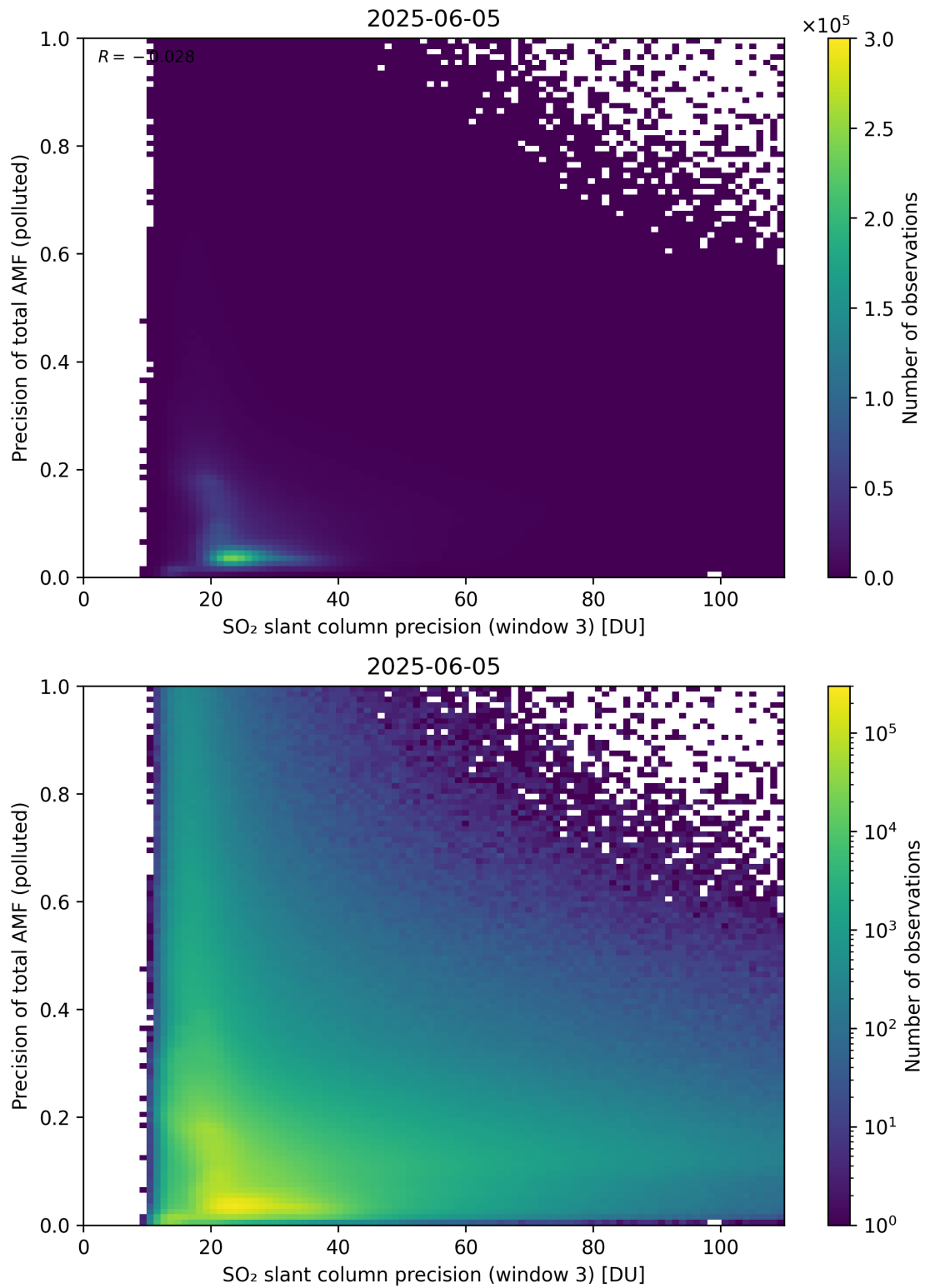
Figure 314: Scatter density plot of “SO 2 slant column precision (window 3)” against “Precision of total AMF (polluted)” for 2025-06-04 to 2025-06-06.
