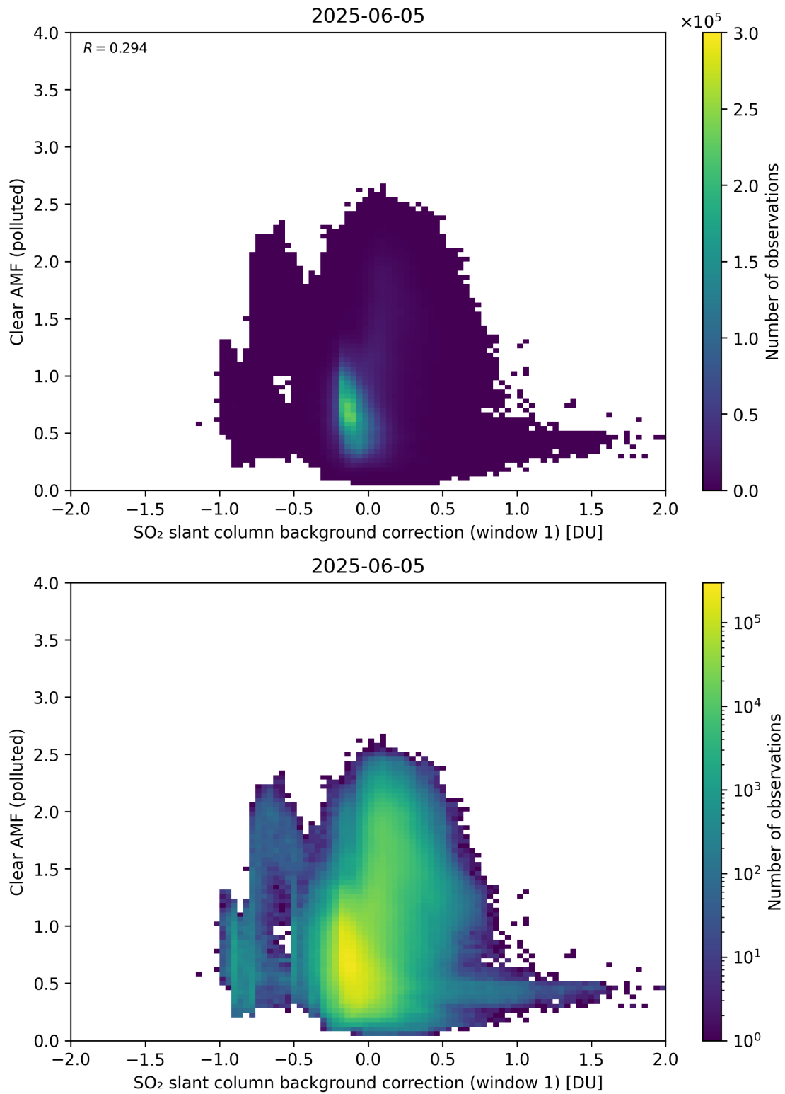
Figure 114: Scatter density plot of “SO 2 slant column background correction (window 1)” against “Clear AMF (polluted)” for 2025-06-04 to 2025-06-06.
