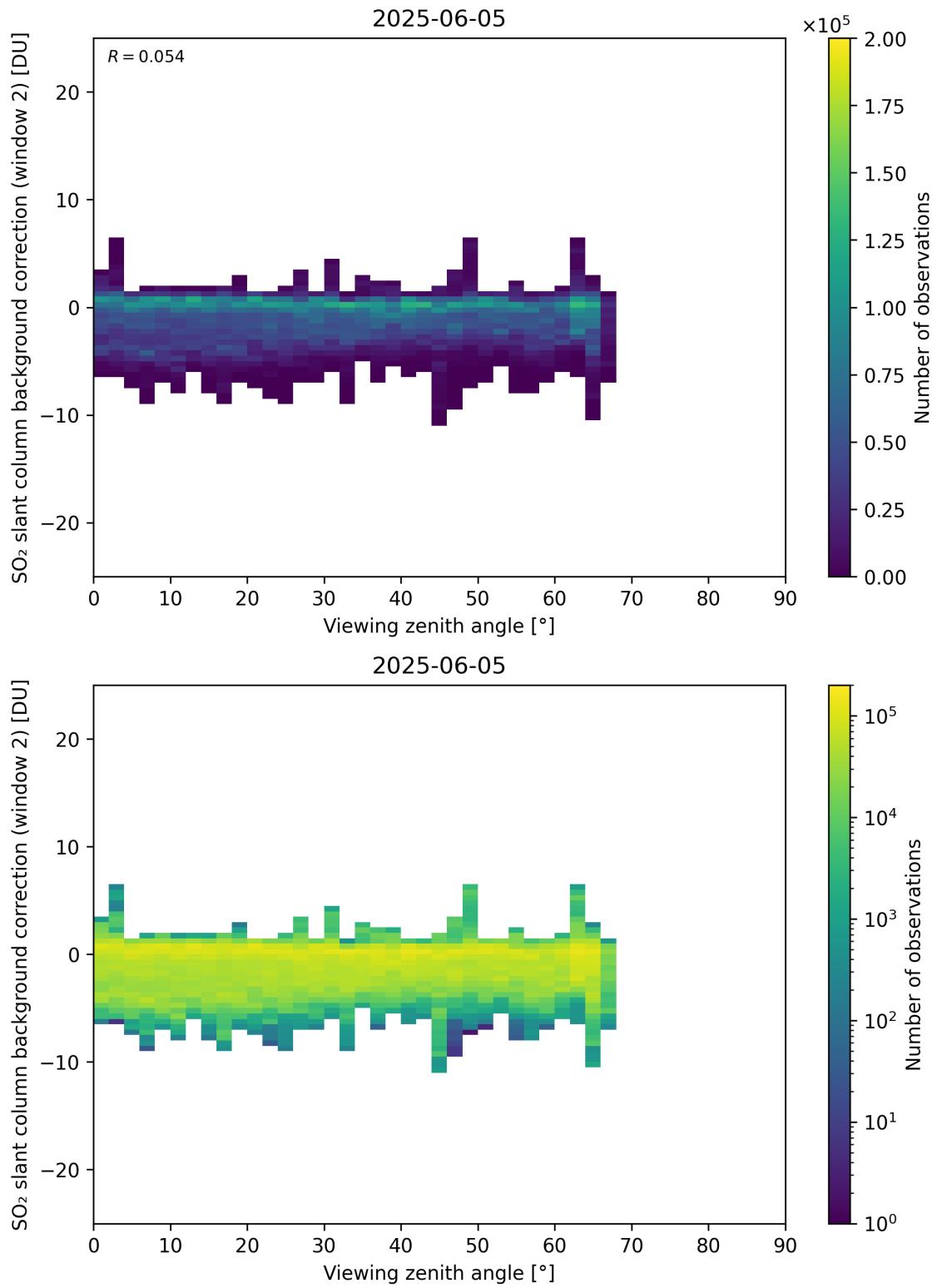
Figure 363: Scatter density plot of “Viewing zenith angle” against “SO 2 slant column background correction (window 2)” for 2025-06-04 to 2025-06-06.
