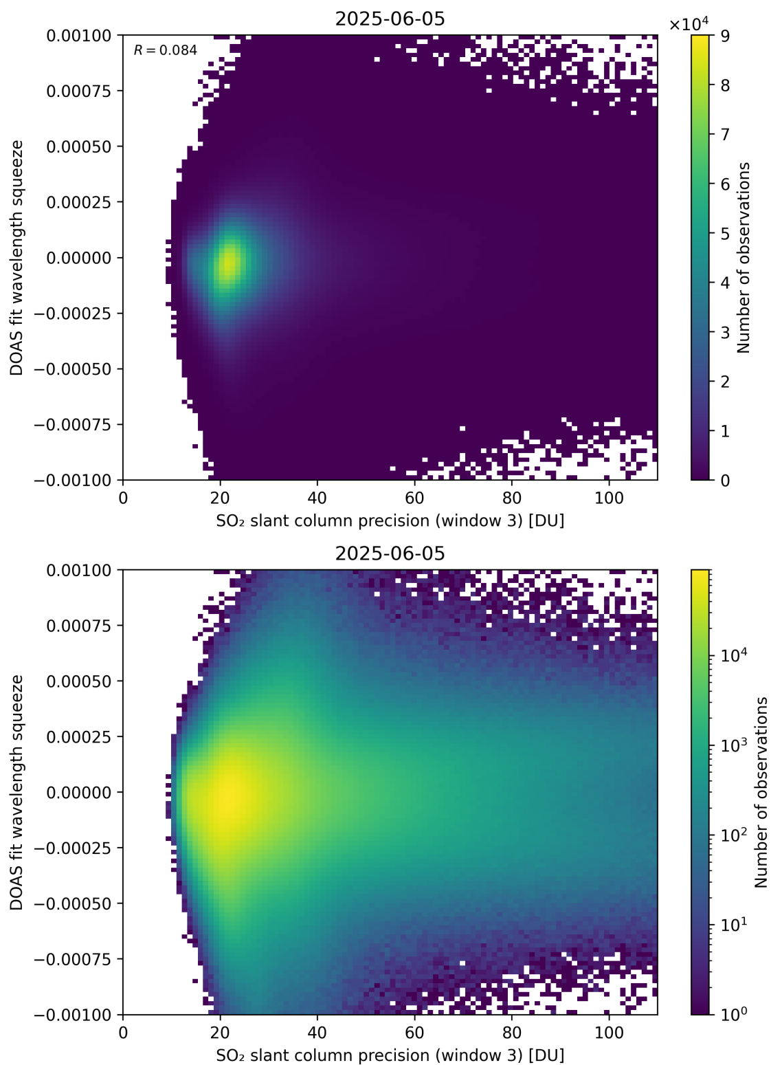
Figure 309: Scatter density plot of “SO 2 slant column precision (window 3)” against “DOAS fit wavelength squeeze” for 2025-06-04 to 2025-06-06.
