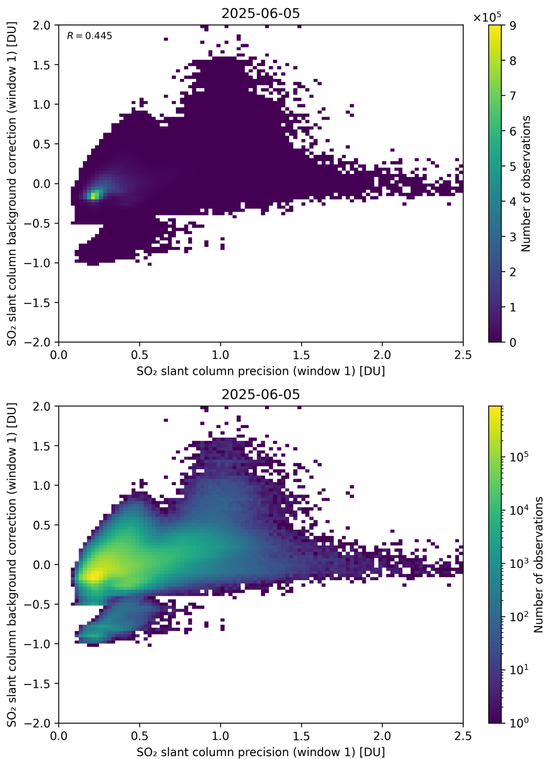
Figure 268: Scatter density plot of “SO 2 slant column precision (window 1)” against “SO 2 slant column background correction (window 1)” for 2025-06-04 to 2025-06-06.
