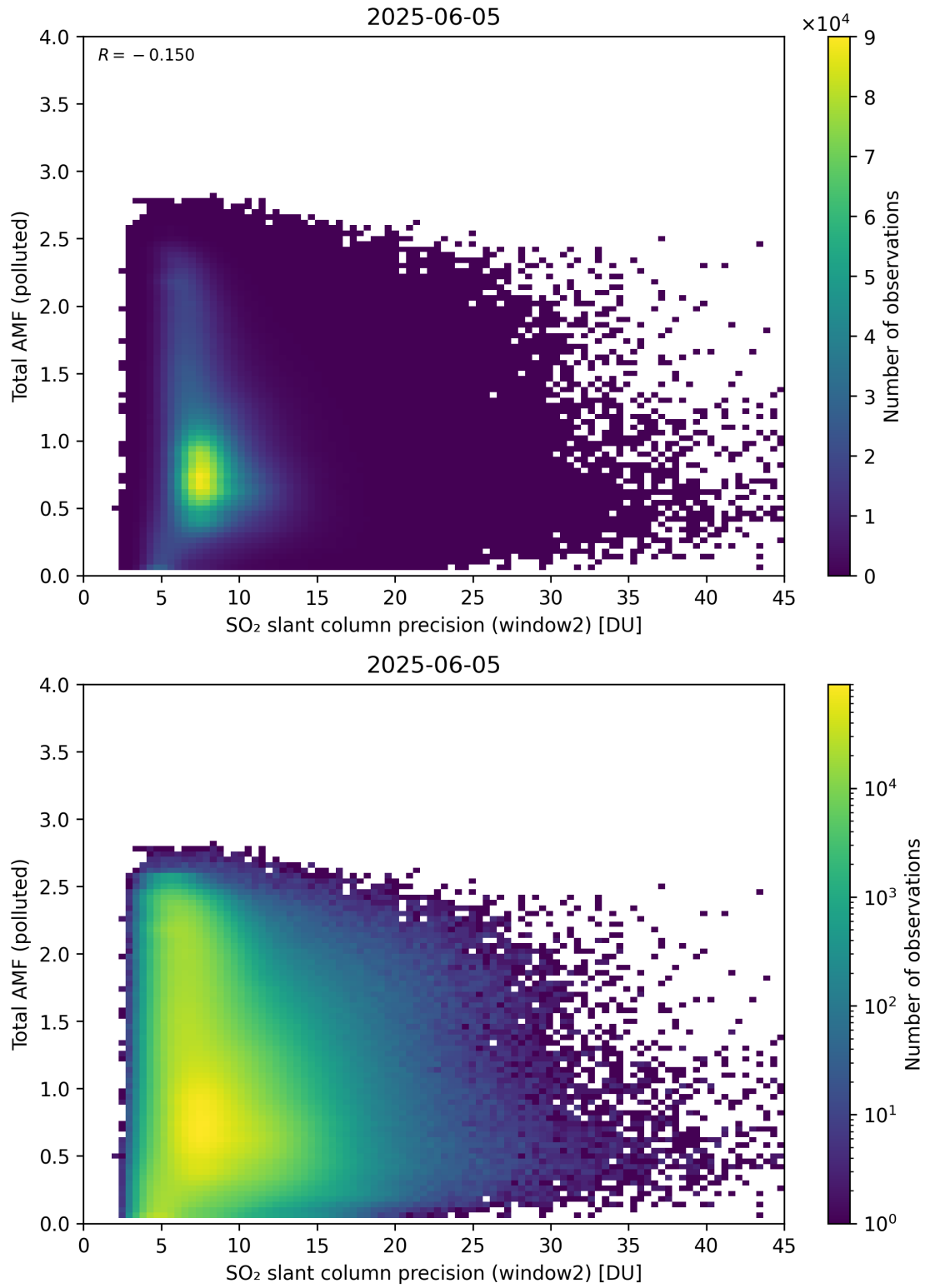
Figure 301: Scatter density plot of “SO 2 slant column precision (window2)” against “Total AMF (polluted)” for 2025-06-04 to 2025-06-06.
