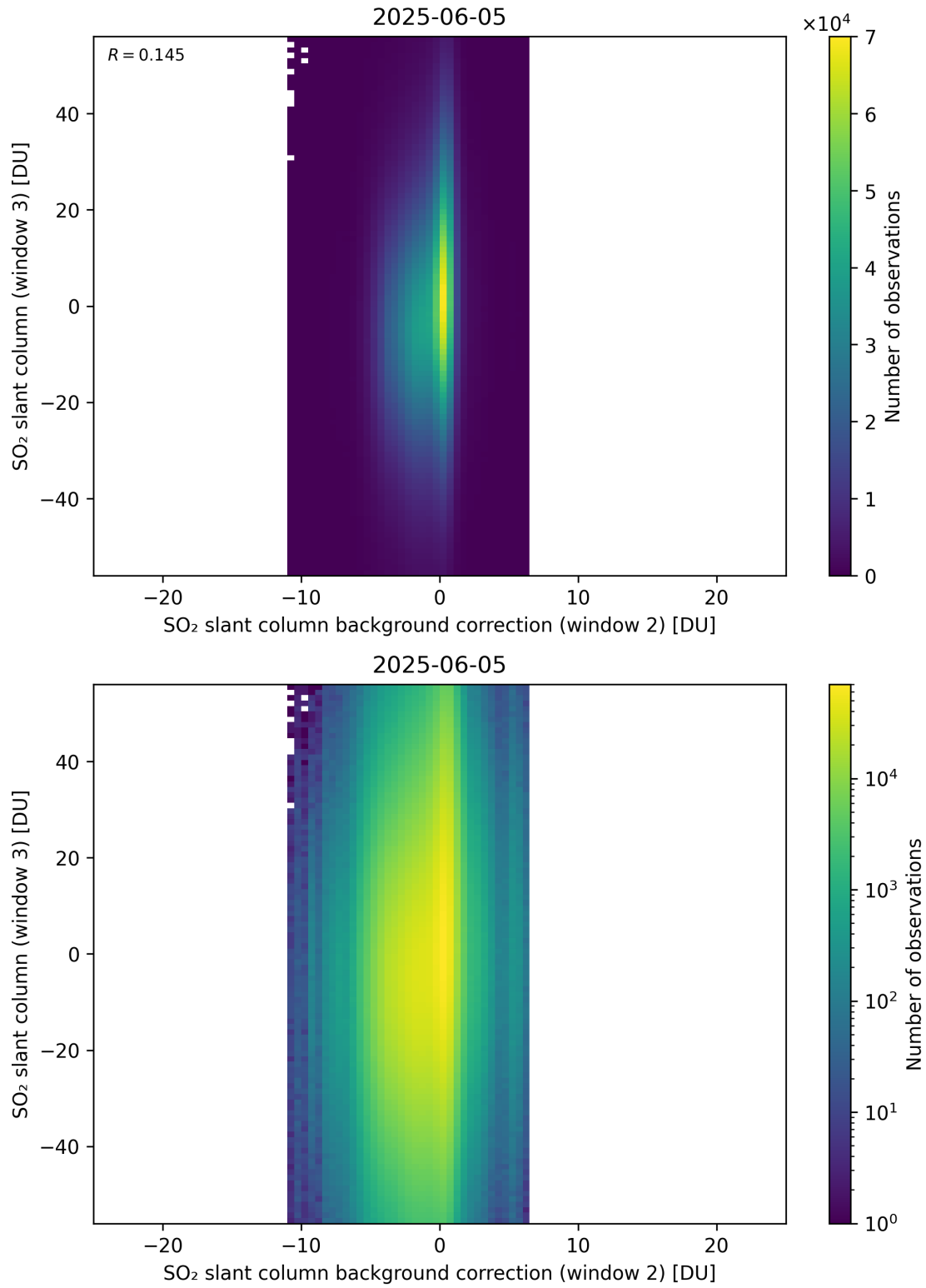
Figure 128: Scatter density plot of “SO 2 slant column background correction (window 2)” against “SO 2 slant column (window 3)” for 2025-06-04 to 2025-06-06.
