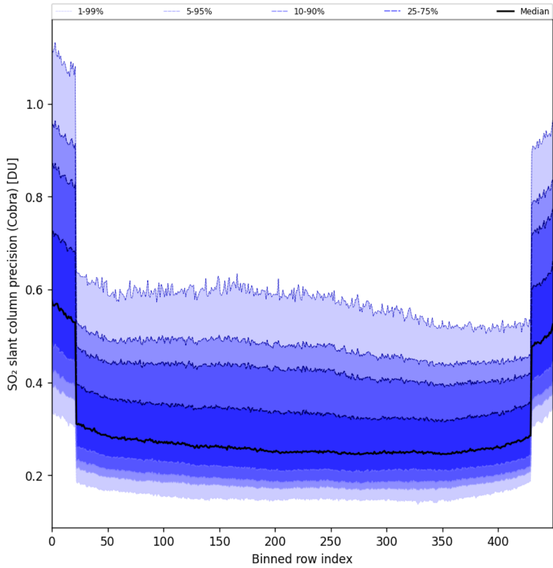
Figure 88: Along track statistics of “SO 2 slant column precision (Cobra)” for 2025-06-04 to 2025-06-06
