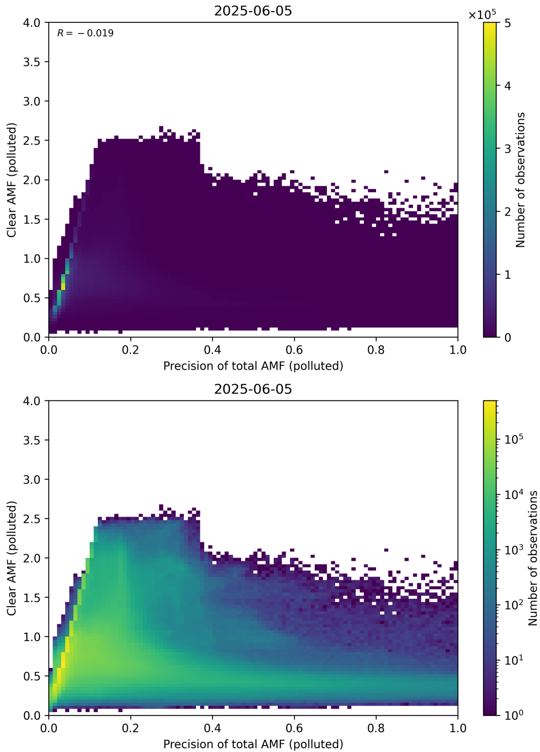
Figure 320: Scatter density plot of “Precision of total AMF (polluted)” against “Clear AMF (polluted)” for 2025-06-04 to 2025-06-06.
