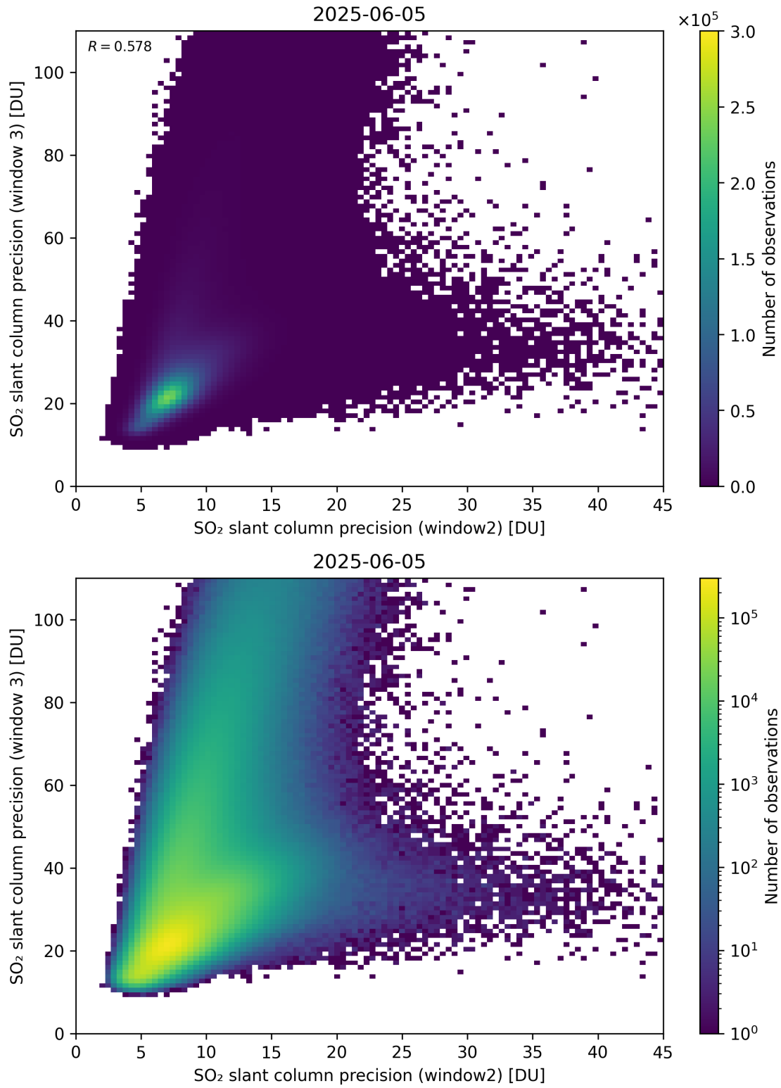
Figure 300: Scatter density plot of “SO 2 slant column precision (window2)” against “SO 2 slant column precision (window 3)” for 2025-06-04 to 2025-06-06.
