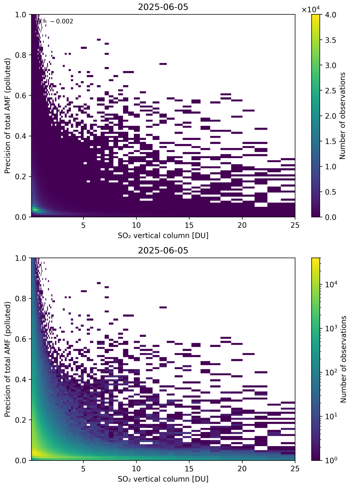
Figure 360: Scatter density plot of “SO 2 vertical column” against “Precision of total AMF (polluted)” for 2025-06-04 to 2025-06-06.
