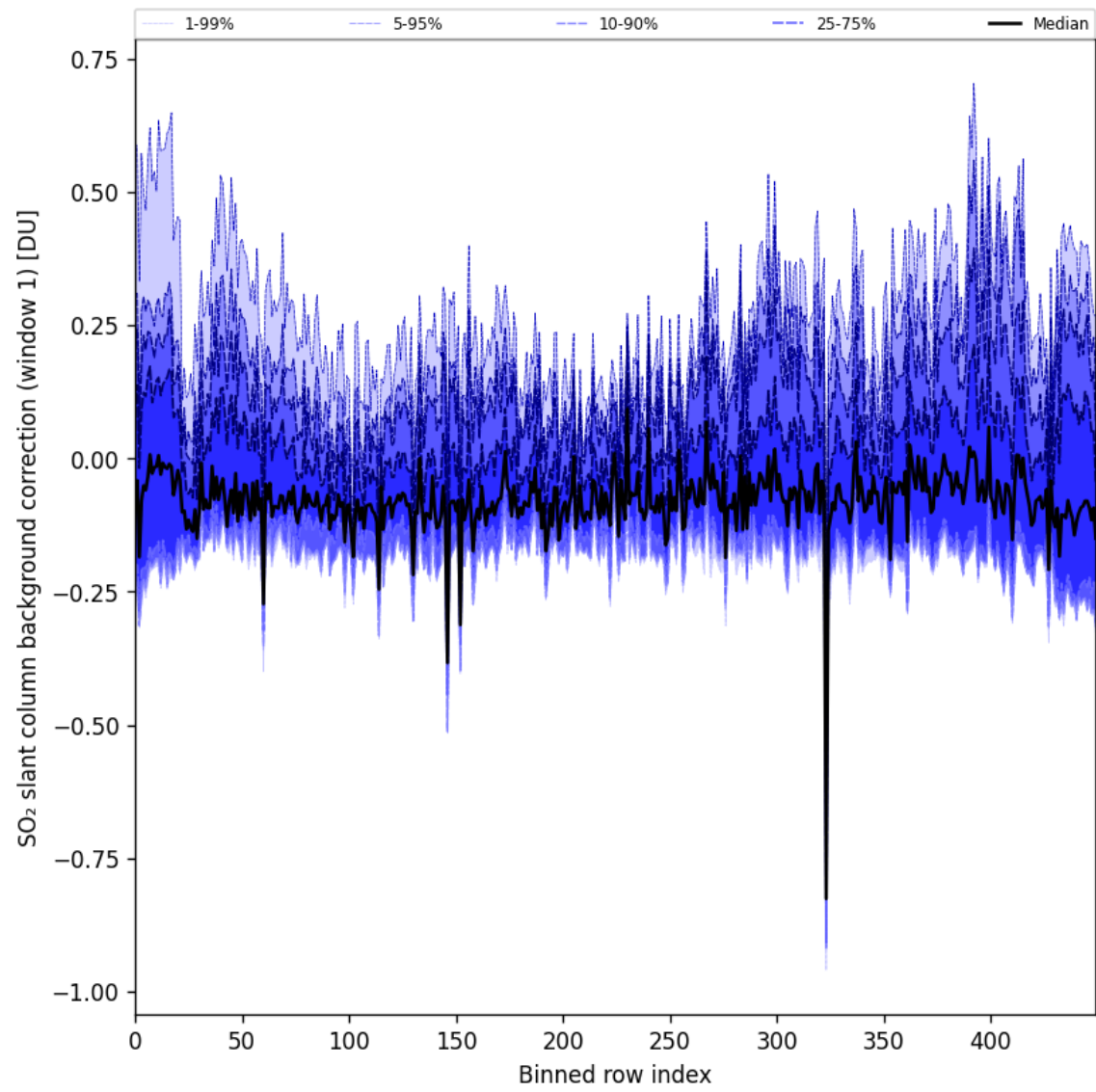
Figure 92: Along track statistics of “SO 2 slant column background correction (window 1)” for 2025-06-04 to 2025-06-06
