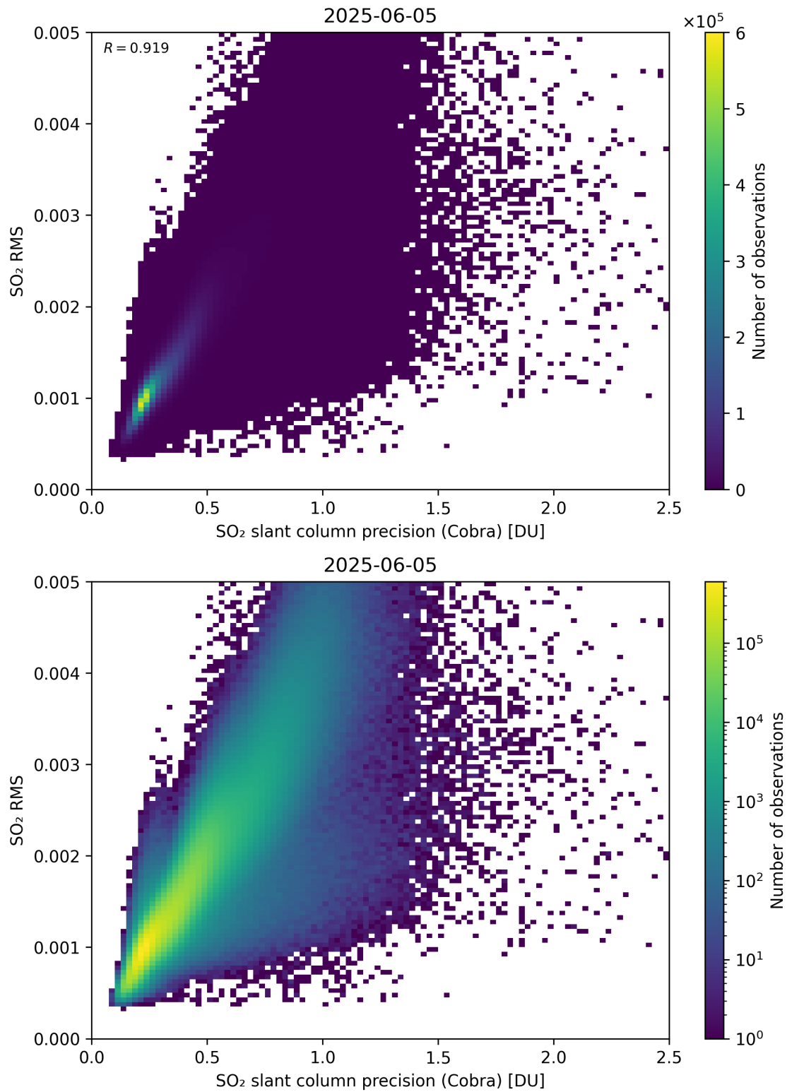
Figure 204: Scatter density plot of “SO 2 slant column precision (Cobra)” against “SO 2 RMS” for 2025-06-04 to 2025-06-06.
