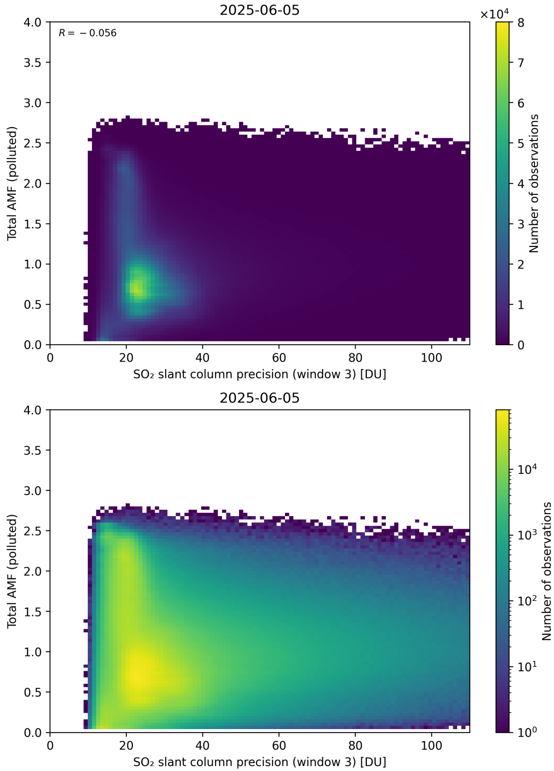
Figure 313: Scatter density plot of “SO 2 slant column precision (window 3)” against “Total AMF (polluted)” for 2025-06-04 to 2025-06-06.
