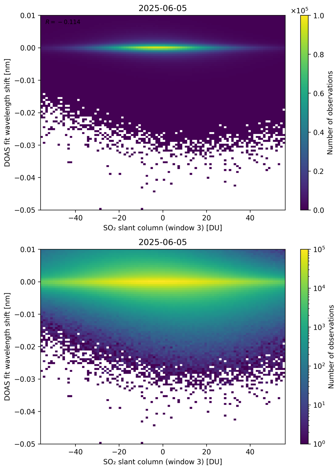
Figure 304: Scatter density plot of “SO 2 slant column (window 3)” against “DOAS fit wavelength shift” for 2025-06-04 to 2025-06-06.
