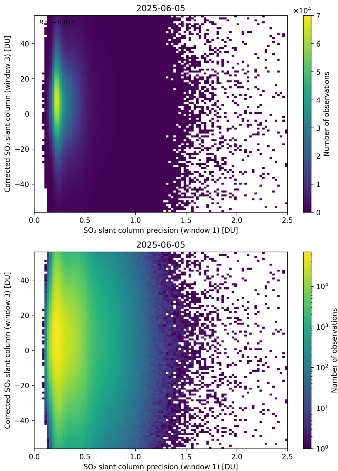
Figure 276: Scatter density plot of “SO 2 slant column precision (window 1)” against “Corrected SO 2 slant column (window 3)” for 2025-06-04 to 2025-06-06.
