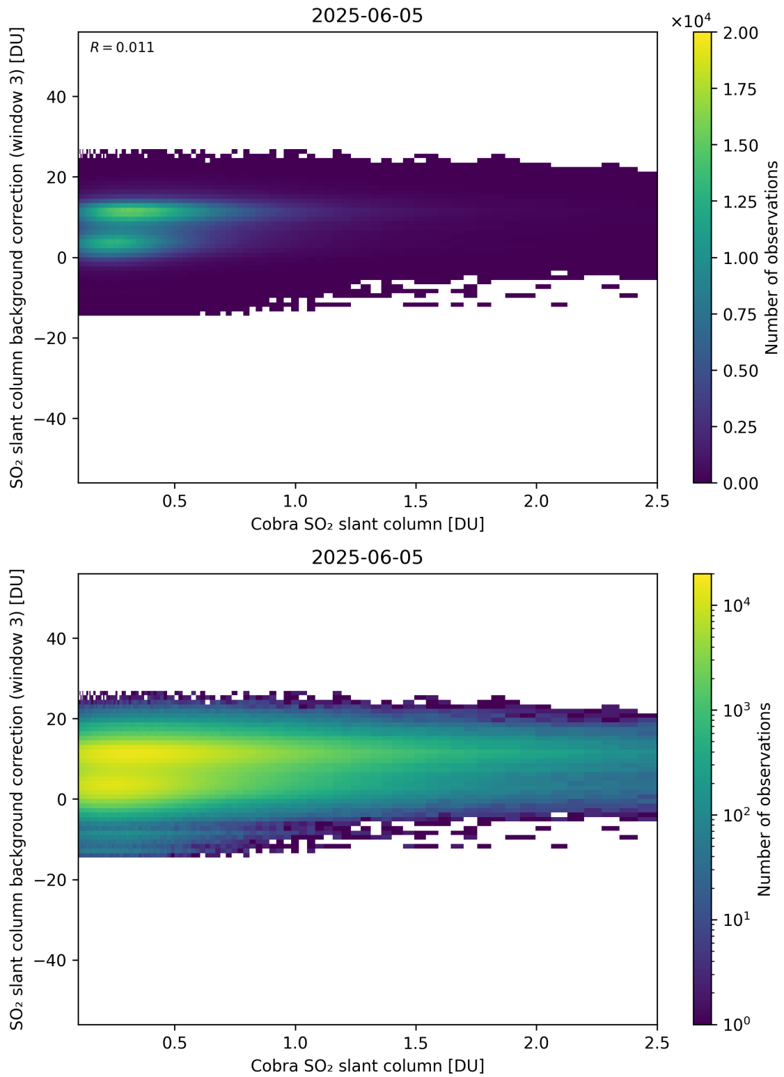
Figure 195: Scatter density plot of “Cobra SO 2 slant column” against “SO 2 slant column background correction (window 3)” for 2025-06-04 to 2025-06-06.
