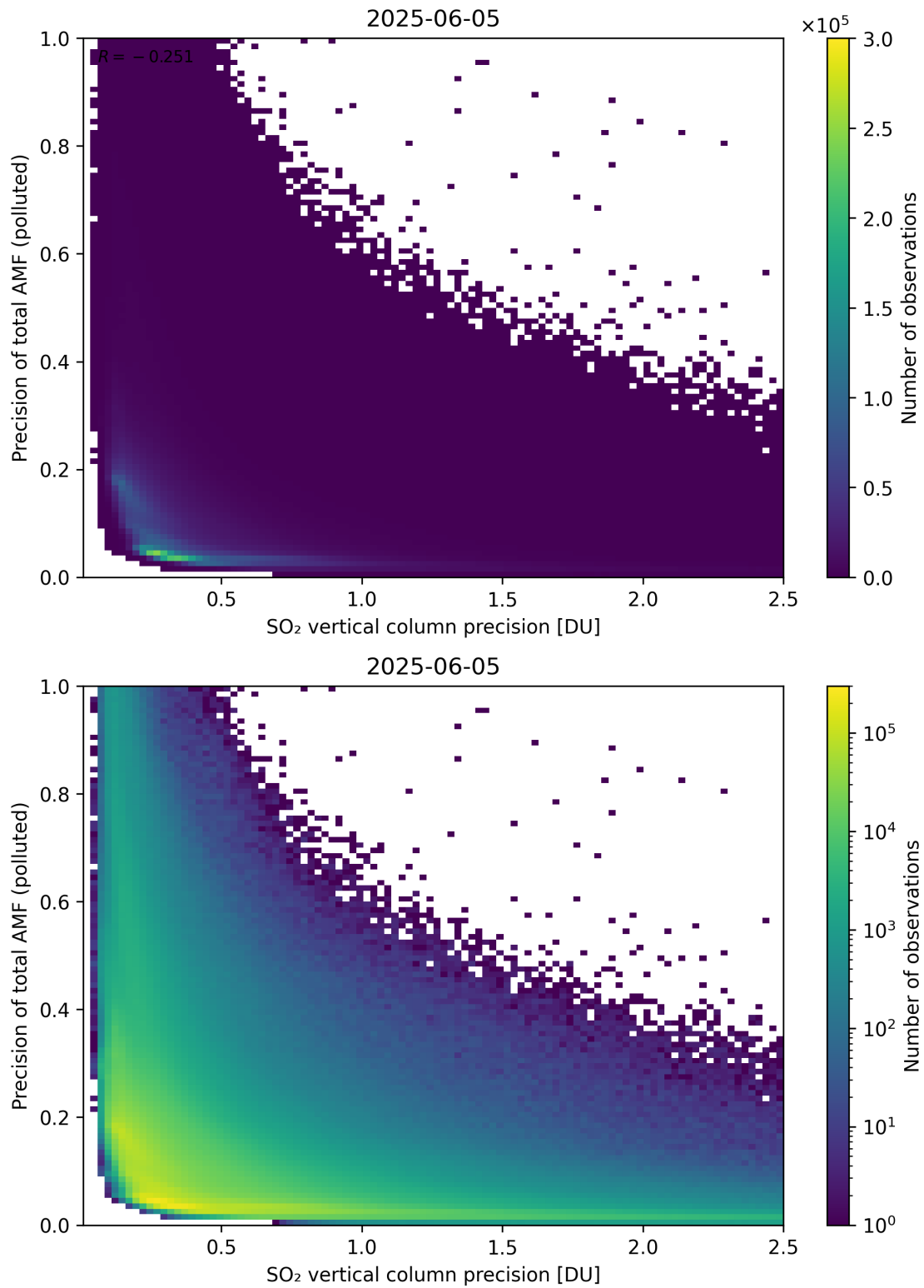
Figure 347: Scatter density plot of “SO 2 vertical column precision” against “Precision of total AMF (polluted)” for 2025-06-04 to 2025-06-06.
