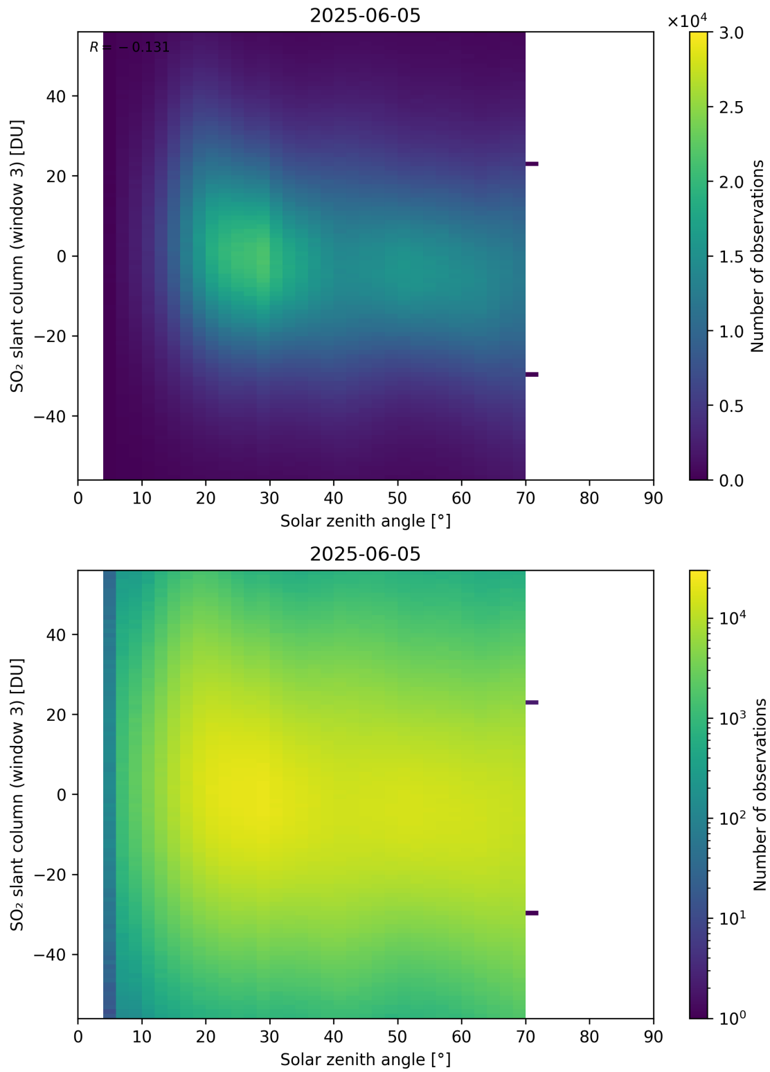
Figure 187: Scatter density plot of “Solar zenith angle” against “SO 2 slant column (window 3)” for 2025-06-04 to 2025-06-06.
