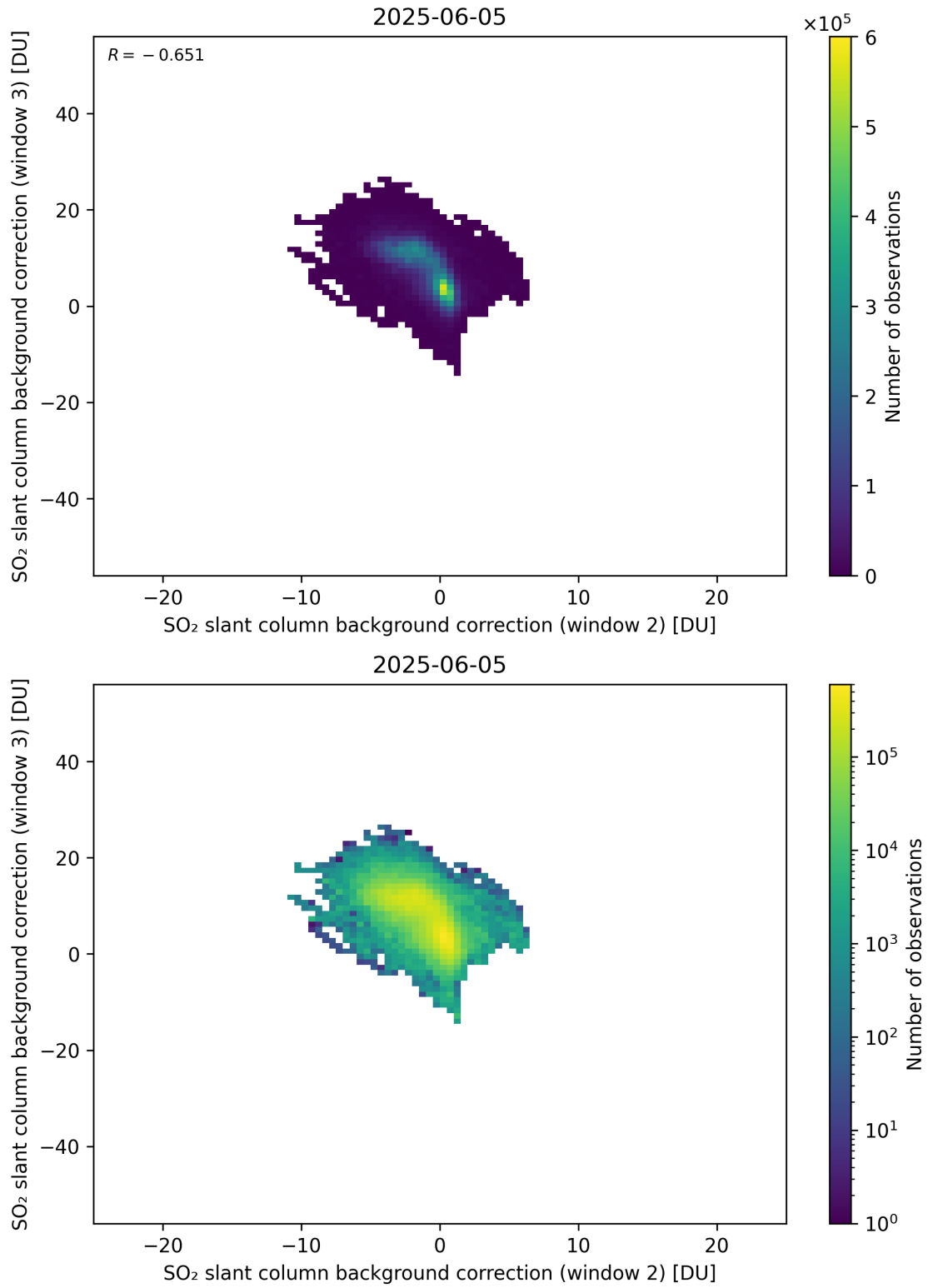
Figure 122: Scatter density plot of “SO 2 slant column background correction (window 2)” against “SO 2 slant column background correction (window 3)” for 2025-06-04 to 2025-06-06.
