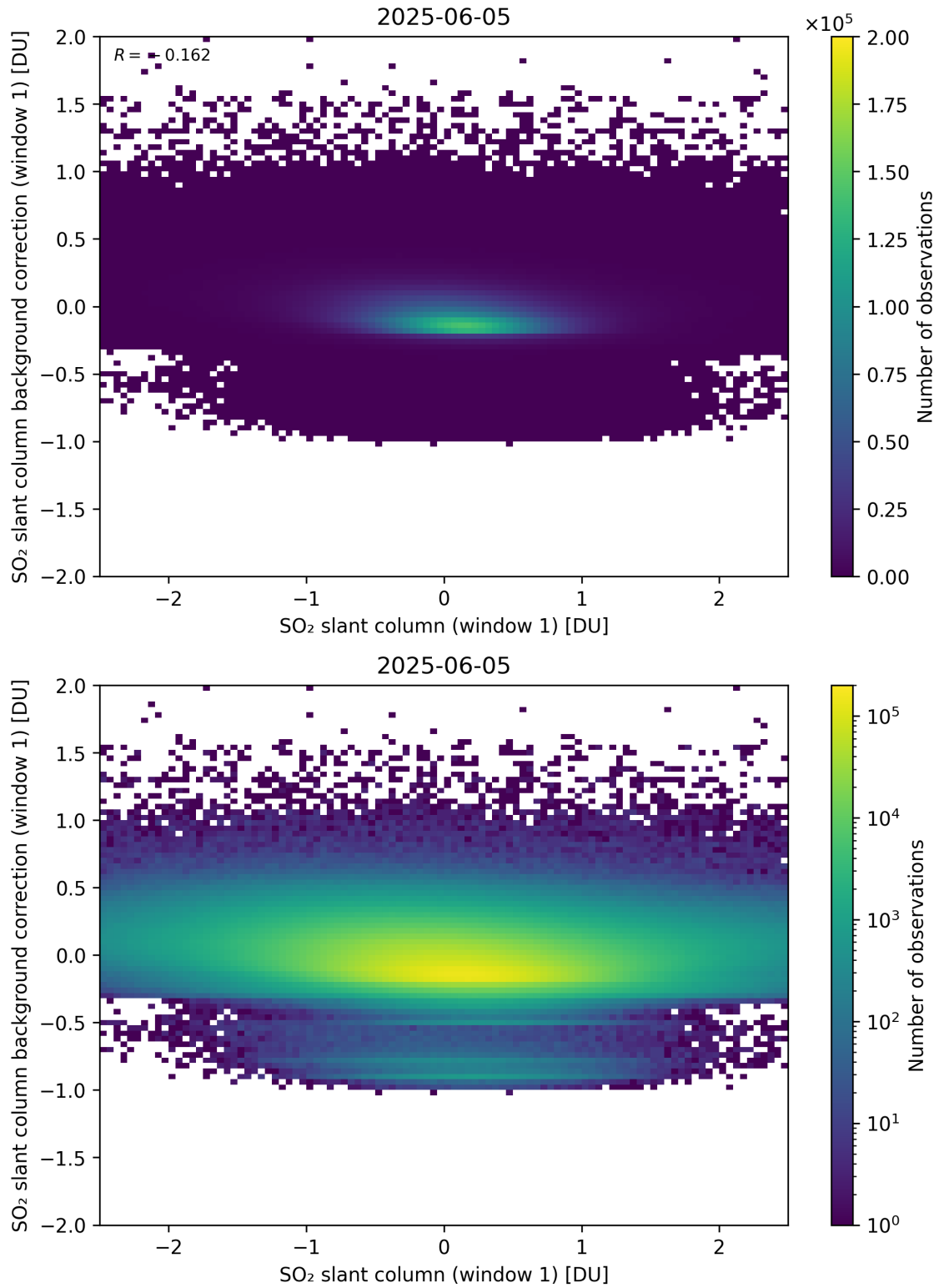
Figure 262: Scatter density plot of “SO 2 slant column (window 1)” against “SO 2 slant column background correction (window 1)” for 2025-06-04 to 2025-06-06.
