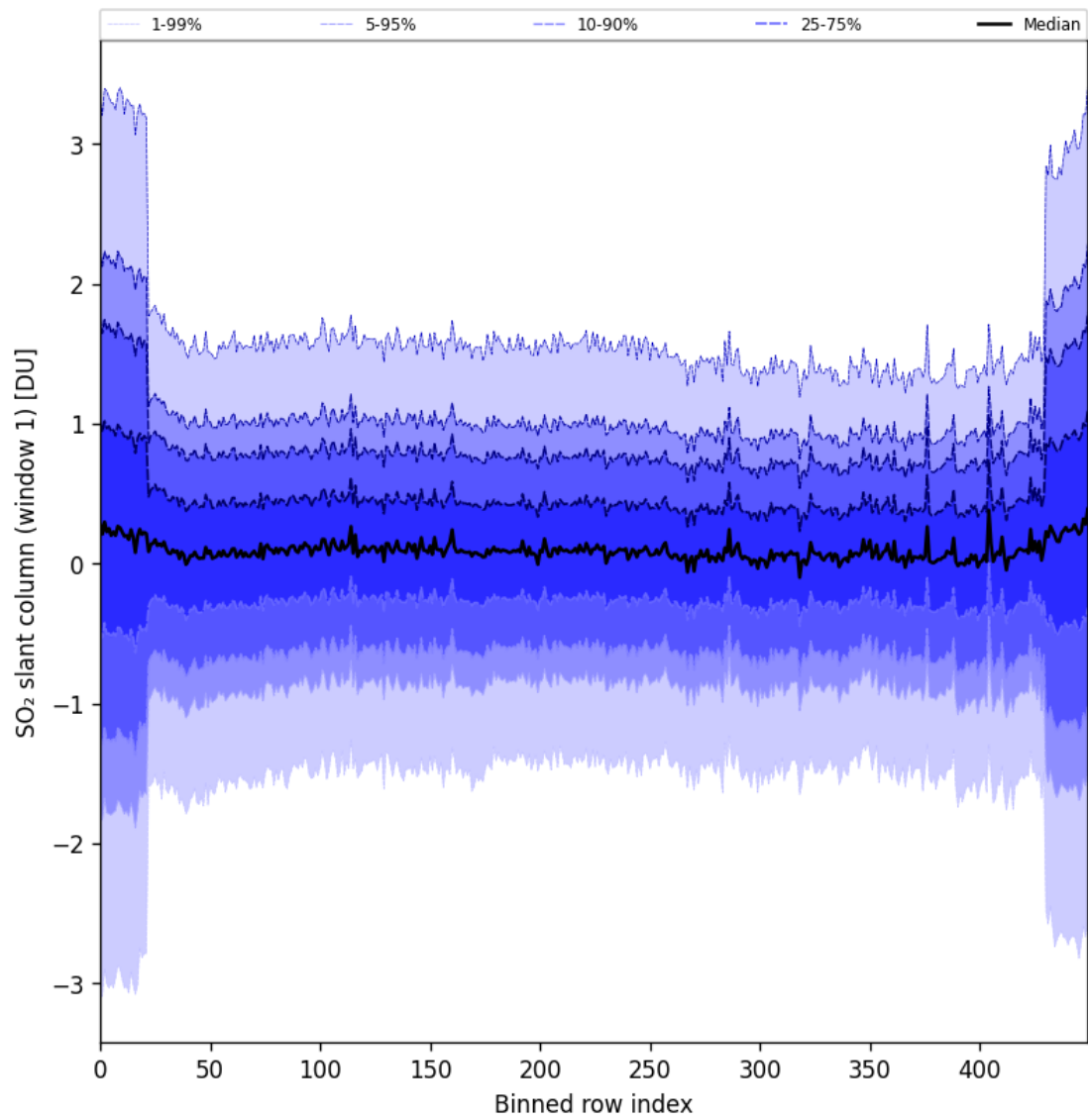
Figure 89: Along track statistics of “SO 2 slant column (window 1)” for 2025-06-04 to 2025-06-06
