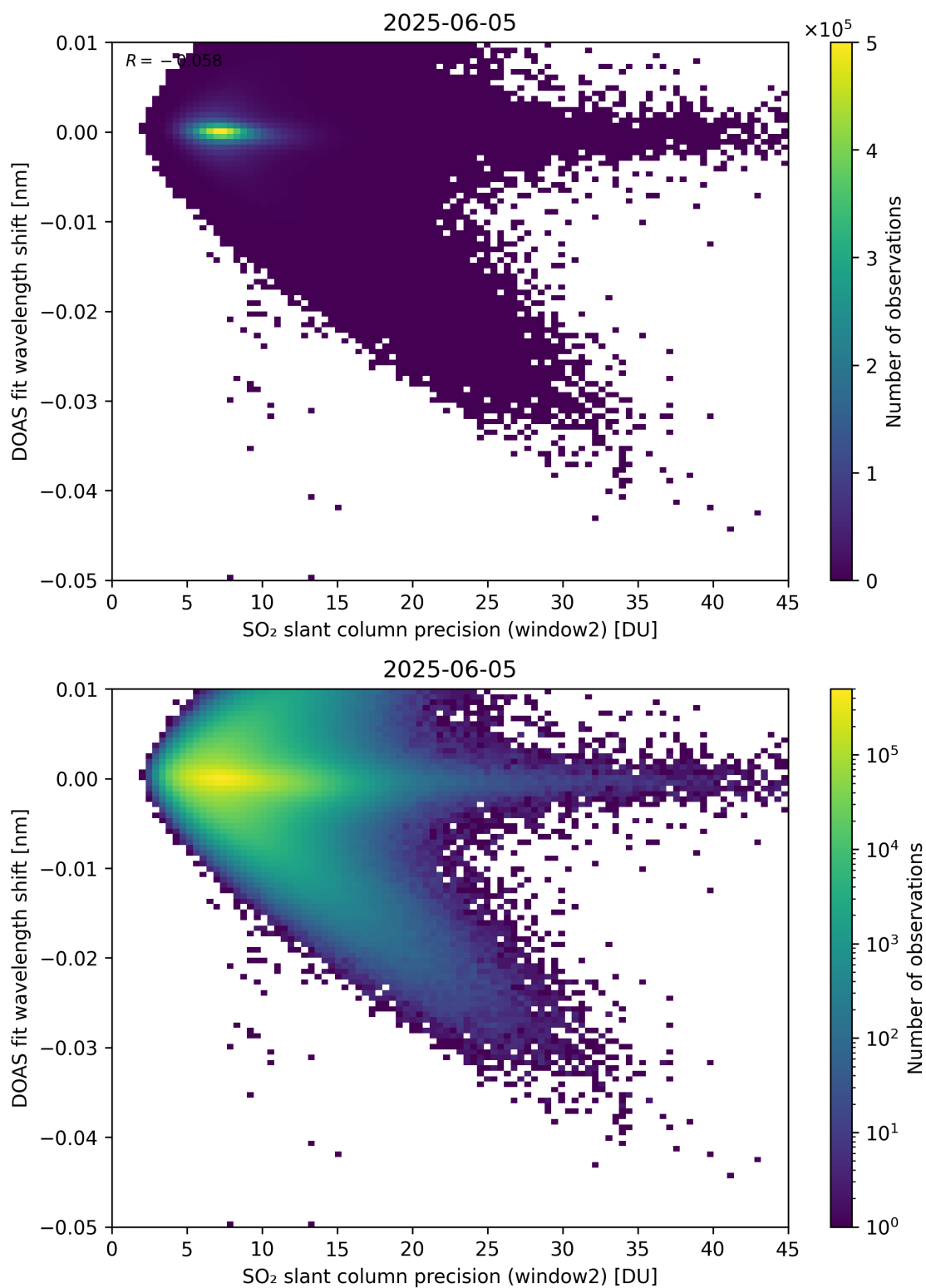
Figure 293: Scatter density plot of “SO 2 slant column precision (window2)” against “DOAS fit wavelength shift” for 2025-06-04 to 2025-06-06.
