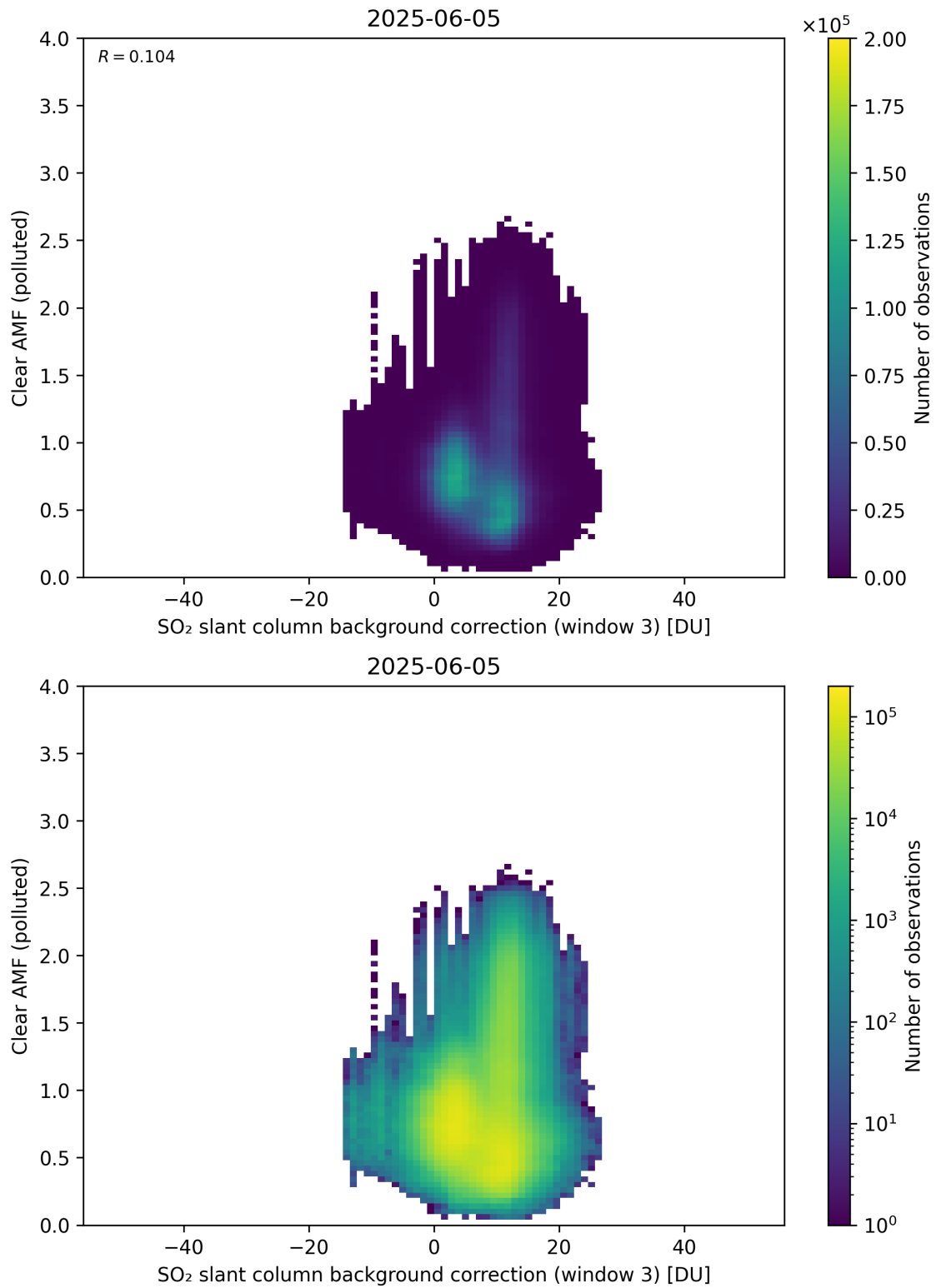
Figure 135: Scatter density plot of “SO 2 slant column background correction (window 3)” against “Clear AMF (polluted)” for 2025-06-04 to 2025-06-06.
