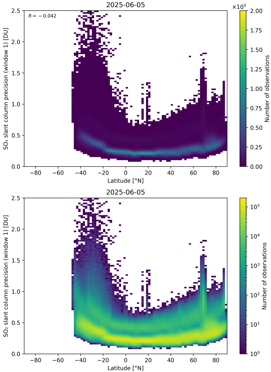
Figure 163: Scatter density plot of “Latitude” against “SO 2 slant column precision (window 1)” for 2025-06-04 to 2025-06-06.
