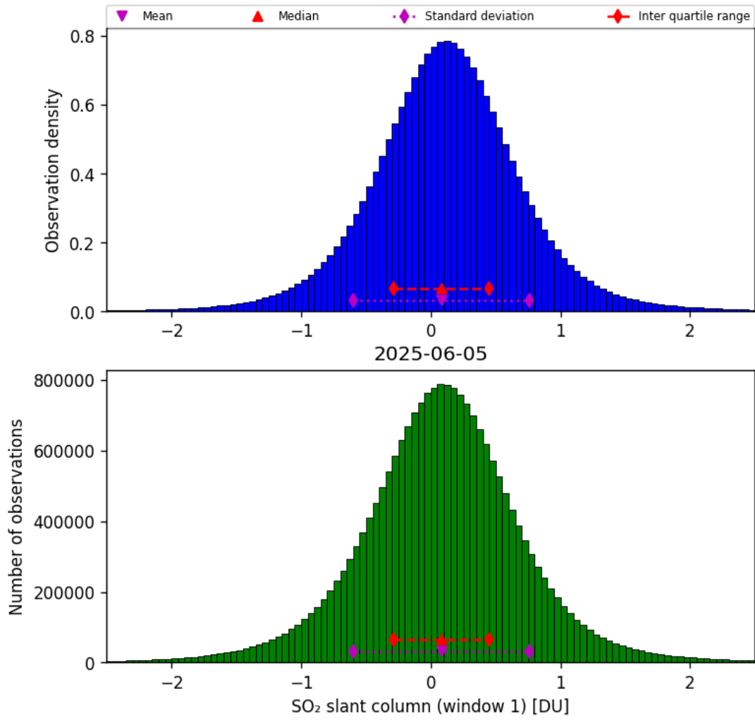
Figure 63: Histogram of “SO 2 slant column (window 1)” for 2025-06-04 to 2025-06-06
