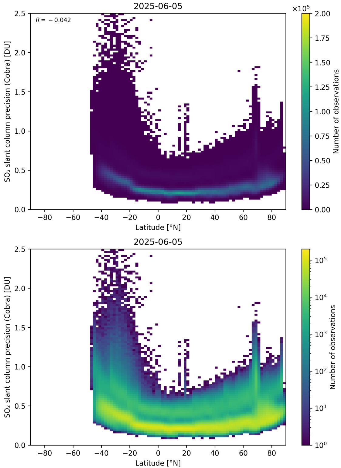
Figure 158: Scatter density plot of “Latitude” against “SO 2 slant column precision (Cobra)” for 2025-06-04 to 2025-06-06.
