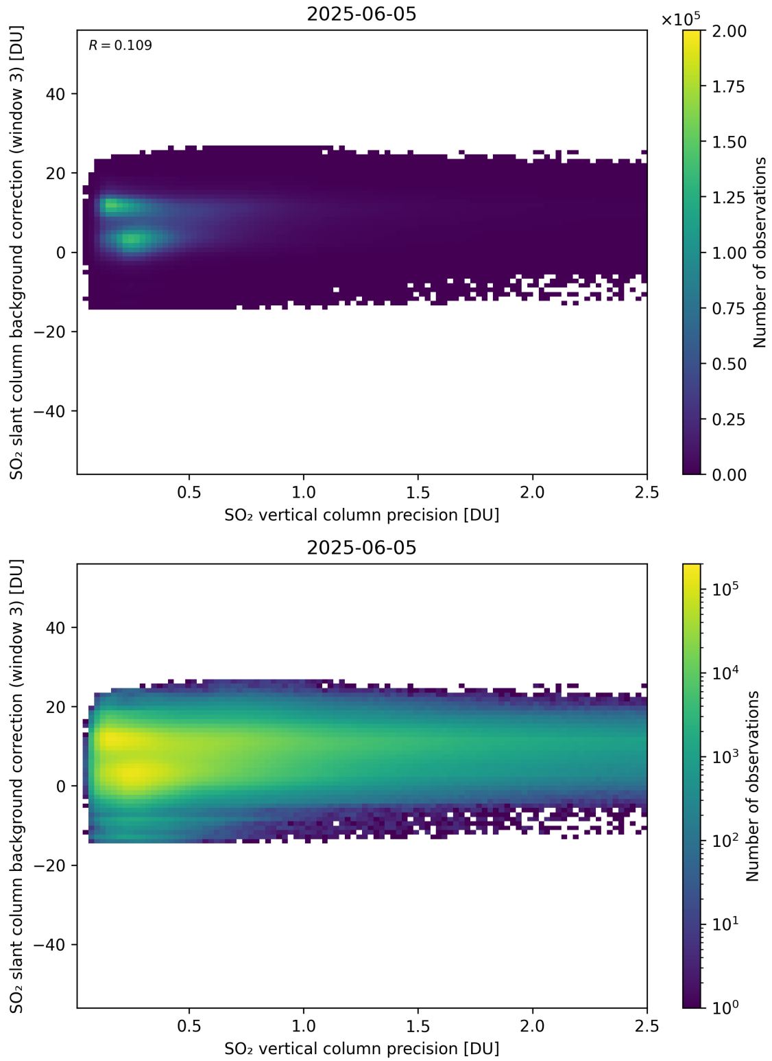
Figure 331: Scatter density plot of “SO 2 vertical column precision” against “SO 2 slant column background correction (window 3)” for 2025-06-04 to 2025-06-06.
