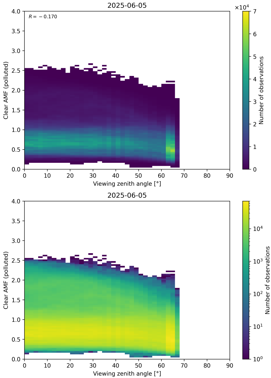
Figure 370: Scatter density plot of “Viewing zenith angle” against “Clear AMF (polluted)” for 2025-06-04 to 2025-06-06.
