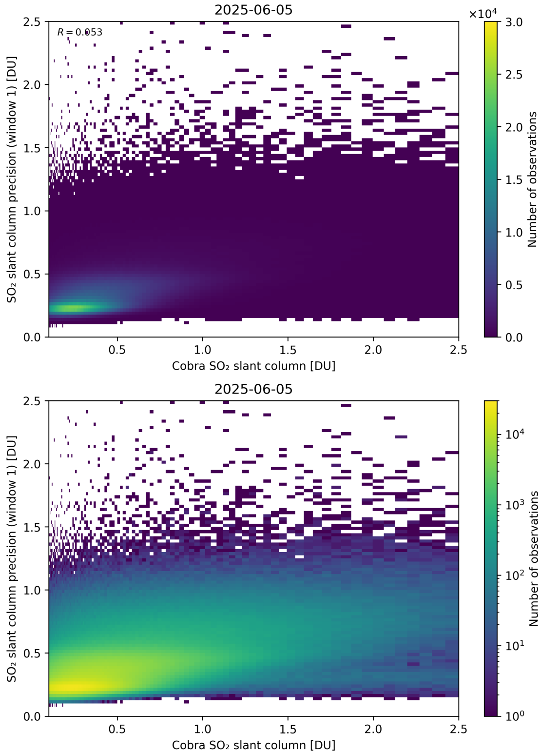
Figure 220: Scatter density plot of “Cobra SO 2 slant column” against “SO 2 slant column precision (window 1)” for 2025-06-04 to 2025-06-06.
