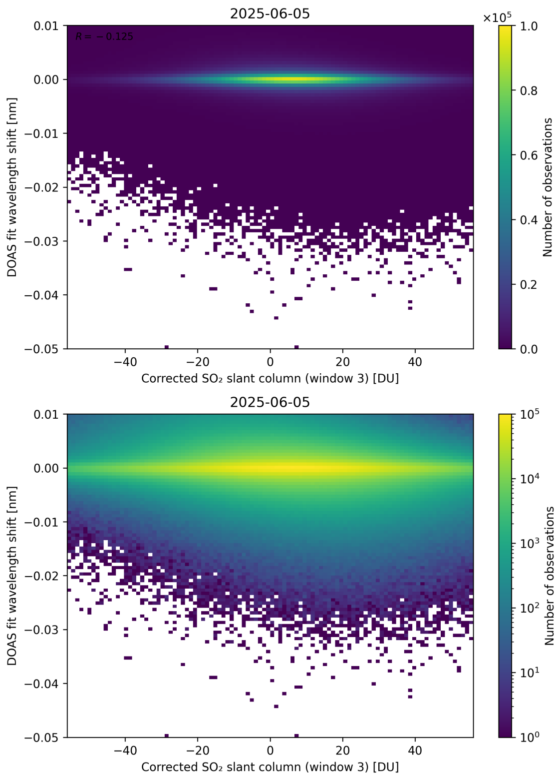
Figure 256: Scatter density plot of “Corrected SO 2 slant column (window 3)” against “DOAS fit wavelength shift” for 2025-06-04 to 2025-06-06.
