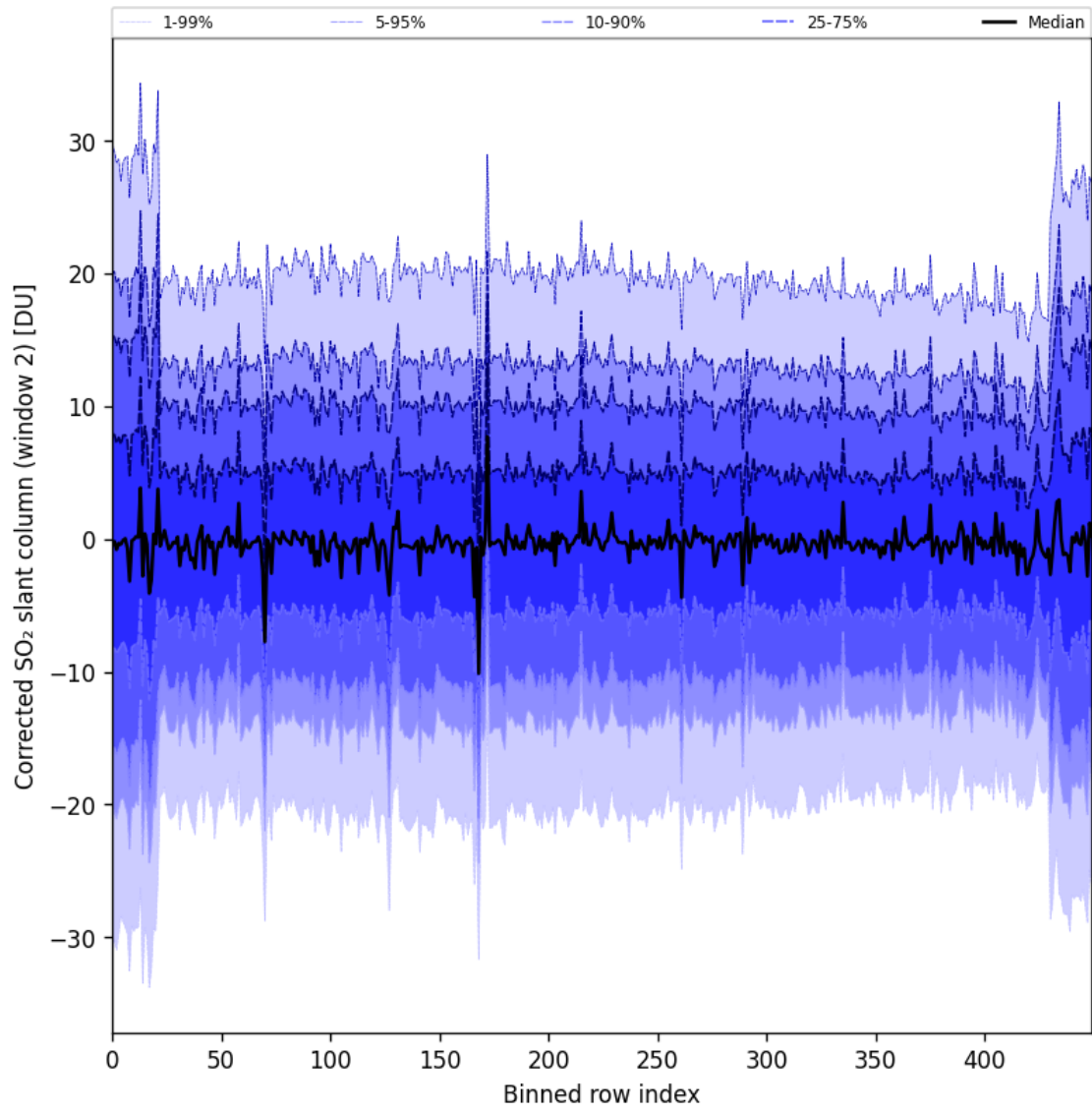
Figure 95: Along track statistics of “Corrected SO 2 slant column (window 2)” for 2025-06-04 to 2025-06-06
