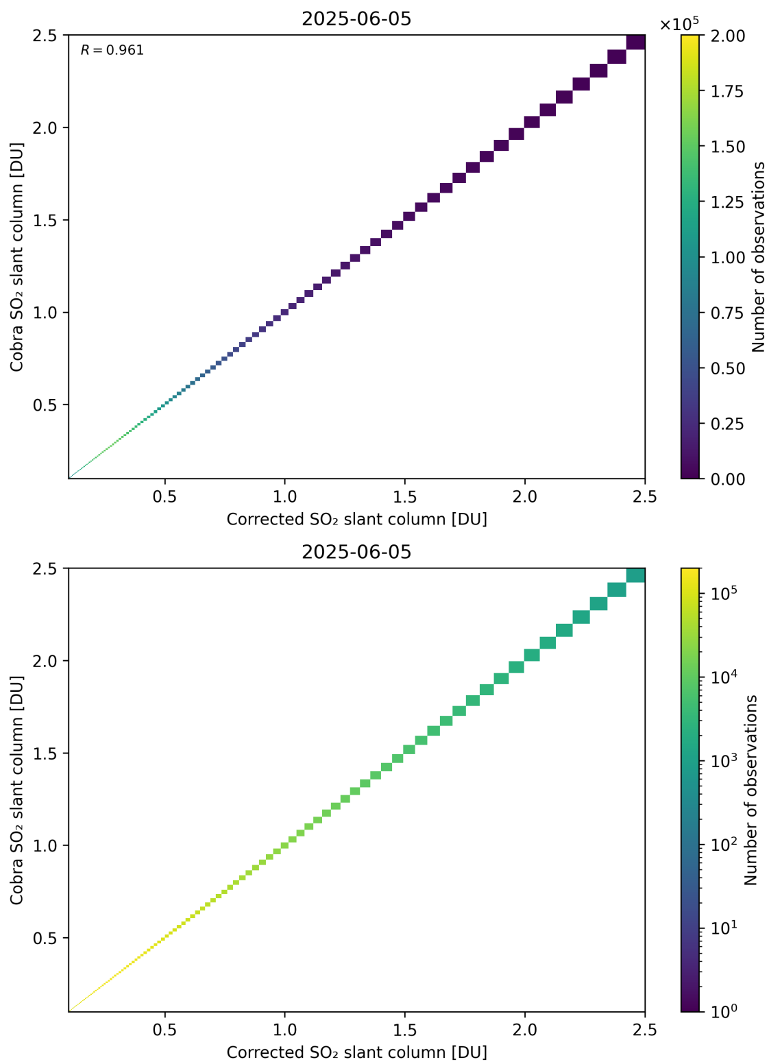
Figure 233: Scatter density plot of “Corrected SO 2 slant column” against “Cobra SO 2 slant column” for 2025-06-04 to 2025-06-06.
