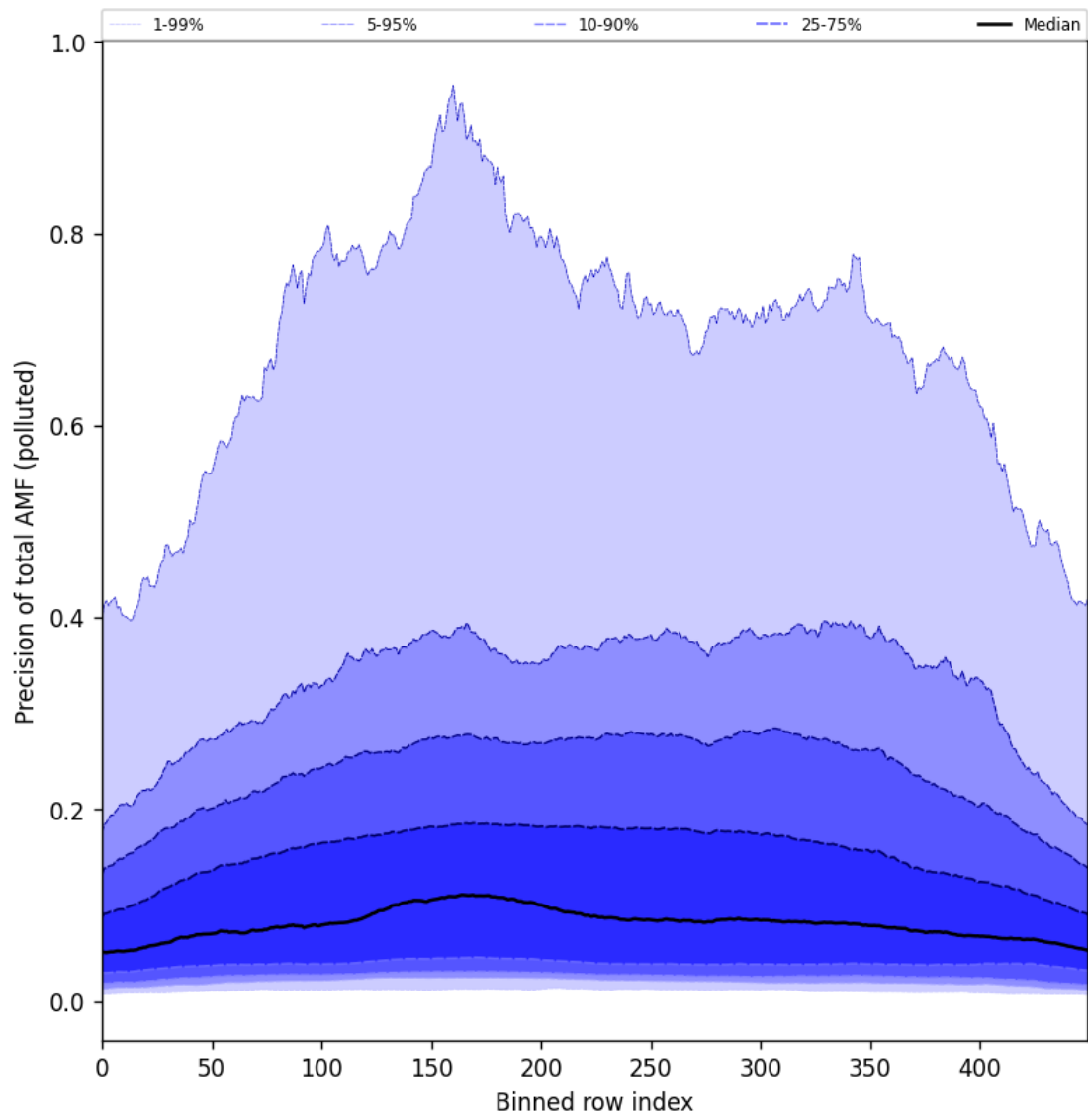
Figure 106: Along track statistics of “Precision of total AMF (polluted)” for 2025-06-04 to 2025-06-06
