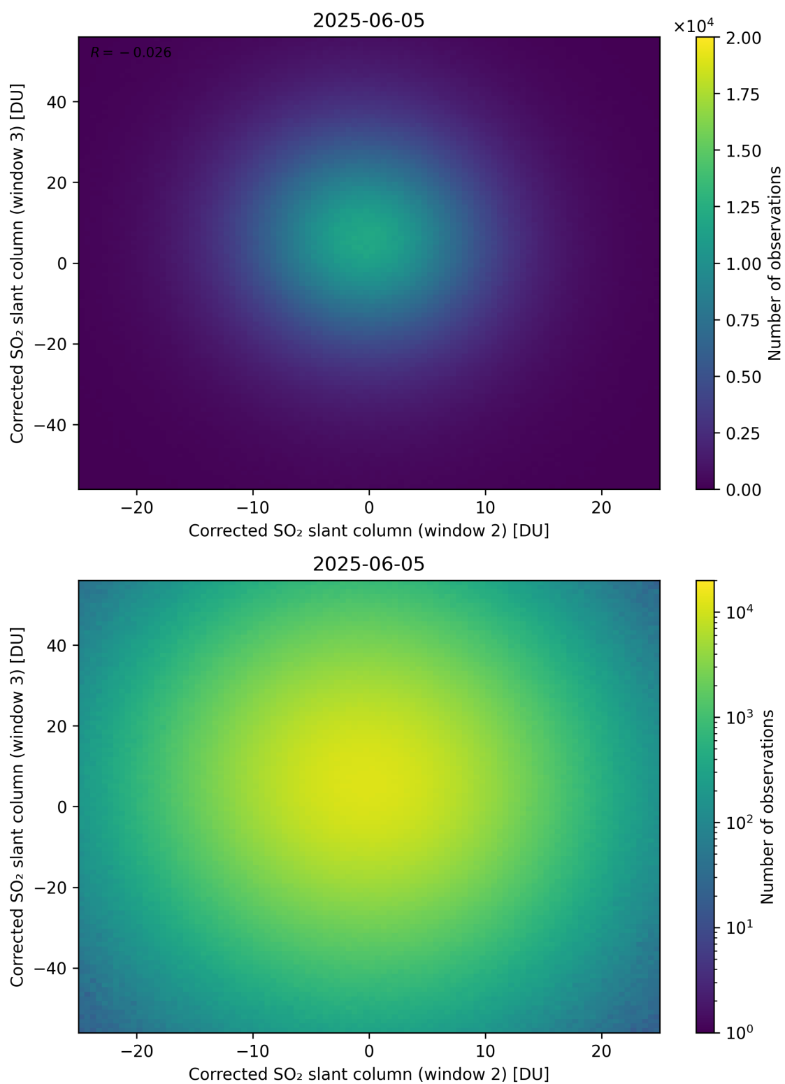
Figure 250: Scatter density plot of “Corrected SO 2 slant column (window 2)” against “Corrected SO 2 slant column (window 3)” for 2025-06-04 to 2025-06-06.
