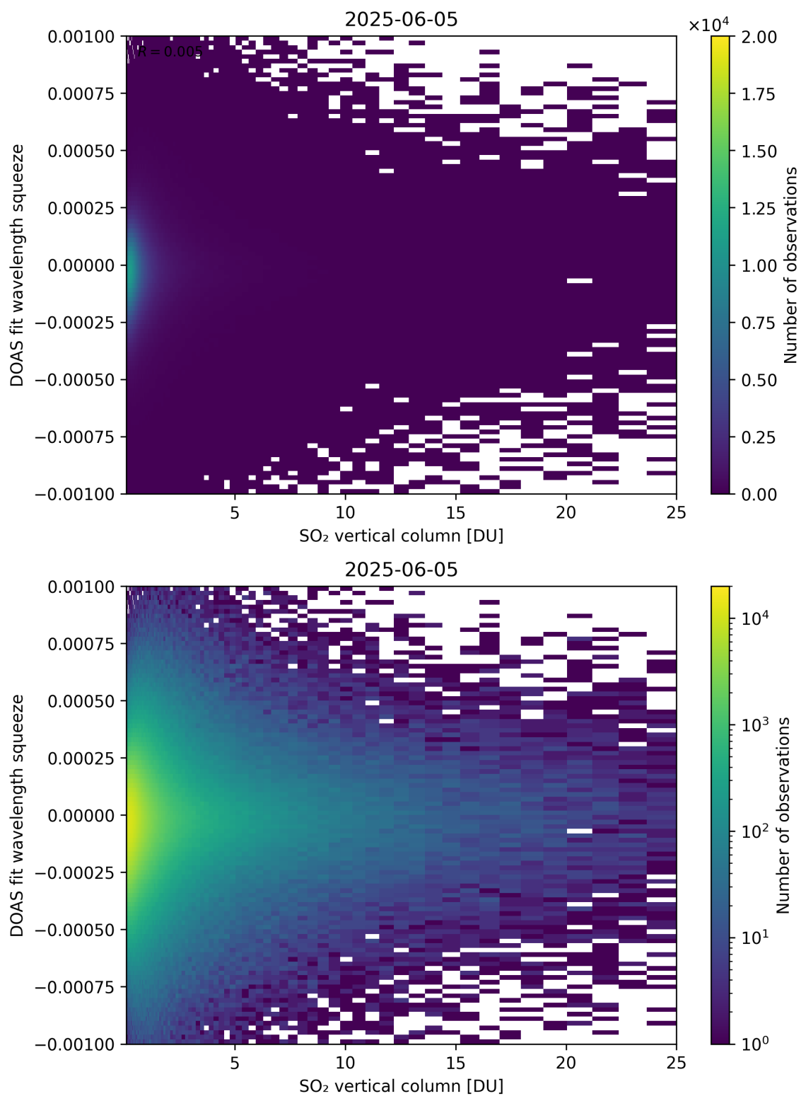
Figure 327: Scatter density plot of “SO 2 vertical column” against “DOAS fit wavelength squeeze” for 2025-06-04 to 2025-06-06.
