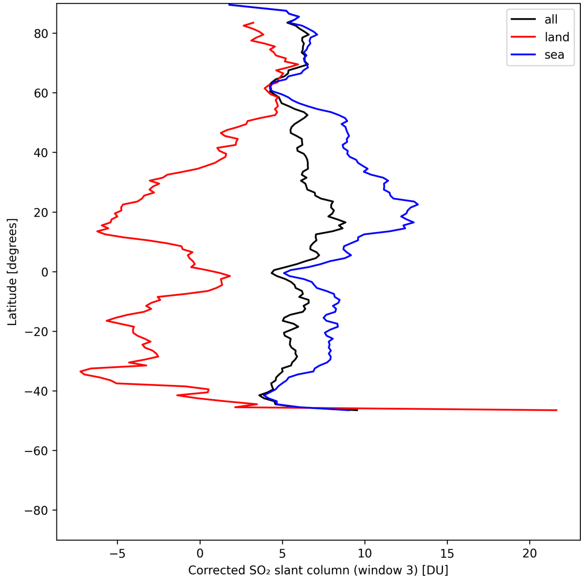
Figure 47: Zonal average of “Corrected SO 2 slant column (window 3)” for 2025-06-04 to 2025-06-06.
