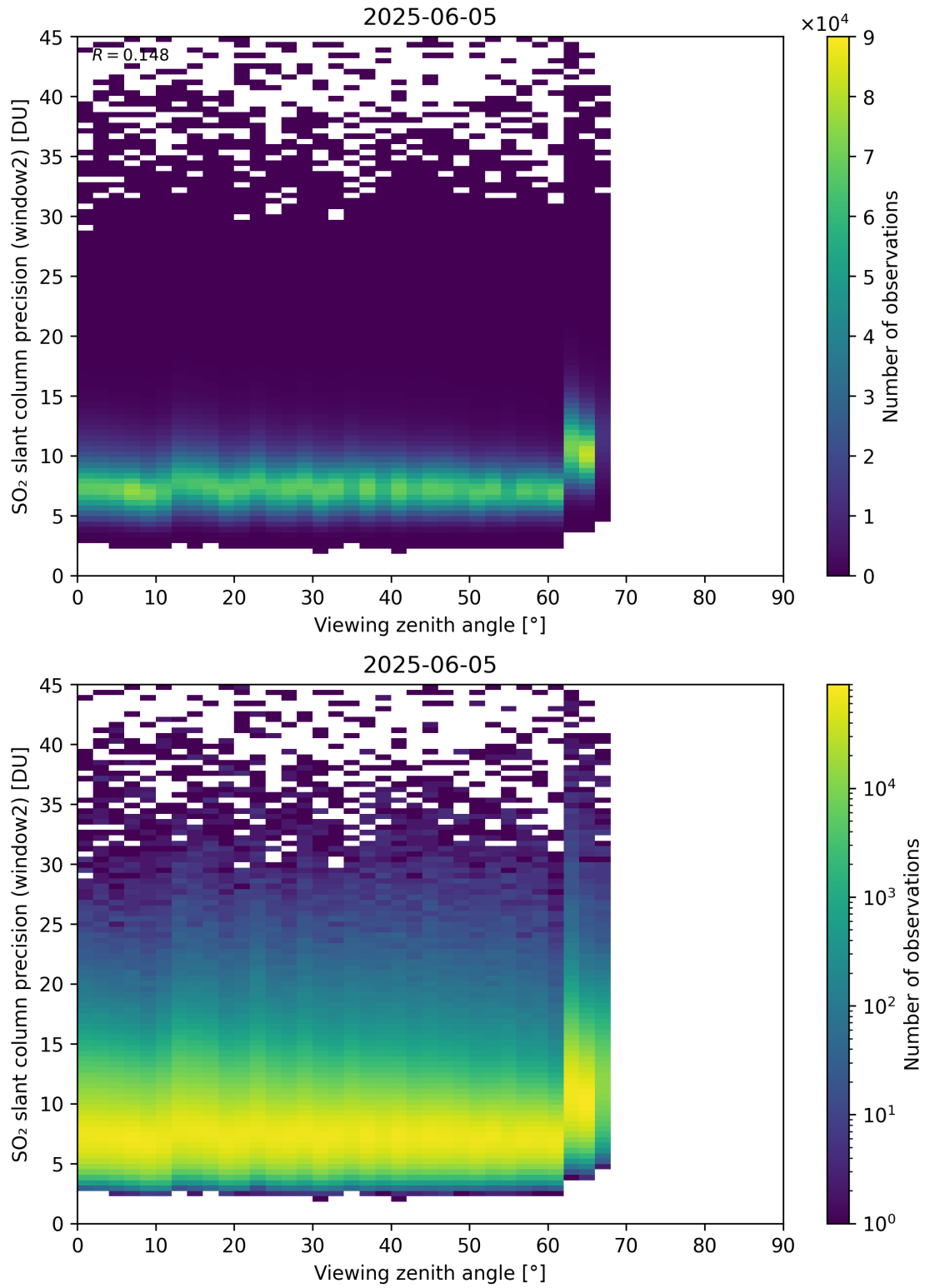
Figure 378: Scatter density plot of “Viewing zenith angle” against “SO 2 slant column precision (window2)” for 2025-06-04 to 2025-06-06.
