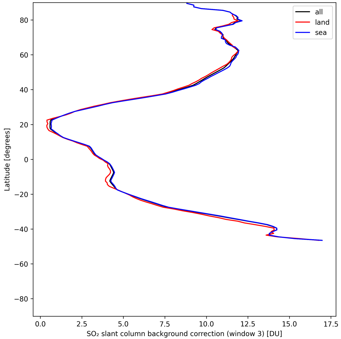
Figure 48: Zonal average of “SO 2 slant column background correction (window 3)” for 2025-06-04 to 2025-06-06.
