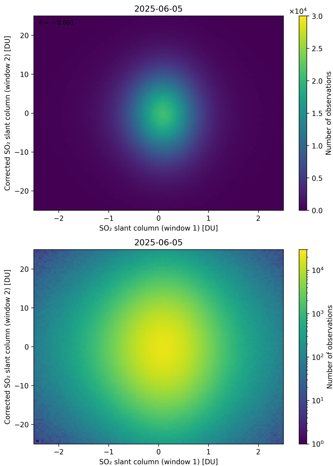
Figure 283: Scatter density plot of “SO 2 slant column (window 1)” against “Corrected SO 2 slant column (window 2)” for 2025-06-04 to 2025-06-06.
