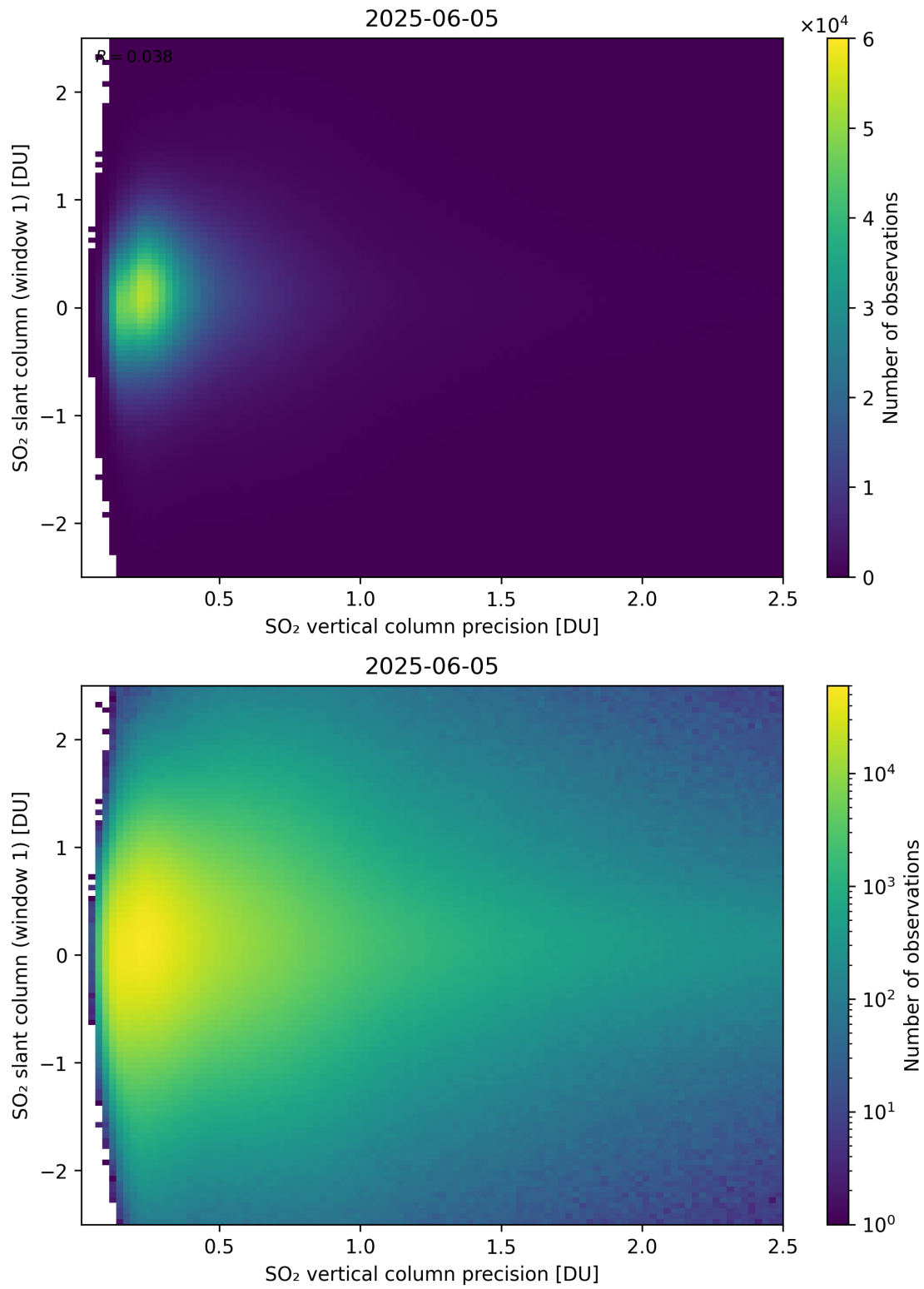
Figure 341: Scatter density plot of “SO 2 vertical column precision” against “SO 2 slant column (window 1)” for 2025-06-04 to 2025-06-06.
