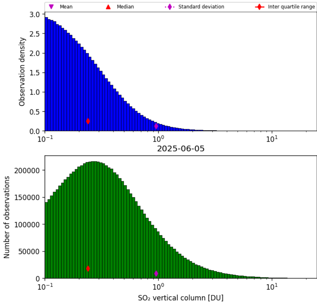
Figure 58: Histogram of “SO 2 vertical column” for 2025-06-04 to 2025-06-06
