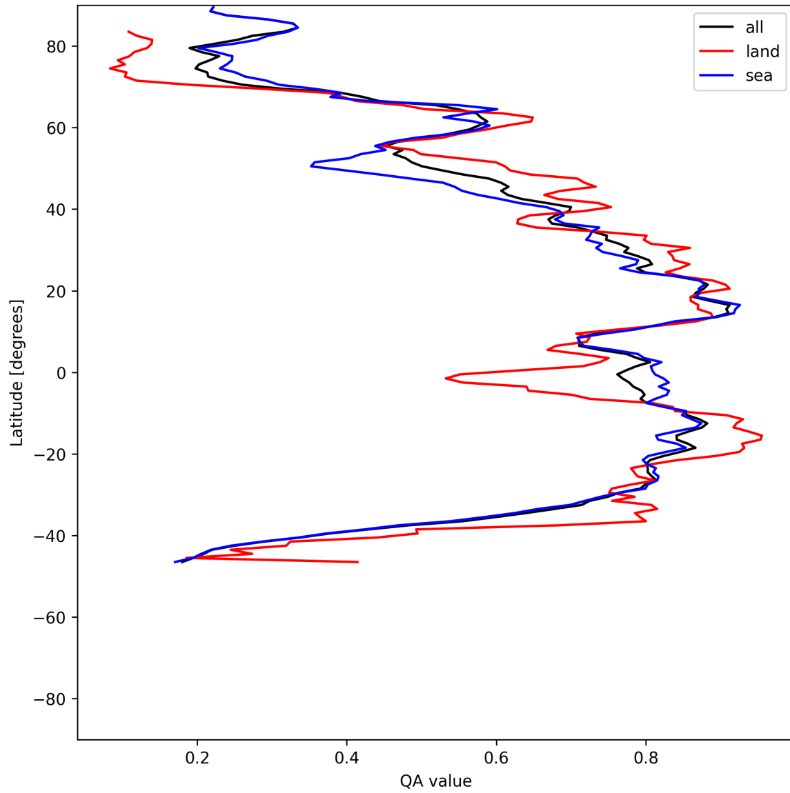
Figure 31: Zonal average of “QA value” for 2025-06-04 to 2025-06-06.
