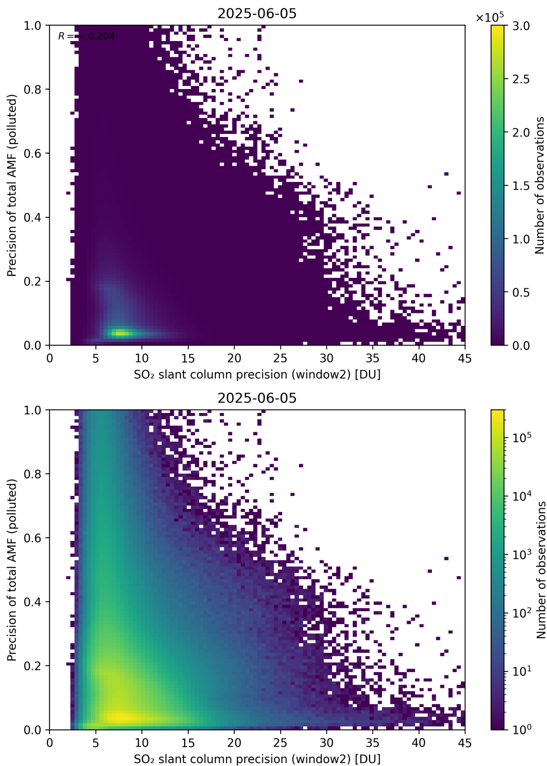
Figure 302: Scatter density plot of “SO 2 slant column precision (window2)” against “Precision of total AMF (polluted)” for 2025-06-04 to 2025-06-06.
