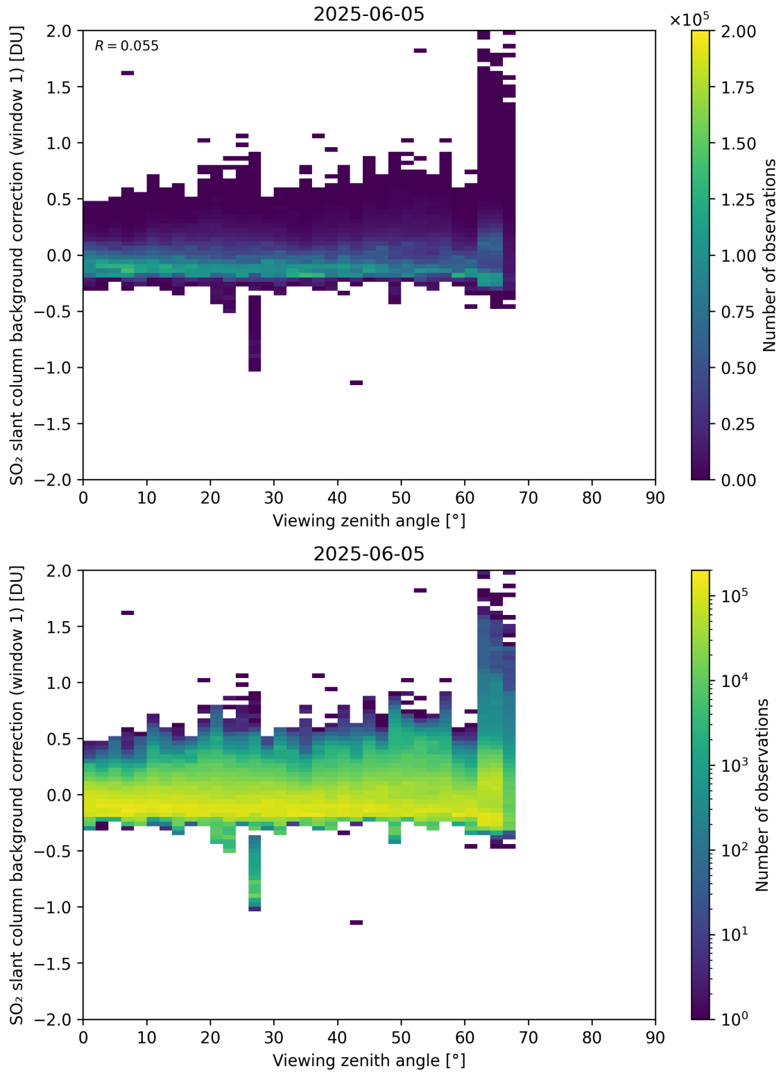
Figure 362: Scatter density plot of “Viewing zenith angle” against “SO 2 slant column background correction (window 1)” for 2025-06-04 to 2025-06-06.
