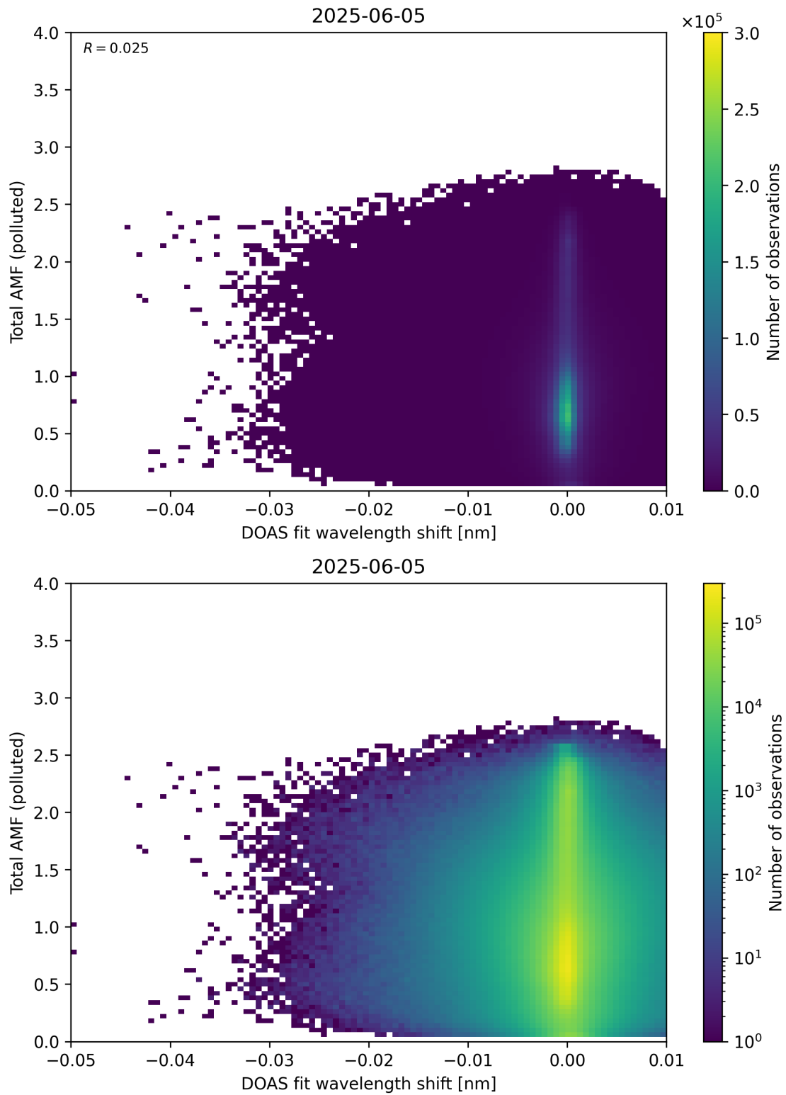
Figure 141: Scatter density plot of “DOAS fit wavelength shift” against “Total AMF (polluted)” for 2025-06-04 to 2025-06-06.
