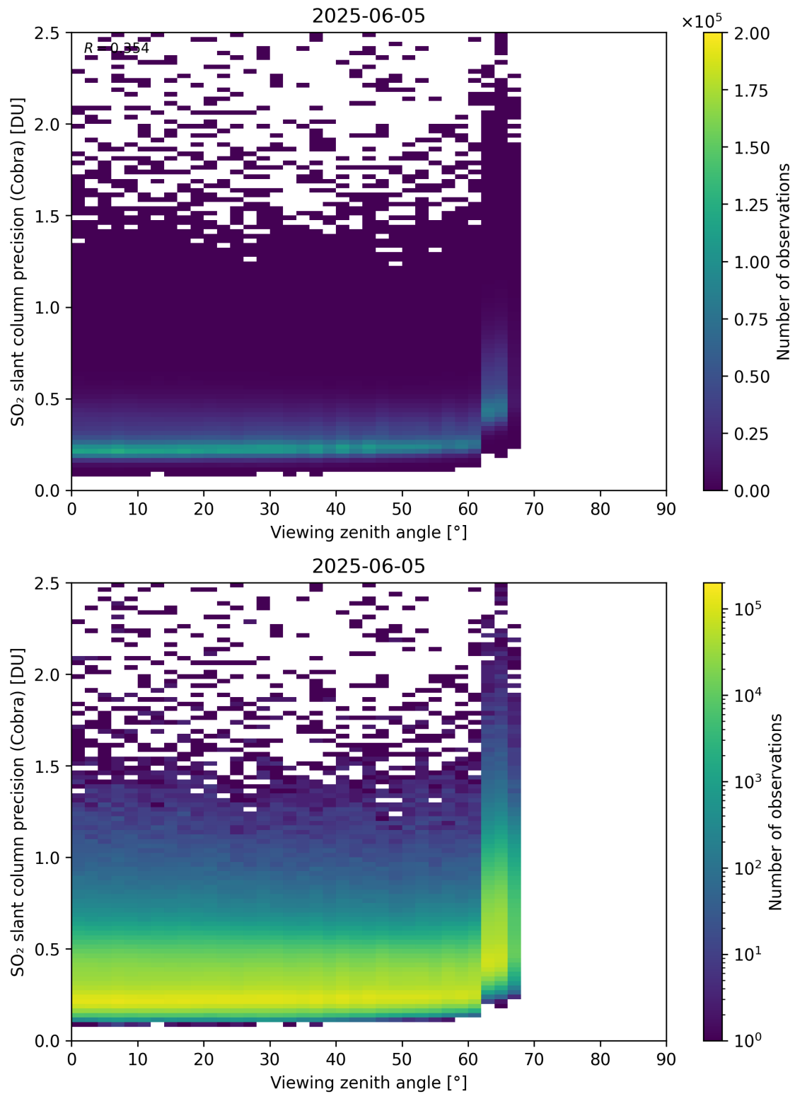
Figure 372: Scatter density plot of “Viewing zenith angle” against “SO 2 slant column precision (Cobra)” for 2025-06-04 to 2025-06-06.
