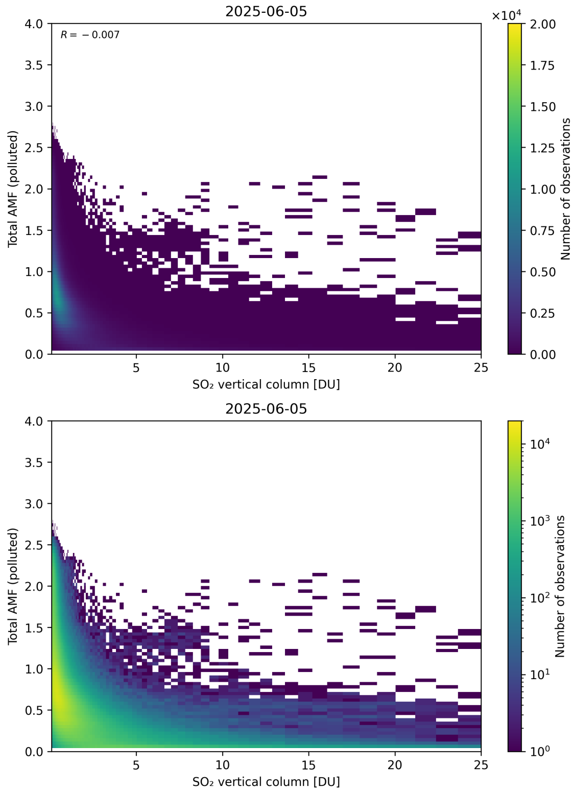
Figure 359: Scatter density plot of “SO 2 vertical column” against “Total AMF (polluted)” for 2025-06-04 to 2025-06-06.
