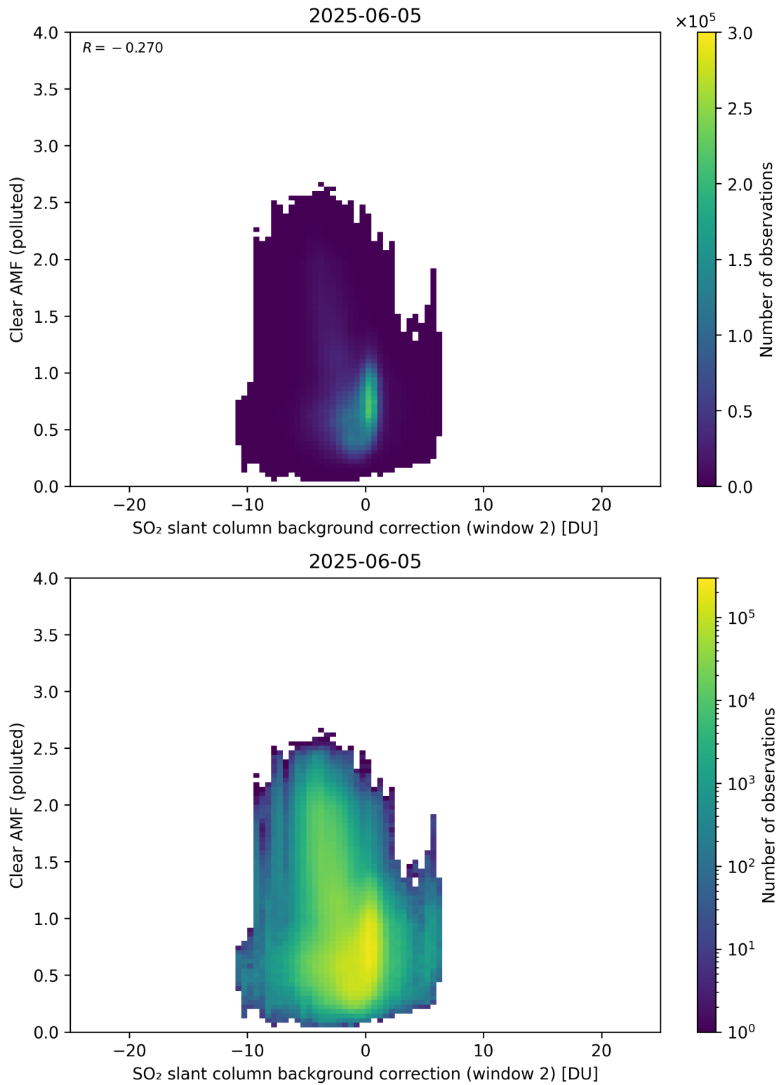
Figure 126: Scatter density plot of “SO 2 slant column background correction (window 2)” against “Clear AMF (polluted)” for 2025-06-04 to 2025-06-06.
