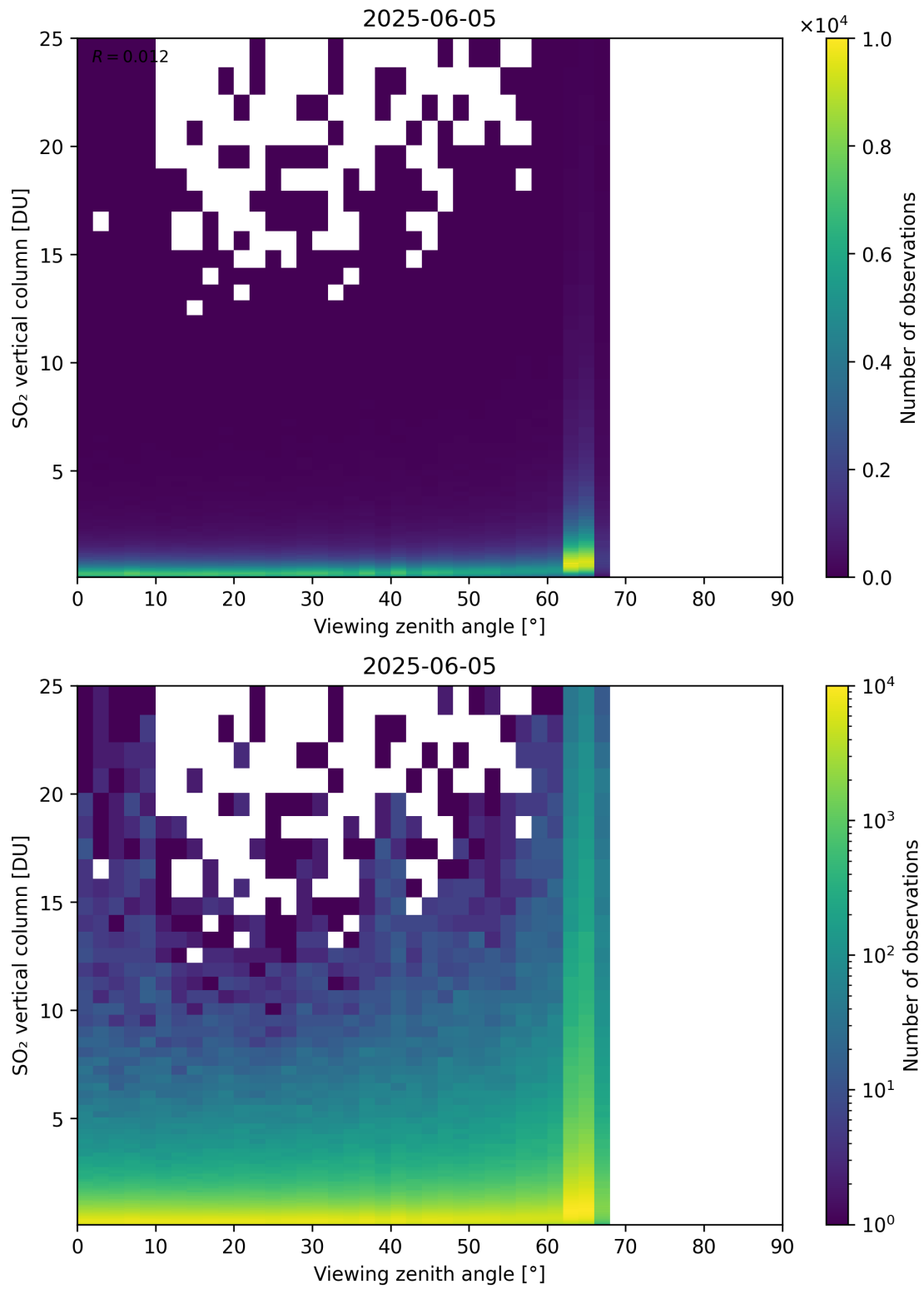
Figure 383: Scatter density plot of “Viewing zenith angle” against “SO 2 vertical column” for 2025-06-04 to 2025-06-06.
