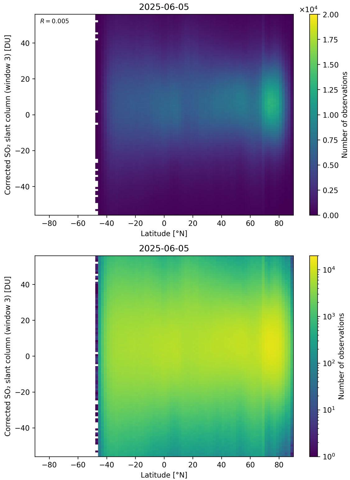
Figure 161: Scatter density plot of “Latitude” against “Corrected SO 2 slant column (window 3)” for 2025-06-04 to 2025-06-06.
