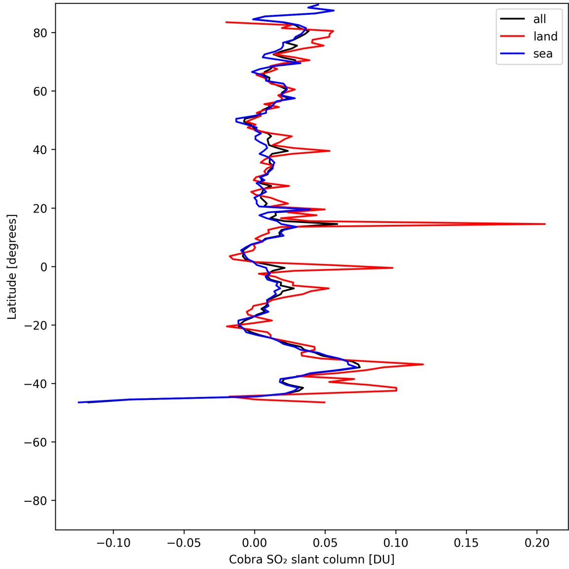
Figure 35: Zonal average of “Cobra SO 2 slant column” for 2025-06-04 to 2025-06-06.
