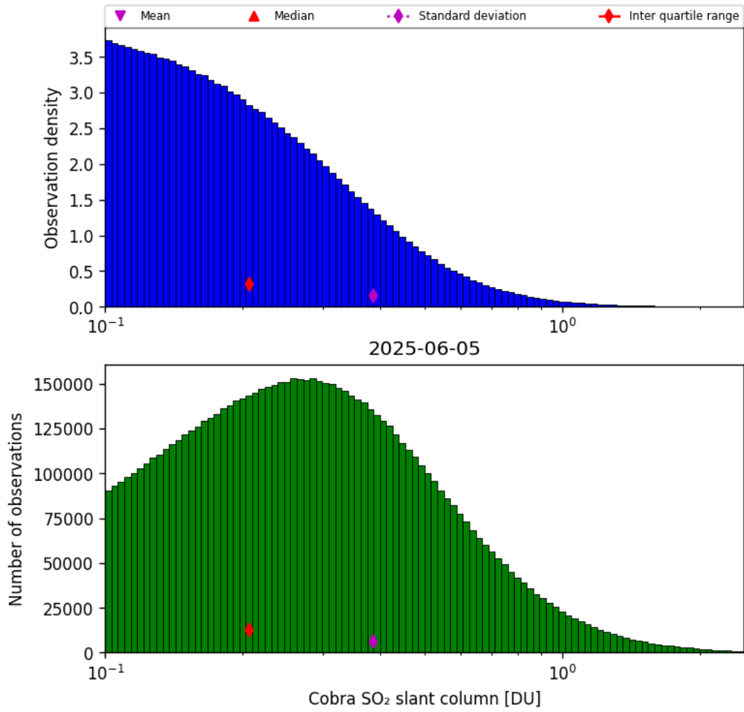
Figure 61: Histogram of “Cobra SO 2 slant column” for 2025-06-04 to 2025-06-06
