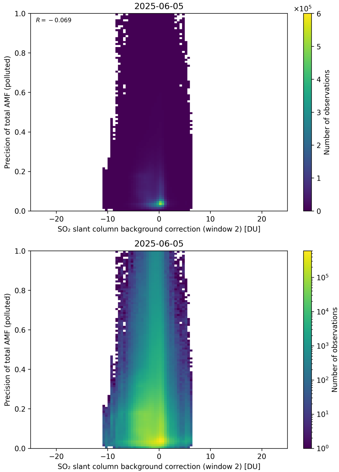
Figure 131: Scatter density plot of “SO 2 slant column background correction (window 2)” against “Precision of total AMF (polluted)” for 2025-06-04 to 2025-06-06.
