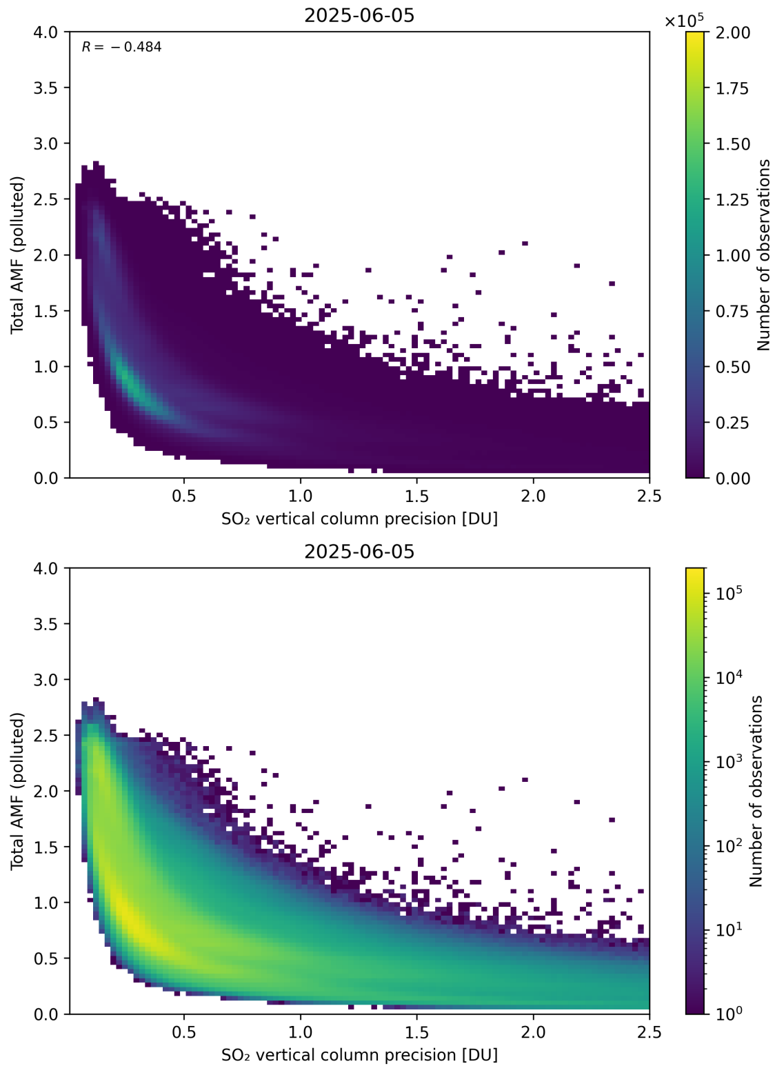
Figure 346: Scatter density plot of “SO 2 vertical column precision” against “Total AMF (polluted)” for 2025-06-04 to 2025-06-06.
