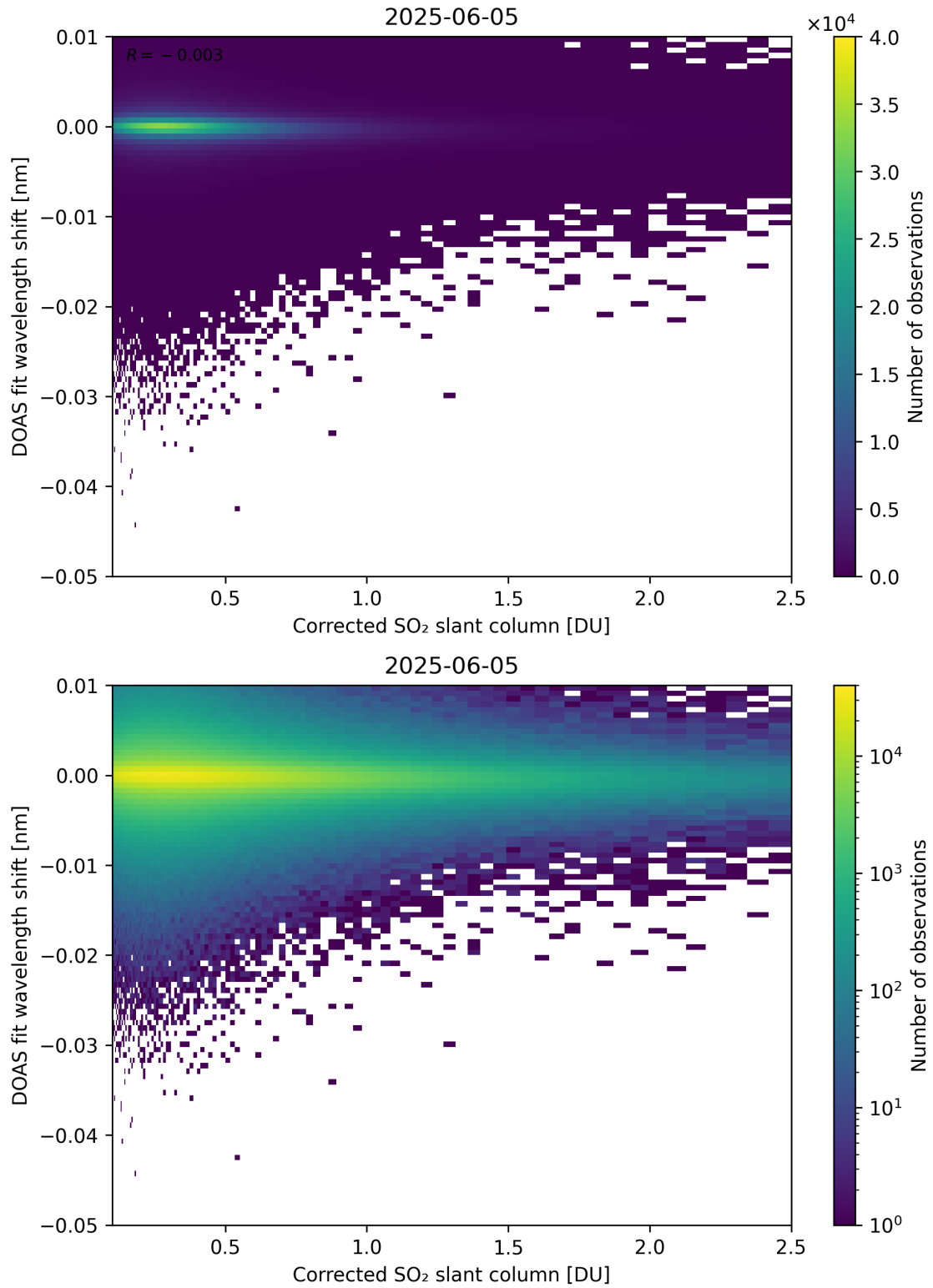
Figure 229: Scatter density plot of “Corrected SO 2 slant column” against “DOAS fit wavelength shift” for 2025-06-04 to 2025-06-06.
