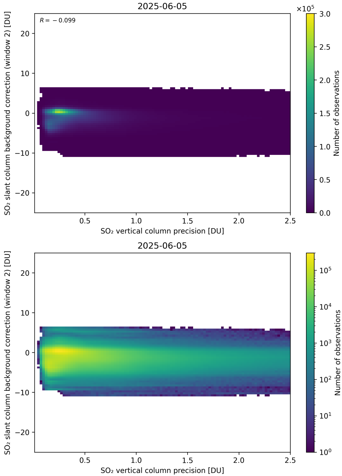
Figure 330: Scatter density plot of “SO 2 vertical column precision” against “SO 2 slant column background correction (window 2)” for 2025-06-04 to 2025-06-06.
