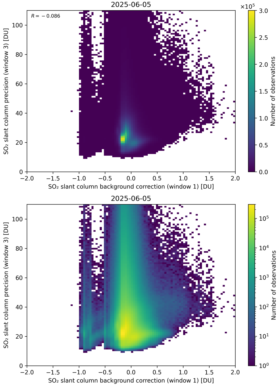
Figure 119: Scatter density plot of “SO 2 slant column background correction (window 1)” against “SO 2 slant column precision (window 3)” for 2025-06-04 to 2025-06-06.
