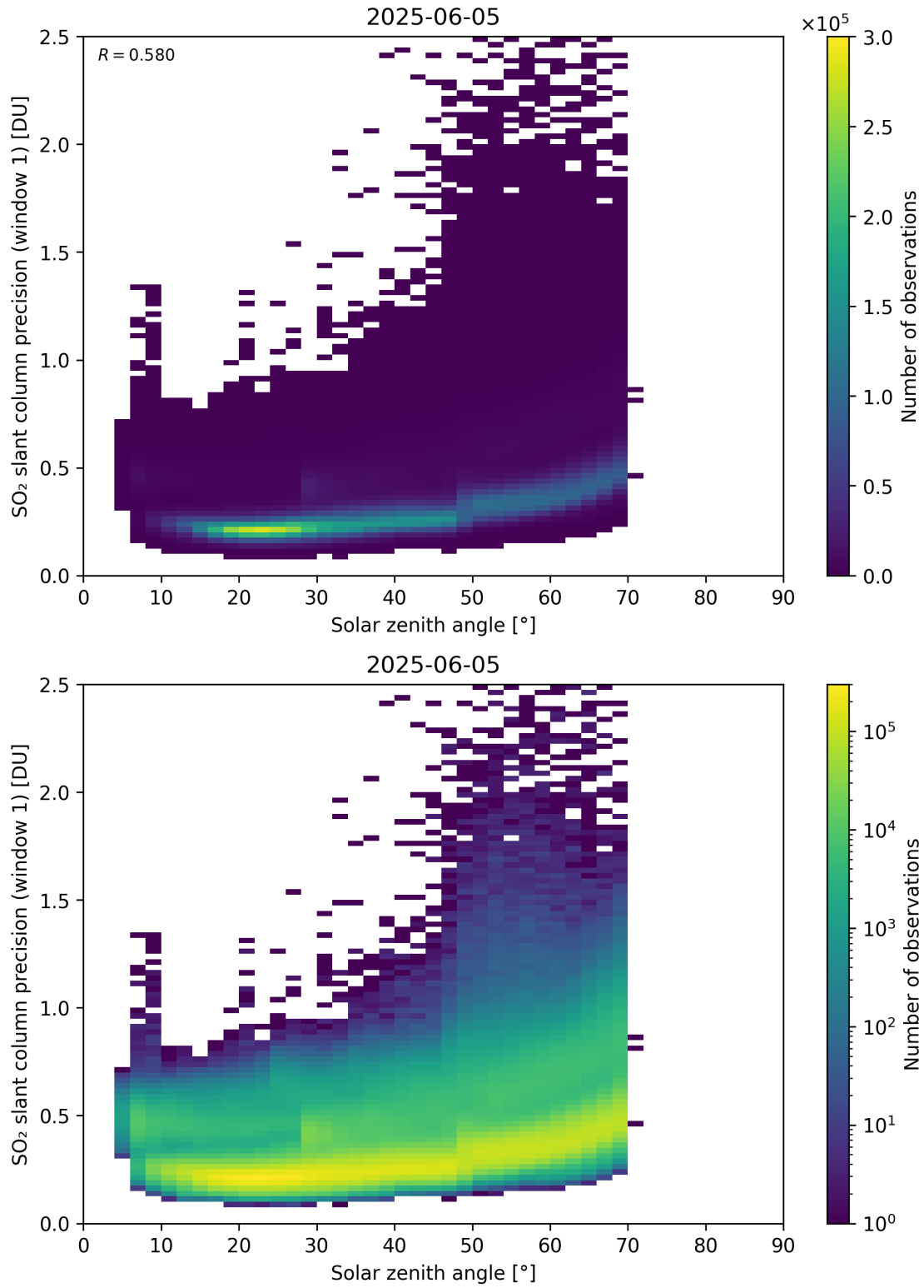
Figure 185: Scatter density plot of “Solar zenith angle” against “SO 2 slant column precision (window 1)” for 2025-06-04 to 2025-06-06.
