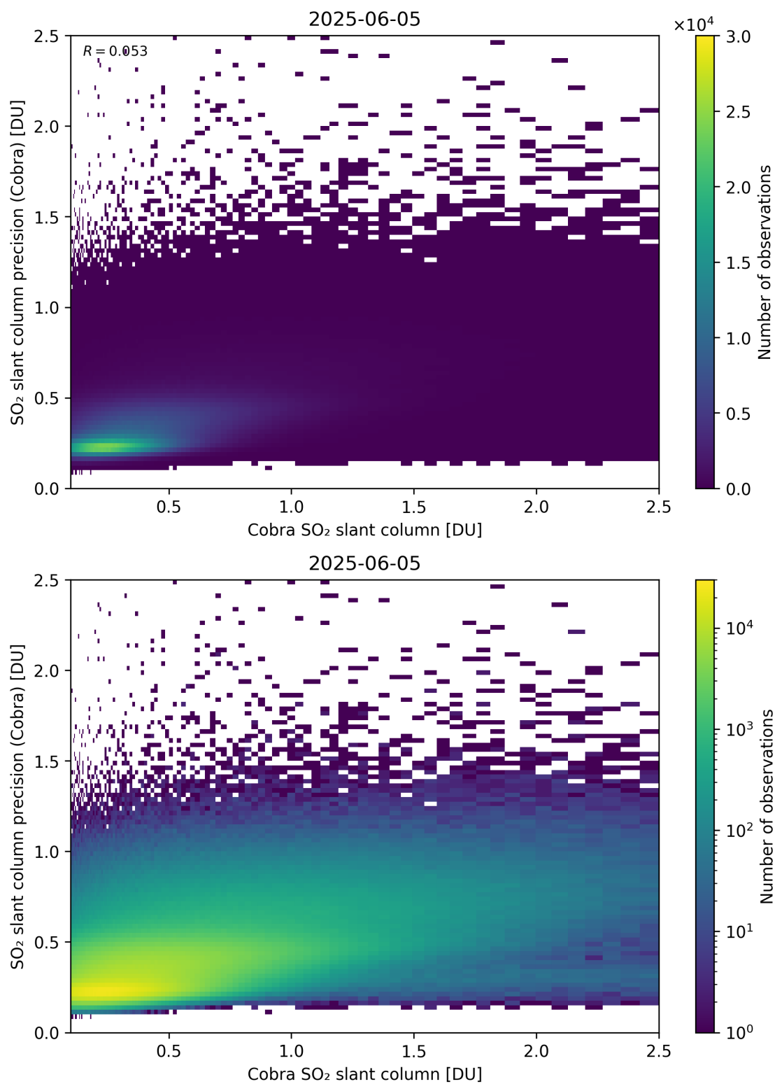
Figure 216: Scatter density plot of “Cobra SO 2 slant column” against “SO 2 slant column precision (Cobra)” for 2025-06-04 to 2025-06-06.
