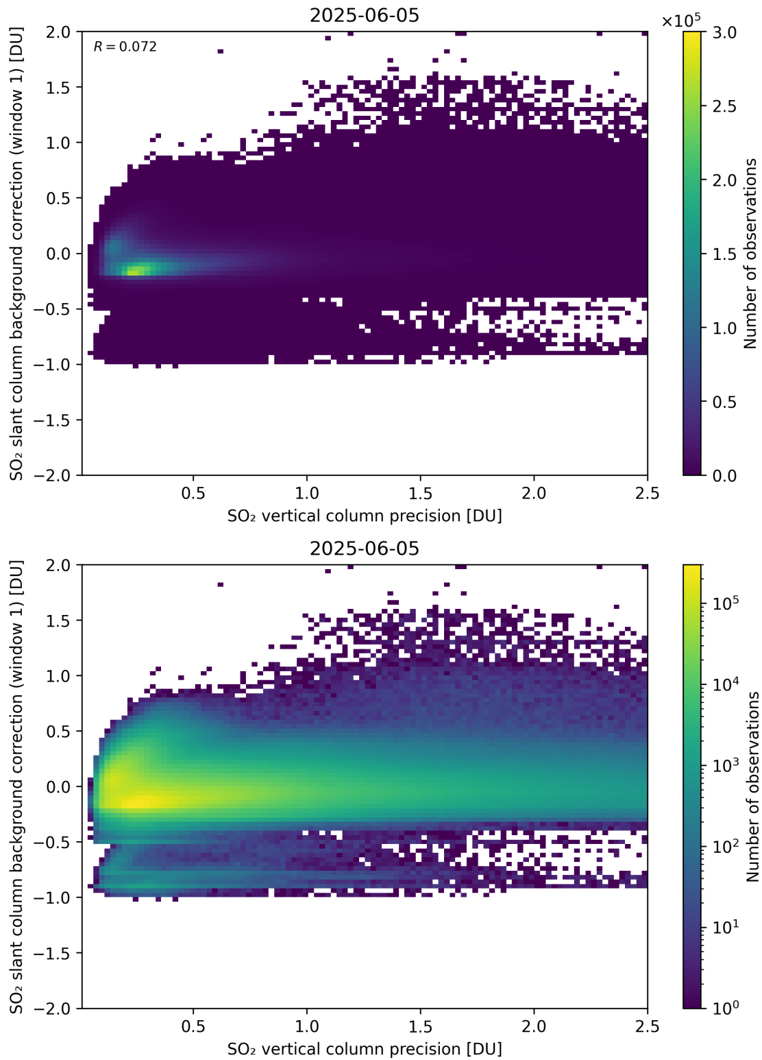
Figure 329: Scatter density plot of “SO 2 vertical column precision” against “SO 2 slant column background correction (window 1)” for 2025-06-04 to 2025-06-06.
