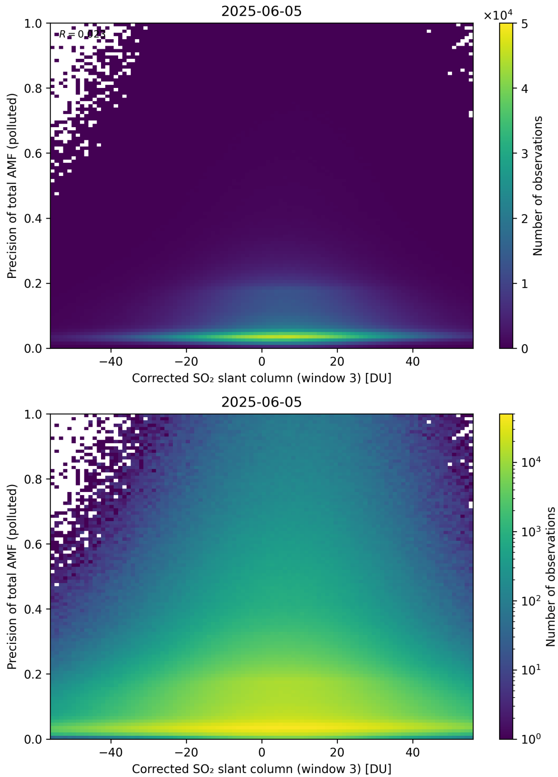
Figure 261: Scatter density plot of “Corrected SO 2 slant column (window 3)” against “Precision of total AMF (polluted)” for 2025-06-04 to 2025-06-06.
