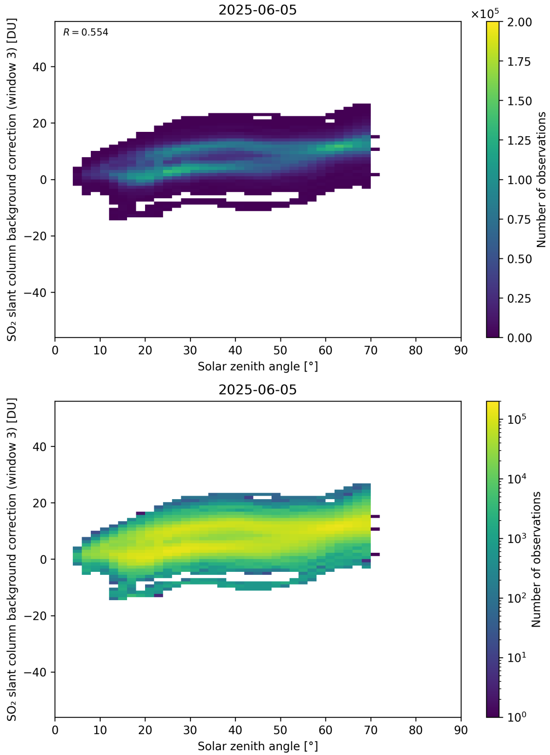
Figure 173: Scatter density plot of “Solar zenith angle” against “SO 2 slant column background correction (window 3)” for 2025-06-04 to 2025-06-06.
