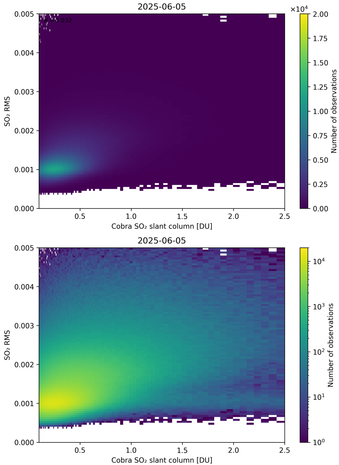
Figure 198: Scatter density plot of “Cobra SO 2 slant column” against “SO 2 RMS” for 2025-06-04 to 2025-06-06.
