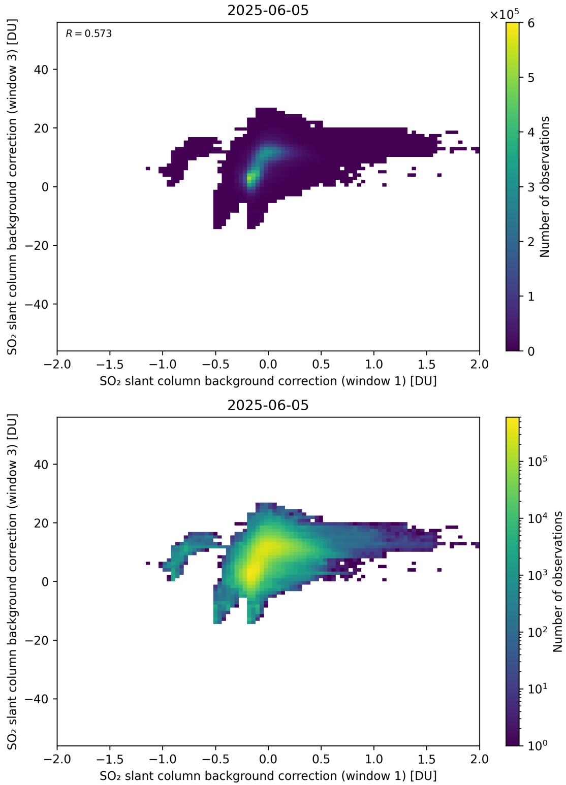
Figure 110: Scatter density plot of “SO 2 slant column background correction (window 1)” against “SO 2 slant column background correction (window 3)” for 2025-06-04 to 2025-06-06.
