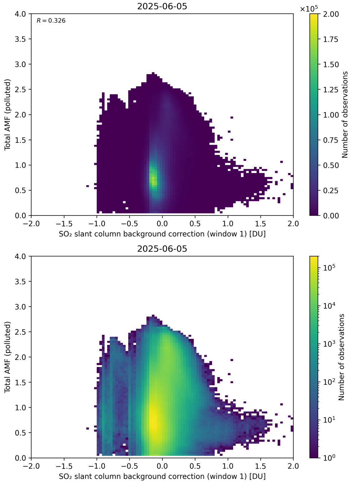
Figure 120: Scatter density plot of “SO 2 slant column background correction (window 1)” against “Total AMF (polluted)” for 2025-06-04 to 2025-06-06.
