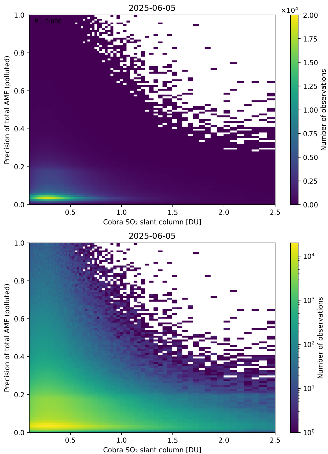
Figure 225: Scatter density plot of “Cobra SO 2 slant column” against “Precision of total AMF (polluted)” for 2025-06-04 to 2025-06-06.
