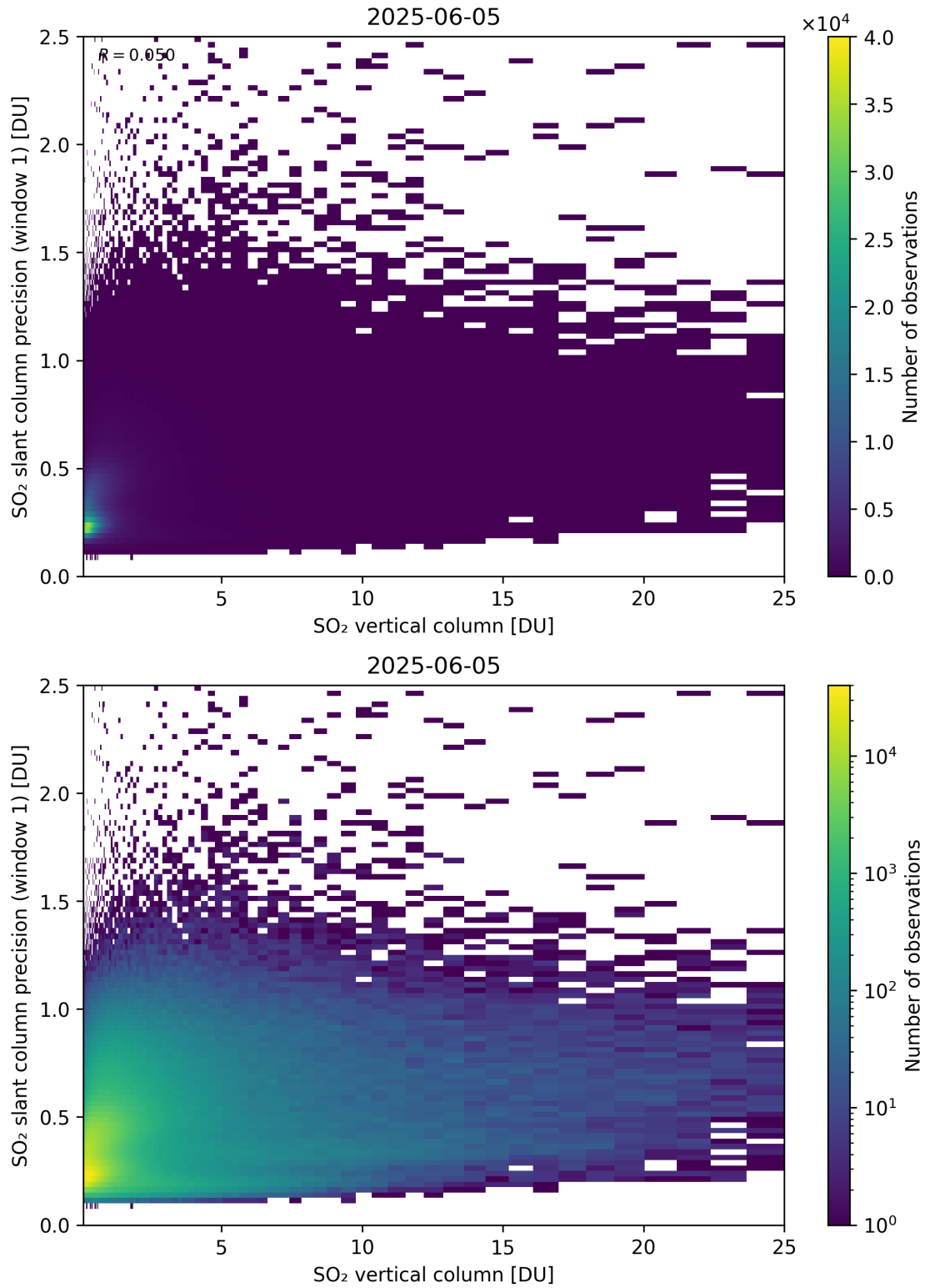
Figure 355: Scatter density plot of “SO 2 vertical column” against “SO 2 slant column precision (window 1)” for 2025-06-04 to 2025-06-06.
