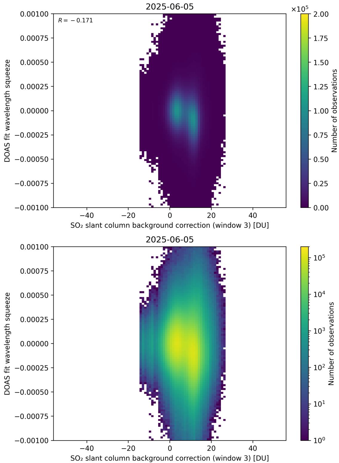
Figure 133: Scatter density plot of “SO 2 slant column background correction (window 3)” against “DOAS fit wavelength squeeze” for 2025-06-04 to 2025-06-06.
