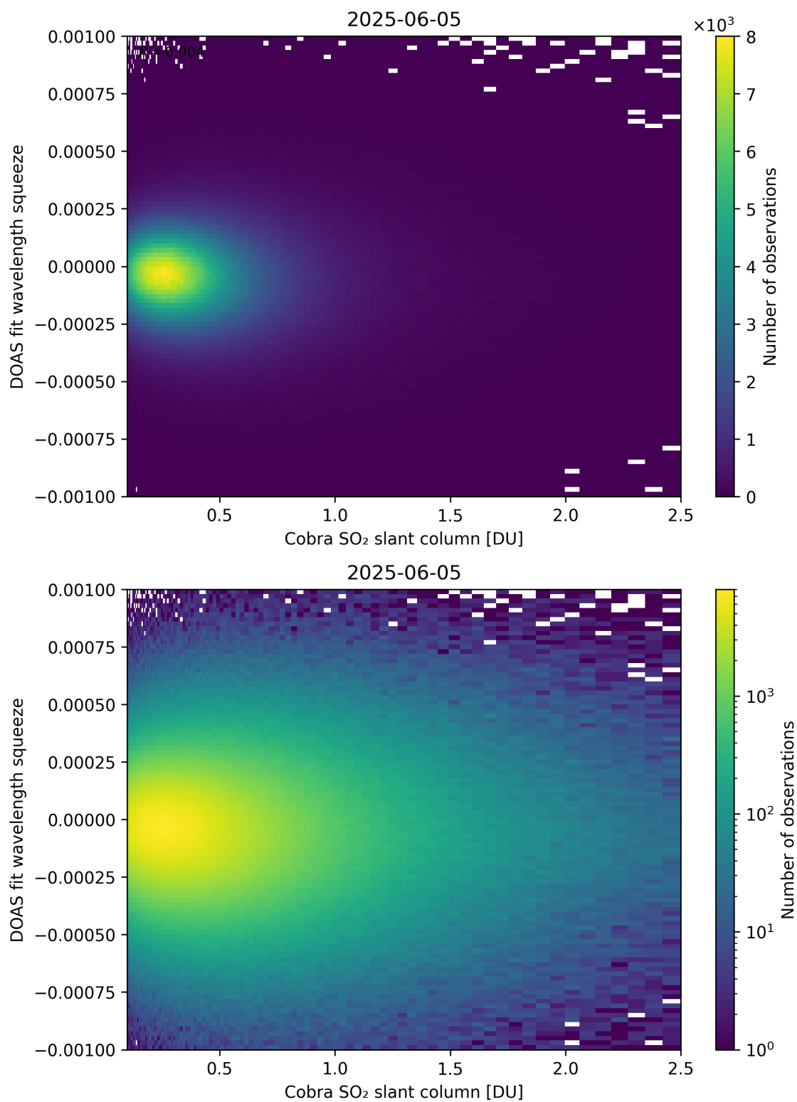
Figure 197: Scatter density plot of “Cobra SO 2 slant column” against “DOAS fit wavelength squeeze” for 2025-06-04 to 2025-06-06.
