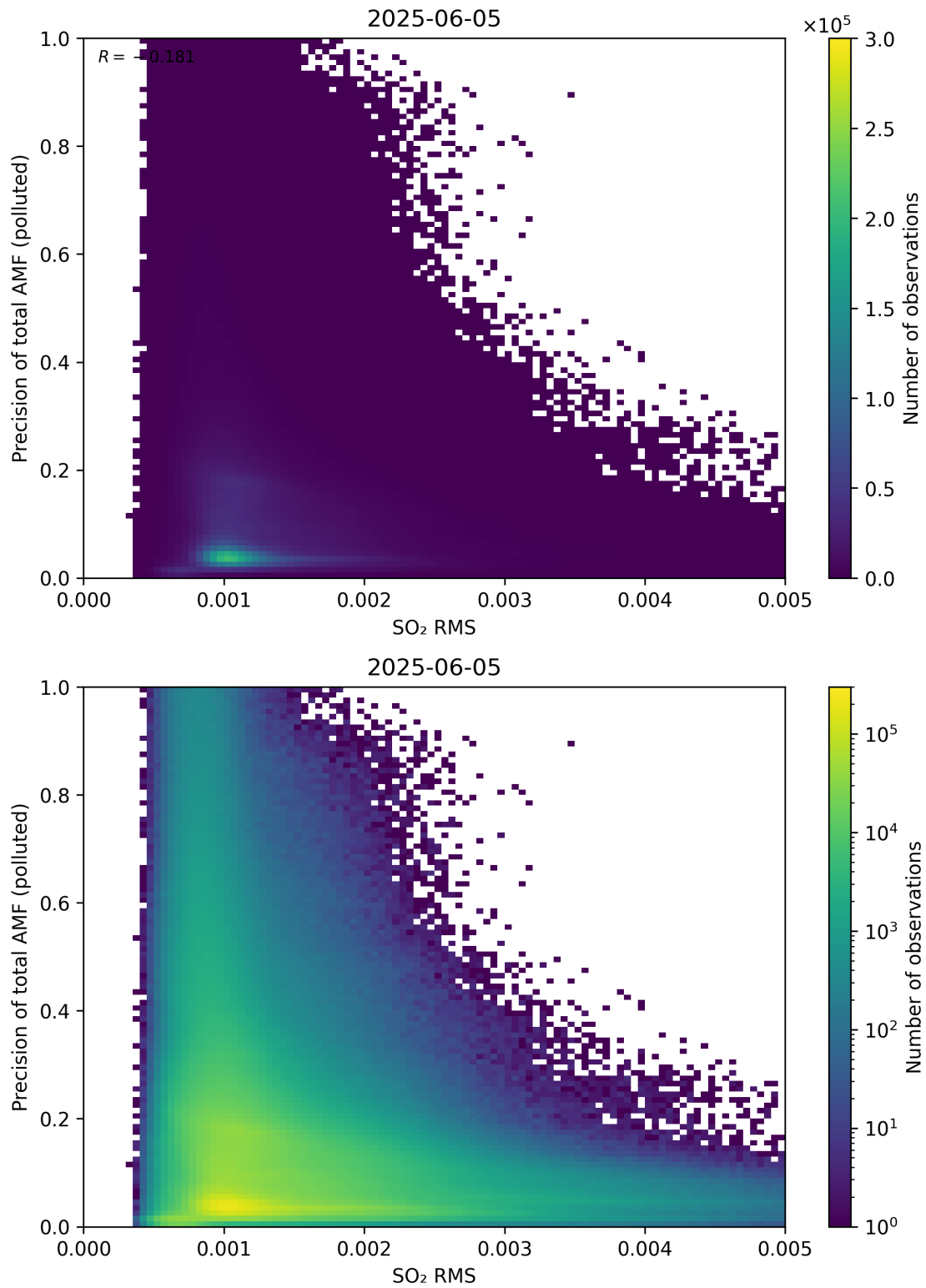
Figure 149: Scatter density plot of “SO 2 RMS” against “Precision of total AMF (polluted)” for 2025-06-04 to 2025-06-06.
