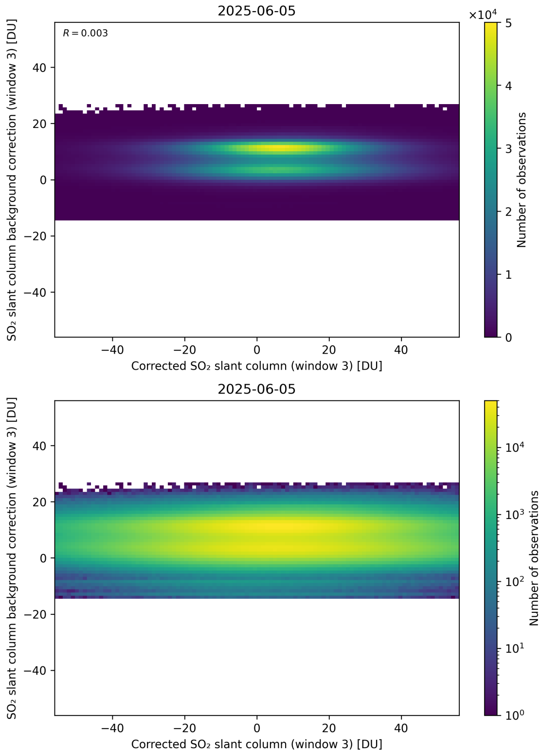
Figure 255: Scatter density plot of “Corrected SO 2 slant column (window 3)” against “SO 2 slant column background correction (window 3)” for 2025-06-04 to 2025-06-06.
