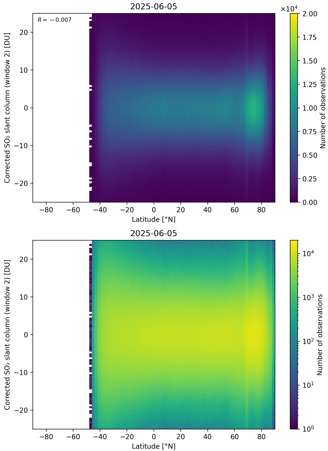
Figure 160: Scatter density plot of “Latitude” against “Corrected SO 2 slant column (window 2)” for 2025-06-04 to 2025-06-06.
