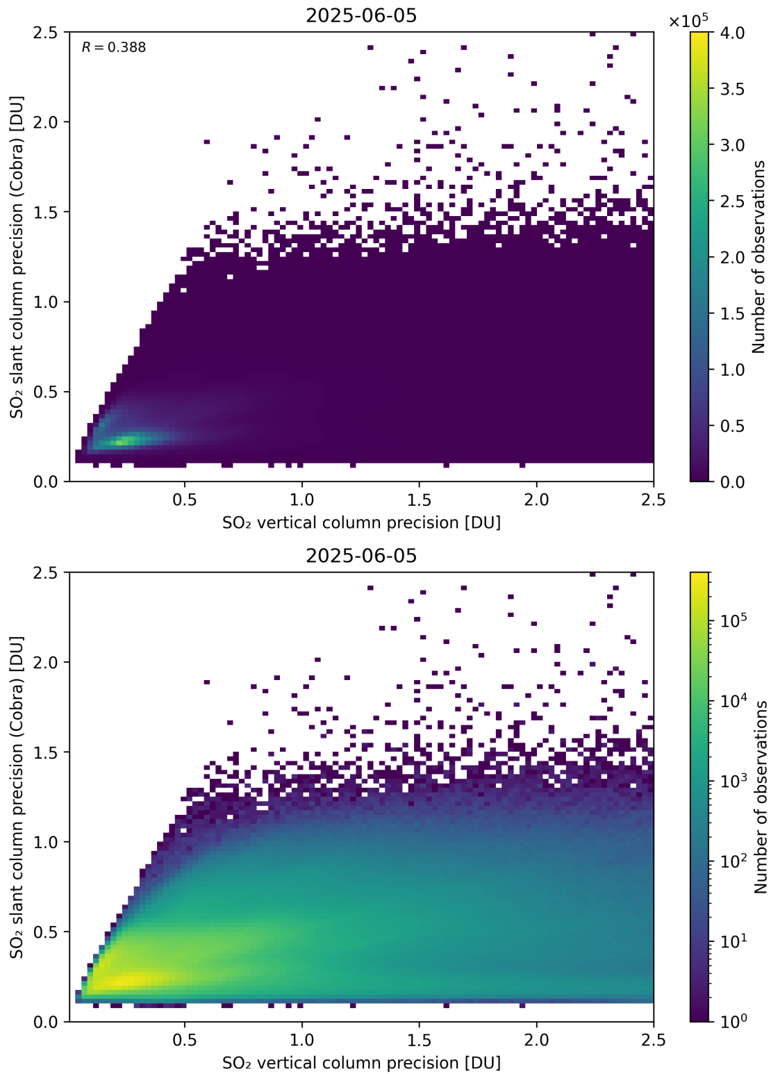
Figure 337: Scatter density plot of “SO 2 vertical column precision” against “SO 2 slant column precision (Cobra)” for 2025-06-04 to 2025-06-06.
