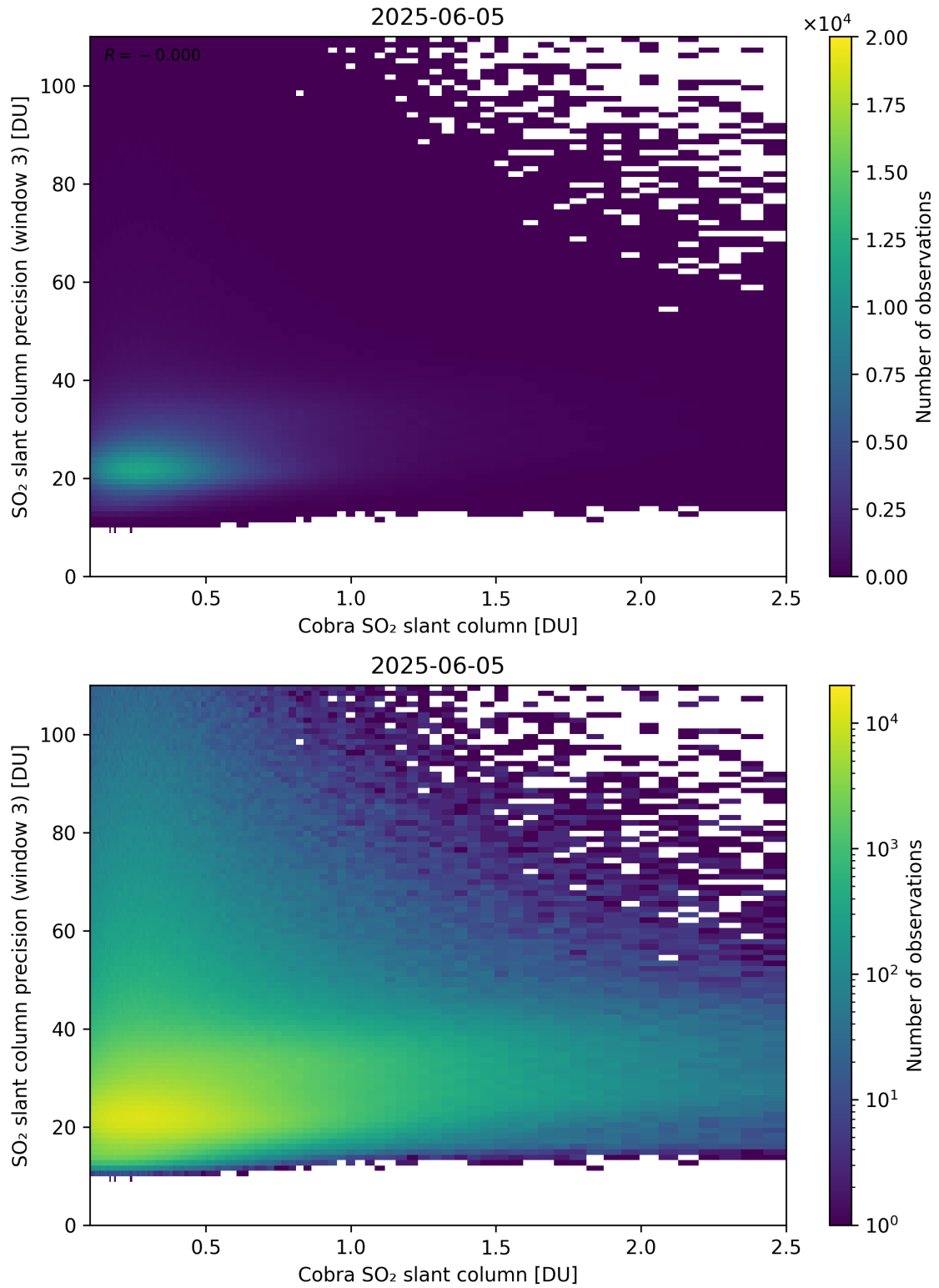
Figure 223: Scatter density plot of “Cobra SO 2 slant column” against “SO 2 slant column precision (window 3)” for 2025-06-04 to 2025-06-06.
