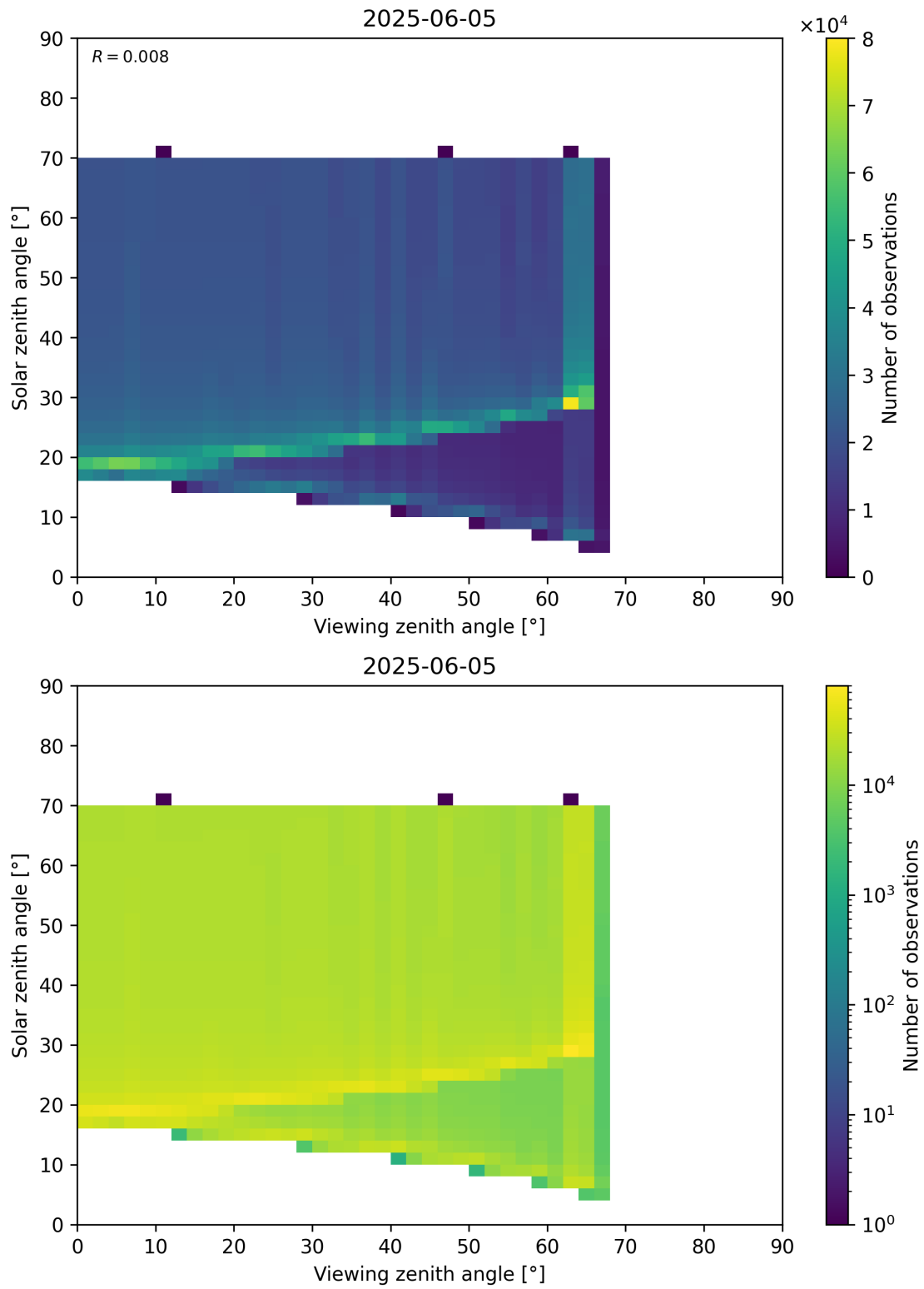
Figure 369: Scatter density plot of “Viewing zenith angle” against “Solar zenith angle” for 2025-06-04 to 2025-06-06.
