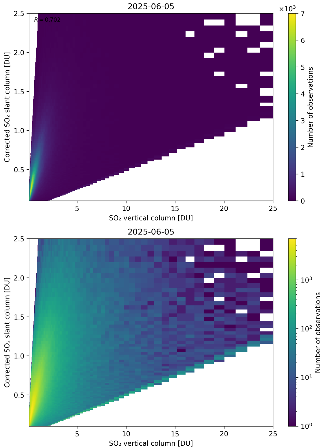
Figure 351: Scatter density plot of “SO 2 vertical column” against “Corrected SO 2 slant column” for 2025-06-04 to 2025-06-06.
