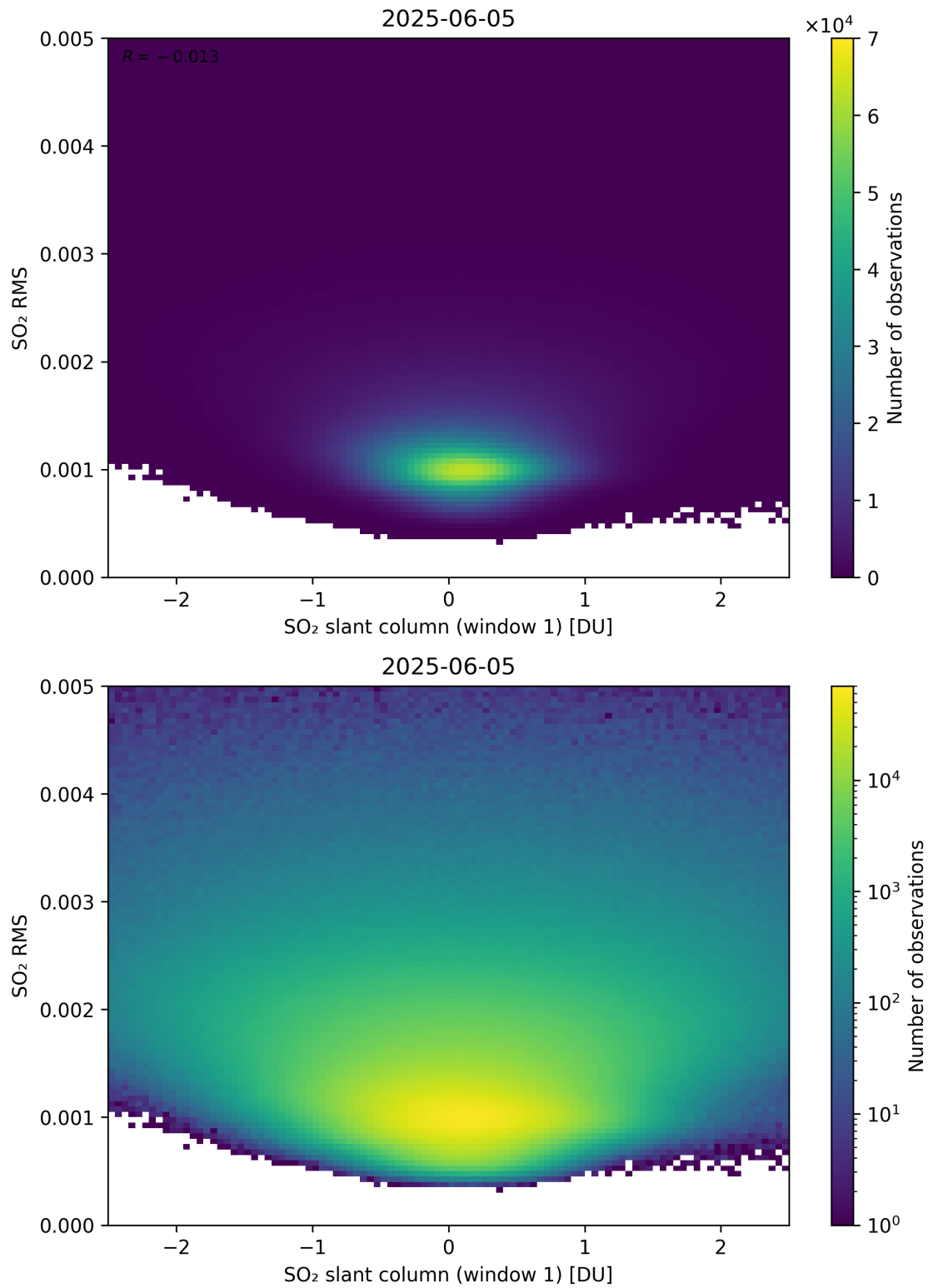
Figure 267: Scatter density plot of “SO 2 slant column (window 1)” against “SO 2 RMS” for 2025-06-04 to 2025-06-06.
