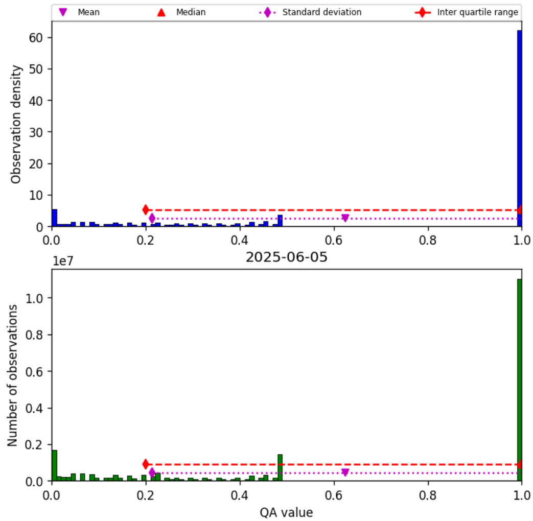
Figure 57: Histogram of “QA value” for 2025-06-04 to 2025-06-06
