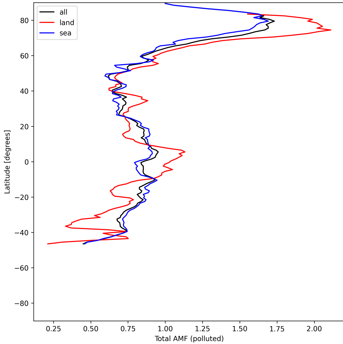
Figure 53: Zonal average of “Total AMF (polluted)” for 2025-06-04 to 2025-06-06.
