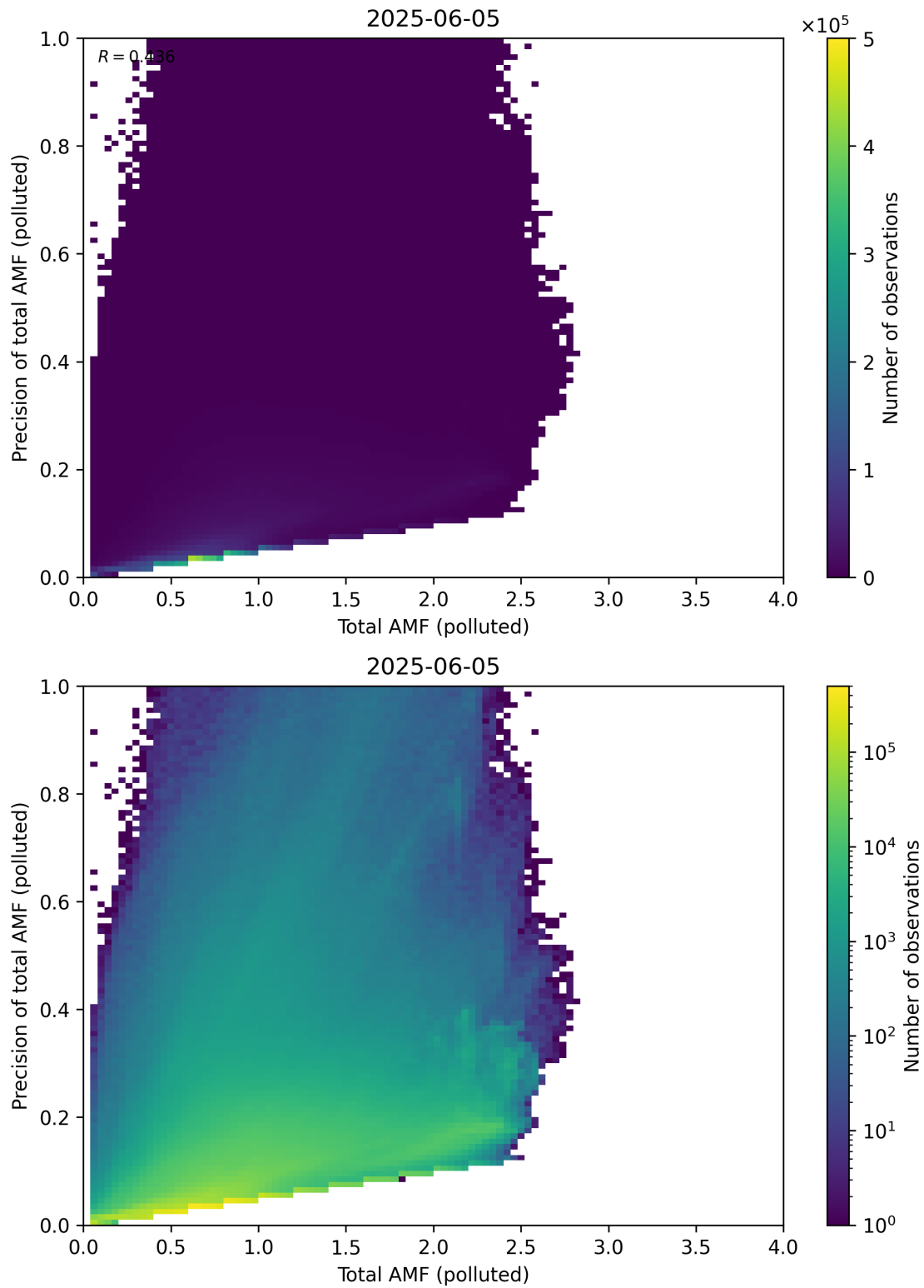
Figure 322: Scatter density plot of “Total AMF (polluted)” against “Precision of total AMF (polluted)” for 2025-06-04 to 2025-06-06.
