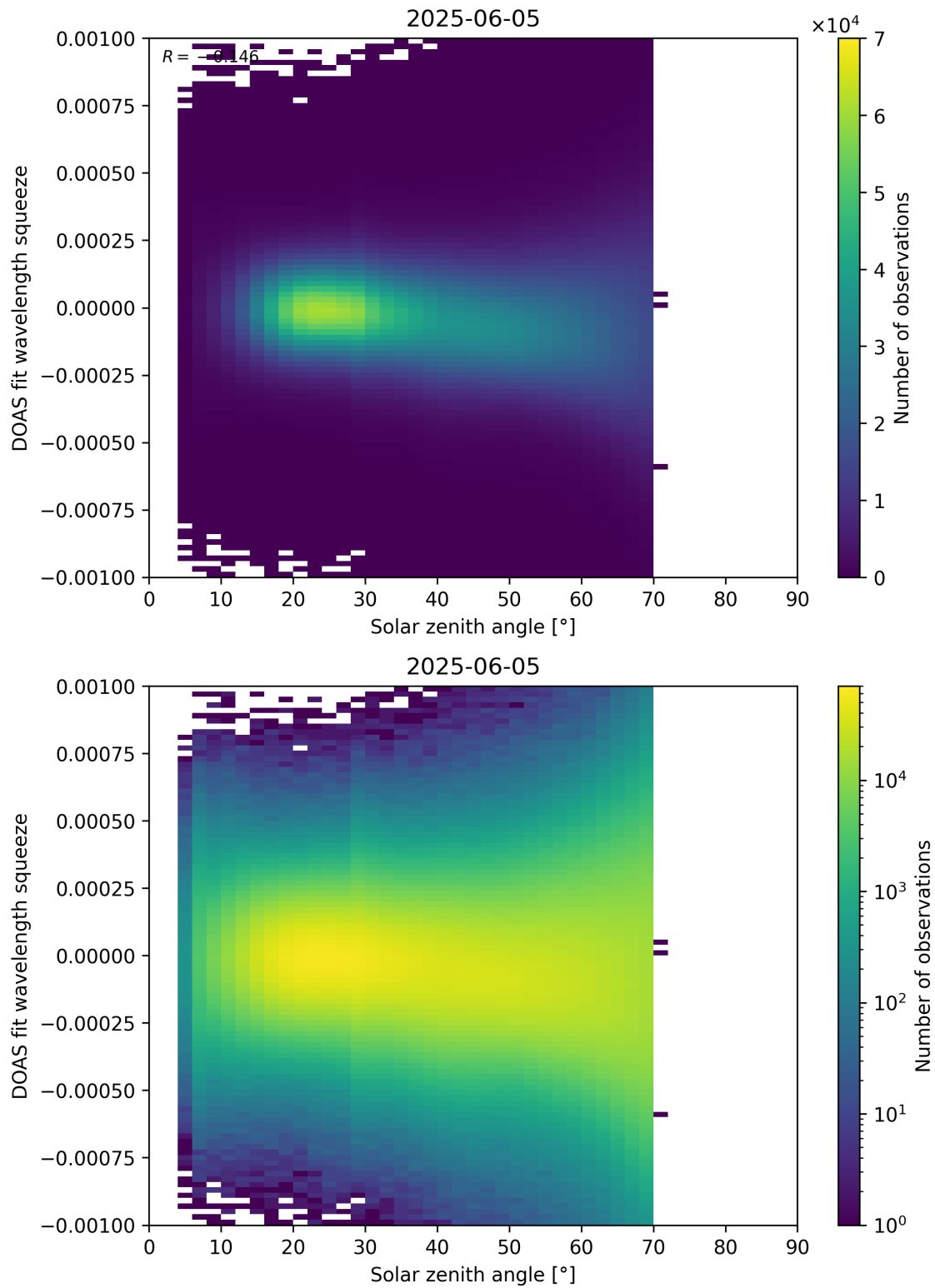
Figure 175: Scatter density plot of “Solar zenith angle” against “DOAS fit wavelength squeeze” for 2025-06-04 to 2025-06-06.
