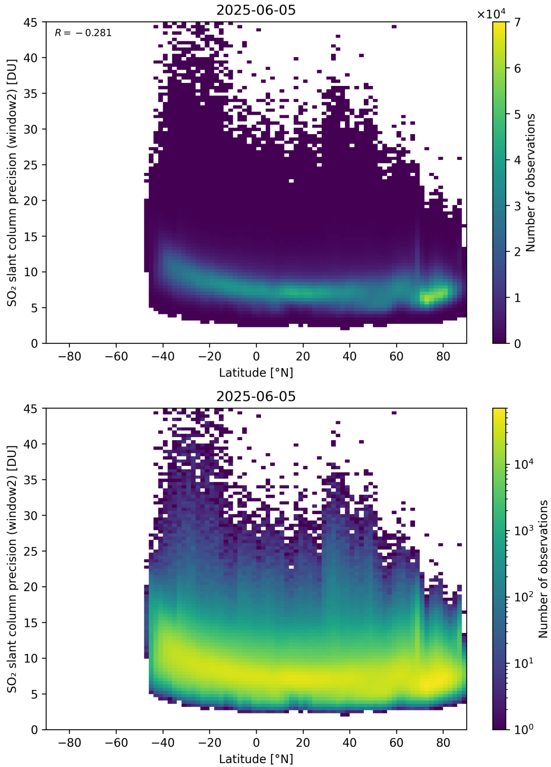
Figure 164: Scatter density plot of “Latitude” against “SO 2 slant column precision (window2)” for 2025-06-04 to 2025-06-06.
