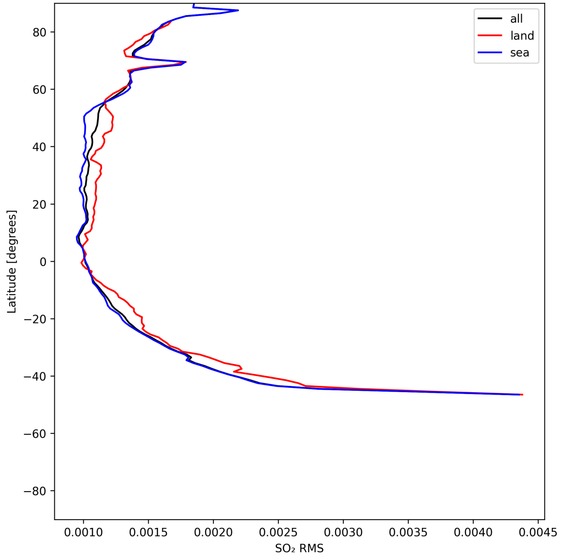
Figure 52: Zonal average of “SO 2 RMS” for 2025-06-04 to 2025-06-06.
