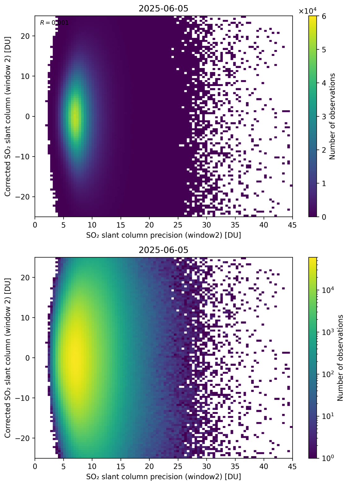
Figure 297: Scatter density plot of “SO 2 slant column precision (window2)” against “Corrected SO 2 slant column (window 2)” for 2025-06-04 to 2025-06-06.
