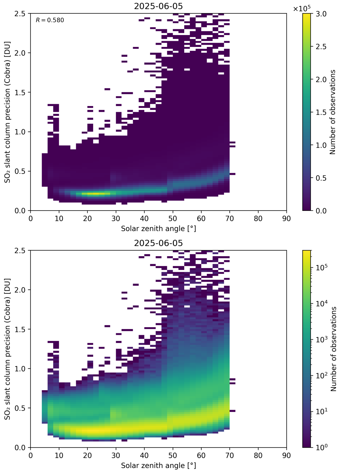
Figure 180: Scatter density plot of “Solar zenith angle” against “SO 2 slant column precision (Cobra)” for 2025-06-04 to 2025-06-06.
