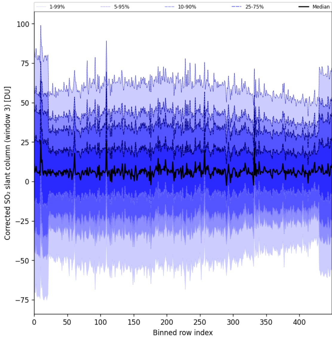
Figure 99: Along track statistics of “Corrected SO 2 slant column (window 3)” for 2025-06-04 to 2025-06-06
