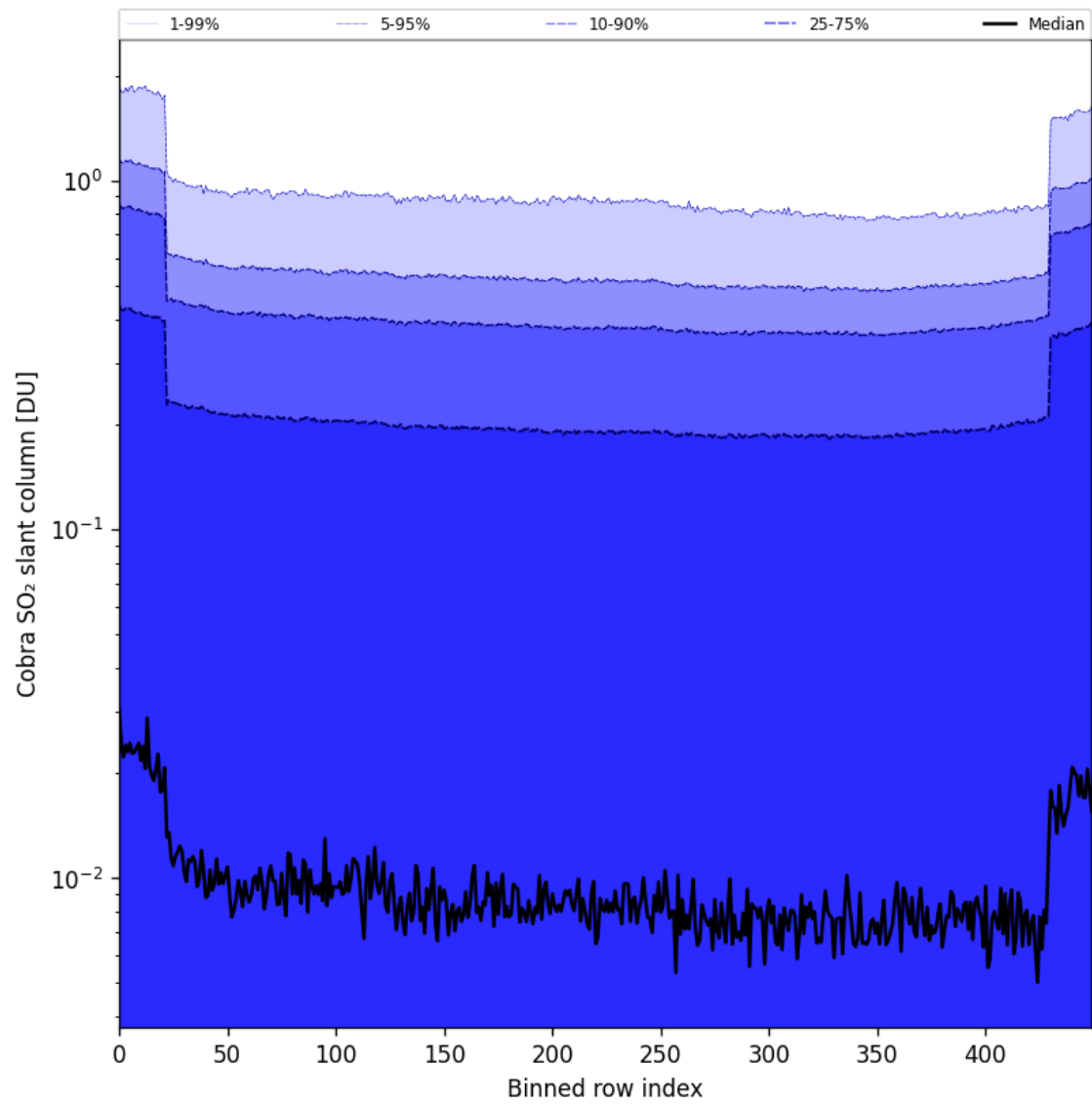
Figure 87: Along track statistics of “Cobra SO 2 slant column” for 2025-06-04 to 2025-06-06
