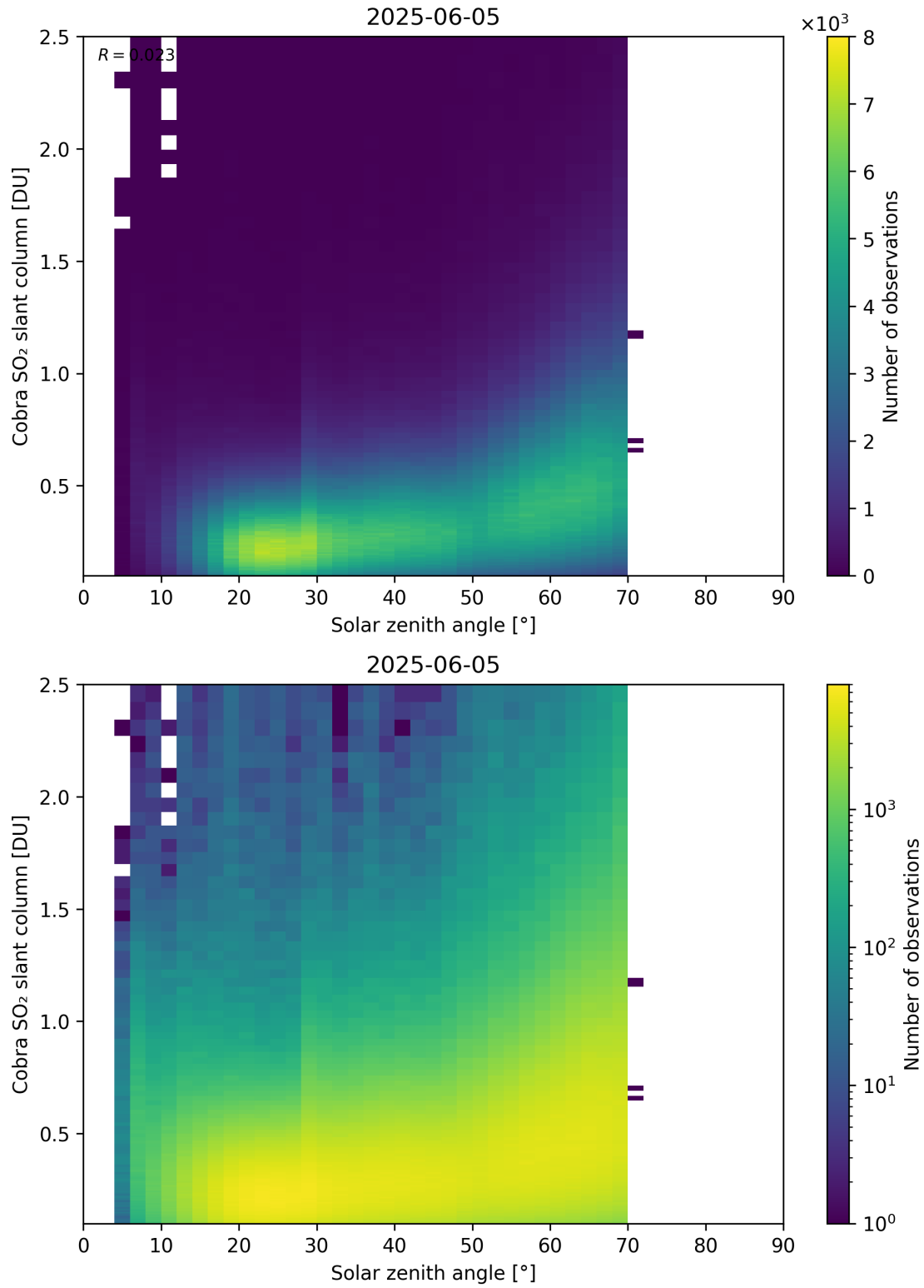
Figure 179: Scatter density plot of “Solar zenith angle” against “Cobra SO 2 slant column” for 2025-06-04 to 2025-06-06.
