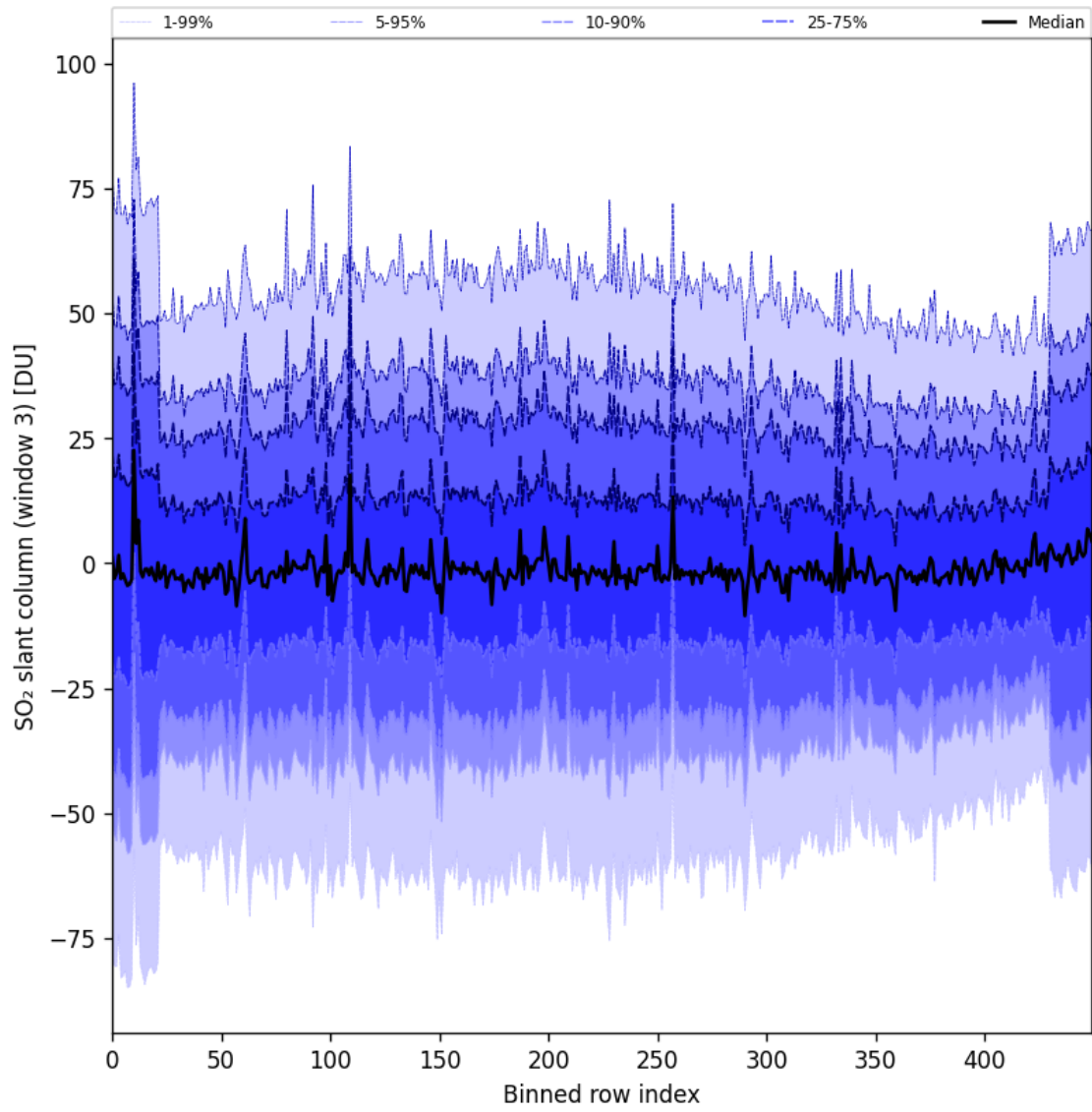
Figure 97: Along track statistics of “SO 2 slant column (window 3)” for 2025-06-04 to 2025-06-06
