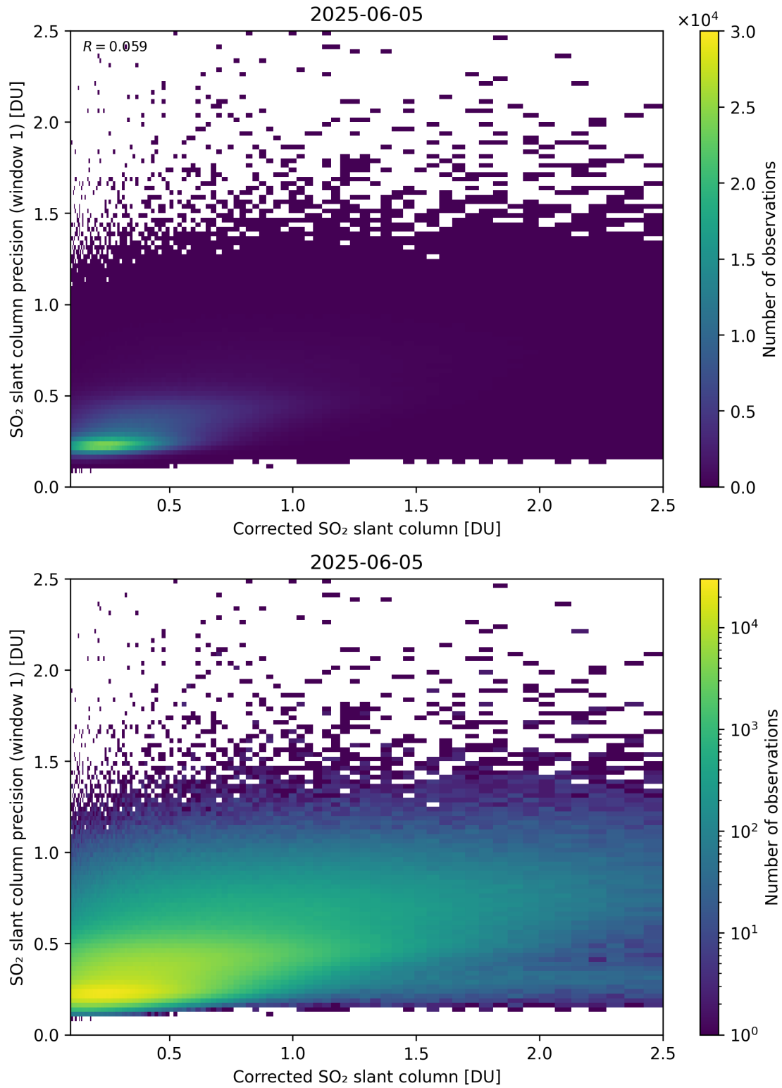
Figure 238: Scatter density plot of “Corrected SO 2 slant column” against “SO 2 slant column precision (window 1)” for 2025-06-04 to 2025-06-06.
