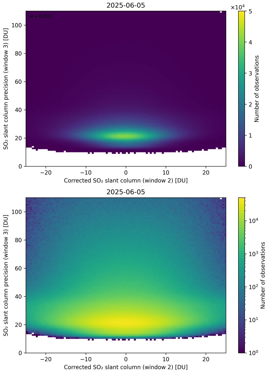
Figure 252: Scatter density plot of “Corrected SO 2 slant column (window 2)” against “SO 2 slant column precision (window 3)” for 2025-06-04 to 2025-06-06.
