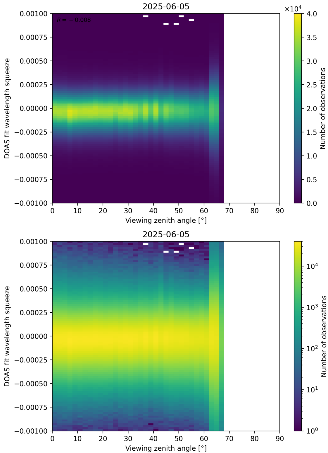
Figure 366: Scatter density plot of “Viewing zenith angle” against “DOAS fit wavelength squeeze” for 2025-06-04 to 2025-06-06.
