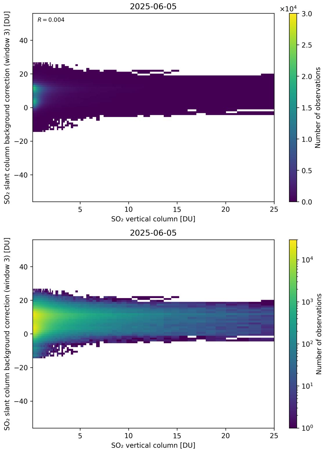
Figure 325: Scatter density plot of “SO 2 vertical column” against “SO 2 slant column background correction (window 3)” for 2025-06-04 to 2025-06-06.
