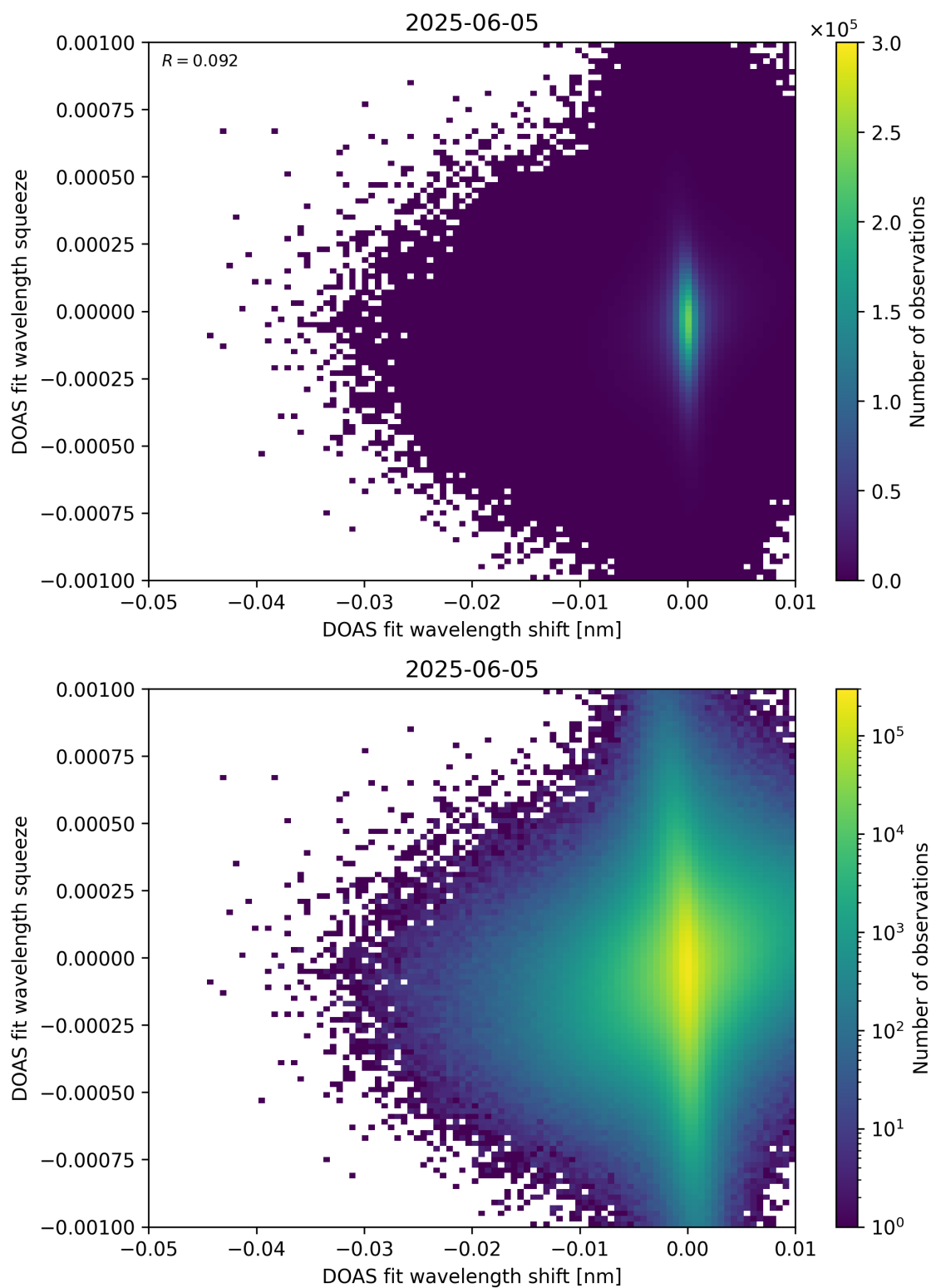
Figure 138: Scatter density plot of “DOAS fit wavelength shift” against “DOAS fit wavelength squeeze” for 2025-06-04 to 2025-06-06.
