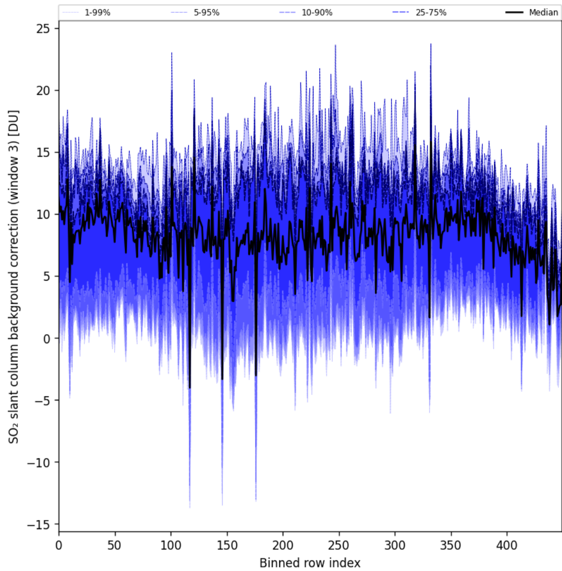
Figure 100: Along track statistics of “SO 2 slant column background correction (window 3)” for 2025-06-04 to 2025-06-06
