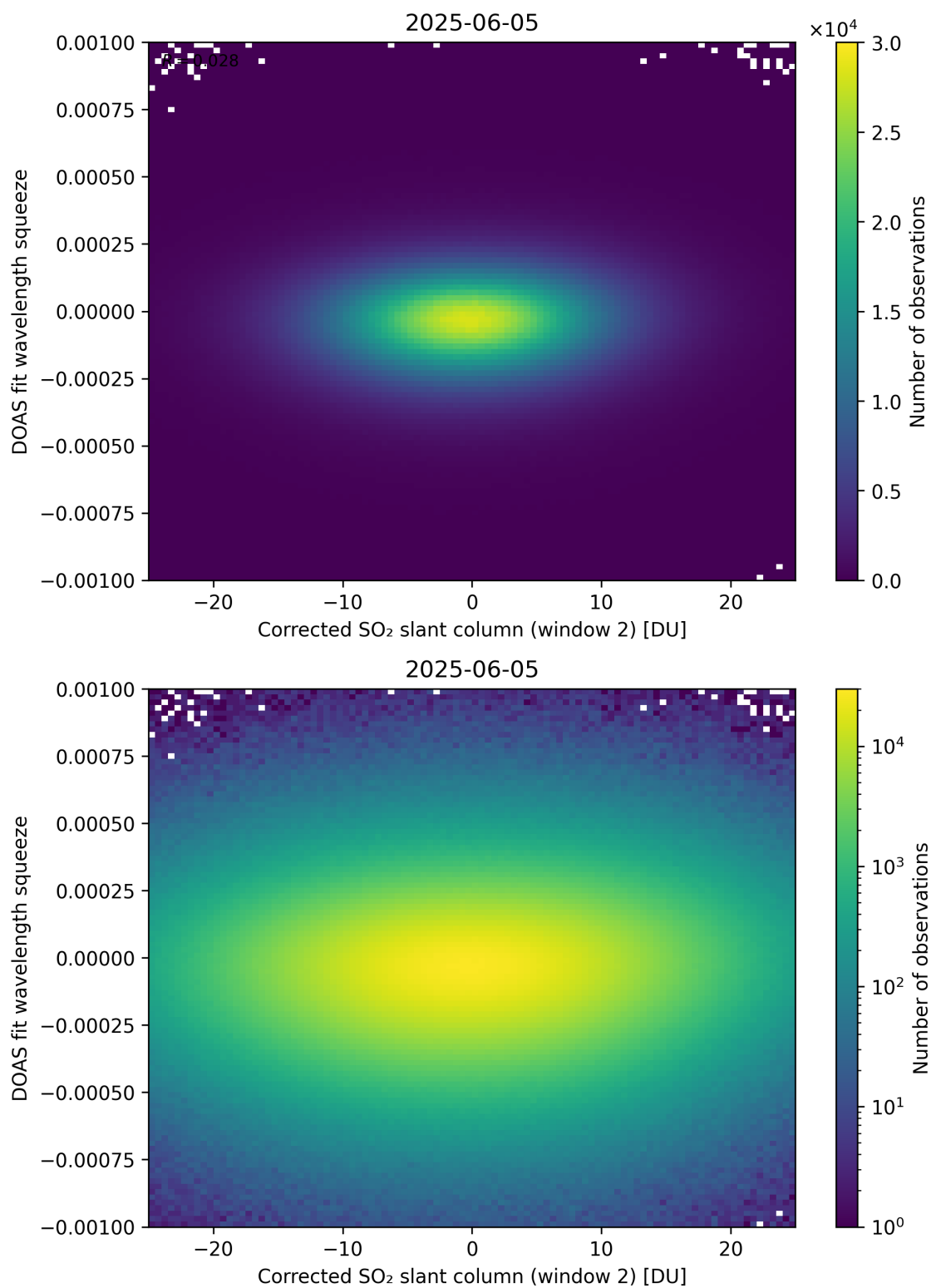
Figure 247: Scatter density plot of “Corrected SO 2 slant column (window 2)” against “DOAS fit wavelength squeeze” for 2025-06-04 to 2025-06-06.
