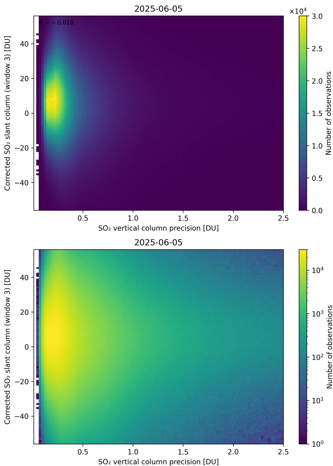
Figure 340: Scatter density plot of “SO 2 vertical column precision” against “Corrected SO 2 slant column (window 3)” for 2025-06-04 to 2025-06-06.
