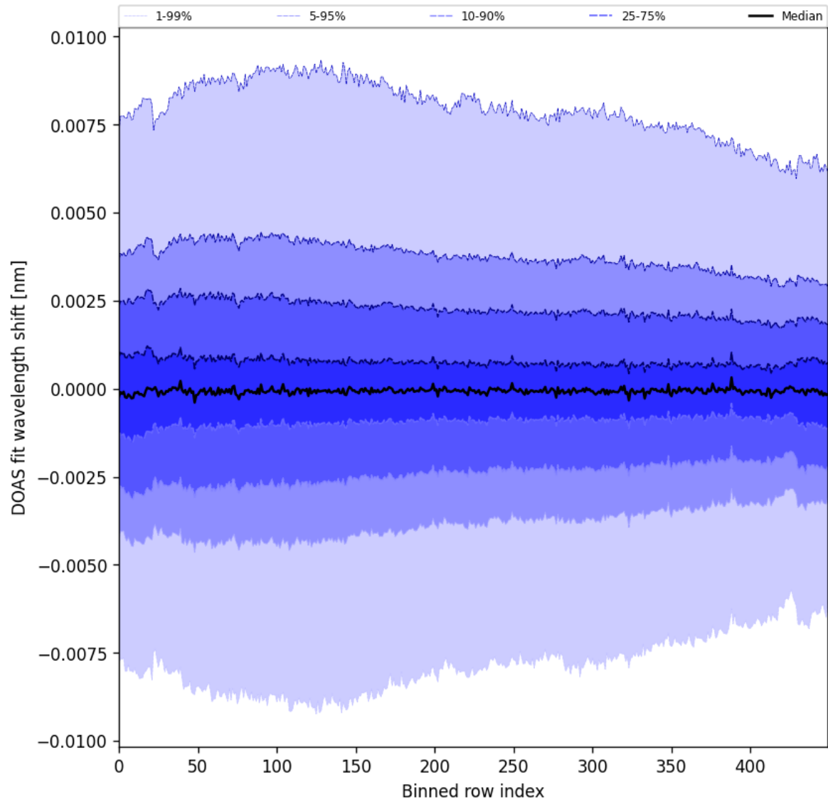
Figure 102: Along track statistics of “DOAS fit wavelength shift” for 2025-06-04 to 2025-06-06
