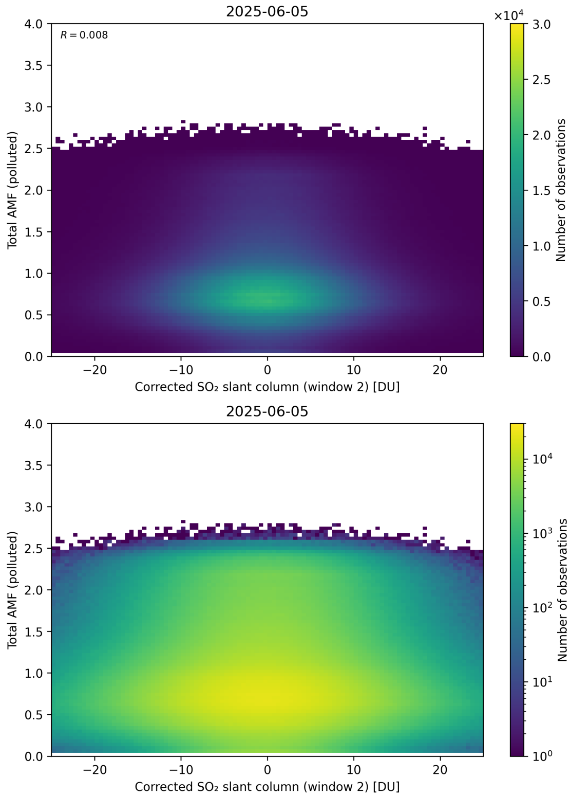
Figure 253: Scatter density plot of “Corrected SO 2 slant column (window 2)” against “Total AMF (polluted)” for 2025-06-04 to 2025-06-06.
