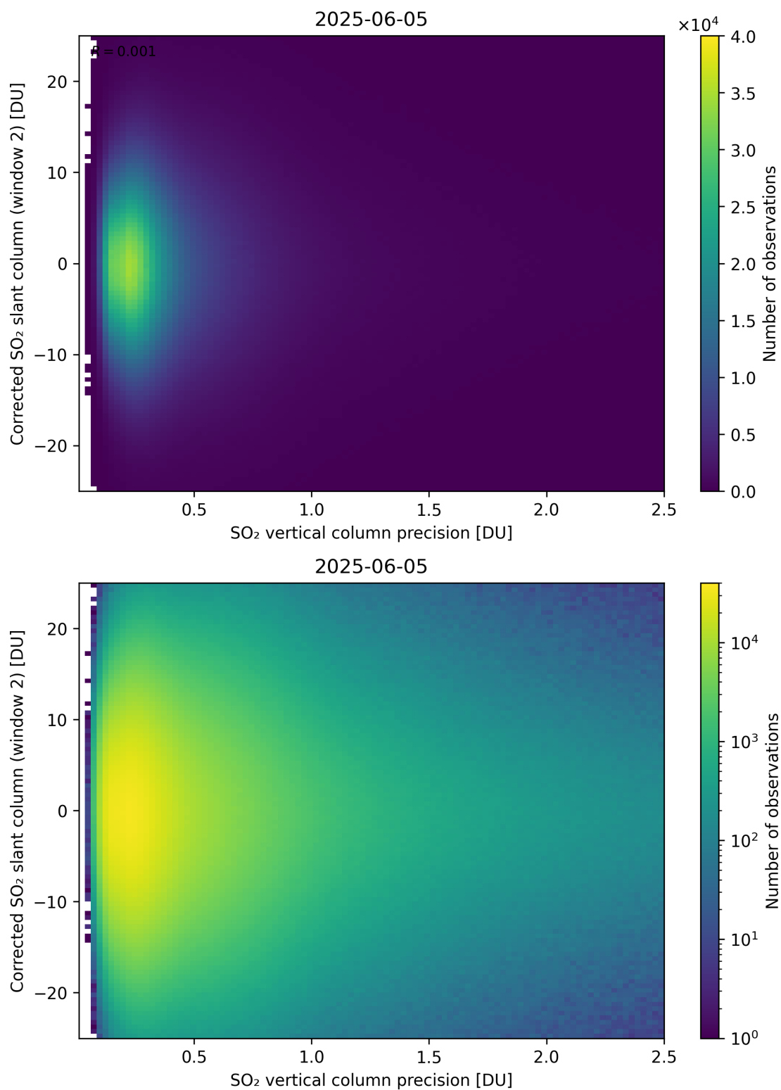
Figure 339: Scatter density plot of “SO 2 vertical column precision” against “Corrected SO 2 slant column (window 2)” for 2025-06-04 to 2025-06-06.
