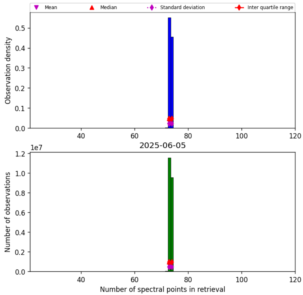
Figure 82: Histogram of “Number of spectral points in retrieval” for 2025-06-04 to 2025-06-06
