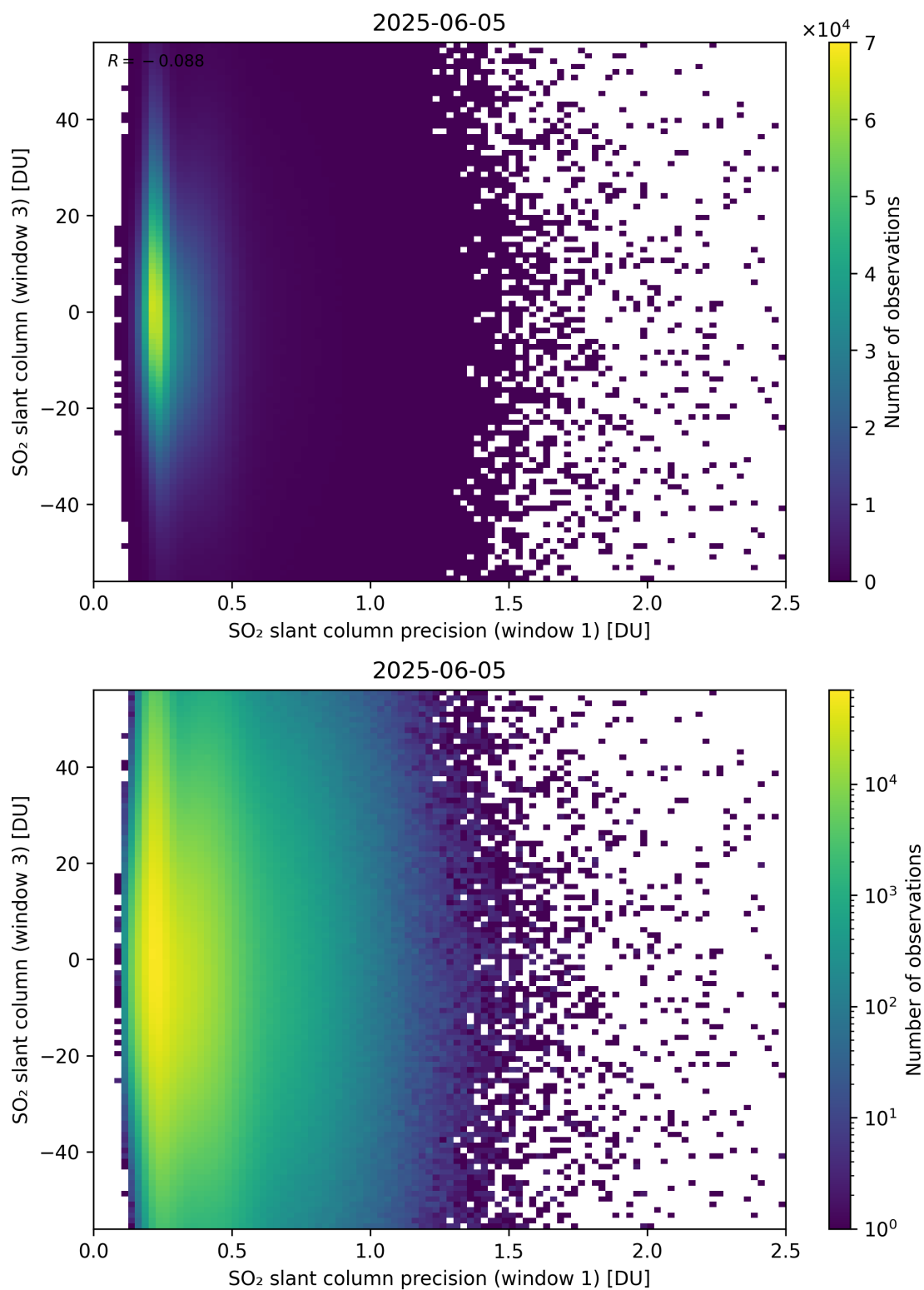
Figure 278: Scatter density plot of “SO 2 slant column precision (window 1)” against “SO 2 slant column (window 3)” for 2025-06-04 to 2025-06-06.
