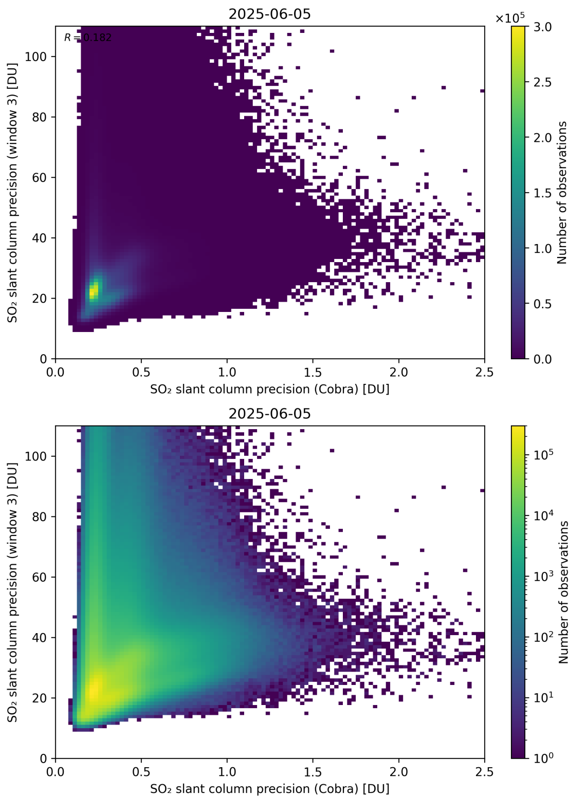
Figure 212: Scatter density plot of “SO 2 slant column precision (Cobra)” against “SO 2 slant column precision (window 3)” for 2025-06-04 to 2025-06-06.
