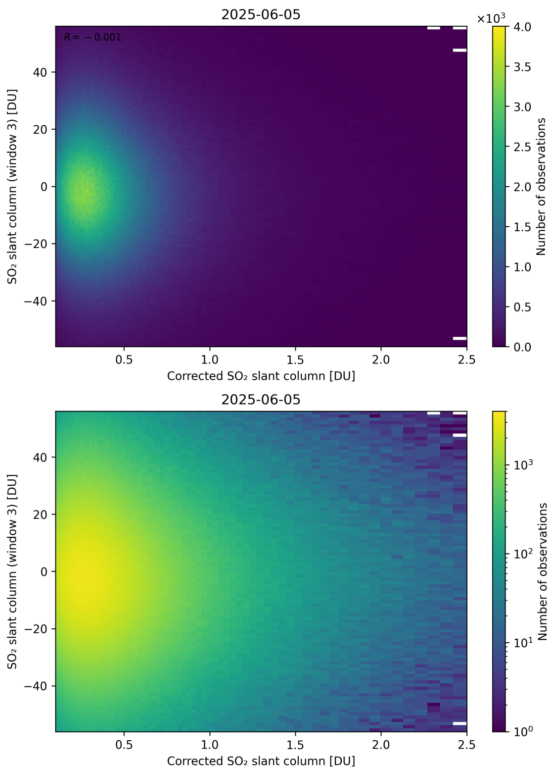
Figure 240: Scatter density plot of “Corrected SO 2 slant column” against “SO 2 slant column (window 3)” for 2025-06-04 to 2025-06-06.
