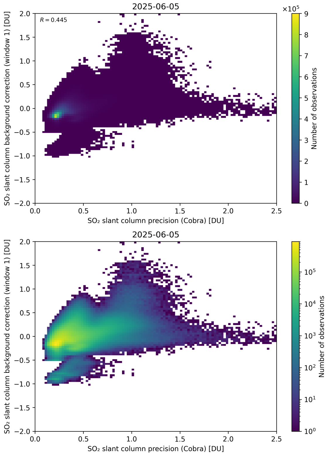
Figure 199: Scatter density plot of “SO 2 slant column precision (Cobra)” against “SO 2 slant column background correction (window 1)” for 2025-06-04 to 2025-06-06.
