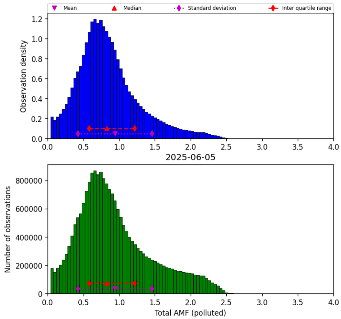
Figure 79: Histogram of “Total AMF (polluted)” for 2025-06-04 to 2025-06-06
