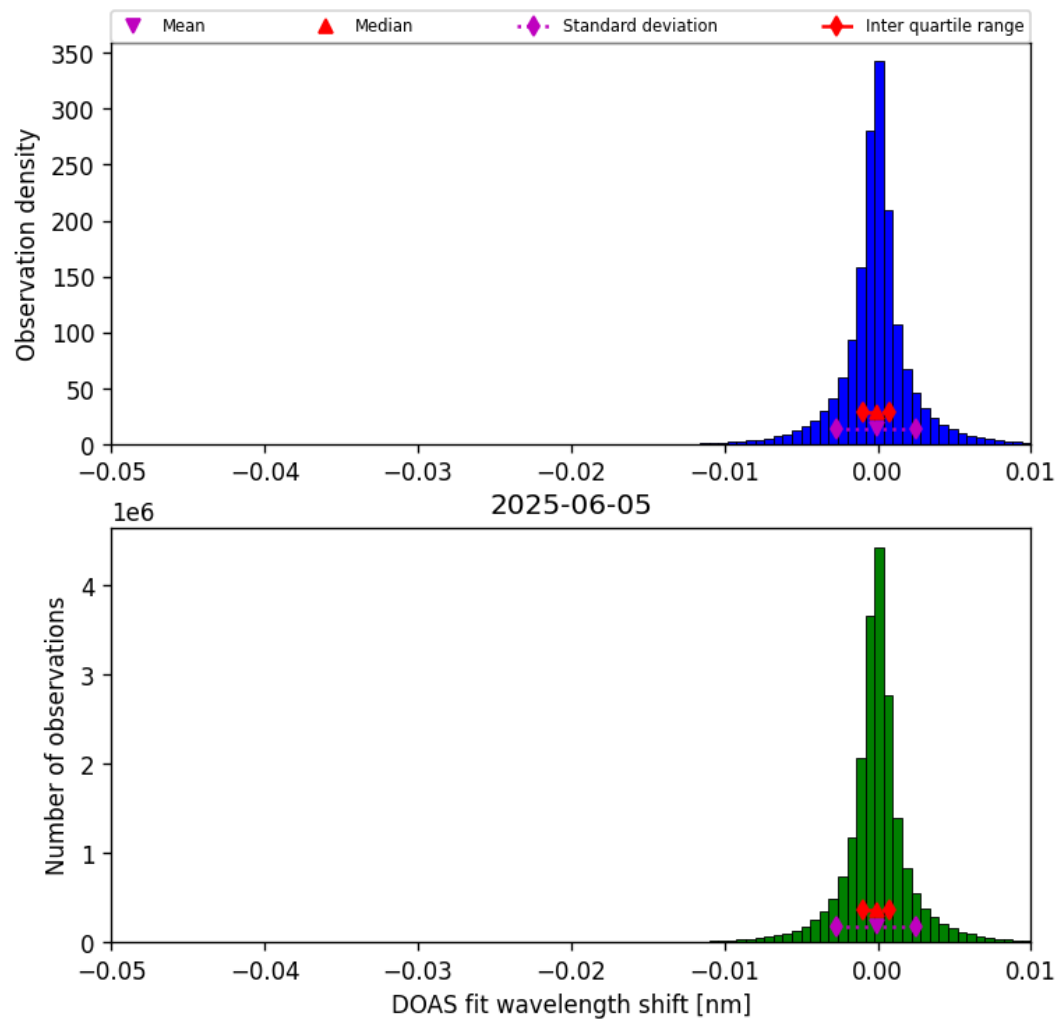
Figure 76: Histogram of “DOAS fit wavelength shift” for 2025-06-04 to 2025-06-06
