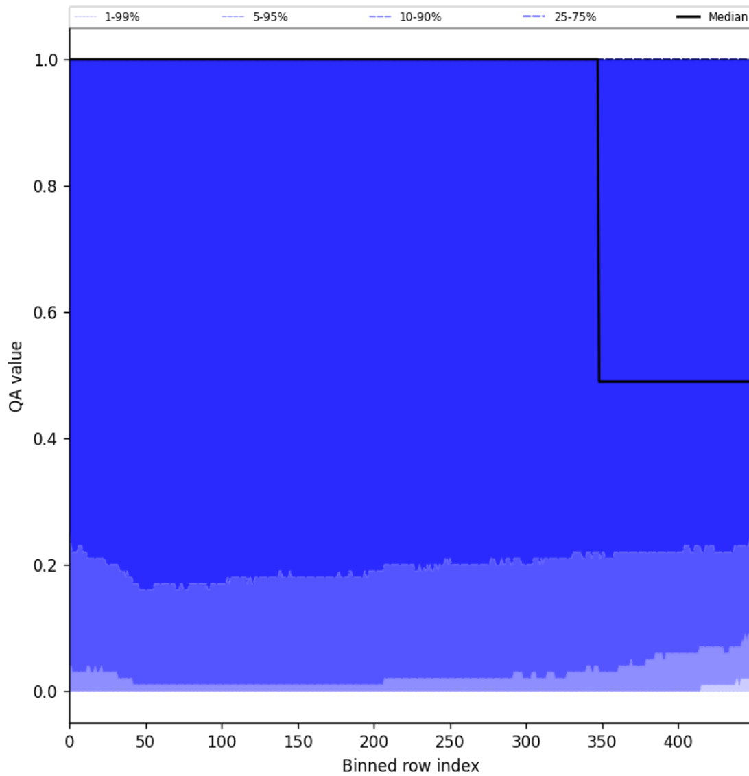
Figure 83: Along track statistics of “QA value” for 2025-06-04 to 2025-06-06
