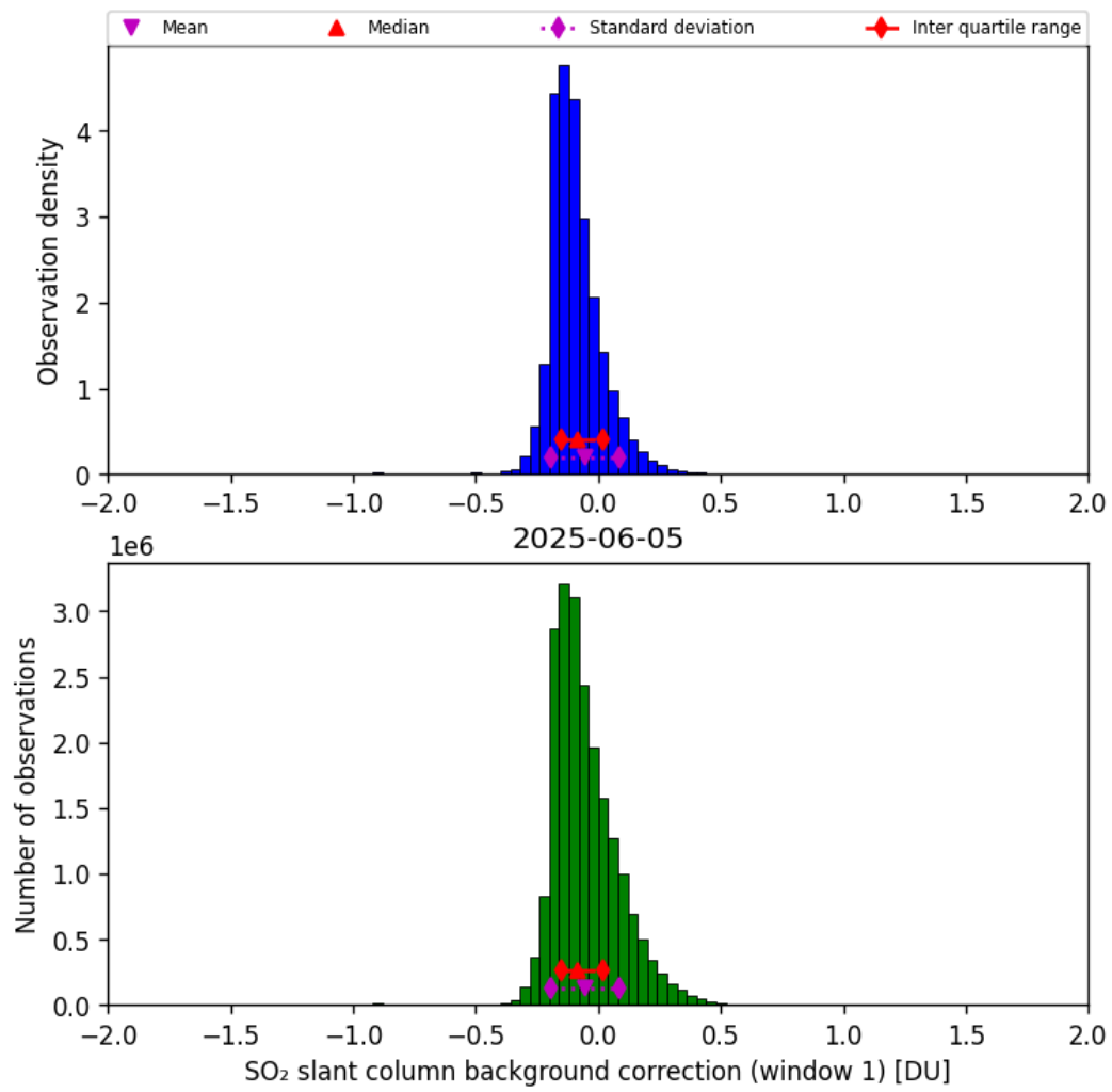
Figure 66: Histogram of “SO 2 slant column background correction (window 1)” for 2025-06-04 to 2025-06-06
