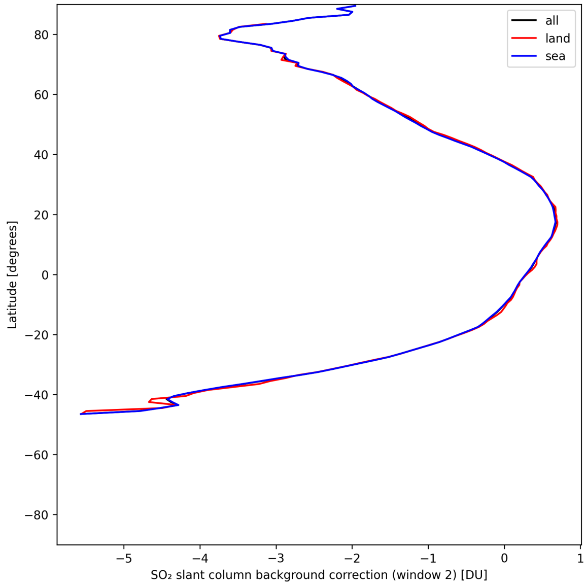
Figure 44: Zonal average of “SO 2 slant column background correction (window 2)” for 2025-06-04 to 2025-06-06.
