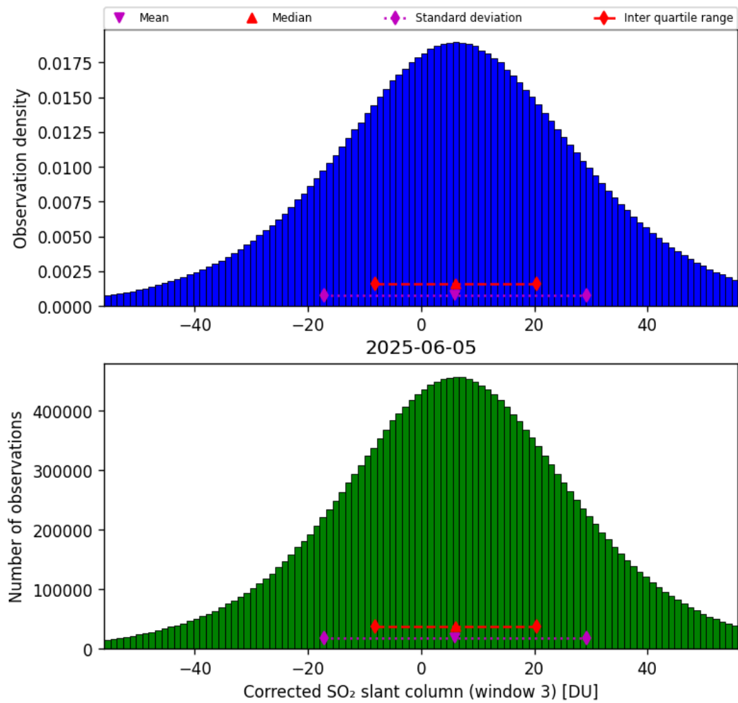
Figure 73: Histogram of “Corrected SO 2 slant column (window 3)” for 2025-06-04 to 2025-06-06
