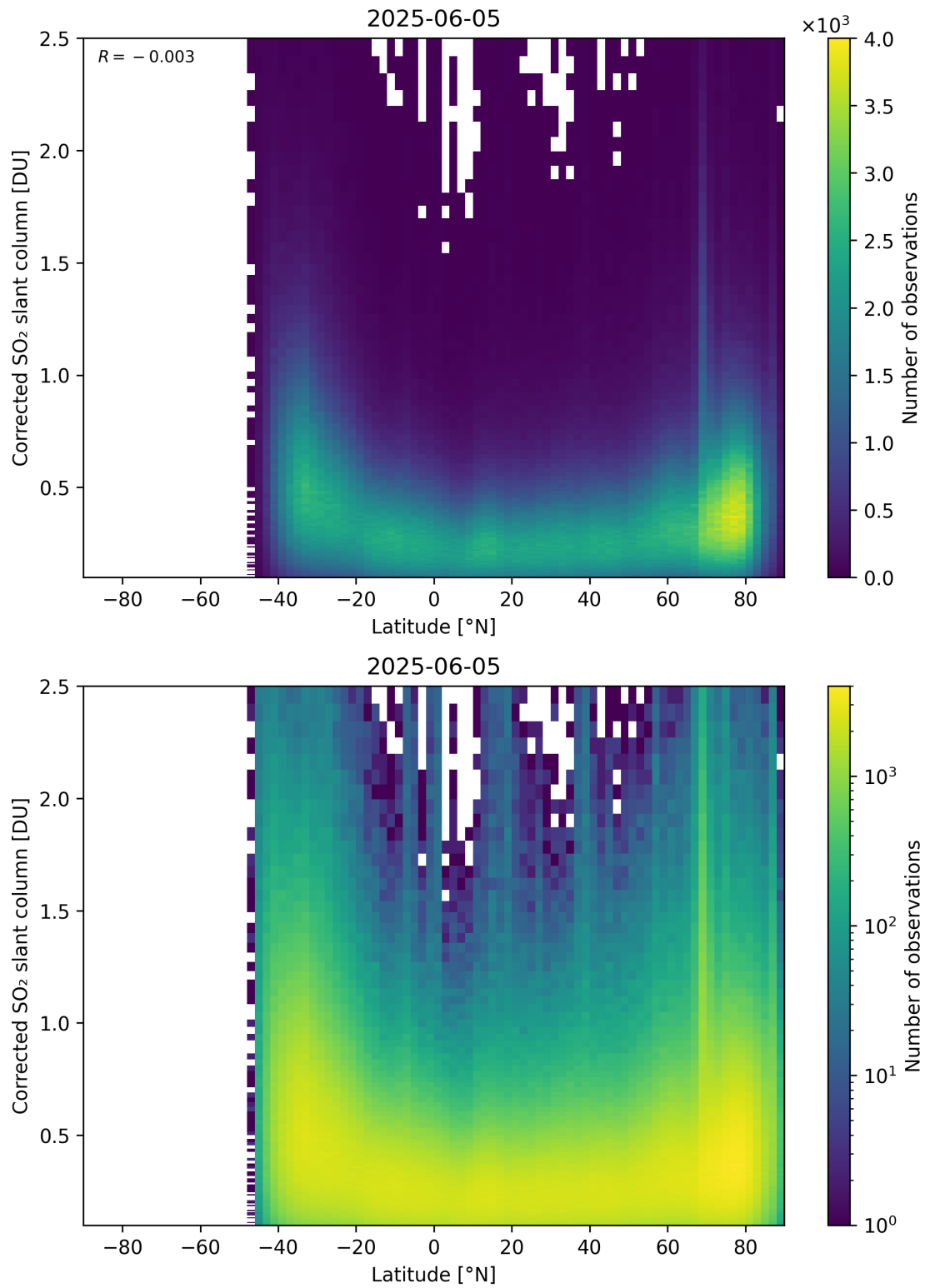
Figure 159: Scatter density plot of “Latitude” against “Corrected SO 2 slant column” for 2025-06-04 to 2025-06-06.
