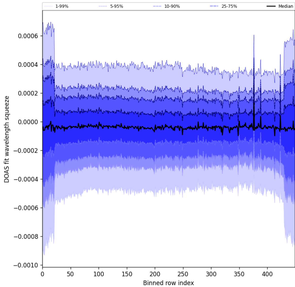
Figure 103: Along track statistics of “DOAS fit wavelength squeeze” for 2025-06-04 to 2025-06-06
