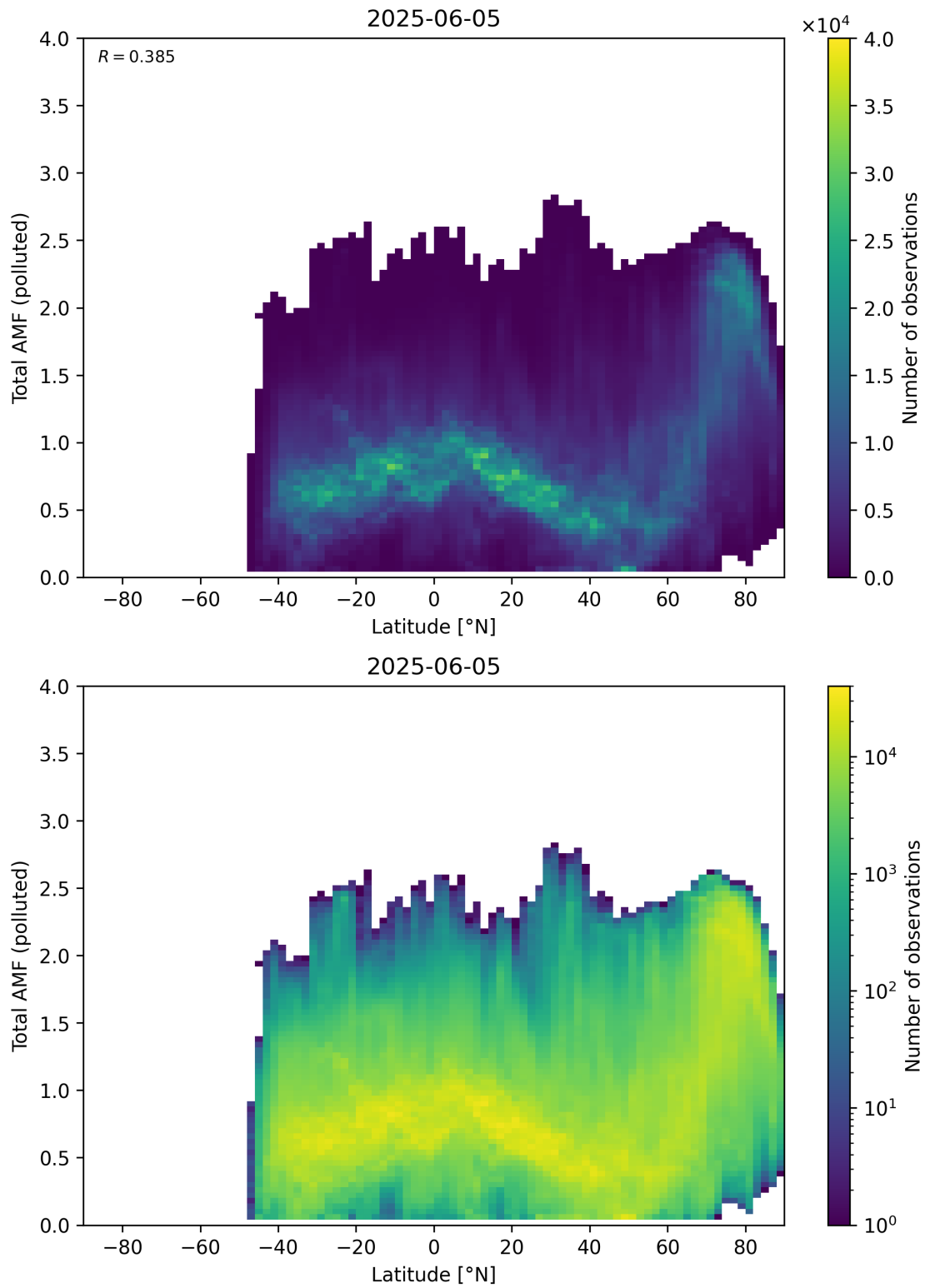
Figure 167: Scatter density plot of “Latitude” against “Total AMF (polluted)” for 2025-06-04 to 2025-06-06.
