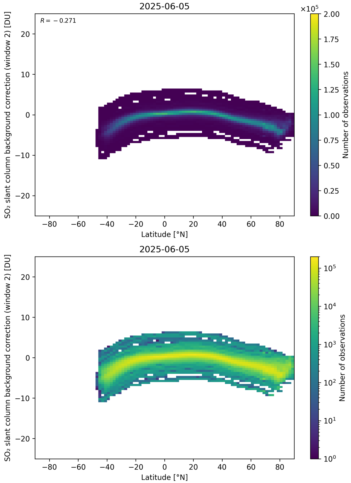
Figure 151: Scatter density plot of “Latitude” against “SO 2 slant column background correction (window 2)” for 2025-06-04 to 2025-06-06.
