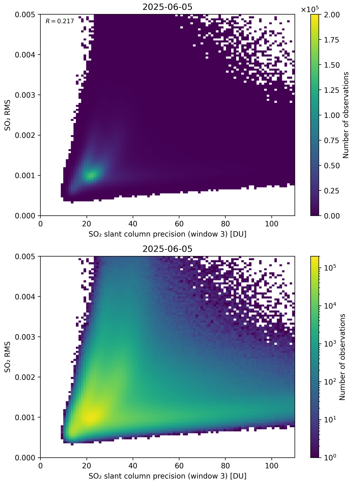
Figure 310: Scatter density plot of “SO 2 slant column precision (window 3)” against “SO 2 RMS” for 2025-06-04 to 2025-06-06.
