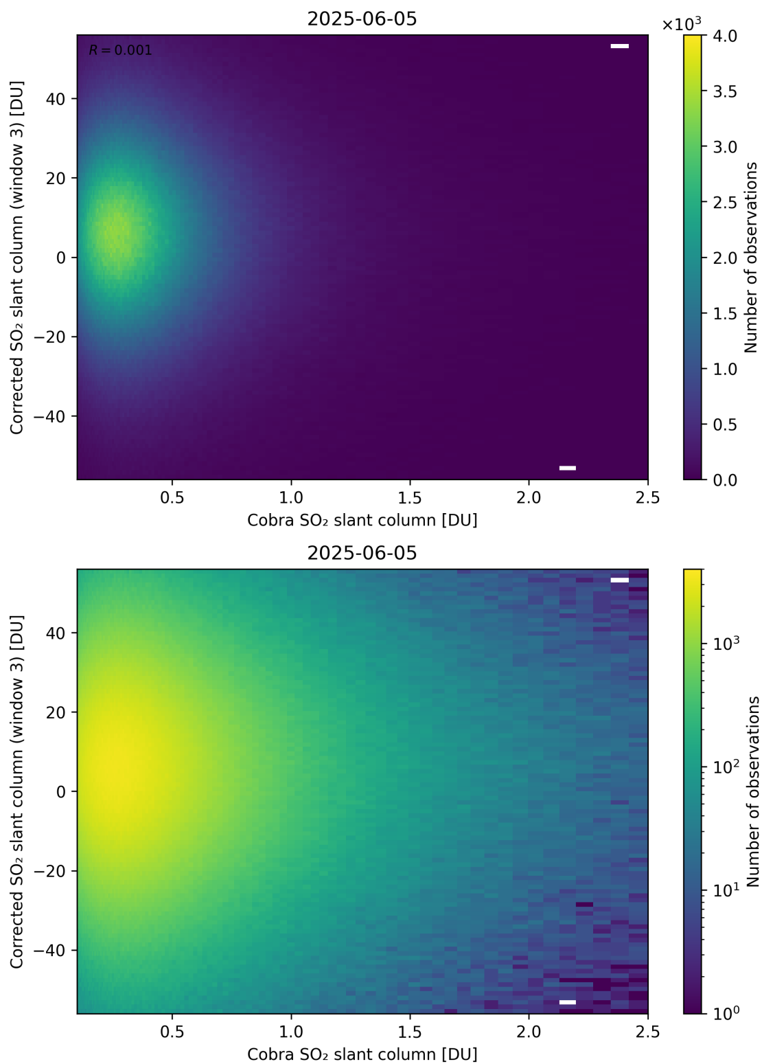
Figure 218: Scatter density plot of “Cobra SO 2 slant column” against “Corrected SO 2 slant column (window 3)” for 2025-06-04 to 2025-06-06.
