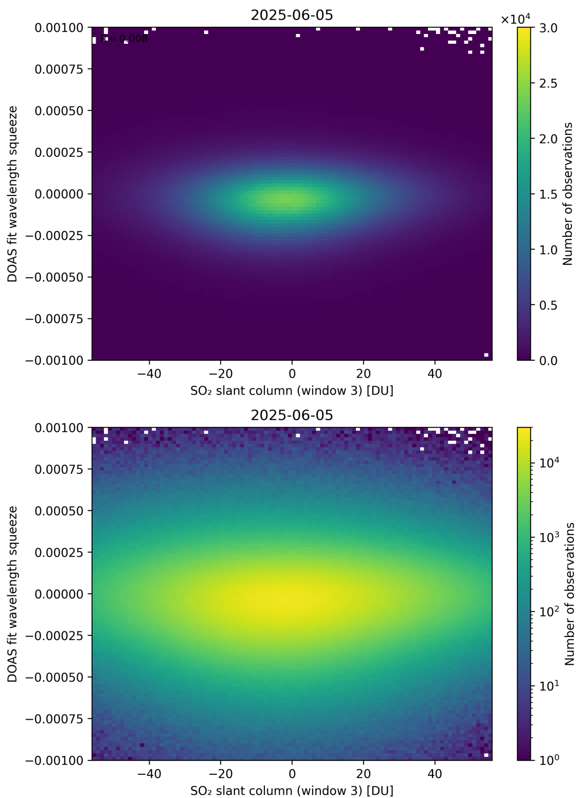
Figure 305: Scatter density plot of “SO 2 slant column (window 3)” against “DOAS fit wavelength squeeze” for 2025-06-04 to 2025-06-06.
