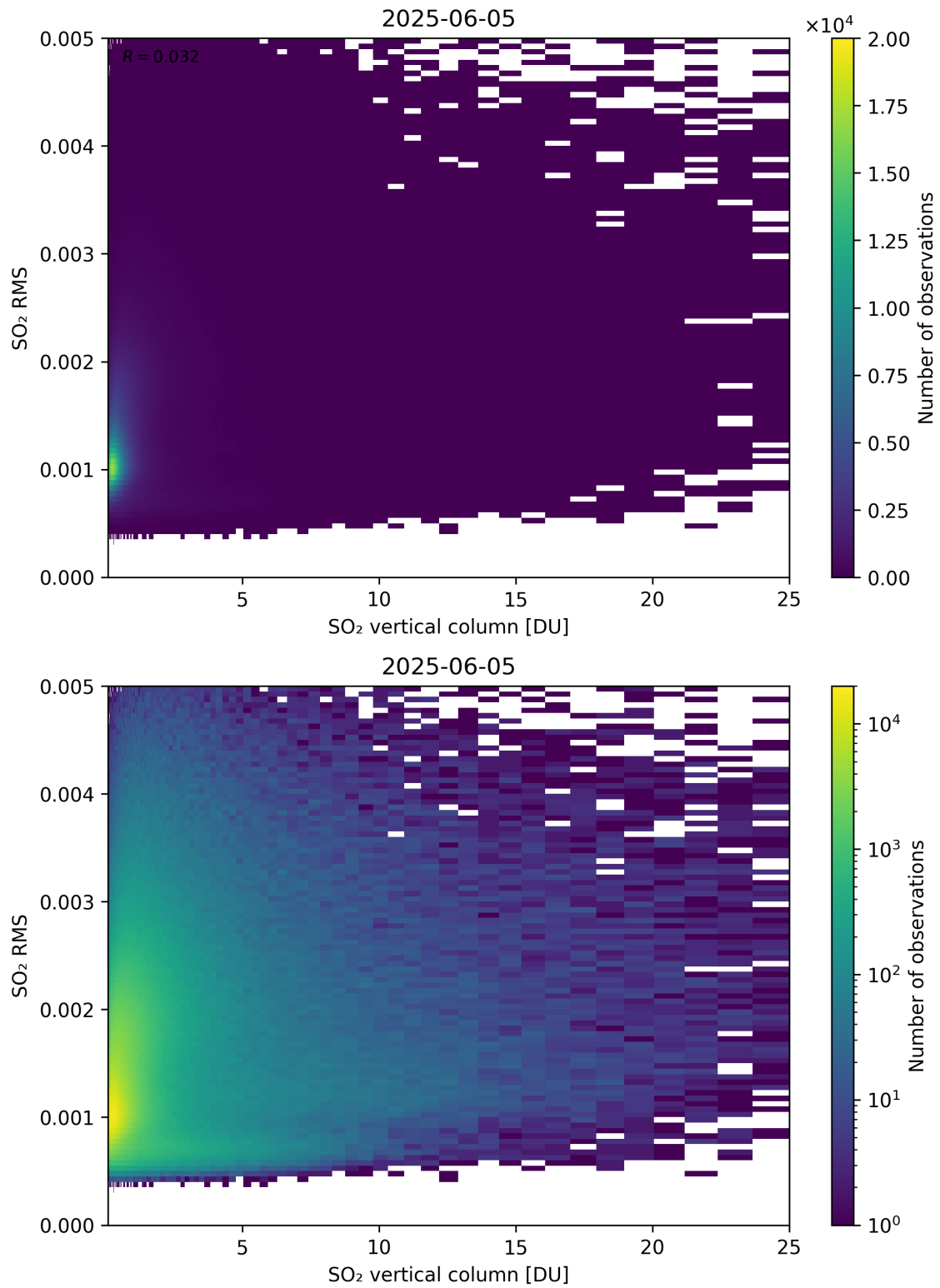
Figure 328: Scatter density plot of “SO 2 vertical column” against “SO 2 RMS” for 2025-06-04 to 2025-06-06.
