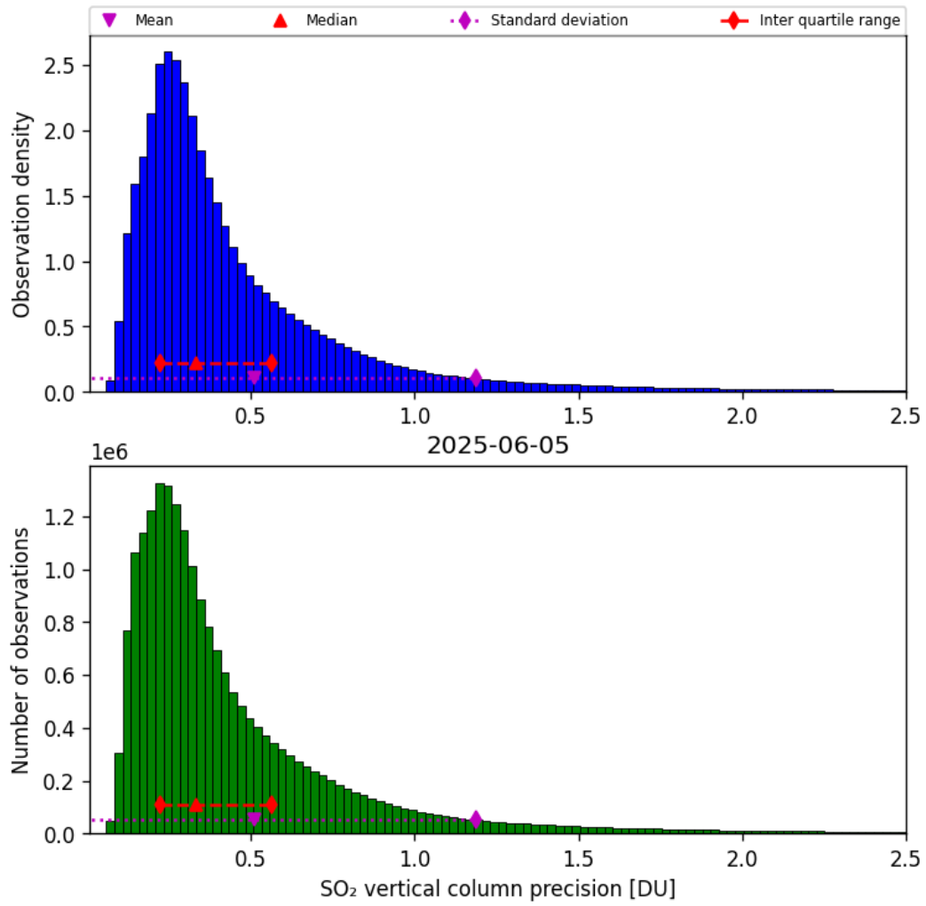
Figure 59: Histogram of “SO 2 vertical column precision” for 2025-06-04 to 2025-06-06
