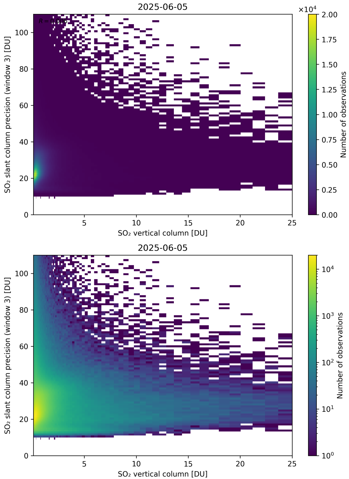
Figure 358: Scatter density plot of “SO 2 vertical column” against “SO 2 slant column precision (window 3)” for 2025-06-04 to 2025-06-06.
