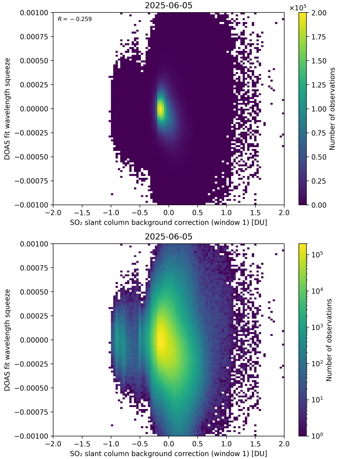
Figure 112: Scatter density plot of “SO 2 slant column background correction (window 1)” against “DOAS fit wavelength squeeze” for 2025-06-04 to 2025-06-06.
