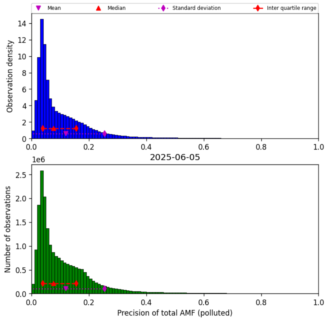
Figure 80: Histogram of “Precision of total AMF (polluted)” for 2025-06-04 to 2025-06-06
