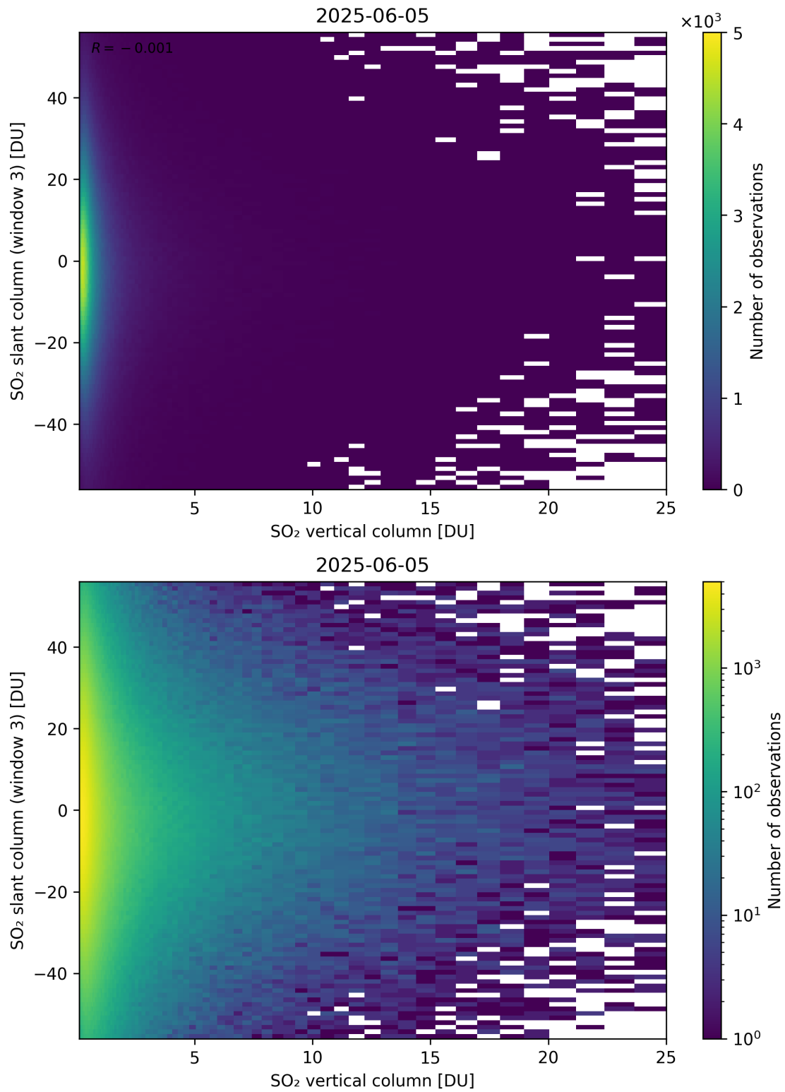
Figure 357: Scatter density plot of “SO 2 vertical column” against “SO 2 slant column (window 3)” for 2025-06-04 to 2025-06-06.
