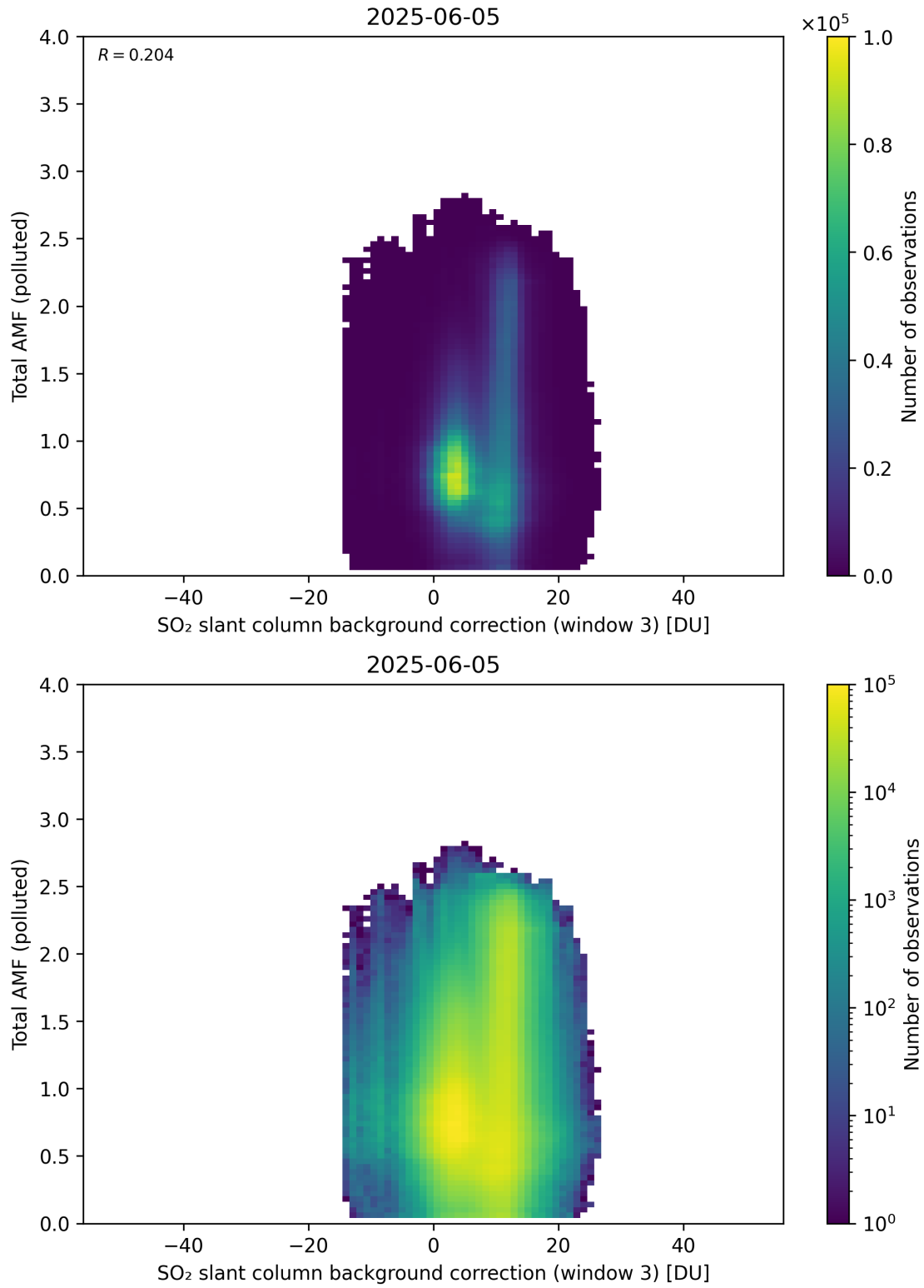
Figure 136: Scatter density plot of “SO 2 slant column background correction (window 3)” against “Total AMF (polluted)” for 2025-06-04 to 2025-06-06.
