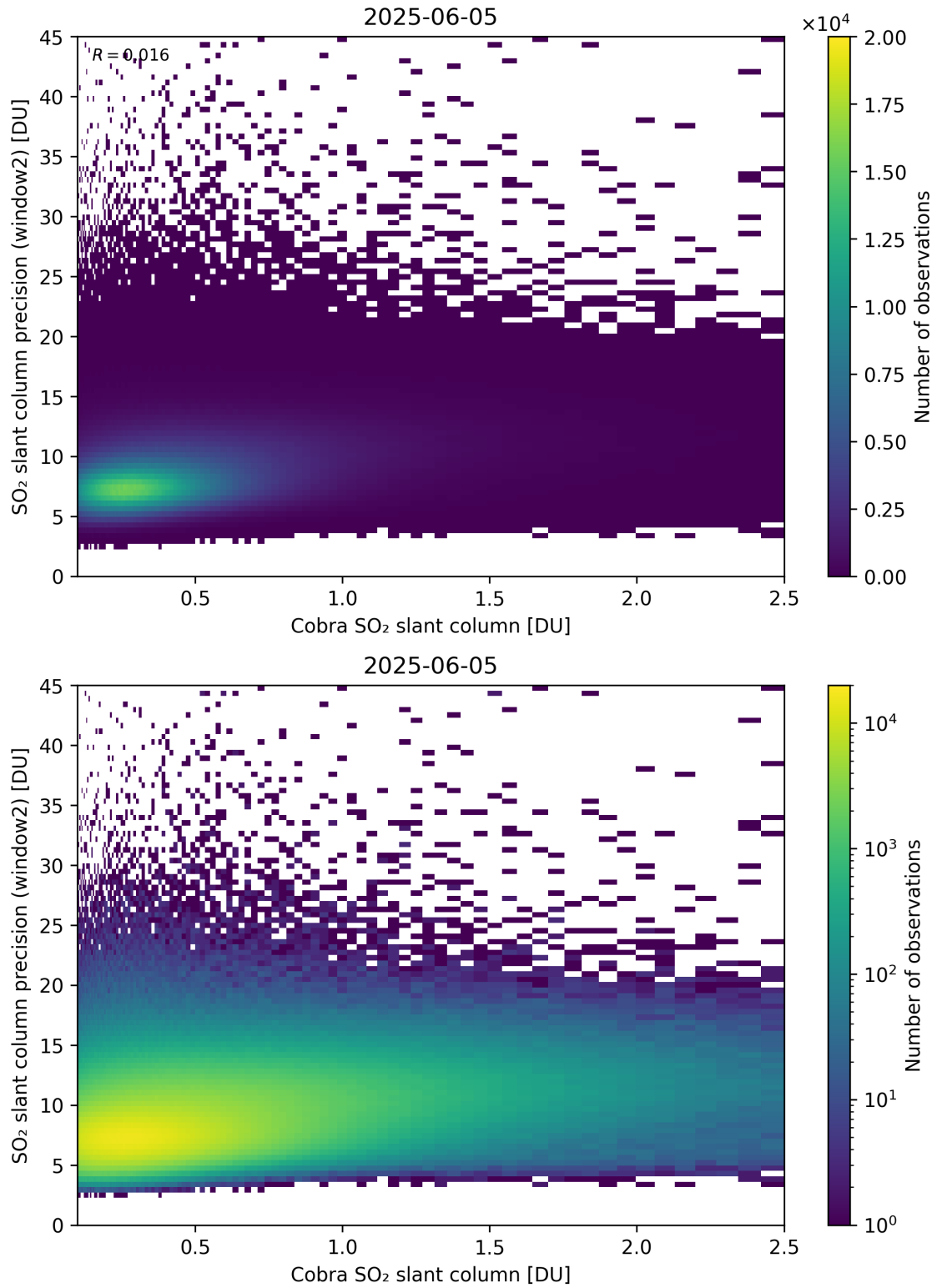
Figure 221: Scatter density plot of “Cobra SO 2 slant column” against “SO 2 slant column precision (window2)” for 2025-06-04 to 2025-06-06.
