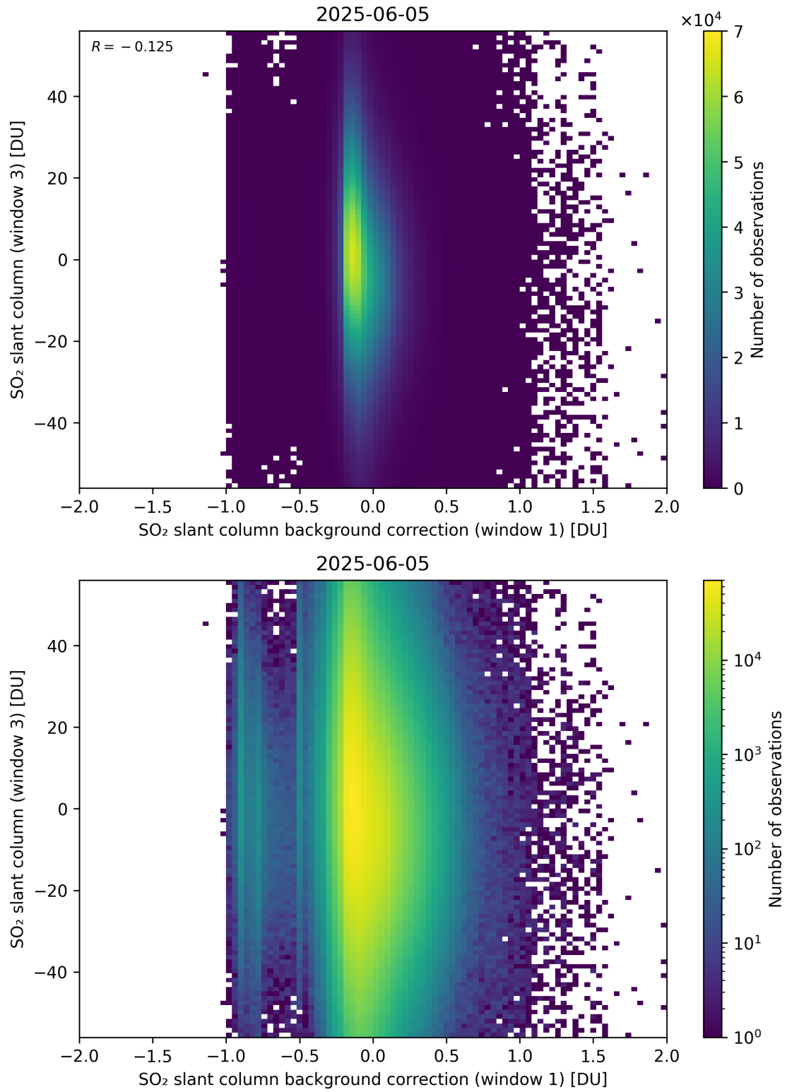
Figure 118: Scatter density plot of “SO 2 slant column background correction (window 1)” against “SO 2 slant column (window 3)” for 2025-06-04 to 2025-06-06.
