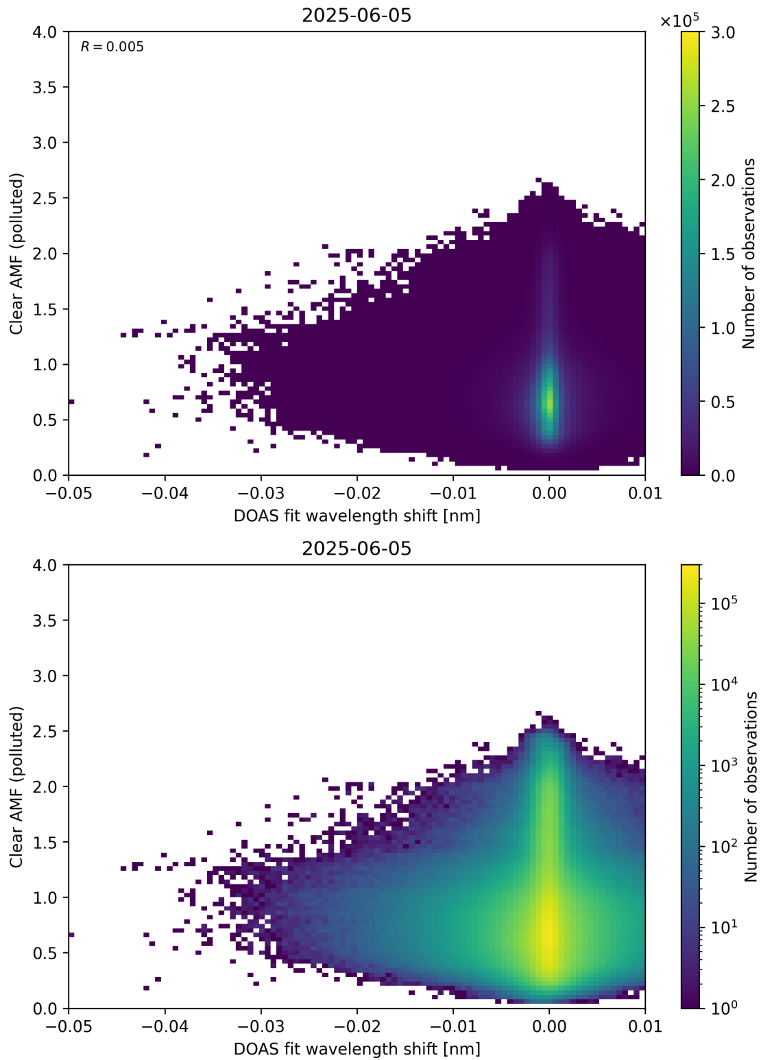
Figure 140: Scatter density plot of “DOAS fit wavelength shift” against “Clear AMF (polluted)” for 2025-06-04 to 2025-06-06.
