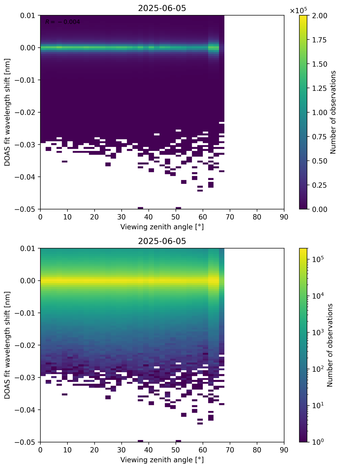
Figure 365: Scatter density plot of “Viewing zenith angle” against “DOAS fit wavelength shift” for 2025-06-04 to 2025-06-06.
