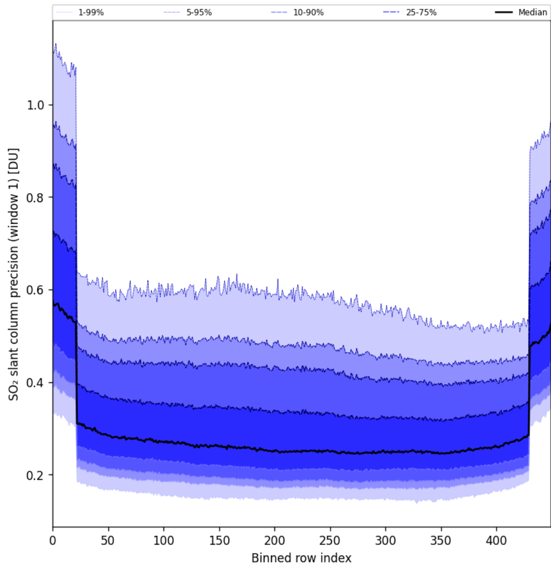
Figure 90: Along track statistics of “SO 2 slant column precision (window 1)” for 2025-06-04 to 2025-06-06
