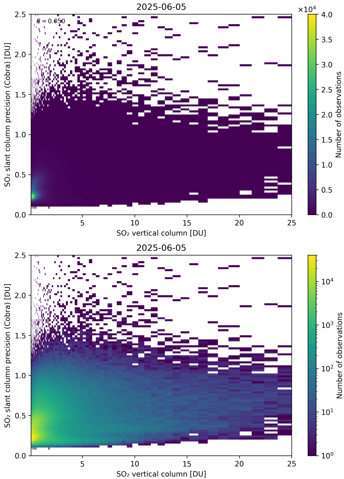
Figure 350: Scatter density plot of “SO 2 vertical column” against “SO 2 slant column precision (Cobra)” for 2025-06-04 to 2025-06-06.
