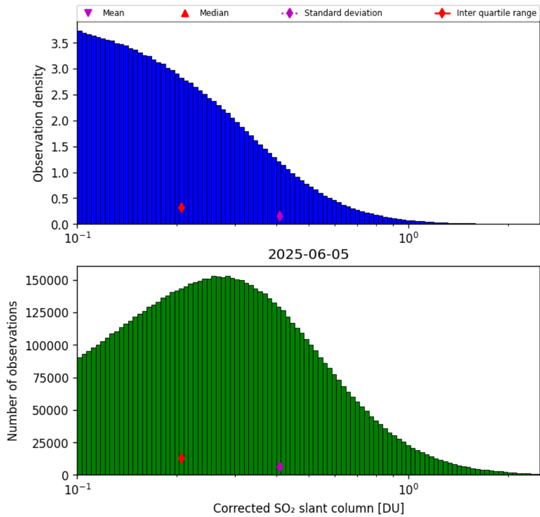
Figure 60: Histogram of "Corrected SO 2 slant column" for 2025-06-04 to 2025-06-06
