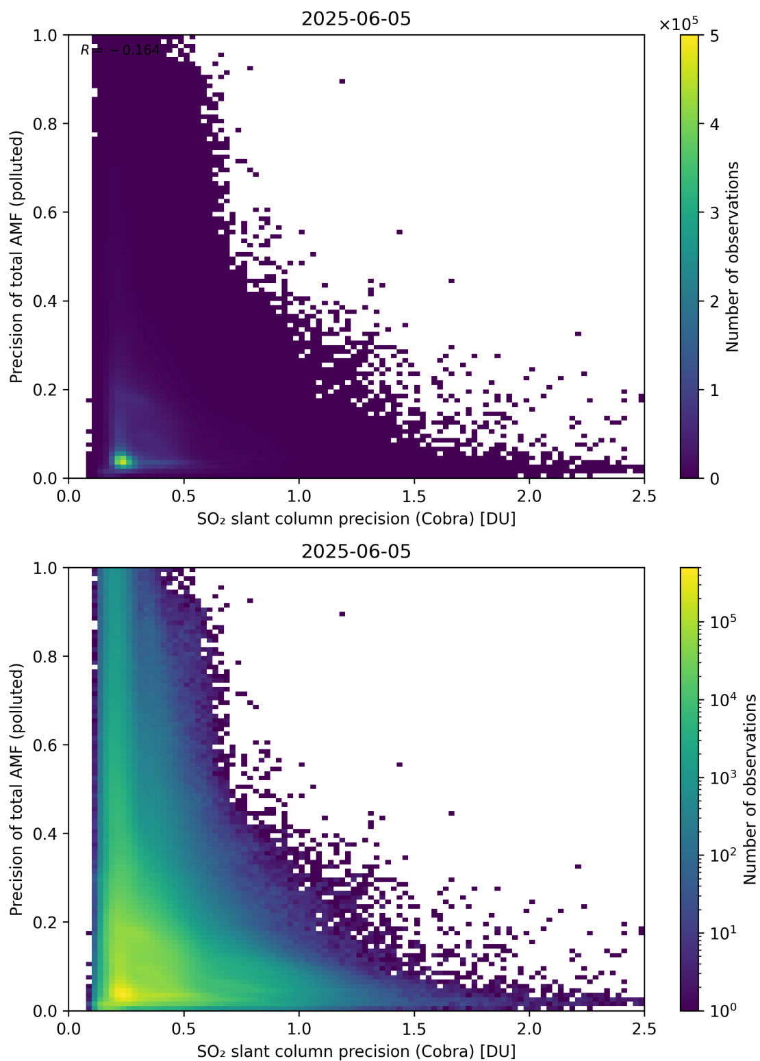
Figure 214: Scatter density plot of “SO 2 slant column precision (Cobra)” against “Precision of total AMF (polluted)” for 2025-06-04 to 2025-06-06.
