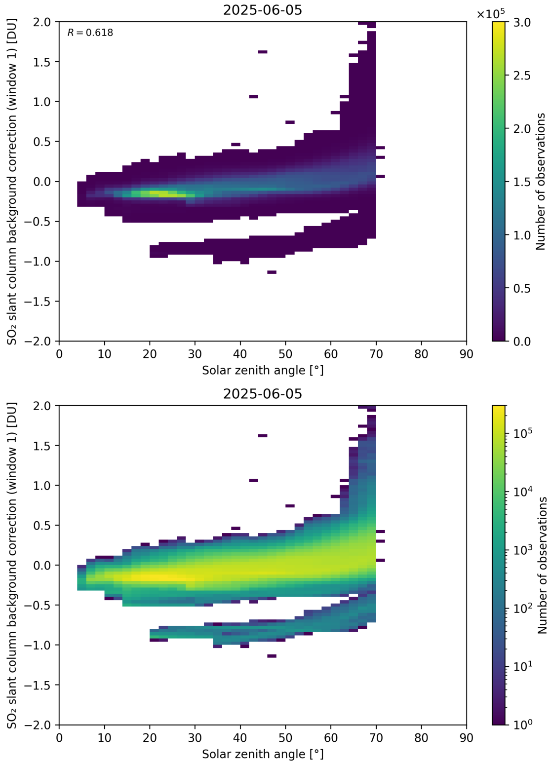
Figure 171: Scatter density plot of “Solar zenith angle” against “SO 2 slant column background correction (window 1)” for 2025-06-04 to 2025-06-06.
