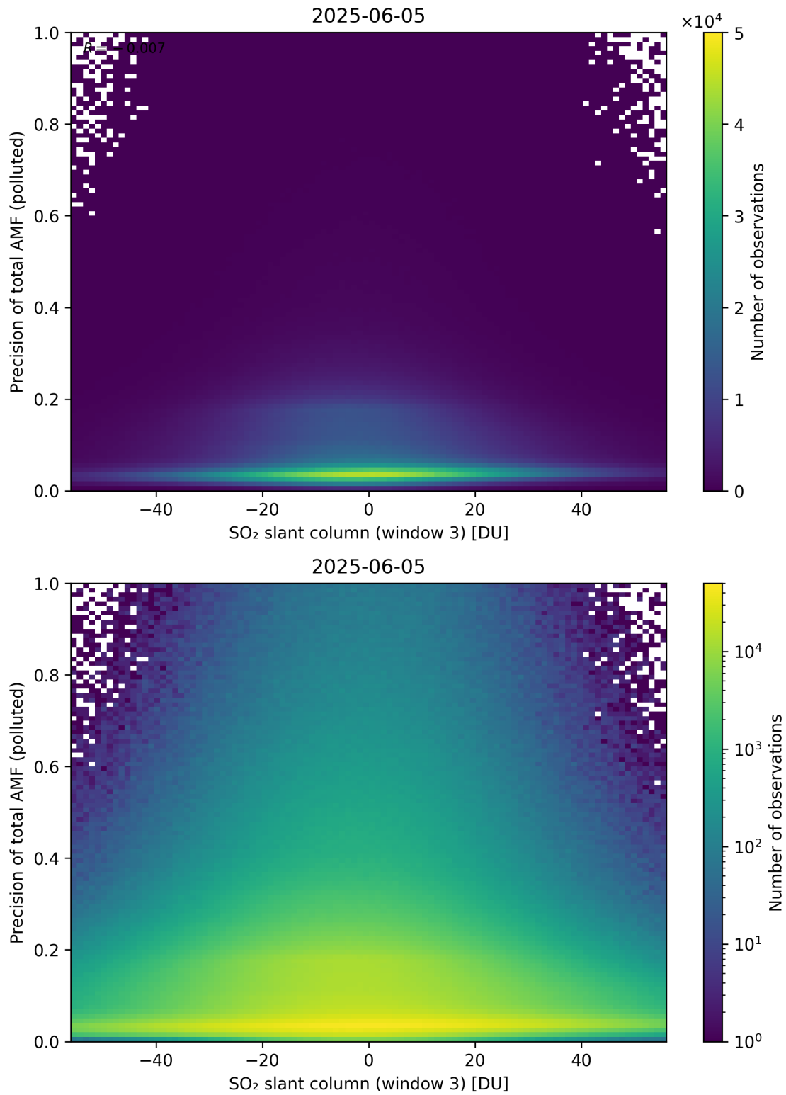
Figure 319: Scatter density plot of “SO 2 slant column (window 3)” against “Precision of total AMF (polluted)” for 2025-06-04 to 2025-06-06.
