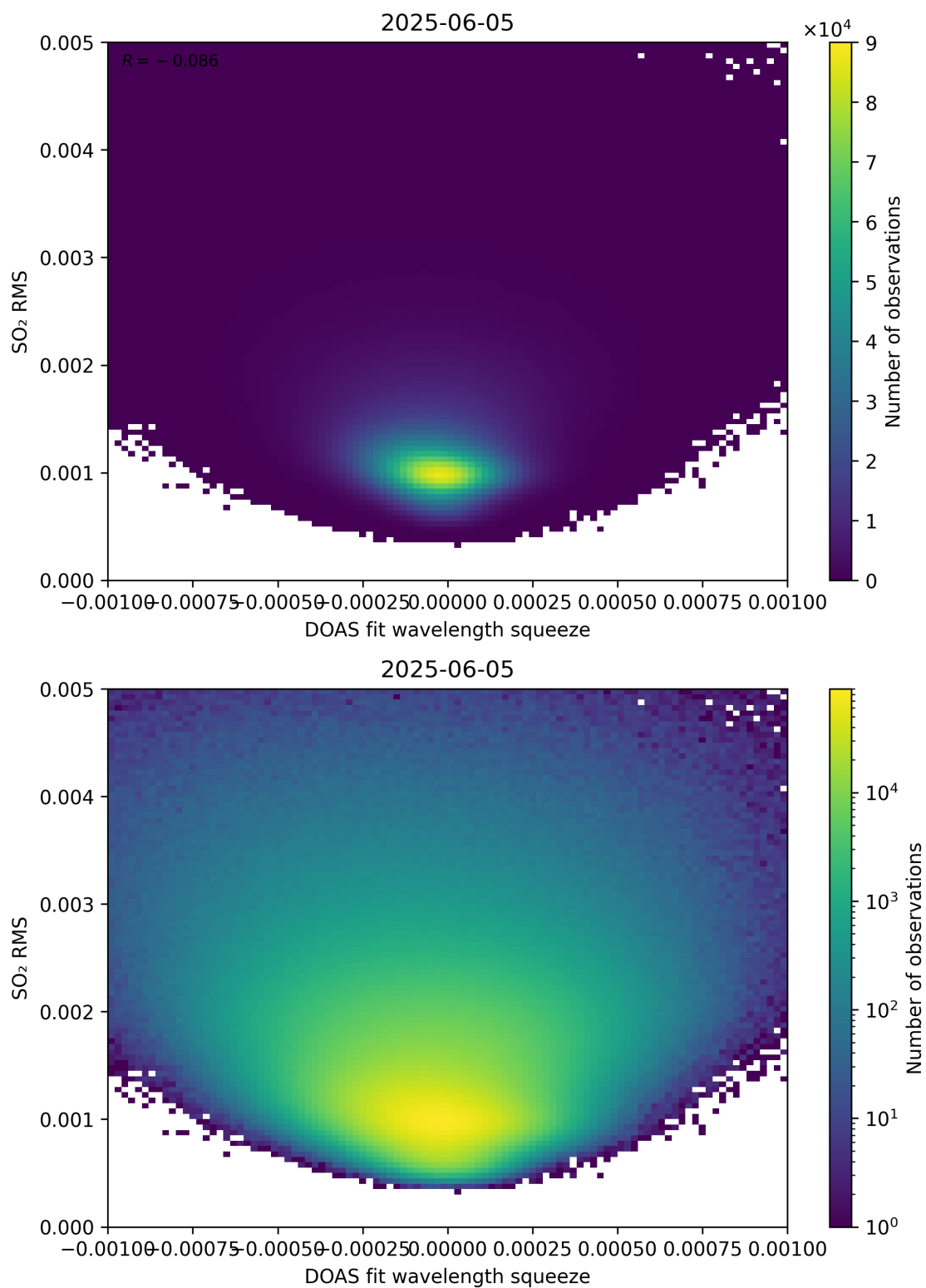
Figure 143: Scatter density plot of “DOAS fit wavelength squeeze” against “SO 2 RMS” for 2025-06-04 to 2025-06-06.
