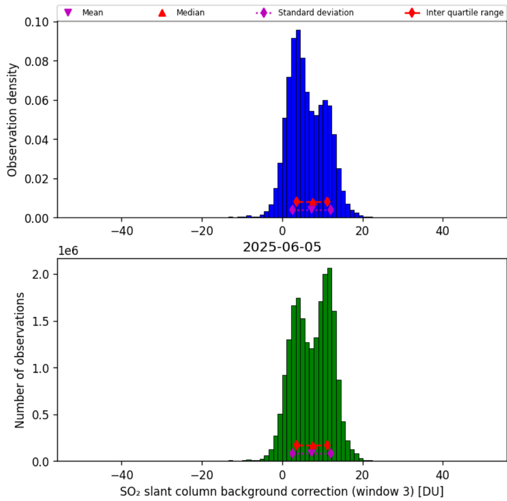
Figure 74: Histogram of “SO 2 slant column background correction (window 3)” for 2025-06-04 to 2025-06-06
