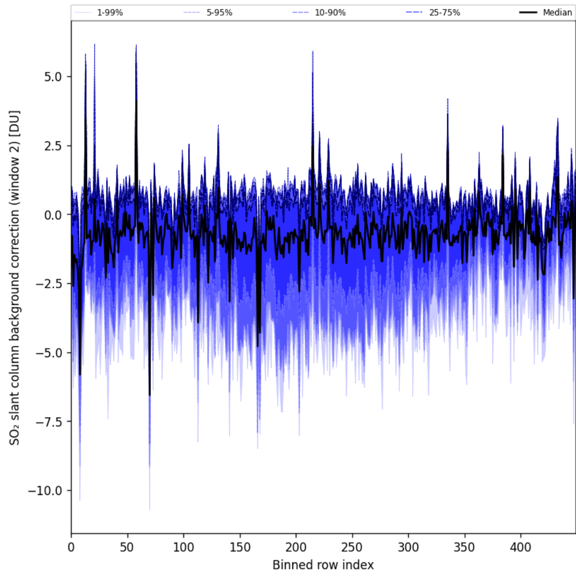
Figure 96: Along track statistics of “SO 2 slant column background correction (window 2)” for 2025-06-04 to 2025-06-06
