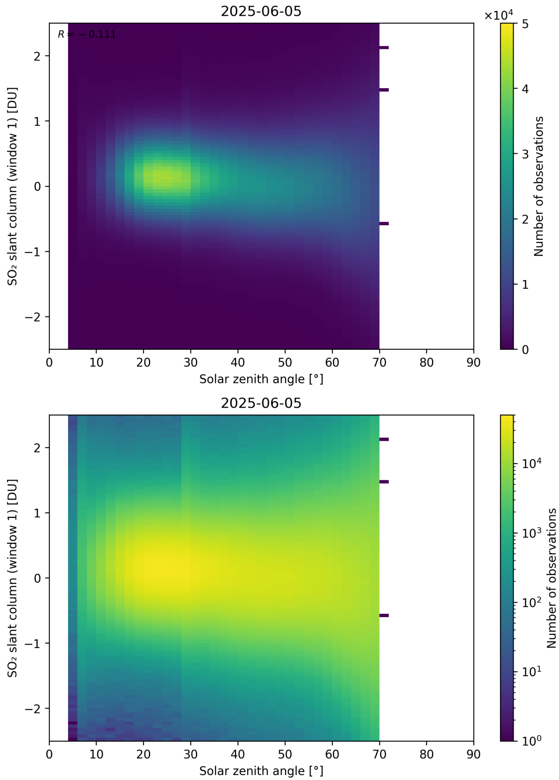
Figure 184: Scatter density plot of “Solar zenith angle” against “SO 2 slant column (window 1)” for 2025-06-04 to 2025-06-06.
