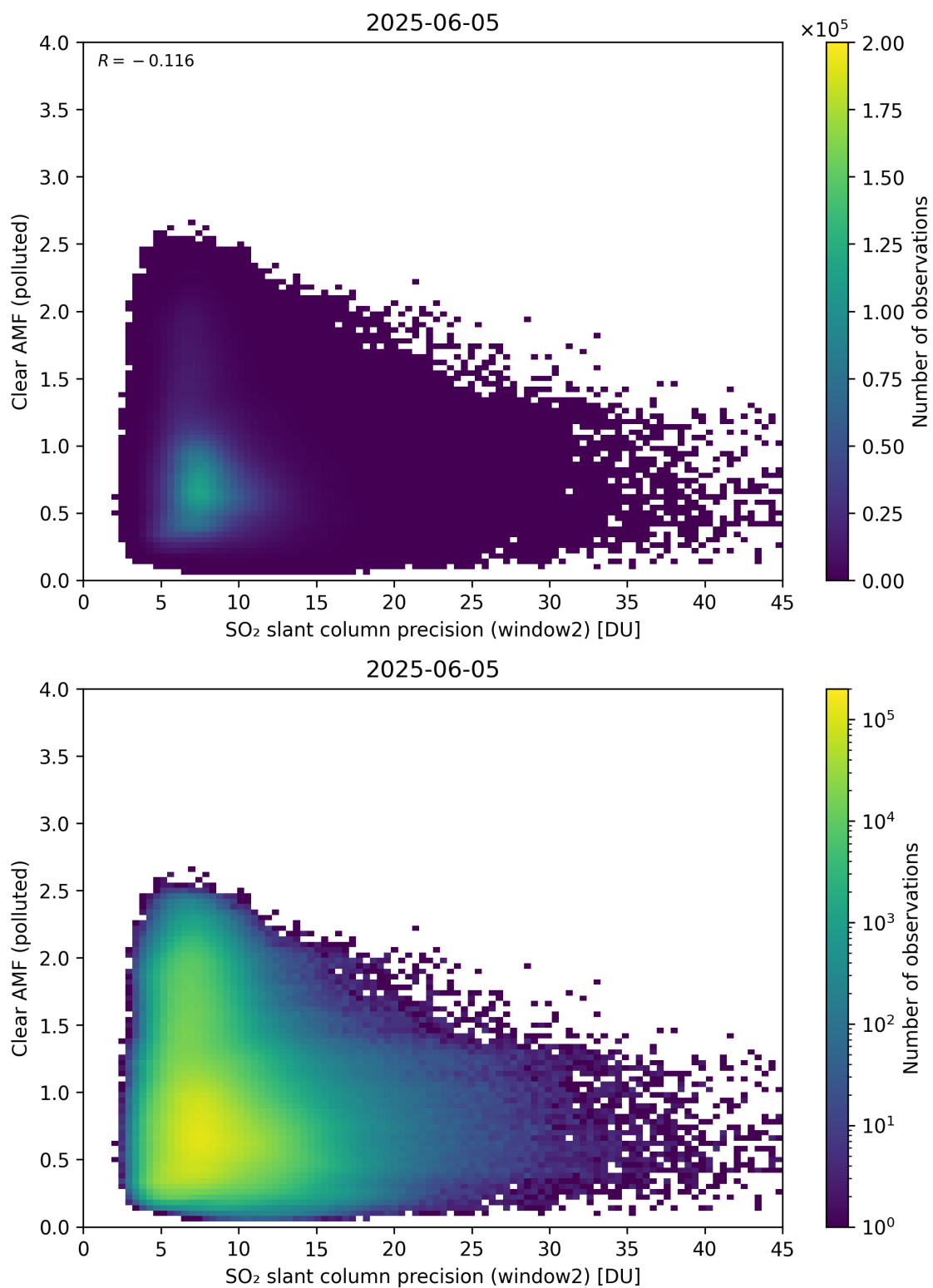
Figure 296: Scatter density plot of “SO 2 slant column precision (window2)” against “Clear AMF (polluted)” for 2025-06-04 to 2025-06-06.
