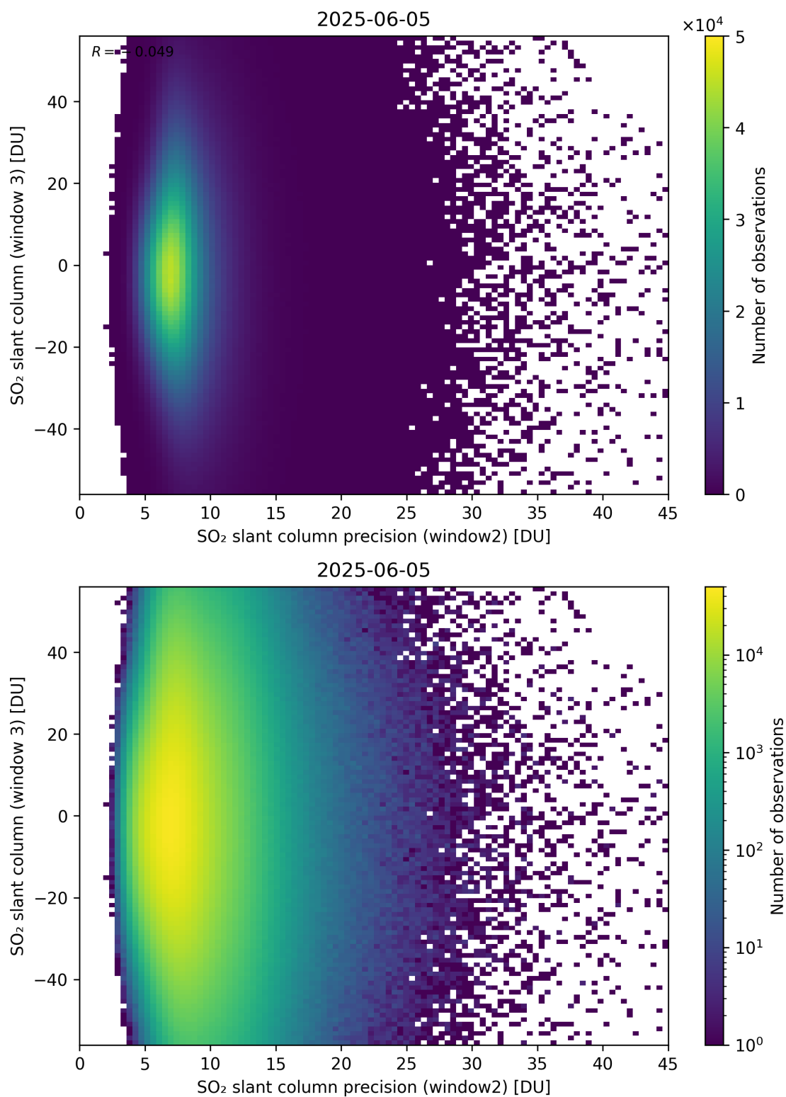
Figure 299: Scatter density plot of “SO 2 slant column precision (window2)” against “SO 2 slant column (window 3)” for 2025-06-04 to 2025-06-06.
