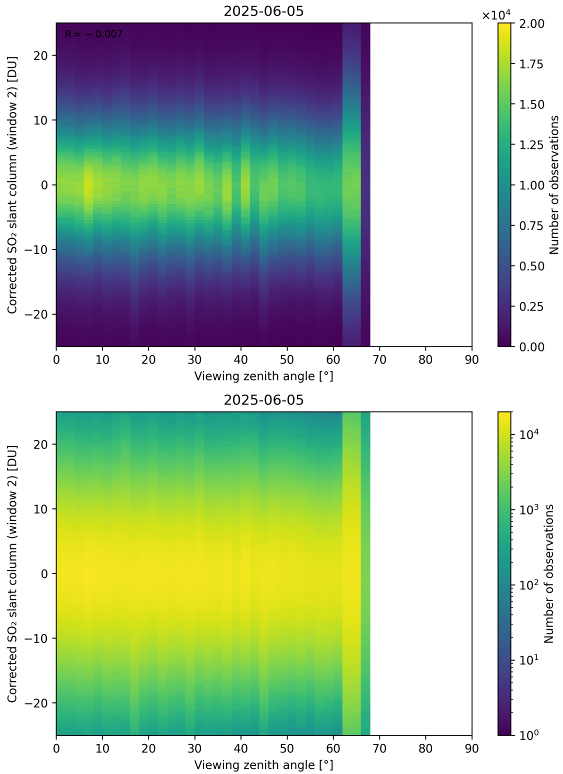
Figure 374: Scatter density plot of “Viewing zenith angle” against “Corrected SO 2 slant column (window 2)” for 2025-06-04 to 2025-06-06.
