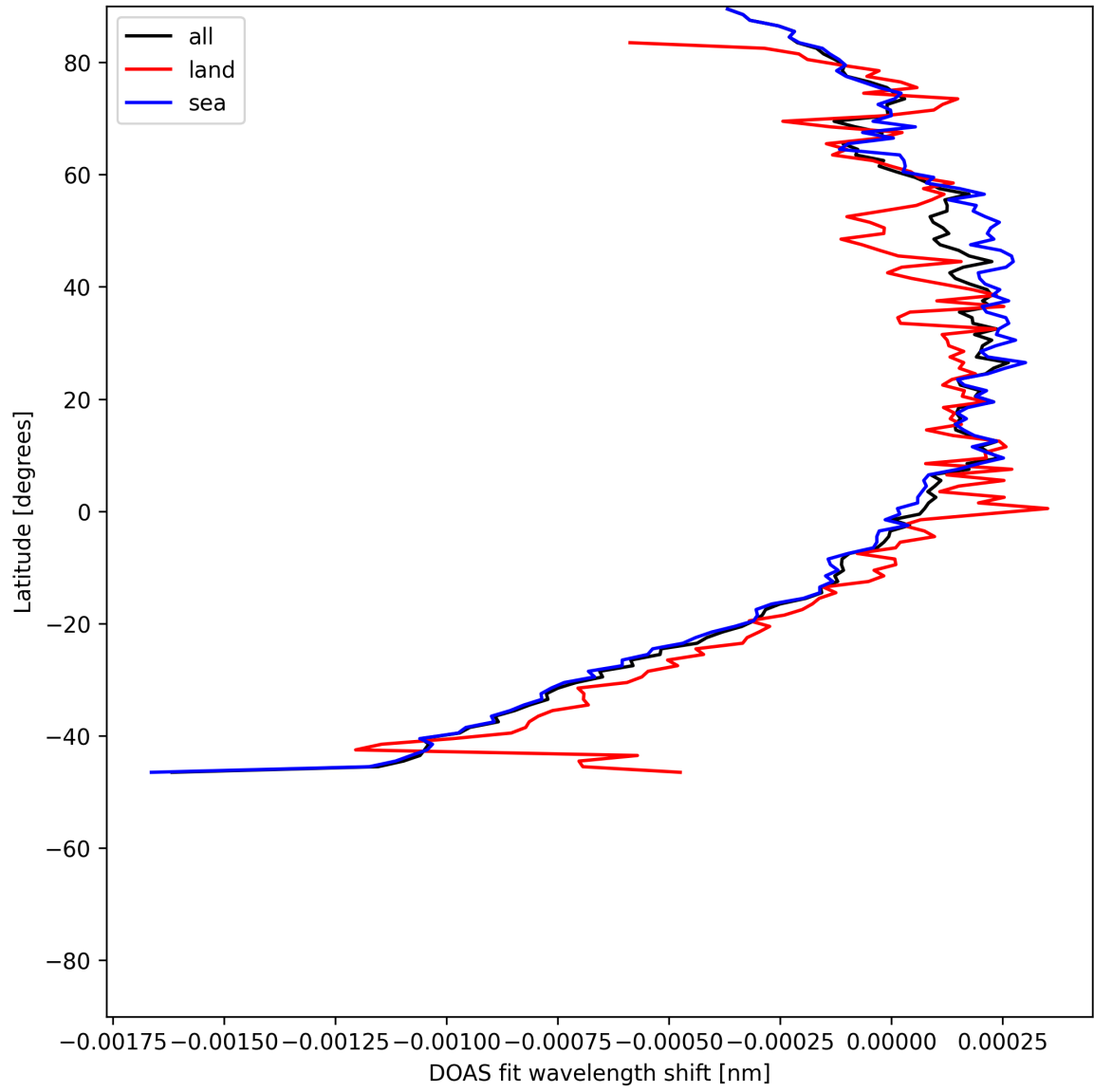
Figure 50: Zonal average of “DOAS fit wavelength shift” for 2025-06-04 to 2025-06-06.
