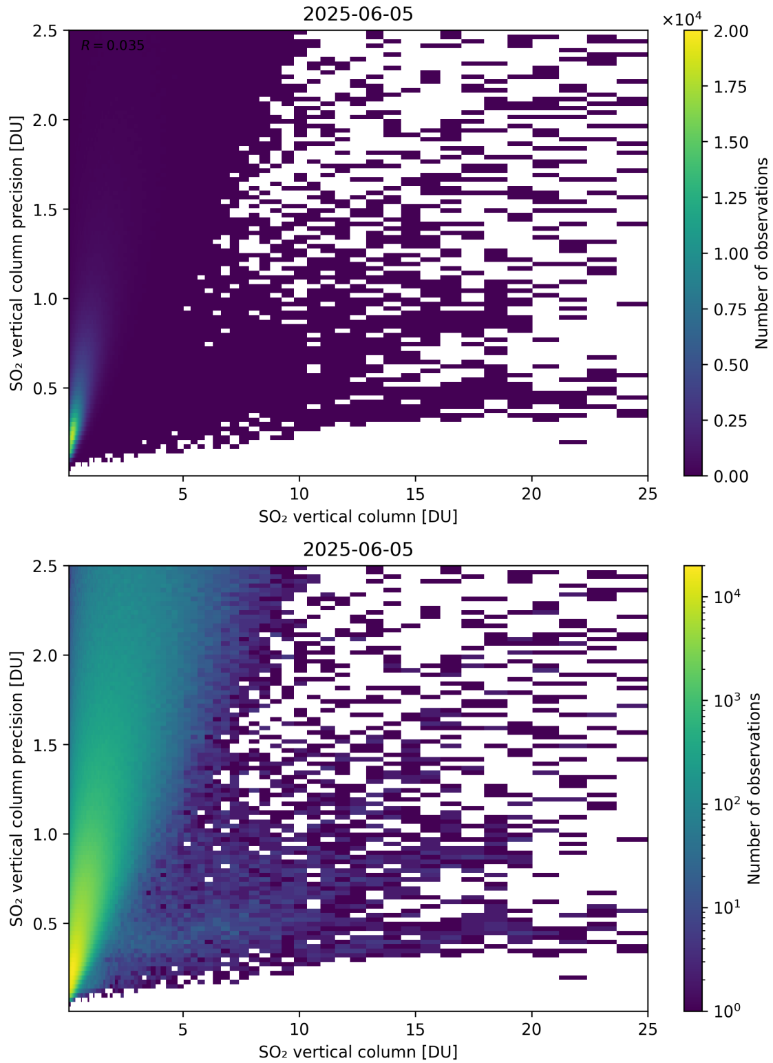
Figure 361: Scatter density plot of “SO 2 vertical column” against “SO 2 vertical column precision” for 2025-06-04 to 2025-06-06.
