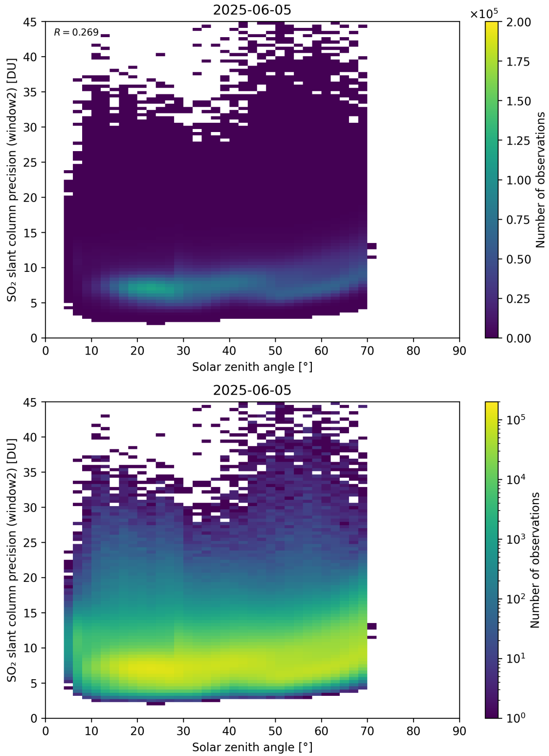
Figure 186: Scatter density plot of “Solar zenith angle” against “SO 2 slant column precision (window2)” for 2025-06-04 to 2025-06-06.
