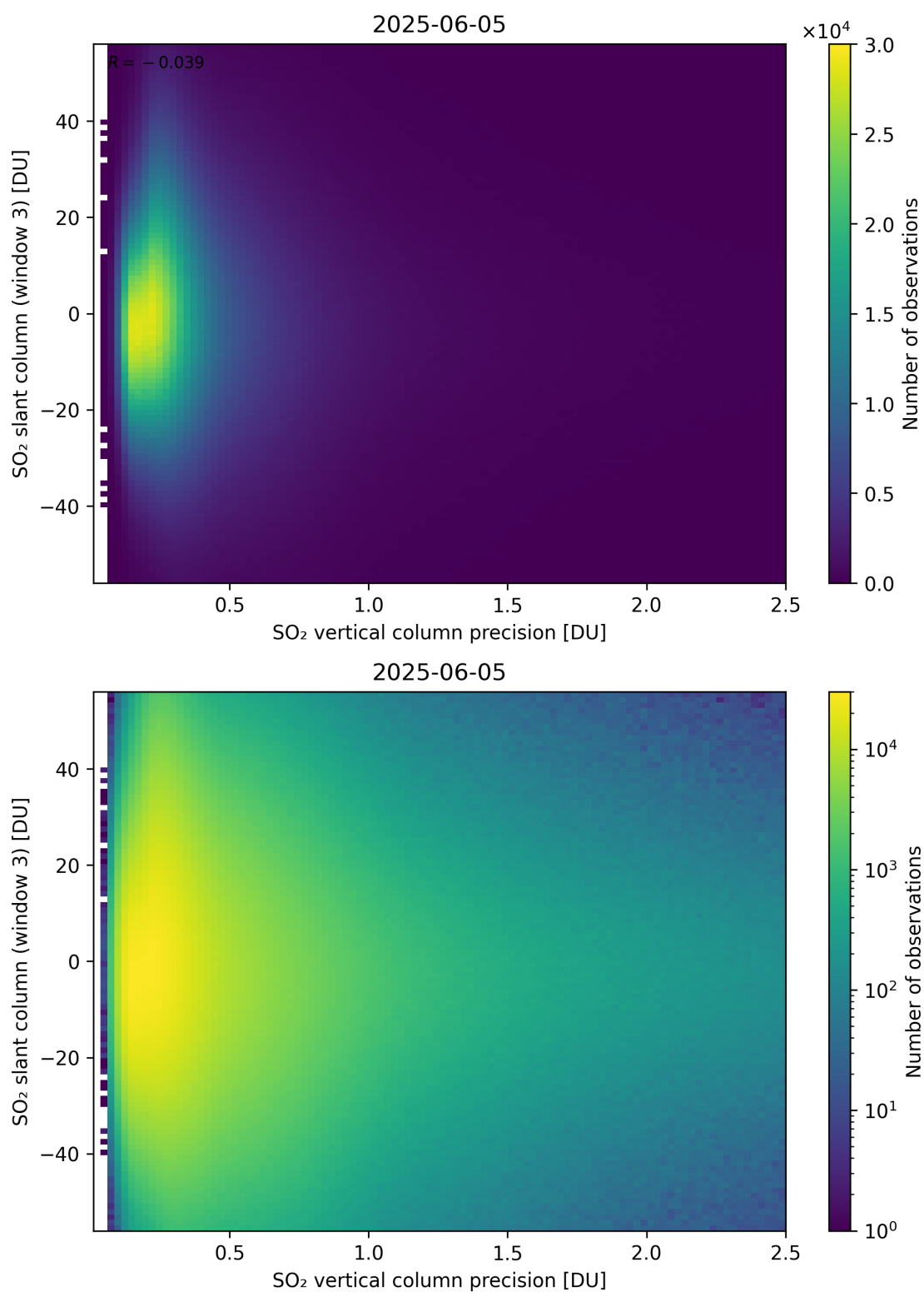
Figure 344: Scatter density plot of “SO 2 vertical column precision” against “SO 2 slant column (window 3)” for 2025-06-04 to 2025-06-06.
