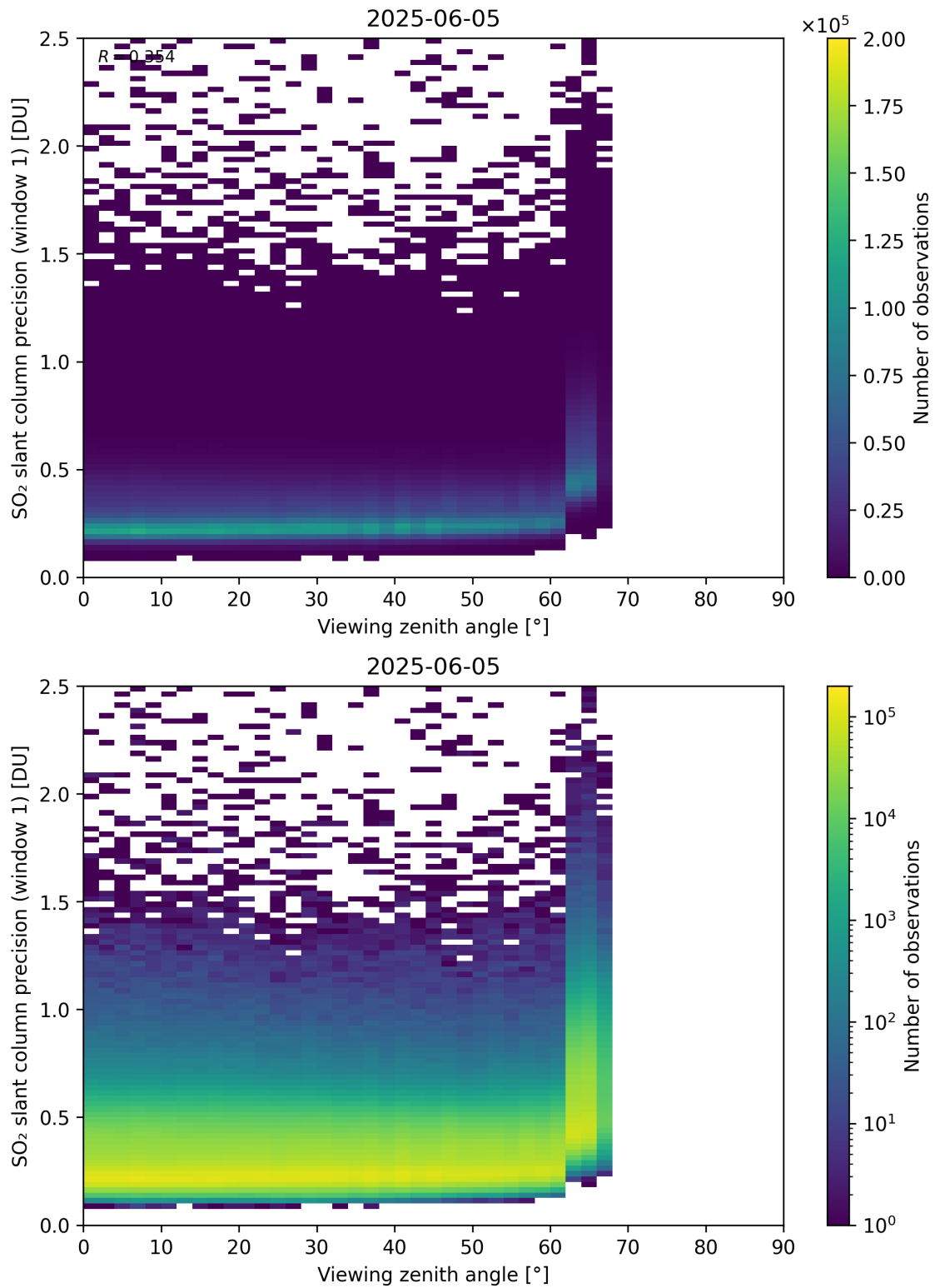
Figure 377: Scatter density plot of “Viewing zenith angle” against “SO 2 slant column precision (window 1)” for 2025-06-04 to 2025-06-06.
