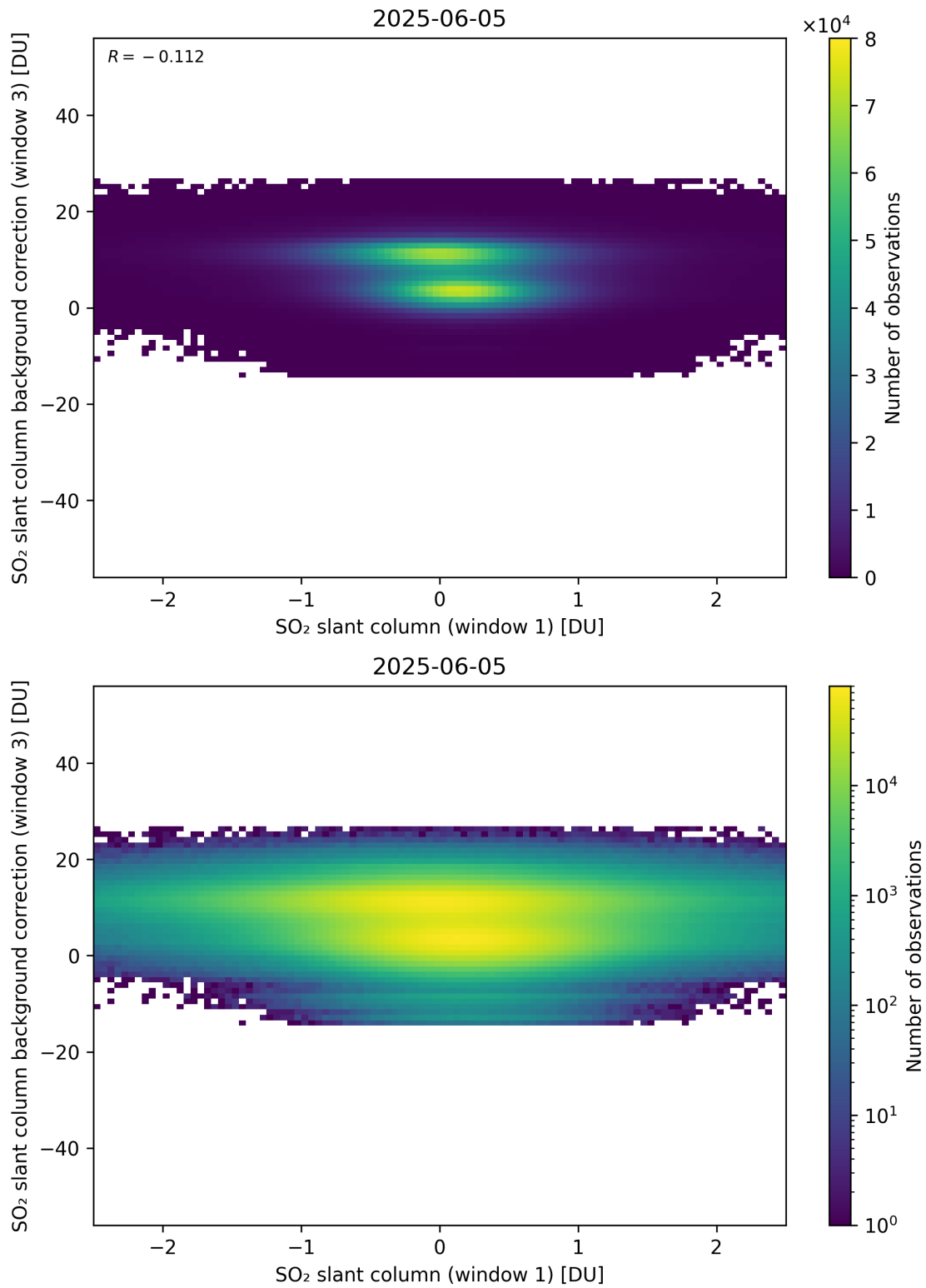
Figure 264: Scatter density plot of “SO 2 slant column (window 1)” against “SO 2 slant column background correction (window 3)” for 2025-06-04 to 2025-06-06.
