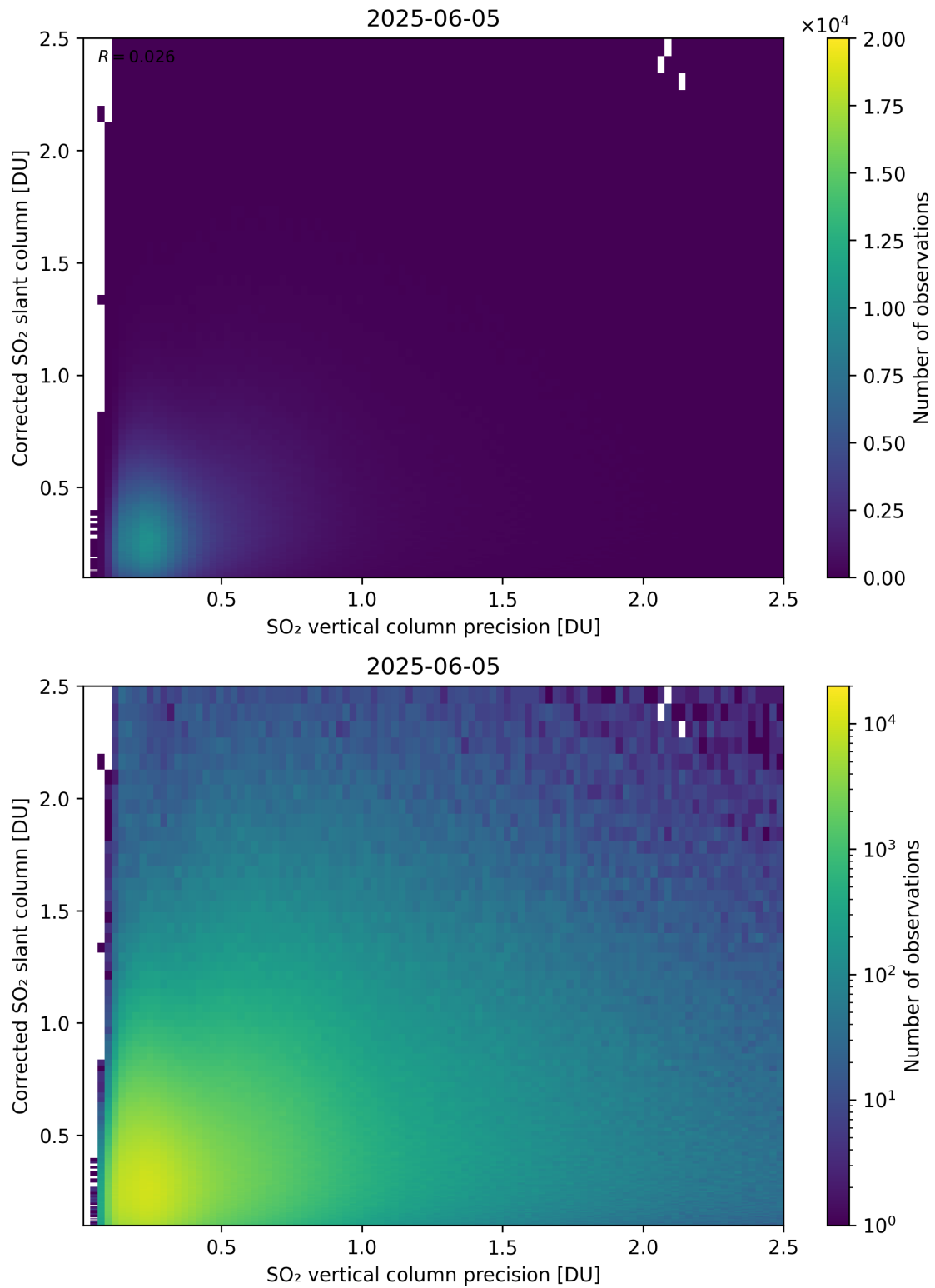
Figure 338: Scatter density plot of “SO 2 vertical column precision” against “Corrected SO 2 slant column” for 2025-06-04 to 2025-06-06.
