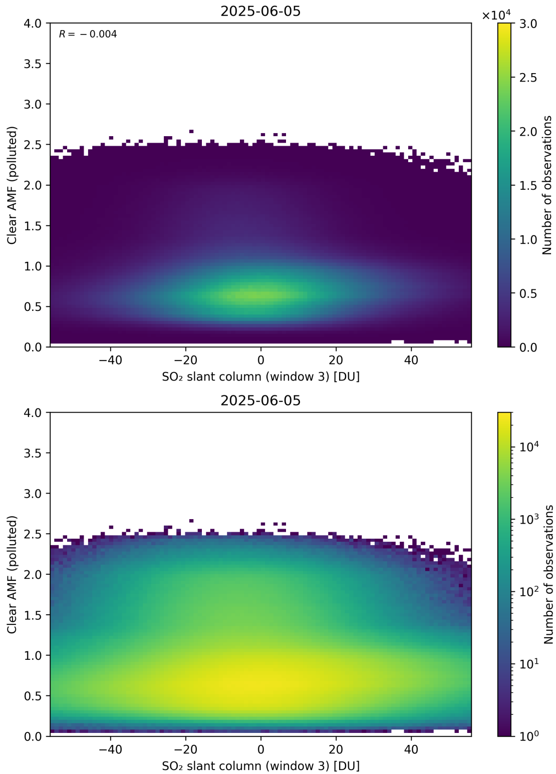
Figure 315: Scatter density plot of “SO 2 slant column (window 3)” against “Clear AMF (polluted)” for 2025-06-04 to 2025-06-06.
