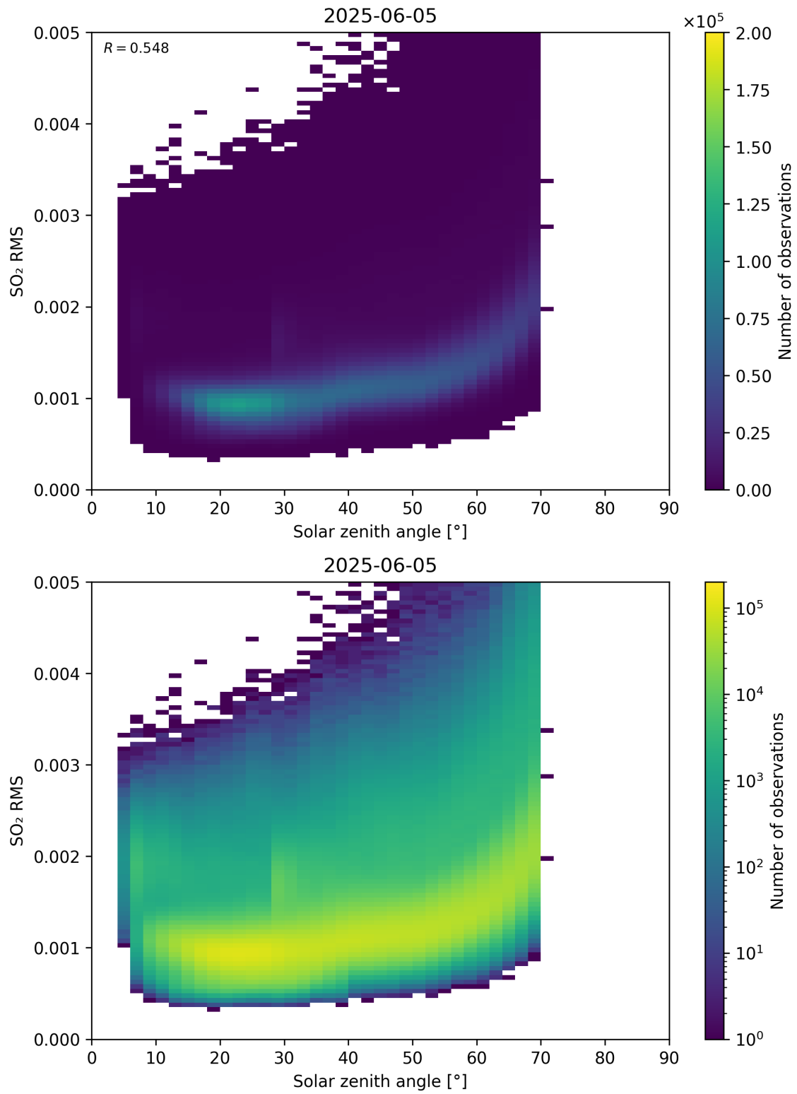
Figure 176: Scatter density plot of “Solar zenith angle” against “SO 2 RMS” for 2025-06-04 to 2025-06-06.
