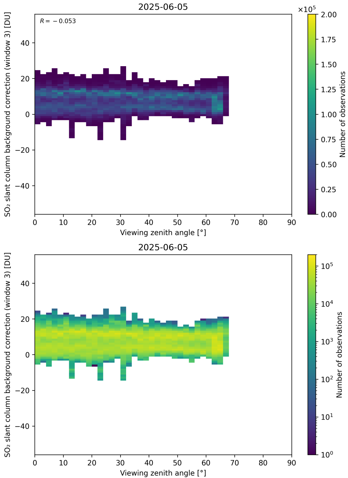
Figure 364: Scatter density plot of “Viewing zenith angle” against “SO 2 slant column background correction (window 3)” for 2025-06-04 to 2025-06-06.
