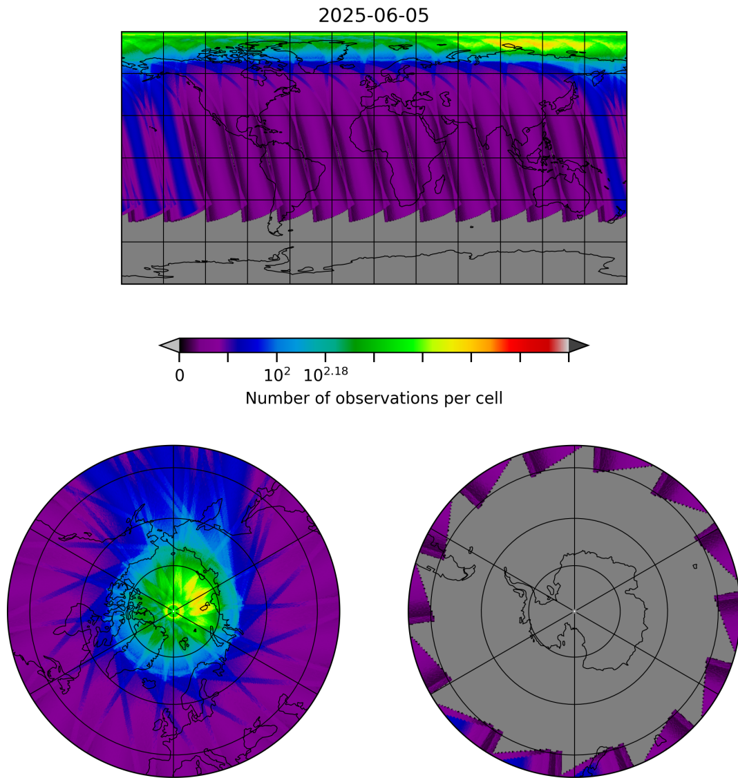
Figure 30: Map of the number of observations for 2025-06-04 to 2025-06-06
