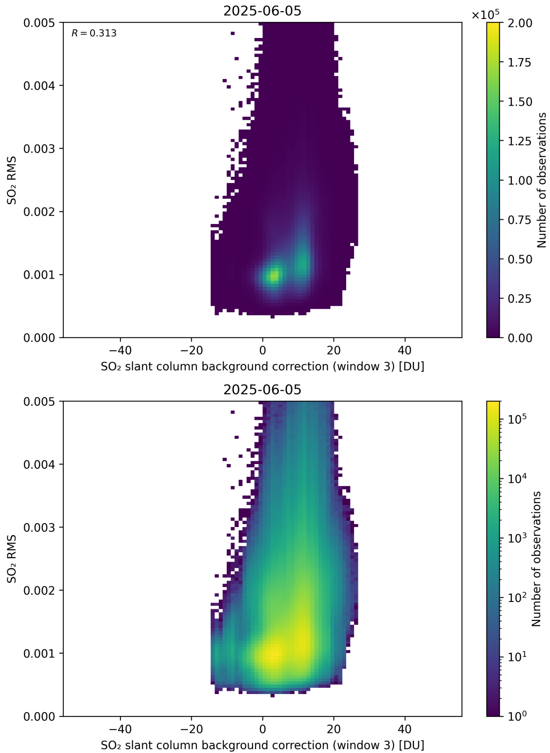
Figure 134: Scatter density plot of “SO 2 slant column background correction (window 3)” against “SO 2 RMS” for 2025-06-04 to 2025-06-06.
