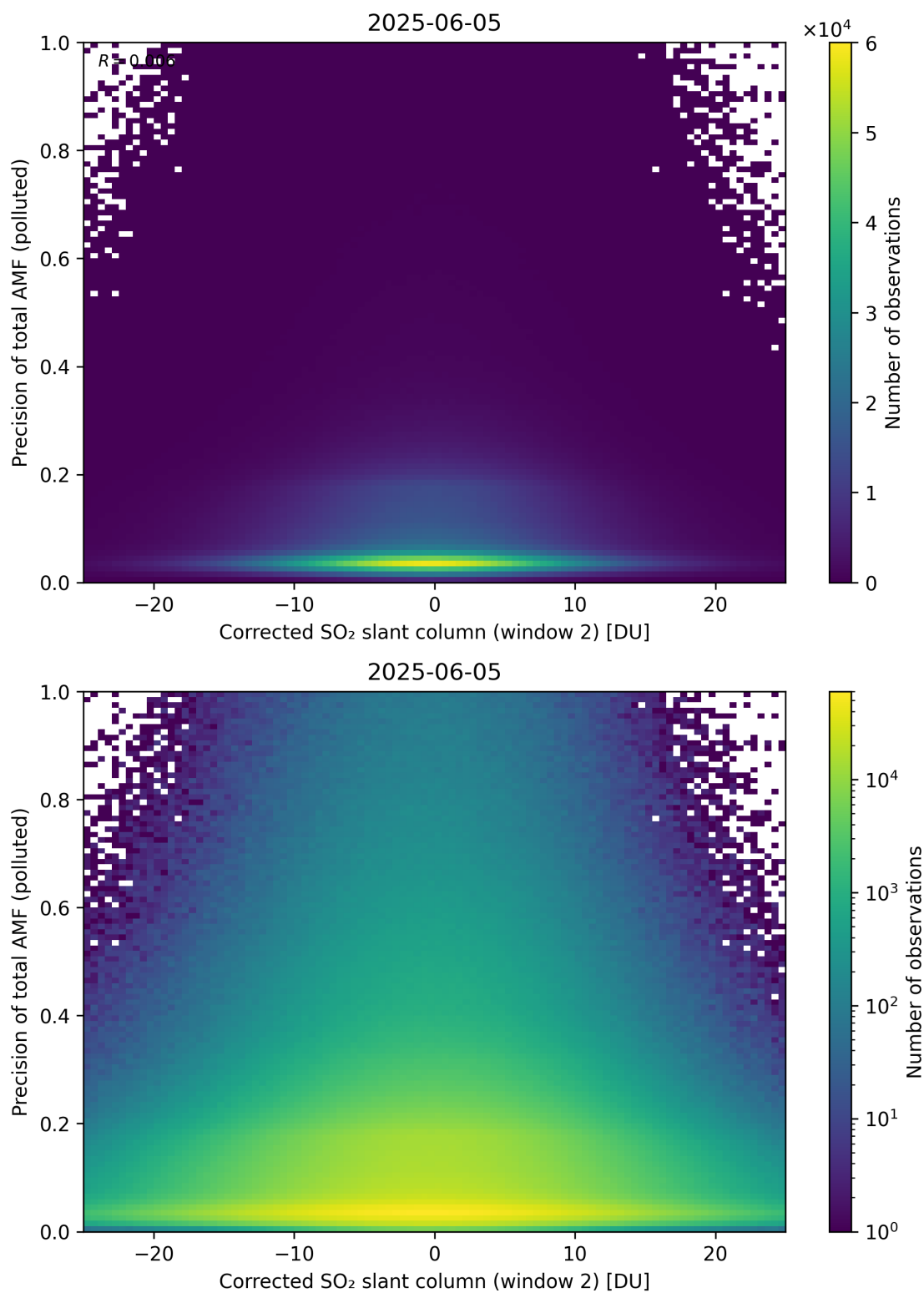
Figure 254: Scatter density plot of “Corrected SO 2 slant column (window 2)” against “Precision of total AMF (polluted)” for 2025-06-04 to 2025-06-06.
