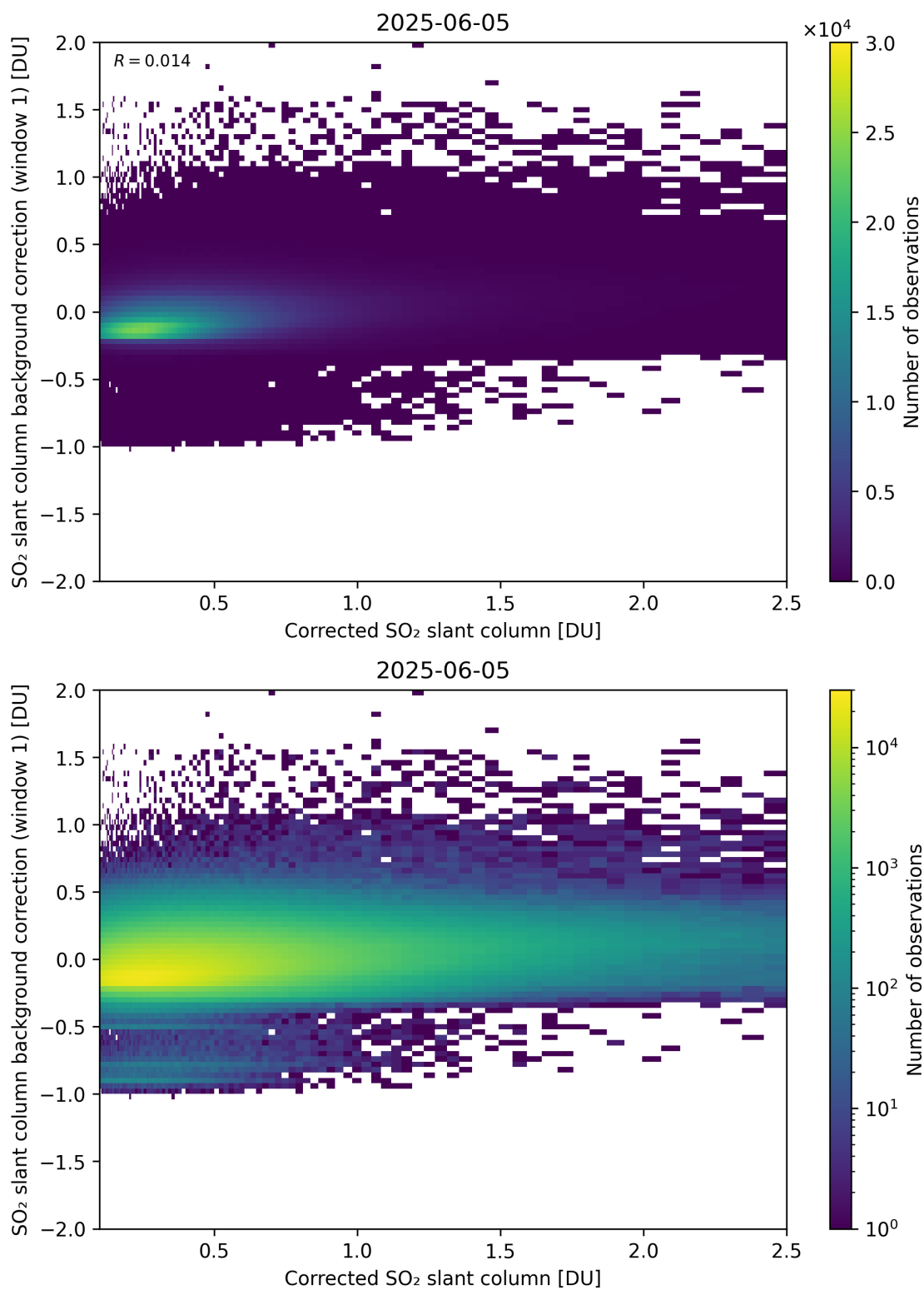
Figure 226: Scatter density plot of “Corrected SO 2 slant column” against “SO 2 slant column background correction (window 1)” for 2025-06-04 to 2025-06-06.
