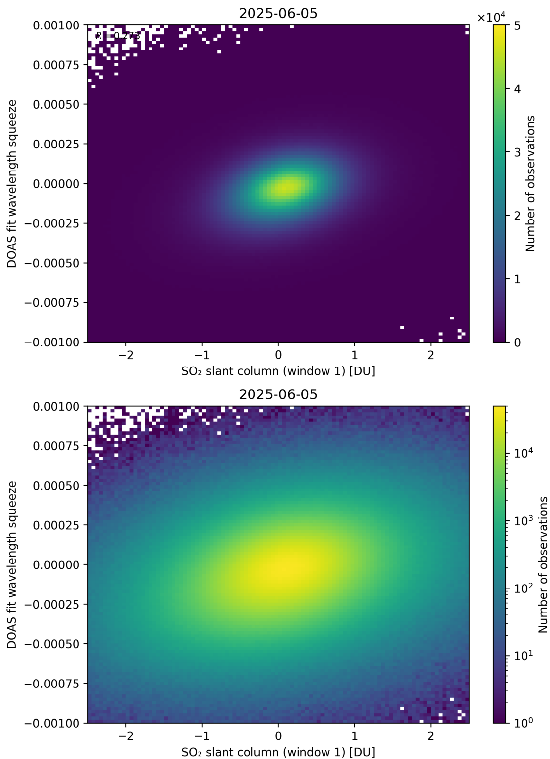
Figure 266: Scatter density plot of “SO 2 slant column (window 1)” against “DOAS fit wavelength squeeze” for 2025-06-04 to 2025-06-06.
