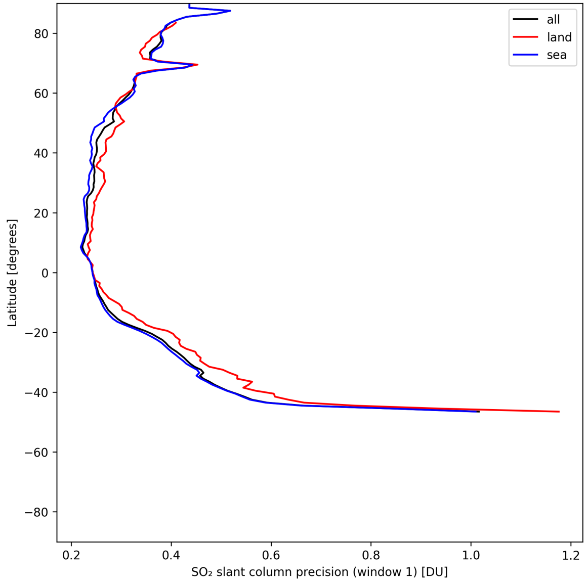
Figure 38: Zonal average of “SO 2 slant column precision (window 1)” for 2025-06-04 to 2025-06-06.
