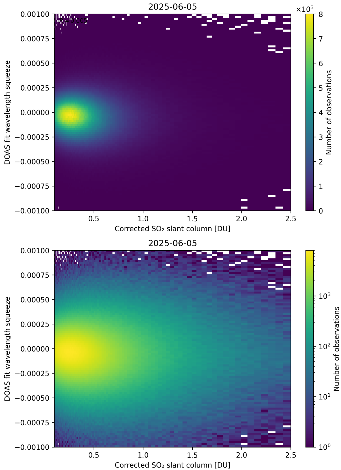
Figure 230: Scatter density plot of “Corrected SO 2 slant column” against “DOAS fit wavelength squeeze” for 2025-06-04 to 2025-06-06.
