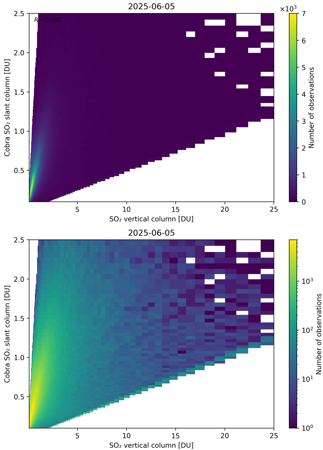
Figure 349: Scatter density plot of “SO 2 vertical column” against “Cobra SO 2 slant column” for 2025-06-04 to 2025-06-06.
