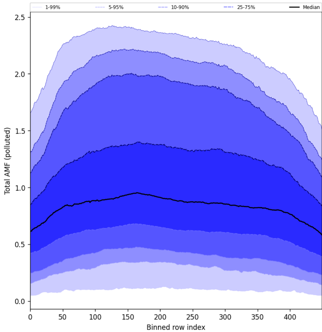
Figure 105: Along track statistics of “Total AMF (polluted)” for 2025-06-04 to 2025-06-06
