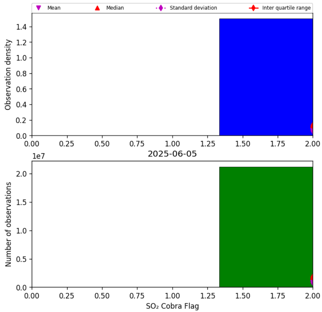
Figure 75: Histogram of “SO 2 Cobra Flag” for 2025-06-04 to 2025-06-06
