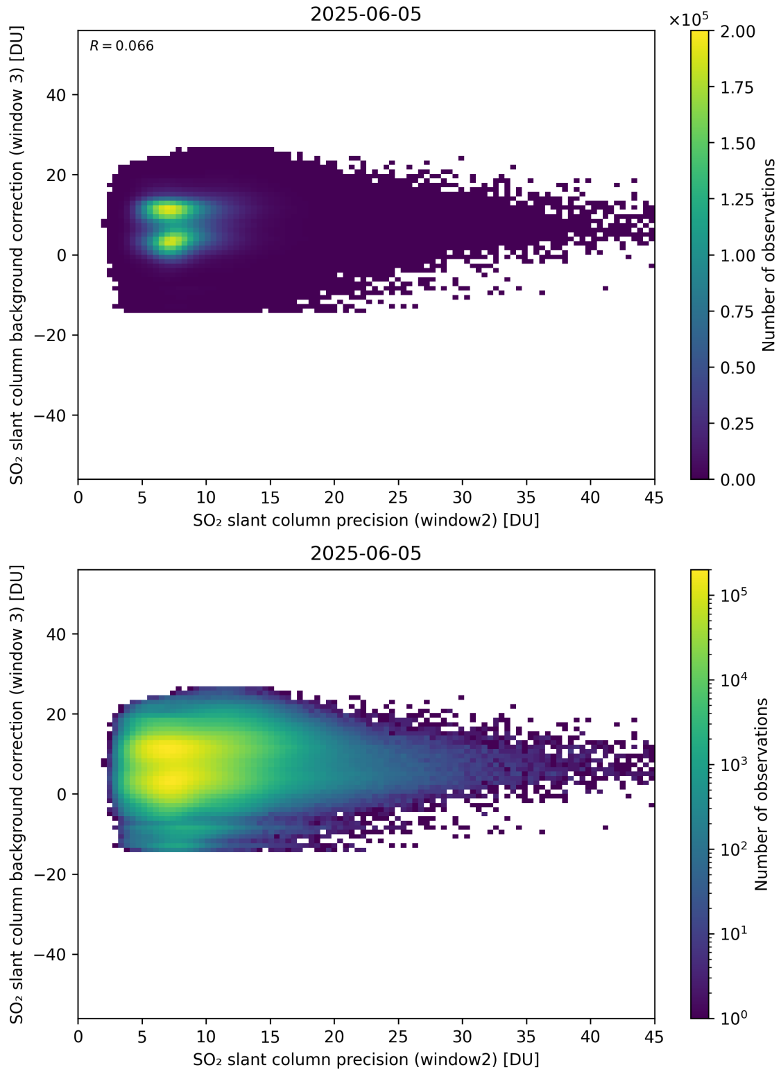
Figure 292: Scatter density plot of “SO 2 slant column precision (window2)” against “SO 2 slant column background correction (window 3)” for 2025-06-04 to 2025-06-06.
