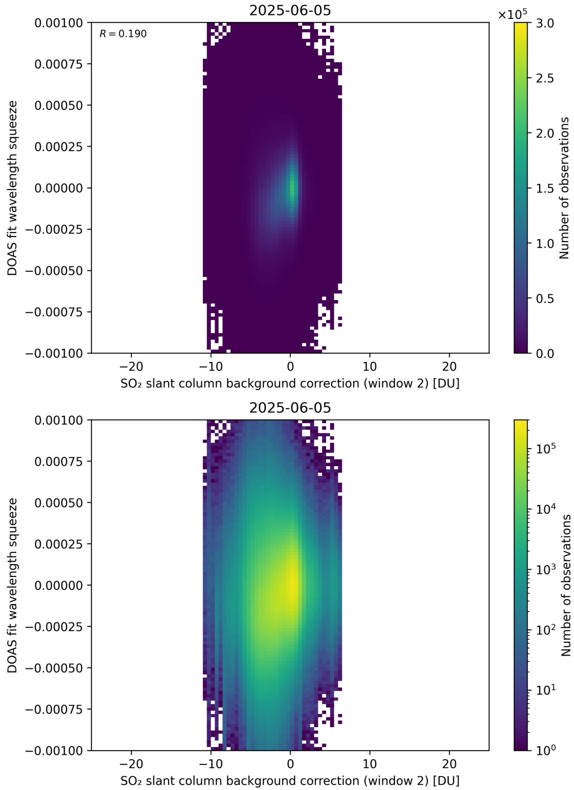
Figure 124: Scatter density plot of “SO 2 slant column background correction (window 2)” against “DOAS fit wavelength squeeze” for 2025-06-04 to 2025-06-06.
