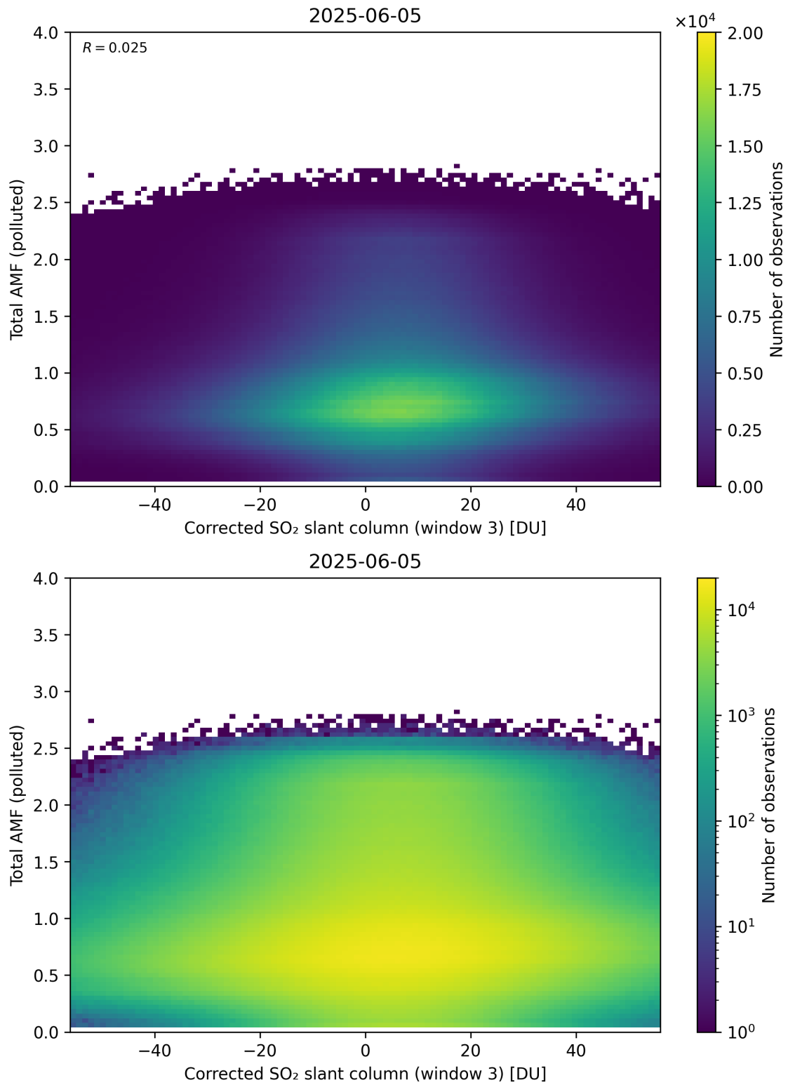
Figure 260: Scatter density plot of “Corrected SO 2 slant column (window 3)” against “Total AMF (polluted)” for 2025-06-04 to 2025-06-06.
