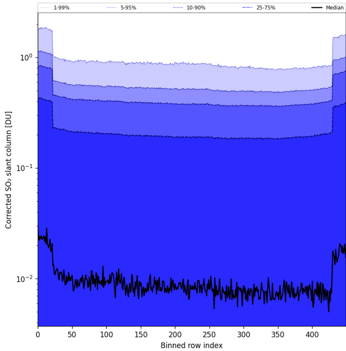
Figure 86: Along track statistics of “Corrected SO 2 slant column” for 2025-06-04 to 2025-06-06
