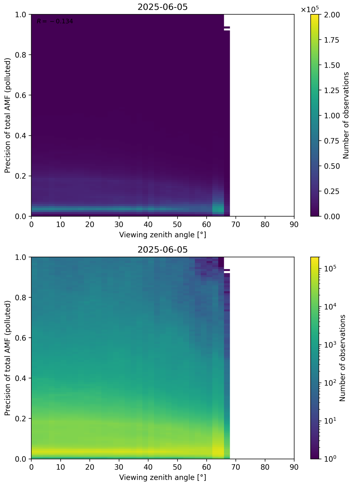
Figure 382: Scatter density plot of “Viewing zenith angle” against “Precision of total AMF (polluted)” for 2025-06-04 to 2025-06-06.
