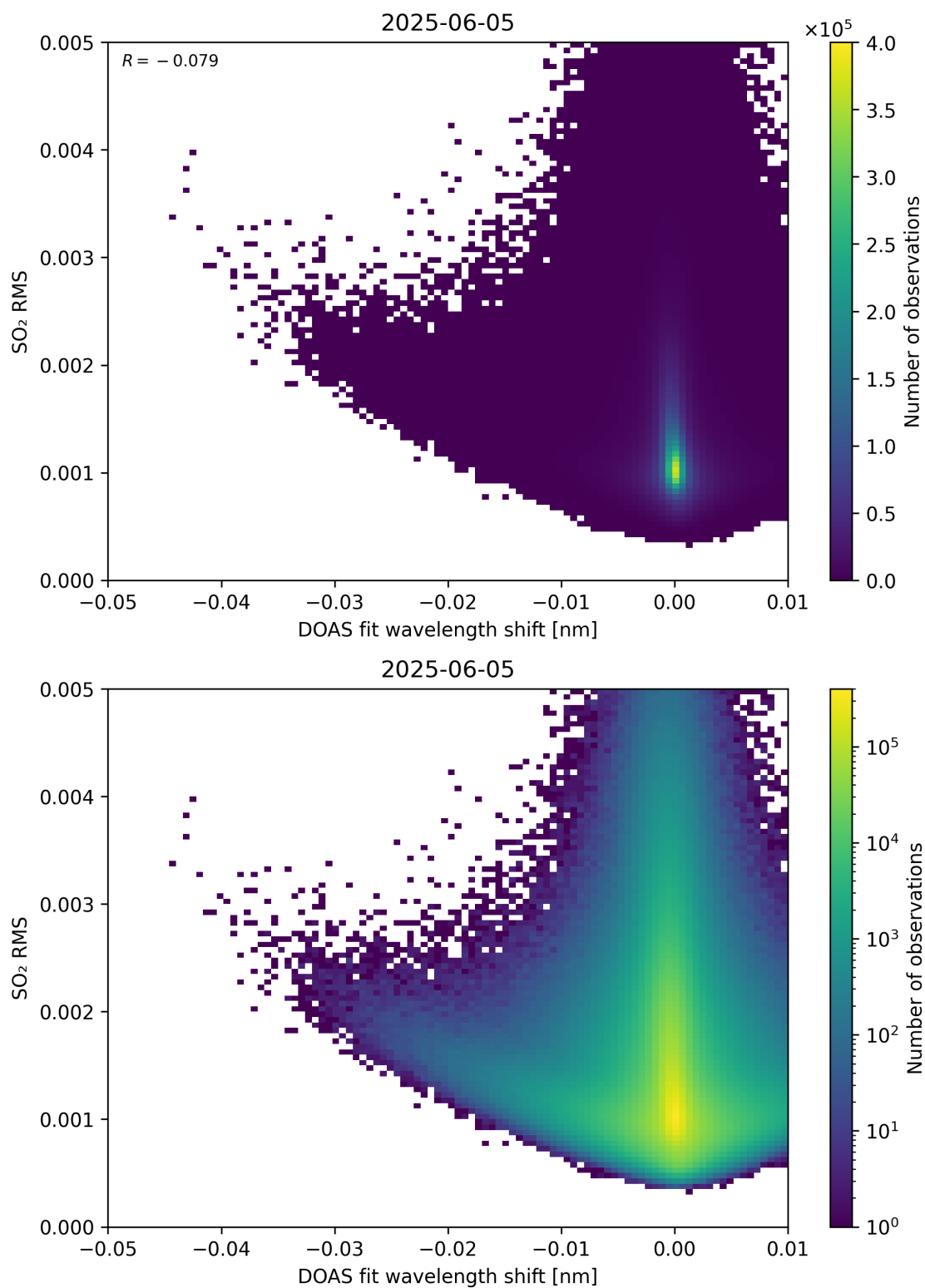
Figure 139: Scatter density plot of “DOAS fit wavelength shift” against “SO 2 RMS” for 2025-06-04 to 2025-06-06.
