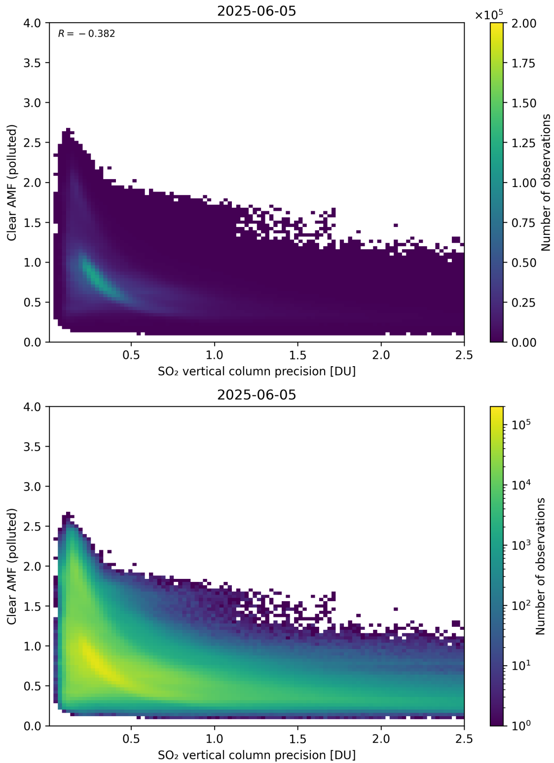
Figure 335: Scatter density plot of “SO 2 vertical column precision” against “Clear AMF (polluted)” for 2025-06-04 to 2025-06-06.
