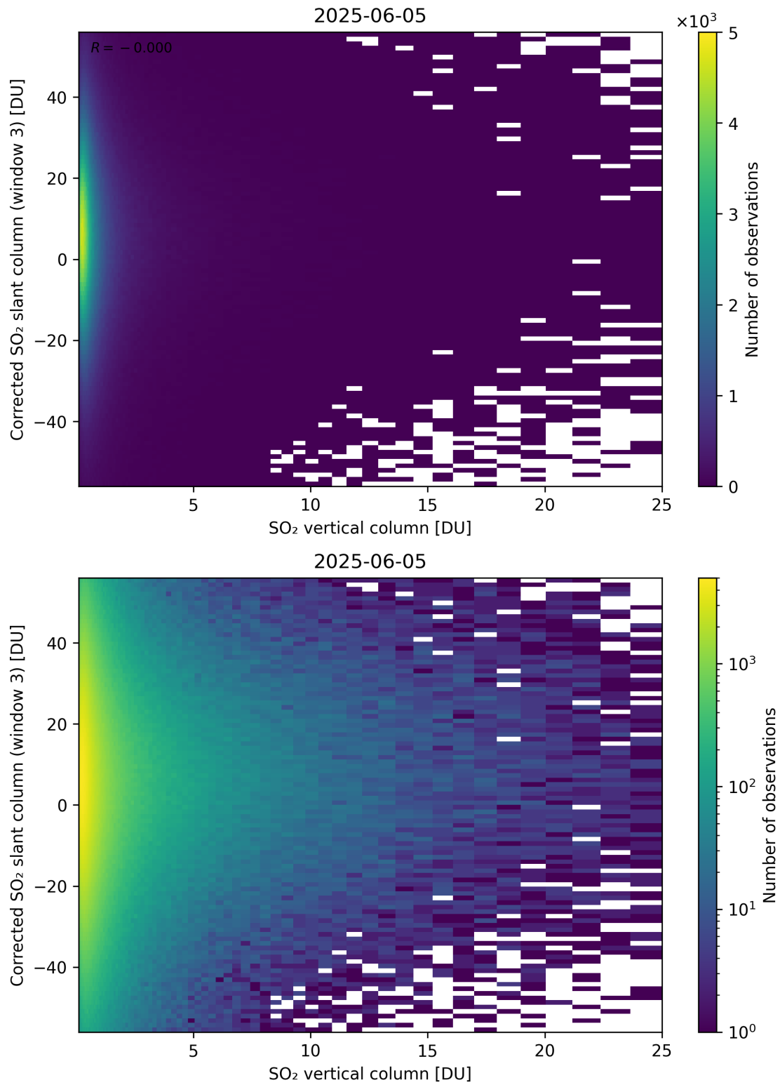
Figure 353: Scatter density plot of “SO 2 vertical column” against “Corrected SO 2 slant column (window 3)” for 2025-06-04 to 2025-06-06.
