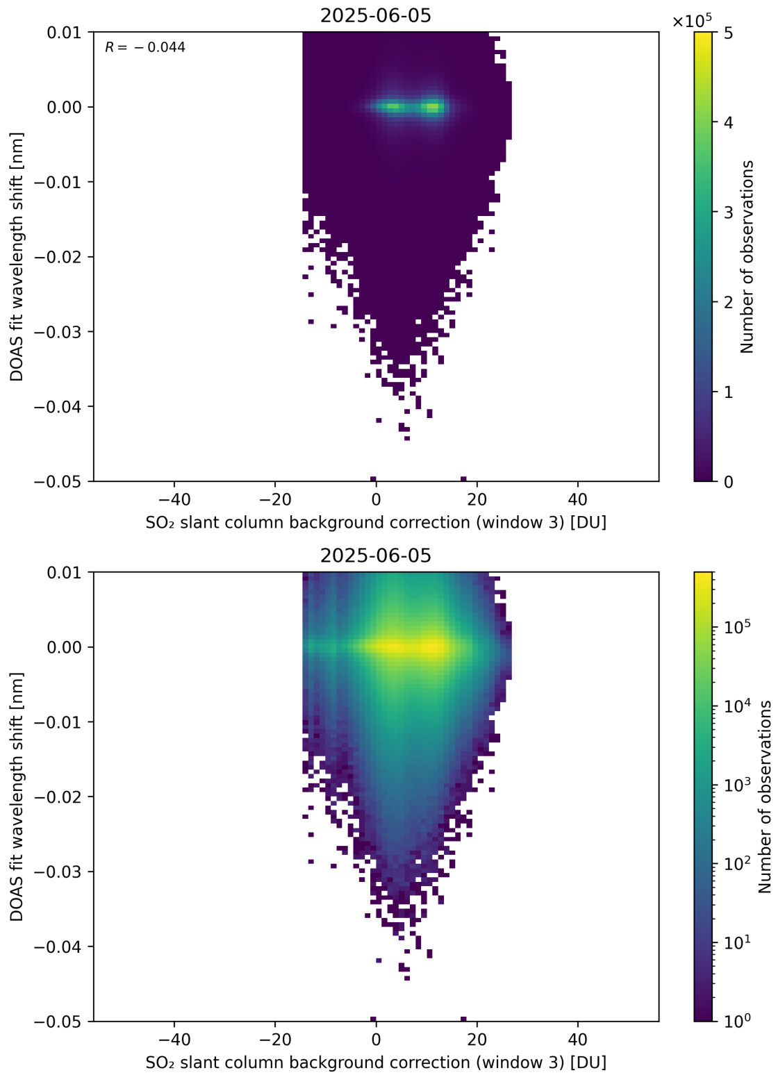
Figure 132: Scatter density plot of “SO 2 slant column background correction (window 3)” against “DOAS fit wavelength shift” for 2025-06-04 to 2025-06-06.
