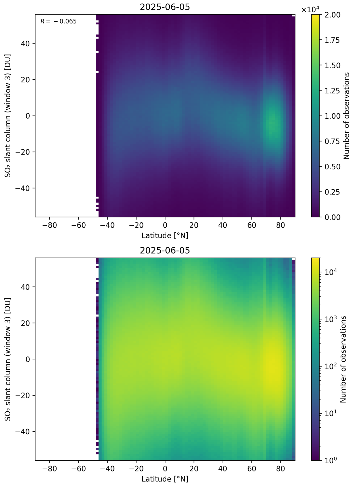
Figure 165: Scatter density plot of “Latitude” against “SO 2 slant column (window 3)” for 2025-06-04 to 2025-06-06.
