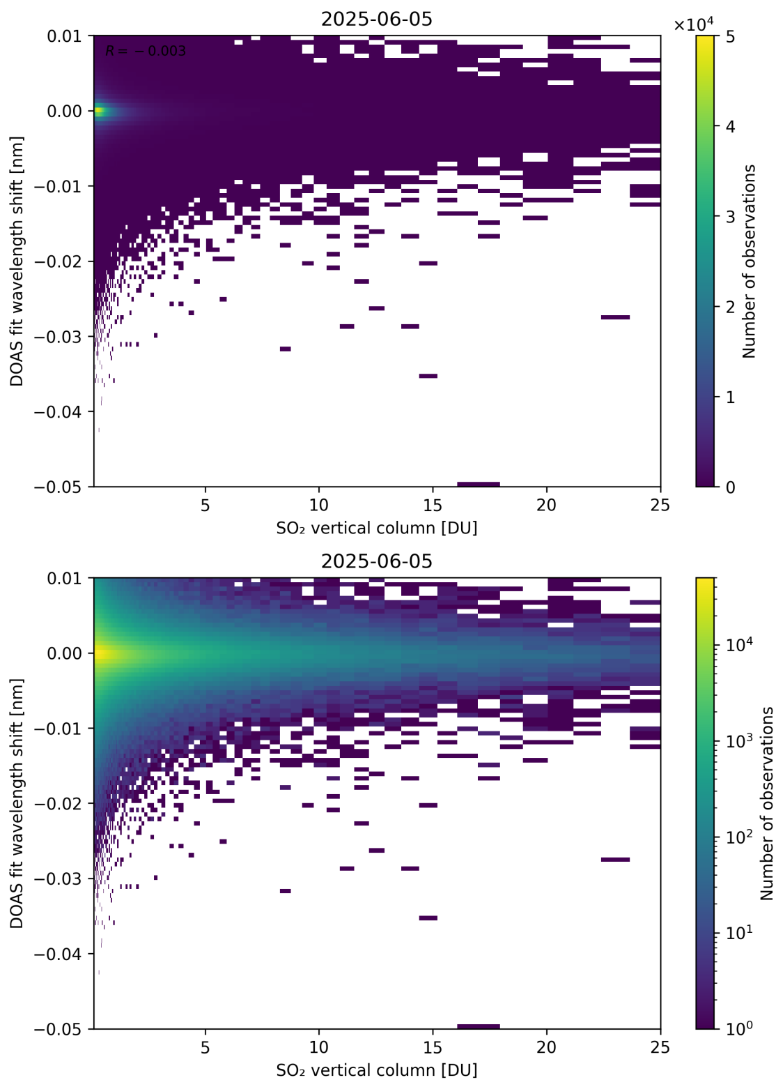
Figure 326: Scatter density plot of “SO 2 vertical column” against “DOAS fit wavelength shift” for 2025-06-04 to 2025-06-06.
