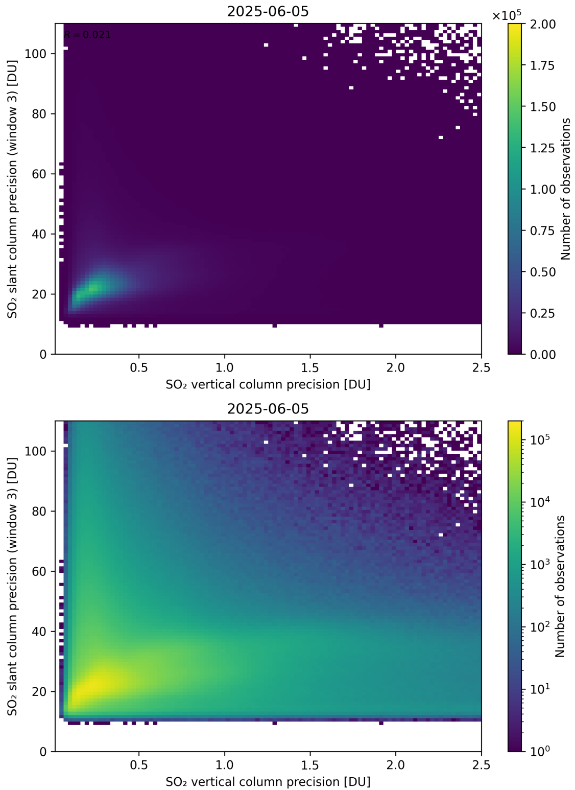
Figure 345: Scatter density plot of “SO 2 vertical column precision” against “SO 2 slant column precision (window 3)” for 2025-06-04 to 2025-06-06.
