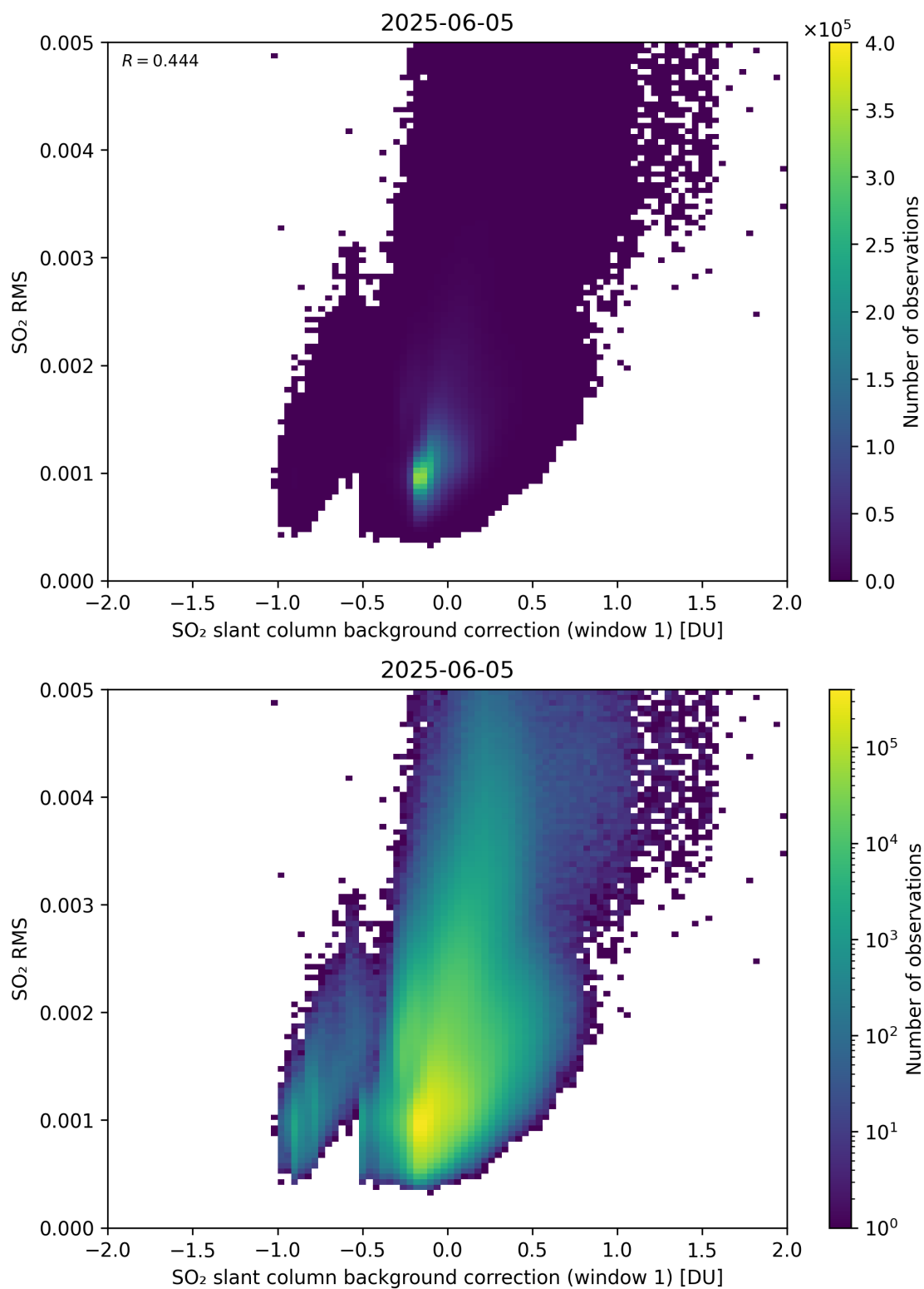
Figure 113: Scatter density plot of “SO 2 slant column background correction (window 1)” against “SO 2 RMS” for 2025-06-04 to 2025-06-06.
