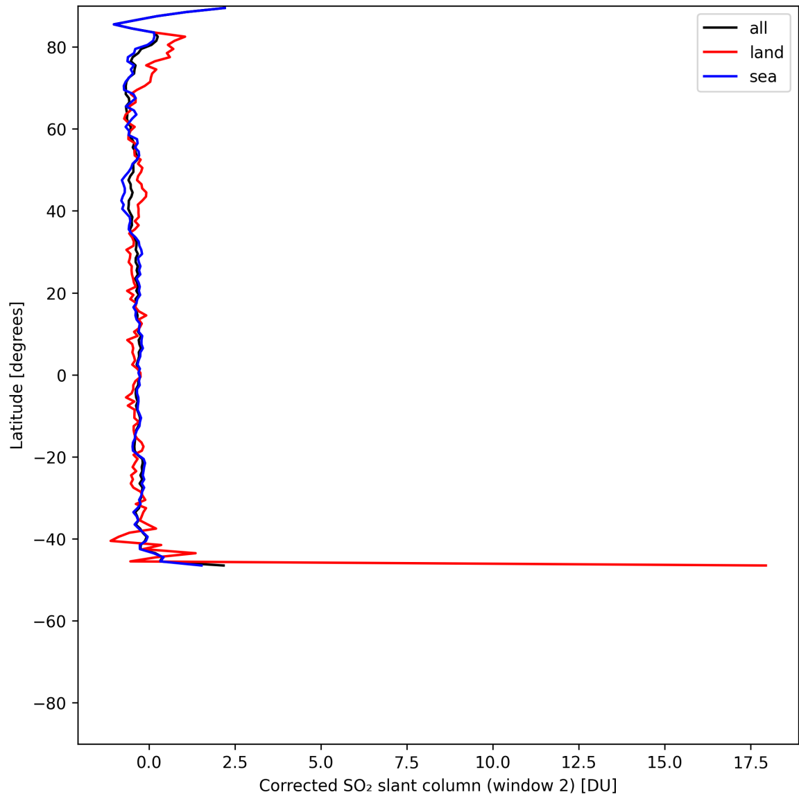
Figure 43: Zonal average of “Corrected SO 2 slant column (window 2)” for 2025-06-04 to 2025-06-06.
