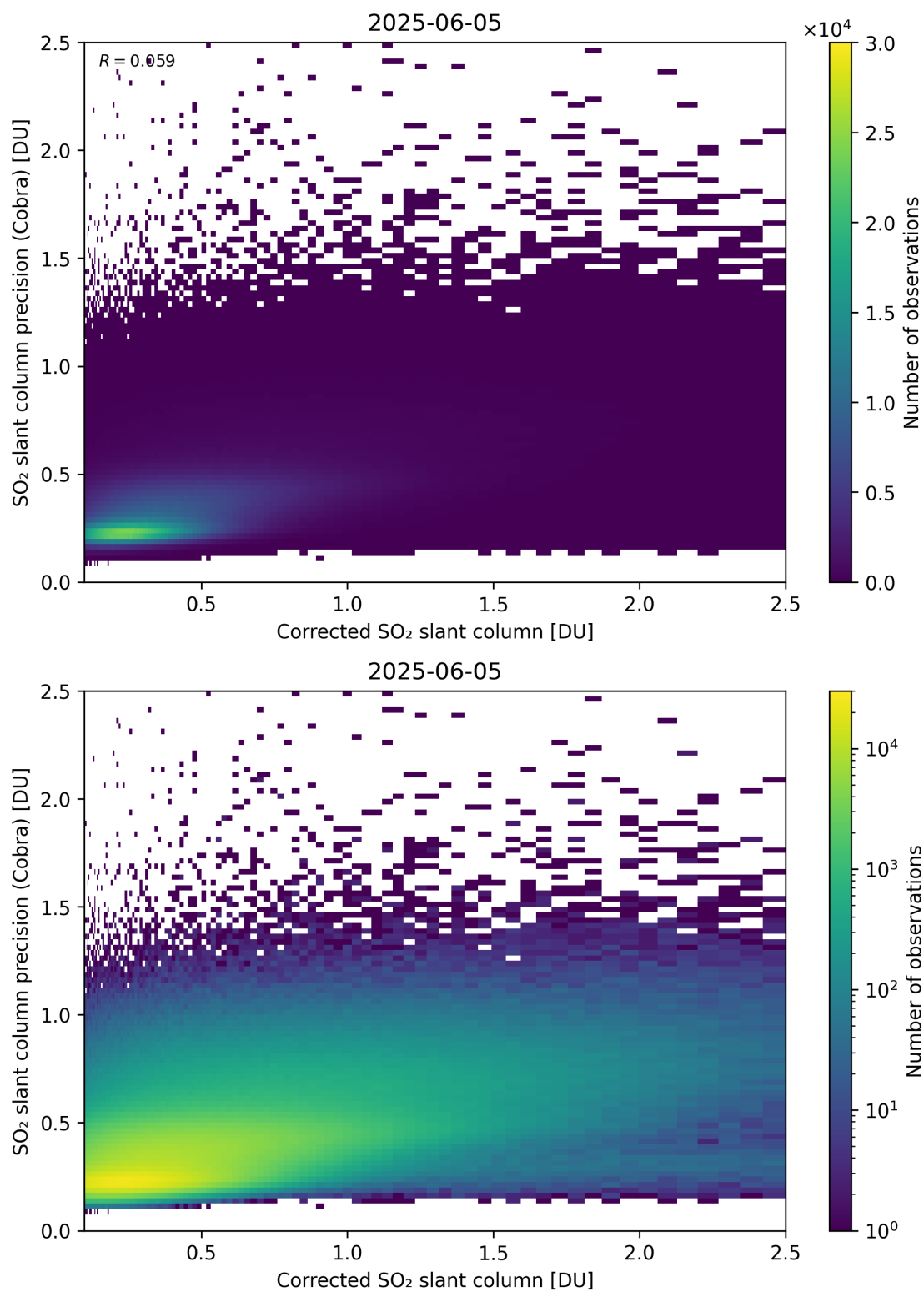
Figure 234: Scatter density plot of “Corrected SO 2 slant column” against “SO 2 slant column precision (Cobra)” for 2025-06-04 to 2025-06-06.
