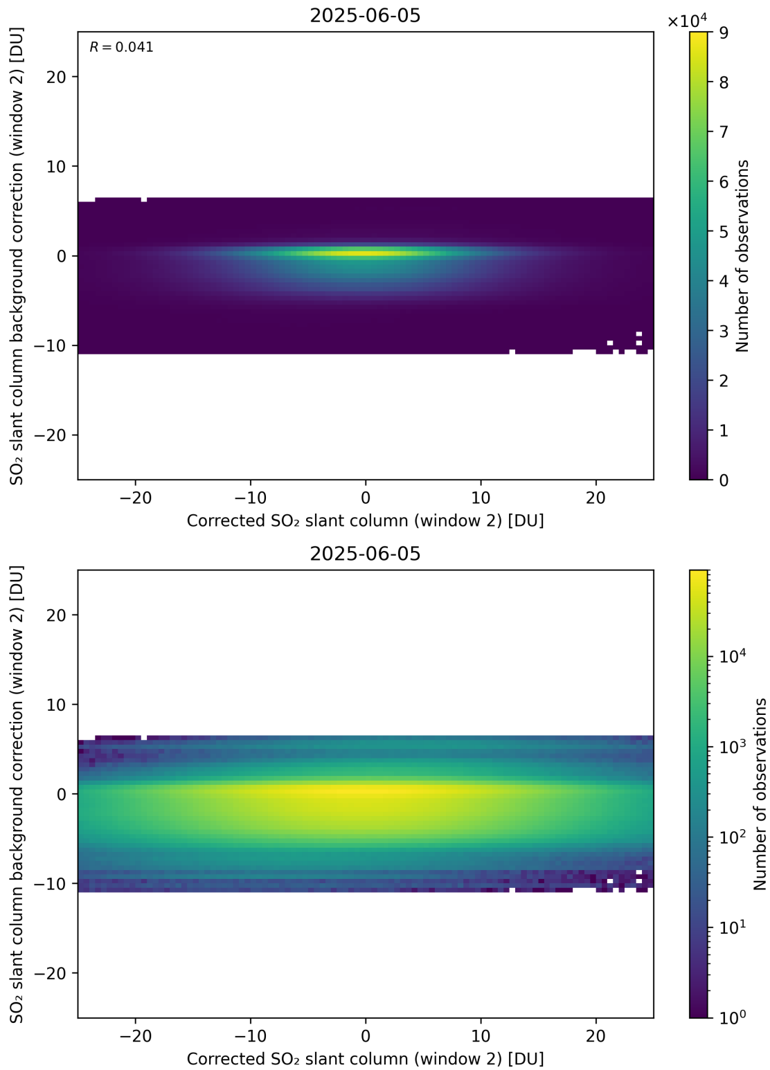
Figure 244: Scatter density plot of “Corrected SO 2 slant column (window 2)” against “SO 2 slant column background correction (window 2)” for 2025-06-04 to 2025-06-06.
