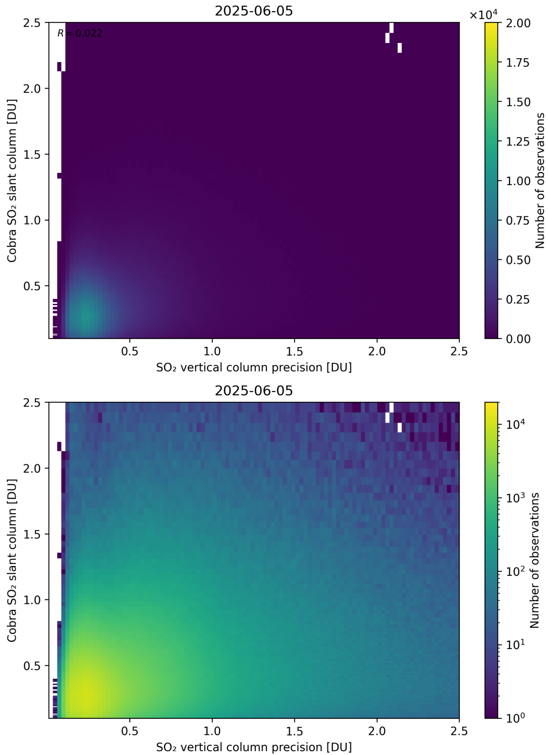
Figure 336: Scatter density plot of “SO 2 vertical column precision” against “Cobra SO 2 slant column” for 2025-06-04 to 2025-06-06.
