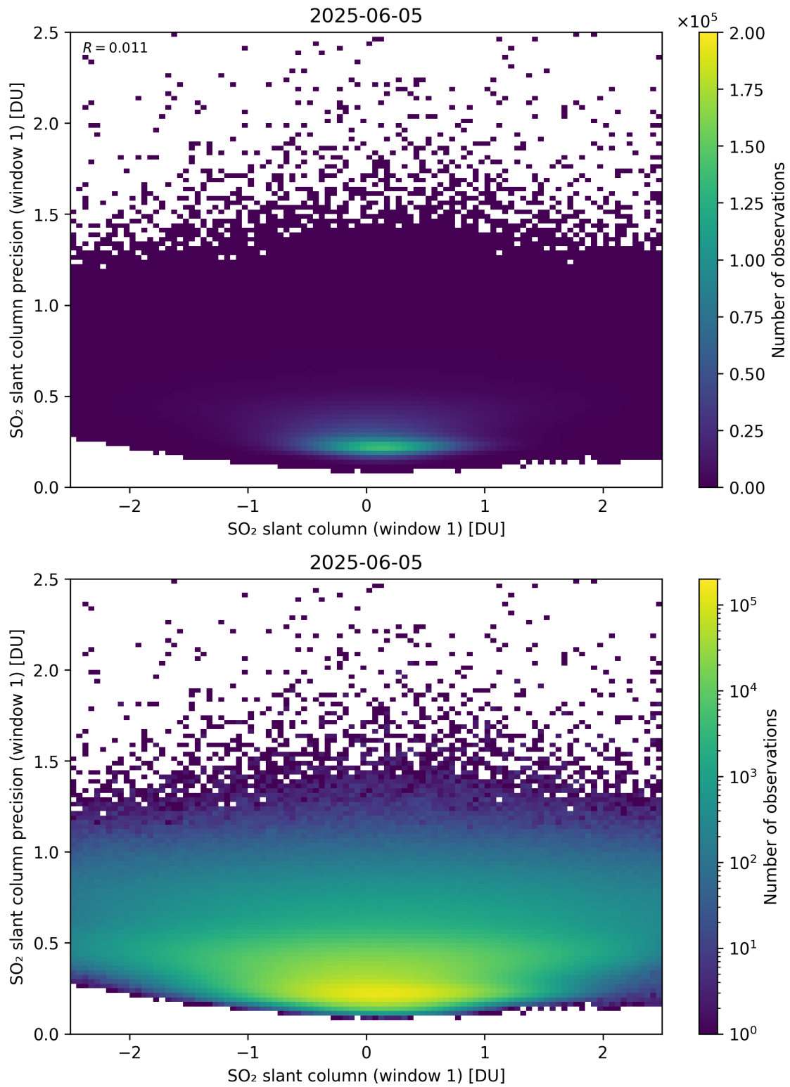
Figure 285: Scatter density plot of “SO 2 slant column (window 1)” against “SO 2 slant column precision (window 1)” for 2025-06-04 to 2025-06-06.
