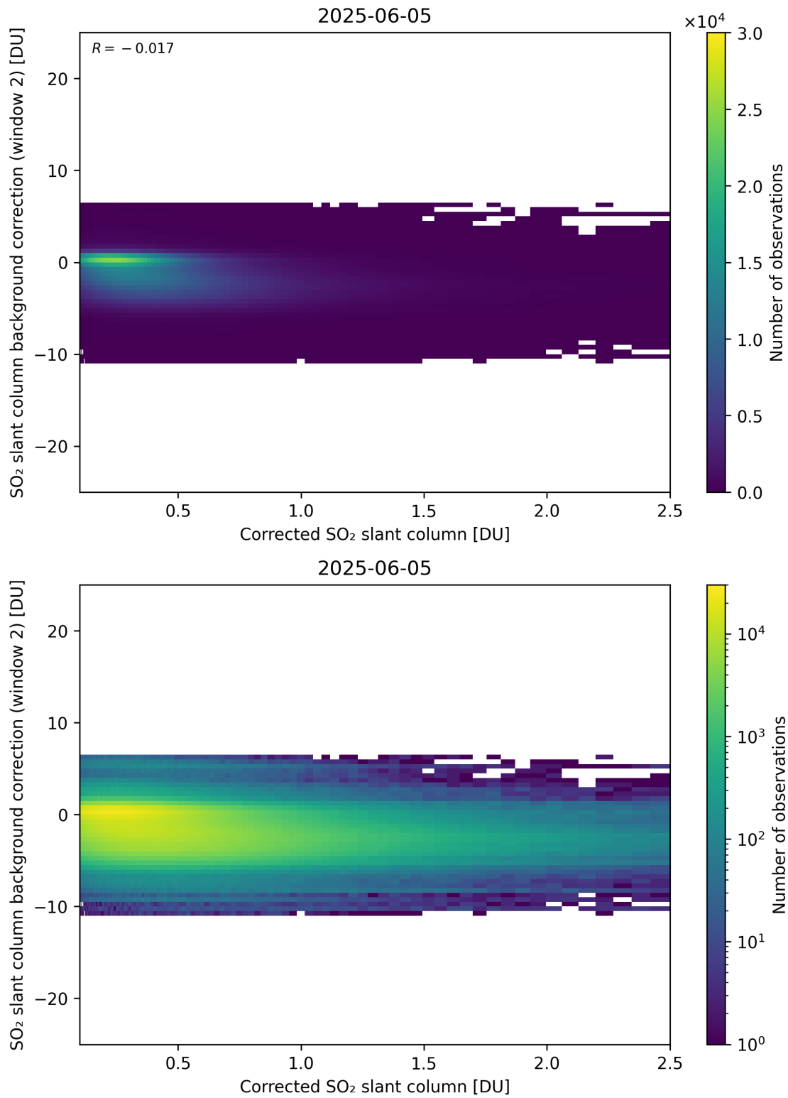
Figure 227: Scatter density plot of “Corrected SO 2 slant column” against “SO 2 slant column background correction (window 2)” for 2025-06-04 to 2025-06-06.
