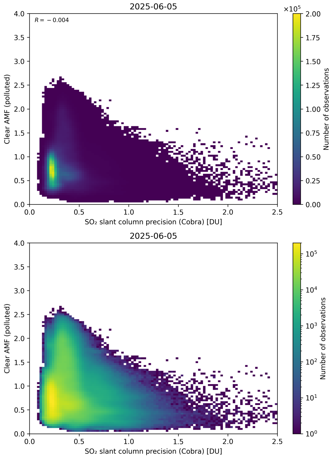
Figure 205: Scatter density plot of “SO 2 slant column precision (Cobra)” against “Clear AMF (polluted)” for 2025-06-04 to 2025-06-06.
