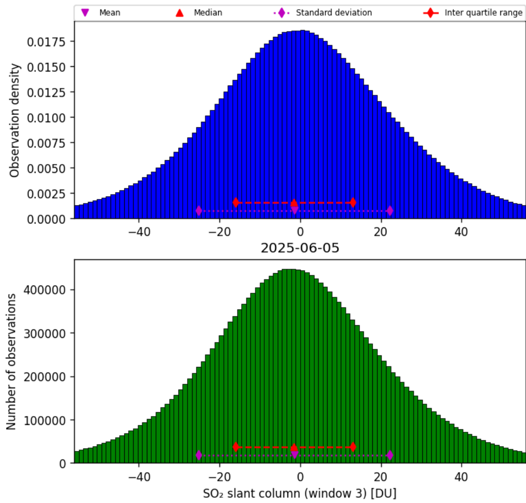
Figure 71: Histogram of “SO 2 slant column (window 3)” for 2025-06-04 to 2025-06-06
