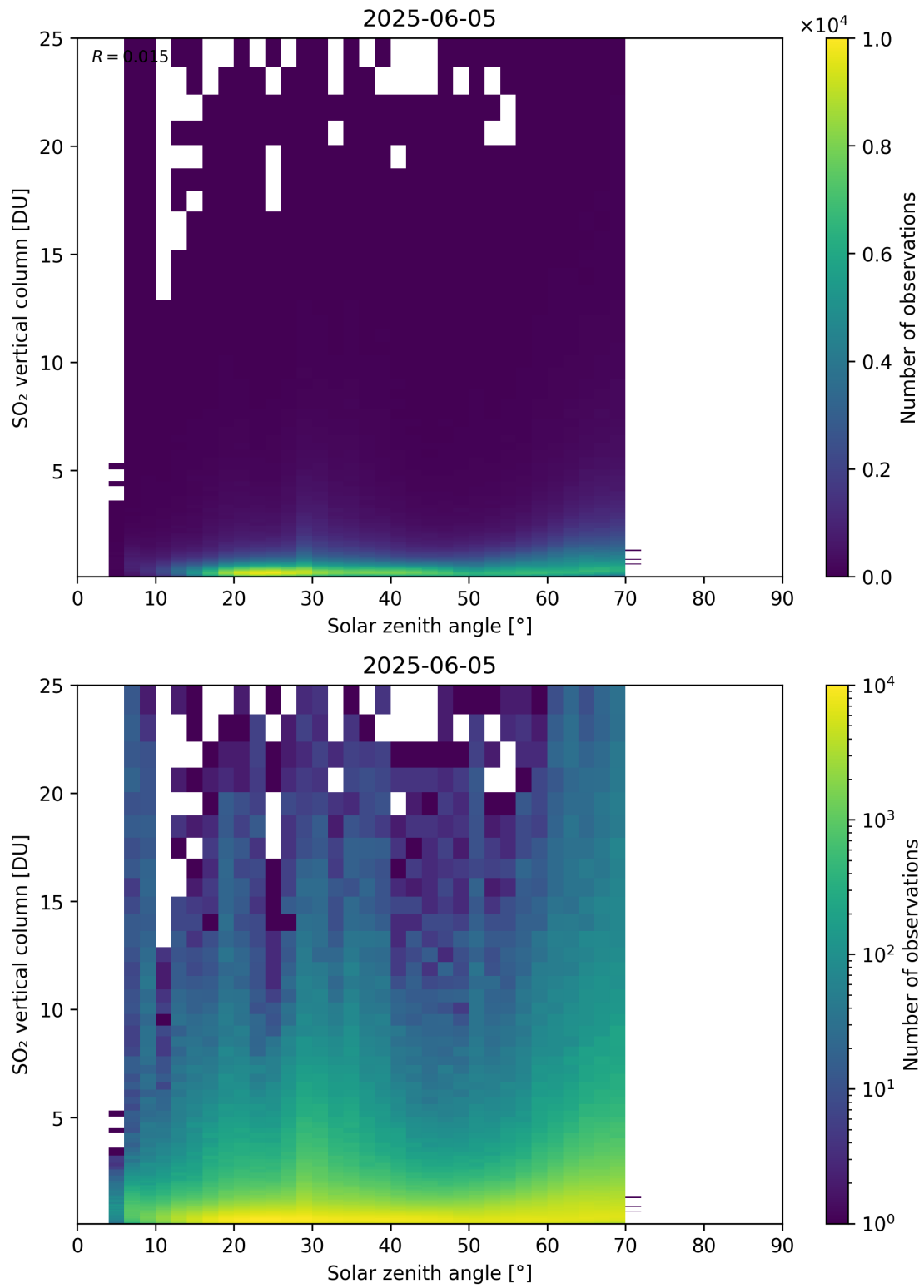
Figure 191: Scatter density plot of “Solar zenith angle” against “SO 2 vertical column” for 2025-06-04 to 2025-06-06.
