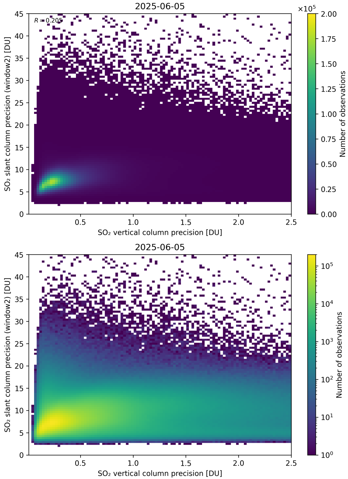
Figure 343: Scatter density plot of “SO 2 vertical column precision” against “SO 2 slant column precision (window2)” for 2025-06-04 to 2025-06-06.
