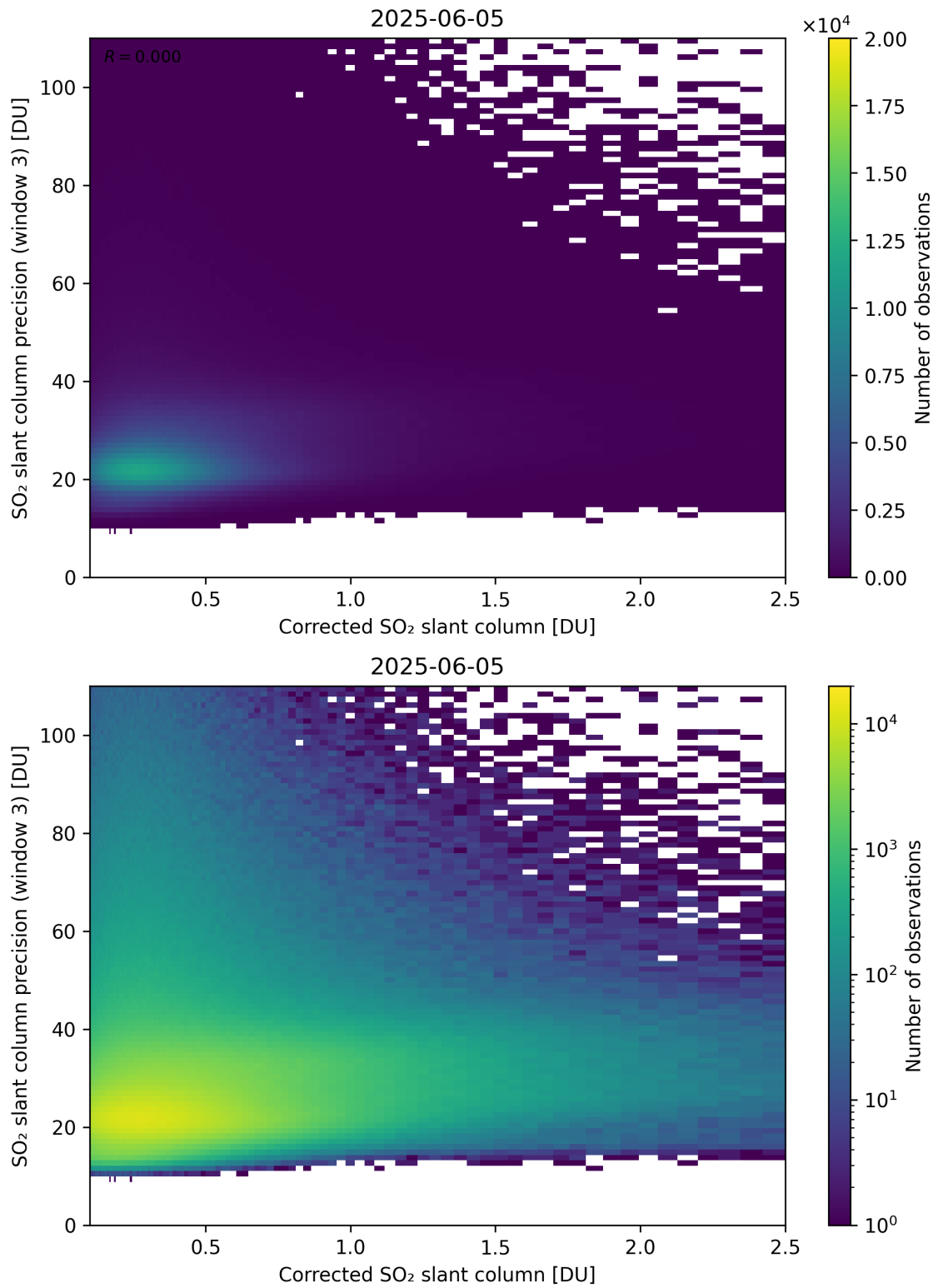
Figure 241: Scatter density plot of “Corrected SO 2 slant column” against “SO 2 slant column precision (window 3)” for 2025-06-04 to 2025-06-06.
