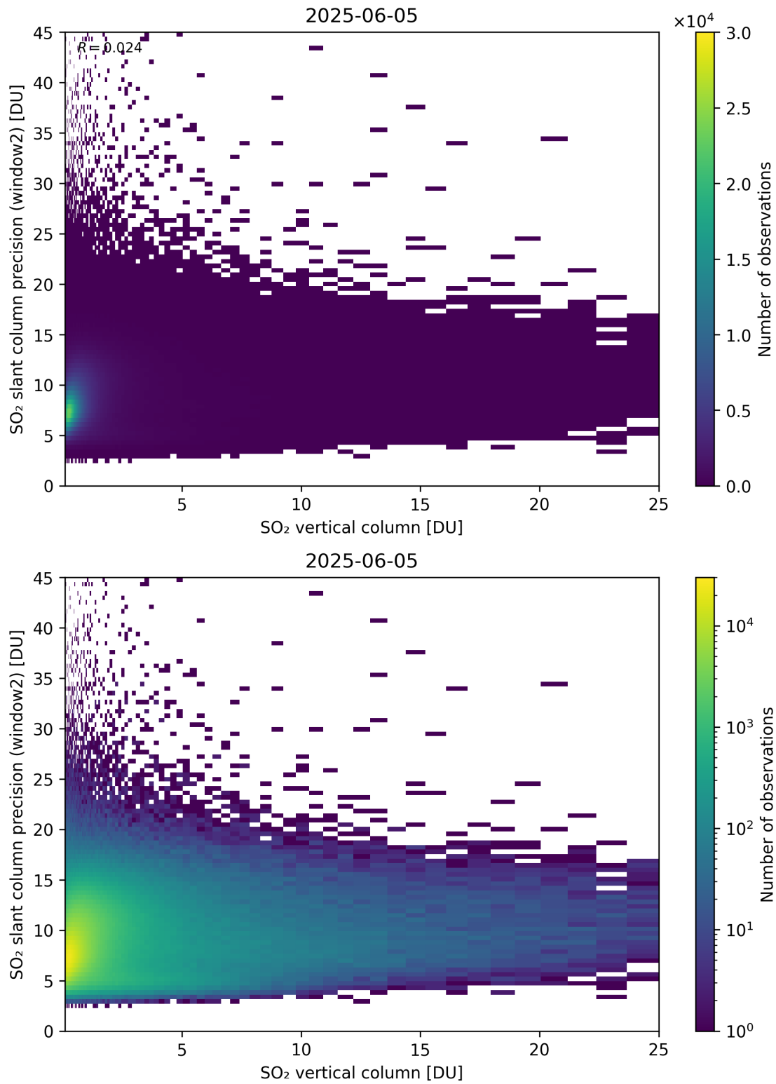
Figure 356: Scatter density plot of “SO 2 vertical column” against “SO 2 slant column precision (window2)” for 2025-06-04 to 2025-06-06.
