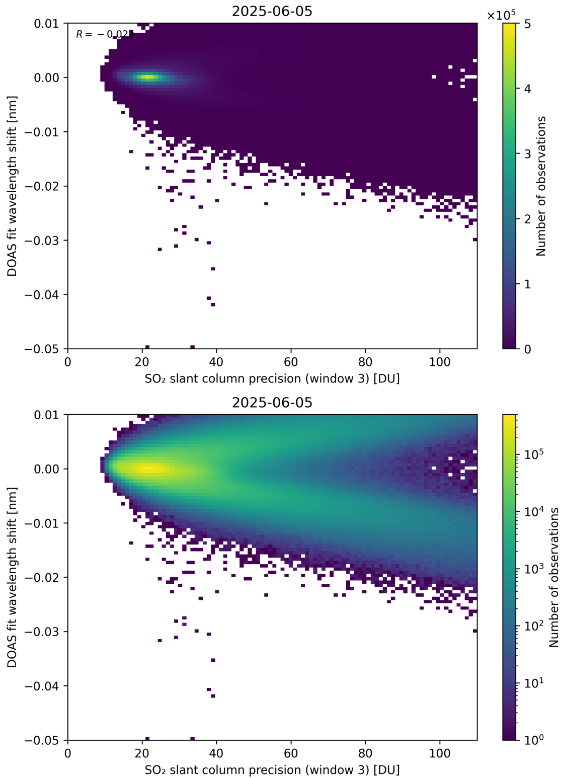
Figure 308: Scatter density plot of “SO 2 slant column precision (window 3)” against “DOAS fit wavelength shift” for 2025-06-04 to 2025-06-06.
