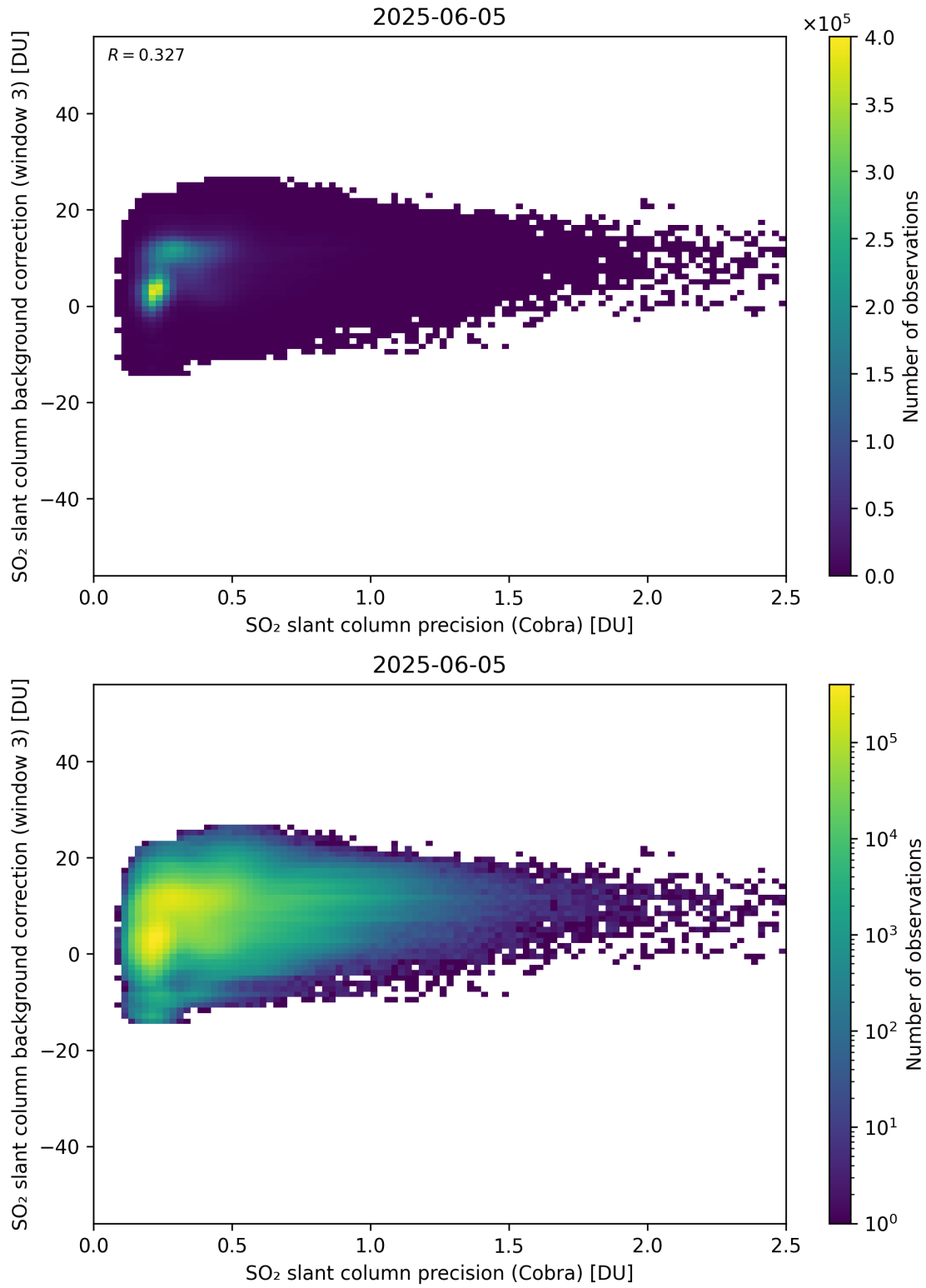
Figure 201: Scatter density plot of “SO 2 slant column precision (Cobra)” against “SO 2 slant column background correction (window 3)” for 2025-06-04 to 2025-06-06.
