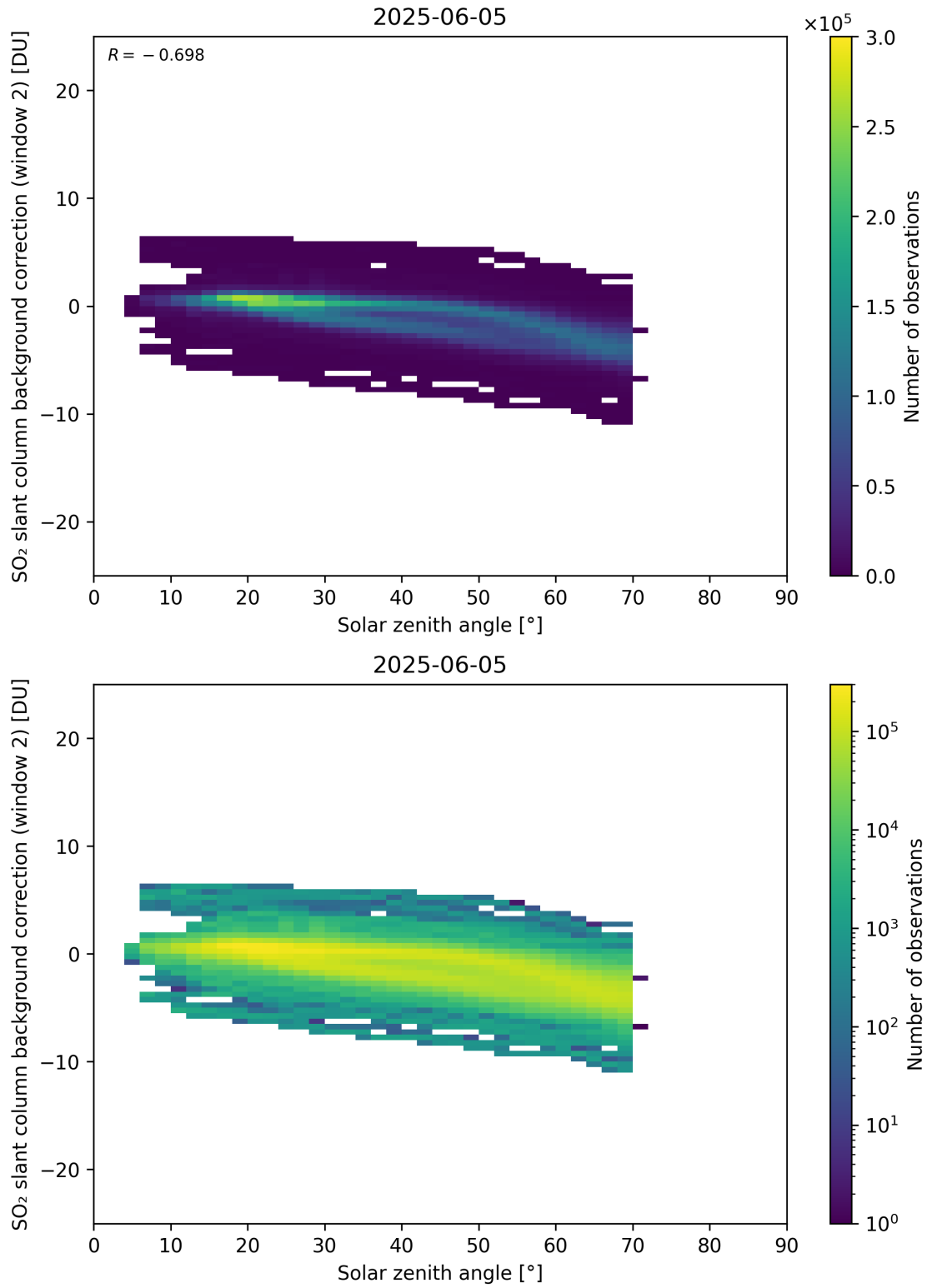
Figure 172: Scatter density plot of “Solar zenith angle” against “SO 2 slant column background correction (window 2)” for 2025-06-04 to 2025-06-06.
