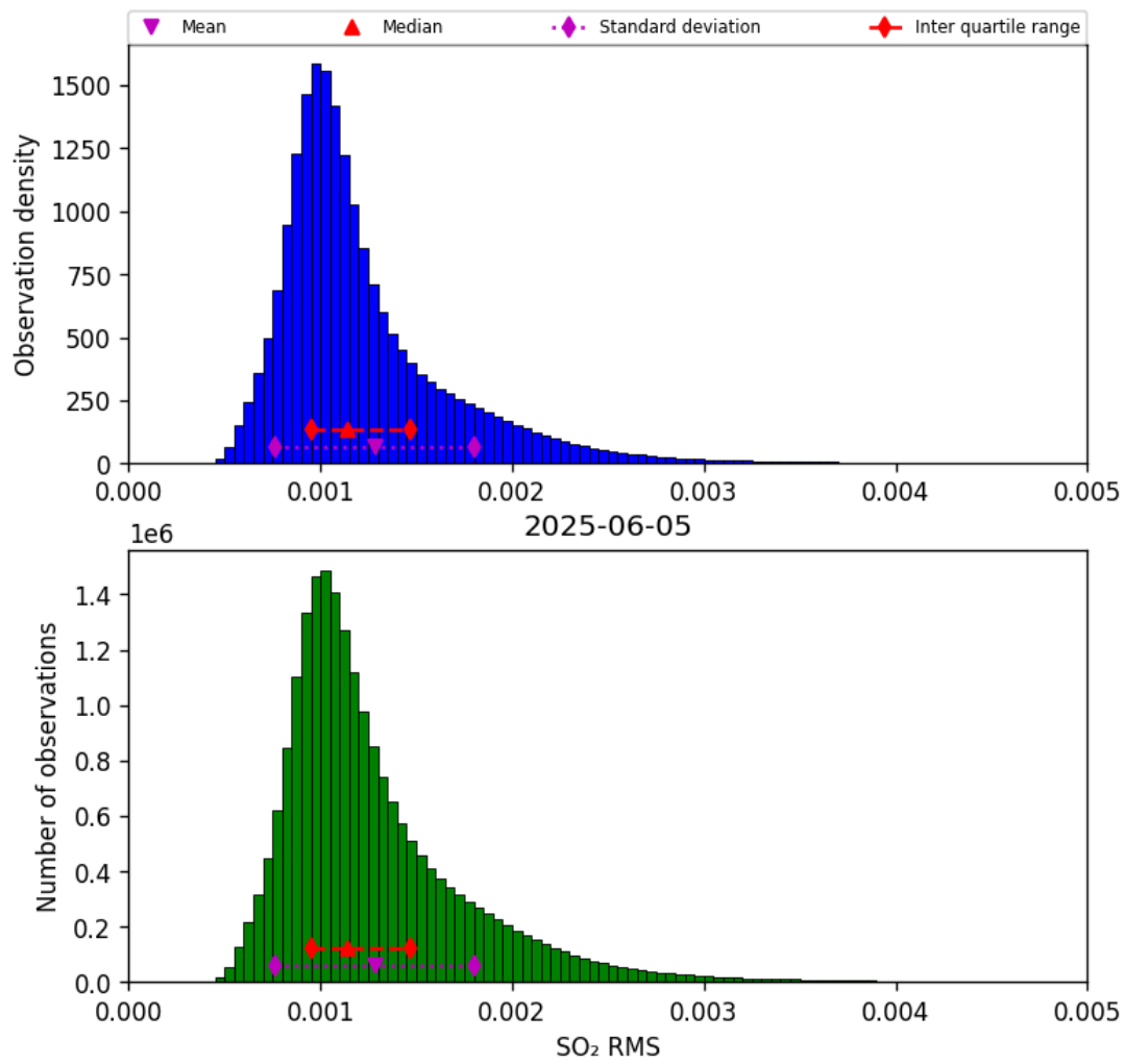
Figure 78: Histogram of “SO 2 RMS” for 2025-06-04 to 2025-06-06
