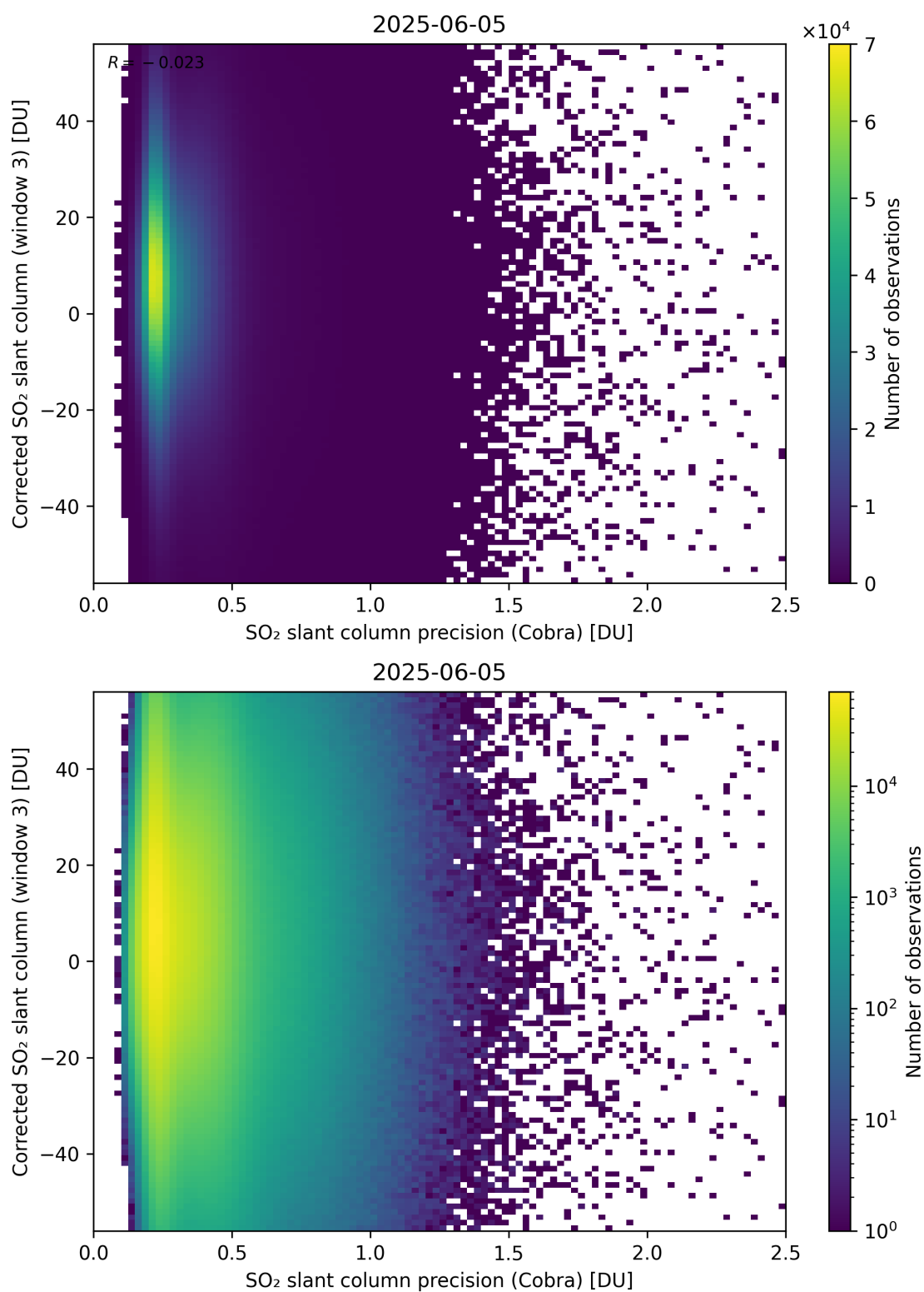
Figure 207: Scatter density plot of “SO 2 slant column precision (Cobra)” against “Corrected SO 2 slant column (window 3)” for 2025-06-04 to 2025-06-06.
