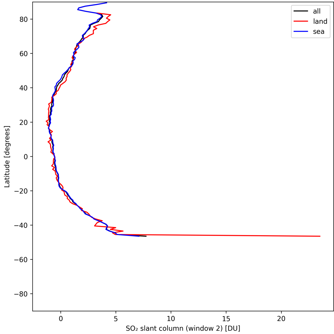
Figure 41: Zonal average of “SO 2 slant column (window 2)” for 2025-06-04 to 2025-06-06.
