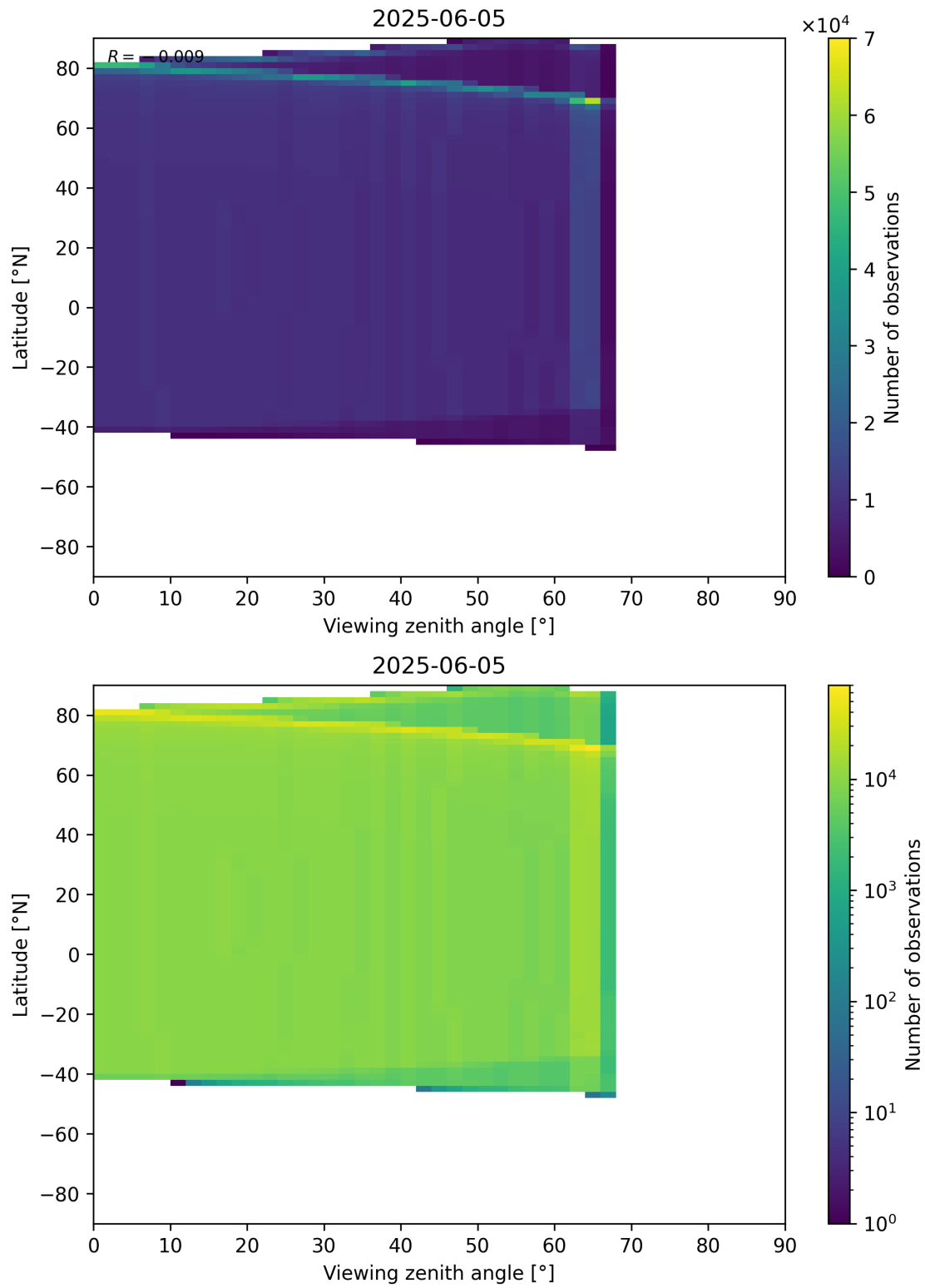
Figure 368: Scatter density plot of “Viewing zenith angle” against “Latitude” for 2025-06-04 to 2025-06-06.
