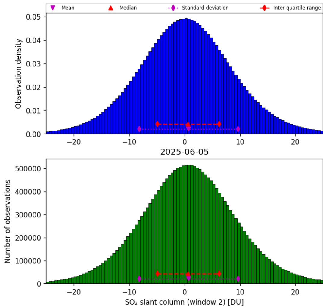
Figure 67: Histogram of “SO 2 slant column (window 2)” for 2025-06-04 to 2025-06-06
