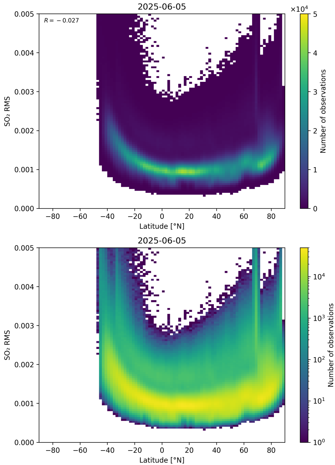
Figure 155: Scatter density plot of “Latitude” against “SO 2 RMS” for 2025-06-04 to 2025-06-06.
