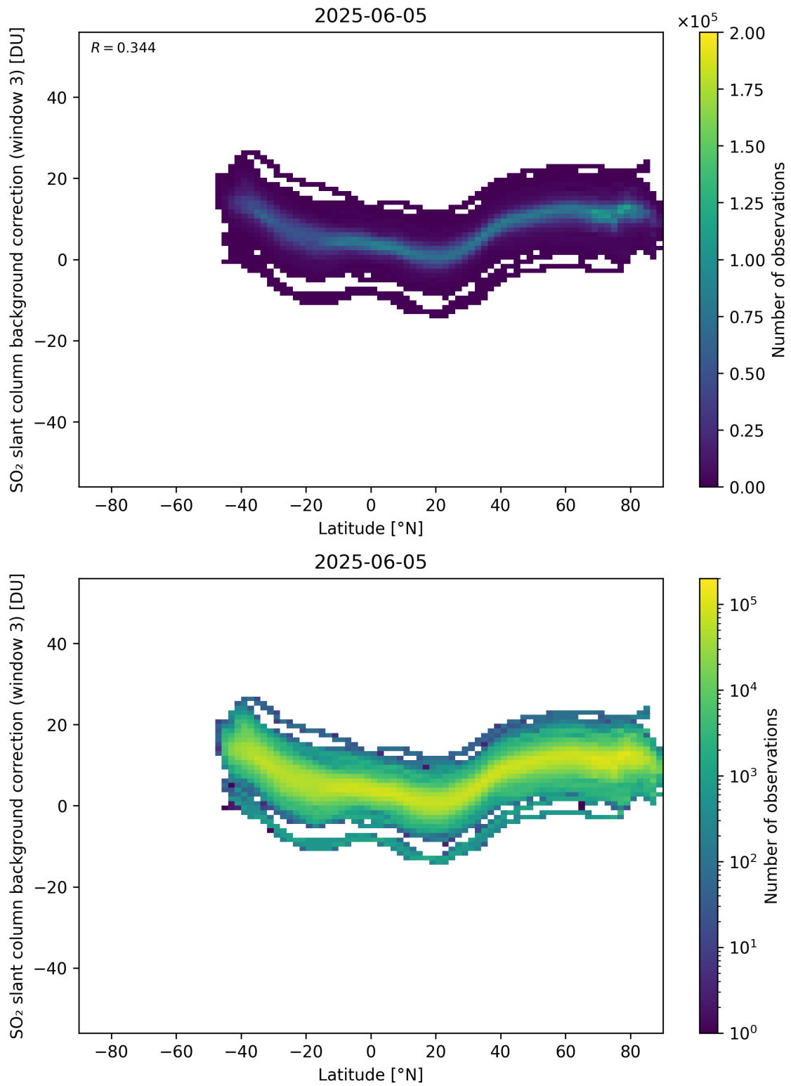
Figure 152: Scatter density plot of “Latitude” against “SO 2 slant column background correction (window 3)” for 2025-06-04 to 2025-06-06.
