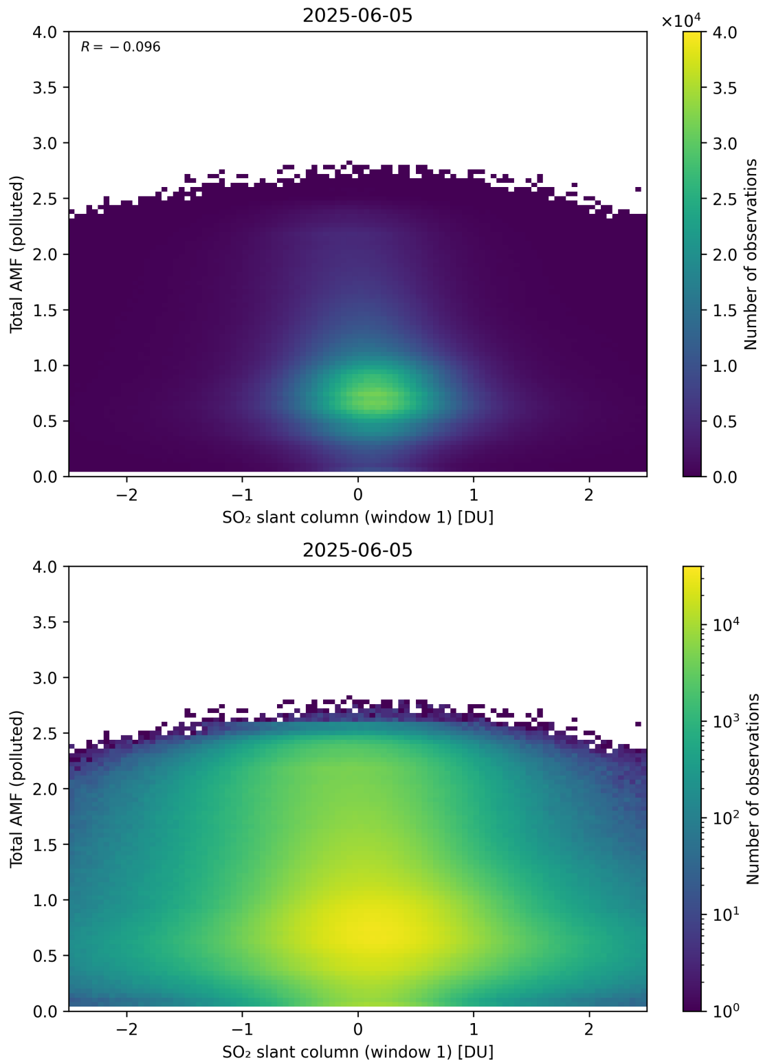
Figure 289: Scatter density plot of “SO 2 slant column (window 1)” against “Total AMF (polluted)” for 2025-06-04 to 2025-06-06.
