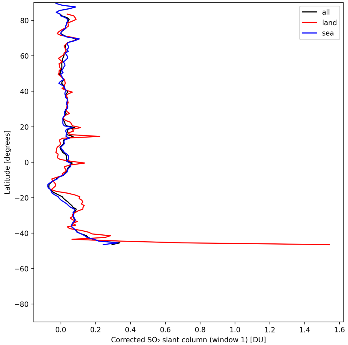
Figure 39: Zonal average of “Corrected SO 2 slant column (window 1)” for 2025-06-04 to 2025-06-06.
