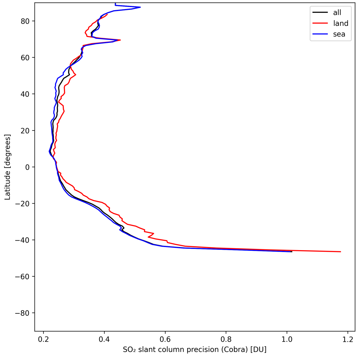
Figure 36: Zonal average of “SO 2 slant column precision (Cobra)” for 2025-06-04 to 2025-06-06.
