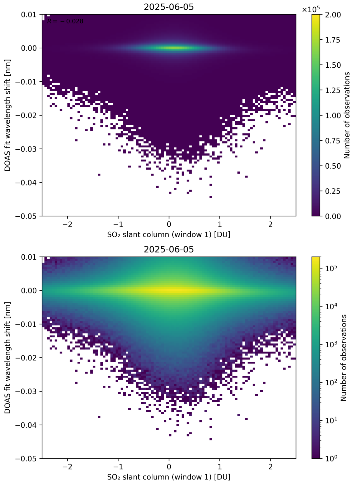
Figure 265: Scatter density plot of “SO 2 slant column (window 1)” against “DOAS fit wavelength shift” for 2025-06-04 to 2025-06-06.
