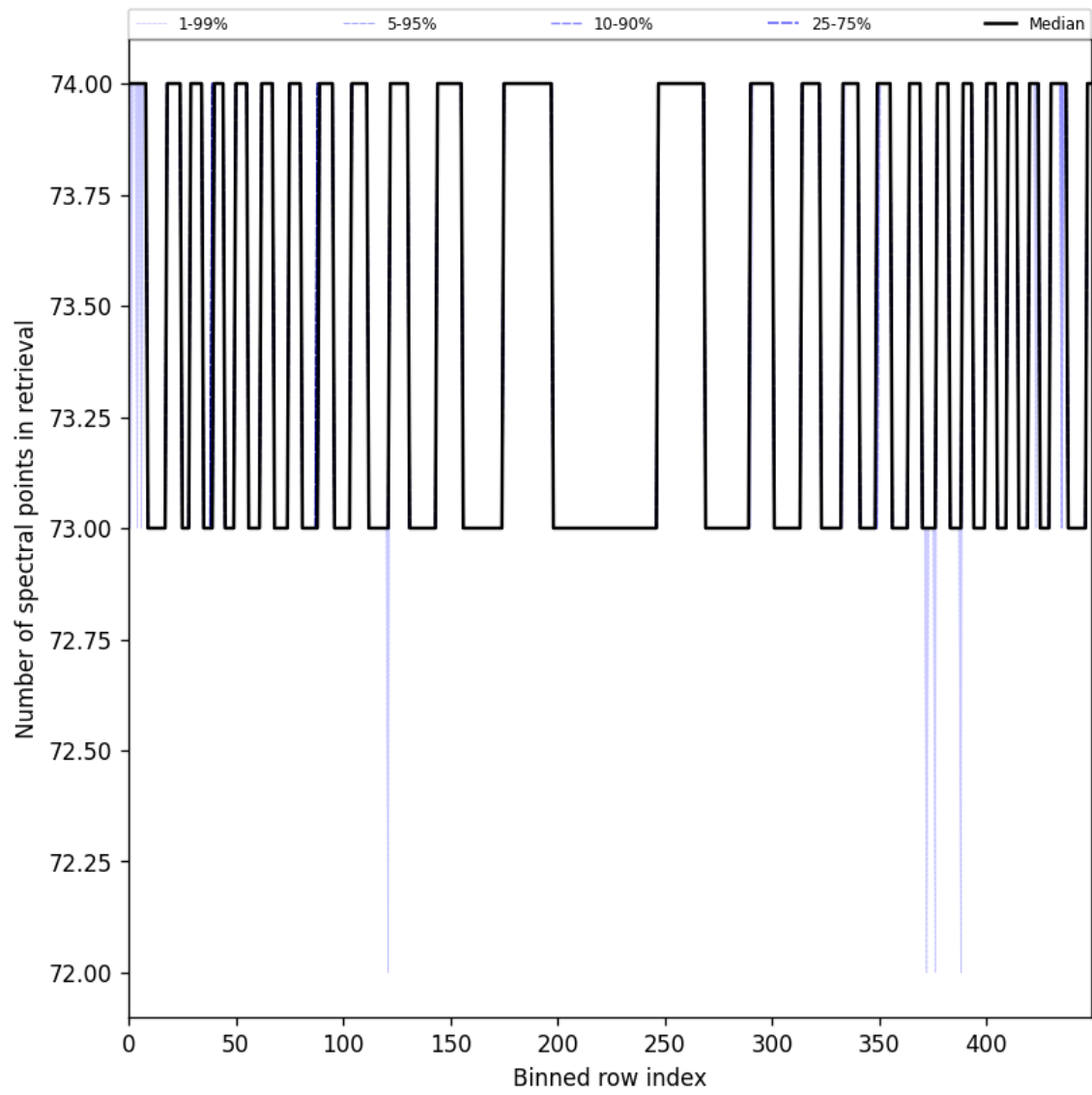
Figure 108: Along track statistics of “Number of spectral points in retrieval” for 2025-06-04 to 2025-06-06
