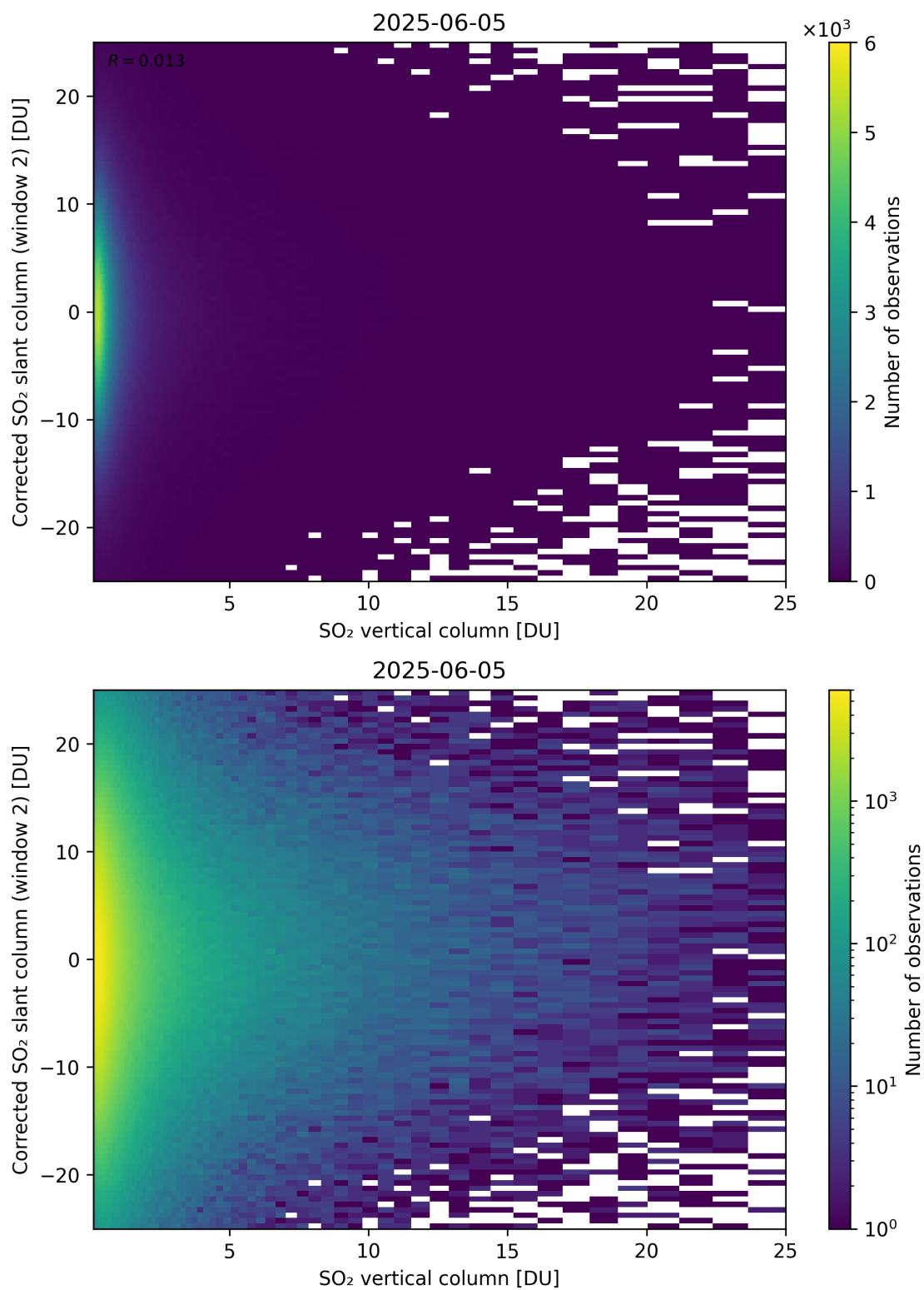
Figure 352: Scatter density plot of “SO 2 vertical column” against “Corrected SO 2 slant column (window 2)” for 2025-06-04 to 2025-06-06.
