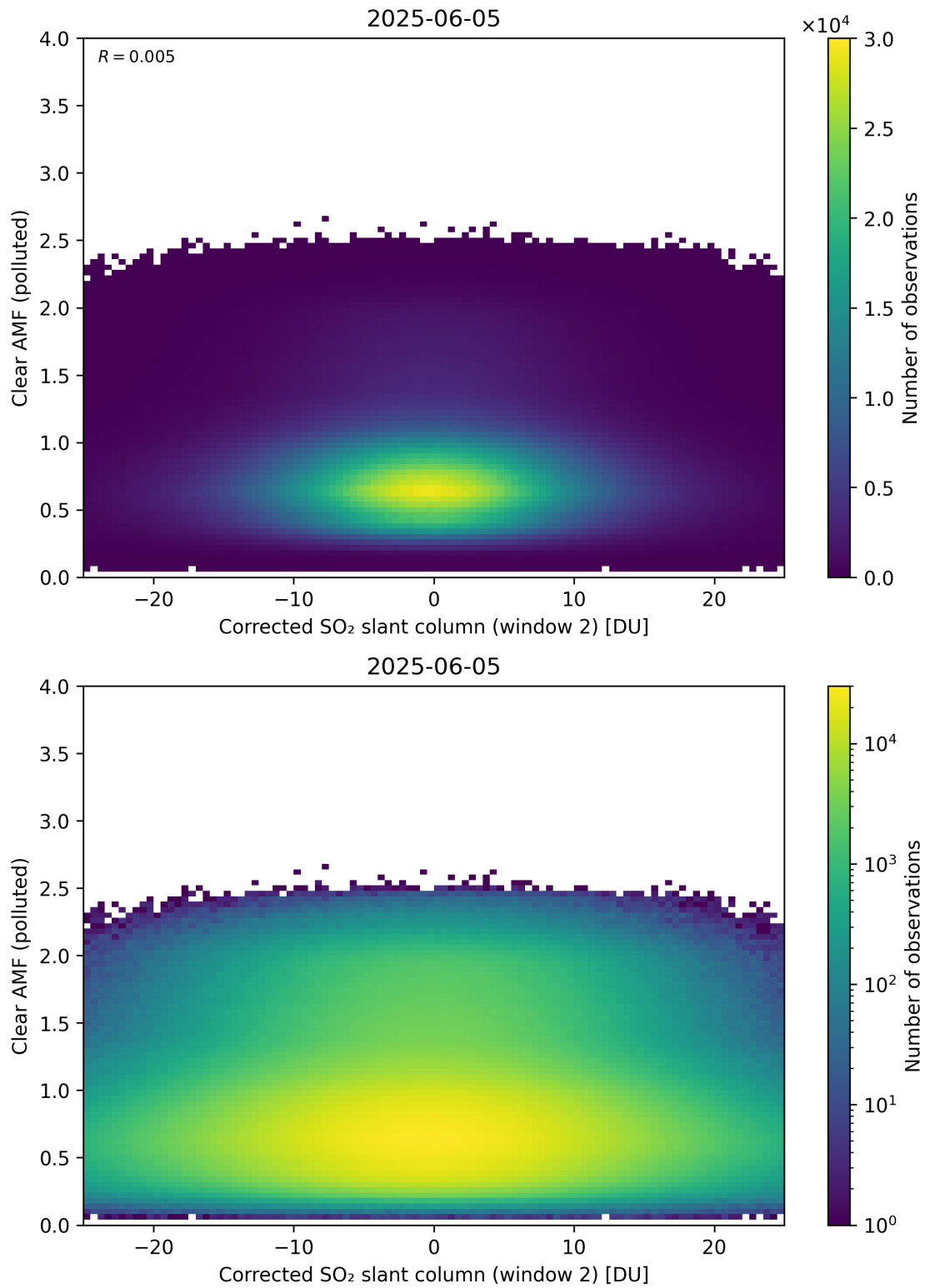
Figure 249: Scatter density plot of “Corrected SO 2 slant column (window 2)” against “Clear AMF (polluted)” for 2025-06-04 to 2025-06-06.
