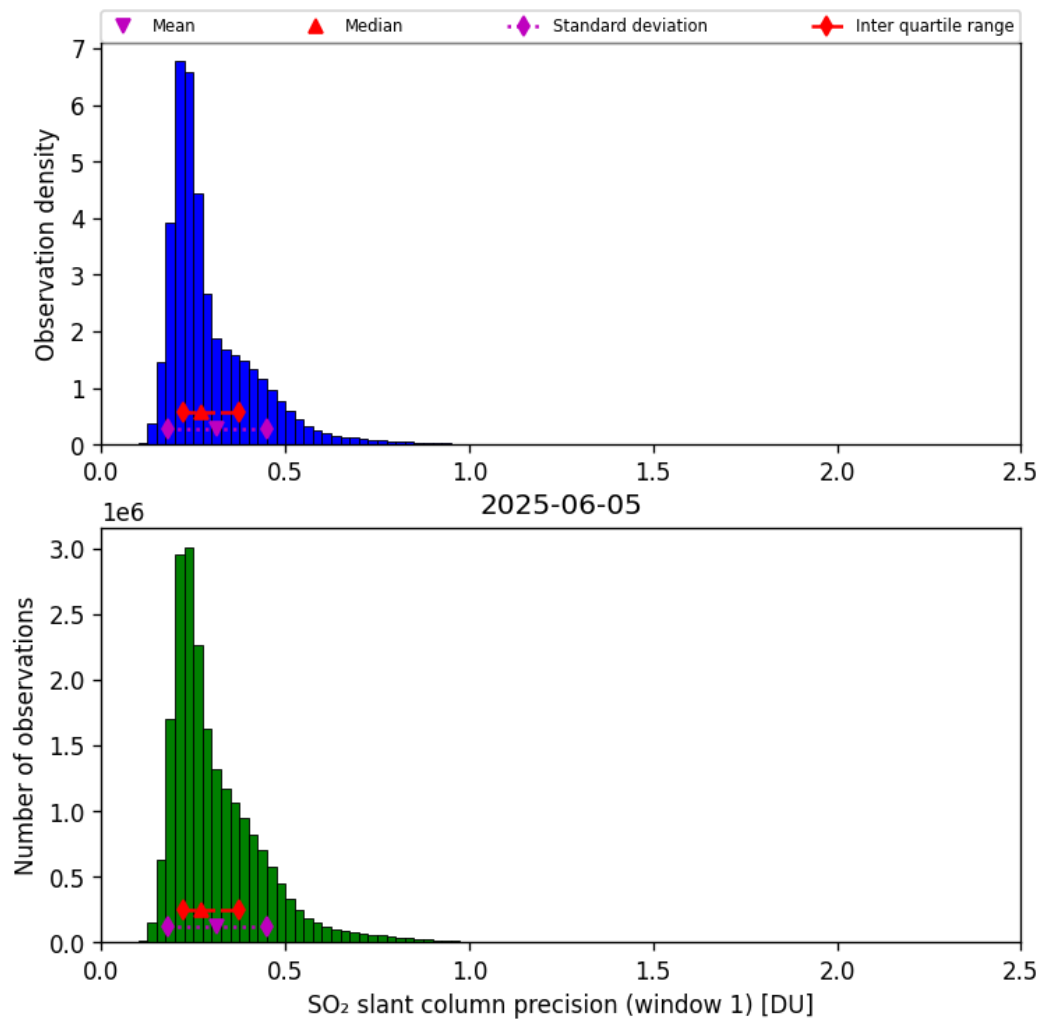
Figure 64: Histogram of “SO 2 slant column precision (window 1)” for 2025-06-04 to 2025-06-06
