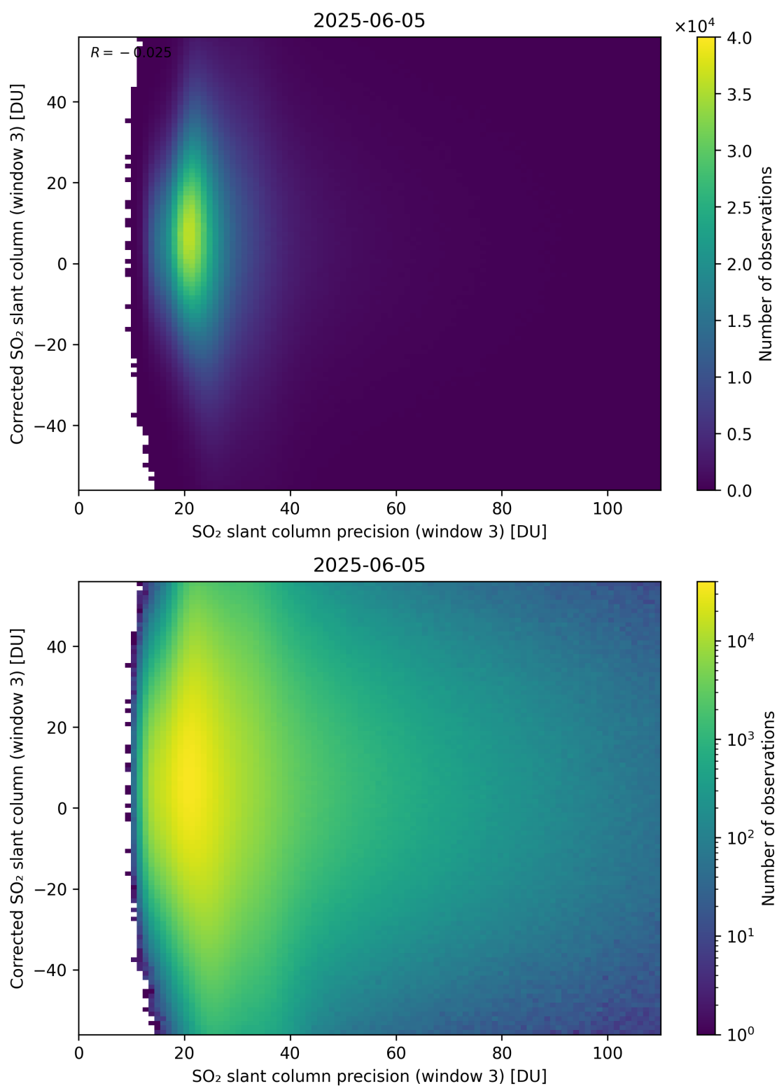
Figure 312: Scatter density plot of “SO 2 slant column precision (window 3)” against “Corrected SO 2 slant column (window 3)” for 2025-06-04 to 2025-06-06.
