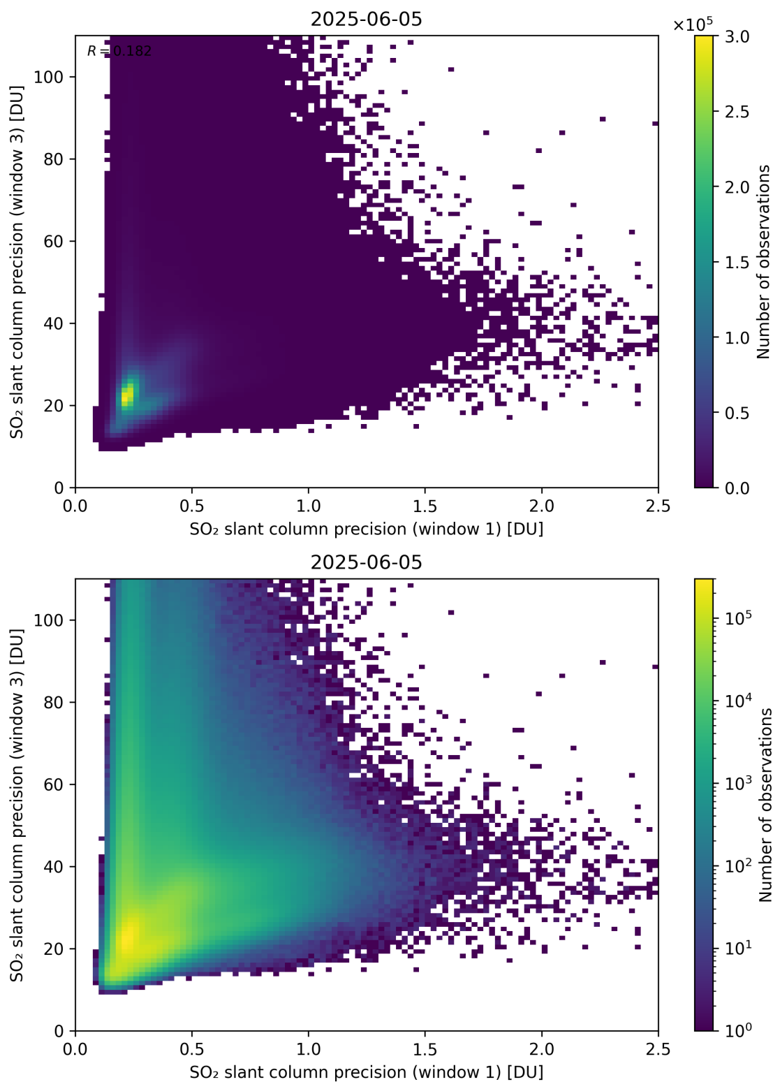
Figure 279: Scatter density plot of “SO 2 slant column precision (window 1)” against “SO 2 slant column precision (window 3)” for 2025-06-04 to 2025-06-06.
