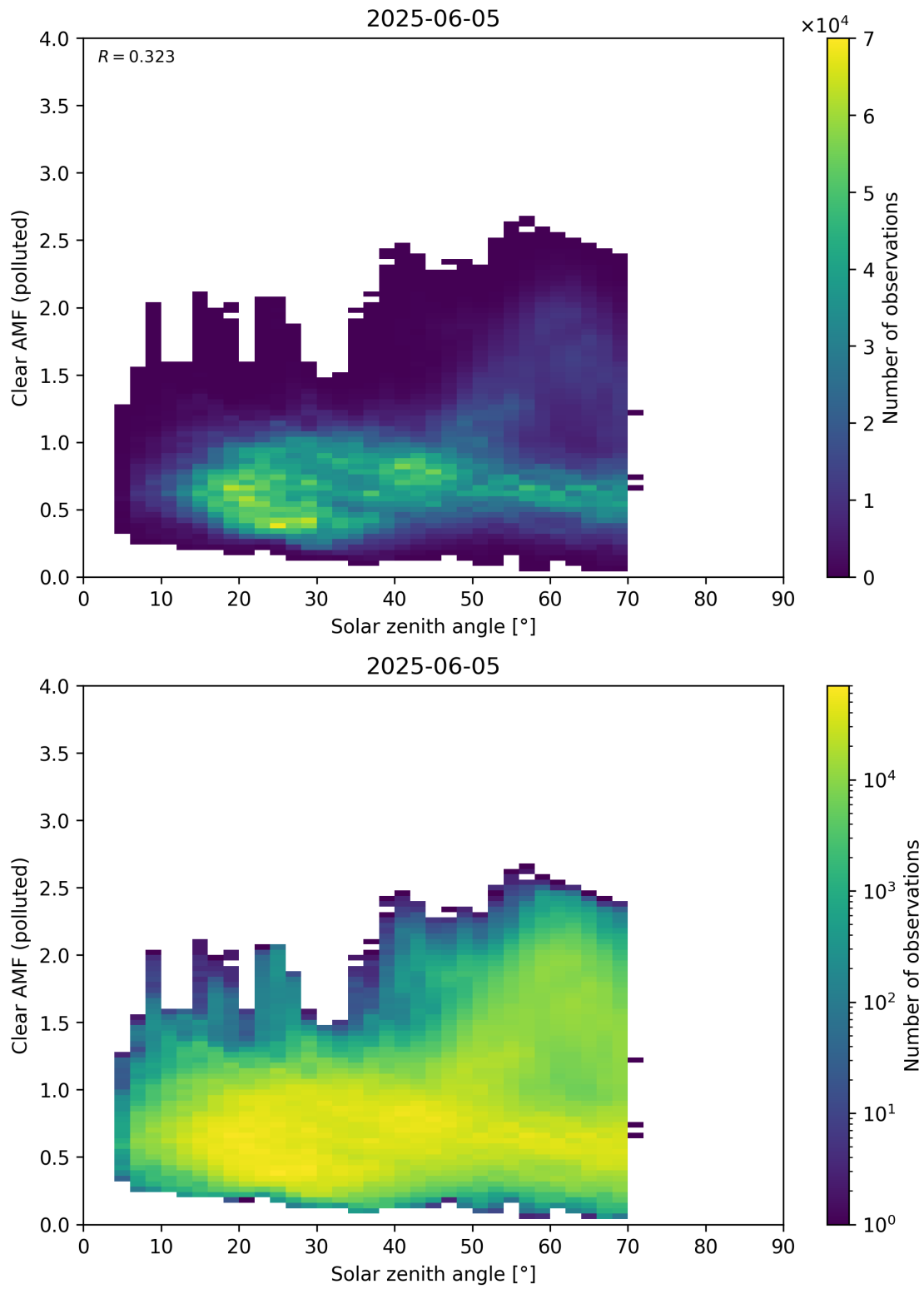
Figure 178: Scatter density plot of “Solar zenith angle” against “Clear AMF (polluted)” for 2025-06-04 to 2025-06-06.
