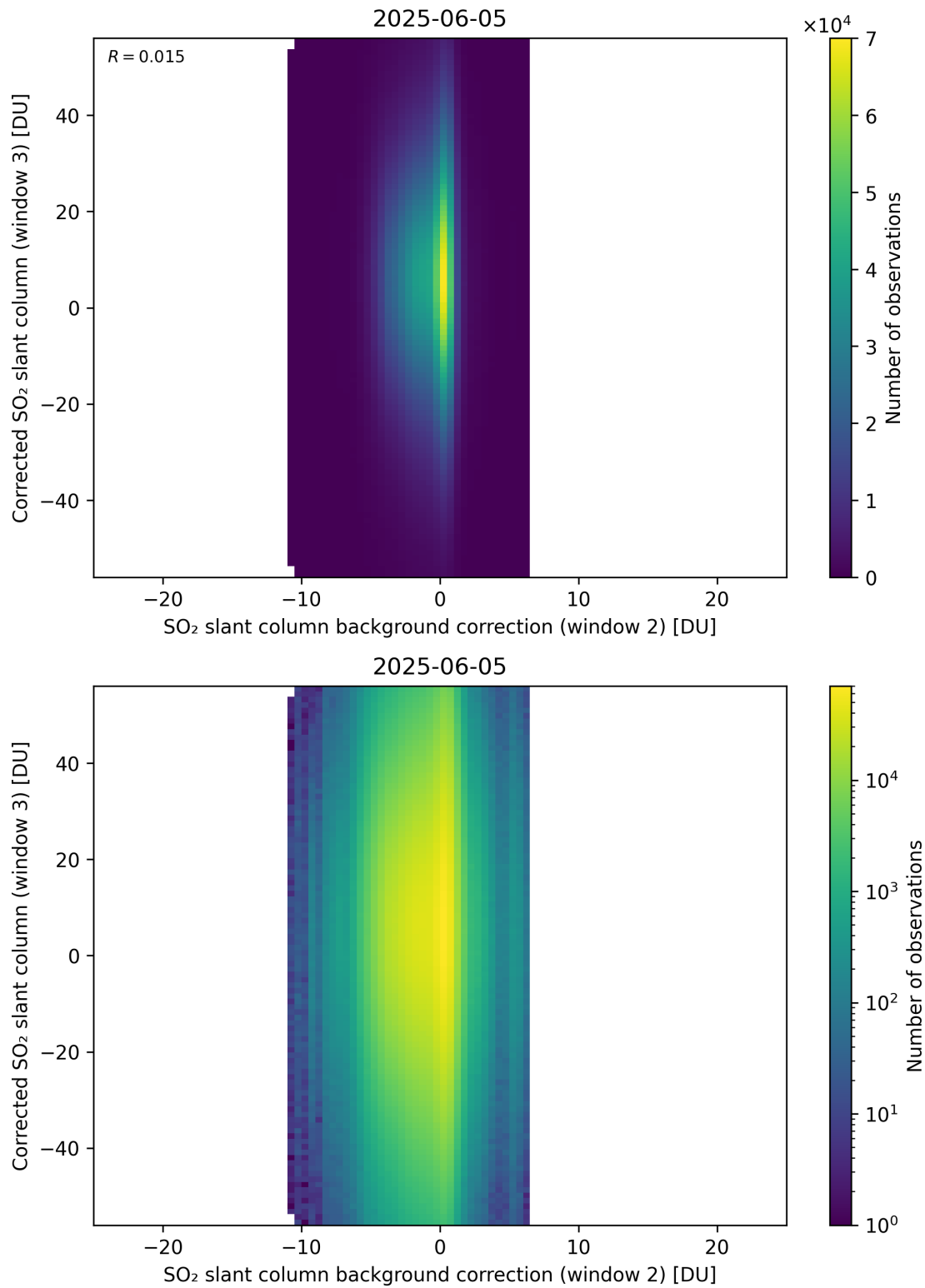
Figure 127: Scatter density plot of “SO 2 slant column background correction (window 2)” against “Corrected SO 2 slant column (window 3)” for 2025-06-04 to 2025-06-06.
