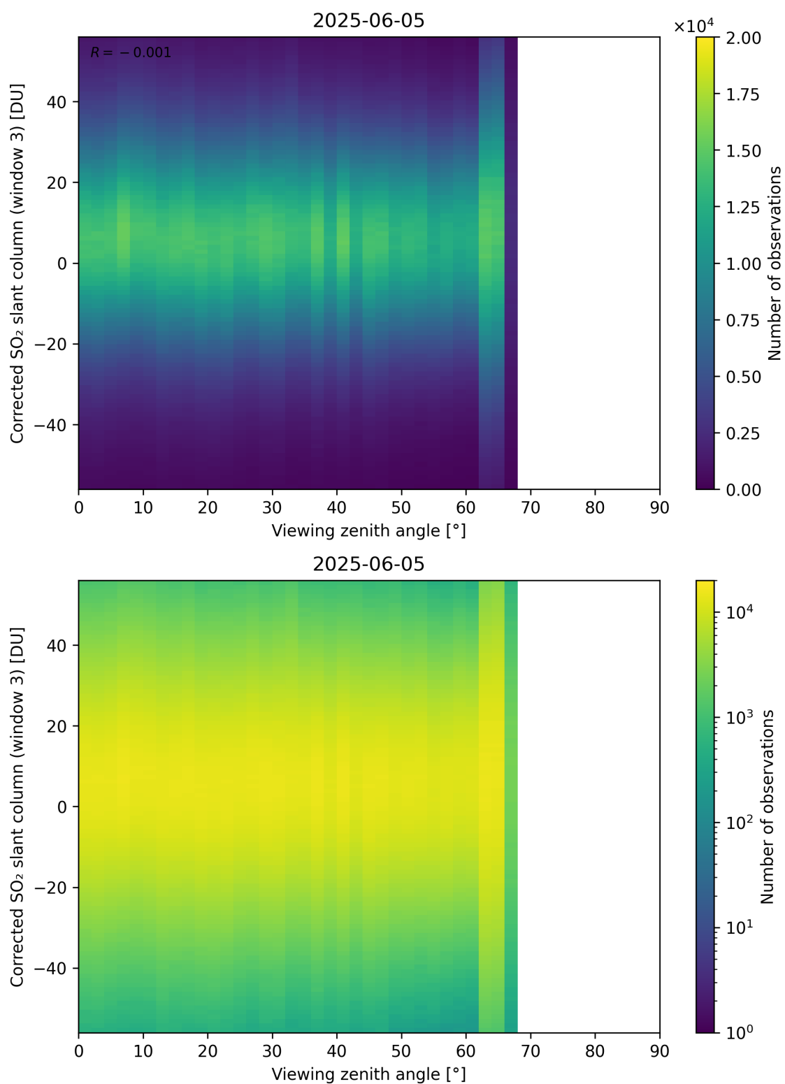
Figure 375: Scatter density plot of “Viewing zenith angle” against “Corrected SO 2 slant column (window 3)” for 2025-06-04 to 2025-06-06.
