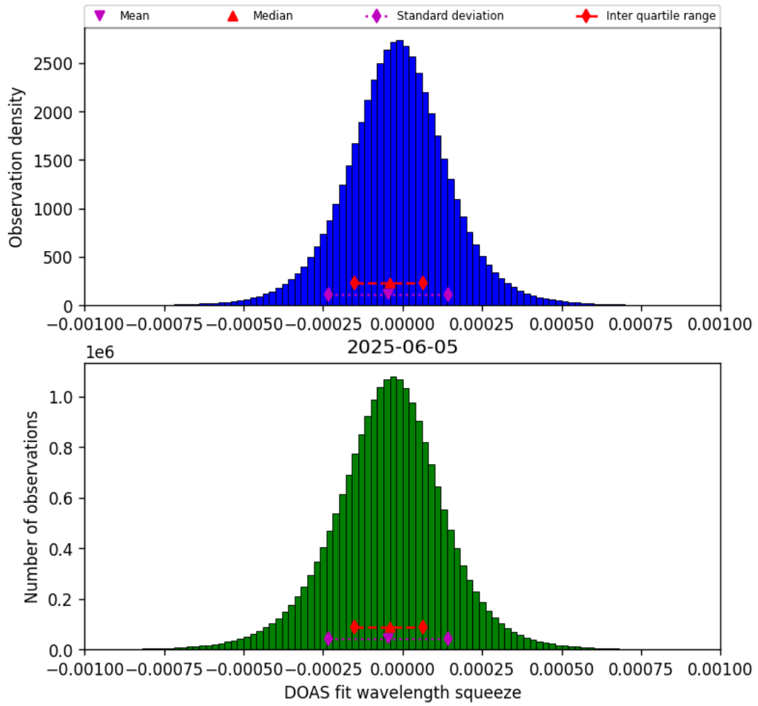
Figure 77: Histogram of “DOAS fit wavelength squeeze” for 2025-06-04 to 2025-06-06
