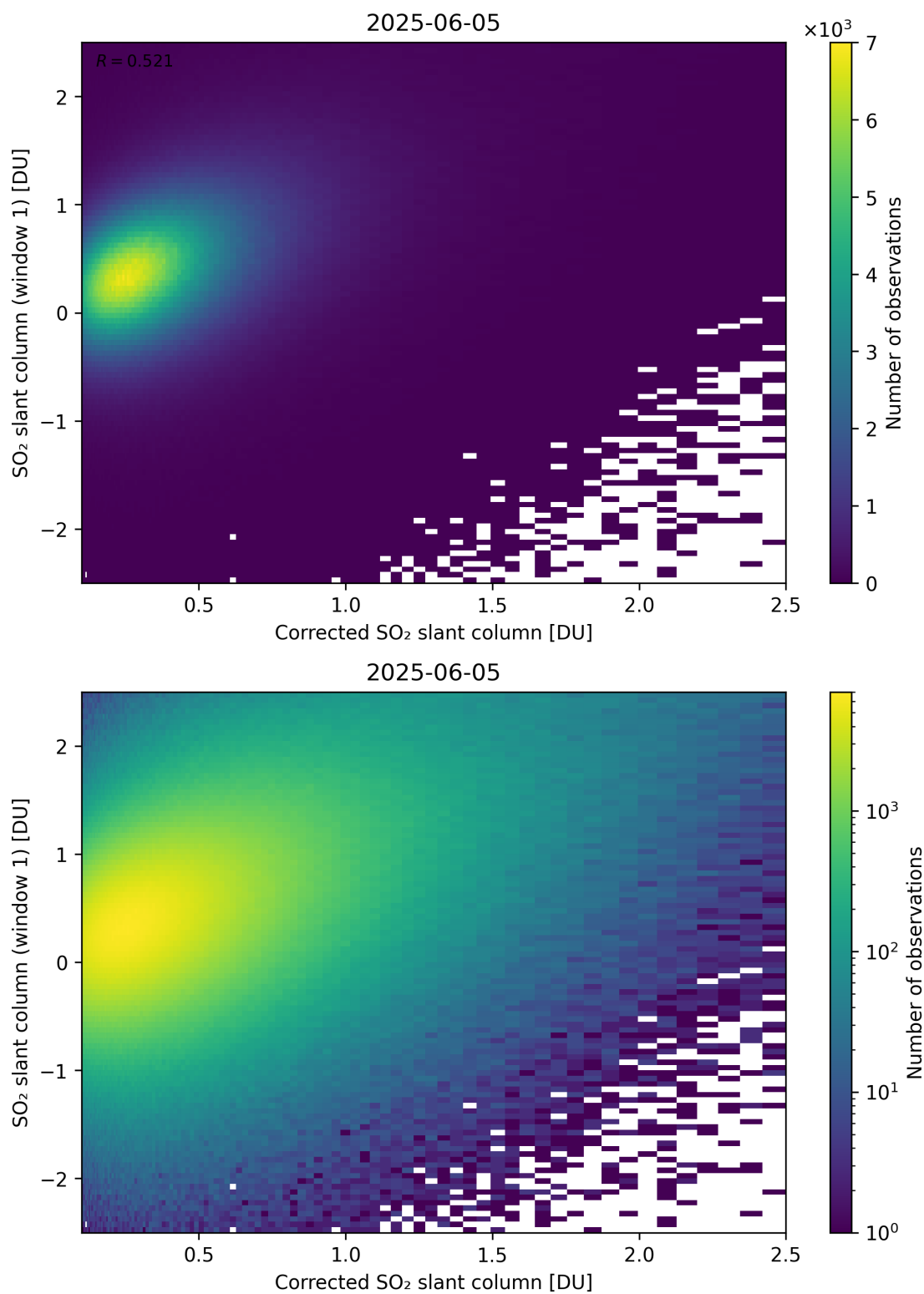
Figure 237: Scatter density plot of “Corrected SO 2 slant column” against “SO 2 slant column (window 1)” for 2025-06-04 to 2025-06-06.
