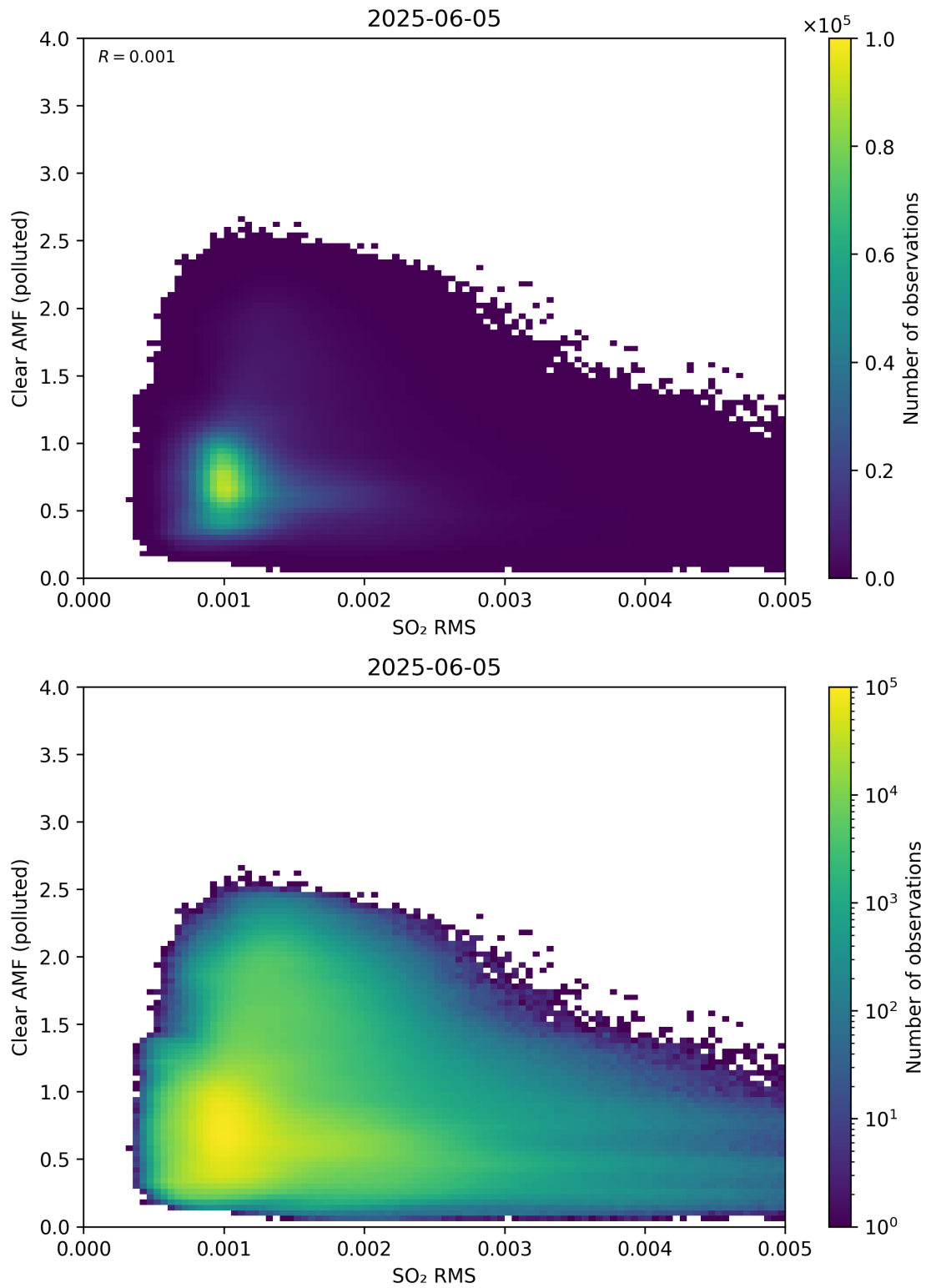
Figure 147: Scatter density plot of “SO 2 RMS” against “Clear AMF (polluted)” for 2025-06-04 to 2025-06-06.
