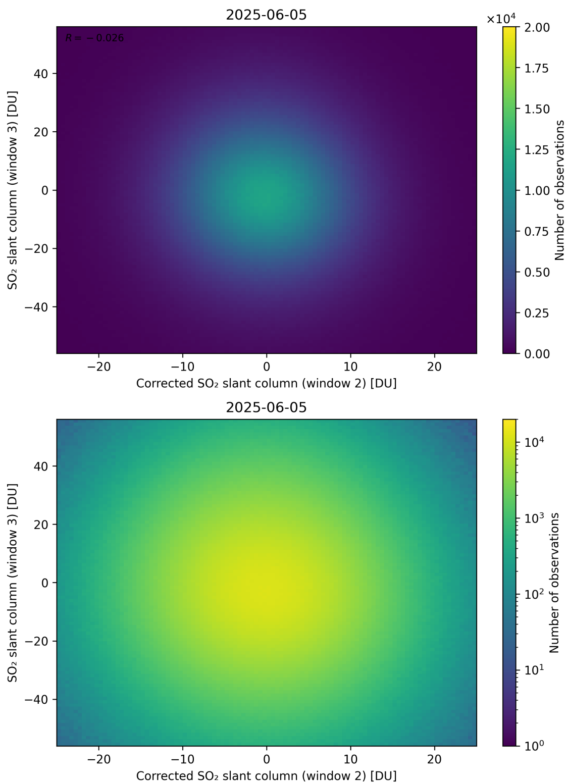
Figure 251: Scatter density plot of “Corrected SO 2 slant column (window 2)” against “SO 2 slant column (window 3)” for 2025-06-04 to 2025-06-06.
