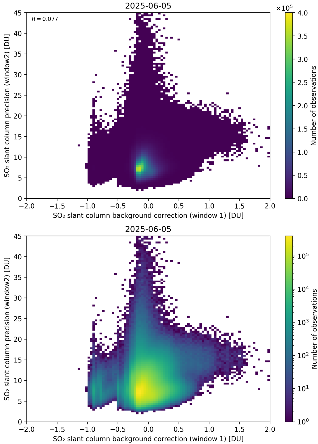
Figure 117: Scatter density plot of “SO 2 slant column background correction (window 1)” against “SO 2 slant column precision (window2)” for 2025-06-04 to 2025-06-06.
