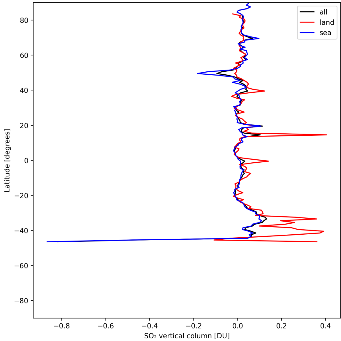
Figure 32: Zonal average of “SO 2 vertical column” for 2025-06-04 to 2025-06-06.
