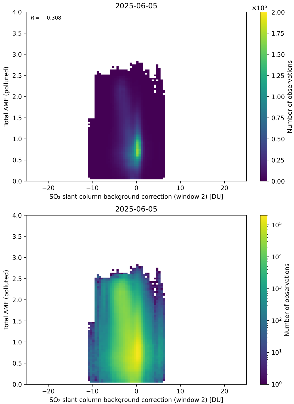
Figure 130: Scatter density plot of “SO 2 slant column background correction (window 2)” against “Total AMF (polluted)” for 2025-06-04 to 2025-06-06.
