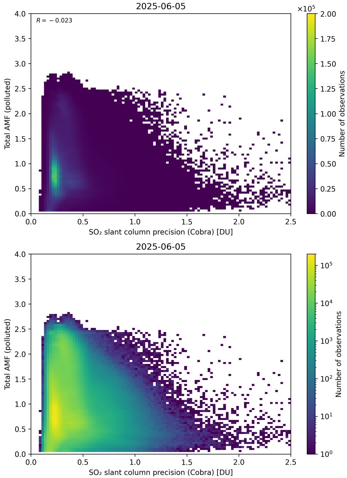
Figure 213: Scatter density plot of “SO 2 slant column precision (Cobra)” against “Total AMF (polluted)” for 2025-06-04 to 2025-06-06.
