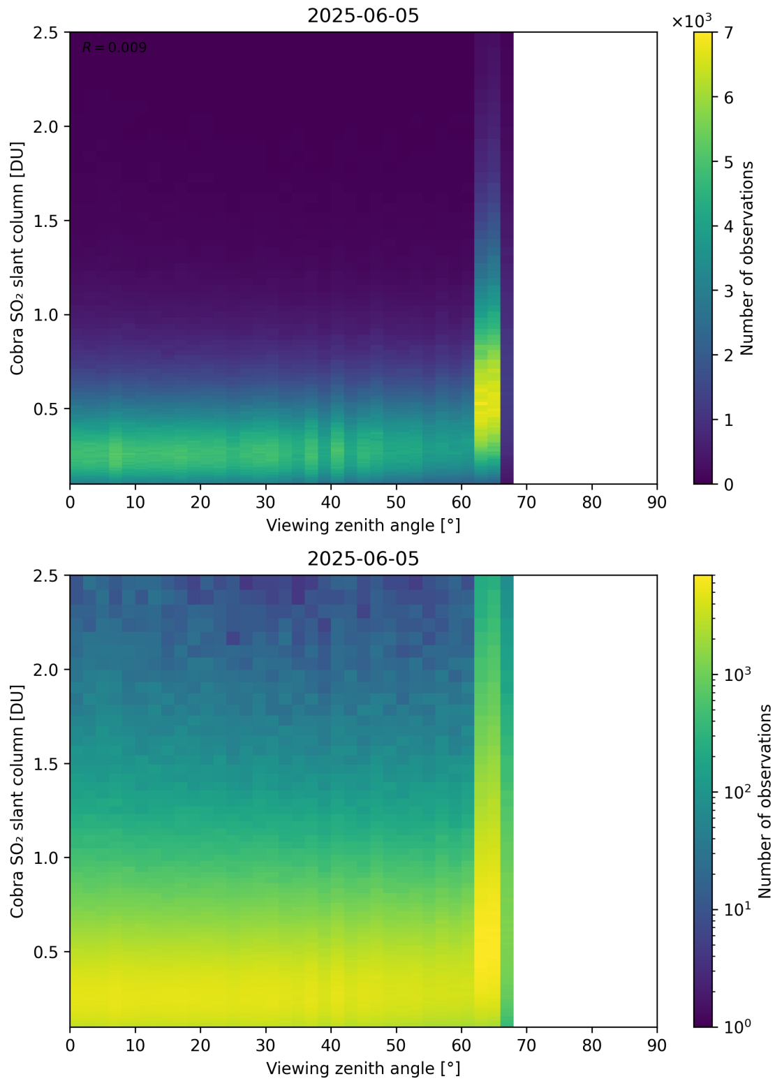
Figure 371: Scatter density plot of “Viewing zenith angle” against “Cobra SO 2 slant column” for 2025-06-04 to 2025-06-06.
