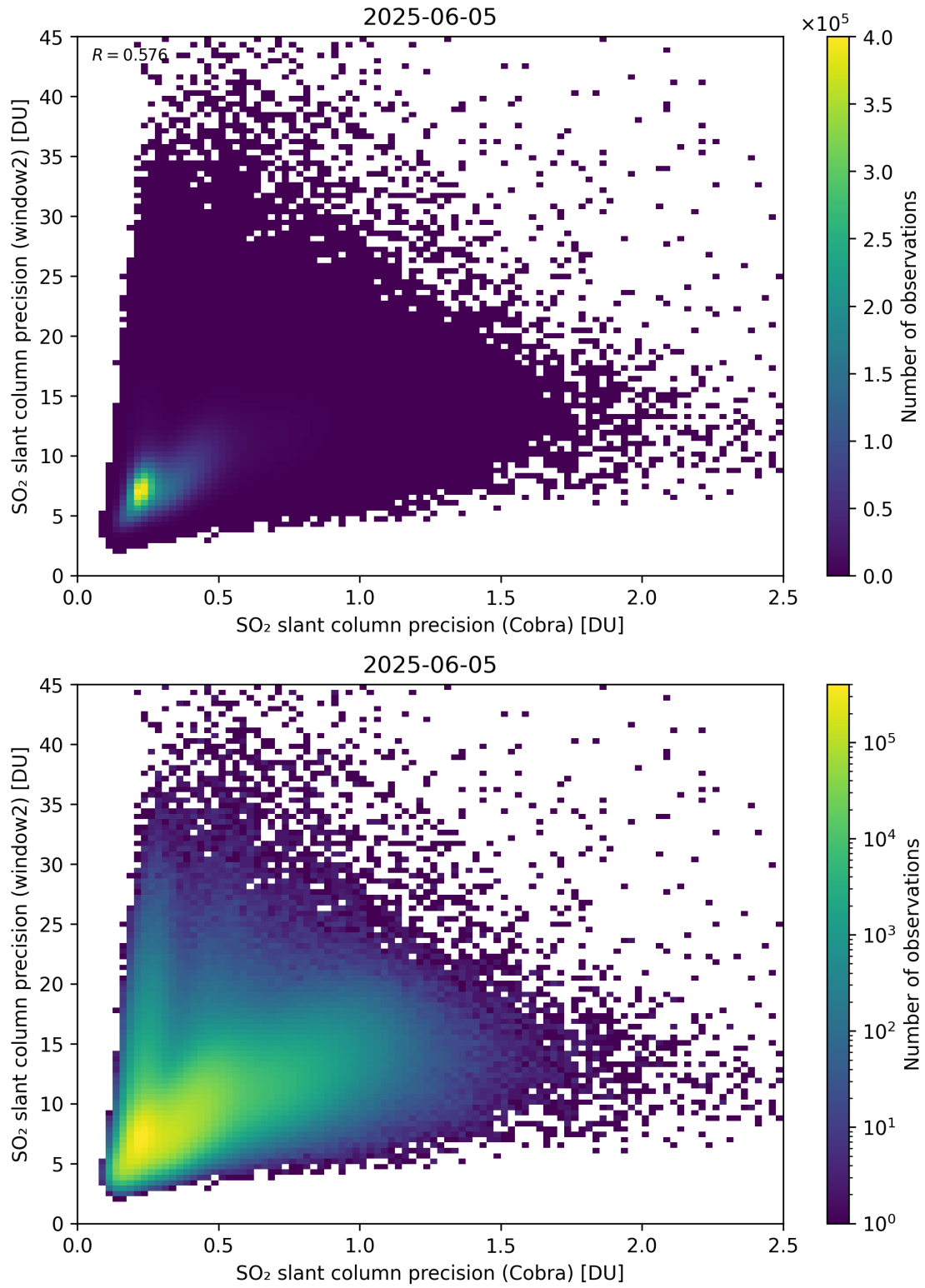
Figure 210: Scatter density plot of “SO 2 slant column precision (Cobra)” against “SO 2 slant column precision (window2)” for 2025-06-04 to 2025-06-06.
