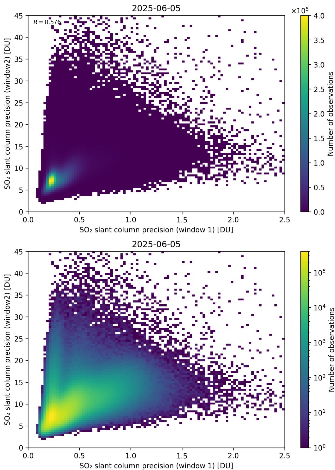
Figure 277: Scatter density plot of “SO 2 slant column precision (window 1)” against “SO 2 slant column precision (window2)” for 2025-06-04 to 2025-06-06.
