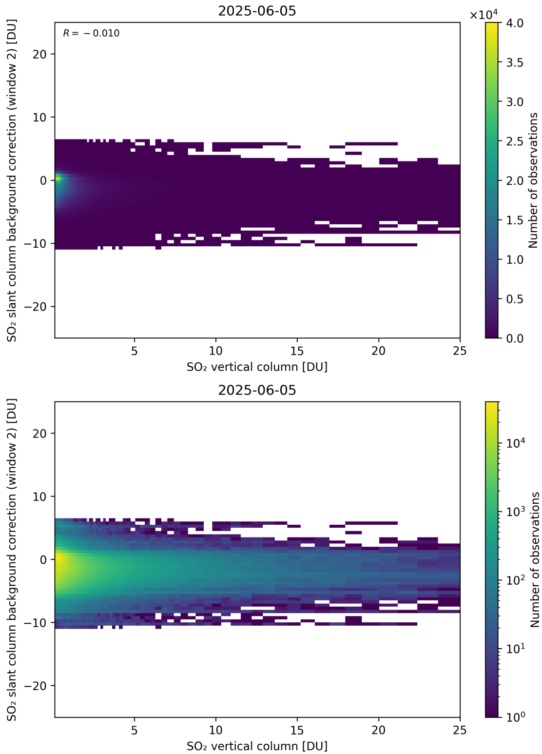
Figure 324: Scatter density plot of “SO 2 vertical column” against “SO 2 slant column background correction (window 2)” for 2025-06-04 to 2025-06-06.
