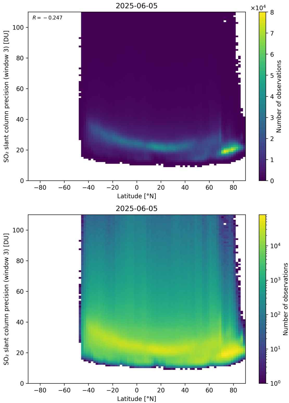
Figure 166: Scatter density plot of “Latitude” against “SO 2 slant column precision (window 3)” for 2025-06-04 to 2025-06-06.
