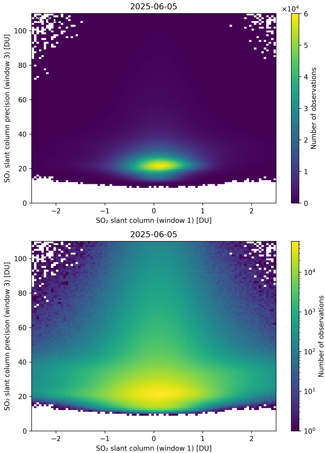
Figure 288: Scatter density plot of “SO 2 slant column (window 1)” against “SO 2 slant column precision (window 3)” for 2025-06-04 to 2025-06-06.
