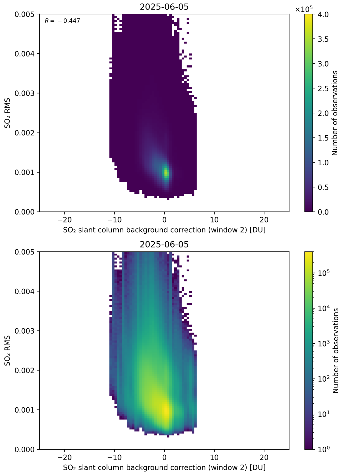
Figure 125: Scatter density plot of “SO 2 slant column background correction (window 2)” against “SO 2 RMS” for 2025-06-04 to 2025-06-06.
