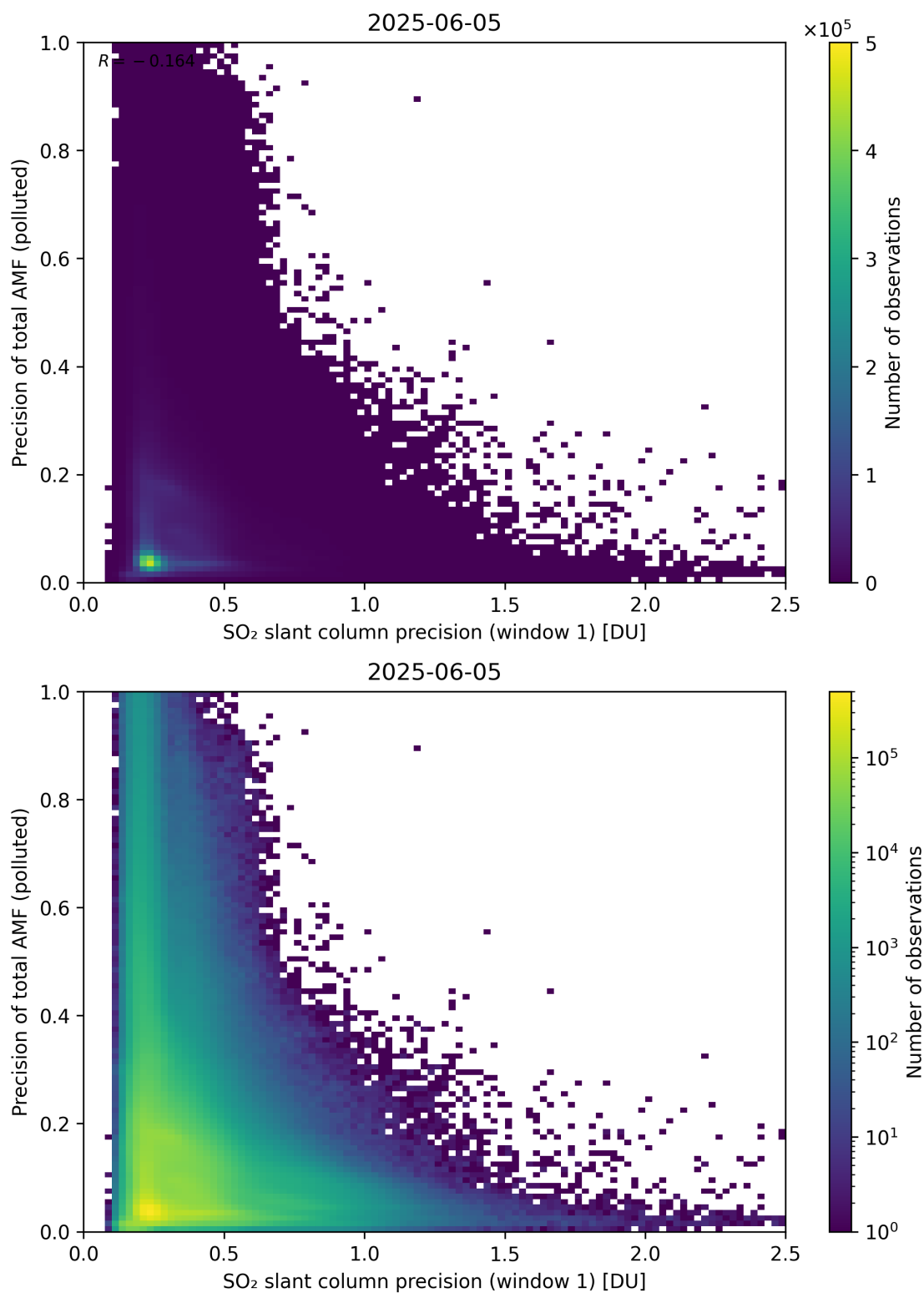
Figure 281: Scatter density plot of “SO 2 slant column precision (window 1)” against “Precision of total AMF (polluted)” for 2025-06-04 to 2025-06-06.
