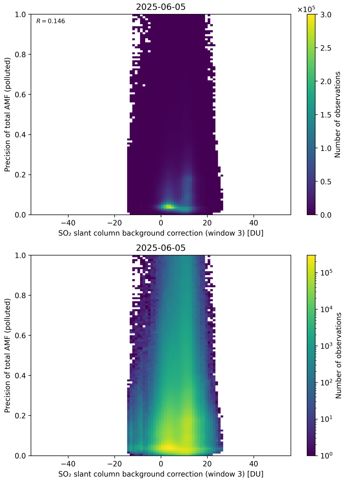
Figure 137: Scatter density plot of “SO 2 slant column background correction (window 3)” against “Precision of total AMF (polluted)” for 2025-06-04 to 2025-06-06.
