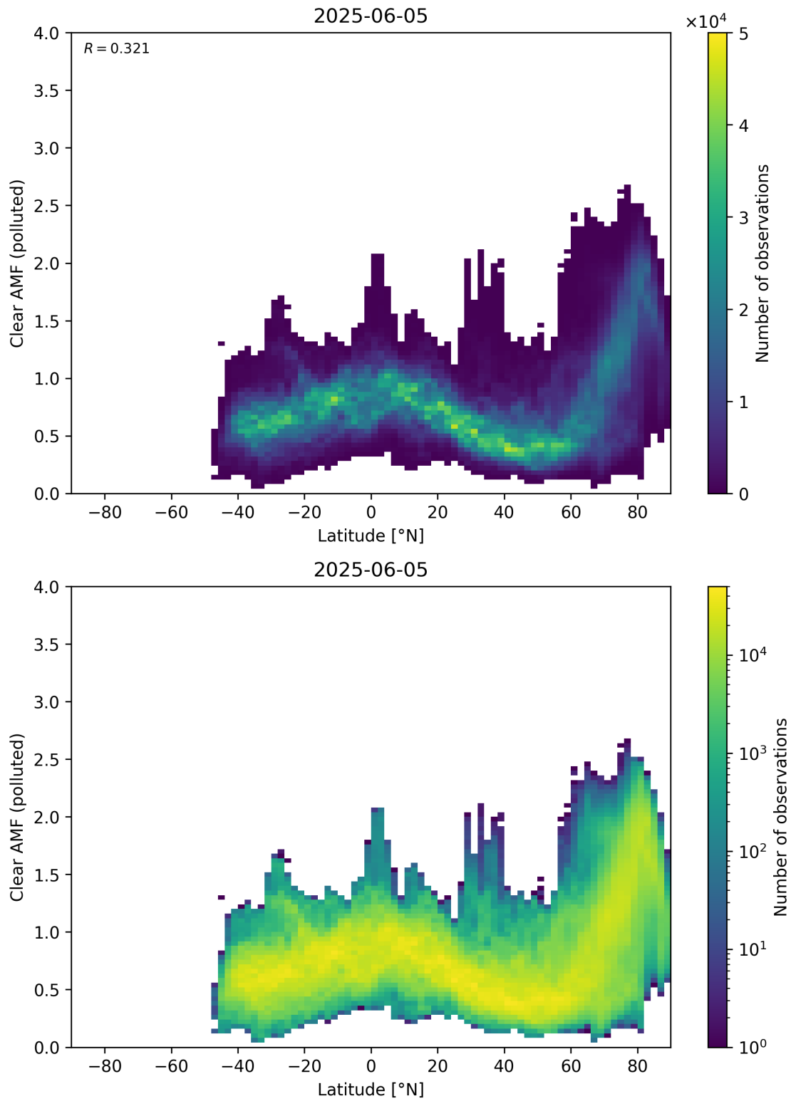
Figure 156: Scatter density plot of “Latitude” against “Clear AMF (polluted)” for 2025-06-04 to 2025-06-06.
