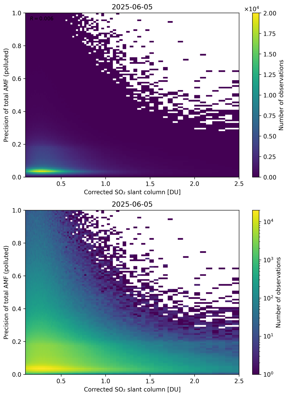
Figure 243: Scatter density plot of “Corrected SO 2 slant column” against “Precision of total AMF (polluted)” for 2025-06-04 to 2025-06-06.
