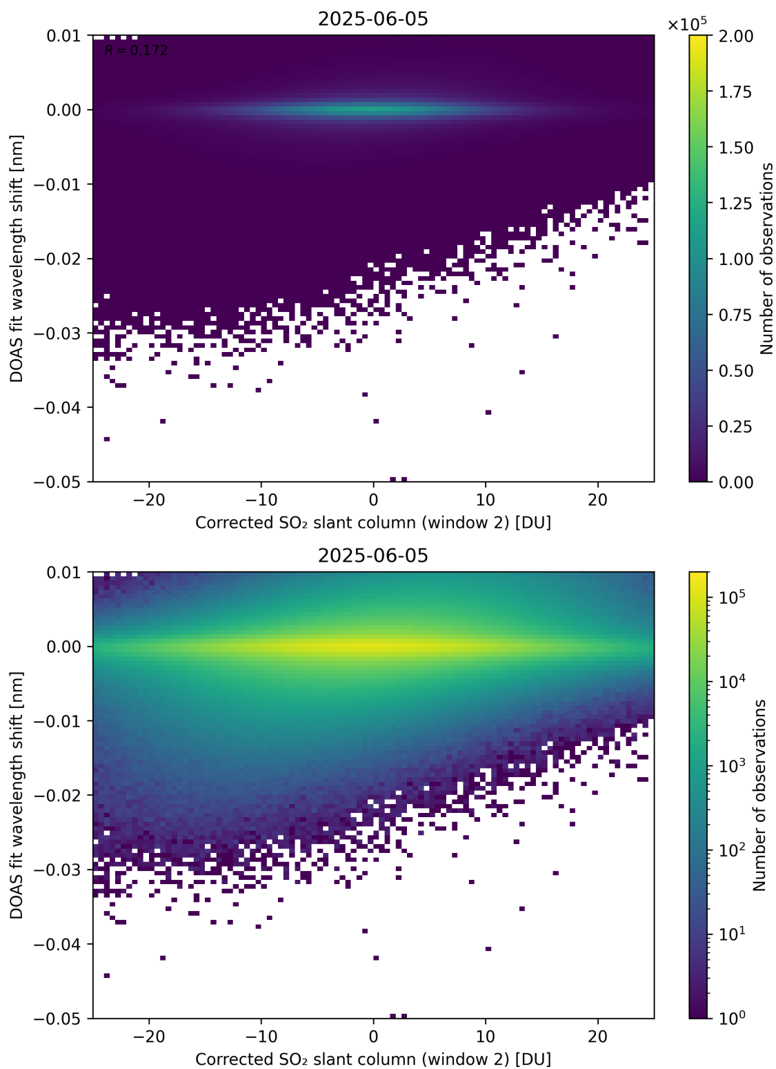
Figure 246: Scatter density plot of “Corrected SO 2 slant column (window 2)” against “DOAS fit wavelength shift” for 2025-06-04 to 2025-06-06.
