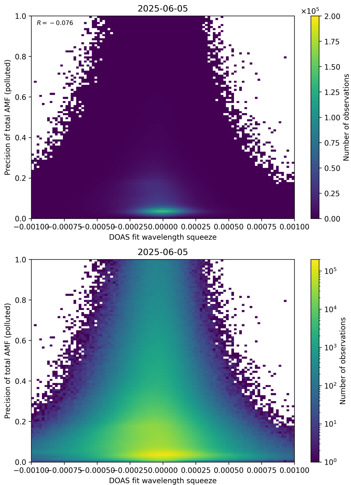
Figure 146: Scatter density plot of “DOAS fit wavelength squeeze” against “Precision of total AMF (polluted)” for 2025-06-04 to 2025-06-06.
