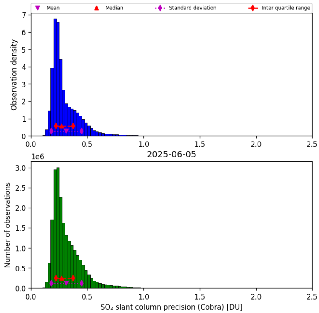
Figure 62: Histogram of “SO 2 slant column precision (Cobra)” for 2025-06-04 to 2025-06-06
