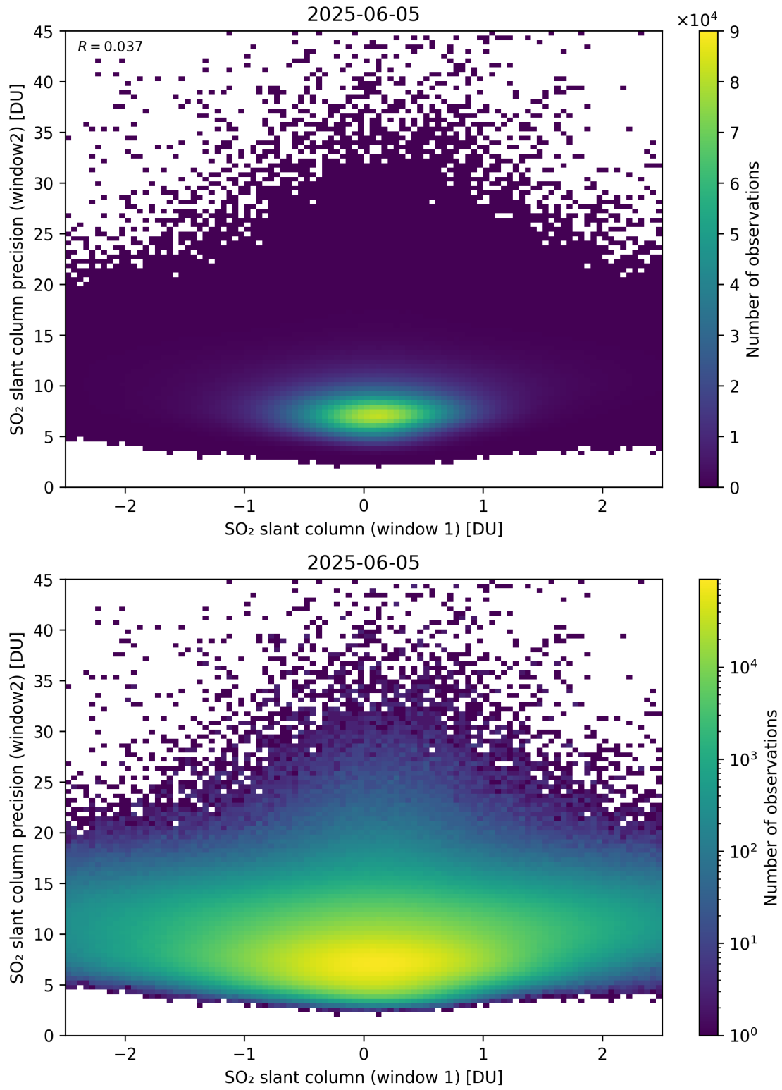
Figure 286: Scatter density plot of “SO 2 slant column (window 1)” against “SO 2 slant column precision (window2)” for 2025-06-04 to 2025-06-06.
