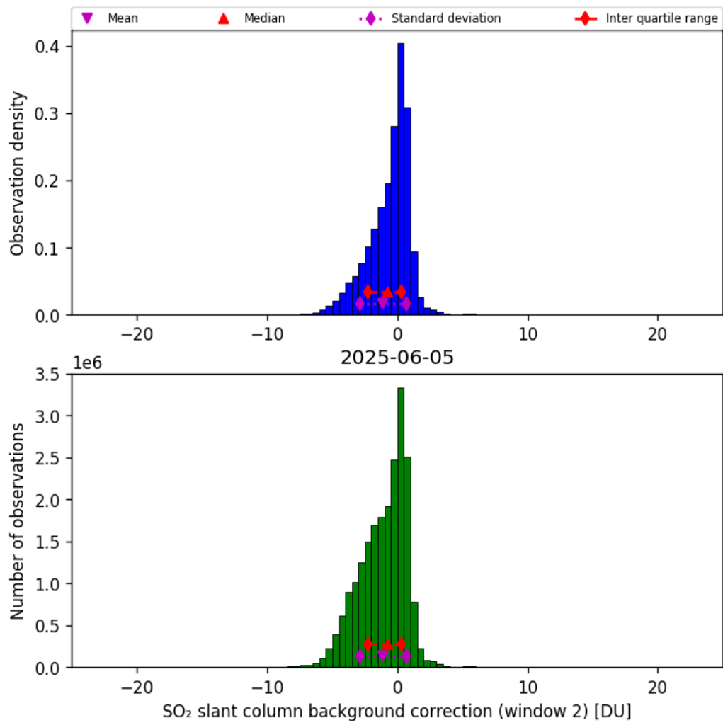
Figure 70: Histogram of “SO 2 slant column background correction (window 2)” for 2025-06-04 to 2025-06-06
