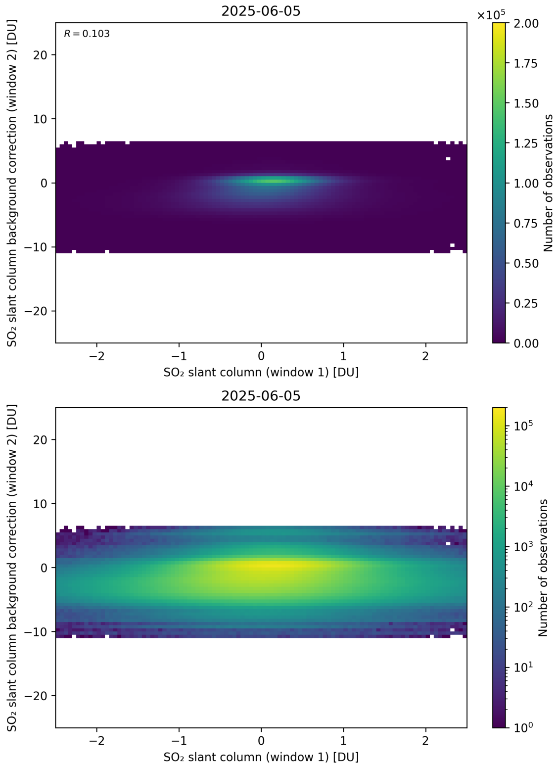
Figure 263: Scatter density plot of “SO 2 slant column (window 1)” against “SO 2 slant column background correction (window 2)” for 2025-06-04 to 2025-06-06.
