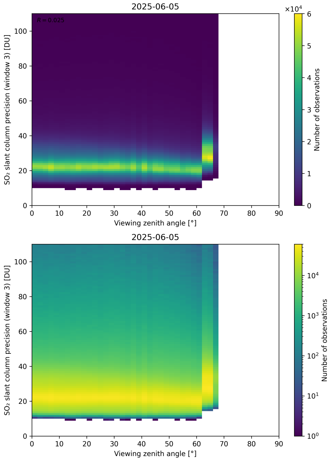
Figure 380: Scatter density plot of “Viewing zenith angle” against “SO 2 slant column precision (window 3)” for 2025-06-04 to 2025-06-06.
