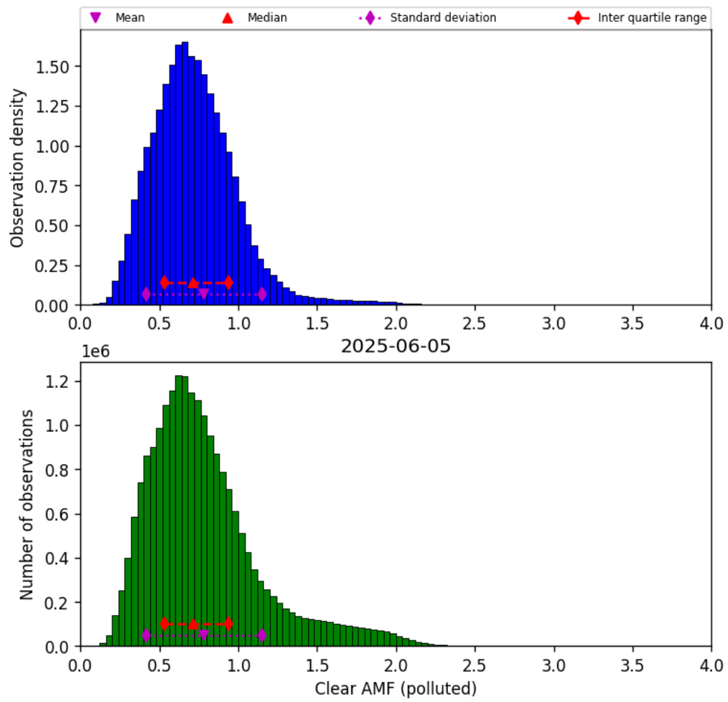
Figure 81: Histogram of “Clear AMF (polluted)” for 2025-06-04 to 2025-06-06
