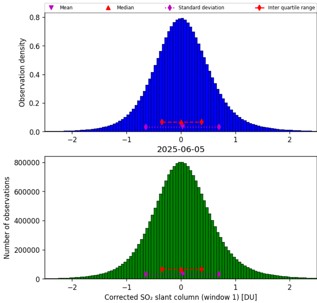
Figure 65: Histogram of “Corrected SO 2 slant column (window 1)” for 2025-06-04 to 2025-06-06
