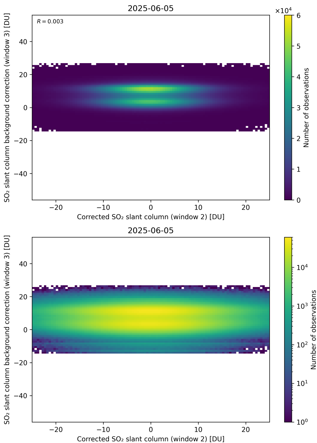
Figure 245: Scatter density plot of “Corrected SO 2 slant column (window 2)” against “SO 2 slant column background correction (window 3)” for 2025-06-04 to 2025-06-06.
