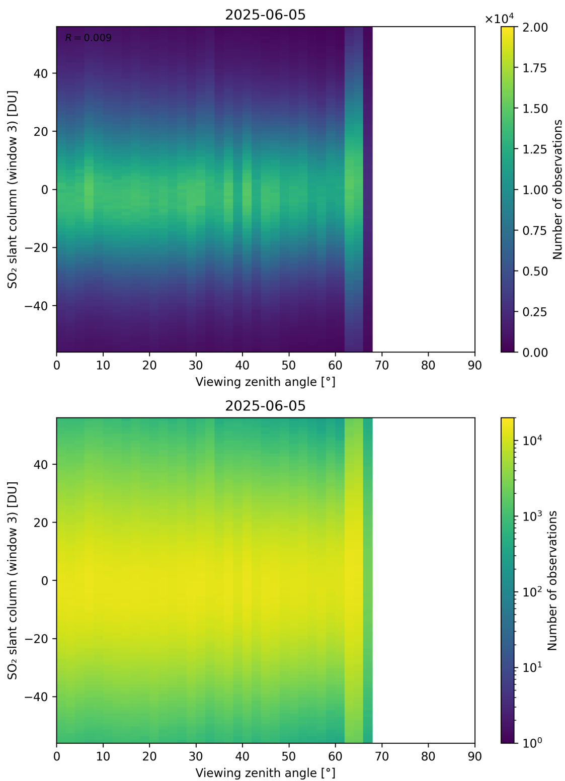
Figure 379: Scatter density plot of “Viewing zenith angle” against “SO 2 slant column (window 3)” for 2025-06-04 to 2025-06-06.
