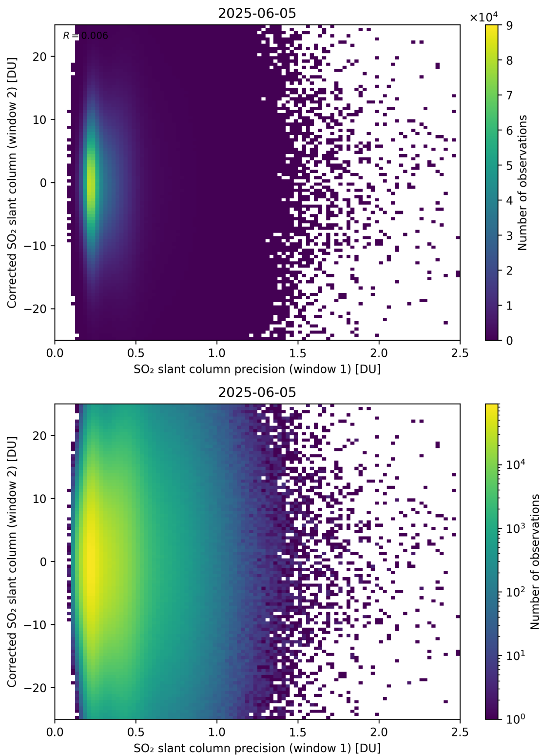
Figure 275: Scatter density plot of “SO 2 slant column precision (window 1)” against “Corrected SO 2 slant column (window 2)” for 2025-06-04 to 2025-06-06.
