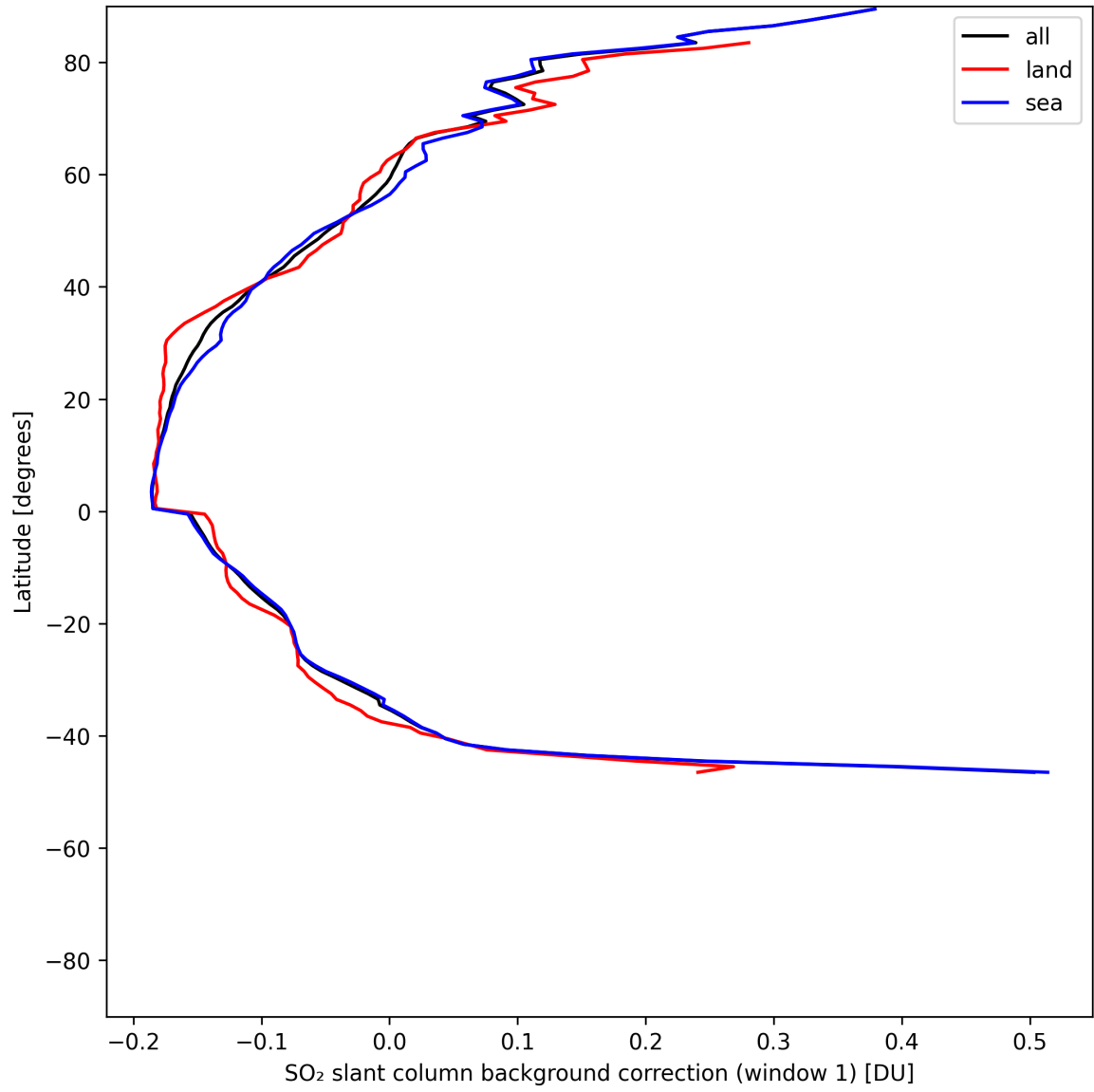
Figure 40: Zonal average of “SO 2 slant column background correction (window 1)” for 2025-06-04 to 2025-06-06.
