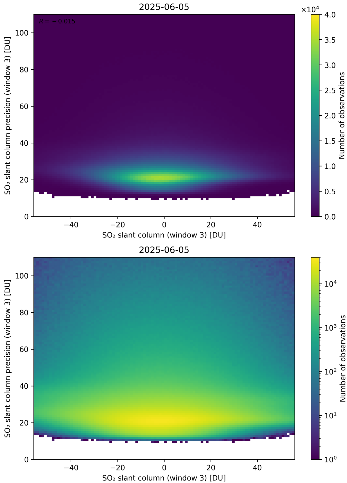
Figure 317: Scatter density plot of “SO 2 slant column (window 3)” against “SO 2 slant column precision (window 3)” for 2025-06-04 to 2025-06-06.
