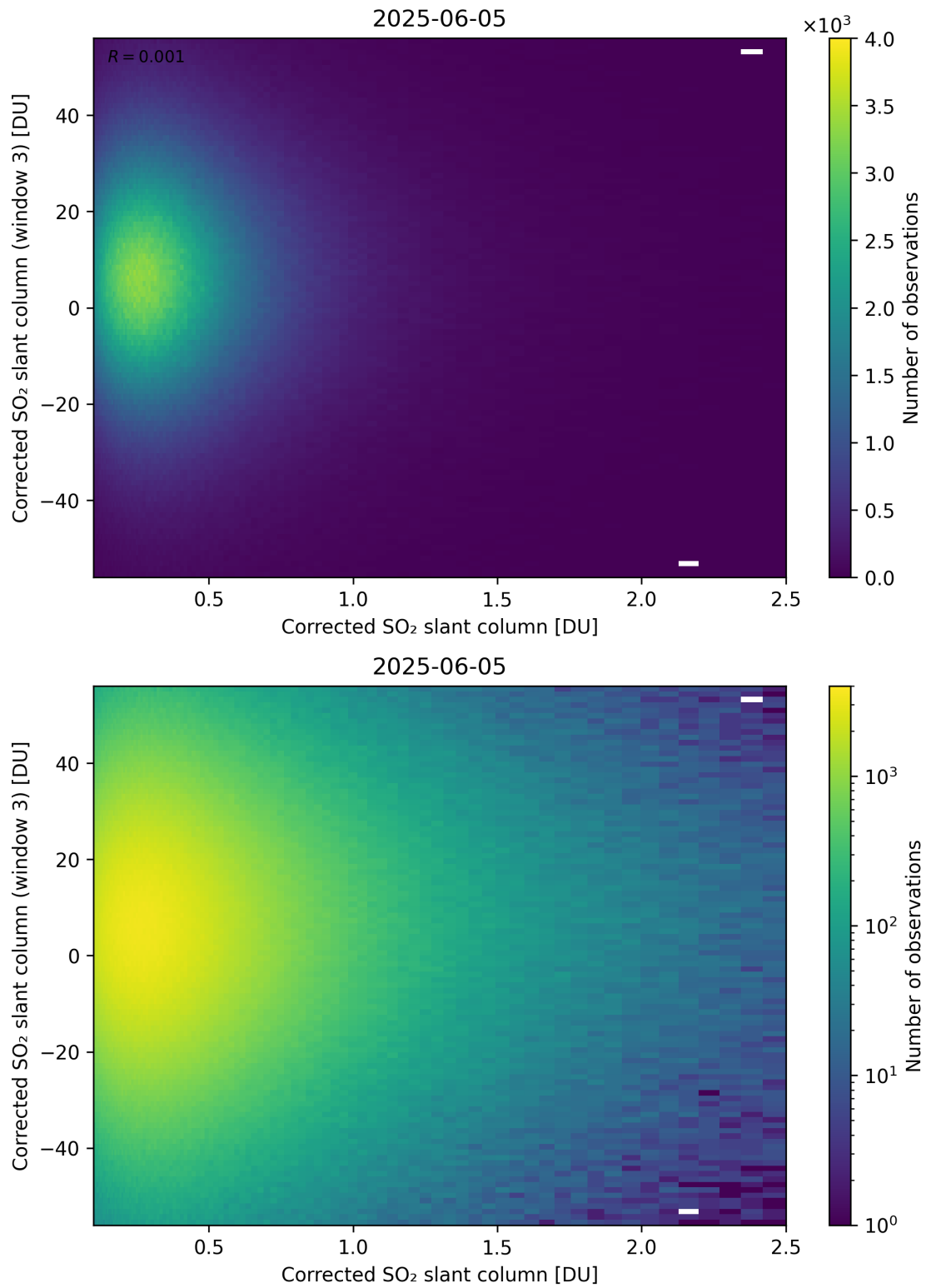
Figure 236: Scatter density plot of “Corrected SO 2 slant column” against “Corrected SO 2 slant column (window 3)” for 2025-06-04 to 2025-06-06.
