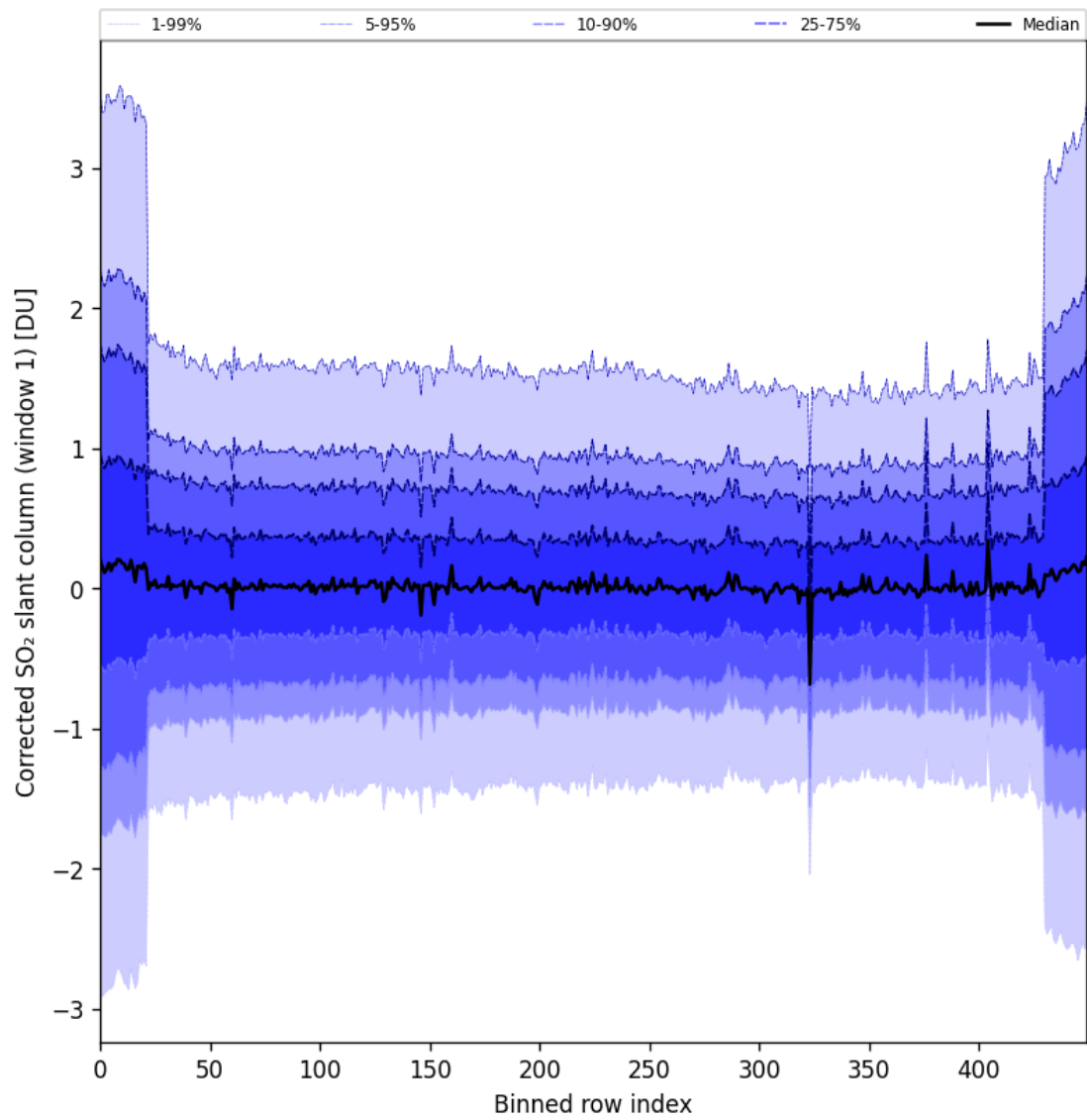
Figure 91: Along track statistics of “Corrected SO 2 slant column (window 1)” for 2025-06-04 to 2025-06-06
