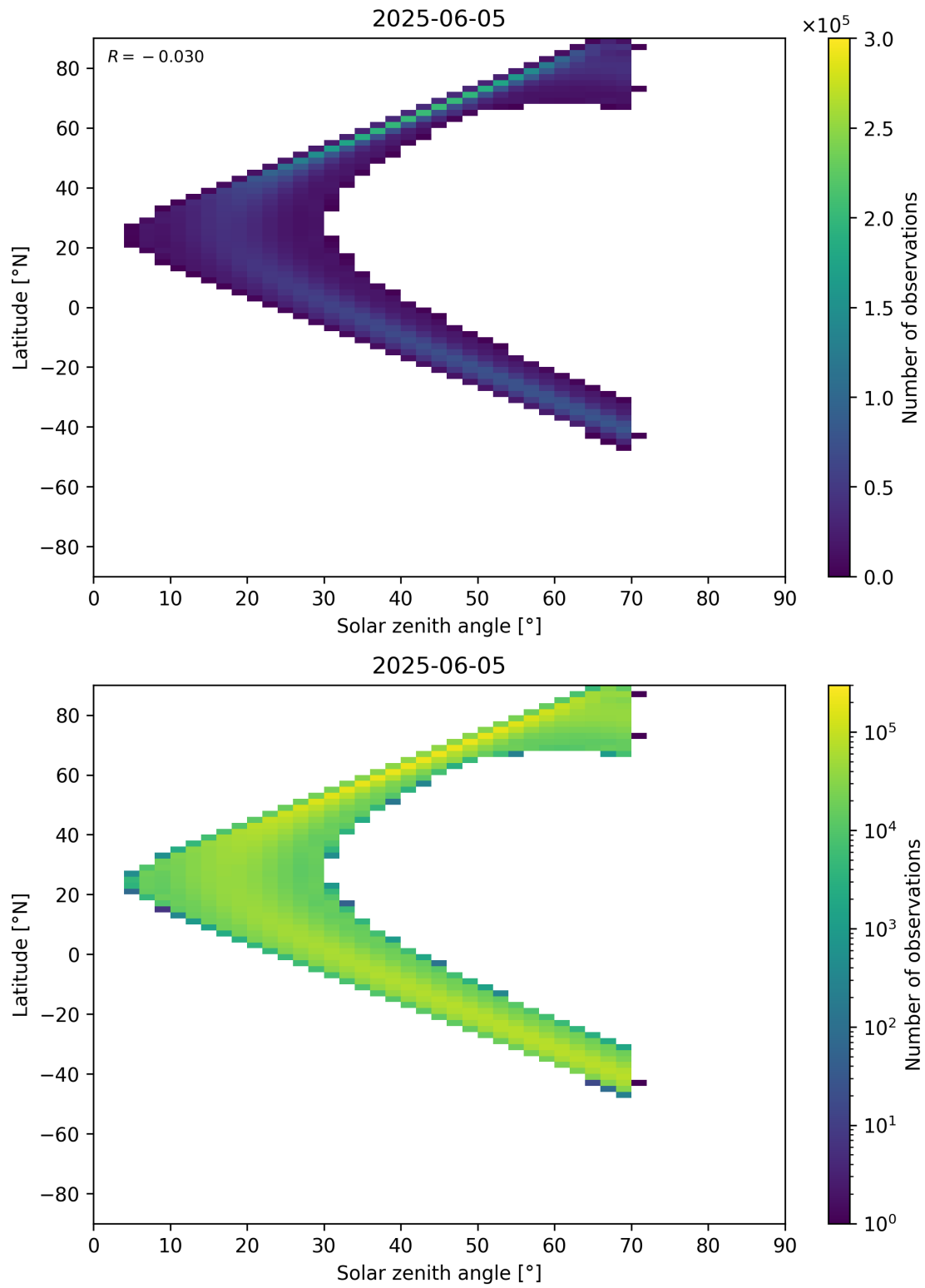
Figure 177: Scatter density plot of “Solar zenith angle” against “Latitude” for 2025-06-04 to 2025-06-06.
