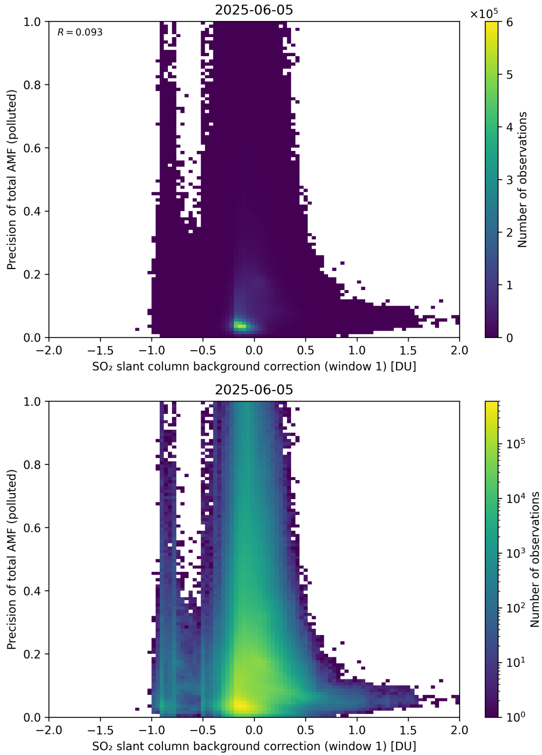
Figure 121: Scatter density plot of “SO 2 slant column background correction (window 1)” against “Precision of total AMF (polluted)” for 2025-06-04 to 2025-06-06.
