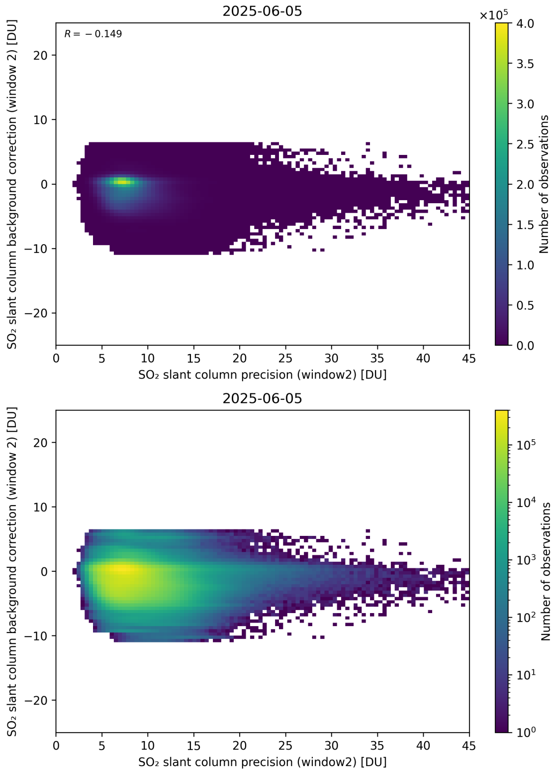
Figure 291: Scatter density plot of “SO 2 slant column precision (window2)” against “SO 2 slant column background correction (window 2)” for 2025-06-04 to 2025-06-06.
