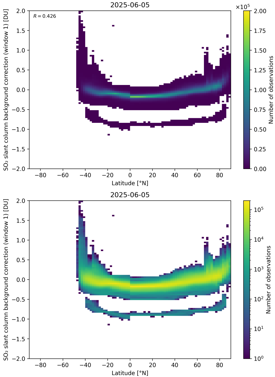
Figure 150: Scatter density plot of “Latitude” against “SO 2 slant column background correction (window 1)” for 2025-06-04 to 2025-06-06.
