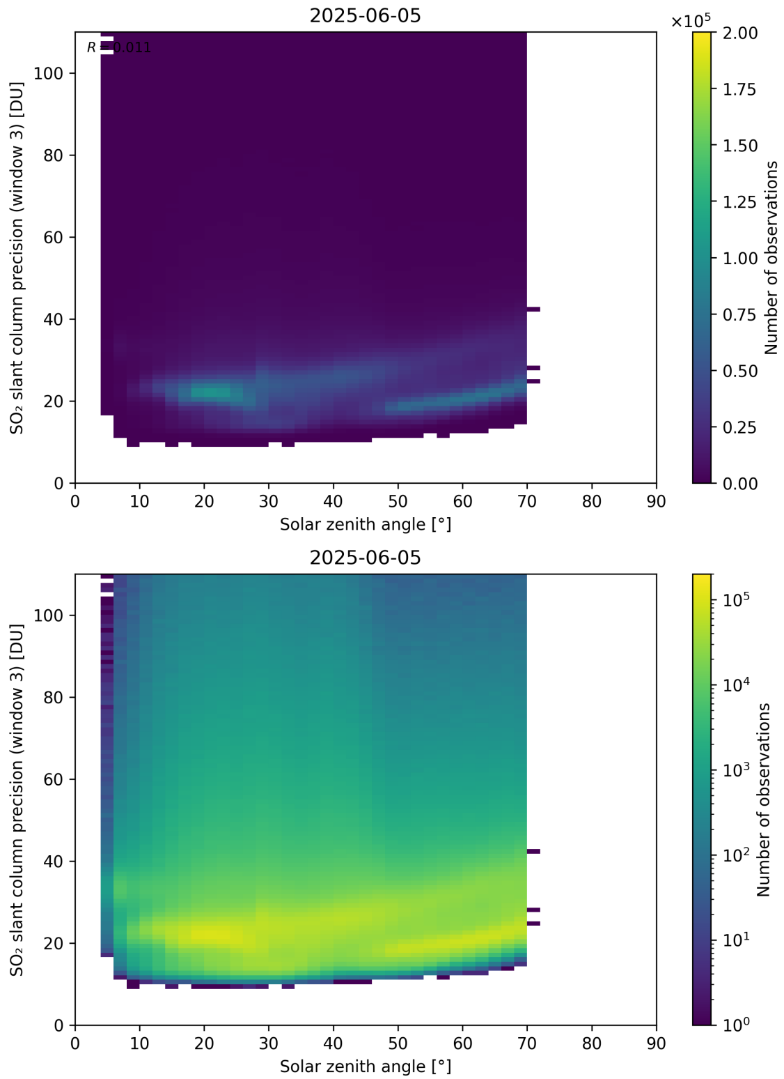
Figure 188: Scatter density plot of “Solar zenith angle” against “SO 2 slant column precision (window 3)” for 2025-06-04 to 2025-06-06.
