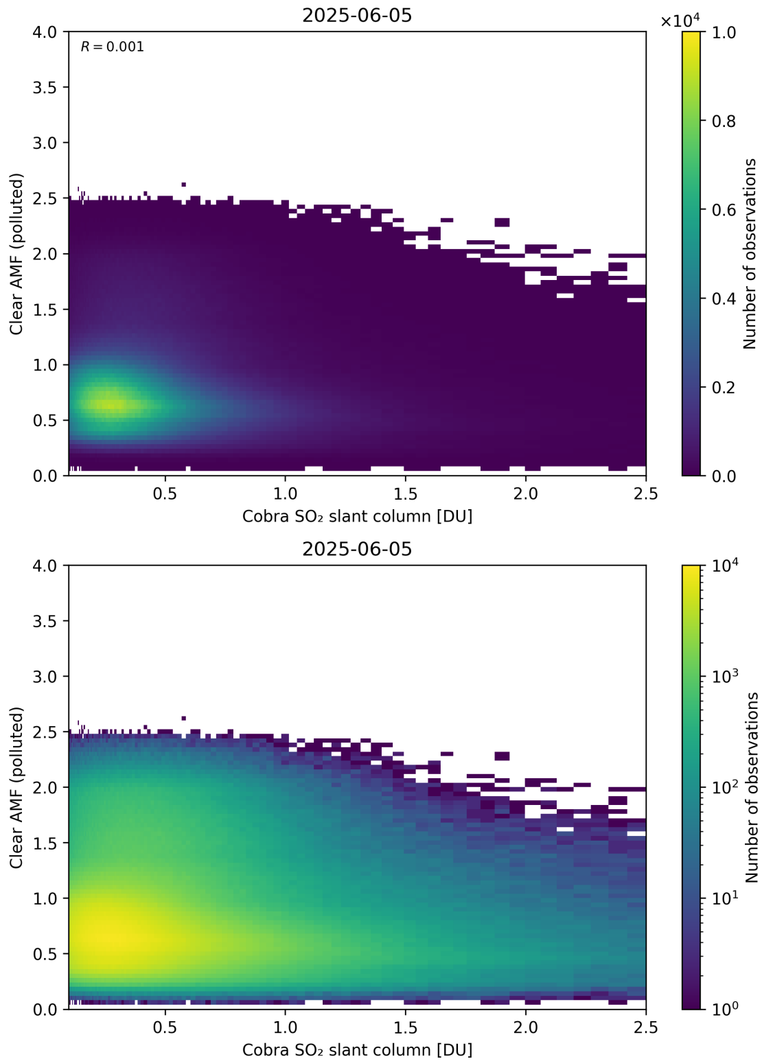
Figure 215: Scatter density plot of “Cobra SO 2 slant column” against “Clear AMF (polluted)” for 2025-06-04 to 2025-06-06.
