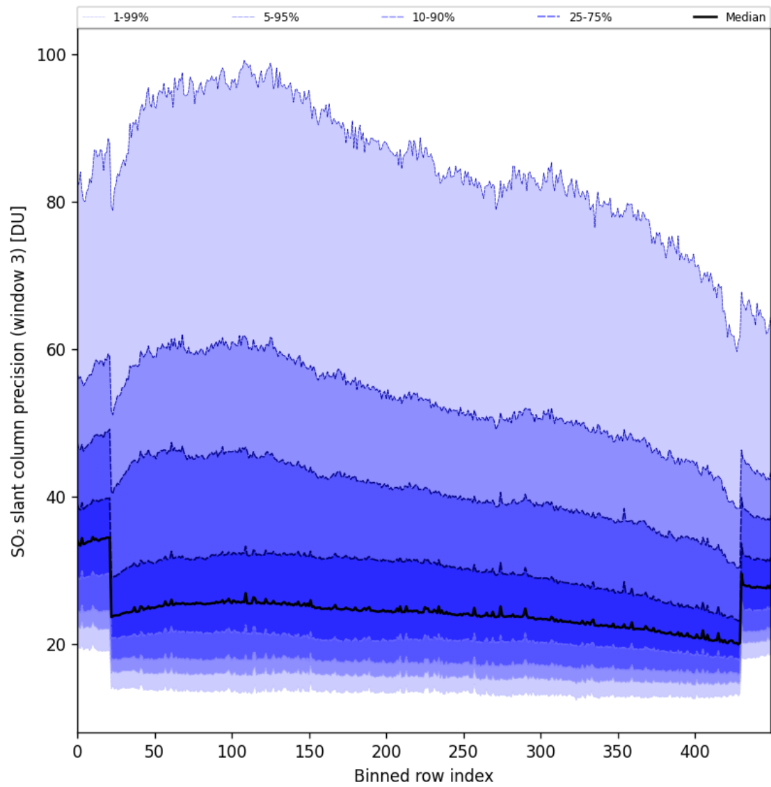
Figure 98: Along track statistics of “SO 2 slant column precision (window 3)” for 2025-06-04 to 2025-06-06
