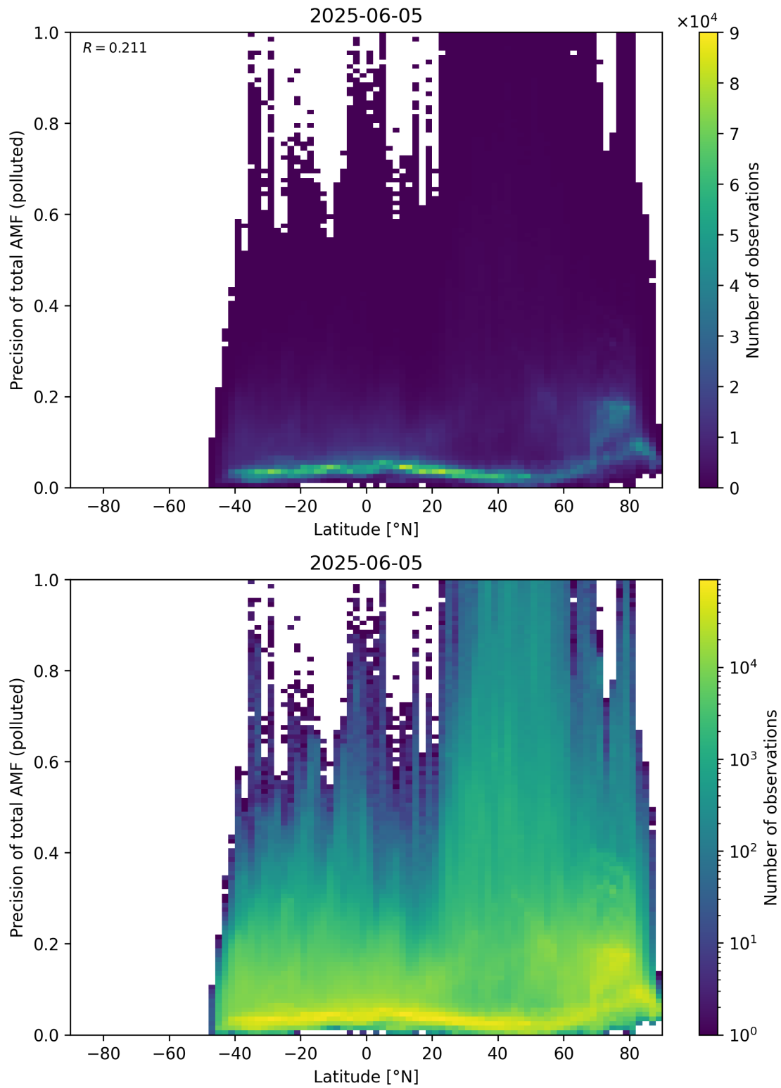
Figure 168: Scatter density plot of “Latitude” against “Precision of total AMF (polluted)” for 2025-06-04 to 2025-06-06.
