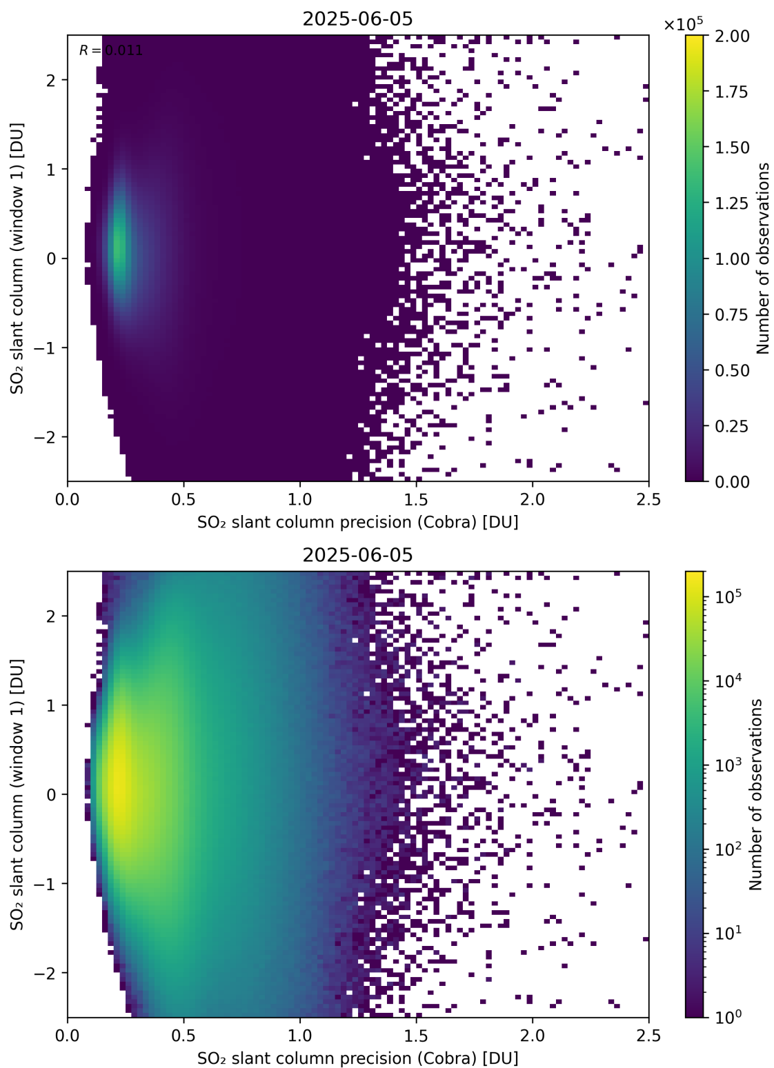
Figure 208: Scatter density plot of “SO 2 slant column precision (Cobra)” against “SO 2 slant column (window 1)” for 2025-06-04 to 2025-06-06.
