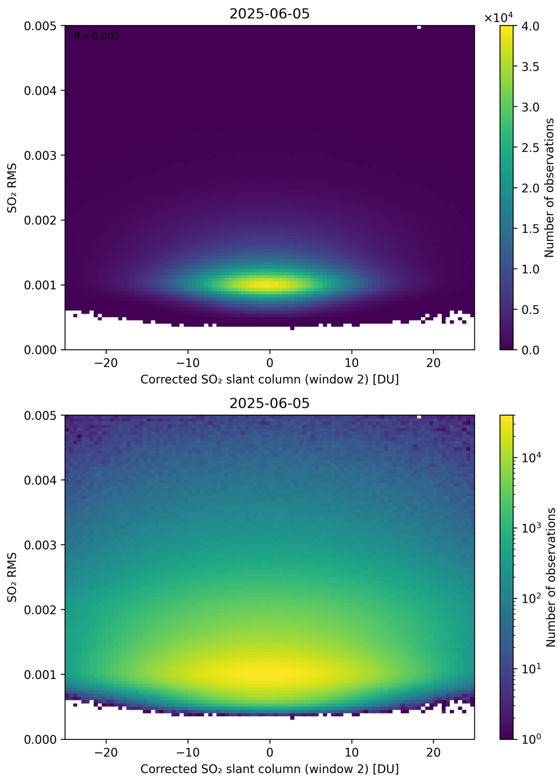
Figure 248: Scatter density plot of “Corrected SO 2 slant column (window 2)” against “SO 2 RMS” for 2025-06-04 to 2025-06-06.
