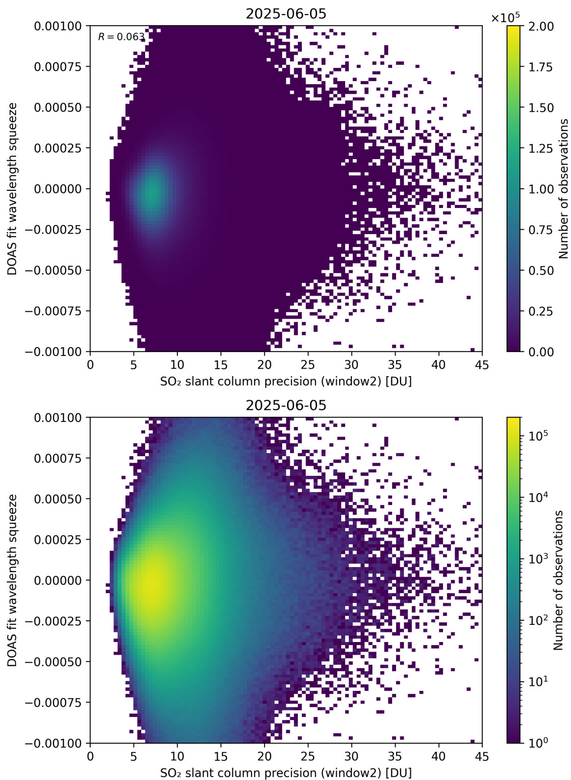
Figure 294: Scatter density plot of “SO 2 slant column precision (window2)” against “DOAS fit wavelength squeeze” for 2025-06-04 to 2025-06-06.
