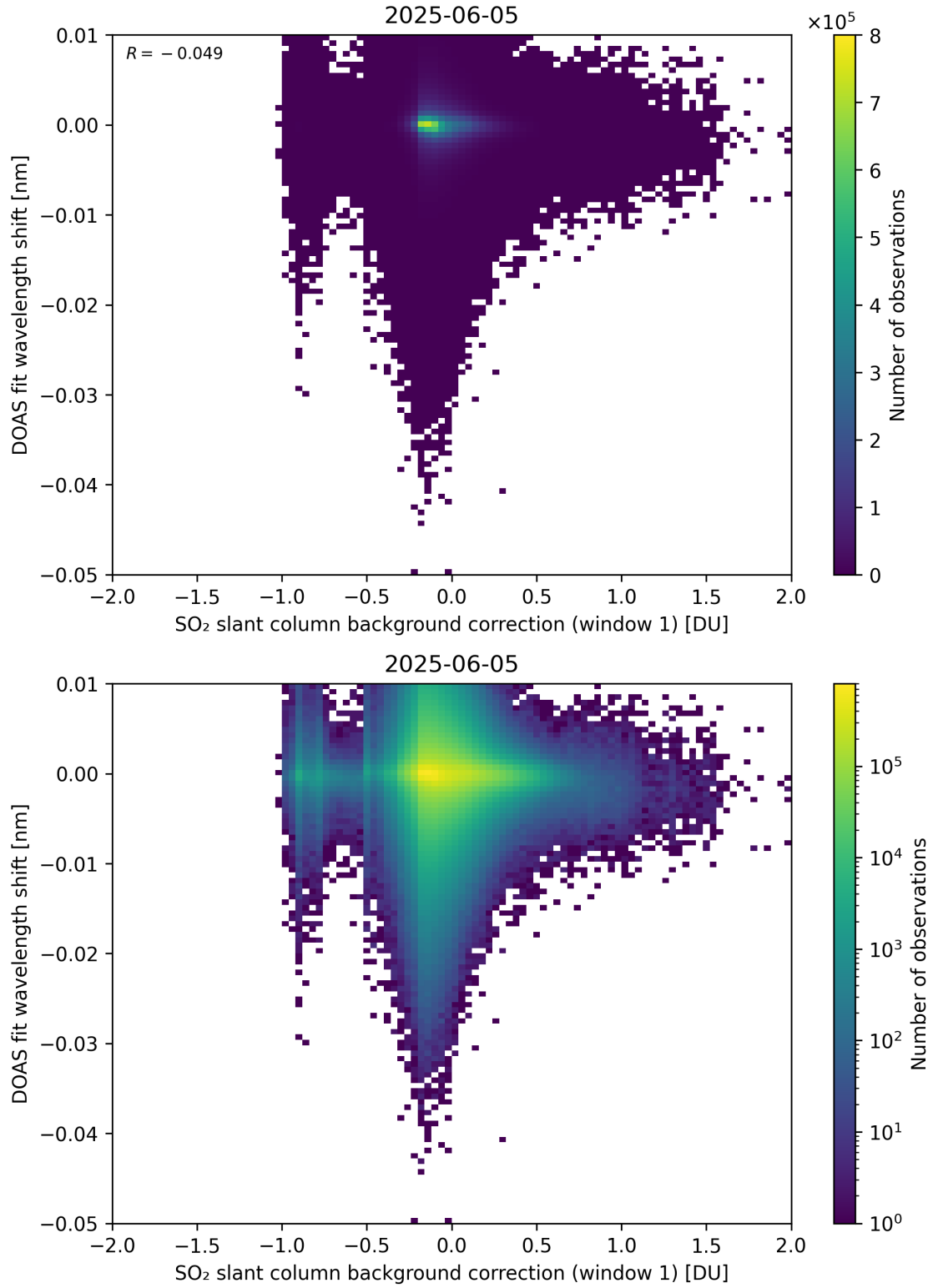
Figure 111: Scatter density plot of “SO 2 slant column background correction (window 1)” against “DOAS fit wavelength shift” for 2025-06-04 to 2025-06-06.
