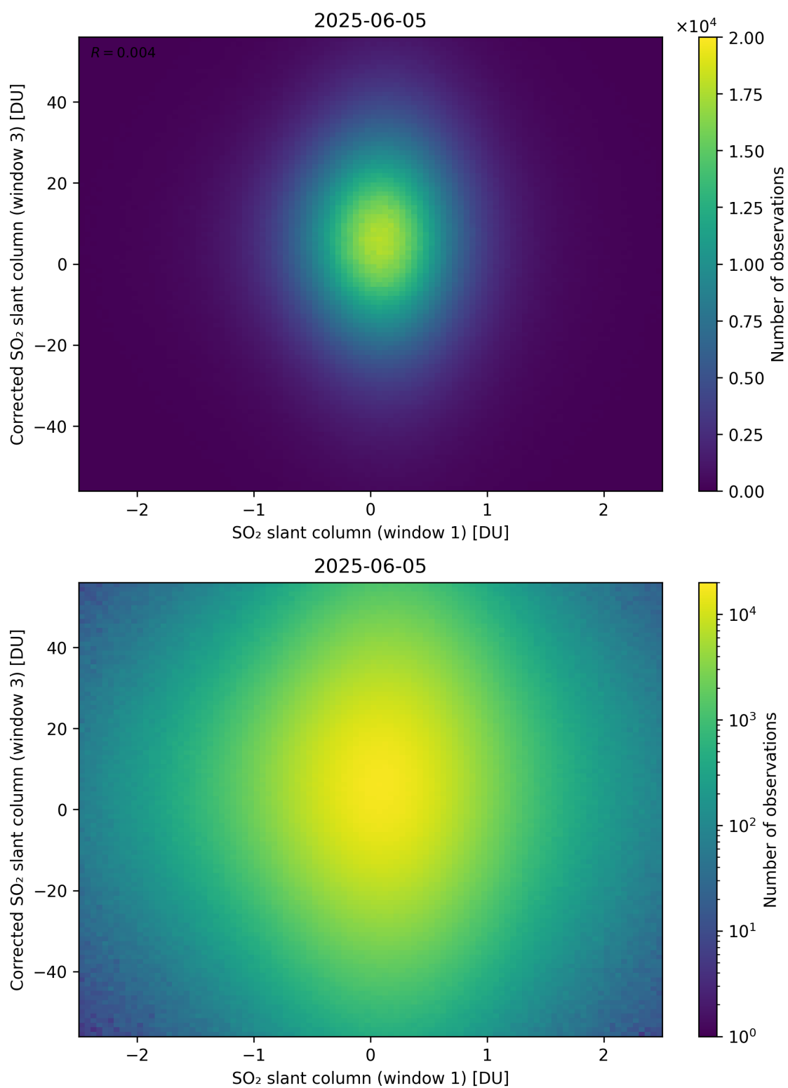
Figure 284: Scatter density plot of “SO 2 slant column (window 1)” against “Corrected SO 2 slant column (window 3)” for 2025-06-04 to 2025-06-06.
