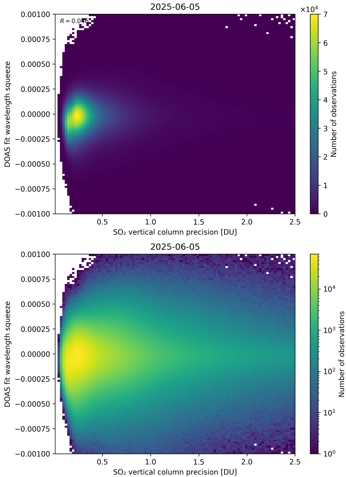
Figure 333: Scatter density plot of “SO 2 vertical column precision” against “DOAS fit wavelength squeeze” for 2025-06-04 to 2025-06-06.
