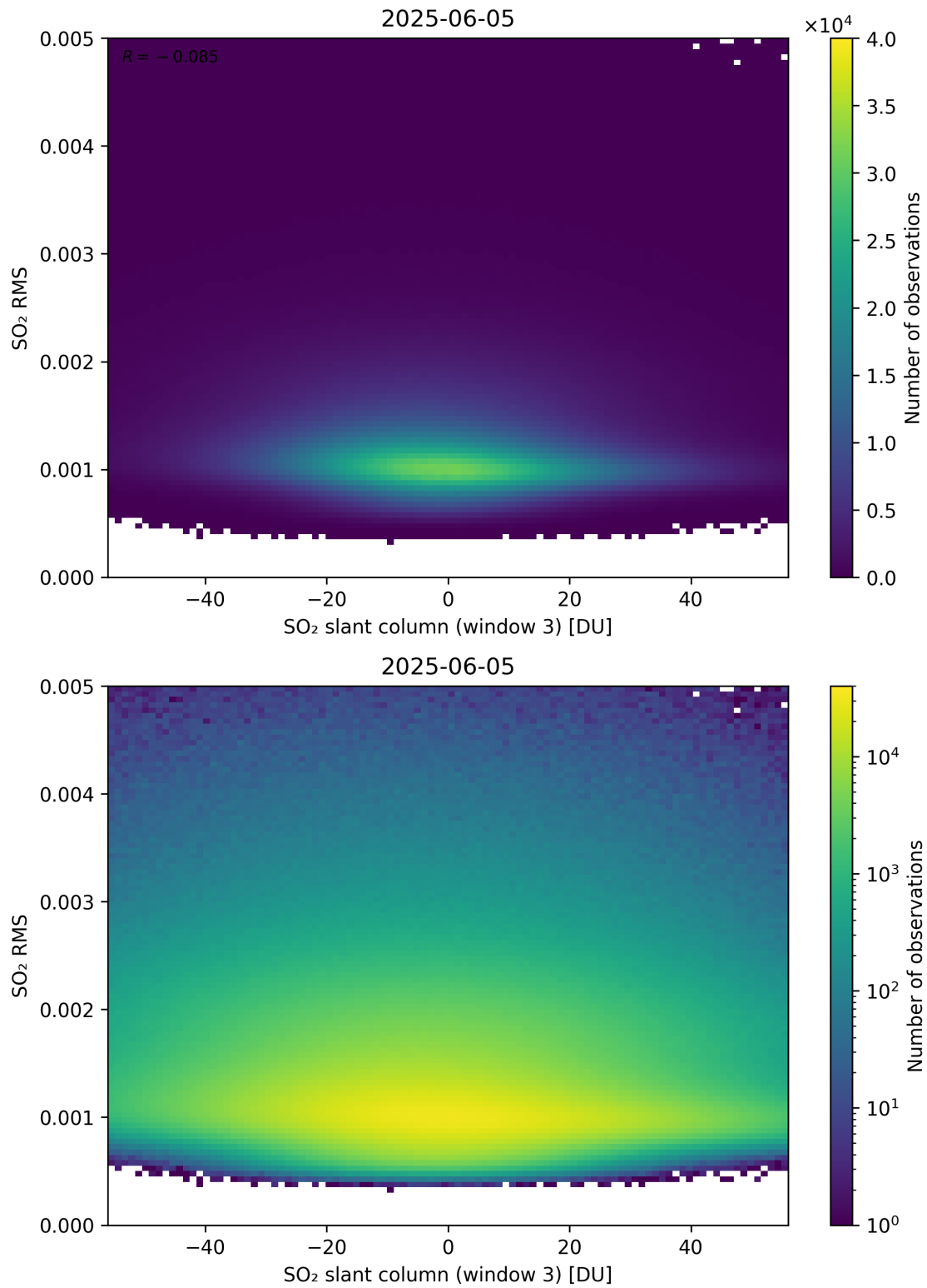
Figure 306: Scatter density plot of “SO 2 slant column (window 3)” against “SO 2 RMS” for 2025-06-04 to 2025-06-06.
