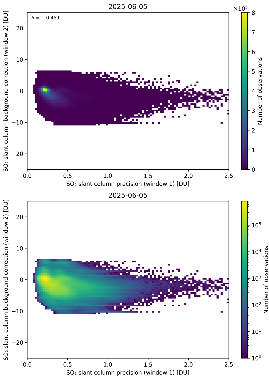
Figure 269: Scatter density plot of “SO 2 slant column precision (window 1)” against “SO 2 slant column background correction (window 2)” for 2025-06-04 to 2025-06-06.
