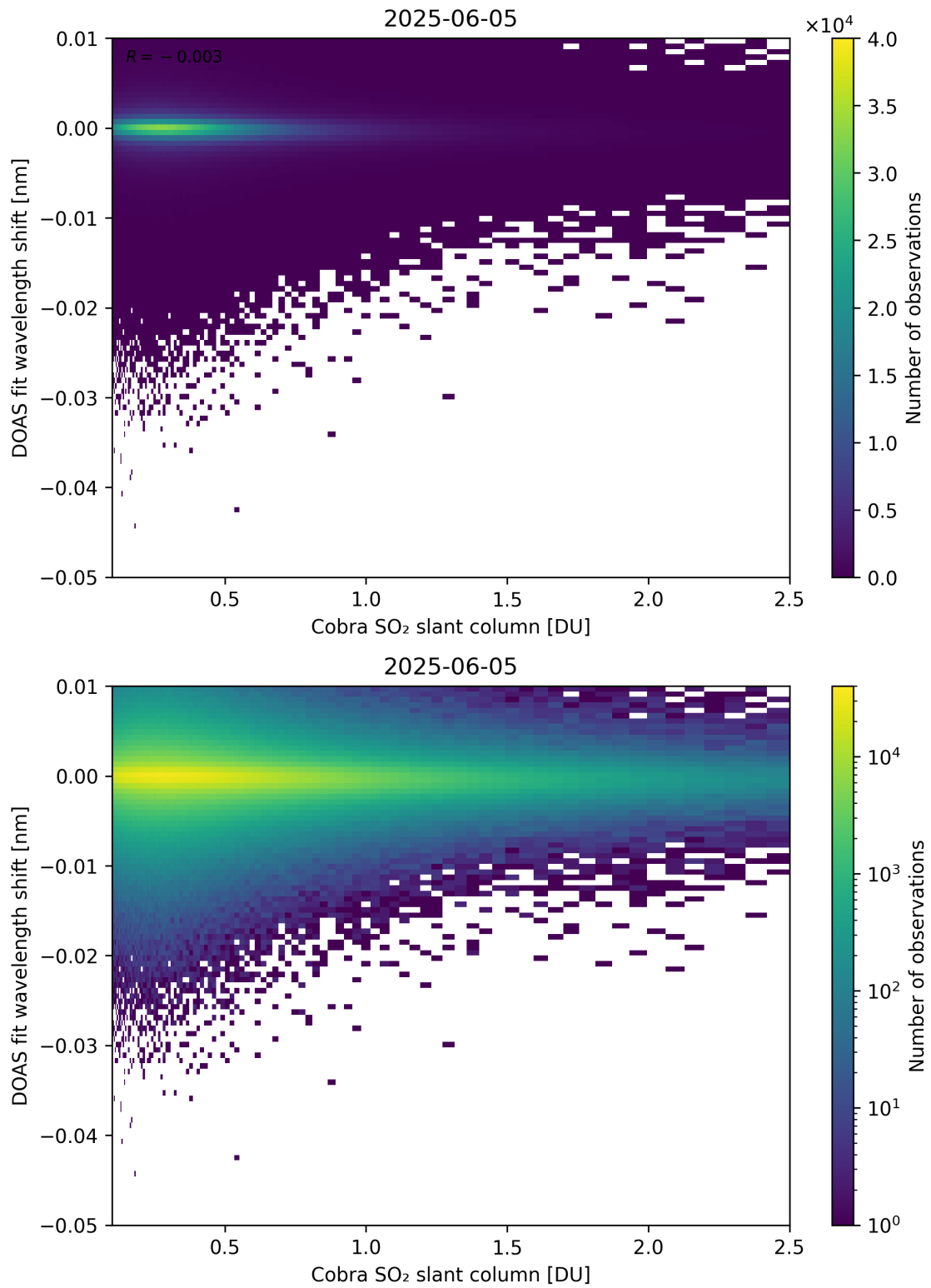
Figure 196: Scatter density plot of “Cobra SO 2 slant column” against “DOAS fit wavelength shift” for 2025-06-04 to 2025-06-06.
