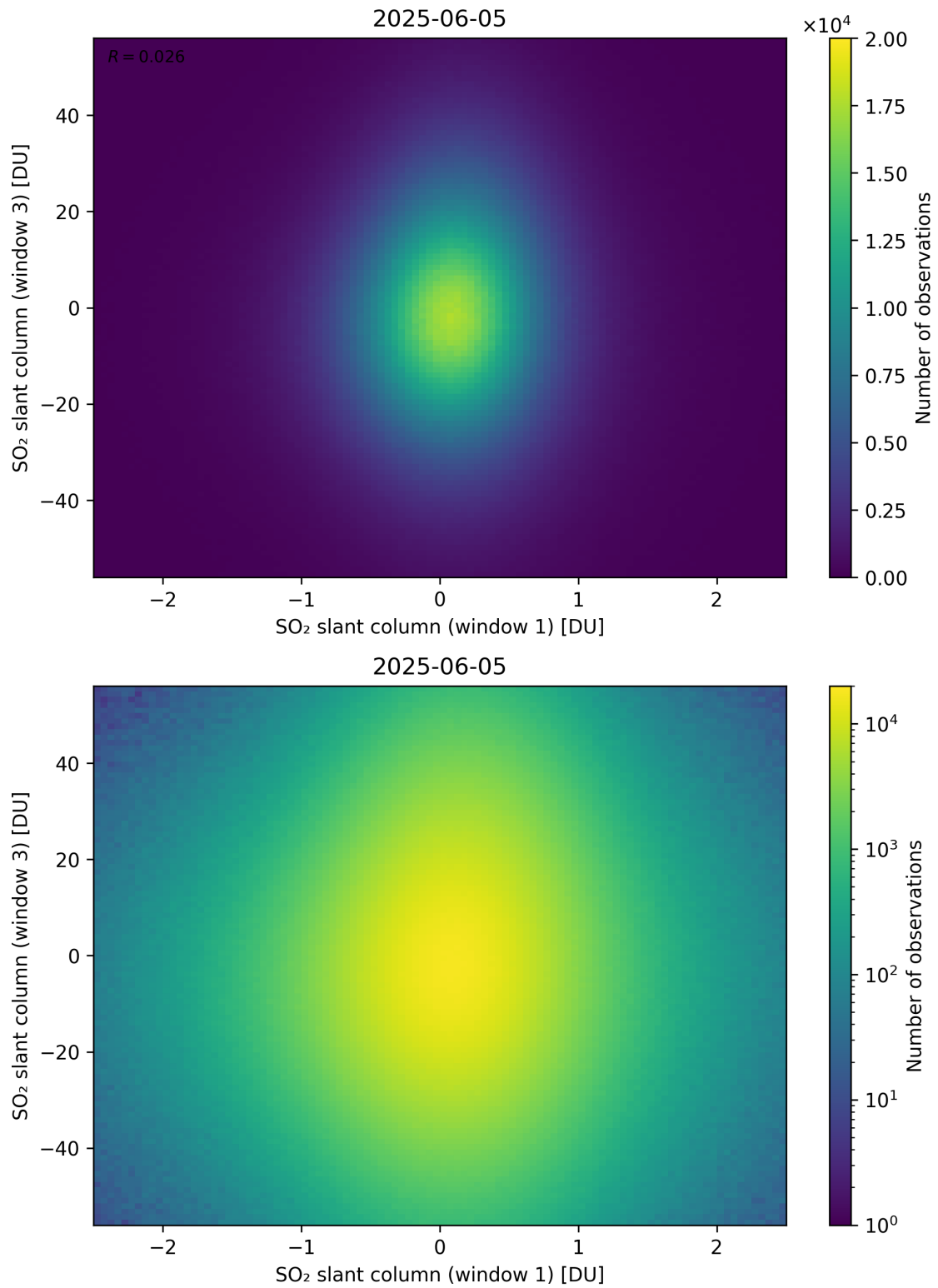
Figure 287: Scatter density plot of “SO 2 slant column (window 1)” against “SO 2 slant column (window 3)” for 2025-06-04 to 2025-06-06.
