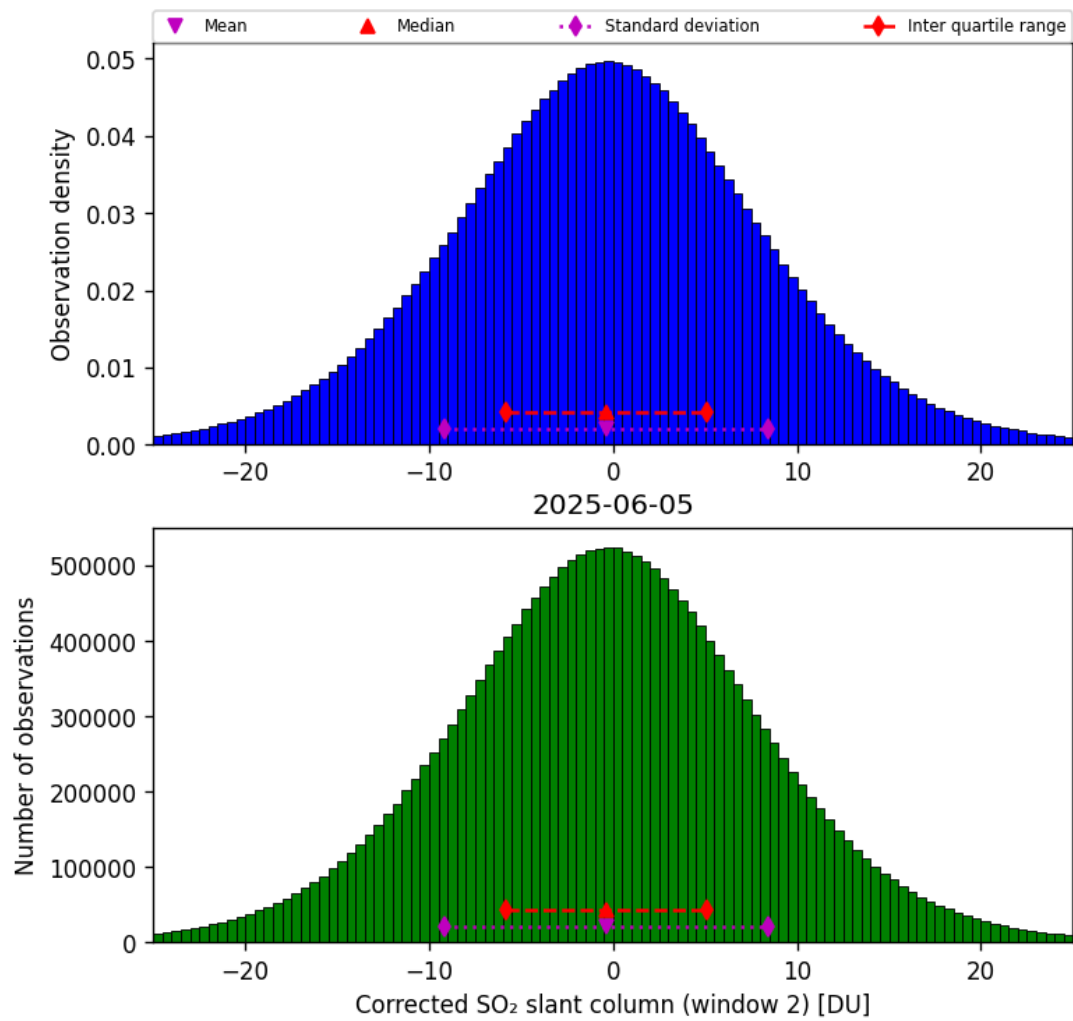
Figure 69: Histogram of “Corrected SO 2 slant column (window 2)” for 2025-06-04 to 2025-06-06
