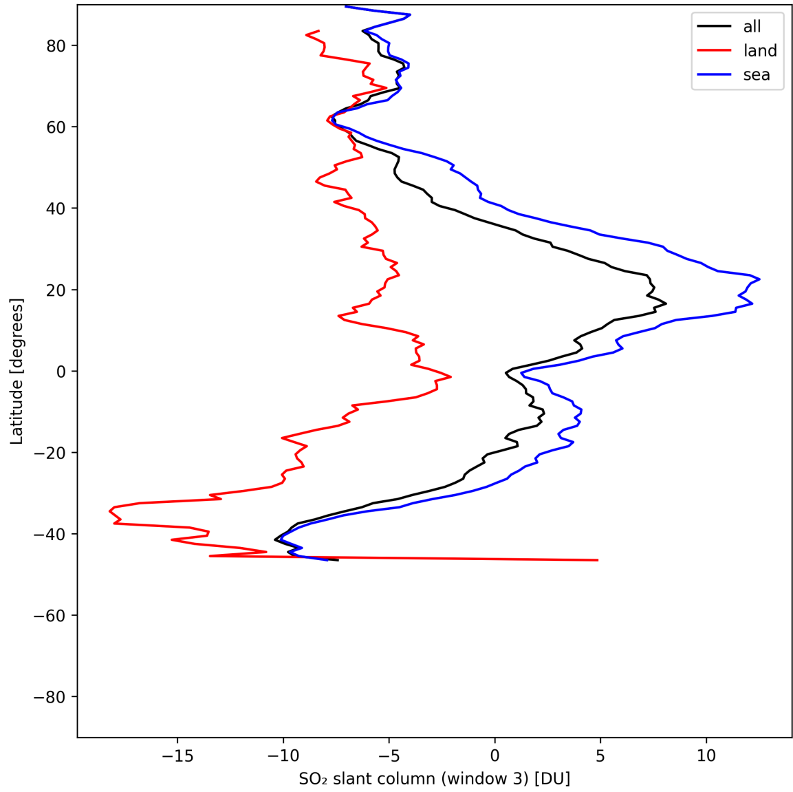
Figure 45: Zonal average of “SO 2 slant column (window 3)” for 2025-06-04 to 2025-06-06.
