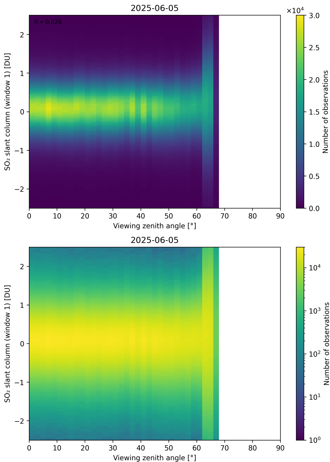
Figure 376: Scatter density plot of “Viewing zenith angle” against “SO 2 slant column (window 1)” for 2025-06-04 to 2025-06-06.
