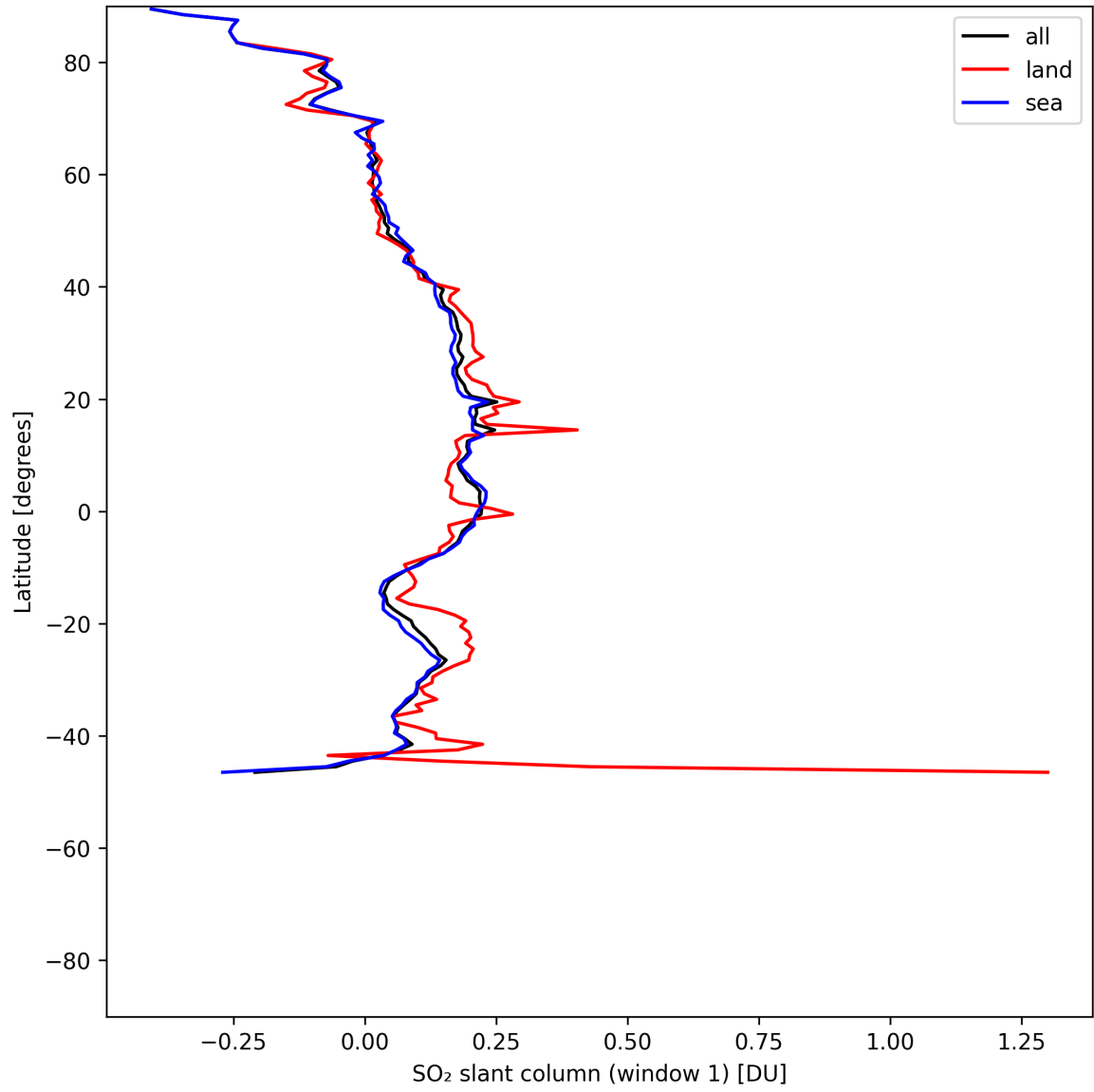
Figure 37: Zonal average of “SO 2 slant column (window 1)” for 2025-06-04 to 2025-06-06.
