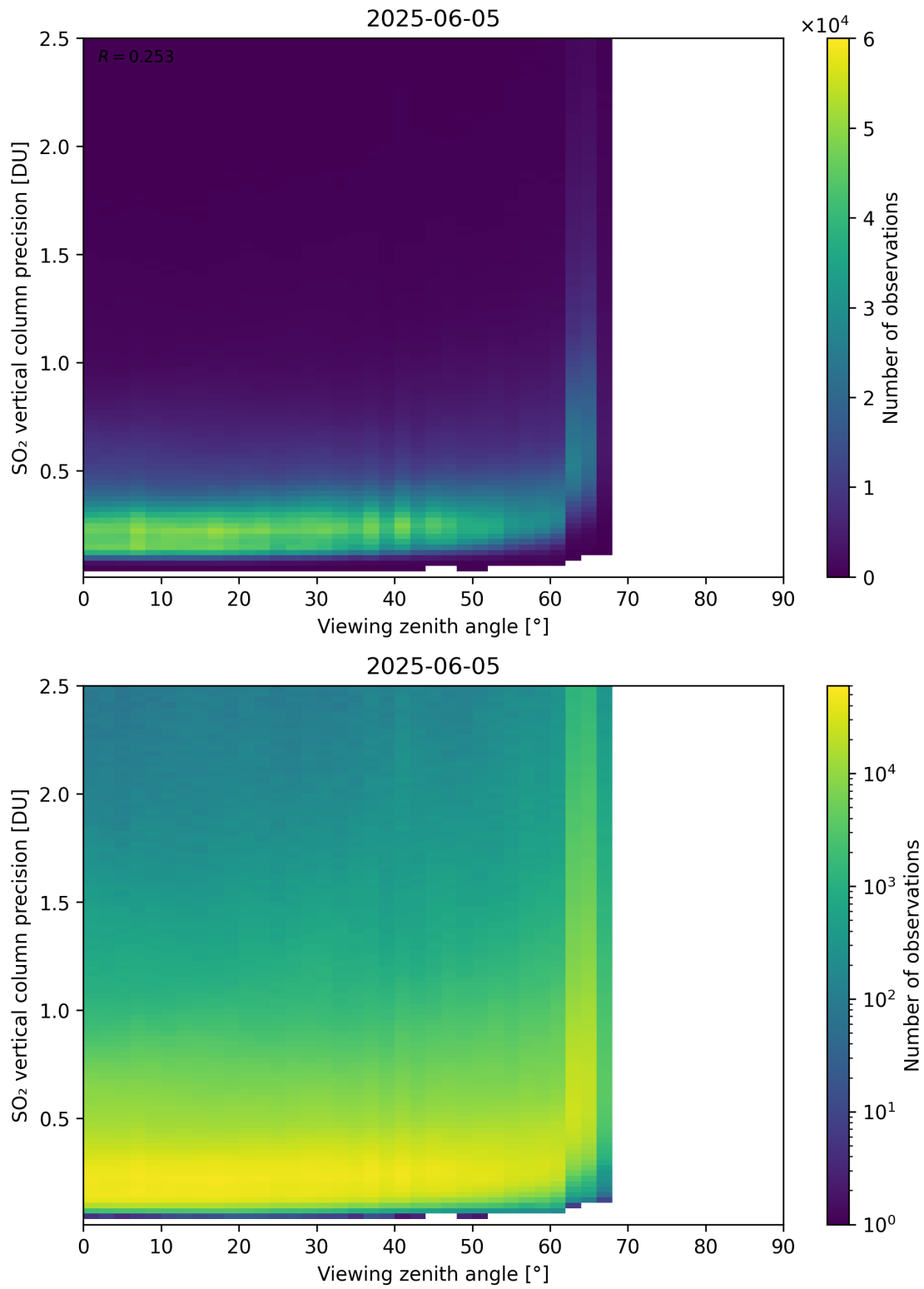
Figure 384: Scatter density plot of “Viewing zenith angle” against “SO 2 vertical column precision” for 2025-06-04 to 2025-06-06.
