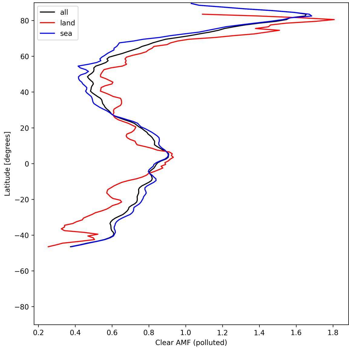
Figure 55: Zonal average of “Clear AMF (polluted)” for 2025-06-04 to 2025-06-06.
