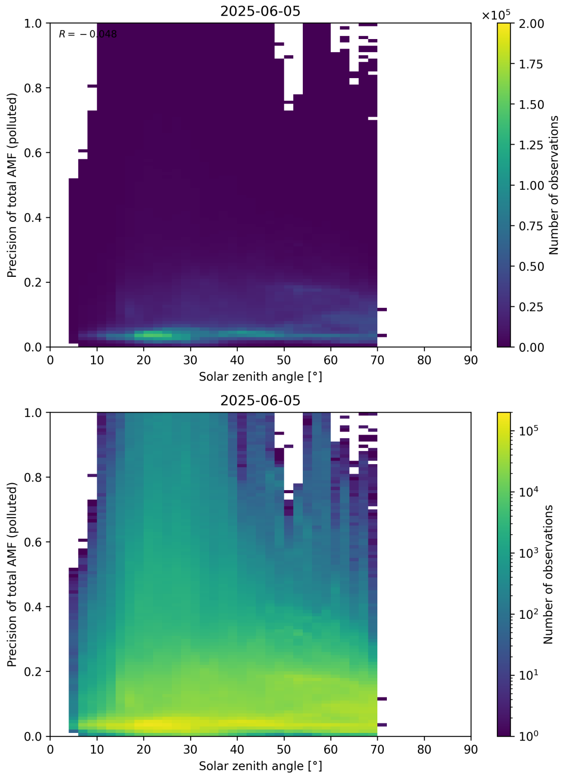
Figure 190: Scatter density plot of “Solar zenith angle” against “Precision of total AMF (polluted)” for 2025-06-04 to 2025-06-06.
