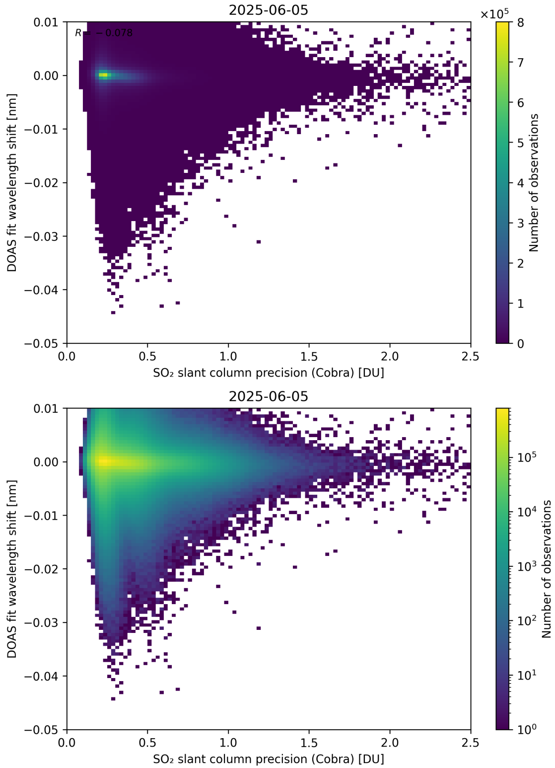
Figure 202: Scatter density plot of “SO 2 slant column precision (Cobra)” against “DOAS fit wavelength shift” for 2025-06-04 to 2025-06-06.
