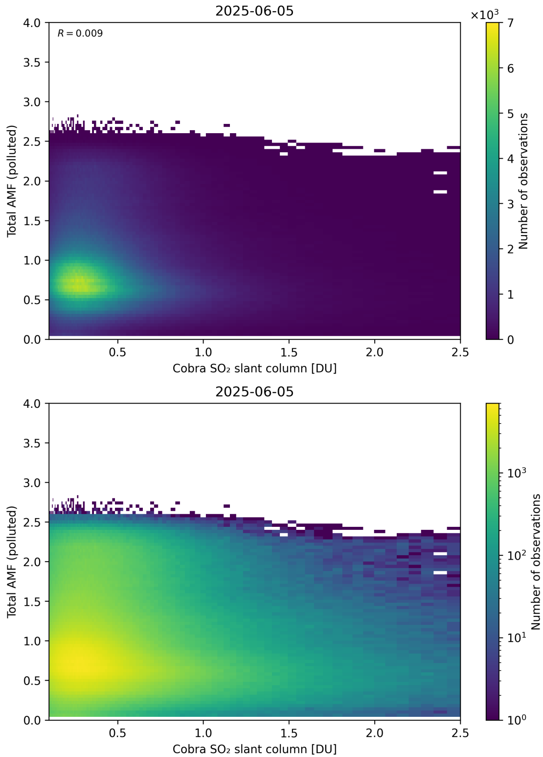
Figure 224: Scatter density plot of “Cobra SO 2 slant column” against “Total AMF (polluted)” for 2025-06-04 to 2025-06-06.
