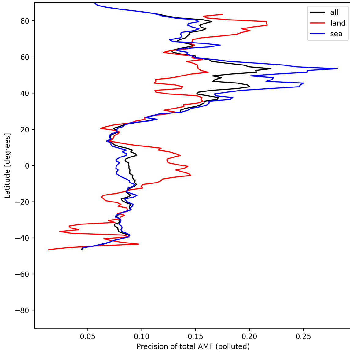
Figure 54: Zonal average of “Precision of total AMF (polluted)” for 2025-06-04 to 2025-06-06.
