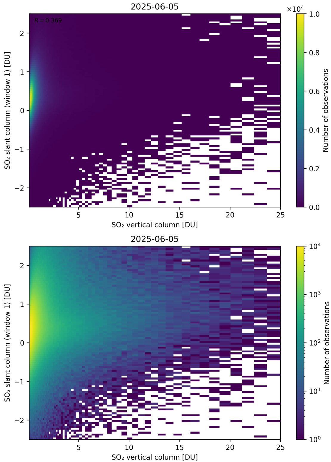
Figure 354: Scatter density plot of “SO 2 vertical column” against “SO 2 slant column (window 1)” for 2025-06-04 to 2025-06-06.
