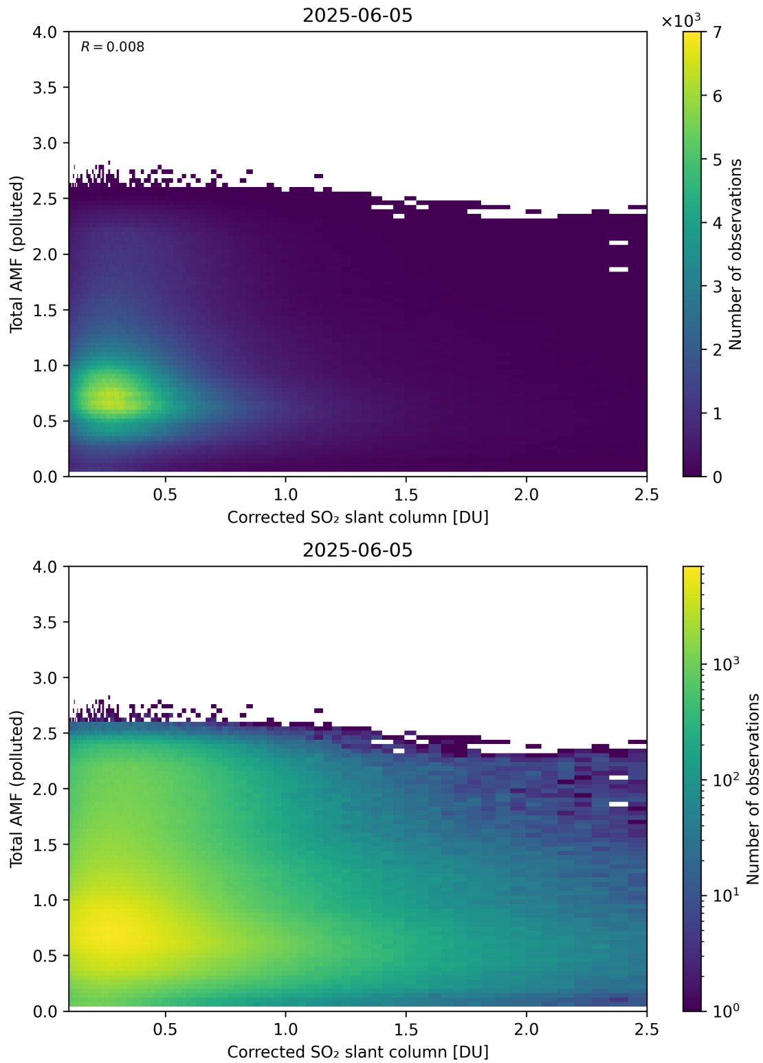
Figure 242: Scatter density plot of “Corrected SO 2 slant column” against “Total AMF (polluted)” for 2025-06-04 to 2025-06-06.
