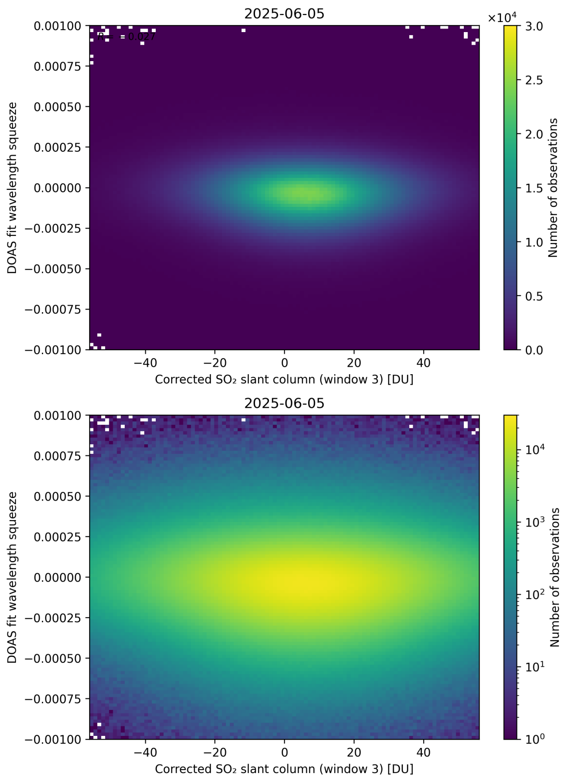
Figure 257: Scatter density plot of “Corrected SO 2 slant column (window 3)” against “DOAS fit wavelength squeeze” for 2025-06-04 to 2025-06-06.
