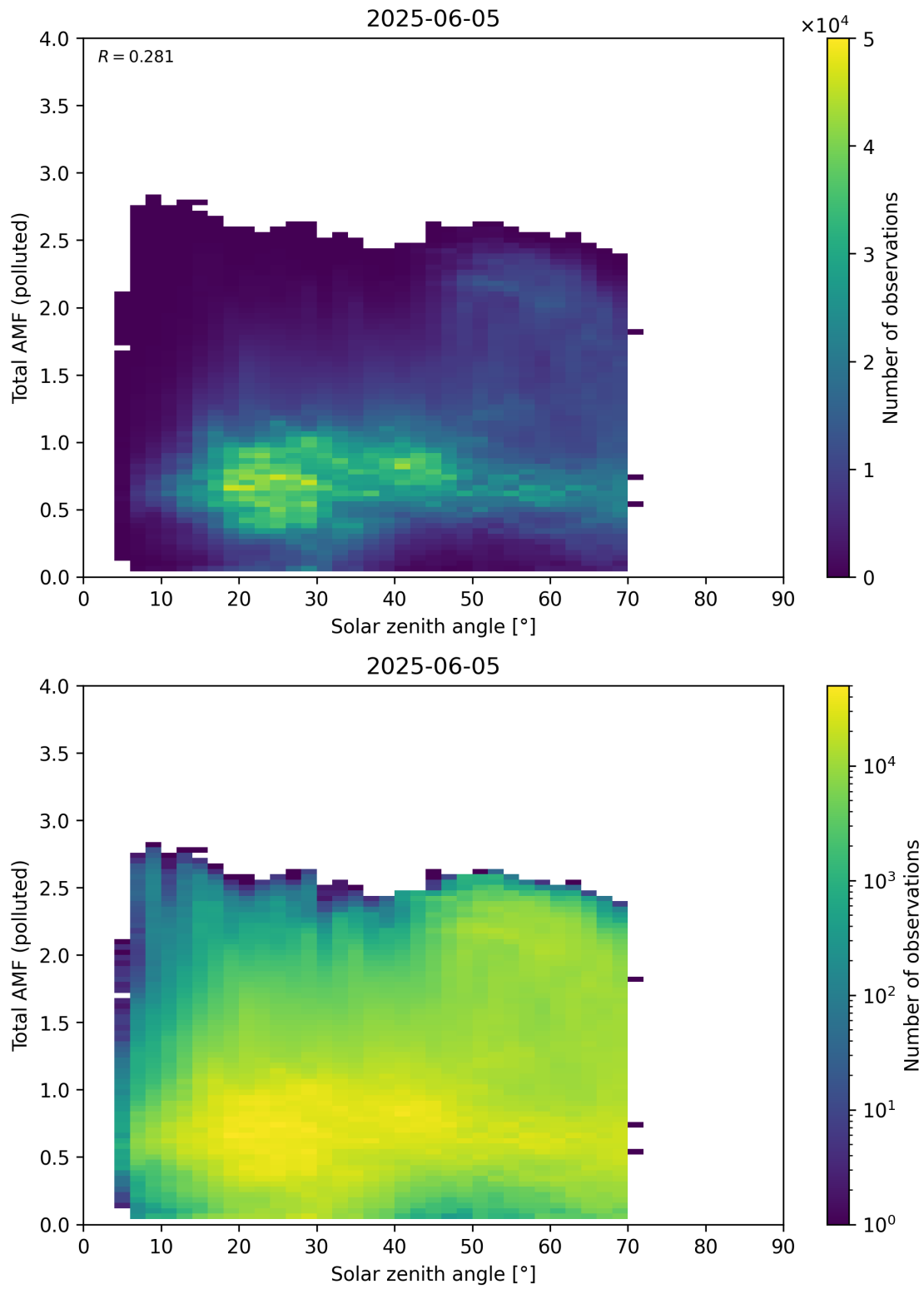
Figure 189: Scatter density plot of “Solar zenith angle” against “Total AMF (polluted)” for 2025-06-04 to 2025-06-06.
