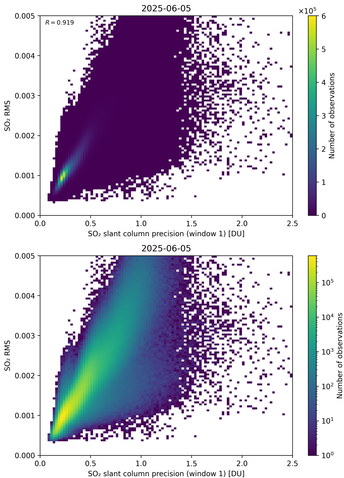
Figure 273: Scatter density plot of “SO 2 slant column precision (window 1)” against “SO 2 RMS” for 2025-06-04 to 2025-06-06.
