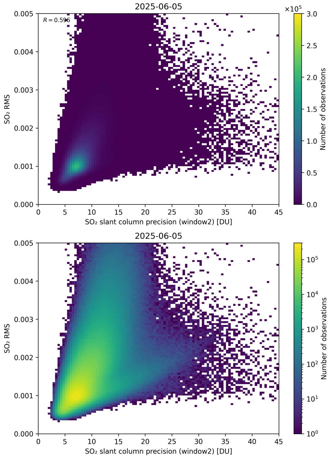
Figure 295: Scatter density plot of “SO 2 slant column precision (window2)” against “SO 2 RMS” for 2025-06-04 to 2025-06-06.
