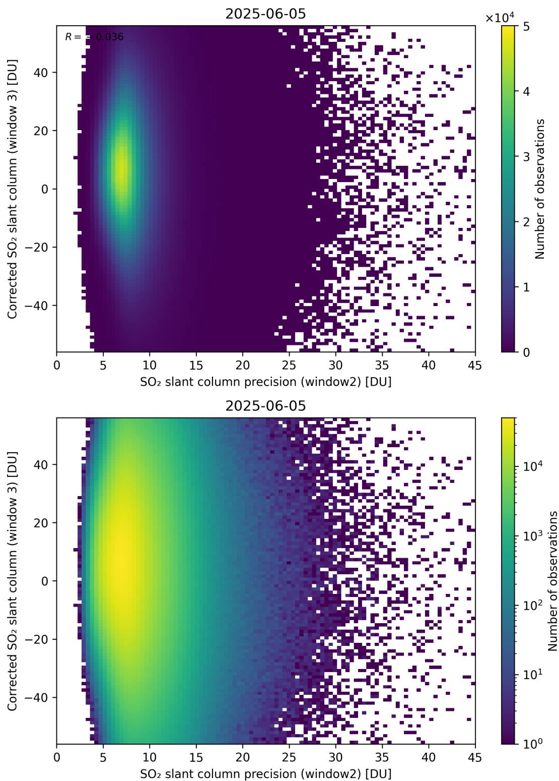
Figure 298: Scatter density plot of “SO 2 slant column precision (window2)” against “Corrected SO 2 slant column (window 3)” for 2025-06-04 to 2025-06-06.
