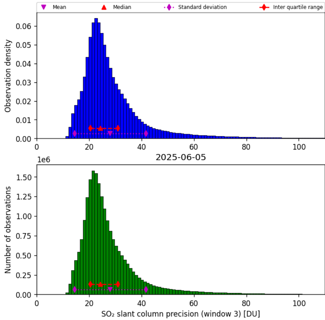
Figure 72: Histogram of “SO 2 slant column precision (window 3)” for 2025-06-04 to 2025-06-06
