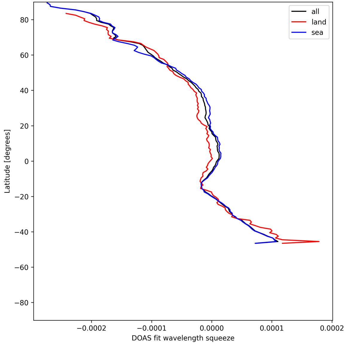
Figure 51: Zonal average of “DOAS fit wavelength squeeze” for 2025-06-04 to 2025-06-06.
