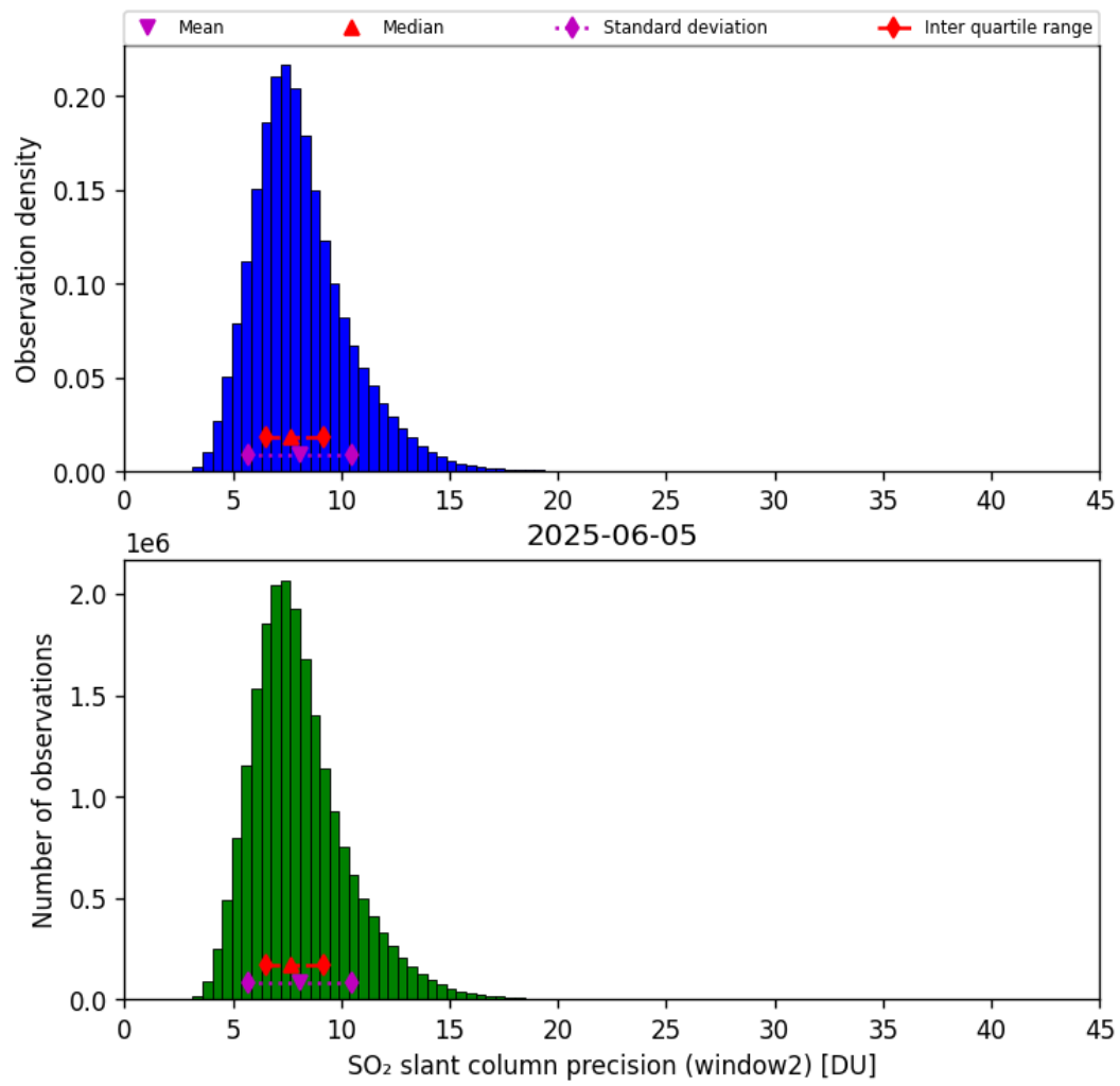
Figure 68: Histogram of “SO 2 slant column precision (window2)” for 2025-06-04 to 2025-06-06
