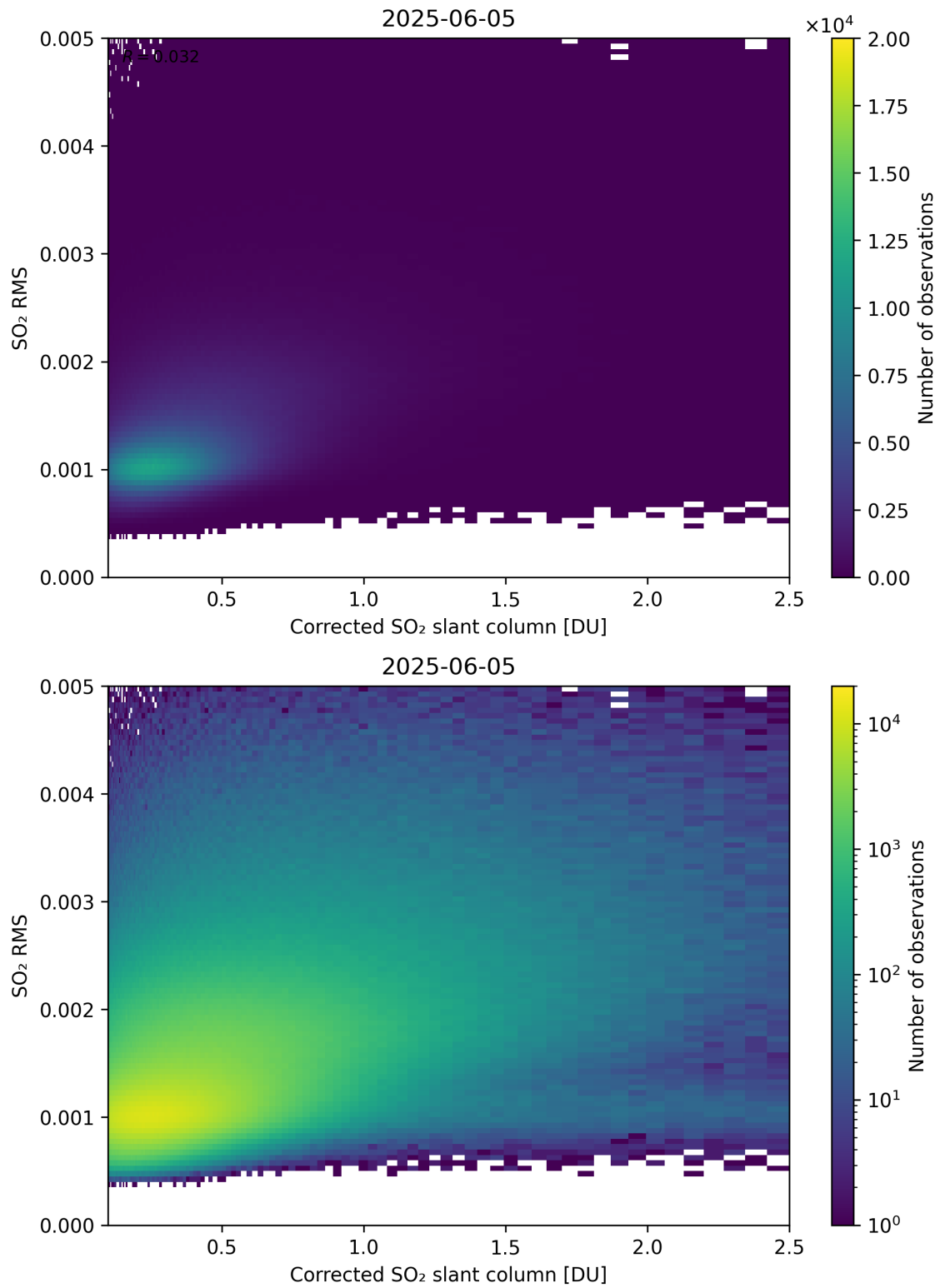
Figure 231: Scatter density plot of “Corrected SO 2 slant column” against “SO 2 RMS” for 2025-06-04 to 2025-06-06.
