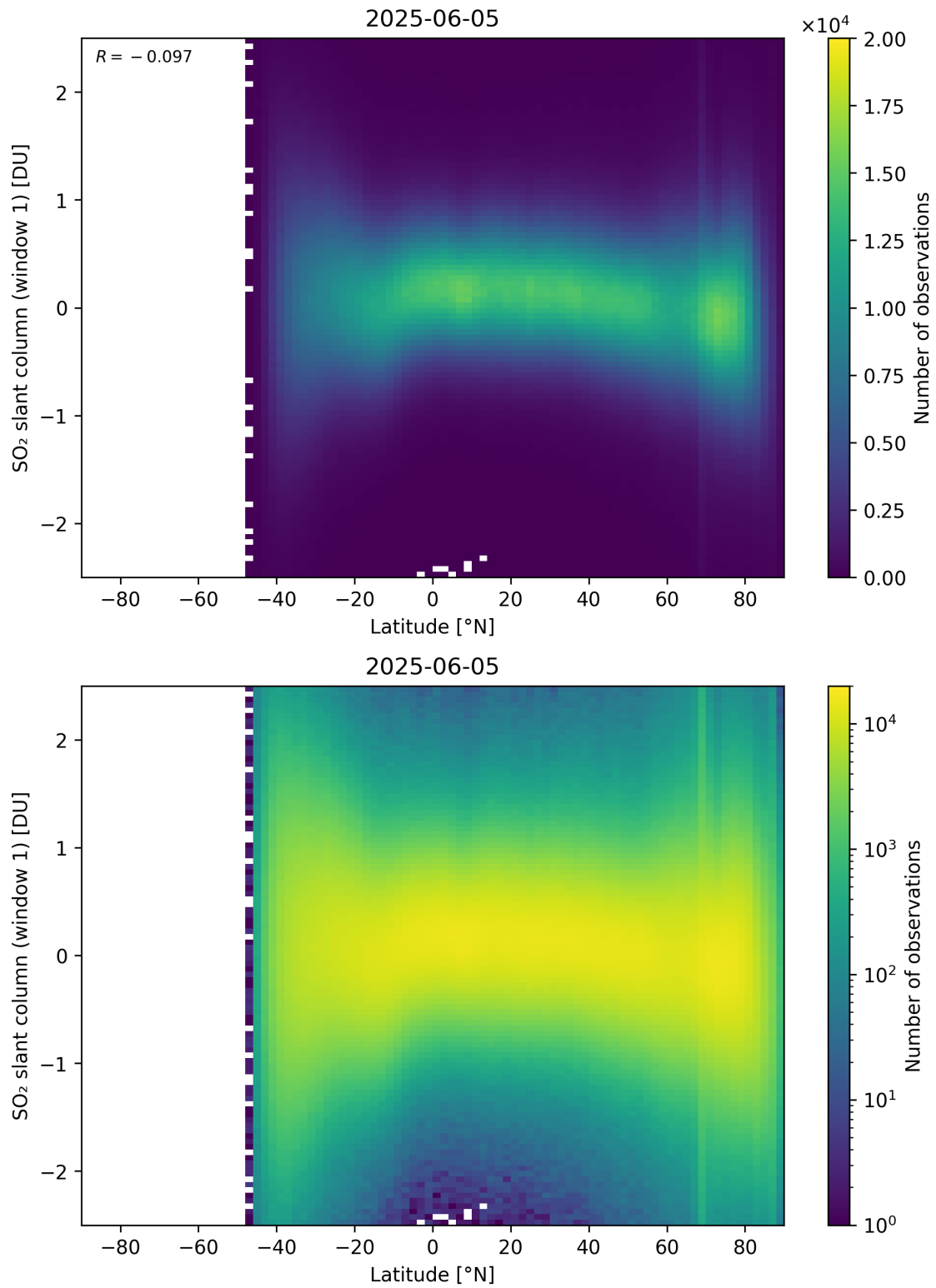
Figure 162: Scatter density plot of “Latitude” against “SO 2 slant column (window 1)” for 2025-06-04 to 2025-06-06.
