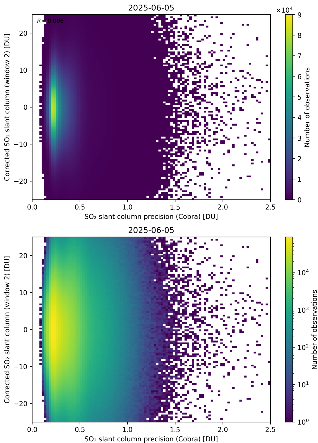
Figure 206: Scatter density plot of “SO 2 slant column precision (Cobra)” against “Corrected SO 2 slant column (window 2)” for 2025-06-04 to 2025-06-06.
