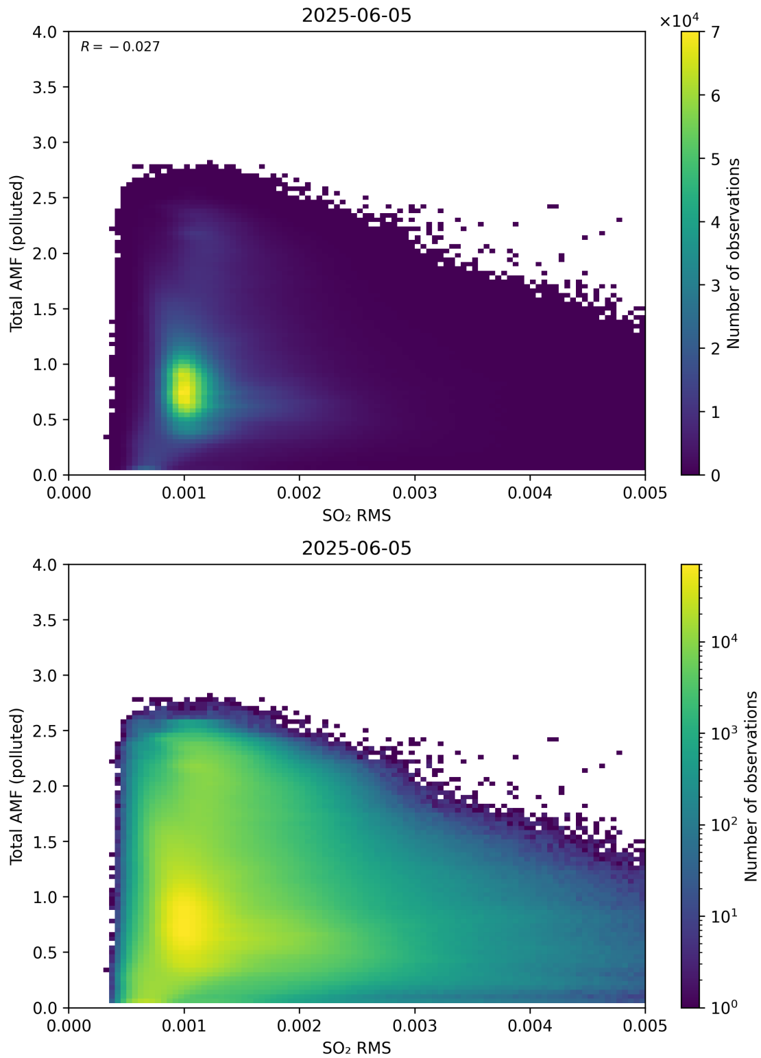
Figure 148: Scatter density plot of “SO 2 RMS” against “Total AMF (polluted)” for 2025-06-04 to 2025-06-06.
