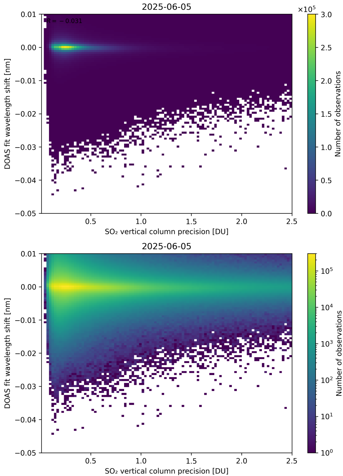
Figure 332: Scatter density plot of “SO 2 vertical column precision” against “DOAS fit wavelength shift” for 2025-06-04 to 2025-06-06.
