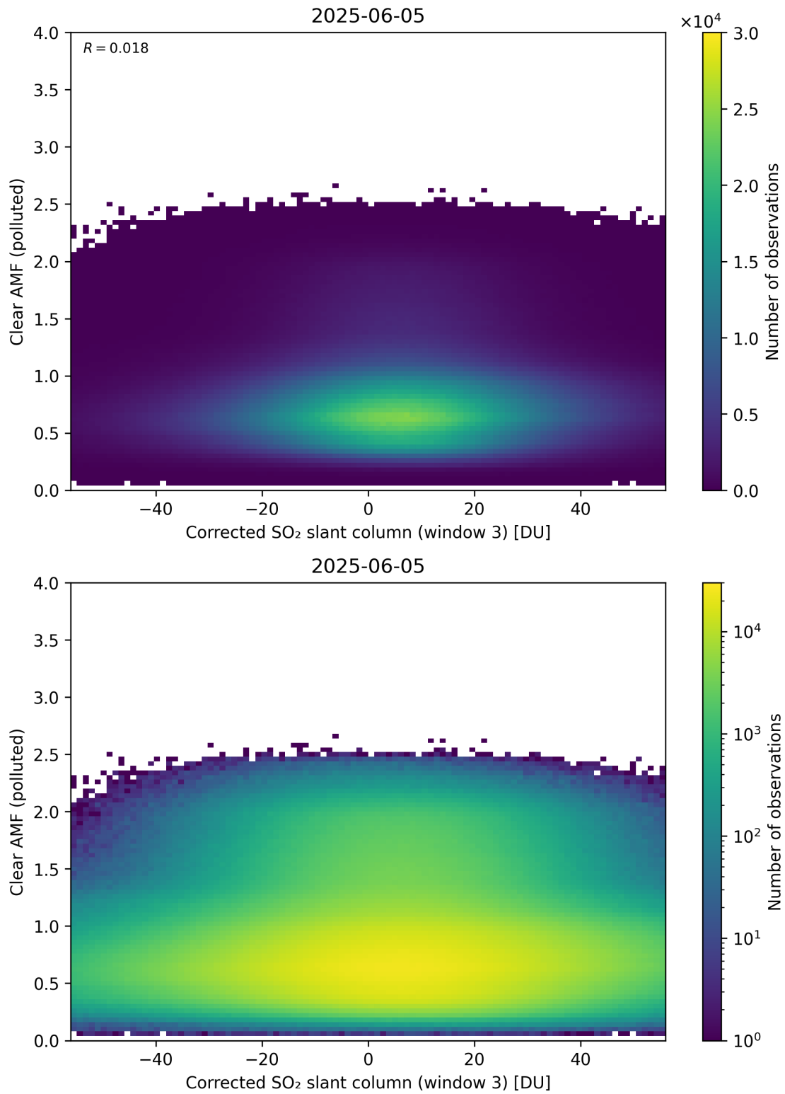
Figure 259: Scatter density plot of “Corrected SO 2 slant column (window 3)” against “Clear AMF (polluted)” for 2025-06-04 to 2025-06-06.
