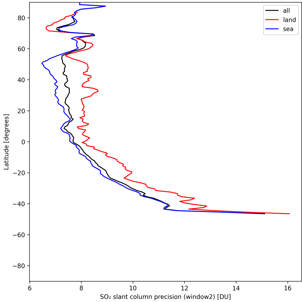
Figure 42: Zonal average of “SO 2 slant column precision (window2)” for 2025-06-04 to 2025-06-06.
