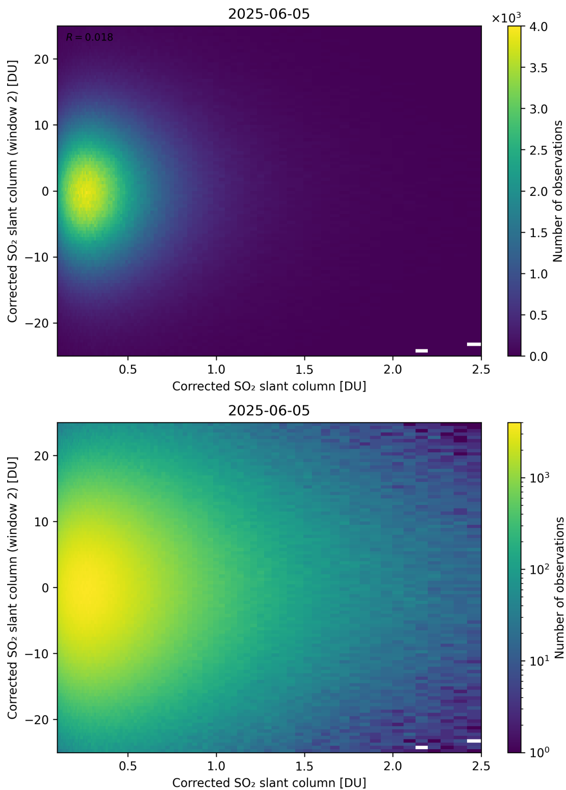
Figure 235: Scatter density plot of “Corrected SO 2 slant column” against “Corrected SO 2 slant column (window 2)” for 2025-06-04 to 2025-06-06.
