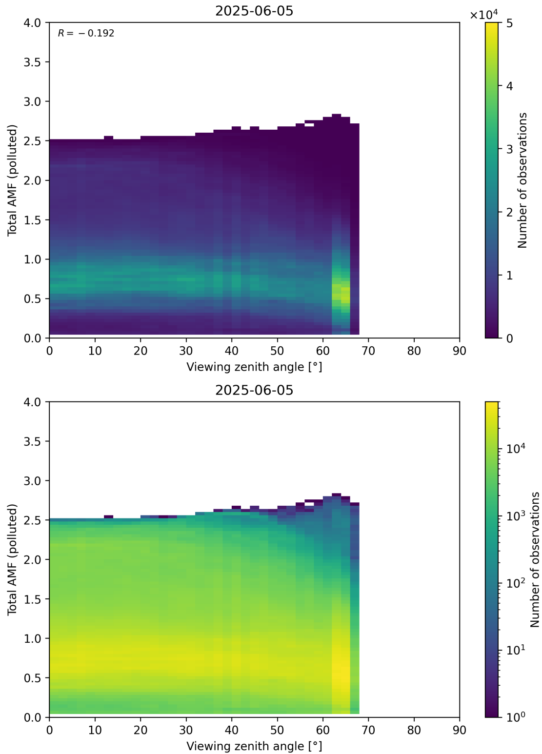
Figure 381: Scatter density plot of “Viewing zenith angle” against “Total AMF (polluted)” for 2025-06-04 to 2025-06-06.
