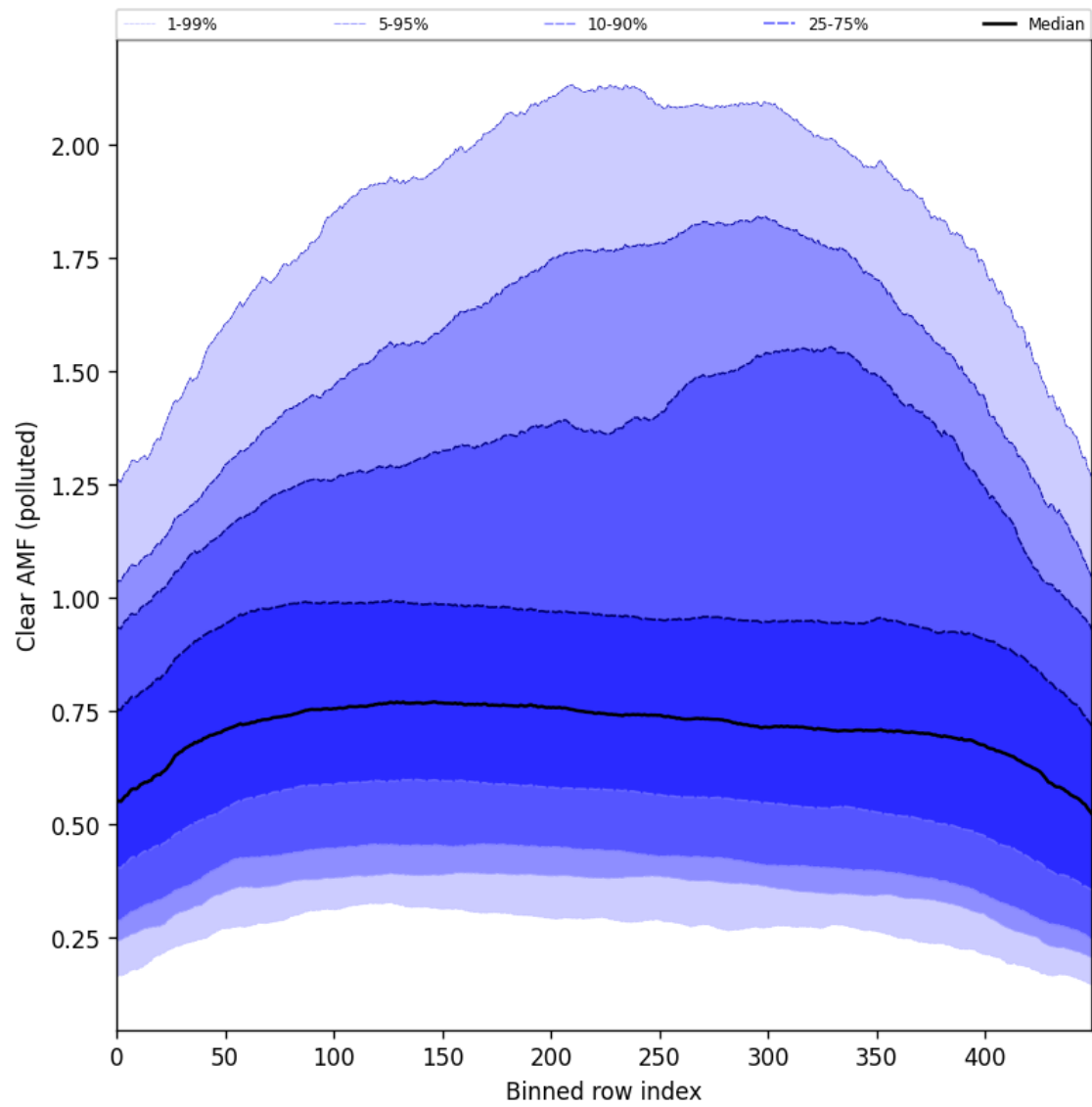
Figure 107: Along track statistics of “Clear AMF (polluted)” for 2025-06-04 to 2025-06-06
