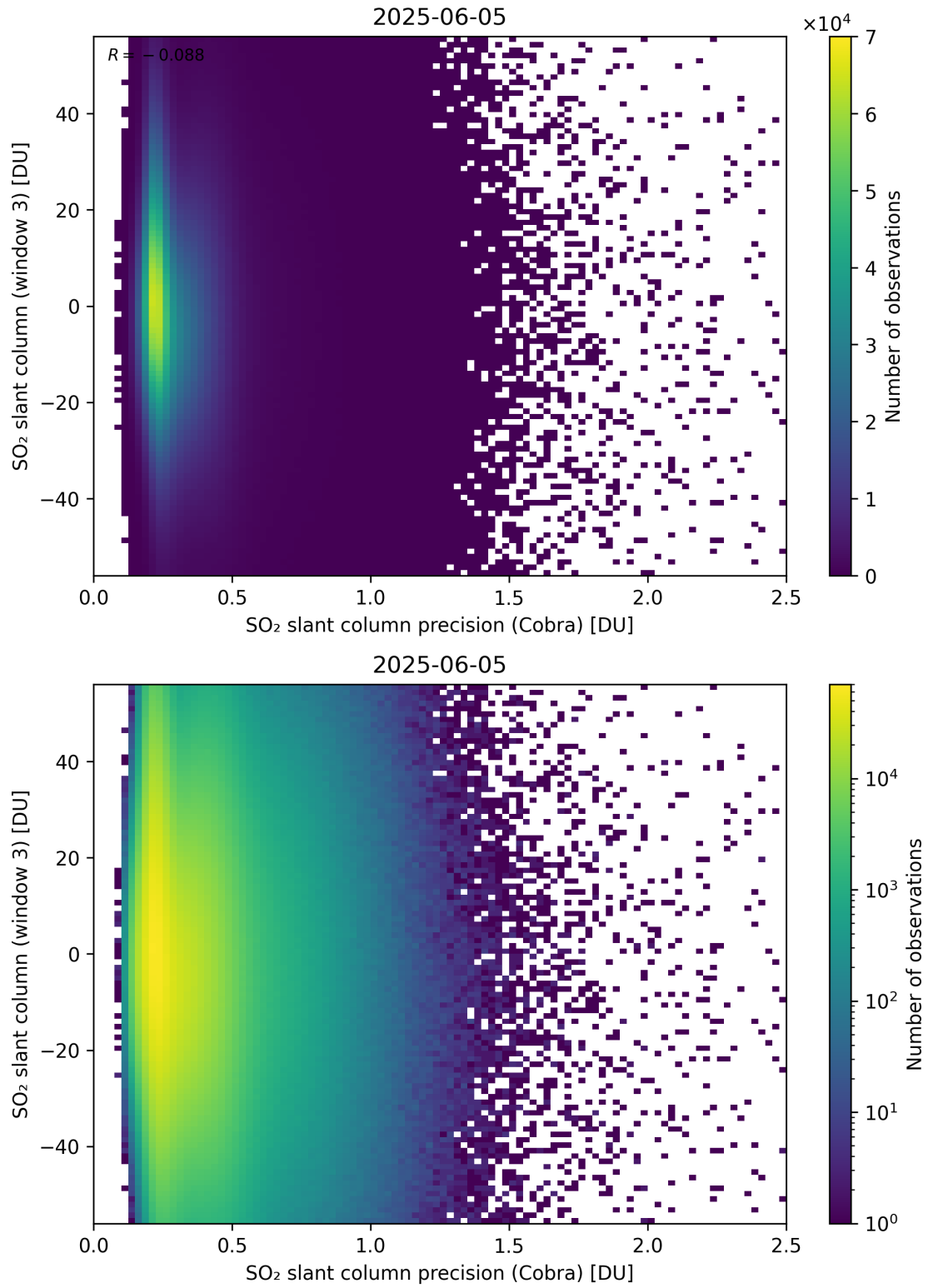
Figure 211: Scatter density plot of “SO 2 slant column precision (Cobra)” against “SO 2 slant column (window 3)” for 2025-06-04 to 2025-06-06.
