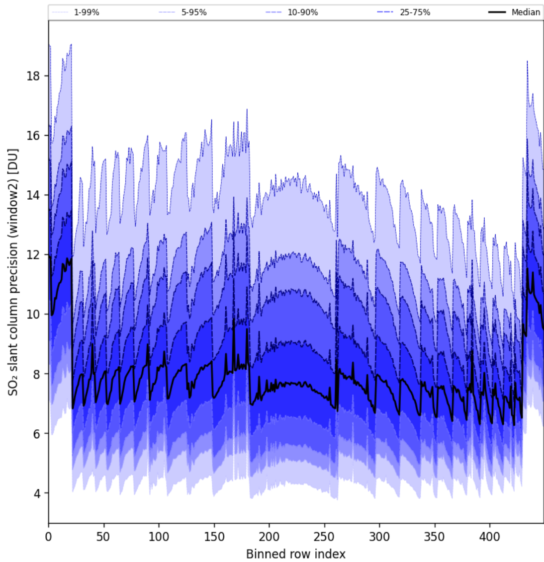
Figure 94: Along track statistics of “SO 2 slant column precision (window2)” for 2025-06-04 to 2025-06-06
