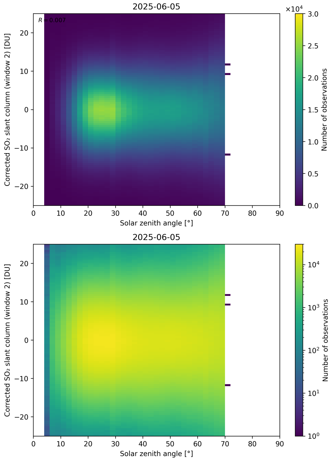
Figure 182: Scatter density plot of “Solar zenith angle” against “Corrected SO 2 slant column (window 2)” for 2025-06-04 to 2025-06-06.
