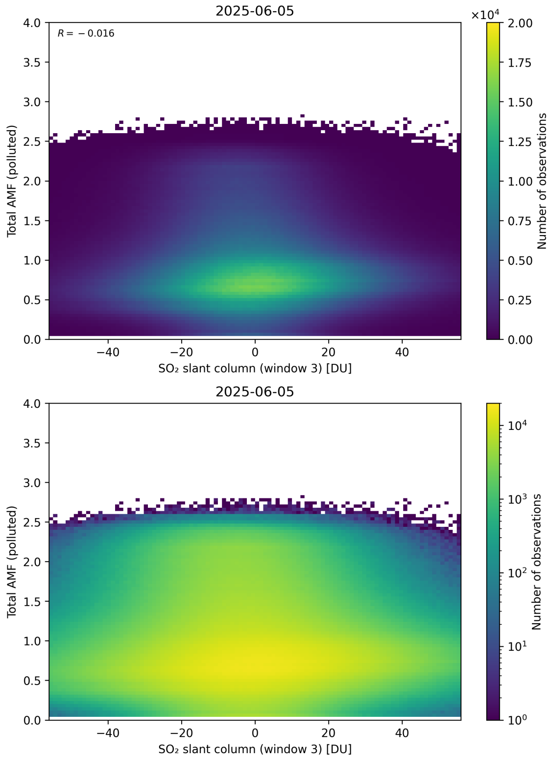
Figure 318: Scatter density plot of “SO 2 slant column (window 3)” against “Total AMF (polluted)” for 2025-06-04 to 2025-06-06.
