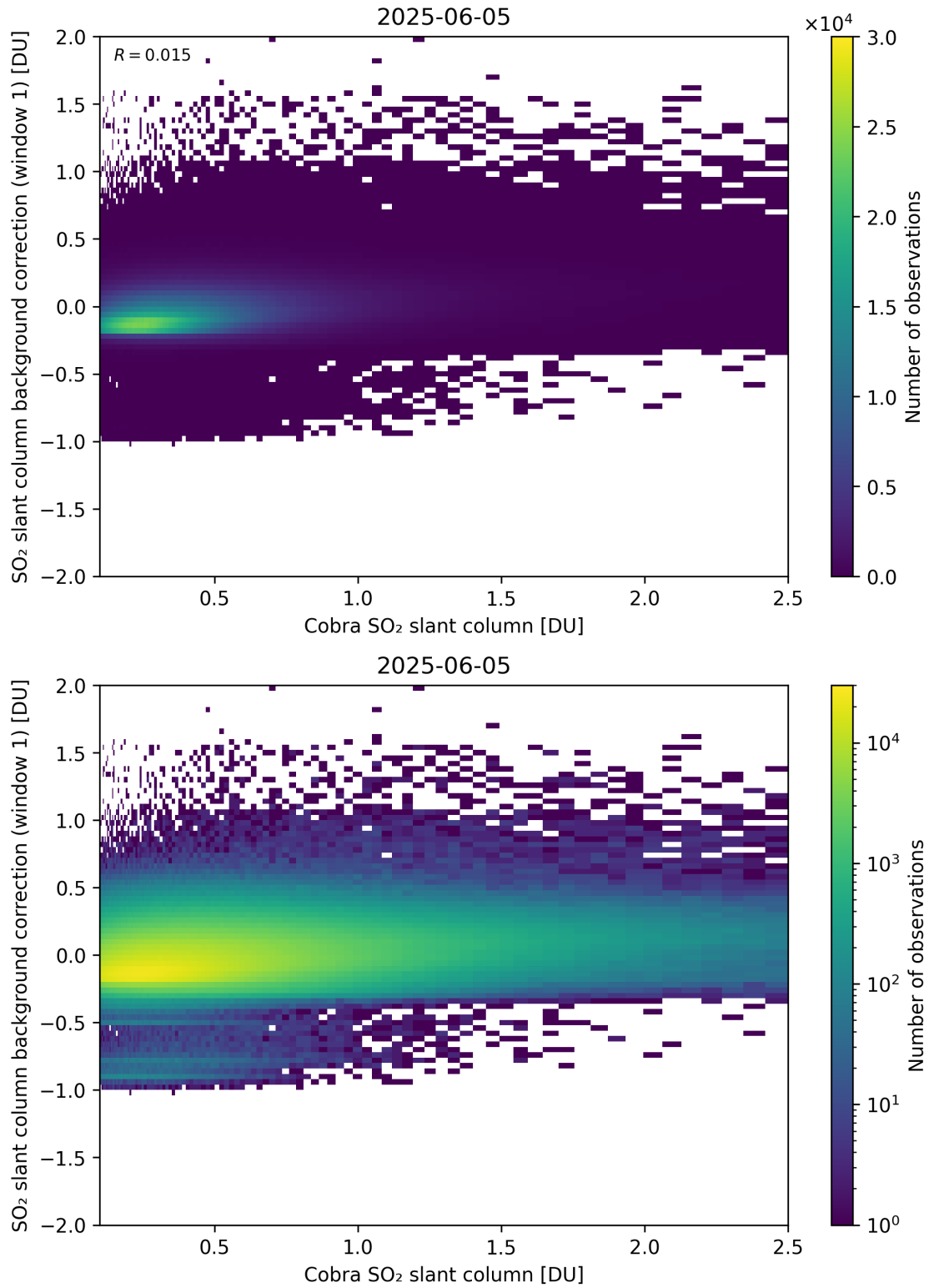
Figure 193: Scatter density plot of “Cobra SO 2 slant column” against “SO 2 slant column background correction (window 1)” for 2025-06-04 to 2025-06-06.
