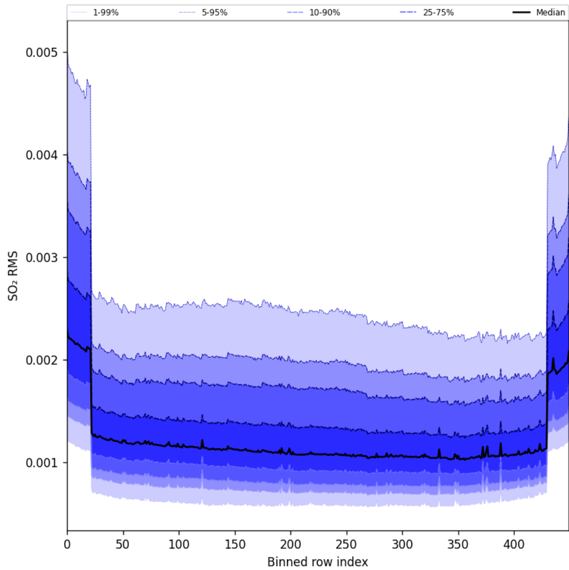
Figure 104: Along track statistics of “SO 2 RMS” for 2025-06-04 to 2025-06-06
