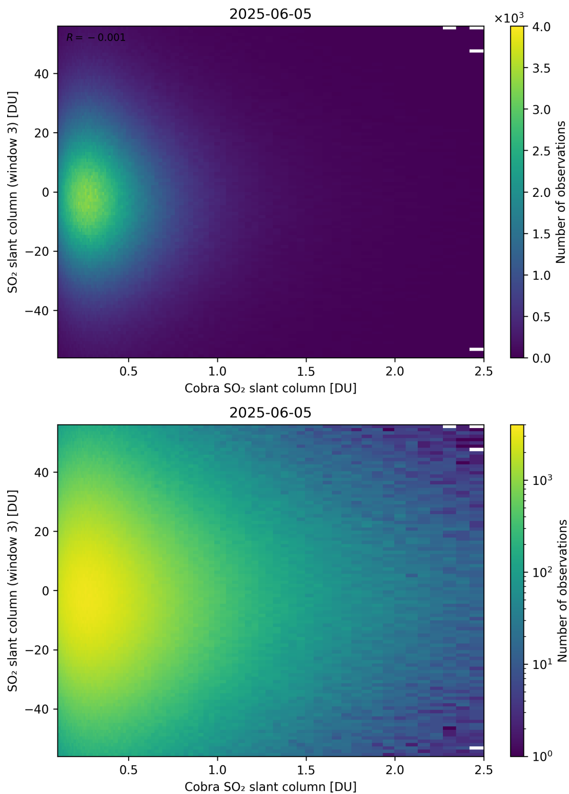
Figure 222: Scatter density plot of “Cobra SO 2 slant column” against “SO 2 slant column (window 3)” for 2025-06-04 to 2025-06-06.
