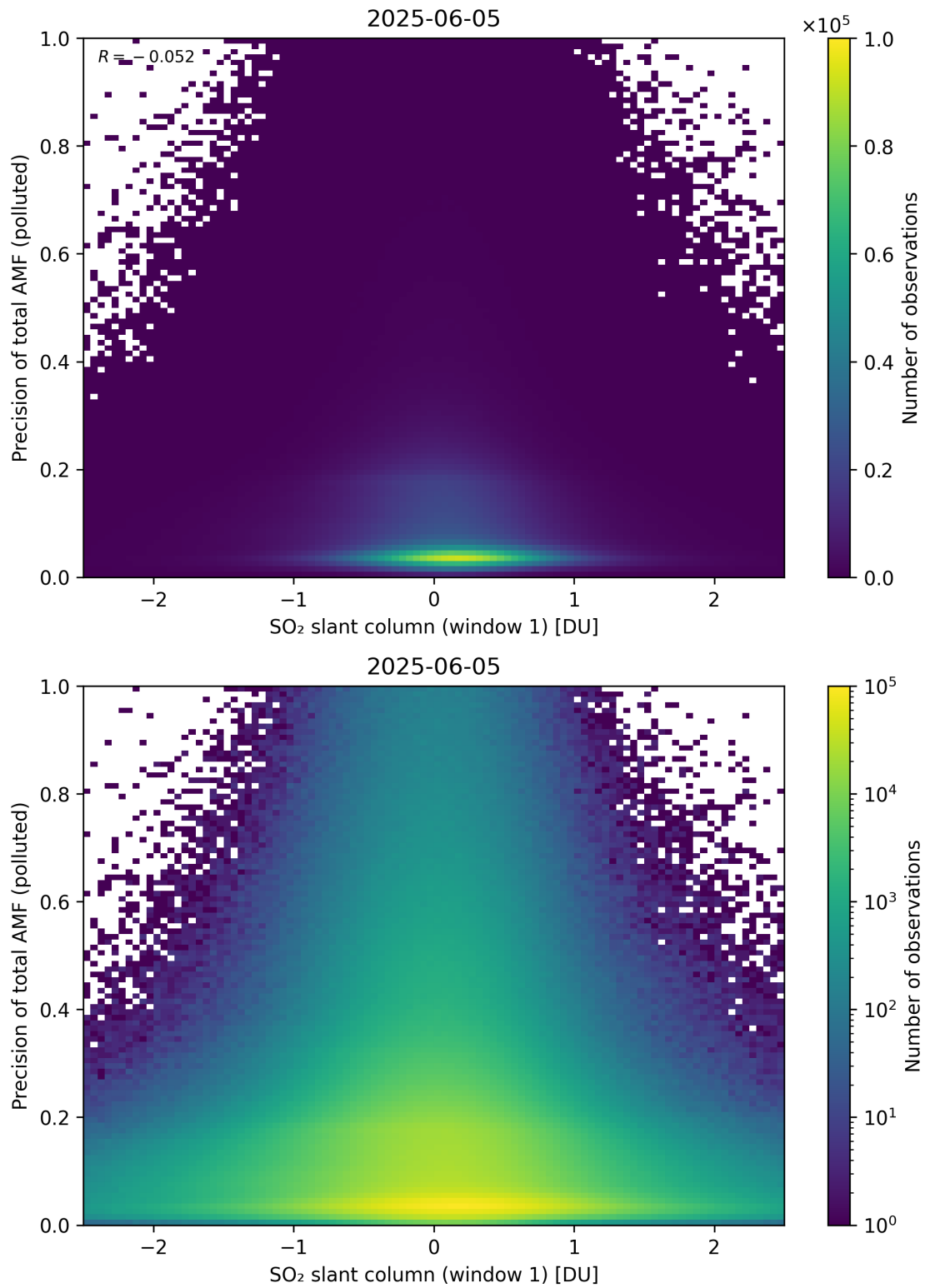
Figure 290: Scatter density plot of “SO 2 slant column (window 1)” against “Precision of total AMF (polluted)” for 2025-06-04 to 2025-06-06.
