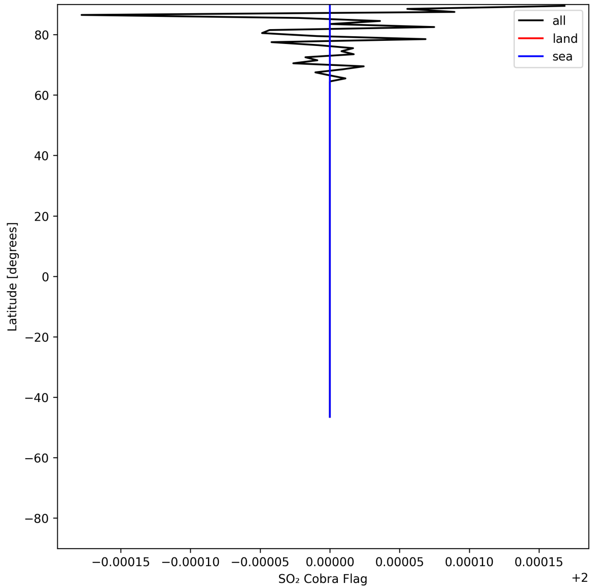
Figure 49: Zonal average of “SO 2 Cobra Flag” for 2025-06-04 to 2025-06-06.
