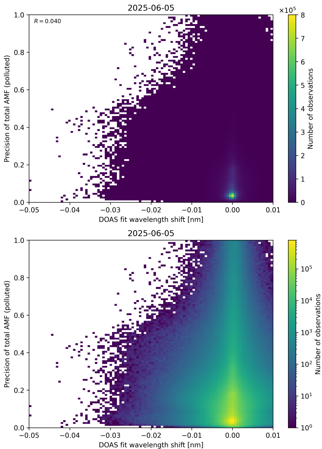
Figure 142: Scatter density plot of “DOAS fit wavelength shift” against “Precision of total AMF (polluted)” for 2025-06-04 to 2025-06-06.
