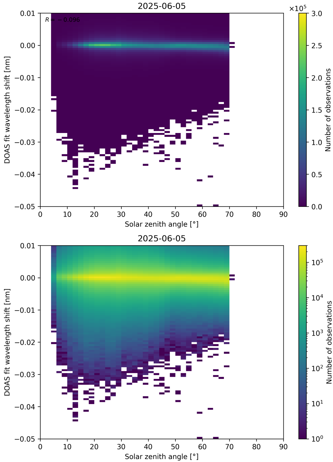
Figure 174: Scatter density plot of “Solar zenith angle” against “DOAS fit wavelength shift” for 2025-06-04 to 2025-06-06.
