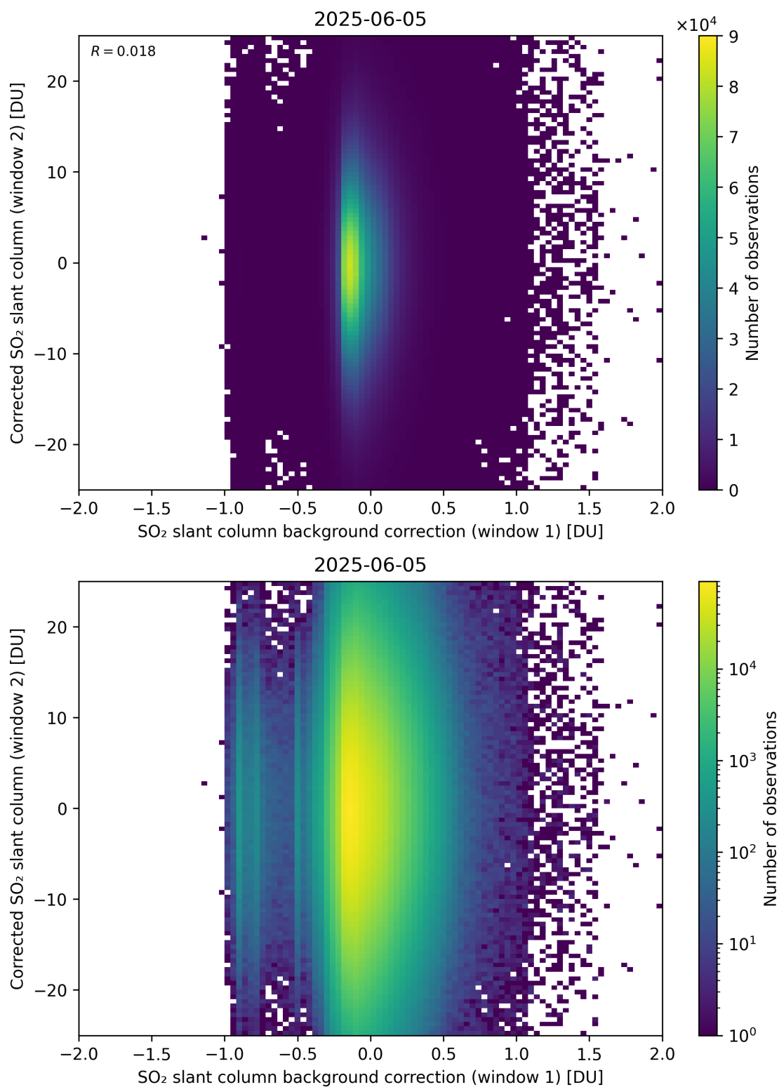
Figure 115: Scatter density plot of “SO 2 slant column background correction (window 1)” against “Corrected SO 2 slant column (window 2)” for 2025-06-04 to 2025-06-06.
