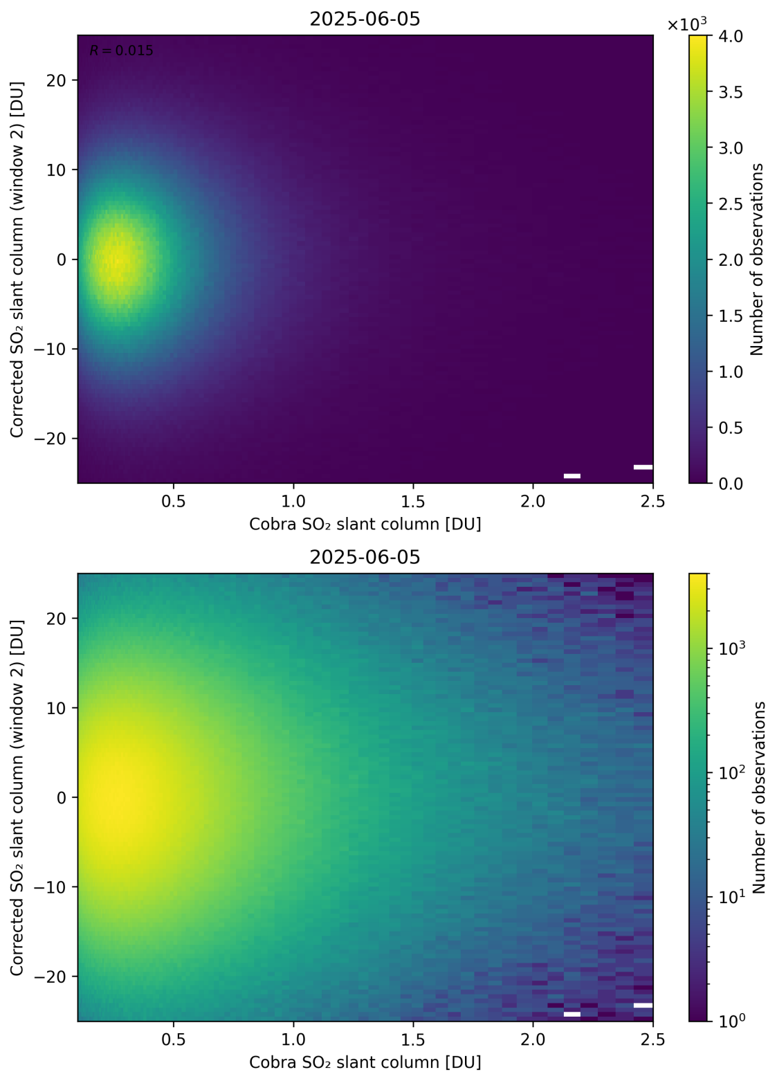
Figure 217: Scatter density plot of “Cobra SO 2 slant column” against “Corrected SO 2 slant column (window 2)” for 2025-06-04 to 2025-06-06.
