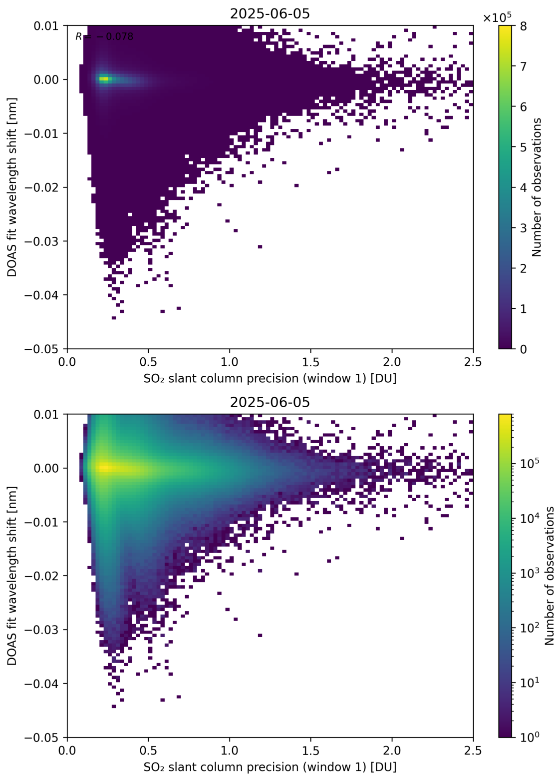
Figure 271: Scatter density plot of “SO 2 slant column precision (window 1)” against “DOAS fit wavelength shift” for 2025-06-04 to 2025-06-06.
