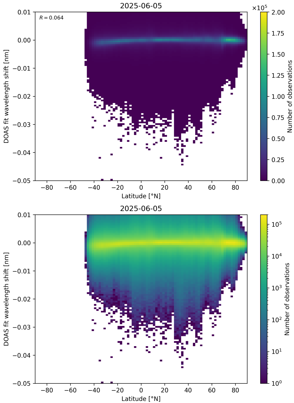
Figure 153: Scatter density plot of “Latitude” against “DOAS fit wavelength shift” for 2025-06-04 to 2025-06-06.
