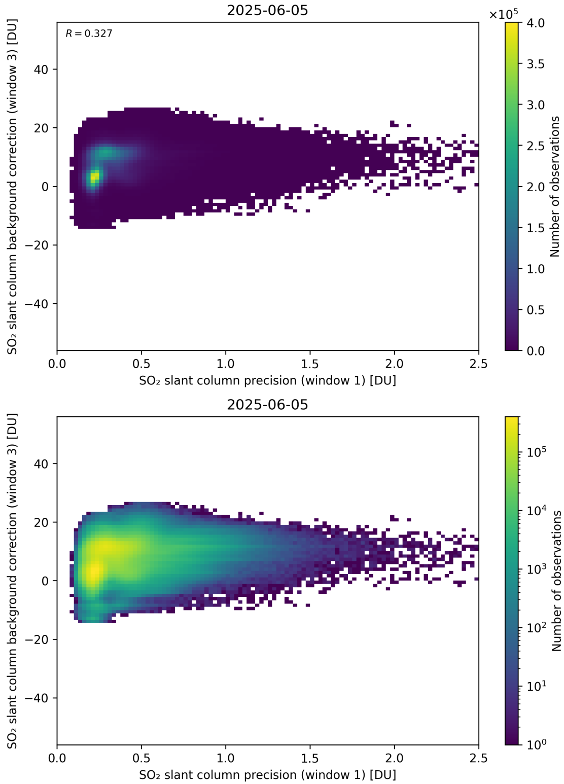
Figure 270: Scatter density plot of “SO 2 slant column precision (window 1)” against “SO 2 slant column background correction (window 3)” for 2025-06-04 to 2025-06-06.
