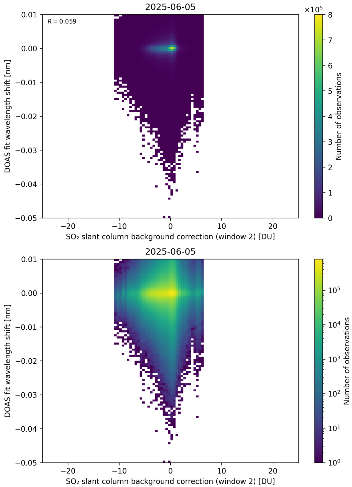
Figure 123: Scatter density plot of “SO 2 slant column background correction (window 2)” against “DOAS fit wavelength shift” for 2025-06-04 to 2025-06-06.
