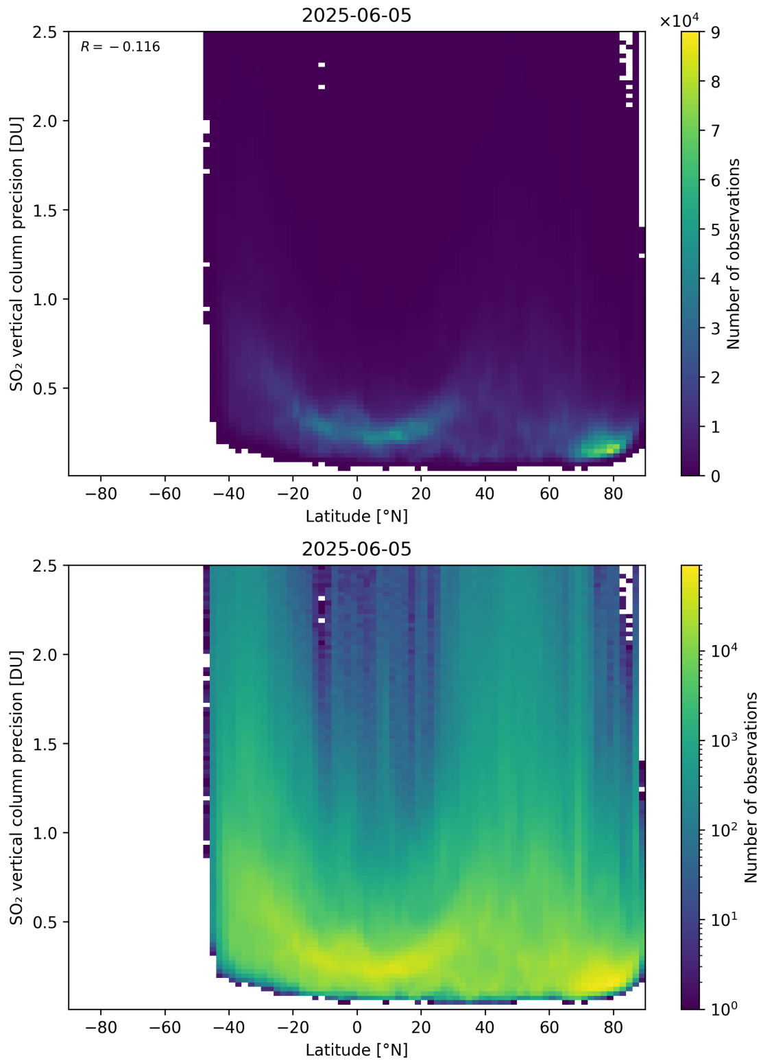
Figure 170: Scatter density plot of “Latitude” against “SO 2 vertical column precision” for 2025-06-04 to 2025-06-06.
