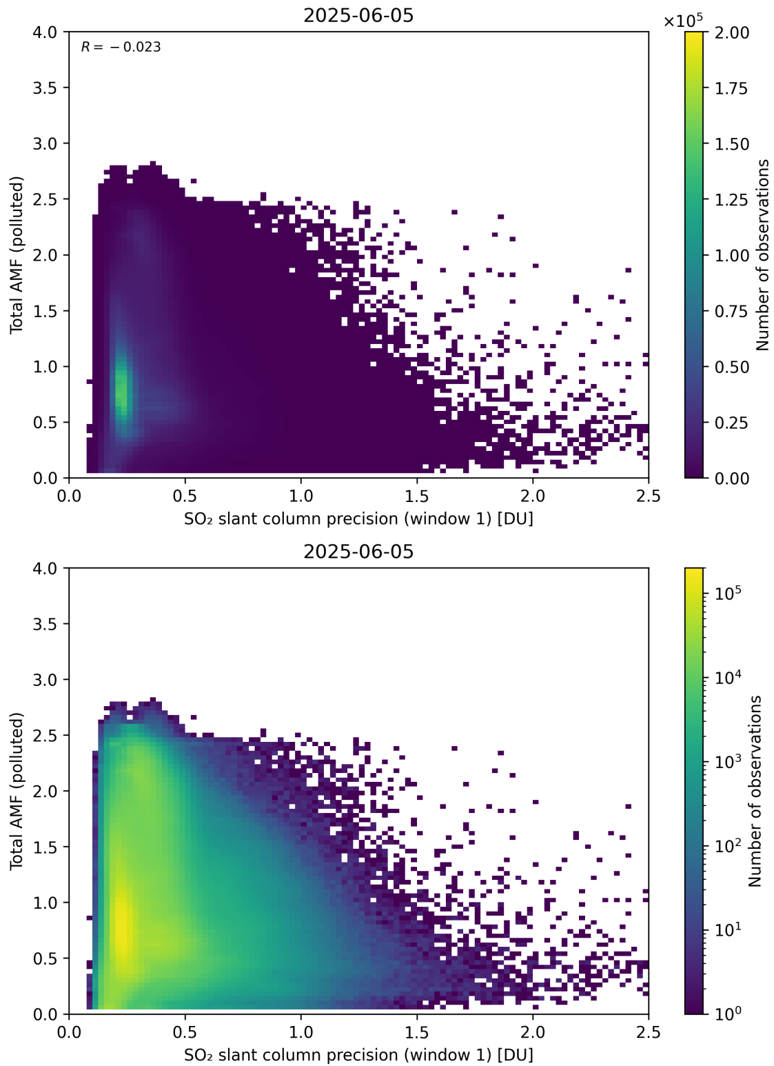
Figure 280: Scatter density plot of “SO 2 slant column precision (window 1)” against “Total AMF (polluted)” for 2025-06-04 to 2025-06-06.
