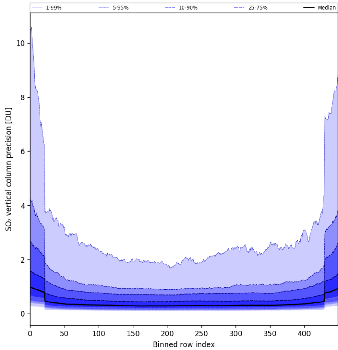
Figure 85: Along track statistics of “SO 2 vertical column precision” for 2025-06-04 to 2025-06-06
