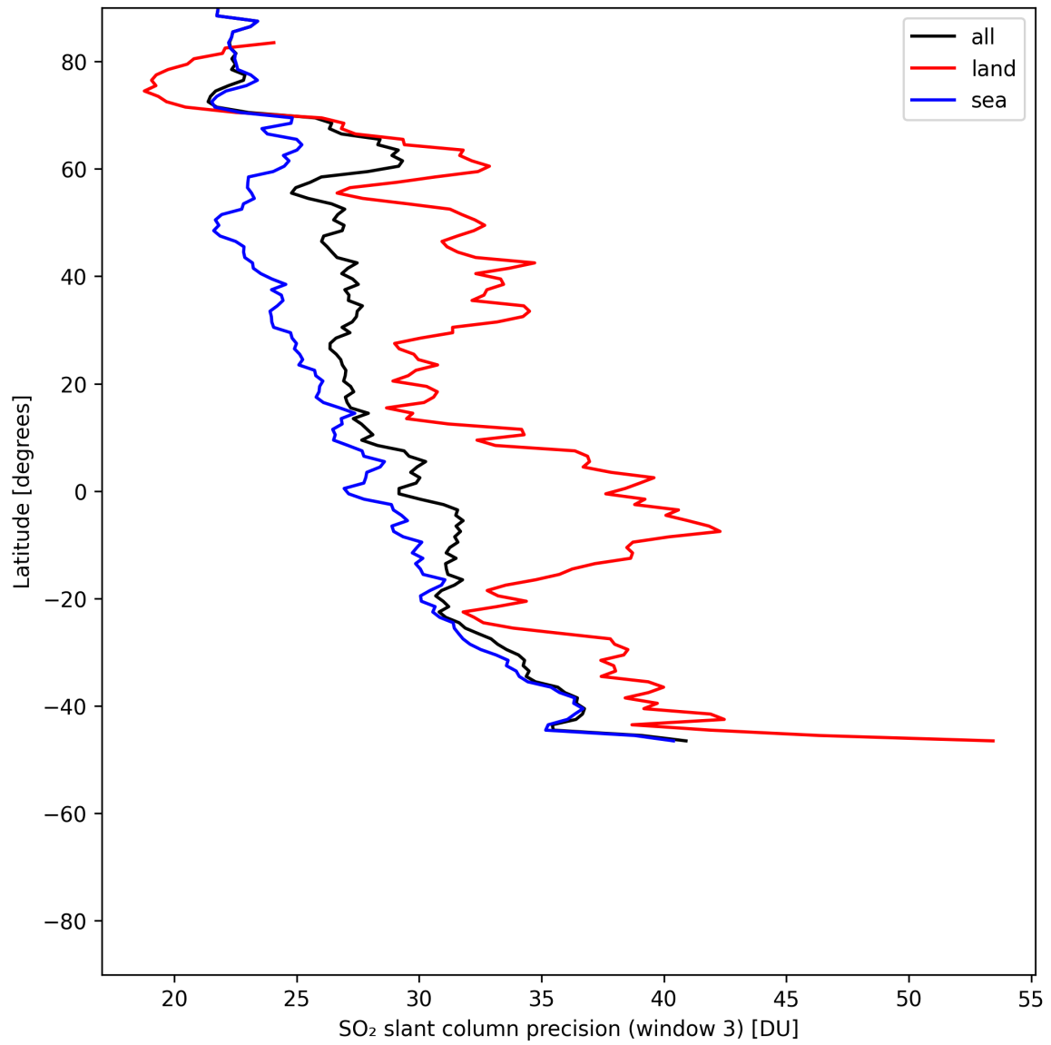
Figure 46: Zonal average of “SO 2 slant column precision (window 3)” for 2025-06-04 to 2025-06-06.
