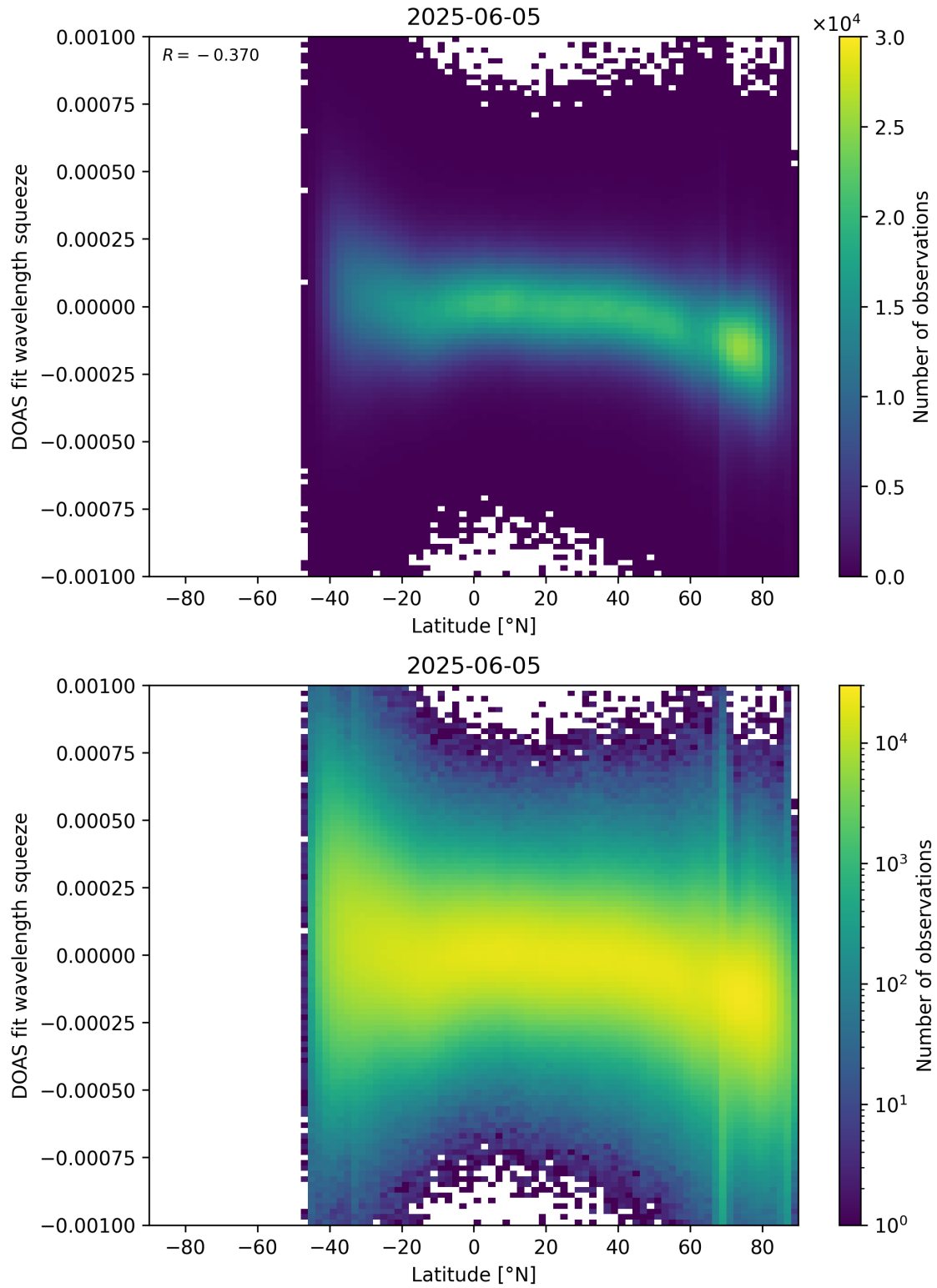
Figure 154: Scatter density plot of “Latitude” against “DOAS fit wavelength squeeze” for 2025-06-04 to 2025-06-06.
