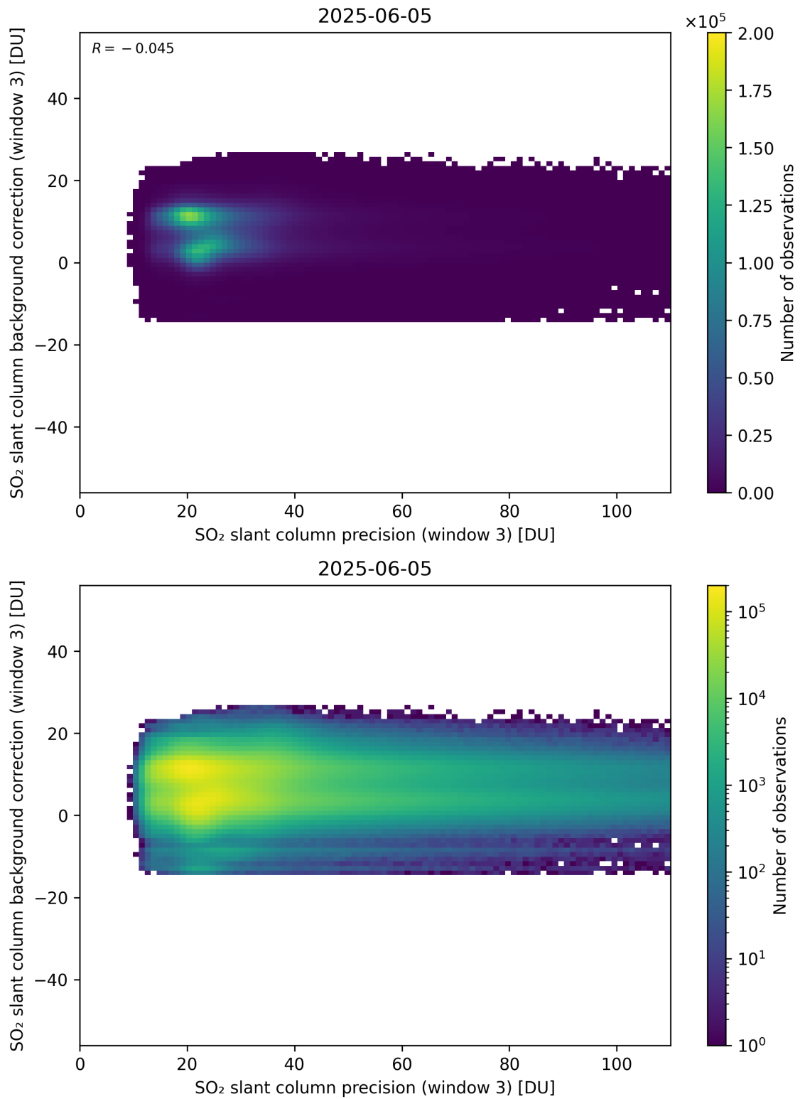
Figure 307: Scatter density plot of “SO 2 slant column precision (window 3)” against “SO 2 slant column background correction (window 3)” for 2025-06-04 to 2025-06-06.
