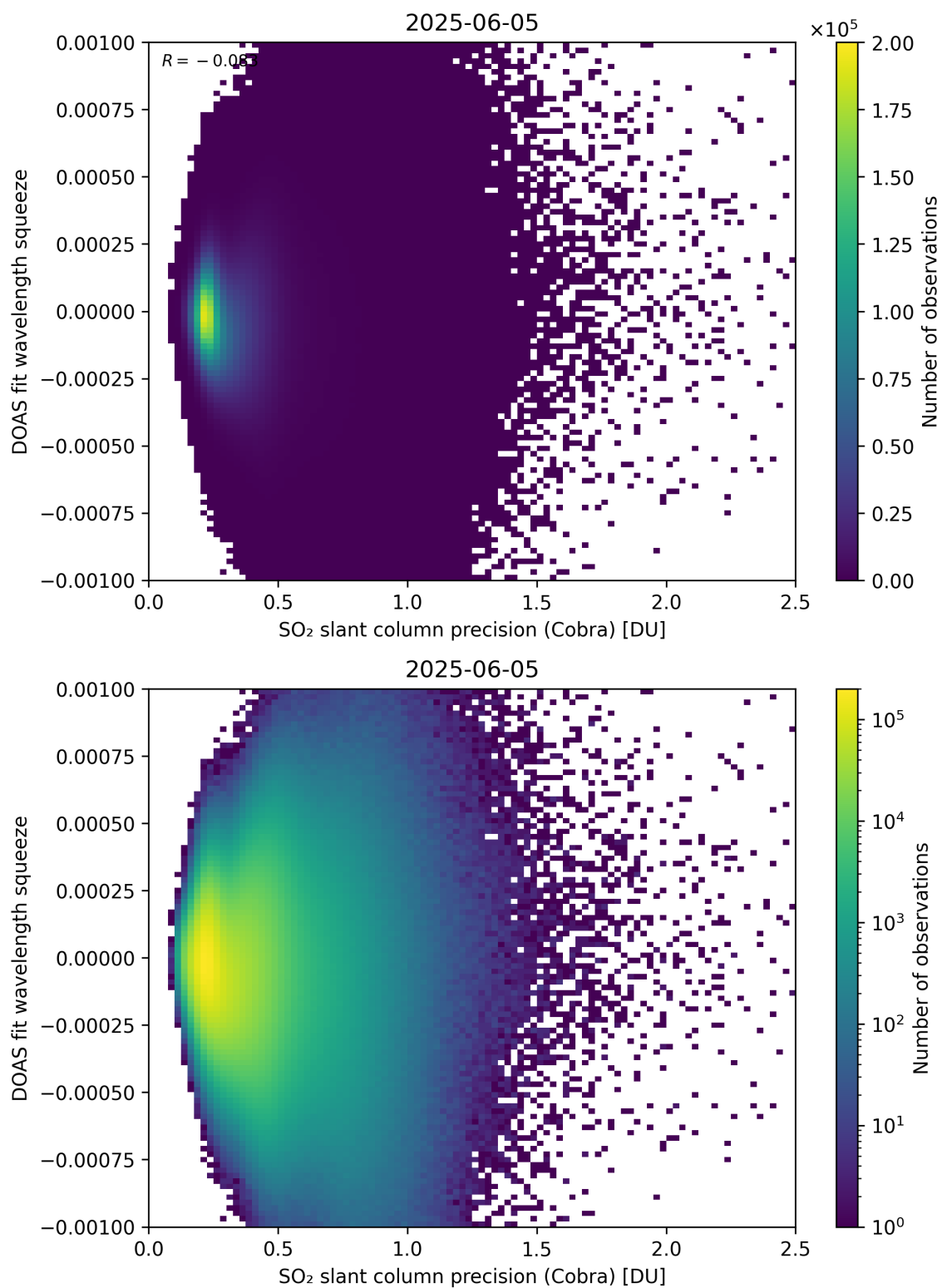
Figure 203: Scatter density plot of “SO 2 slant column precision (Cobra)” against “DOAS fit wavelength squeeze” for 2025-06-04 to 2025-06-06.
