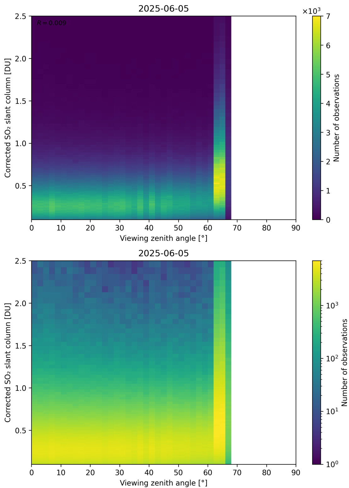
Figure 373: Scatter density plot of “Viewing zenith angle” against “Corrected SO 2 slant column” for 2025-06-04 to 2025-06-06.
