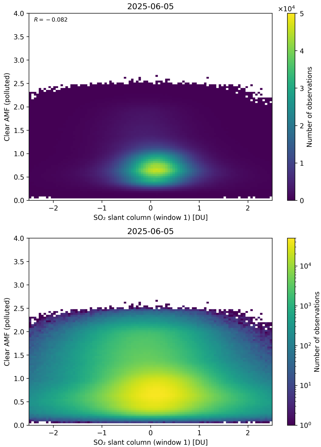
Figure 282: Scatter density plot of “SO 2 slant column (window 1)” against “Clear AMF (polluted)” for 2025-06-04 to 2025-06-06.
