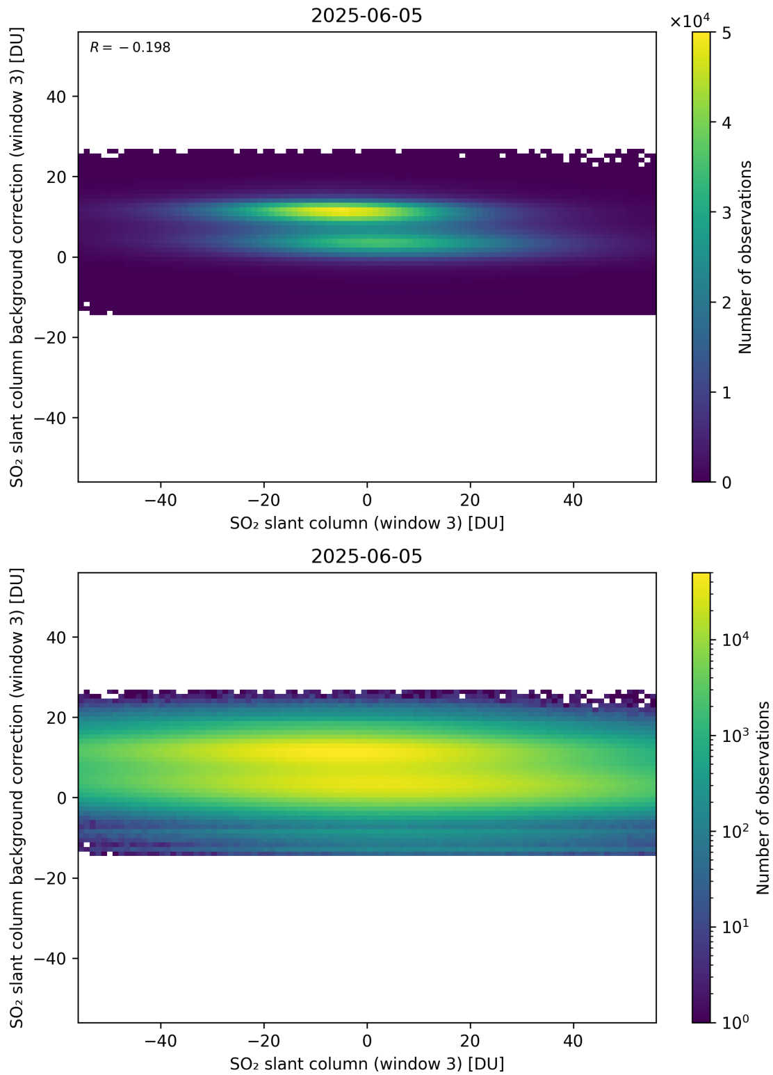
Figure 303: Scatter density plot of “SO 2 slant column (window 3)” against “SO 2 slant column background correction (window 3)” for 2025-06-04 to 2025-06-06.
