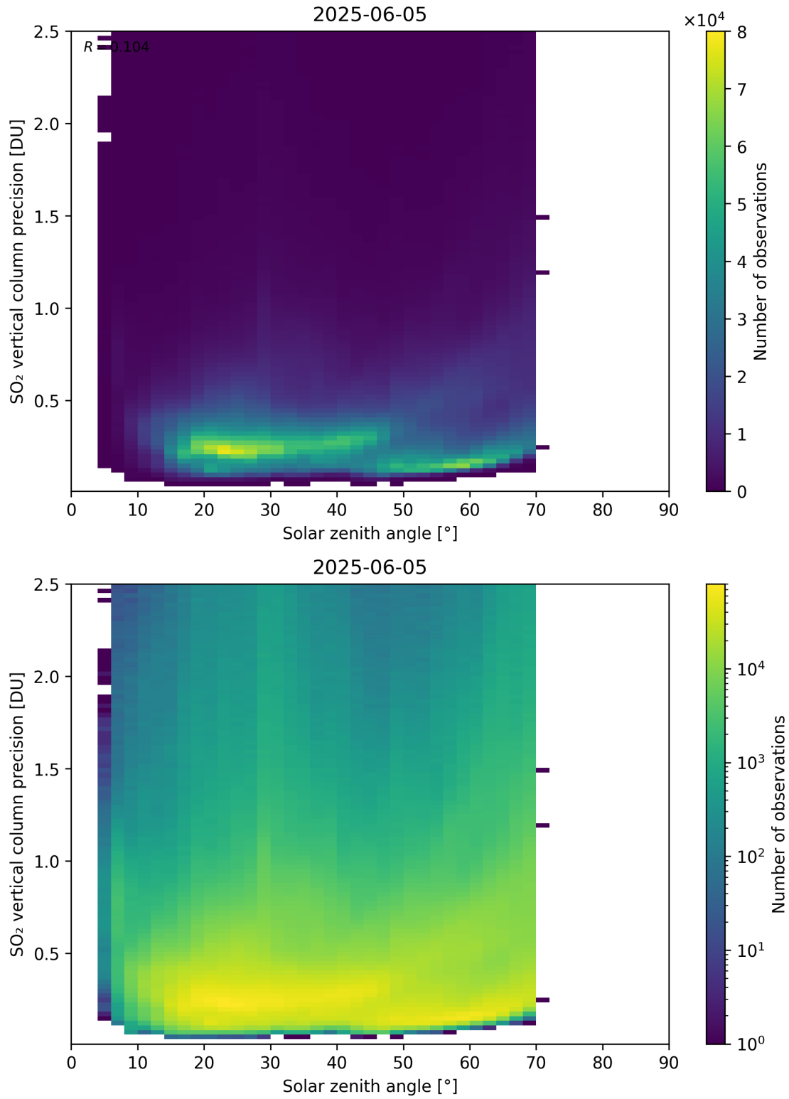
Figure 192: Scatter density plot of “Solar zenith angle” against “SO 2 vertical column precision” for 2025-06-04 to 2025-06-06.
