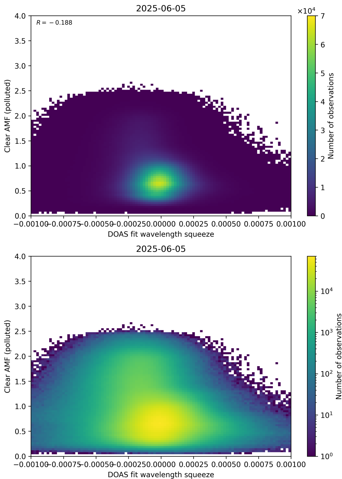
Figure 144: Scatter density plot of “DOAS fit wavelength squeeze” against “Clear AMF (polluted)” for 2025-06-04 to 2025-06-06.
