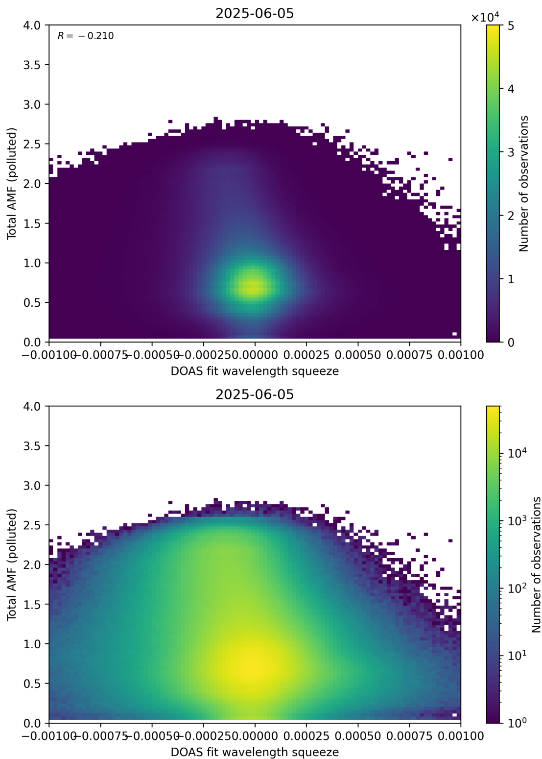
Figure 145: Scatter density plot of “DOAS fit wavelength squeeze” against “Total AMF (polluted)” for 2025-06-04 to 2025-06-06.
