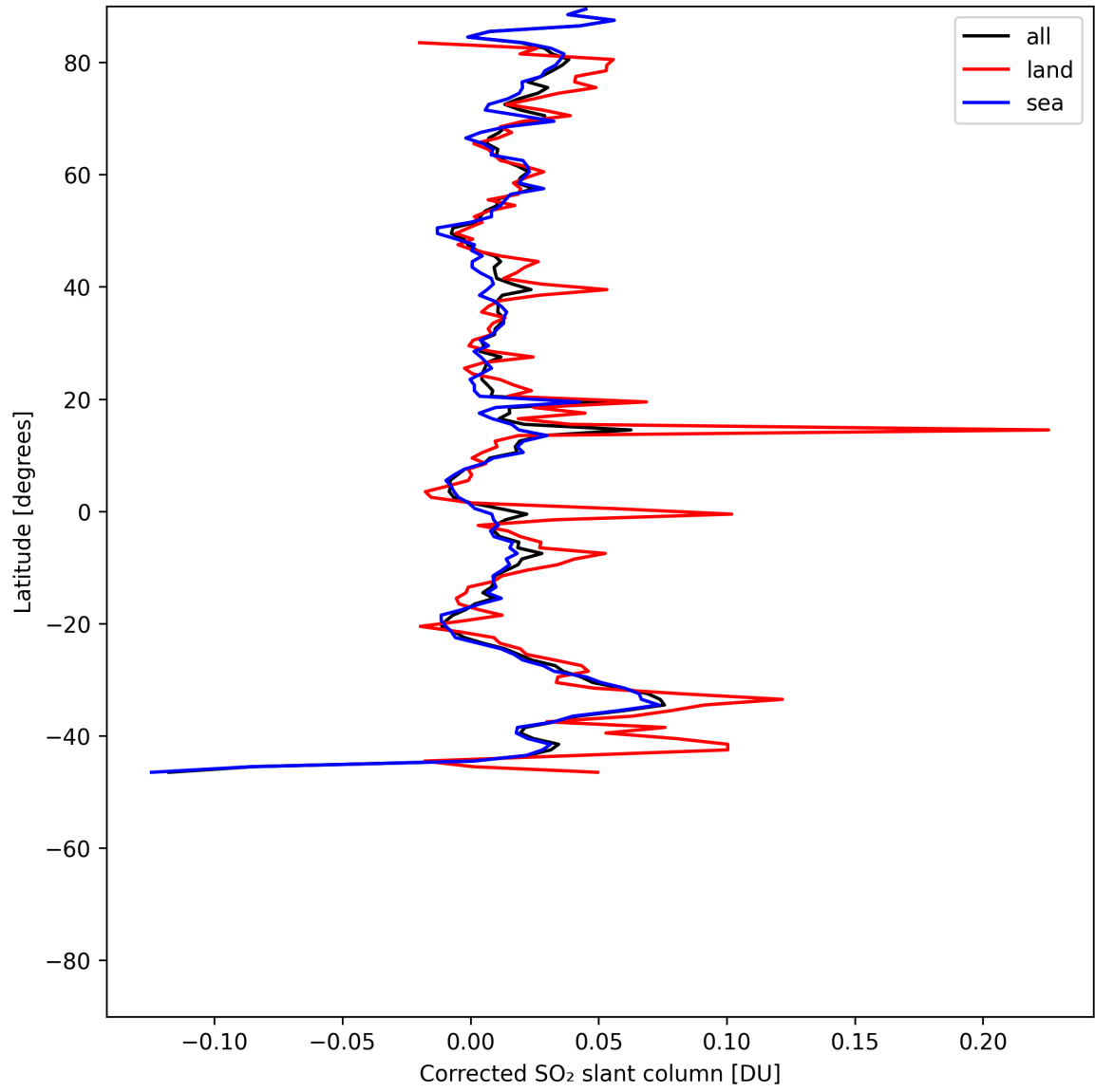
Figure 34: Zonal average of “Corrected SO 2 slant column” for 2025-06-04 to 2025-06-06.
