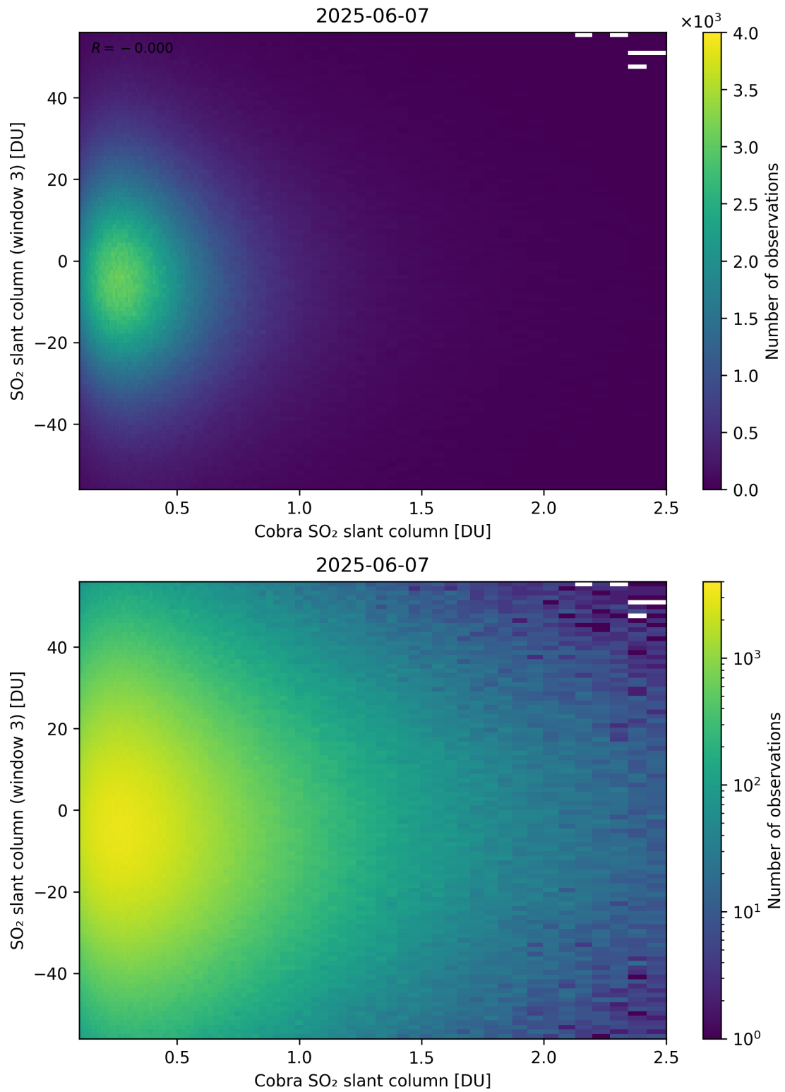
Figure 222: Scatter density plot of “Cobra SO 2 slant column” against “SO 2 slant column (window 3)” for 2025-06-06 to 2025-06-08.
