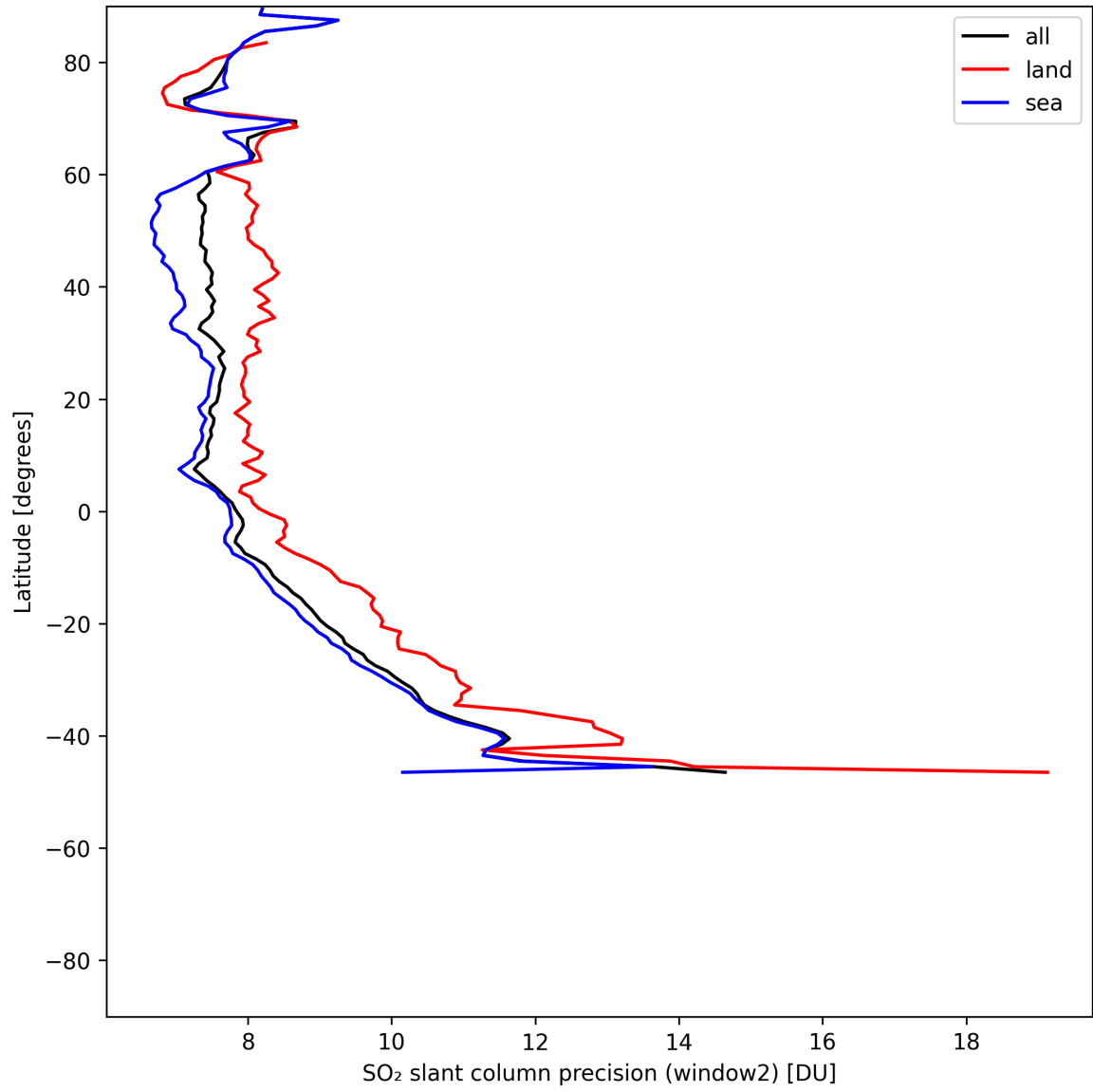
Figure 42: Zonal average of “SO 2 slant column precision (window2)” for 2025-06-06 to 2025-06-08.
