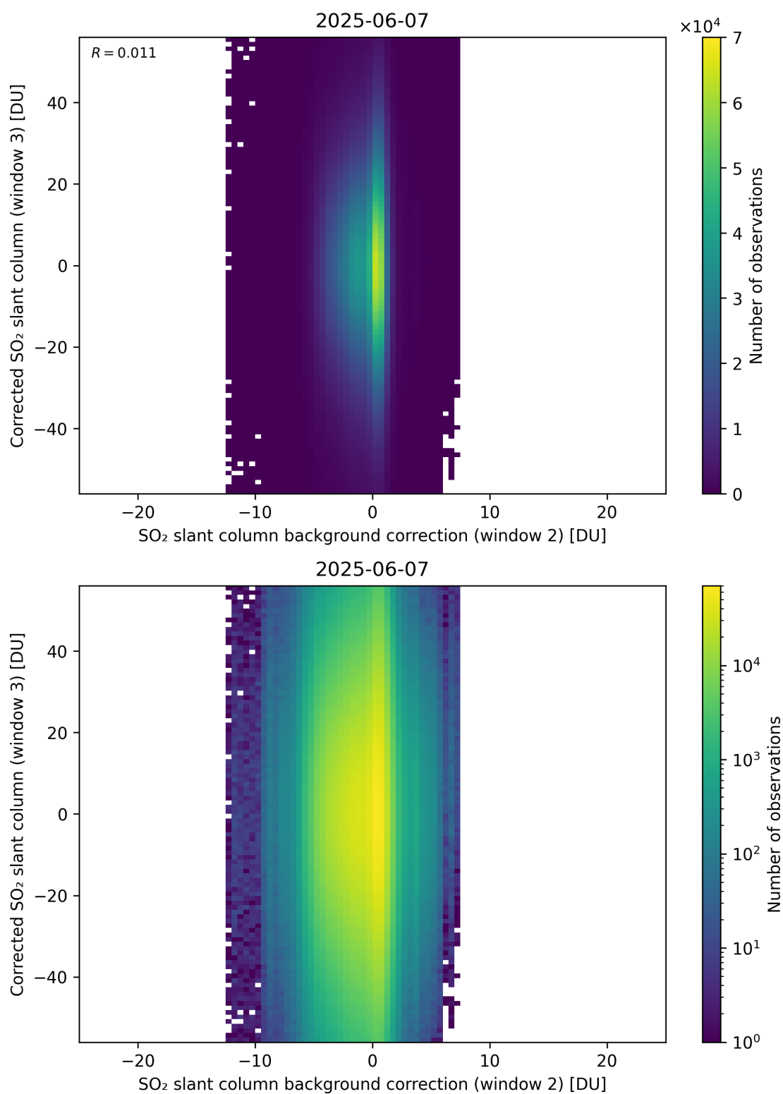
Figure 127: Scatter density plot of “SO 2 slant column background correction (window 2)” against “Corrected SO 2 slant column (window 3)” for 2025-06-06 to 2025-06-08.
