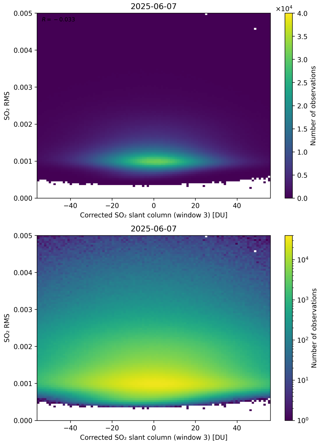
Figure 258: Scatter density plot of “Corrected SO 2 slant column (window 3)” against “SO 2 RMS” for 2025-06-06 to 2025-06-08.
