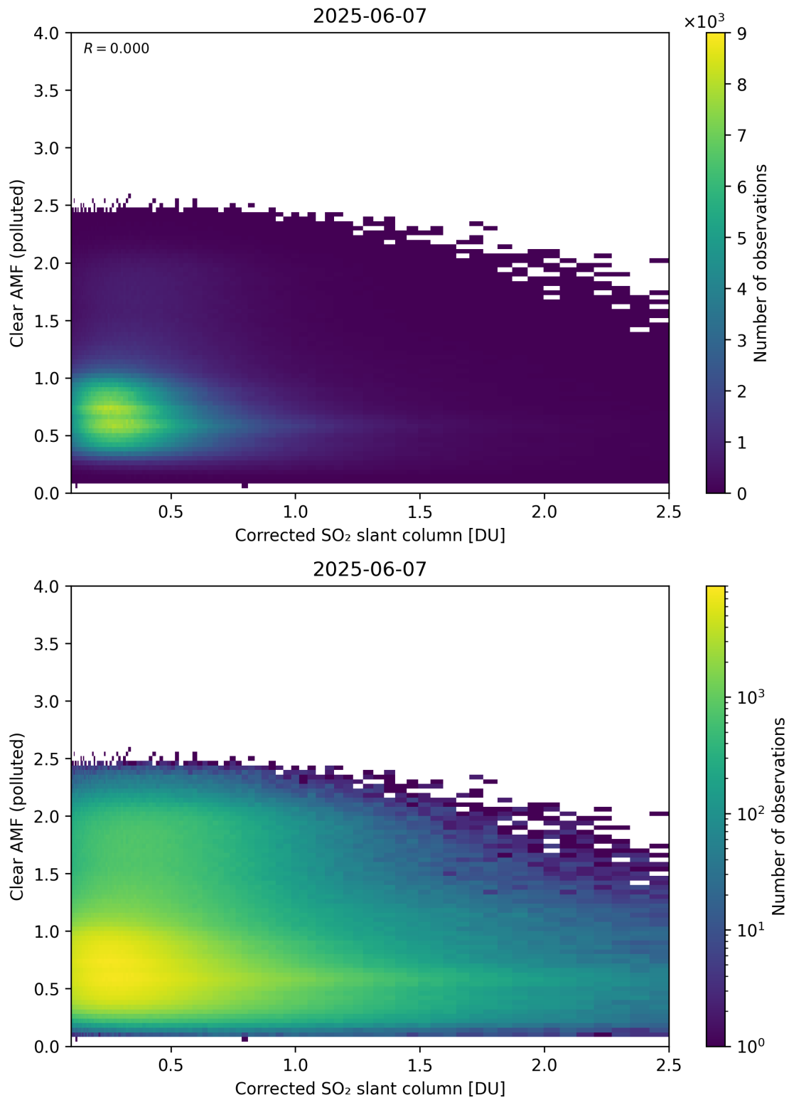
Figure 232: Scatter density plot of “Corrected SO 2 slant column” against “Clear AMF (polluted)” for 2025-06-06 to 2025-06-08.
