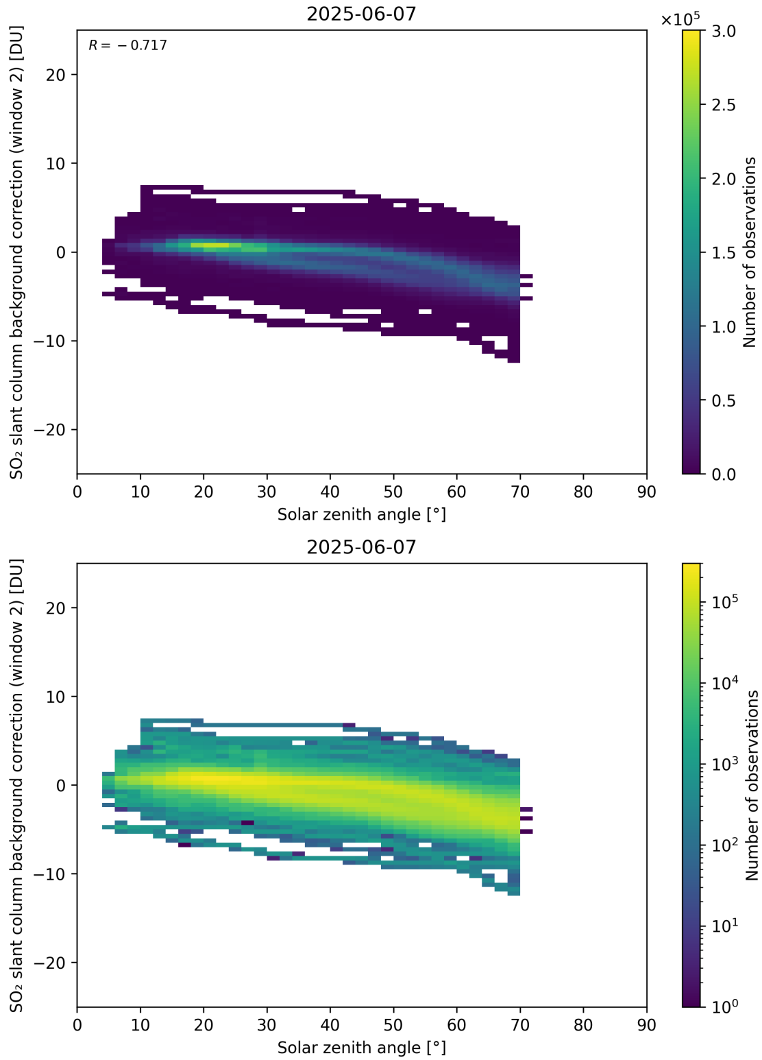
Figure 172: Scatter density plot of “Solar zenith angle” against “SO 2 slant column background correction (window 2)” for 2025-06-06 to 2025-06-08.
