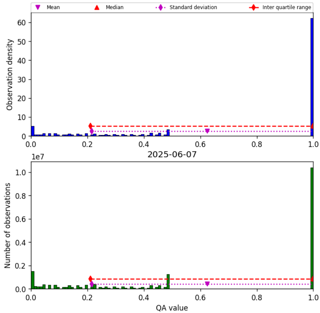
Figure 57: Histogram of “QA value” for 2025-06-06 to 2025-06-08
