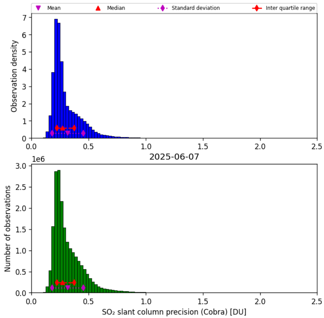
Figure 62: Histogram of “SO 2 slant column precision (Cobra)” for 2025-06-06 to 2025-06-08
