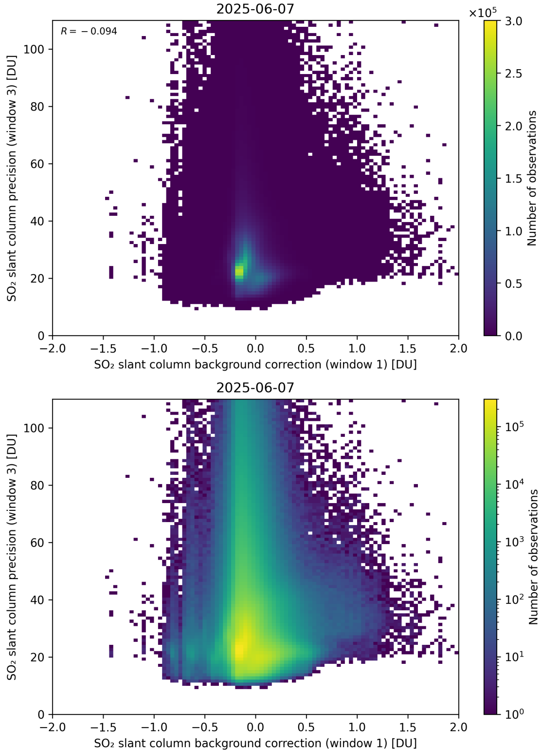
Figure 119: Scatter density plot of “SO 2 slant column background correction (window 1)” against “SO 2 slant column precision (window 3)” for 2025-06-06 to 2025-06-08.
