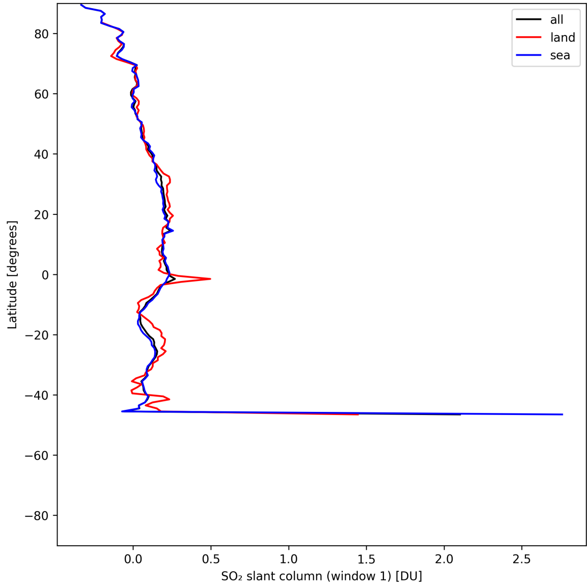
Figure 37: Zonal average of “SO 2 slant column (window 1)” for 2025-06-06 to 2025-06-08.
