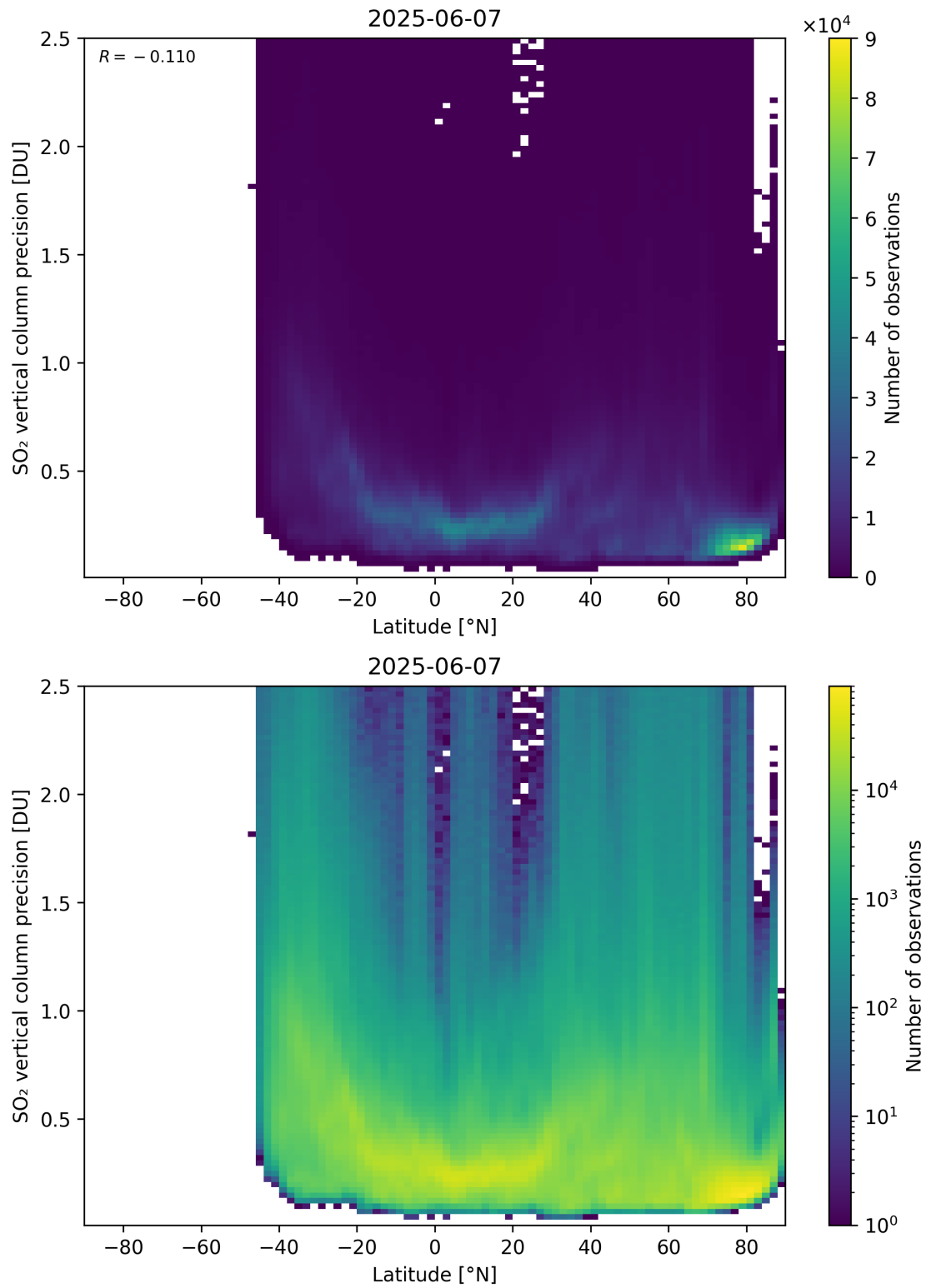
Figure 170: Scatter density plot of “Latitude” against “SO 2 vertical column precision” for 2025-06-06 to 2025-06-08.
