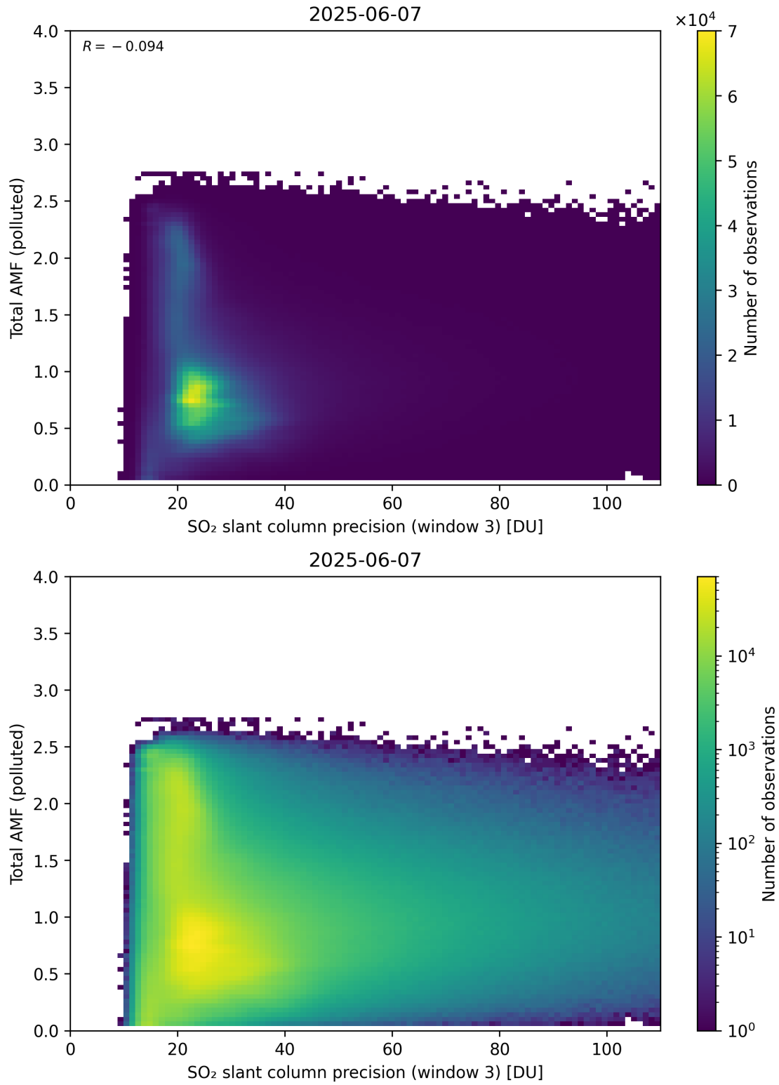
Figure 313: Scatter density plot of “SO 2 slant column precision (window 3)” against “Total AMF (polluted)” for 2025-06-06 to 2025-06-08.
