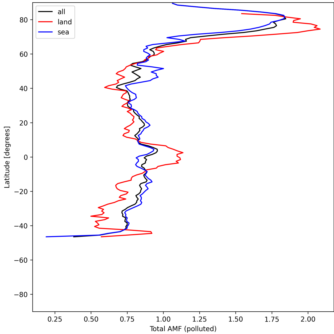
Figure 53: Zonal average of “Total AMF (polluted)” for 2025-06-06 to 2025-06-08.
