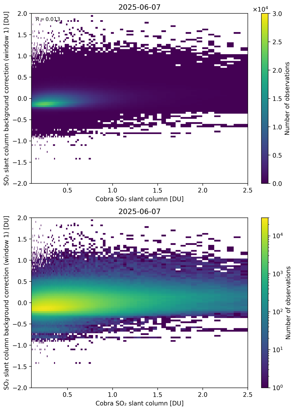
Figure 193: Scatter density plot of “Cobra SO 2 slant column” against “SO 2 slant column background correction (window 1)” for 2025-06-06 to 2025-06-08.
