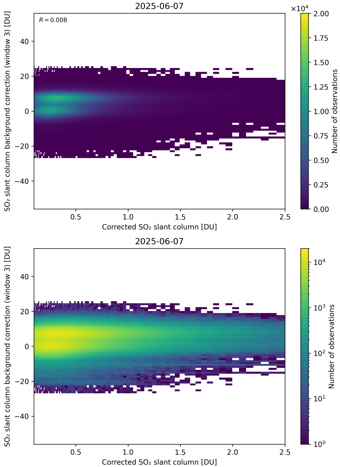
Figure 228: Scatter density plot of “Corrected SO 2 slant column” against “SO 2 slant column background correction (window 3)” for 2025-06-06 to 2025-06-08.
