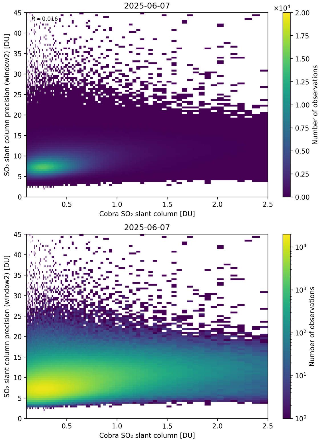
Figure 221: Scatter density plot of “Cobra SO 2 slant column” against “SO 2 slant column precision (window2)” for 2025-06-06 to 2025-06-08.
