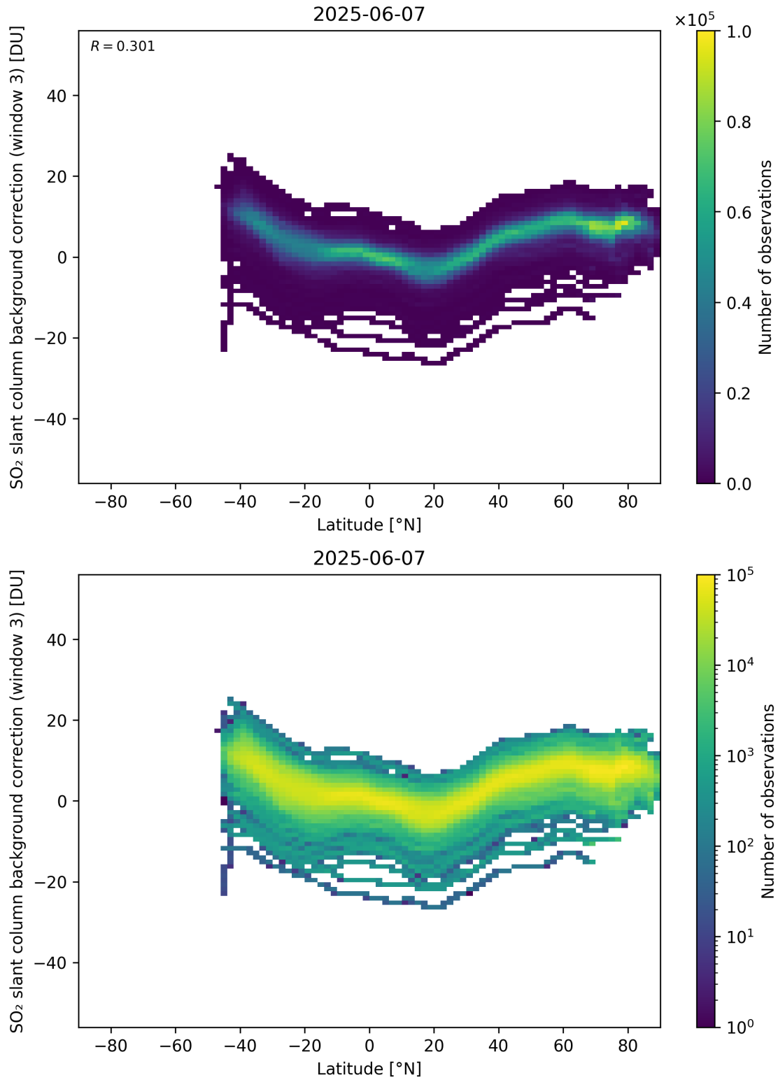
Figure 152: Scatter density plot of “Latitude” against “SO 2 slant column background correction (window 3)” for 2025-06-06 to 2025-06-08.
