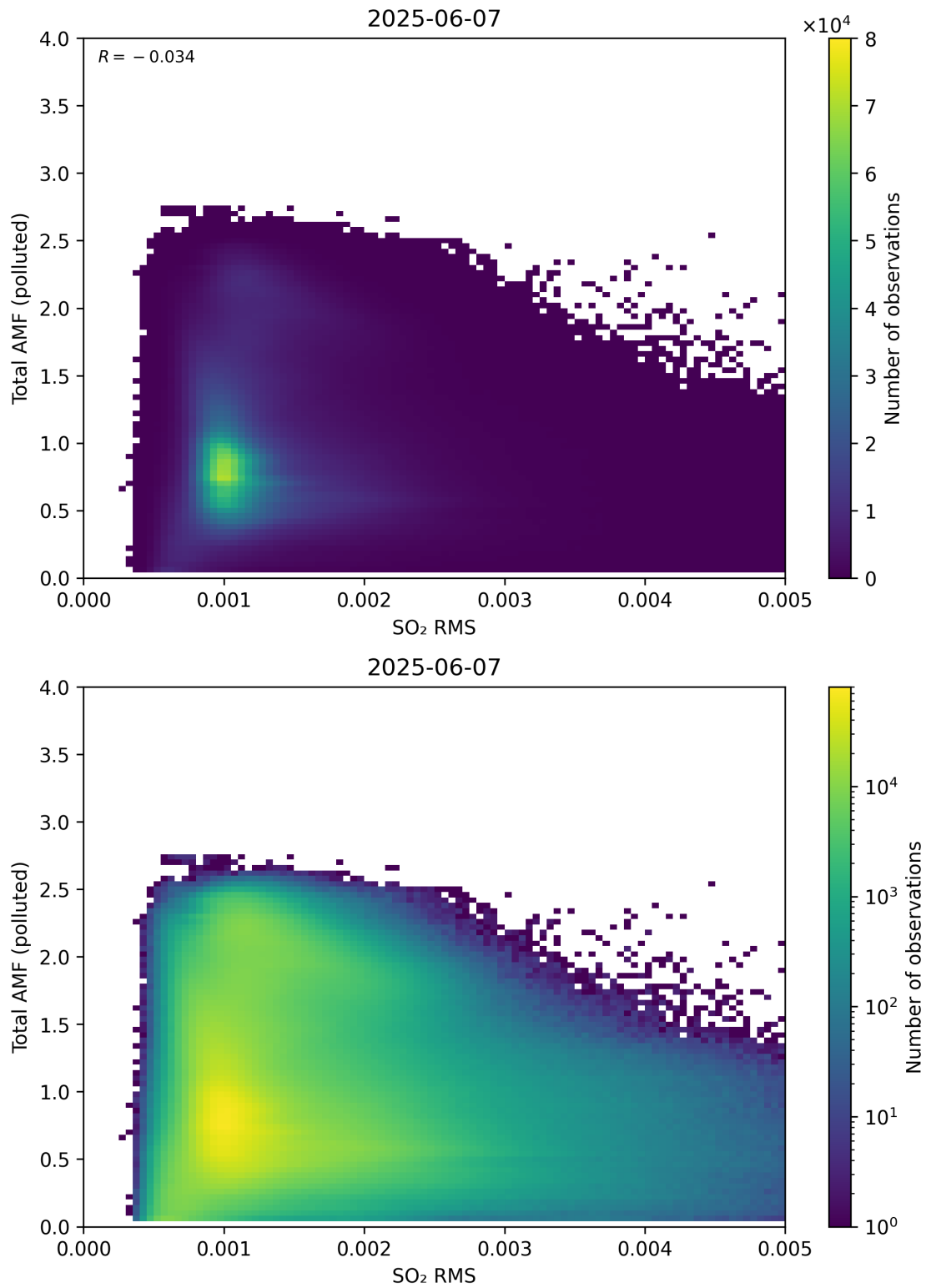
Figure 148: Scatter density plot of “SO 2 RMS” against “Total AMF (polluted)” for 2025-06-06 to 2025-06-08.
