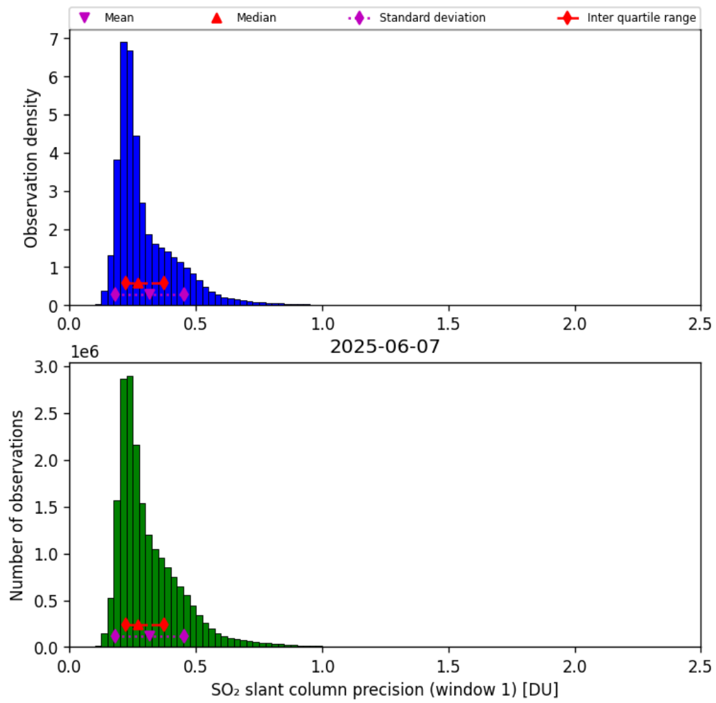
Figure 64: Histogram of “SO 2 slant column precision (window 1)” for 2025-06-06 to 2025-06-08
