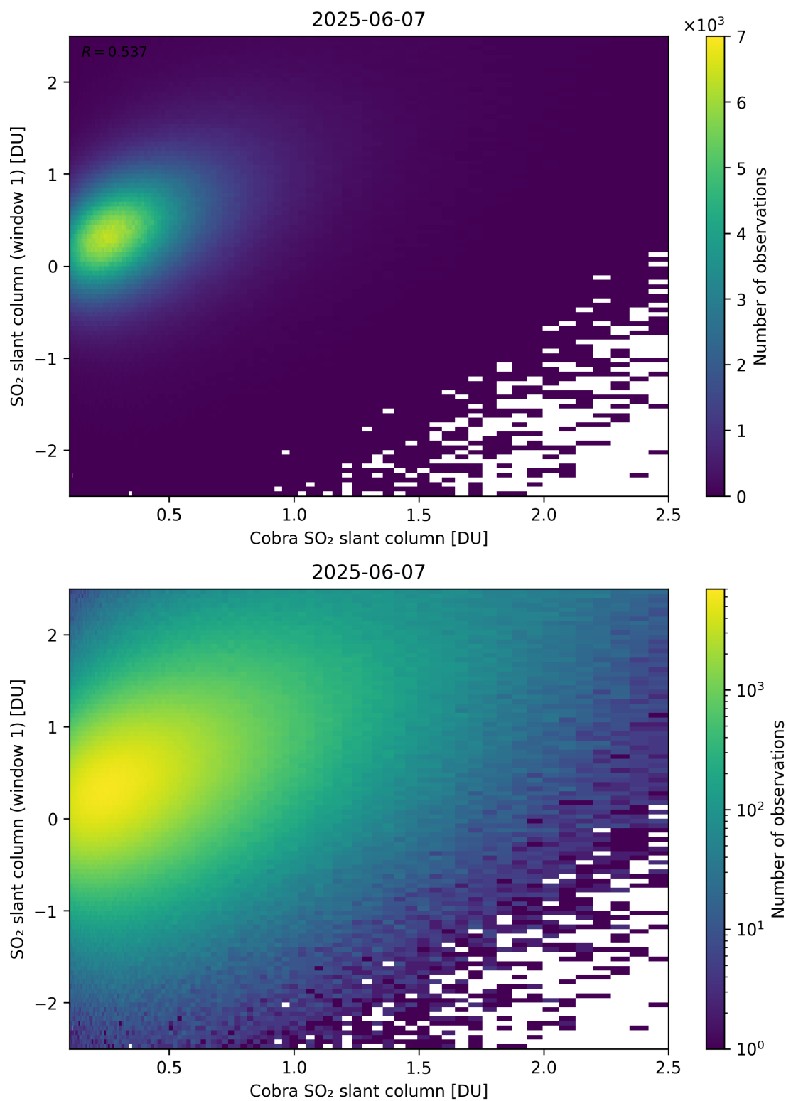
Figure 219: Scatter density plot of “Cobra SO 2 slant column” against “SO 2 slant column (window 1)” for 2025-06-06 to 2025-06-08.
