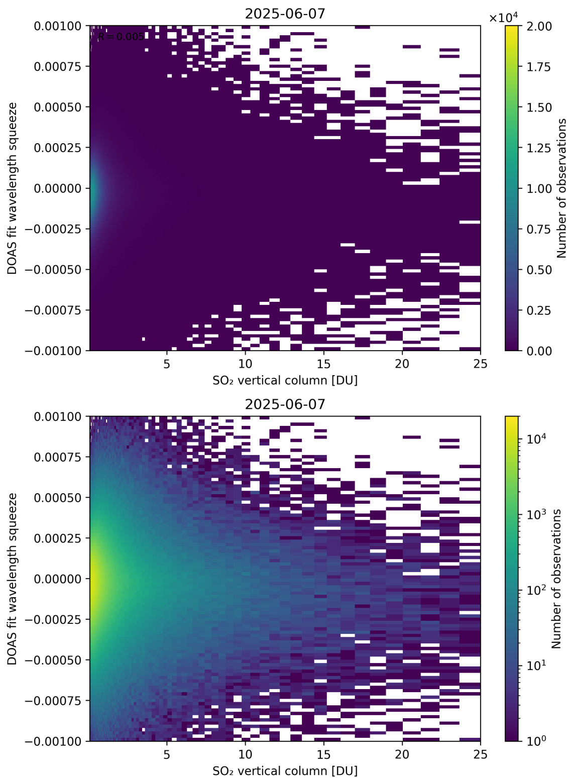
Figure 327: Scatter density plot of “SO 2 vertical column” against “DOAS fit wavelength squeeze” for 2025-06-06 to 2025-06-08.
