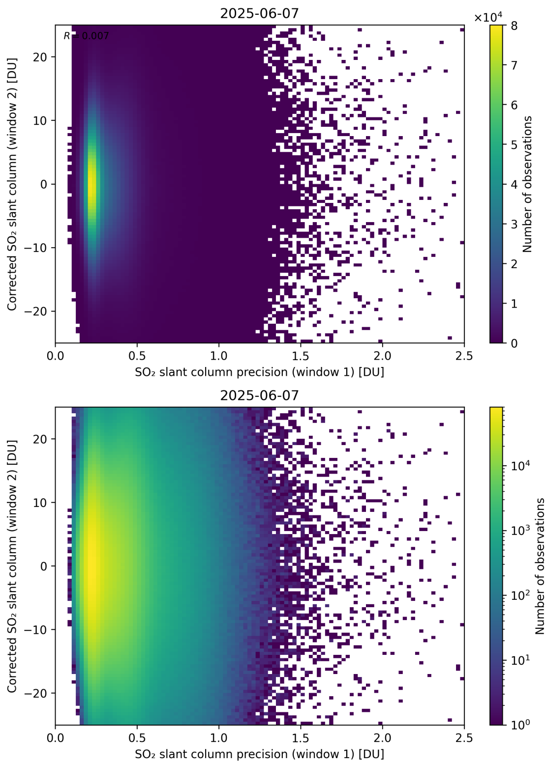
Figure 275: Scatter density plot of “SO 2 slant column precision (window 1)” against “Corrected SO 2 slant column (window 2)” for 2025-06-06 to 2025-06-08.
