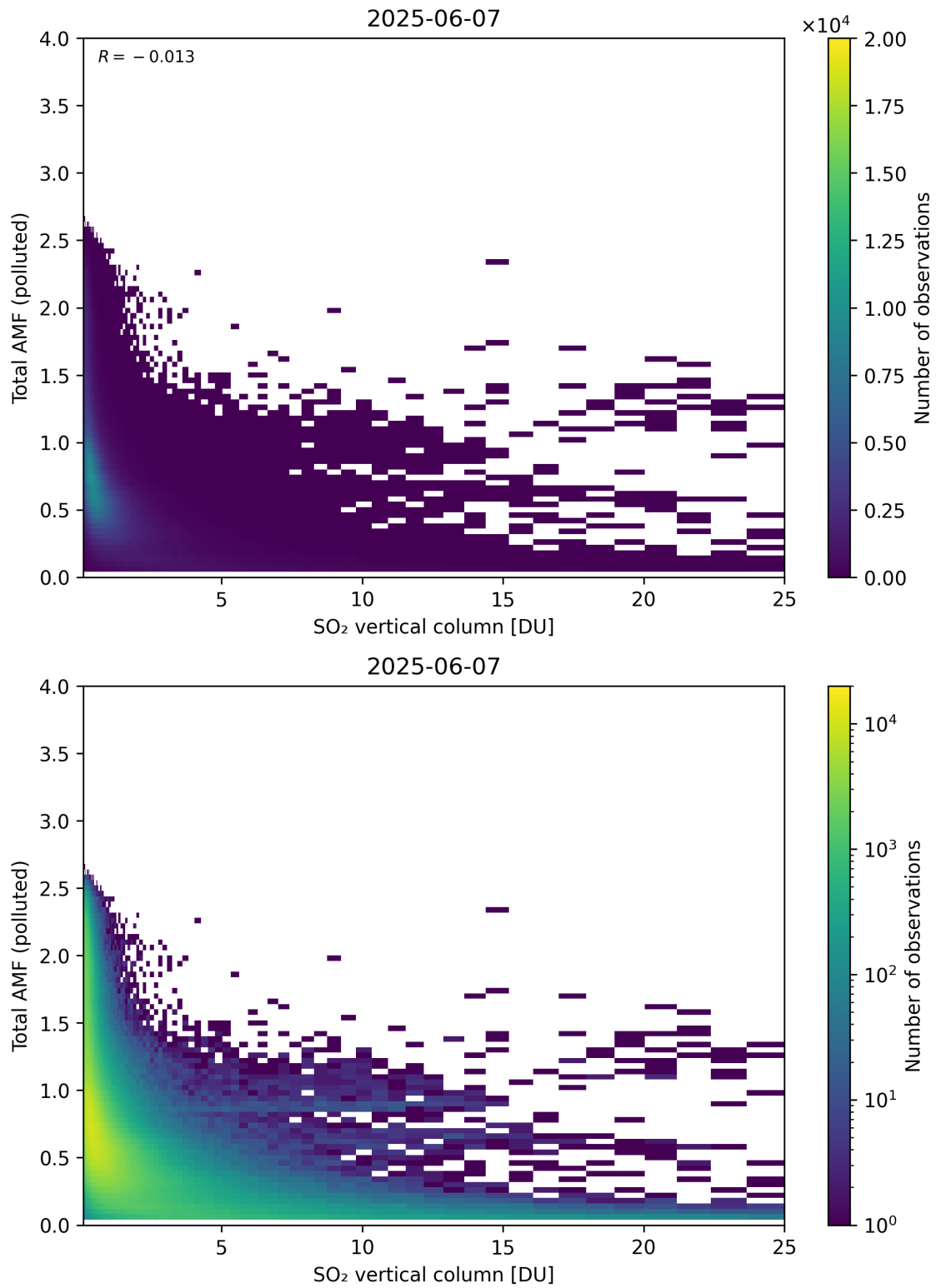
Figure 359: Scatter density plot of “SO 2 vertical column” against “Total AMF (polluted)” for 2025-06-06 to 2025-06-08.
