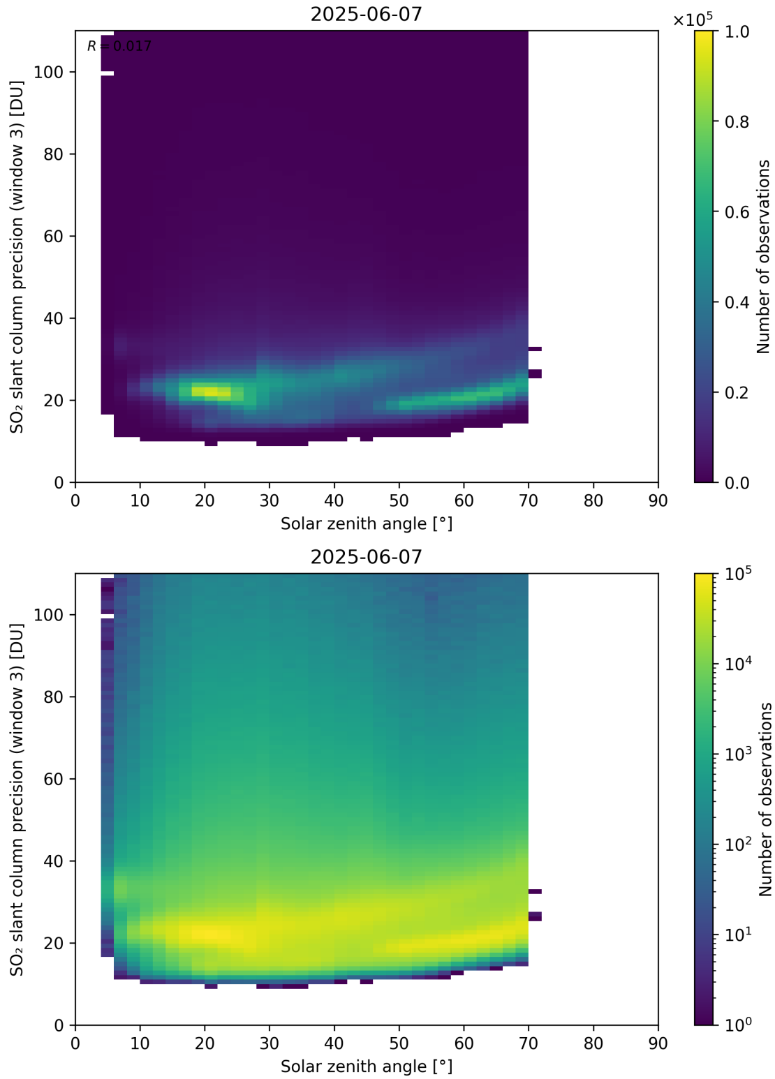
Figure 188: Scatter density plot of “Solar zenith angle” against “SO 2 slant column precision (window 3)” for 2025-06-06 to 2025-06-08.
