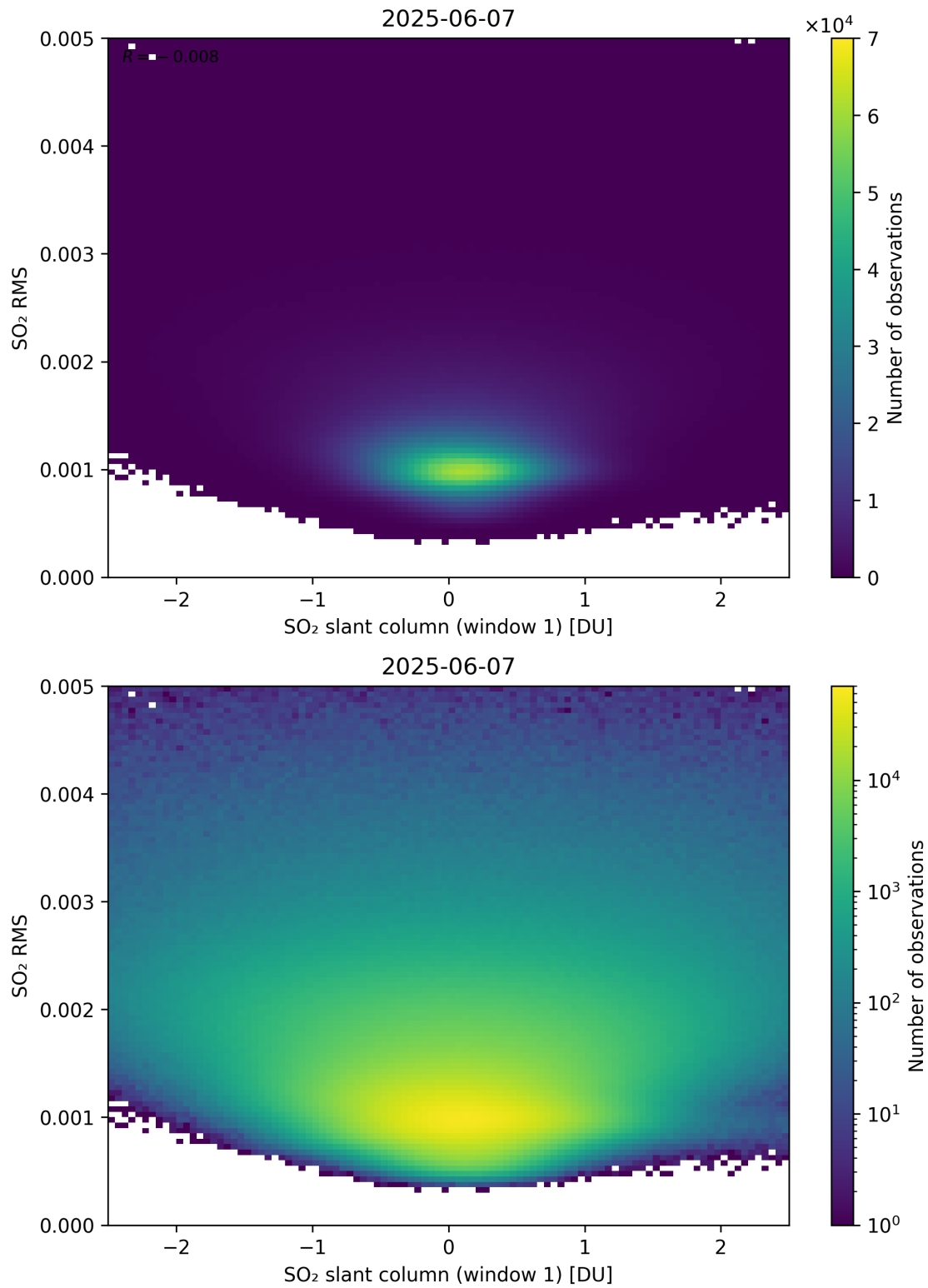
Figure 267: Scatter density plot of “SO 2 slant column (window 1)” against “SO 2 RMS” for 2025-06-06 to 2025-06-08.
