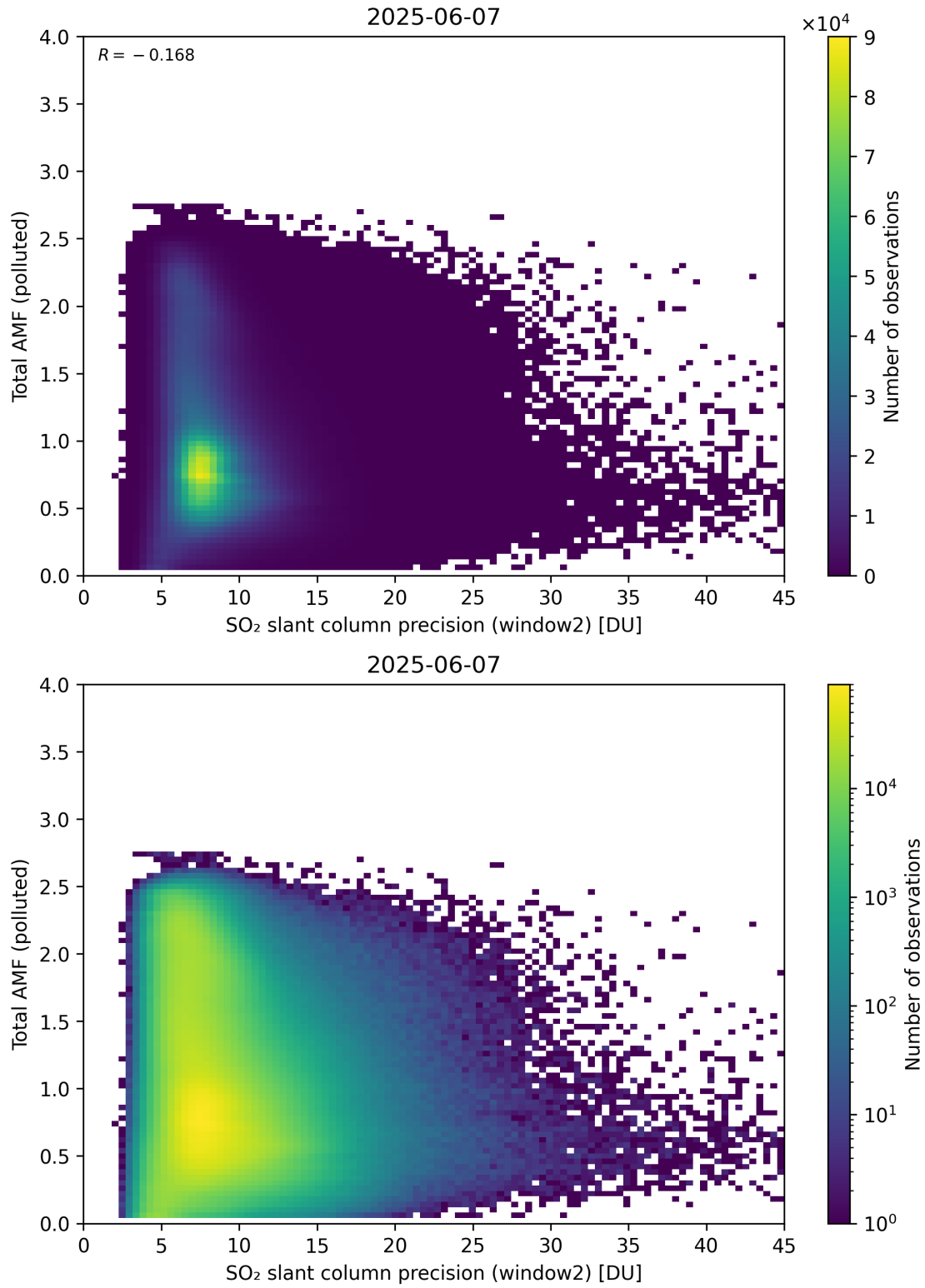
Figure 301: Scatter density plot of “SO 2 slant column precision (window2)” against “Total AMF (polluted)” for 2025-06-06 to 2025-06-08.
