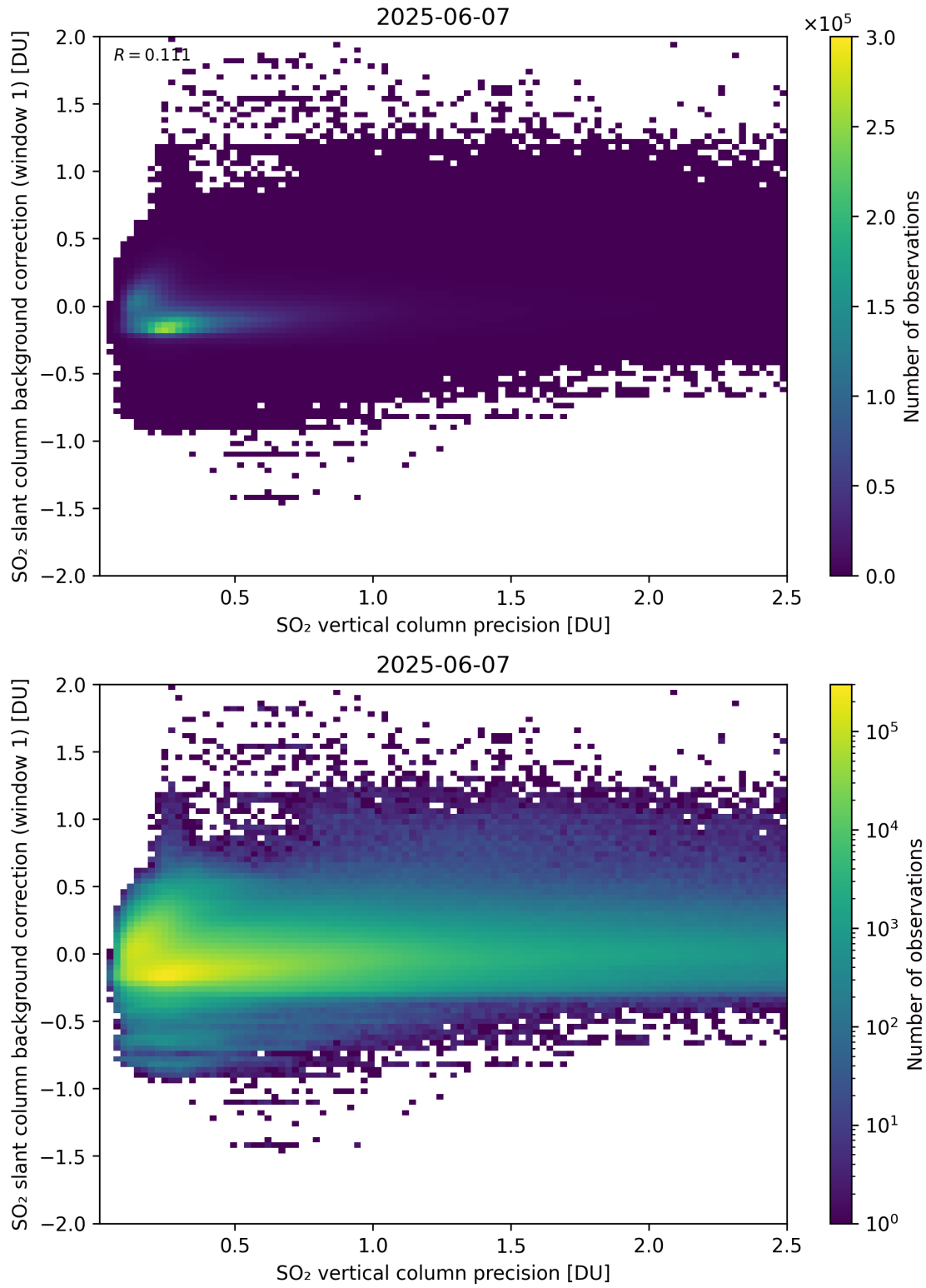
Figure 329: Scatter density plot of “SO 2 vertical column precision” against “SO 2 slant column background correction (window 1)” for 2025-06-06 to 2025-06-08.
