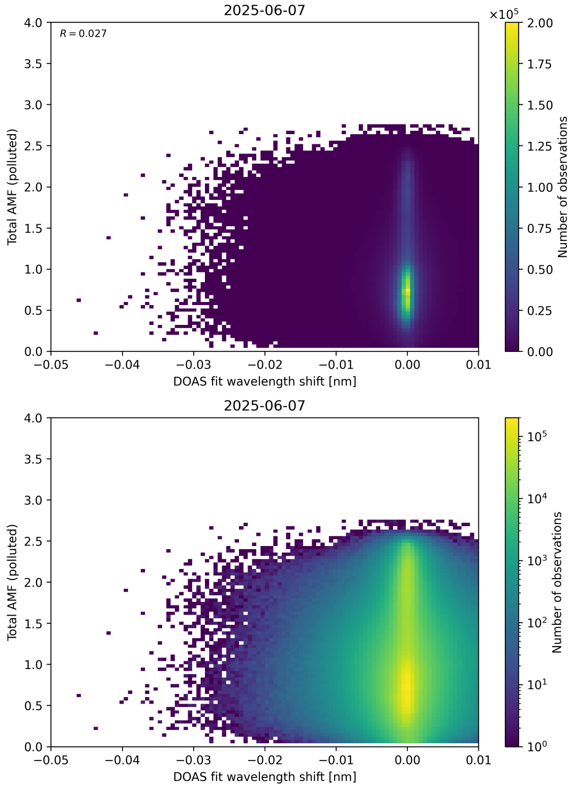
Figure 141: Scatter density plot of “DOAS fit wavelength shift” against “Total AMF (polluted)” for 2025-06-06 to 2025-06-08.
