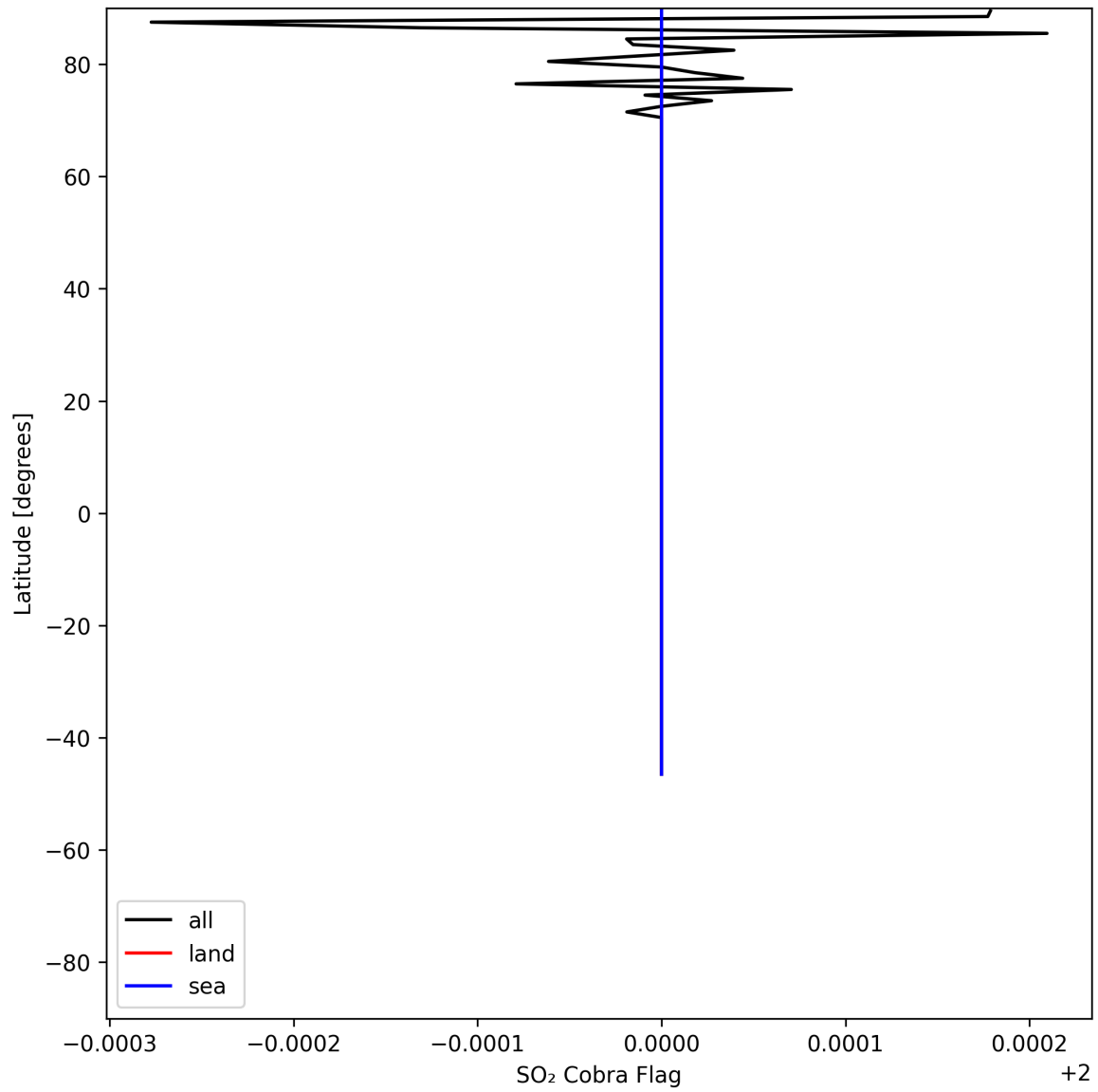
Figure 49: Zonal average of “SO 2 Cobra Flag” for 2025-06-06 to 2025-06-08.
