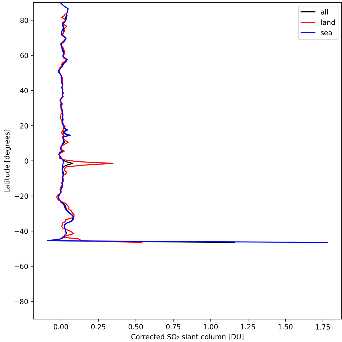
Figure 34: Zonal average of “Corrected SO 2 slant column” for 2025-06-06 to 2025-06-08.
