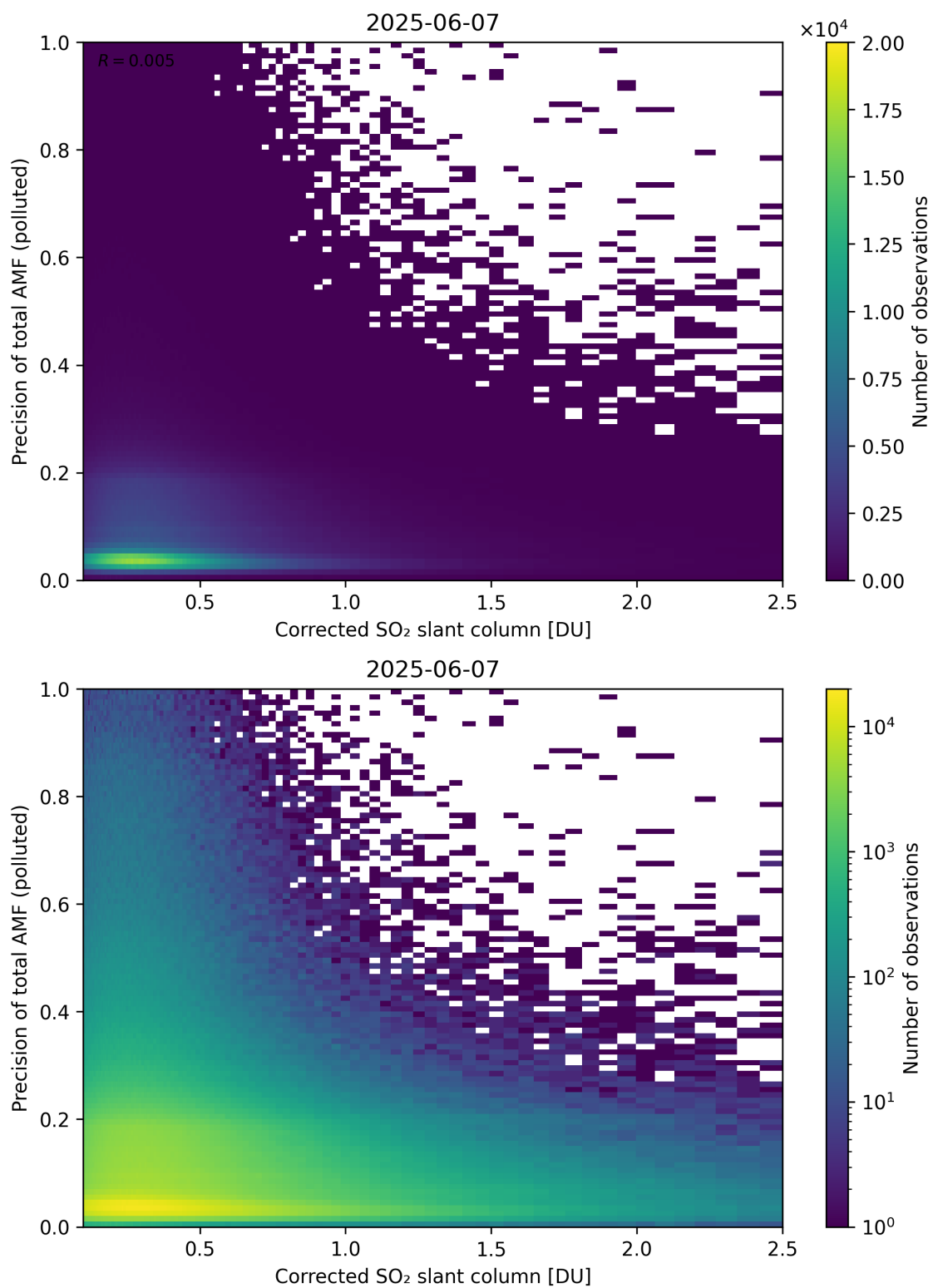
Figure 243: Scatter density plot of “Corrected SO 2 slant column” against “Precision of total AMF (polluted)” for 2025-06-06 to 2025-06-08.
