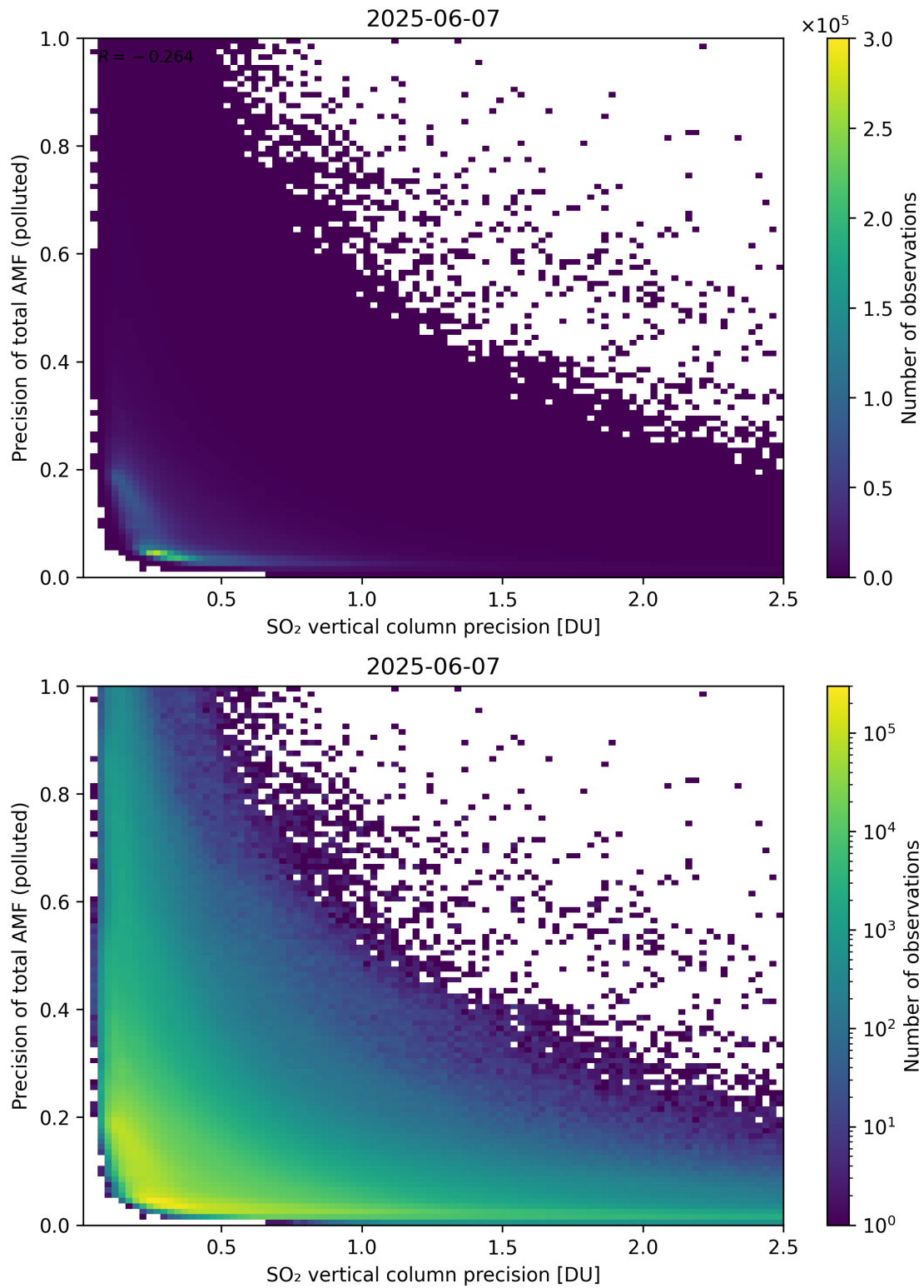
Figure 347: Scatter density plot of “SO 2 vertical column precision” against “Precision of total AMF (polluted)” for 2025-06-06 to 2025-06-08.
