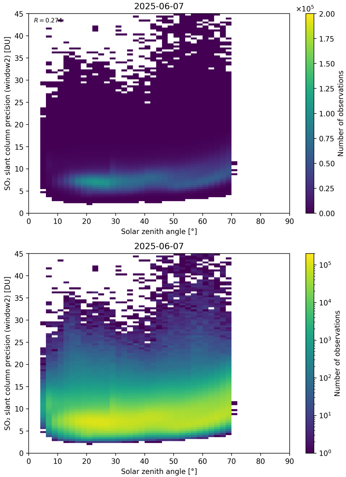
Figure 186: Scatter density plot of “Solar zenith angle” against “SO 2 slant column precision (window2)” for 2025-06-06 to 2025-06-08.
