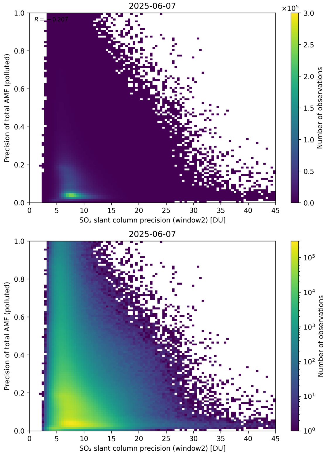
Figure 302: Scatter density plot of “SO 2 slant column precision (window2)” against “Precision of total AMF (polluted)” for 2025-06-06 to 2025-06-08.
