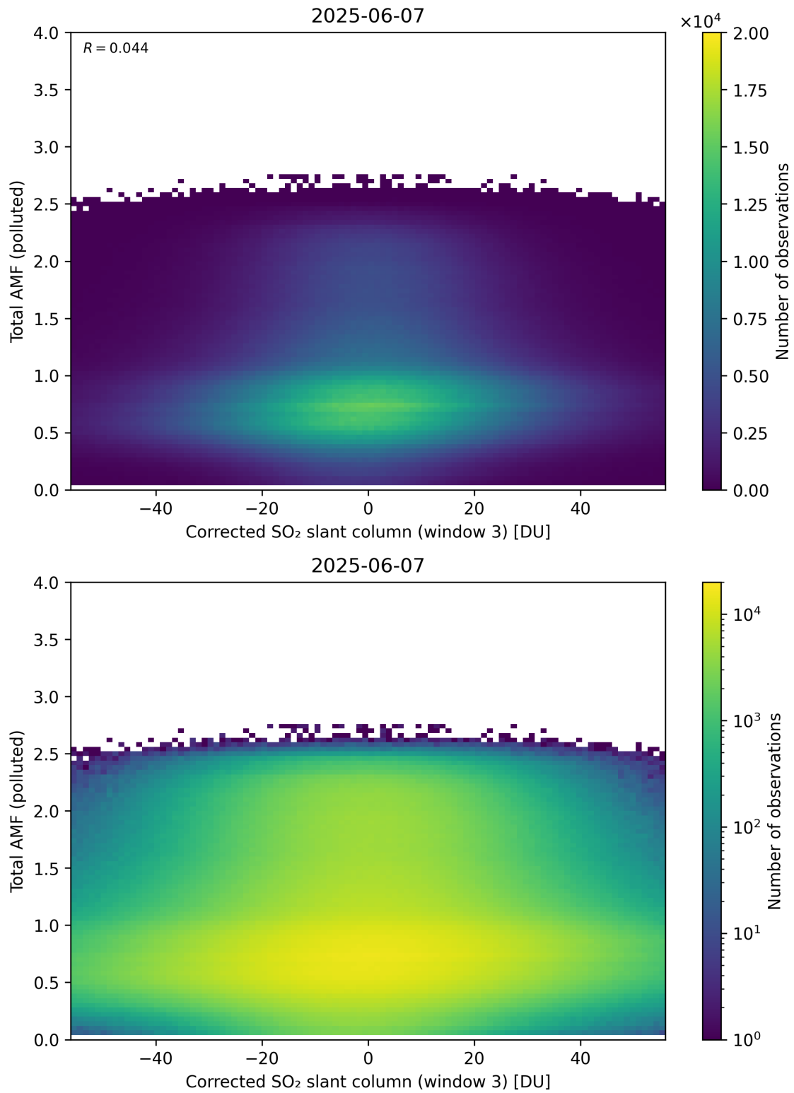
Figure 260: Scatter density plot of “Corrected SO 2 slant column (window 3)” against “Total AMF (polluted)” for 2025-06-06 to 2025-06-08.
