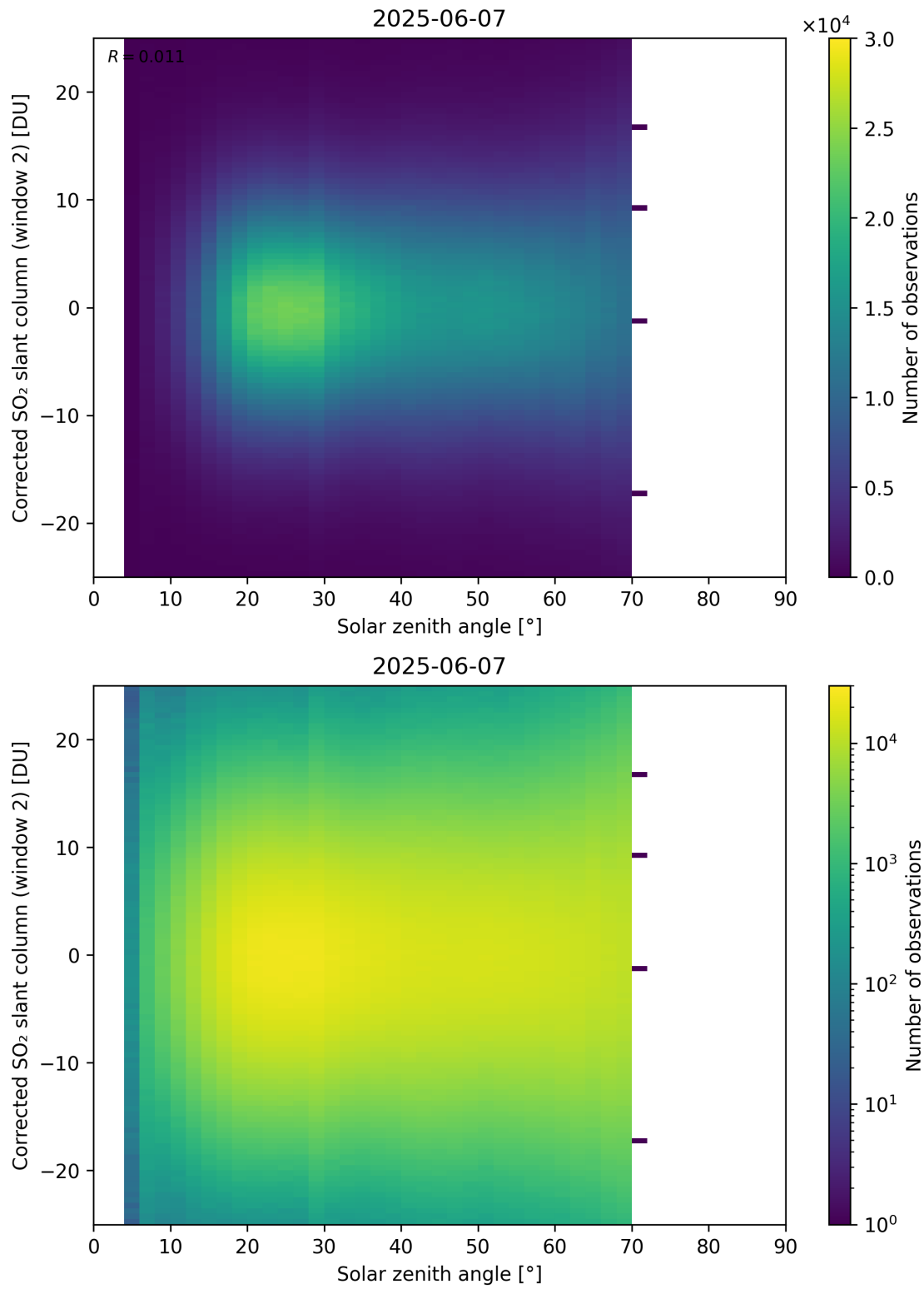
Figure 182: Scatter density plot of “Solar zenith angle” against “Corrected SO 2 slant column (window 2)” for 2025-06-06 to 2025-06-08.
