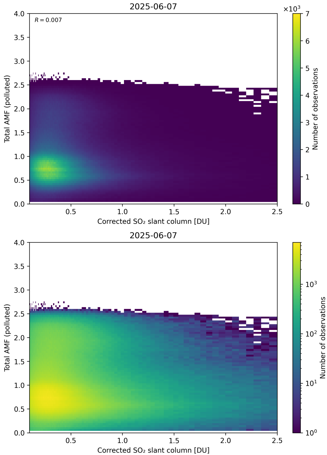
Figure 242: Scatter density plot of “Corrected SO 2 slant column” against “Total AMF (polluted)” for 2025-06-06 to 2025-06-08.
