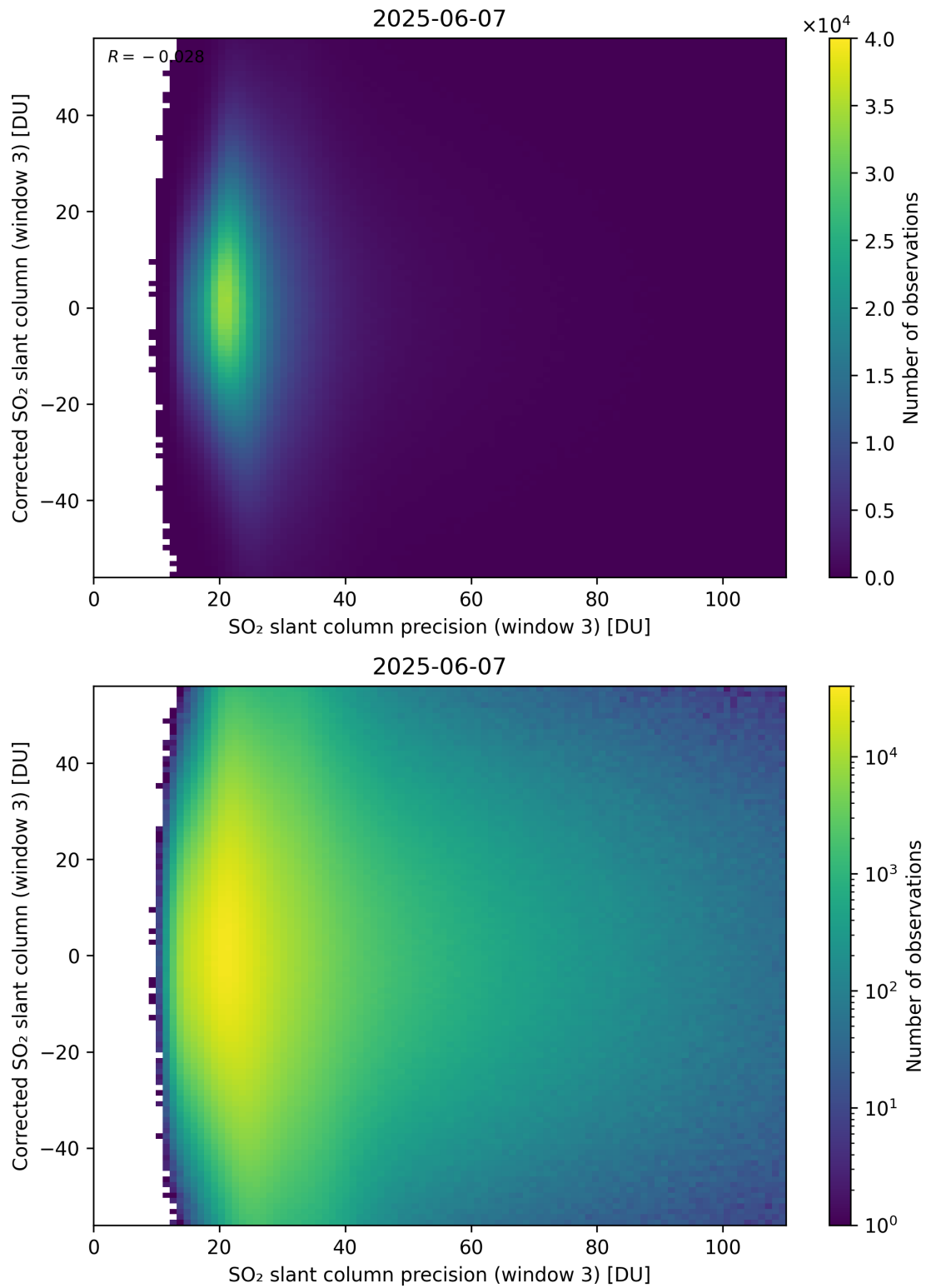
Figure 312: Scatter density plot of “SO 2 slant column precision (window 3)” against “Corrected SO 2 slant column (window 3)” for 2025-06-06 to 2025-06-08.
