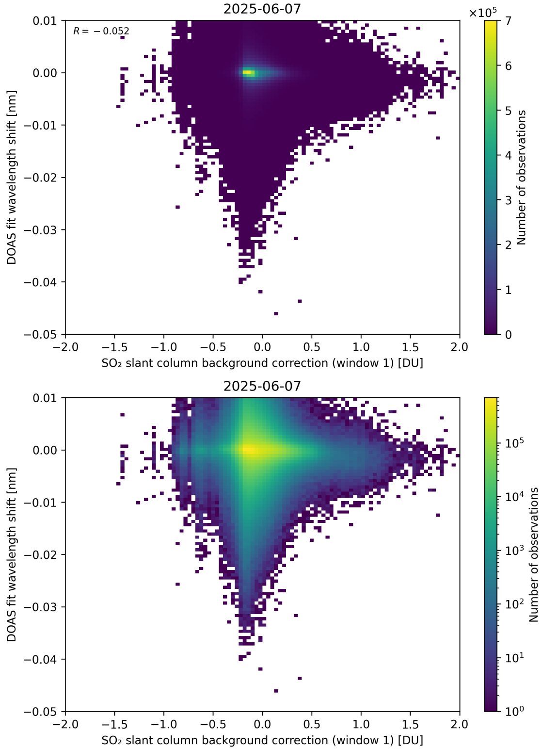
Figure 111: Scatter density plot of “SO 2 slant column background correction (window 1)” against “DOAS fit wavelength shift” for 2025-06-06 to 2025-06-08.
