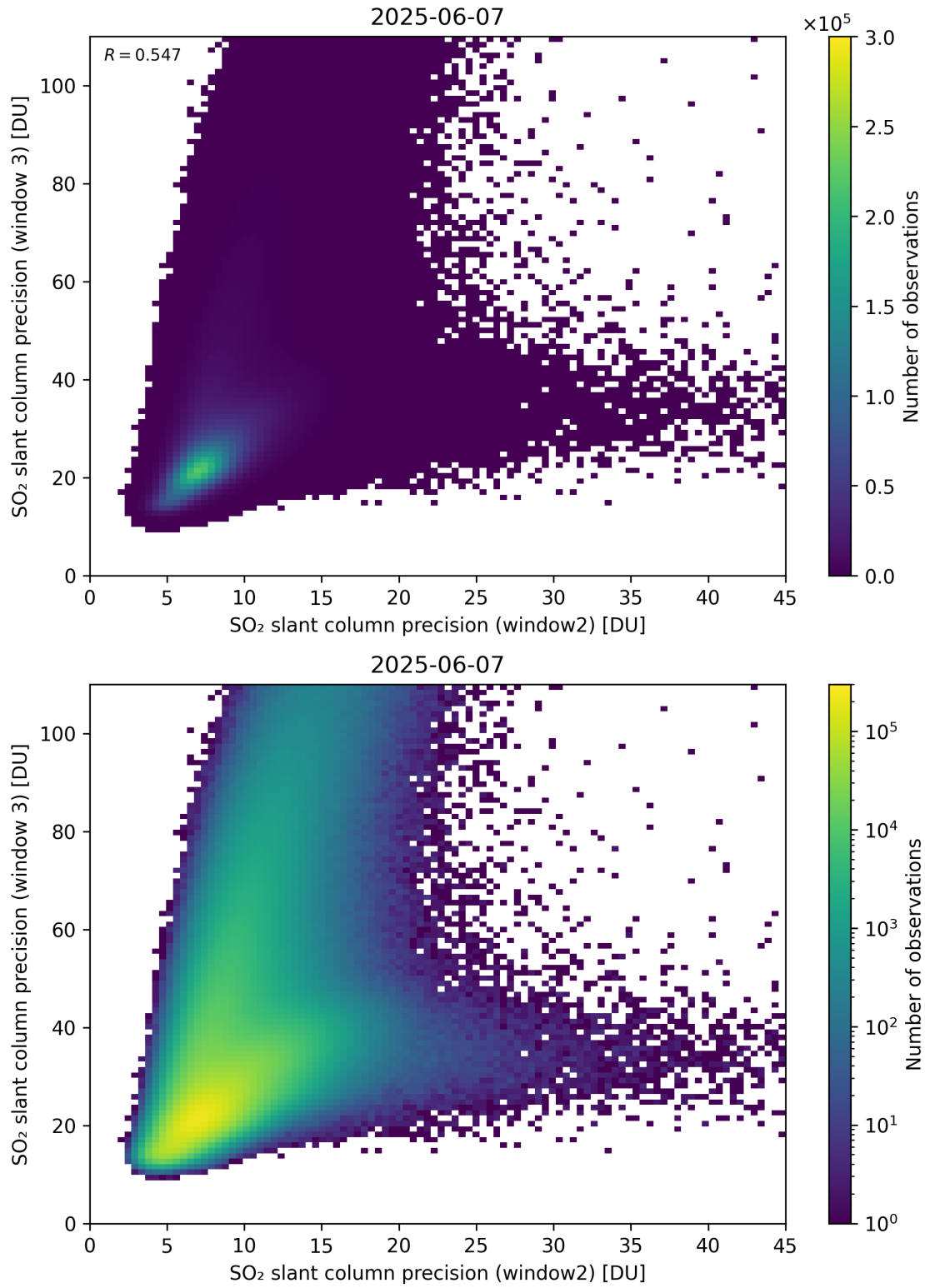
Figure 300: Scatter density plot of “SO 2 slant column precision (window2)” against “SO 2 slant column precision (window 3)” for 2025-06-06 to 2025-06-08.
