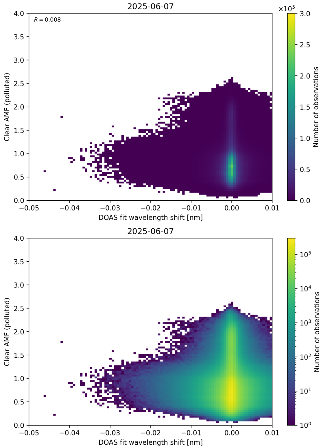
Figure 140: Scatter density plot of “DOAS fit wavelength shift” against “Clear AMF (polluted)” for 2025-06-06 to 2025-06-08.
