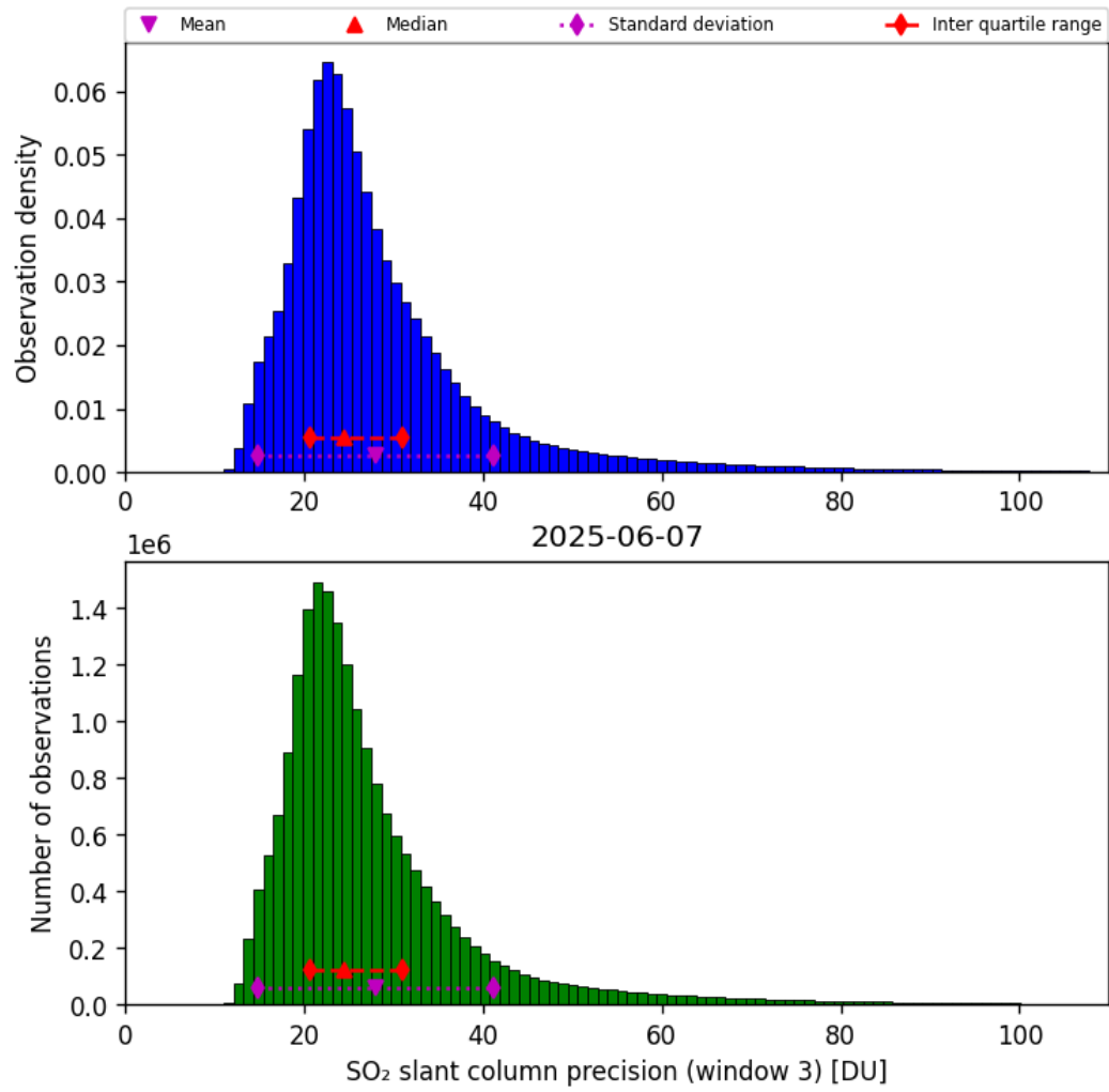
Figure 72: Histogram of “SO 2 slant column precision (window 3)” for 2025-06-06 to 2025-06-08
