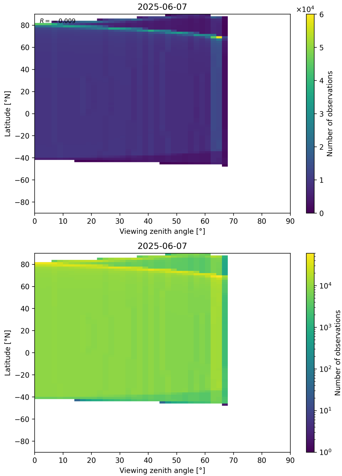
Figure 368: Scatter density plot of “Viewing zenith angle” against “Latitude” for 2025-06-06 to 2025-06-08.
