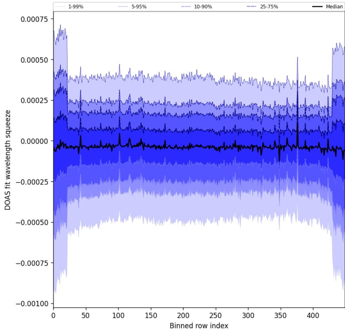
Figure 103: Along track statistics of “DOAS fit wavelength squeeze” for 2025-06-06 to 2025-06-08
