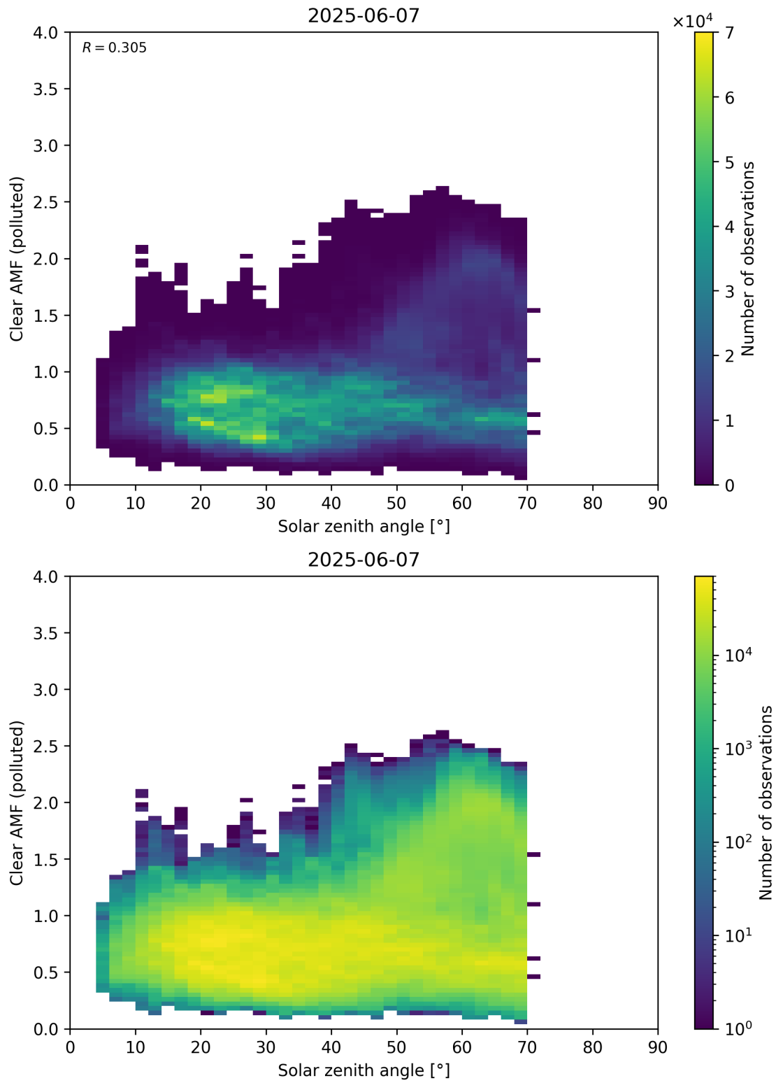
Figure 178: Scatter density plot of “Solar zenith angle” against “Clear AMF (polluted)” for 2025-06-06 to 2025-06-08.
