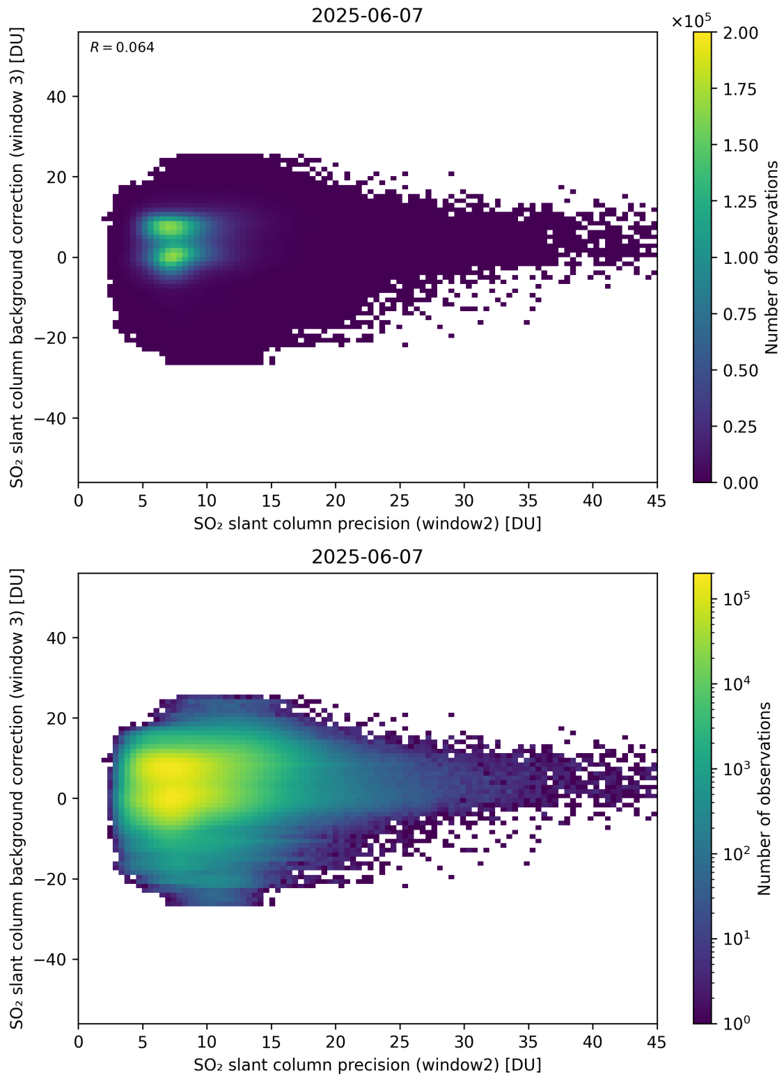
Figure 292: Scatter density plot of “SO 2 slant column precision (window2)” against “SO 2 slant column background correction (window 3)” for 2025-06-06 to 2025-06-08.
