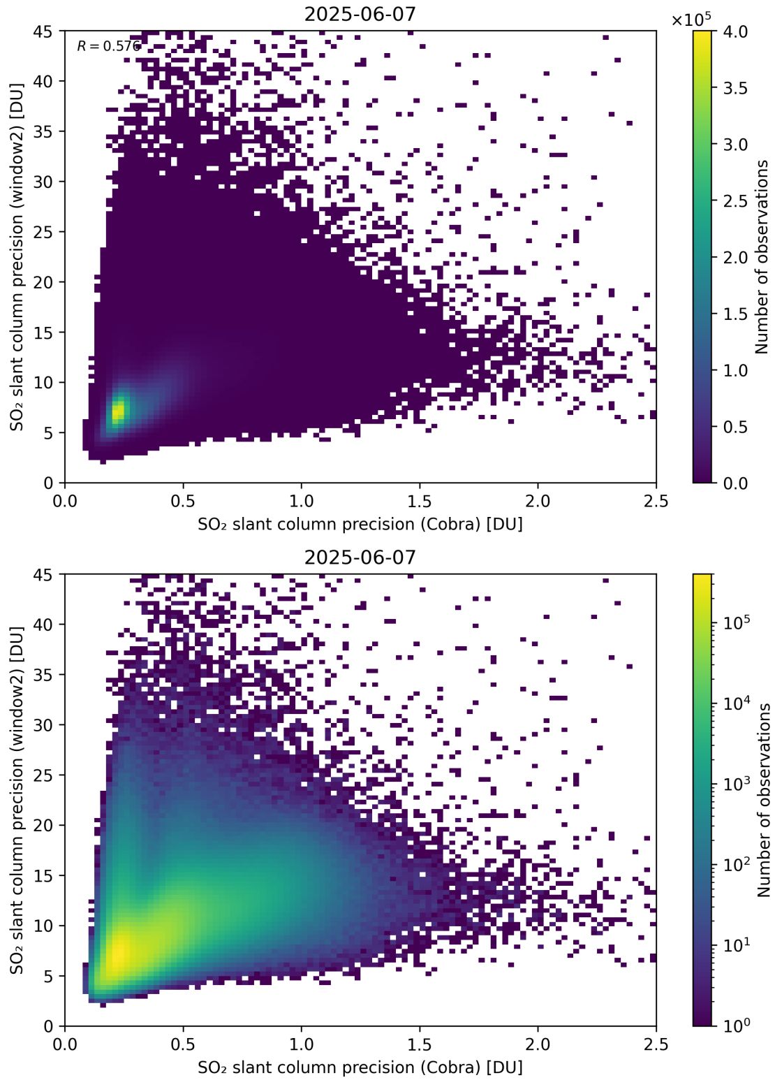
Figure 210: Scatter density plot of “SO 2 slant column precision (Cobra)” against “SO 2 slant column precision (window2)” for 2025-06-06 to 2025-06-08.
