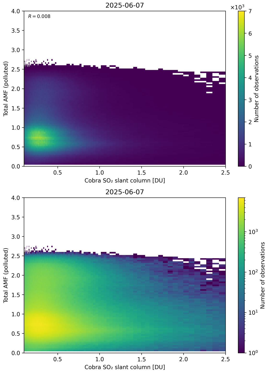
Figure 224: Scatter density plot of “Cobra SO 2 slant column” against “Total AMF (polluted)” for 2025-06-06 to 2025-06-08.
