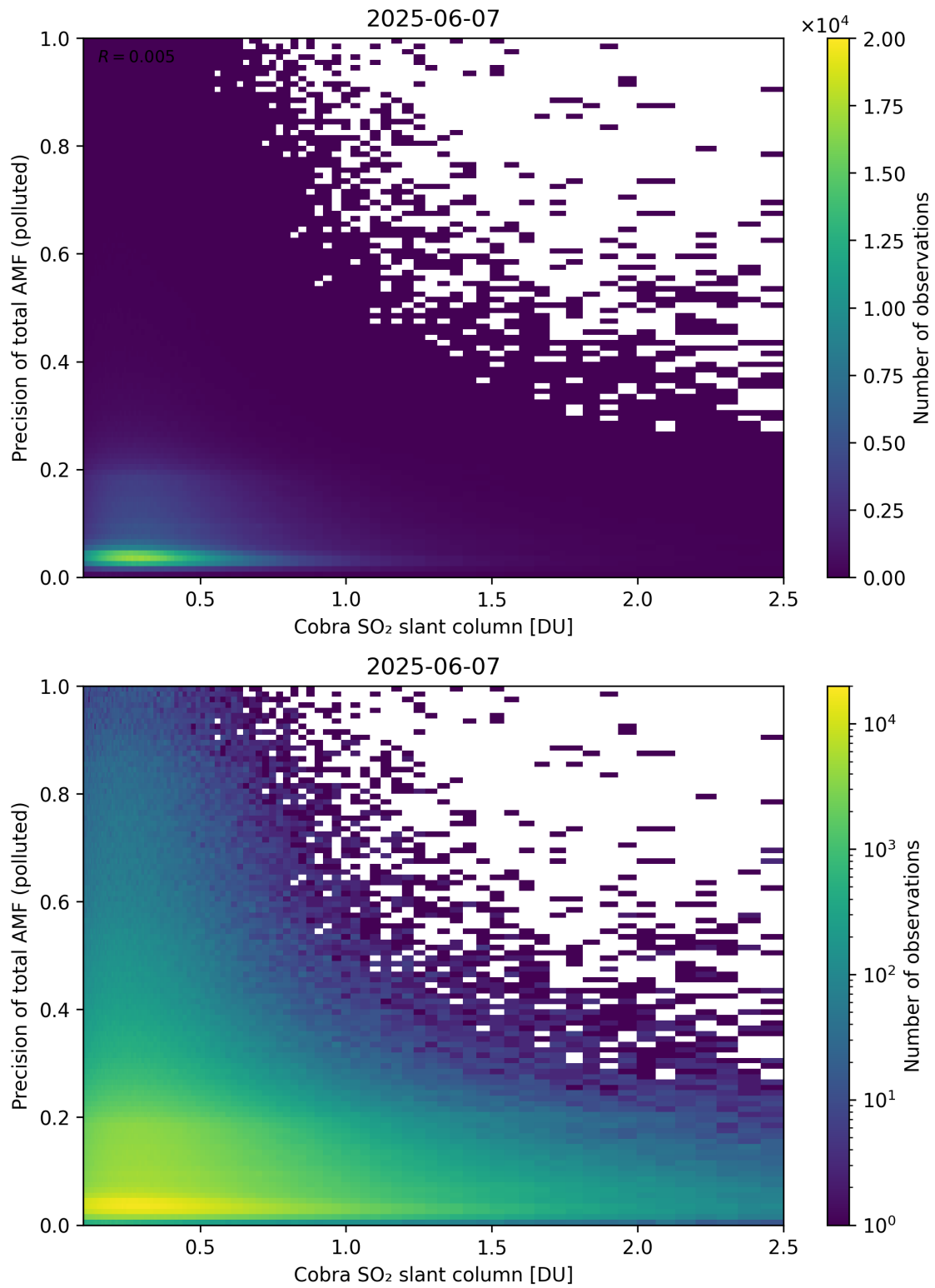
Figure 225: Scatter density plot of “Cobra SO 2 slant column” against “Precision of total AMF (polluted)” for 2025-06-06 to 2025-06-08.
