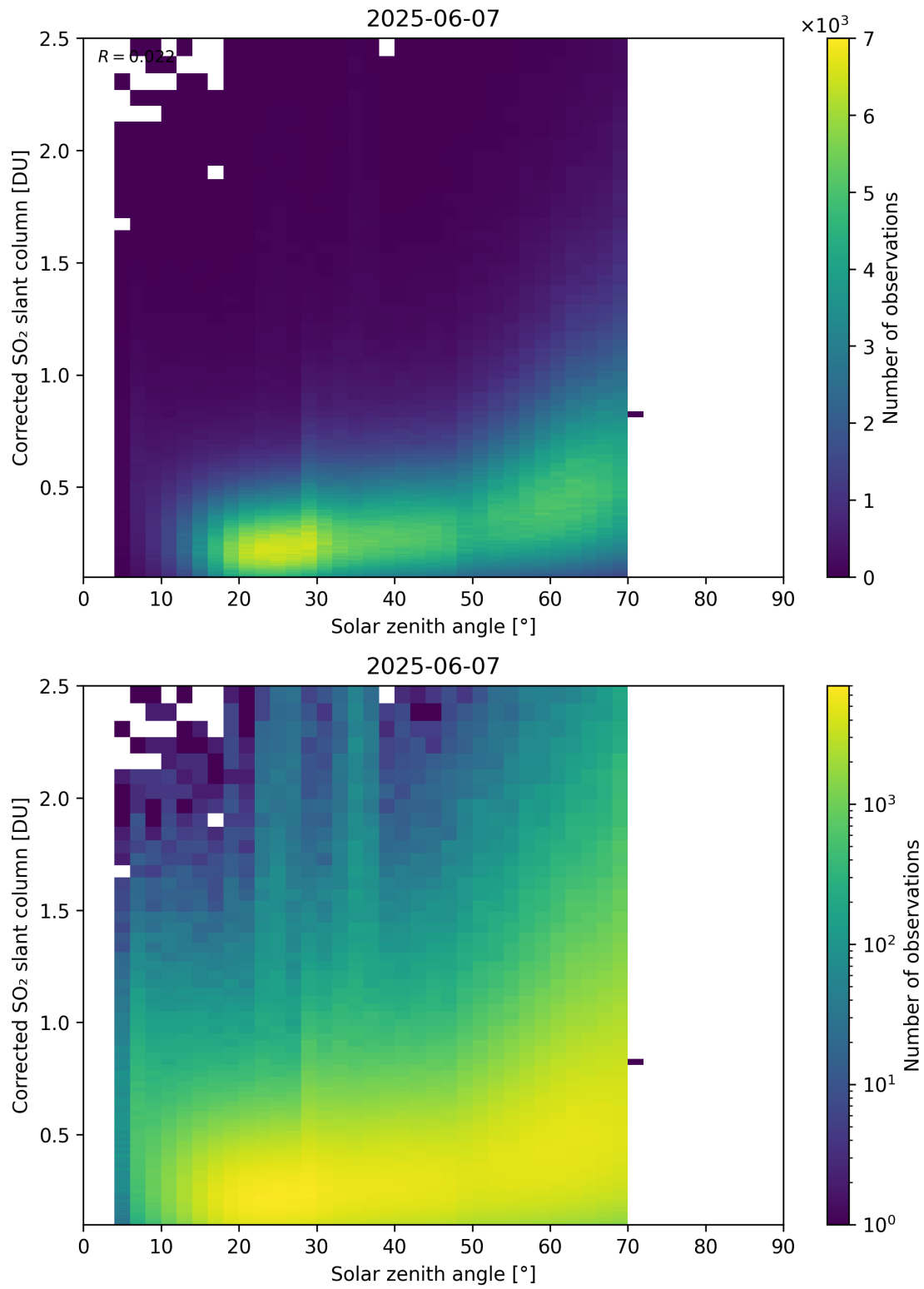
Figure 181: Scatter density plot of “Solar zenith angle” against “Corrected SO 2 slant column” for 2025-06-06 to 2025-06-08.
