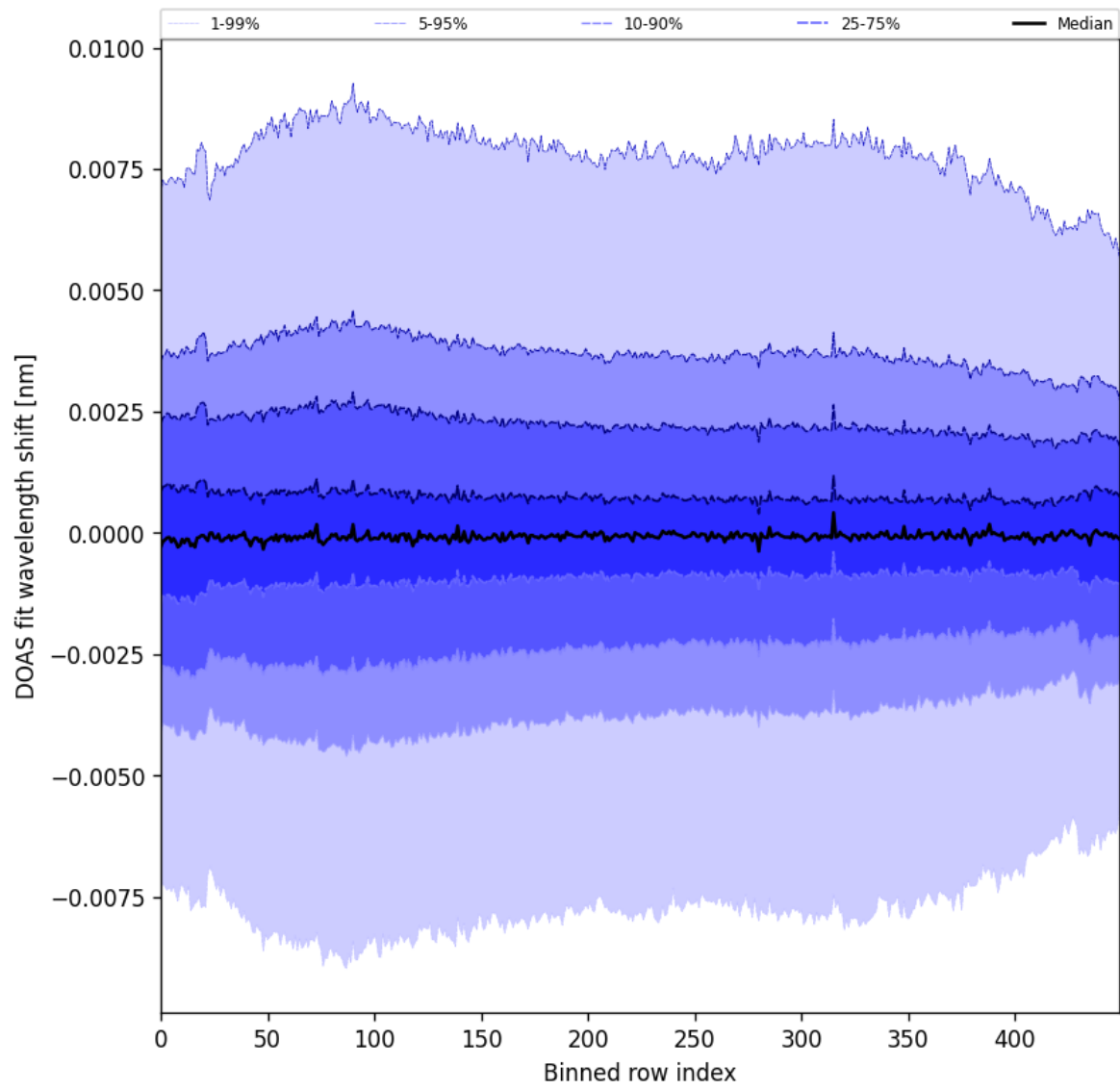
Figure 102: Along track statistics of “DOAS fit wavelength shift” for 2025-06-06 to 2025-06-08
