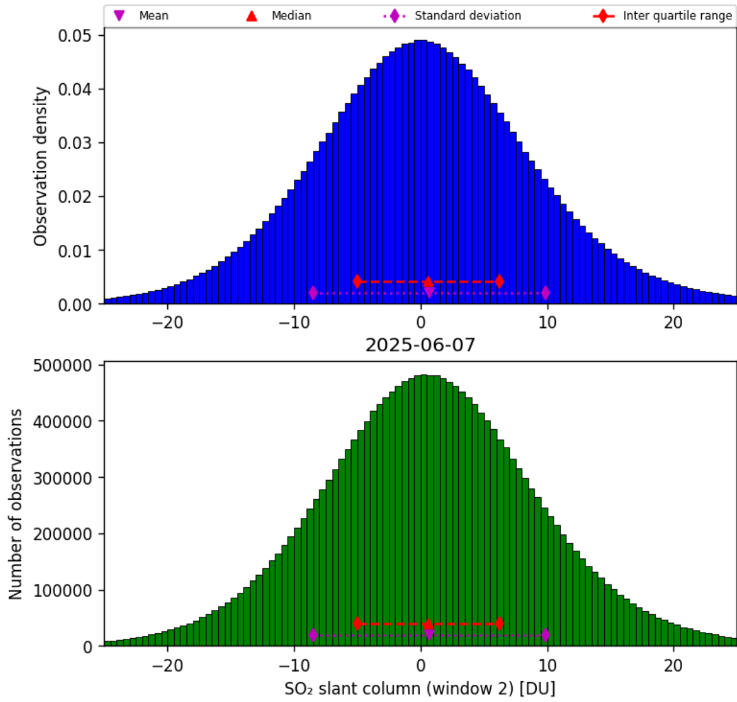
Figure 67: Histogram of “SO 2 slant column (window 2)” for 2025-06-06 to 2025-06-08
