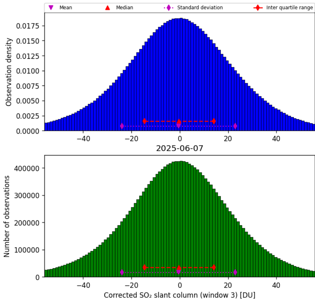
Figure 73: Histogram of “Corrected SO 2 slant column (window 3)” for 2025-06-06 to 2025-06-08
