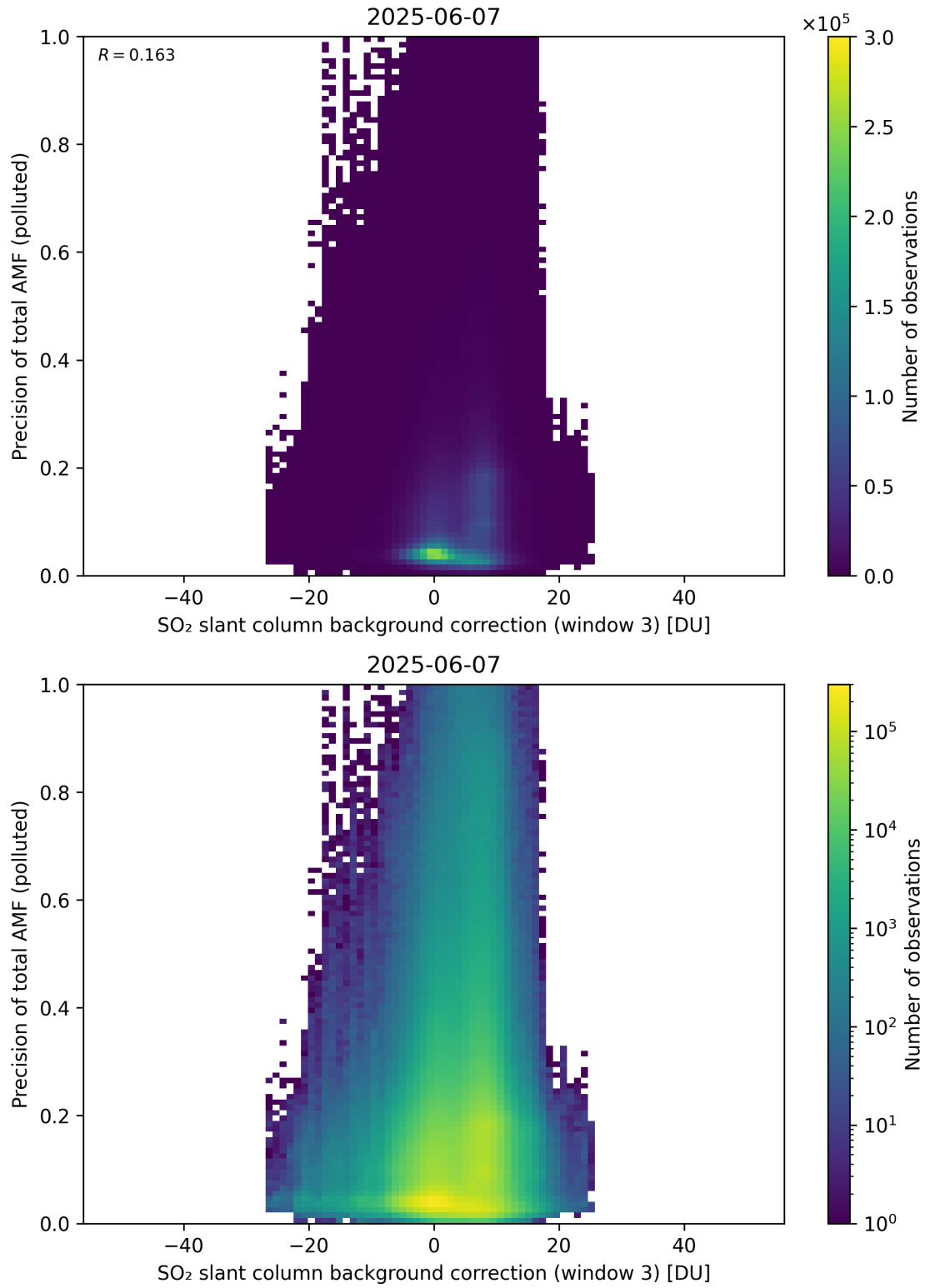
Figure 137: Scatter density plot of “SO 2 slant column background correction (window 3)” against “Precision of total AMF (polluted)” for 2025-06-06 to 2025-06-08.
