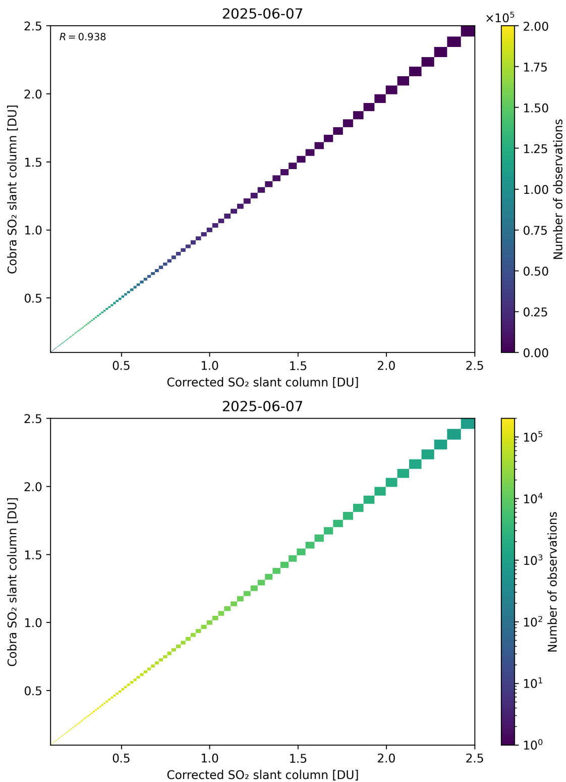
Figure 233: Scatter density plot of “Corrected SO 2 slant column” against “Cobra SO 2 slant column” for 2025-06-06 to 2025-06-08.
