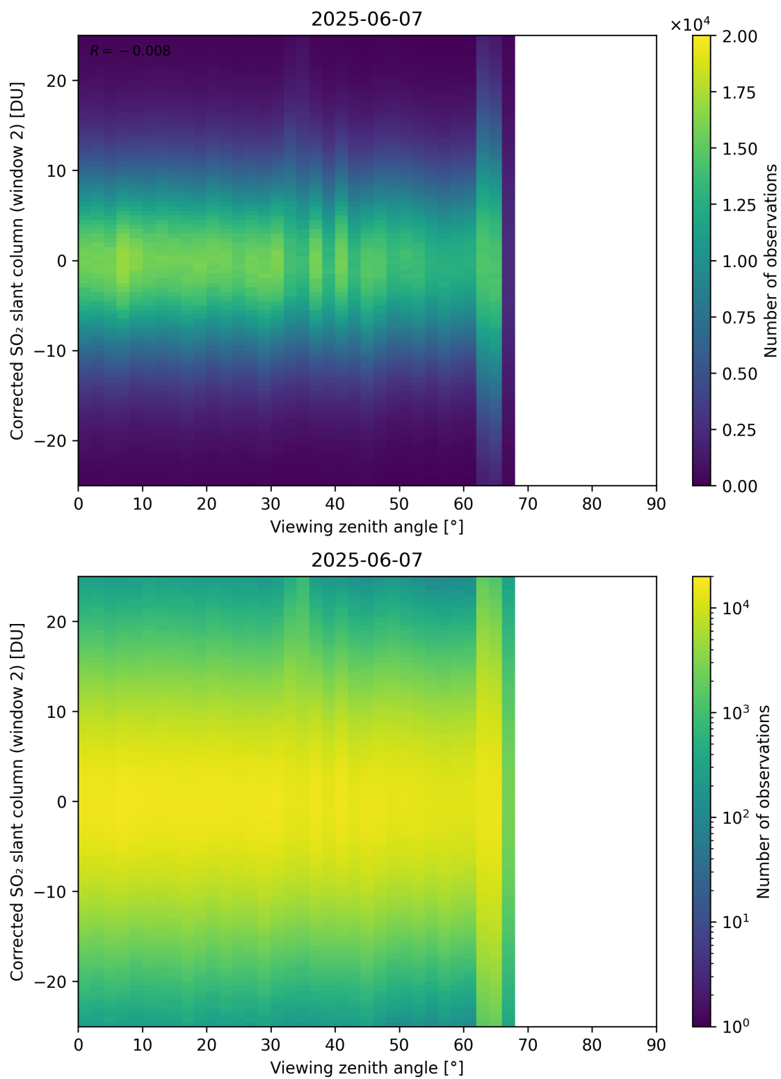
Figure 374: Scatter density plot of “Viewing zenith angle” against “Corrected SO 2 slant column (window 2)” for 2025-06-06 to 2025-06-08.
