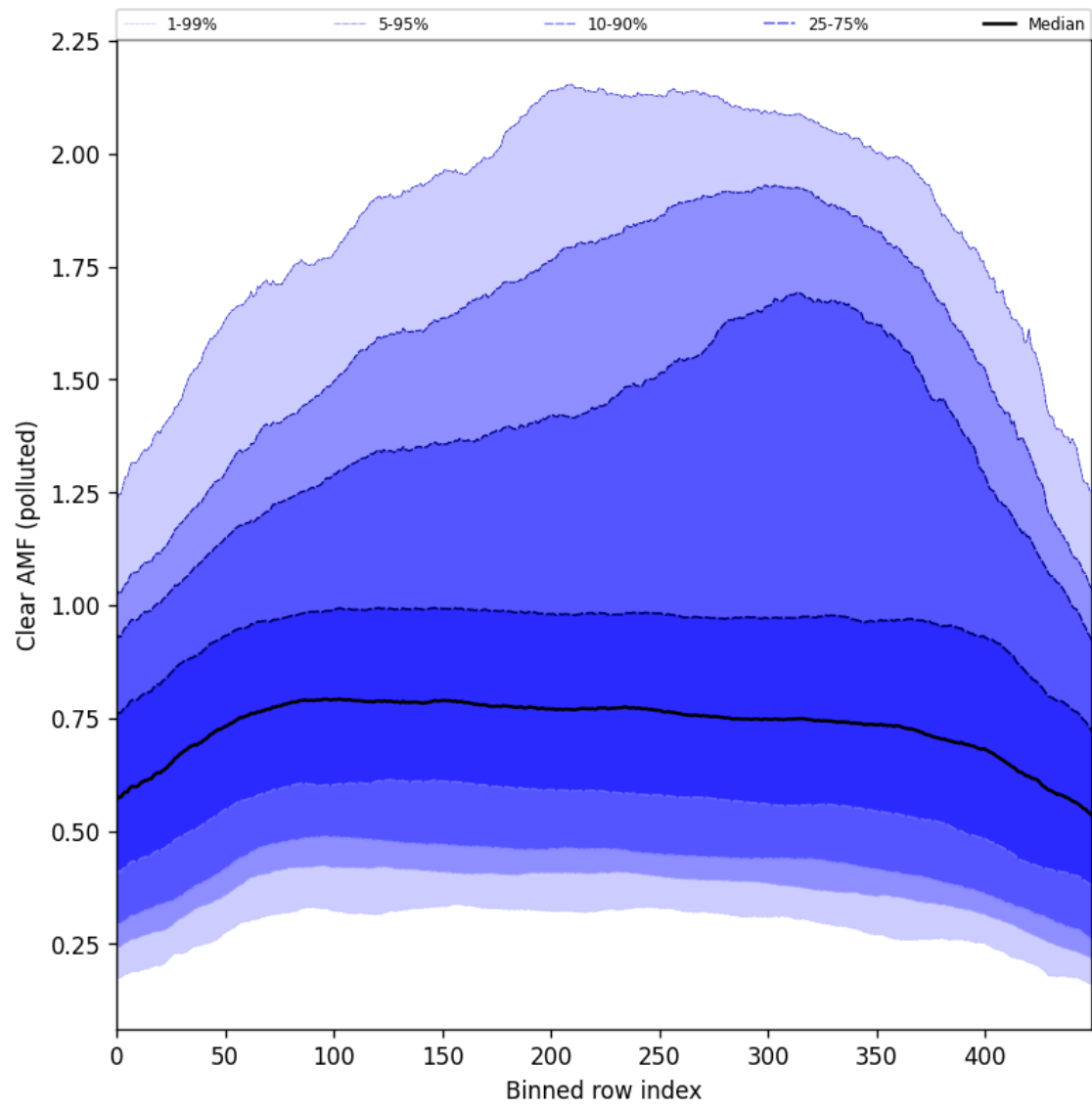
Figure 107: Along track statistics of “Clear AMF (polluted)” for 2025-06-06 to 2025-06-08
