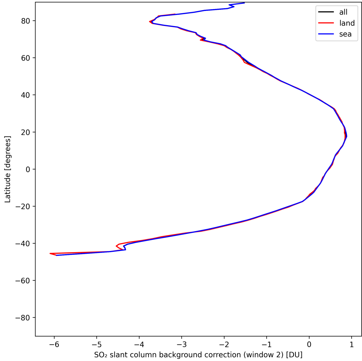
Figure 44: Zonal average of “SO 2 slant column background correction (window 2)” for 2025-06-06 to 2025-06-08.
