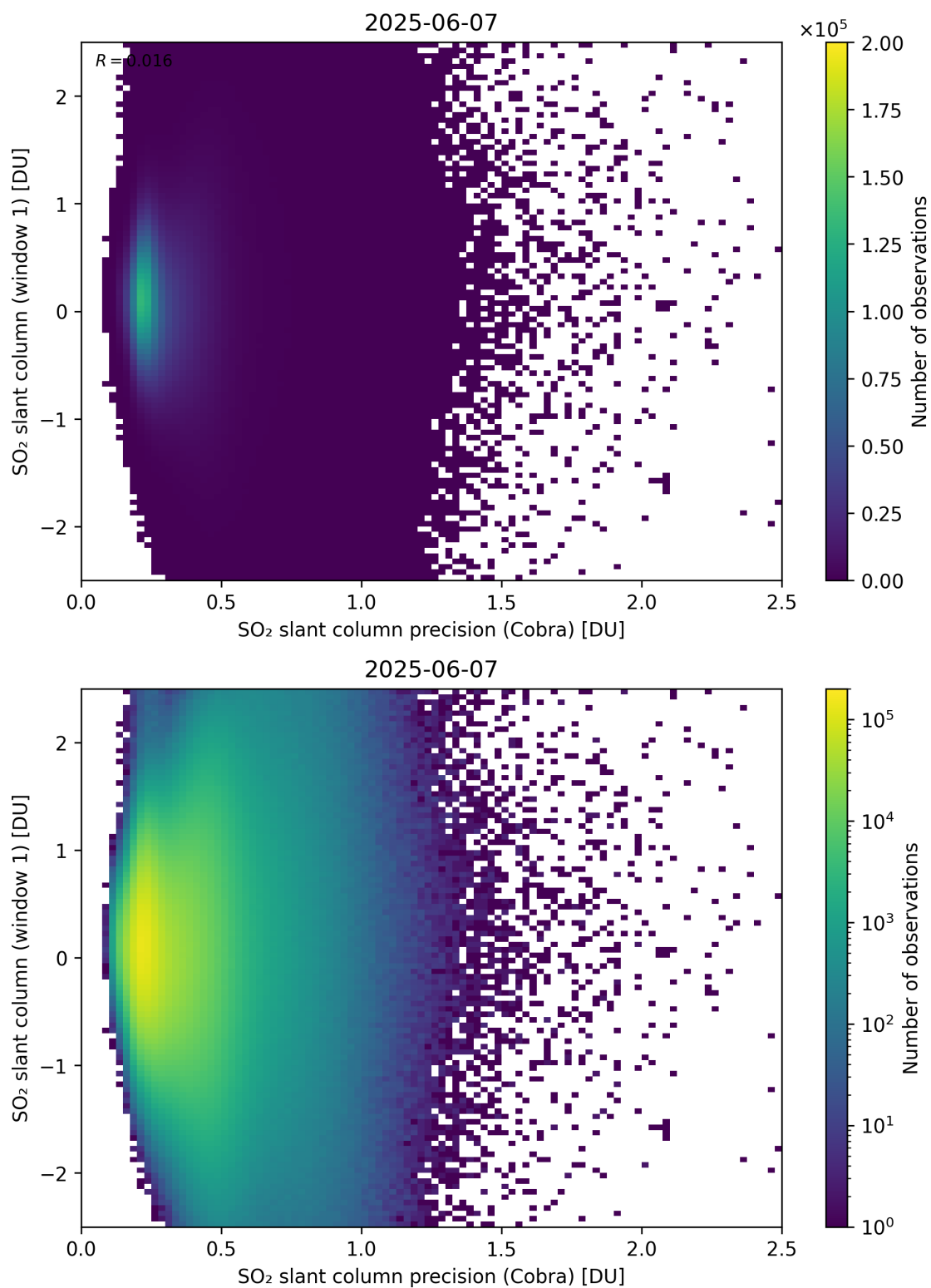
Figure 208: Scatter density plot of “SO 2 slant column precision (Cobra)” against “SO 2 slant column (window 1)” for 2025-06-06 to 2025-06-08.
