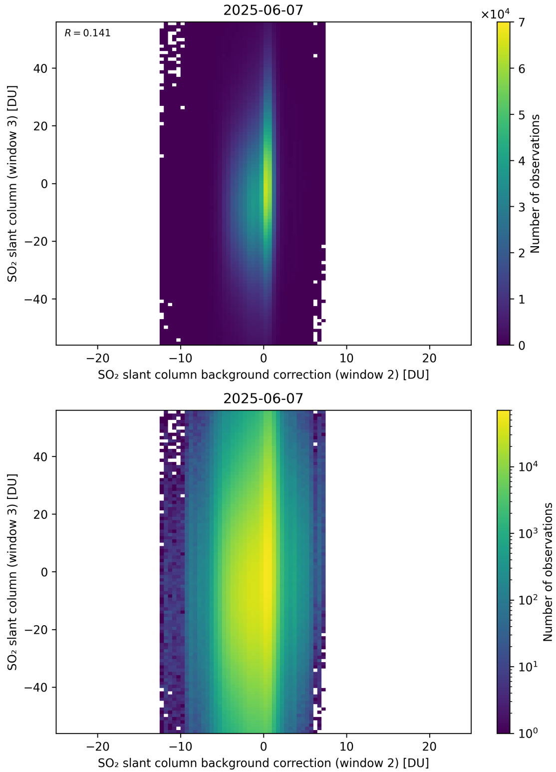
Figure 128: Scatter density plot of “SO 2 slant column background correction (window 2)” against “SO 2 slant column (window 3)” for 2025-06-06 to 2025-06-08.
