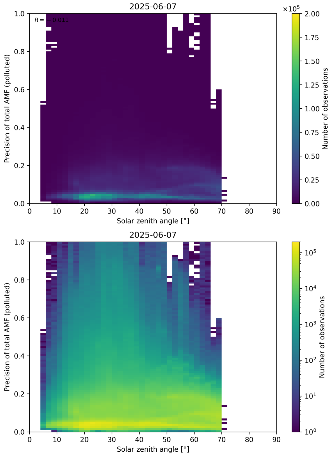
Figure 190: Scatter density plot of “Solar zenith angle” against “Precision of total AMF (polluted)” for 2025-06-06 to 2025-06-08.
