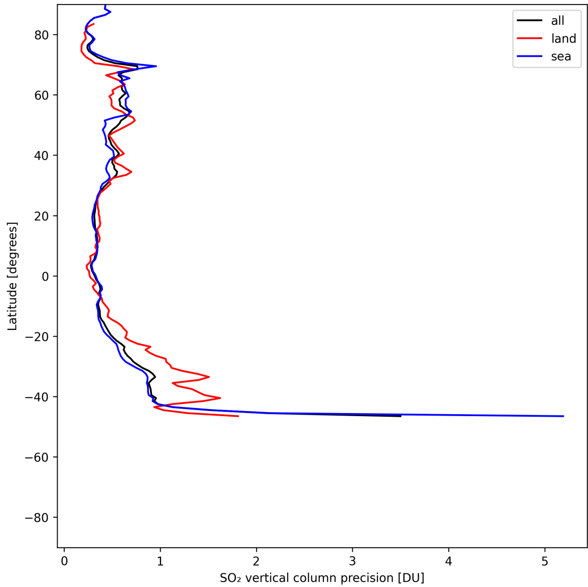
Figure 33: Zonal average of “SO 2 vertical column precision” for 2025-06-06 to 2025-06-08.
