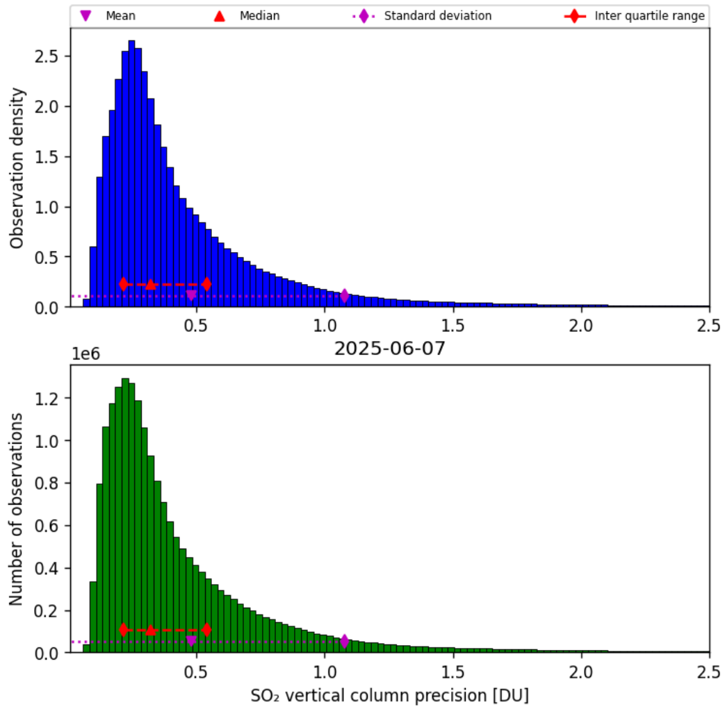
Figure 59: Histogram of “SO 2 vertical column precision” for 2025-06-06 to 2025-06-08
