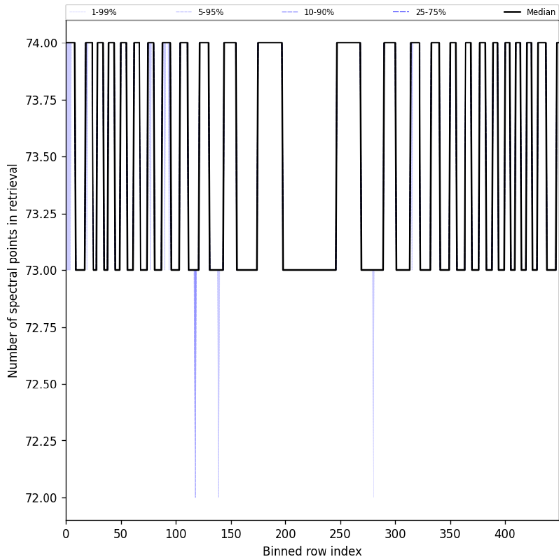
Figure 108: Along track statistics of “Number of spectral points in retrieval” for 2025-06-06 to 2025-06-08
