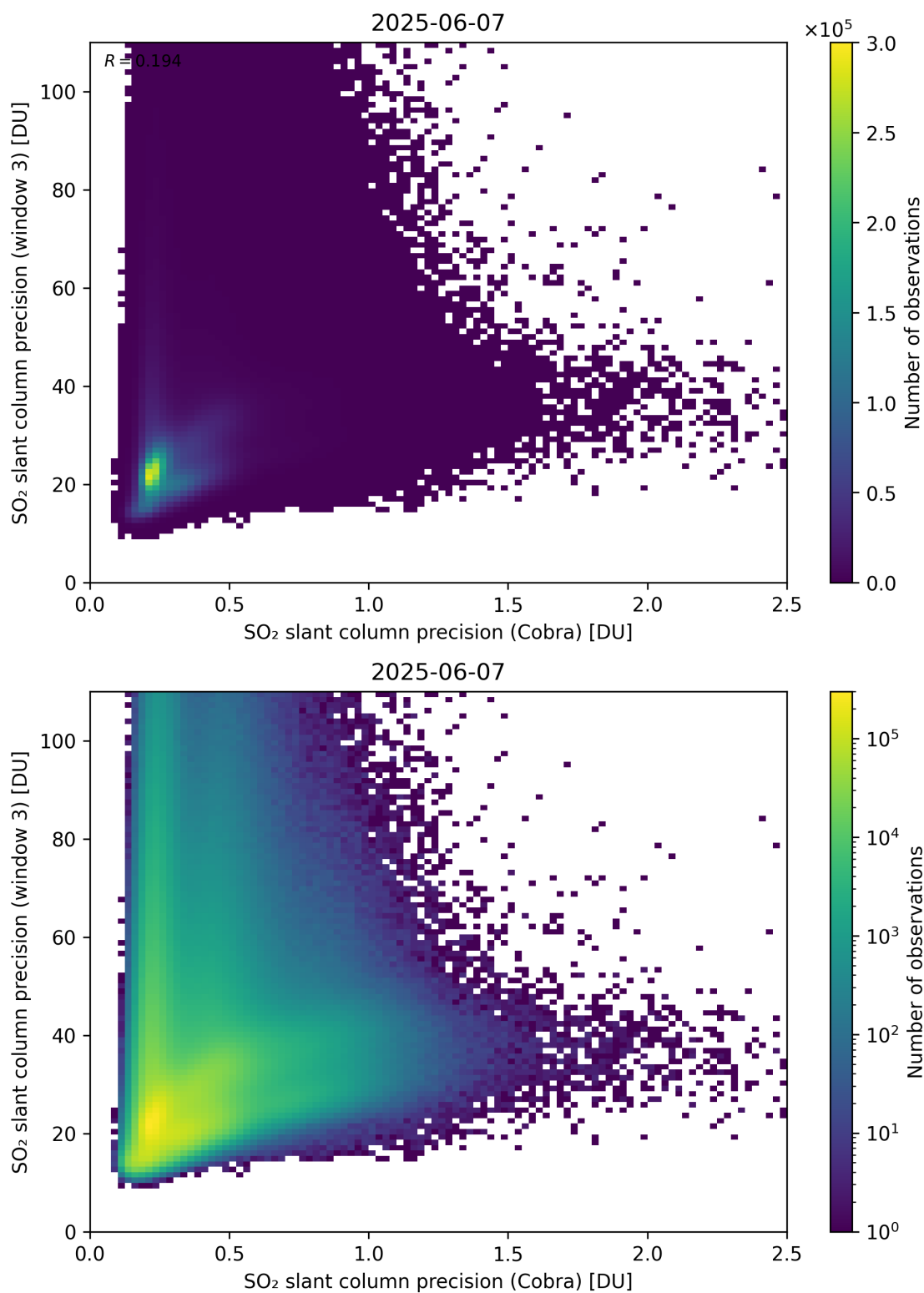
Figure 212: Scatter density plot of “SO 2 slant column precision (Cobra)” against “SO 2 slant column precision (window 3)” for 2025-06-06 to 2025-06-08.
