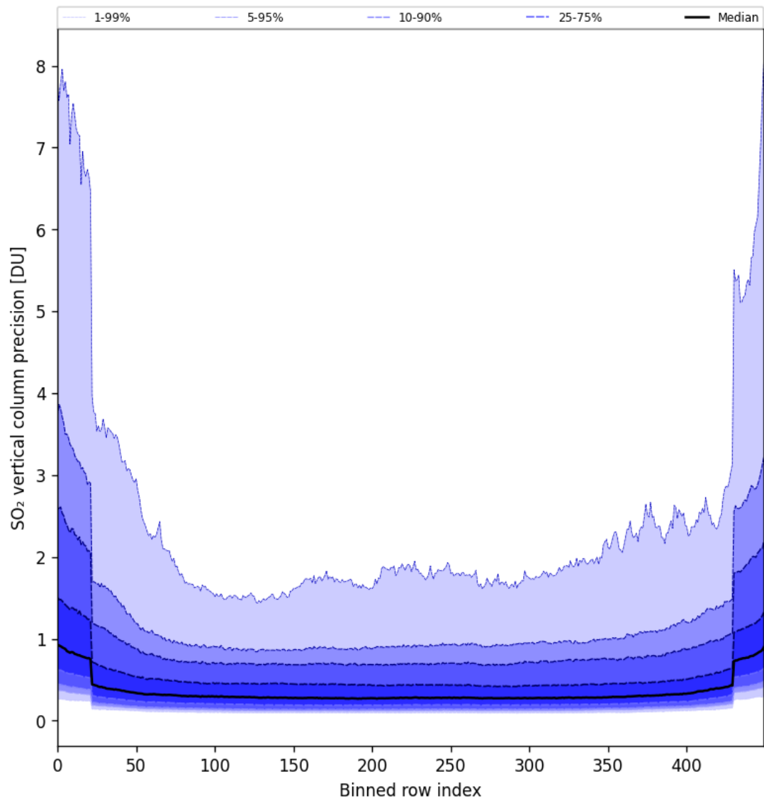
Figure 85: Along track statistics of “SO 2 vertical column precision” for 2025-06-06 to 2025-06-08
