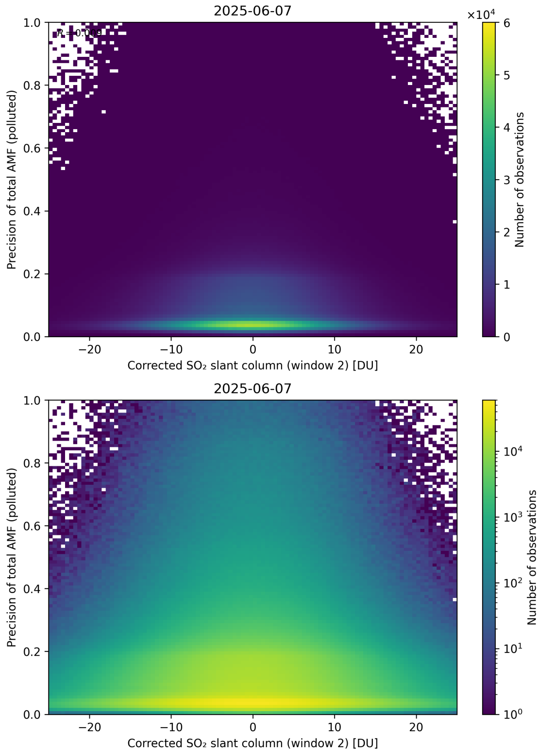
Figure 254: Scatter density plot of “Corrected SO 2 slant column (window 2)” against “Precision of total AMF (polluted)” for 2025-06-06 to 2025-06-08.
