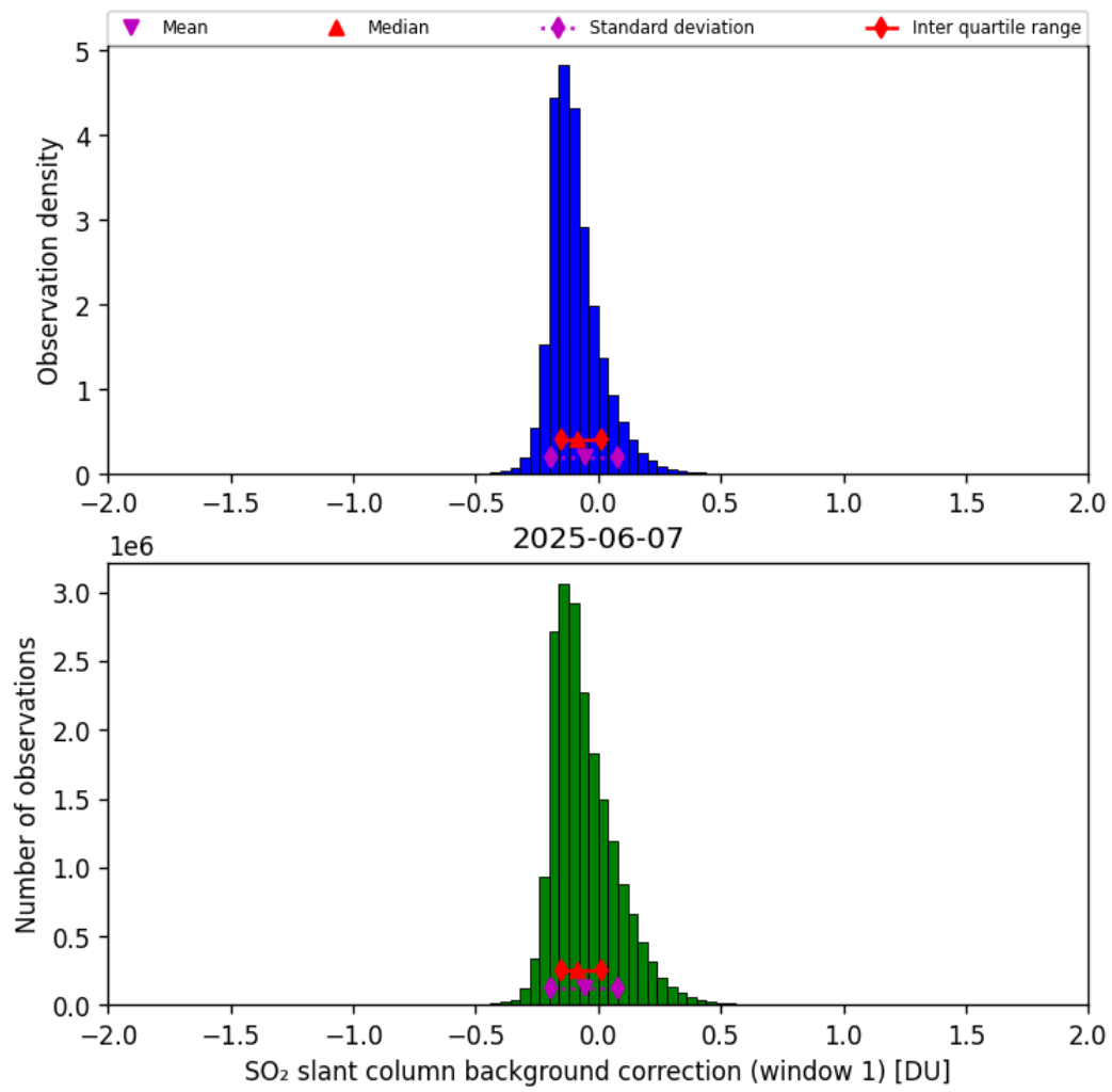
Figure 66: Histogram of “SO 2 slant column background correction (window 1)” for 2025-06-06 to 2025-06-08
