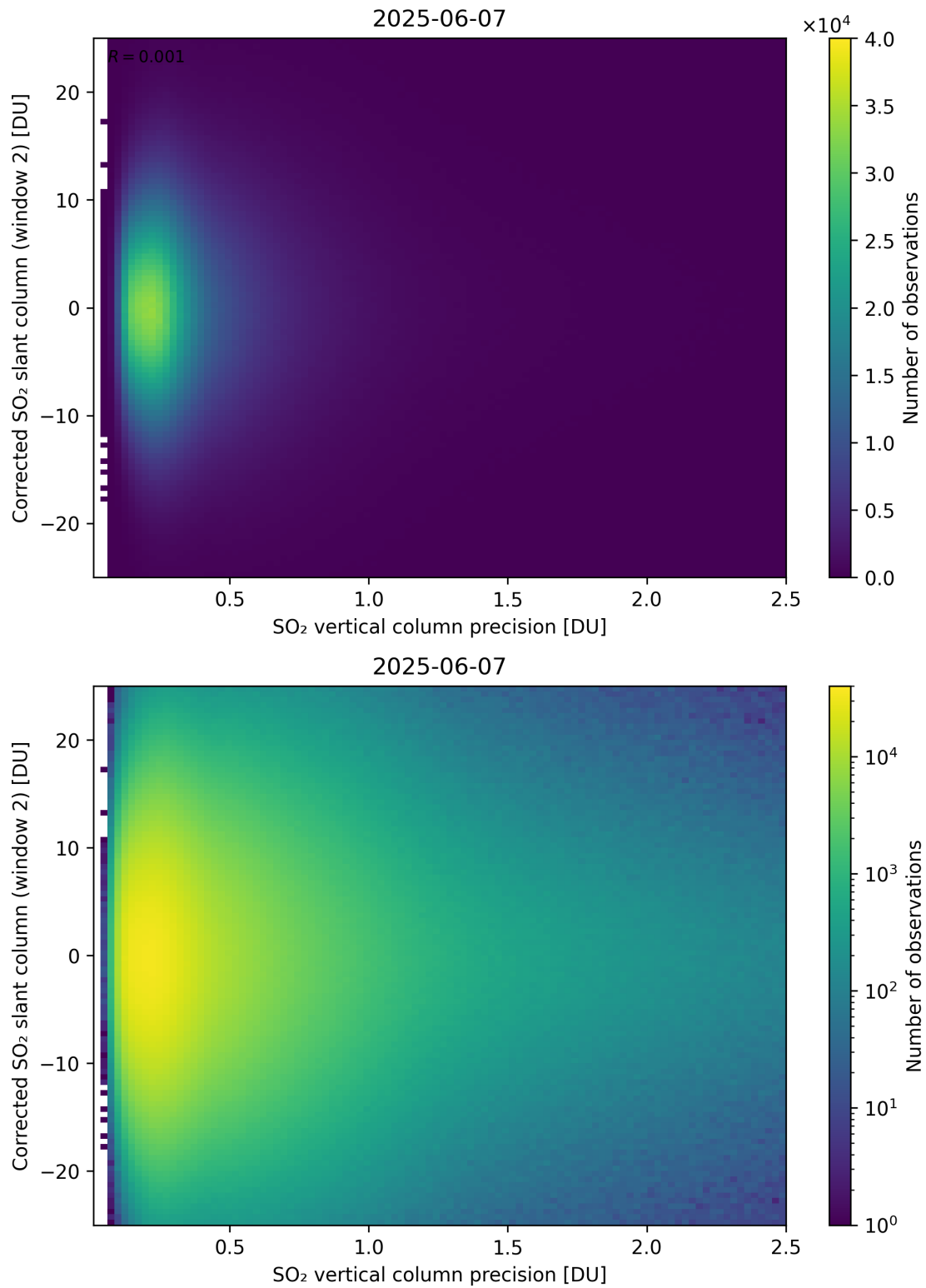
Figure 339: Scatter density plot of “SO 2 vertical column precision” against “Corrected SO 2 slant column (window 2)” for 2025-06-06 to 2025-06-08.
