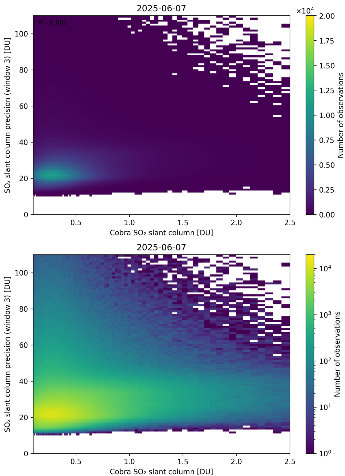
Figure 223: Scatter density plot of “Cobra SO 2 slant column” against “SO 2 slant column precision (window 3)” for 2025-06-06 to 2025-06-08.
