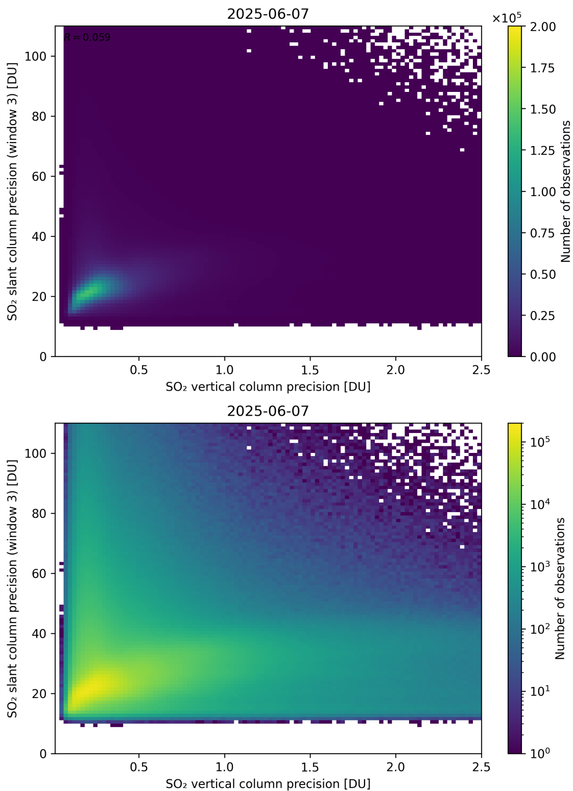
Figure 345: Scatter density plot of “SO 2 vertical column precision” against “SO 2 slant column precision (window 3)” for 2025-06-06 to 2025-06-08.
