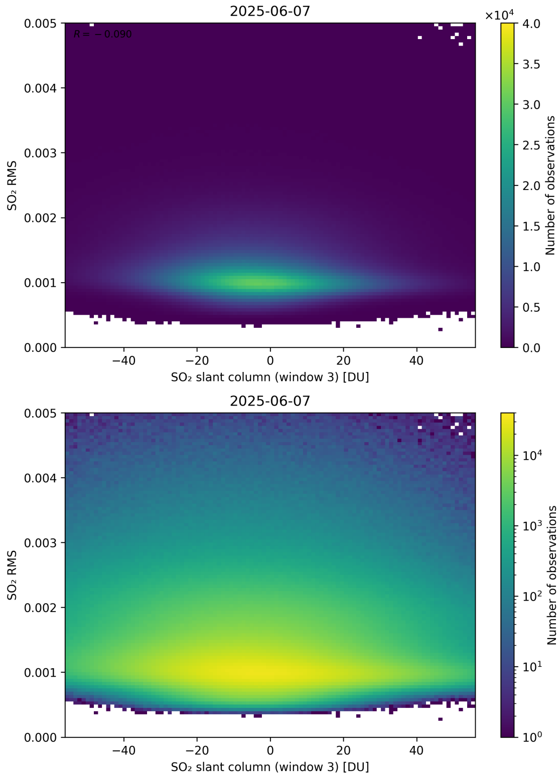
Figure 306: Scatter density plot of “SO 2 slant column (window 3)” against “SO 2 RMS” for 2025-06-06 to 2025-06-08.
