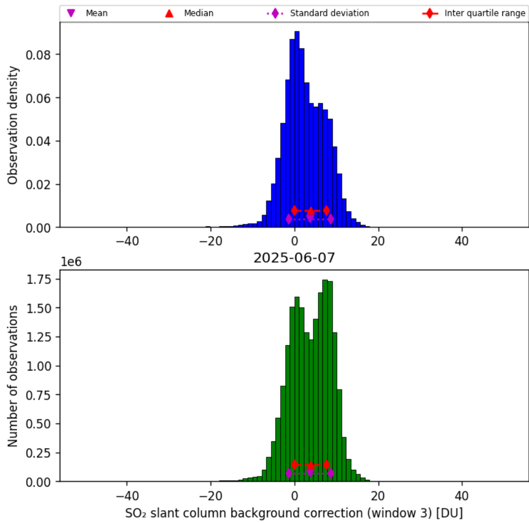
Figure 74: Histogram of “SO 2 slant column background correction (window 3)” for 2025-06-06 to 2025-06-08
