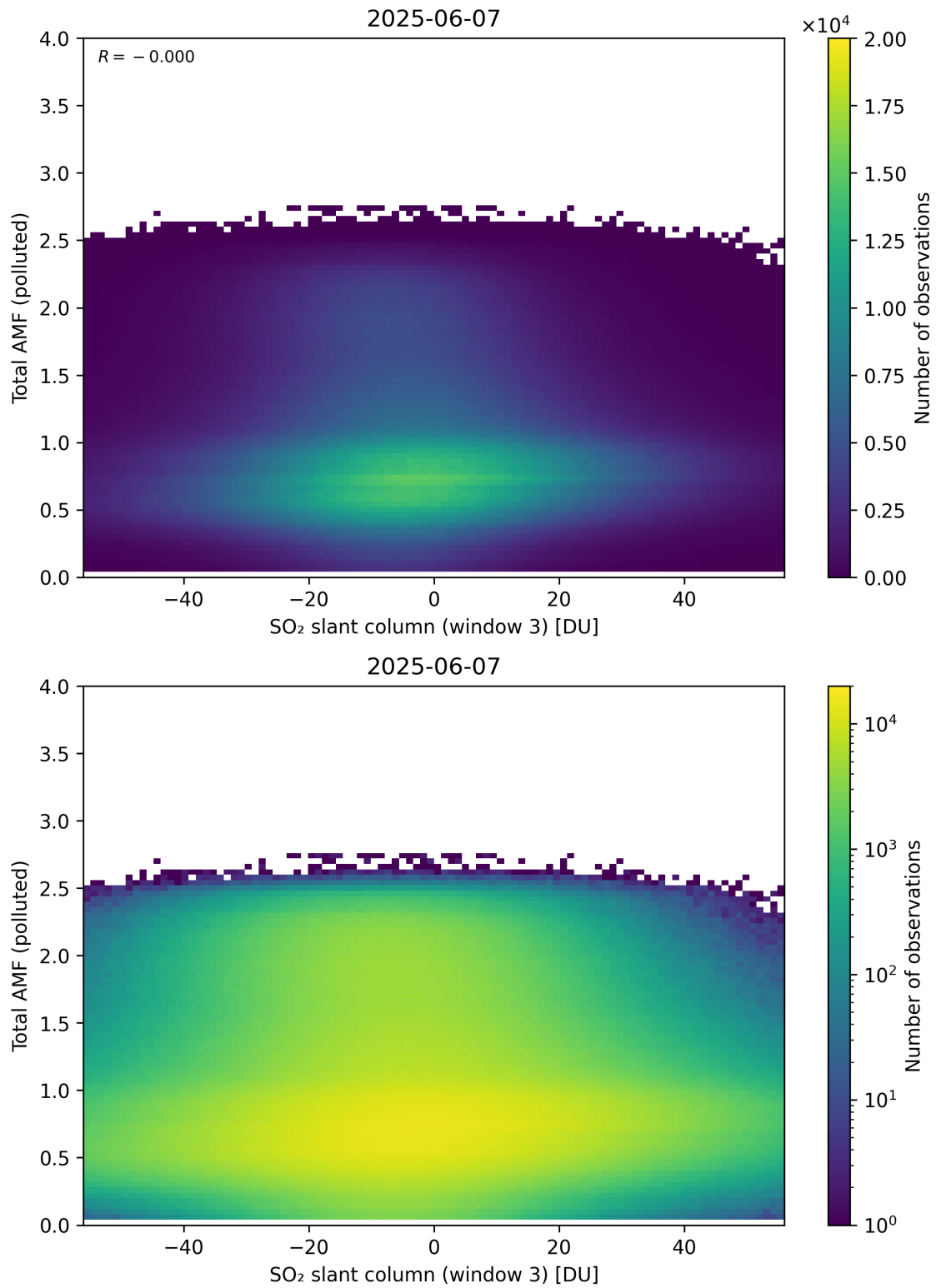
Figure 318: Scatter density plot of “SO 2 slant column (window 3)” against “Total AMF (polluted)” for 2025-06-06 to 2025-06-08.
