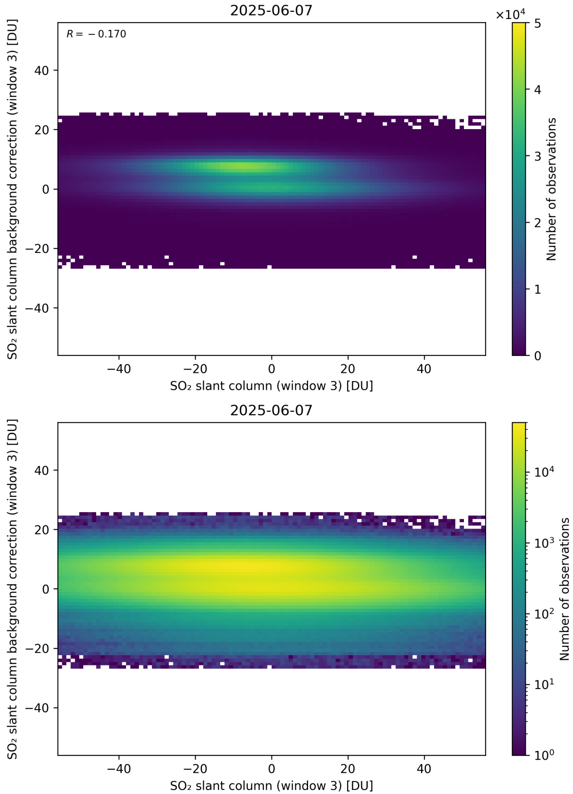
Figure 303: Scatter density plot of “SO 2 slant column (window 3)” against “SO 2 slant column background correction (window 3)” for 2025-06-06 to 2025-06-08.
