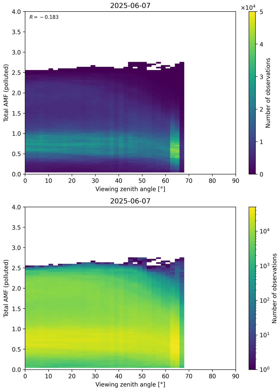
Figure 381: Scatter density plot of “Viewing zenith angle” against “Total AMF (polluted)” for 2025-06-06 to 2025-06-08.
