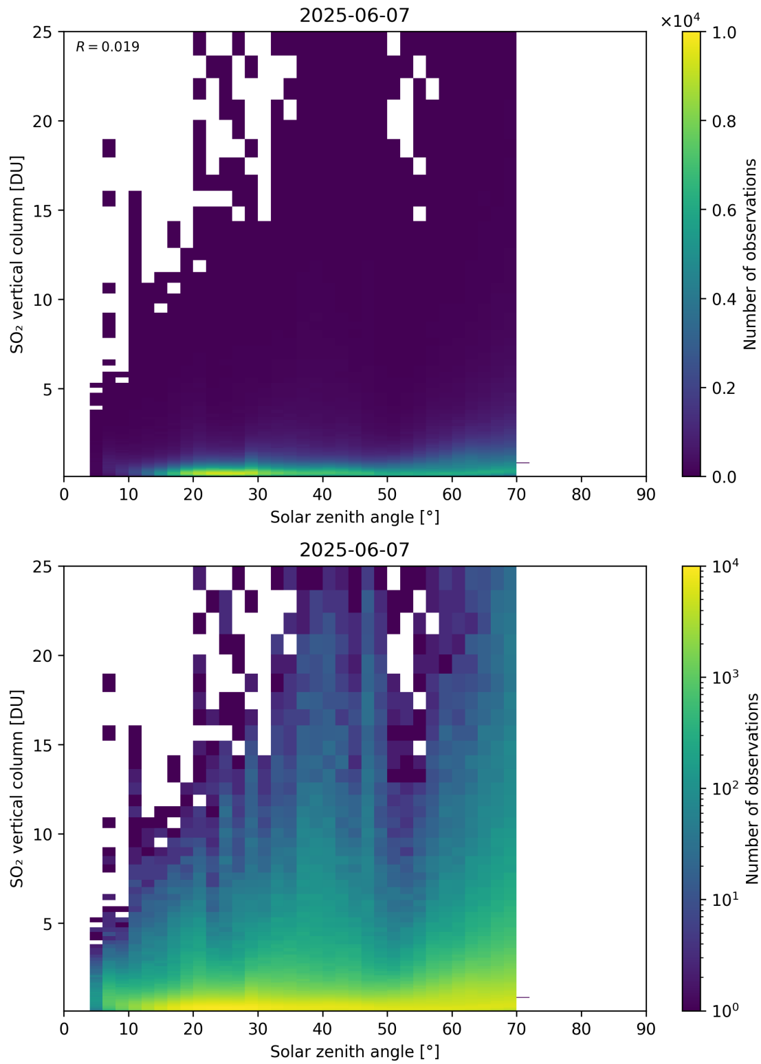
Figure 191: Scatter density plot of “Solar zenith angle” against “SO 2 vertical column” for 2025-06-06 to 2025-06-08.
