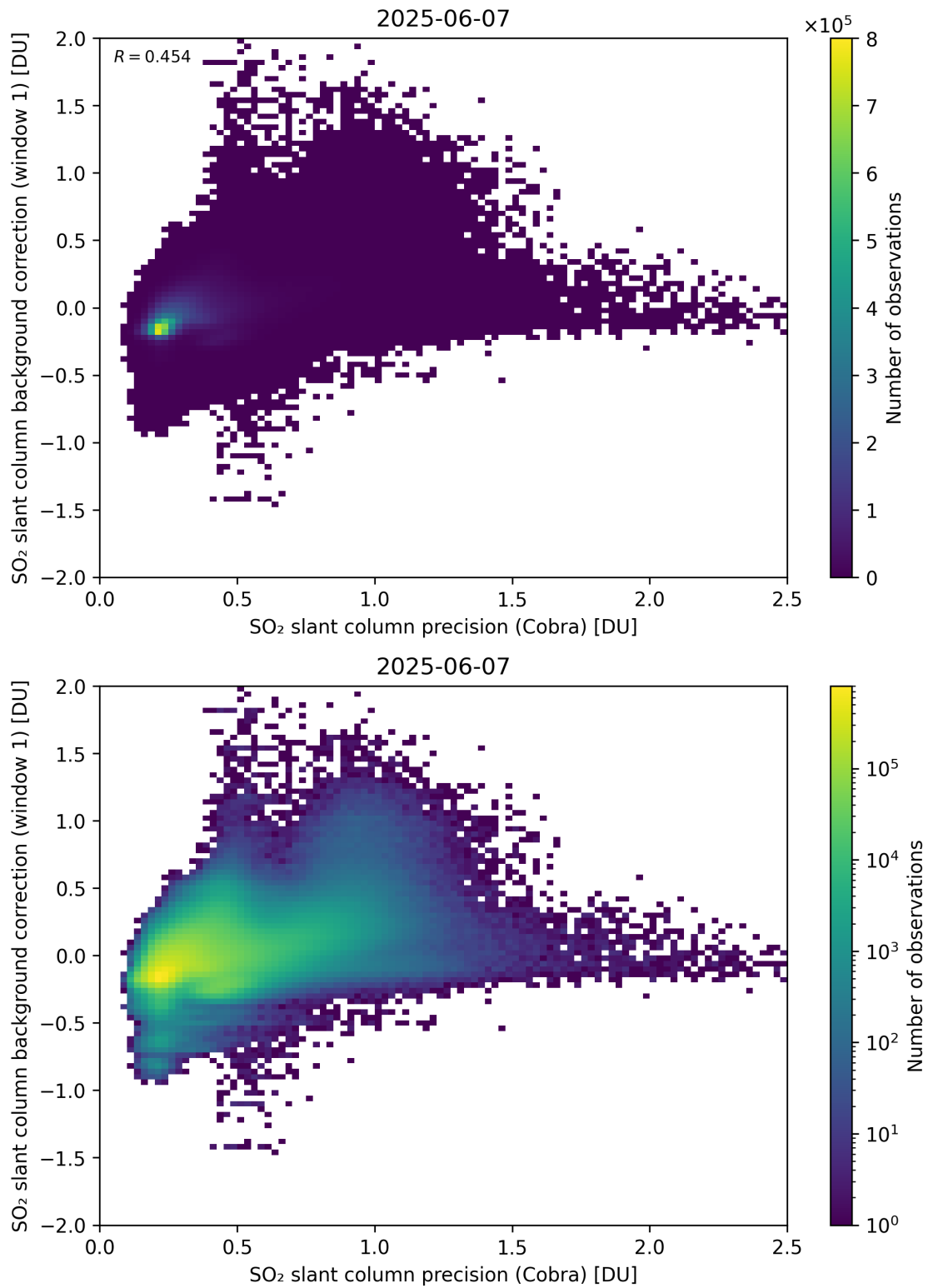
Figure 199: Scatter density plot of “SO 2 slant column precision (Cobra)” against “SO 2 slant column background correction (window 1)” for 2025-06-06 to 2025-06-08.
