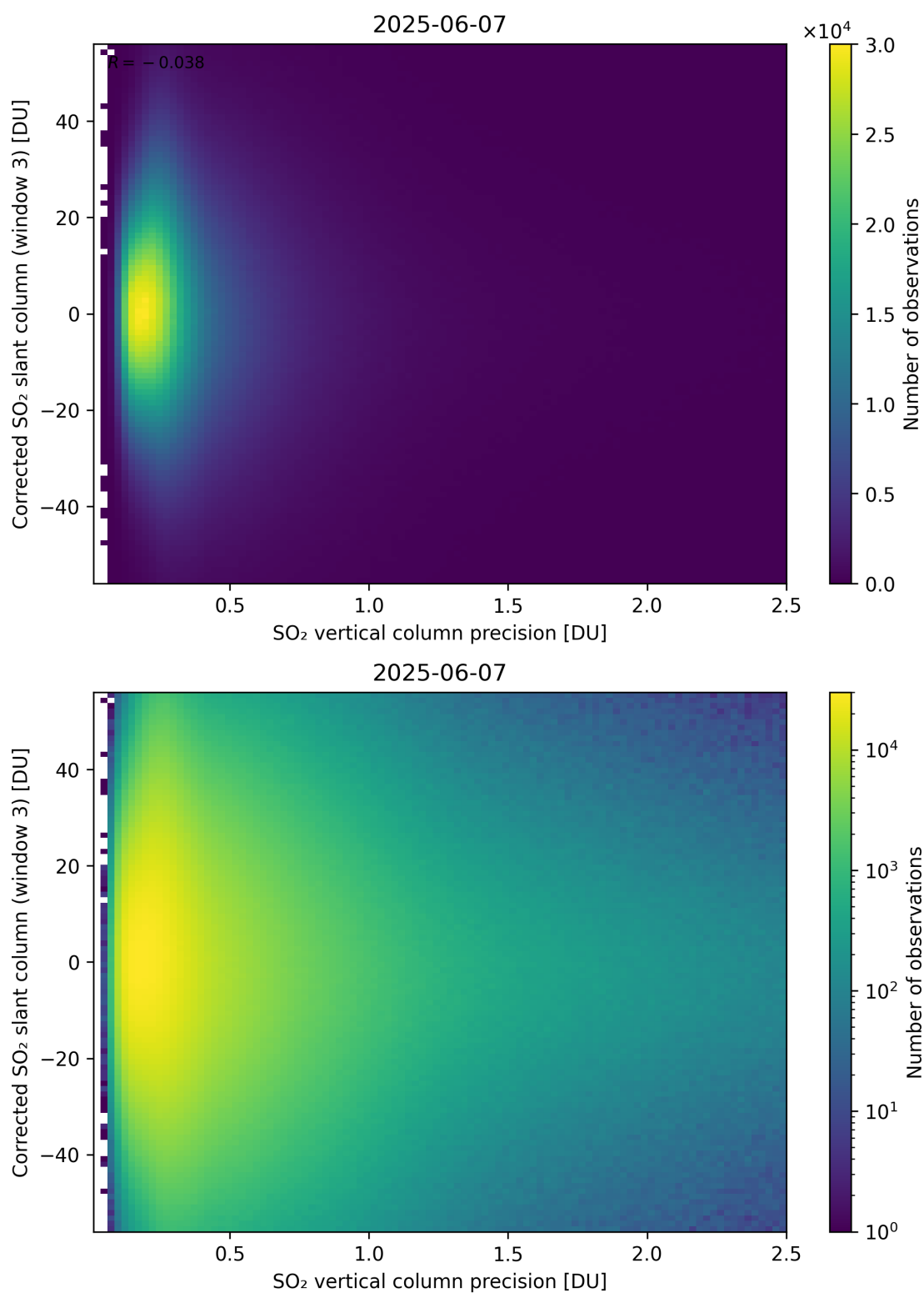
Figure 340: Scatter density plot of “SO 2 vertical column precision” against “Corrected SO 2 slant column (window 3)” for 2025-06-06 to 2025-06-08.
