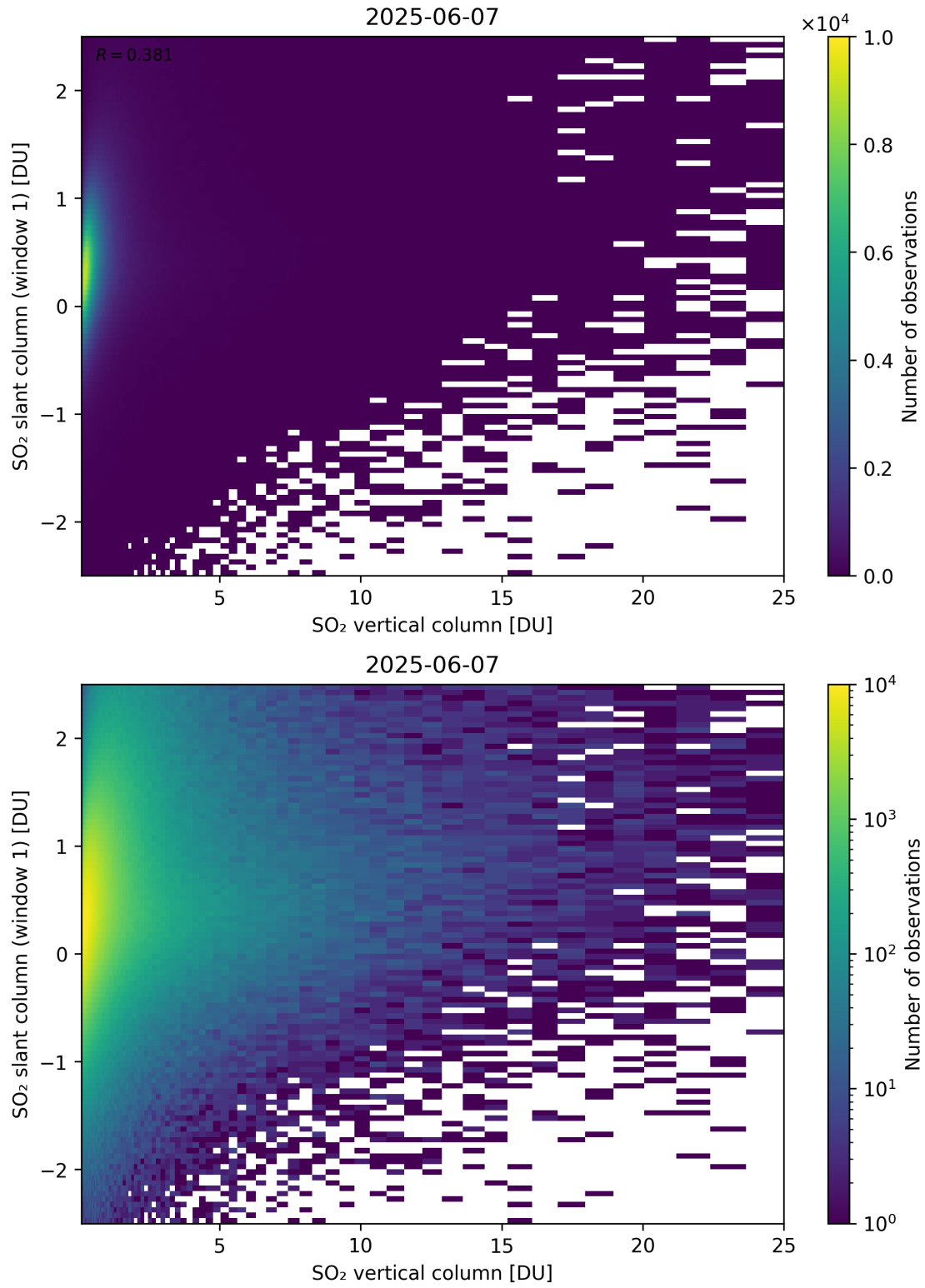
Figure 354: Scatter density plot of “SO 2 vertical column” against “SO 2 slant column (window 1)” for 2025-06-06 to 2025-06-08.
