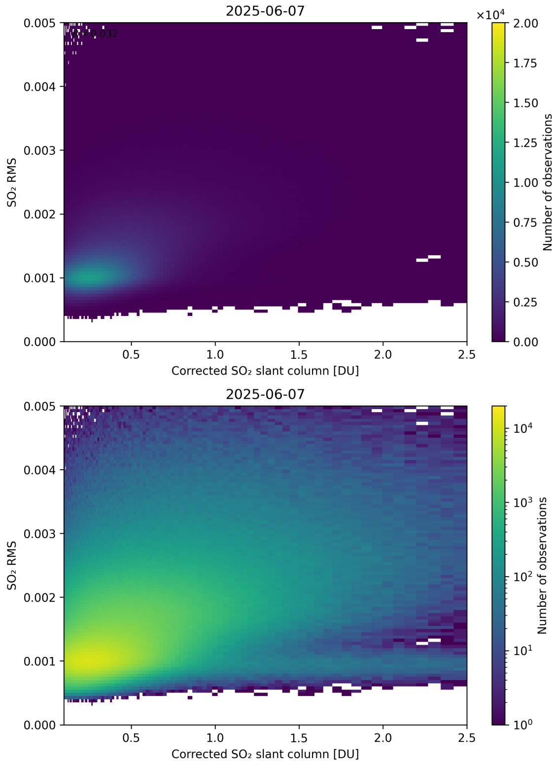
Figure 231: Scatter density plot of “Corrected SO 2 slant column” against “SO 2 RMS” for 2025-06-06 to 2025-06-08.
