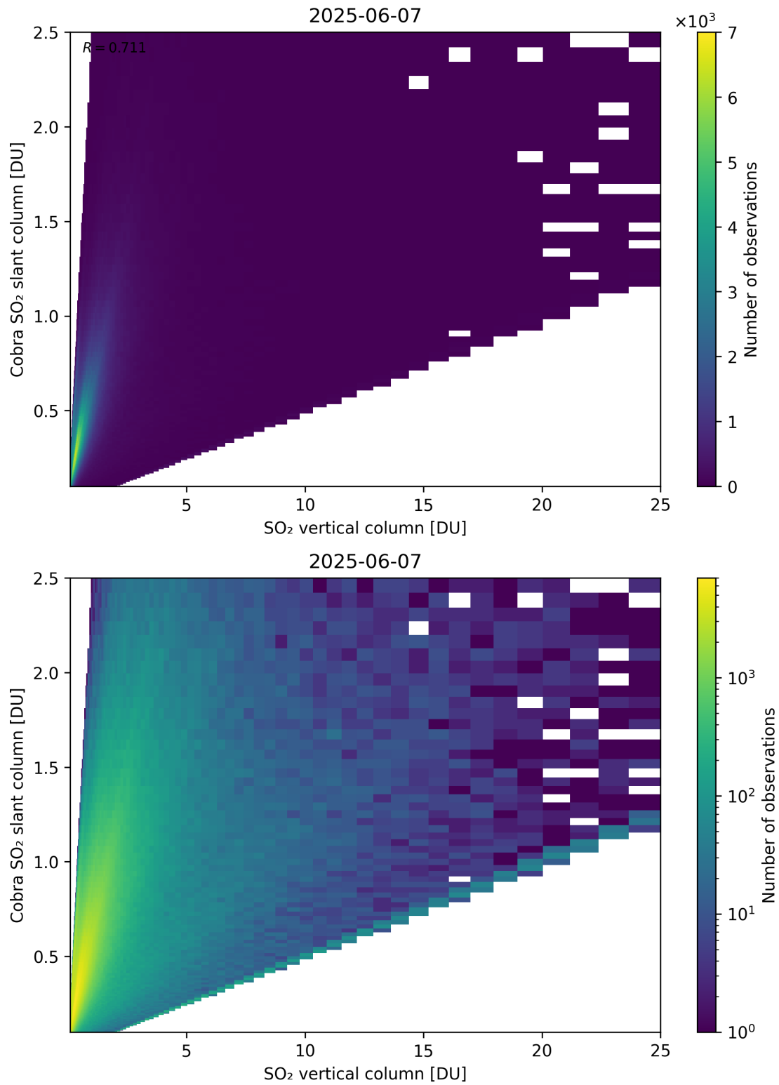
Figure 349: Scatter density plot of “SO 2 vertical column” against “Cobra SO 2 slant column” for 2025-06-06 to 2025-06-08.
