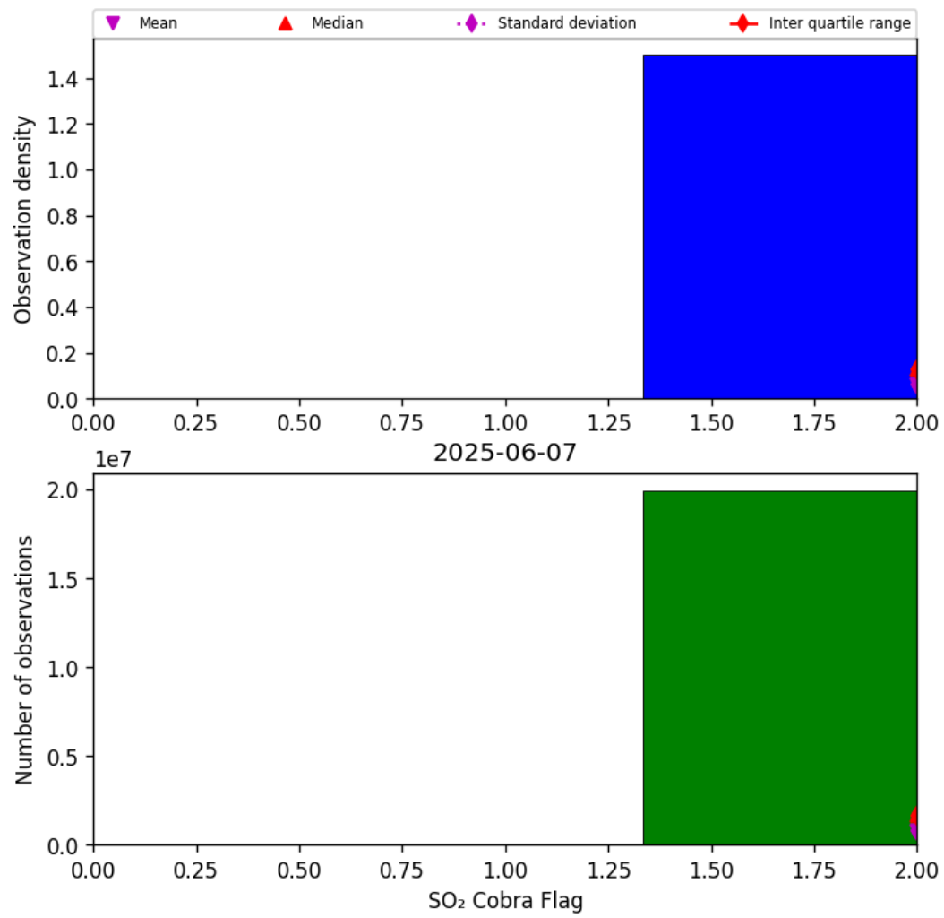
Figure 75: Histogram of “SO 2 Cobra Flag” for 2025-06-06 to 2025-06-08
