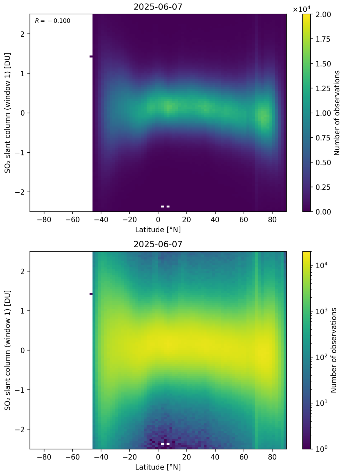
Figure 162: Scatter density plot of “Latitude” against “SO 2 slant column (window 1)” for 2025-06-06 to 2025-06-08.
