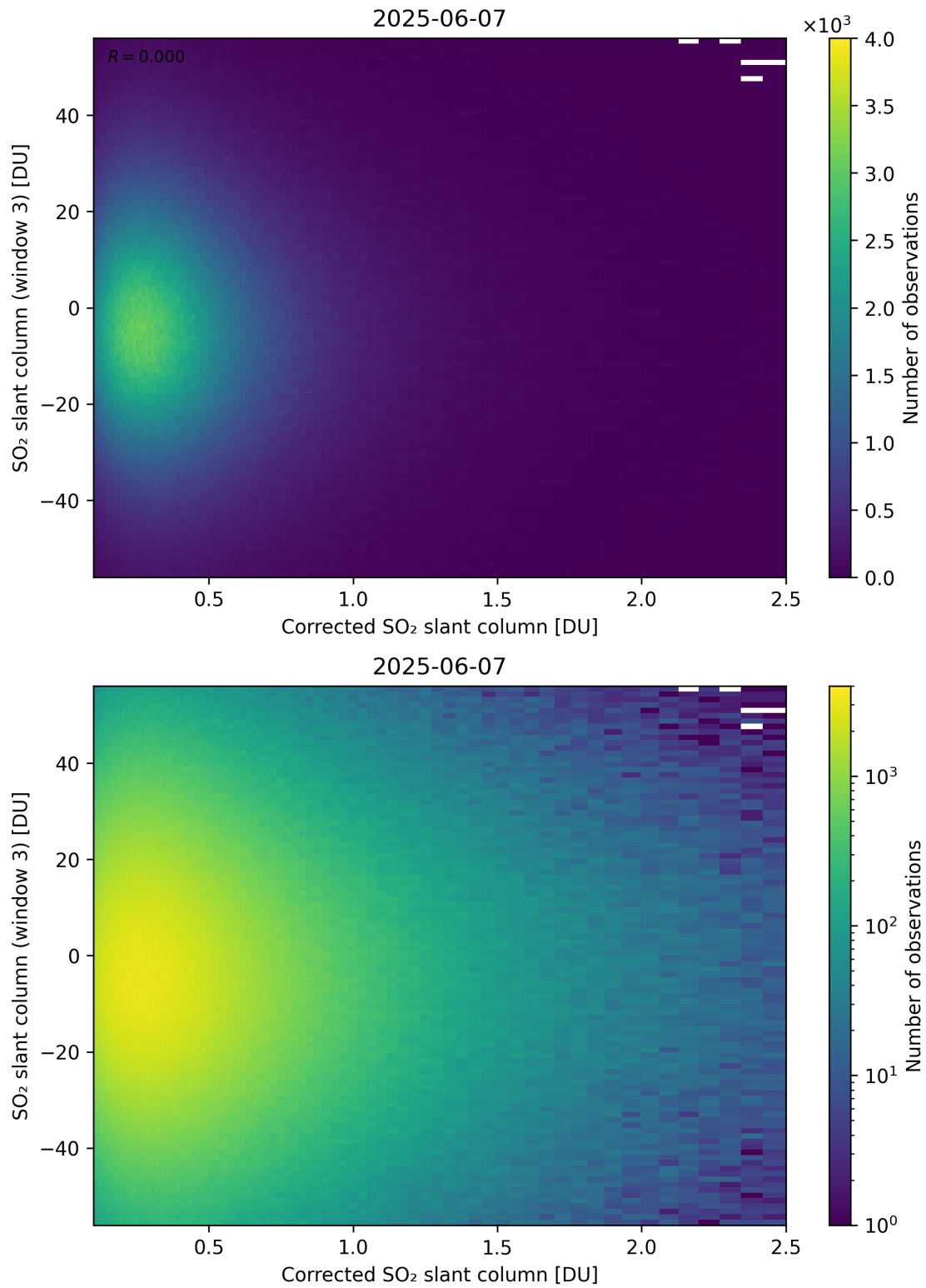
Figure 240: Scatter density plot of “Corrected SO 2 slant column” against “SO 2 slant column (window 3)” for 2025-06-06 to 2025-06-08.
