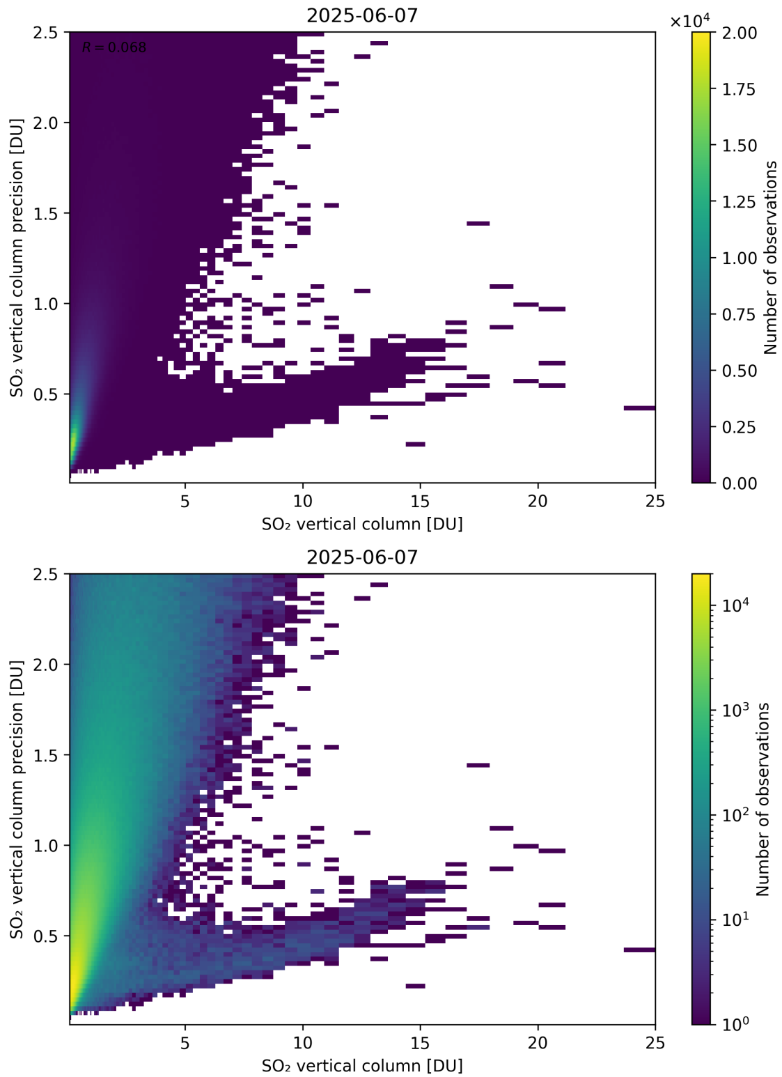
Figure 361: Scatter density plot of “SO 2 vertical column” against “SO 2 vertical column precision” for 2025-06-06 to 2025-06-08.
