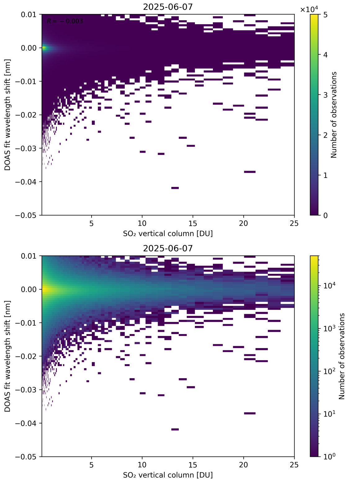
Figure 326: Scatter density plot of “SO 2 vertical column” against “DOAS fit wavelength shift” for 2025-06-06 to 2025-06-08.
