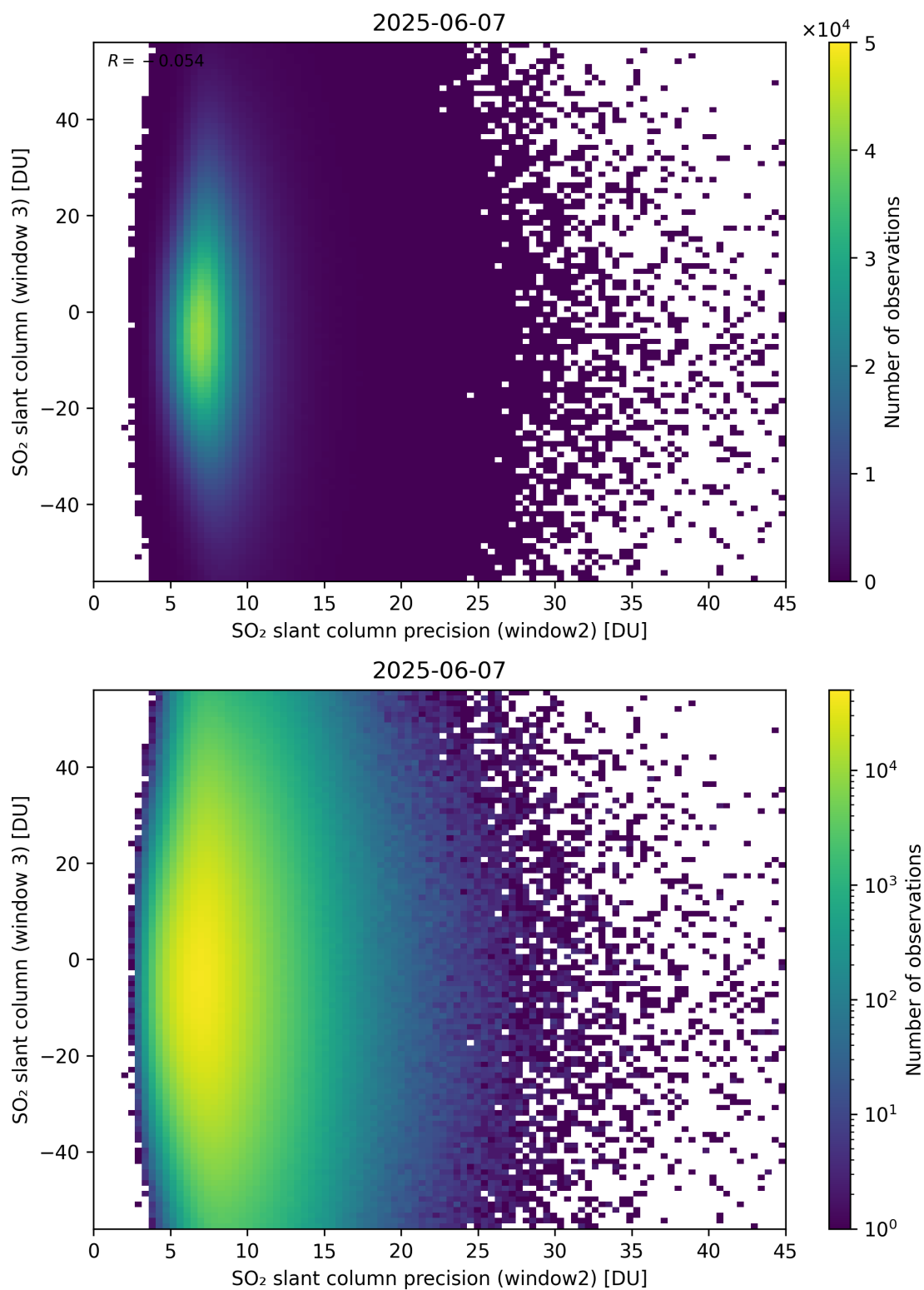
Figure 299: Scatter density plot of “SO 2 slant column precision (window2)” against “SO 2 slant column (window 3)” for 2025-06-06 to 2025-06-08.
