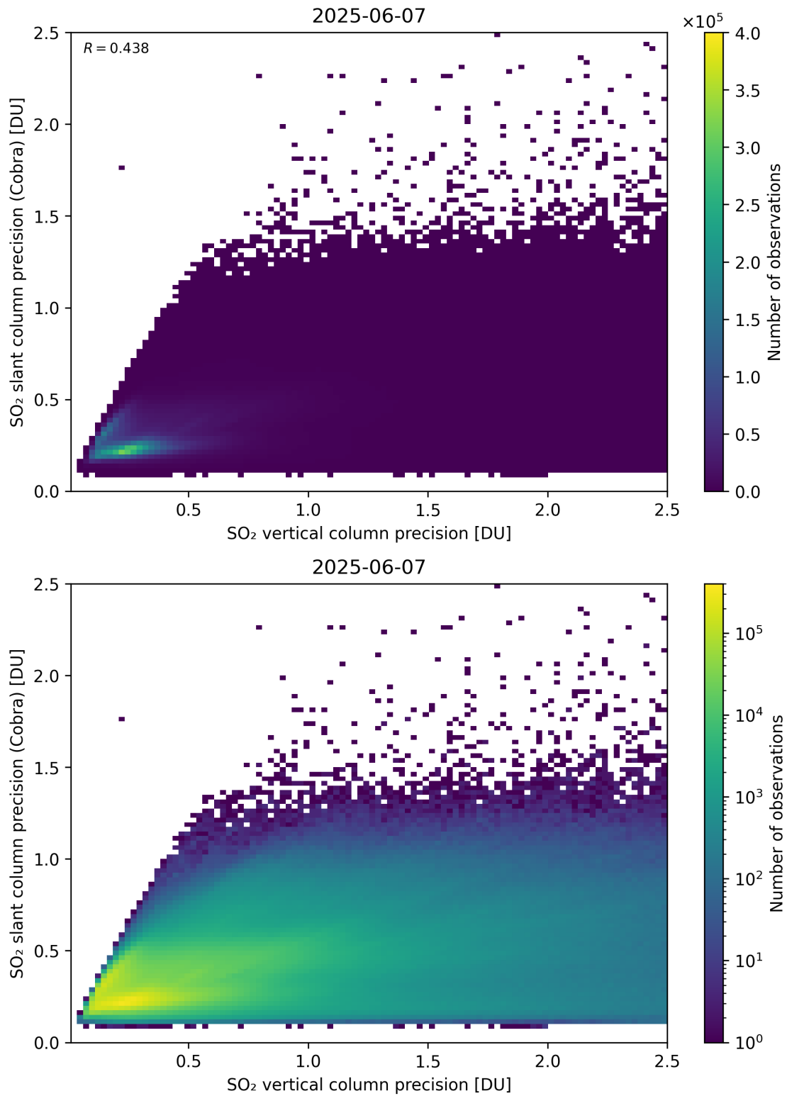
Figure 337: Scatter density plot of “SO 2 vertical column precision” against “SO 2 slant column precision (Cobra)” for 2025-06-06 to 2025-06-08.
