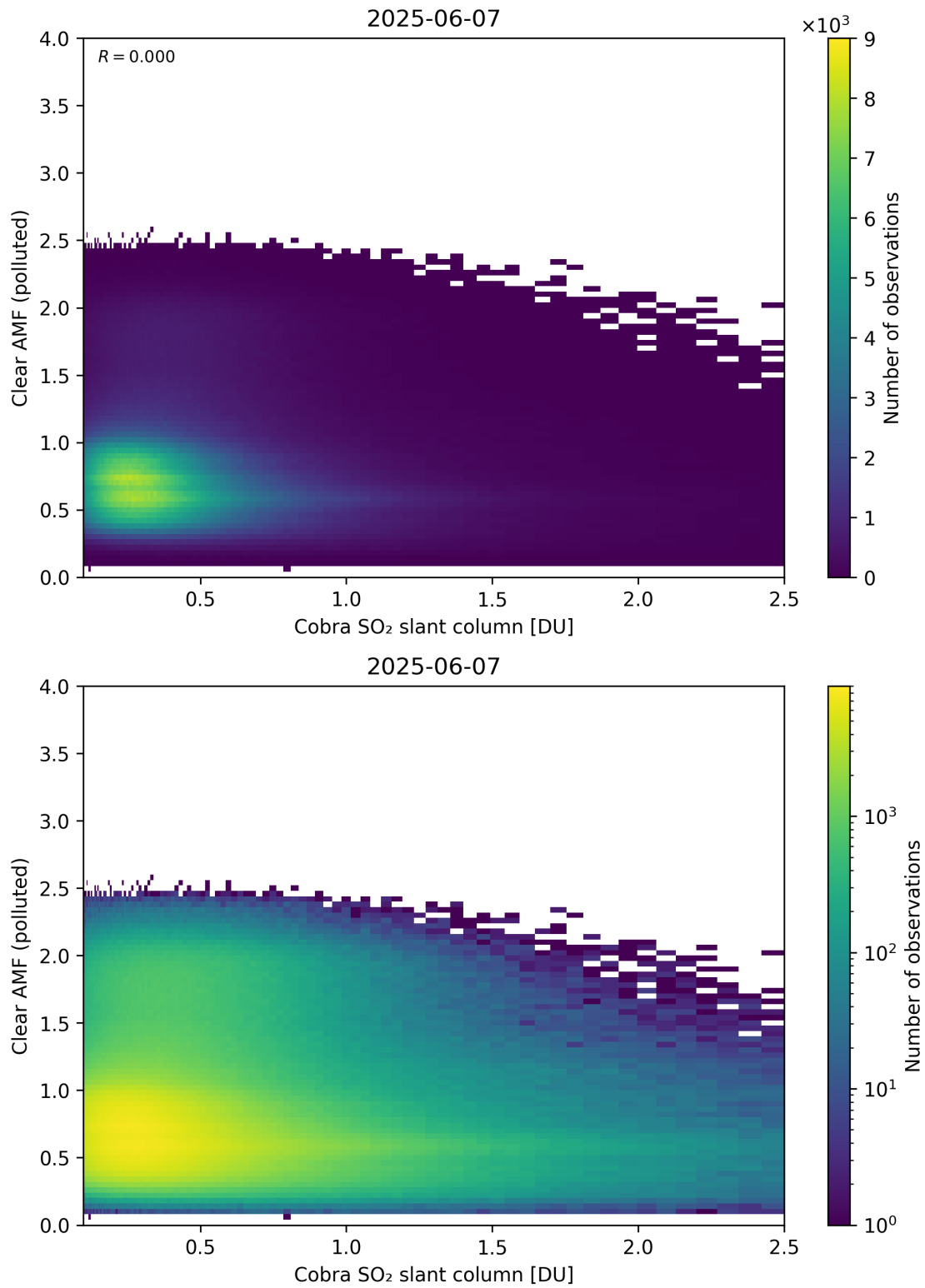
Figure 215: Scatter density plot of “Cobra SO 2 slant column” against “Clear AMF (polluted)” for 2025-06-06 to 2025-06-08.
