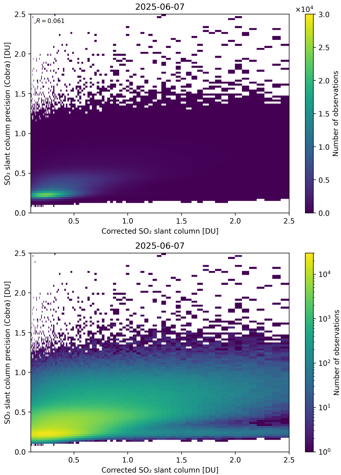
Figure 234: Scatter density plot of “Corrected SO 2 slant column” against “SO 2 slant column precision (Cobra)” for 2025-06-06 to 2025-06-08.
