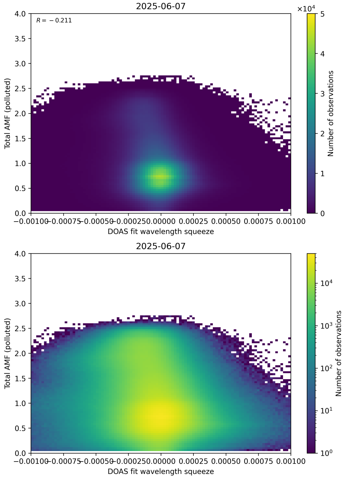
Figure 145: Scatter density plot of “DOAS fit wavelength squeeze” against “Total AMF (polluted)” for 2025-06-06 to 2025-06-08.
