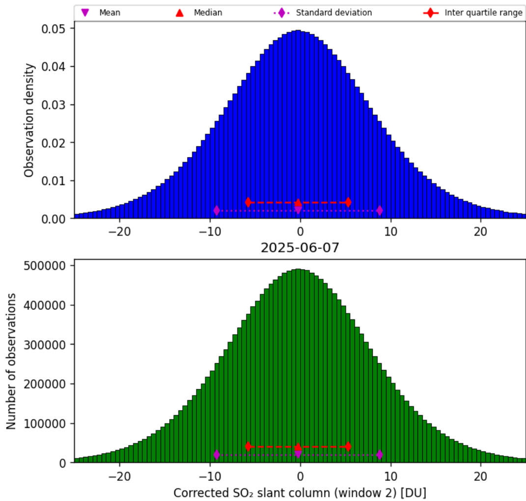
Figure 69: Histogram of “Corrected SO 2 slant column (window 2)” for 2025-06-06 to 2025-06-08
