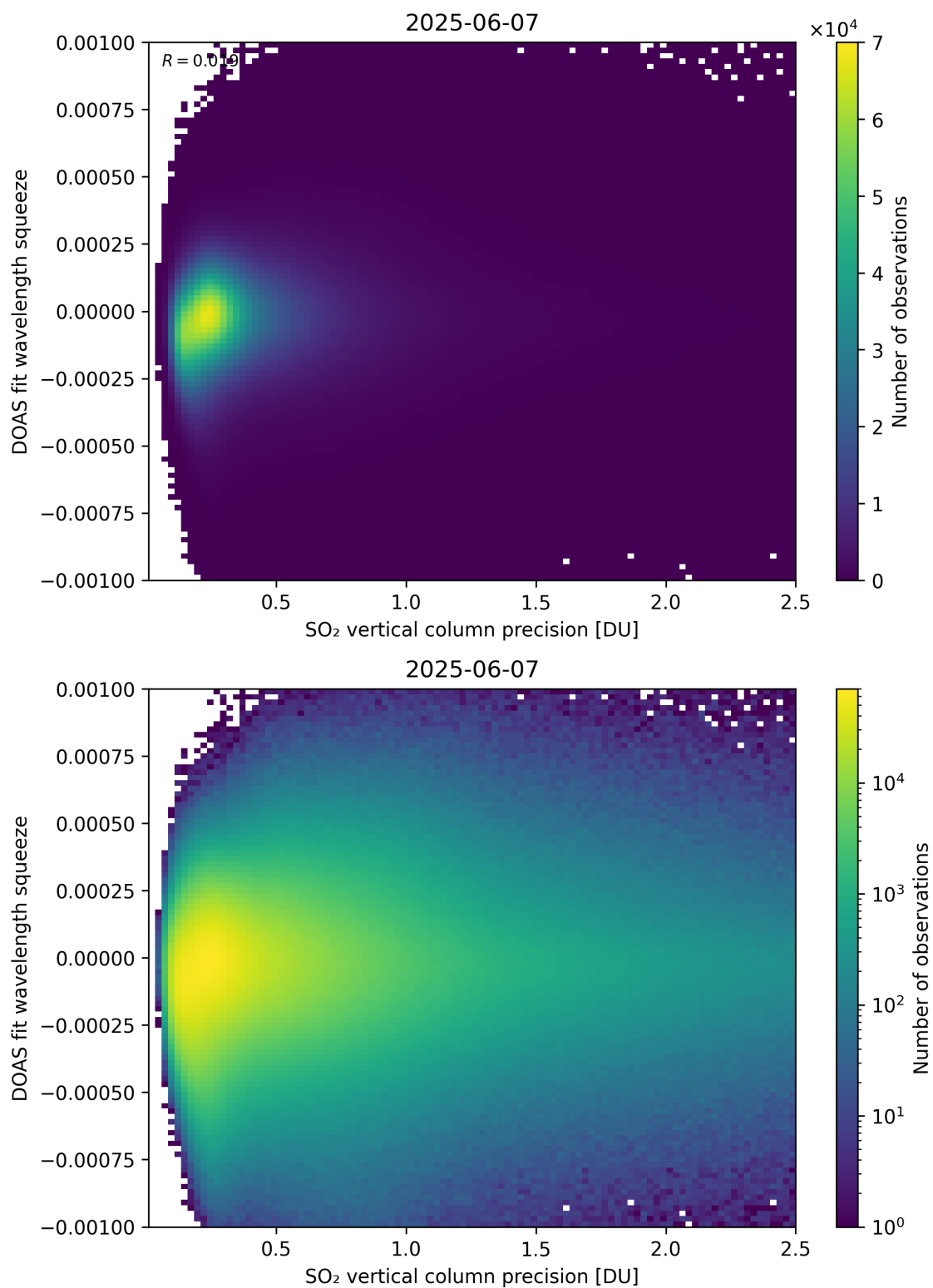
Figure 333: Scatter density plot of “SO 2 vertical column precision” against “DOAS fit wavelength squeeze” for 2025-06-06 to 2025-06-08.
