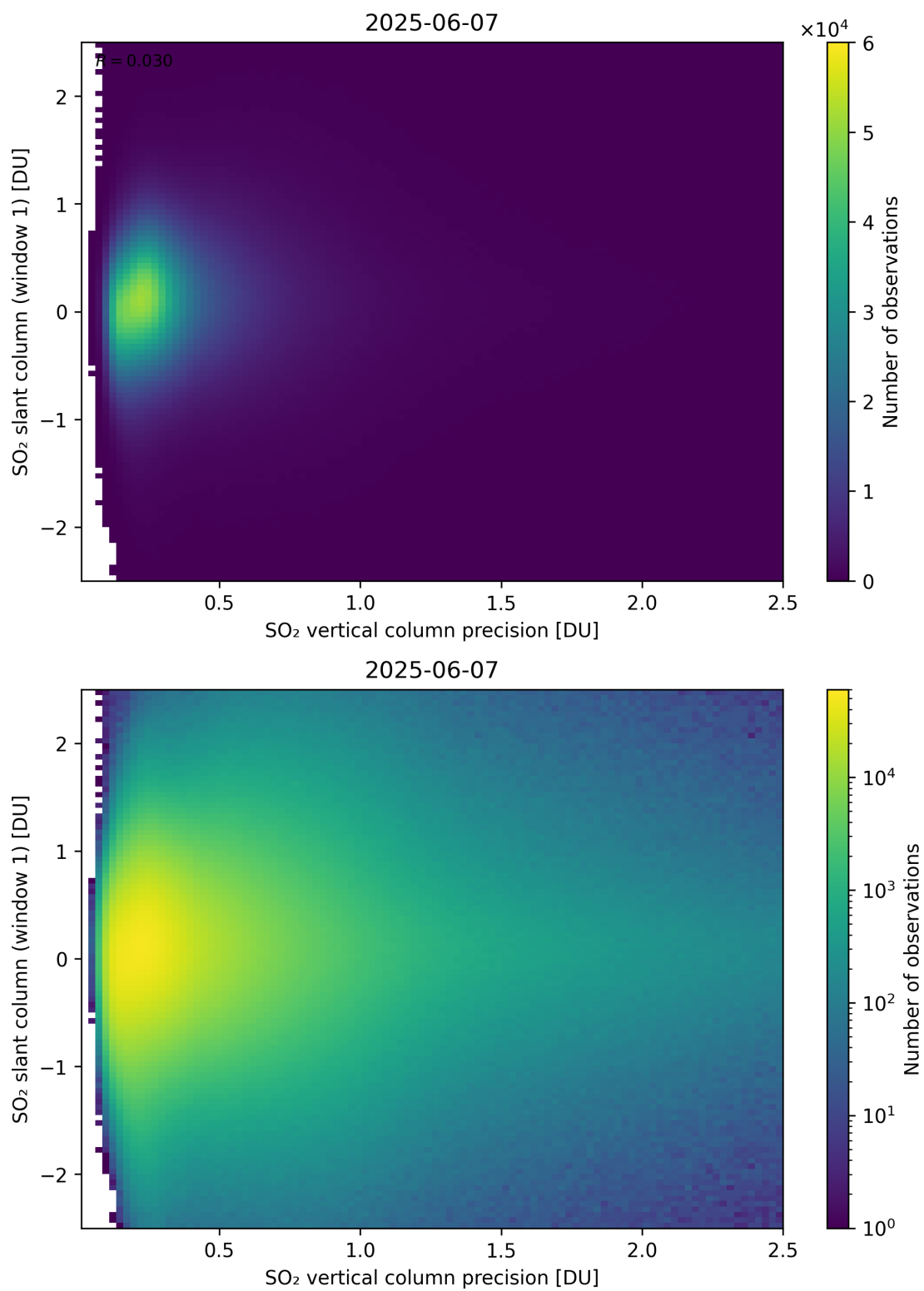
Figure 341: Scatter density plot of “SO 2 vertical column precision” against “SO 2 slant column (window 1)” for 2025-06-06 to 2025-06-08.
