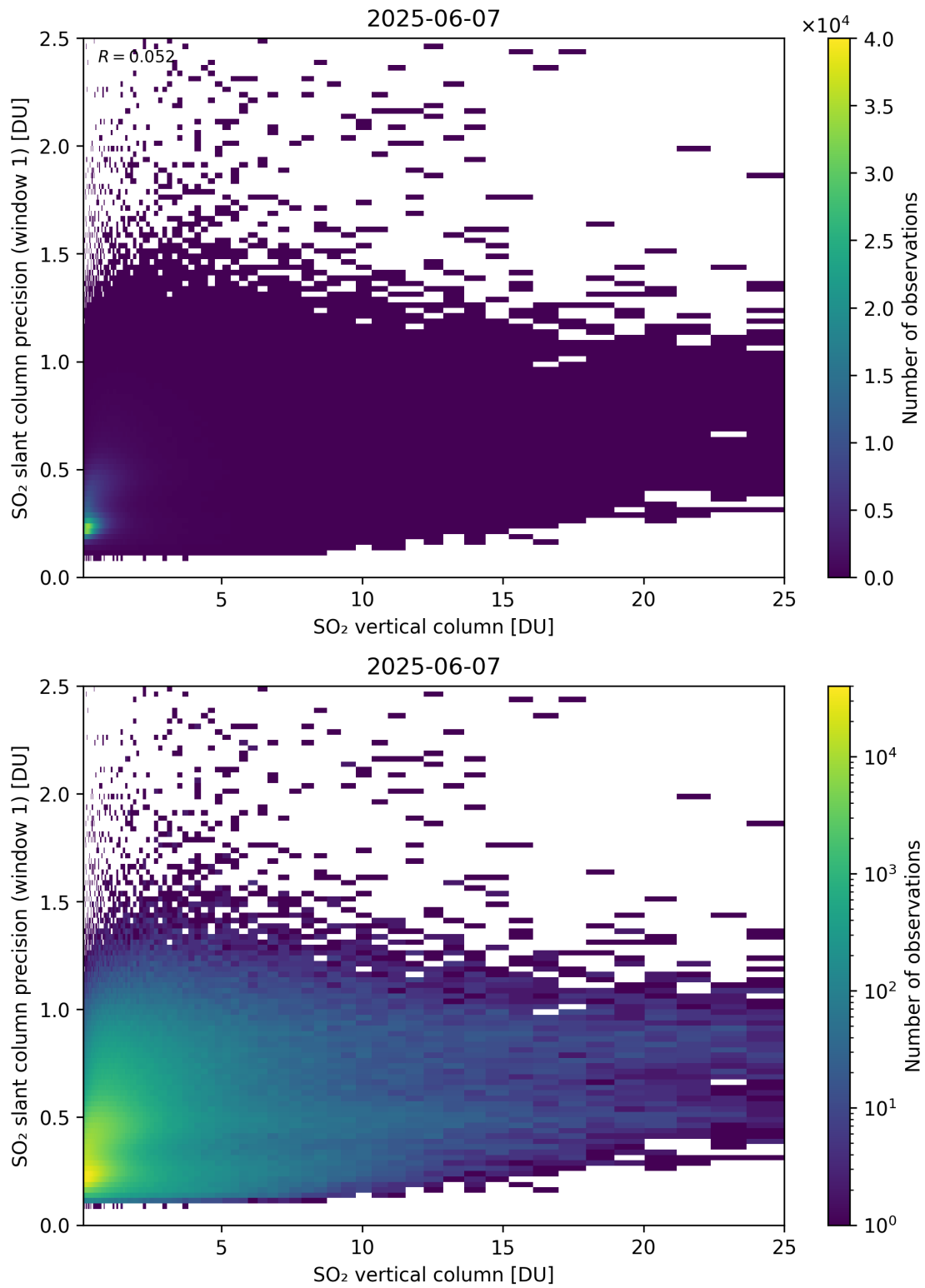
Figure 355: Scatter density plot of “SO 2 vertical column” against “SO 2 slant column precision (window 1)” for 2025-06-06 to 2025-06-08.
