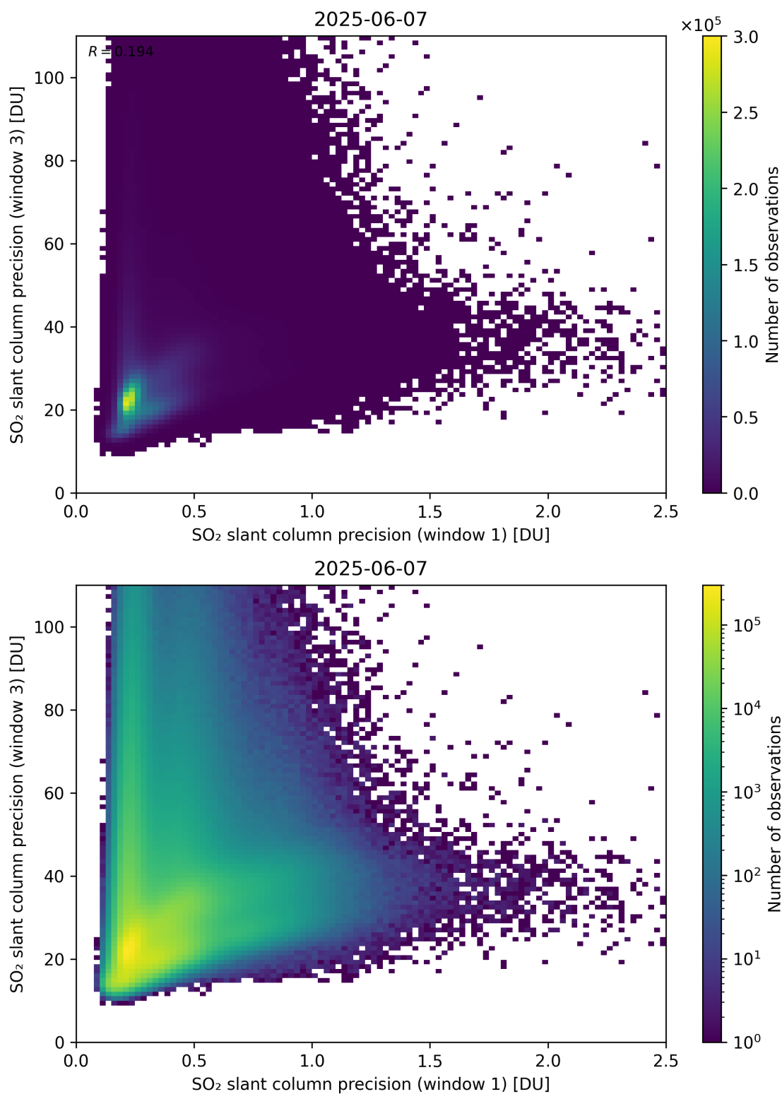
Figure 279: Scatter density plot of “SO 2 slant column precision (window 1)” against “SO 2 slant column precision (window 3)” for 2025-06-06 to 2025-06-08.
