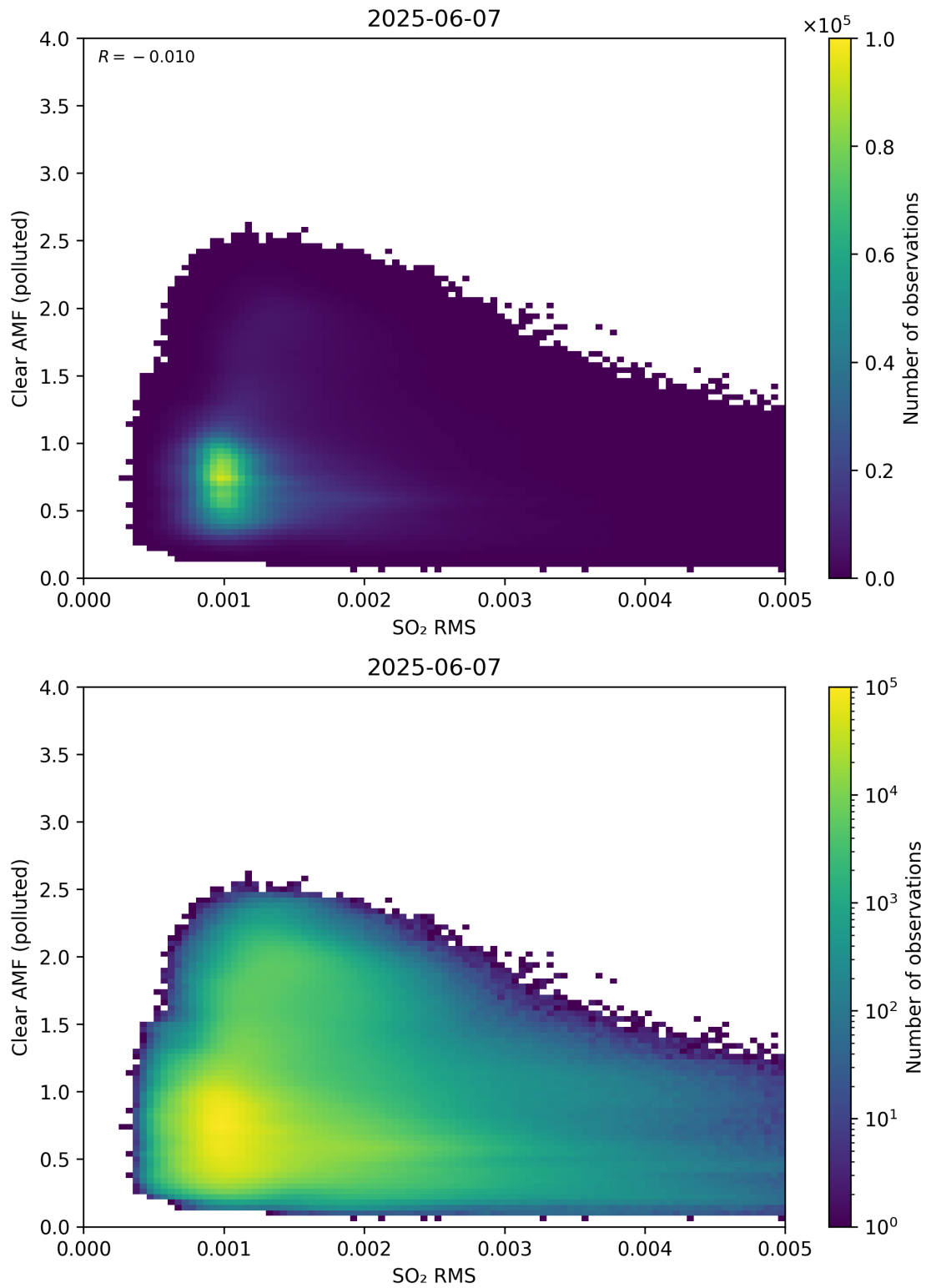
Figure 147: Scatter density plot of “SO 2 RMS” against “Clear AMF (polluted)” for 2025-06-06 to 2025-06-08.
