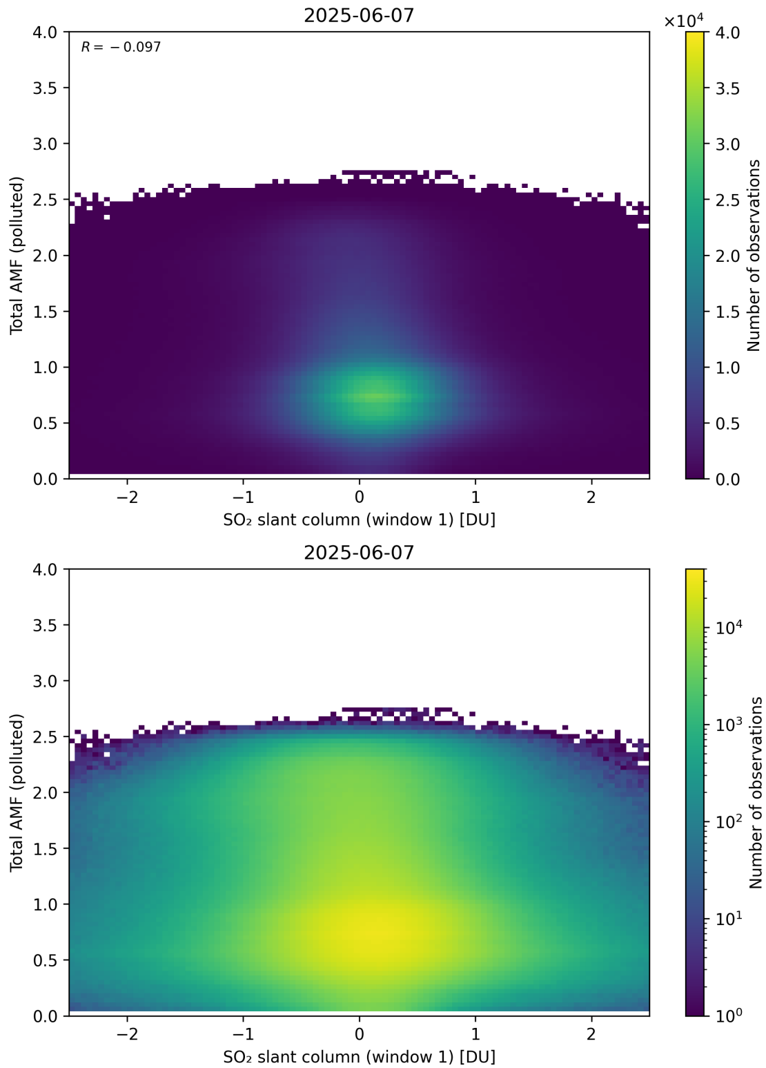
Figure 289: Scatter density plot of “SO 2 slant column (window 1)” against “Total AMF (polluted)” for 2025-06-06 to 2025-06-08.
