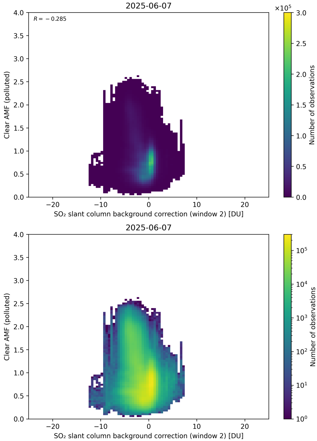
Figure 126: Scatter density plot of “SO 2 slant column background correction (window 2)” against “Clear AMF (polluted)” for 2025-06-06 to 2025-06-08.
