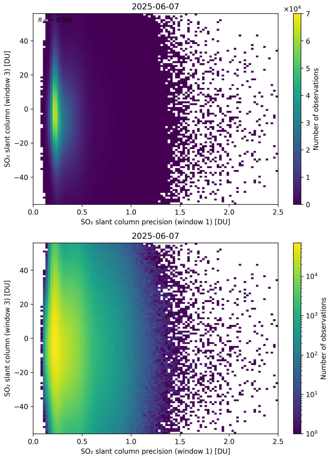
Figure 278: Scatter density plot of “SO 2 slant column precision (window 1)” against “SO 2 slant column (window 3)” for 2025-06-06 to 2025-06-08.
