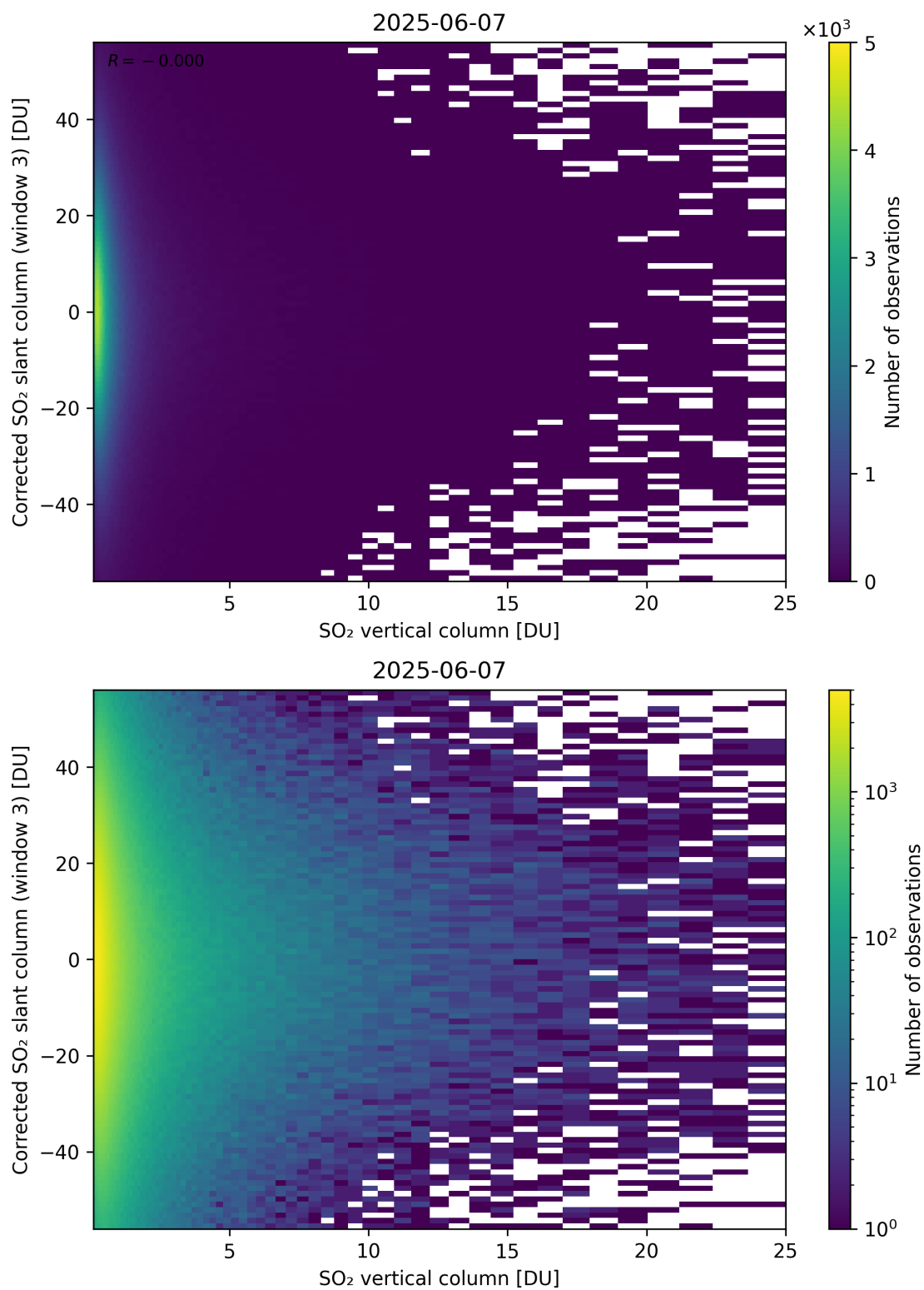
Figure 353: Scatter density plot of “SO 2 vertical column” against “Corrected SO 2 slant column (window 3)” for 2025-06-06 to 2025-06-08.
