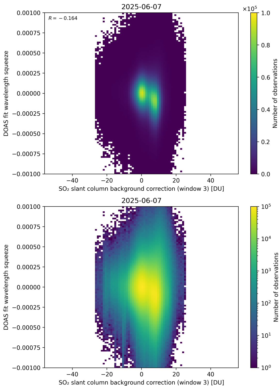
Figure 133: Scatter density plot of “SO 2 slant column background correction (window 3)” against “DOAS fit wavelength squeeze” for 2025-06-06 to 2025-06-08.
