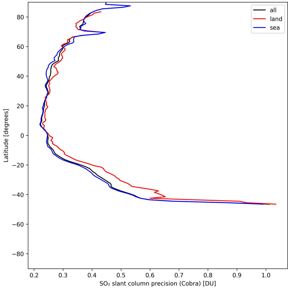
Figure 36: Zonal average of “SO 2 slant column precision (Cobra)” for 2025-06-06 to 2025-06-08.
