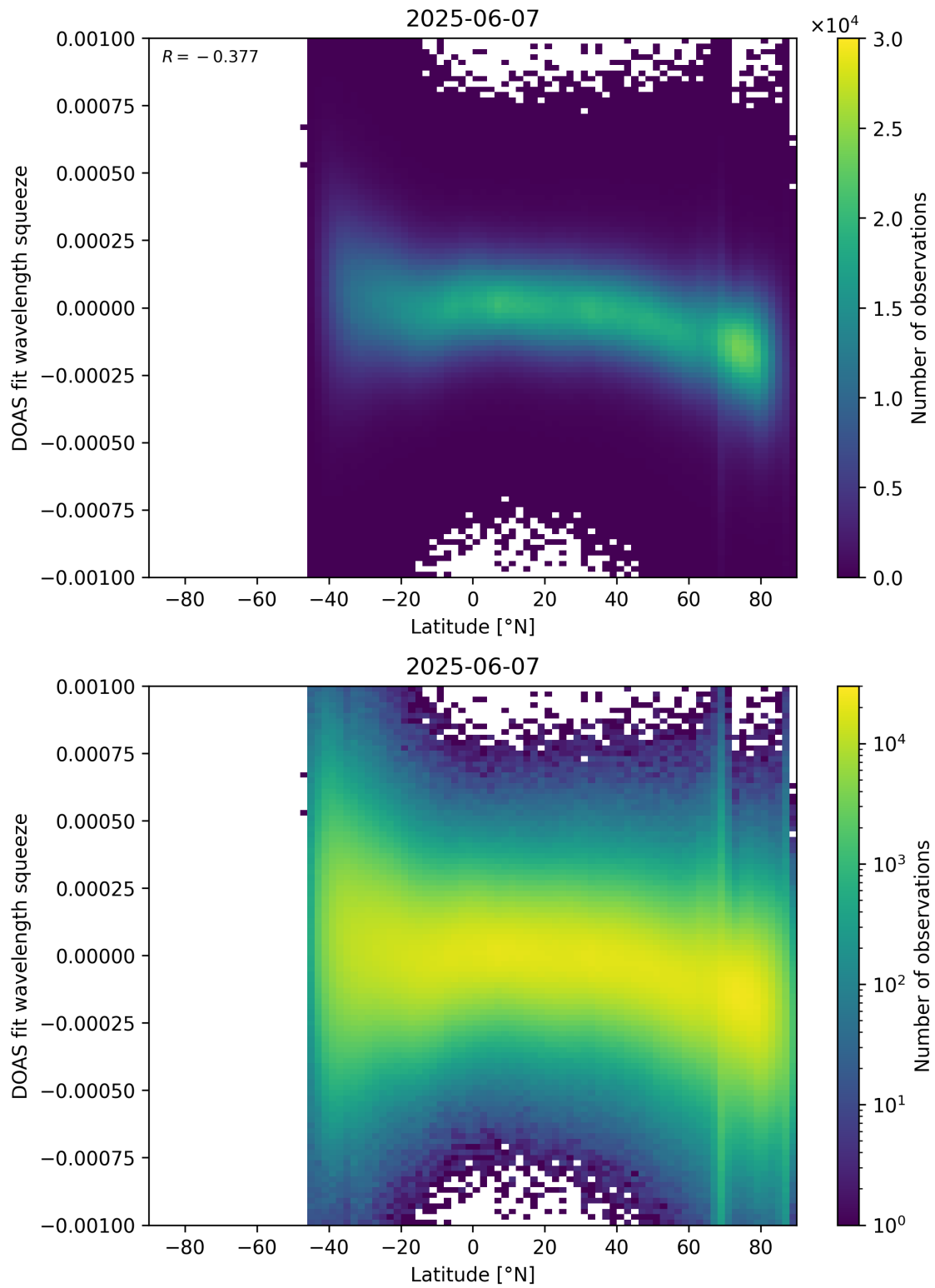
Figure 154: Scatter density plot of “Latitude” against “DOAS fit wavelength squeeze” for 2025-06-06 to 2025-06-08.
