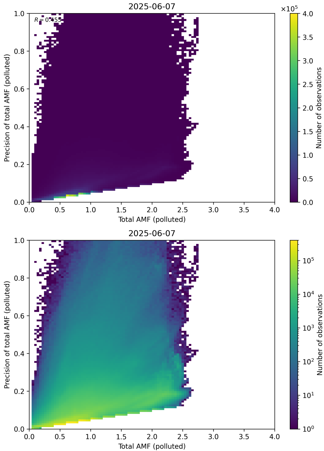
Figure 322: Scatter density plot of “Total AMF (polluted)” against “Precision of total AMF (polluted)” for 2025-06-06 to 2025-06-08.
