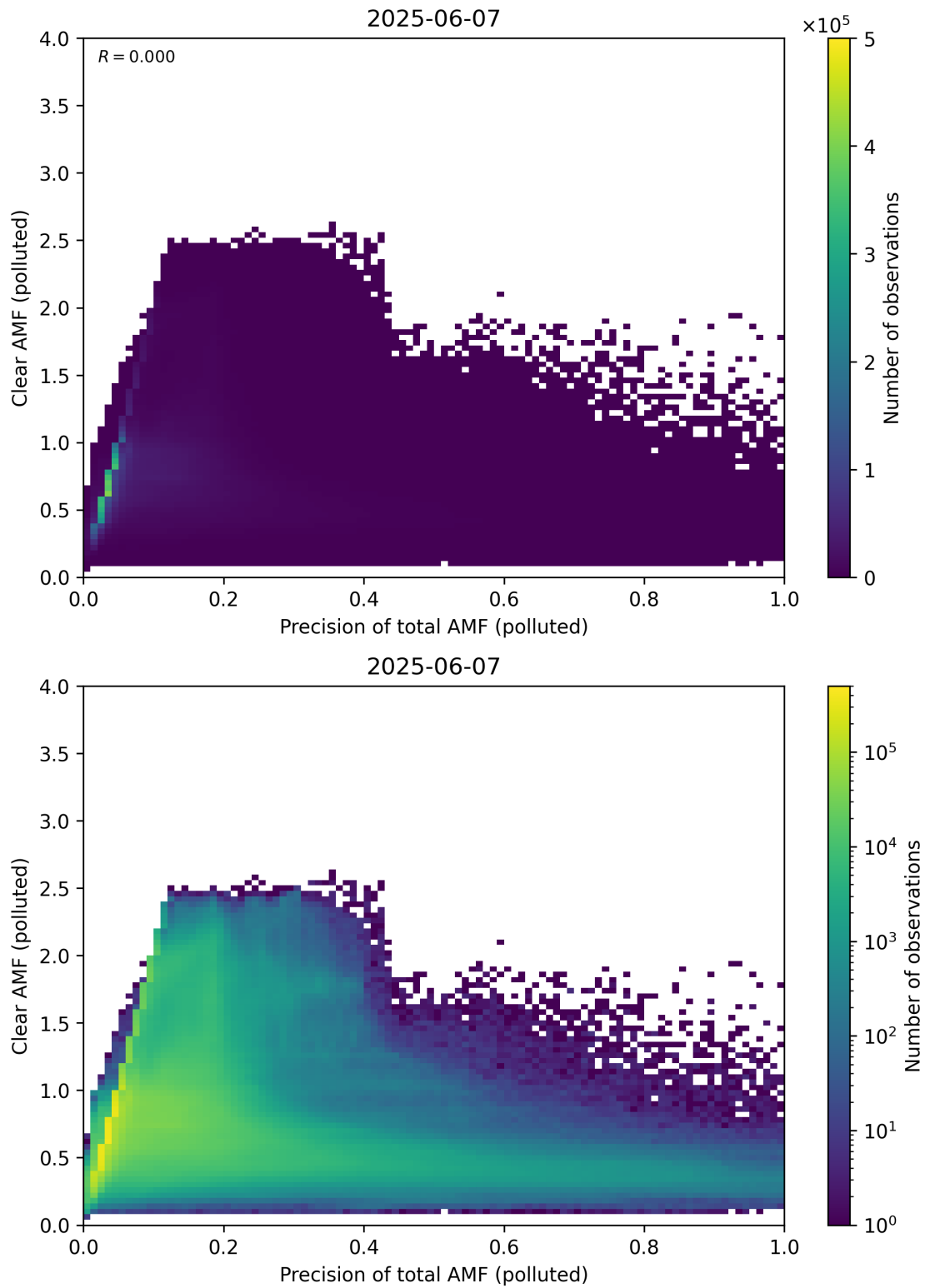
Figure 320: Scatter density plot of “Precision of total AMF (polluted)” against “Clear AMF (polluted)” for 2025-06-06 to 2025-06-08.
