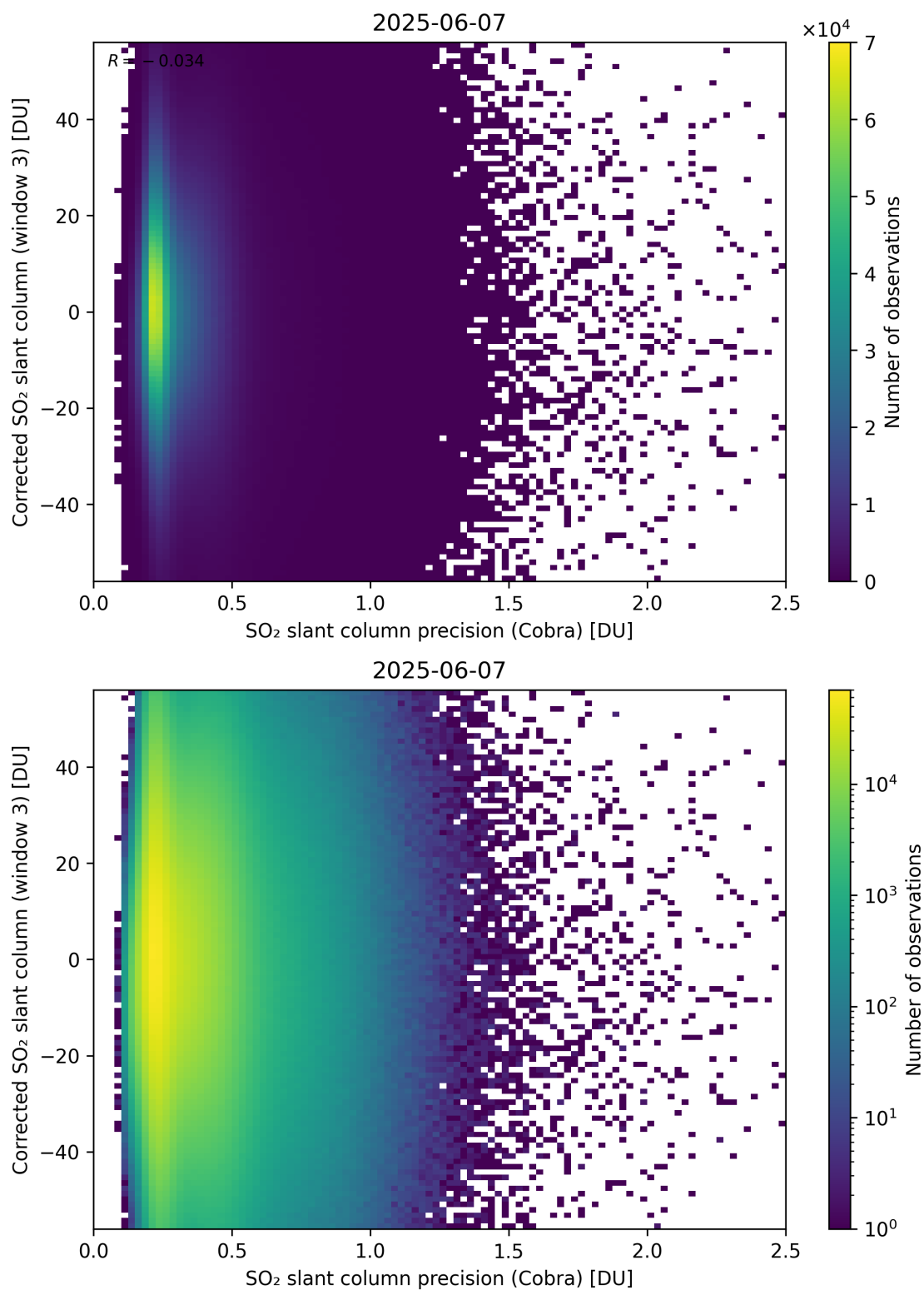
Figure 207: Scatter density plot of “SO 2 slant column precision (Cobra)” against “Corrected SO 2 slant column (window 3)” for 2025-06-06 to 2025-06-08.
