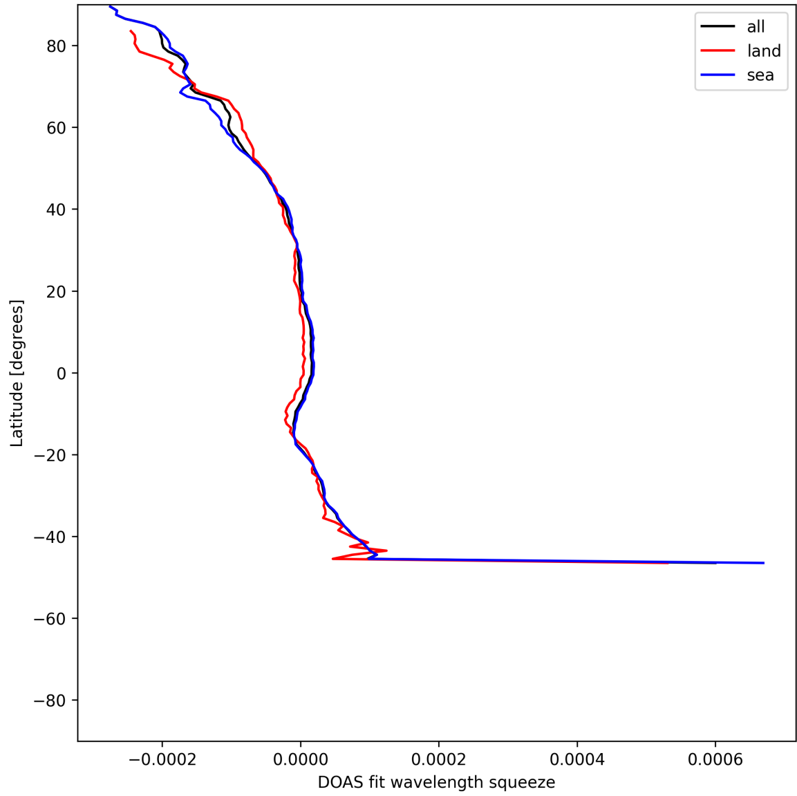
Figure 51: Zonal average of “DOAS fit wavelength squeeze” for 2025-06-06 to 2025-06-08.
