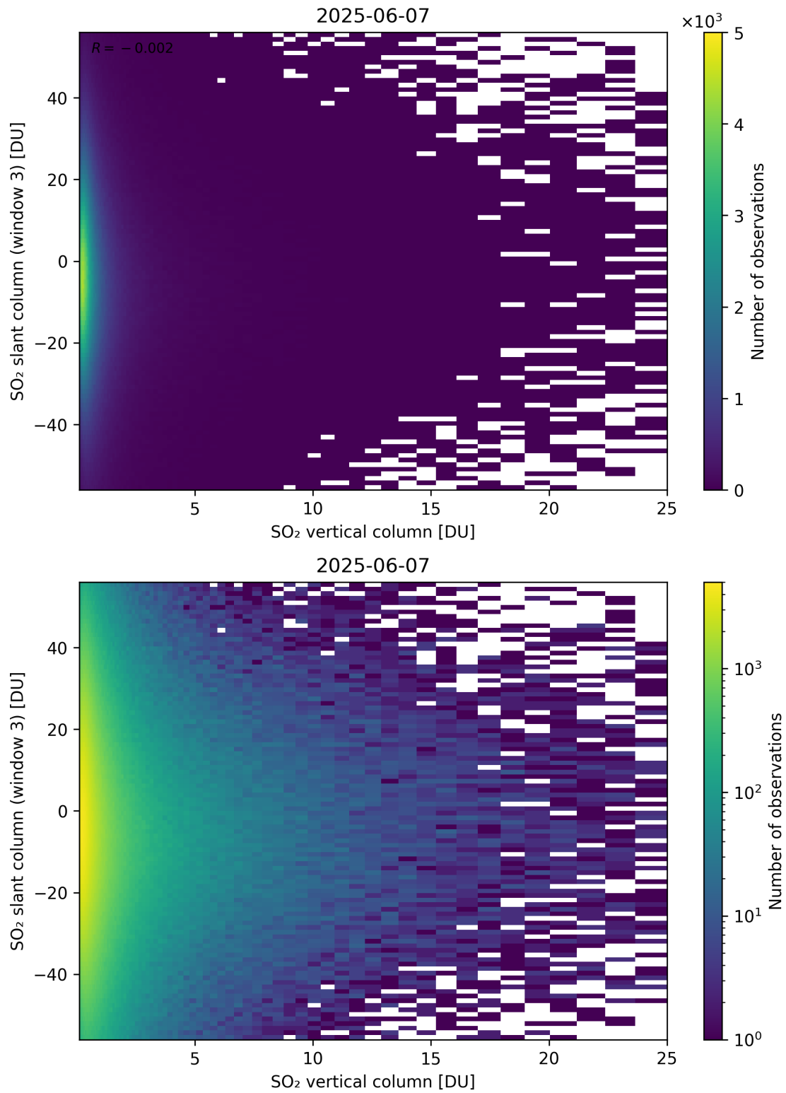
Figure 357: Scatter density plot of “SO 2 vertical column” against “SO 2 slant column (window 3)” for 2025-06-06 to 2025-06-08.
