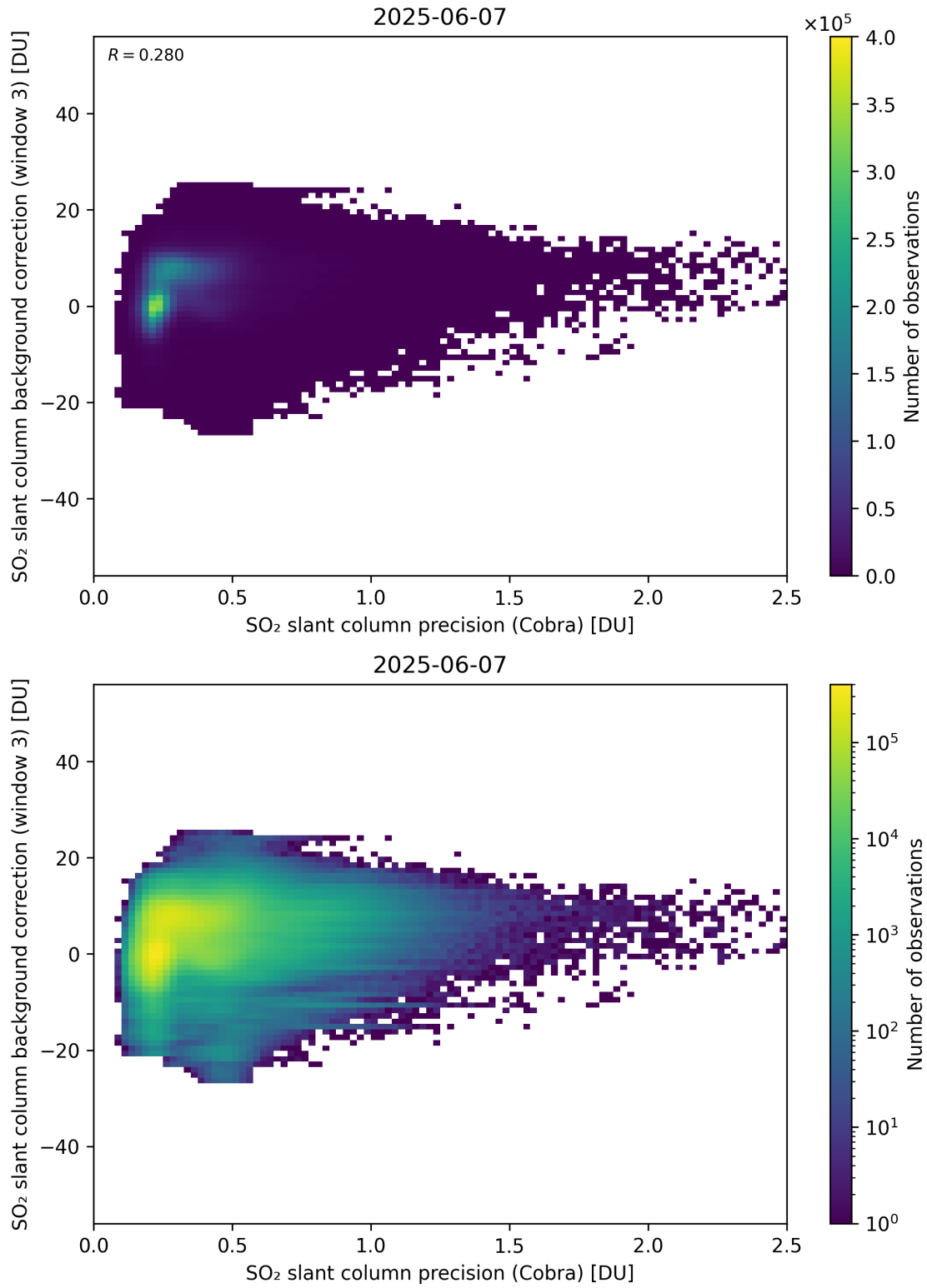
Figure 201: Scatter density plot of “SO 2 slant column precision (Cobra)” against “SO 2 slant column background correction (window 3)” for 2025-06-06 to 2025-06-08.
