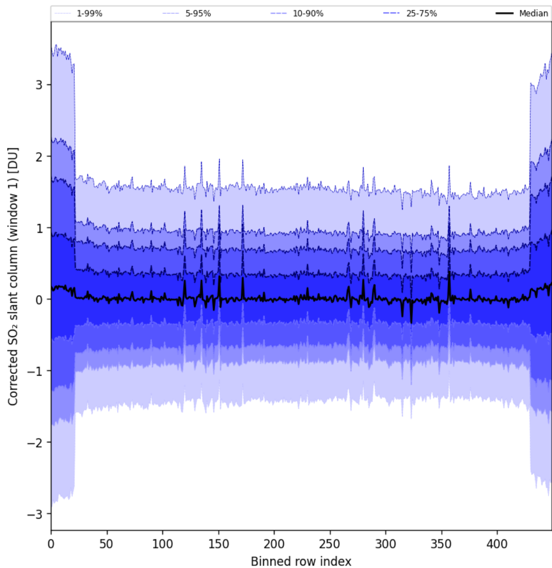
Figure 91: Along track statistics of “Corrected SO 2 slant column (window 1)” for 2025-06-06 to 2025-06-08
