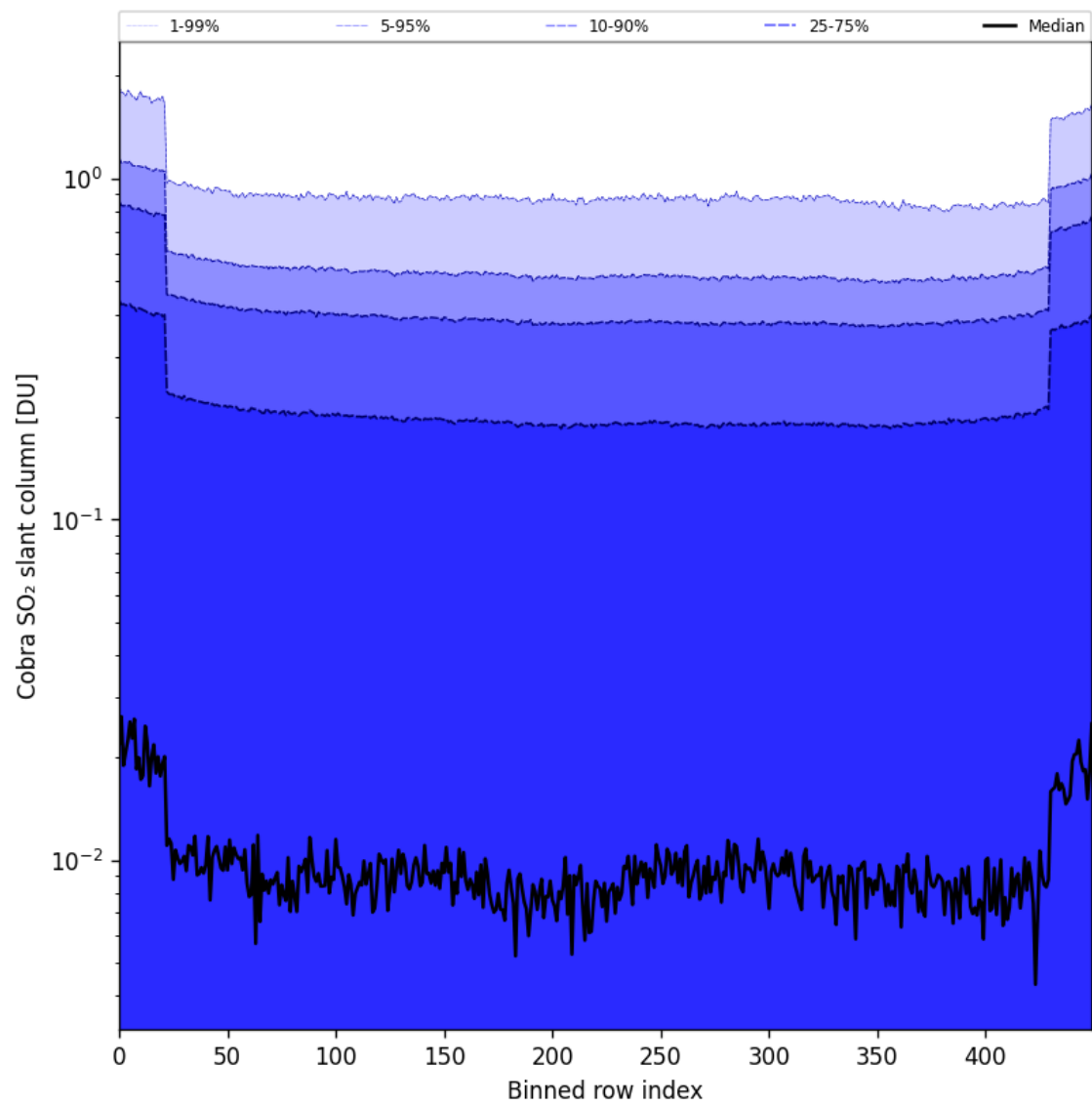
Figure 87: Along track statistics of "Cobra SO 2 slant column" for 2025-06-06 to 2025-06-08
