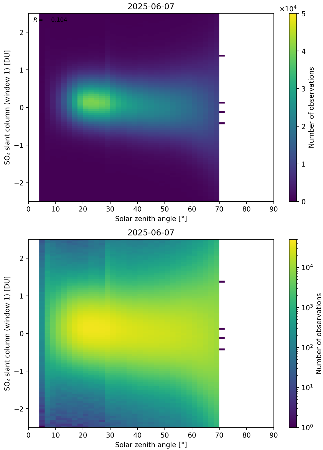
Figure 184: Scatter density plot of “Solar zenith angle” against “SO 2 slant column (window 1)” for 2025-06-06 to 2025-06-08.
