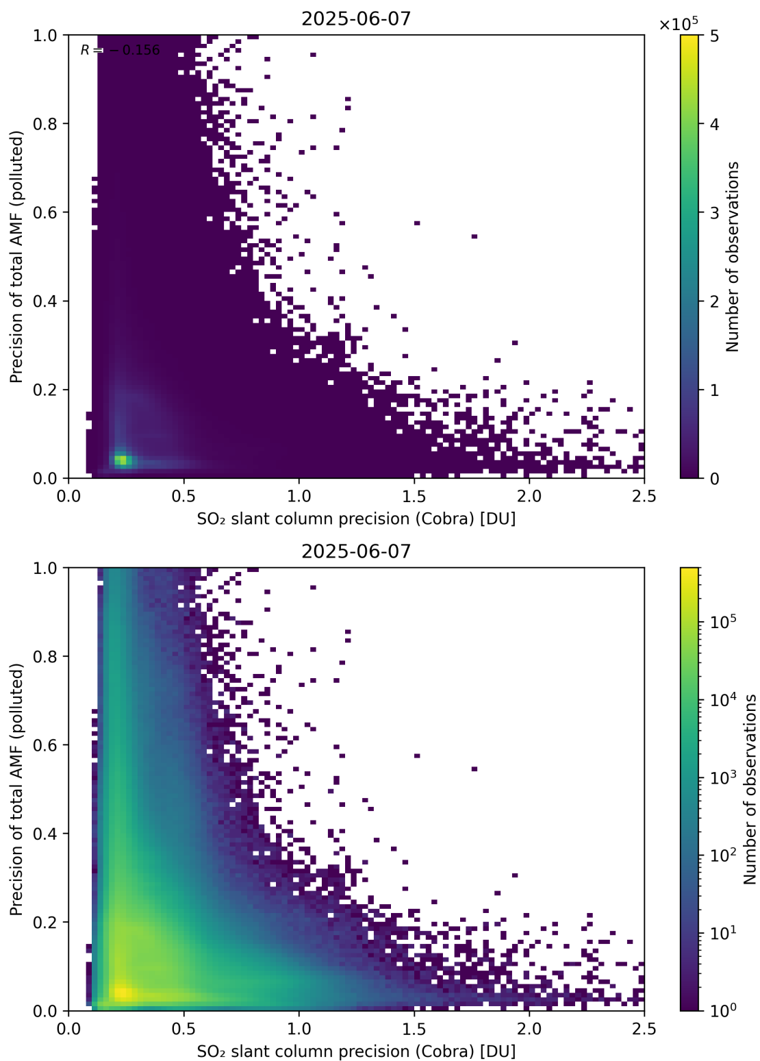
Figure 214: Scatter density plot of “SO 2 slant column precision (Cobra)” against “Precision of total AMF (polluted)” for 2025-06-06 to 2025-06-08.
