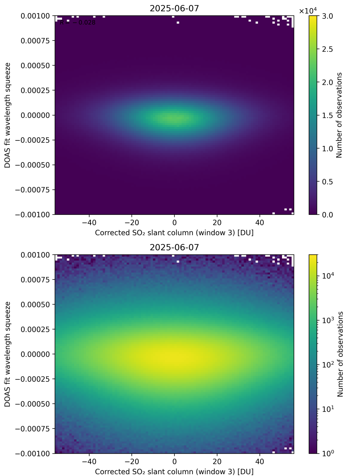
Figure 257: Scatter density plot of “Corrected SO 2 slant column (window 3)” against “DOAS fit wavelength squeeze” for 2025-06-06 to 2025-06-08.
