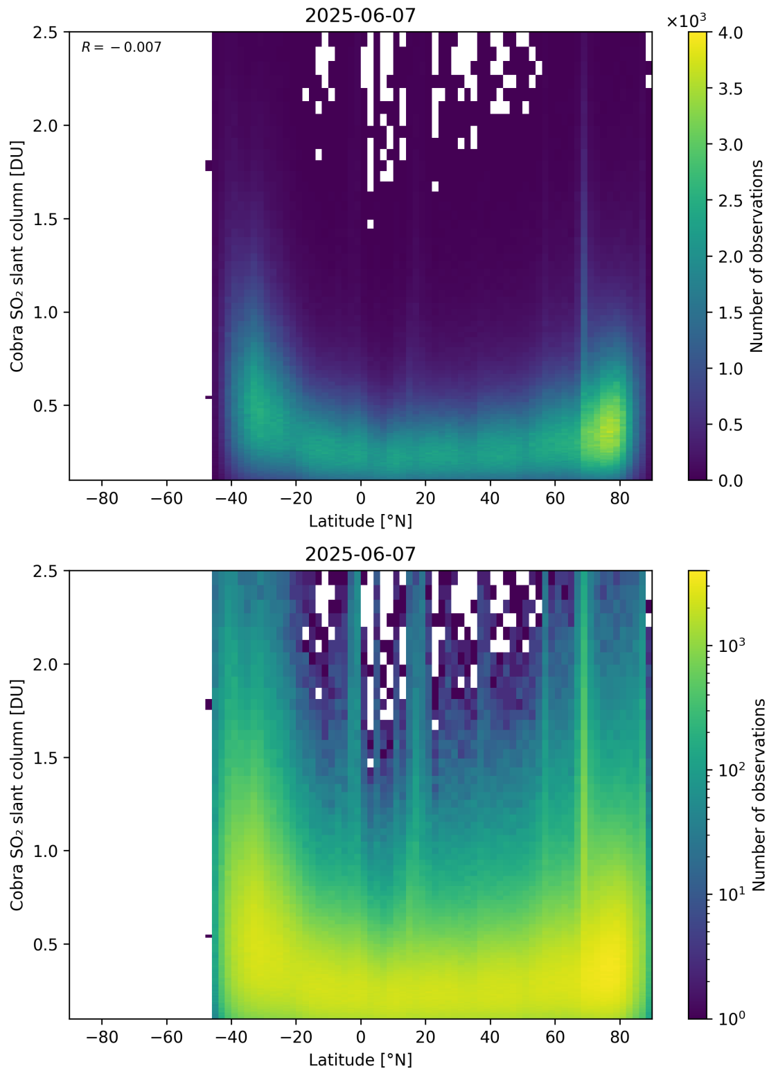
Figure 157: Scatter density plot of “Latitude” against “Cobra SO 2 slant column” for 2025-06-06 to 2025-06-08.
