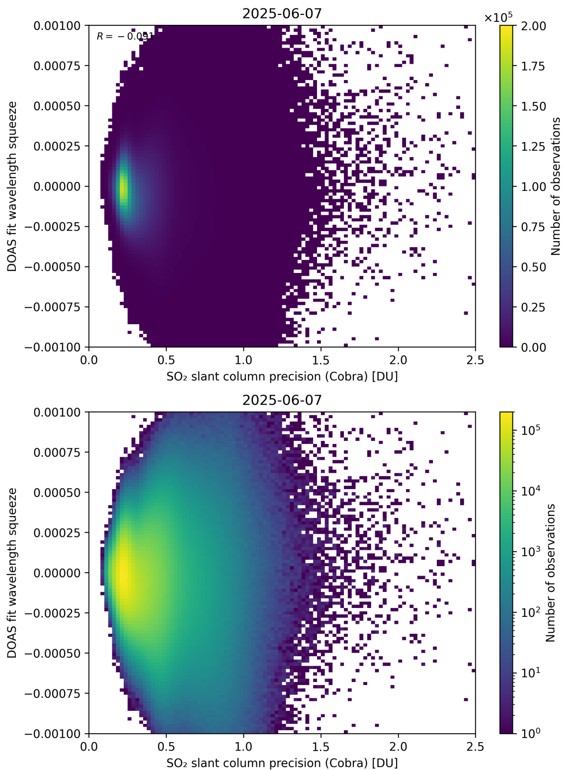
Figure 203: Scatter density plot of “SO 2 slant column precision (Cobra)” against “DOAS fit wavelength squeeze” for 2025-06-06 to 2025-06-08.
