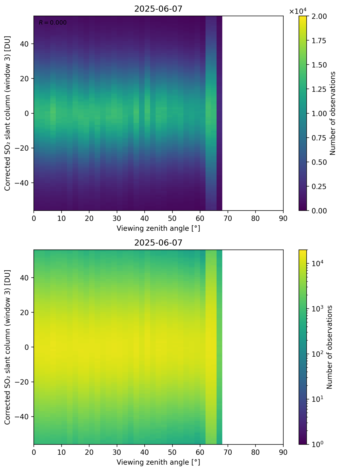
Figure 375: Scatter density plot of “Viewing zenith angle” against “Corrected SO 2 slant column (window 3)” for 2025-06-06 to 2025-06-08.
