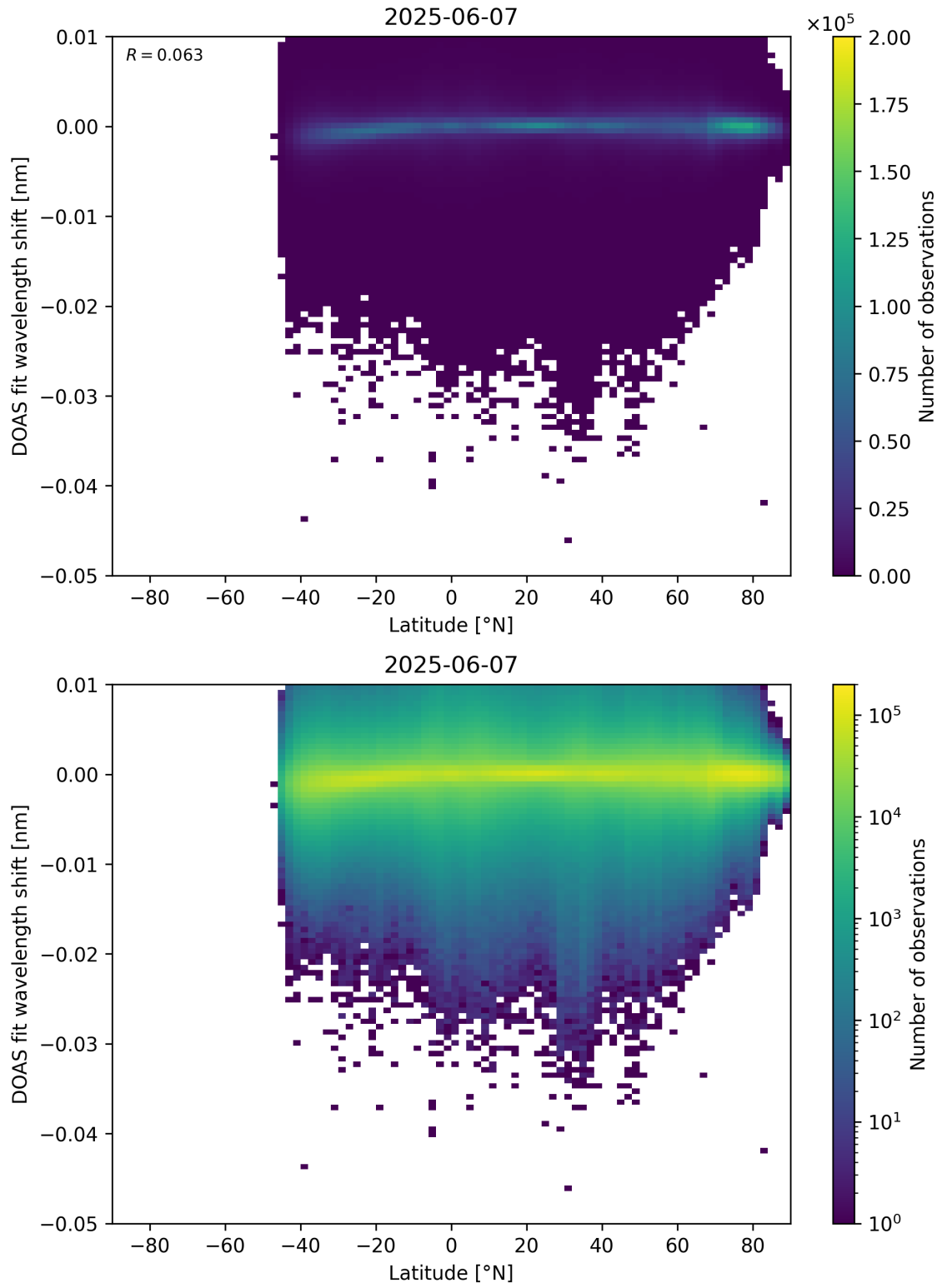
Figure 153: Scatter density plot of “Latitude” against “DOAS fit wavelength shift” for 2025-06-06 to 2025-06-08.
