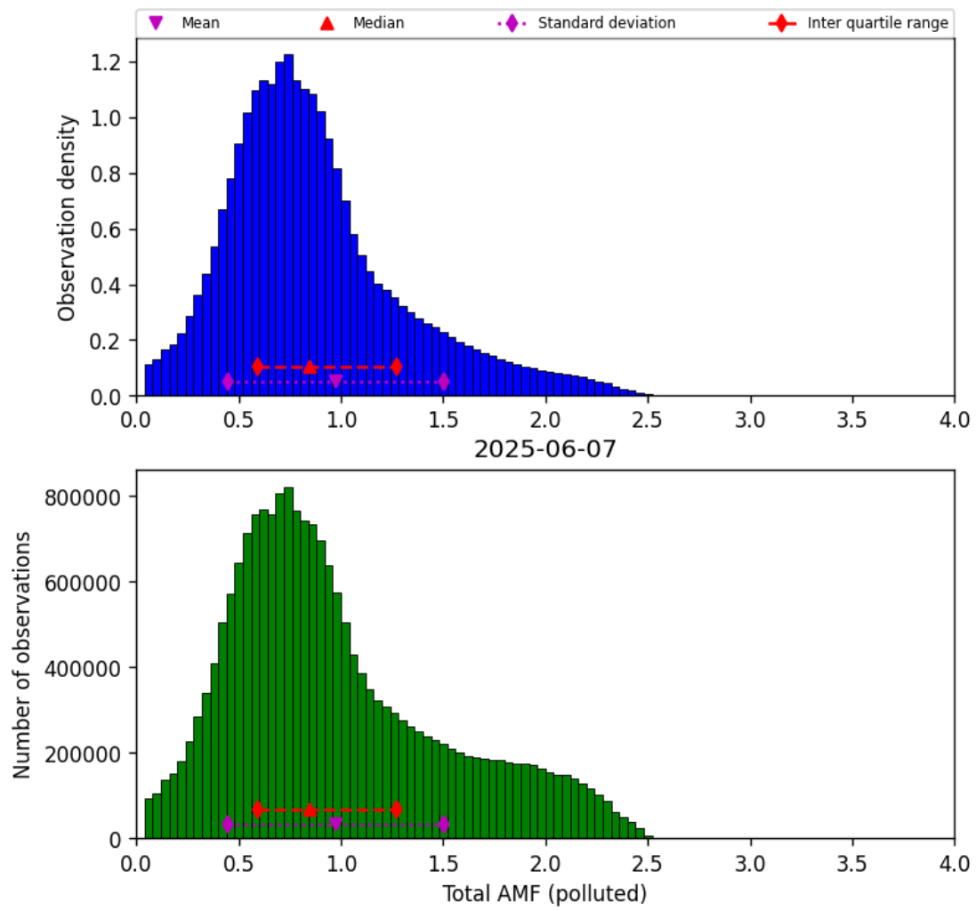
Figure 79: Histogram of “Total AMF (polluted)” for 2025-06-06 to 2025-06-08
