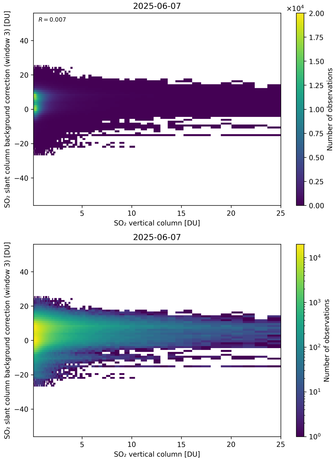
Figure 325: Scatter density plot of “SO 2 vertical column” against “SO 2 slant column background correction (window 3)” for 2025-06-06 to 2025-06-08.
