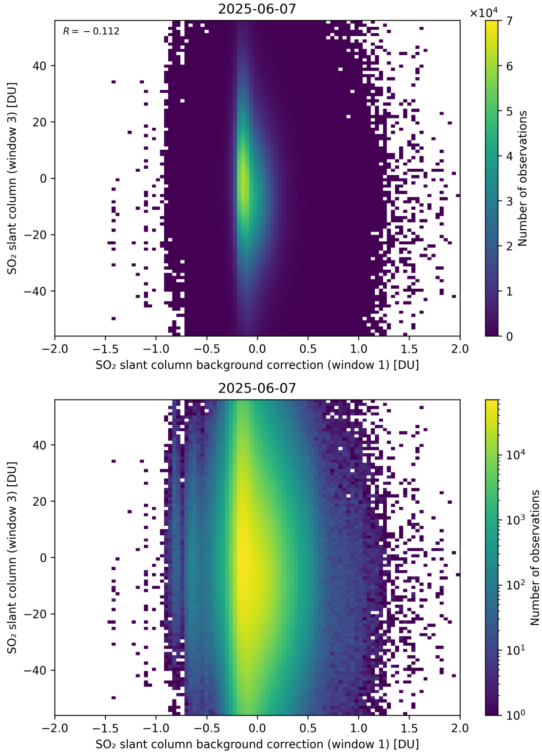
Figure 118: Scatter density plot of “SO 2 slant column background correction (window 1)” against “SO 2 slant column (window 3)” for 2025-06-06 to 2025-06-08.
