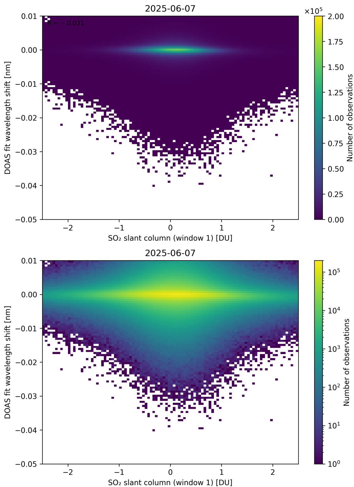
Figure 265: Scatter density plot of “SO 2 slant column (window 1)” against “DOAS fit wavelength shift” for 2025-06-06 to 2025-06-08.
