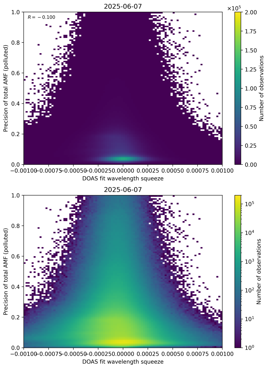
Figure 146: Scatter density plot of “DOAS fit wavelength squeeze” against “Precision of total AMF (polluted)” for 2025-06-06 to 2025-06-08.
