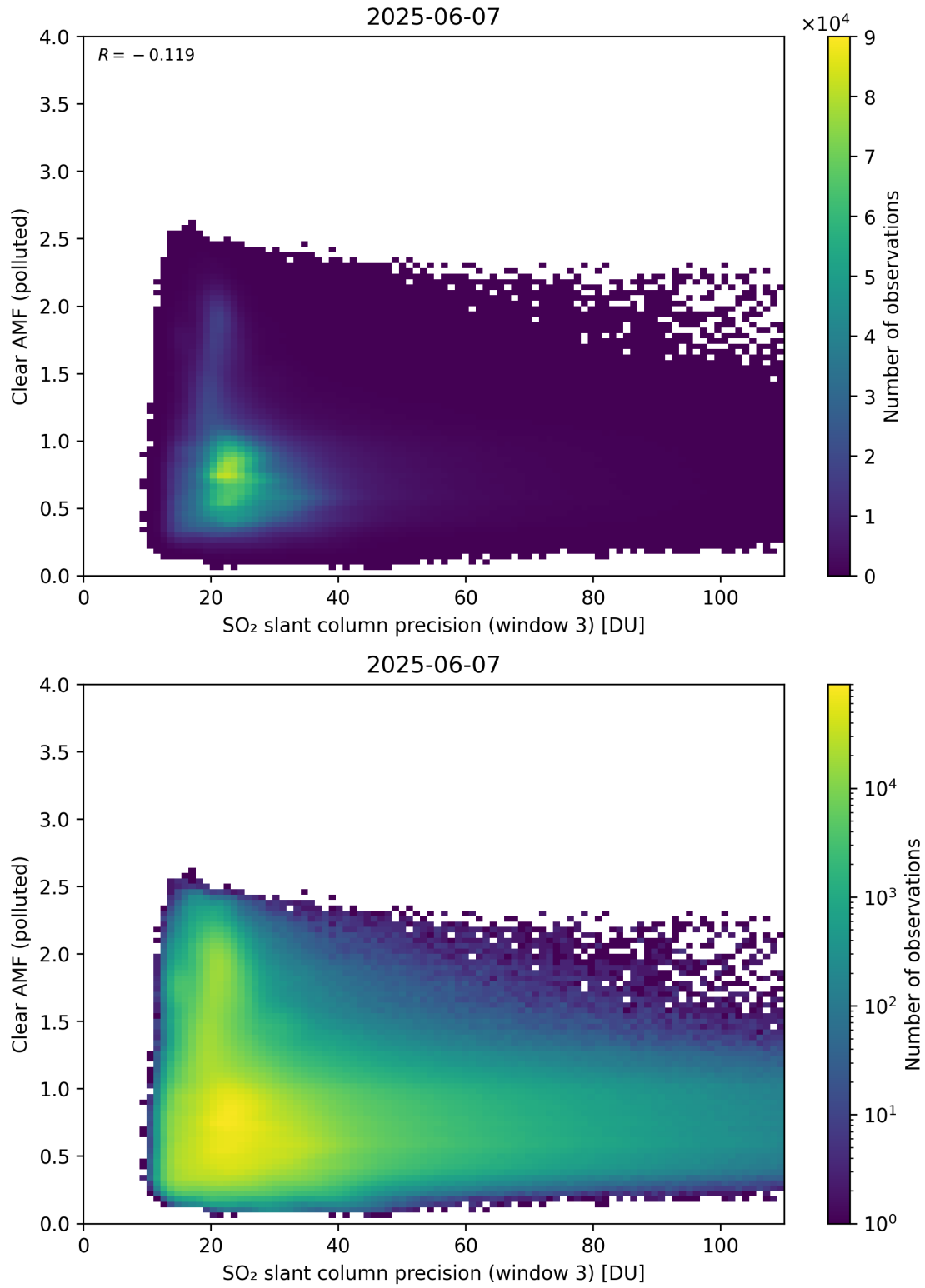
Figure 311: Scatter density plot of “SO 2 slant column precision (window 3)” against “Clear AMF (polluted)” for 2025-06-06 to 2025-06-08.
