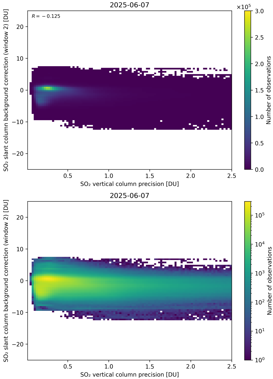
Figure 330: Scatter density plot of “SO 2 vertical column precision” against “SO 2 slant column background correction (window 2)” for 2025-06-06 to 2025-06-08.
