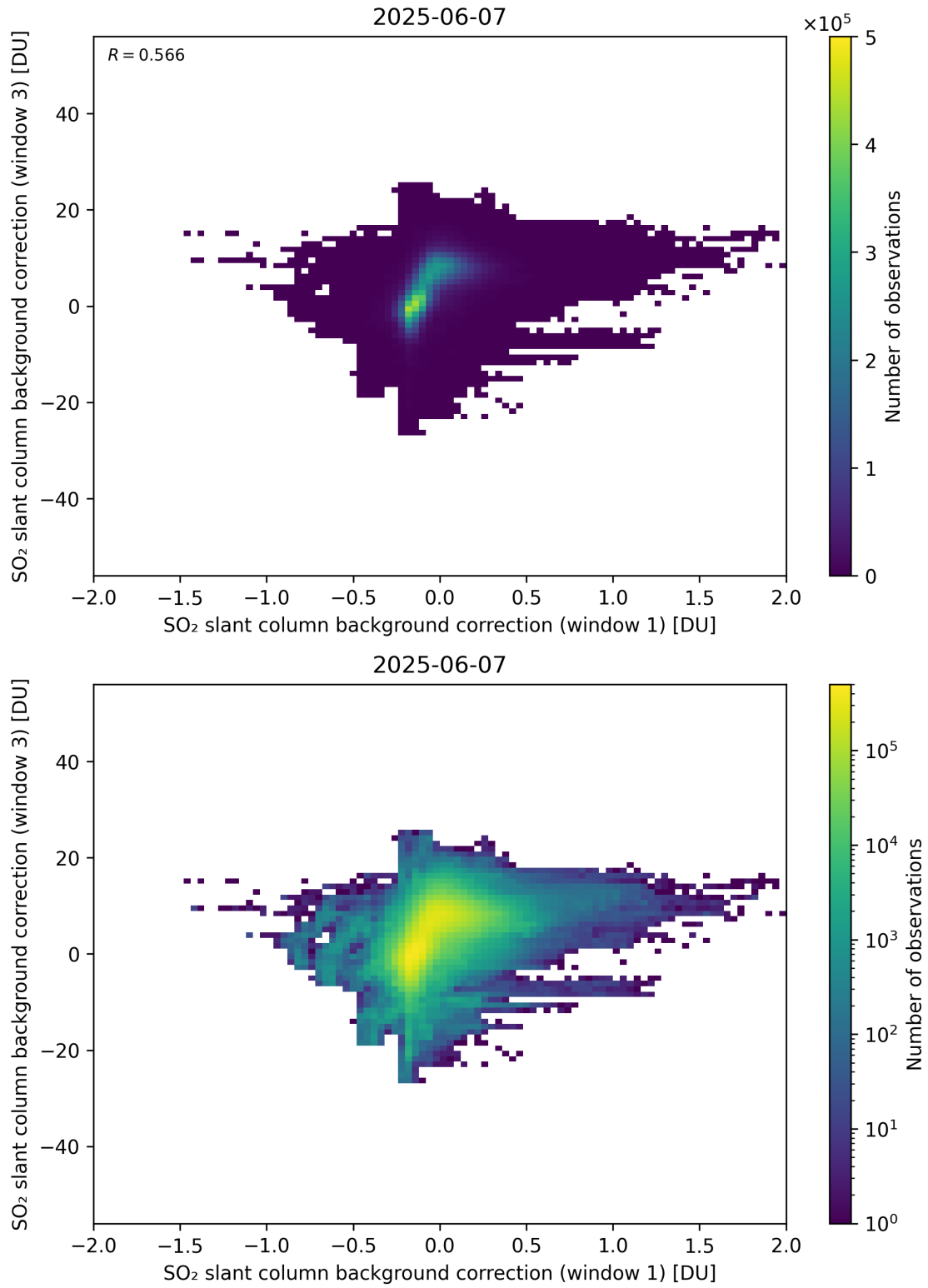
Figure 110: Scatter density plot of “SO 2 slant column background correction (window 1)” against “SO 2 slant column background correction (window 3)” for 2025-06-06 to 2025-06-08.
