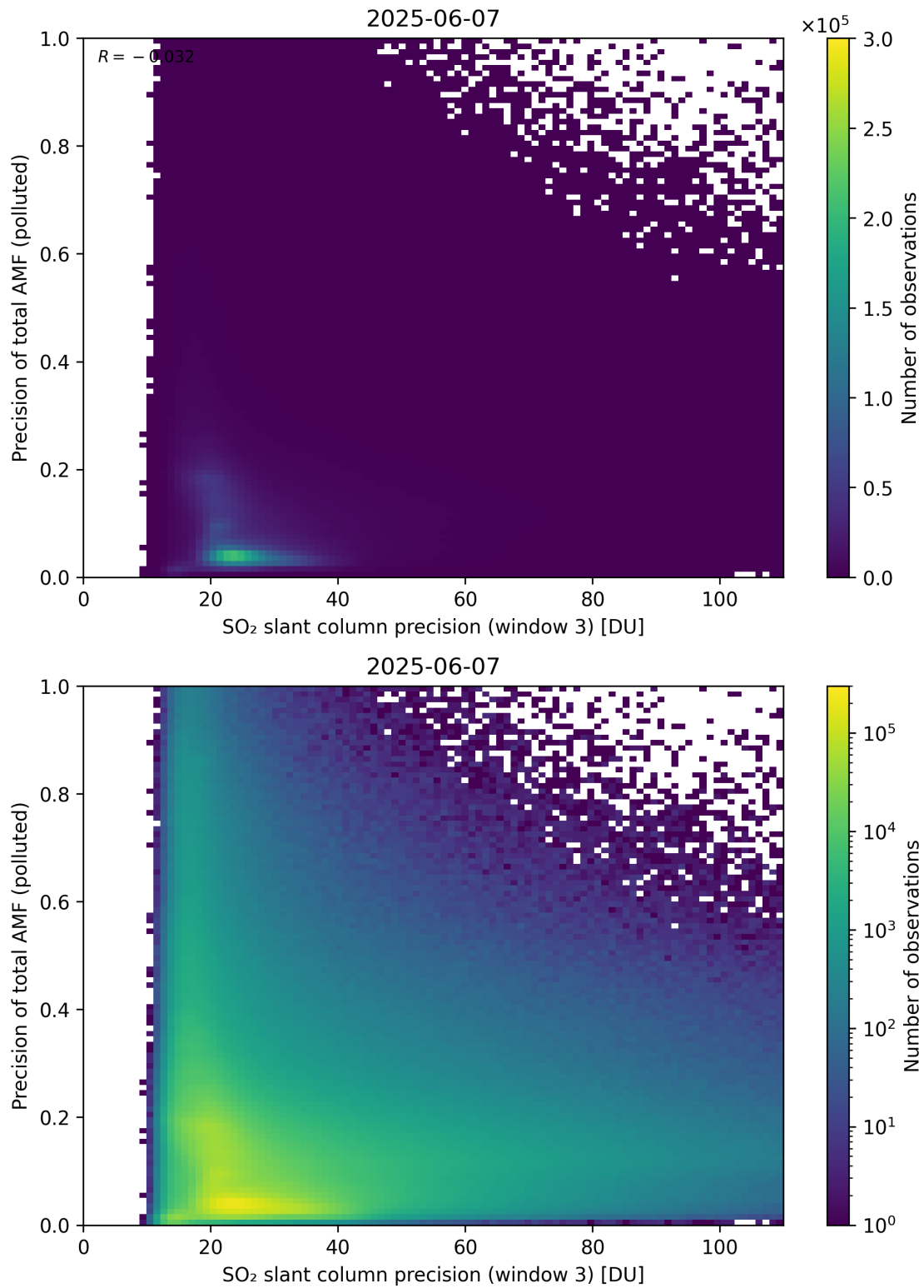
Figure 314: Scatter density plot of “SO 2 slant column precision (window 3)” against “Precision of total AMF (polluted)” for 2025-06-06 to 2025-06-08.
