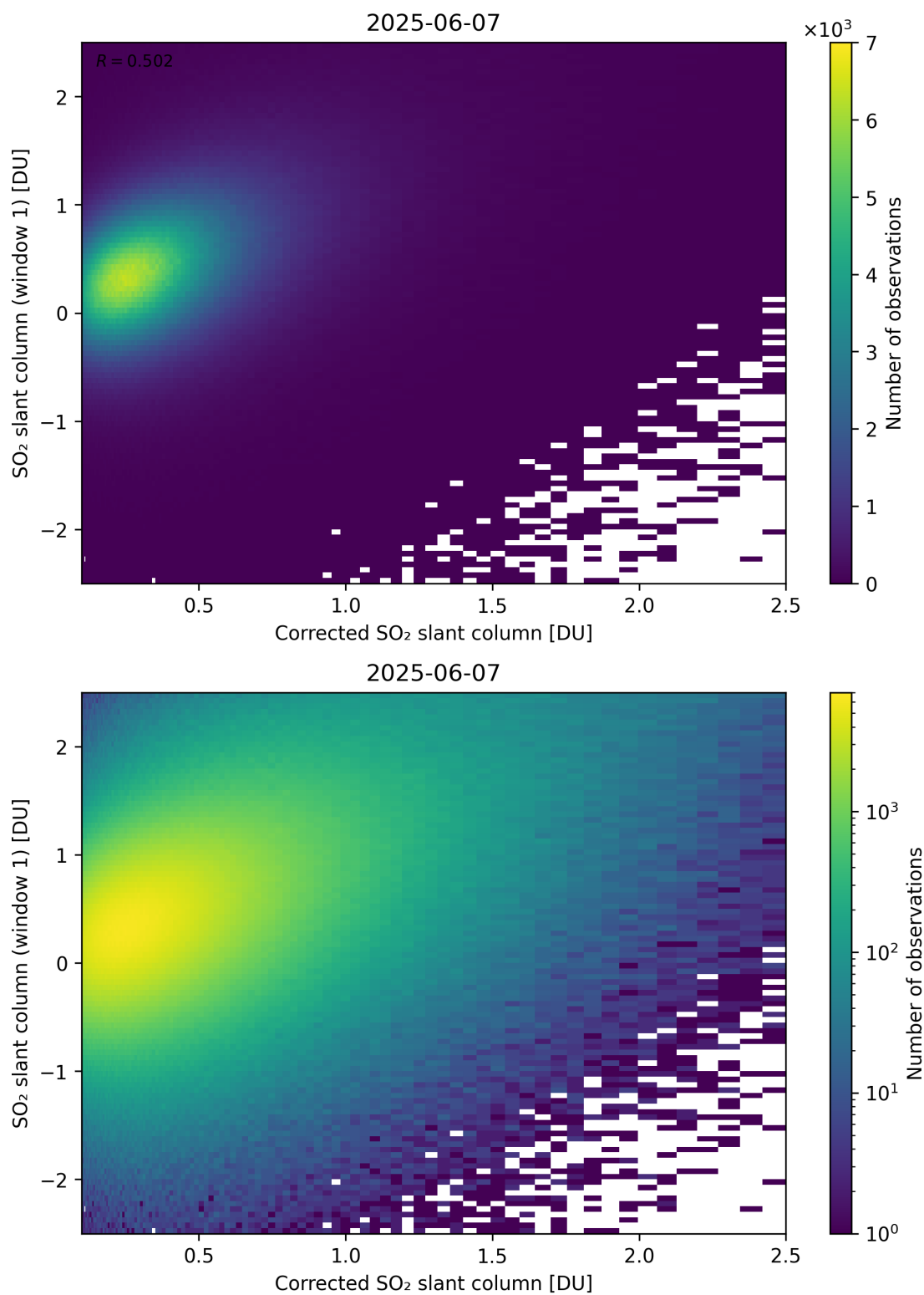
Figure 237: Scatter density plot of “Corrected SO 2 slant column” against “SO 2 slant column (window 1)” for 2025-06-06 to 2025-06-08.
