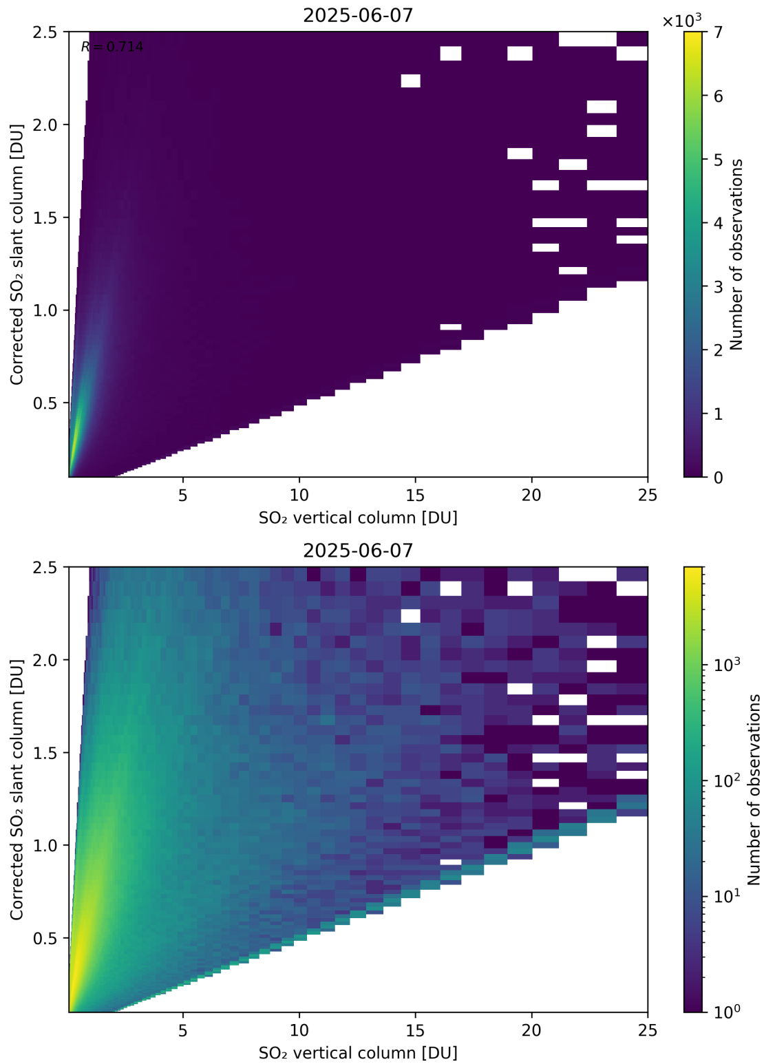
Figure 351: Scatter density plot of “SO 2 vertical column” against “Corrected SO 2 slant column” for 2025-06-06 to 2025-06-08.
