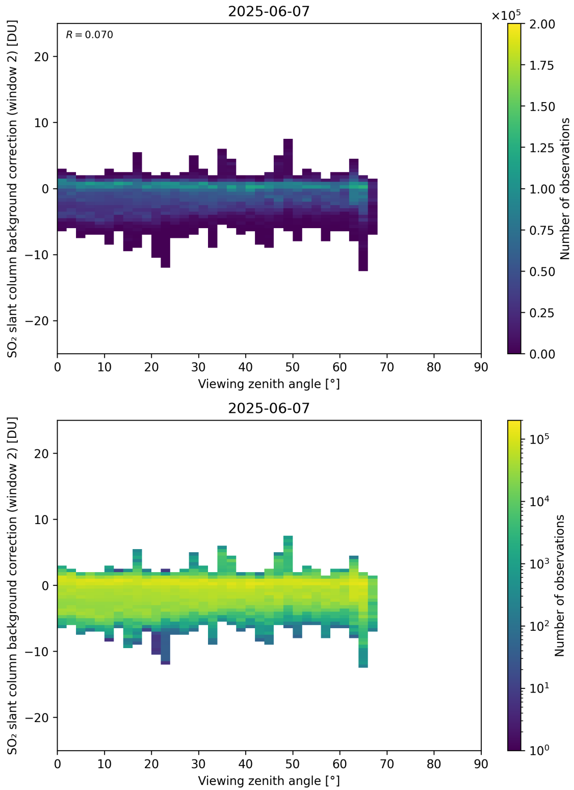
Figure 363: Scatter density plot of “Viewing zenith angle” against “SO 2 slant column background correction (window 2)” for 2025-06-06 to 2025-06-08.
