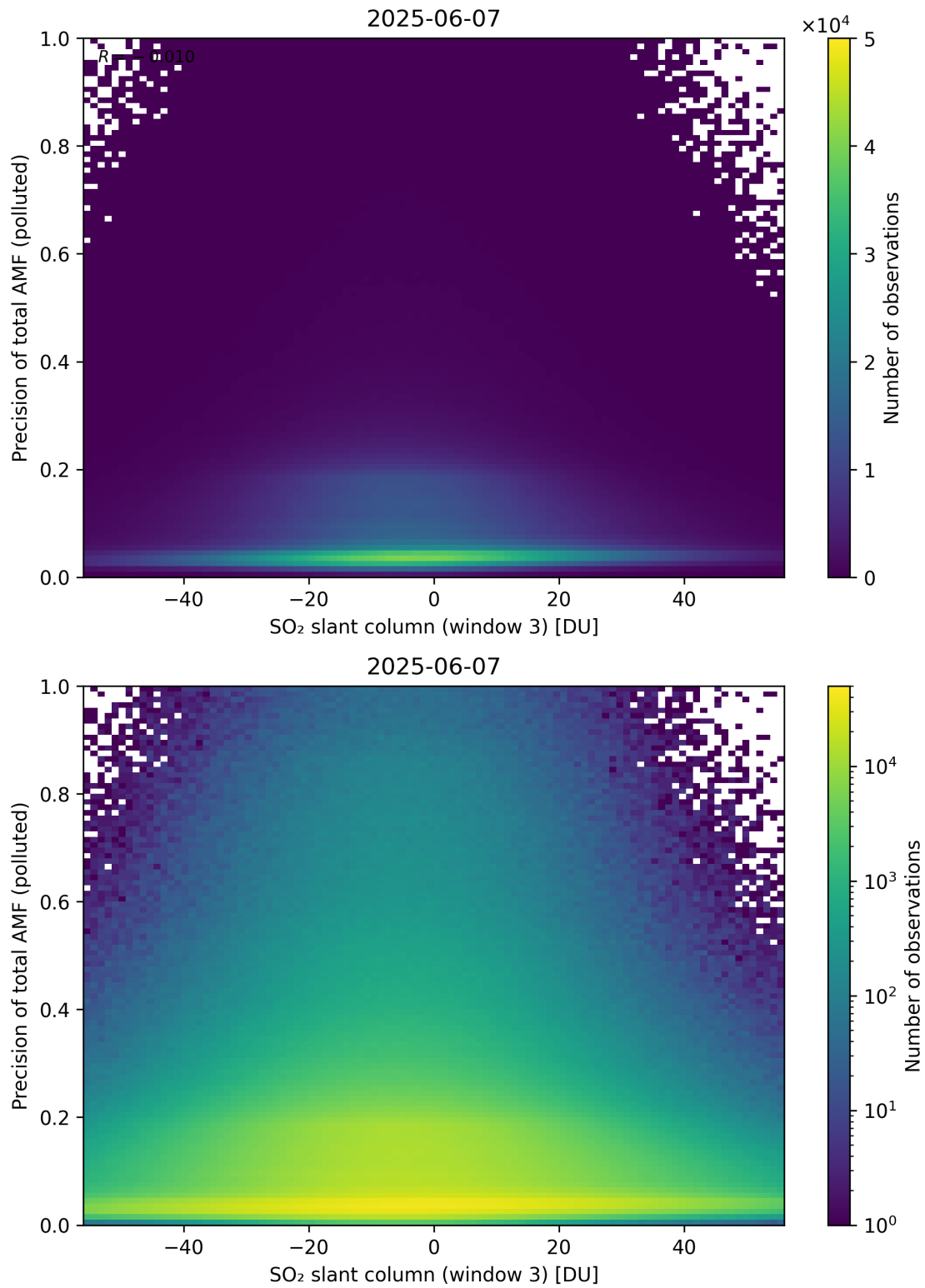
Figure 319: Scatter density plot of “SO 2 slant column (window 3)” against “Precision of total AMF (polluted)” for 2025-06-06 to 2025-06-08.
