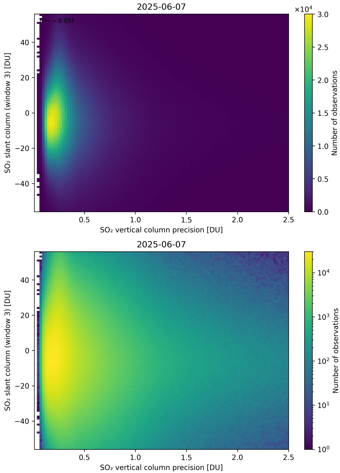
Figure 344: Scatter density plot of “SO 2 vertical column precision” against “SO 2 slant column (window 3)” for 2025-06-06 to 2025-06-08.
