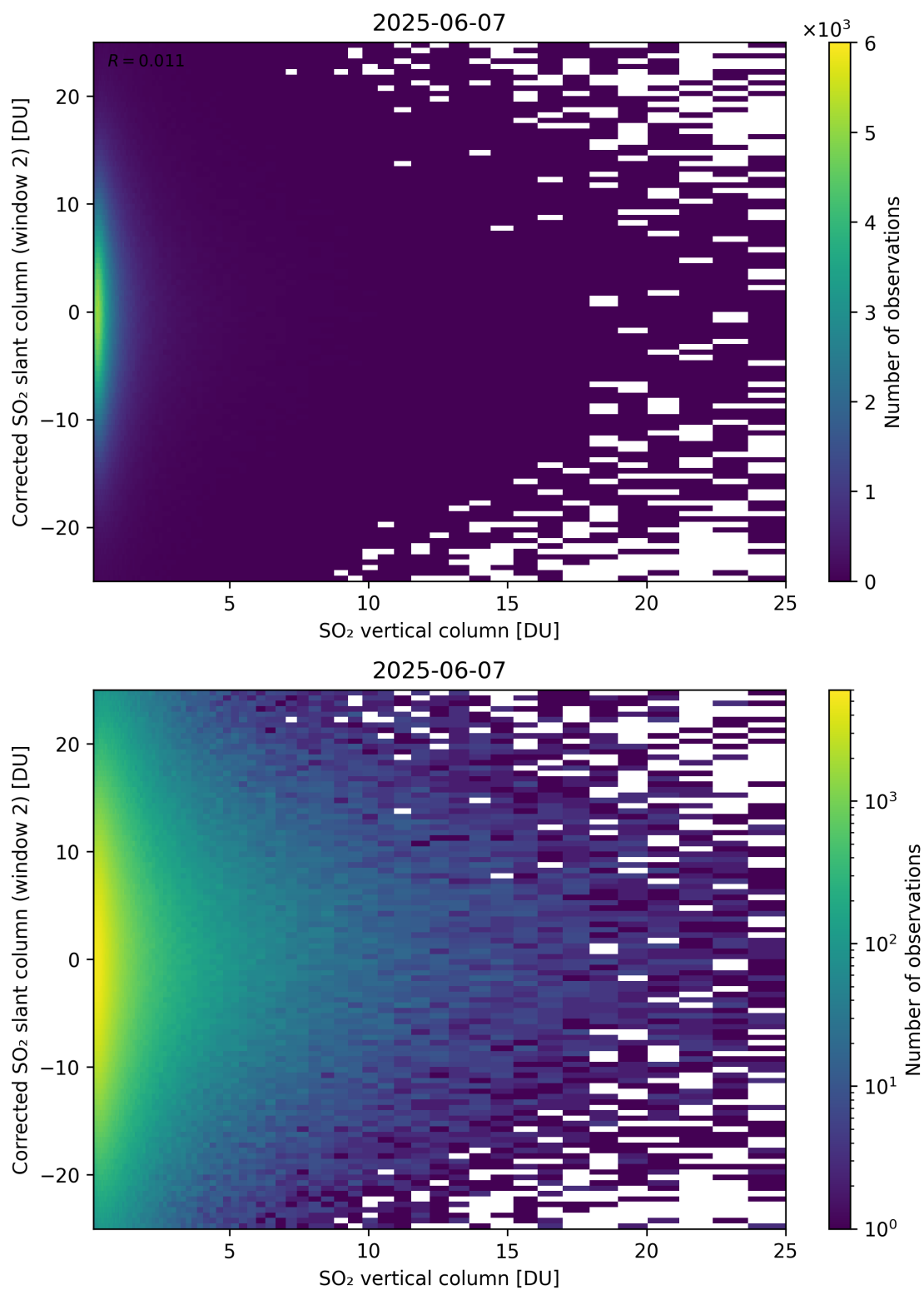
Figure 352: Scatter density plot of “SO 2 vertical column” against “Corrected SO 2 slant column (window 2)” for 2025-06-06 to 2025-06-08.
