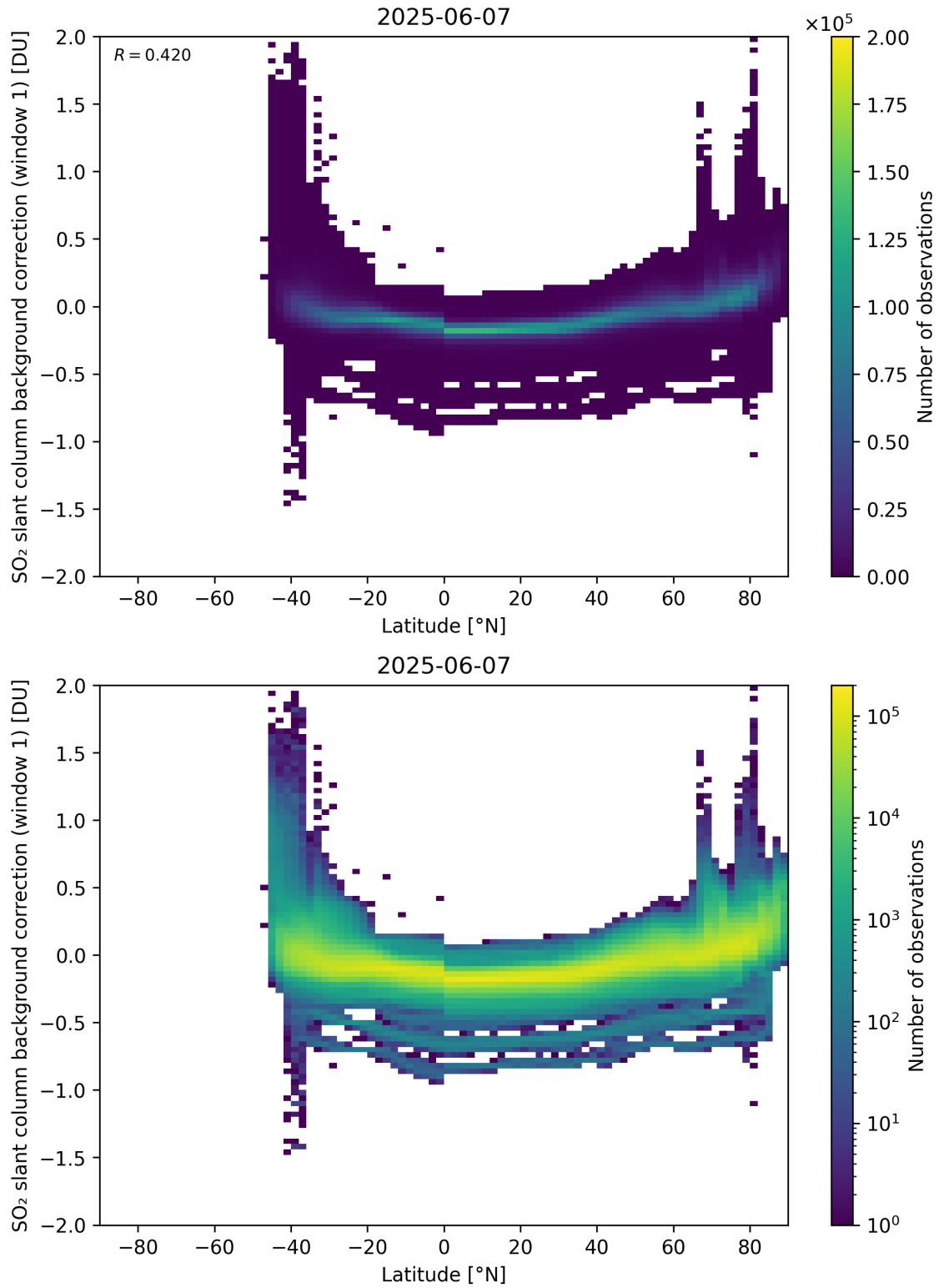
Figure 150: Scatter density plot of “Latitude” against “SO 2 slant column background correction (window 1)” for 2025-06-06 to 2025-06-08.
