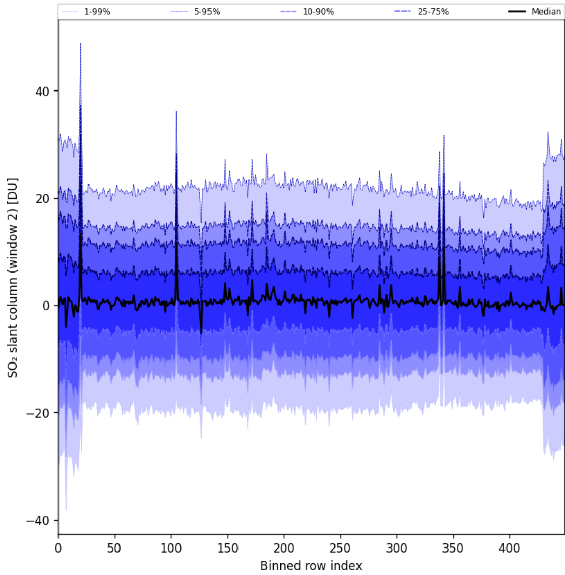
Figure 93: Along track statistics of "SO 2 slant column (window 2)" for 2025-06-06 to 2025-06-08
