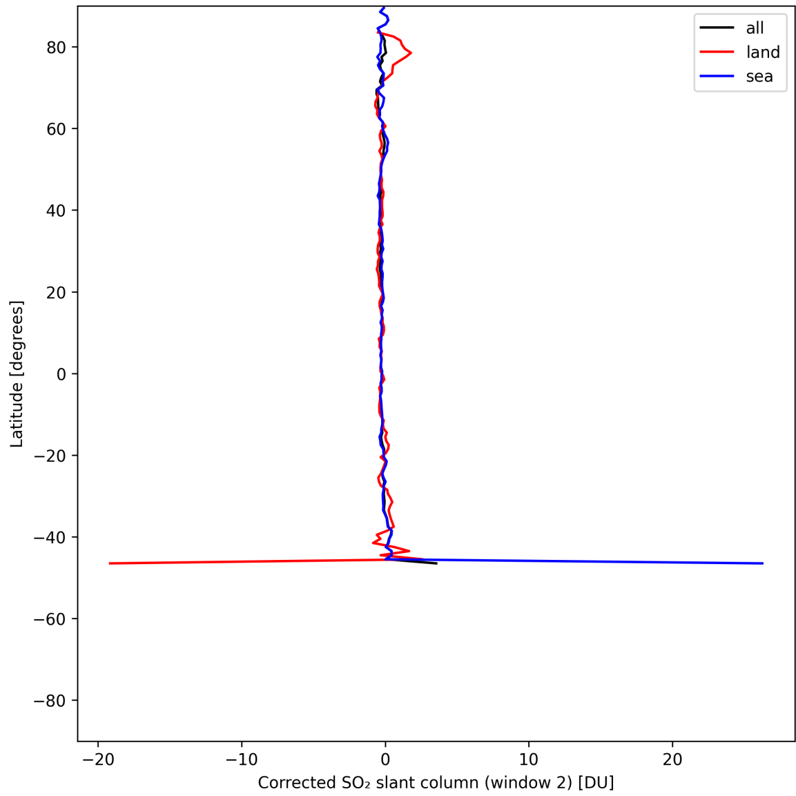
Figure 43: Zonal average of “Corrected SO 2 slant column (window 2)” for 2025-06-06 to 2025-06-08.
