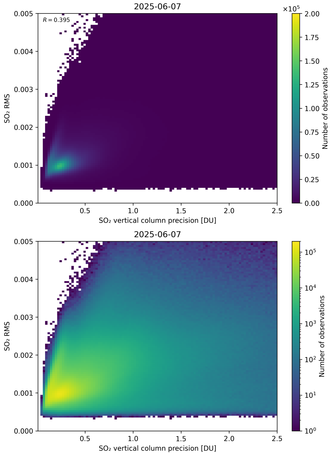
Figure 334: Scatter density plot of “SO 2 vertical column precision” against “SO 2 RMS” for 2025-06-06 to 2025-06-08.
