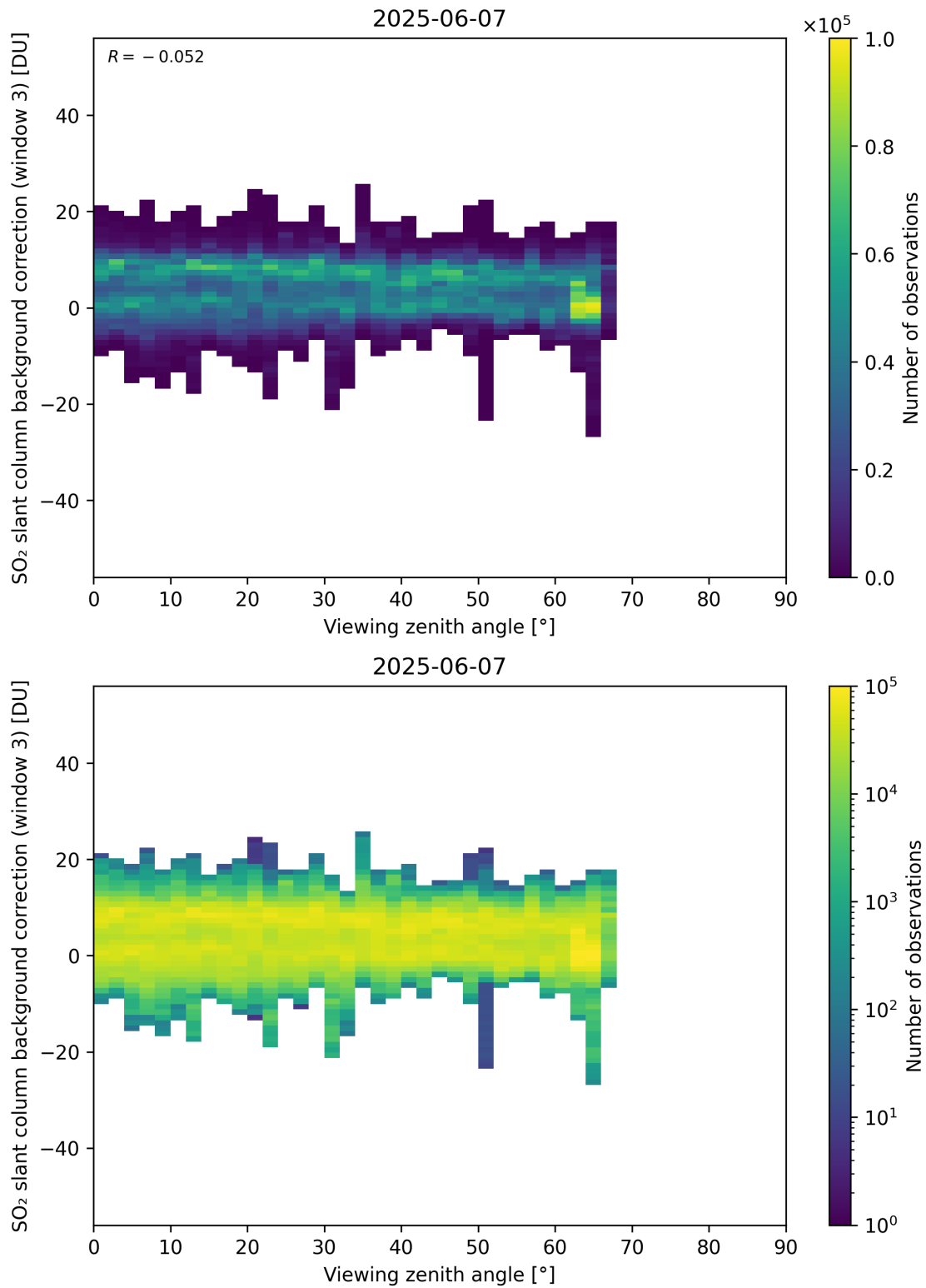
Figure 364: Scatter density plot of “Viewing zenith angle” against “SO 2 slant column background correction (window 3)” for 2025-06-06 to 2025-06-08.
