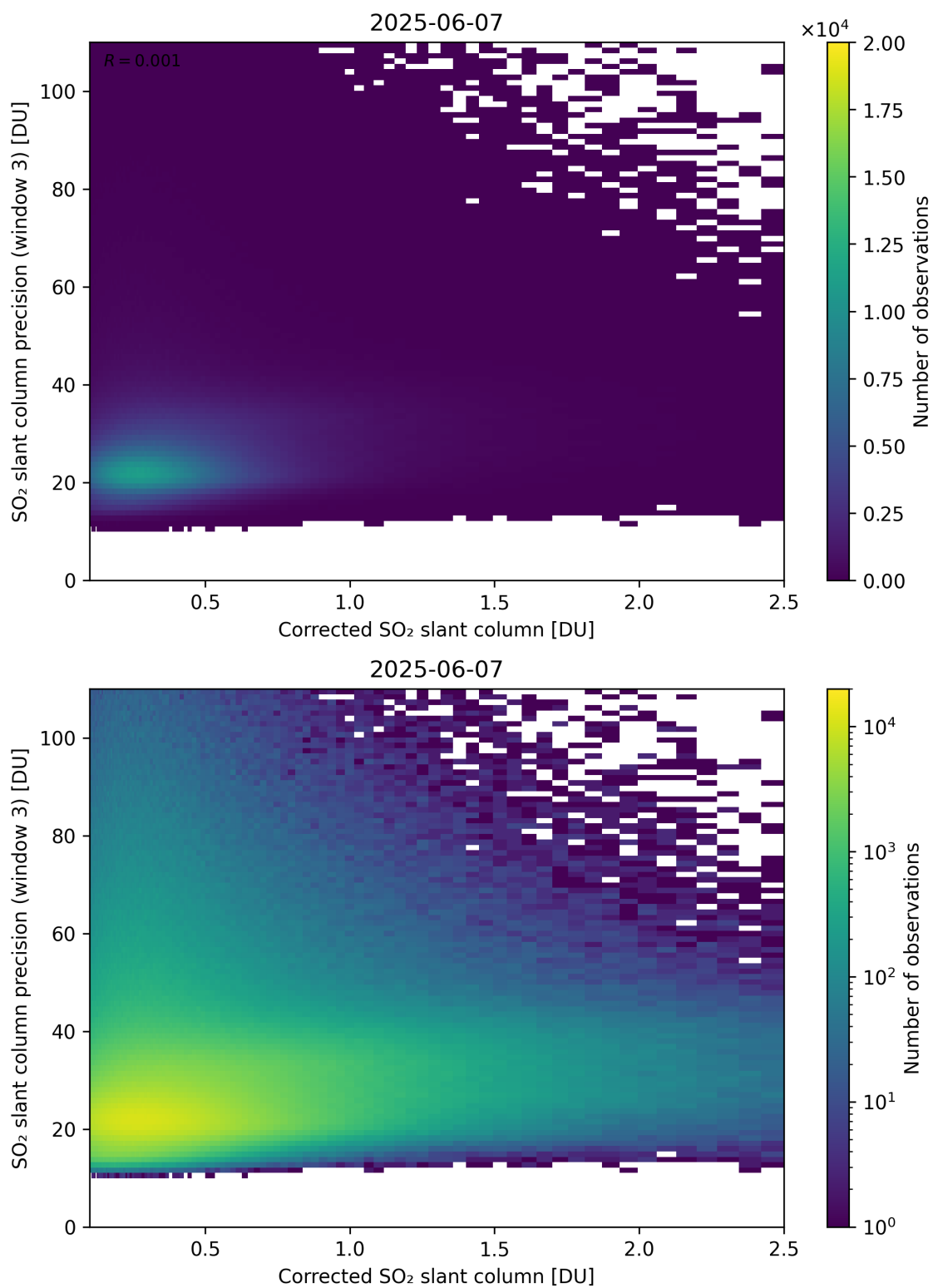
Figure 241: Scatter density plot of “Corrected SO 2 slant column” against “SO 2 slant column precision (window 3)” for 2025-06-06 to 2025-06-08.
