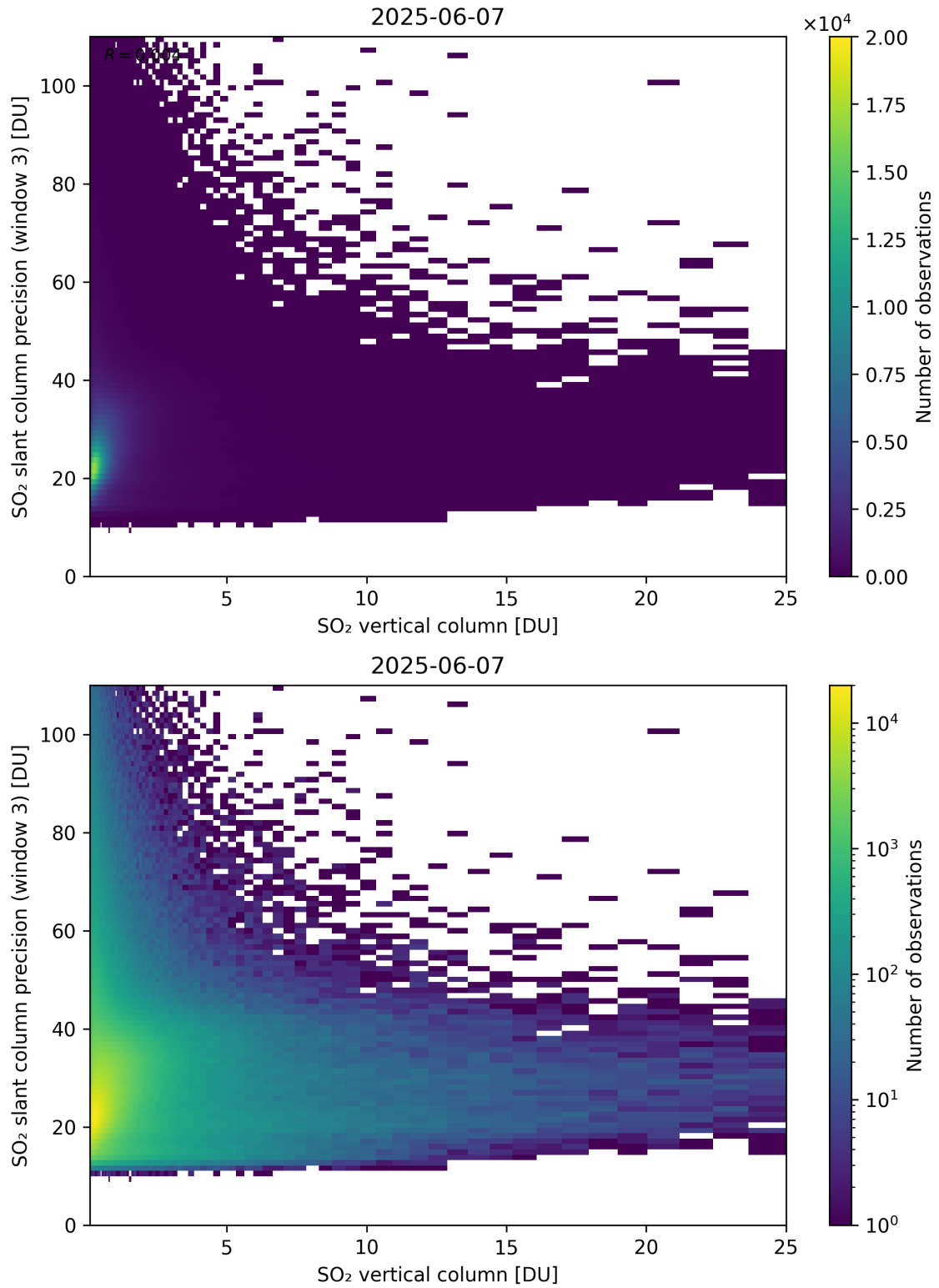
Figure 358: Scatter density plot of “SO 2 vertical column” against “SO 2 slant column precision (window 3)” for 2025-06-06 to 2025-06-08.
