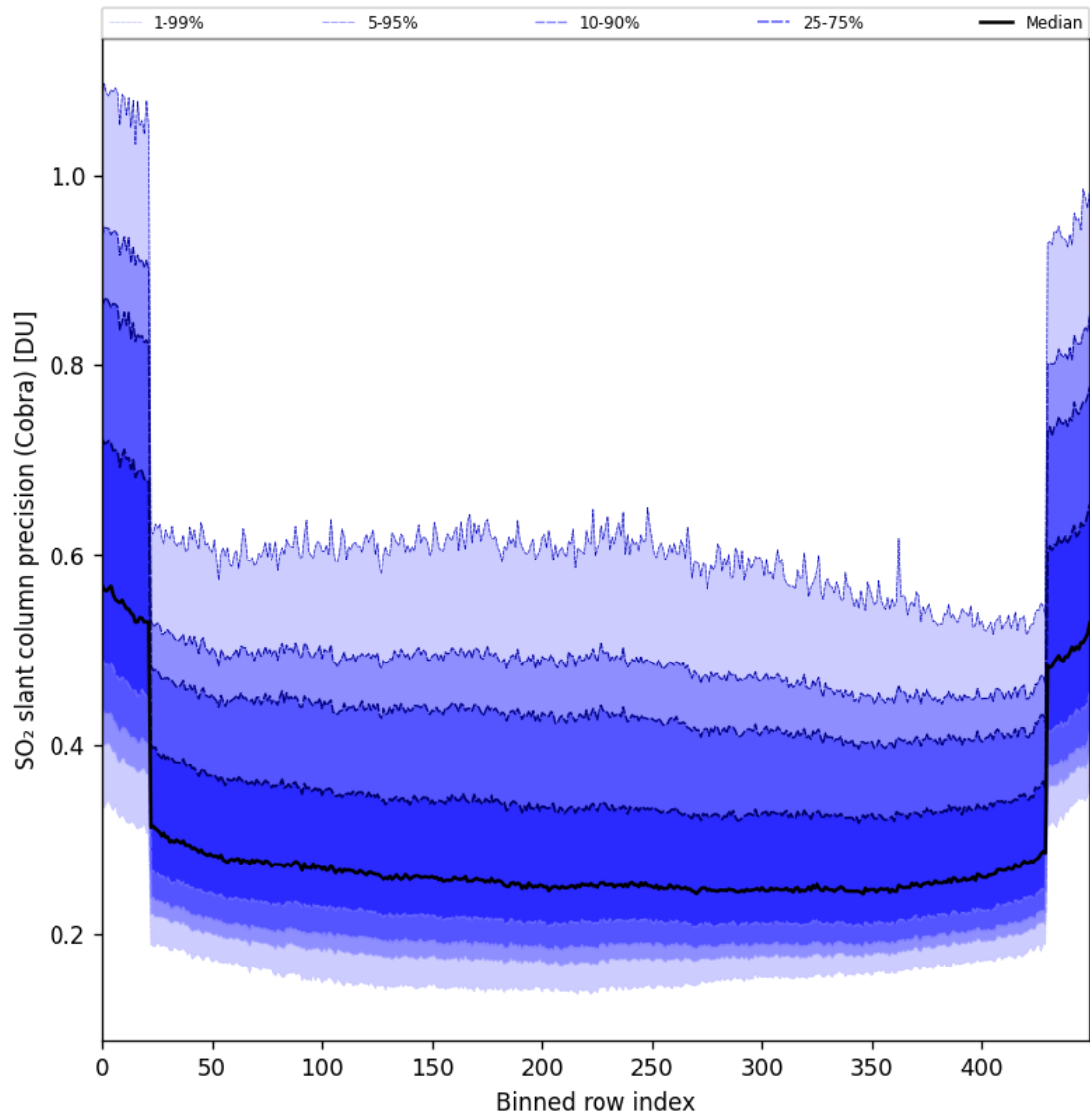
Figure 88: Along track statistics of “SO 2 slant column precision (Cobra)” for 2025-06-06 to 2025-06-08
