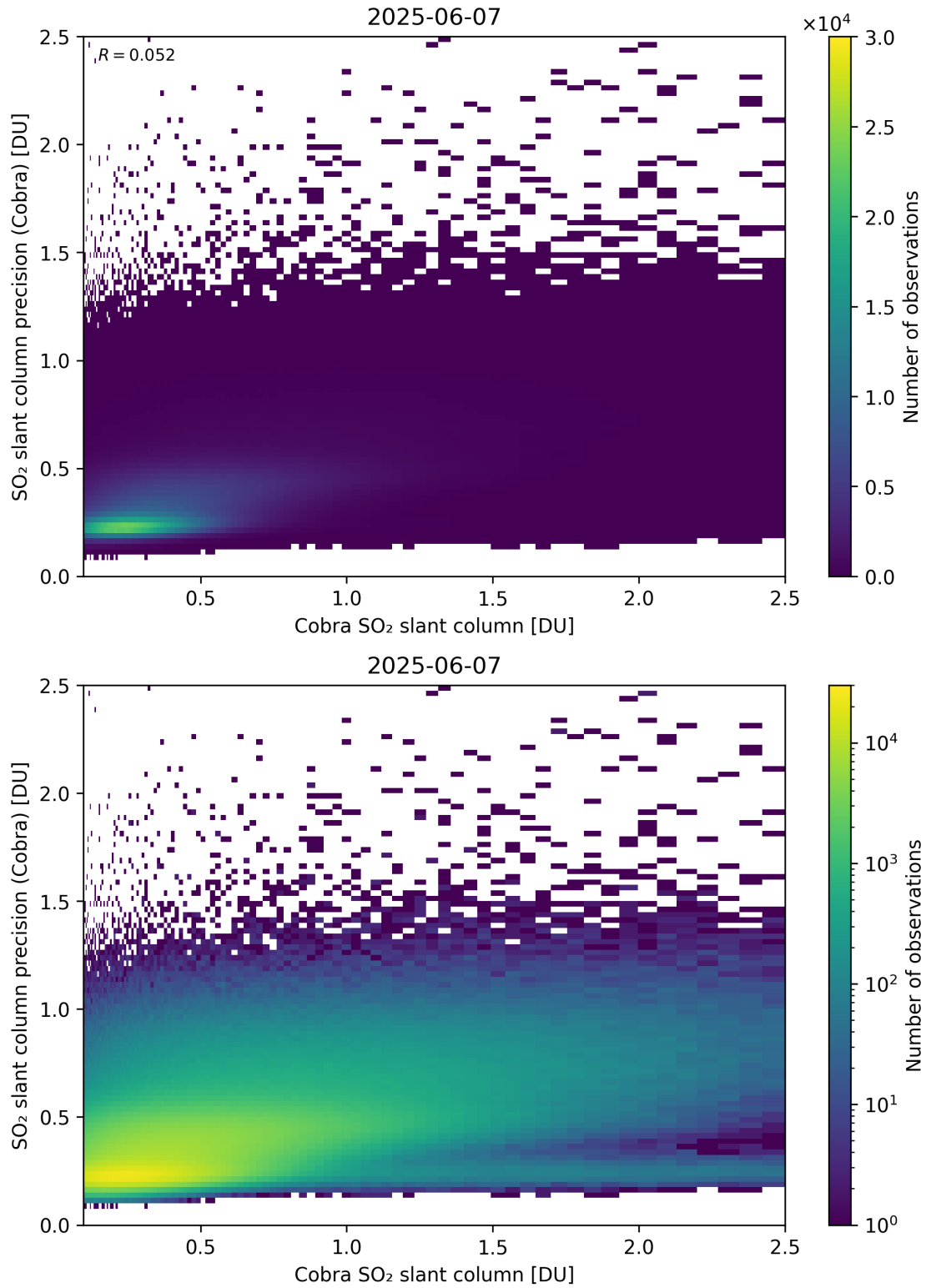
Figure 216: Scatter density plot of “Cobra SO 2 slant column” against “SO 2 slant column precision (Cobra)” for 2025-06-06 to 2025-06-08.
