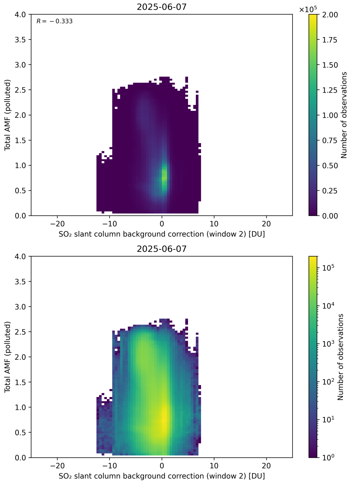
Figure 130: Scatter density plot of “SO 2 slant column background correction (window 2)” against “Total AMF (polluted)” for 2025-06-06 to 2025-06-08.
