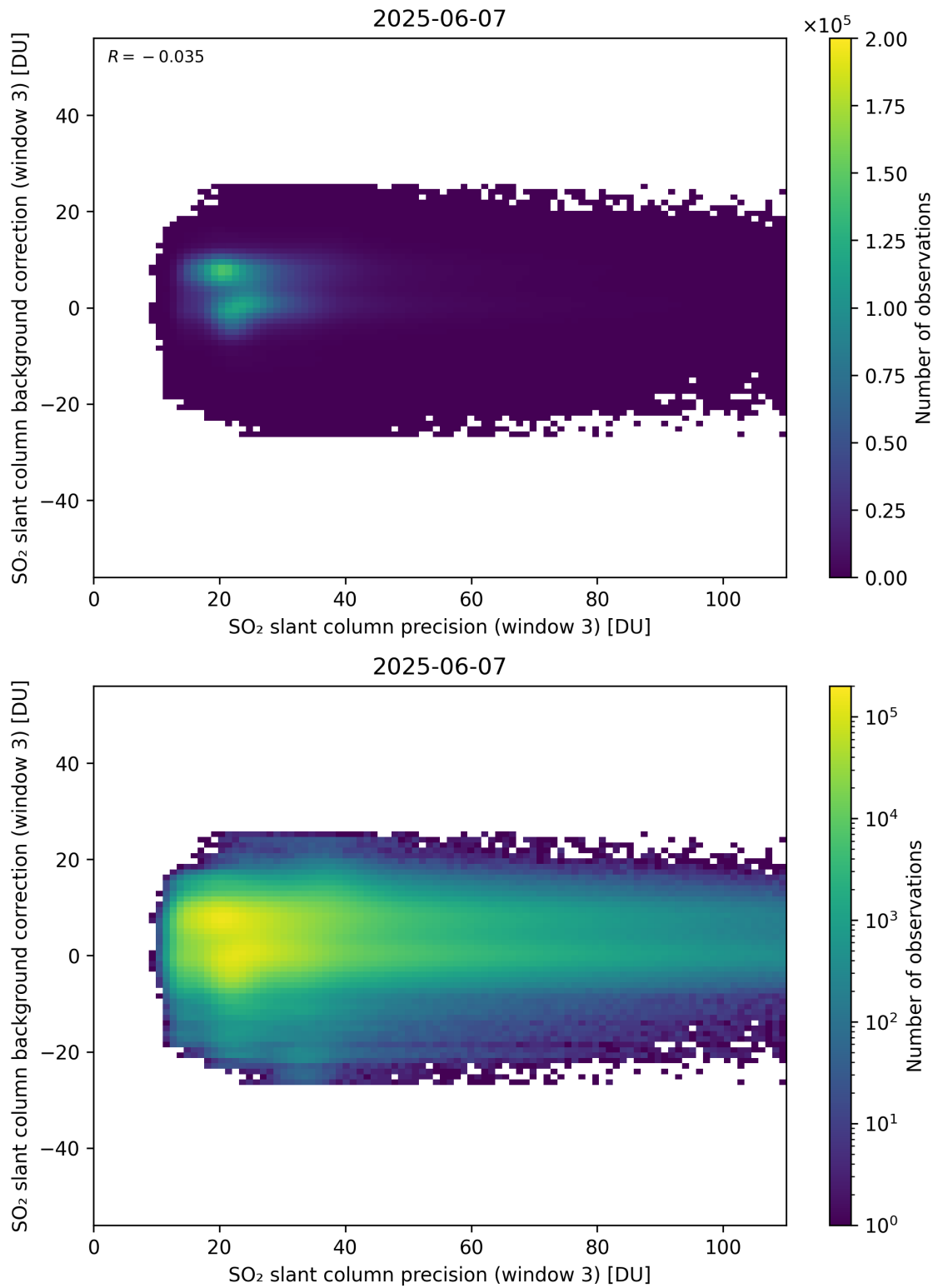
Figure 307: Scatter density plot of “SO 2 slant column precision (window 3)” against “SO 2 slant column background correction (window 3)” for 2025-06-06 to 2025-06-08.
