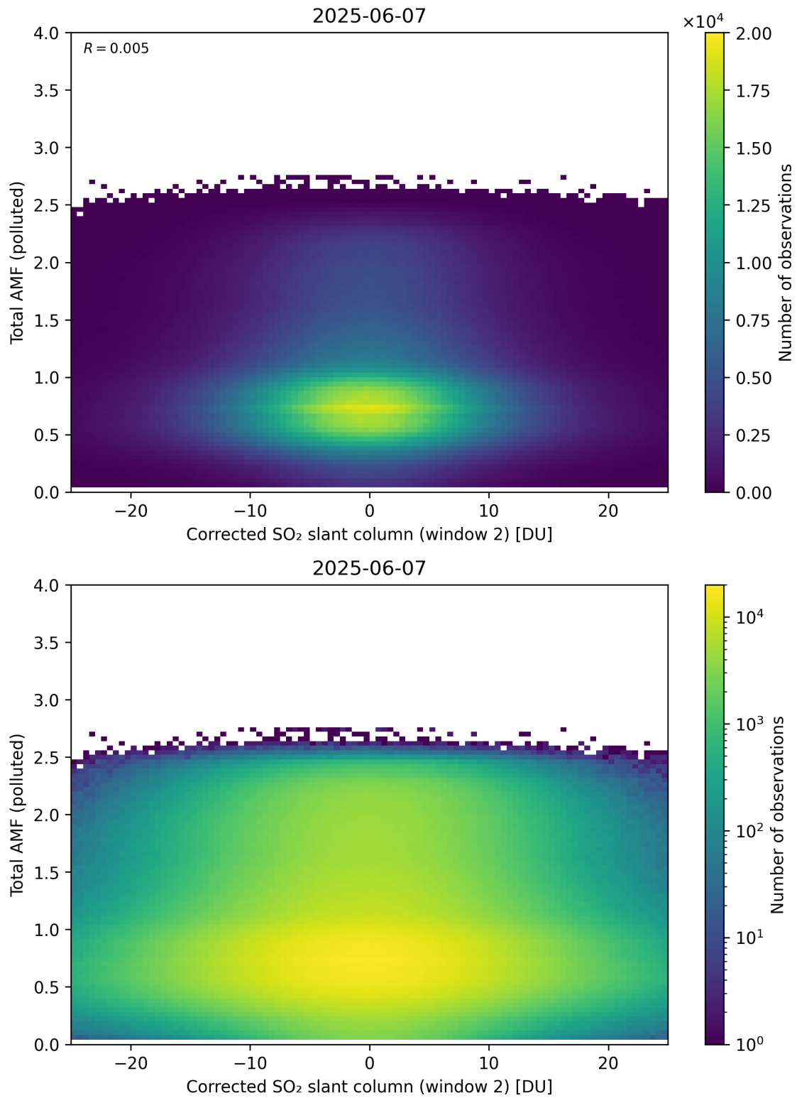
Figure 253: Scatter density plot of “Corrected SO 2 slant column (window 2)” against “Total AMF (polluted)” for 2025-06-06 to 2025-06-08.
