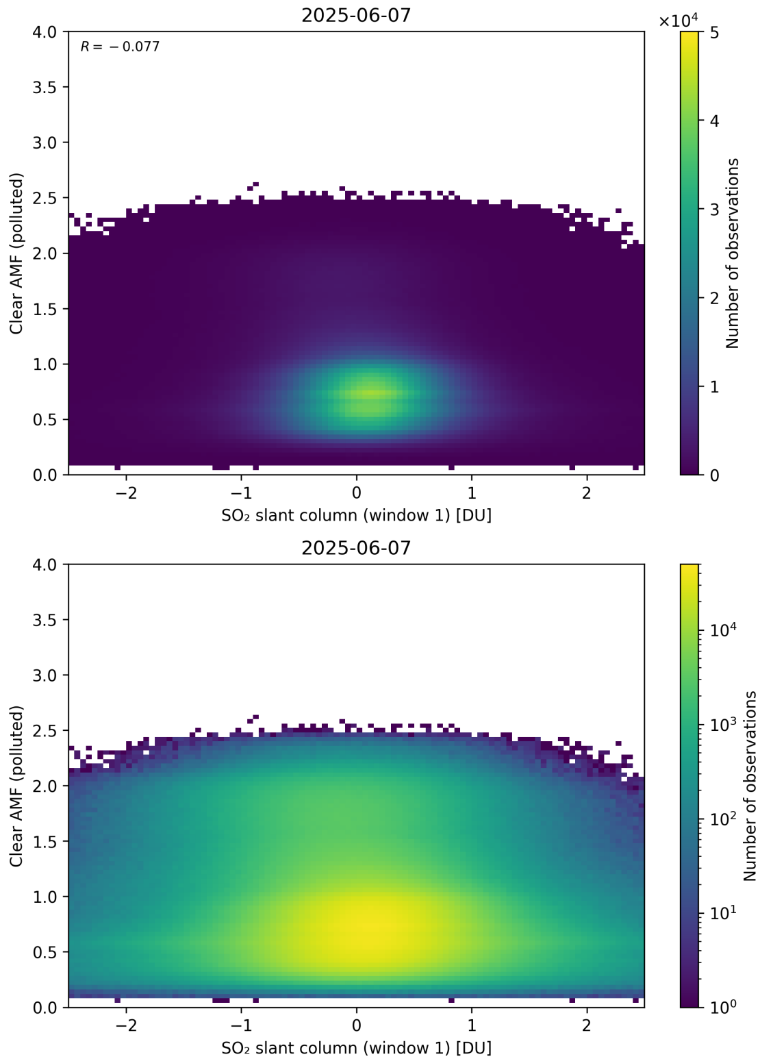
Figure 282: Scatter density plot of “SO 2 slant column (window 1)” against “Clear AMF (polluted)” for 2025-06-06 to 2025-06-08.
