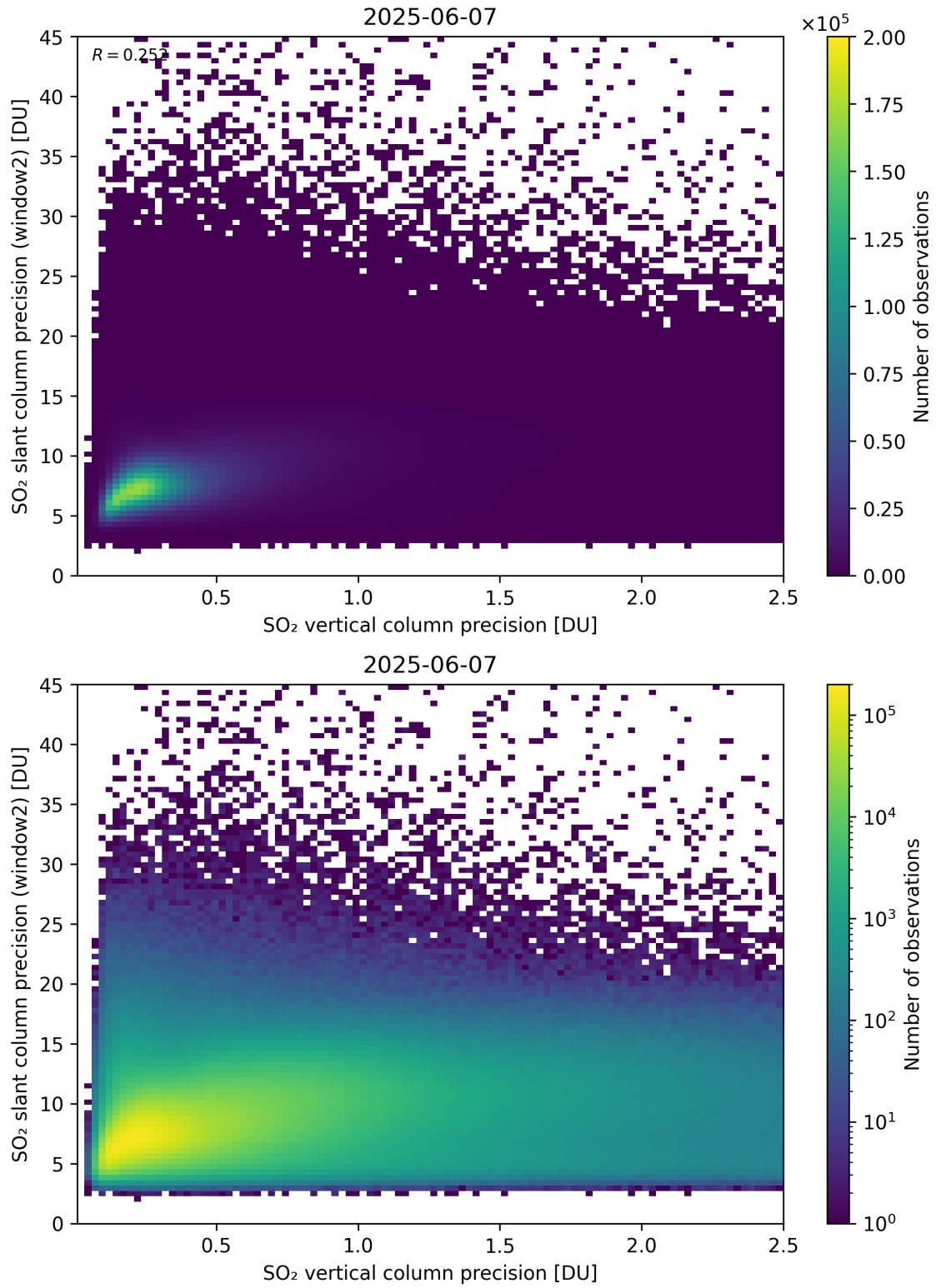
Figure 343: Scatter density plot of “SO 2 vertical column precision” against “SO 2 slant column precision (window2)” for 2025-06-06 to 2025-06-08.
