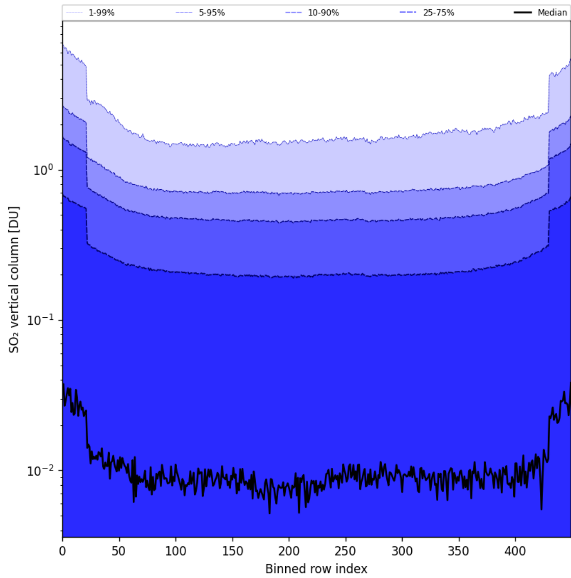
Figure 84: Along track statistics of “SO 2 vertical column” for 2025-06-06 to 2025-06-08
