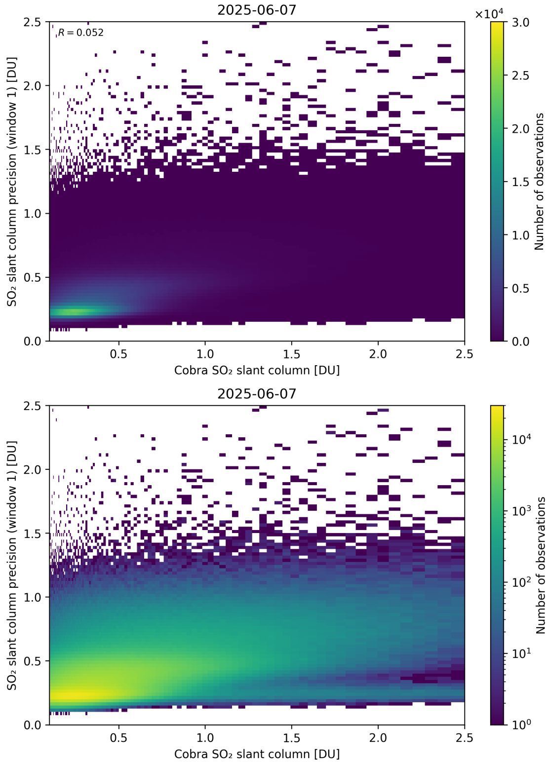
Figure 220: Scatter density plot of “Cobra SO 2 slant column” against “SO 2 slant column precision (window 1)” for 2025-06-06 to 2025-06-08.
