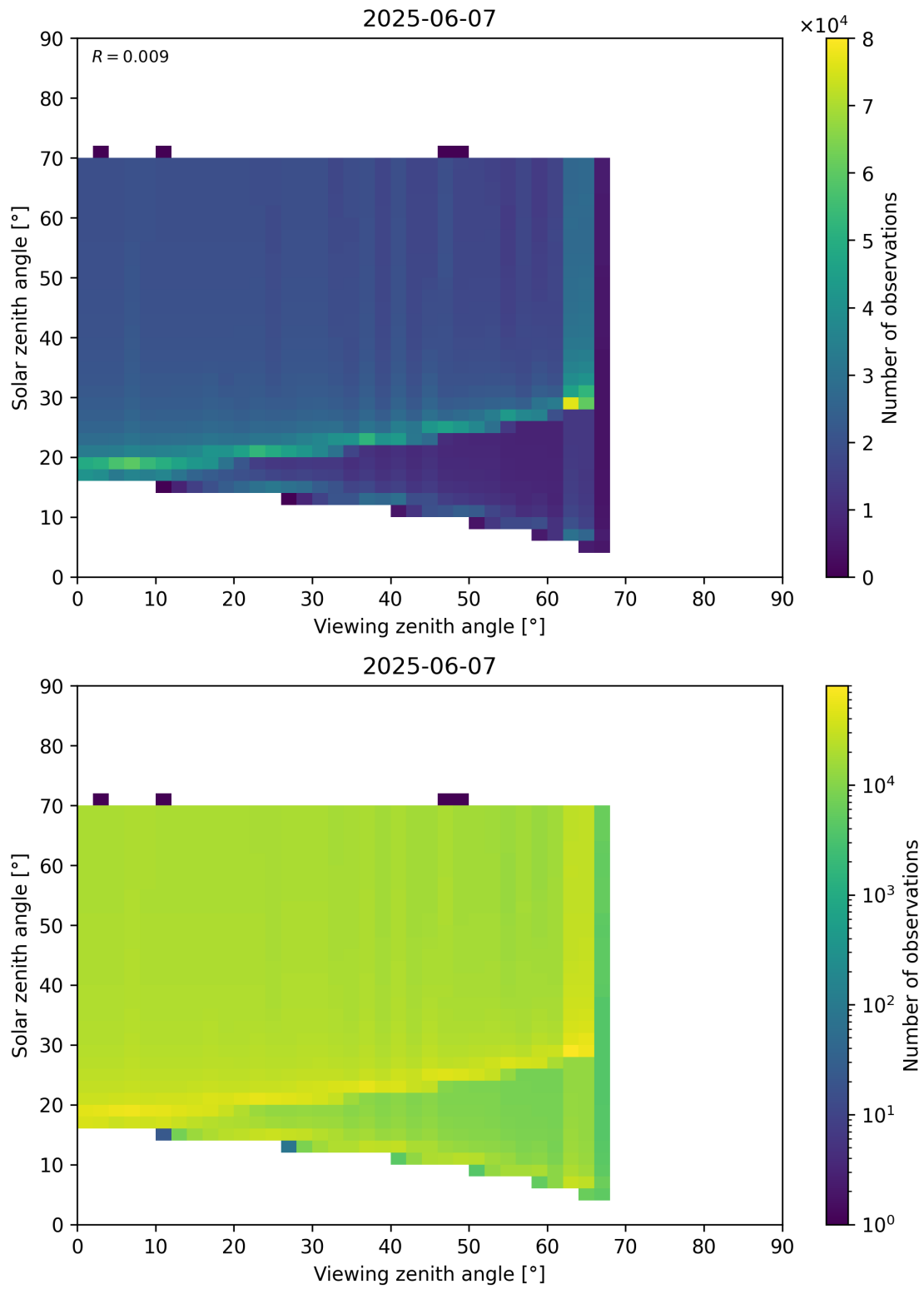
Figure 369: Scatter density plot of “Viewing zenith angle” against “Solar zenith angle” for 2025-06-06 to 2025-06-08.
