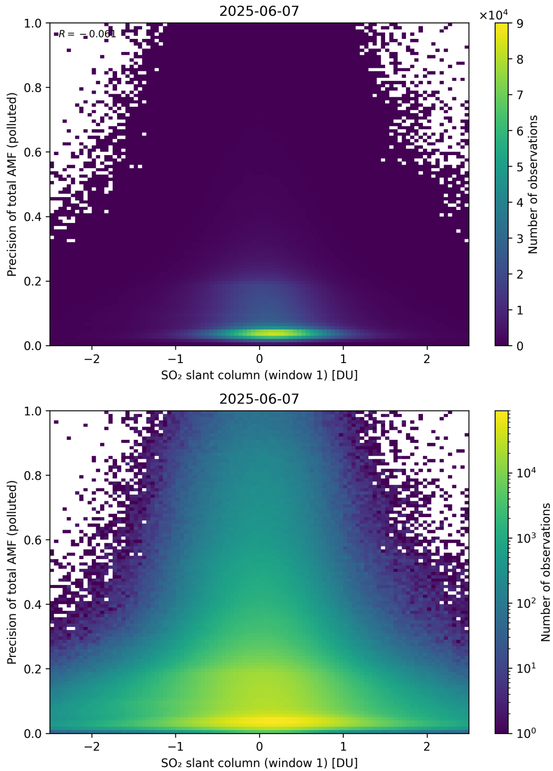
Figure 290: Scatter density plot of “SO 2 slant column (window 1)” against “Precision of total AMF (polluted)” for 2025-06-06 to 2025-06-08.
