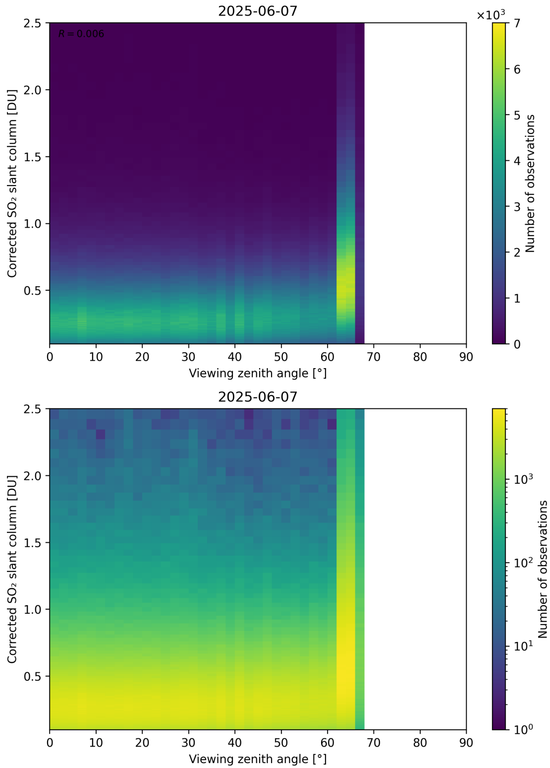
Figure 373: Scatter density plot of “Viewing zenith angle” against “Corrected SO 2 slant column” for 2025-06-06 to 2025-06-08.
