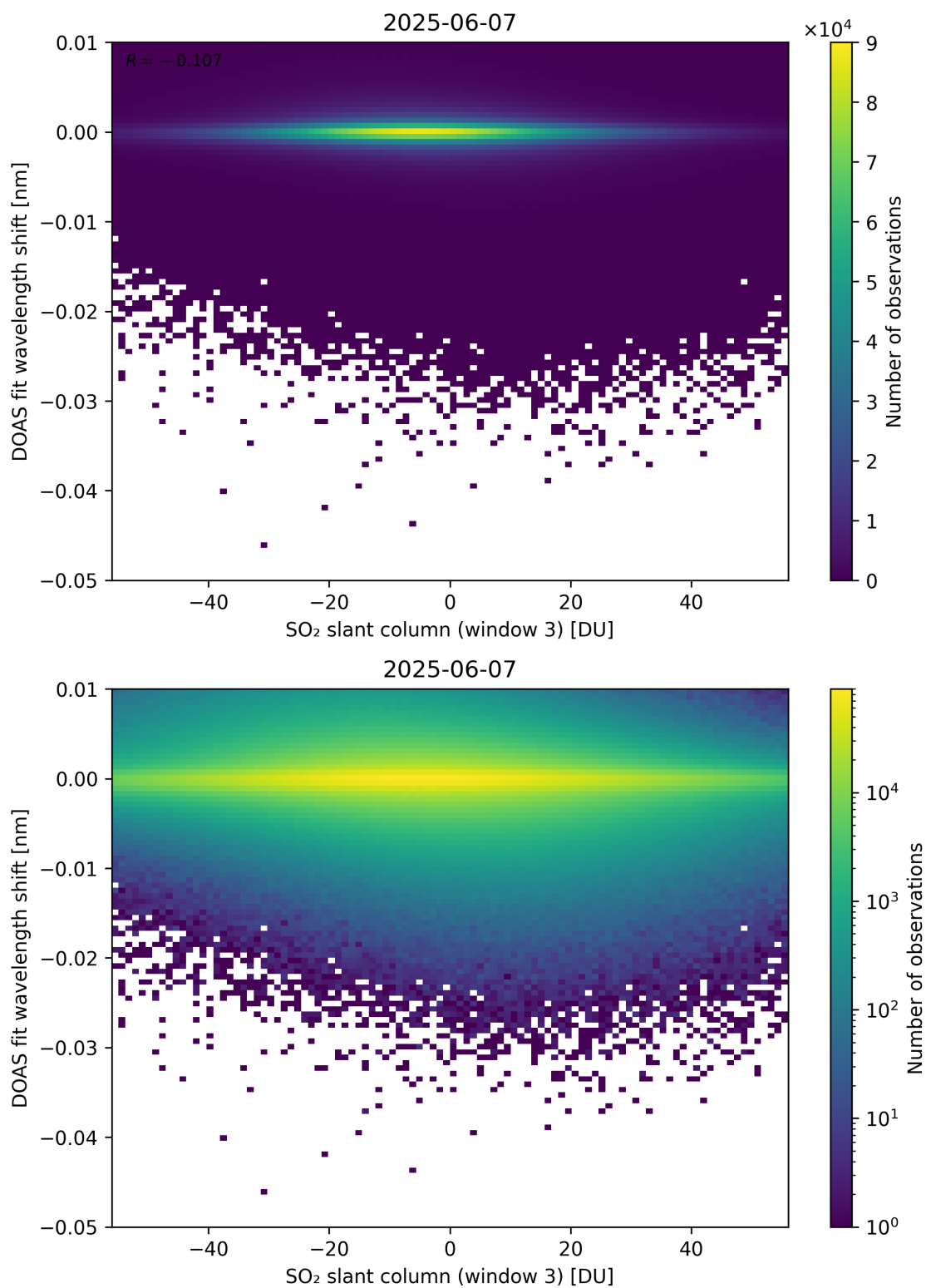
Figure 304: Scatter density plot of “SO 2 slant column (window 3)” against “DOAS fit wavelength shift” for 2025-06-06 to 2025-06-08.
