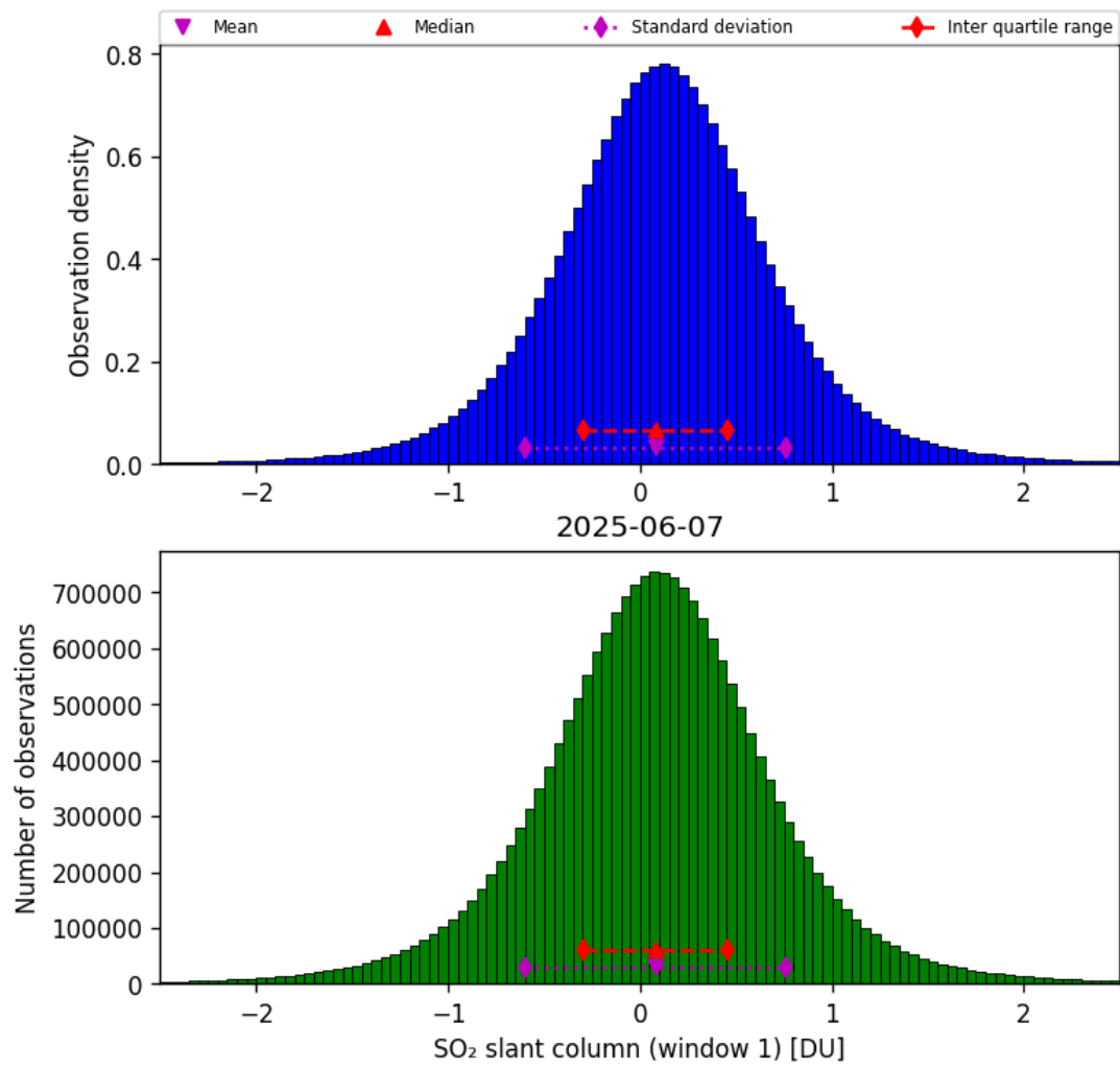
Figure 63: Histogram of “SO 2 slant column (window 1)” for 2025-06-06 to 2025-06-08
