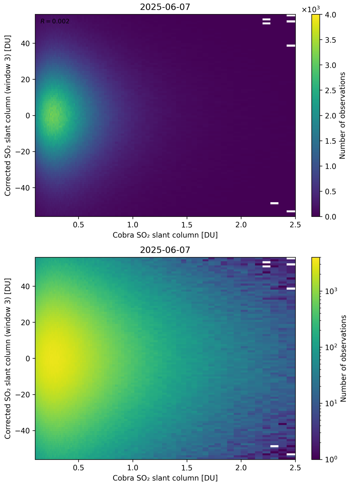
Figure 218: Scatter density plot of “Cobra SO 2 slant column” against “Corrected SO 2 slant column (window 3)” for 2025-06-06 to 2025-06-08.
