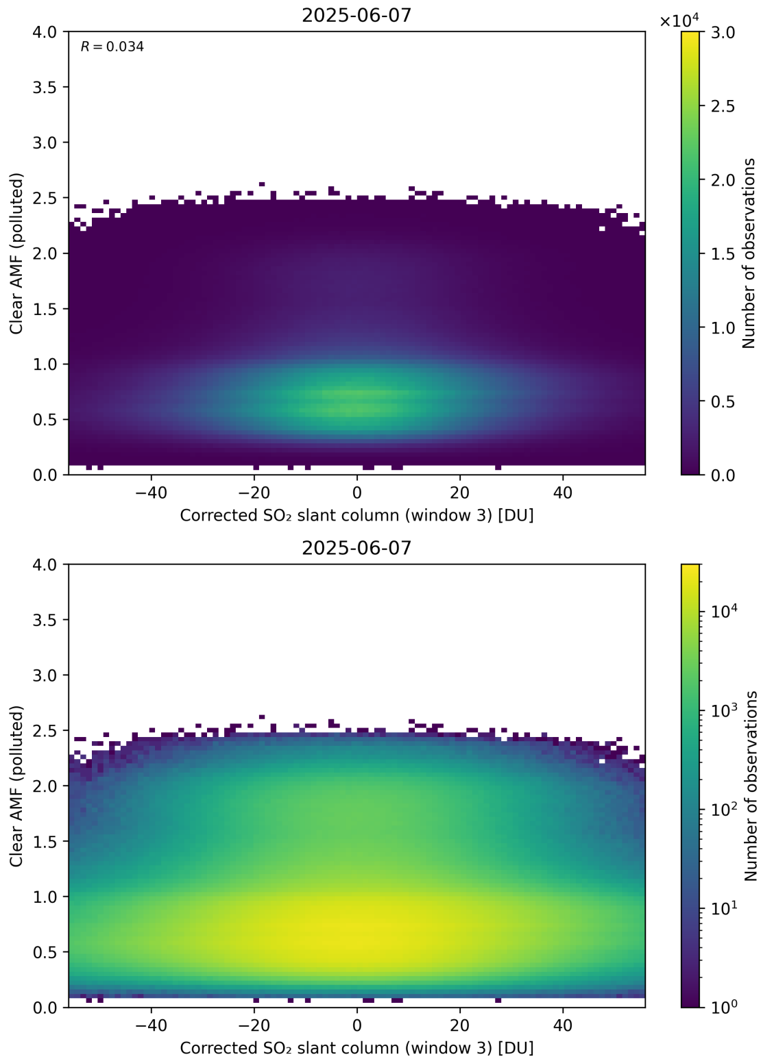
Figure 259: Scatter density plot of “Corrected SO 2 slant column (window 3)” against “Clear AMF (polluted)” for 2025-06-06 to 2025-06-08.
