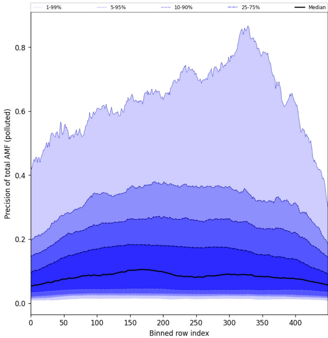
Figure 106: Along track statistics of “Precision of total AMF (polluted)” for 2025-06-06 to 2025-06-08
