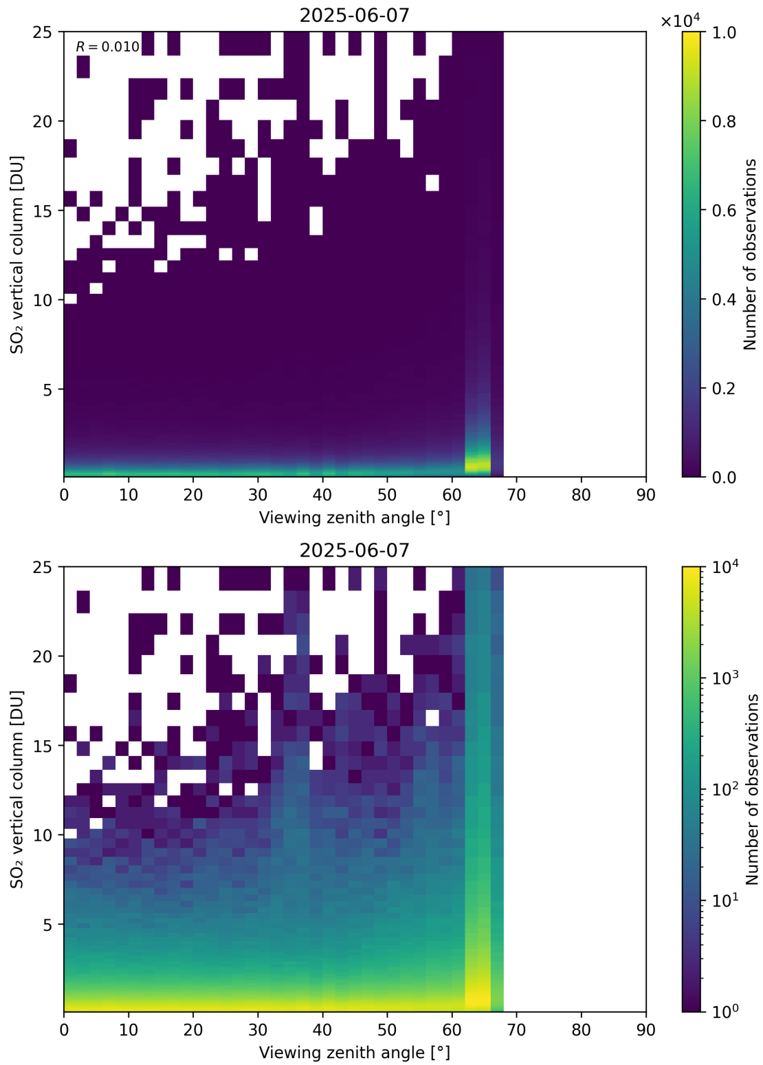
Figure 383: Scatter density plot of “Viewing zenith angle” against “SO 2 vertical column” for 2025-06-06 to 2025-06-08.
