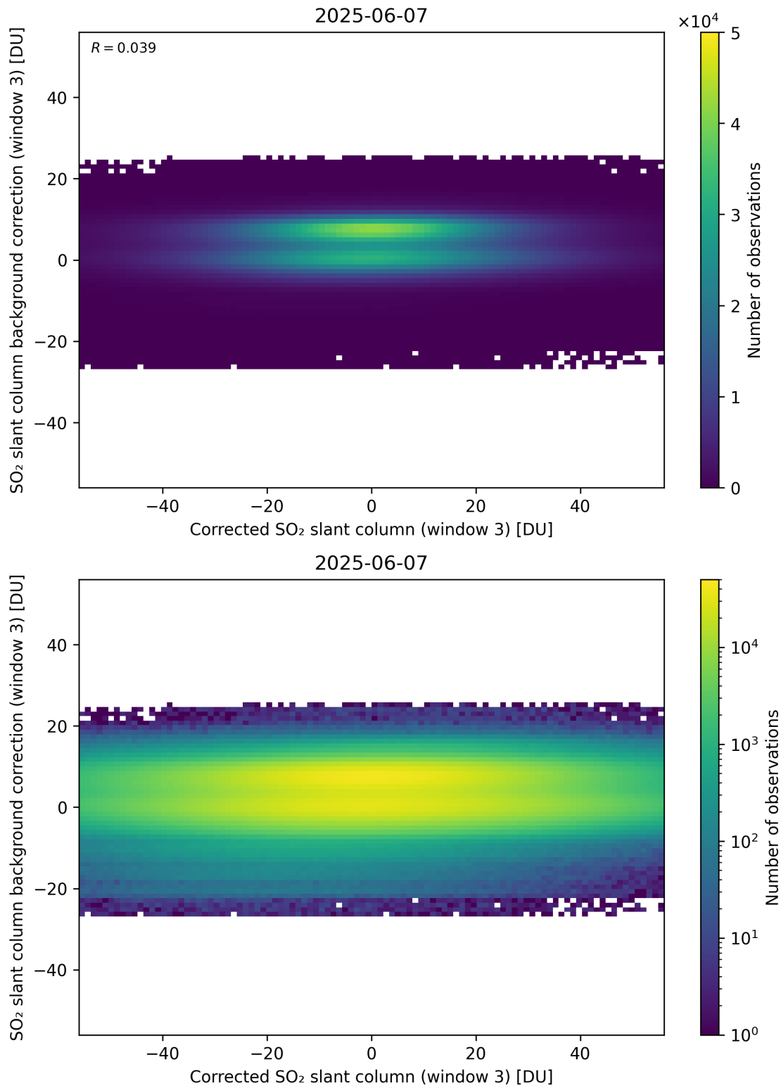
Figure 255: Scatter density plot of “Corrected SO 2 slant column (window 3)” against “SO 2 slant column background correction (window 3)” for 2025-06-06 to 2025-06-08.
