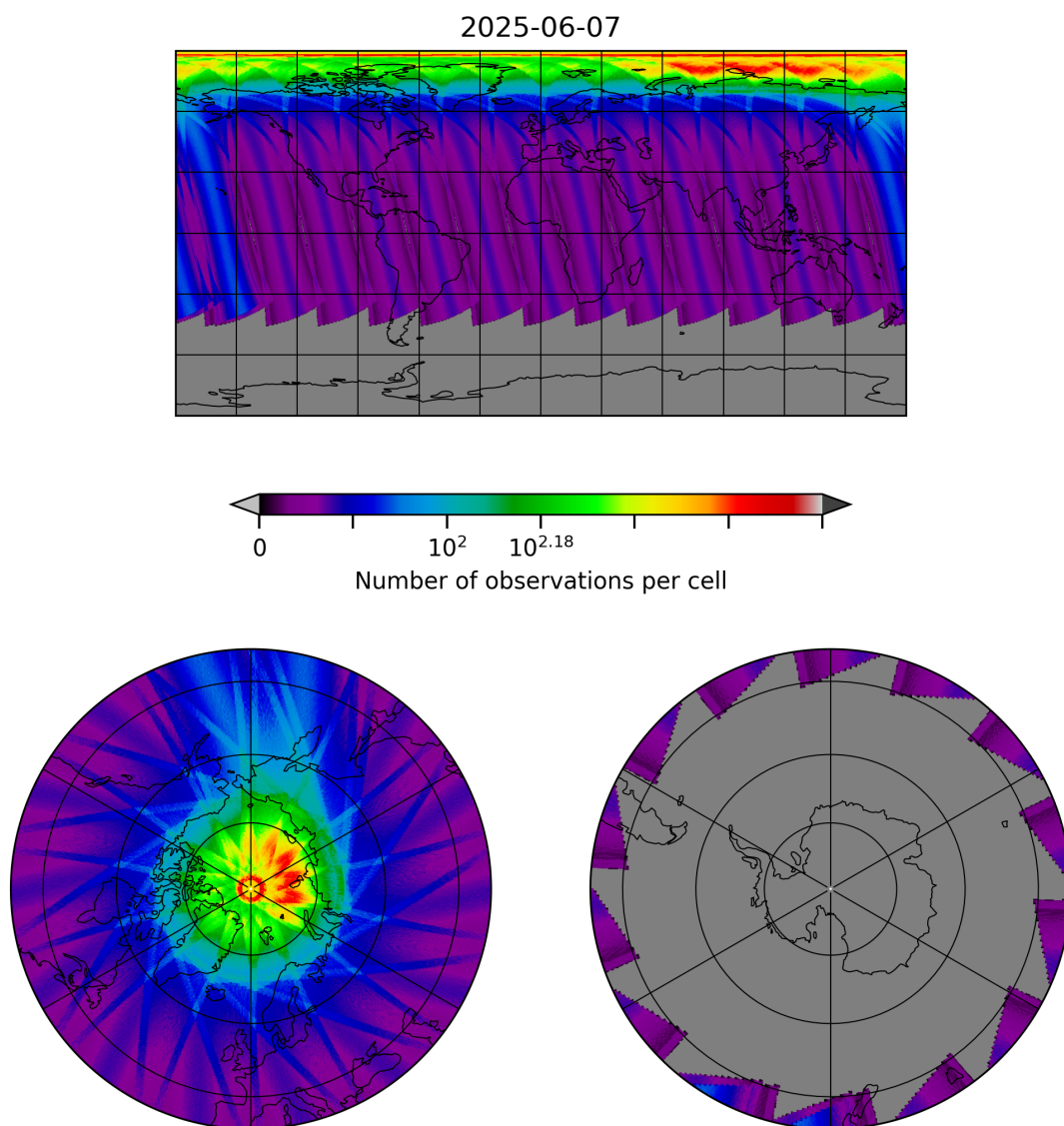
Figure 30: Map of the number of observations for 2025-06-06 to 2025-06-08
