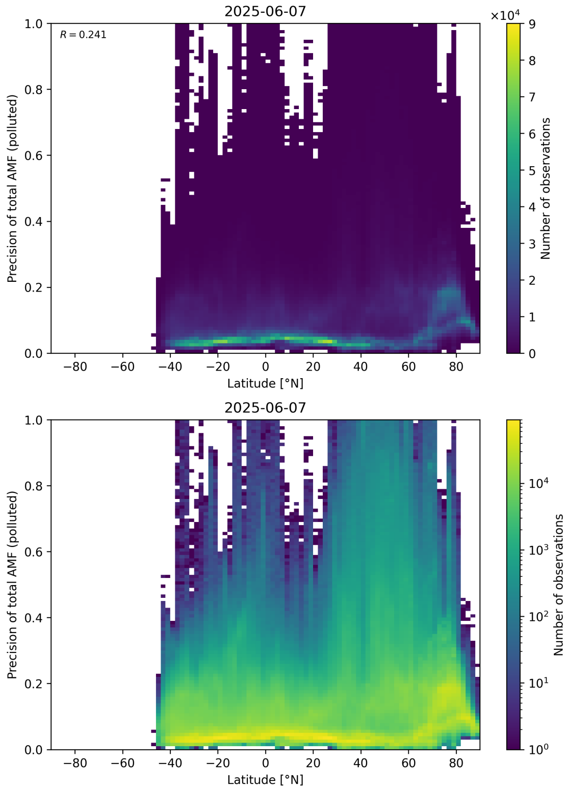
Figure 168: Scatter density plot of “Latitude” against “Precision of total AMF (polluted)” for 2025-06-06 to 2025-06-08.
