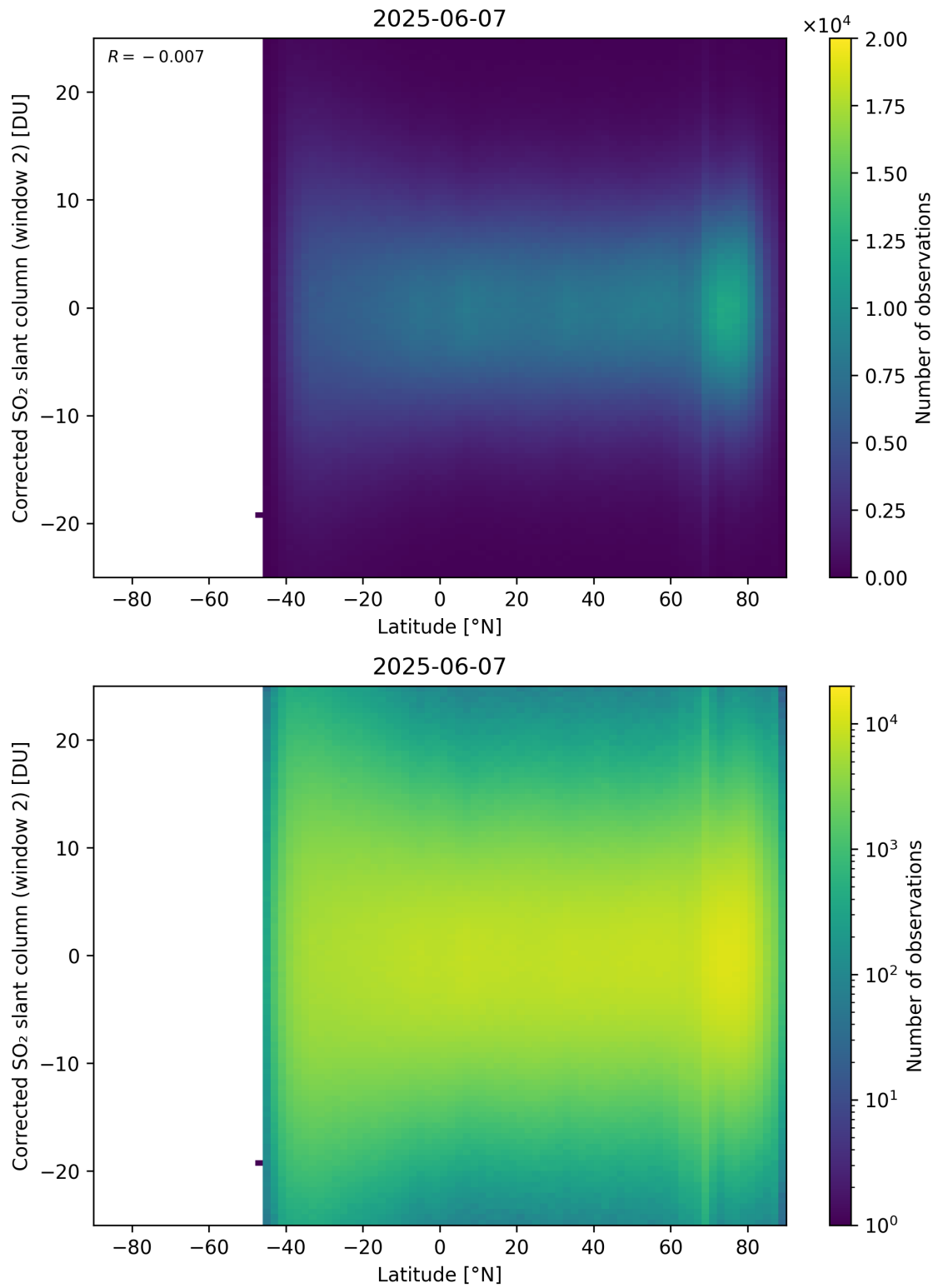
Figure 160: Scatter density plot of “Latitude” against “Corrected SO 2 slant column (window 2)” for 2025-06-06 to 2025-06-08.
