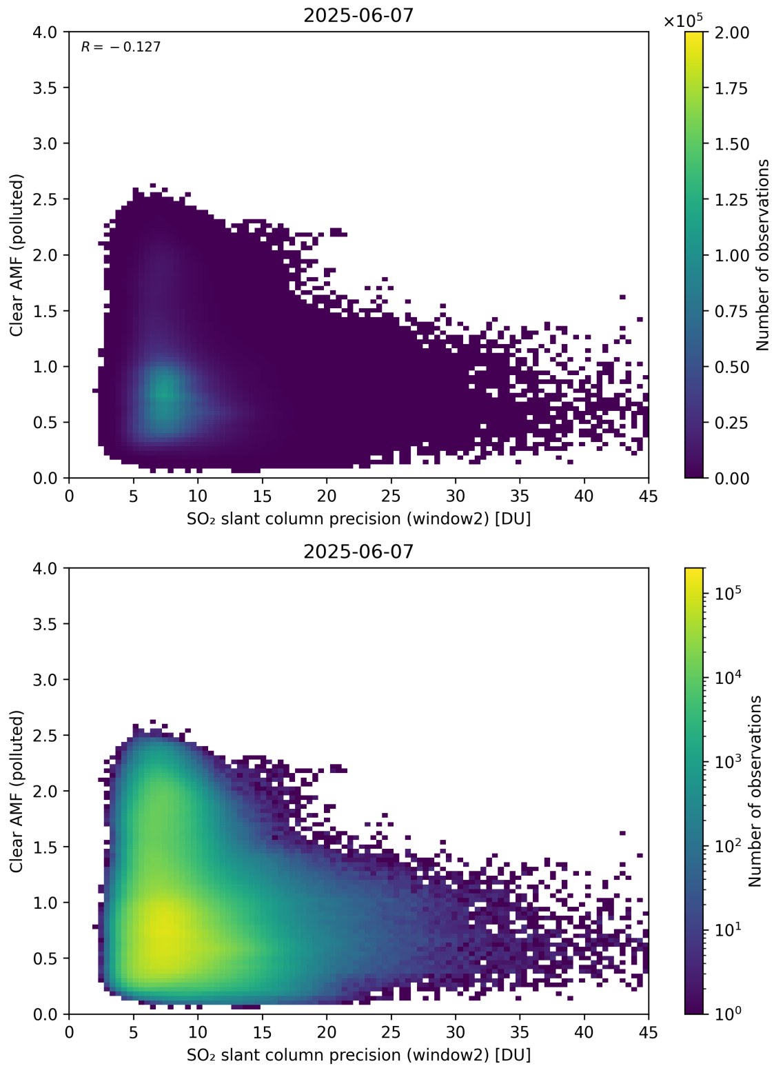
Figure 296: Scatter density plot of “SO 2 slant column precision (window2)” against “Clear AMF (polluted)” for 2025-06-06 to 2025-06-08.
