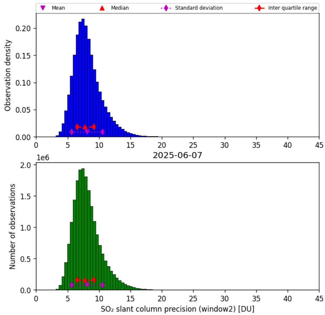
Figure 68: Histogram of “SO 2 slant column precision (window2)” for 2025-06-06 to 2025-06-08
