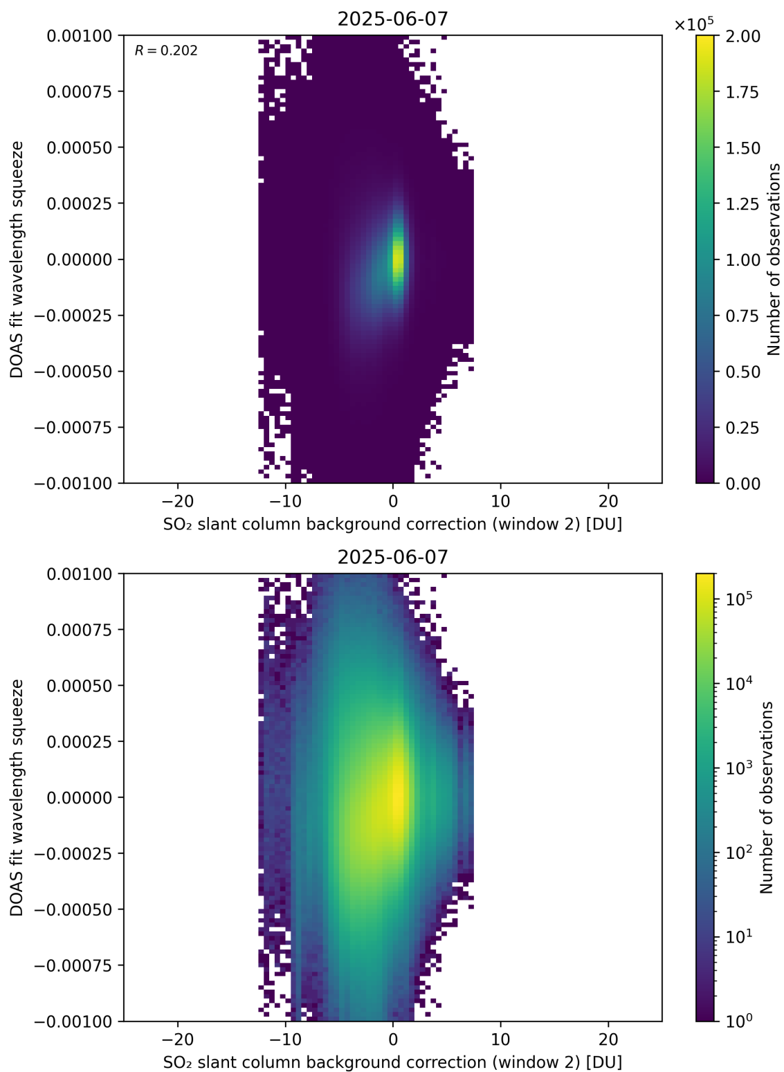
Figure 124: Scatter density plot of “SO 2 slant column background correction (window 2)” against “DOAS fit wavelength squeeze” for 2025-06-06 to 2025-06-08.
