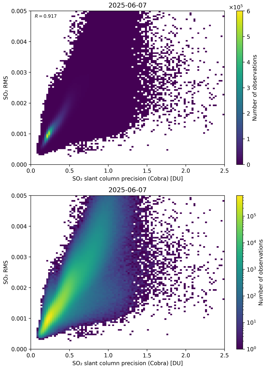
Figure 204: Scatter density plot of “SO 2 slant column precision (Cobra)” against “SO 2 RMS” for 2025-06-06 to 2025-06-08.
