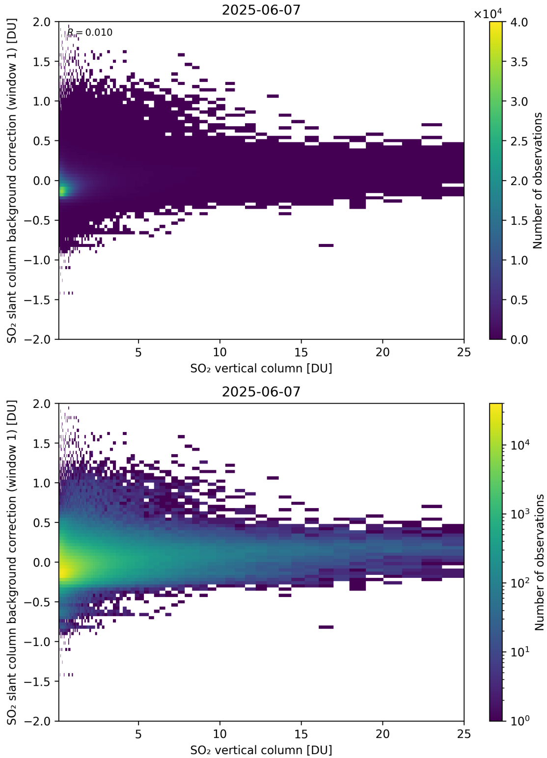
Figure 323: Scatter density plot of “SO 2 vertical column” against “SO 2 slant column background correction (window 1)” for 2025-06-06 to 2025-06-08.
