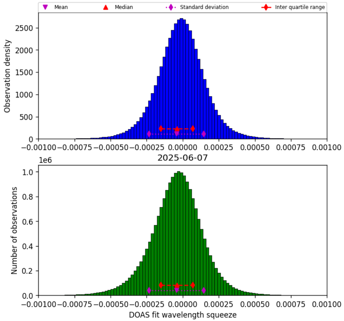
Figure 77: Histogram of “DOAS fit wavelength squeeze” for 2025-06-06 to 2025-06-08
