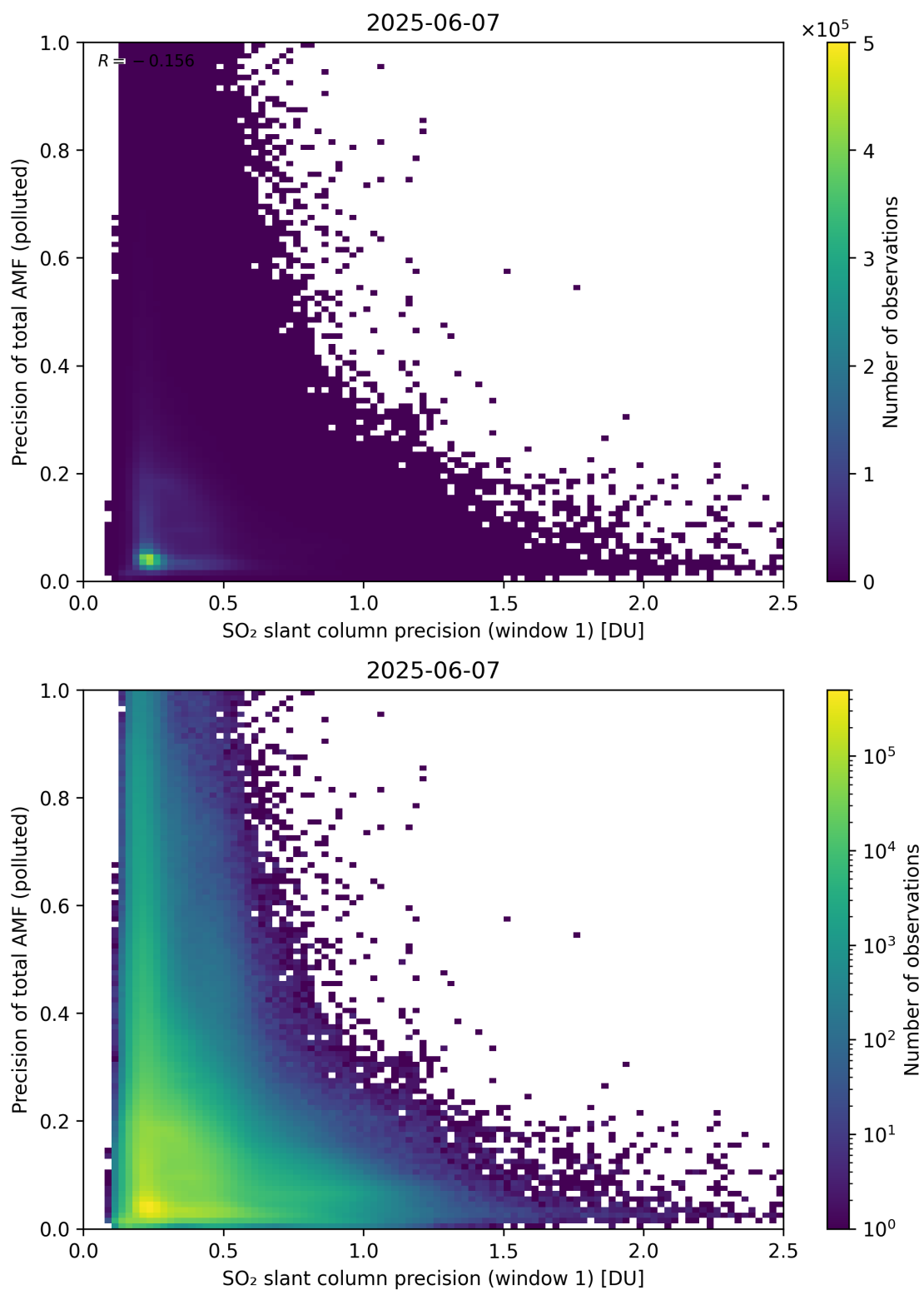
Figure 281: Scatter density plot of “SO 2 slant column precision (window 1)” against “Precision of total AMF (polluted)” for 2025-06-06 to 2025-06-08.
