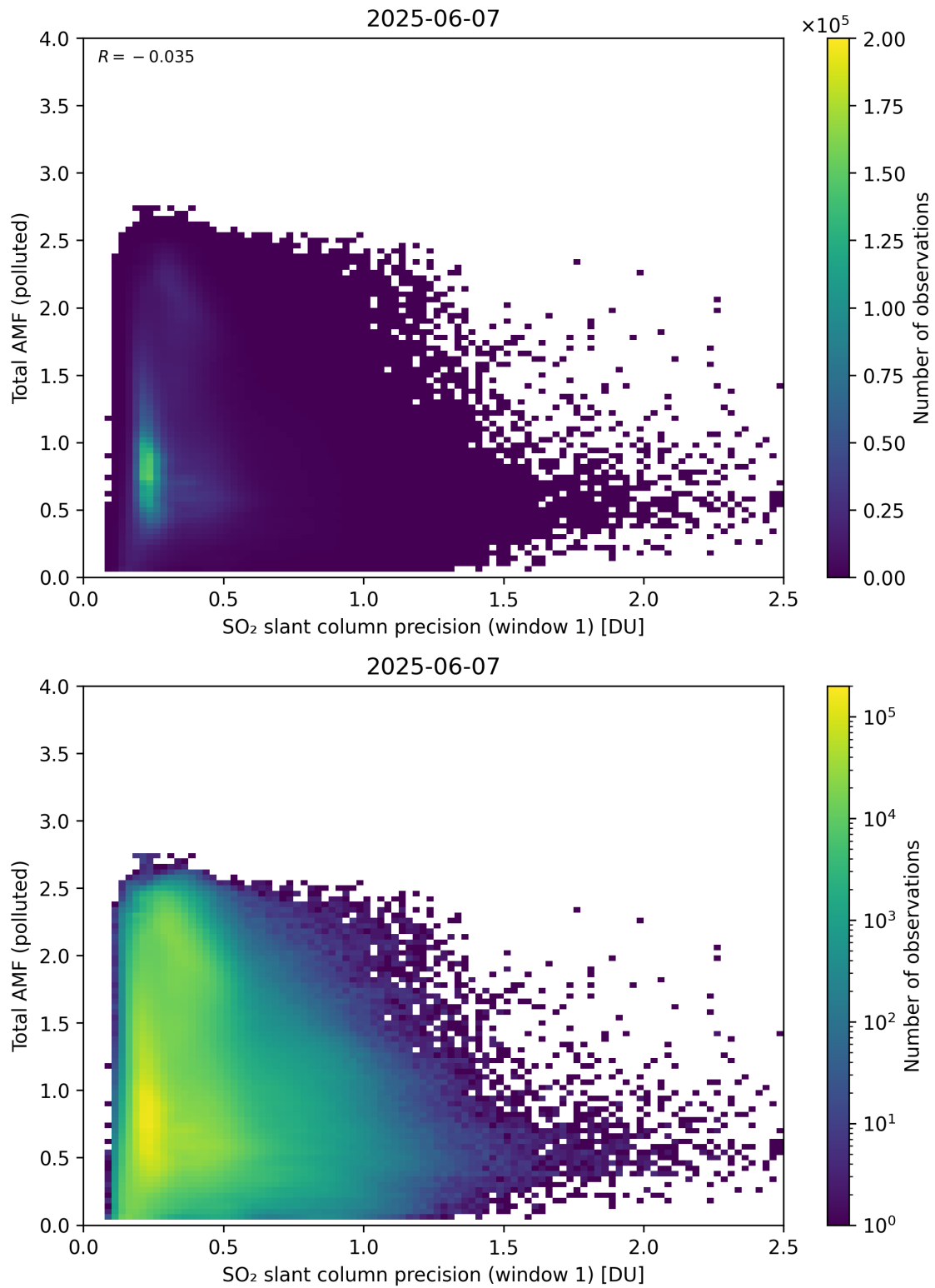
Figure 280: Scatter density plot of “SO 2 slant column precision (window 1)” against “Total AMF (polluted)” for 2025-06-06 to 2025-06-08.
