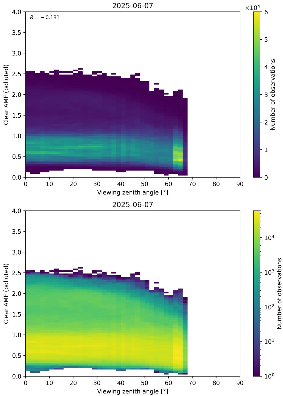
Figure 370: Scatter density plot of “Viewing zenith angle” against “Clear AMF (polluted)” for 2025-06-06 to 2025-06-08.
