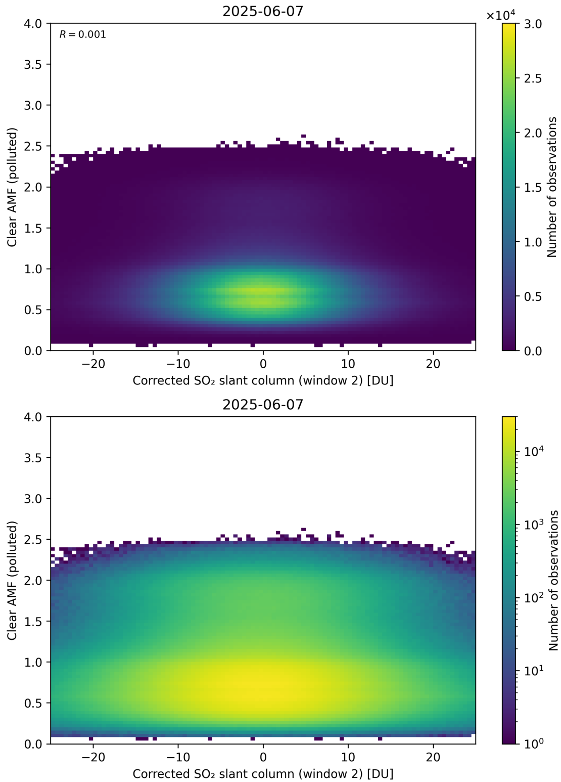
Figure 249: Scatter density plot of “Corrected SO 2 slant column (window 2)” against “Clear AMF (polluted)” for 2025-06-06 to 2025-06-08.
