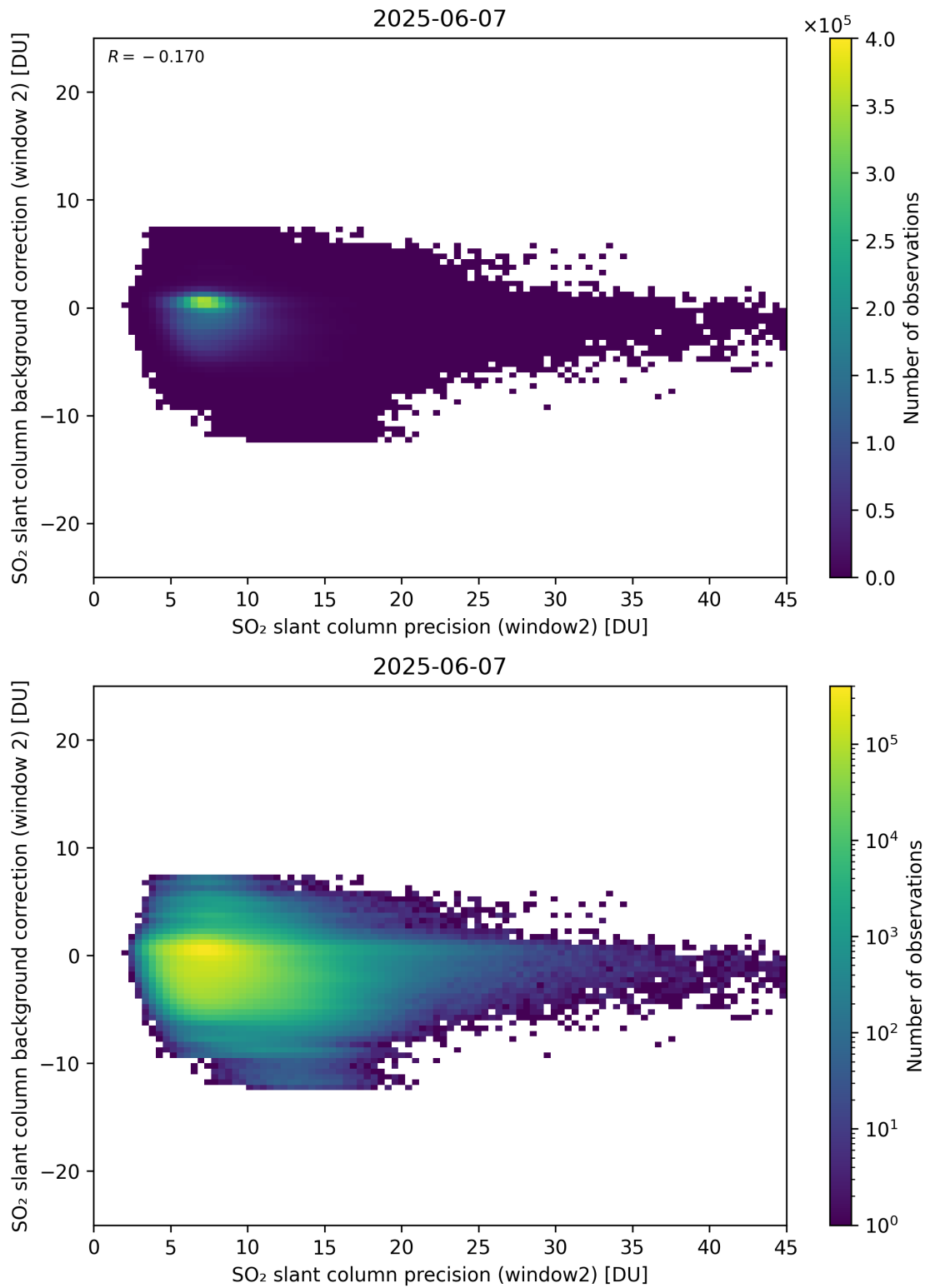
Figure 291: Scatter density plot of “SO 2 slant column precision (window2)” against “SO 2 slant column background correction (window 2)” for 2025-06-06 to 2025-06-08.
