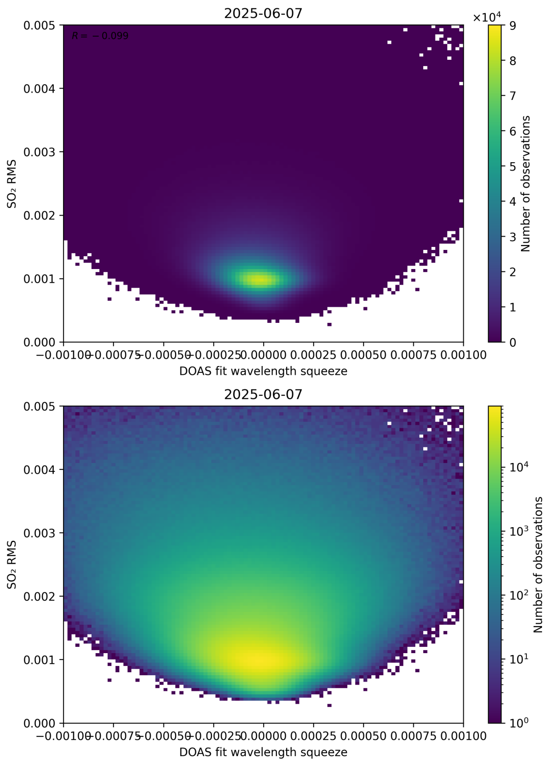
Figure 143: Scatter density plot of “DOAS fit wavelength squeeze” against “SO 2 RMS” for 2025-06-06 to 2025-06-08.
