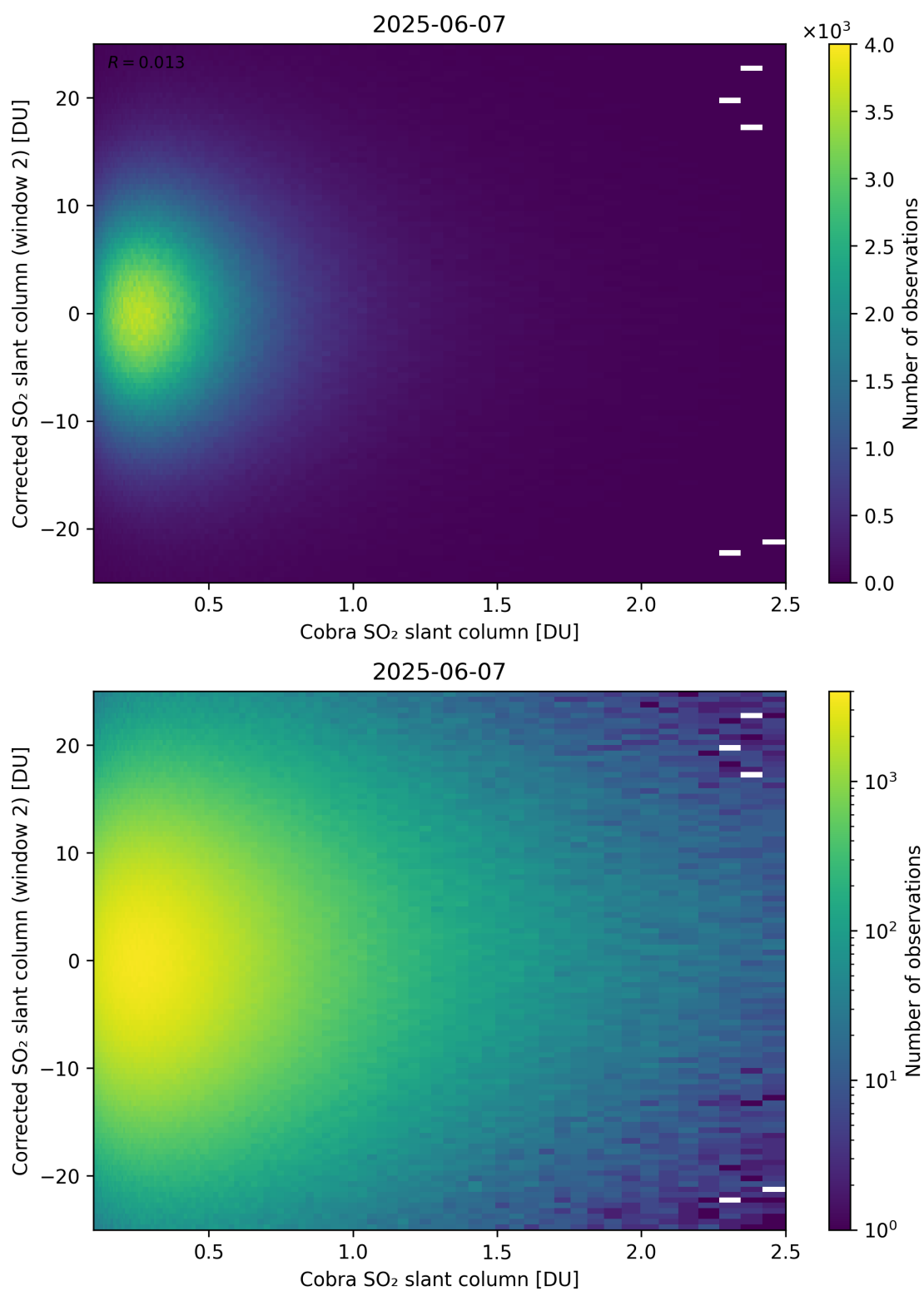
Figure 217: Scatter density plot of “Cobra SO 2 slant column” against “Corrected SO 2 slant column (window 2)” for 2025-06-06 to 2025-06-08.
