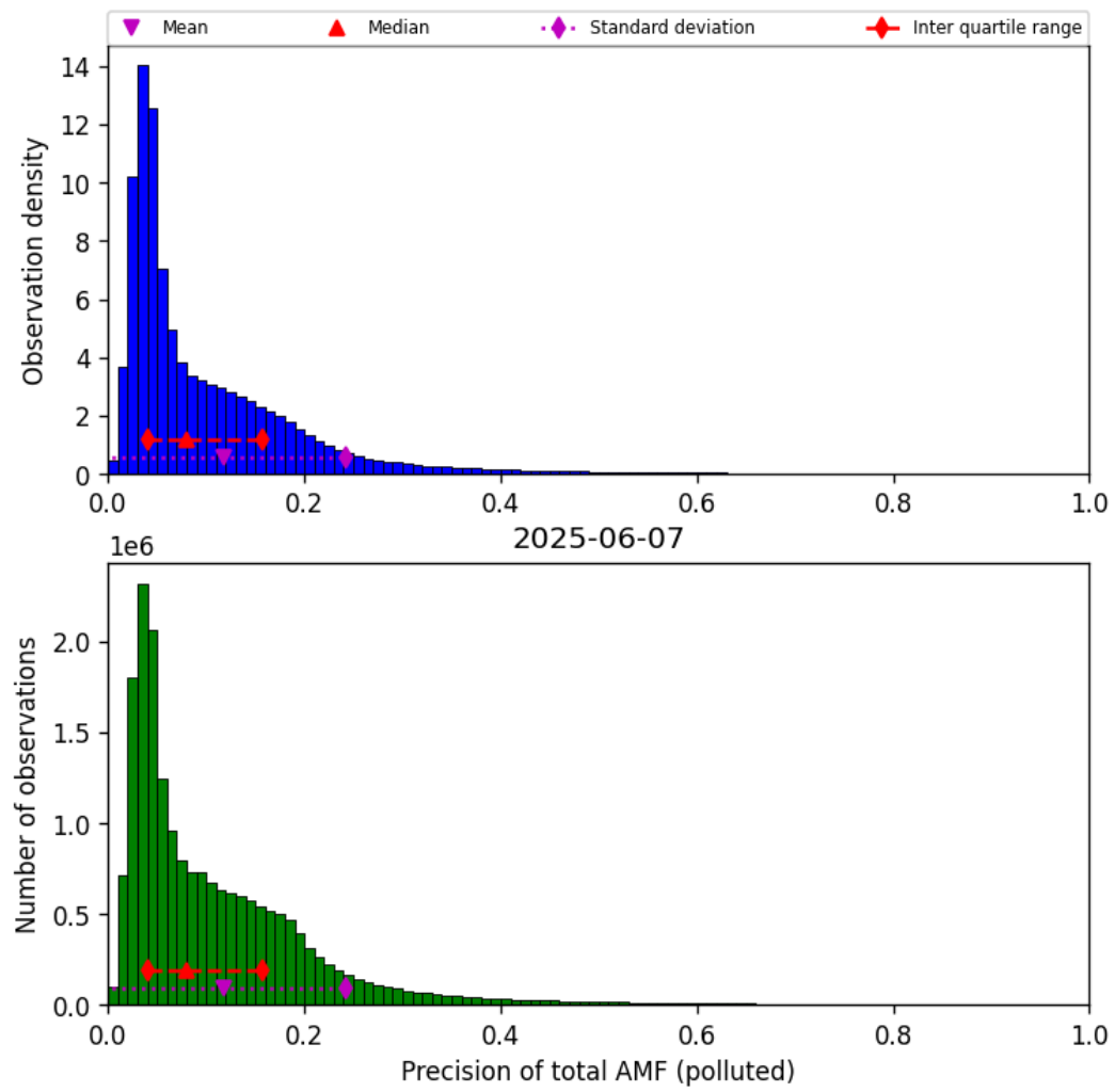
Figure 80: Histogram of “Precision of total AMF (polluted)” for 2025-06-06 to 2025-06-08
