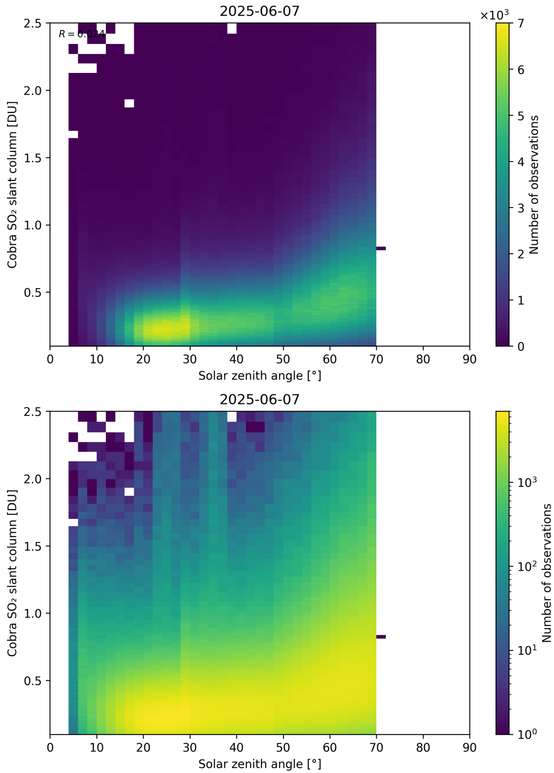
Figure 179: Scatter density plot of “Solar zenith angle” against “Cobra SO 2 slant column” for 2025-06-06 to 2025-06-08.
