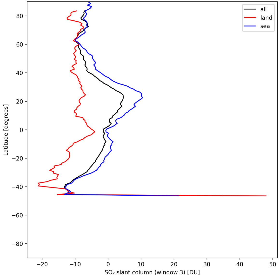
Figure 45: Zonal average of “SO 2 slant column (window 3)” for 2025-06-06 to 2025-06-08.
