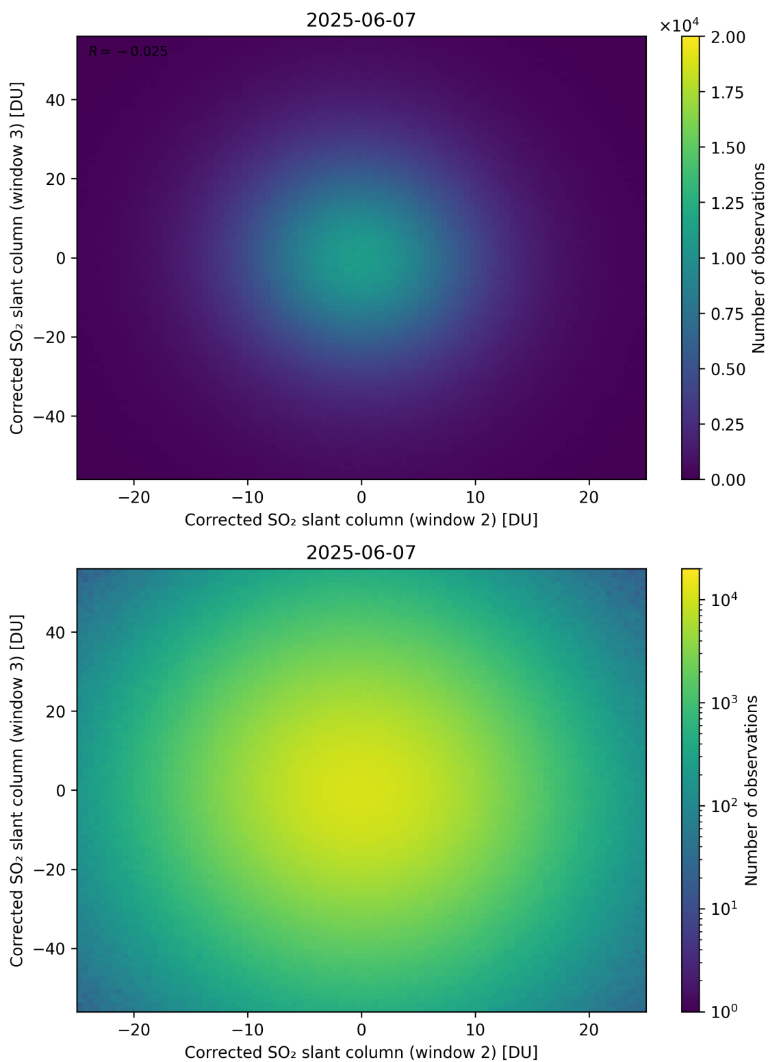
Figure 250: Scatter density plot of “Corrected SO 2 slant column (window 2)” against “Corrected SO 2 slant column (window 3)” for 2025-06-06 to 2025-06-08.
