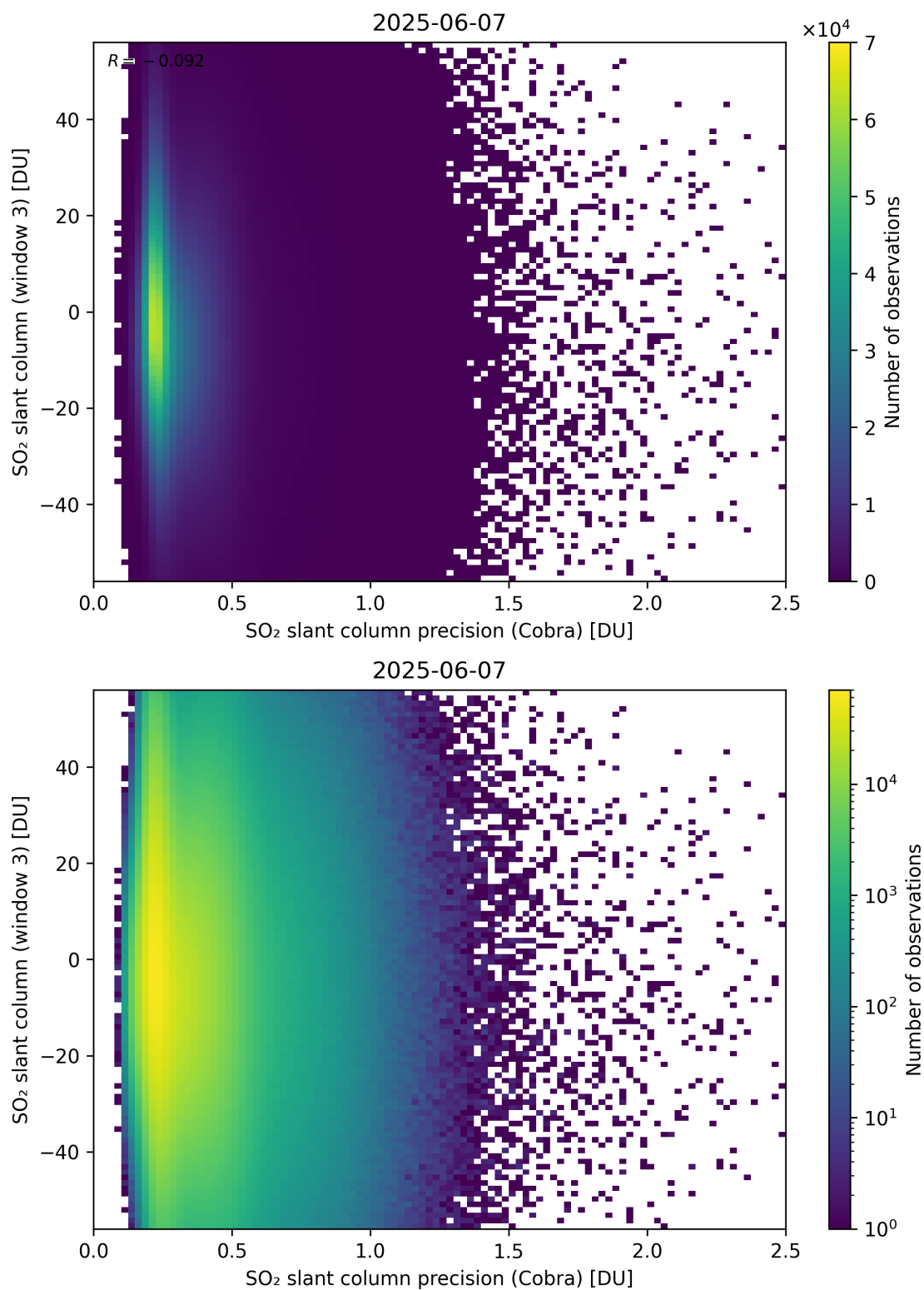
Figure 211: Scatter density plot of “SO 2 slant column precision (Cobra)” against “SO 2 slant column (window 3)” for 2025-06-06 to 2025-06-08.
