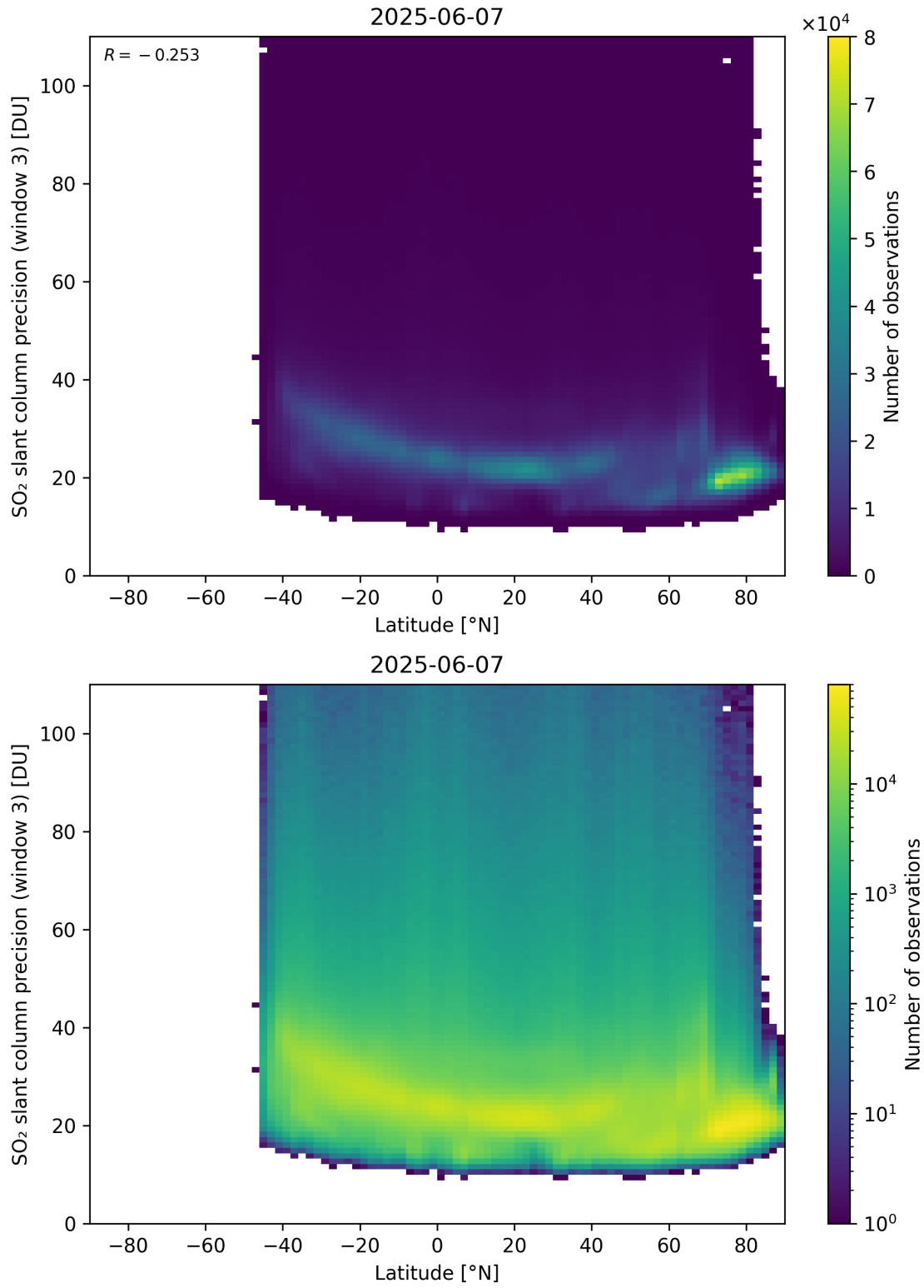
Figure 166: Scatter density plot of “Latitude” against “SO 2 slant column precision (window 3)” for 2025-06-06 to 2025-06-08.
