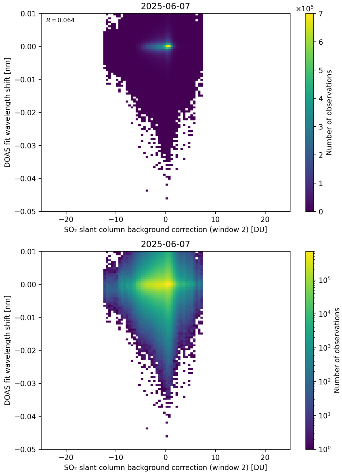
Figure 123: Scatter density plot of “SO 2 slant column background correction (window 2)” against “DOAS fit wavelength shift” for 2025-06-06 to 2025-06-08.
