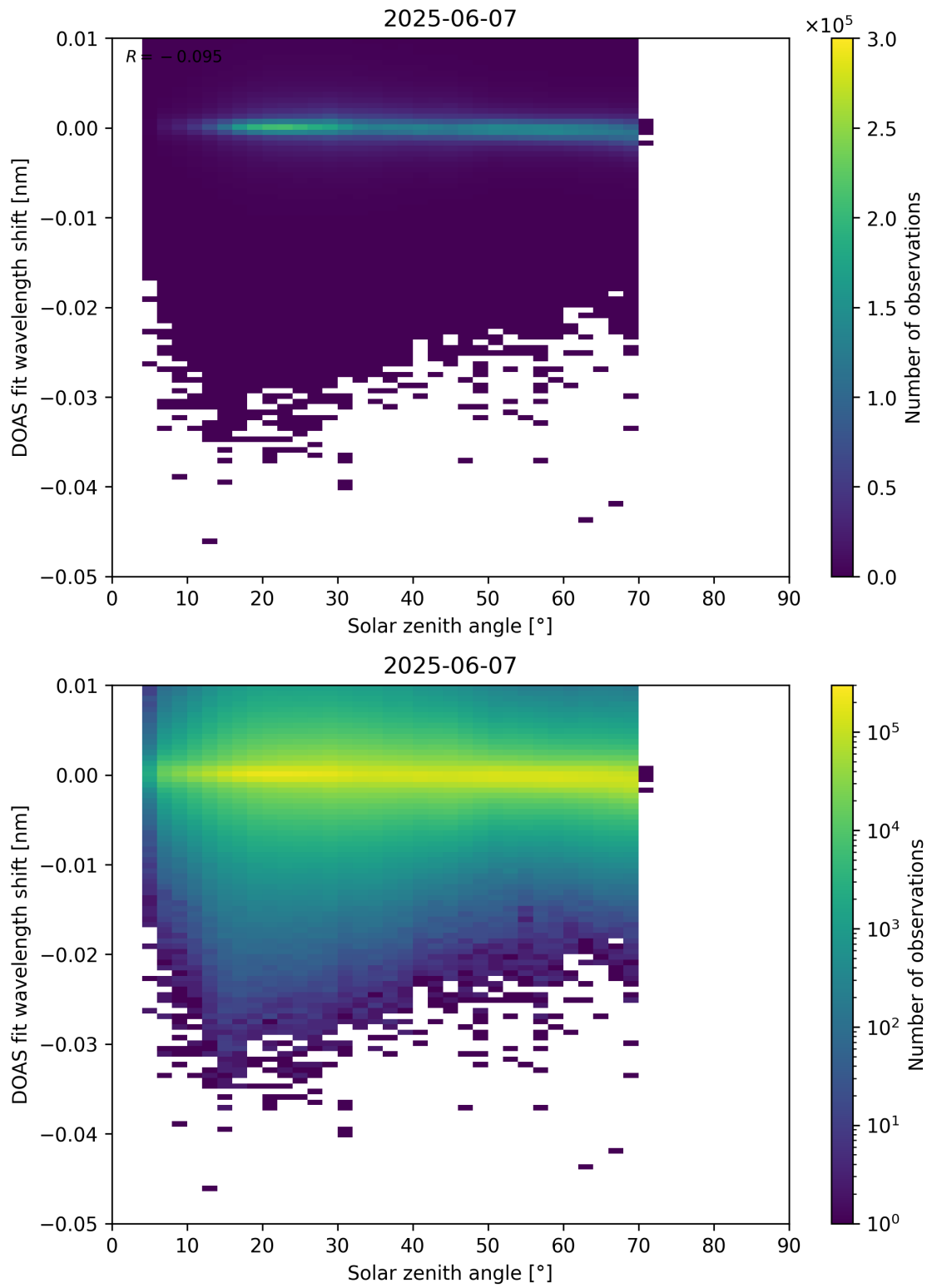
Figure 174: Scatter density plot of “Solar zenith angle” against “DOAS fit wavelength shift” for 2025-06-06 to 2025-06-08.
