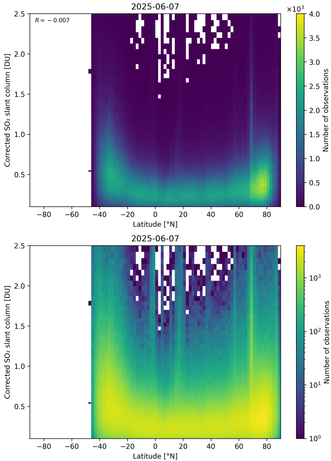
Figure 159: Scatter density plot of “Latitude” against “Corrected SO 2 slant column” for 2025-06-06 to 2025-06-08.
