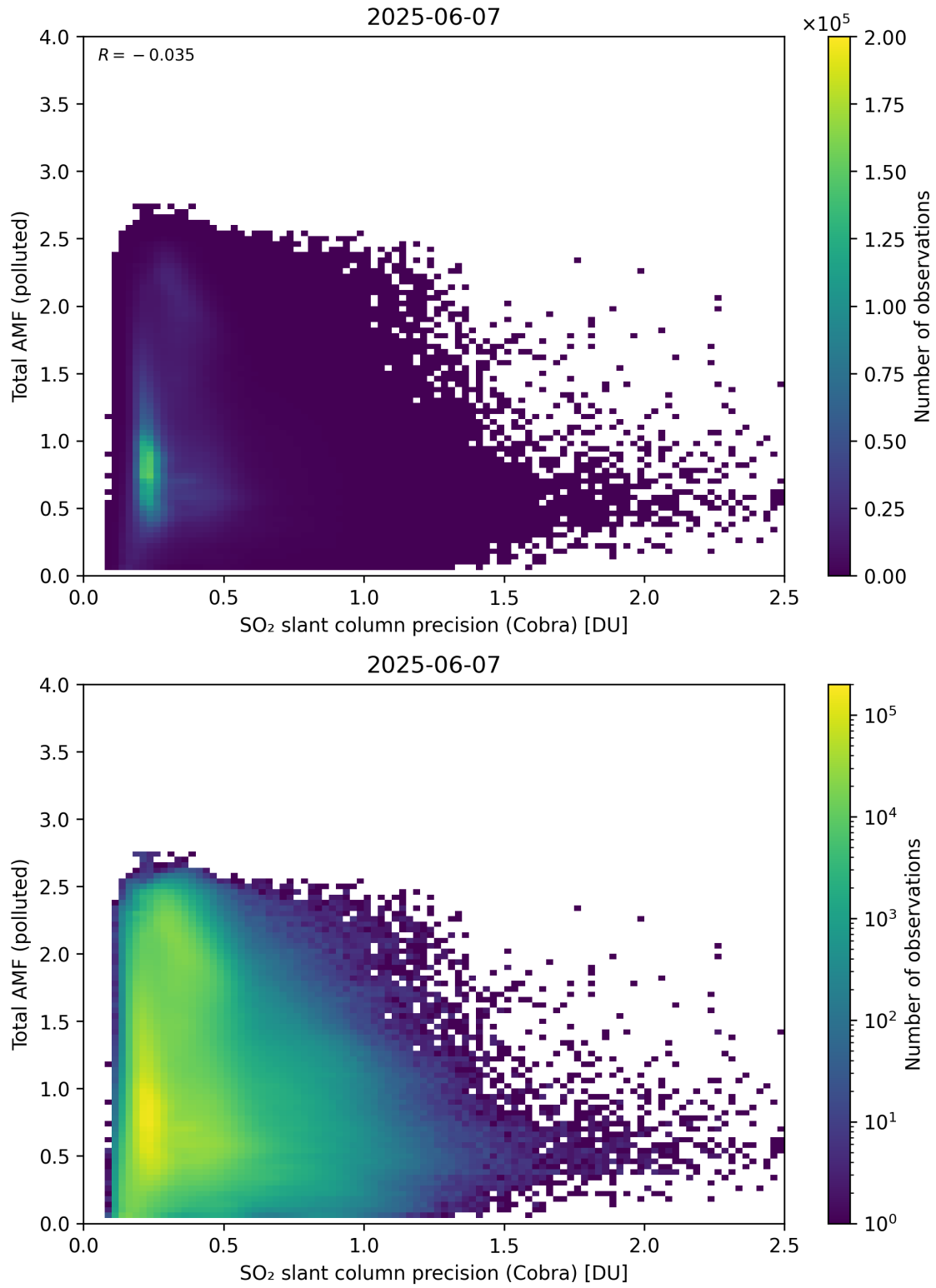
Figure 213: Scatter density plot of “SO 2 slant column precision (Cobra)” against “Total AMF (polluted)” for 2025-06-06 to 2025-06-08.
