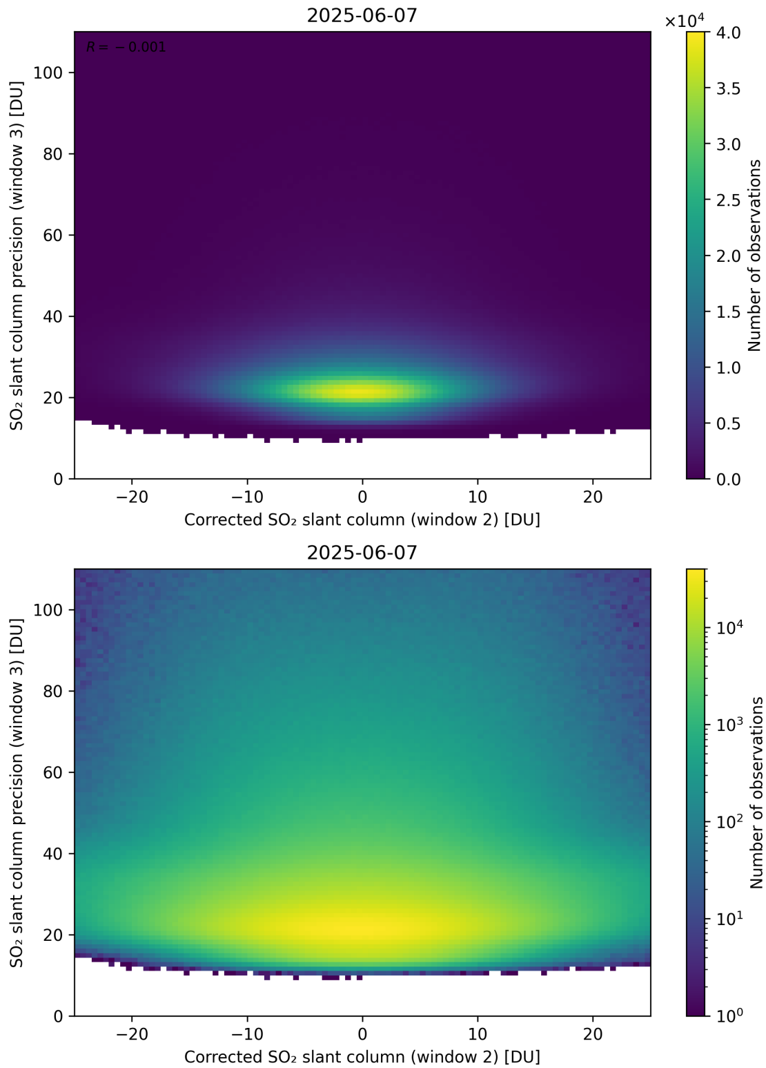
Figure 252: Scatter density plot of “Corrected SO 2 slant column (window 2)” against “SO 2 slant column precision (window 3)” for 2025-06-06 to 2025-06-08.
