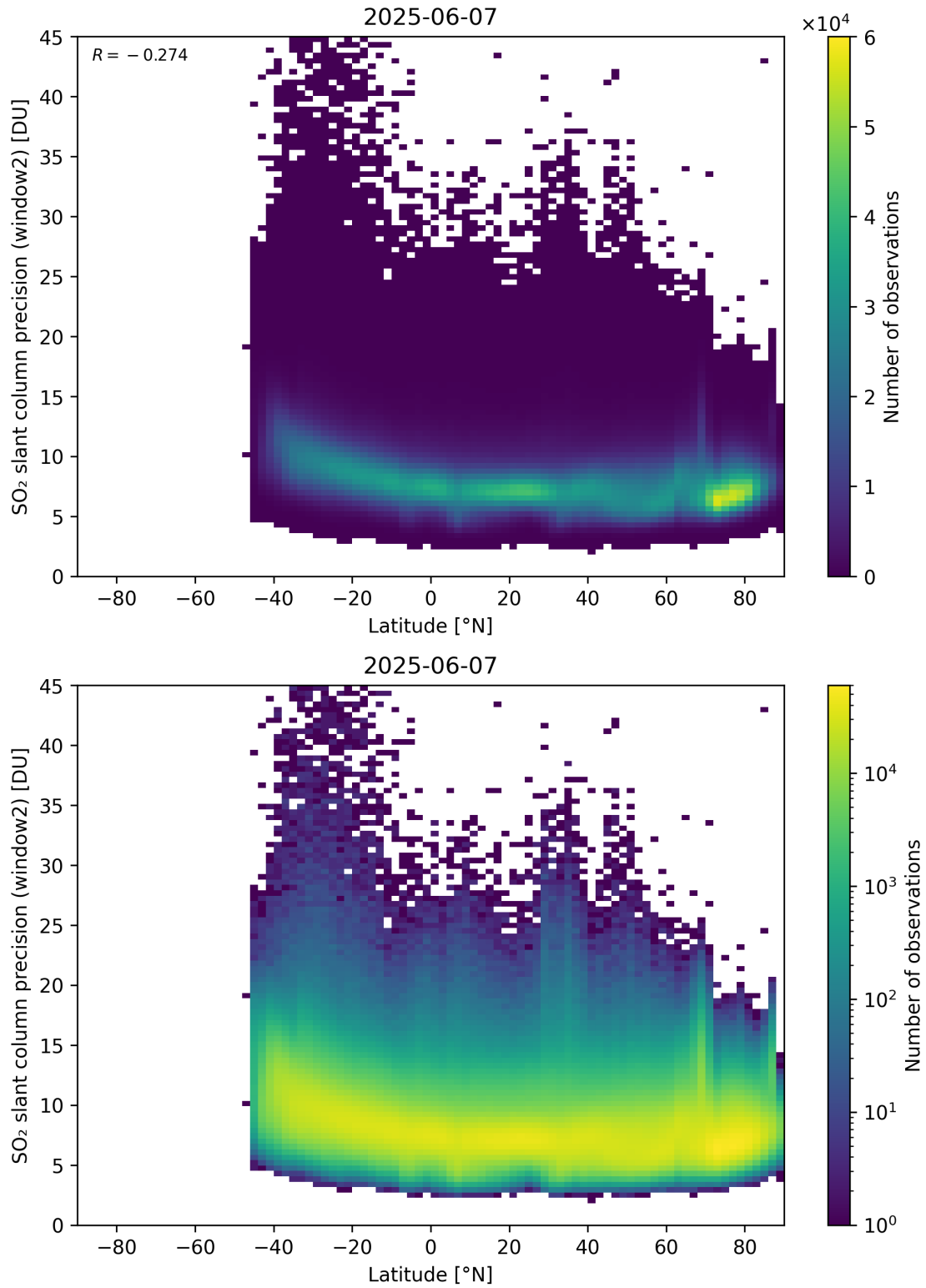
Figure 164: Scatter density plot of “Latitude” against “SO 2 slant column precision (window2)” for 2025-06-06 to 2025-06-08.
