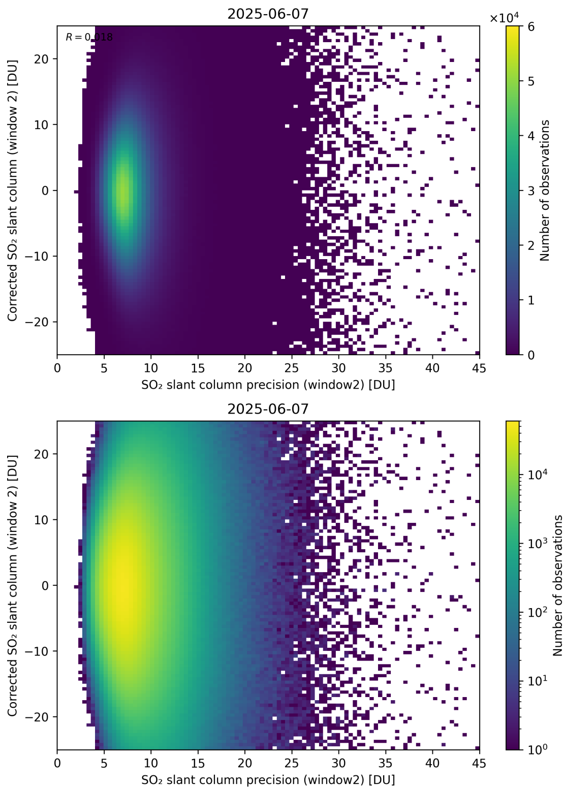
Figure 297: Scatter density plot of “SO 2 slant column precision (window2)” against “Corrected SO 2 slant column (window 2)” for 2025-06-06 to 2025-06-08.
