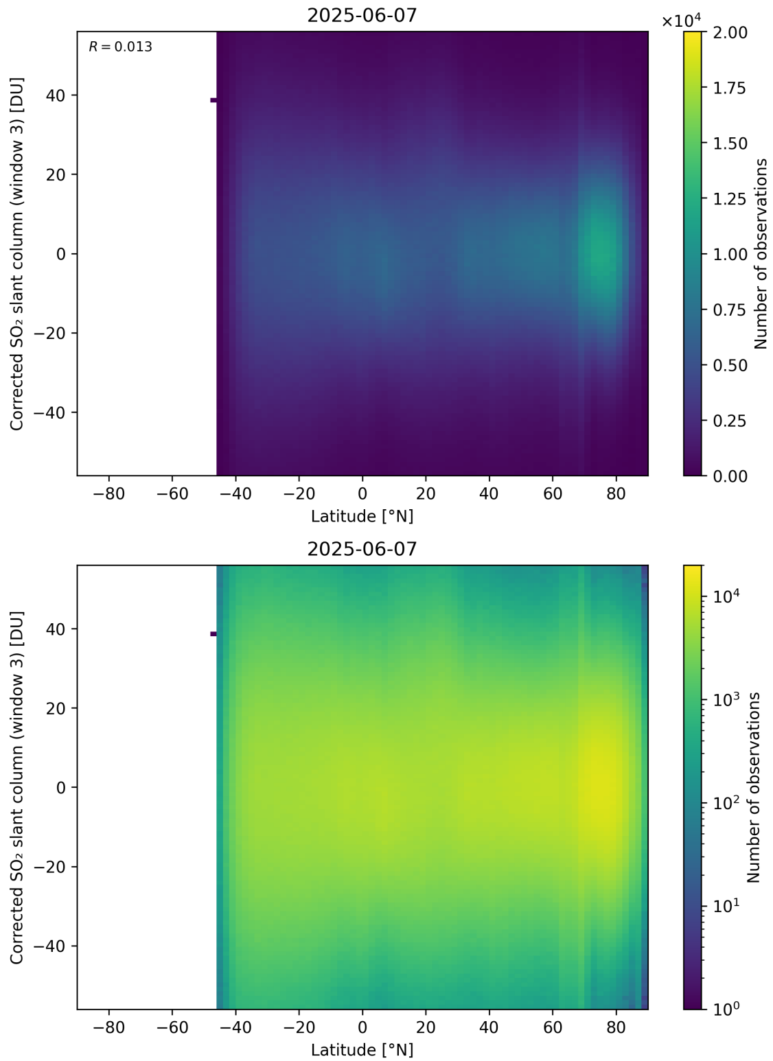
Figure 161: Scatter density plot of “Latitude” against “Corrected SO 2 slant column (window 3)” for 2025-06-06 to 2025-06-08.
