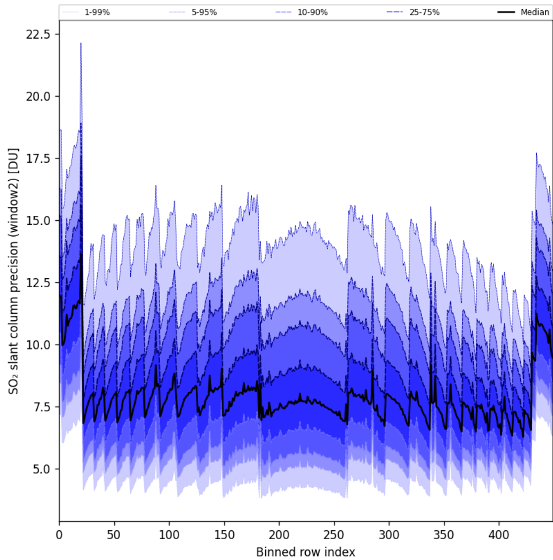
Figure 94: Along track statistics of “SO 2 slant column precision (window2)” for 2025-06-06 to 2025-06-08
