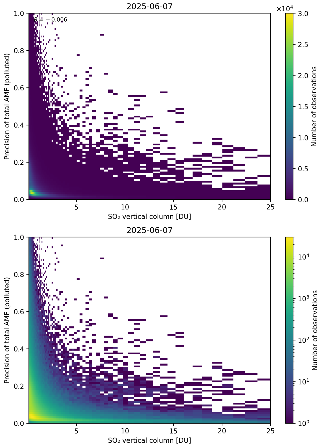
Figure 360: Scatter density plot of “SO 2 vertical column” against “Precision of total AMF (polluted)” for 2025-06-06 to 2025-06-08.
