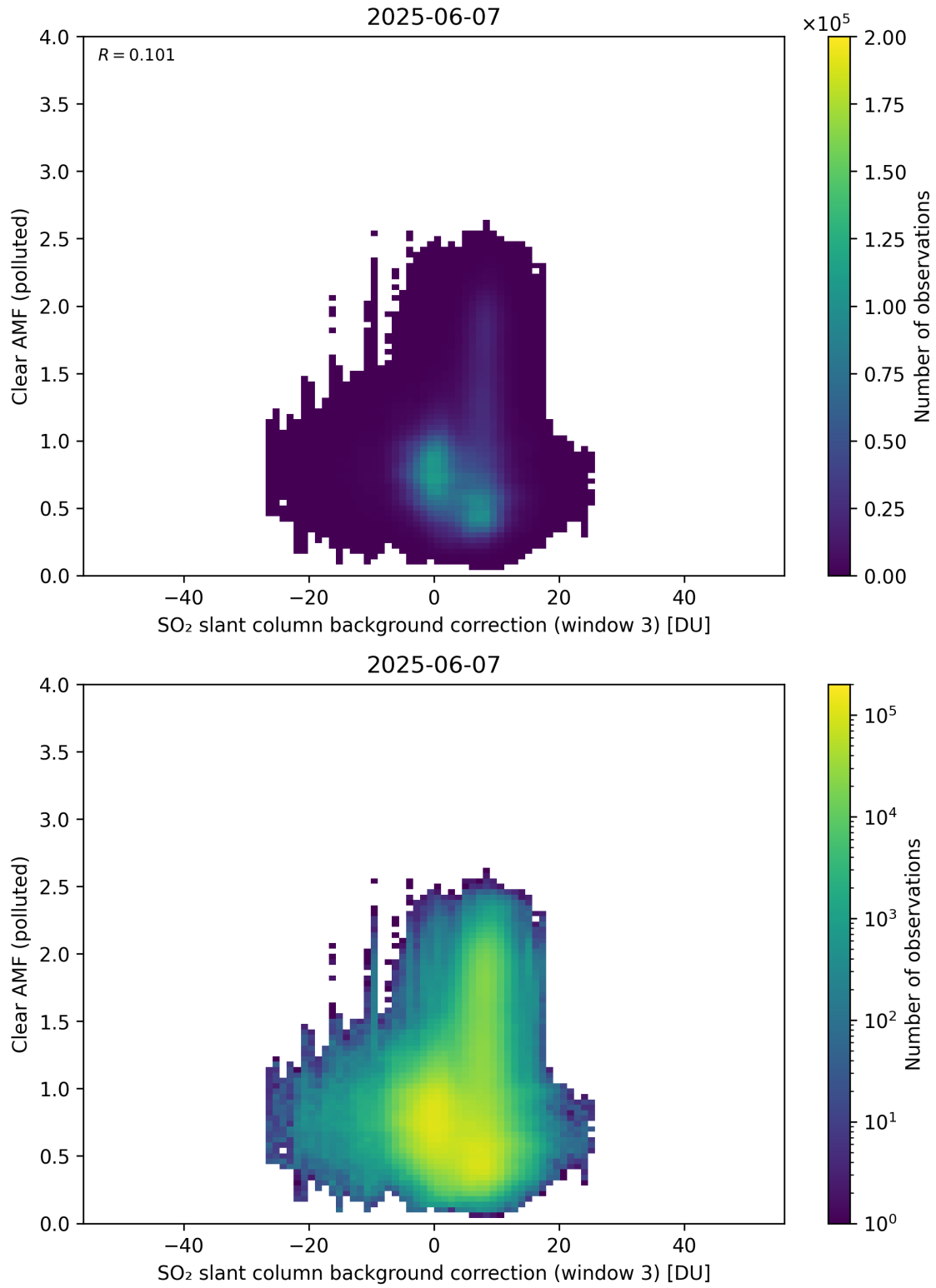
Figure 135: Scatter density plot of “SO 2 slant column background correction (window 3)” against “Clear AMF (polluted)” for 2025-06-06 to 2025-06-08.
