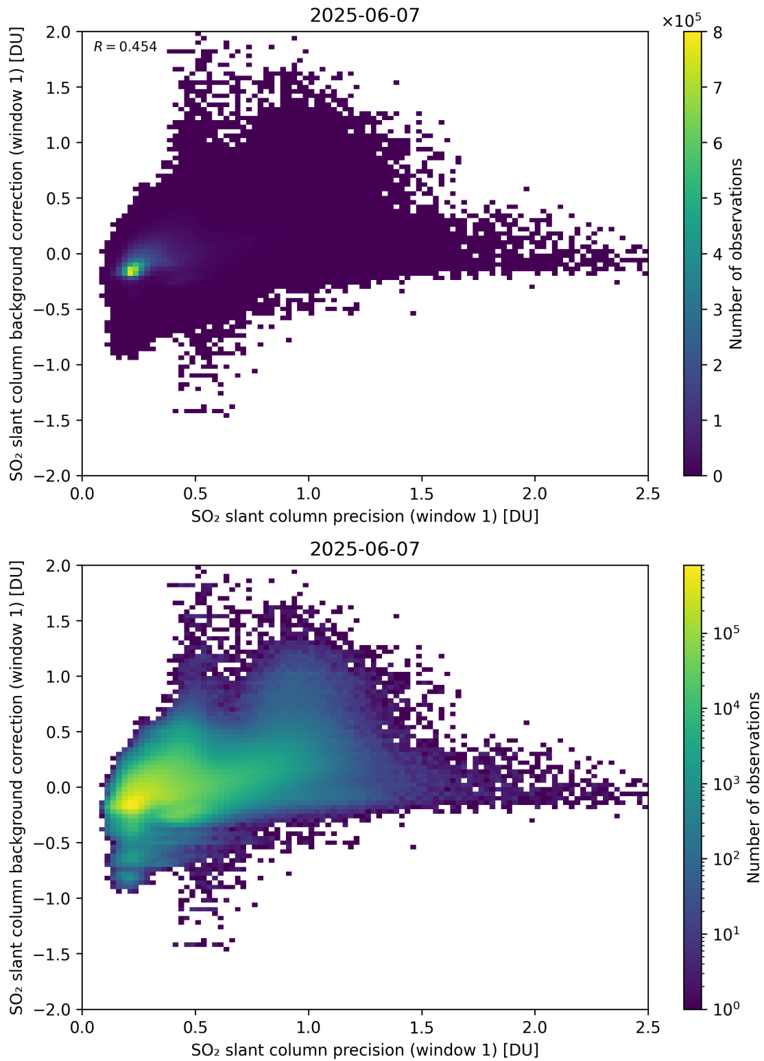
Figure 268: Scatter density plot of “SO 2 slant column precision (window 1)” against “SO 2 slant column background correction (window 1)” for 2025-06-06 to 2025-06-08.
