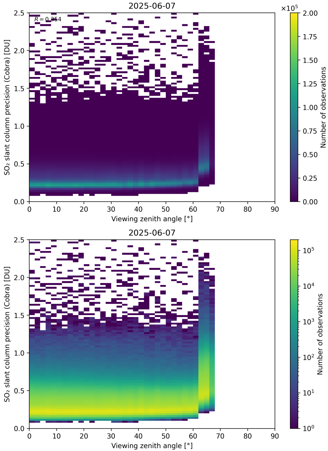
Figure 372: Scatter density plot of “Viewing zenith angle” against “SO 2 slant column precision (Cobra)” for 2025-06-06 to 2025-06-08.
