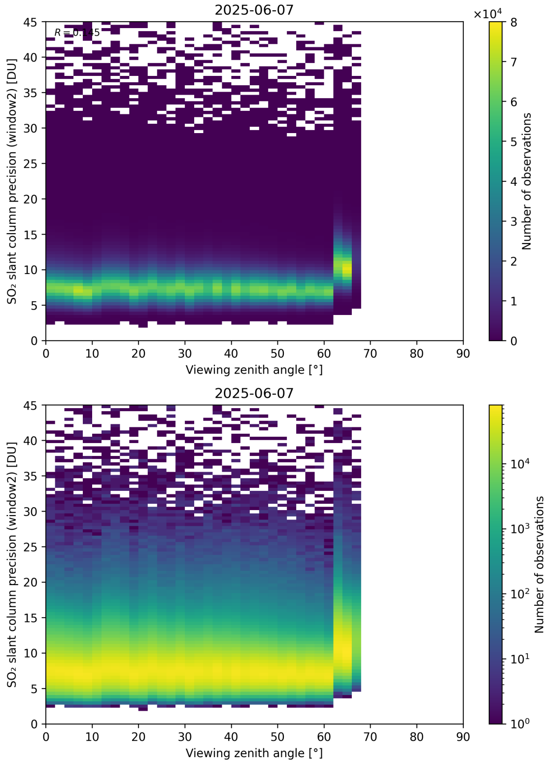
Figure 378: Scatter density plot of “Viewing zenith angle” against “SO 2 slant column precision (window2)” for 2025-06-06 to 2025-06-08.
