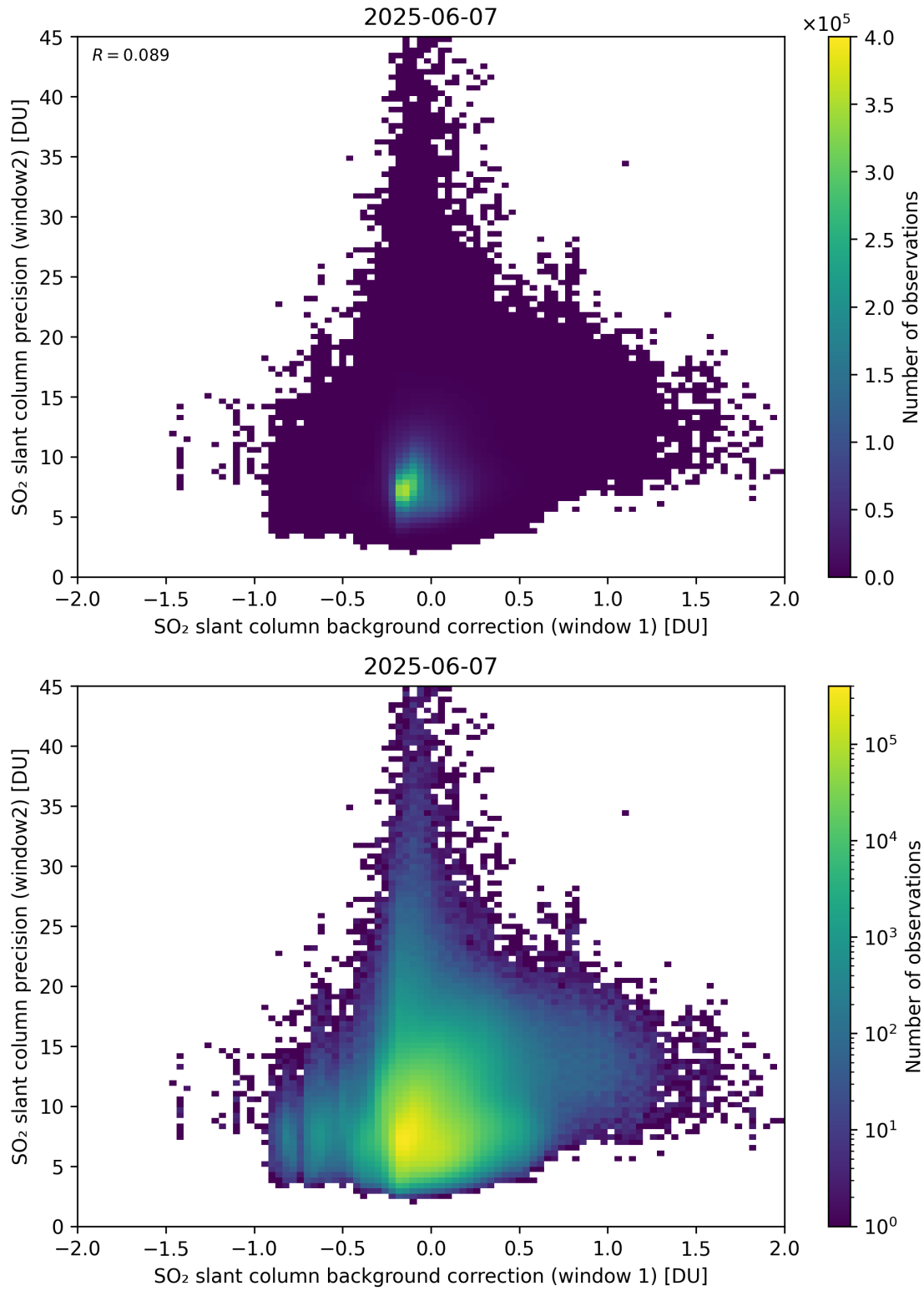
Figure 117: Scatter density plot of “SO 2 slant column background correction (window 1)” against “SO 2 slant column precision (window2)” for 2025-06-06 to 2025-06-08.
