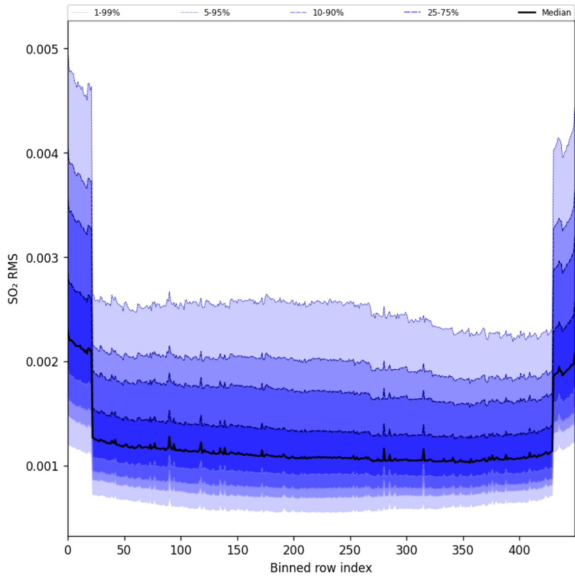
Figure 104: Along track statistics of “SO 2 RMS” for 2025-06-06 to 2025-06-08
