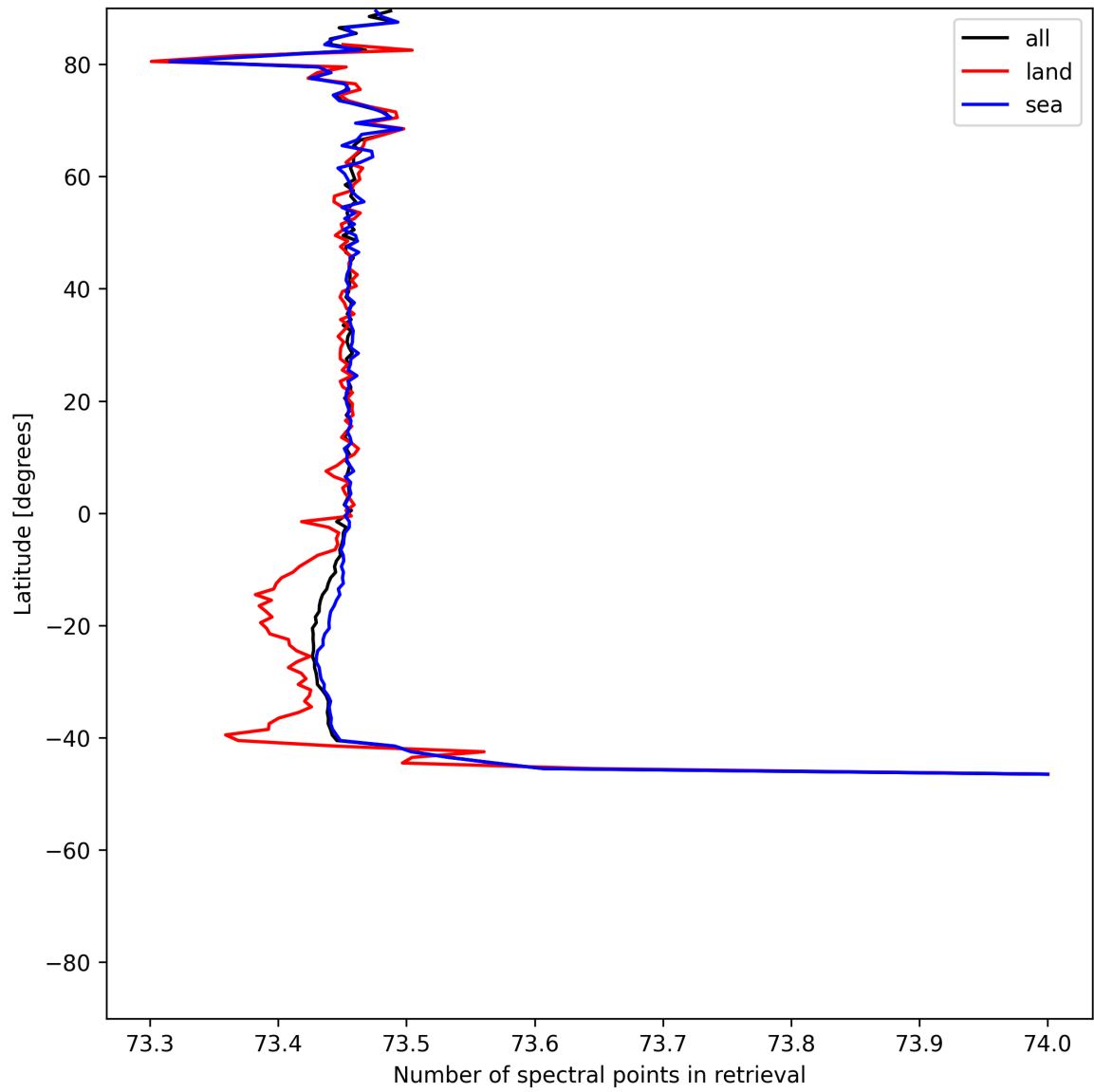
Figure 56: Zonal average of “Number of spectral points in retrieval” for 2025-06-06 to 2025-06-08.
