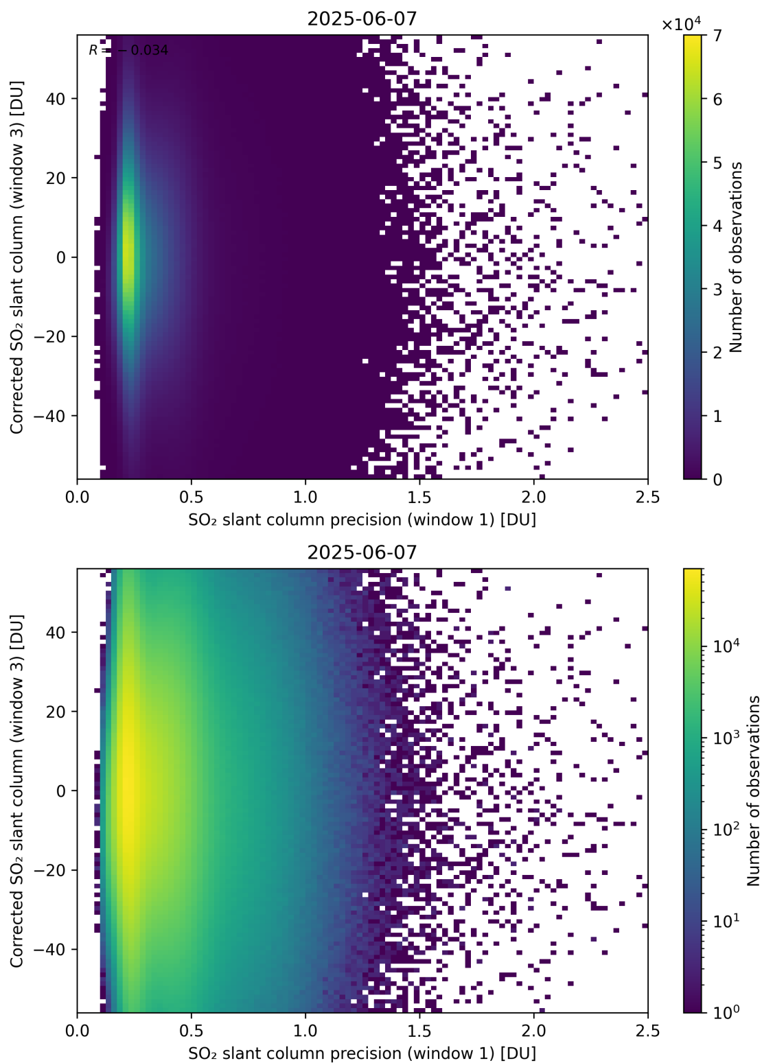
Figure 276: Scatter density plot of “SO 2 slant column precision (window 1)” against “Corrected SO 2 slant column (window 3)” for 2025-06-06 to 2025-06-08.
