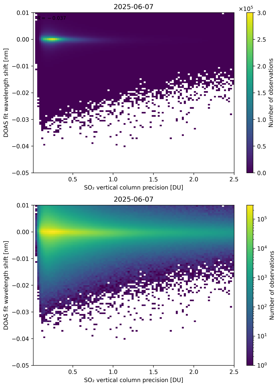
Figure 332: Scatter density plot of “SO 2 vertical column precision” against “DOAS fit wavelength shift” for 2025-06-06 to 2025-06-08.
