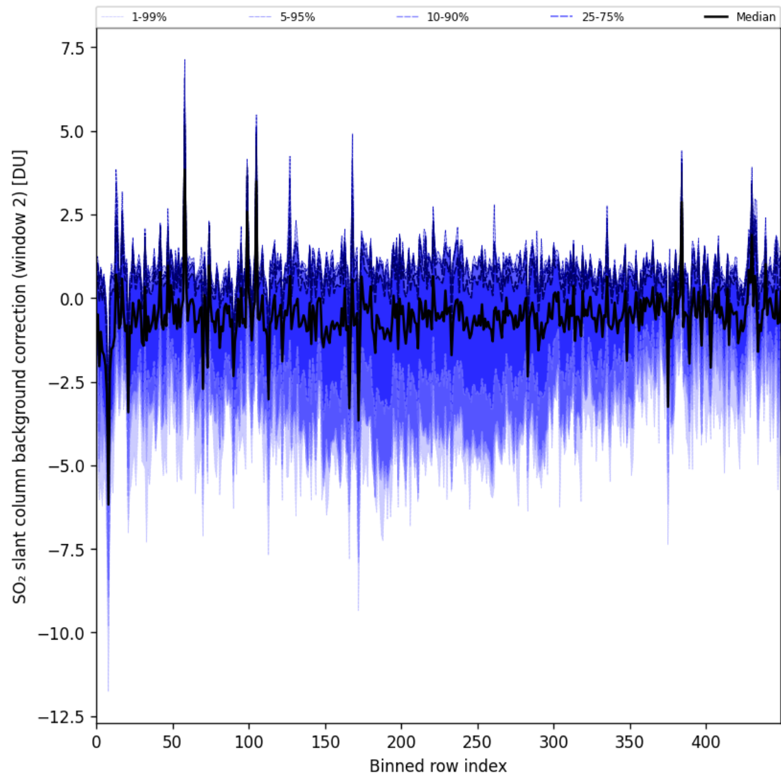
Figure 96: Along track statistics of “SO 2 slant column background correction (window 2)” for 2025-06-06 to 2025-06-08
