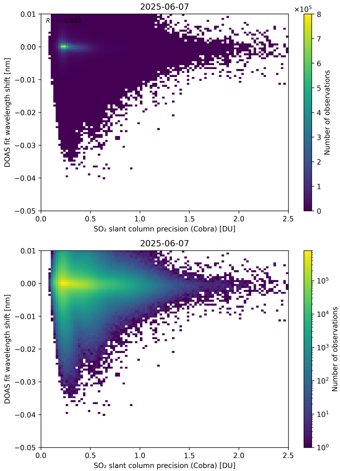
Figure 202: Scatter density plot of “SO 2 slant column precision (Cobra)” against “DOAS fit wavelength shift” for 2025-06-06 to 2025-06-08.
