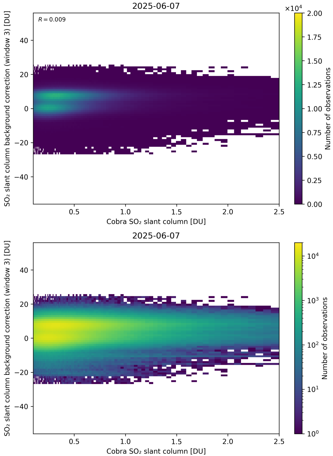
Figure 195: Scatter density plot of “Cobra SO 2 slant column” against “SO 2 slant column background correction (window 3)” for 2025-06-06 to 2025-06-08.
