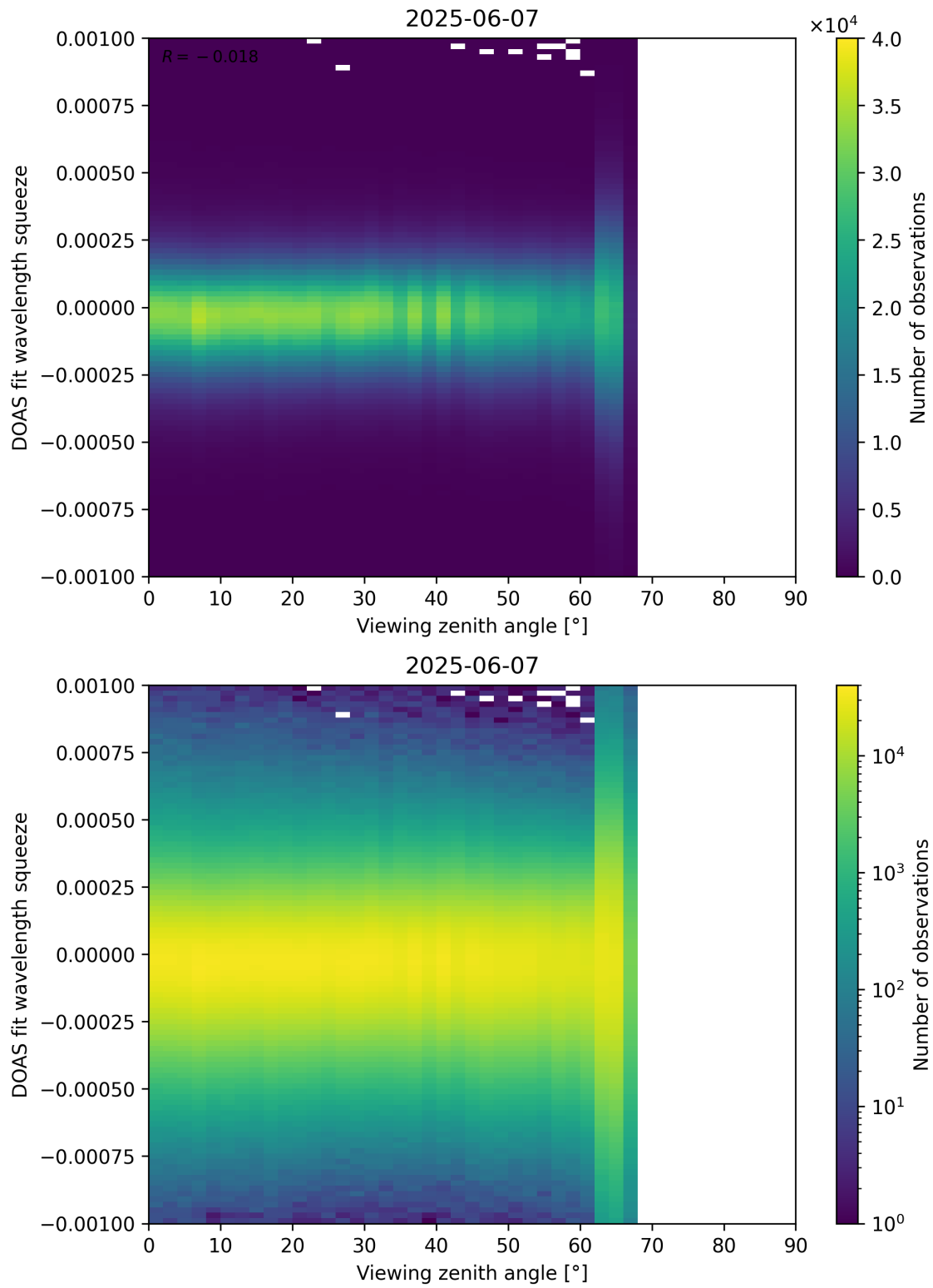
Figure 366: Scatter density plot of “Viewing zenith angle” against “DOAS fit wavelength squeeze” for 2025-06-06 to 2025-06-08.
