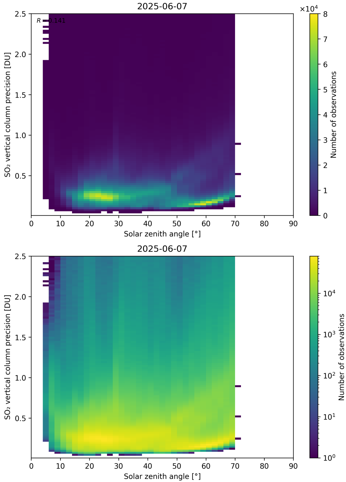
Figure 192: Scatter density plot of “Solar zenith angle” against “SO 2 vertical column precision” for 2025-06-06 to 2025-06-08.
