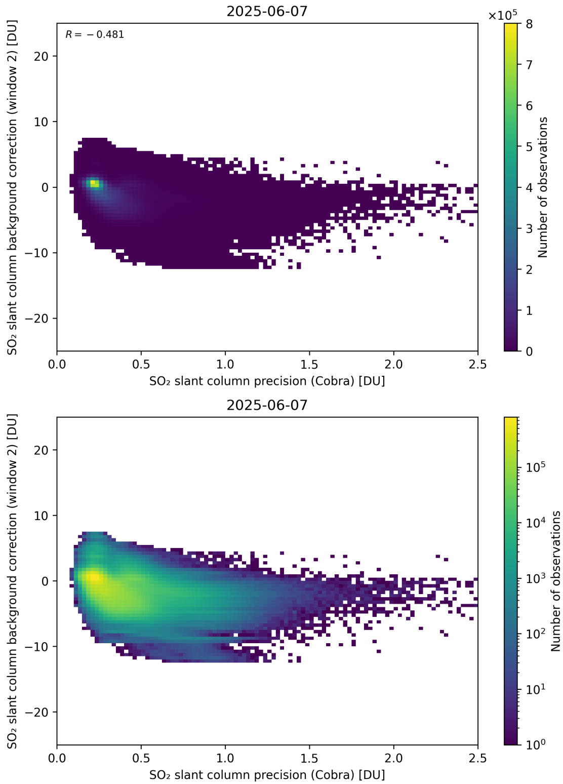
Figure 200: Scatter density plot of “SO 2 slant column precision (Cobra)” against “SO 2 slant column background correction (window 2)” for 2025-06-06 to 2025-06-08.
