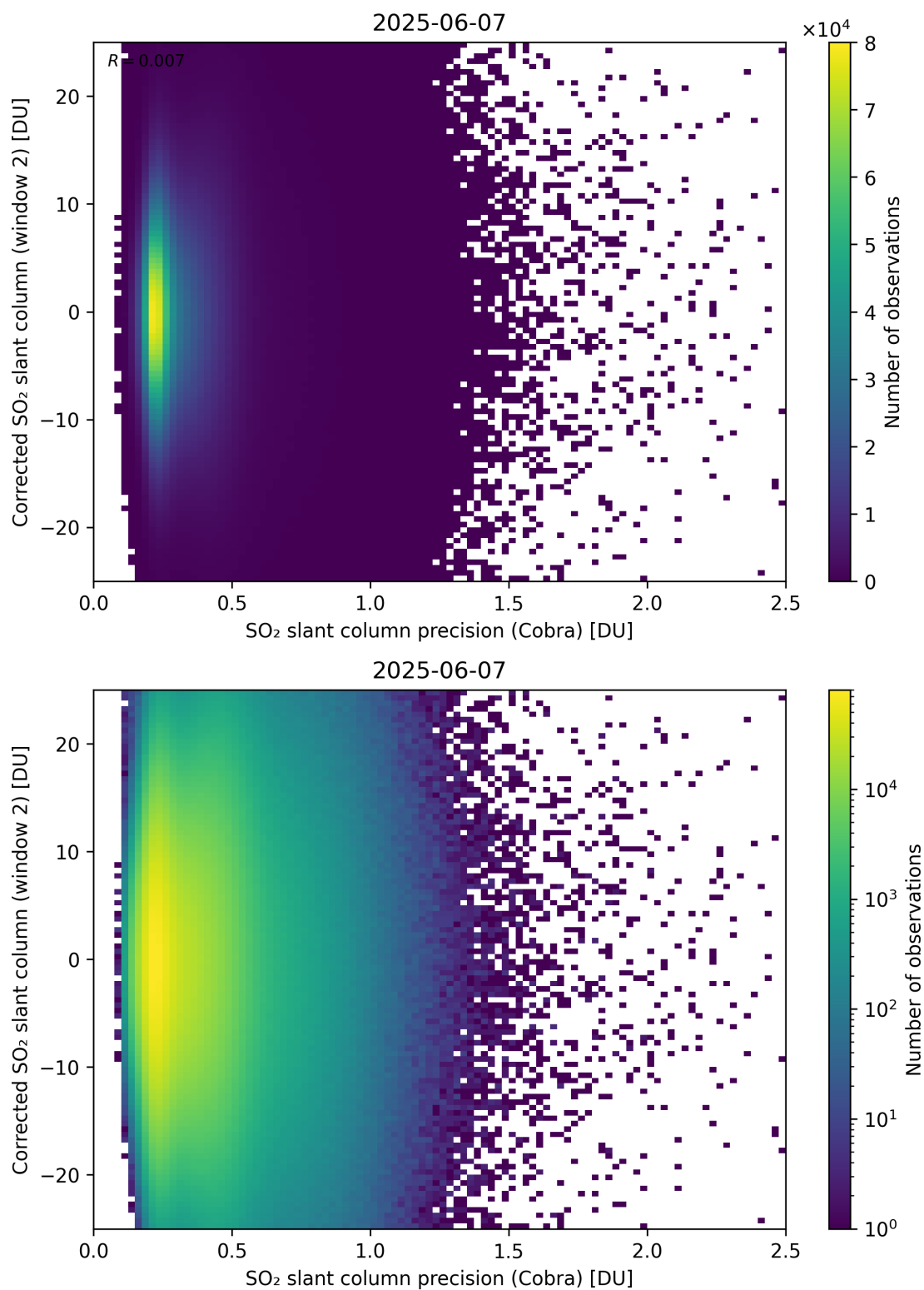
Figure 206: Scatter density plot of “SO 2 slant column precision (Cobra)” against “Corrected SO 2 slant column (window 2)” for 2025-06-06 to 2025-06-08.
