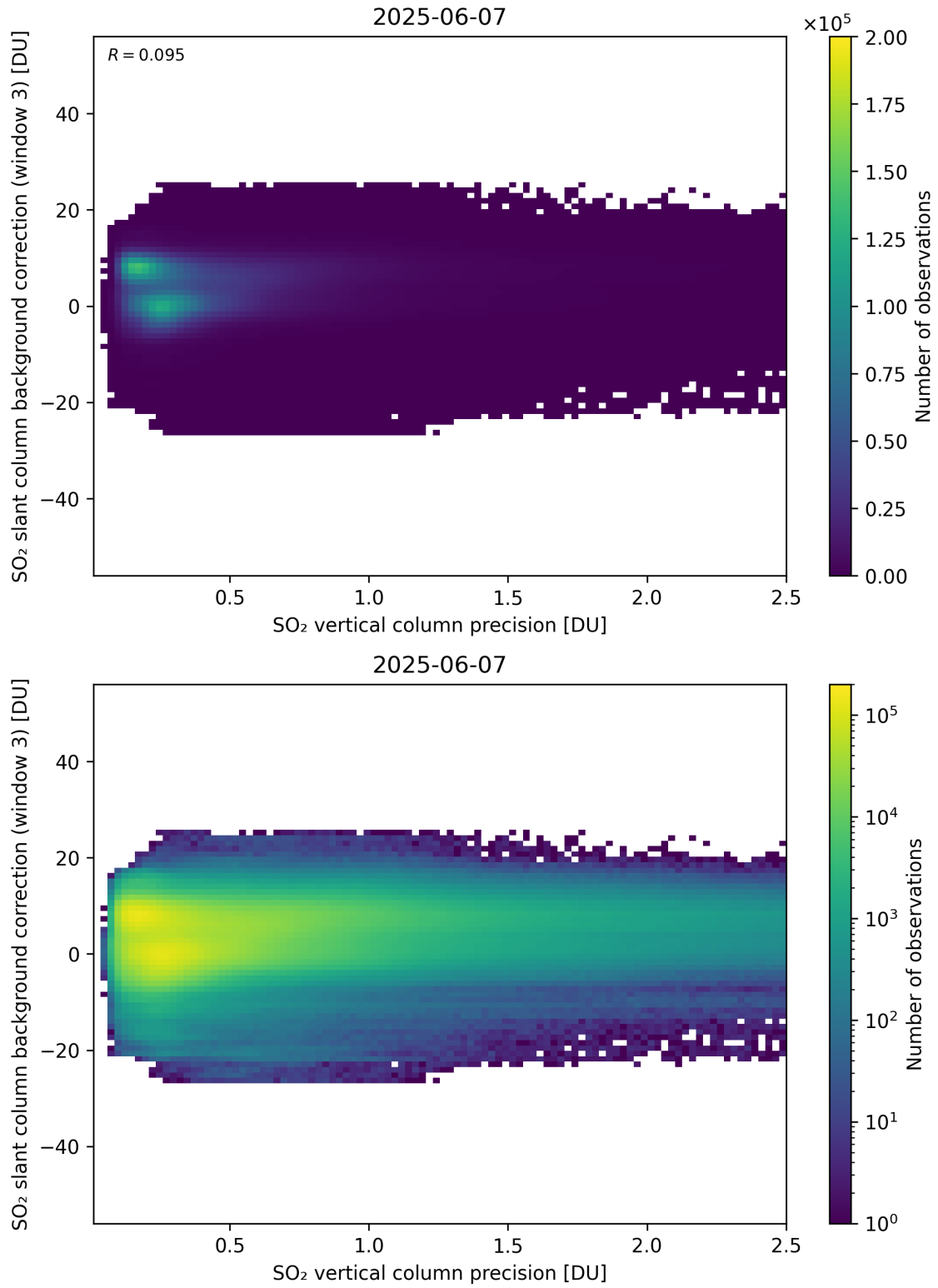
Figure 331: Scatter density plot of “SO 2 vertical column precision” against “SO 2 slant column background correction (window 3)” for 2025-06-06 to 2025-06-08.
