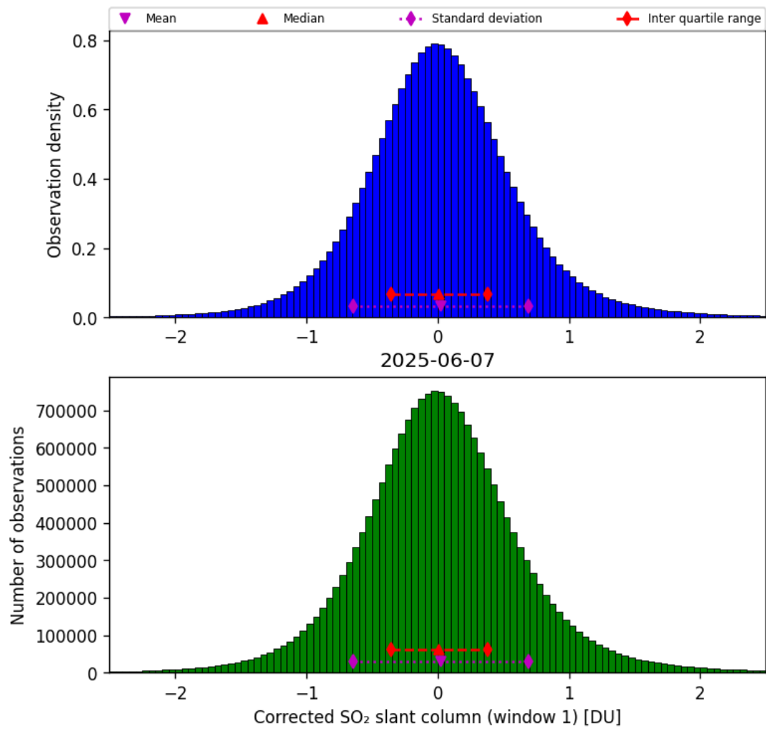
Figure 65: Histogram of “Corrected SO 2 slant column (window 1)” for 2025-06-06 to 2025-06-08
