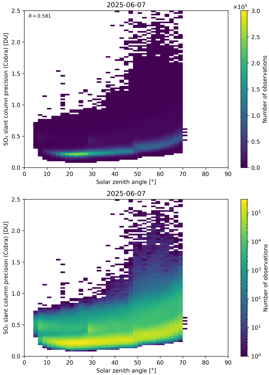
Figure 180: Scatter density plot of “Solar zenith angle” against “SO 2 slant column precision (Cobra)” for 2025-06-06 to 2025-06-08.
