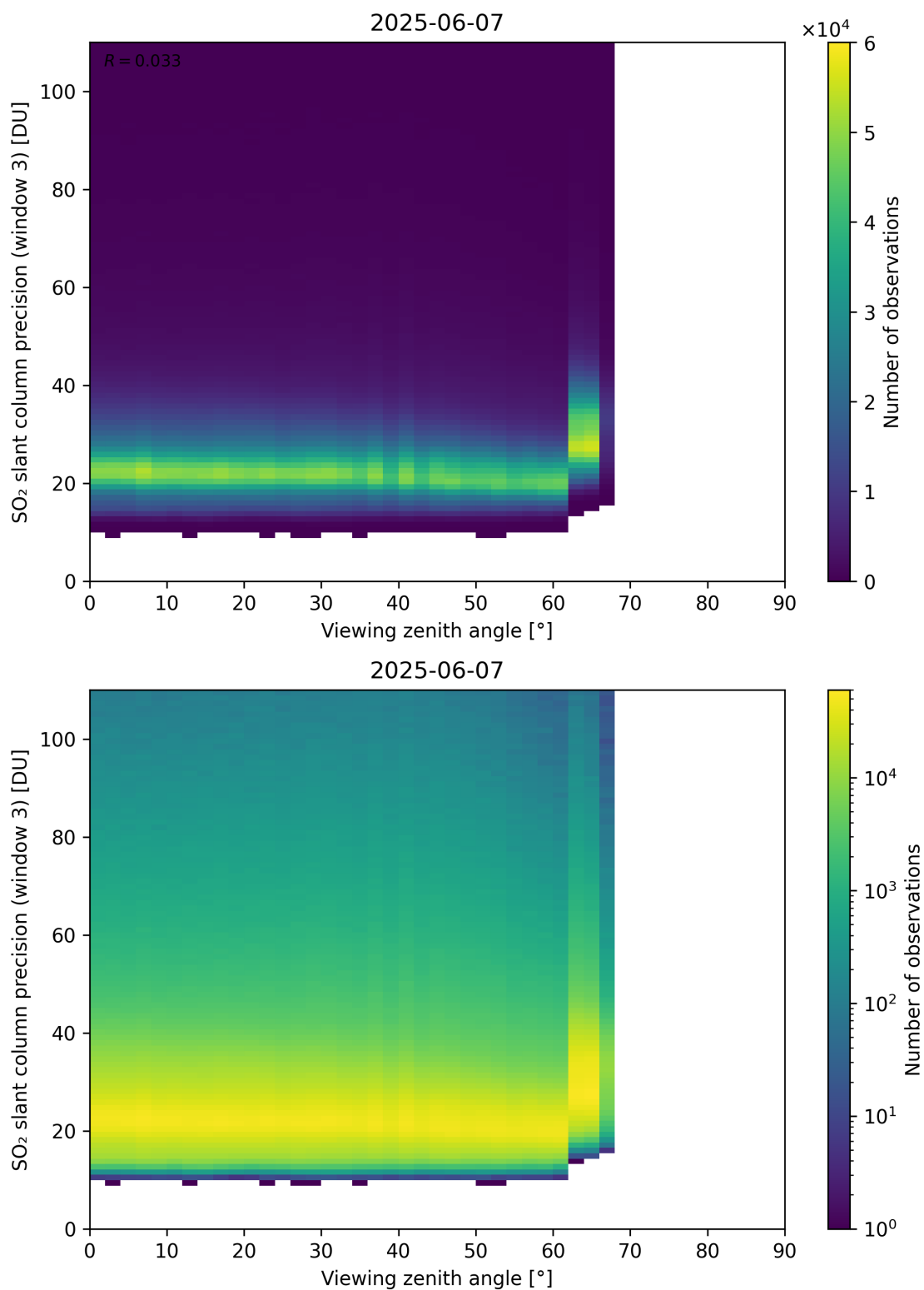
Figure 380: Scatter density plot of “Viewing zenith angle” against “SO 2 slant column precision (window 3)” for 2025-06-06 to 2025-06-08.
