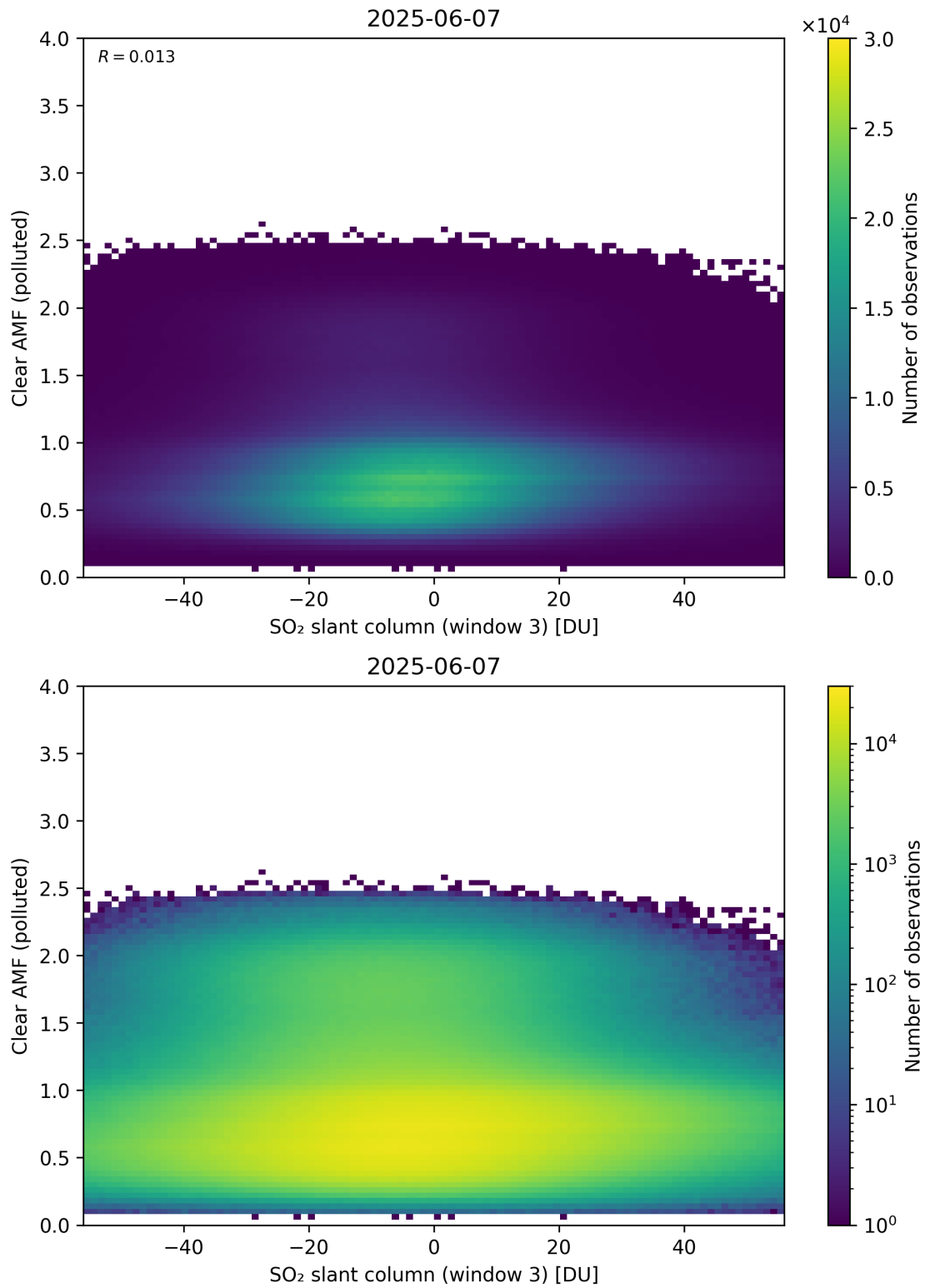
Figure 315: Scatter density plot of “SO 2 slant column (window 3)” against “Clear AMF (polluted)” for 2025-06-06 to 2025-06-08.
