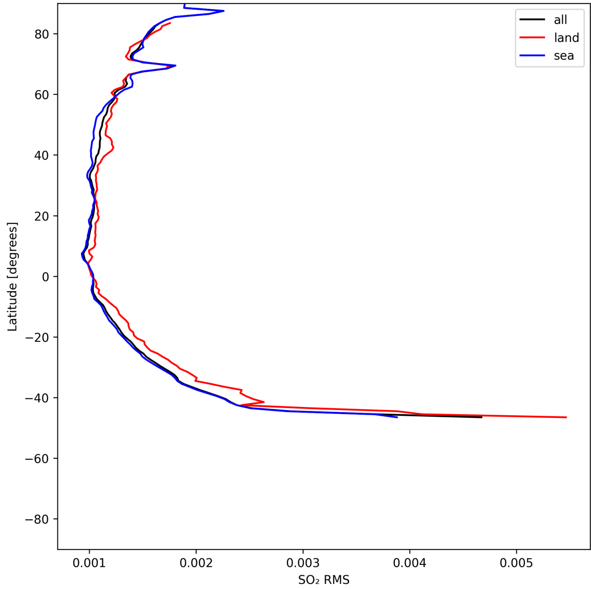
Figure 52: Zonal average of “SO 2 RMS” for 2025-06-06 to 2025-06-08.
