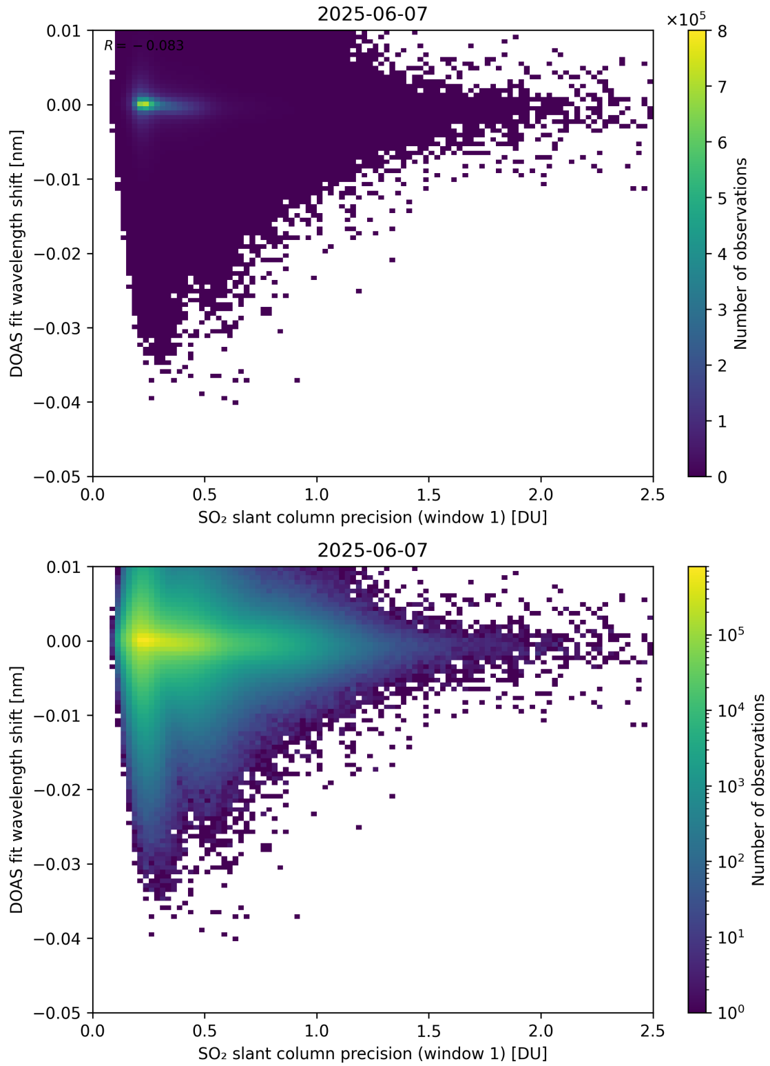
Figure 271: Scatter density plot of “SO 2 slant column precision (window 1)” against “DOAS fit wavelength shift” for 2025-06-06 to 2025-06-08.
