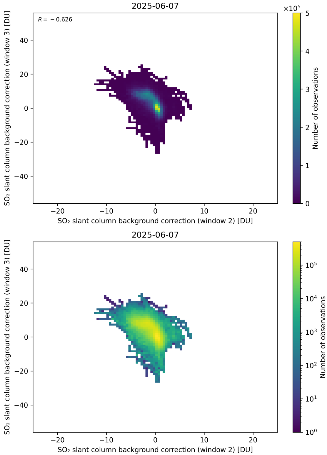
Figure 122: Scatter density plot of “SO 2 slant column background correction (window 2)” against “SO 2 slant column background correction (window 3)” for 2025-06-06 to 2025-06-08.
