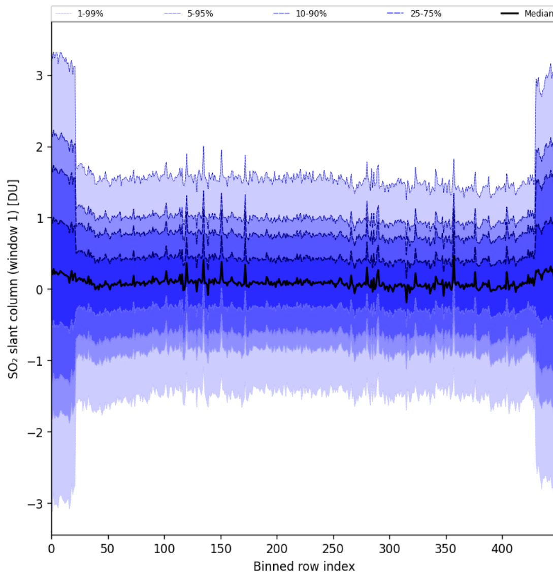
Figure 89: Along track statistics of “SO 2 slant column (window 1)” for 2025-06-06 to 2025-06-08
