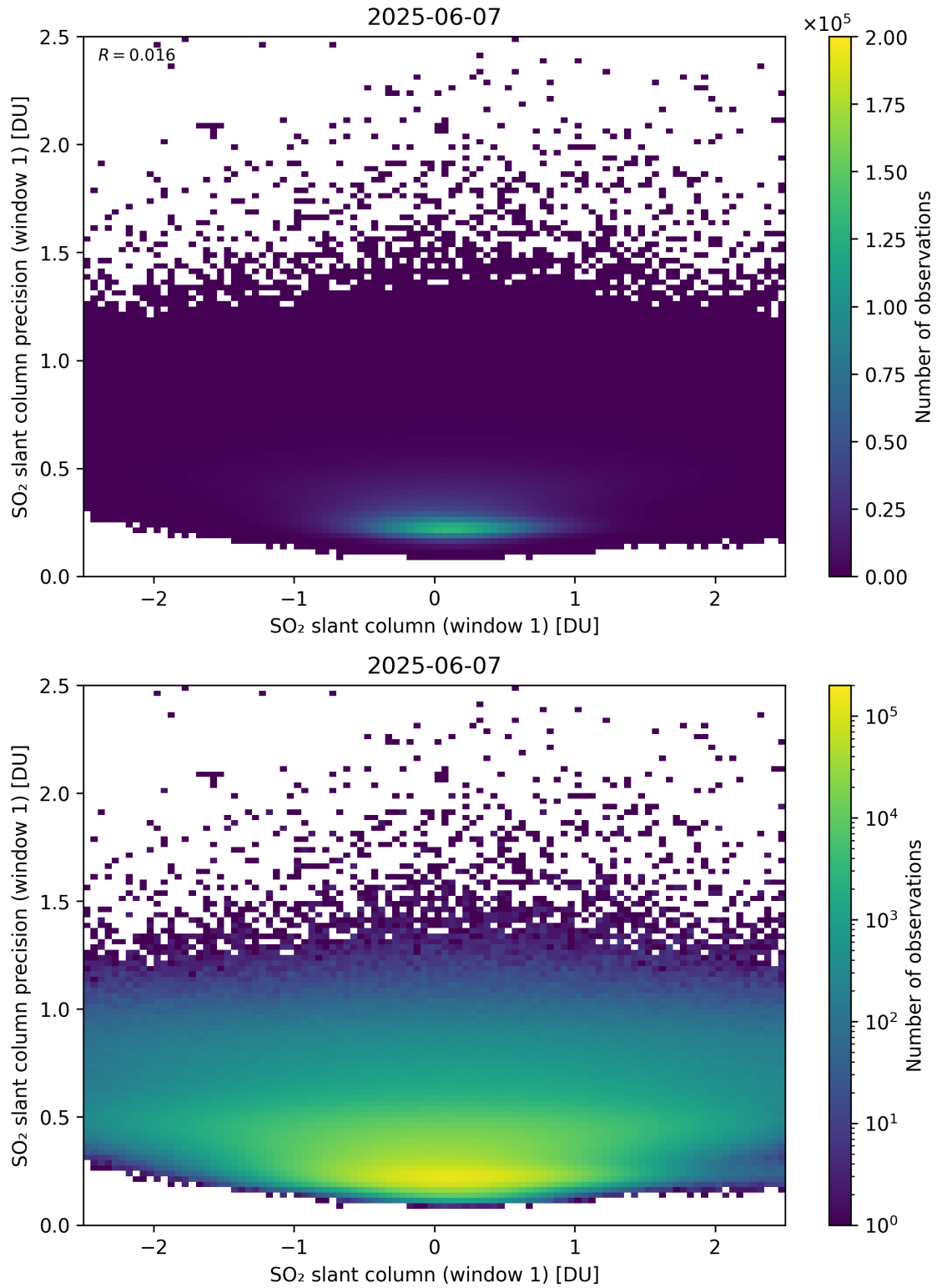
Figure 285: Scatter density plot of “SO 2 slant column (window 1)” against “SO 2 slant column precision (window 1)” for 2025-06-06 to 2025-06-08.
