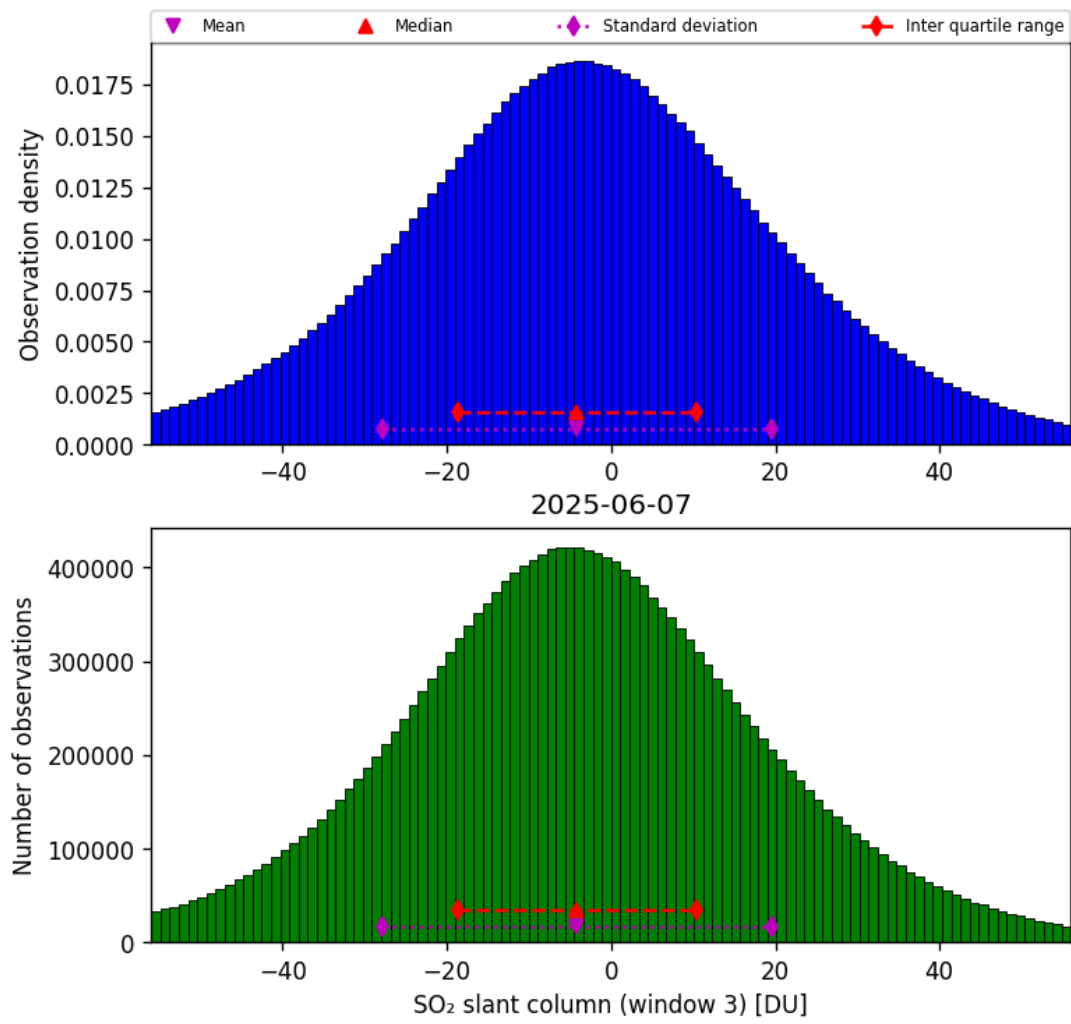
Figure 71: Histogram of “SO 2 slant column (window 3)” for 2025-06-06 to 2025-06-08
