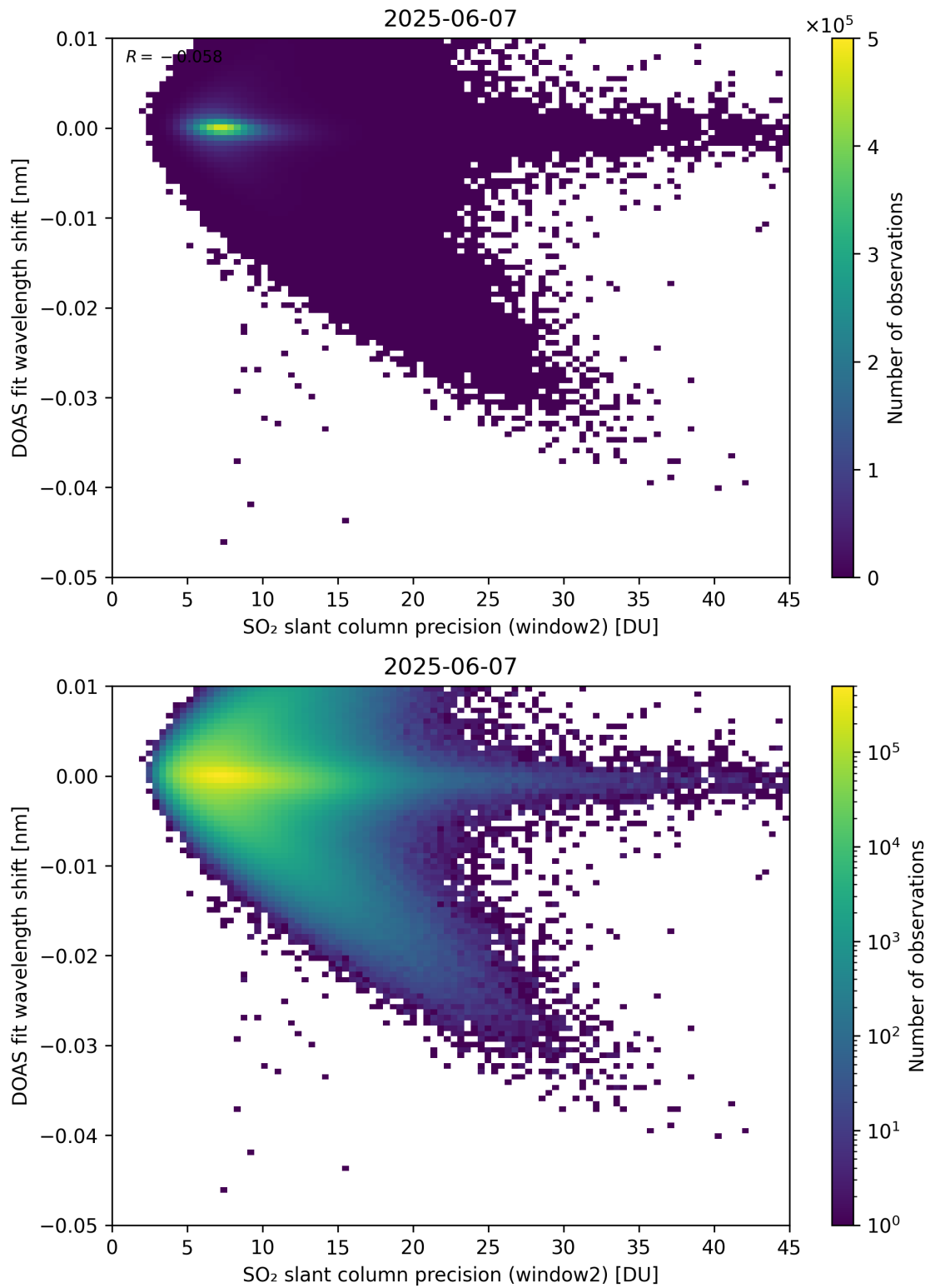
Figure 293: Scatter density plot of “SO 2 slant column precision (window2)” against “DOAS fit wavelength shift” for 2025-06-06 to 2025-06-08.
