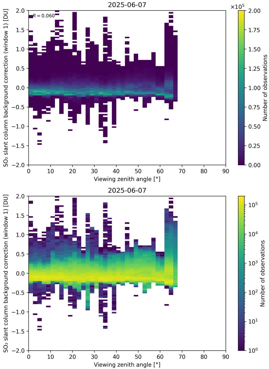
Figure 362: Scatter density plot of “Viewing zenith angle” against “SO 2 slant column background correction (window 1)” for 2025-06-06 to 2025-06-08.
