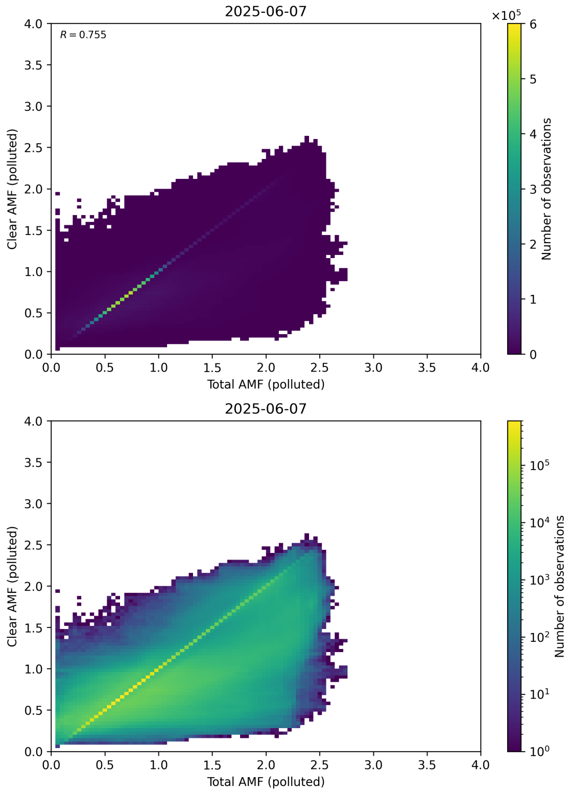
Figure 321: Scatter density plot of “Total AMF (polluted)” against “Clear AMF (polluted)” for 2025-06-06 to 2025-06-08.
