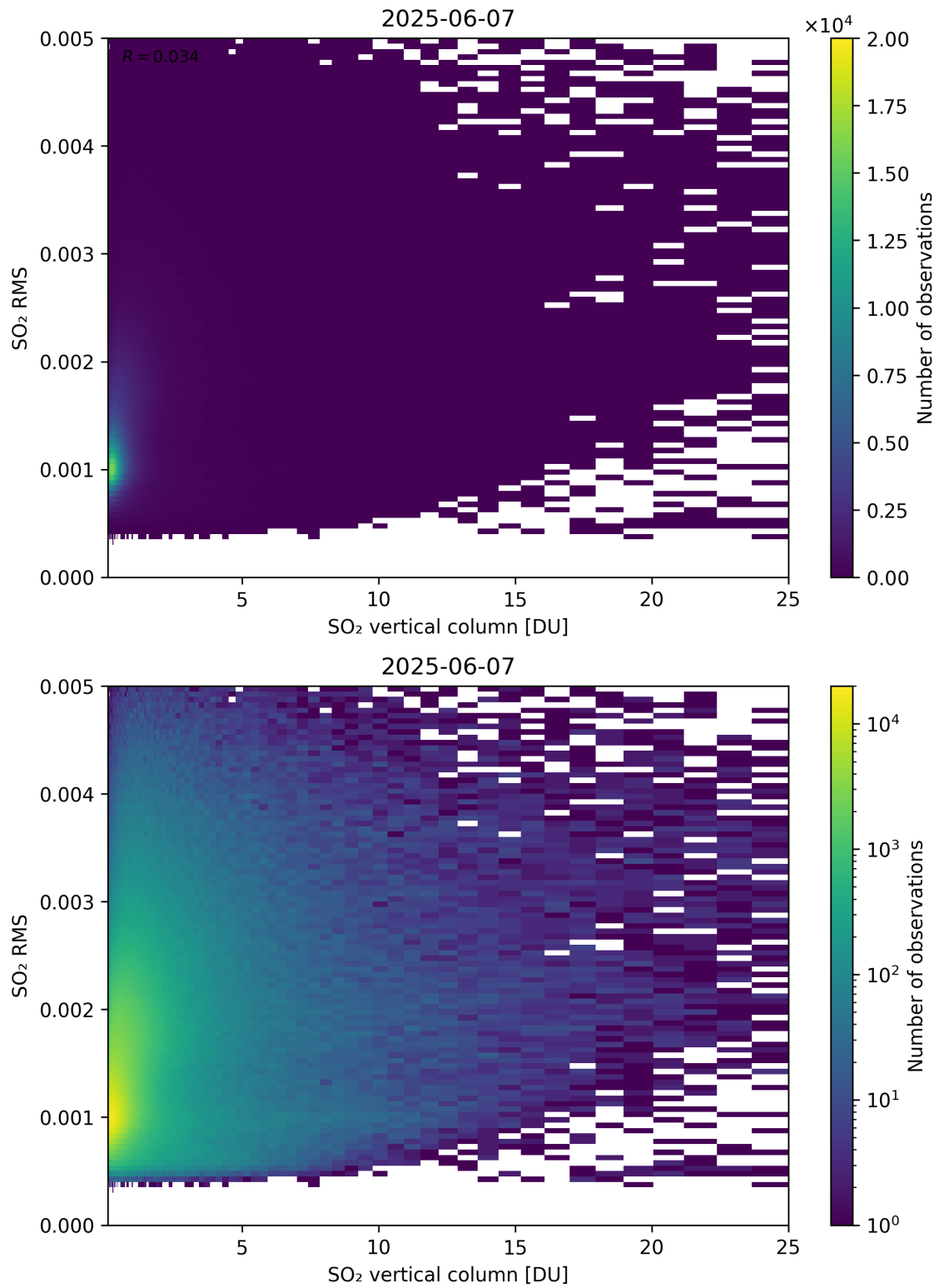
Figure 328: Scatter density plot of “SO 2 vertical column” against “SO 2 RMS” for 2025-06-06 to 2025-06-08.
