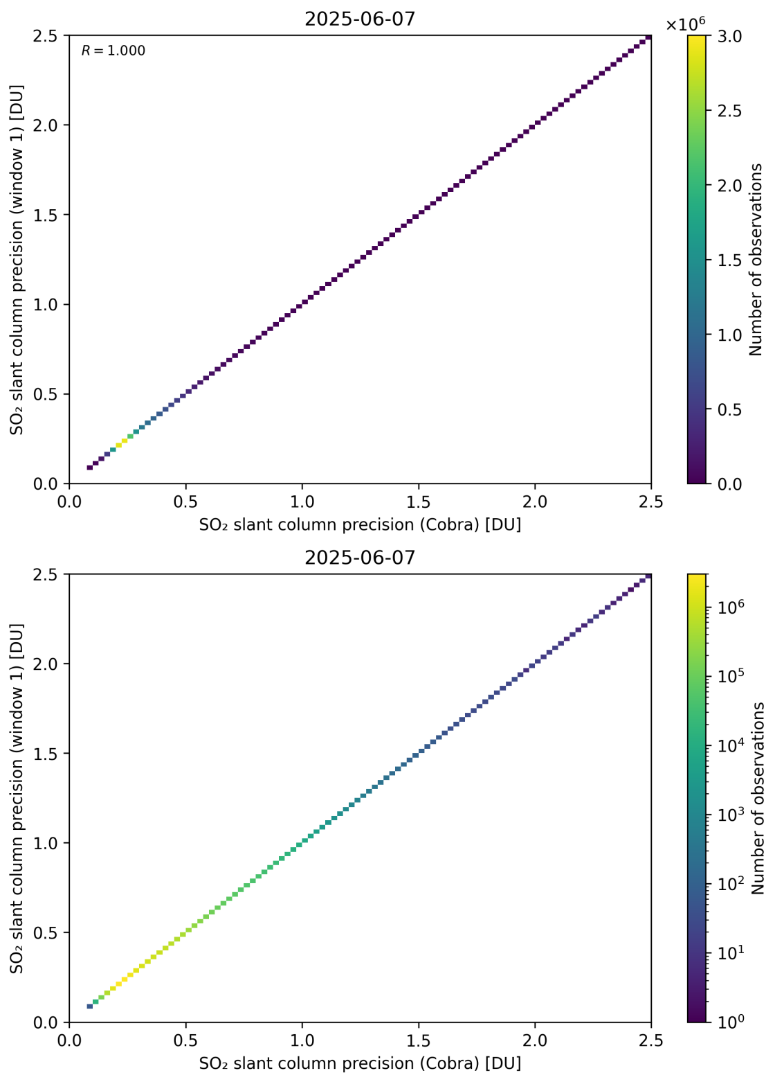
Figure 209: Scatter density plot of “SO 2 slant column precision (Cobra)” against “SO 2 slant column precision (window 1)” for 2025-06-06 to 2025-06-08.
