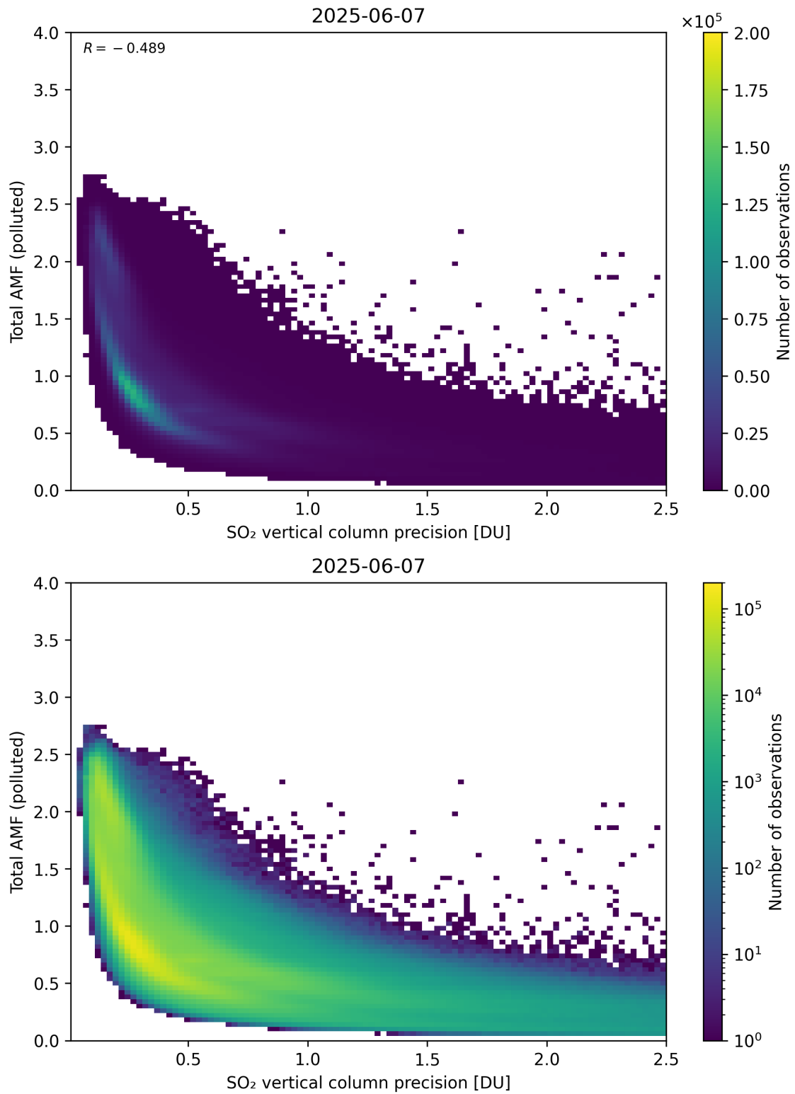
Figure 346: Scatter density plot of “SO 2 vertical column precision” against “Total AMF (polluted)” for 2025-06-06 to 2025-06-08.
