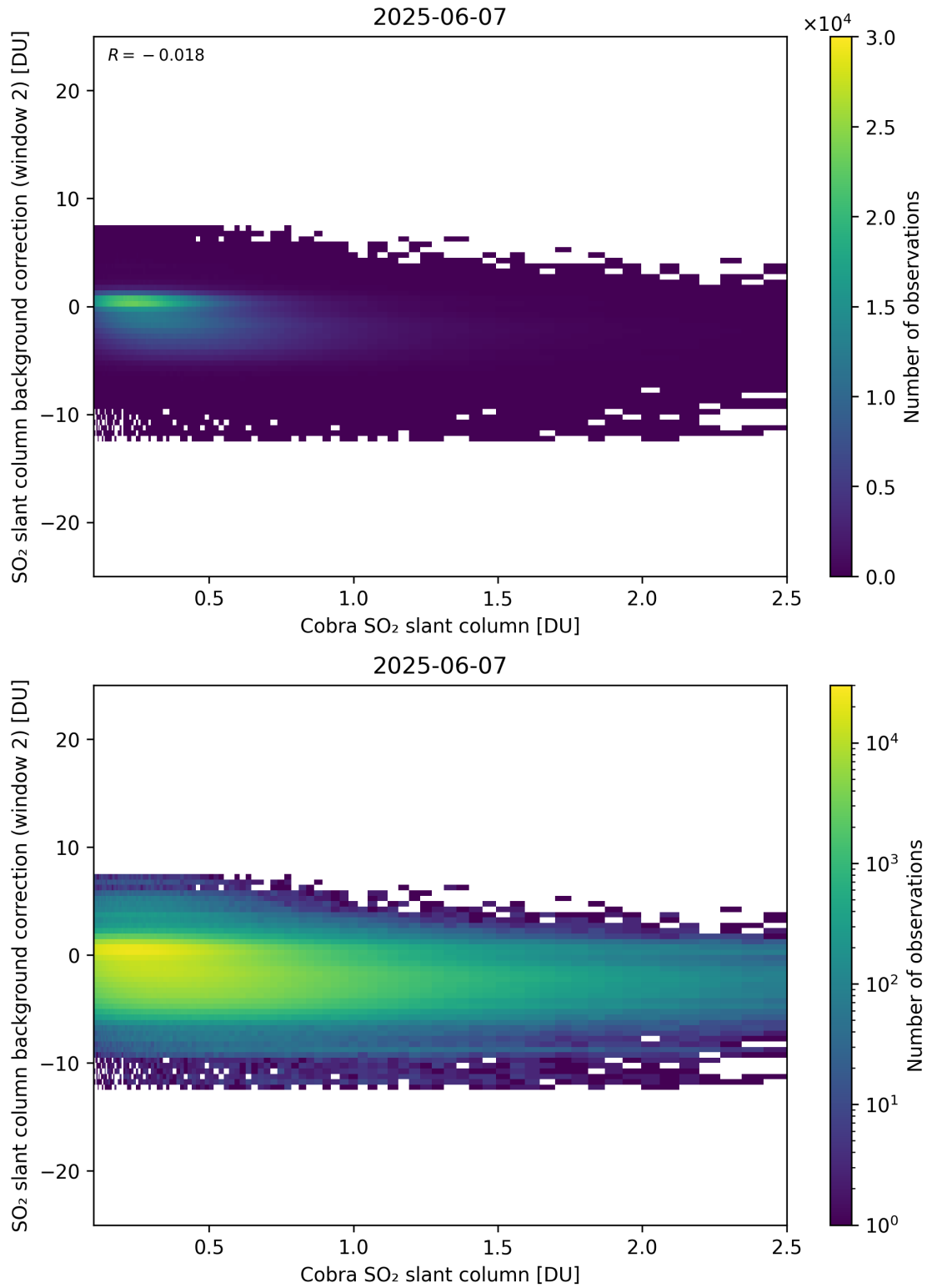
Figure 194: Scatter density plot of “Cobra SO 2 slant column” against “SO 2 slant column background correction (window 2)” for 2025-06-06 to 2025-06-08.
