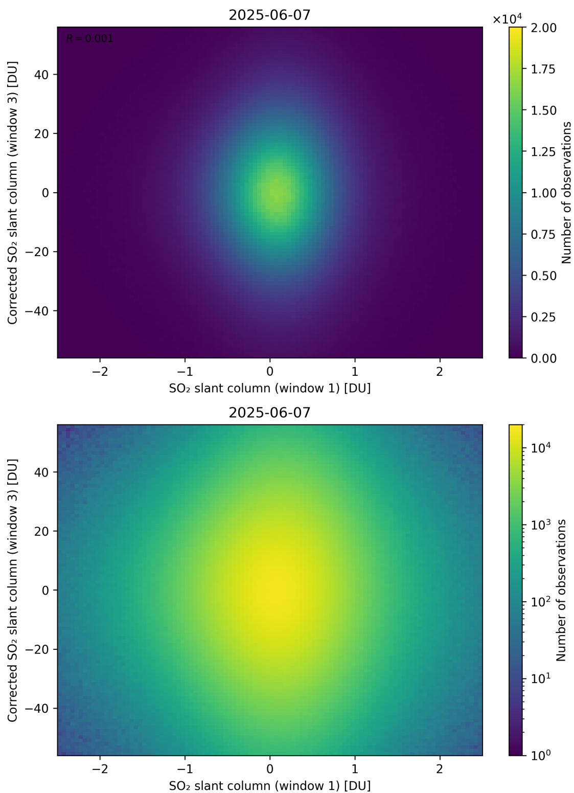
Figure 284: Scatter density plot of “SO 2 slant column (window 1)” against “Corrected SO 2 slant column (window 3)” for 2025-06-06 to 2025-06-08.
