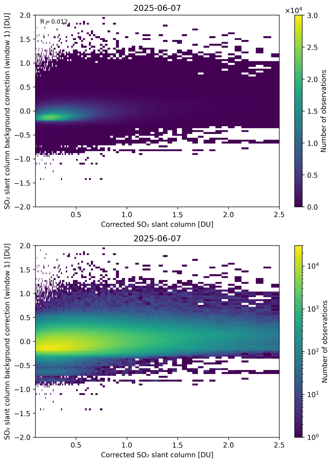
Figure 226: Scatter density plot of “Corrected SO 2 slant column” against “SO 2 slant column background correction (window 1)” for 2025-06-06 to 2025-06-08.
