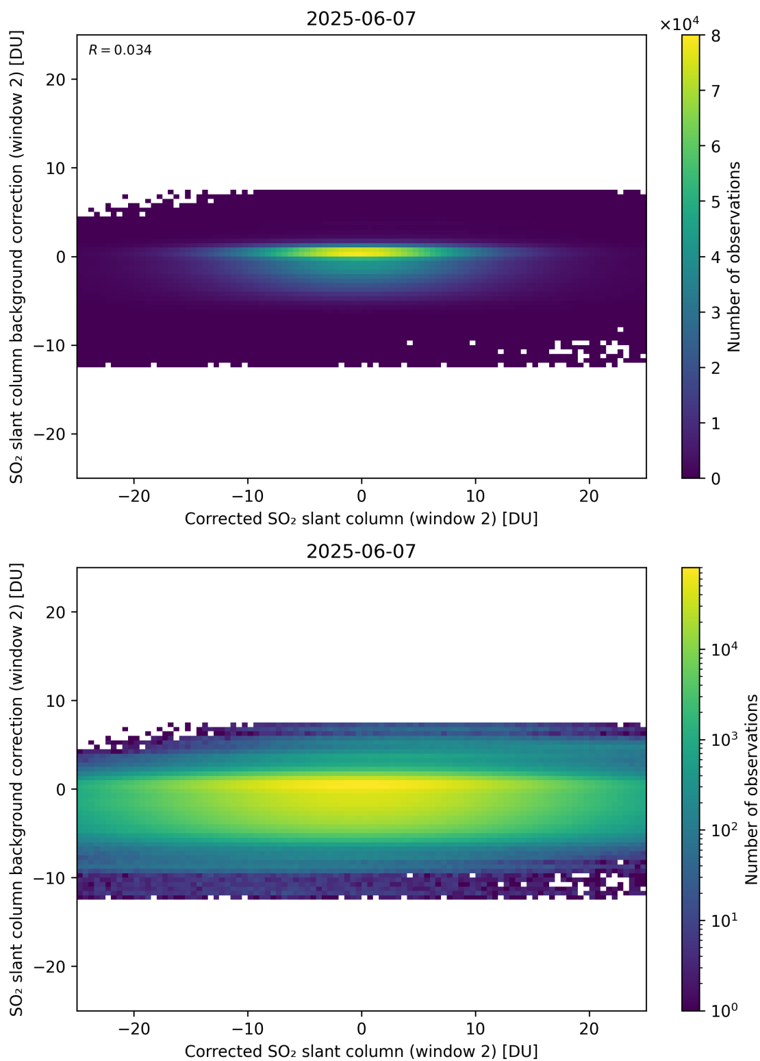
Figure 244: Scatter density plot of “Corrected SO 2 slant column (window 2)” against “SO 2 slant column background correction (window 2)” for 2025-06-06 to 2025-06-08.
