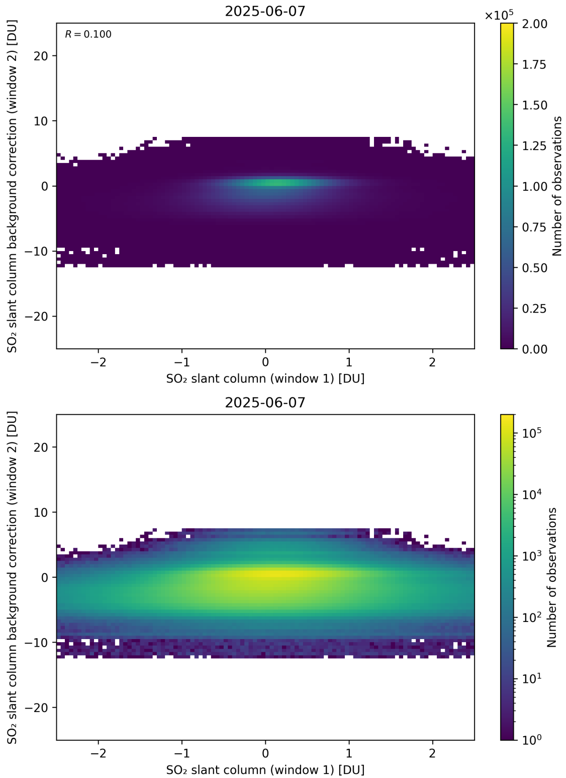
Figure 263: Scatter density plot of “SO 2 slant column (window 1)” against “SO 2 slant column background correction (window 2)” for 2025-06-06 to 2025-06-08.
