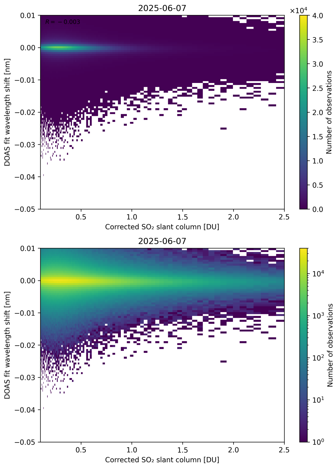
Figure 229: Scatter density plot of “Corrected SO 2 slant column” against “DOAS fit wavelength shift” for 2025-06-06 to 2025-06-08.
