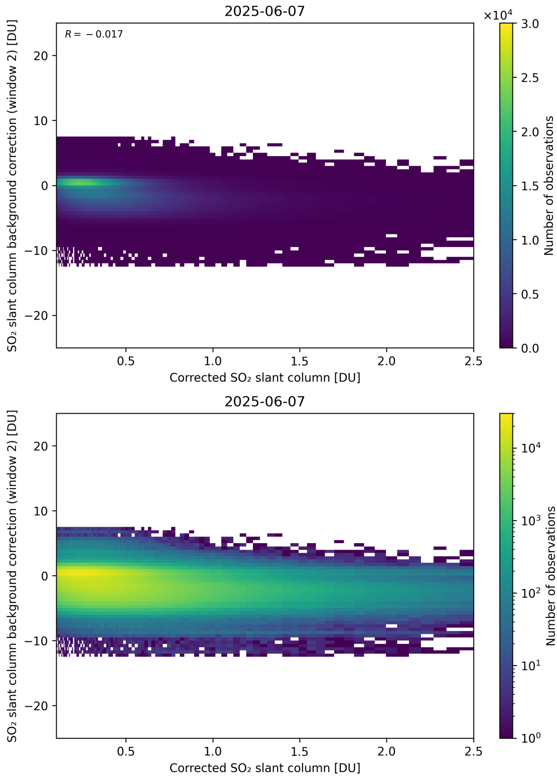
Figure 227: Scatter density plot of “Corrected SO 2 slant column” against “SO 2 slant column background correction (window 2)” for 2025-06-06 to 2025-06-08.
