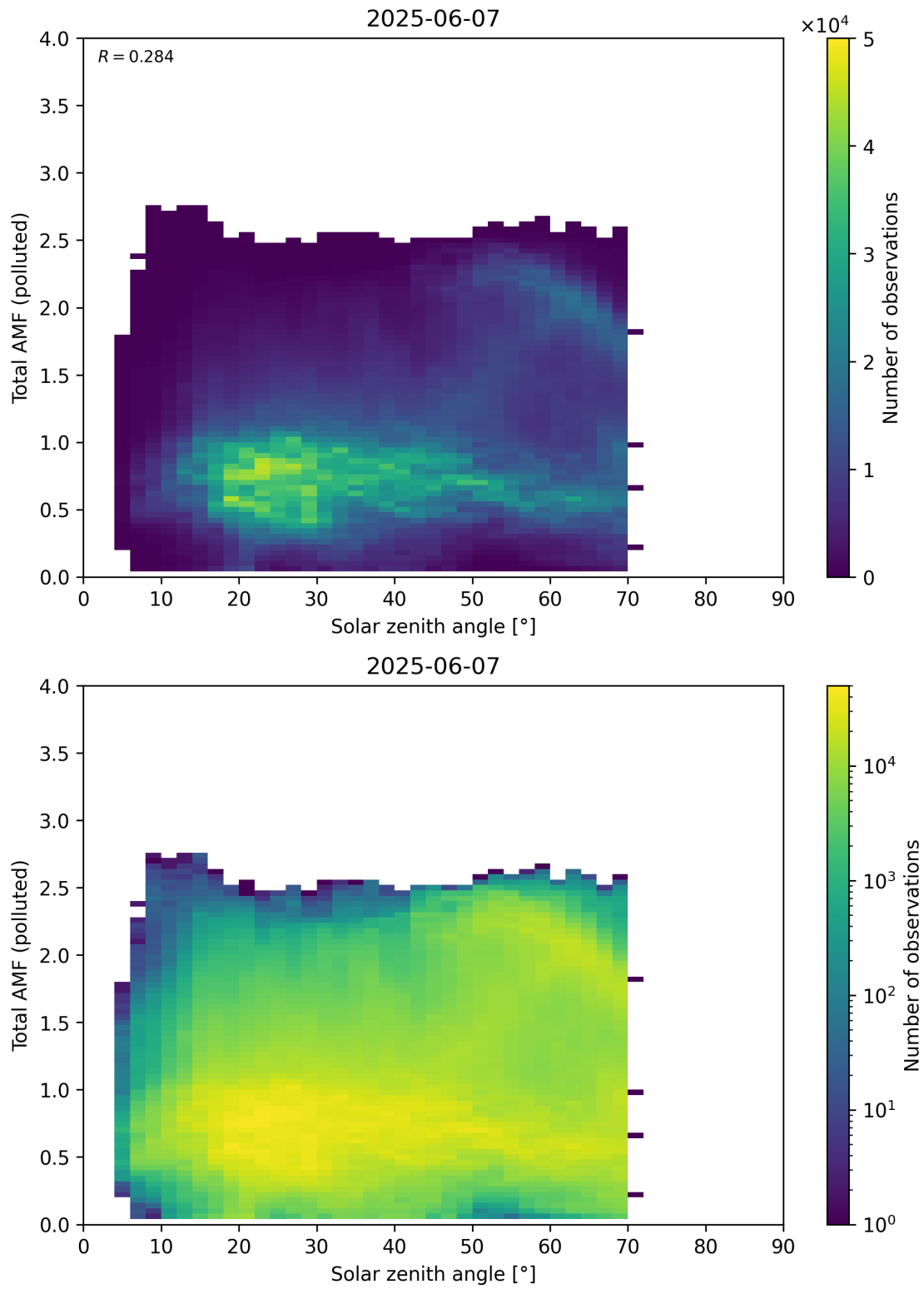
Figure 189: Scatter density plot of “Solar zenith angle” against “Total AMF (polluted)” for 2025-06-06 to 2025-06-08.
