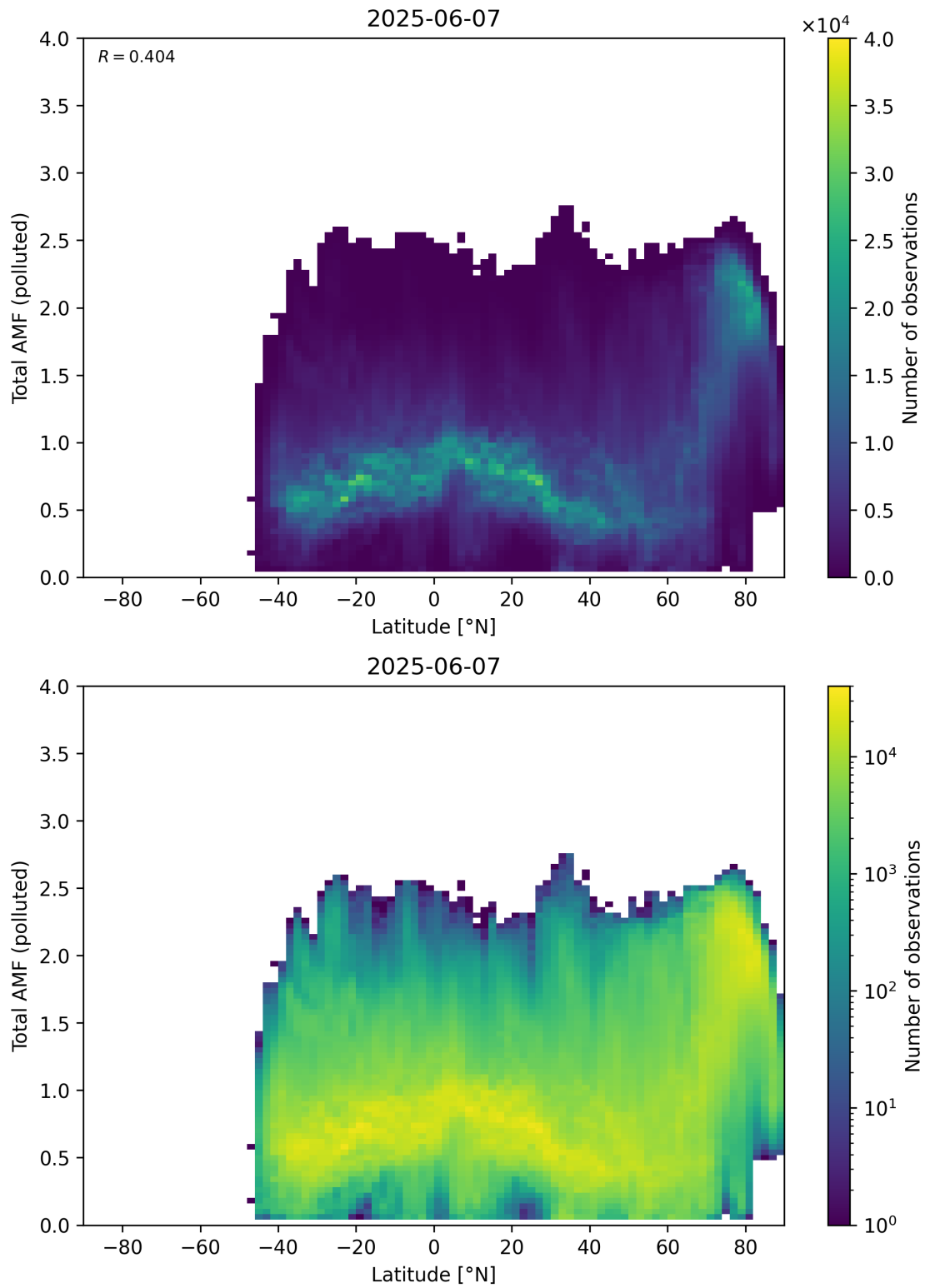
Figure 167: Scatter density plot of “Latitude” against “Total AMF (polluted)” for 2025-06-06 to 2025-06-08.
