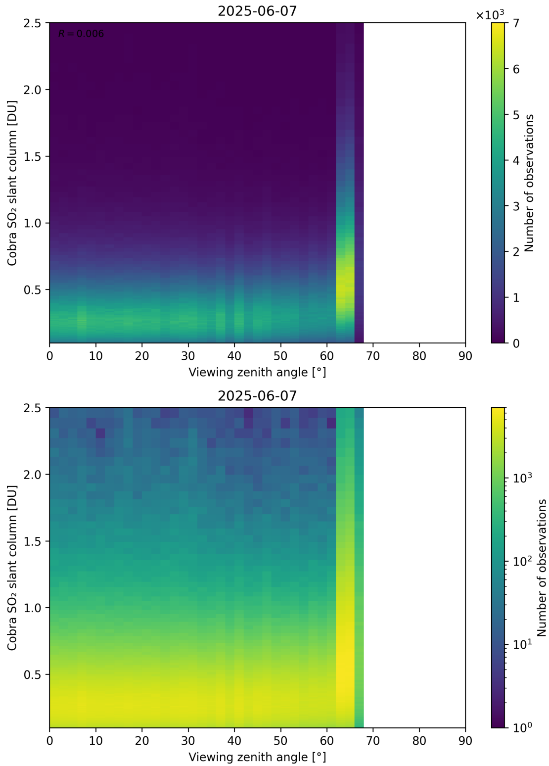
Figure 371: Scatter density plot of “Viewing zenith angle” against “Cobra SO 2 slant column” for 2025-06-06 to 2025-06-08.
