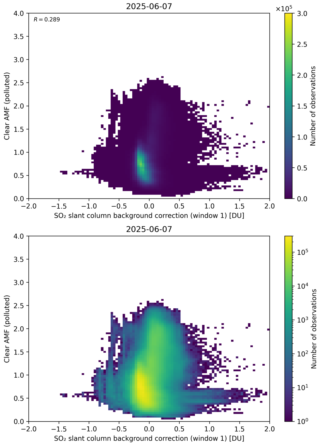
Figure 114: Scatter density plot of “SO 2 slant column background correction (window 1)” against “Clear AMF (polluted)” for 2025-06-06 to 2025-06-08.
