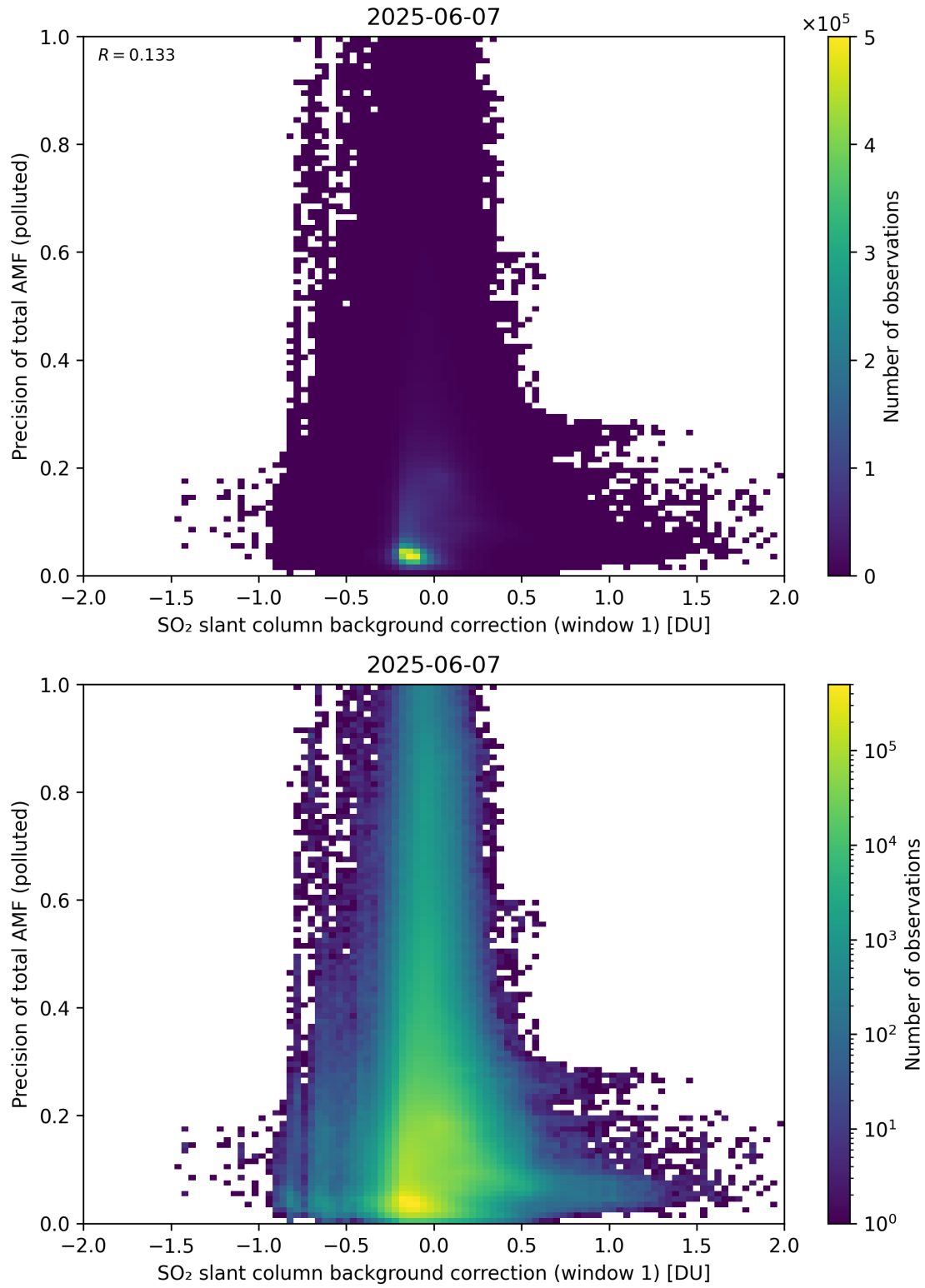
Figure 121: Scatter density plot of “SO 2 slant column background correction (window 1)” against “Precision of total AMF (polluted)” for 2025-06-06 to 2025-06-08.
