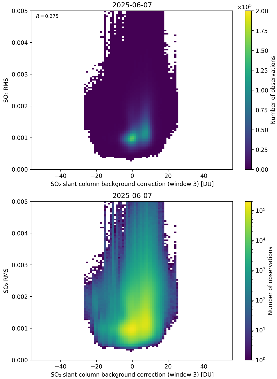
Figure 134: Scatter density plot of “SO 2 slant column background correction (window 3)” against “SO 2 RMS” for 2025-06-06 to 2025-06-08.
