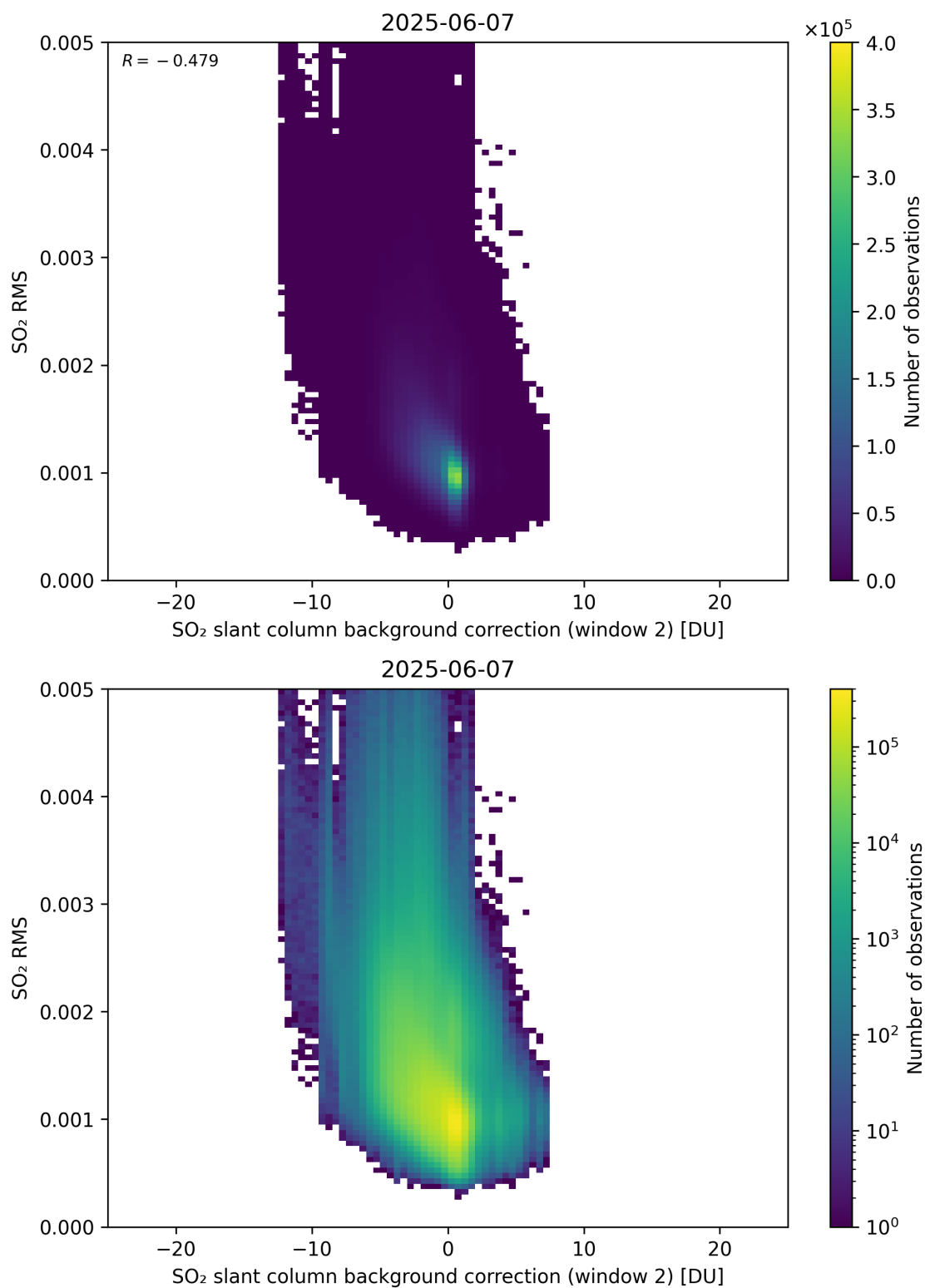
Figure 125: Scatter density plot of “SO 2 slant column background correction (window 2)” against “SO 2 RMS” for 2025-06-06 to 2025-06-08.
