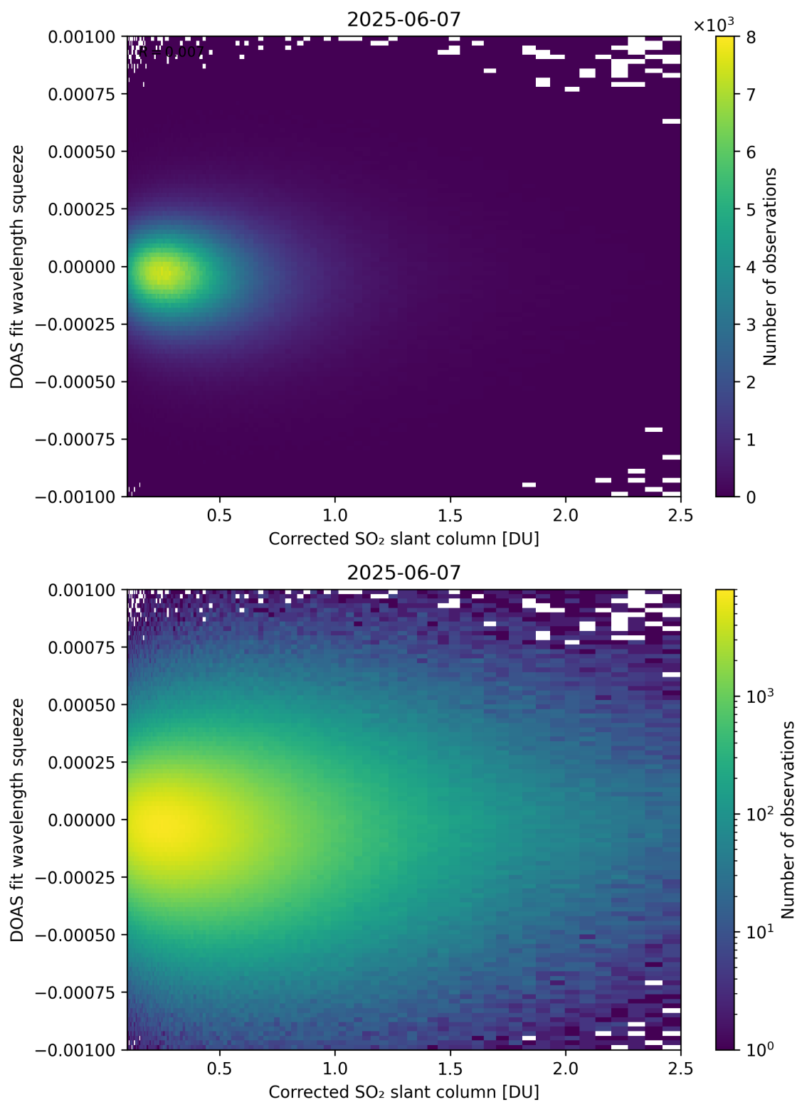
Figure 230: Scatter density plot of “Corrected SO 2 slant column” against “DOAS fit wavelength squeeze” for 2025-06-06 to 2025-06-08.
