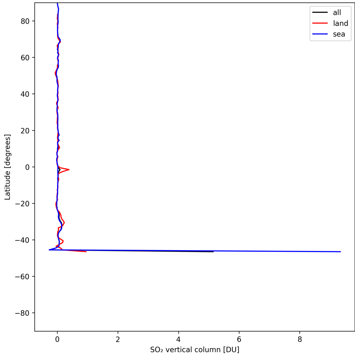
Figure 32: Zonal average of “SO 2 vertical column” for 2025-06-06 to 2025-06-08.
