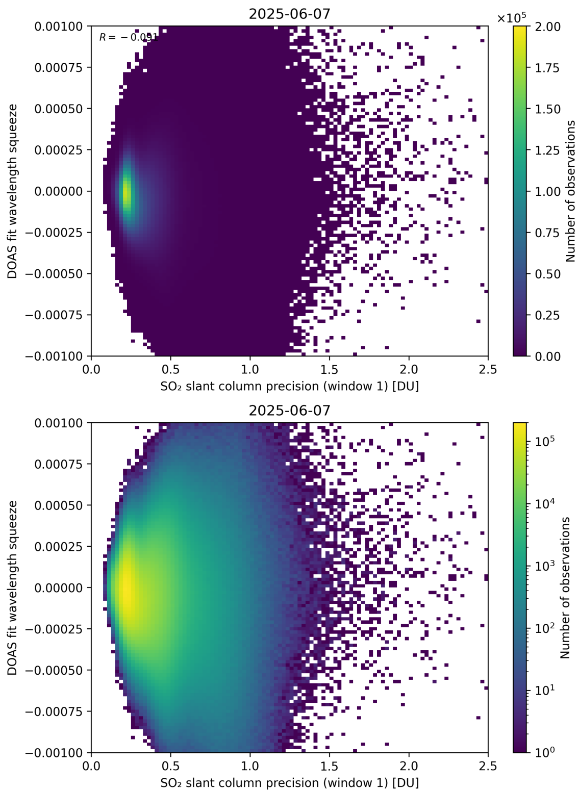
Figure 272: Scatter density plot of “SO 2 slant column precision (window 1)” against “DOAS fit wavelength squeeze” for 2025-06-06 to 2025-06-08.
