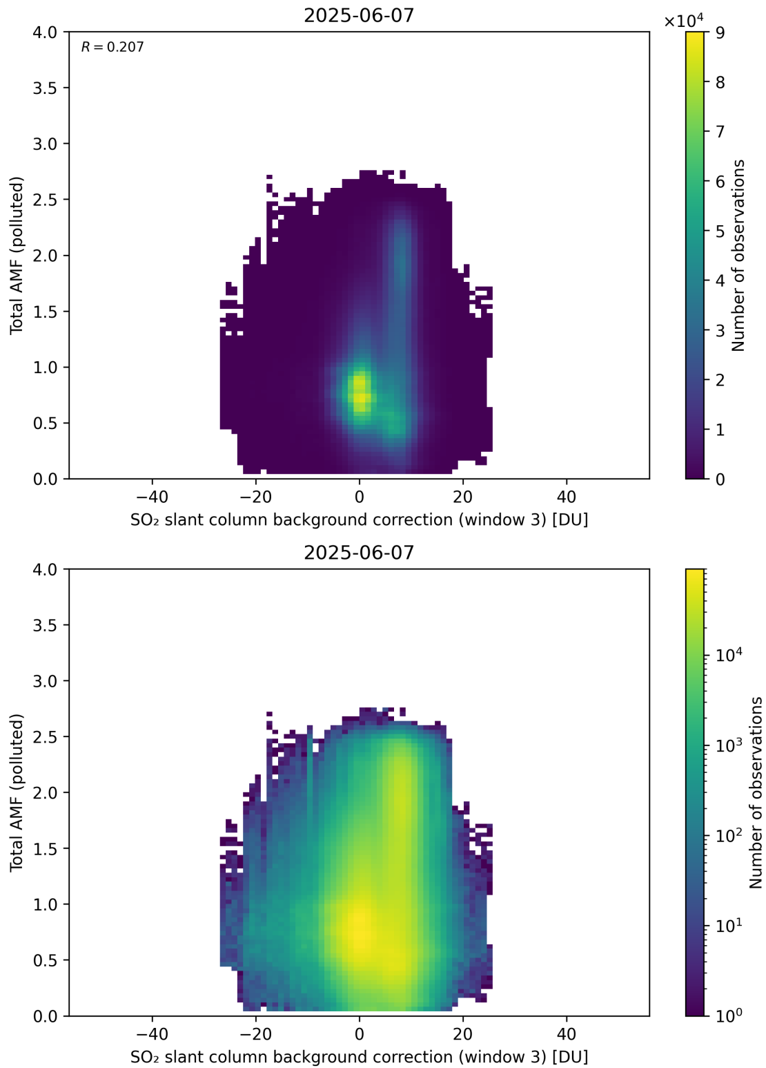
Figure 136: Scatter density plot of “SO 2 slant column background correction (window 3)” against “Total AMF (polluted)” for 2025-06-06 to 2025-06-08.
