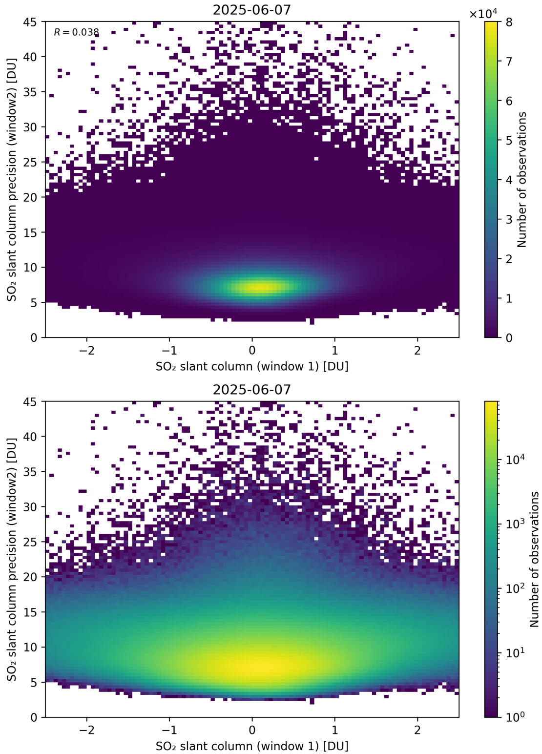
Figure 286: Scatter density plot of “SO 2 slant column (window 1)” against “SO 2 slant column precision (window2)” for 2025-06-06 to 2025-06-08.
