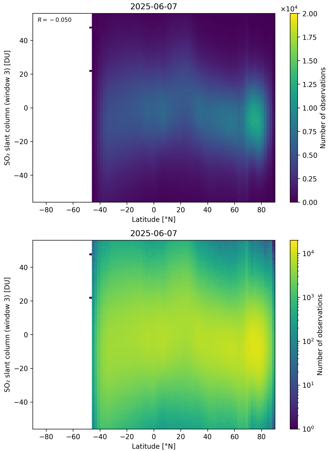
Figure 165: Scatter density plot of “Latitude” against “SO 2 slant column (window 3)” for 2025-06-06 to 2025-06-08.
