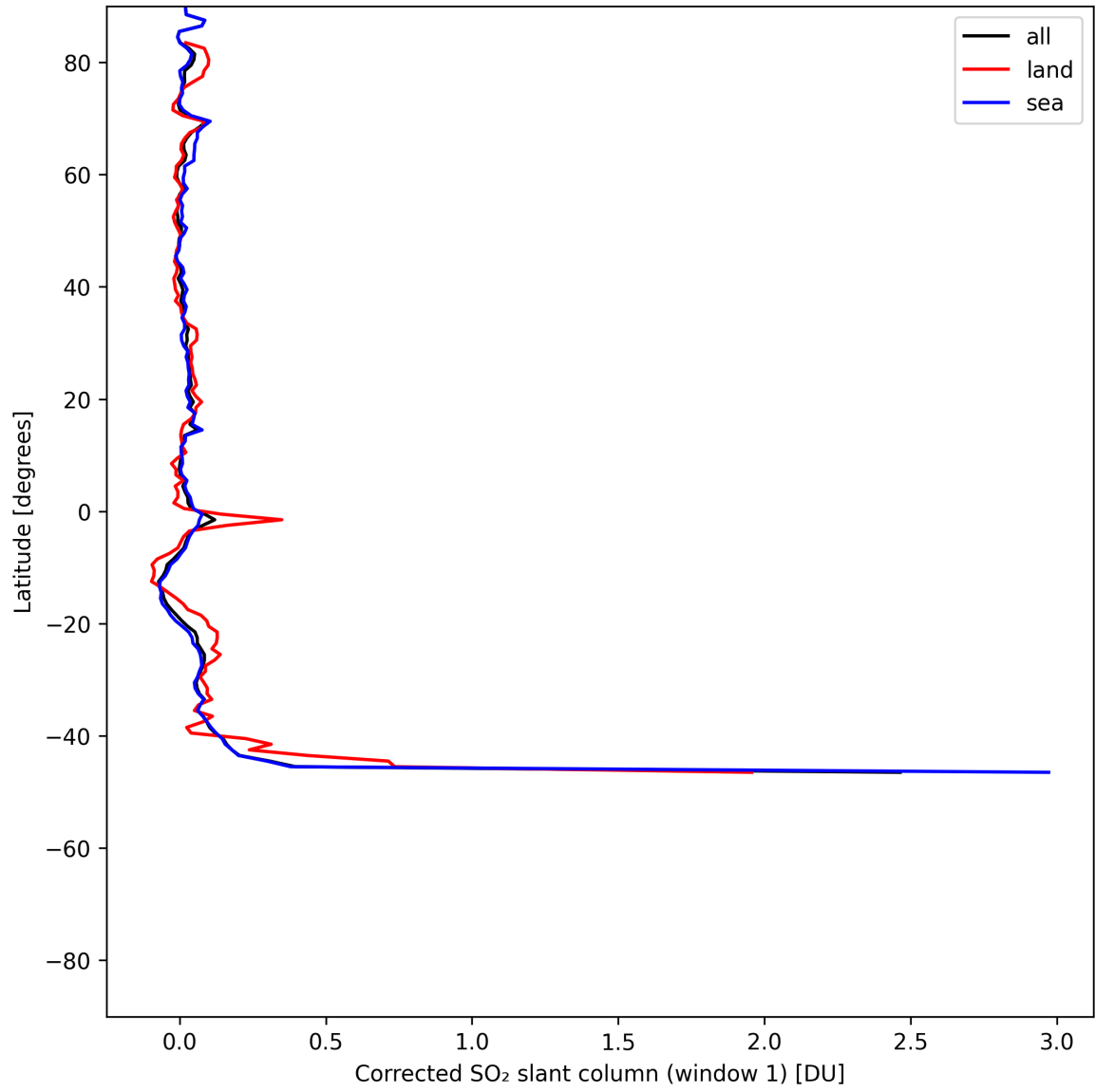
Figure 39: Zonal average of “Corrected SO 2 slant column (window 1)” for 2025-06-06 to 2025-06-08.
