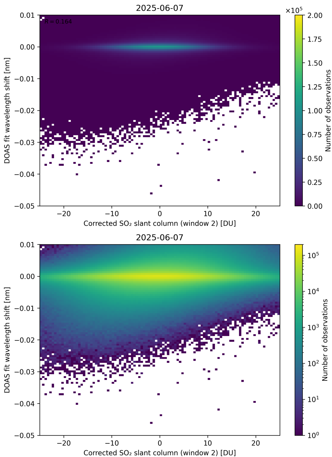
Figure 246: Scatter density plot of “Corrected SO 2 slant column (window 2)” against “DOAS fit wavelength shift” for 2025-06-06 to 2025-06-08.
