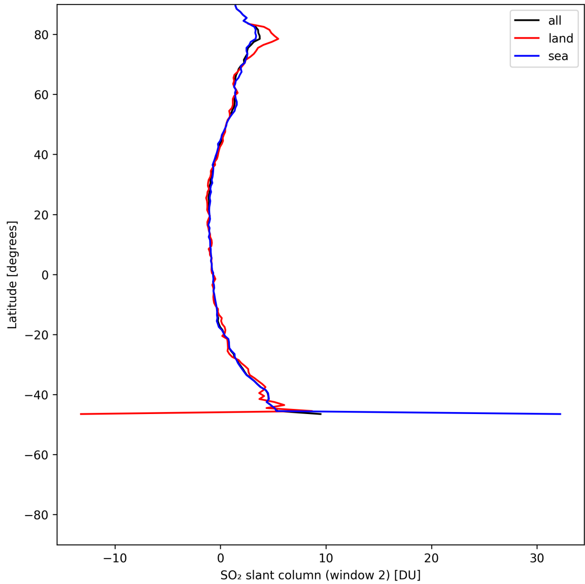
Figure 41: Zonal average of “SO 2 slant column (window 2)” for 2025-06-06 to 2025-06-08.
