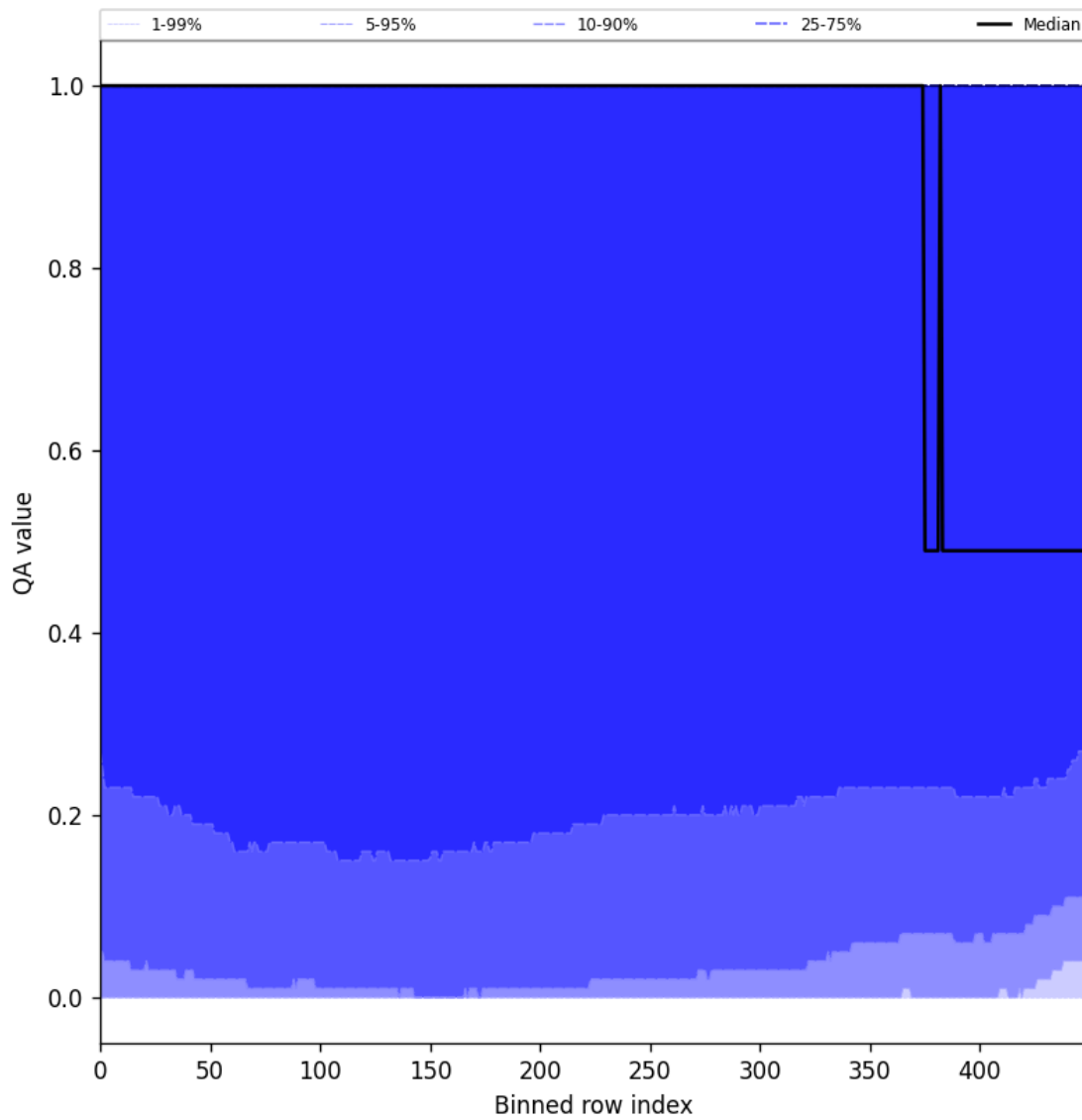
Figure 83: Along track statistics of “QA value” for 2025-06-06 to 2025-06-08
