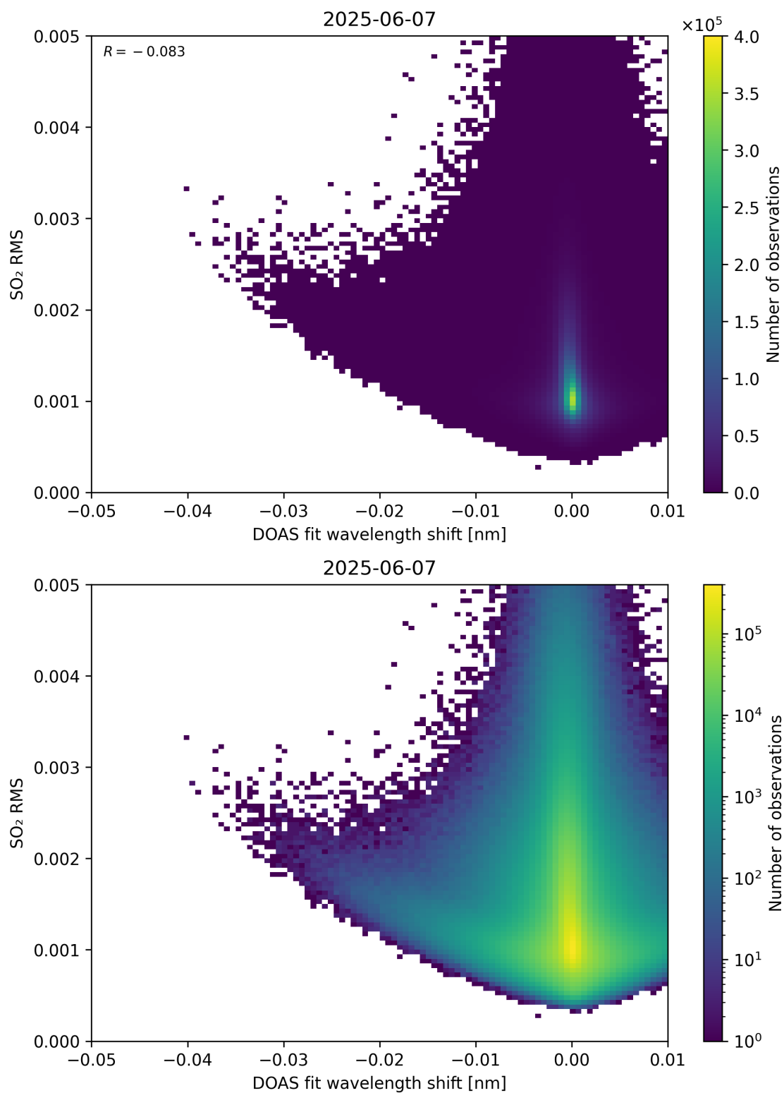
Figure 139: Scatter density plot of “DOAS fit wavelength shift” against “SO 2 RMS” for 2025-06-06 to 2025-06-08.
