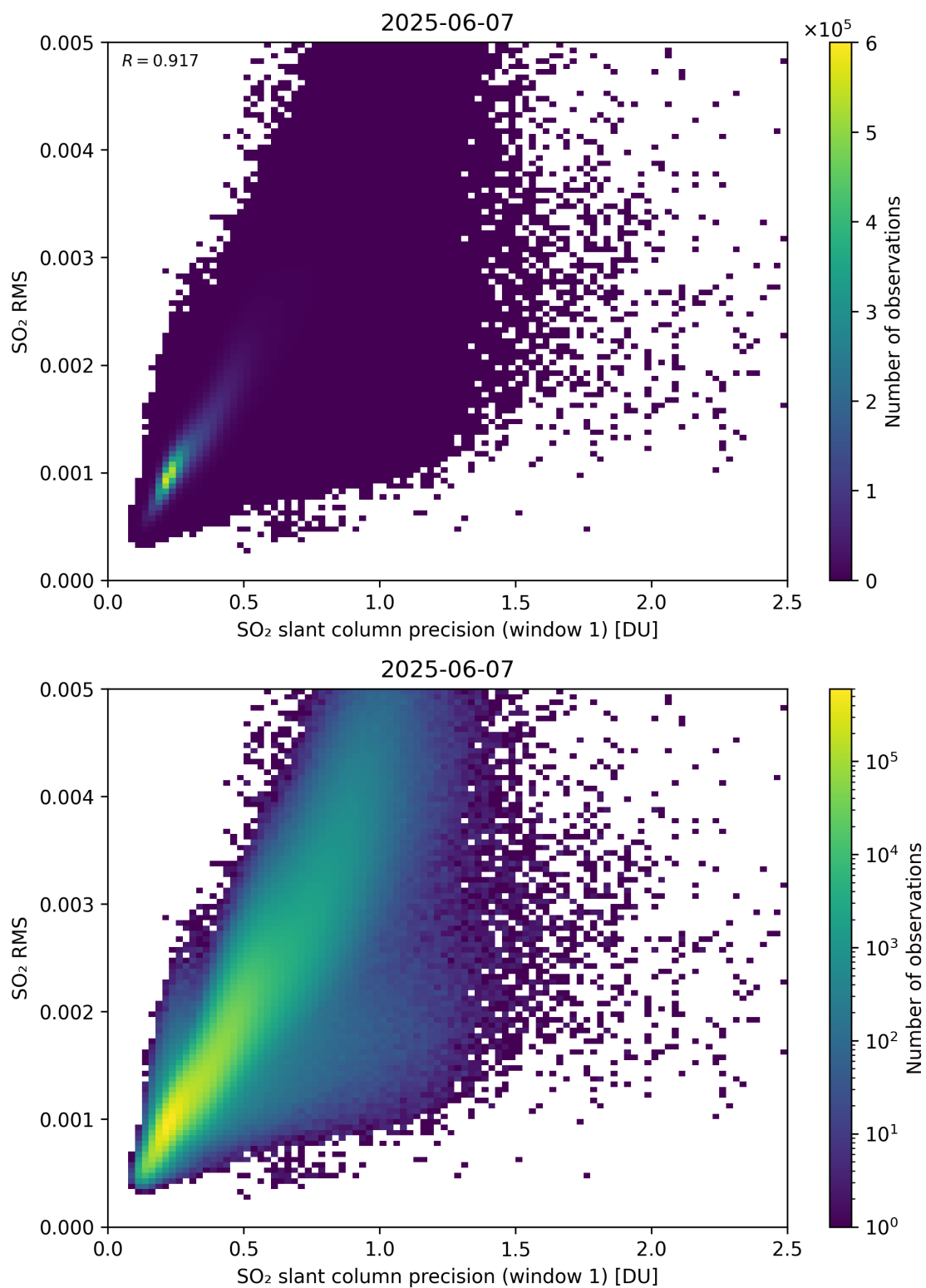
Figure 273: Scatter density plot of “SO 2 slant column precision (window 1)” against “SO 2 RMS” for 2025-06-06 to 2025-06-08.
