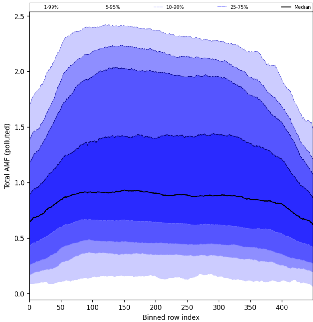
Figure 105: Along track statistics of “Total AMF (polluted)” for 2025-06-06 to 2025-06-08
