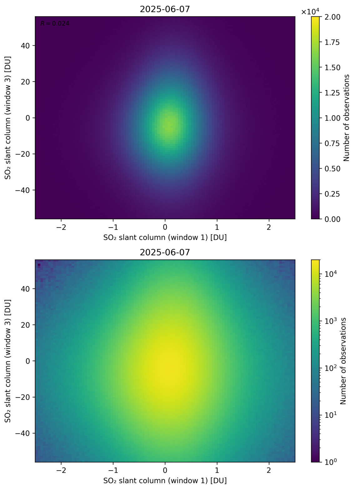
Figure 287: Scatter density plot of “SO 2 slant column (window 1)” against “SO 2 slant column (window 3)” for 2025-06-06 to 2025-06-08.
