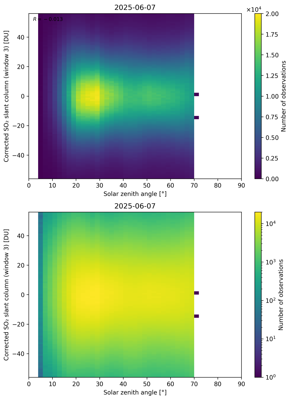
Figure 183: Scatter density plot of “Solar zenith angle” against “Corrected SO 2 slant column (window 3)” for 2025-06-06 to 2025-06-08.
