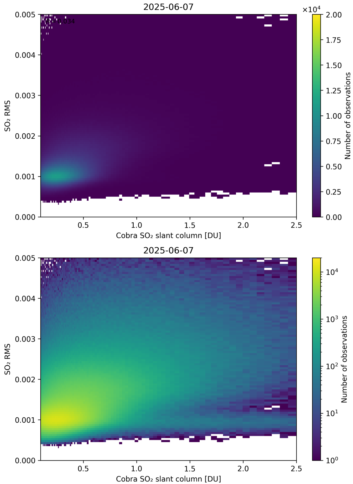
Figure 198: Scatter density plot of “Cobra SO 2 slant column” against “SO 2 RMS” for 2025-06-06 to 2025-06-08.
