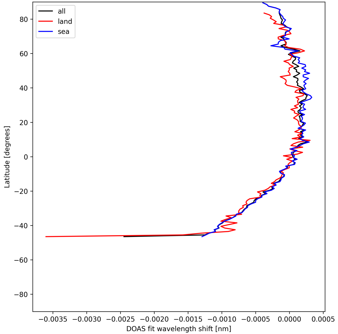
Figure 50: Zonal average of “DOAS fit wavelength shift” for 2025-06-06 to 2025-06-08.
