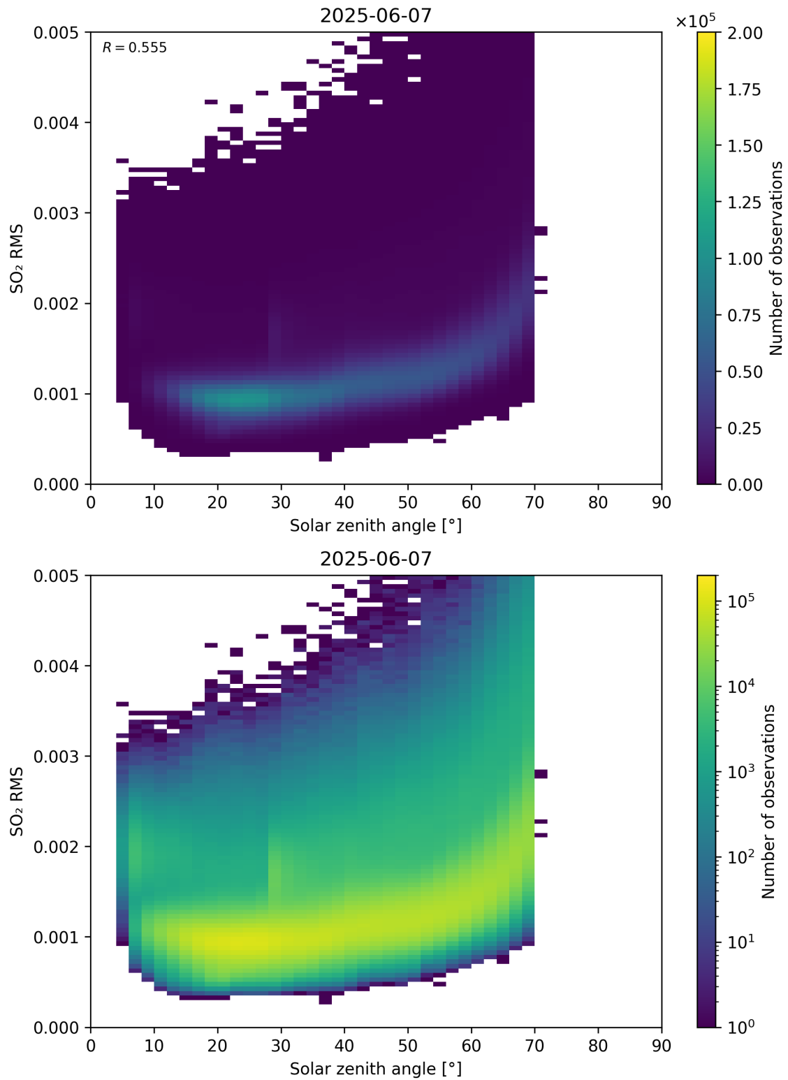
Figure 176: Scatter density plot of “Solar zenith angle” against “SO 2 RMS” for 2025-06-06 to 2025-06-08.
