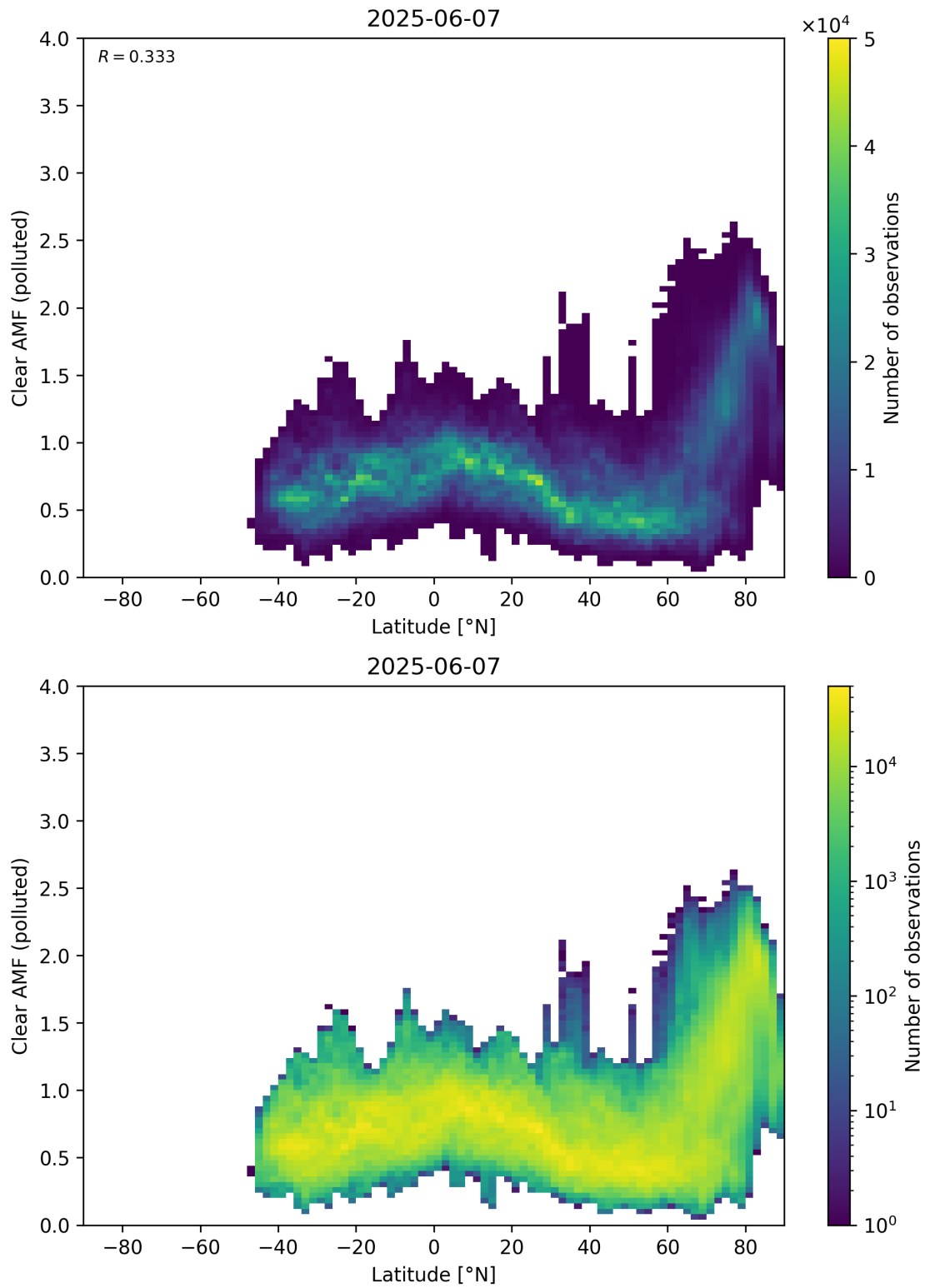
Figure 156: Scatter density plot of “Latitude” against “Clear AMF (polluted)” for 2025-06-06 to 2025-06-08.
