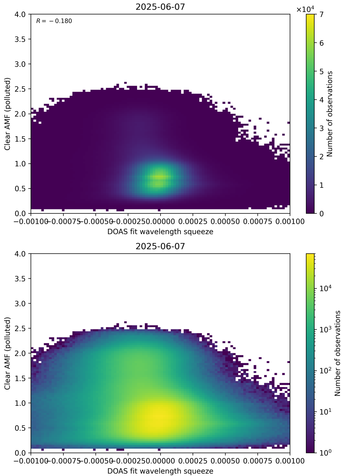
Figure 144: Scatter density plot of “DOAS fit wavelength squeeze” against “Clear AMF (polluted)” for 2025-06-06 to 2025-06-08.
