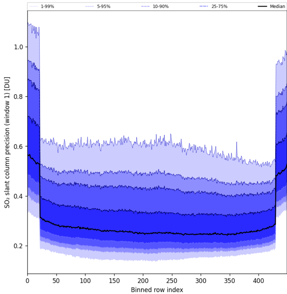
Figure 90: Along track statistics of “SO 2 slant column precision (window 1)” for 2025-06-06 to 2025-06-08
