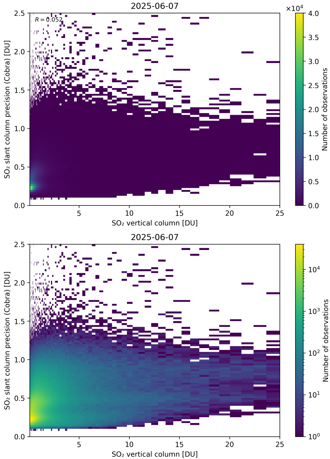
Figure 350: Scatter density plot of “SO 2 vertical column” against “SO 2 slant column precision (Cobra)” for 2025-06-06 to 2025-06-08.
