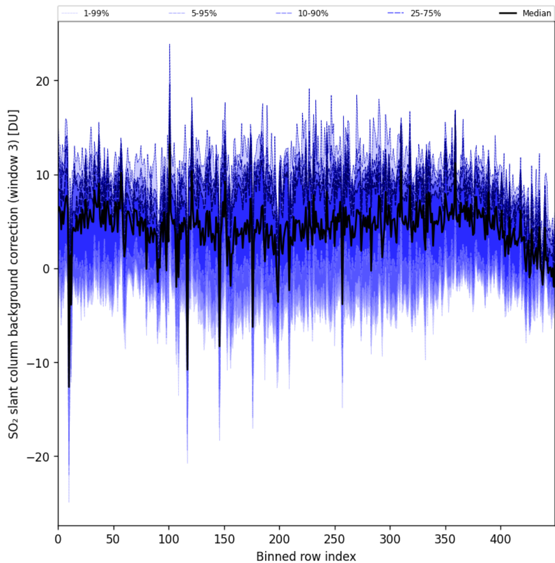
Figure 100: Along track statistics of "SO 2 slant column background correction (window 3)" for 2025-06-06 to 2025-06-08
