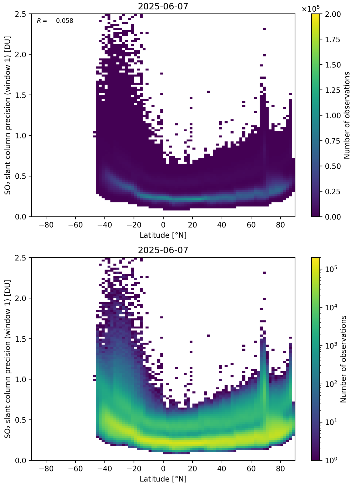
Figure 163: Scatter density plot of “Latitude” against “SO 2 slant column precision (window 1)” for 2025-06-06 to 2025-06-08.
