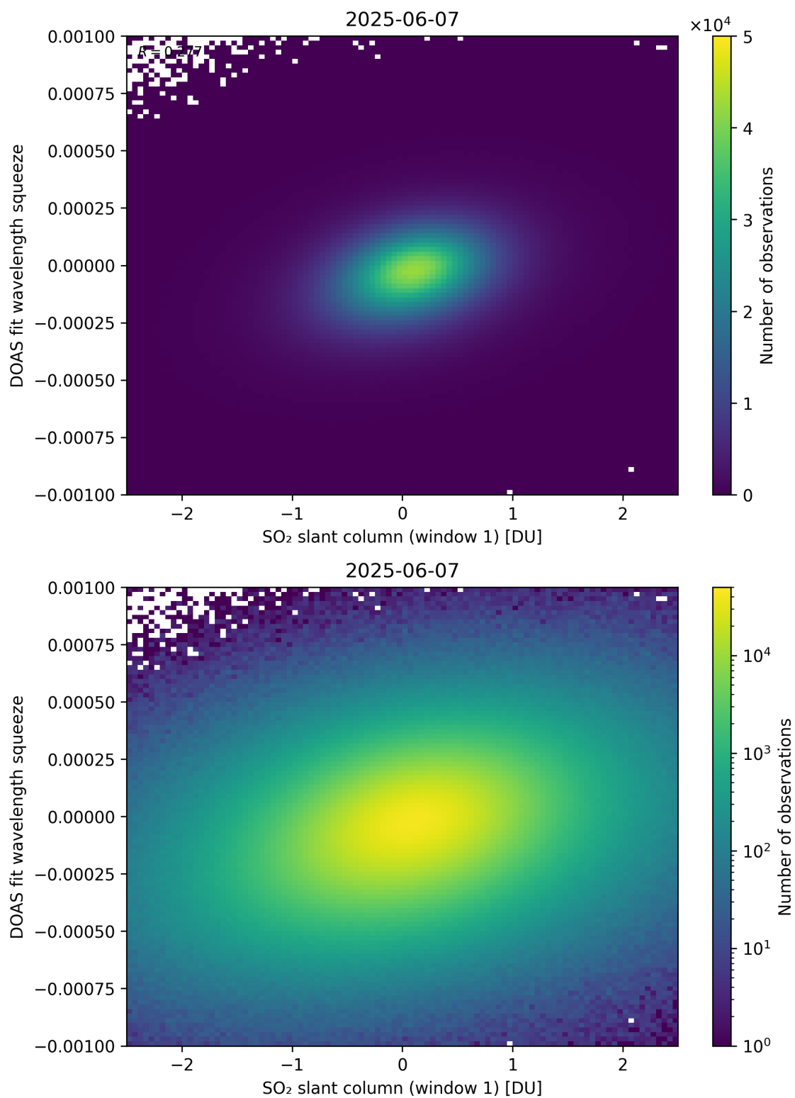
Figure 266: Scatter density plot of “SO 2 slant column (window 1)” against “DOAS fit wavelength squeeze” for 2025-06-06 to 2025-06-08.
