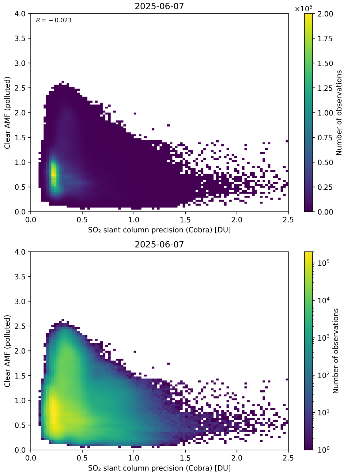
Figure 205: Scatter density plot of “SO 2 slant column precision (Cobra)” against “Clear AMF (polluted)” for 2025-06-06 to 2025-06-08.
