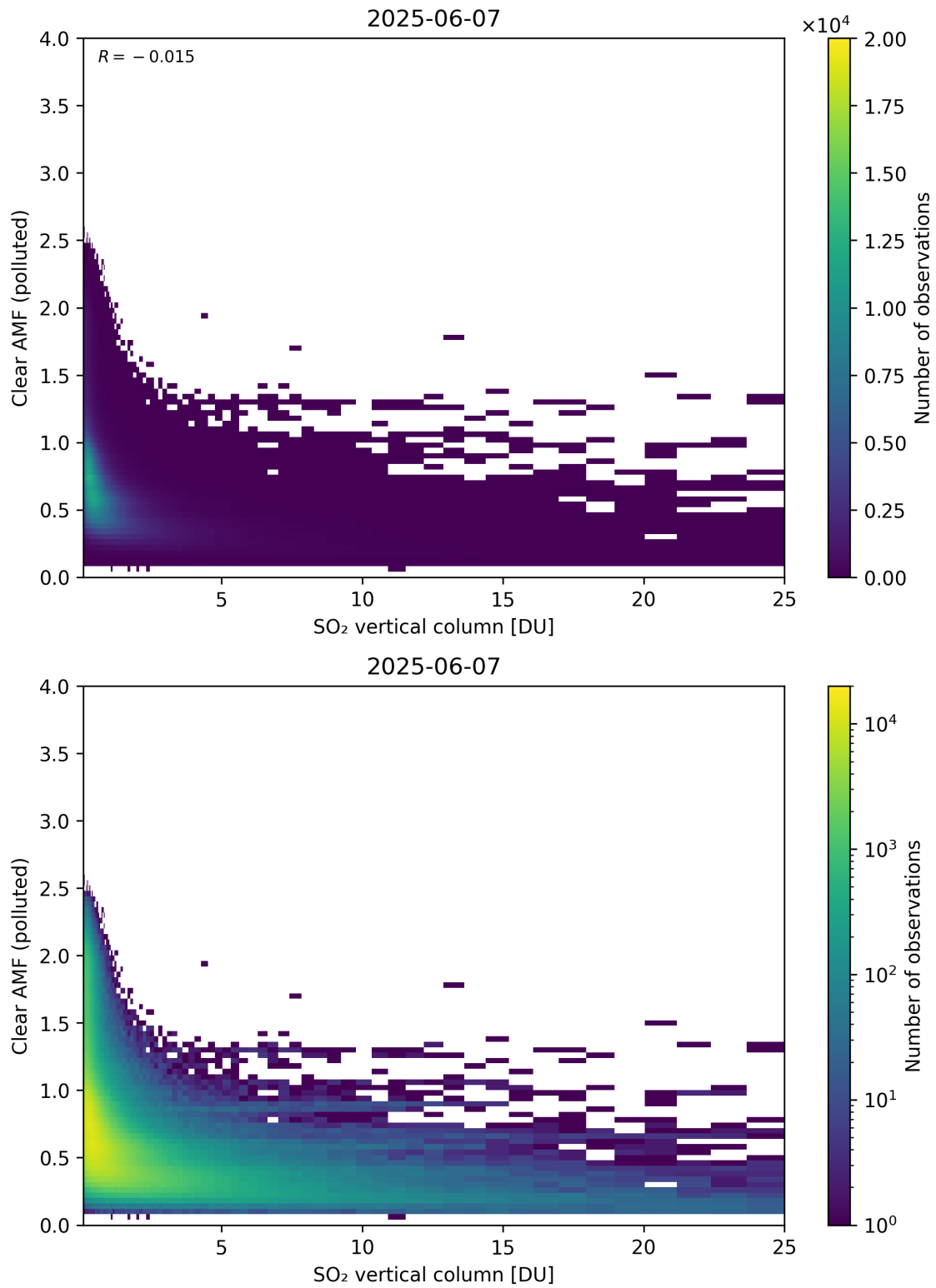
Figure 348: Scatter density plot of “SO 2 vertical column” against “Clear AMF (polluted)” for 2025-06-06 to 2025-06-08.
