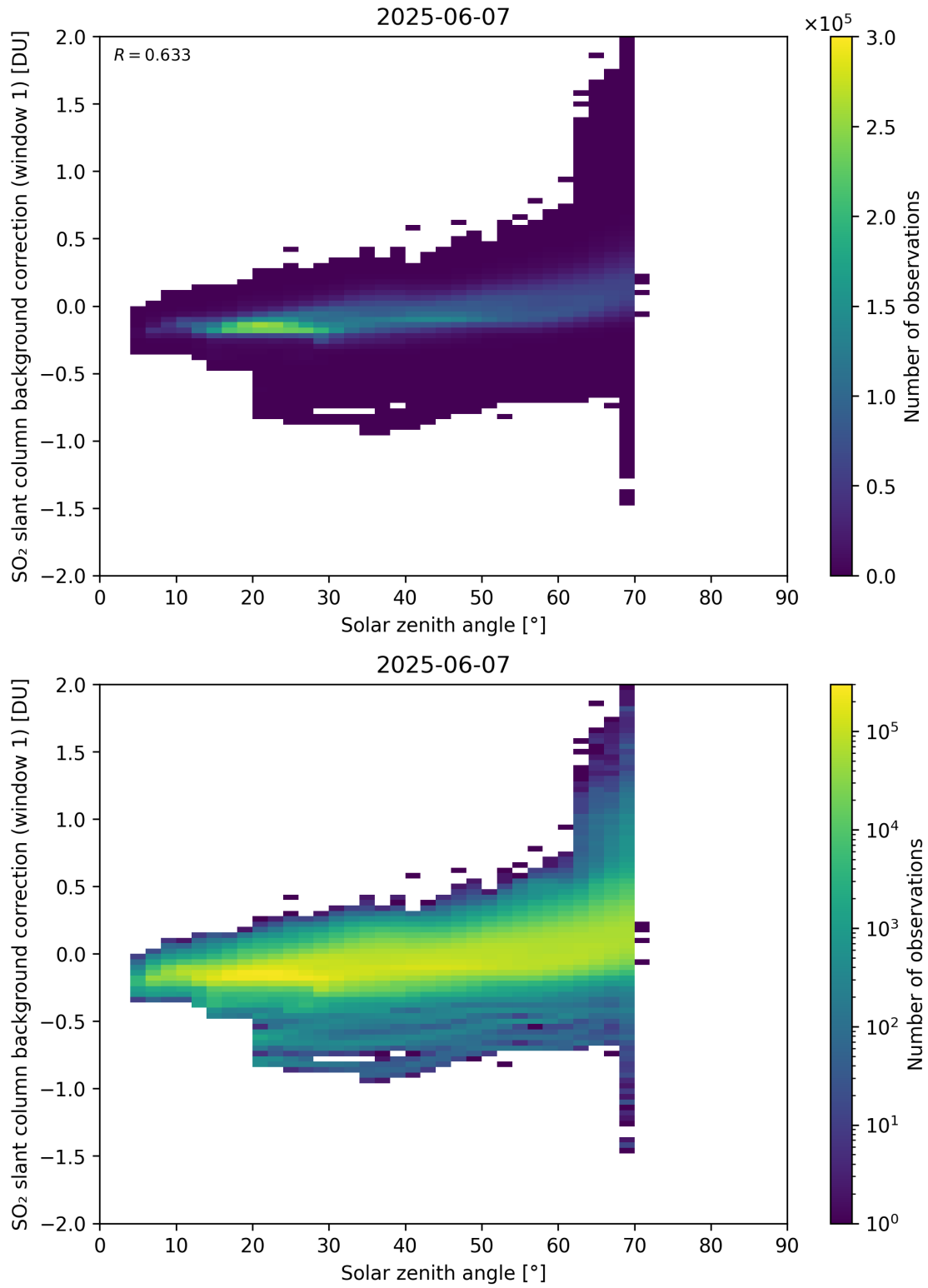
Figure 171: Scatter density plot of “Solar zenith angle” against “SO 2 slant column background correction (window 1)” for 2025-06-06 to 2025-06-08.
