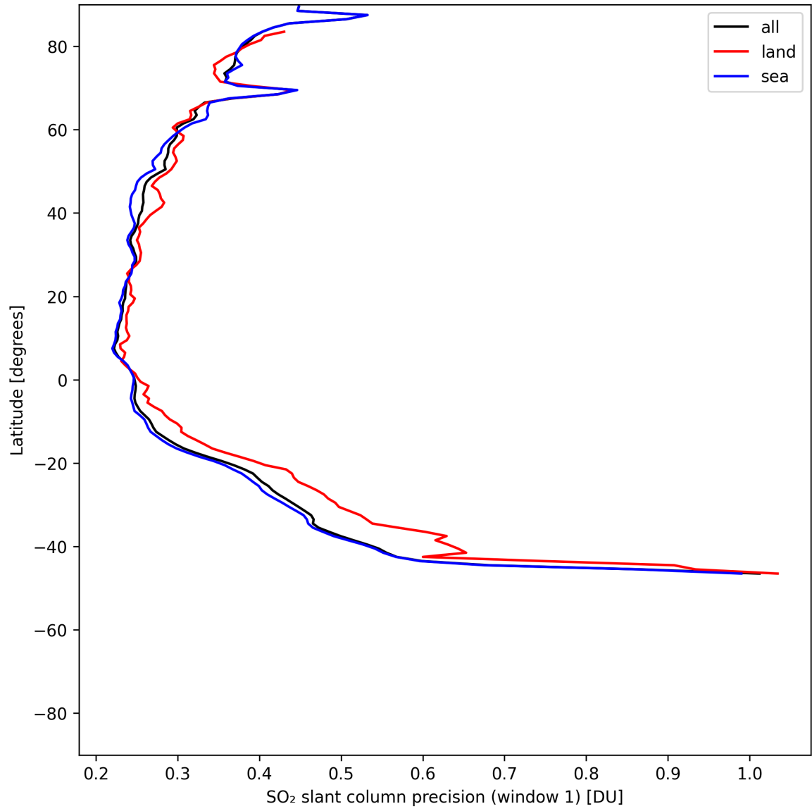
Figure 38: Zonal average of “SO 2 slant column precision (window 1)” for 2025-06-06 to 2025-06-08.
