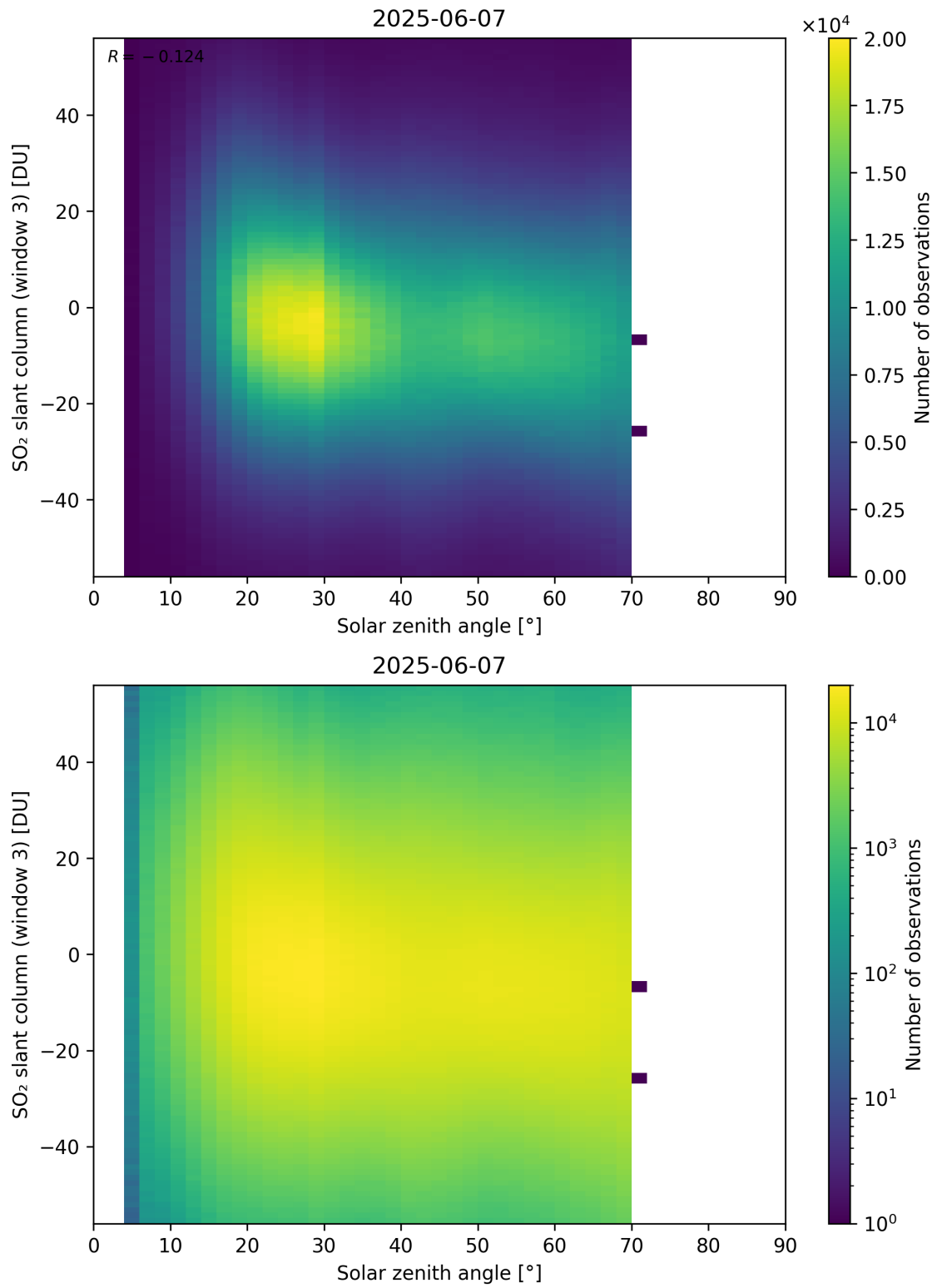
Figure 187: Scatter density plot of “Solar zenith angle” against “SO 2 slant column (window 3)” for 2025-06-06 to 2025-06-08.
