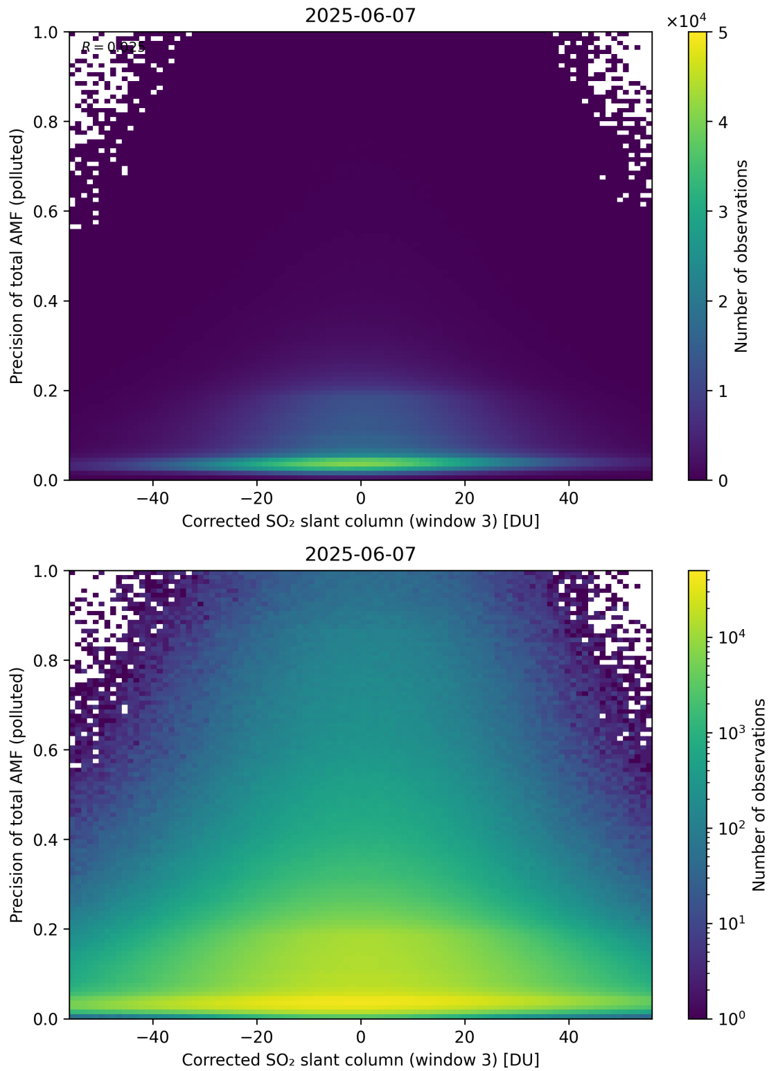
Figure 261: Scatter density plot of “Corrected SO 2 slant column (window 3)” against “Precision of total AMF (polluted)” for 2025-06-06 to 2025-06-08.
