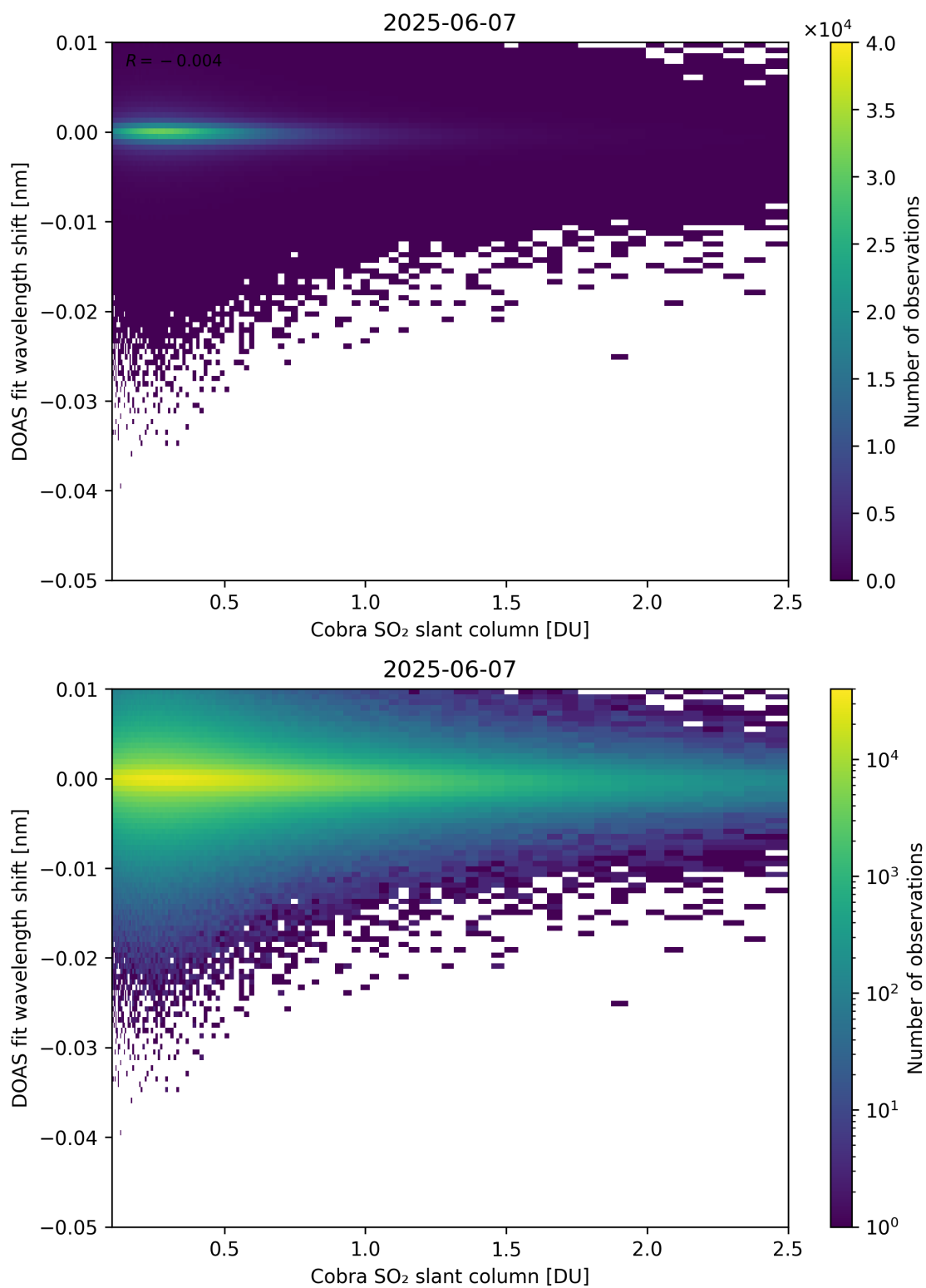
Figure 196: Scatter density plot of “Cobra SO 2 slant column” against “DOAS fit wavelength shift” for 2025-06-06 to 2025-06-08.
