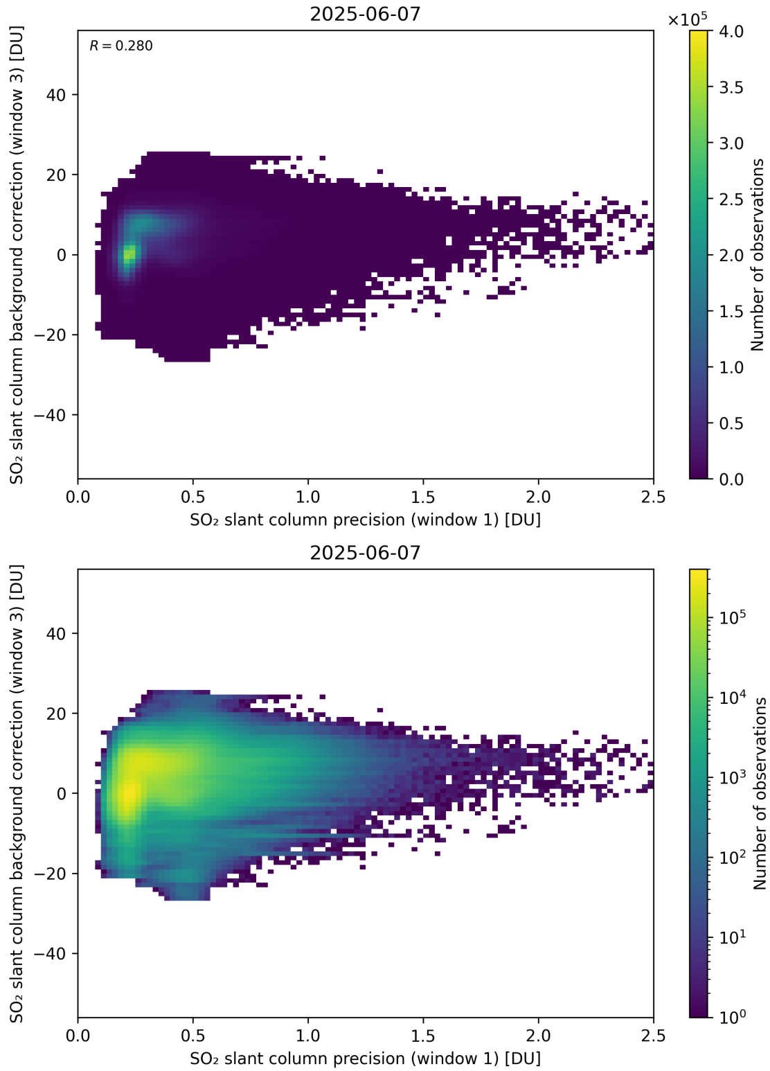
Figure 270: Scatter density plot of “SO 2 slant column precision (window 1)” against “SO 2 slant column background correction (window 3)” for 2025-06-06 to 2025-06-08.
