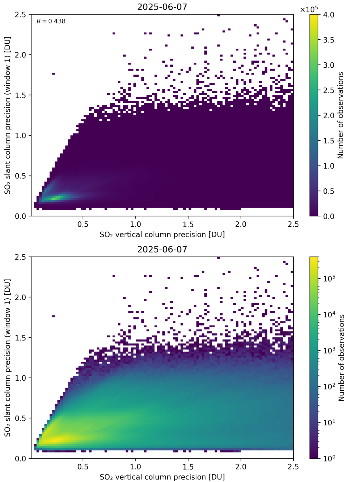
Figure 342: Scatter density plot of “SO 2 vertical column precision” against “SO 2 slant column precision (window 1)” for 2025-06-06 to 2025-06-08.
