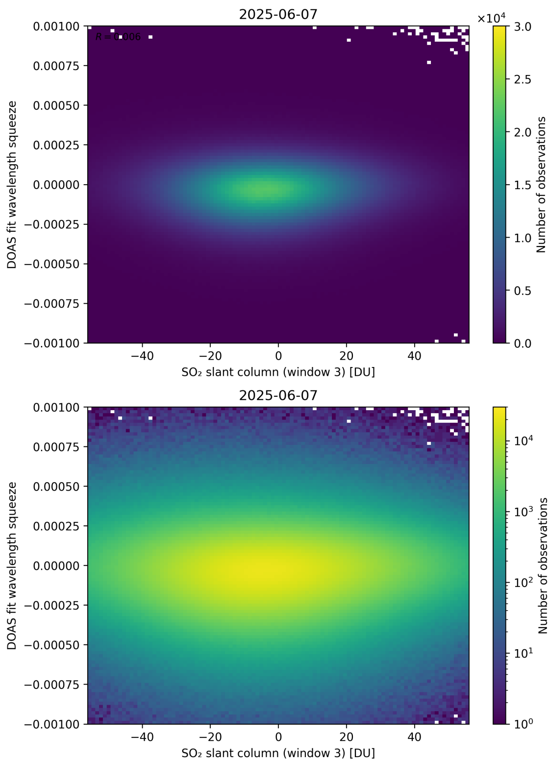
Figure 305: Scatter density plot of “SO 2 slant column (window 3)” against “DOAS fit wavelength squeeze” for 2025-06-06 to 2025-06-08.
