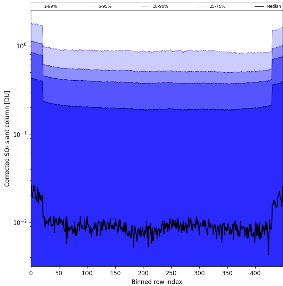
Figure 86: Along track statistics of “Corrected SO 2 slant column” for 2025-06-06 to 2025-06-08
