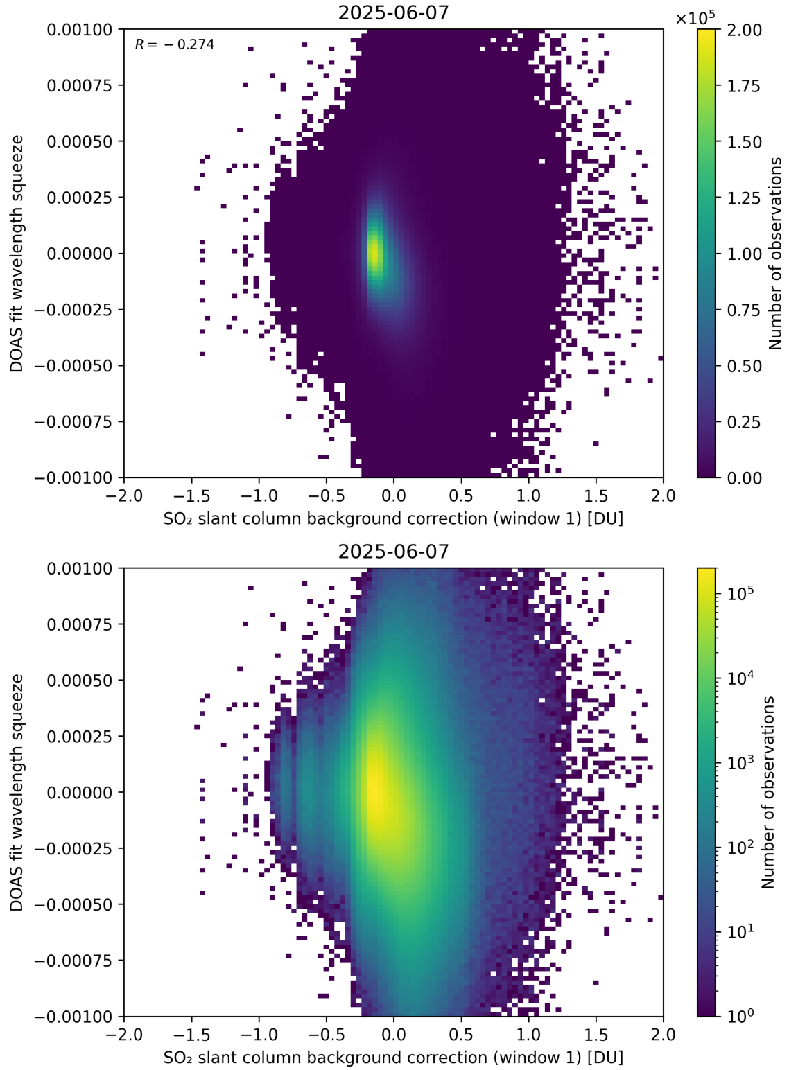
Figure 112: Scatter density plot of “SO 2 slant column background correction (window 1)” against “DOAS fit wavelength squeeze” for 2025-06-06 to 2025-06-08.
