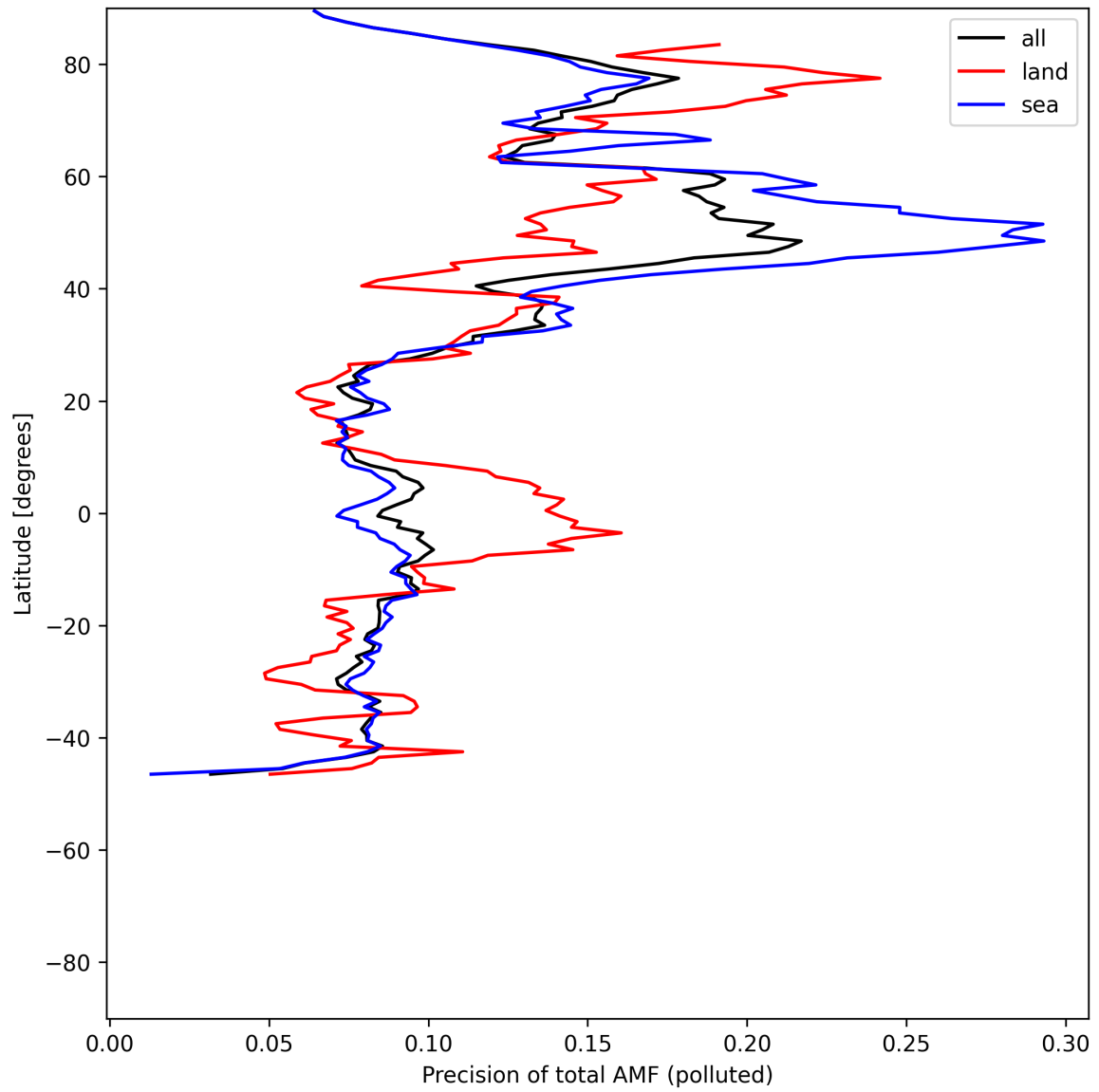
Figure 54: Zonal average of “Precision of total AMF (polluted)” for 2025-06-06 to 2025-06-08.
