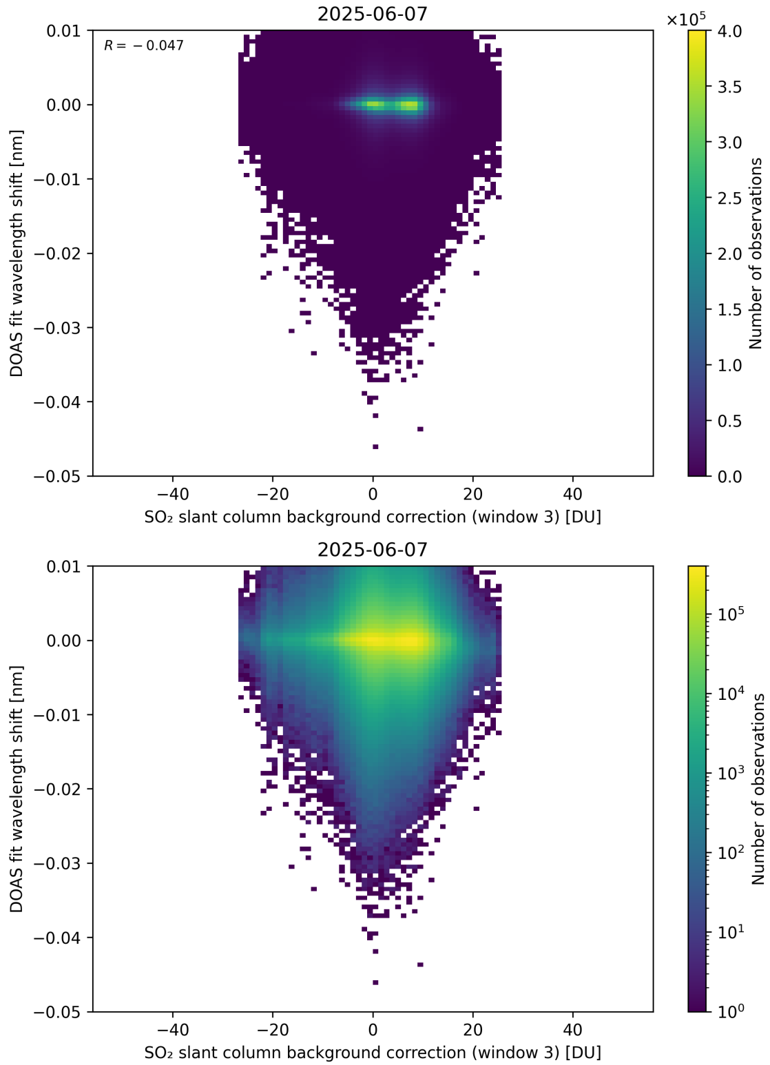
Figure 132: Scatter density plot of “SO 2 slant column background correction (window 3)” against “DOAS fit wavelength shift” for 2025-06-06 to 2025-06-08.
