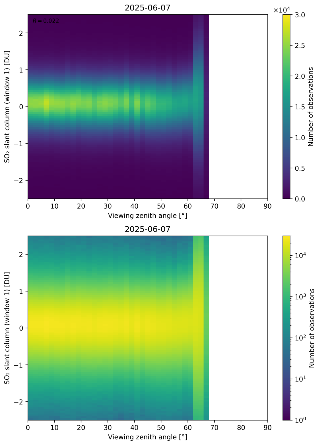
Figure 376: Scatter density plot of “Viewing zenith angle” against “SO 2 slant column (window 1)” for 2025-06-06 to 2025-06-08.
