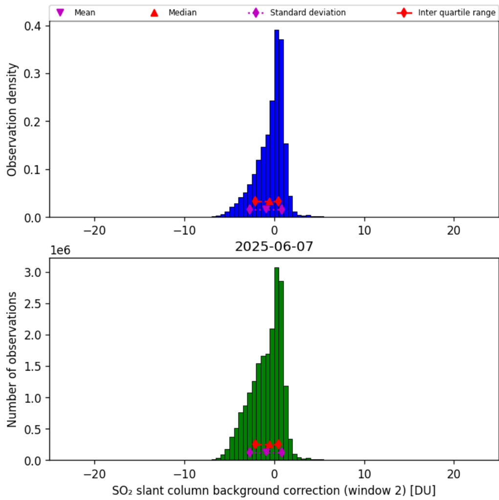
Figure 70: Histogram of “SO 2 slant column background correction (window 2)” for 2025-06-06 to 2025-06-08
