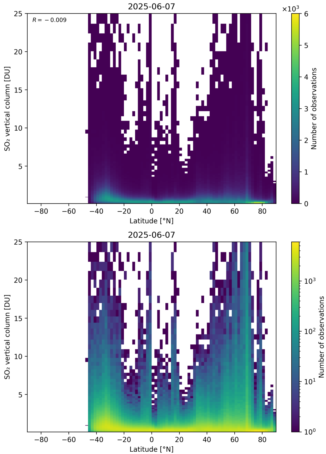
Figure 169: Scatter density plot of “Latitude” against “SO 2 vertical column” for 2025-06-06 to 2025-06-08.
