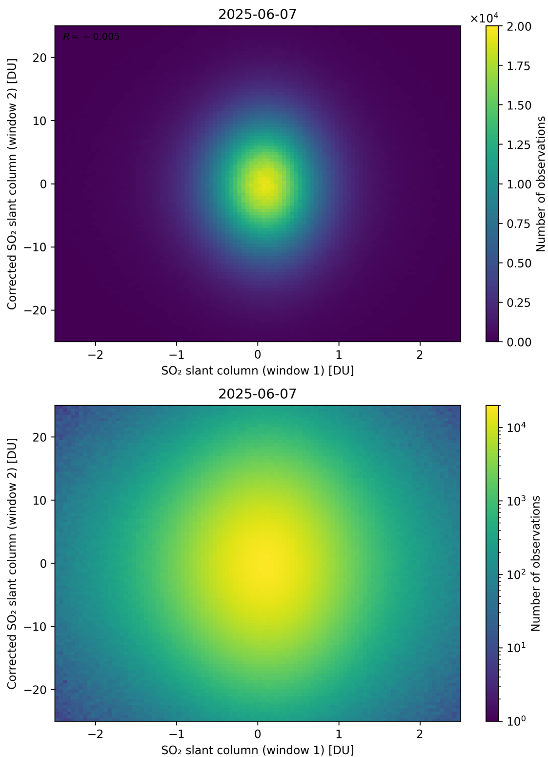
Figure 283: Scatter density plot of “SO 2 slant column (window 1)” against “Corrected SO 2 slant column (window 2)” for 2025-06-06 to 2025-06-08.
