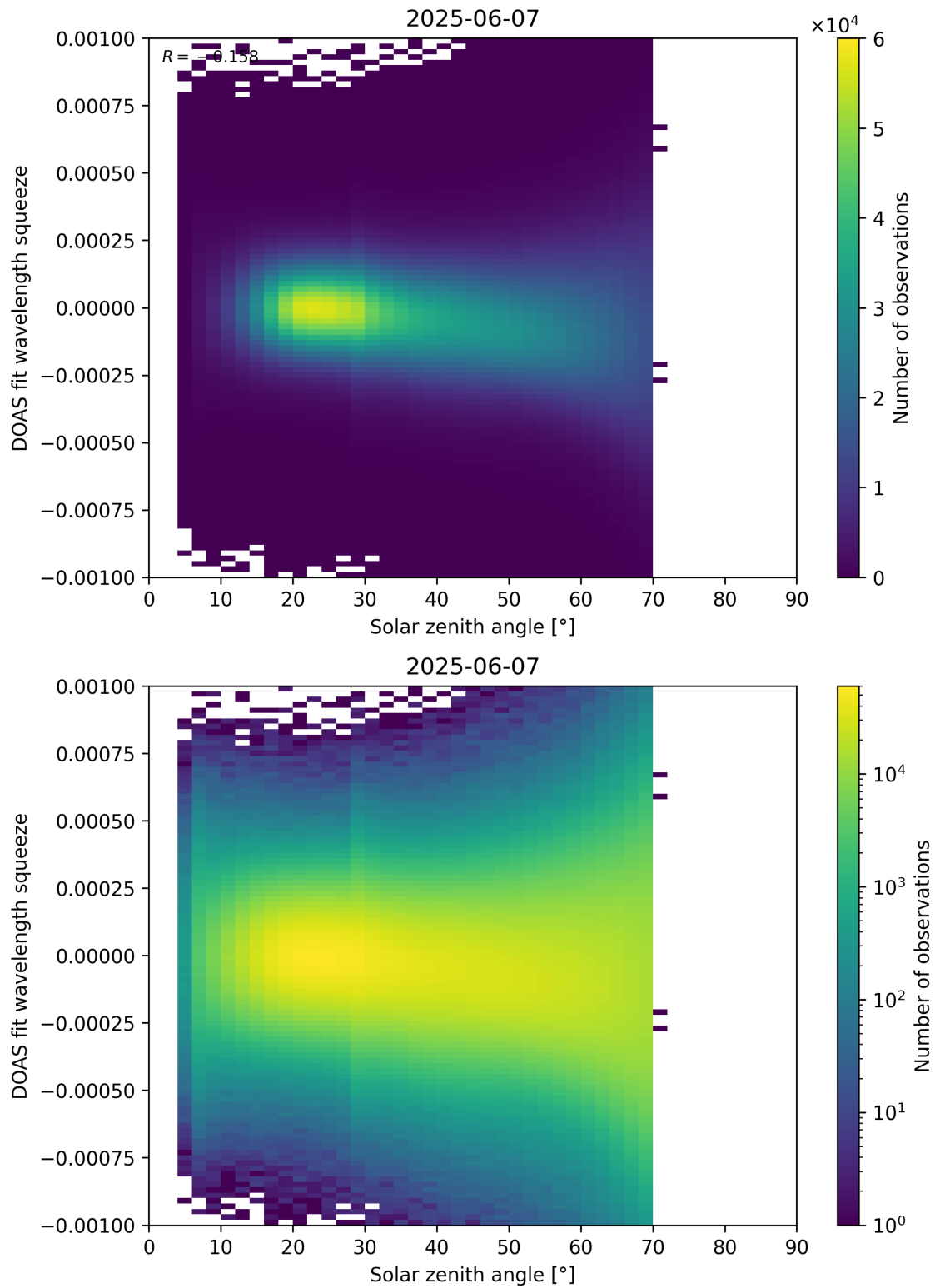
Figure 175: Scatter density plot of “Solar zenith angle” against “DOAS fit wavelength squeeze” for 2025-06-06 to 2025-06-08.
