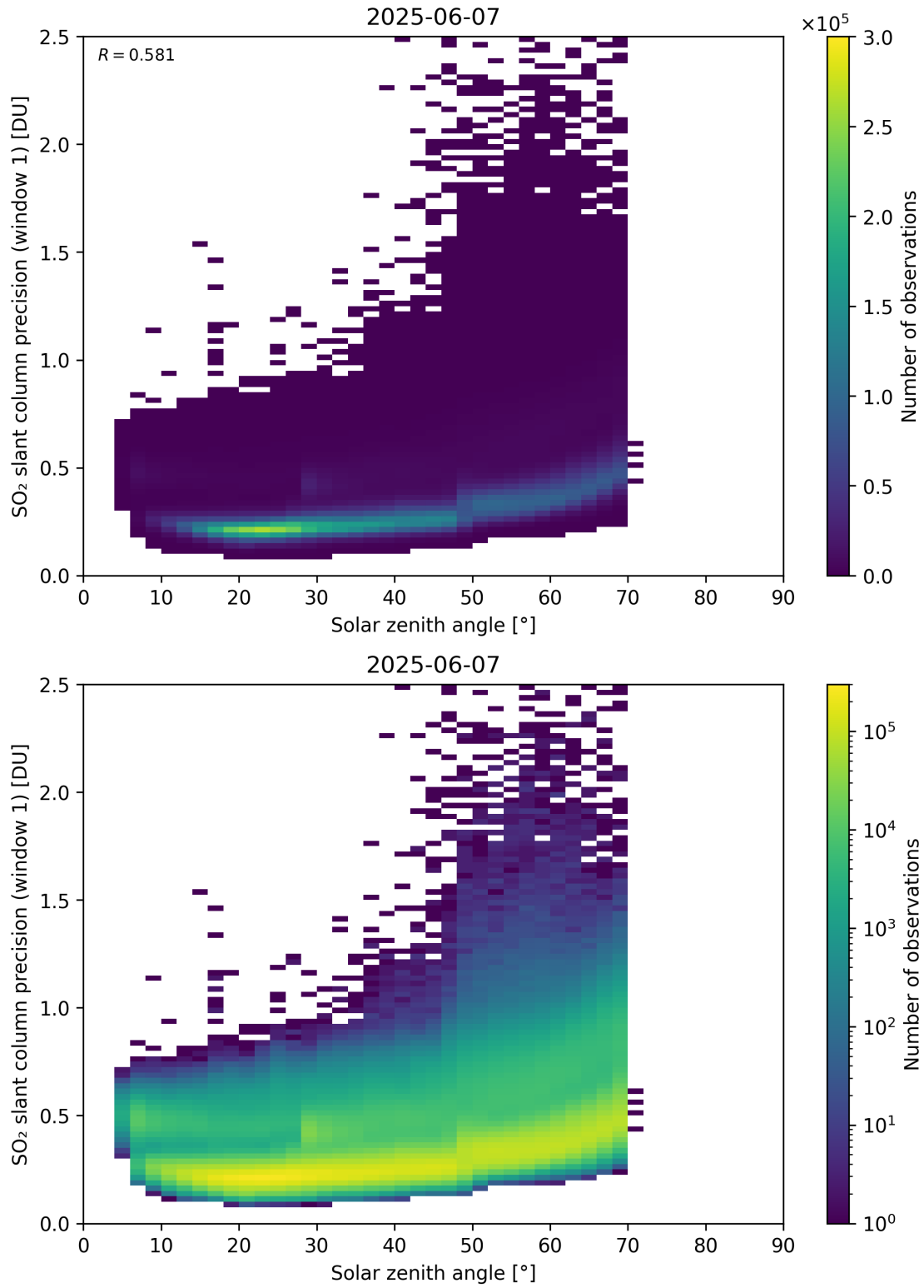
Figure 185: Scatter density plot of “Solar zenith angle” against “SO 2 slant column precision (window 1)” for 2025-06-06 to 2025-06-08.
