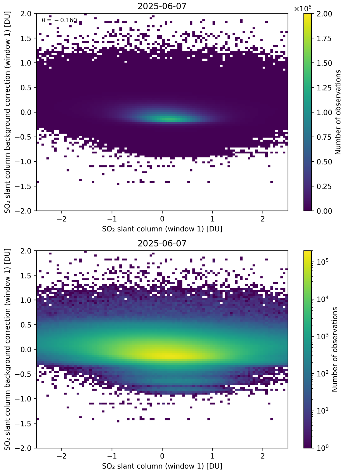
Figure 262: Scatter density plot of “SO 2 slant column (window 1)” against “SO 2 slant column background correction (window 1)” for 2025-06-06 to 2025-06-08.
