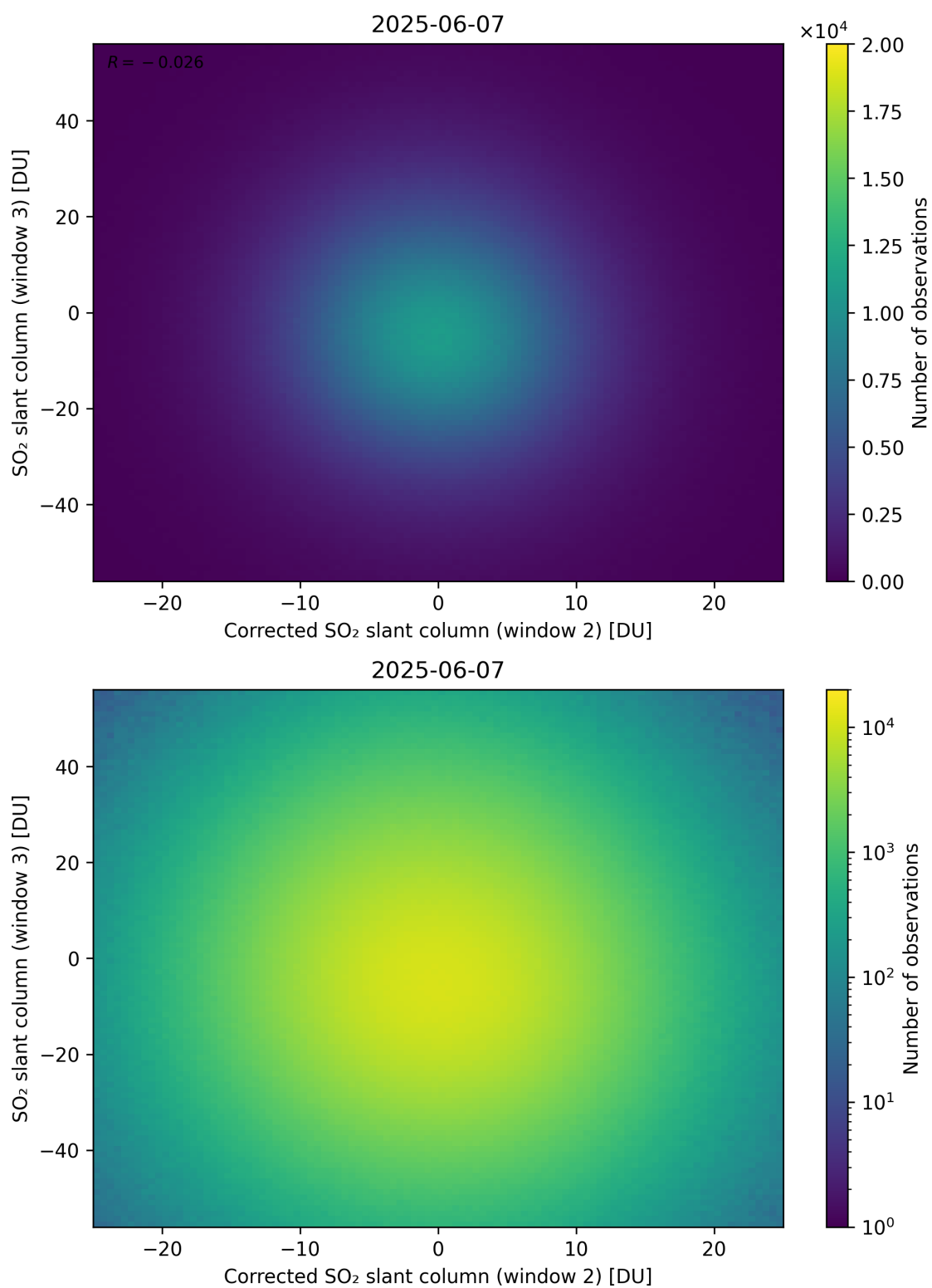
Figure 251: Scatter density plot of “Corrected SO 2 slant column (window 2)” against “SO 2 slant column (window 3)” for 2025-06-06 to 2025-06-08.
