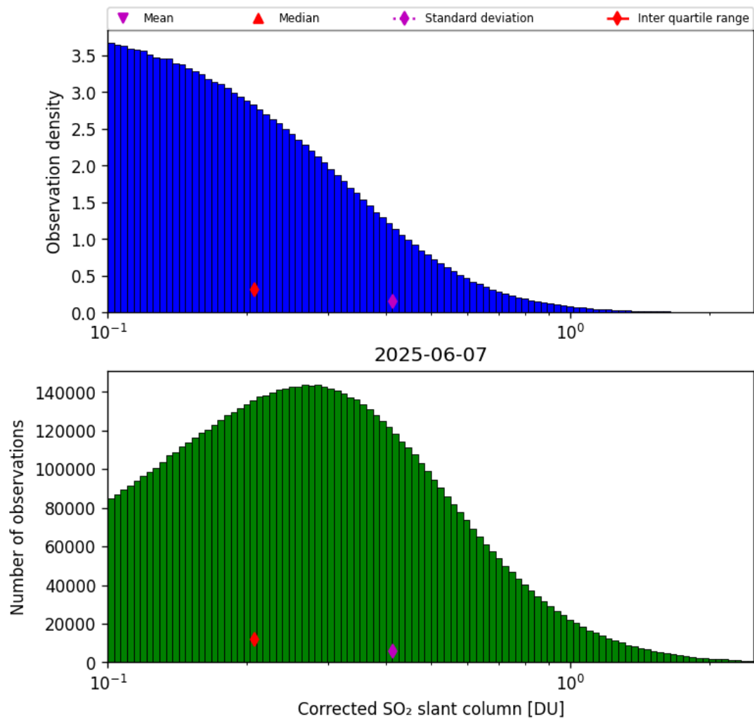
Figure 60: Histogram of “Corrected SO 2 slant column” for 2025-06-06 to 2025-06-08
