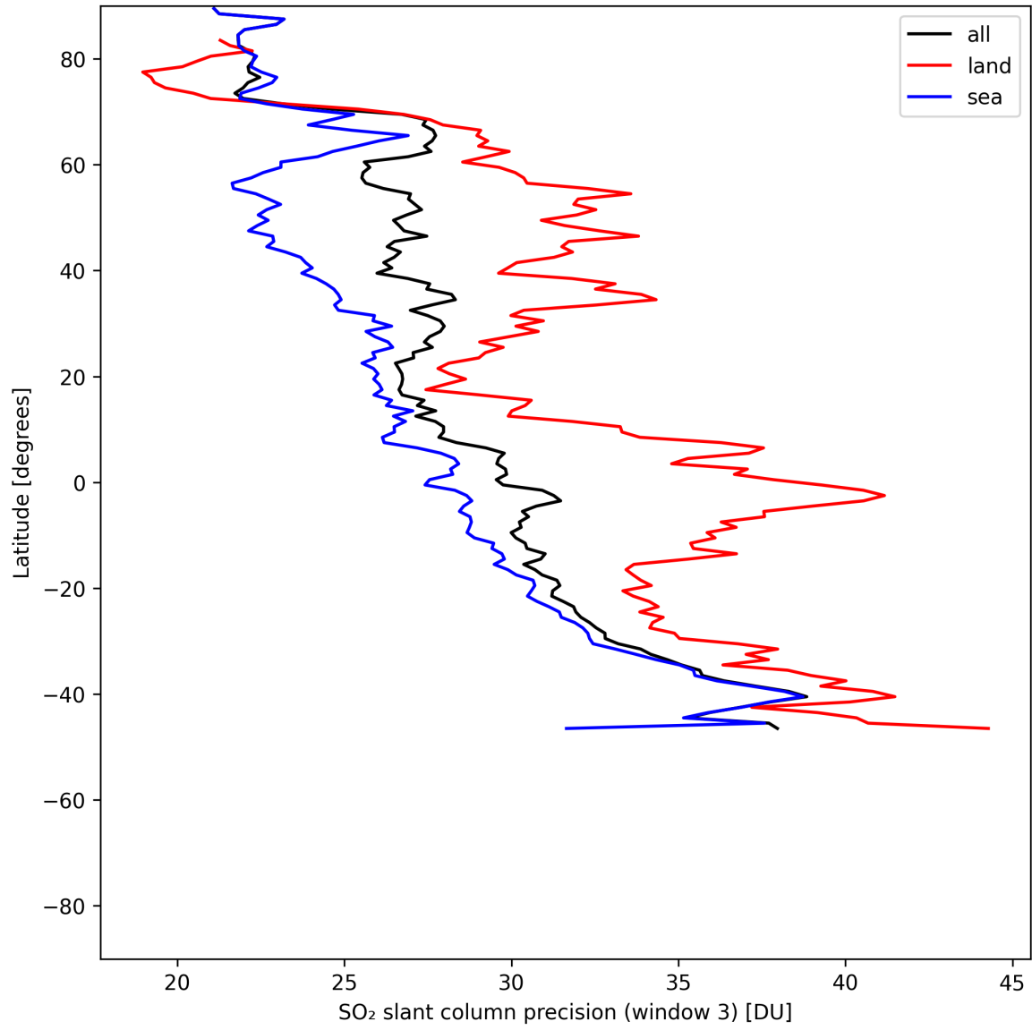
Figure 46: Zonal average of “SO 2 slant column precision (window 3)” for 2025-06-06 to 2025-06-08.
