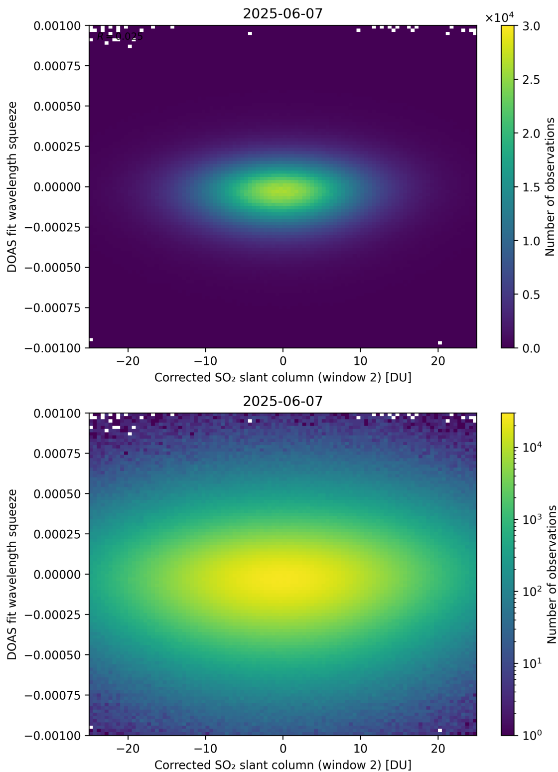
Figure 247: Scatter density plot of “Corrected SO 2 slant column (window 2)” against “DOAS fit wavelength squeeze” for 2025-06-06 to 2025-06-08.
