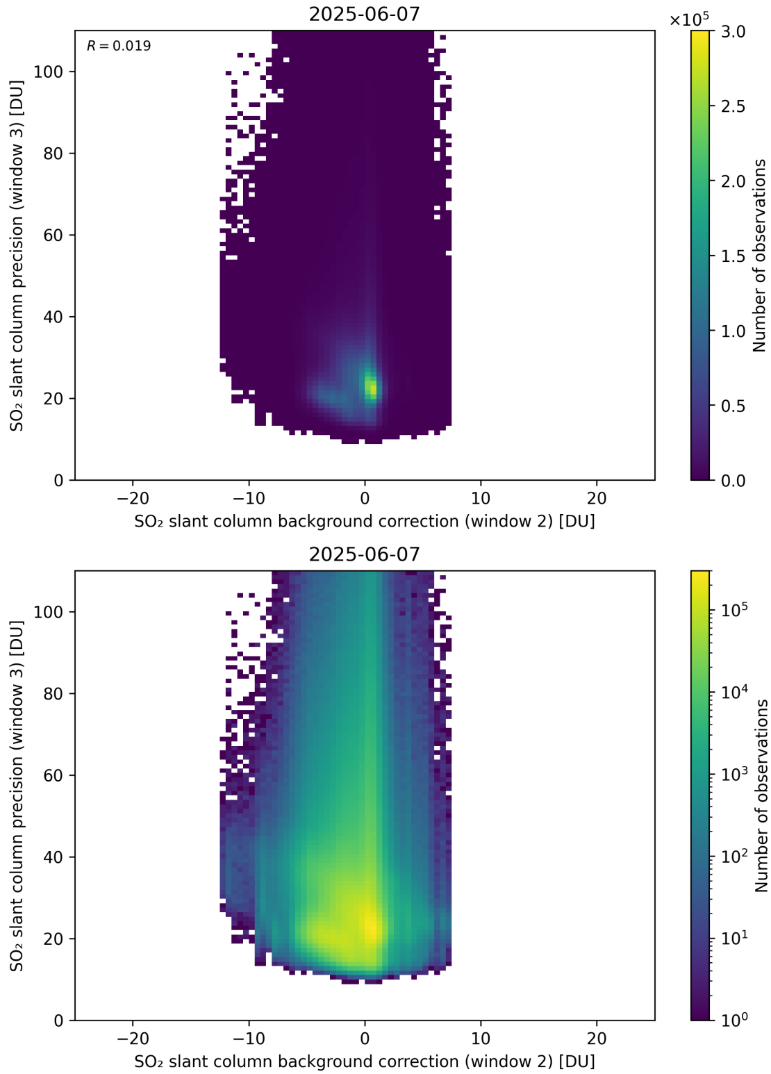
Figure 129: Scatter density plot of “SO 2 slant column background correction (window 2)” against “SO 2 slant column precision (window 3)” for 2025-06-06 to 2025-06-08.
