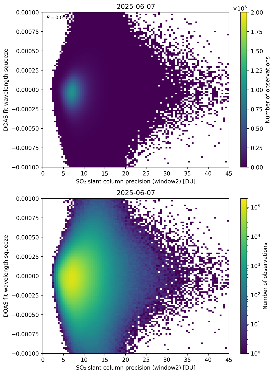
Figure 294: Scatter density plot of “SO 2 slant column precision (window2)” against “DOAS fit wavelength squeeze” for 2025-06-06 to 2025-06-08.
