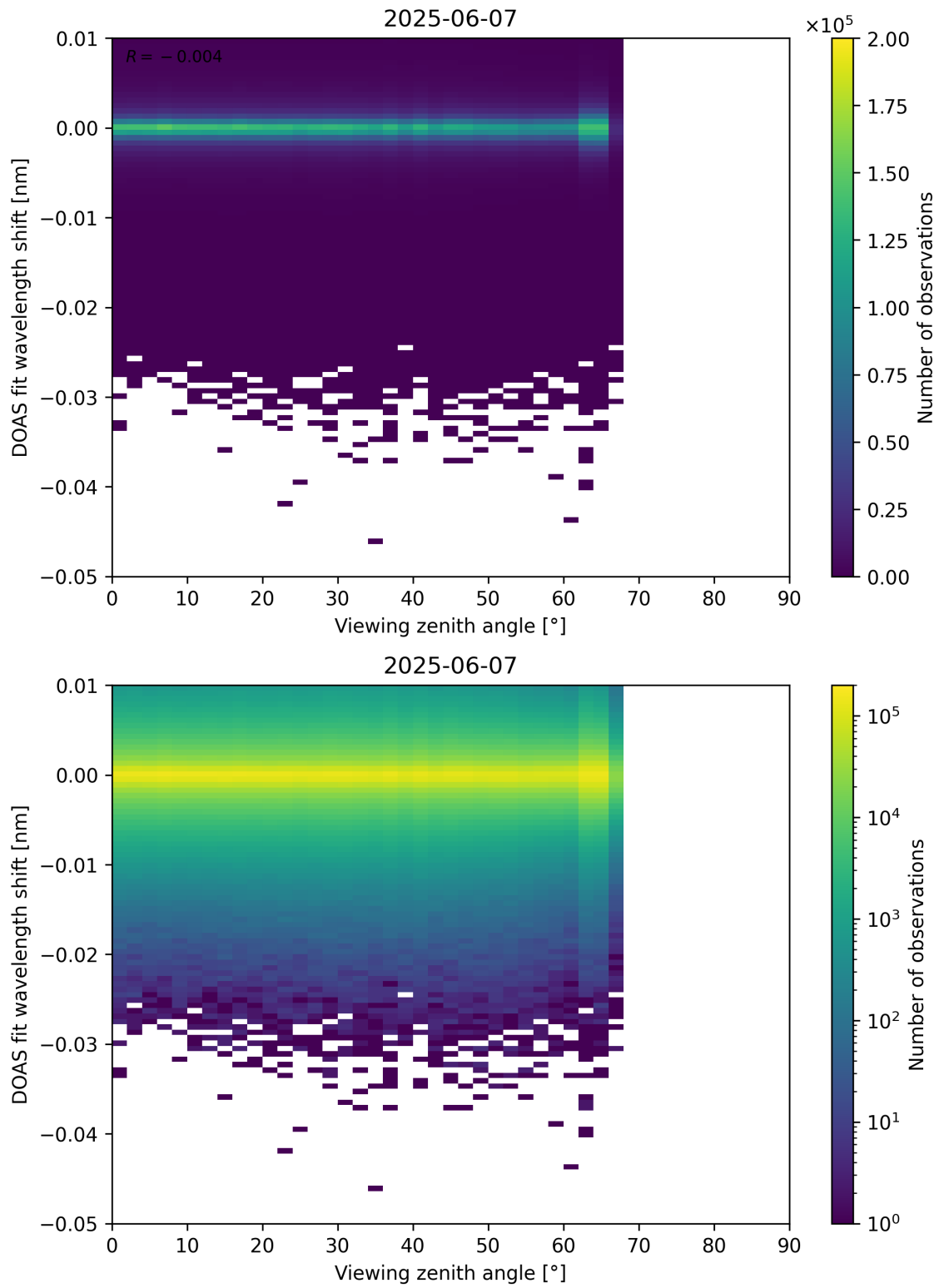
Figure 365: Scatter density plot of “Viewing zenith angle” against “DOAS fit wavelength shift” for 2025-06-06 to 2025-06-08.
