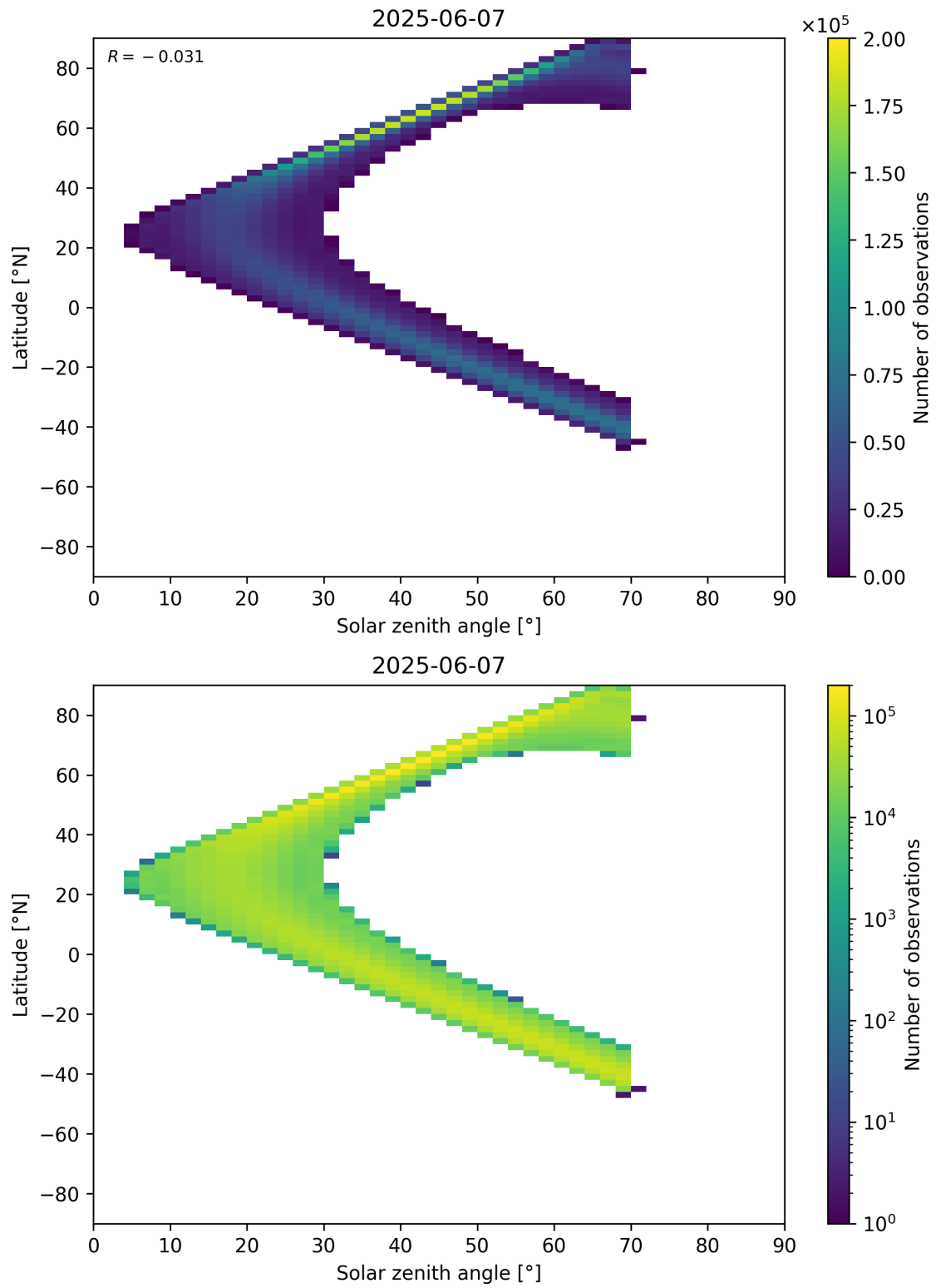
Figure 177: Scatter density plot of “Solar zenith angle” against “Latitude” for 2025-06-06 to 2025-06-08.
