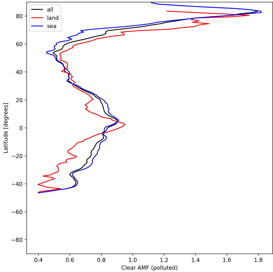
Figure 55: Zonal average of “Clear AMF (polluted)” for 2025-06-06 to 2025-06-08.
