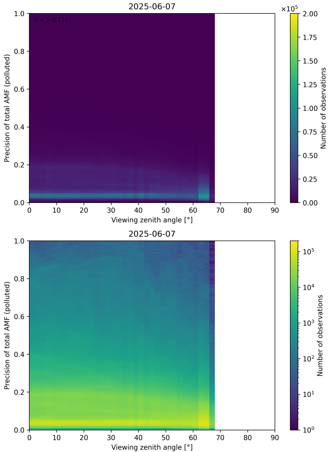
Figure 382: Scatter density plot of “Viewing zenith angle” against “Precision of total AMF (polluted)” for 2025-06-06 to 2025-06-08.
