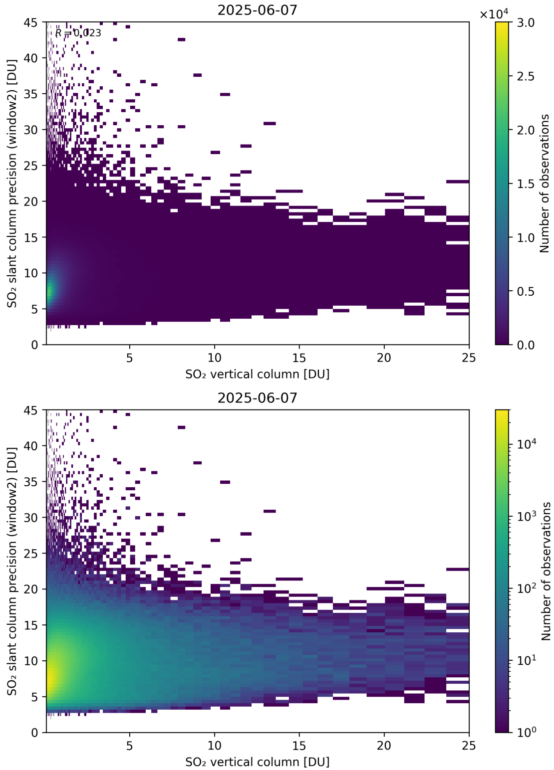
Figure 356: Scatter density plot of “SO 2 vertical column” against “SO 2 slant column precision (window2)” for 2025-06-06 to 2025-06-08.
