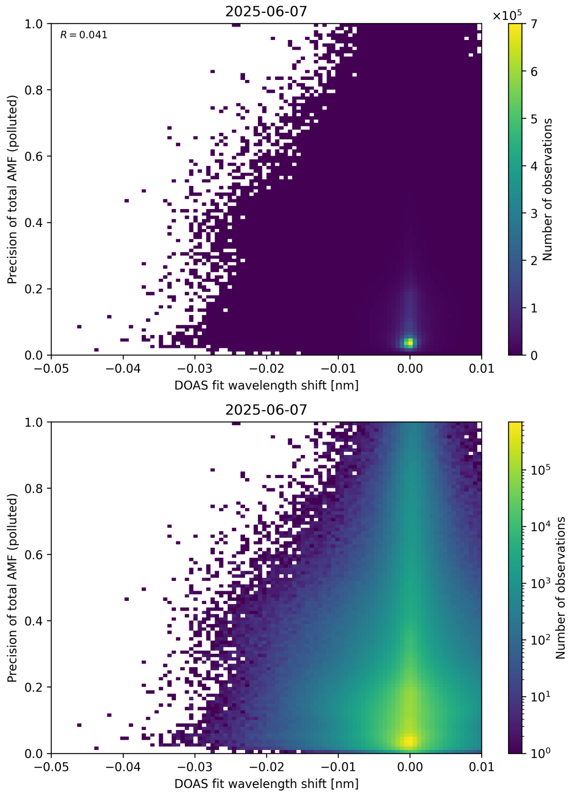
Figure 142: Scatter density plot of “DOAS fit wavelength shift” against “Precision of total AMF (polluted)” for 2025-06-06 to 2025-06-08.
