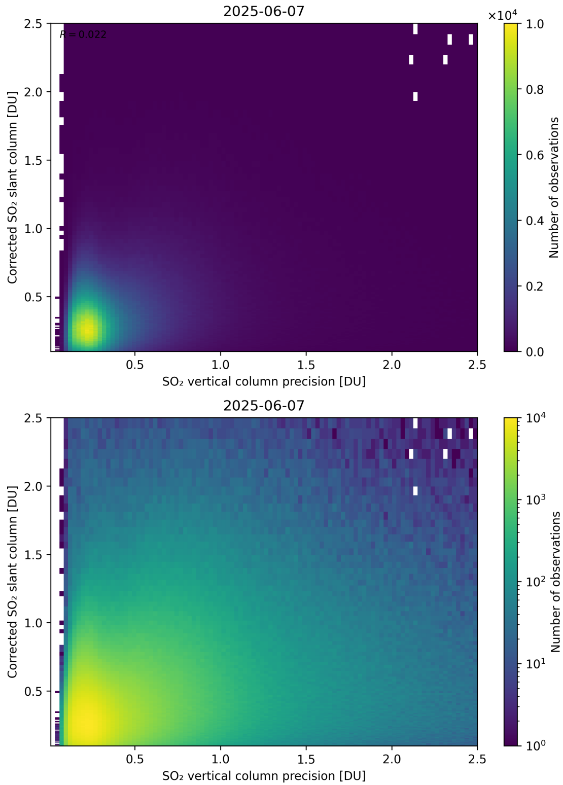
Figure 338: Scatter density plot of “SO 2 vertical column precision” against “Corrected SO 2 slant column” for 2025-06-06 to 2025-06-08.
