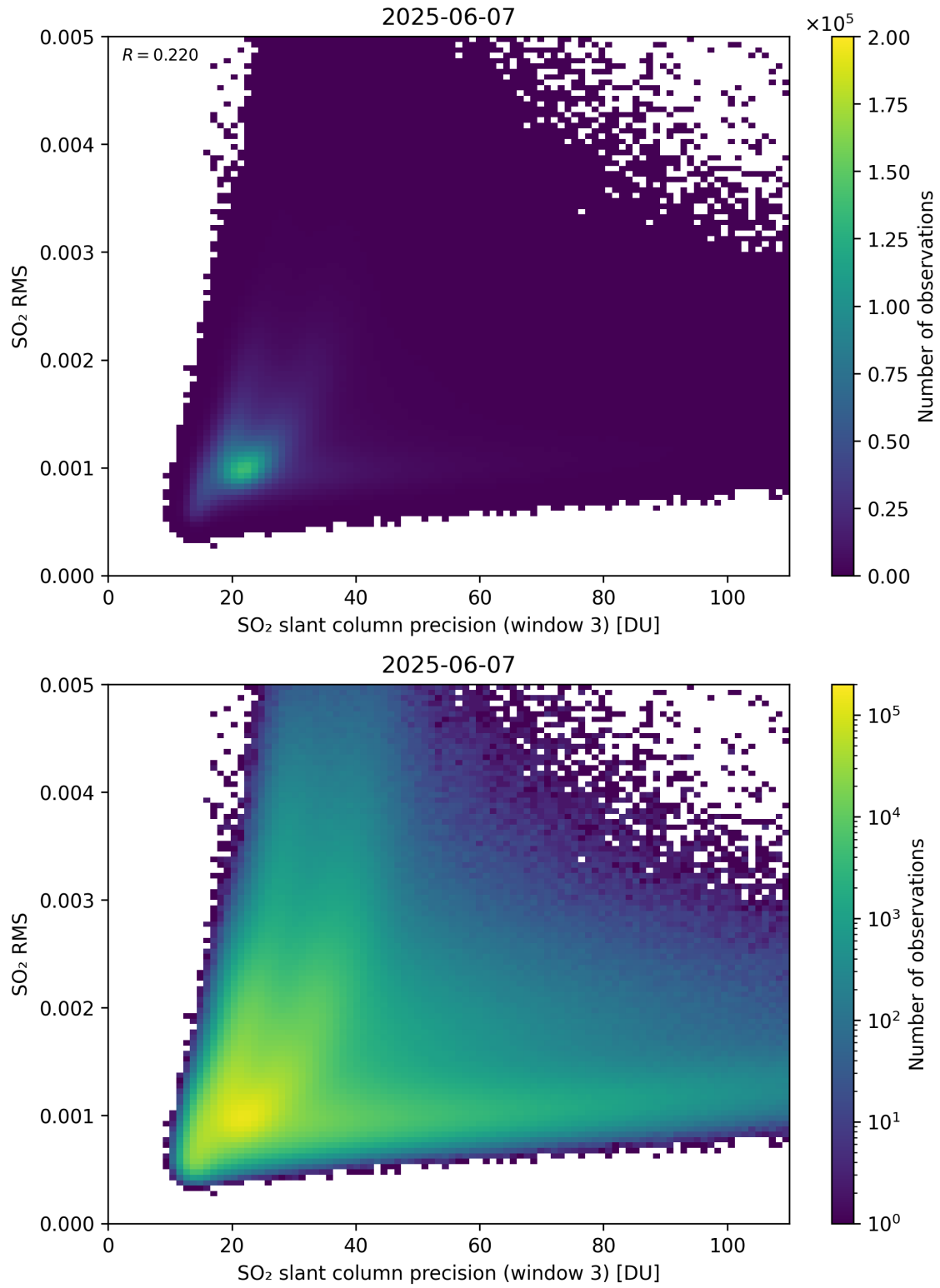
Figure 310: Scatter density plot of “SO 2 slant column precision (window 3)” against “SO 2 RMS” for 2025-06-06 to 2025-06-08.
