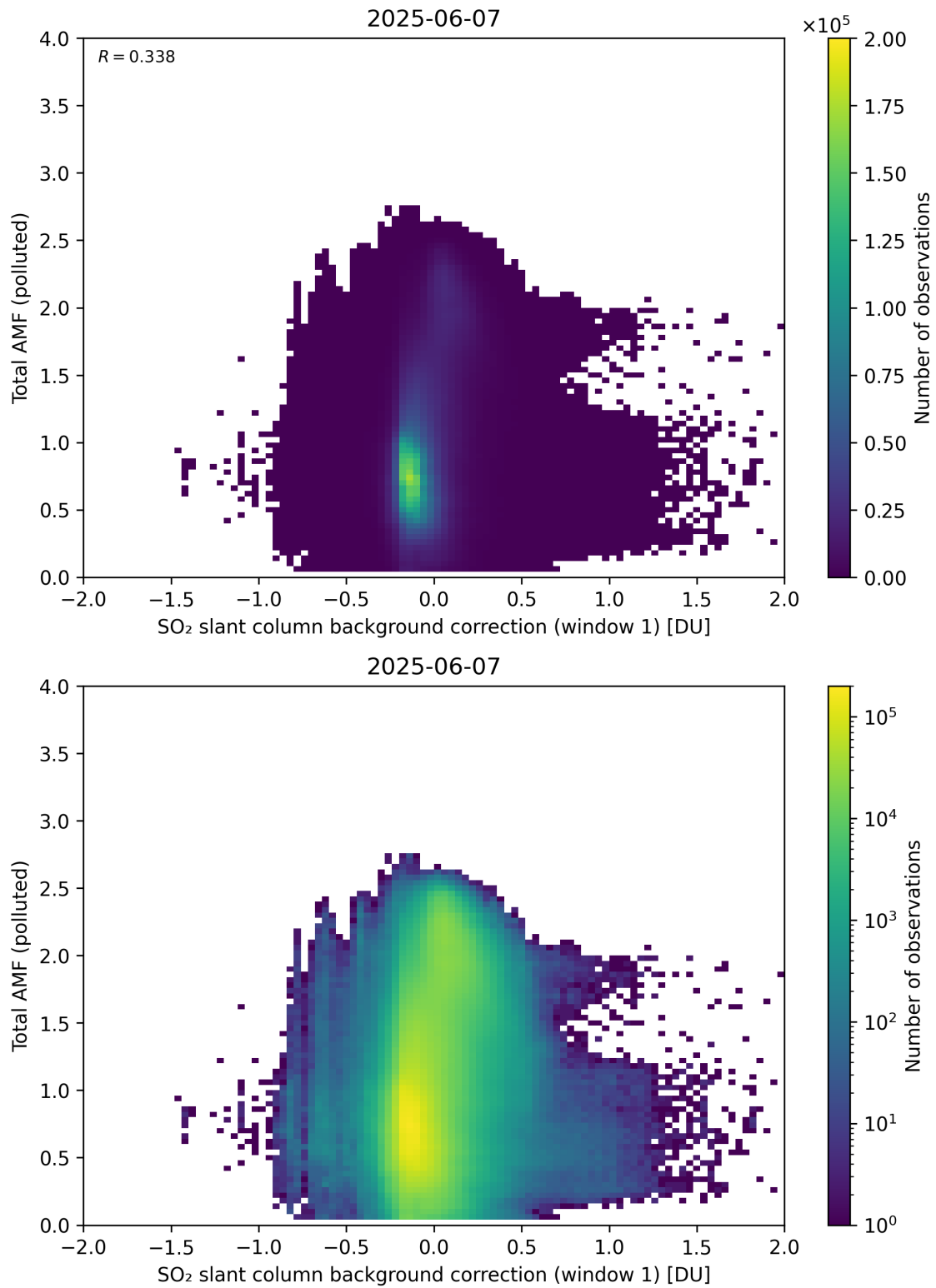
Figure 120: Scatter density plot of “SO 2 slant column background correction (window 1)” against “Total AMF (polluted)” for 2025-06-06 to 2025-06-08.
