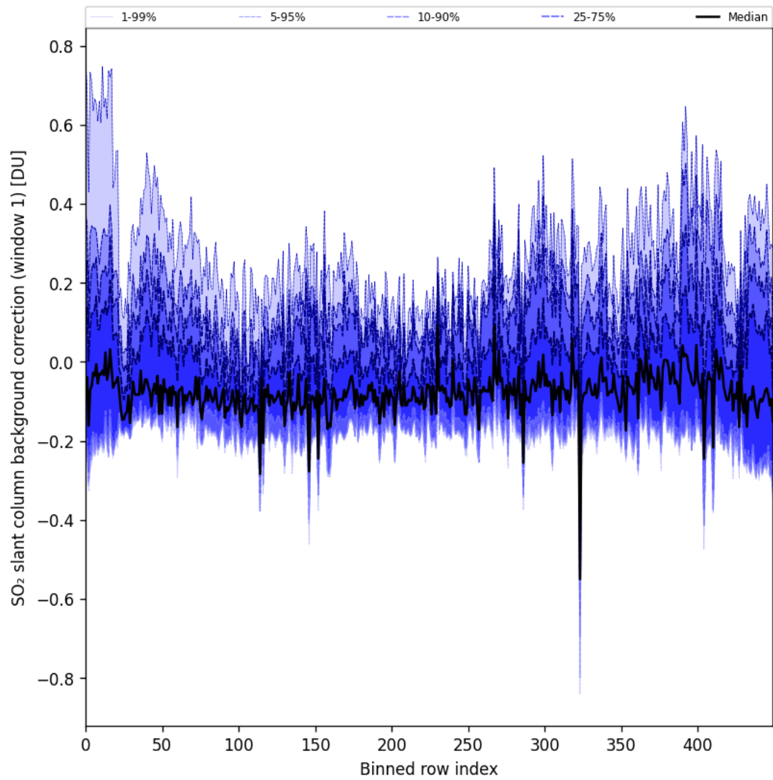
Figure 92: Along track statistics of “SO 2 slant column background correction (window 1)” for 2025-06-06 to 2025-06-08
