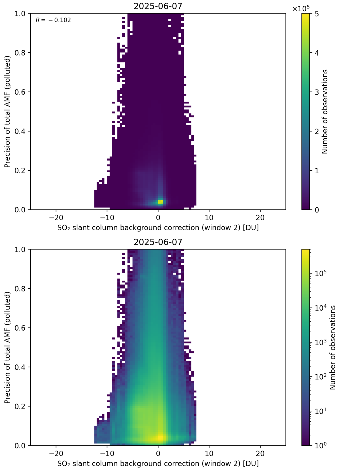
Figure 131: Scatter density plot of “SO 2 slant column background correction (window 2)” against “Precision of total AMF (polluted)” for 2025-06-06 to 2025-06-08.
