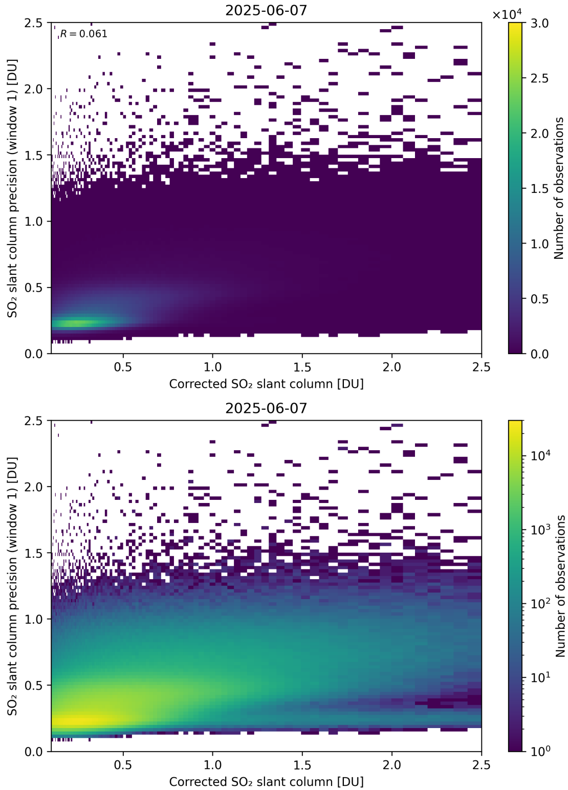
Figure 238: Scatter density plot of “Corrected SO 2 slant column” against “SO 2 slant column precision (window 1)” for 2025-06-06 to 2025-06-08.
