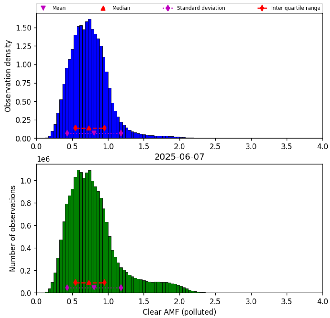
Figure 81: Histogram of “Clear AMF (polluted)” for 2025-06-06 to 2025-06-08
