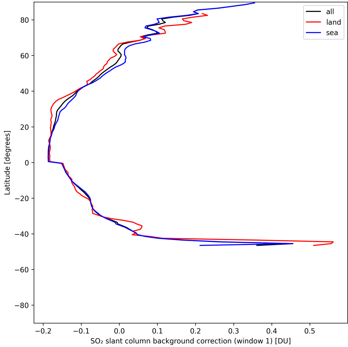
Figure 40: Zonal average of “SO 2 slant column background correction (window 1)” for 2025-06-06 to 2025-06-08.
