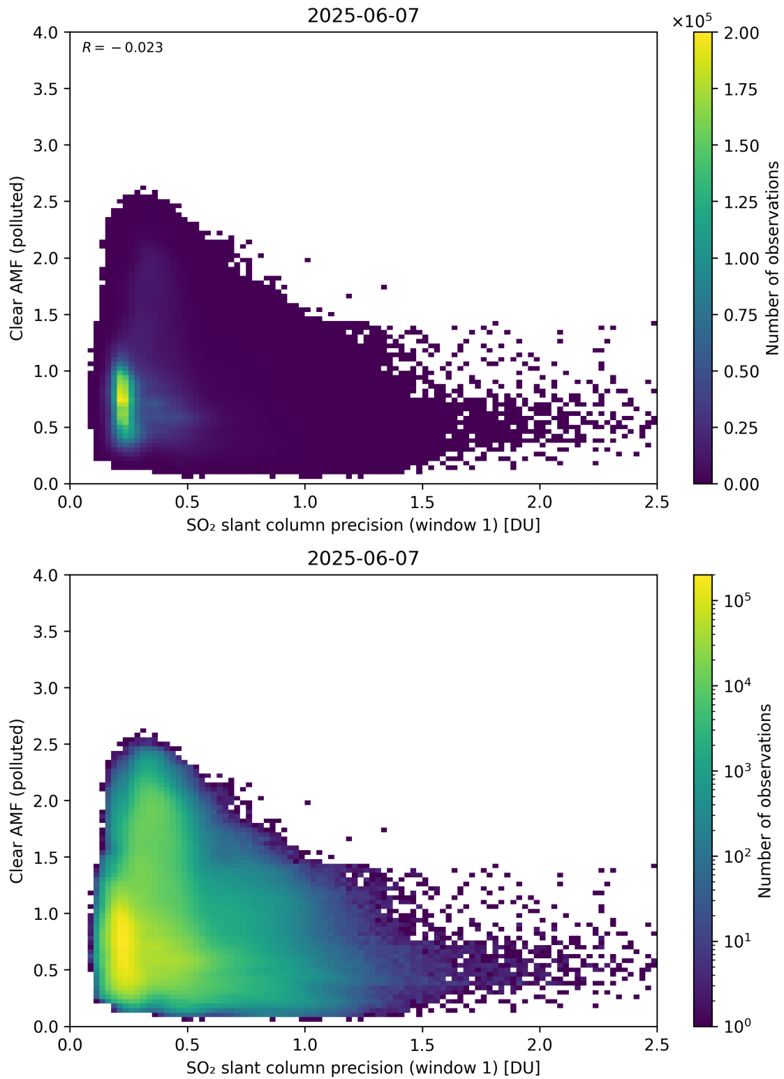
Figure 274: Scatter density plot of “SO 2 slant column precision (window 1)” against “Clear AMF (polluted)” for 2025-06-06 to 2025-06-08.
