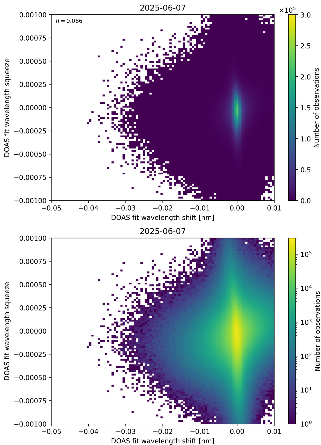
Figure 138: Scatter density plot of “DOAS fit wavelength shift” against “DOAS fit wavelength squeeze” for 2025-06-06 to 2025-06-08.
