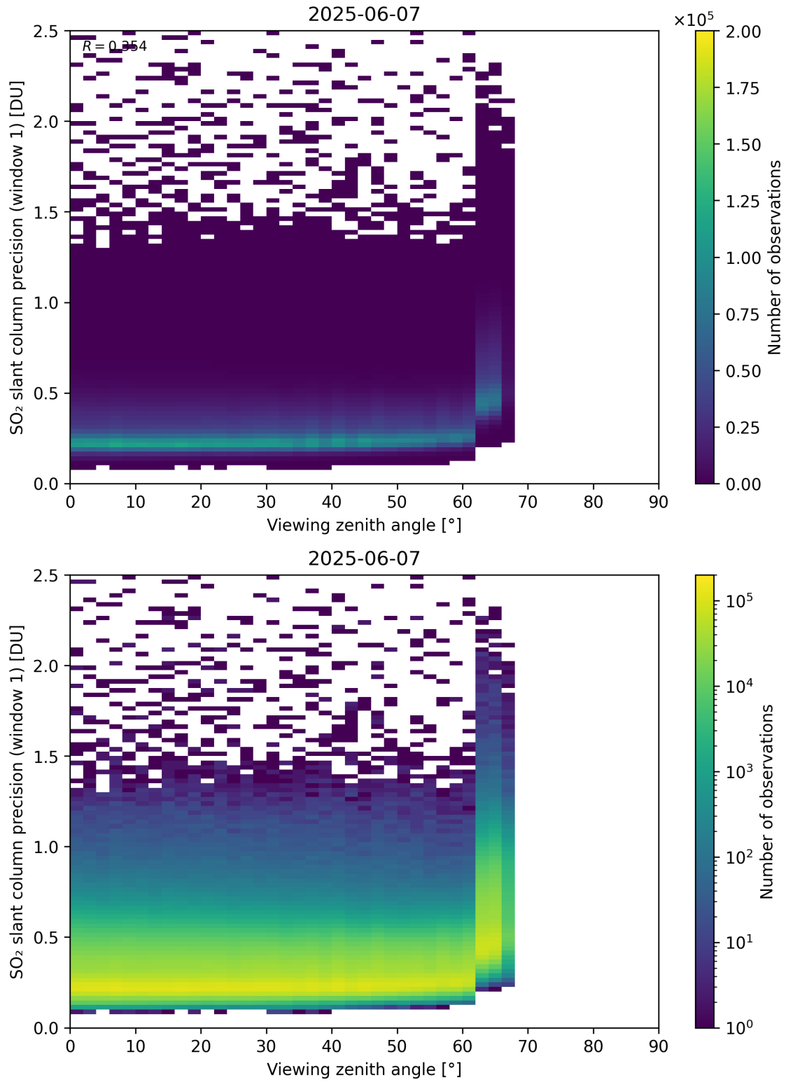
Figure 377: Scatter density plot of “Viewing zenith angle” against “SO 2 slant column precision (window 1)” for 2025-06-06 to 2025-06-08.
