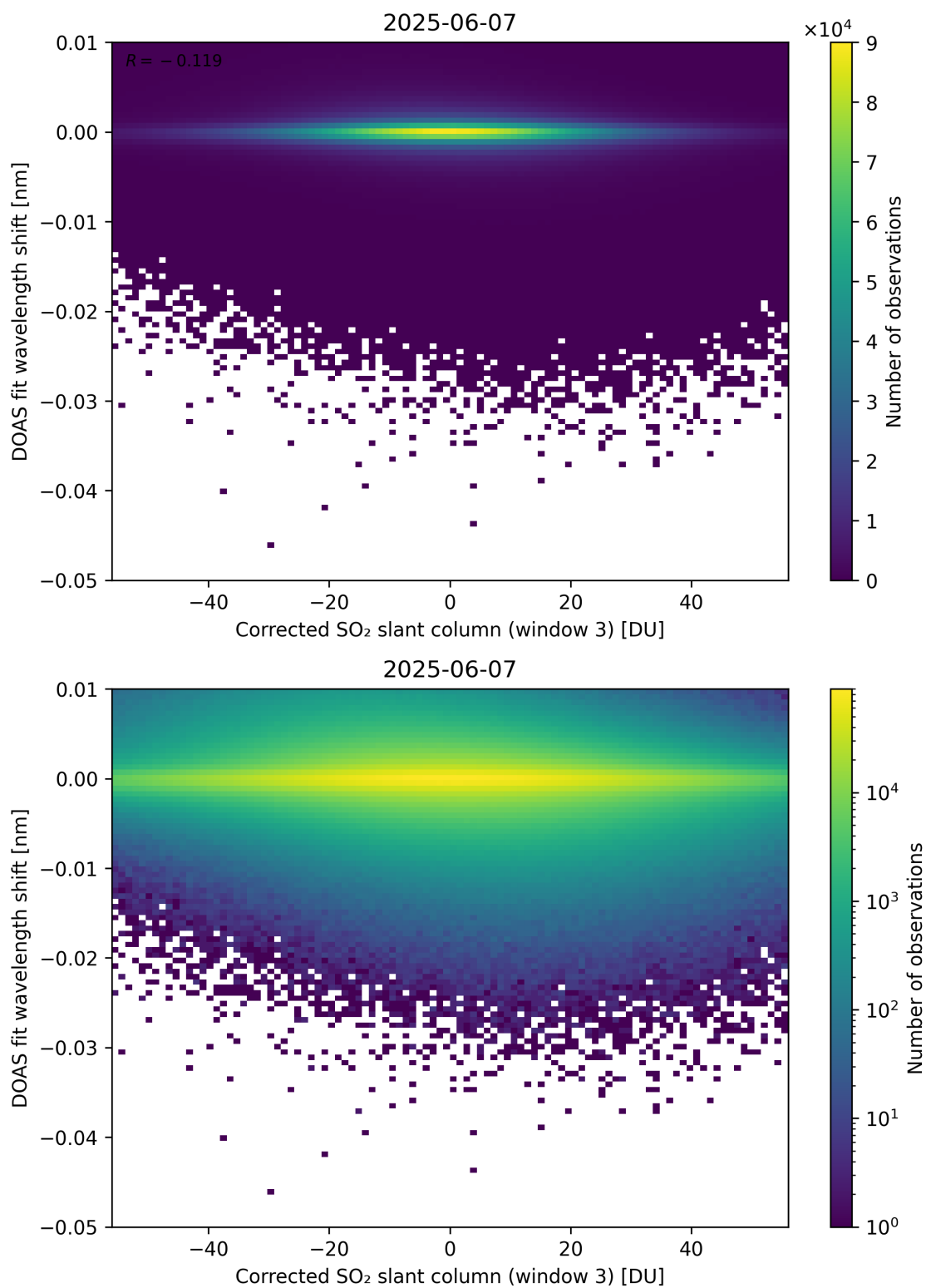
Figure 256: Scatter density plot of “Corrected SO 2 slant column (window 3)” against “DOAS fit wavelength shift” for 2025-06-06 to 2025-06-08.
