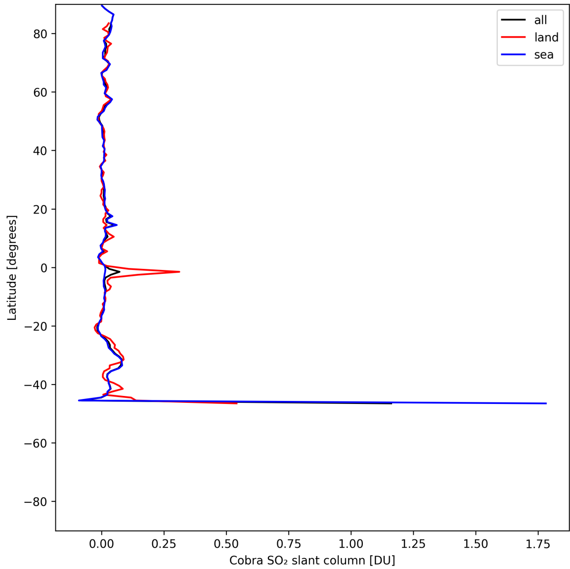
Figure 35: Zonal average of “Cobra SO 2 slant column” for 2025-06-06 to 2025-06-08.
