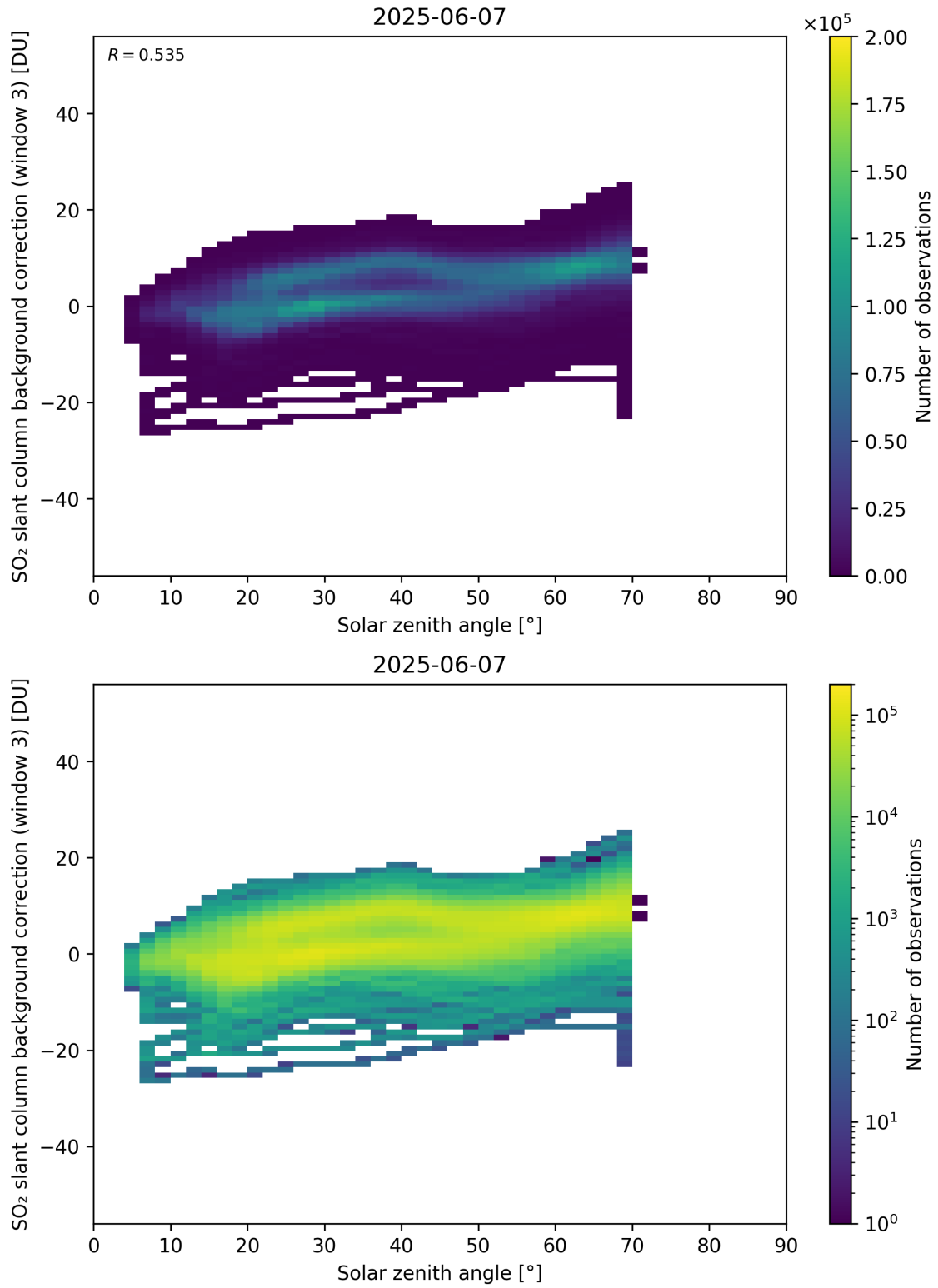
Figure 173: Scatter density plot of “Solar zenith angle” against “SO 2 slant column background correction (window 3)” for 2025-06-06 to 2025-06-08.
