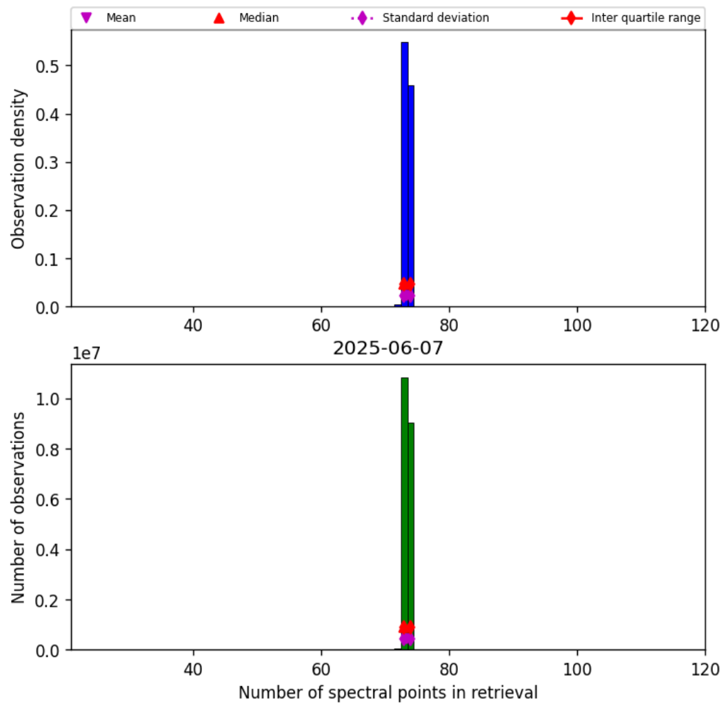
Figure 82: Histogram of “Number of spectral points in retrieval” for 2025-06-06 to 2025-06-08
