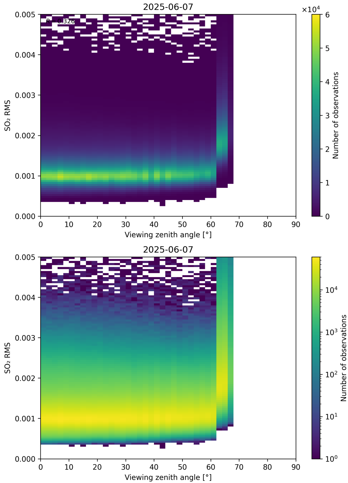
Figure 367: Scatter density plot of “Viewing zenith angle” against “SO 2 RMS” for 2025-06-06 to 2025-06-08.
