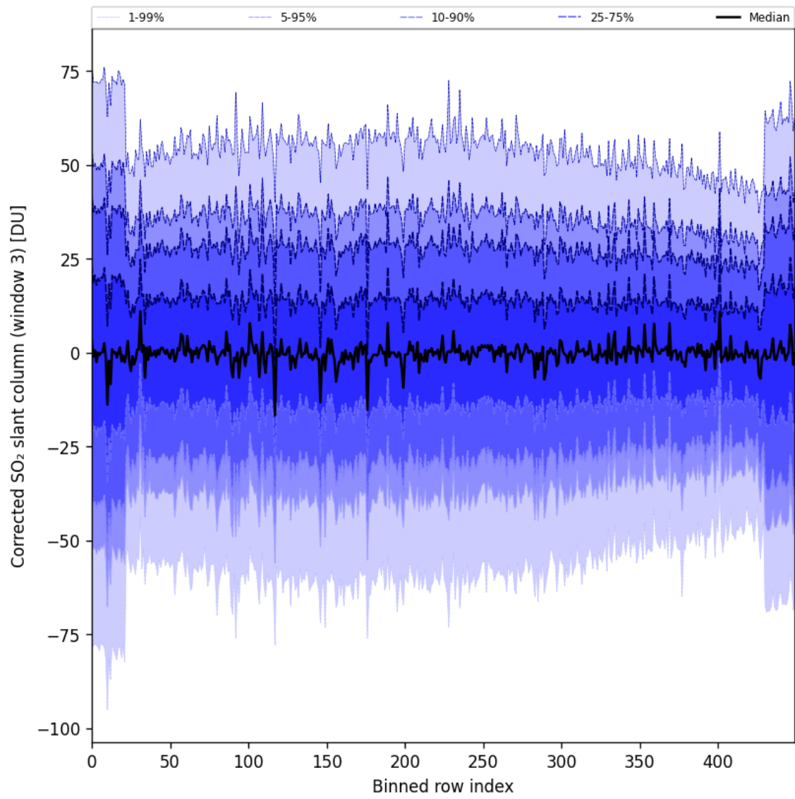
Figure 99: Along track statistics of “Corrected SO 2 slant column (window 3)” for 2025-06-06 to 2025-06-08
