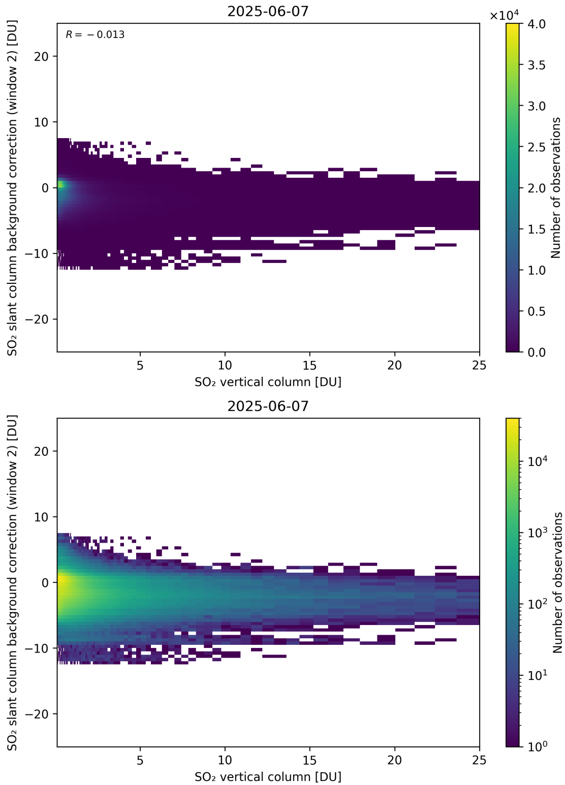
Figure 324: Scatter density plot of “SO 2 vertical column” against “SO 2 slant column background correction (window 2)” for 2025-06-06 to 2025-06-08.
