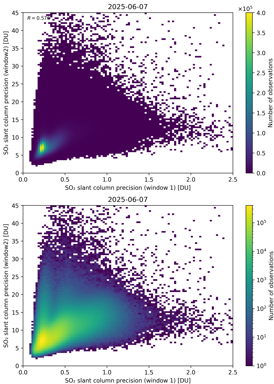
Figure 277: Scatter density plot of “SO 2 slant column precision (window 1)” against “SO 2 slant column precision (window2)” for 2025-06-06 to 2025-06-08.
