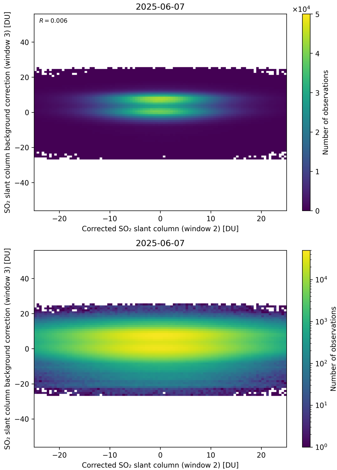
Figure 245: Scatter density plot of “Corrected SO 2 slant column (window 2)” against “SO 2 slant column background correction (window 3)” for 2025-06-06 to 2025-06-08.
