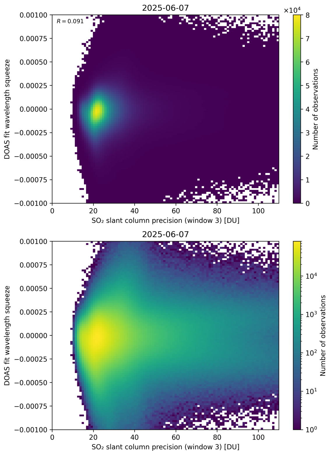
Figure 309: Scatter density plot of “SO 2 slant column precision (window 3)” against “DOAS fit wavelength squeeze” for 2025-06-06 to 2025-06-08.
