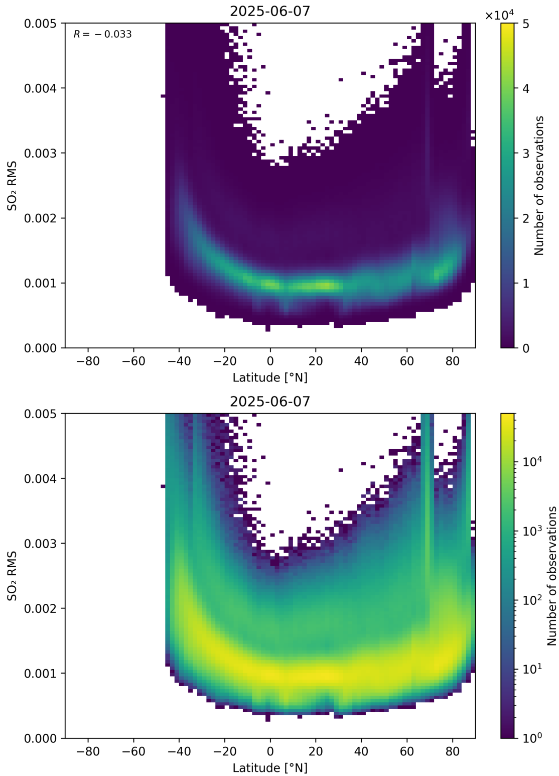
Figure 155: Scatter density plot of “Latitude” against “SO 2 RMS” for 2025-06-06 to 2025-06-08.
