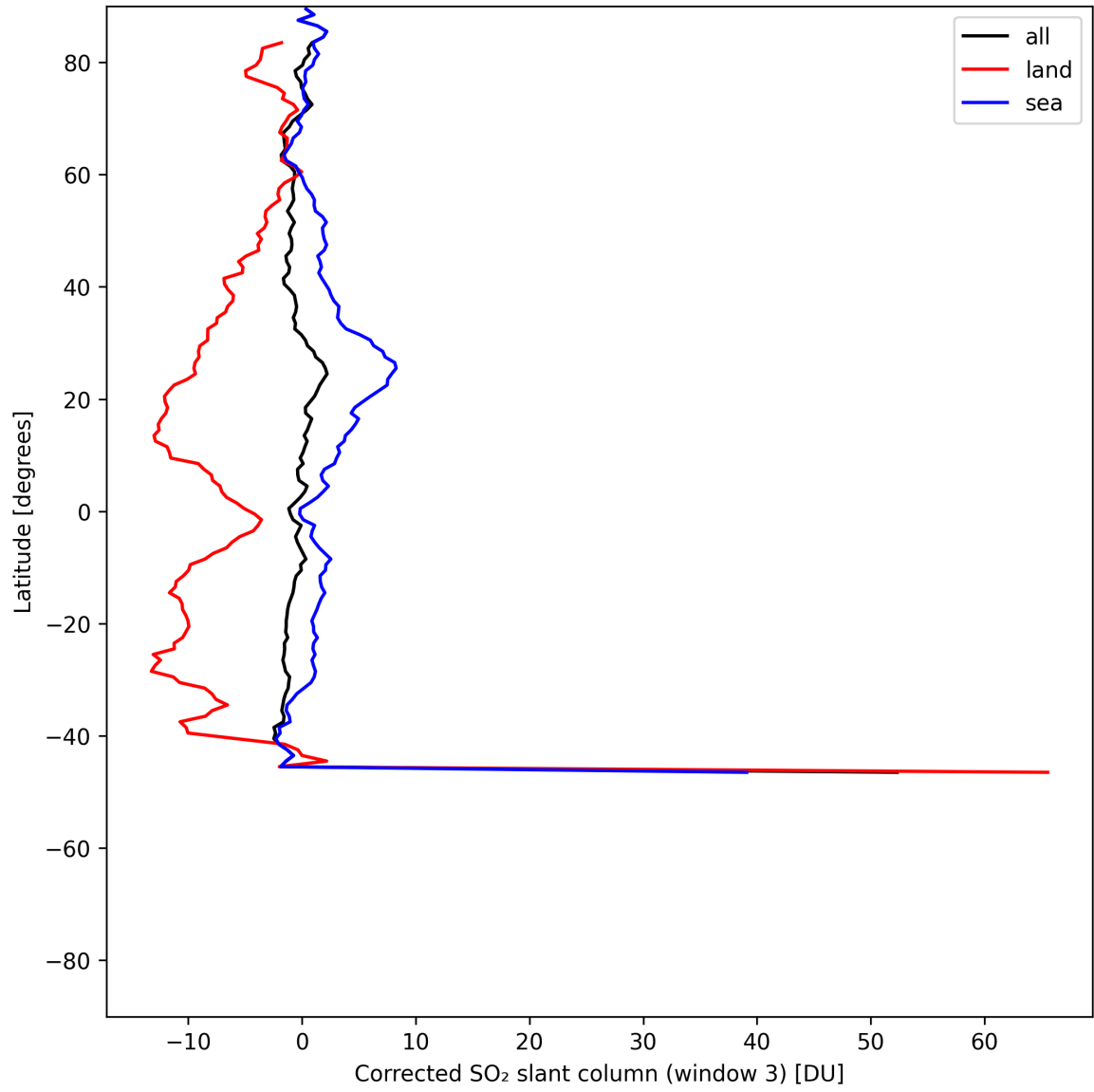
Figure 47: Zonal average of “Corrected SO 2 slant column (window 3)” for 2025-06-06 to 2025-06-08.
