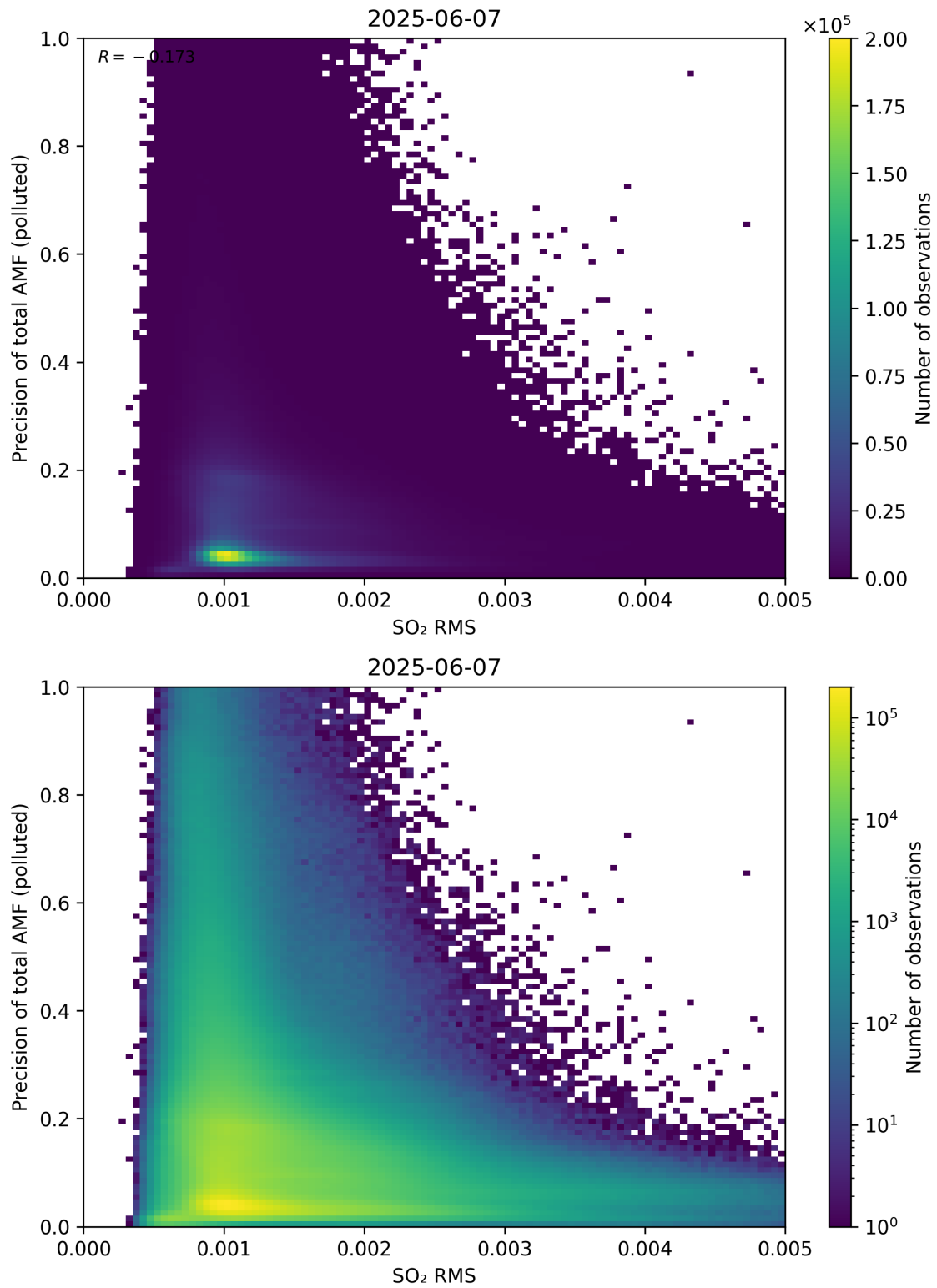
Figure 149: Scatter density plot of “SO 2 RMS” against “Precision of total AMF (polluted)” for 2025-06-06 to 2025-06-08.
