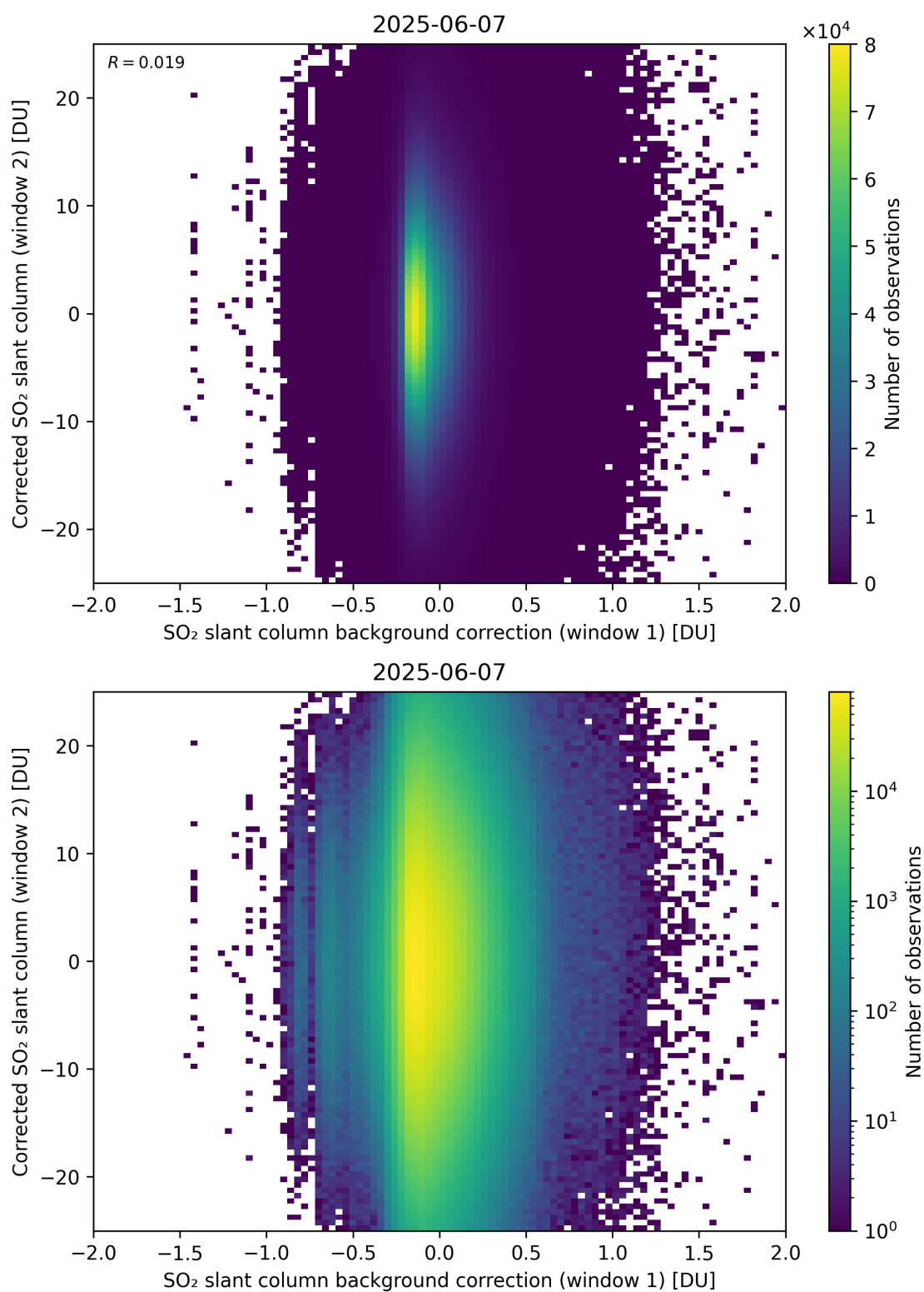
Figure 115: Scatter density plot of “SO 2 slant column background correction (window 1)” against “Corrected SO 2 slant column (window 2)” for 2025-06-06 to 2025-06-08.
