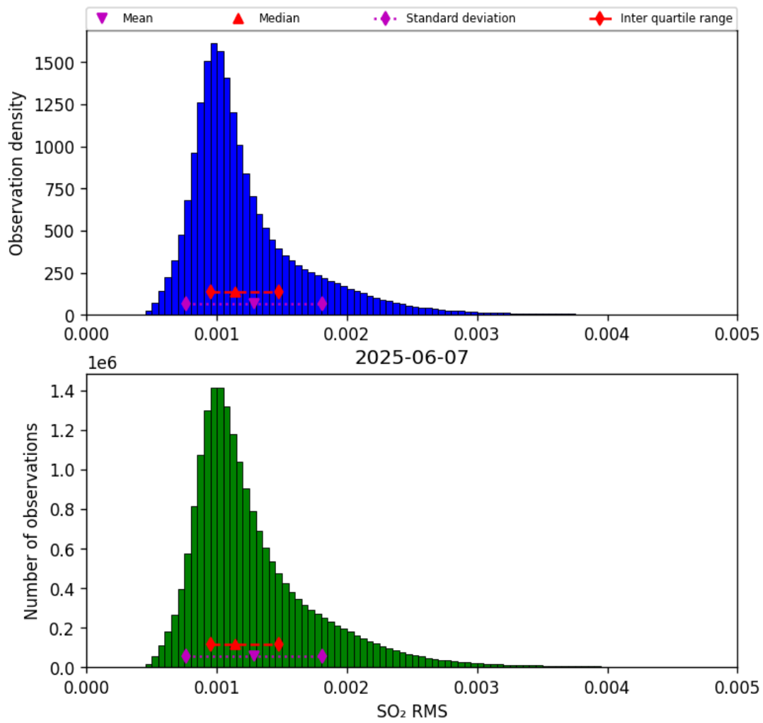
Figure 78: Histogram of “SO 2 RMS” for 2025-06-06 to 2025-06-08
