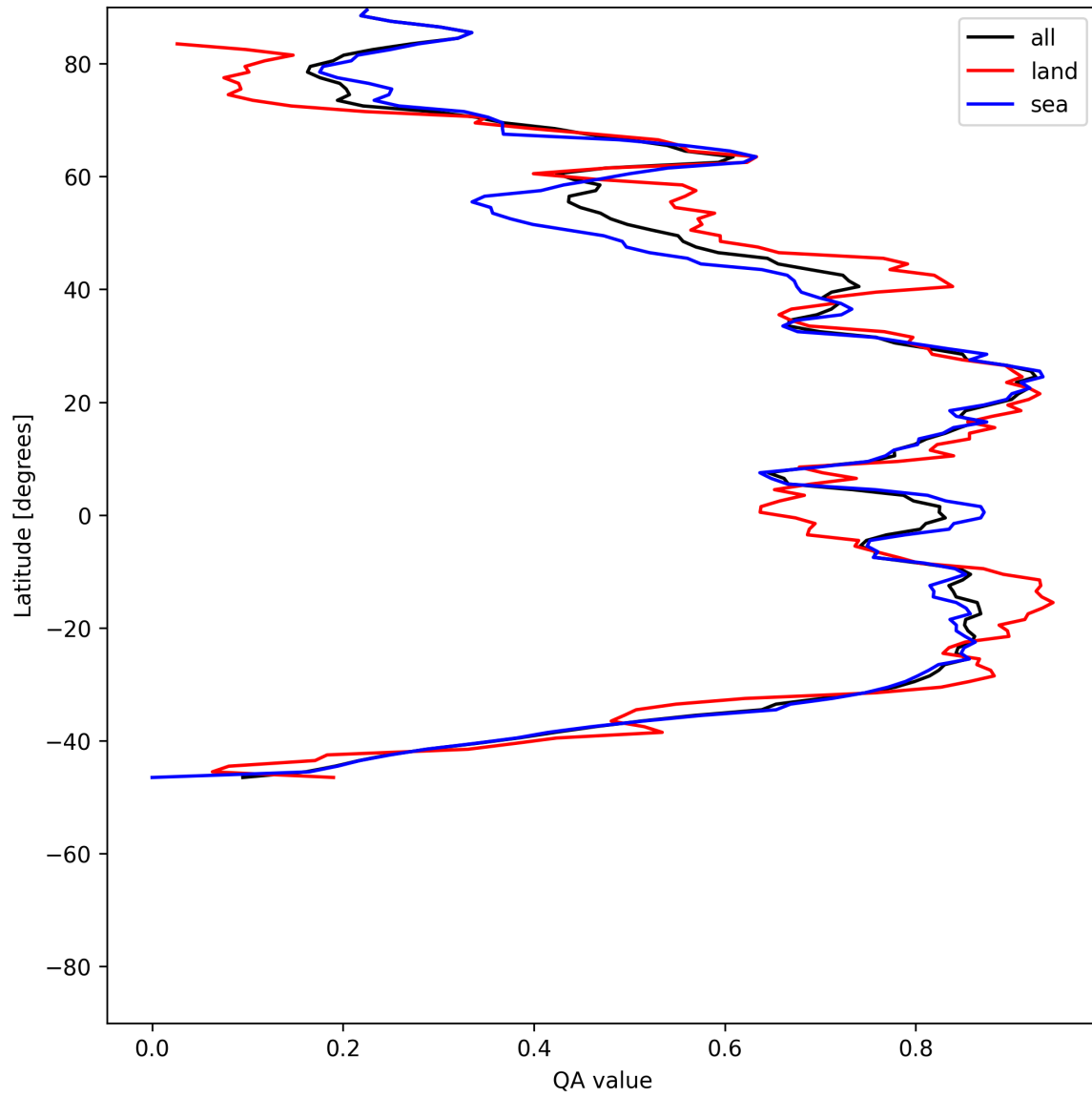
Figure 31: Zonal average of “QA value” for 2025-06-06 to 2025-06-08.
