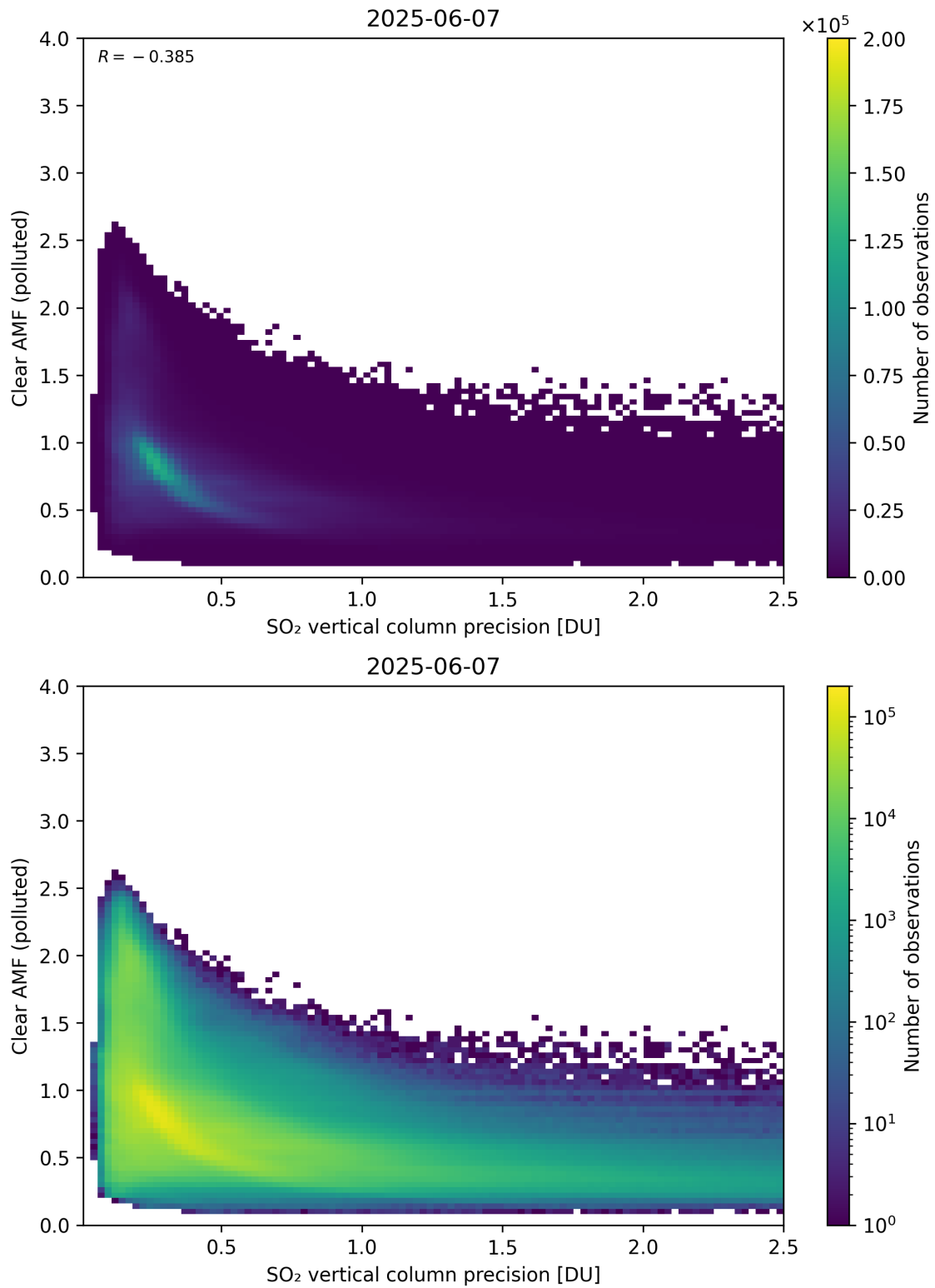
Figure 335: Scatter density plot of “SO 2 vertical column precision” against “Clear AMF (polluted)” for 2025-06-06 to 2025-06-08.
