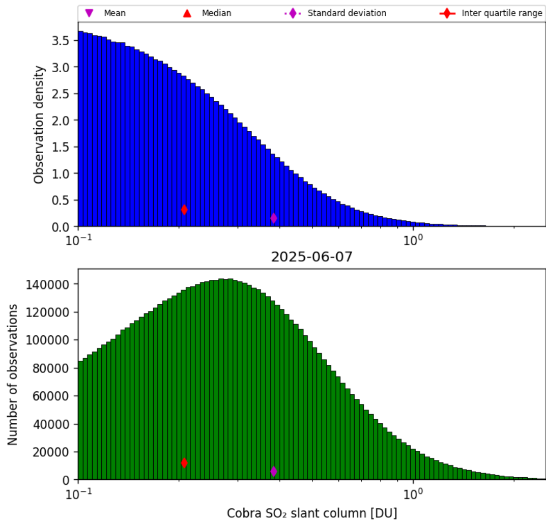
Figure 61: Histogram of “Cobra SO 2 slant column” for 2025-06-06 to 2025-06-08
