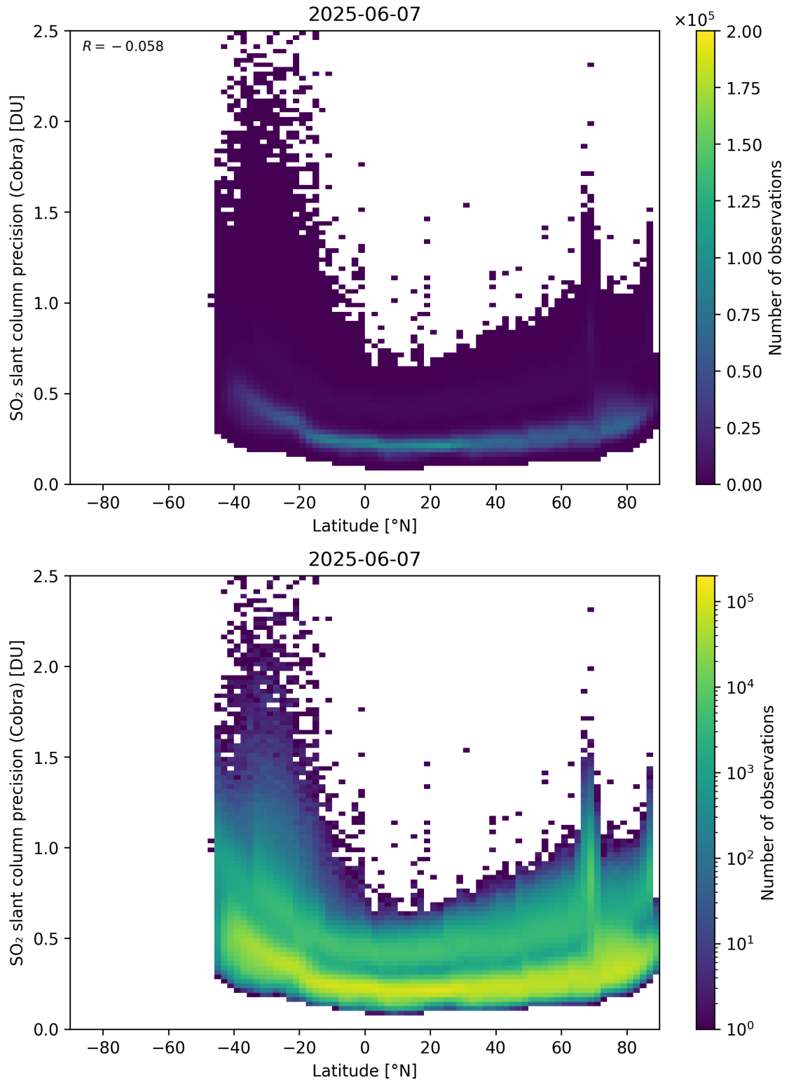
Figure 158: Scatter density plot of “Latitude” against “SO 2 slant column precision (Cobra)” for 2025-06-06 to 2025-06-08.
