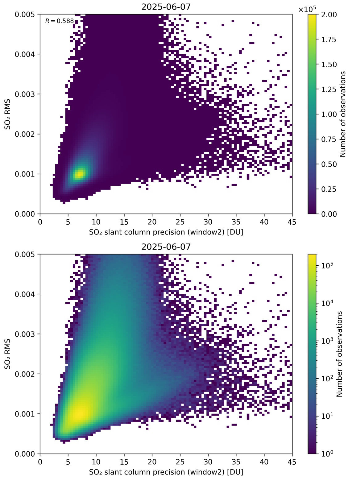
Figure 295: Scatter density plot of “SO 2 slant column precision (window2)” against “SO 2 RMS” for 2025-06-06 to 2025-06-08.
