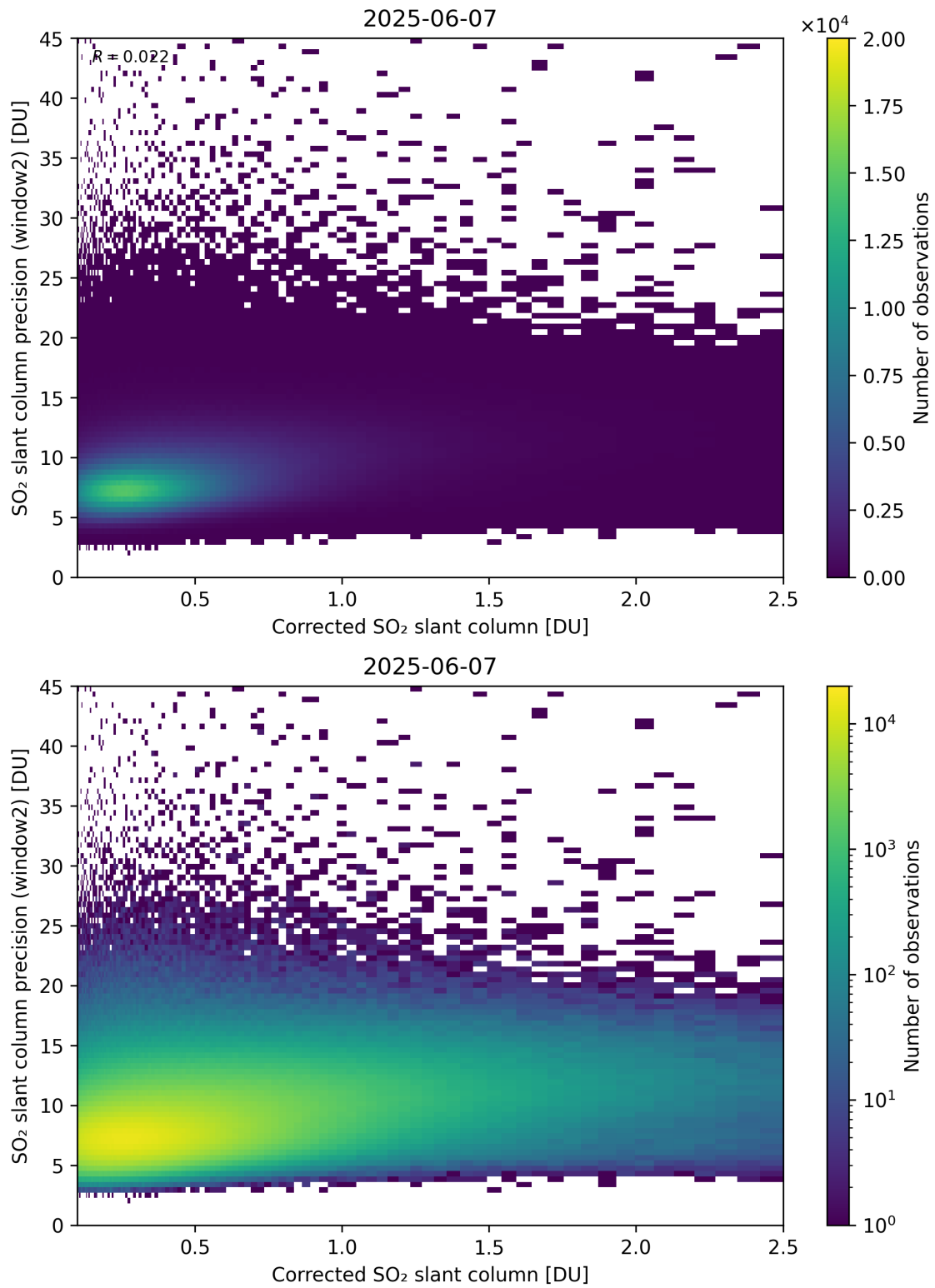
Figure 239: Scatter density plot of “Corrected SO 2 slant column” against “SO 2 slant column precision (window2)” for 2025-06-06 to 2025-06-08.
