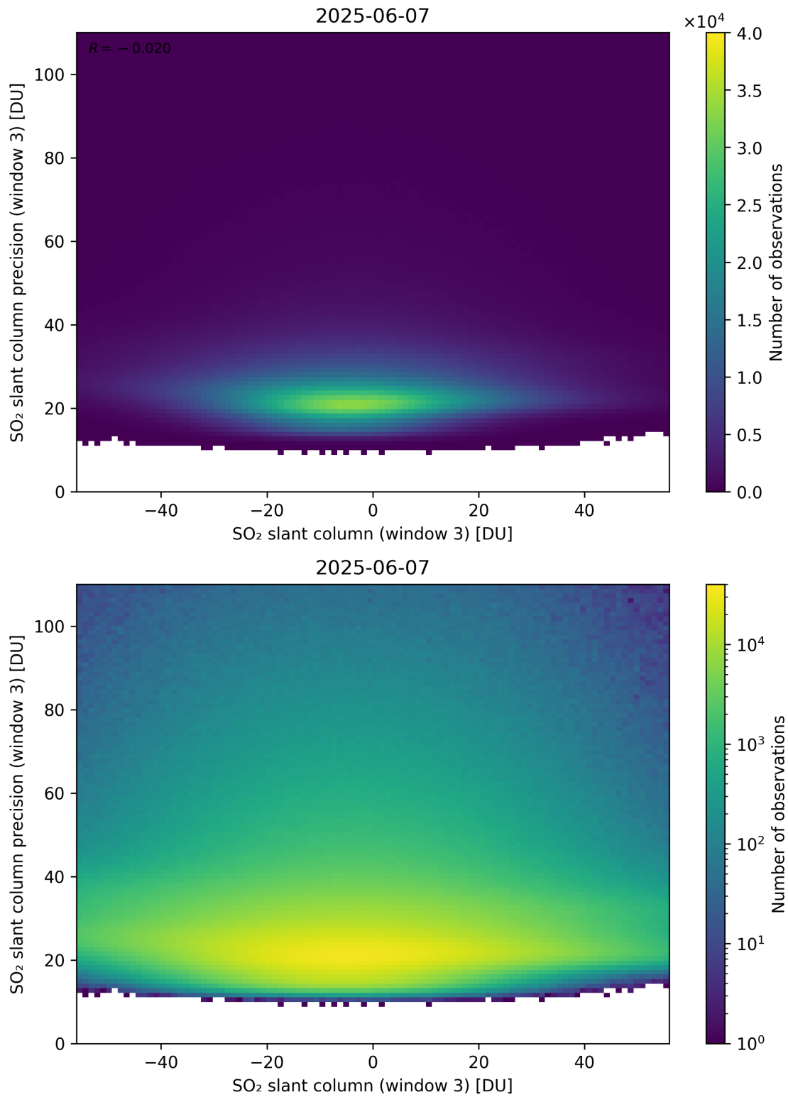
Figure 317: Scatter density plot of “SO 2 slant column (window 3)” against “SO 2 slant column precision (window 3)” for 2025-06-06 to 2025-06-08.
