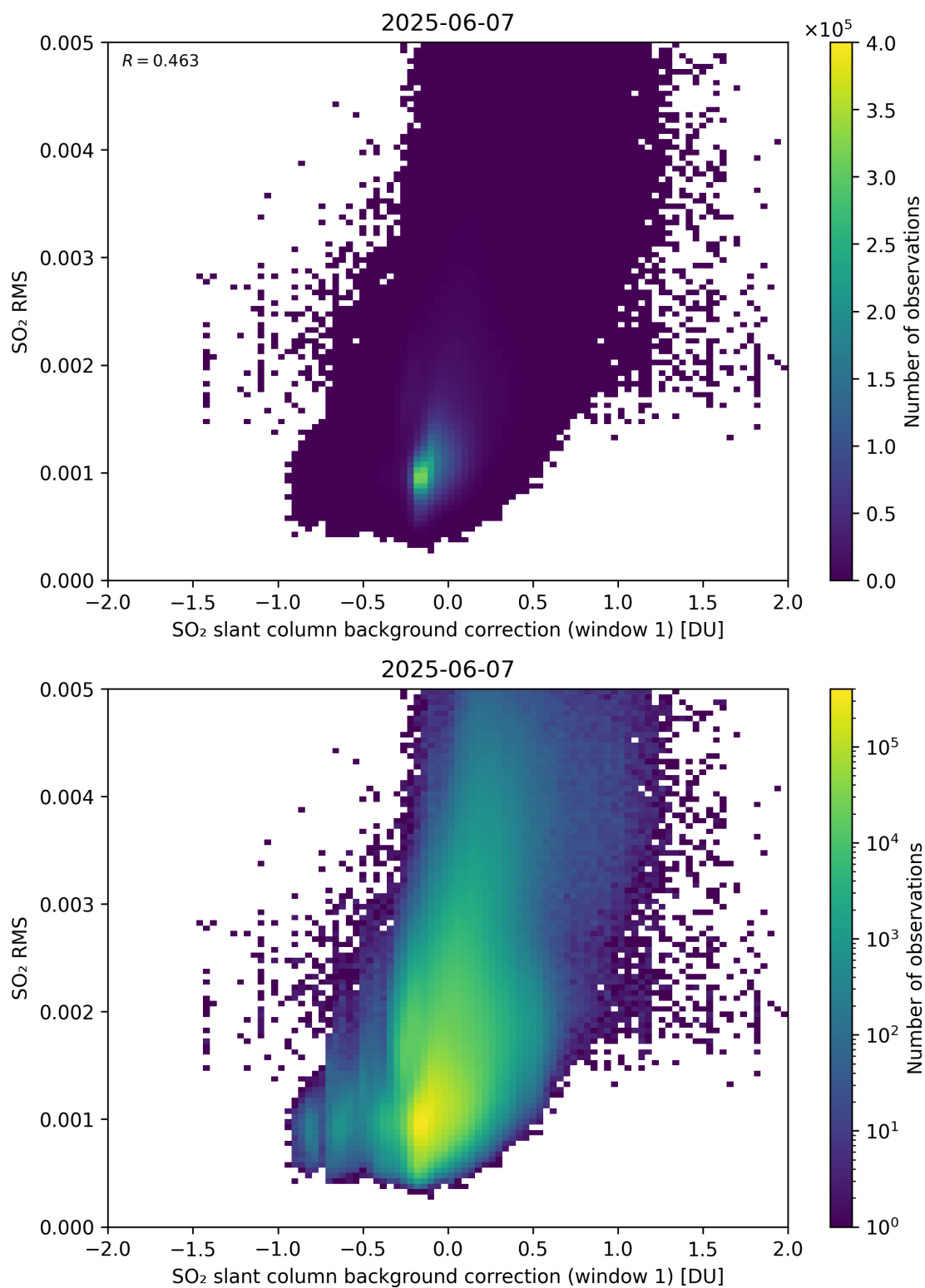
Figure 113: Scatter density plot of “SO 2 slant column background correction (window 1)” against “SO 2 RMS” for 2025-06-06 to 2025-06-08.
