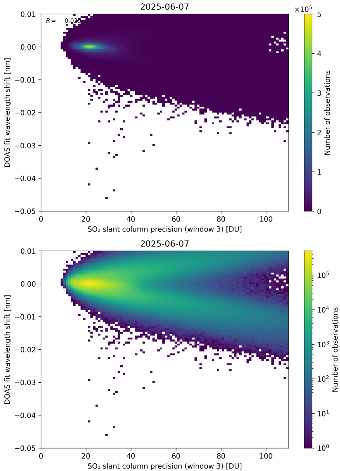
Figure 308: Scatter density plot of “SO 2 slant column precision (window 3)” against “DOAS fit wavelength shift” for 2025-06-06 to 2025-06-08.
