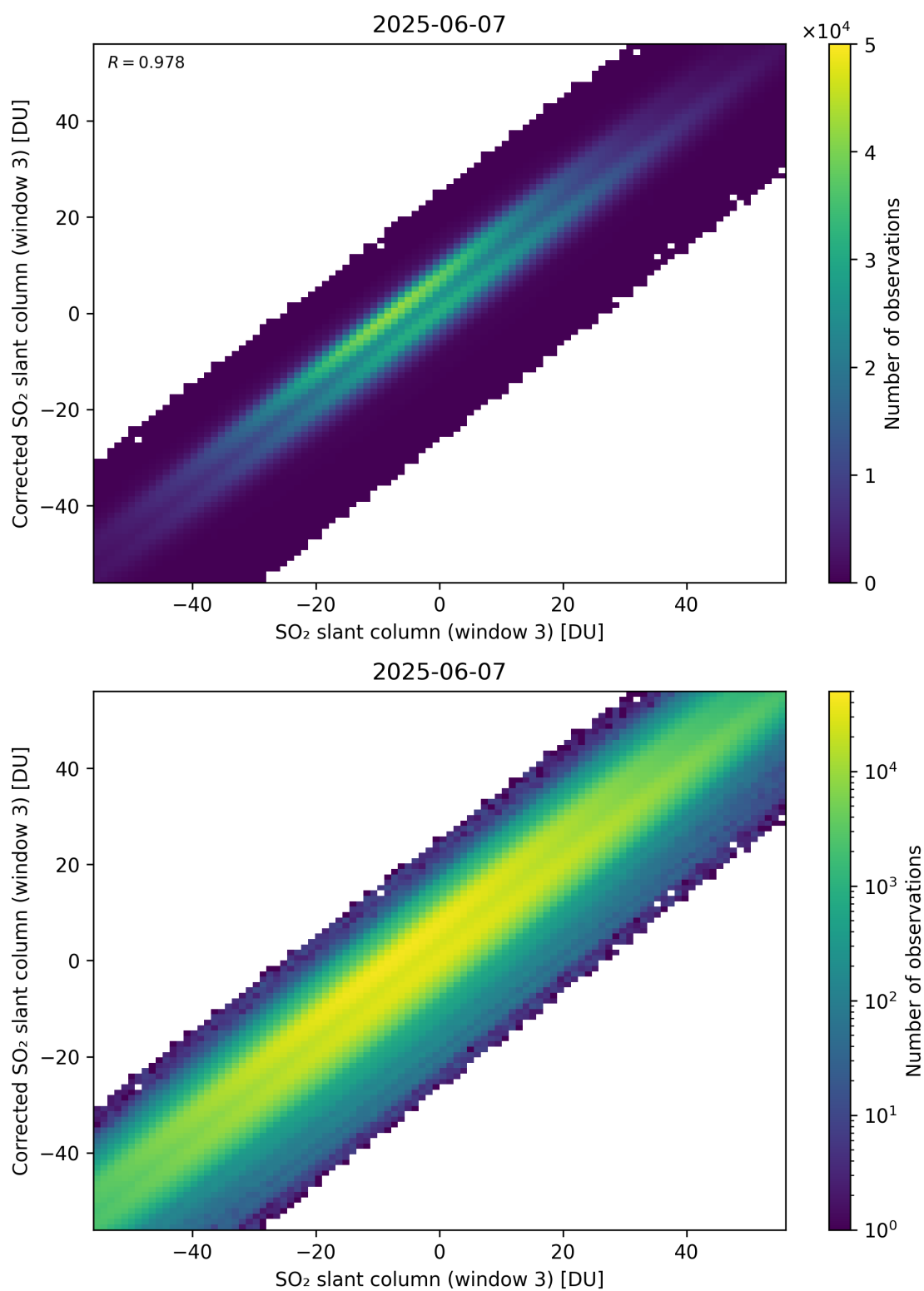
Figure 316: Scatter density plot of “SO 2 slant column (window 3)” against “Corrected SO 2 slant column (window 3)” for 2025-06-06 to 2025-06-08.
