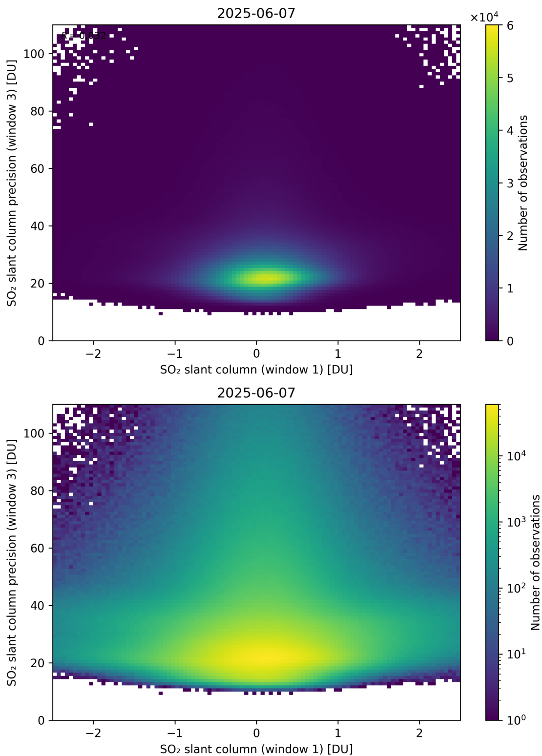
Figure 288: Scatter density plot of “SO 2 slant column (window 1)” against “SO 2 slant column precision (window 3)” for 2025-06-06 to 2025-06-08.
