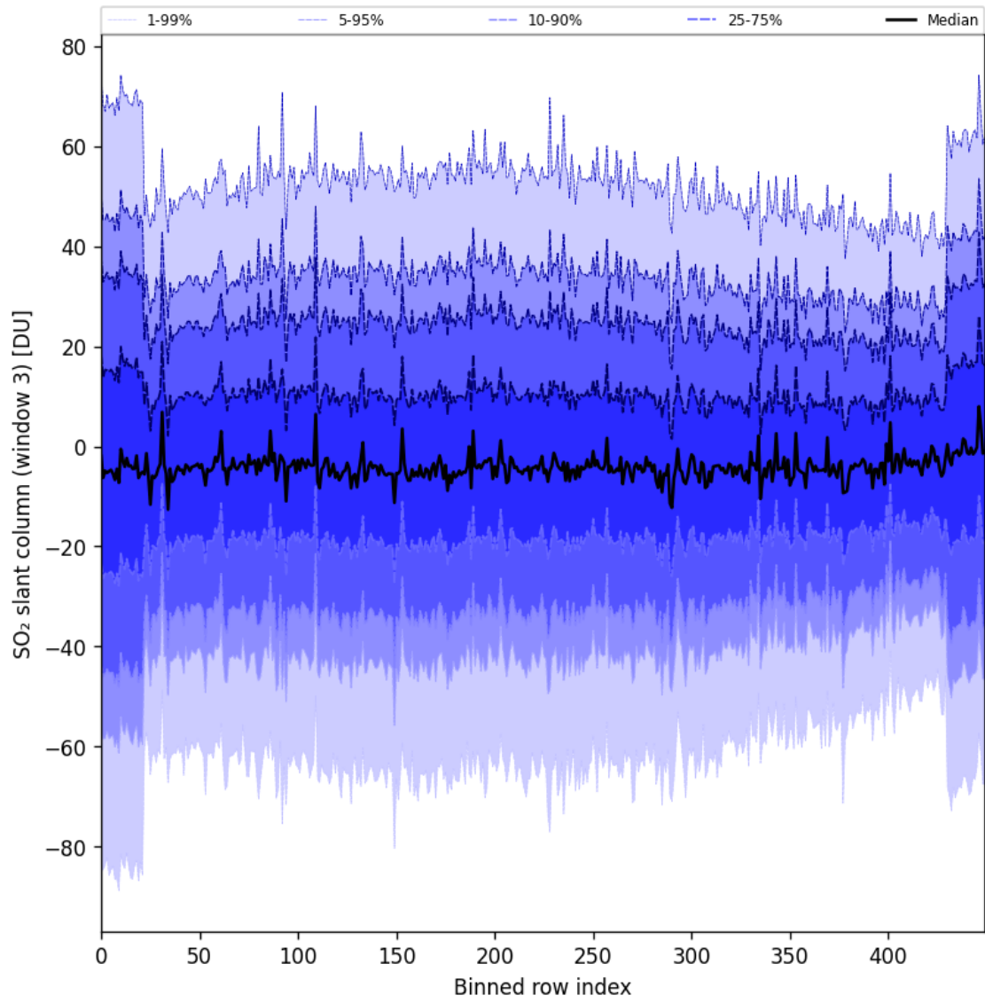
Figure 97: Along track statistics of “SO 2 slant column (window 3)” for 2025-06-06 to 2025-06-08
