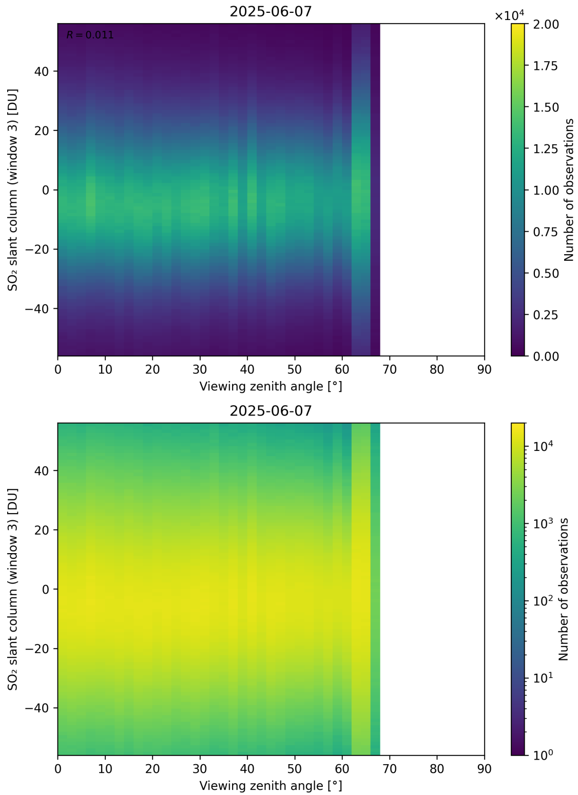
Figure 379: Scatter density plot of “Viewing zenith angle” against “SO 2 slant column (window 3)” for 2025-06-06 to 2025-06-08.
