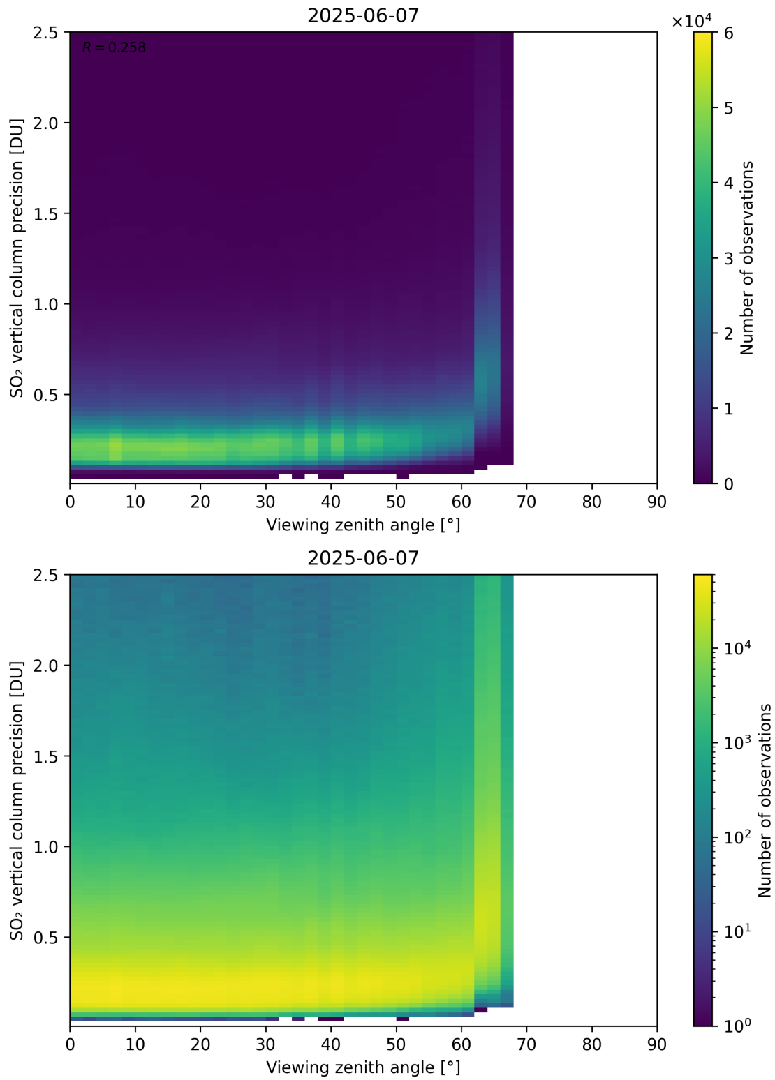
Figure 384: Scatter density plot of “Viewing zenith angle” against “SO 2 vertical column precision” for 2025-06-06 to 2025-06-08.
