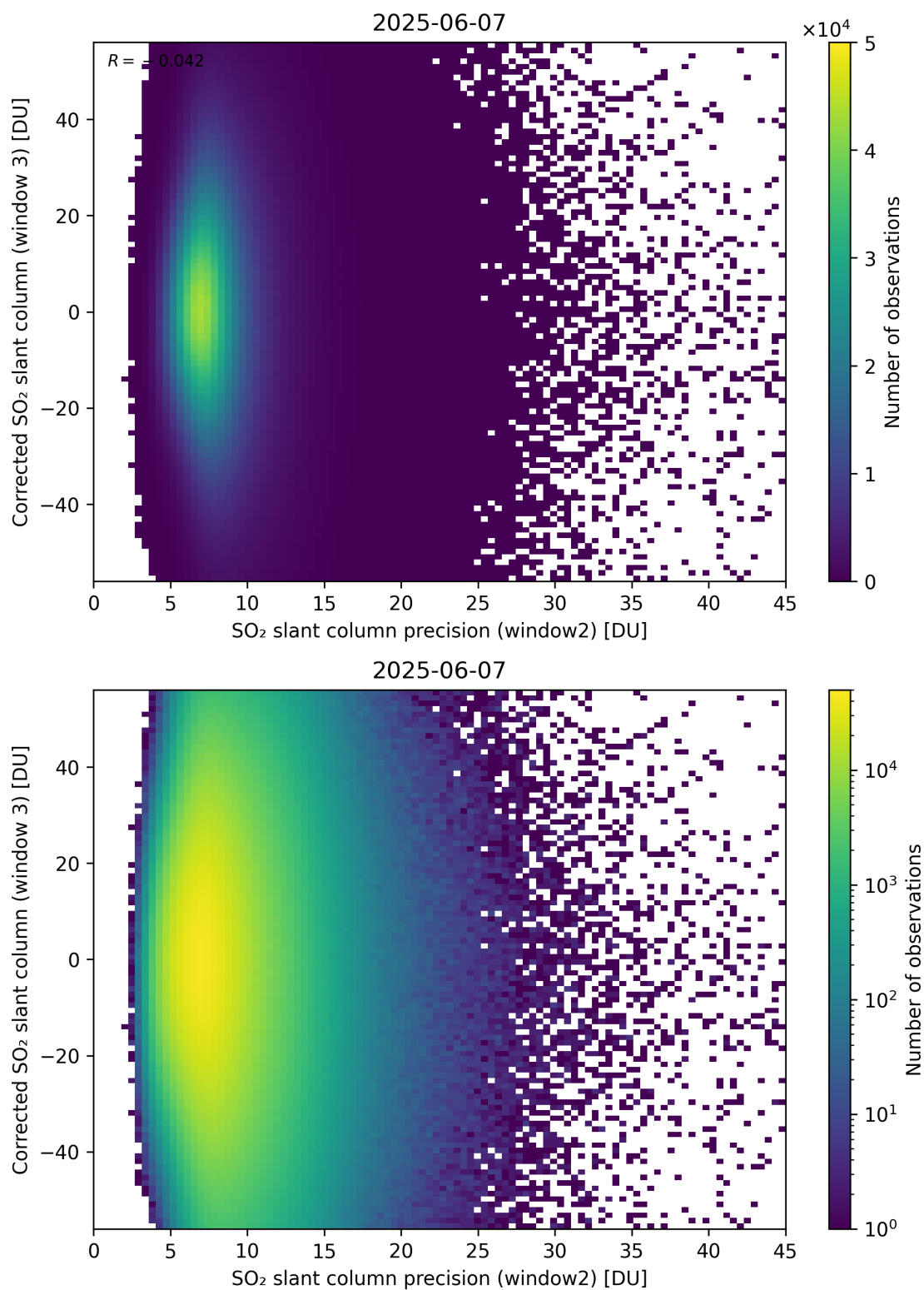
Figure 298: Scatter density plot of “SO 2 slant column precision (window2)” against “Corrected SO 2 slant column (window 3)” for 2025-06-06 to 2025-06-08.
