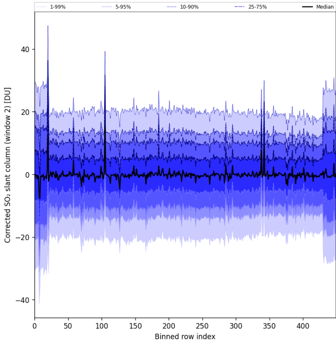
Figure 95: Along track statistics of “Corrected SO 2 slant column (window 2)” for 2025-06-06 to 2025-06-08
