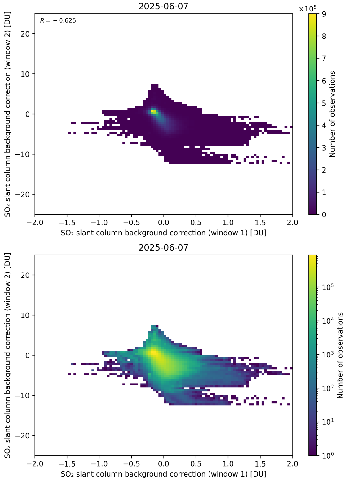
Figure 109: Scatter density plot of “SO 2 slant column background correction (window 1)” against “SO 2 slant column background correction (window 2)” for 2025-06-06 to 2025-06-08.
