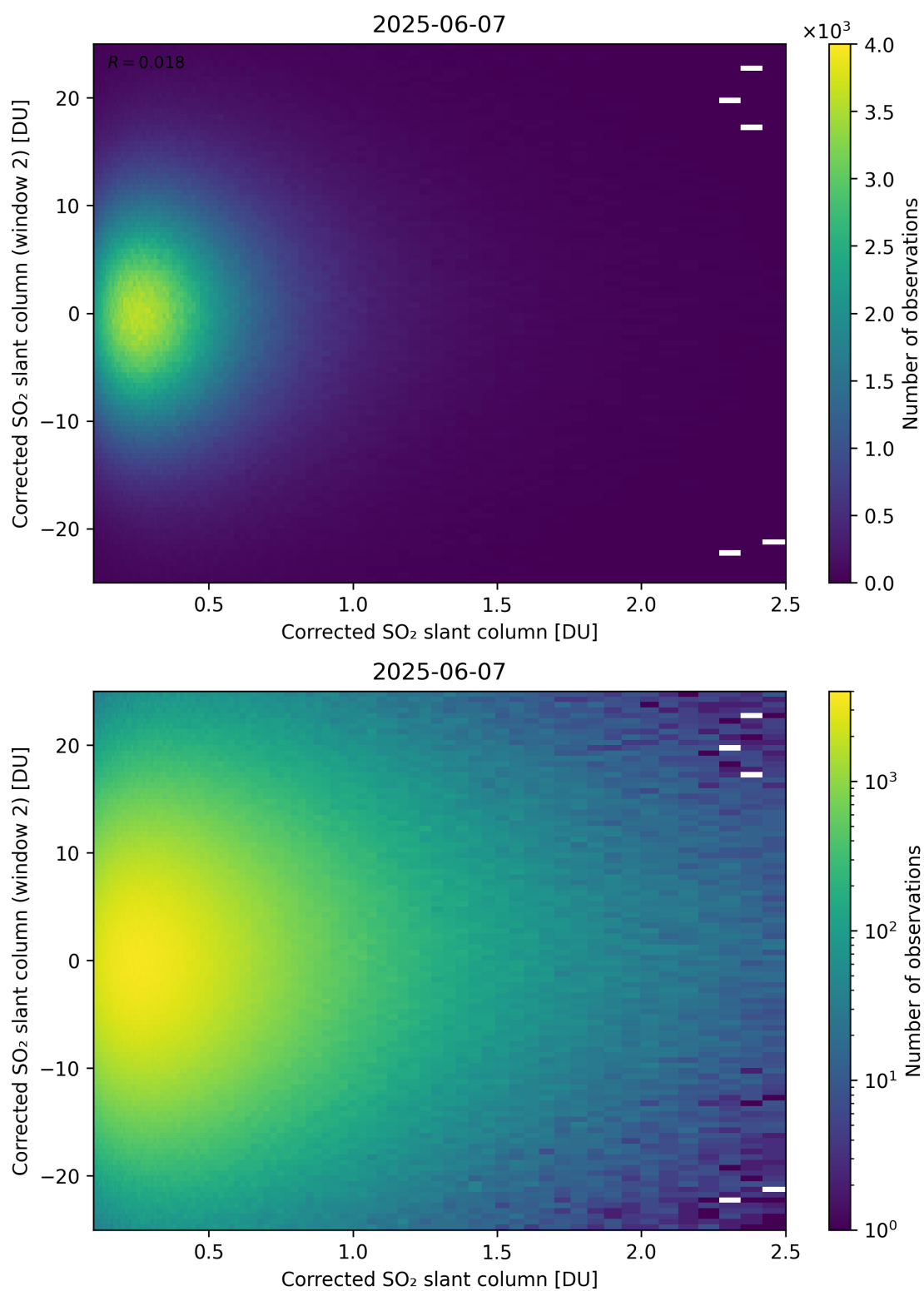
Figure 235: Scatter density plot of “Corrected SO 2 slant column” against “Corrected SO 2 slant column (window 2)” for 2025-06-06 to 2025-06-08.
