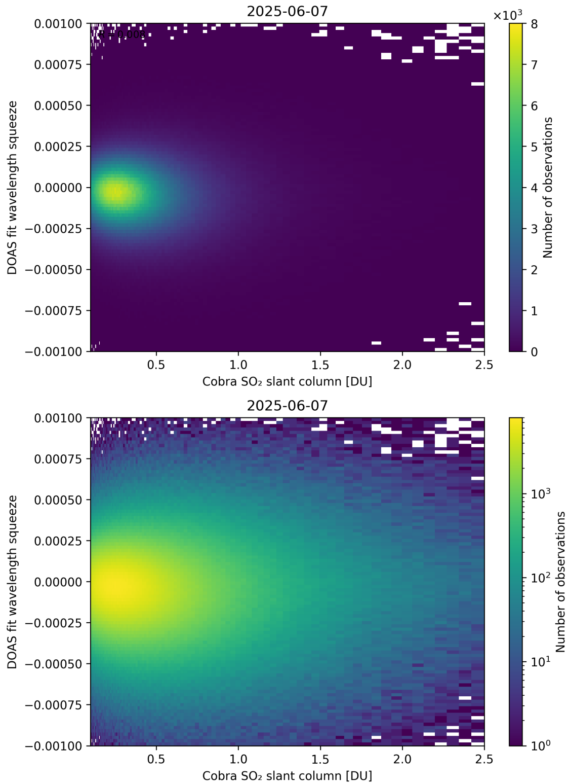
Figure 197: Scatter density plot of “Cobra SO 2 slant column” against “DOAS fit wavelength squeeze” for 2025-06-06 to 2025-06-08.
