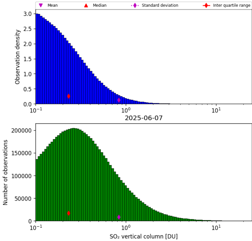
Figure 58: Histogram of “SO 2 vertical column” for 2025-06-06 to 2025-06-08
