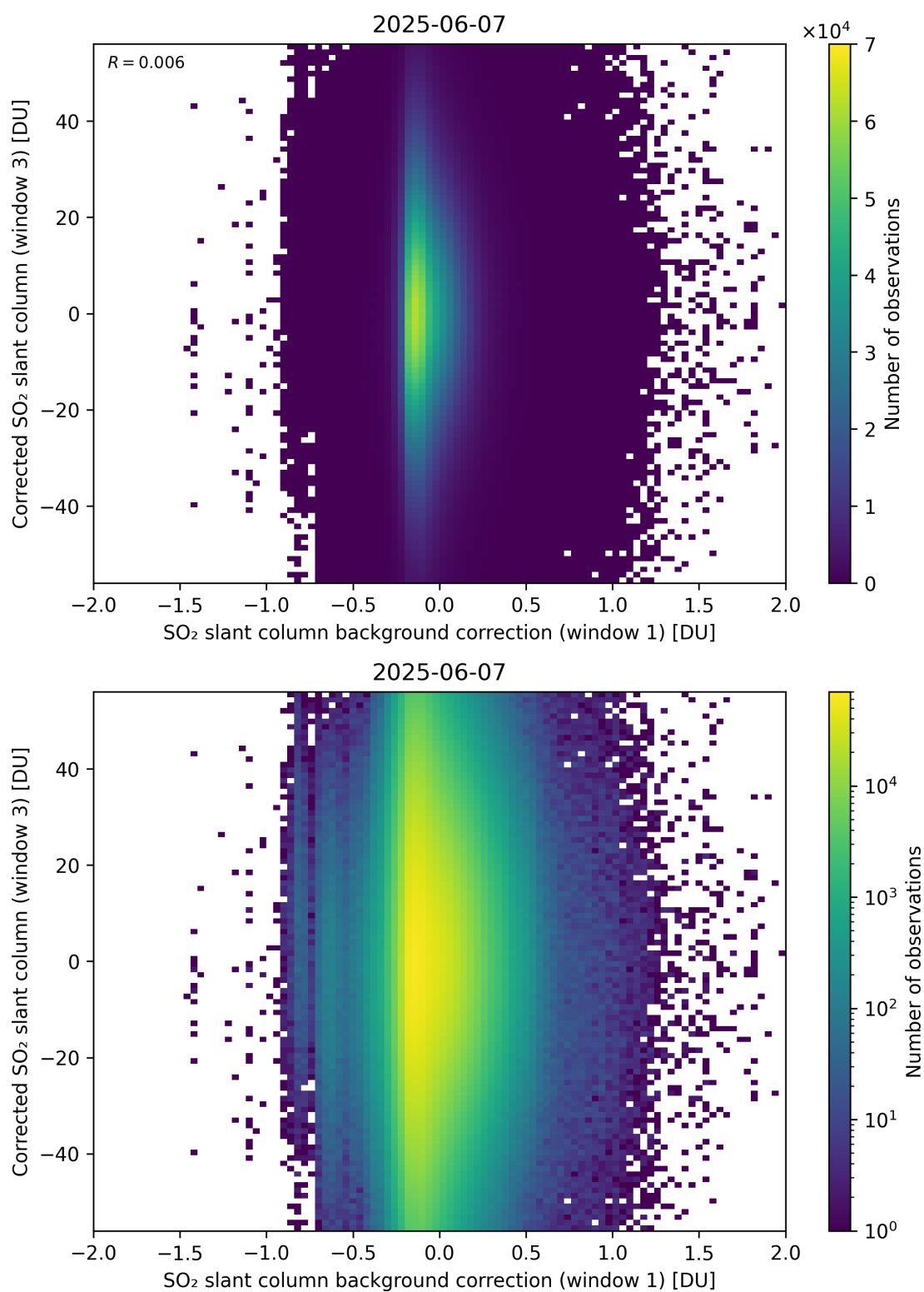
Figure 116: Scatter density plot of “SO 2 slant column background correction (window 1)” against “Corrected SO 2 slant column (window 3)” for 2025-06-06 to 2025-06-08.
