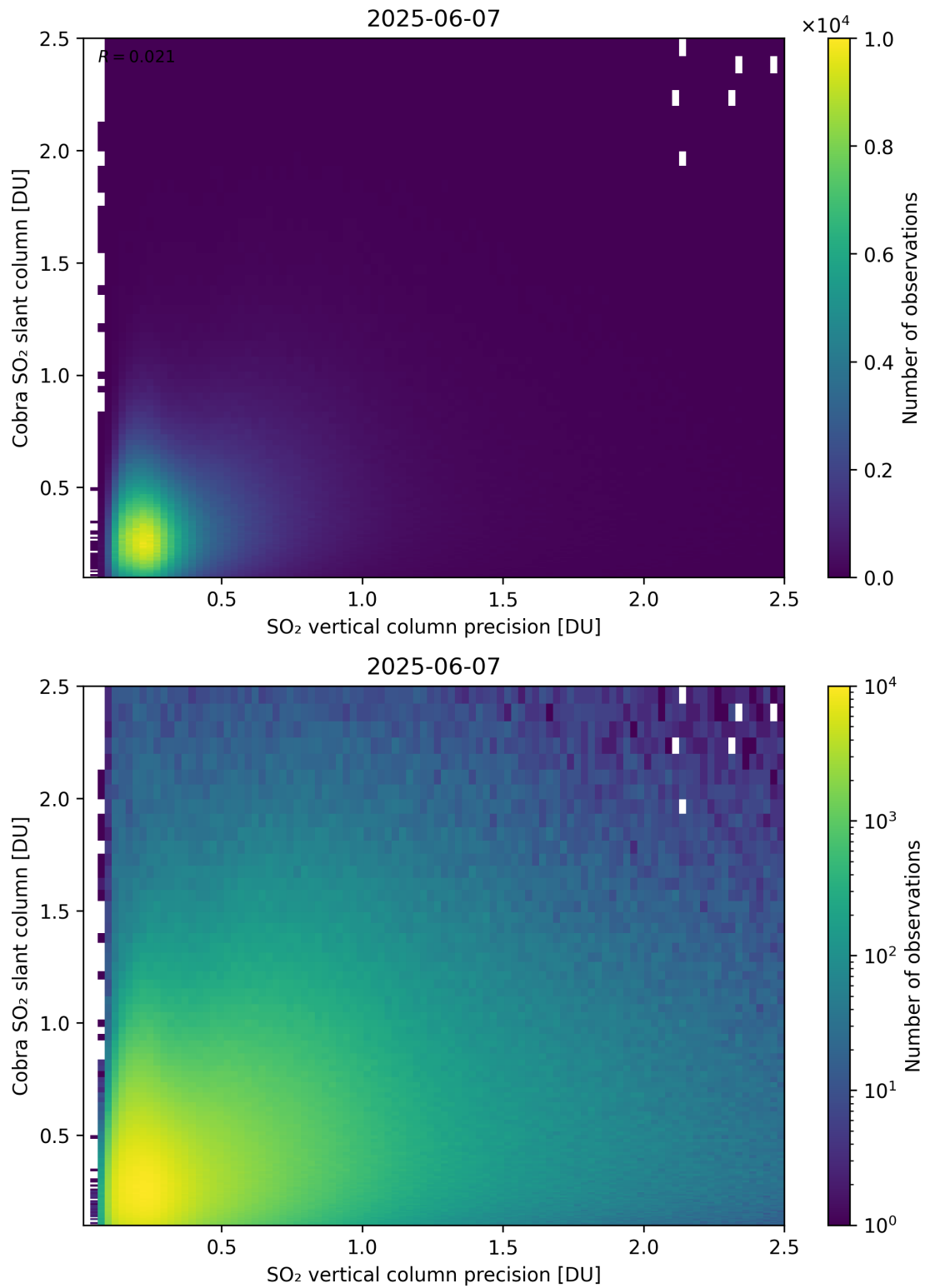
Figure 336: Scatter density plot of “SO 2 vertical column precision” against “Cobra SO 2 slant column” for 2025-06-06 to 2025-06-08.
