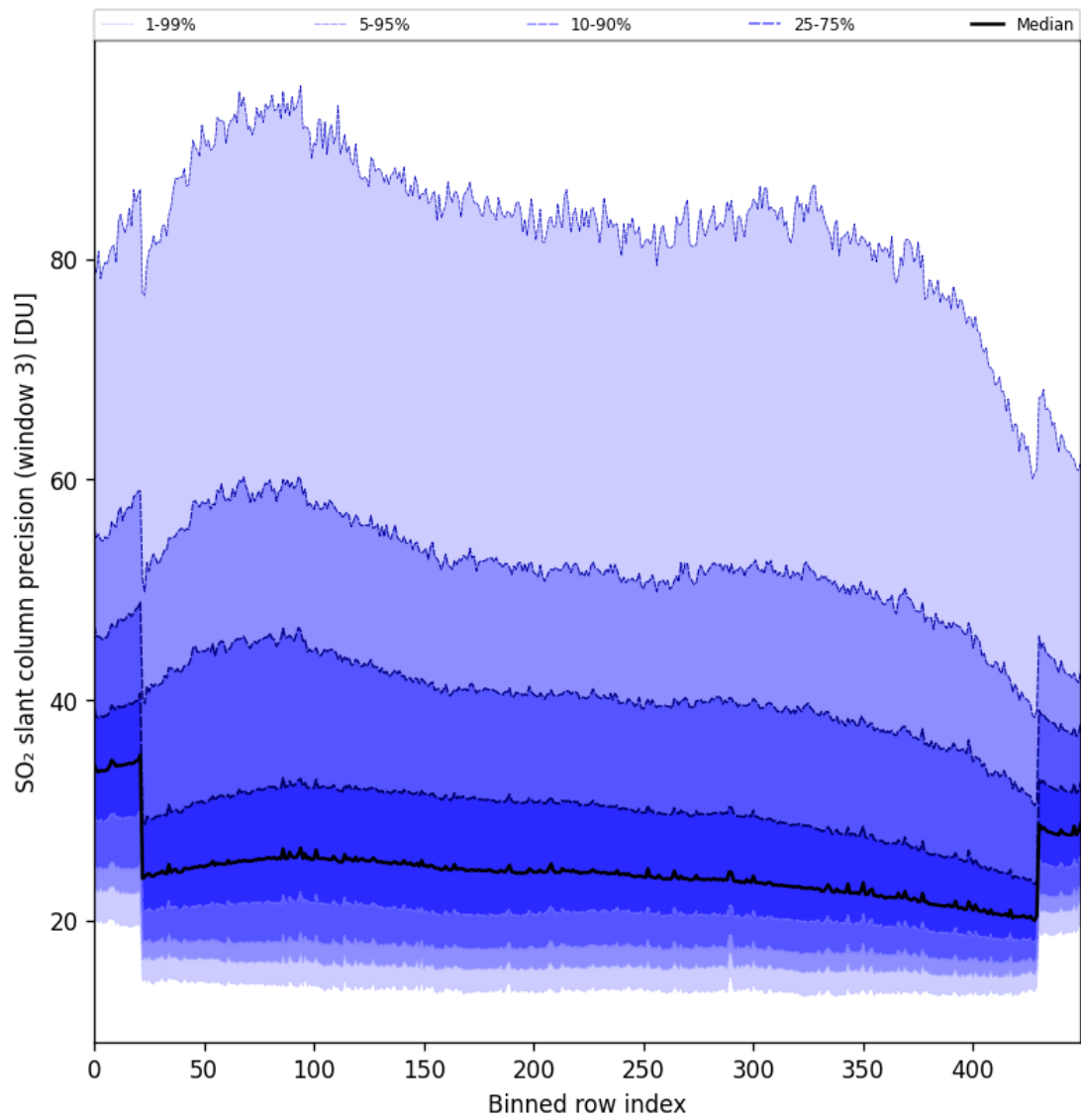
Figure 98: Along track statistics of “SO 2 slant column precision (window 3)” for 2025-06-06 to 2025-06-08
