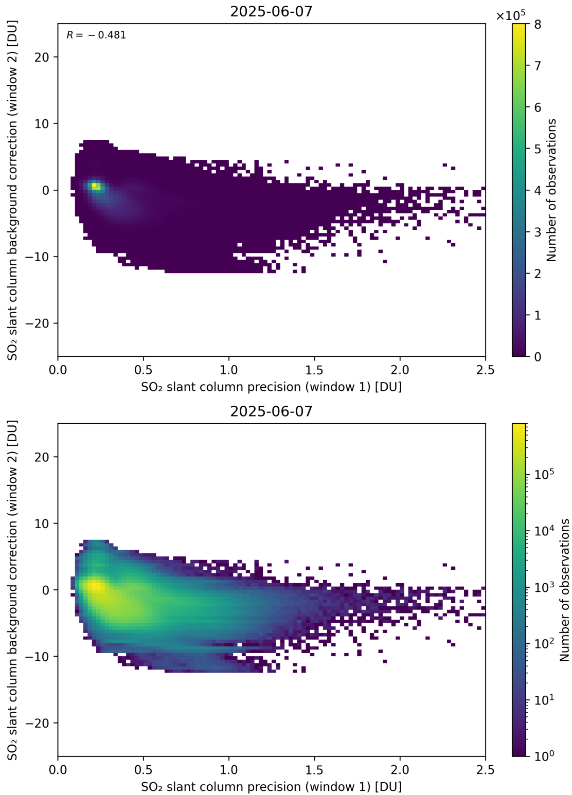
Figure 269: Scatter density plot of “SO 2 slant column precision (window 1)” against “SO 2 slant column background correction (window 2)” for 2025-06-06 to 2025-06-08.
