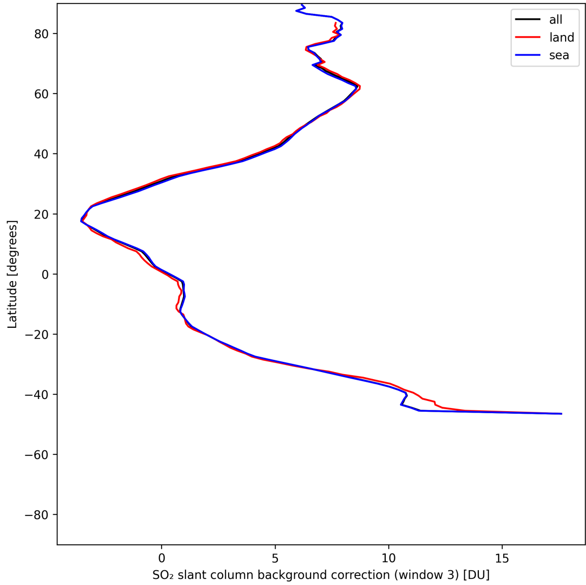
Figure 48: Zonal average of “SO 2 slant column background correction (window 3)” for 2025-06-06 to 2025-06-08.
