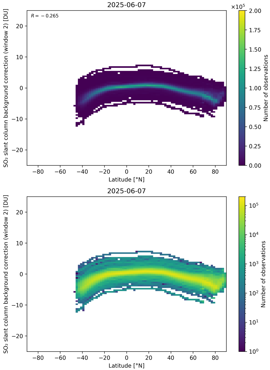
Figure 151: Scatter density plot of “Latitude” against “SO 2 slant column background correction (window 2)” for 2025-06-06 to 2025-06-08.
