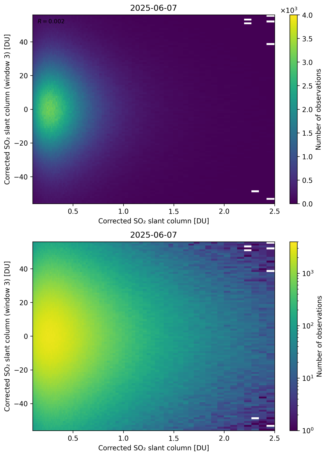
Figure 236: Scatter density plot of “Corrected SO 2 slant column” against “Corrected SO 2 slant column (window 3)” for 2025-06-06 to 2025-06-08.
