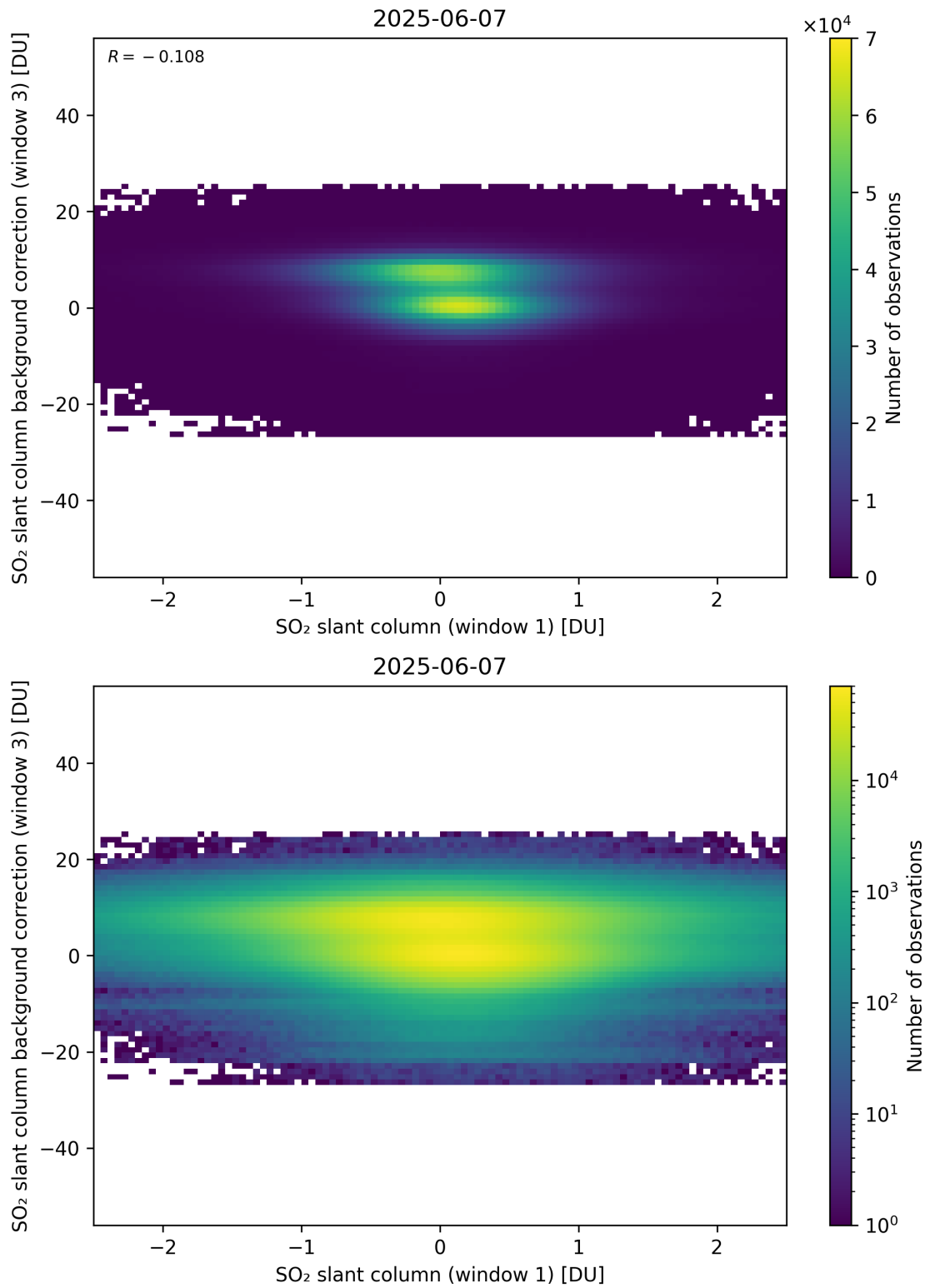
Figure 264: Scatter density plot of “SO 2 slant column (window 1)” against “SO 2 slant column background correction (window 3)” for 2025-06-06 to 2025-06-08.
