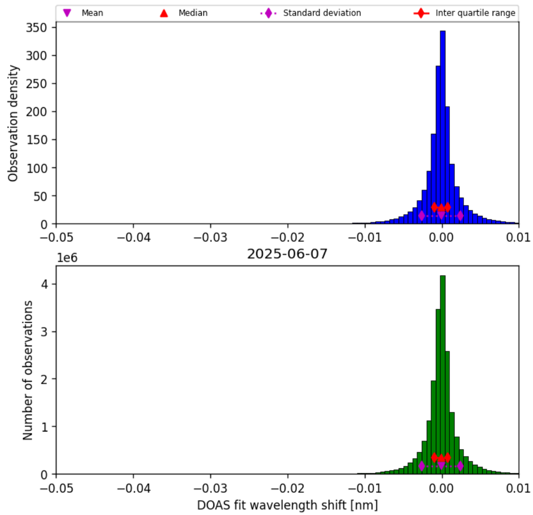
Figure 76: Histogram of “DOAS fit wavelength shift” for 2025-06-06 to 2025-06-08
