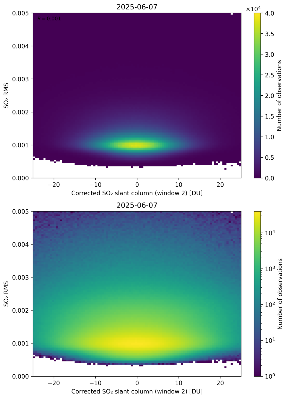
Figure 248: Scatter density plot of “Corrected SO 2 slant column (window 2)” against “SO 2 RMS” for 2025-06-06 to 2025-06-08.
