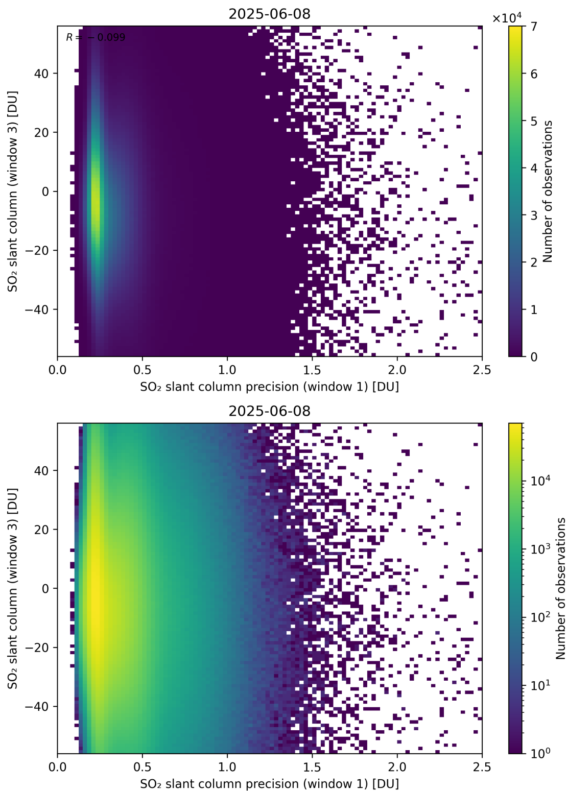
Figure 278: Scatter density plot of “SO 2 slant column precision (window 1)” against “SO 2 slant column (window 3)” for 2025-06-07 to 2025-06-09.
