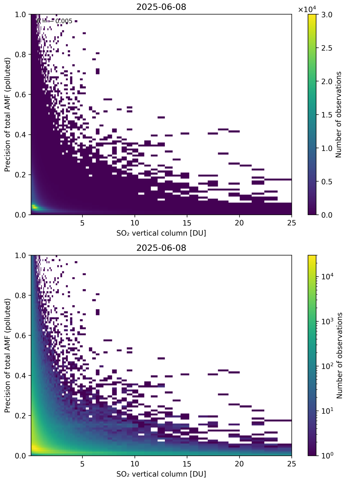
Figure 360: Scatter density plot of “SO 2 vertical column” against “Precision of total AMF (polluted)” for 2025-06-07 to 2025-06-09.
