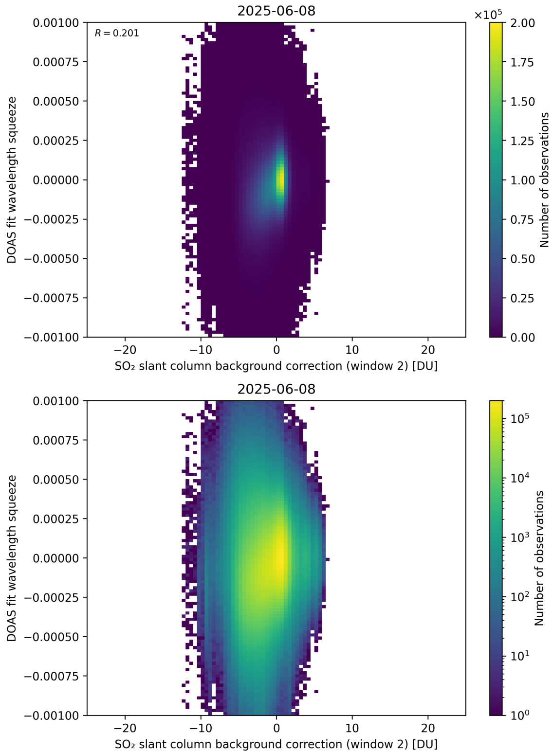
Figure 124: Scatter density plot of “SO 2 slant column background correction (window 2)” against “DOAS fit wavelength squeeze” for 2025-06-07 to 2025-06-09.
