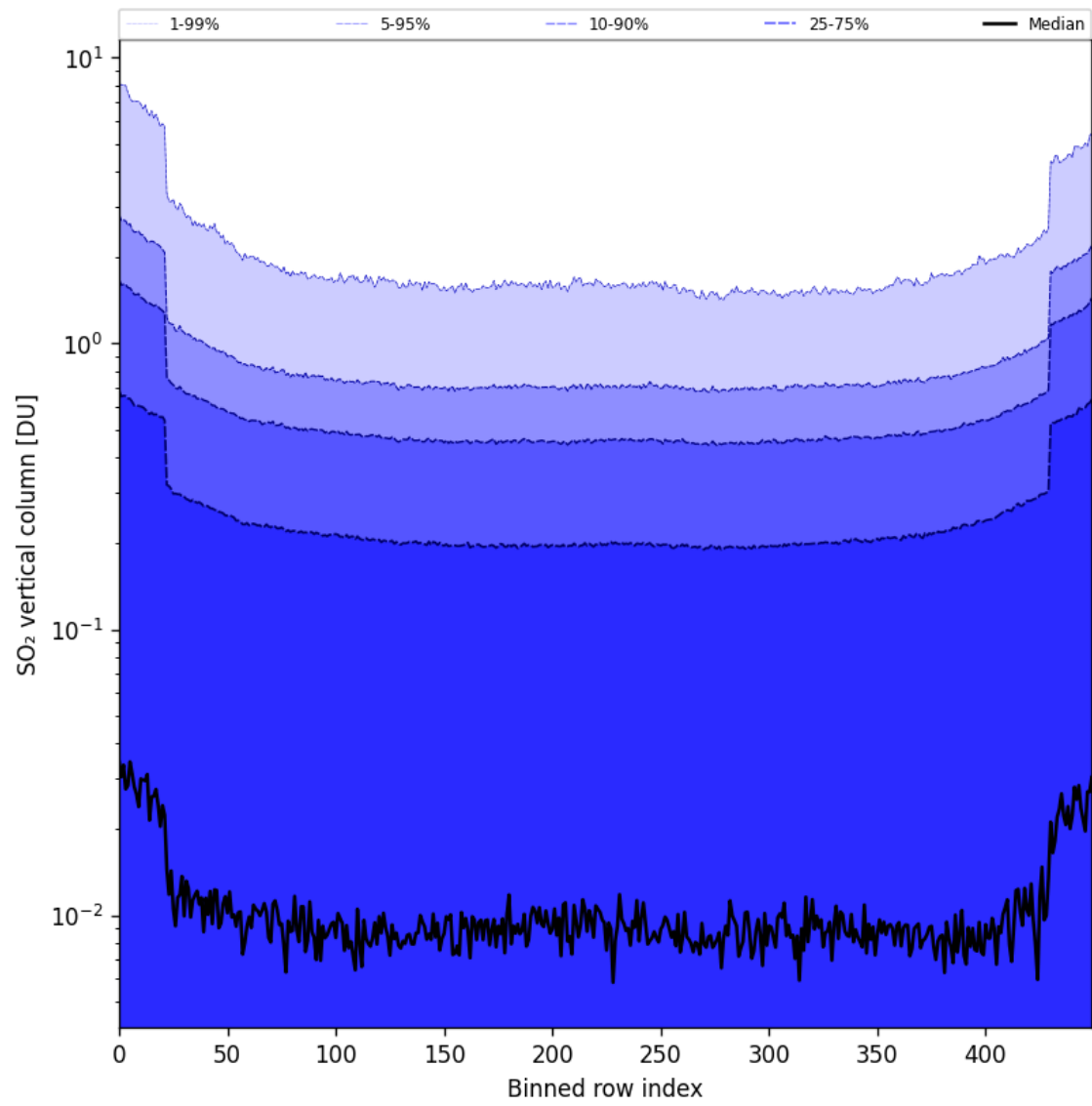
Figure 84: Along track statistics of “SO 2 vertical column” for 2025-06-07 to 2025-06-09
