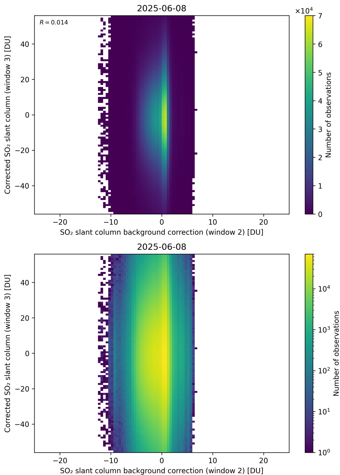
Figure 127: Scatter density plot of “SO 2 slant column background correction (window 2)” against “Corrected SO 2 slant column (window 3)” for 2025-06-07 to 2025-06-09.
