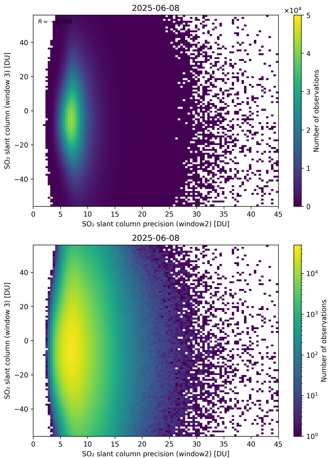
Figure 299: Scatter density plot of “SO 2 slant column precision (window2)” against “SO 2 slant column (window 3)” for 2025-06-07 to 2025-06-09.
