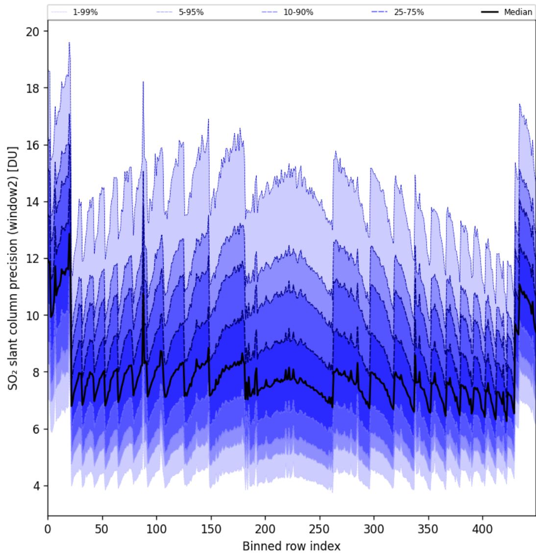
Figure 94: Along track statistics of “SO 2 slant column precision (window2)” for 2025-06-07 to 2025-06-09
