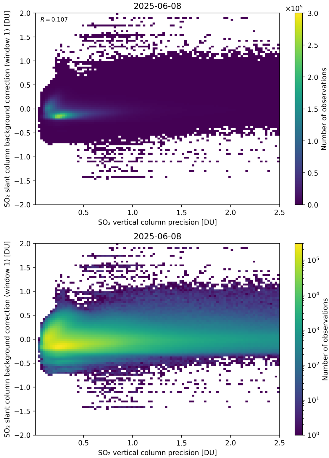
Figure 329: Scatter density plot of “SO 2 vertical column precision” against “SO 2 slant column background correction (window 1)” for 2025-06-07 to 2025-06-09.
