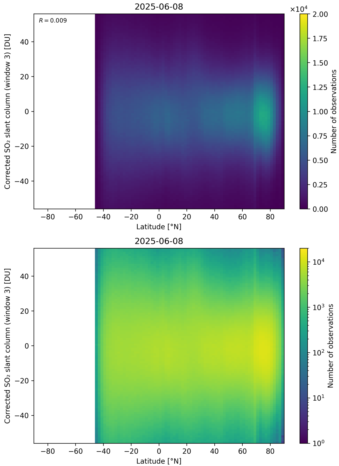
Figure 161: Scatter density plot of “Latitude” against “Corrected SO 2 slant column (window 3)” for 2025-06-07 to 2025-06-09.
