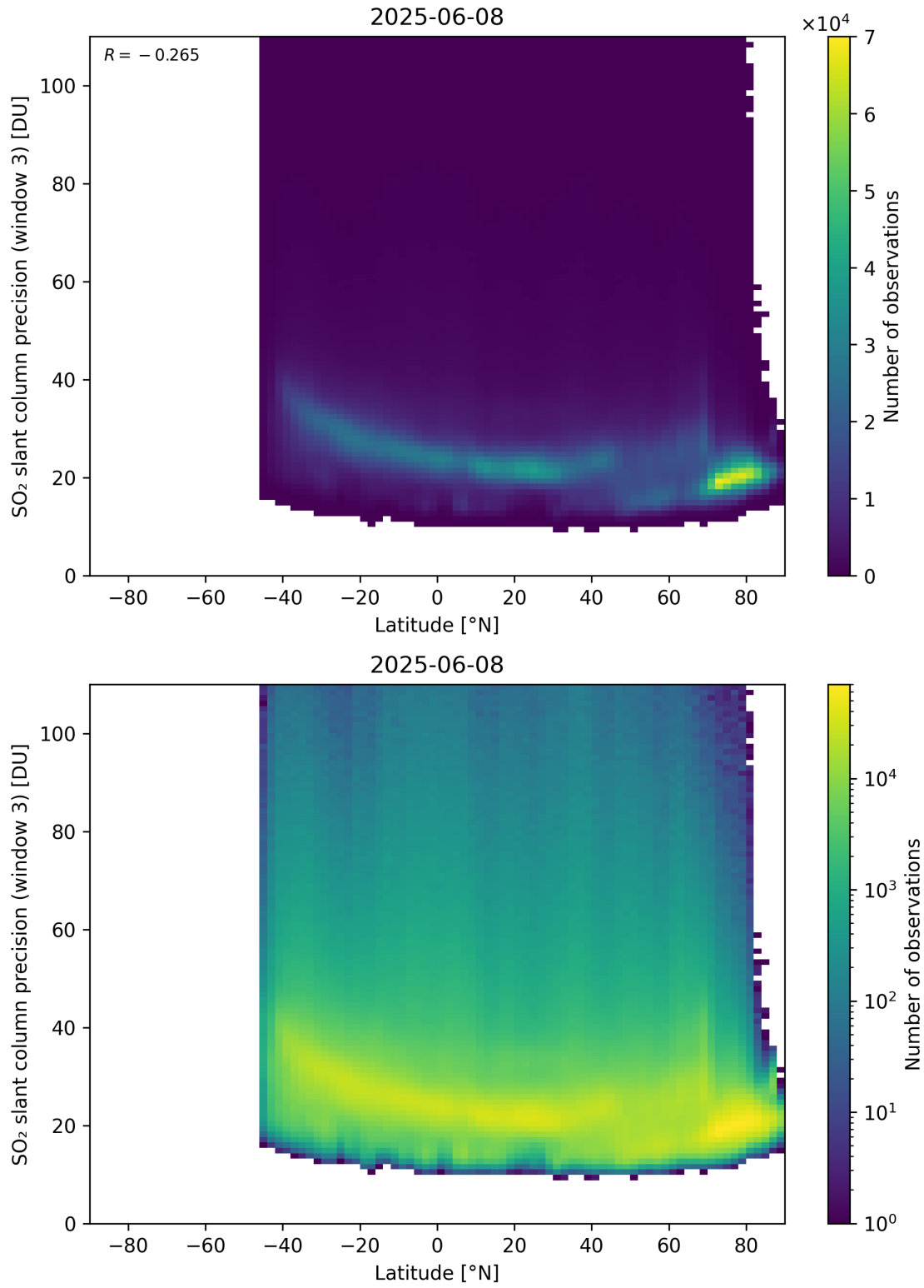
Figure 166: Scatter density plot of “Latitude” against “SO 2 slant column precision (window 3)” for 2025-06-07 to 2025-06-09.
