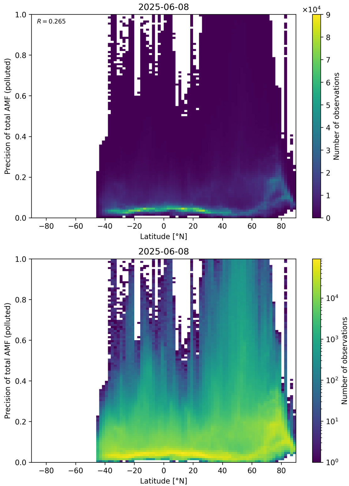
Figure 168: Scatter density plot of “Latitude” against “Precision of total AMF (polluted)” for 2025-06-07 to 2025-06-09.
