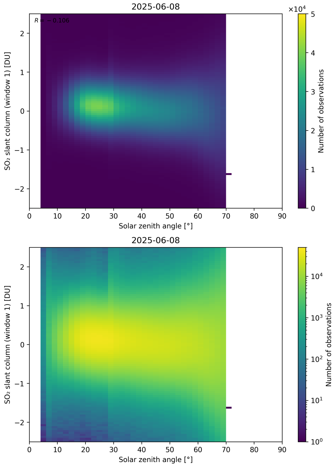
Figure 184: Scatter density plot of “Solar zenith angle” against “SO 2 slant column (window 1)” for 2025-06-07 to 2025-06-09.
