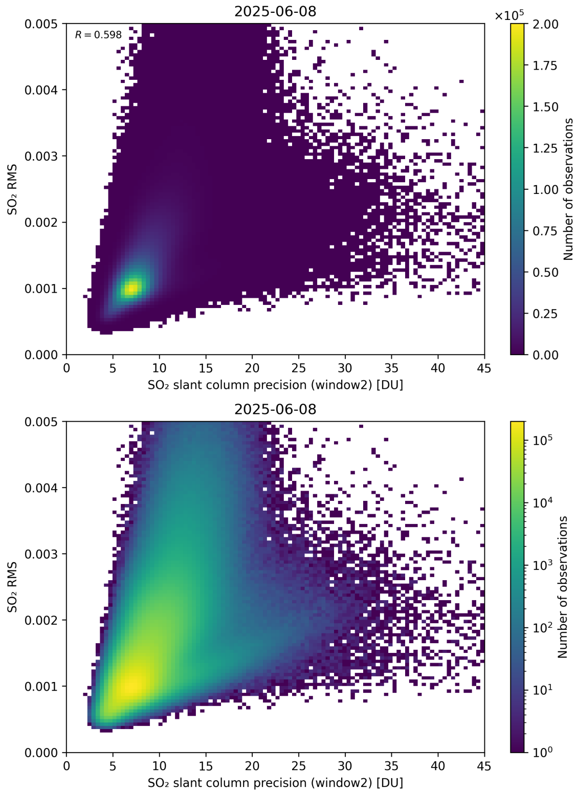
Figure 295: Scatter density plot of “SO 2 slant column precision (window2)” against “SO 2 RMS” for 2025-06-07 to 2025-06-09.
