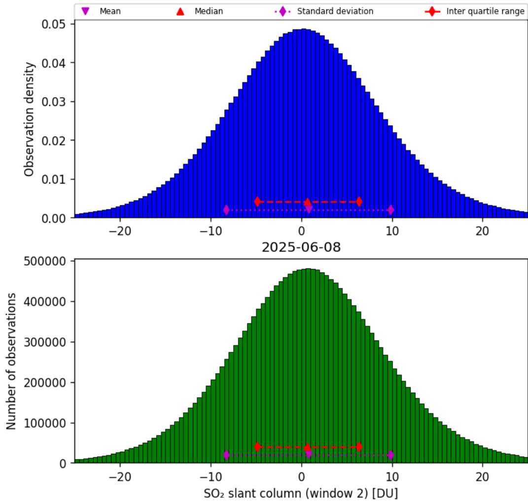
Figure 67: Histogram of “SO 2 slant column (window 2)” for 2025-06-07 to 2025-06-09
