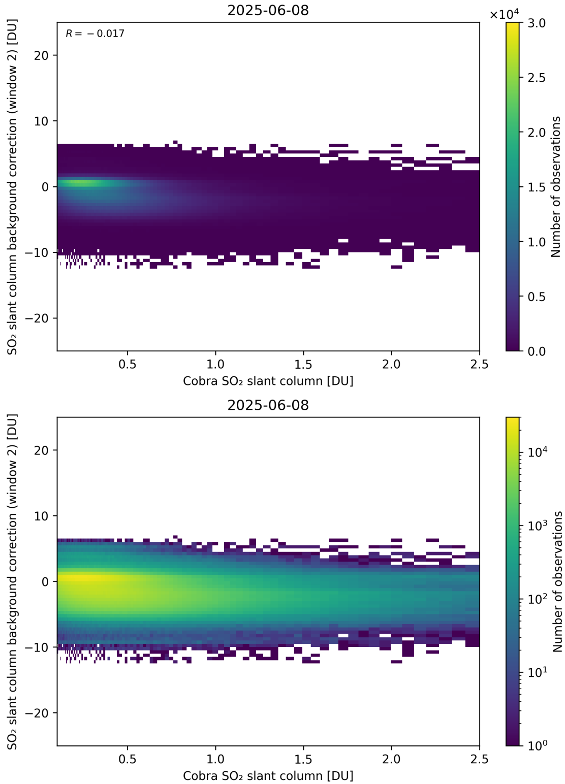
Figure 194: Scatter density plot of “Cobra SO 2 slant column” against “SO 2 slant column background correction (window 2)” for 2025-06-07 to 2025-06-09.
