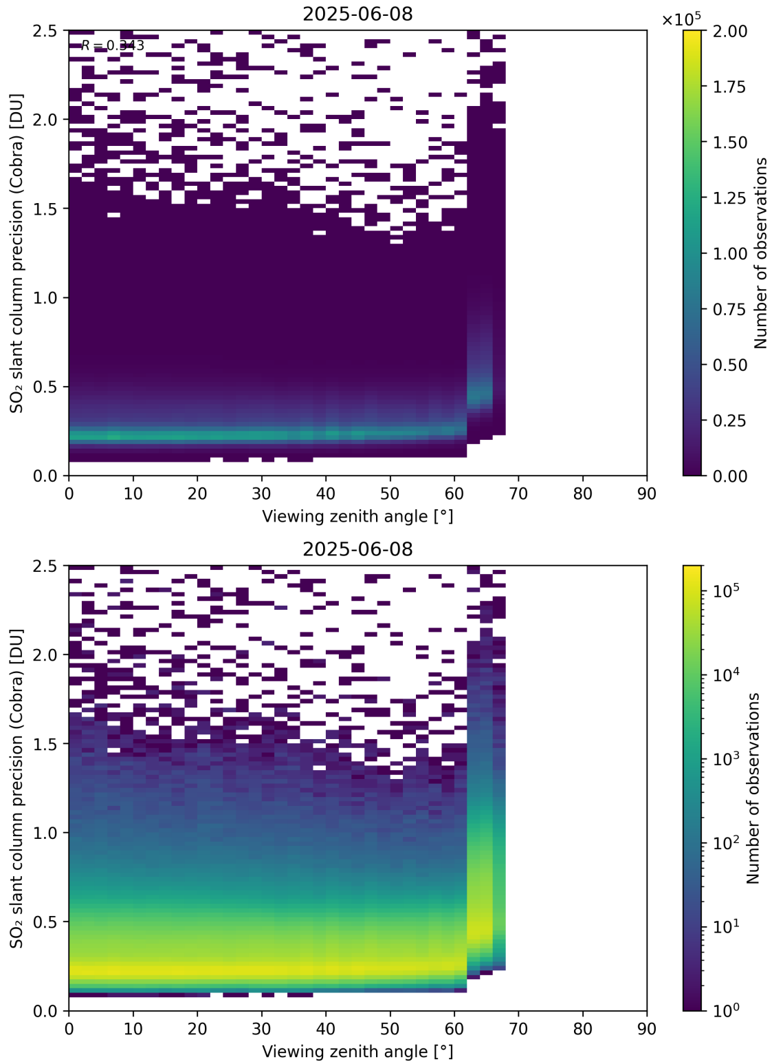
Figure 372: Scatter density plot of “Viewing zenith angle” against “SO 2 slant column precision (Cobra)” for 2025-06-07 to 2025-06-09.
