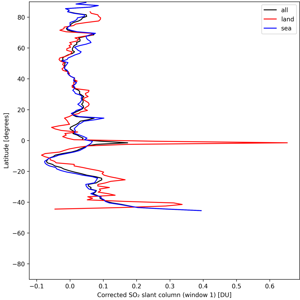
Figure 39: Zonal average of “Corrected SO 2 slant column (window 1)” for 2025-06-07 to 2025-06-09.
