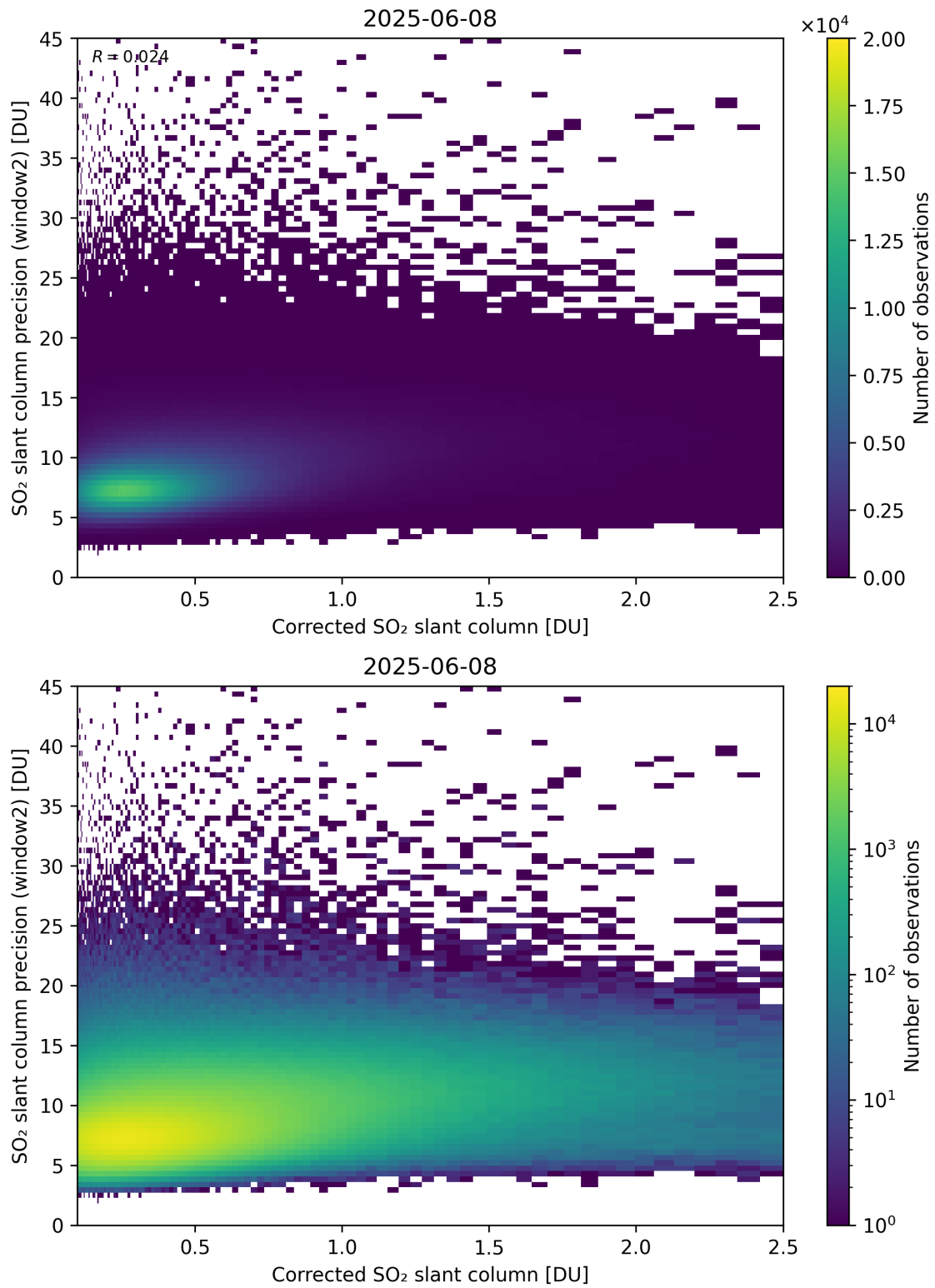
Figure 239: Scatter density plot of “Corrected SO 2 slant column” against “SO 2 slant column precision (window2)” for 2025-06-07 to 2025-06-09.
