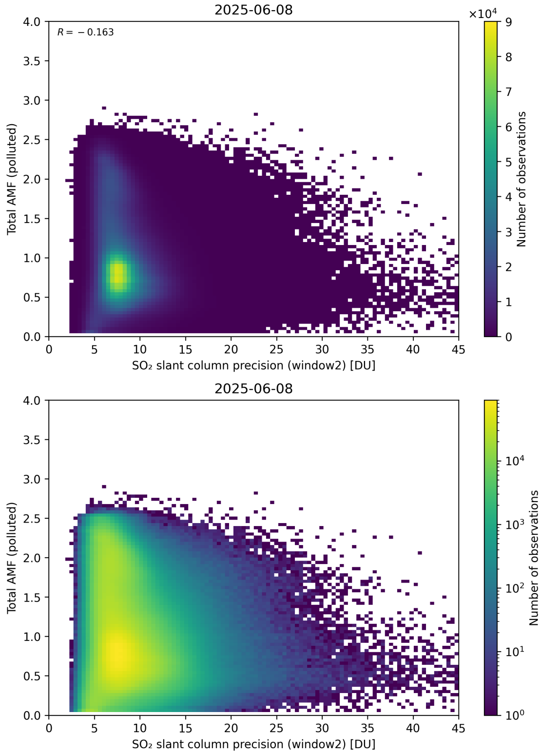
Figure 301: Scatter density plot of “SO 2 slant column precision (window2)” against “Total AMF (polluted)” for 2025-06-07 to 2025-06-09.
