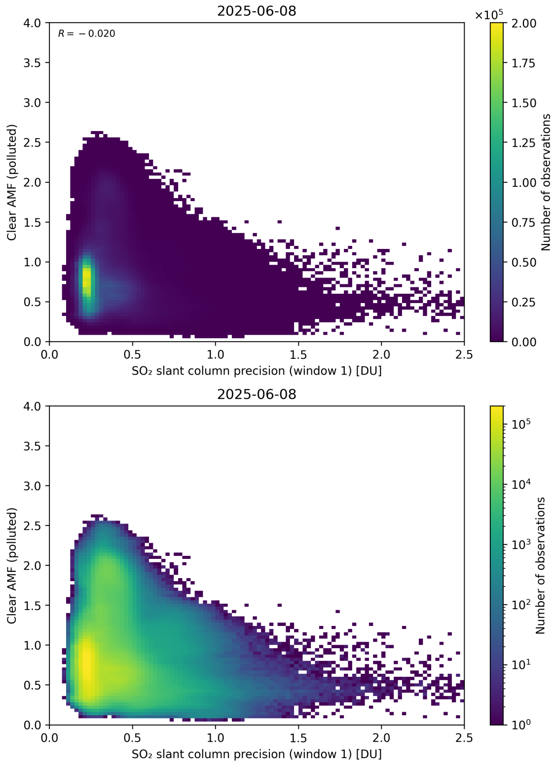
Figure 274: Scatter density plot of “SO 2 slant column precision (window 1)” against “Clear AMF (polluted)” for 2025-06-07 to 2025-06-09.
