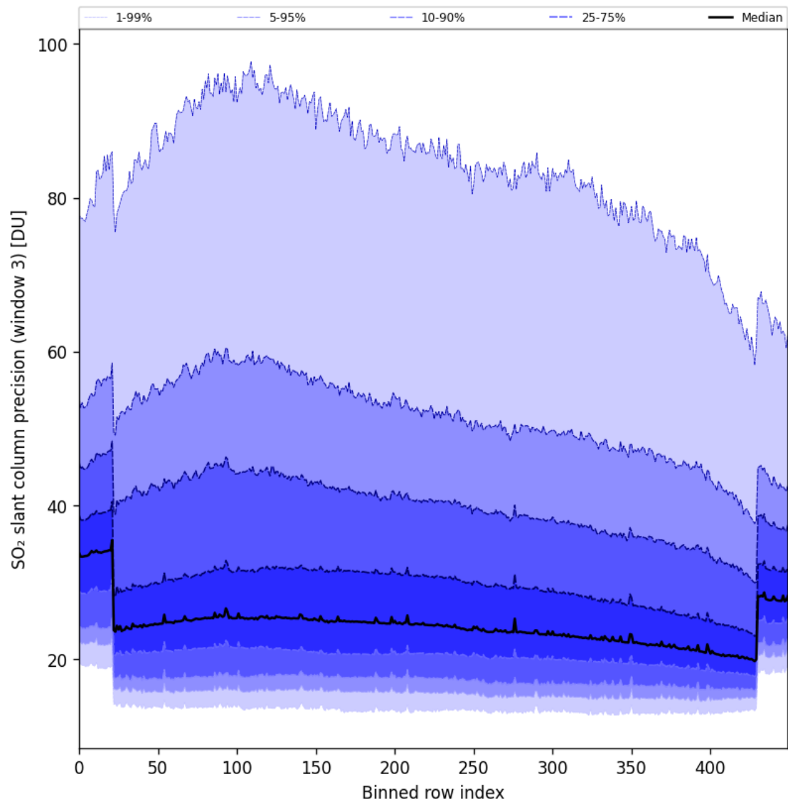
Figure 98: Along track statistics of “SO 2 slant column precision (window 3)” for 2025-06-07 to 2025-06-09
