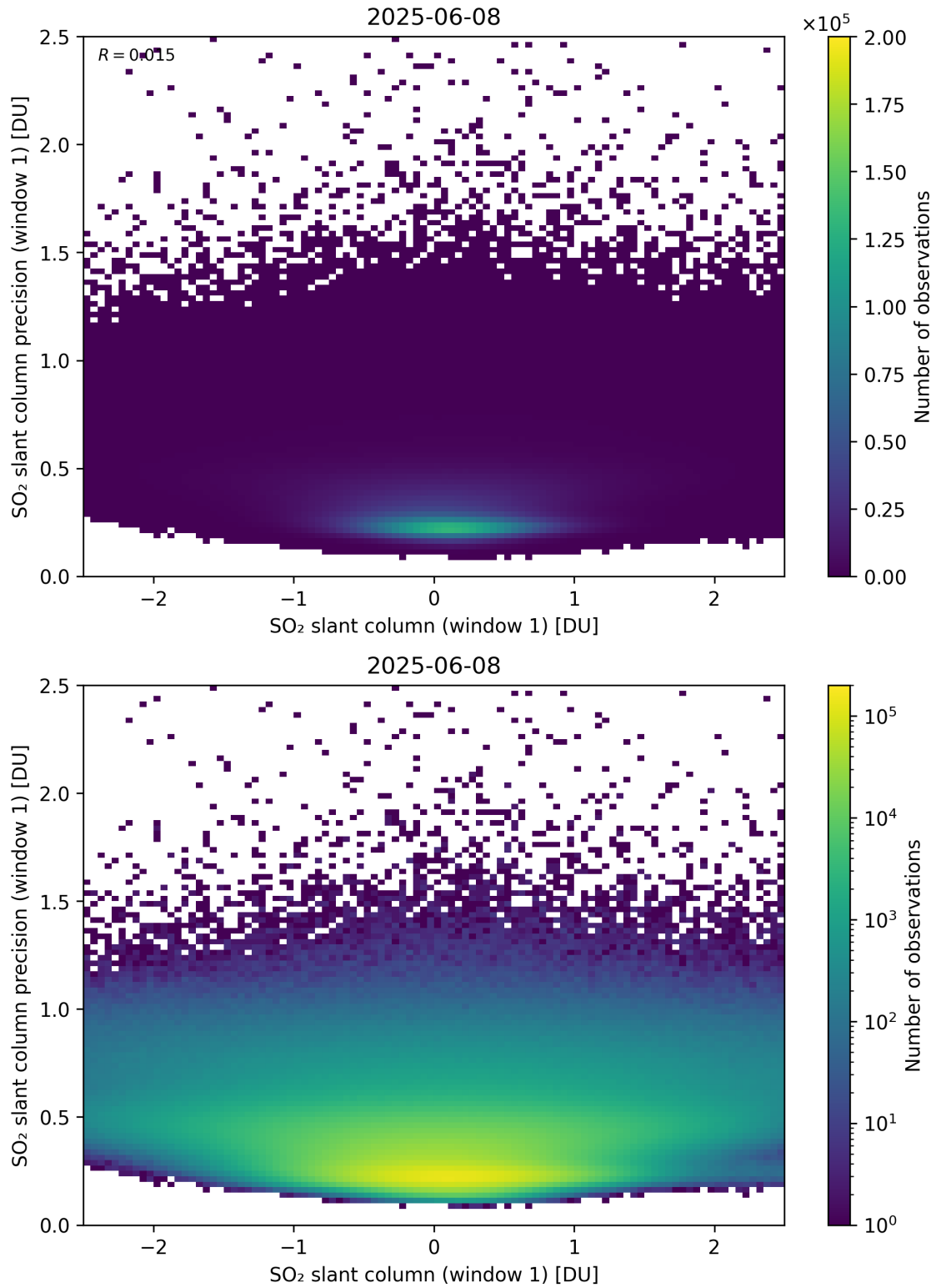
Figure 285: Scatter density plot of “SO 2 slant column (window 1)” against “SO 2 slant column precision (window 1)” for 2025-06-07 to 2025-06-09.
