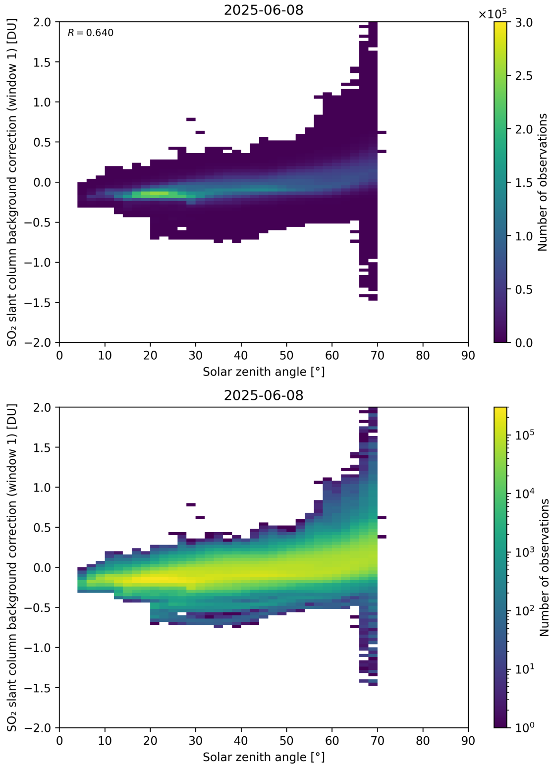
Figure 171: Scatter density plot of “Solar zenith angle” against “SO 2 slant column background correction (window 1)” for 2025-06-07 to 2025-06-09.
