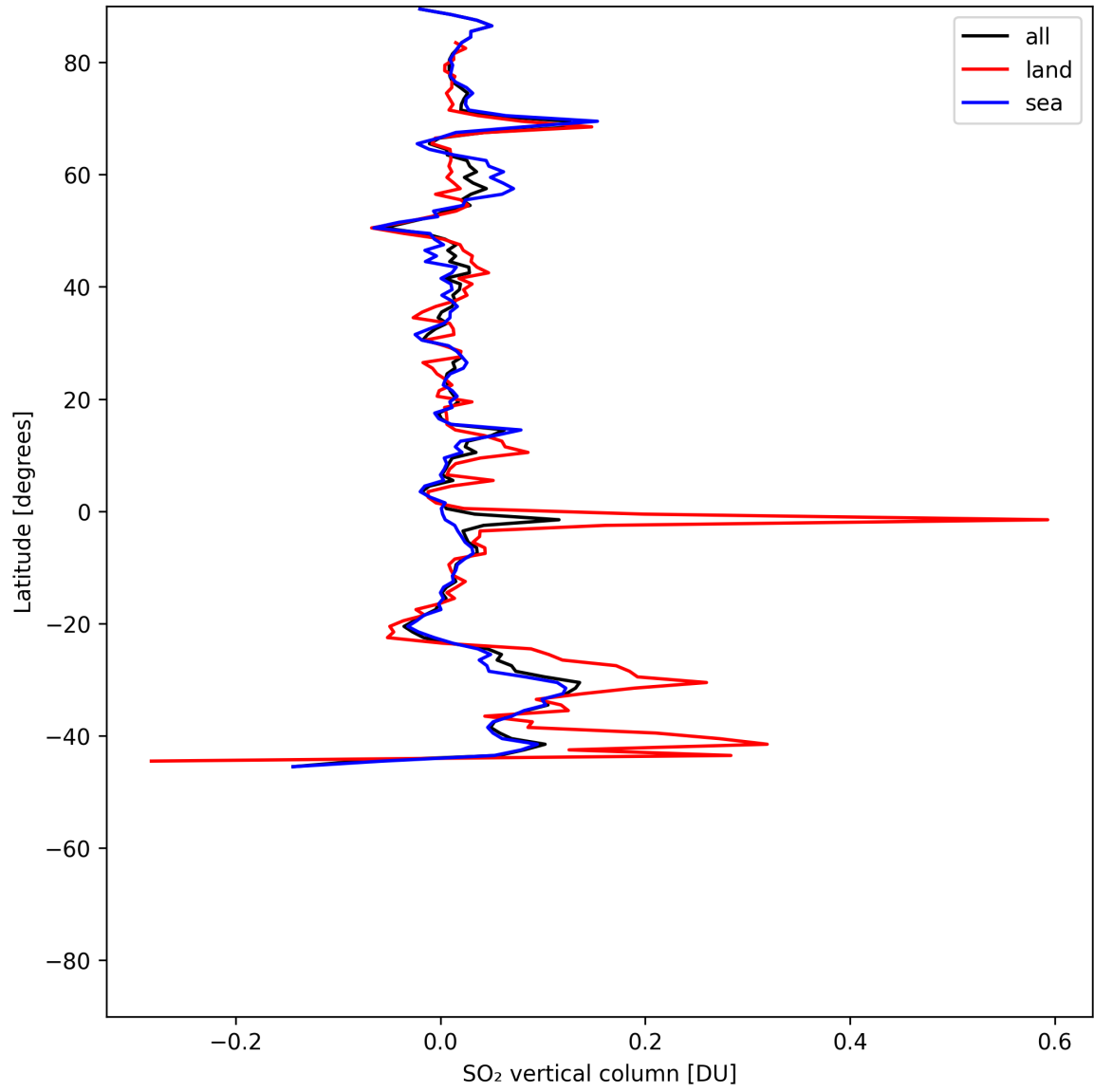
Figure 32: Zonal average of “SO 2 vertical column” for 2025-06-07 to 2025-06-09.
