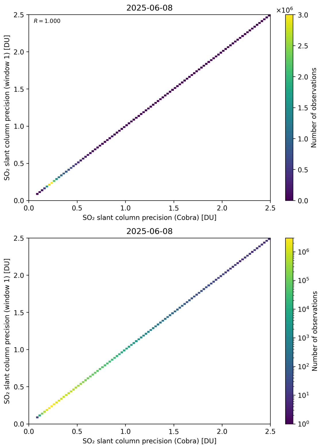
Figure 209: Scatter density plot of “SO 2 slant column precision (Cobra)” against “SO 2 slant column precision (window 1)” for 2025-06-07 to 2025-06-09.
