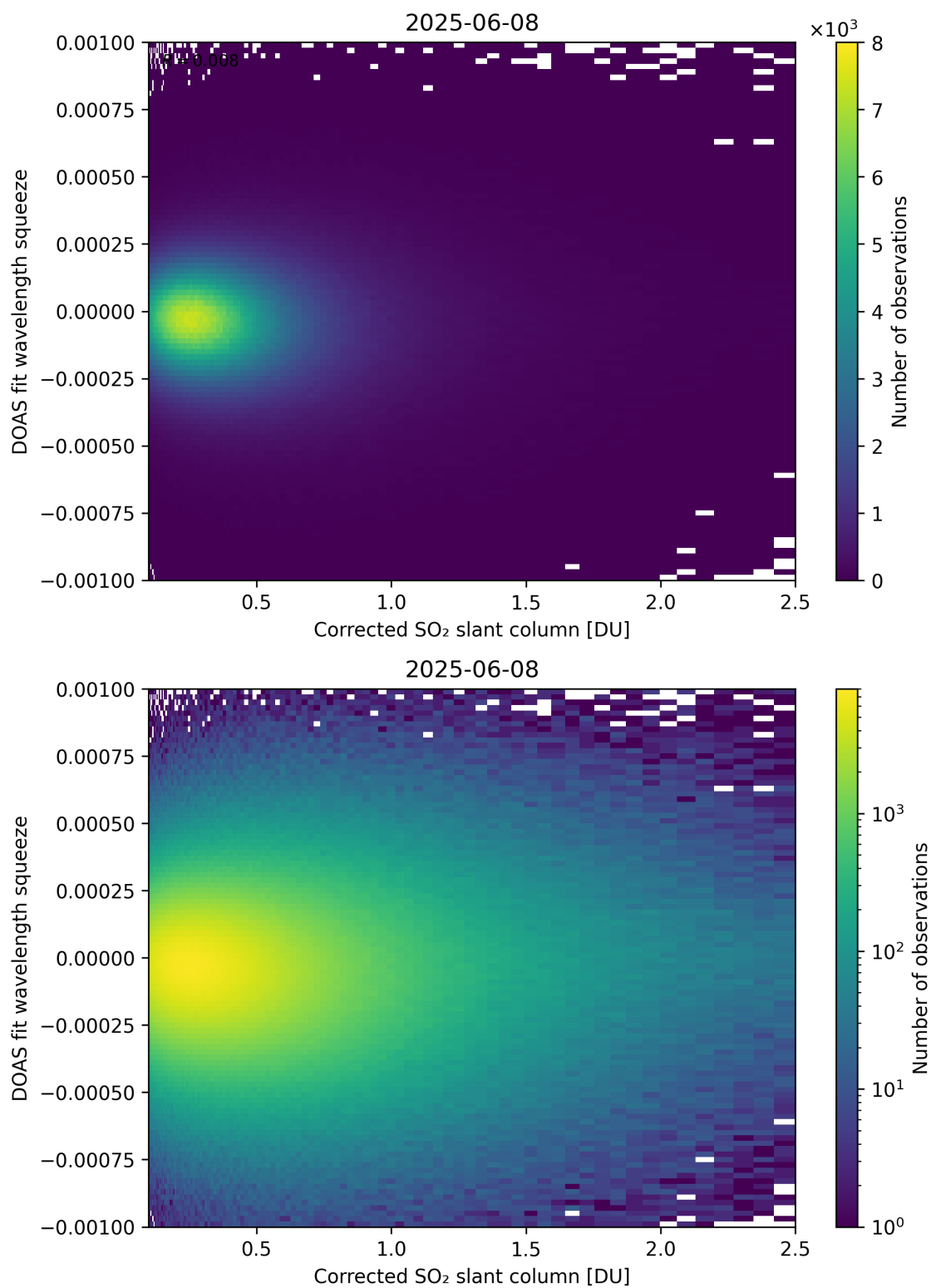
Figure 230: Scatter density plot of “Corrected SO 2 slant column” against “DOAS fit wavelength squeeze” for 2025-06-07 to 2025-06-09.
