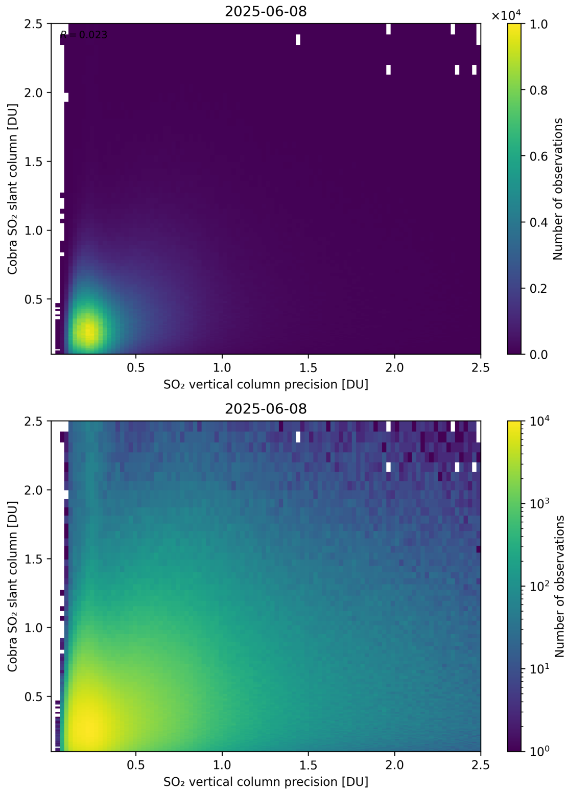
Figure 336: Scatter density plot of “SO 2 vertical column precision” against “Cobra SO 2 slant column” for 2025-06-07 to 2025-06-09.
