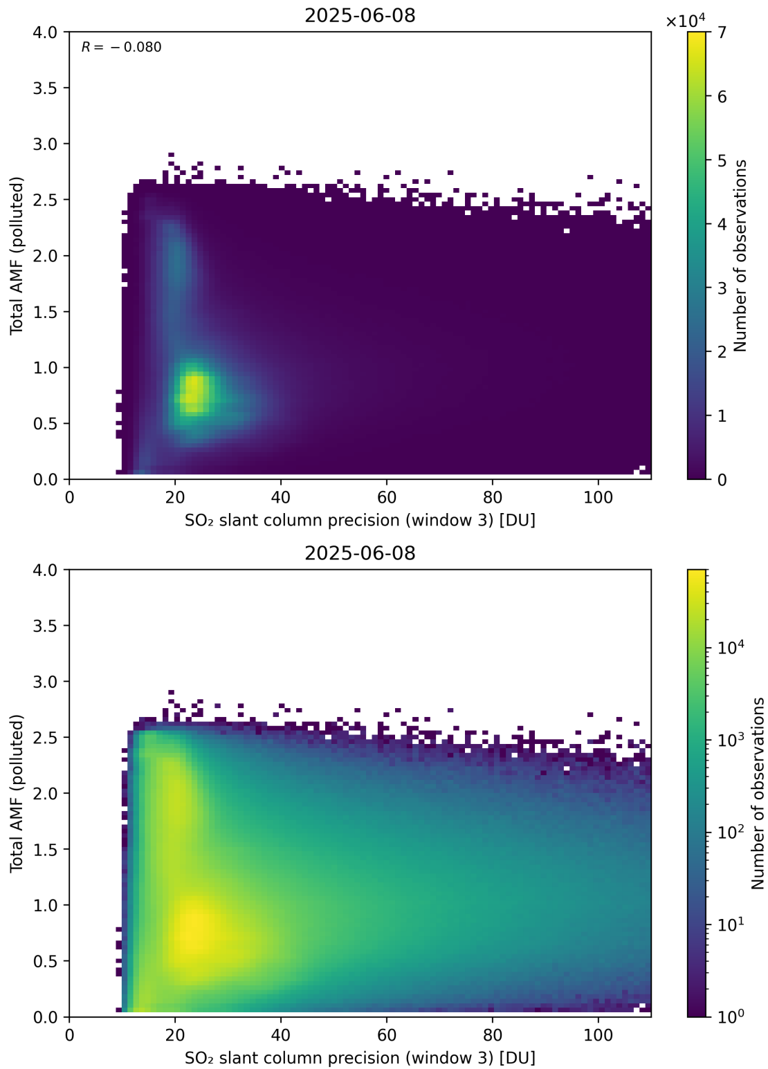
Figure 313: Scatter density plot of “SO 2 slant column precision (window 3)” against “Total AMF (polluted)” for 2025-06-07 to 2025-06-09.
