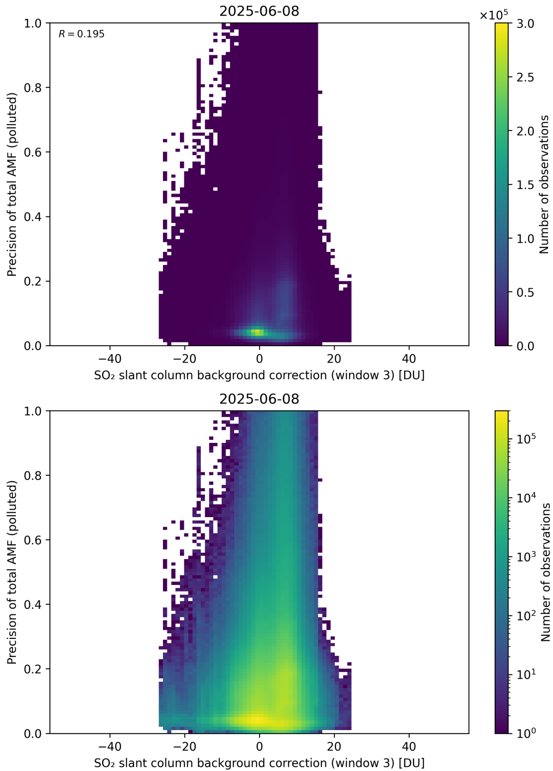
Figure 137: Scatter density plot of “SO 2 slant column background correction (window 3)” against “Precision of total AMF (polluted)” for 2025-06-07 to 2025-06-09.
