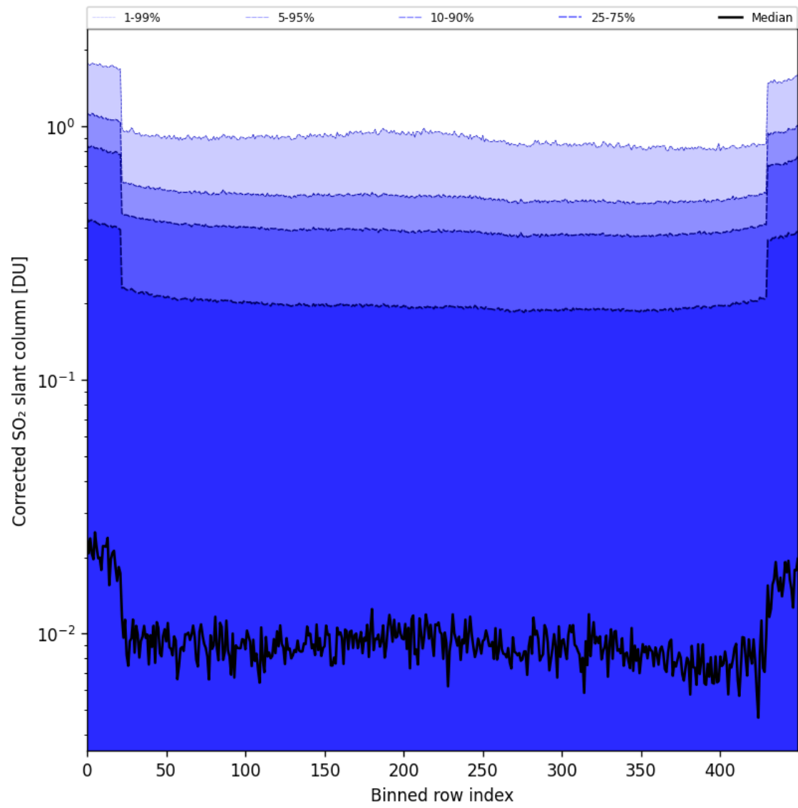
Figure 86: Along track statistics of “Corrected SO 2 slant column” for 2025-06-07 to 2025-06-09
