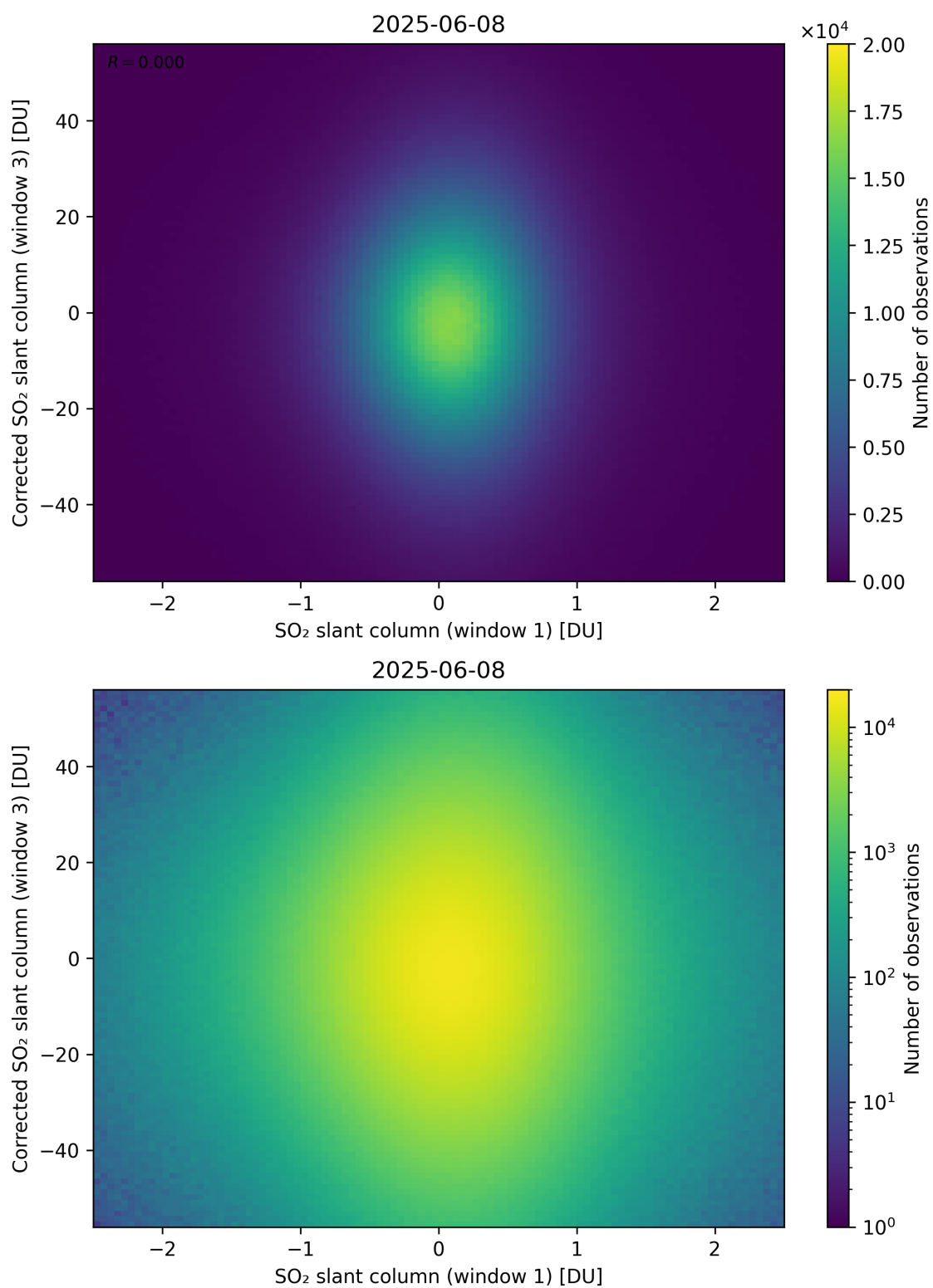
Figure 284: Scatter density plot of “SO 2 slant column (window 1)” against “Corrected SO 2 slant column (window 3)” for 2025-06-07 to 2025-06-09.
