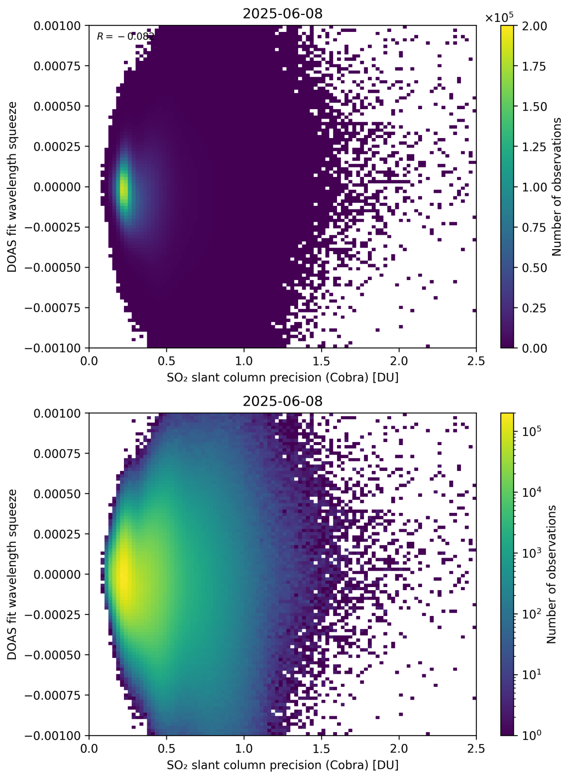
Figure 203: Scatter density plot of “SO 2 slant column precision (Cobra)” against “DOAS fit wavelength squeeze” for 2025-06-07 to 2025-06-09.
