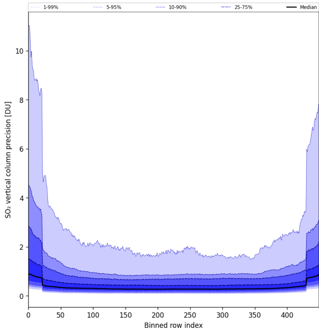
Figure 85: Along track statistics of “SO 2 vertical column precision” for 2025-06-07 to 2025-06-09
