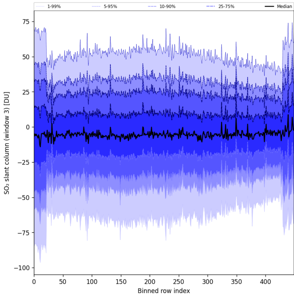
Figure 97: Along track statistics of “SO 2 slant column (window 3)” for 2025-06-07 to 2025-06-09
