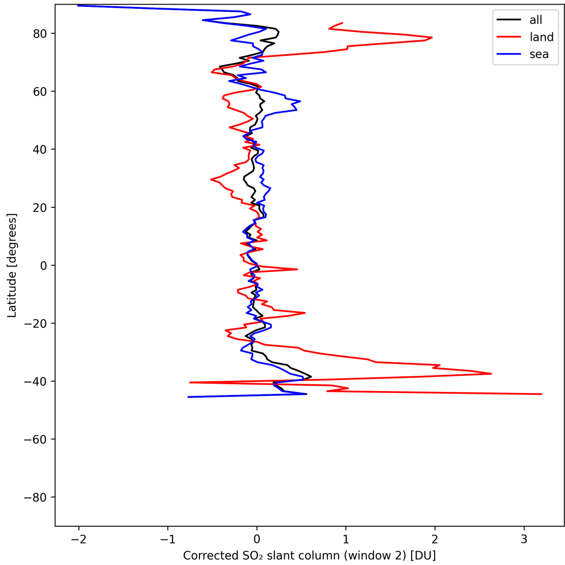
Figure 43: Zonal average of “Corrected SO 2 slant column (window 2)” for 2025-06-07 to 2025-06-09.
