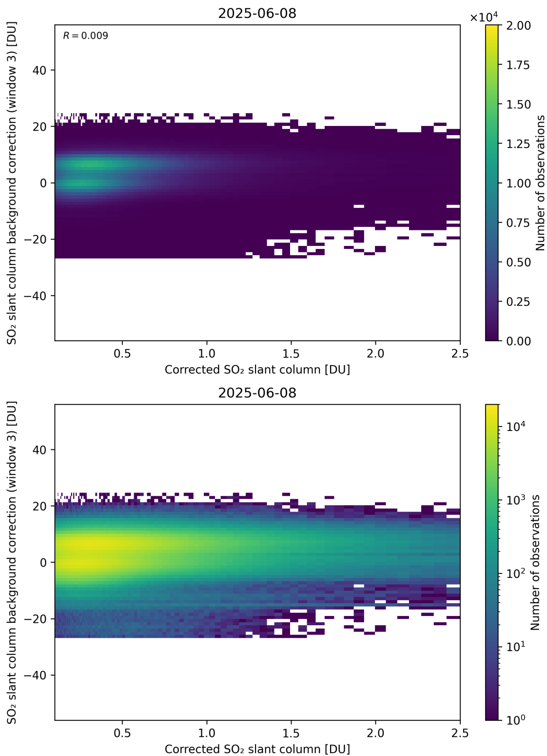
Figure 228: Scatter density plot of “Corrected SO 2 slant column” against “SO 2 slant column background correction (window 3)” for 2025-06-07 to 2025-06-09.
