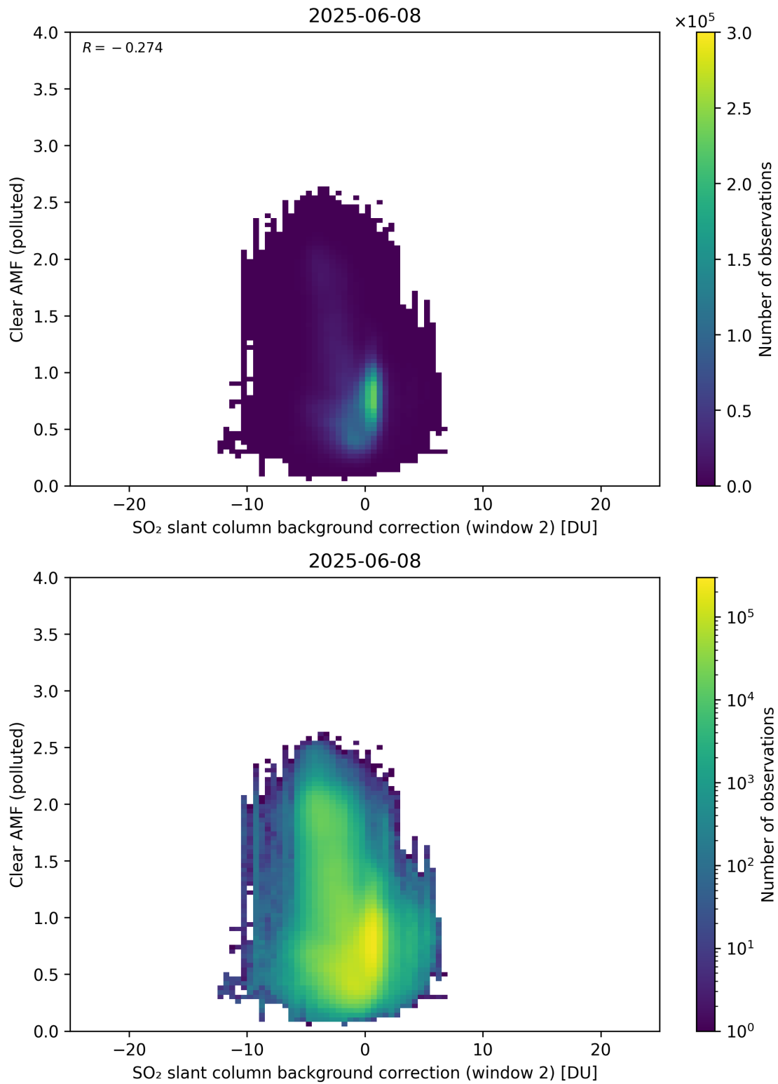
Figure 126: Scatter density plot of “SO 2 slant column background correction (window 2)” against “Clear AMF (polluted)” for 2025-06-07 to 2025-06-09.
