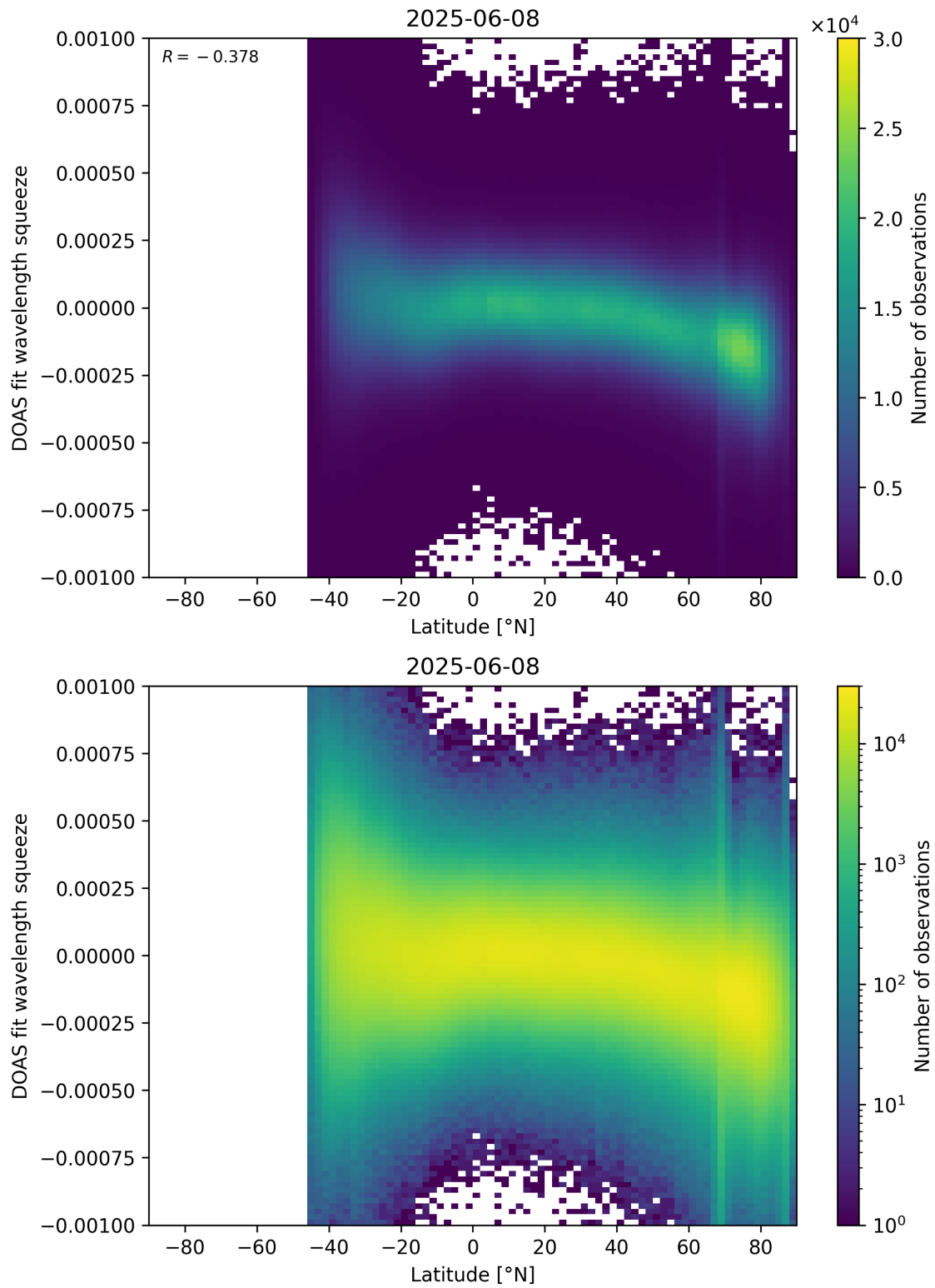
Figure 154: Scatter density plot of “Latitude” against “DOAS fit wavelength squeeze” for 2025-06-07 to 2025-06-09.
