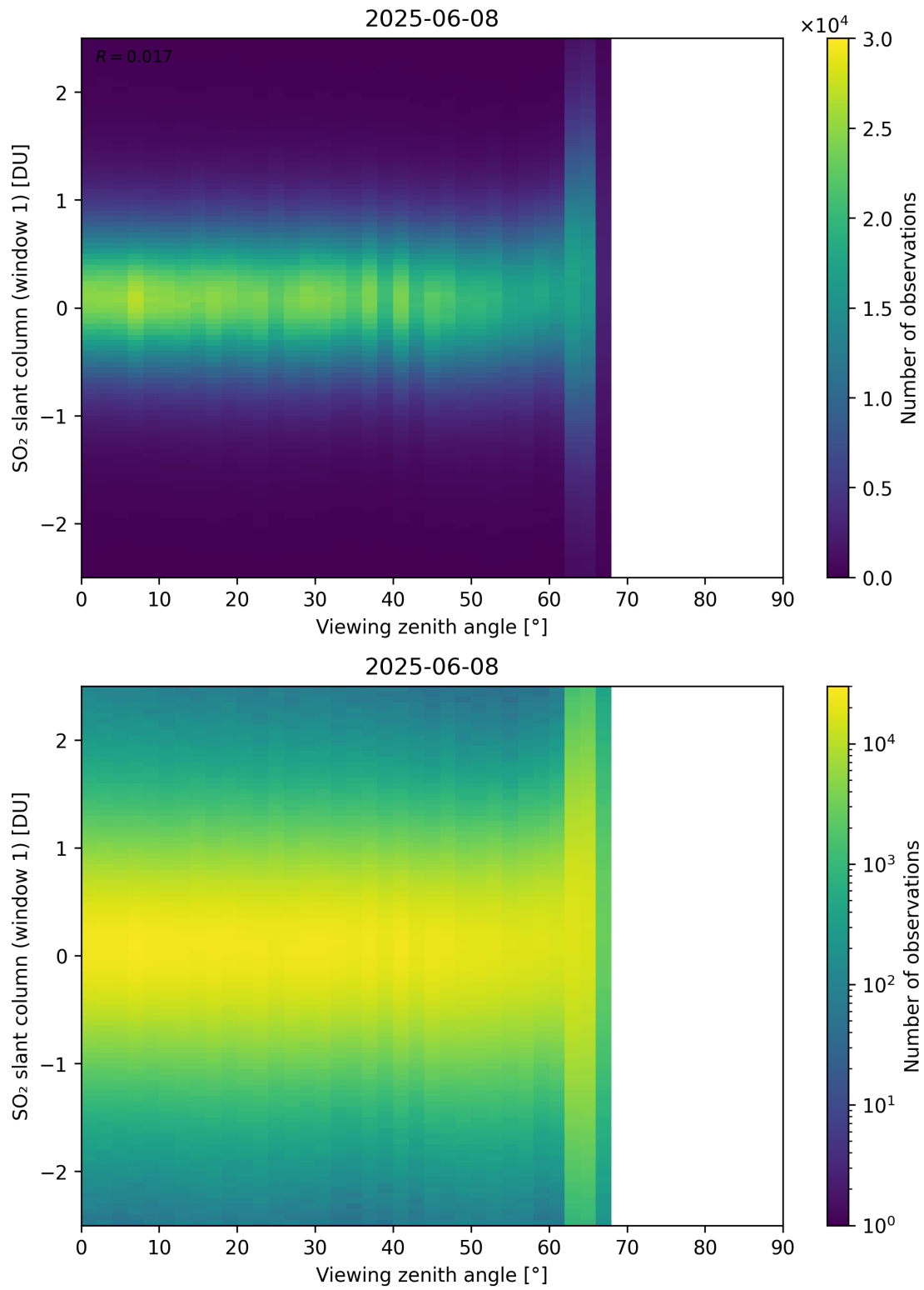
Figure 376: Scatter density plot of “Viewing zenith angle” against “SO 2 slant column (window 1)” for 2025-06-07 to 2025-06-09.
