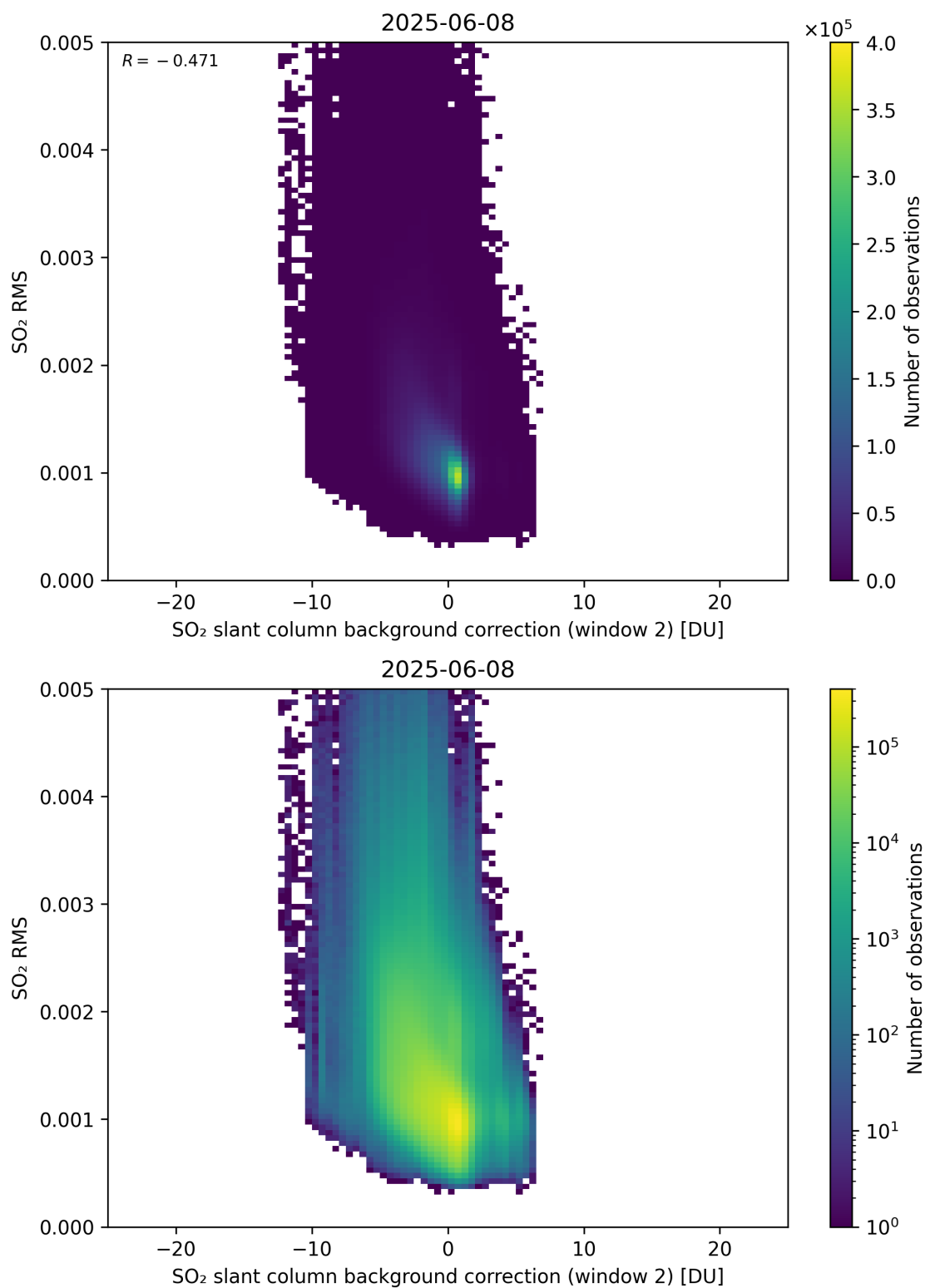
Figure 125: Scatter density plot of “SO 2 slant column background correction (window 2)” against “SO 2 RMS” for 2025-06-07 to 2025-06-09.
