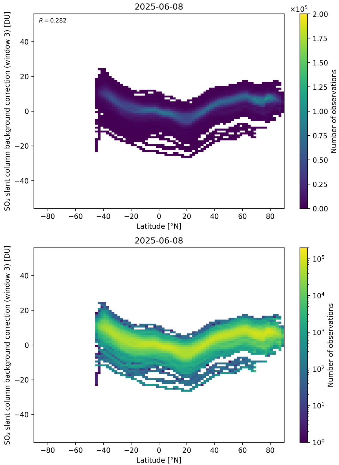
Figure 152: Scatter density plot of “Latitude” against “SO 2 slant column background correction (window 3)” for 2025-06-07 to 2025-06-09.
