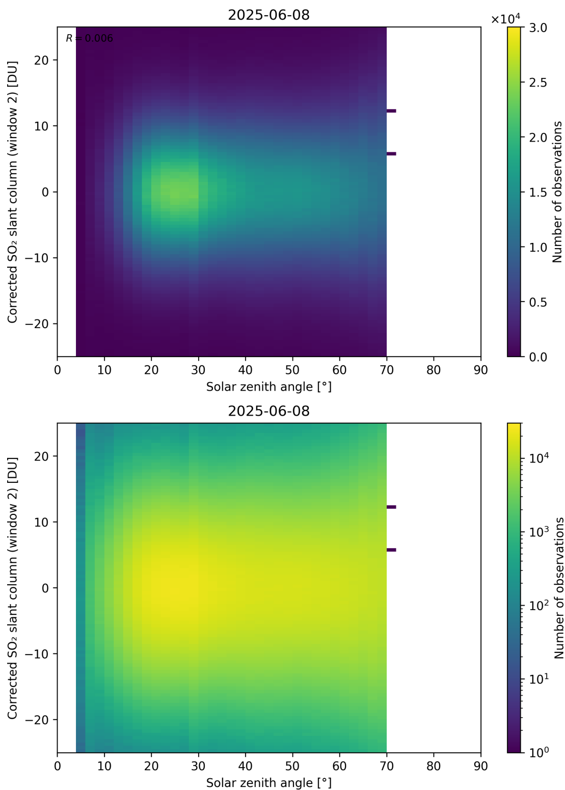
Figure 182: Scatter density plot of “Solar zenith angle” against “Corrected SO 2 slant column (window 2)” for 2025-06-07 to 2025-06-09.
