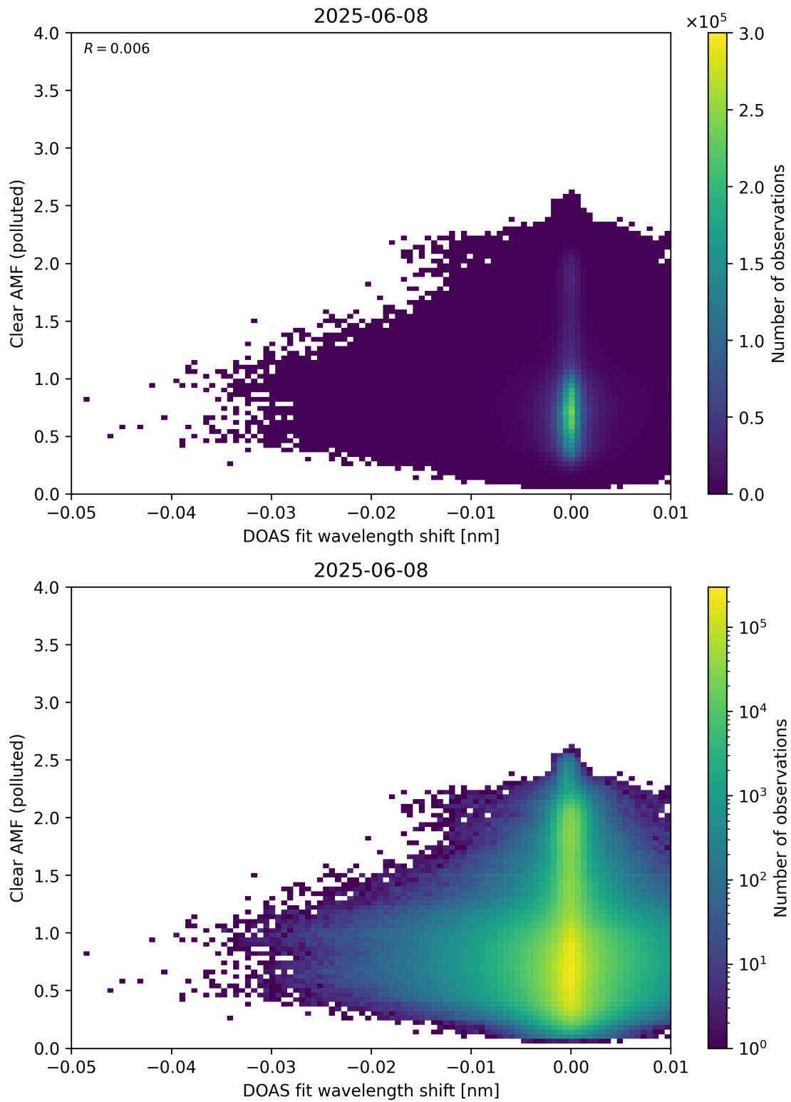
Figure 140: Scatter density plot of “DOAS fit wavelength shift” against “Clear AMF (polluted)” for 2025-06-07 to 2025-06-09.
