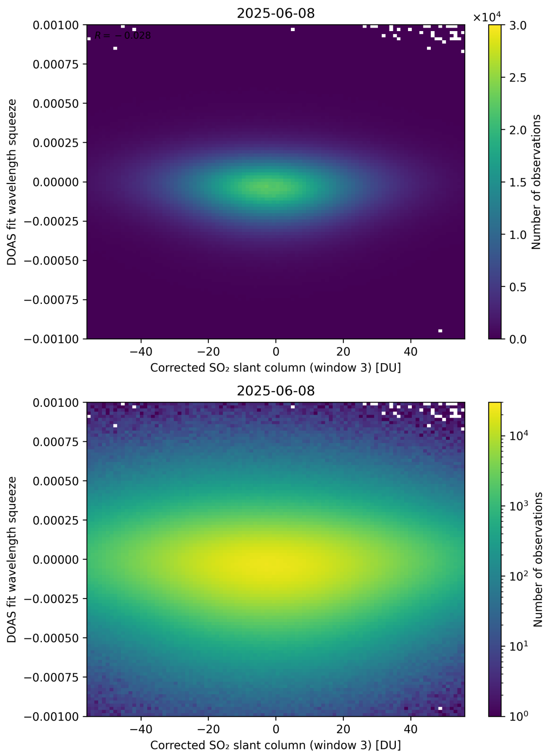
Figure 257: Scatter density plot of “Corrected SO 2 slant column (window 3)” against “DOAS fit wavelength squeeze” for 2025-06-07 to 2025-06-09.
