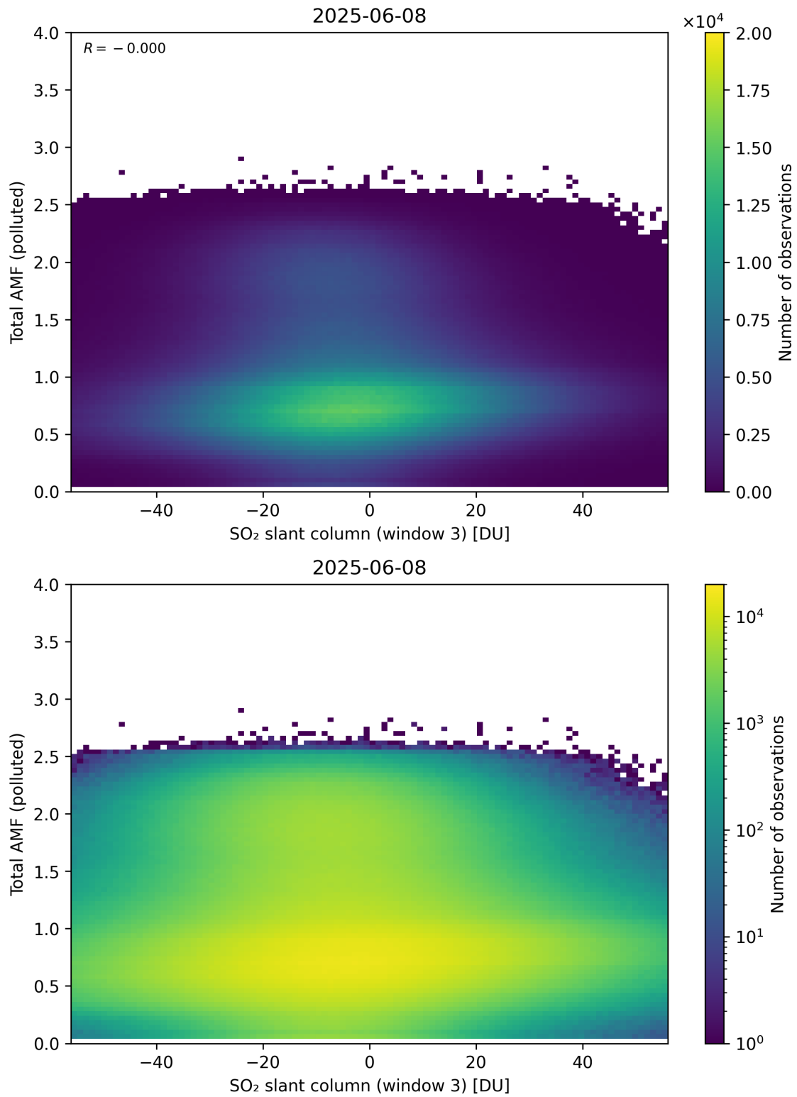
Figure 318: Scatter density plot of “SO 2 slant column (window 3)” against “Total AMF (polluted)” for 2025-06-07 to 2025-06-09.
