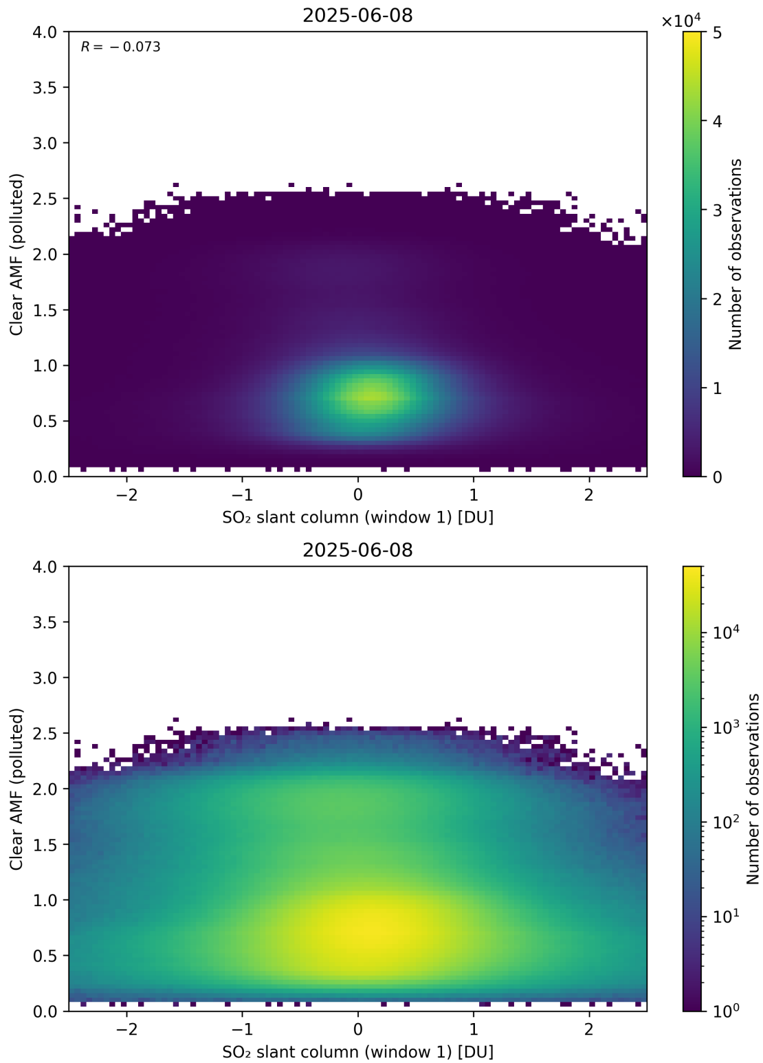
Figure 282: Scatter density plot of “SO 2 slant column (window 1)” against “Clear AMF (polluted)” for 2025-06-07 to 2025-06-09.
