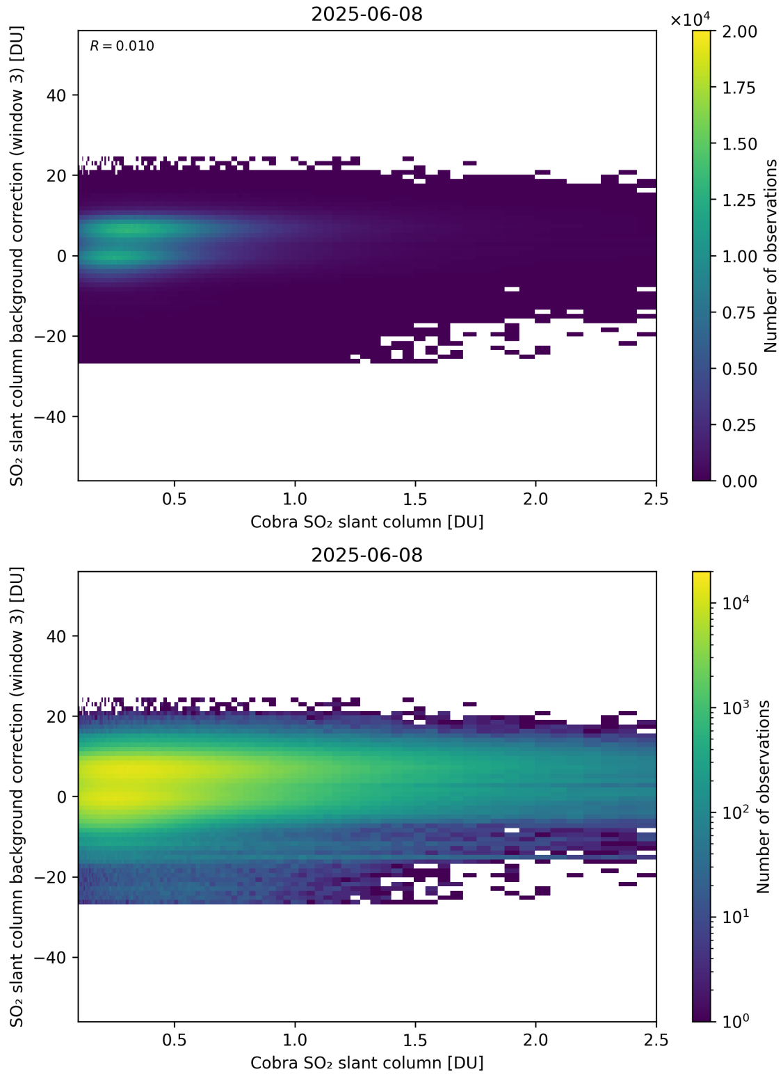
Figure 195: Scatter density plot of “Cobra SO 2 slant column” against “SO 2 slant column background correction (window 3)” for 2025-06-07 to 2025-06-09.
