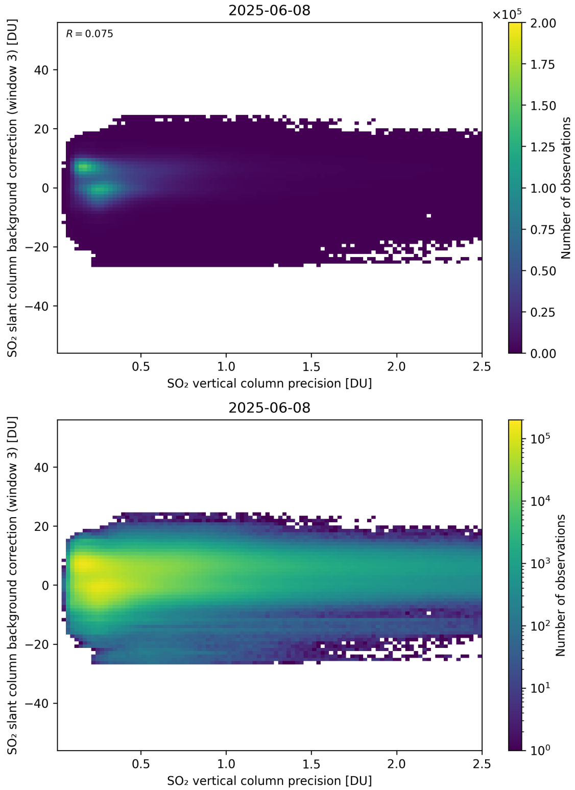
Figure 331: Scatter density plot of “SO 2 vertical column precision” against “SO 2 slant column background correction (window 3)” for 2025-06-07 to 2025-06-09.
