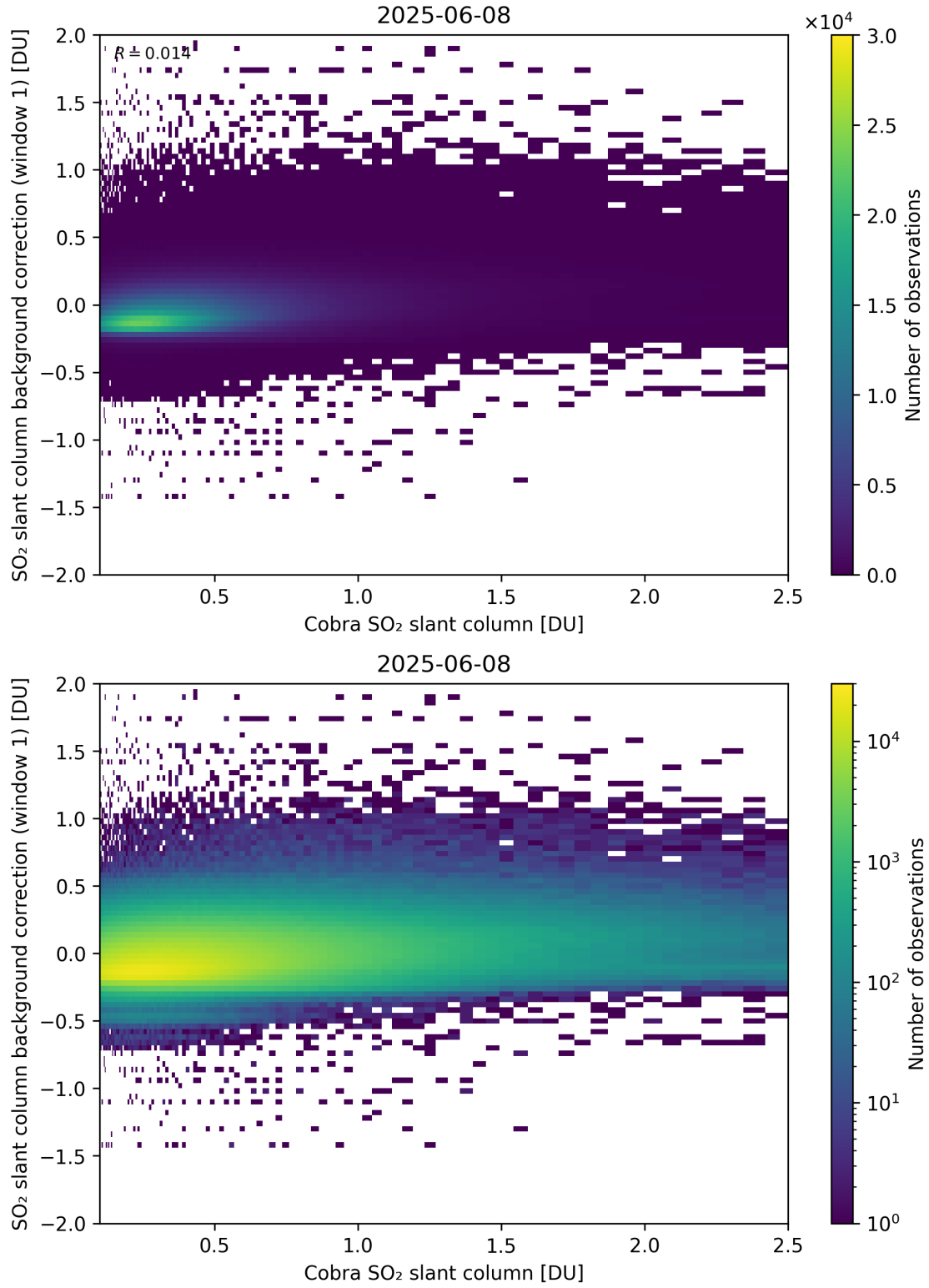
Figure 193: Scatter density plot of “Cobra SO 2 slant column” against “SO 2 slant column background correction (window 1)” for 2025-06-07 to 2025-06-09.
