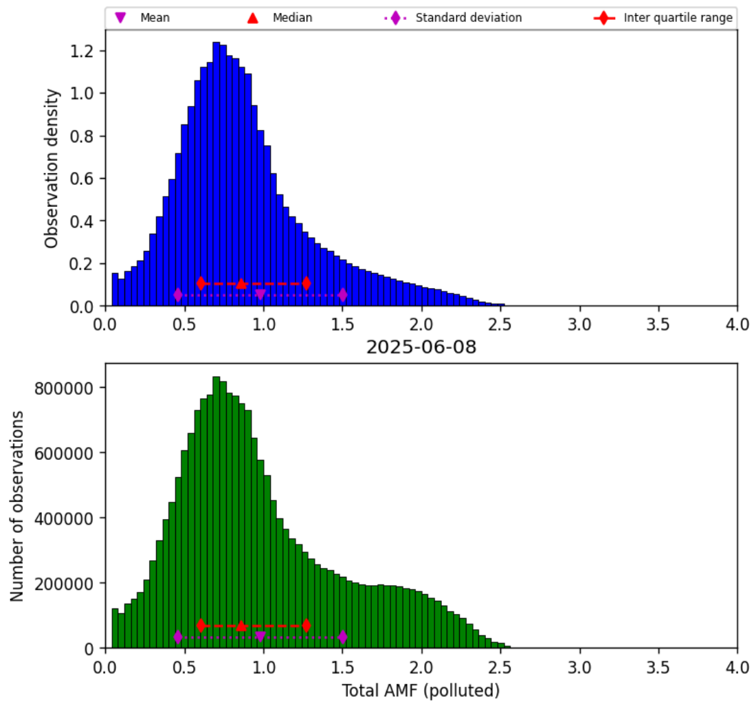
Figure 79: Histogram of “Total AMF (polluted)” for 2025-06-07 to 2025-06-09
