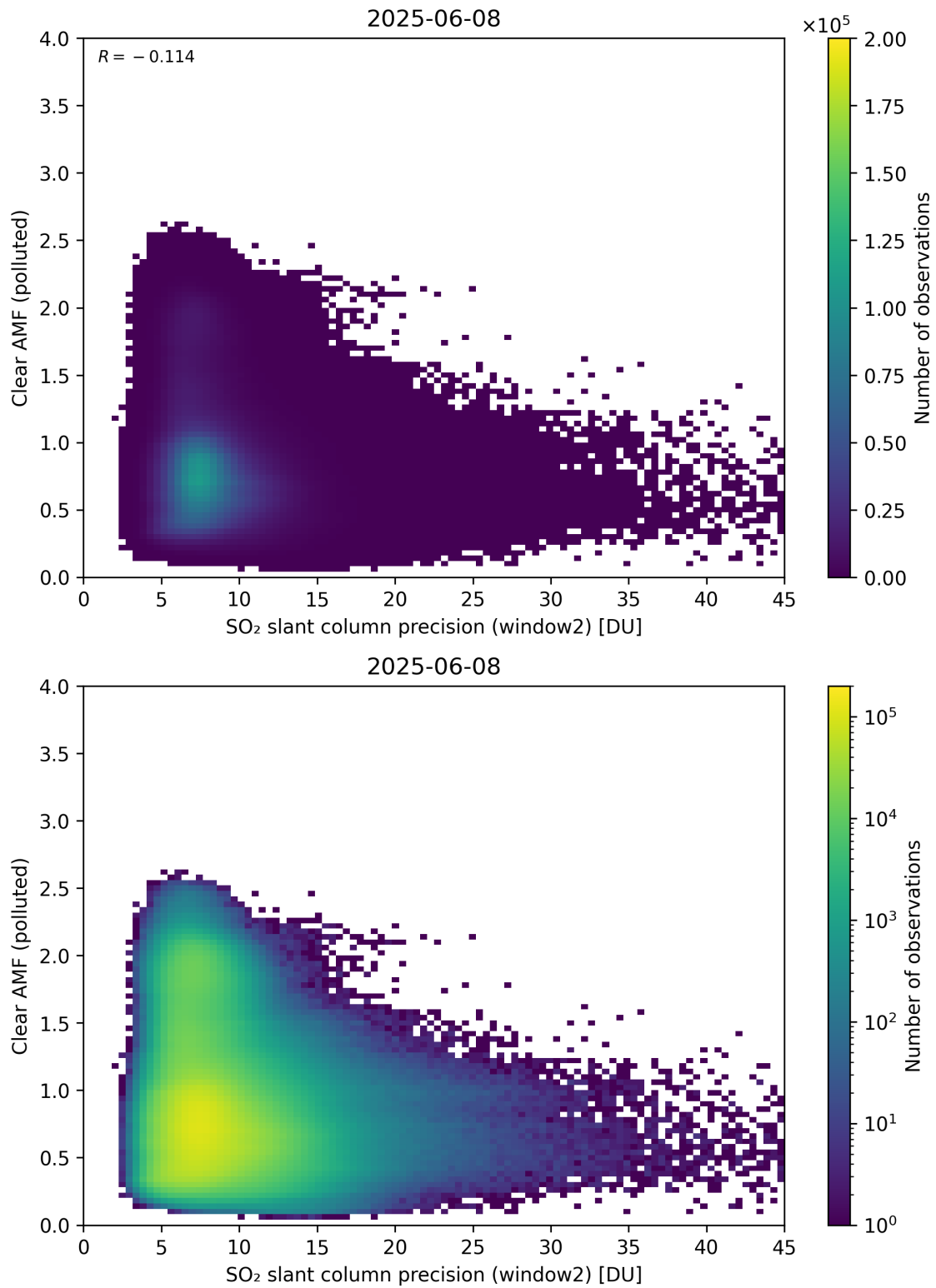
Figure 296: Scatter density plot of “SO 2 slant column precision (window2)” against “Clear AMF (polluted)” for 2025-06-07 to 2025-06-09.
