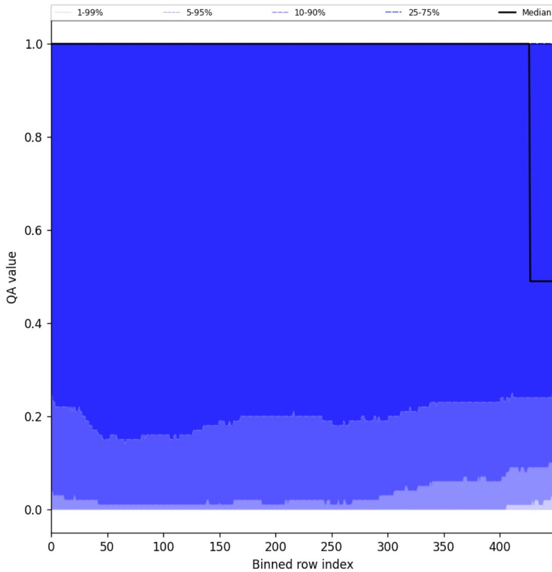
Figure 83: Along track statistics of “QA value” for 2025-06-07 to 2025-06-09
