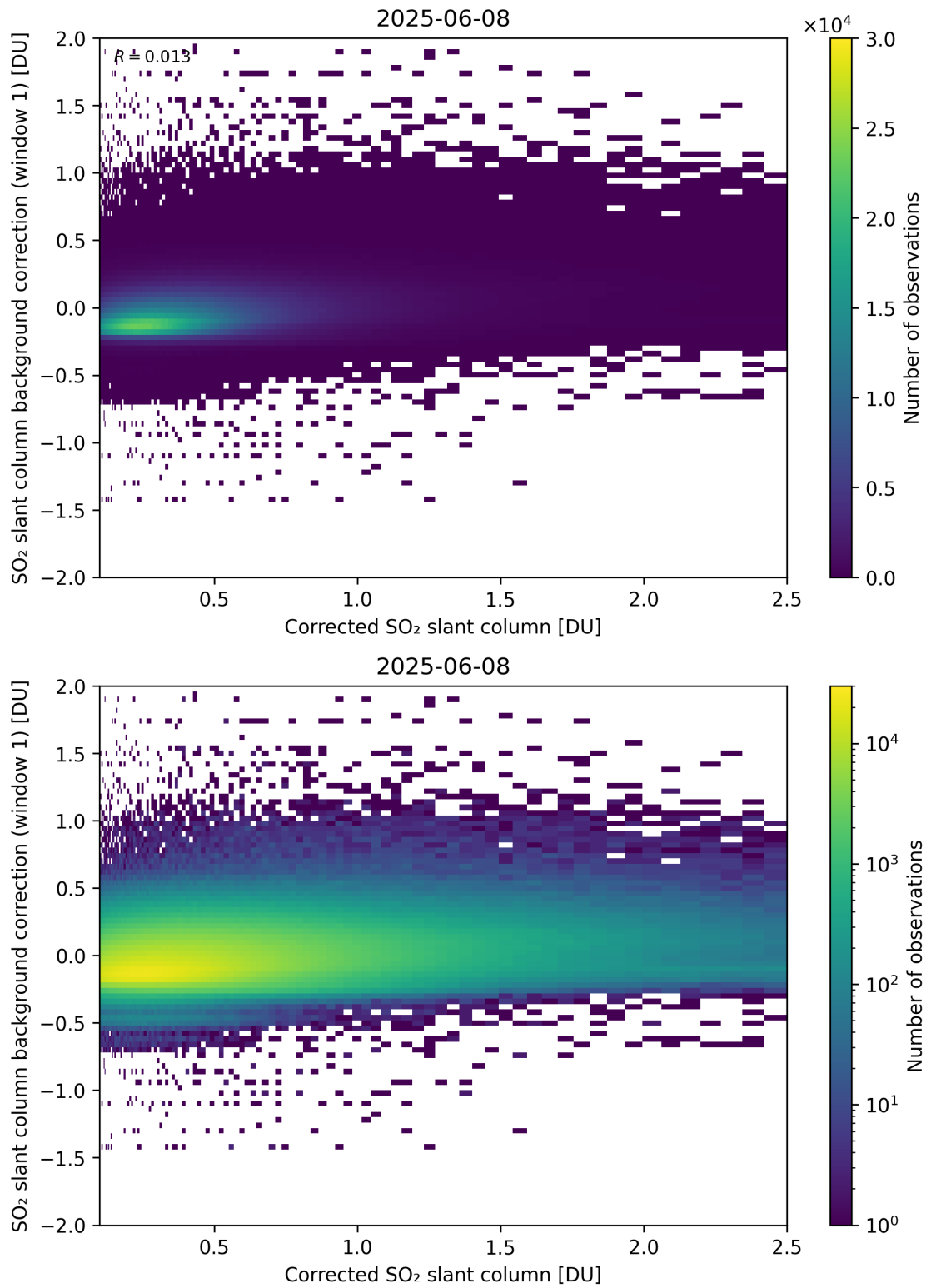
Figure 226: Scatter density plot of “Corrected SO 2 slant column” against “SO 2 slant column background correction (window 1)” for 2025-06-07 to 2025-06-09.
