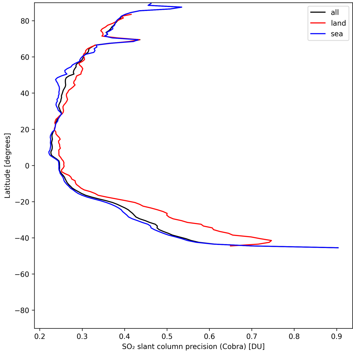
Figure 36: Zonal average of “SO 2 slant column precision (Cobra)” for 2025-06-07 to 2025-06-09.
