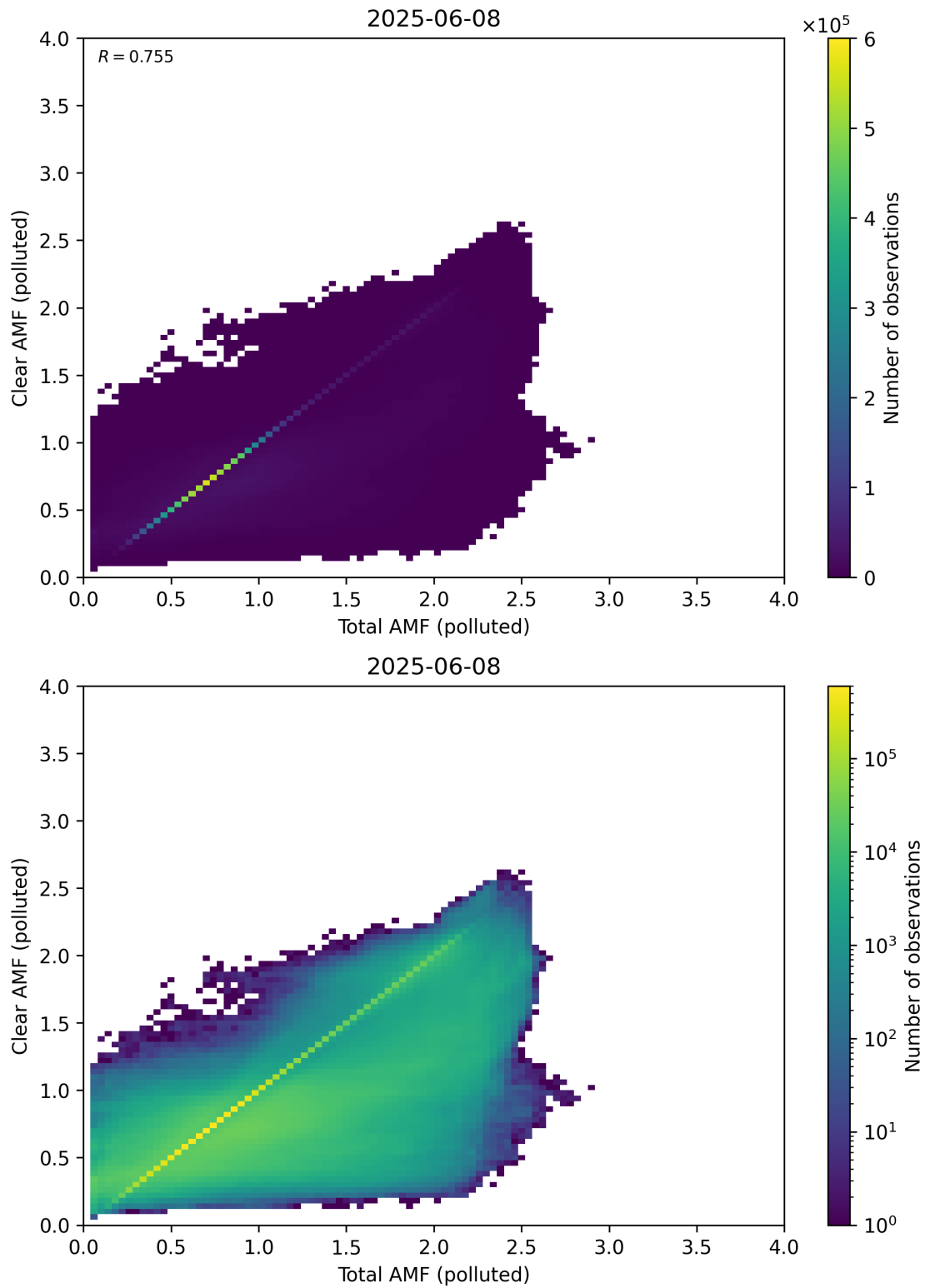
Figure 321: Scatter density plot of “Total AMF (polluted)” against “Clear AMF (polluted)” for 2025-06-07 to 2025-06-09.
