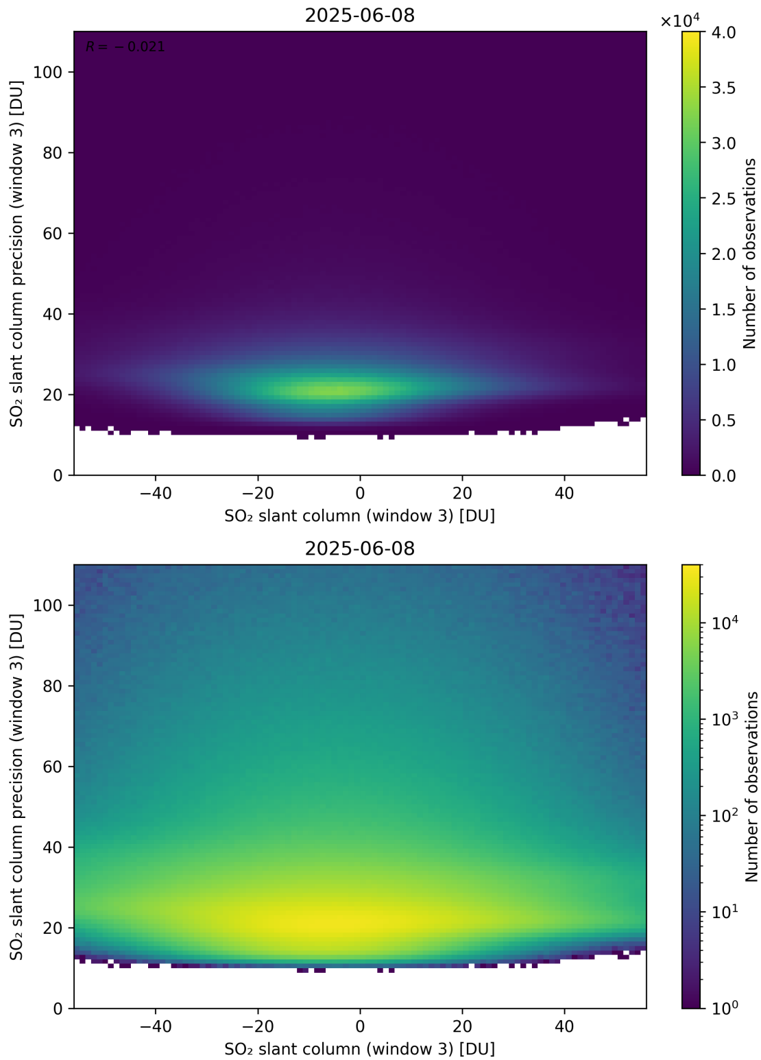
Figure 317: Scatter density plot of “SO 2 slant column (window 3)” against “SO 2 slant column precision (window 3)” for 2025-06-07 to 2025-06-09.
