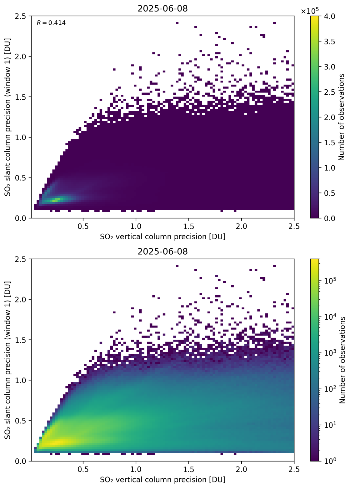
Figure 342: Scatter density plot of “SO 2 vertical column precision” against “SO 2 slant column precision (window 1)” for 2025-06-07 to 2025-06-09.
