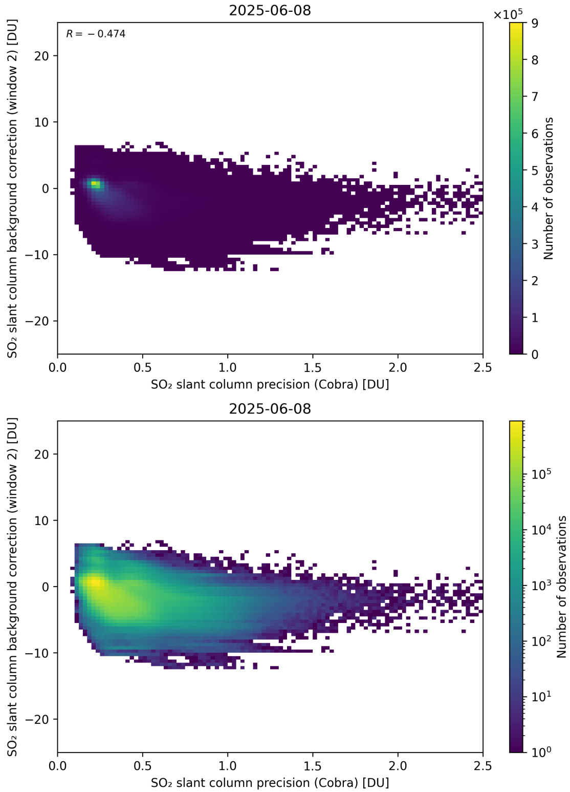
Figure 200: Scatter density plot of “SO 2 slant column precision (Cobra)” against “SO 2 slant column background correction (window 2)” for 2025-06-07 to 2025-06-09.
