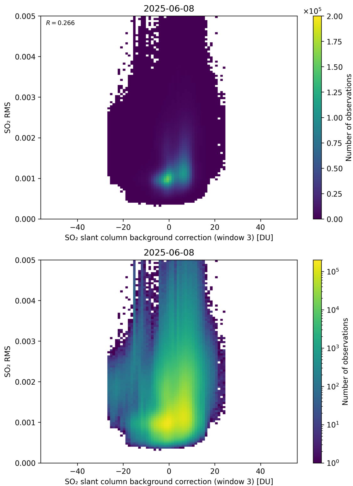
Figure 134: Scatter density plot of “SO 2 slant column background correction (window 3)” against “SO 2 RMS” for 2025-06-07 to 2025-06-09.
