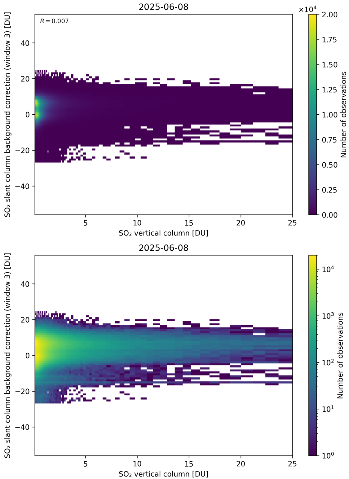
Figure 325: Scatter density plot of “SO 2 vertical column” against “SO 2 slant column background correction (window 3)” for 2025-06-07 to 2025-06-09.
