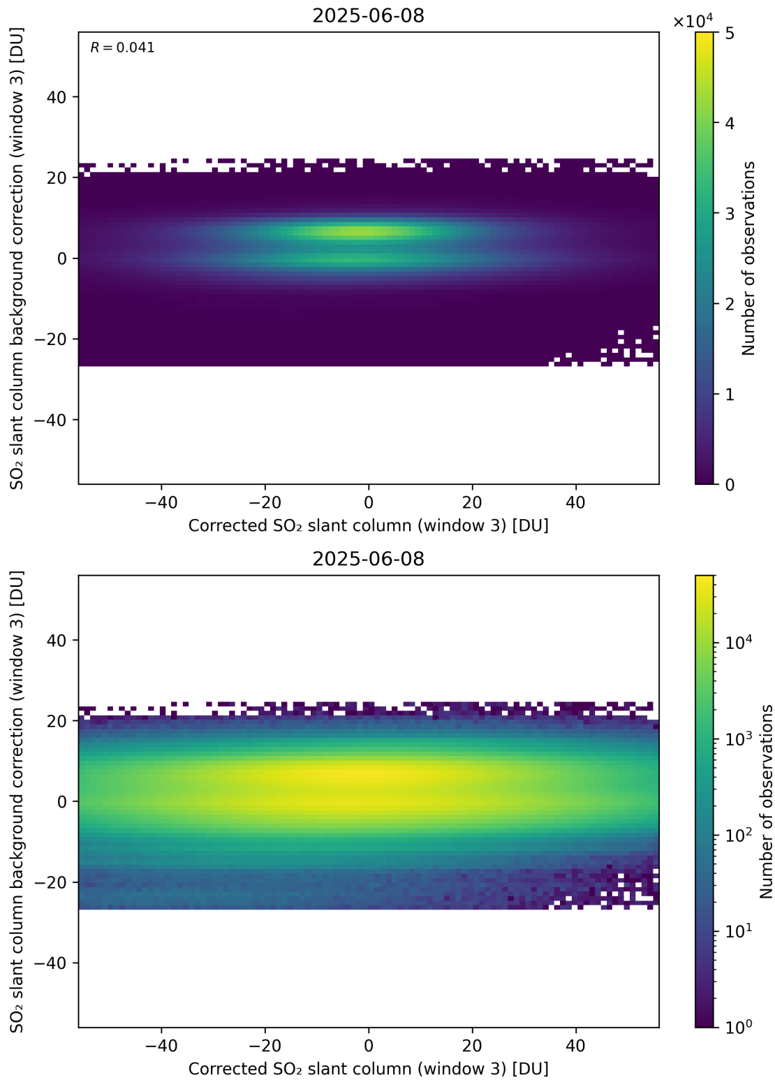
Figure 255: Scatter density plot of “Corrected SO 2 slant column (window 3)” against “SO 2 slant column background correction (window 3)” for 2025-06-07 to 2025-06-09.
