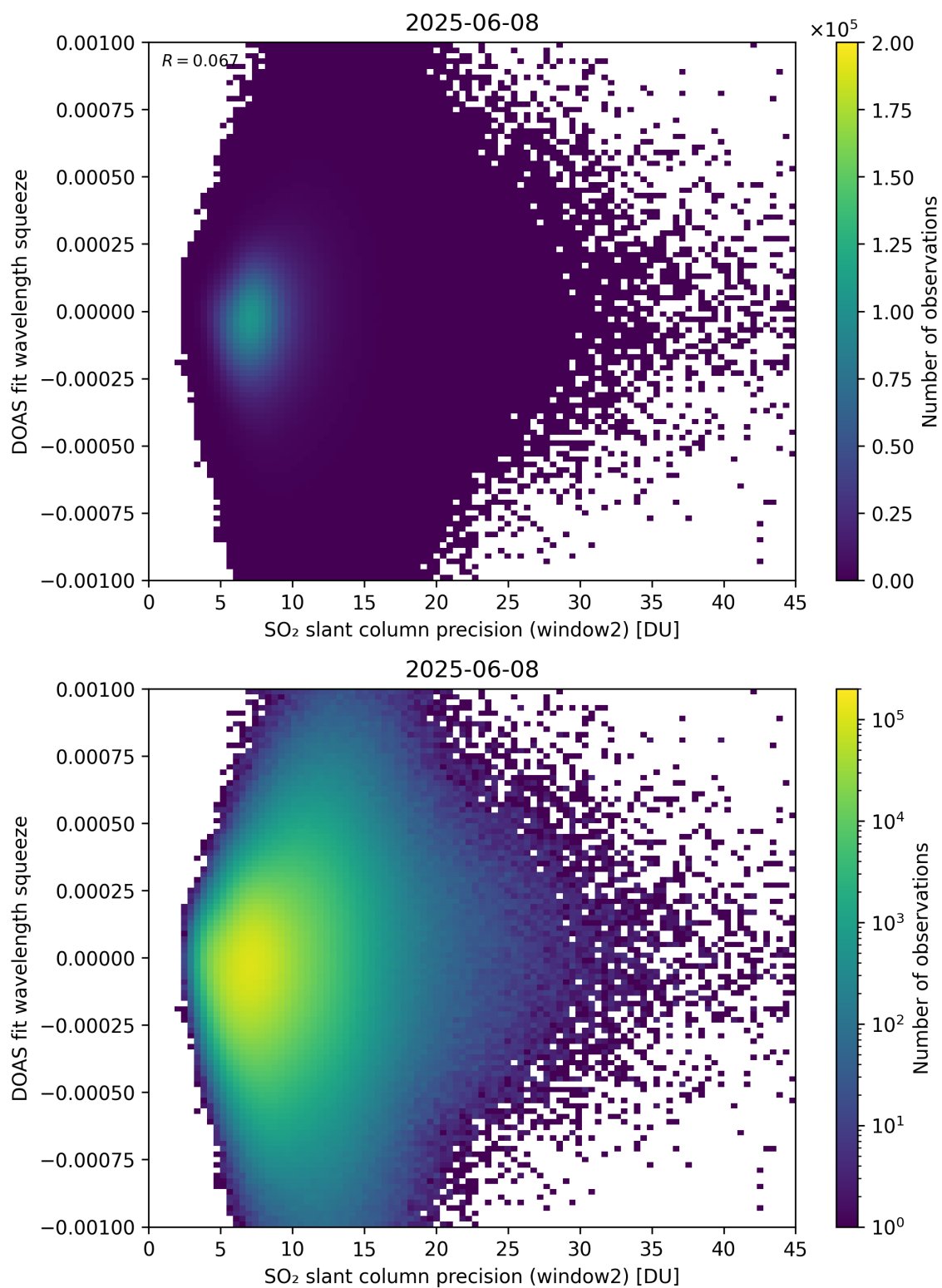
Figure 294: Scatter density plot of “SO 2 slant column precision (window2)” against “DOAS fit wavelength squeeze” for 2025-06-07 to 2025-06-09.
