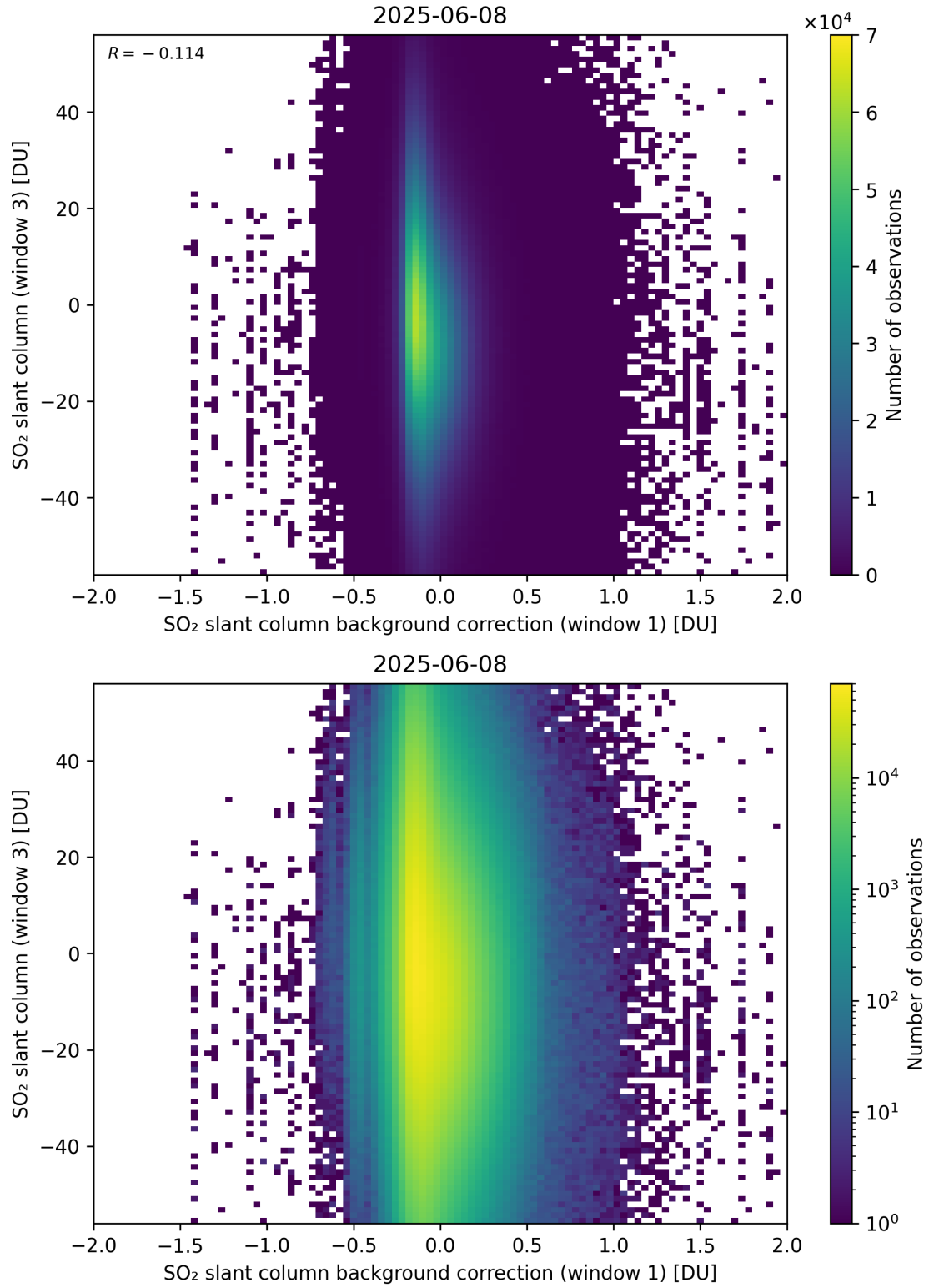
Figure 118: Scatter density plot of “SO 2 slant column background correction (window 1)” against “SO 2 slant column (window 3)” for 2025-06-07 to 2025-06-09.
