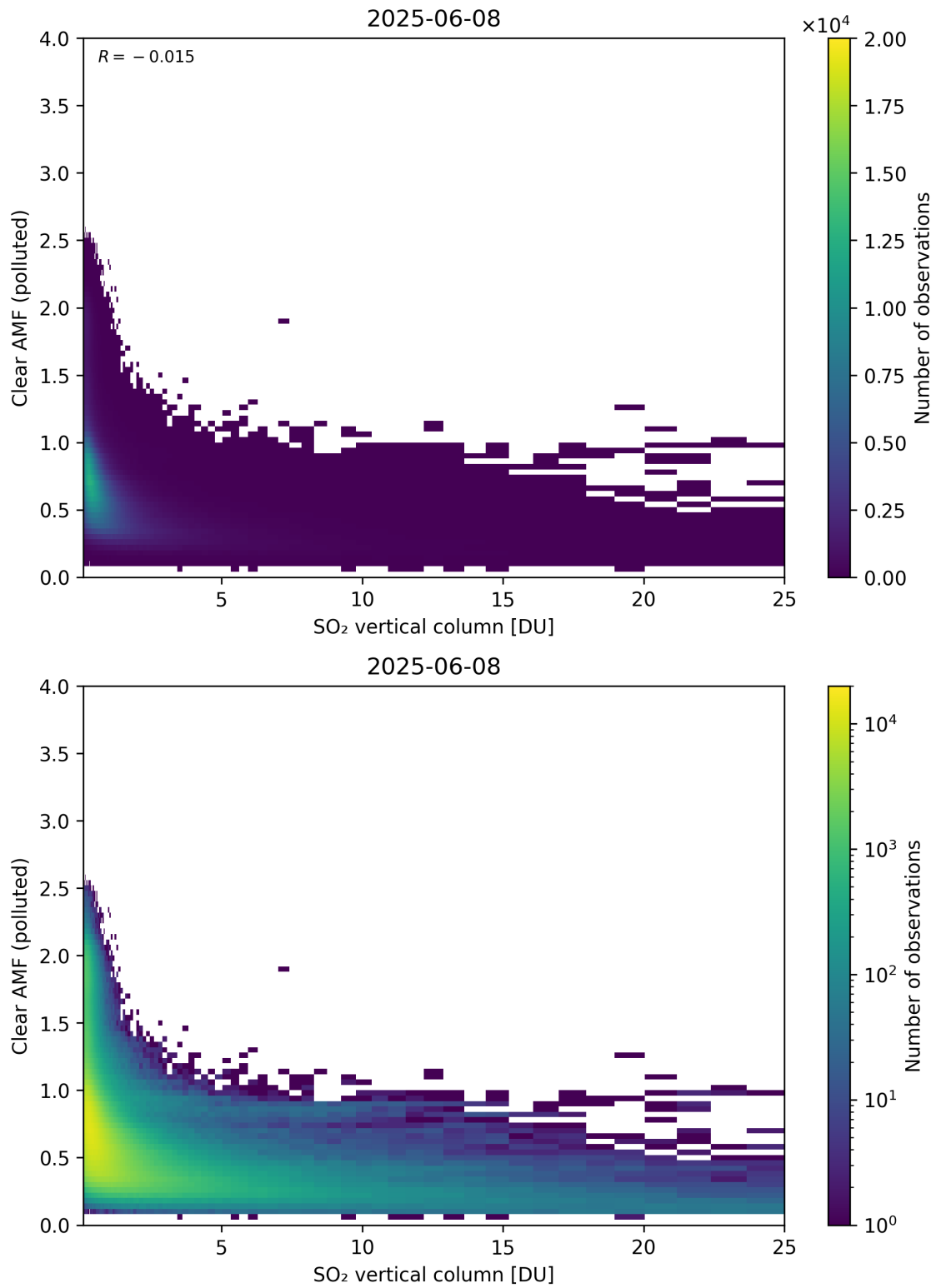
Figure 348: Scatter density plot of “SO 2 vertical column” against “Clear AMF (polluted)” for 2025-06-07 to 2025-06-09.
