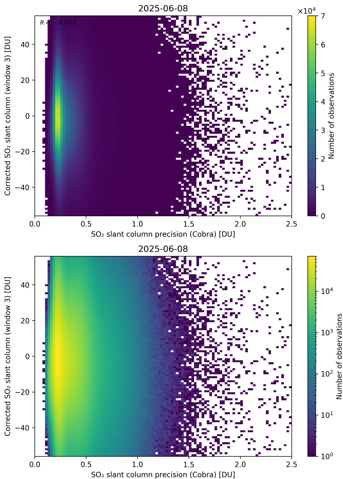
Figure 207: Scatter density plot of “SO 2 slant column precision (Cobra)” against “Corrected SO 2 slant column (window 3)” for 2025-06-07 to 2025-06-09.
