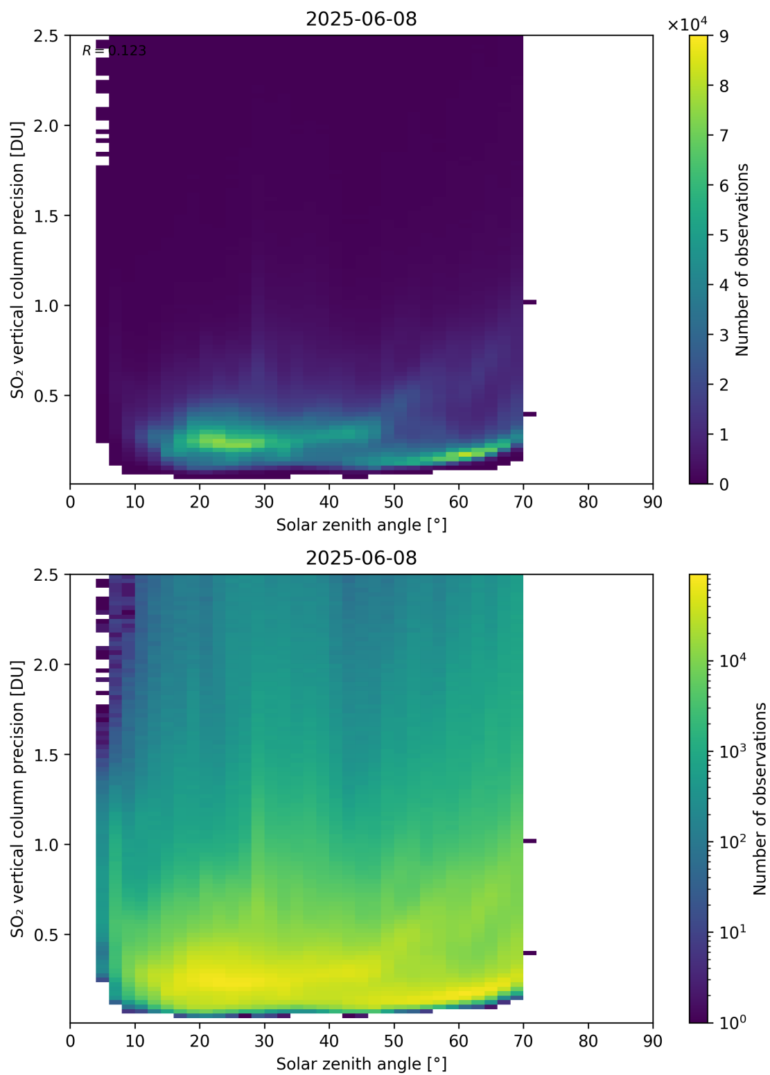
Figure 192: Scatter density plot of “Solar zenith angle” against “SO 2 vertical column precision” for 2025-06-07 to 2025-06-09.
