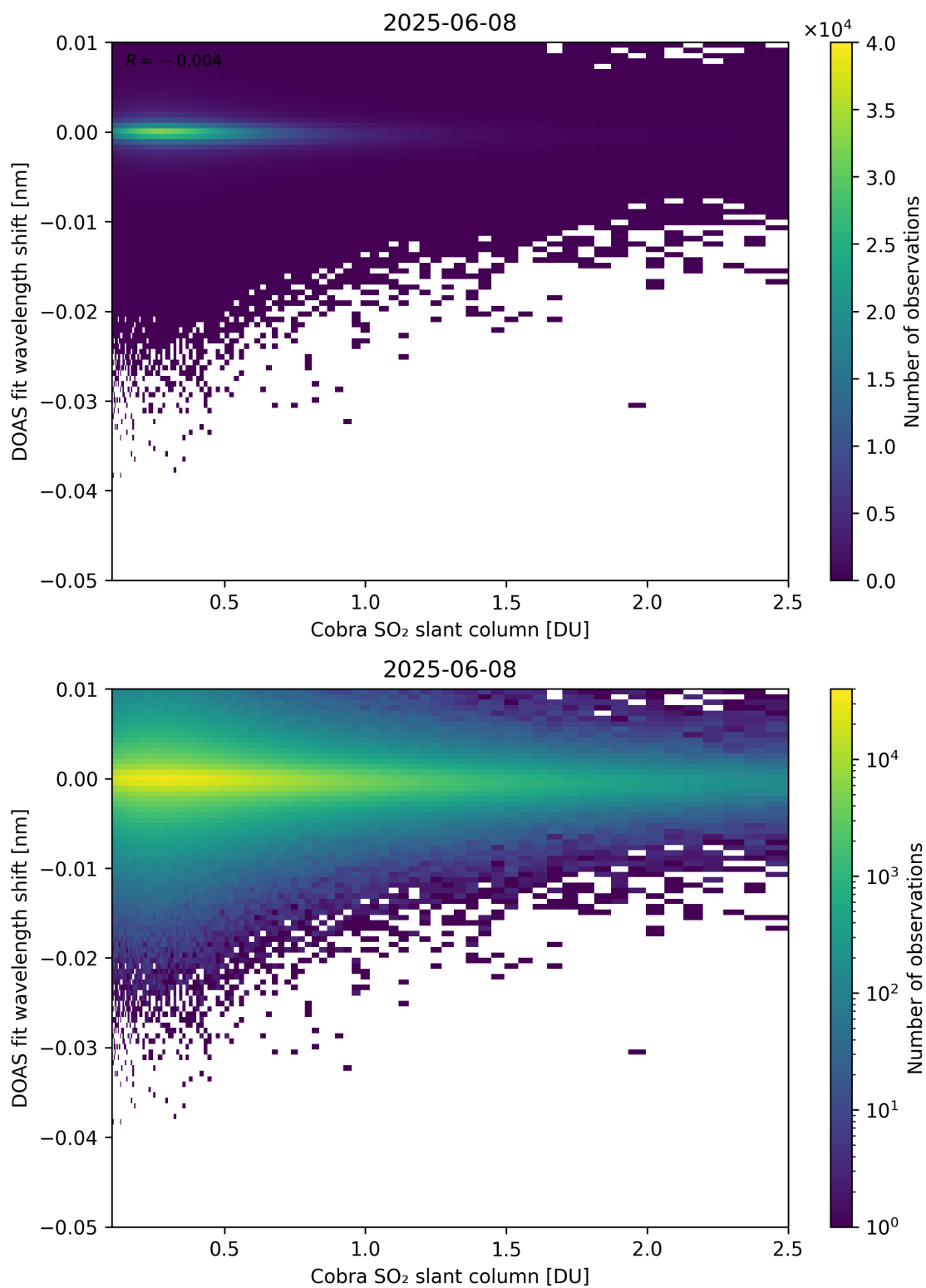
Figure 196: Scatter density plot of “Cobra SO 2 slant column” against “DOAS fit wavelength shift” for 2025-06-07 to 2025-06-09.
