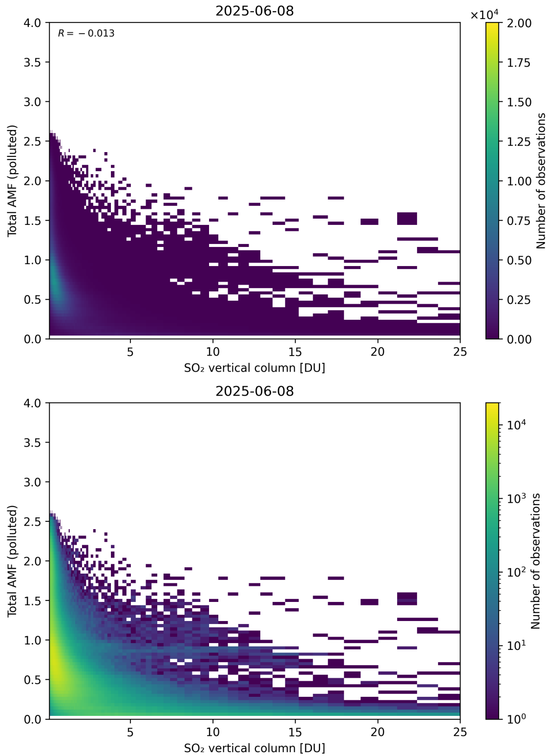
Figure 359: Scatter density plot of “SO 2 vertical column” against “Total AMF (polluted)” for 2025-06-07 to 2025-06-09.
