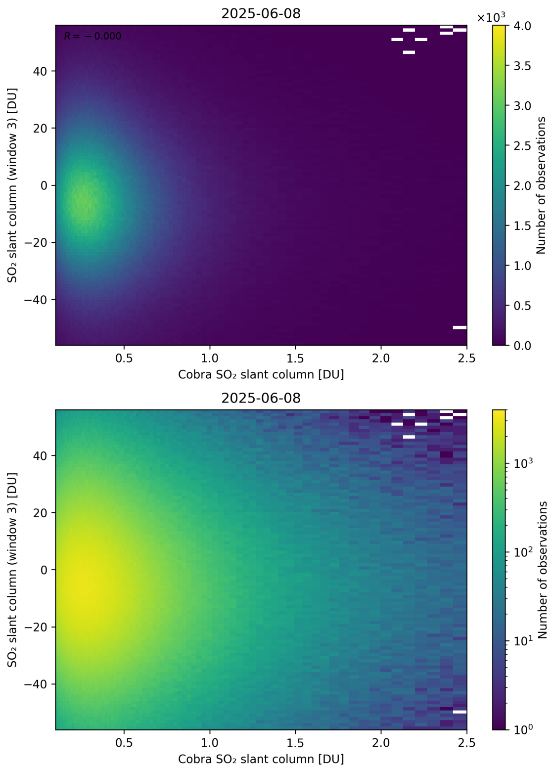
Figure 222: Scatter density plot of “Cobra SO 2 slant column” against “SO 2 slant column (window 3)” for 2025-06-07 to 2025-06-09.
