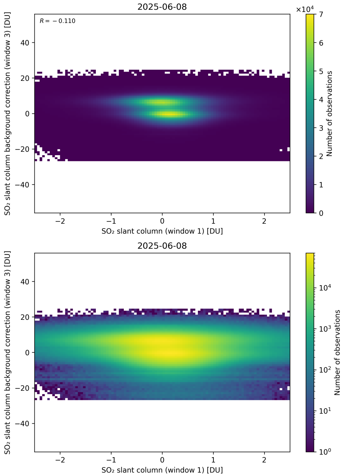
Figure 264: Scatter density plot of “SO 2 slant column (window 1)” against “SO 2 slant column background correction (window 3)” for 2025-06-07 to 2025-06-09.
