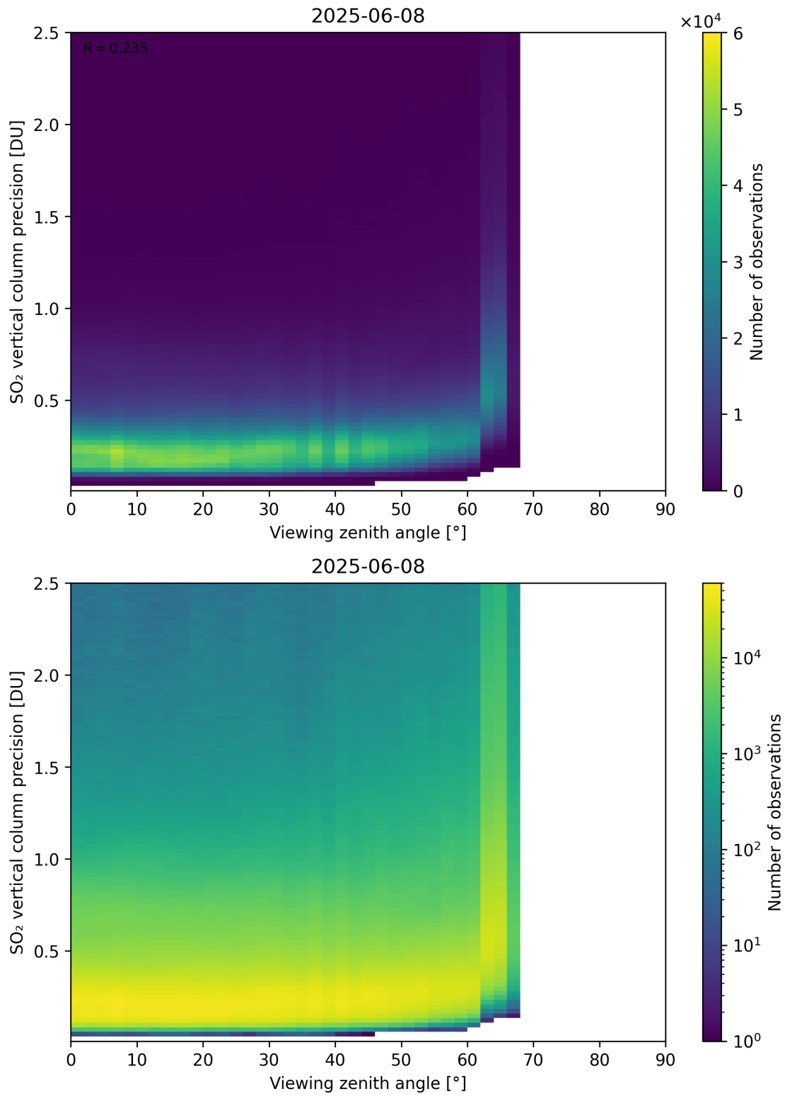
Figure 384: Scatter density plot of “Viewing zenith angle” against “SO 2 vertical column precision” for 2025-06-07 to 2025-06-09.
