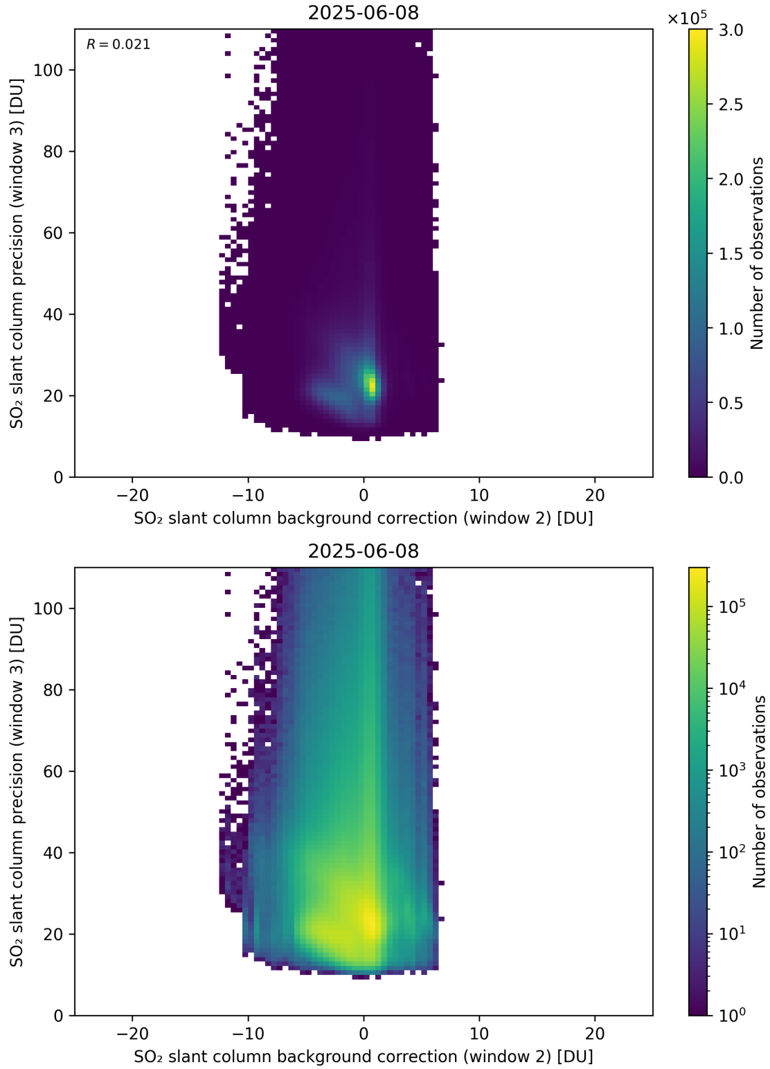
Figure 129: Scatter density plot of “SO 2 slant column background correction (window 2)” against “SO 2 slant column precision (window 3)” for 2025-06-07 to 2025-06-09.
