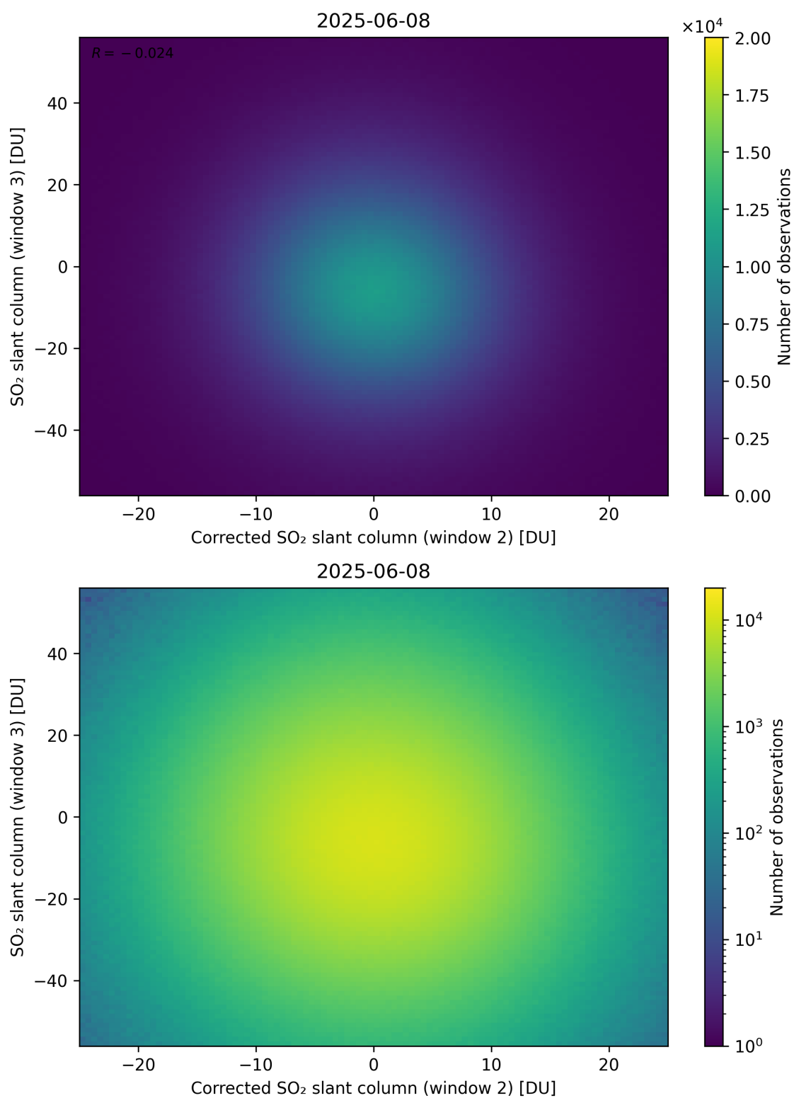
Figure 251: Scatter density plot of “Corrected SO 2 slant column (window 2)” against “SO 2 slant column (window 3)” for 2025-06-07 to 2025-06-09.
