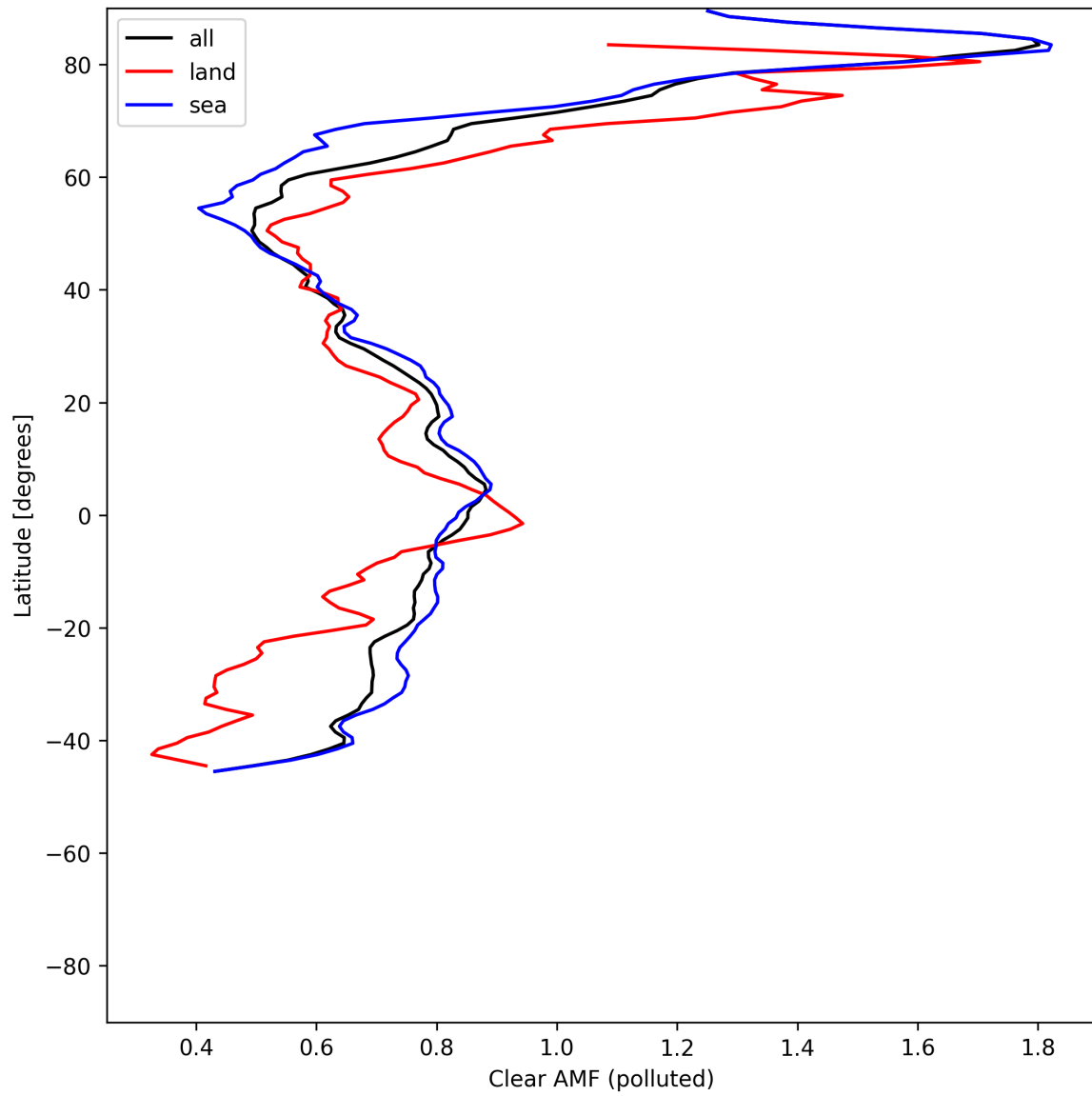
Figure 55: Zonal average of “Clear AMF (polluted)” for 2025-06-07 to 2025-06-09.
