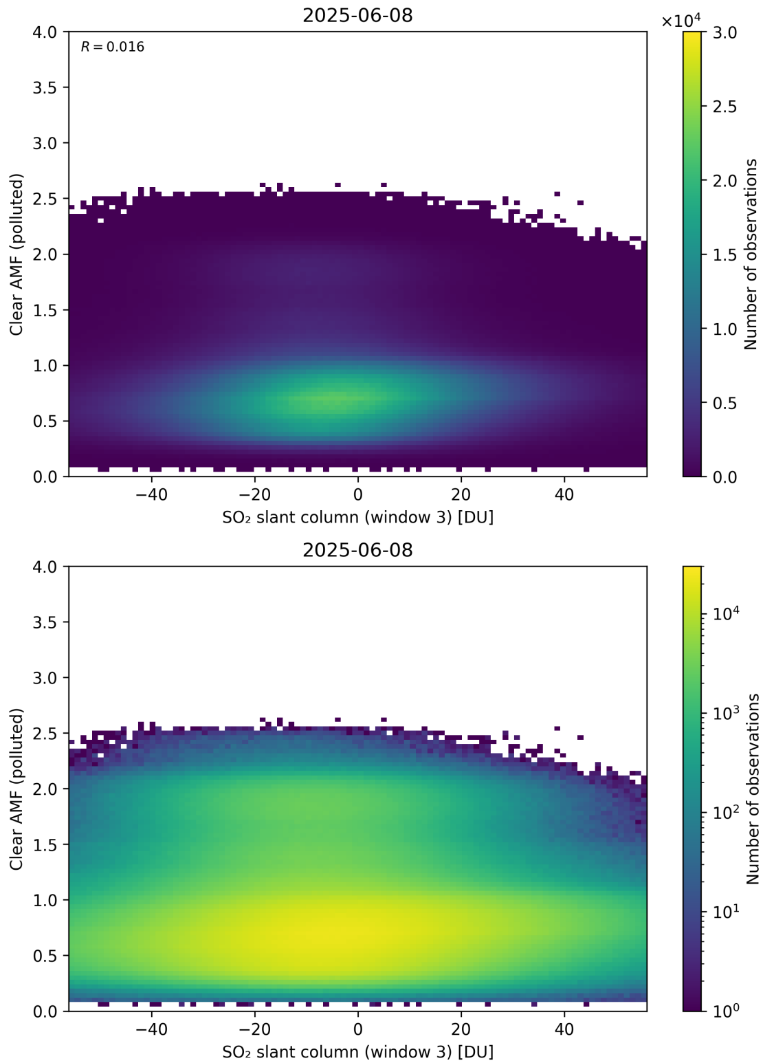
Figure 315: Scatter density plot of “SO 2 slant column (window 3)” against “Clear AMF (polluted)” for 2025-06-07 to 2025-06-09.
