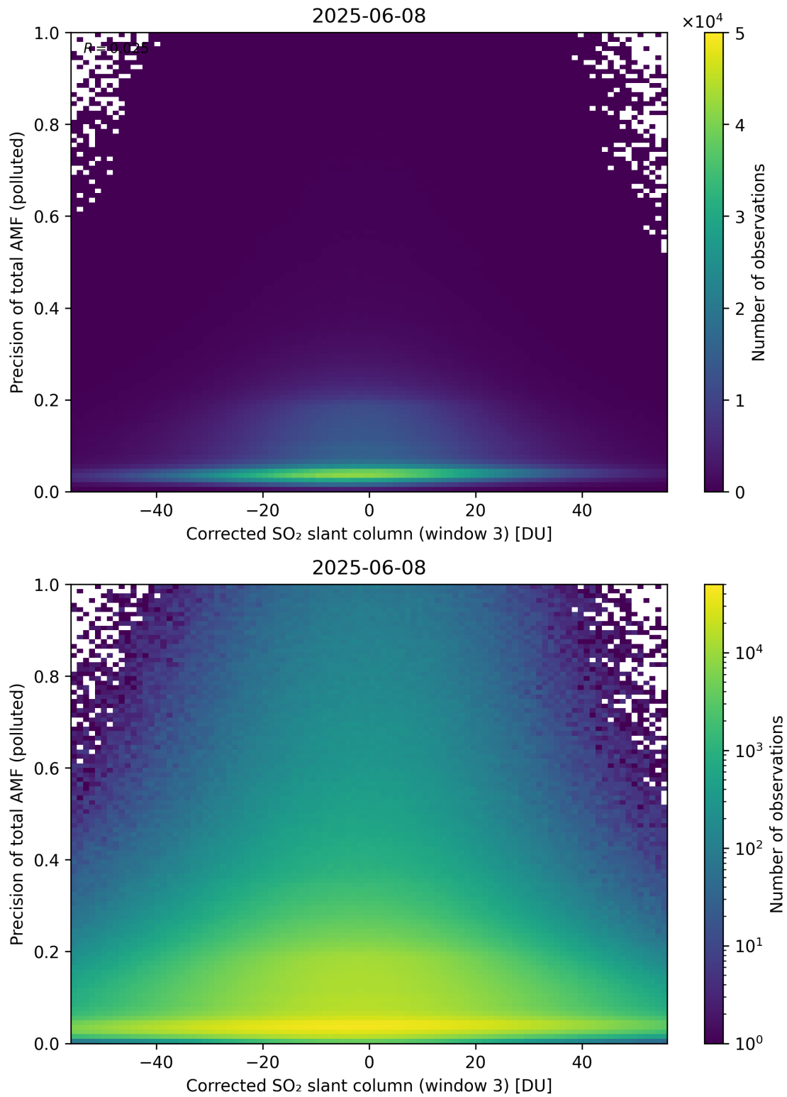
Figure 261: Scatter density plot of “Corrected SO 2 slant column (window 3)” against “Precision of total AMF (polluted)” for 2025-06-07 to 2025-06-09.
