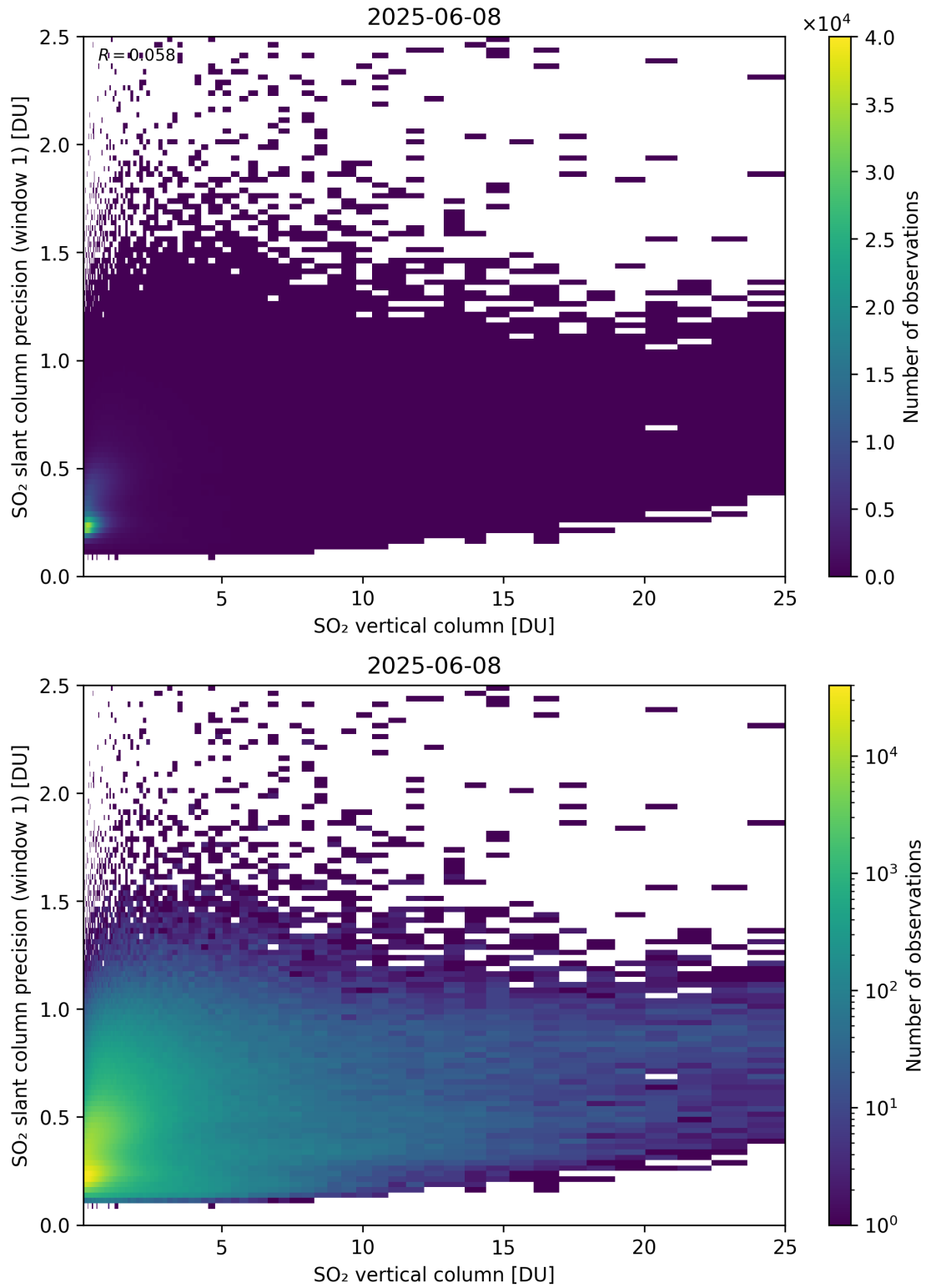
Figure 355: Scatter density plot of “SO 2 vertical column” against “SO 2 slant column precision (window 1)” for 2025-06-07 to 2025-06-09.
