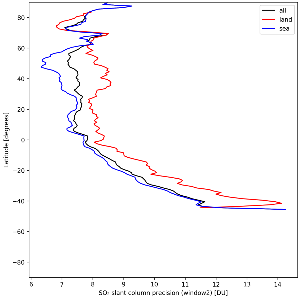
Figure 42: Zonal average of “SO 2 slant column precision (window2)” for 2025-06-07 to 2025-06-09.
