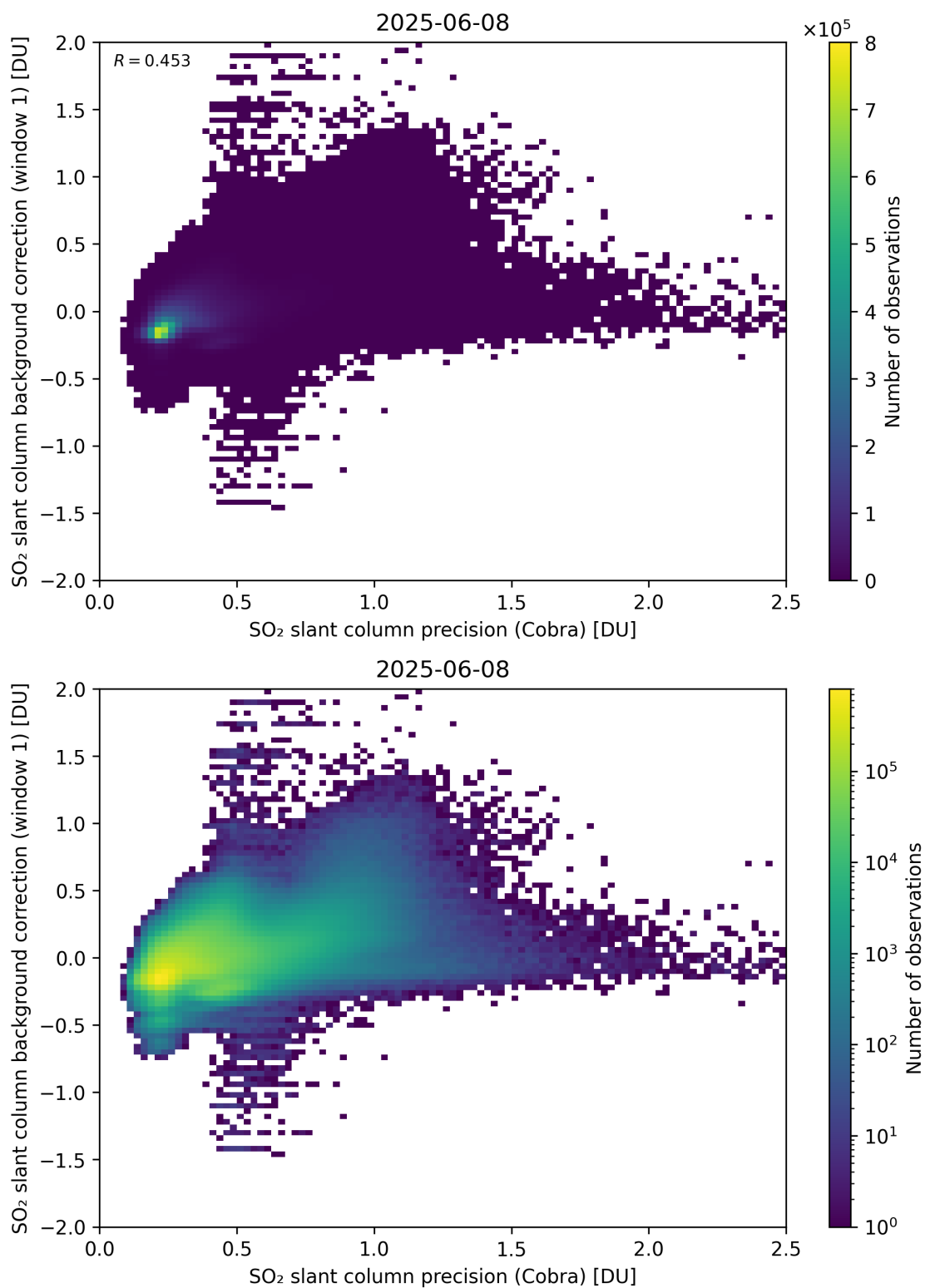
Figure 199: Scatter density plot of “SO 2 slant column precision (Cobra)” against “SO 2 slant column background correction (window 1)” for 2025-06-07 to 2025-06-09.
