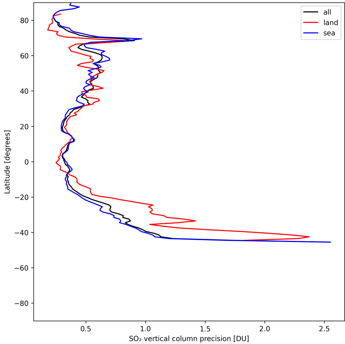
Figure 33: Zonal average of “SO 2 vertical column precision” for 2025-06-07 to 2025-06-09.
