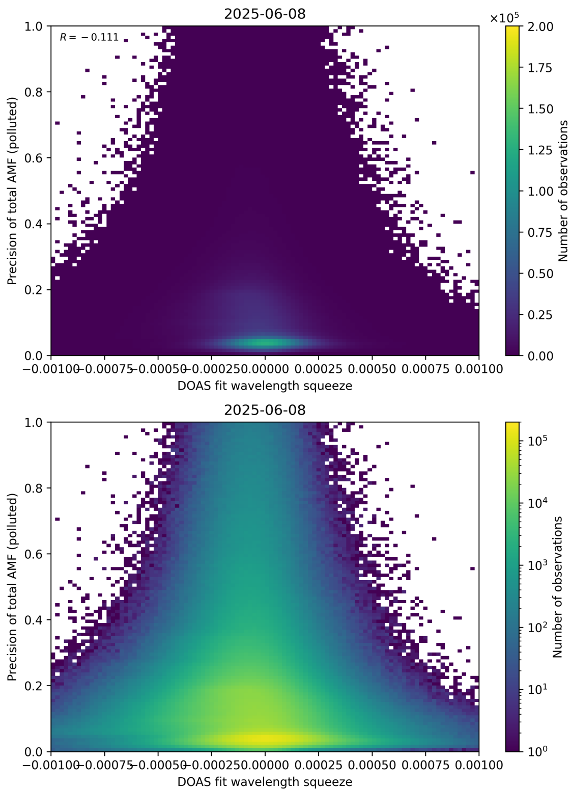
Figure 146: Scatter density plot of “DOAS fit wavelength squeeze” against “Precision of total AMF (polluted)” for 2025-06-07 to 2025-06-09.
