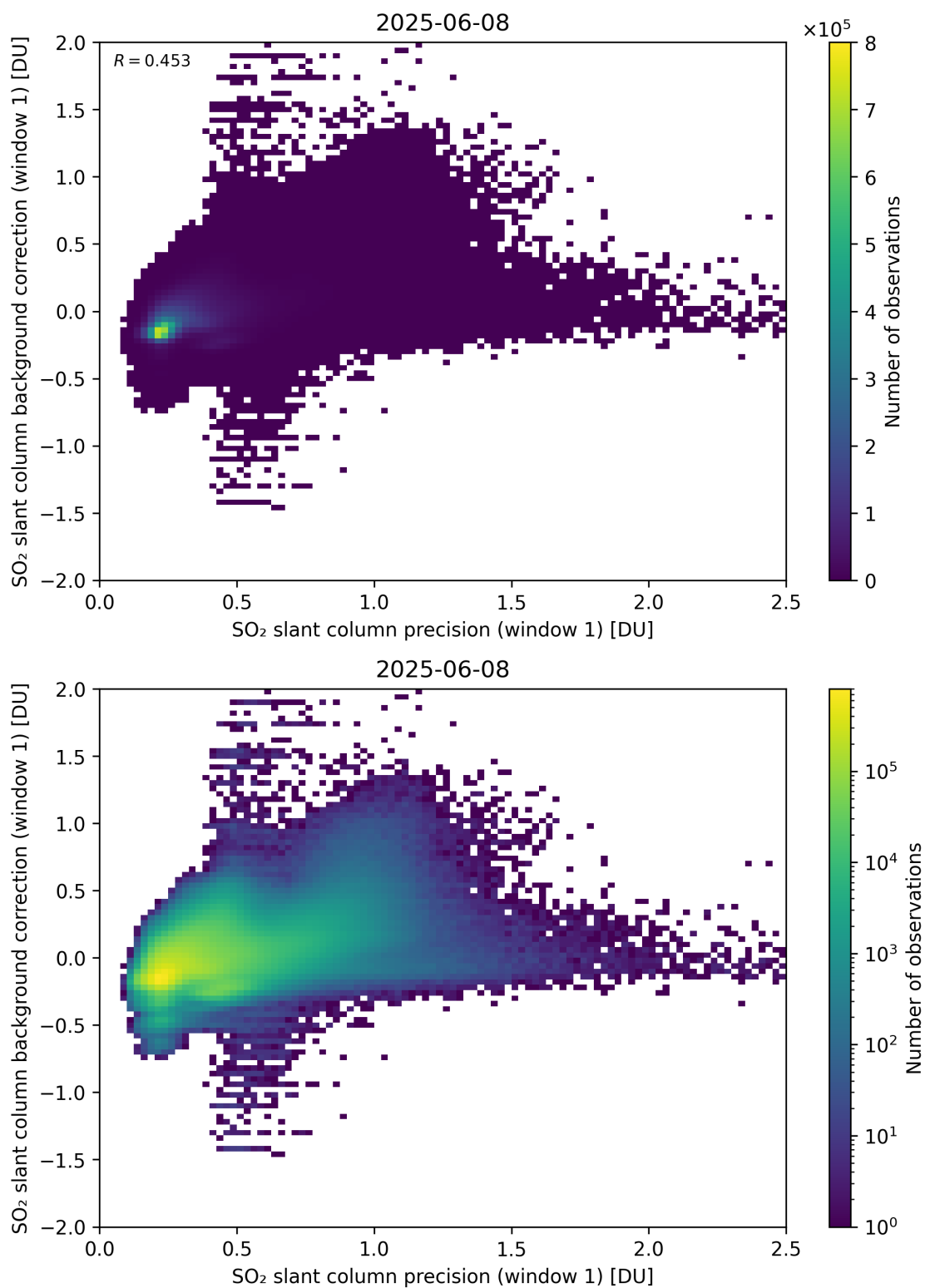
Figure 268: Scatter density plot of “SO 2 slant column precision (window 1)” against “SO 2 slant column background correction (window 1)” for 2025-06-07 to 2025-06-09.
