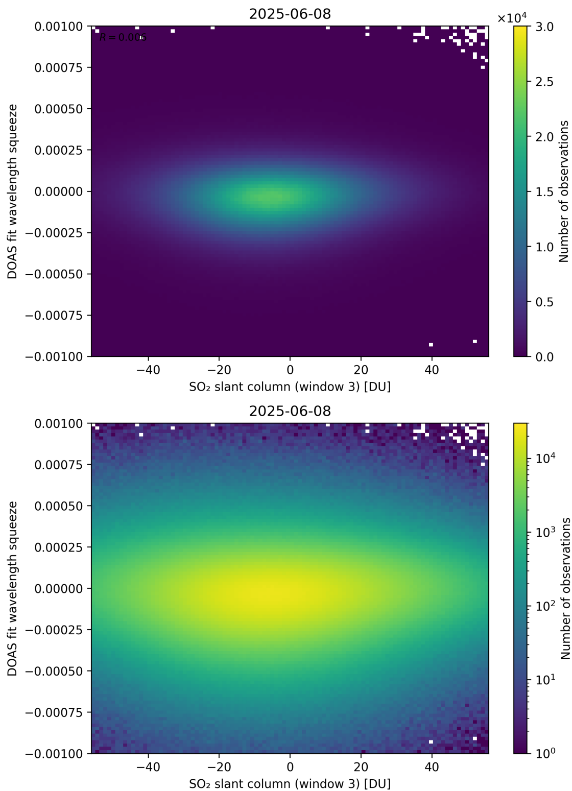
Figure 305: Scatter density plot of “SO 2 slant column (window 3)” against “DOAS fit wavelength squeeze” for 2025-06-07 to 2025-06-09.
