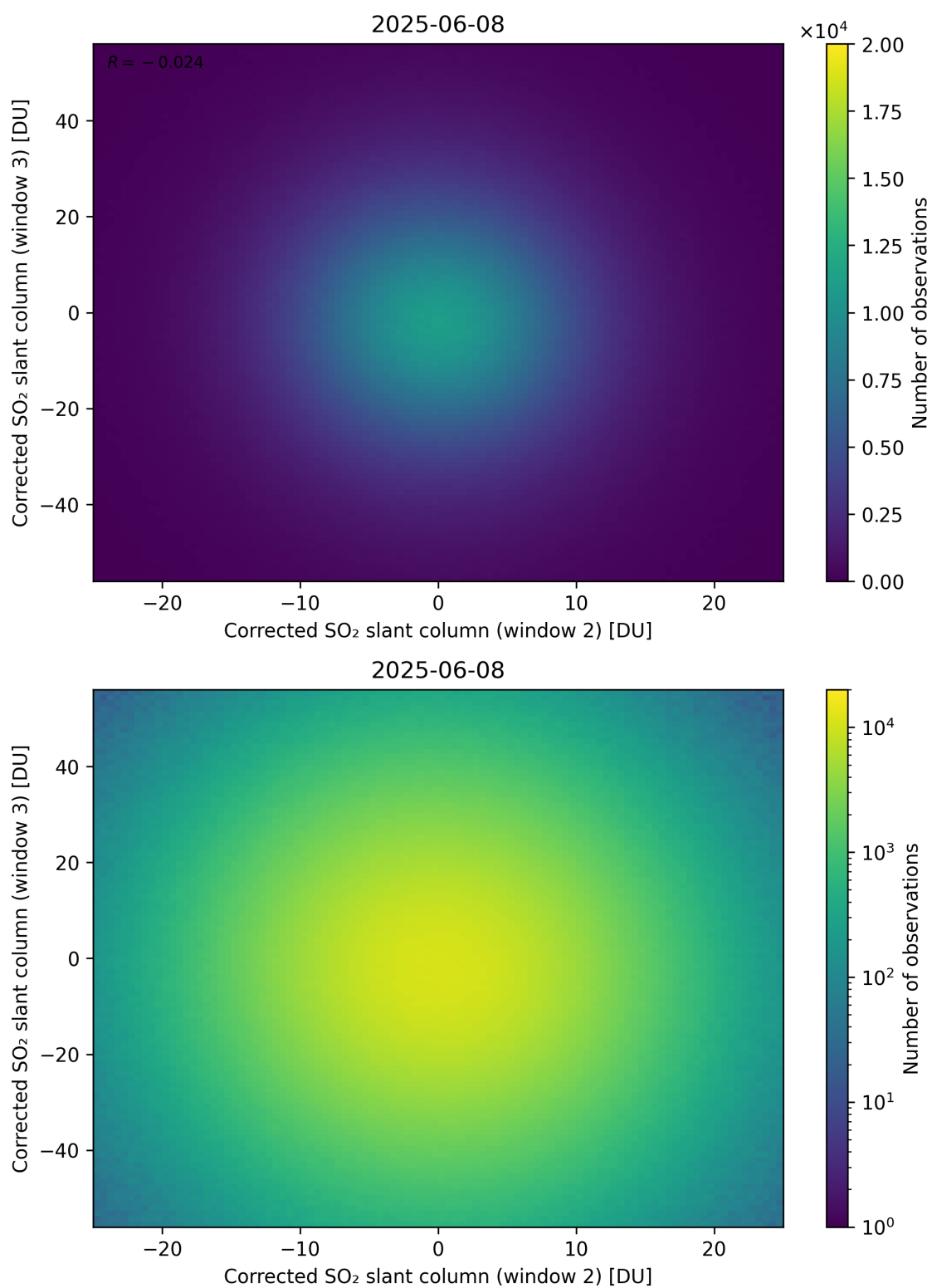
Figure 250: Scatter density plot of “Corrected SO 2 slant column (window 2)” against “Corrected SO 2 slant column (window 3)” for 2025-06-07 to 2025-06-09.
