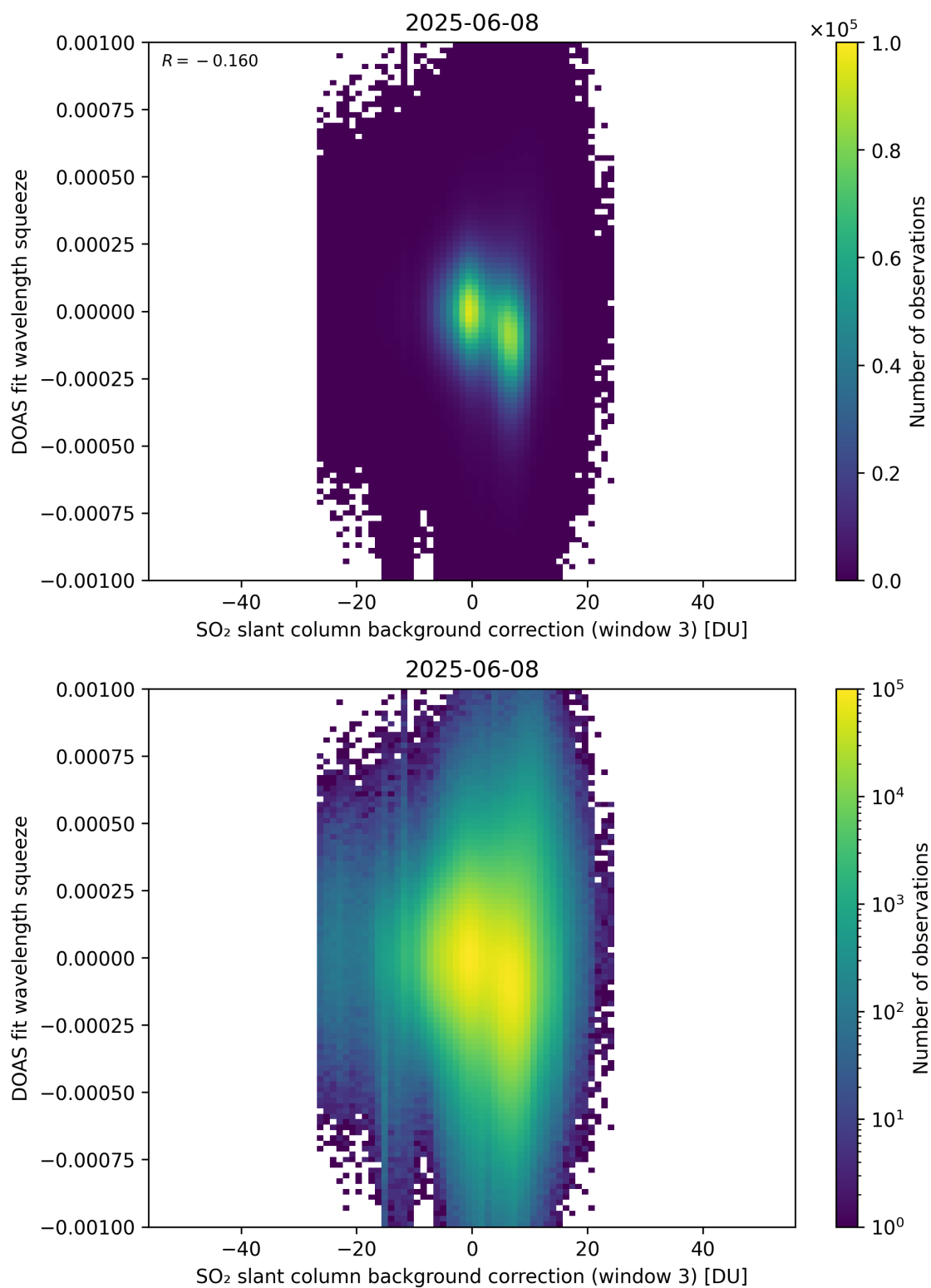
Figure 133: Scatter density plot of “SO 2 slant column background correction (window 3)” against “DOAS fit wavelength squeeze” for 2025-06-07 to 2025-06-09.
