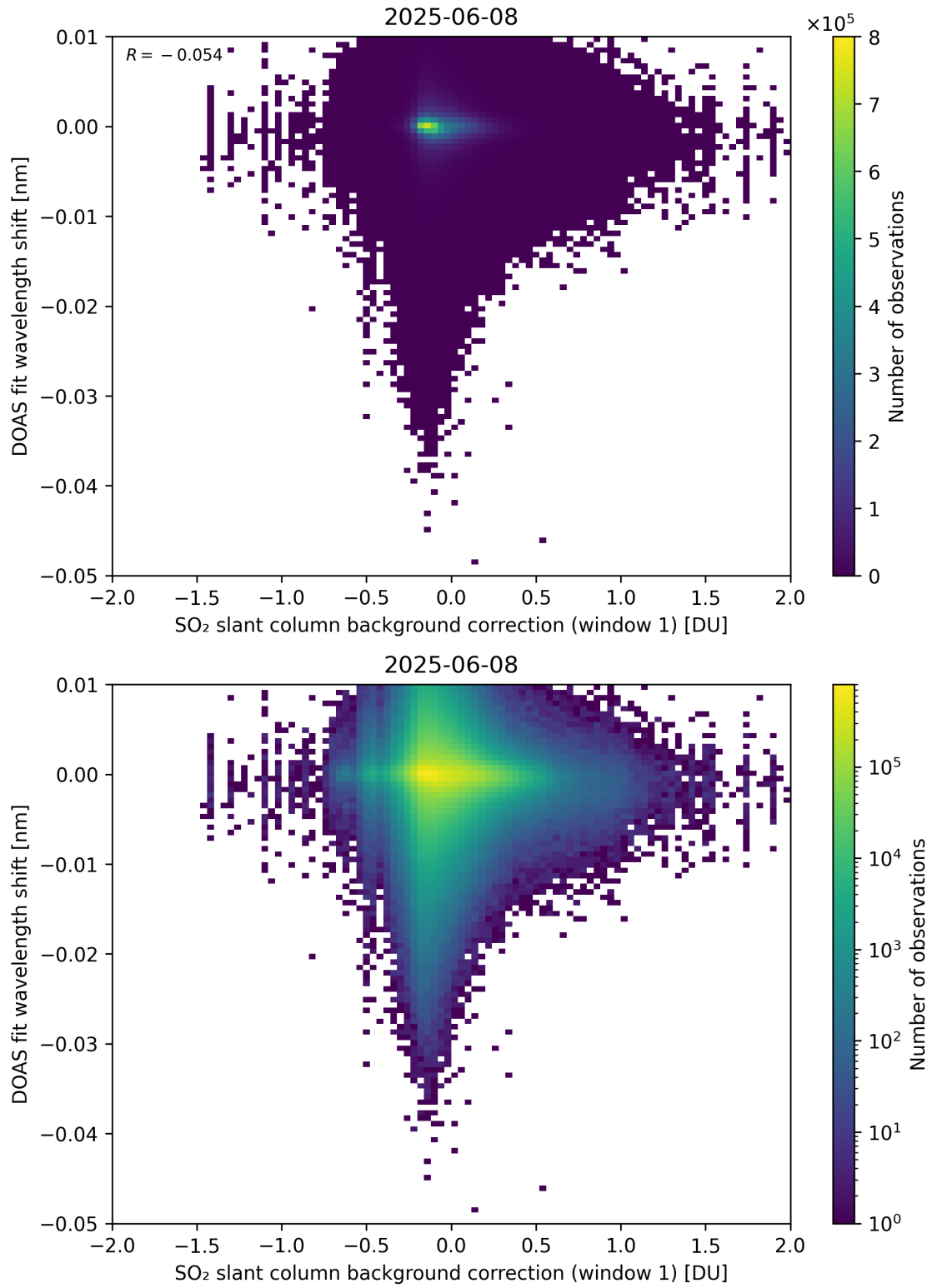
Figure 111: Scatter density plot of “SO 2 slant column background correction (window 1)” against “DOAS fit wavelength shift” for 2025-06-07 to 2025-06-09.
