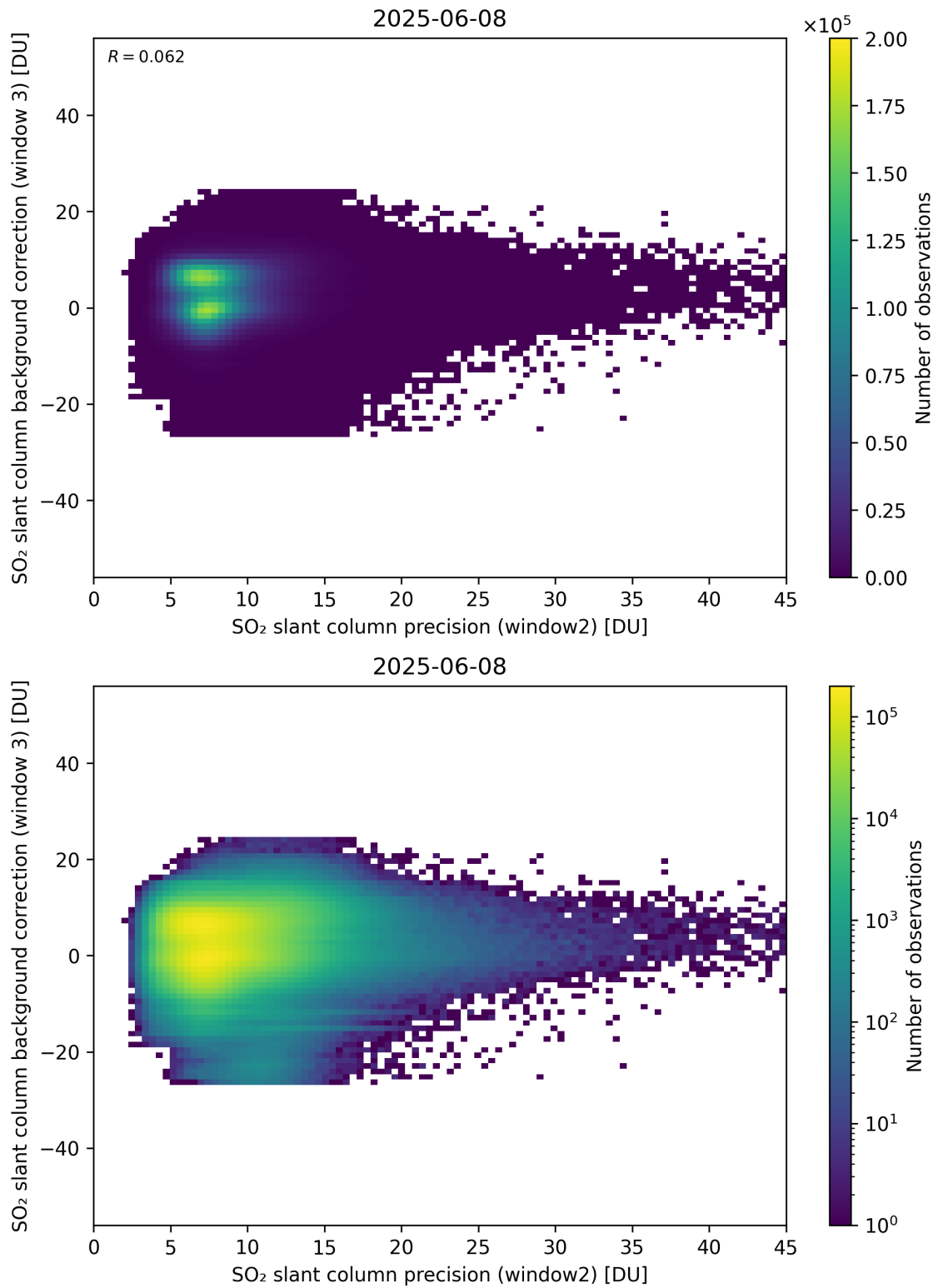
Figure 292: Scatter density plot of “SO 2 slant column precision (window2)” against “SO 2 slant column background correction (window 3)” for 2025-06-07 to 2025-06-09.
