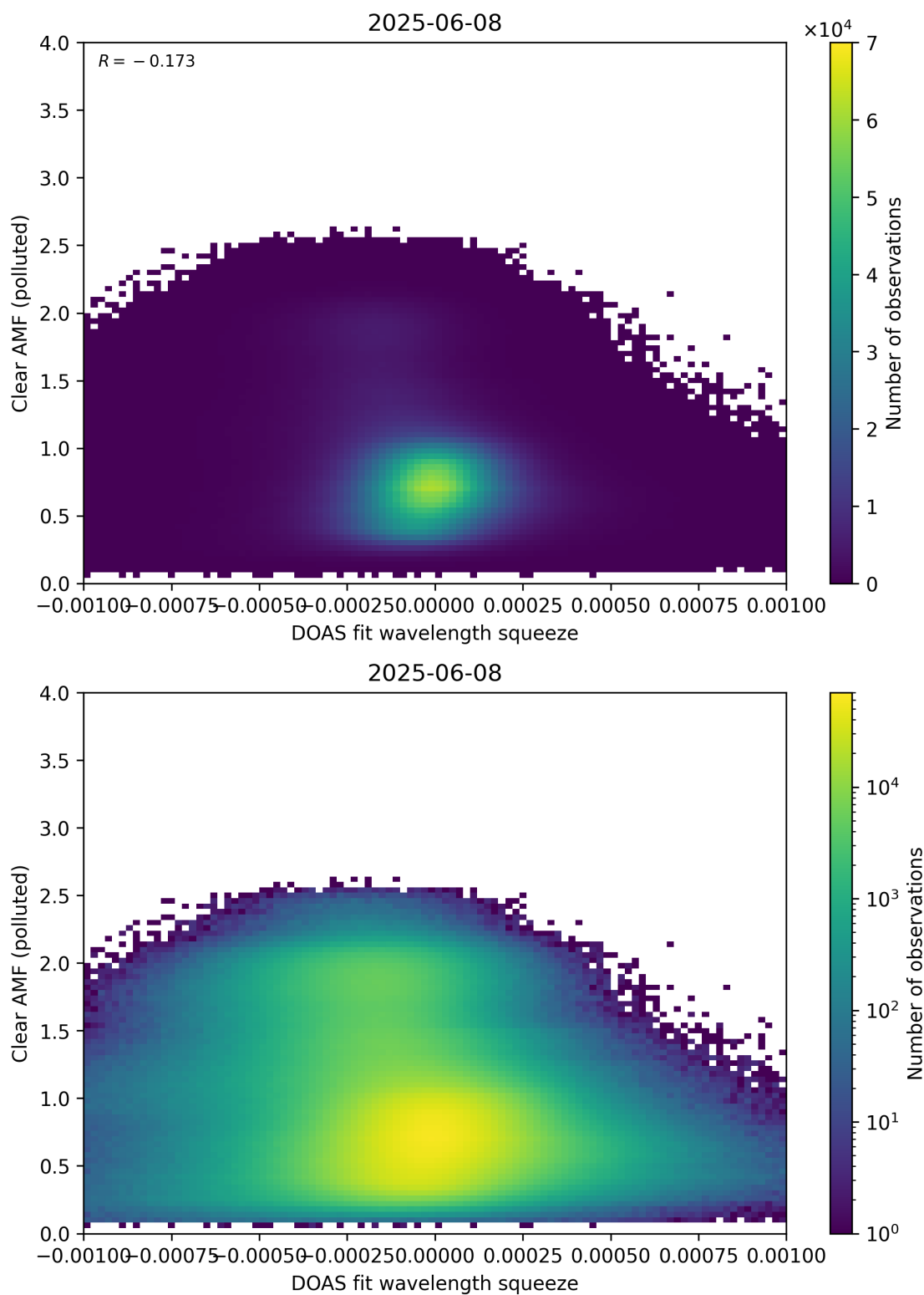
Figure 144: Scatter density plot of “DOAS fit wavelength squeeze” against “Clear AMF (polluted)” for 2025-06-07 to 2025-06-09.
