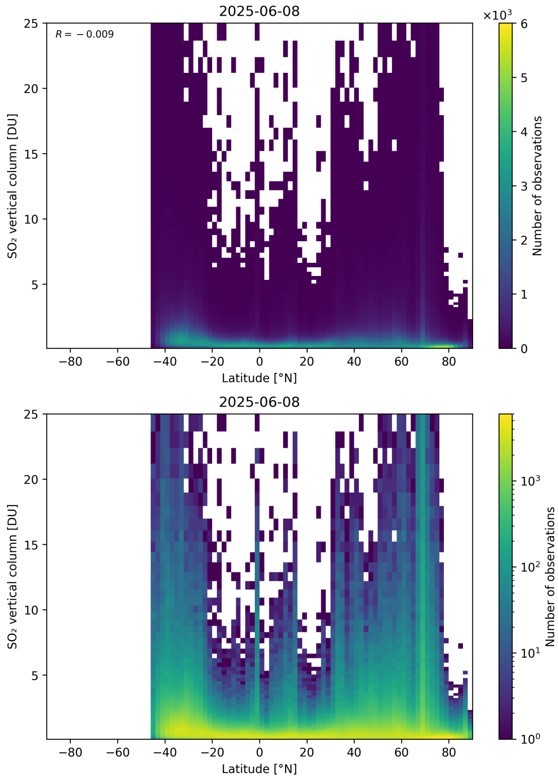
Figure 169: Scatter density plot of “Latitude” against “SO 2 vertical column” for 2025-06-07 to 2025-06-09.
