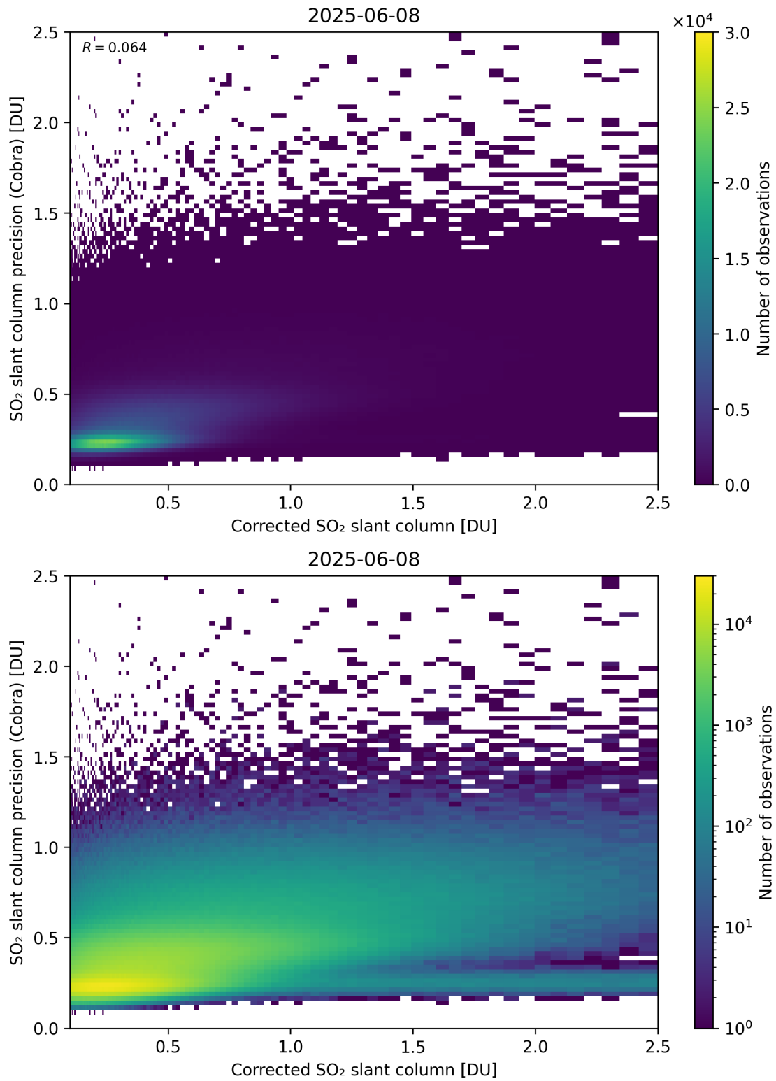
Figure 234: Scatter density plot of “Corrected SO 2 slant column” against “SO 2 slant column precision (Cobra)” for 2025-06-07 to 2025-06-09.
