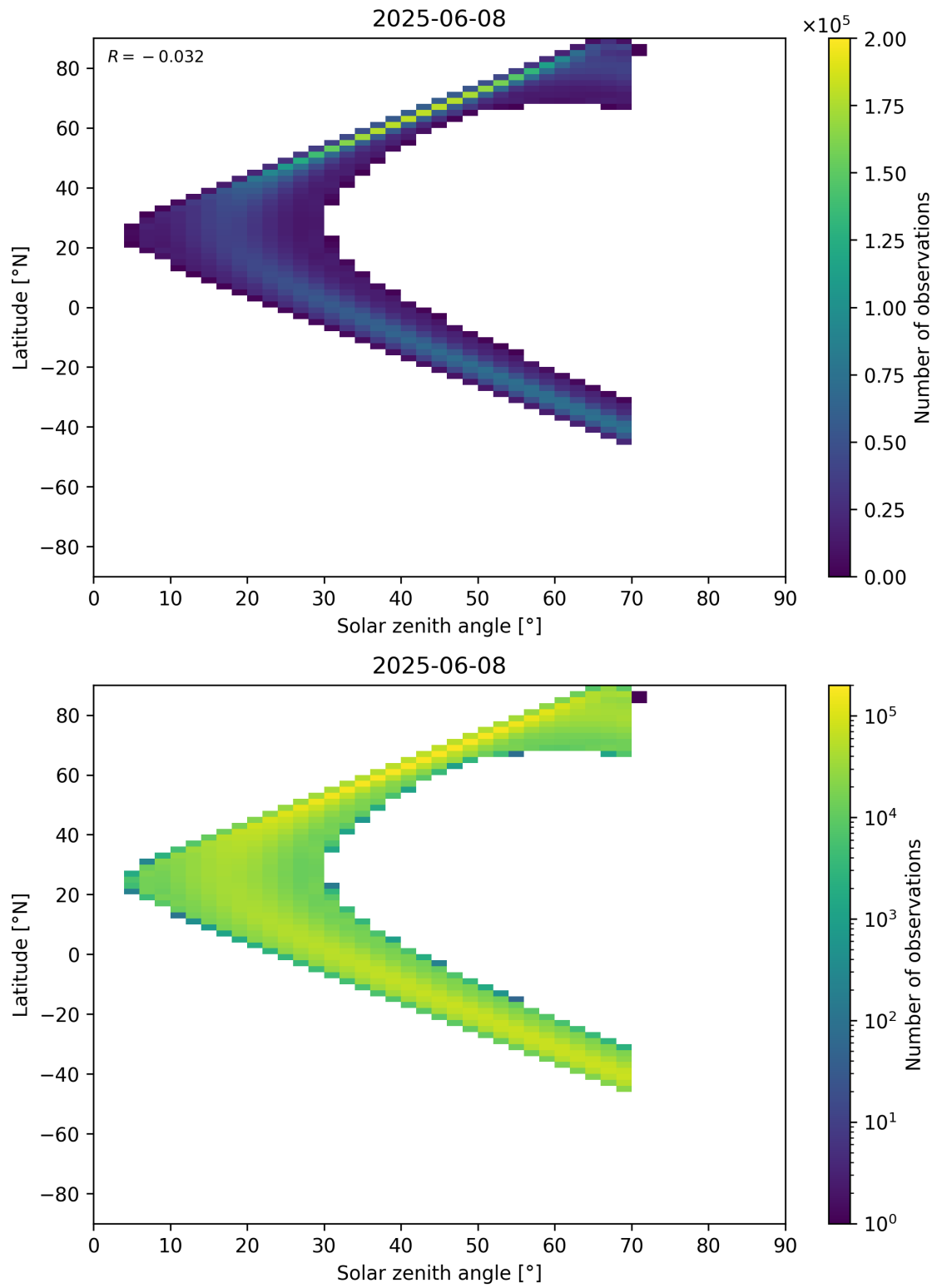
Figure 177: Scatter density plot of “Solar zenith angle” against “Latitude” for 2025-06-07 to 2025-06-09.
