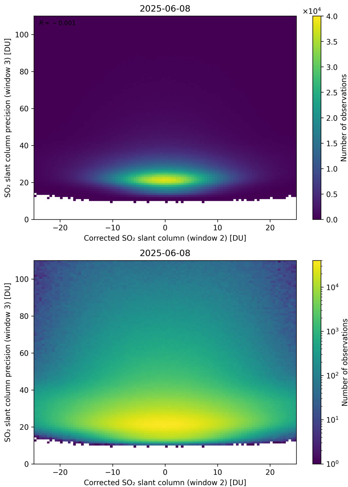
Figure 252: Scatter density plot of “Corrected SO 2 slant column (window 2)” against “SO 2 slant column precision (window 3)” for 2025-06-07 to 2025-06-09.
