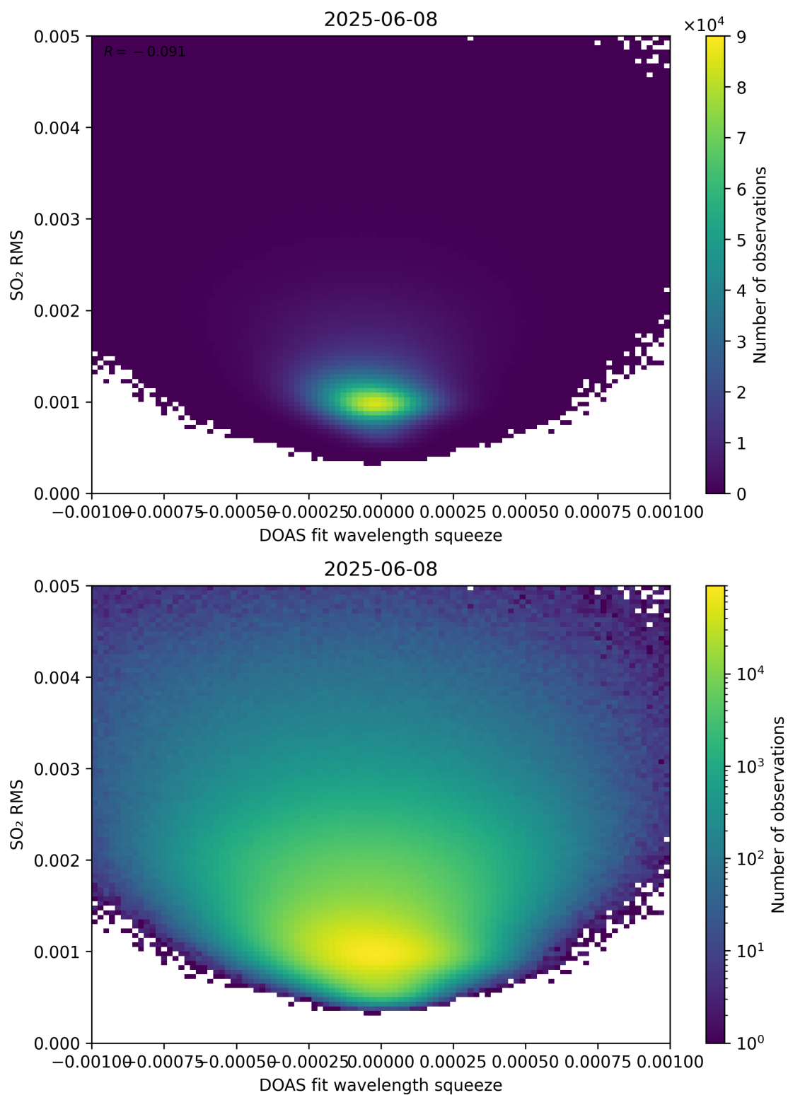
Figure 143: Scatter density plot of “DOAS fit wavelength squeeze” against “SO 2 RMS” for 2025-06-07 to 2025-06-09.
