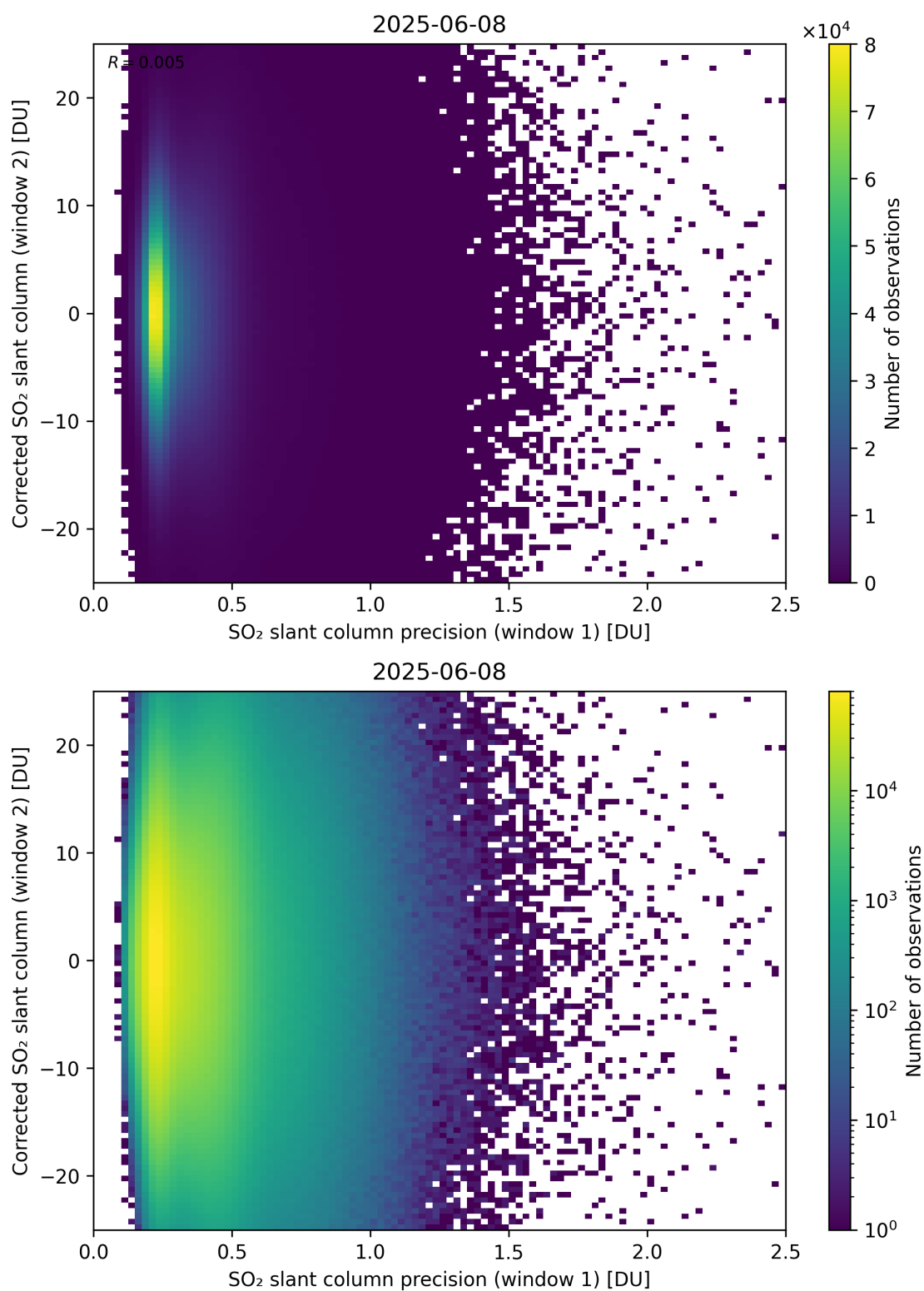
Figure 275: Scatter density plot of “SO 2 slant column precision (window 1)” against “Corrected SO 2 slant column (window 2)” for 2025-06-07 to 2025-06-09.
