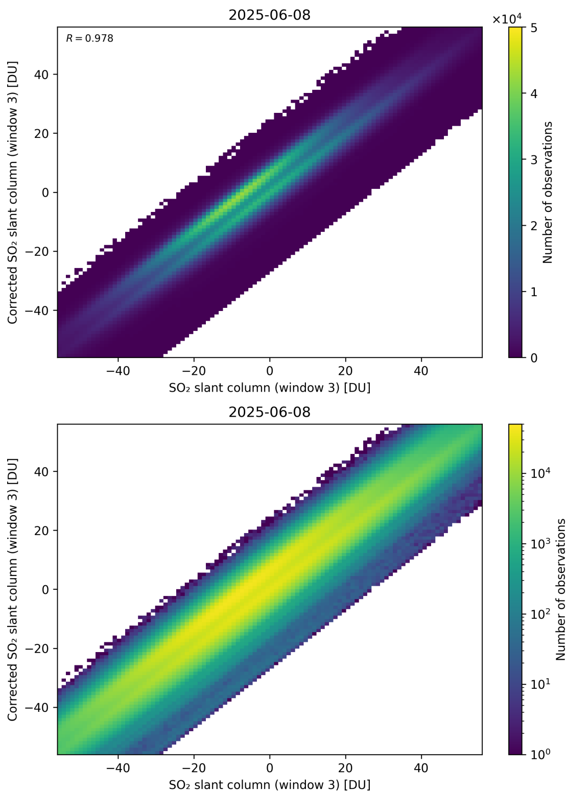
Figure 316: Scatter density plot of “SO 2 slant column (window 3)” against “Corrected SO 2 slant column (window 3)” for 2025-06-07 to 2025-06-09.
