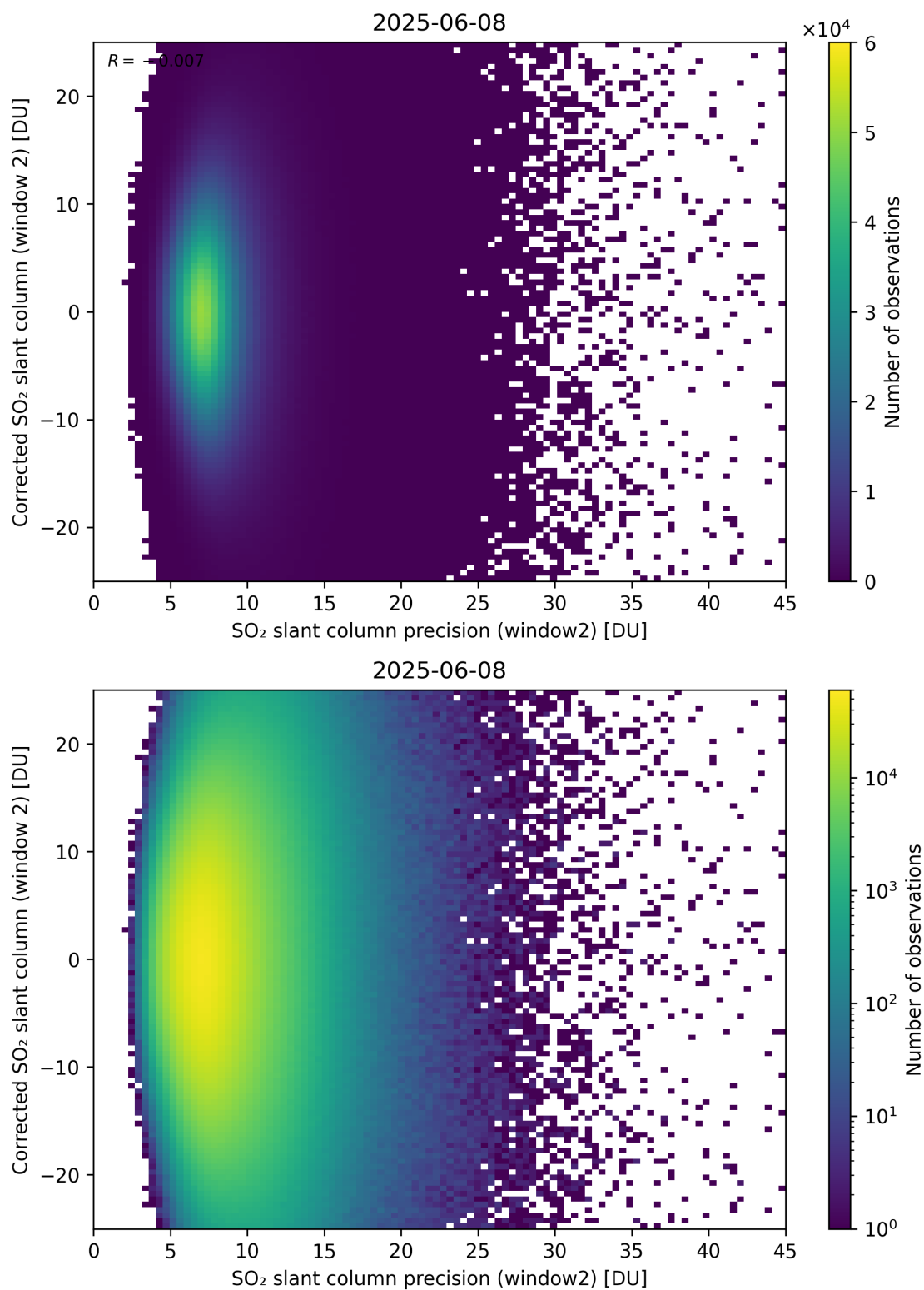
Figure 297: Scatter density plot of “SO 2 slant column precision (window2)” against “Corrected SO 2 slant column (window 2)” for 2025-06-07 to 2025-06-09.
