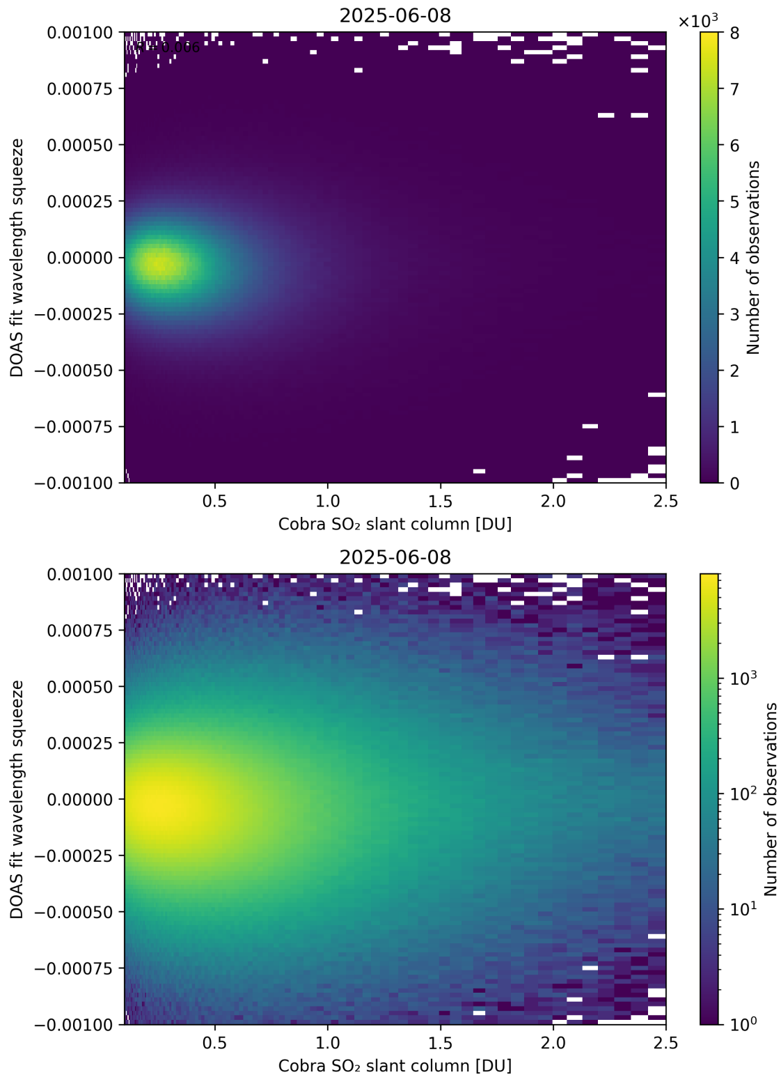
Figure 197: Scatter density plot of “Cobra SO 2 slant column” against “DOAS fit wavelength squeeze” for 2025-06-07 to 2025-06-09.
