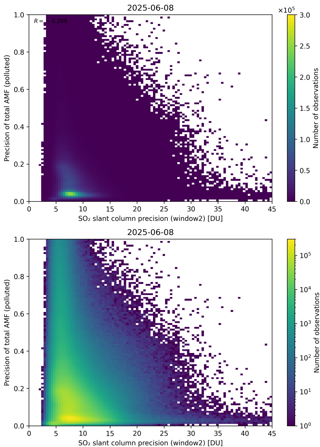
Figure 302: Scatter density plot of “SO 2 slant column precision (window2)” against “Precision of total AMF (polluted)” for 2025-06-07 to 2025-06-09.
