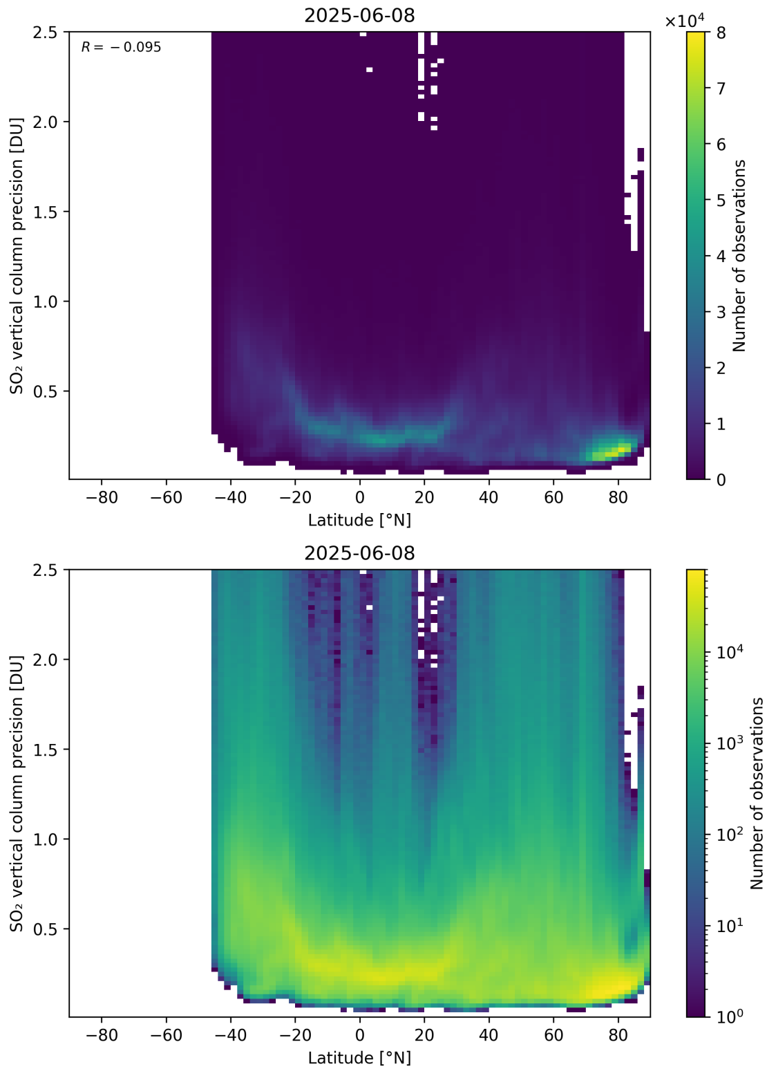
Figure 170: Scatter density plot of “Latitude” against “SO 2 vertical column precision” for 2025-06-07 to 2025-06-09.
