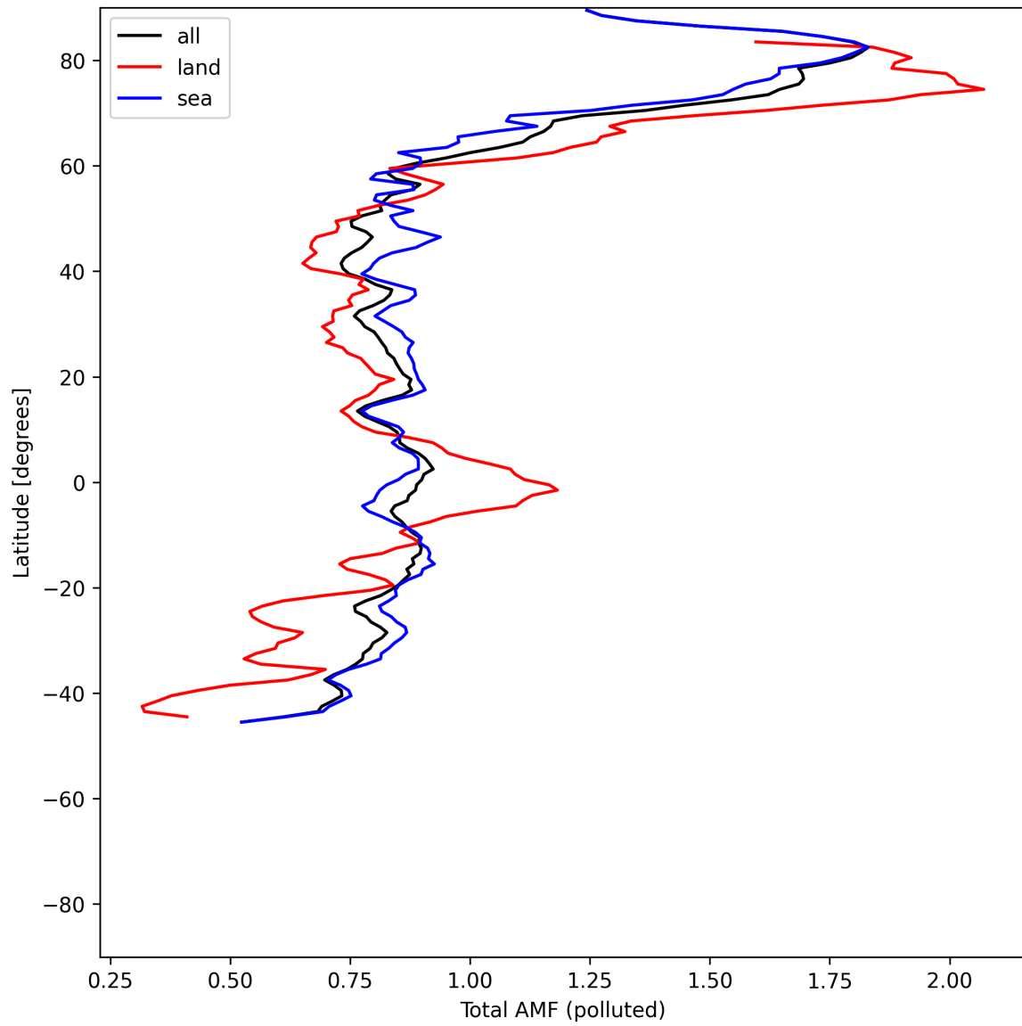
Figure 53: Zonal average of “Total AMF (polluted)” for 2025-06-07 to 2025-06-09.
