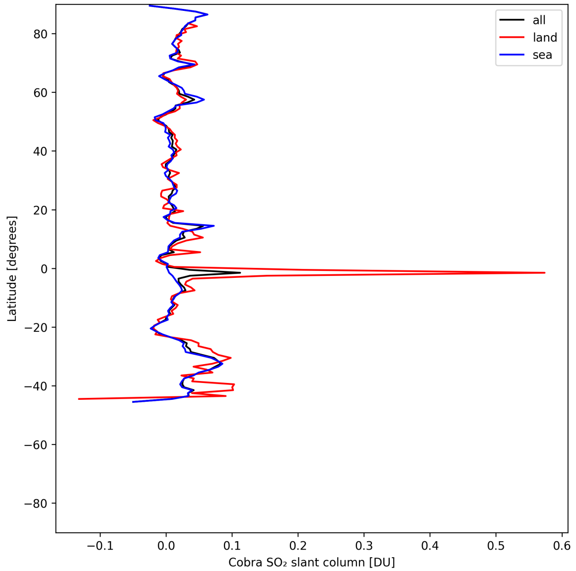
Figure 35: Zonal average of “Cobra SO 2 slant column” for 2025-06-07 to 2025-06-09.
