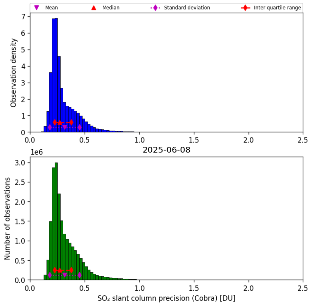
Figure 62: Histogram of “SO 2 slant column precision (Cobra)” for 2025-06-07 to 2025-06-09
