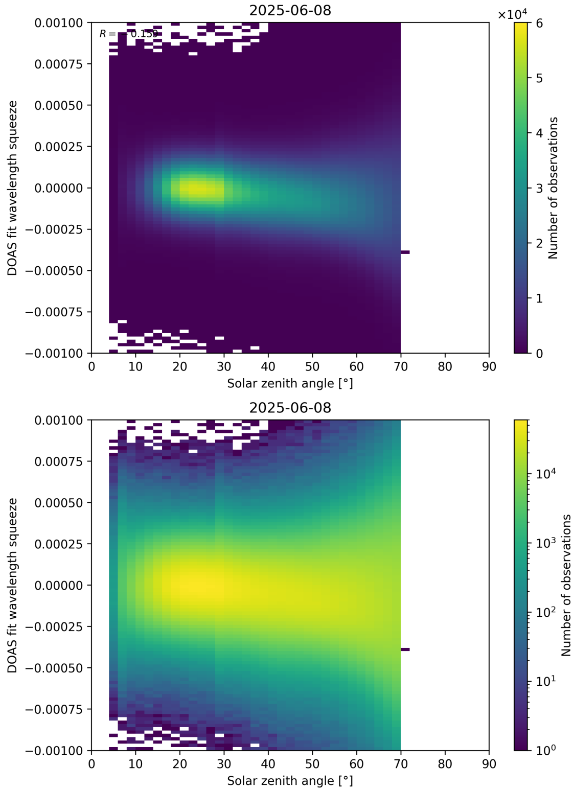
Figure 175: Scatter density plot of “Solar zenith angle” against “DOAS fit wavelength squeeze” for 2025-06-07 to 2025-06-09.
