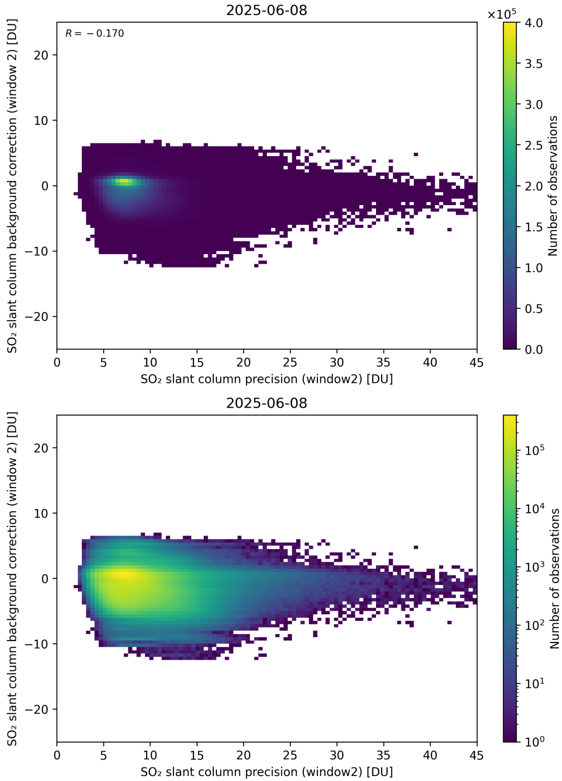
Figure 291: Scatter density plot of “SO 2 slant column precision (window2)” against “SO 2 slant column background correction (window 2)” for 2025-06-07 to 2025-06-09.
