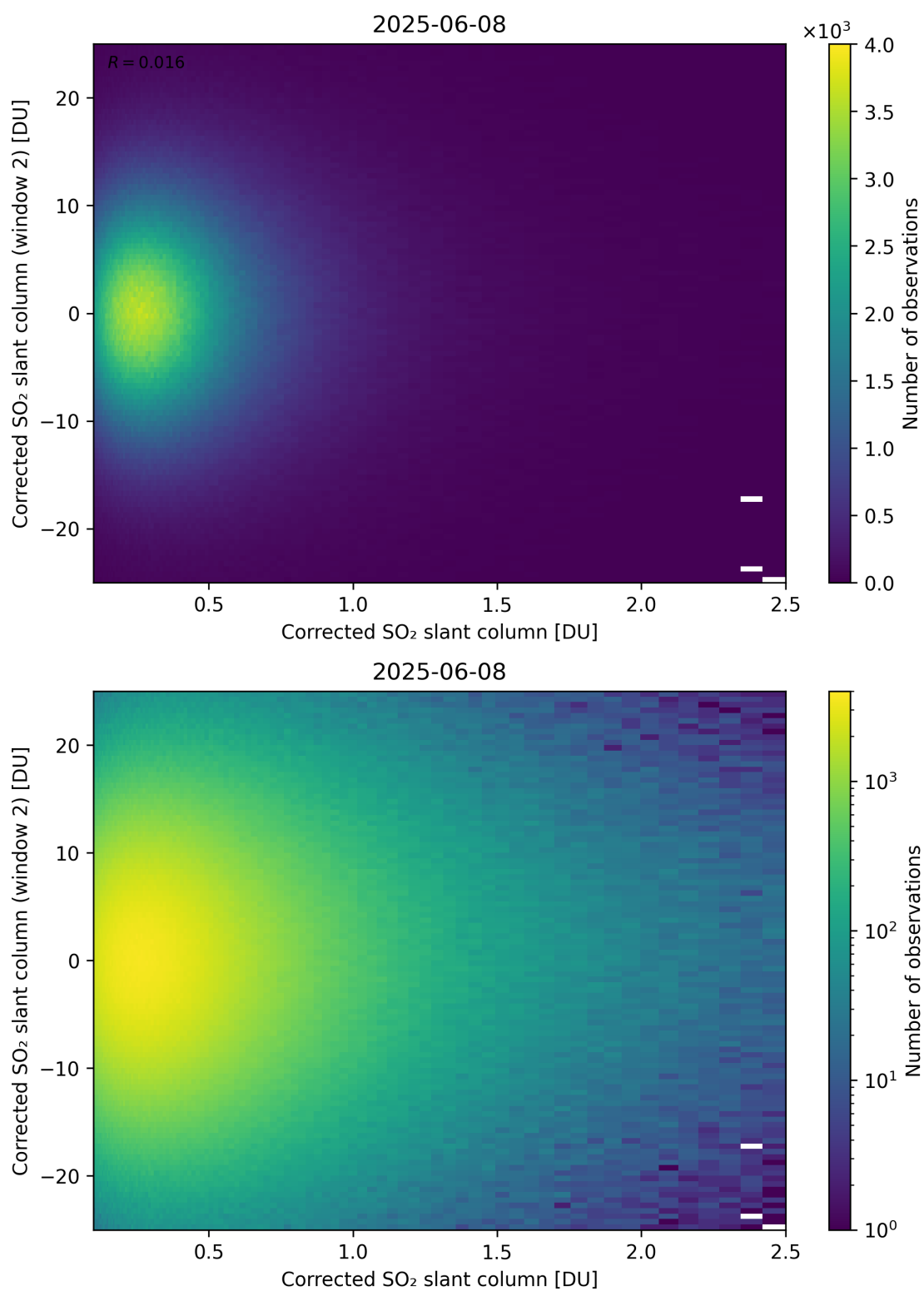
Figure 235: Scatter density plot of “Corrected SO 2 slant column” against “Corrected SO 2 slant column (window 2)” for 2025-06-07 to 2025-06-09.
