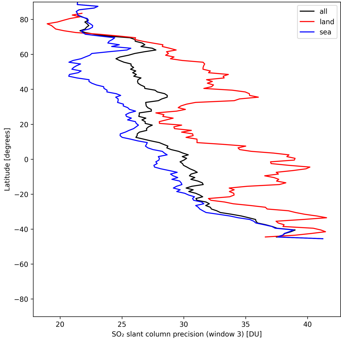
Figure 46: Zonal average of “SO 2 slant column precision (window 3)” for 2025-06-07 to 2025-06-09.
