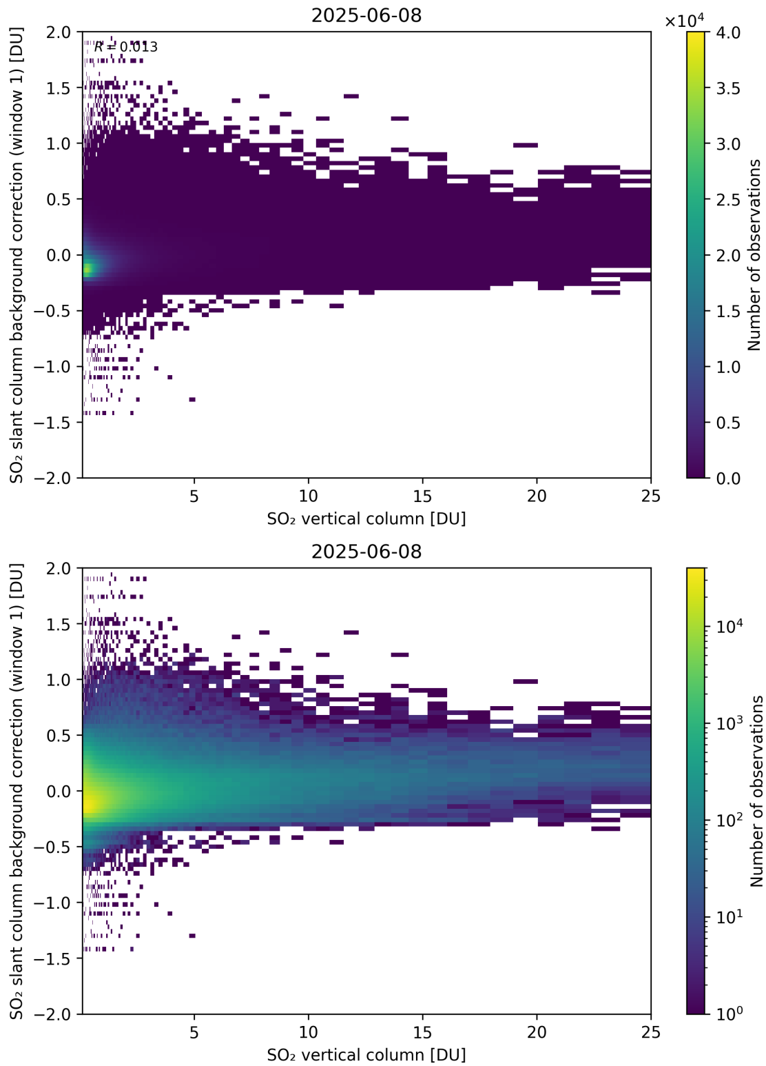
Figure 323: Scatter density plot of “SO 2 vertical column” against “SO 2 slant column background correction (window 1)” for 2025-06-07 to 2025-06-09.
