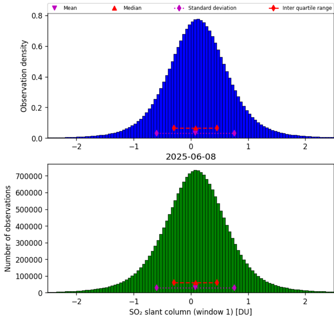
Figure 63: Histogram of “SO 2 slant column (window 1)” for 2025-06-07 to 2025-06-09
