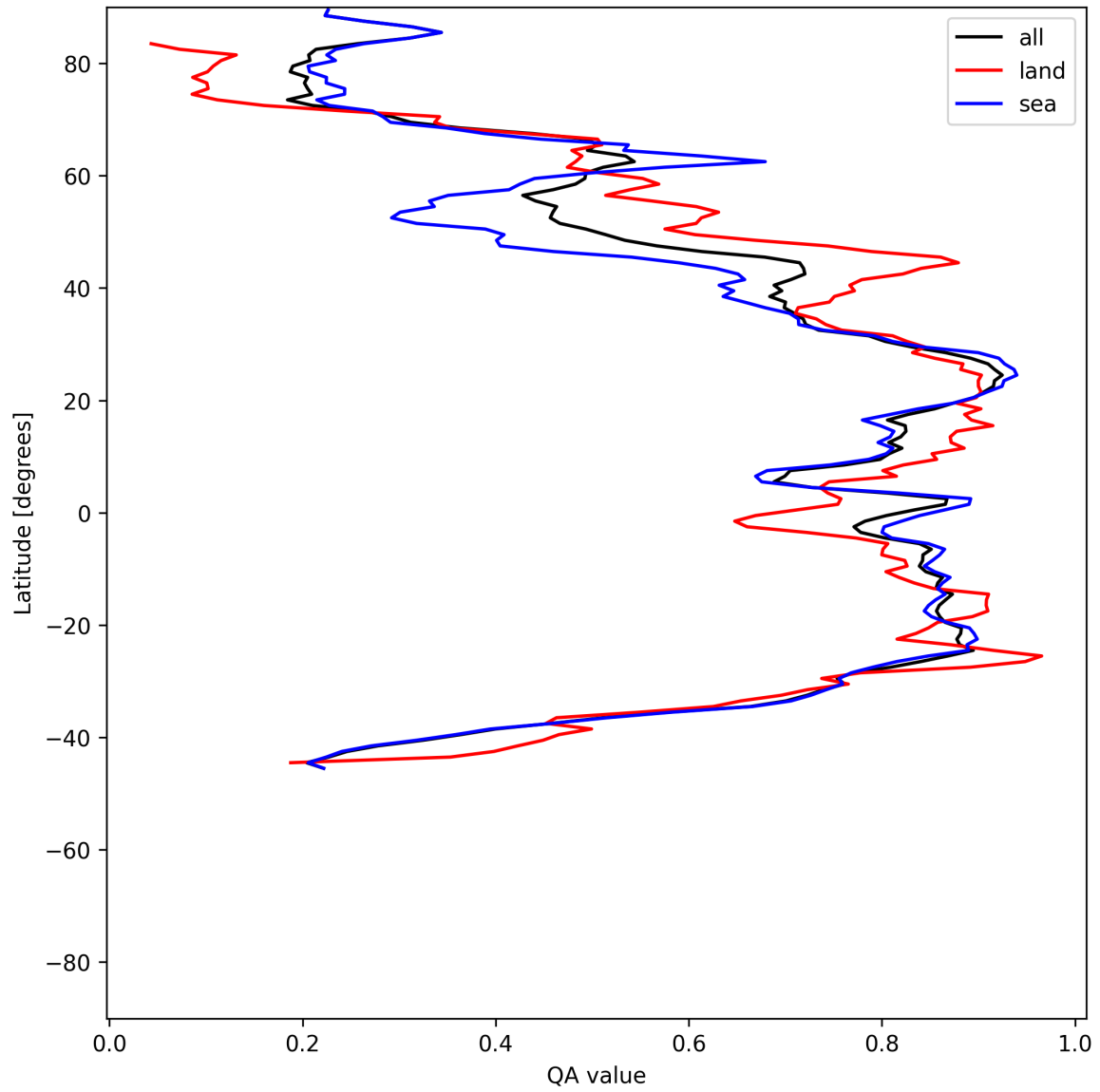
Figure 31: Zonal average of “QA value” for 2025-06-07 to 2025-06-09.
