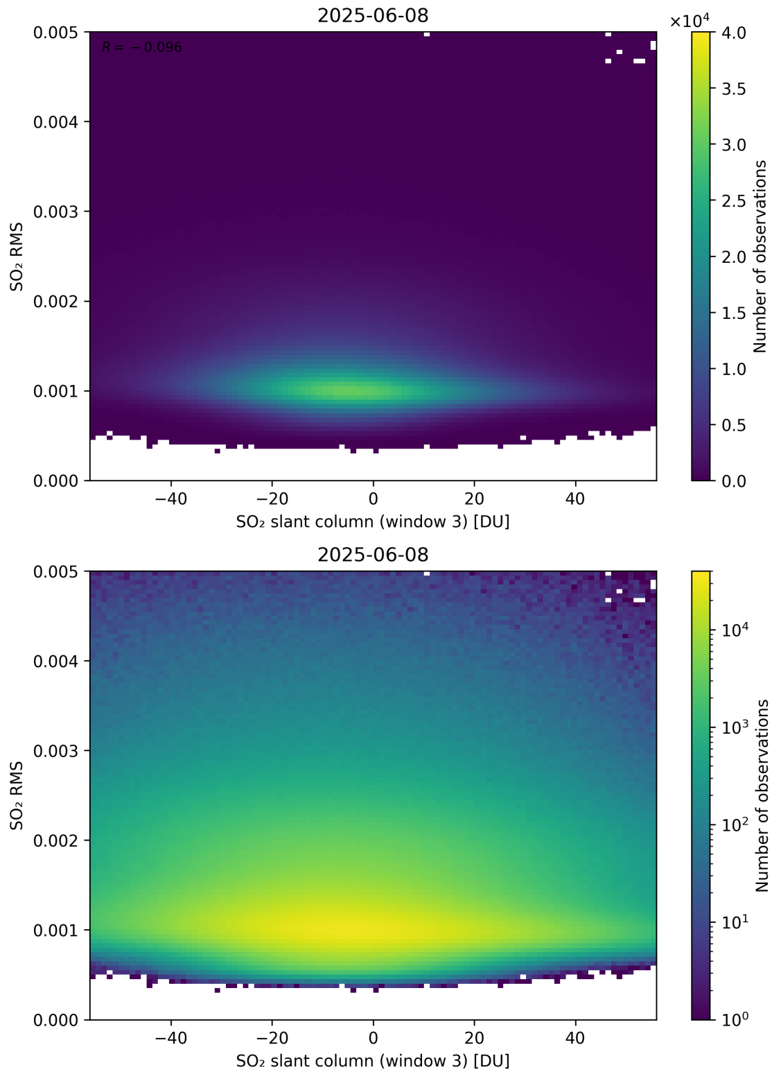
Figure 306: Scatter density plot of “SO 2 slant column (window 3)” against “SO 2 RMS” for 2025-06-07 to 2025-06-09.
