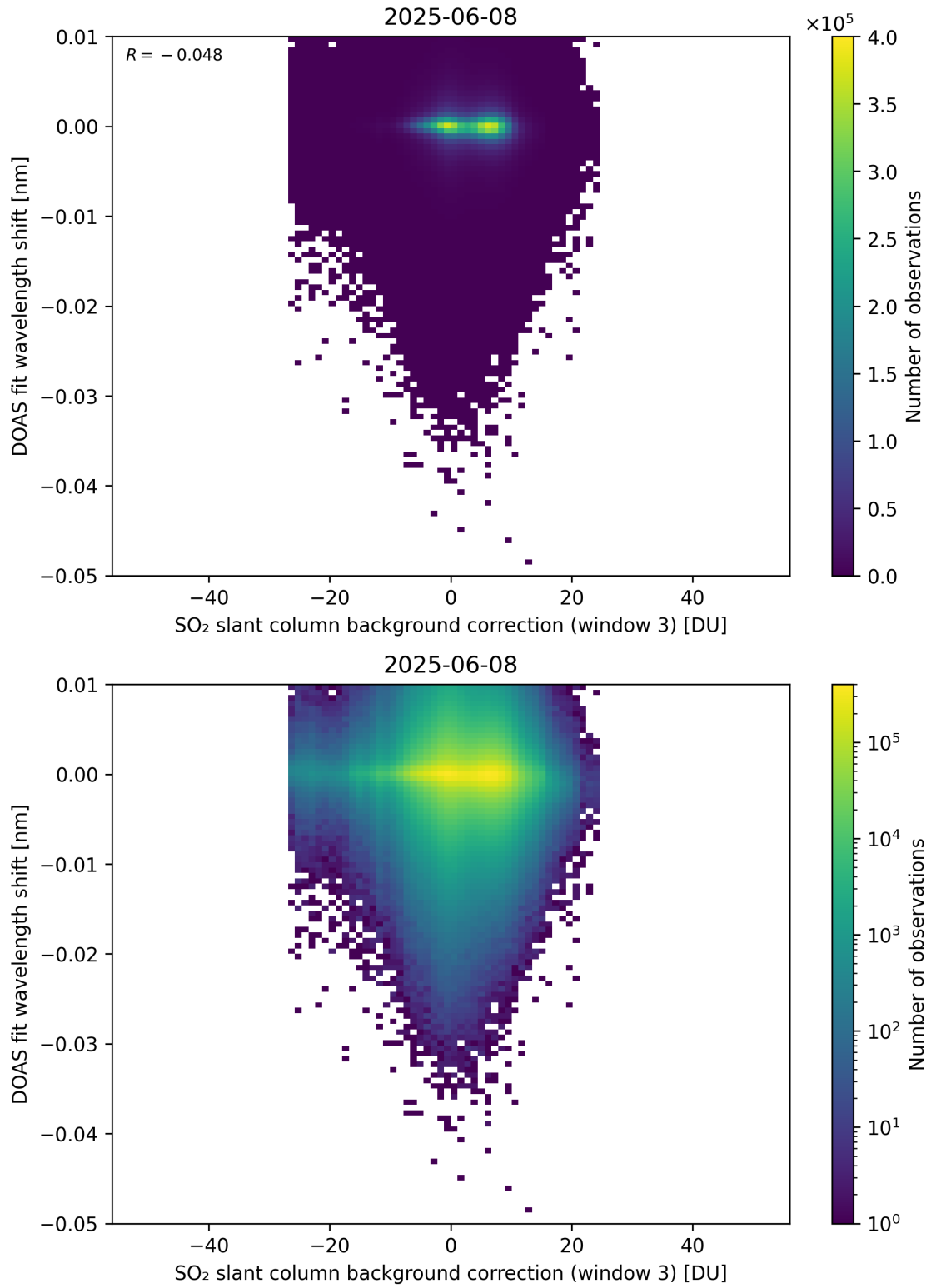
Figure 132: Scatter density plot of “SO 2 slant column background correction (window 3)” against “DOAS fit wavelength shift” for 2025-06-07 to 2025-06-09.
