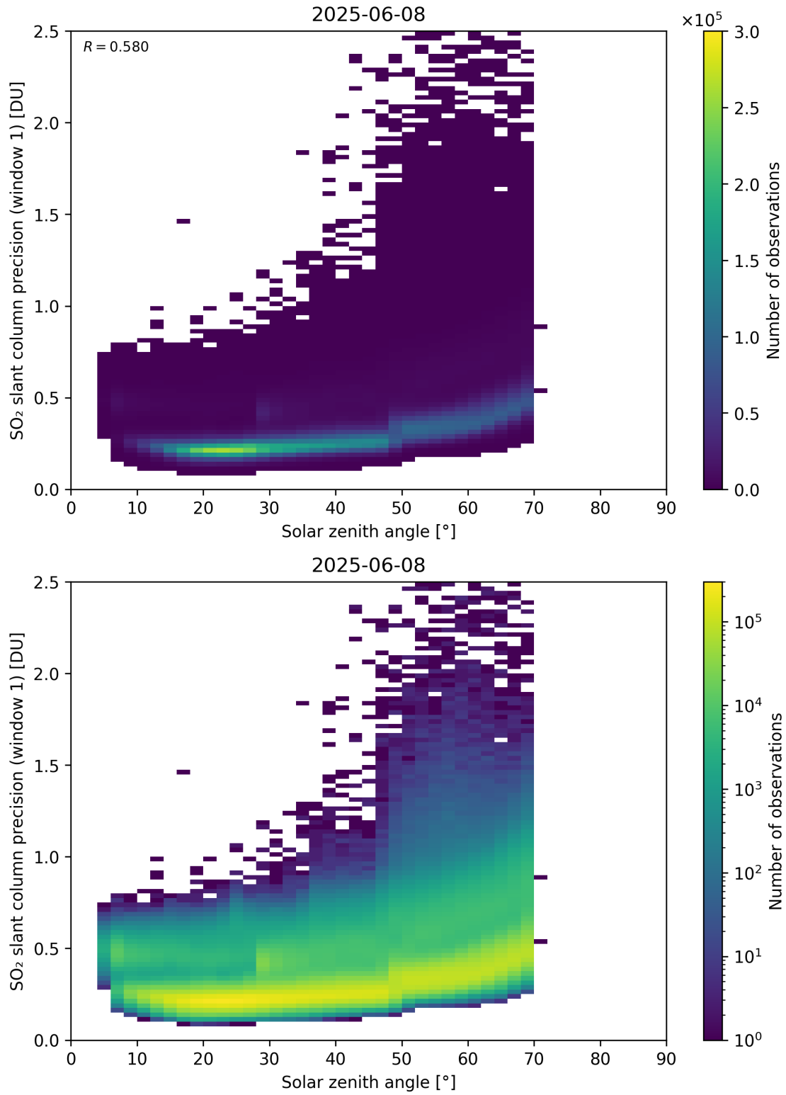
Figure 185: Scatter density plot of “Solar zenith angle” against “SO 2 slant column precision (window 1)” for 2025-06-07 to 2025-06-09.
