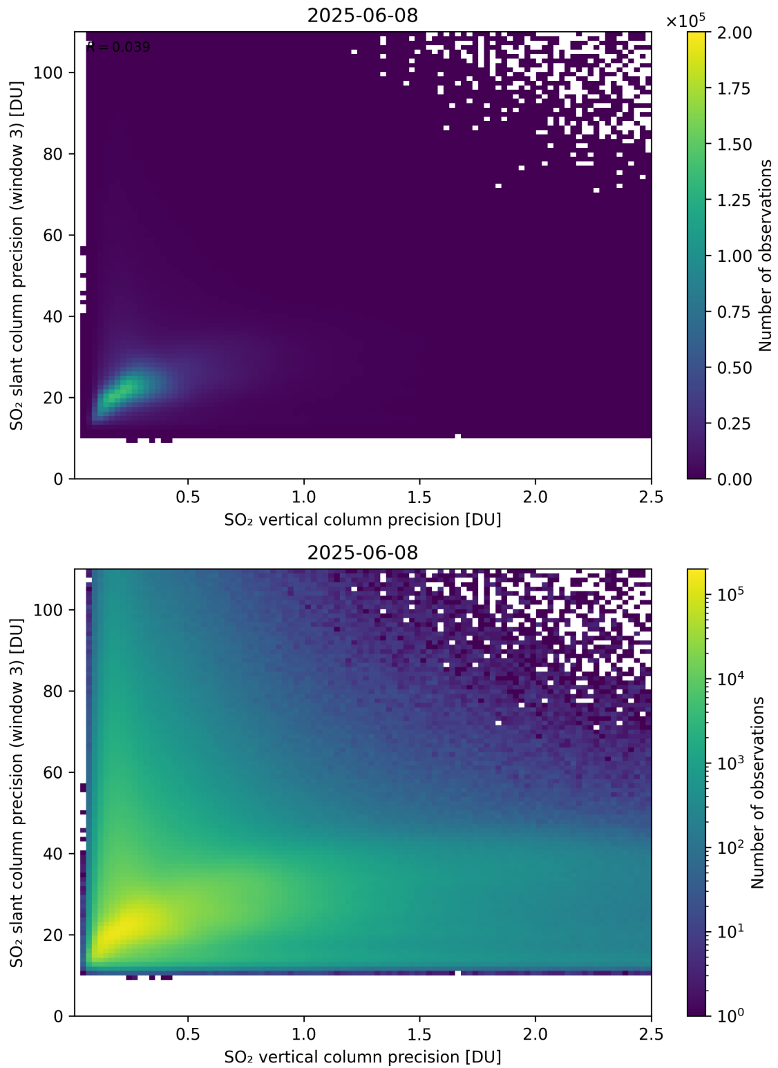
Figure 345: Scatter density plot of “SO 2 vertical column precision” against “SO 2 slant column precision (window 3)” for 2025-06-07 to 2025-06-09.
