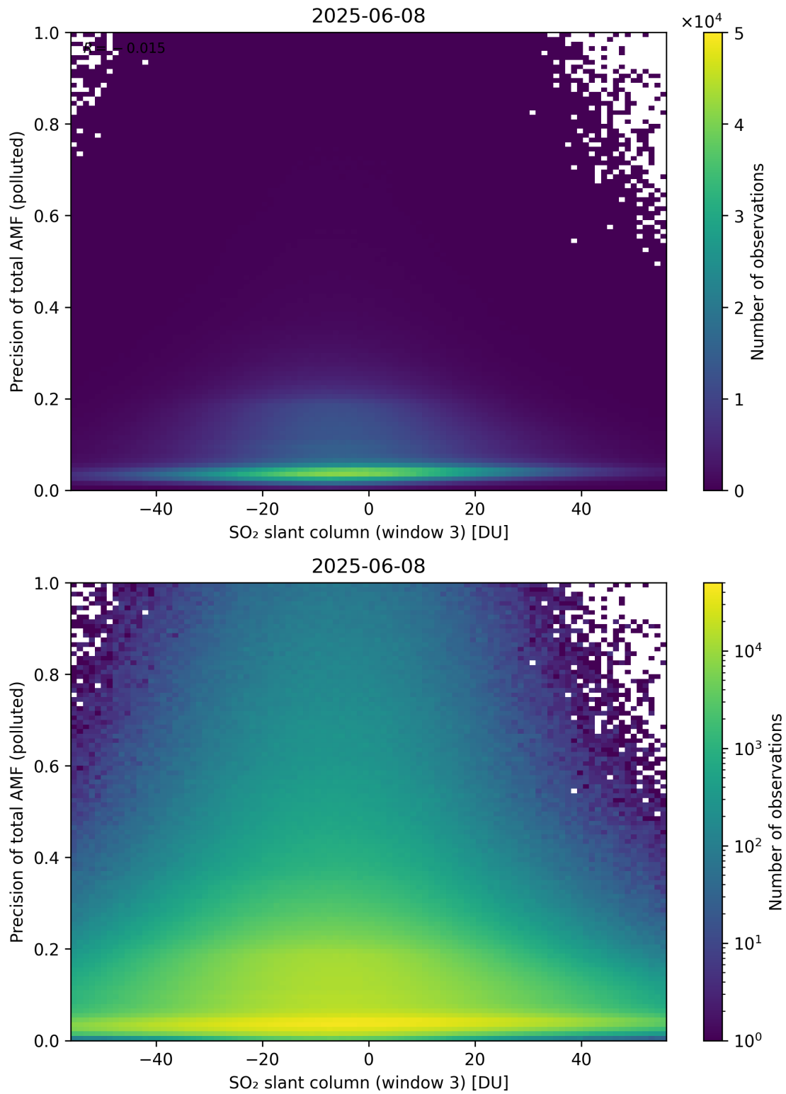
Figure 319: Scatter density plot of “SO 2 slant column (window 3)” against “Precision of total AMF (polluted)” for 2025-06-07 to 2025-06-09.
