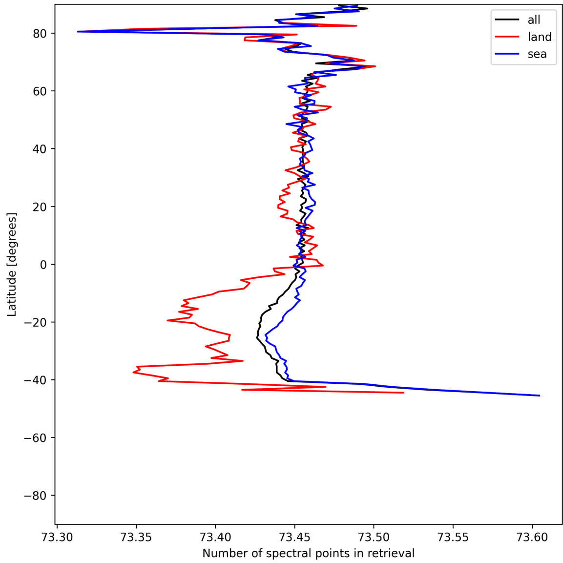
Figure 56: Zonal average of “Number of spectral points in retrieval” for 2025-06-07 to 2025-06-09.
