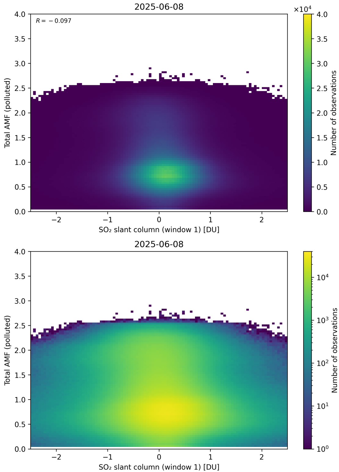
Figure 289: Scatter density plot of “SO 2 slant column (window 1)” against “Total AMF (polluted)” for 2025-06-07 to 2025-06-09.
