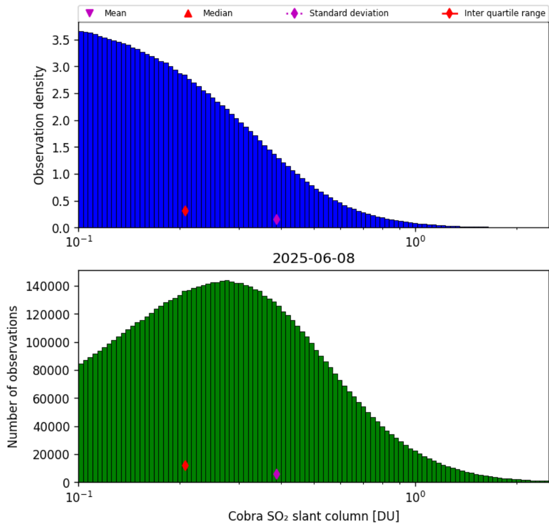
Figure 61: Histogram of “Cobra SO 2 slant column” for 2025-06-07 to 2025-06-09
