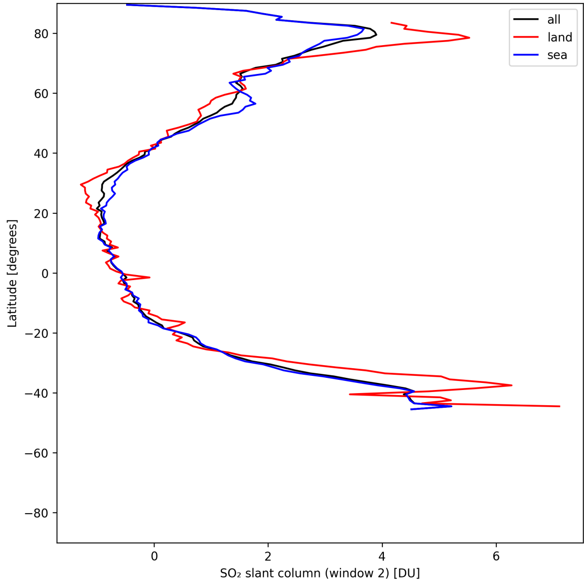
Figure 41: Zonal average of “SO 2 slant column (window 2)” for 2025-06-07 to 2025-06-09.
