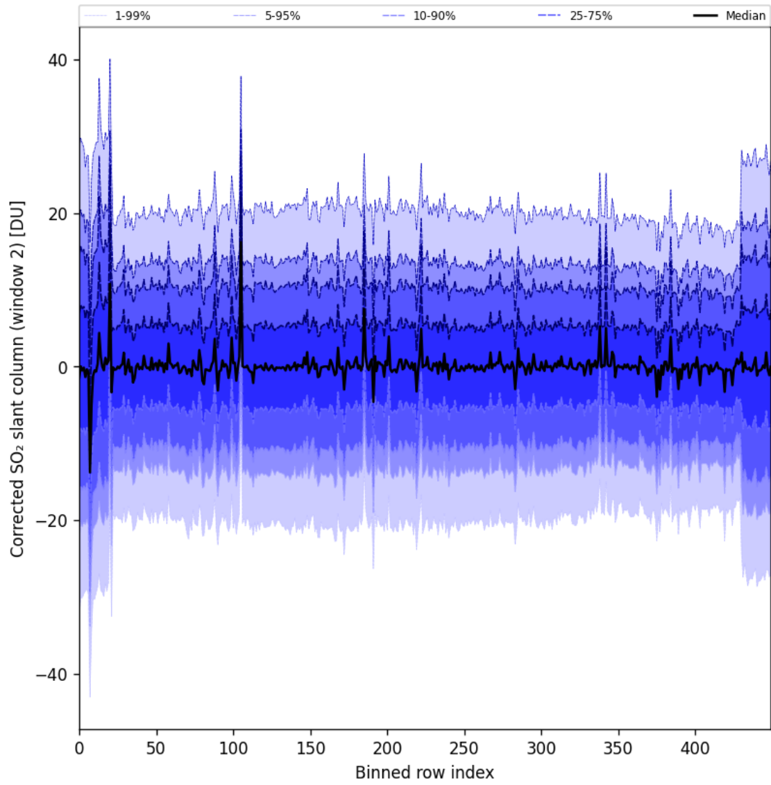
Figure 95: Along track statistics of “Corrected SO 2 slant column (window 2)” for 2025-06-07 to 2025-06-09
