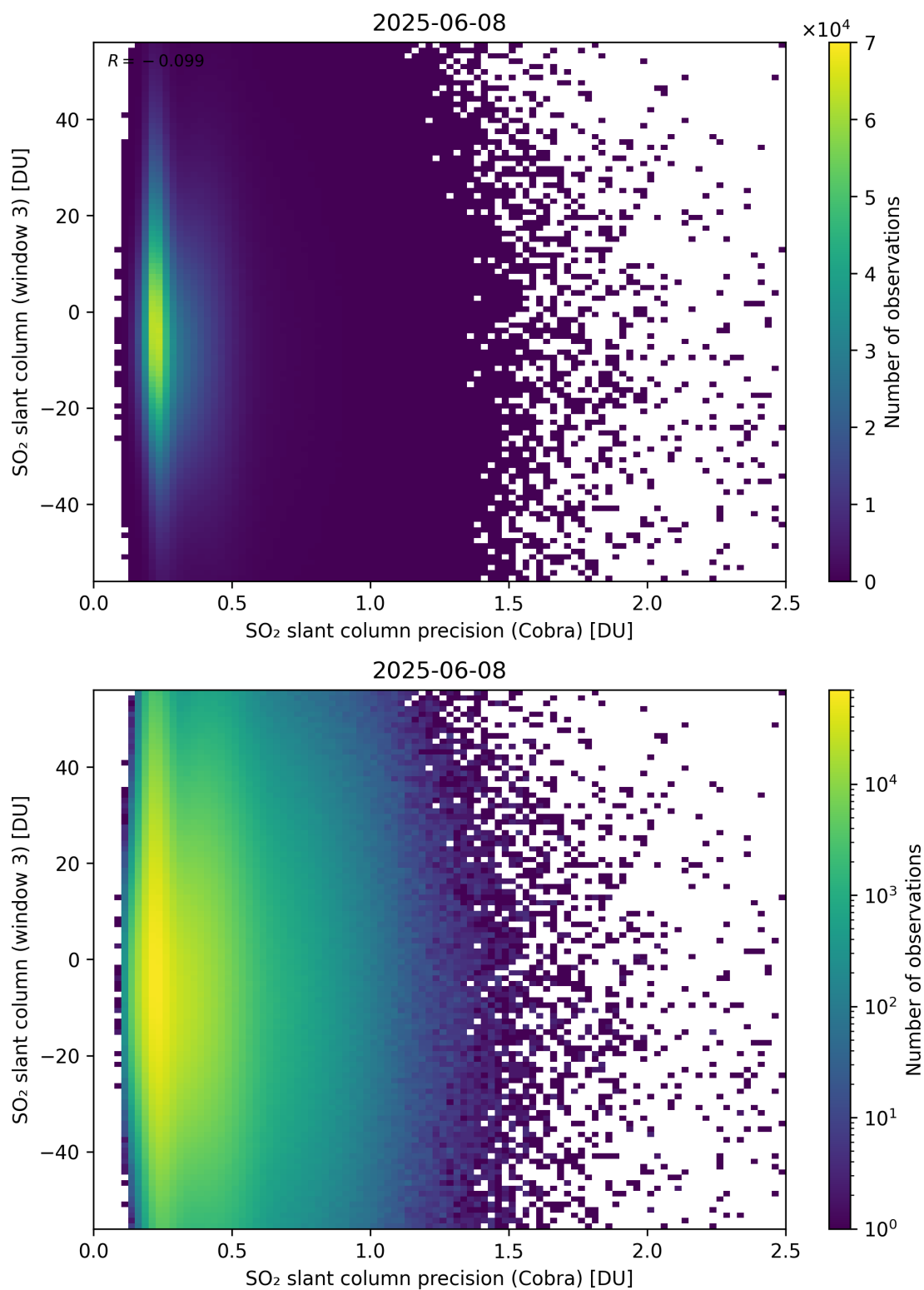
Figure 211: Scatter density plot of “SO 2 slant column precision (Cobra)” against “SO 2 slant column (window 3)” for 2025-06-07 to 2025-06-09.
