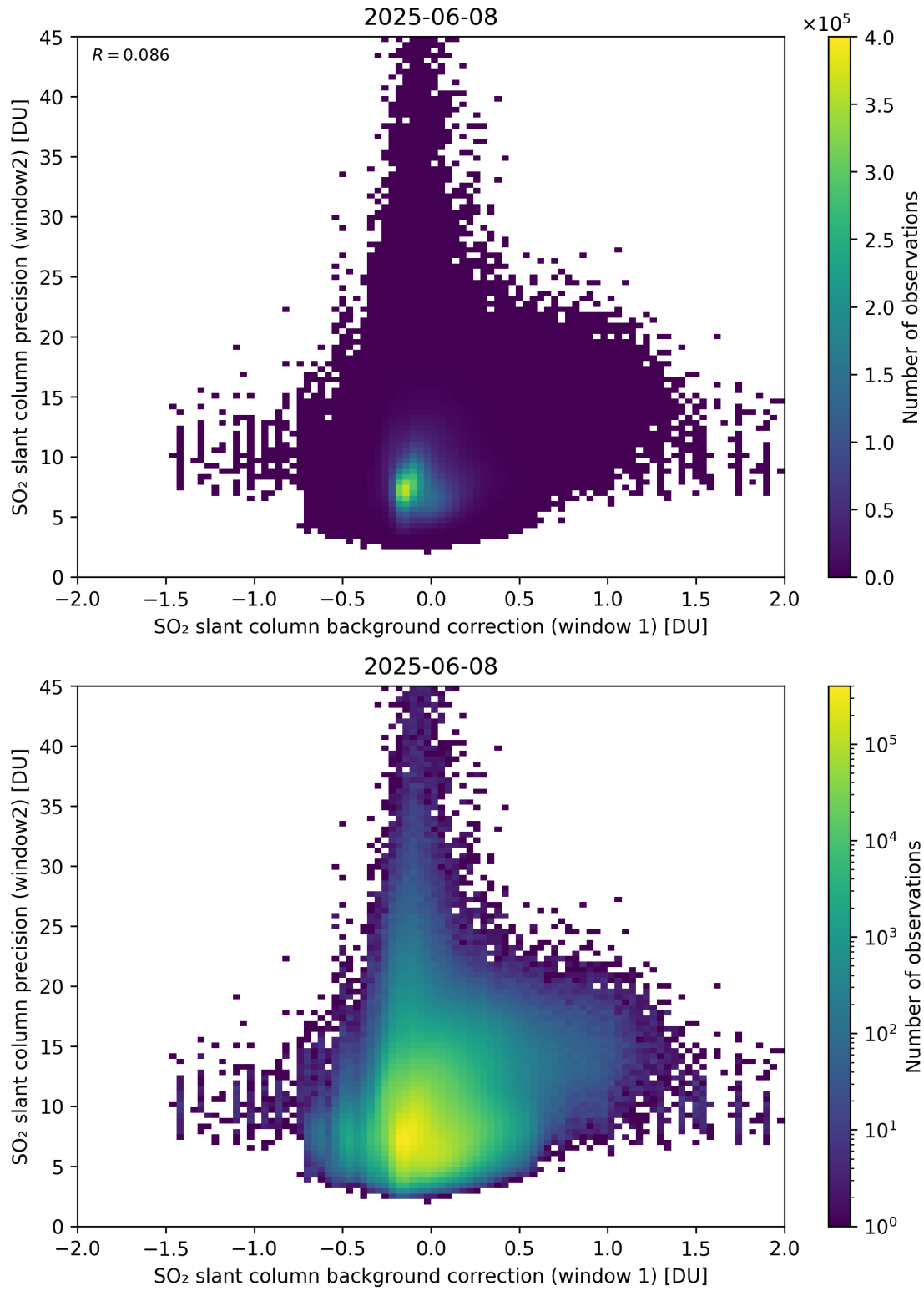
Figure 117: Scatter density plot of “SO 2 slant column background correction (window 1)” against “SO 2 slant column precision (window2)” for 2025-06-07 to 2025-06-09.
