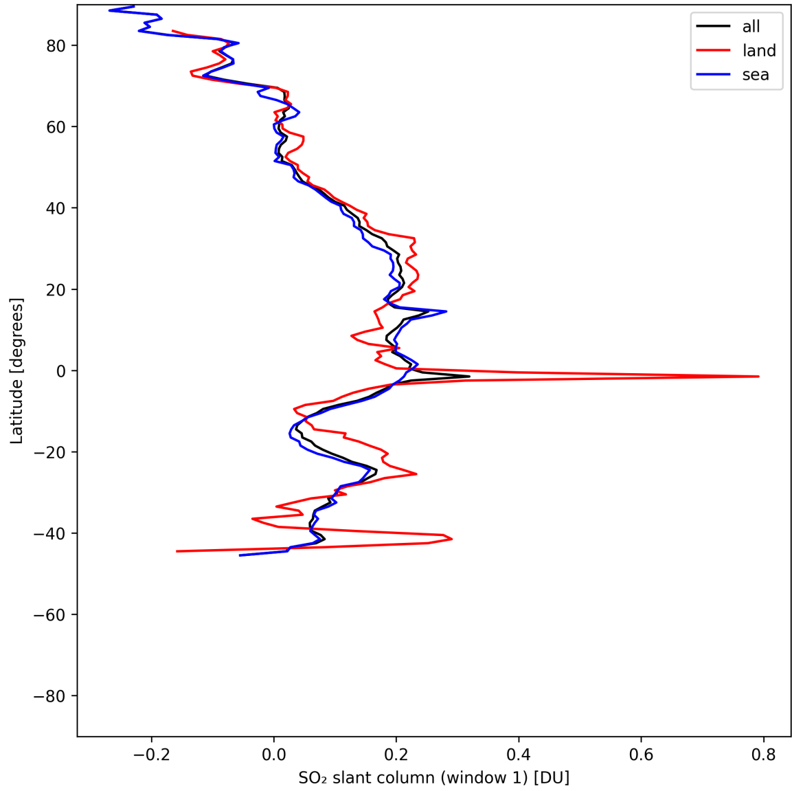
Figure 37: Zonal average of “SO 2 slant column (window 1)” for 2025-06-07 to 2025-06-09.
