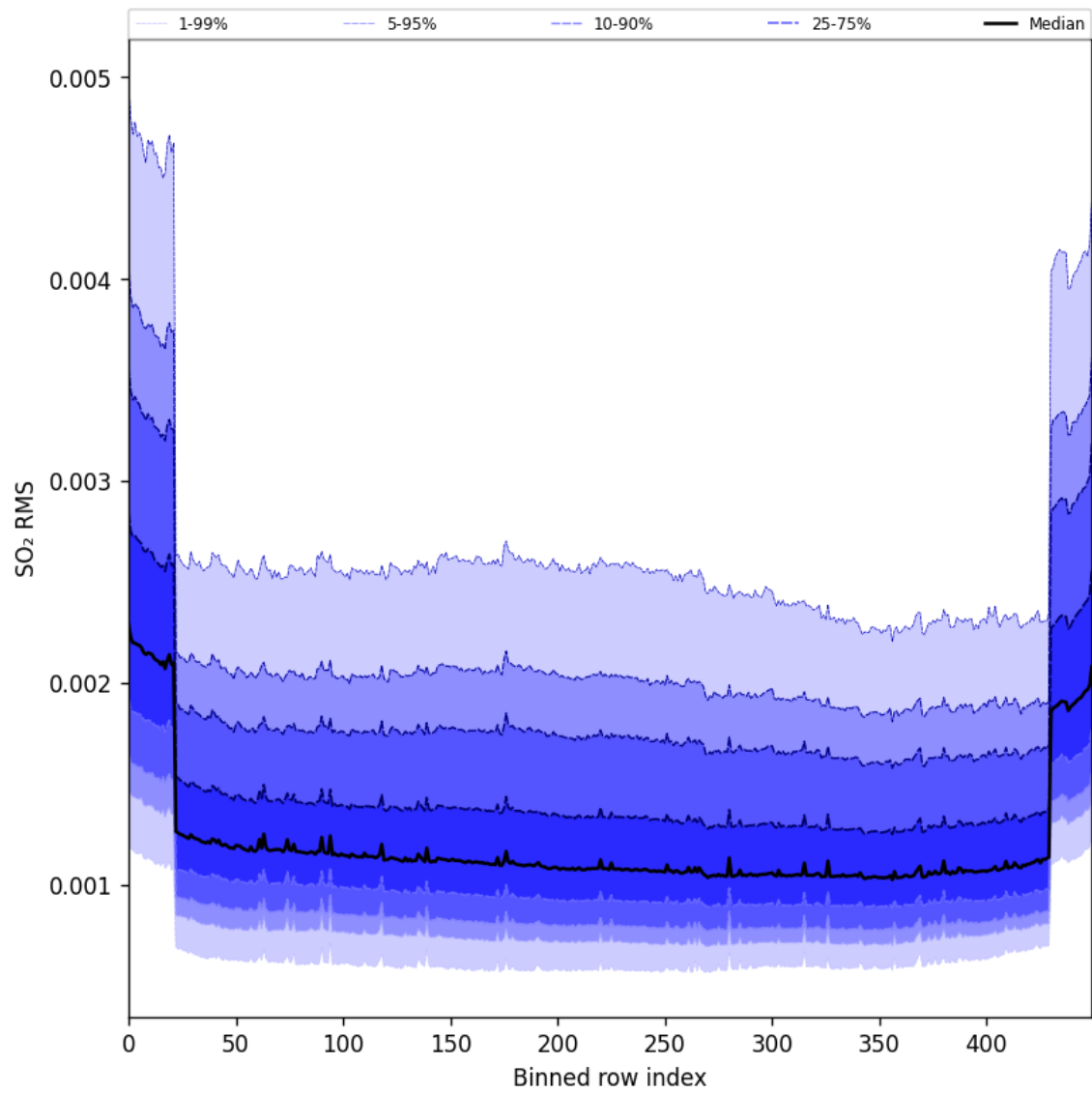
Figure 104: Along track statistics of “SO 2 RMS” for 2025-06-07 to 2025-06-09
