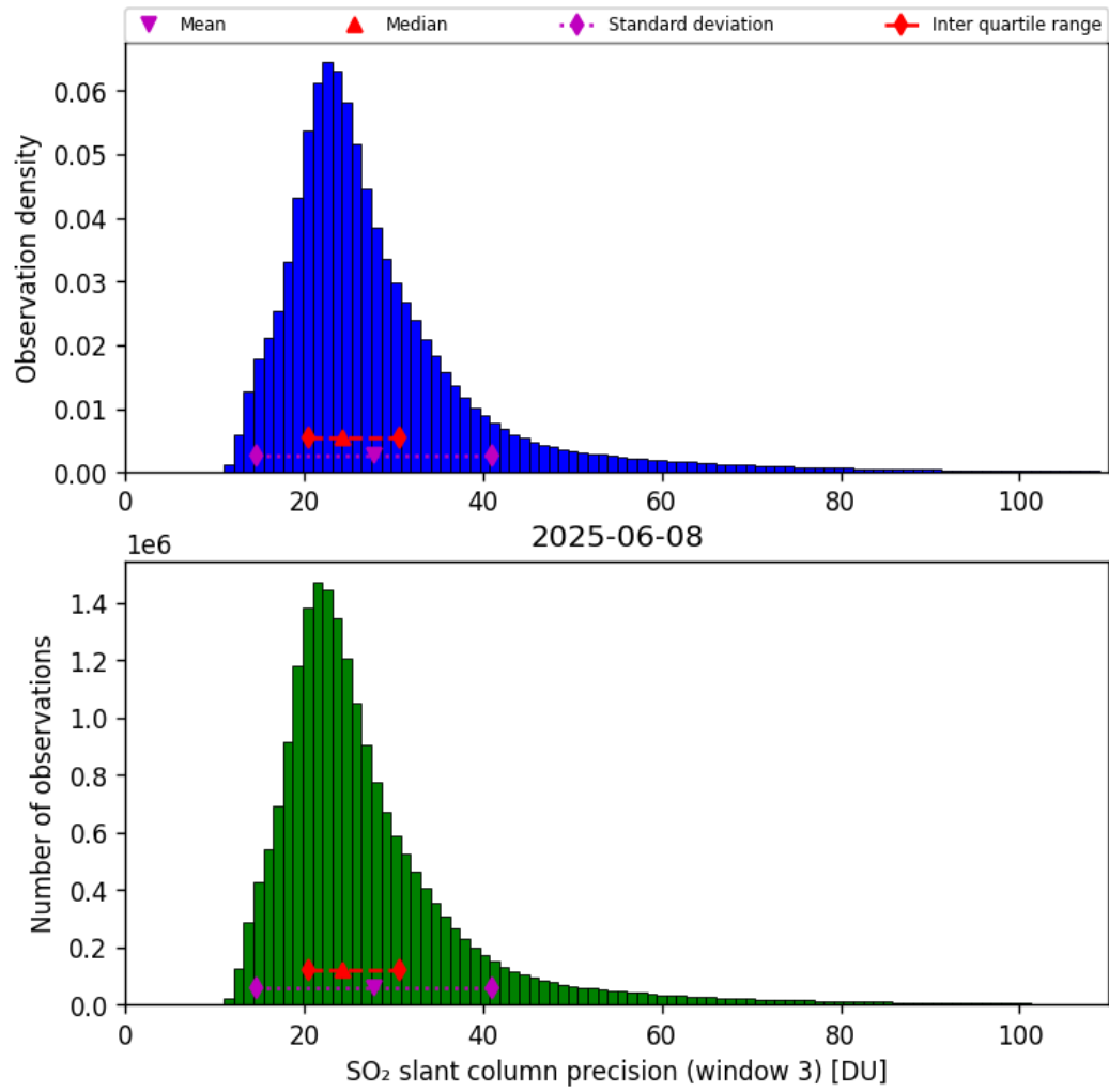
Figure 72: Histogram of “SO 2 slant column precision (window 3)” for 2025-06-07 to 2025-06-09
