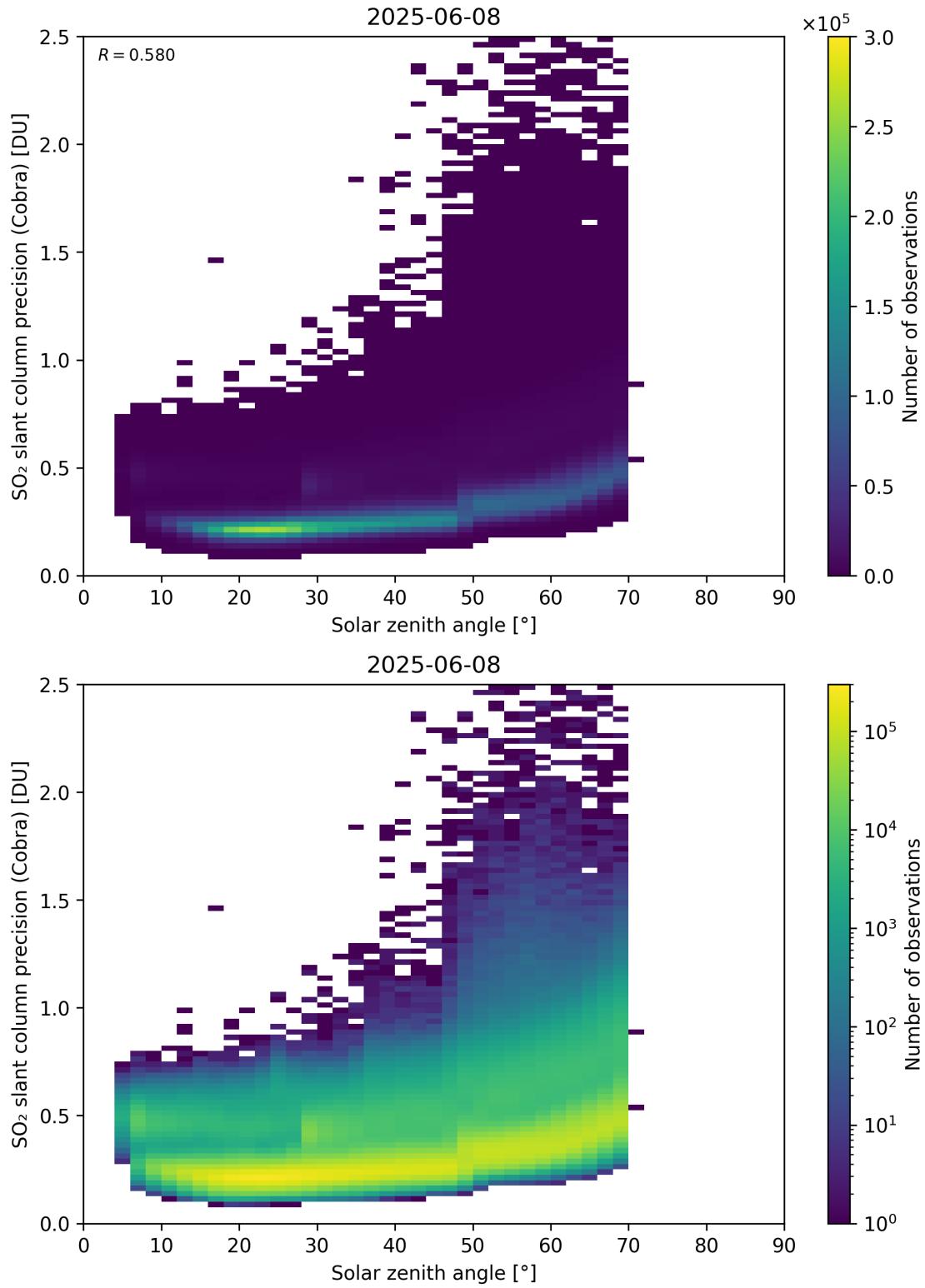
Figure 180: Scatter density plot of “Solar zenith angle” against “SO 2 slant column precision (Cobra)” for 2025-06-07 to 2025-06-09.
