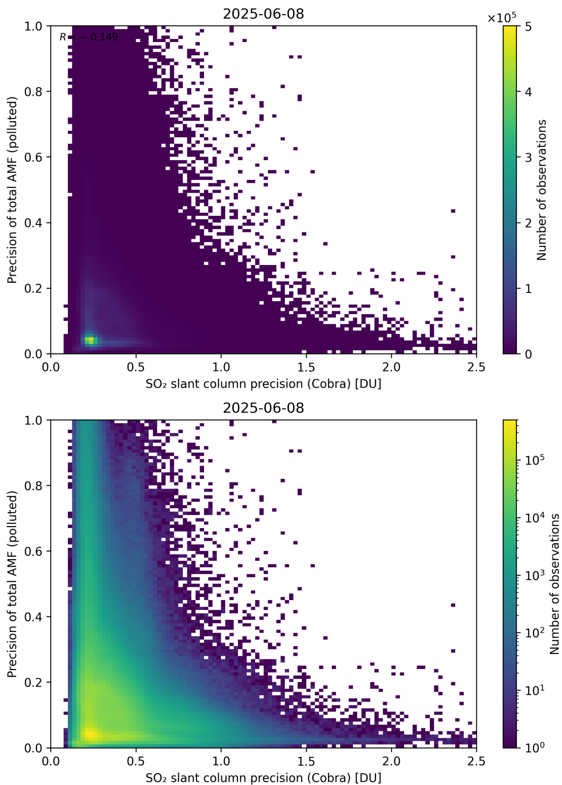
Figure 214: Scatter density plot of “SO 2 slant column precision (Cobra)” against “Precision of total AMF (polluted)” for 2025-06-07 to 2025-06-09.
