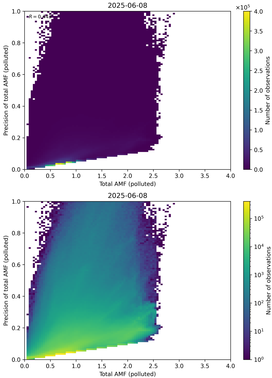
Figure 322: Scatter density plot of “Total AMF (polluted)” against “Precision of total AMF (polluted)” for 2025-06-07 to 2025-06-09.
