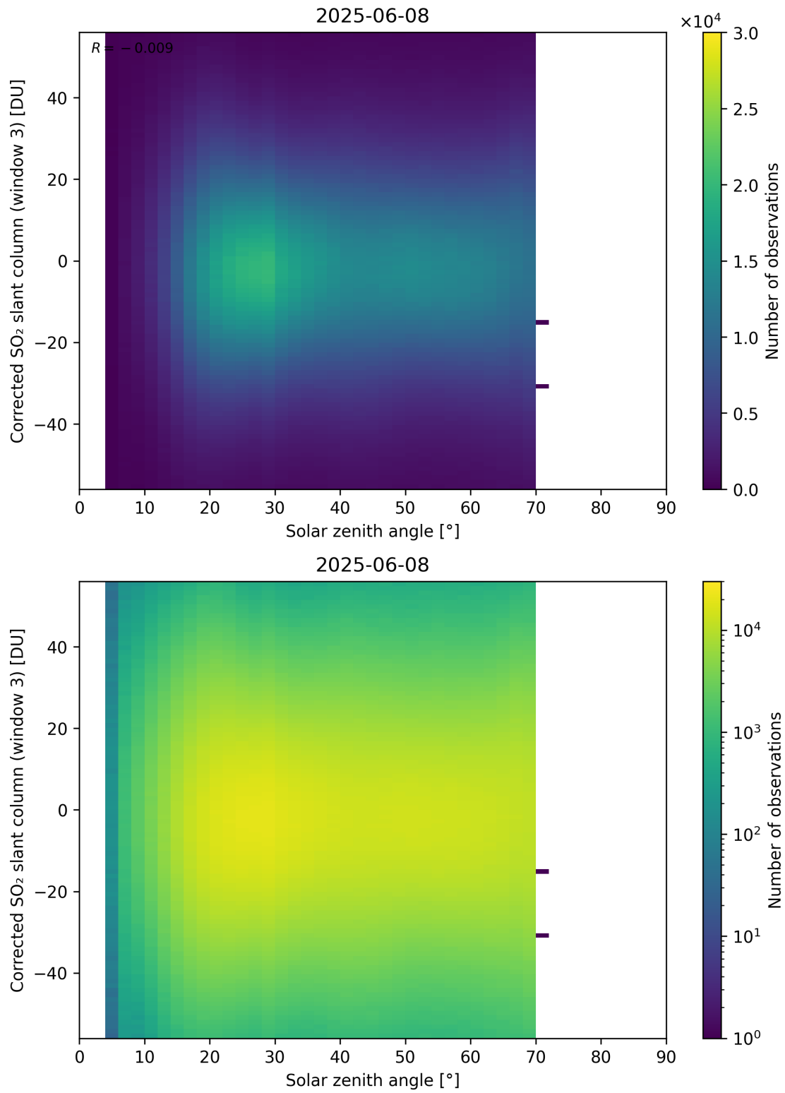
Figure 183: Scatter density plot of “Solar zenith angle” against “Corrected SO 2 slant column (window 3)” for 2025-06-07 to 2025-06-09.
