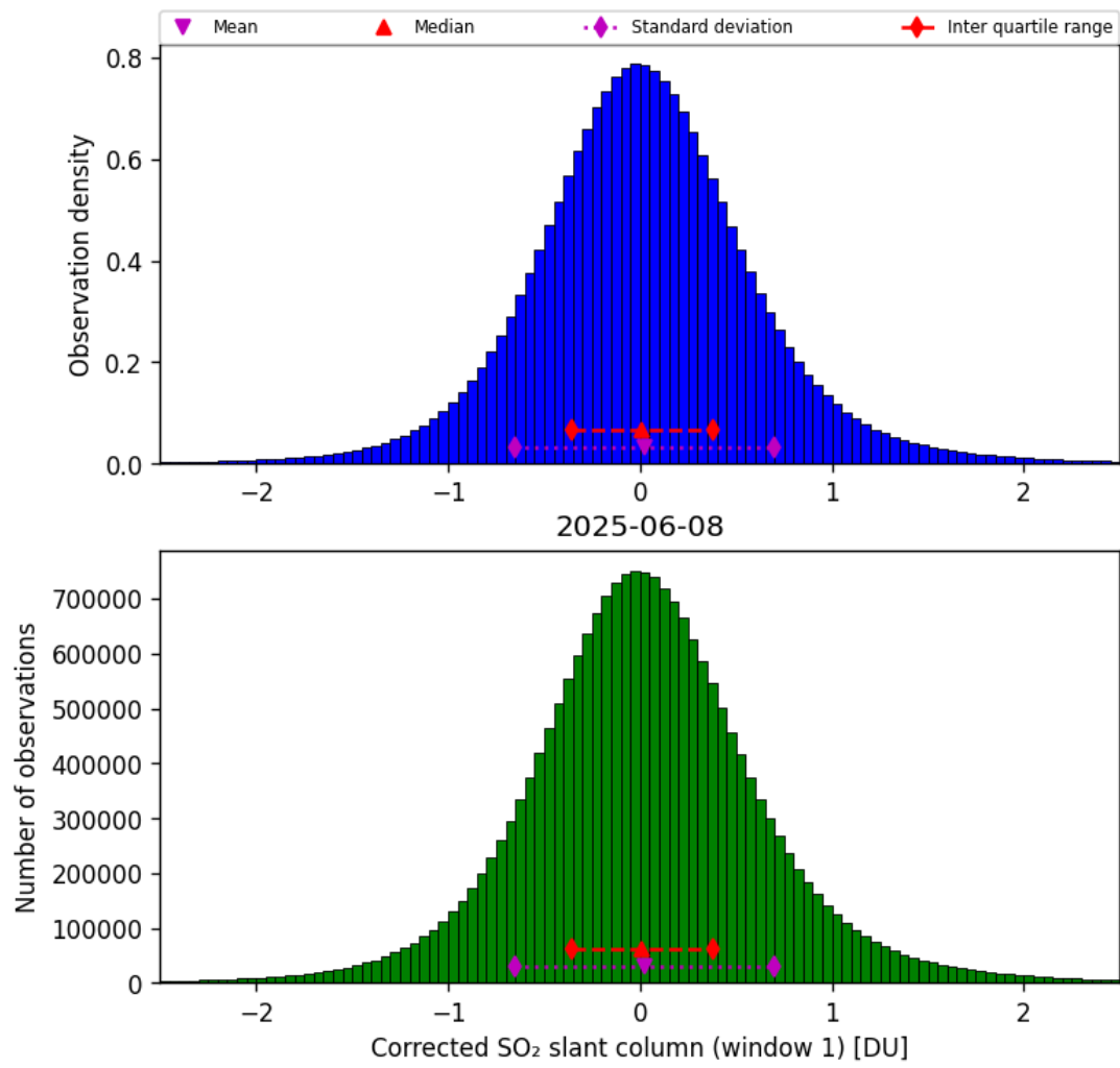
Figure 65: Histogram of “Corrected SO 2 slant column (window 1)” for 2025-06-07 to 2025-06-09
