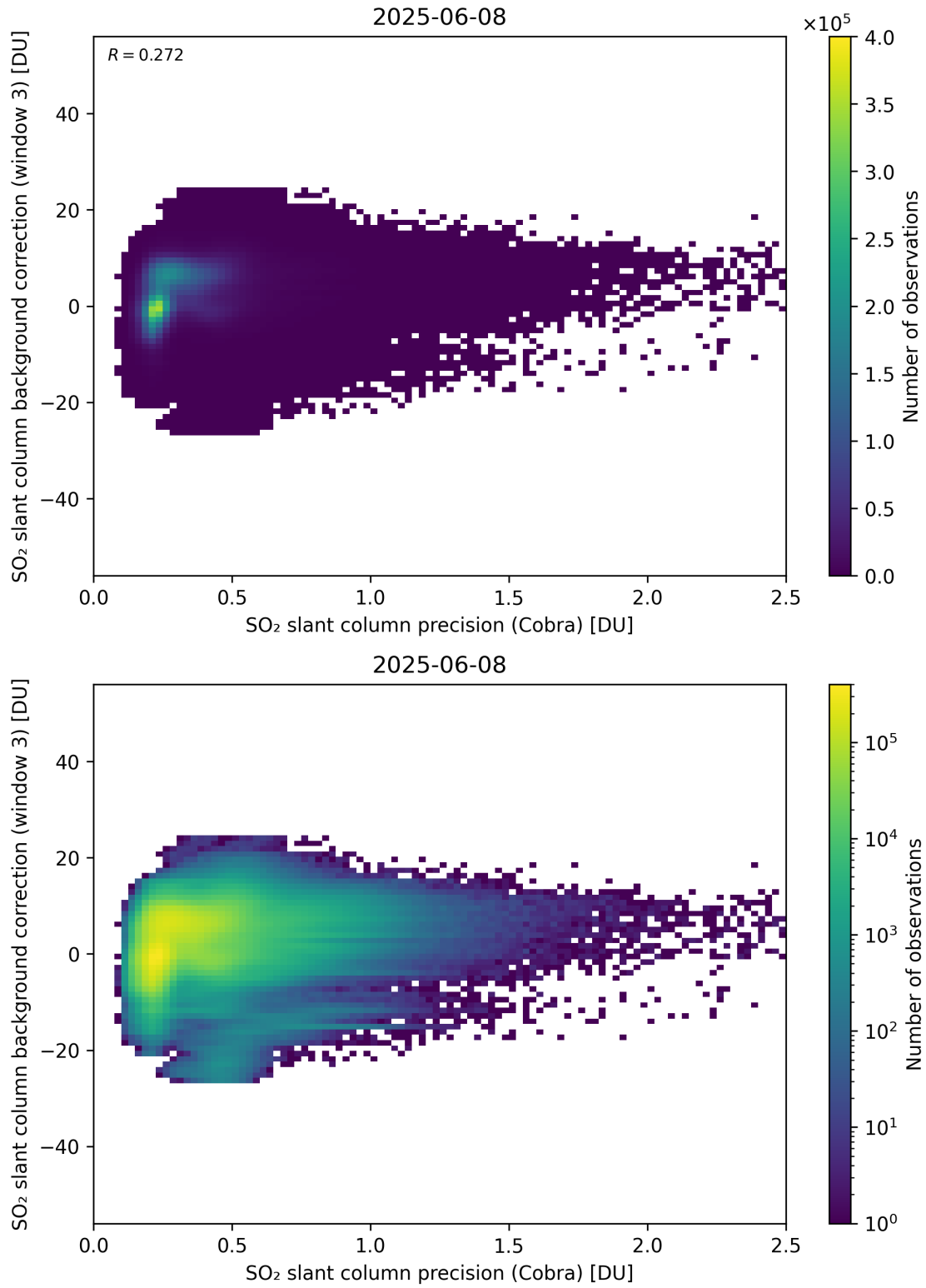
Figure 201: Scatter density plot of “SO 2 slant column precision (Cobra)” against “SO 2 slant column background correction (window 3)” for 2025-06-07 to 2025-06-09.
