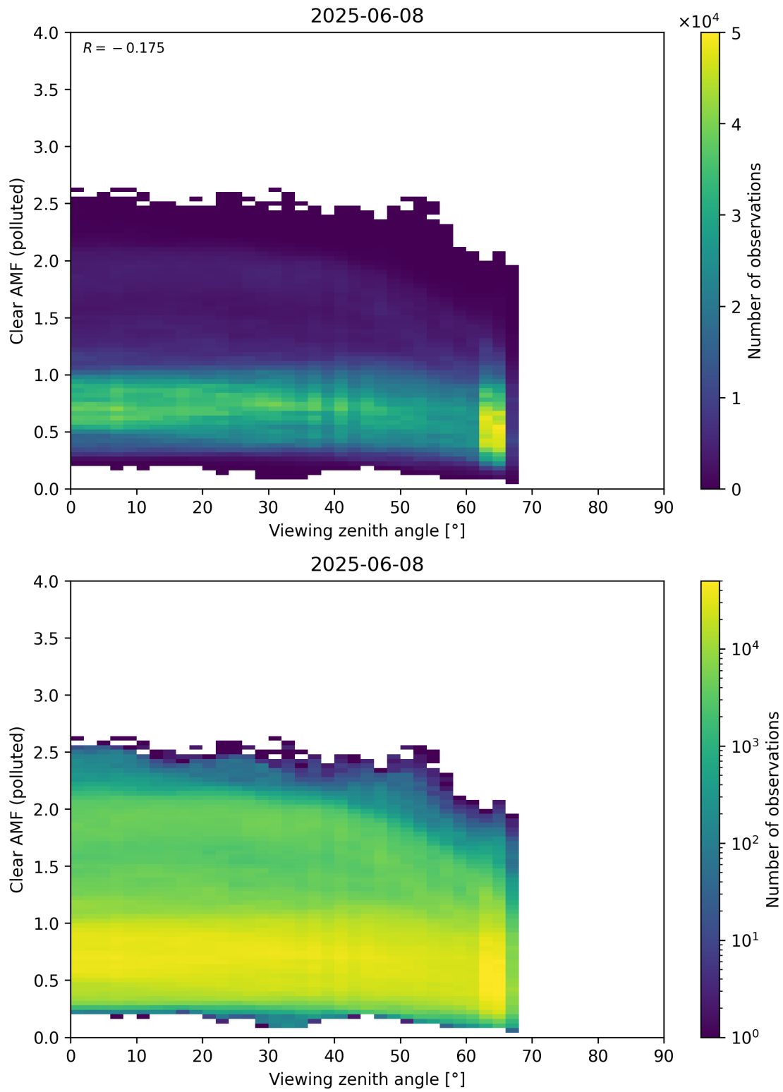
Figure 370: Scatter density plot of “Viewing zenith angle” against “Clear AMF (polluted)” for 2025-06-07 to 2025-06-09.
