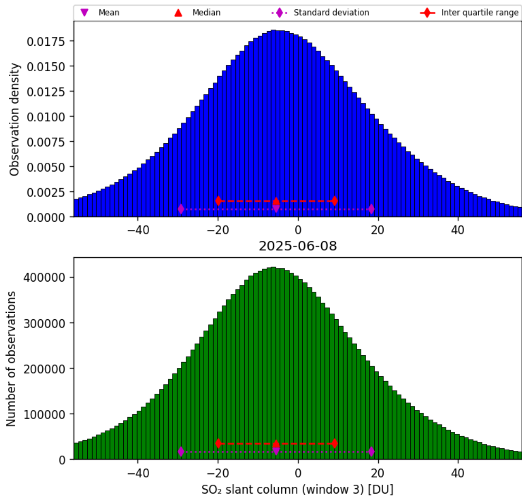
Figure 71: Histogram of “SO 2 slant column (window 3)” for 2025-06-07 to 2025-06-09
