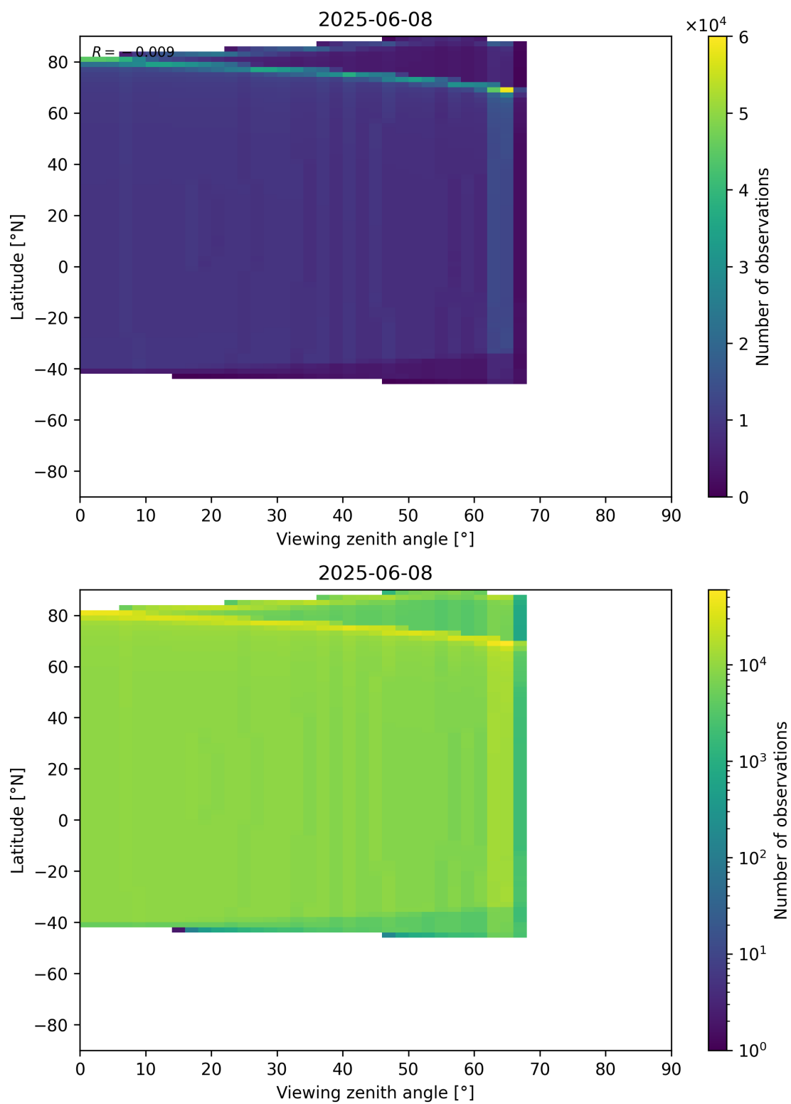
Figure 368: Scatter density plot of “Viewing zenith angle” against “Latitude” for 2025-06-07 to 2025-06-09.
