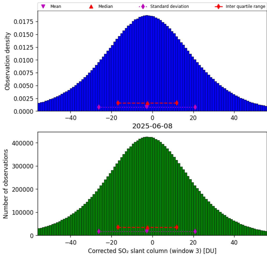
Figure 73: Histogram of “Corrected SO 2 slant column (window 3)” for 2025-06-07 to 2025-06-09
