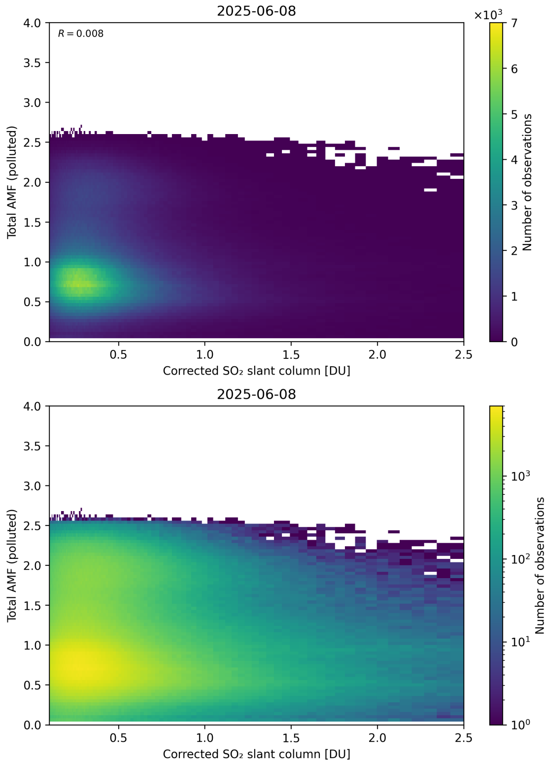
Figure 242: Scatter density plot of “Corrected SO 2 slant column” against “Total AMF (polluted)” for 2025-06-07 to 2025-06-09.
