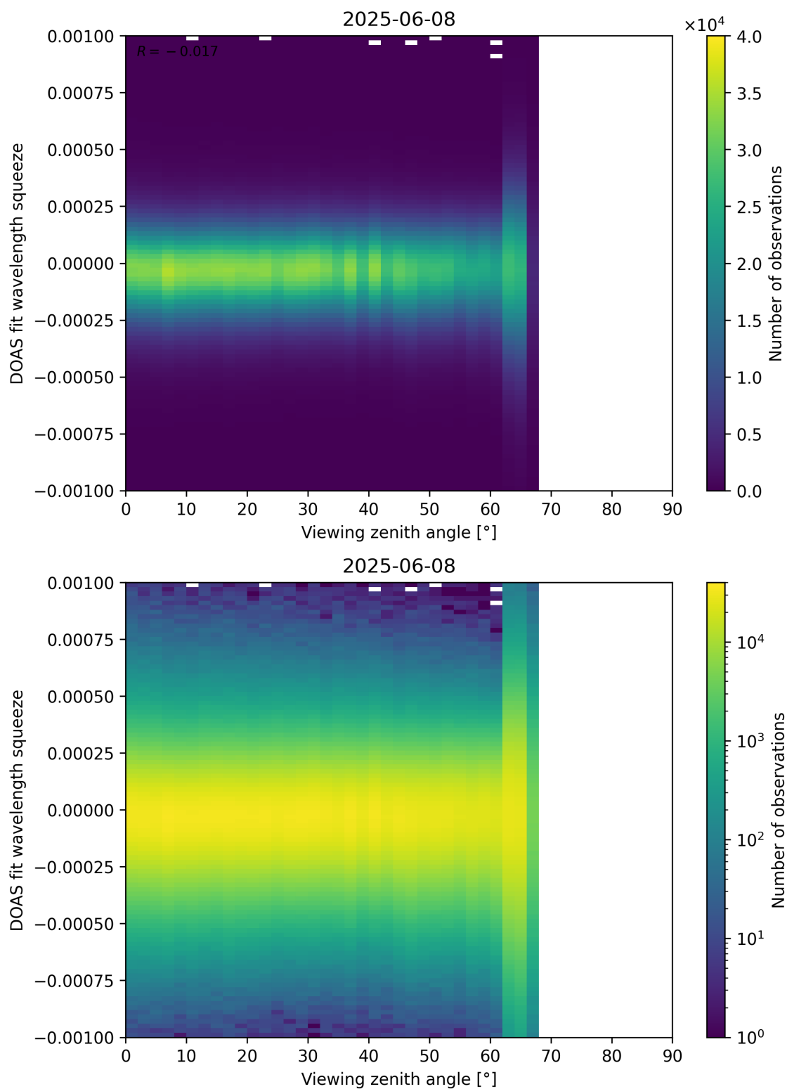
Figure 366: Scatter density plot of “Viewing zenith angle” against “DOAS fit wavelength squeeze” for 2025-06-07 to 2025-06-09.
