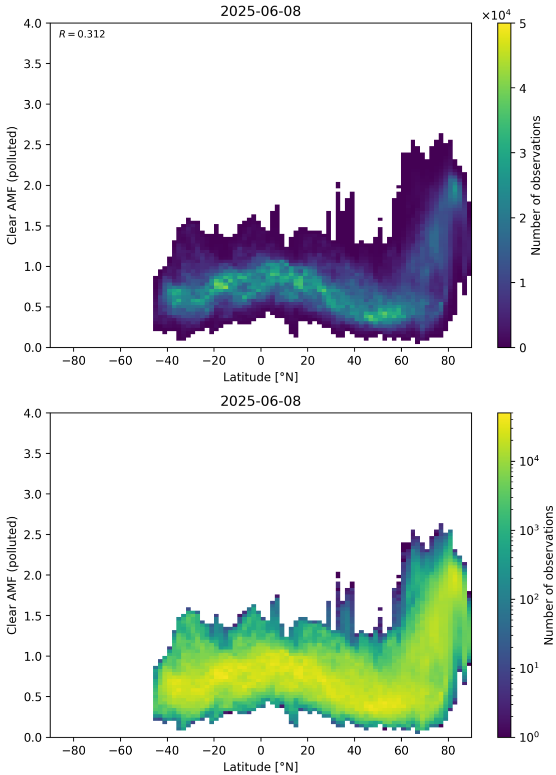
Figure 156: Scatter density plot of “Latitude” against “Clear AMF (polluted)” for 2025-06-07 to 2025-06-09.
