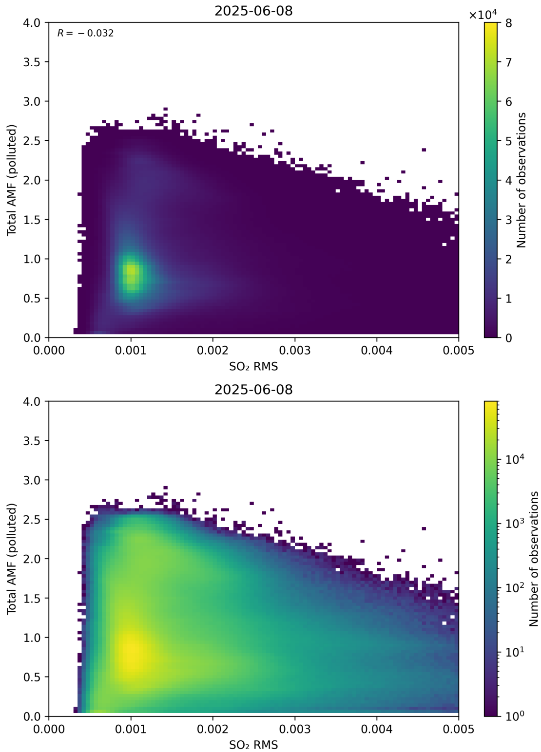
Figure 148: Scatter density plot of “SO 2 RMS” against “Total AMF (polluted)” for 2025-06-07 to 2025-06-09.
