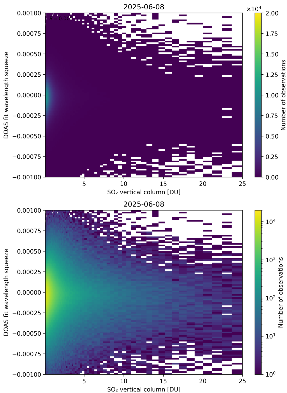
Figure 327: Scatter density plot of “SO 2 vertical column” against “DOAS fit wavelength squeeze” for 2025-06-07 to 2025-06-09.
