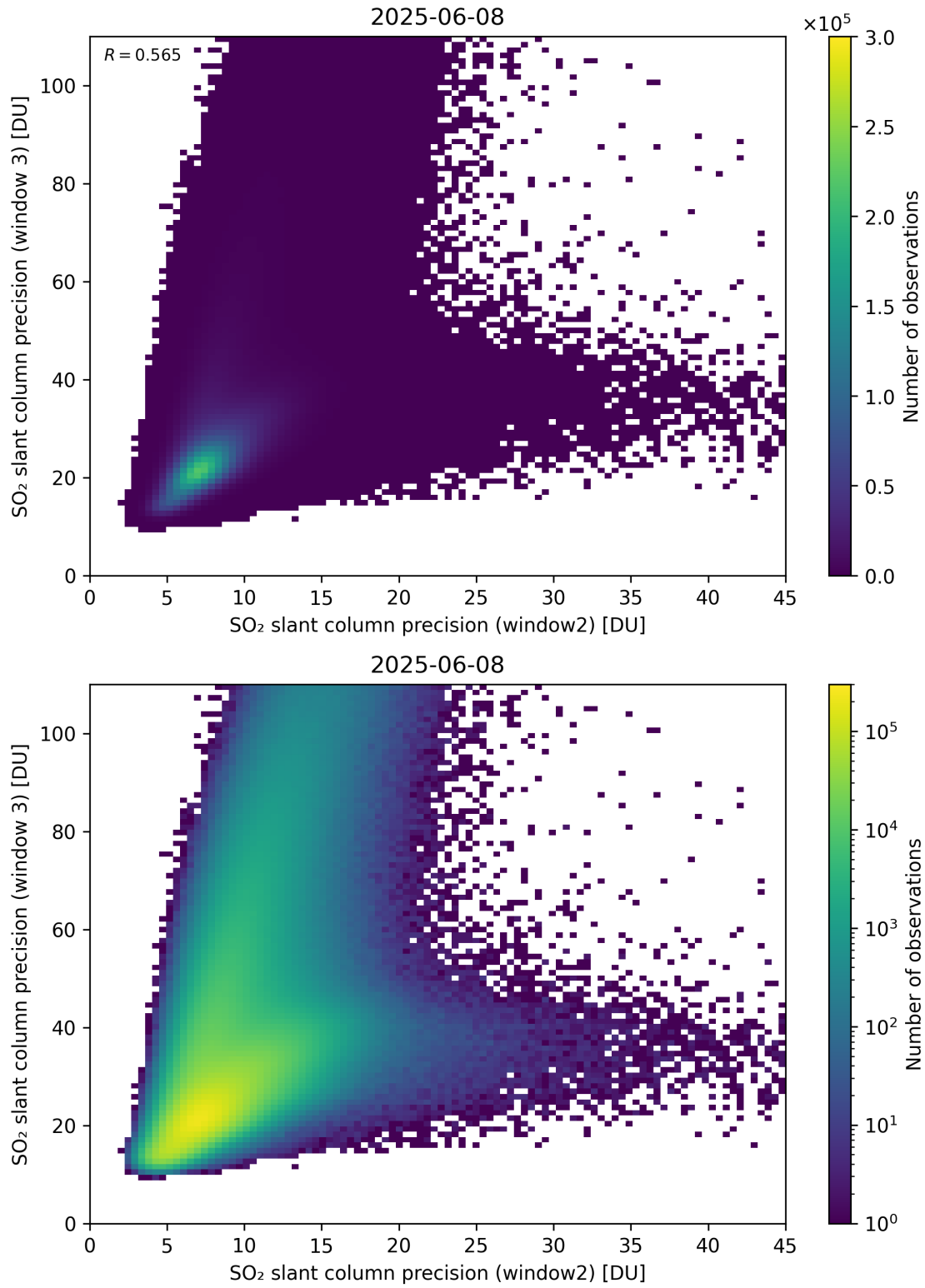
Figure 300: Scatter density plot of “SO 2 slant column precision (window2)” against “SO 2 slant column precision (window 3)” for 2025-06-07 to 2025-06-09.
