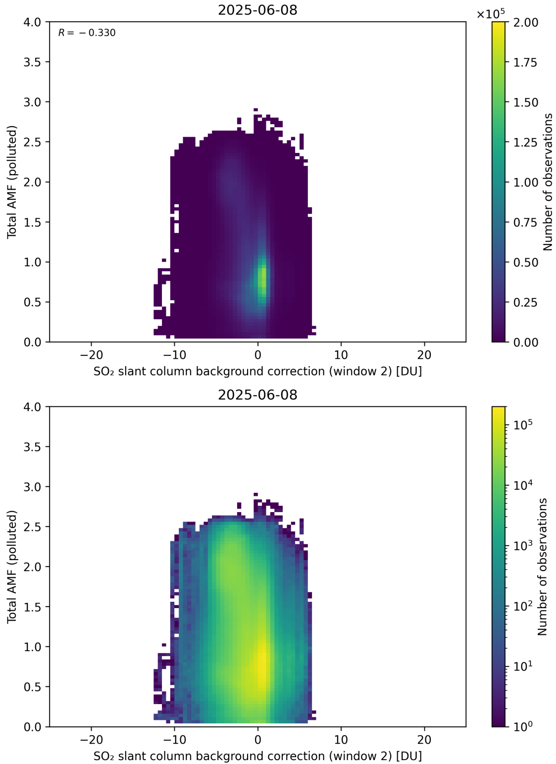
Figure 130: Scatter density plot of “SO 2 slant column background correction (window 2)” against “Total AMF (polluted)” for 2025-06-07 to 2025-06-09.
