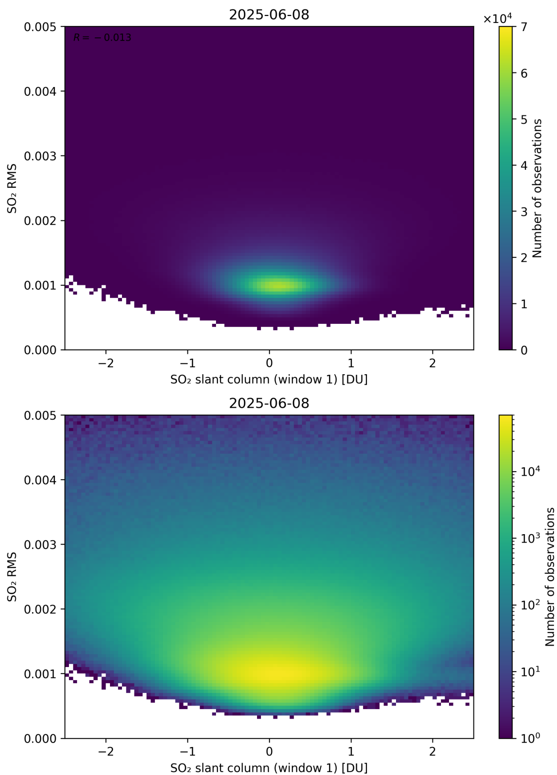
Figure 267: Scatter density plot of “SO 2 slant column (window 1)” against “SO 2 RMS” for 2025-06-07 to 2025-06-09.
