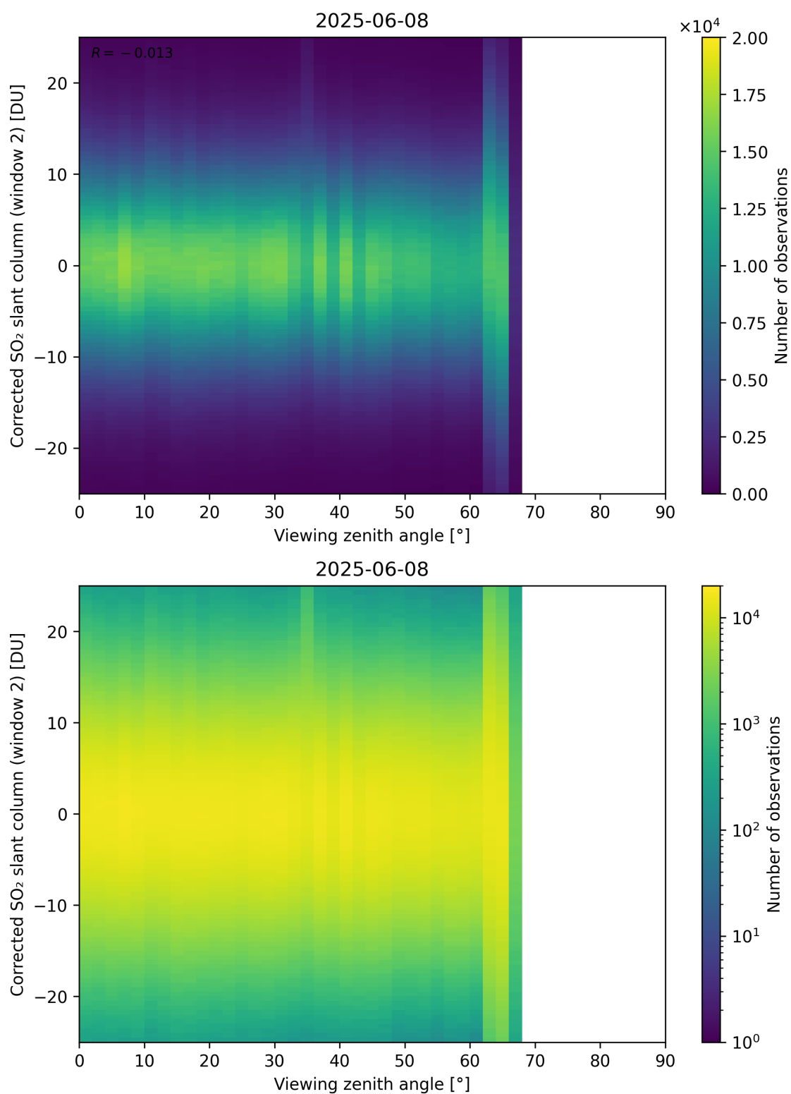
Figure 374: Scatter density plot of “Viewing zenith angle” against “Corrected SO 2 slant column (window 2)” for 2025-06-07 to 2025-06-09.
