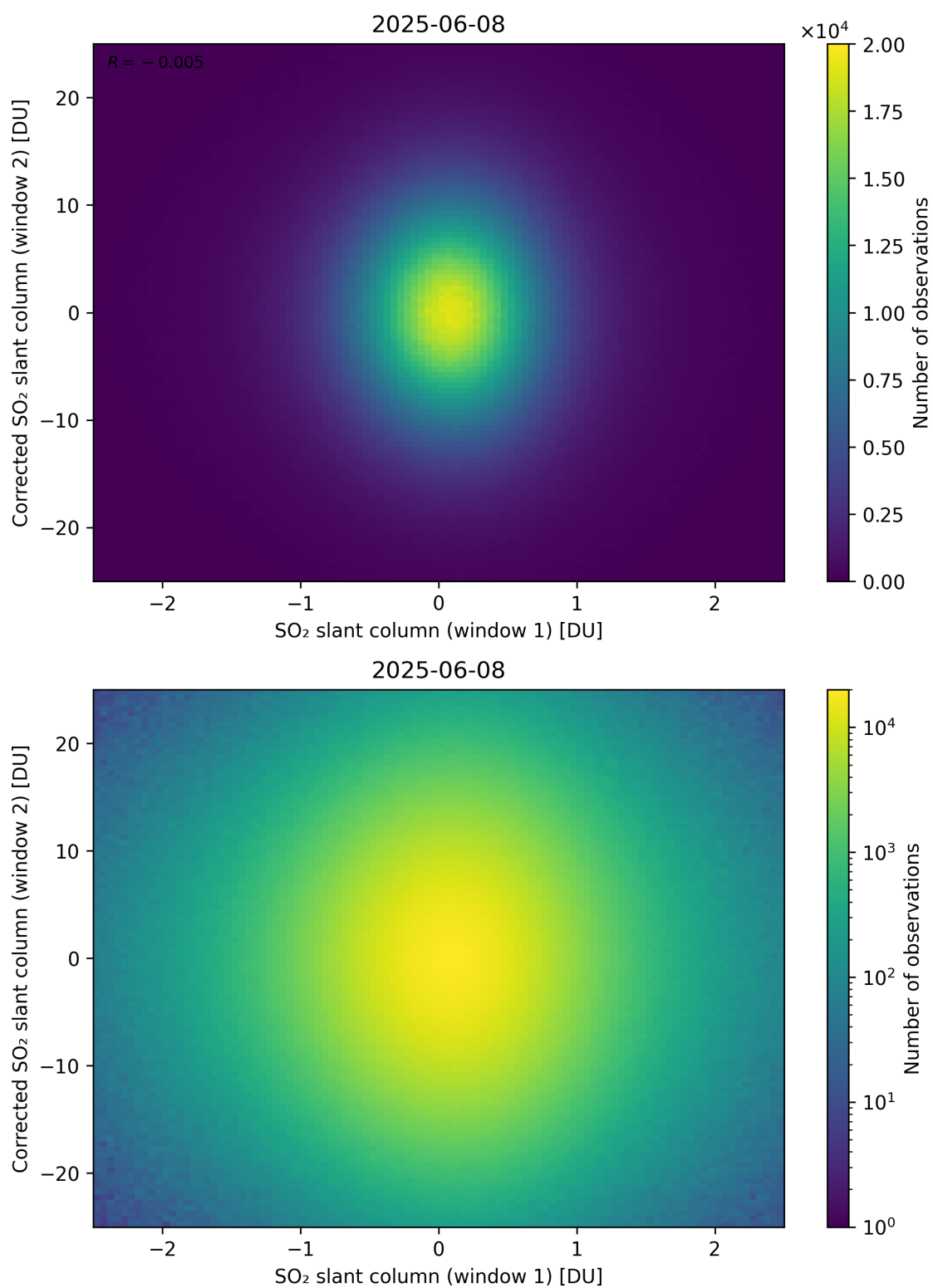
Figure 283: Scatter density plot of “SO 2 slant column (window 1)” against “Corrected SO 2 slant column (window 2)” for 2025-06-07 to 2025-06-09.
