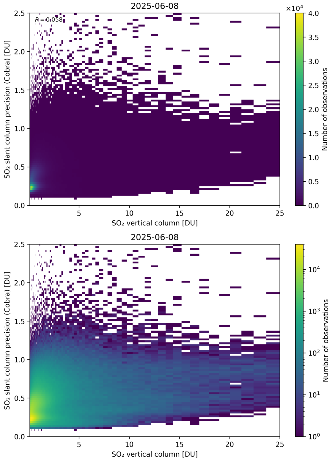
Figure 350: Scatter density plot of “SO 2 vertical column” against “SO 2 slant column precision (Cobra)” for 2025-06-07 to 2025-06-09.
