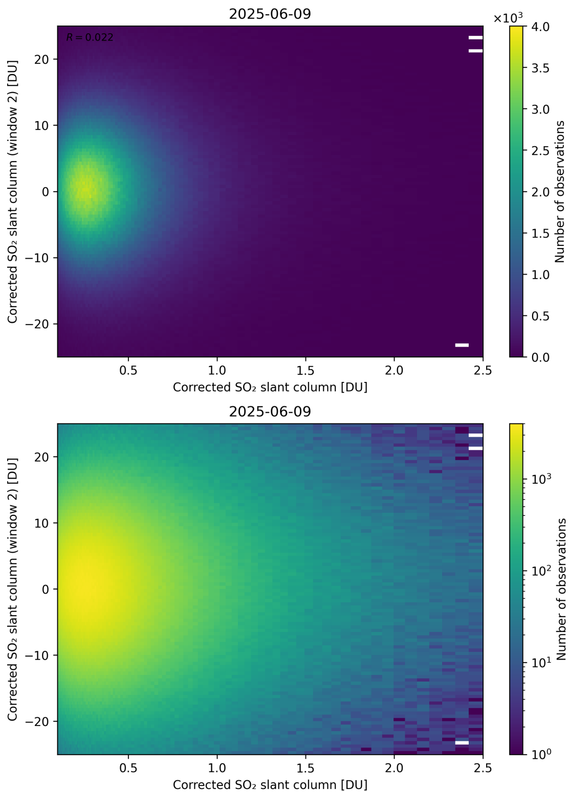
Figure 235: Scatter density plot of “Corrected SO 2 slant column” against “Corrected SO 2 slant column (window 2)” for 2025-06-08 to 2025-06-10.
