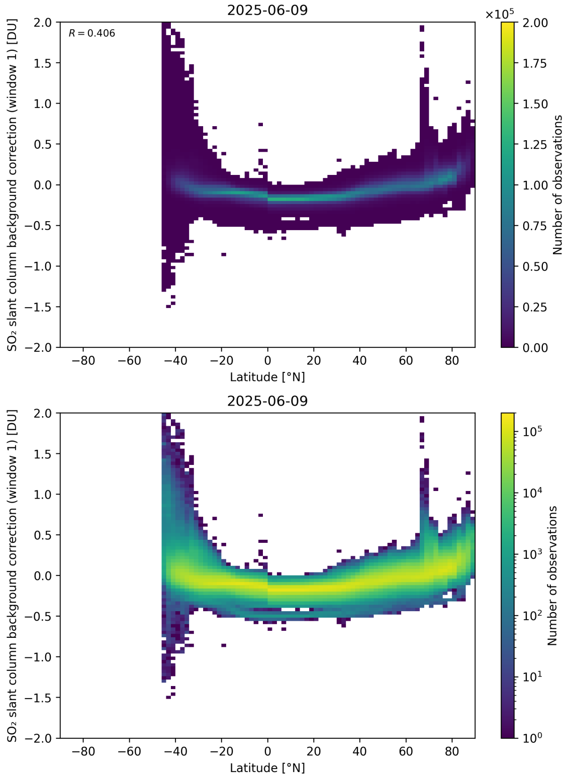
Figure 150: Scatter density plot of “Latitude” against “SO 2 slant column background correction (window 1)” for 2025-06-08 to 2025-06-10.
