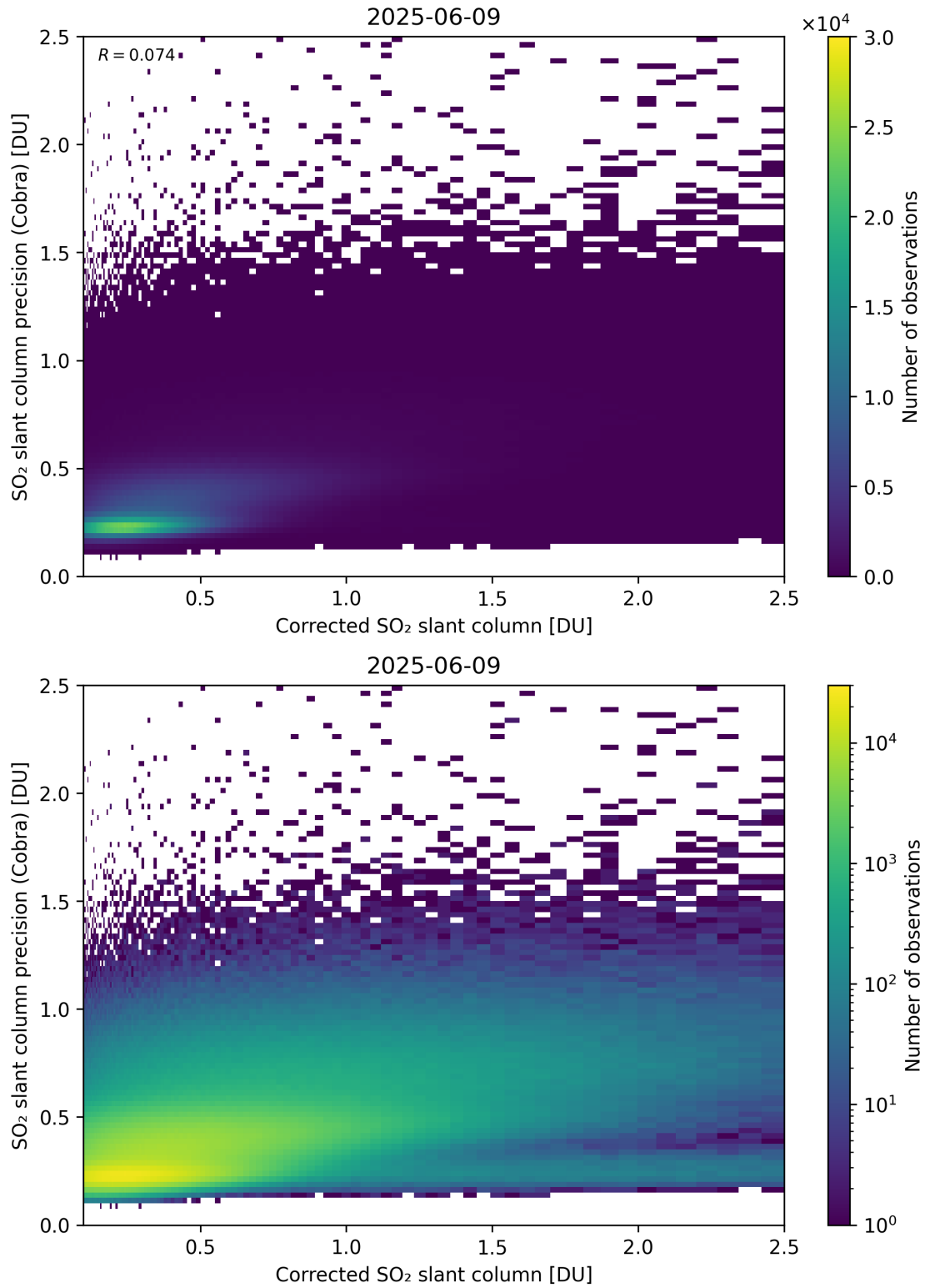
Figure 234: Scatter density plot of “Corrected SO 2 slant column” against “SO 2 slant column precision (Cobra)” for 2025-06-08 to 2025-06-10.
