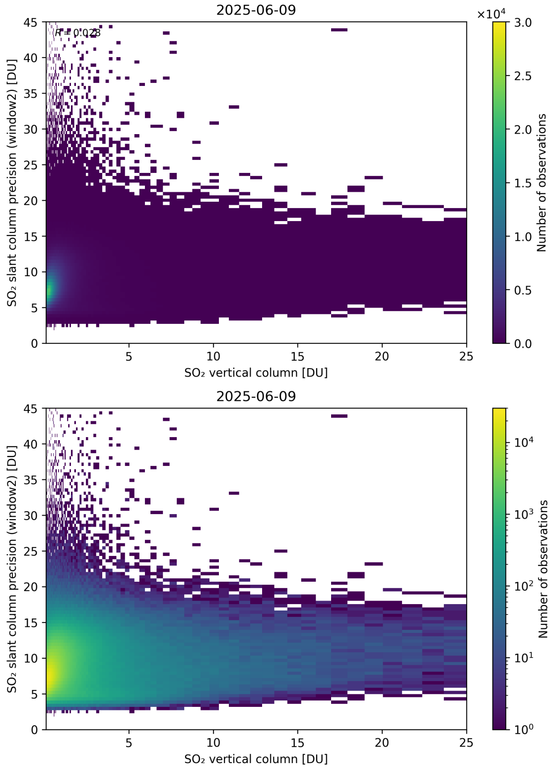
Figure 356: Scatter density plot of “SO 2 vertical column” against “SO 2 slant column precision (window2)” for 2025-06-08 to 2025-06-10.
