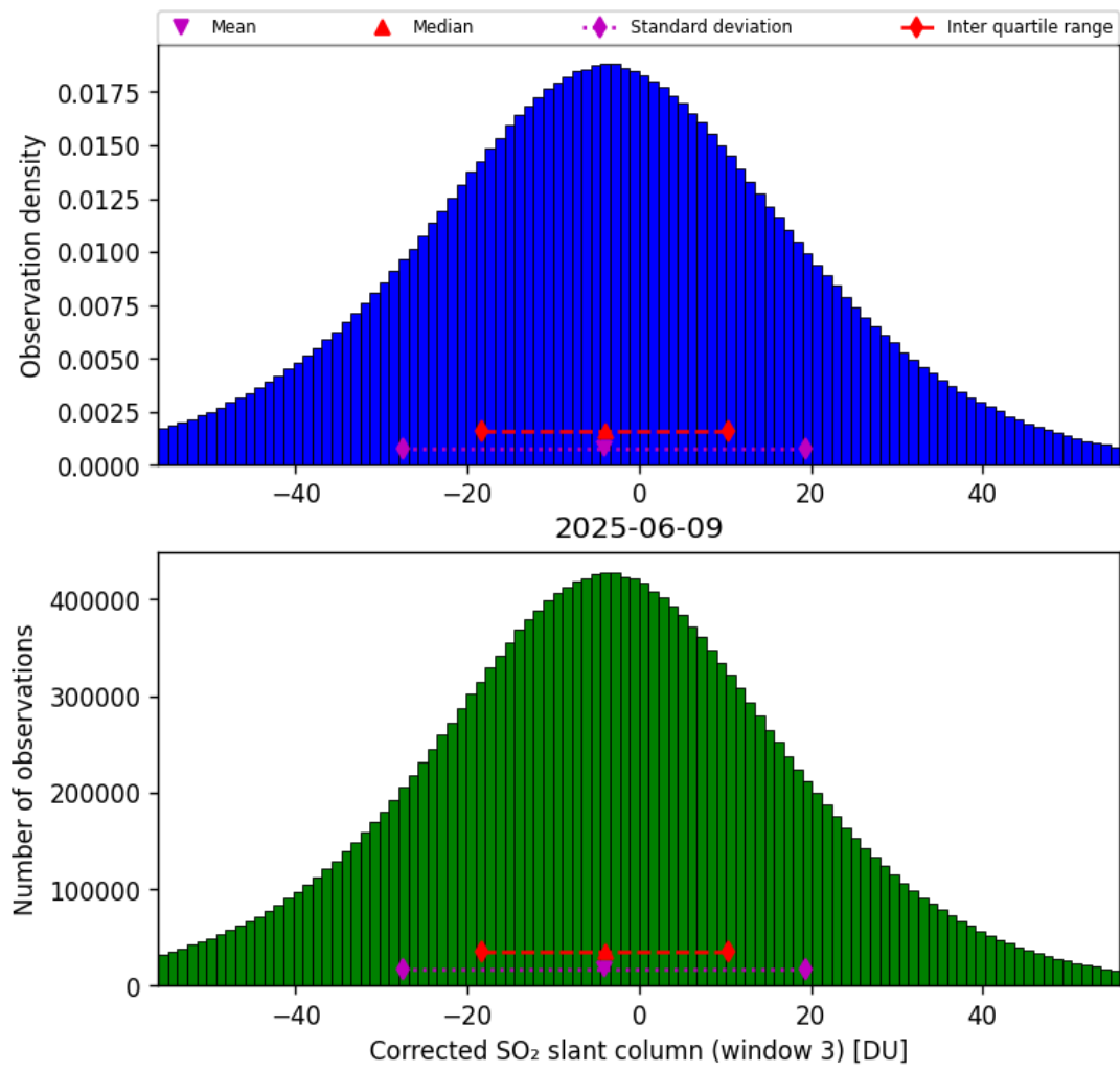
Figure 73: Histogram of “Corrected SO 2 slant column (window 3)” for 2025-06-08 to 2025-06-10
