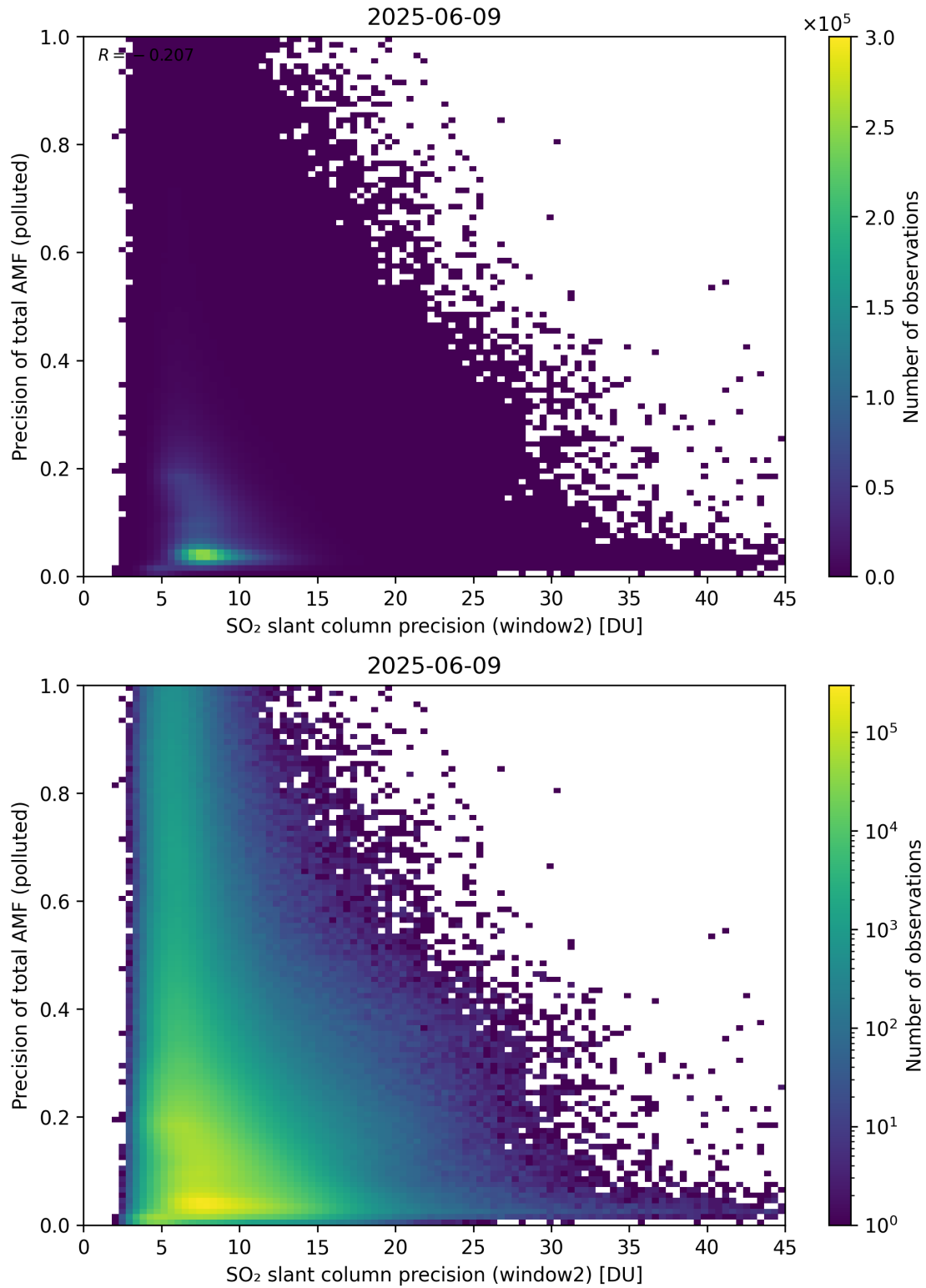
Figure 302: Scatter density plot of “SO 2 slant column precision (window2)” against “Precision of total AMF (polluted)” for 2025-06-08 to 2025-06-10.
