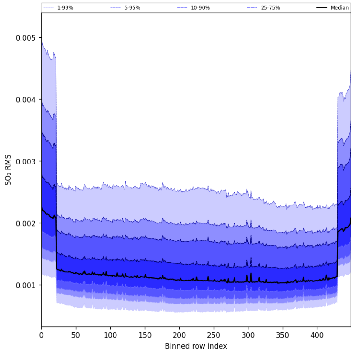
Figure 104: Along track statistics of “SO 2 RMS” for 2025-06-08 to 2025-06-10
