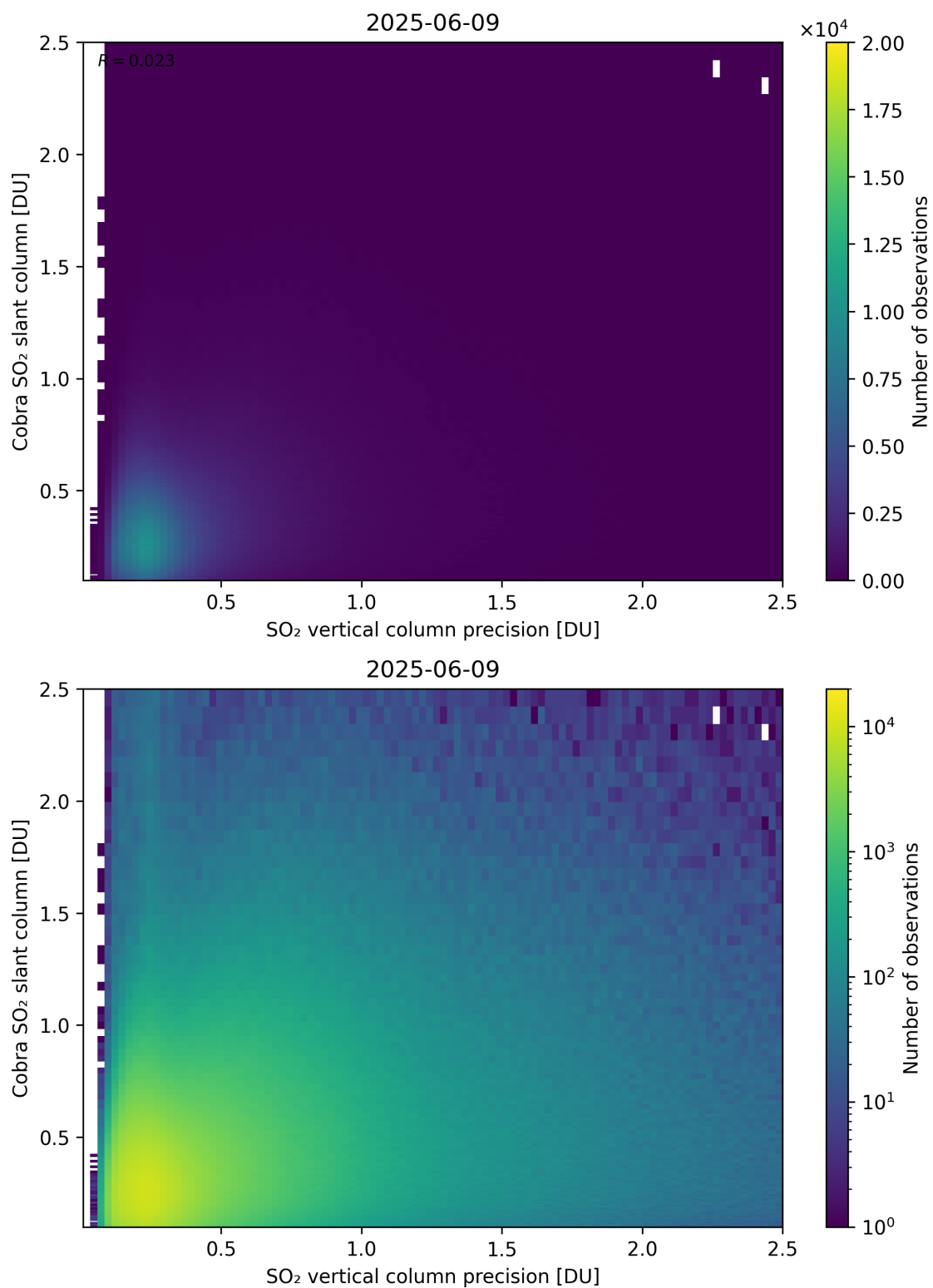
Figure 336: Scatter density plot of “SO 2 vertical column precision” against “Cobra SO 2 slant column” for 2025-06-08 to 2025-06-10.
