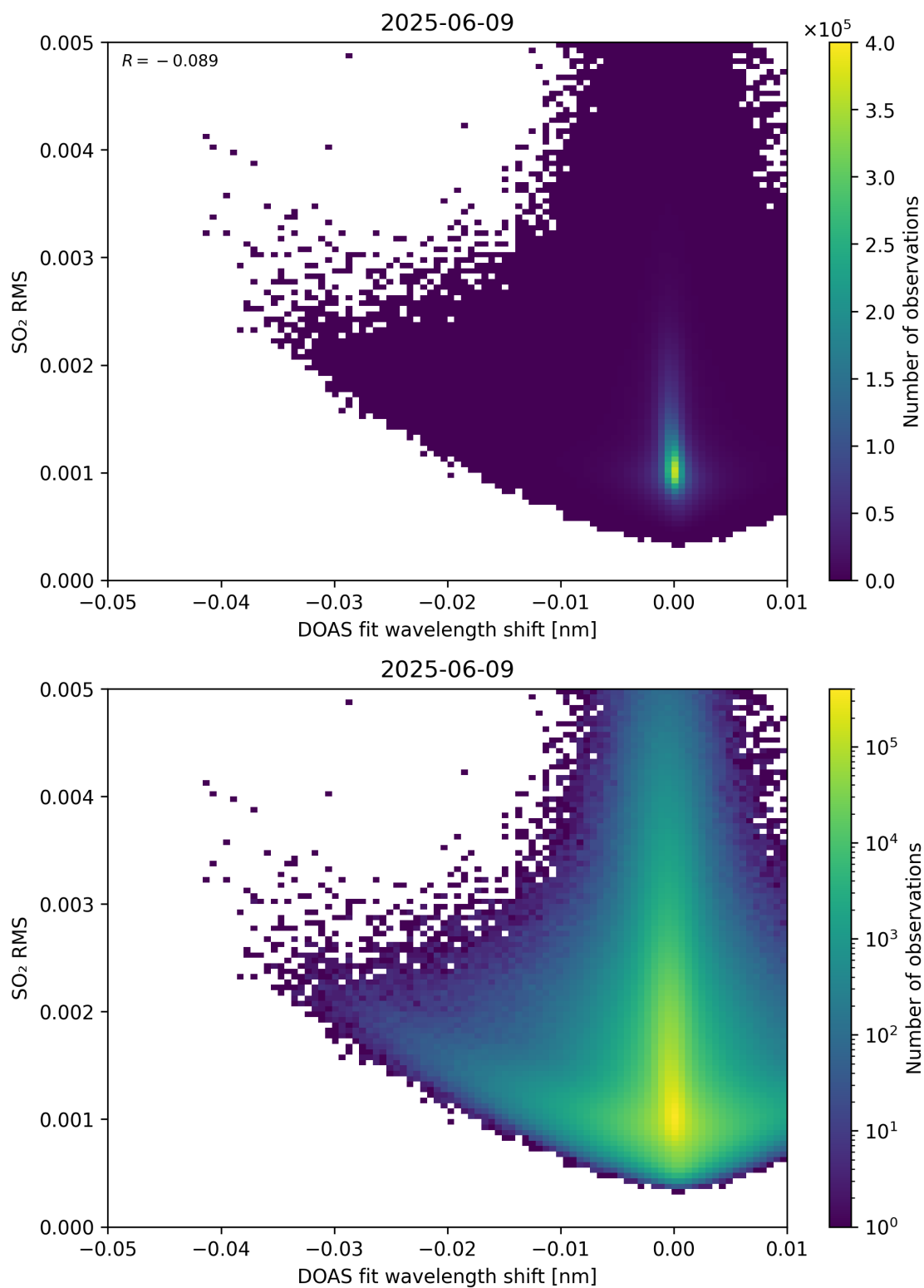
Figure 139: Scatter density plot of “DOAS fit wavelength shift” against “SO 2 RMS” for 2025-06-08 to 2025-06-10.
