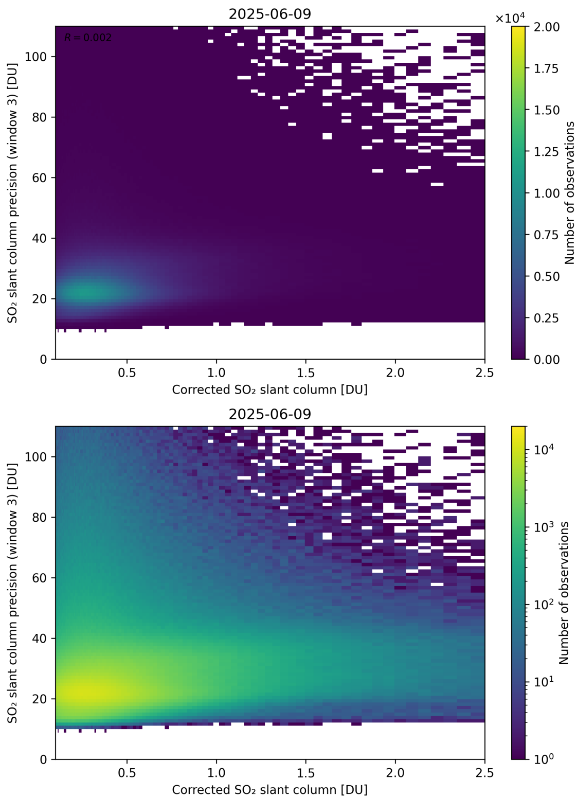
Figure 241: Scatter density plot of “Corrected SO 2 slant column” against “SO 2 slant column precision (window 3)” for 2025-06-08 to 2025-06-10.
