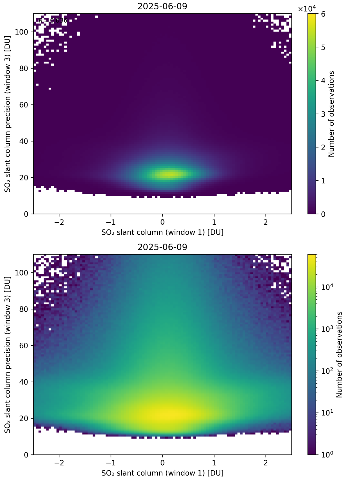
Figure 288: Scatter density plot of “SO 2 slant column (window 1)” against “SO 2 slant column precision (window 3)” for 2025-06-08 to 2025-06-10.
