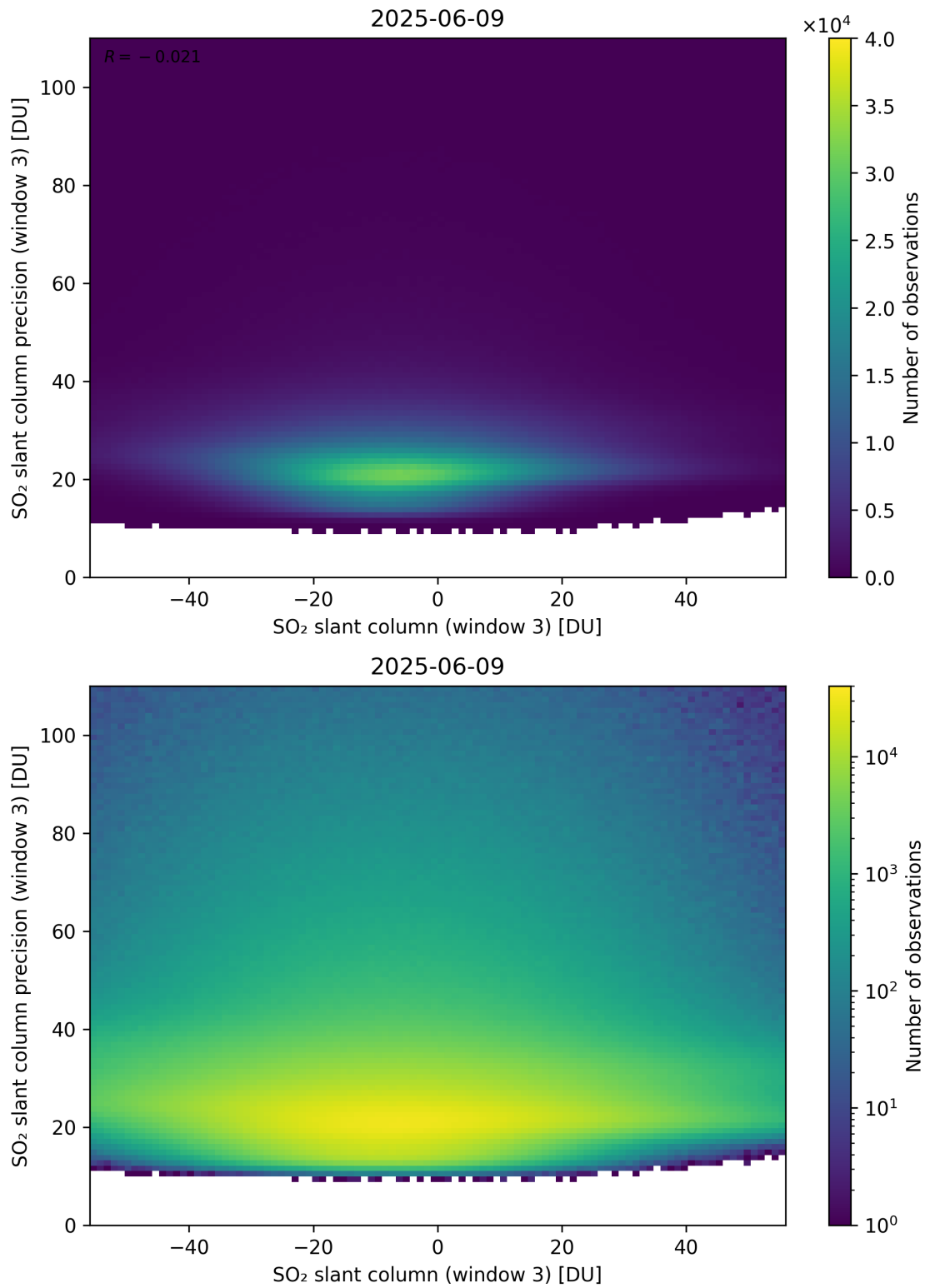
Figure 317: Scatter density plot of “SO 2 slant column (window 3)” against “SO 2 slant column precision (window 3)” for 2025-06-08 to 2025-06-10.
