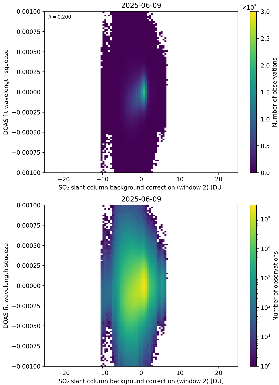
Figure 124: Scatter density plot of “SO 2 slant column background correction (window 2)” against “DOAS fit wavelength squeeze” for 2025-06-08 to 2025-06-10.
