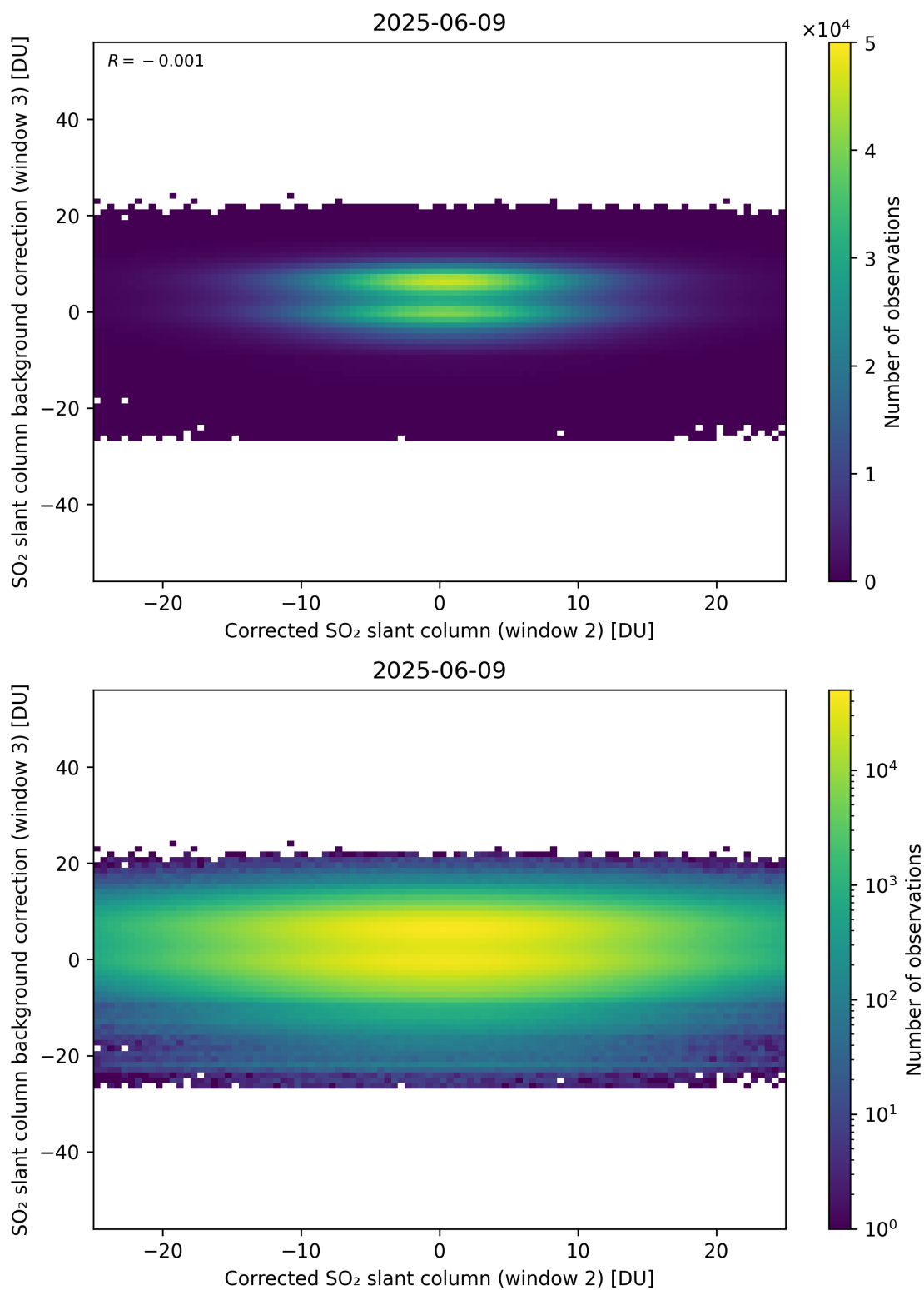
Figure 245: Scatter density plot of “Corrected SO 2 slant column (window 2)” against “SO 2 slant column background correction (window 3)” for 2025-06-08 to 2025-06-10.
