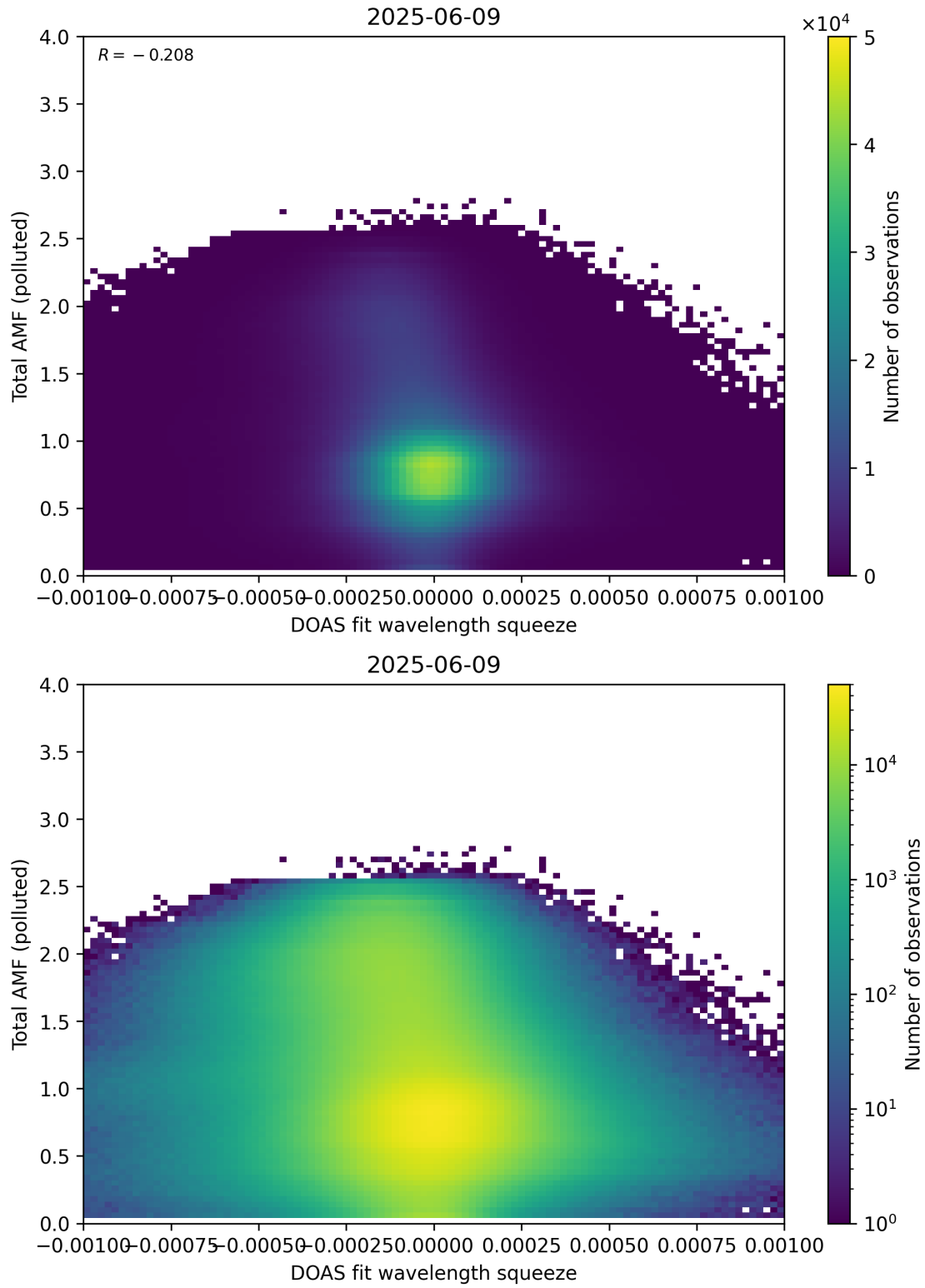
Figure 145: Scatter density plot of “DOAS fit wavelength squeeze” against “Total AMF (polluted)” for 2025-06-08 to 2025-06-10.
