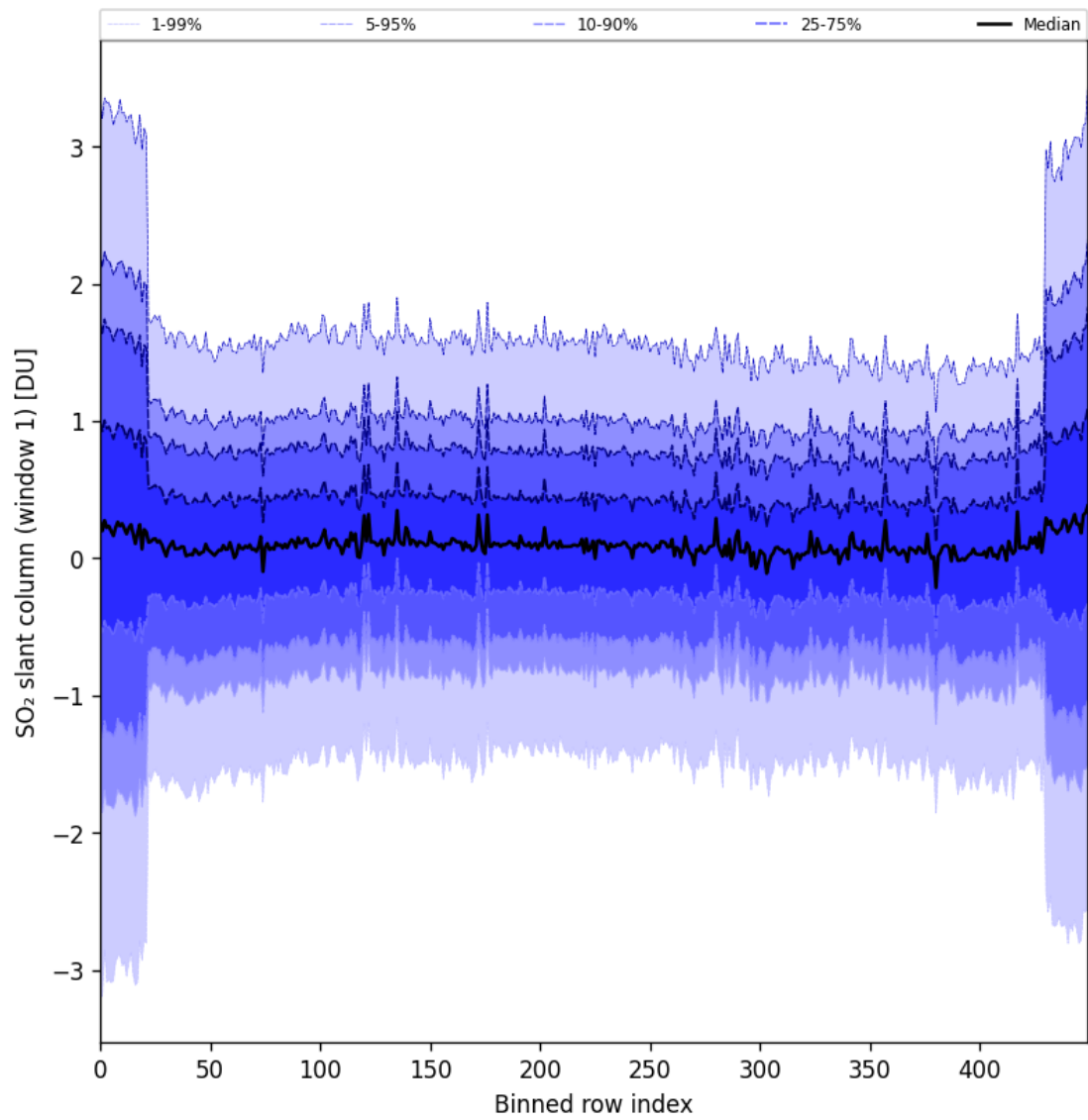
Figure 89: Along track statistics of “SO 2 slant column (window 1)” for 2025-06-08 to 2025-06-10
