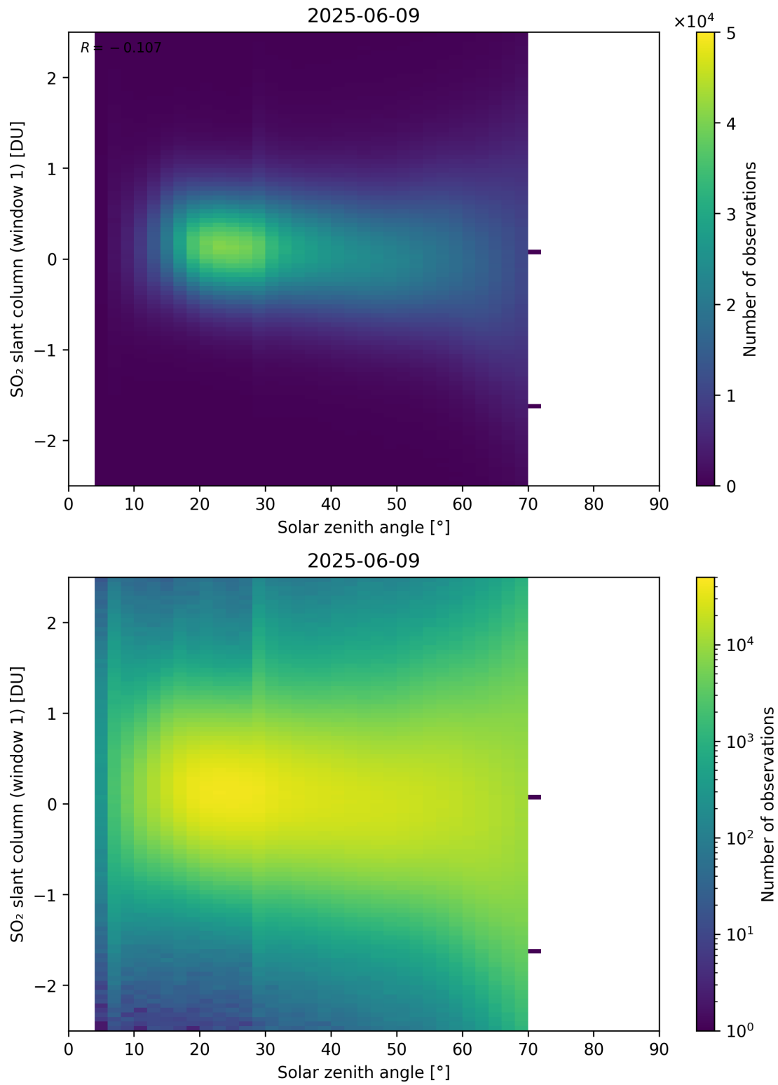
Figure 184: Scatter density plot of “Solar zenith angle” against “SO 2 slant column (window 1)” for 2025-06-08 to 2025-06-10.
