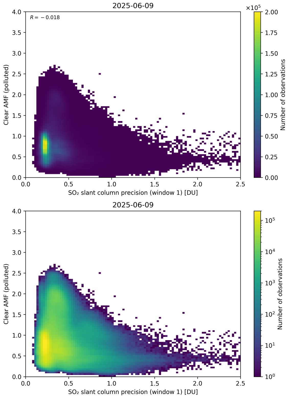
Figure 274: Scatter density plot of “SO 2 slant column precision (window 1)” against “Clear AMF (polluted)” for 2025-06-08 to 2025-06-10.
