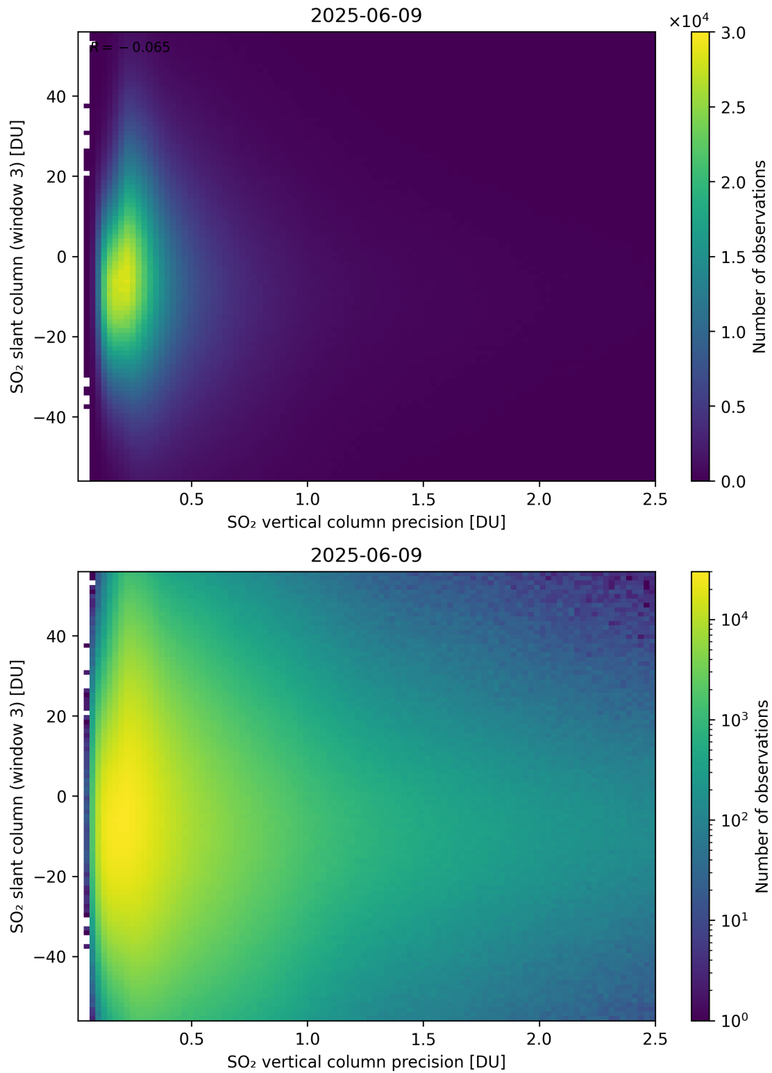
Figure 344: Scatter density plot of “SO 2 vertical column precision” against “SO 2 slant column (window 3)” for 2025-06-08 to 2025-06-10.
