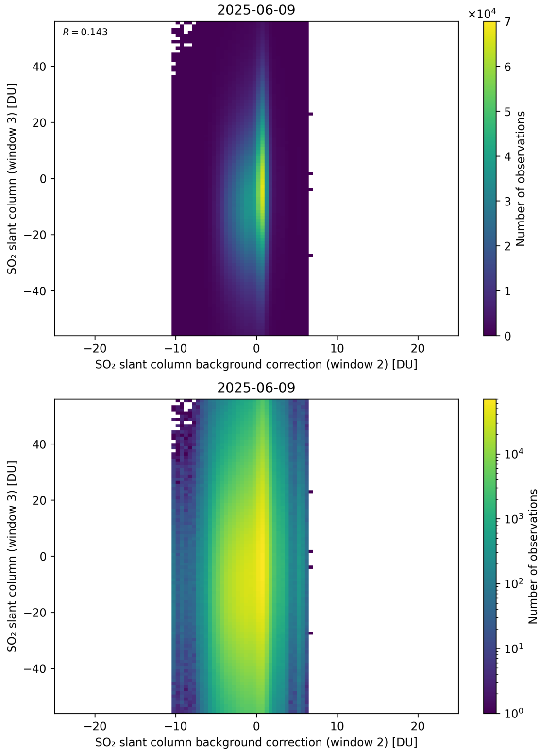
Figure 128: Scatter density plot of “SO 2 slant column background correction (window 2)” against “SO 2 slant column (window 3)” for 2025-06-08 to 2025-06-10.
