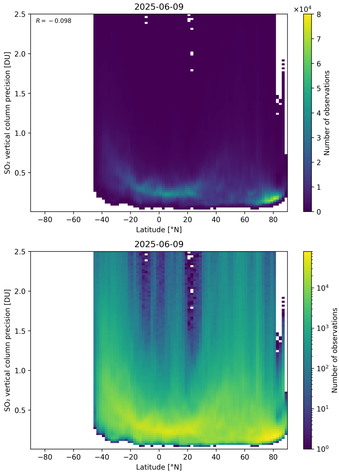
Figure 170: Scatter density plot of “Latitude” against “SO 2 vertical column precision” for 2025-06-08 to 2025-06-10.
