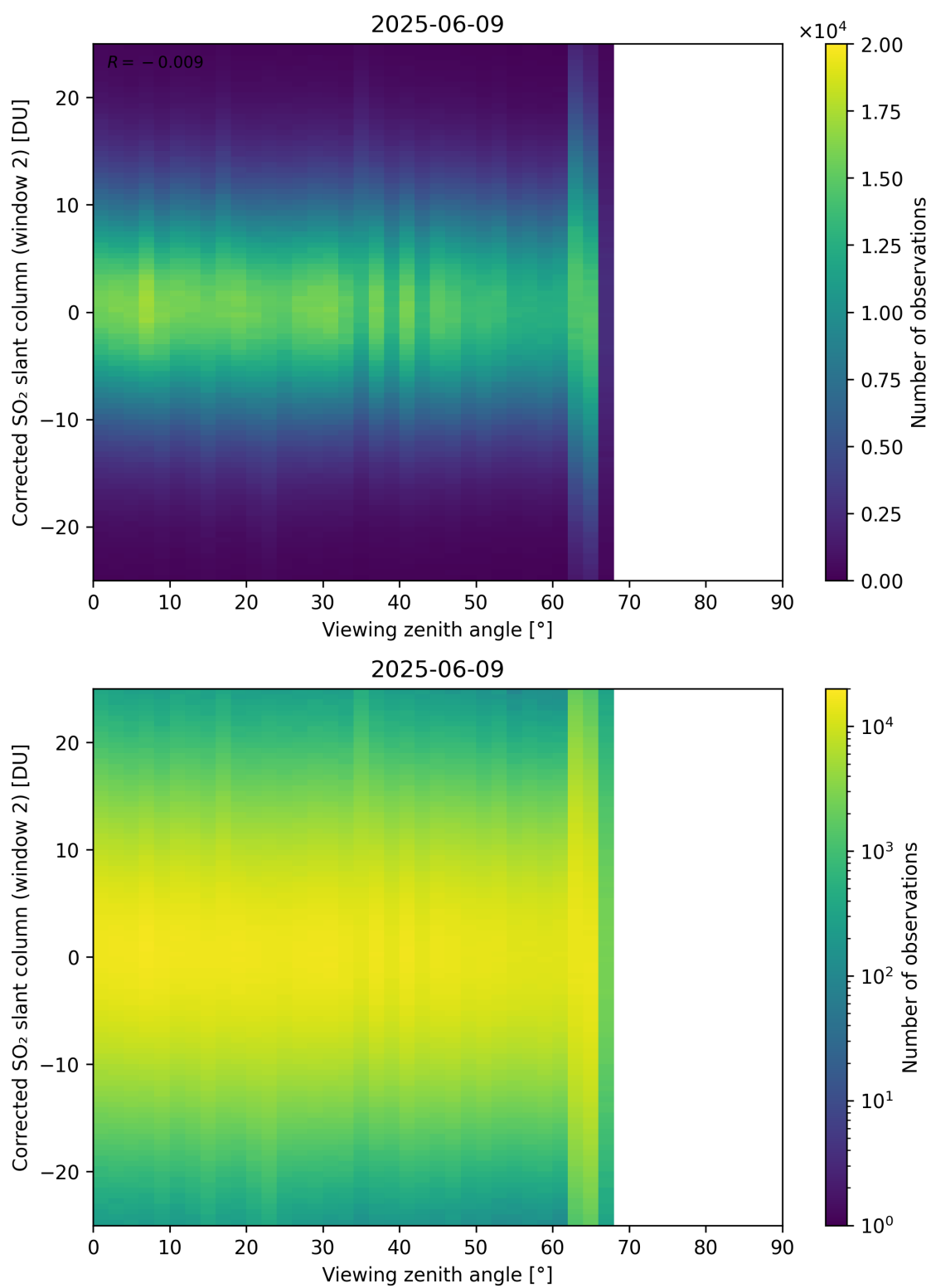
Figure 374: Scatter density plot of “Viewing zenith angle” against “Corrected SO 2 slant column (window 2)” for 2025-06-08 to 2025-06-10.
