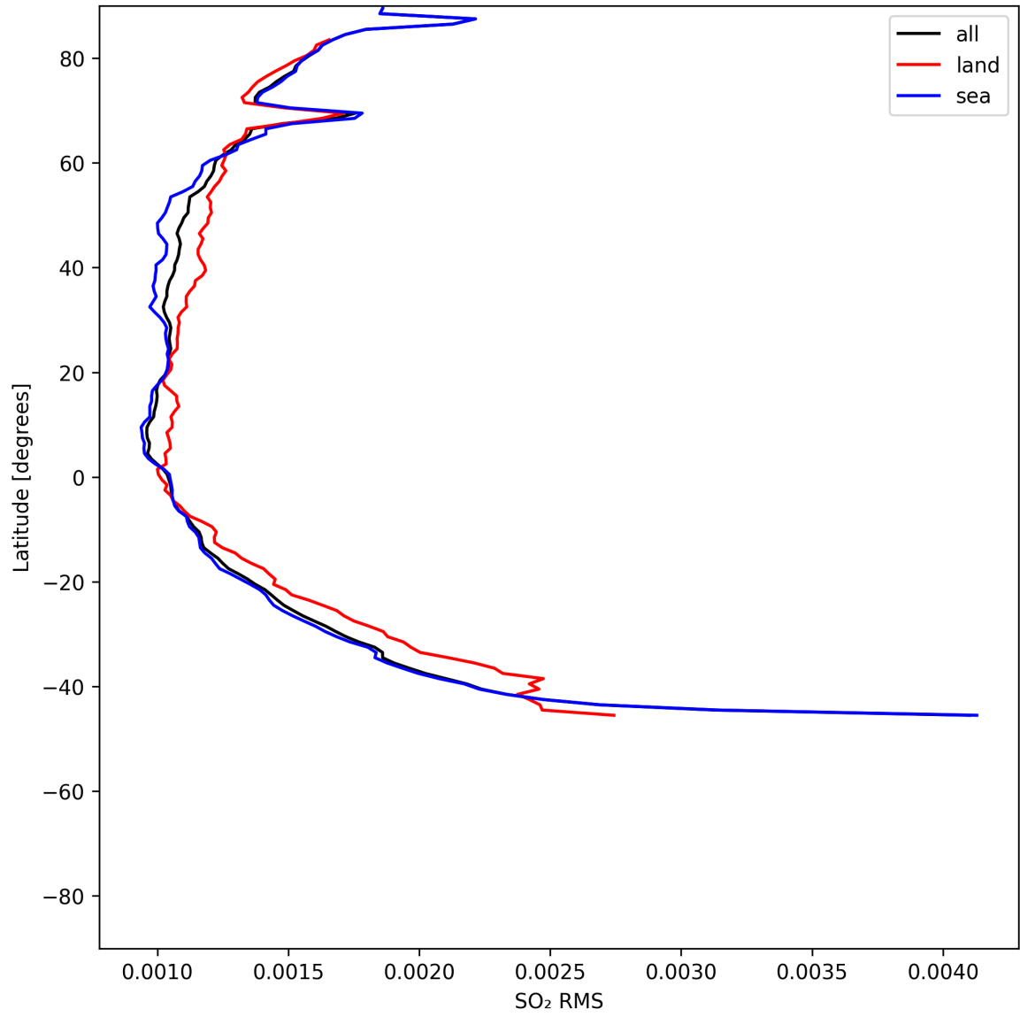
Figure 52: Zonal average of “SO 2 RMS” for 2025-06-08 to 2025-06-10.
