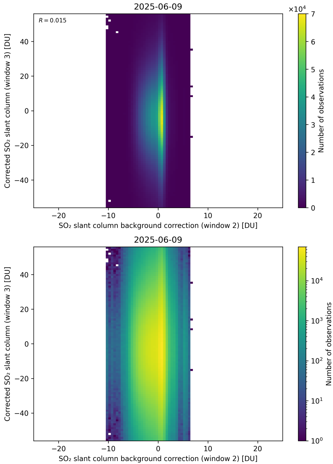
Figure 127: Scatter density plot of “SO 2 slant column background correction (window 2)” against “Corrected SO 2 slant column (window 3)” for 2025-06-08 to 2025-06-10.
