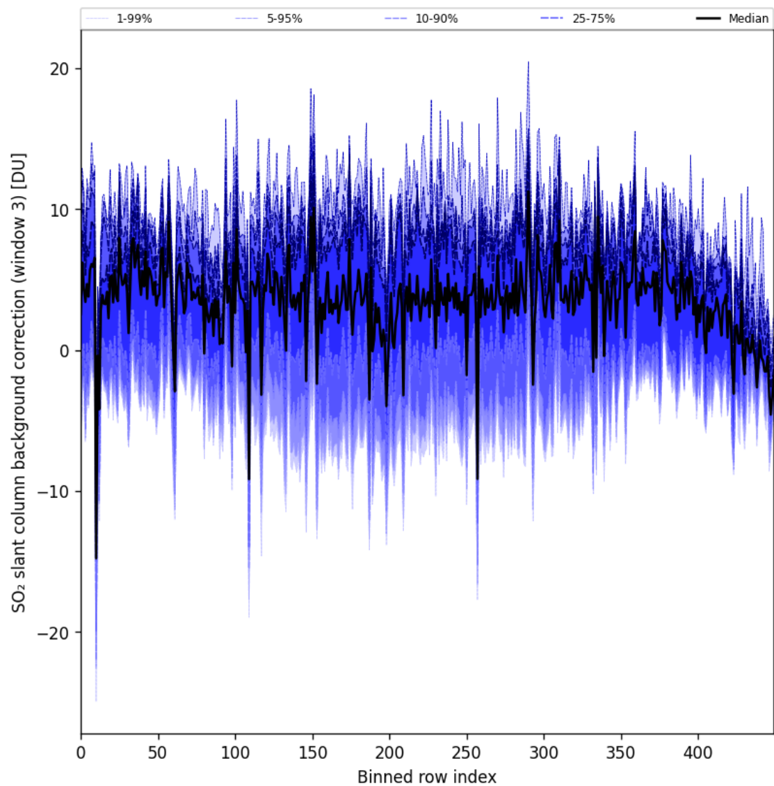
Figure 100: Along track statistics of “SO 2 slant column background correction (window 3)” for 2025-06-08 to 2025-06-10
