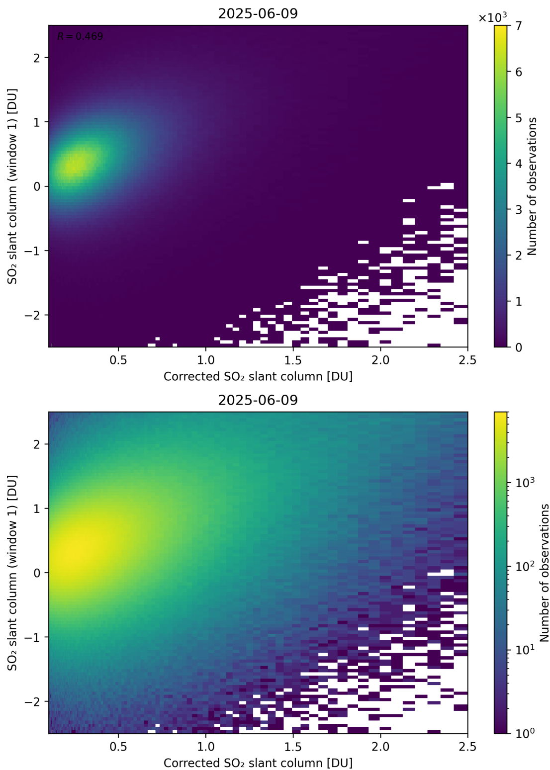
Figure 237: Scatter density plot of “Corrected SO 2 slant column” against “SO 2 slant column (window 1)” for 2025-06-08 to 2025-06-10.
