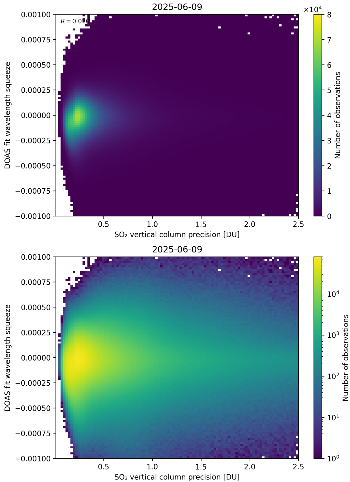
Figure 333: Scatter density plot of “SO 2 vertical column precision” against “DOAS fit wavelength squeeze” for 2025-06-08 to 2025-06-10.
