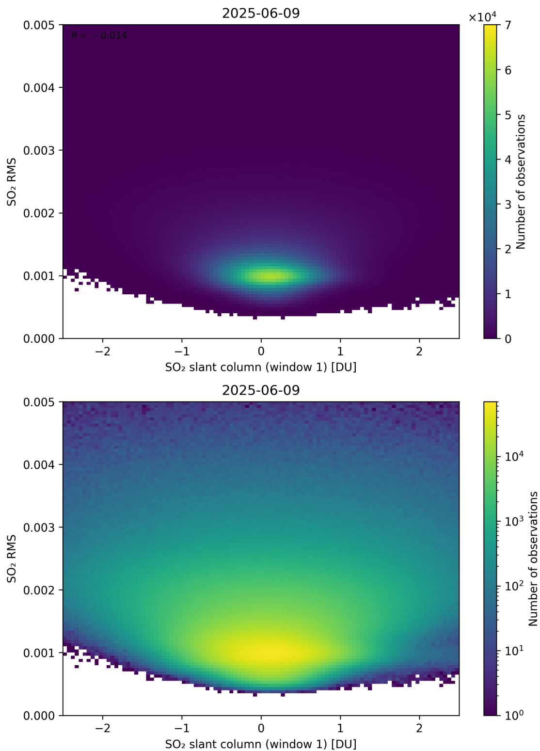
Figure 267: Scatter density plot of “SO 2 slant column (window 1)” against “SO 2 RMS” for 2025-06-08 to 2025-06-10.
