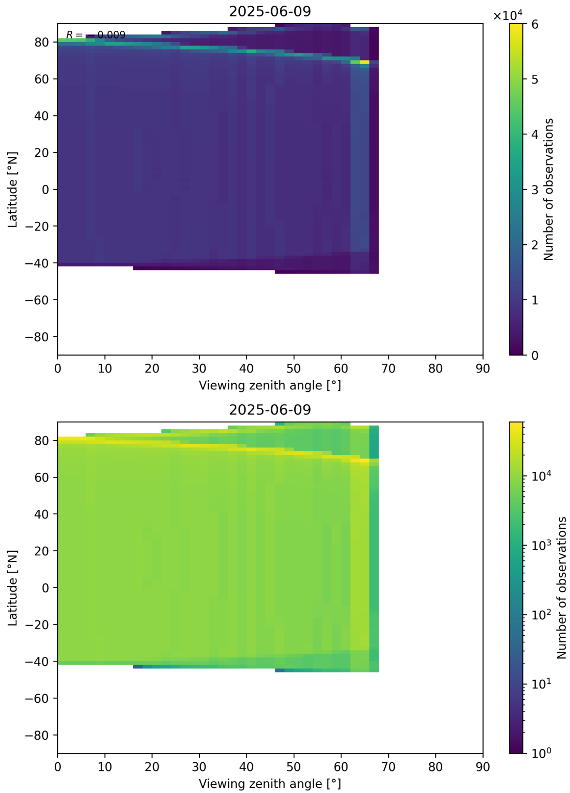
Figure 368: Scatter density plot of “Viewing zenith angle” against “Latitude” for 2025-06-08 to 2025-06-10.
