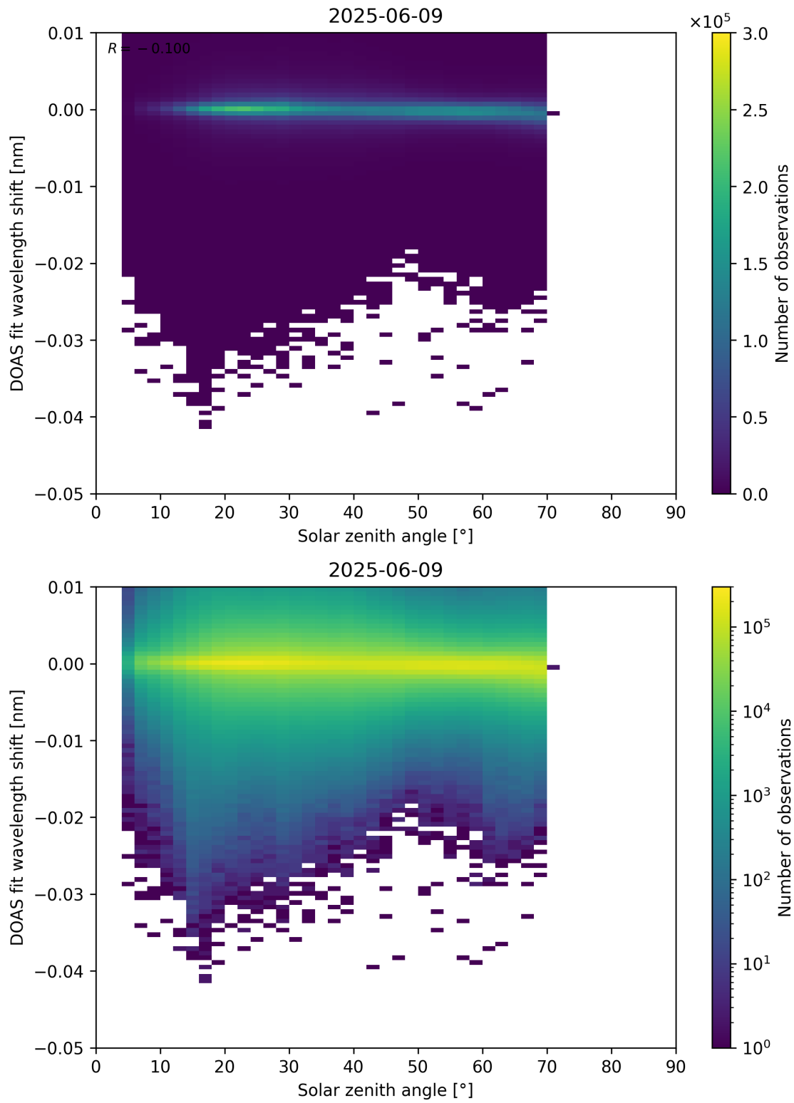
Figure 174: Scatter density plot of “Solar zenith angle” against “DOAS fit wavelength shift” for 2025-06-08 to 2025-06-10.
