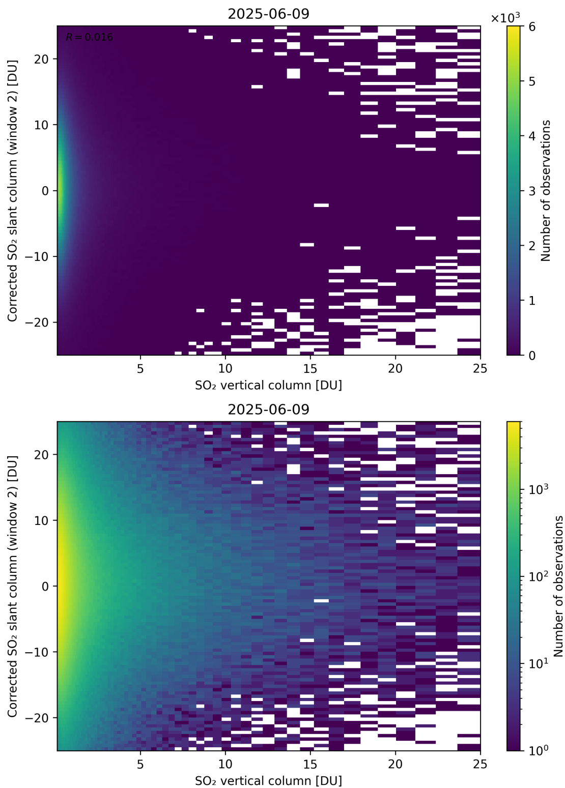
Figure 352: Scatter density plot of “SO 2 vertical column” against “Corrected SO 2 slant column (window 2)” for 2025-06-08 to 2025-06-10.
