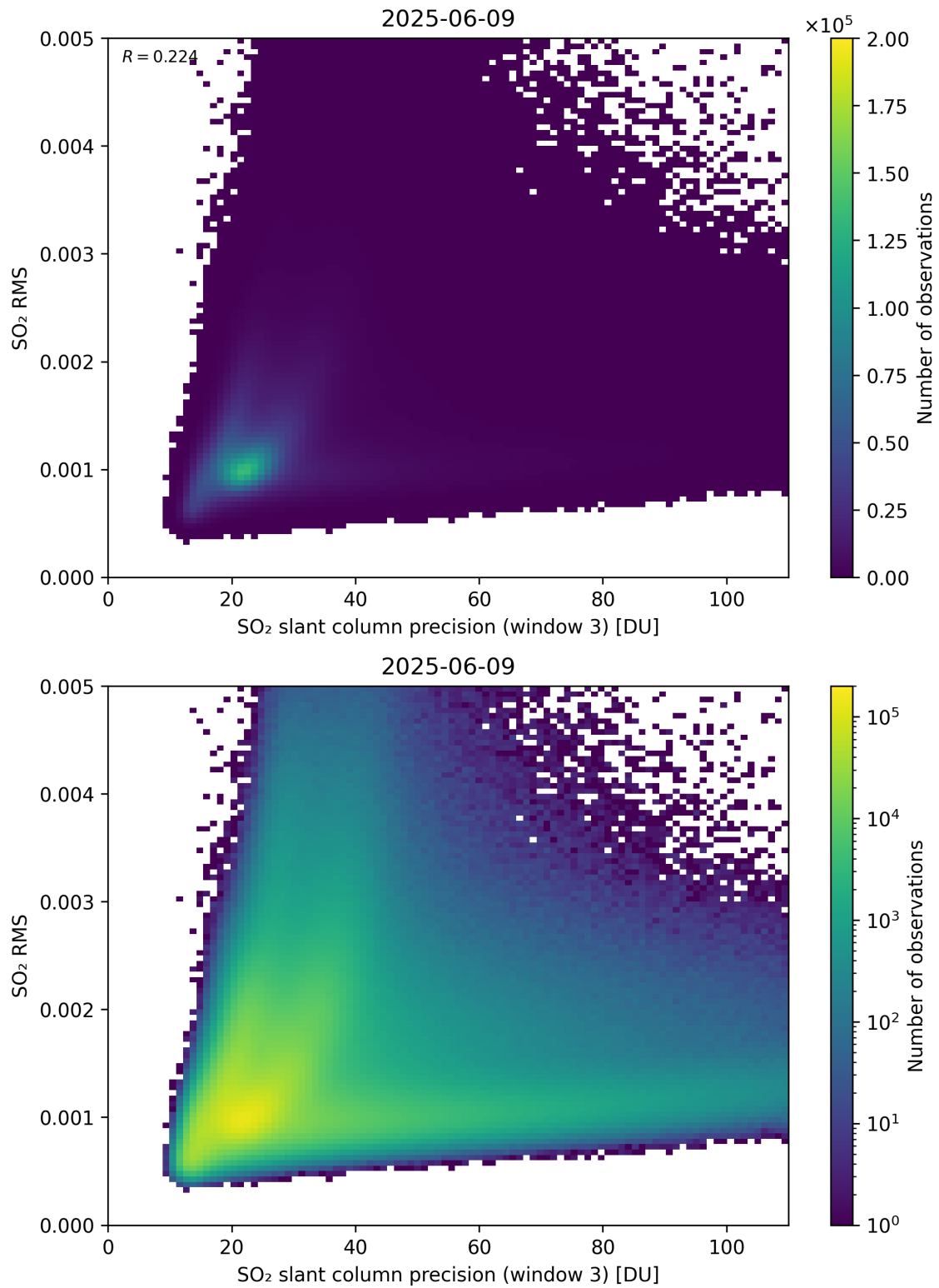
Figure 310: Scatter density plot of “SO 2 slant column precision (window 3)” against “SO 2 RMS” for 2025-06-08 to 2025-06-10.
