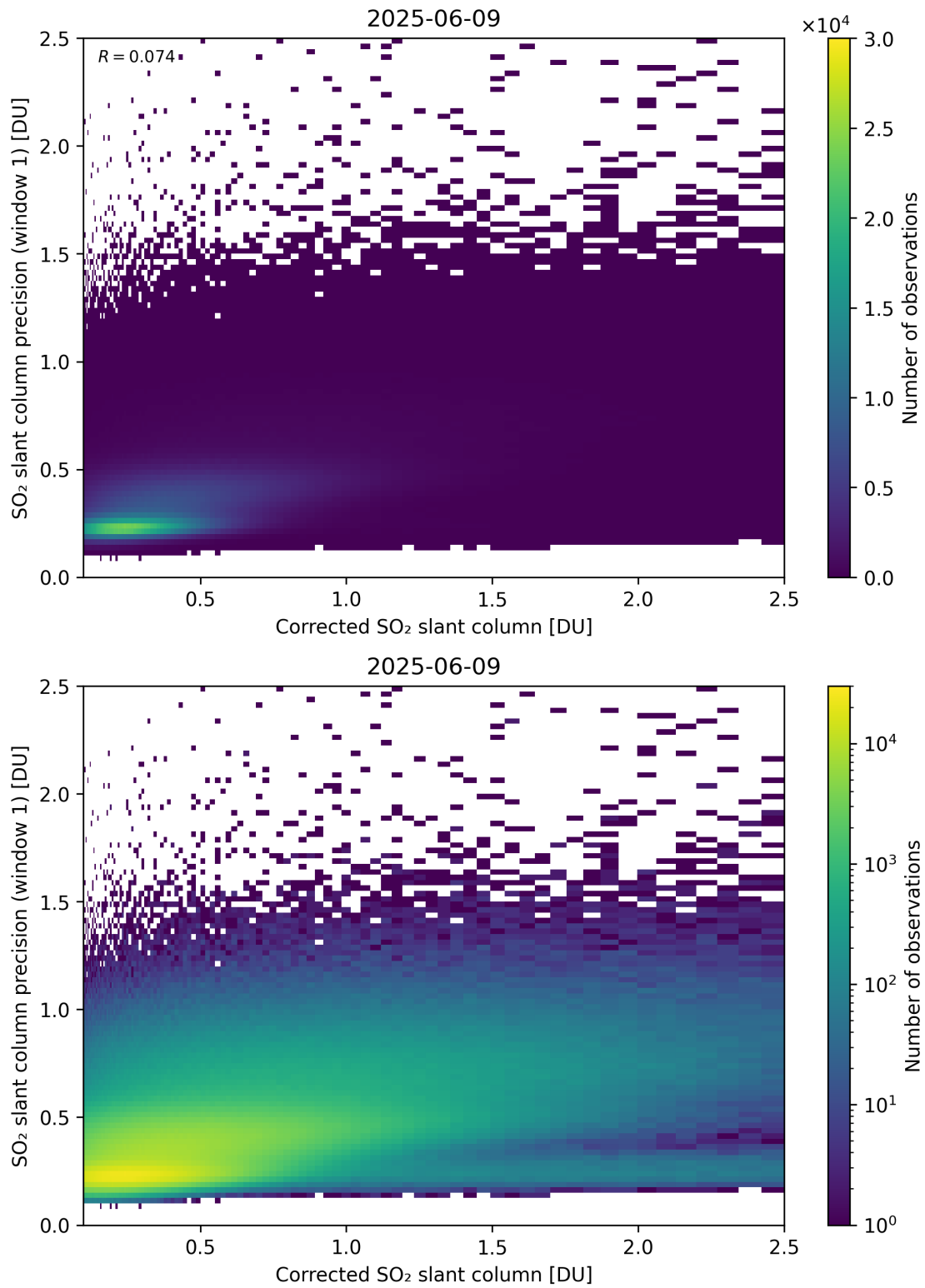
Figure 238: Scatter density plot of “Corrected SO 2 slant column” against “SO 2 slant column precision (window 1)” for 2025-06-08 to 2025-06-10.
