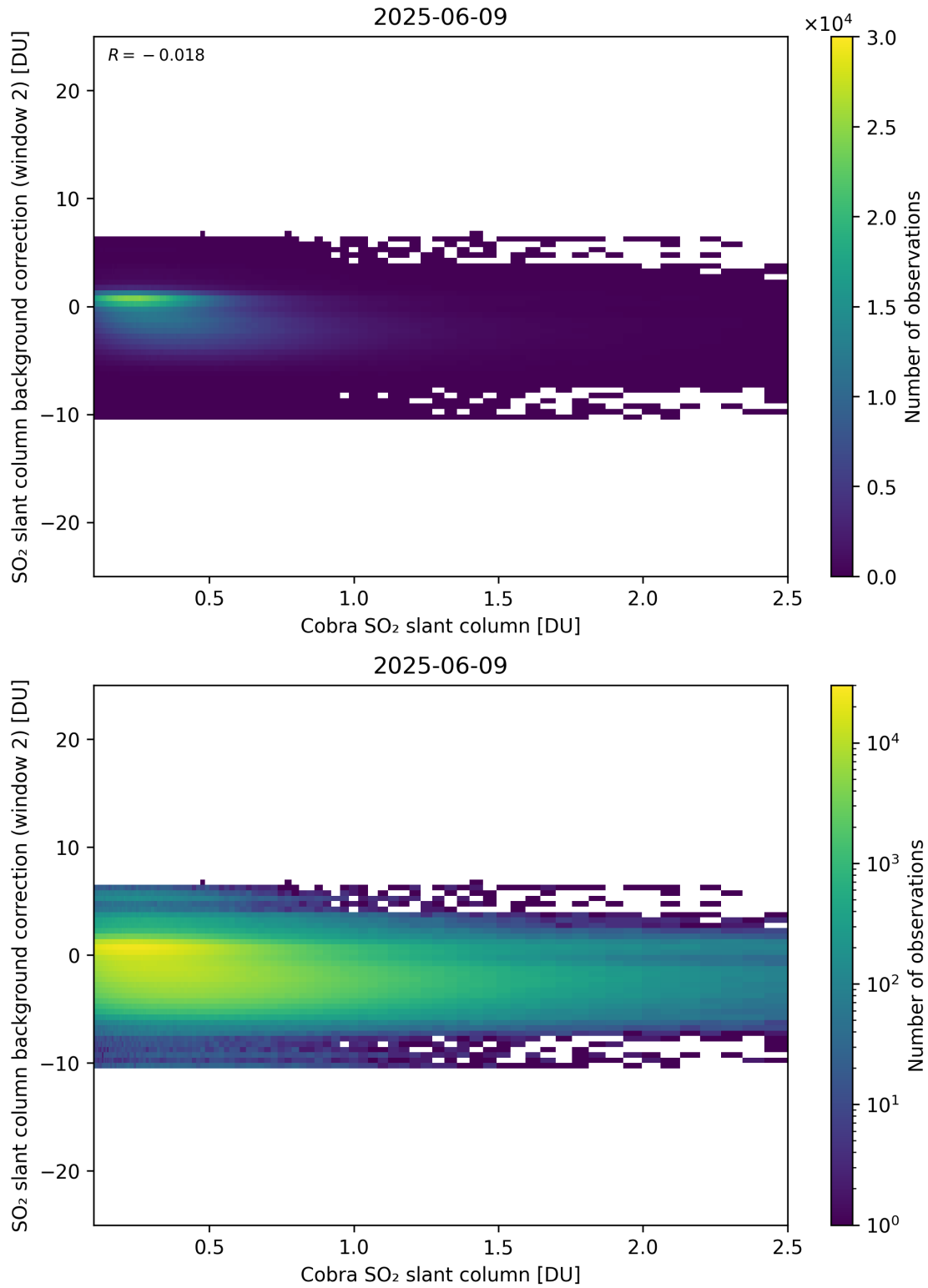
Figure 194: Scatter density plot of “Cobra SO 2 slant column” against “SO 2 slant column background correction (window 2)” for 2025-06-08 to 2025-06-10.
