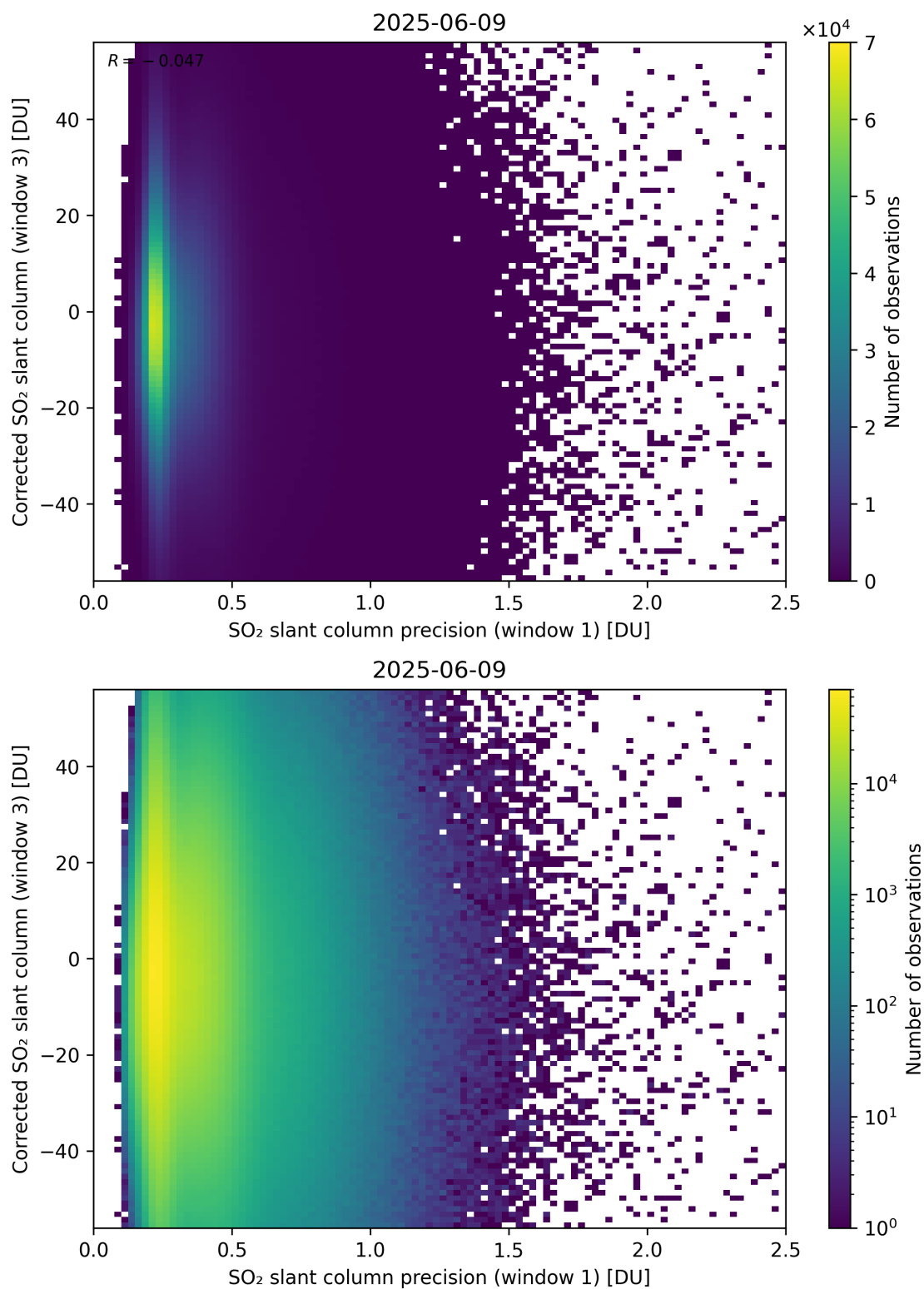
Figure 276: Scatter density plot of “SO 2 slant column precision (window 1)” against “Corrected SO 2 slant column (window 3)” for 2025-06-08 to 2025-06-10.
