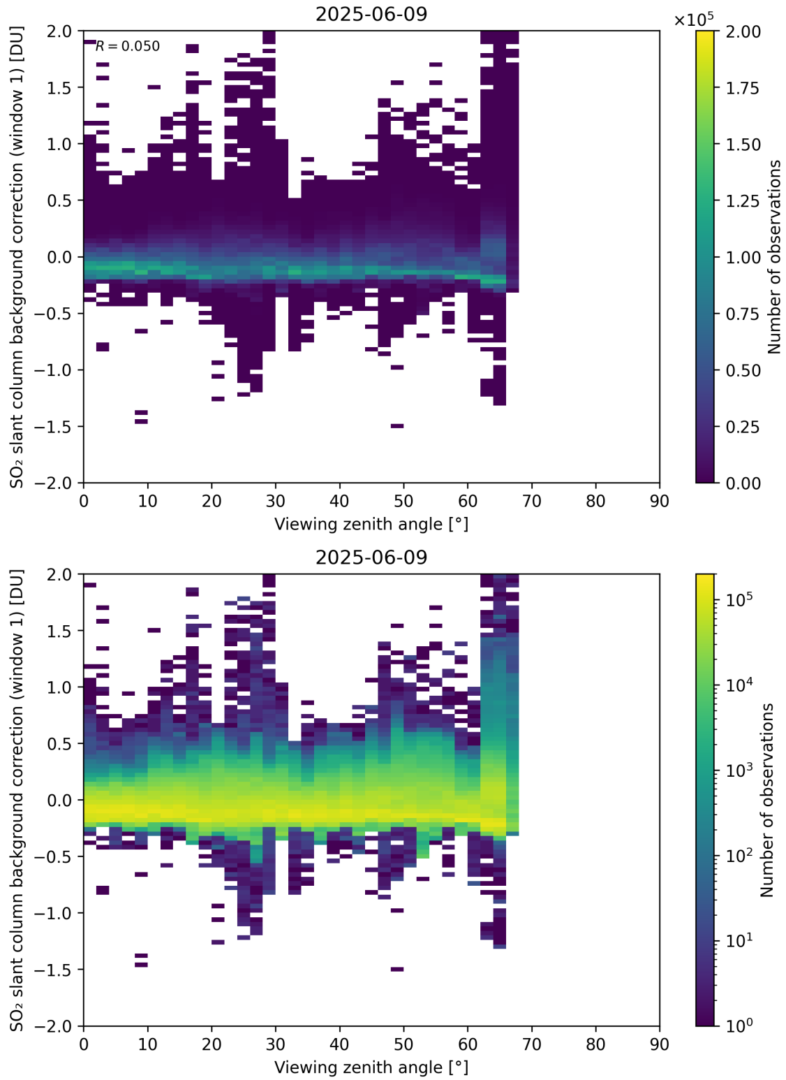
Figure 362: Scatter density plot of “Viewing zenith angle” against “SO 2 slant column background correction (window 1)” for 2025-06-08 to 2025-06-10.
