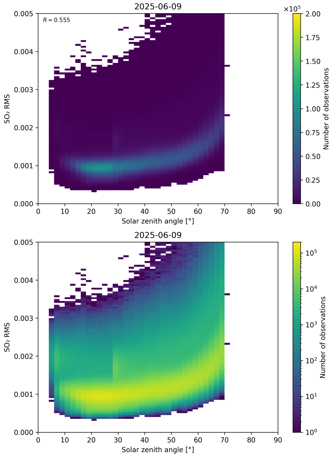
Figure 176: Scatter density plot of “Solar zenith angle” against “SO 2 RMS” for 2025-06-08 to 2025-06-10.
