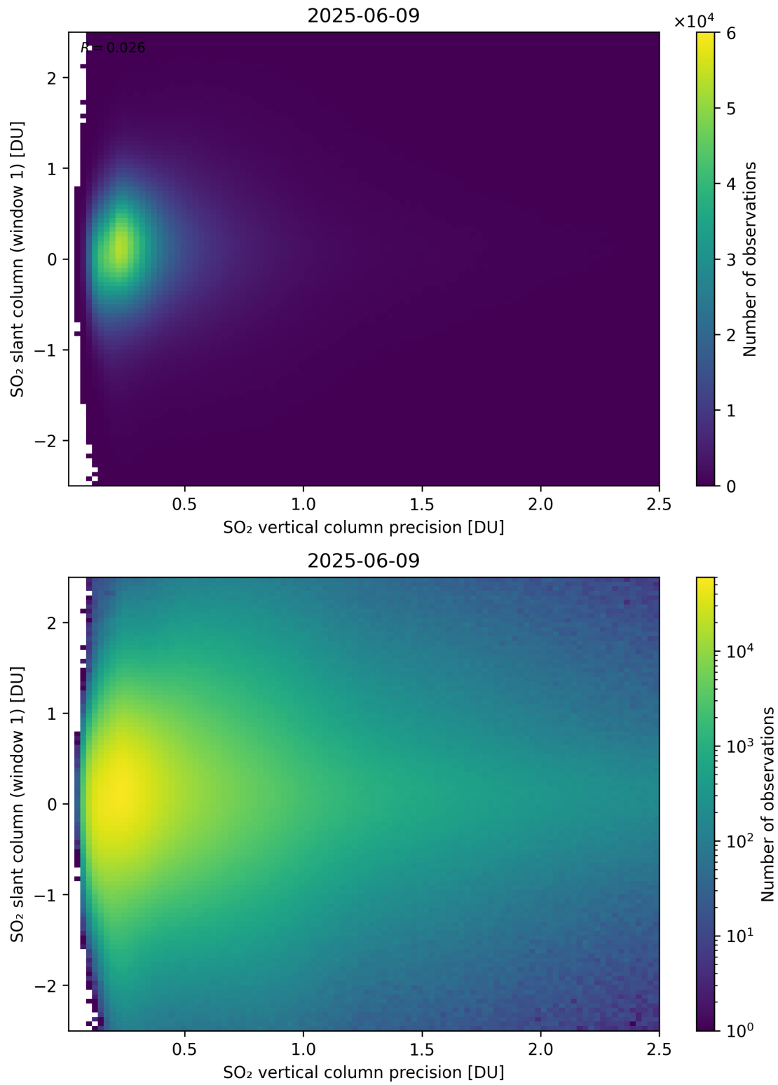
Figure 341: Scatter density plot of “SO 2 vertical column precision” against “SO 2 slant column (window 1)” for 2025-06-08 to 2025-06-10.
