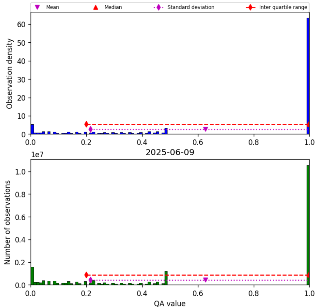
Figure 57: Histogram of “QA value” for 2025-06-08 to 2025-06-10
