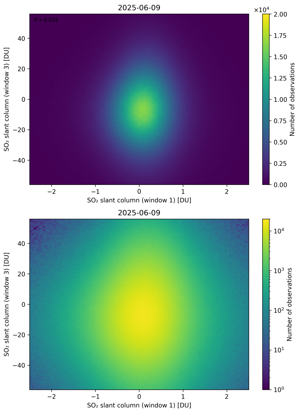
Figure 287: Scatter density plot of “SO 2 slant column (window 1)” against “SO 2 slant column (window 3)” for 2025-06-08 to 2025-06-10.
