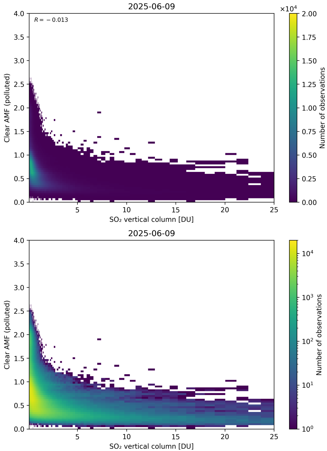
Figure 348: Scatter density plot of “SO 2 vertical column” against “Clear AMF (polluted)” for 2025-06-08 to 2025-06-10.
