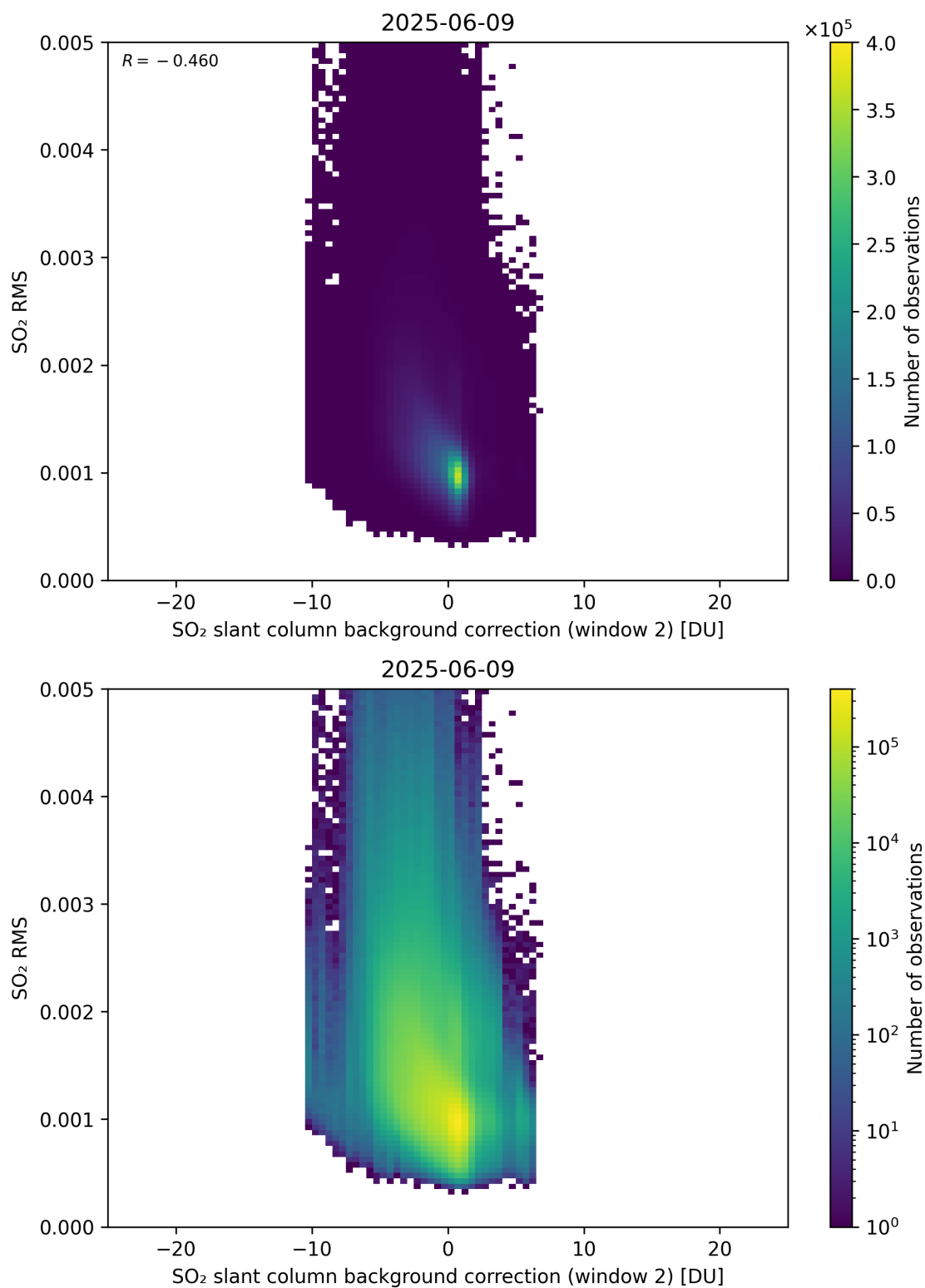
Figure 125: Scatter density plot of “SO 2 slant column background correction (window 2)” against “SO 2 RMS” for 2025-06-08 to 2025-06-10.
