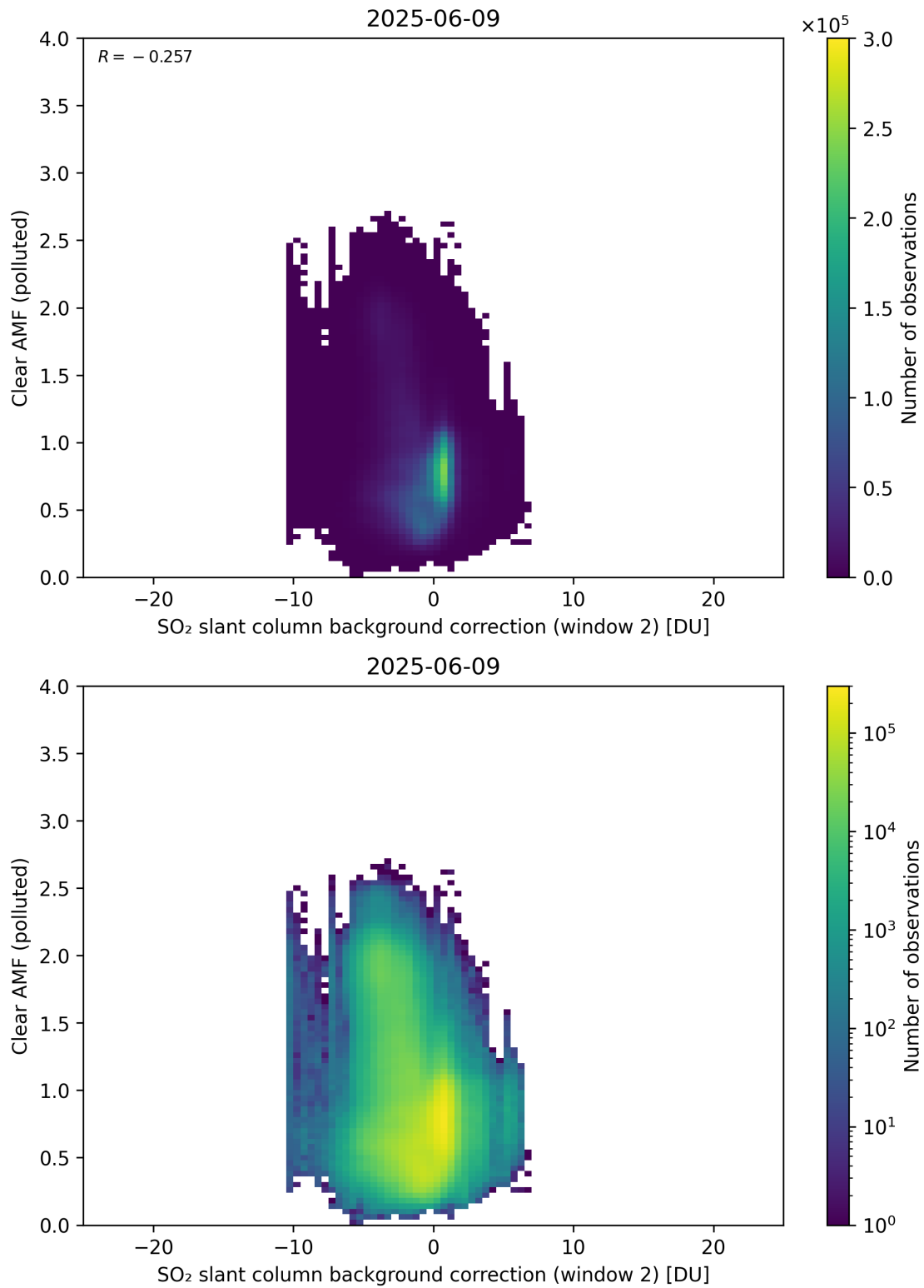
Figure 126: Scatter density plot of “SO 2 slant column background correction (window 2)” against “Clear AMF (polluted)” for 2025-06-08 to 2025-06-10.
