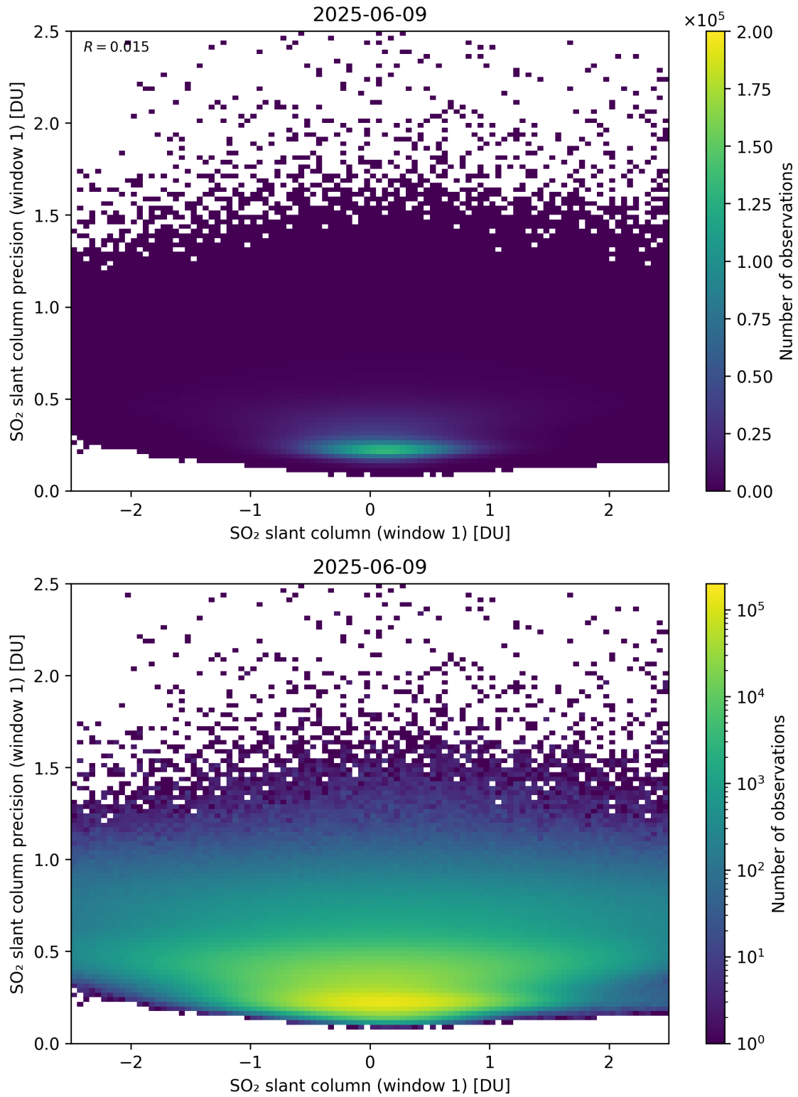
Figure 285: Scatter density plot of “SO 2 slant column (window 1)” against “SO 2 slant column precision (window 1)” for 2025-06-08 to 2025-06-10.
