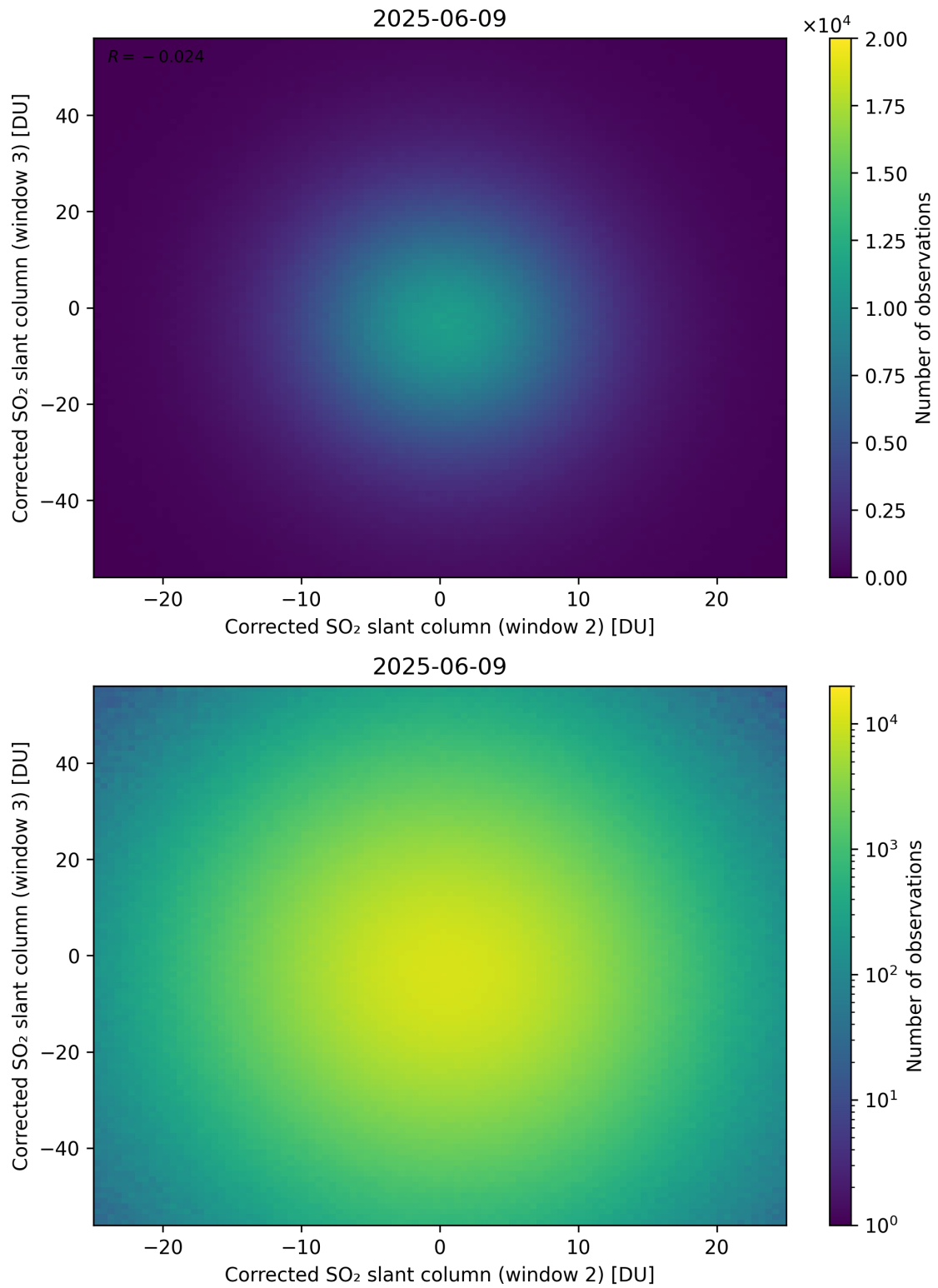
Figure 250: Scatter density plot of “Corrected SO 2 slant column (window 2)” against “Corrected SO 2 slant column (window 3)” for 2025-06-08 to 2025-06-10.
