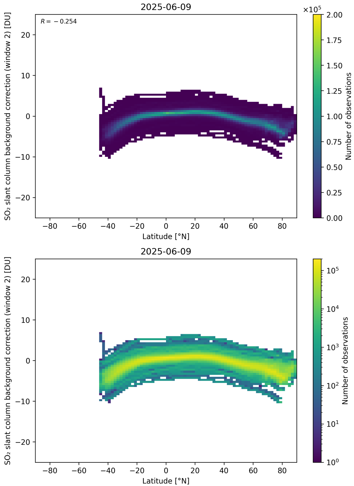
Figure 151: Scatter density plot of “Latitude” against “SO 2 slant column background correction (window 2)” for 2025-06-08 to 2025-06-10.
