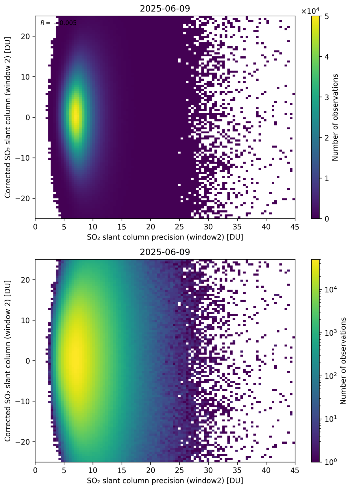
Figure 297: Scatter density plot of “SO 2 slant column precision (window2)” against “Corrected SO 2 slant column (window 2)” for 2025-06-08 to 2025-06-10.
