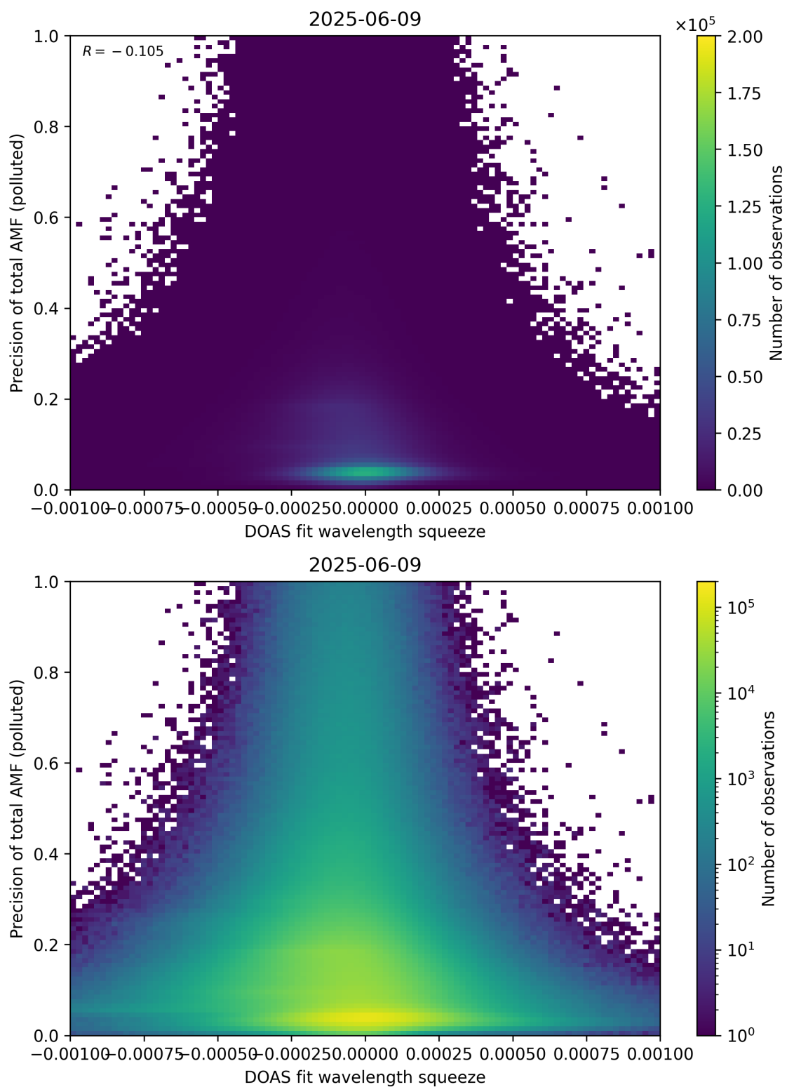
Figure 146: Scatter density plot of “DOAS fit wavelength squeeze” against “Precision of total AMF (polluted)” for 2025-06-08 to 2025-06-10.
