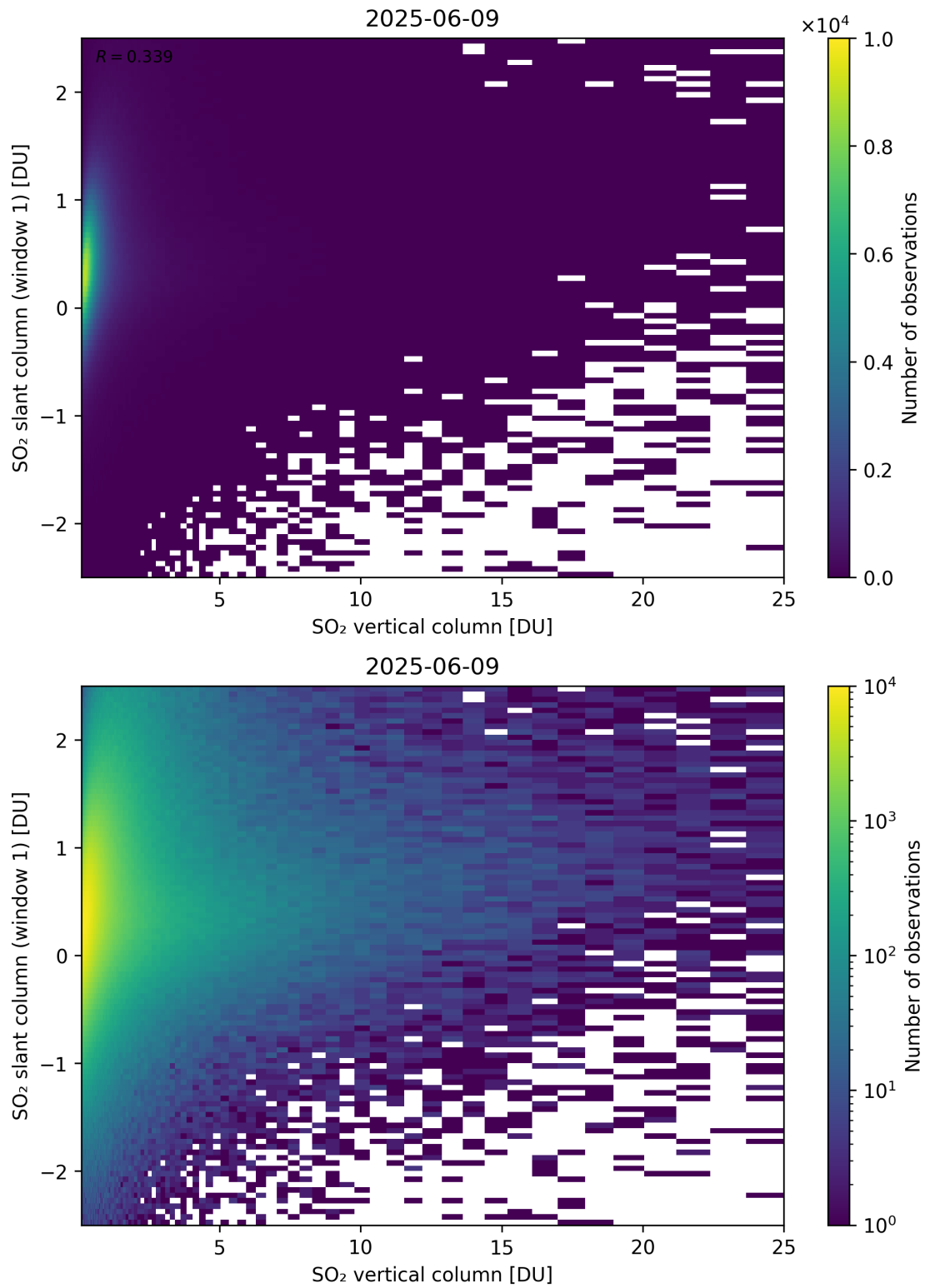
Figure 354: Scatter density plot of “SO 2 vertical column” against “SO 2 slant column (window 1)” for 2025-06-08 to 2025-06-10.
