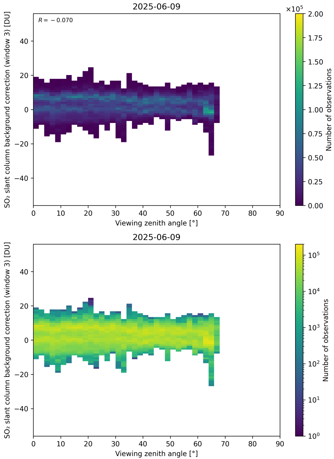
Figure 364: Scatter density plot of “Viewing zenith angle” against “SO 2 slant column background correction (window 3)” for 2025-06-08 to 2025-06-10.
