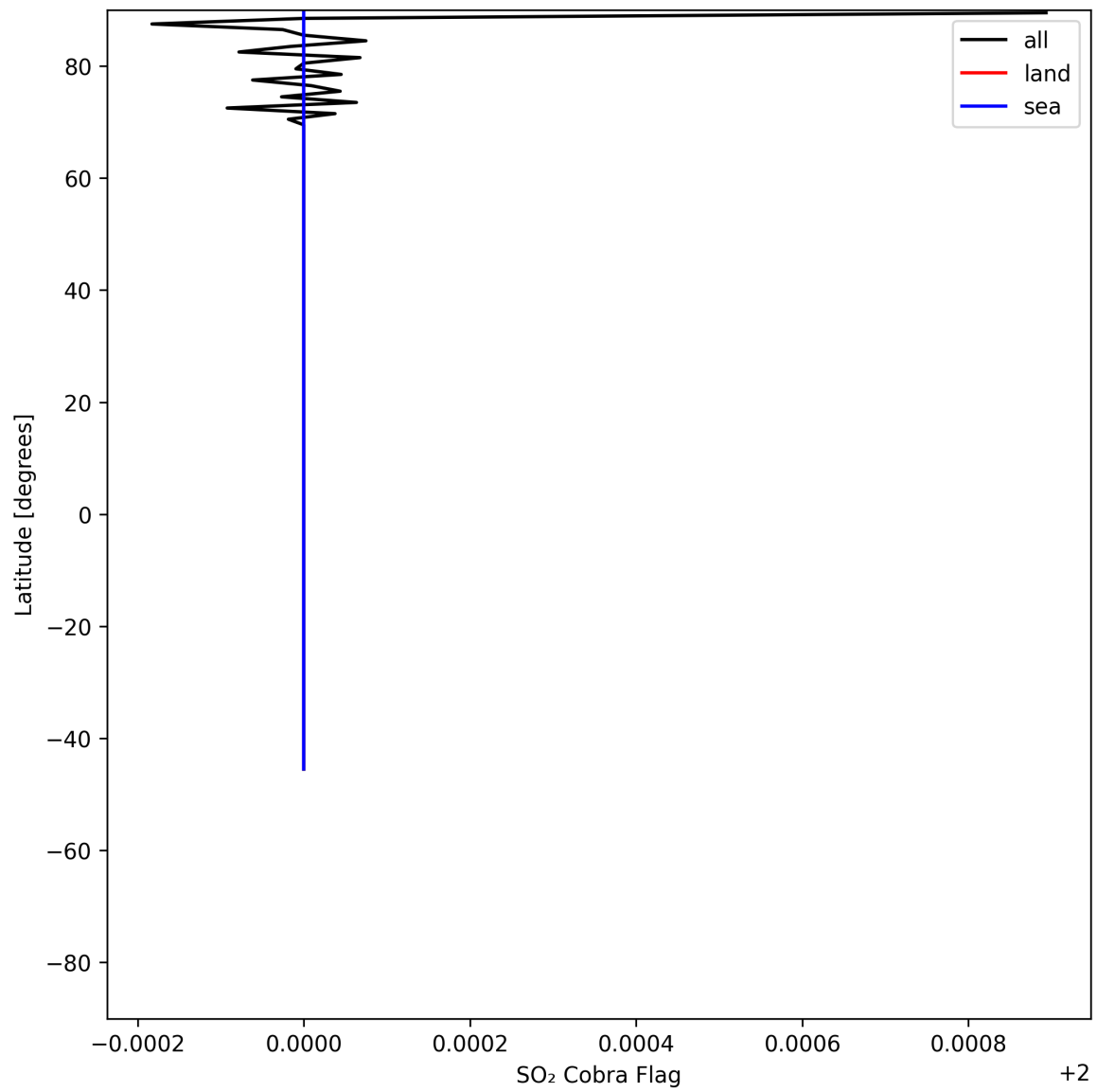
Figure 49: Zonal average of “SO 2 Cobra Flag” for 2025-06-08 to 2025-06-10.
