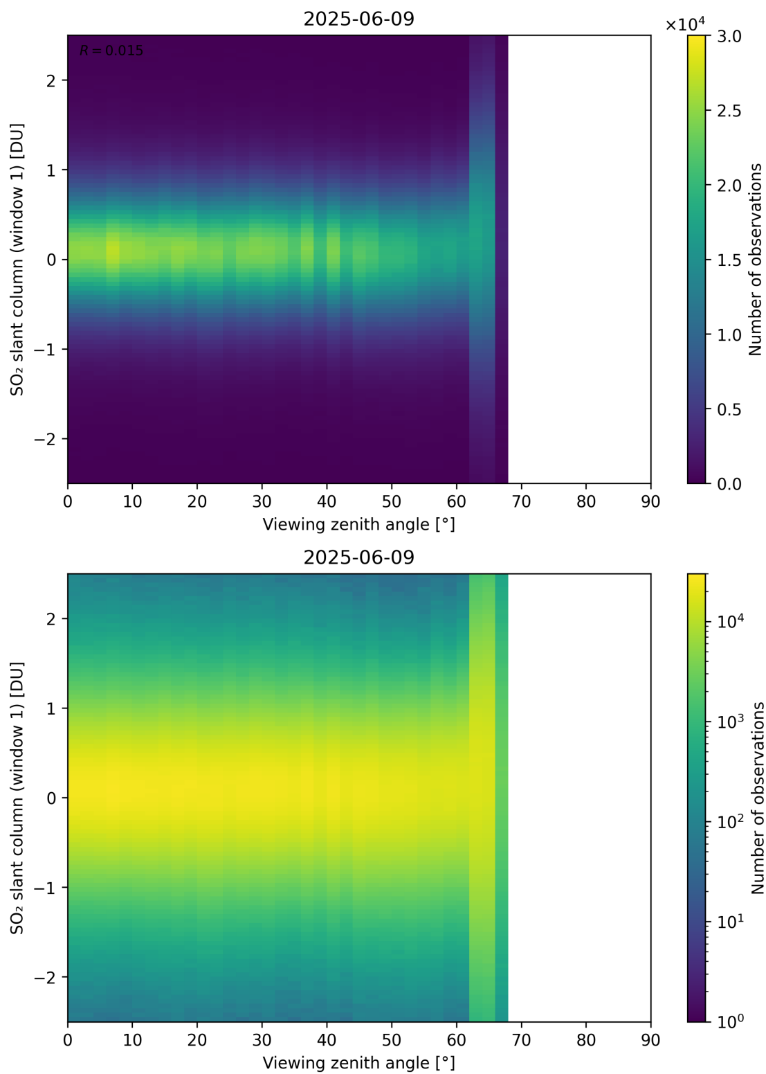
Figure 376: Scatter density plot of “Viewing zenith angle” against “SO 2 slant column (window 1)” for 2025-06-08 to 2025-06-10.
