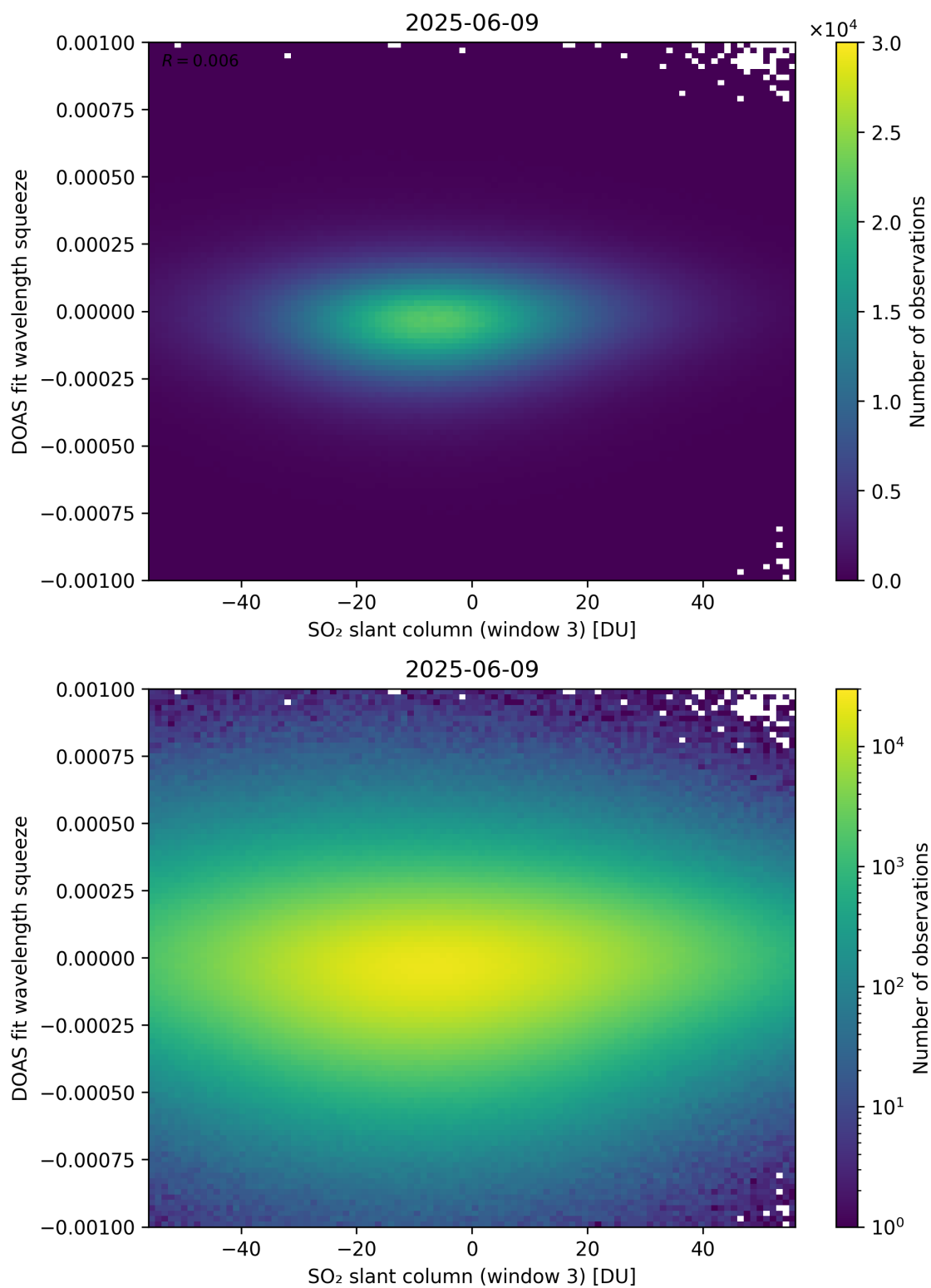
Figure 305: Scatter density plot of “SO 2 slant column (window 3)” against “DOAS fit wavelength squeeze” for 2025-06-08 to 2025-06-10.
