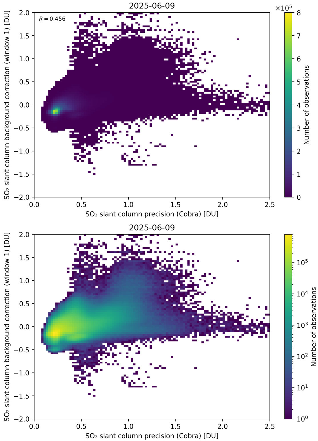
Figure 199: Scatter density plot of “SO 2 slant column precision (Cobra)” against “SO 2 slant column background correction (window 1)” for 2025-06-08 to 2025-06-10.
