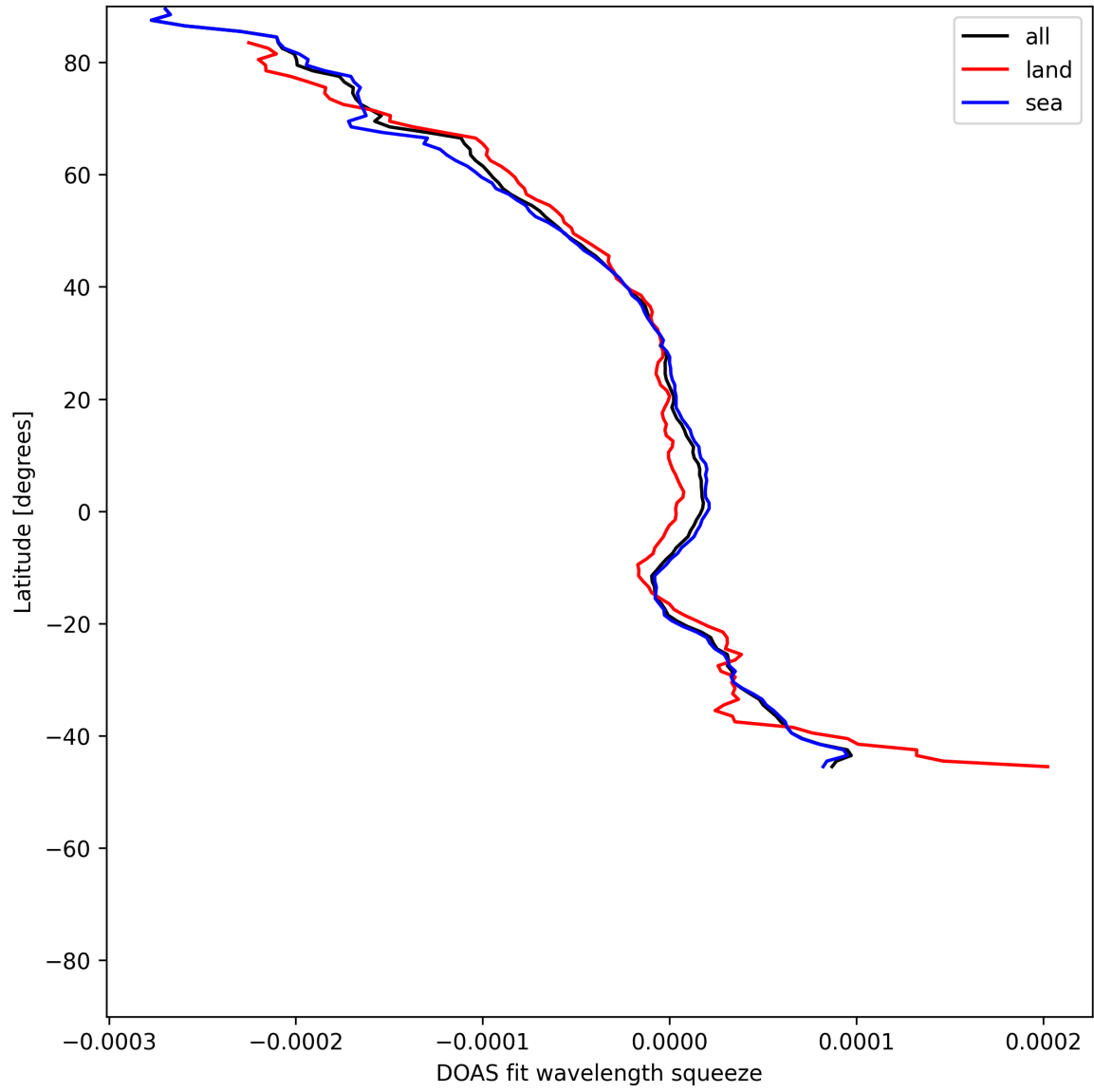
Figure 51: Zonal average of “DOAS fit wavelength squeeze” for 2025-06-08 to 2025-06-10.
