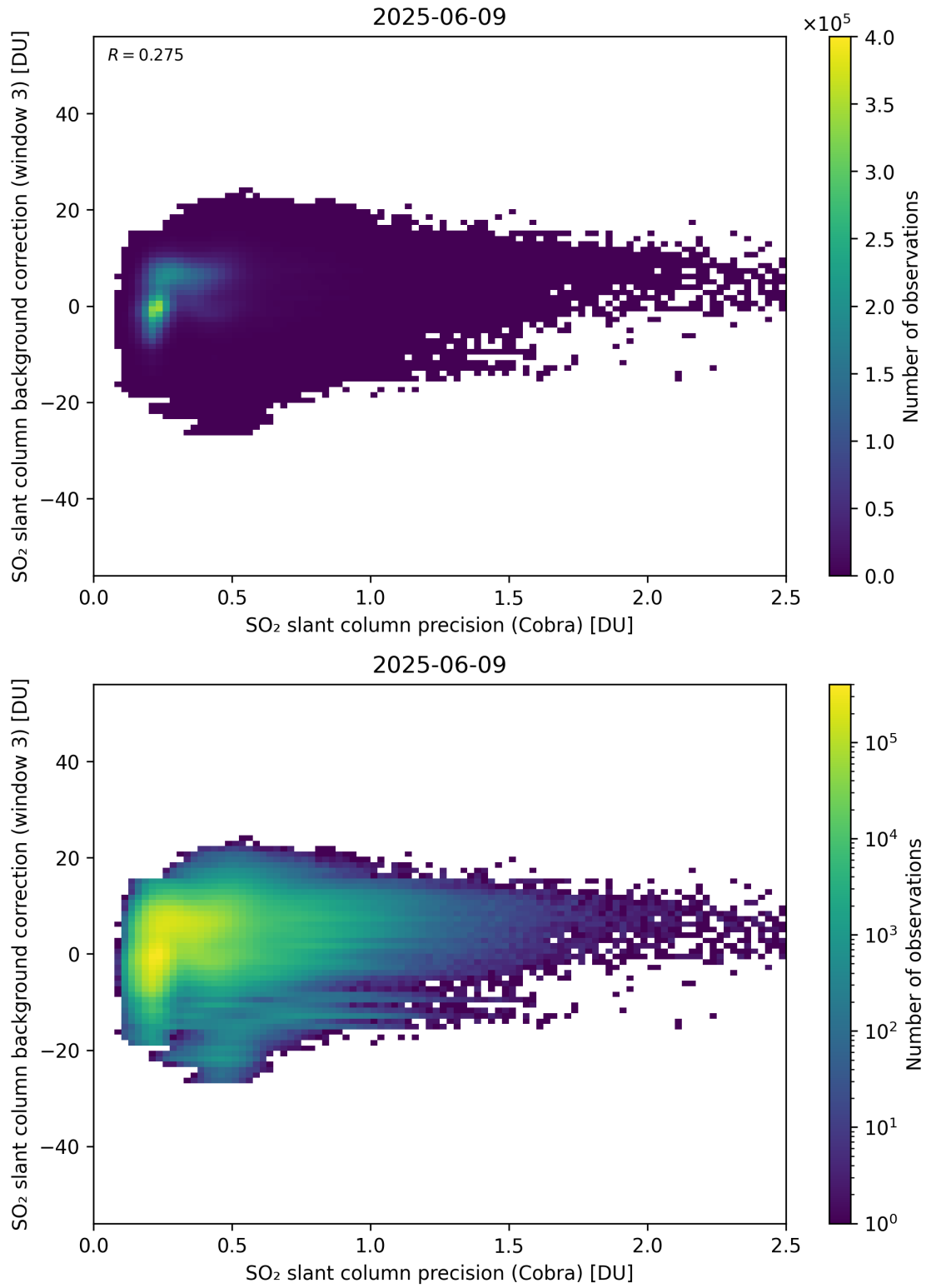
Figure 201: Scatter density plot of “SO 2 slant column precision (Cobra)” against “SO 2 slant column background correction (window 3)” for 2025-06-08 to 2025-06-10.
