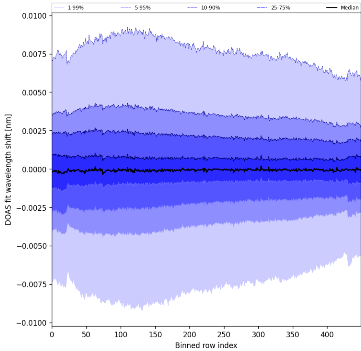
Figure 102: Along track statistics of “DOAS fit wavelength shift” for 2025-06-08 to 2025-06-10
