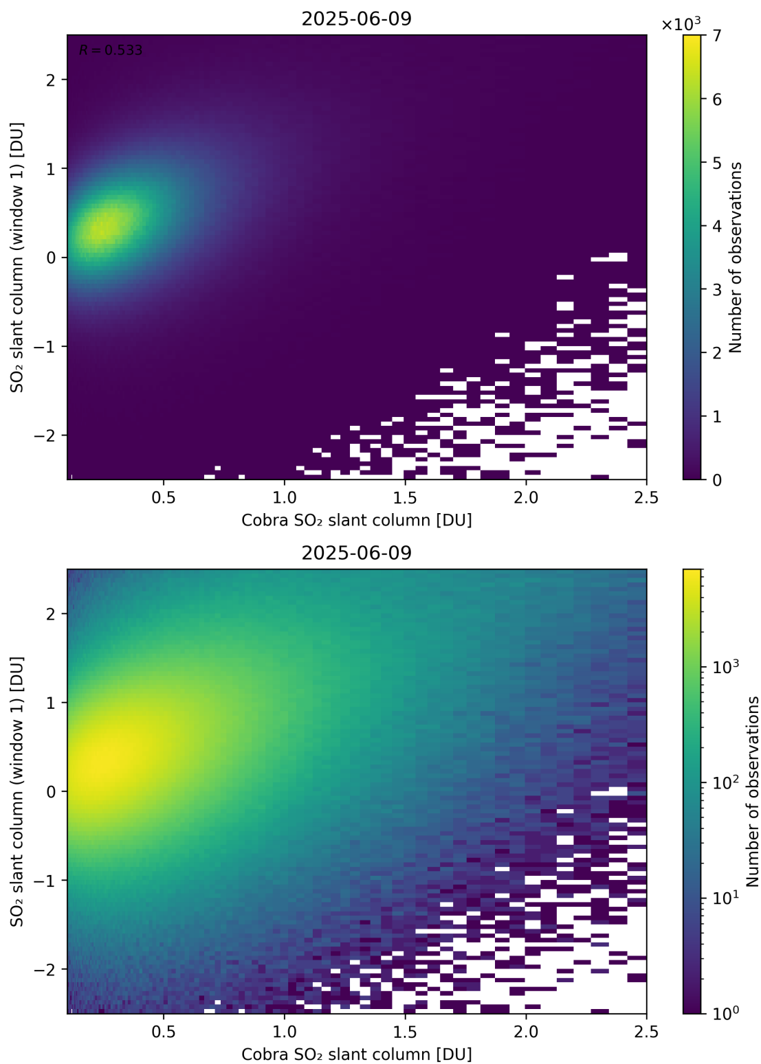
Figure 219: Scatter density plot of “Cobra SO 2 slant column” against “SO 2 slant column (window 1)” for 2025-06-08 to 2025-06-10.
