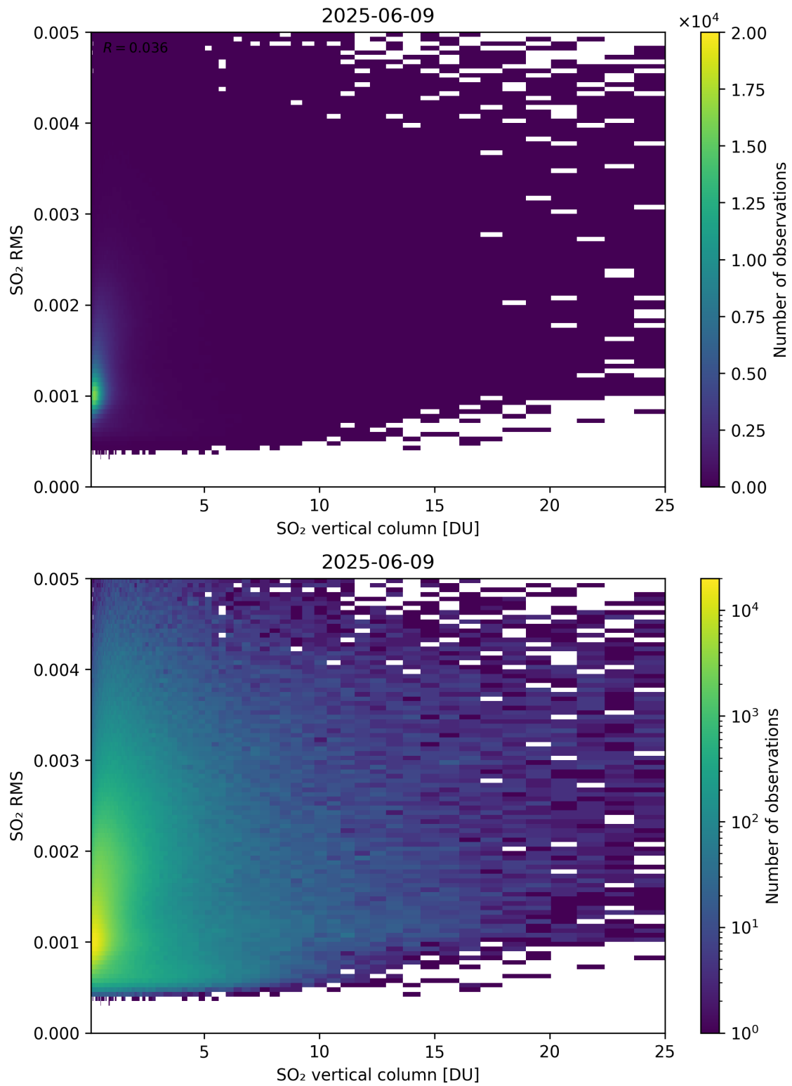
Figure 328: Scatter density plot of “SO 2 vertical column” against “SO 2 RMS” for 2025-06-08 to 2025-06-10.
