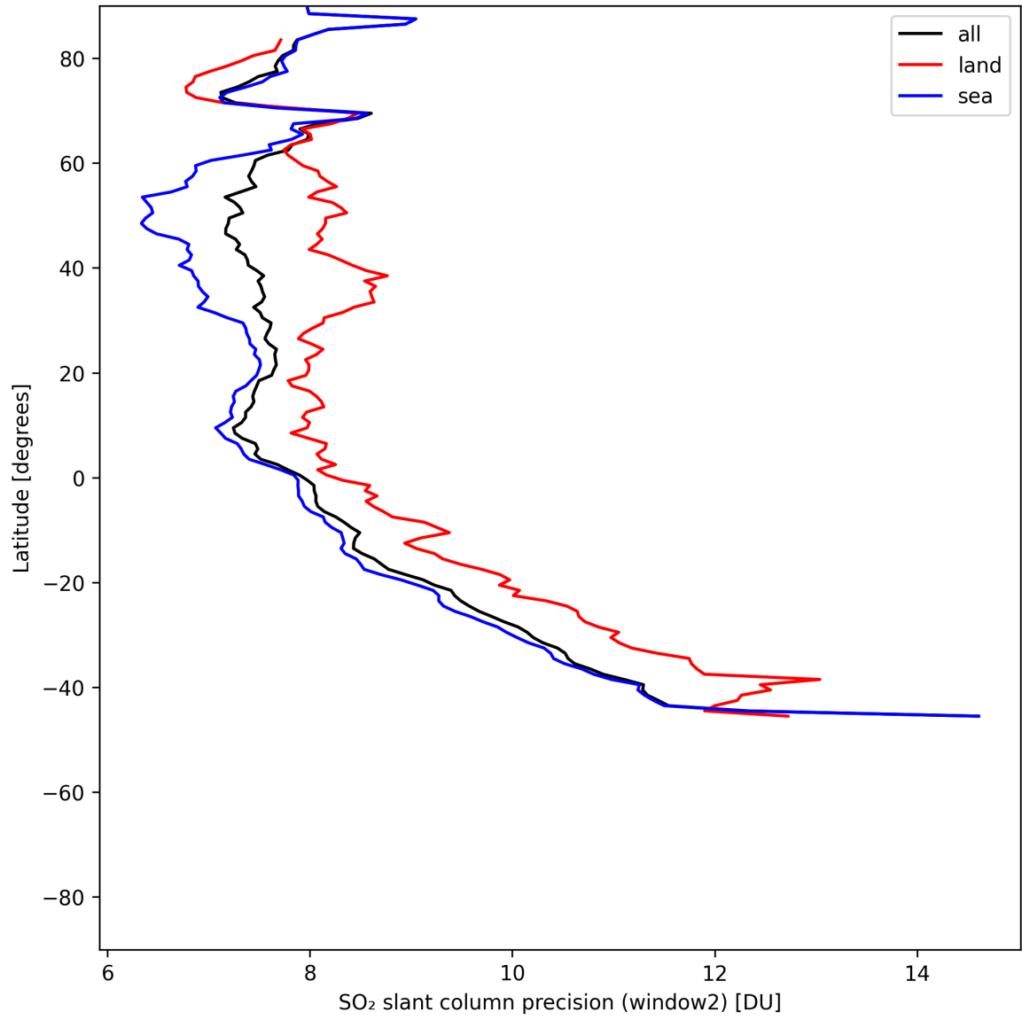
Figure 42: Zonal average of “SO 2 slant column precision (window2)” for 2025-06-08 to 2025-06-10.
