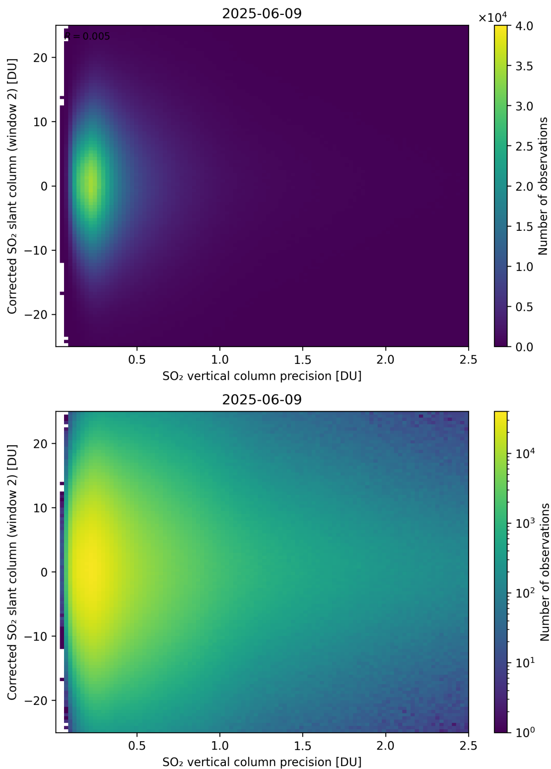
Figure 339: Scatter density plot of “SO 2 vertical column precision” against “Corrected SO 2 slant column (window 2)” for 2025-06-08 to 2025-06-10.
