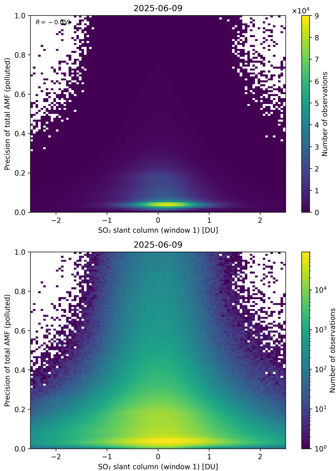
Figure 290: Scatter density plot of “SO 2 slant column (window 1)” against “Precision of total AMF (polluted)” for 2025-06-08 to 2025-06-10.
