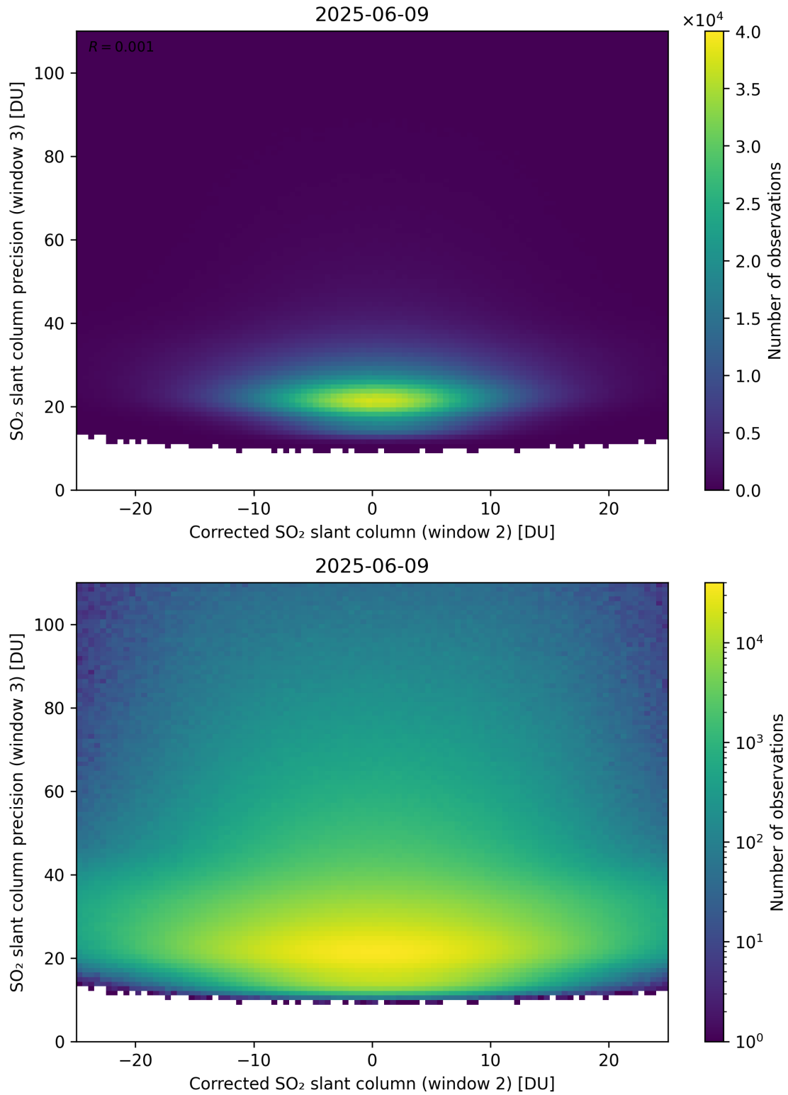
Figure 252: Scatter density plot of “Corrected SO 2 slant column (window 2)” against “SO 2 slant column precision (window 3)” for 2025-06-08 to 2025-06-10.
