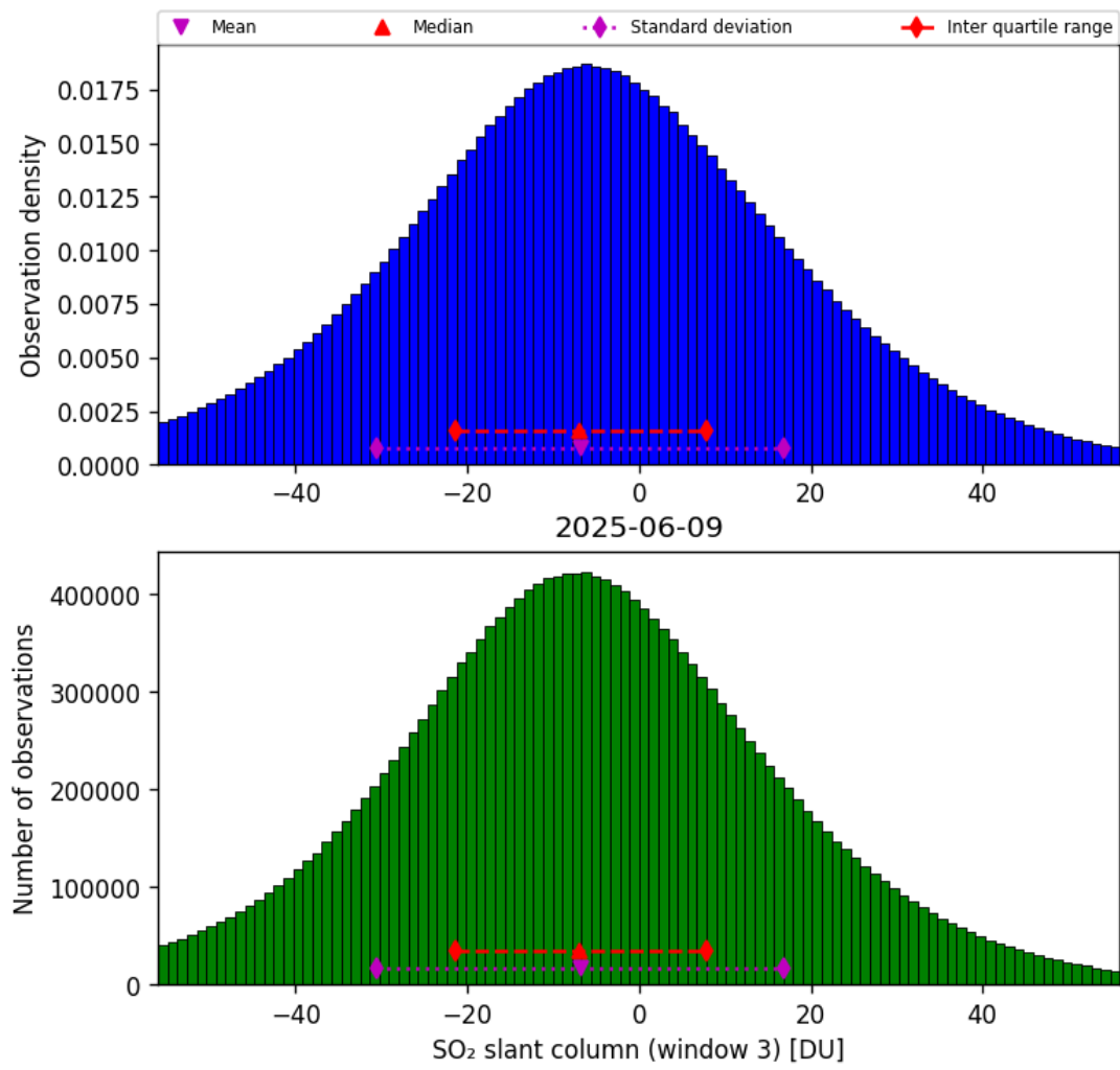
Figure 71: Histogram of “SO 2 slant column (window 3)” for 2025-06-08 to 2025-06-10
