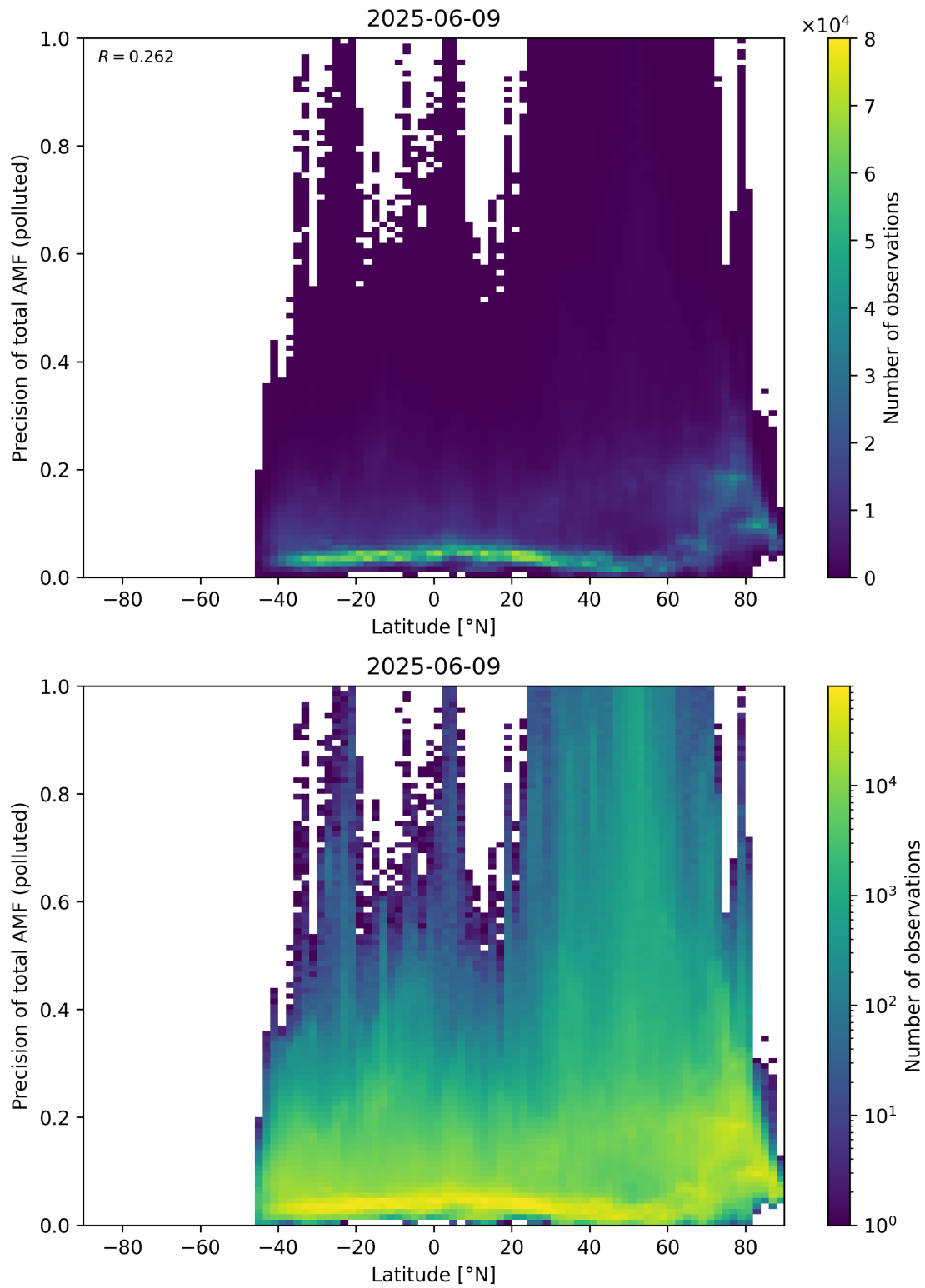
Figure 168: Scatter density plot of “Latitude” against “Precision of total AMF (polluted)” for 2025-06-08 to 2025-06-10.
