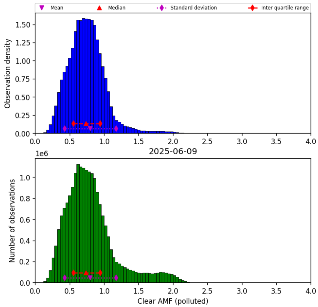
Figure 81: Histogram of “Clear AMF (polluted)” for 2025-06-08 to 2025-06-10
