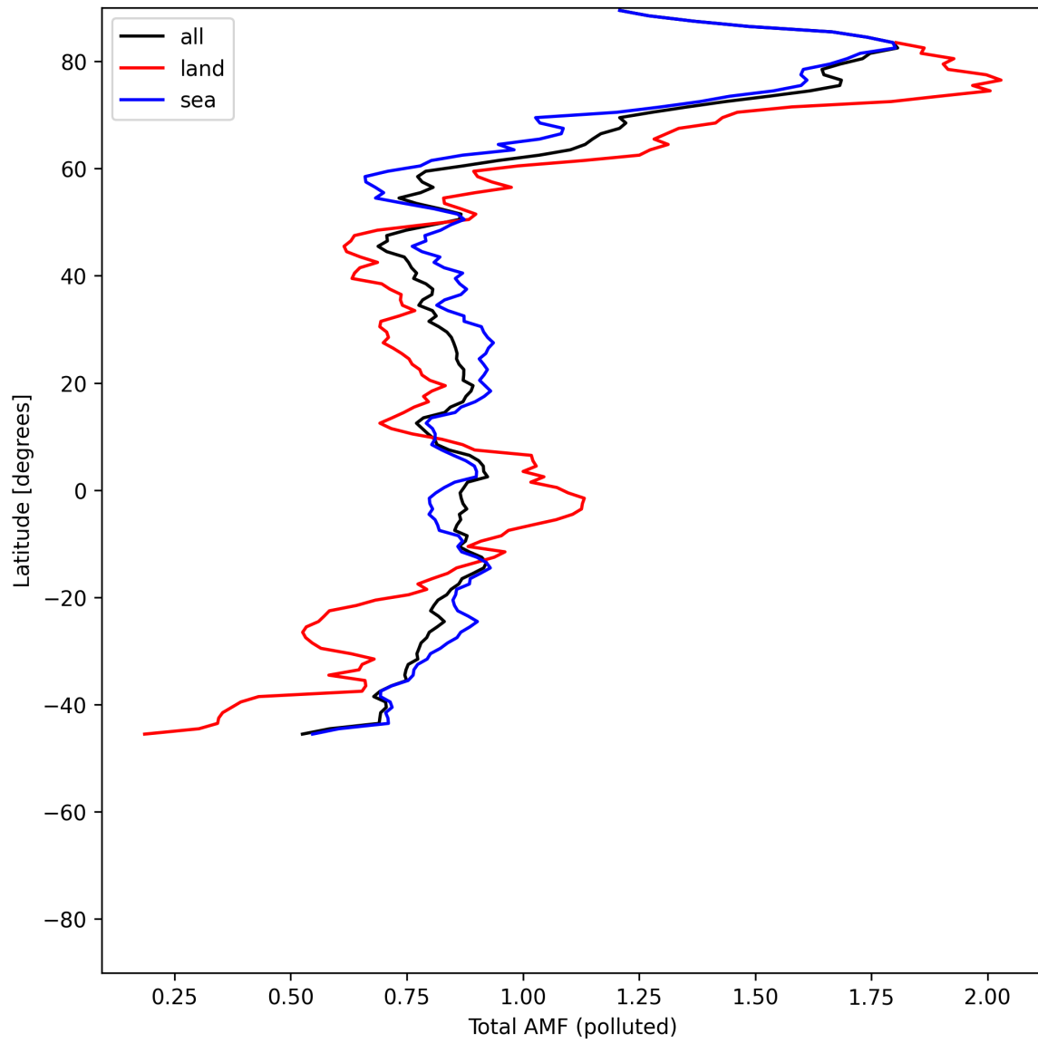
Figure 53: Zonal average of “Total AMF (polluted)” for 2025-06-08 to 2025-06-10.
