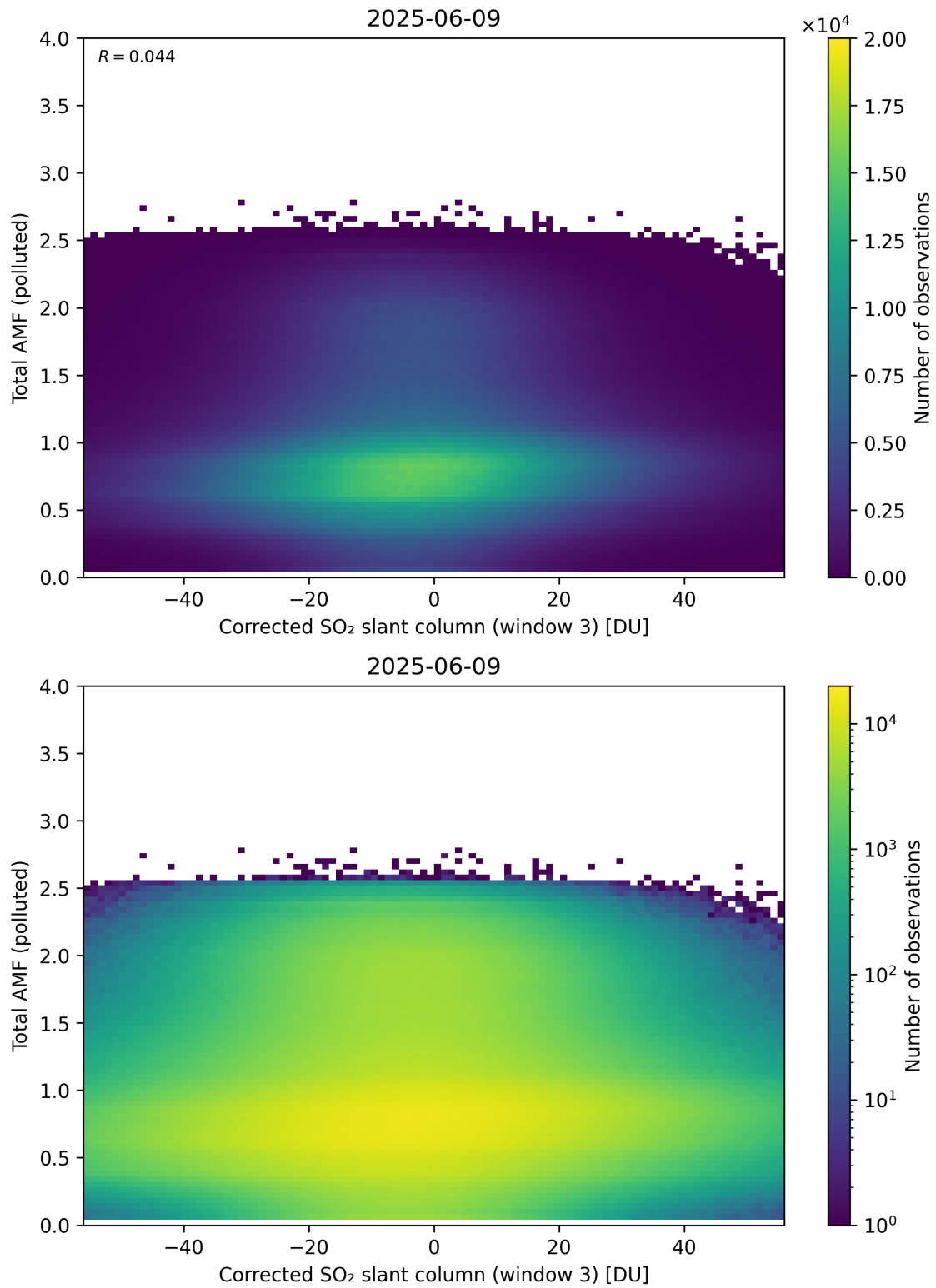
Figure 260: Scatter density plot of “Corrected SO 2 slant column (window 3)” against “Total AMF (polluted)” for 2025-06-08 to 2025-06-10.
