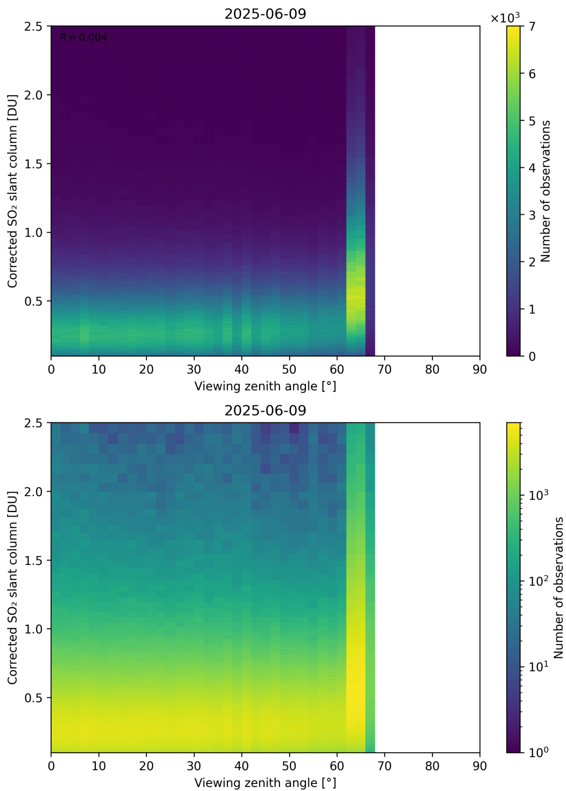
Figure 373: Scatter density plot of “Viewing zenith angle” against “Corrected SO 2 slant column” for 2025-06-08 to 2025-06-10.
