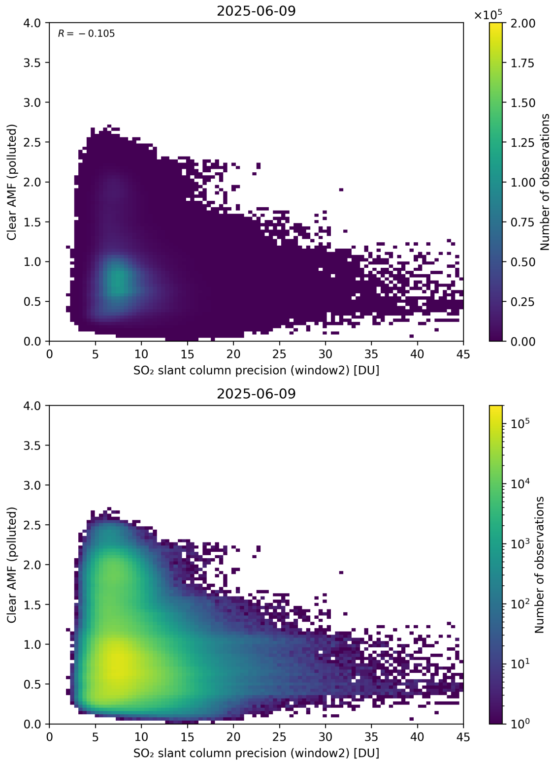
Figure 296: Scatter density plot of “SO 2 slant column precision (window2)” against “Clear AMF (polluted)” for 2025-06-08 to 2025-06-10.
