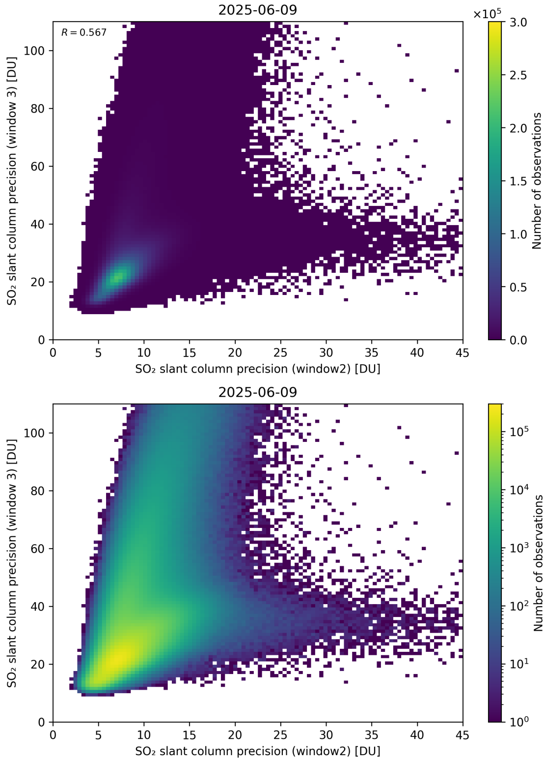
Figure 300: Scatter density plot of “SO 2 slant column precision (window2)” against “SO 2 slant column precision (window 3)” for 2025-06-08 to 2025-06-10.
