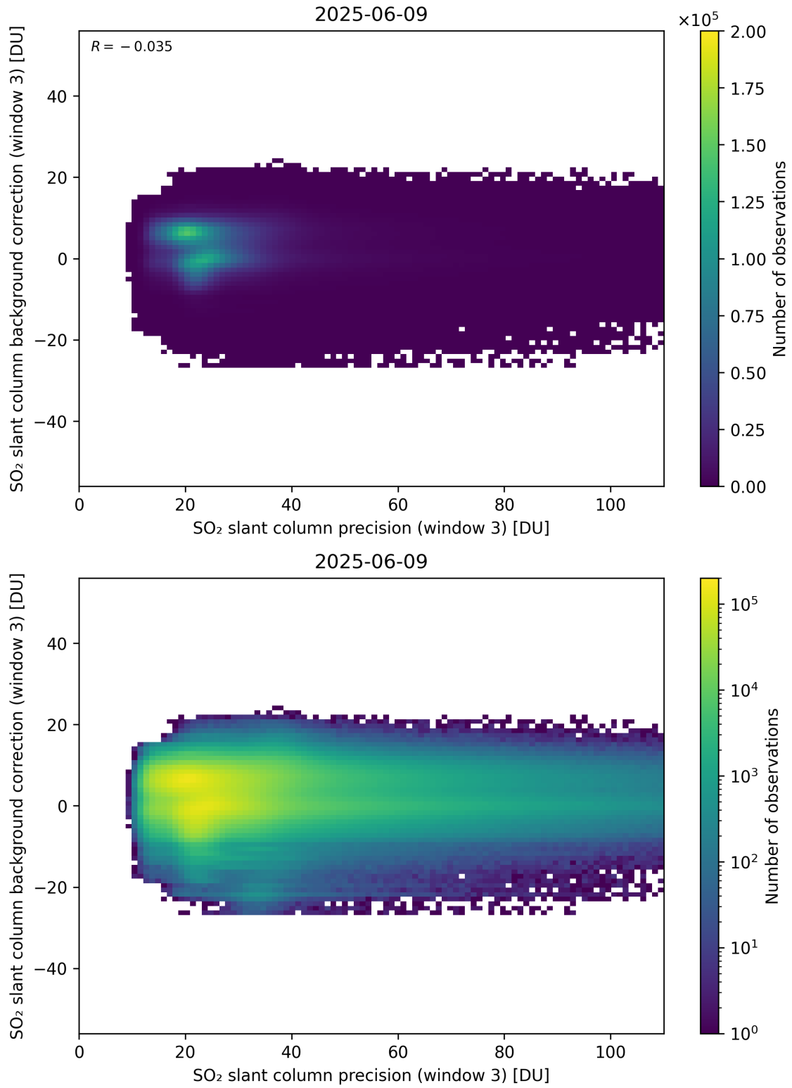
Figure 307: Scatter density plot of “SO 2 slant column precision (window 3)” against “SO 2 slant column background correction (window 3)” for 2025-06-08 to 2025-06-10.
