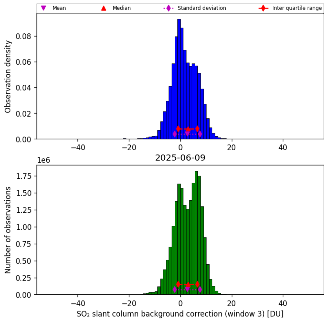
Figure 74: Histogram of “SO 2 slant column background correction (window 3)” for 2025-06-08 to 2025-06-10
