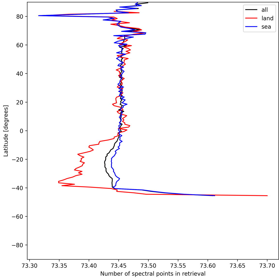
Figure 56: Zonal average of “Number of spectral points in retrieval” for 2025-06-08 to 2025-06-10.
