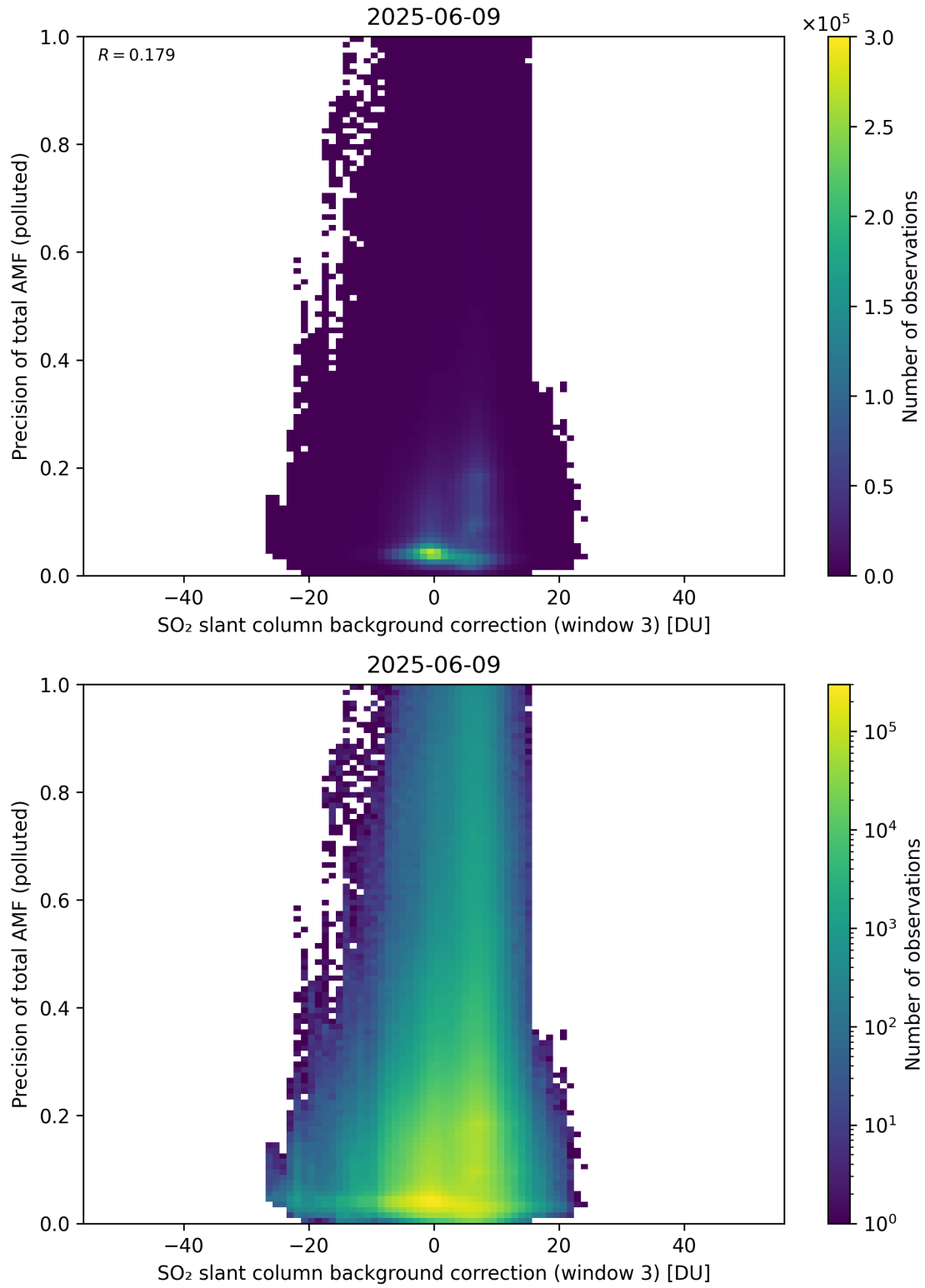
Figure 137: Scatter density plot of “SO 2 slant column background correction (window 3)” against “Precision of total AMF (polluted)” for 2025-06-08 to 2025-06-10.
