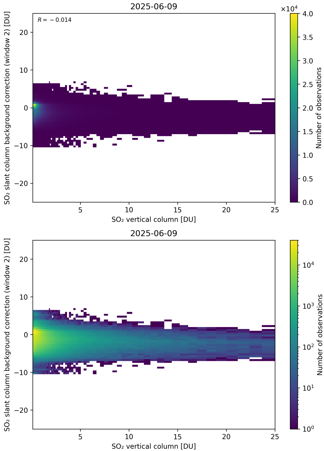
Figure 324: Scatter density plot of “SO 2 vertical column” against “SO 2 slant column background correction (window 2)” for 2025-06-08 to 2025-06-10.
