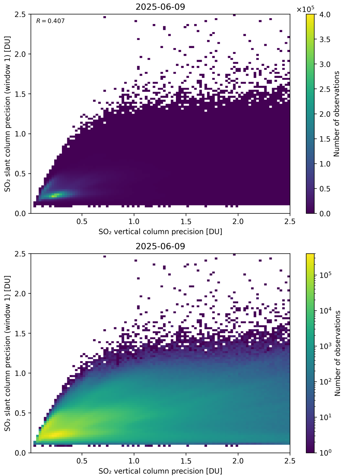
Figure 342: Scatter density plot of “SO 2 vertical column precision” against “SO 2 slant column precision (window 1)” for 2025-06-08 to 2025-06-10.
