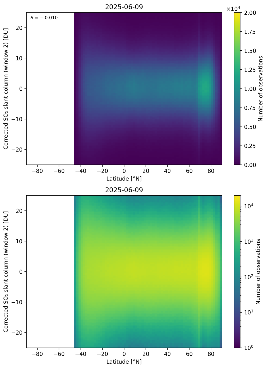
Figure 160: Scatter density plot of “Latitude” against “Corrected SO 2 slant column (window 2)” for 2025-06-08 to 2025-06-10.
