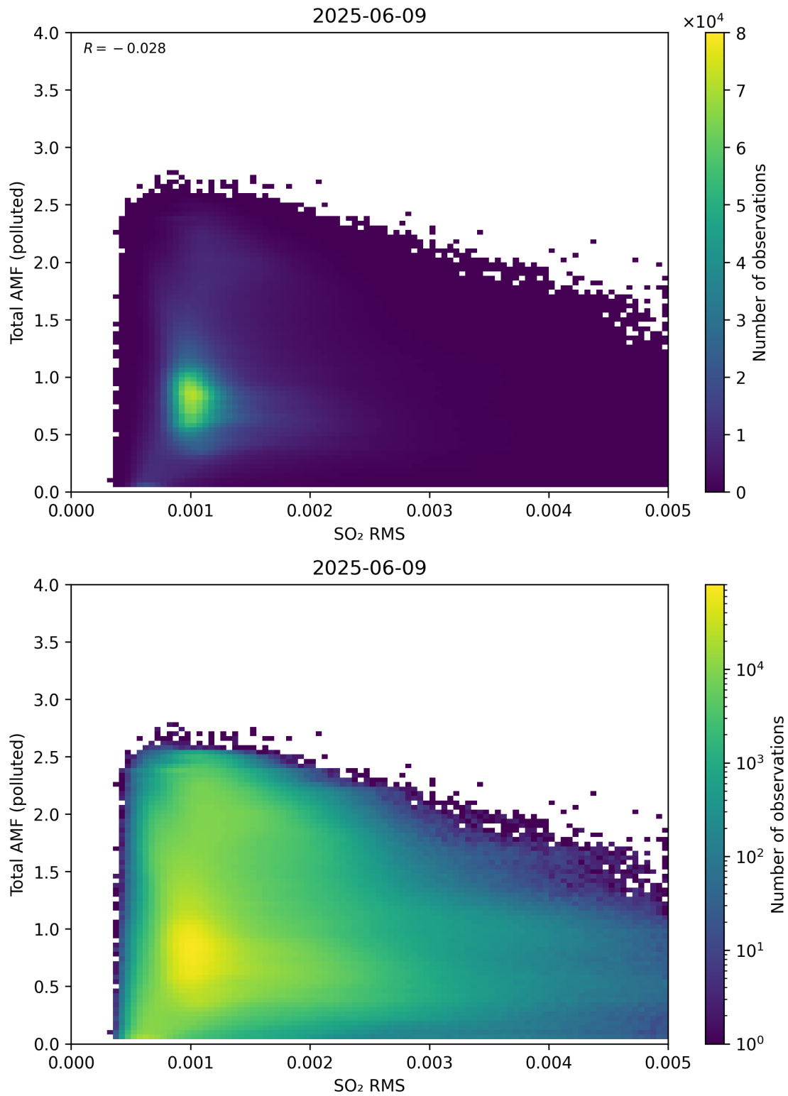
Figure 148: Scatter density plot of “SO 2 RMS” against “Total AMF (polluted)” for 2025-06-08 to 2025-06-10.
