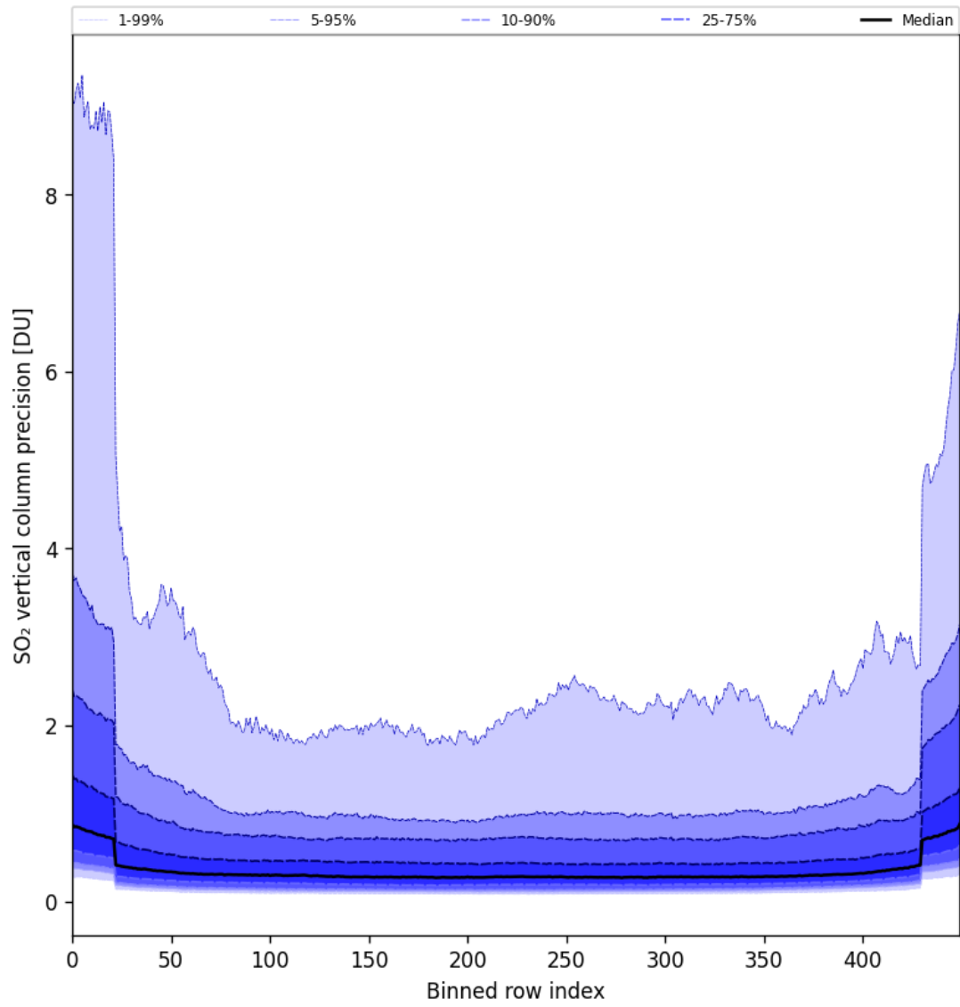
Figure 85: Along track statistics of “SO 2 vertical column precision” for 2025-06-08 to 2025-06-10
