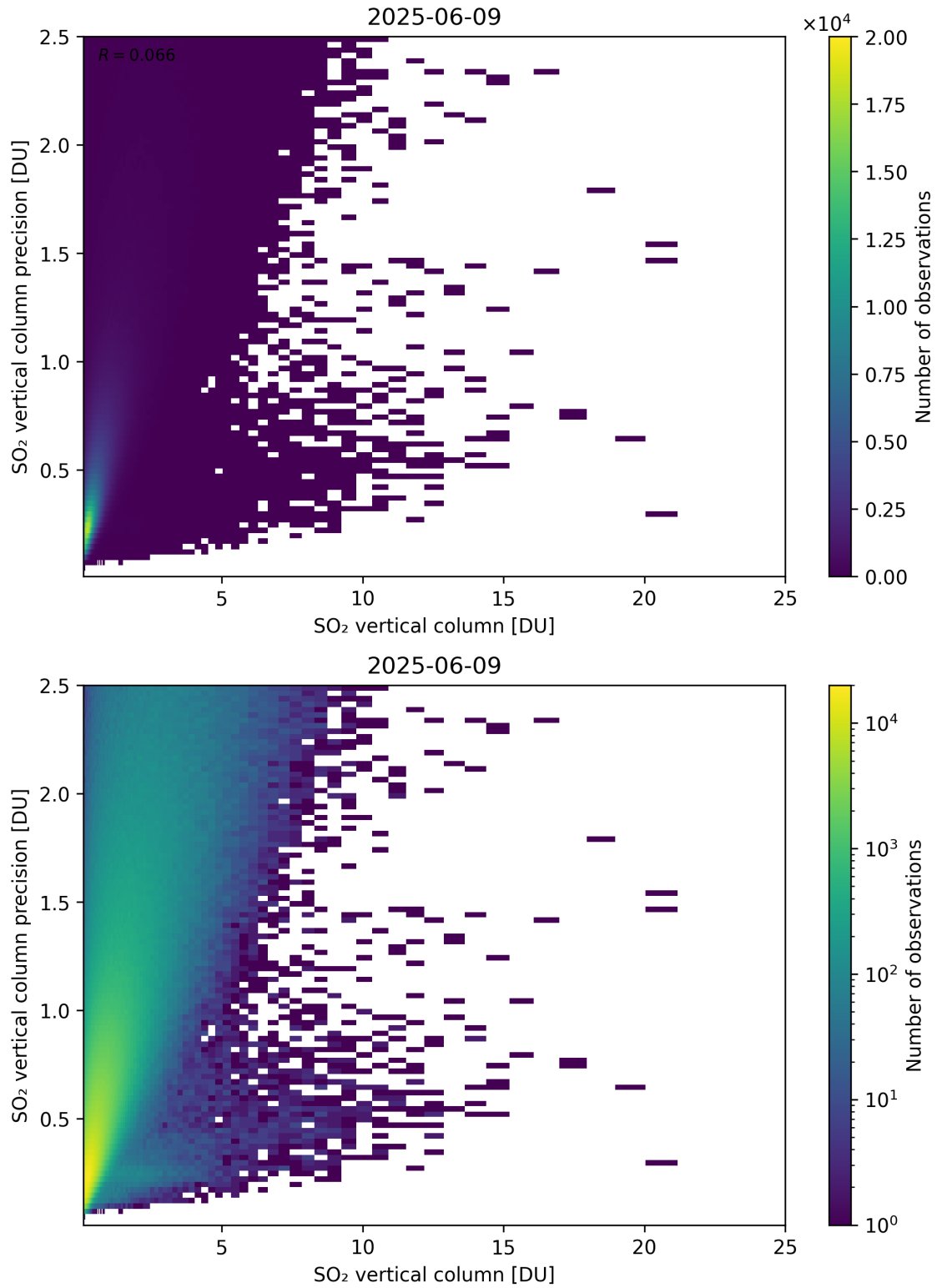
Figure 361: Scatter density plot of “SO 2 vertical column” against “SO 2 vertical column precision” for 2025-06-08 to 2025-06-10.
