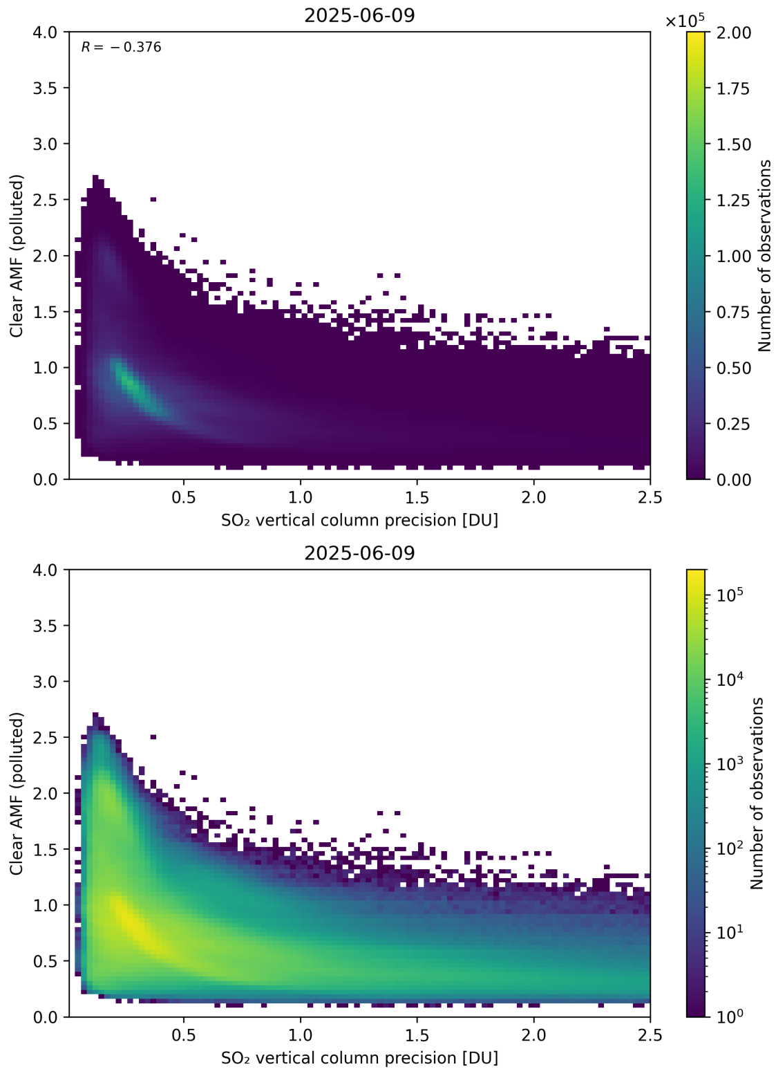
Figure 335: Scatter density plot of “SO 2 vertical column precision” against “Clear AMF (polluted)” for 2025-06-08 to 2025-06-10.
