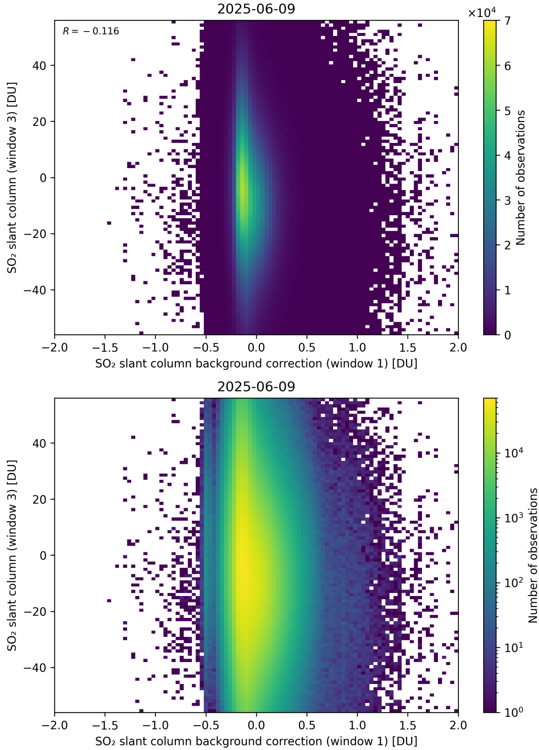
Figure 118: Scatter density plot of “SO 2 slant column background correction (window 1)” against “SO 2 slant column (window 3)” for 2025-06-08 to 2025-06-10.
