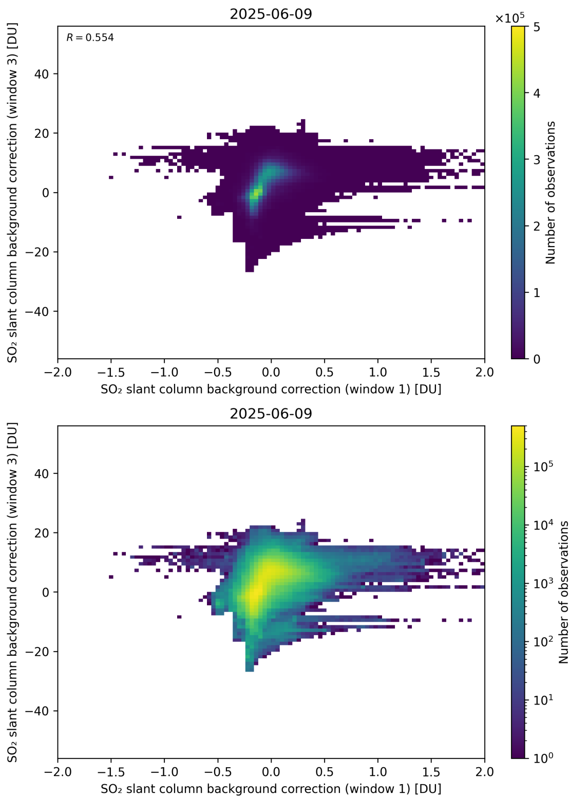
Figure 110: Scatter density plot of “SO 2 slant column background correction (window 1)” against “SO 2 slant column background correction (window 3)” for 2025-06-08 to 2025-06-10.
