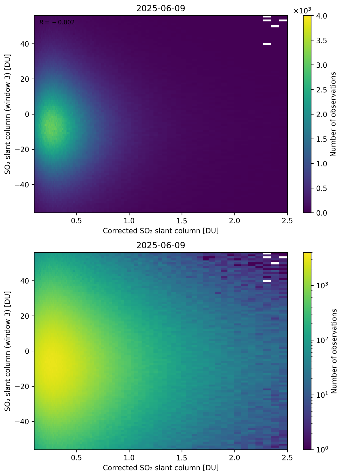
Figure 240: Scatter density plot of “Corrected SO 2 slant column” against “SO 2 slant column (window 3)” for 2025-06-08 to 2025-06-10.
