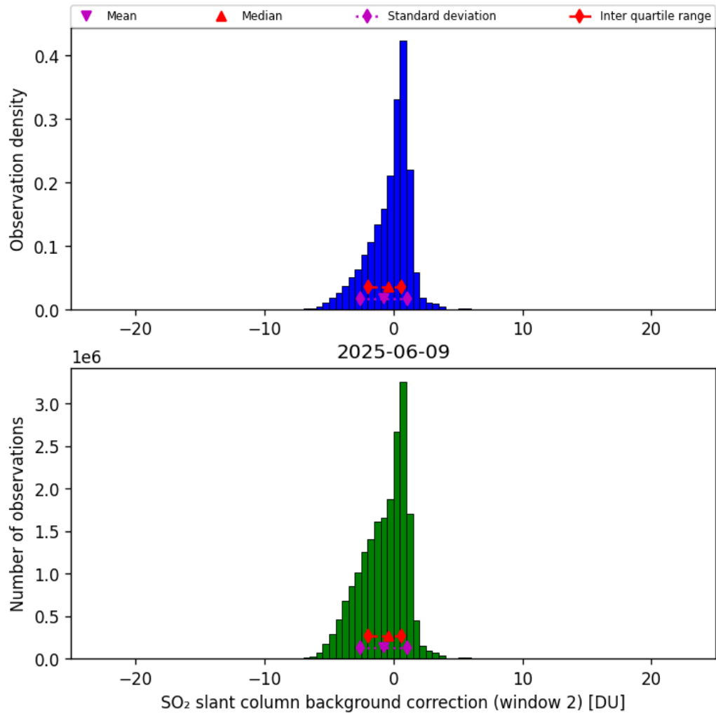
Figure 70: Histogram of “SO 2 slant column background correction (window 2)” for 2025-06-08 to 2025-06-10
