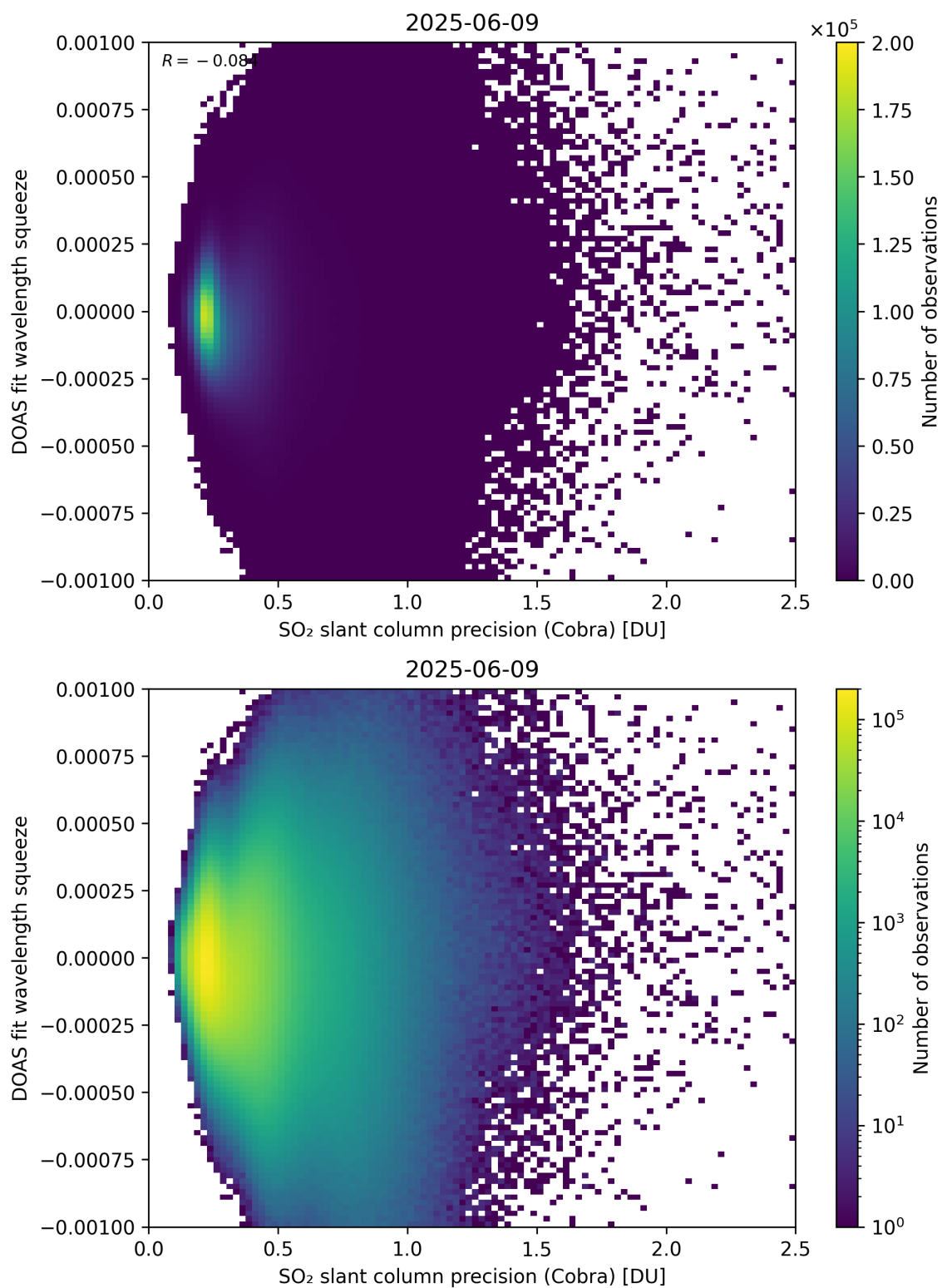
Figure 203: Scatter density plot of “SO 2 slant column precision (Cobra)” against “DOAS fit wavelength squeeze” for 2025-06-08 to 2025-06-10.
