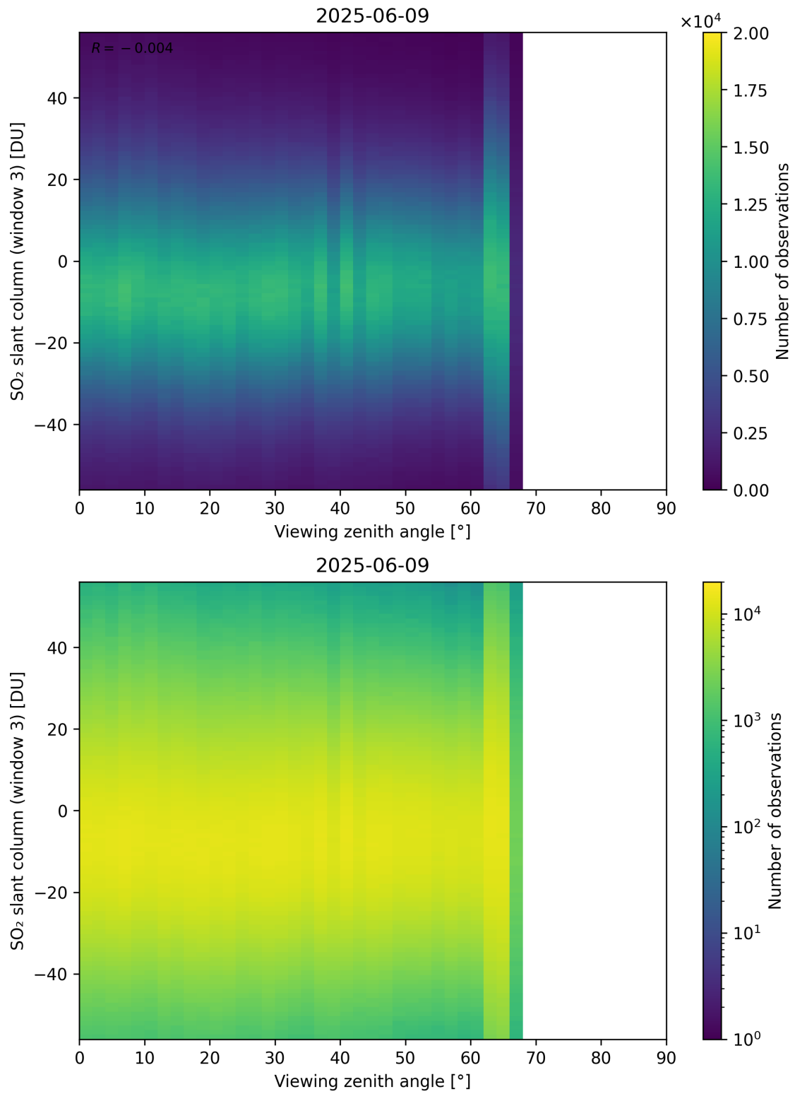
Figure 379: Scatter density plot of “Viewing zenith angle” against “SO 2 slant column (window 3)” for 2025-06-08 to 2025-06-10.
