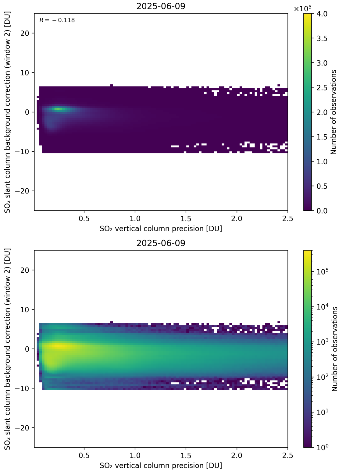
Figure 330: Scatter density plot of “SO 2 vertical column precision” against “SO 2 slant column background correction (window 2)” for 2025-06-08 to 2025-06-10.
