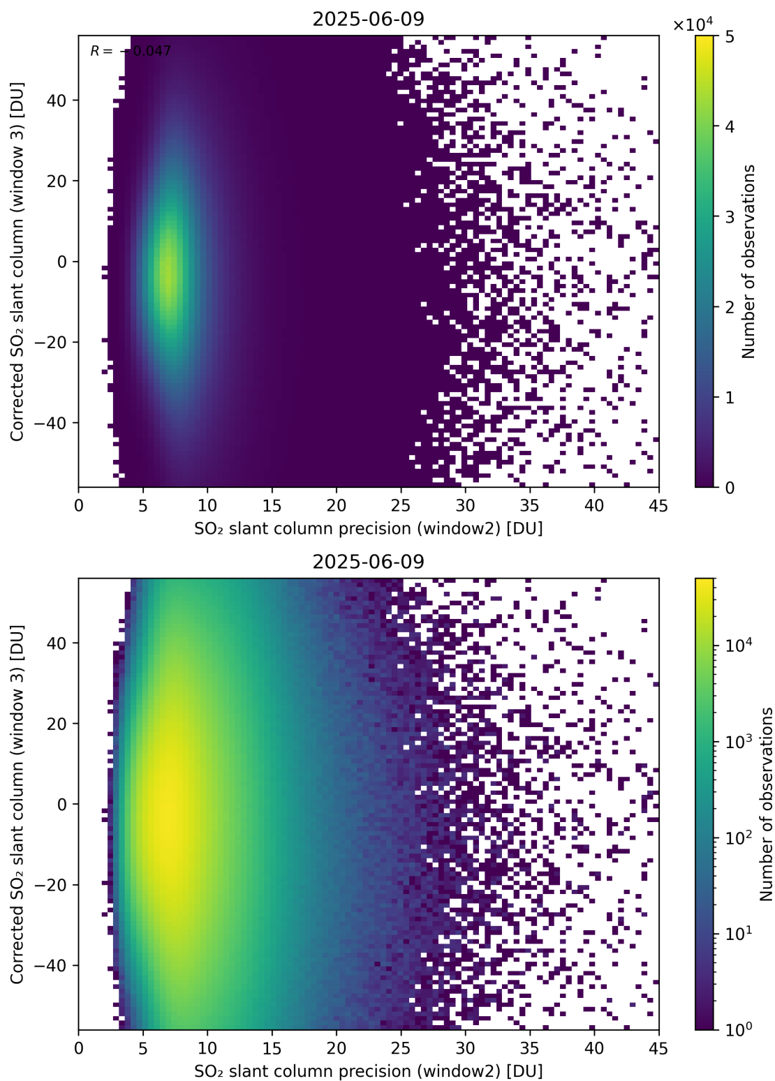
Figure 298: Scatter density plot of “SO 2 slant column precision (window2)” against “Corrected SO 2 slant column (window 3)” for 2025-06-08 to 2025-06-10.
