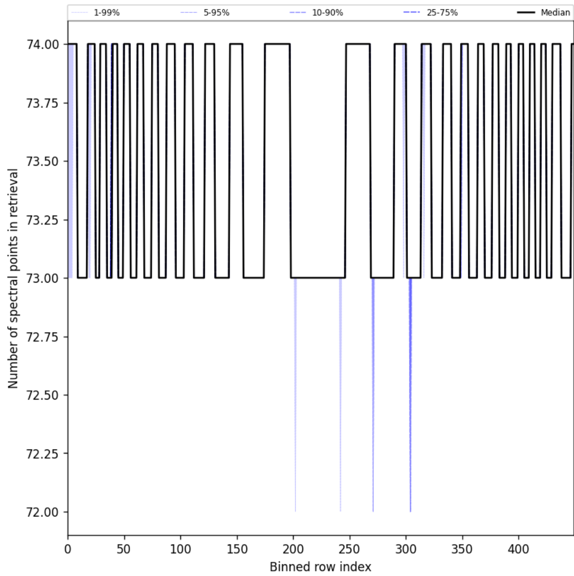
Figure 108: Along track statistics of “Number of spectral points in retrieval” for 2025-06-08 to 2025-06-10
