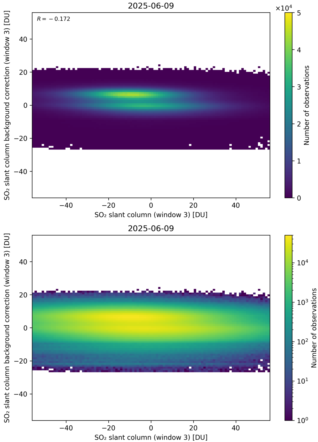
Figure 303: Scatter density plot of “SO 2 slant column (window 3)” against “SO 2 slant column background correction (window 3)” for 2025-06-08 to 2025-06-10.
