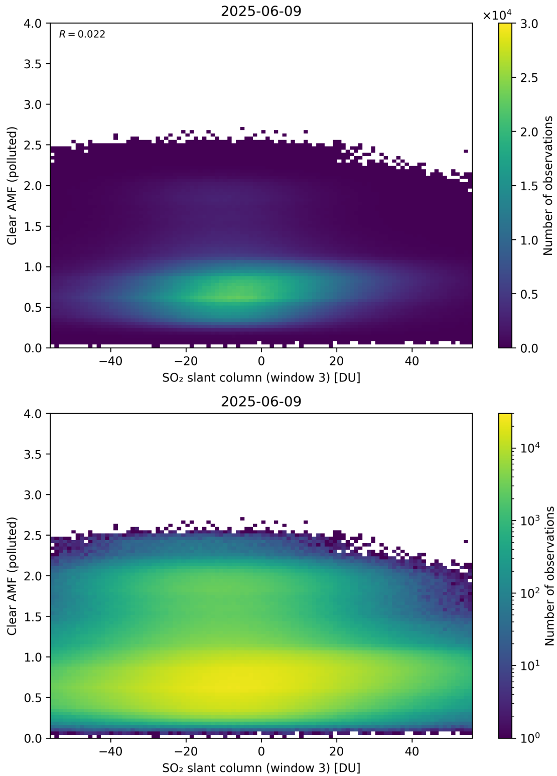
Figure 315: Scatter density plot of “SO 2 slant column (window 3)” against “Clear AMF (polluted)” for 2025-06-08 to 2025-06-10.
