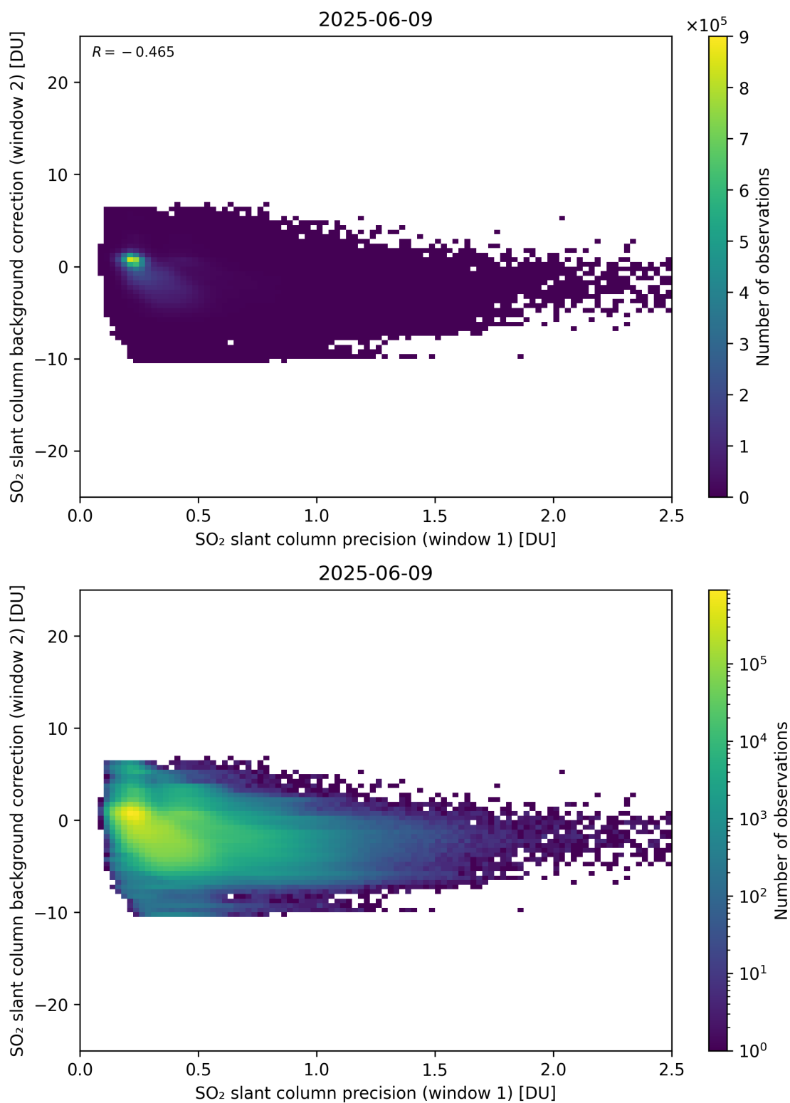
Figure 269: Scatter density plot of “SO 2 slant column precision (window 1)” against “SO 2 slant column background correction (window 2)” for 2025-06-08 to 2025-06-10.
