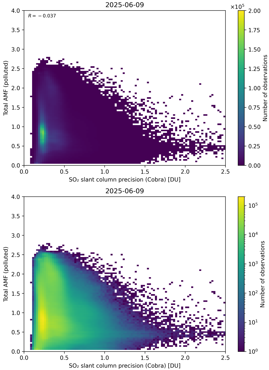
Figure 213: Scatter density plot of “SO 2 slant column precision (Cobra)” against “Total AMF (polluted)” for 2025-06-08 to 2025-06-10.
