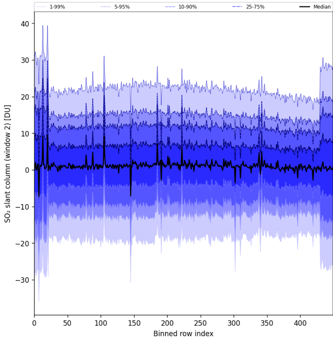
Figure 93: Along track statistics of “SO 2 slant column (window 2)” for 2025-06-08 to 2025-06-10
