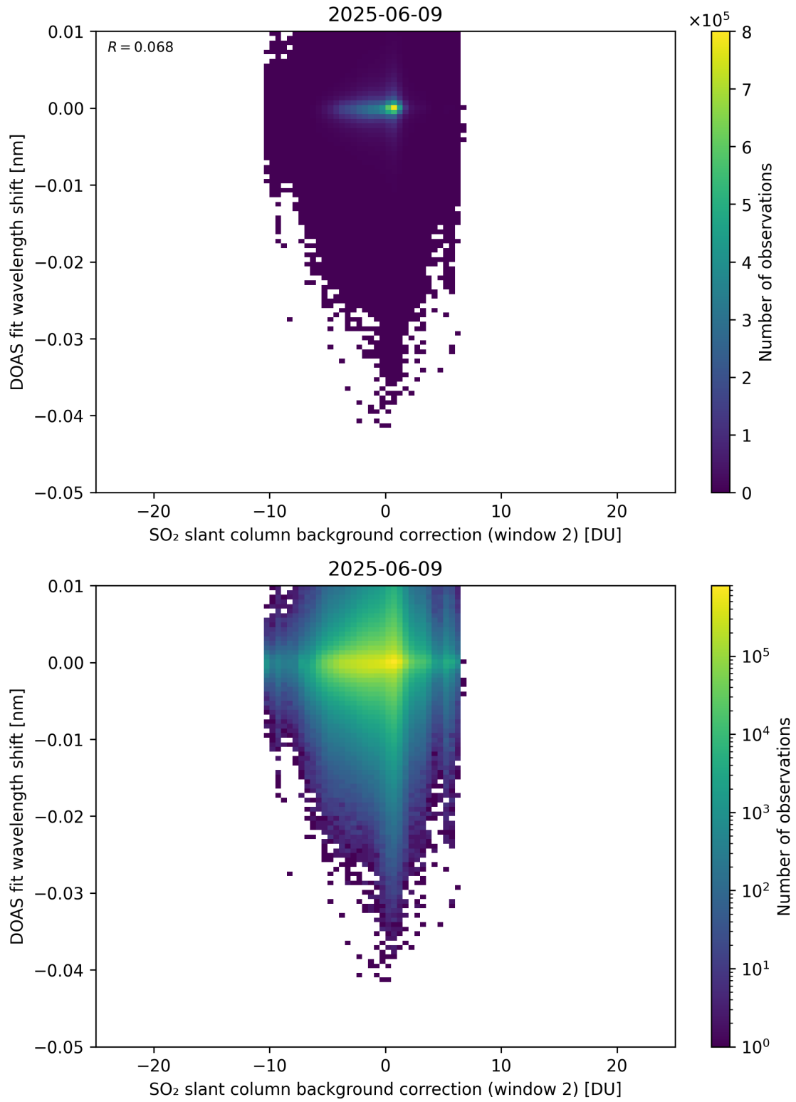
Figure 123: Scatter density plot of “SO 2 slant column background correction (window 2)” against “DOAS fit wavelength shift” for 2025-06-08 to 2025-06-10.
