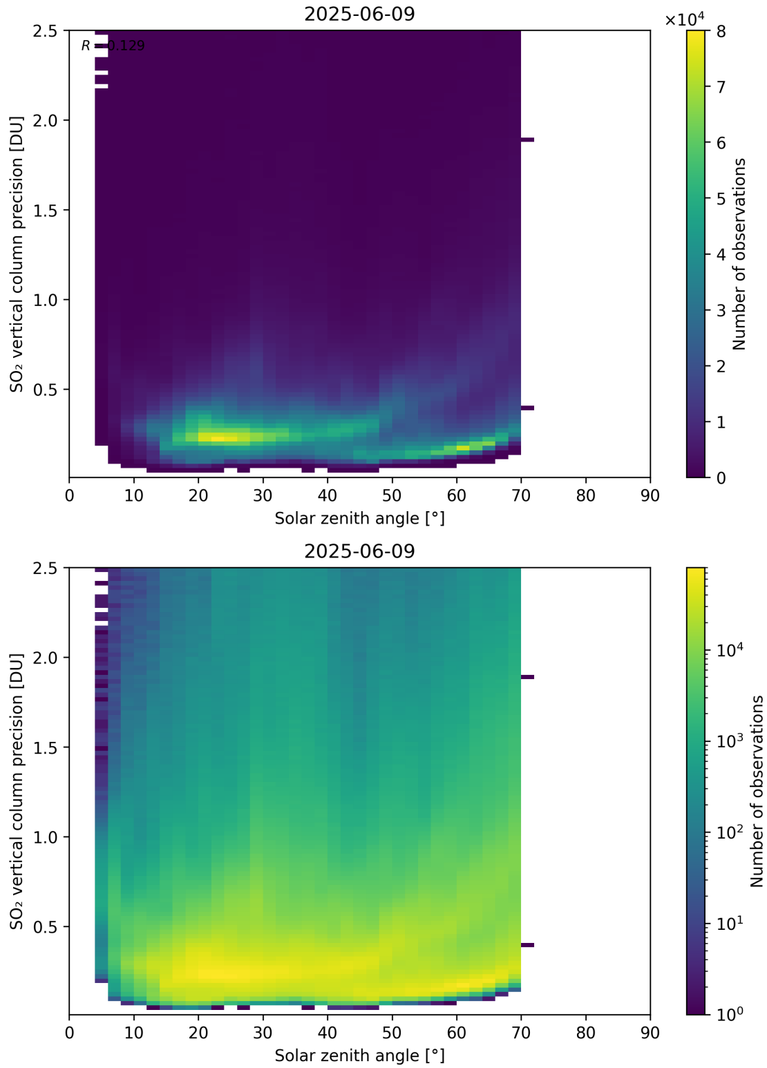
Figure 192: Scatter density plot of “Solar zenith angle” against “SO 2 vertical column precision” for 2025-06-08 to 2025-06-10.
