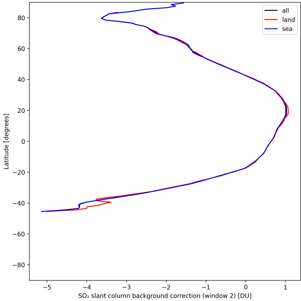
Figure 44: Zonal average of “SO 2 slant column background correction (window 2)” for 2025-06-08 to 2025-06-10.
