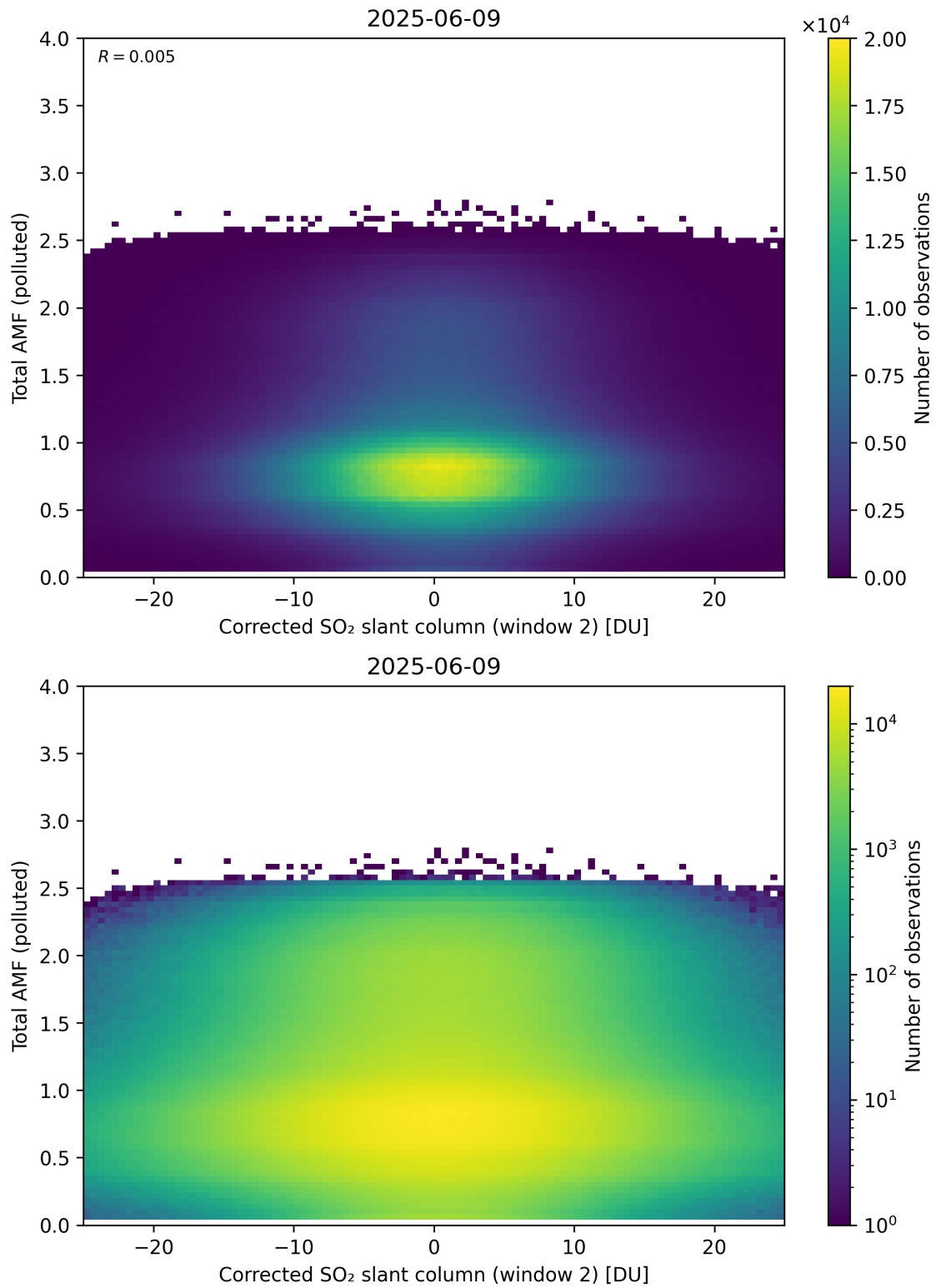
Figure 253: Scatter density plot of “Corrected SO 2 slant column (window 2)” against “Total AMF (polluted)” for 2025-06-08 to 2025-06-10.
