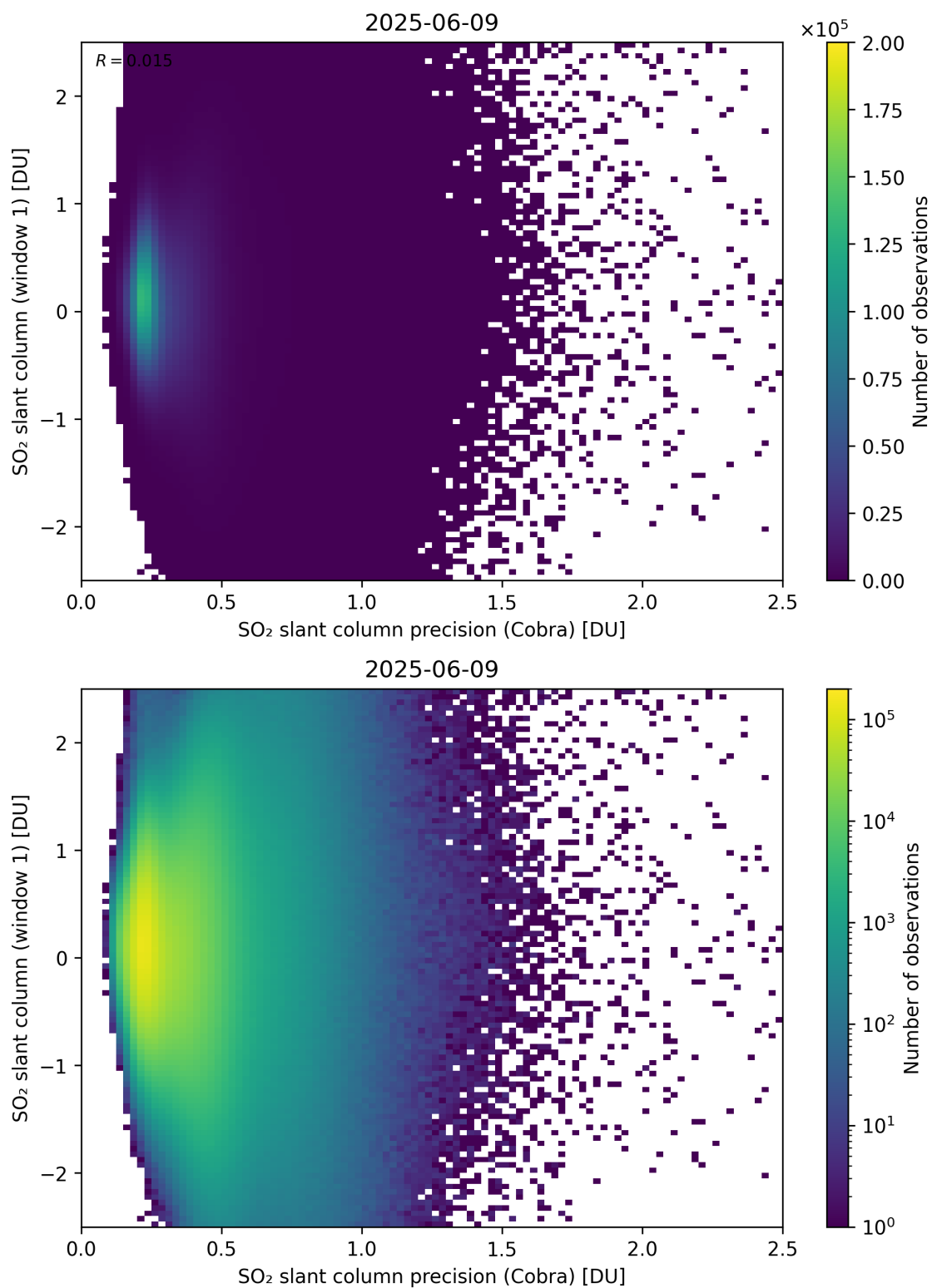
Figure 208: Scatter density plot of “SO 2 slant column precision (Cobra)” against “SO 2 slant column (window 1)” for 2025-06-08 to 2025-06-10.
