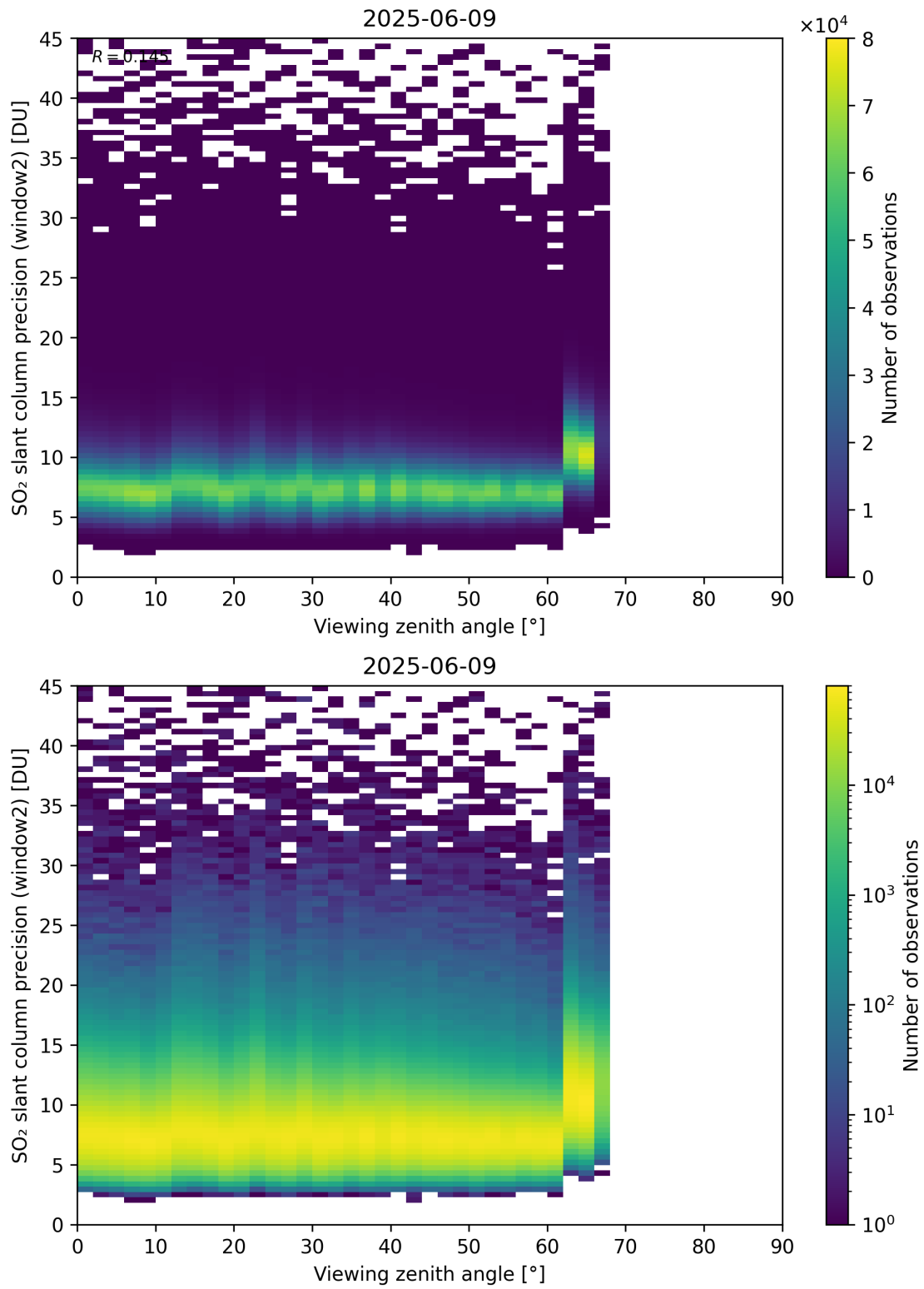
Figure 378: Scatter density plot of “Viewing zenith angle” against “SO 2 slant column precision (window2)” for 2025-06-08 to 2025-06-10.
