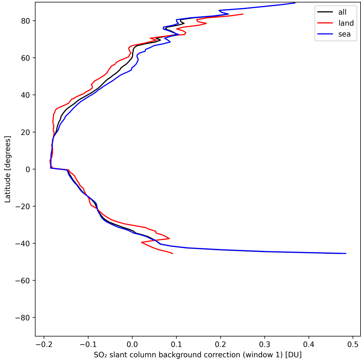
Figure 40: Zonal average of “SO 2 slant column background correction (window 1)” for 2025-06-08 to 2025-06-10.
