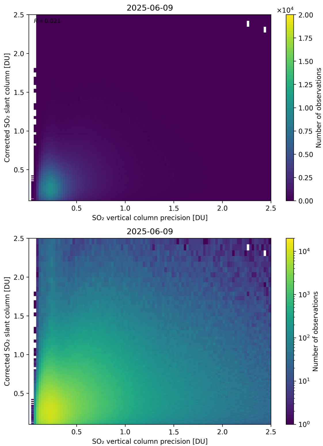
Figure 338: Scatter density plot of “SO 2 vertical column precision” against “Corrected SO 2 slant column” for 2025-06-08 to 2025-06-10.
