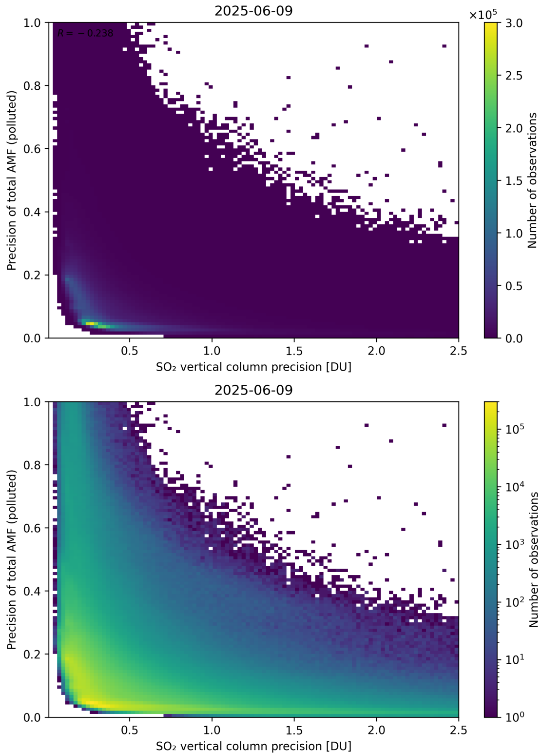
Figure 347: Scatter density plot of “SO 2 vertical column precision” against “Precision of total AMF (polluted)” for 2025-06-08 to 2025-06-10.
