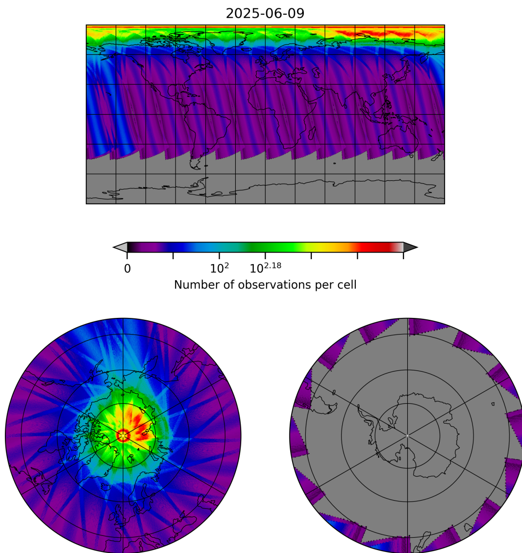
Figure 30: Map of the number of observations for 2025-06-08 to 2025-06-10
