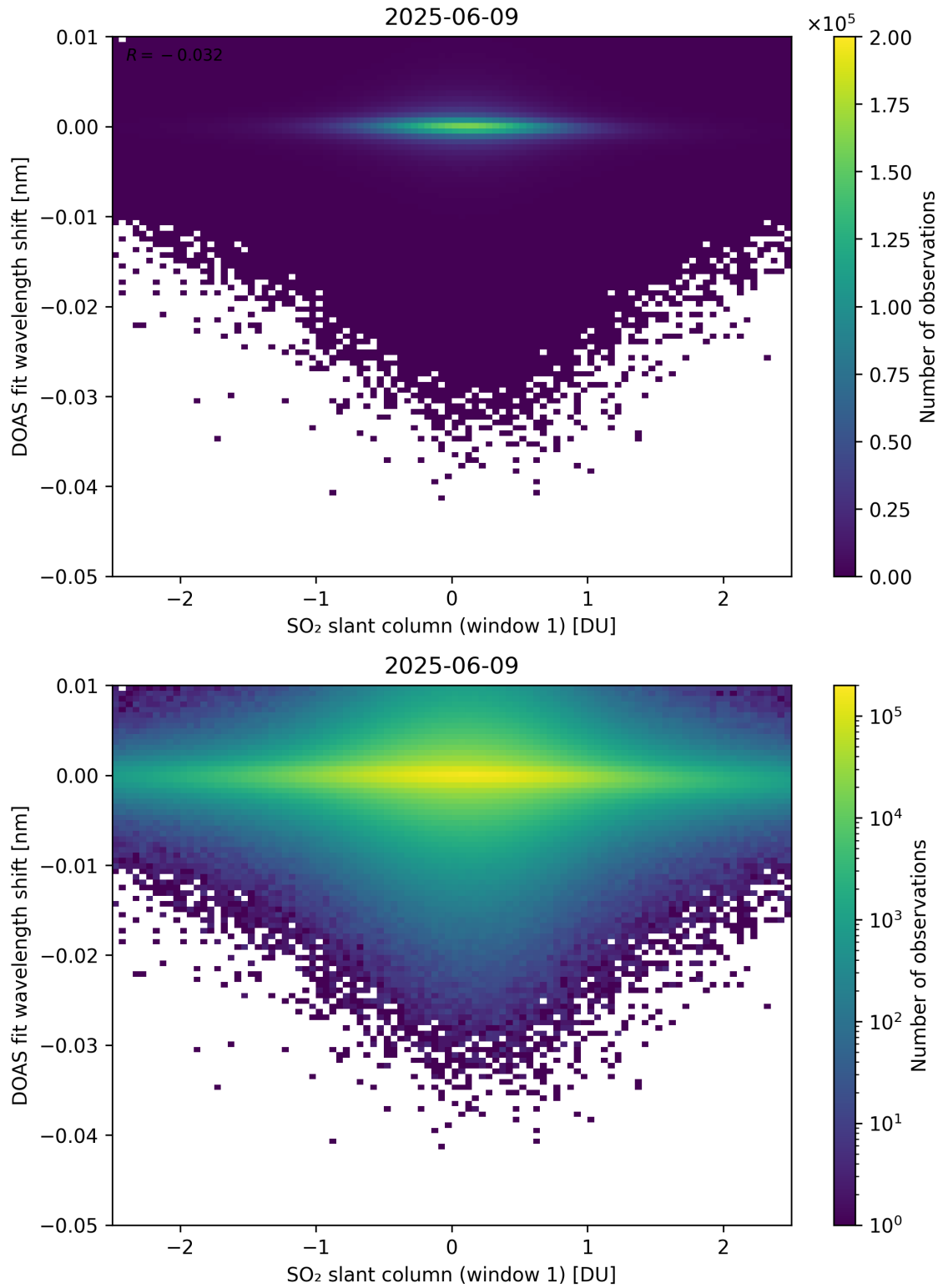
Figure 265: Scatter density plot of “SO 2 slant column (window 1)” against “DOAS fit wavelength shift” for 2025-06-08 to 2025-06-10.
