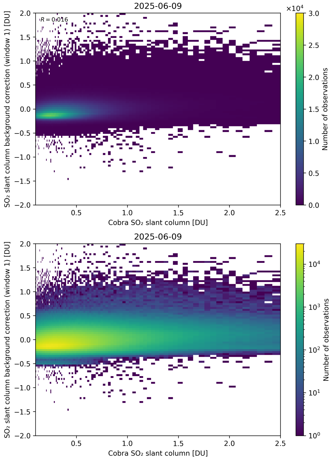
Figure 193: Scatter density plot of “Cobra SO 2 slant column” against “SO 2 slant column background correction (window 1)” for 2025-06-08 to 2025-06-10.
