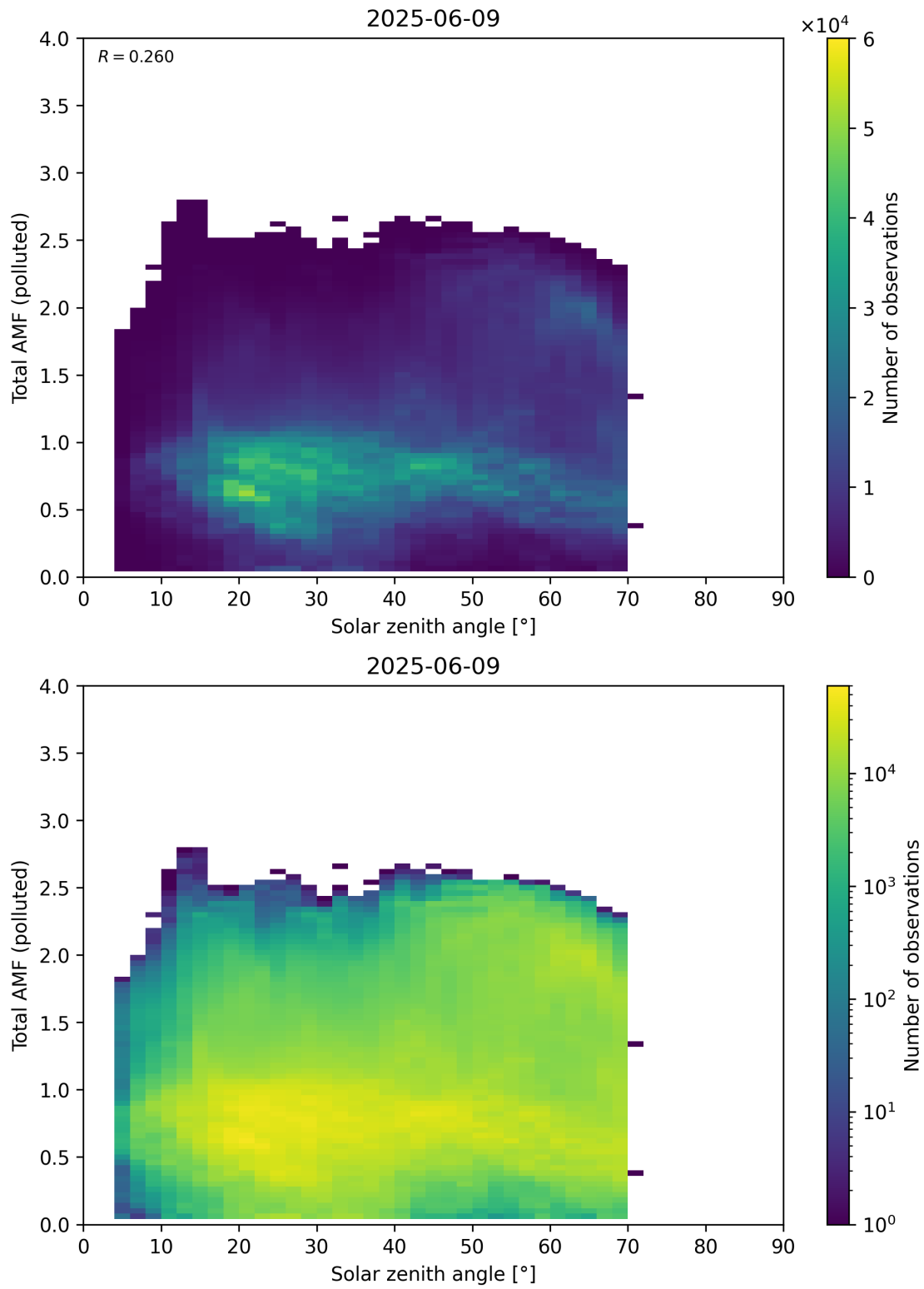
Figure 189: Scatter density plot of “Solar zenith angle” against “Total AMF (polluted)” for 2025-06-08 to 2025-06-10.
