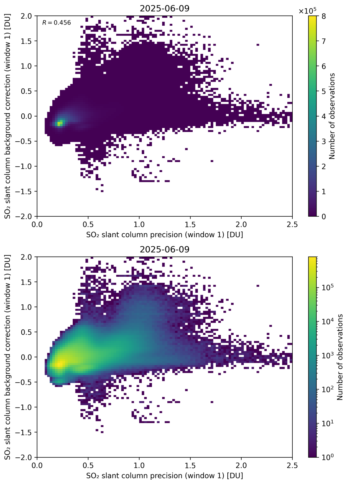
Figure 268: Scatter density plot of “SO 2 slant column precision (window 1)” against “SO 2 slant column background correction (window 1)” for 2025-06-08 to 2025-06-10.
