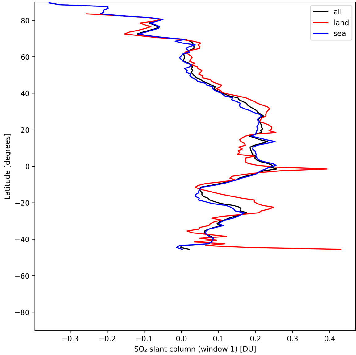
Figure 37: Zonal average of “SO 2 slant column (window 1)” for 2025-06-08 to 2025-06-10.
