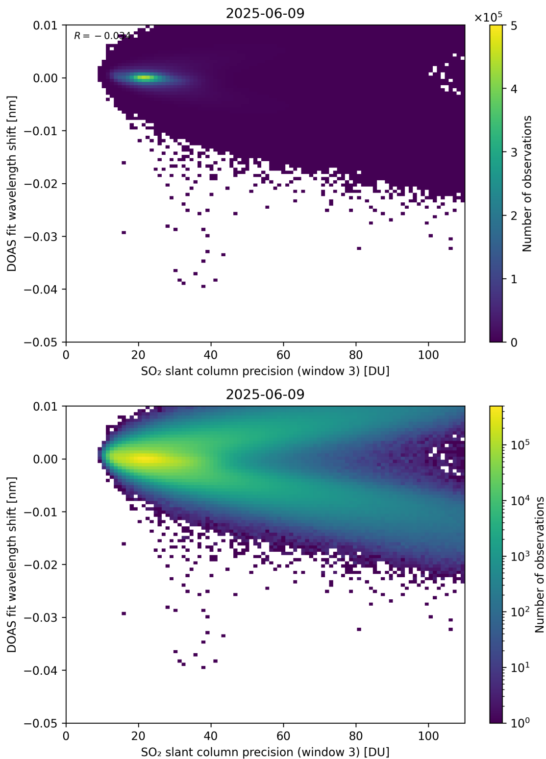
Figure 308: Scatter density plot of “SO 2 slant column precision (window 3)” against “DOAS fit wavelength shift” for 2025-06-08 to 2025-06-10.
