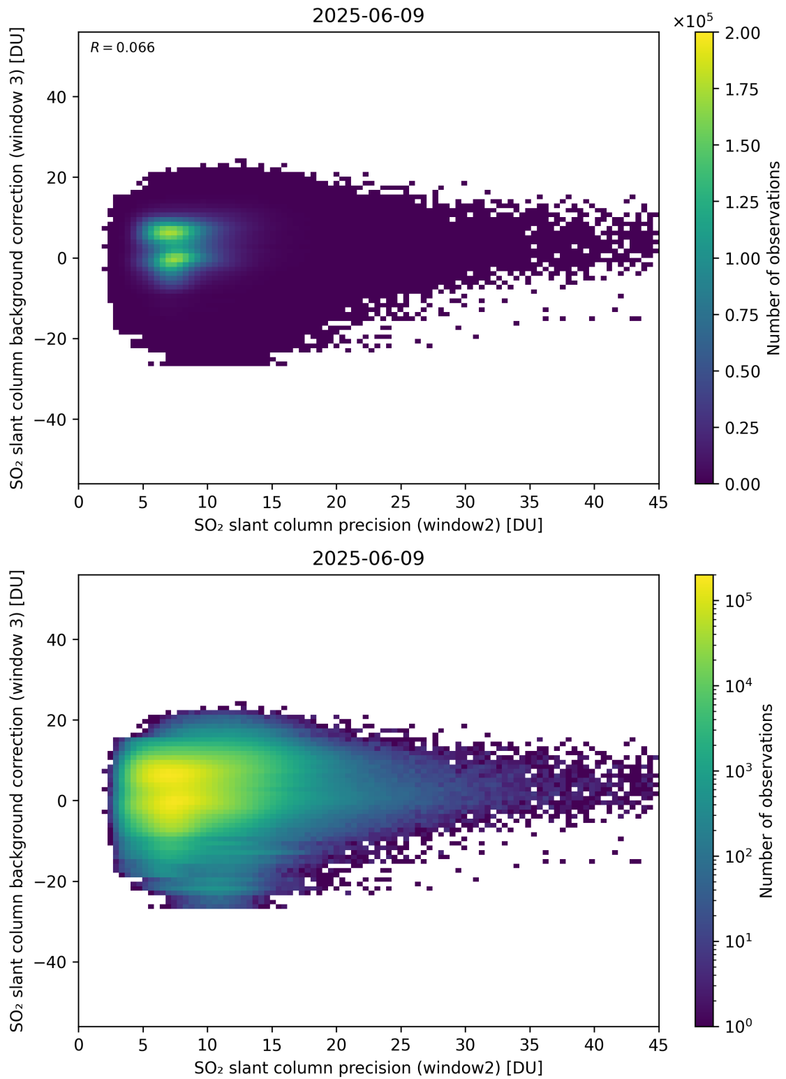
Figure 292: Scatter density plot of “SO 2 slant column precision (window2)” against “SO 2 slant column background correction (window 3)” for 2025-06-08 to 2025-06-10.
