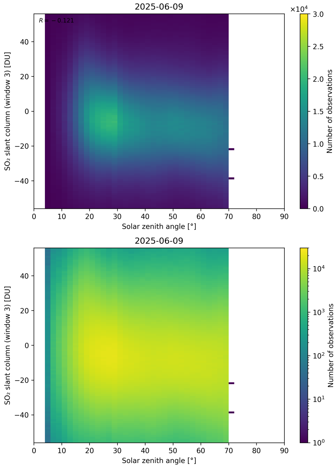
Figure 187: Scatter density plot of “Solar zenith angle” against “SO 2 slant column (window 3)” for 2025-06-08 to 2025-06-10.
