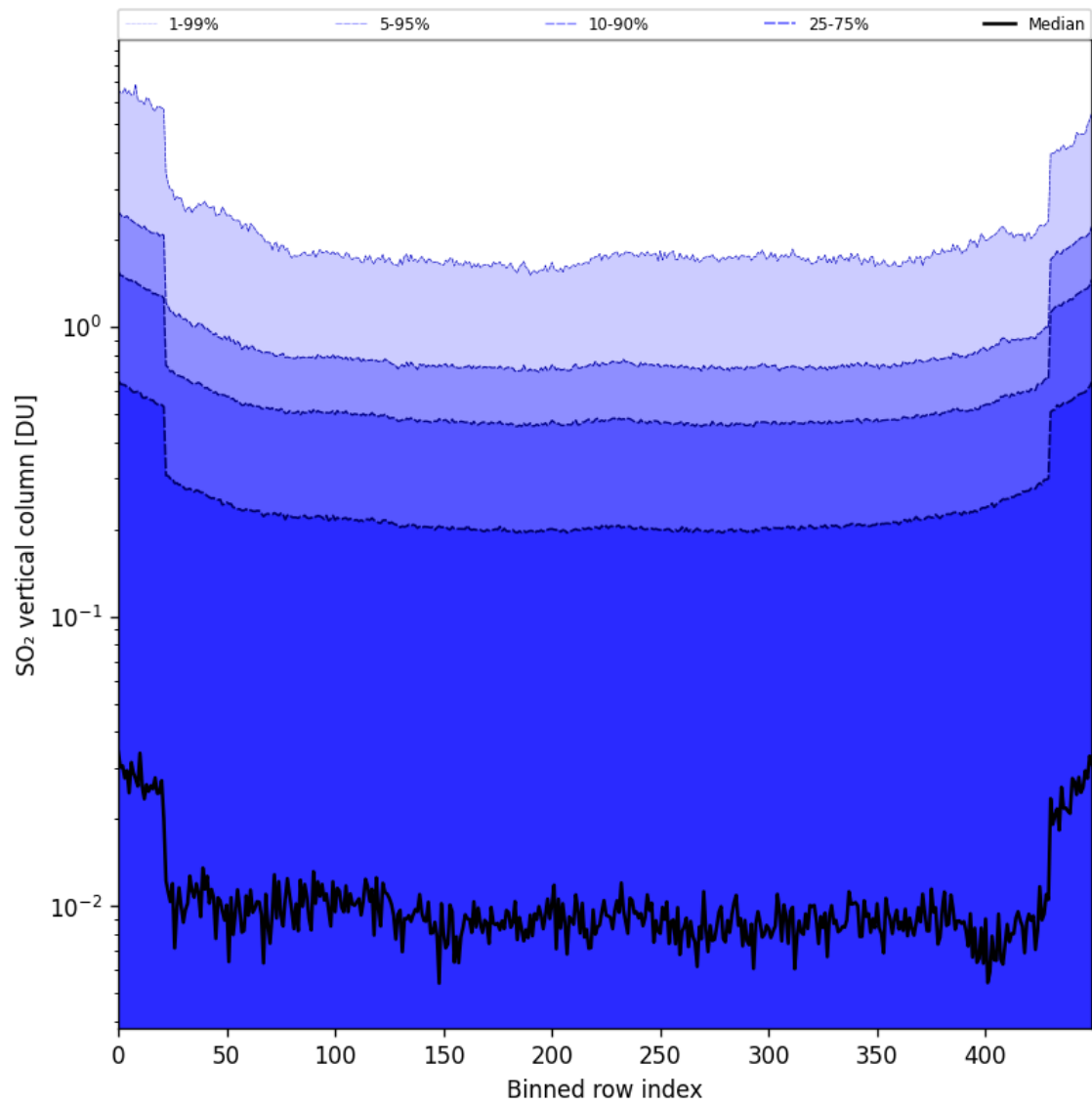
Figure 84: Along track statistics of “SO 2 vertical column” for 2025-06-08 to 2025-06-10
