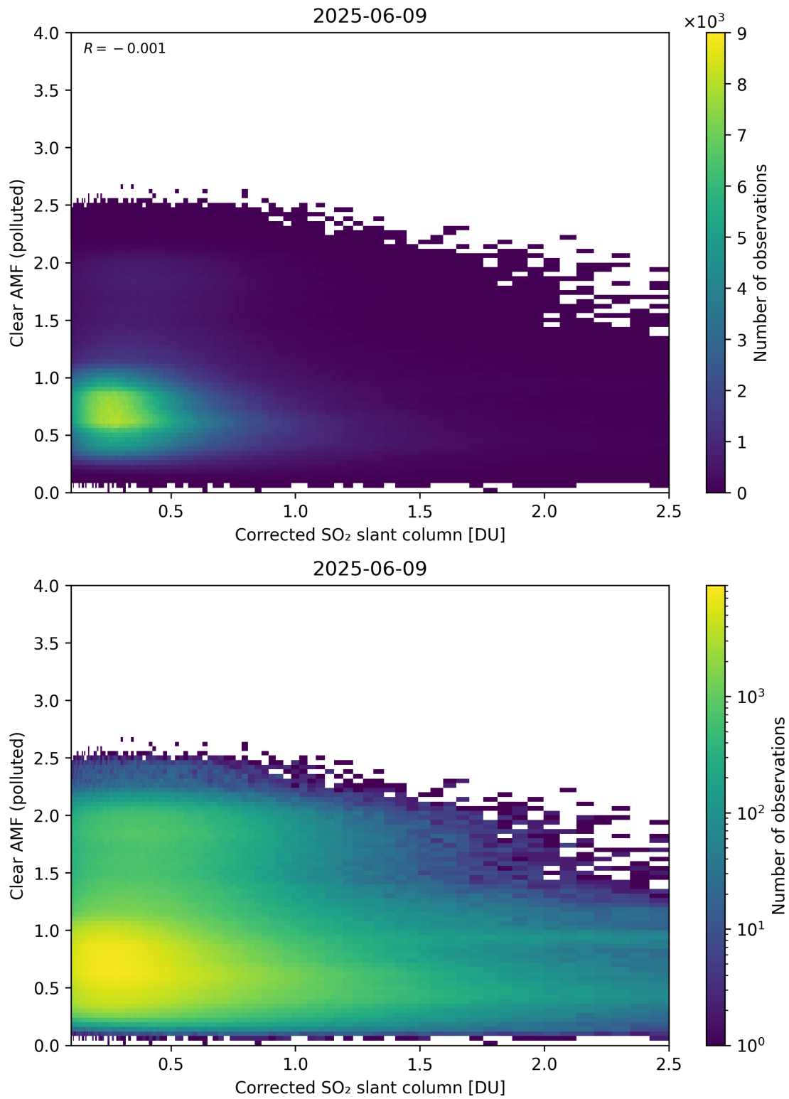
Figure 232: Scatter density plot of “Corrected SO 2 slant column” against “Clear AMF (polluted)” for 2025-06-08 to 2025-06-10.
