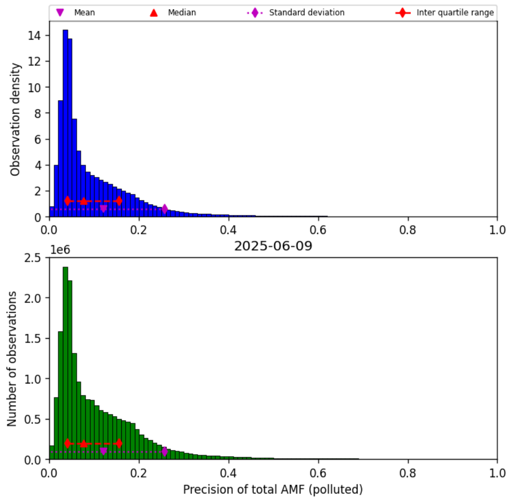
Figure 80: Histogram of “Precision of total AMF (polluted)” for 2025-06-08 to 2025-06-10
