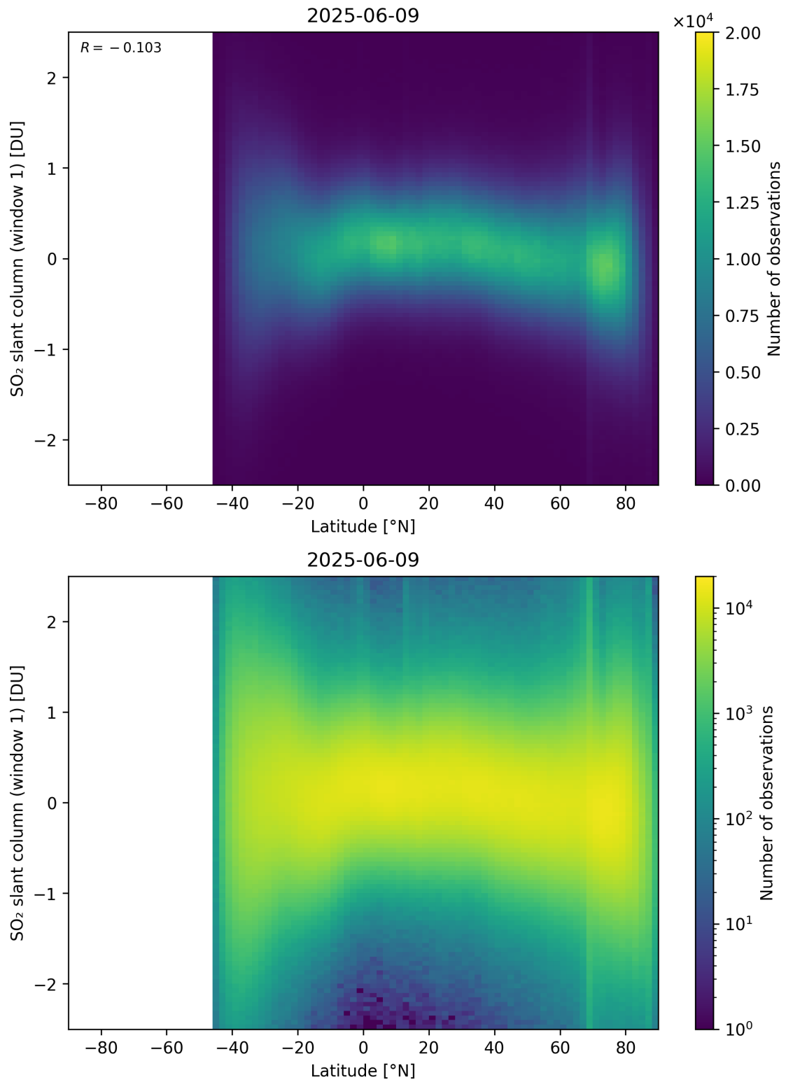
Figure 162: Scatter density plot of “Latitude” against “SO 2 slant column (window 1)” for 2025-06-08 to 2025-06-10.
