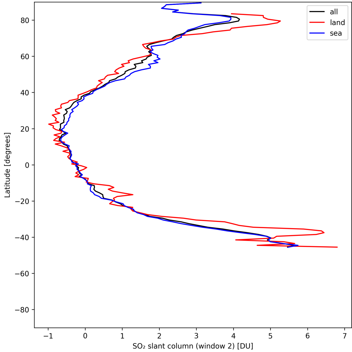
Figure 41: Zonal average of “SO 2 slant column (window 2)” for 2025-06-08 to 2025-06-10.
