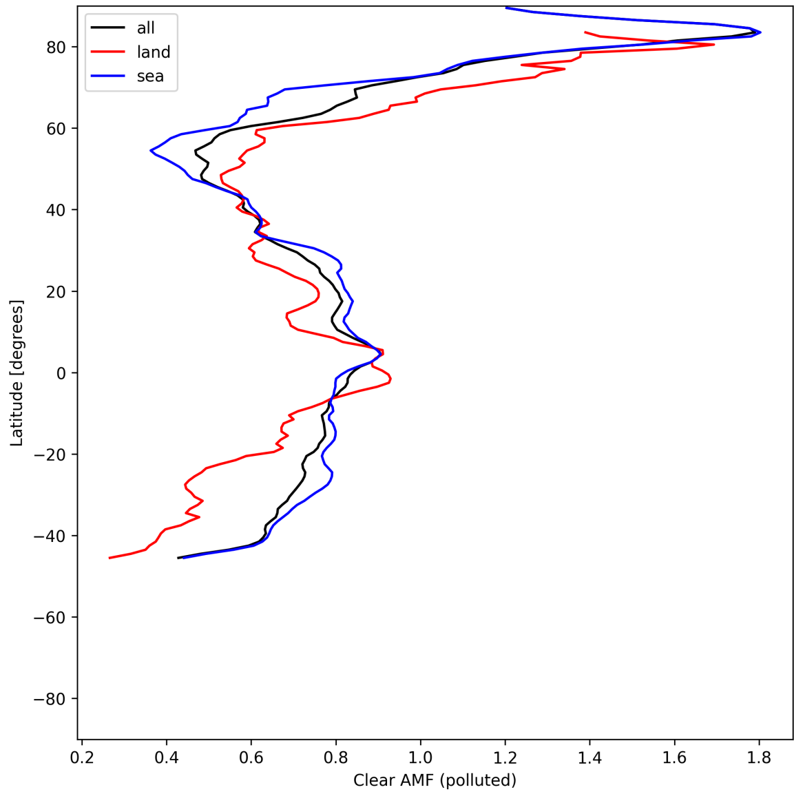
Figure 55: Zonal average of “Clear AMF (polluted)” for 2025-06-08 to 2025-06-10.
