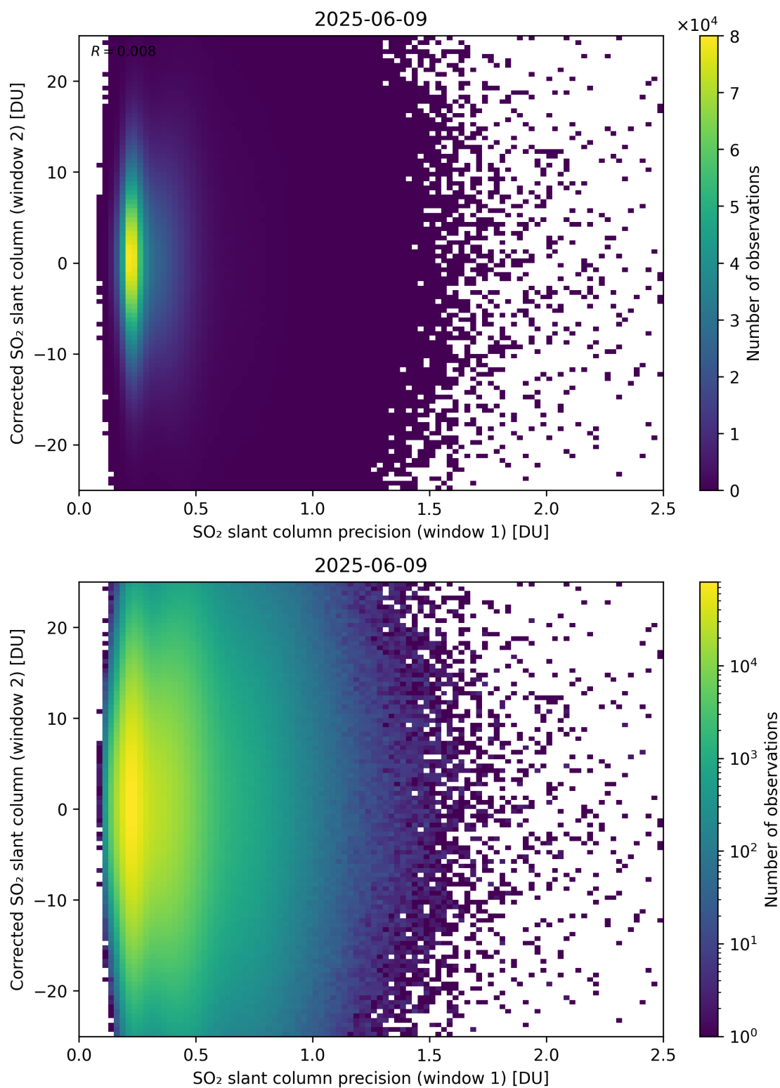
Figure 275: Scatter density plot of “SO 2 slant column precision (window 1)” against “Corrected SO 2 slant column (window 2)” for 2025-06-08 to 2025-06-10.
