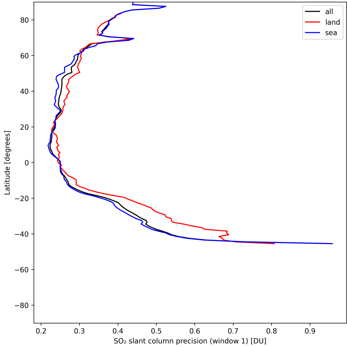
Figure 38: Zonal average of “SO 2 slant column precision (window 1)” for 2025-06-08 to 2025-06-10.
