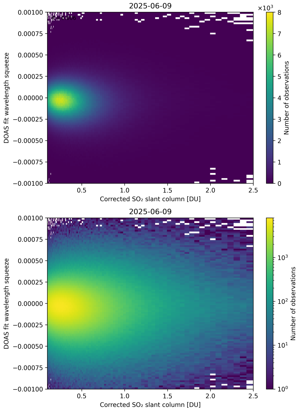
Figure 230: Scatter density plot of "Corrected SO 2 slant column" against "DOAS fit wavelength squeeze" for 2025-06-08 to 2025-06-10.
