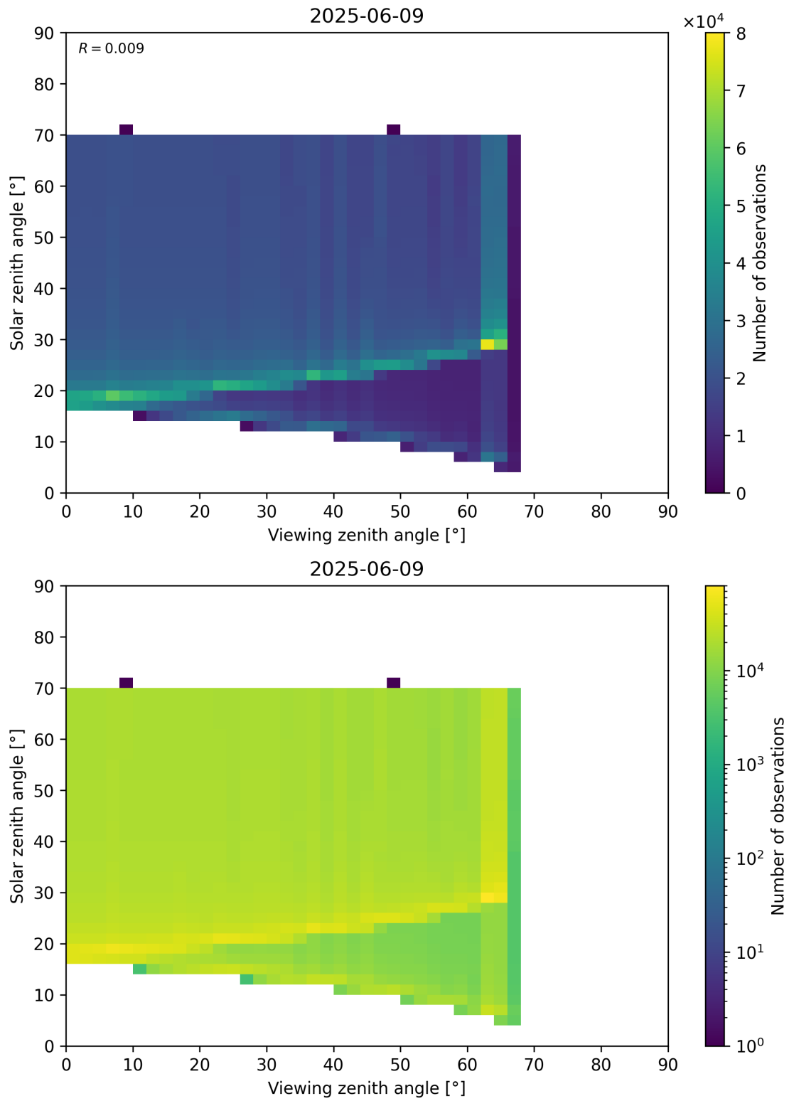
Figure 369: Scatter density plot of “Viewing zenith angle” against “Solar zenith angle” for 2025-06-08 to 2025-06-10.
