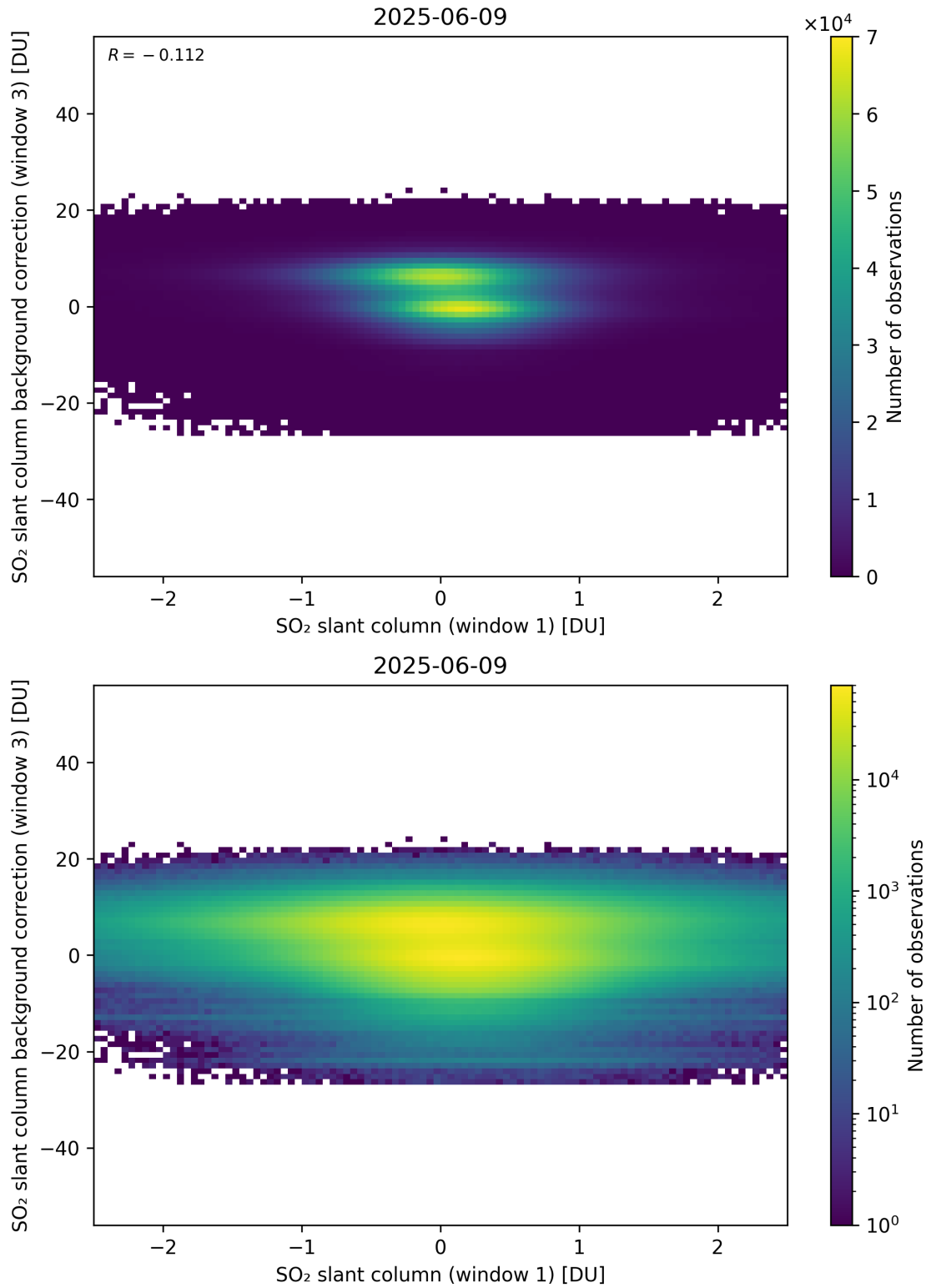
Figure 264: Scatter density plot of “SO 2 slant column (window 1)” against “SO 2 slant column background correction (window 3)” for 2025-06-08 to 2025-06-10.
