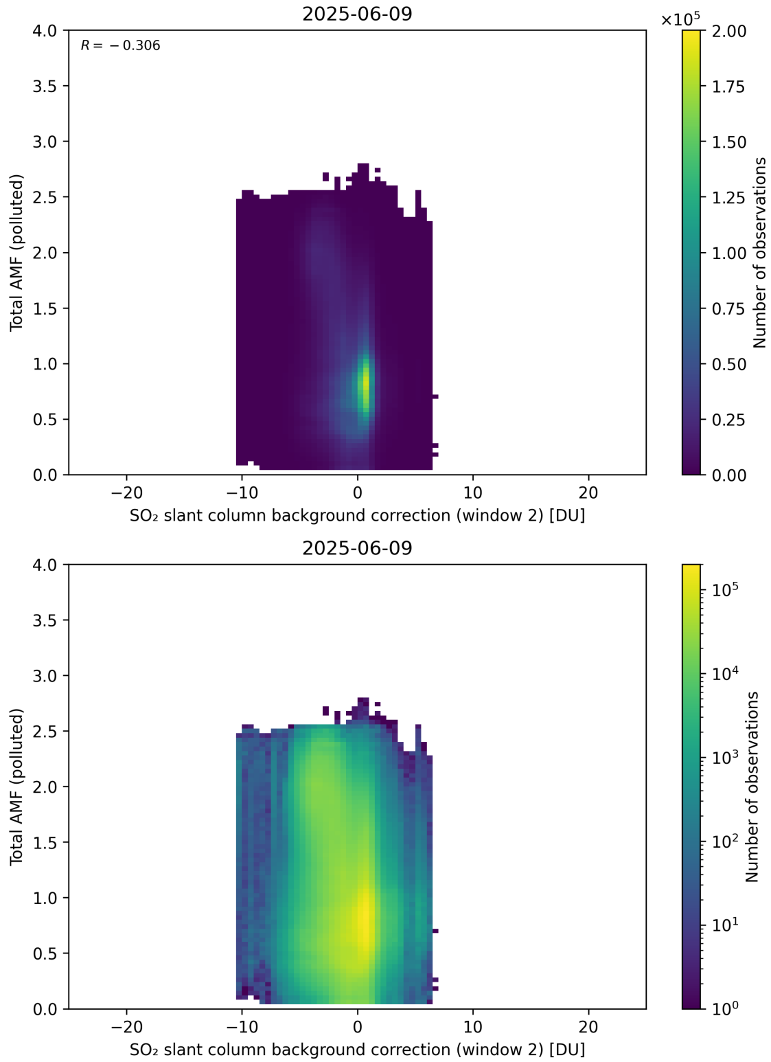
Figure 130: Scatter density plot of “SO 2 slant column background correction (window 2)” against “Total AMF (polluted)” for 2025-06-08 to 2025-06-10.
