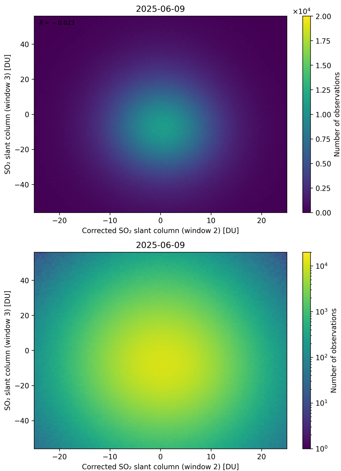
Figure 251: Scatter density plot of “Corrected SO 2 slant column (window 2)” against “SO 2 slant column (window 3)” for 2025-06-08 to 2025-06-10.
