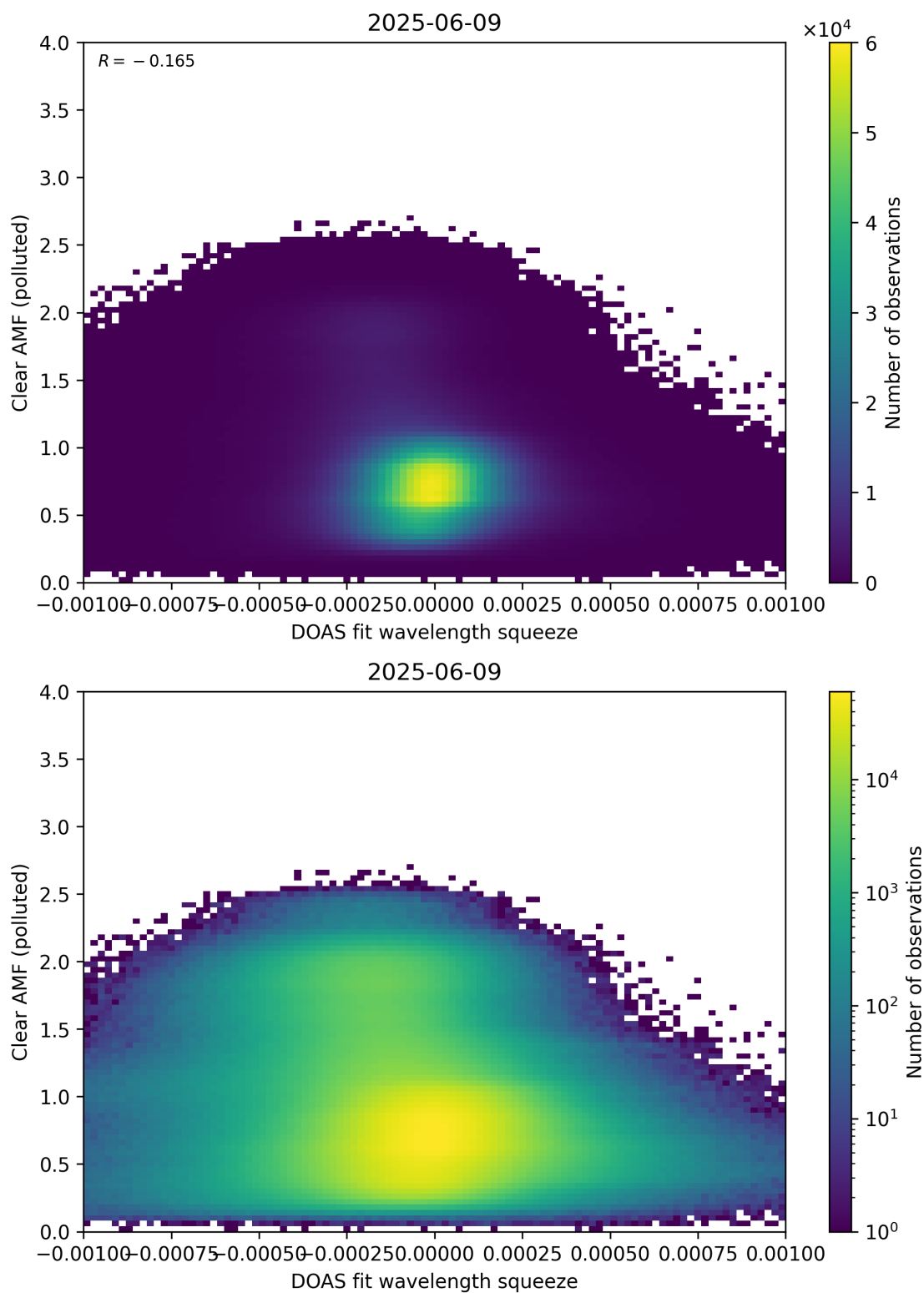
Figure 144: Scatter density plot of “DOAS fit wavelength squeeze” against “Clear AMF (polluted)” for 2025-06-08 to 2025-06-10.
