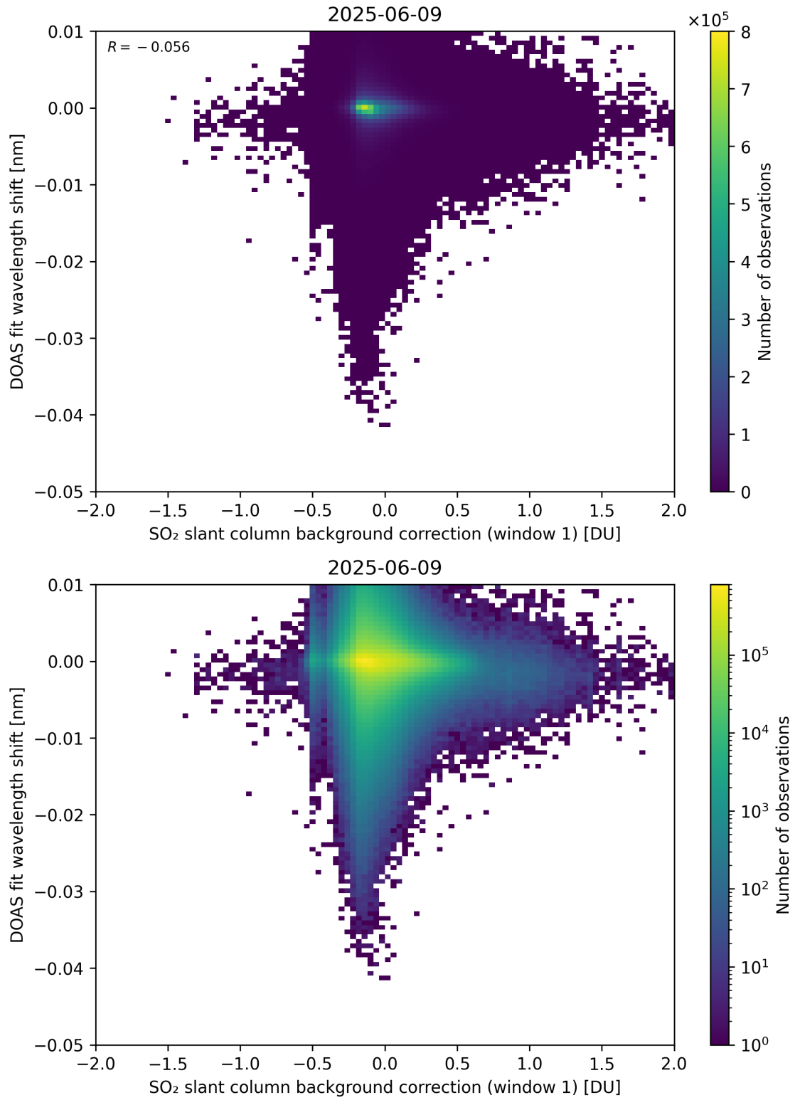
Figure 111: Scatter density plot of “SO 2 slant column background correction (window 1)” against “DOAS fit wavelength shift” for 2025-06-08 to 2025-06-10.
