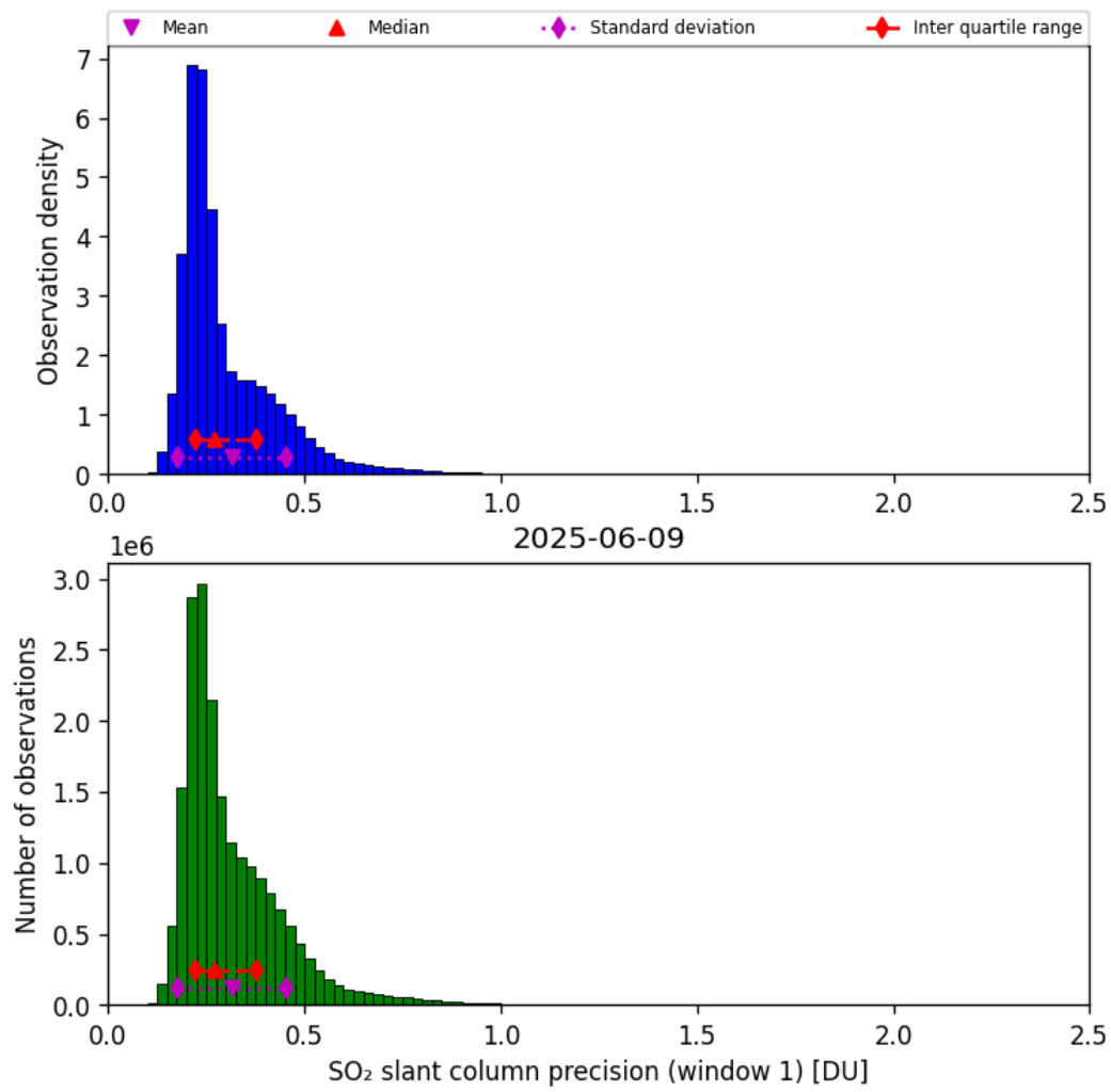
Figure 64: Histogram of “SO 2 slant column precision (window 1)” for 2025-06-08 to 2025-06-10
