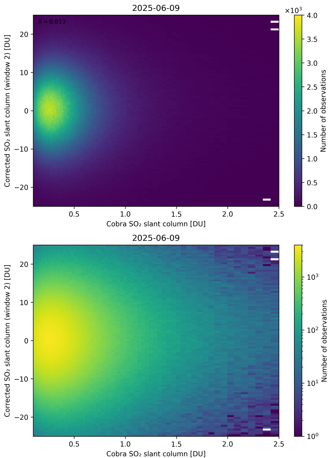
Figure 217: Scatter density plot of “Cobra SO 2 slant column” against “Corrected SO 2 slant column (window 2)” for 2025-06-08 to 2025-06-10.
