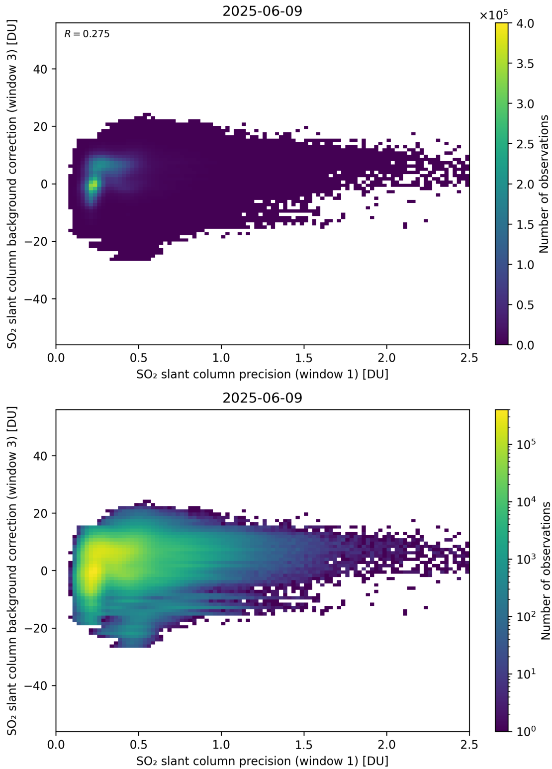
Figure 270: Scatter density plot of “SO 2 slant column precision (window 1)” against “SO 2 slant column background correction (window 3)” for 2025-06-08 to 2025-06-10.
