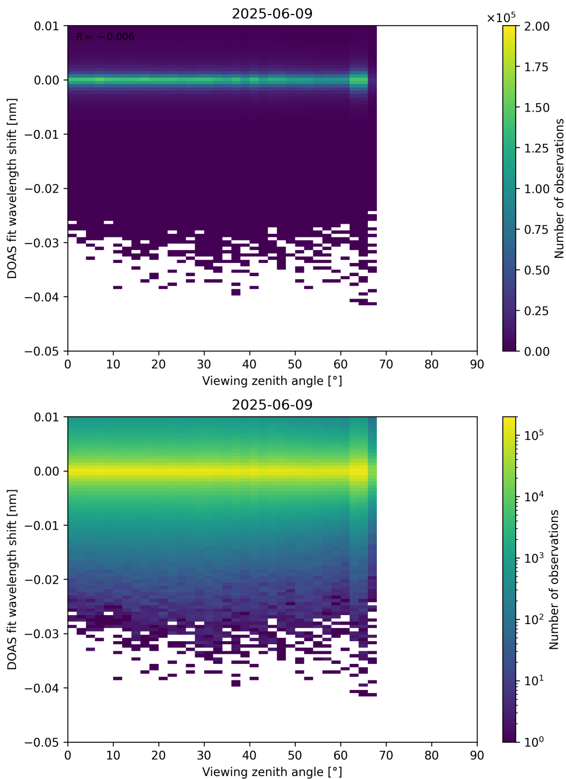
Figure 365: Scatter density plot of “Viewing zenith angle” against “DOAS fit wavelength shift” for 2025-06-08 to 2025-06-10.
