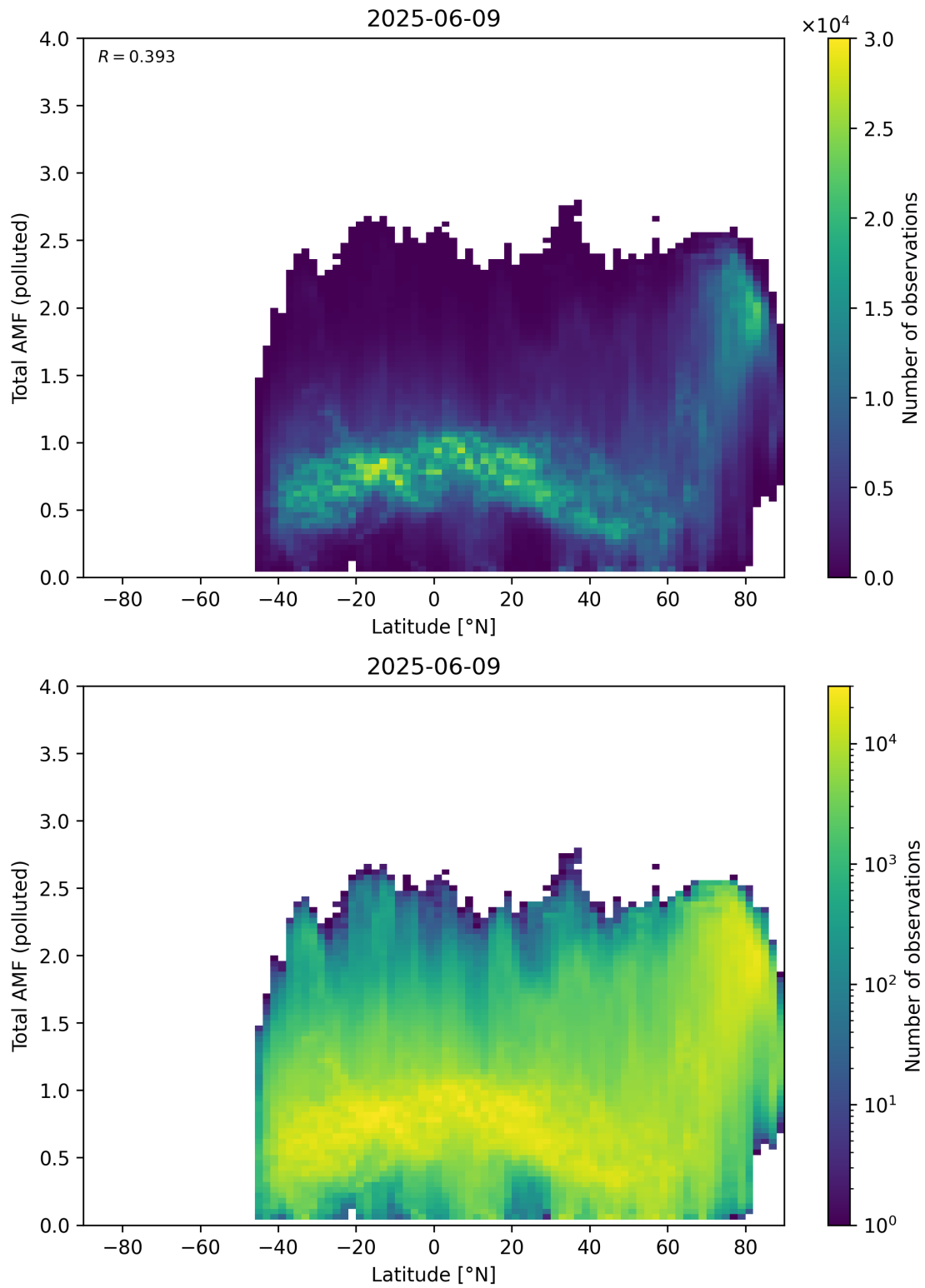
Figure 167: Scatter density plot of “Latitude” against “Total AMF (polluted)” for 2025-06-08 to 2025-06-10.
