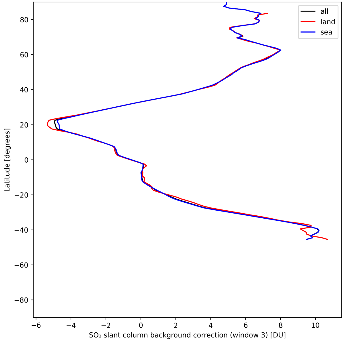
Figure 48: Zonal average of “SO 2 slant column background correction (window 3)” for 2025-06-08 to 2025-06-10.
