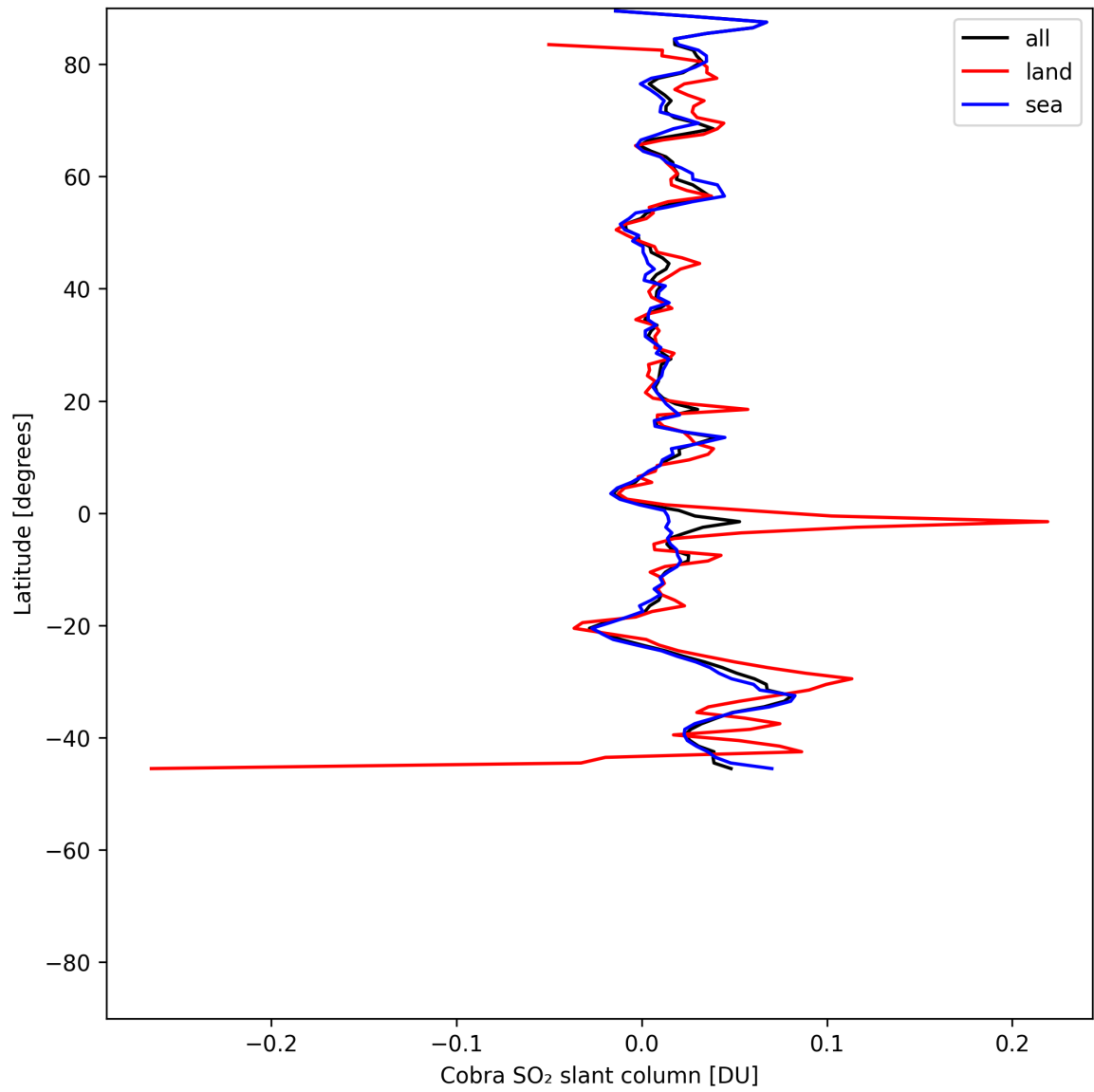
Figure 35: Zonal average of “Cobra SO 2 slant column” for 2025-06-08 to 2025-06-10.
