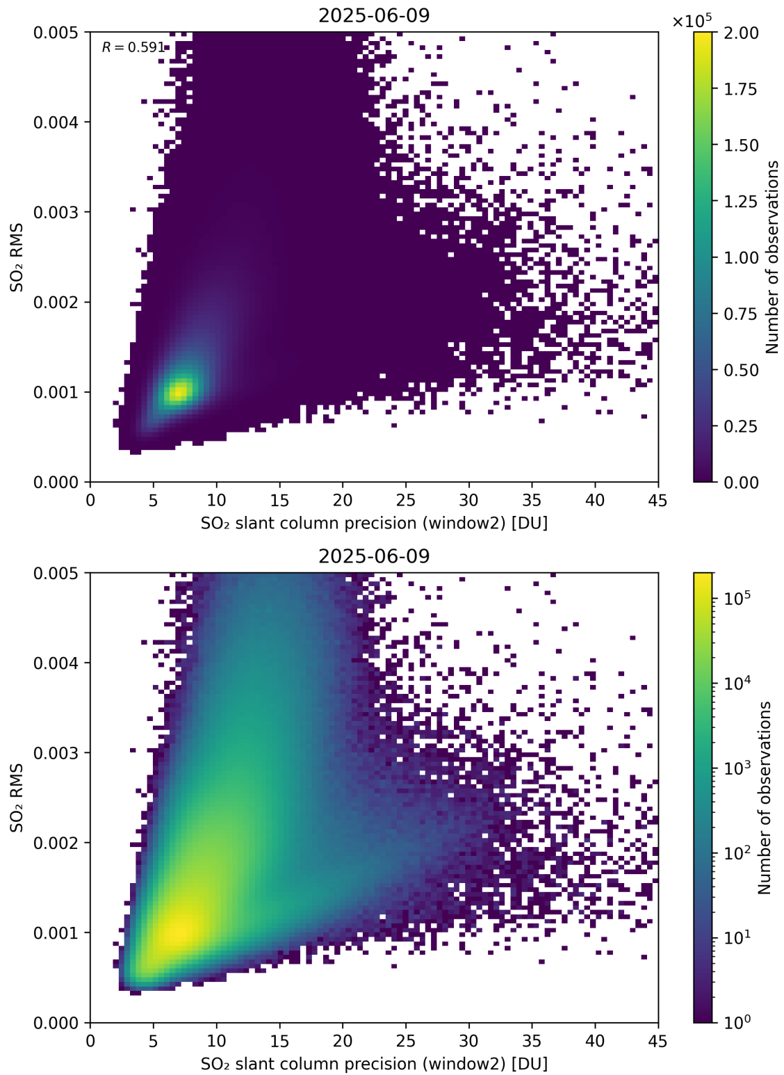
Figure 295: Scatter density plot of “SO 2 slant column precision (window2)” against “SO 2 RMS” for 2025-06-08 to 2025-06-10.
