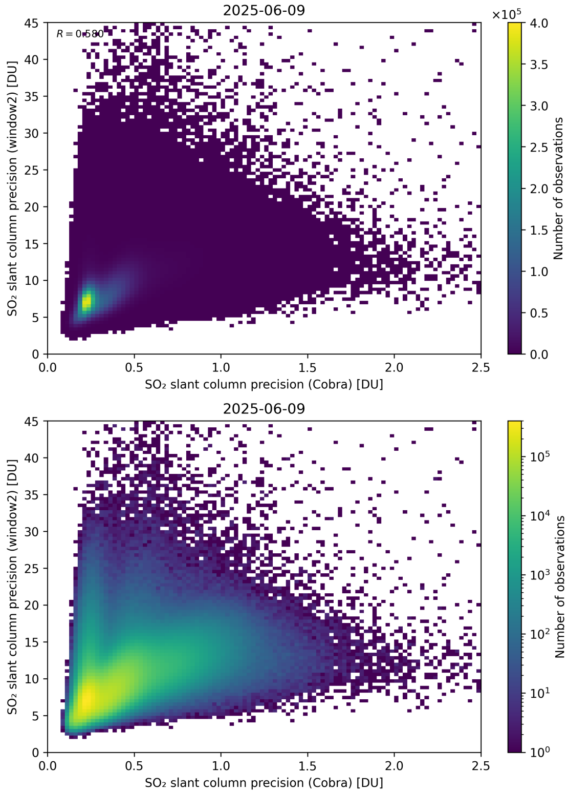
Figure 210: Scatter density plot of “SO 2 slant column precision (Cobra)” against “SO 2 slant column precision (window2)” for 2025-06-08 to 2025-06-10.
