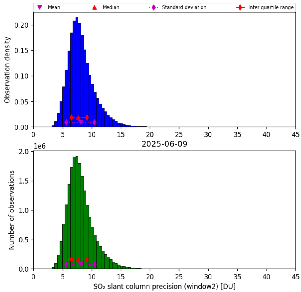
Figure 68: Histogram of “SO 2 slant column precision (window2)” for 2025-06-08 to 2025-06-10
