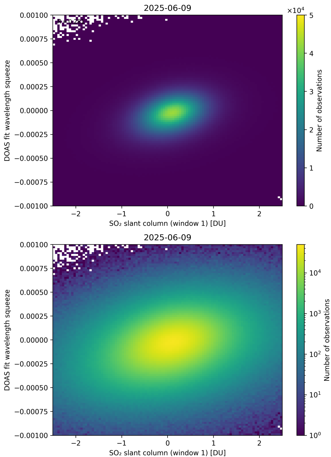
Figure 266: Scatter density plot of “SO 2 slant column (window 1)” against “DOAS fit wavelength squeeze” for 2025-06-08 to 2025-06-10.
