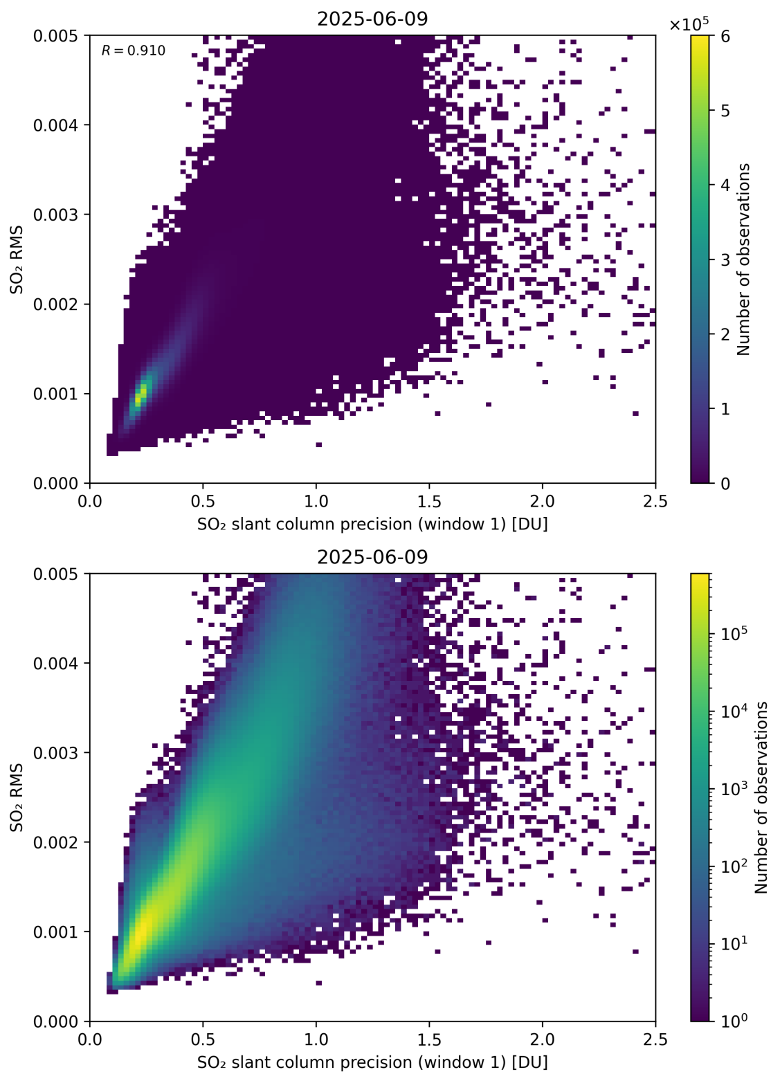
Figure 273: Scatter density plot of “SO 2 slant column precision (window 1)” against “SO 2 RMS” for 2025-06-08 to 2025-06-10.
