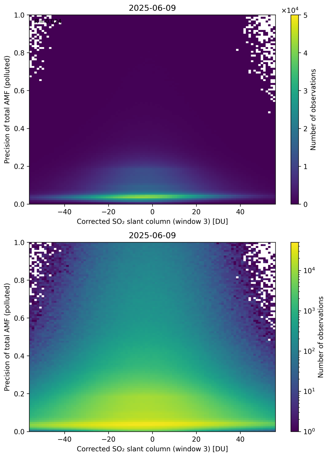
Figure 261: Scatter density plot of “Corrected SO 2 slant column (window 3)” against “Precision of total AMF (polluted)” for 2025-06-08 to 2025-06-10.
