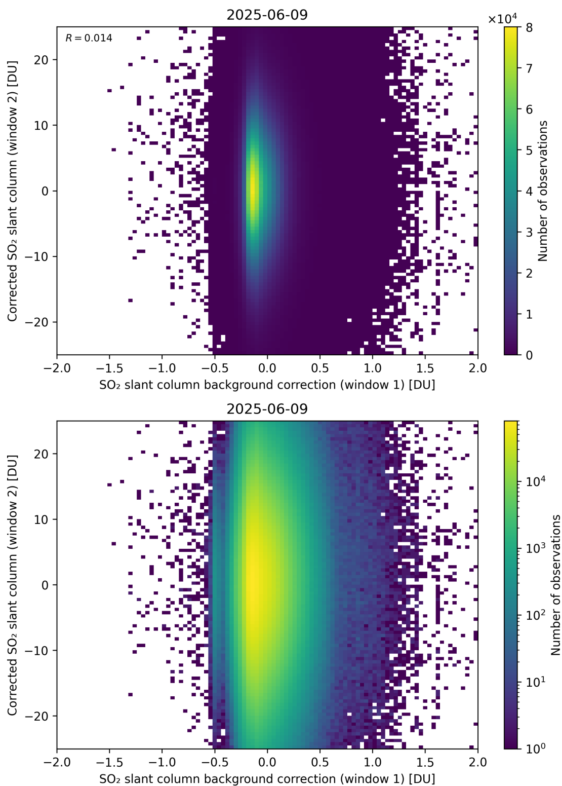
Figure 115: Scatter density plot of “SO 2 slant column background correction (window 1)” against “Corrected SO 2 slant column (window 2)” for 2025-06-08 to 2025-06-10.
