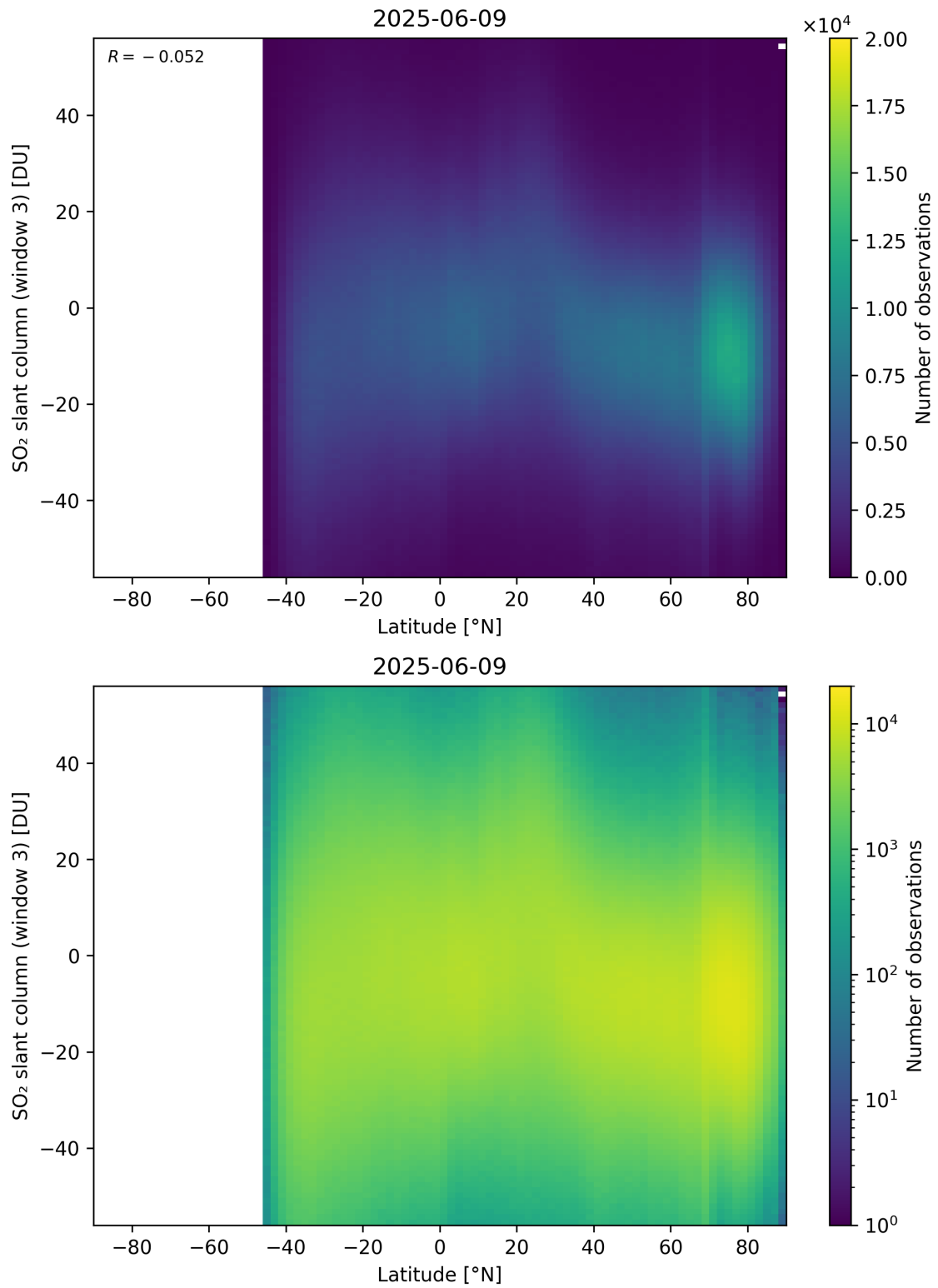
Figure 165: Scatter density plot of “Latitude” against “SO 2 slant column (window 3)” for 2025-06-08 to 2025-06-10.
