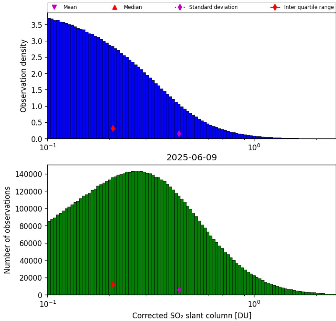
Figure 60: Histogram of “Corrected SO 2 slant column” for 2025-06-08 to 2025-06-10
