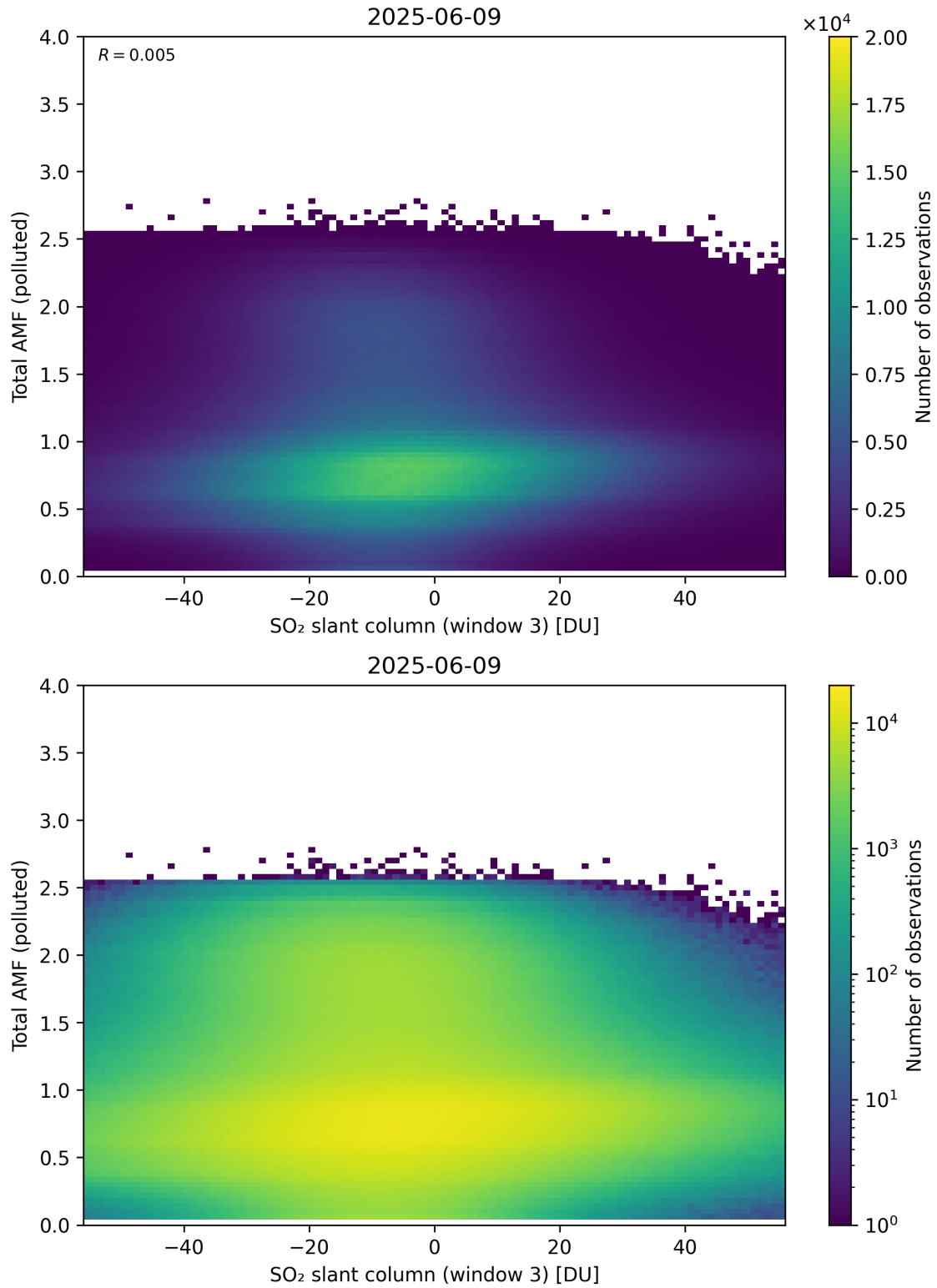
Figure 318: Scatter density plot of “SO 2 slant column (window 3)” against “Total AMF (polluted)” for 2025-06-08 to 2025-06-10.
