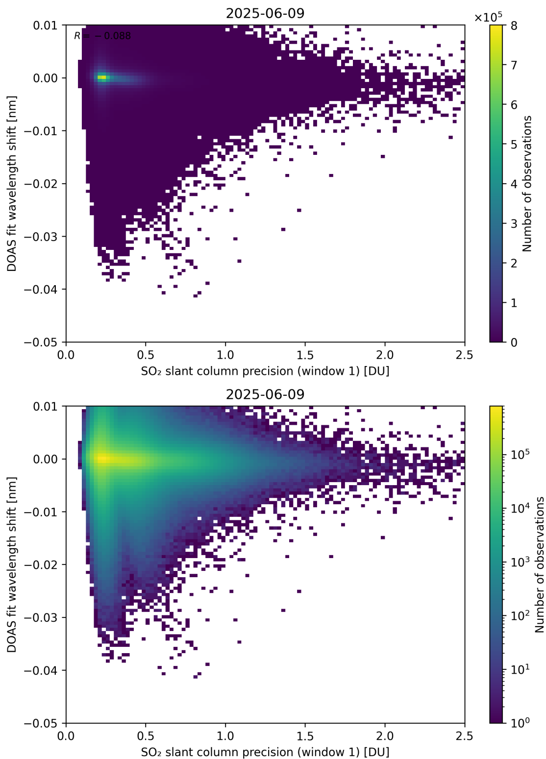
Figure 271: Scatter density plot of “SO 2 slant column precision (window 1)” against “DOAS fit wavelength shift” for 2025-06-08 to 2025-06-10.
