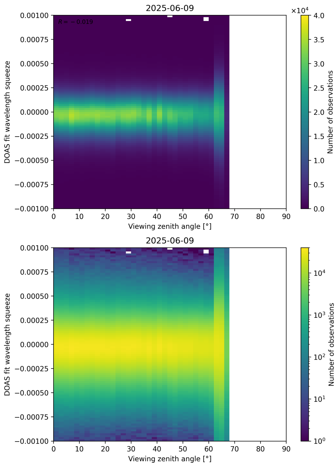
Figure 366: Scatter density plot of “Viewing zenith angle” against “DOAS fit wavelength squeeze” for 2025-06-08 to 2025-06-10.
