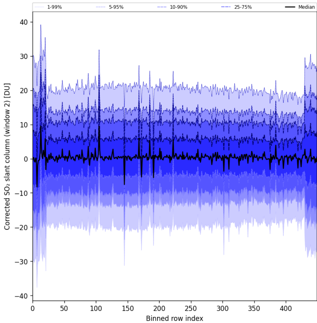
Figure 95: Along track statistics of “Corrected SO 2 slant column (window 2)” for 2025-06-08 to 2025-06-10
