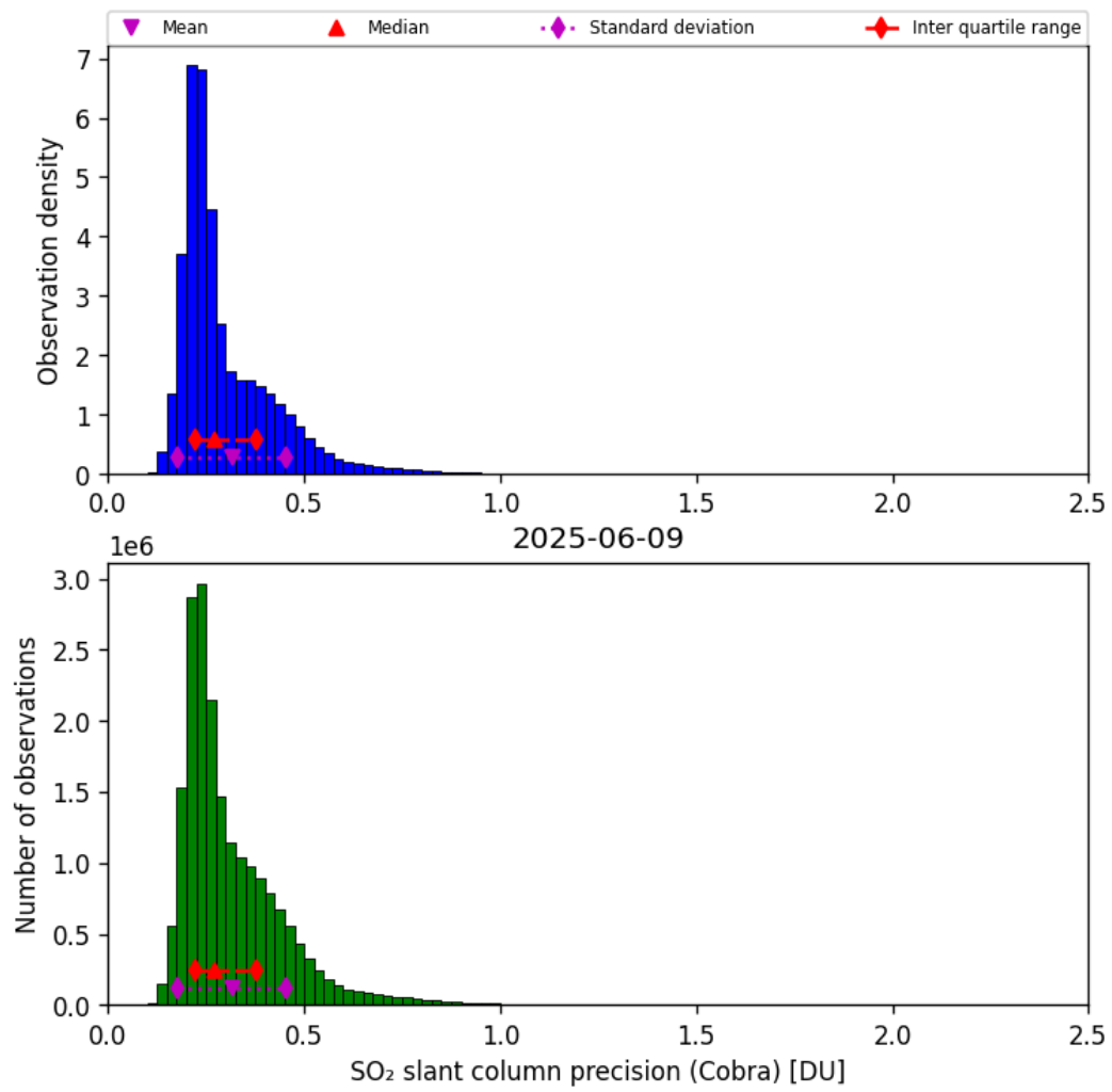
Figure 62: Histogram of “SO 2 slant column precision (Cobra)” for 2025-06-08 to 2025-06-10
