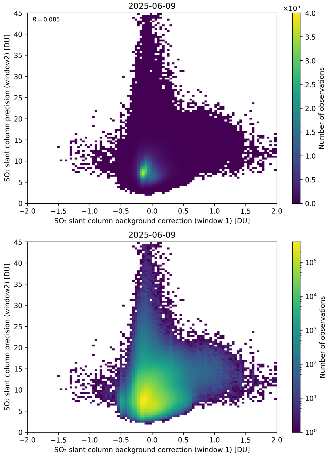
Figure 117: Scatter density plot of “SO 2 slant column background correction (window 1)” against “SO 2 slant column precision (window2)” for 2025-06-08 to 2025-06-10.
