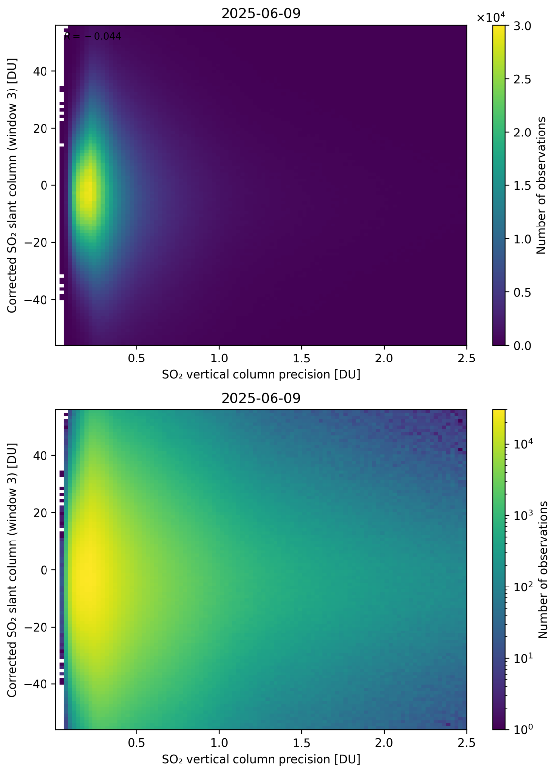
Figure 340: Scatter density plot of “SO 2 vertical column precision” against “Corrected SO 2 slant column (window 3)” for 2025-06-08 to 2025-06-10.
