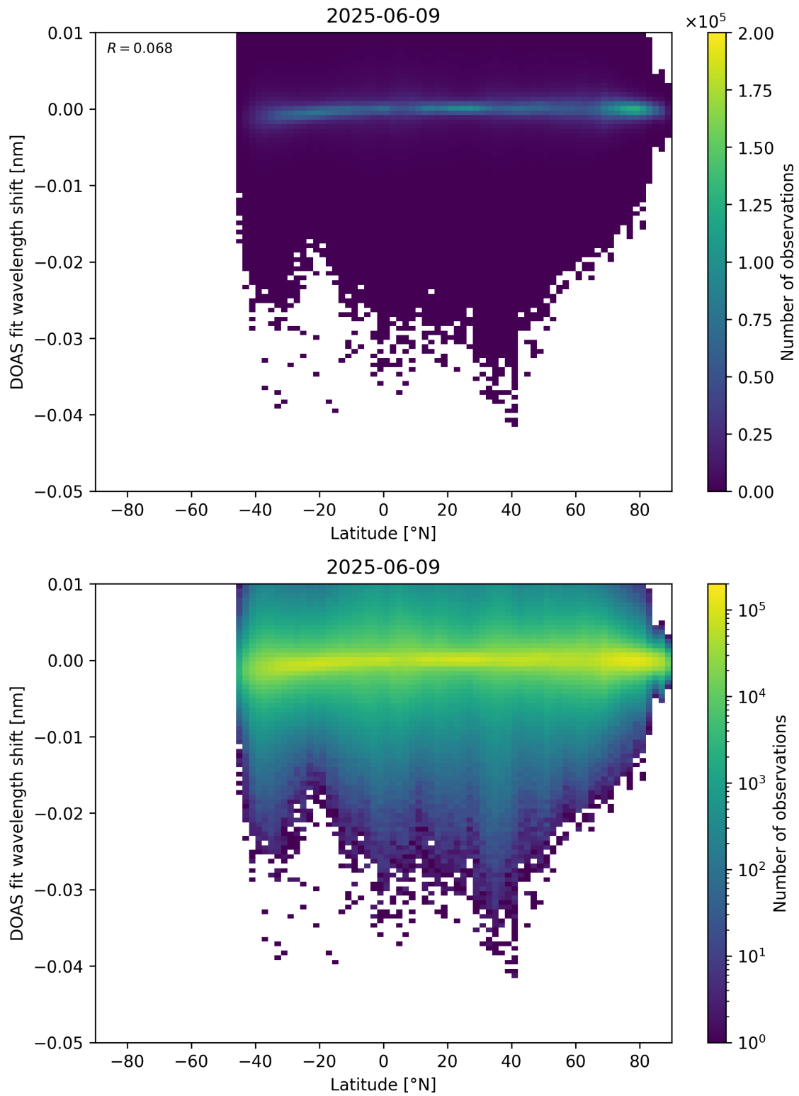
Figure 153: Scatter density plot of “Latitude” against “DOAS fit wavelength shift” for 2025-06-08 to 2025-06-10.
