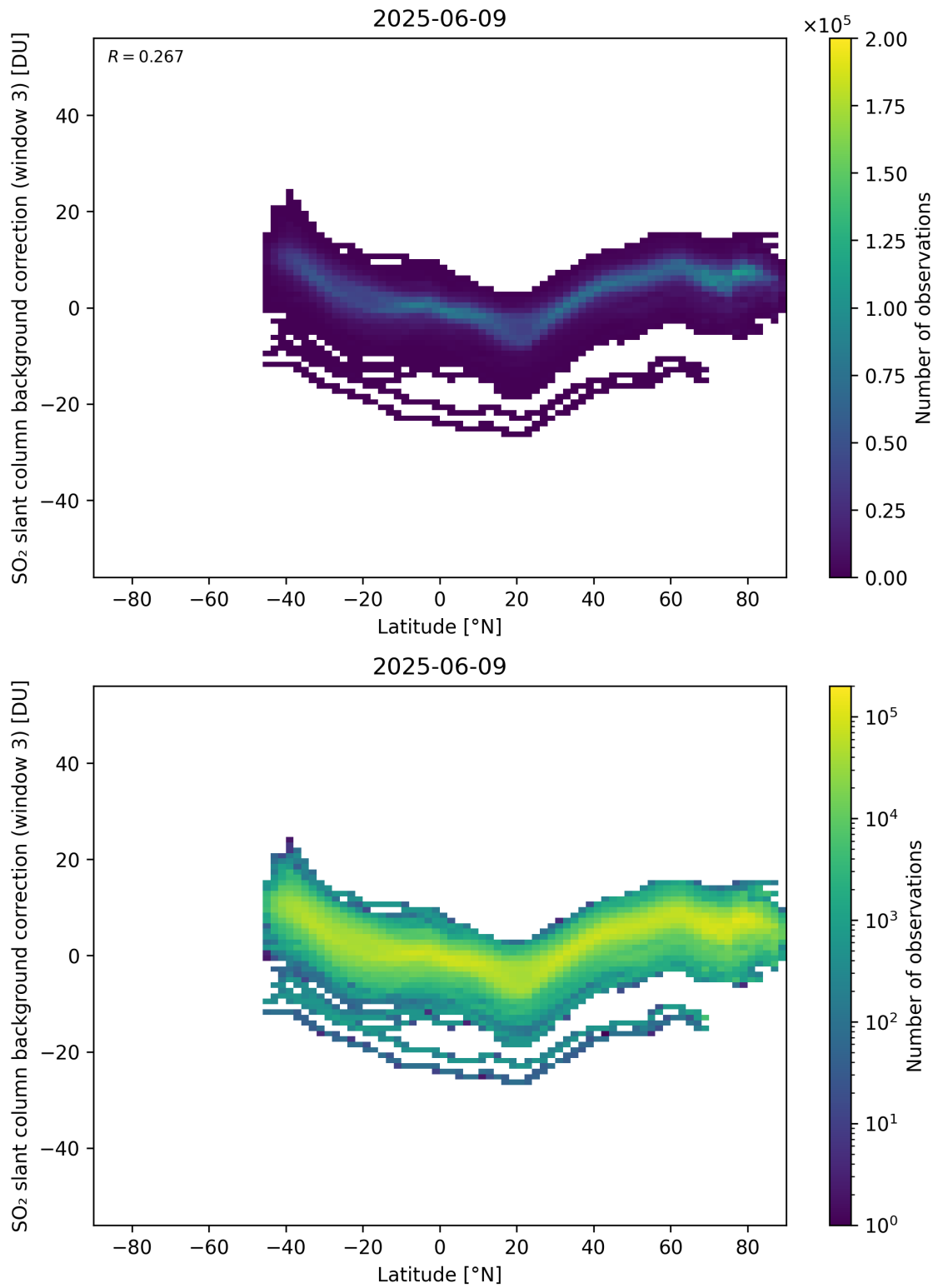
Figure 152: Scatter density plot of “Latitude” against “SO 2 slant column background correction (window 3)” for 2025-06-08 to 2025-06-10.
