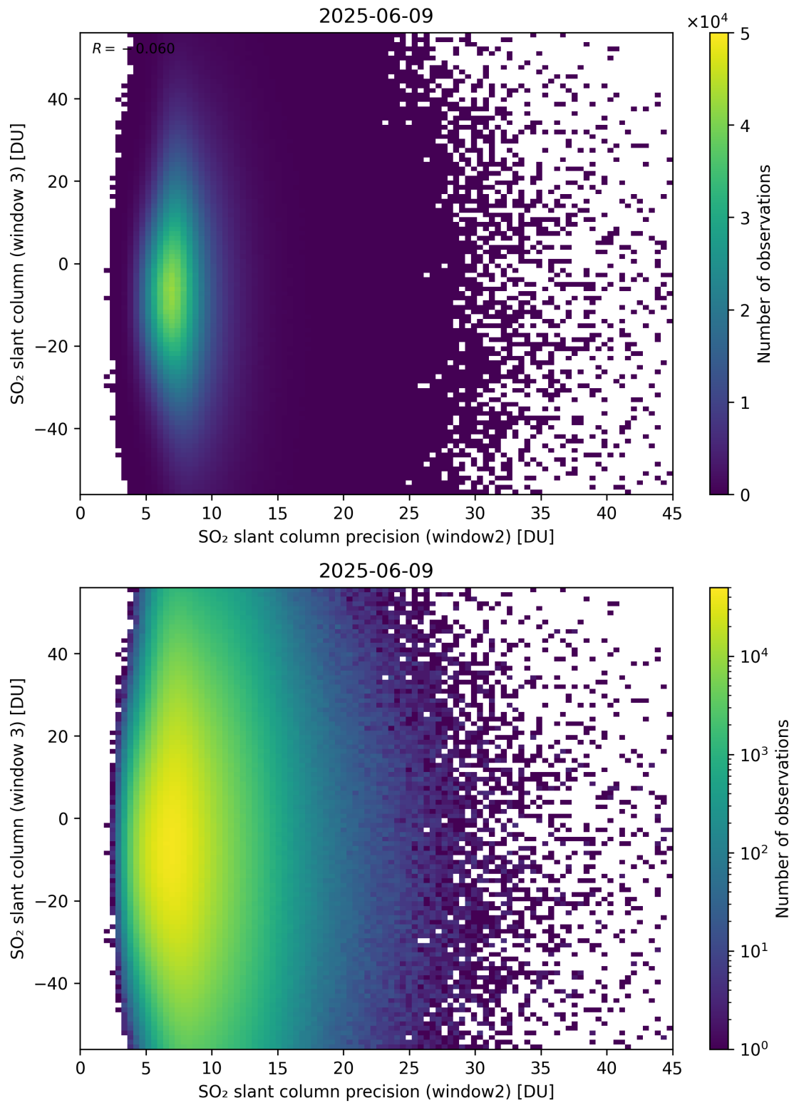
Figure 299: Scatter density plot of “SO 2 slant column precision (window2)” against “SO 2 slant column (window 3)” for 2025-06-08 to 2025-06-10.
