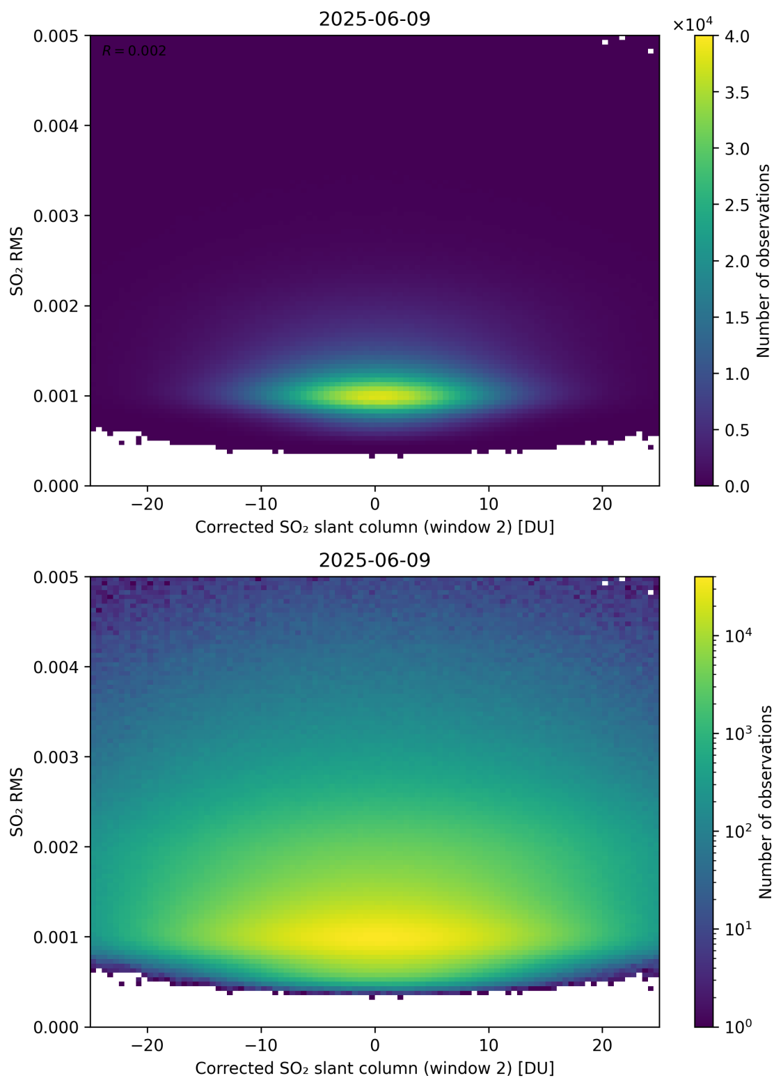
Figure 248: Scatter density plot of “Corrected SO 2 slant column (window 2)” against “SO 2 RMS” for 2025-06-08 to 2025-06-10.
