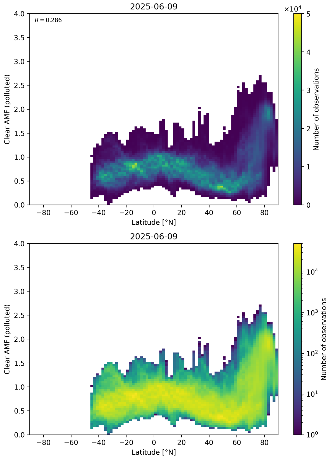
Figure 156: Scatter density plot of “Latitude” against “Clear AMF (polluted)” for 2025-06-08 to 2025-06-10.
