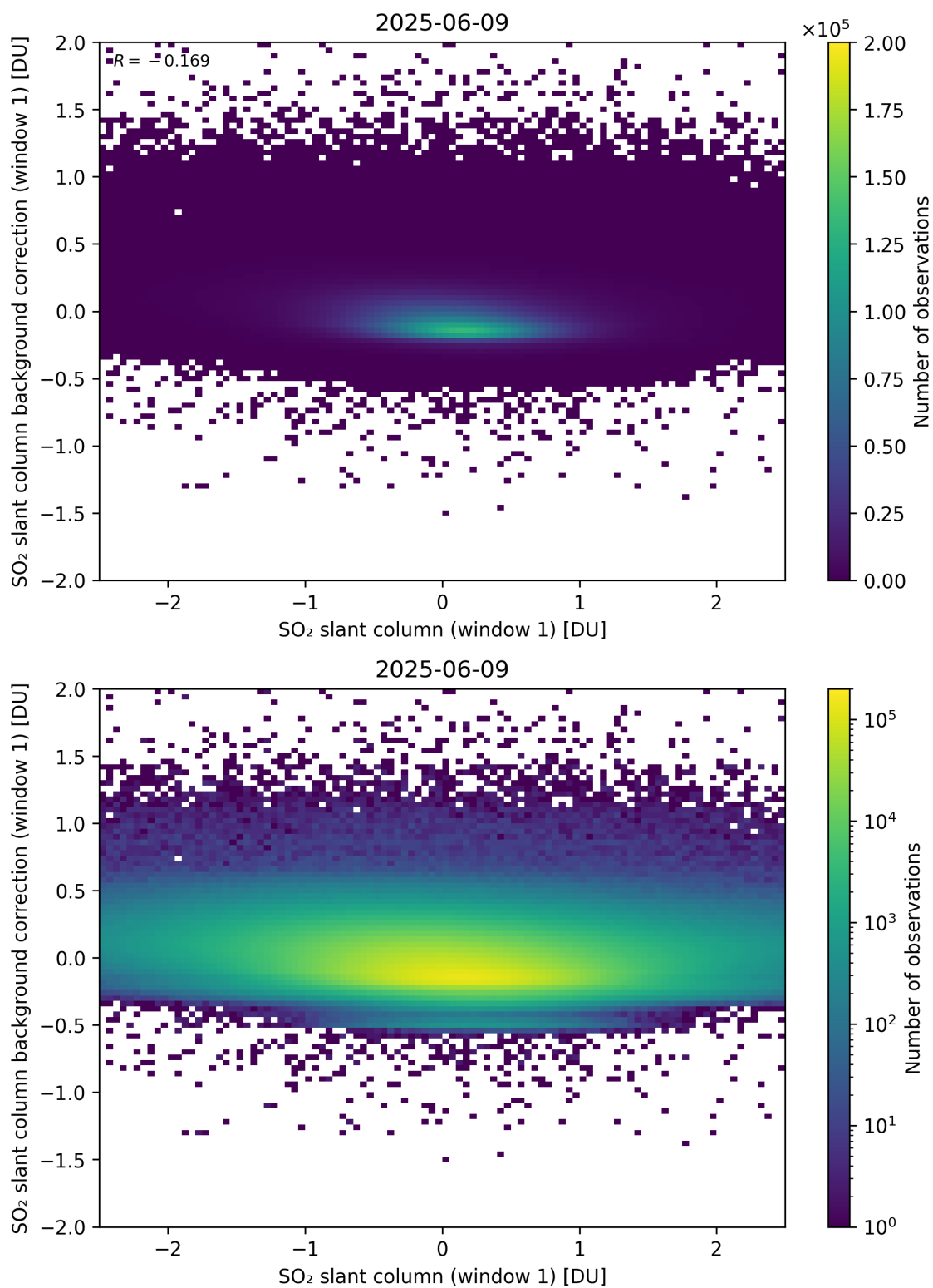
Figure 262: Scatter density plot of “SO 2 slant column (window 1)” against “SO 2 slant column background correction (window 1)” for 2025-06-08 to 2025-06-10.
