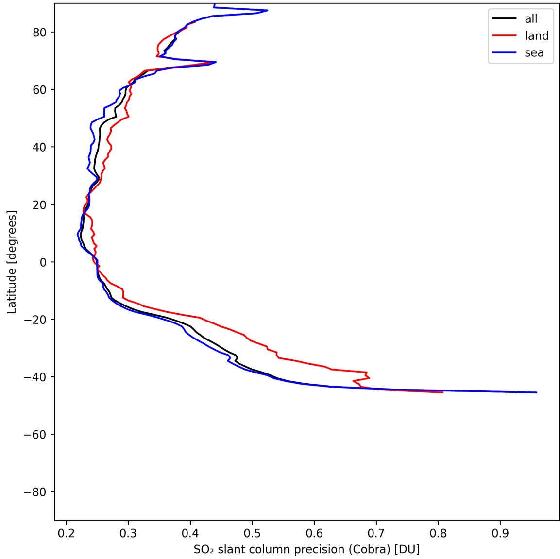
Figure 36: Zonal average of “SO 2 slant column precision (Cobra)” for 2025-06-08 to 2025-06-10.
