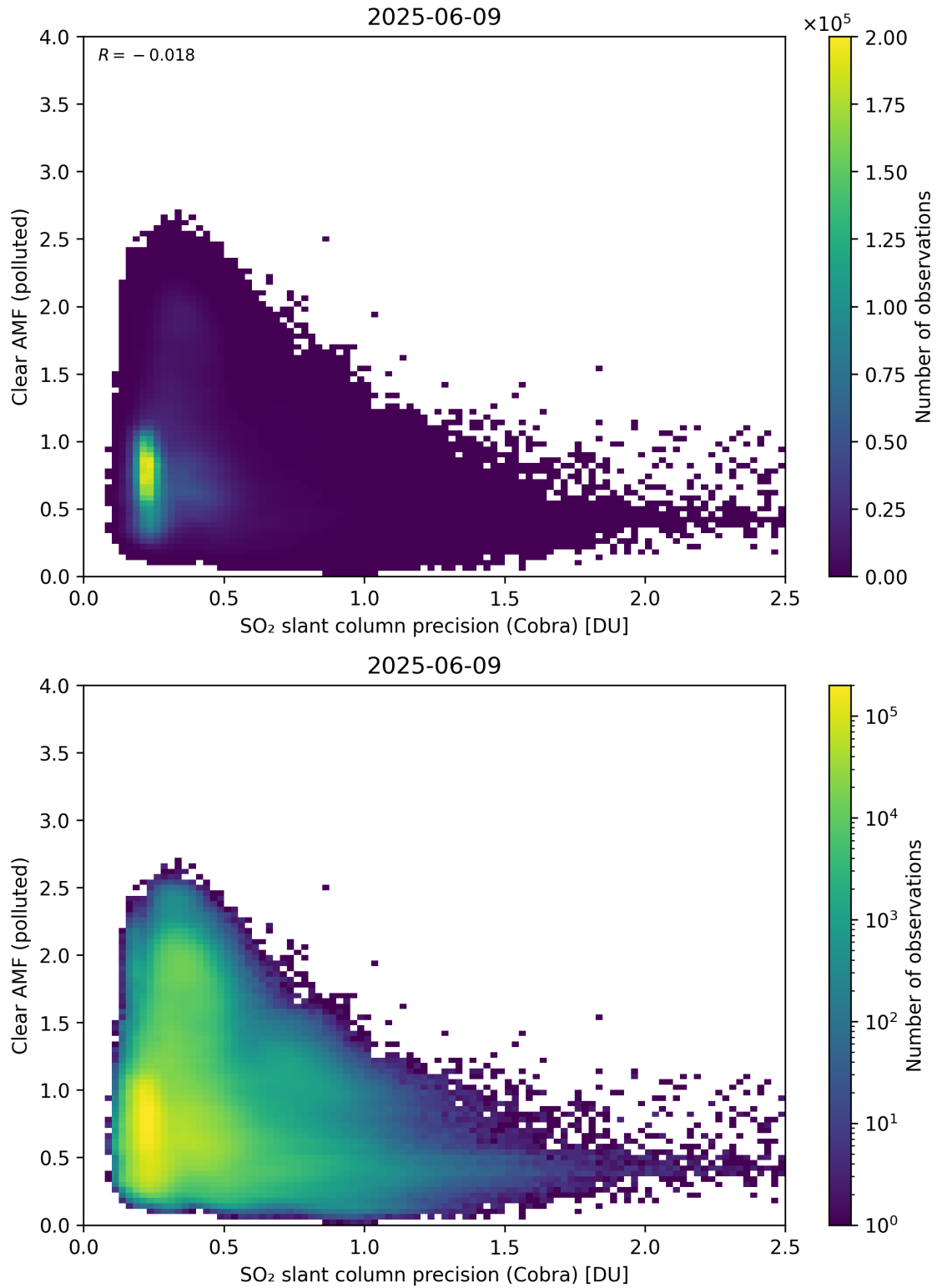
Figure 205: Scatter density plot of “SO 2 slant column precision (Cobra)” against “Clear AMF (polluted)” for 2025-06-08 to 2025-06-10.
