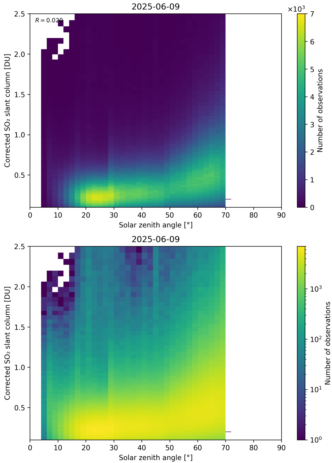
Figure 181: Scatter density plot of “Solar zenith angle” against “Corrected SO 2 slant column” for 2025-06-08 to 2025-06-10.
