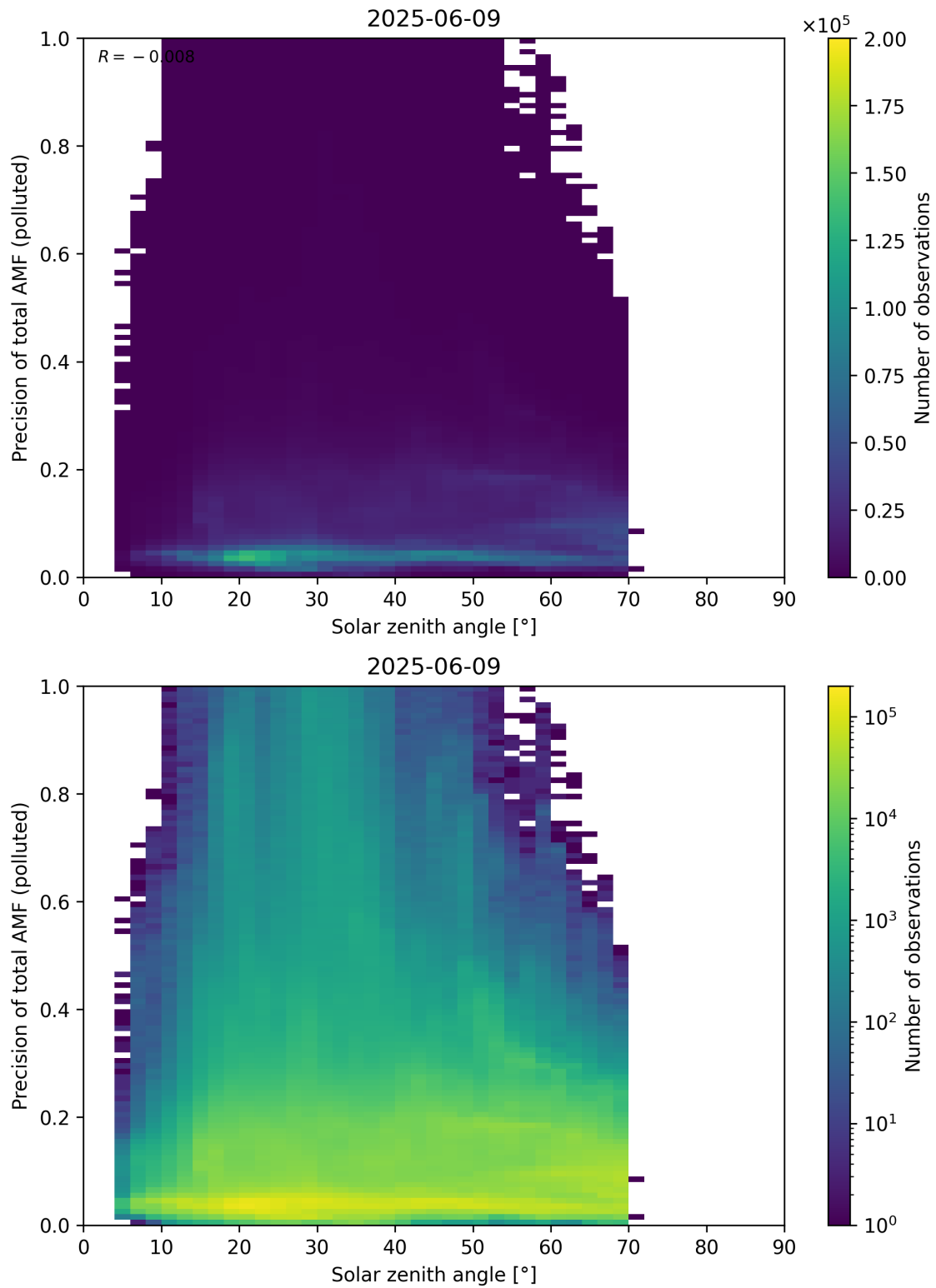
Figure 190: Scatter density plot of “Solar zenith angle” against “Precision of total AMF (polluted)” for 2025-06-08 to 2025-06-10.
