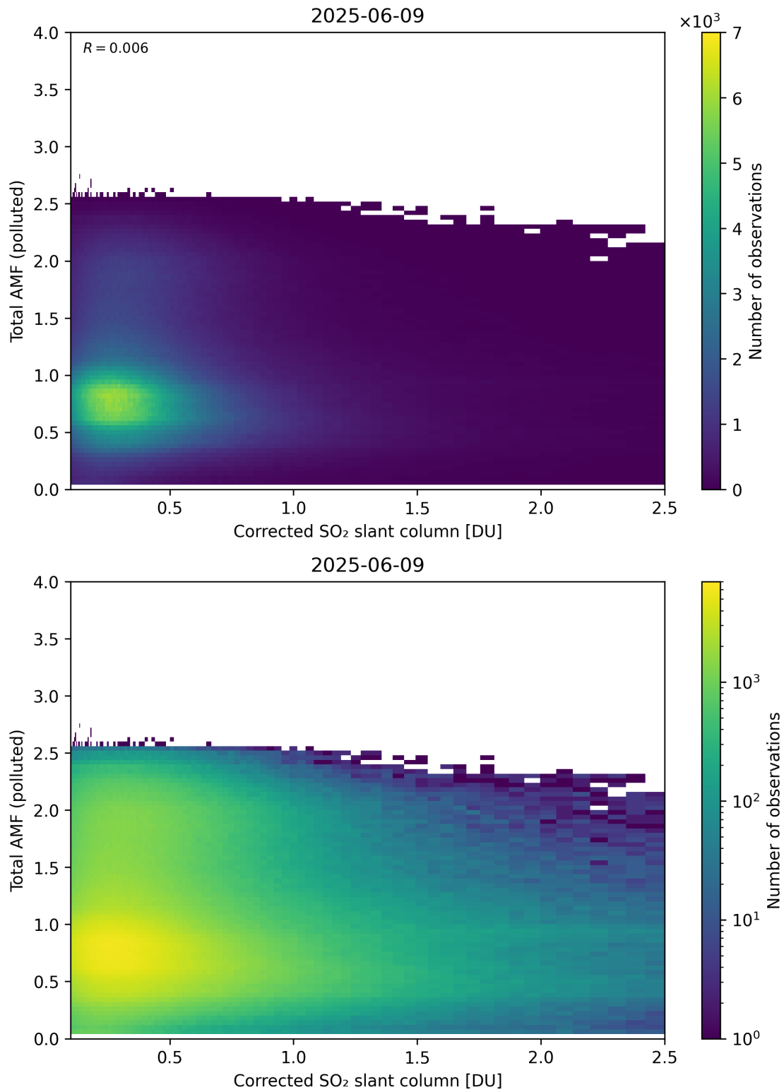
Figure 242: Scatter density plot of “Corrected SO 2 slant column” against “Total AMF (polluted)” for 2025-06-08 to 2025-06-10.
