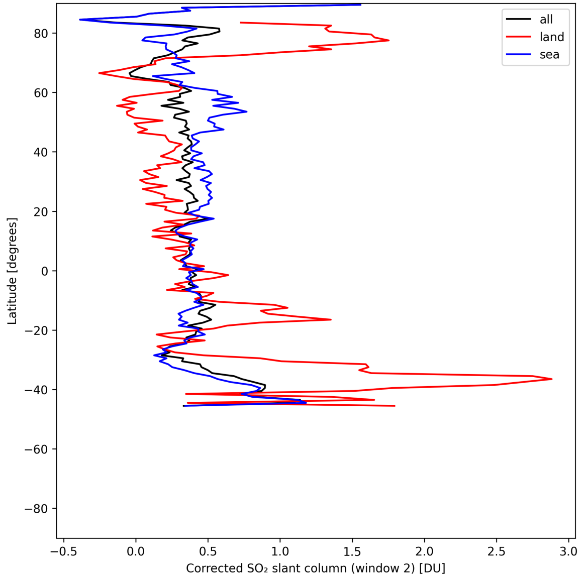
Figure 43: Zonal average of “Corrected SO 2 slant column (window 2)” for 2025-06-08 to 2025-06-10.
