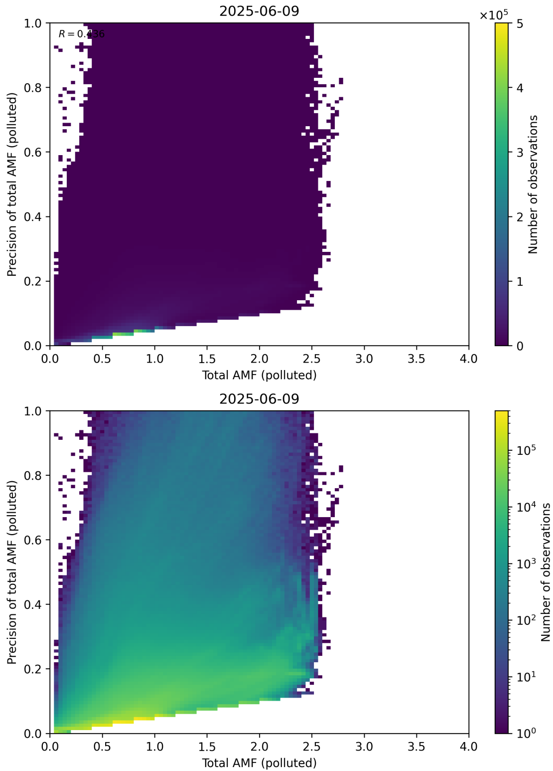
Figure 322: Scatter density plot of “Total AMF (polluted)” against “Precision of total AMF (polluted)” for 2025-06-08 to 2025-06-10.
