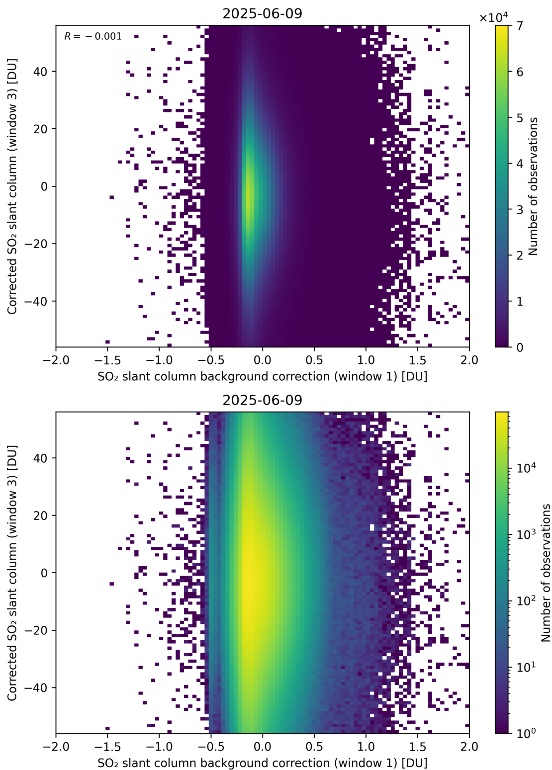
Figure 116: Scatter density plot of “SO 2 slant column background correction (window 1)” against “Corrected SO 2 slant column (window 3)” for 2025-06-08 to 2025-06-10.
