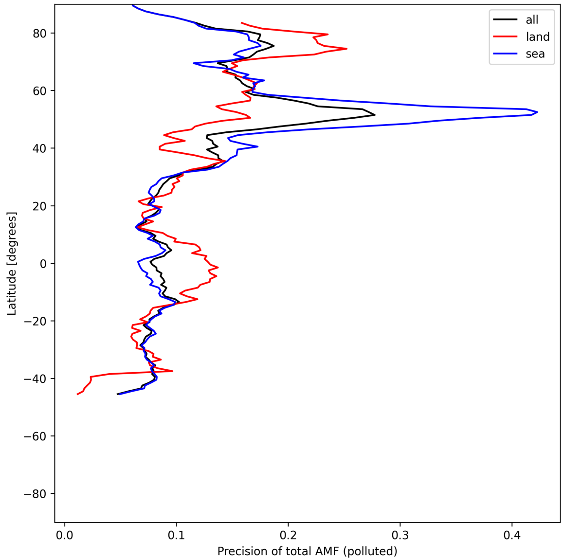
Figure 54: Zonal average of “Precision of total AMF (polluted)” for 2025-06-08 to 2025-06-10.
