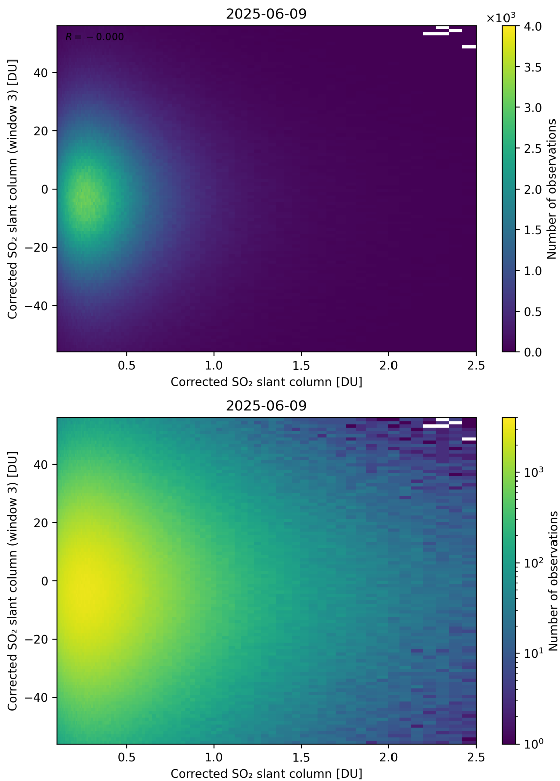
Figure 236: Scatter density plot of “Corrected SO 2 slant column” against “Corrected SO 2 slant column (window 3)” for 2025-06-08 to 2025-06-10.
