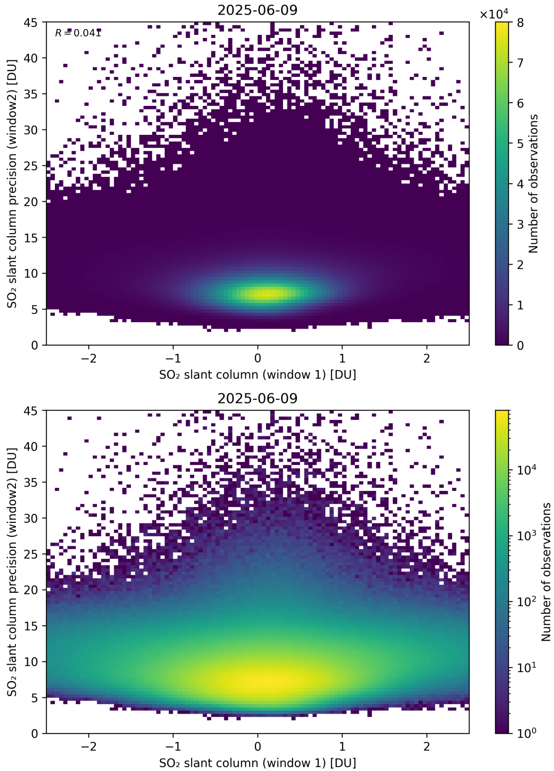
Figure 286: Scatter density plot of “SO 2 slant column (window 1)” against “SO 2 slant column precision (window2)” for 2025-06-08 to 2025-06-10.
