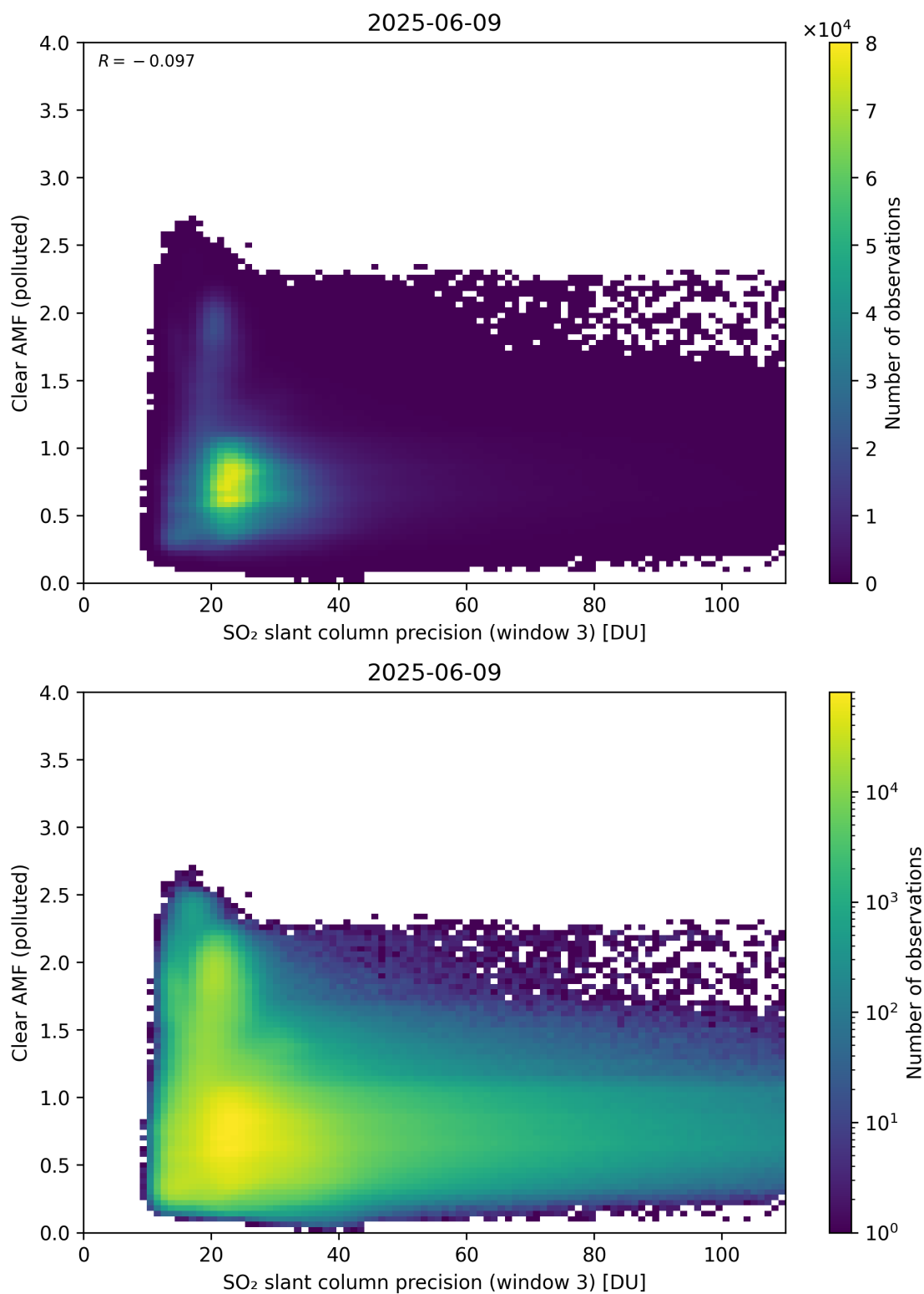
Figure 311: Scatter density plot of “SO 2 slant column precision (window 3)” against “Clear AMF (polluted)” for 2025-06-08 to 2025-06-10.
