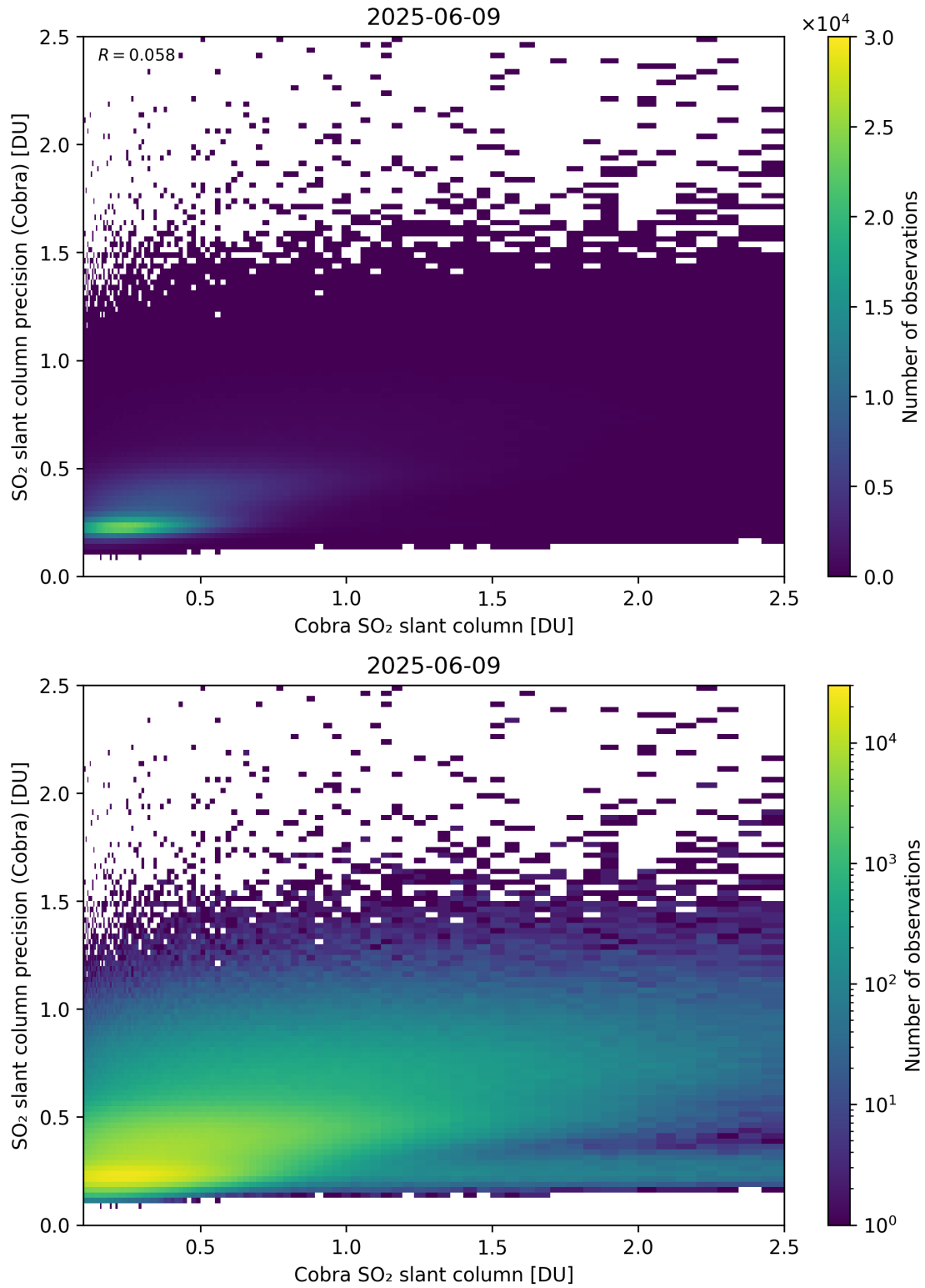
Figure 216: Scatter density plot of “Cobra SO 2 slant column” against “SO 2 slant column precision (Cobra)” for 2025-06-08 to 2025-06-10.
