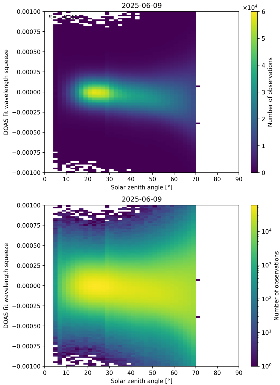
Figure 175: Scatter density plot of “Solar zenith angle” against “DOAS fit wavelength squeeze” for 2025-06-08 to 2025-06-10.
