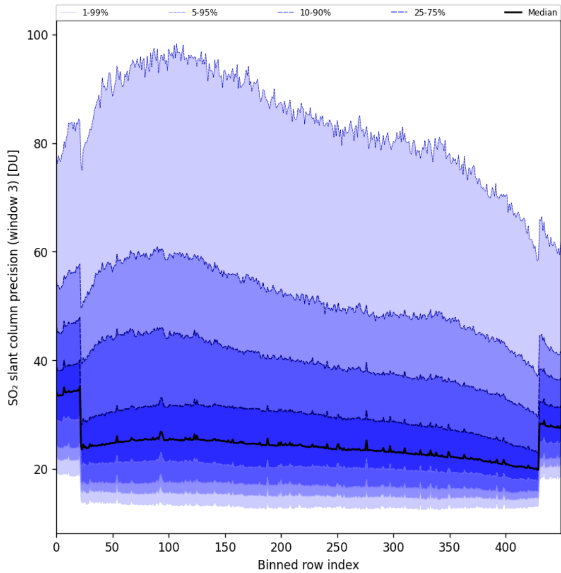
Figure 98: Along track statistics of “SO 2 slant column precision (window 3)” for 2025-06-08 to 2025-06-10
