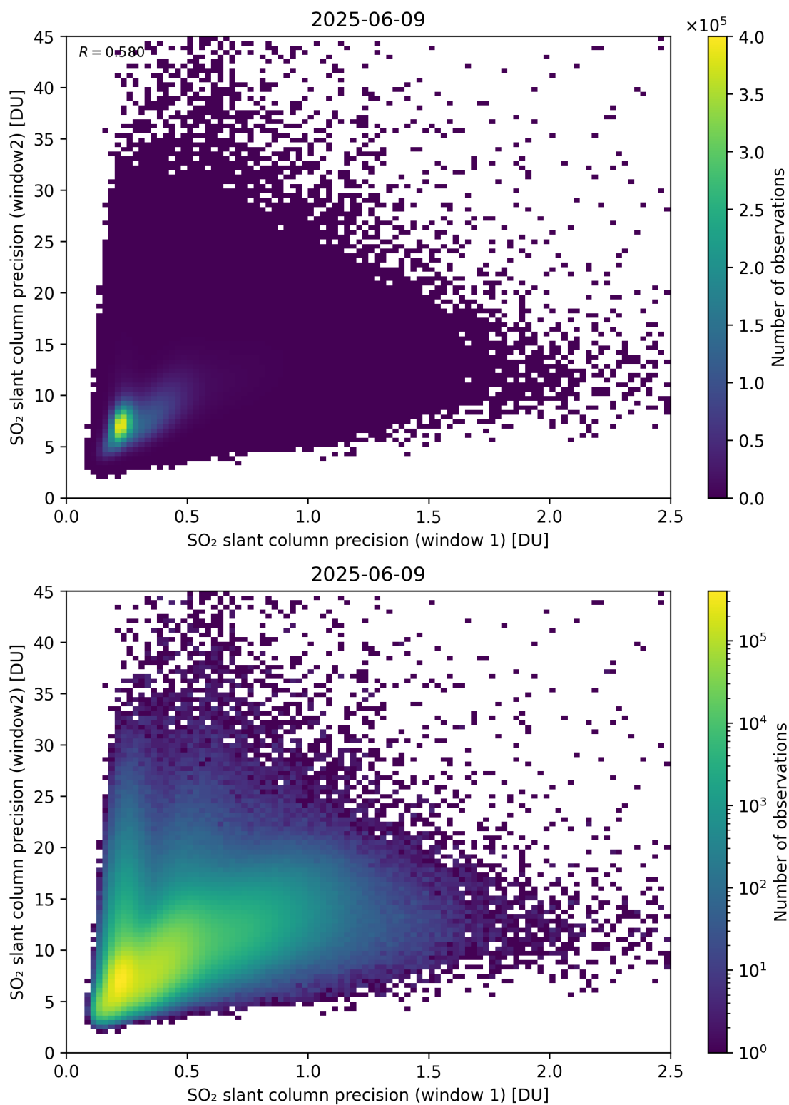
Figure 277: Scatter density plot of “SO 2 slant column precision (window 1)” against “SO 2 slant column precision (window2)” for 2025-06-08 to 2025-06-10.
