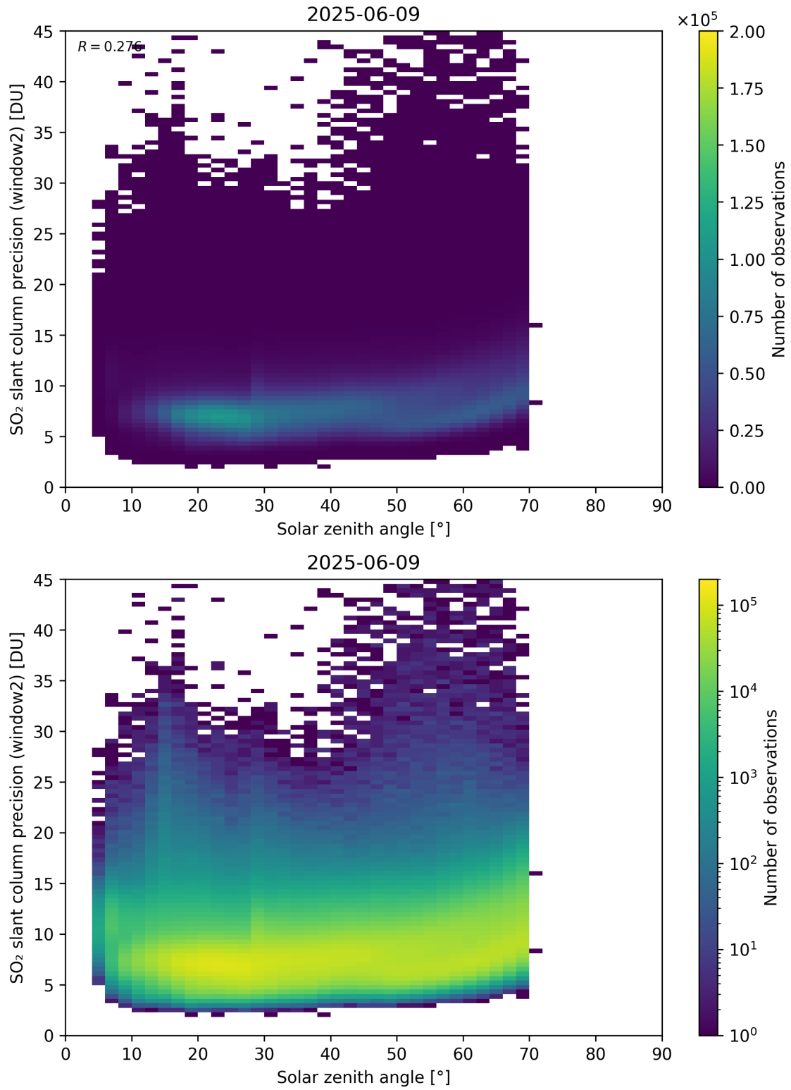
Figure 186: Scatter density plot of “Solar zenith angle” against “SO 2 slant column precision (window2)” for 2025-06-08 to 2025-06-10.
