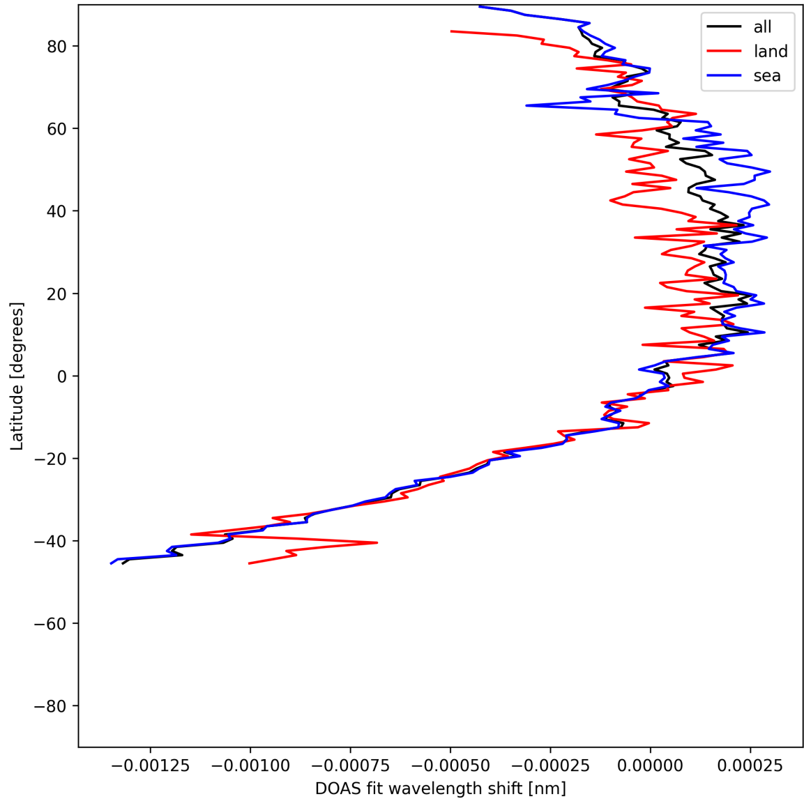
Figure 50: Zonal average of “DOAS fit wavelength shift” for 2025-06-08 to 2025-06-10.
