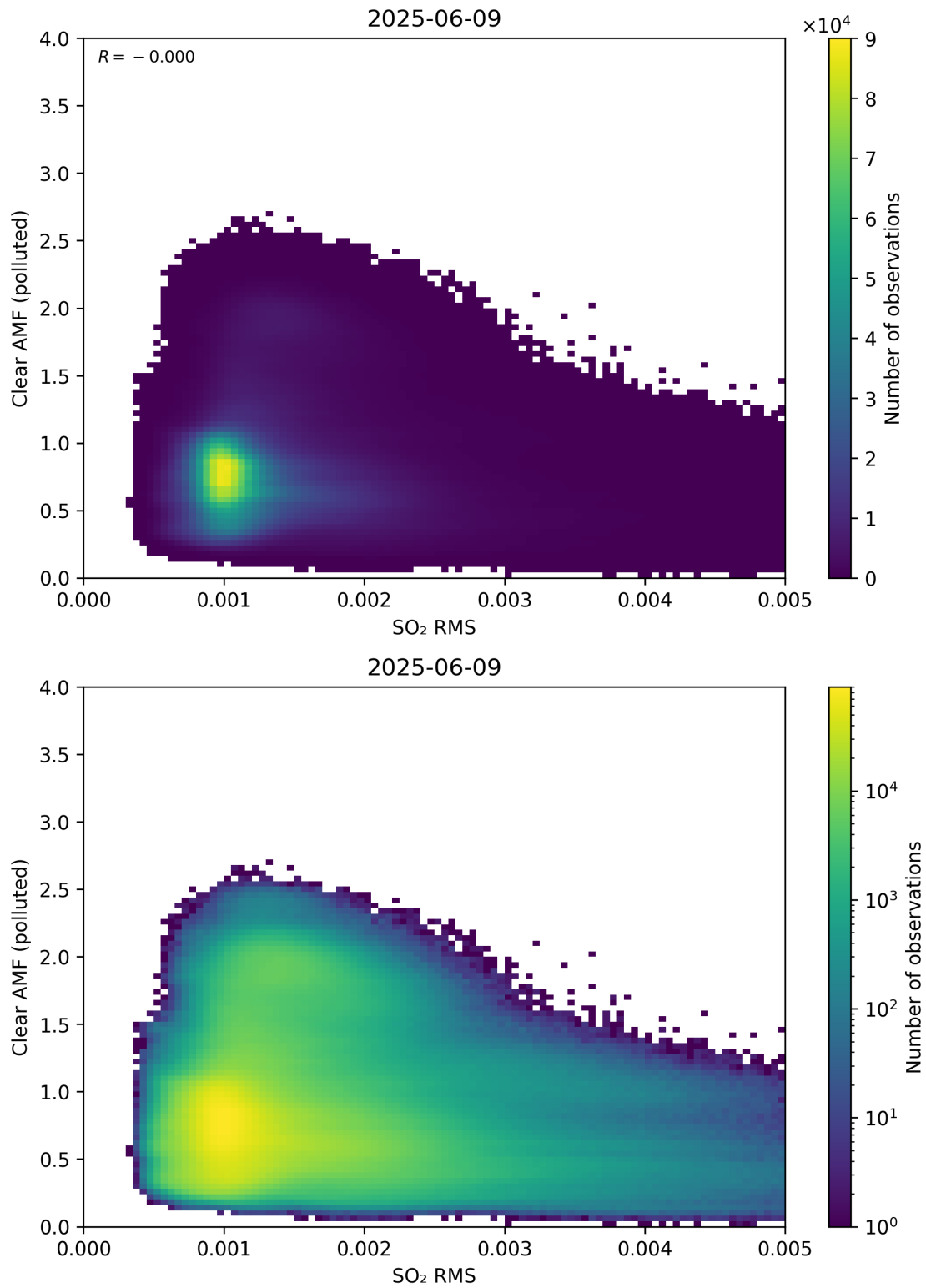
Figure 147: Scatter density plot of “SO 2 RMS” against “Clear AMF (polluted)” for 2025-06-08 to 2025-06-10.
