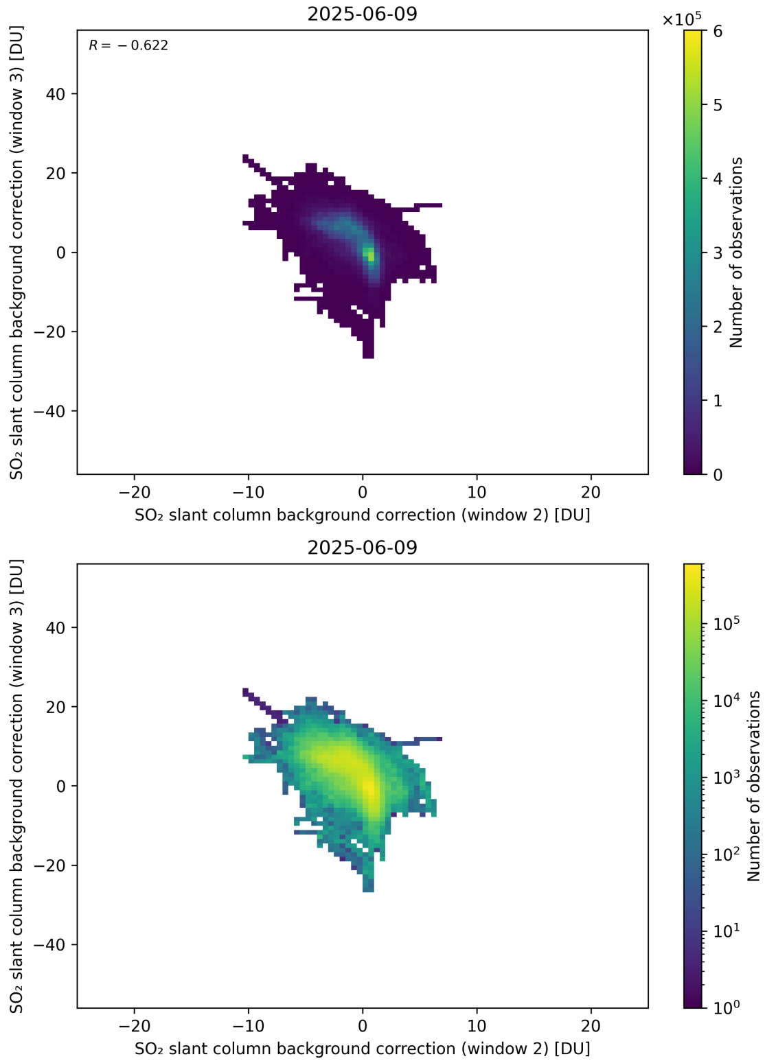
Figure 122: Scatter density plot of “SO 2 slant column background correction (window 2)” against “SO 2 slant column background correction (window 3)” for 2025-06-08 to 2025-06-10.
