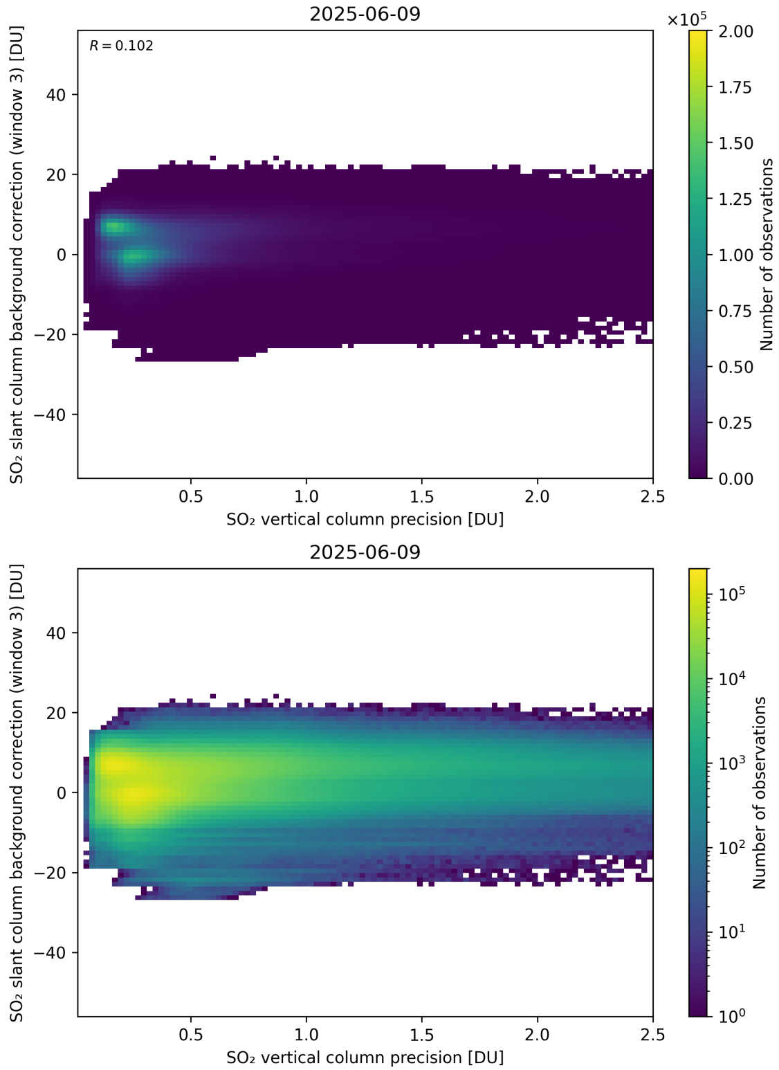
Figure 331: Scatter density plot of “SO 2 vertical column precision” against “SO 2 slant column background correction (window 3)” for 2025-06-08 to 2025-06-10.
