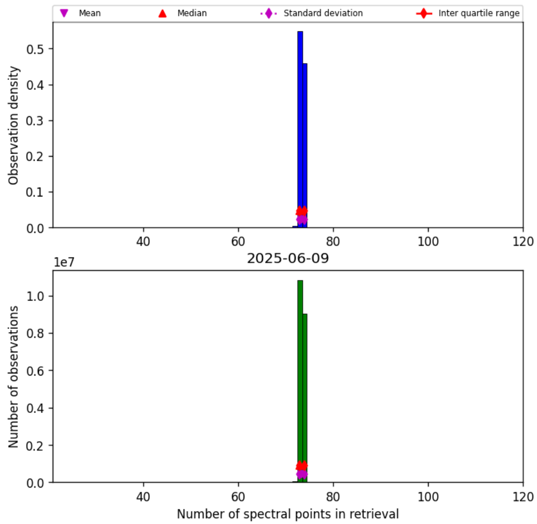
Figure 82: Histogram of “Number of spectral points in retrieval” for 2025-06-08 to 2025-06-10
