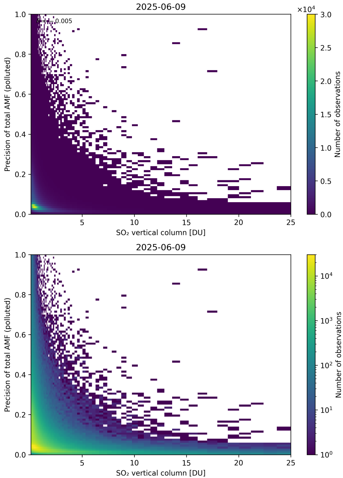
Figure 360: Scatter density plot of “SO 2 vertical column” against “Precision of total AMF (polluted)” for 2025-06-08 to 2025-06-10.
