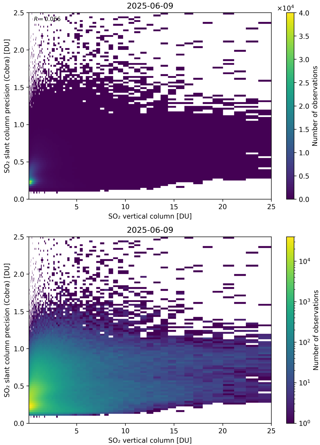
Figure 350: Scatter density plot of “SO 2 vertical column” against “SO 2 slant column precision (Cobra)” for 2025-06-08 to 2025-06-10.
