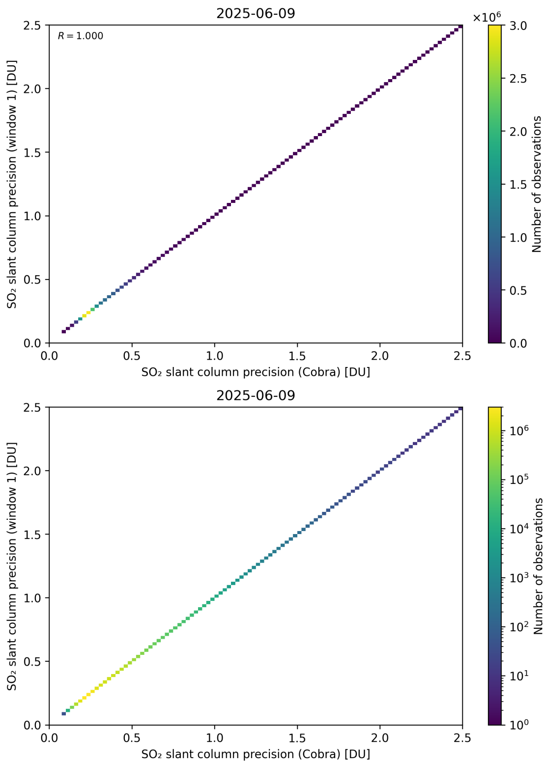
Figure 209: Scatter density plot of “SO 2 slant column precision (Cobra)” against “SO 2 slant column precision (window 1)” for 2025-06-08 to 2025-06-10.
