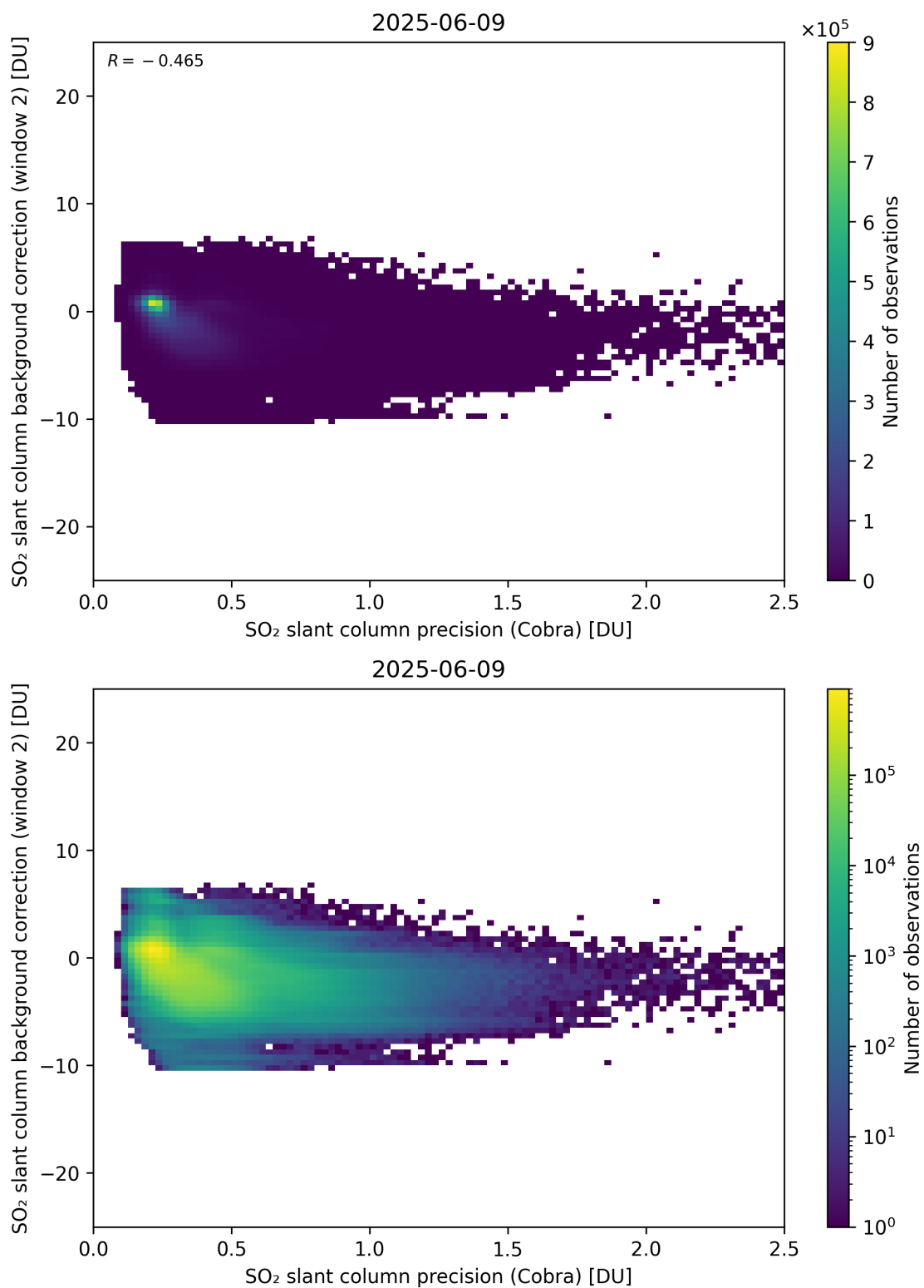
Figure 200: Scatter density plot of “SO 2 slant column precision (Cobra)” against “SO 2 slant column background correction (window 2)” for 2025-06-08 to 2025-06-10.
