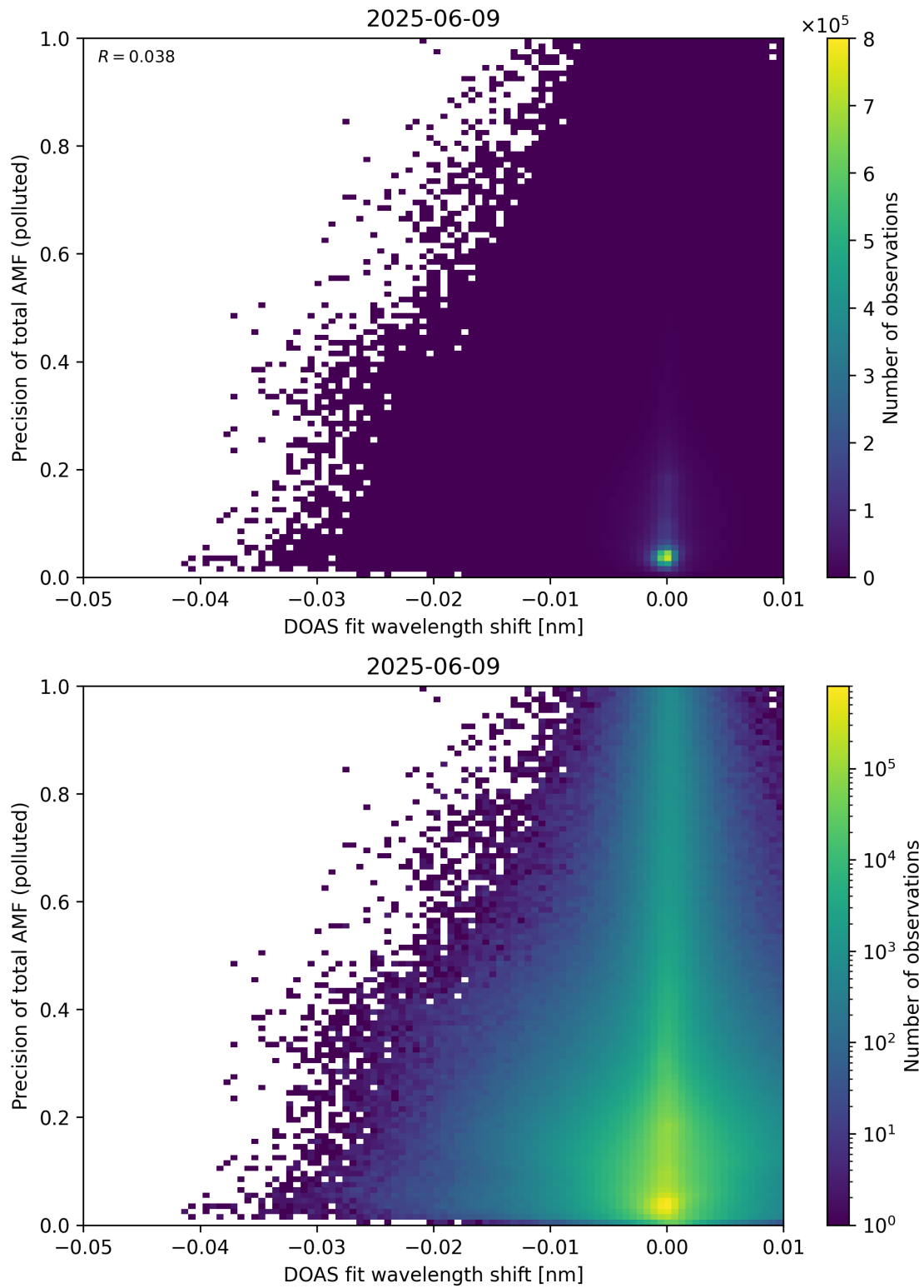
Figure 142: Scatter density plot of “DOAS fit wavelength shift” against “Precision of total AMF (polluted)” for 2025-06-08 to 2025-06-10.
