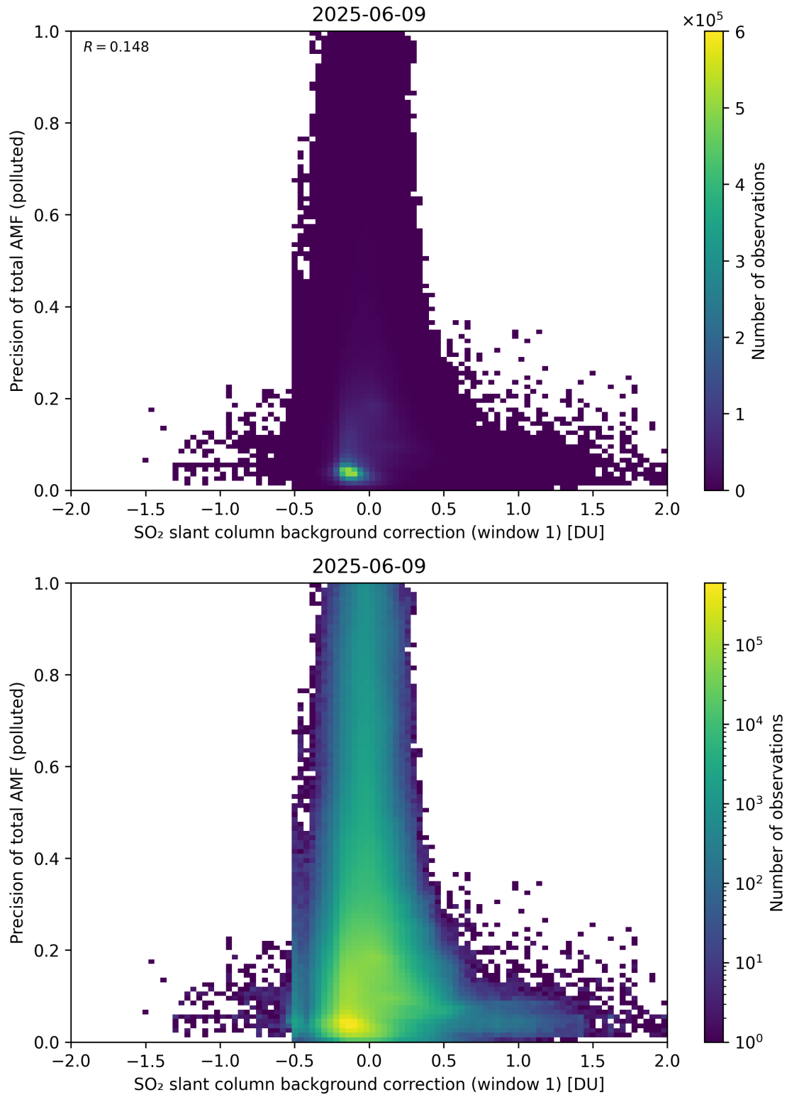
Figure 121: Scatter density plot of “SO 2 slant column background correction (window 1)” against “Precision of total AMF (polluted)” for 2025-06-08 to 2025-06-10.
