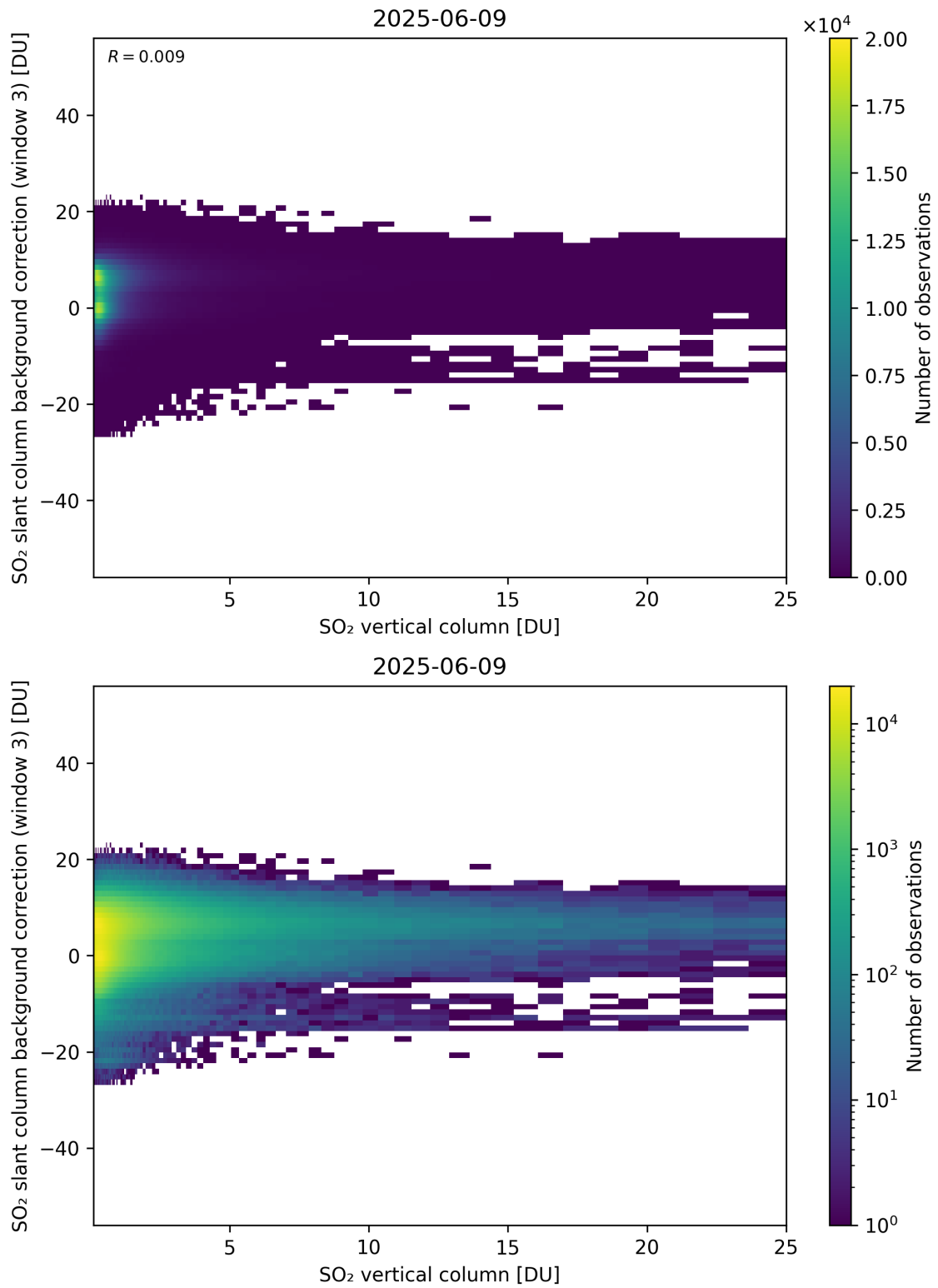
Figure 325: Scatter density plot of “SO 2 vertical column” against “SO 2 slant column background correction (window 3)” for 2025-06-08 to 2025-06-10.
