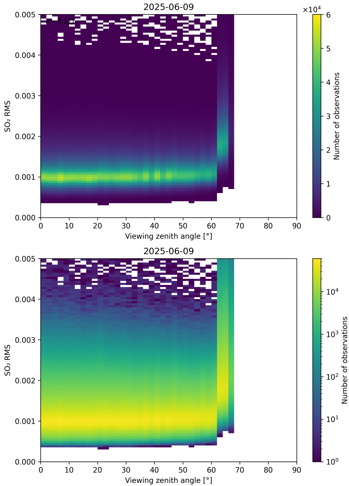
Figure 367: Scatter density plot of “Viewing zenith angle” against “SO 2 RMS” for 2025-06-08 to 2025-06-10.
