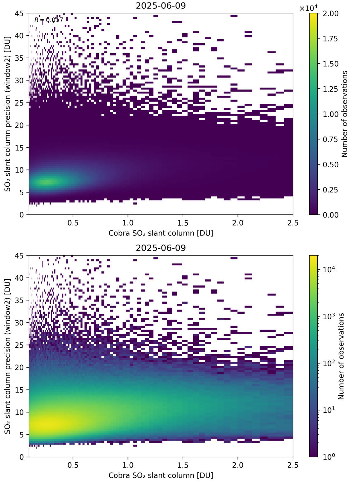
Figure 221: Scatter density plot of “Cobra SO 2 slant column” against “SO 2 slant column precision (window2)” for 2025-06-08 to 2025-06-10.
