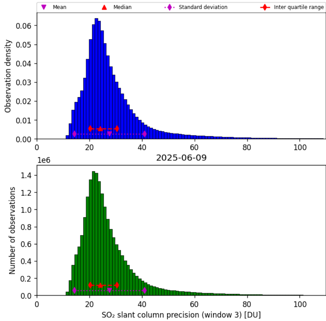
Figure 72: Histogram of “SO 2 slant column precision (window 3)” for 2025-06-08 to 2025-06-10
