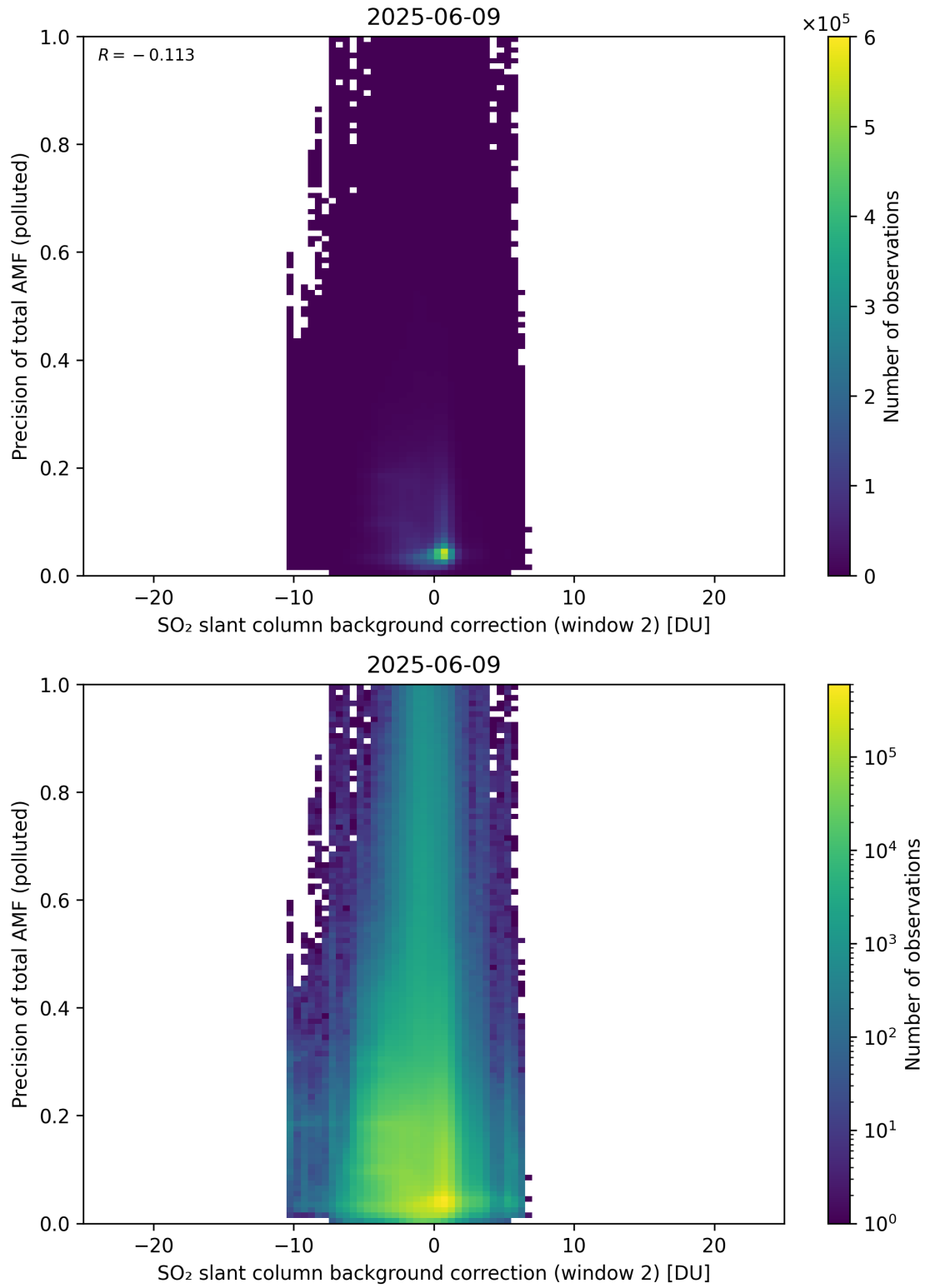
Figure 131: Scatter density plot of “SO 2 slant column background correction (window 2)” against “Precision of total AMF (polluted)” for 2025-06-08 to 2025-06-10.
