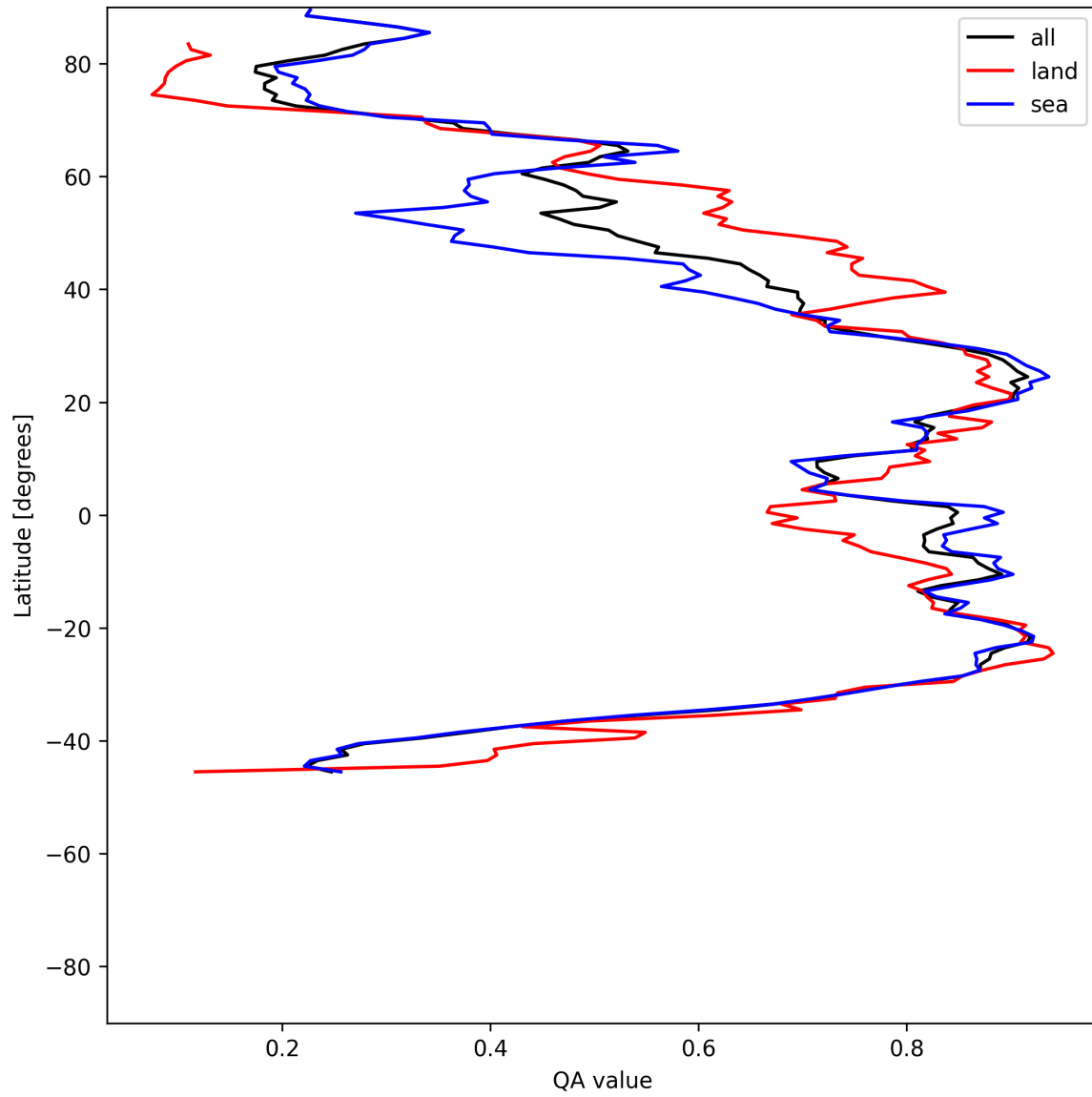
Figure 31: Zonal average of “QA value” for 2025-06-08 to 2025-06-10.
