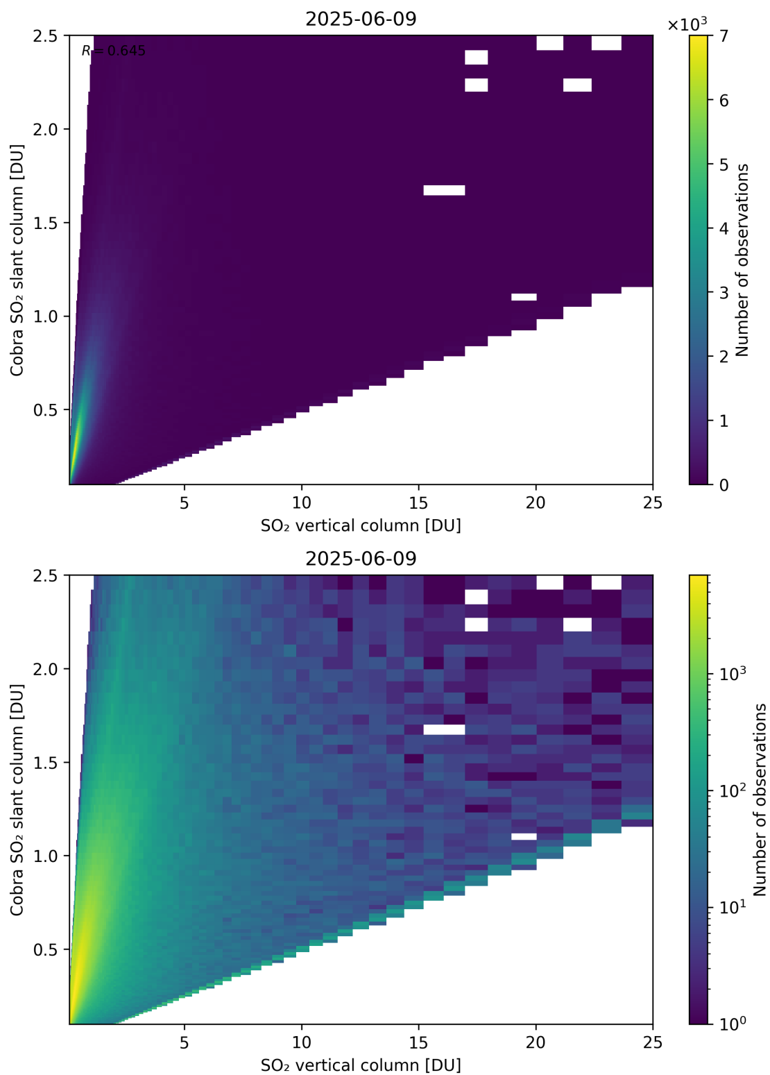
Figure 349: Scatter density plot of “SO 2 vertical column” against “Cobra SO 2 slant column” for 2025-06-08 to 2025-06-10.
