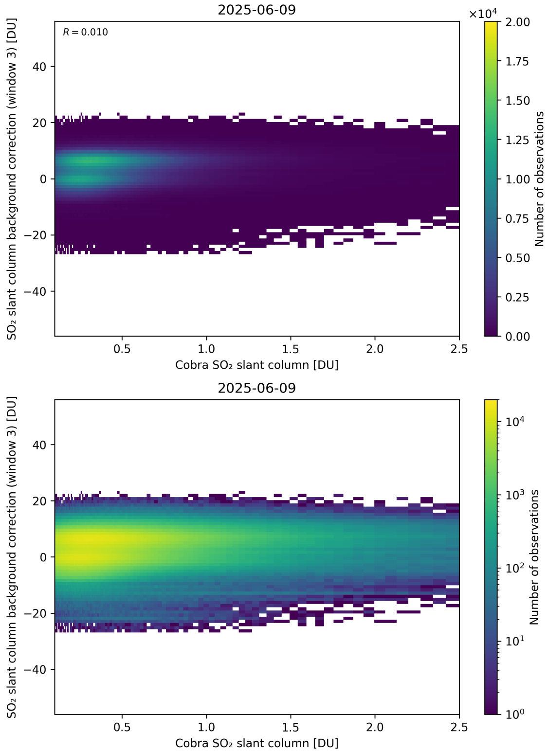
Figure 195: Scatter density plot of “Cobra SO 2 slant column” against “SO 2 slant column background correction (window 3)” for 2025-06-08 to 2025-06-10.
