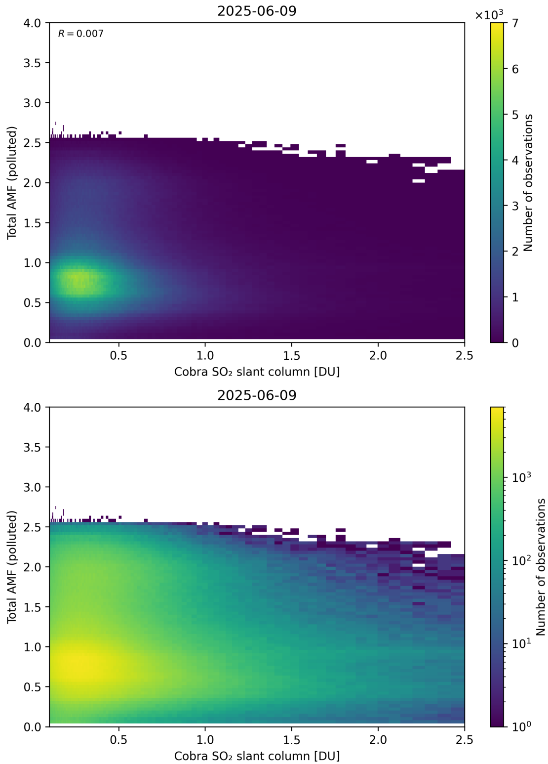
Figure 224: Scatter density plot of “Cobra SO 2 slant column” against “Total AMF (polluted)” for 2025-06-08 to 2025-06-10.
