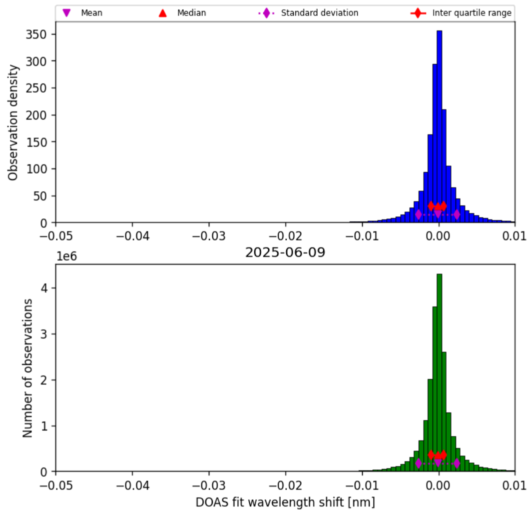
Figure 76: Histogram of “DOAS fit wavelength shift” for 2025-06-08 to 2025-06-10
