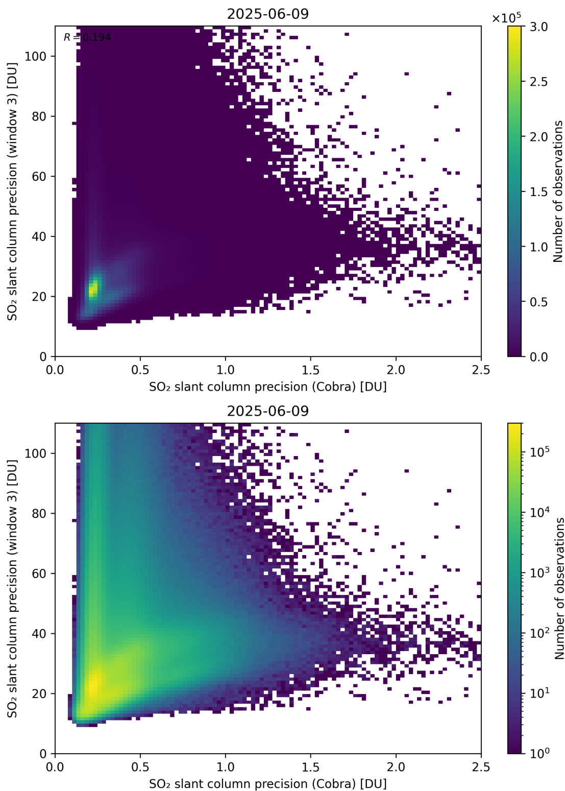
Figure 212: Scatter density plot of “SO 2 slant column precision (Cobra)” against “SO 2 slant column precision (window 3)” for 2025-06-08 to 2025-06-10.
