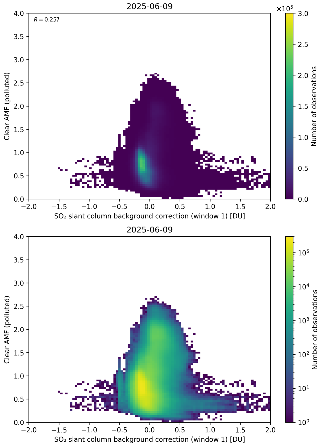
Figure 114: Scatter density plot of “SO 2 slant column background correction (window 1)” against “Clear AMF (polluted)” for 2025-06-08 to 2025-06-10.
