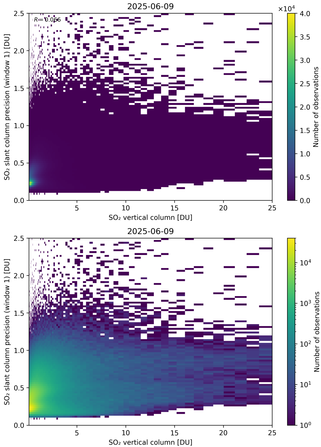
Figure 355: Scatter density plot of “SO 2 vertical column” against “SO 2 slant column precision (window 1)” for 2025-06-08 to 2025-06-10.
