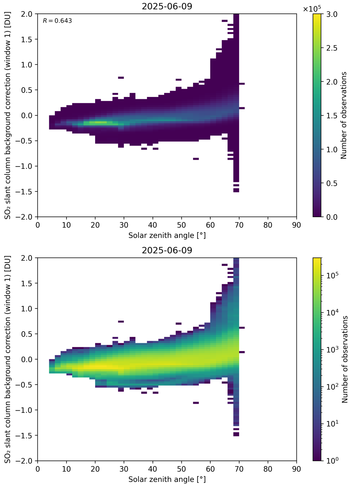
Figure 171: Scatter density plot of “Solar zenith angle” against “SO 2 slant column background correction (window 1)” for 2025-06-08 to 2025-06-10.
