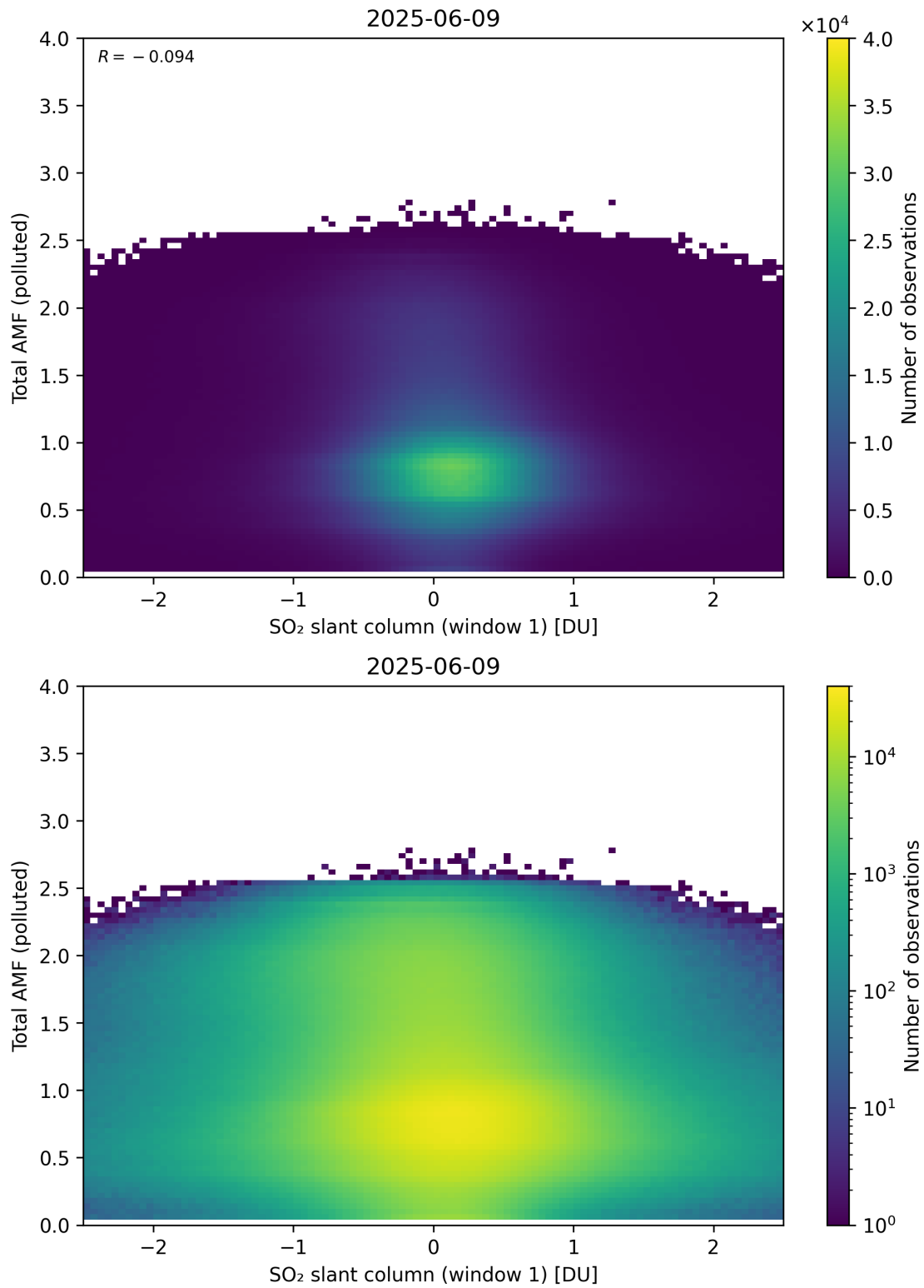
Figure 289: Scatter density plot of “SO 2 slant column (window 1)” against “Total AMF (polluted)” for 2025-06-08 to 2025-06-10.
