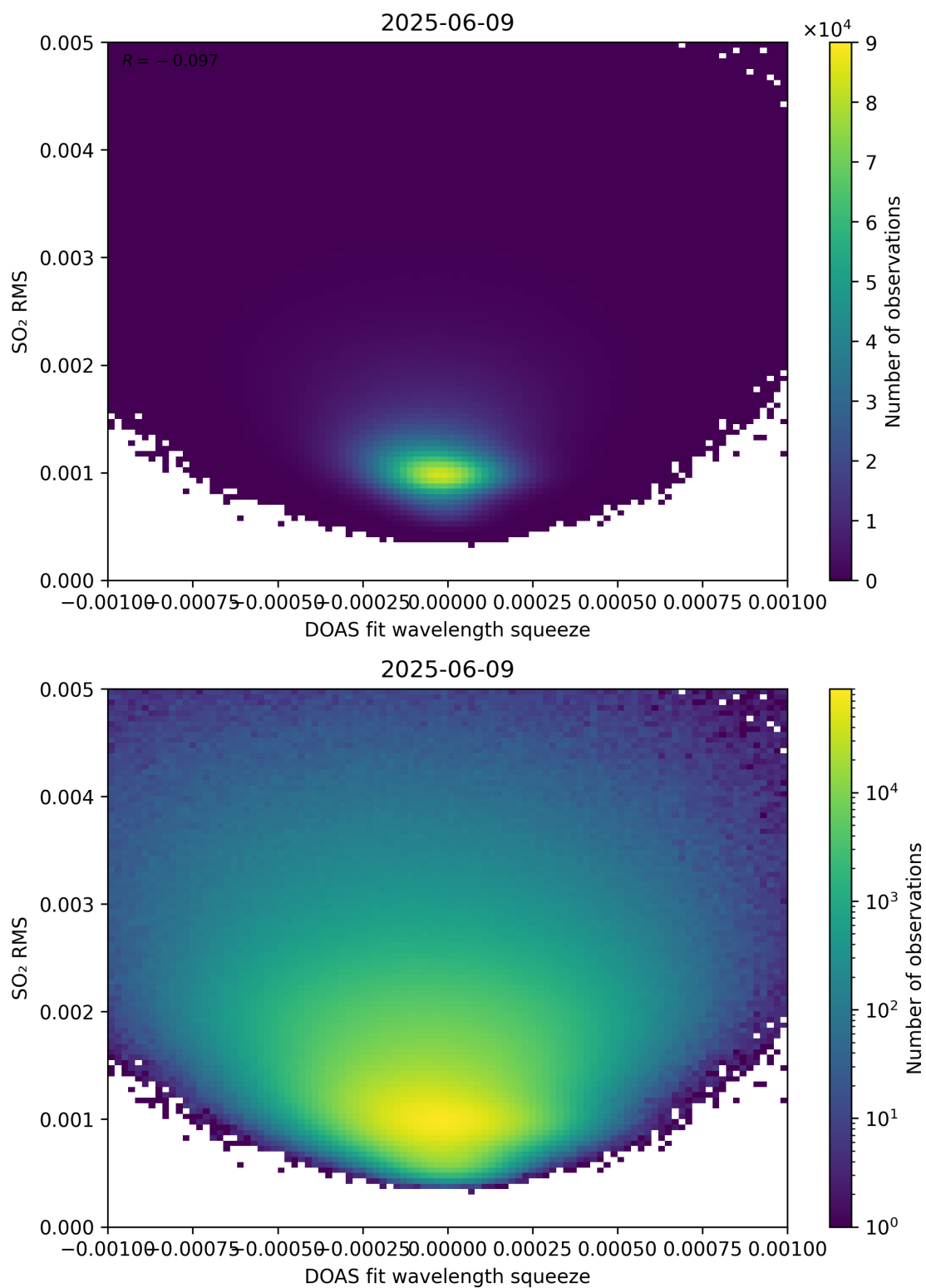
Figure 143: Scatter density plot of “DOAS fit wavelength squeeze” against “SO 2 RMS” for 2025-06-08 to 2025-06-10.
