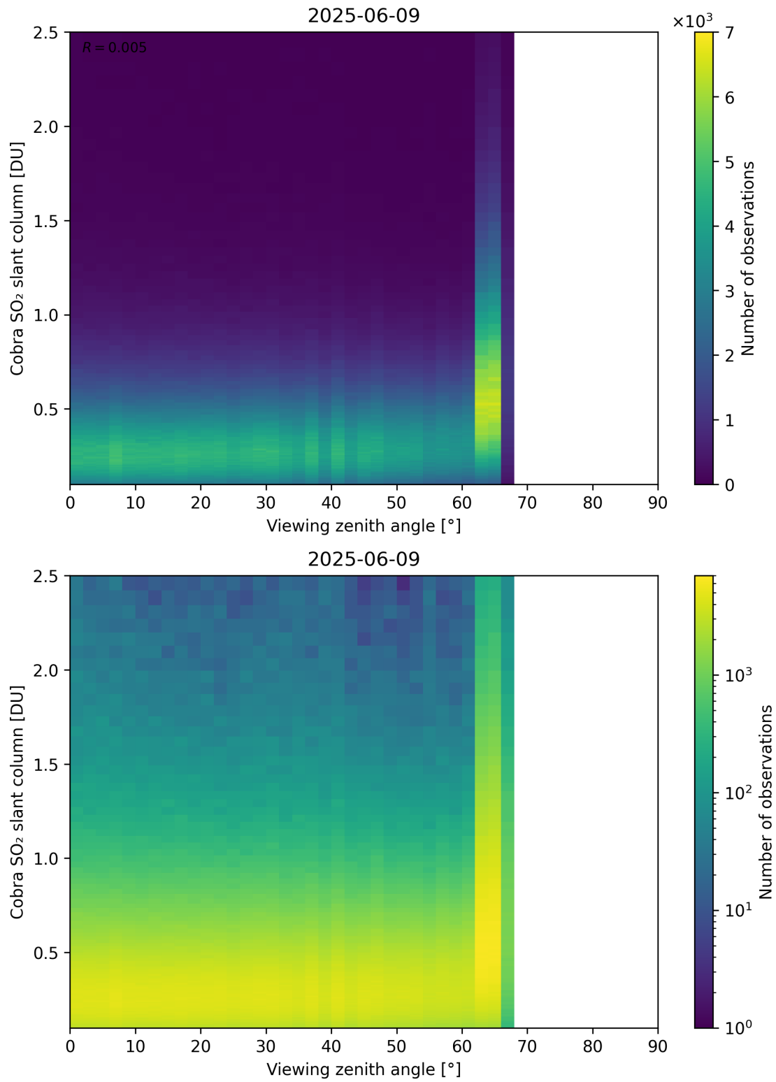
Figure 371: Scatter density plot of “Viewing zenith angle” against “Cobra SO 2 slant column” for 2025-06-08 to 2025-06-10.
