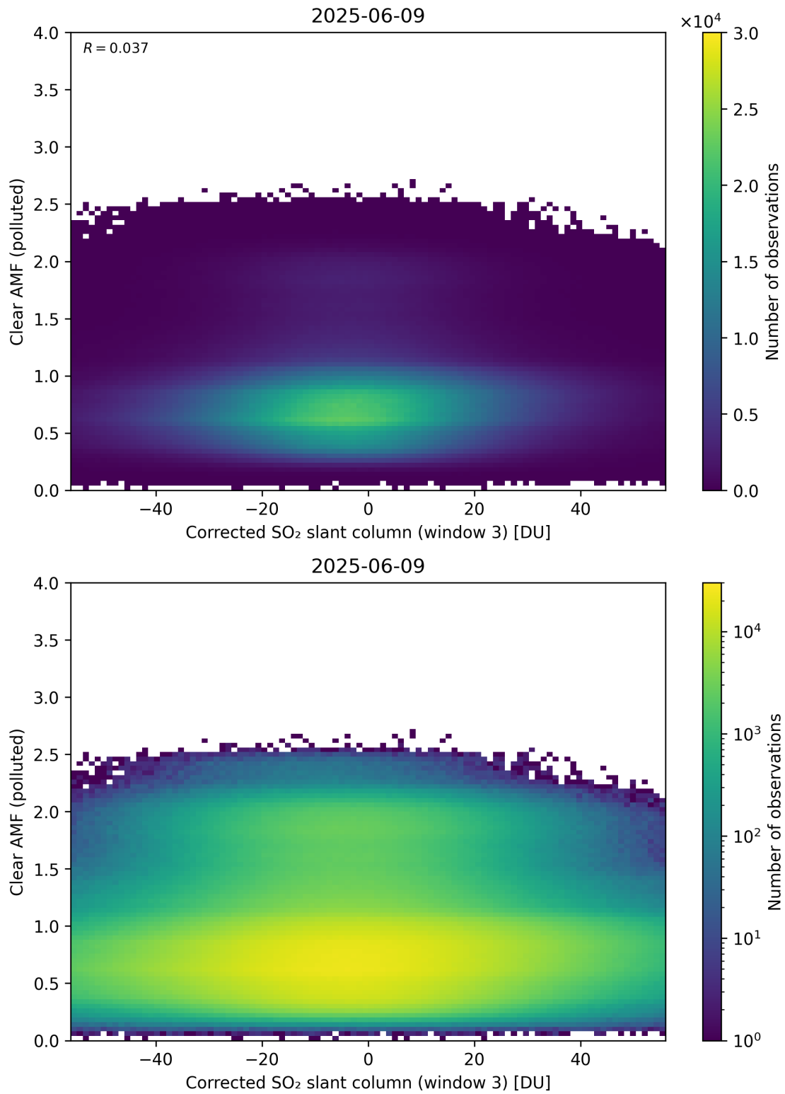
Figure 259: Scatter density plot of “Corrected SO 2 slant column (window 3)” against “Clear AMF (polluted)” for 2025-06-08 to 2025-06-10.
