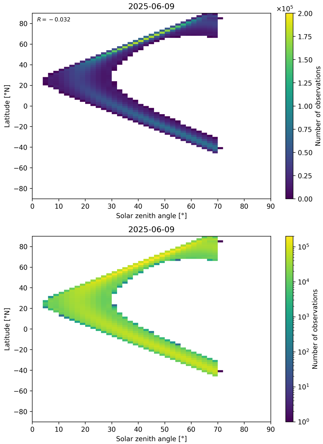
Figure 177: Scatter density plot of “Solar zenith angle” against “Latitude” for 2025-06-08 to 2025-06-10.
