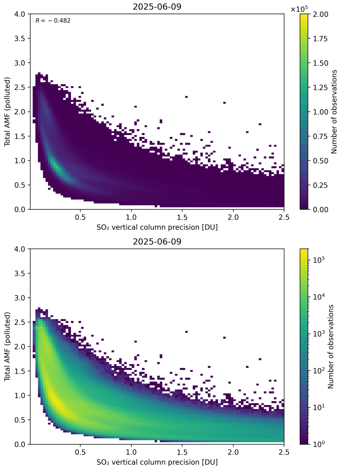
Figure 346: Scatter density plot of “SO 2 vertical column precision” against “Total AMF (polluted)” for 2025-06-08 to 2025-06-10.
