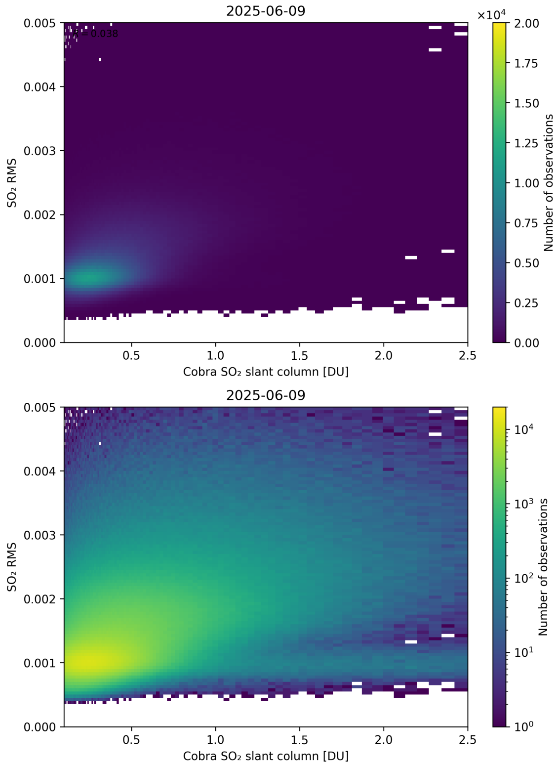
Figure 198: Scatter density plot of “Cobra SO 2 slant column” against “SO 2 RMS” for 2025-06-08 to 2025-06-10.
