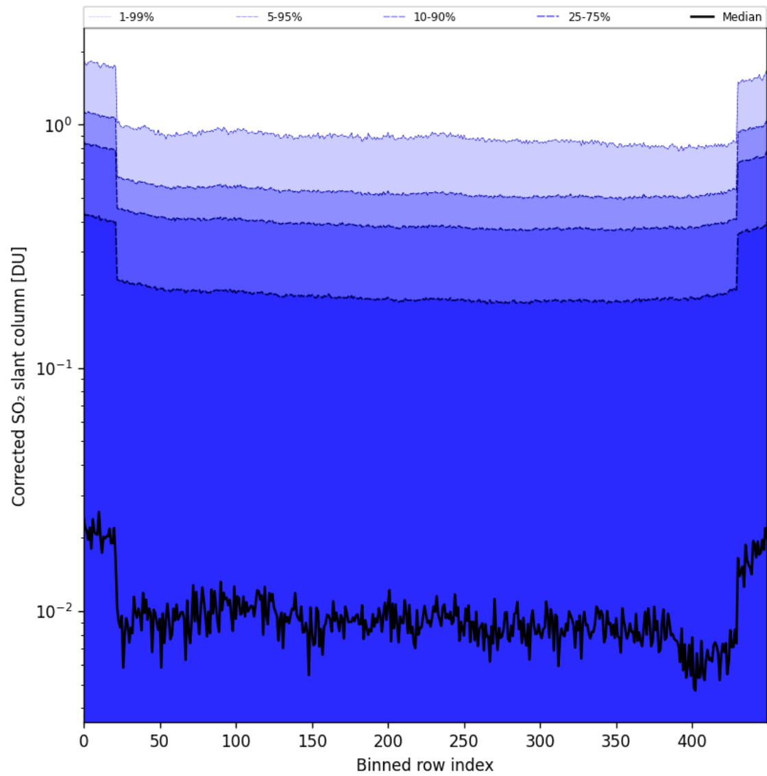
Figure 86: Along track statistics of “Corrected SO 2 slant column” for 2025-06-08 to 2025-06-10
