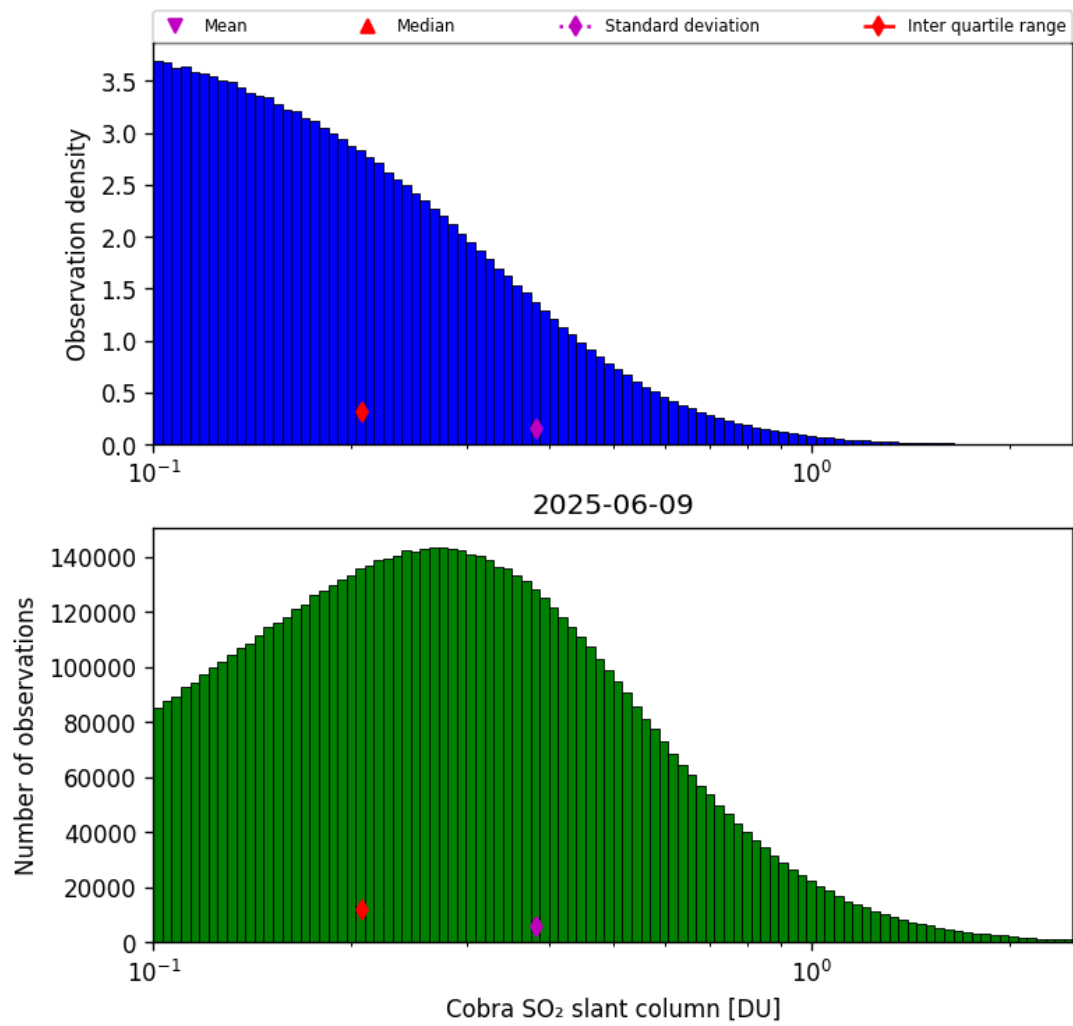
Figure 61: Histogram of “Cobra SO 2 slant column” for 2025-06-08 to 2025-06-10
