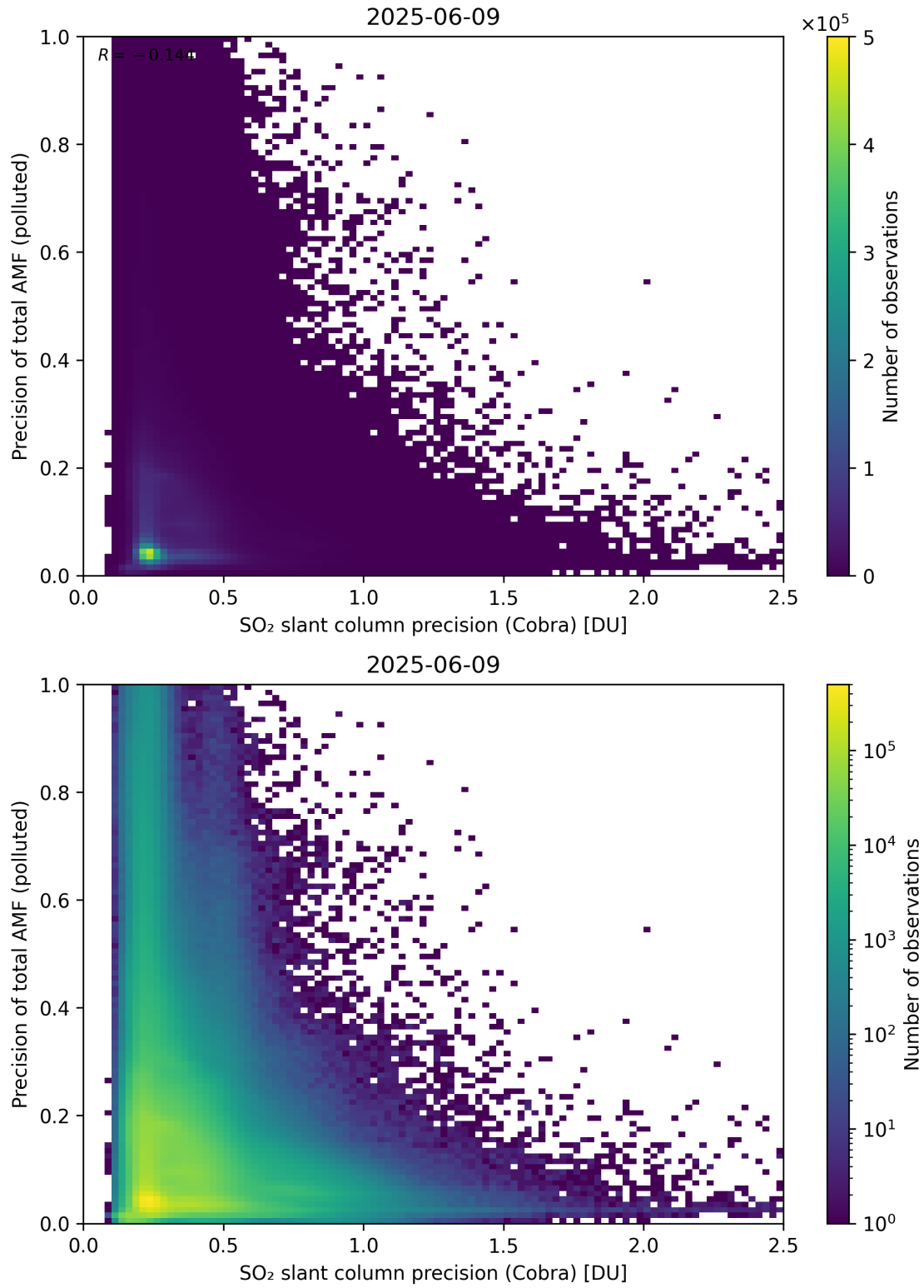
Figure 214: Scatter density plot of “SO 2 slant column precision (Cobra)” against “Precision of total AMF (polluted)” for 2025-06-08 to 2025-06-10.
