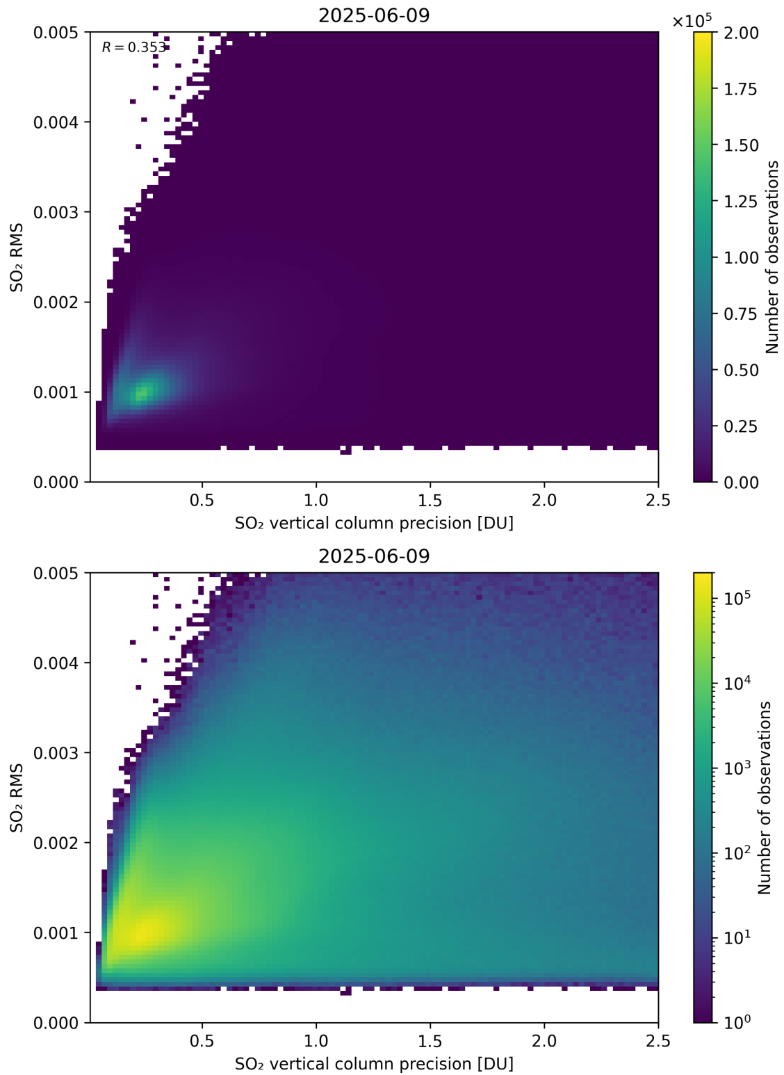
Figure 334: Scatter density plot of “SO 2 vertical column precision” against “SO 2 RMS” for 2025-06-08 to 2025-06-10.
