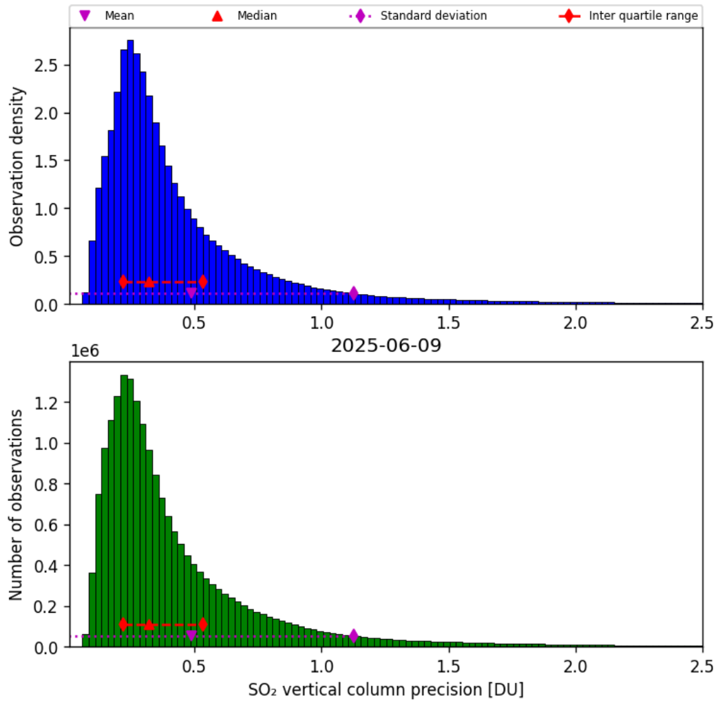
Figure 59: Histogram of “SO 2 vertical column precision” for 2025-06-08 to 2025-06-10
