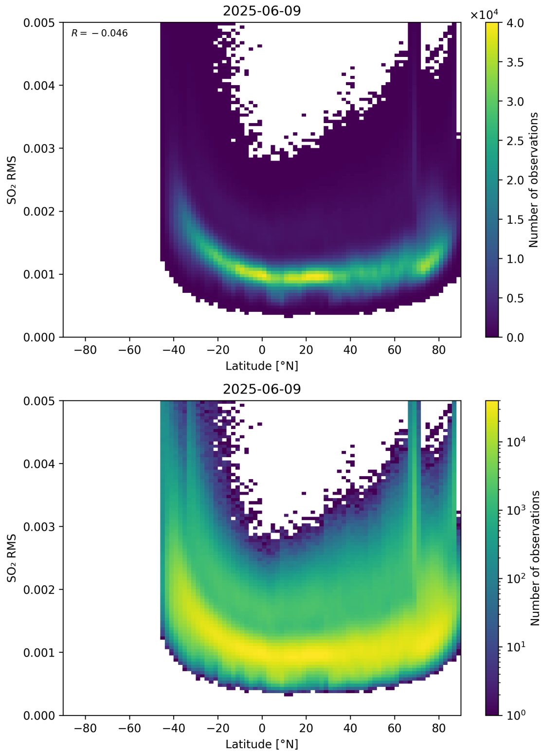
Figure 155: Scatter density plot of “Latitude” against “SO 2 RMS” for 2025-06-08 to 2025-06-10.
