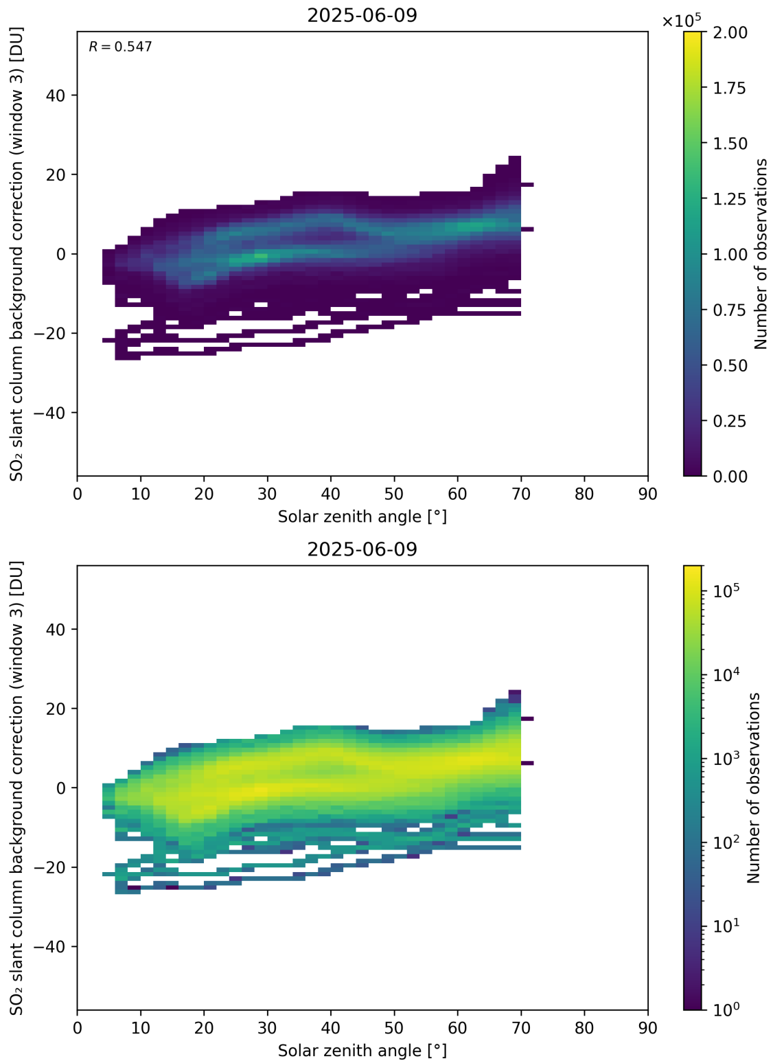
Figure 173: Scatter density plot of “Solar zenith angle” against “SO 2 slant column background correction (window 3)” for 2025-06-08 to 2025-06-10.
