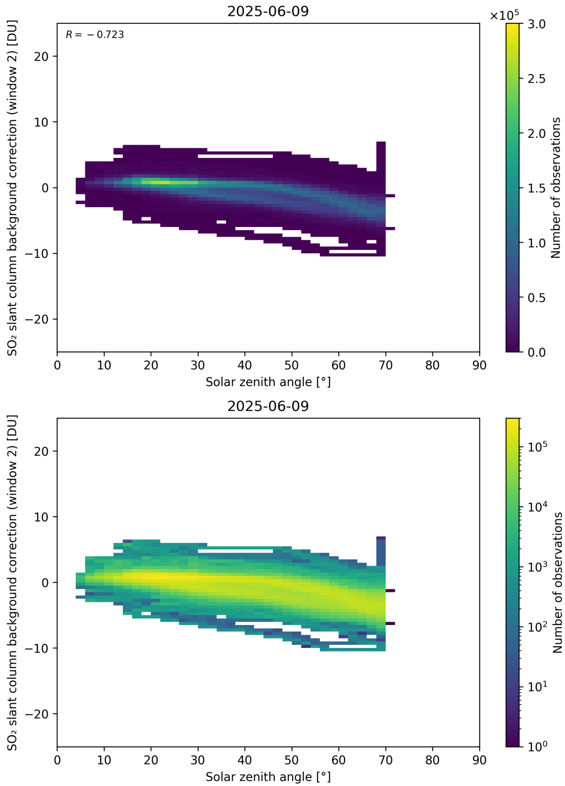
Figure 172: Scatter density plot of “Solar zenith angle” against “SO 2 slant column background correction (window 2)” for 2025-06-08 to 2025-06-10.
