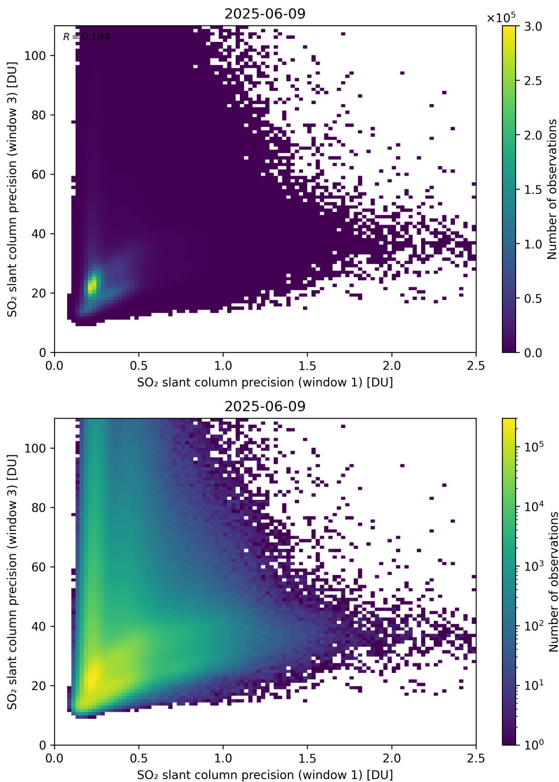
Figure 279: Scatter density plot of “SO 2 slant column precision (window 1)” against “SO 2 slant column precision (window 3)” for 2025-06-08 to 2025-06-10.
