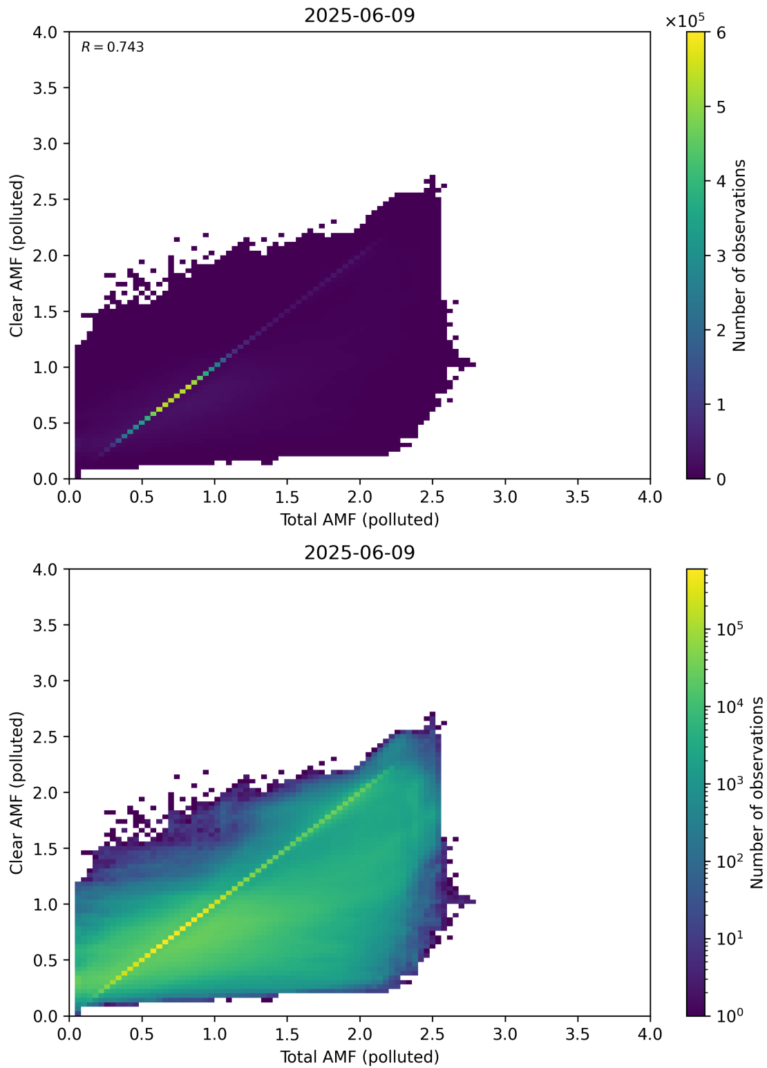
Figure 321: Scatter density plot of “Total AMF (polluted)” against “Clear AMF (polluted)” for 2025-06-08 to 2025-06-10.
