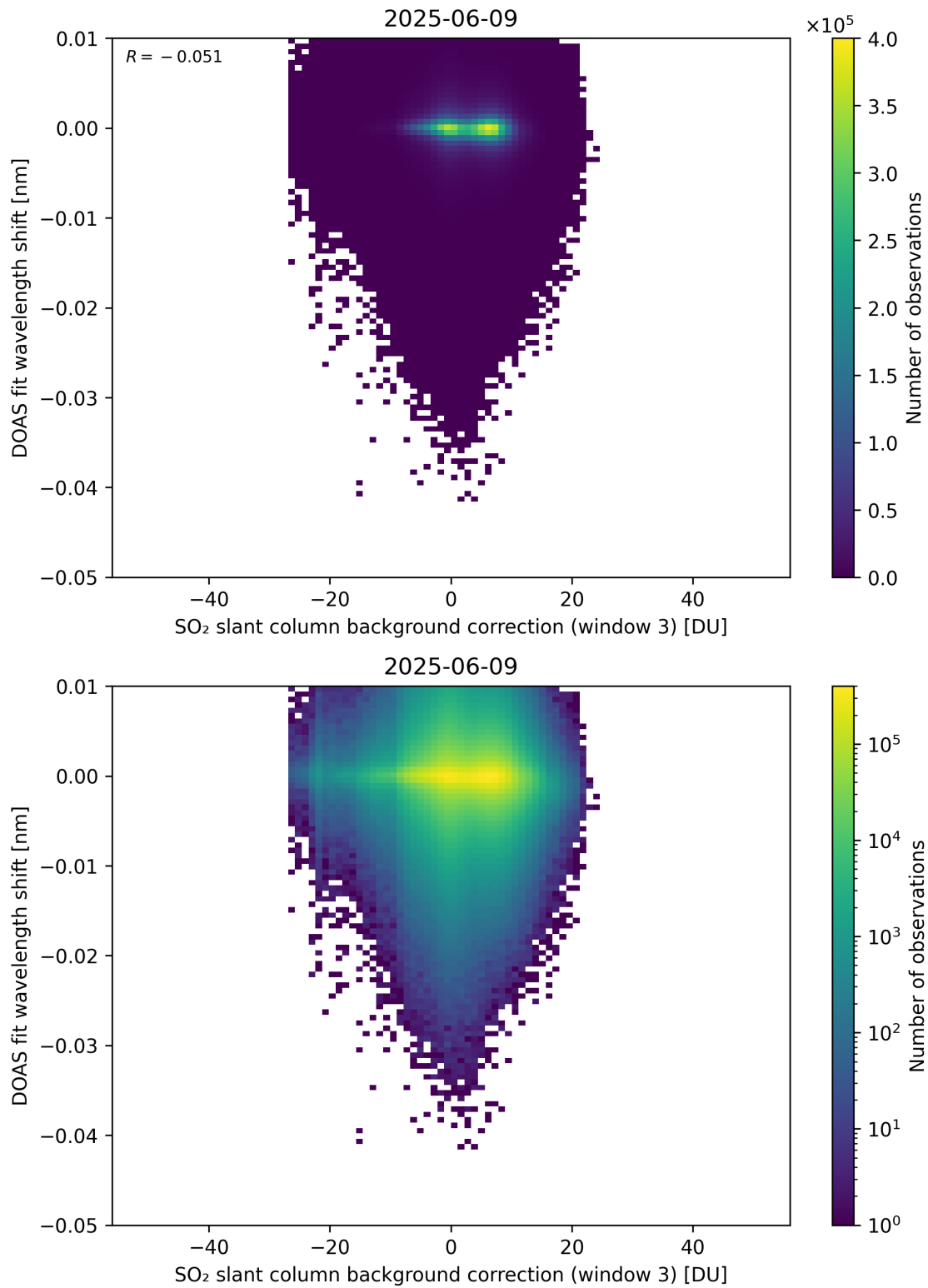
Figure 132: Scatter density plot of “SO 2 slant column background correction (window 3)” against “DOAS fit wavelength shift” for 2025-06-08 to 2025-06-10.
