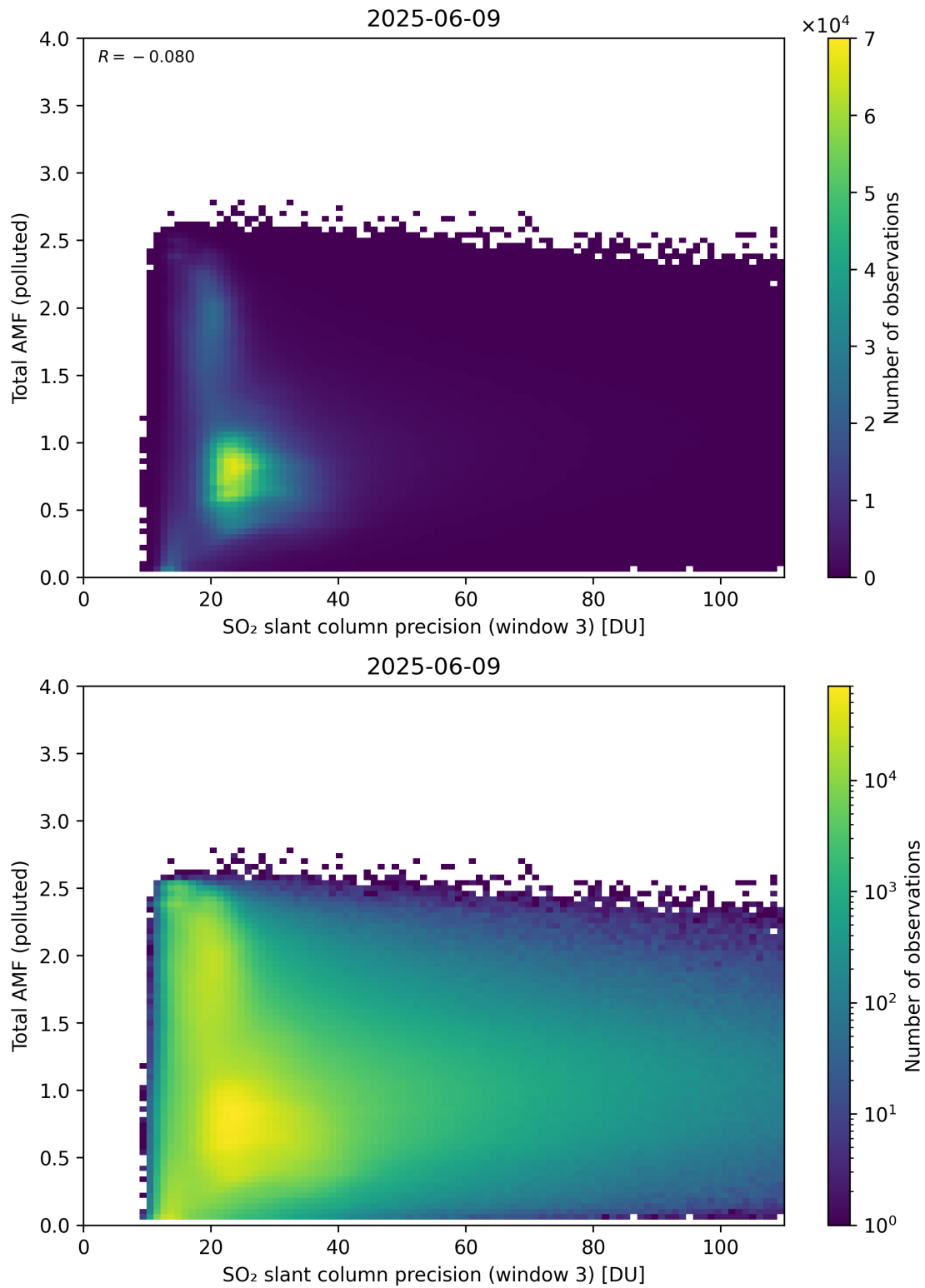
Figure 313: Scatter density plot of “SO 2 slant column precision (window 3)” against “Total AMF (polluted)” for 2025-06-08 to 2025-06-10.
