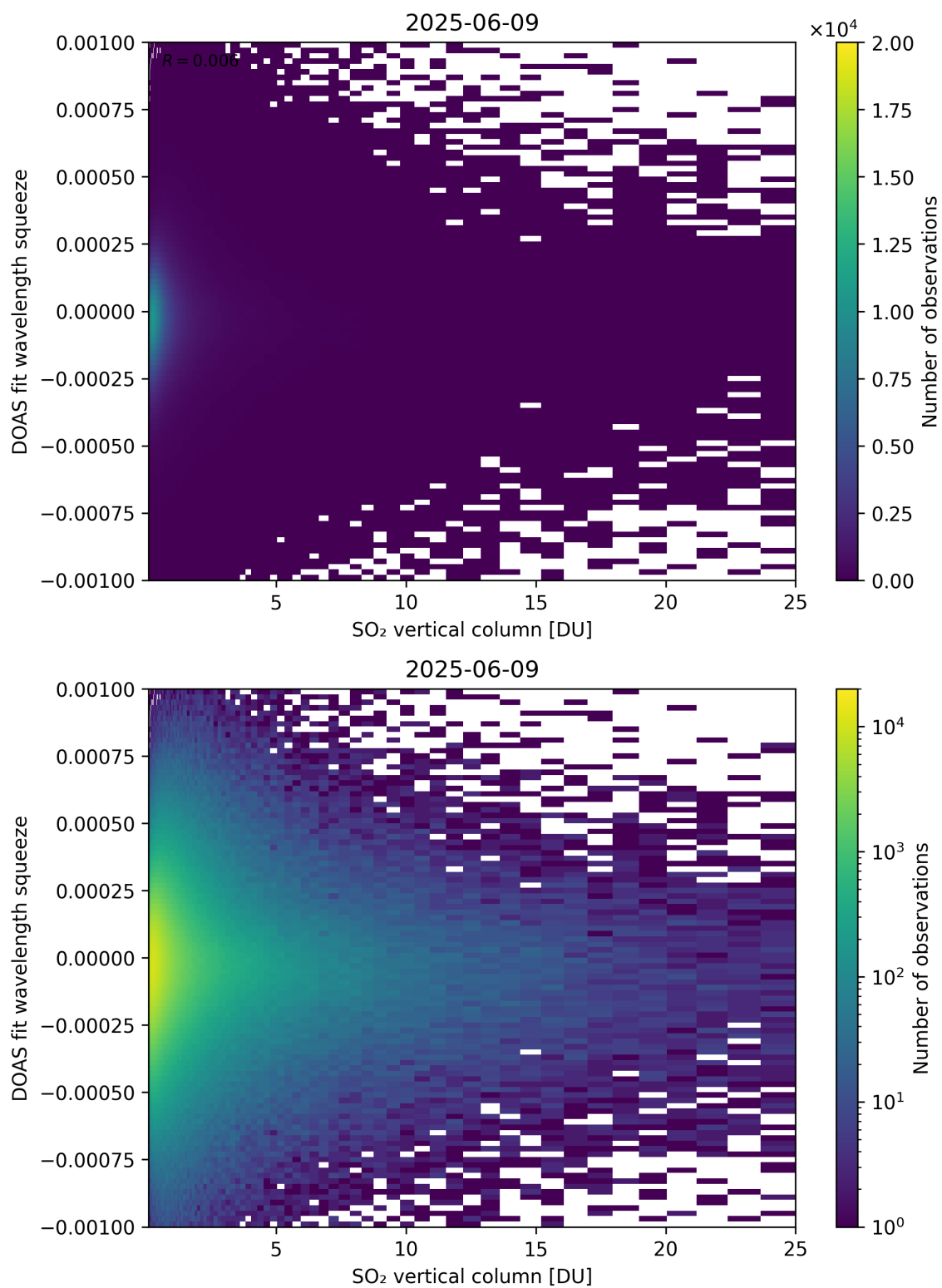
Figure 327: Scatter density plot of “SO 2 vertical column” against “DOAS fit wavelength squeeze” for 2025-06-08 to 2025-06-10.
