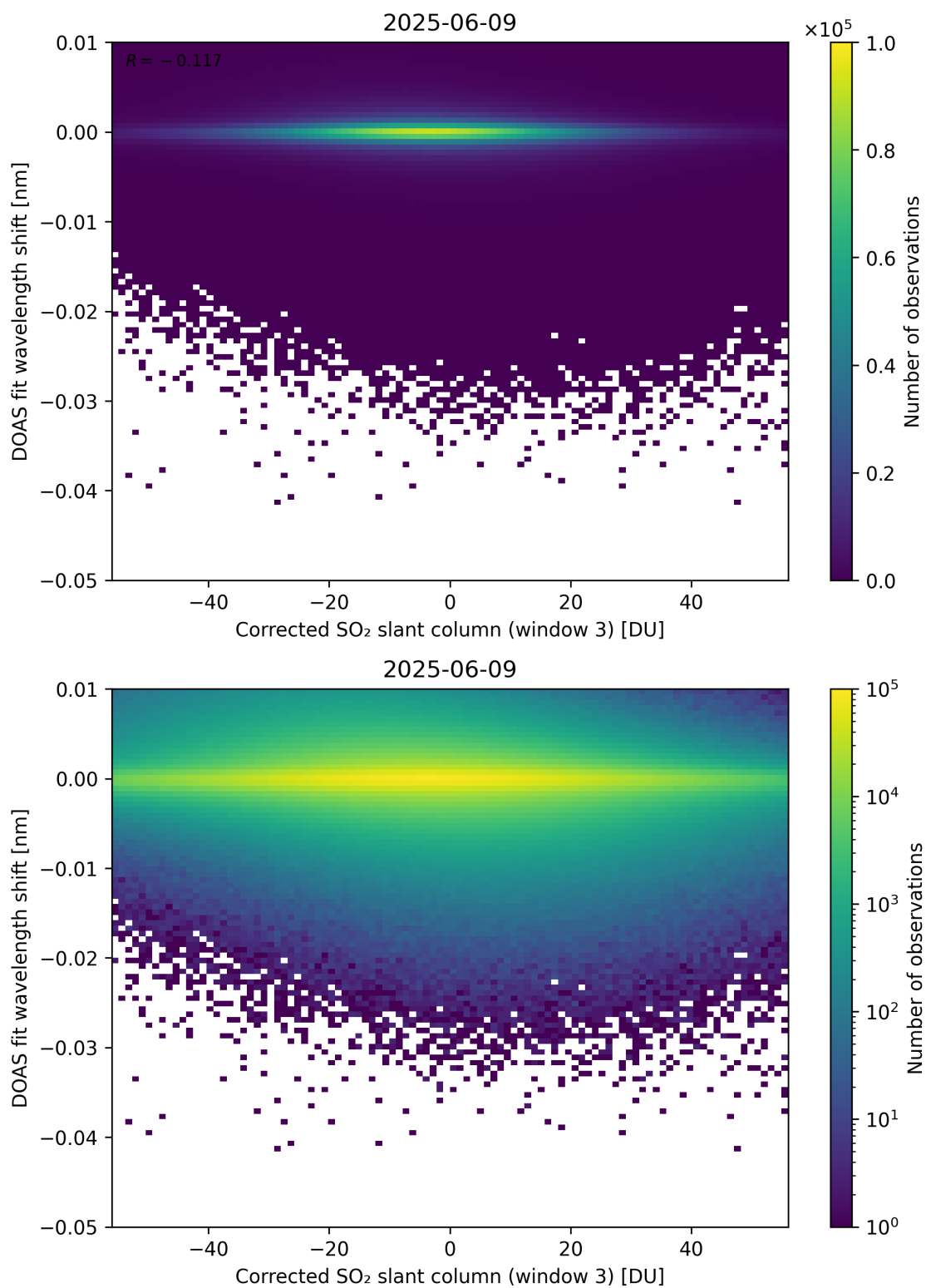
Figure 256: Scatter density plot of “Corrected SO 2 slant column (window 3)” against “DOAS fit wavelength shift” for 2025-06-08 to 2025-06-10.
