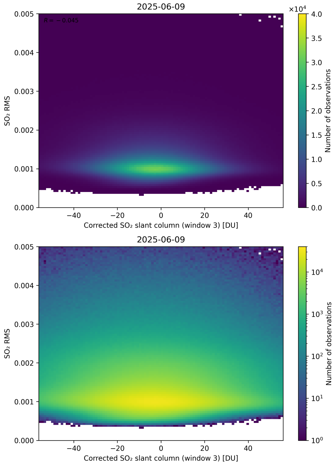
Figure 258: Scatter density plot of “Corrected SO 2 slant column (window 3)” against “SO 2 RMS” for 2025-06-08 to 2025-06-10.
