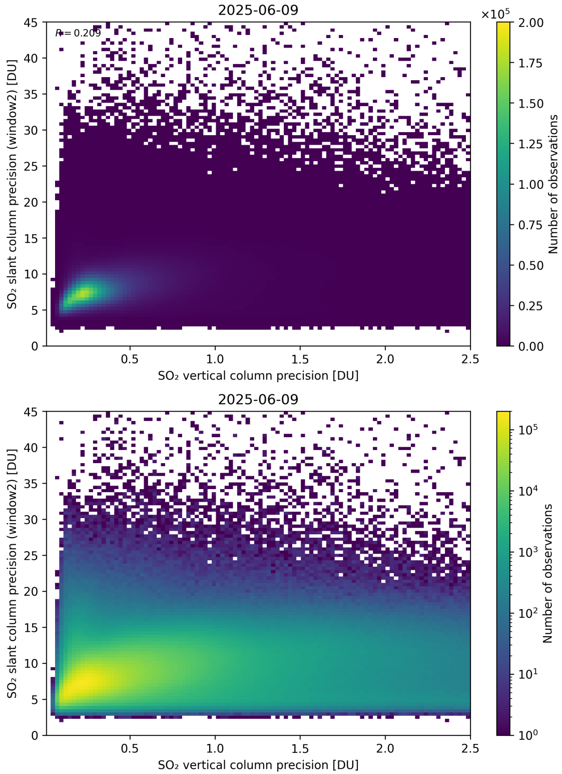
Figure 343: Scatter density plot of “SO 2 vertical column precision” against “SO 2 slant column precision (window2)” for 2025-06-08 to 2025-06-10.
