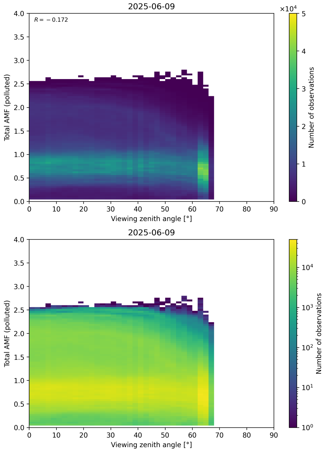
Figure 381: Scatter density plot of “Viewing zenith angle” against “Total AMF (polluted)” for 2025-06-08 to 2025-06-10.
