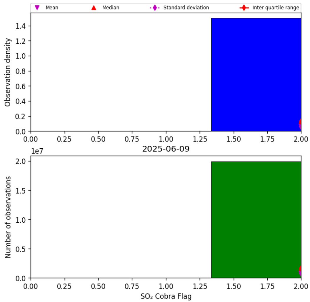
Figure 75: Histogram of “SO 2 Cobra Flag” for 2025-06-08 to 2025-06-10
