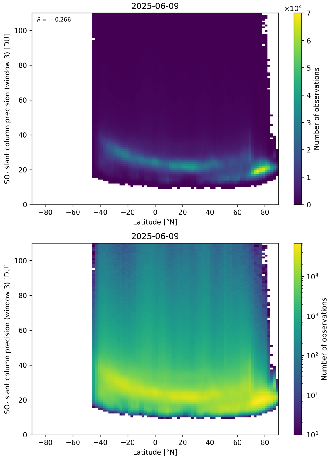
Figure 166: Scatter density plot of “Latitude” against “SO 2 slant column precision (window 3)” for 2025-06-08 to 2025-06-10.
