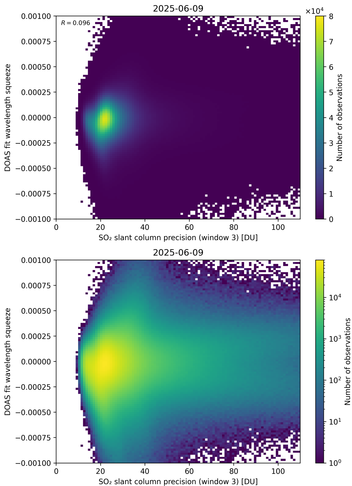
Figure 309: Scatter density plot of “SO 2 slant column precision (window 3)” against “DOAS fit wavelength squeeze” for 2025-06-08 to 2025-06-10.
