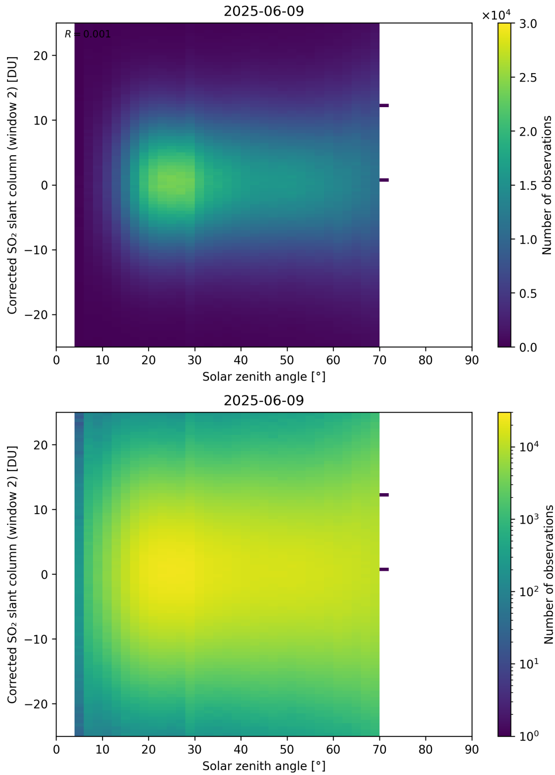
Figure 182: Scatter density plot of “Solar zenith angle” against “Corrected SO 2 slant column (window 2)” for 2025-06-08 to 2025-06-10.
