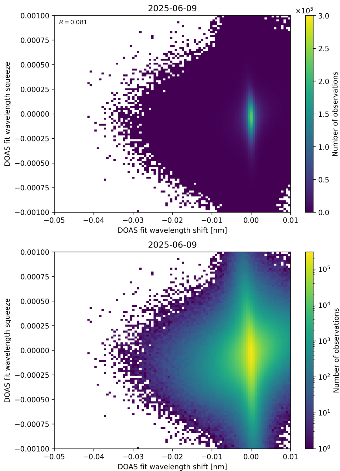
Figure 138: Scatter density plot of “DOAS fit wavelength shift” against “DOAS fit wavelength squeeze” for 2025-06-08 to 2025-06-10.
