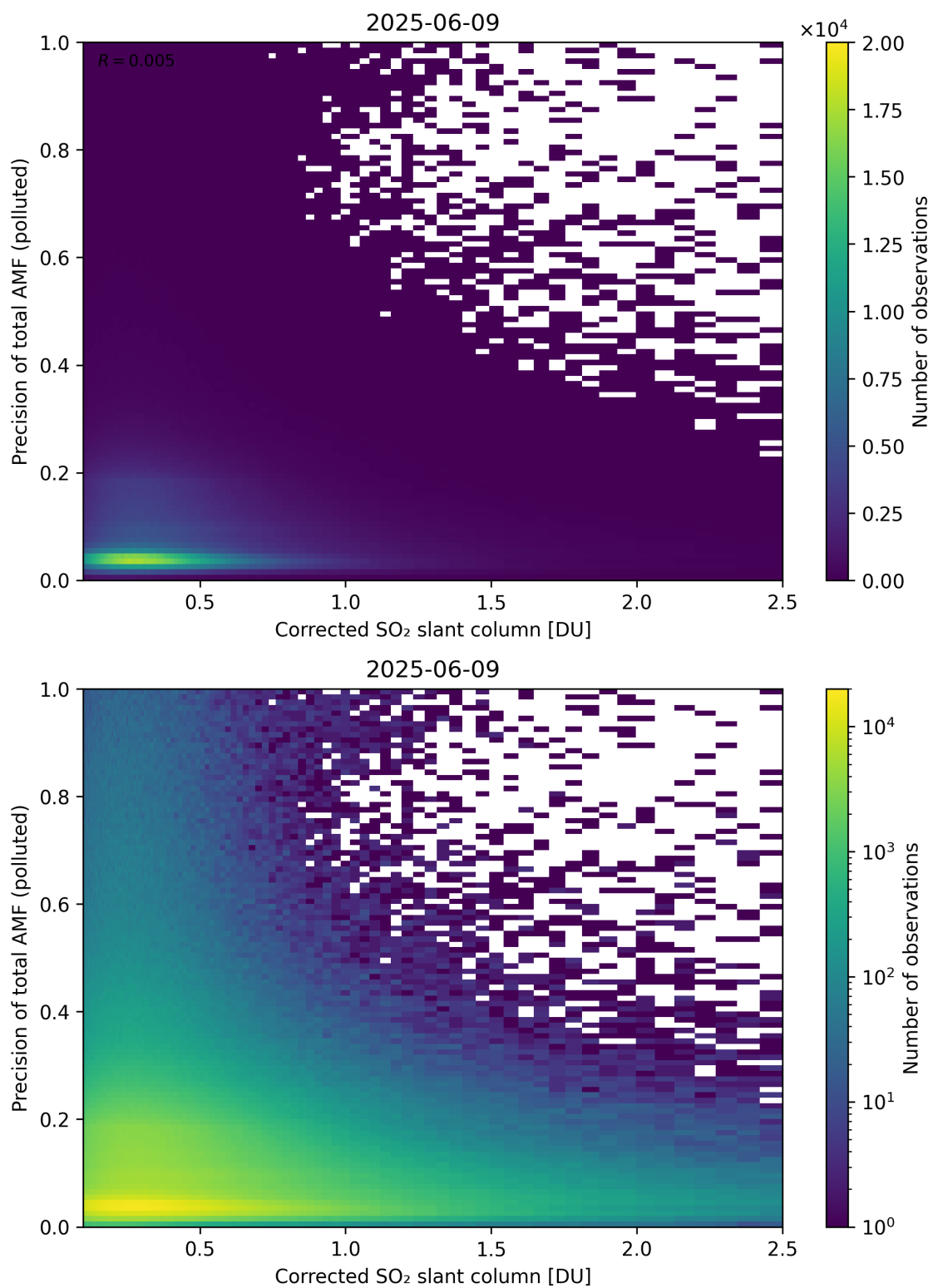
Figure 243: Scatter density plot of “Corrected SO 2 slant column” against “Precision of total AMF (polluted)” for 2025-06-08 to 2025-06-10.
