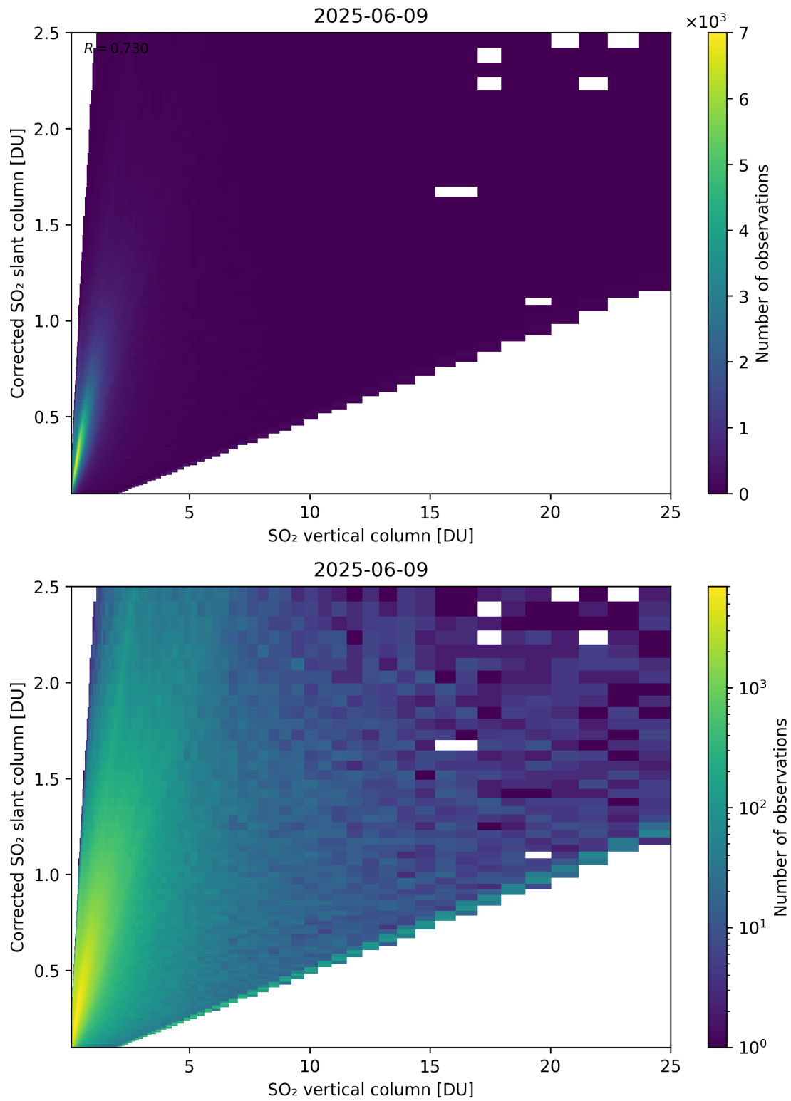
Figure 351: Scatter density plot of “SO 2 vertical column” against “Corrected SO 2 slant column” for 2025-06-08 to 2025-06-10.
