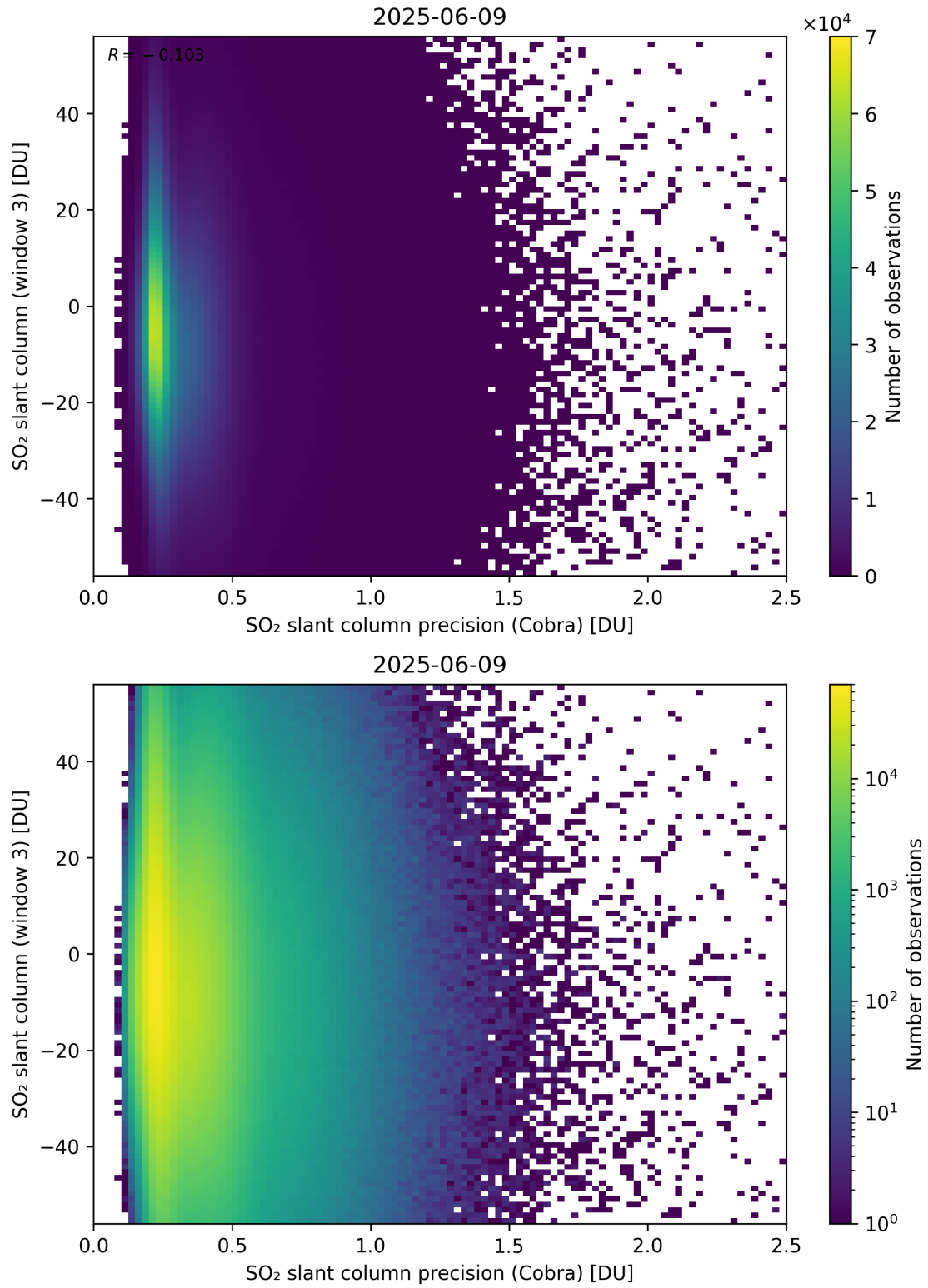
Figure 211: Scatter density plot of “SO 2 slant column precision (Cobra)” against “SO 2 slant column (window 3)” for 2025-06-08 to 2025-06-10.
