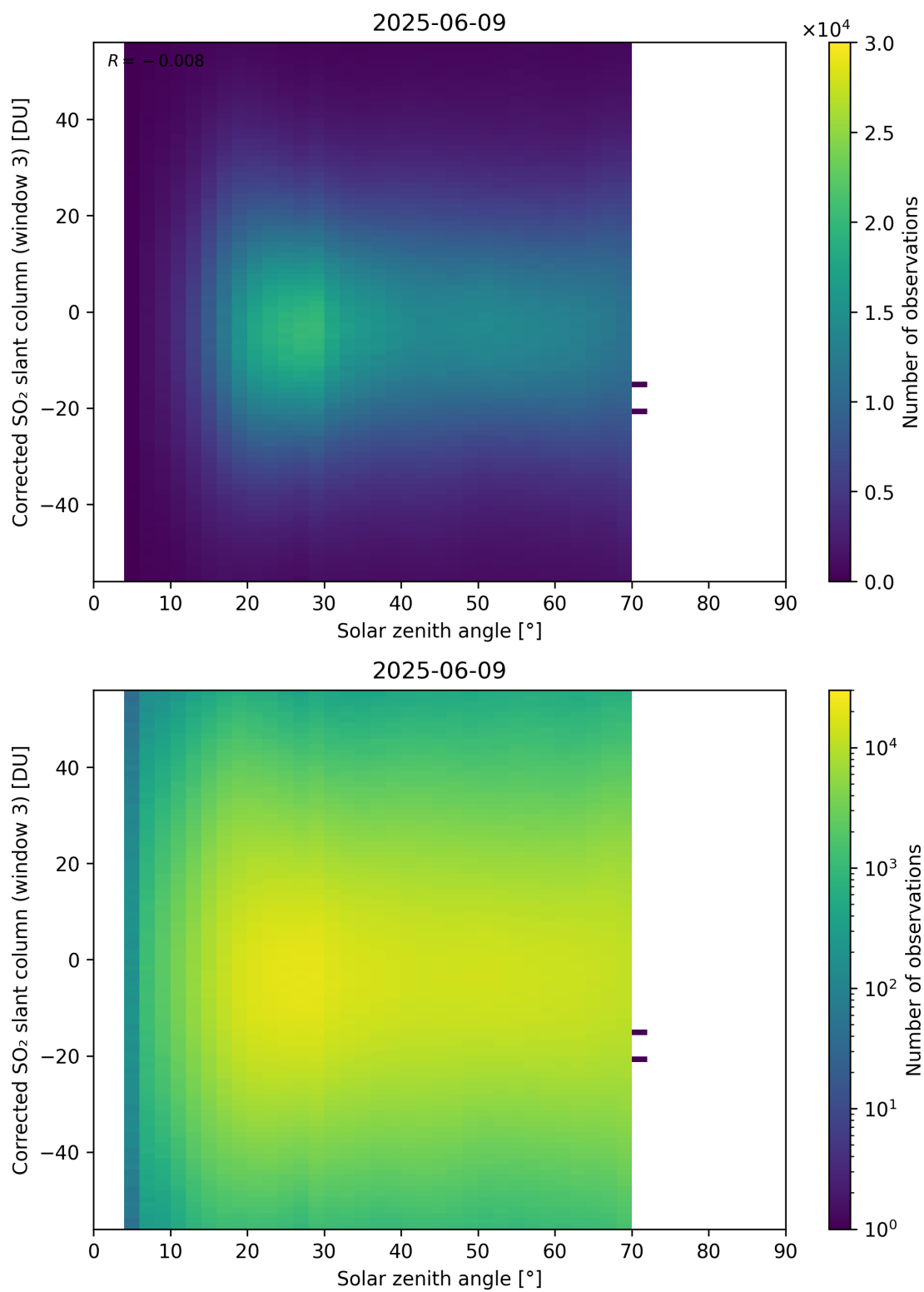
Figure 183: Scatter density plot of “Solar zenith angle” against “Corrected SO 2 slant column (window 3)” for 2025-06-08 to 2025-06-10.
