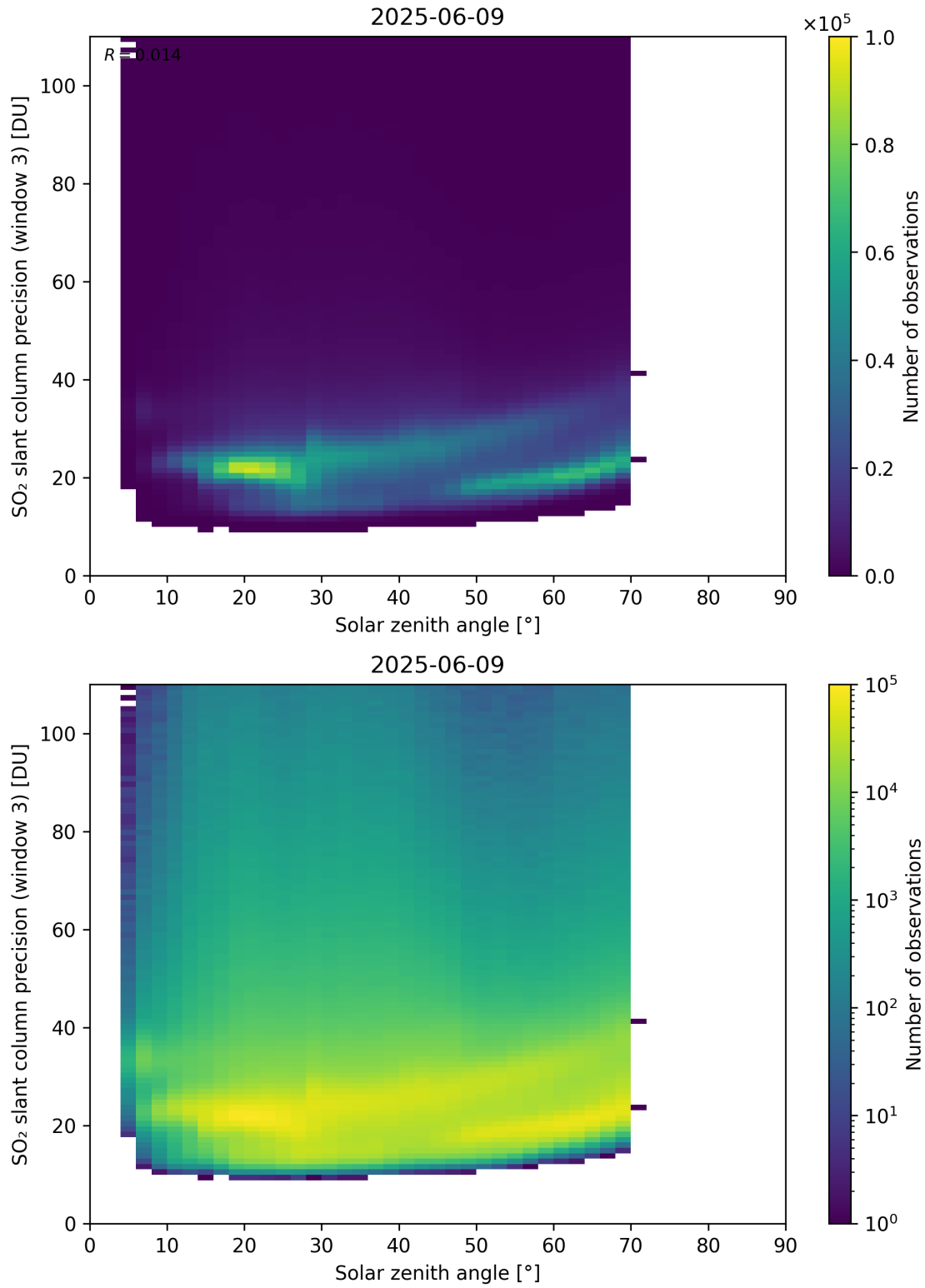
Figure 188: Scatter density plot of “Solar zenith angle” against “SO 2 slant column precision (window 3)” for 2025-06-08 to 2025-06-10.
