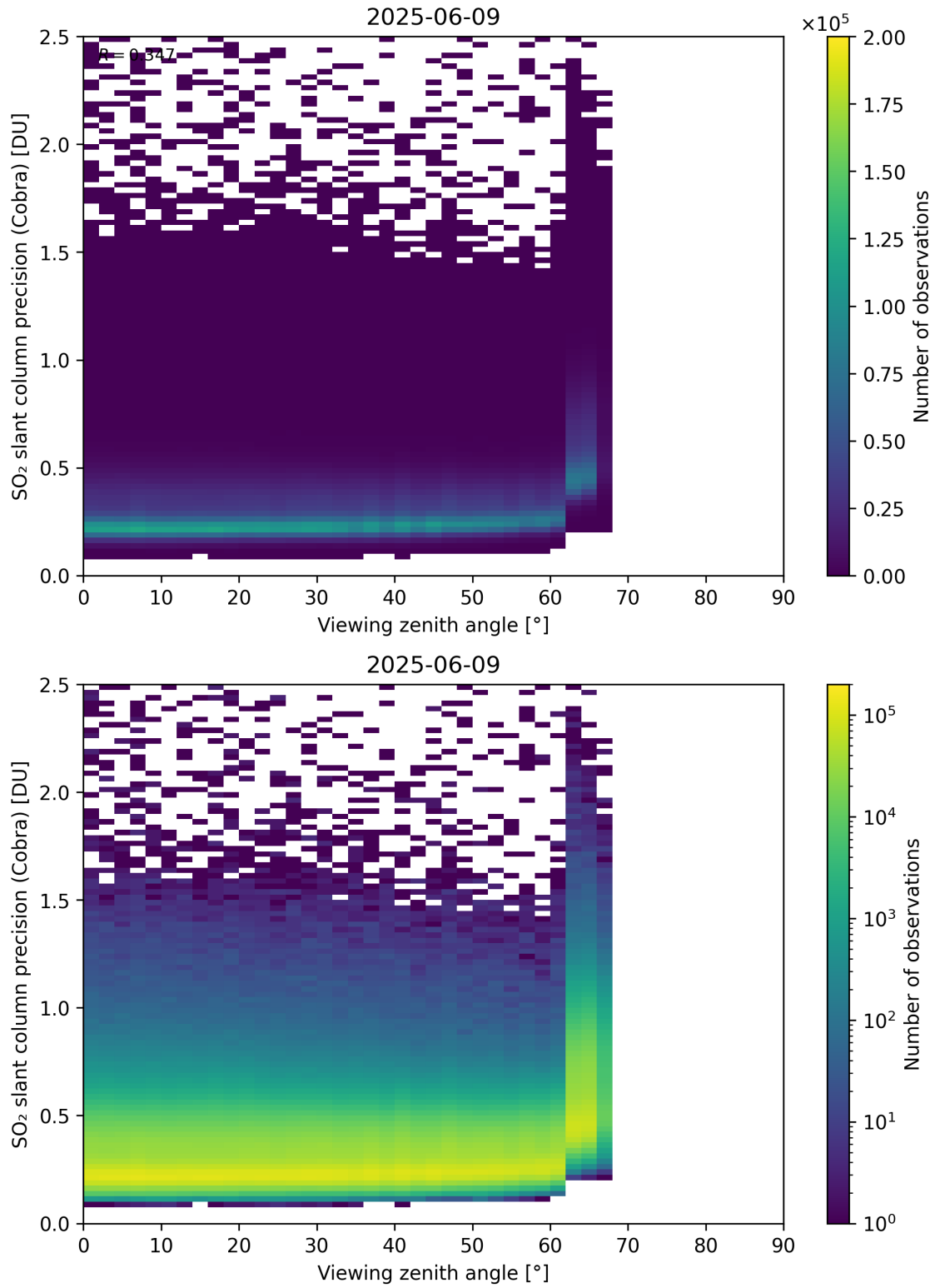
Figure 372: Scatter density plot of “Viewing zenith angle” against “SO 2 slant column precision (Cobra)” for 2025-06-08 to 2025-06-10.
