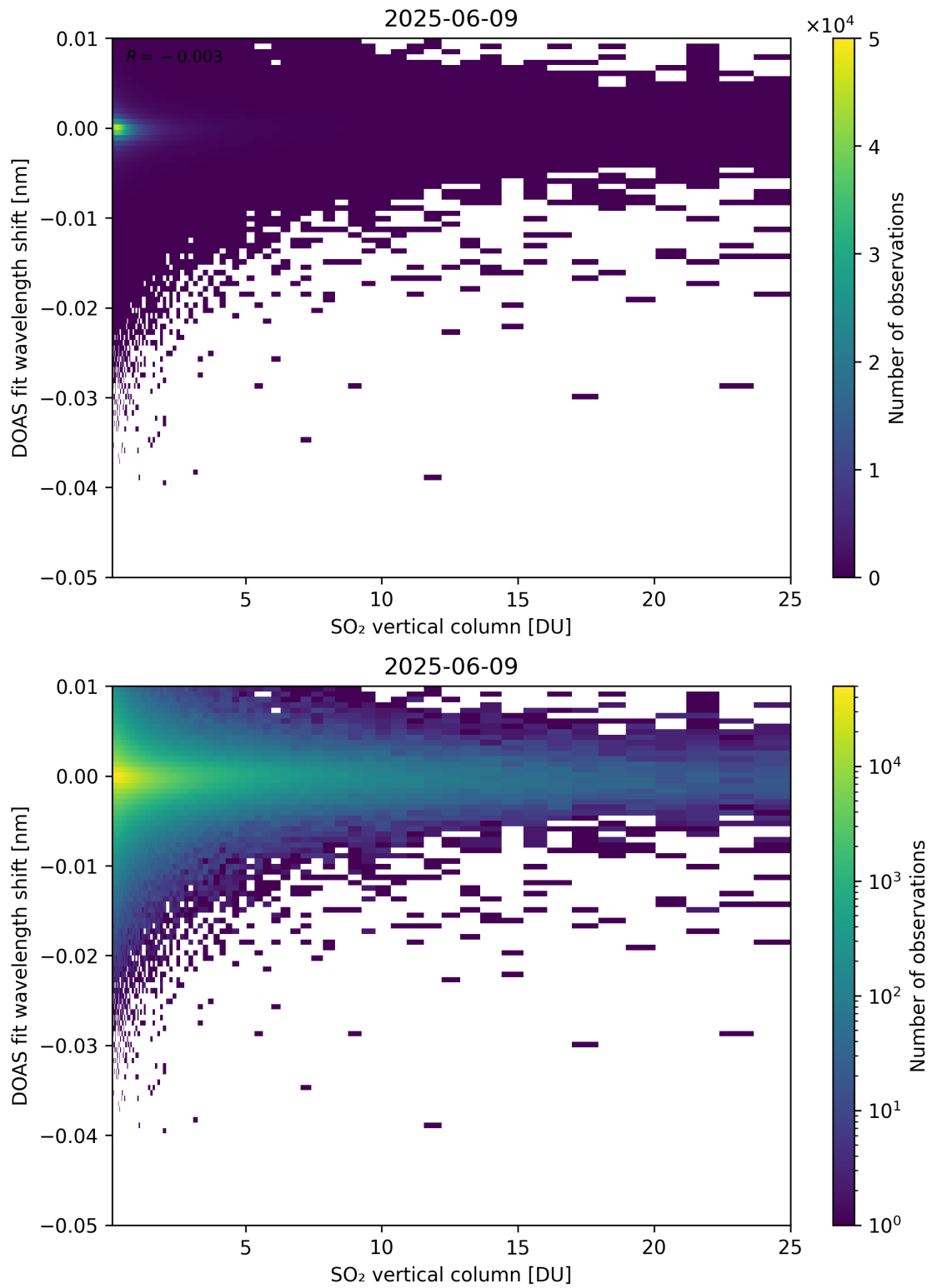
Figure 326: Scatter density plot of “SO 2 vertical column” against “DOAS fit wavelength shift” for 2025-06-08 to 2025-06-10.
