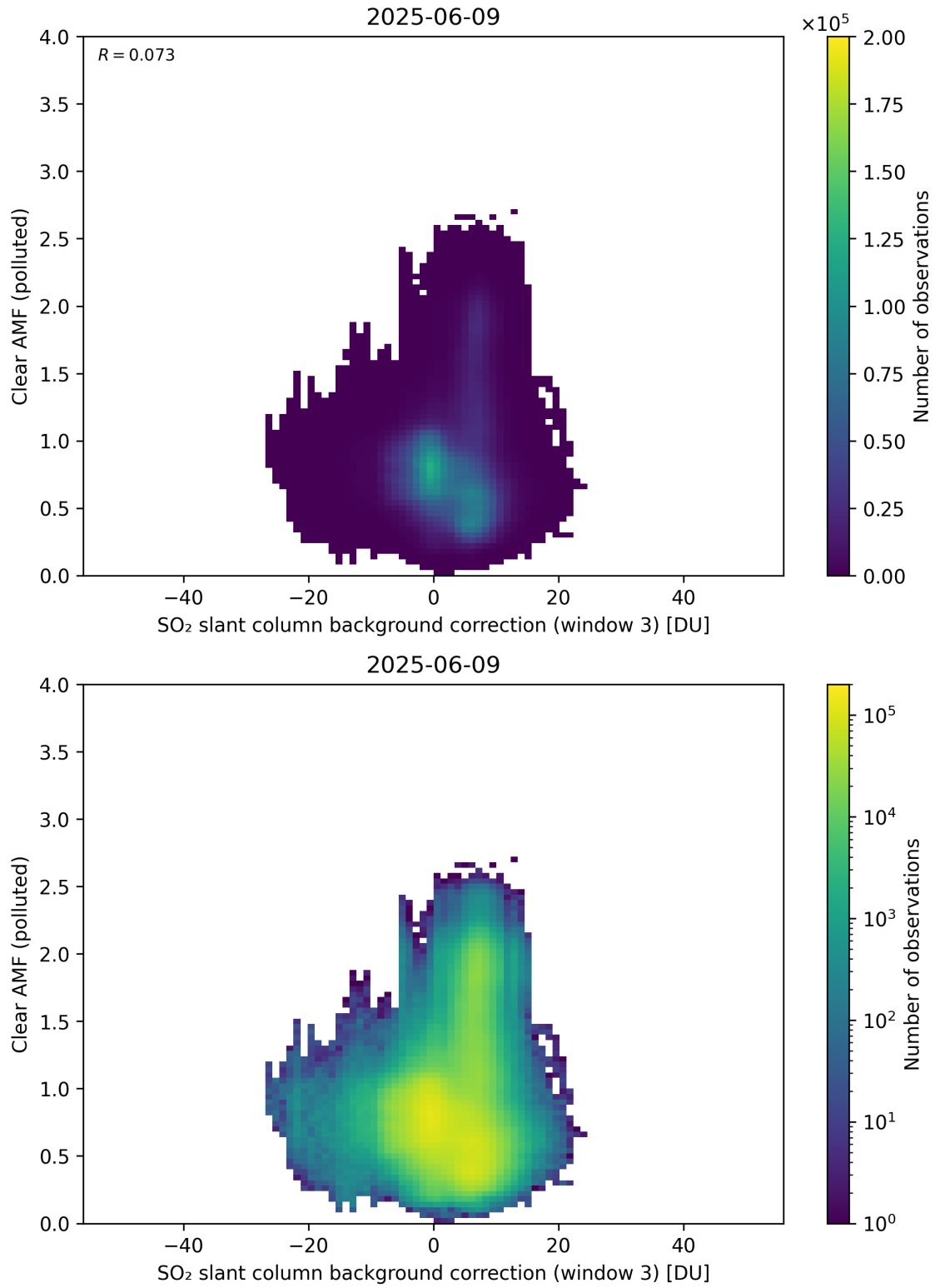
Figure 135: Scatter density plot of “SO 2 slant column background correction (window 3)” against “Clear AMF (polluted)” for 2025-06-08 to 2025-06-10.
