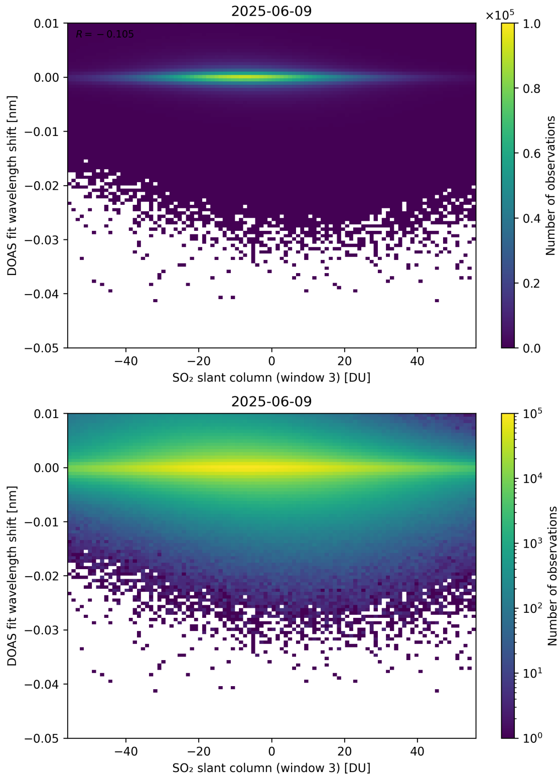
Figure 304: Scatter density plot of “SO 2 slant column (window 3)” against “DOAS fit wavelength shift” for 2025-06-08 to 2025-06-10.
