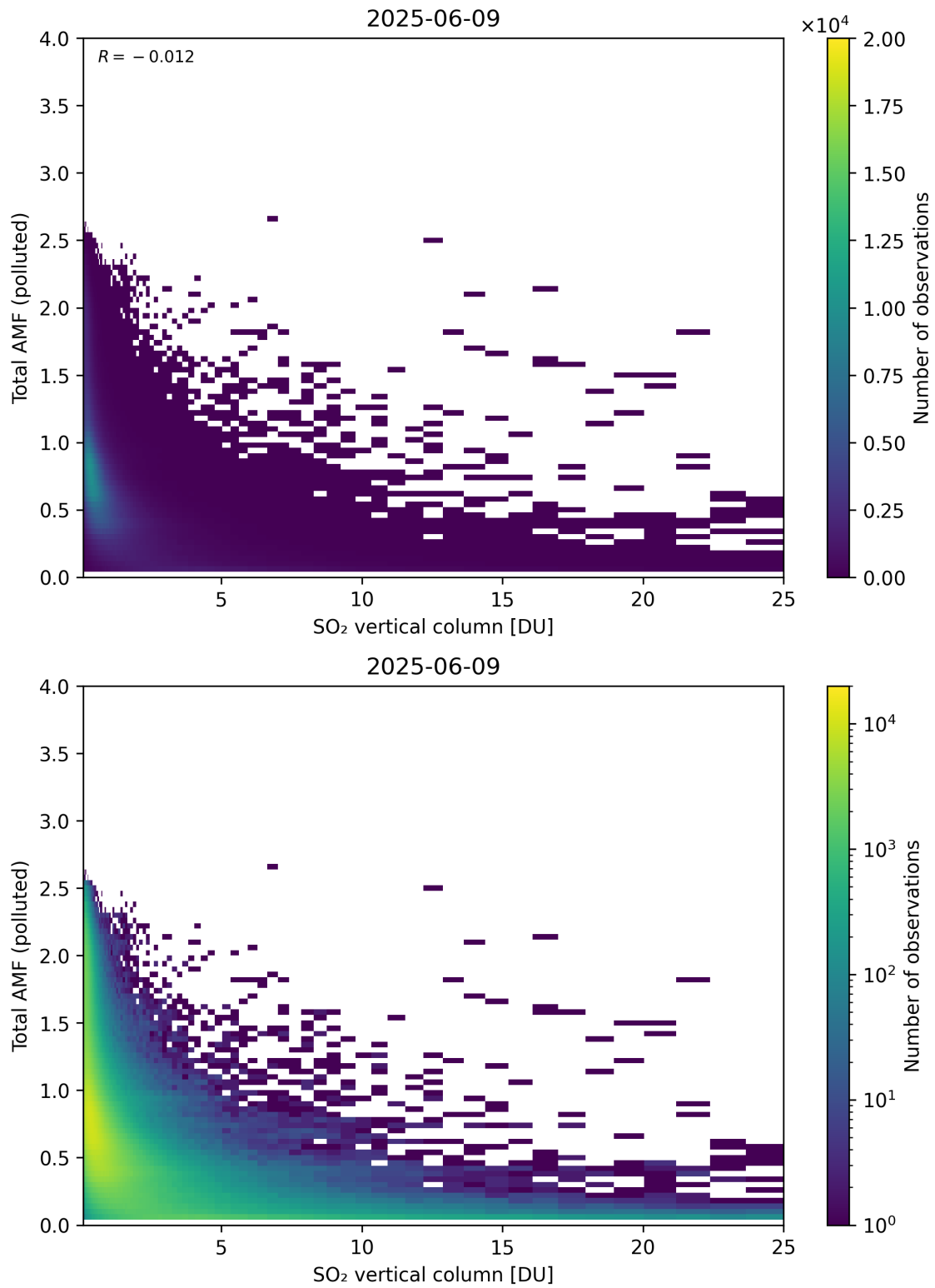
Figure 359: Scatter density plot of “SO 2 vertical column” against “Total AMF (polluted)” for 2025-06-08 to 2025-06-10.
