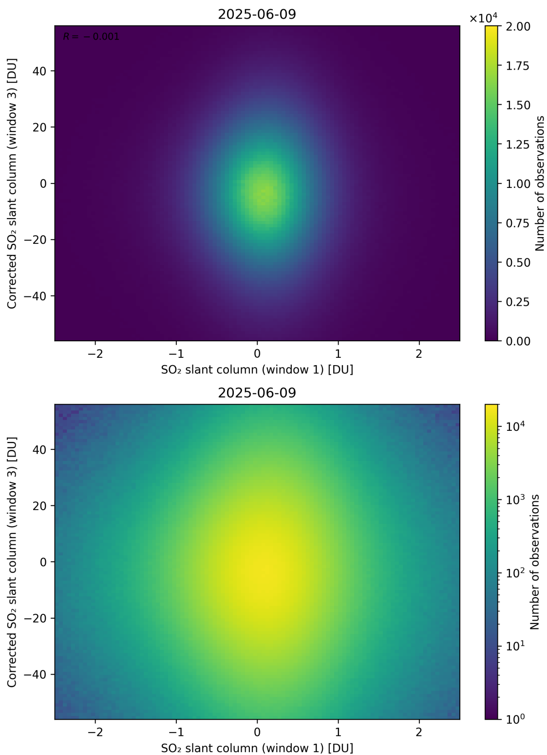
Figure 284: Scatter density plot of “SO 2 slant column (window 1)” against “Corrected SO 2 slant column (window 3)” for 2025-06-08 to 2025-06-10.
