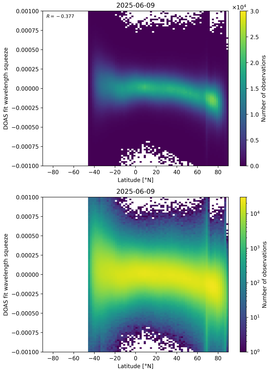
Figure 154: Scatter density plot of “Latitude” against “DOAS fit wavelength squeeze” for 2025-06-08 to 2025-06-10.
