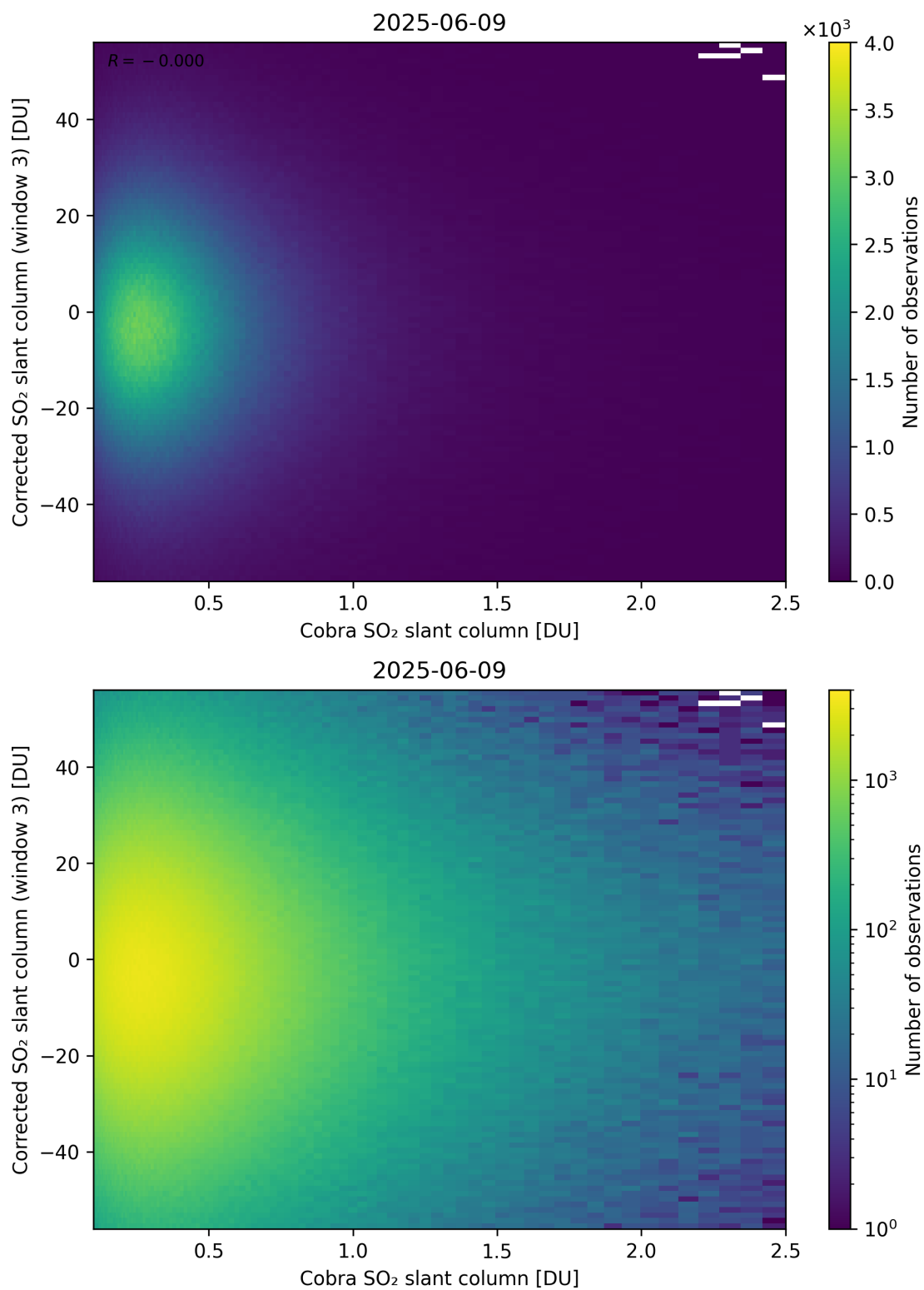
Figure 218: Scatter density plot of “Cobra SO 2 slant column” against “Corrected SO 2 slant column (window 3)” for 2025-06-08 to 2025-06-10.
