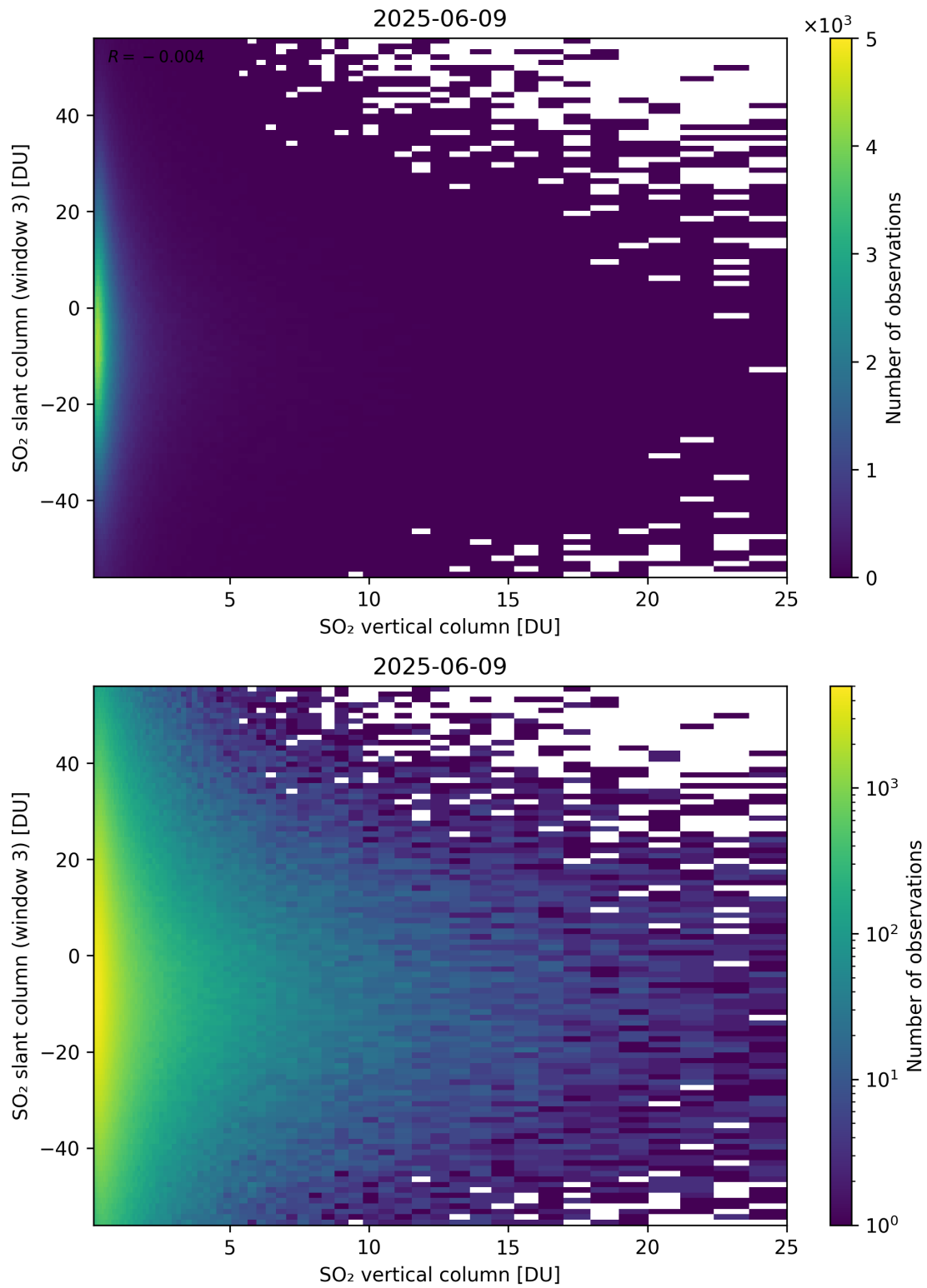
Figure 357: Scatter density plot of “SO 2 vertical column” against “SO 2 slant column (window 3)” for 2025-06-08 to 2025-06-10.
