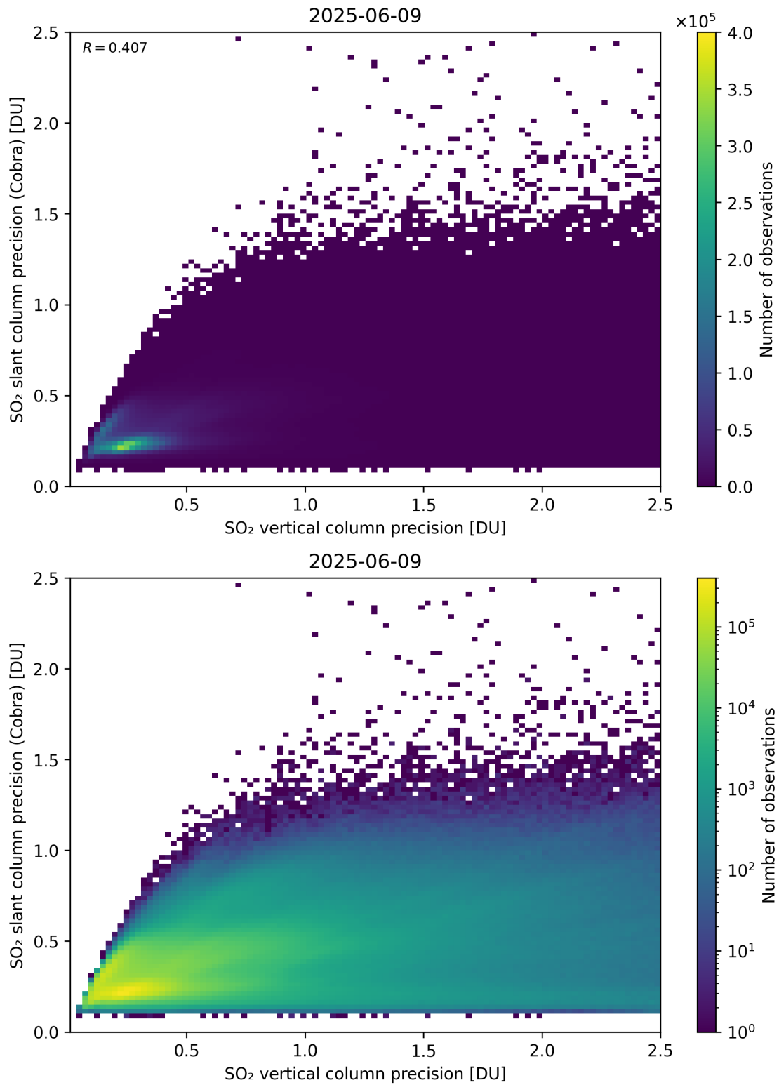
Figure 337: Scatter density plot of “SO 2 vertical column precision” against “SO 2 slant column precision (Cobra)” for 2025-06-08 to 2025-06-10.
