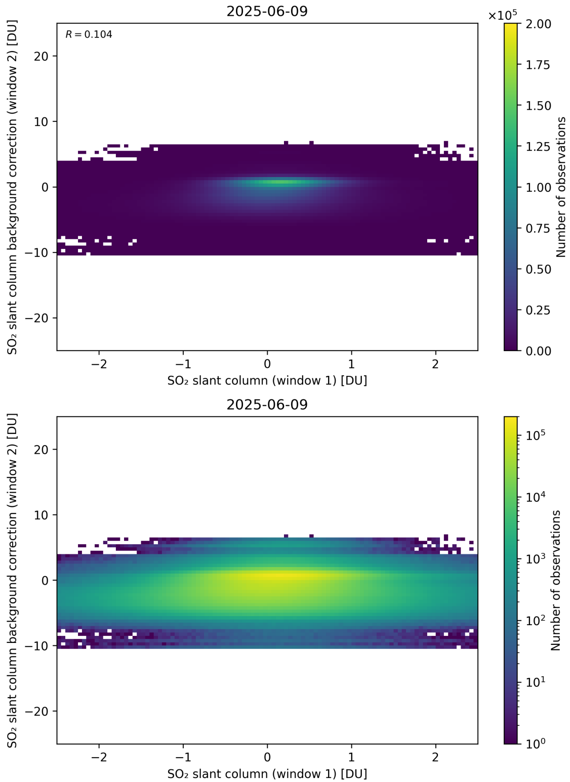
Figure 263: Scatter density plot of “SO 2 slant column (window 1)” against “SO 2 slant column background correction (window 2)” for 2025-06-08 to 2025-06-10.
