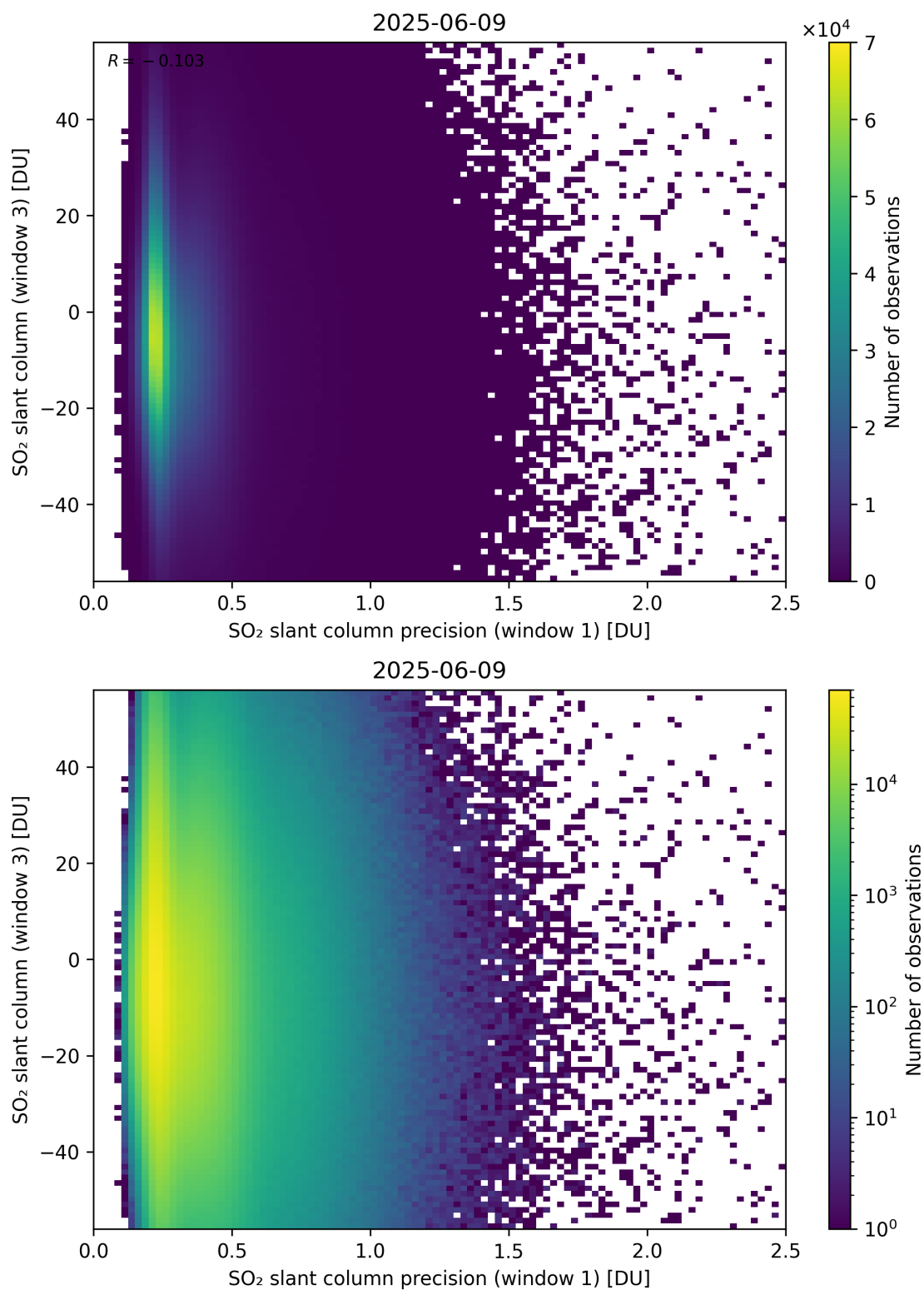
Figure 278: Scatter density plot of “SO 2 slant column precision (window 1)” against “SO 2 slant column (window 3)” for 2025-06-08 to 2025-06-10.
