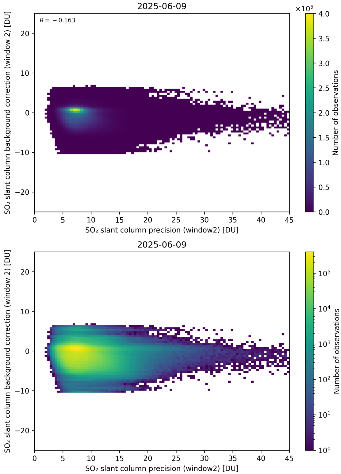
Figure 291: Scatter density plot of “SO 2 slant column precision (window2)” against “SO 2 slant column background correction (window 2)” for 2025-06-08 to 2025-06-10.
