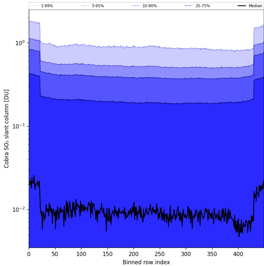
Figure 87: Along track statistics of “Cobra SO 2 slant column” for 2025-06-08 to 2025-06-10
