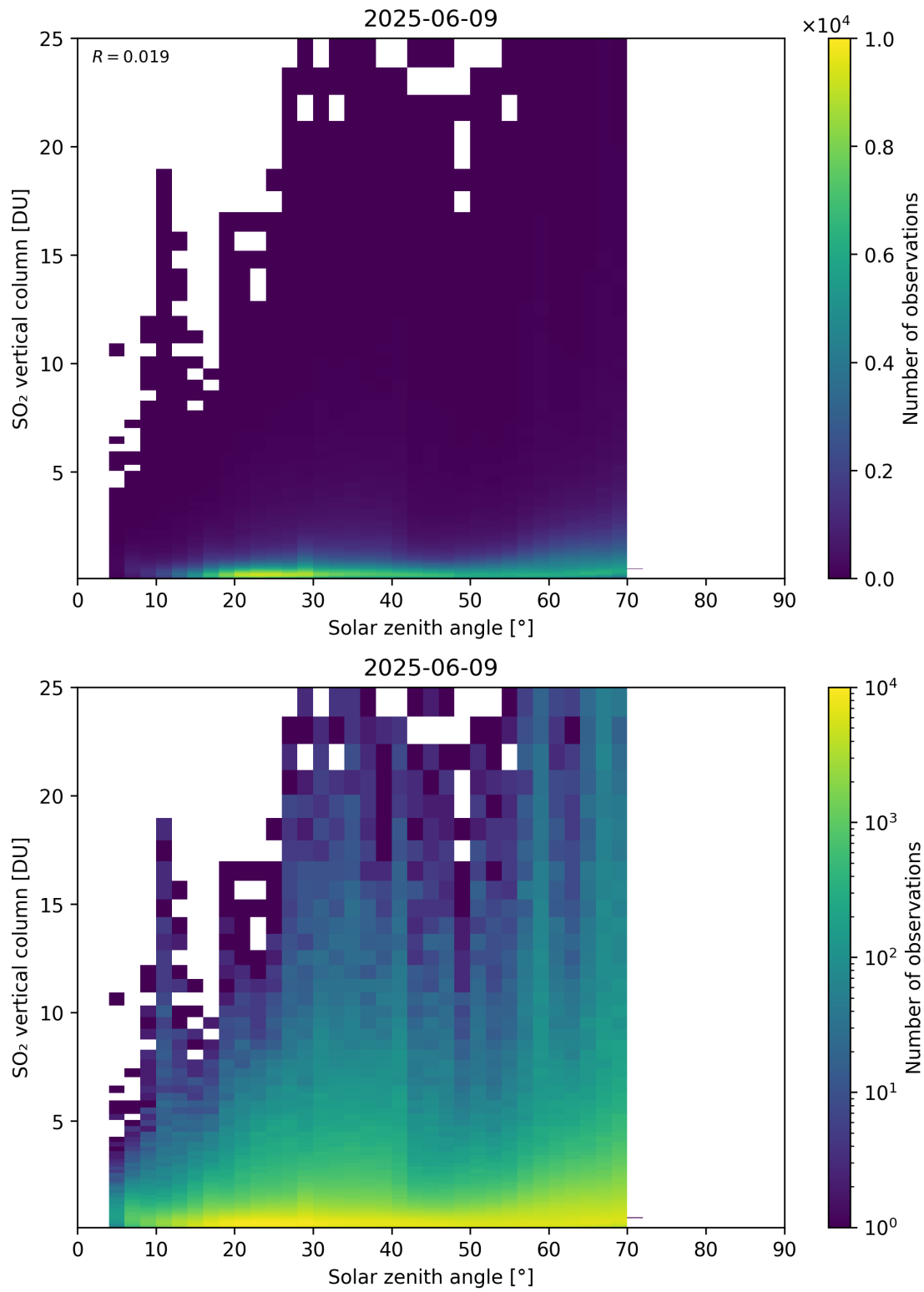
Figure 191: Scatter density plot of “Solar zenith angle” against “SO 2 vertical column” for 2025-06-08 to 2025-06-10.
