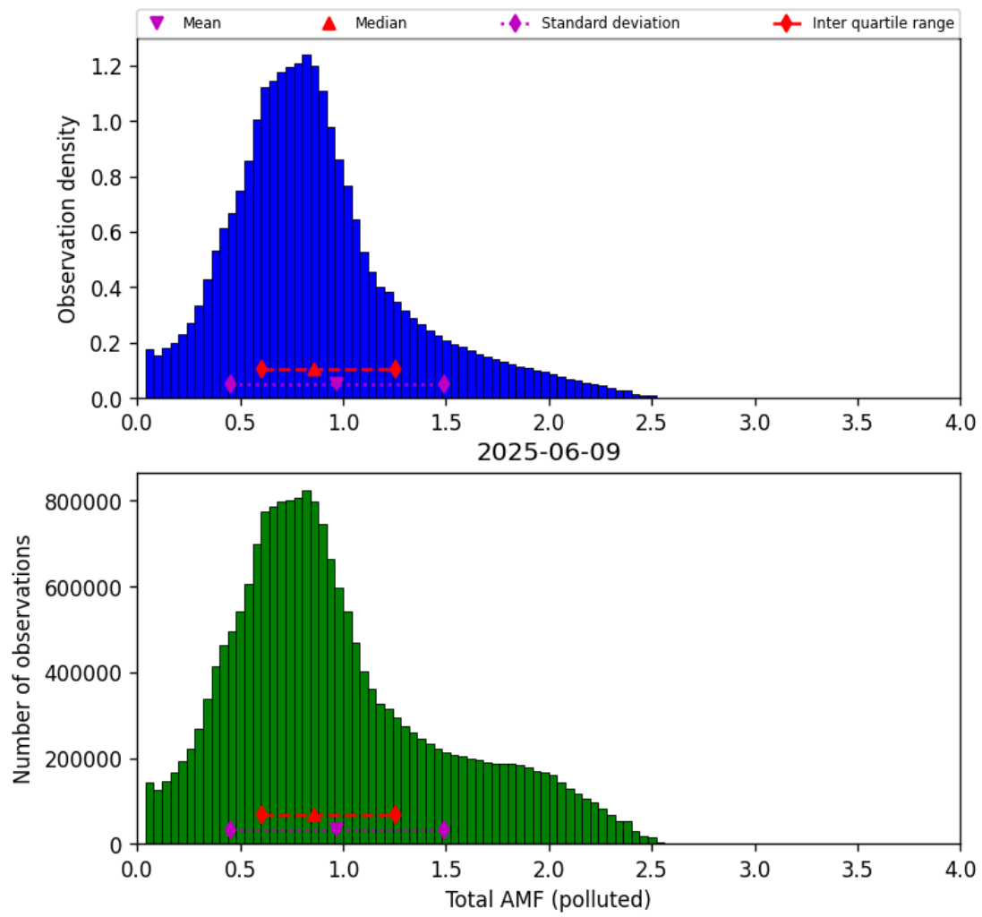
Figure 79: Histogram of “Total AMF (polluted)” for 2025-06-08 to 2025-06-10
