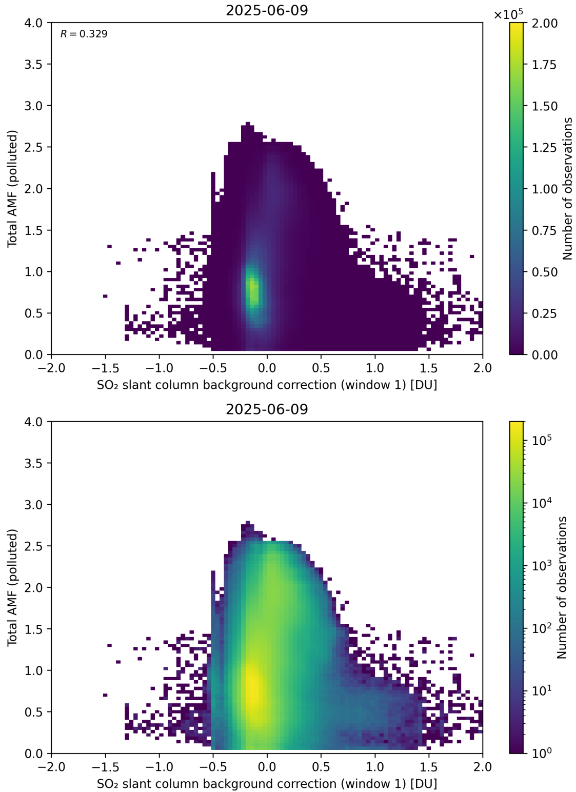
Figure 120: Scatter density plot of “SO 2 slant column background correction (window 1)” against “Total AMF (polluted)” for 2025-06-08 to 2025-06-10.
