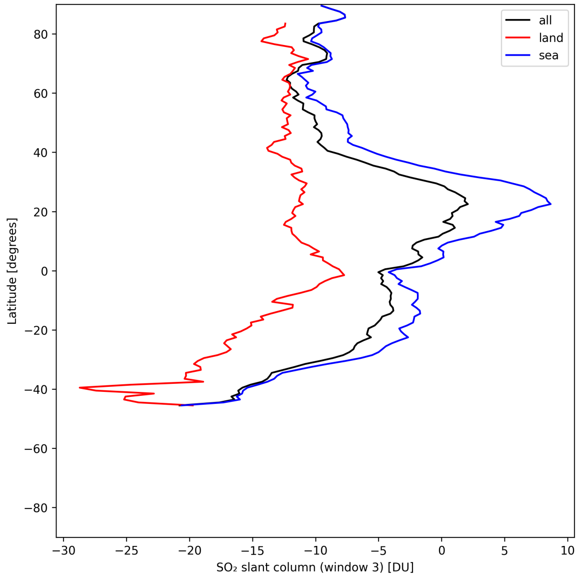
Figure 45: Zonal average of “SO 2 slant column (window 3)” for 2025-06-08 to 2025-06-10.
