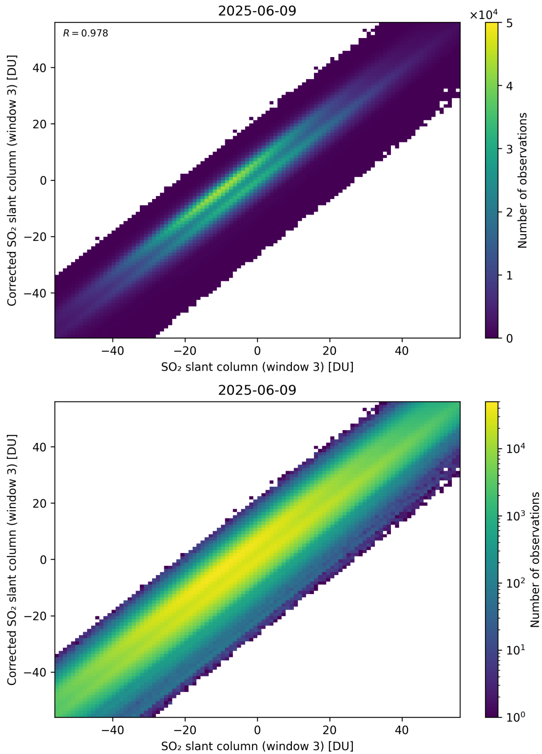
Figure 316: Scatter density plot of “SO 2 slant column (window 3)” against “Corrected SO 2 slant column (window 3)” for 2025-06-08 to 2025-06-10.
