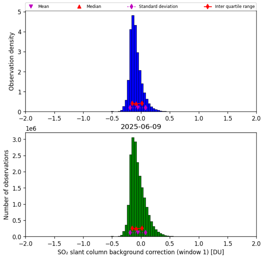
Figure 66: Histogram of “SO 2 slant column background correction (window 1)” for 2025-06-08 to 2025-06-10
