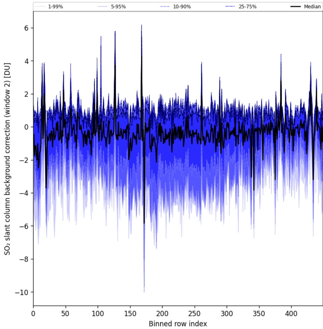
Figure 96: Along track statistics of “SO 2 slant column background correction (window 2)” for 2025-06-08 to 2025-06-10
