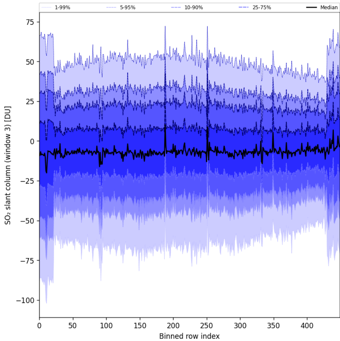
Figure 97: Along track statistics of “SO 2 slant column (window 3)” for 2025-06-08 to 2025-06-10
