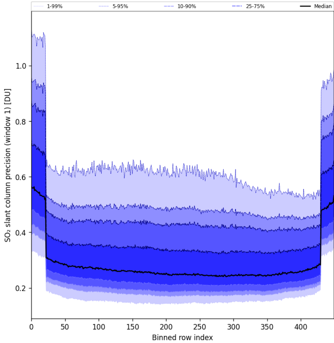
Figure 90: Along track statistics of “SO 2 slant column precision (window 1)” for 2025-06-08 to 2025-06-10
