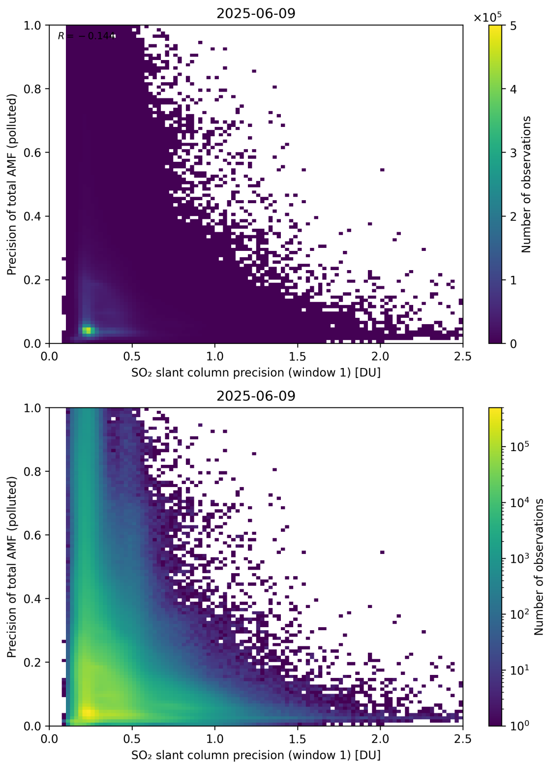
Figure 281: Scatter density plot of “SO 2 slant column precision (window 1)” against “Precision of total AMF (polluted)” for 2025-06-08 to 2025-06-10.
