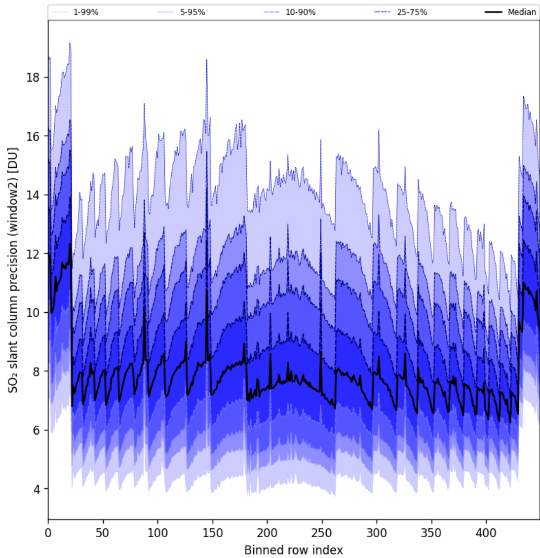
Figure 94: Along track statistics of “SO 2 slant column precision (window2)” for 2025-06-08 to 2025-06-10
