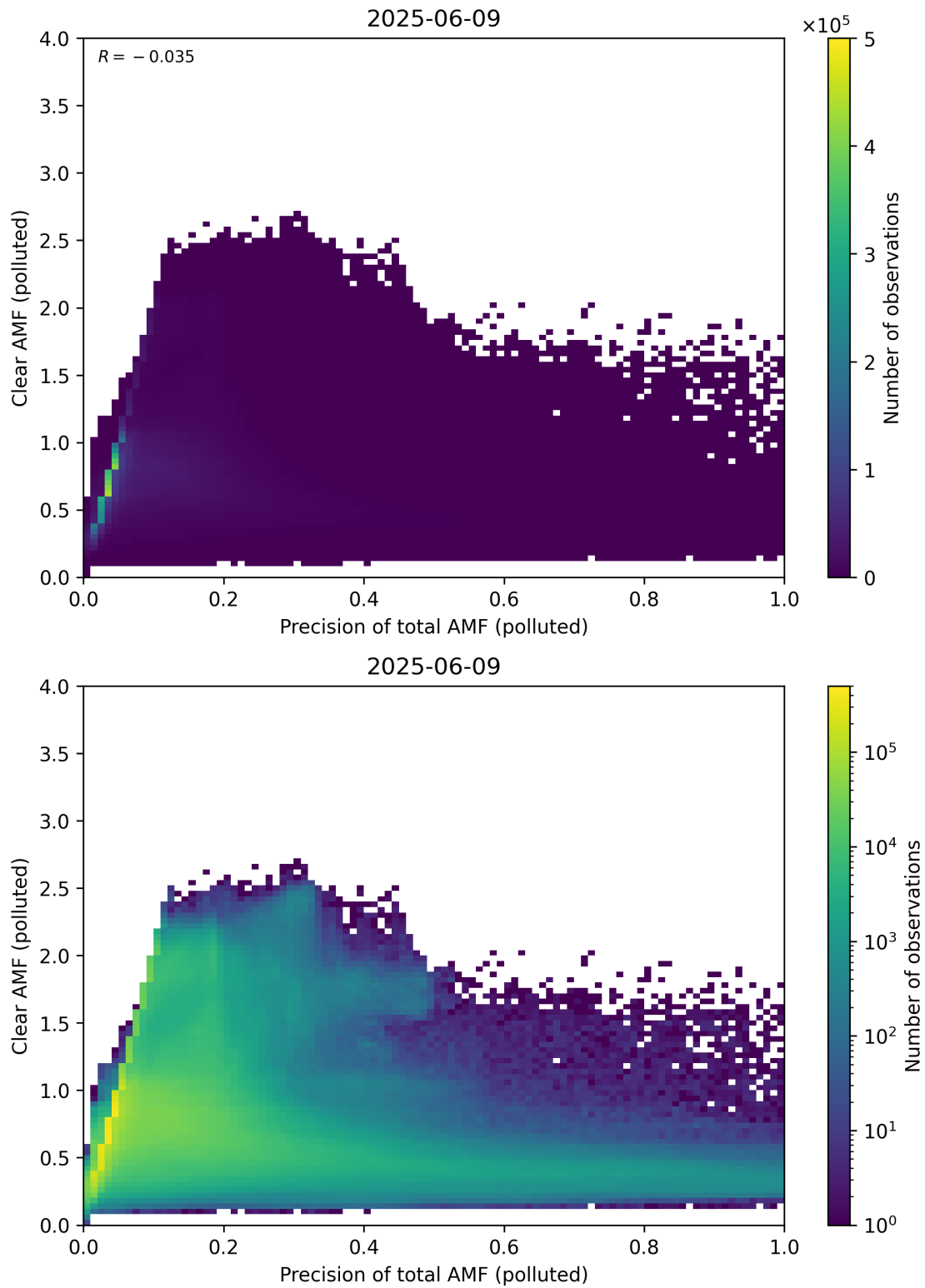
Figure 320: Scatter density plot of “Precision of total AMF (polluted)” against “Clear AMF (polluted)” for 2025-06-08 to 2025-06-10.
