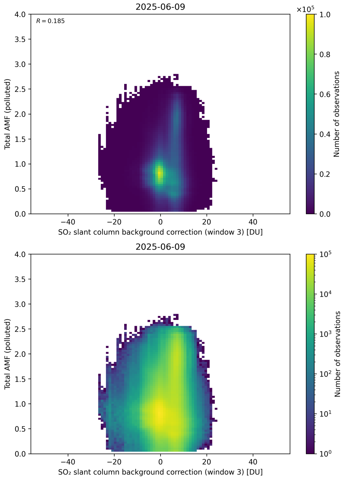
Figure 136: Scatter density plot of “SO 2 slant column background correction (window 3)” against “Total AMF (polluted)” for 2025-06-08 to 2025-06-10.
