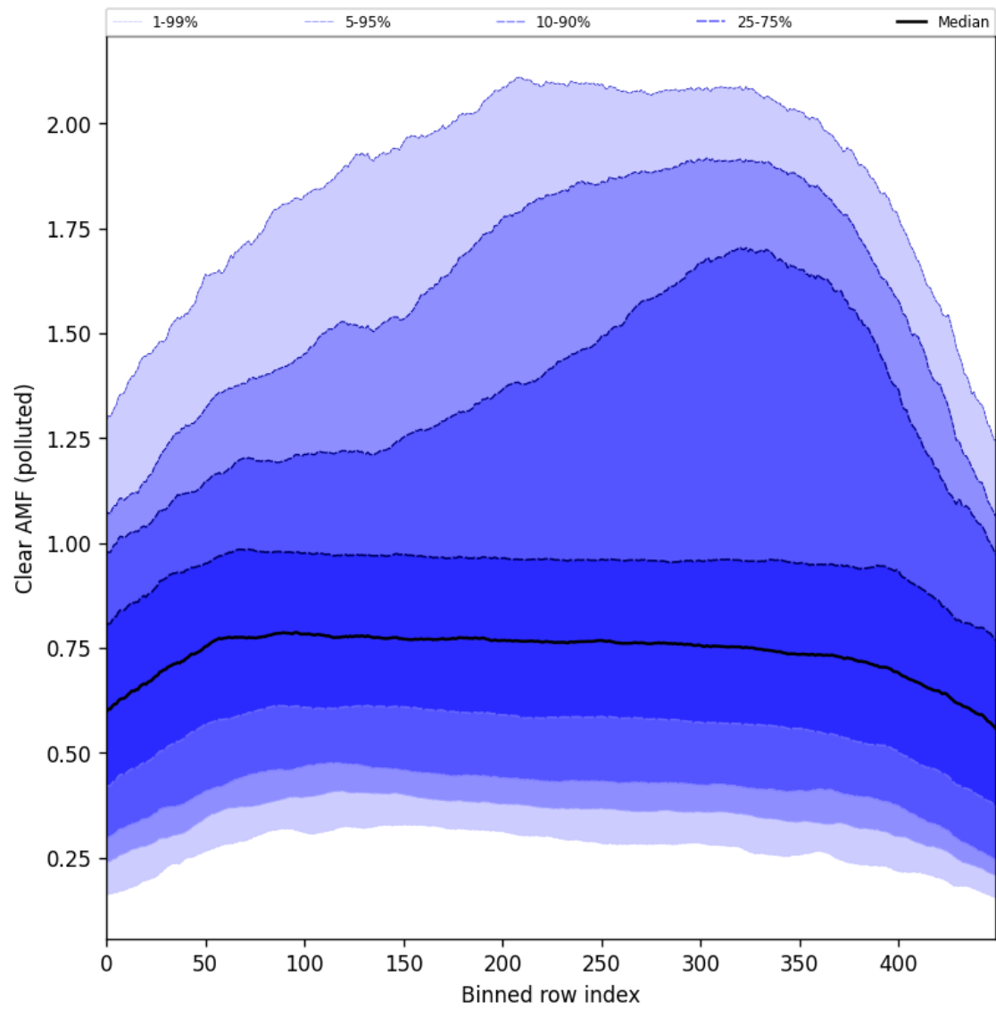
Figure 107: Along track statistics of “Clear AMF (polluted)” for 2025-06-08 to 2025-06-10
