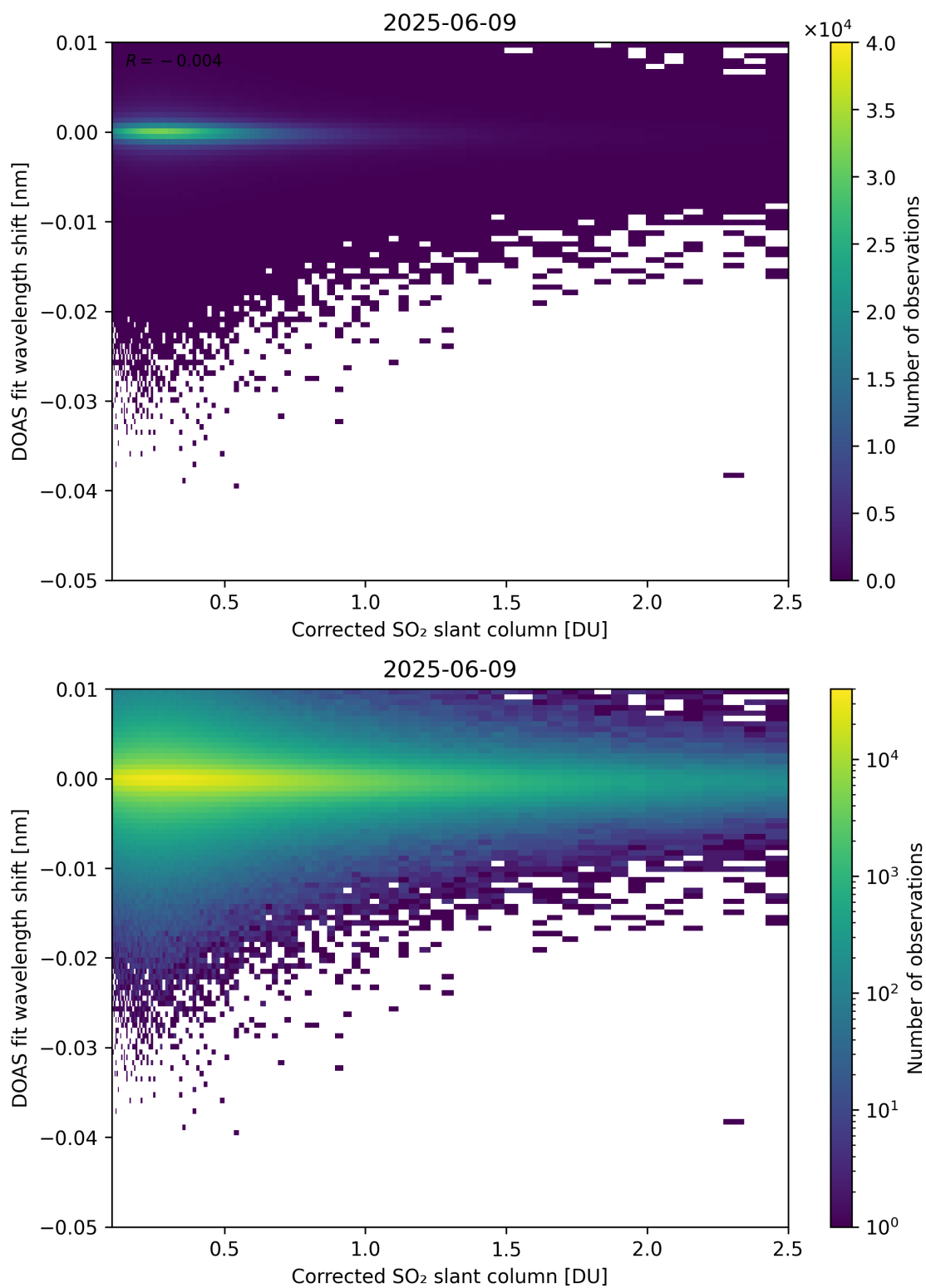
Figure 229: Scatter density plot of “Corrected SO 2 slant column” against “DOAS fit wavelength shift” for 2025-06-08 to 2025-06-10.
