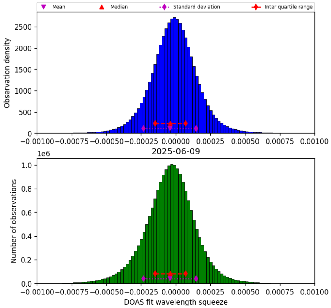
Figure 77: Histogram of “DOAS fit wavelength squeeze” for 2025-06-08 to 2025-06-10
