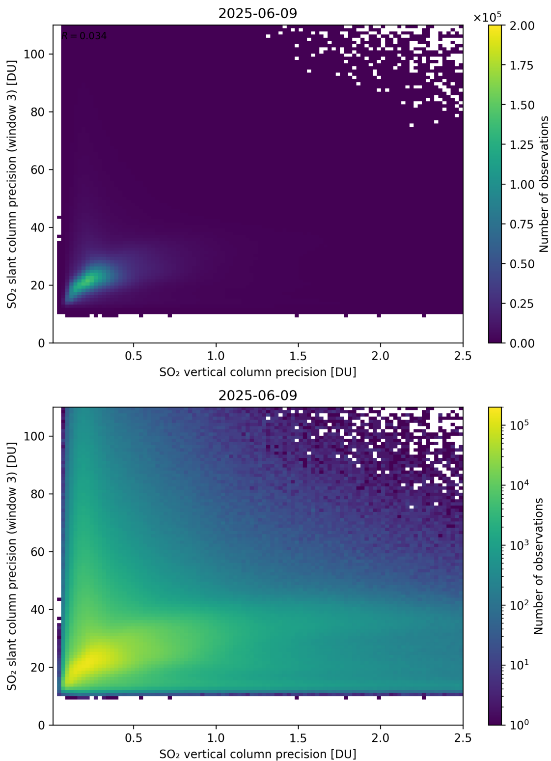
Figure 345: Scatter density plot of “SO 2 vertical column precision” against “SO 2 slant column precision (window 3)” for 2025-06-08 to 2025-06-10.
