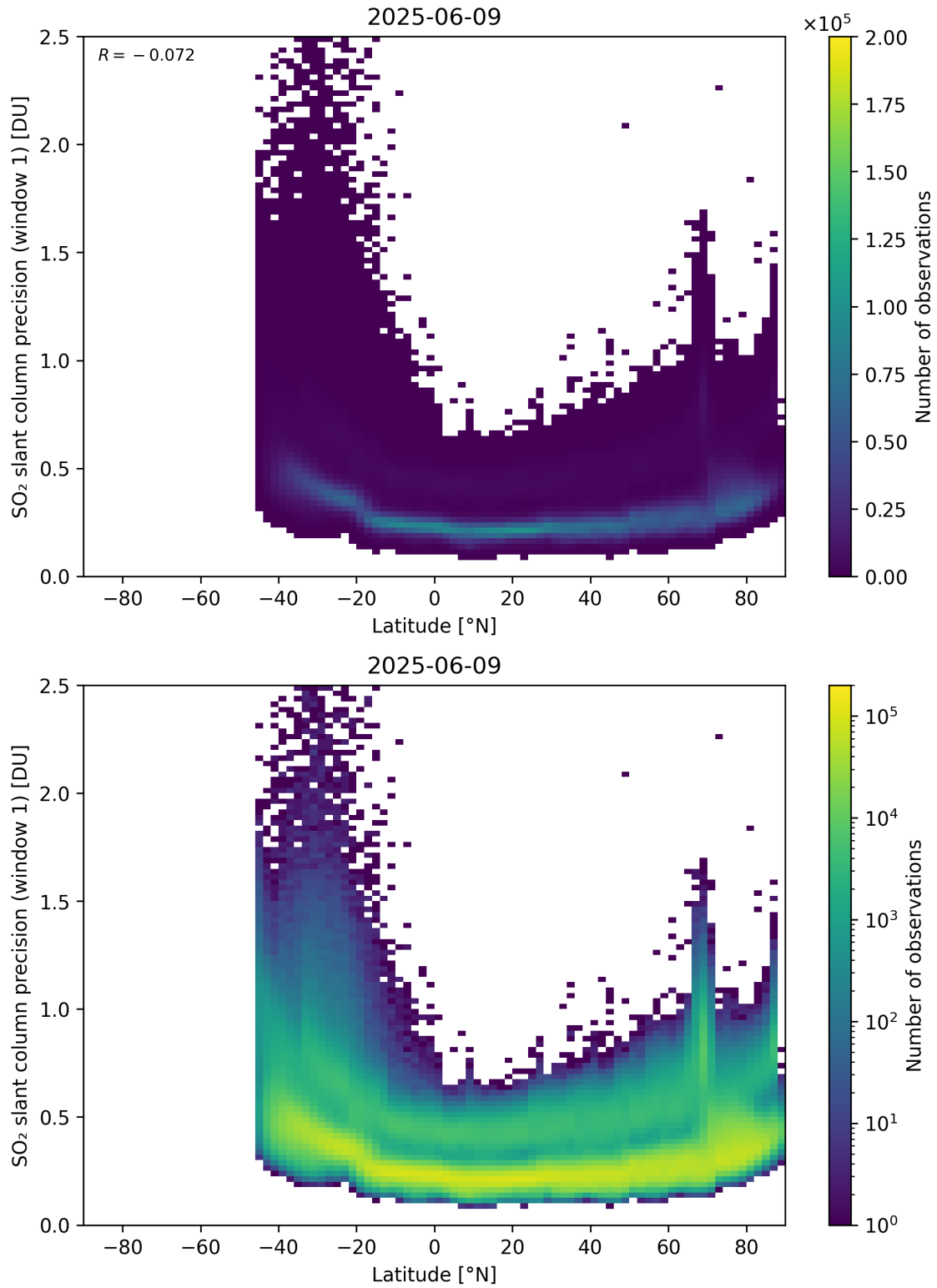
Figure 163: Scatter density plot of “Latitude” against “SO 2 slant column precision (window 1)” for 2025-06-08 to 2025-06-10.
