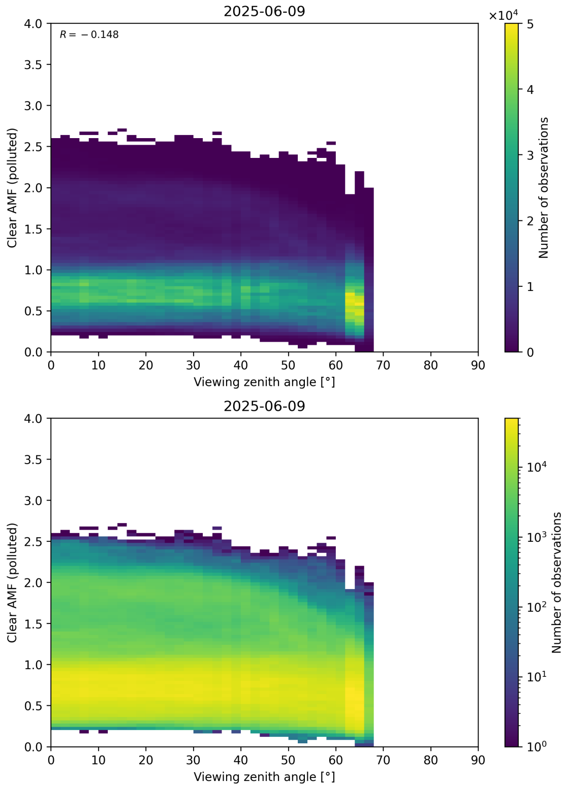
Figure 370: Scatter density plot of “Viewing zenith angle” against “Clear AMF (polluted)” for 2025-06-08 to 2025-06-10.
