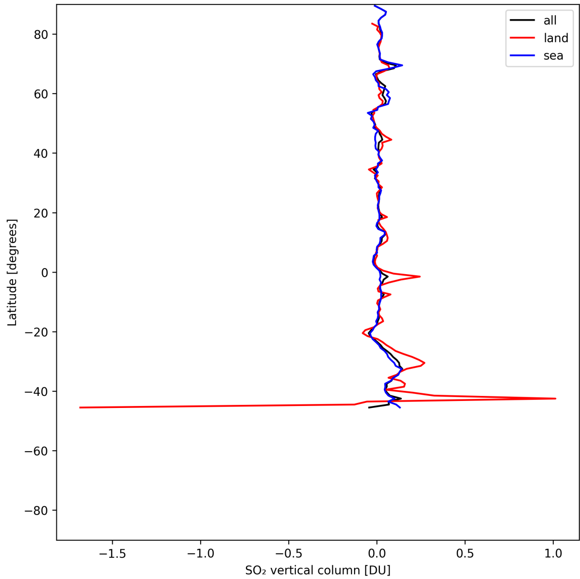
Figure 32: Zonal average of “SO 2 vertical column” for 2025-06-08 to 2025-06-10.
