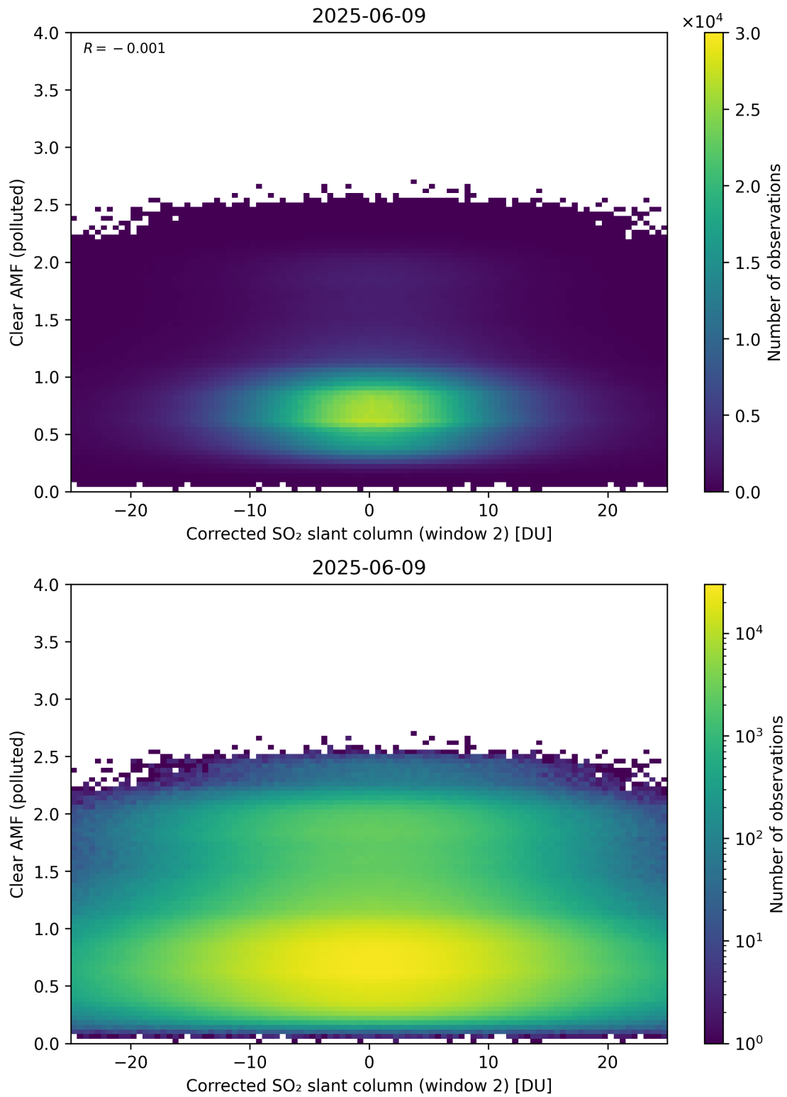
Figure 249: Scatter density plot of “Corrected SO 2 slant column (window 2)” against “Clear AMF (polluted)” for 2025-06-08 to 2025-06-10.
