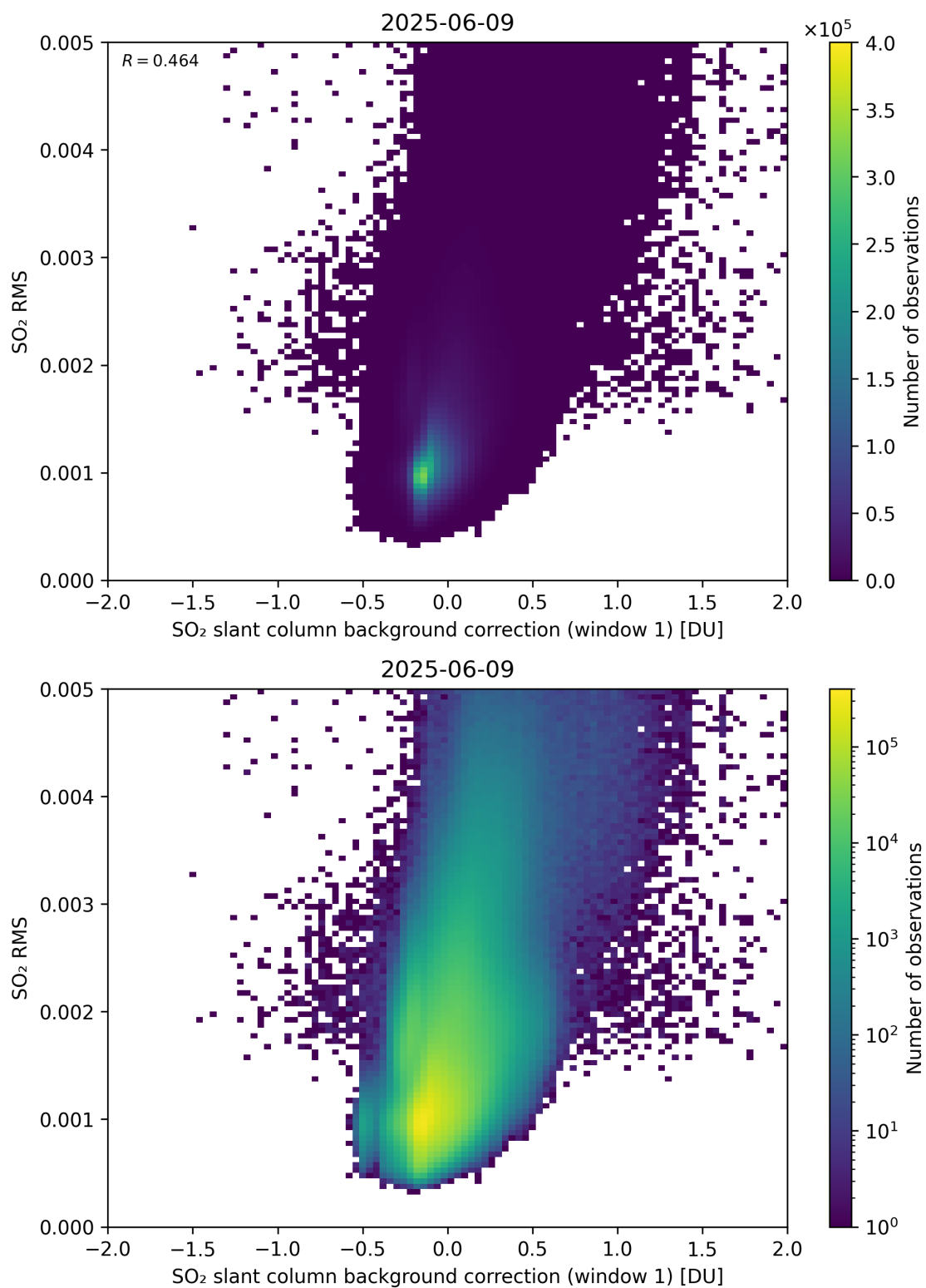
Figure 113: Scatter density plot of “SO 2 slant column background correction (window 1)” against “SO 2 RMS” for 2025-06-08 to 2025-06-10.
