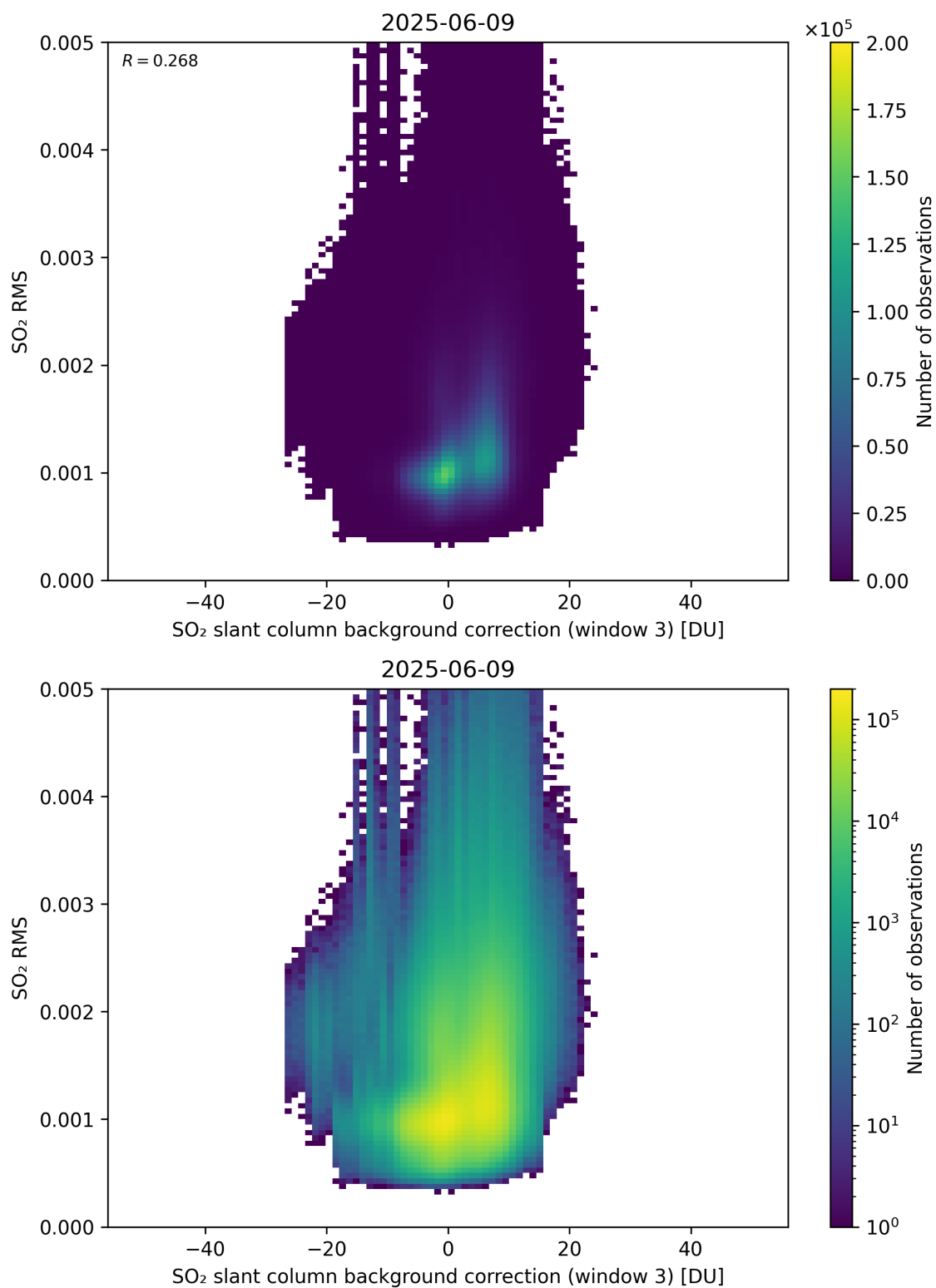
Figure 134: Scatter density plot of “SO 2 slant column background correction (window 3)” against “SO 2 RMS” for 2025-06-08 to 2025-06-10.
