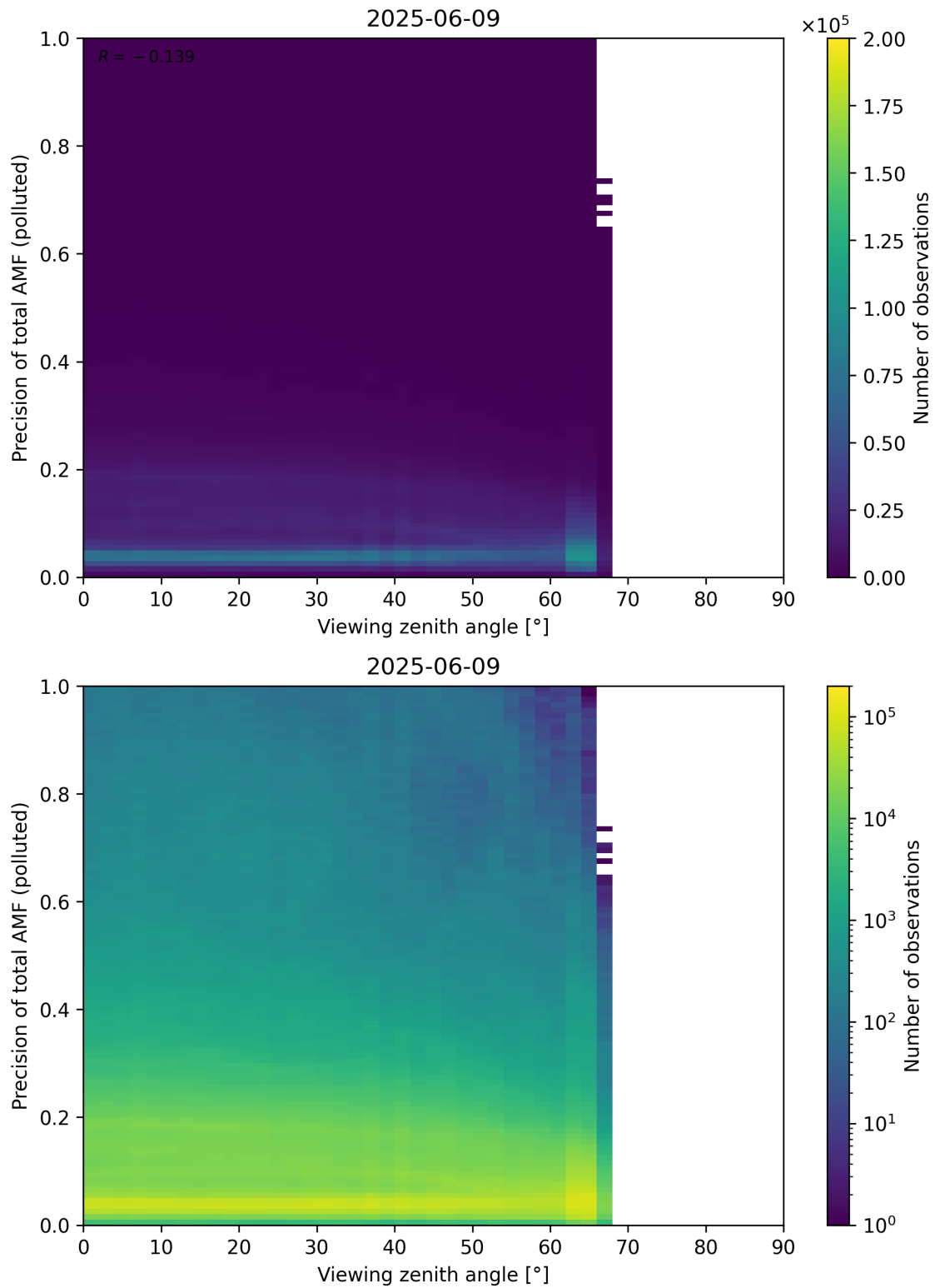
Figure 382: Scatter density plot of “Viewing zenith angle” against “Precision of total AMF (polluted)” for 2025-06-08 to 2025-06-10.
