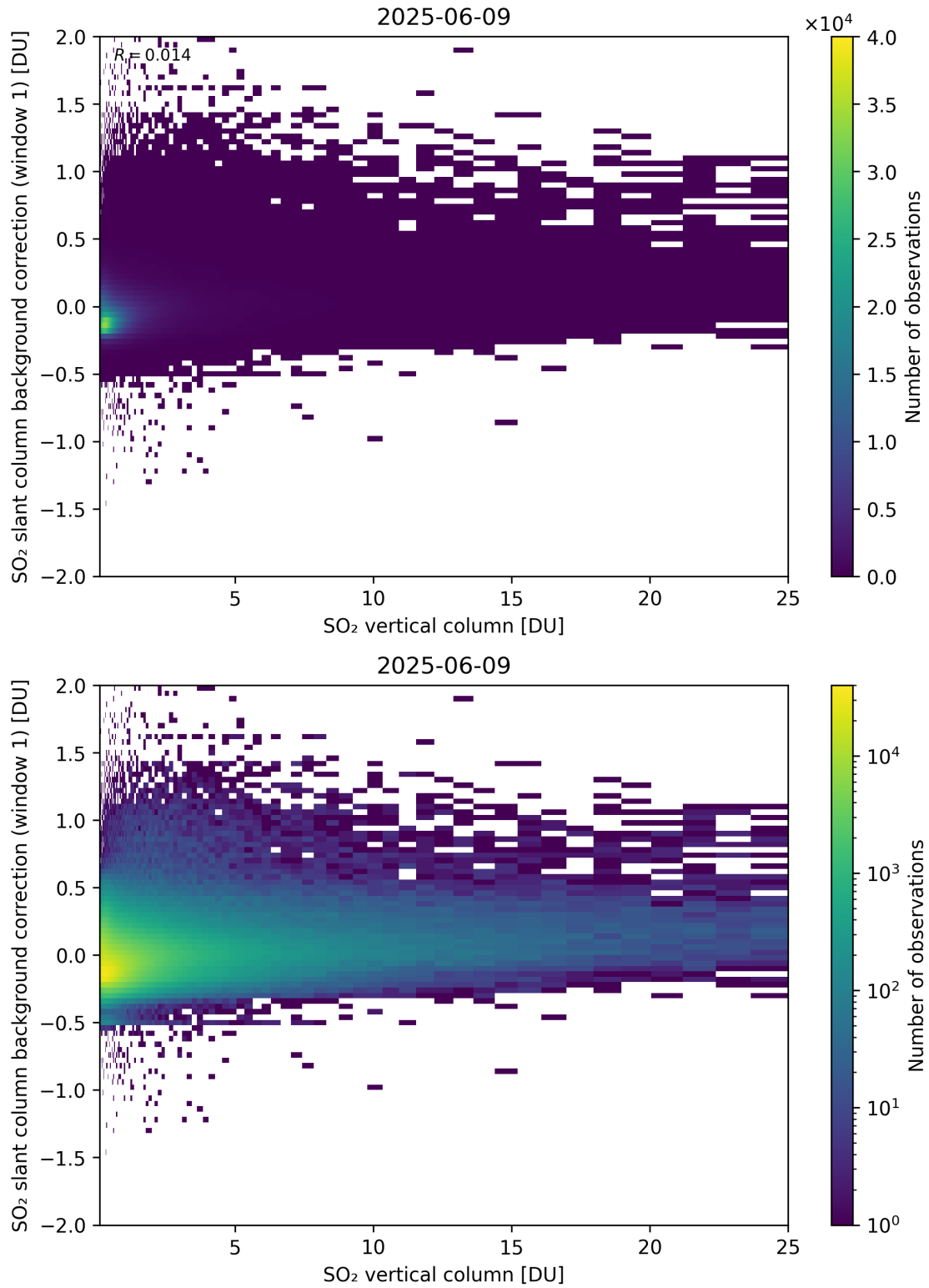
Figure 323: Scatter density plot of “SO 2 vertical column” against “SO 2 slant column background correction (window 1)” for 2025-06-08 to 2025-06-10.
