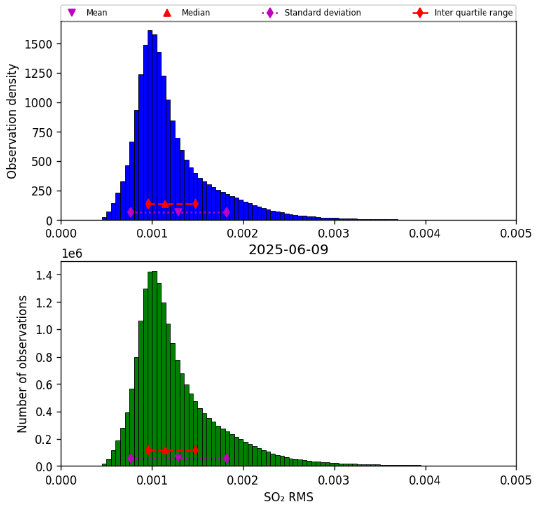
Figure 78: Histogram of “SO 2 RMS” for 2025-06-08 to 2025-06-10
