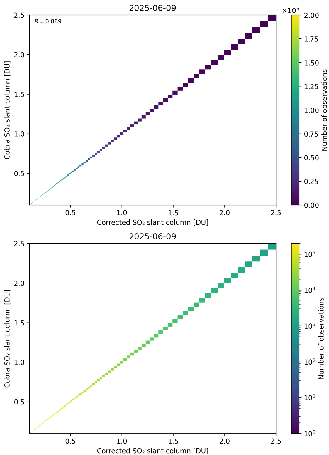
Figure 233: Scatter density plot of “Corrected SO 2 slant column” against “Cobra SO 2 slant column” for 2025-06-08 to 2025-06-10.
