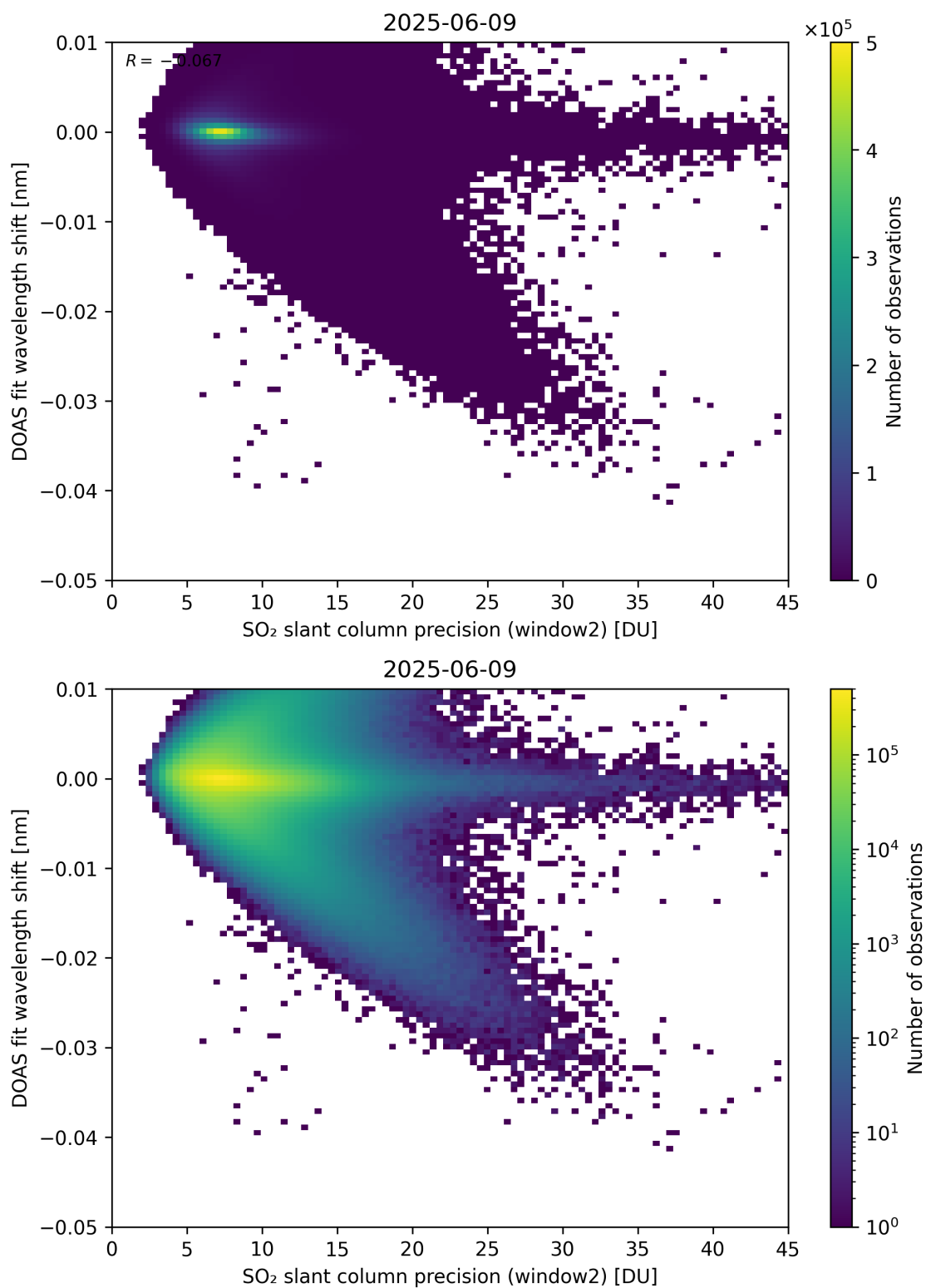
Figure 293: Scatter density plot of “SO 2 slant column precision (window2)” against “DOAS fit wavelength shift” for 2025-06-08 to 2025-06-10.
