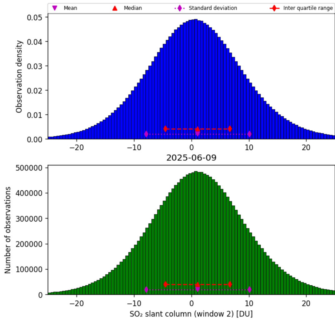
Figure 67: Histogram of “SO 2 slant column (window 2)” for 2025-06-08 to 2025-06-10
