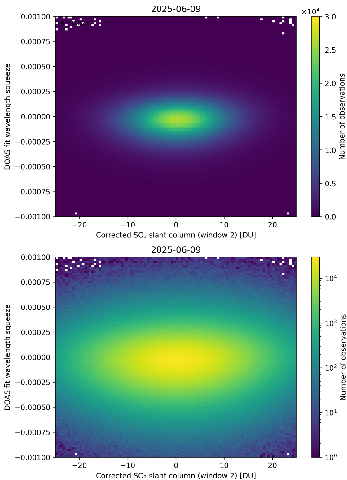
Figure 247: Scatter density plot of “Corrected SO 2 slant column (window 2)” against “DOAS fit wavelength squeeze” for 2025-06-08 to 2025-06-10.
