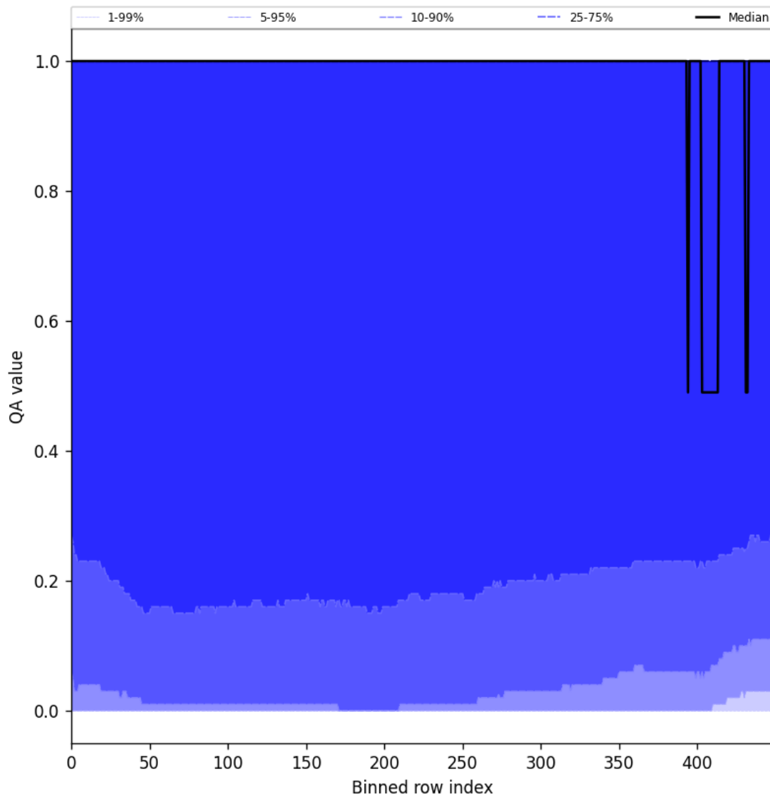
Figure 83: Along track statistics of “QA value” for 2025-06-08 to 2025-06-10
