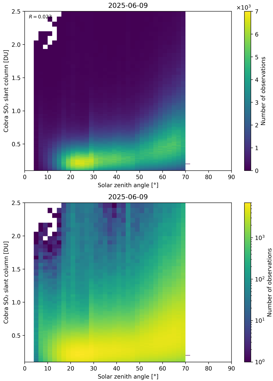
Figure 179: Scatter density plot of “Solar zenith angle” against “Cobra SO 2 slant column” for 2025-06-08 to 2025-06-10.
