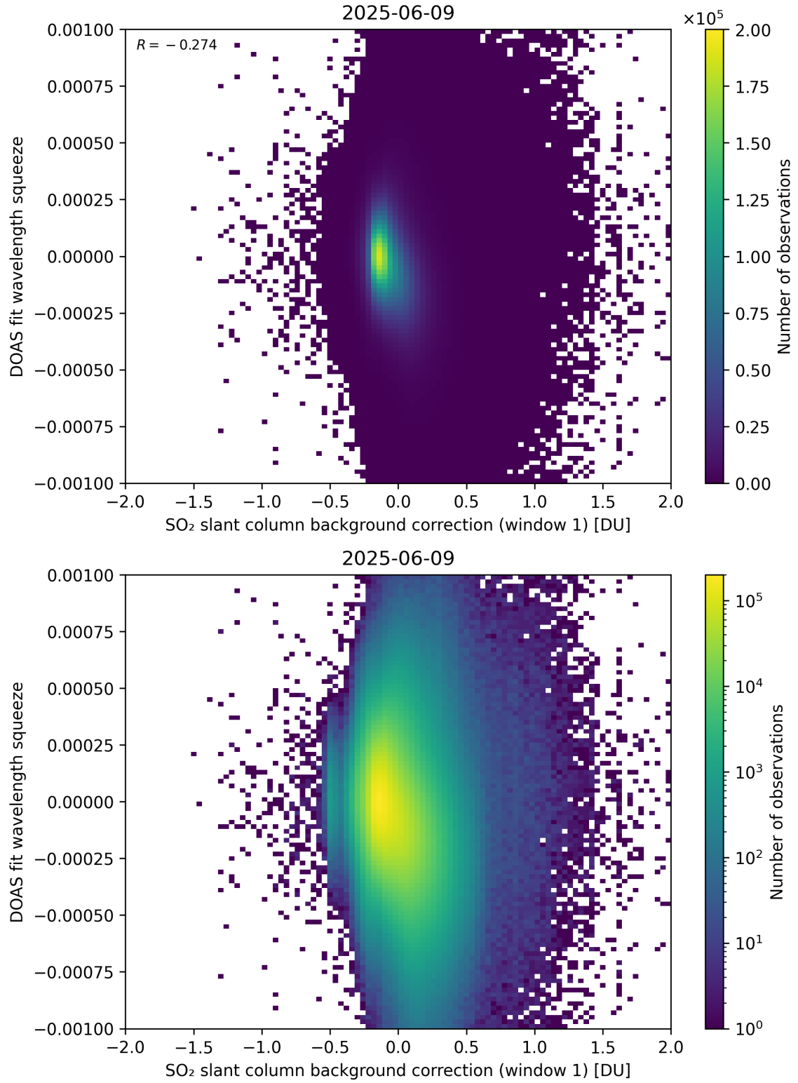
Figure 112: Scatter density plot of “SO 2 slant column background correction (window 1)” against “DOAS fit wavelength squeeze” for 2025-06-08 to 2025-06-10.
