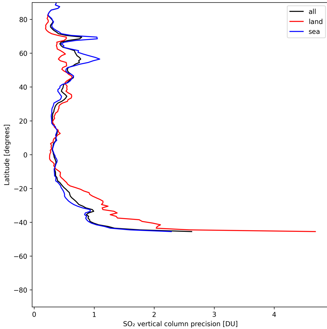
Figure 33: Zonal average of “SO 2 vertical column precision” for 2025-06-08 to 2025-06-10.
