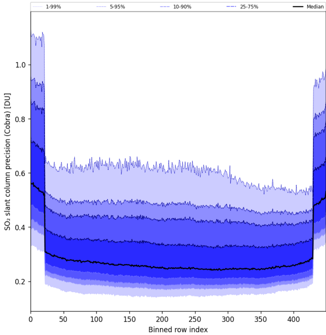
Figure 88: Along track statistics of “SO 2 slant column precision (Cobra)” for 2025-06-08 to 2025-06-10
