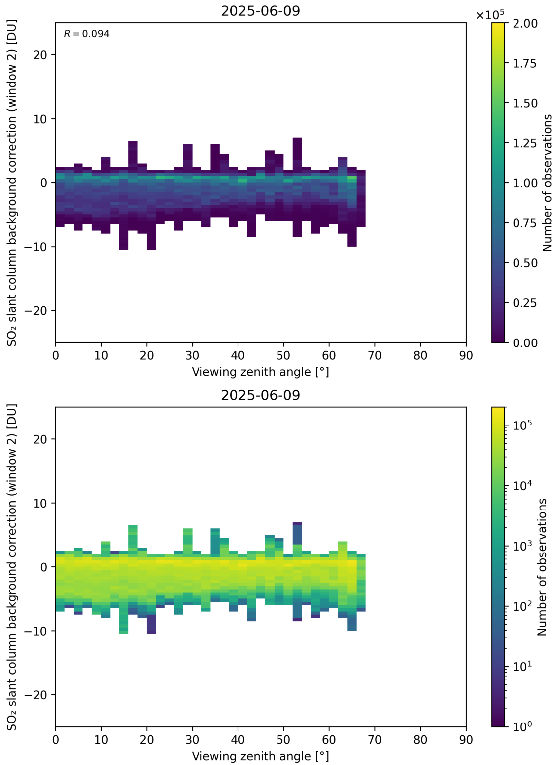
Figure 363: Scatter density plot of “Viewing zenith angle” against “SO 2 slant column background correction (window 2)” for 2025-06-08 to 2025-06-10.
