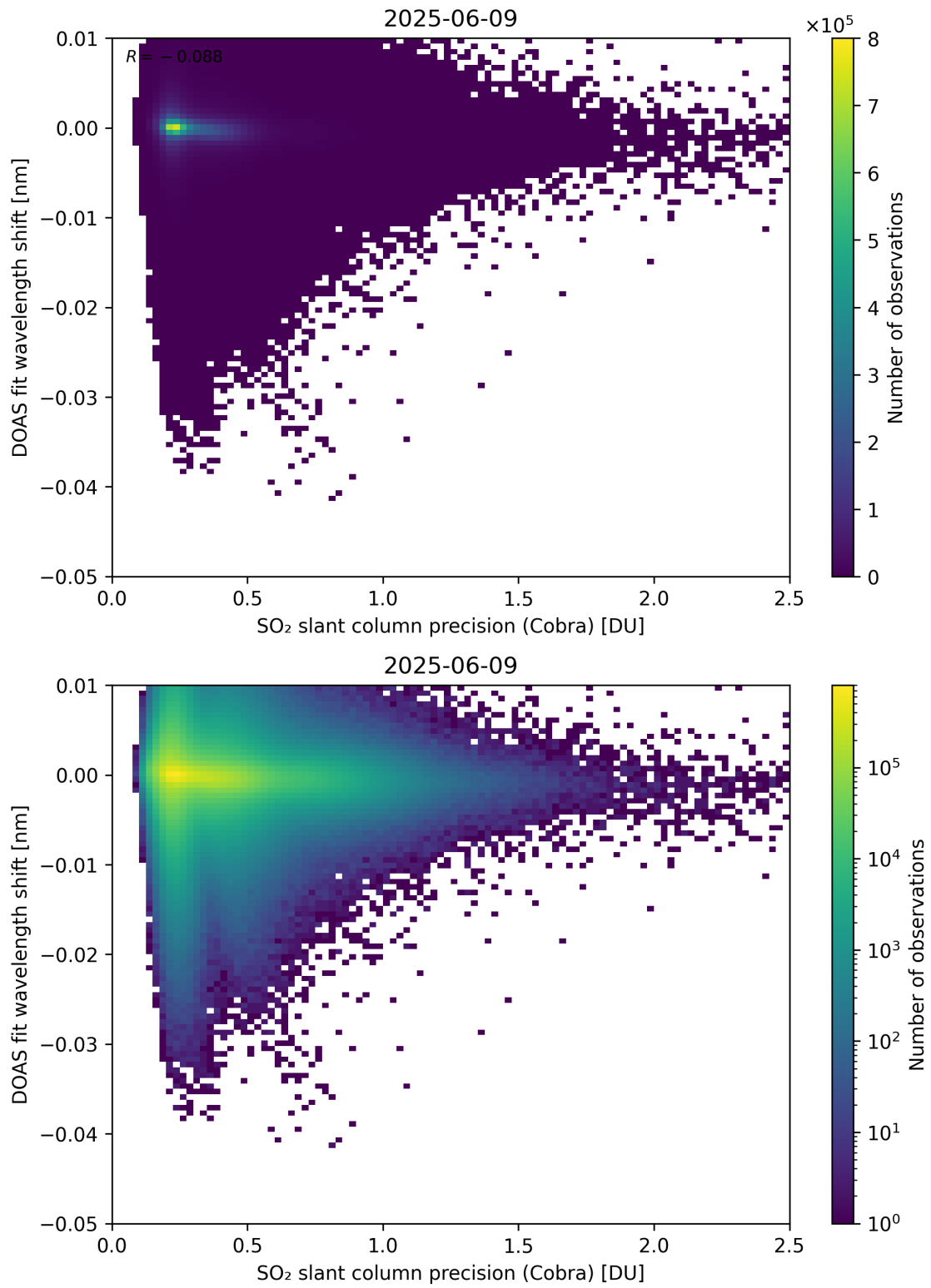
Figure 202: Scatter density plot of “SO 2 slant column precision (Cobra)” against “DOAS fit wavelength shift” for 2025-06-08 to 2025-06-10.
