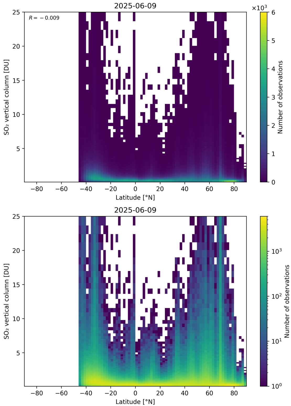
Figure 169: Scatter density plot of “Latitude” against “SO 2 vertical column” for 2025-06-08 to 2025-06-10.
