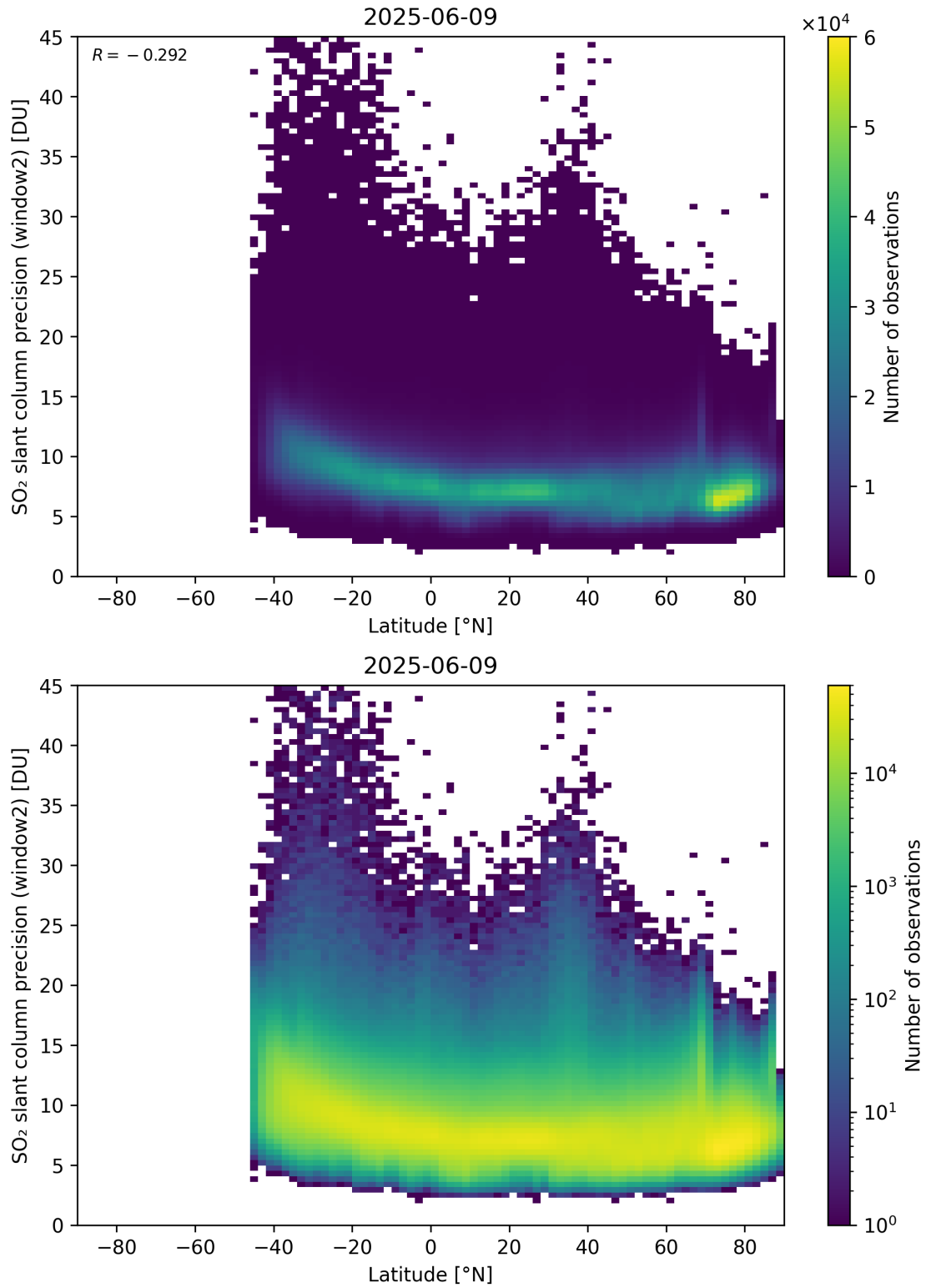
Figure 164: Scatter density plot of “Latitude” against “SO 2 slant column precision (window2)” for 2025-06-08 to 2025-06-10.
