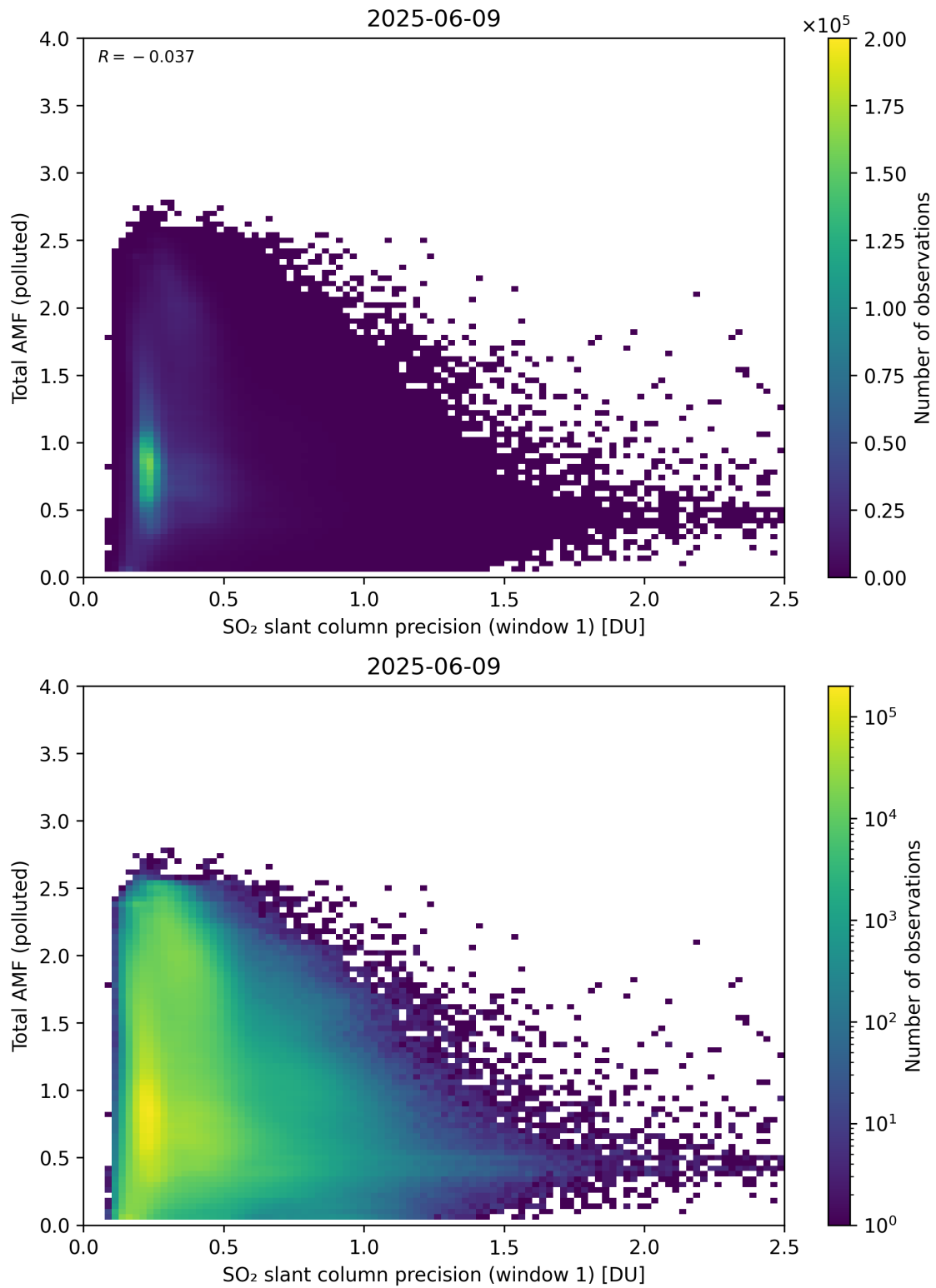
Figure 280: Scatter density plot of “SO 2 slant column precision (window 1)” against “Total AMF (polluted)” for 2025-06-08 to 2025-06-10.
