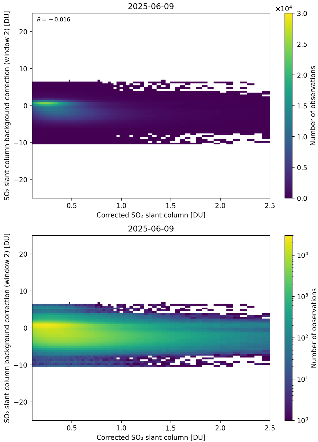
Figure 227: Scatter density plot of “Corrected SO 2 slant column” against “SO 2 slant column background correction (window 2)” for 2025-06-08 to 2025-06-10.
