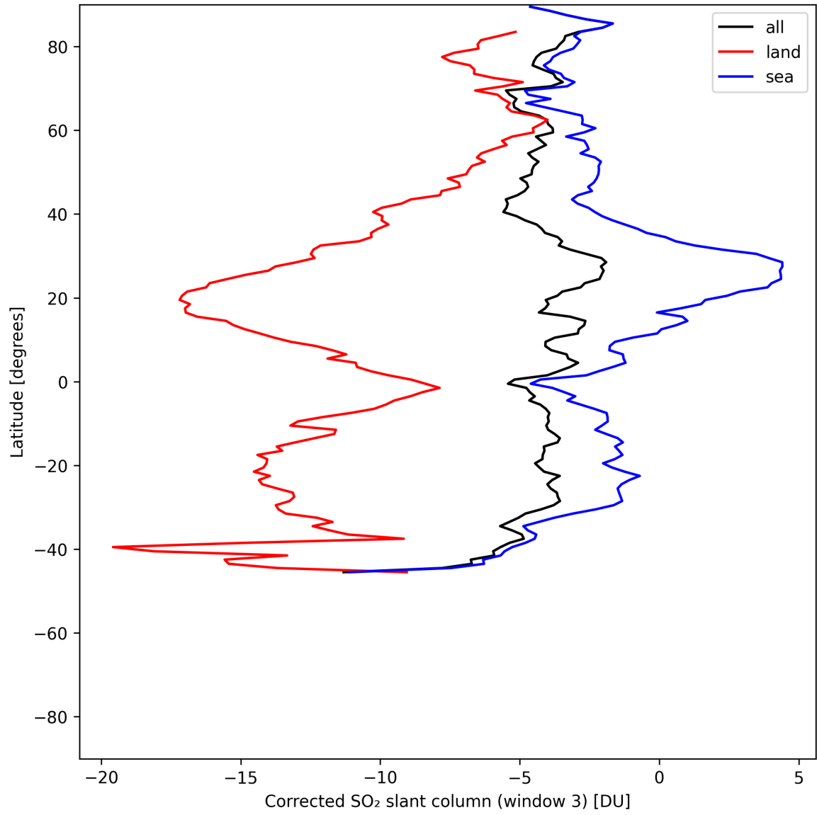
Figure 47: Zonal average of “Corrected SO 2 slant column (window 3)” for 2025-06-08 to 2025-06-10.
