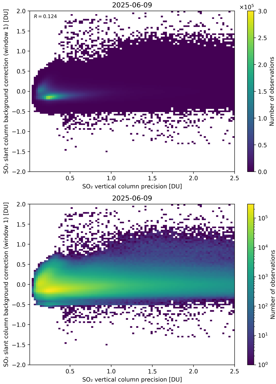
Figure 329: Scatter density plot of “SO 2 vertical column precision” against “SO 2 slant column background correction (window 1)” for 2025-06-08 to 2025-06-10.
