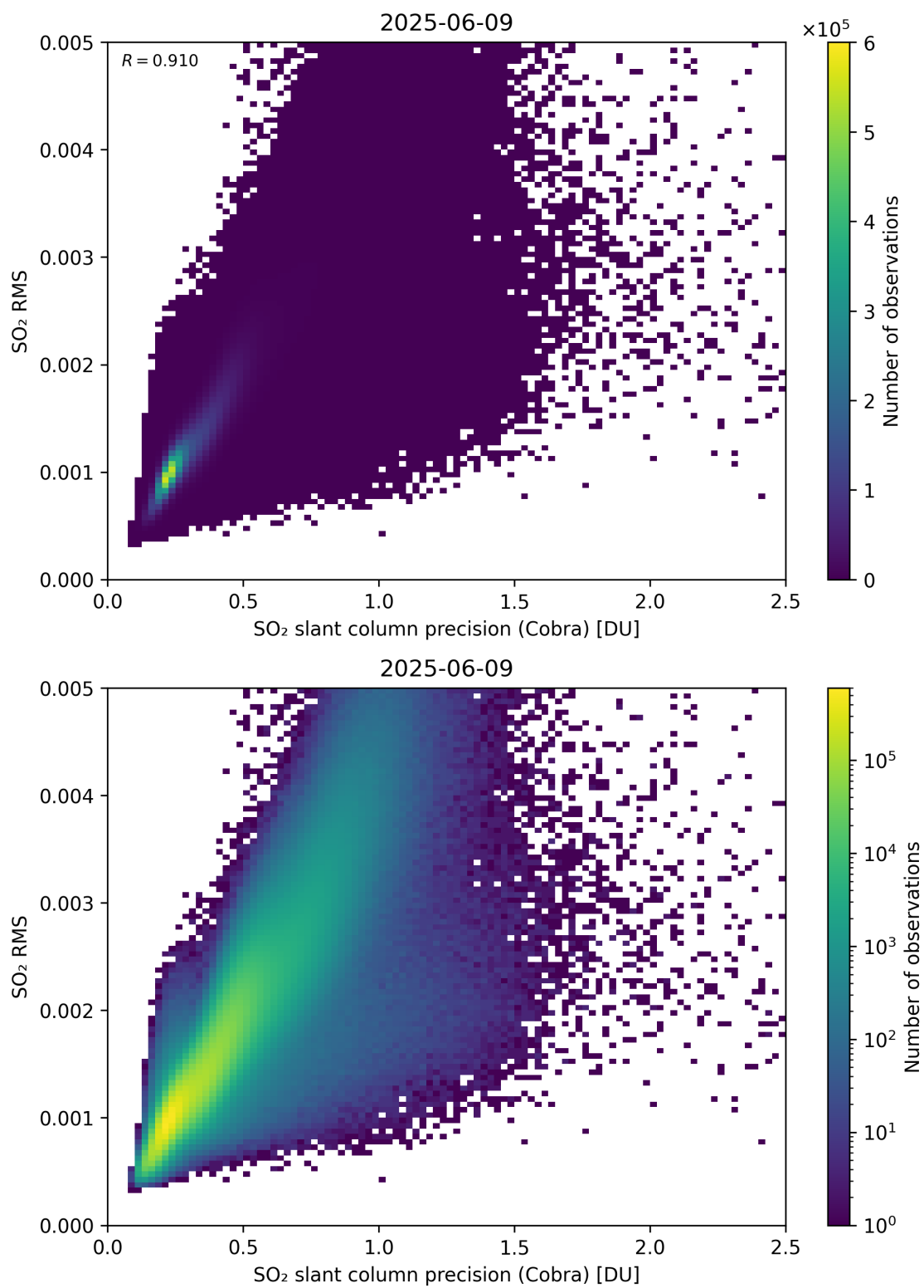
Figure 204: Scatter density plot of “SO 2 slant column precision (Cobra)” against “SO 2 RMS” for 2025-06-08 to 2025-06-10.
