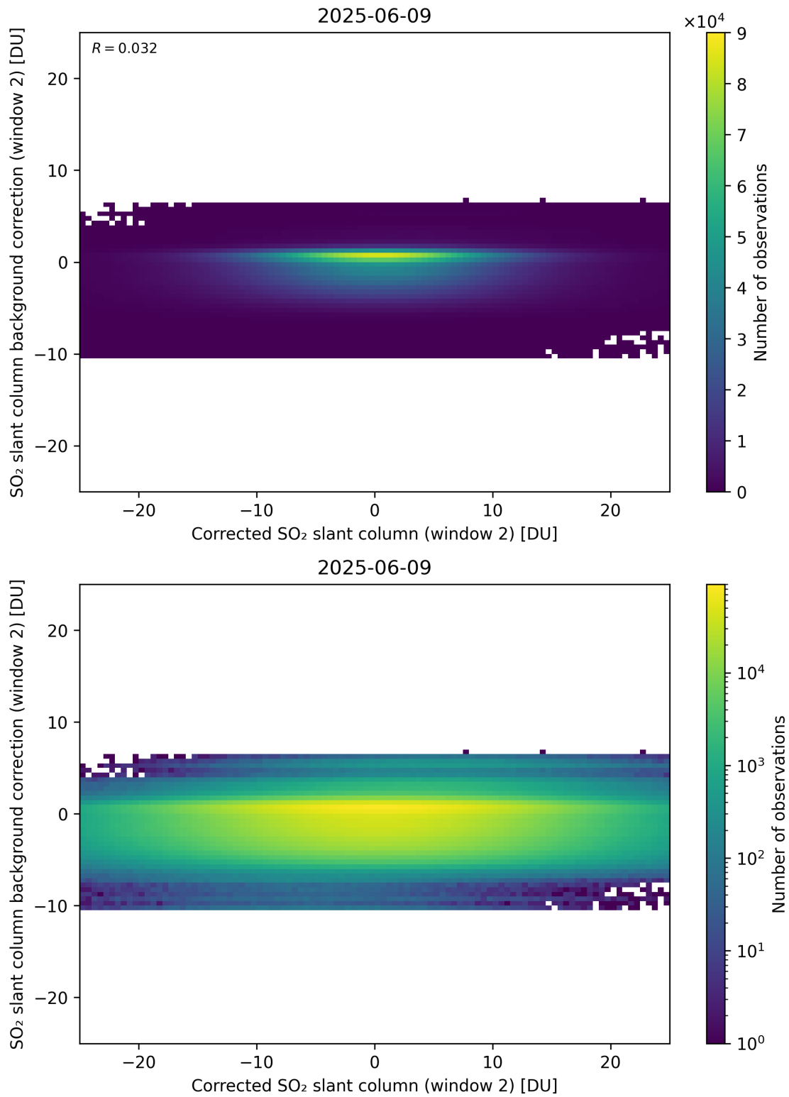
Figure 244: Scatter density plot of “Corrected SO 2 slant column (window 2)” against “SO 2 slant column background correction (window 2)” for 2025-06-08 to 2025-06-10.
