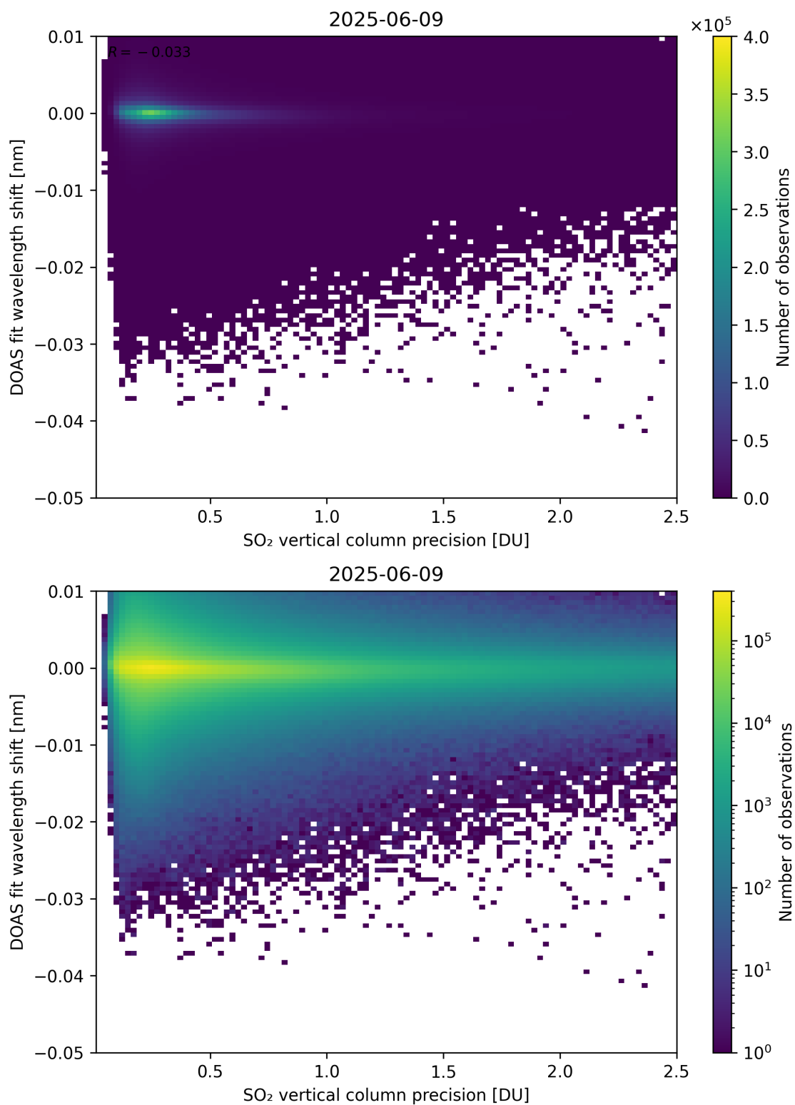
Figure 332: Scatter density plot of “SO 2 vertical column precision” against “DOAS fit wavelength shift” for 2025-06-08 to 2025-06-10.
