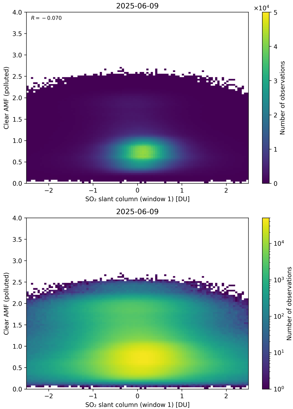
Figure 282: Scatter density plot of “SO 2 slant column (window 1)” against “Clear AMF (polluted)” for 2025-06-08 to 2025-06-10.
