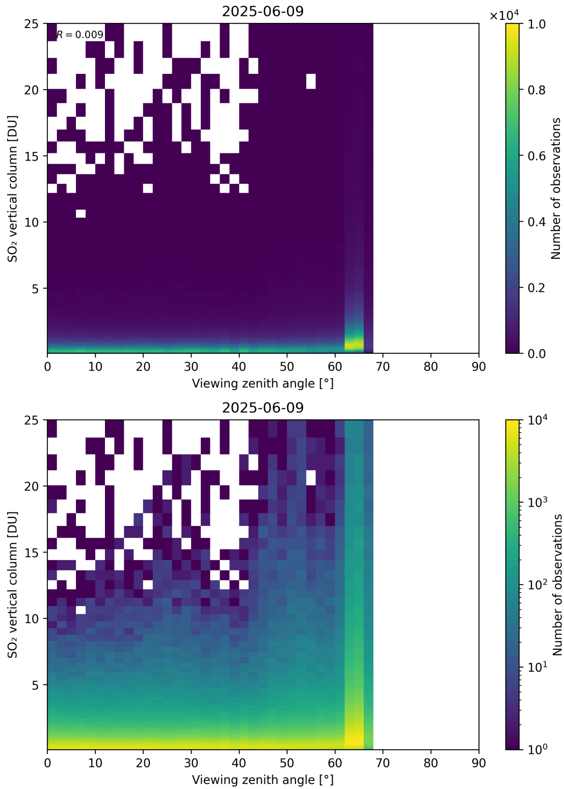
Figure 383: Scatter density plot of “Viewing zenith angle” against “SO 2 vertical column” for 2025-06-08 to 2025-06-10.
