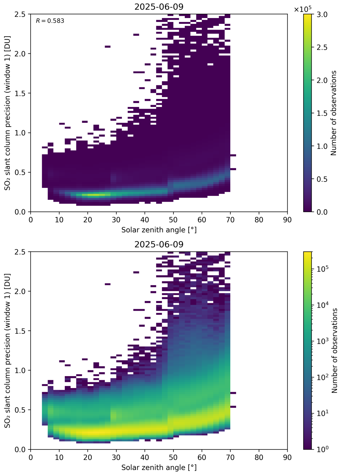
Figure 185: Scatter density plot of “Solar zenith angle” against “SO 2 slant column precision (window 1)” for 2025-06-08 to 2025-06-10.
