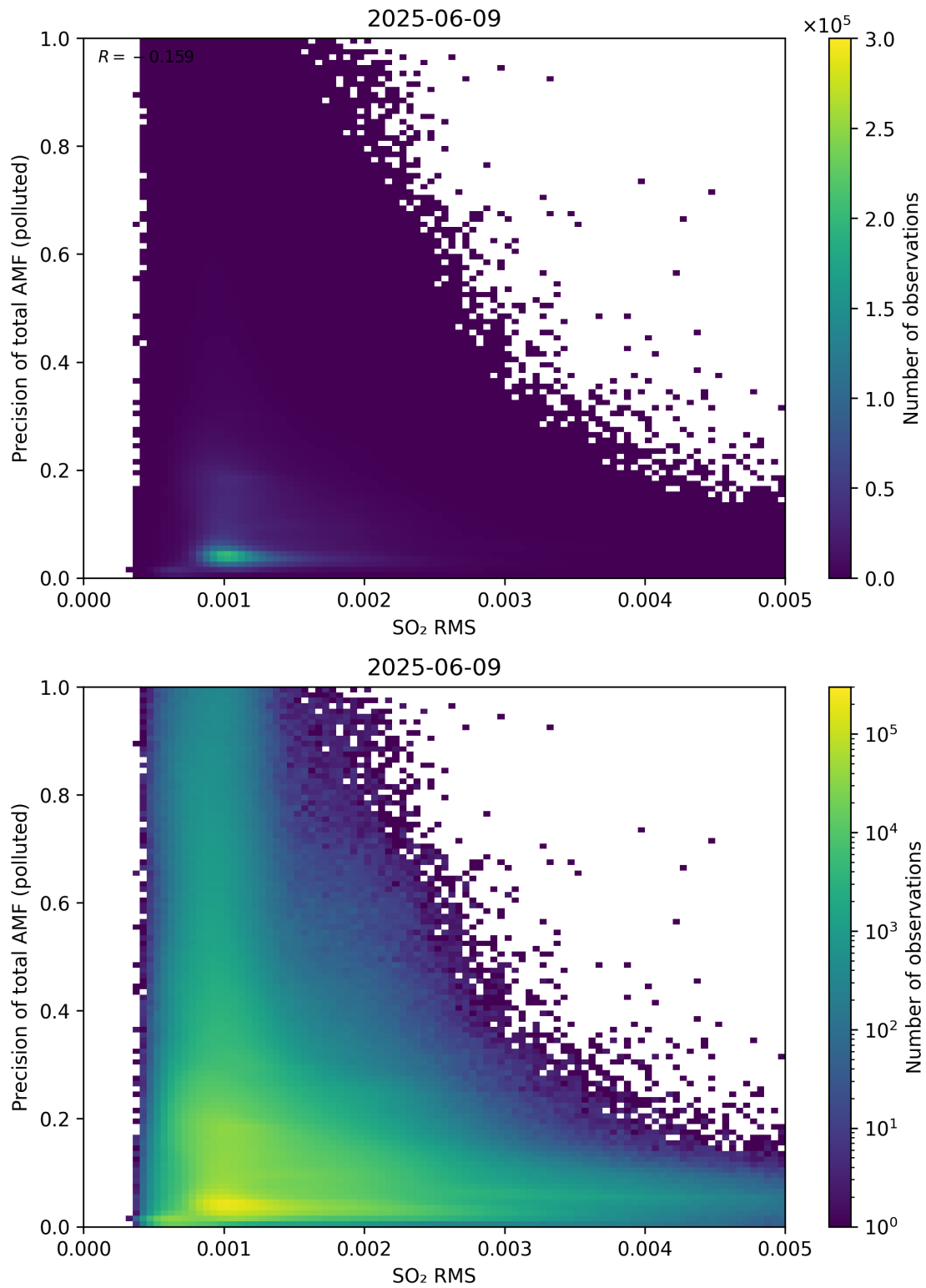
Figure 149: Scatter density plot of “SO 2 RMS” against “Precision of total AMF (polluted)” for 2025-06-08 to 2025-06-10.
