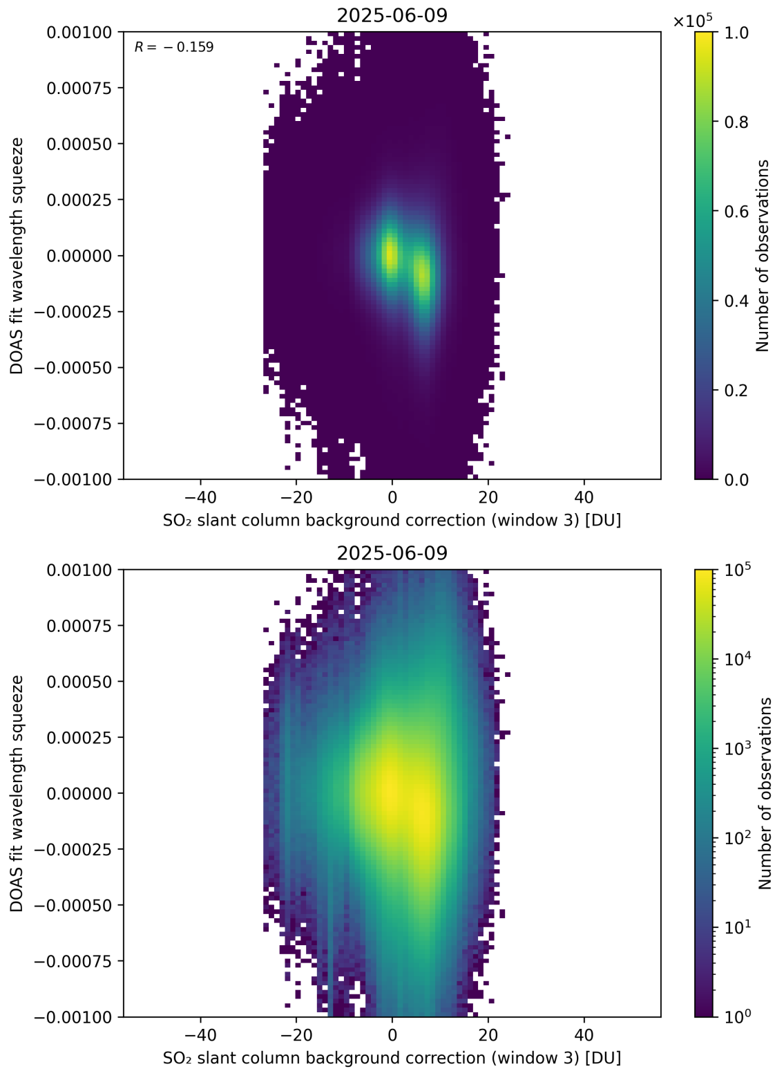
Figure 133: Scatter density plot of “SO 2 slant column background correction (window 3)” against “DOAS fit wavelength squeeze” for 2025-06-08 to 2025-06-10.
