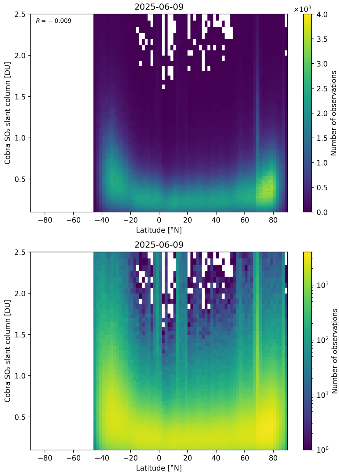
Figure 157: Scatter density plot of “Latitude” against “Cobra SO 2 slant column” for 2025-06-08 to 2025-06-10.
