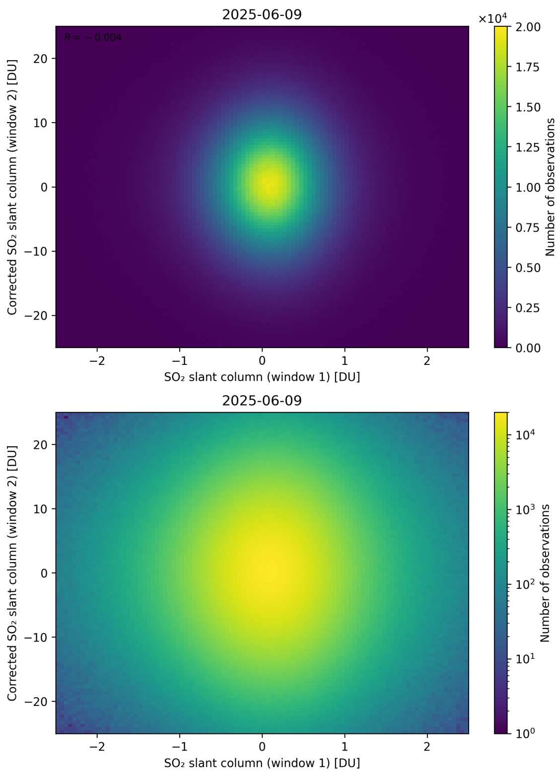
Figure 283: Scatter density plot of “SO 2 slant column (window 1)” against “Corrected SO 2 slant column (window 2)” for 2025-06-08 to 2025-06-10.
