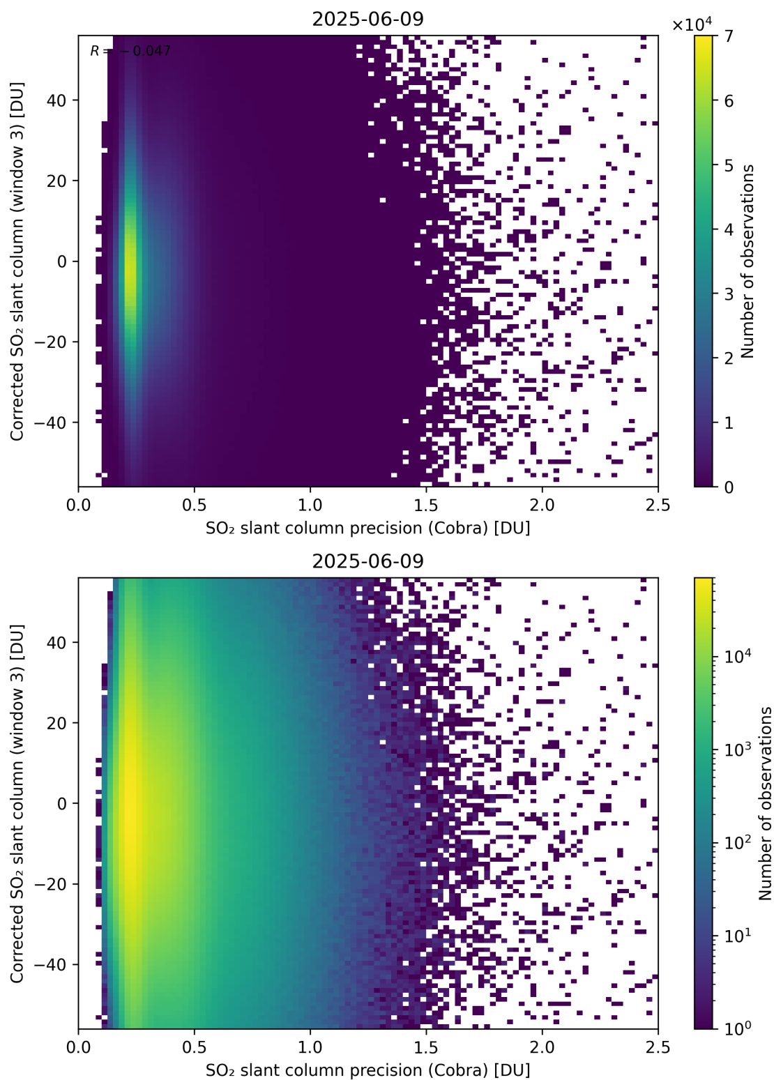
Figure 207: Scatter density plot of “SO 2 slant column precision (Cobra)” against “Corrected SO 2 slant column (window 3)” for 2025-06-08 to 2025-06-10.
