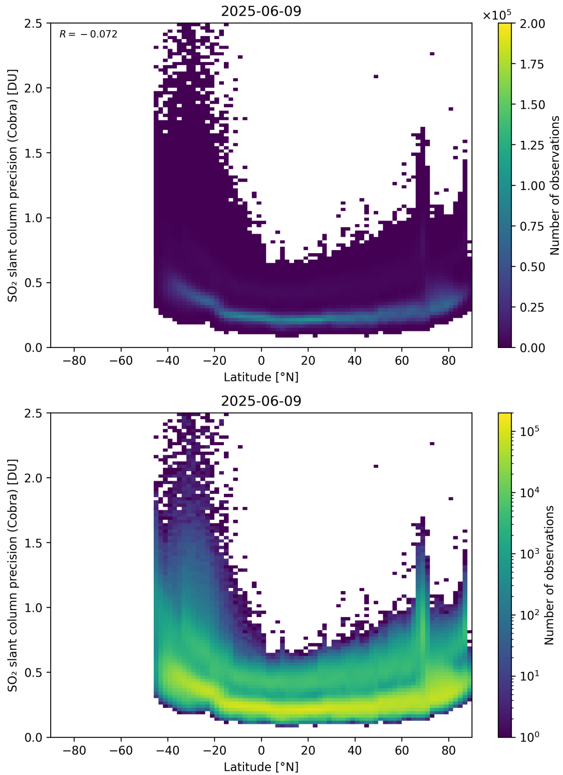
Figure 158: Scatter density plot of “Latitude” against “SO 2 slant column precision (Cobra)” for 2025-06-08 to 2025-06-10.
