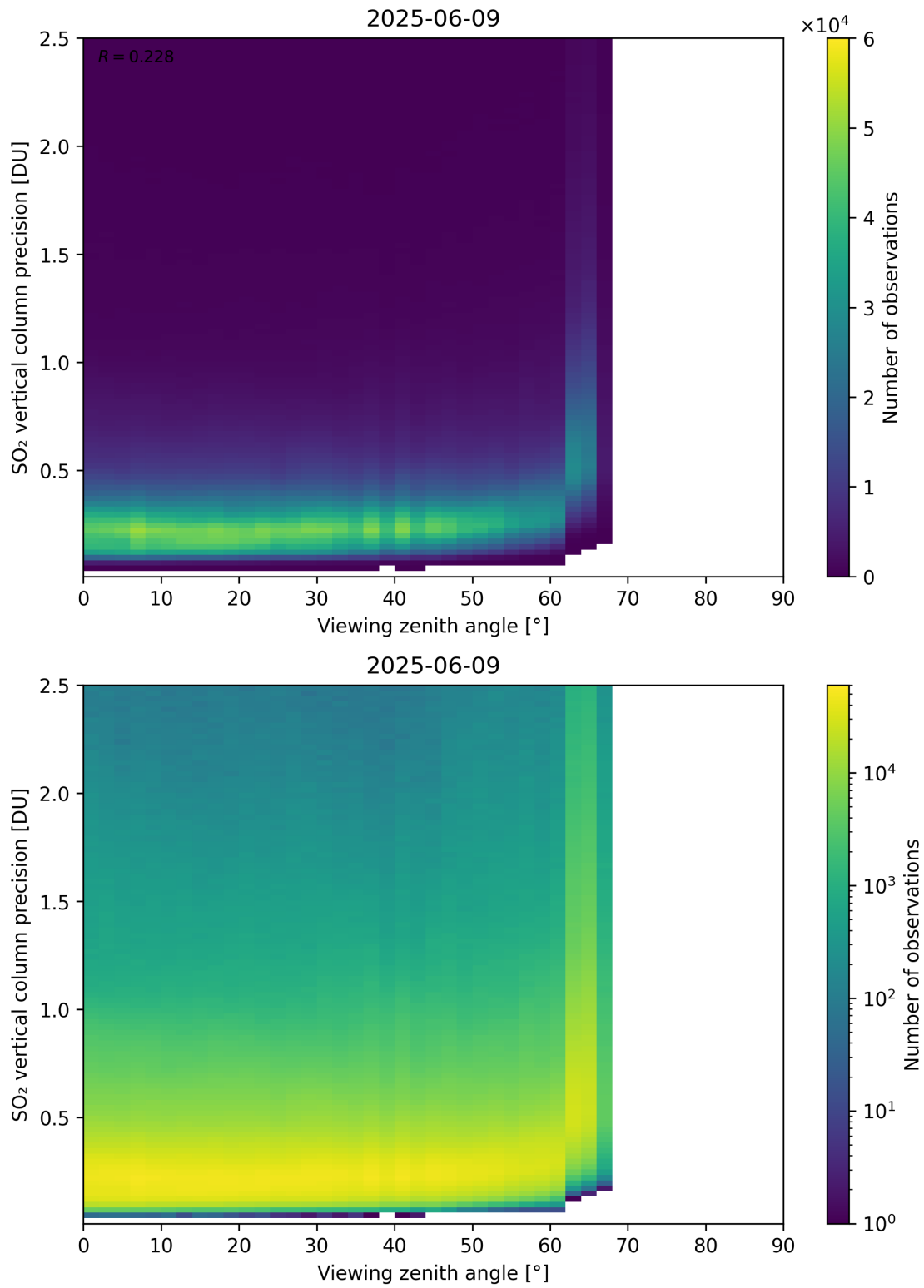
Figure 384: Scatter density plot of “Viewing zenith angle” against “SO 2 vertical column precision” for 2025-06-08 to 2025-06-10.
