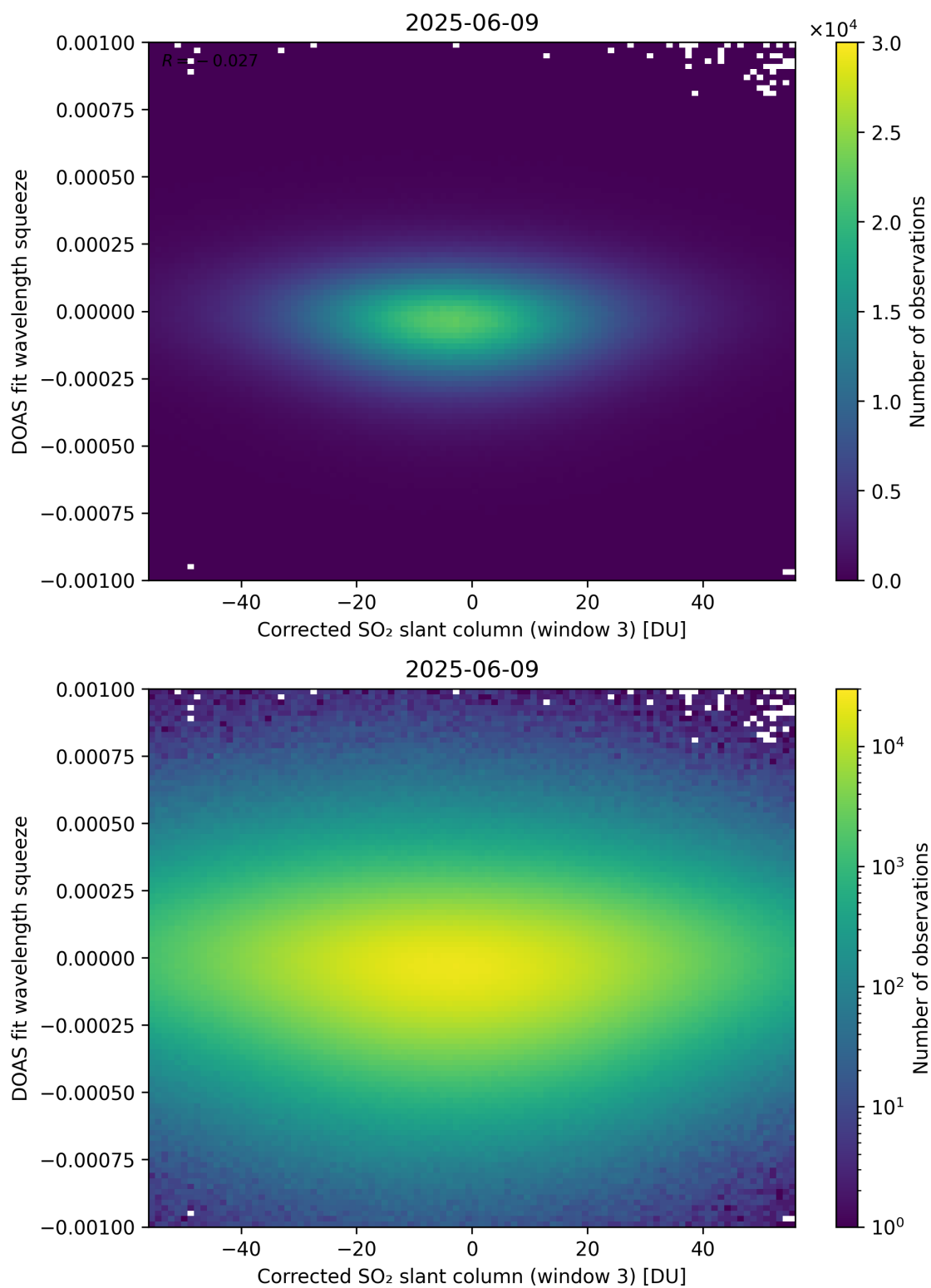
Figure 257: Scatter density plot of “Corrected SO 2 slant column (window 3)” against “DOAS fit wavelength squeeze” for 2025-06-08 to 2025-06-10.
