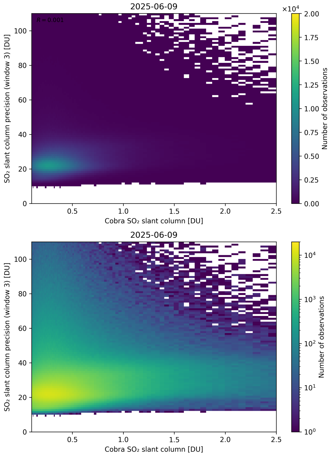
Figure 223: Scatter density plot of “Cobra SO 2 slant column” against “SO 2 slant column precision (window 3)” for 2025-06-08 to 2025-06-10.
