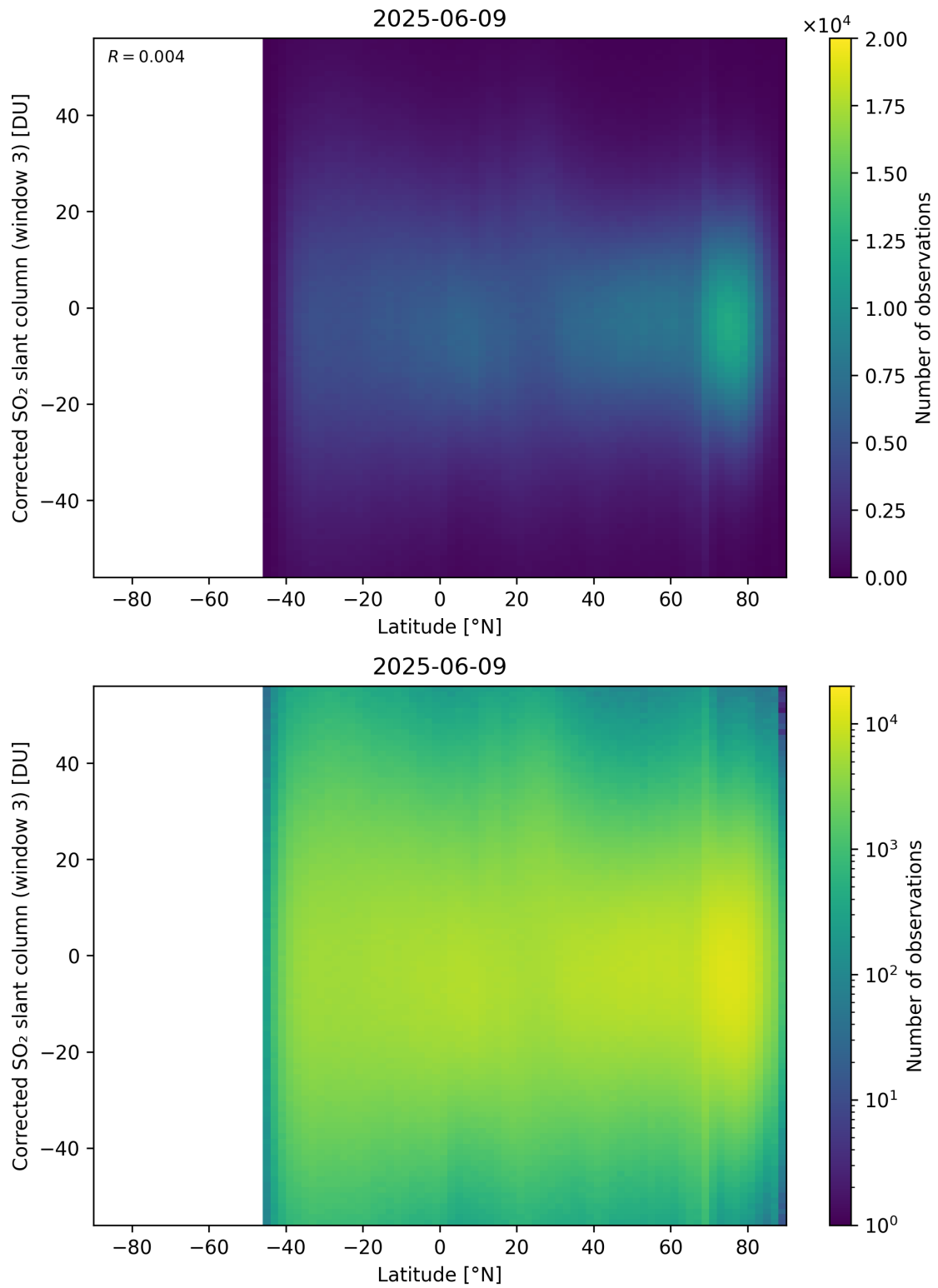
Figure 161: Scatter density plot of “Latitude” against “Corrected SO 2 slant column (window 3)” for 2025-06-08 to 2025-06-10.
