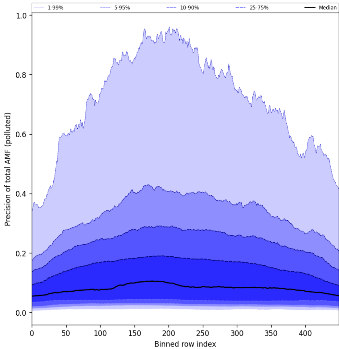
Figure 106: Along track statistics of “Precision of total AMF (polluted)” for 2025-06-08 to 2025-06-10
