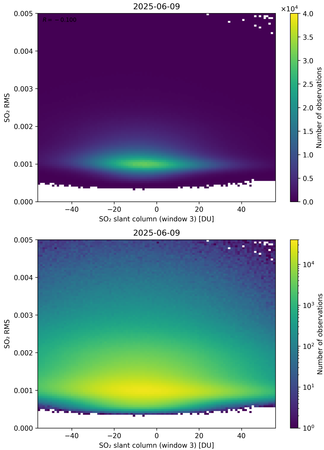
Figure 306: Scatter density plot of “SO 2 slant column (window 3)” against “SO 2 RMS” for 2025-06-08 to 2025-06-10.
