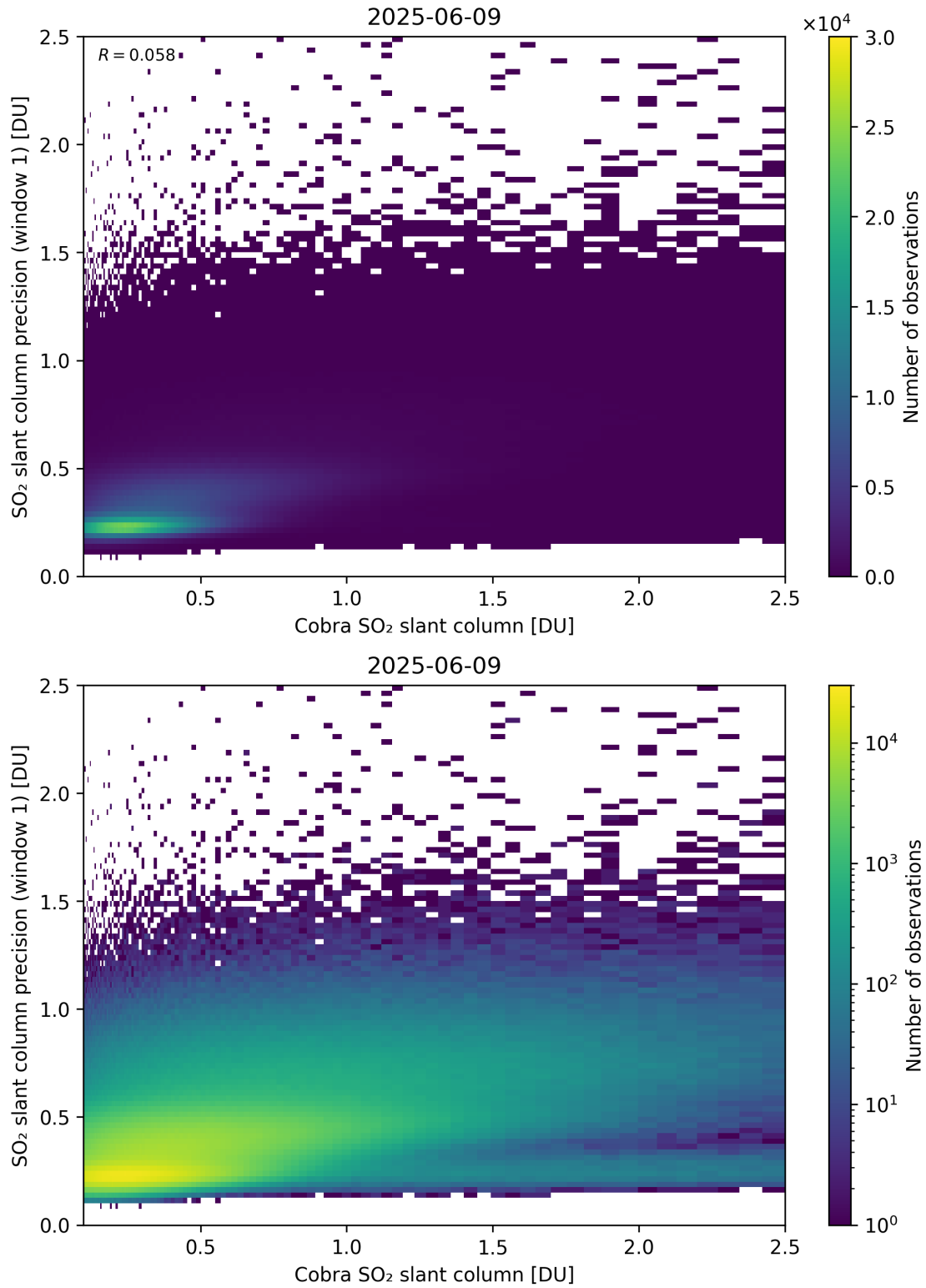
Figure 220: Scatter density plot of “Cobra SO 2 slant column” against “SO 2 slant column precision (window 1)” for 2025-06-08 to 2025-06-10.
