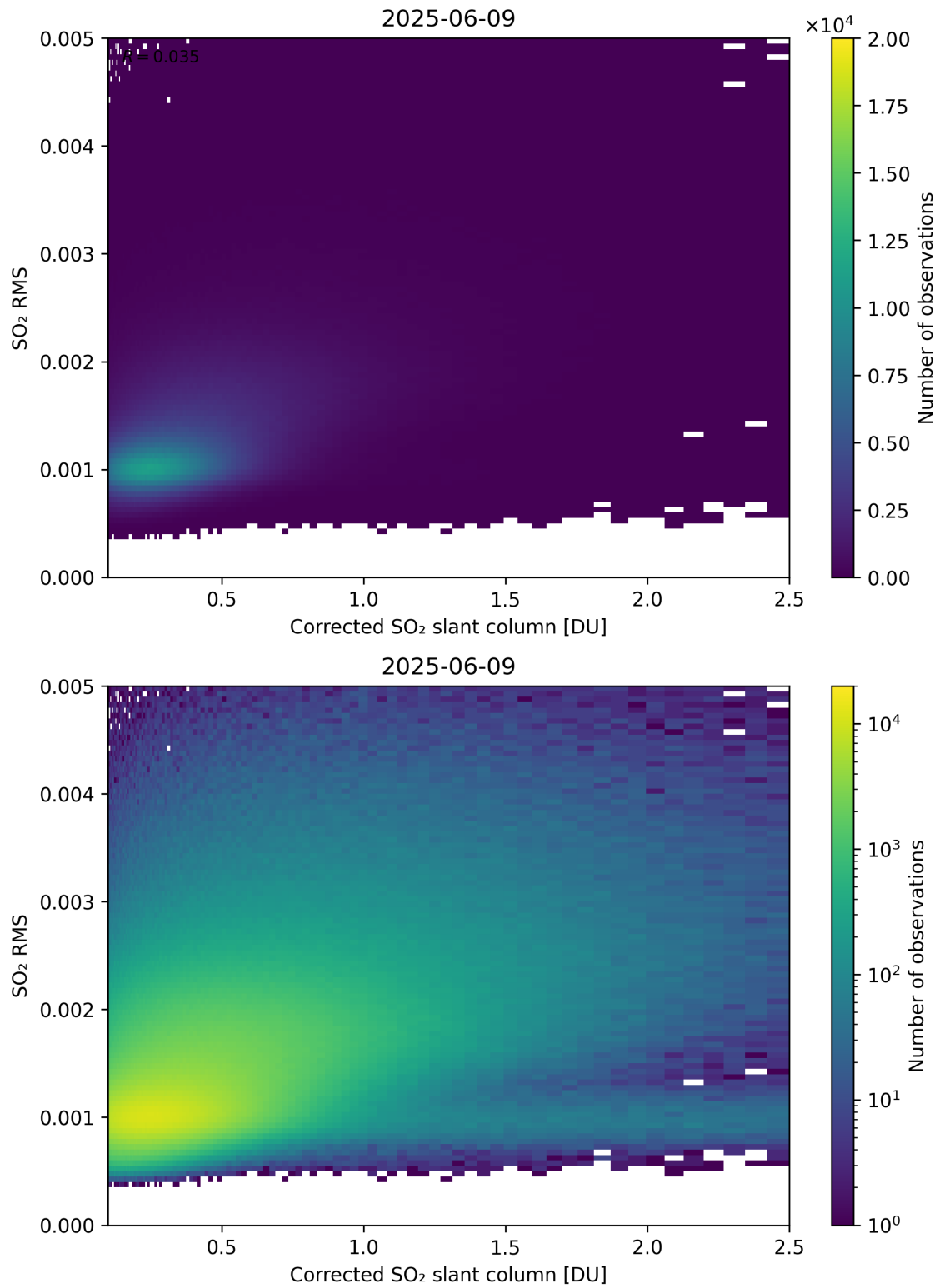
Figure 231: Scatter density plot of “Corrected SO 2 slant column” against “SO 2 RMS” for 2025-06-08 to 2025-06-10.
