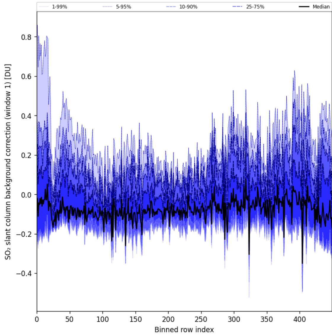
Figure 92: Along track statistics of “SO 2 slant column background correction (window 1)” for 2025-06-08 to 2025-06-10
