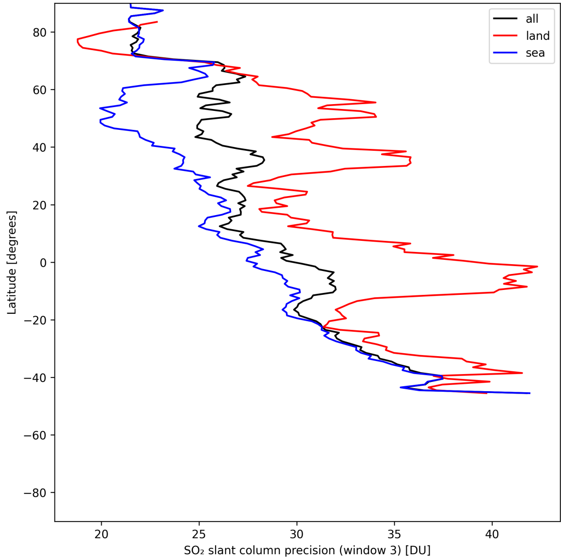
Figure 46: Zonal average of “SO 2 slant column precision (window 3)” for 2025-06-08 to 2025-06-10.
