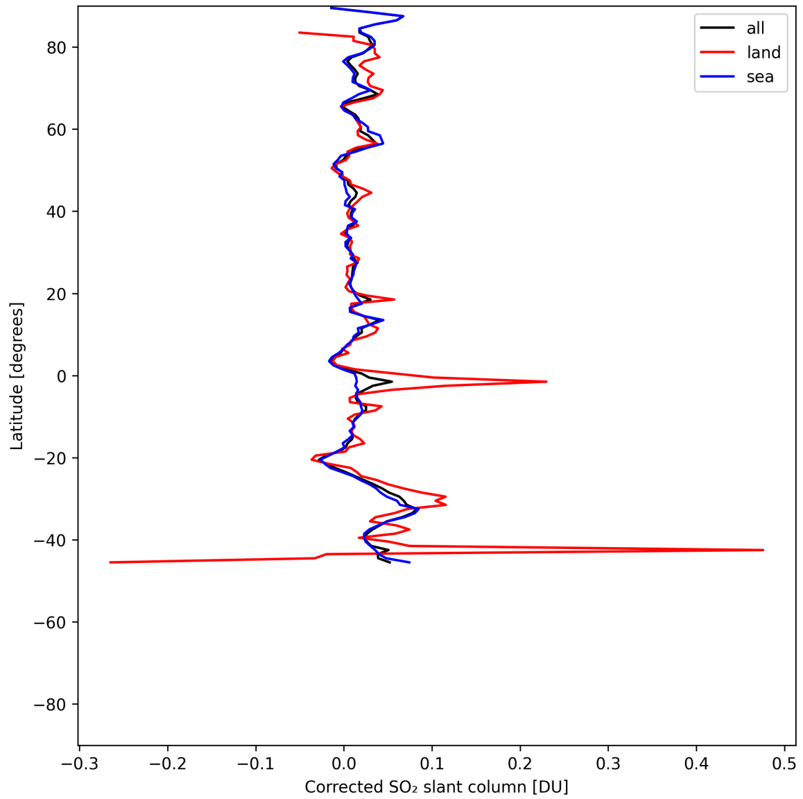
Figure 34: Zonal average of "Corrected SO 2 slant column" for 2025-06-08 to 2025-06-10.
