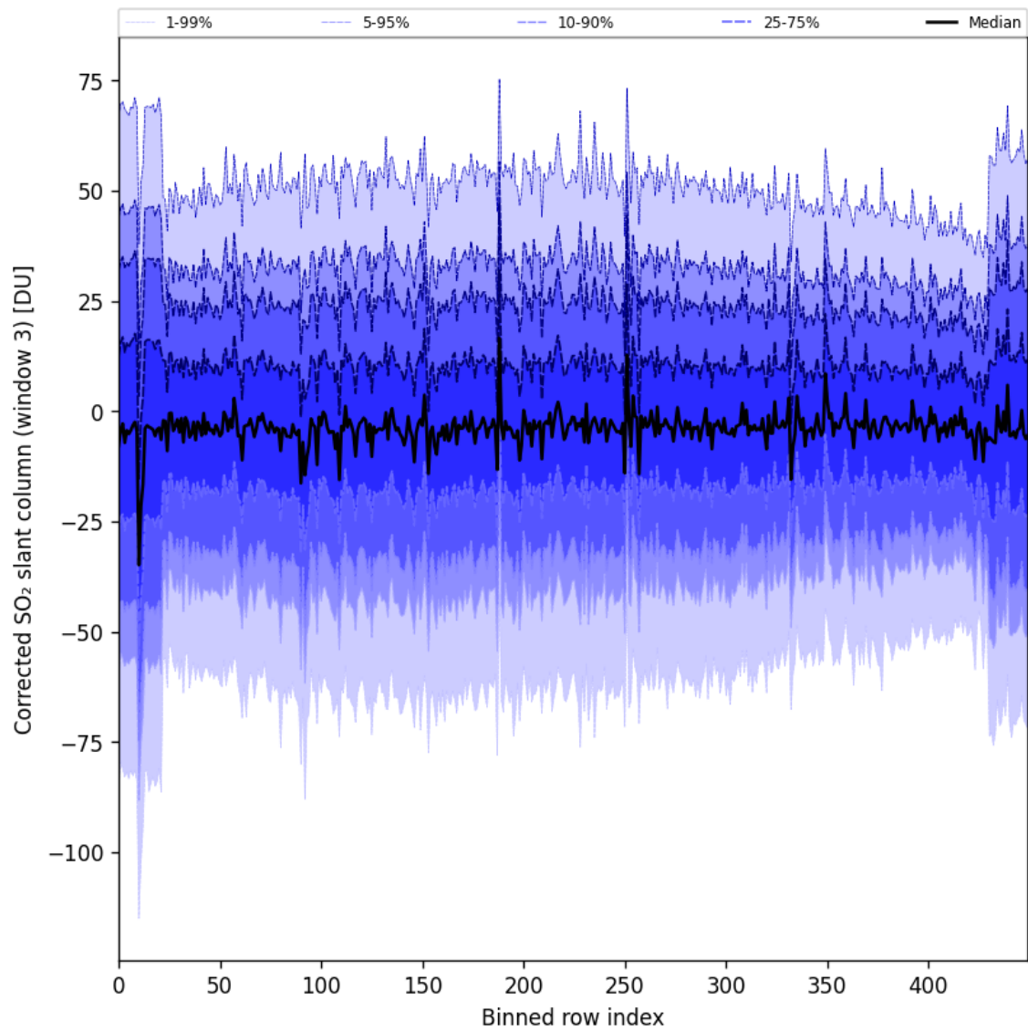
Figure 99: Along track statistics of “Corrected SO 2 slant column (window 3)” for 2025-06-08 to 2025-06-10
