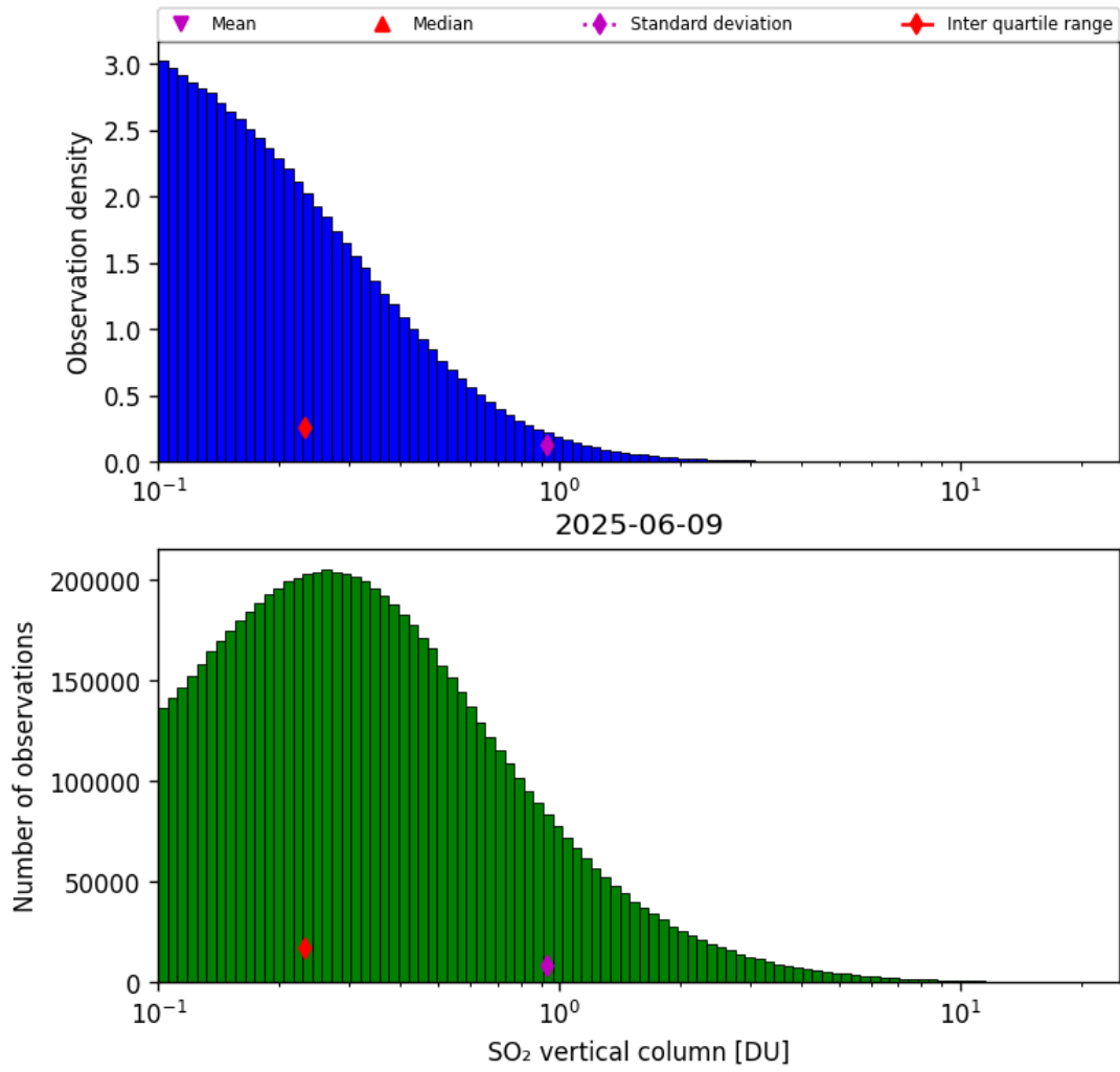
Figure 58: Histogram of “SO 2 vertical column” for 2025-06-08 to 2025-06-10
