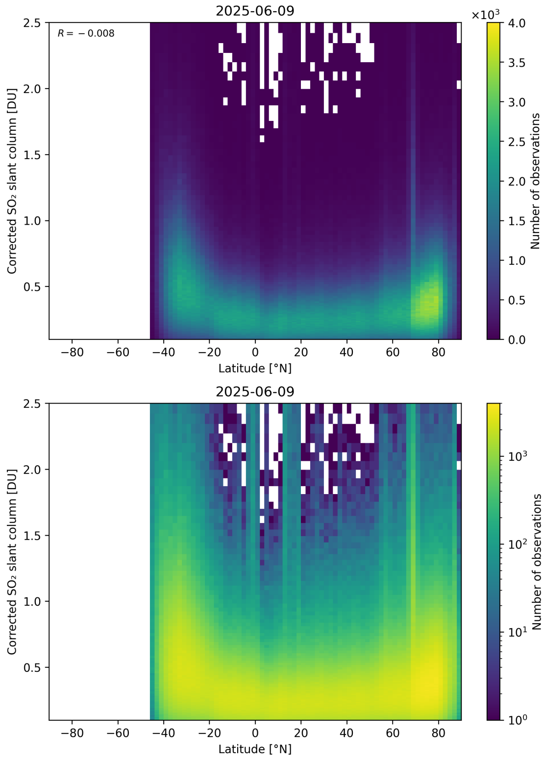
Figure 159: Scatter density plot of “Latitude” against “Corrected SO 2 slant column” for 2025-06-08 to 2025-06-10.
