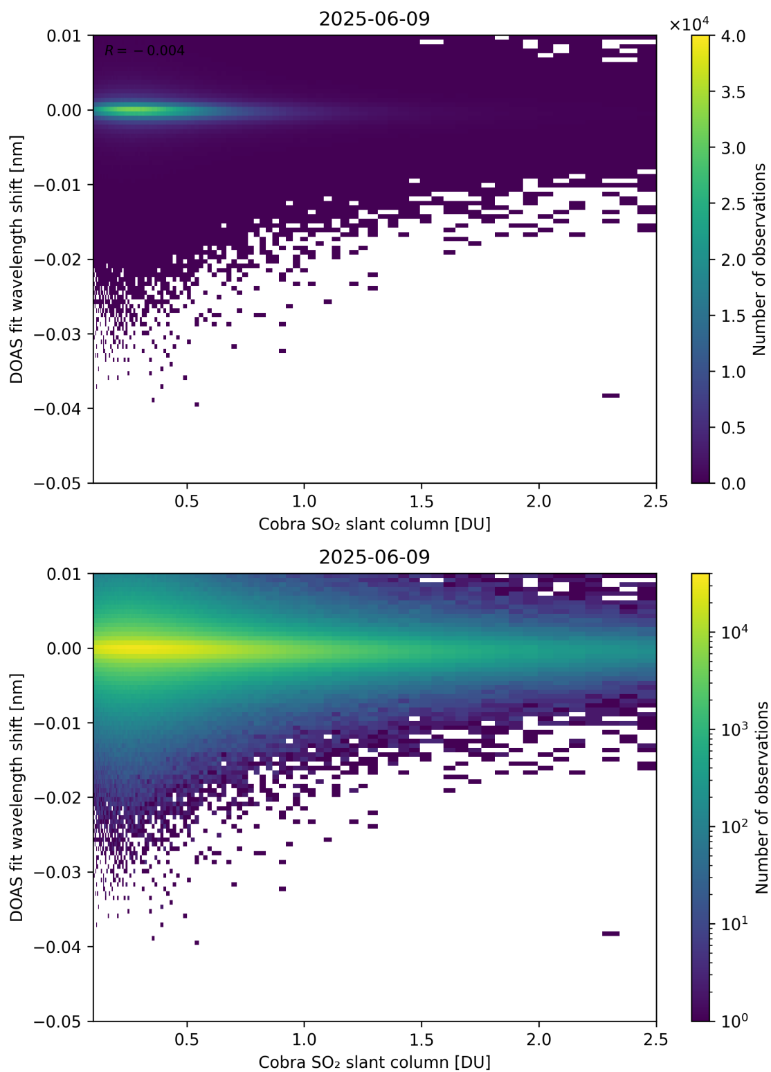
Figure 196: Scatter density plot of “Cobra SO 2 slant column” against “DOAS fit wavelength shift” for 2025-06-08 to 2025-06-10.
