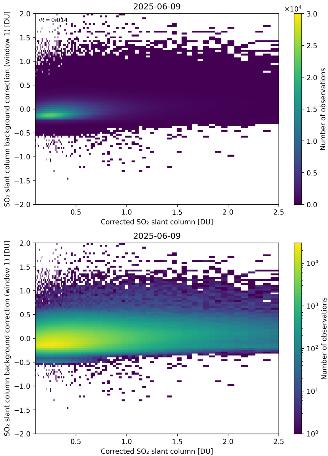
Figure 226: Scatter density plot of “Corrected SO 2 slant column” against “SO 2 slant column background correction (window 1)” for 2025-06-08 to 2025-06-10.
