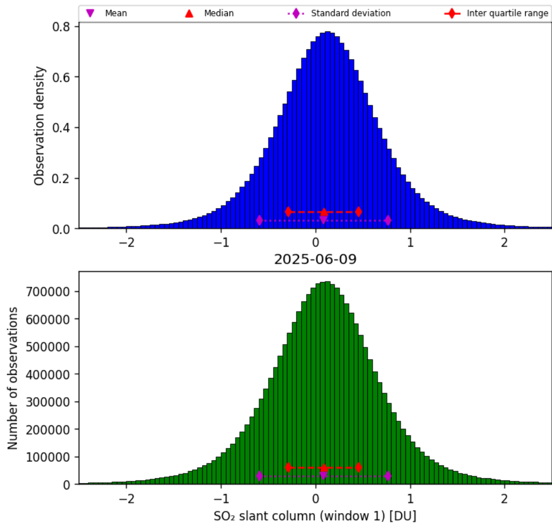
Figure 63: Histogram of “SO 2 slant column (window 1)” for 2025-06-08 to 2025-06-10
