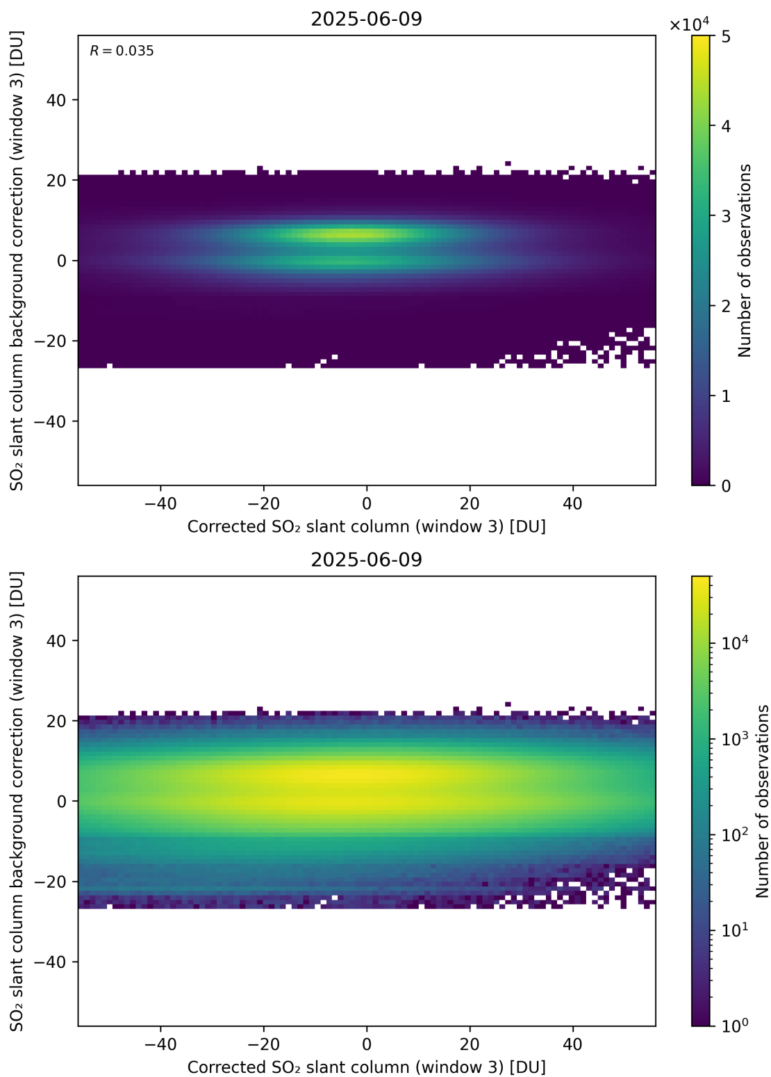
Figure 255: Scatter density plot of “Corrected SO 2 slant column (window 3)” against “SO 2 slant column background correction (window 3)” for 2025-06-08 to 2025-06-10.
