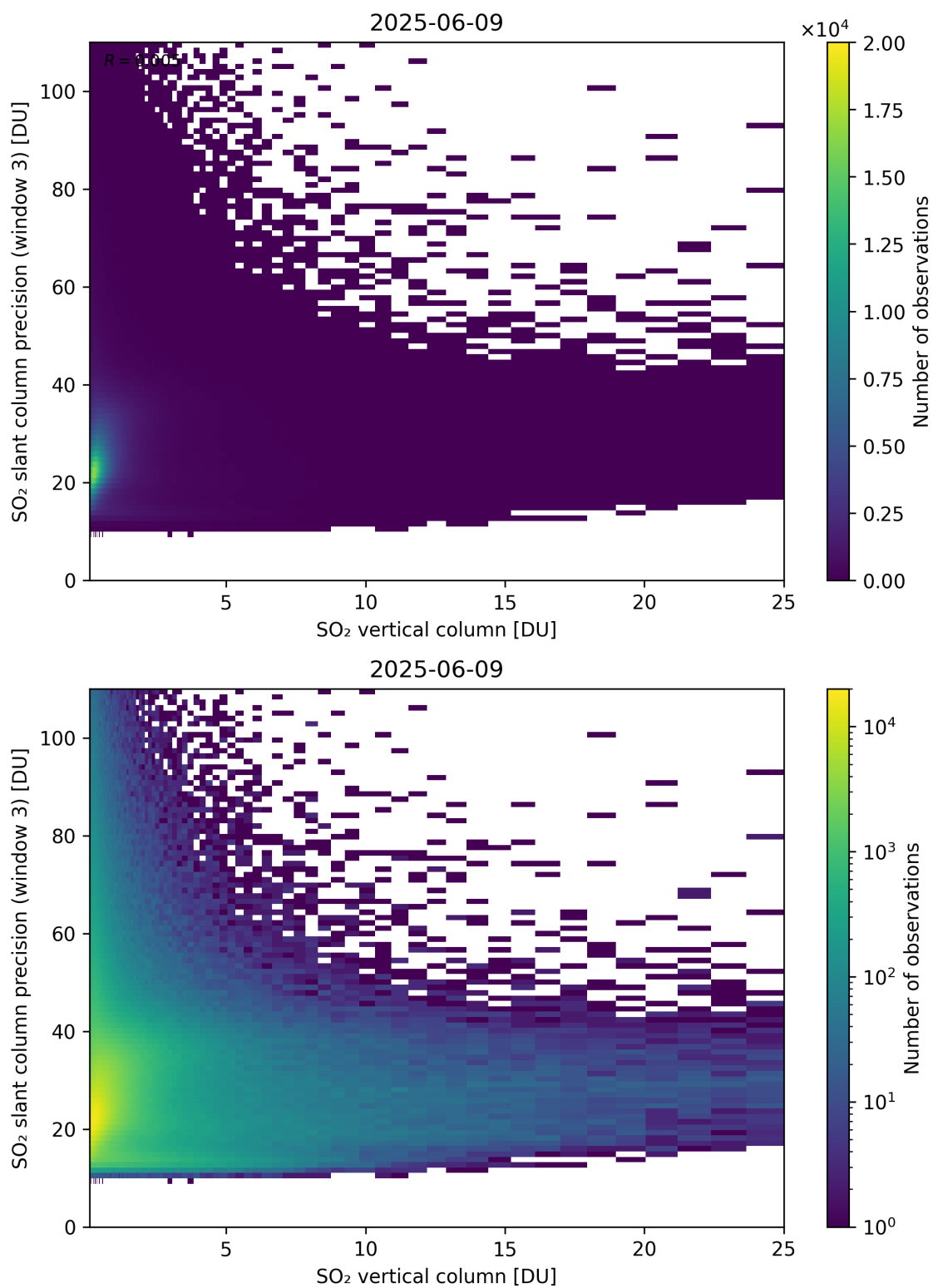
Figure 358: Scatter density plot of “SO 2 vertical column” against “SO 2 slant column precision (window 3)” for 2025-06-08 to 2025-06-10.
