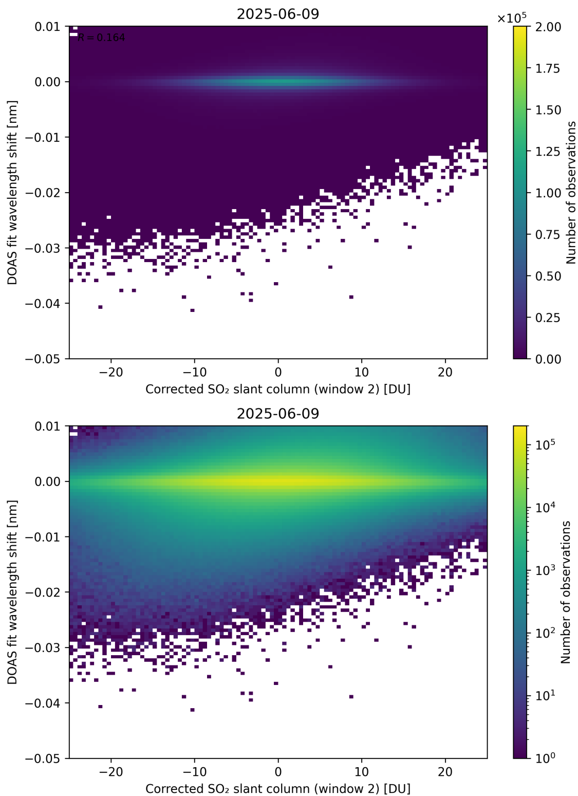
Figure 246: Scatter density plot of “Corrected SO 2 slant column (window 2)” against “DOAS fit wavelength shift” for 2025-06-08 to 2025-06-10.
