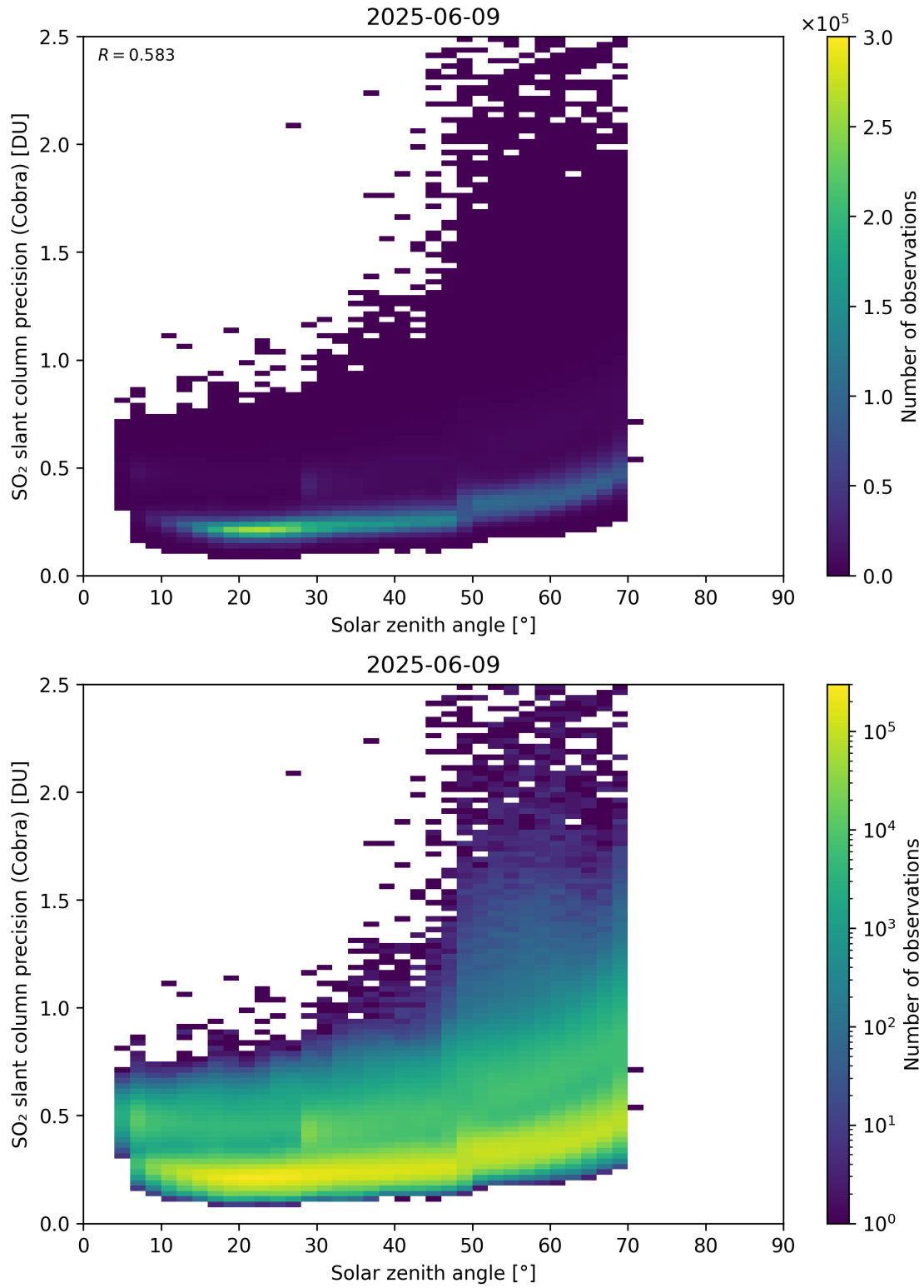
Figure 180: Scatter density plot of “Solar zenith angle” against “SO 2 slant column precision (Cobra)” for 2025-06-08 to 2025-06-10.
