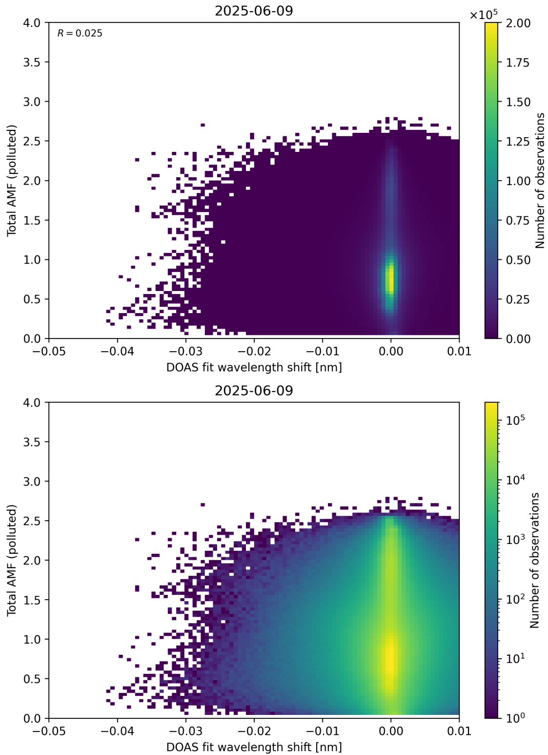
Figure 141: Scatter density plot of “DOAS fit wavelength shift” against “Total AMF (polluted)” for 2025-06-08 to 2025-06-10.
