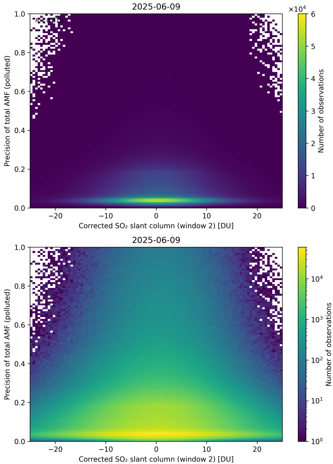
Figure 254: Scatter density plot of “Corrected SO 2 slant column (window 2)” against “Precision of total AMF (polluted)” for 2025-06-08 to 2025-06-10.
