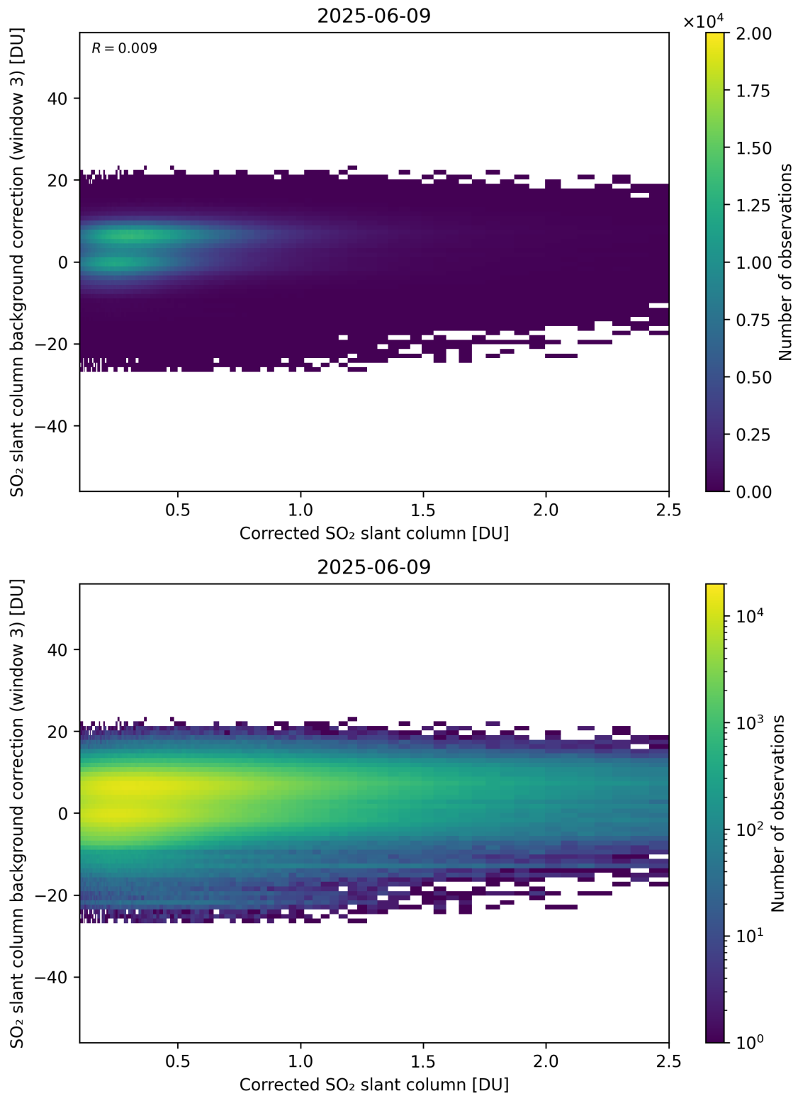
Figure 228: Scatter density plot of “Corrected SO 2 slant column” against “SO 2 slant column background correction (window 3)” for 2025-06-08 to 2025-06-10.
