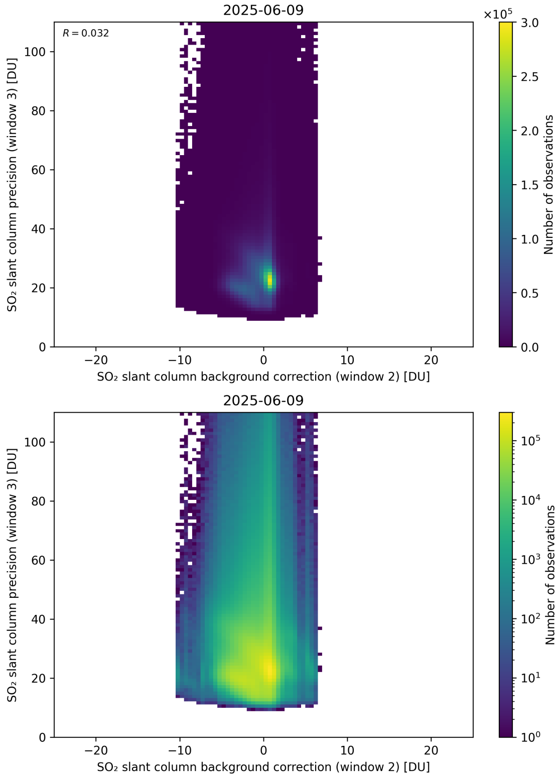
Figure 129: Scatter density plot of “SO 2 slant column background correction (window 2)” against “SO 2 slant column precision (window 3)” for 2025-06-08 to 2025-06-10.
