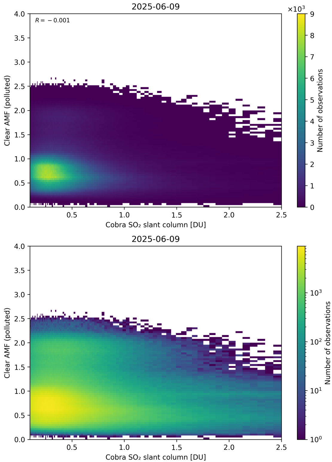
Figure 215: Scatter density plot of “Cobra SO 2 slant column” against “Clear AMF (polluted)” for 2025-06-08 to 2025-06-10.
