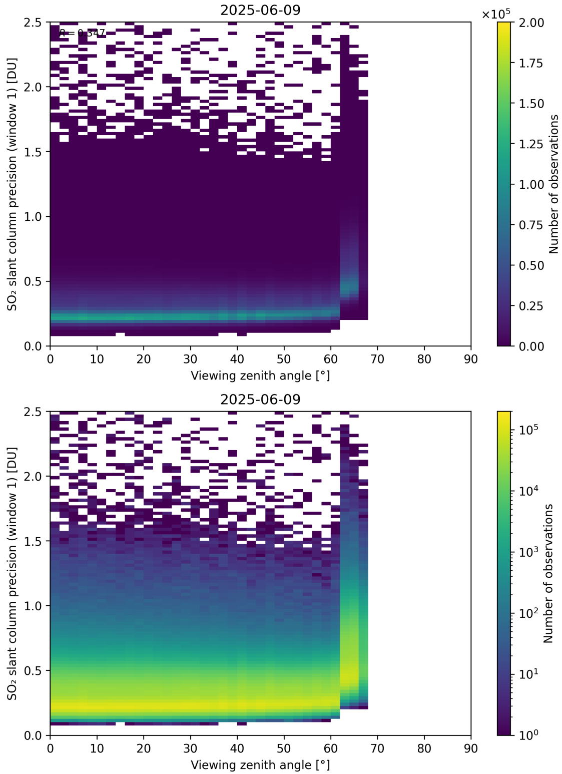
Figure 377: Scatter density plot of “Viewing zenith angle” against “SO 2 slant column precision (window 1)” for 2025-06-08 to 2025-06-10.
