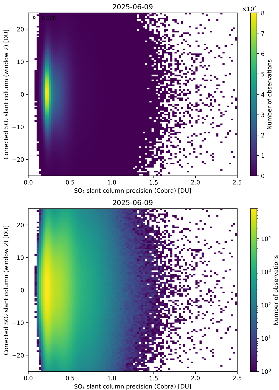
Figure 206: Scatter density plot of “SO 2 slant column precision (Cobra)” against “Corrected SO 2 slant column (window 2)” for 2025-06-08 to 2025-06-10.
