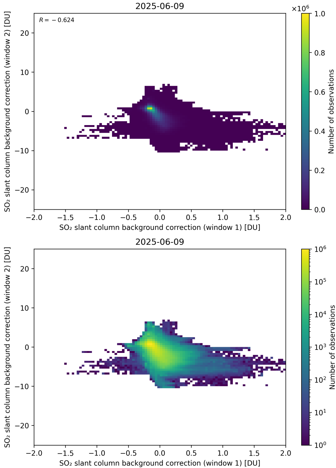
Figure 109: Scatter density plot of “SO 2 slant column background correction (window 1)” against “SO 2 slant column background correction (window 2)” for 2025-06-08 to 2025-06-10.
