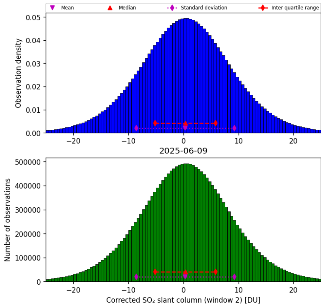
Figure 69: Histogram of “Corrected SO 2 slant column (window 2)” for 2025-06-08 to 2025-06-10
