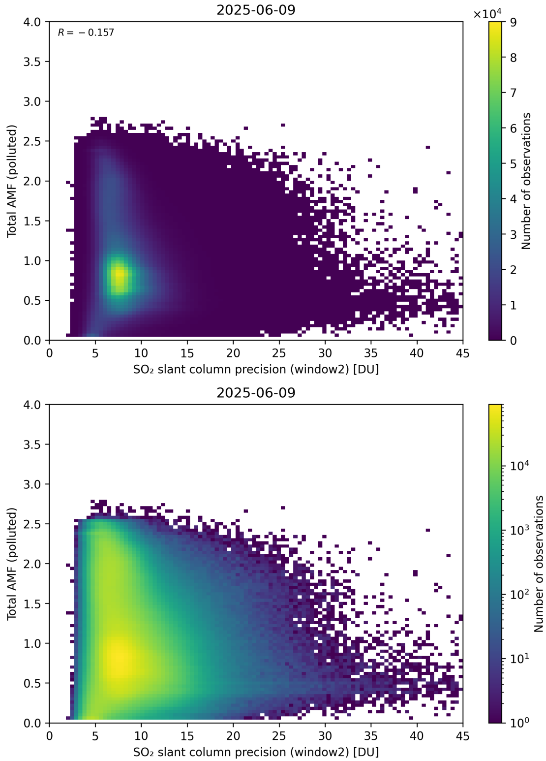
Figure 301: Scatter density plot of “SO 2 slant column precision (window2)” against “Total AMF (polluted)” for 2025-06-08 to 2025-06-10.
