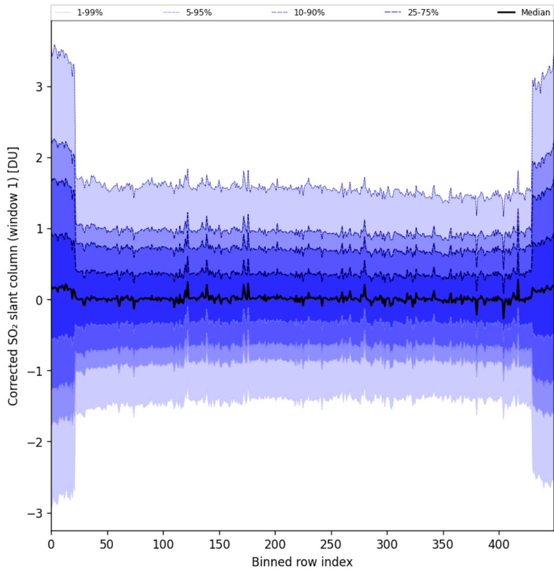
Figure 91: Along track statistics of “Corrected SO 2 slant column (window 1)” for 2025-06-08 to 2025-06-10
