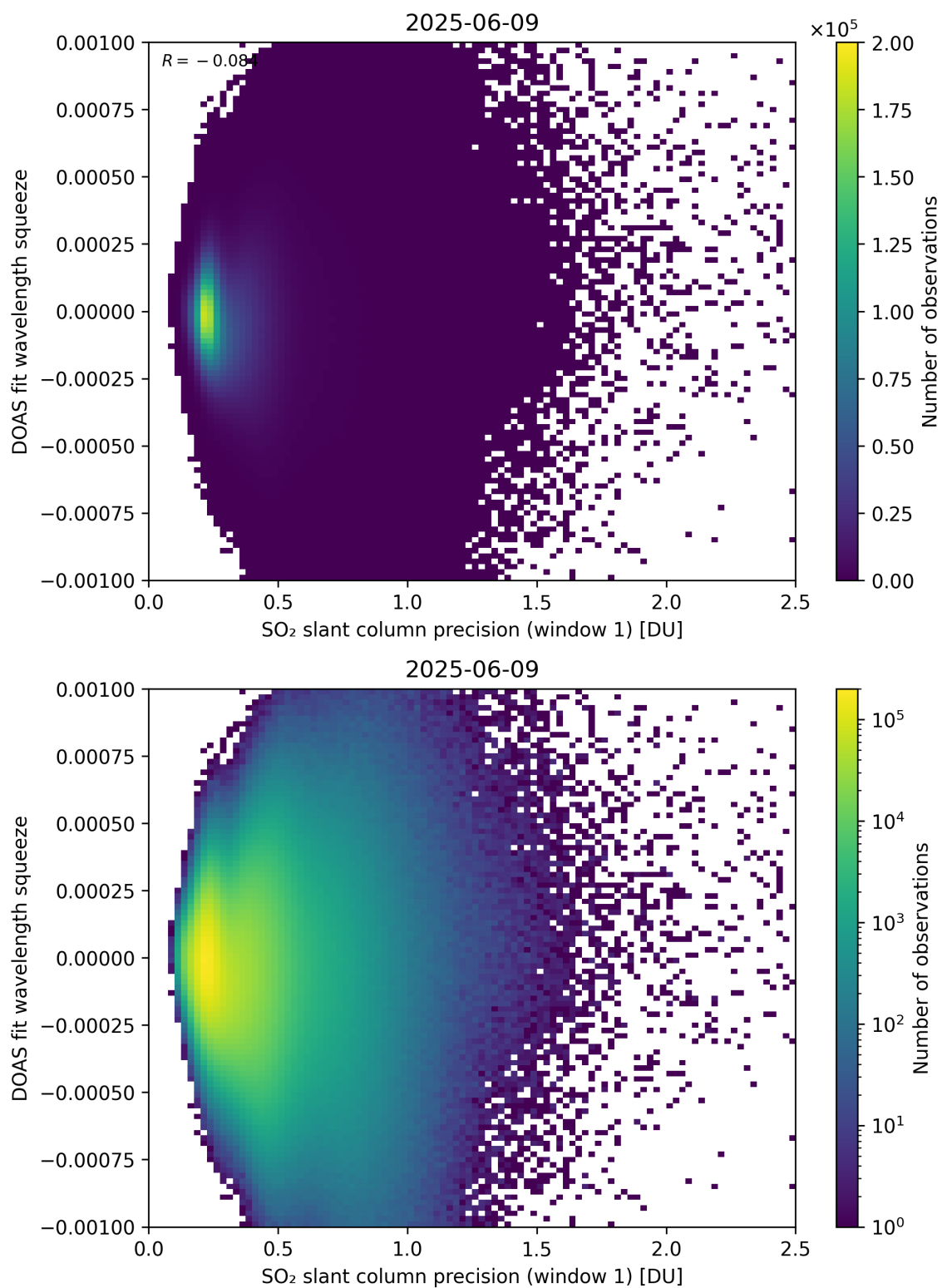
Figure 272: Scatter density plot of “SO 2 slant column precision (window 1)” against “DOAS fit wavelength squeeze” for 2025-06-08 to 2025-06-10.
