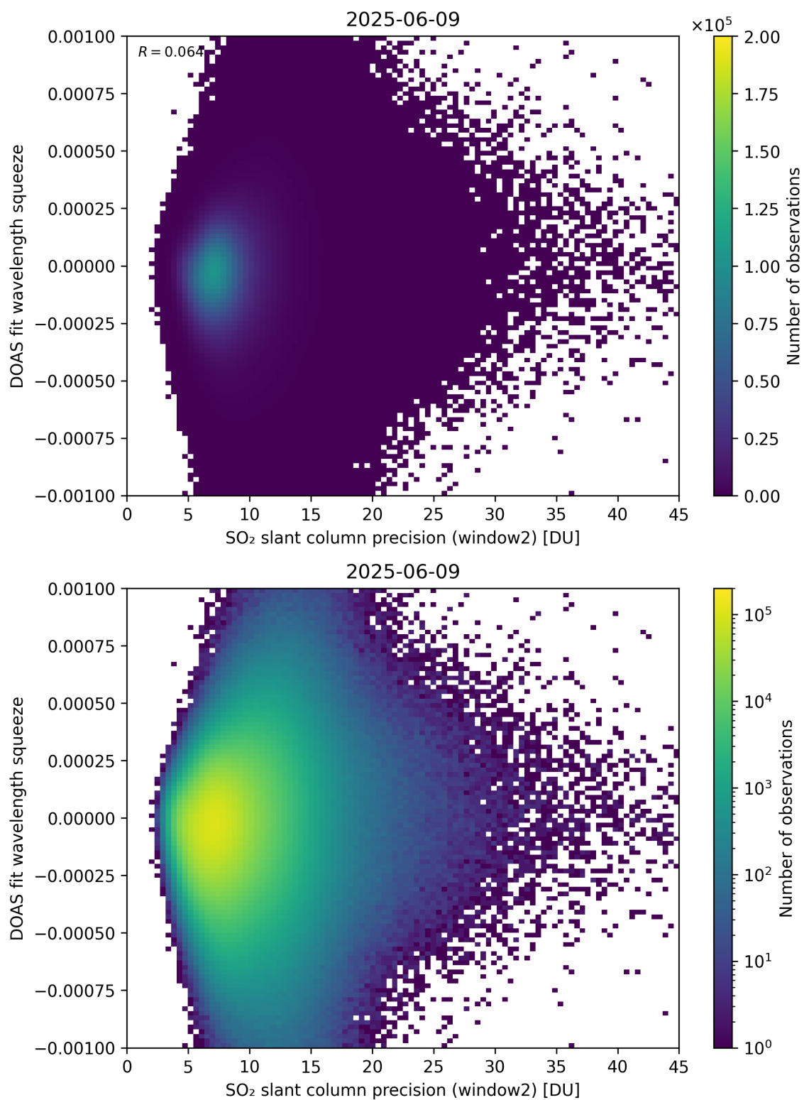
Figure 294: Scatter density plot of “SO 2 slant column precision (window2)” against “DOAS fit wavelength squeeze” for 2025-06-08 to 2025-06-10.
