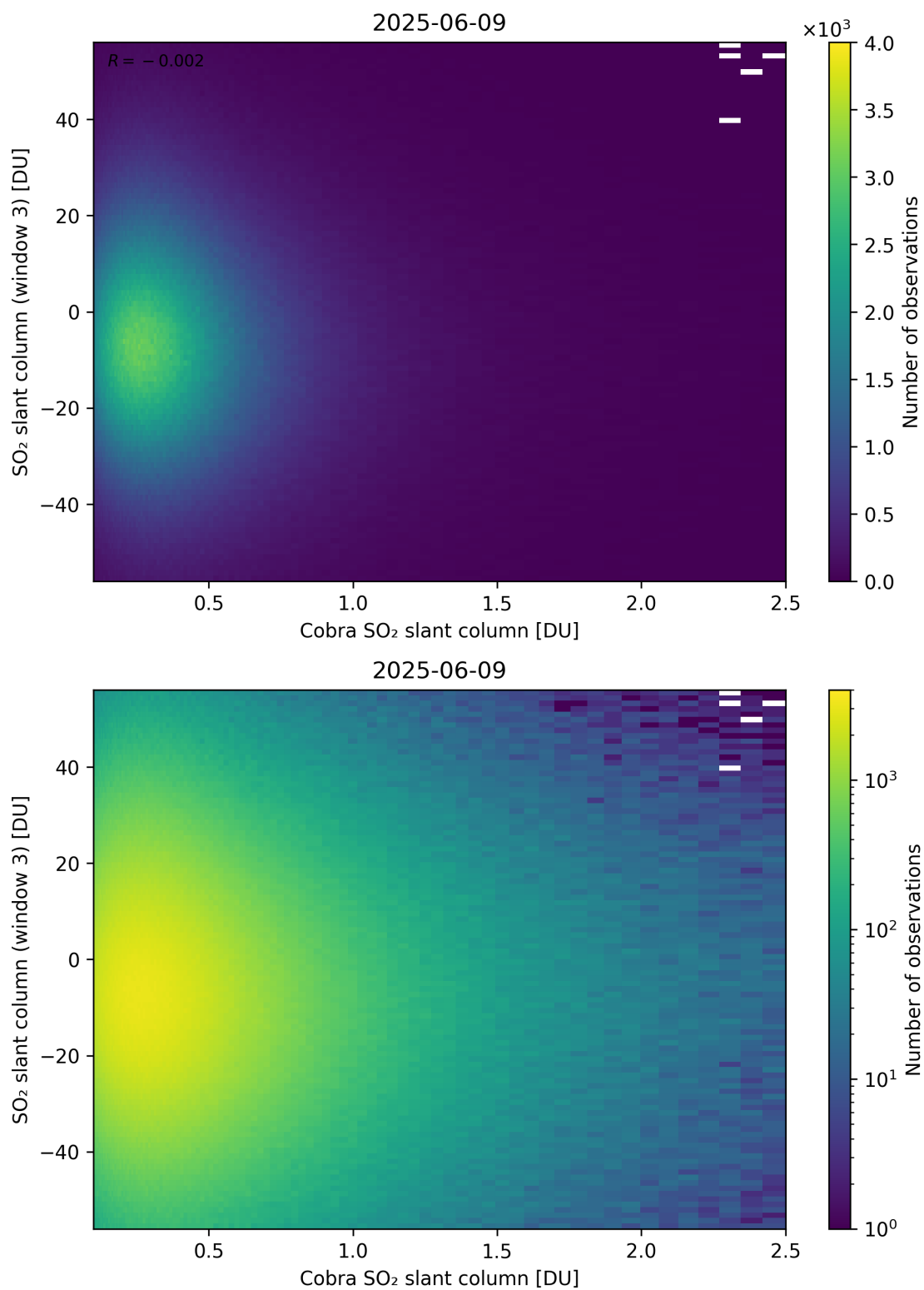
Figure 222: Scatter density plot of “Cobra SO 2 slant column” against “SO 2 slant column (window 3)” for 2025-06-08 to 2025-06-10.
