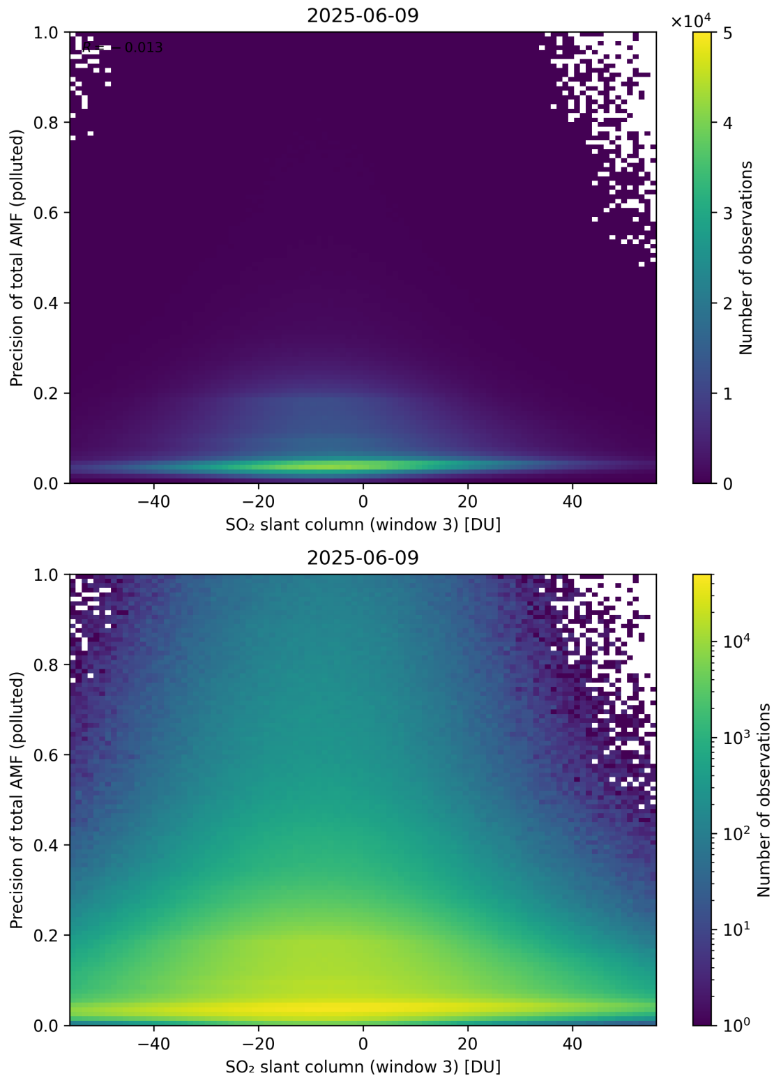
Figure 319: Scatter density plot of “SO 2 slant column (window 3)” against “Precision of total AMF (polluted)” for 2025-06-08 to 2025-06-10.
