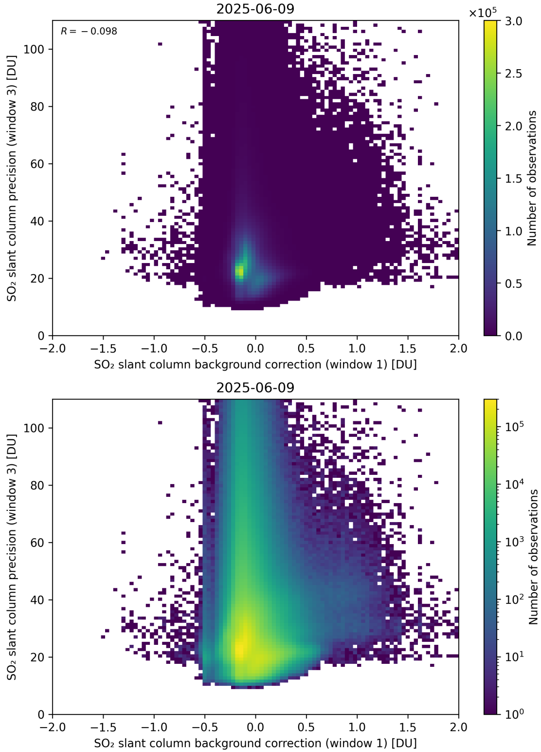
Figure 119: Scatter density plot of “SO 2 slant column background correction (window 1)” against “SO 2 slant column precision (window 3)” for 2025-06-08 to 2025-06-10.
