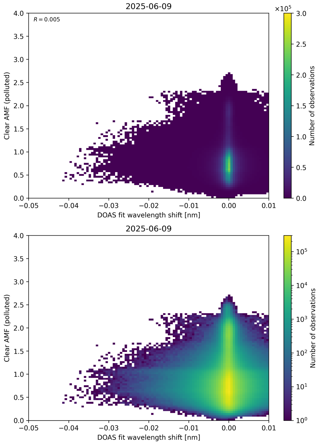
Figure 140: Scatter density plot of “DOAS fit wavelength shift” against “Clear AMF (polluted)” for 2025-06-08 to 2025-06-10.
