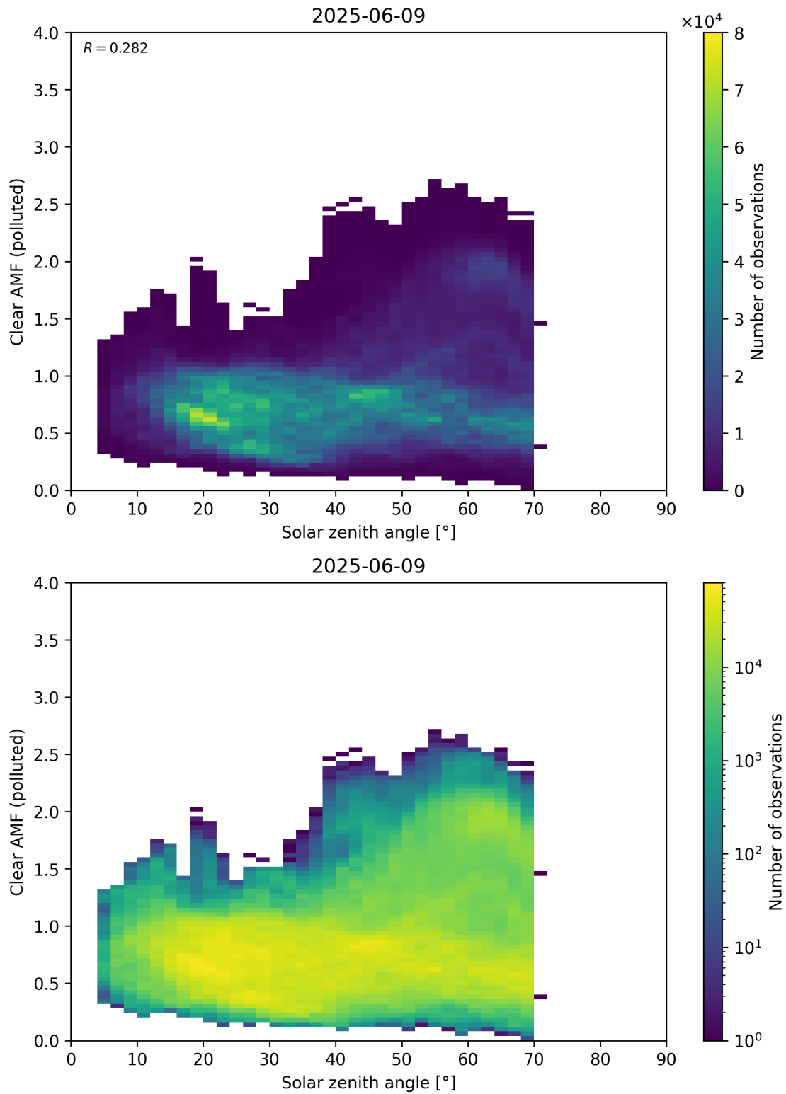
Figure 178: Scatter density plot of “Solar zenith angle” against “Clear AMF (polluted)” for 2025-06-08 to 2025-06-10.
