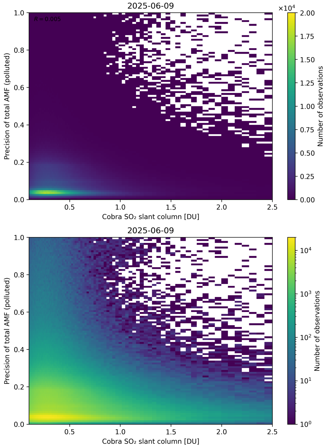
Figure 225: Scatter density plot of “Cobra SO 2 slant column” against “Precision of total AMF (polluted)” for 2025-06-08 to 2025-06-10.
