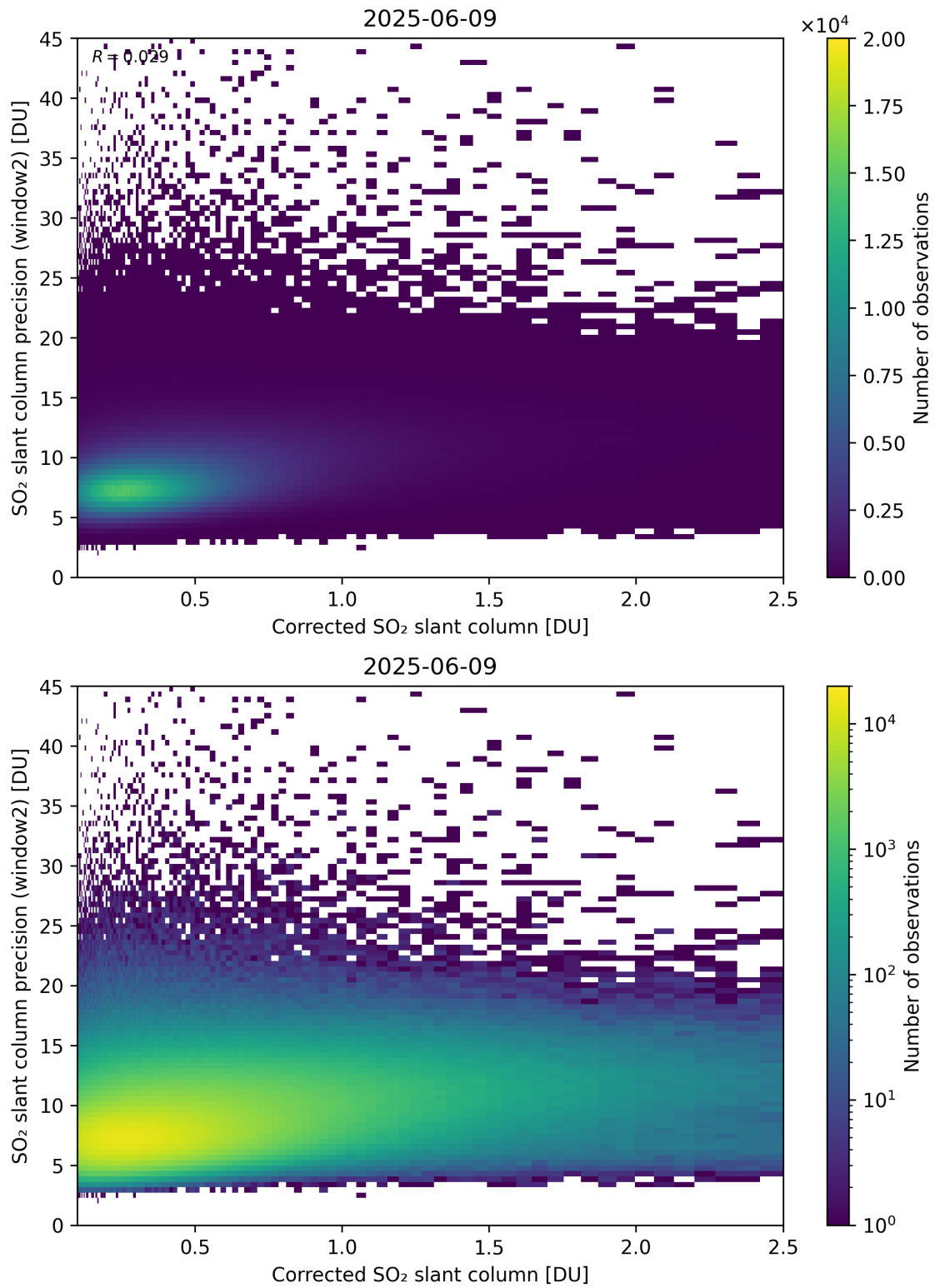
Figure 239: Scatter density plot of “Corrected SO 2 slant column” against “SO 2 slant column precision (window2)” for 2025-06-08 to 2025-06-10.
