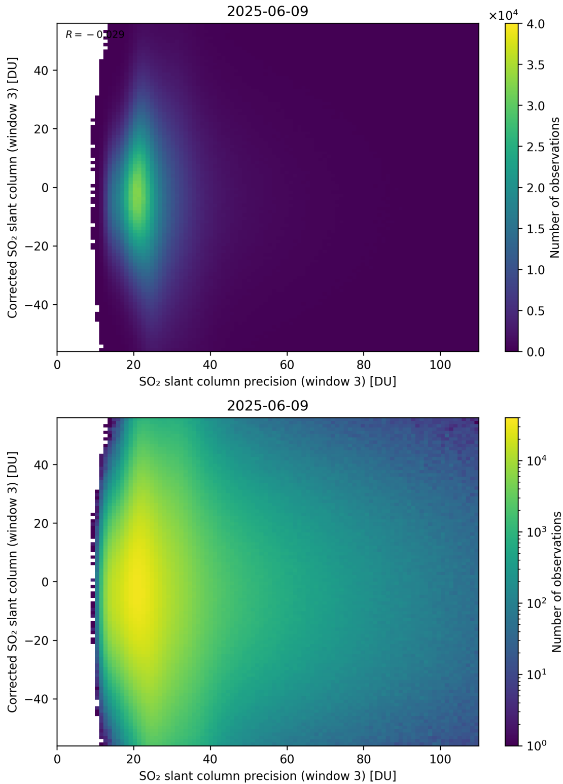
Figure 312: Scatter density plot of “SO 2 slant column precision (window 3)” against “Corrected SO 2 slant column (window 3)” for 2025-06-08 to 2025-06-10.
