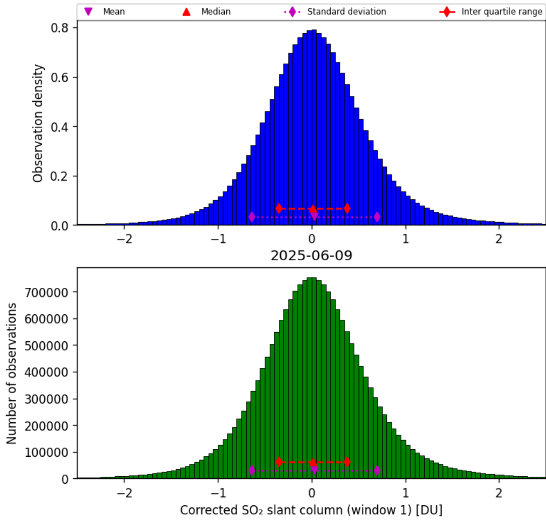
Figure 65: Histogram of “Corrected SO 2 slant column (window 1)” for 2025-06-08 to 2025-06-10
