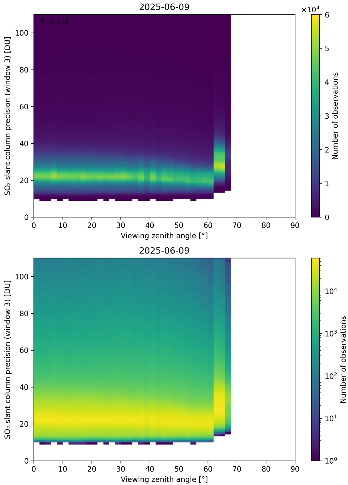
Figure 380: Scatter density plot of “Viewing zenith angle” against “SO 2 slant column precision (window 3)” for 2025-06-08 to 2025-06-10.
