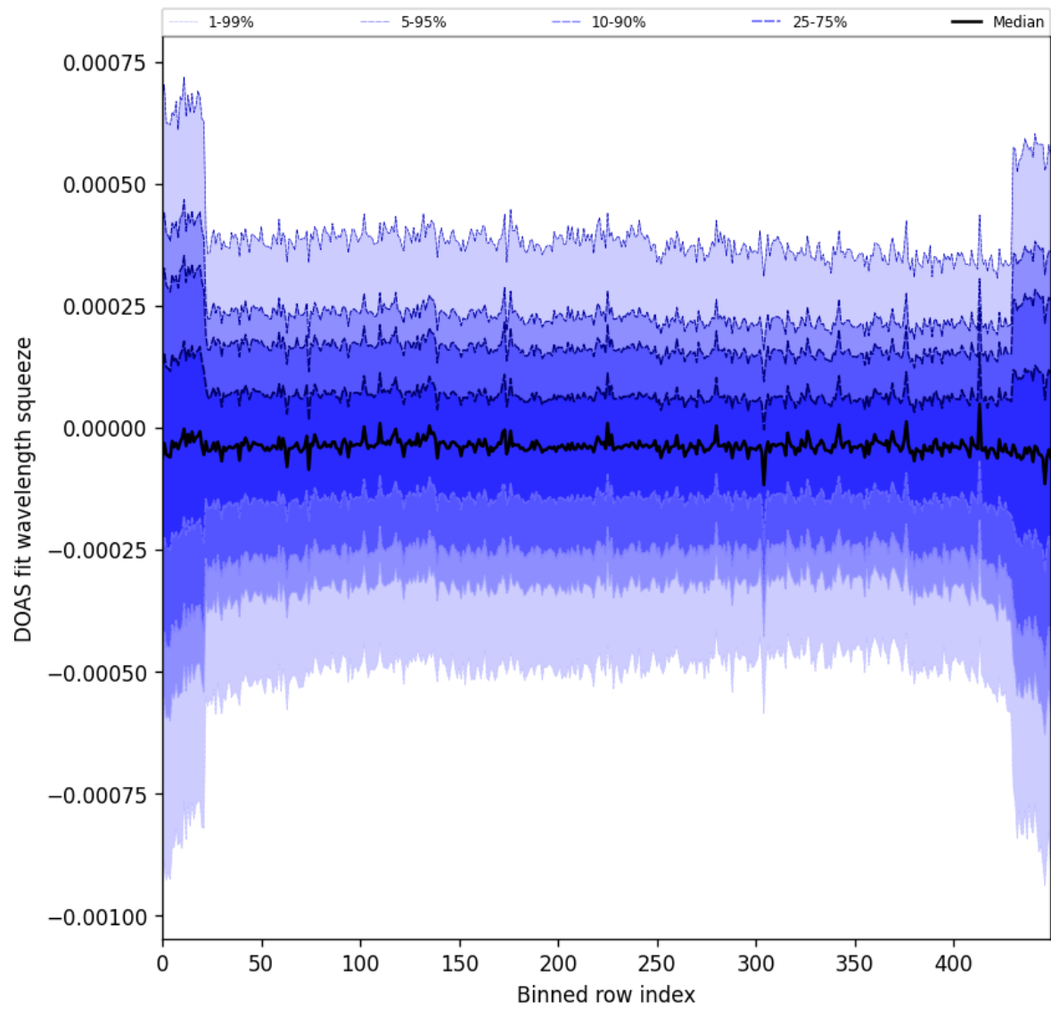
Figure 103: Along track statistics of “DOAS fit wavelength squeeze” for 2025-06-08 to 2025-06-10
