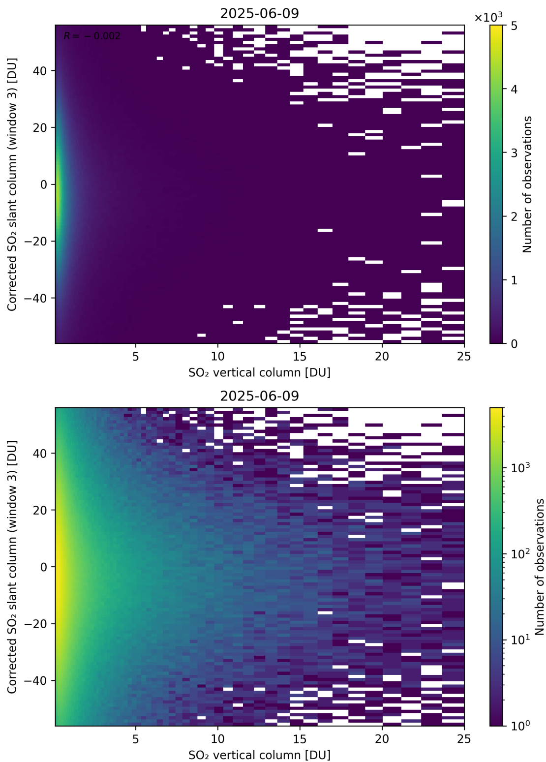
Figure 353: Scatter density plot of “SO 2 vertical column” against “Corrected SO 2 slant column (window 3)” for 2025-06-08 to 2025-06-10.
