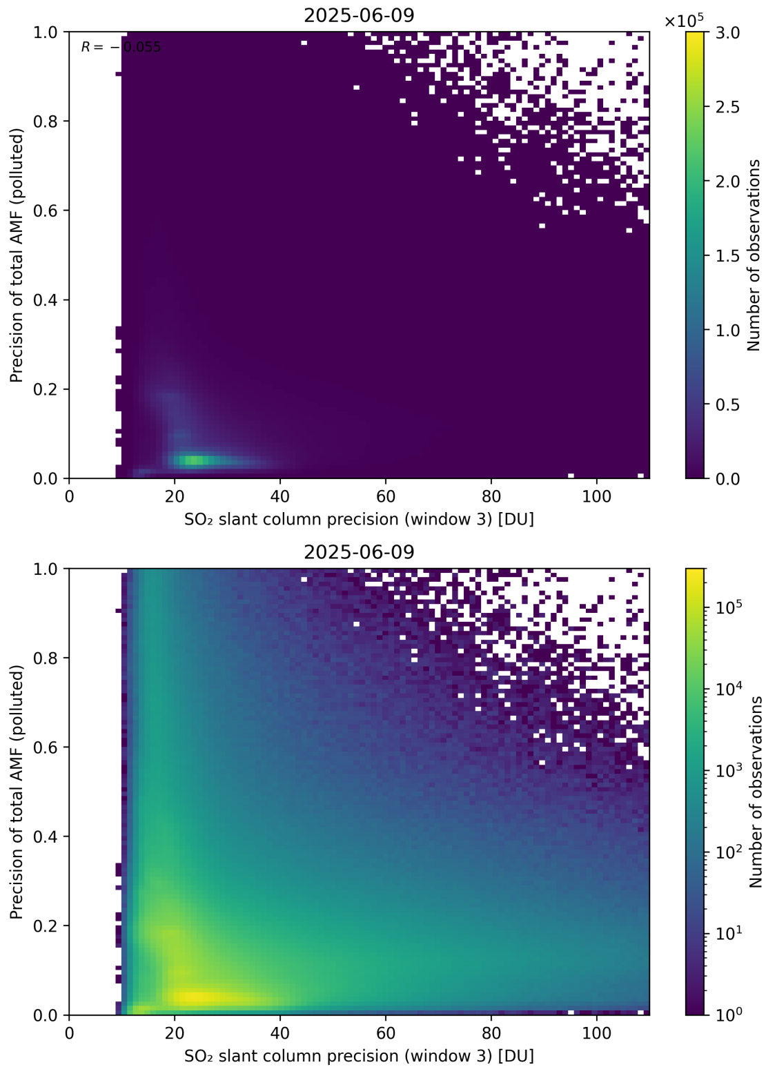
Figure 314: Scatter density plot of “SO 2 slant column precision (window 3)” against “Precision of total AMF (polluted)” for 2025-06-08 to 2025-06-10.
