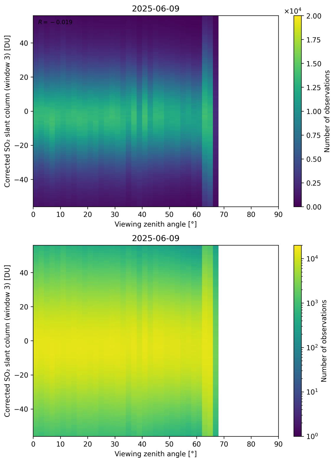
Figure 375: Scatter density plot of “Viewing zenith angle” against “Corrected SO 2 slant column (window 3)” for 2025-06-08 to 2025-06-10.
