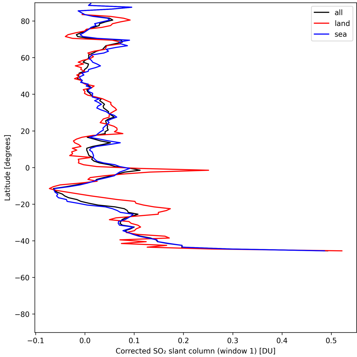
Figure 39: Zonal average of "Corrected SO 2 slant column (window 1)" for 2025-06-08 to 2025-06-10.
