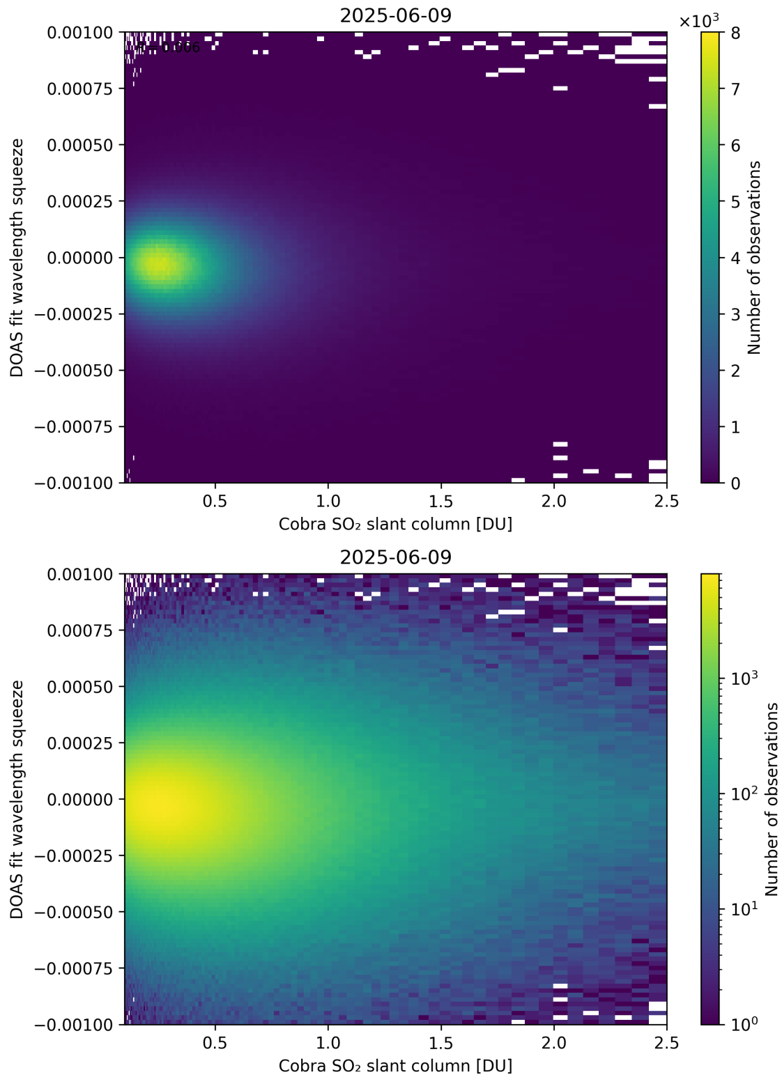
Figure 197: Scatter density plot of “Cobra SO 2 slant column” against “DOAS fit wavelength squeeze” for 2025-06-08 to 2025-06-10.
