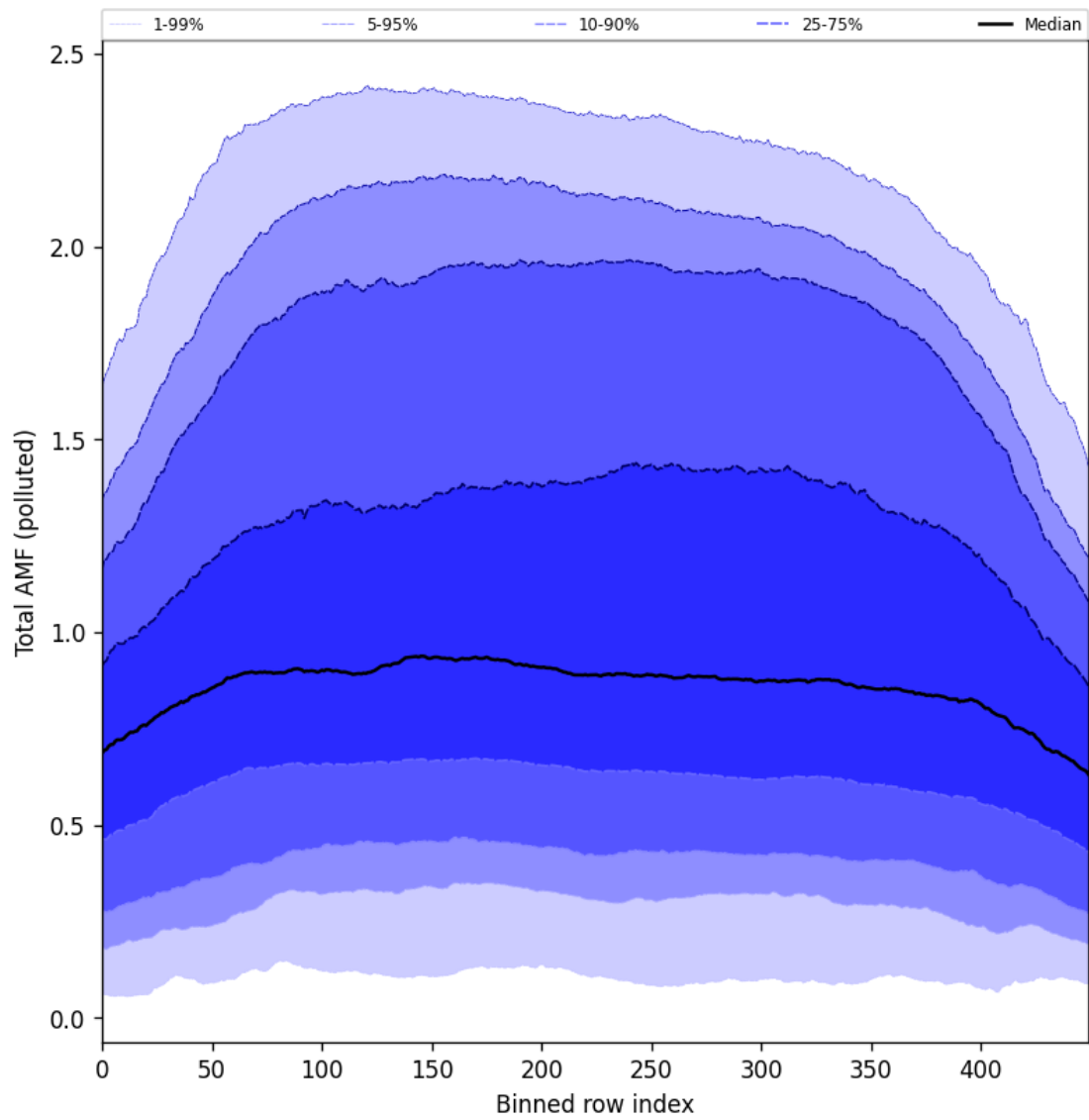
Figure 105: Along track statistics of “Total AMF (polluted)” for 2025-06-08 to 2025-06-10
