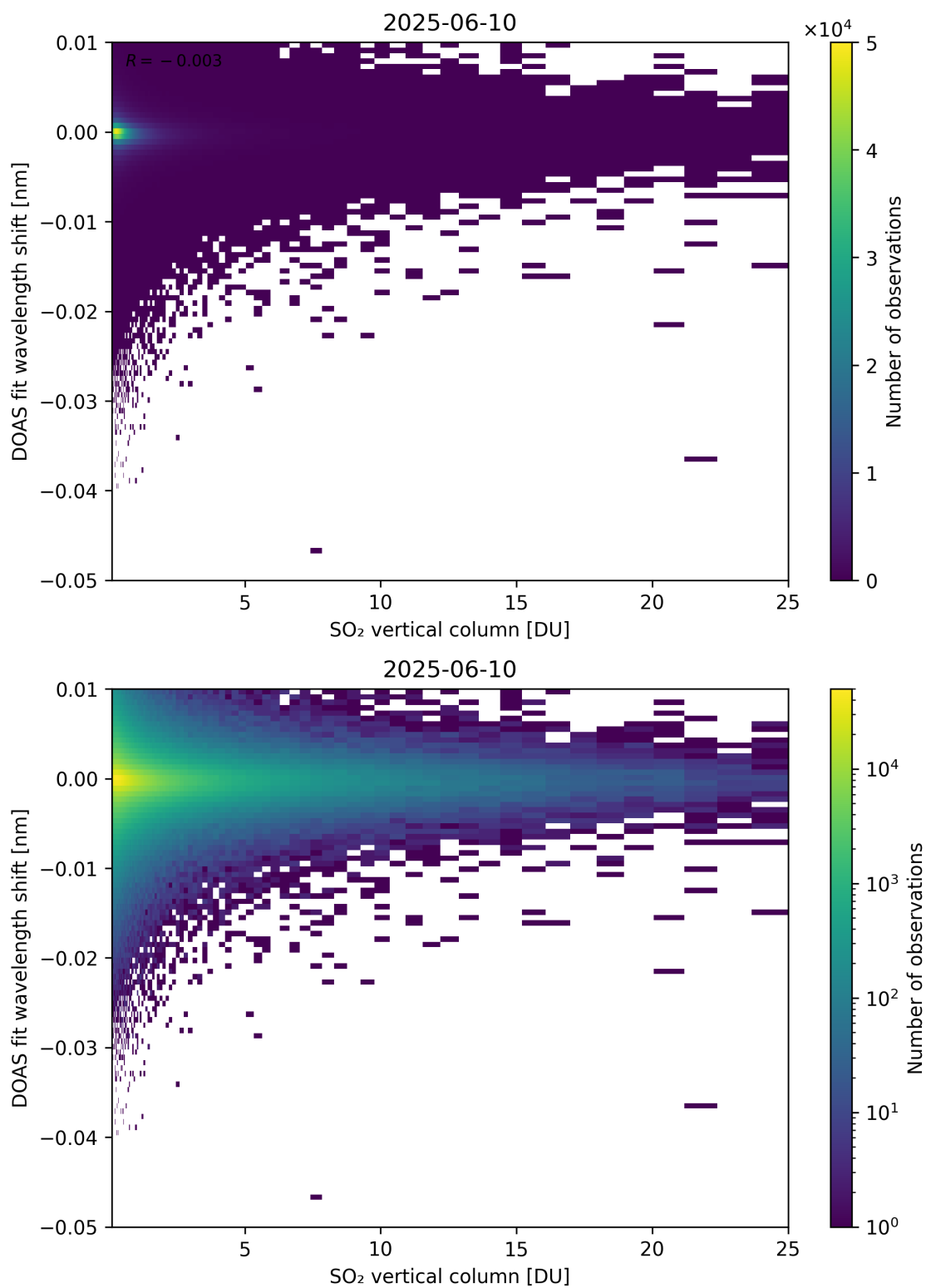
Figure 326: Scatter density plot of “SO 2 vertical column” against “DOAS fit wavelength shift” for 2025-06-09 to 2025-06-11.
