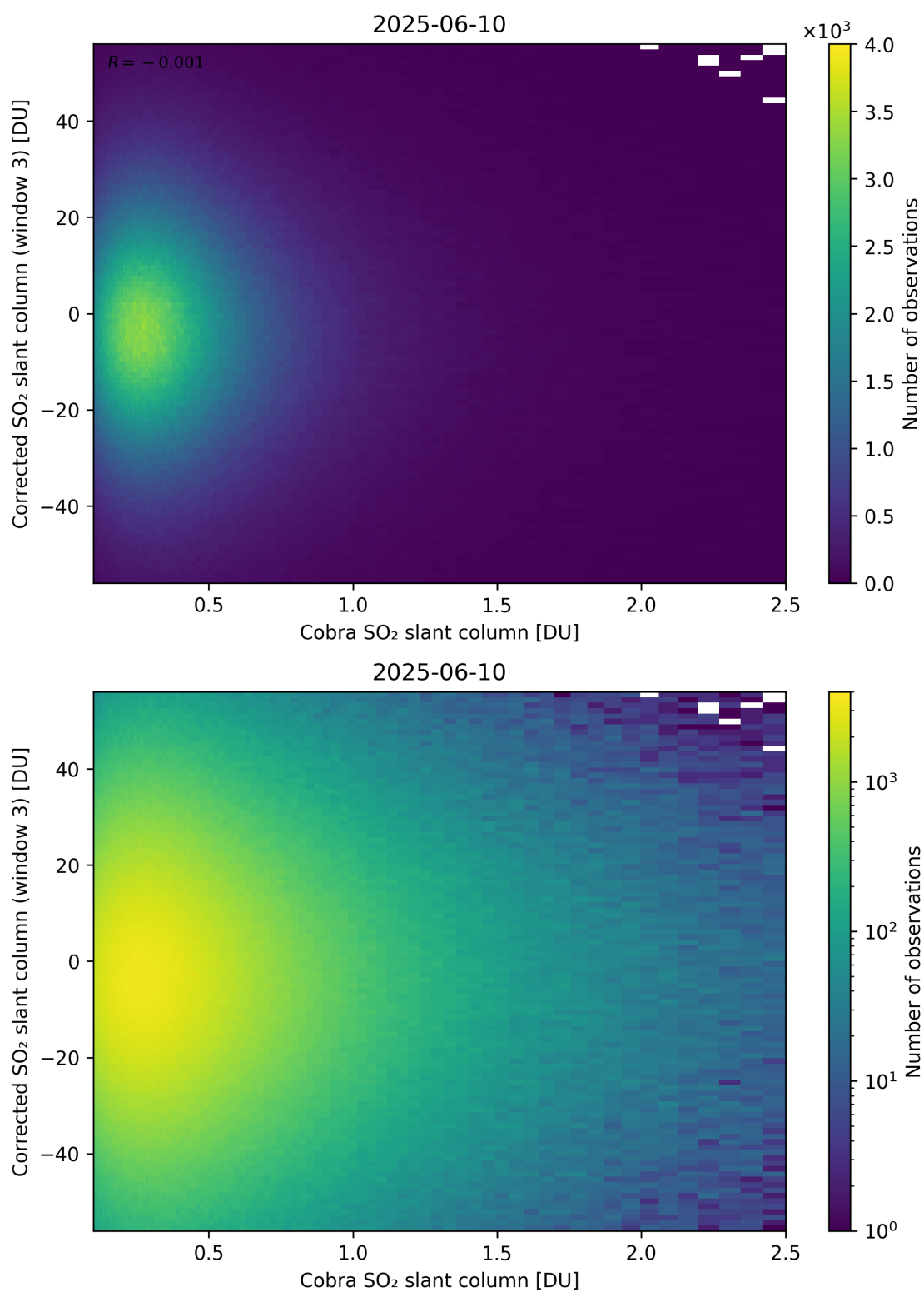
Figure 218: Scatter density plot of “Cobra SO 2 slant column” against “Corrected SO 2 slant column (window 3)” for 2025-06-09 to 2025-06-11.
