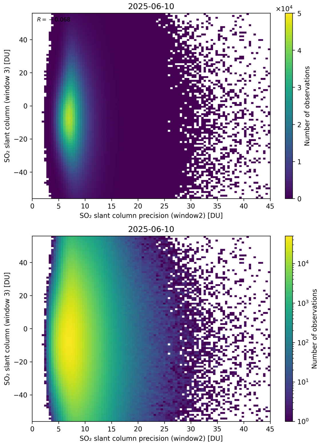
Figure 299: Scatter density plot of “SO 2 slant column precision (window2)” against “SO 2 slant column (window 3)” for 2025-06-09 to 2025-06-11.
