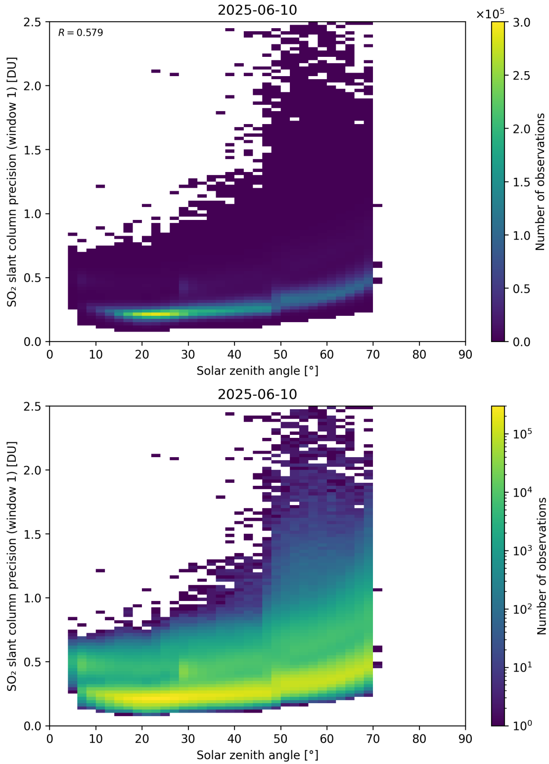
Figure 185: Scatter density plot of “Solar zenith angle” against “SO 2 slant column precision (window 1)” for 2025-06-09 to 2025-06-11.
