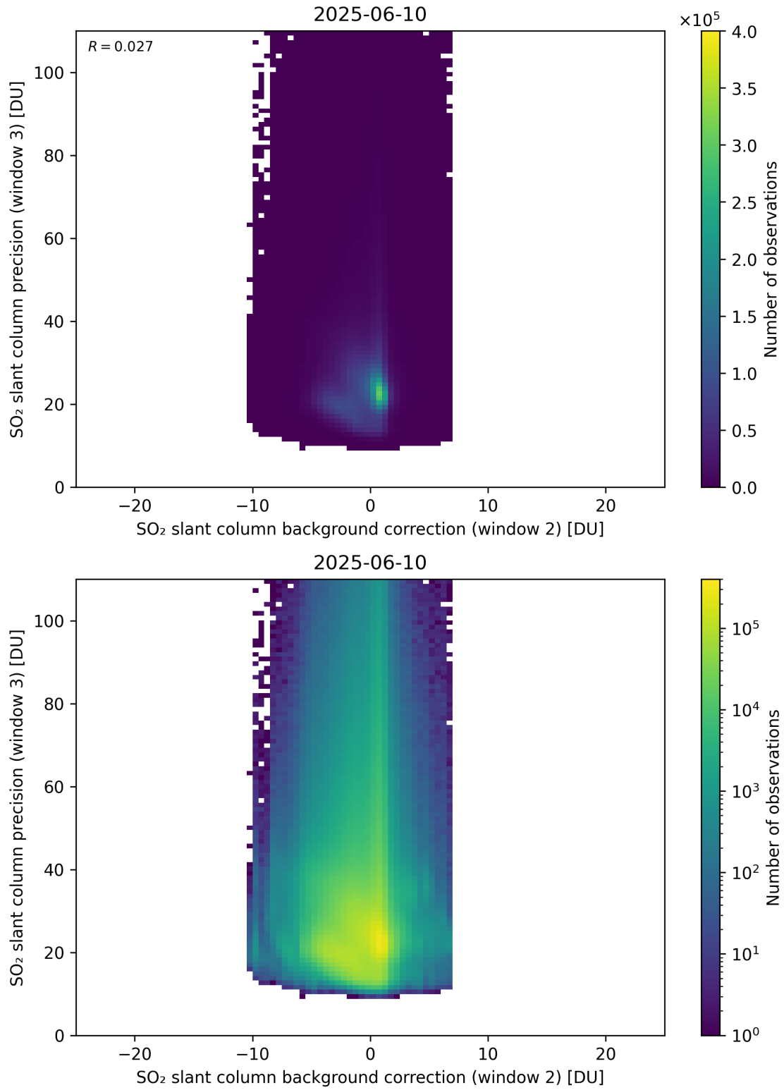
Figure 129: Scatter density plot of “SO 2 slant column background correction (window 2)” against “SO 2 slant column precision (window 3)” for 2025-06-09 to 2025-06-11.
