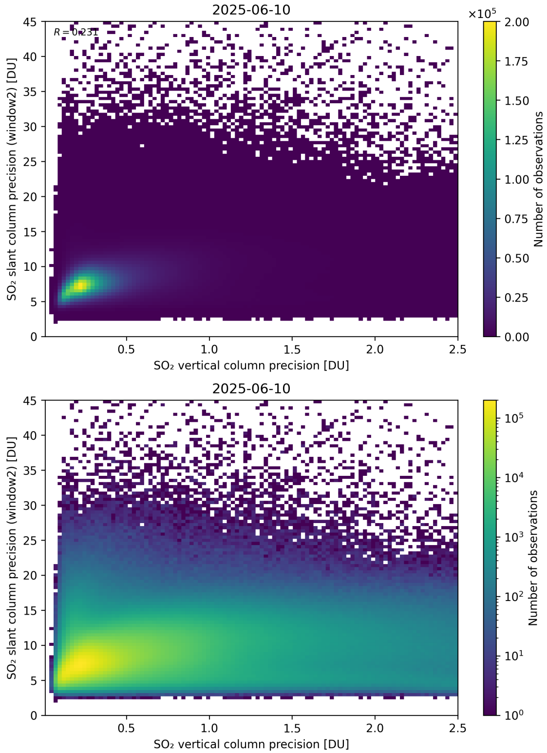
Figure 343: Scatter density plot of “SO 2 vertical column precision” against “SO 2 slant column precision (window2)” for 2025-06-09 to 2025-06-11.
