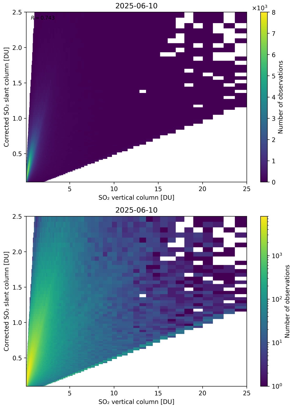
Figure 351: Scatter density plot of “SO 2 vertical column” against “Corrected SO 2 slant column” for 2025-06-09 to 2025-06-11.
