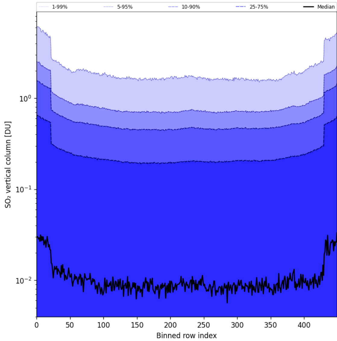
Figure 84: Along track statistics of “SO 2 vertical column” for 2025-06-09 to 2025-06-11
