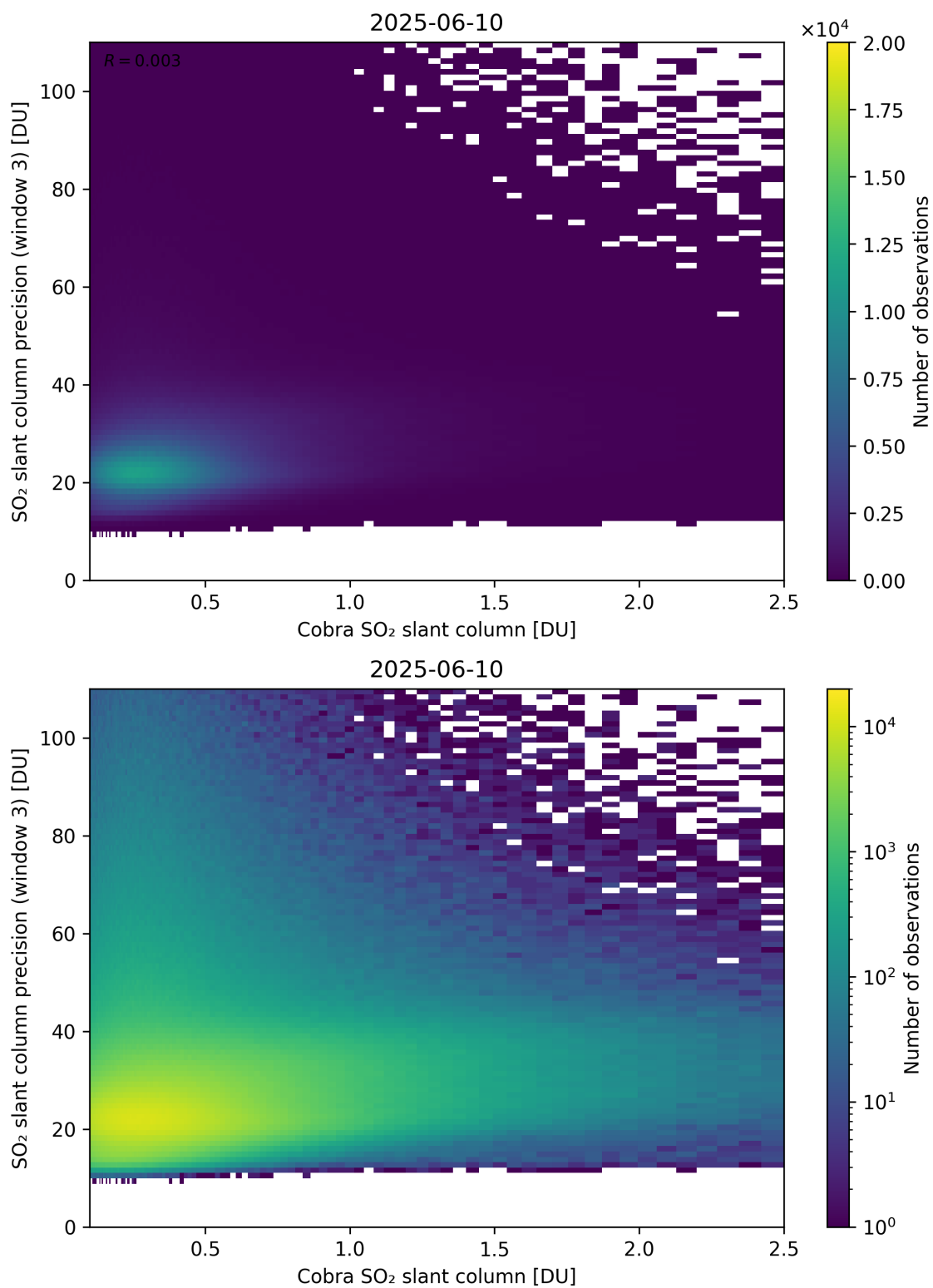
Figure 223: Scatter density plot of “Cobra SO 2 slant column” against “SO 2 slant column precision (window 3)” for 2025-06-09 to 2025-06-11.
