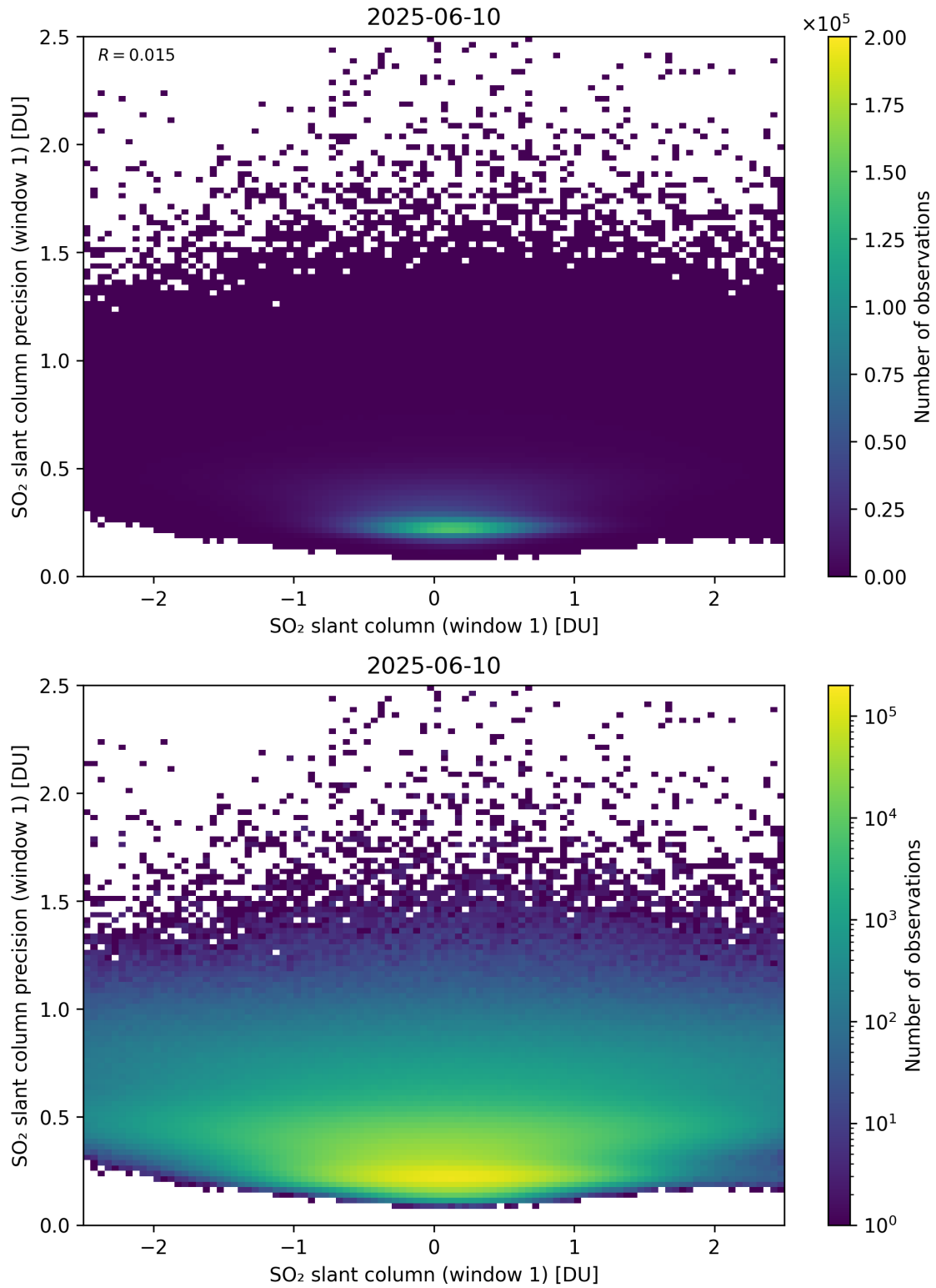
Figure 285: Scatter density plot of “SO 2 slant column (window 1)” against “SO 2 slant column precision (window 1)” for 2025-06-09 to 2025-06-11.
