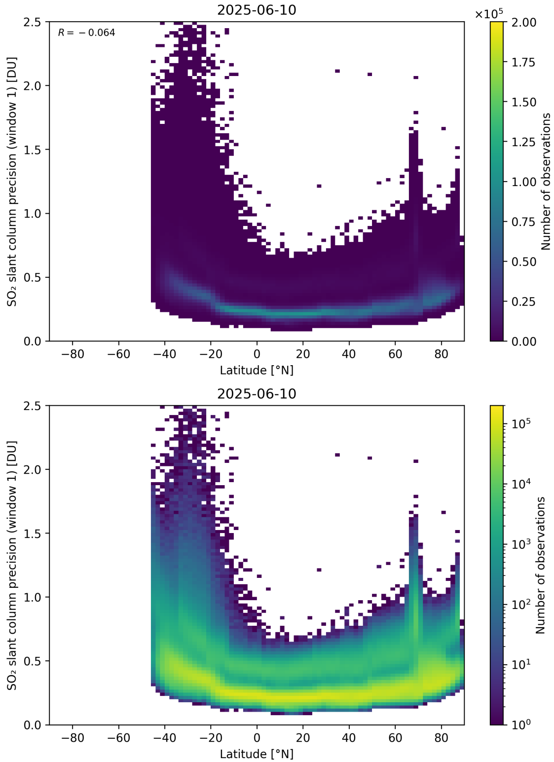
Figure 163: Scatter density plot of “Latitude” against “SO 2 slant column precision (window 1)” for 2025-06-09 to 2025-06-11.
