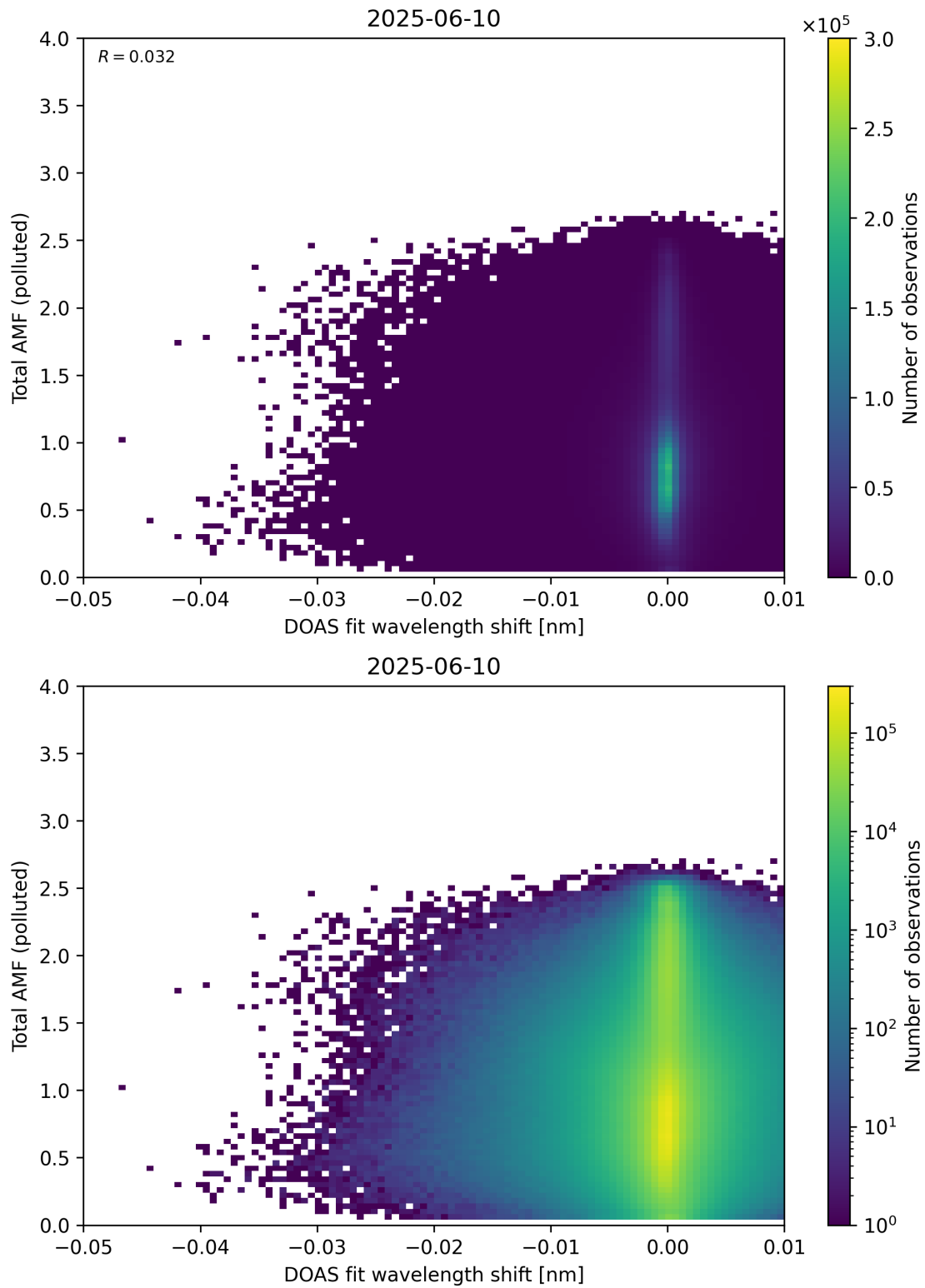
Figure 141: Scatter density plot of “DOAS fit wavelength shift” against “Total AMF (polluted)” for 2025-06-09 to 2025-06-11.
