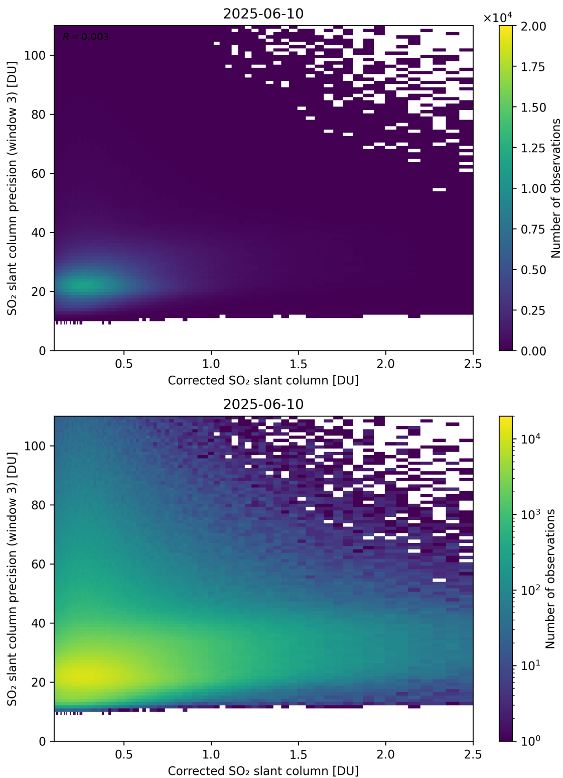
Figure 241: Scatter density plot of “Corrected SO 2 slant column” against “SO 2 slant column precision (window 3)” for 2025-06-09 to 2025-06-11.
