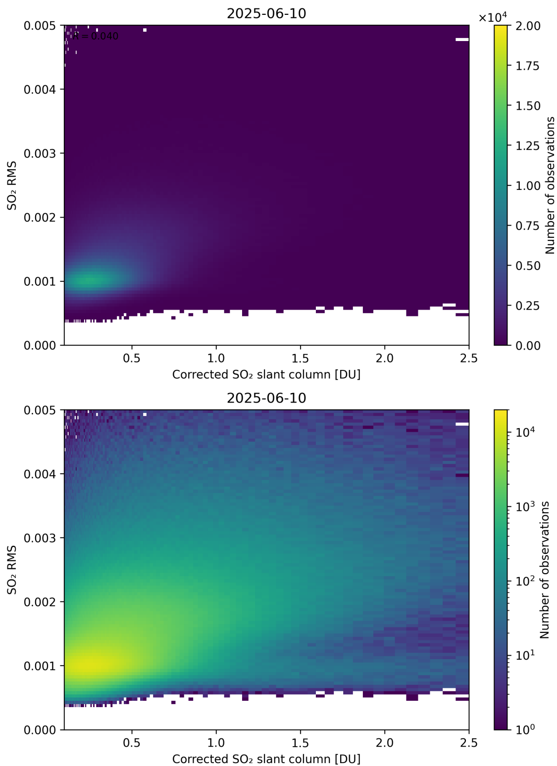
Figure 231: Scatter density plot of “Corrected SO 2 slant column” against “SO 2 RMS” for 2025-06-09 to 2025-06-11.
