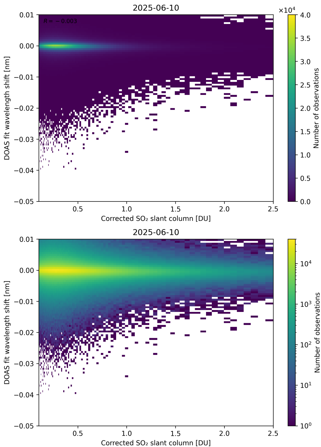
Figure 229: Scatter density plot of “Corrected SO 2 slant column” against “DOAS fit wavelength shift” for 2025-06-09 to 2025-06-11.
