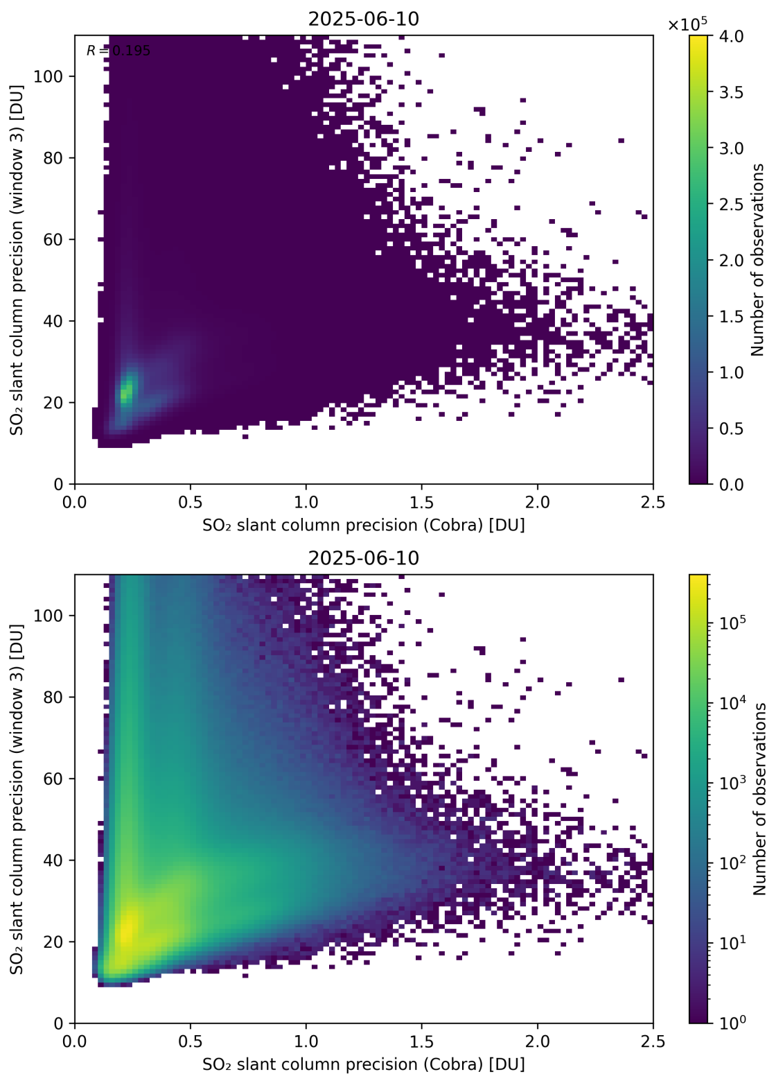
Figure 212: Scatter density plot of “SO 2 slant column precision (Cobra)” against “SO 2 slant column precision (window 3)” for 2025-06-09 to 2025-06-11.
