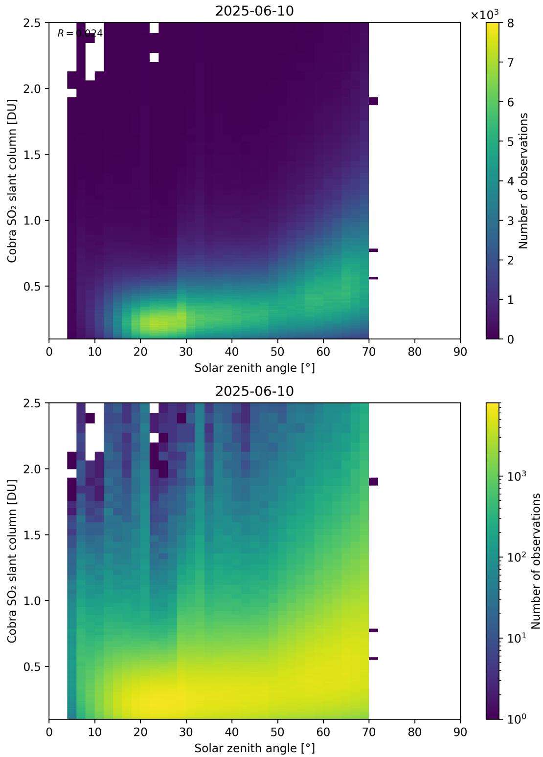
Figure 179: Scatter density plot of “Solar zenith angle” against “Cobra SO 2 slant column” for 2025-06-09 to 2025-06-11.
