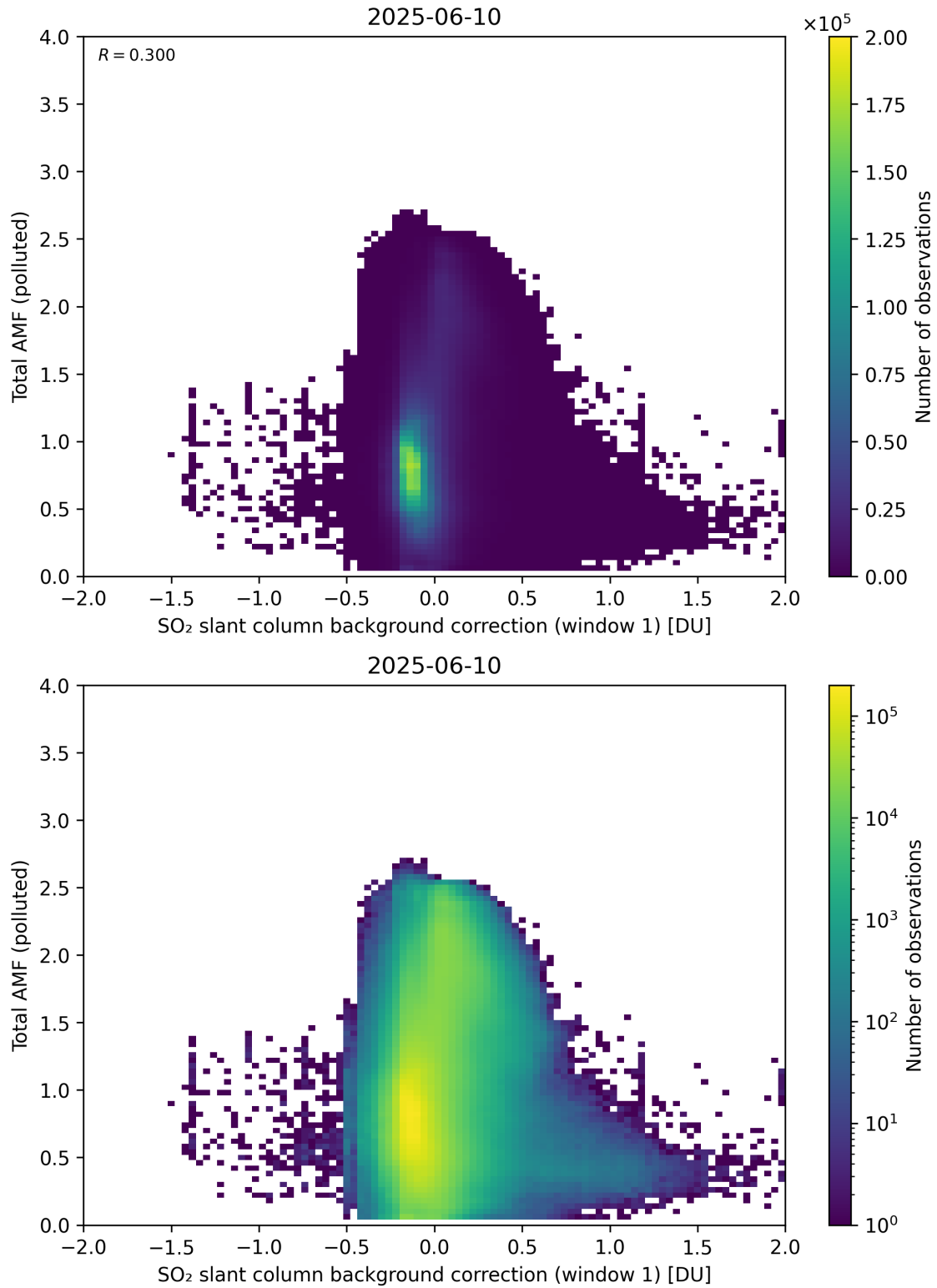
Figure 120: Scatter density plot of “SO 2 slant column background correction (window 1)” against “Total AMF (polluted)” for 2025-06-09 to 2025-06-11.
