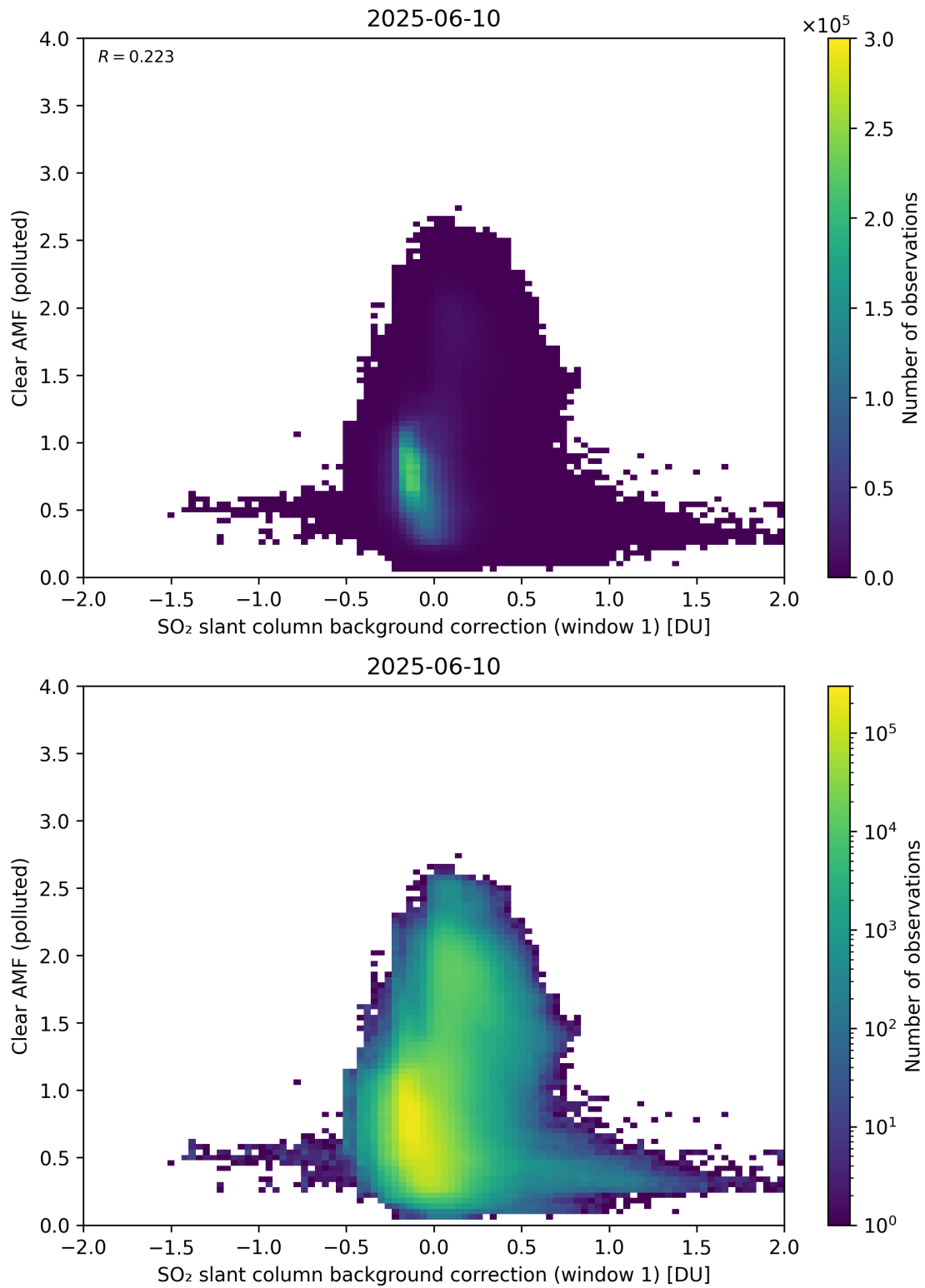
Figure 114: Scatter density plot of “SO 2 slant column background correction (window 1)” against “Clear AMF (polluted)” for 2025-06-09 to 2025-06-11.
