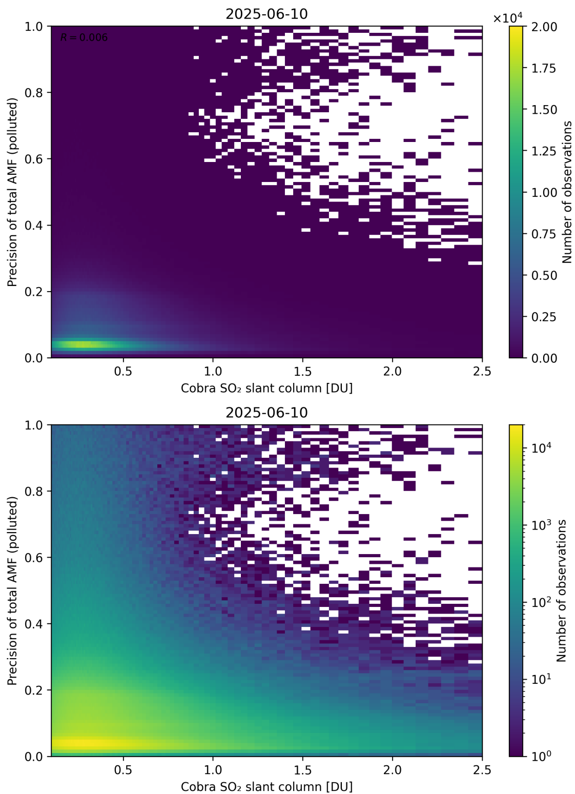
Figure 225: Scatter density plot of “Cobra SO 2 slant column” against “Precision of total AMF (polluted)” for 2025-06-09 to 2025-06-11.
