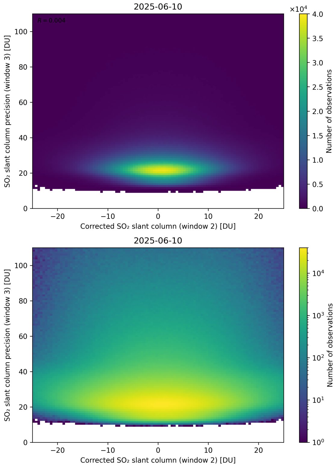
Figure 252: Scatter density plot of “Corrected SO 2 slant column (window 2)” against “SO 2 slant column precision (window 3)” for 2025-06-09 to 2025-06-11.
