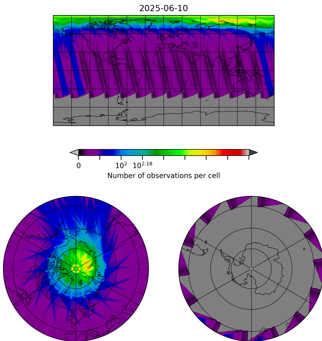
Figure 30: Map of the number of observations for 2025-06-09 to 2025-06-11
