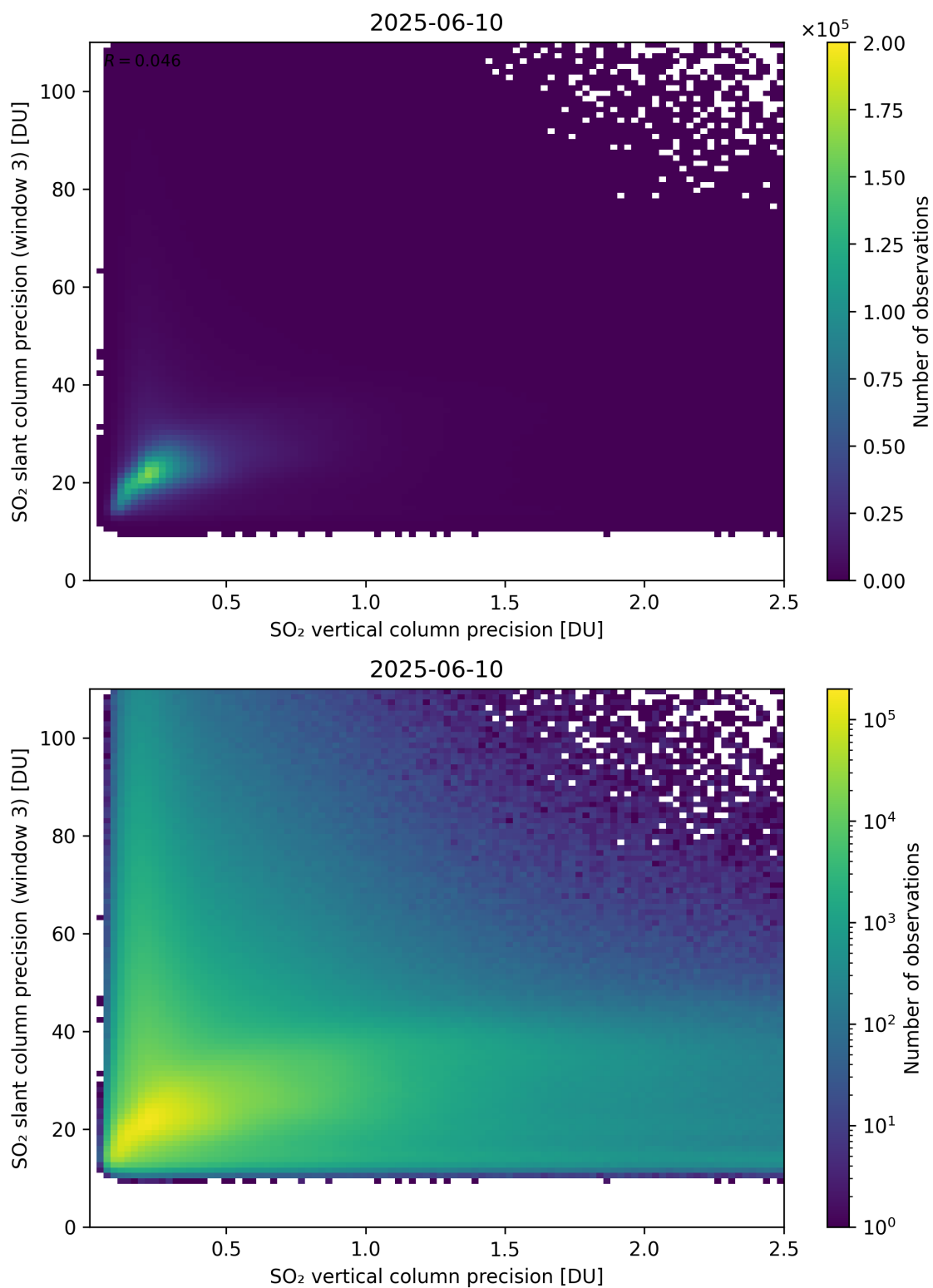
Figure 345: Scatter density plot of “SO 2 vertical column precision” against “SO 2 slant column precision (window 3)” for 2025-06-09 to 2025-06-11.
