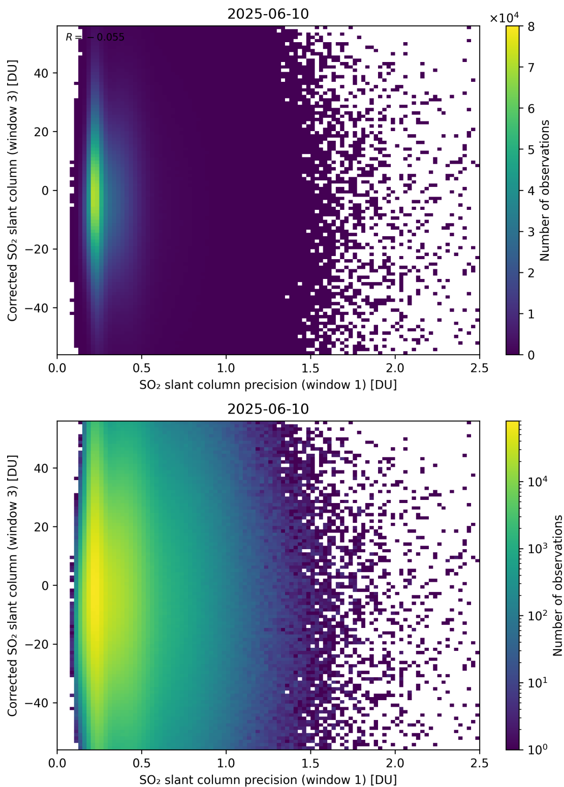
Figure 276: Scatter density plot of “SO 2 slant column precision (window 1)” against “Corrected SO 2 slant column (window 3)” for 2025-06-09 to 2025-06-11.
