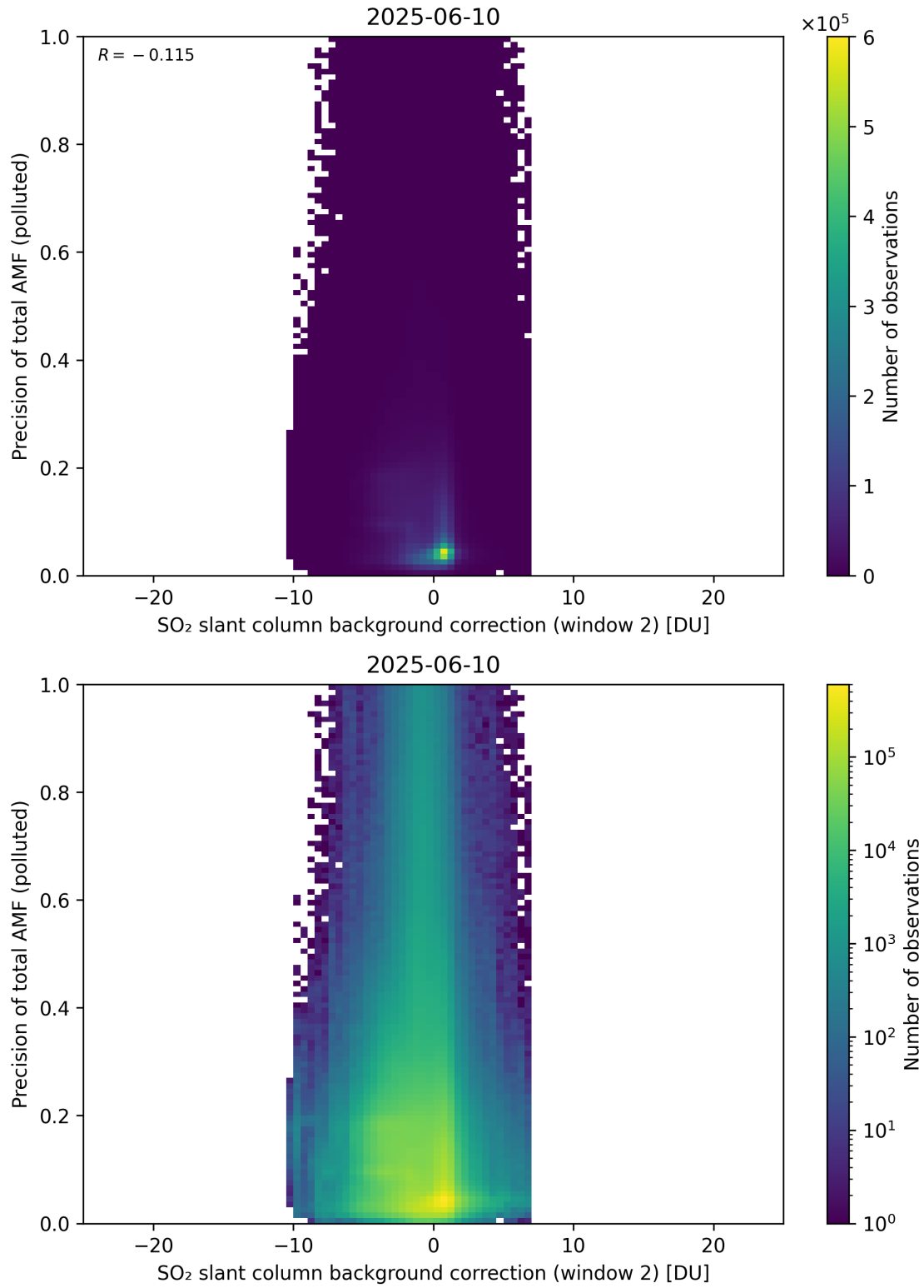
Figure 131: Scatter density plot of “SO 2 slant column background correction (window 2)” against “Precision of total AMF (polluted)” for 2025-06-09 to 2025-06-11.
