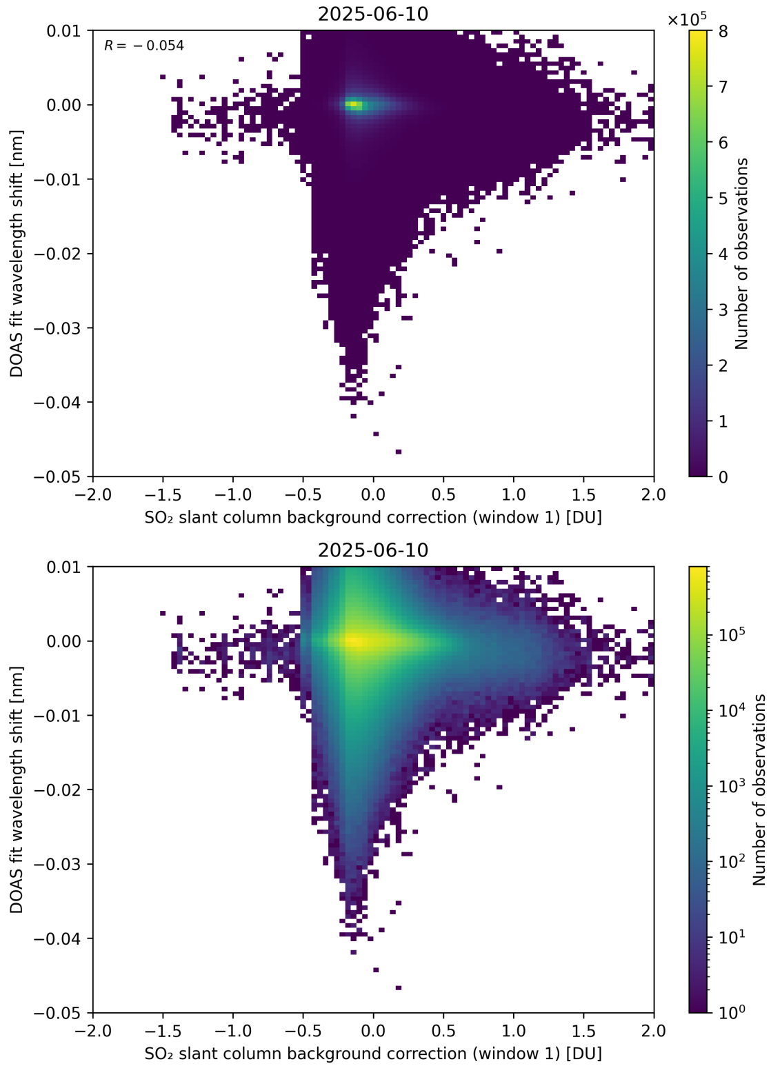
Figure 111: Scatter density plot of “SO 2 slant column background correction (window 1)” against “DOAS fit wavelength shift” for 2025-06-09 to 2025-06-11.
