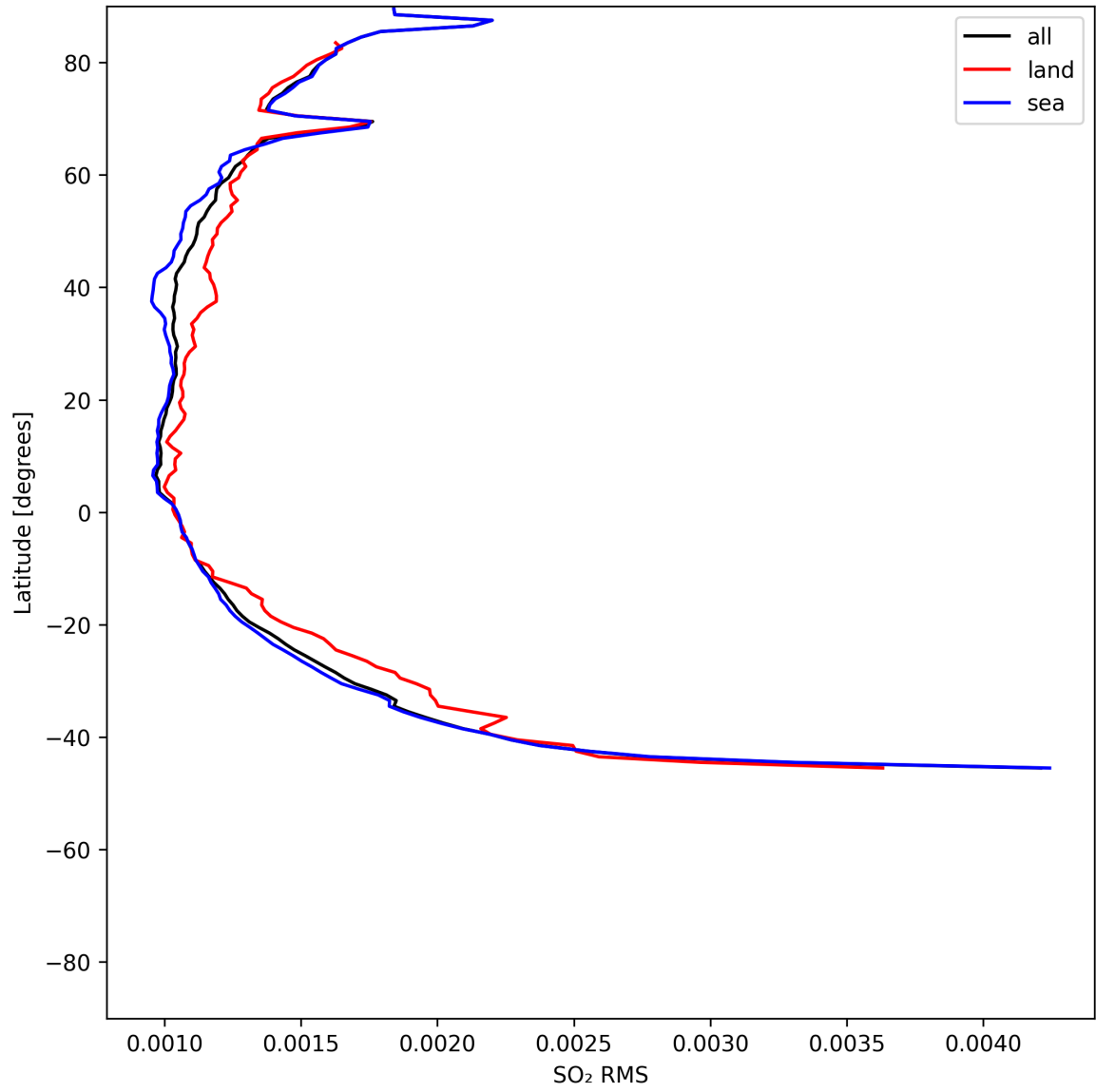
Figure 52: Zonal average of “SO 2 RMS” for 2025-06-09 to 2025-06-11.
