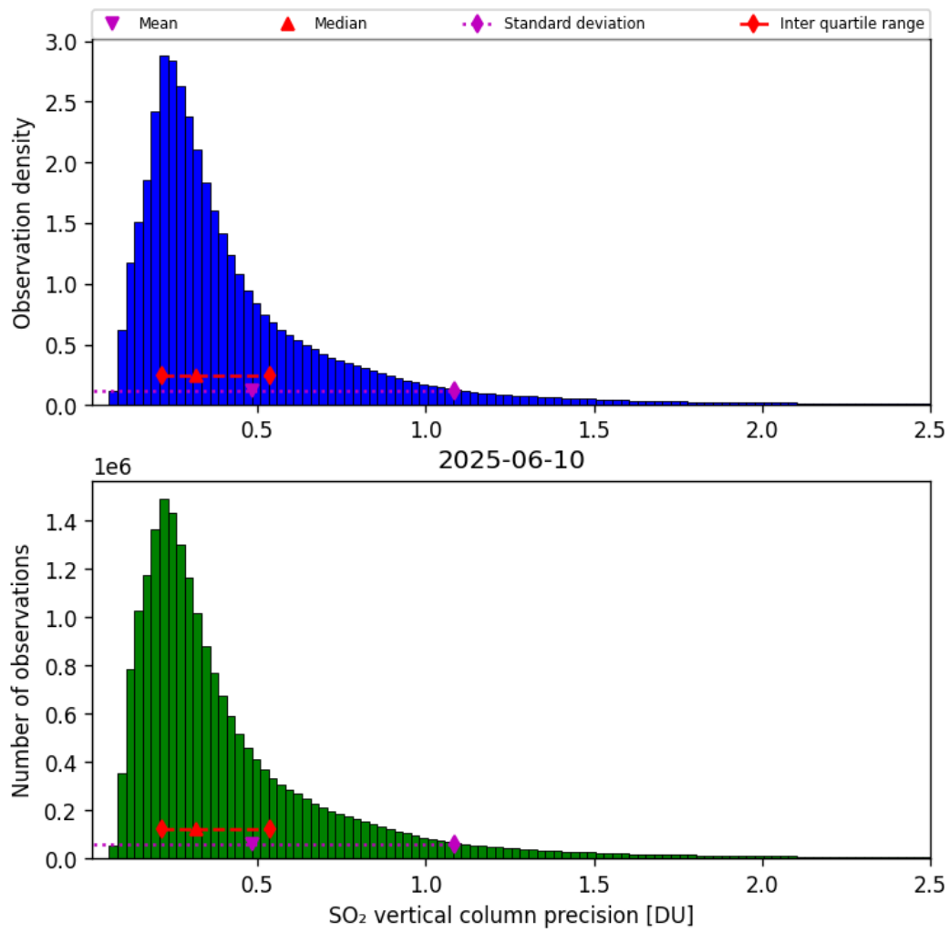
Figure 59: Histogram of “SO 2 vertical column precision” for 2025-06-09 to 2025-06-11
