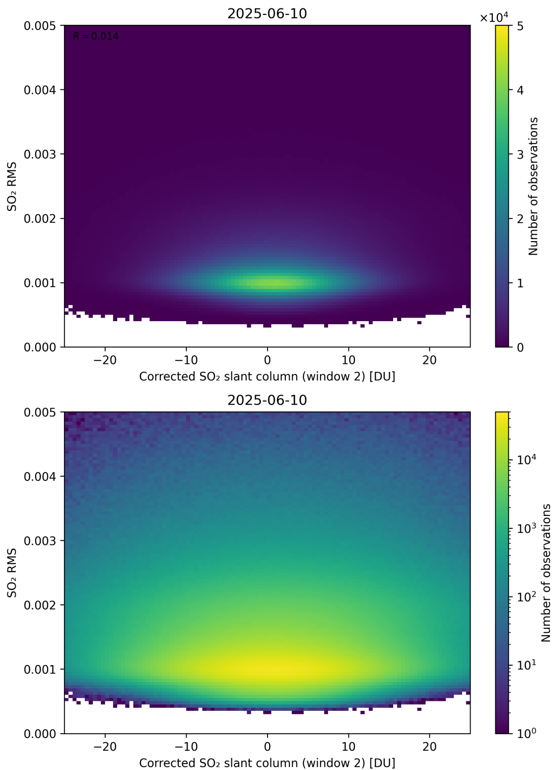
Figure 248: Scatter density plot of “Corrected SO 2 slant column (window 2)” against “SO 2 RMS” for 2025-06-09 to 2025-06-11.
