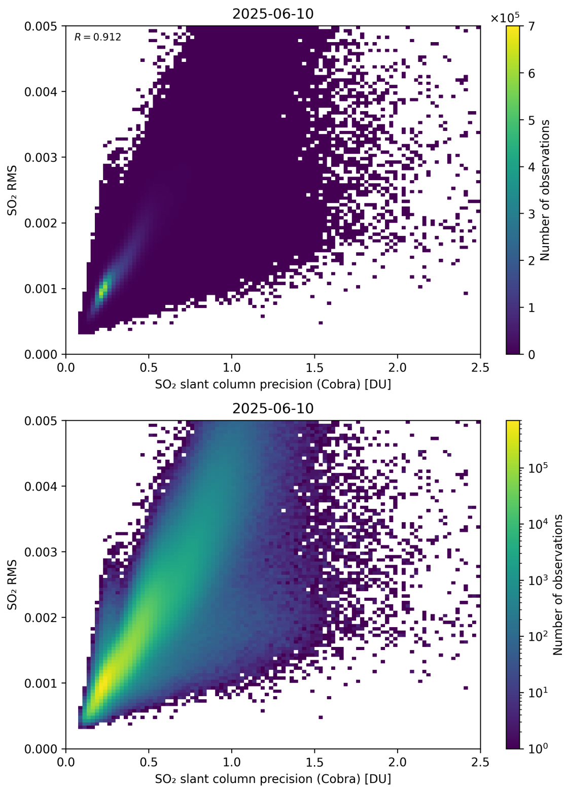
Figure 204: Scatter density plot of “SO 2 slant column precision (Cobra)” against “SO 2 RMS” for 2025-06-09 to 2025-06-11.
