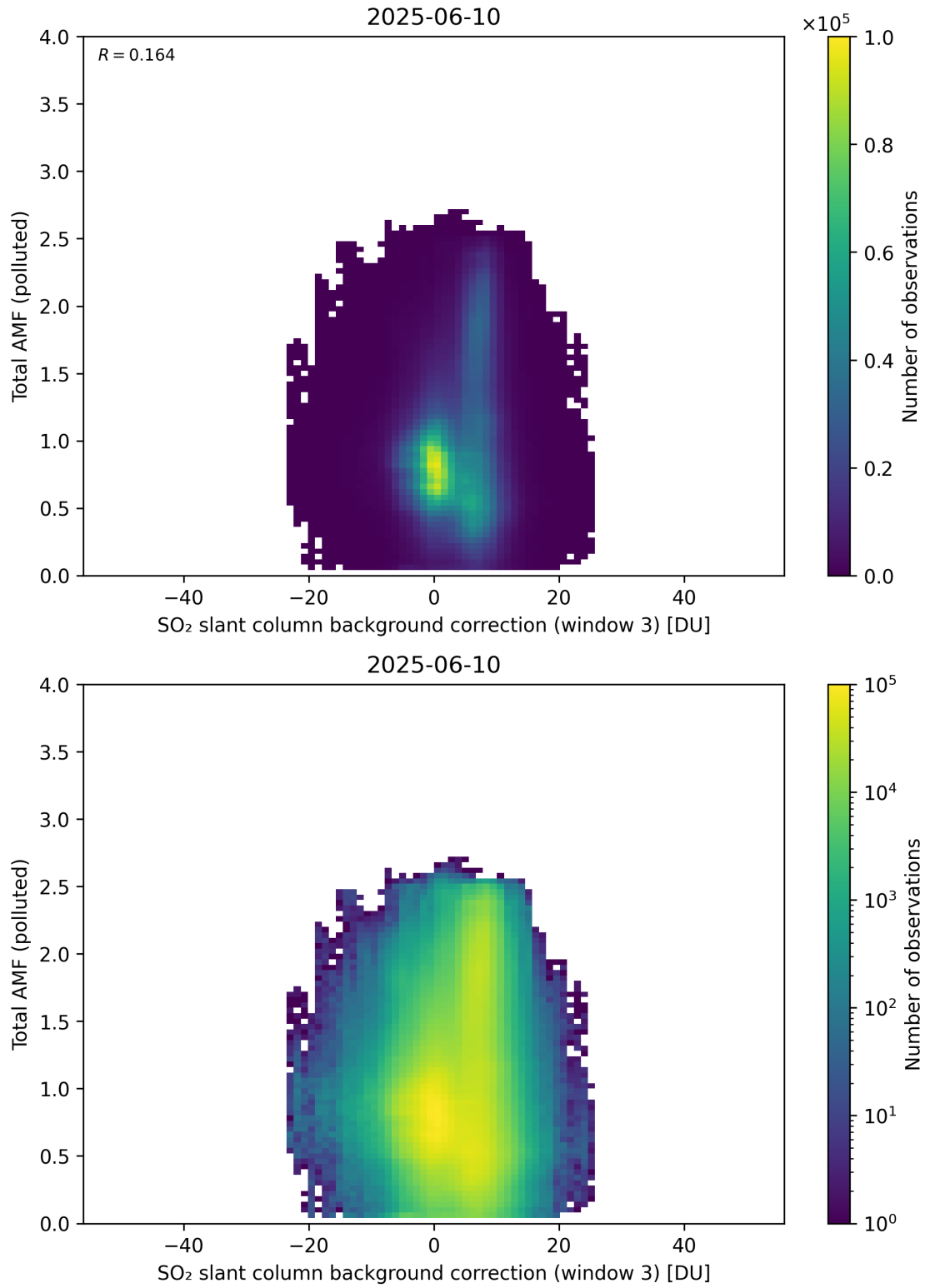
Figure 136: Scatter density plot of “SO 2 slant column background correction (window 3)” against “Total AMF (polluted)” for 2025-06-09 to 2025-06-11.
