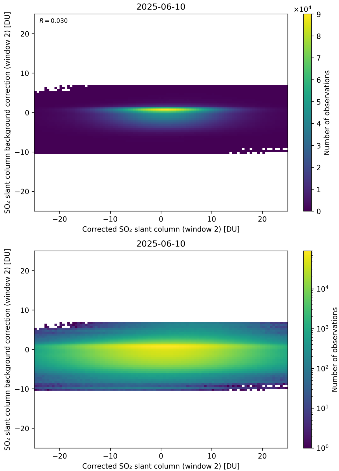
Figure 244: Scatter density plot of “Corrected SO 2 slant column (window 2)” against “SO 2 slant column background correction (window 2)” for 2025-06-09 to 2025-06-11.
