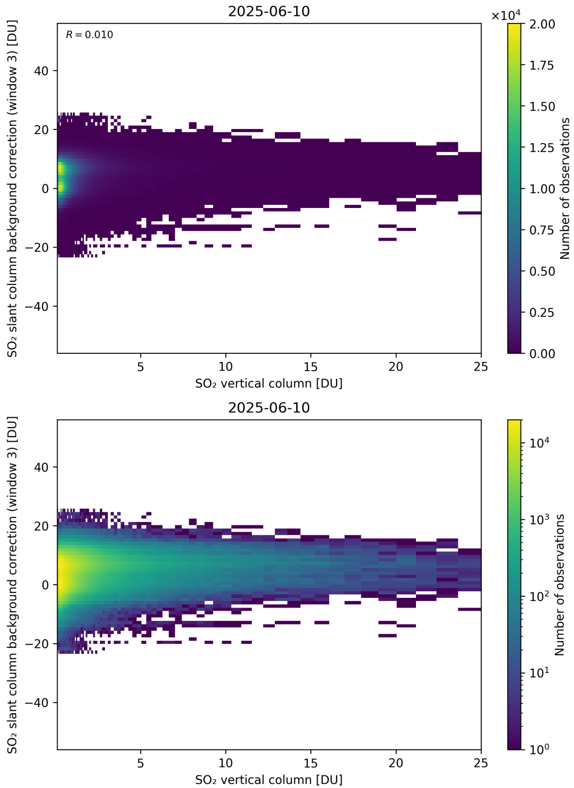
Figure 325: Scatter density plot of “SO 2 vertical column” against “SO 2 slant column background correction (window 3)” for 2025-06-09 to 2025-06-11.
