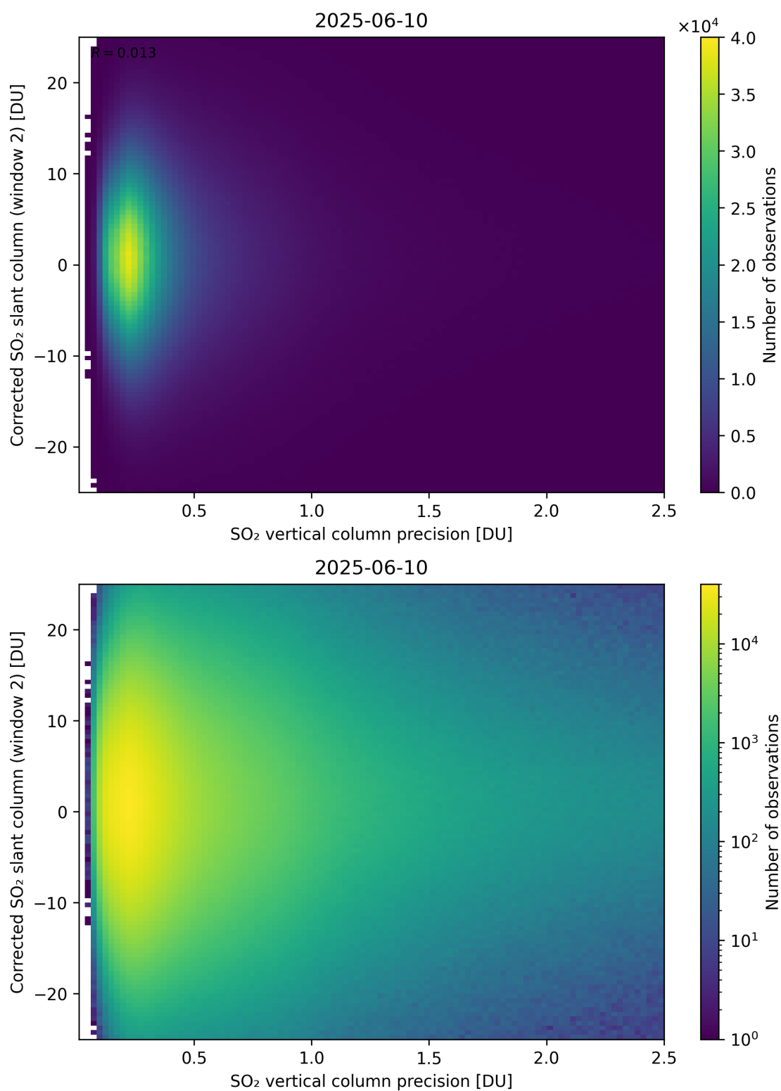
Figure 339: Scatter density plot of “SO 2 vertical column precision” against “Corrected SO 2 slant column (window 2)” for 2025-06-09 to 2025-06-11.
