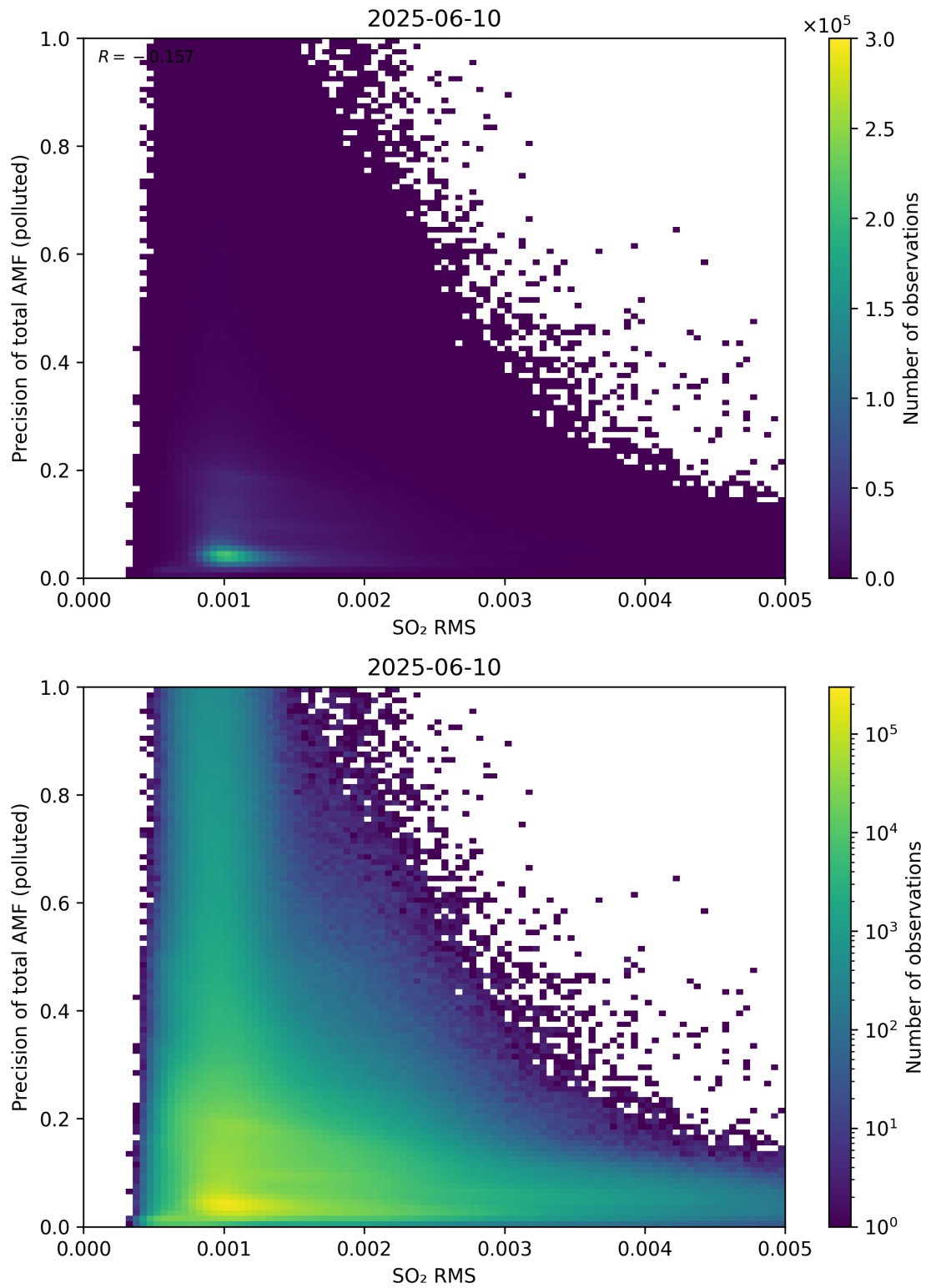
Figure 149: Scatter density plot of “SO 2 RMS” against “Precision of total AMF (polluted)” for 2025-06-09 to 2025-06-11.
