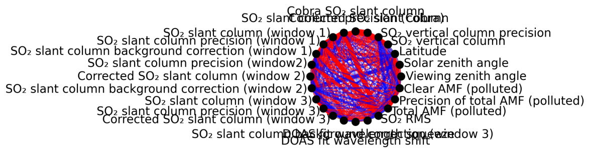
Figure 1: Map of correlation graph for 2025-06-09 to 2025-06-11.
