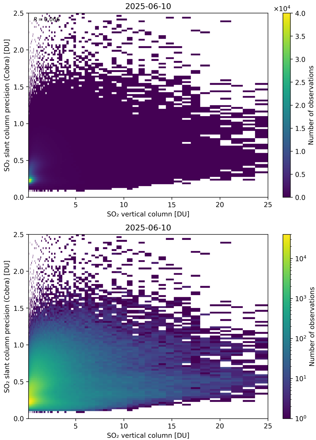
Figure 350: Scatter density plot of “SO 2 vertical column” against “SO 2 slant column precision (Cobra)” for 2025-06-09 to 2025-06-11.
