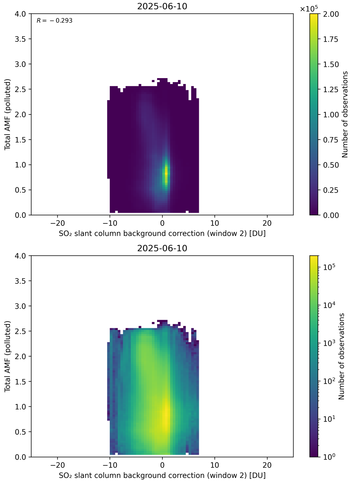
Figure 130: Scatter density plot of “SO 2 slant column background correction (window 2)” against “Total AMF (polluted)” for 2025-06-09 to 2025-06-11.
