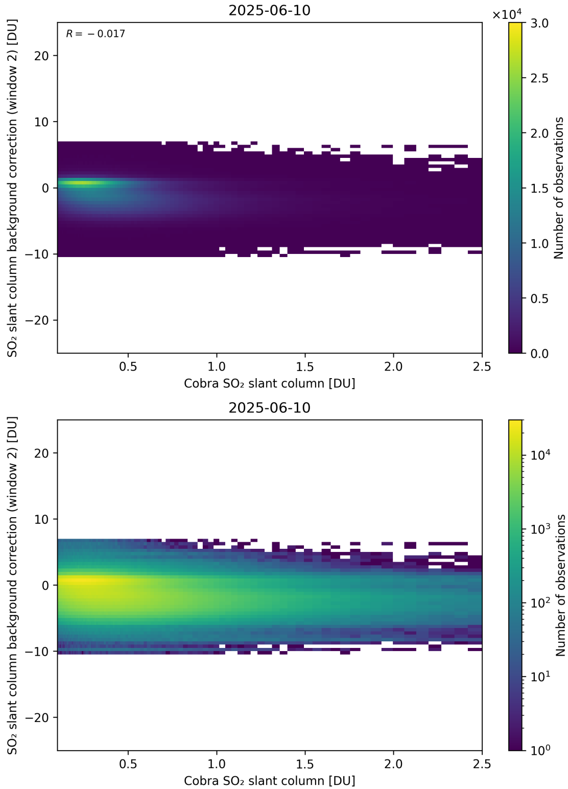
Figure 194: Scatter density plot of “Cobra SO 2 slant column” against “SO 2 slant column background correction (window 2)” for 2025-06-09 to 2025-06-11.
