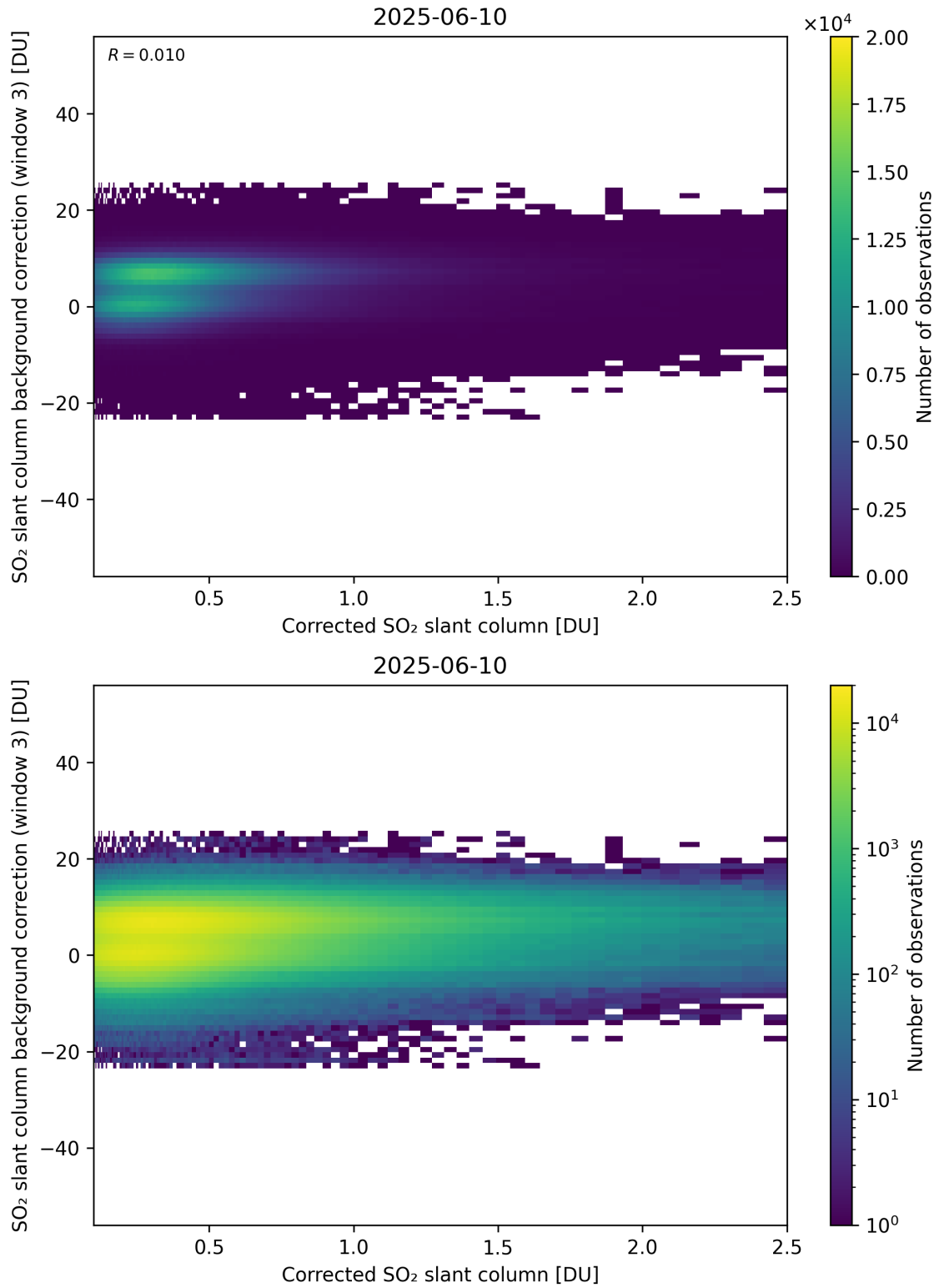
Figure 228: Scatter density plot of “Corrected SO 2 slant column” against “SO 2 slant column background correction (window 3)” for 2025-06-09 to 2025-06-11.
