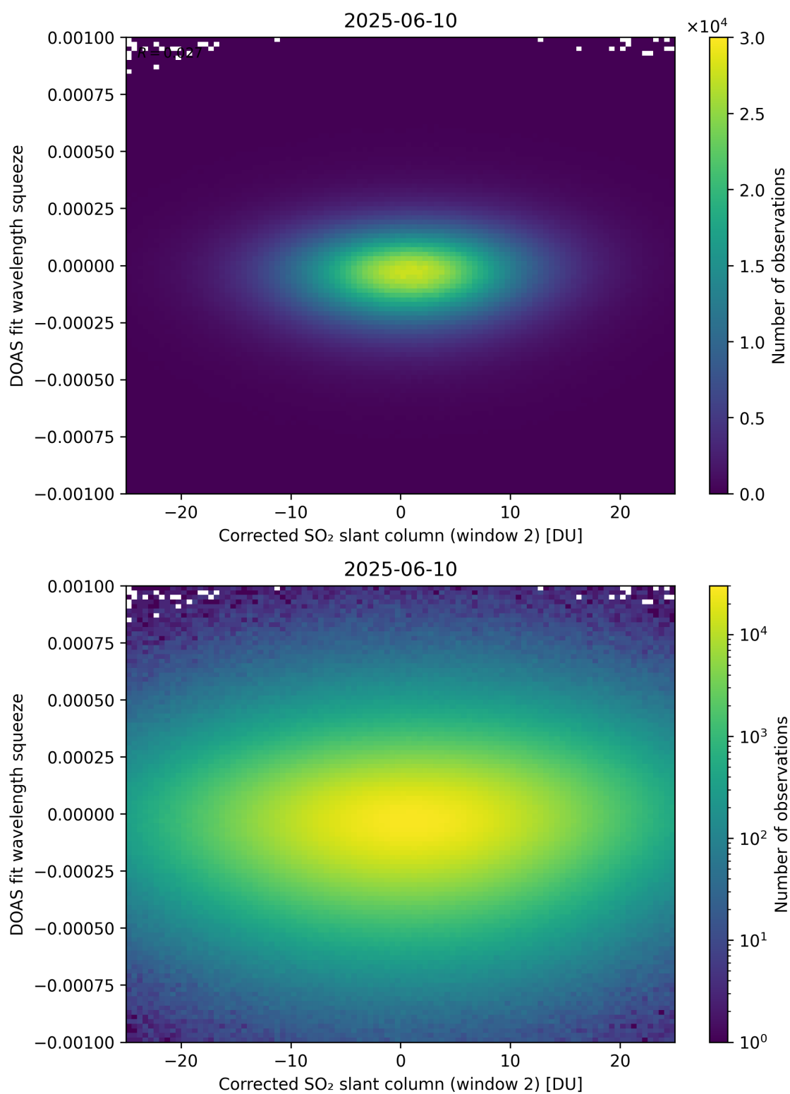
Figure 247: Scatter density plot of “Corrected SO 2 slant column (window 2)” against “DOAS fit wavelength squeeze” for 2025-06-09 to 2025-06-11.
