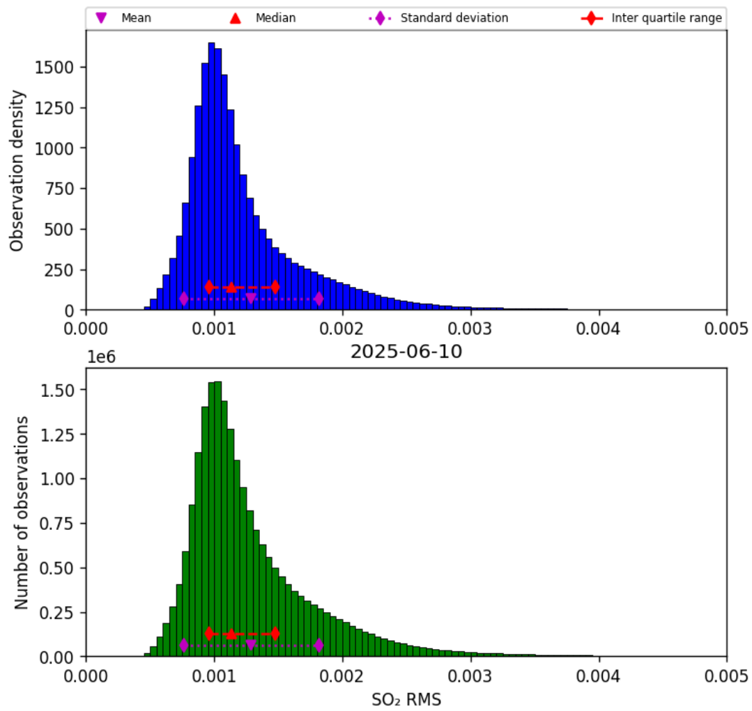
Figure 78: Histogram of “SO 2 RMS” for 2025-06-09 to 2025-06-11
