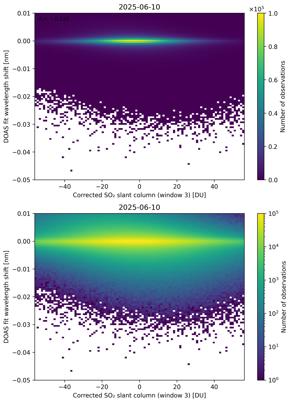
Figure 256: Scatter density plot of “Corrected SO 2 slant column (window 3)” against “DOAS fit wavelength shift” for 2025-06-09 to 2025-06-11.
