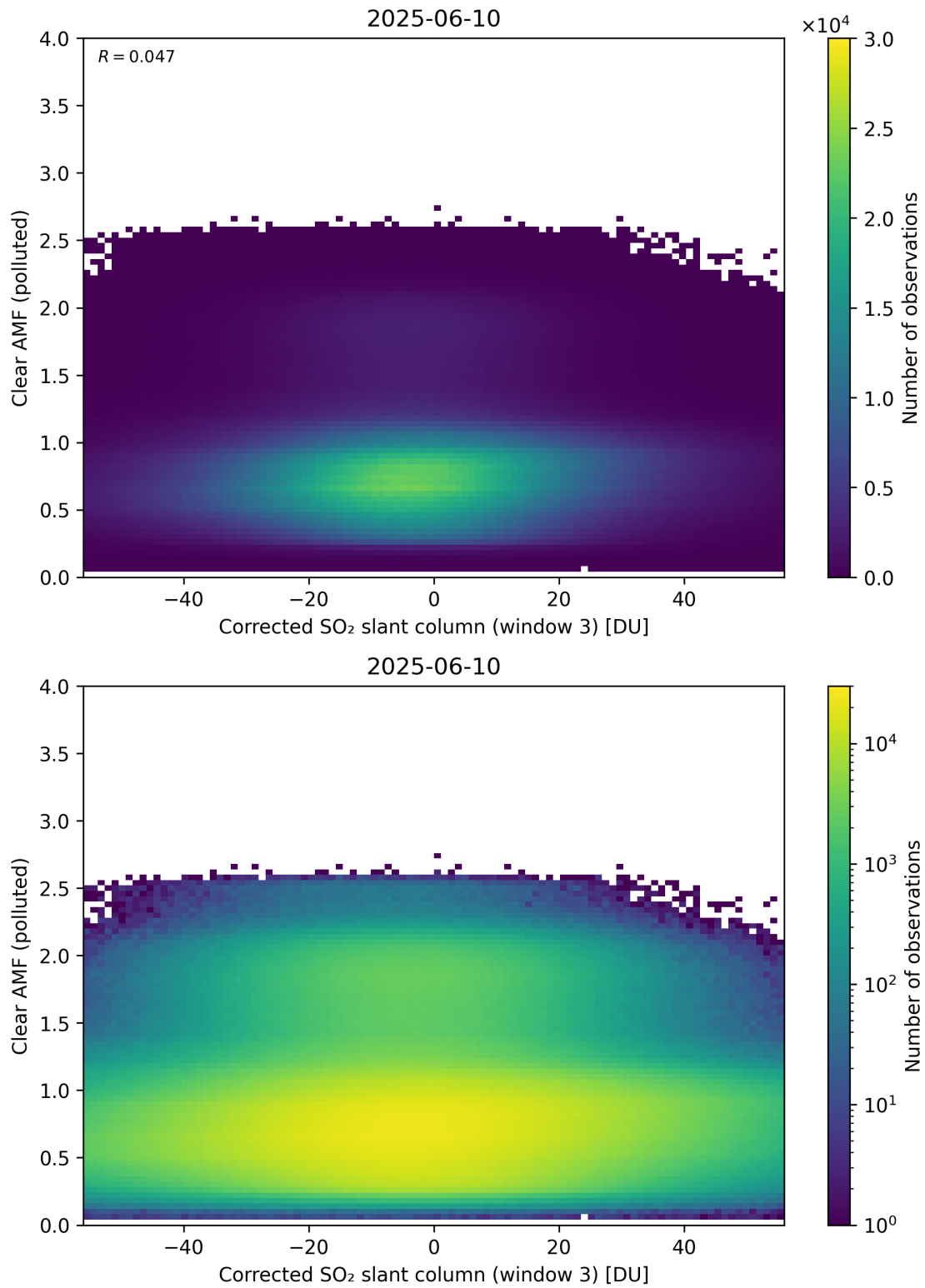
Figure 259: Scatter density plot of “Corrected SO 2 slant column (window 3)” against “Clear AMF (polluted)” for 2025-06-09 to 2025-06-11.
