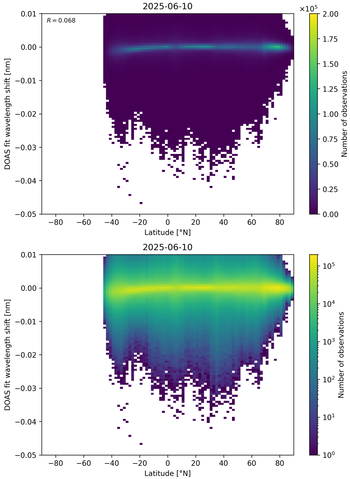
Figure 153: Scatter density plot of “Latitude” against “DOAS fit wavelength shift” for 2025-06-09 to 2025-06-11.
