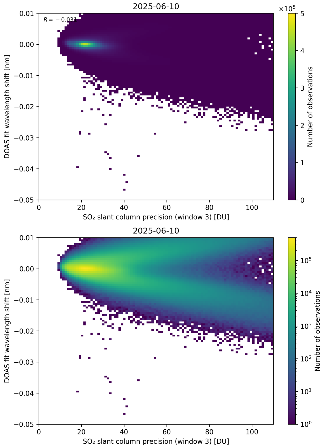
Figure 308: Scatter density plot of “SO 2 slant column precision (window 3)” against “DOAS fit wavelength shift” for 2025-06-09 to 2025-06-11.
