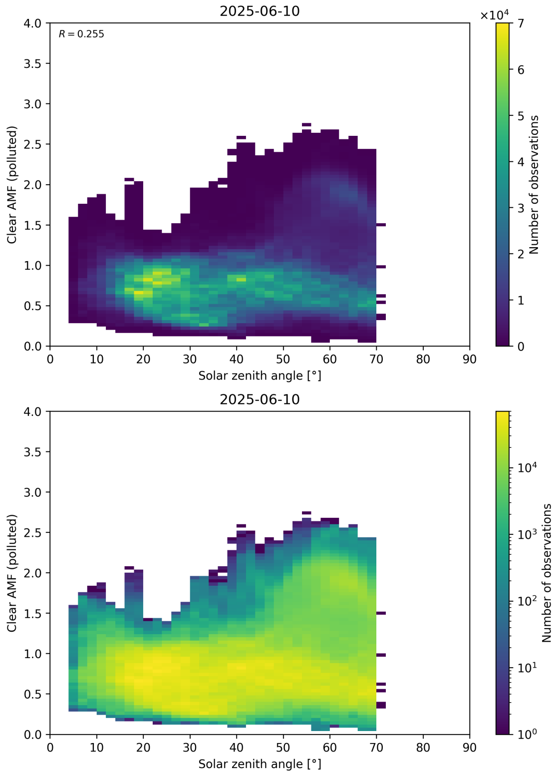
Figure 178: Scatter density plot of “Solar zenith angle” against “Clear AMF (polluted)” for 2025-06-09 to 2025-06-11.
