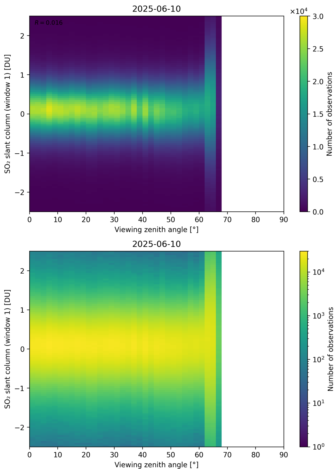
Figure 376: Scatter density plot of “Viewing zenith angle” against “SO 2 slant column (window 1)” for 2025-06-09 to 2025-06-11.
