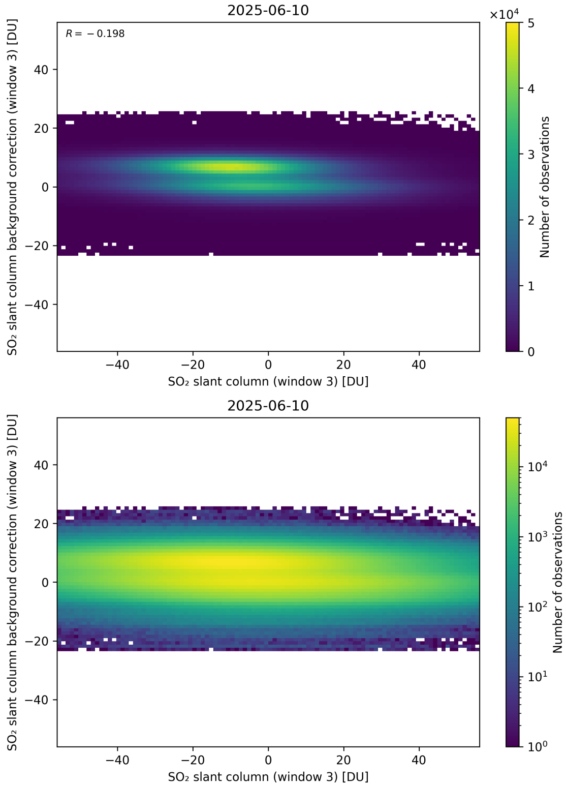
Figure 303: Scatter density plot of “SO 2 slant column (window 3)” against “SO 2 slant column background correction (window 3)” for 2025-06-09 to 2025-06-11.
