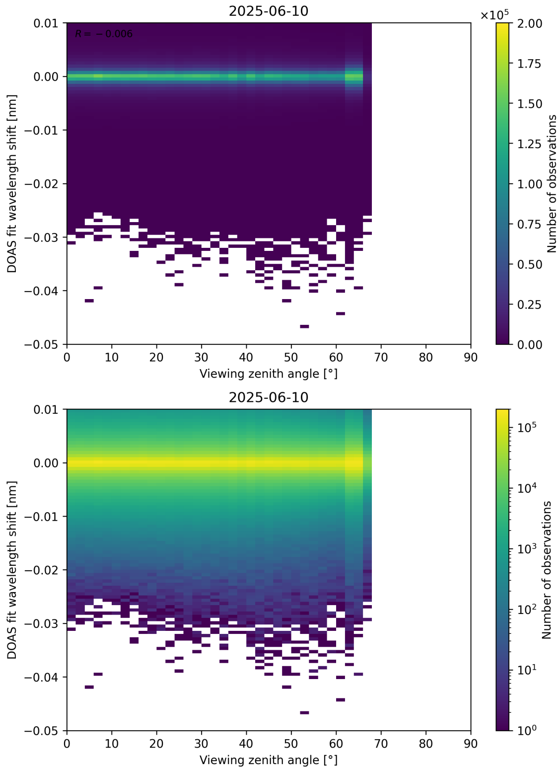
Figure 365: Scatter density plot of “Viewing zenith angle” against “DOAS fit wavelength shift” for 2025-06-09 to 2025-06-11.
