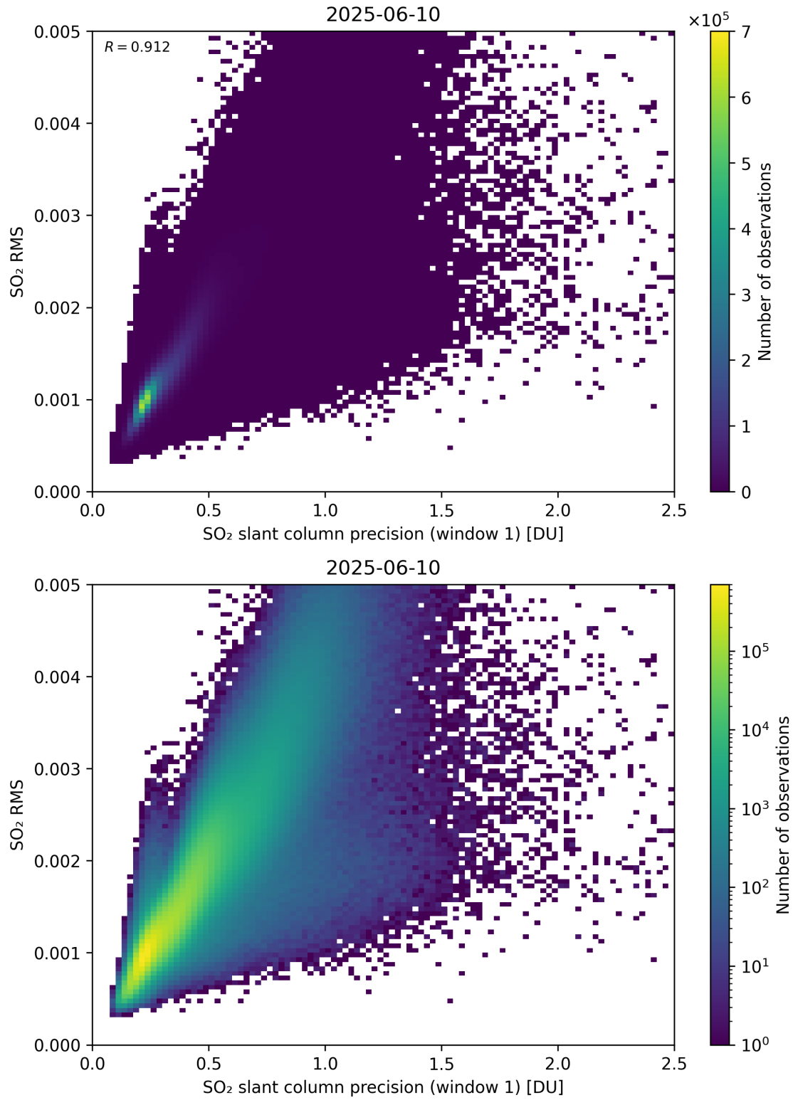
Figure 273: Scatter density plot of “SO 2 slant column precision (window 1)” against “SO 2 RMS” for 2025-06-09 to 2025-06-11.
