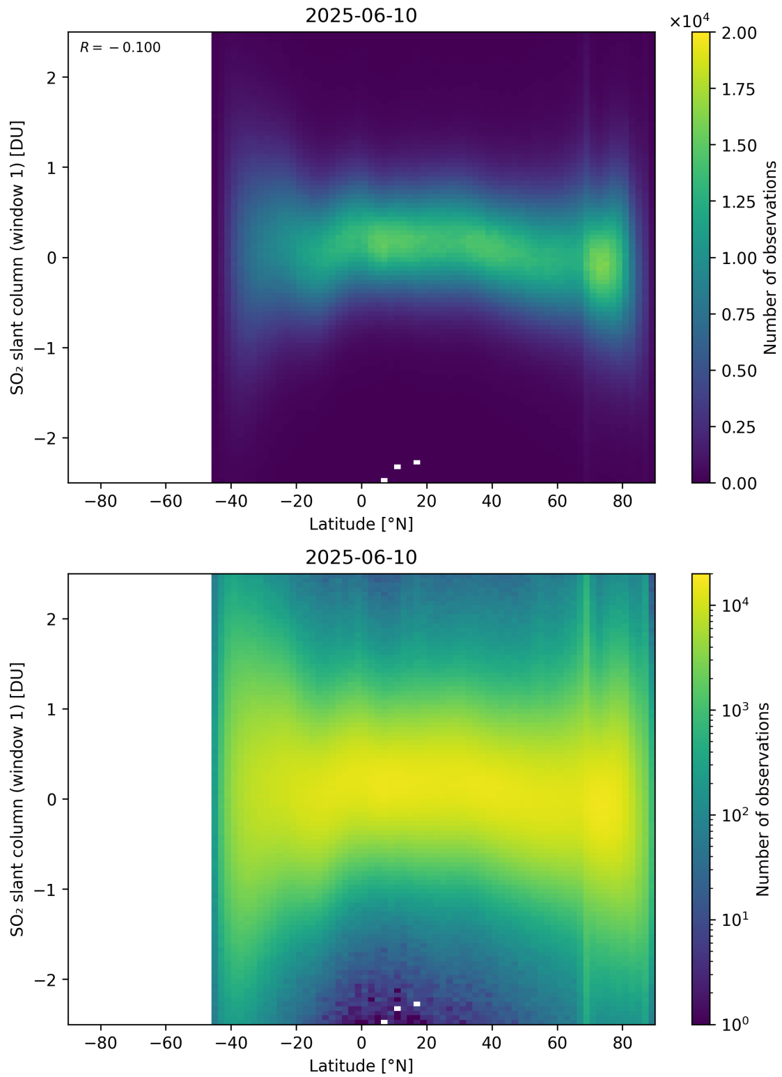
Figure 162: Scatter density plot of “Latitude” against “SO 2 slant column (window 1)” for 2025-06-09 to 2025-06-11.
