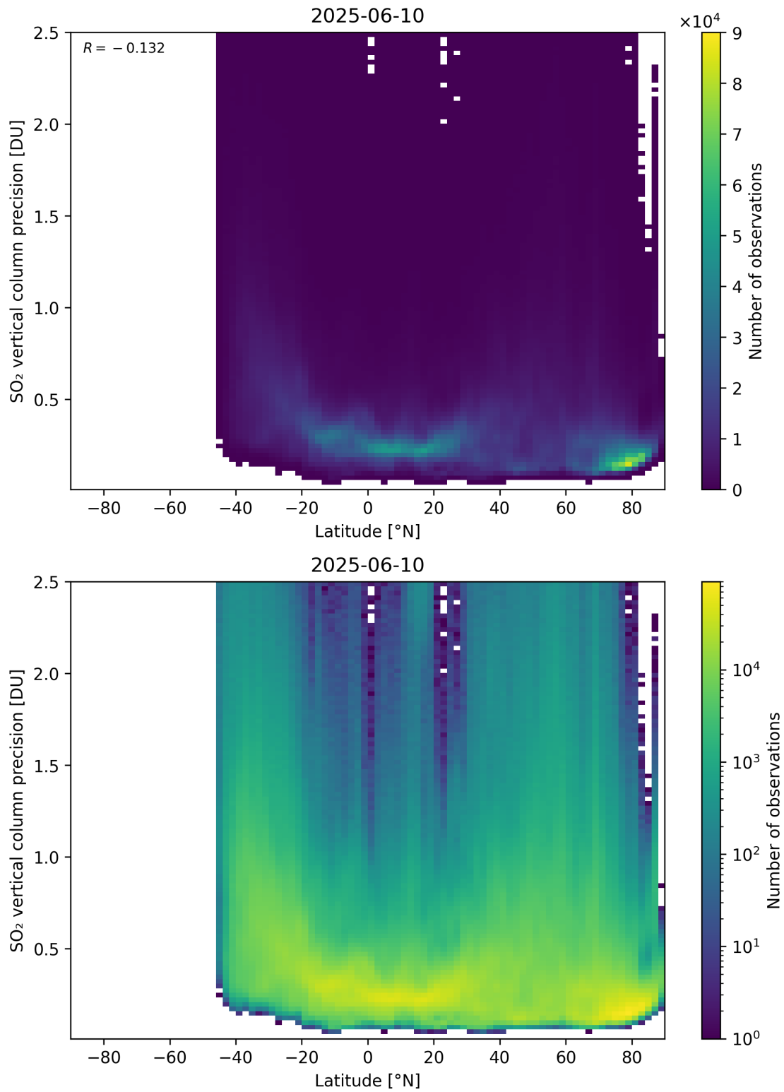
Figure 170: Scatter density plot of “Latitude” against “SO 2 vertical column precision” for 2025-06-09 to 2025-06-11.
