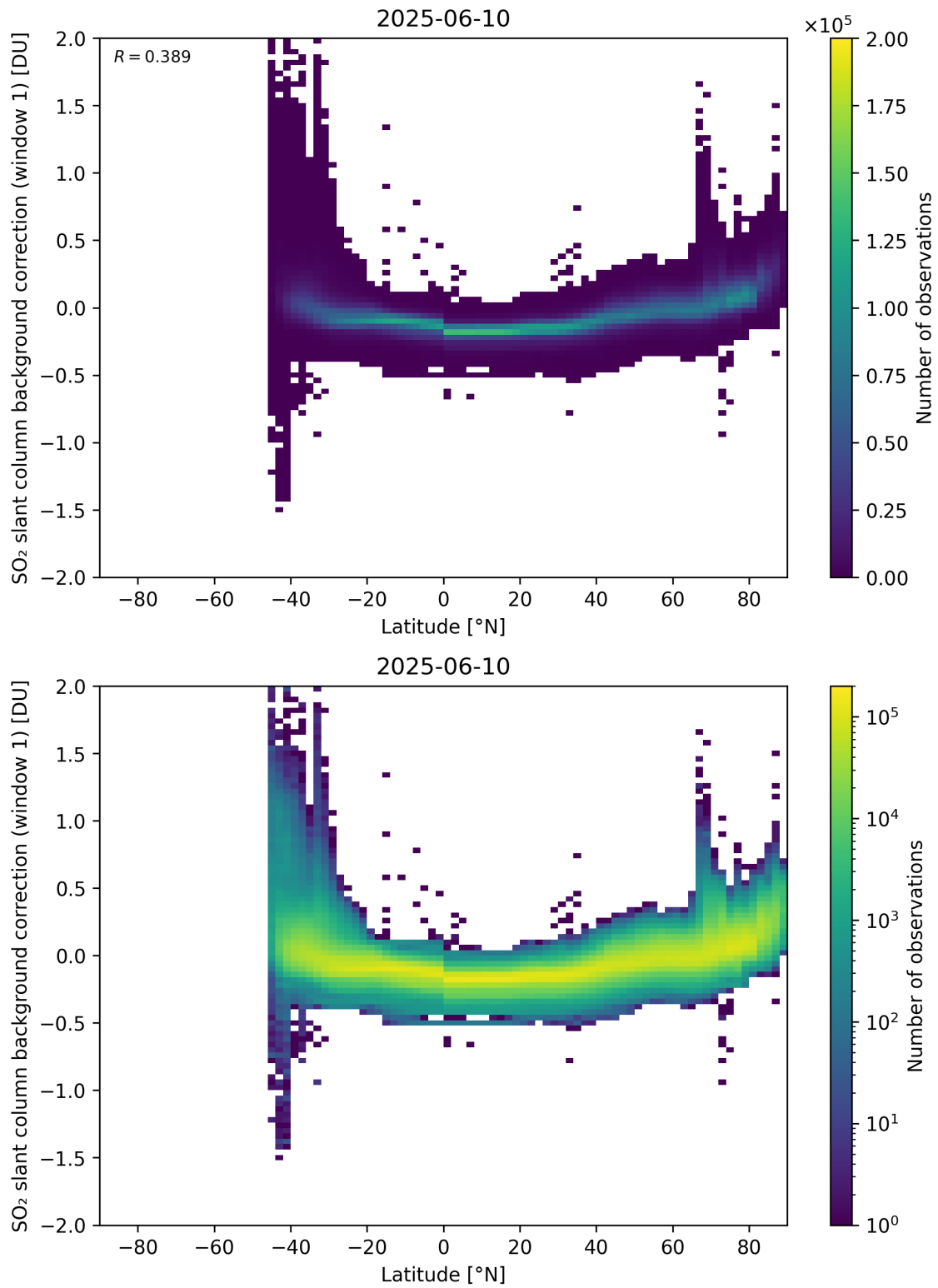
Figure 150: Scatter density plot of “Latitude” against “SO 2 slant column background correction (window 1)” for 2025-06-09 to 2025-06-11.
