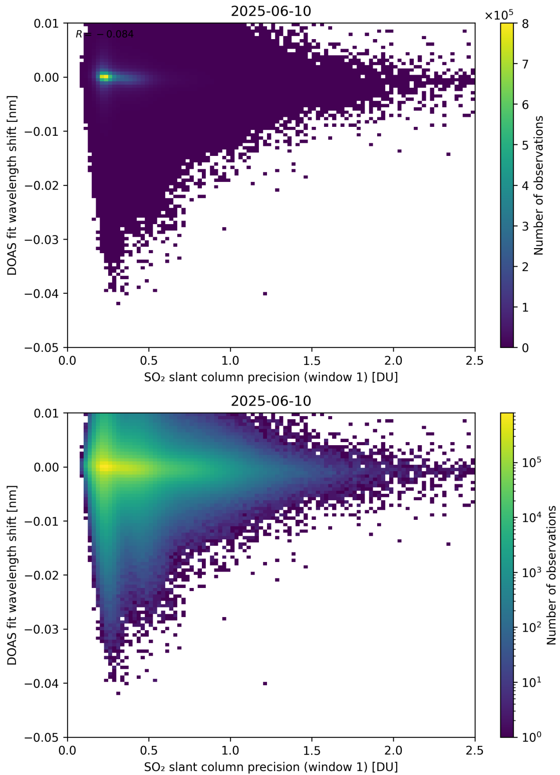
Figure 271: Scatter density plot of “SO 2 slant column precision (window 1)” against “DOAS fit wavelength shift” for 2025-06-09 to 2025-06-11.
