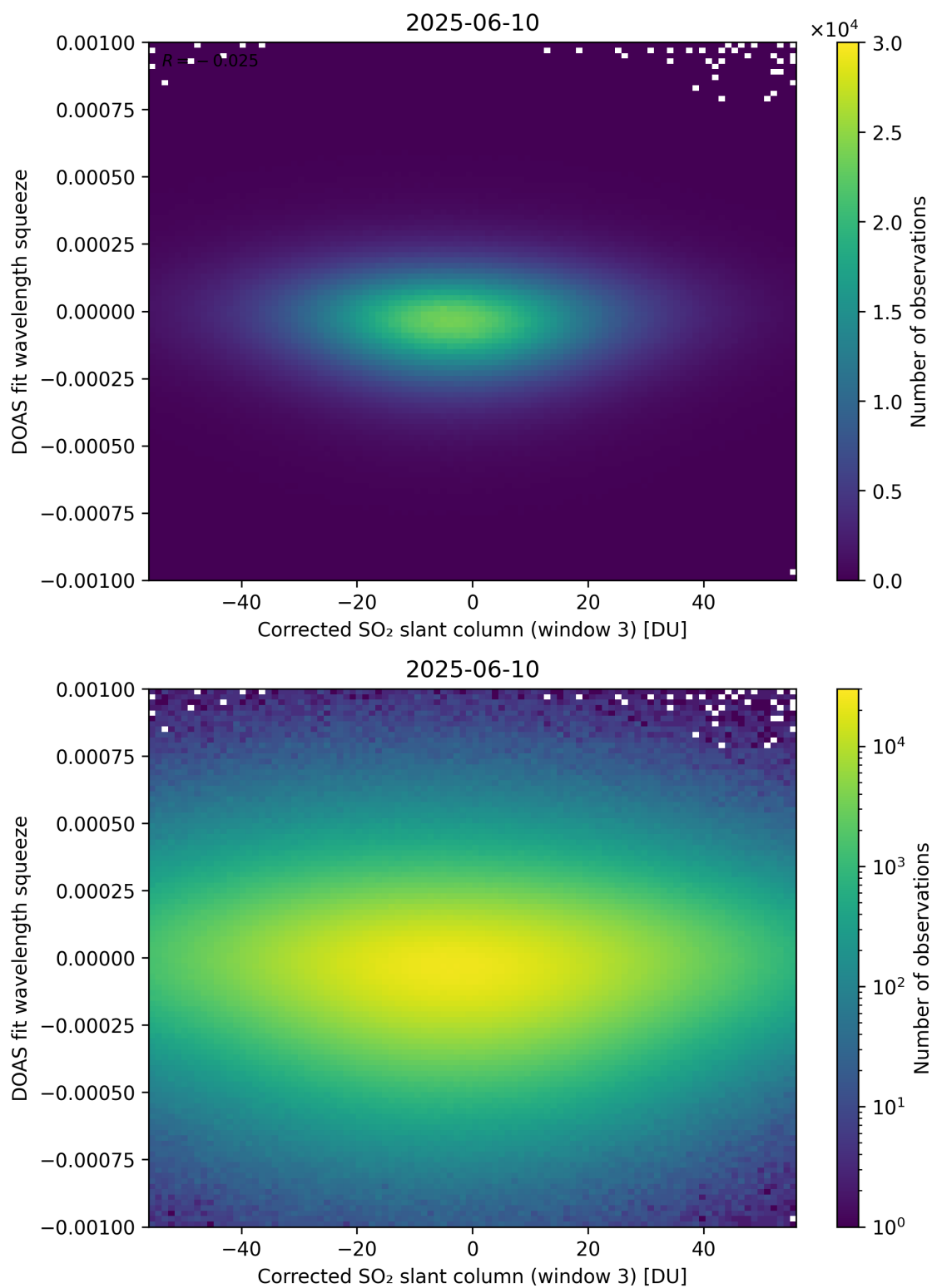
Figure 257: Scatter density plot of “Corrected SO 2 slant column (window 3)” against “DOAS fit wavelength squeeze” for 2025-06-09 to 2025-06-11.
