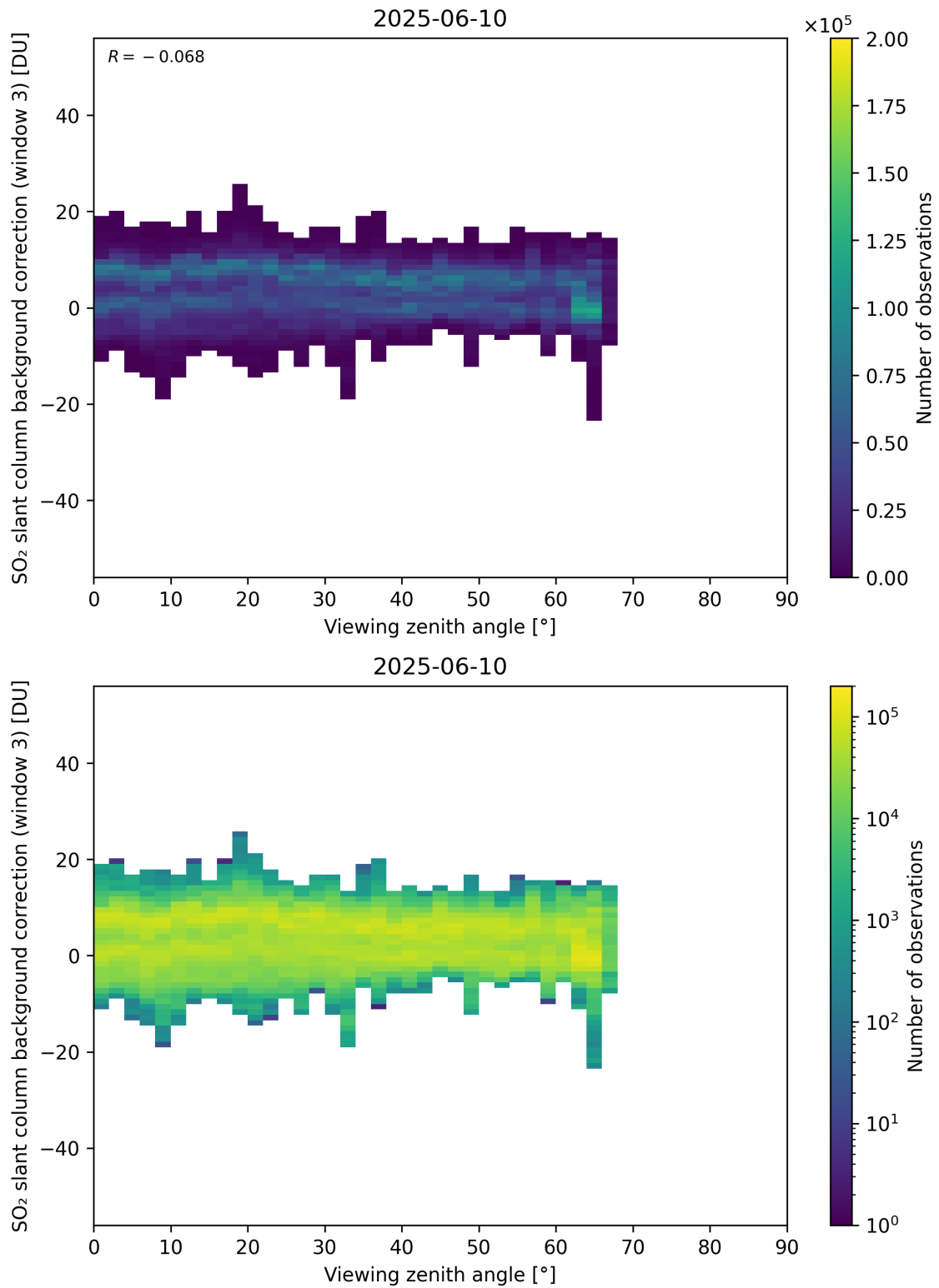
Figure 364: Scatter density plot of “Viewing zenith angle” against “SO 2 slant column background correction (window 3)” for 2025-06-09 to 2025-06-11.
