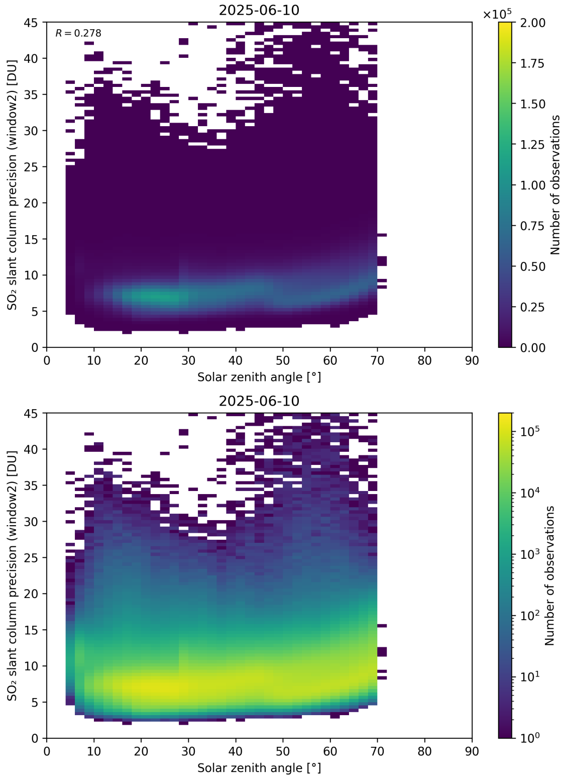
Figure 186: Scatter density plot of “Solar zenith angle” against “SO 2 slant column precision (window2)” for 2025-06-09 to 2025-06-11.
