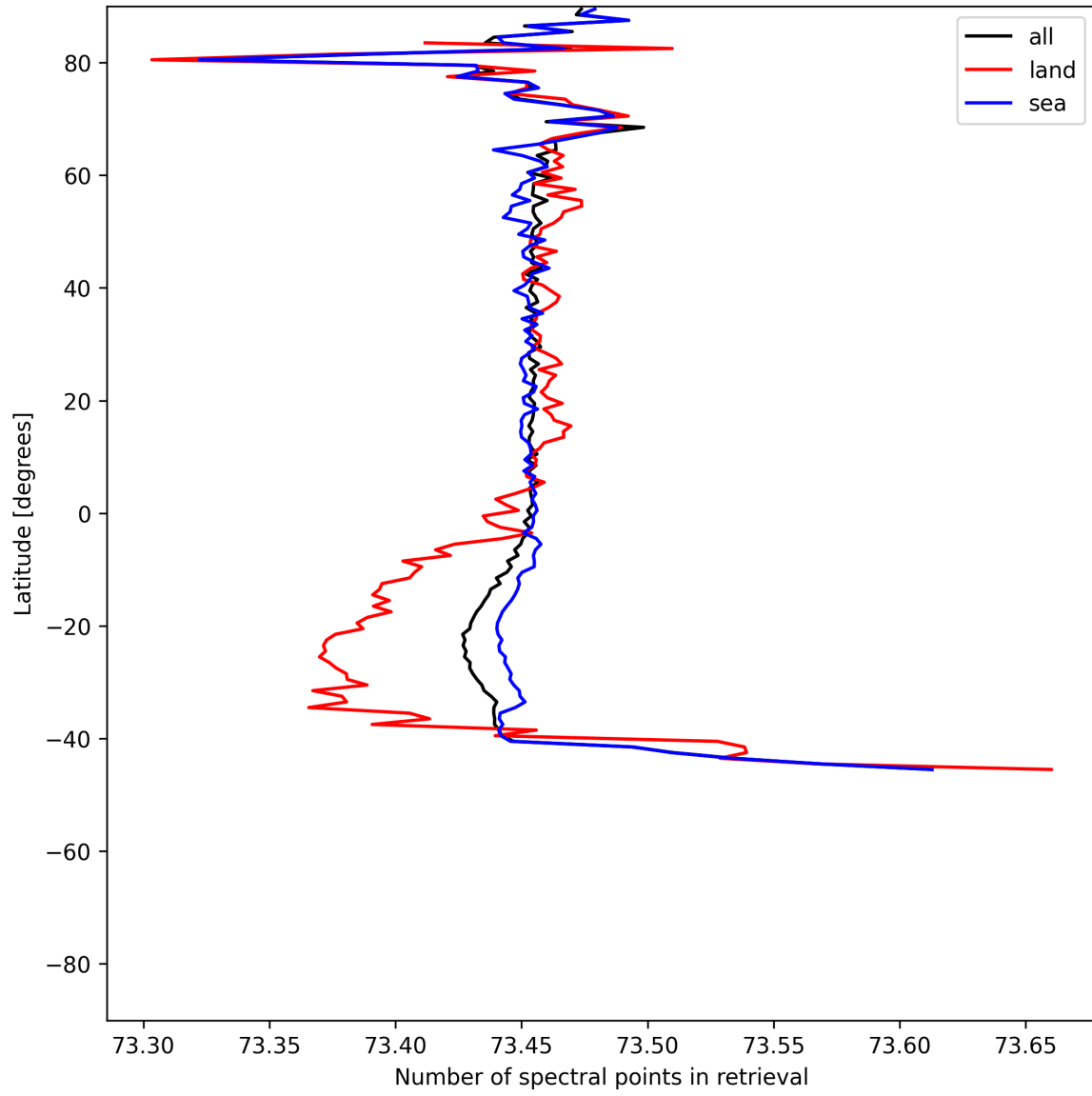
Figure 56: Zonal average of “Number of spectral points in retrieval” for 2025-06-09 to 2025-06-11.
