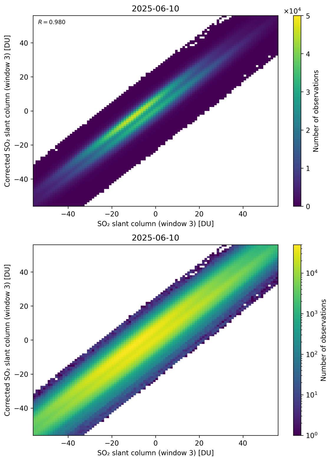
Figure 316: Scatter density plot of “SO 2 slant column (window 3)” against “Corrected SO 2 slant column (window 3)” for 2025-06-09 to 2025-06-11.
