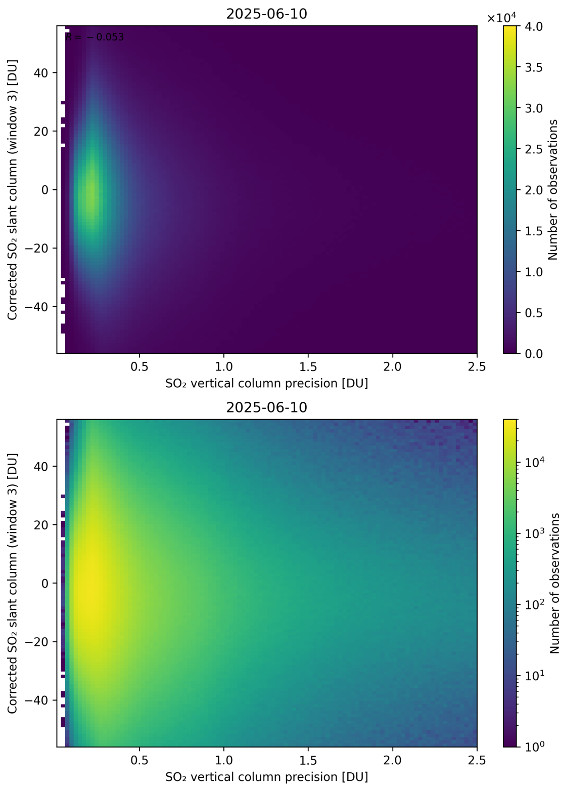
Figure 340: Scatter density plot of “SO 2 vertical column precision” against “Corrected SO 2 slant column (window 3)” for 2025-06-09 to 2025-06-11.
