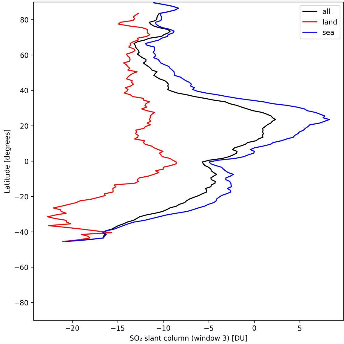
Figure 45: Zonal average of “SO 2 slant column (window 3)” for 2025-06-09 to 2025-06-11.
