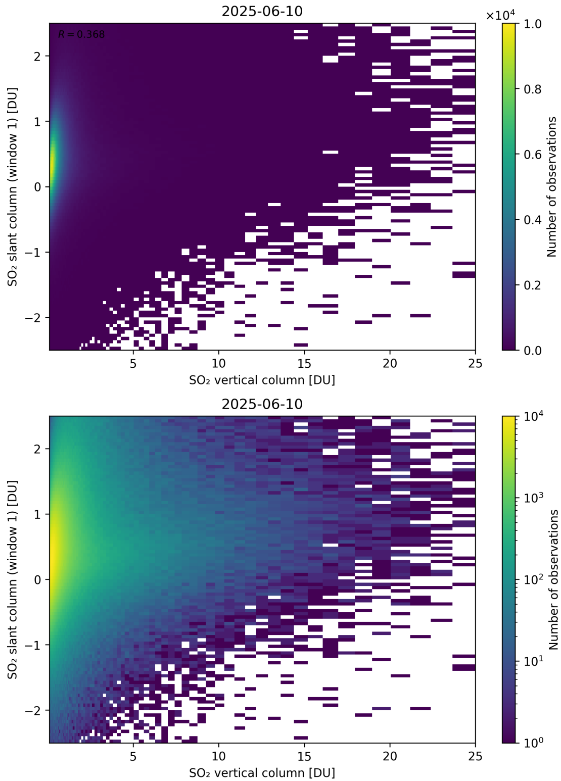
Figure 354: Scatter density plot of “SO 2 vertical column” against “SO 2 slant column (window 1)” for 2025-06-09 to 2025-06-11.
