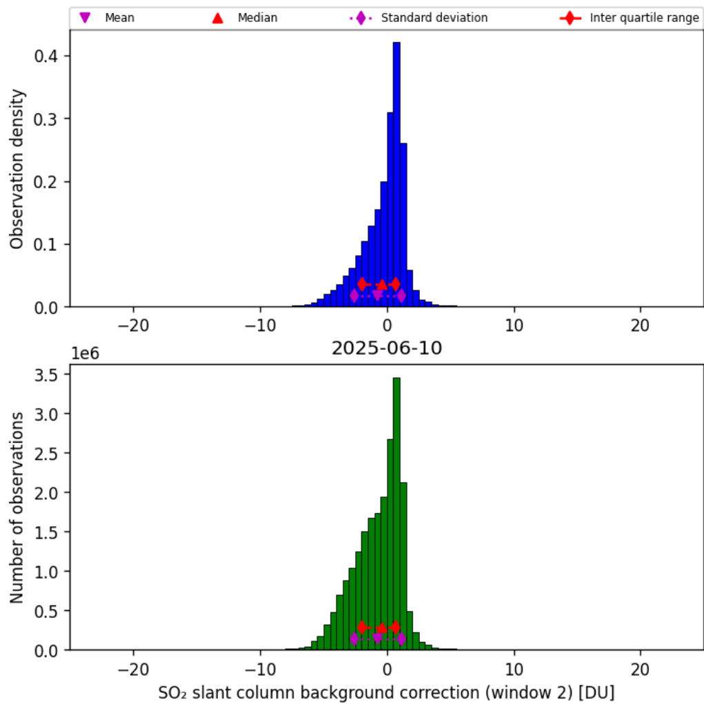
Figure 70: Histogram of “SO 2 slant column background correction (window 2)” for 2025-06-09 to 2025-06-11
