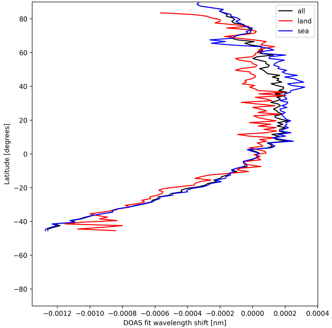
Figure 50: Zonal average of “DOAS fit wavelength shift” for 2025-06-09 to 2025-06-11.
