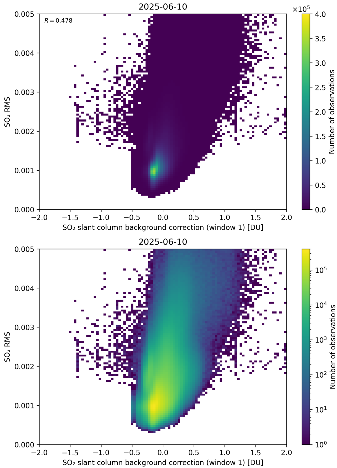
Figure 113: Scatter density plot of “SO 2 slant column background correction (window 1)” against “SO 2 RMS” for 2025-06-09 to 2025-06-11.
