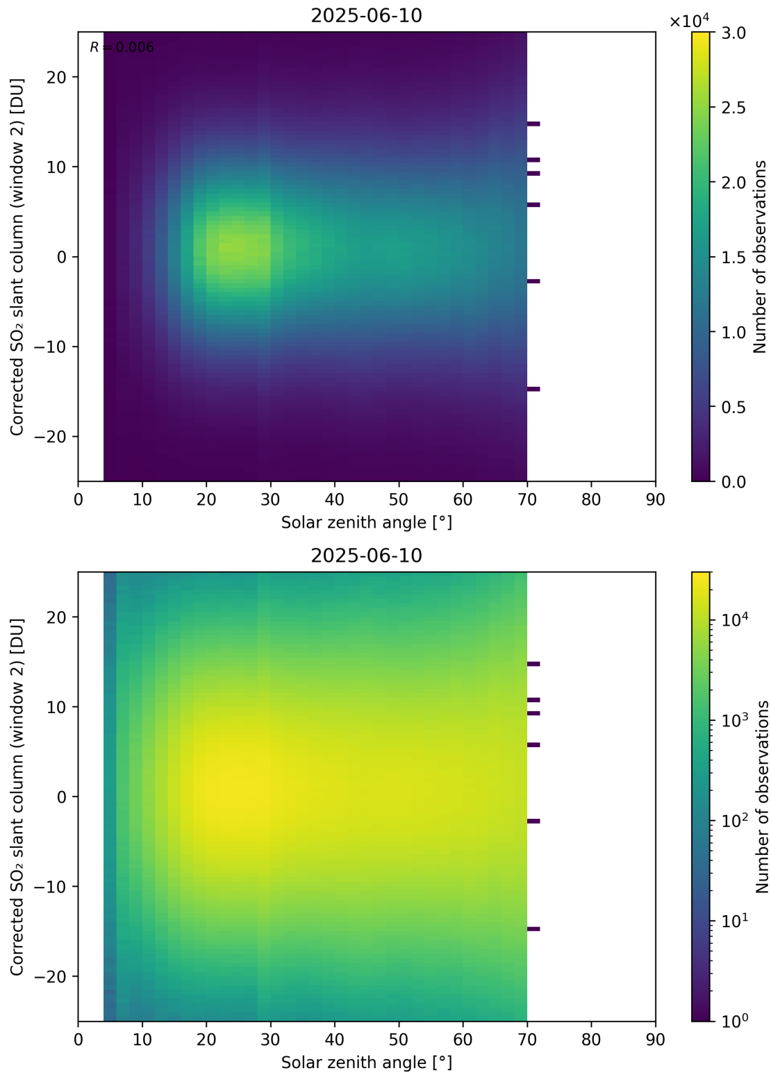
Figure 182: Scatter density plot of “Solar zenith angle” against “Corrected SO 2 slant column (window 2)” for 2025-06-09 to 2025-06-11.
