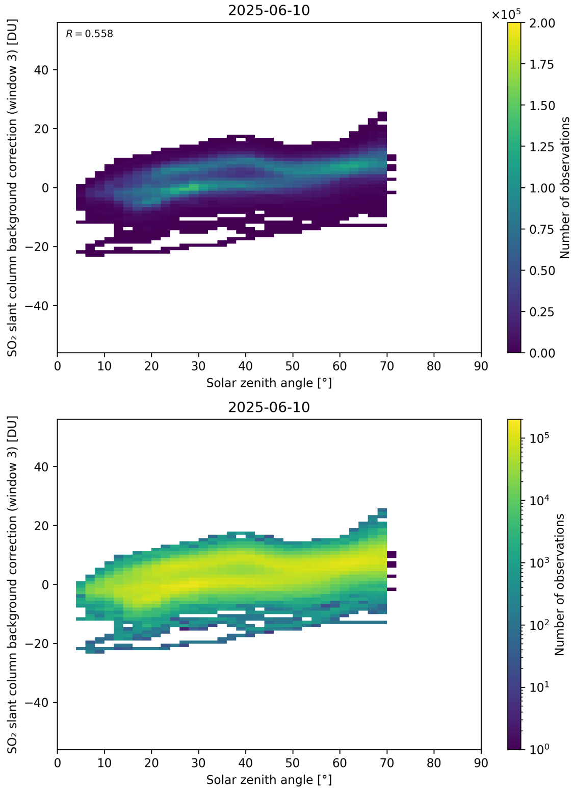
Figure 173: Scatter density plot of “Solar zenith angle” against “SO 2 slant column background correction (window 3)” for 2025-06-09 to 2025-06-11.
