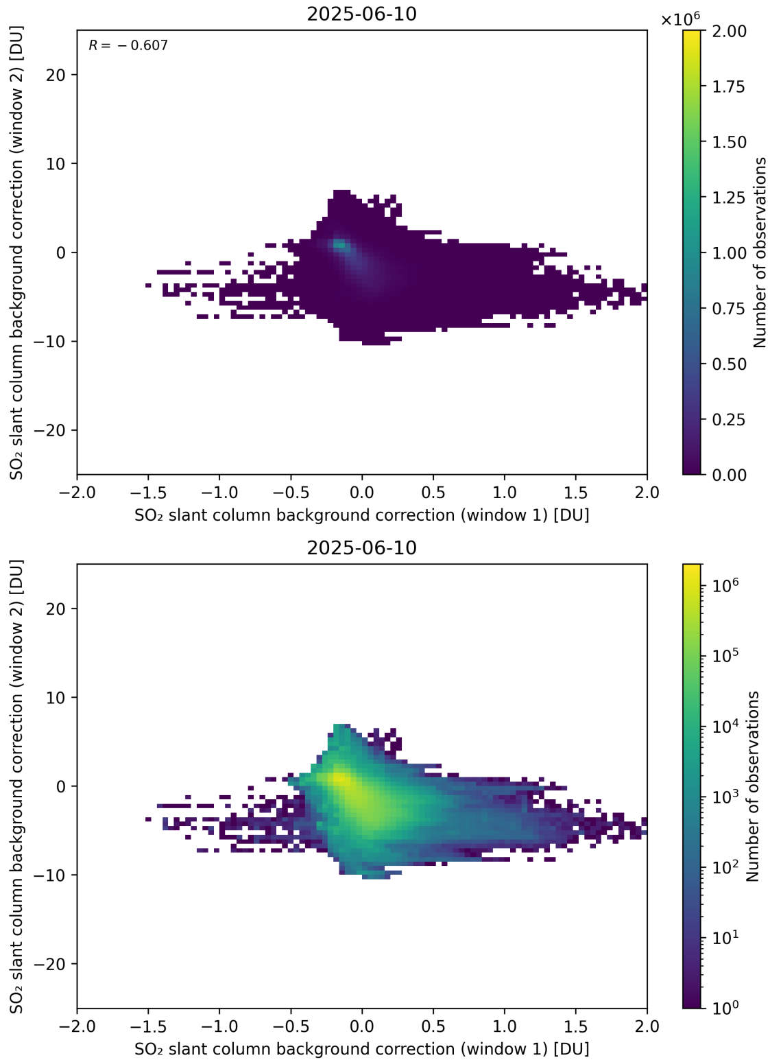
Figure 109: Scatter density plot of “SO 2 slant column background correction (window 1)” against “SO 2 slant column background correction (window 2)” for 2025-06-09 to 2025-06-11.
