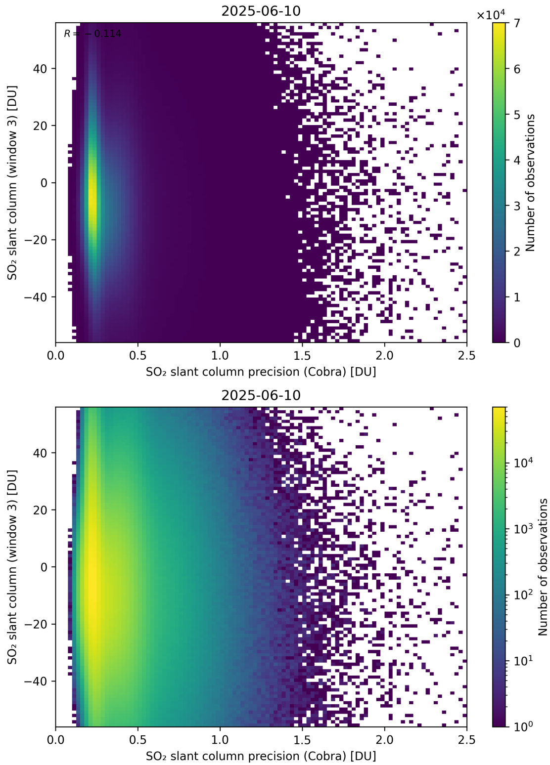
Figure 211: Scatter density plot of “SO 2 slant column precision (Cobra)” against “SO 2 slant column (window 3)” for 2025-06-09 to 2025-06-11.
