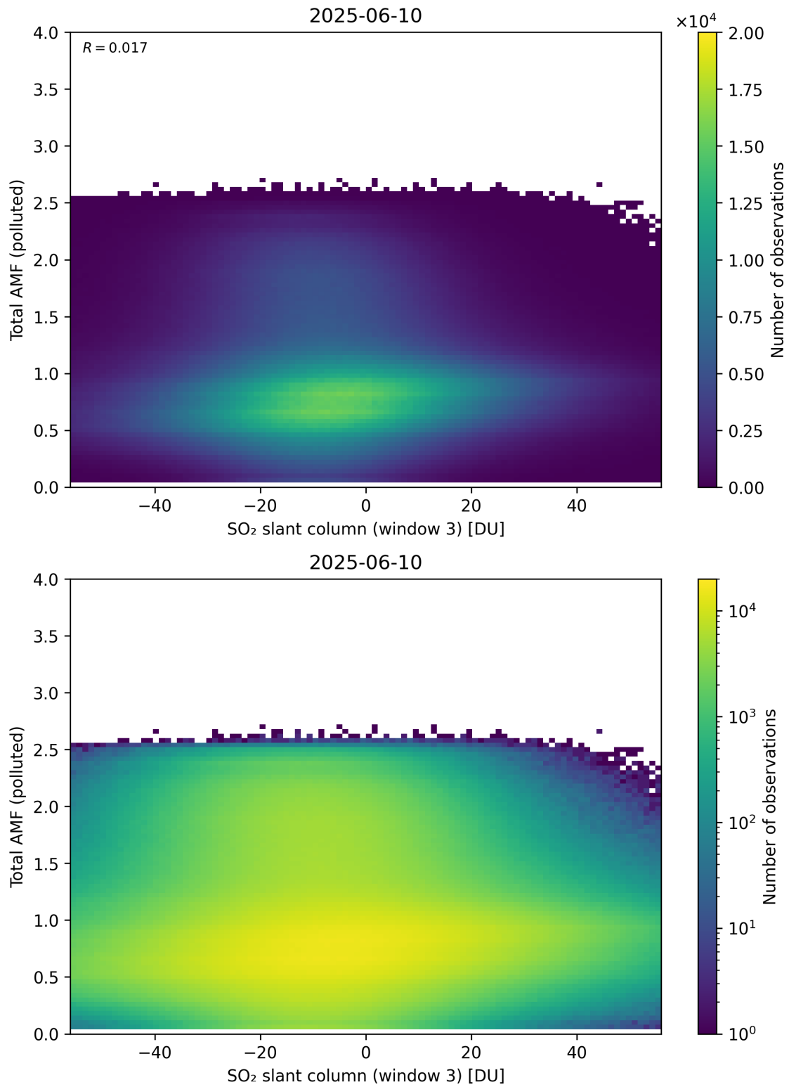
Figure 318: Scatter density plot of “SO 2 slant column (window 3)” against “Total AMF (polluted)” for 2025-06-09 to 2025-06-11.
