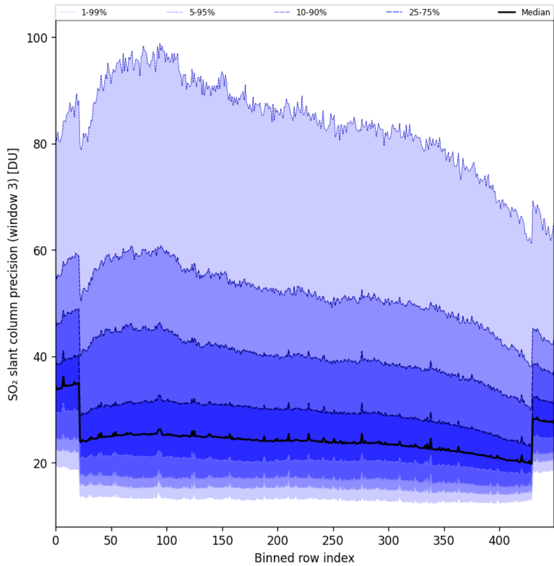
Figure 98: Along track statistics of “SO 2 slant column precision (window 3)” for 2025-06-09 to 2025-06-11
