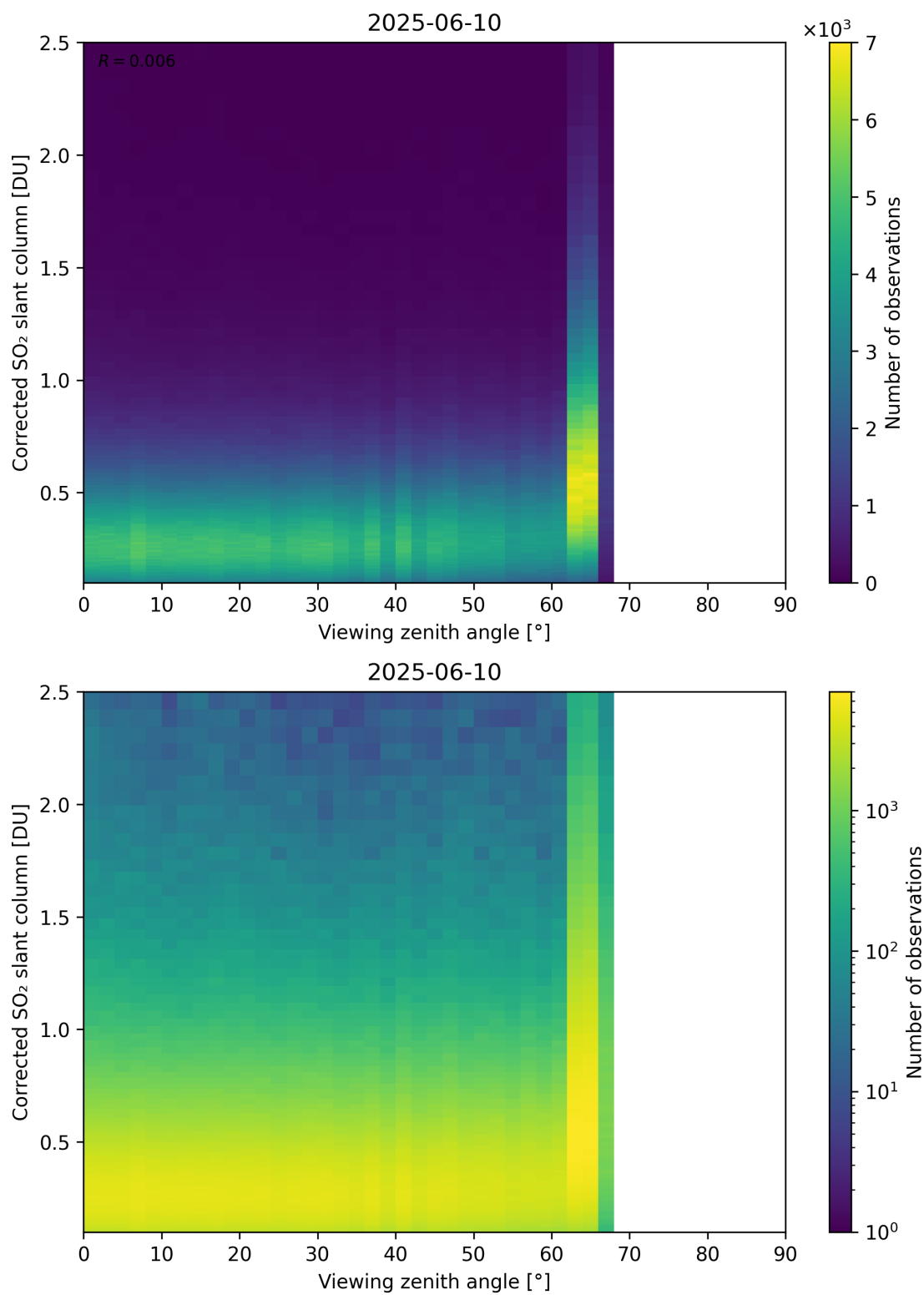
Figure 373: Scatter density plot of “Viewing zenith angle” against “Corrected SO 2 slant column” for 2025-06-09 to 2025-06-11.
