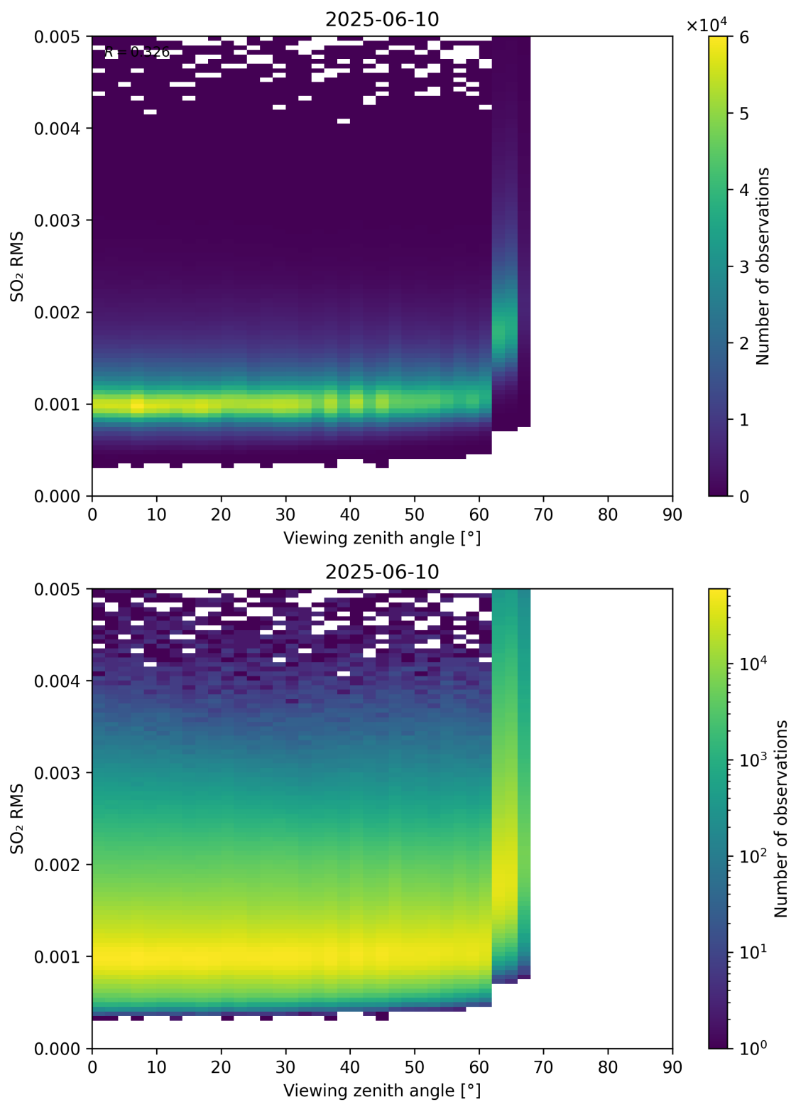
Figure 367: Scatter density plot of “Viewing zenith angle” against “SO 2 RMS” for 2025-06-09 to 2025-06-11.
