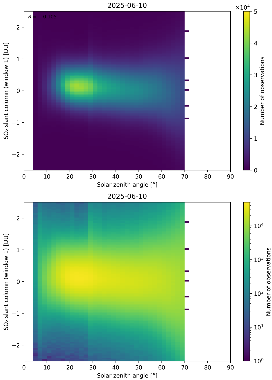
Figure 184: Scatter density plot of “Solar zenith angle” against “SO 2 slant column (window 1)” for 2025-06-09 to 2025-06-11.
