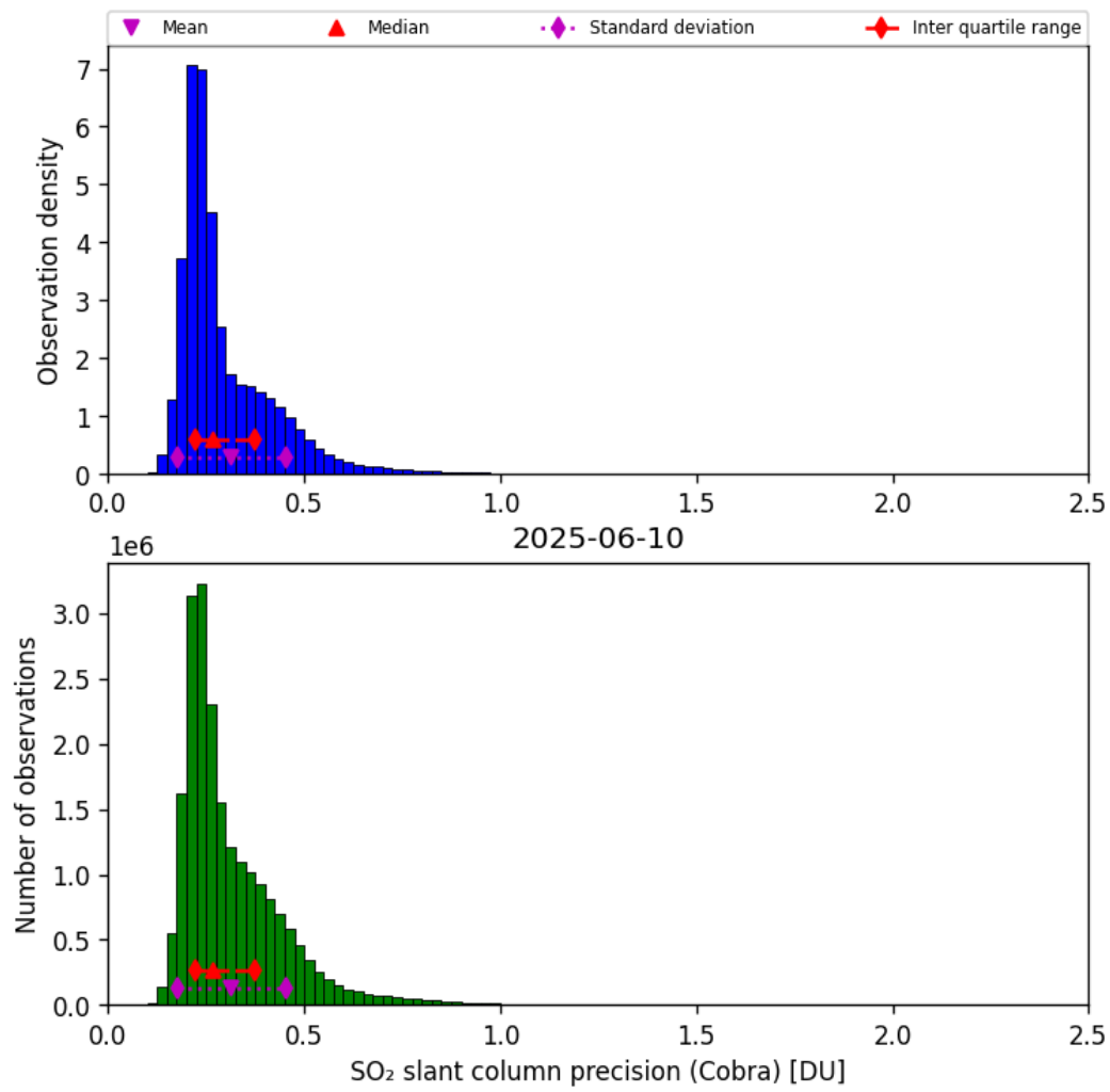
Figure 62: Histogram of “SO 2 slant column precision (Cobra)” for 2025-06-09 to 2025-06-11
