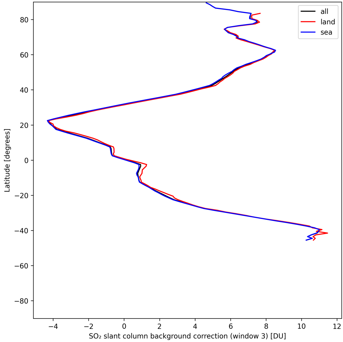
Figure 48: Zonal average of “SO 2 slant column background correction (window 3)” for 2025-06-09 to 2025-06-11.
