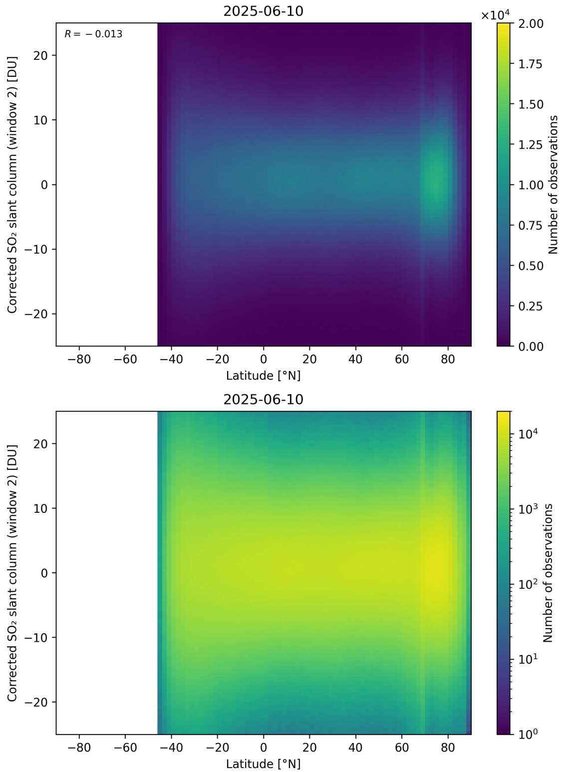
Figure 160: Scatter density plot of “Latitude” against “Corrected SO 2 slant column (window 2)” for 2025-06-09 to 2025-06-11.
