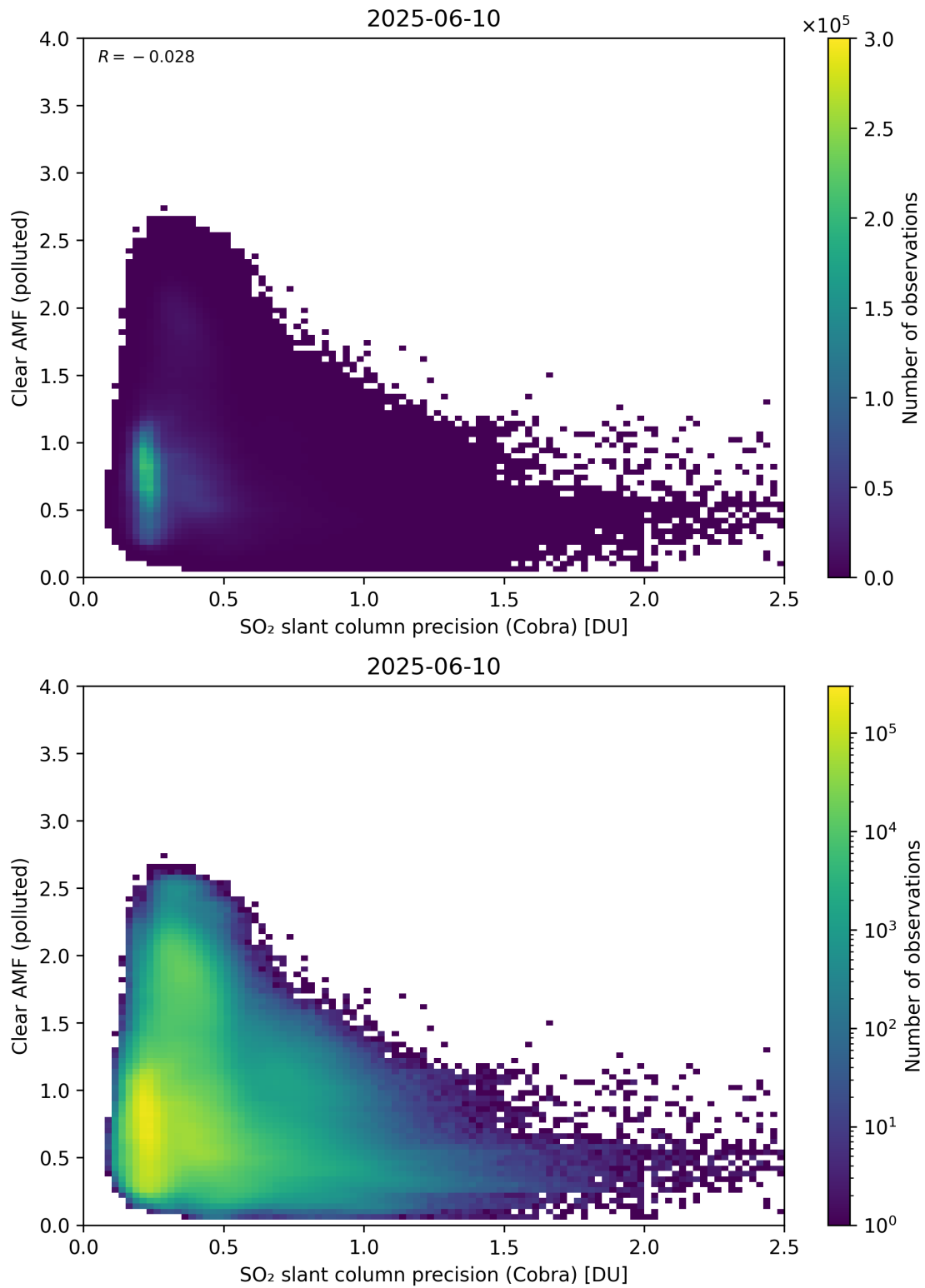
Figure 205: Scatter density plot of “SO 2 slant column precision (Cobra)” against “Clear AMF (polluted)” for 2025-06-09 to 2025-06-11.
