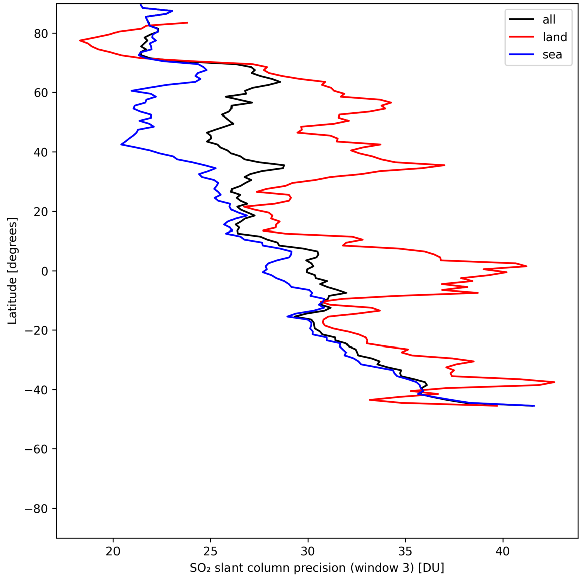
Figure 46: Zonal average of “SO 2 slant column precision (window 3)” for 2025-06-09 to 2025-06-11.
