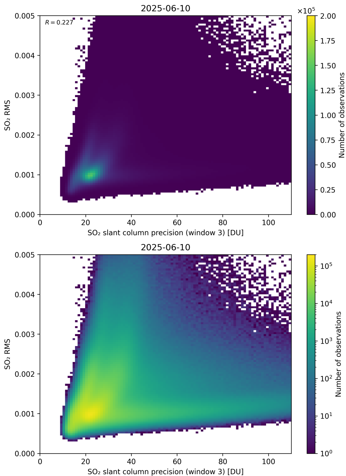
Figure 310: Scatter density plot of “SO 2 slant column precision (window 3)” against “SO 2 RMS” for 2025-06-09 to 2025-06-11.
