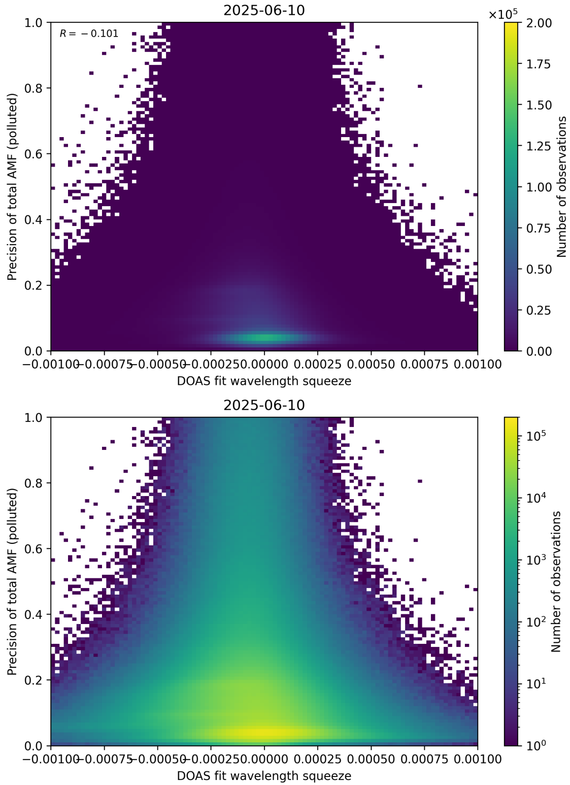
Figure 146: Scatter density plot of “DOAS fit wavelength squeeze” against “Precision of total AMF (polluted)” for 2025-06-09 to 2025-06-11.
