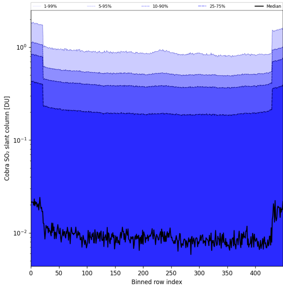
Figure 87: Along track statistics of “Cobra SO 2 slant column” for 2025-06-09 to 2025-06-11
