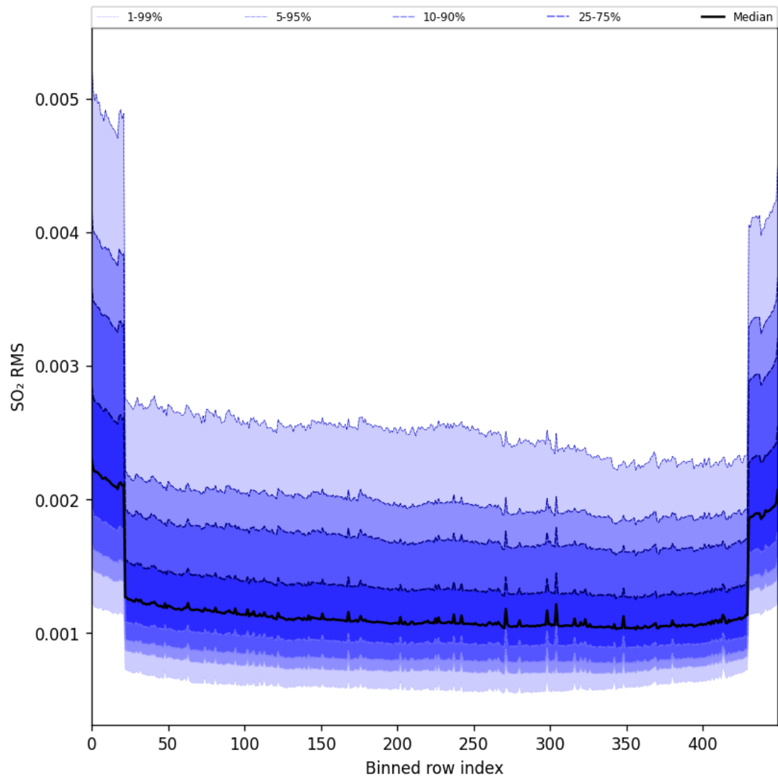
Figure 104: Along track statistics of “SO 2 RMS” for 2025-06-09 to 2025-06-11
