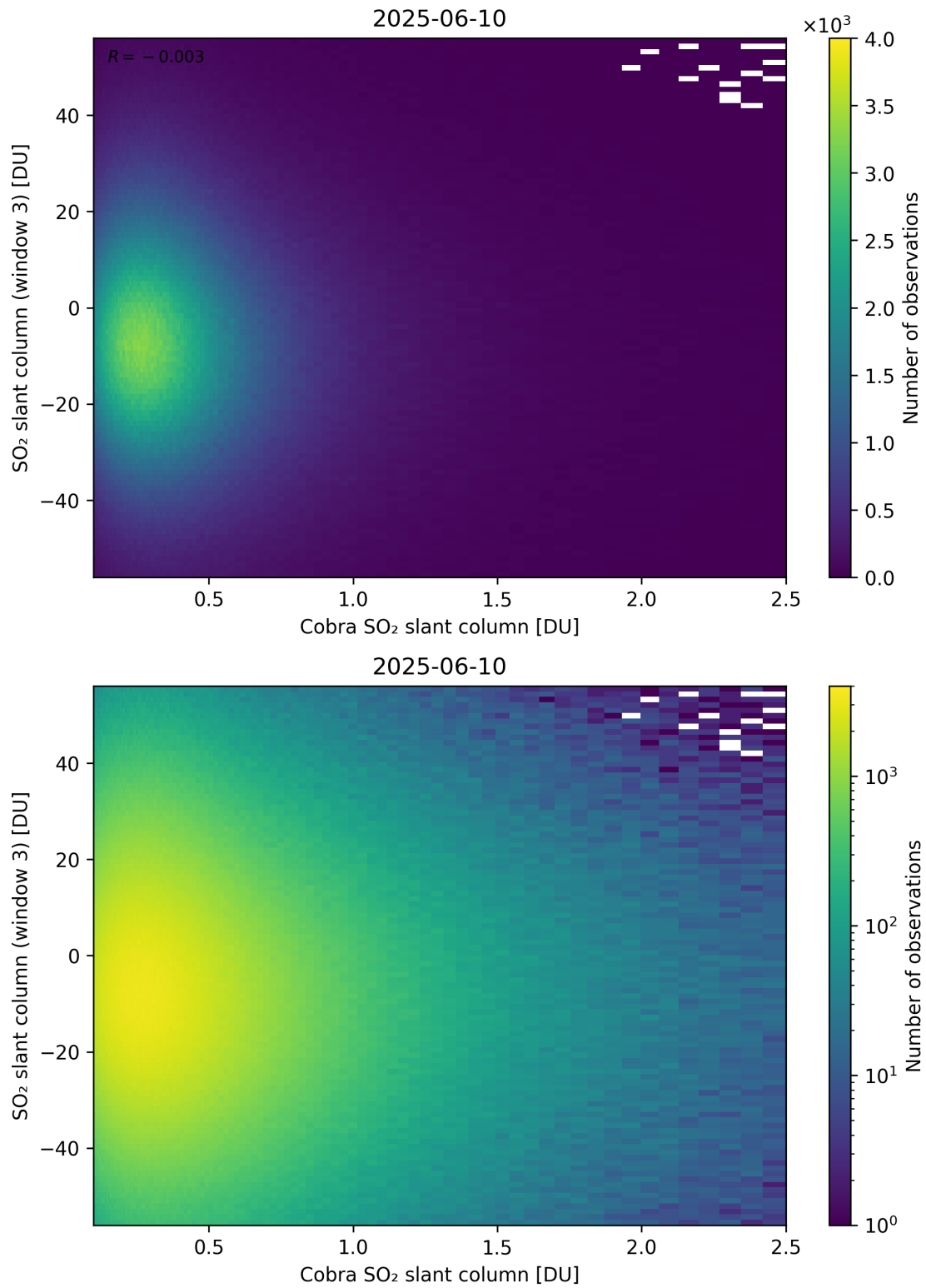
Figure 222: Scatter density plot of “Cobra SO 2 slant column” against “SO 2 slant column (window 3)” for 2025-06-09 to 2025-06-11.
