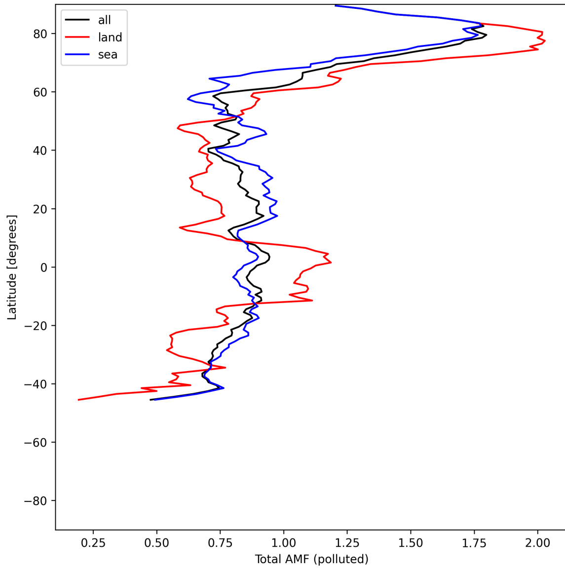
Figure 53: Zonal average of “Total AMF (polluted)” for 2025-06-09 to 2025-06-11.
