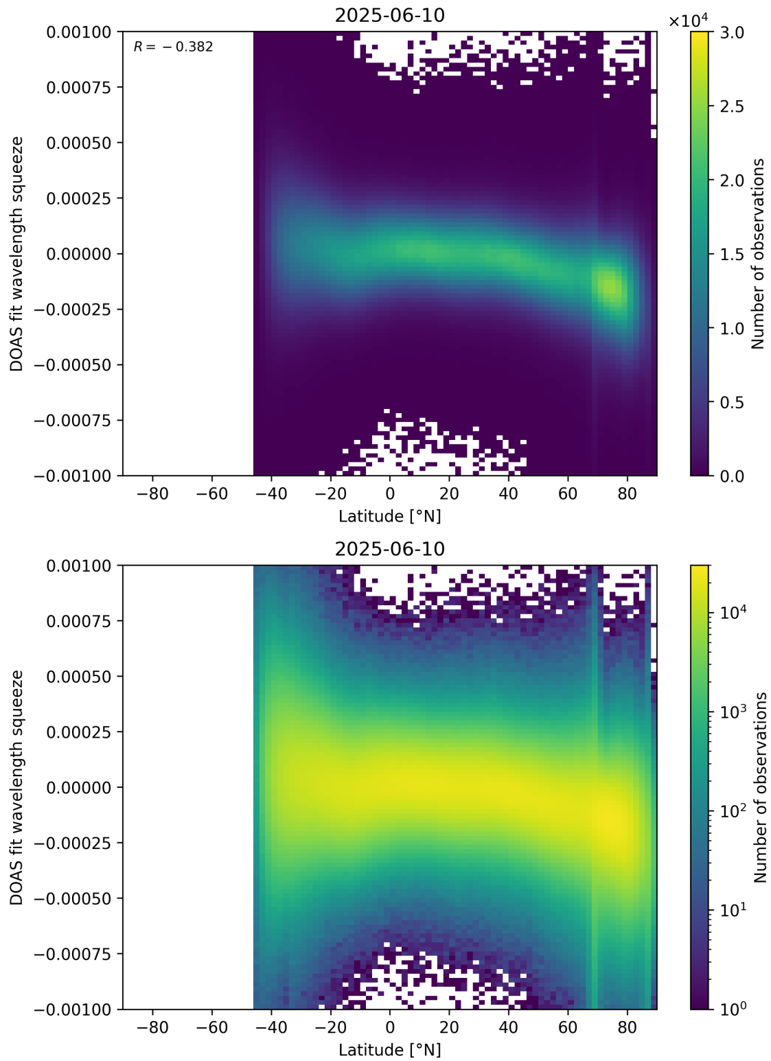
Figure 154: Scatter density plot of “Latitude” against “DOAS fit wavelength squeeze” for 2025-06-09 to 2025-06-11.
