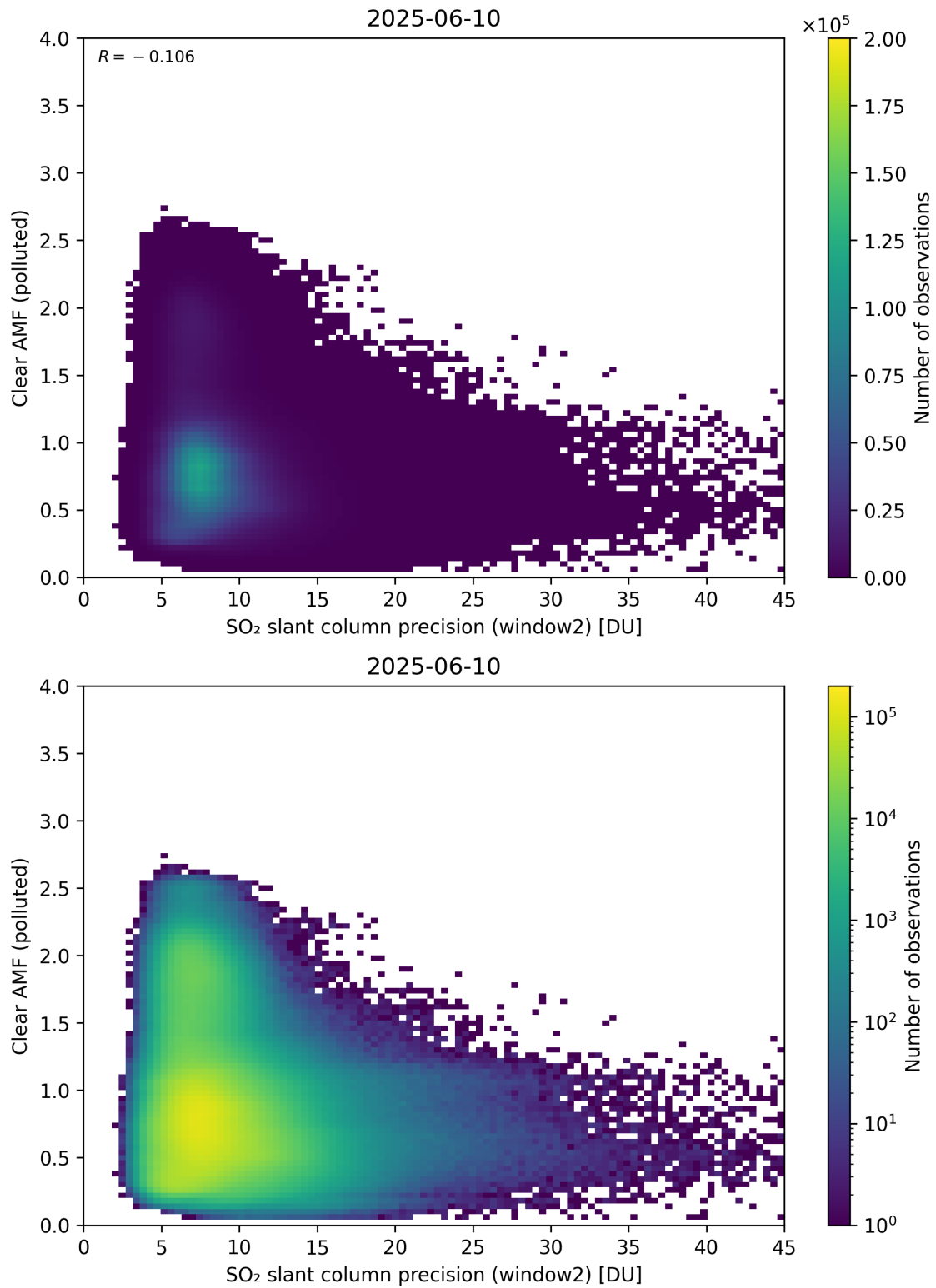
Figure 296: Scatter density plot of “SO 2 slant column precision (window2)” against “Clear AMF (polluted)” for 2025-06-09 to 2025-06-11.
