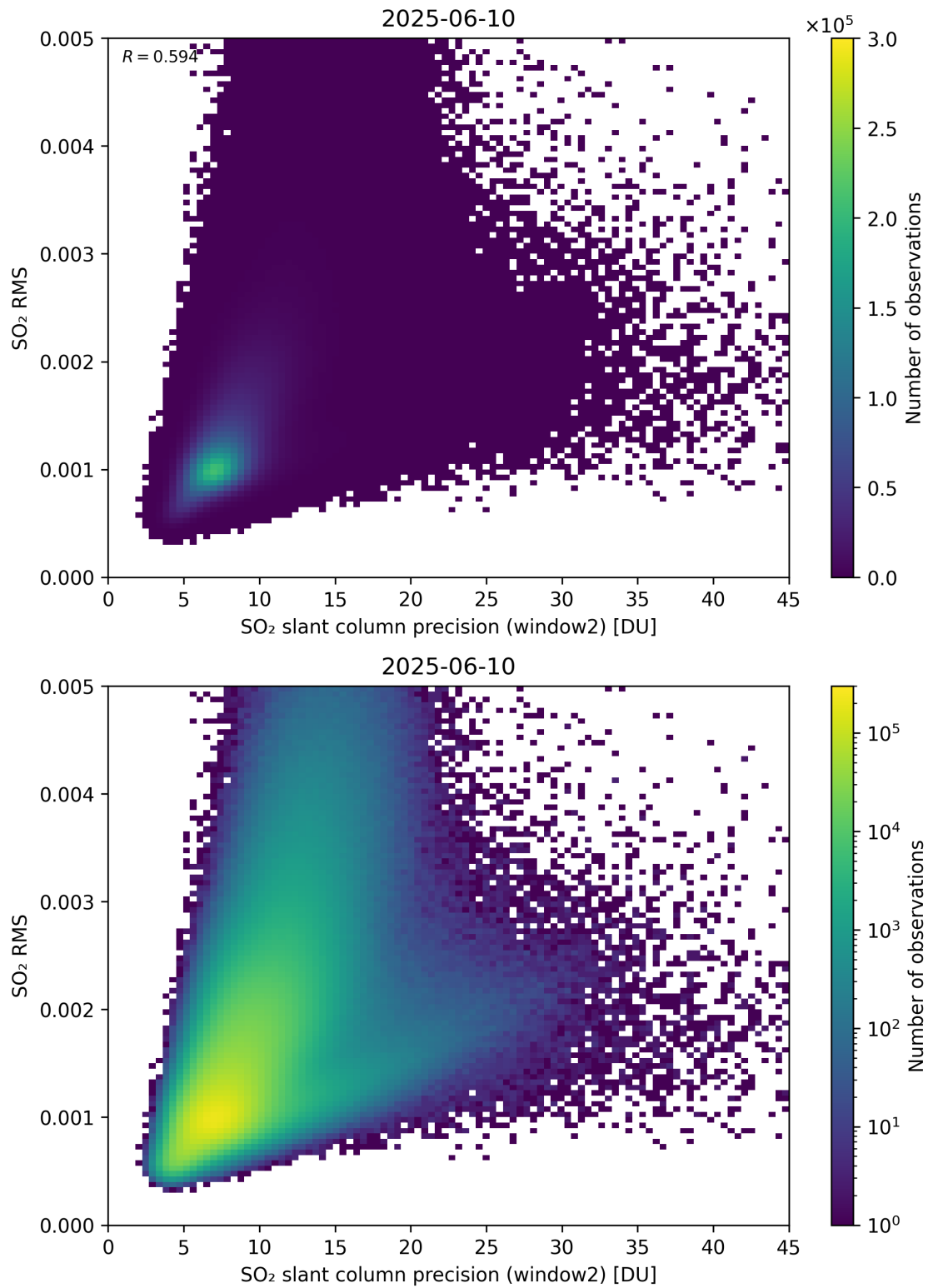
Figure 295: Scatter density plot of “SO 2 slant column precision (window2)” against “SO 2 RMS” for 2025-06-09 to 2025-06-11.
