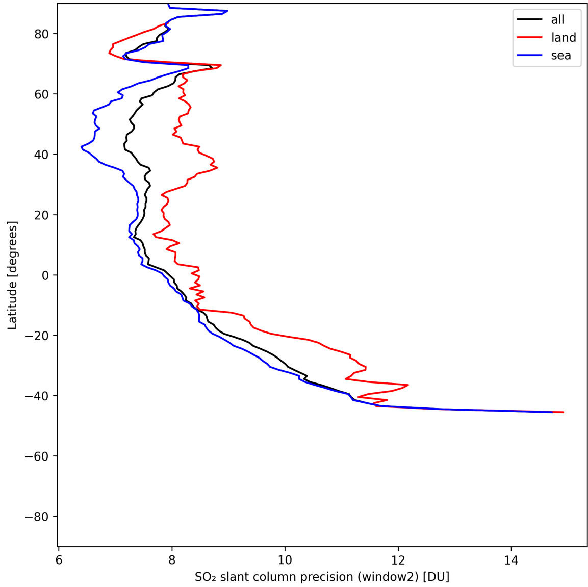
Figure 42: Zonal average of “SO 2 slant column precision (window2)” for 2025-06-09 to 2025-06-11.
