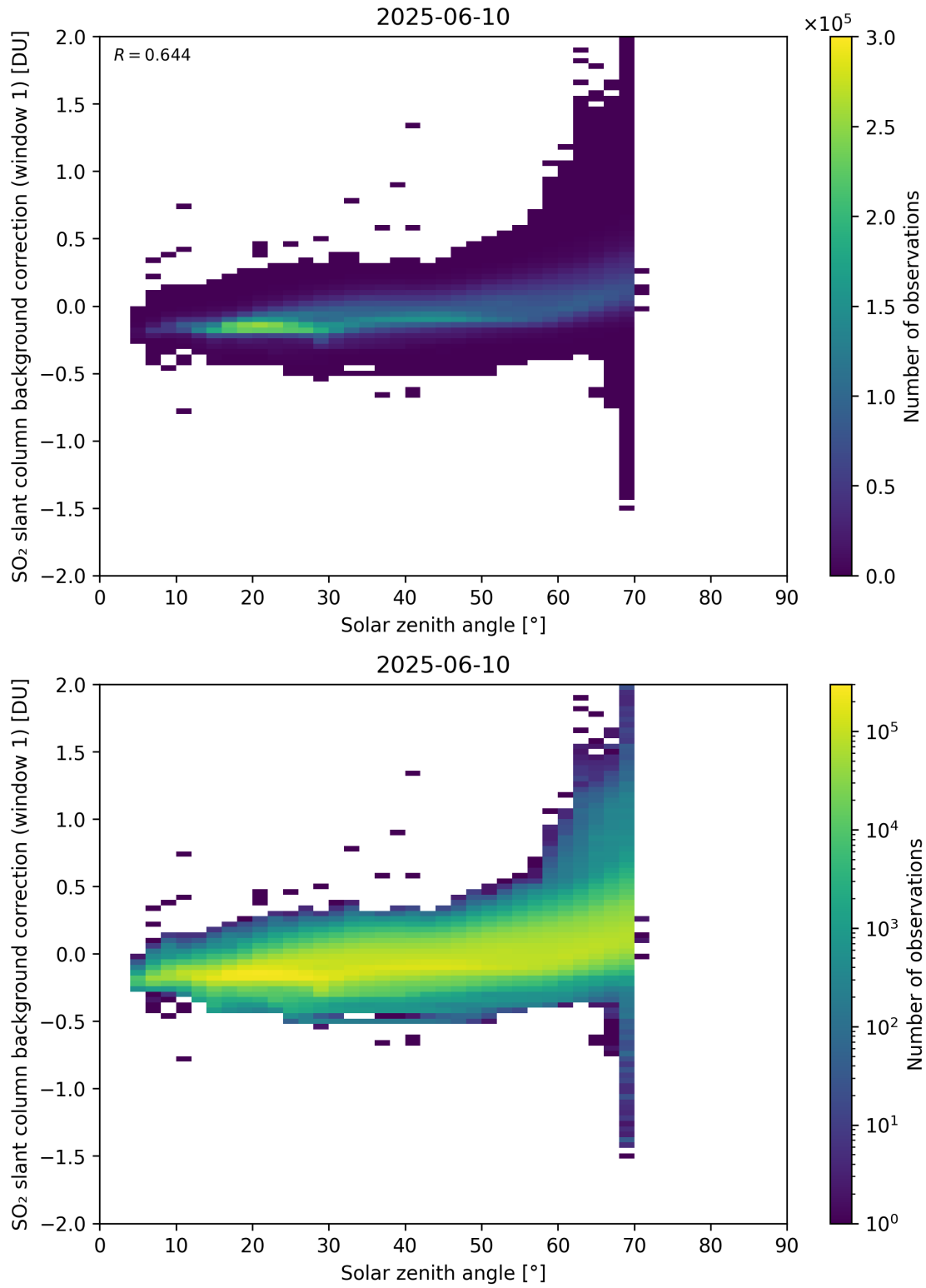
Figure 171: Scatter density plot of “Solar zenith angle” against “SO 2 slant column background correction (window 1)” for 2025-06-09 to 2025-06-11.
