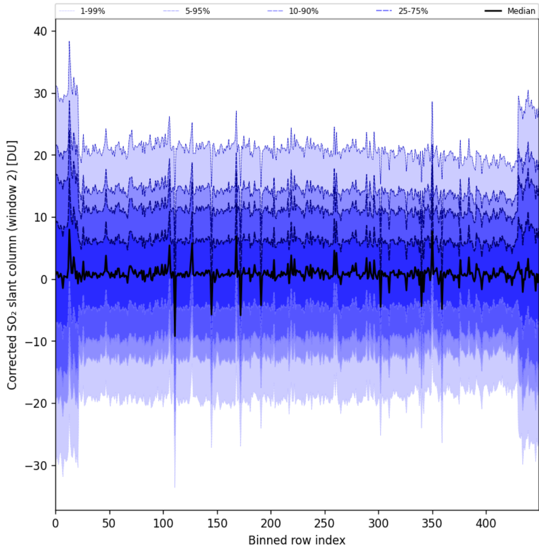
Figure 95: Along track statistics of “Corrected SO 2 slant column (window 2)” for 2025-06-09 to 2025-06-11
