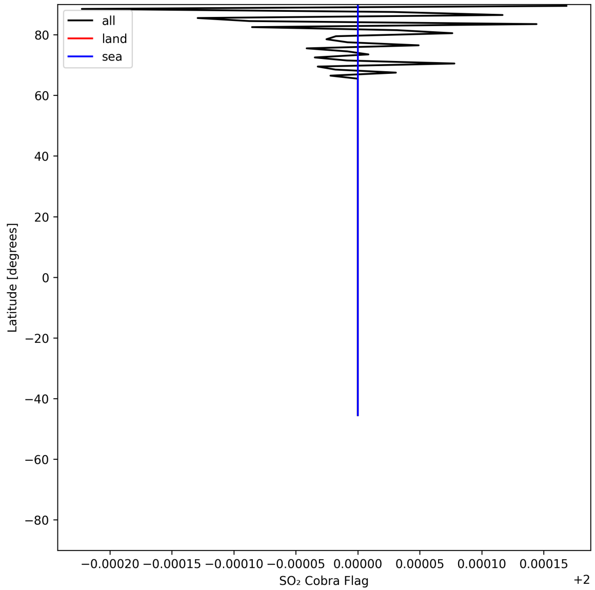
Figure 49: Zonal average of “SO 2 Cobra Flag” for 2025-06-09 to 2025-06-11.
