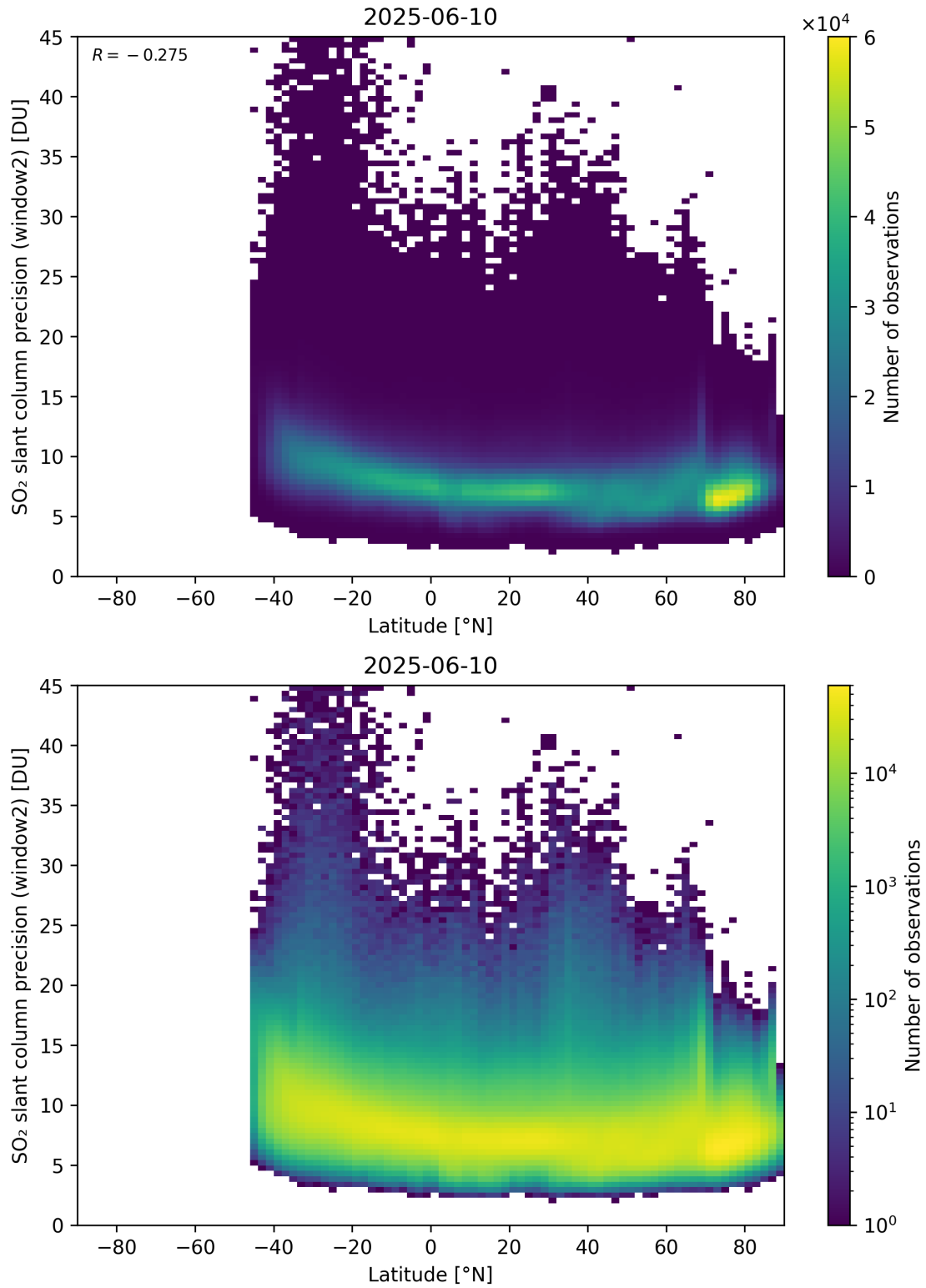
Figure 164: Scatter density plot of “Latitude” against “SO 2 slant column precision (window2)” for 2025-06-09 to 2025-06-11.
