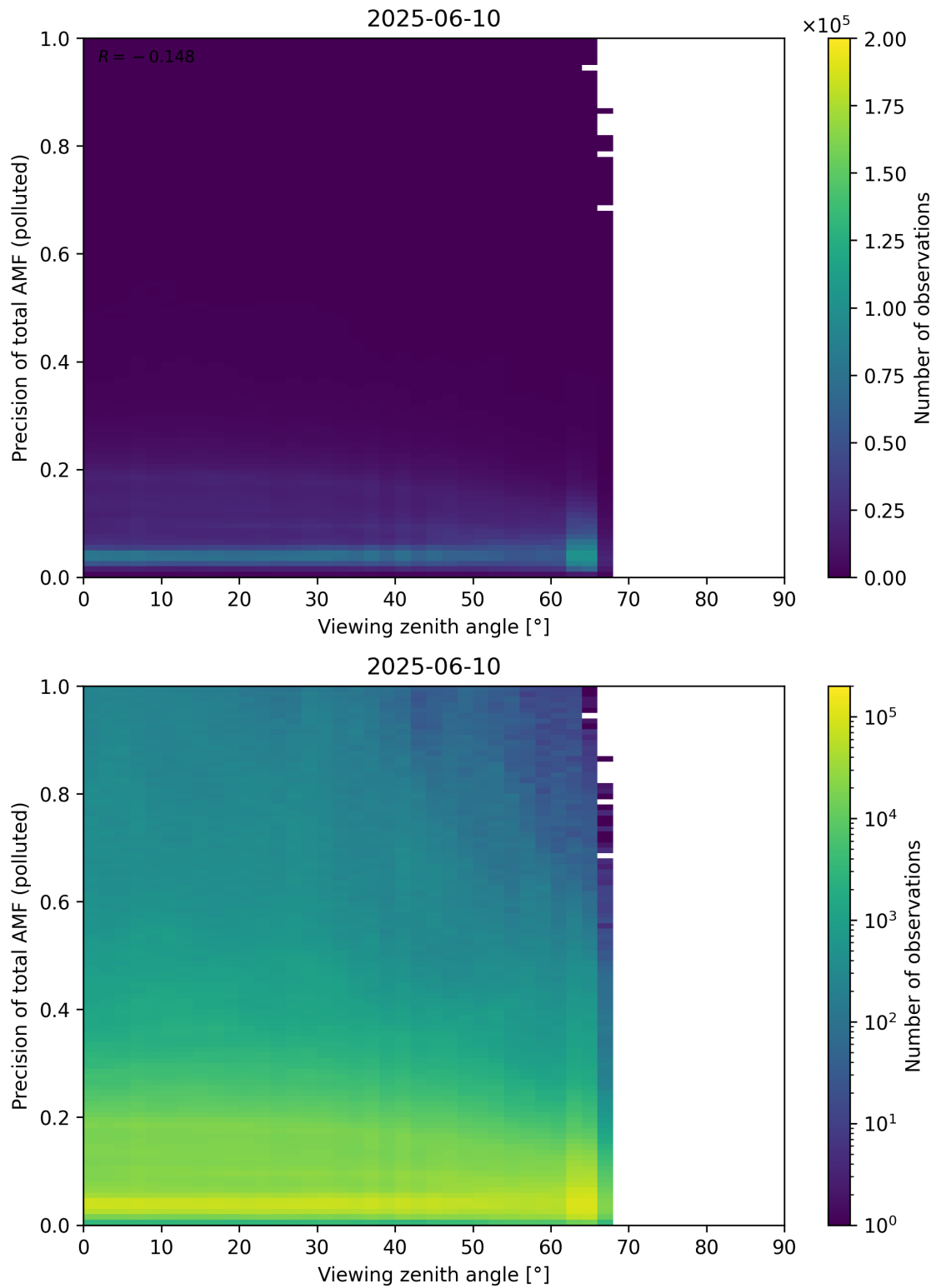
Figure 382: Scatter density plot of “Viewing zenith angle” against “Precision of total AMF (polluted)” for 2025-06-09 to 2025-06-11.
