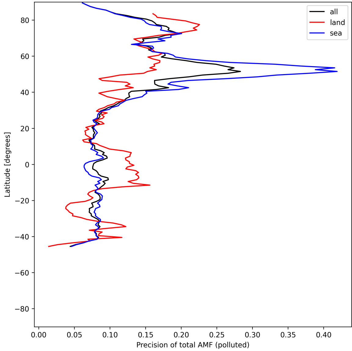
Figure 54: Zonal average of “Precision of total AMF (polluted)” for 2025-06-09 to 2025-06-11.
