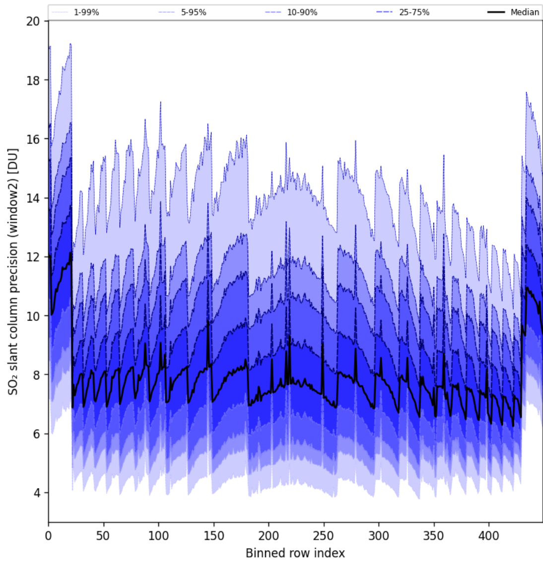
Figure 94: Along track statistics of “SO 2 slant column precision (window2)” for 2025-06-09 to 2025-06-11
