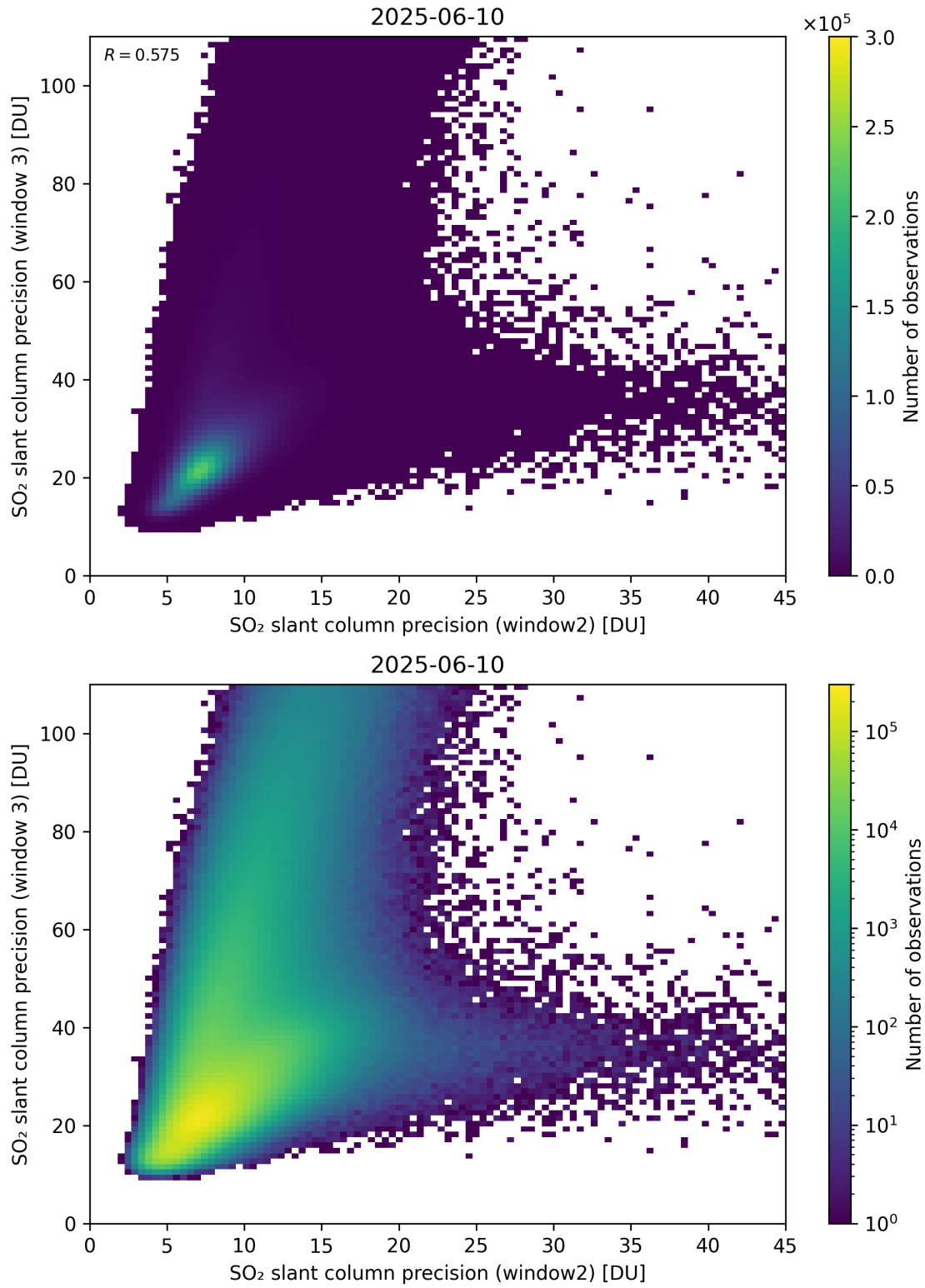
Figure 300: Scatter density plot of “SO 2 slant column precision (window2)” against “SO 2 slant column precision (window 3)” for 2025-06-09 to 2025-06-11.
