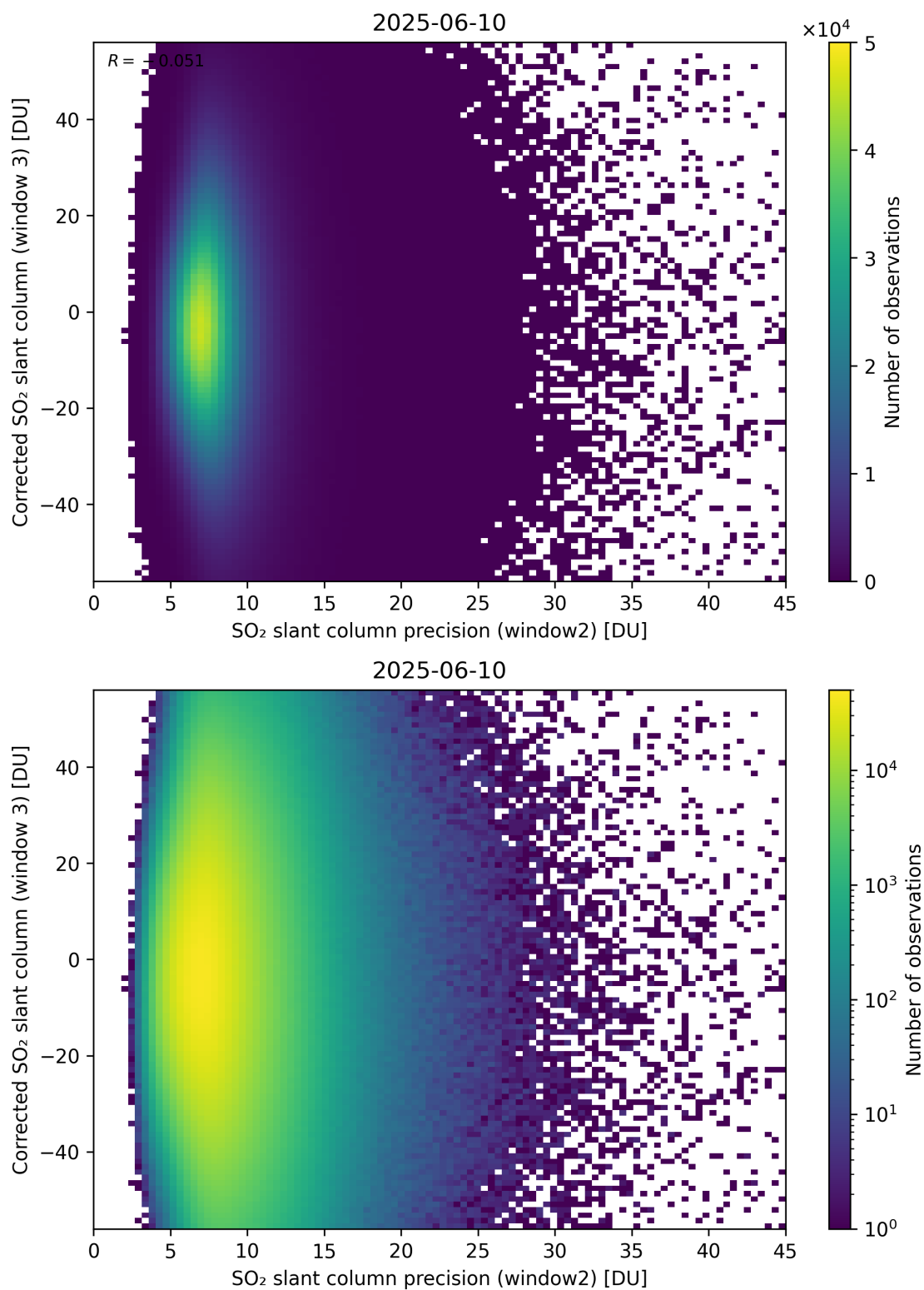
Figure 298: Scatter density plot of “SO 2 slant column precision (window2)” against “Corrected SO 2 slant column (window 3)” for 2025-06-09 to 2025-06-11.
