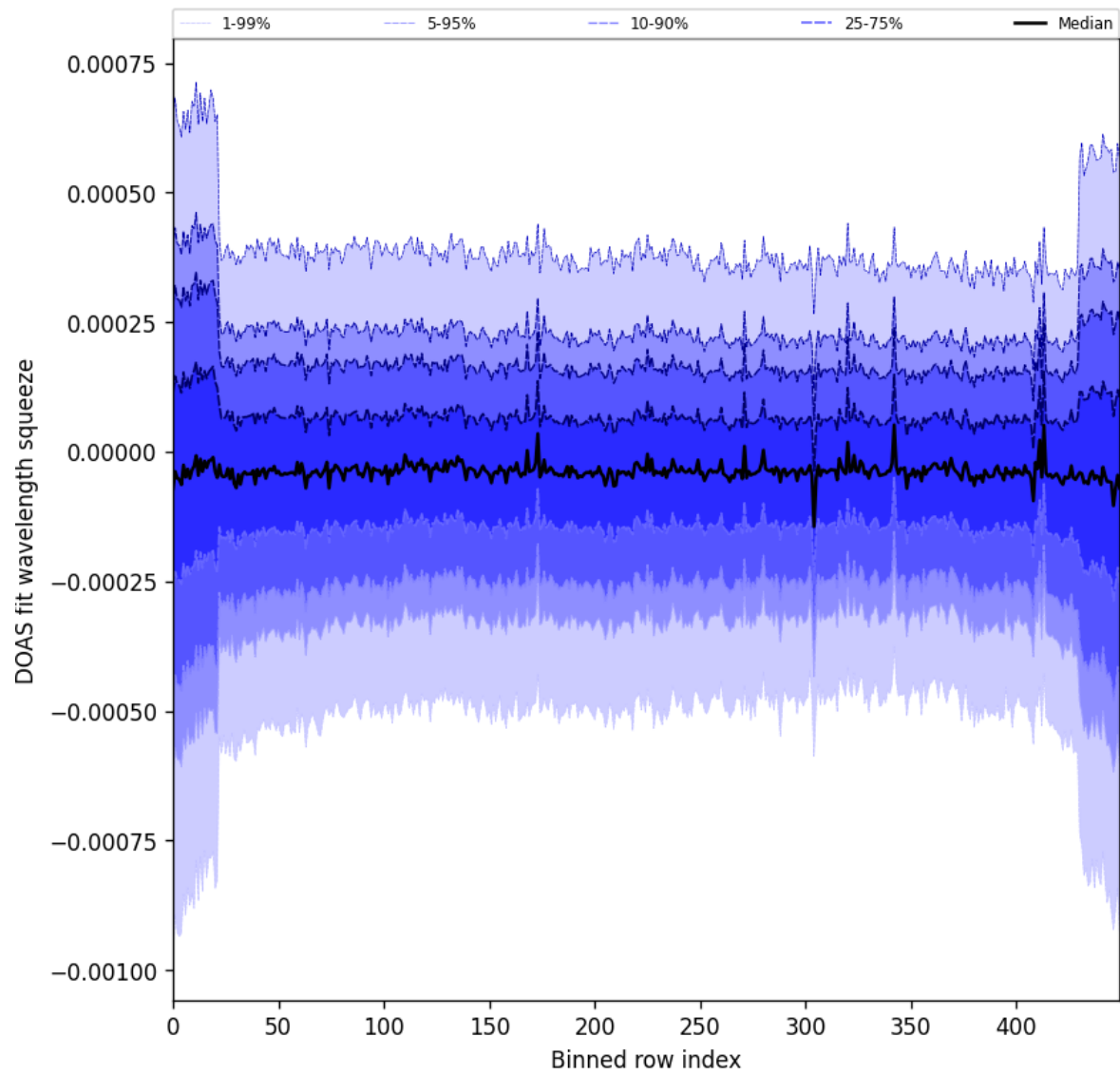
Figure 103: Along track statistics of “DOAS fit wavelength squeeze” for 2025-06-09 to 2025-06-11
