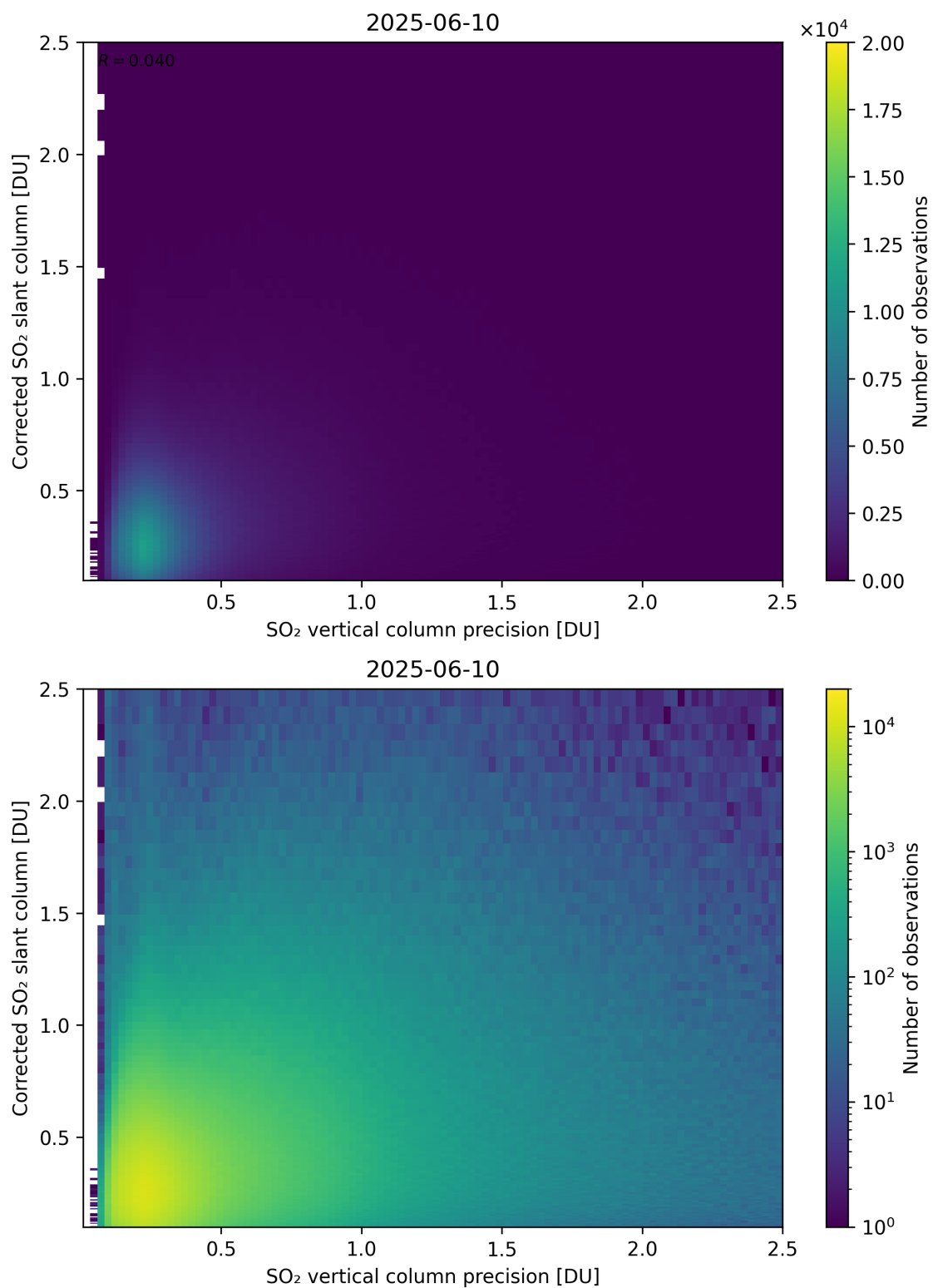
Figure 338: Scatter density plot of “SO 2 vertical column precision” against “Corrected SO 2 slant column” for 2025-06-09 to 2025-06-11.
