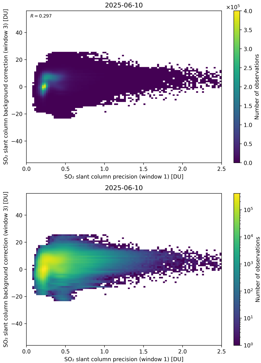
Figure 270: Scatter density plot of “SO 2 slant column precision (window 1)” against “SO 2 slant column background correction (window 3)” for 2025-06-09 to 2025-06-11.
