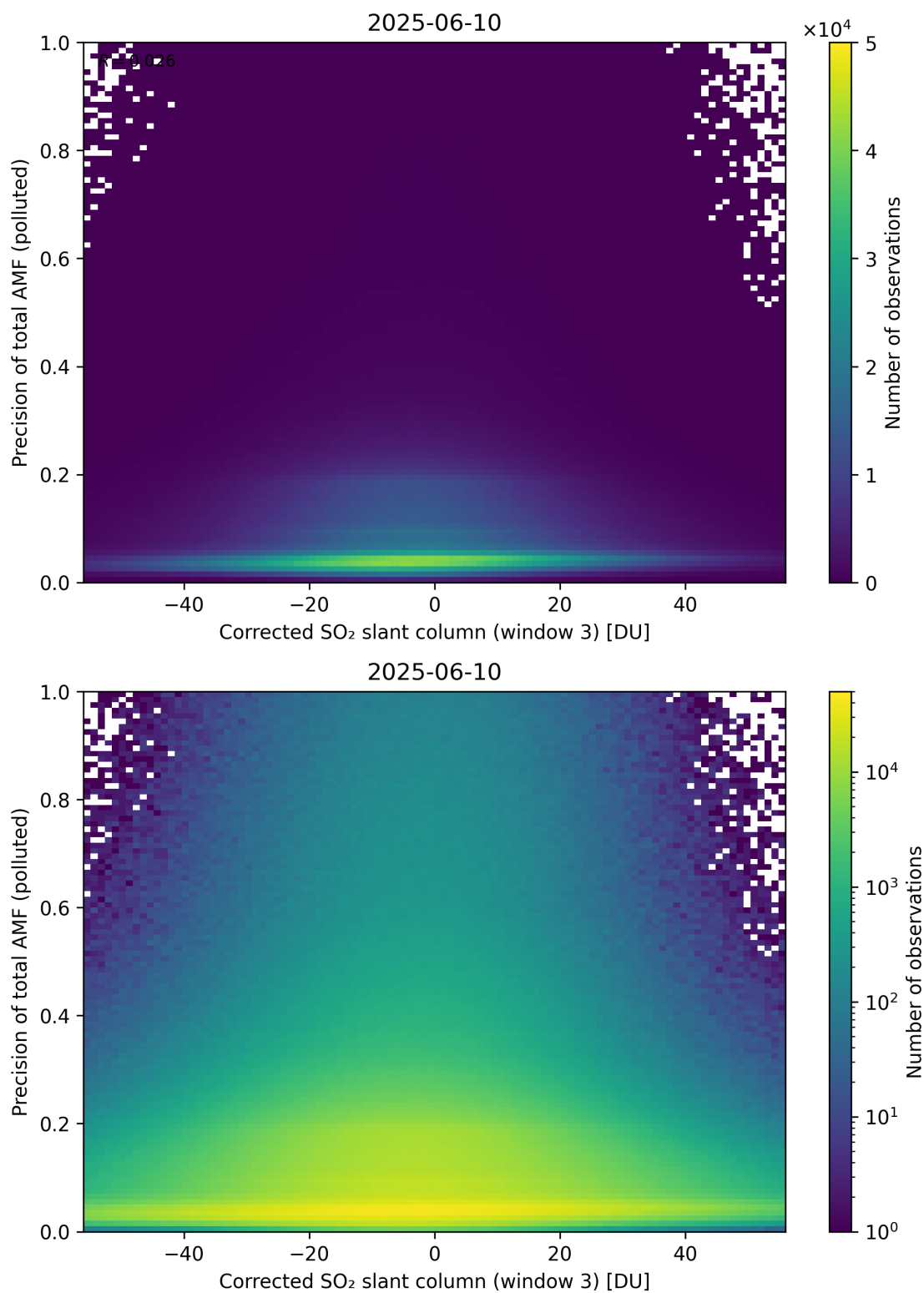
Figure 261: Scatter density plot of “Corrected SO 2 slant column (window 3)” against “Precision of total AMF (polluted)” for 2025-06-09 to 2025-06-11.
