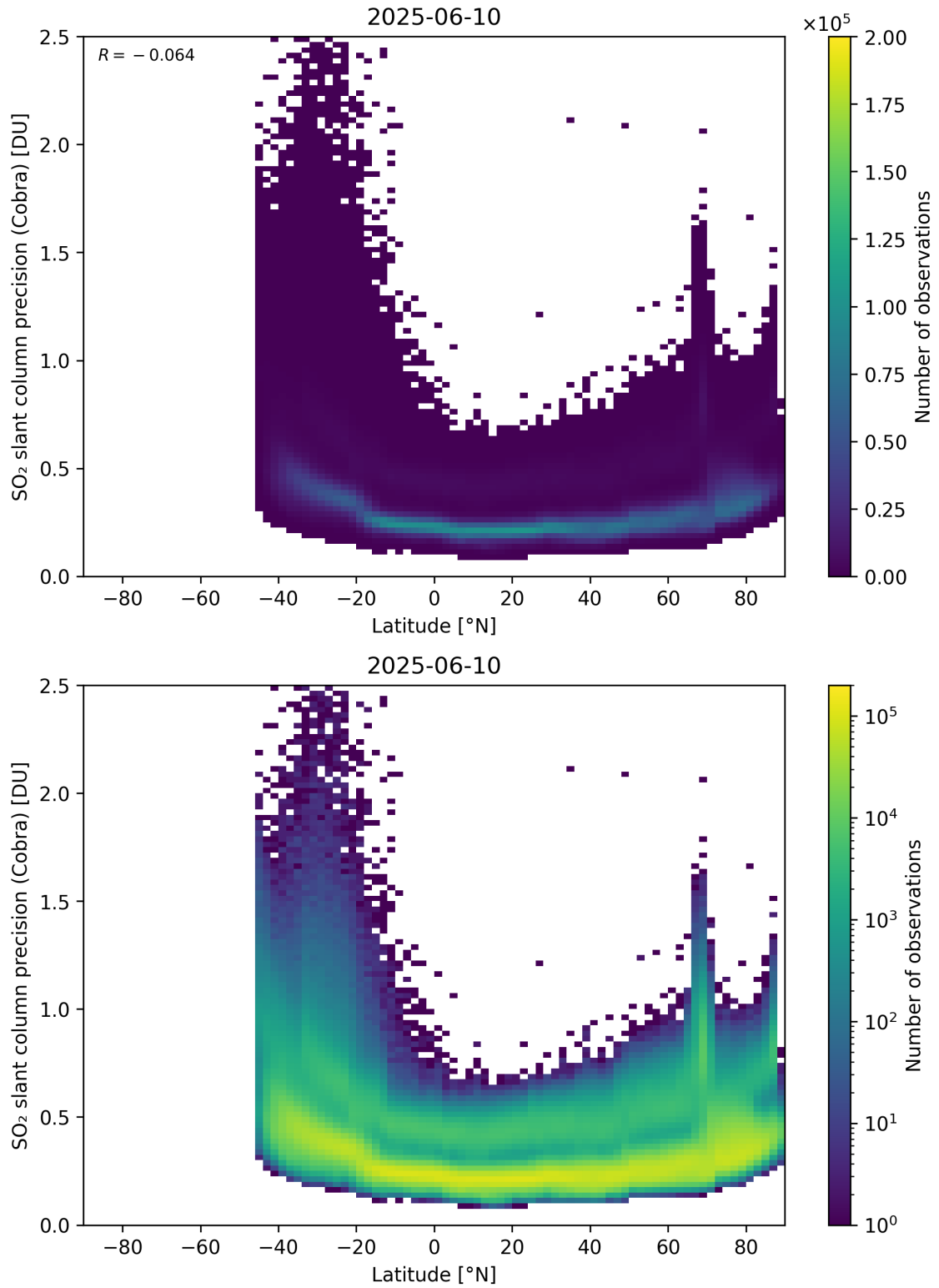
Figure 158: Scatter density plot of “Latitude” against “SO 2 slant column precision (Cobra)” for 2025-06-09 to 2025-06-11.
