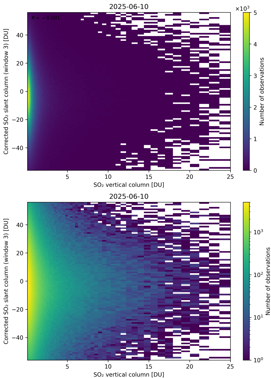
Figure 353: Scatter density plot of “SO 2 vertical column” against “Corrected SO 2 slant column (window 3)” for 2025-06-09 to 2025-06-11.
