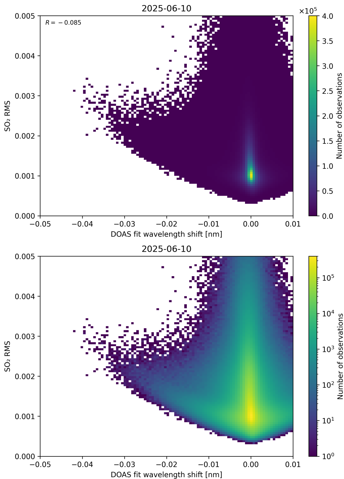
Figure 139: Scatter density plot of “DOAS fit wavelength shift” against “SO 2 RMS” for 2025-06-09 to 2025-06-11.
