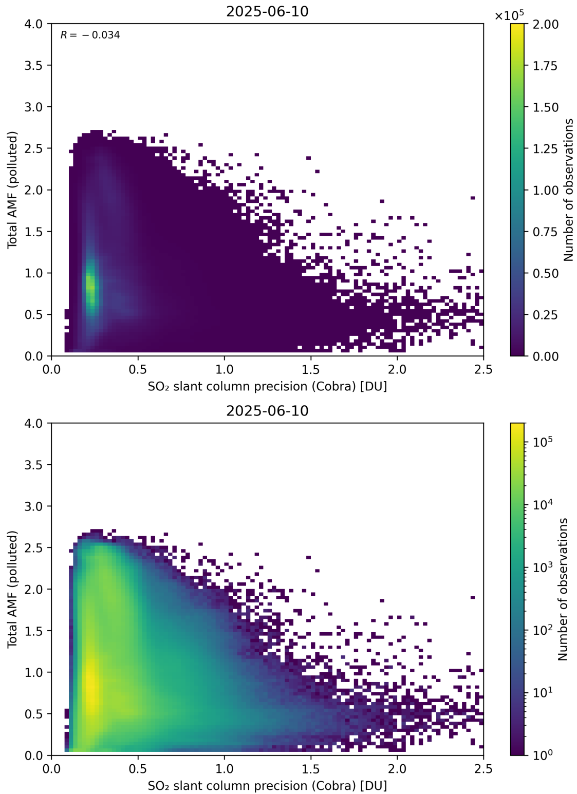
Figure 213: Scatter density plot of “SO 2 slant column precision (Cobra)” against “Total AMF (polluted)” for 2025-06-09 to 2025-06-11.
