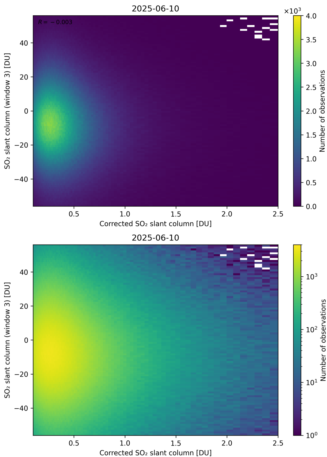
Figure 240: Scatter density plot of “Corrected SO 2 slant column” against “SO 2 slant column (window 3)” for 2025-06-09 to 2025-06-11.
