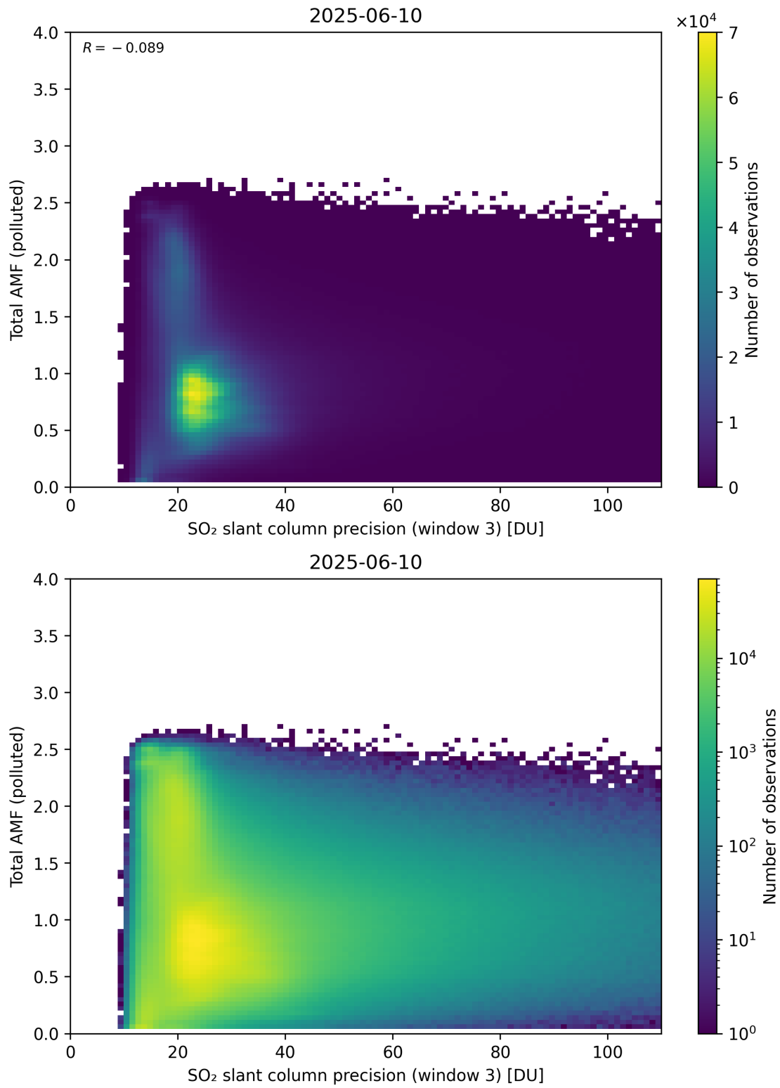
Figure 313: Scatter density plot of “SO 2 slant column precision (window 3)” against “Total AMF (polluted)” for 2025-06-09 to 2025-06-11.
