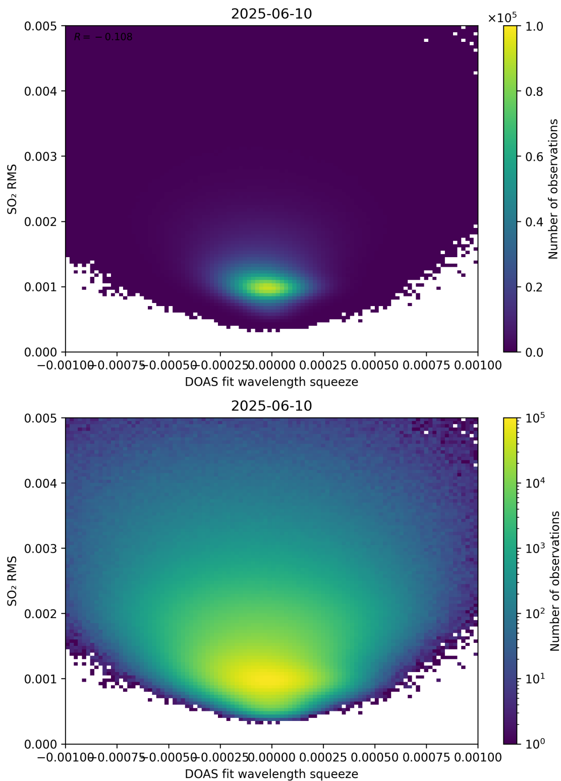
Figure 143: Scatter density plot of “DOAS fit wavelength squeeze” against “SO 2 RMS” for 2025-06-09 to 2025-06-11.
