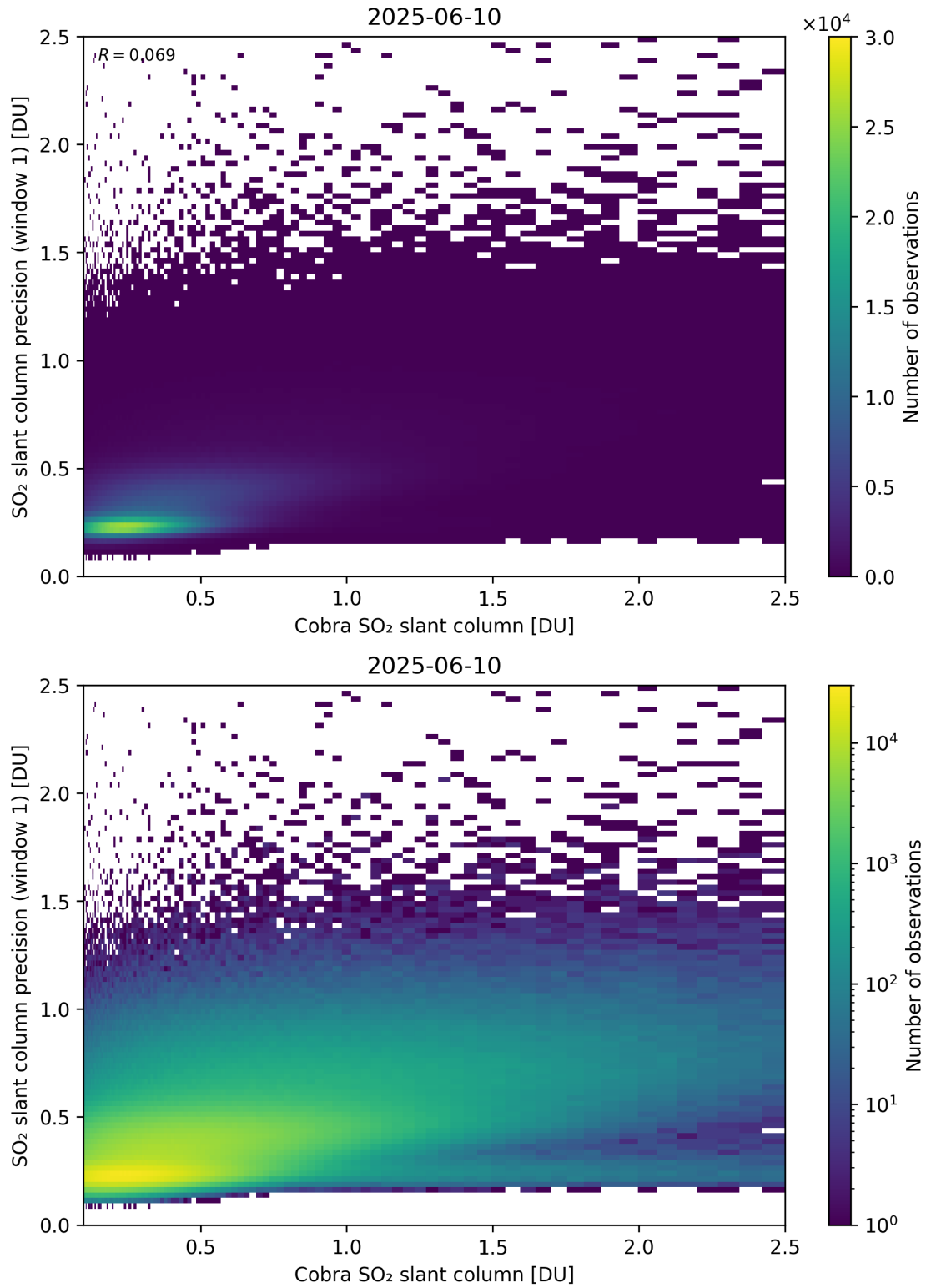
Figure 220: Scatter density plot of “Cobra SO 2 slant column” against “SO 2 slant column precision (window 1)” for 2025-06-09 to 2025-06-11.
