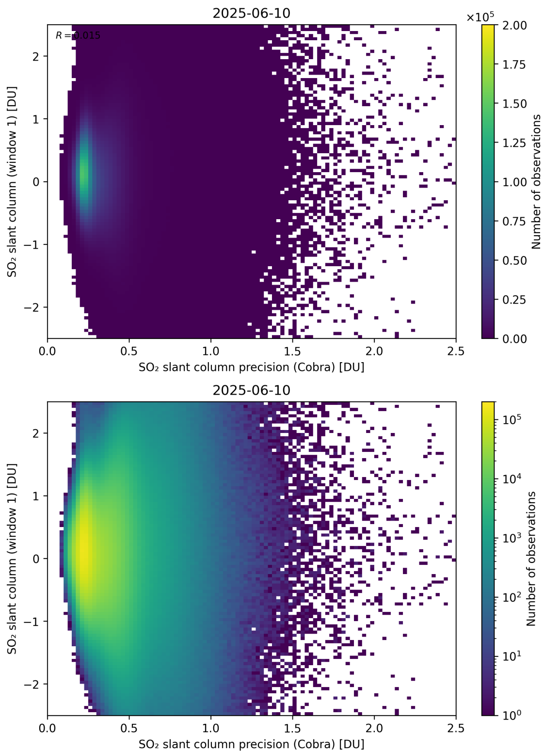
Figure 208: Scatter density plot of “SO 2 slant column precision (Cobra)” against “SO 2 slant column (window 1)” for 2025-06-09 to 2025-06-11.
