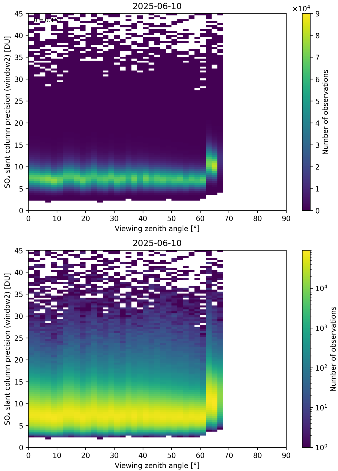
Figure 378: Scatter density plot of “Viewing zenith angle” against “SO 2 slant column precision (window2)” for 2025-06-09 to 2025-06-11.
