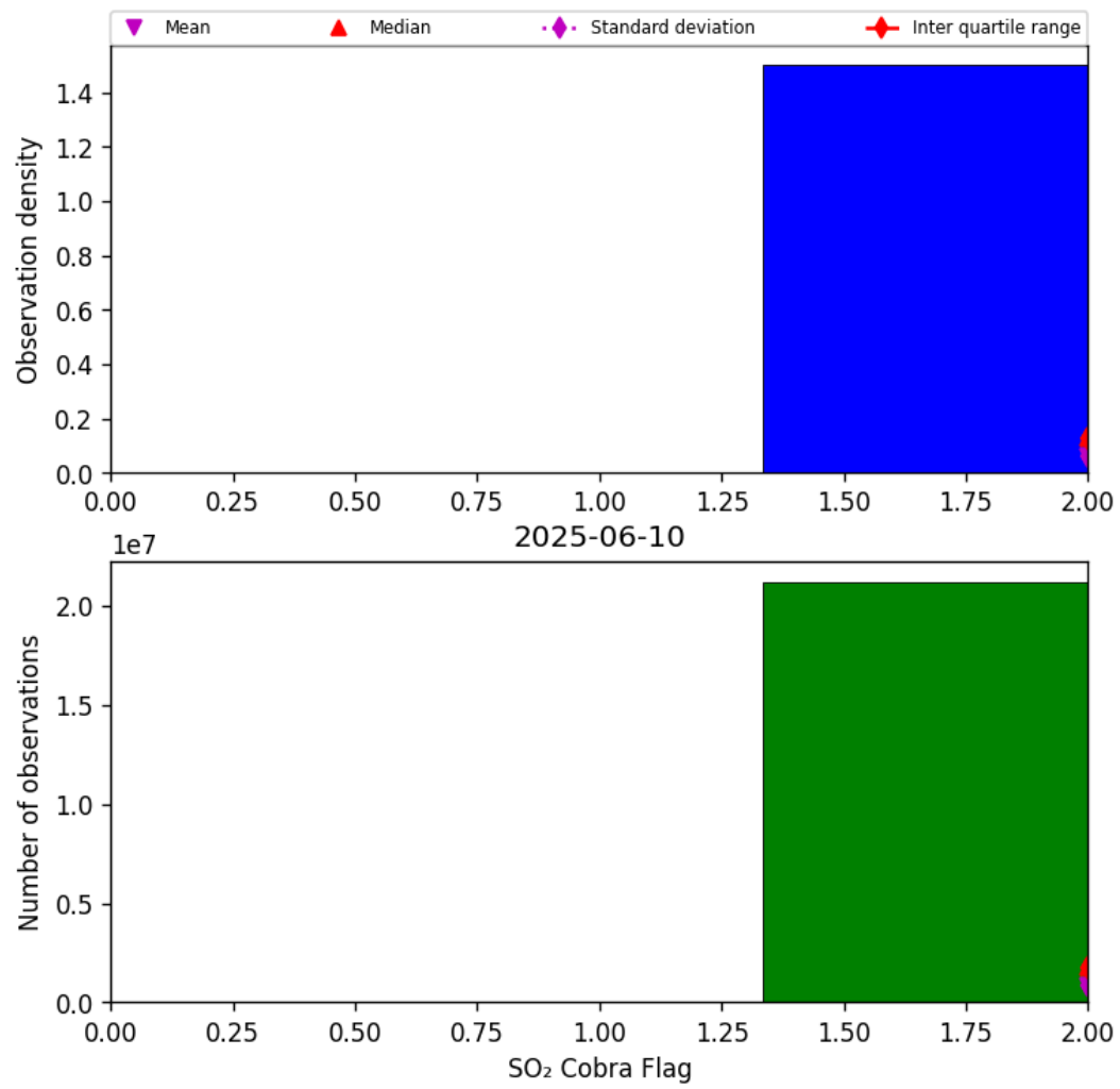
Figure 75: Histogram of “SO 2 Cobra Flag” for 2025-06-09 to 2025-06-11
