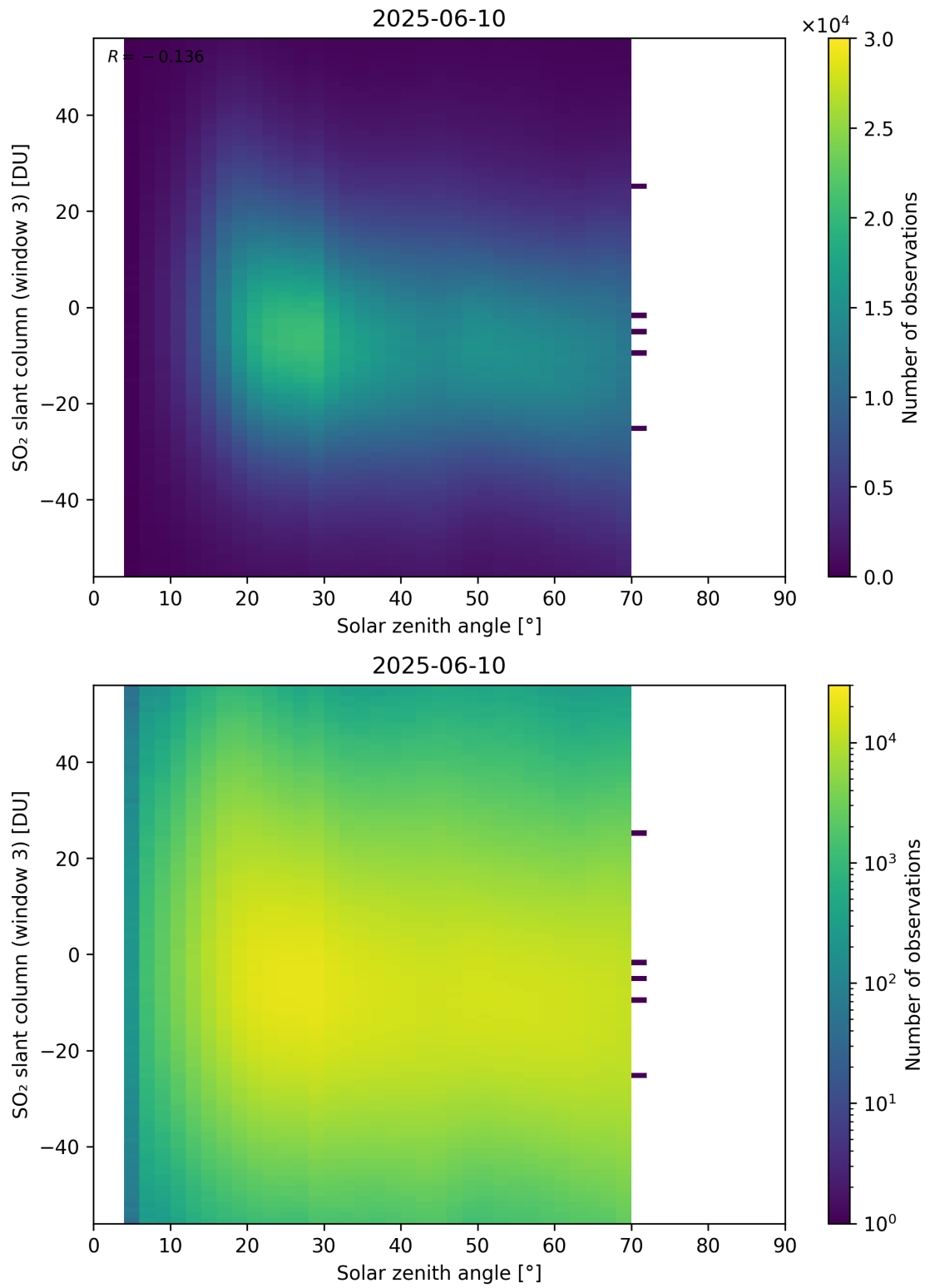
Figure 187: Scatter density plot of “Solar zenith angle” against “SO 2 slant column (window 3)” for 2025-06-09 to 2025-06-11.
