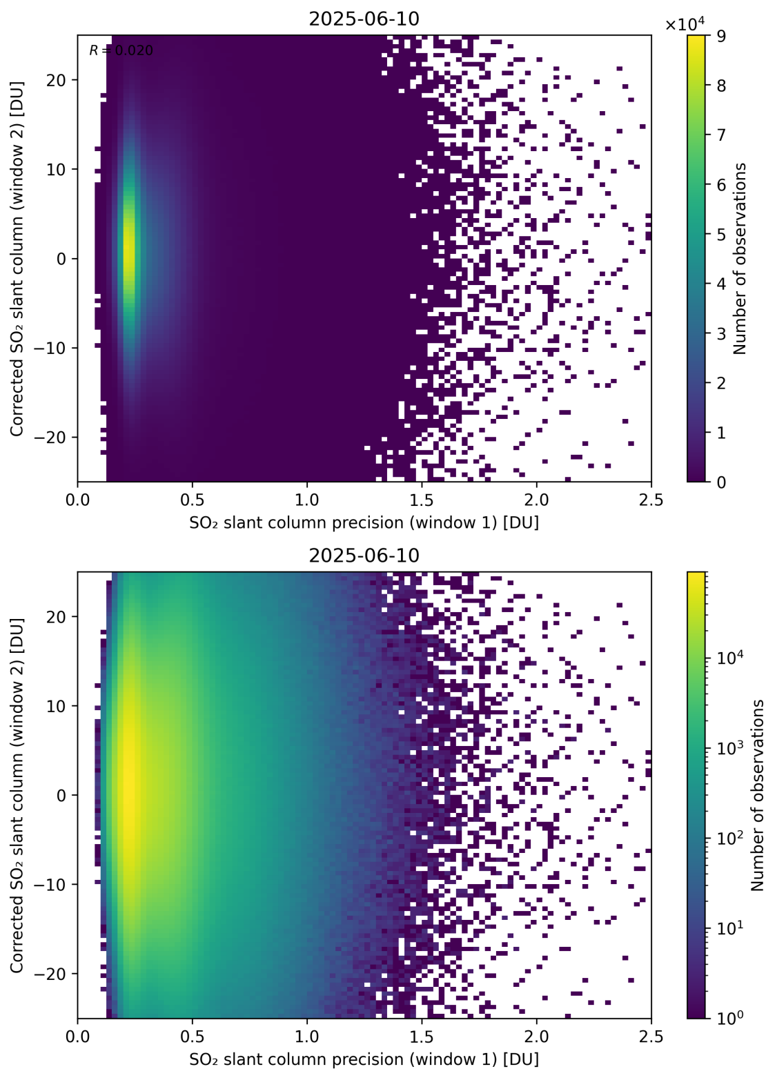
Figure 275: Scatter density plot of “SO 2 slant column precision (window 1)” against “Corrected SO 2 slant column (window 2)” for 2025-06-09 to 2025-06-11.
