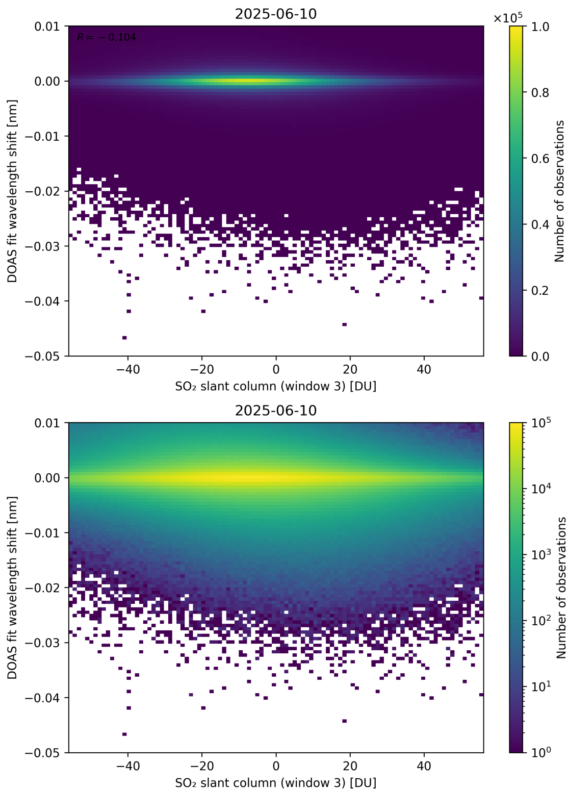
Figure 304: Scatter density plot of “SO 2 slant column (window 3)” against “DOAS fit wavelength shift” for 2025-06-09 to 2025-06-11.
