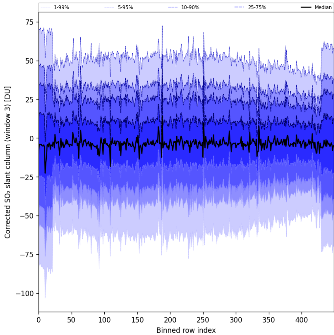
Figure 99: Along track statistics of “Corrected SO 2 slant column (window 3)” for 2025-06-09 to 2025-06-11
