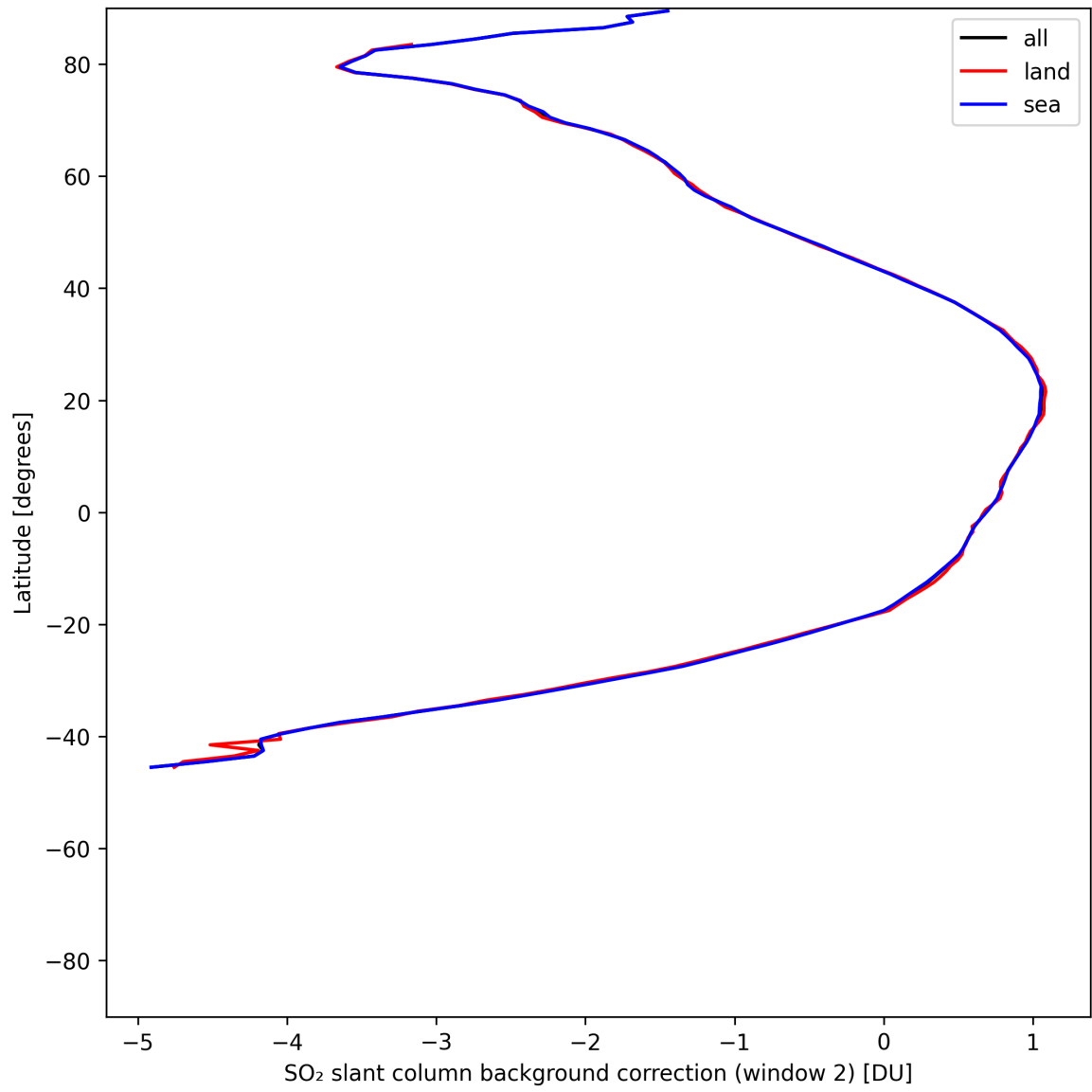
Figure 44: Zonal average of “SO 2 slant column background correction (window 2)” for 2025-06-09 to 2025-06-11.
