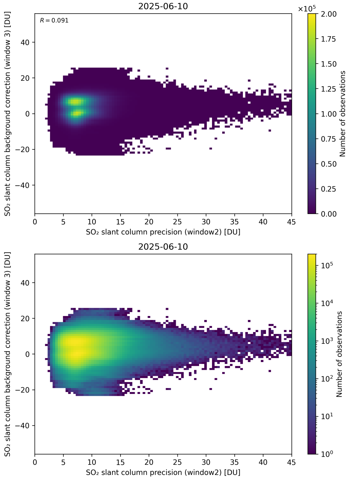
Figure 292: Scatter density plot of “SO 2 slant column precision (window2)” against “SO 2 slant column background correction (window 3)” for 2025-06-09 to 2025-06-11.
