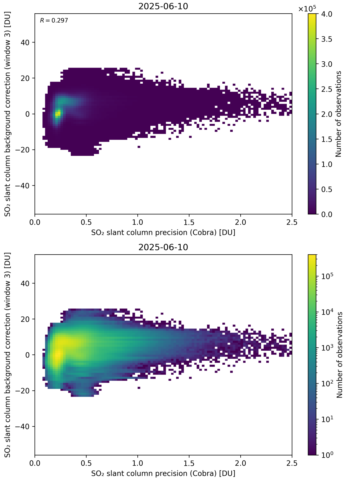
Figure 201: Scatter density plot of “SO 2 slant column precision (Cobra)” against “SO 2 slant column background correction (window 3)” for 2025-06-09 to 2025-06-11.
