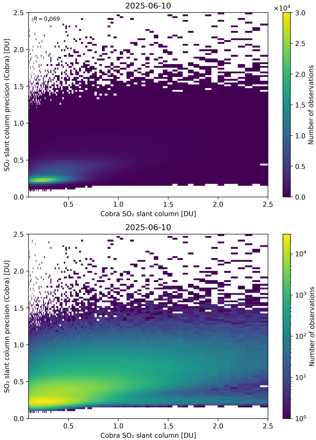
Figure 216: Scatter density plot of “Cobra SO 2 slant column” against “SO 2 slant column precision (Cobra)” for 2025-06-09 to 2025-06-11.
