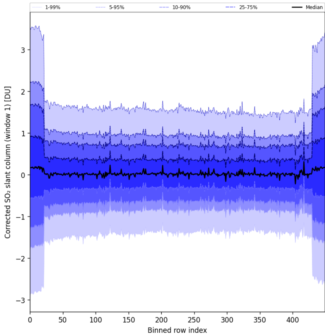
Figure 91: Along track statistics of “Corrected SO 2 slant column (window 1)” for 2025-06-09 to 2025-06-11
