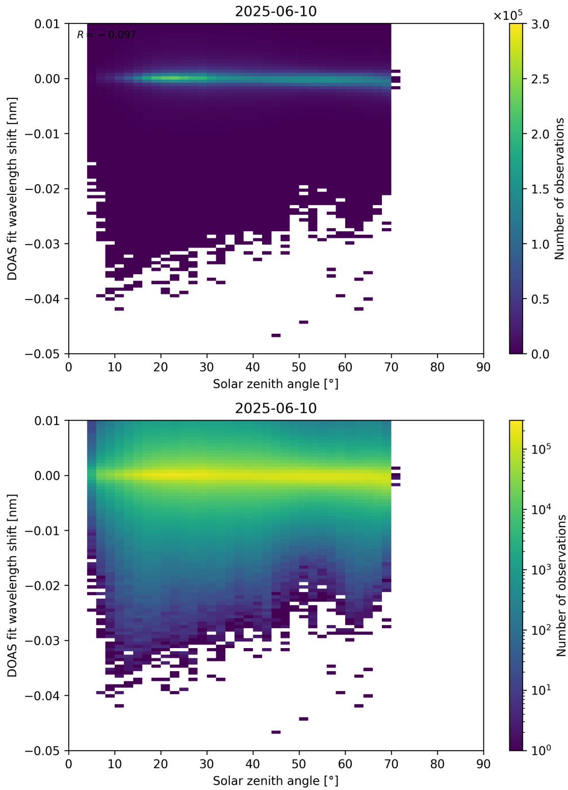
Figure 174: Scatter density plot of “Solar zenith angle” against “DOAS fit wavelength shift” for 2025-06-09 to 2025-06-11.
