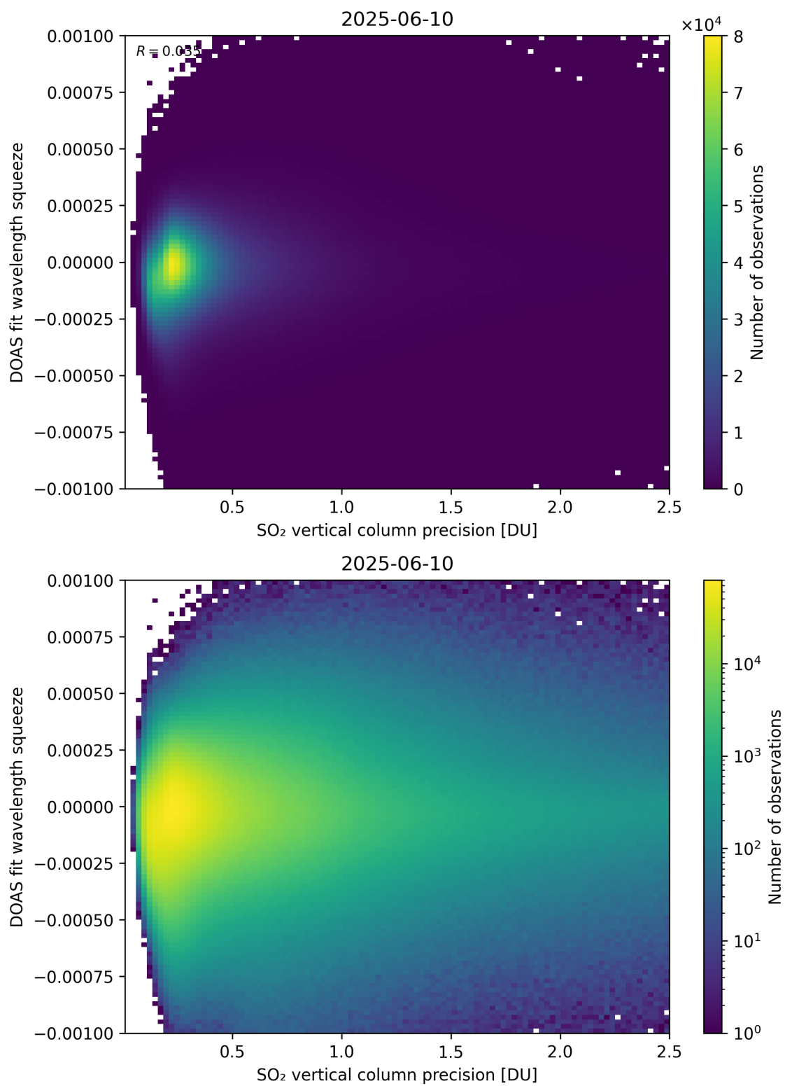
Figure 333: Scatter density plot of “SO 2 vertical column precision” against “DOAS fit wavelength squeeze” for 2025-06-09 to 2025-06-11.
