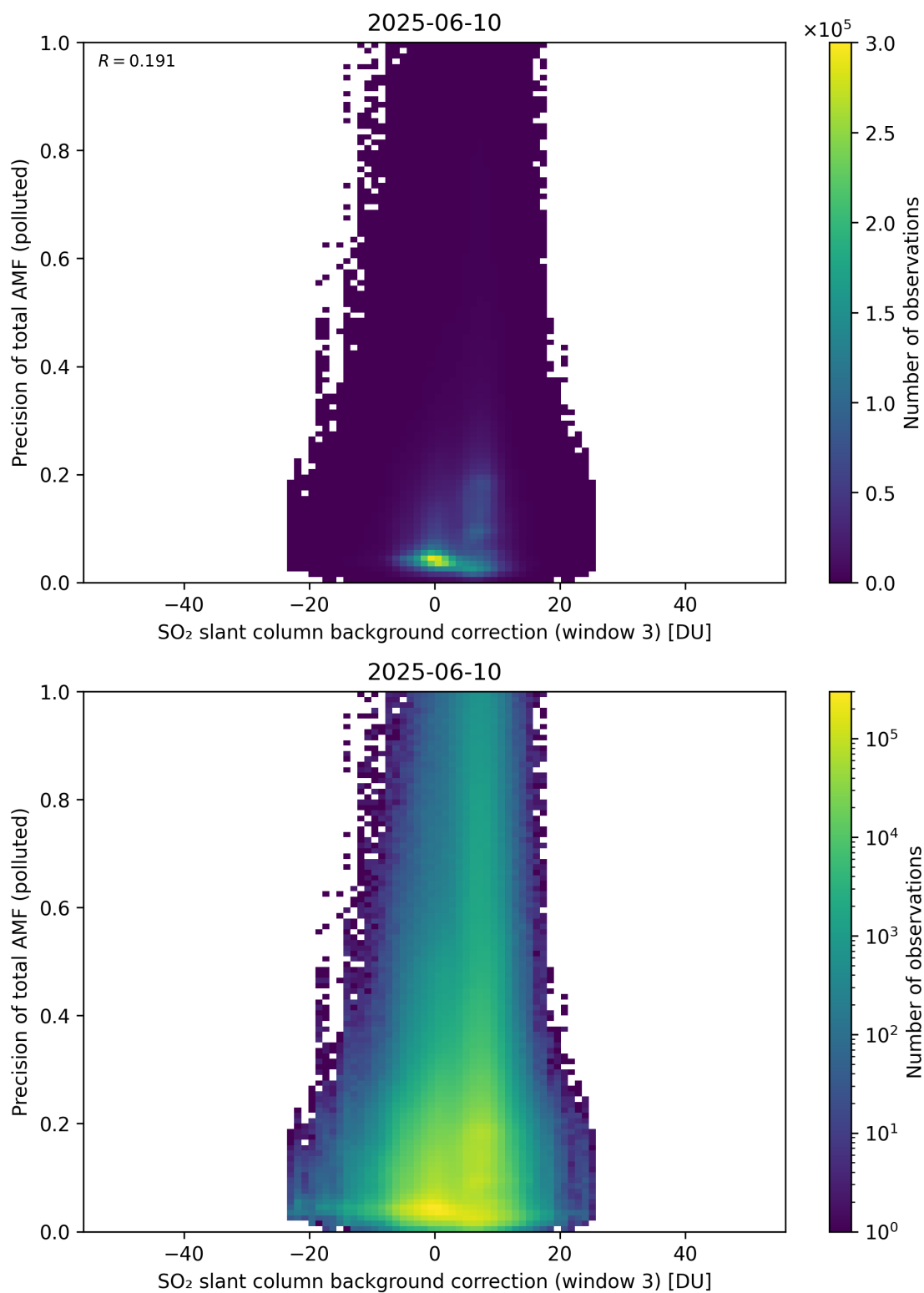
Figure 137: Scatter density plot of “SO 2 slant column background correction (window 3)” against “Precision of total AMF (polluted)” for 2025-06-09 to 2025-06-11.
