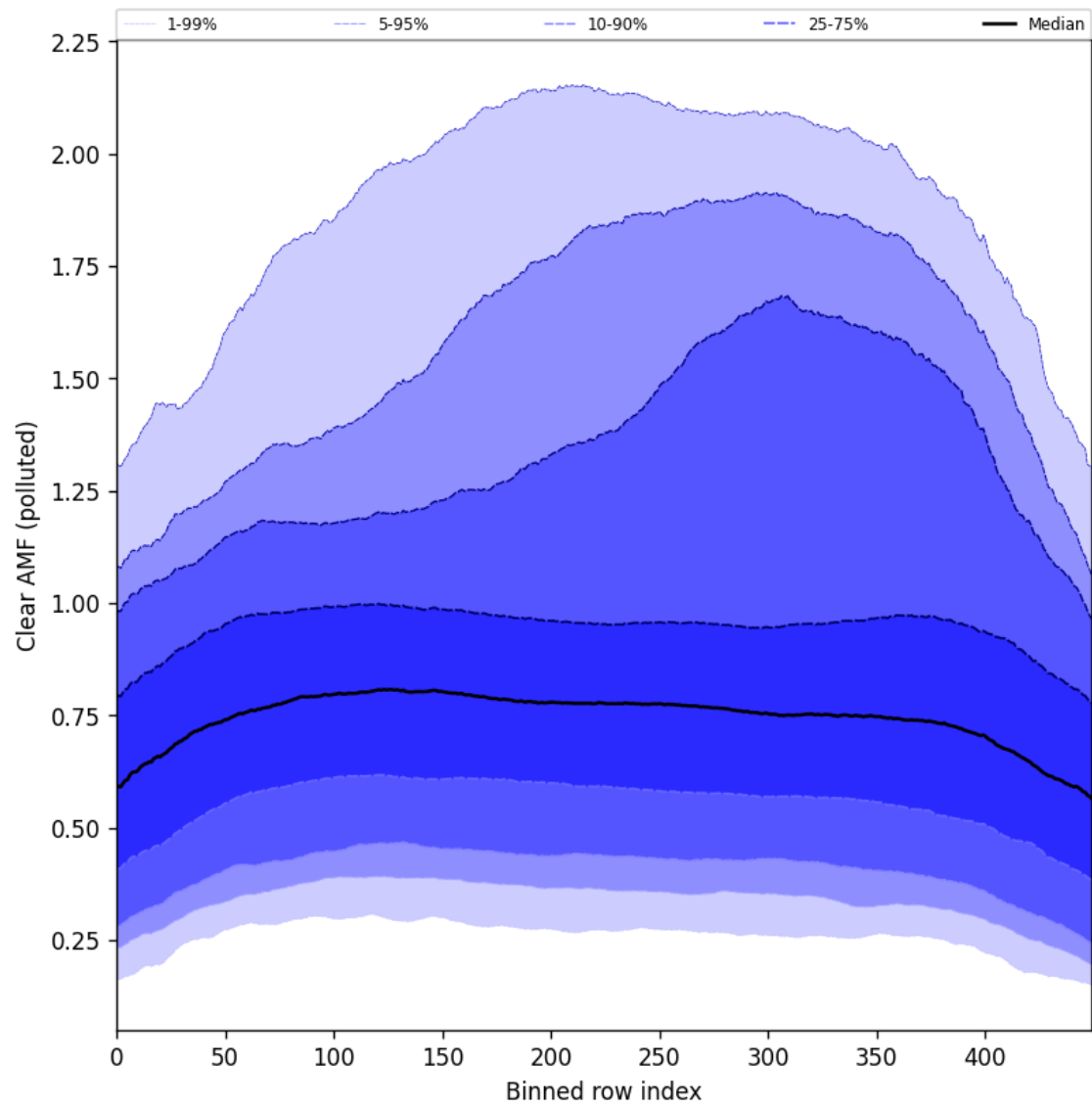
Figure 107: Along track statistics of “Clear AMF (polluted)” for 2025-06-09 to 2025-06-11
