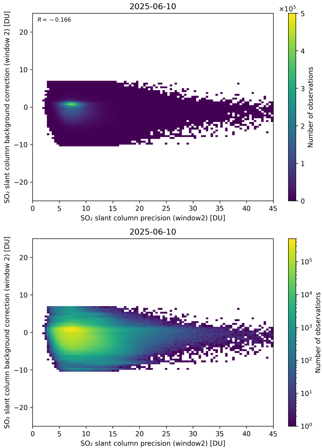
Figure 291: Scatter density plot of “SO 2 slant column precision (window2)” against “SO 2 slant column background correction (window 2)” for 2025-06-09 to 2025-06-11.
