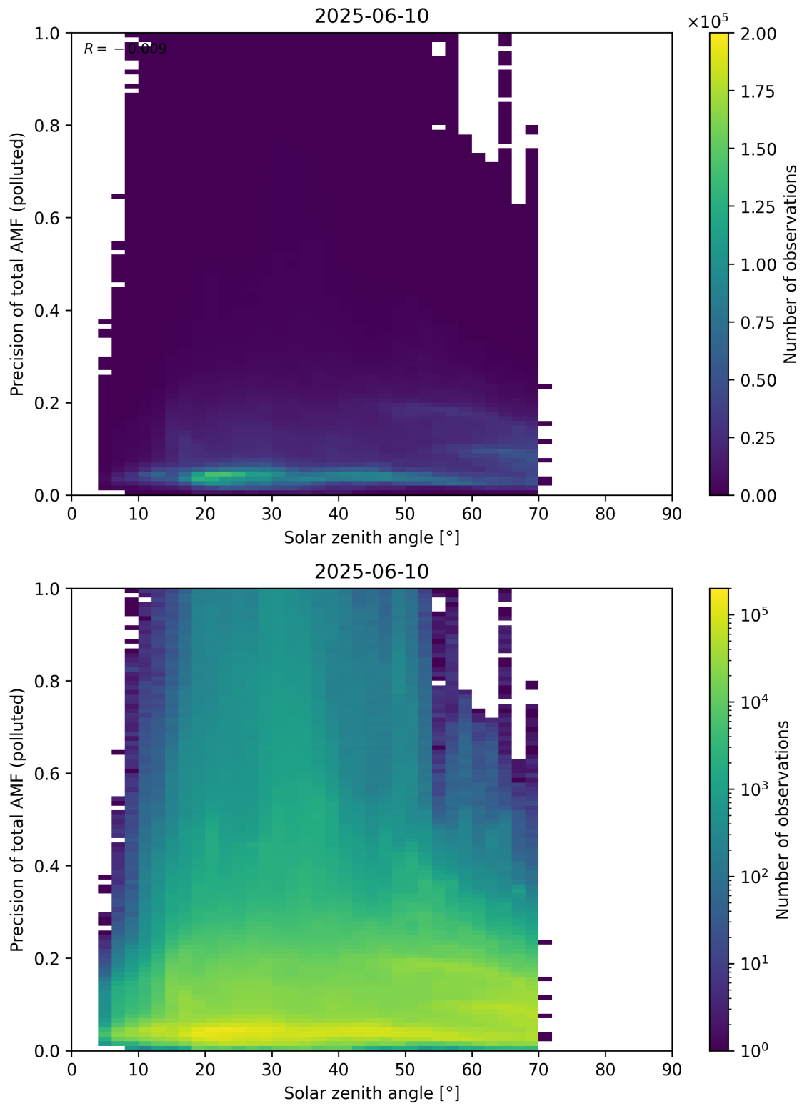
Figure 190: Scatter density plot of “Solar zenith angle” against “Precision of total AMF (polluted)” for 2025-06-09 to 2025-06-11.
