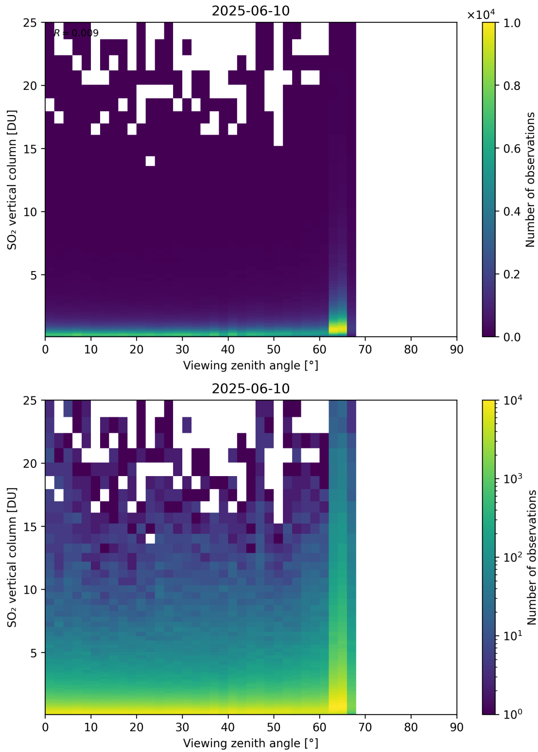
Figure 383: Scatter density plot of “Viewing zenith angle” against “SO 2 vertical column” for 2025-06-09 to 2025-06-11.
