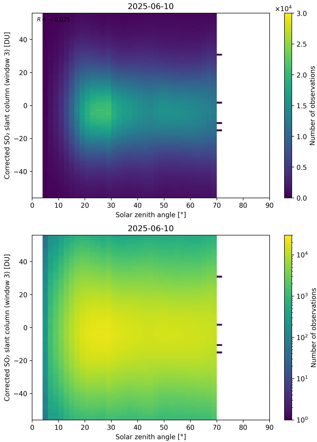
Figure 183: Scatter density plot of “Solar zenith angle” against “Corrected SO 2 slant column (window 3)” for 2025-06-09 to 2025-06-11.
