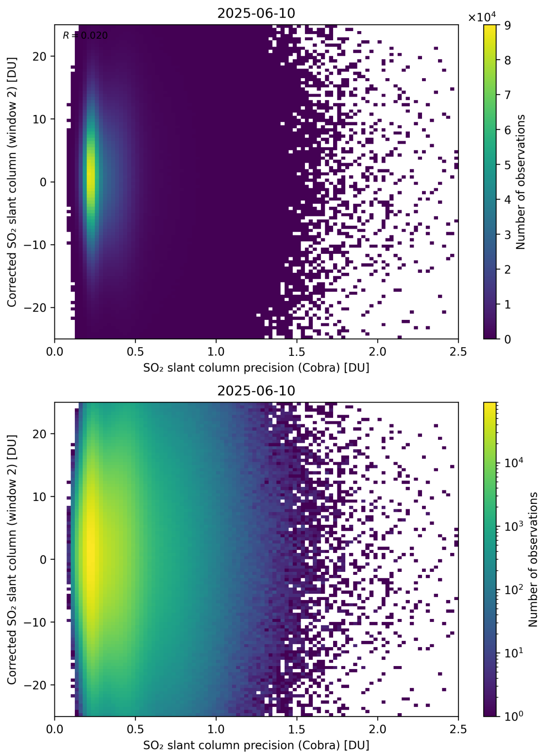
Figure 206: Scatter density plot of “SO 2 slant column precision (Cobra)” against “Corrected SO 2 slant column (window 2)” for 2025-06-09 to 2025-06-11.
