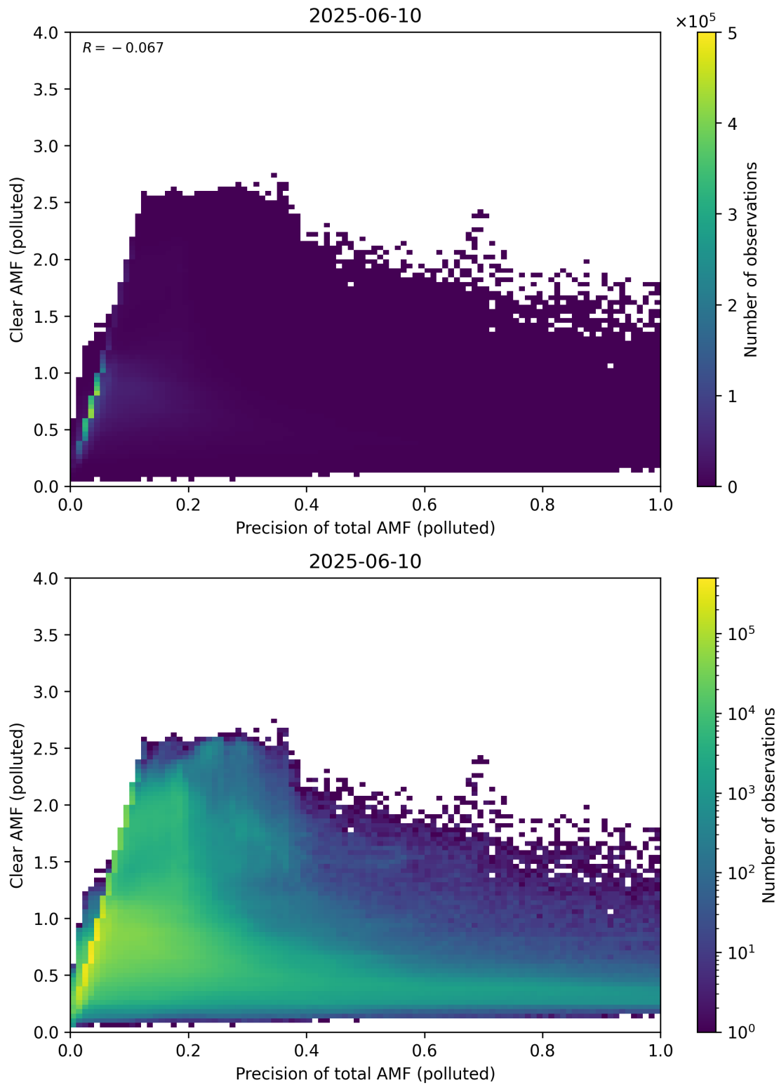
Figure 320: Scatter density plot of “Precision of total AMF (polluted)” against “Clear AMF (polluted)” for 2025-06-09 to 2025-06-11.
