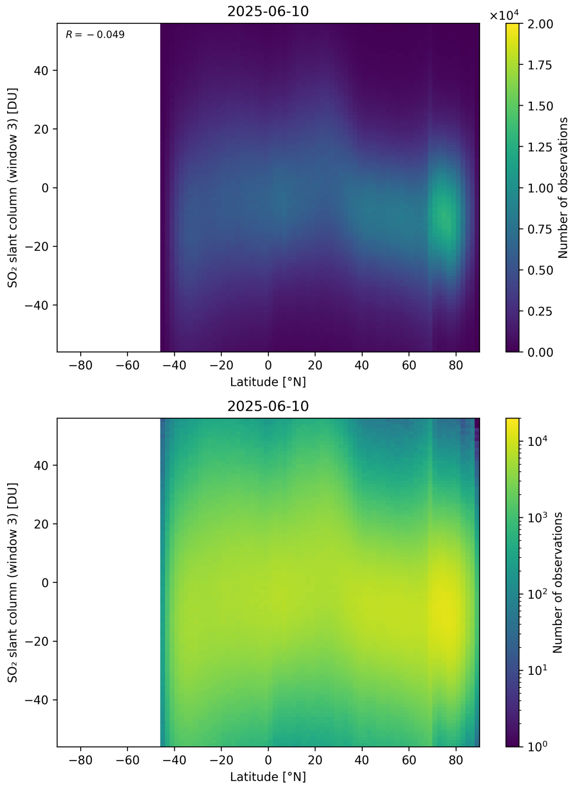
Figure 165: Scatter density plot of “Latitude” against “SO 2 slant column (window 3)” for 2025-06-09 to 2025-06-11.
