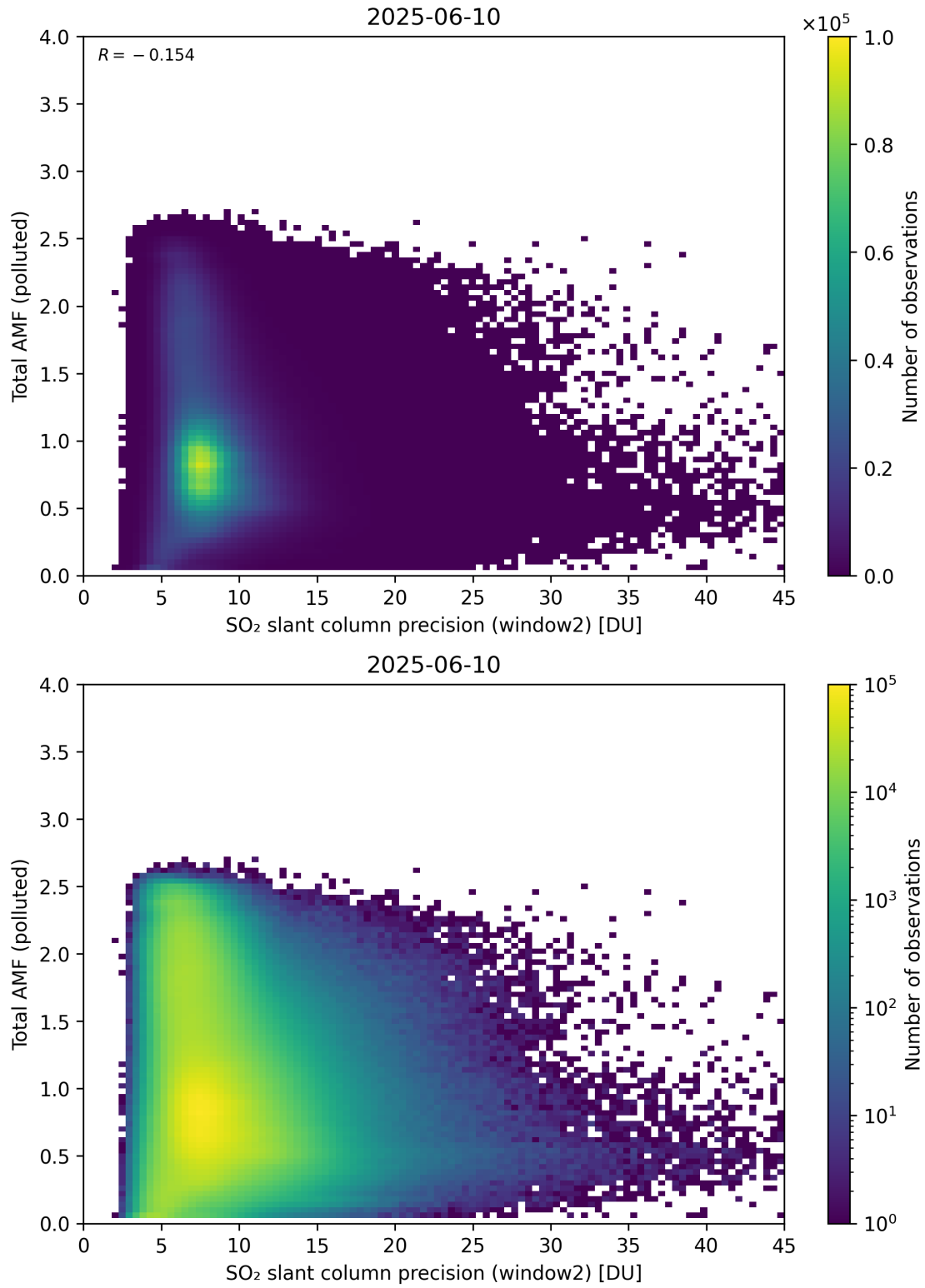
Figure 301: Scatter density plot of “SO 2 slant column precision (window2)” against “Total AMF (polluted)” for 2025-06-09 to 2025-06-11.
