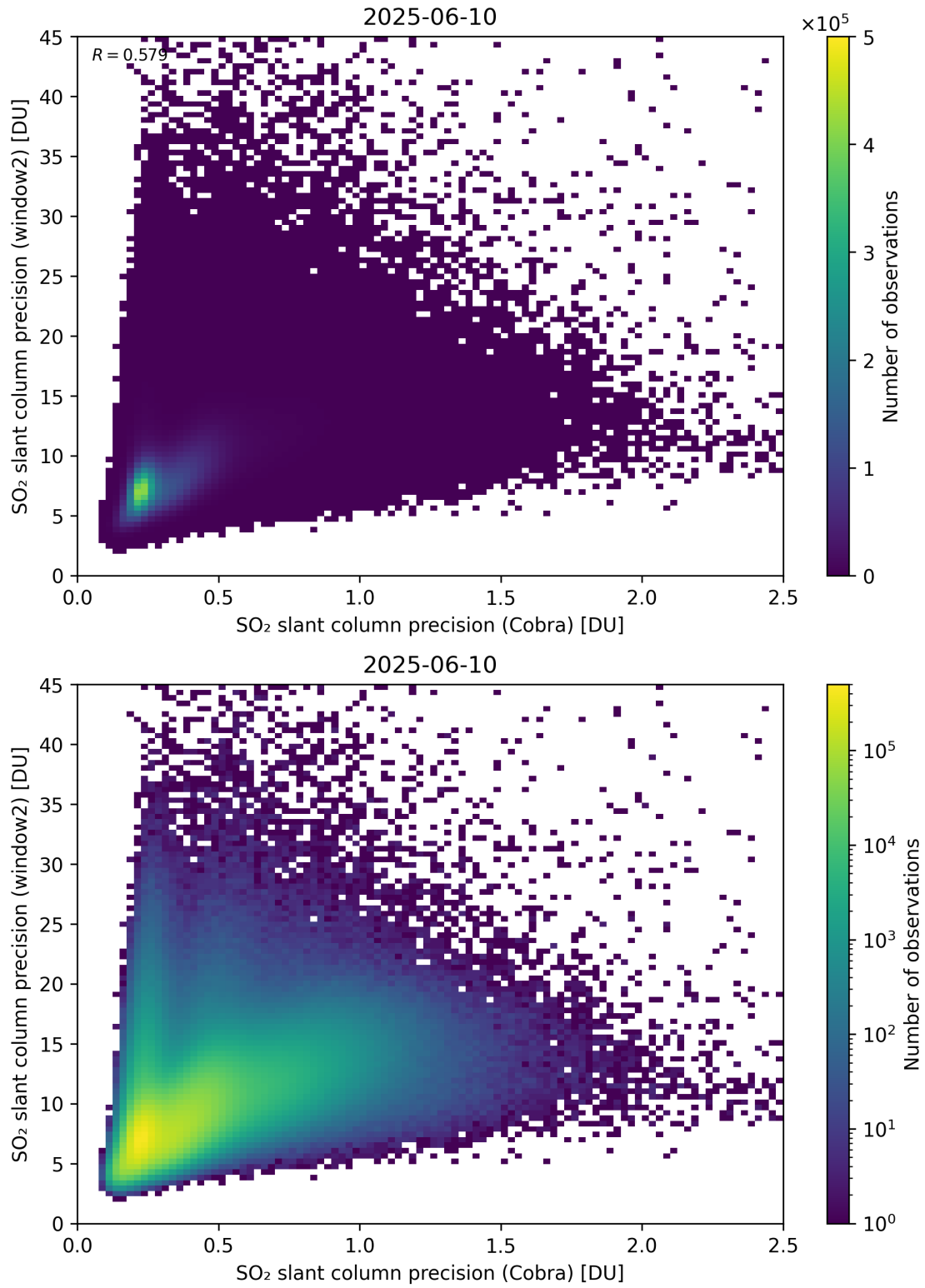
Figure 210: Scatter density plot of “SO 2 slant column precision (Cobra)” against “SO 2 slant column precision (window2)” for 2025-06-09 to 2025-06-11.
