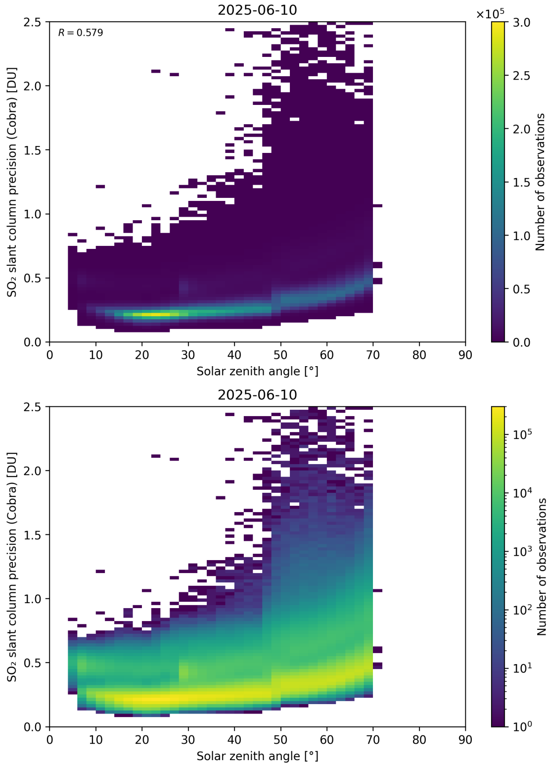
Figure 180: Scatter density plot of “Solar zenith angle” against “SO 2 slant column precision (Cobra)” for 2025-06-09 to 2025-06-11.
