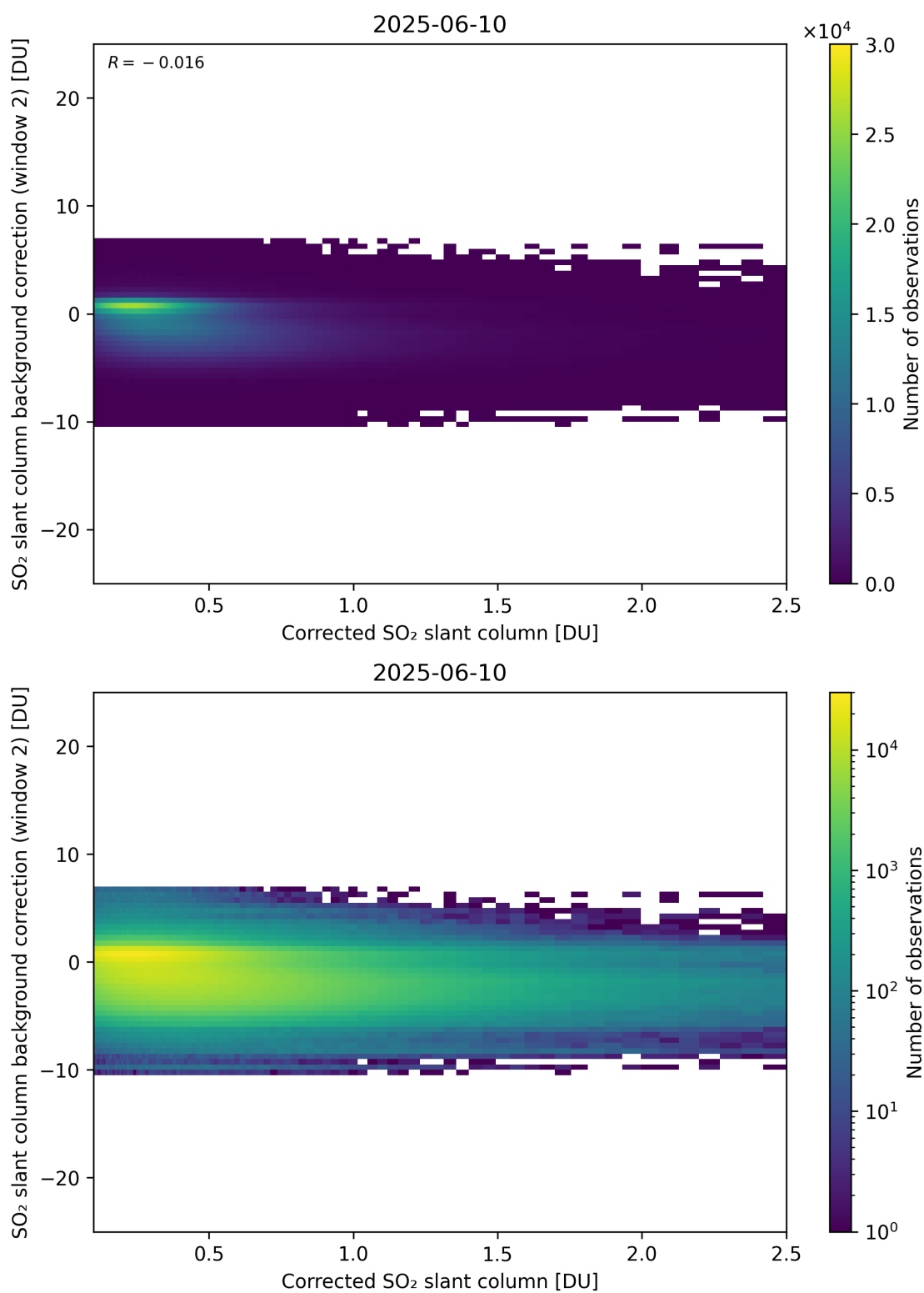
Figure 227: Scatter density plot of “Corrected SO 2 slant column” against “SO 2 slant column background correction (window 2)” for 2025-06-09 to 2025-06-11.
