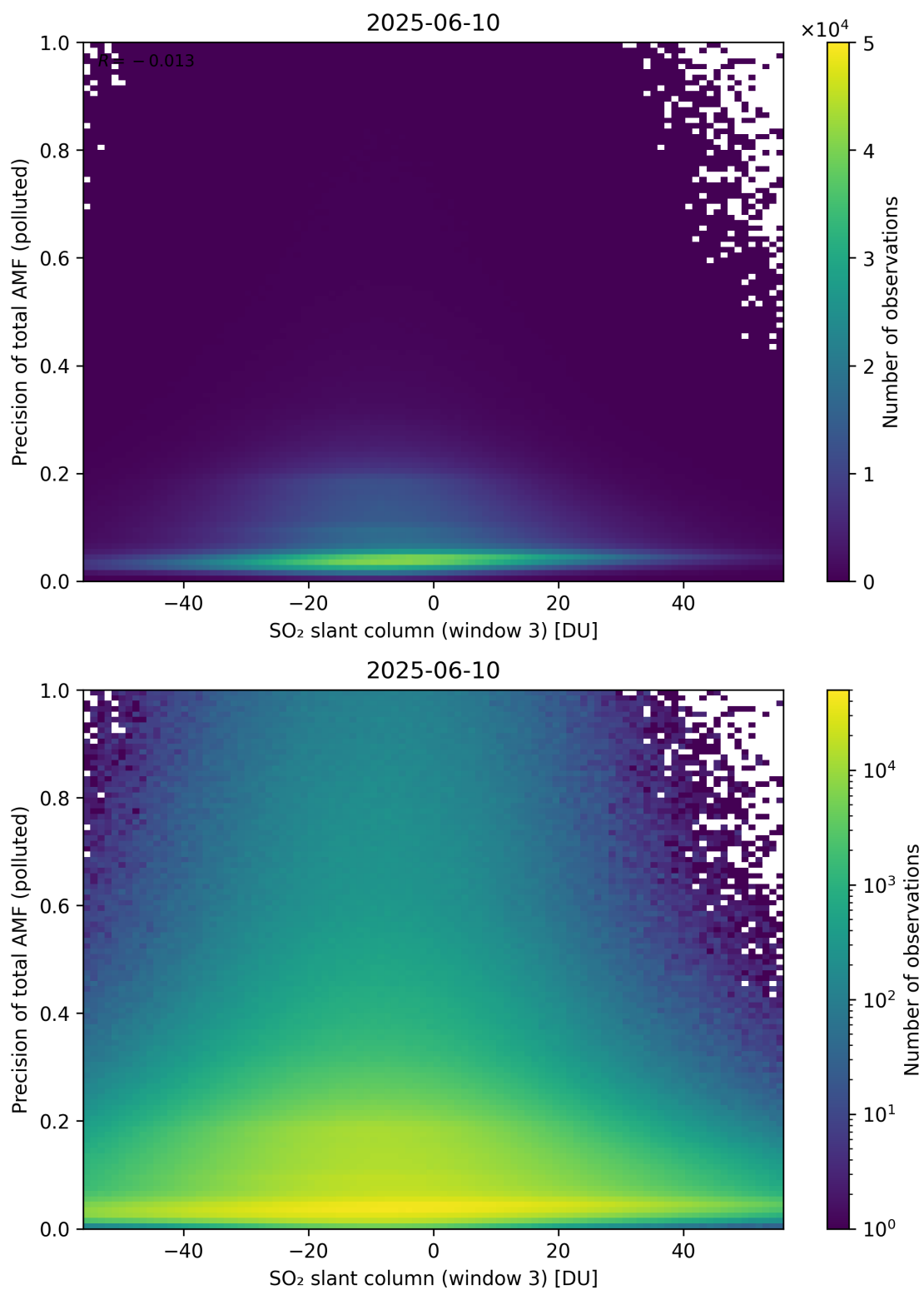
Figure 319: Scatter density plot of “SO 2 slant column (window 3)” against “Precision of total AMF (polluted)” for 2025-06-09 to 2025-06-11.
