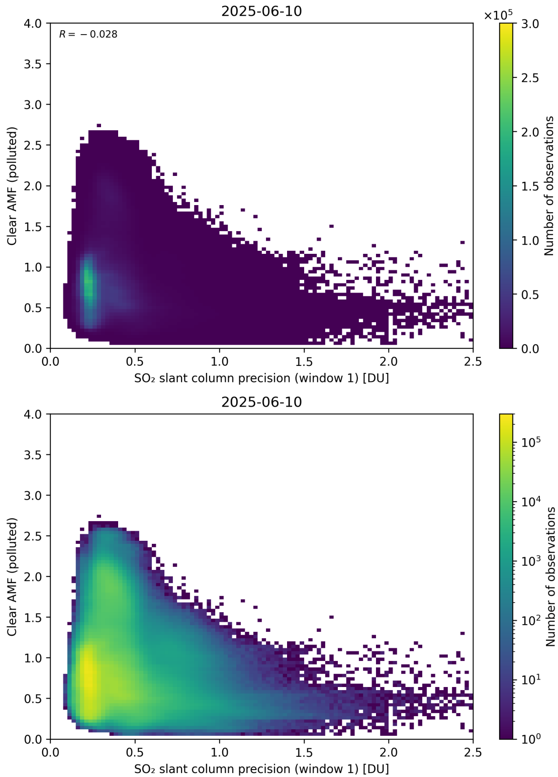
Figure 274: Scatter density plot of “SO 2 slant column precision (window 1)” against “Clear AMF (polluted)” for 2025-06-09 to 2025-06-11.
