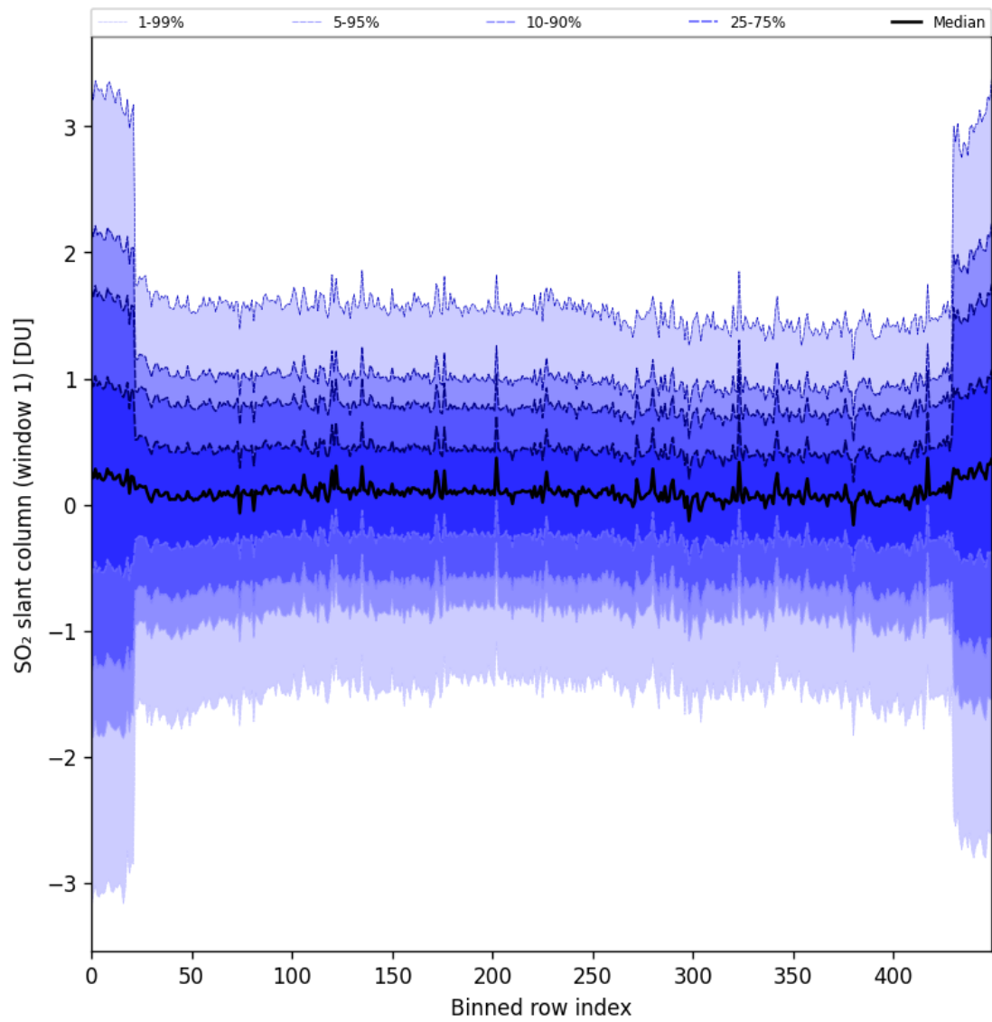
Figure 89: Along track statistics of “SO 2 slant column (window 1)” for 2025-06-09 to 2025-06-11
