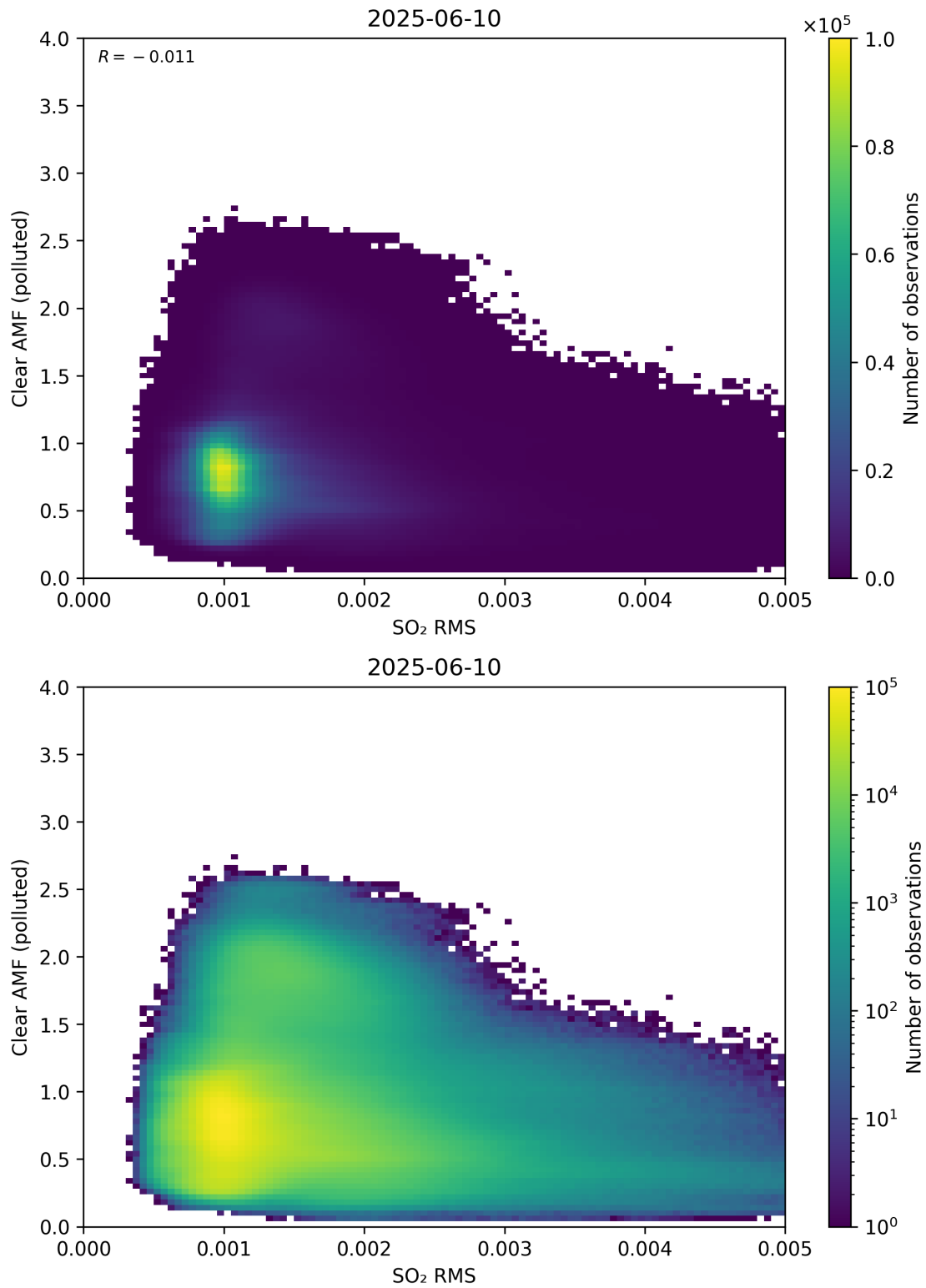
Figure 147: Scatter density plot of “SO 2 RMS” against “Clear AMF (polluted)” for 2025-06-09 to 2025-06-11.
