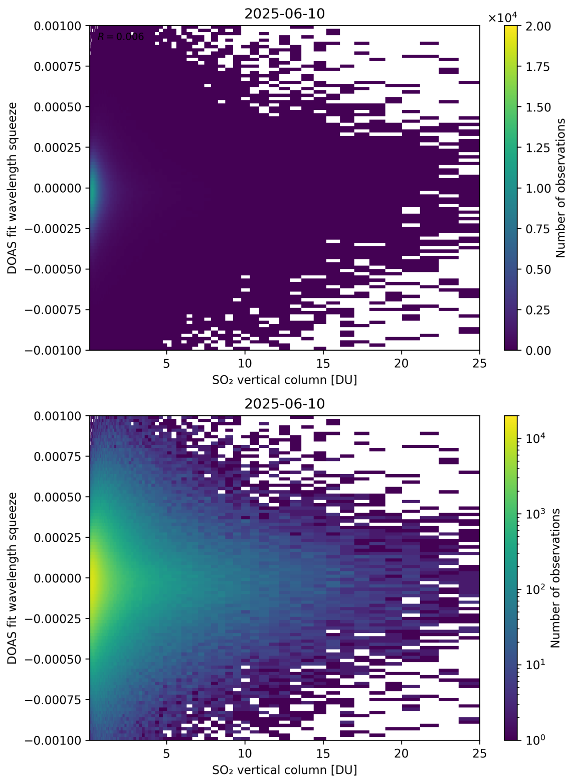
Figure 327: Scatter density plot of “SO 2 vertical column” against “DOAS fit wavelength squeeze” for 2025-06-09 to 2025-06-11.
