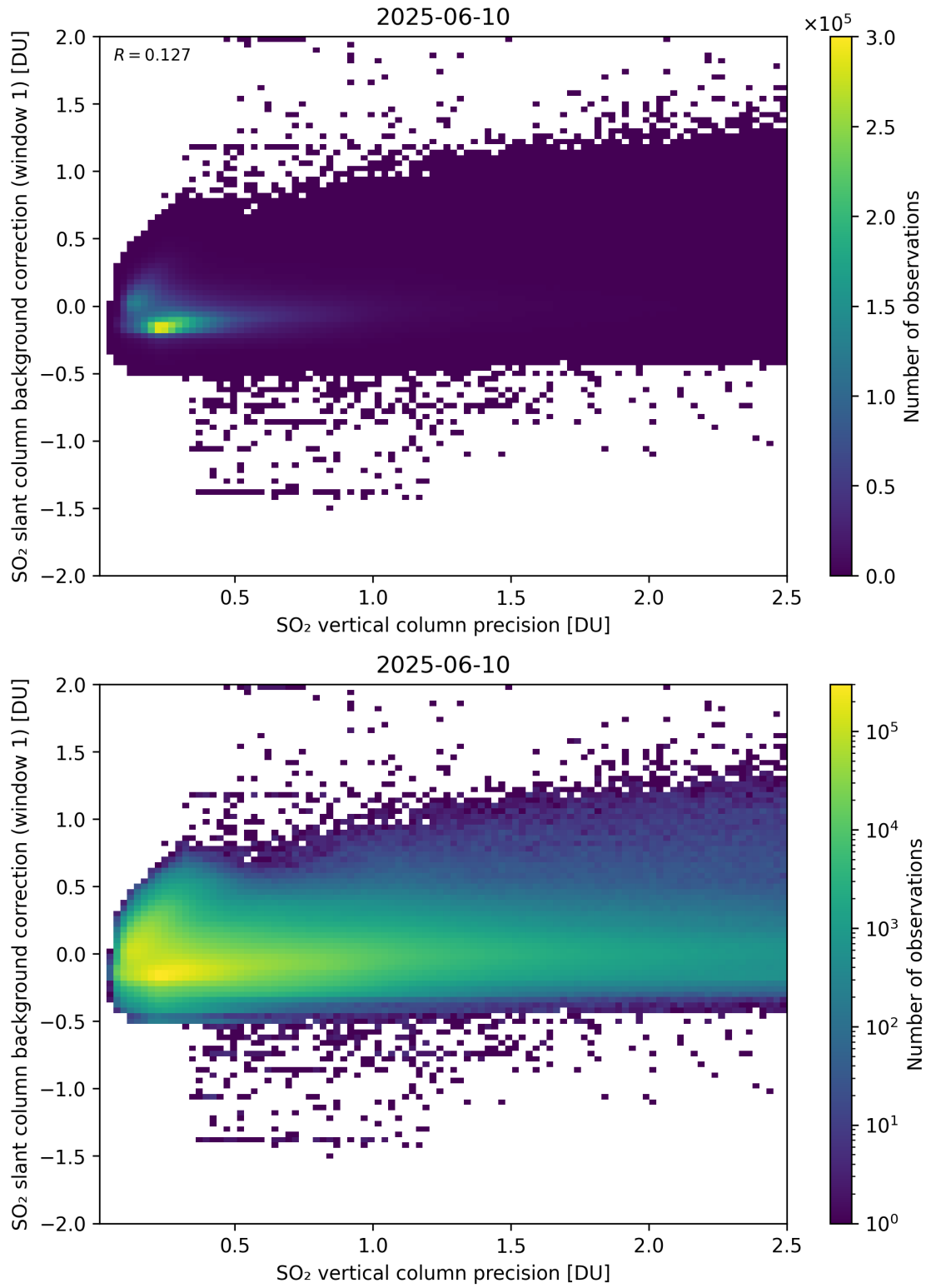
Figure 329: Scatter density plot of “SO 2 vertical column precision” against “SO 2 slant column background correction (window 1)” for 2025-06-09 to 2025-06-11.
