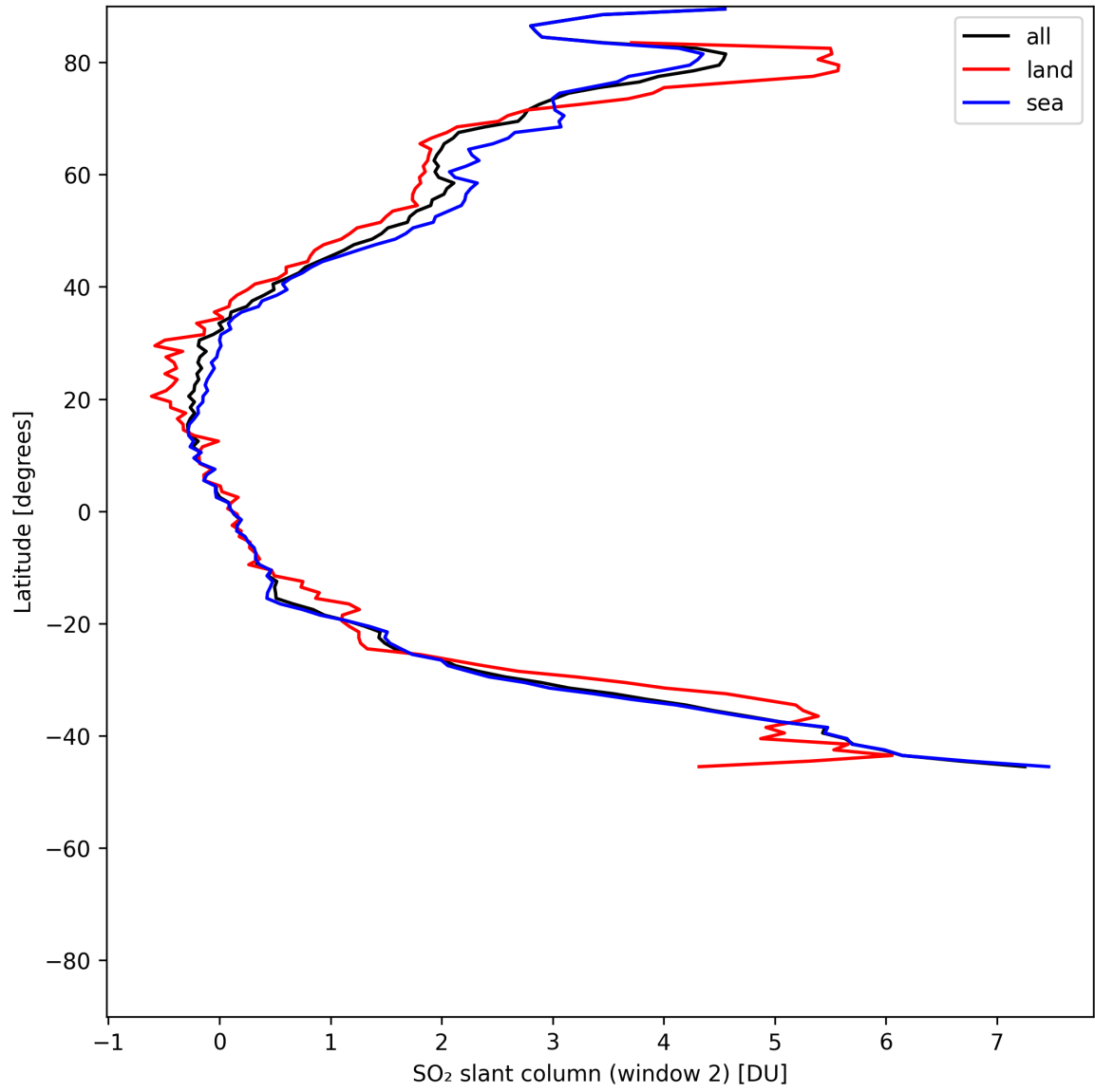
Figure 41: Zonal average of “SO 2 slant column (window 2)” for 2025-06-09 to 2025-06-11.
