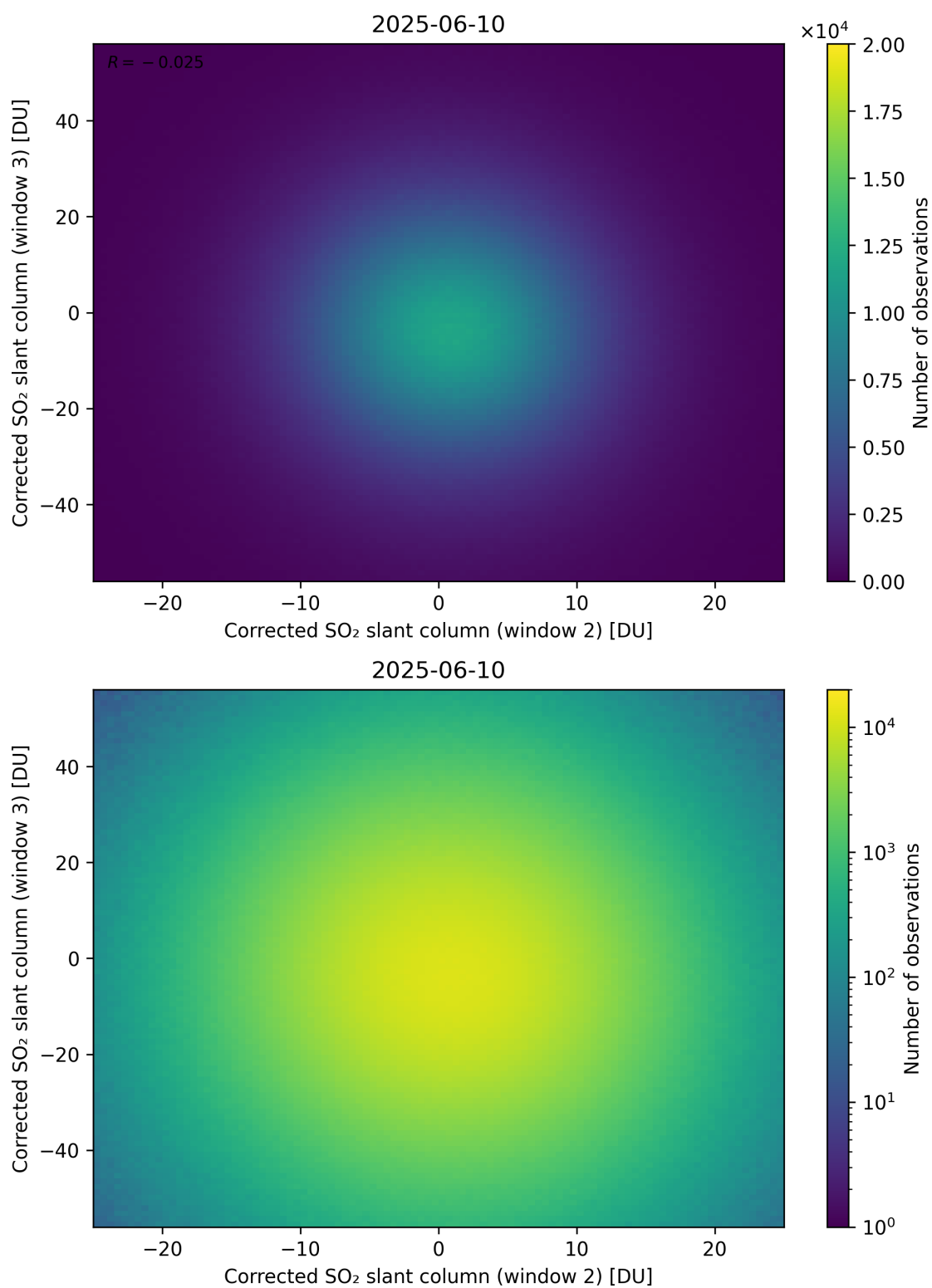
Figure 250: Scatter density plot of “Corrected SO 2 slant column (window 2)” against “Corrected SO 2 slant column (window 3)” for 2025-06-09 to 2025-06-11.
