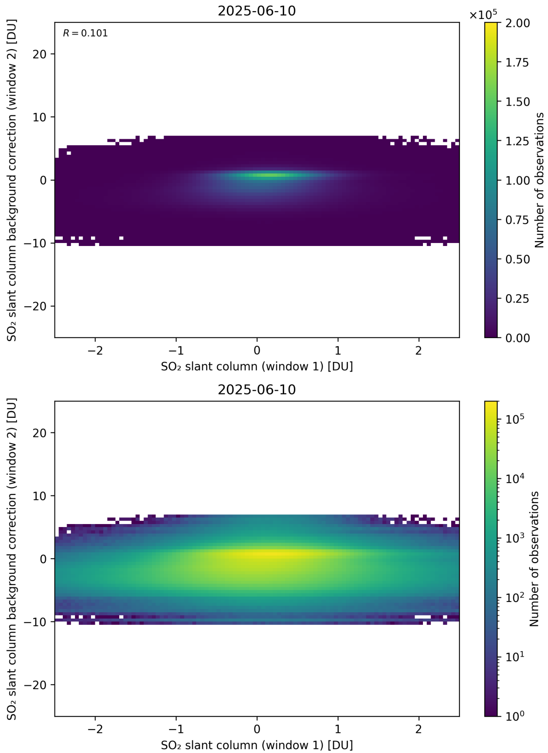
Figure 263: Scatter density plot of “SO 2 slant column (window 1)” against “SO 2 slant column background correction (window 2)” for 2025-06-09 to 2025-06-11.
