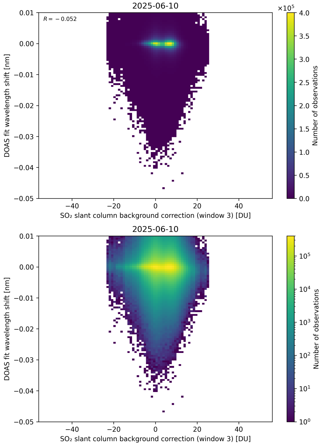
Figure 132: Scatter density plot of “SO 2 slant column background correction (window 3)” against “DOAS fit wavelength shift” for 2025-06-09 to 2025-06-11.
