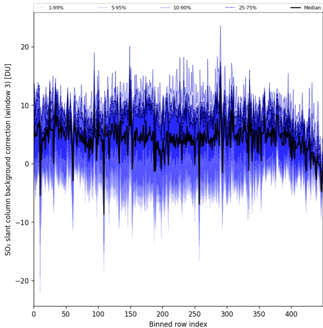
Figure 100: Along track statistics of “SO 2 slant column background correction (window 3)” for 2025-06-09 to 2025-06-11
