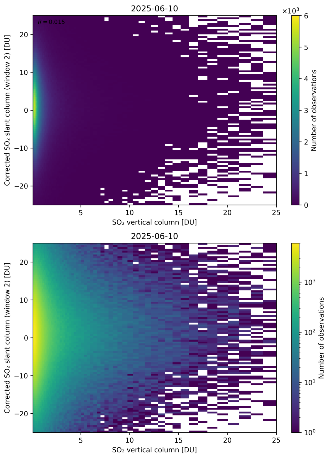
Figure 352: Scatter density plot of “SO 2 vertical column” against “Corrected SO 2 slant column (window 2)” for 2025-06-09 to 2025-06-11.
