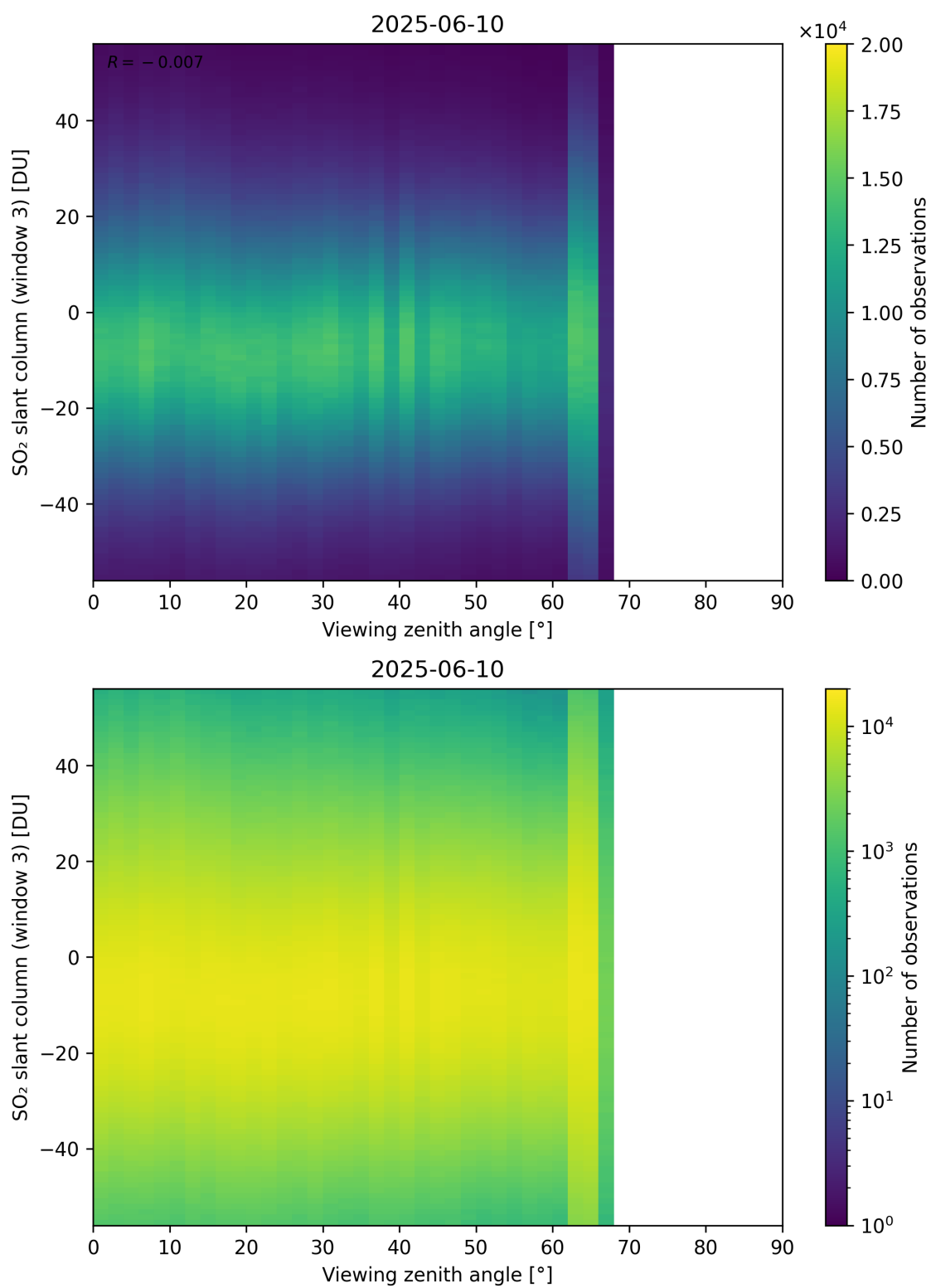
Figure 379: Scatter density plot of “Viewing zenith angle” against “SO 2 slant column (window 3)” for 2025-06-09 to 2025-06-11.
