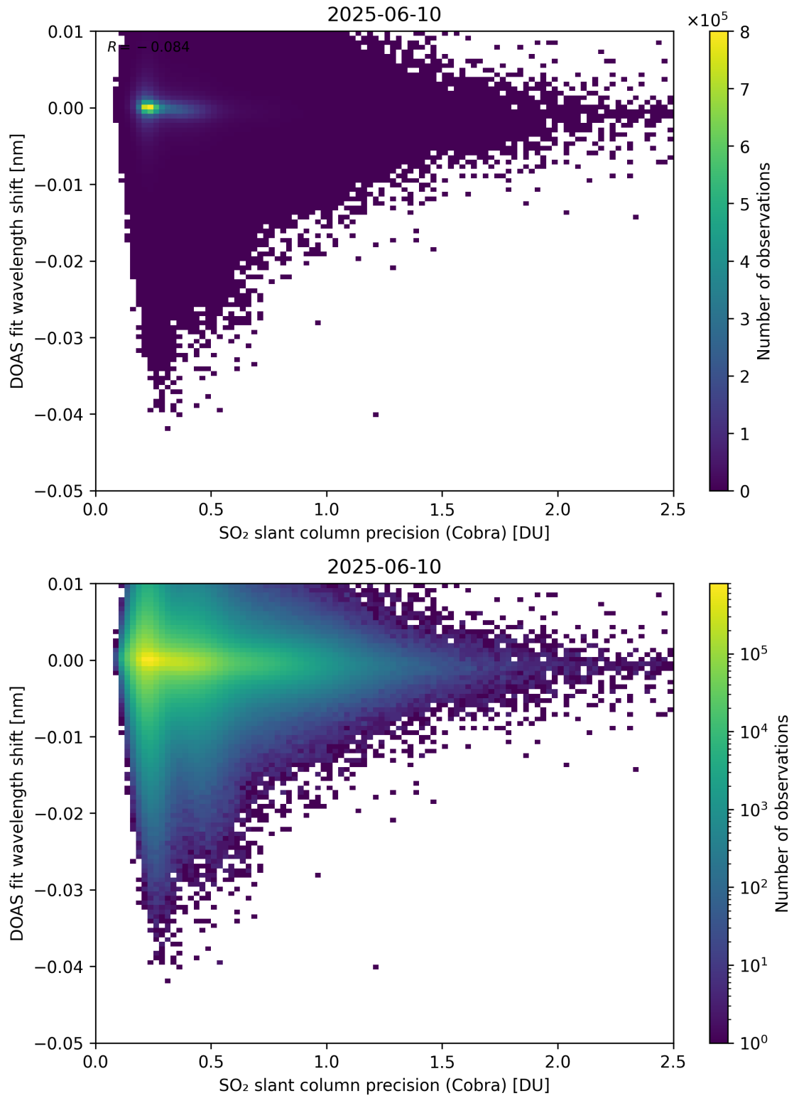
Figure 202: Scatter density plot of “SO 2 slant column precision (Cobra)” against “DOAS fit wavelength shift” for 2025-06-09 to 2025-06-11.
