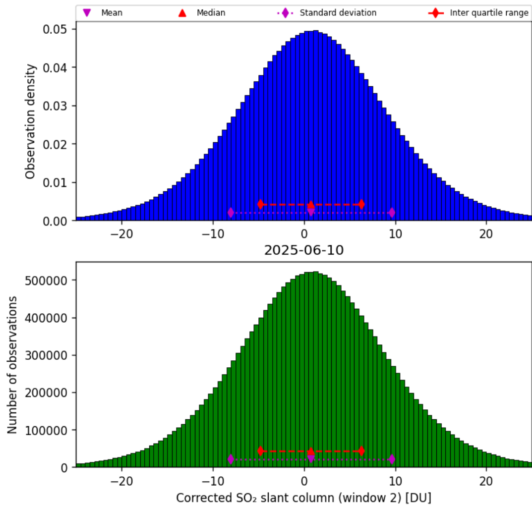
Figure 69: Histogram of “Corrected SO 2 slant column (window 2)” for 2025-06-09 to 2025-06-11
