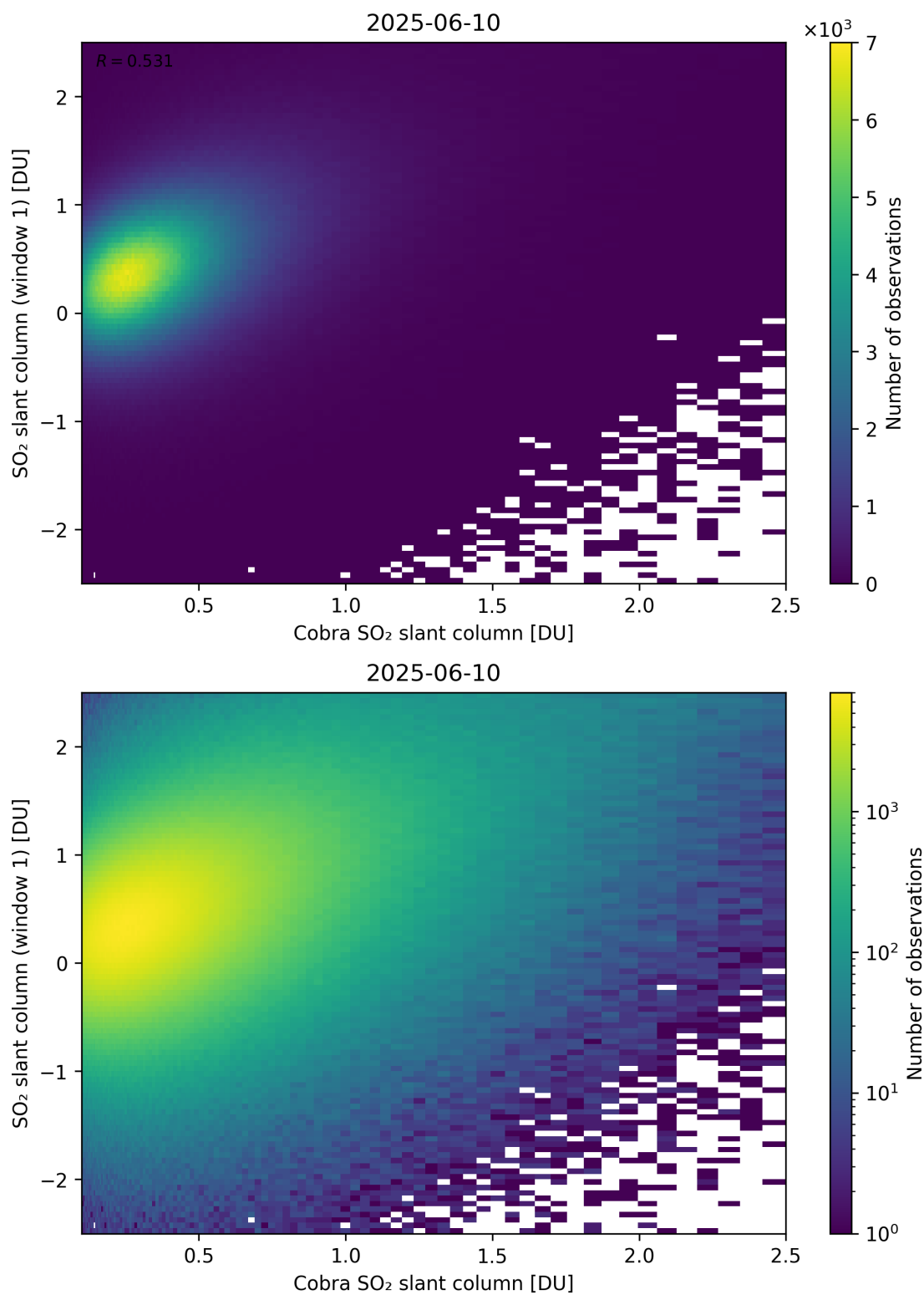
Figure 219: Scatter density plot of “Cobra SO 2 slant column” against “SO 2 slant column (window 1)” for 2025-06-09 to 2025-06-11.
