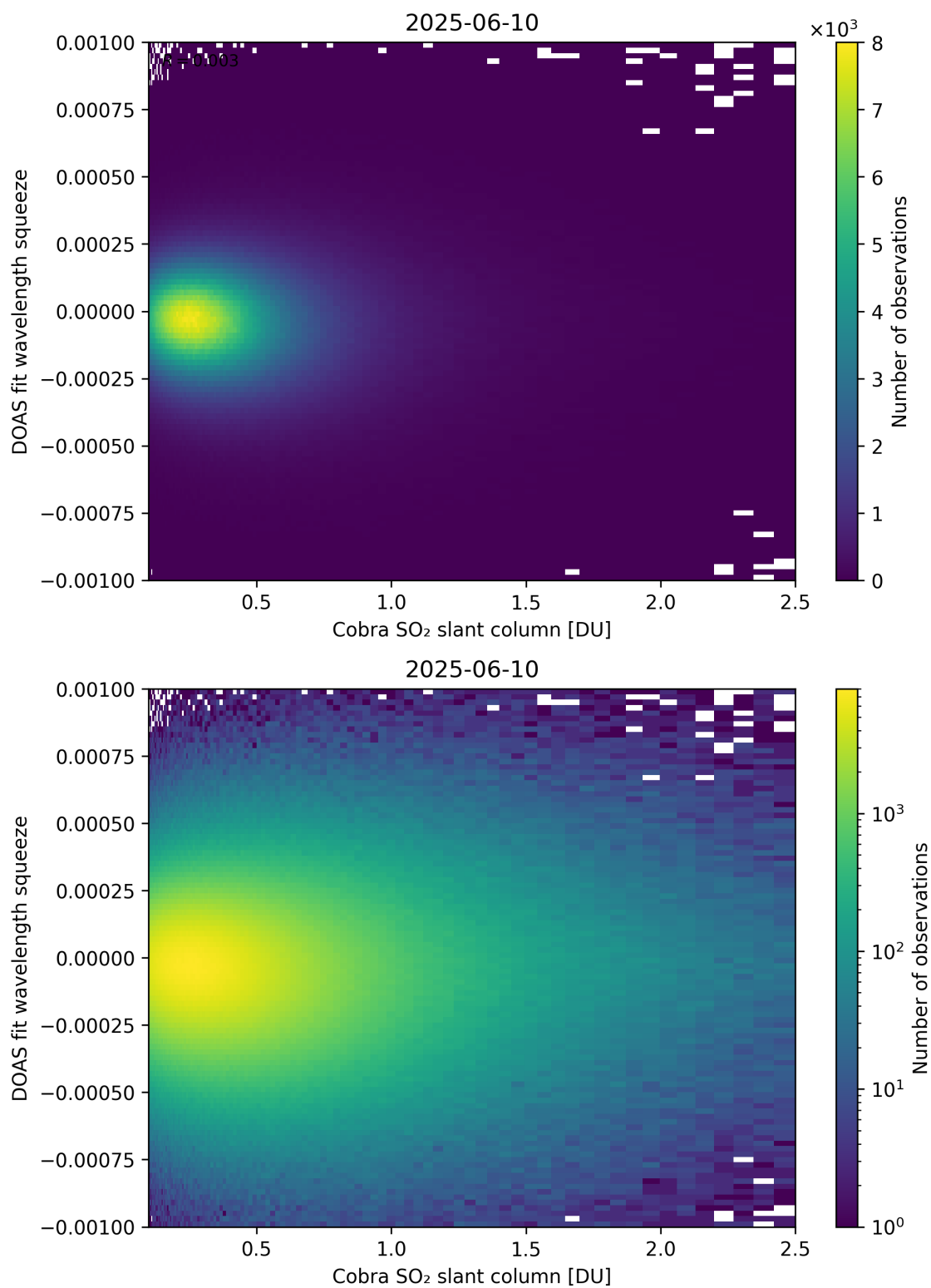
Figure 197: Scatter density plot of “Cobra SO 2 slant column” against “DOAS fit wavelength squeeze” for 2025-06-09 to 2025-06-11.
