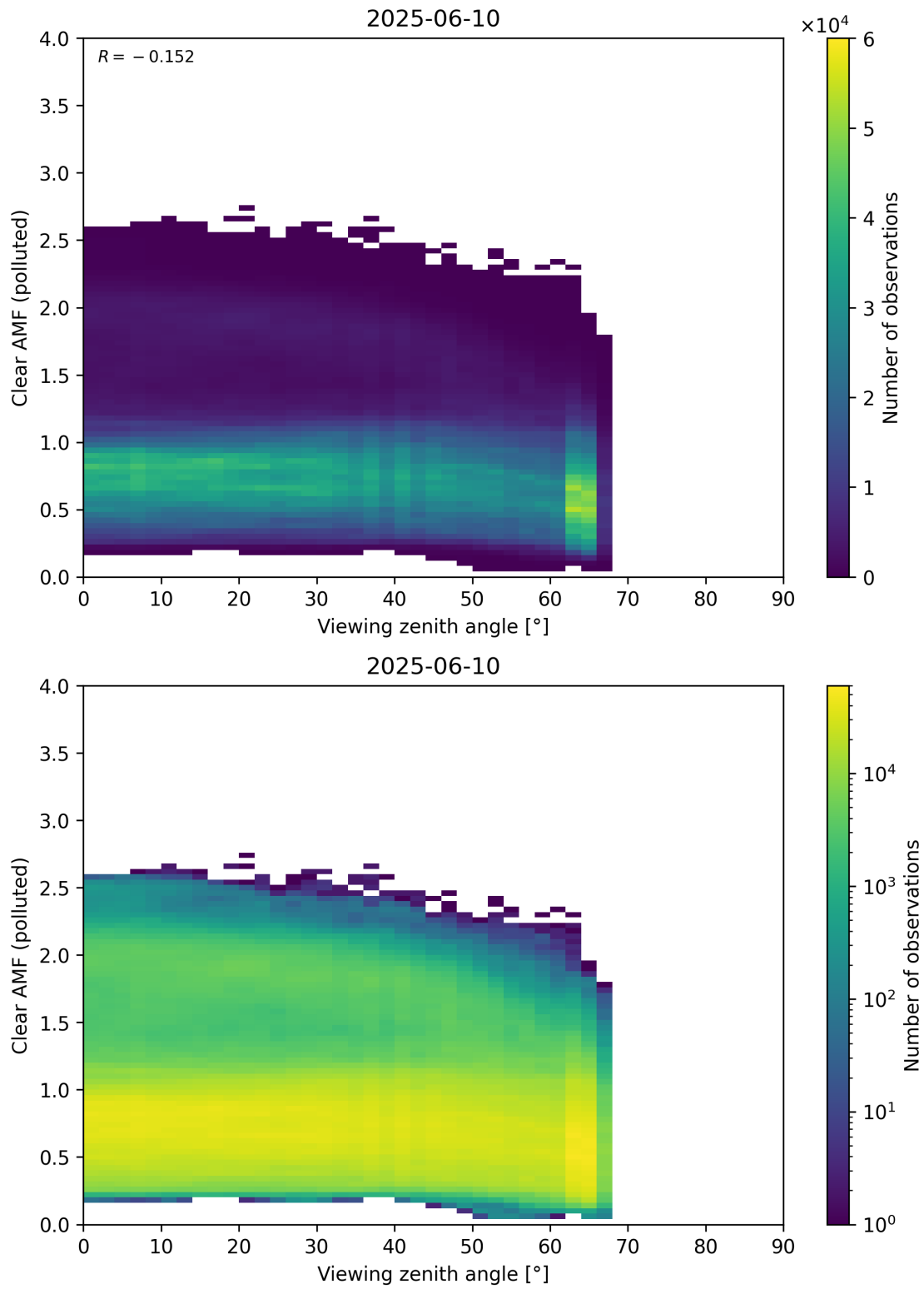
Figure 370: Scatter density plot of “Viewing zenith angle” against “Clear AMF (polluted)” for 2025-06-09 to 2025-06-11.
