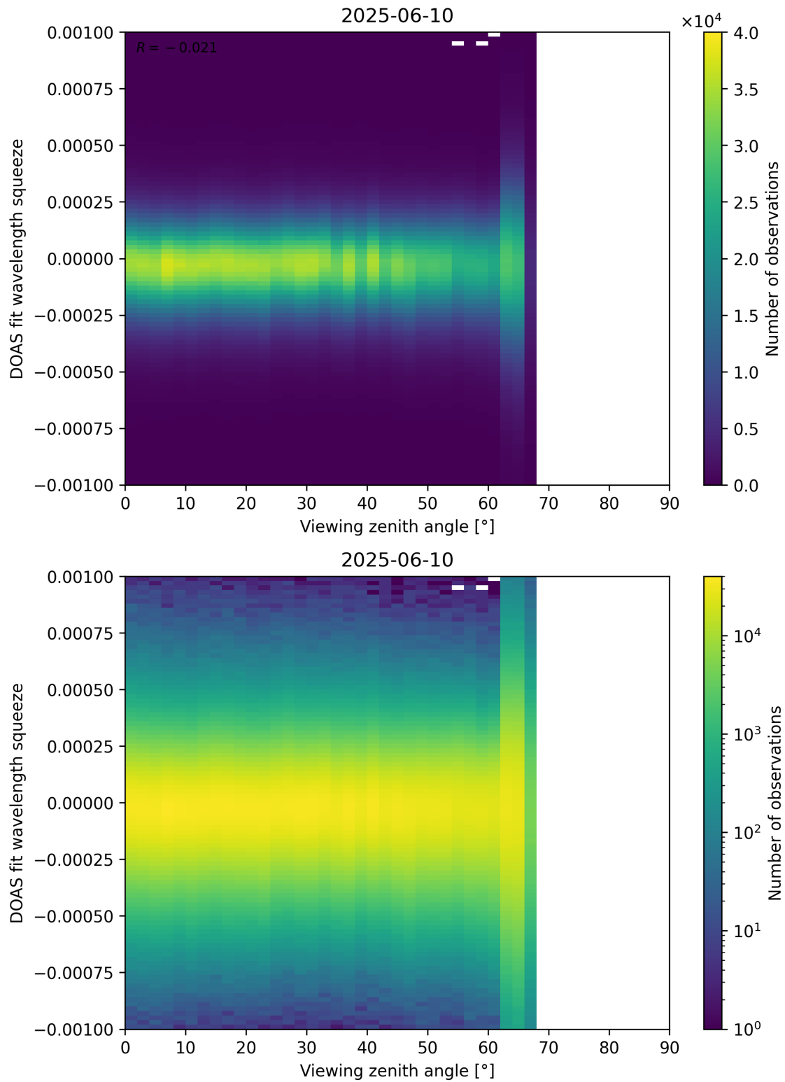
Figure 366: Scatter density plot of “Viewing zenith angle” against “DOAS fit wavelength squeeze” for 2025-06-09 to 2025-06-11.
