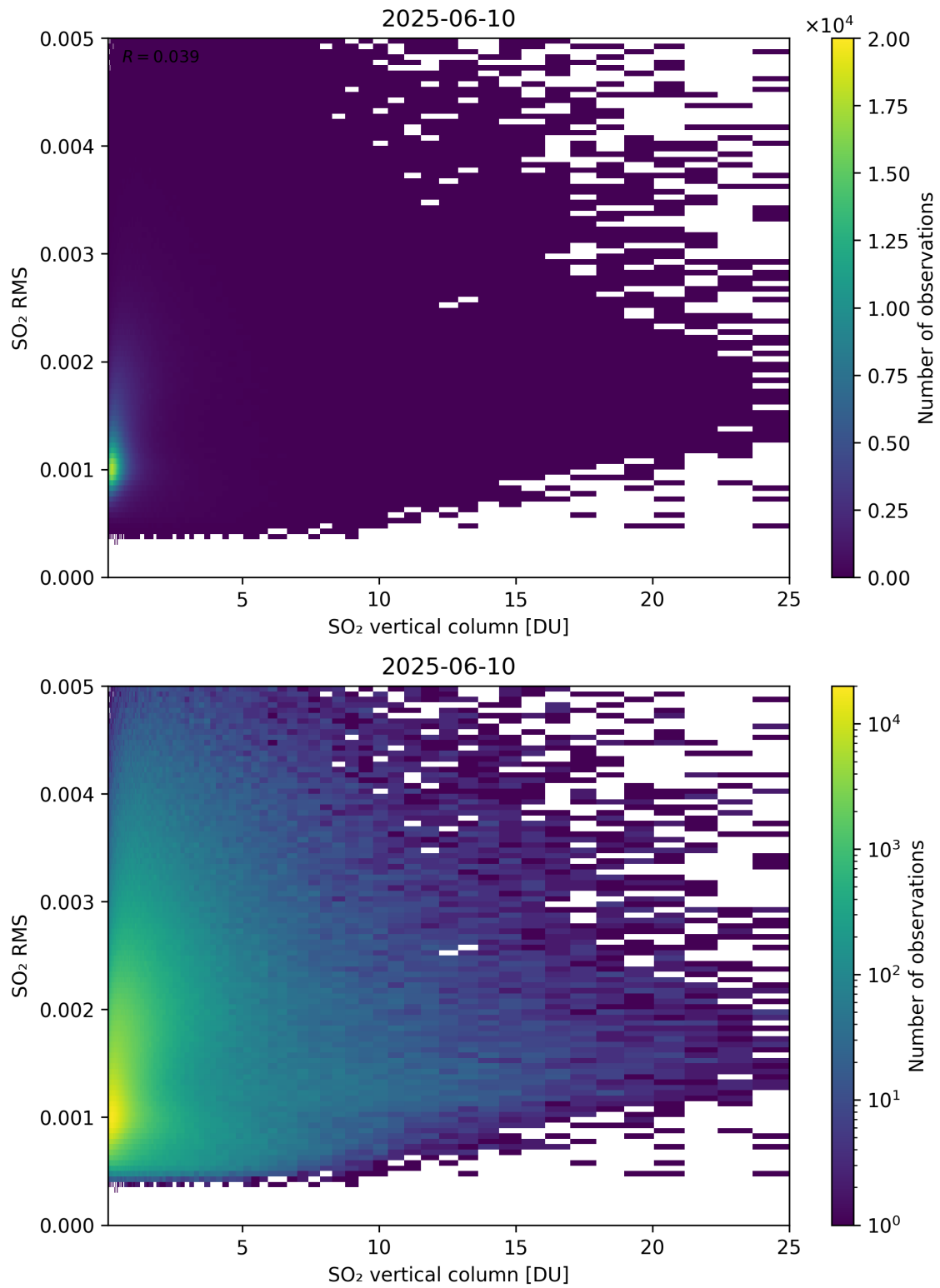
Figure 328: Scatter density plot of “SO 2 vertical column” against “SO 2 RMS” for 2025-06-09 to 2025-06-11.
