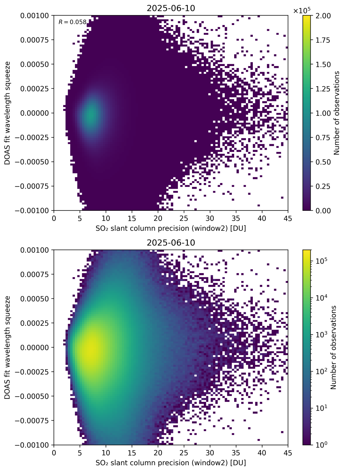
Figure 294: Scatter density plot of “SO 2 slant column precision (window2)” against “DOAS fit wavelength squeeze” for 2025-06-09 to 2025-06-11.
