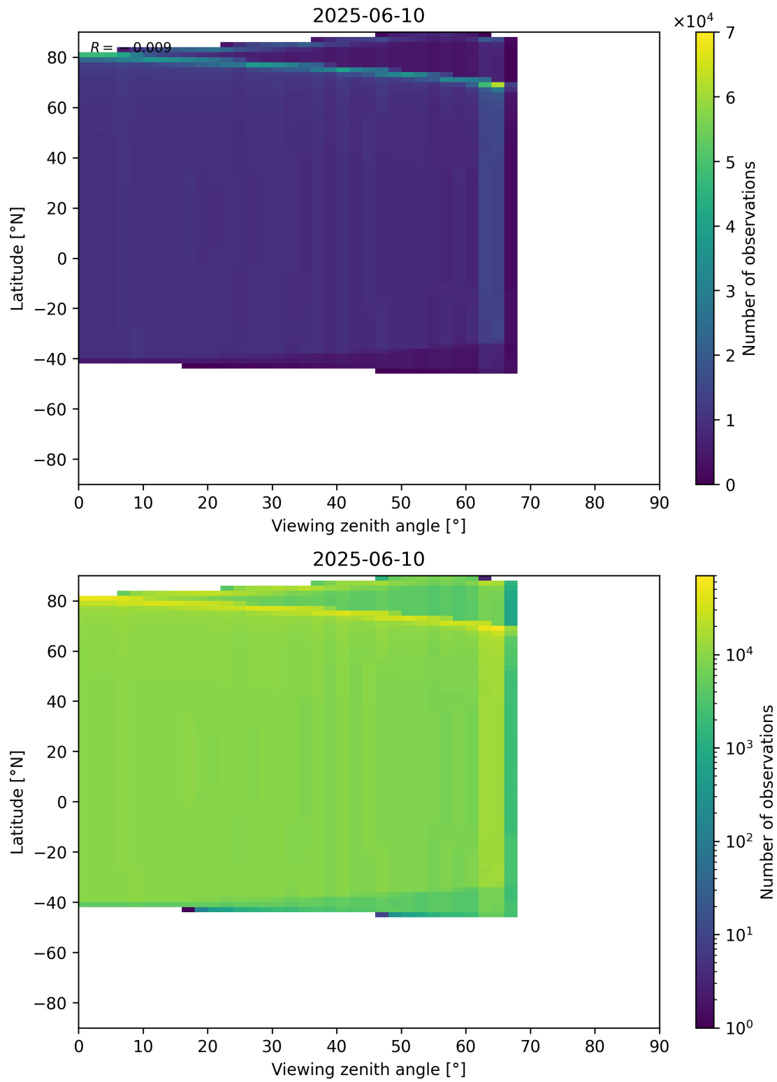
Figure 368: Scatter density plot of “Viewing zenith angle” against “Latitude” for 2025-06-09 to 2025-06-11.
