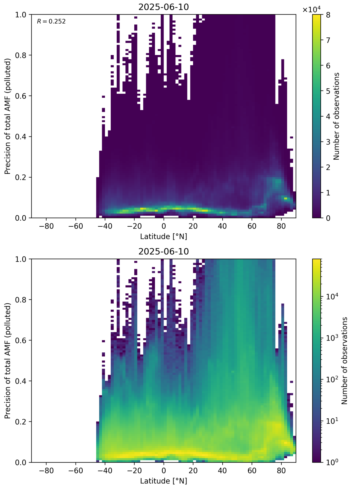
Figure 168: Scatter density plot of “Latitude” against “Precision of total AMF (polluted)” for 2025-06-09 to 2025-06-11.
