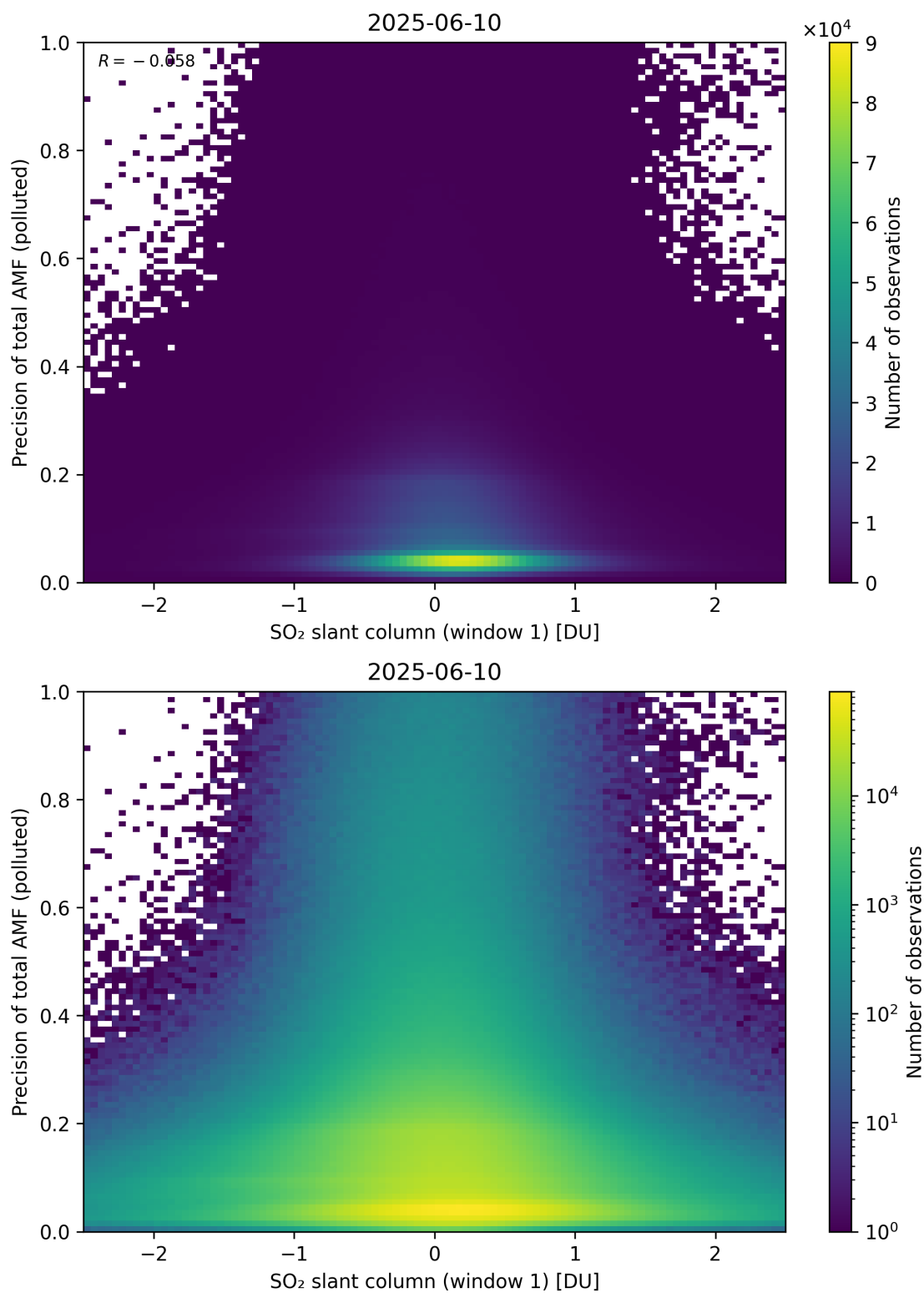
Figure 290: Scatter density plot of “SO 2 slant column (window 1)” against “Precision of total AMF (polluted)” for 2025-06-09 to 2025-06-11.
