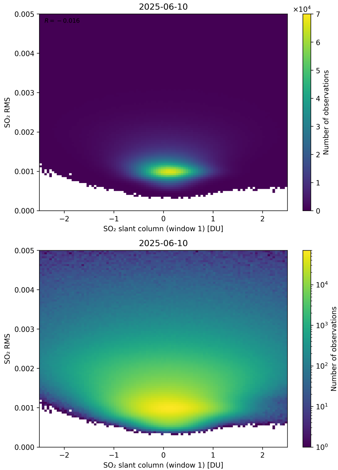
Figure 267: Scatter density plot of “SO 2 slant column (window 1)” against “SO 2 RMS” for 2025-06-09 to 2025-06-11.
