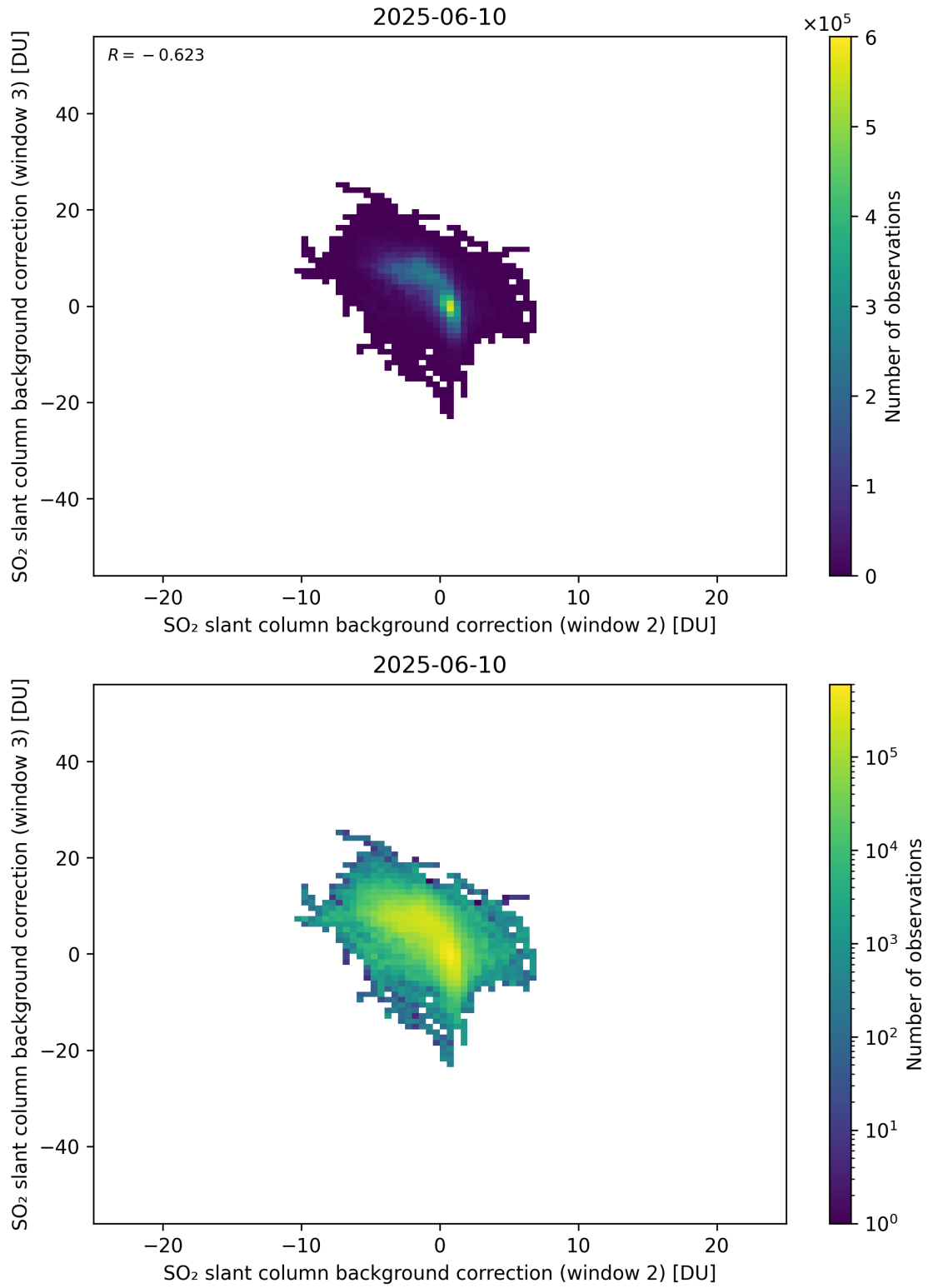
Figure 122: Scatter density plot of “SO 2 slant column background correction (window 2)” against “SO 2 slant column background correction (window 3)” for 2025-06-09 to 2025-06-11.
