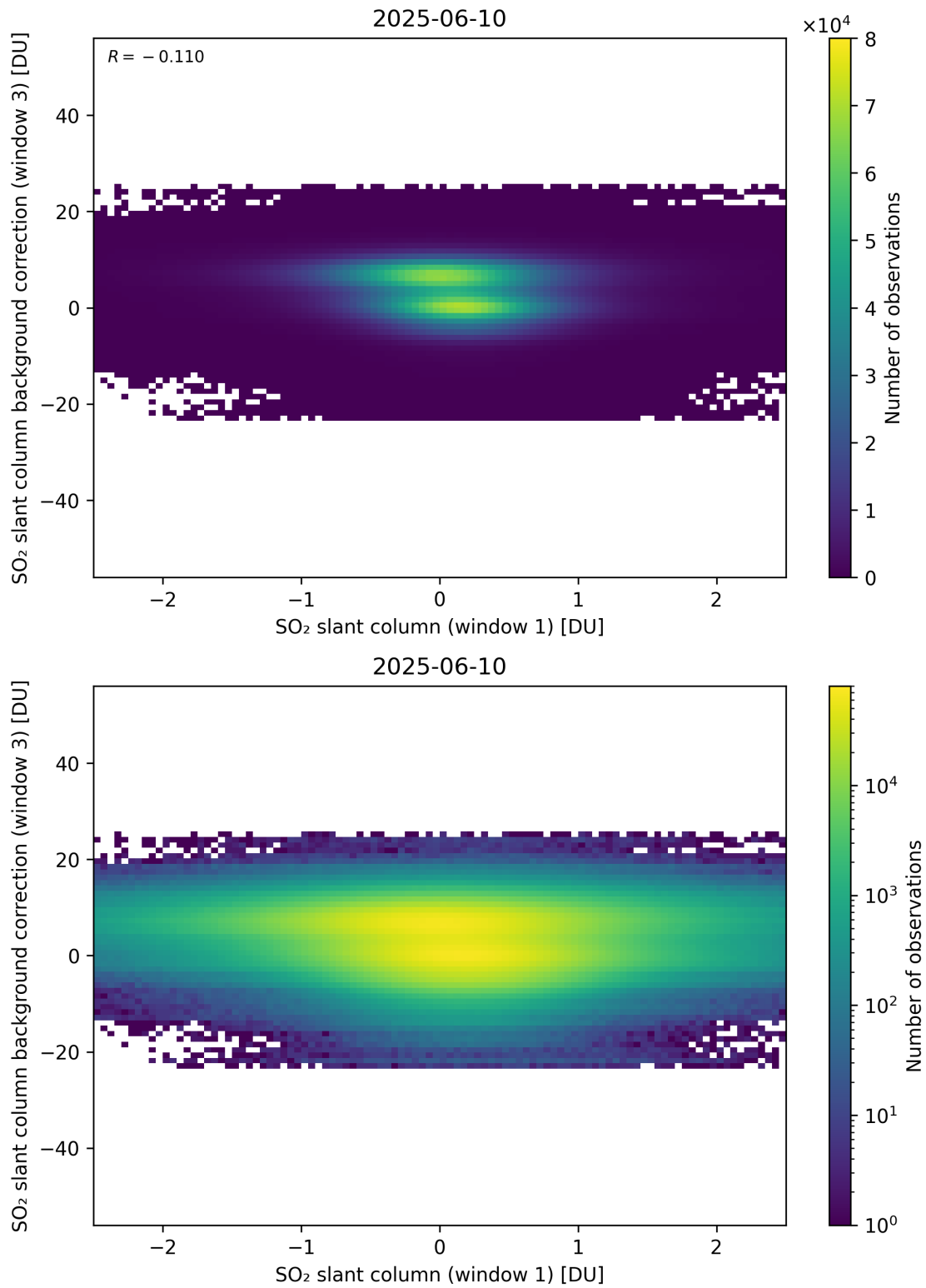
Figure 264: Scatter density plot of “SO 2 slant column (window 1)” against “SO 2 slant column background correction (window 3)” for 2025-06-09 to 2025-06-11.
