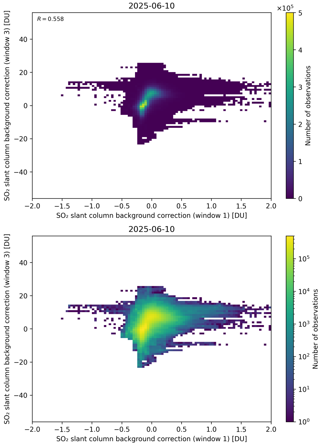
Figure 110: Scatter density plot of “SO 2 slant column background correction (window 1)” against “SO 2 slant column background correction (window 3)” for 2025-06-09 to 2025-06-11.
