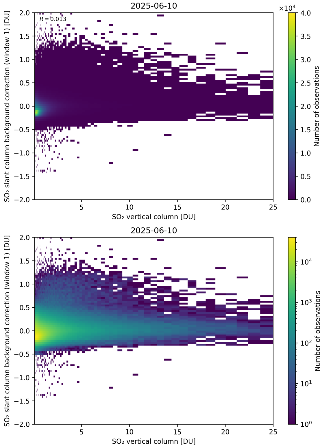
Figure 323: Scatter density plot of “SO 2 vertical column” against “SO 2 slant column background correction (window 1)” for 2025-06-09 to 2025-06-11.
