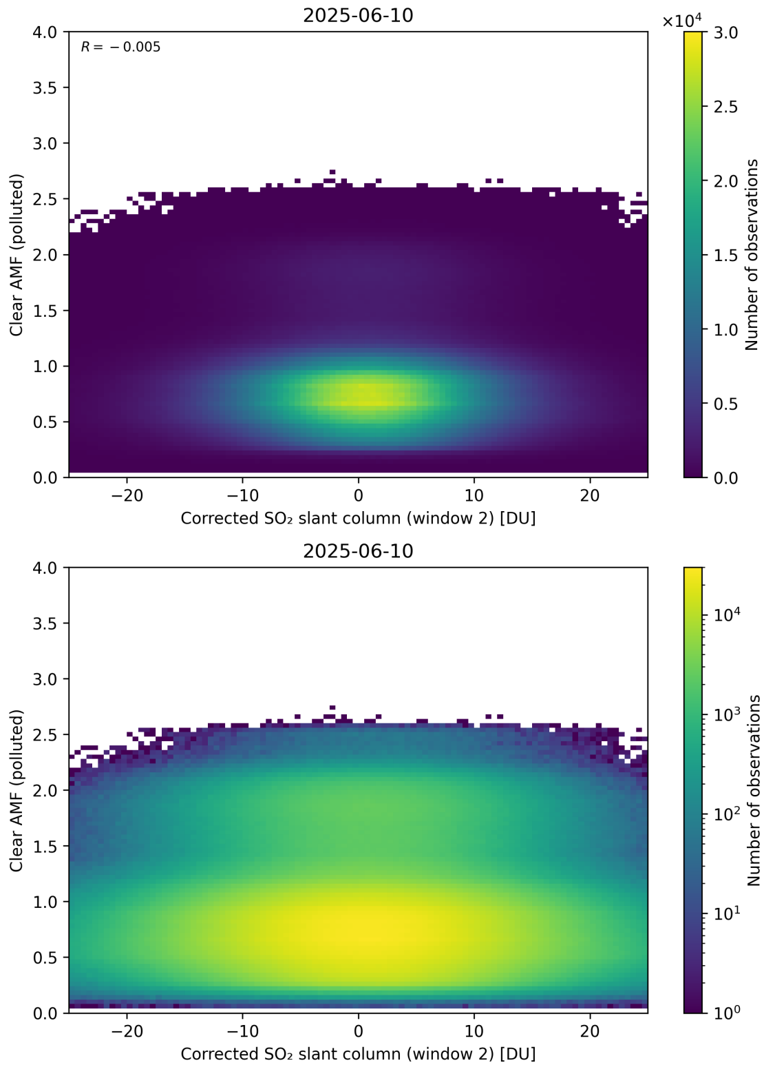
Figure 249: Scatter density plot of “Corrected SO 2 slant column (window 2)” against “Clear AMF (polluted)” for 2025-06-09 to 2025-06-11.
