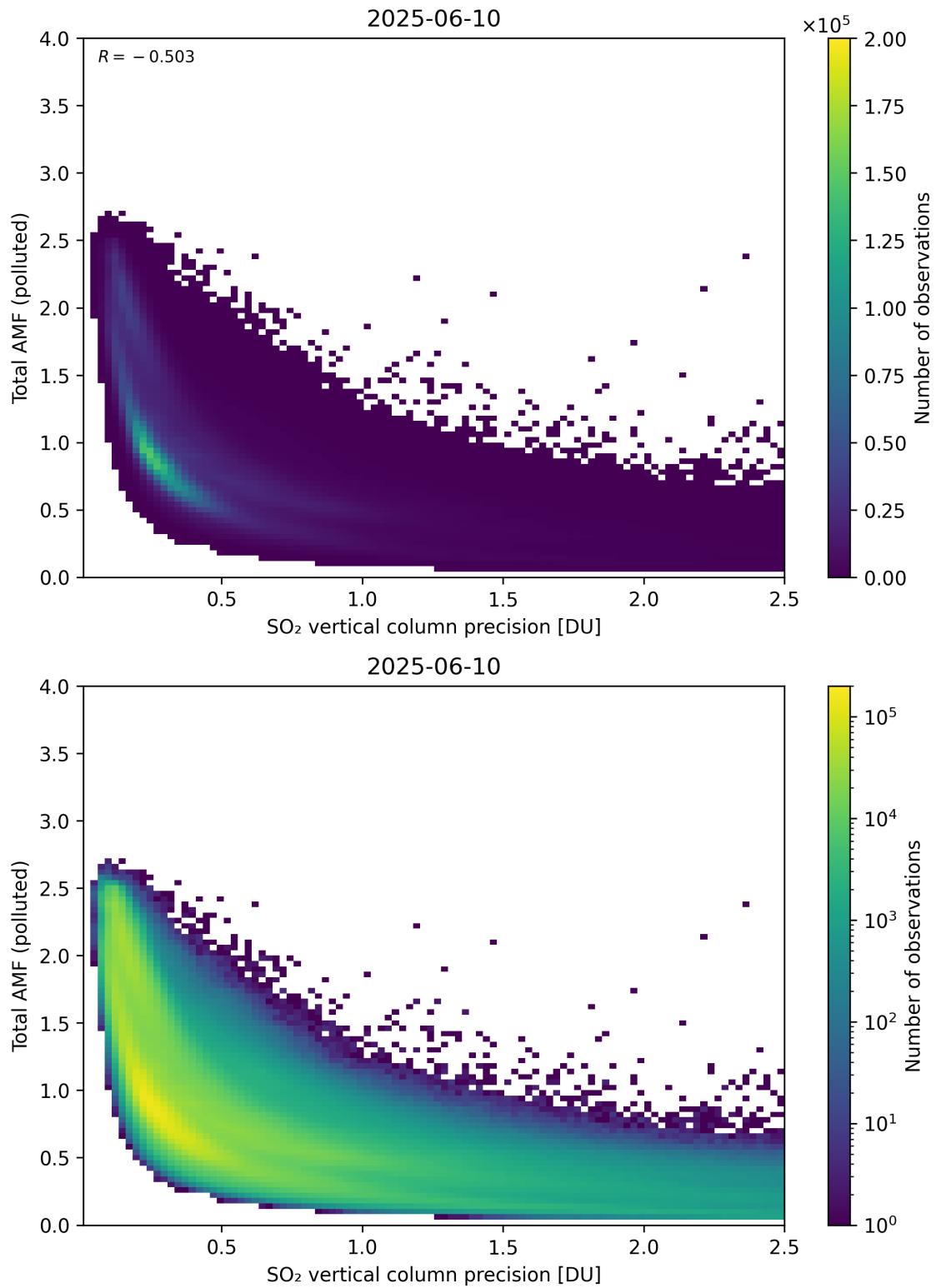
Figure 346: Scatter density plot of “SO 2 vertical column precision” against “Total AMF (polluted)” for 2025-06-09 to 2025-06-11.
