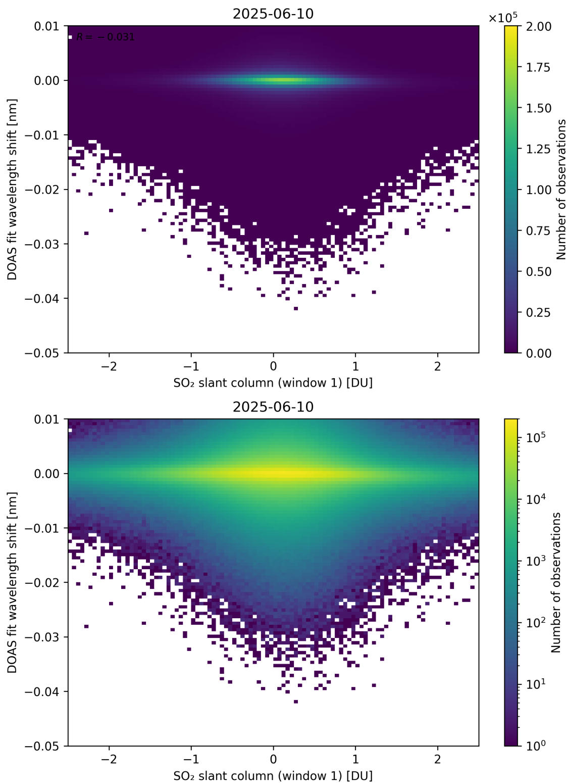
Figure 265: Scatter density plot of “SO 2 slant column (window 1)” against “DOAS fit wavelength shift” for 2025-06-09 to 2025-06-11.
