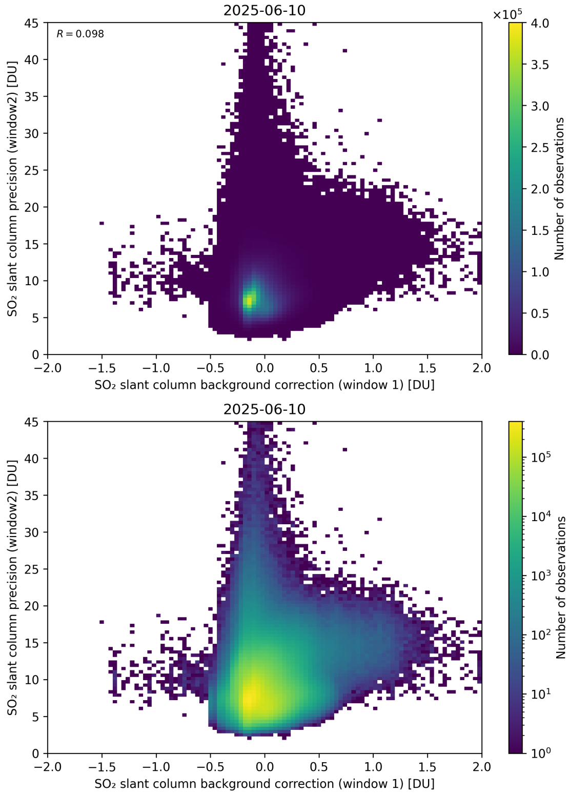
Figure 117: Scatter density plot of “SO 2 slant column background correction (window 1)” against “SO 2 slant column precision (window2)” for 2025-06-09 to 2025-06-11.
