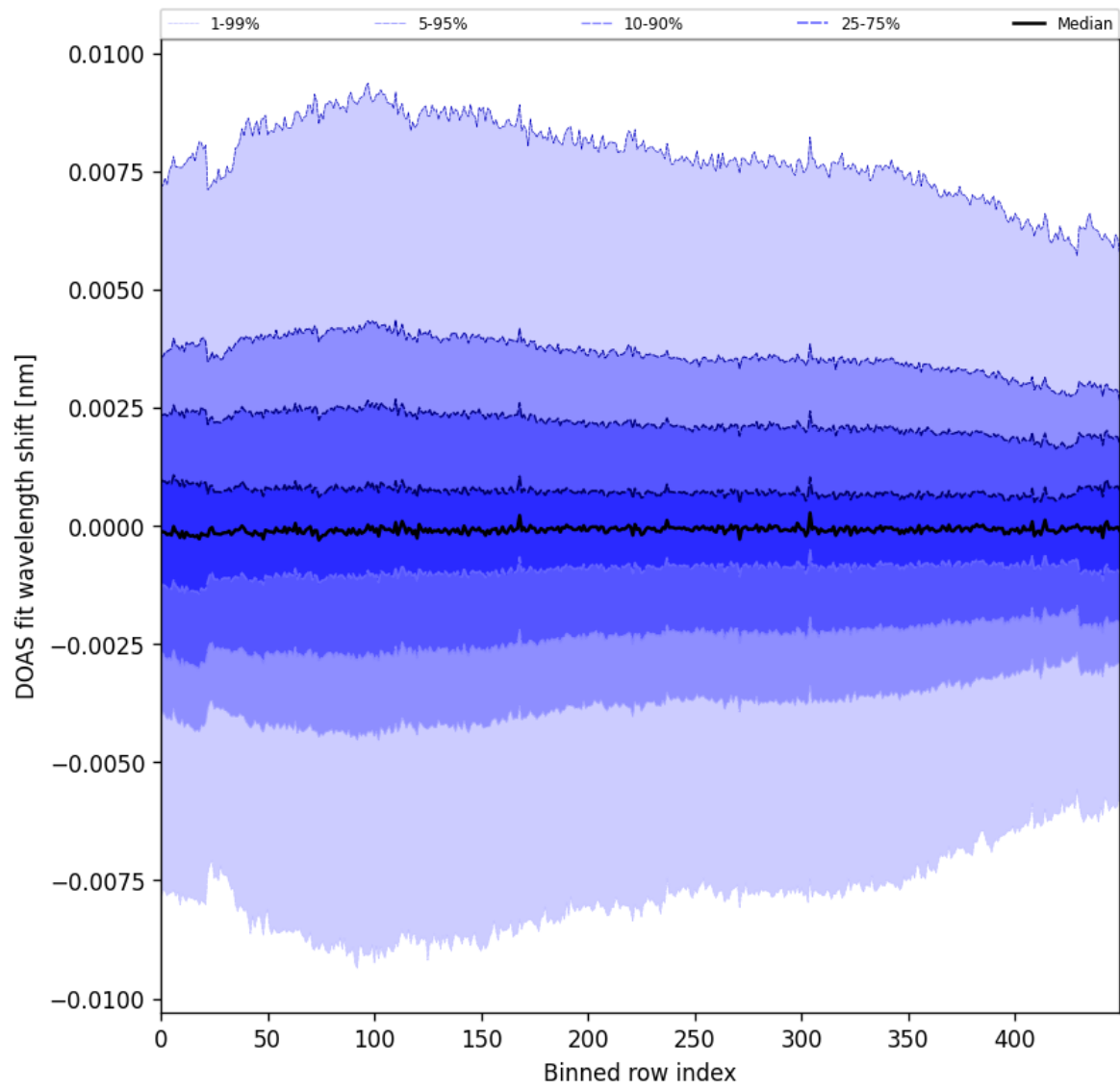
Figure 102: Along track statistics of “DOAS fit wavelength shift” for 2025-06-09 to 2025-06-11
