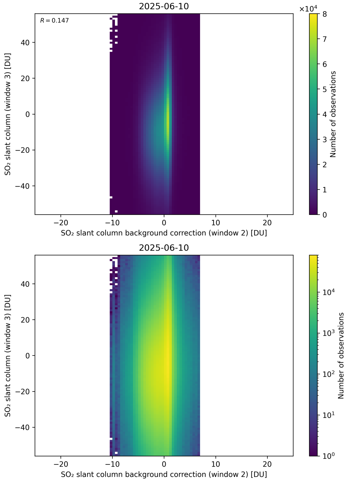
Figure 128: Scatter density plot of “SO 2 slant column background correction (window 2)” against “SO 2 slant column (window 3)” for 2025-06-09 to 2025-06-11.
