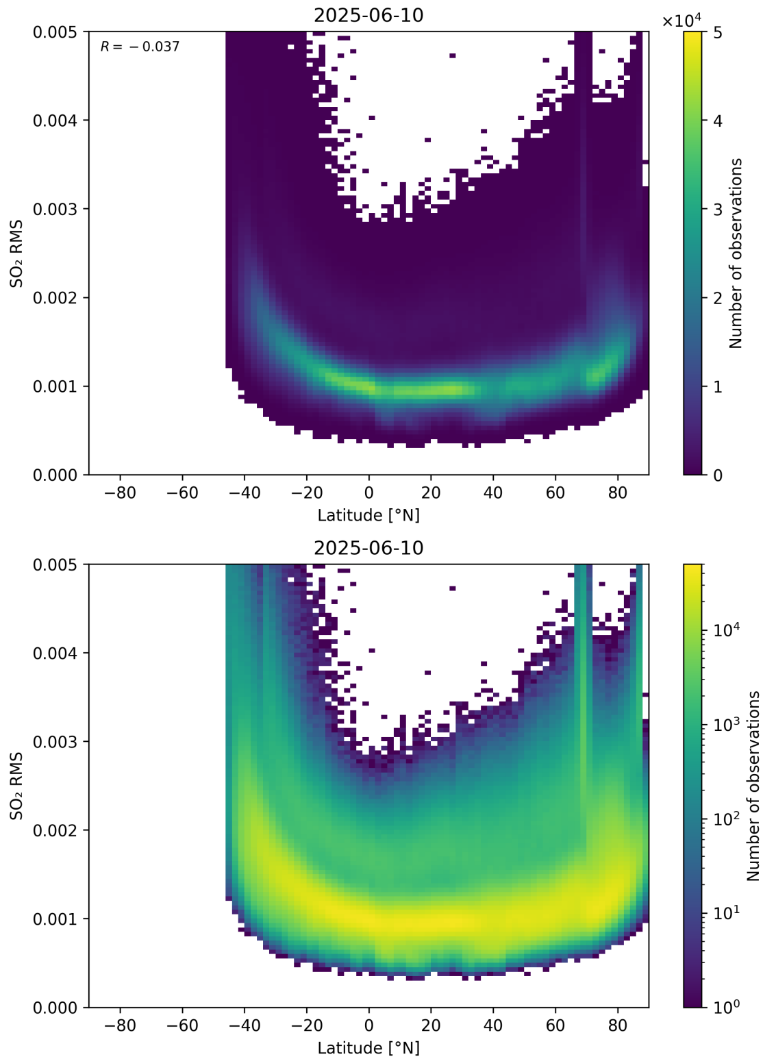
Figure 155: Scatter density plot of “Latitude” against “SO 2 RMS” for 2025-06-09 to 2025-06-11.
