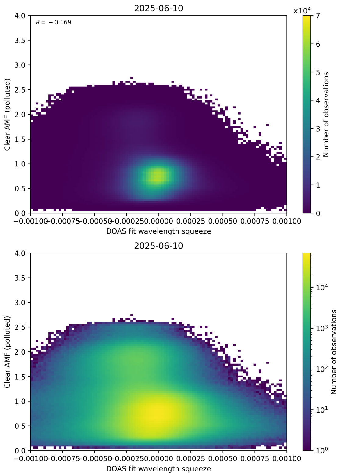
Figure 144: Scatter density plot of “DOAS fit wavelength squeeze” against “Clear AMF (polluted)” for 2025-06-09 to 2025-06-11.
