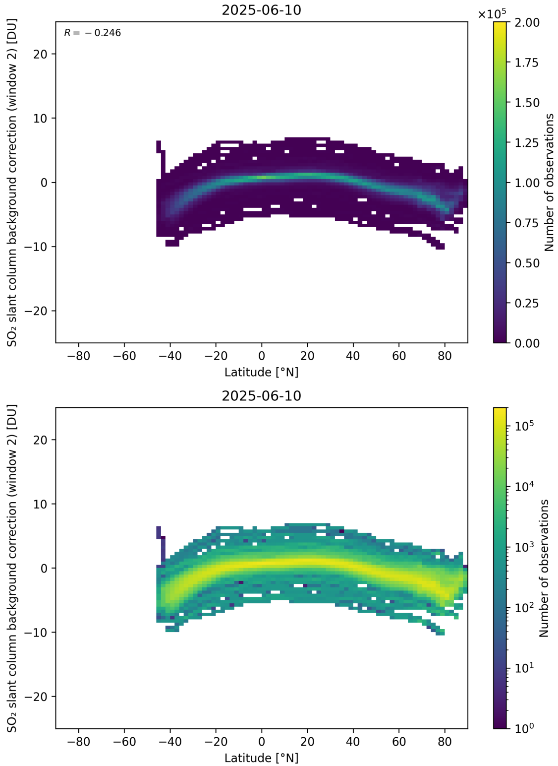
Figure 151: Scatter density plot of “Latitude” against “SO 2 slant column background correction (window 2)” for 2025-06-09 to 2025-06-11.
