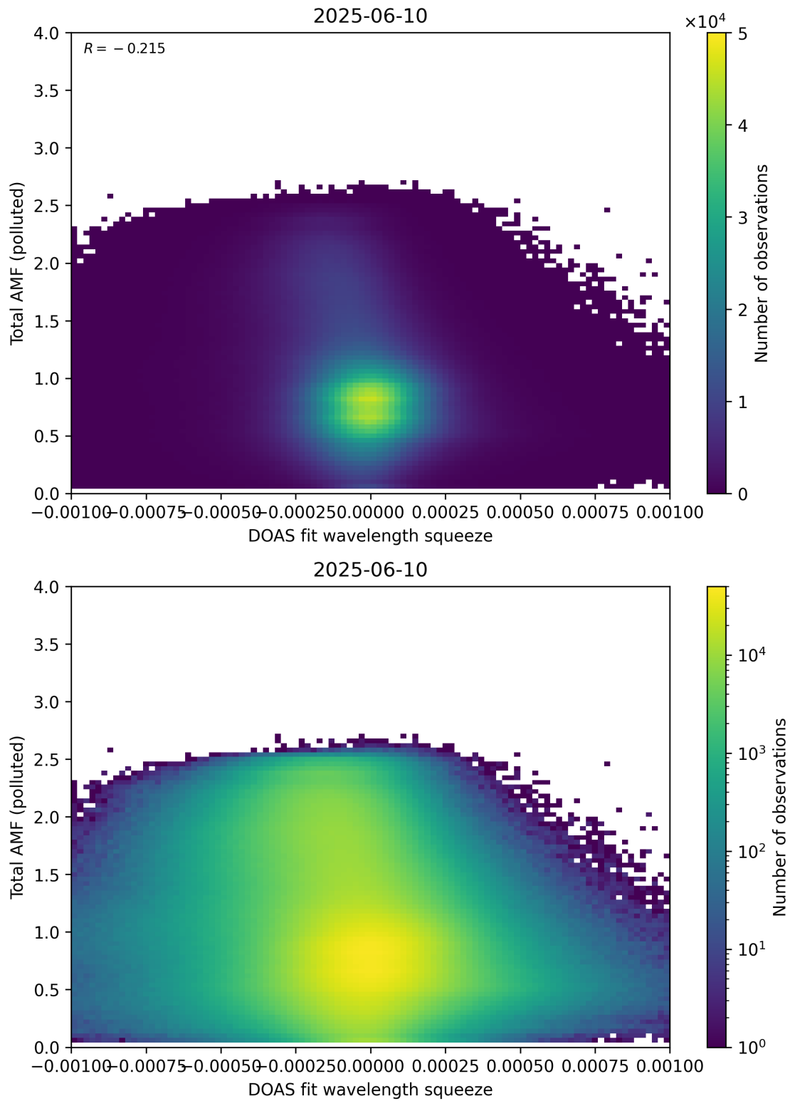
Figure 145: Scatter density plot of “DOAS fit wavelength squeeze” against “Total AMF (polluted)” for 2025-06-09 to 2025-06-11.
