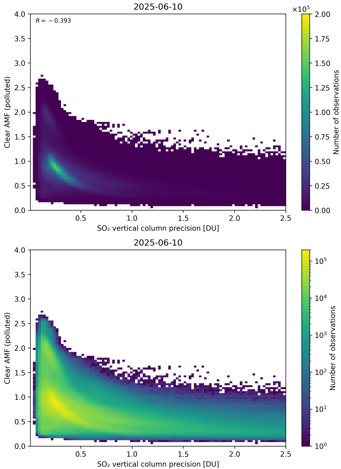
Figure 335: Scatter density plot of “SO 2 vertical column precision” against “Clear AMF (polluted)” for 2025-06-09 to 2025-06-11.
