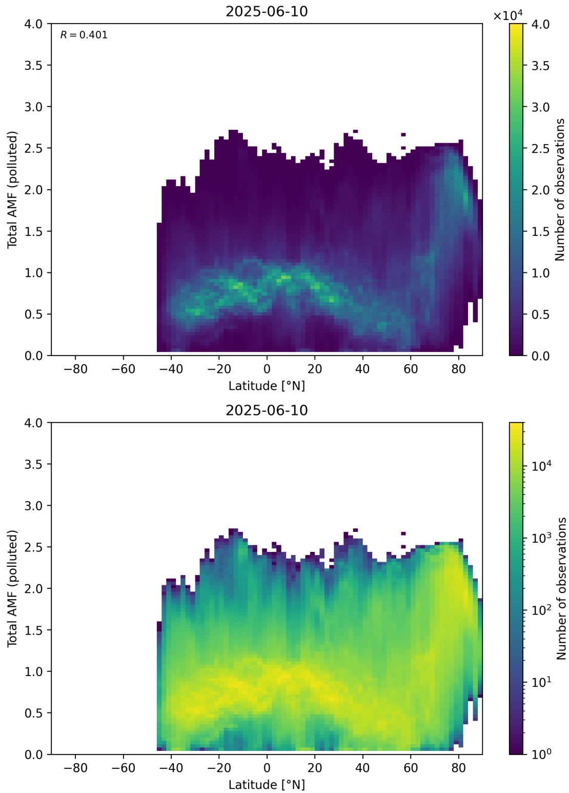
Figure 167: Scatter density plot of “Latitude” against “Total AMF (polluted)” for 2025-06-09 to 2025-06-11.
