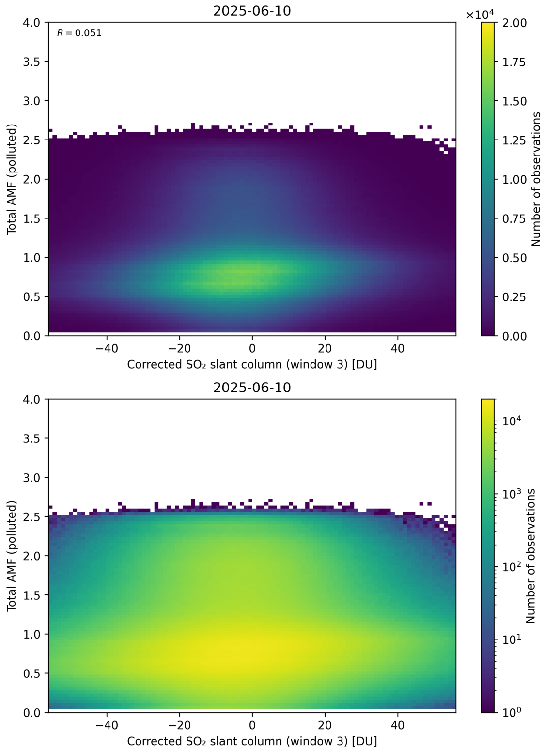
Figure 260: Scatter density plot of “Corrected SO 2 slant column (window 3)” against “Total AMF (polluted)” for 2025-06-09 to 2025-06-11.
