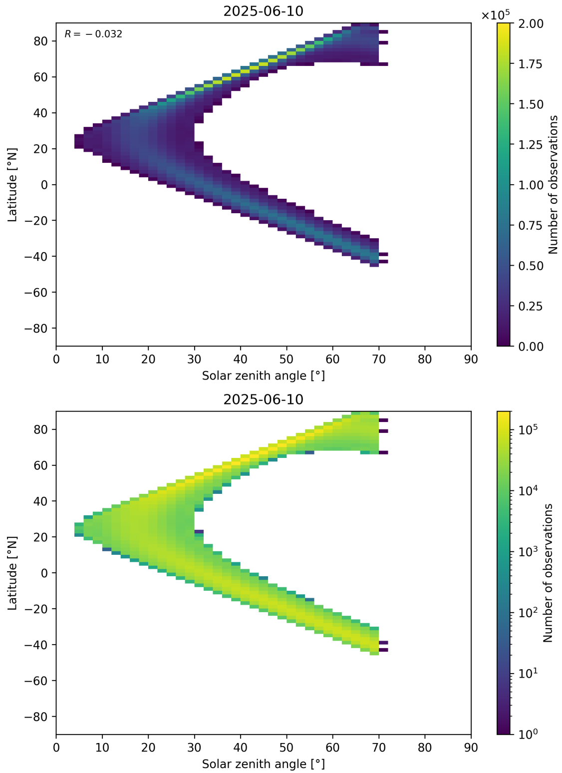
Figure 177: Scatter density plot of “Solar zenith angle” against “Latitude” for 2025-06-09 to 2025-06-11.
