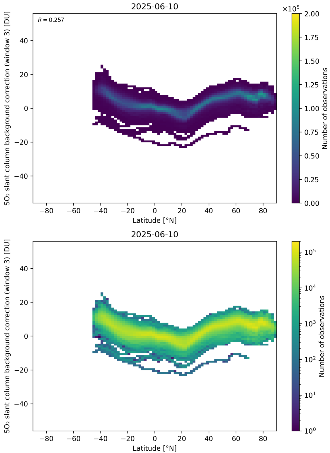
Figure 152: Scatter density plot of “Latitude” against “SO 2 slant column background correction (window 3)” for 2025-06-09 to 2025-06-11.
