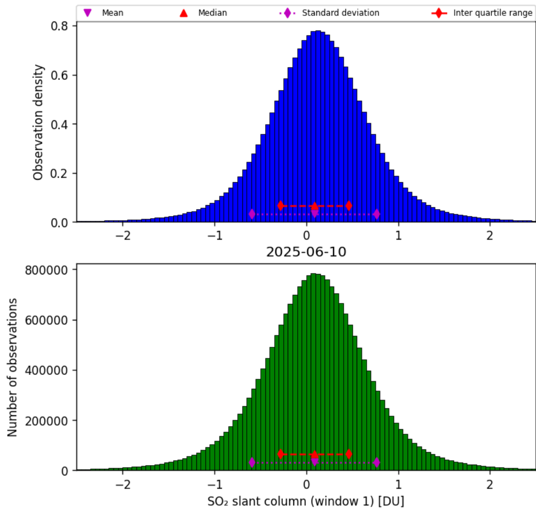
Figure 63: Histogram of “SO 2 slant column (window 1)” for 2025-06-09 to 2025-06-11
