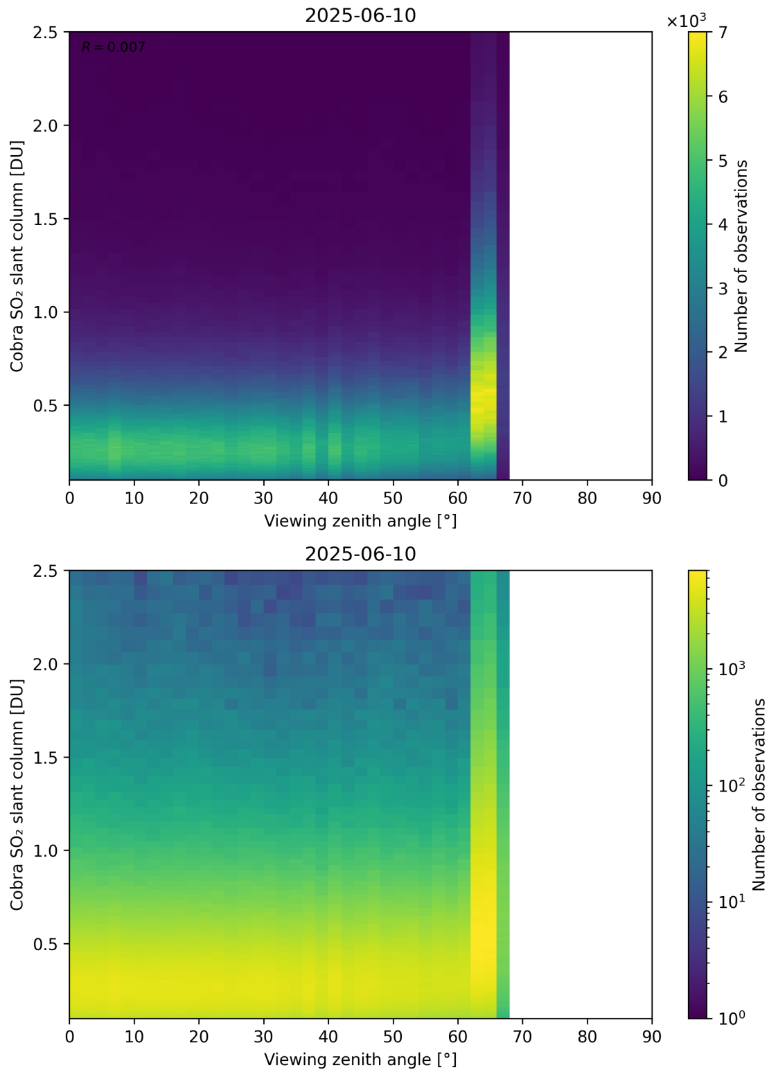
Figure 371: Scatter density plot of “Viewing zenith angle” against “Cobra SO 2 slant column” for 2025-06-09 to 2025-06-11.
