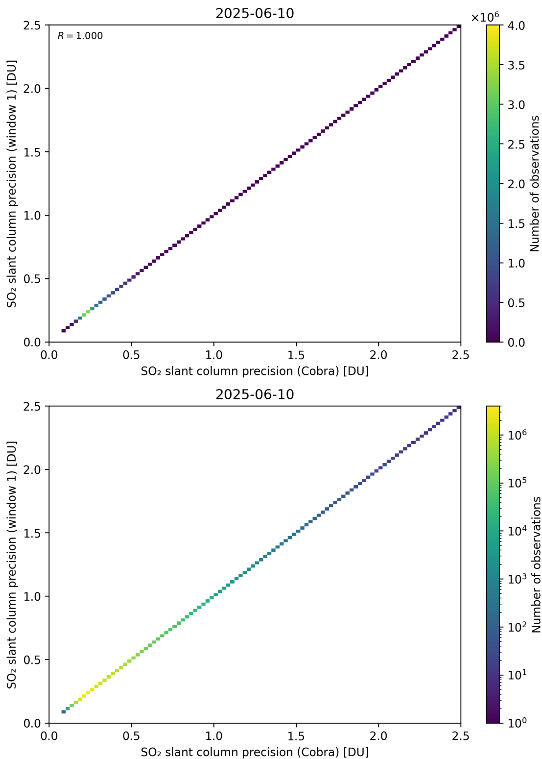
Figure 209: Scatter density plot of “SO 2 slant column precision (Cobra)” against “SO 2 slant column precision (window 1)” for 2025-06-09 to 2025-06-11.
