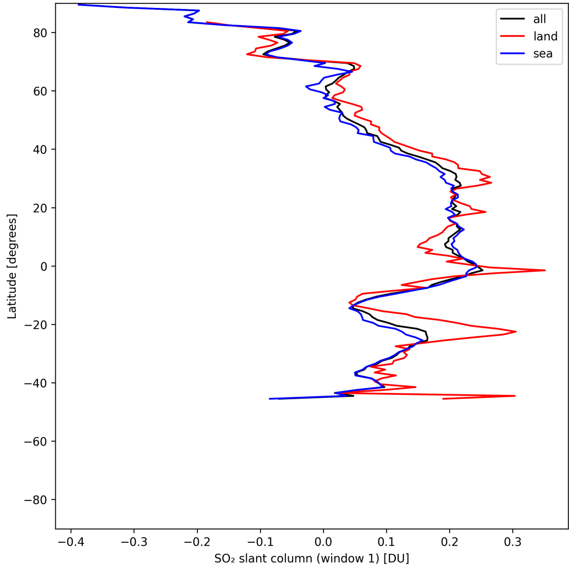
Figure 37: Zonal average of “SO 2 slant column (window 1)” for 2025-06-09 to 2025-06-11.
