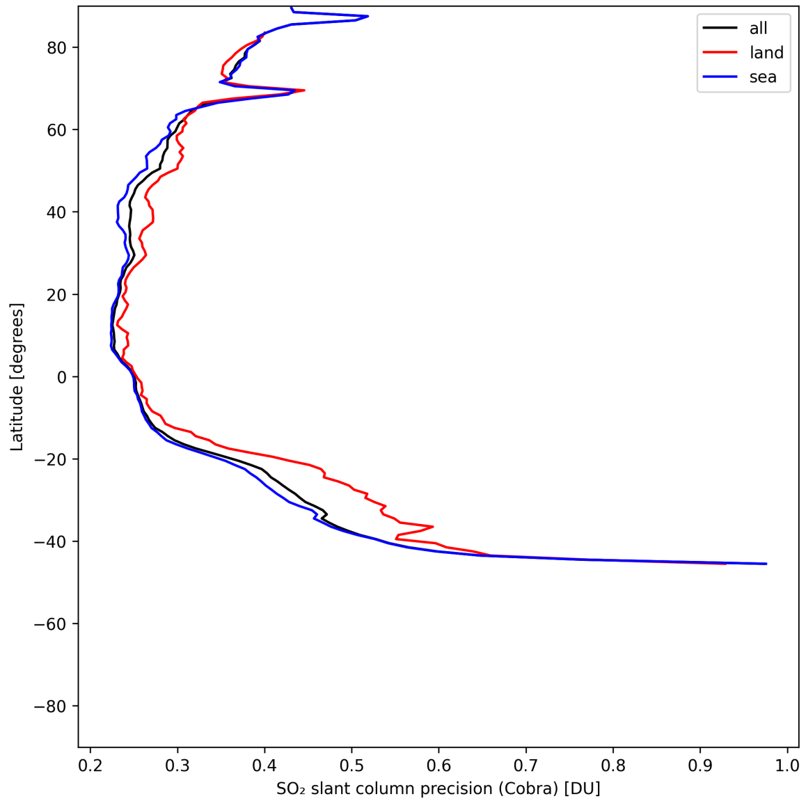
Figure 36: Zonal average of "SO 2 slant column precision (Cobra)" for 2025-06-09 to 2025-06-11.
