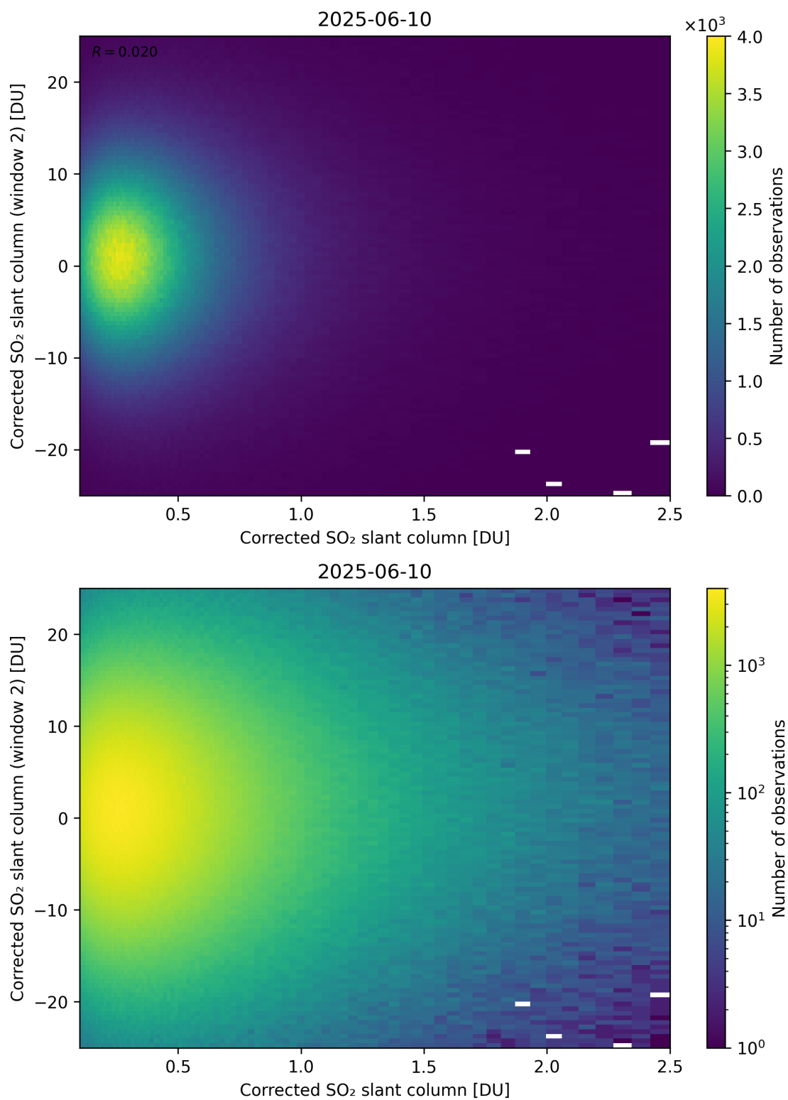
Figure 235: Scatter density plot of “Corrected SO 2 slant column” against “Corrected SO 2 slant column (window 2)” for 2025-06-09 to 2025-06-11.
