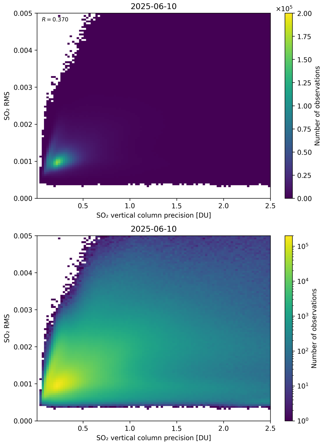
Figure 334: Scatter density plot of “SO 2 vertical column precision” against “SO 2 RMS” for 2025-06-09 to 2025-06-11.
