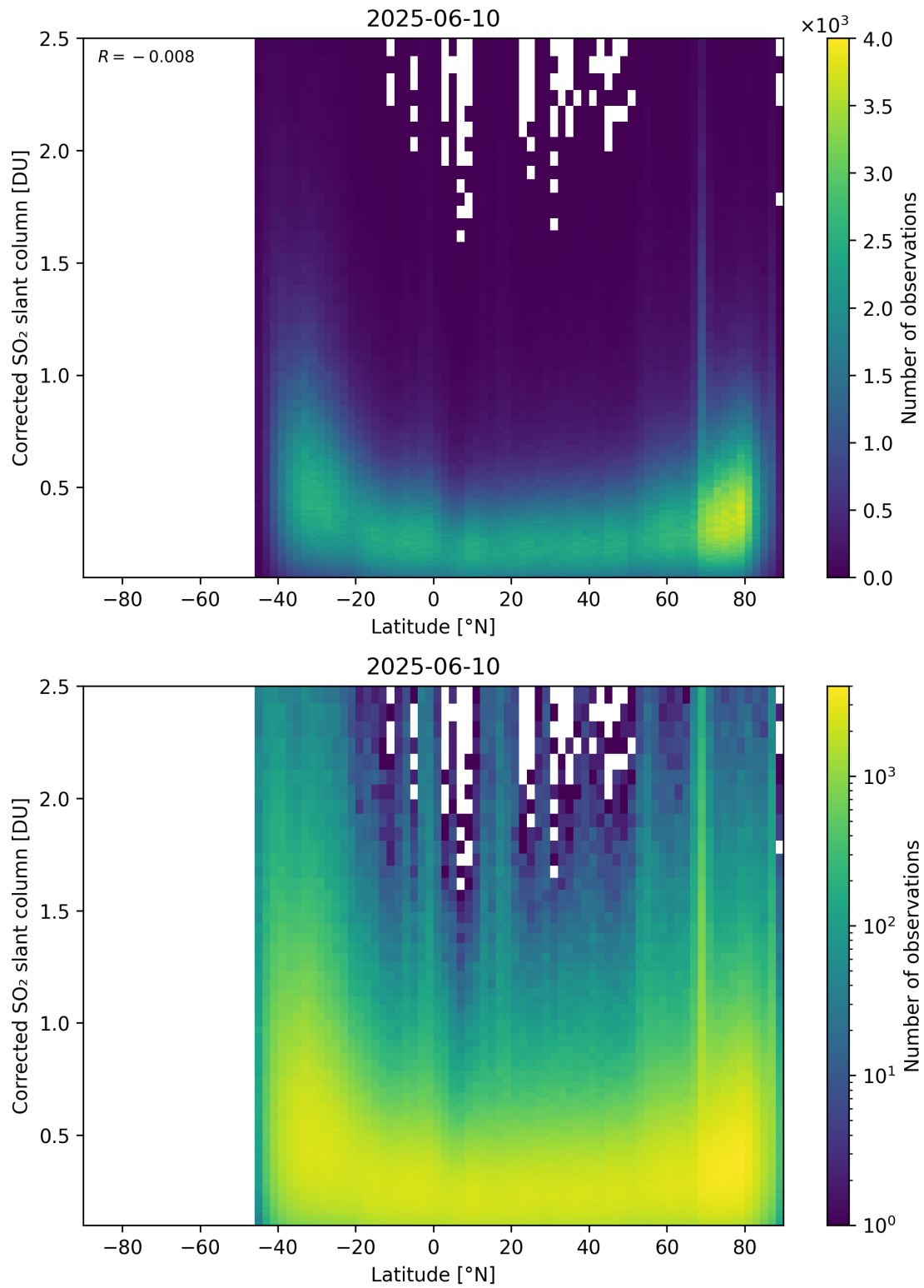
Figure 159: Scatter density plot of “Latitude” against “Corrected SO 2 slant column” for 2025-06-09 to 2025-06-11.
