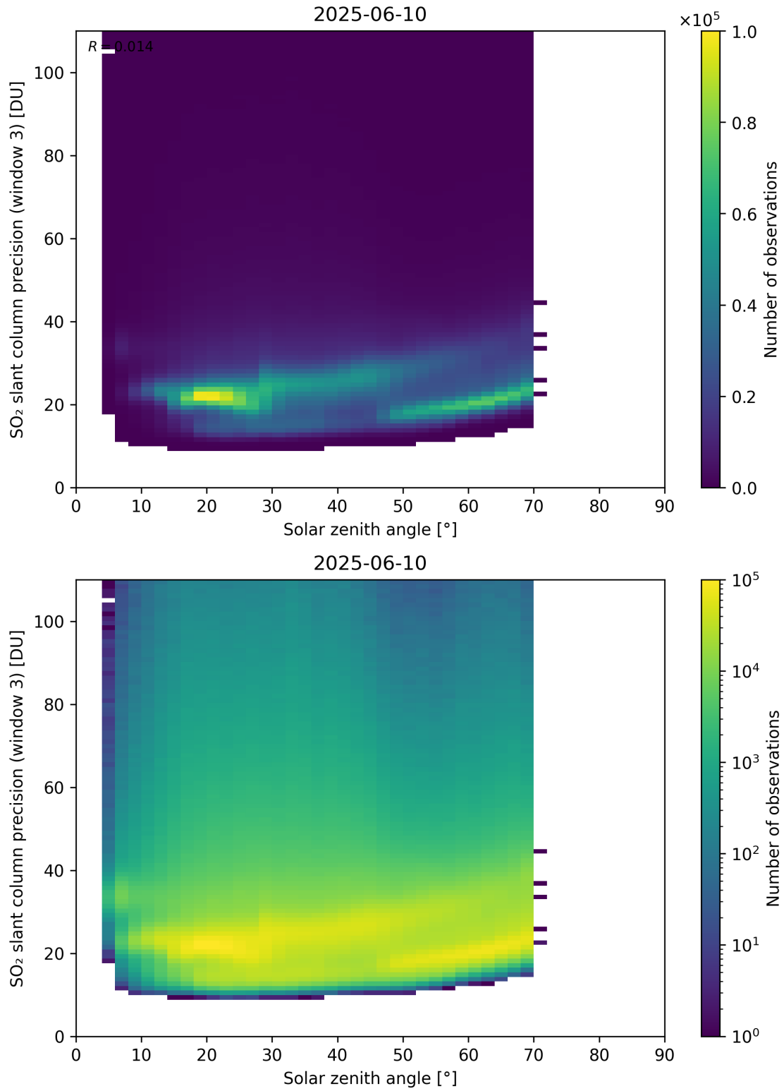
Figure 188: Scatter density plot of “Solar zenith angle” against “SO 2 slant column precision (window 3)” for 2025-06-09 to 2025-06-11.
