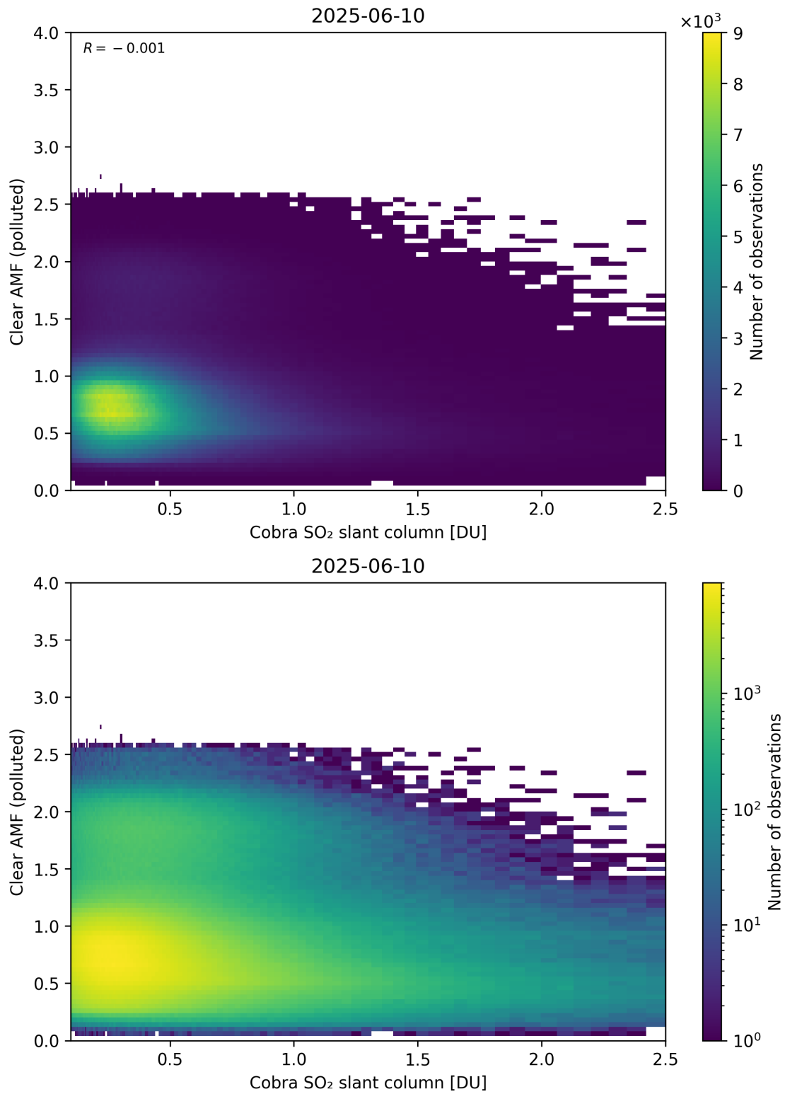
Figure 215: Scatter density plot of “Cobra SO 2 slant column” against “Clear AMF (polluted)” for 2025-06-09 to 2025-06-11.
