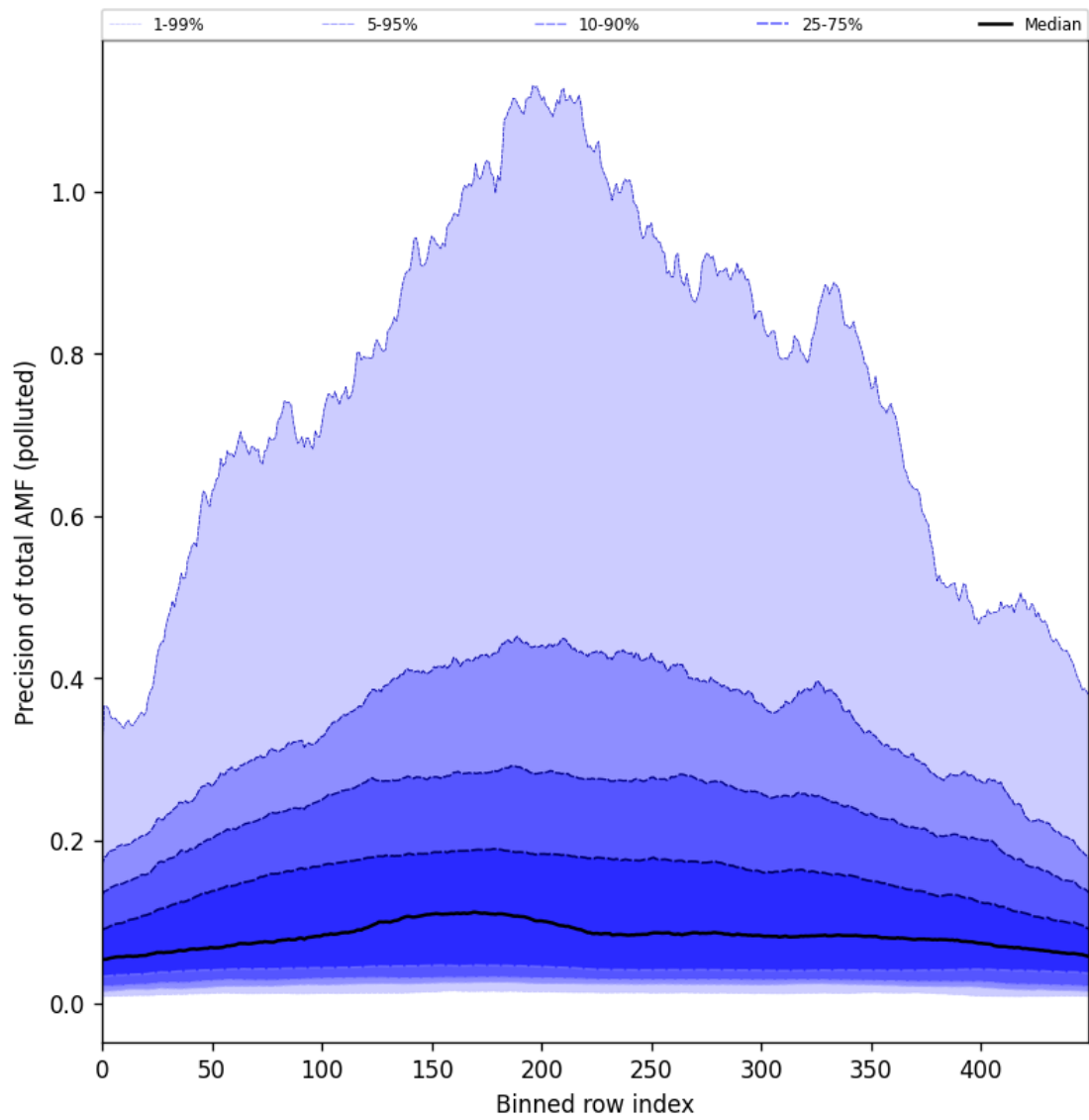
Figure 106: Along track statistics of “Precision of total AMF (polluted)” for 2025-06-09 to 2025-06-11
