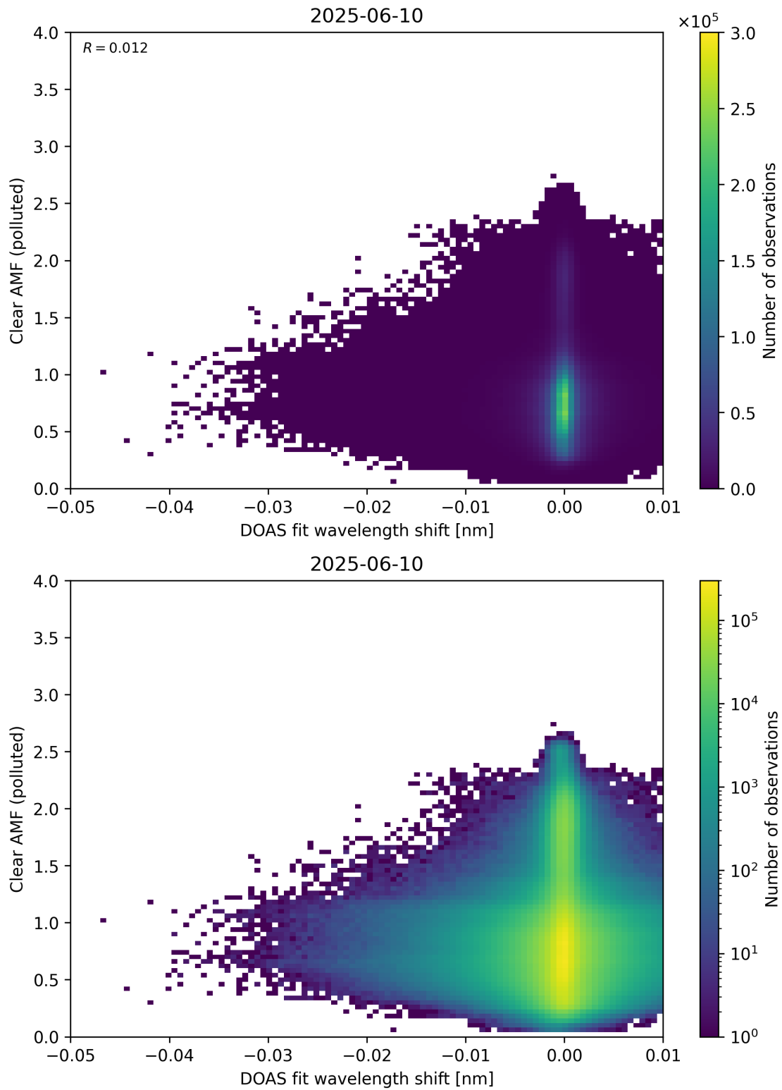
Figure 140: Scatter density plot of “DOAS fit wavelength shift” against “Clear AMF (polluted)” for 2025-06-09 to 2025-06-11.
