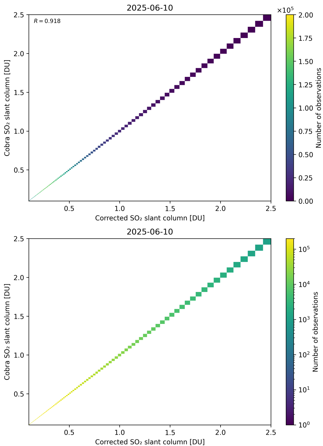
Figure 233: Scatter density plot of “Corrected SO 2 slant column” against “Cobra SO 2 slant column” for 2025-06-09 to 2025-06-11.
