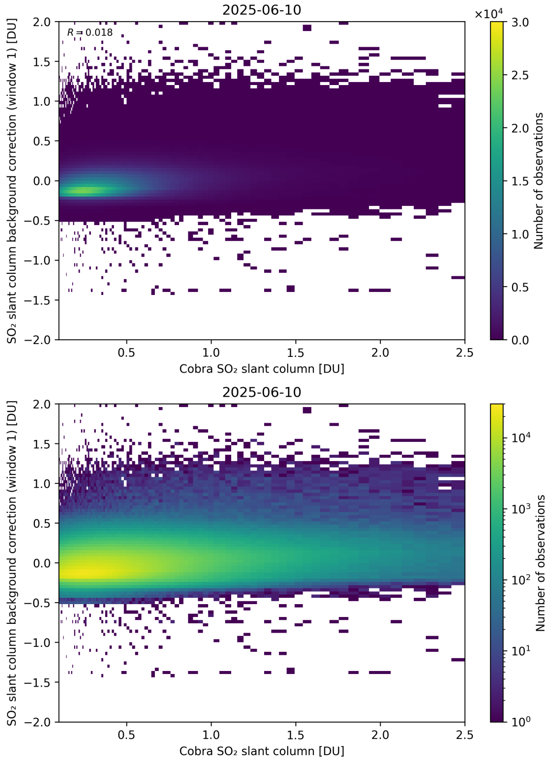
Figure 193: Scatter density plot of “Cobra SO 2 slant column” against “SO 2 slant column background correction (window 1)” for 2025-06-09 to 2025-06-11.
