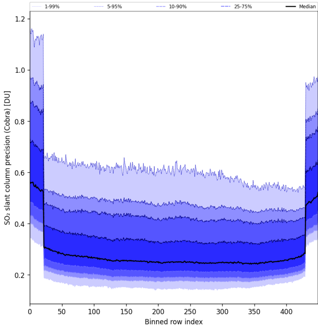
Figure 88: Along track statistics of “SO 2 slant column precision (Cobra)” for 2025-06-09 to 2025-06-11
