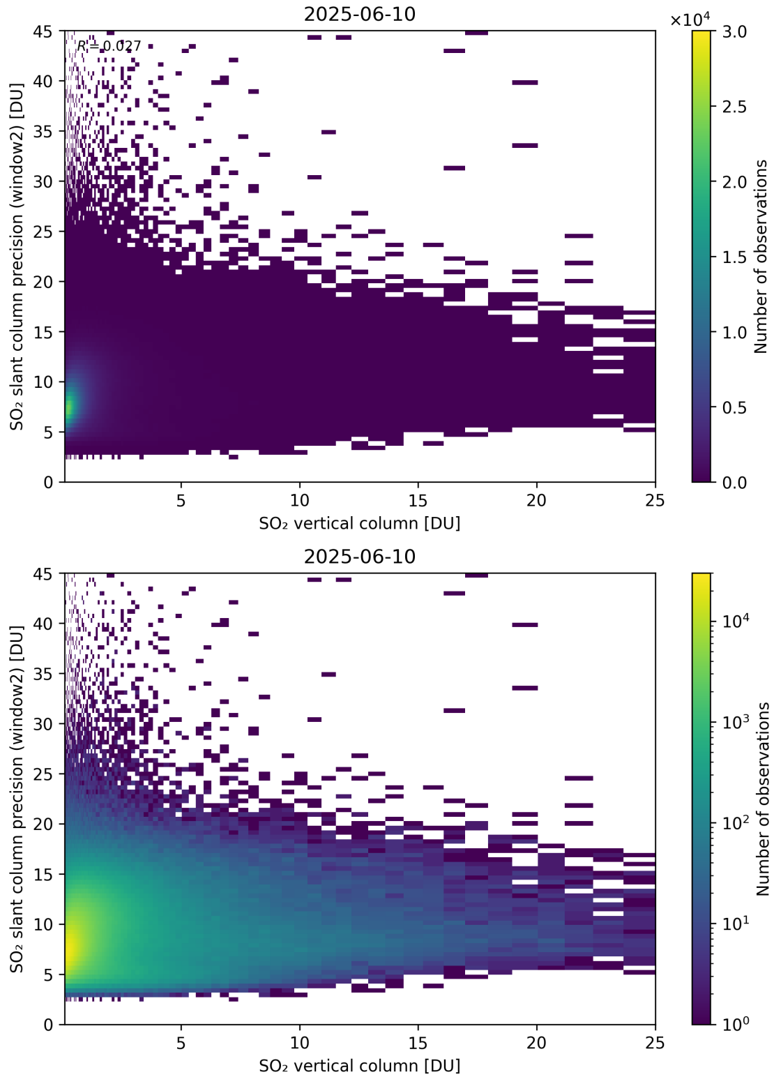
Figure 356: Scatter density plot of “SO 2 vertical column” against “SO 2 slant column precision (window2)” for 2025-06-09 to 2025-06-11.
