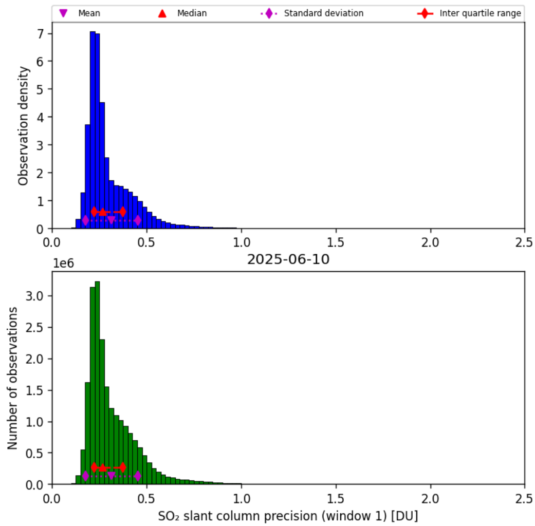
Figure 64: Histogram of “SO 2 slant column precision (window 1)” for 2025-06-09 to 2025-06-11
