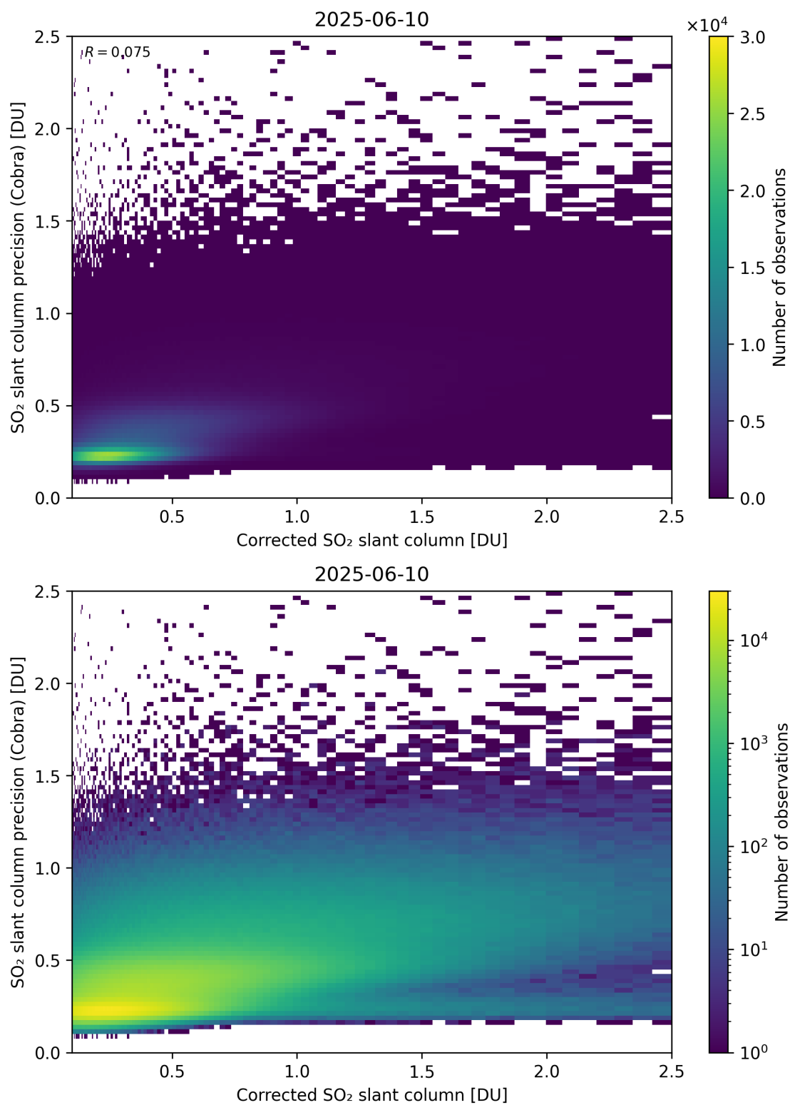
Figure 234: Scatter density plot of “Corrected SO 2 slant column” against “SO 2 slant column precision (Cobra)” for 2025-06-09 to 2025-06-11.
