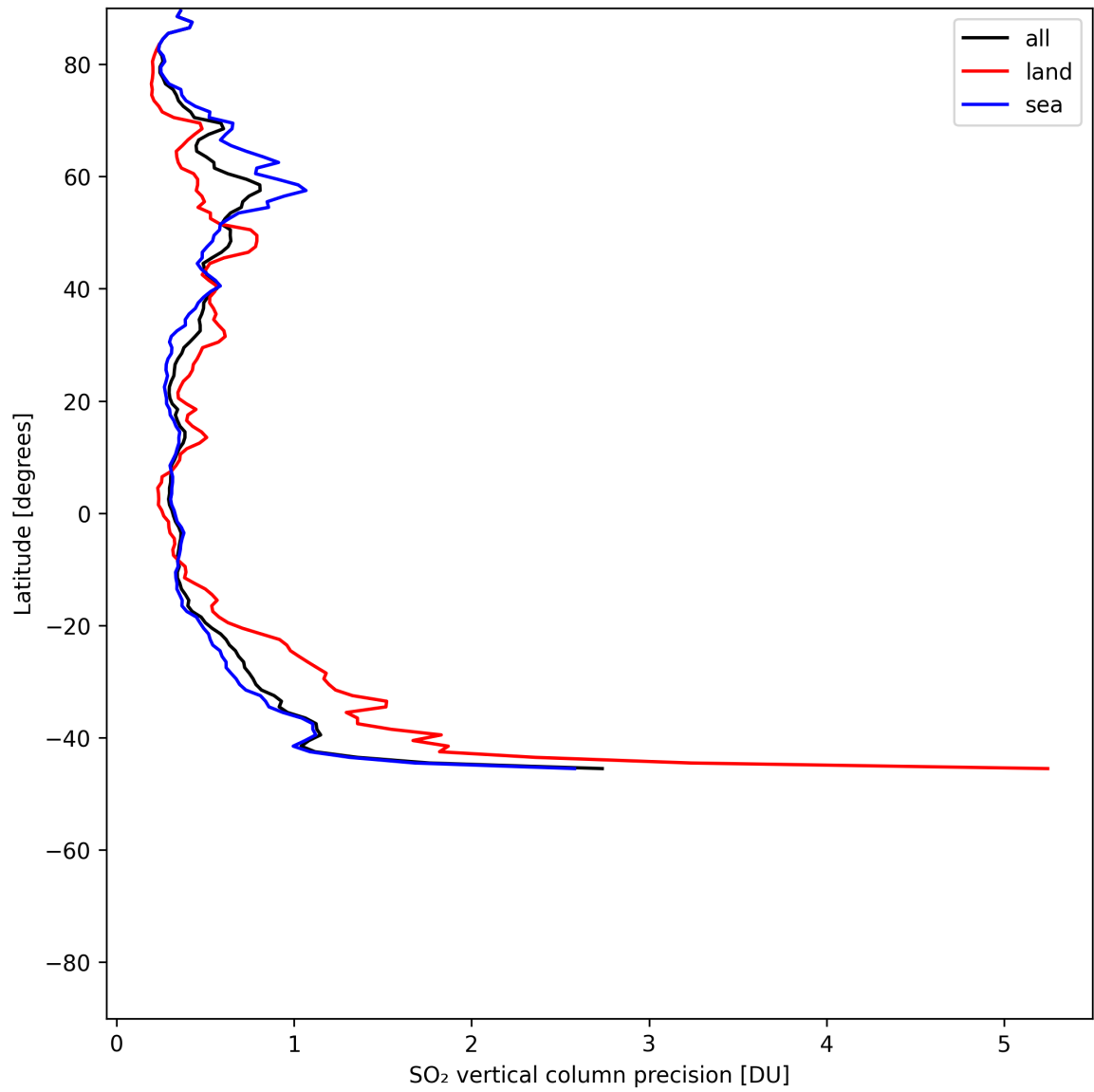
Figure 33: Zonal average of “SO 2 vertical column precision” for 2025-06-09 to 2025-06-11.
