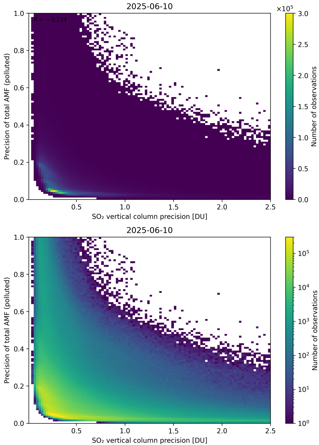
Figure 347: Scatter density plot of “SO 2 vertical column precision” against “Precision of total AMF (polluted)” for 2025-06-09 to 2025-06-11.
