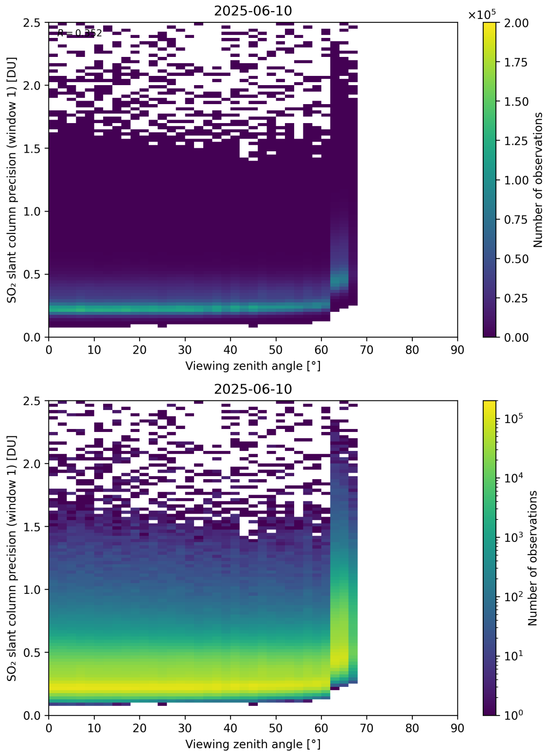
Figure 377: Scatter density plot of “Viewing zenith angle” against “SO 2 slant column precision (window 1)” for 2025-06-09 to 2025-06-11.
