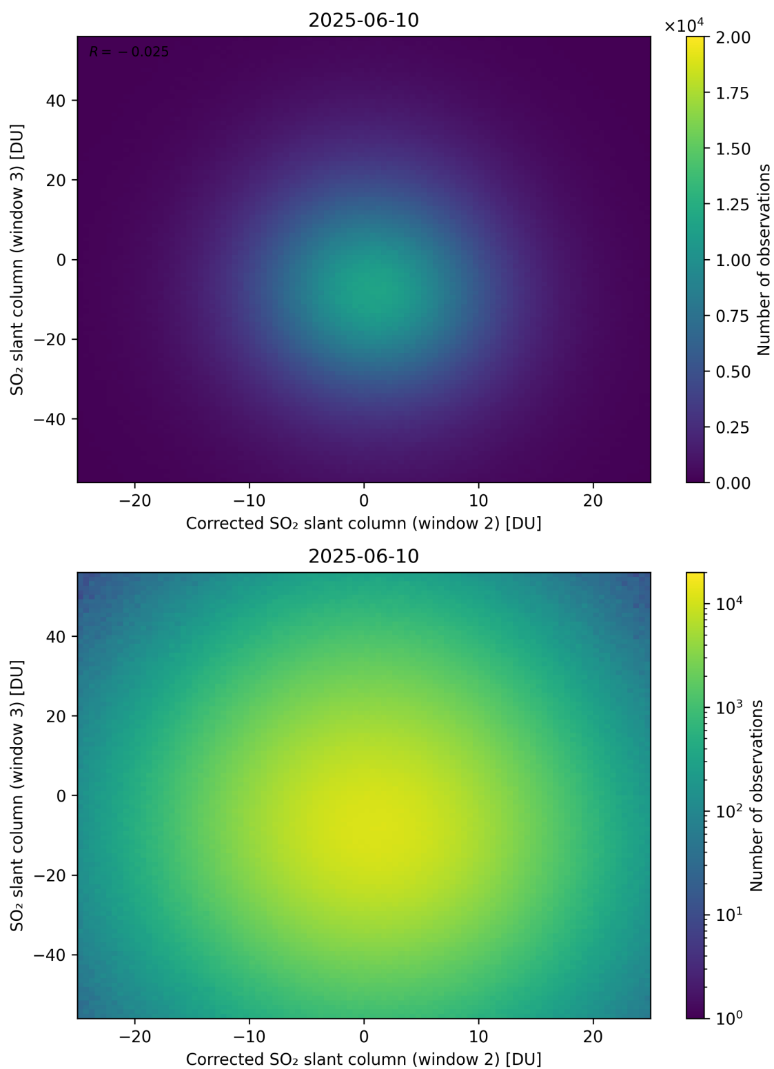
Figure 251: Scatter density plot of “Corrected SO 2 slant column (window 2)” against “SO 2 slant column (window 3)” for 2025-06-09 to 2025-06-11.
