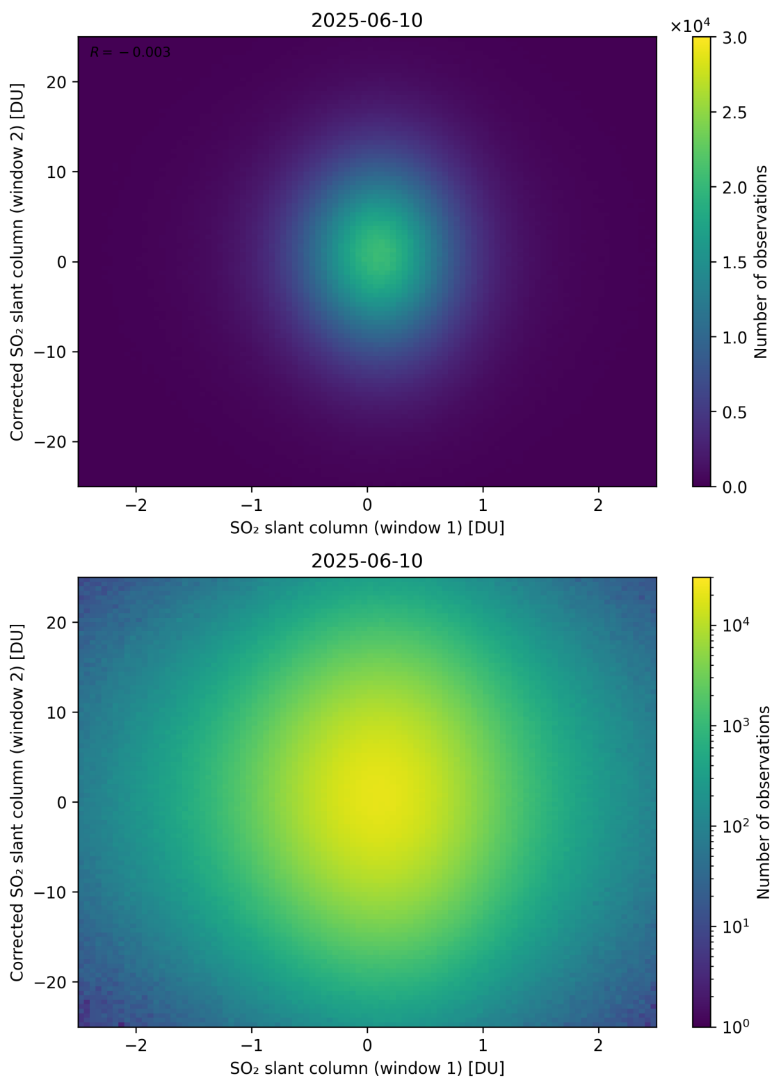
Figure 283: Scatter density plot of “SO 2 slant column (window 1)” against “Corrected SO 2 slant column (window 2)” for 2025-06-09 to 2025-06-11.
