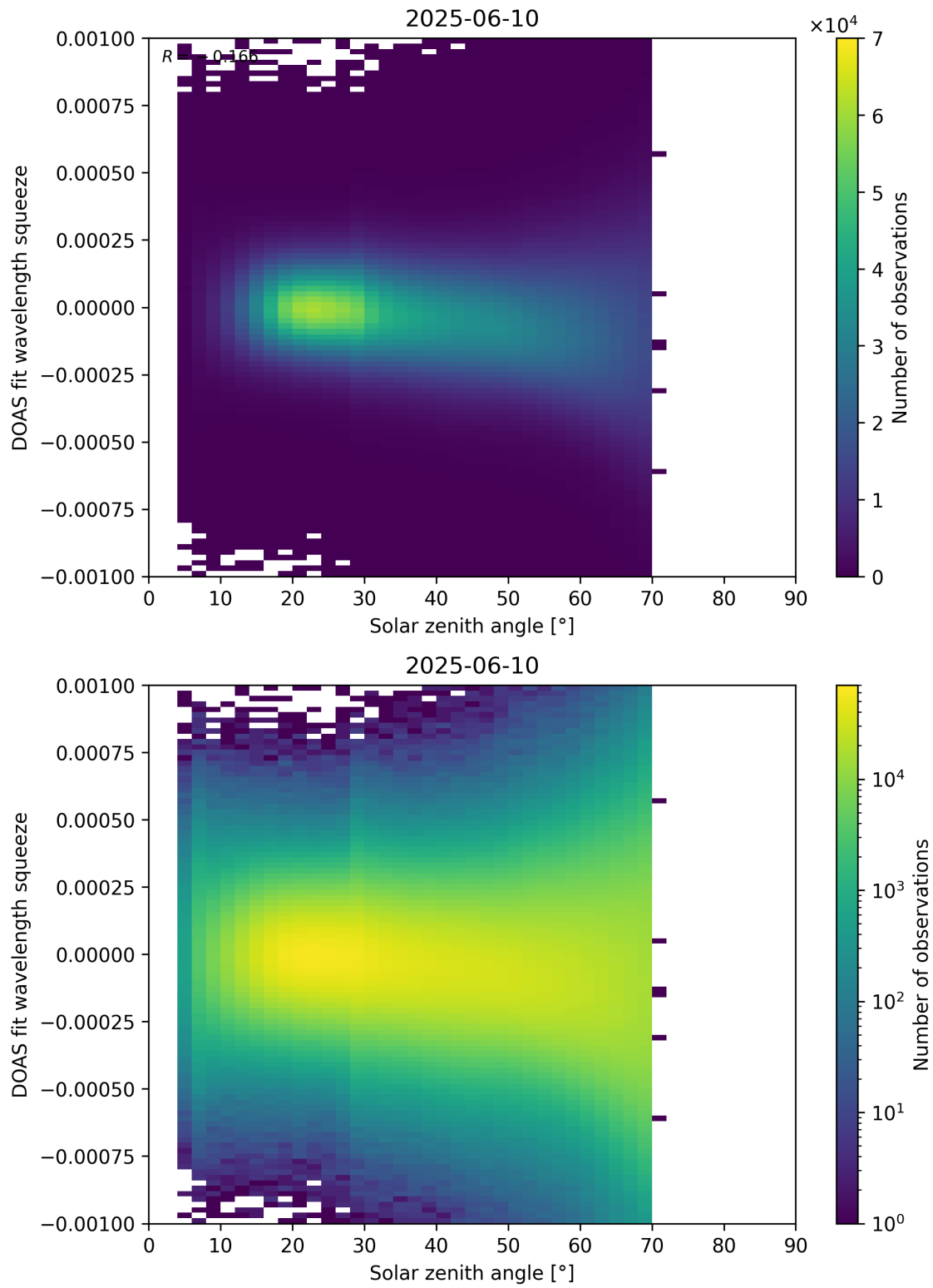
Figure 175: Scatter density plot of “Solar zenith angle” against “DOAS fit wavelength squeeze” for 2025-06-09 to 2025-06-11.
