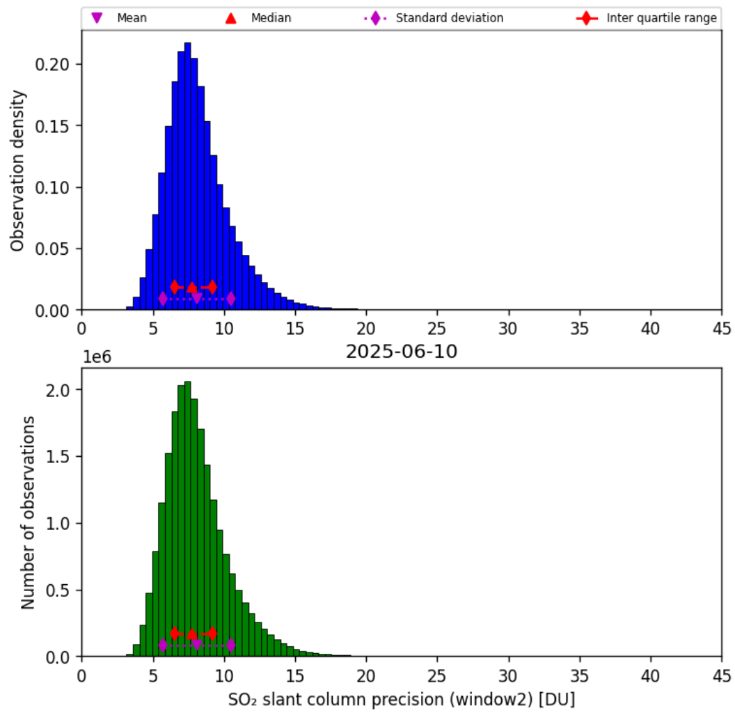
Figure 68: Histogram of “SO 2 slant column precision (window2)” for 2025-06-09 to 2025-06-11
