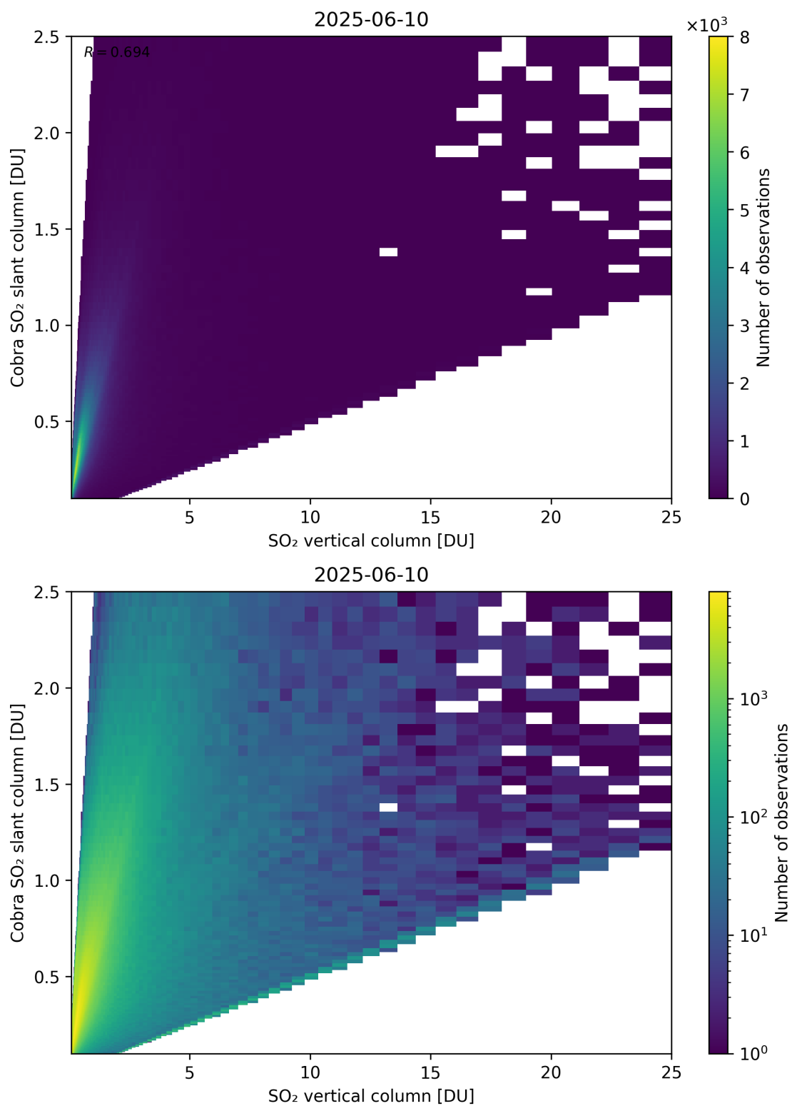
Figure 349: Scatter density plot of “SO 2 vertical column” against “Cobra SO 2 slant column” for 2025-06-09 to 2025-06-11.
