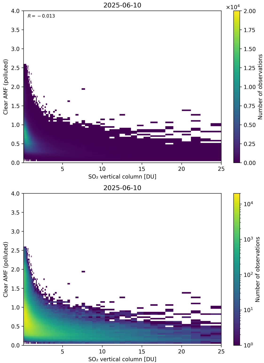
Figure 348: Scatter density plot of “SO 2 vertical column” against “Clear AMF (polluted)” for 2025-06-09 to 2025-06-11.
