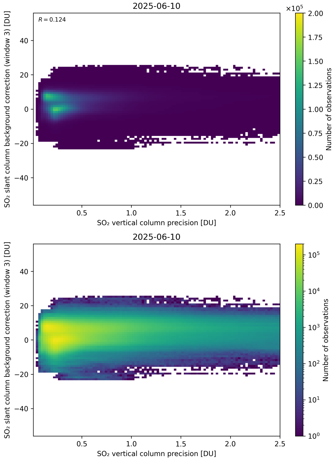
Figure 331: Scatter density plot of “SO 2 vertical column precision” against “SO 2 slant column background correction (window 3)” for 2025-06-09 to 2025-06-11.
