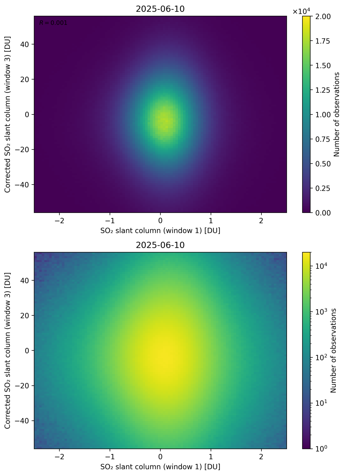
Figure 284: Scatter density plot of “SO 2 slant column (window 1)” against “Corrected SO 2 slant column (window 3)” for 2025-06-09 to 2025-06-11.
