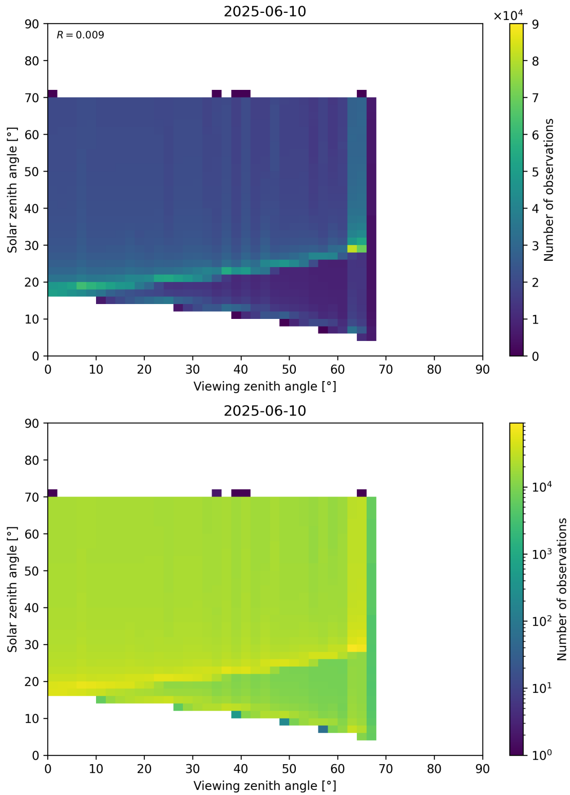
Figure 369: Scatter density plot of “Viewing zenith angle” against “Solar zenith angle” for 2025-06-09 to 2025-06-11.
