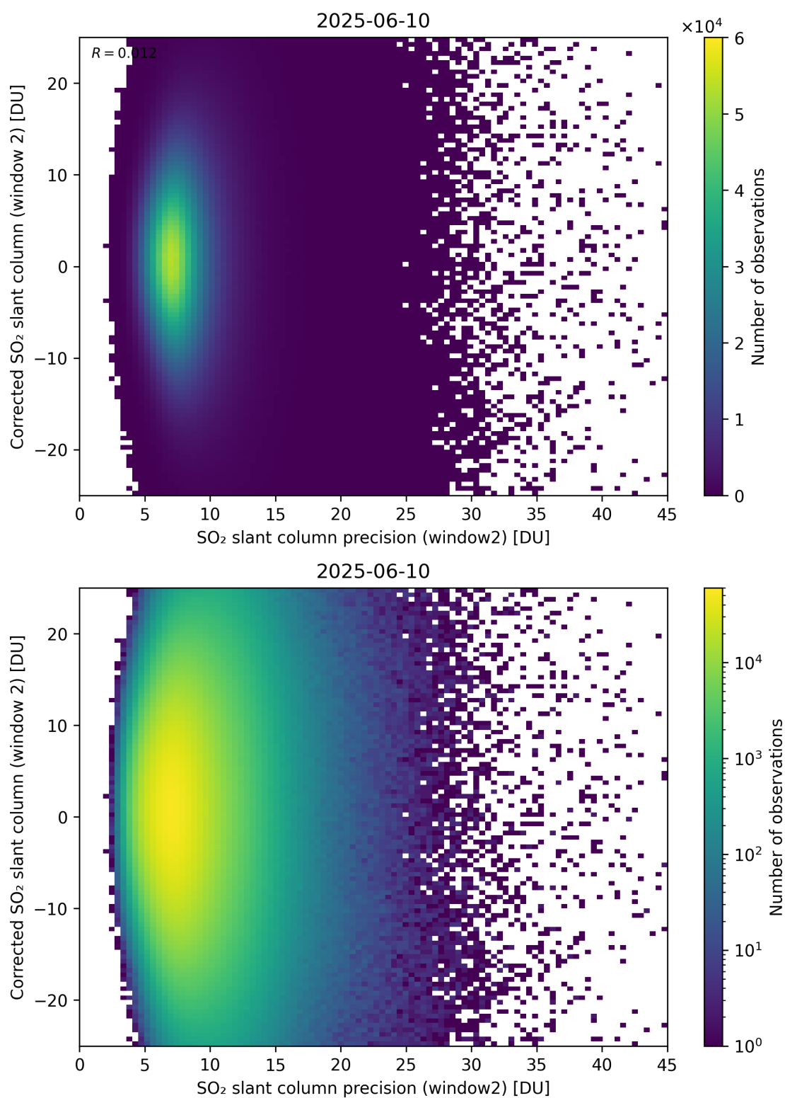
Figure 297: Scatter density plot of “SO 2 slant column precision (window2)” against “Corrected SO 2 slant column (window 2)” for 2025-06-09 to 2025-06-11.
