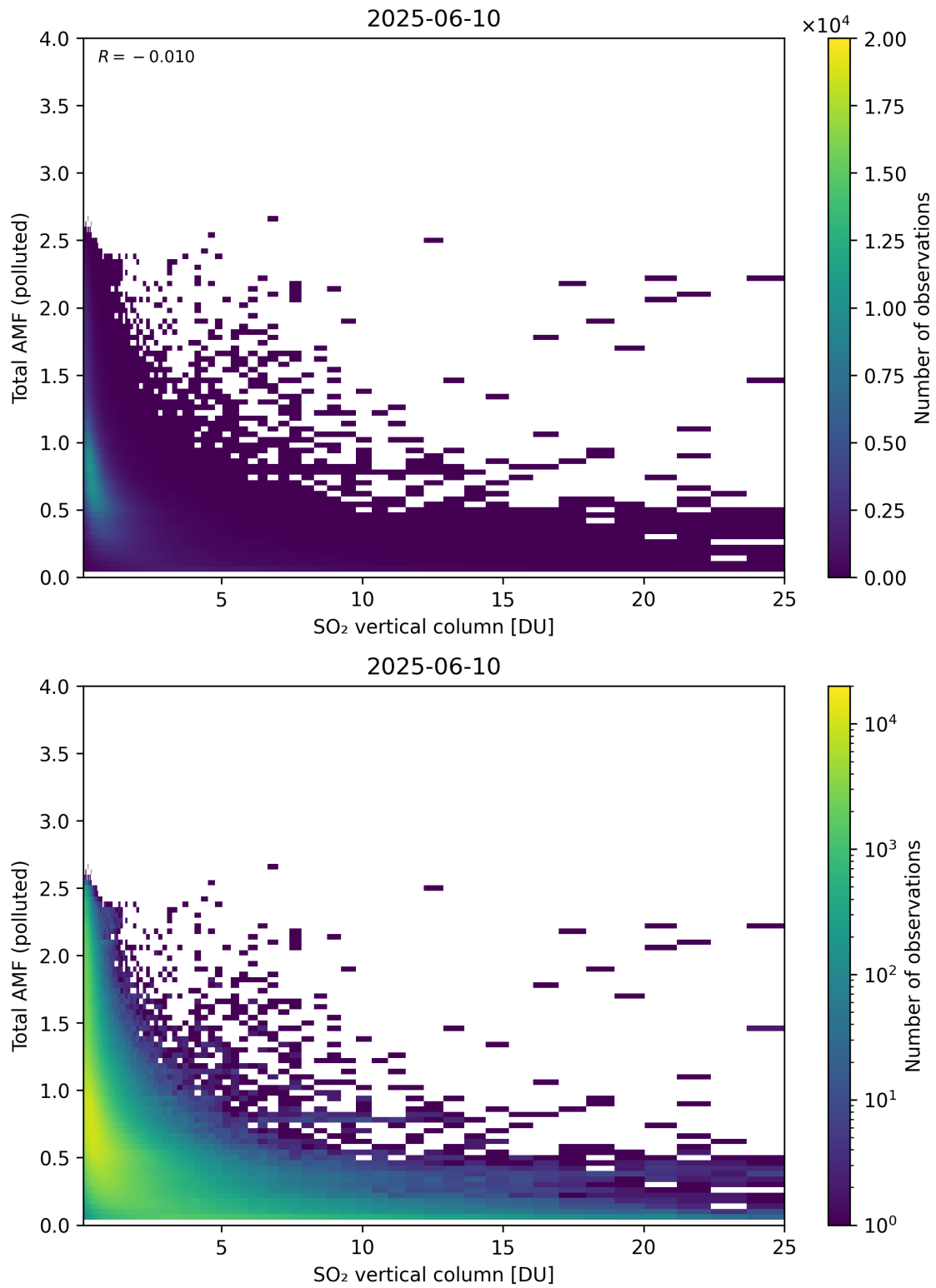
Figure 359: Scatter density plot of “SO 2 vertical column” against “Total AMF (polluted)” for 2025-06-09 to 2025-06-11.
