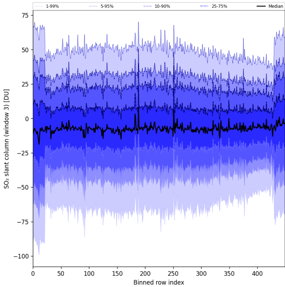
Figure 97: Along track statistics of “SO 2 slant column (window 3)” for 2025-06-09 to 2025-06-11
