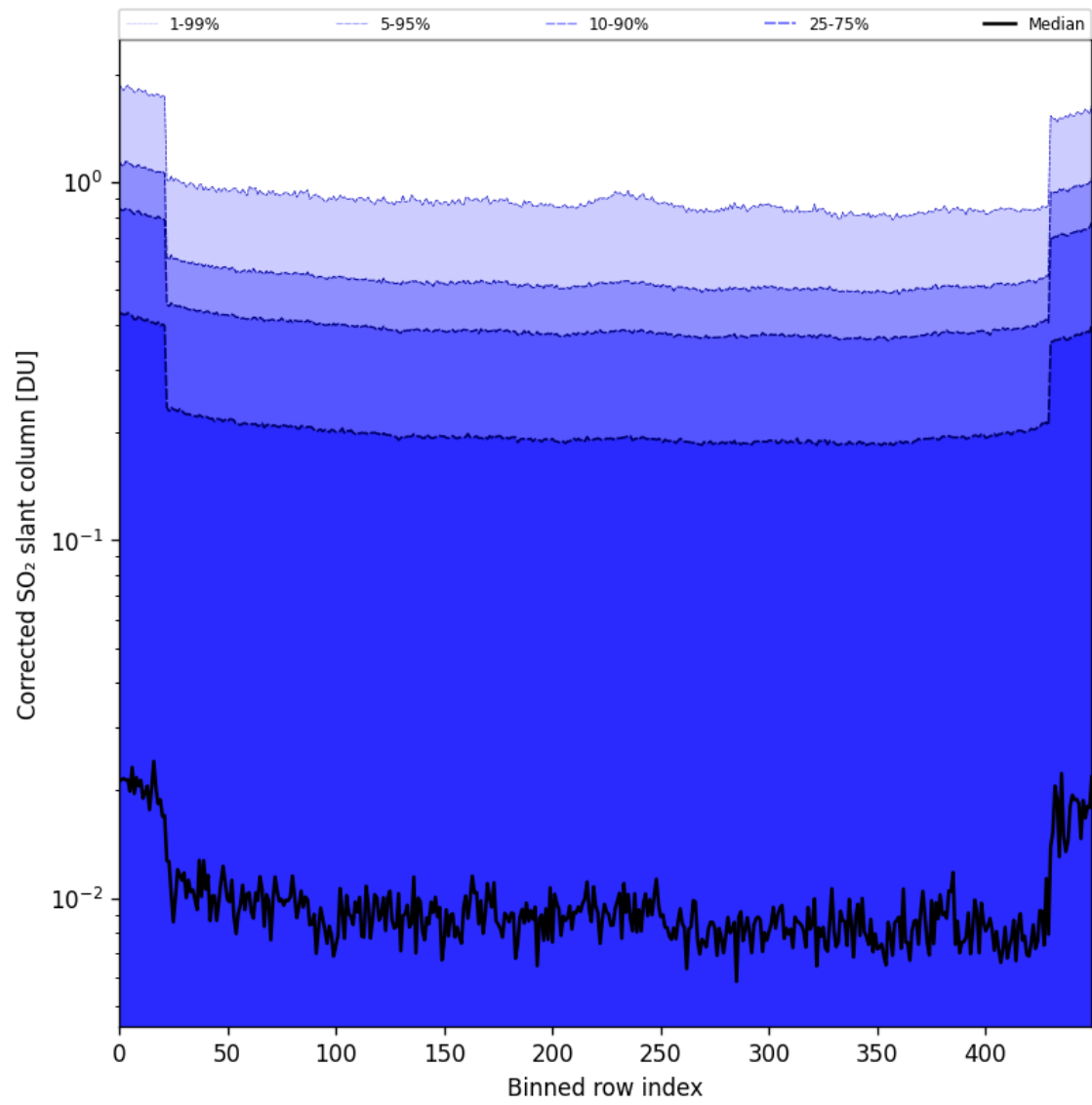
Figure 86: Along track statistics of “Corrected SO 2 slant column” for 2025-06-09 to 2025-06-11
