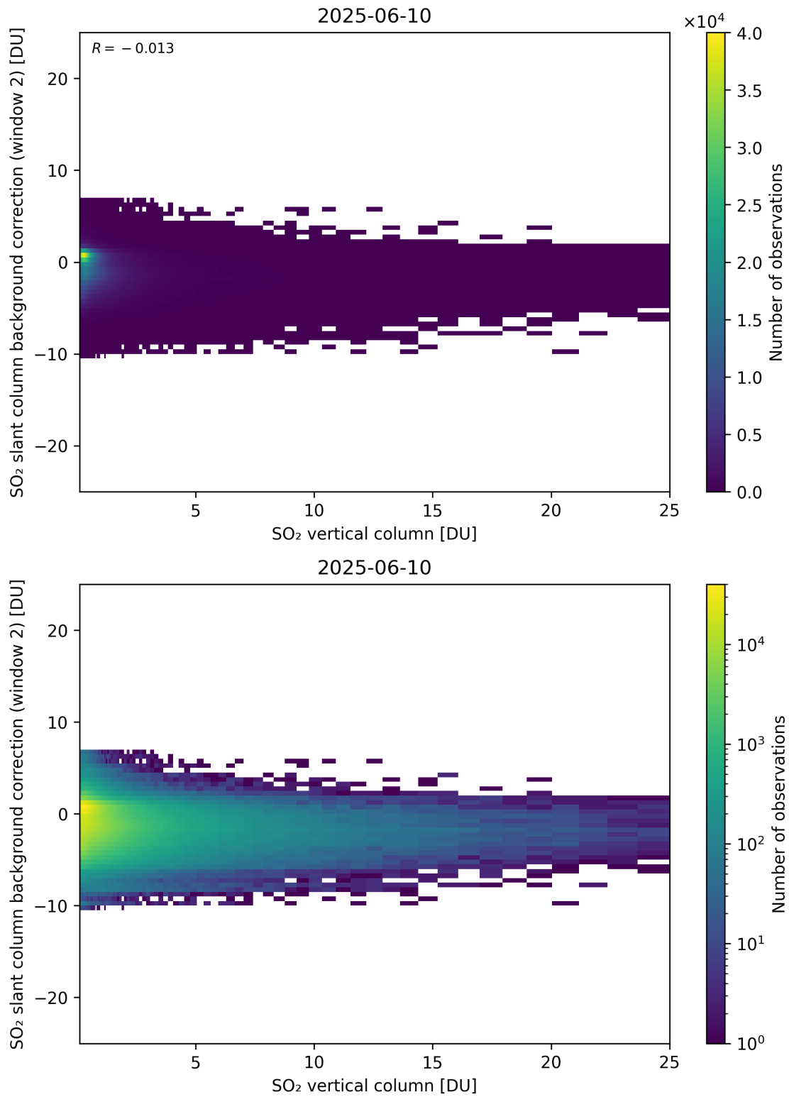
Figure 324: Scatter density plot of “SO 2 vertical column” against “SO 2 slant column background correction (window 2)” for 2025-06-09 to 2025-06-11.
