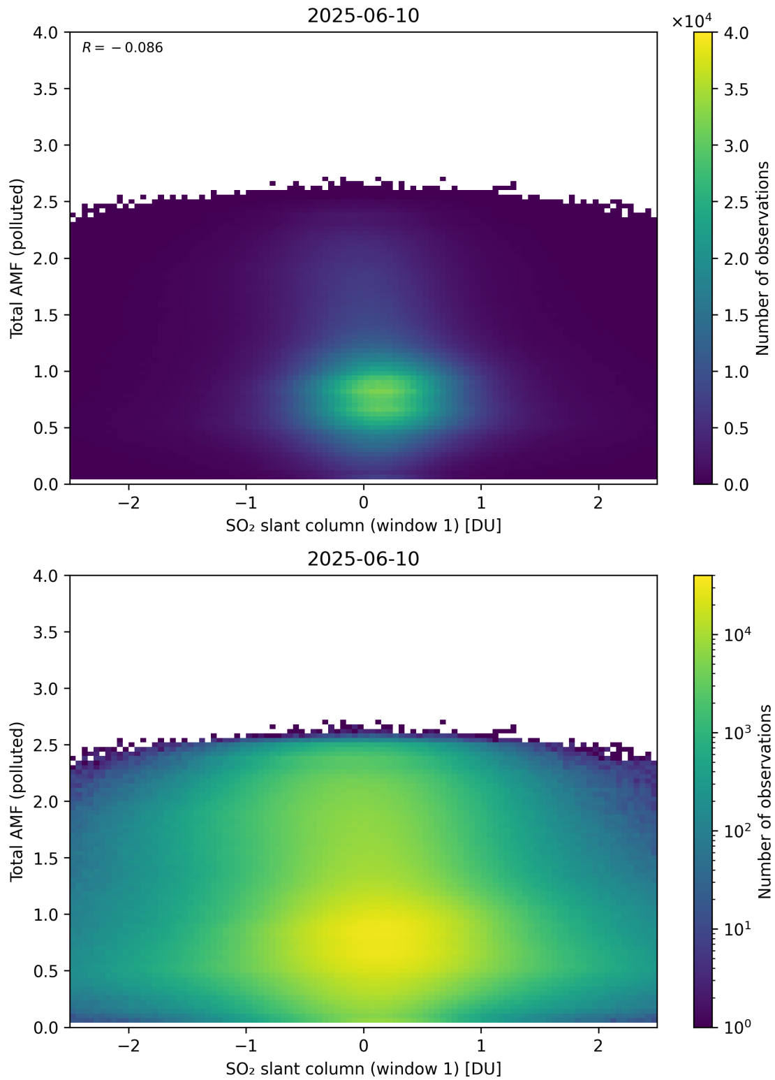
Figure 289: Scatter density plot of “SO 2 slant column (window 1)” against “Total AMF (polluted)” for 2025-06-09 to 2025-06-11.
