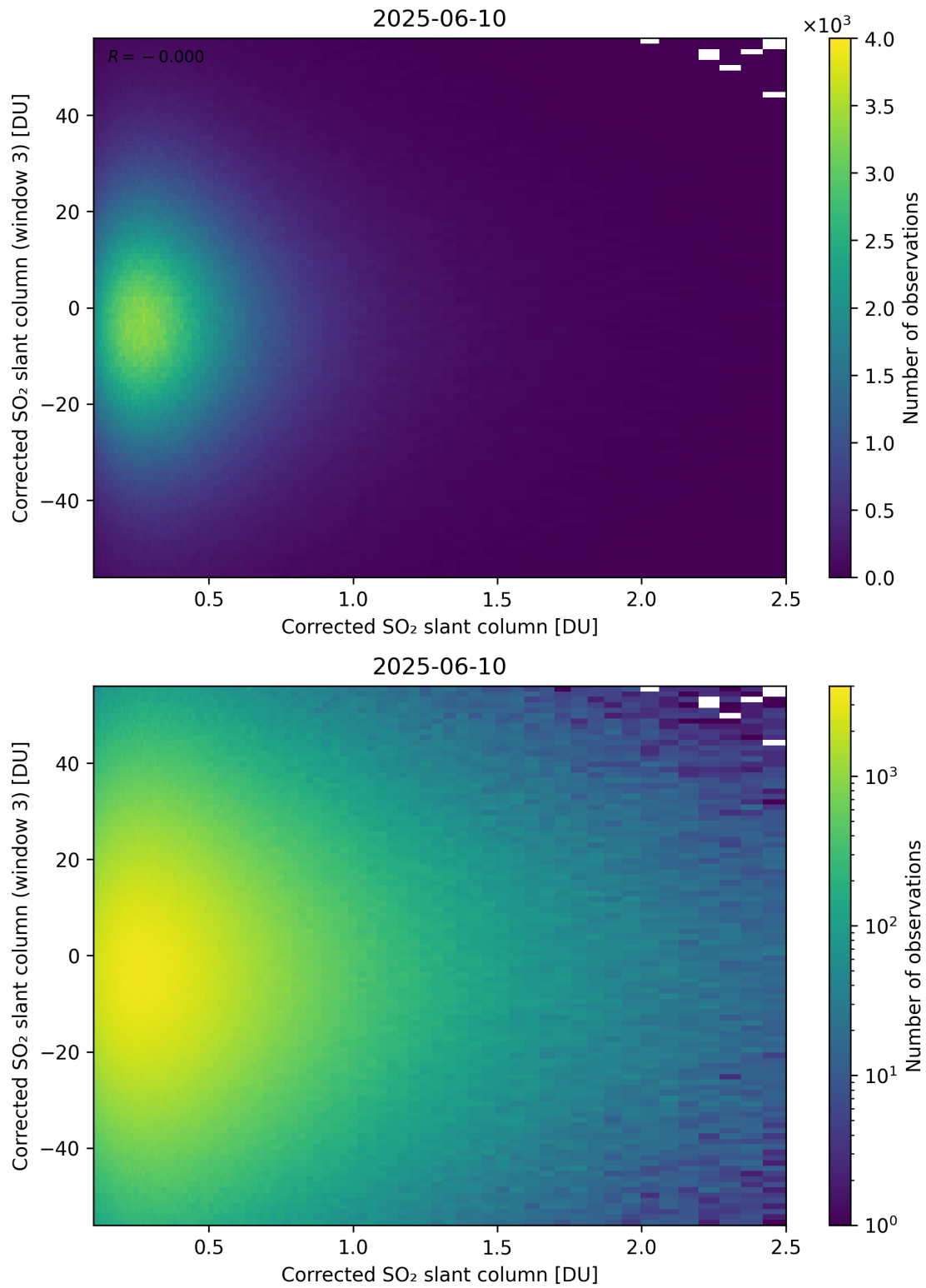
Figure 236: Scatter density plot of “Corrected SO 2 slant column” against “Corrected SO 2 slant column (window 3)” for 2025-06-09 to 2025-06-11.
