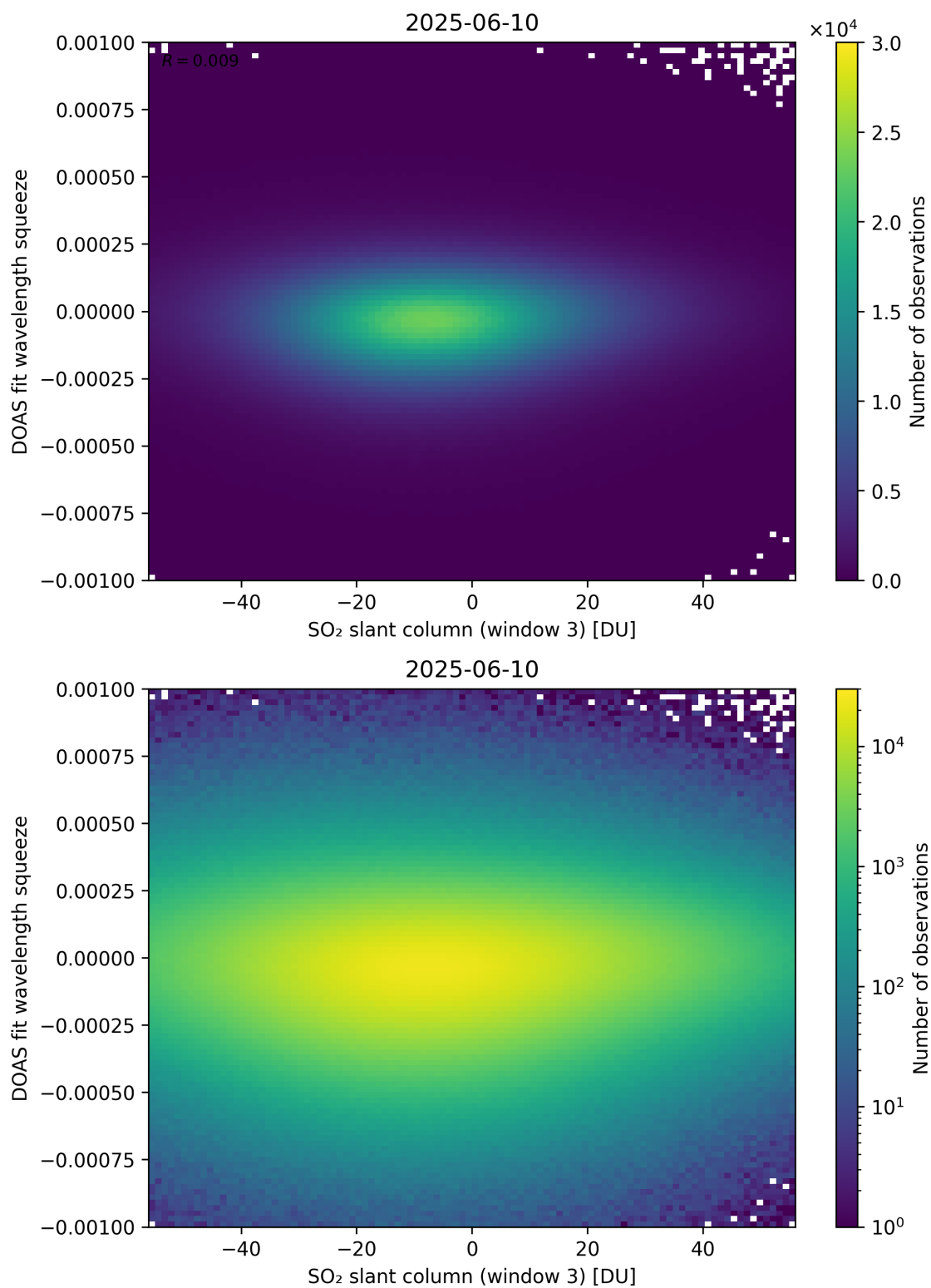
Figure 305: Scatter density plot of “SO 2 slant column (window 3)” against “DOAS fit wavelength squeeze” for 2025-06-09 to 2025-06-11.
