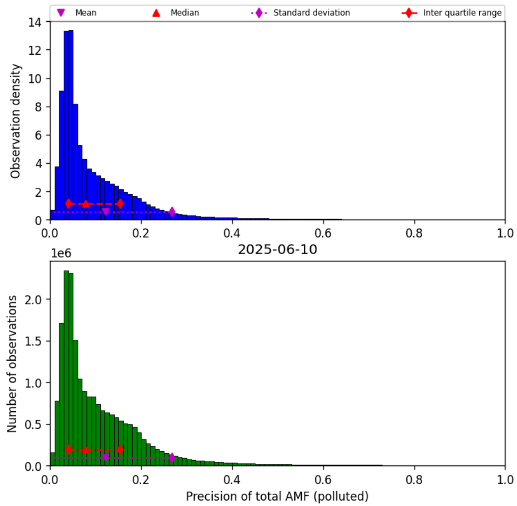
Figure 80: Histogram of “Precision of total AMF (polluted)” for 2025-06-09 to 2025-06-11
