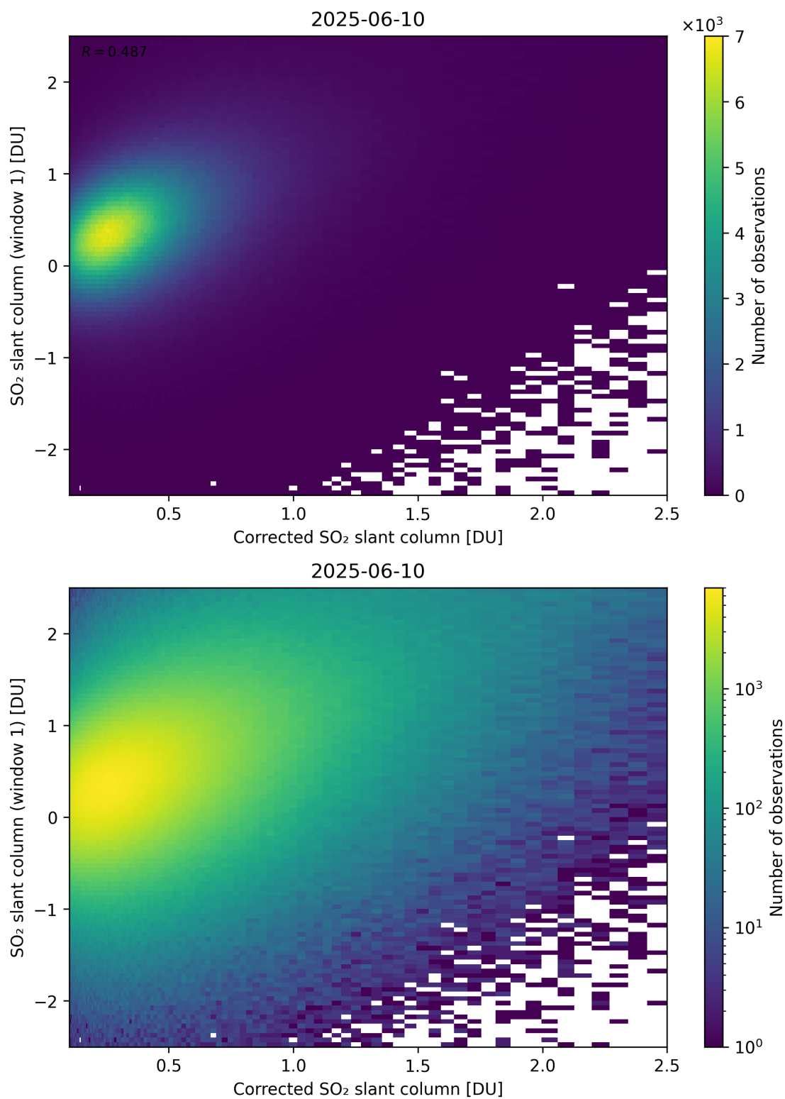
Figure 237: Scatter density plot of “Corrected SO 2 slant column” against “SO 2 slant column (window 1)” for 2025-06-09 to 2025-06-11.
