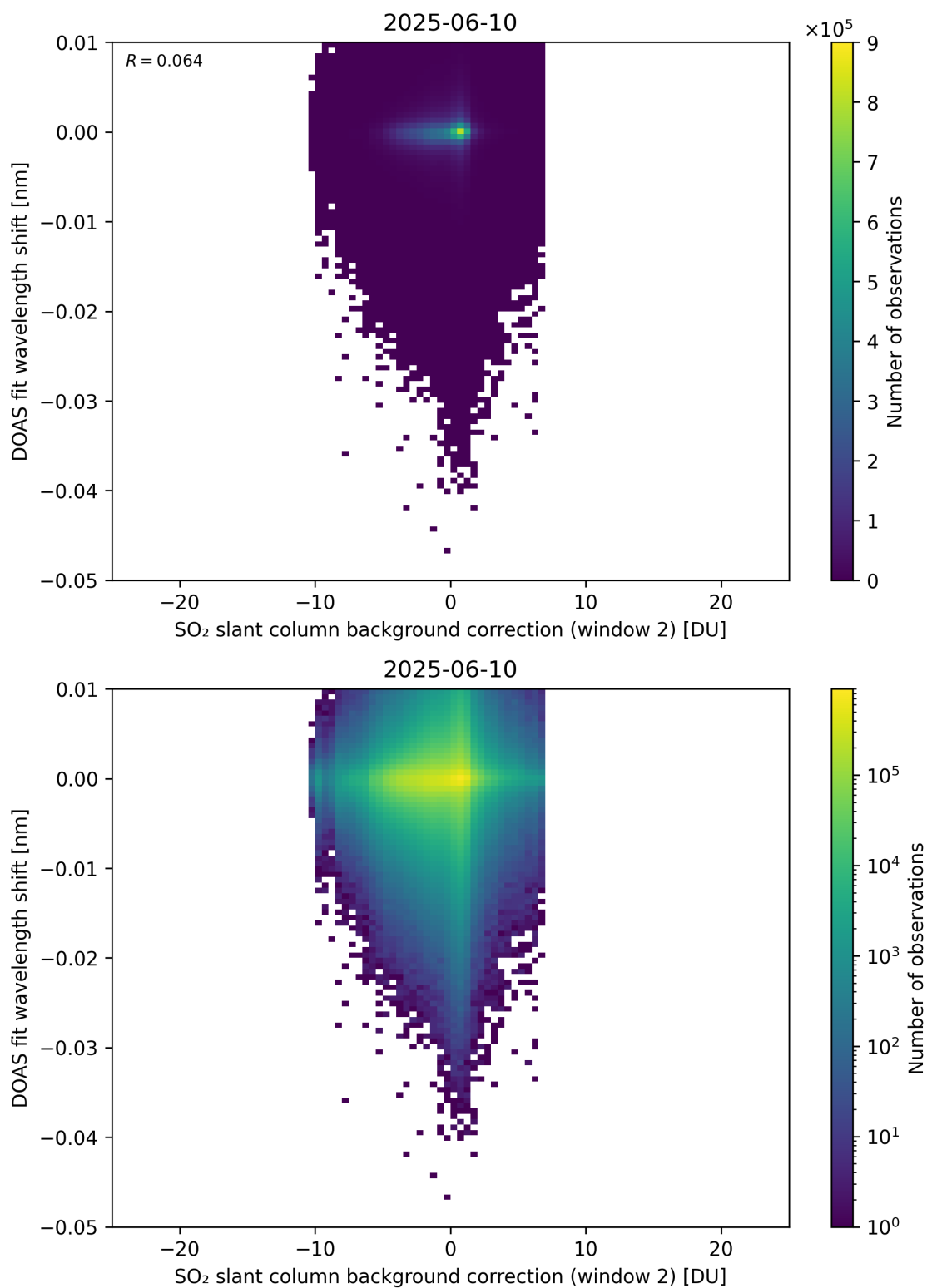
Figure 123: Scatter density plot of “SO 2 slant column background correction (window 2)” against “DOAS fit wavelength shift” for 2025-06-09 to 2025-06-11.
