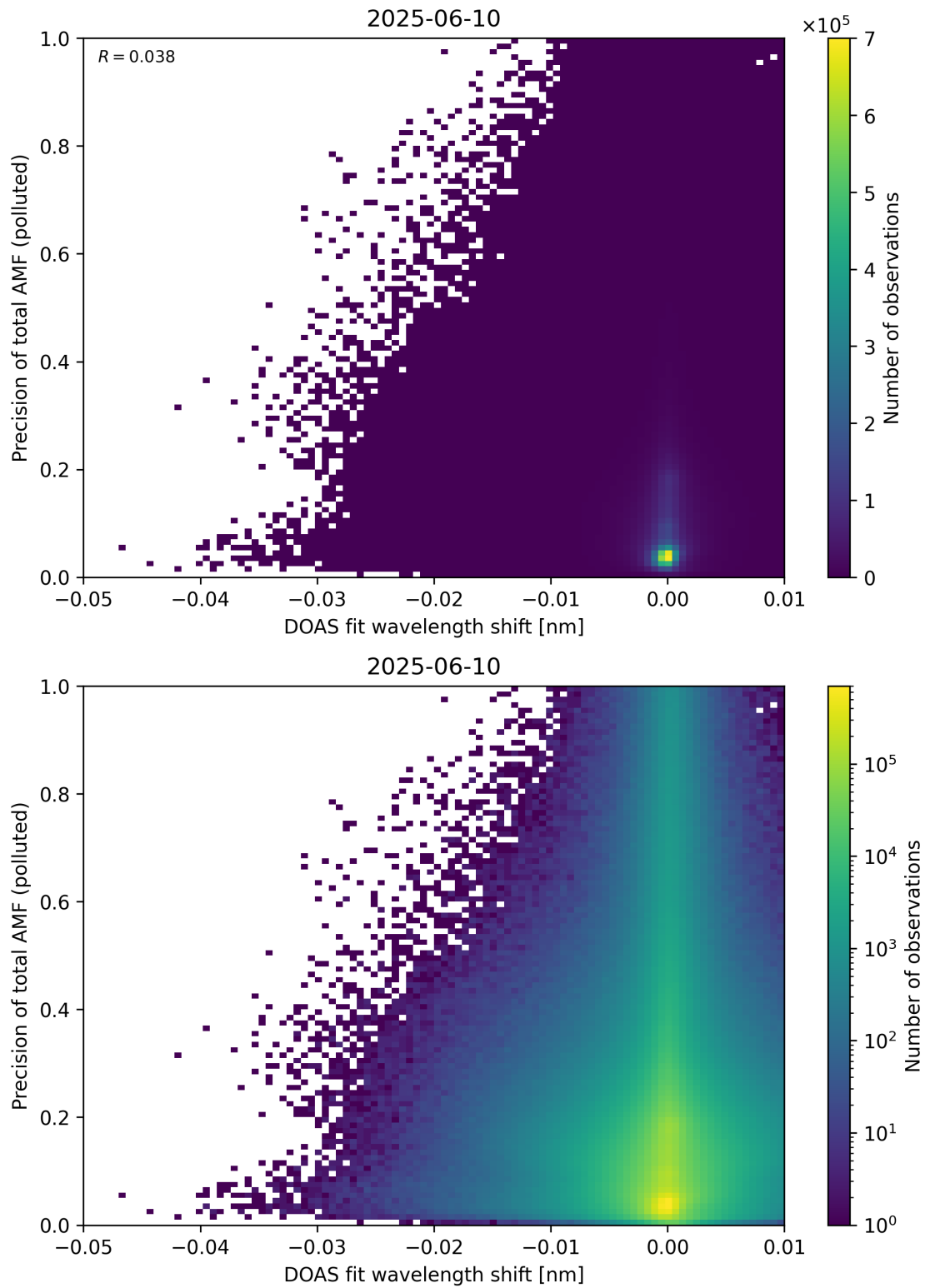
Figure 142: Scatter density plot of “DOAS fit wavelength shift” against “Precision of total AMF (polluted)” for 2025-06-09 to 2025-06-11.
