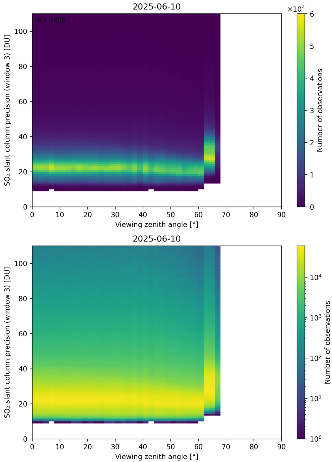
Figure 380: Scatter density plot of “Viewing zenith angle” against “SO 2 slant column precision (window 3)” for 2025-06-09 to 2025-06-11.
