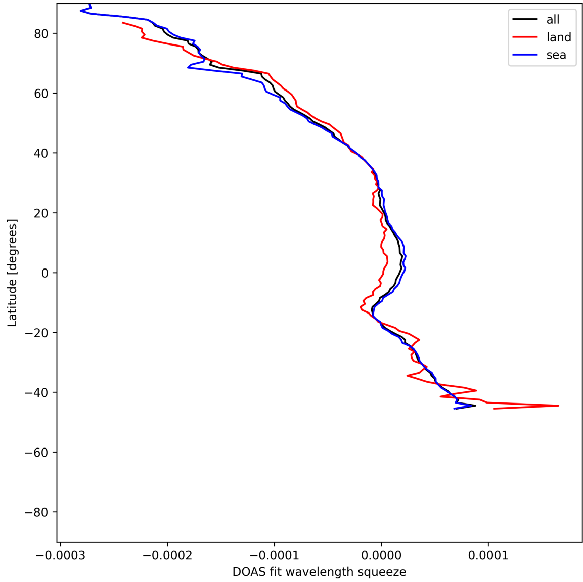
Figure 51: Zonal average of “DOAS fit wavelength squeeze” for 2025-06-09 to 2025-06-11.
