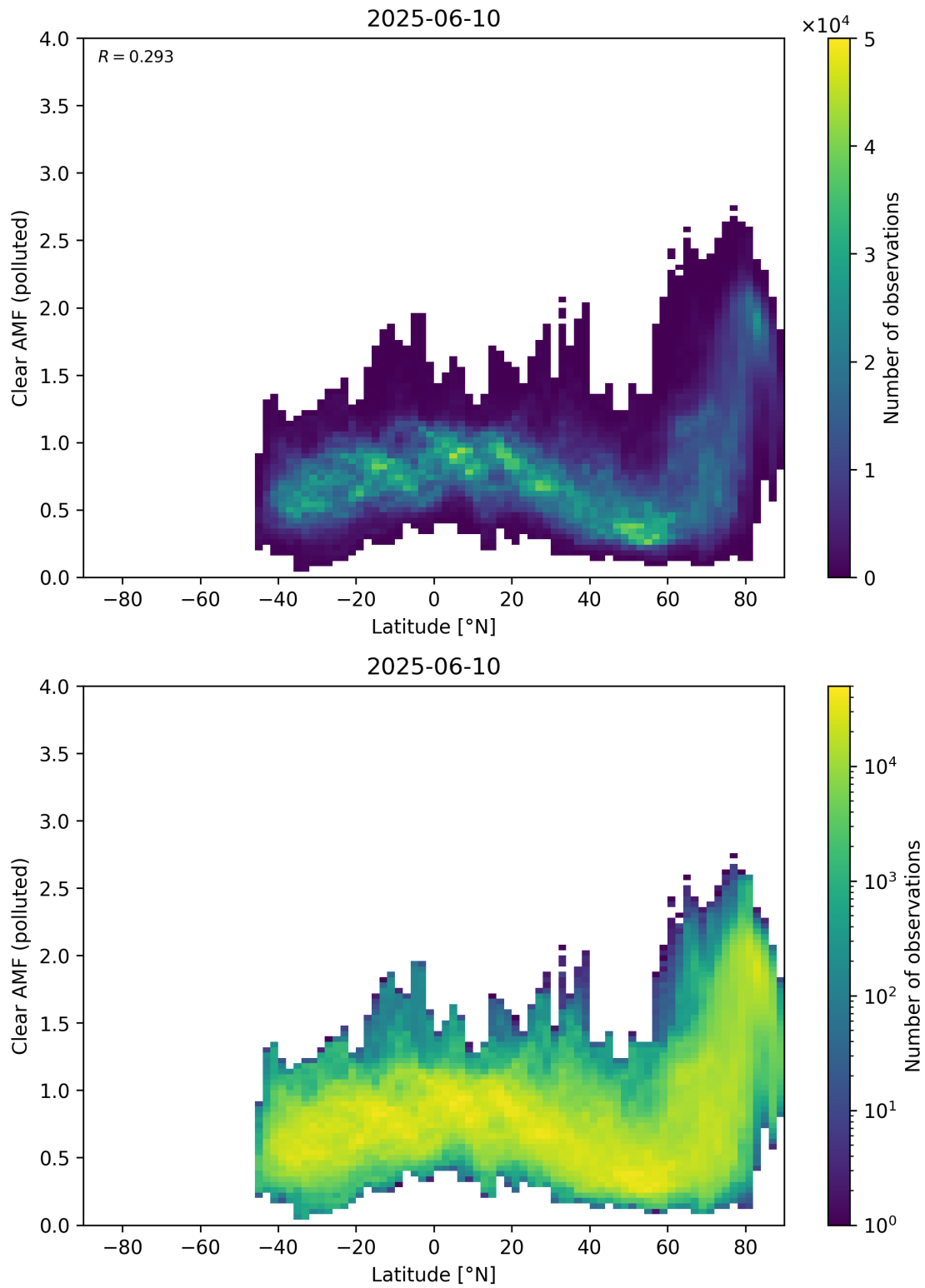
Figure 156: Scatter density plot of “Latitude” against “Clear AMF (polluted)” for 2025-06-09 to 2025-06-11.
