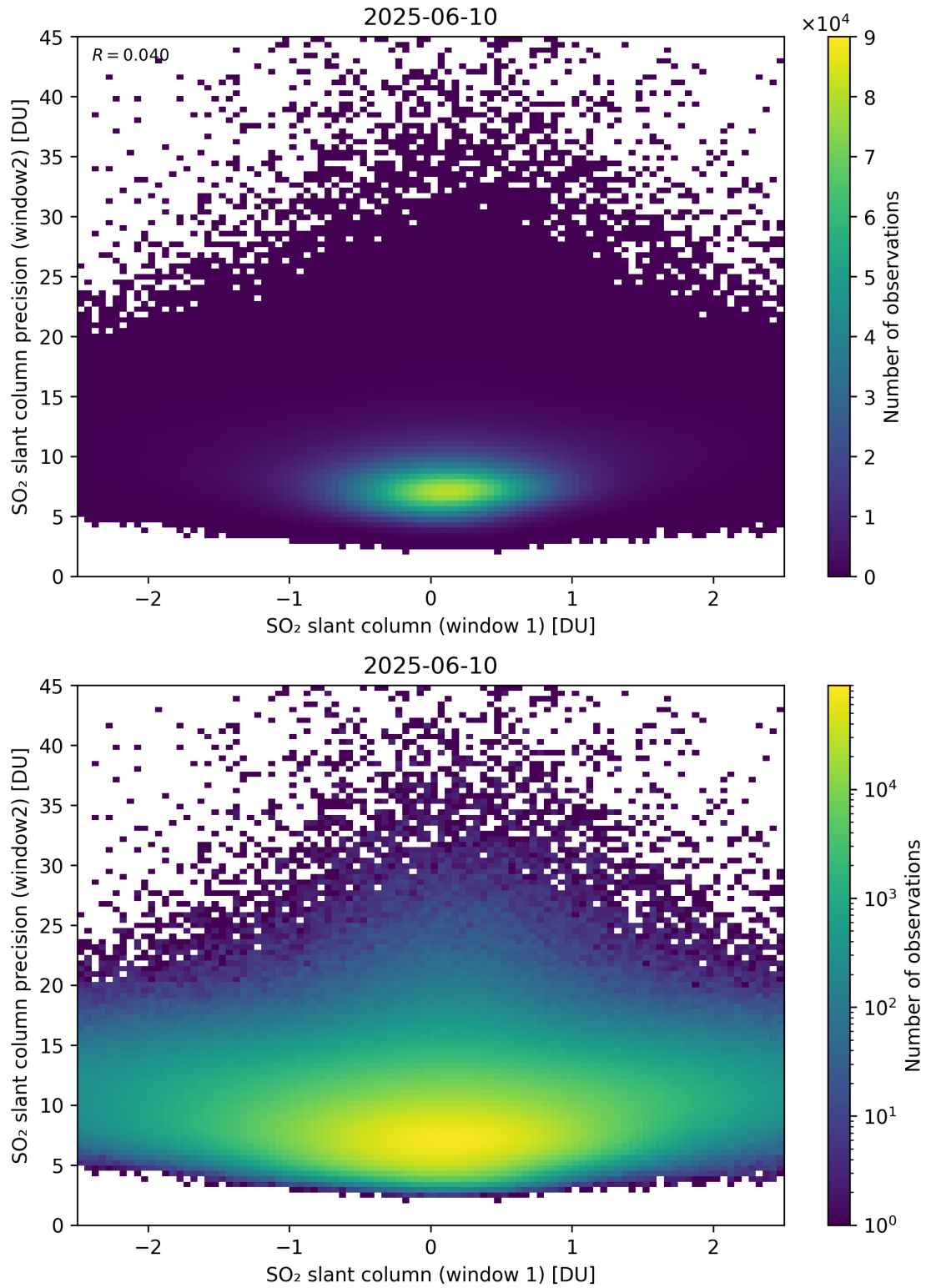
Figure 286: Scatter density plot of “SO 2 slant column (window 1)” against “SO 2 slant column precision (window2)” for 2025-06-09 to 2025-06-11.
