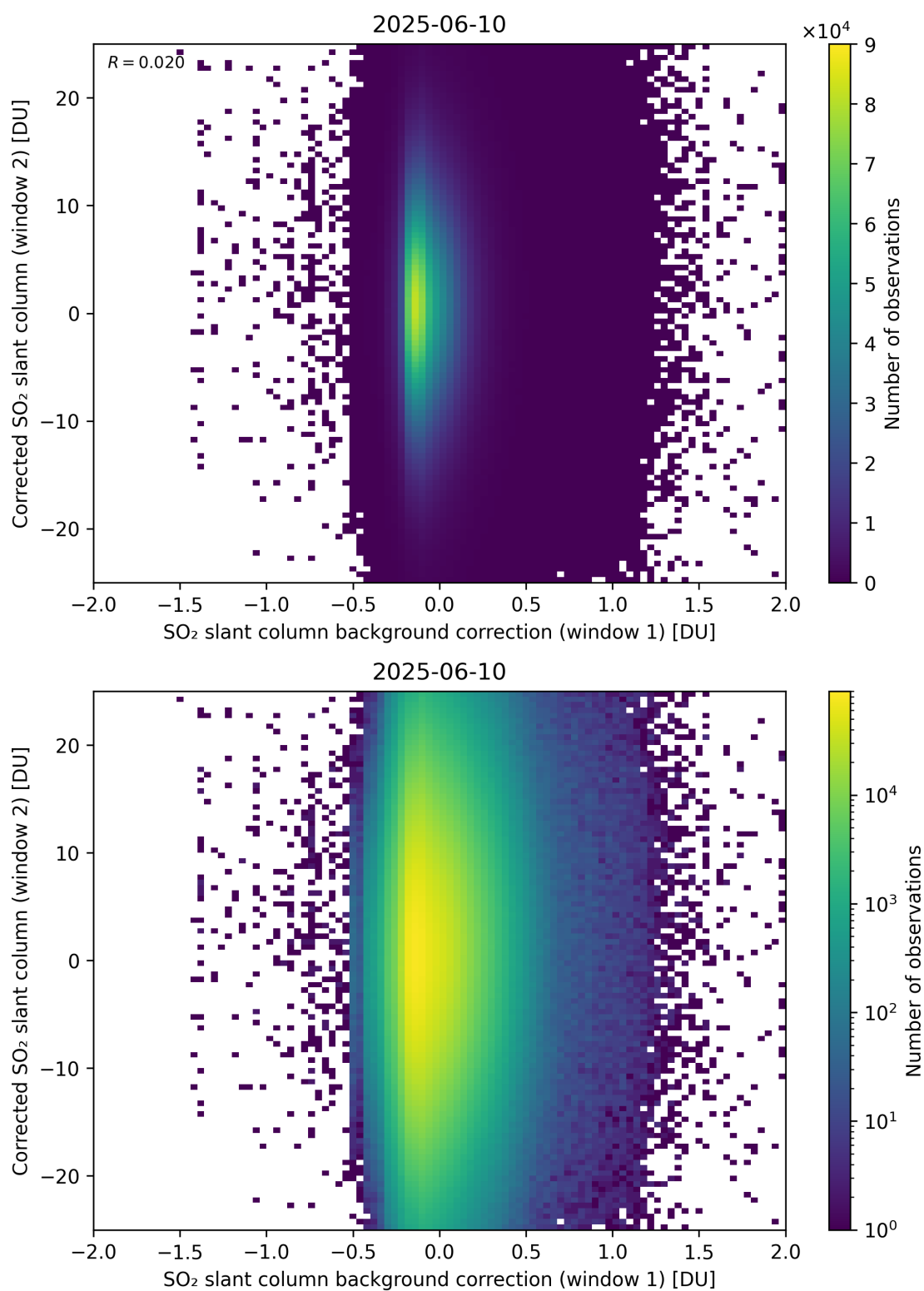
Figure 115: Scatter density plot of “SO 2 slant column background correction (window 1)” against “Corrected SO 2 slant column (window 2)” for 2025-06-09 to 2025-06-11.
