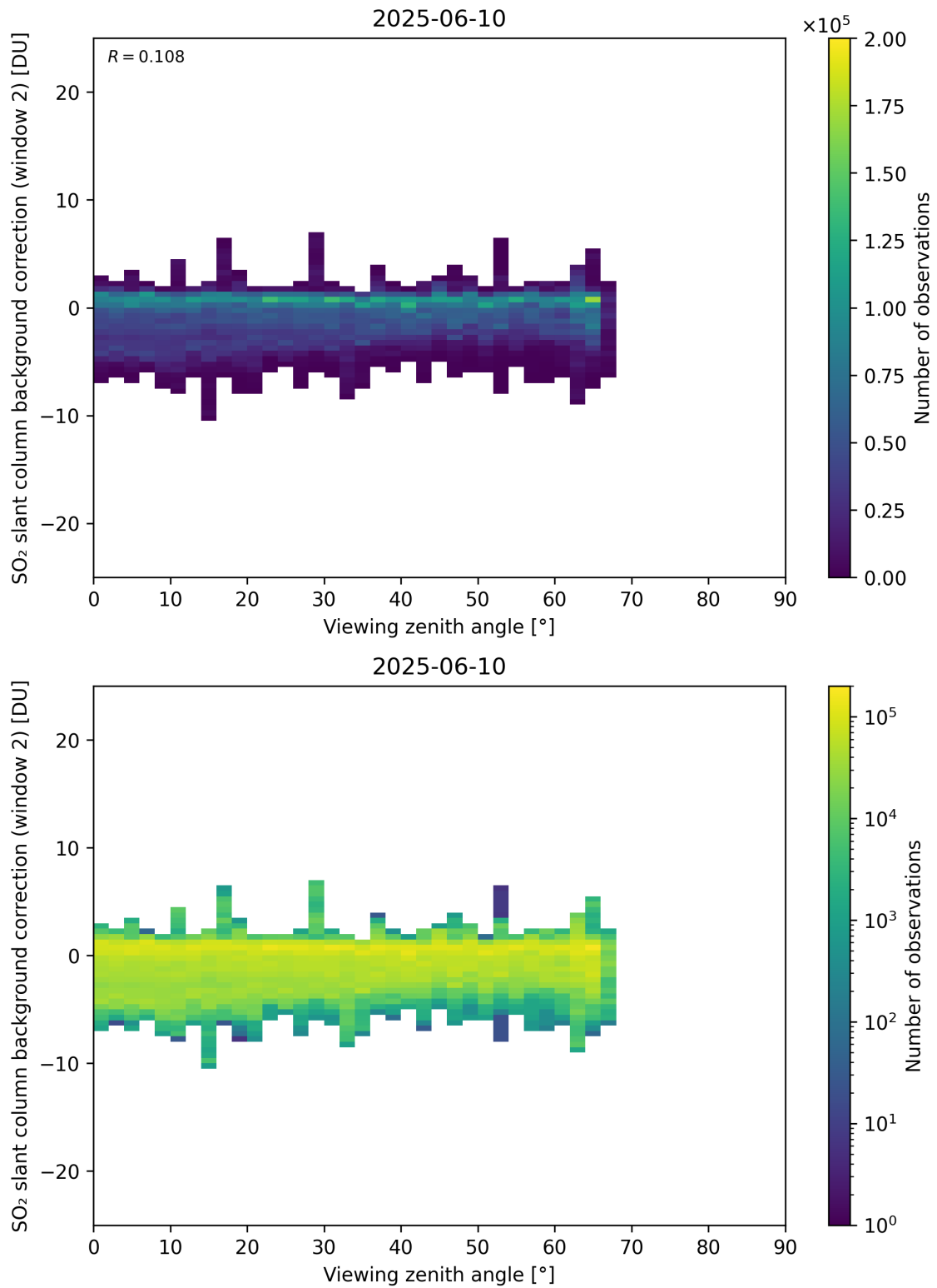
Figure 363: Scatter density plot of “Viewing zenith angle” against “SO 2 slant column background correction (window 2)” for 2025-06-09 to 2025-06-11.
