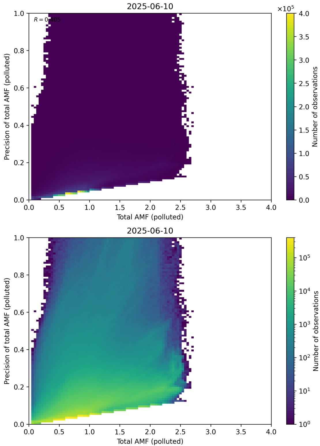
Figure 322: Scatter density plot of “Total AMF (polluted)” against “Precision of total AMF (polluted)” for 2025-06-09 to 2025-06-11.
