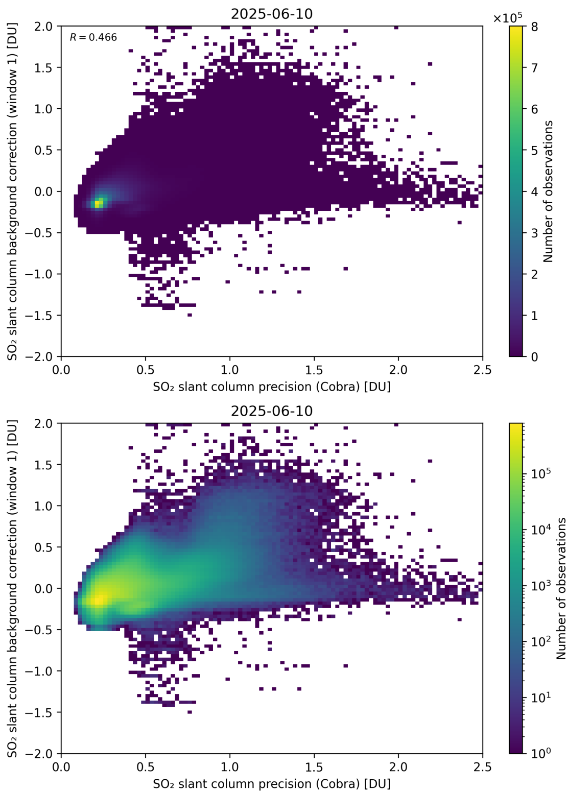
Figure 199: Scatter density plot of “SO 2 slant column precision (Cobra)” against “SO 2 slant column background correction (window 1)” for 2025-06-09 to 2025-06-11.
