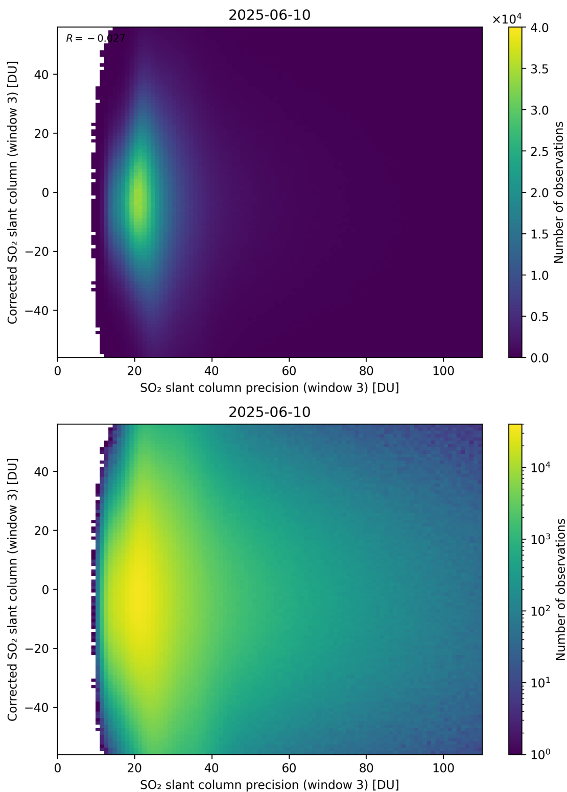
Figure 312: Scatter density plot of “SO 2 slant column precision (window 3)” against “Corrected SO 2 slant column (window 3)” for 2025-06-09 to 2025-06-11.
