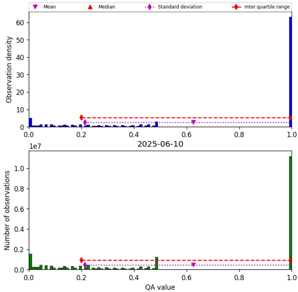
Figure 57: Histogram of “QA value” for 2025-06-09 to 2025-06-11
