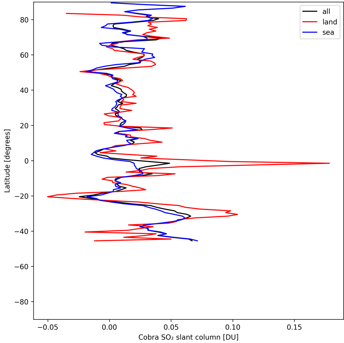
Figure 35: Zonal average of “Cobra SO 2 slant column” for 2025-06-09 to 2025-06-11.
