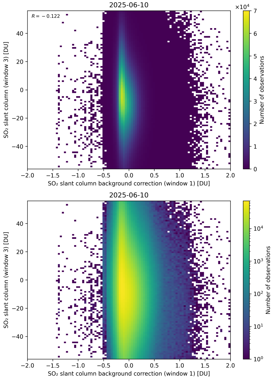
Figure 118: Scatter density plot of “SO 2 slant column background correction (window 1)” against “SO 2 slant column (window 3)” for 2025-06-09 to 2025-06-11.
