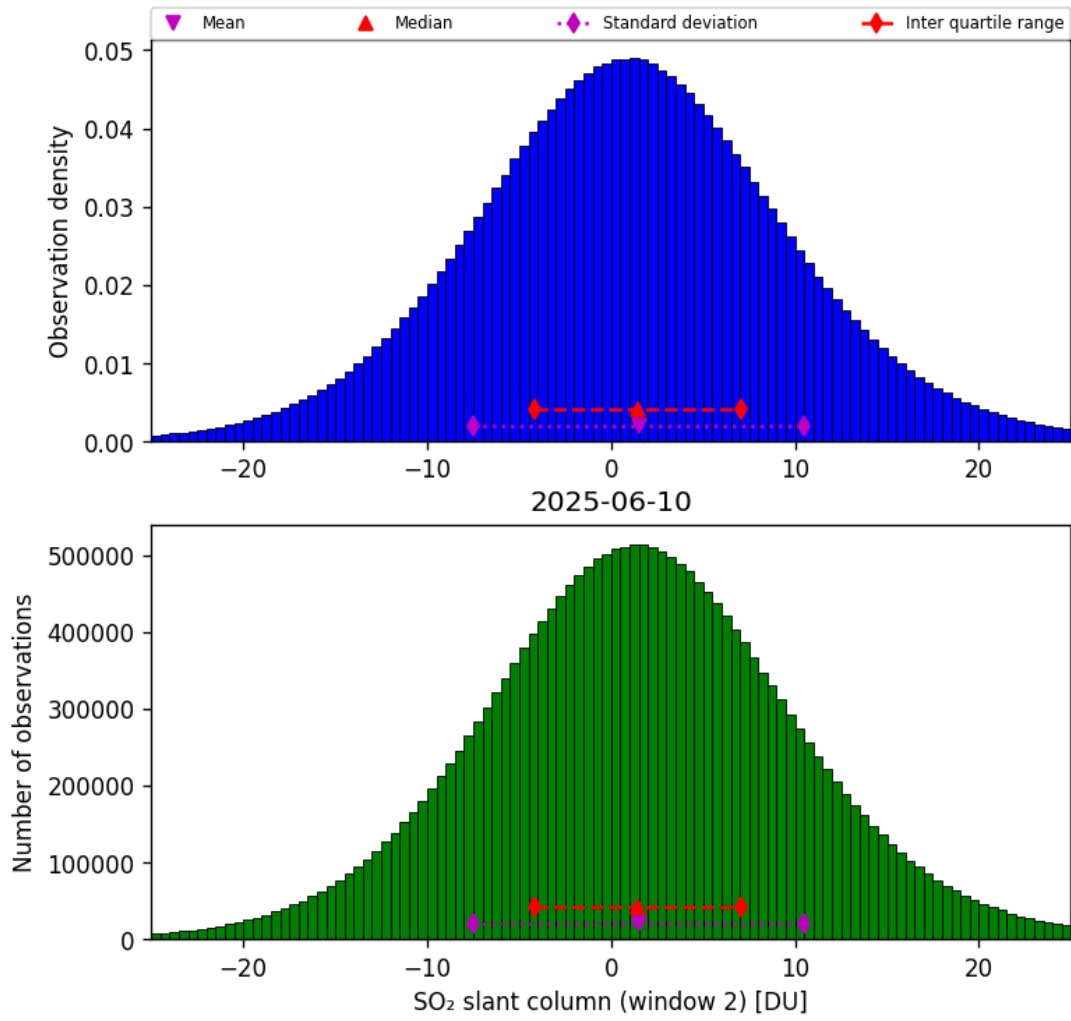
Figure 67: Histogram of “SO 2 slant column (window 2)” for 2025-06-09 to 2025-06-11
