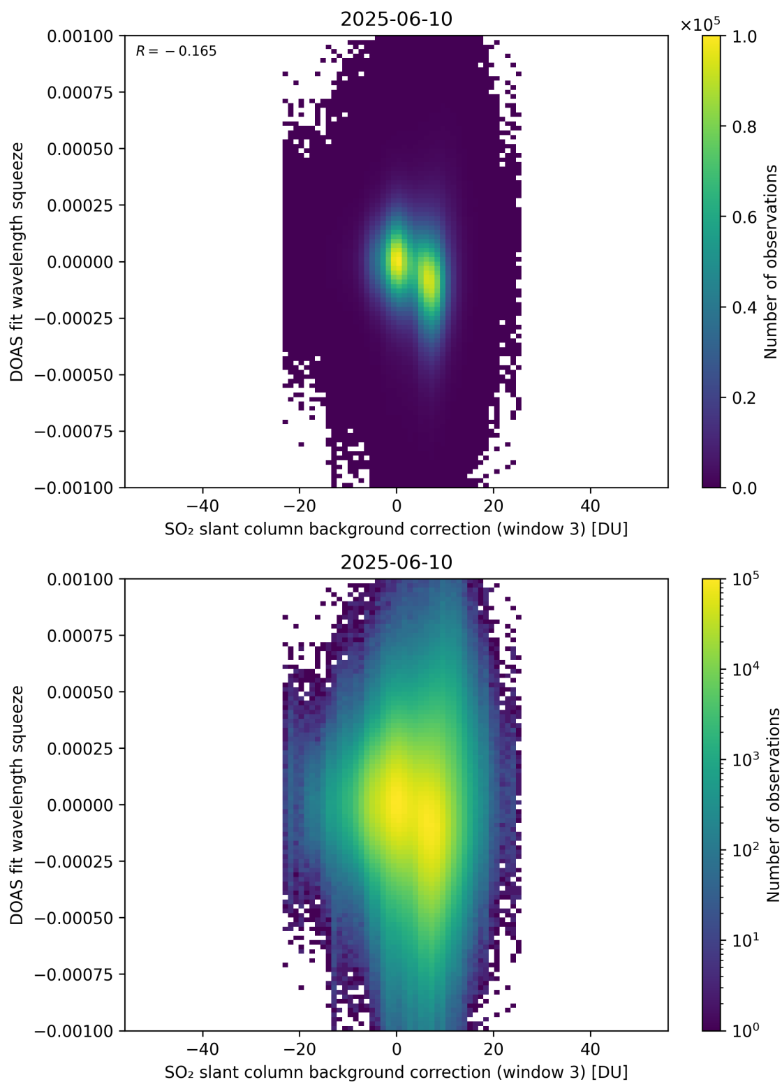
Figure 133: Scatter density plot of “SO 2 slant column background correction (window 3)” against “DOAS fit wavelength squeeze” for 2025-06-09 to 2025-06-11.
