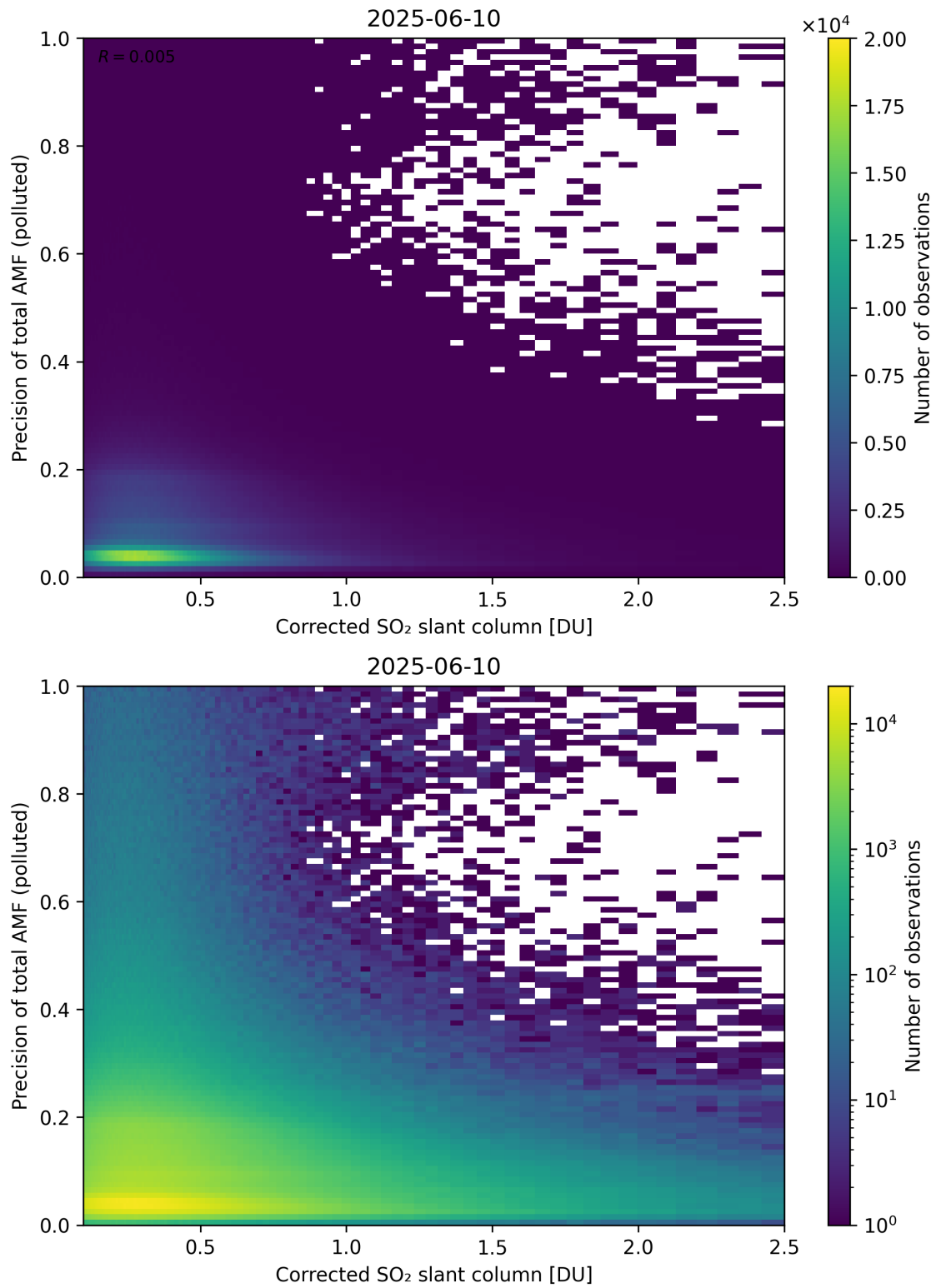
Figure 243: Scatter density plot of “Corrected SO 2 slant column” against “Precision of total AMF (polluted)” for 2025-06-09 to 2025-06-11.
