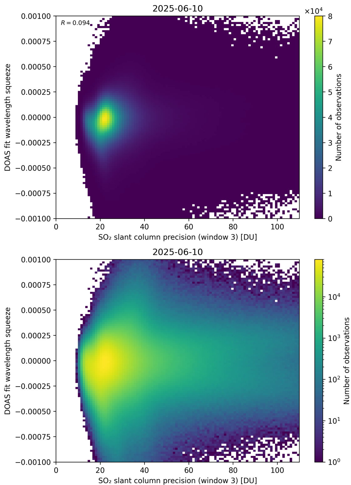
Figure 309: Scatter density plot of “SO 2 slant column precision (window 3)” against “DOAS fit wavelength squeeze” for 2025-06-09 to 2025-06-11.
