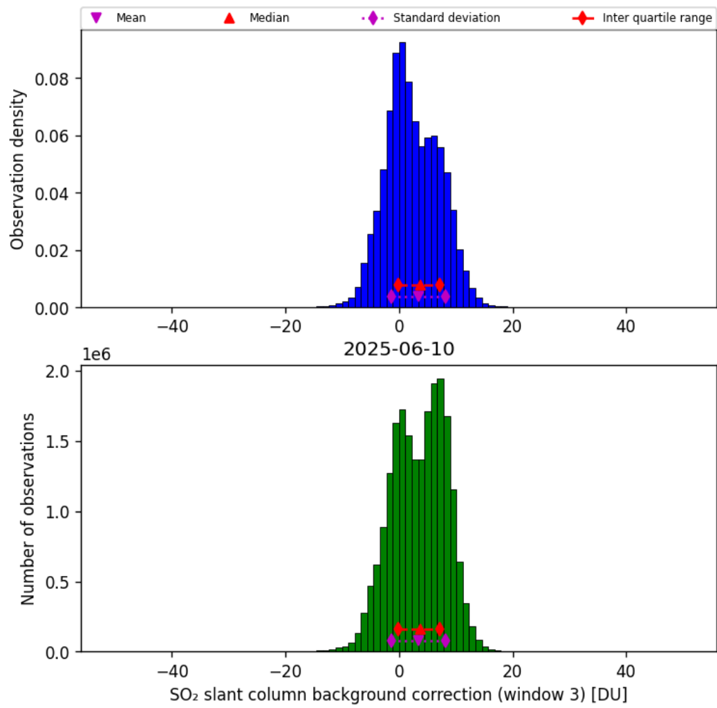
Figure 74: Histogram of “SO 2 slant column background correction (window 3)” for 2025-06-09 to 2025-06-11
