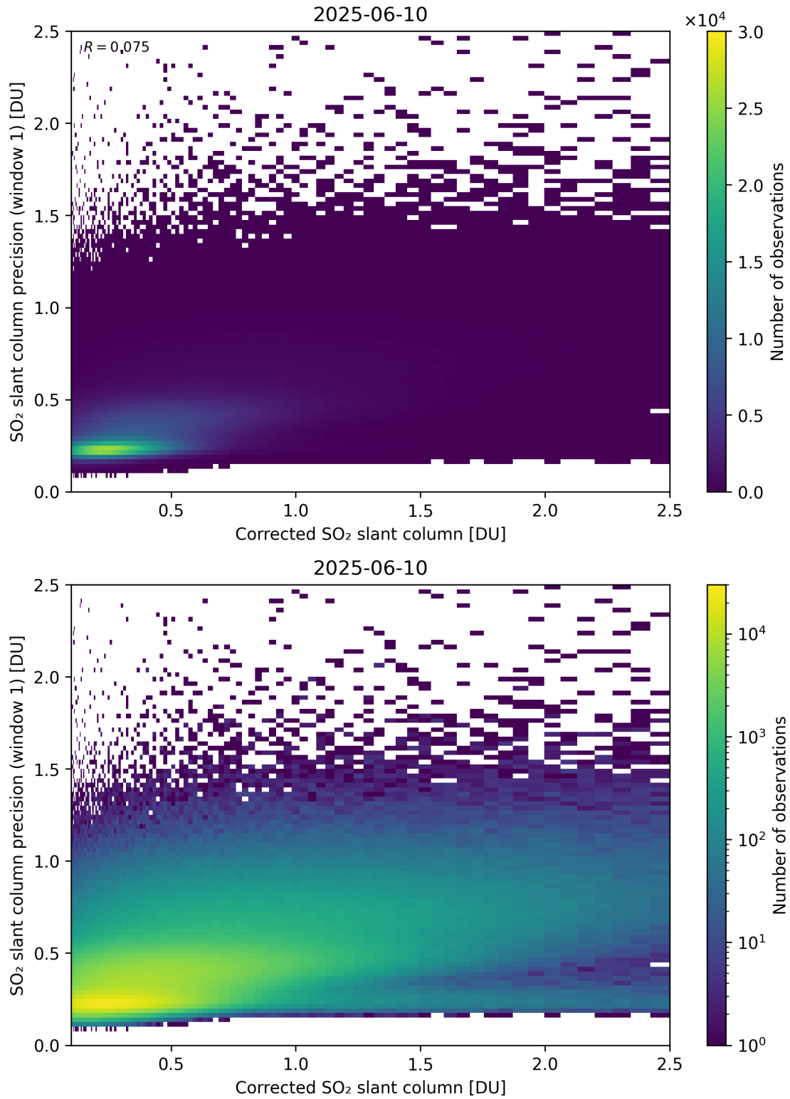
Figure 238: Scatter density plot of “Corrected SO 2 slant column” against “SO 2 slant column precision (window 1)” for 2025-06-09 to 2025-06-11.
