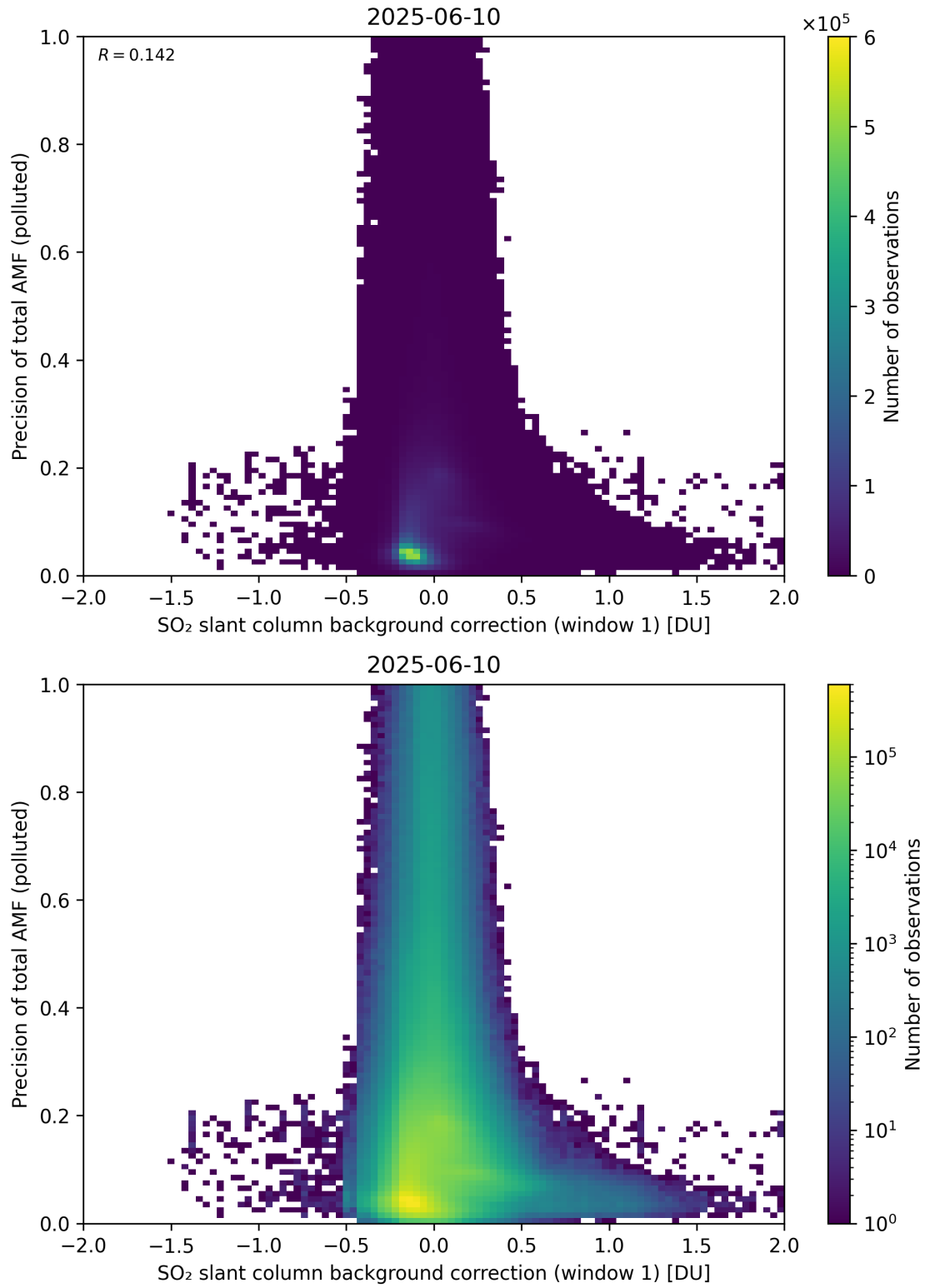
Figure 121: Scatter density plot of “SO 2 slant column background correction (window 1)” against “Precision of total AMF (polluted)” for 2025-06-09 to 2025-06-11.
