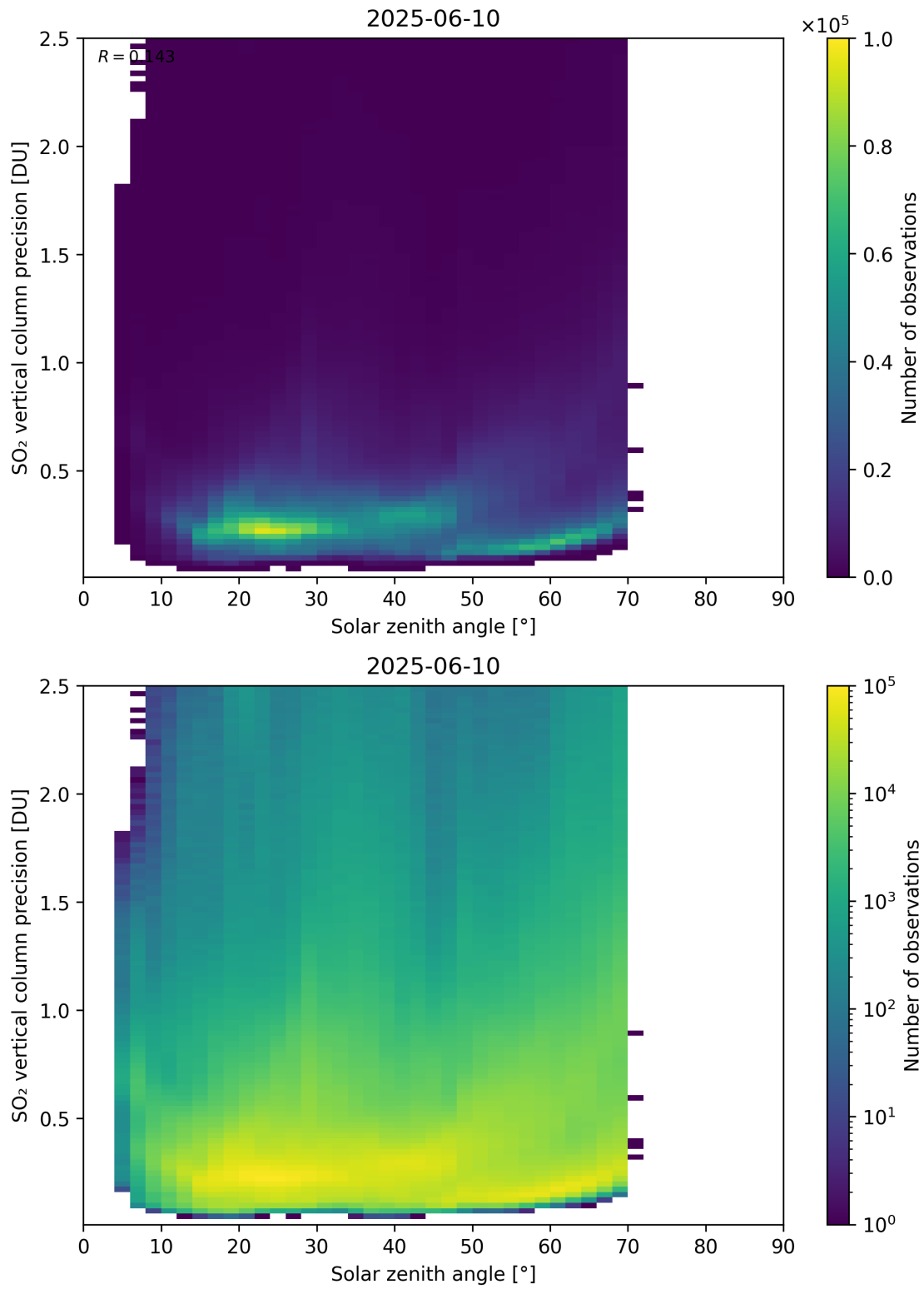
Figure 192: Scatter density plot of “Solar zenith angle” against “SO 2 vertical column precision” for 2025-06-09 to 2025-06-11.
