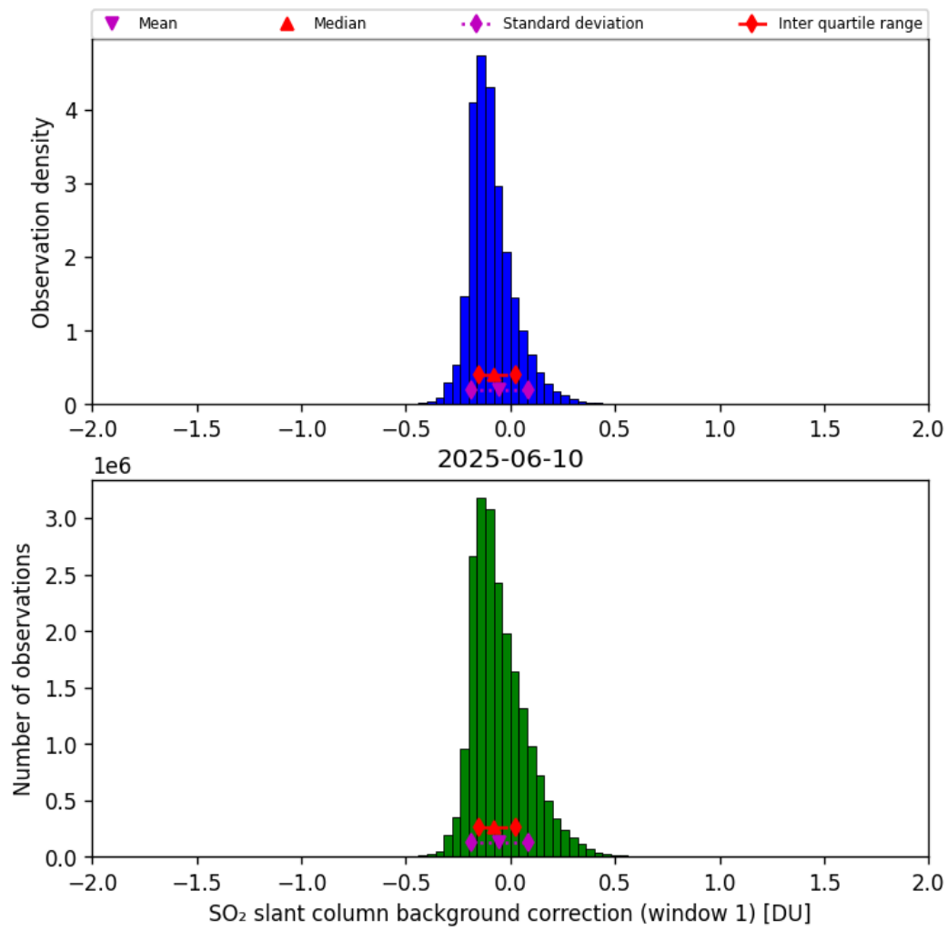
Figure 66: Histogram of “SO 2 slant column background correction (window 1)” for 2025-06-09 to 2025-06-11
