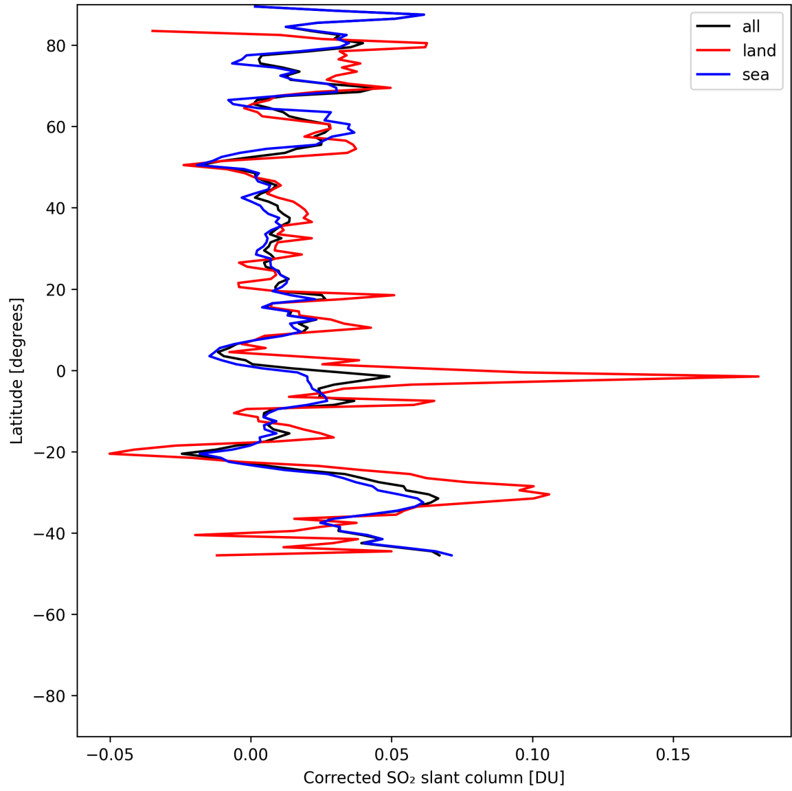
Figure 34: Zonal average of “Corrected SO 2 slant column” for 2025-06-09 to 2025-06-11.
