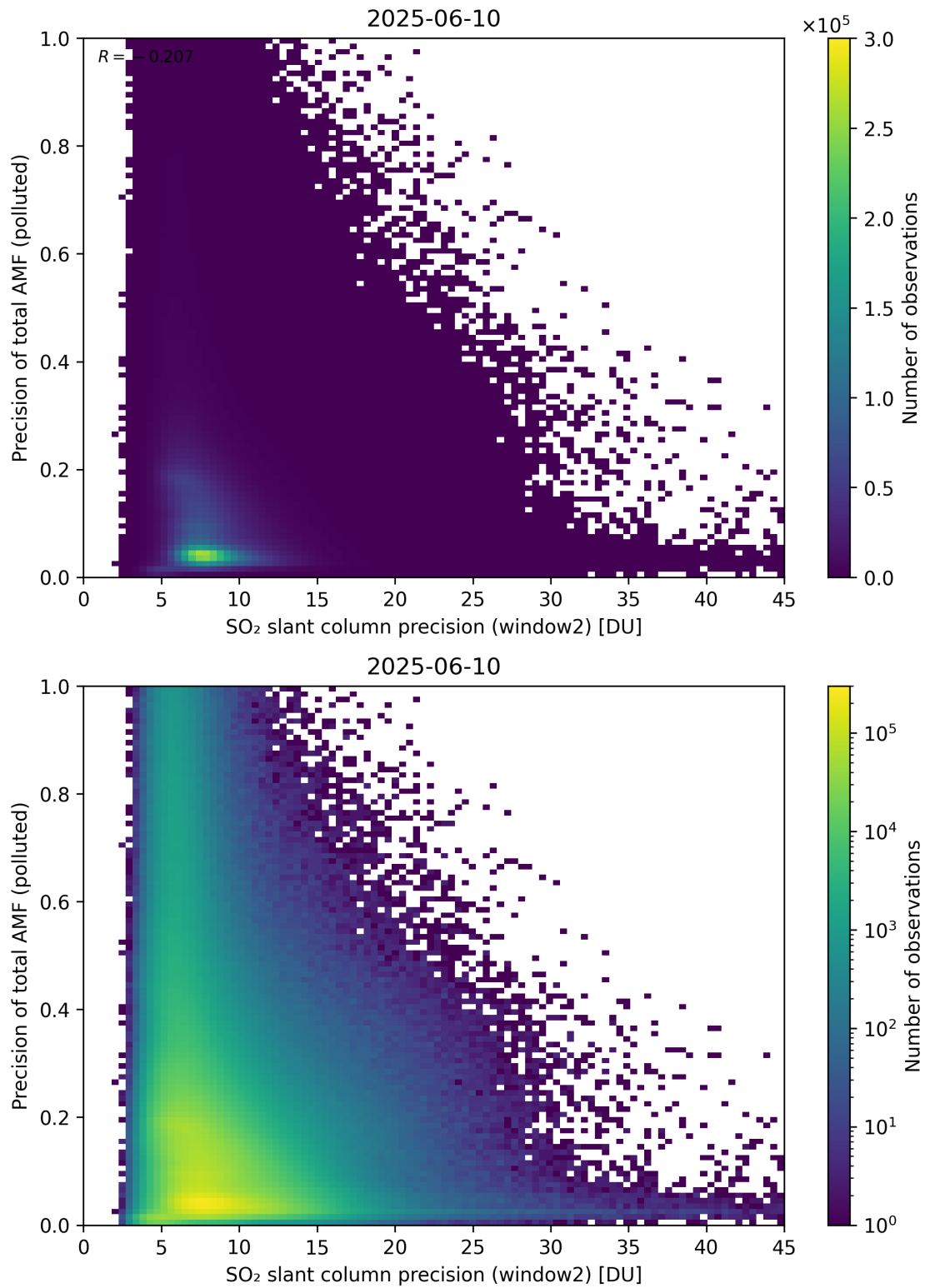
Figure 302: Scatter density plot of “SO 2 slant column precision (window2)” against “Precision of total AMF (polluted)” for 2025-06-09 to 2025-06-11.
