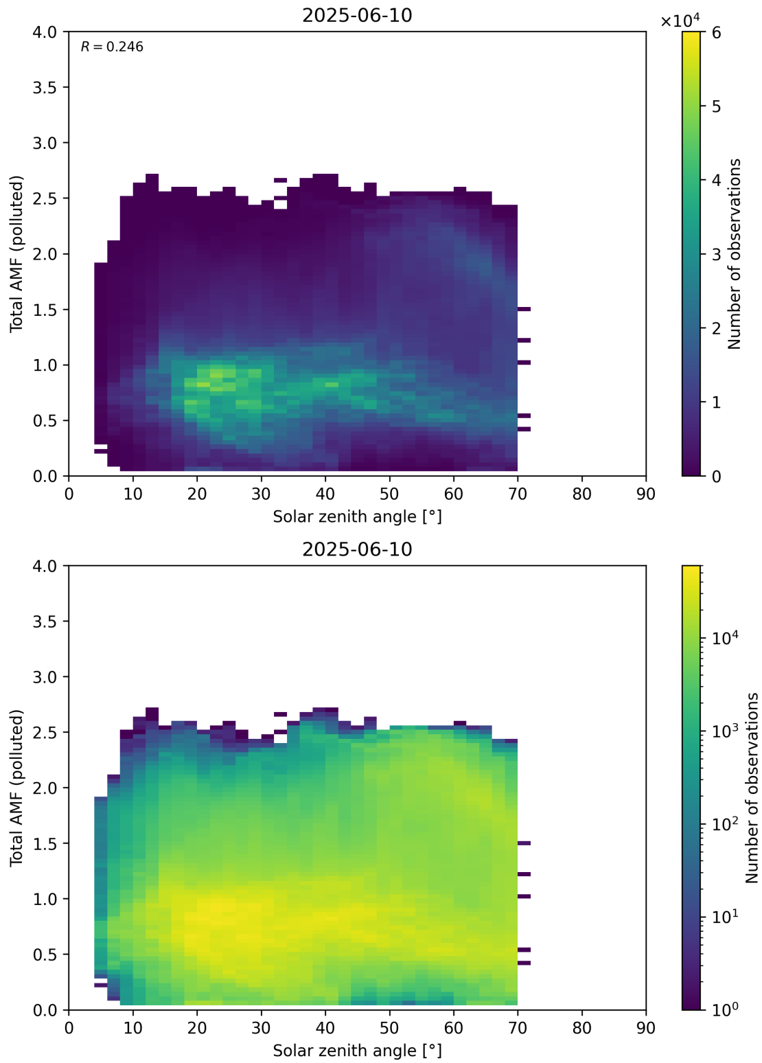
Figure 189: Scatter density plot of “Solar zenith angle” against “Total AMF (polluted)” for 2025-06-09 to 2025-06-11.
