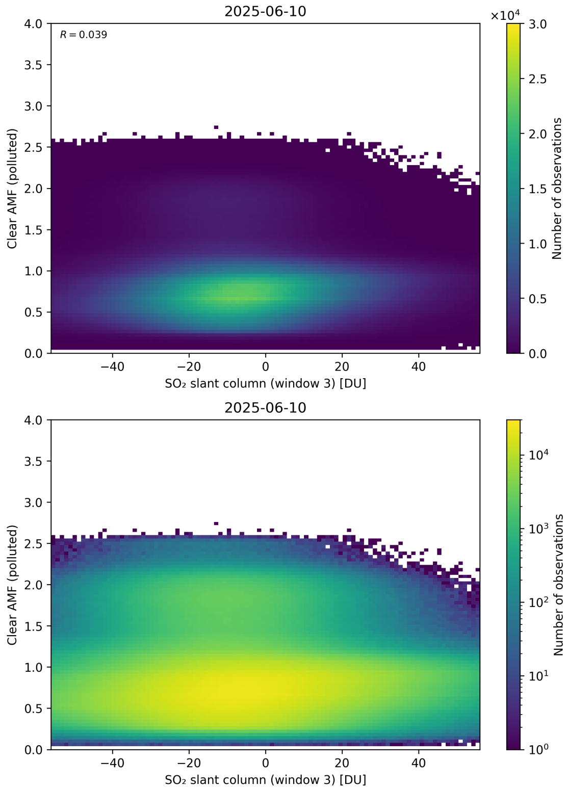
Figure 315: Scatter density plot of “SO 2 slant column (window 3)” against “Clear AMF (polluted)” for 2025-06-09 to 2025-06-11.
