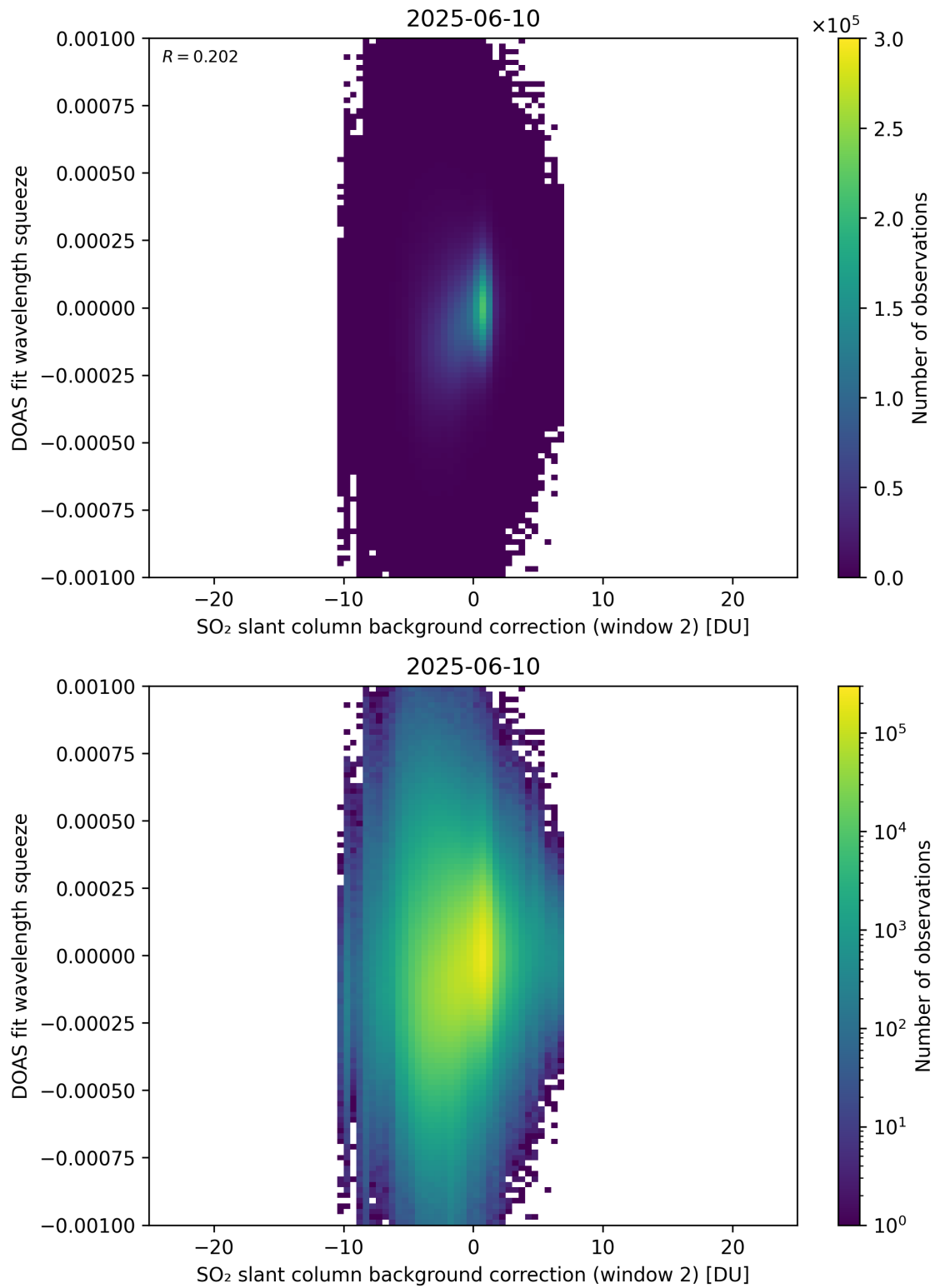
Figure 124: Scatter density plot of “SO 2 slant column background correction (window 2)” against “DOAS fit wavelength squeeze” for 2025-06-09 to 2025-06-11.
