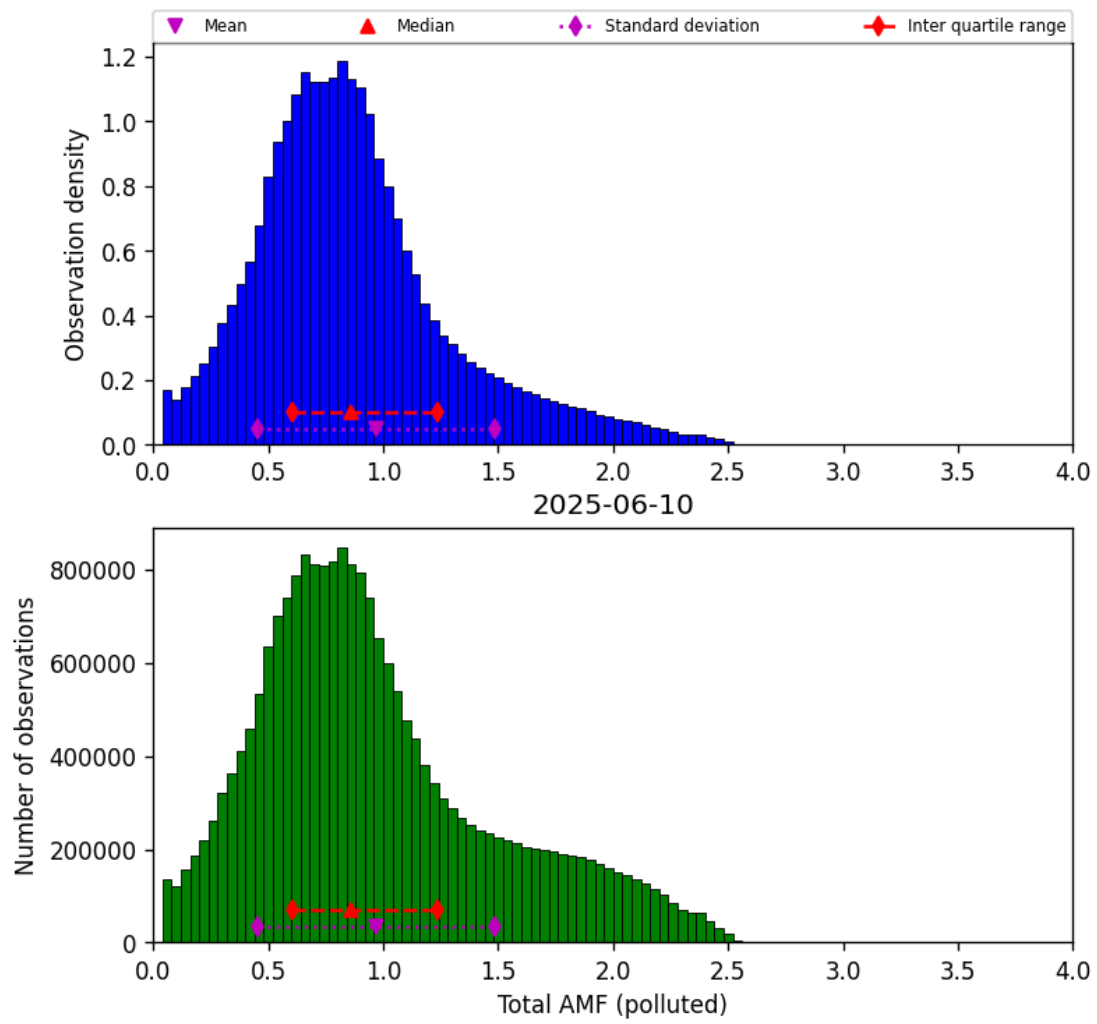
Figure 79: Histogram of “Total AMF (polluted)” for 2025-06-09 to 2025-06-11
