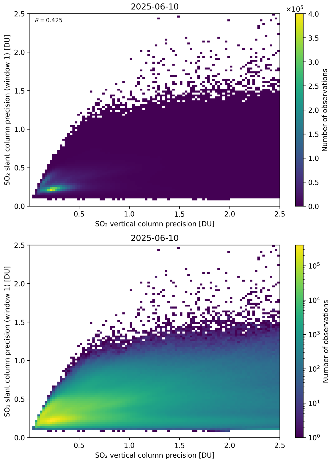
Figure 342: Scatter density plot of “SO 2 vertical column precision” against “SO 2 slant column precision (window 1)” for 2025-06-09 to 2025-06-11.
