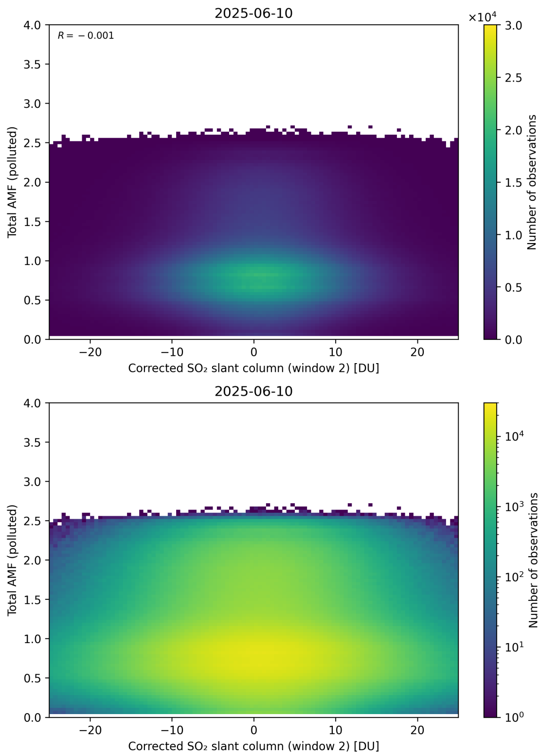
Figure 253: Scatter density plot of “Corrected SO 2 slant column (window 2)” against “Total AMF (polluted)” for 2025-06-09 to 2025-06-11.
