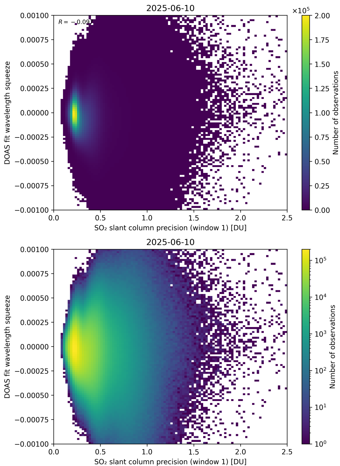
Figure 272: Scatter density plot of “SO 2 slant column precision (window 1)” against “DOAS fit wavelength squeeze” for 2025-06-09 to 2025-06-11.
