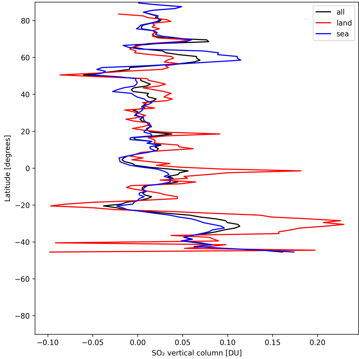
Figure 32: Zonal average of “SO 2 vertical column” for 2025-06-09 to 2025-06-11.
