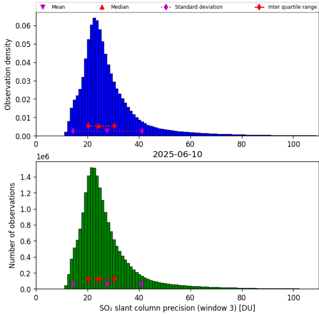
Figure 72: Histogram of “SO 2 slant column precision (window 3)” for 2025-06-09 to 2025-06-11
