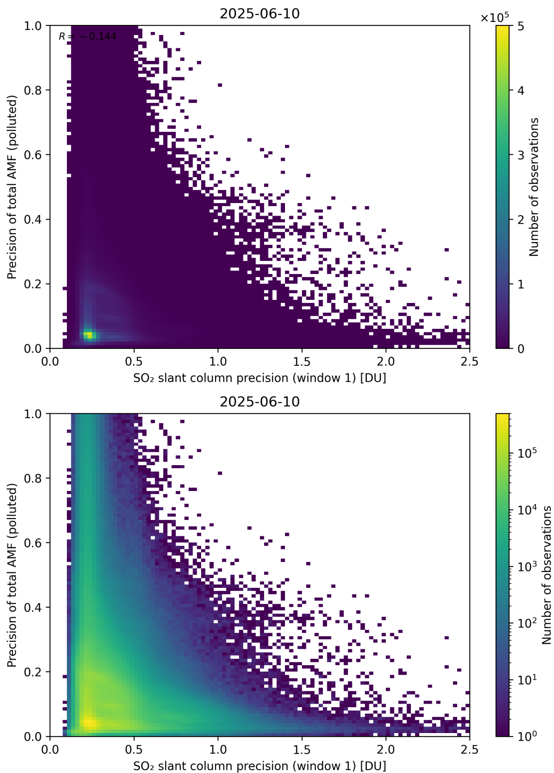
Figure 281: Scatter density plot of “SO 2 slant column precision (window 1)” against “Precision of total AMF (polluted)” for 2025-06-09 to 2025-06-11.
