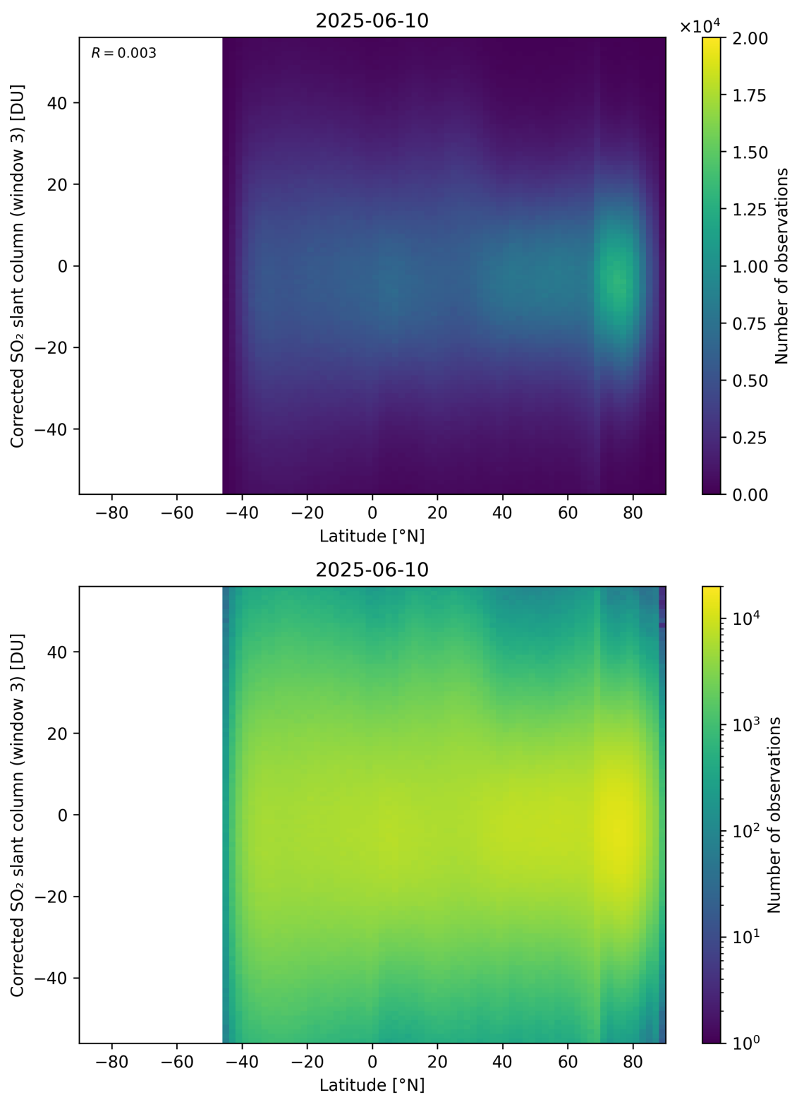
Figure 161: Scatter density plot of “Latitude” against “Corrected SO 2 slant column (window 3)” for 2025-06-09 to 2025-06-11.
