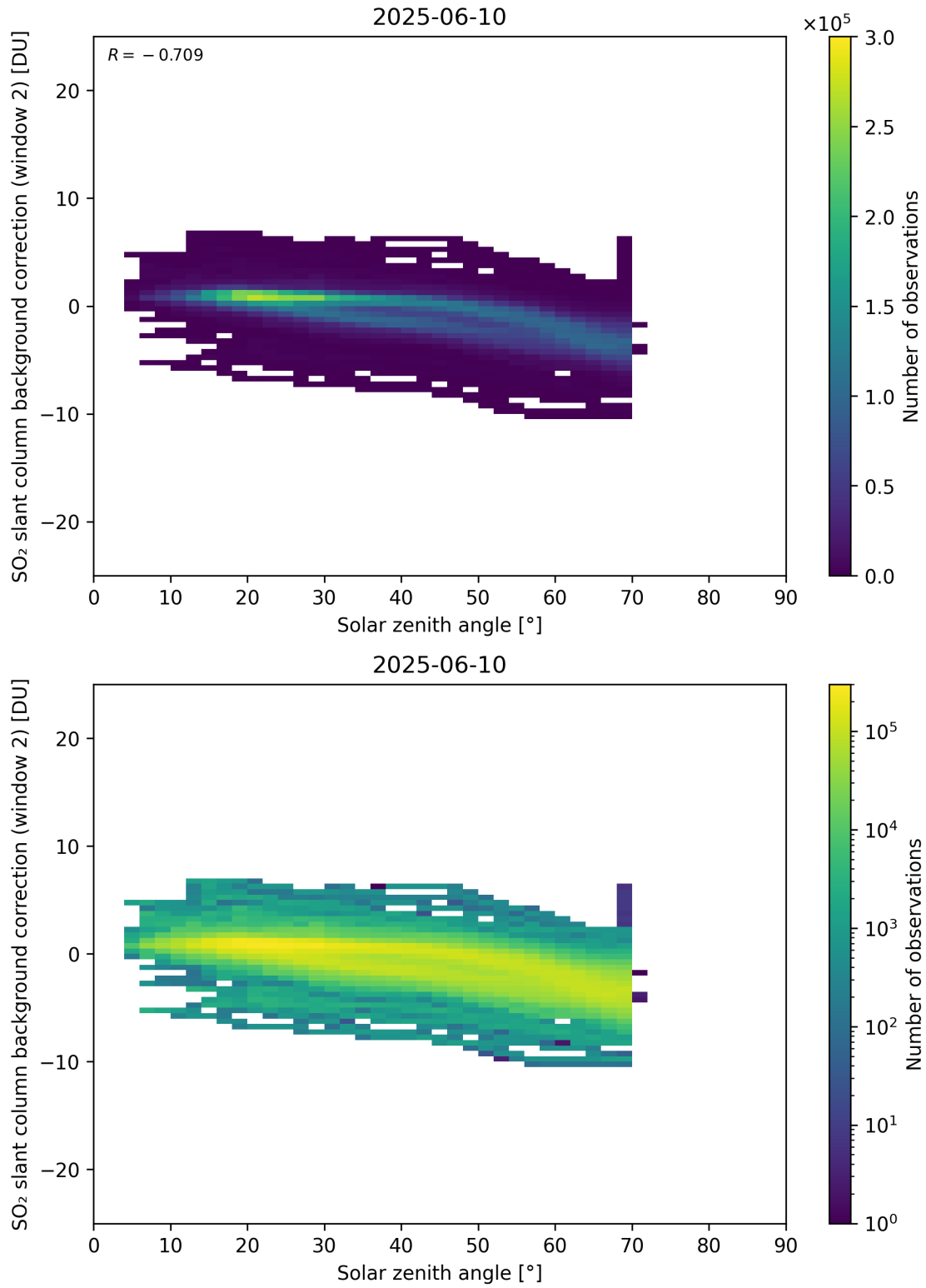
Figure 172: Scatter density plot of “Solar zenith angle” against “SO 2 slant column background correction (window 2)” for 2025-06-09 to 2025-06-11.
