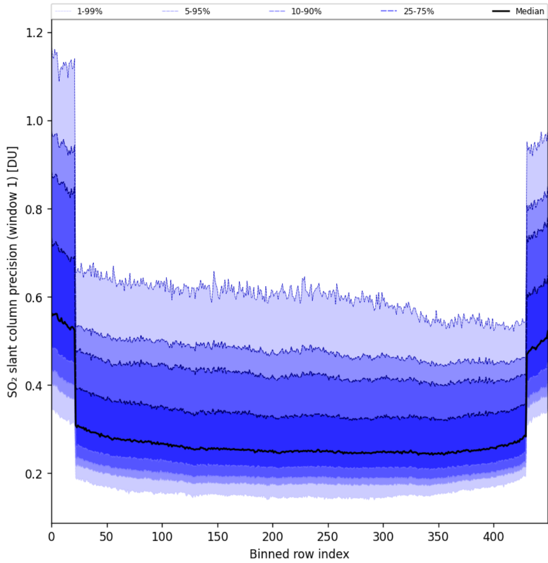
Figure 90: Along track statistics of "SO 2 slant column precision (window 1)" for 2025-06-09 to 2025-06-11
