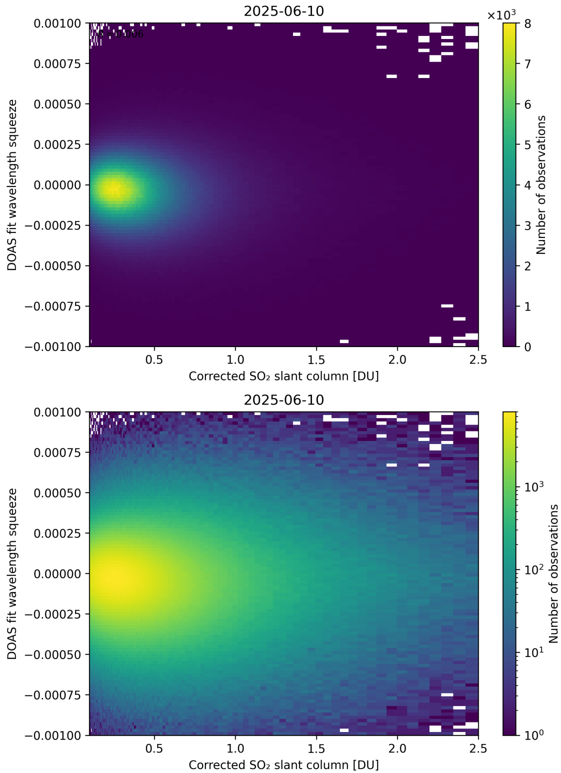
Figure 230: Scatter density plot of “Corrected SO 2 slant column” against “DOAS fit wavelength squeeze” for 2025-06-09 to 2025-06-11.
