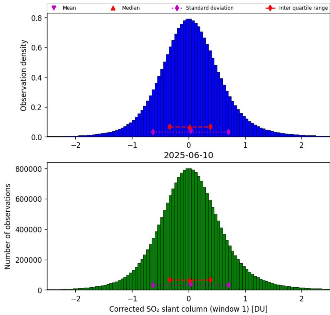
Figure 65: Histogram of “Corrected SO 2 slant column (window 1)” for 2025-06-09 to 2025-06-11
