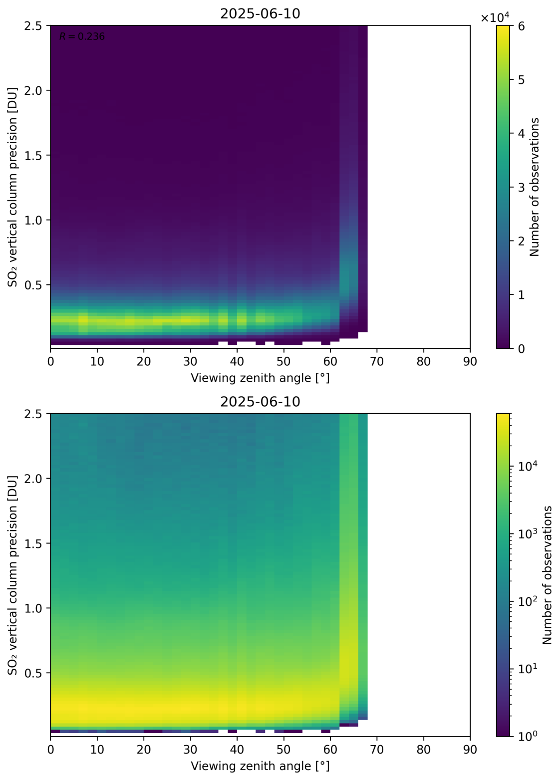
Figure 384: Scatter density plot of “Viewing zenith angle” against “SO 2 vertical column precision” for 2025-06-09 to 2025-06-11.
