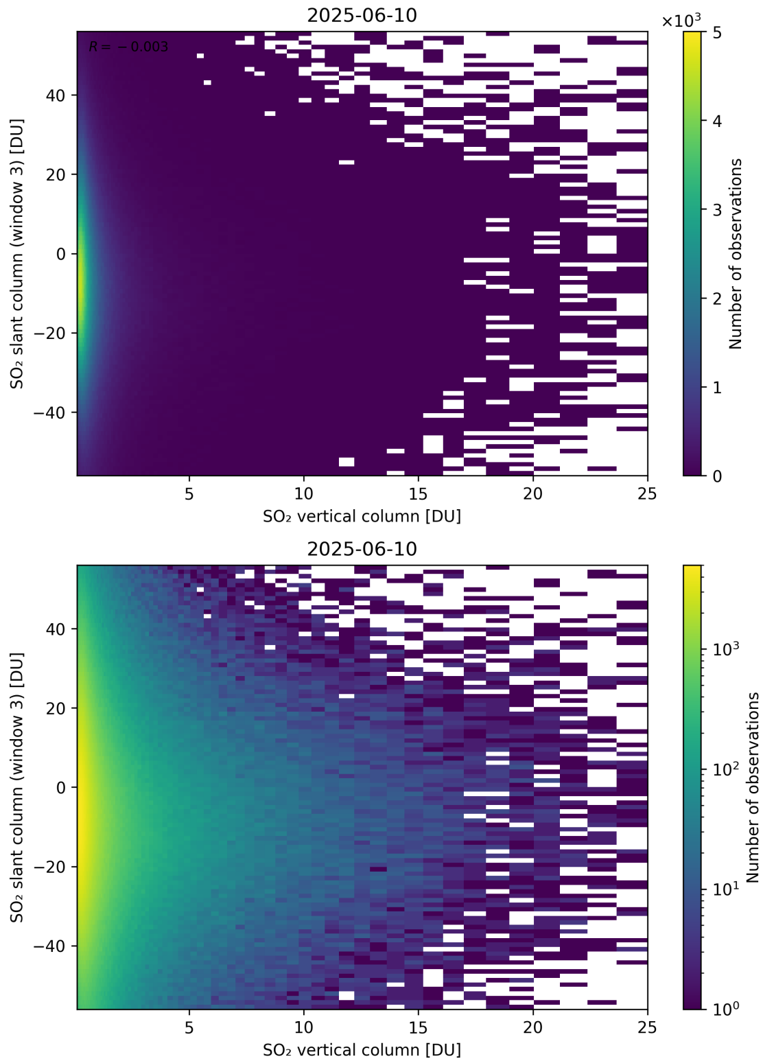
Figure 357: Scatter density plot of “SO 2 vertical column” against “SO 2 slant column (window 3)” for 2025-06-09 to 2025-06-11.
