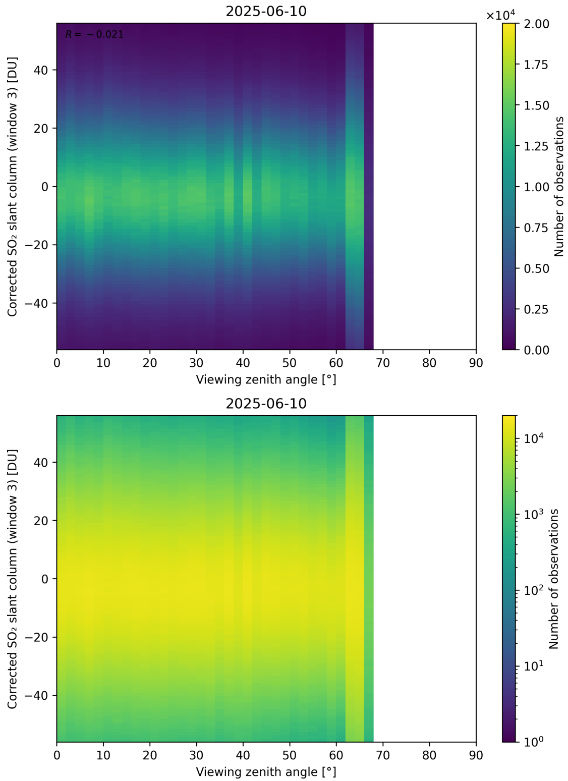
Figure 375: Scatter density plot of “Viewing zenith angle” against “Corrected SO 2 slant column (window 3)” for 2025-06-09 to 2025-06-11.
