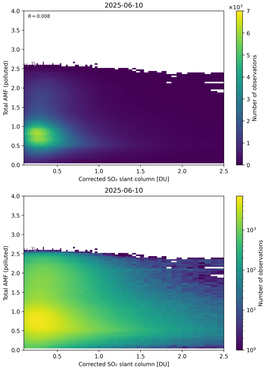
Figure 242: Scatter density plot of “Corrected SO 2 slant column” against “Total AMF (polluted)” for 2025-06-09 to 2025-06-11.
