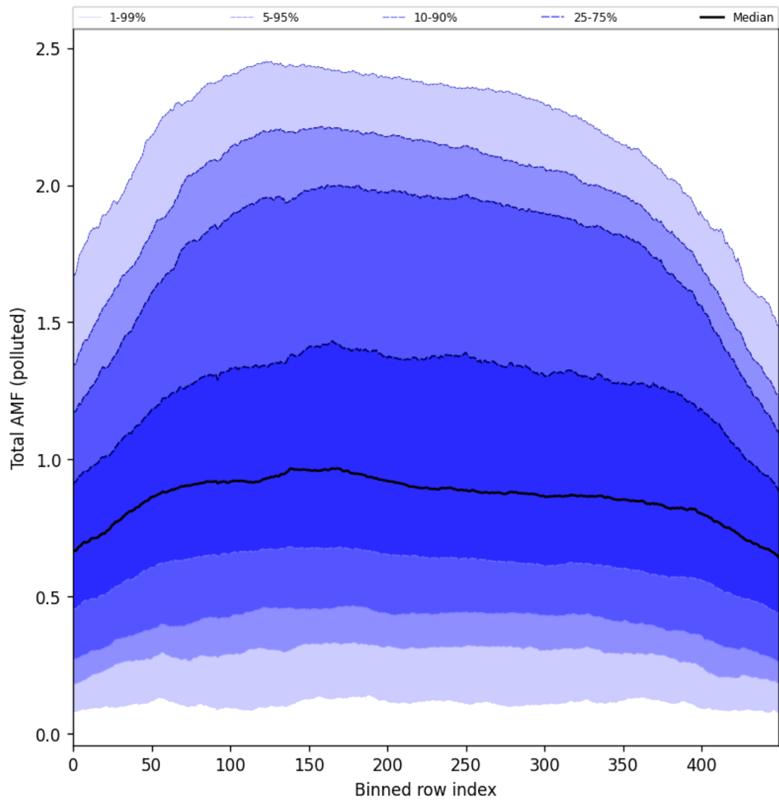
Figure 105: Along track statistics of “Total AMF (polluted)” for 2025-06-09 to 2025-06-11
