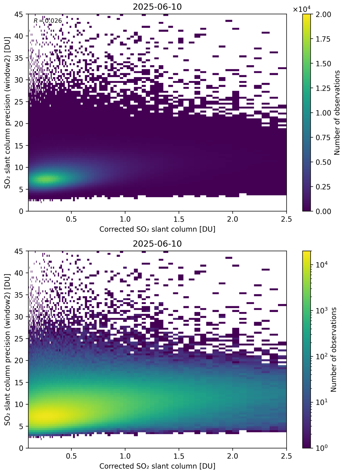
Figure 239: Scatter density plot of “Corrected SO 2 slant column” against “SO 2 slant column precision (window2)” for 2025-06-09 to 2025-06-11.
