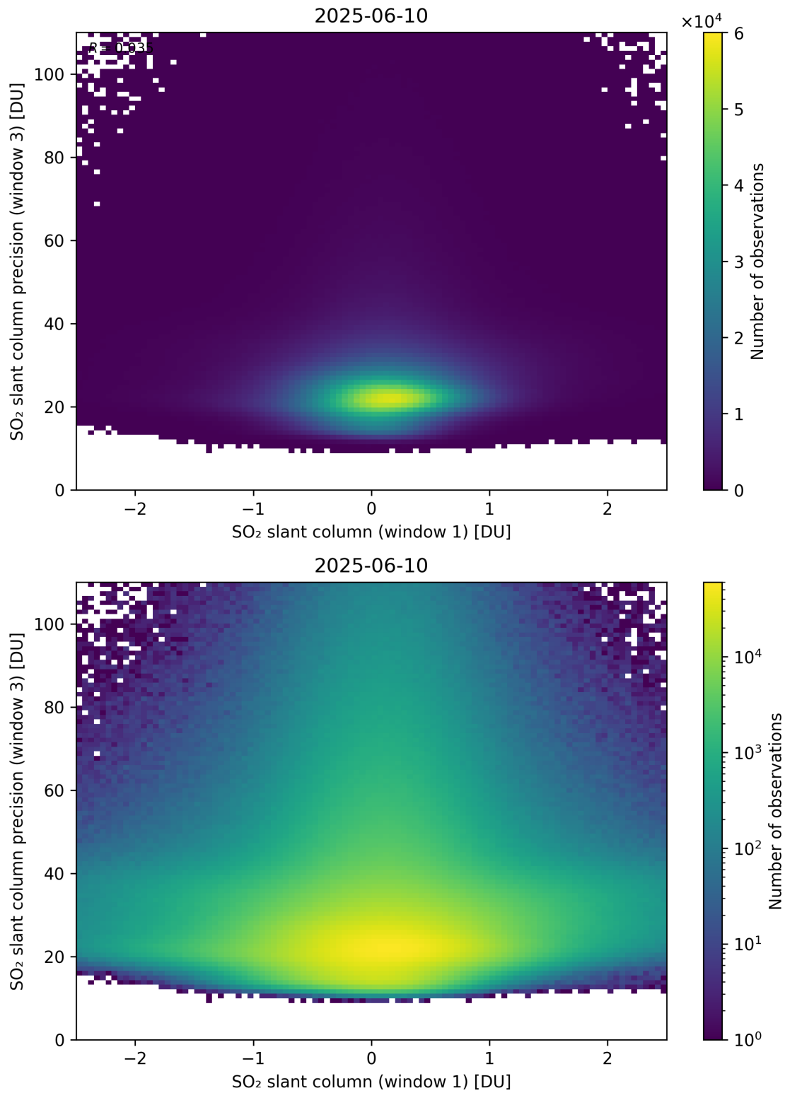
Figure 288: Scatter density plot of “SO 2 slant column (window 1)” against “SO 2 slant column precision (window 3)” for 2025-06-09 to 2025-06-11.
