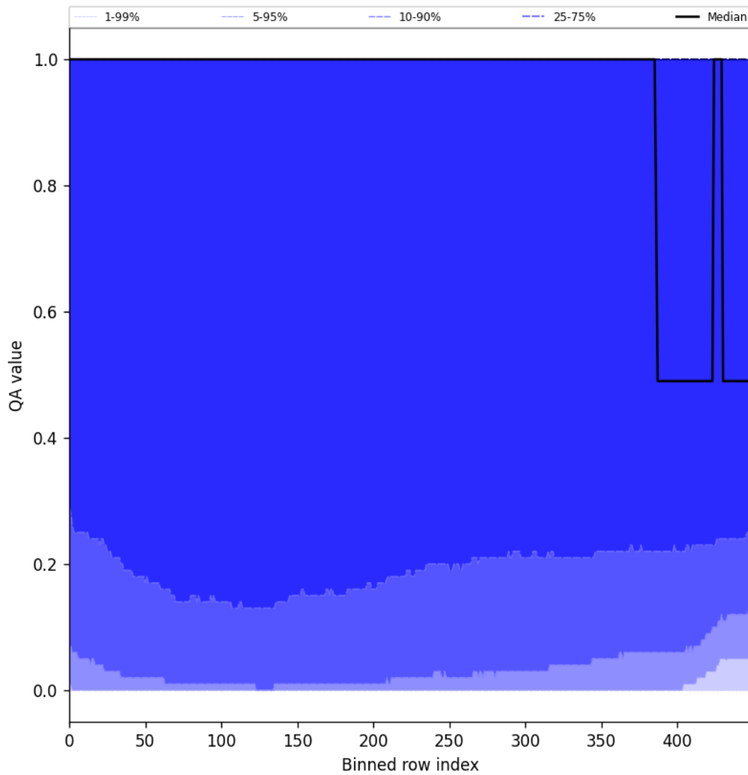
Figure 83: Along track statistics of “QA value” for 2025-06-09 to 2025-06-11
