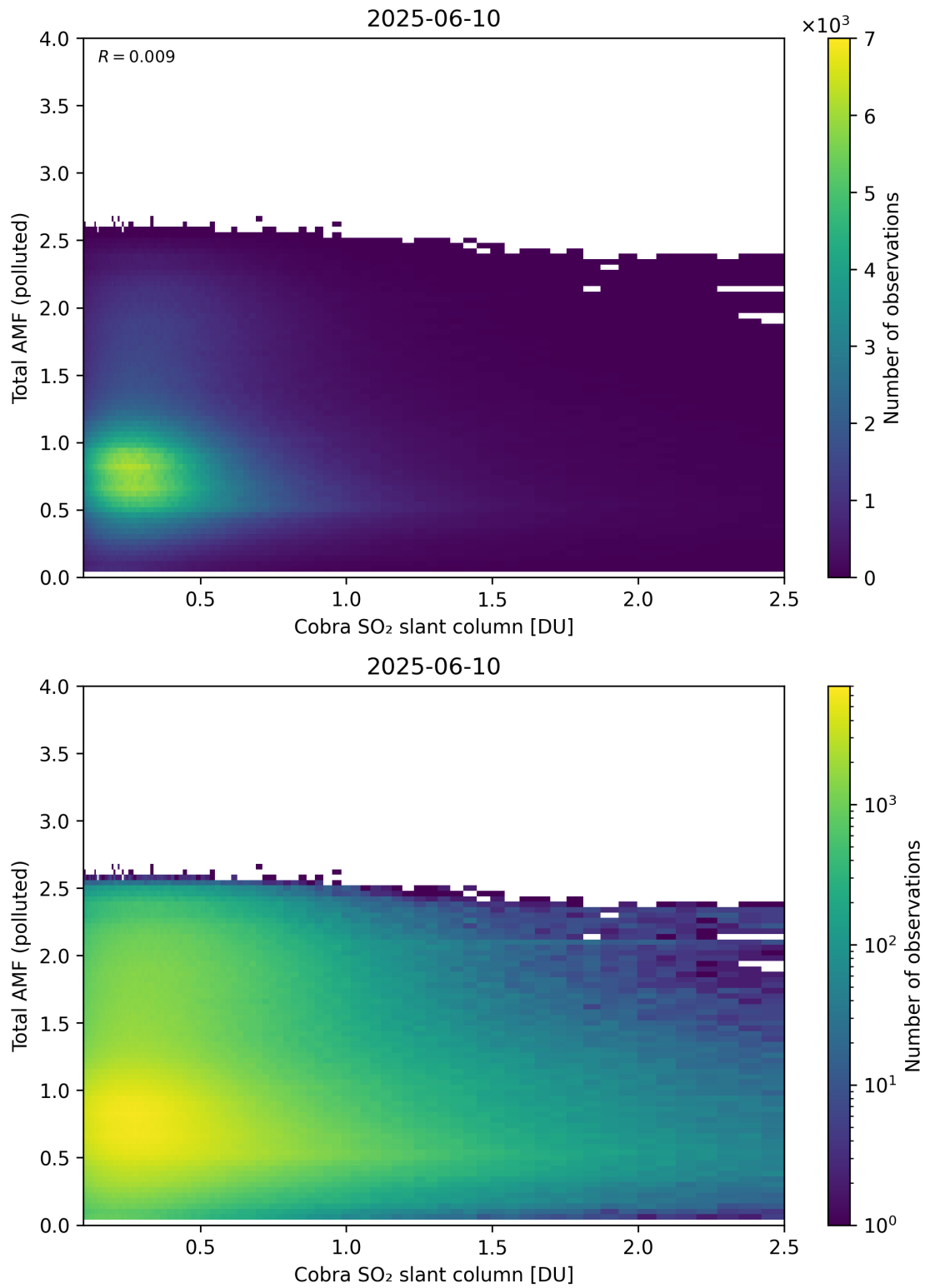
Figure 224: Scatter density plot of “Cobra SO 2 slant column” against “Total AMF (polluted)” for 2025-06-09 to 2025-06-11.
