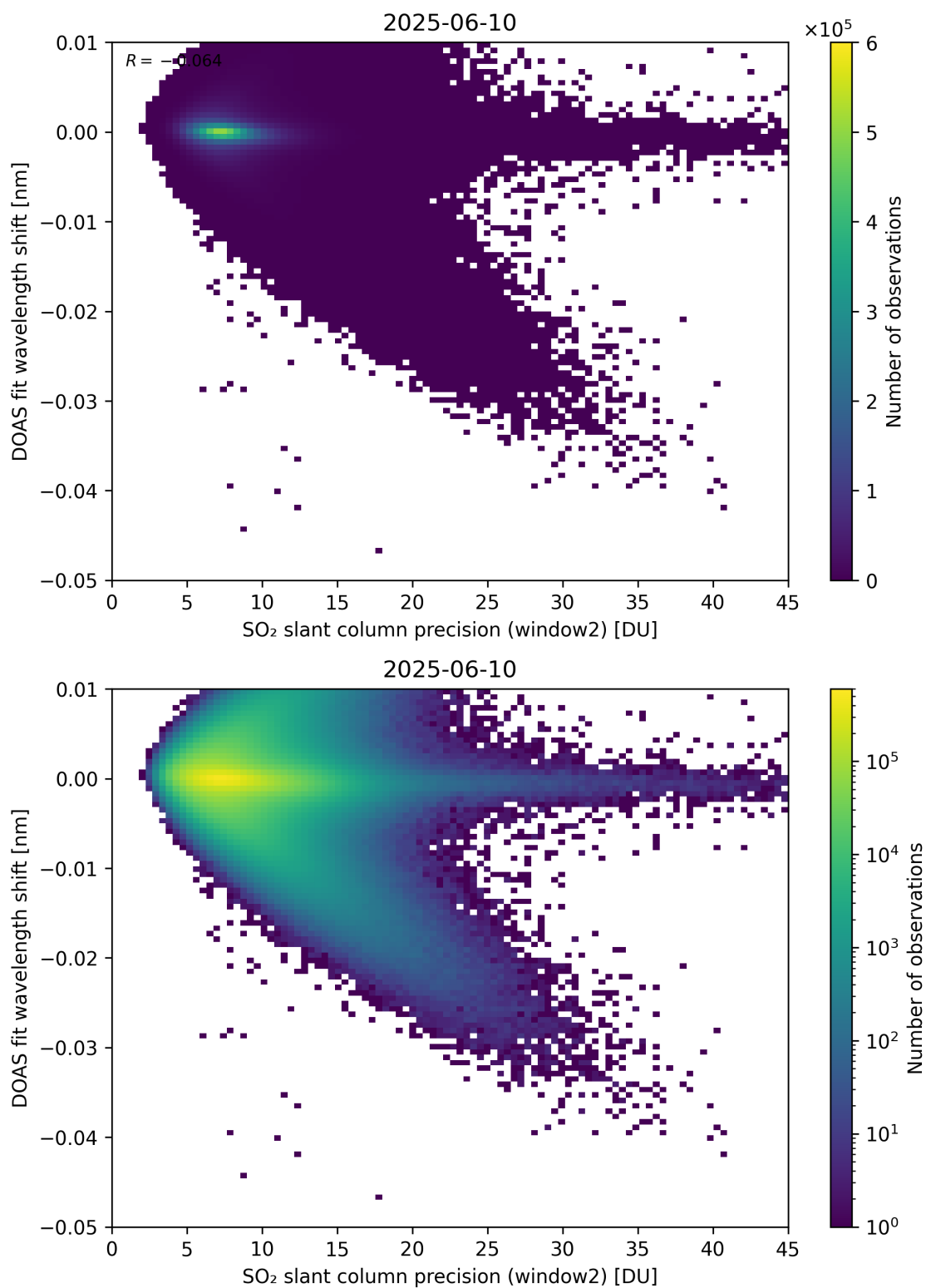
Figure 293: Scatter density plot of “SO 2 slant column precision (window2)” against “DOAS fit wavelength shift” for 2025-06-09 to 2025-06-11.
