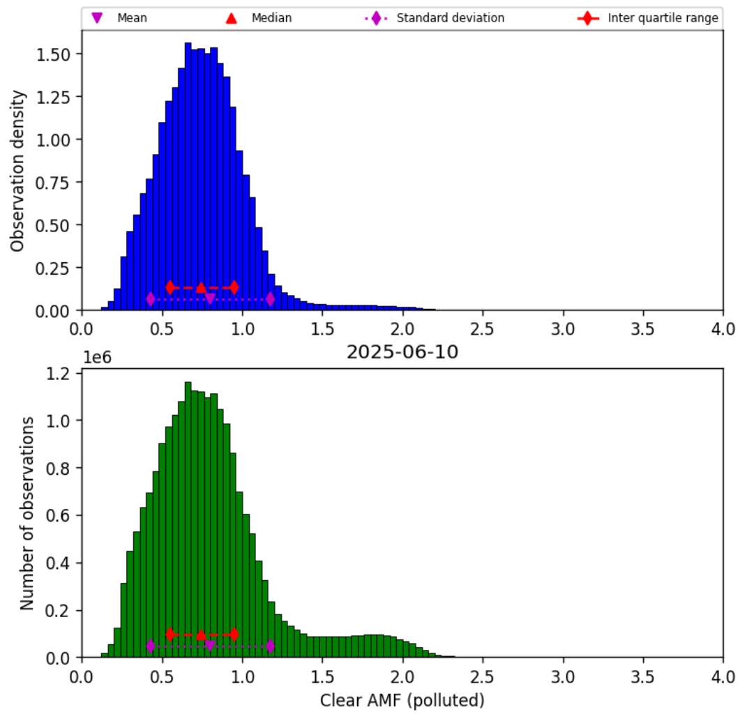
Figure 81: Histogram of “Clear AMF (polluted)” for 2025-06-09 to 2025-06-11
