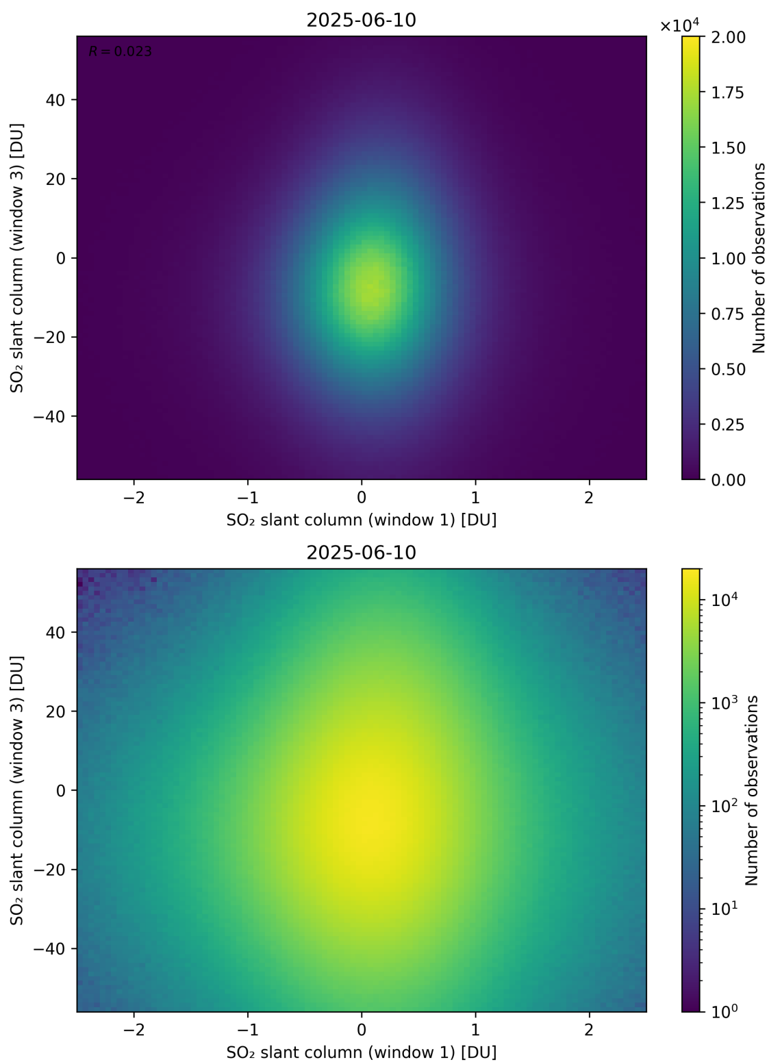
Figure 287: Scatter density plot of “SO 2 slant column (window 1)” against “SO 2 slant column (window 3)” for 2025-06-09 to 2025-06-11.
