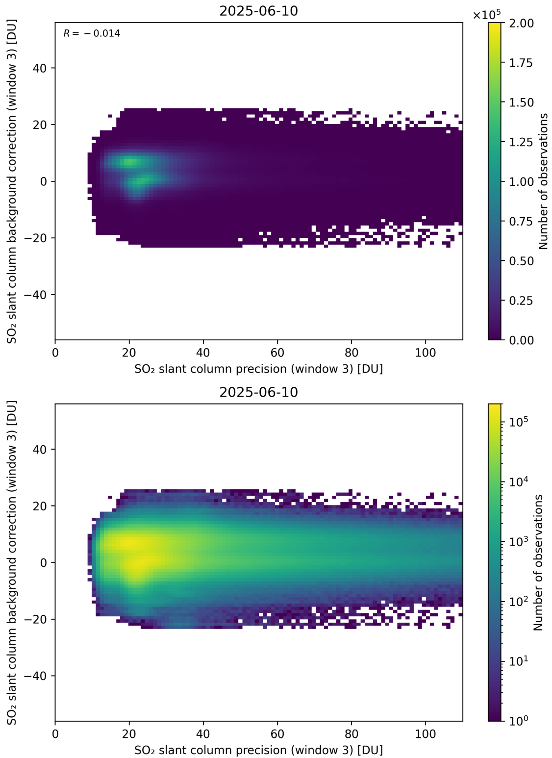
Figure 307: Scatter density plot of “SO 2 slant column precision (window 3)” against “SO 2 slant column background correction (window 3)” for 2025-06-09 to 2025-06-11.
