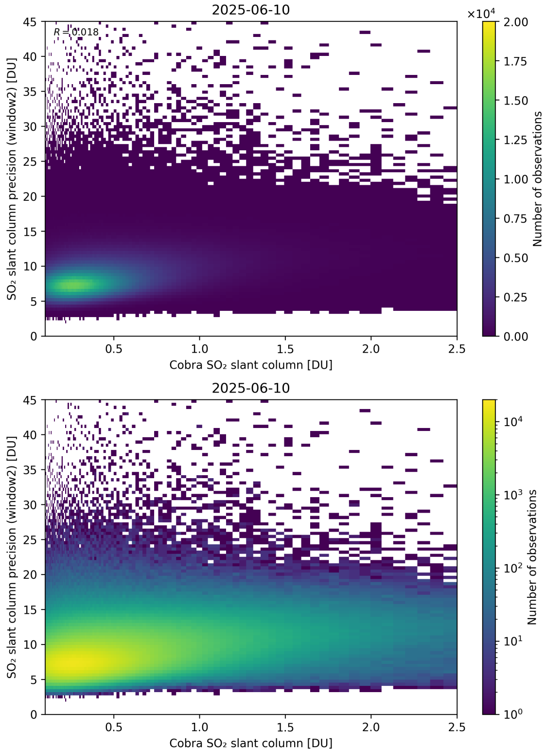
Figure 221: Scatter density plot of “Cobra SO 2 slant column” against “SO 2 slant column precision (window2)” for 2025-06-09 to 2025-06-11.
