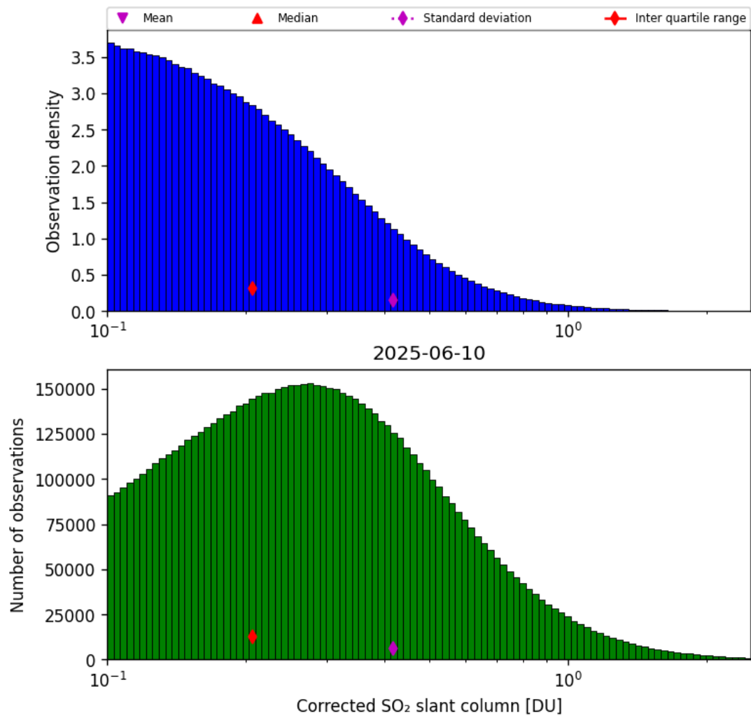
Figure 60: Histogram of “Corrected SO 2 slant column” for 2025-06-09 to 2025-06-11
