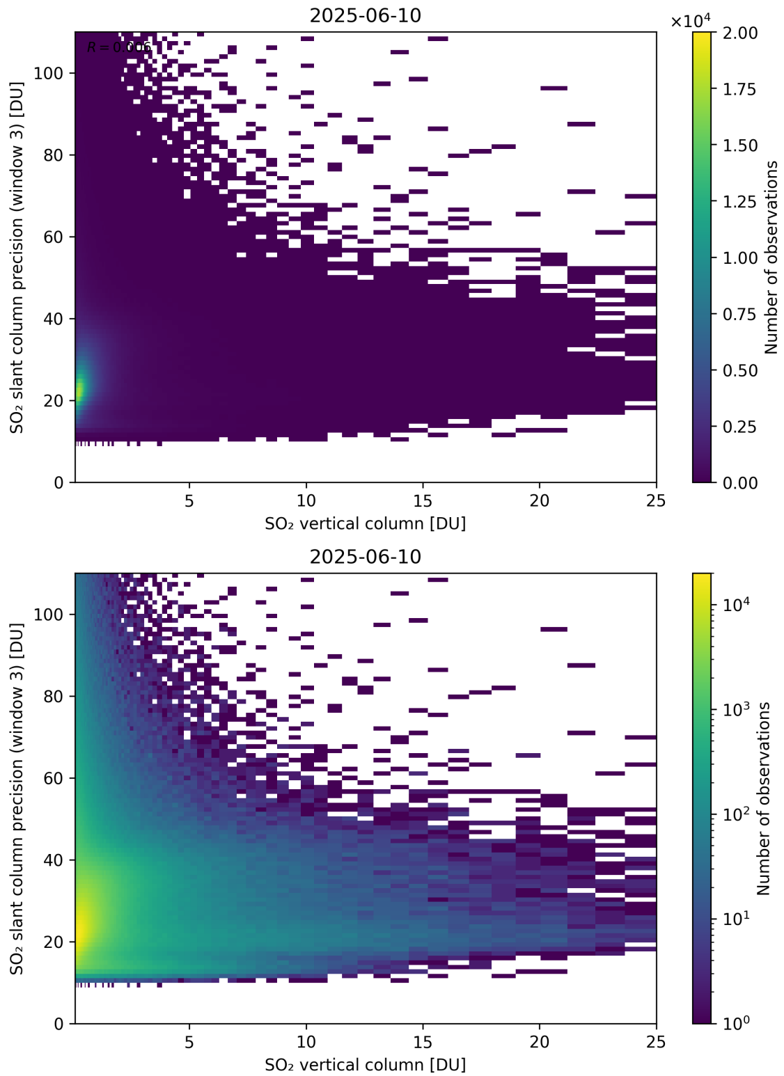
Figure 358: Scatter density plot of “SO 2 vertical column” against “SO 2 slant column precision (window 3)” for 2025-06-09 to 2025-06-11.
