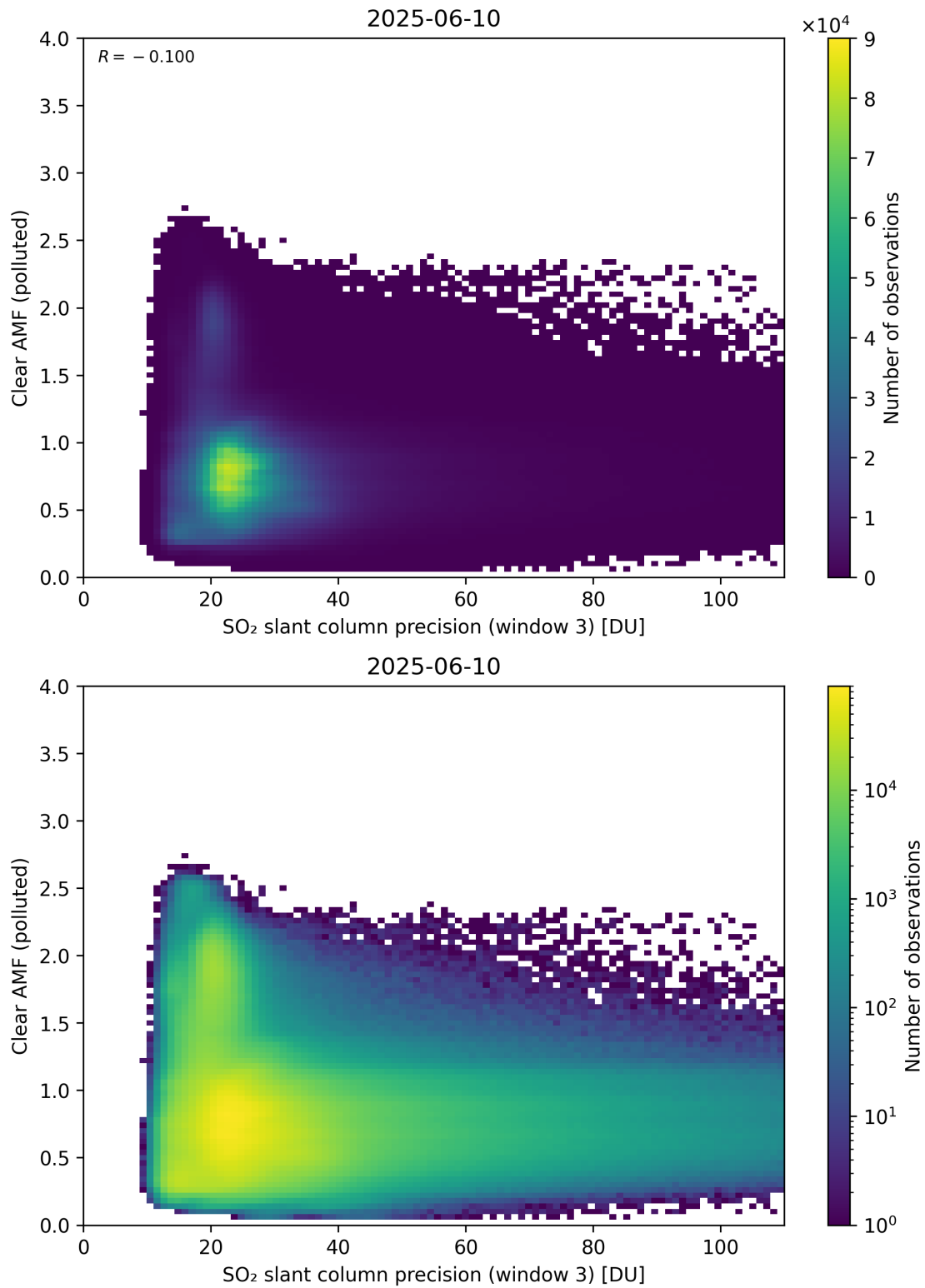
Figure 311: Scatter density plot of “SO 2 slant column precision (window 3)” against “Clear AMF (polluted)” for 2025-06-09 to 2025-06-11.
