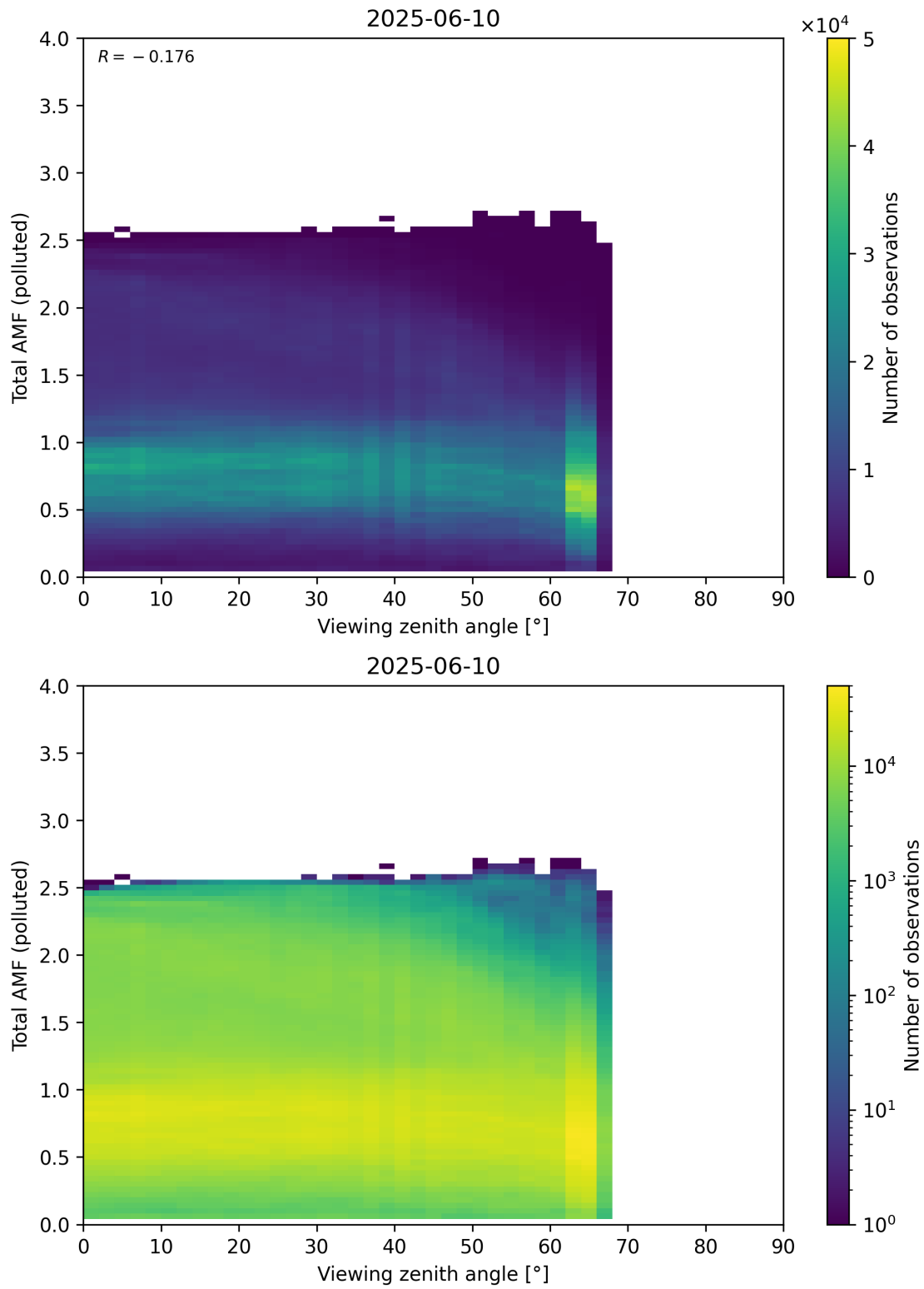
Figure 381: Scatter density plot of “Viewing zenith angle” against “Total AMF (polluted)” for 2025-06-09 to 2025-06-11.
