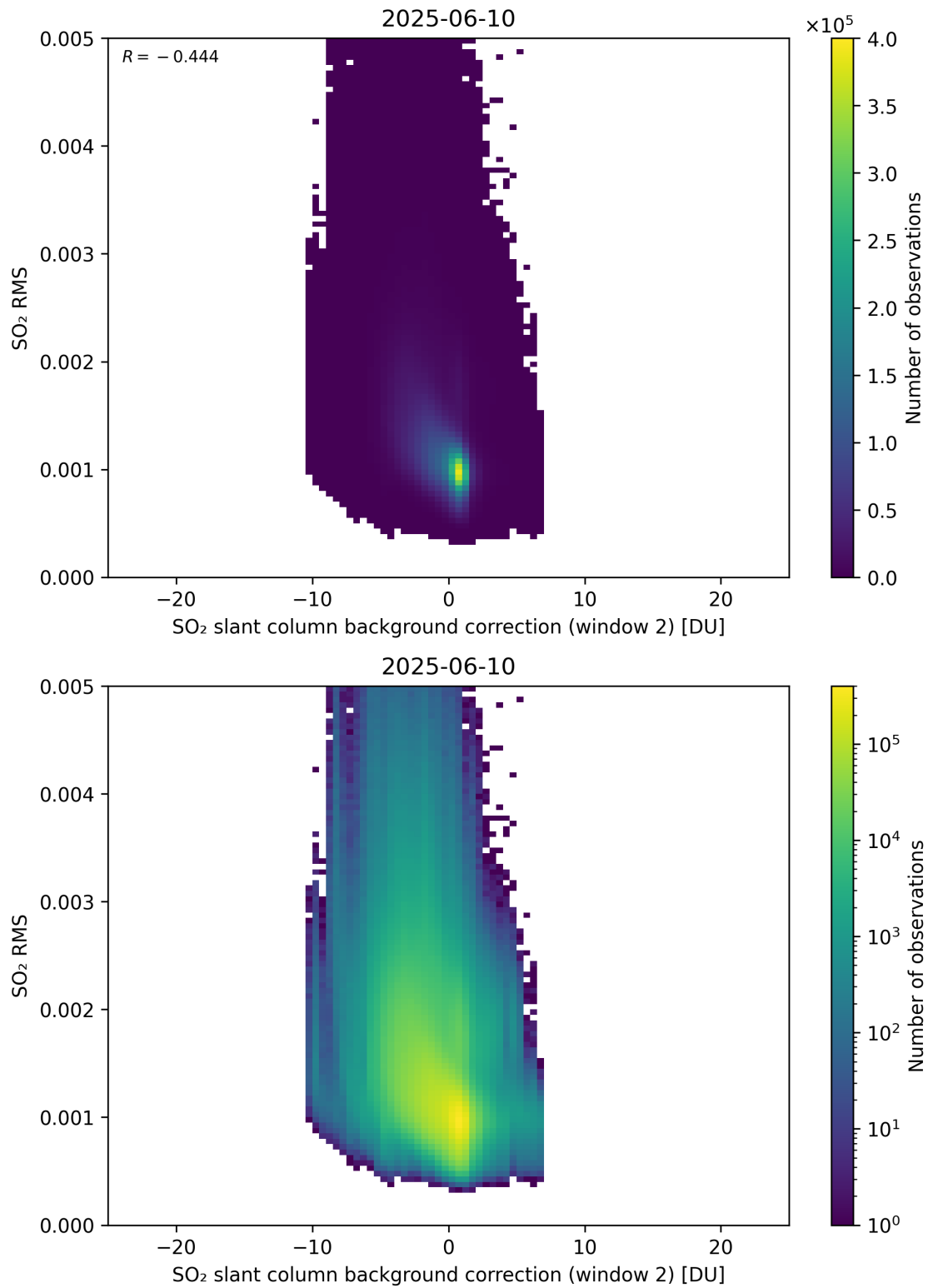
Figure 125: Scatter density plot of “SO 2 slant column background correction (window 2)” against “SO 2 RMS” for 2025-06-09 to 2025-06-11.
