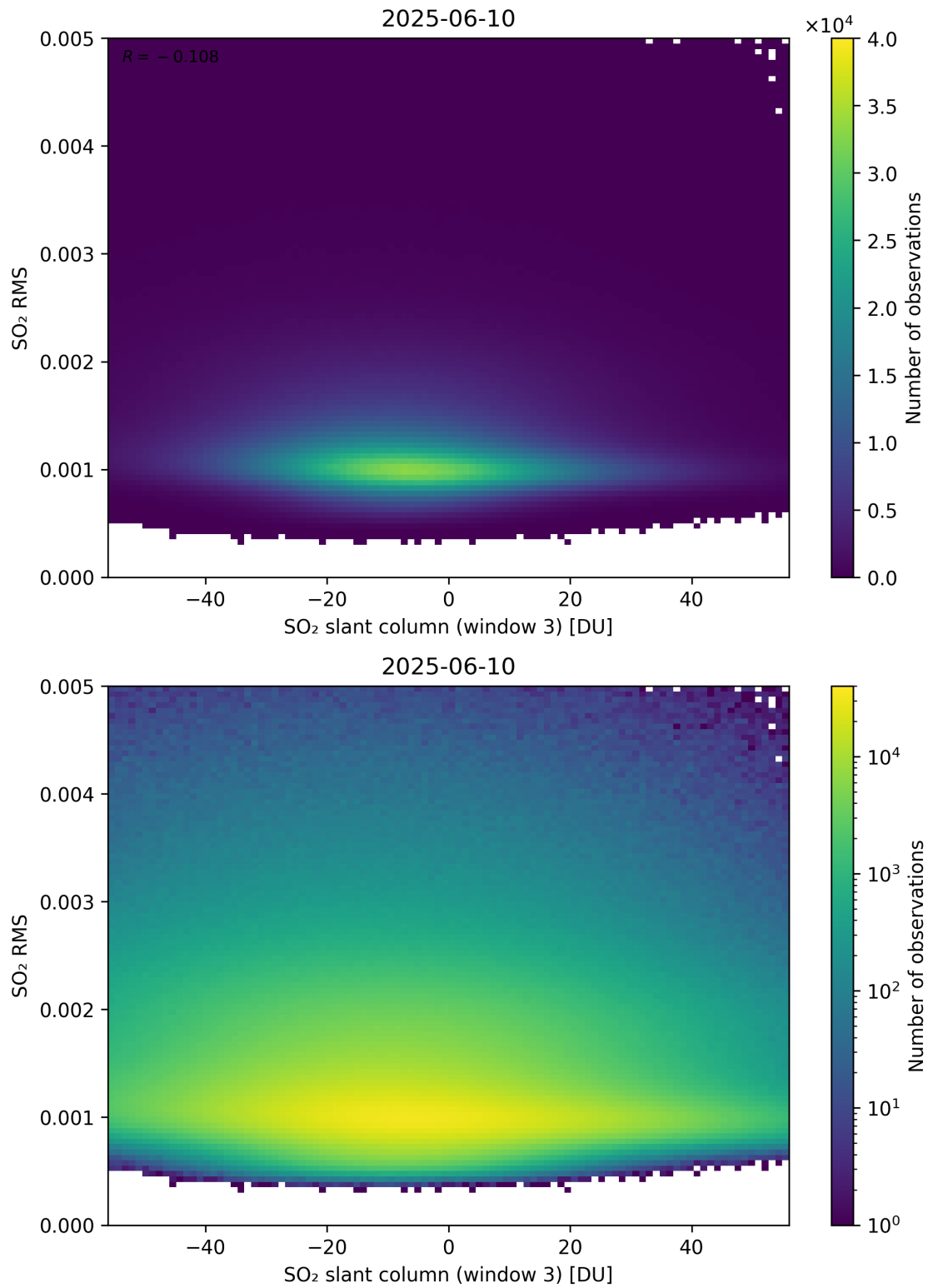
Figure 306: Scatter density plot of “SO 2 slant column (window 3)” against “SO 2 RMS” for 2025-06-09 to 2025-06-11.
