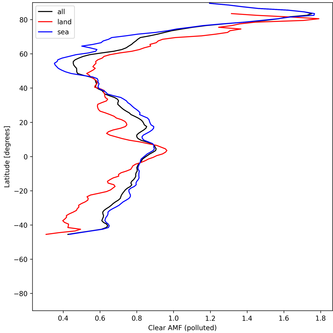
Figure 55: Zonal average of “Clear AMF (polluted)” for 2025-06-09 to 2025-06-11.
