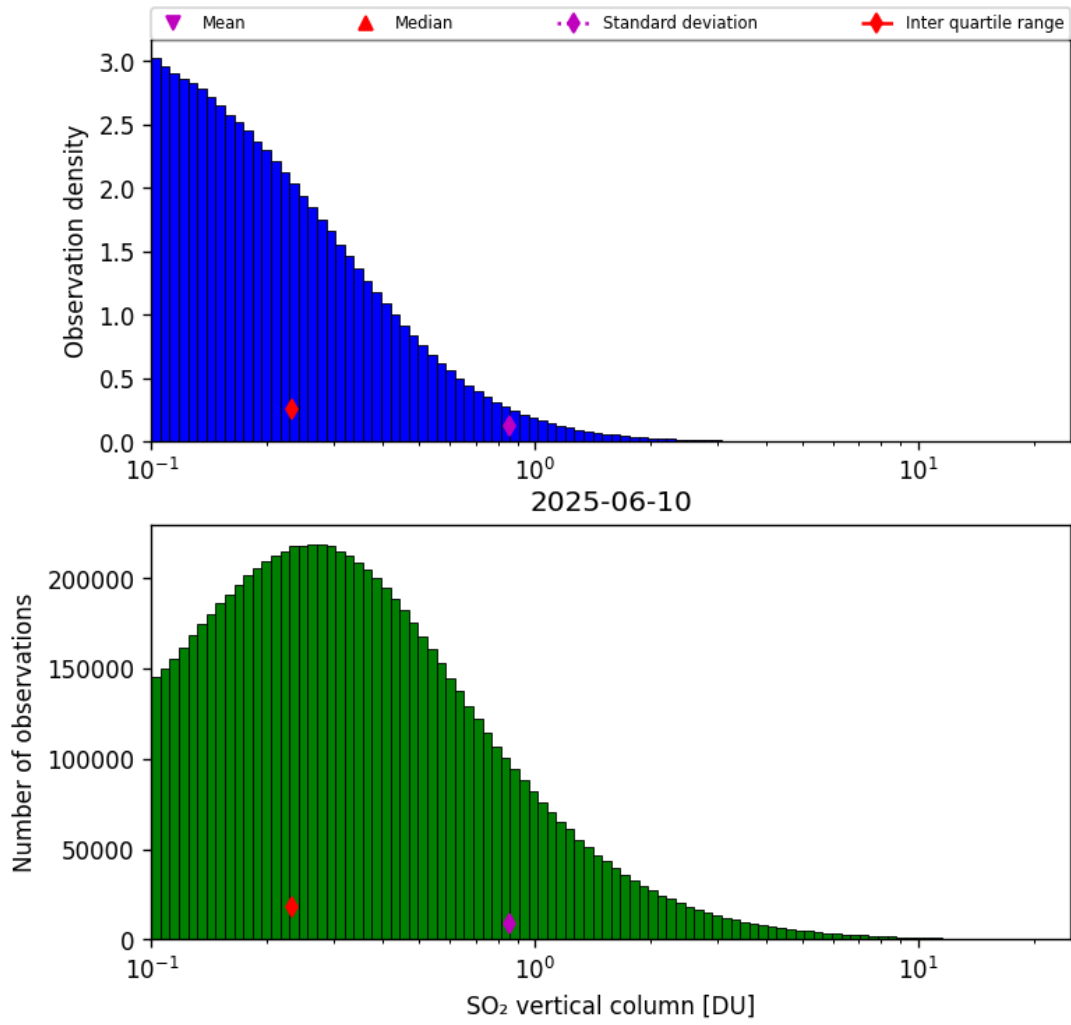
Figure 58: Histogram of “SO 2 vertical column” for 2025-06-09 to 2025-06-11
