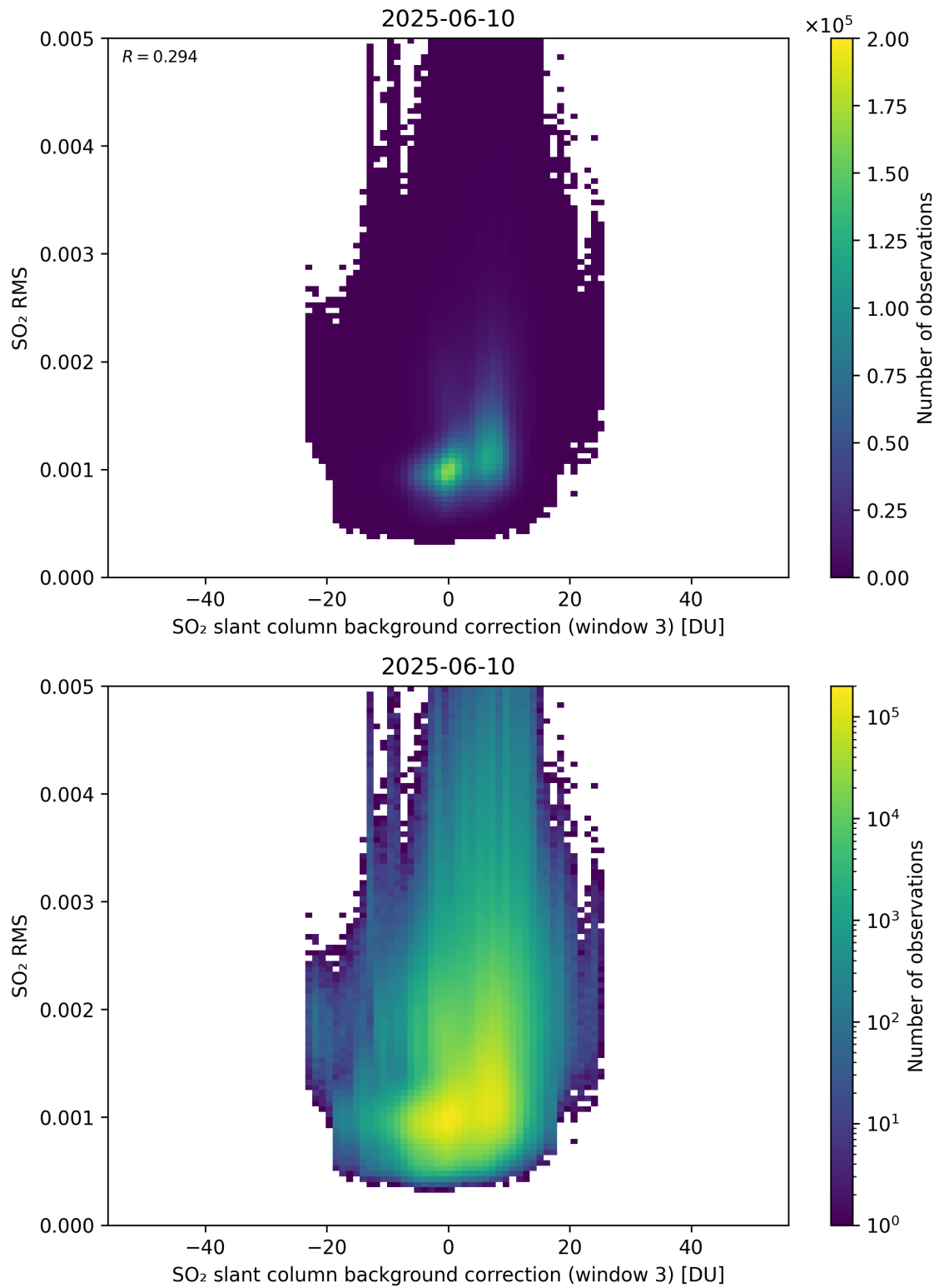
Figure 134: Scatter density plot of “SO 2 slant column background correction (window 3)” against “SO 2 RMS” for 2025-06-09 to 2025-06-11.
