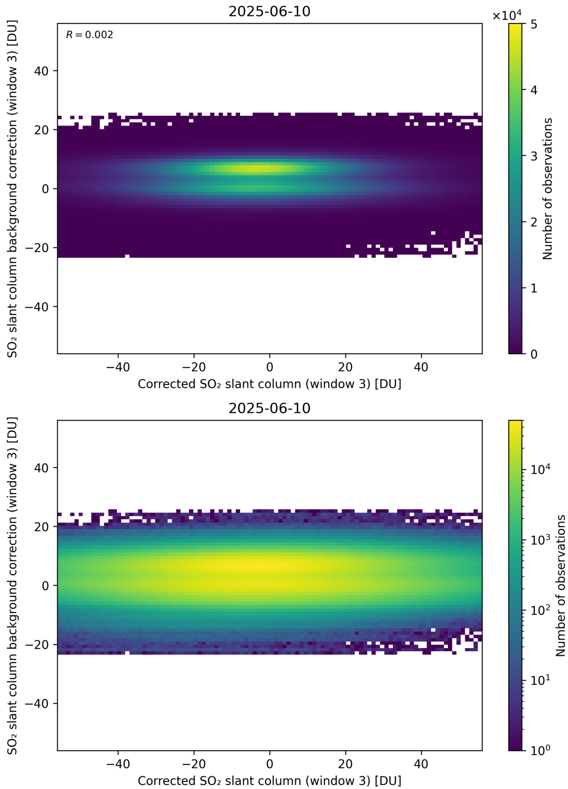
Figure 255: Scatter density plot of “Corrected SO 2 slant column (window 3)” against “SO 2 slant column background correction (window 3)” for 2025-06-09 to 2025-06-11.
