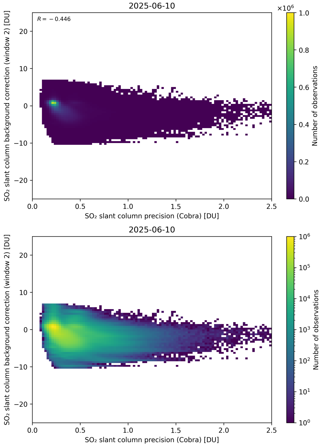
Figure 200: Scatter density plot of “SO 2 slant column precision (Cobra)” against “SO 2 slant column background correction (window 2)” for 2025-06-09 to 2025-06-11.
