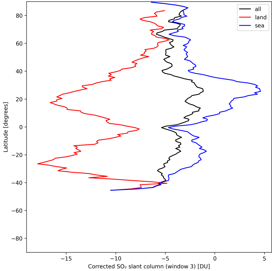
Figure 47: Zonal average of “Corrected SO 2 slant column (window 3)” for 2025-06-09 to 2025-06-11.
