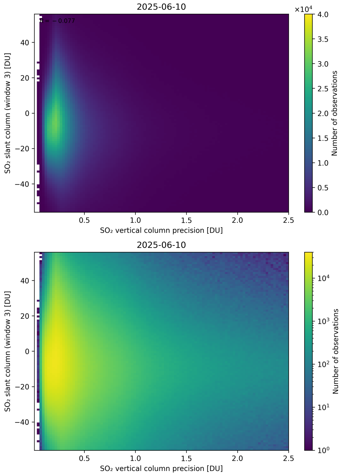
Figure 344: Scatter density plot of “SO 2 vertical column precision” against “SO 2 slant column (window 3)” for 2025-06-09 to 2025-06-11.
