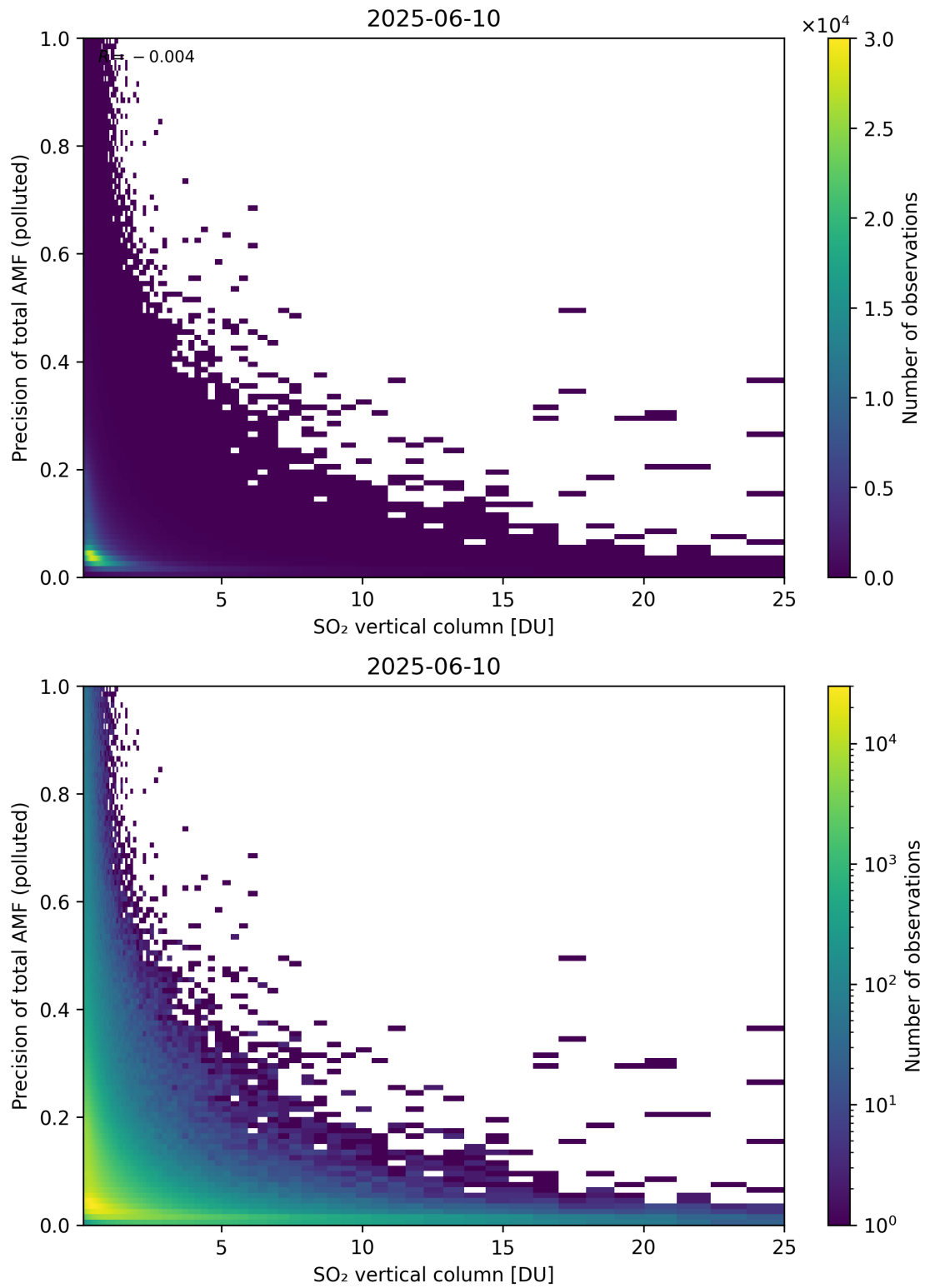
Figure 360: Scatter density plot of “SO 2 vertical column” against “Precision of total AMF (polluted)” for 2025-06-09 to 2025-06-11.
