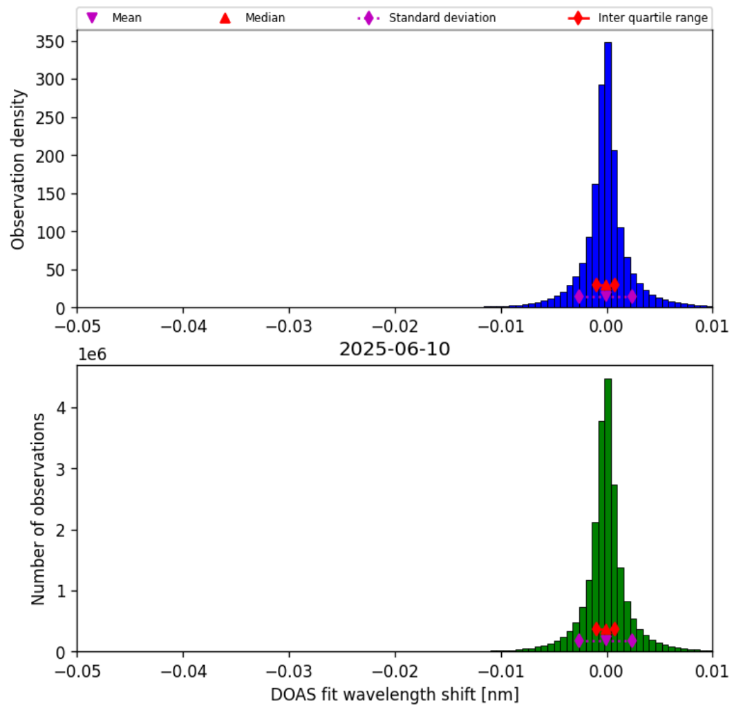
Figure 76: Histogram of “DOAS fit wavelength shift” for 2025-06-09 to 2025-06-11
