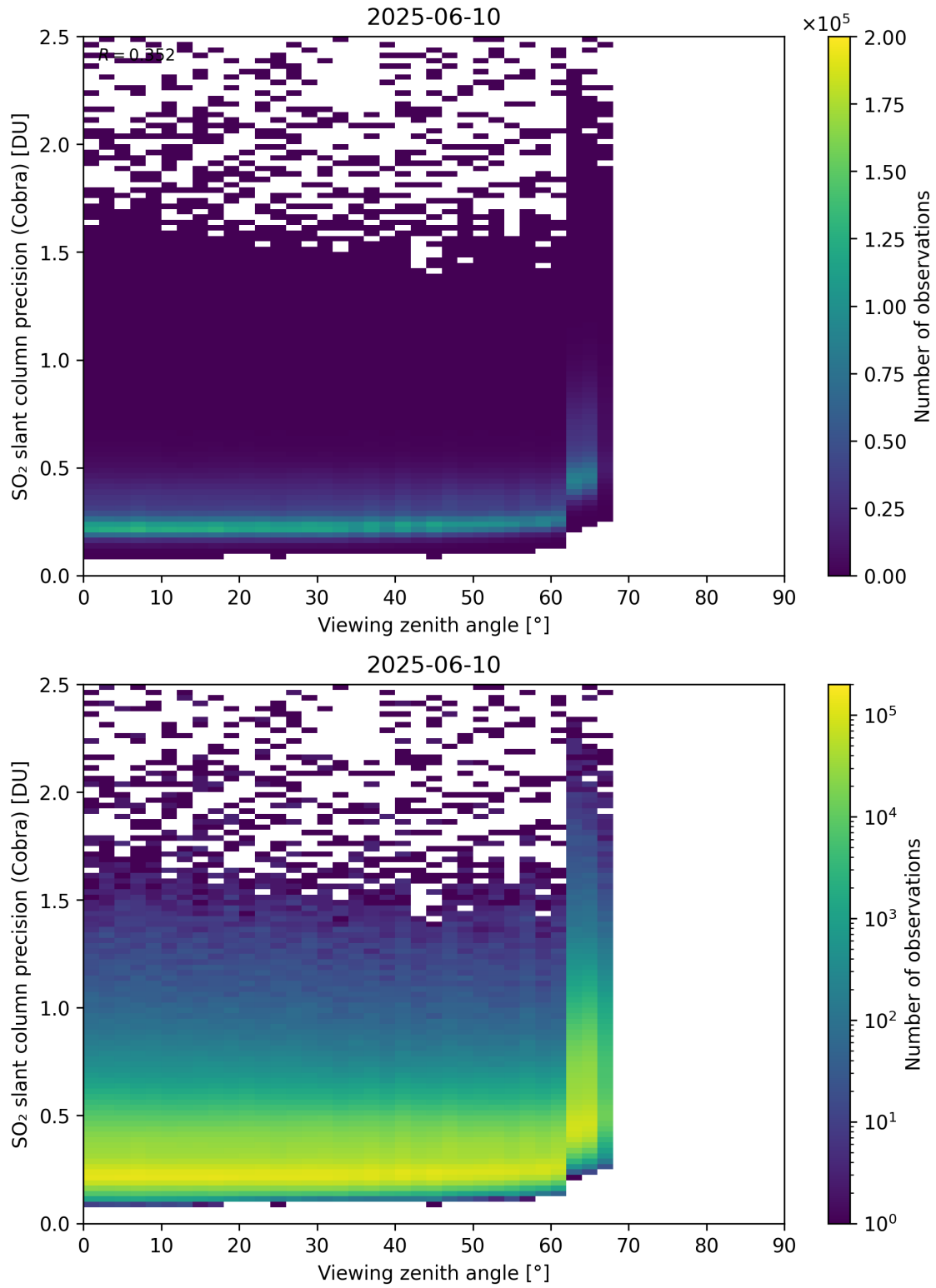
Figure 372: Scatter density plot of “Viewing zenith angle” against “SO 2 slant column precision (Cobra)” for 2025-06-09 to 2025-06-11.
