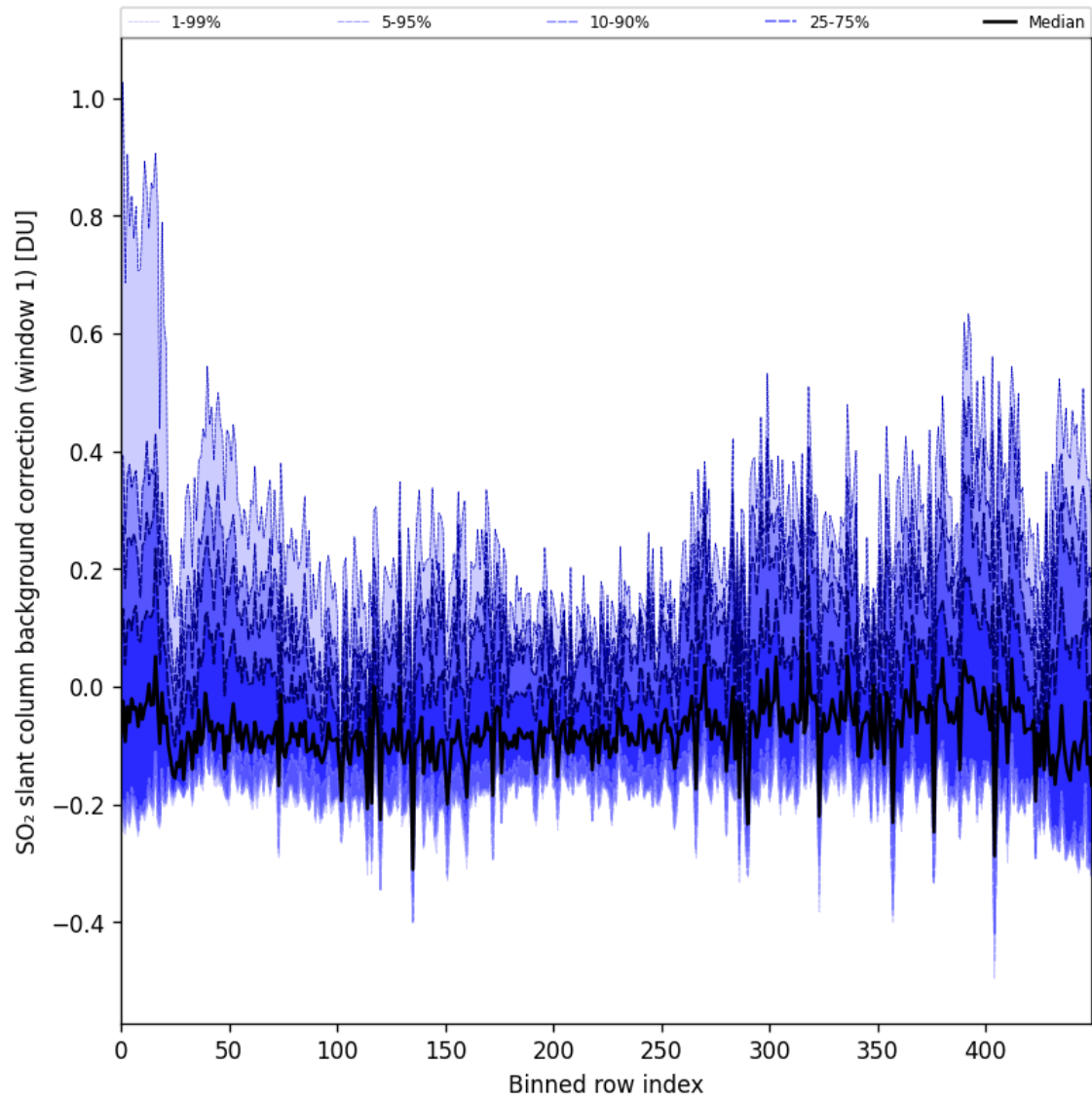
Figure 92: Along track statistics of “SO 2 slant column background correction (window 1)” for 2025-06-09 to 2025-06-11
