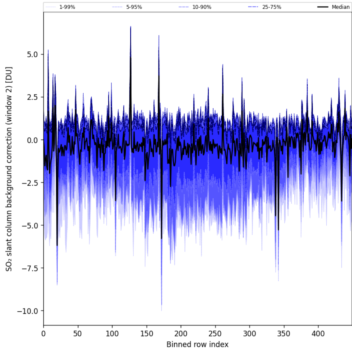
Figure 96: Along track statistics of “SO 2 slant column background correction (window 2)” for 2025-06-09 to 2025-06-11
