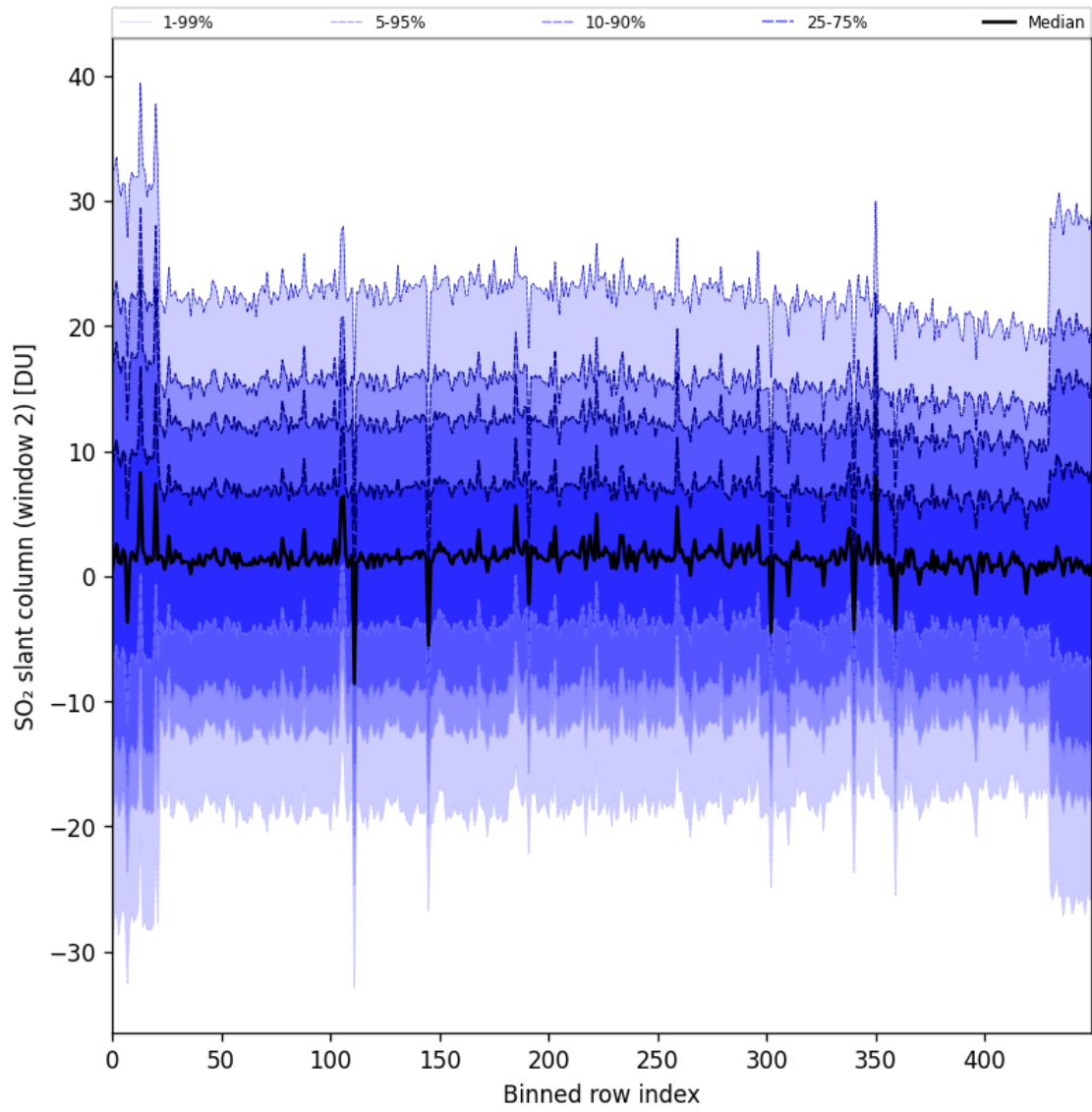
Figure 93: Along track statistics of “SO 2 slant column (window 2)” for 2025-06-09 to 2025-06-11
