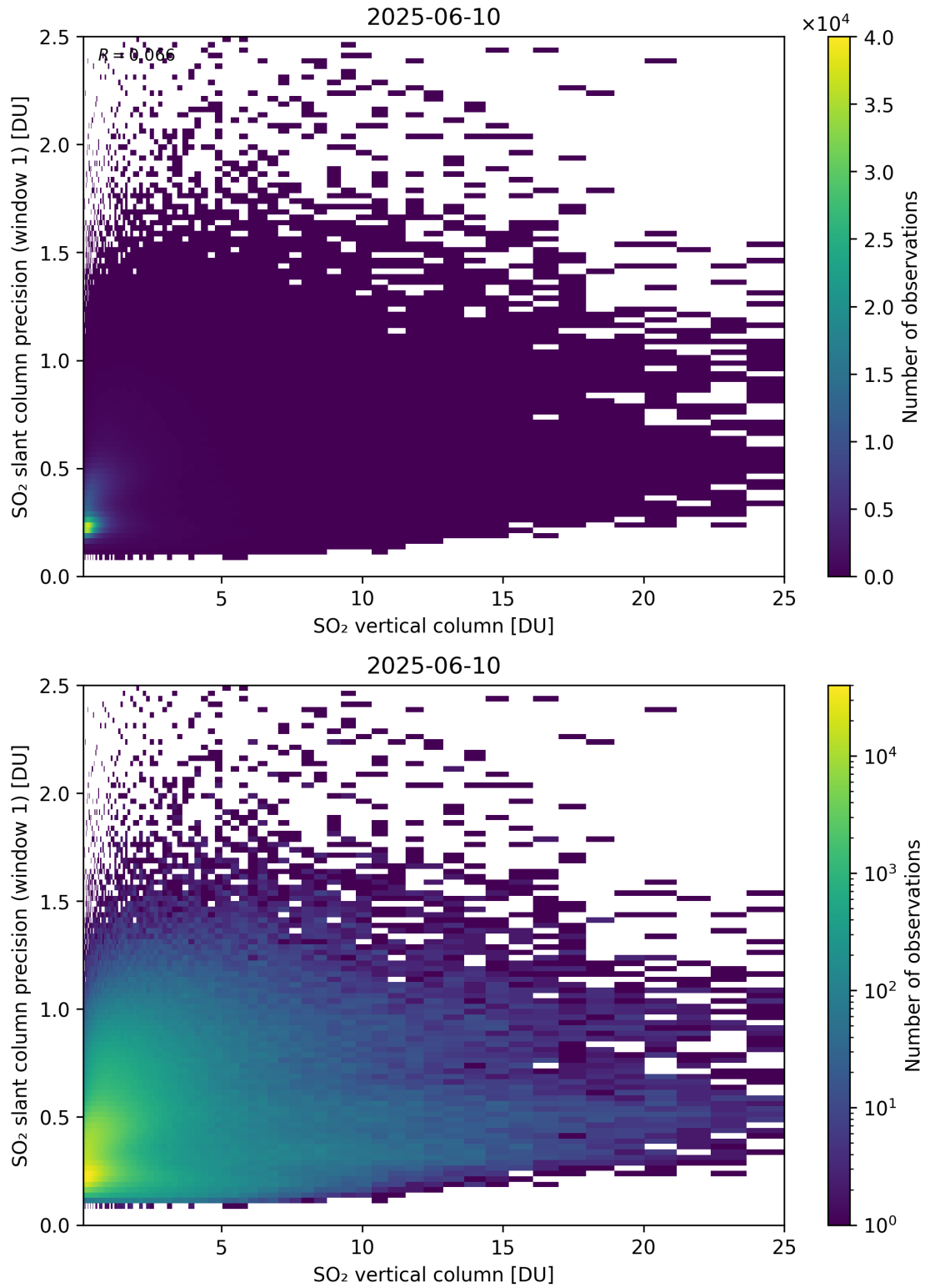
Figure 355: Scatter density plot of “SO 2 vertical column” against “SO 2 slant column precision (window 1)” for 2025-06-09 to 2025-06-11.
