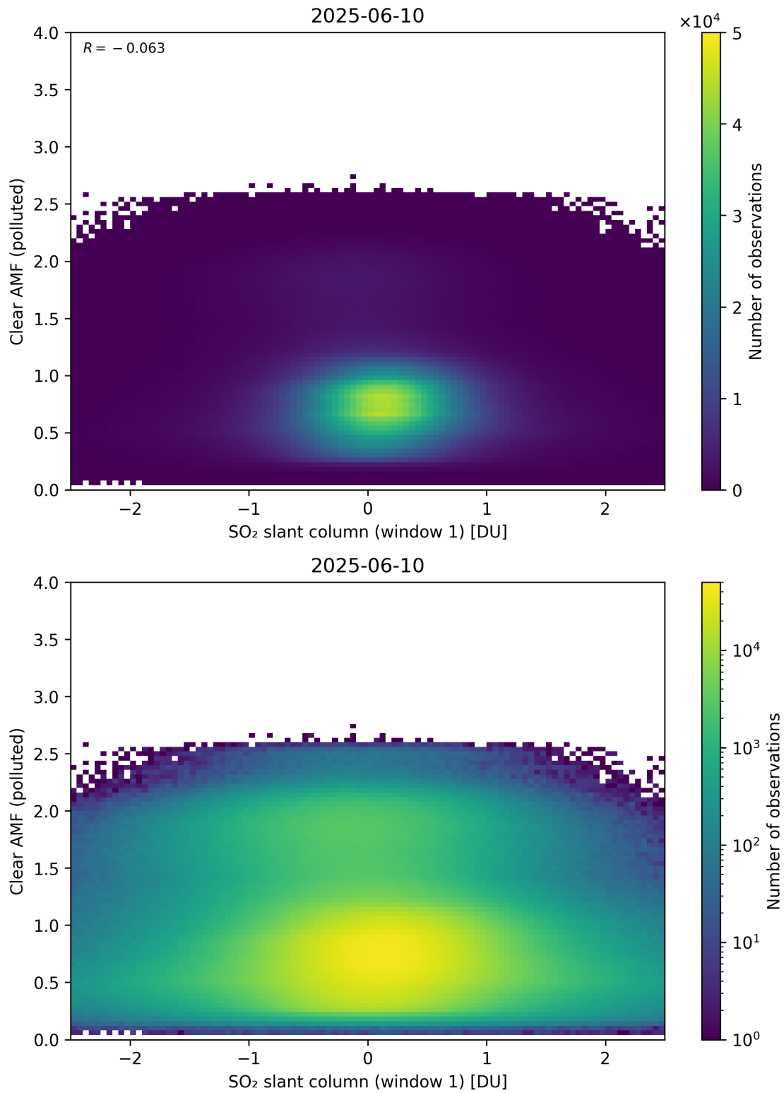
Figure 282: Scatter density plot of “SO 2 slant column (window 1)” against “Clear AMF (polluted)” for 2025-06-09 to 2025-06-11.
