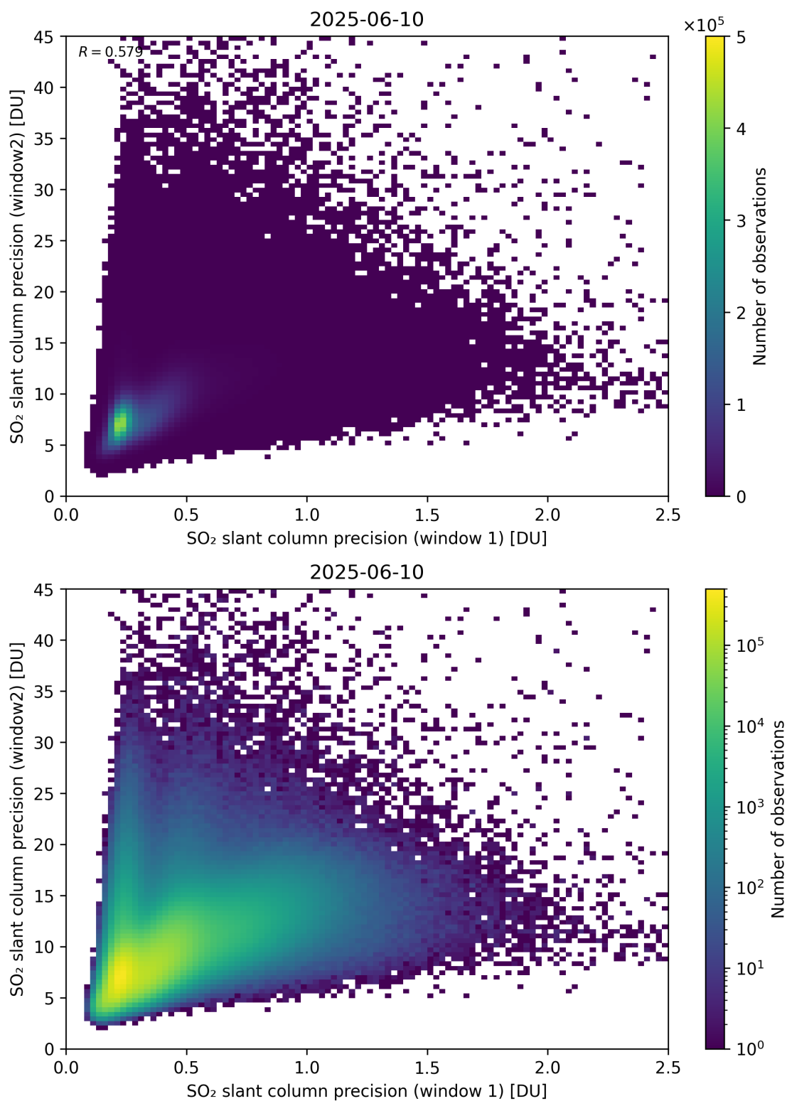
Figure 277: Scatter density plot of “SO 2 slant column precision (window 1)” against “SO 2 slant column precision (window2)” for 2025-06-09 to 2025-06-11.
