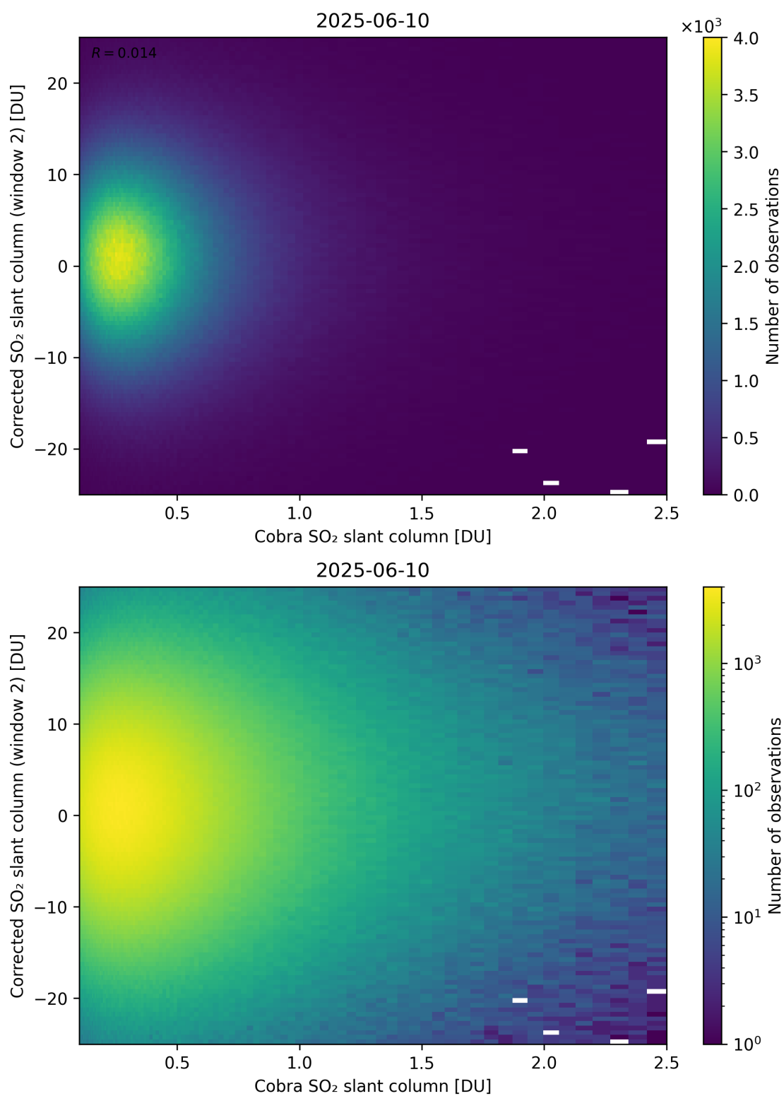
Figure 217: Scatter density plot of “Cobra SO 2 slant column” against “Corrected SO 2 slant column (window 2)” for 2025-06-09 to 2025-06-11.
