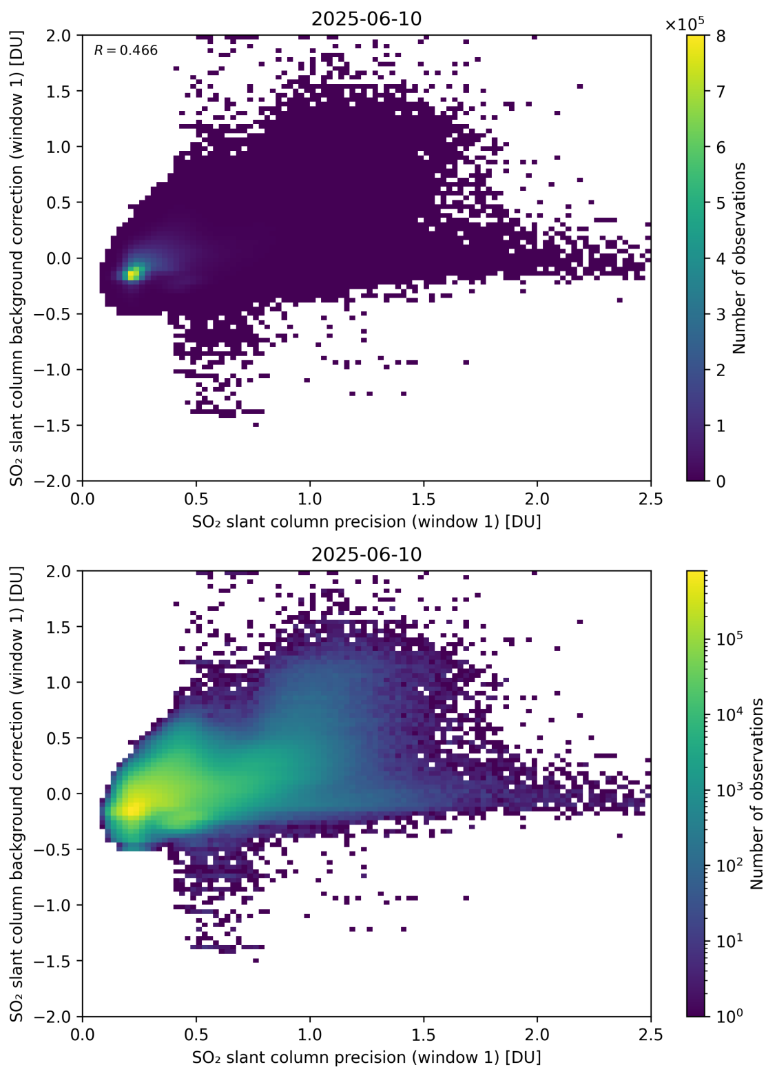
Figure 268: Scatter density plot of “SO 2 slant column precision (window 1)” against “SO 2 slant column background correction (window 1)” for 2025-06-09 to 2025-06-11.
