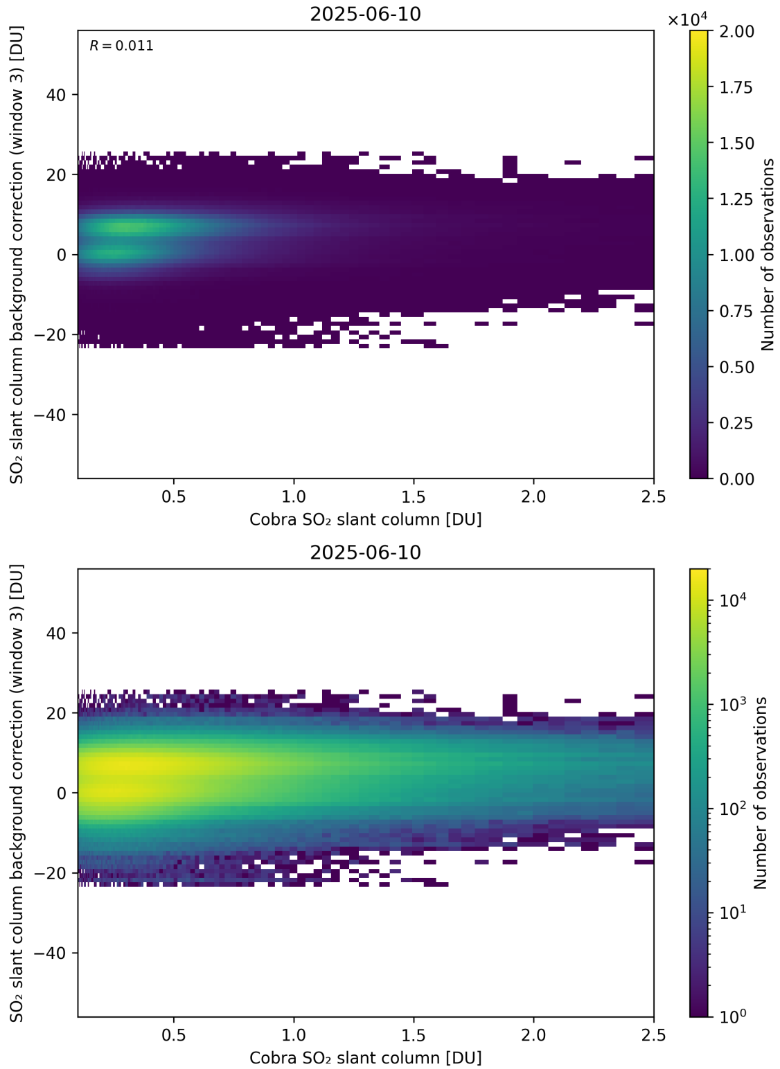
Figure 195: Scatter density plot of “Cobra SO 2 slant column” against “SO 2 slant column background correction (window 3)” for 2025-06-09 to 2025-06-11.
