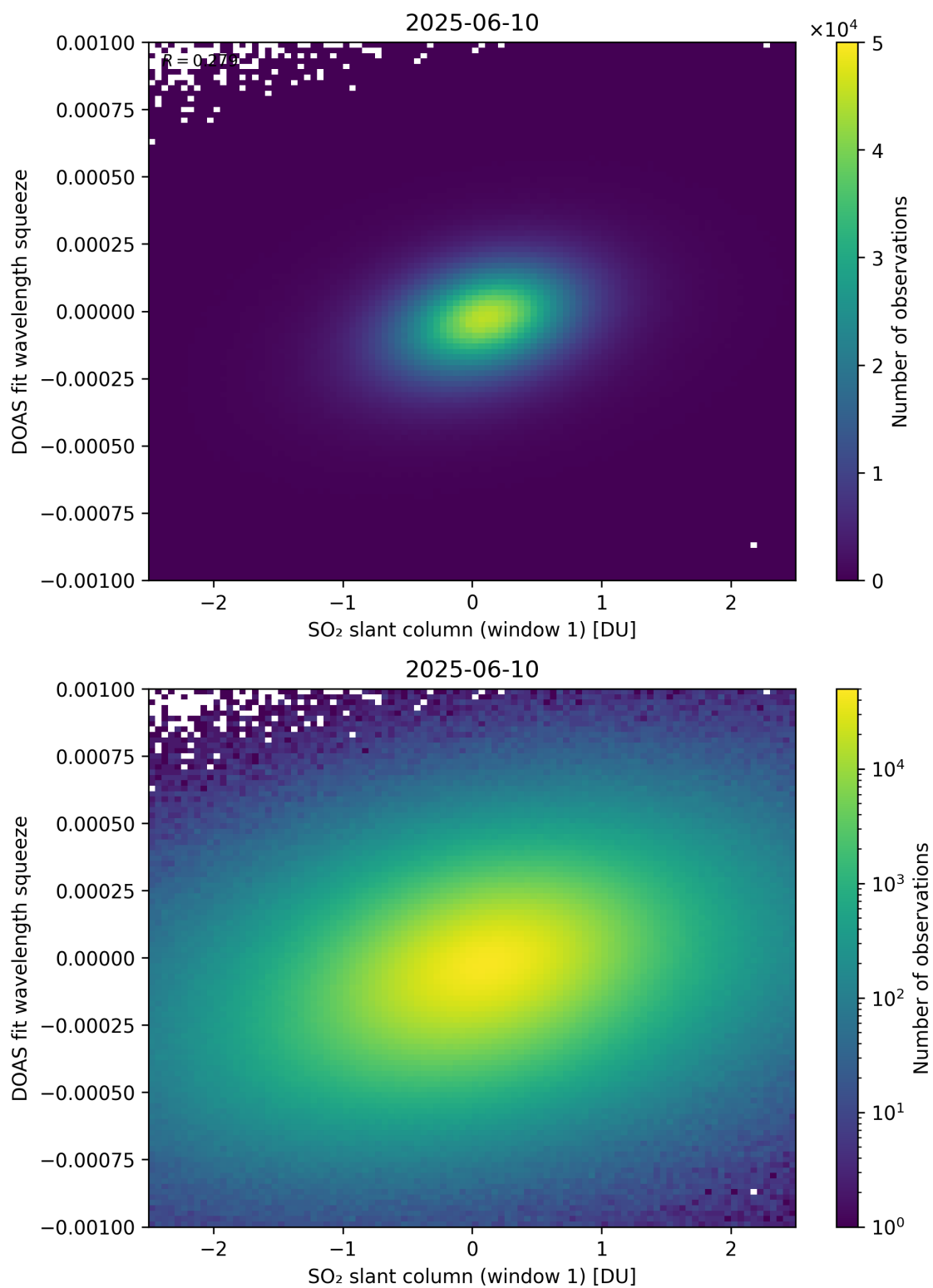
Figure 266: Scatter density plot of “SO 2 slant column (window 1)” against “DOAS fit wavelength squeeze” for 2025-06-09 to 2025-06-11.
