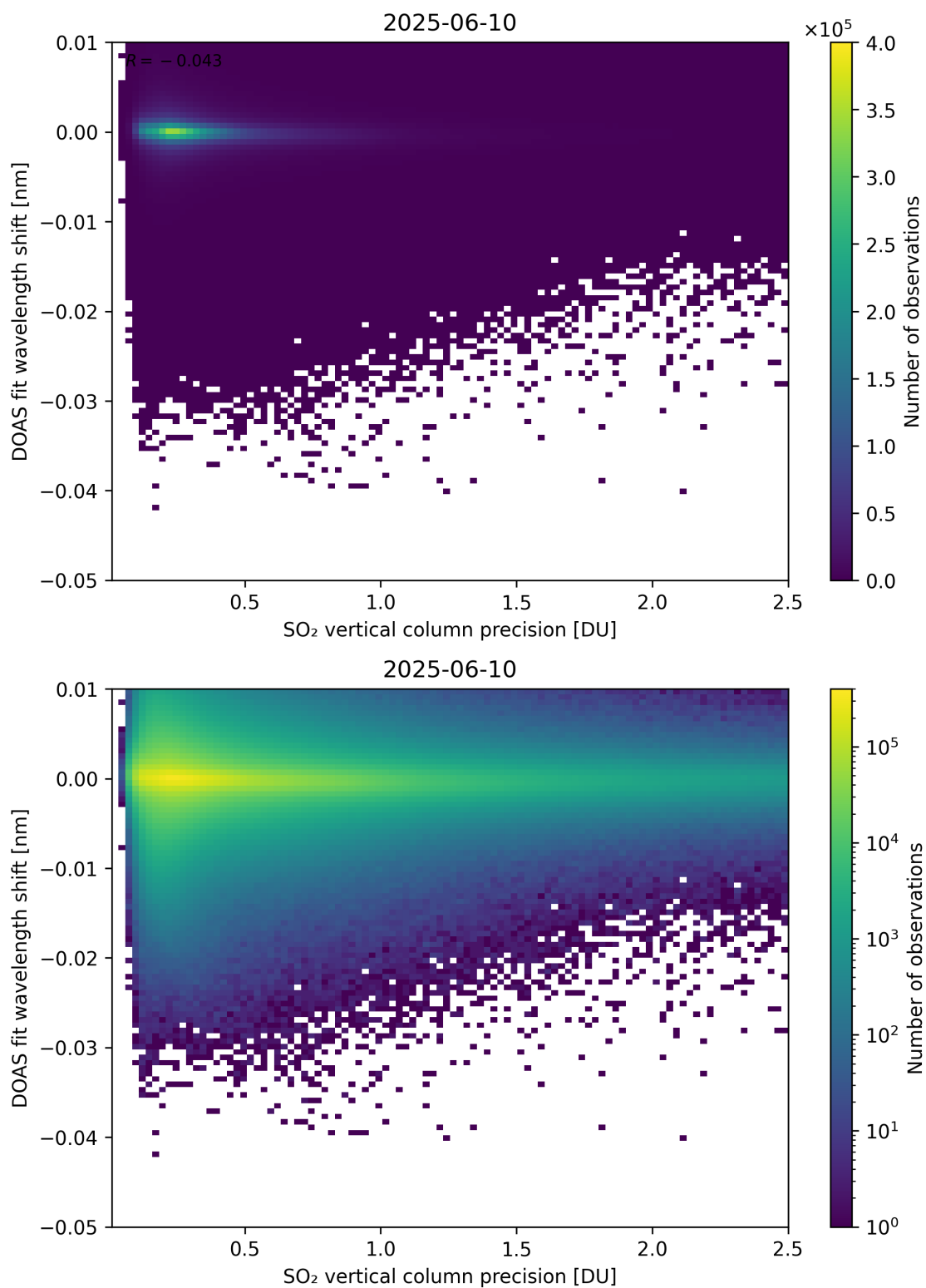
Figure 332: Scatter density plot of “SO 2 vertical column precision” against “DOAS fit wavelength shift” for 2025-06-09 to 2025-06-11.
