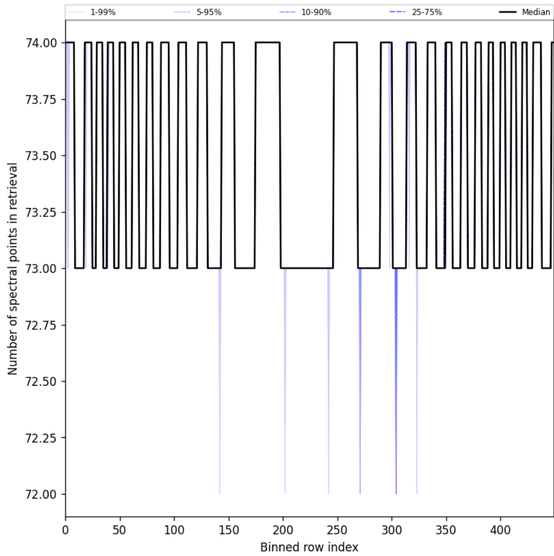
Figure 108: Along track statistics of “Number of spectral points in retrieval” for 2025-06-09 to 2025-06-11
