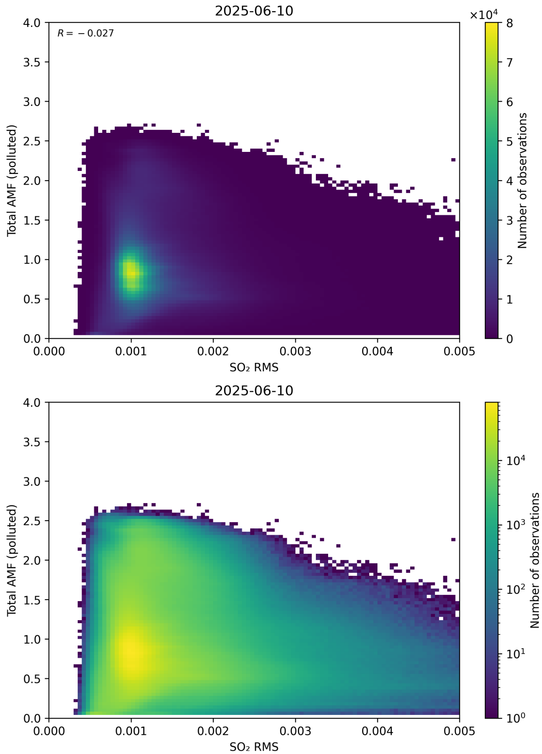
Figure 148: Scatter density plot of “SO 2 RMS” against “Total AMF (polluted)” for 2025-06-09 to 2025-06-11.
