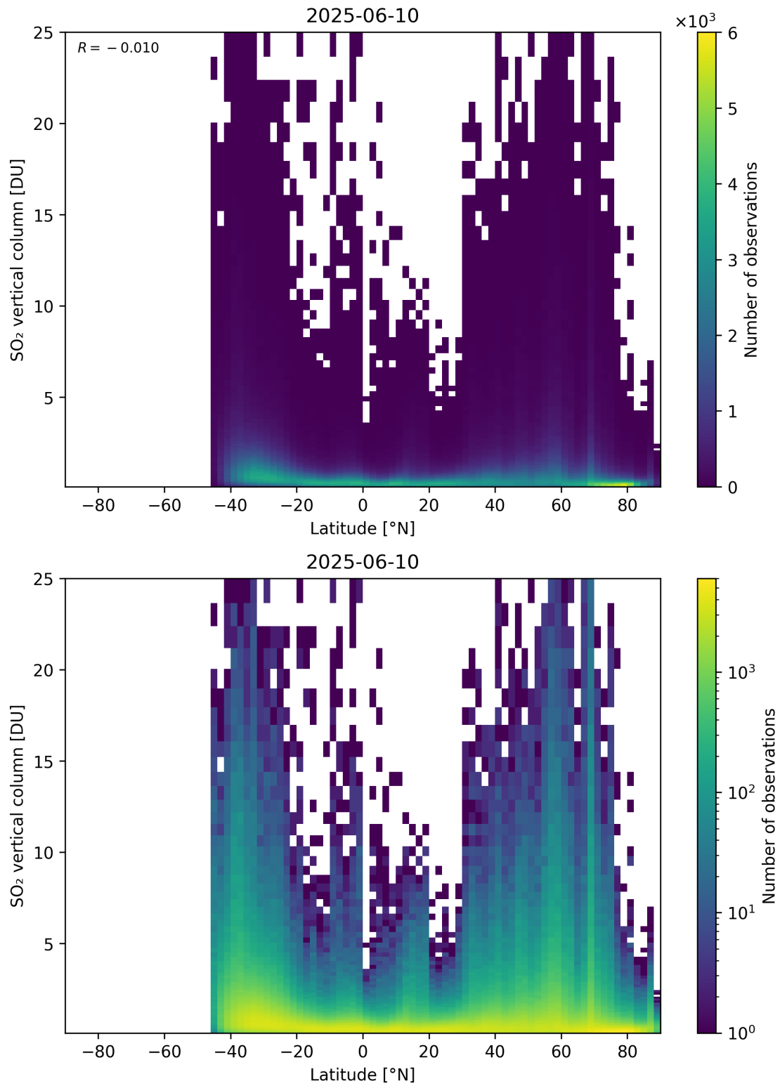
Figure 169: Scatter density plot of “Latitude” against “SO 2 vertical column” for 2025-06-09 to 2025-06-11.
