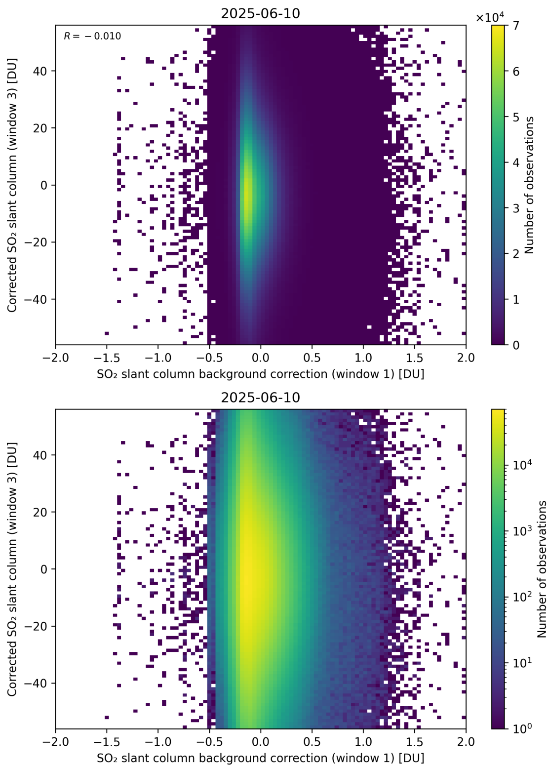
Figure 116: Scatter density plot of “SO 2 slant column background correction (window 1)” against “Corrected SO 2 slant column (window 3)” for 2025-06-09 to 2025-06-11.
