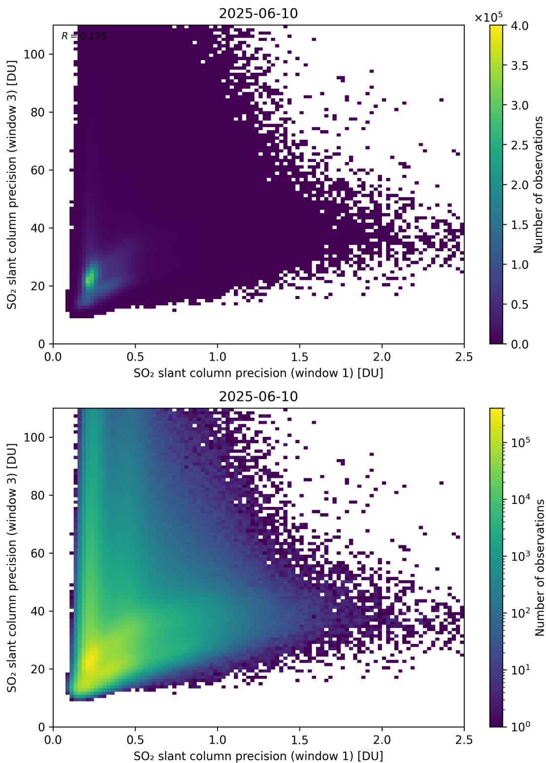
Figure 279: Scatter density plot of “SO 2 slant column precision (window 1)” against “SO 2 slant column precision (window 3)” for 2025-06-09 to 2025-06-11.
