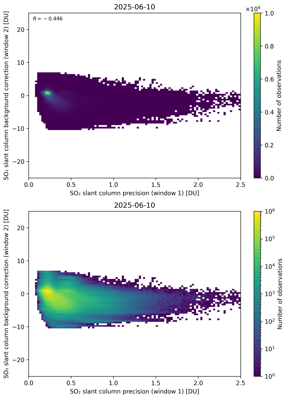
Figure 269: Scatter density plot of “SO 2 slant column precision (window 1)” against “SO 2 slant column background correction (window 2)” for 2025-06-09 to 2025-06-11.
