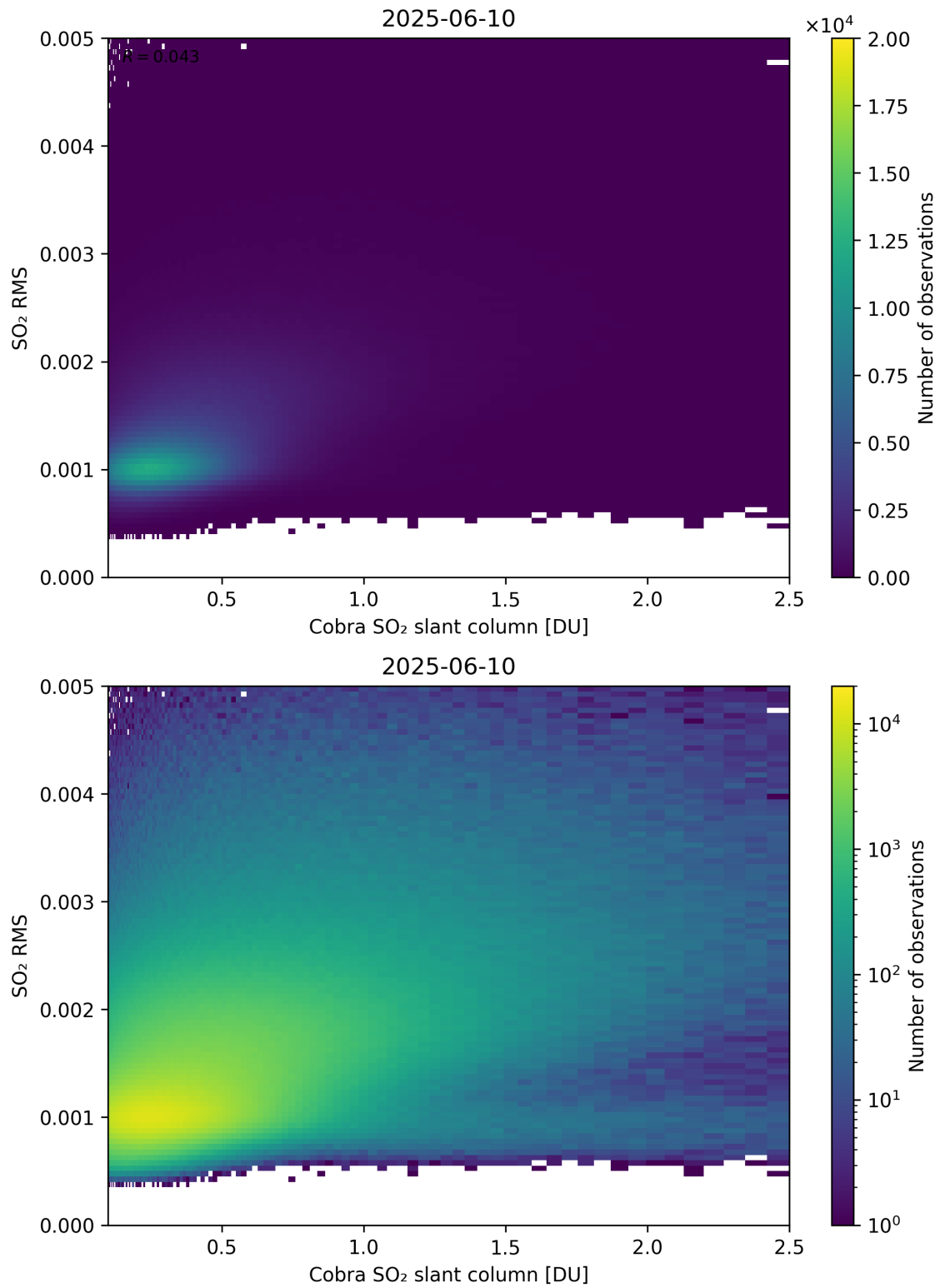
Figure 198: Scatter density plot of “Cobra SO 2 slant column” against “SO 2 RMS” for 2025-06-09 to 2025-06-11.
