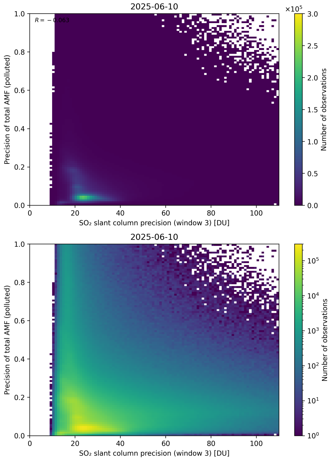
Figure 314: Scatter density plot of “SO 2 slant column precision (window 3)” against “Precision of total AMF (polluted)” for 2025-06-09 to 2025-06-11.
