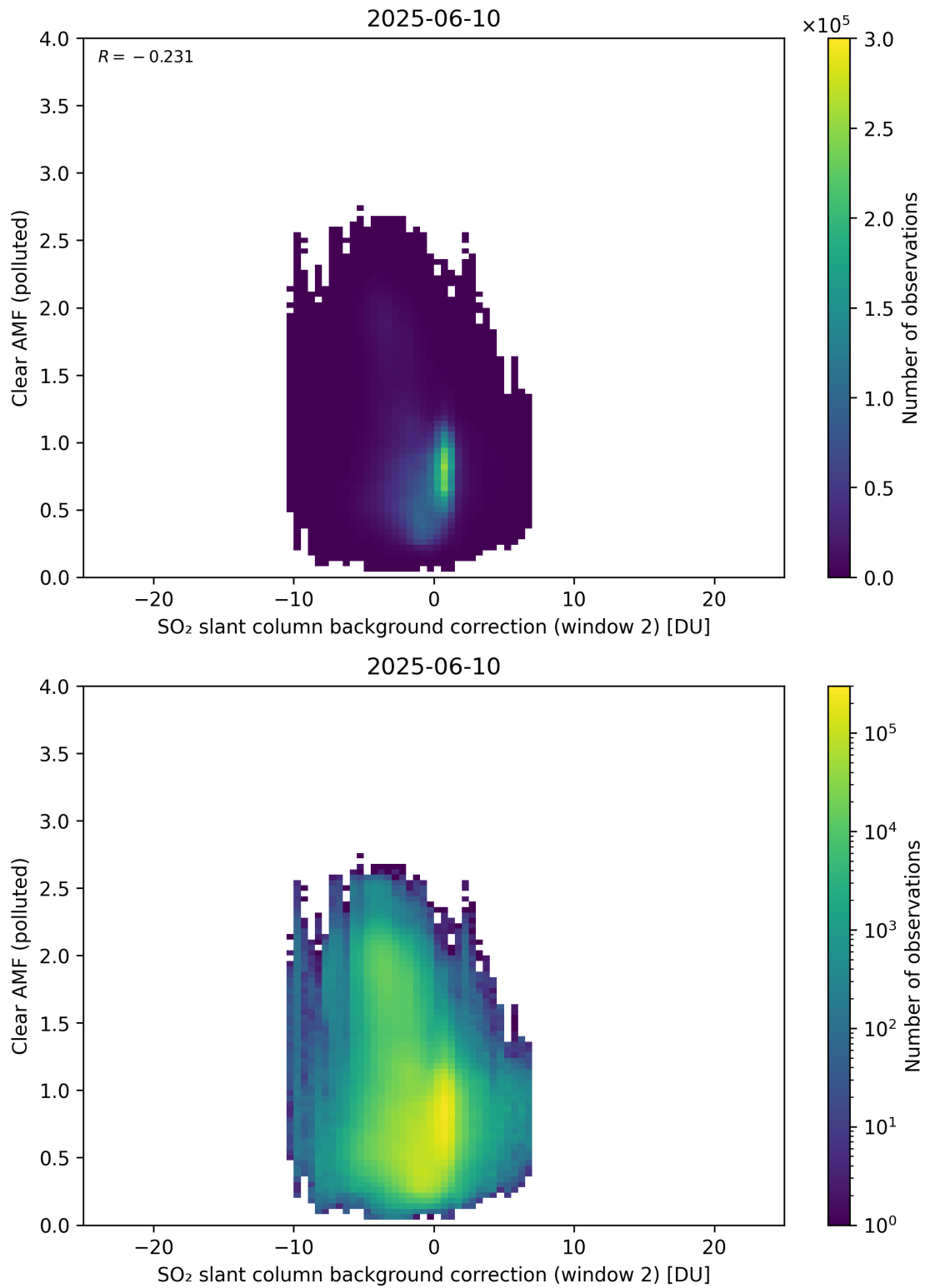
Figure 126: Scatter density plot of “SO 2 slant column background correction (window 2)” against “Clear AMF (polluted)” for 2025-06-09 to 2025-06-11.
