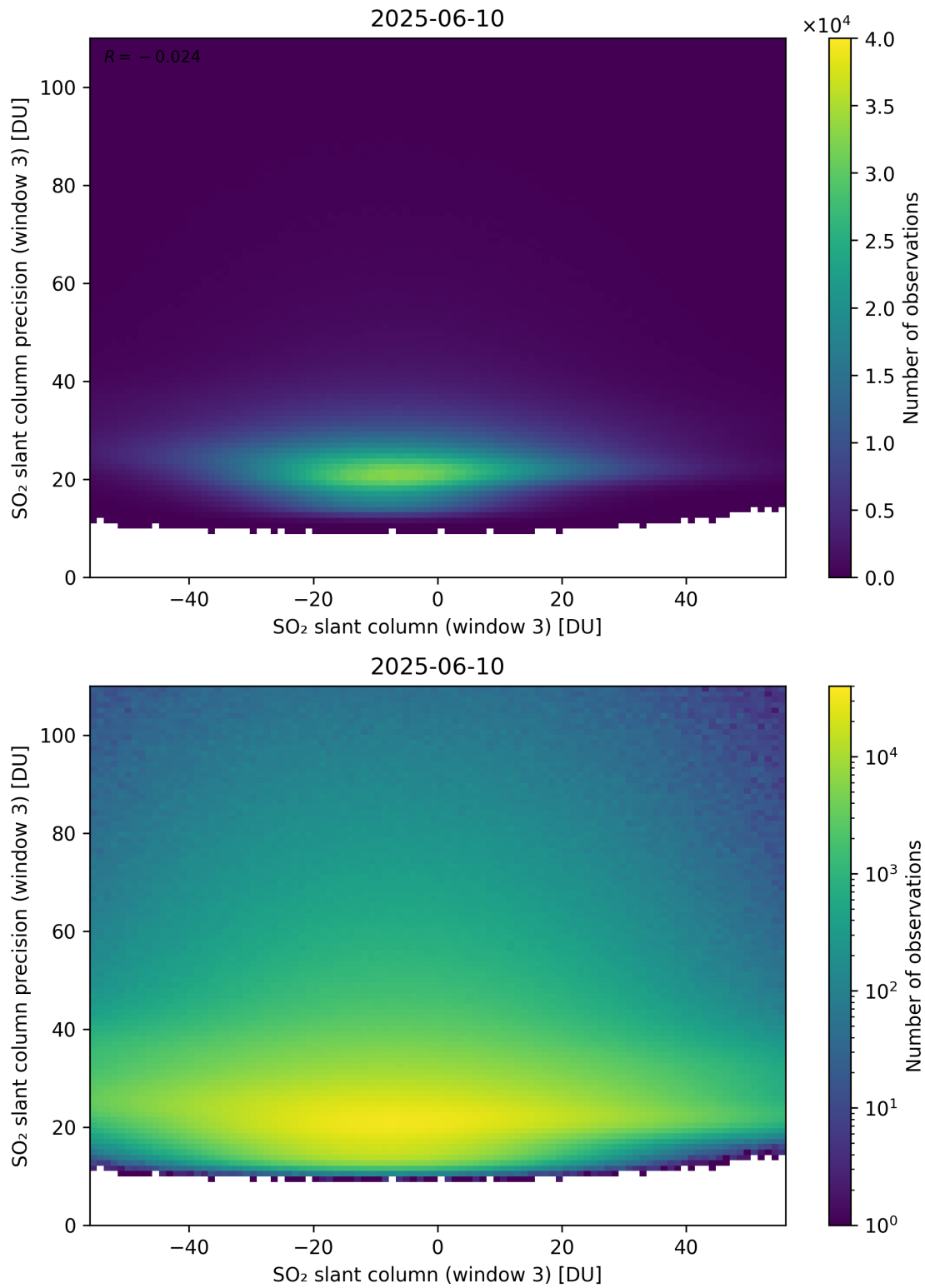
Figure 317: Scatter density plot of “SO 2 slant column (window 3)” against “SO 2 slant column precision (window 3)” for 2025-06-09 to 2025-06-11.
