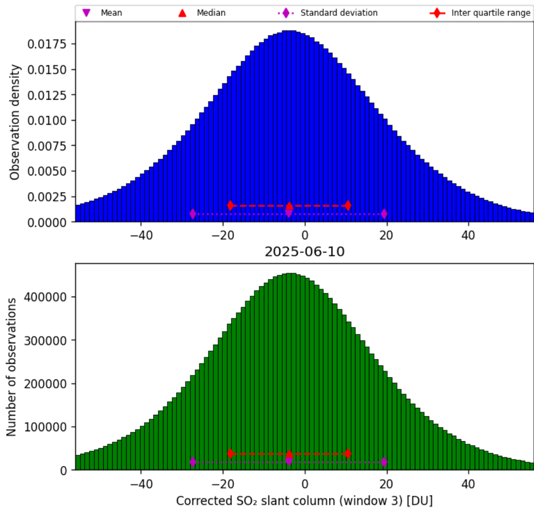
Figure 73: Histogram of “Corrected SO 2 slant column (window 3)” for 2025-06-09 to 2025-06-11
