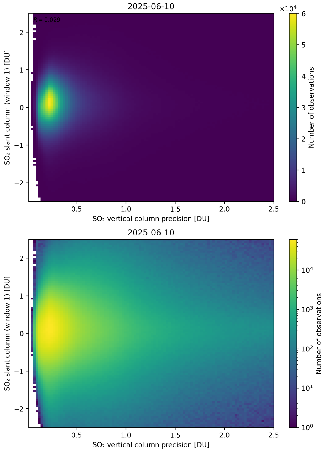
Figure 341: Scatter density plot of “SO 2 vertical column precision” against “SO 2 slant column (window 1)” for 2025-06-09 to 2025-06-11.
