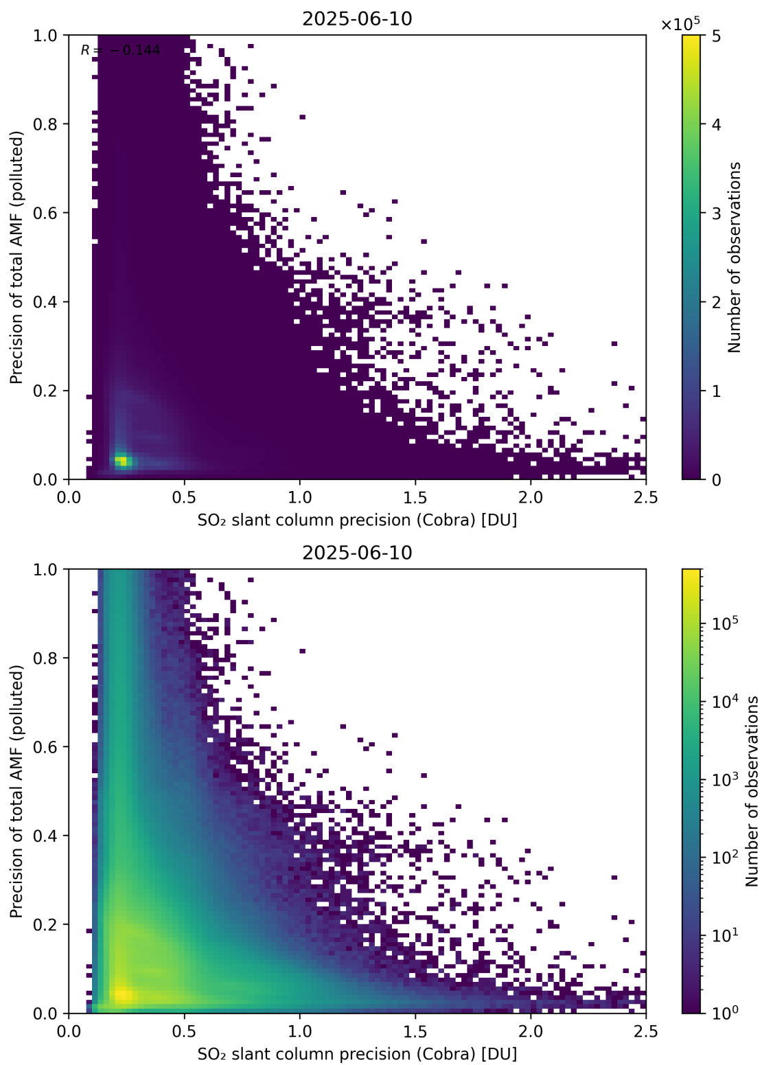
Figure 214: Scatter density plot of “SO 2 slant column precision (Cobra)” against “Precision of total AMF (polluted)” for 2025-06-09 to 2025-06-11.
