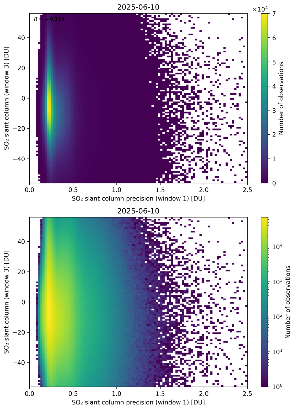
Figure 278: Scatter density plot of “SO 2 slant column precision (window 1)” against “SO 2 slant column (window 3)” for 2025-06-09 to 2025-06-11.
