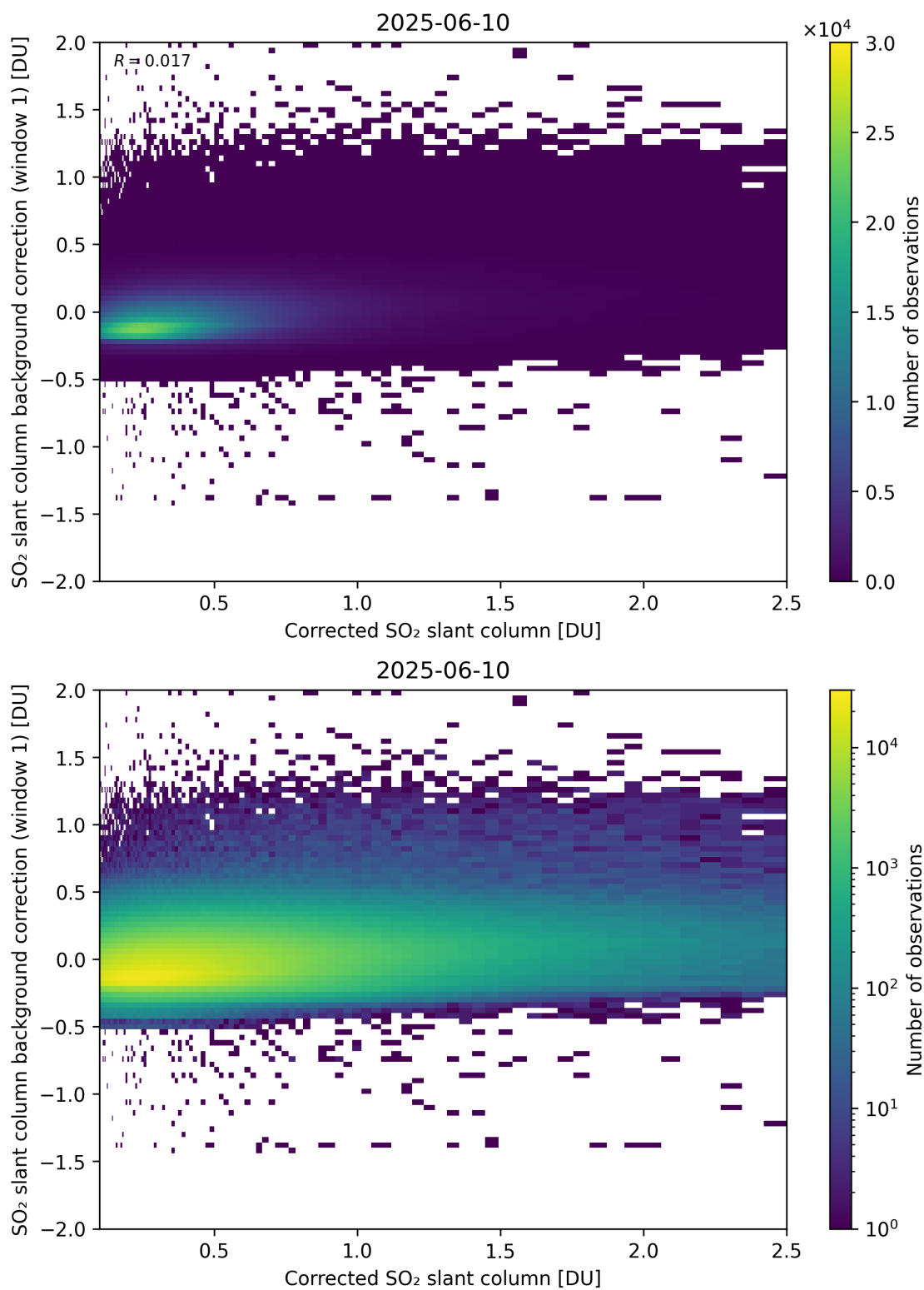
Figure 226: Scatter density plot of “Corrected SO 2 slant column” against “SO 2 slant column background correction (window 1)” for 2025-06-09 to 2025-06-11.
