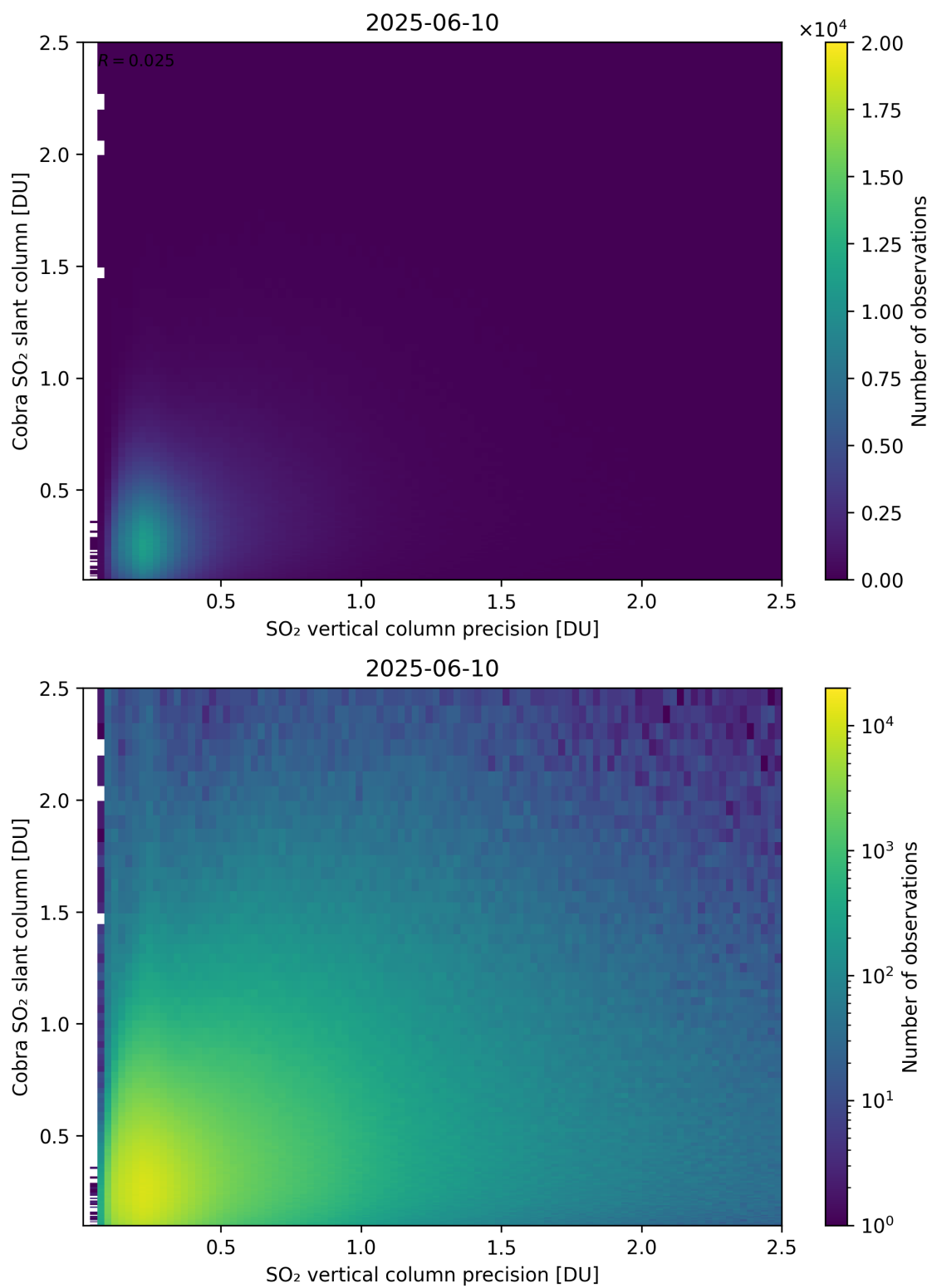
Figure 336: Scatter density plot of “SO 2 vertical column precision” against “Cobra SO 2 slant column” for 2025-06-09 to 2025-06-11.
