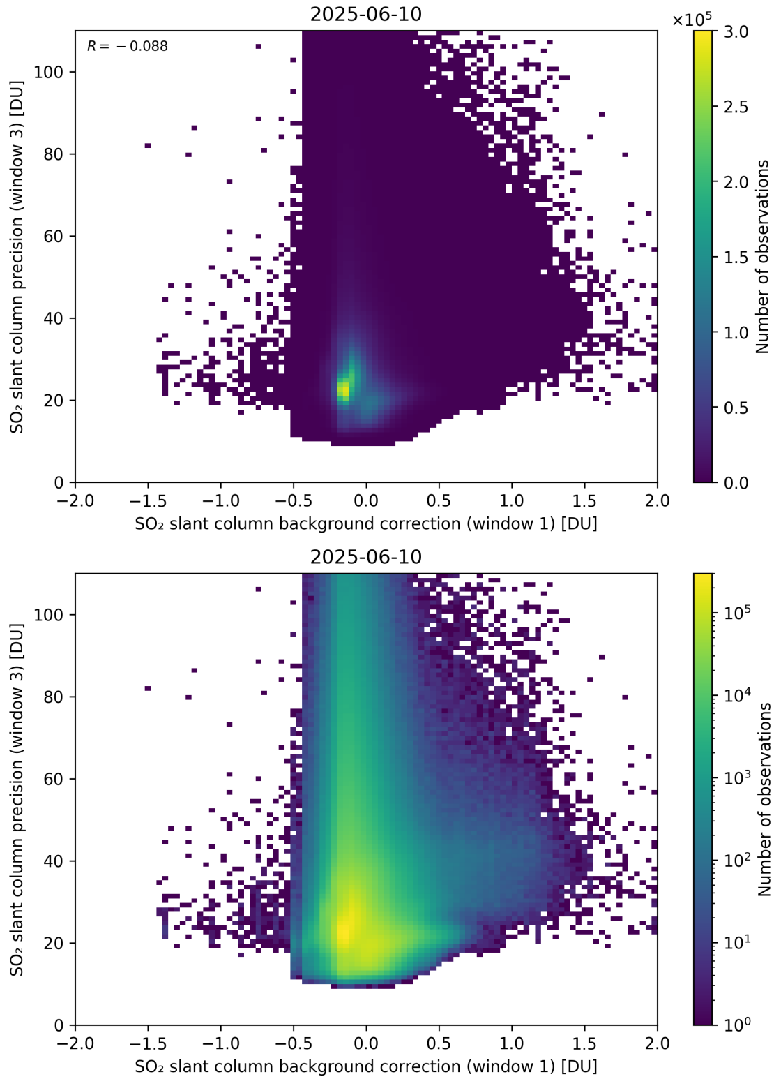
Figure 119: Scatter density plot of “SO 2 slant column background correction (window 1)” against “SO 2 slant column precision (window 3)” for 2025-06-09 to 2025-06-11.
