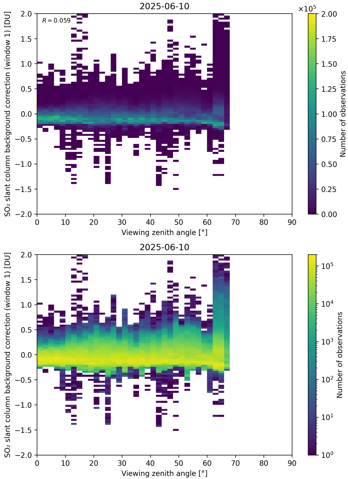
Figure 362: Scatter density plot of “Viewing zenith angle” against “SO 2 slant column background correction (window 1)” for 2025-06-09 to 2025-06-11.
