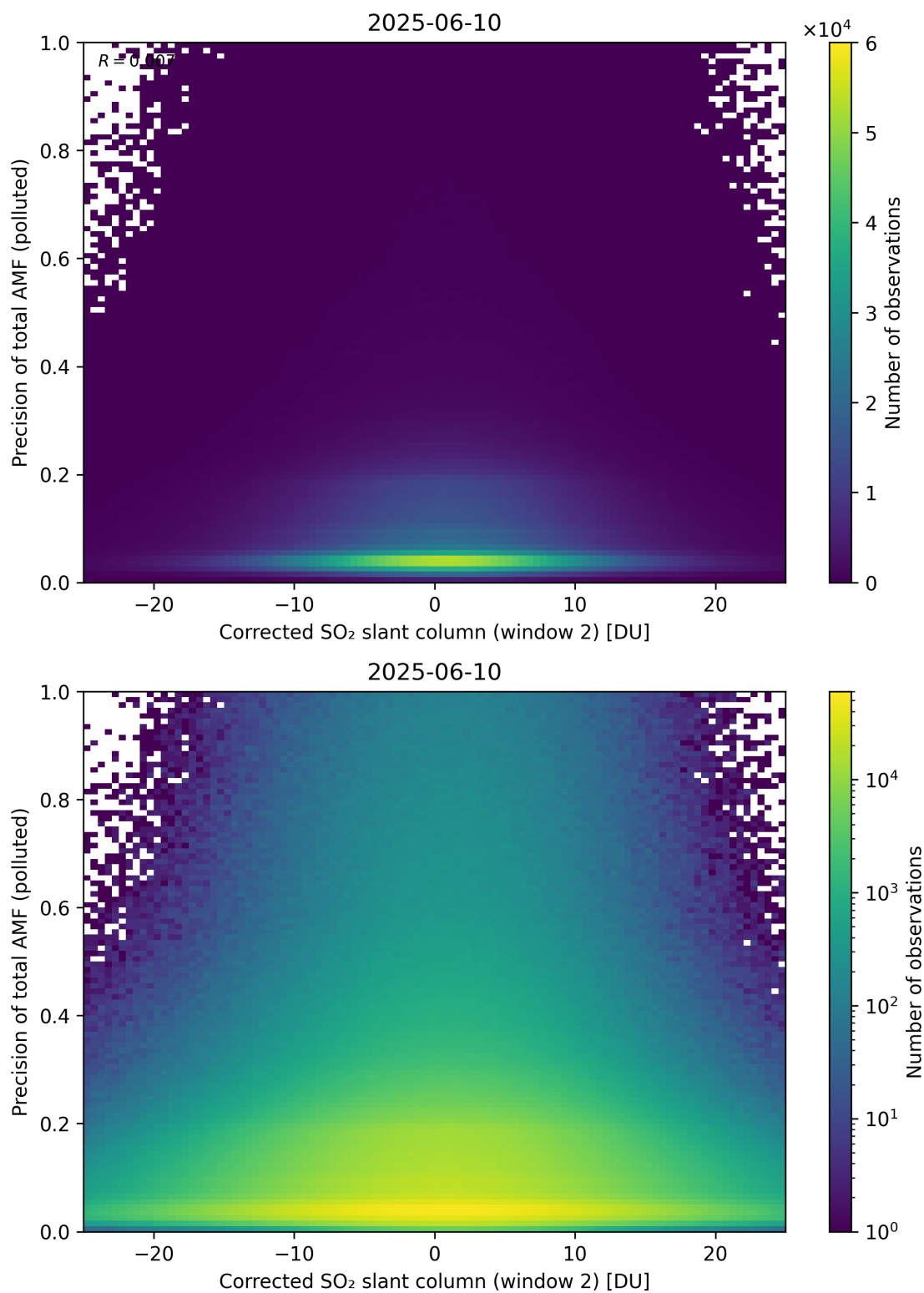
Figure 254: Scatter density plot of “Corrected SO 2 slant column (window 2)” against “Precision of total AMF (polluted)” for 2025-06-09 to 2025-06-11.
