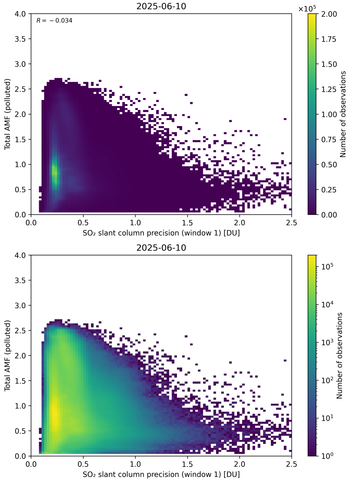
Figure 280: Scatter density plot of “SO 2 slant column precision (window 1)” against “Total AMF (polluted)” for 2025-06-09 to 2025-06-11.
