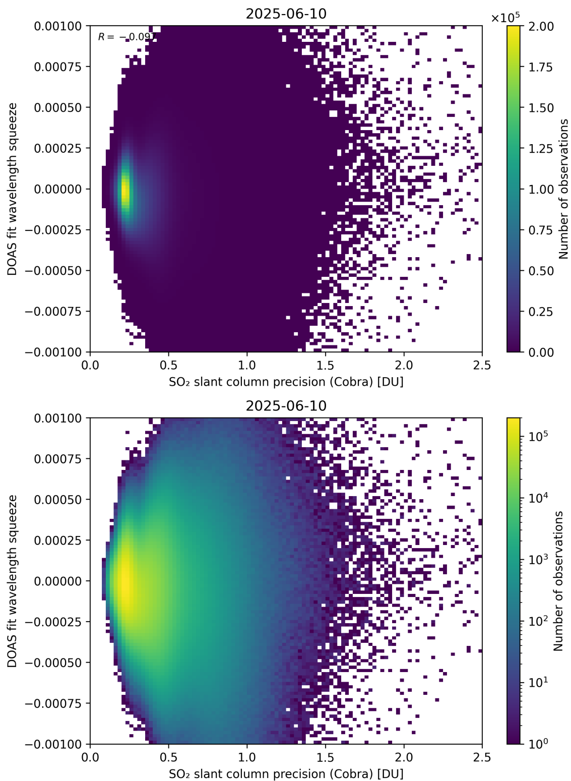
Figure 203: Scatter density plot of “SO 2 slant column precision (Cobra)” against “DOAS fit wavelength squeeze” for 2025-06-09 to 2025-06-11.
