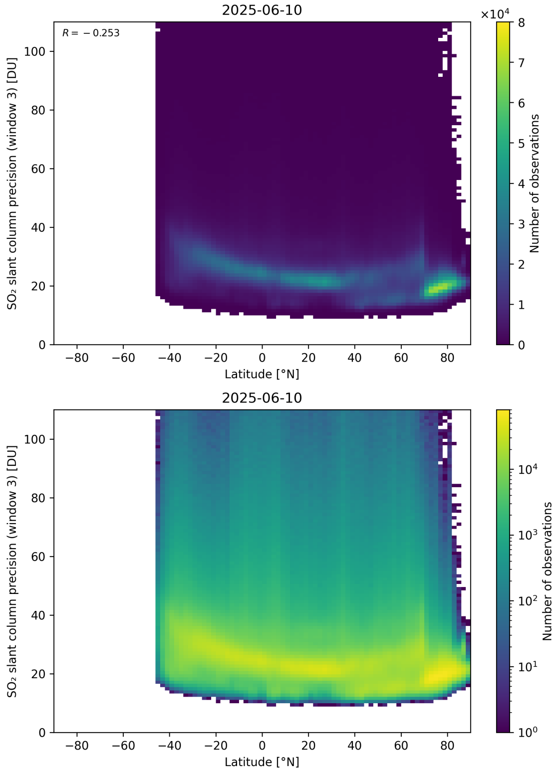
Figure 166: Scatter density plot of “Latitude” against “SO 2 slant column precision (window 3)” for 2025-06-09 to 2025-06-11.
