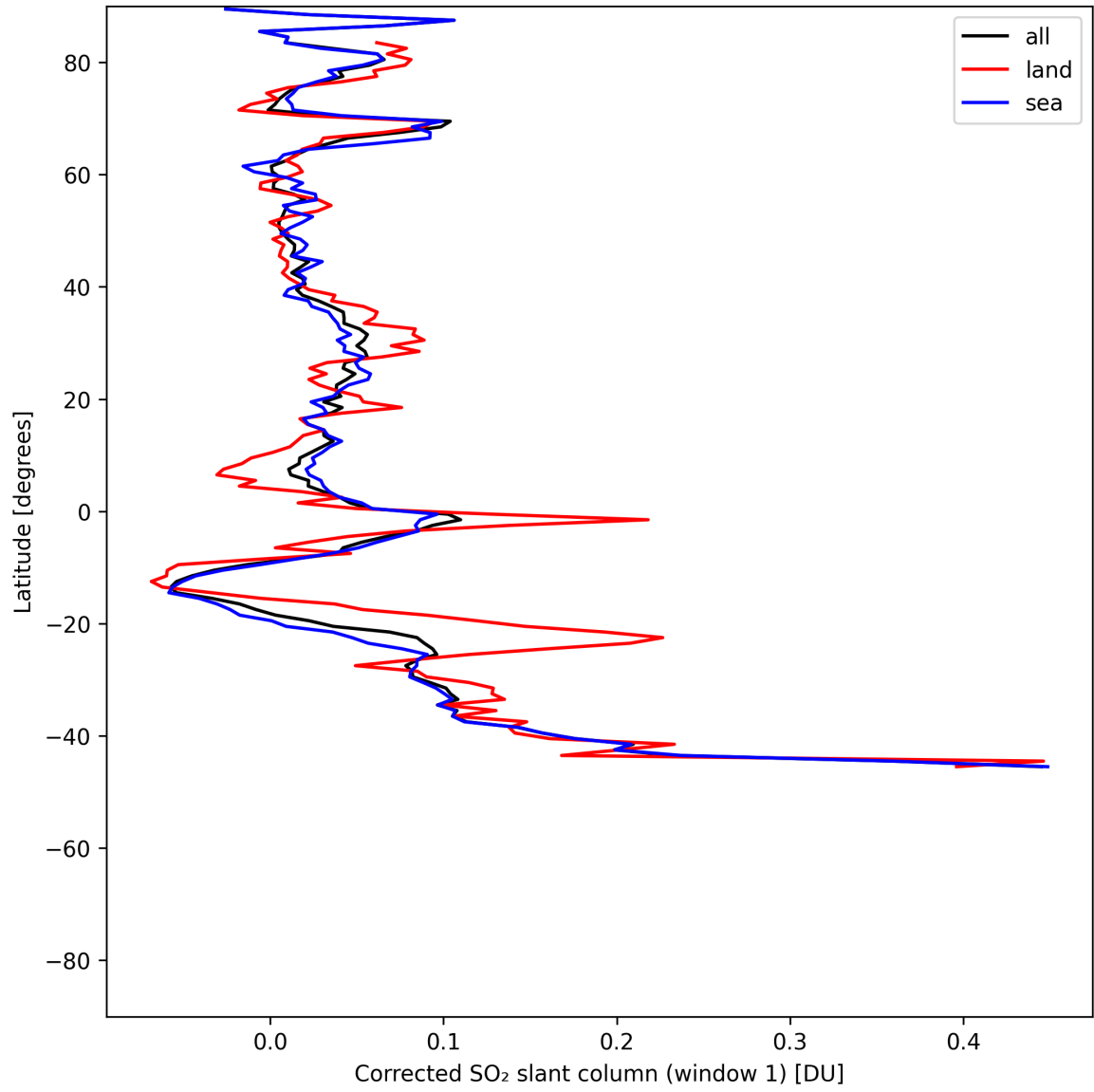
Figure 39: Zonal average of “Corrected SO 2 slant column (window 1)” for 2025-06-09 to 2025-06-11.
