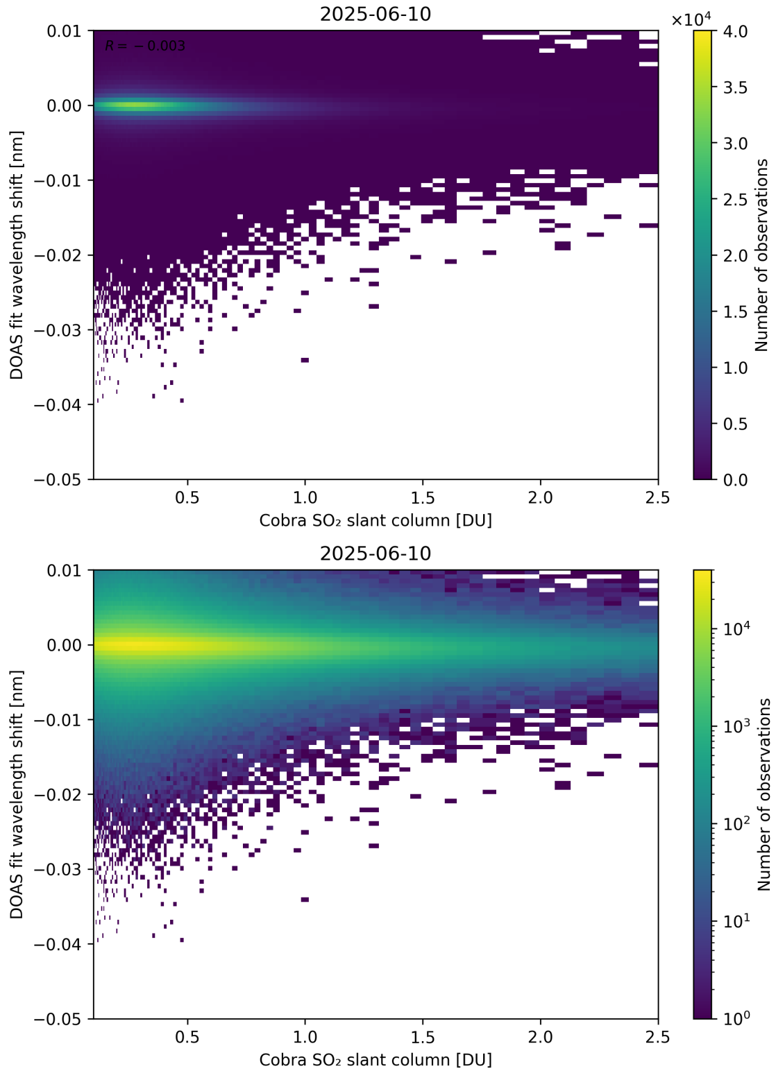
Figure 196: Scatter density plot of “Cobra SO 2 slant column” against “DOAS fit wavelength shift” for 2025-06-09 to 2025-06-11.
