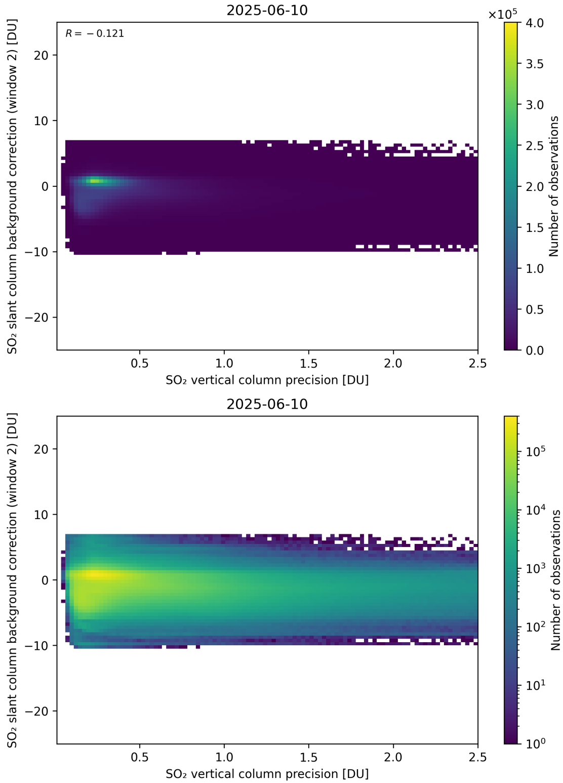
Figure 330: Scatter density plot of “SO 2 vertical column precision” against “SO 2 slant column background correction (window 2)” for 2025-06-09 to 2025-06-11.
