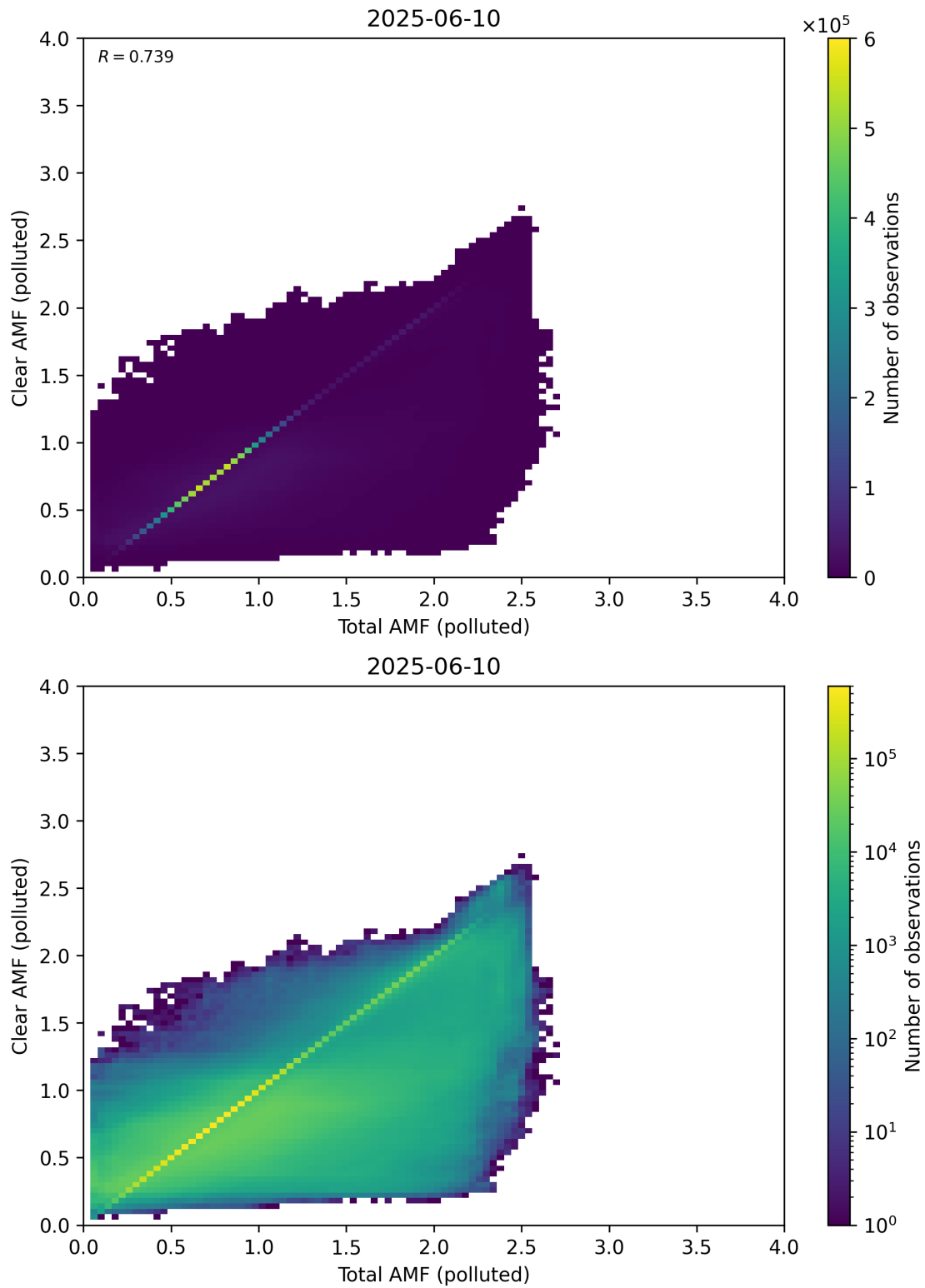
Figure 321: Scatter density plot of “Total AMF (polluted)” against “Clear AMF (polluted)” for 2025-06-09 to 2025-06-11.
