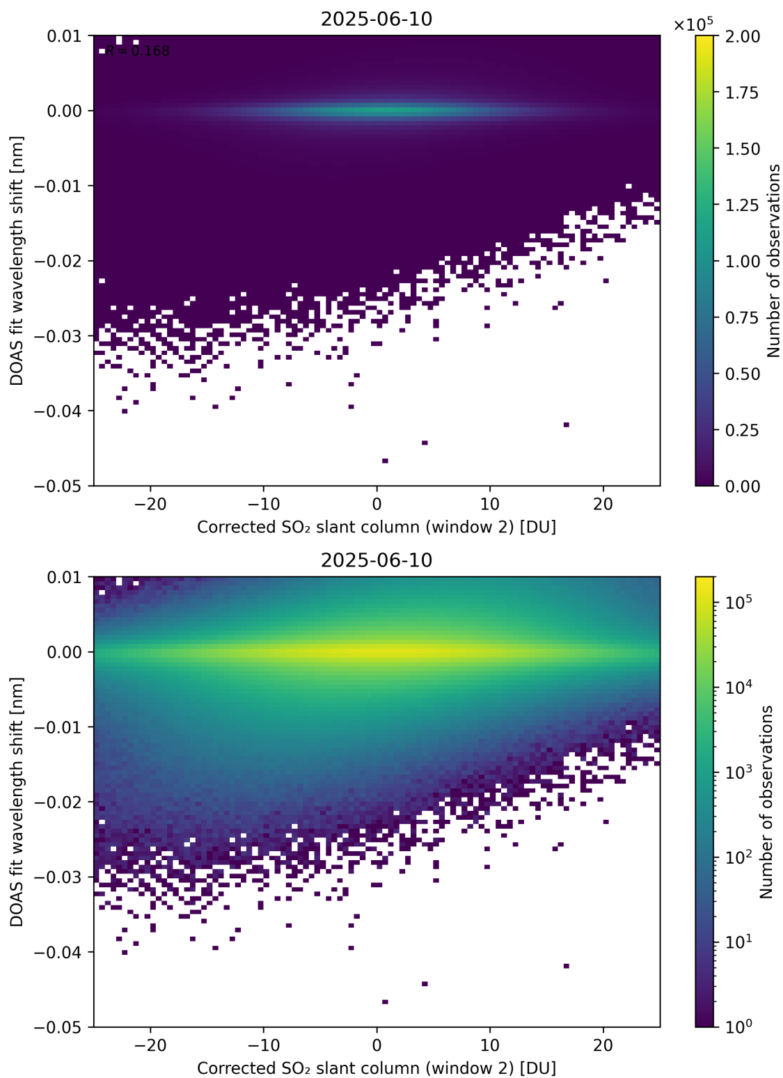
Figure 246: Scatter density plot of “Corrected SO 2 slant column (window 2)” against “DOAS fit wavelength shift” for 2025-06-09 to 2025-06-11.
