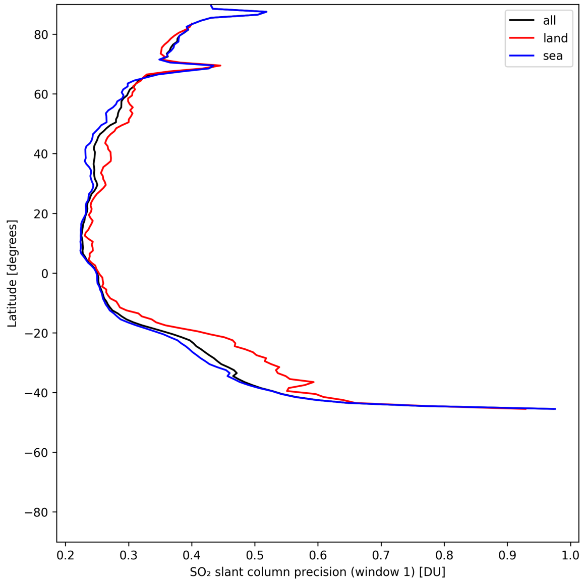
Figure 38: Zonal average of “SO 2 slant column precision (window 1)” for 2025-06-09 to 2025-06-11.
