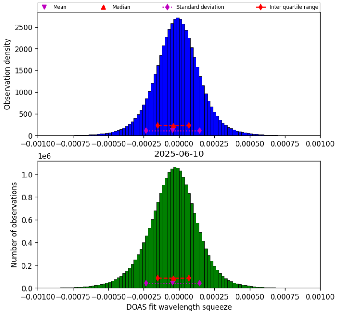
Figure 77: Histogram of “DOAS fit wavelength squeeze” for 2025-06-09 to 2025-06-11
