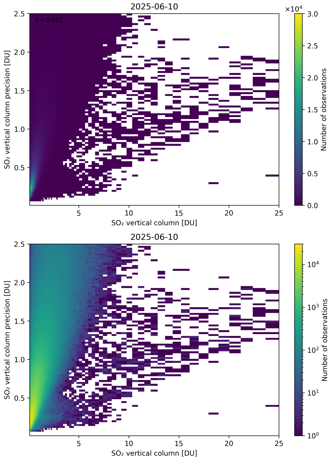
Figure 361: Scatter density plot of “SO 2 vertical column” against “SO 2 vertical column precision” for 2025-06-09 to 2025-06-11.
