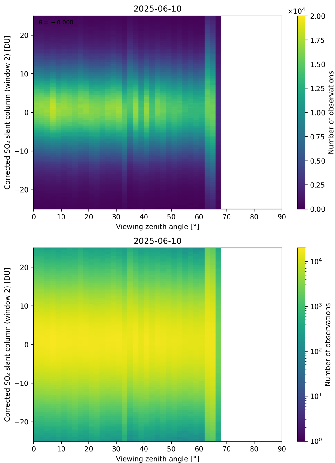
Figure 374: Scatter density plot of “Viewing zenith angle” against “Corrected SO 2 slant column (window 2)” for 2025-06-09 to 2025-06-11.
