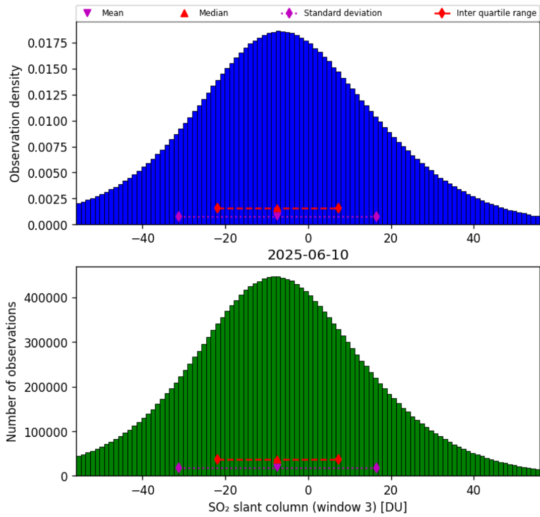
Figure 71: Histogram of “SO 2 slant column (window 3)” for 2025-06-09 to 2025-06-11
