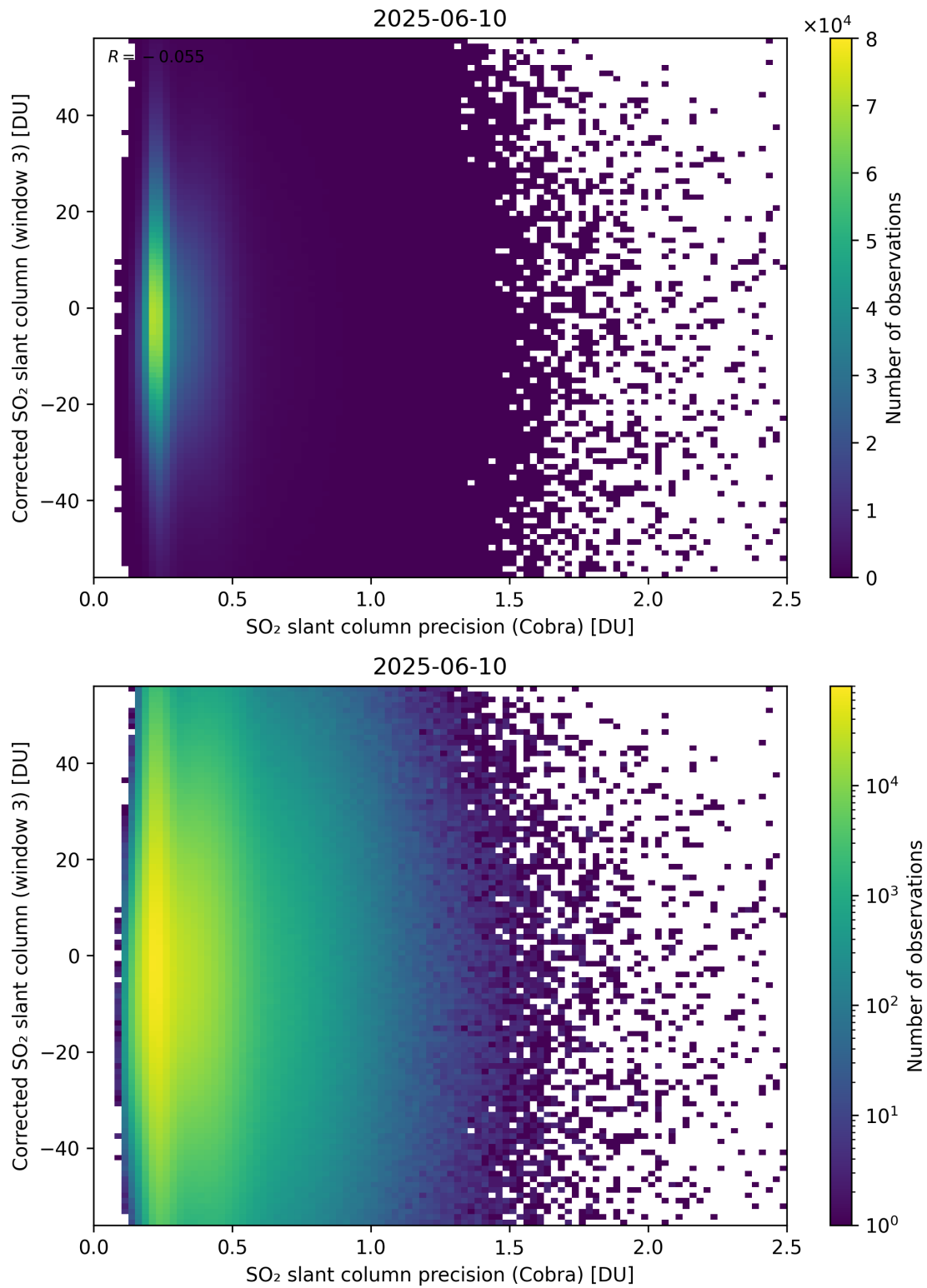
Figure 207: Scatter density plot of “SO 2 slant column precision (Cobra)” against “Corrected SO 2 slant column (window 3)” for 2025-06-09 to 2025-06-11.
