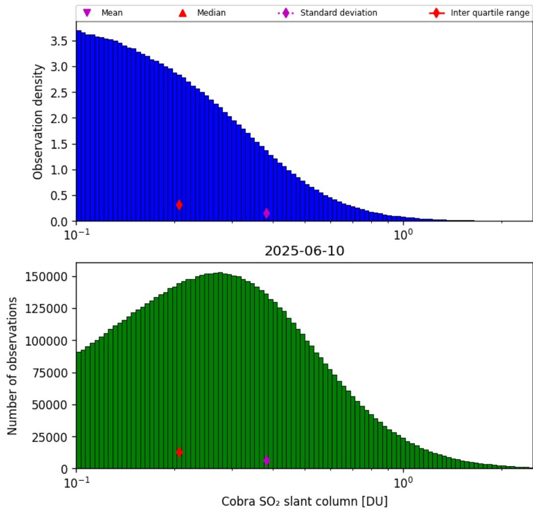
Figure 61: Histogram of “Cobra SO 2 slant column” for 2025-06-09 to 2025-06-11
