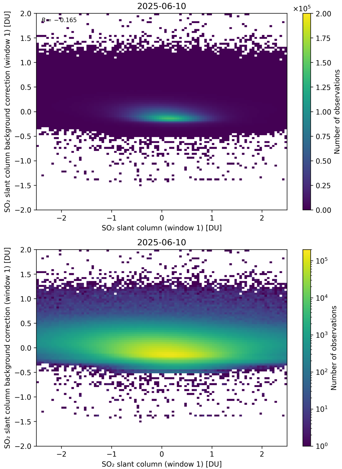
Figure 262: Scatter density plot of “SO 2 slant column (window 1)” against “SO 2 slant column background correction (window 1)” for 2025-06-09 to 2025-06-11.
