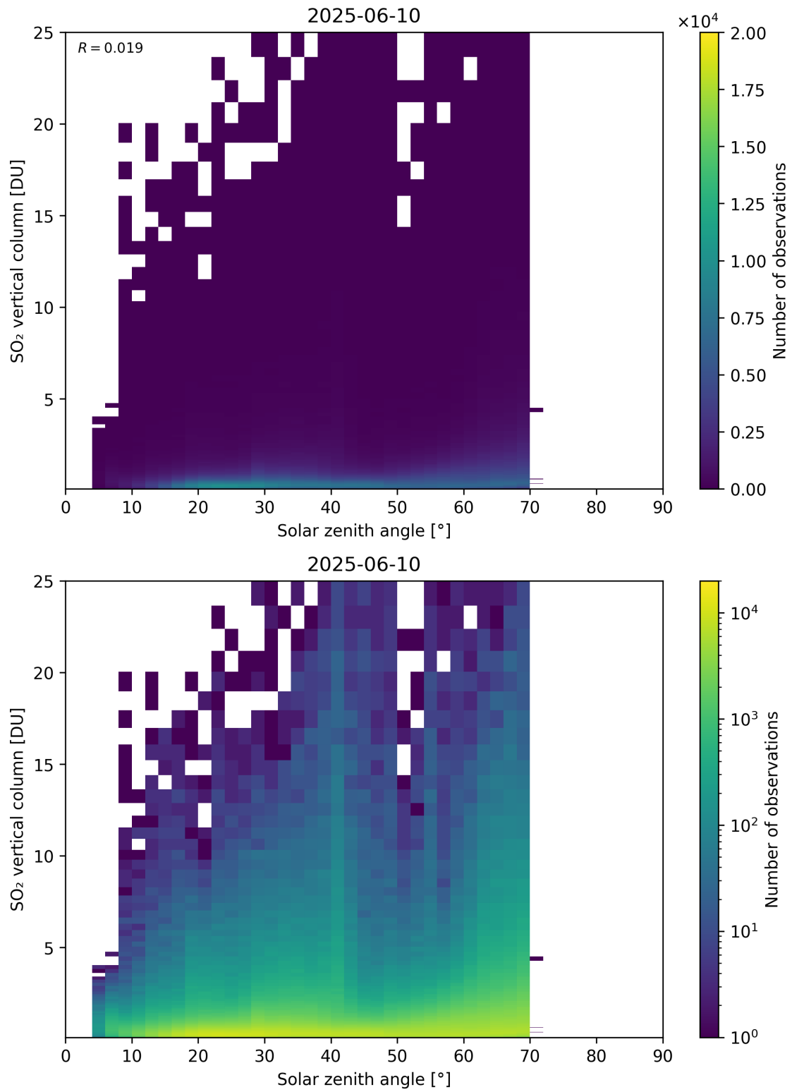
Figure 191: Scatter density plot of “Solar zenith angle” against “SO 2 vertical column” for 2025-06-09 to 2025-06-11.
