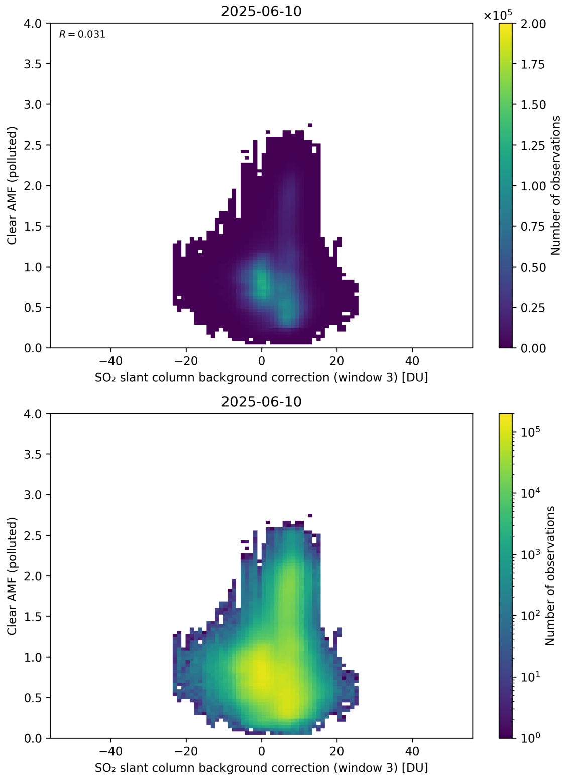
Figure 135: Scatter density plot of “SO 2 slant column background correction (window 3)” against “Clear AMF (polluted)” for 2025-06-09 to 2025-06-11.
