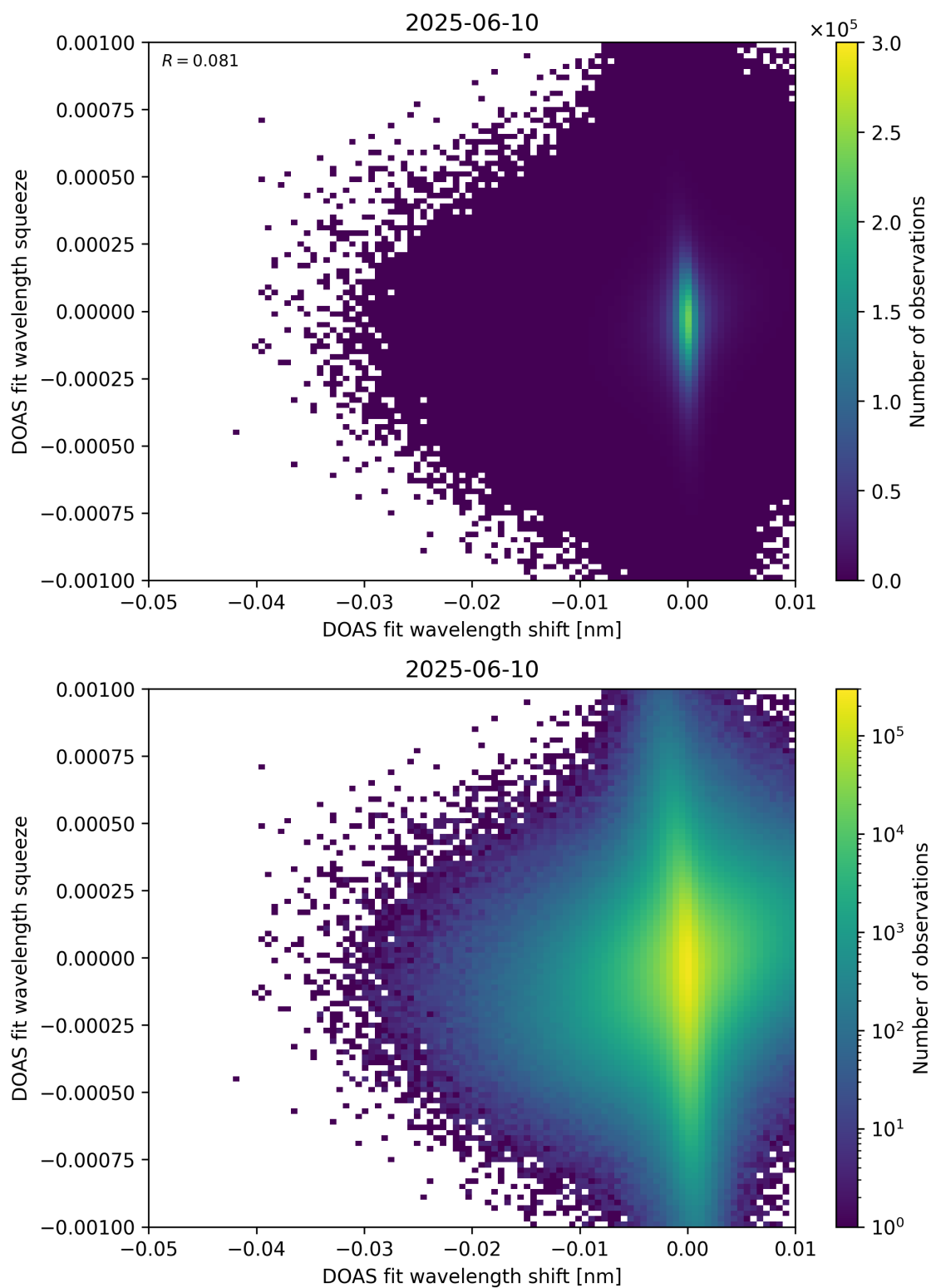
Figure 138: Scatter density plot of “DOAS fit wavelength shift” against “DOAS fit wavelength squeeze” for 2025-06-09 to 2025-06-11.
