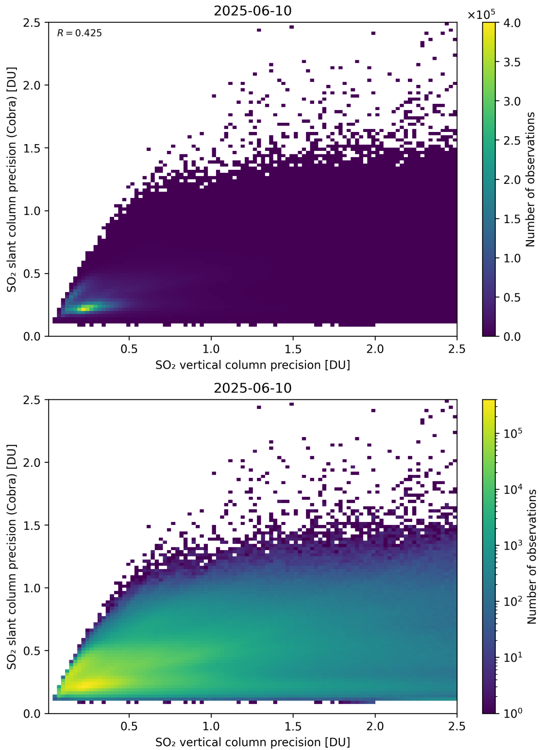
Figure 337: Scatter density plot of “SO 2 vertical column precision” against “SO 2 slant column precision (Cobra)” for 2025-06-09 to 2025-06-11.
