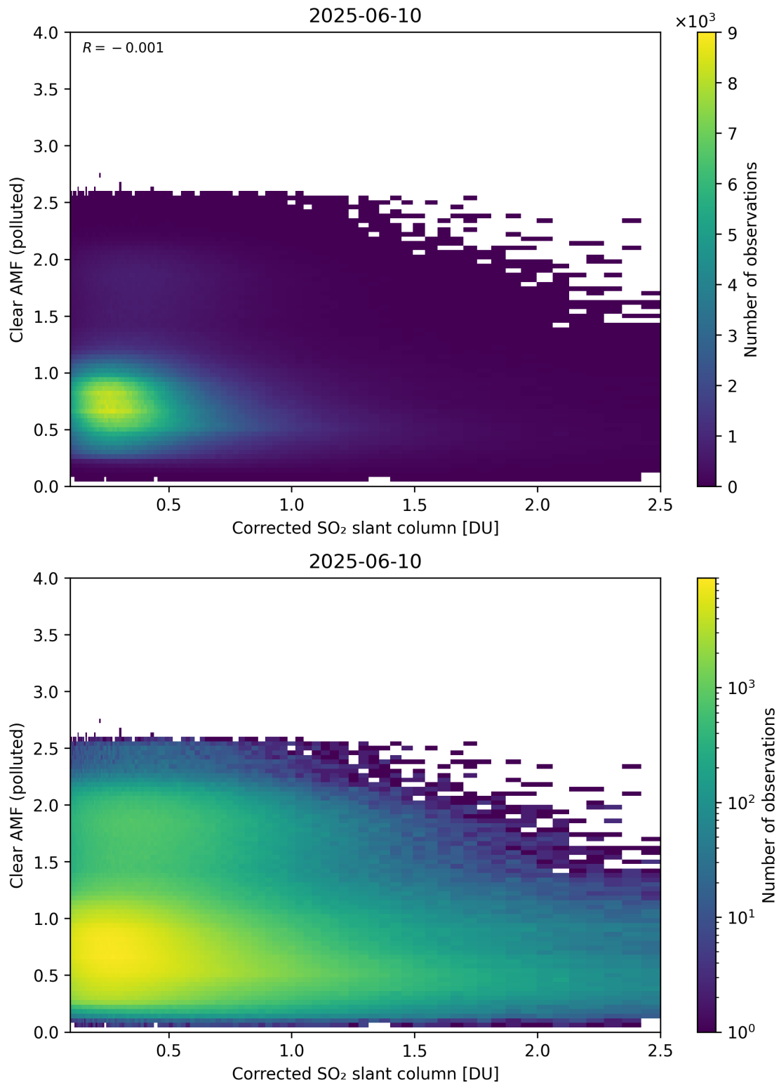
Figure 232: Scatter density plot of “Corrected SO 2 slant column” against “Clear AMF (polluted)” for 2025-06-09 to 2025-06-11.
