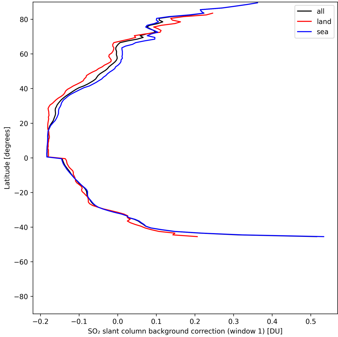
Figure 40: Zonal average of “SO 2 slant column background correction (window 1)” for 2025-06-09 to 2025-06-11.
