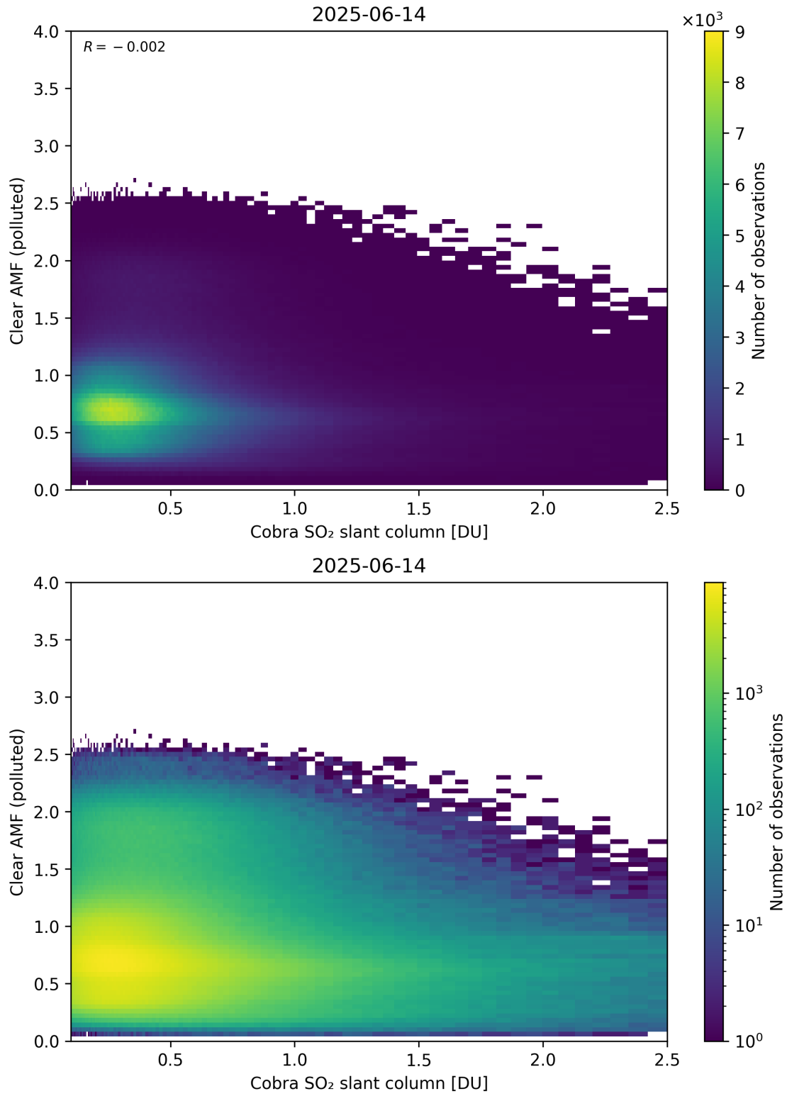
Figure 215: Scatter density plot of “Cobra SO 2 slant column” against “Clear AMF (polluted)” for 2025-06-13 to 2025-06-15.
