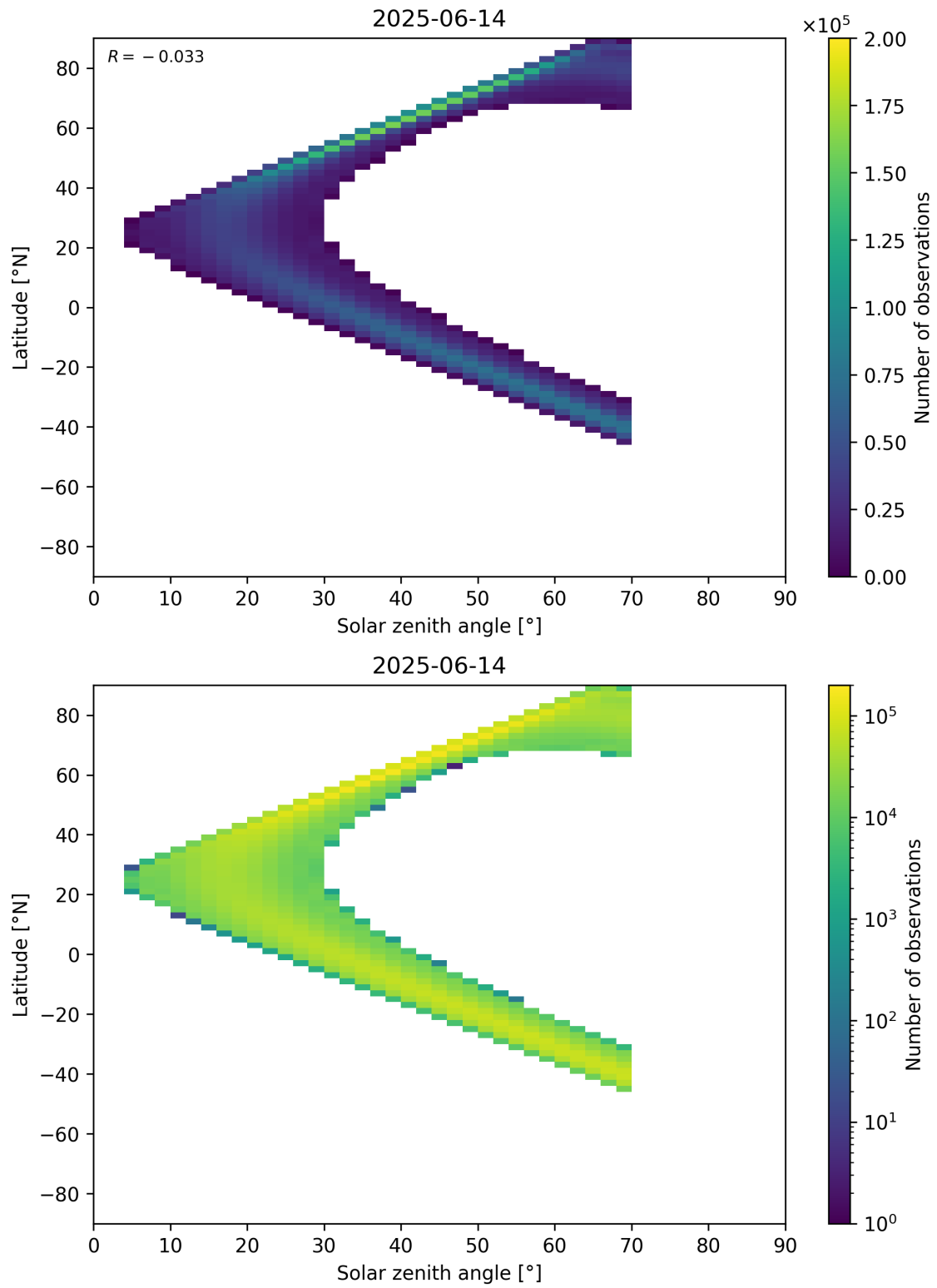
Figure 177: Scatter density plot of “Solar zenith angle” against “Latitude” for 2025-06-13 to 2025-06-15.
