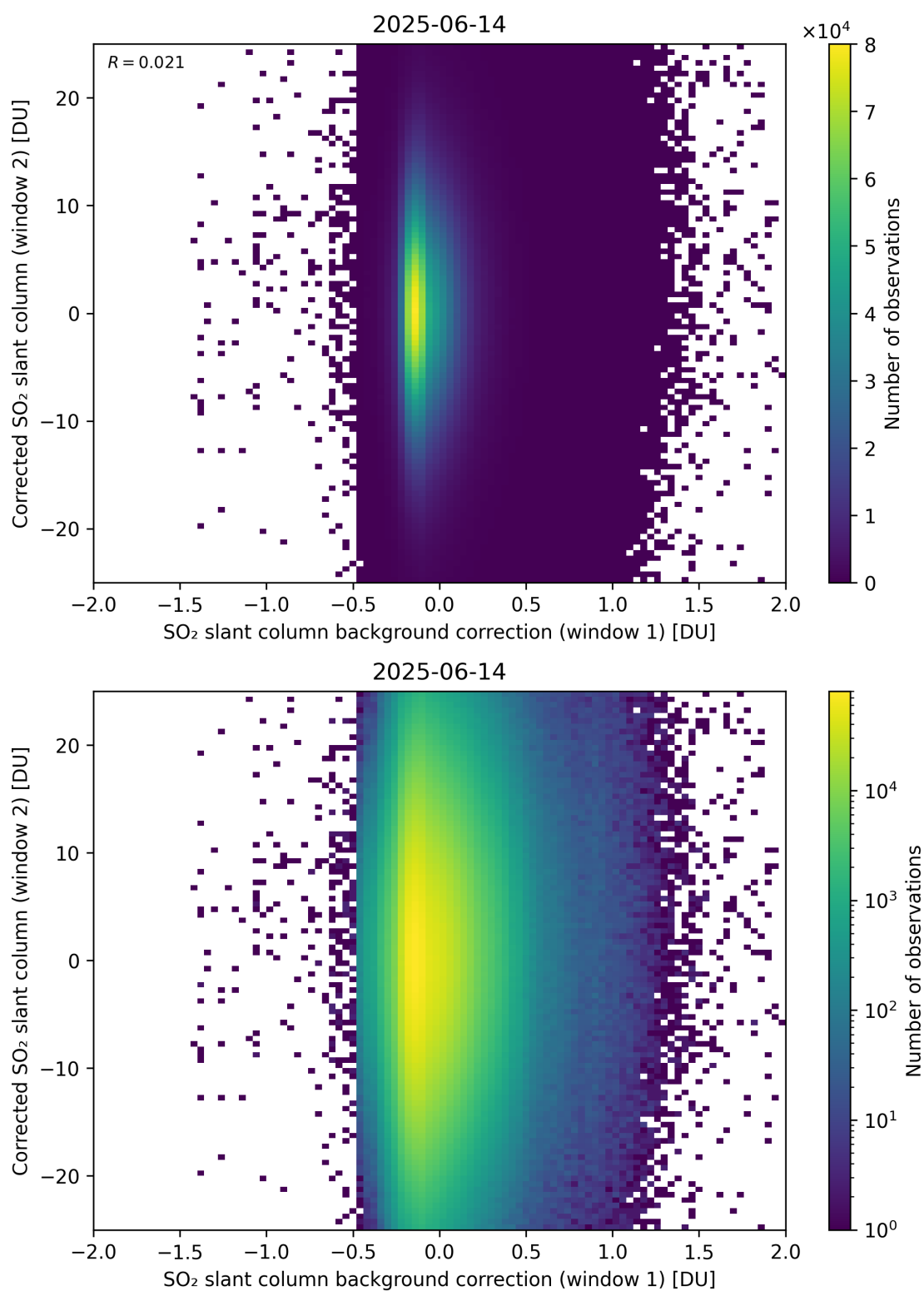
Figure 115: Scatter density plot of “SO 2 slant column background correction (window 1)” against “Corrected SO 2 slant column (window 2)” for 2025-06-13 to 2025-06-15.
