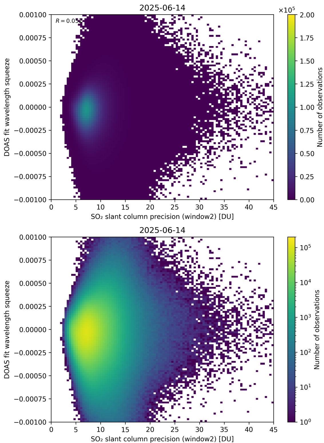
Figure 294: Scatter density plot of “SO 2 slant column precision (window2)” against “DOAS fit wavelength squeeze” for 2025-06-13 to 2025-06-15.
