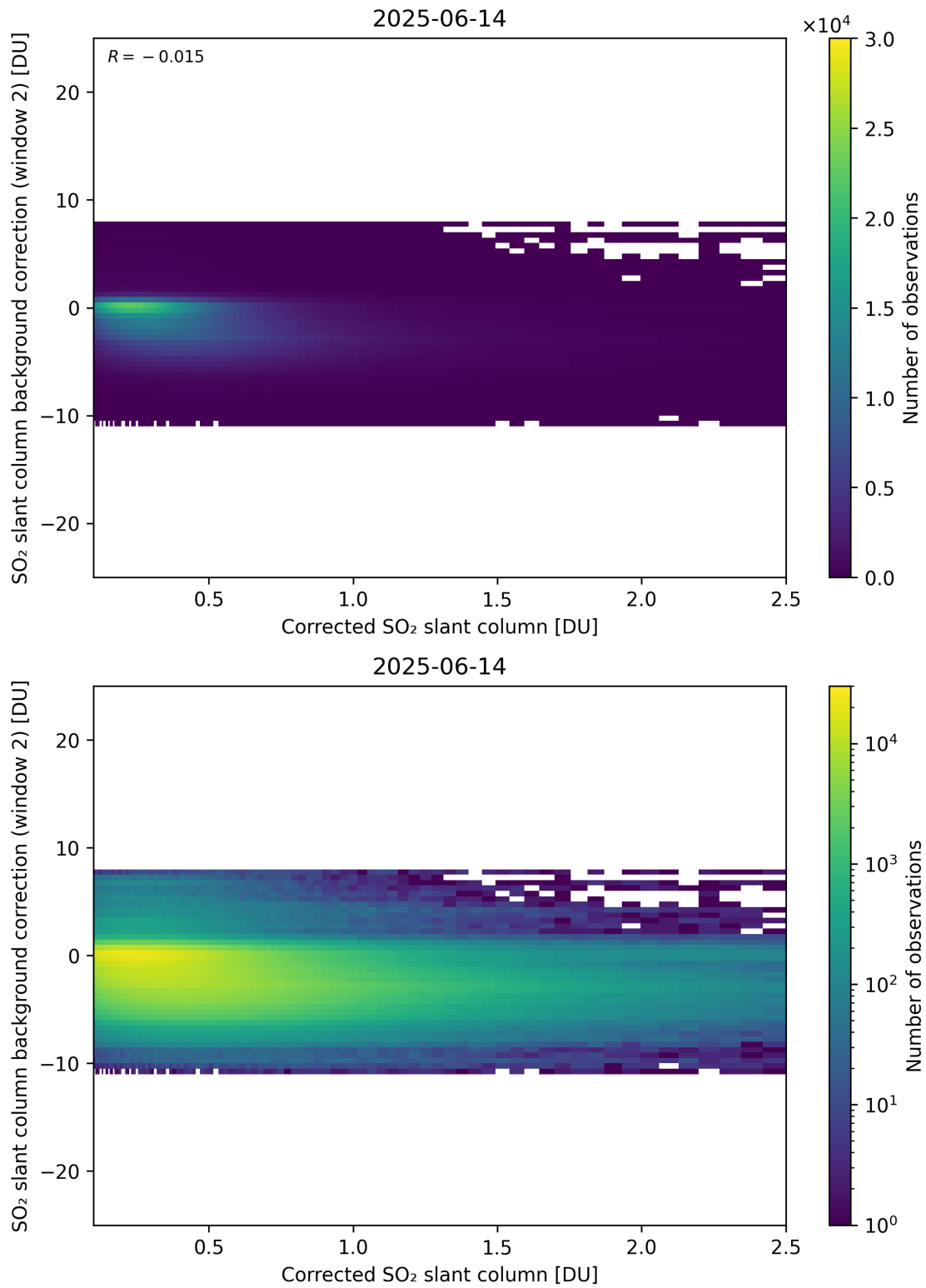
Figure 227: Scatter density plot of “Corrected SO 2 slant column” against “SO 2 slant column background correction (window 2)” for 2025-06-13 to 2025-06-15.
