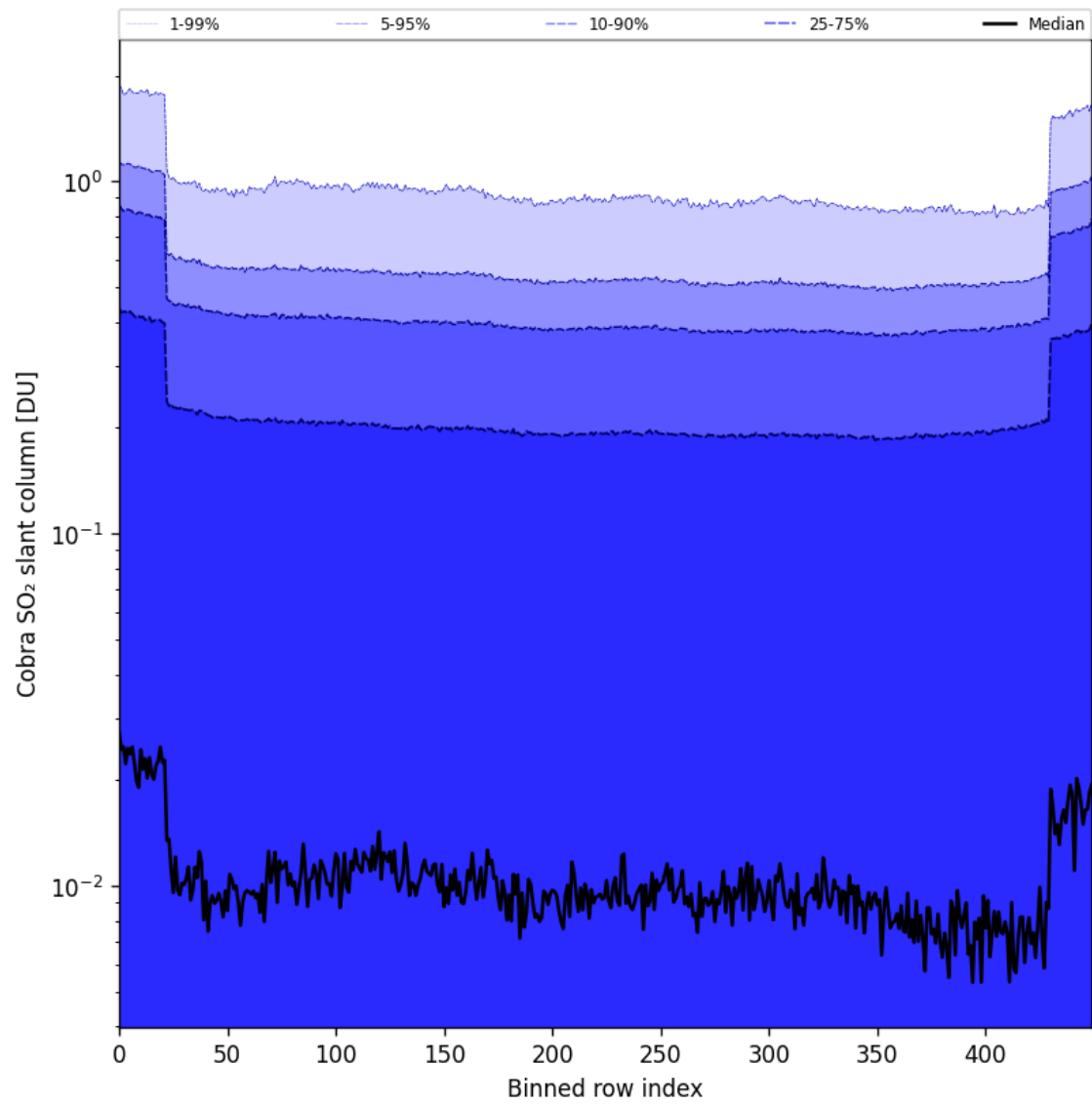
Figure 87: Along track statistics of “Cobra SO 2 slant column” for 2025-06-13 to 2025-06-15
