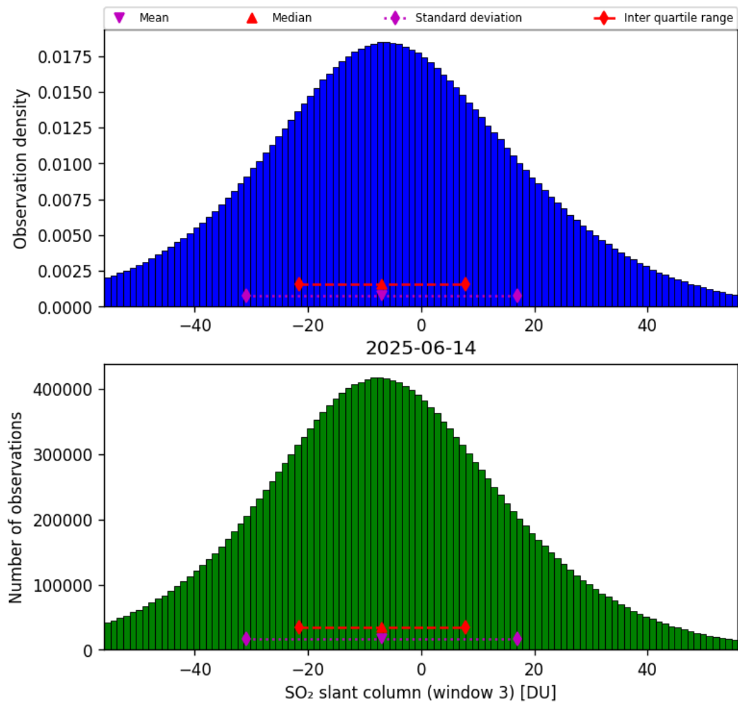
Figure 71: Histogram of “SO 2 slant column (window 3)” for 2025-06-13 to 2025-06-15
