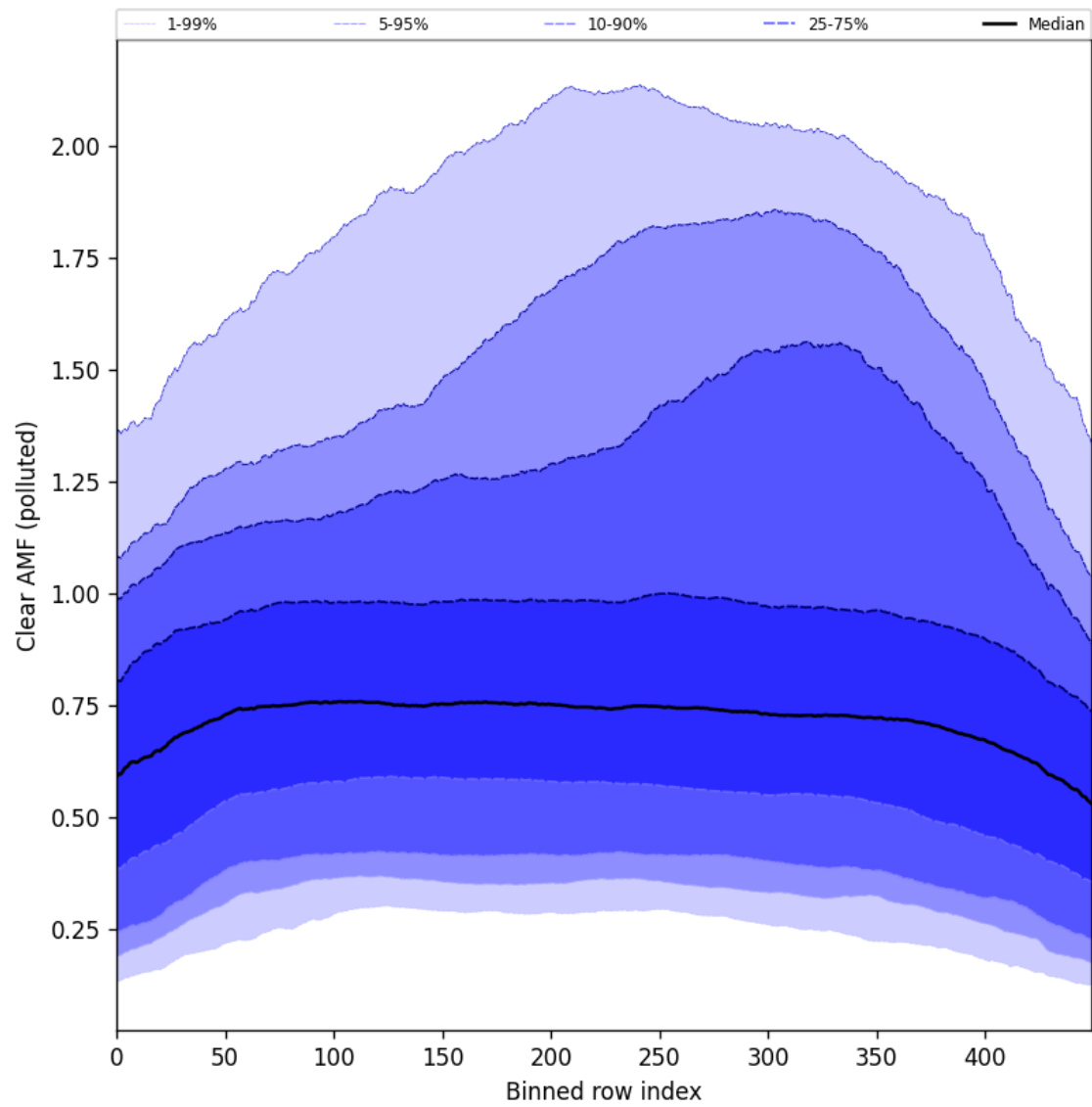
Figure 107: Along track statistics of “Clear AMF (polluted)” for 2025-06-13 to 2025-06-15
