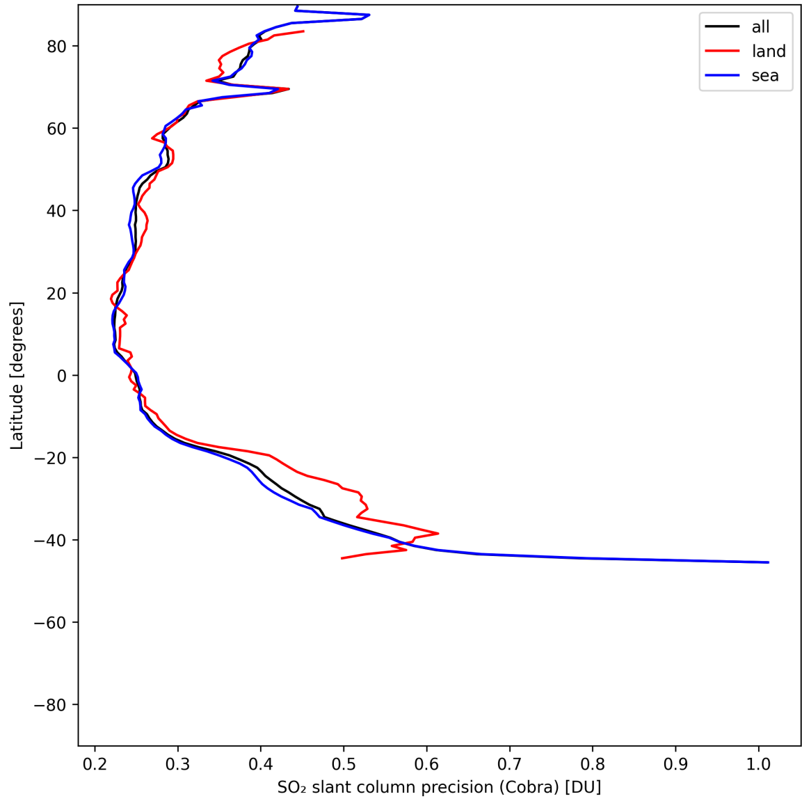
Figure 36: Zonal average of "SO 2 slant column precision (Cobra)" for 2025-06-13 to 2025-06-15.
