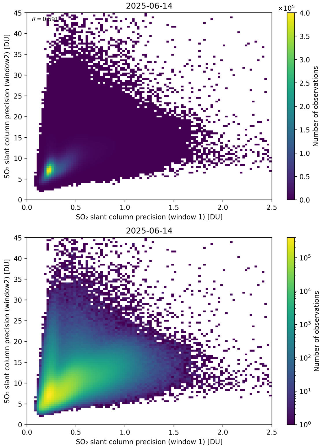
Figure 277: Scatter density plot of “SO 2 slant column precision (window 1)” against “SO 2 slant column precision (window2)” for 2025-06-13 to 2025-06-15.
