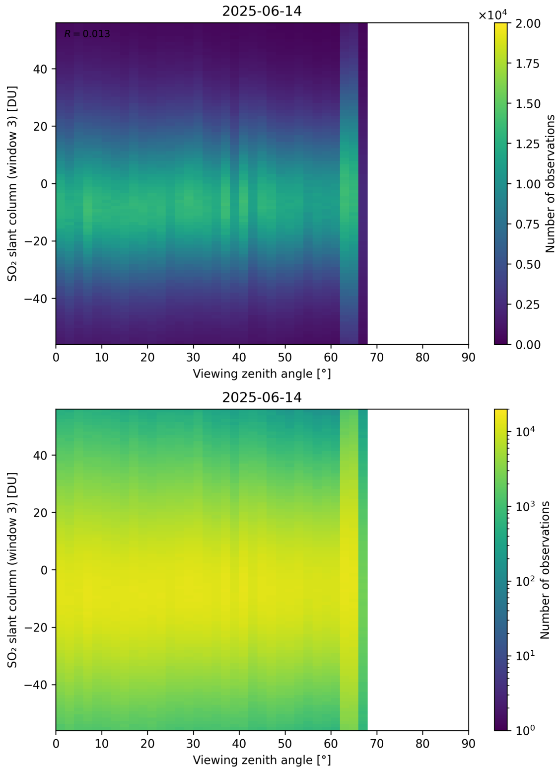
Figure 379: Scatter density plot of “Viewing zenith angle” against “SO 2 slant column (window 3)” for 2025-06-13 to 2025-06-15.
