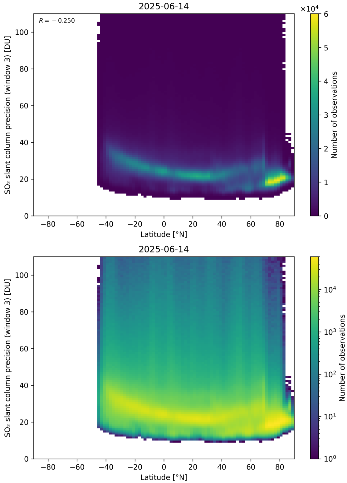
Figure 166: Scatter density plot of “Latitude” against “SO 2 slant column precision (window 3)” for 2025-06-13 to 2025-06-15.
