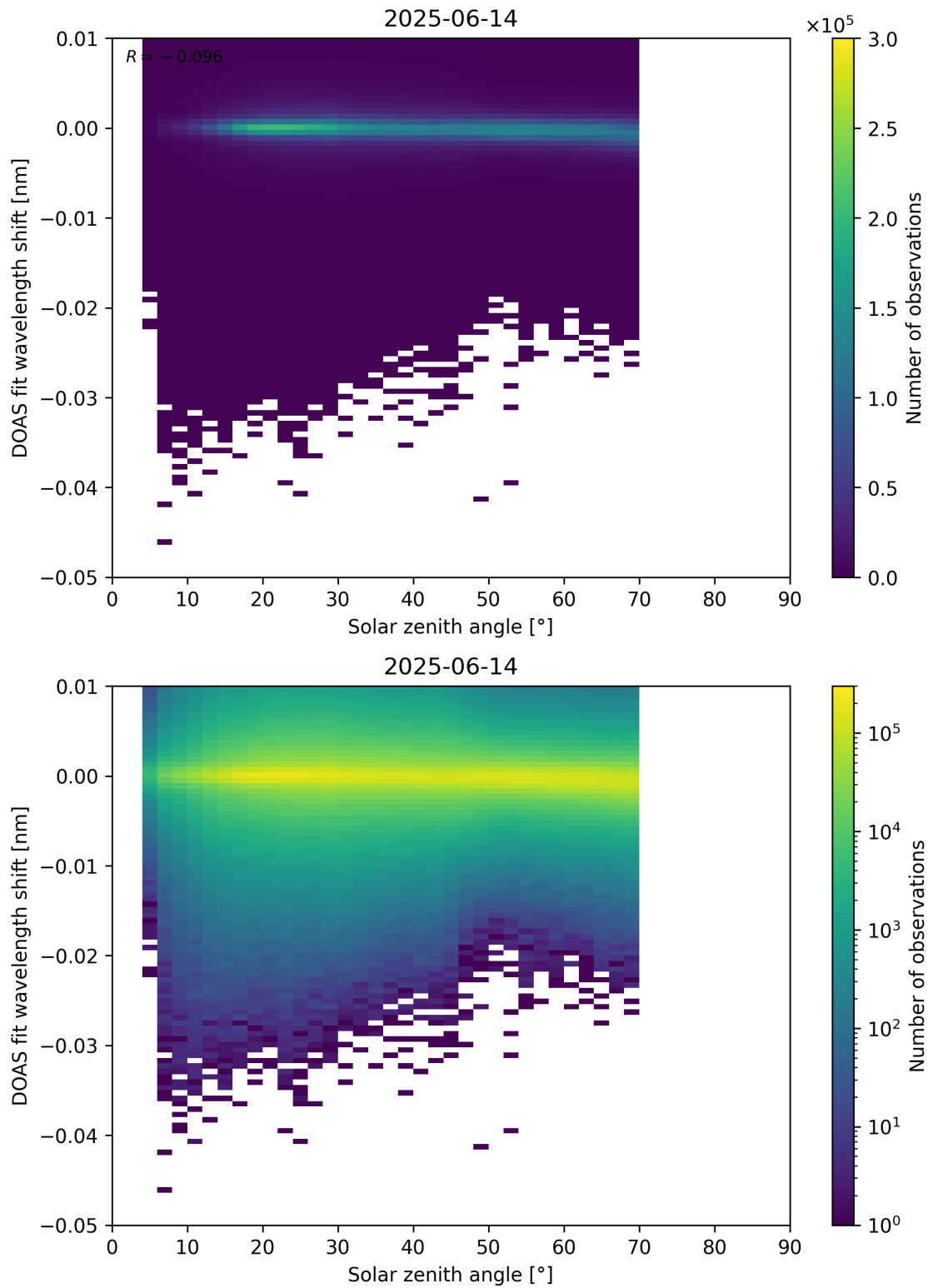
Figure 174: Scatter density plot of “Solar zenith angle” against “DOAS fit wavelength shift” for 2025-06-13 to 2025-06-15.
