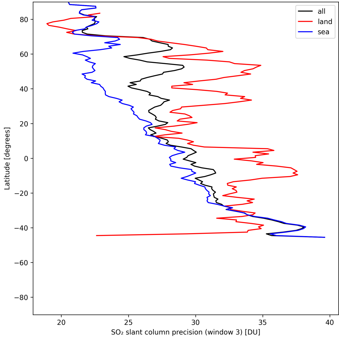
Figure 46: Zonal average of “SO 2 slant column precision (window 3)” for 2025-06-13 to 2025-06-15.
