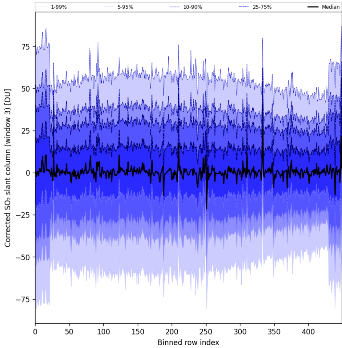
Figure 99: Along track statistics of “Corrected SO 2 slant column (window 3)” for 2025-06-13 to 2025-06-15
