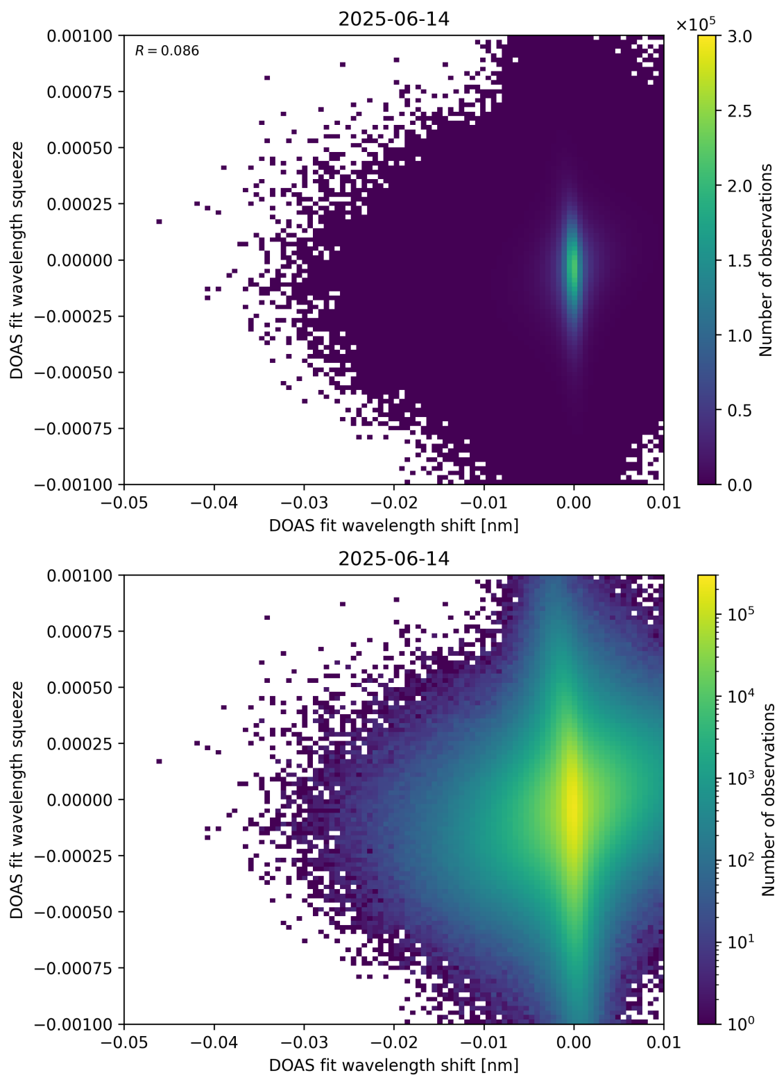
Figure 138: Scatter density plot of “DOAS fit wavelength shift” against “DOAS fit wavelength squeeze” for 2025-06-13 to 2025-06-15.
