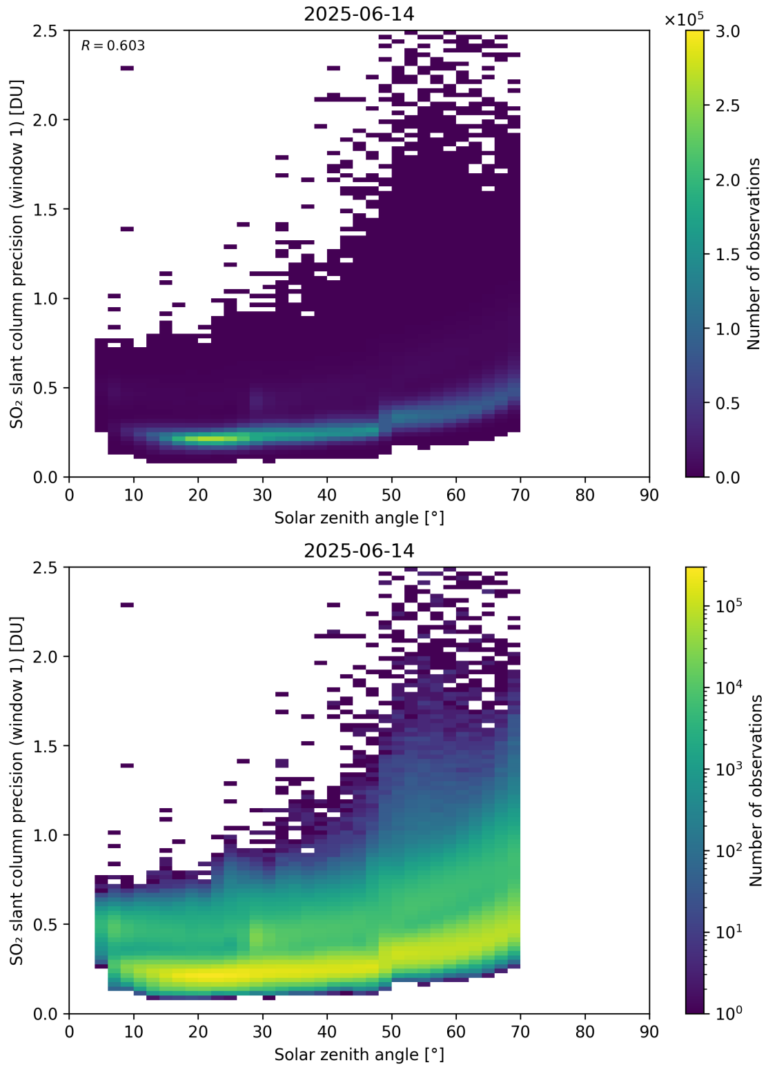
Figure 185: Scatter density plot of “Solar zenith angle” against “SO 2 slant column precision (window 1)” for 2025-06-13 to 2025-06-15.
