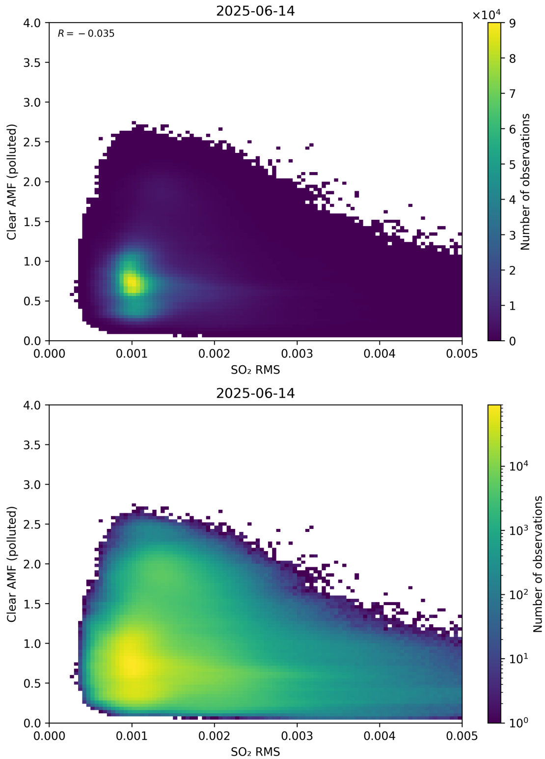
Figure 147: Scatter density plot of “SO 2 RMS” against “Clear AMF (polluted)” for 2025-06-13 to 2025-06-15.
