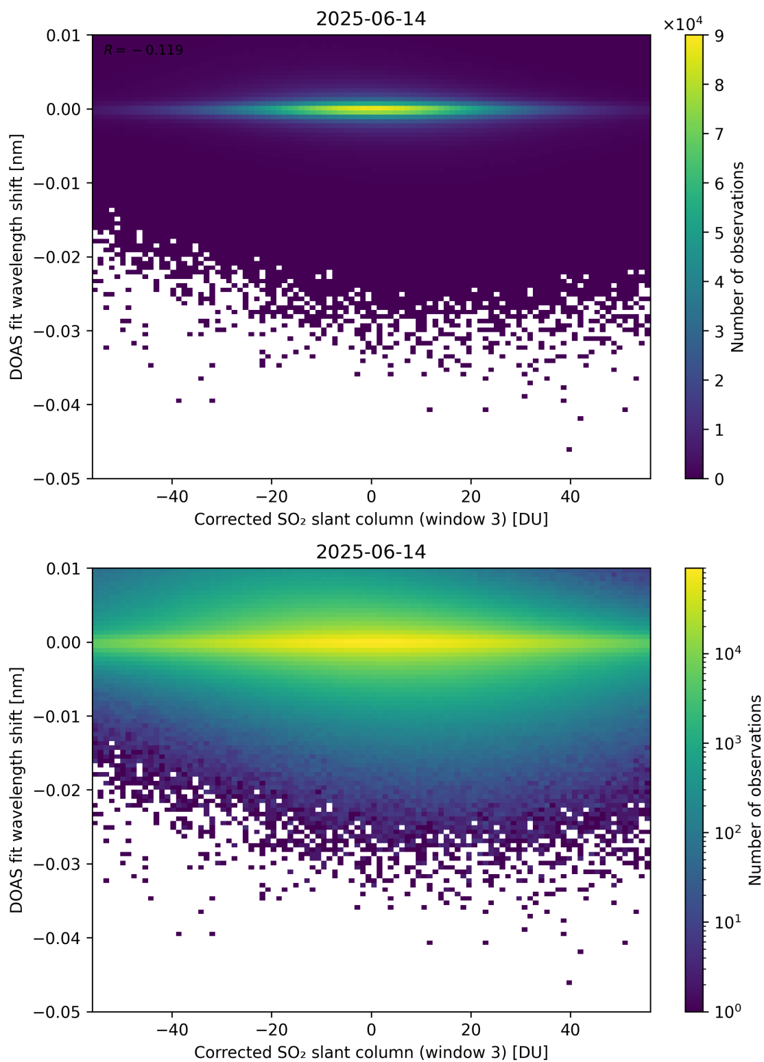
Figure 256: Scatter density plot of “Corrected SO 2 slant column (window 3)” against “DOAS fit wavelength shift” for 2025-06-13 to 2025-06-15.
