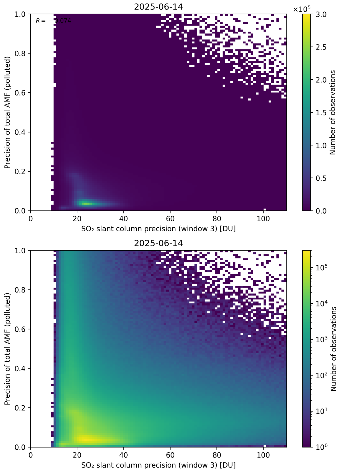
Figure 314: Scatter density plot of “SO 2 slant column precision (window 3)” against “Precision of total AMF (polluted)” for 2025-06-13 to 2025-06-15.
