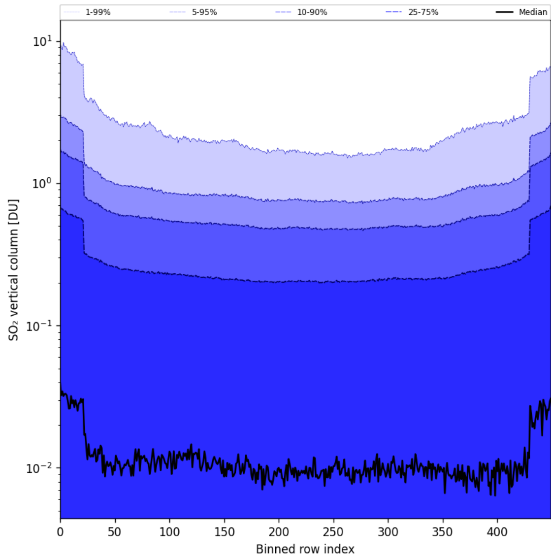
Figure 84: Along track statistics of “SO 2 vertical column” for 2025-06-13 to 2025-06-15
