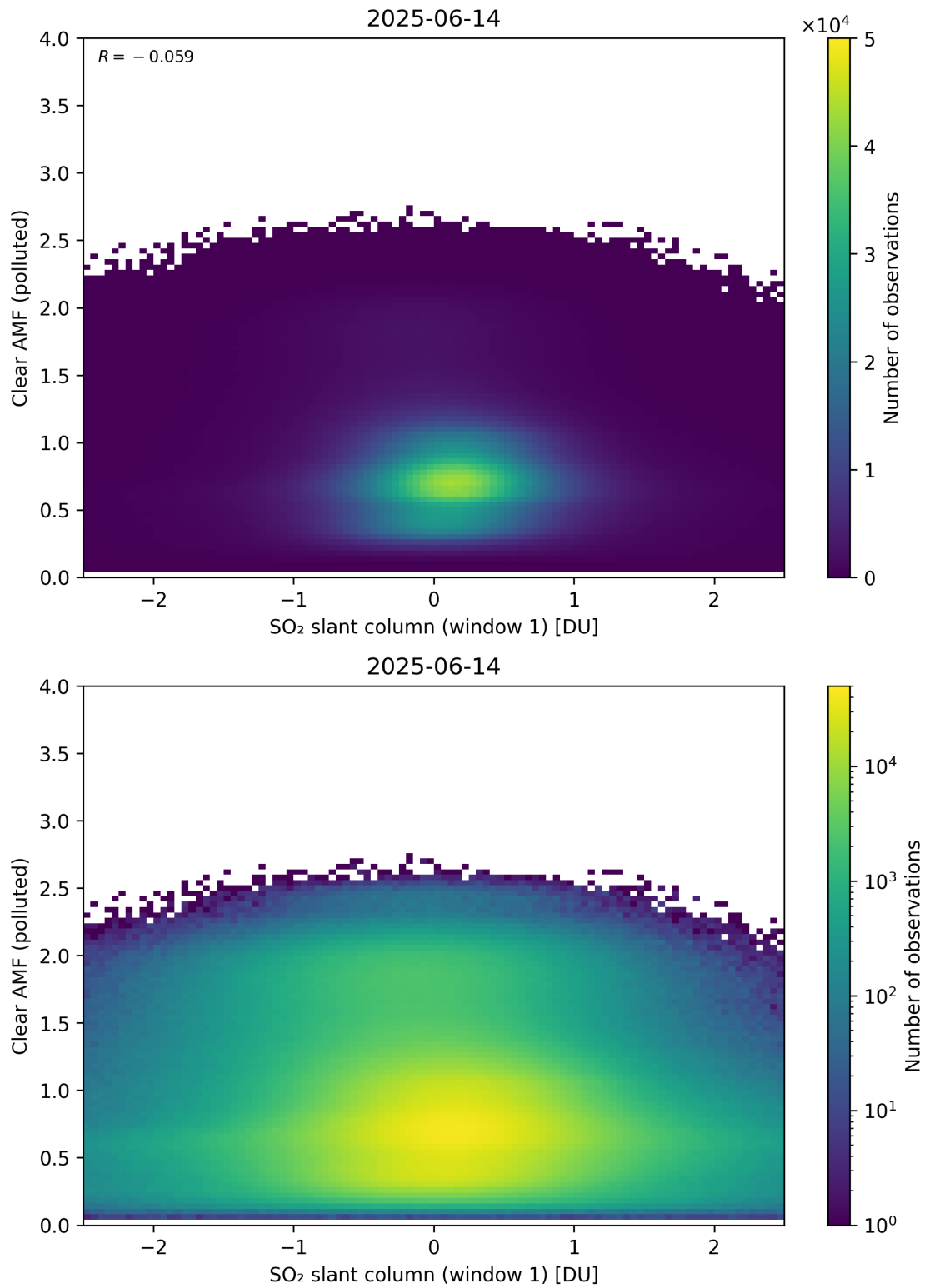
Figure 282: Scatter density plot of “SO 2 slant column (window 1)” against “Clear AMF (polluted)” for 2025-06-13 to 2025-06-15.
