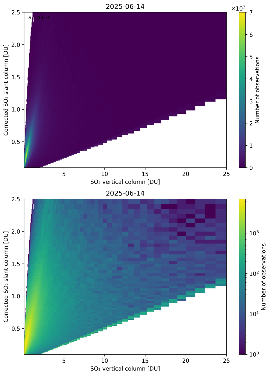
Figure 351: Scatter density plot of “SO 2 vertical column” against “Corrected SO 2 slant column” for 2025-06-13 to 2025-06-15.
