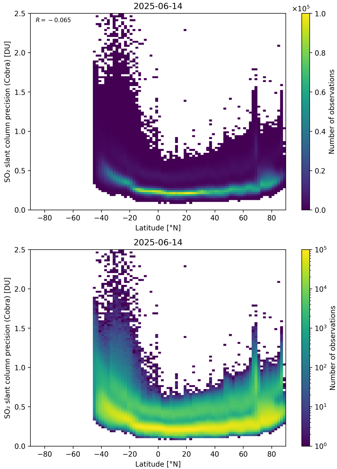
Figure 158: Scatter density plot of “Latitude” against “SO 2 slant column precision (Cobra)” for 2025-06-13 to 2025-06-15.
