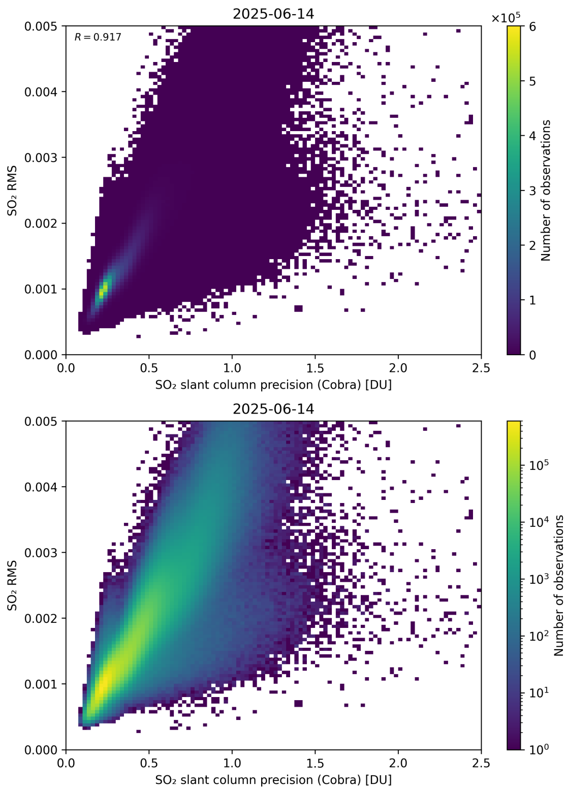
Figure 204: Scatter density plot of “SO 2 slant column precision (Cobra)” against “SO 2 RMS” for 2025-06-13 to 2025-06-15.
