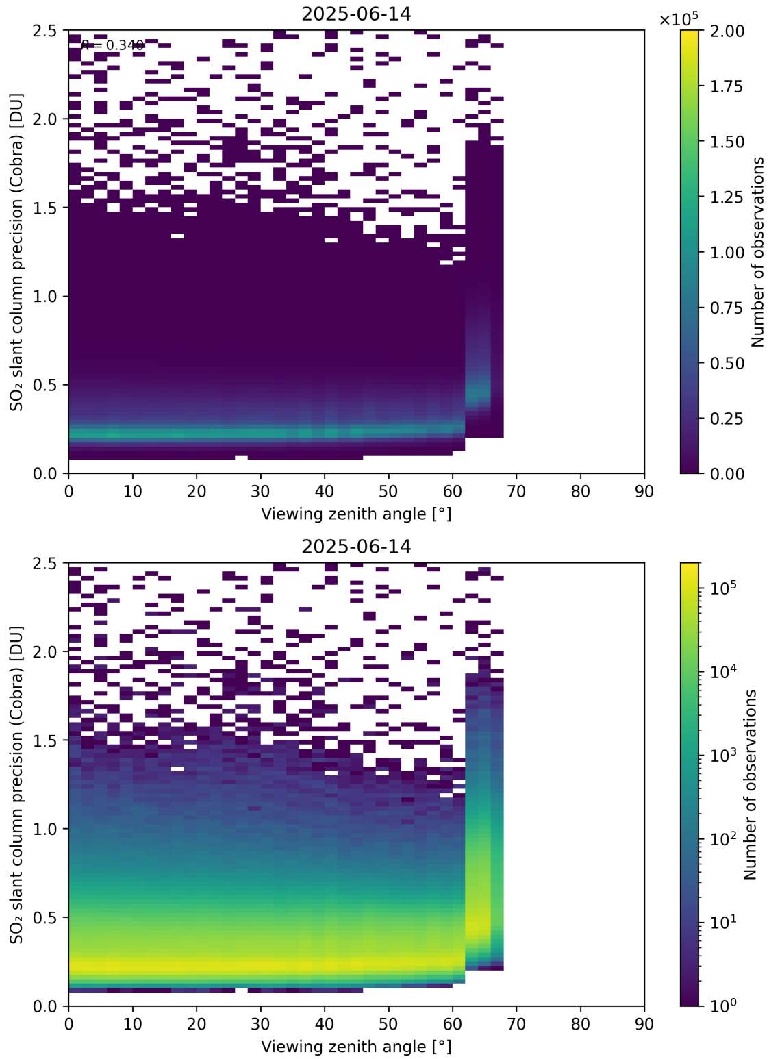
Figure 372: Scatter density plot of “Viewing zenith angle” against “SO 2 slant column precision (Cobra)” for 2025-06-13 to 2025-06-15.
