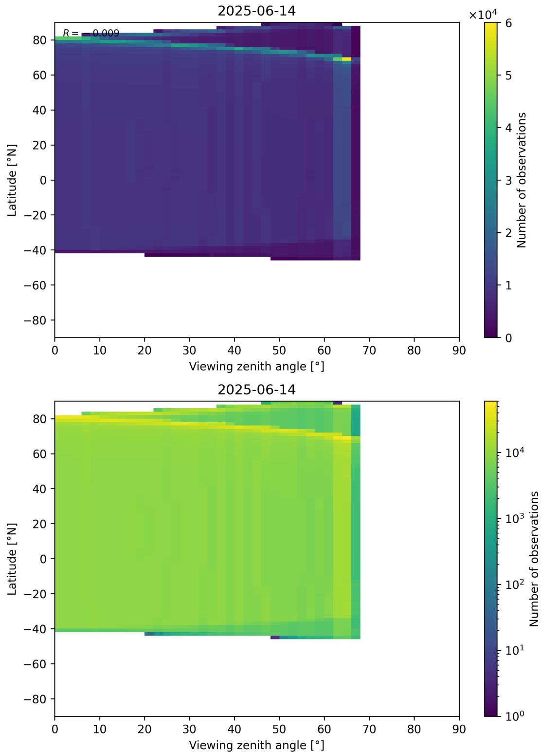
Figure 368: Scatter density plot of “Viewing zenith angle” against “Latitude” for 2025-06-13 to 2025-06-15.
