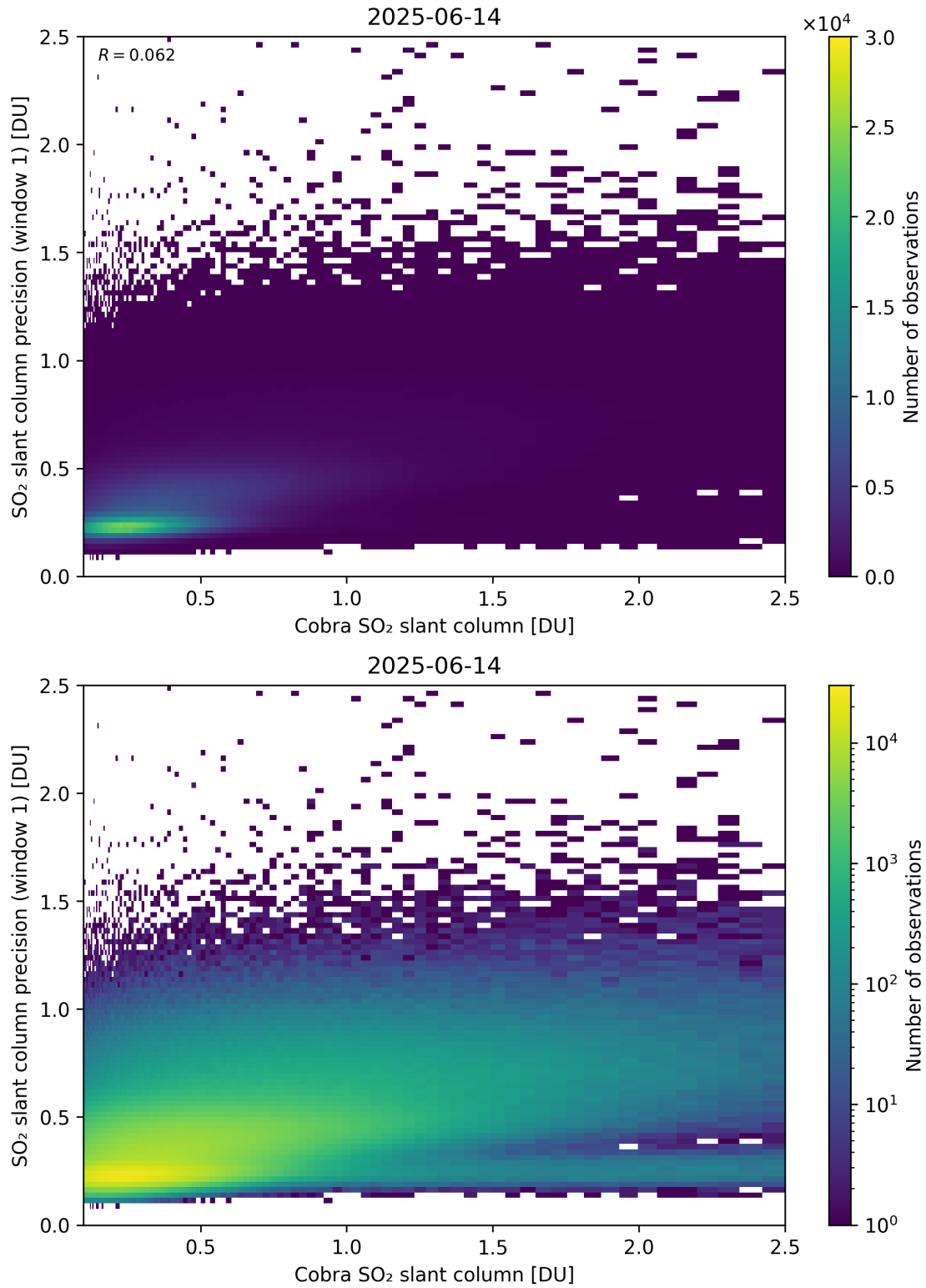
Figure 220: Scatter density plot of “Cobra SO 2 slant column” against “SO 2 slant column precision (window 1)” for 2025-06-13 to 2025-06-15.
