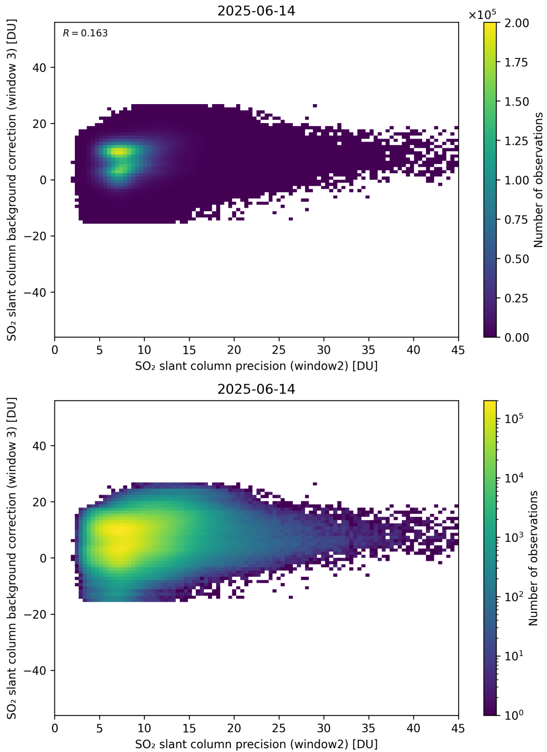
Figure 292: Scatter density plot of “SO 2 slant column precision (window2)” against “SO 2 slant column background correction (window 3)” for 2025-06-13 to 2025-06-15.
