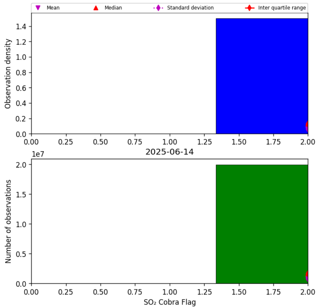
Figure 75: Histogram of “SO 2 Cobra Flag” for 2025-06-13 to 2025-06-15
