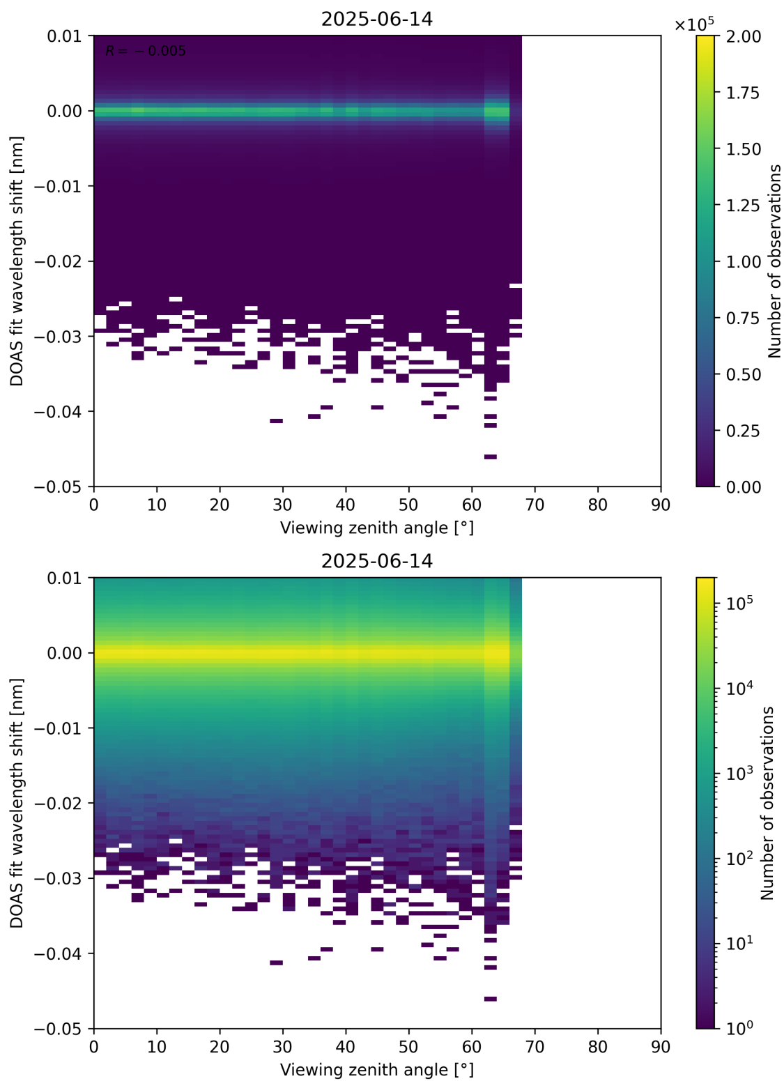
Figure 365: Scatter density plot of “Viewing zenith angle” against “DOAS fit wavelength shift” for 2025-06-13 to 2025-06-15.
