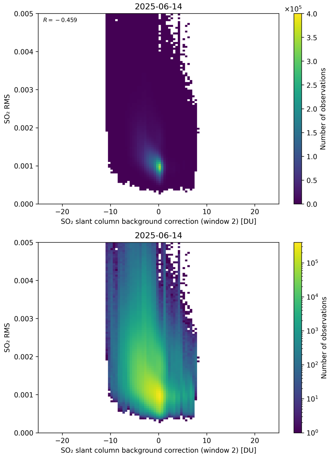
Figure 125: Scatter density plot of “SO 2 slant column background correction (window 2)” against “SO 2 RMS” for 2025-06-13 to 2025-06-15.
