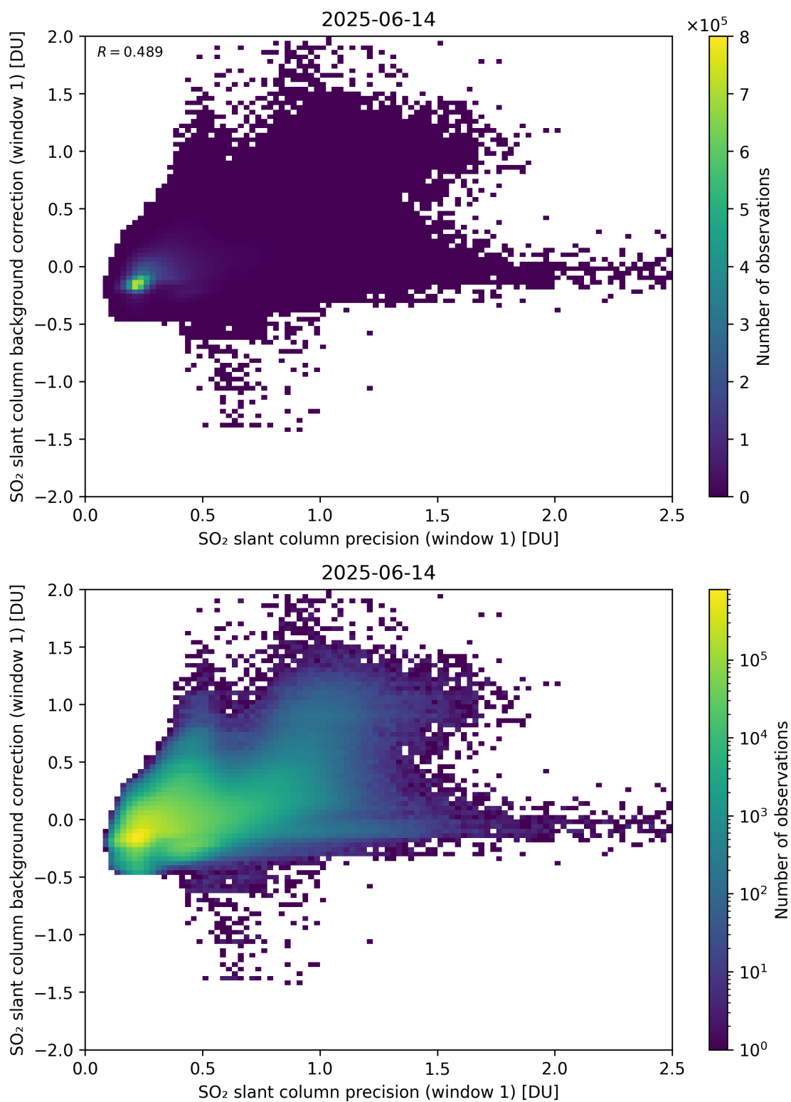
Figure 268: Scatter density plot of “SO 2 slant column precision (window 1)” against “SO 2 slant column background correction (window 1)” for 2025-06-13 to 2025-06-15.
