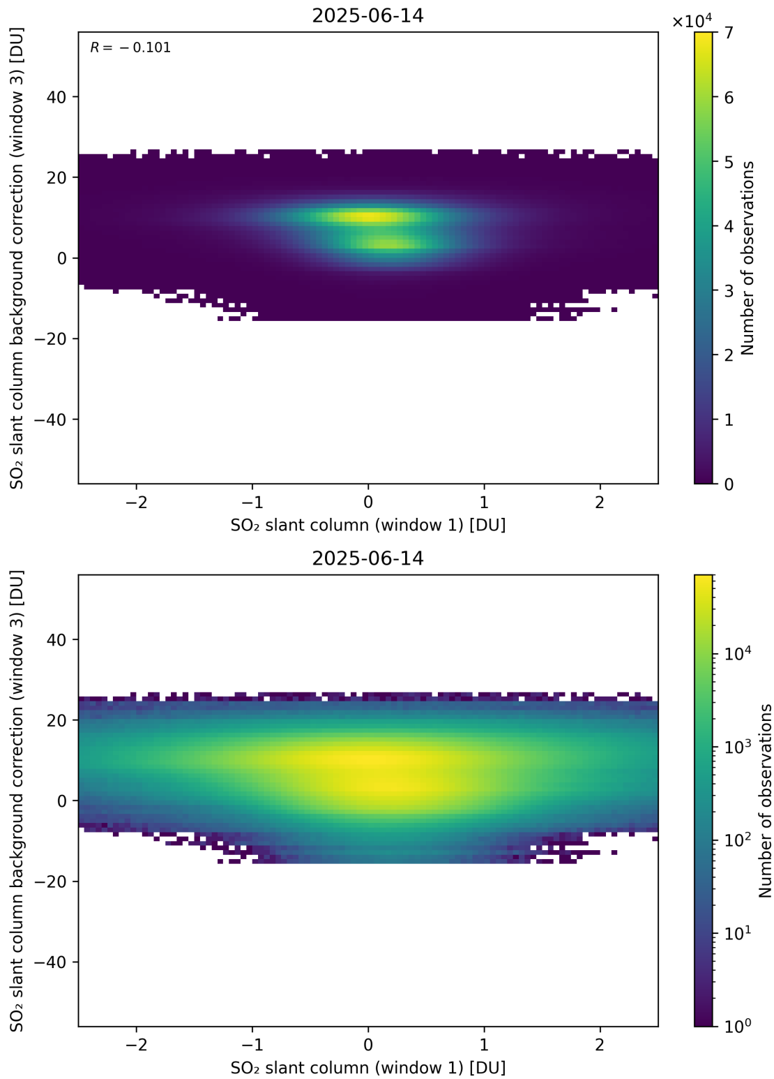
Figure 264: Scatter density plot of “SO 2 slant column (window 1)” against “SO 2 slant column background correction (window 3)” for 2025-06-13 to 2025-06-15.
