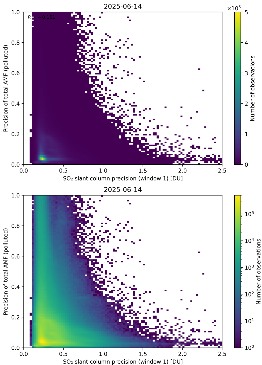
Figure 281: Scatter density plot of “SO 2 slant column precision (window 1)” against “Precision of total AMF (polluted)” for 2025-06-13 to 2025-06-15.
