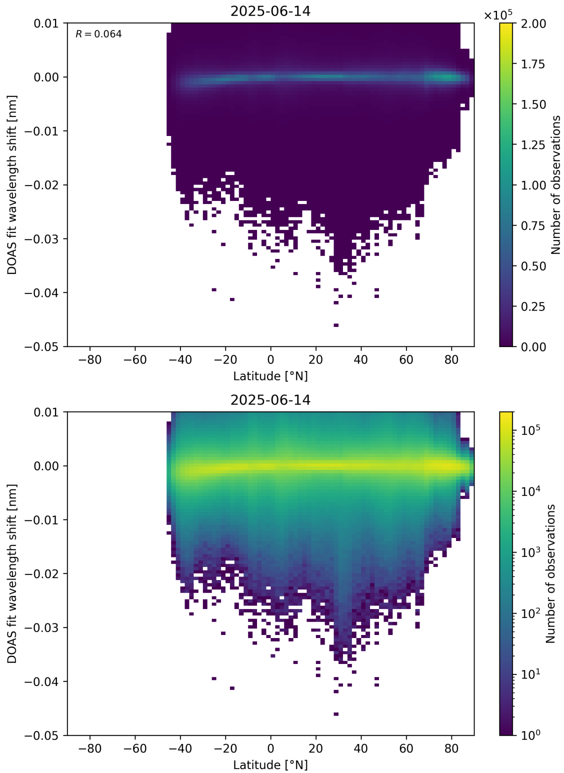
Figure 153: Scatter density plot of “Latitude” against “DOAS fit wavelength shift” for 2025-06-13 to 2025-06-15.
