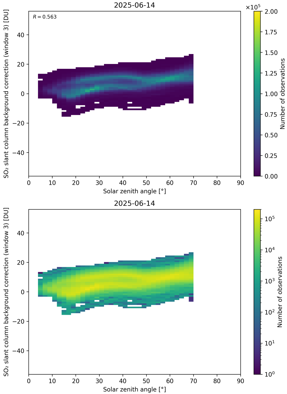
Figure 173: Scatter density plot of “Solar zenith angle” against “SO 2 slant column background correction (window 3)” for 2025-06-13 to 2025-06-15.
