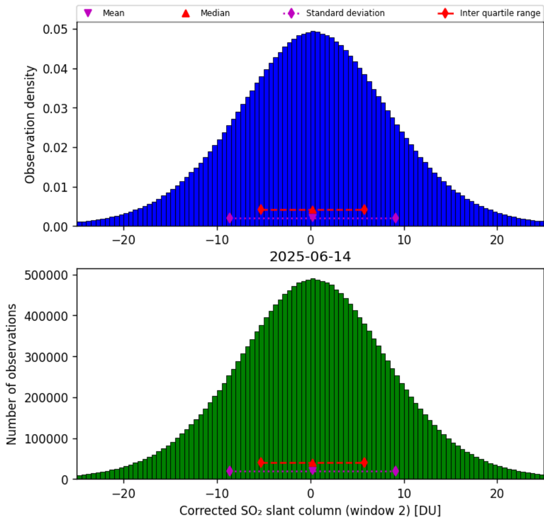
Figure 69: Histogram of “Corrected SO 2 slant column (window 2)” for 2025-06-13 to 2025-06-15
