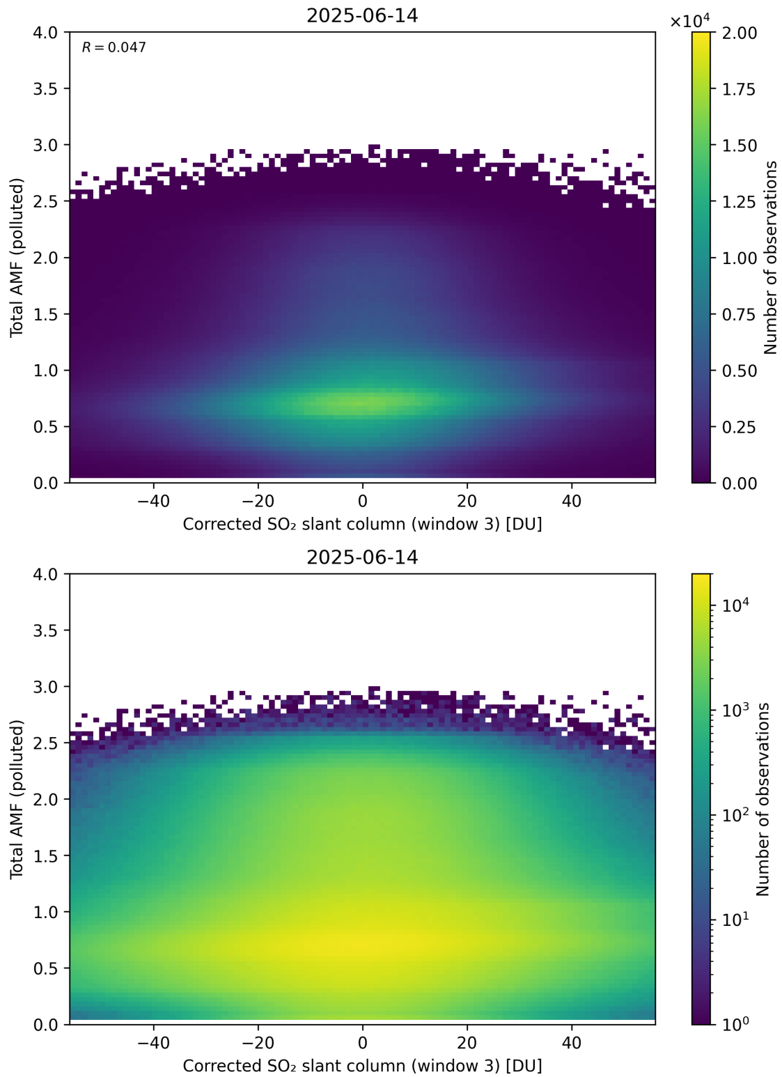
Figure 260: Scatter density plot of “Corrected SO 2 slant column (window 3)” against “Total AMF (polluted)” for 2025-06-13 to 2025-06-15.
