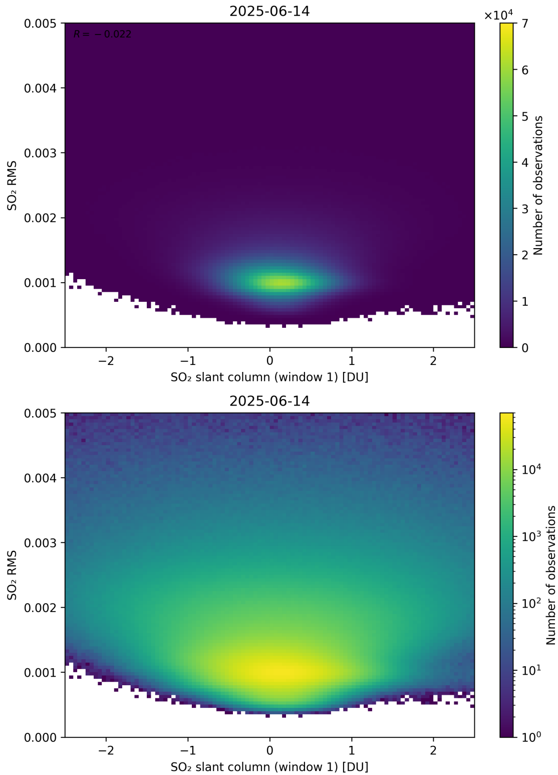
Figure 267: Scatter density plot of “SO 2 slant column (window 1)” against “SO 2 RMS” for 2025-06-13 to 2025-06-15.
