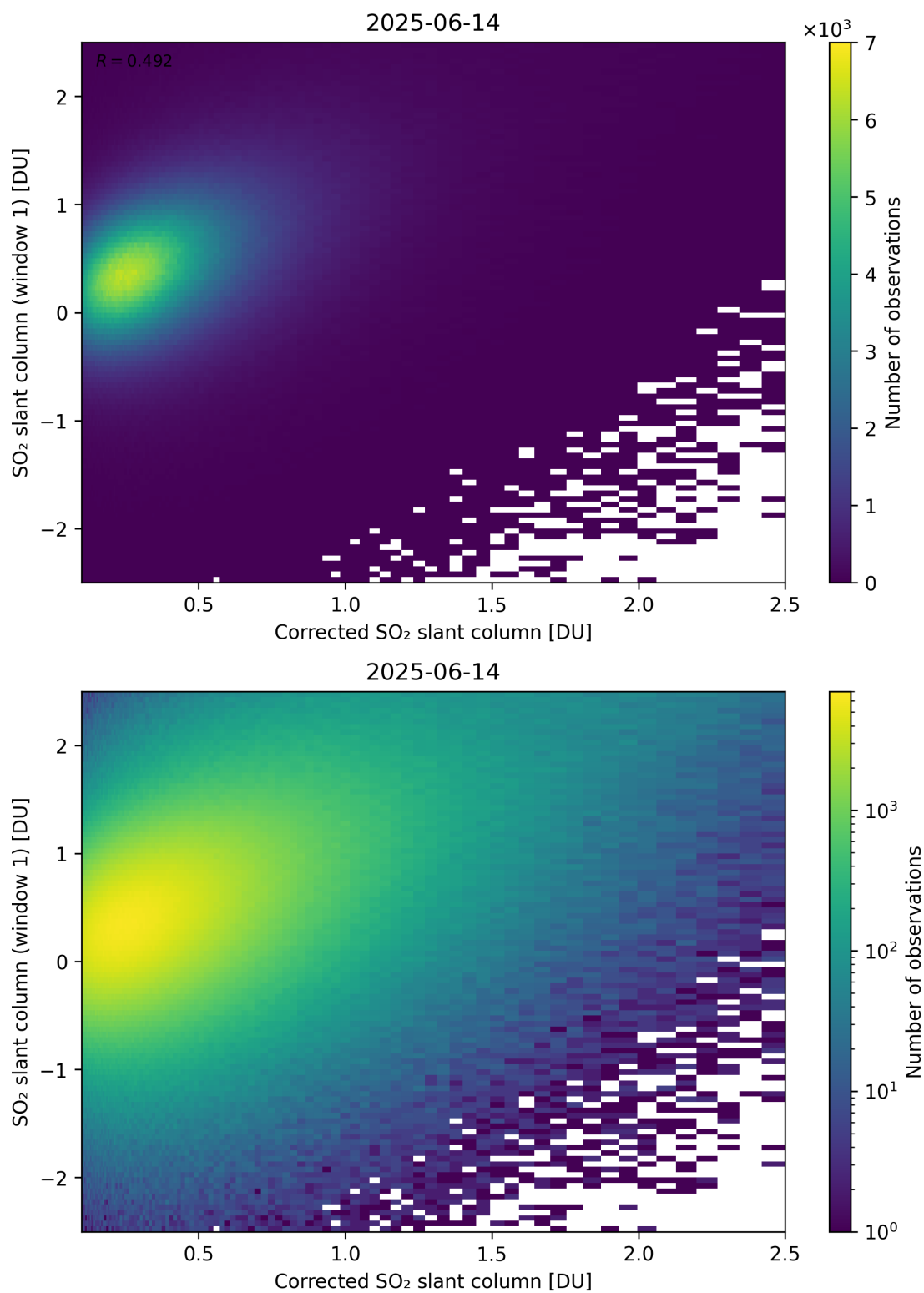
Figure 237: Scatter density plot of “Corrected SO 2 slant column” against “SO 2 slant column (window 1)” for 2025-06-13 to 2025-06-15.
