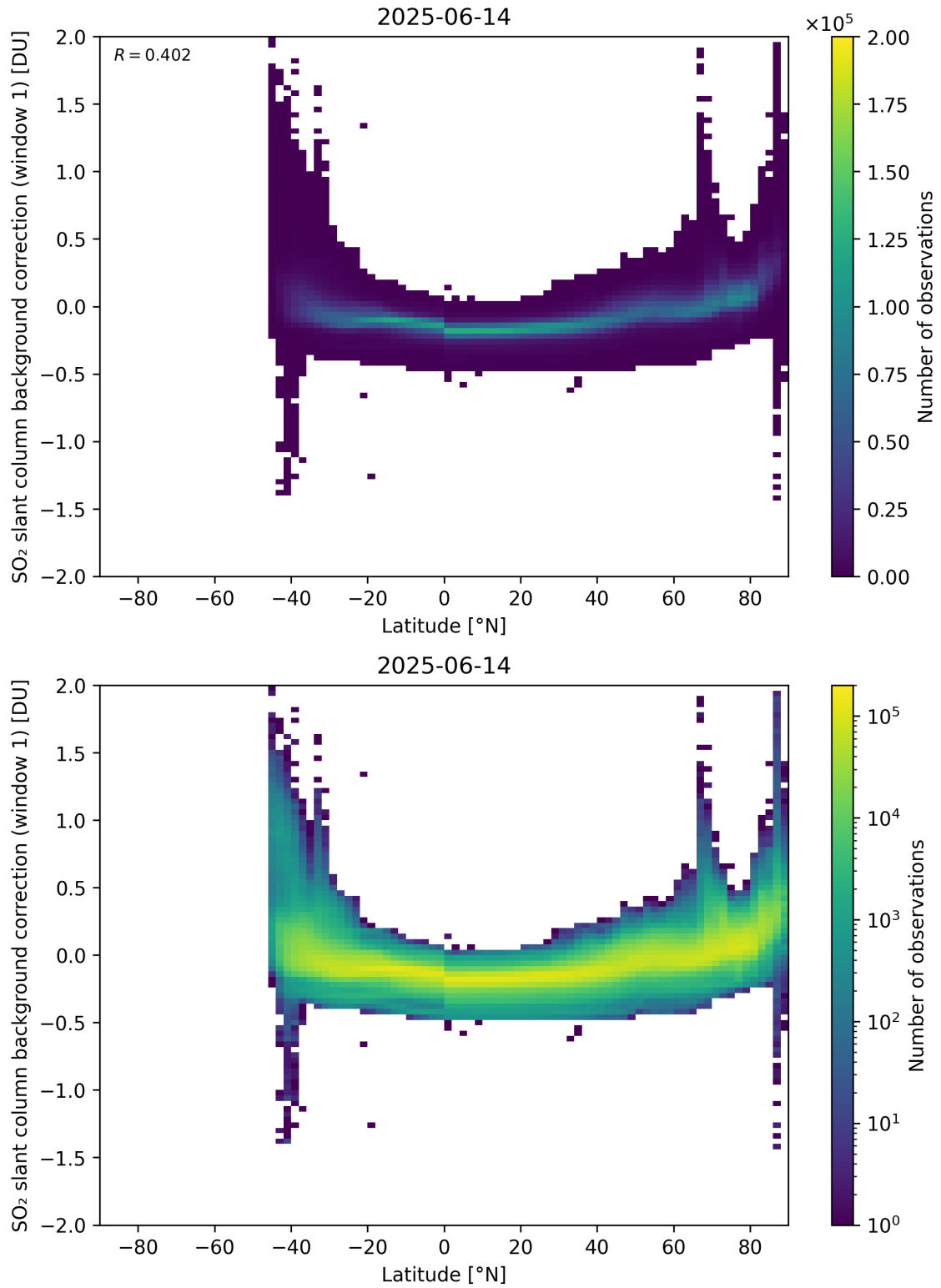
Figure 150: Scatter density plot of “Latitude” against “SO 2 slant column background correction (window 1)” for 2025-06-13 to 2025-06-15.
