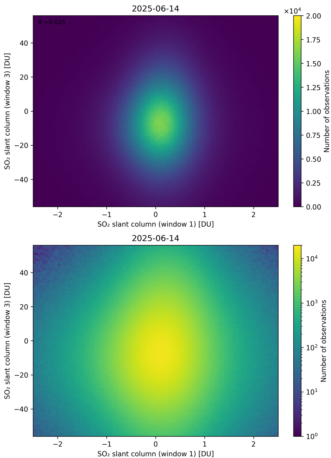
Figure 287: Scatter density plot of “SO 2 slant column (window 1)” against “SO 2 slant column (window 3)” for 2025-06-13 to 2025-06-15.
