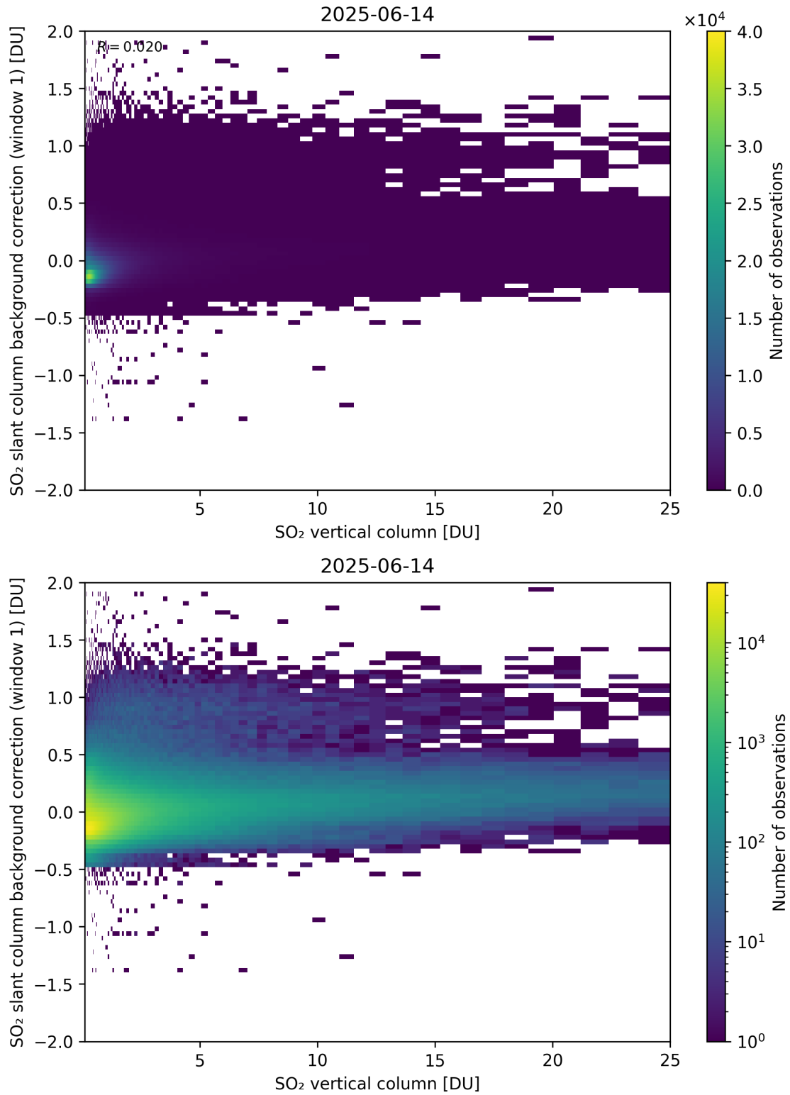
Figure 323: Scatter density plot of “SO 2 vertical column” against “SO 2 slant column background correction (window 1)” for 2025-06-13 to 2025-06-15.
