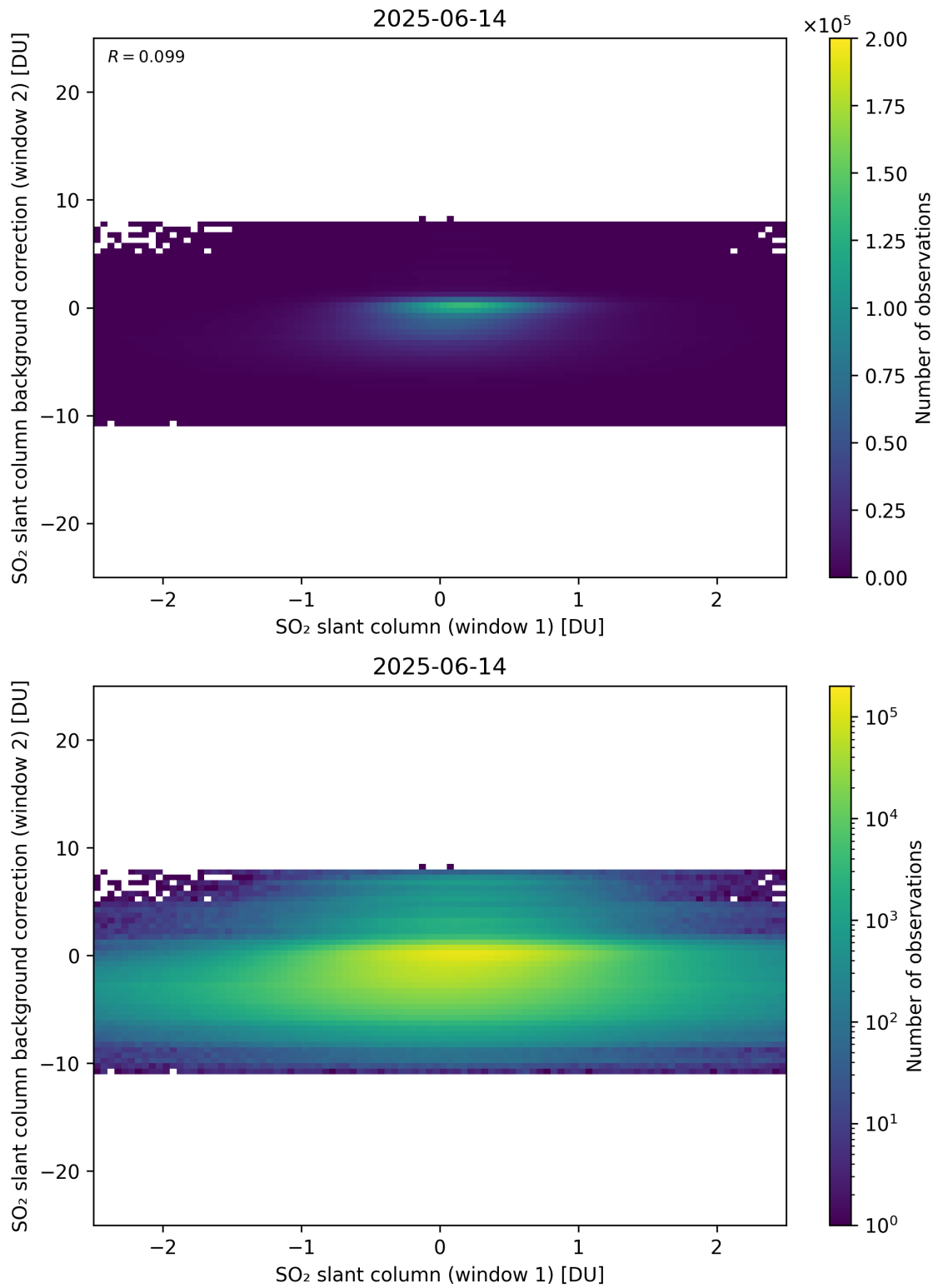
Figure 263: Scatter density plot of “SO 2 slant column (window 1)” against “SO 2 slant column background correction (window 2)” for 2025-06-13 to 2025-06-15.
