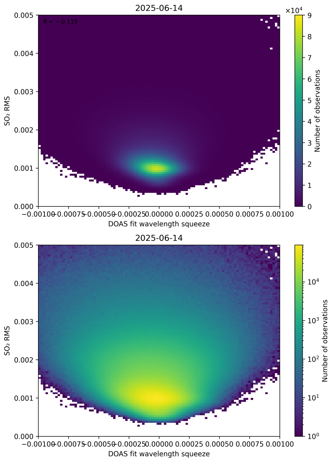
Figure 143: Scatter density plot of “DOAS fit wavelength squeeze” against “SO 2 RMS” for 2025-06-13 to 2025-06-15.
