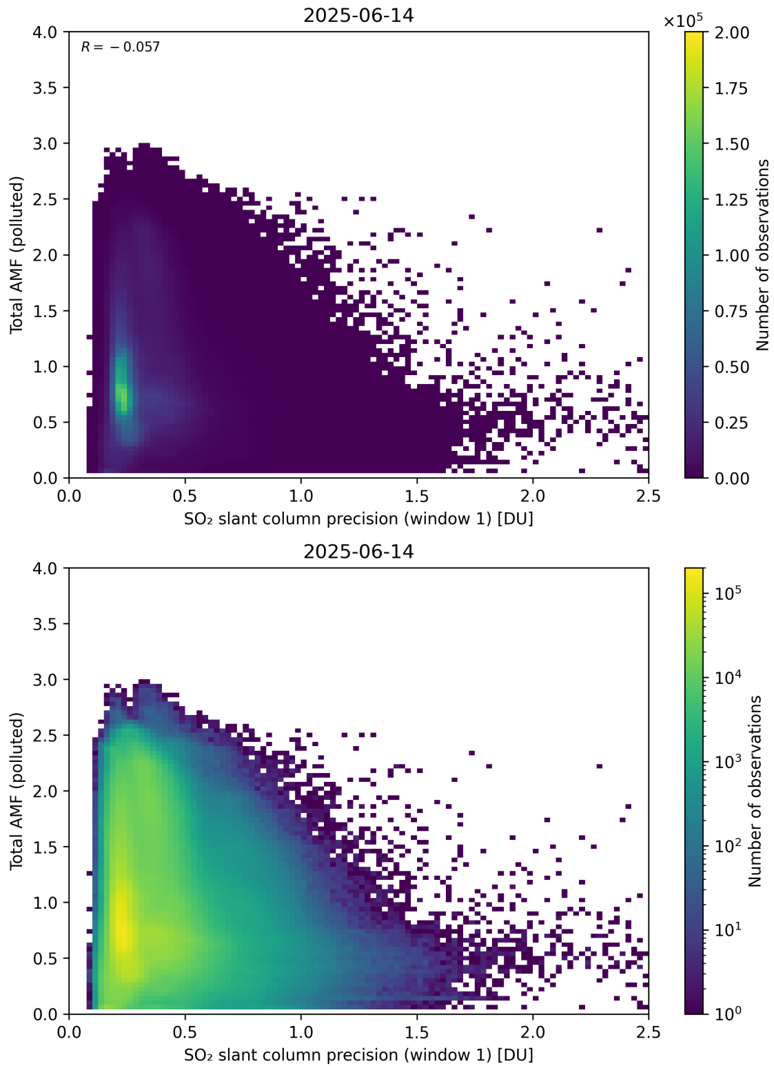
Figure 280: Scatter density plot of “SO 2 slant column precision (window 1)” against “Total AMF (polluted)” for 2025-06-13 to 2025-06-15.
