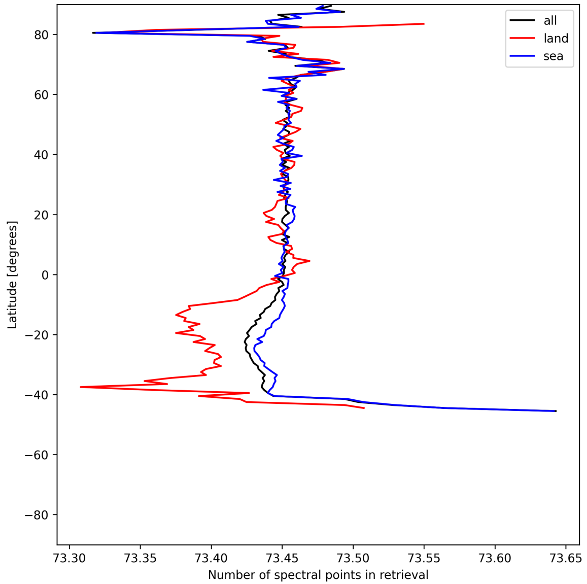
Figure 56: Zonal average of “Number of spectral points in retrieval” for 2025-06-13 to 2025-06-15.
