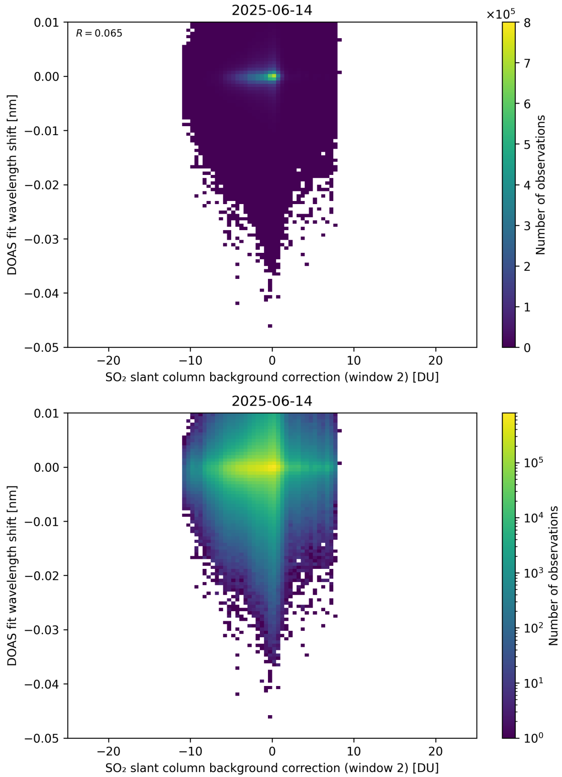
Figure 123: Scatter density plot of “SO 2 slant column background correction (window 2)” against “DOAS fit wavelength shift” for 2025-06-13 to 2025-06-15.
