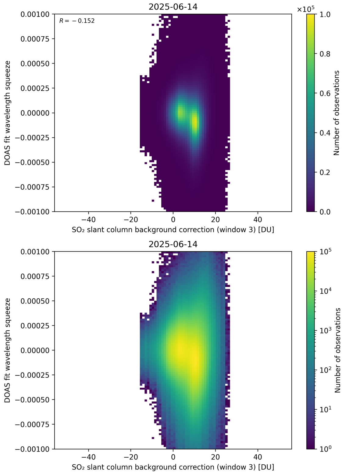
Figure 133: Scatter density plot of “SO 2 slant column background correction (window 3)” against “DOAS fit wavelength squeeze” for 2025-06-13 to 2025-06-15.
