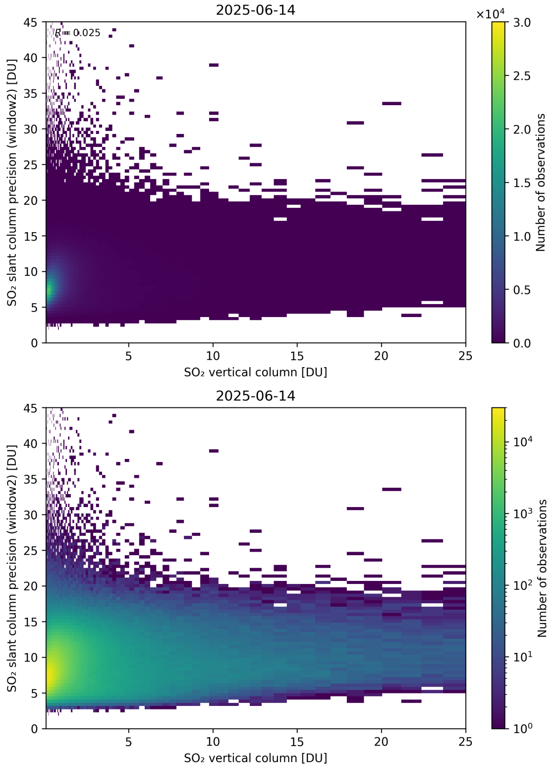
Figure 356: Scatter density plot of “SO 2 vertical column” against “SO 2 slant column precision (window2)” for 2025-06-13 to 2025-06-15.
