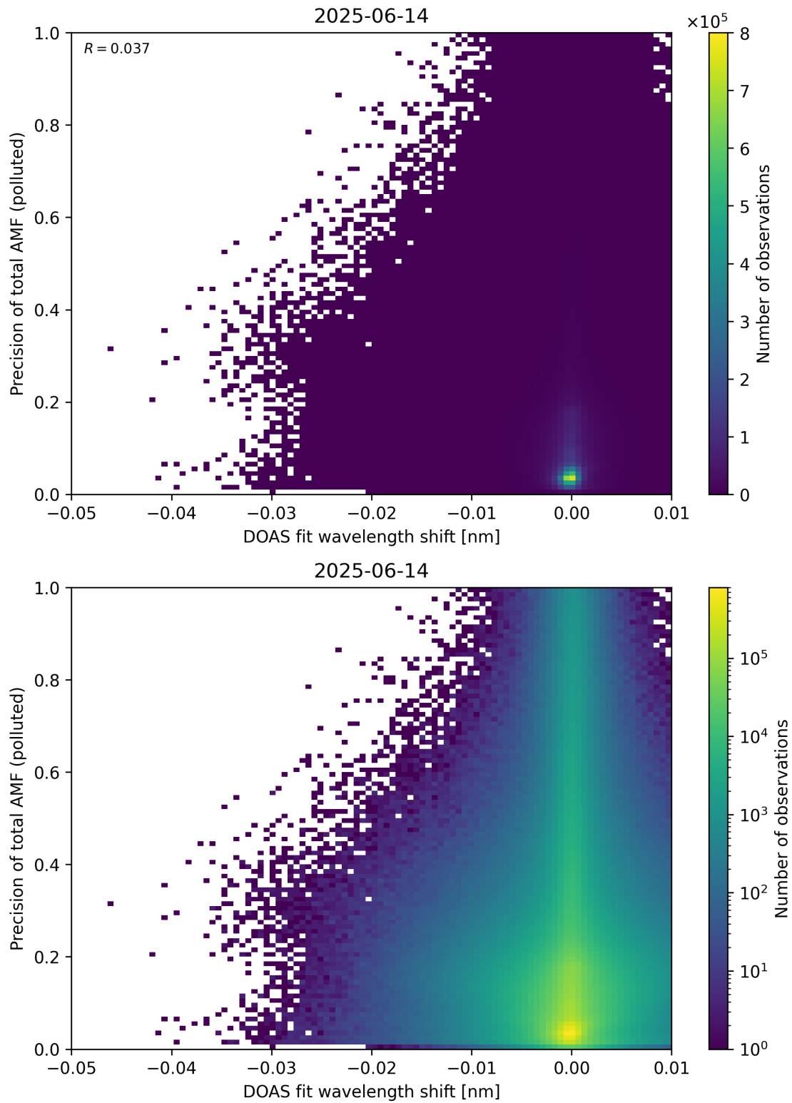
Figure 142: Scatter density plot of “DOAS fit wavelength shift” against “Precision of total AMF (polluted)” for 2025-06-13 to 2025-06-15.
