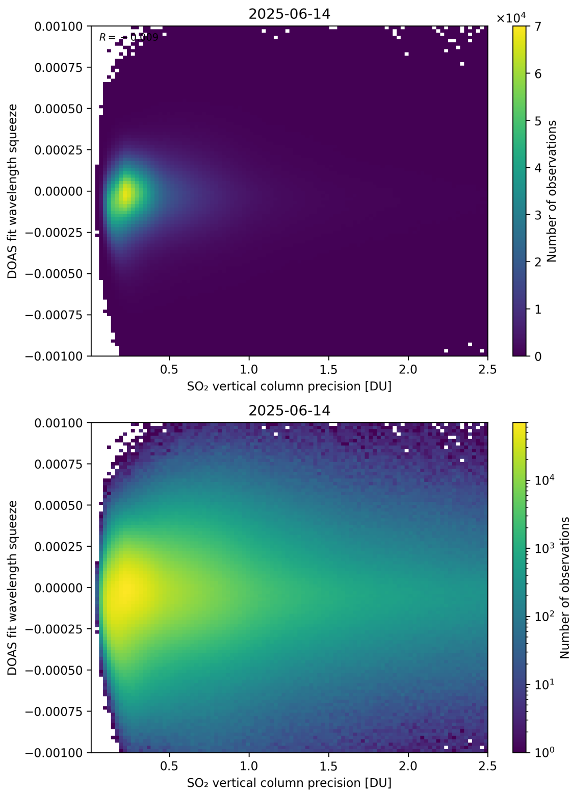
Figure 333: Scatter density plot of “SO 2 vertical column precision” against “DOAS fit wavelength squeeze” for 2025-06-13 to 2025-06-15.
