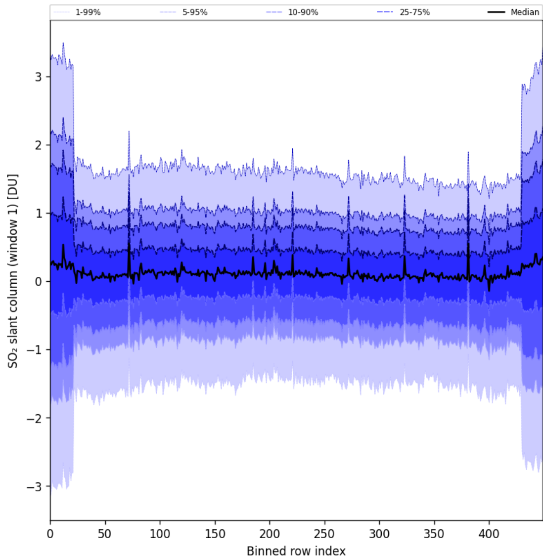
Figure 89: Along track statistics of “SO 2 slant column (window 1)” for 2025-06-13 to 2025-06-15
