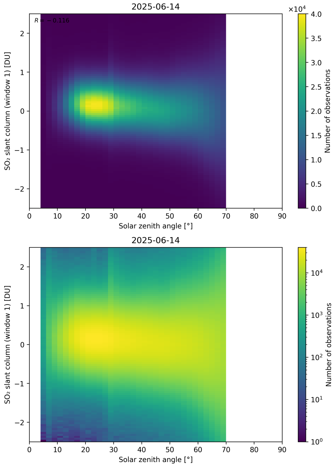
Figure 184: Scatter density plot of “Solar zenith angle” against “SO 2 slant column (window 1)” for 2025-06-13 to 2025-06-15.
