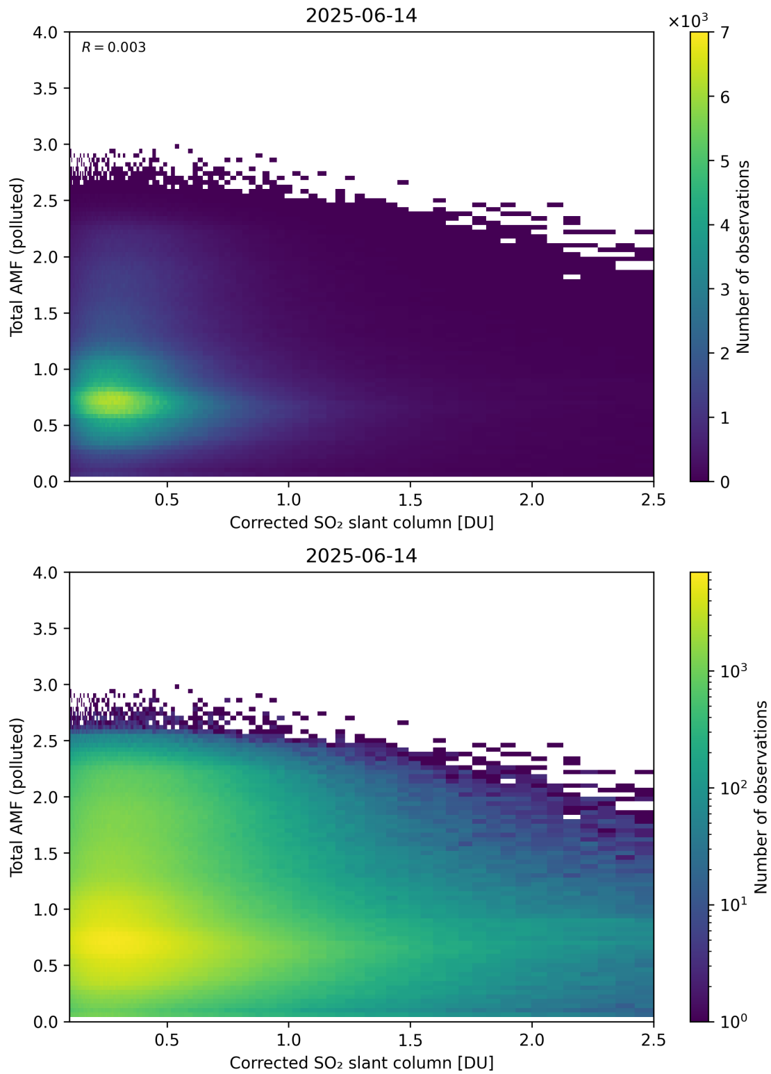
Figure 242: Scatter density plot of “Corrected SO 2 slant column” against “Total AMF (polluted)” for 2025-06-13 to 2025-06-15.
