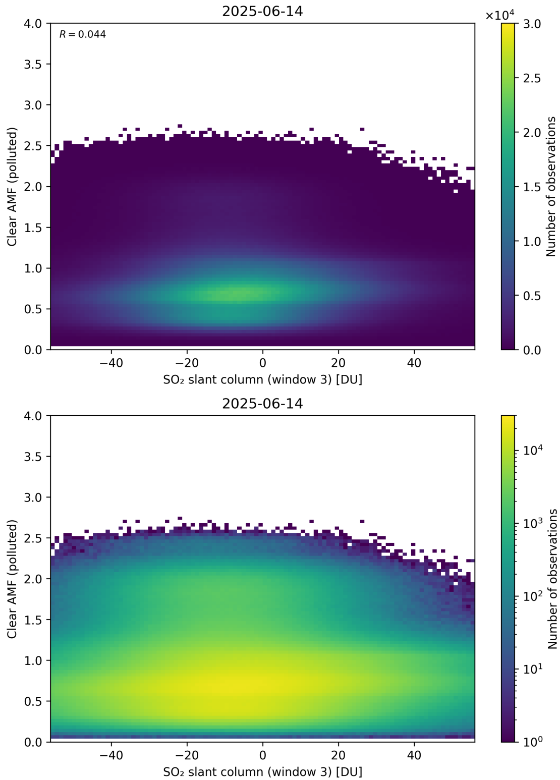
Figure 315: Scatter density plot of “SO 2 slant column (window 3)” against “Clear AMF (polluted)” for 2025-06-13 to 2025-06-15.
