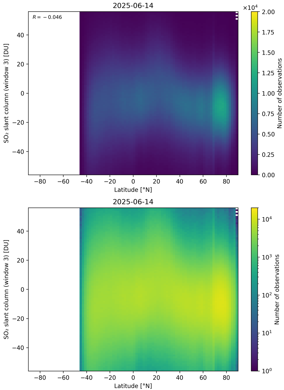
Figure 165: Scatter density plot of “Latitude” against “SO 2 slant column (window 3)” for 2025-06-13 to 2025-06-15.
