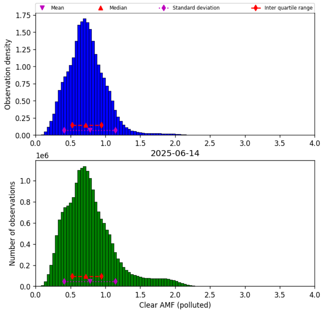
Figure 81: Histogram of “Clear AMF (polluted)” for 2025-06-13 to 2025-06-15
