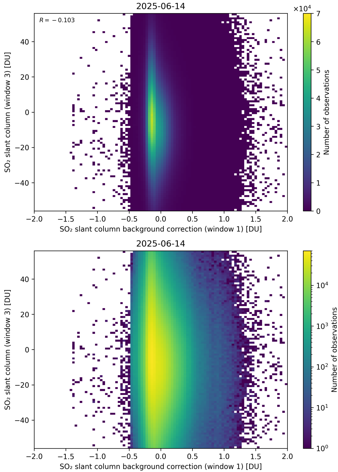
Figure 118: Scatter density plot of “SO 2 slant column background correction (window 1)” against “SO 2 slant column (window 3)” for 2025-06-13 to 2025-06-15.
