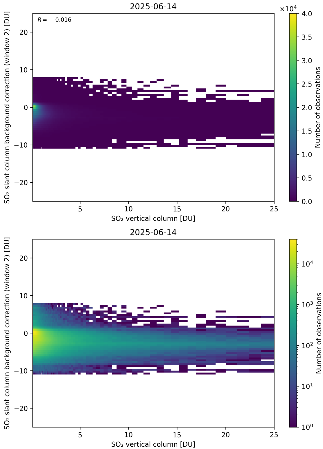
Figure 324: Scatter density plot of “SO 2 vertical column” against “SO 2 slant column background correction (window 2)” for 2025-06-13 to 2025-06-15.
