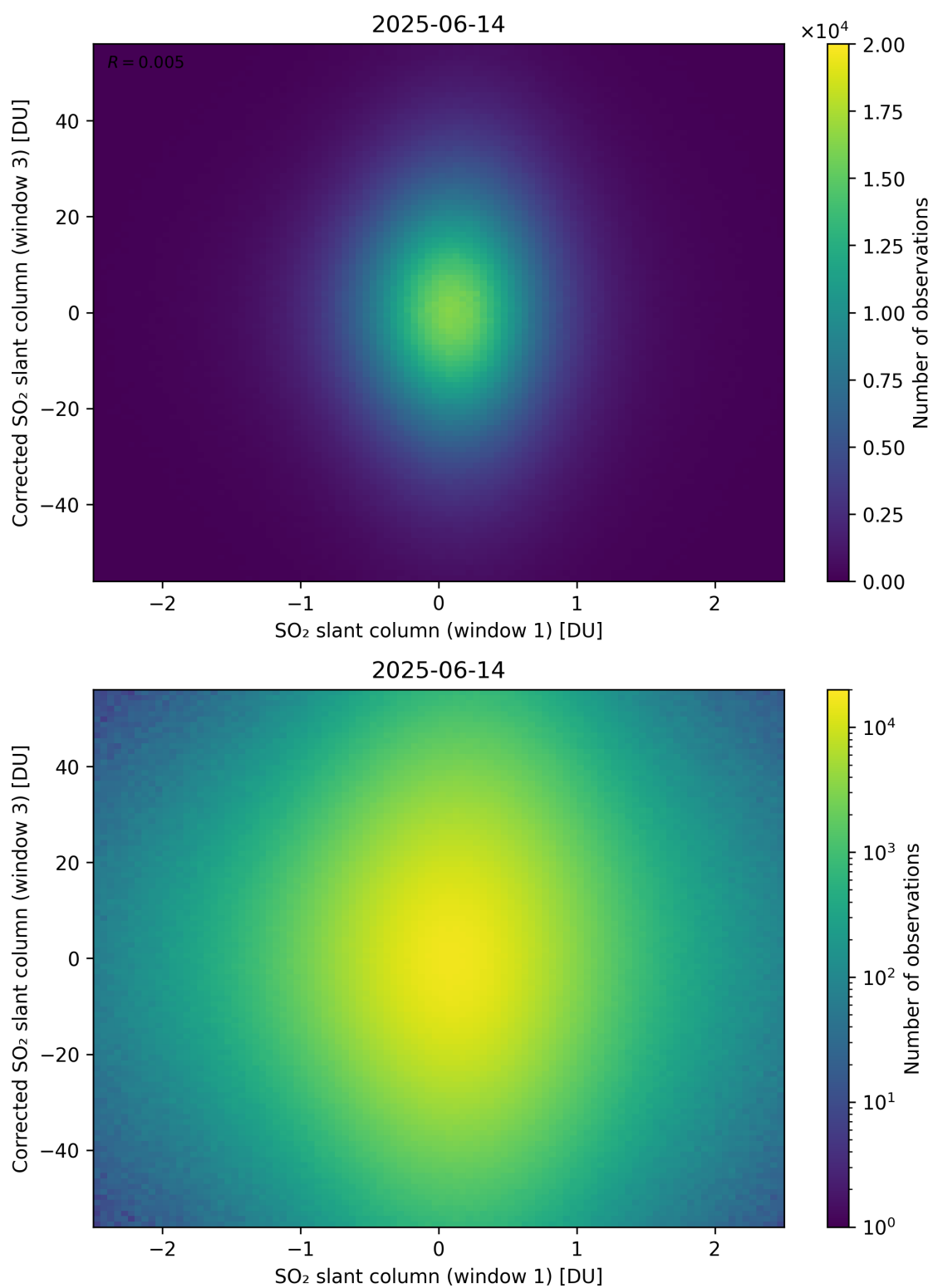
Figure 284: Scatter density plot of “SO 2 slant column (window 1)” against “Corrected SO 2 slant column (window 3)” for 2025-06-13 to 2025-06-15.
