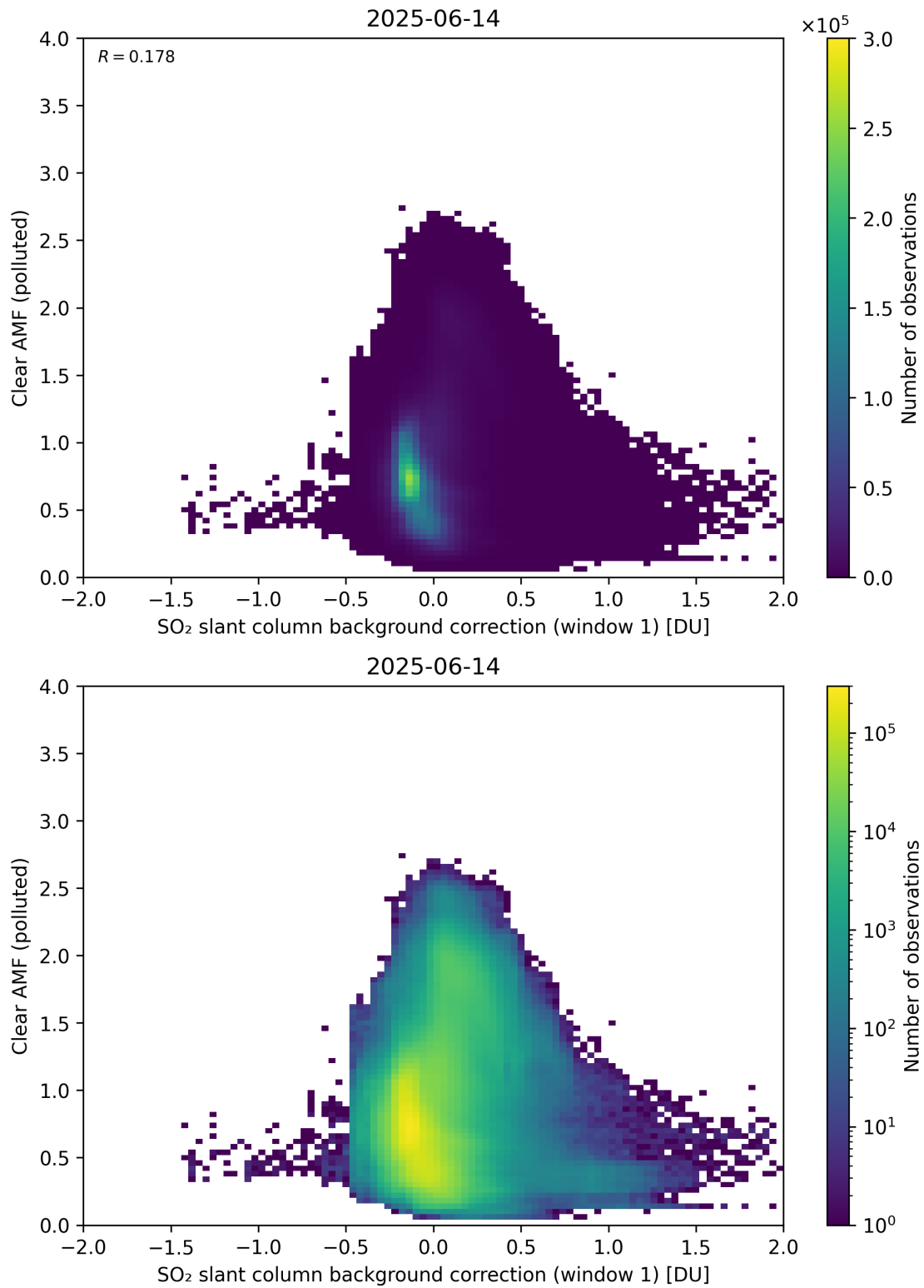
Figure 114: Scatter density plot of “SO 2 slant column background correction (window 1)” against “Clear AMF (polluted)” for 2025-06-13 to 2025-06-15.
