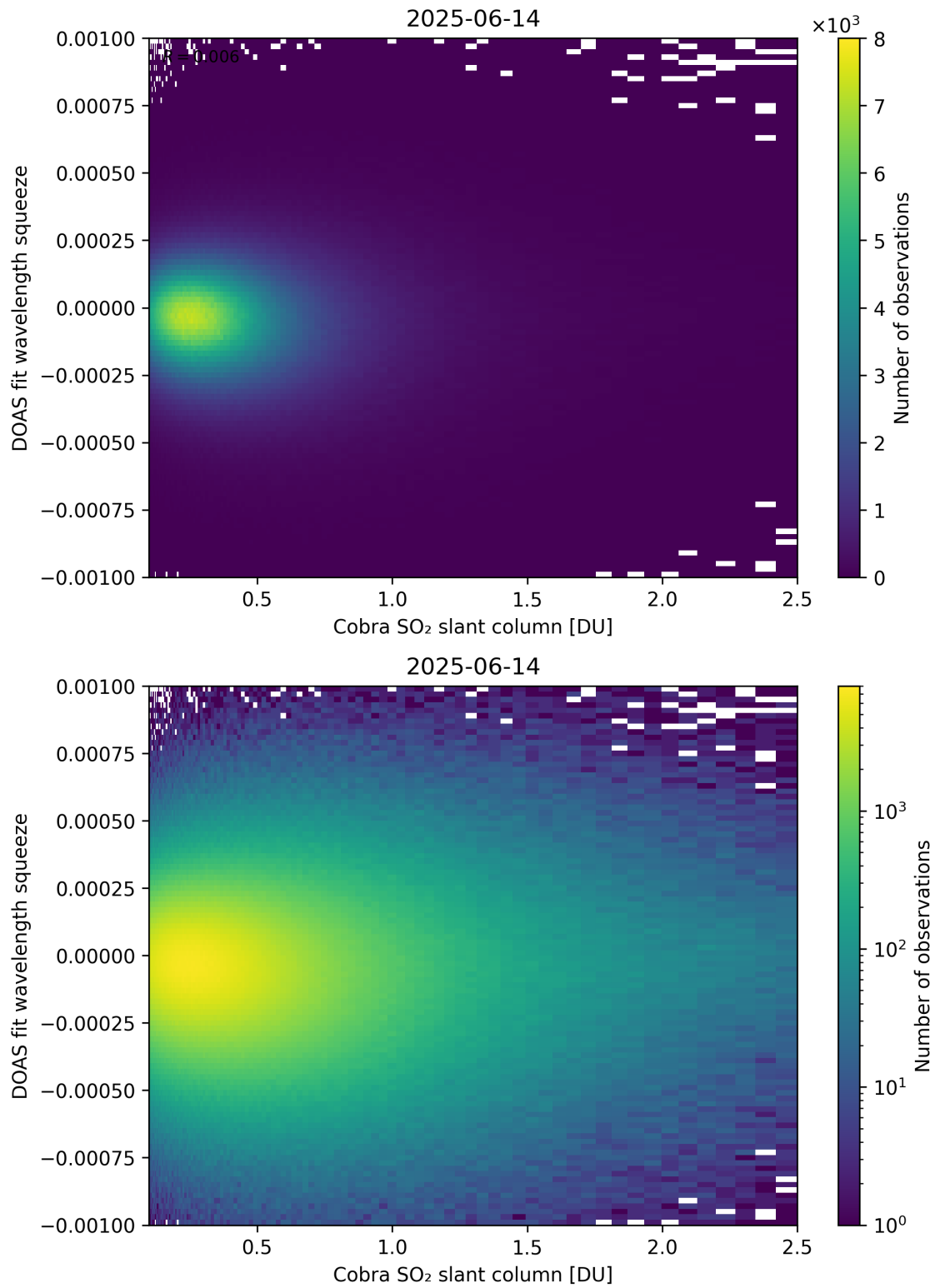
Figure 197: Scatter density plot of “Cobra SO 2 slant column” against “DOAS fit wavelength squeeze” for 2025-06-13 to 2025-06-15.
