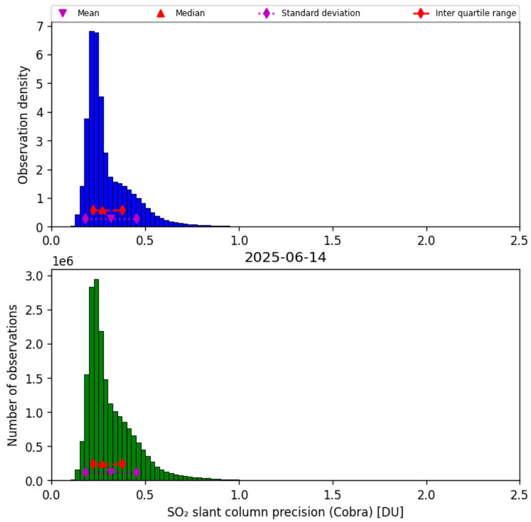
Figure 62: Histogram of “SO 2 slant column precision (Cobra)” for 2025-06-13 to 2025-06-15
