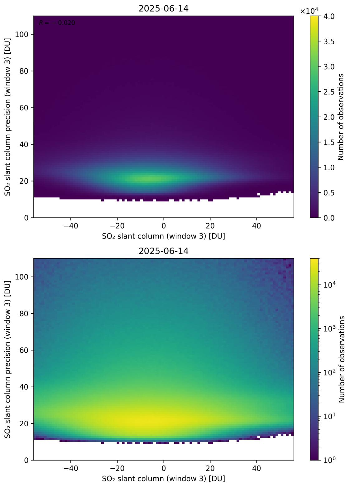
Figure 317: Scatter density plot of “SO 2 slant column (window 3)” against “SO 2 slant column precision (window 3)” for 2025-06-13 to 2025-06-15.
