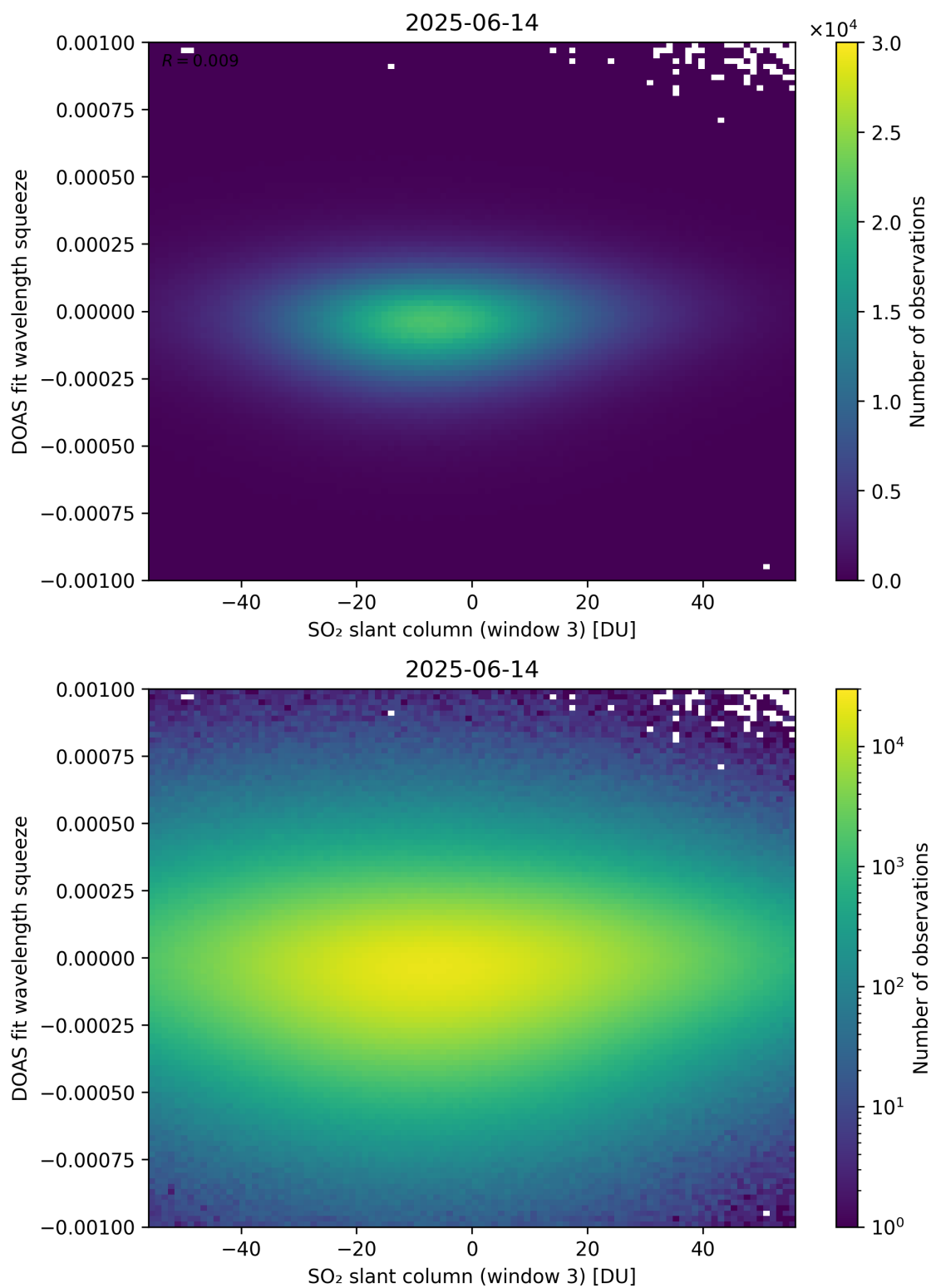
Figure 305: Scatter density plot of “SO 2 slant column (window 3)” against “DOAS fit wavelength squeeze” for 2025-06-13 to 2025-06-15.
