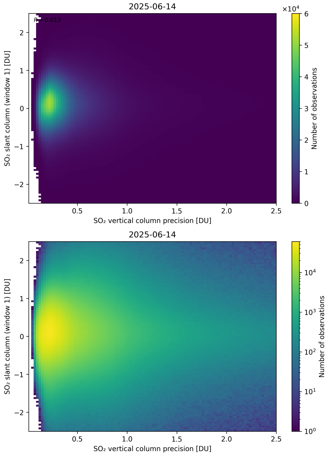
Figure 341: Scatter density plot of “SO 2 vertical column precision” against “SO 2 slant column (window 1)” for 2025-06-13 to 2025-06-15.
