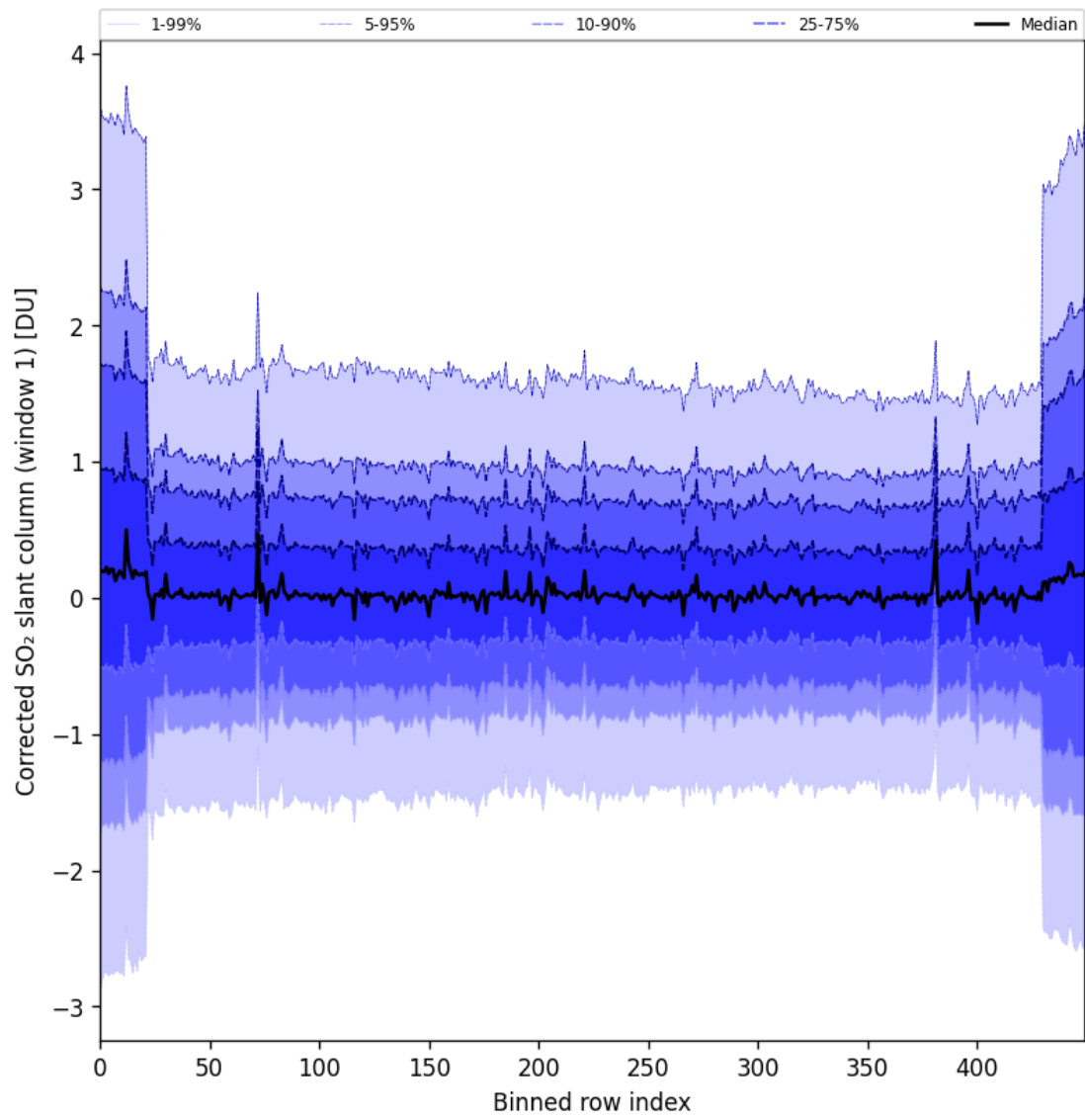
Figure 91: Along track statistics of “Corrected SO 2 slant column (window 1)” for 2025-06-13 to 2025-06-15
