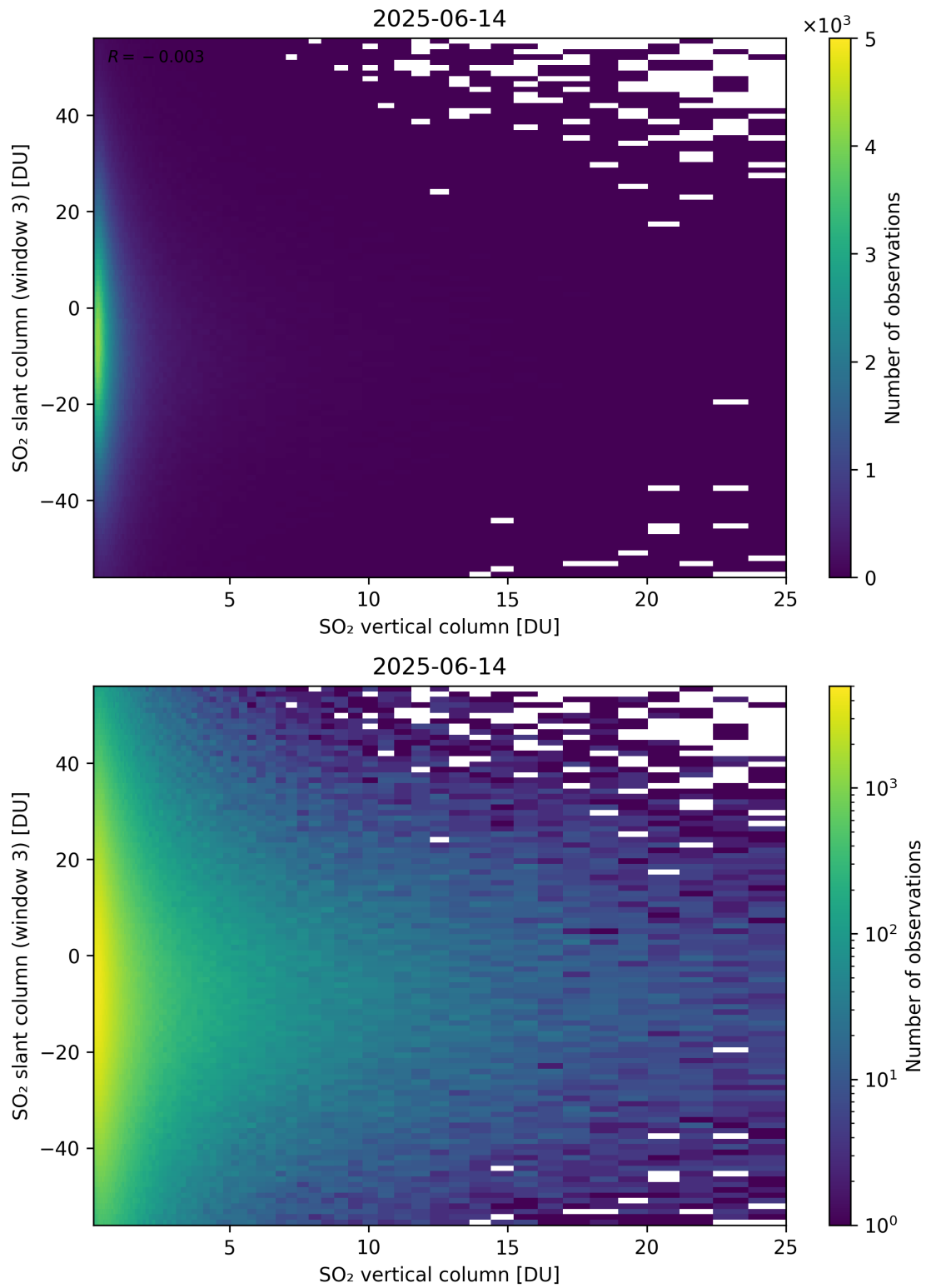
Figure 357: Scatter density plot of “SO 2 vertical column” against “SO 2 slant column (window 3)” for 2025-06-13 to 2025-06-15.
