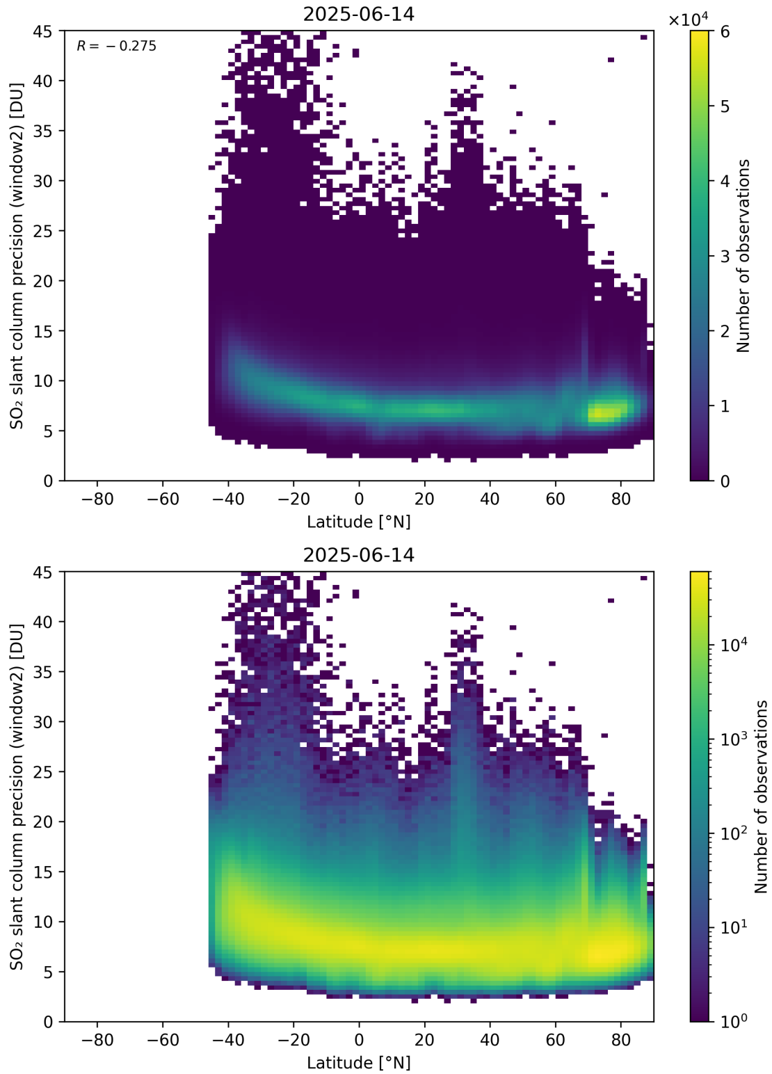
Figure 164: Scatter density plot of “Latitude” against “SO 2 slant column precision (window2)” for 2025-06-13 to 2025-06-15.
