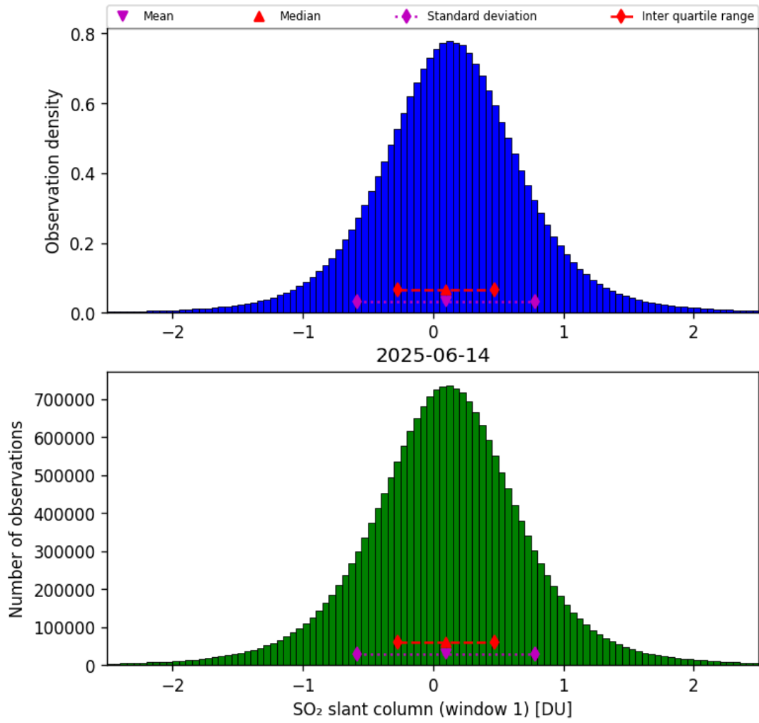
Figure 63: Histogram of “SO 2 slant column (window 1)” for 2025-06-13 to 2025-06-15
