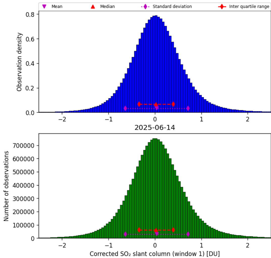
Figure 65: Histogram of “Corrected SO 2 slant column (window 1)” for 2025-06-13 to 2025-06-15
