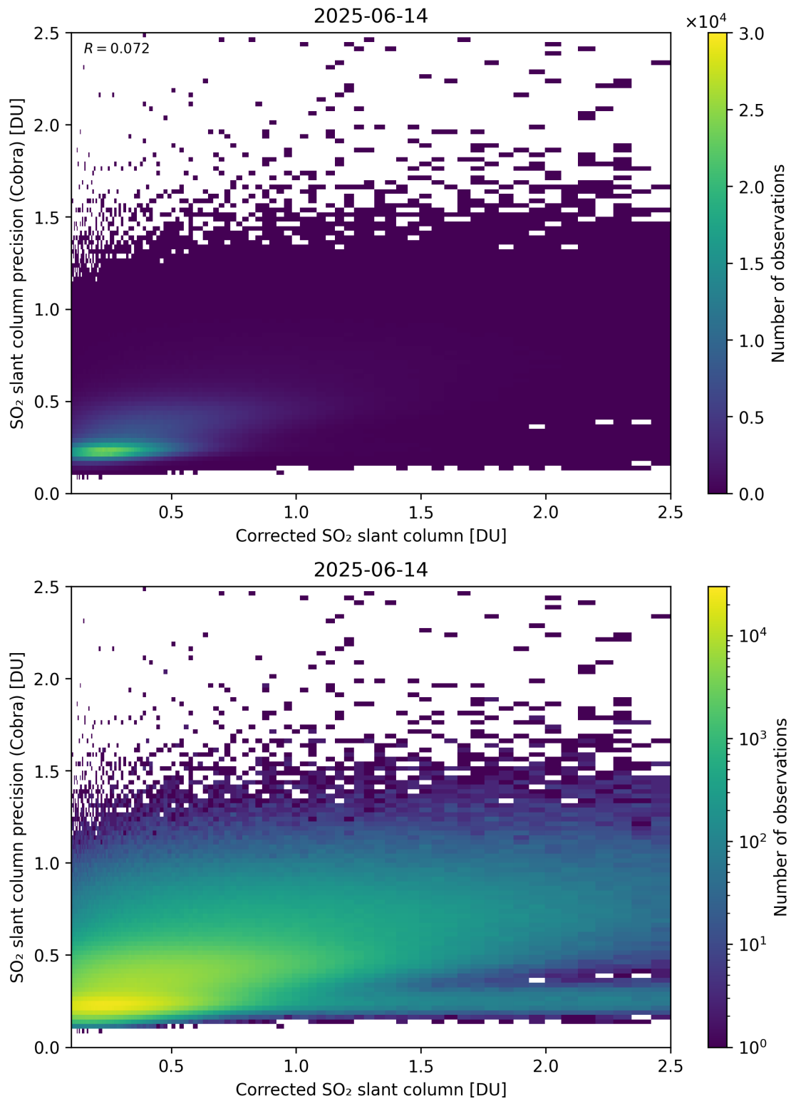
Figure 234: Scatter density plot of “Corrected SO 2 slant column” against “SO 2 slant column precision (Cobra)” for 2025-06-13 to 2025-06-15.
