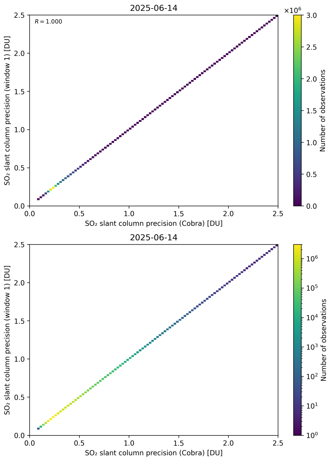
Figure 209: Scatter density plot of “SO 2 slant column precision (Cobra)” against “SO 2 slant column precision (window 1)” for 2025-06-13 to 2025-06-15.
