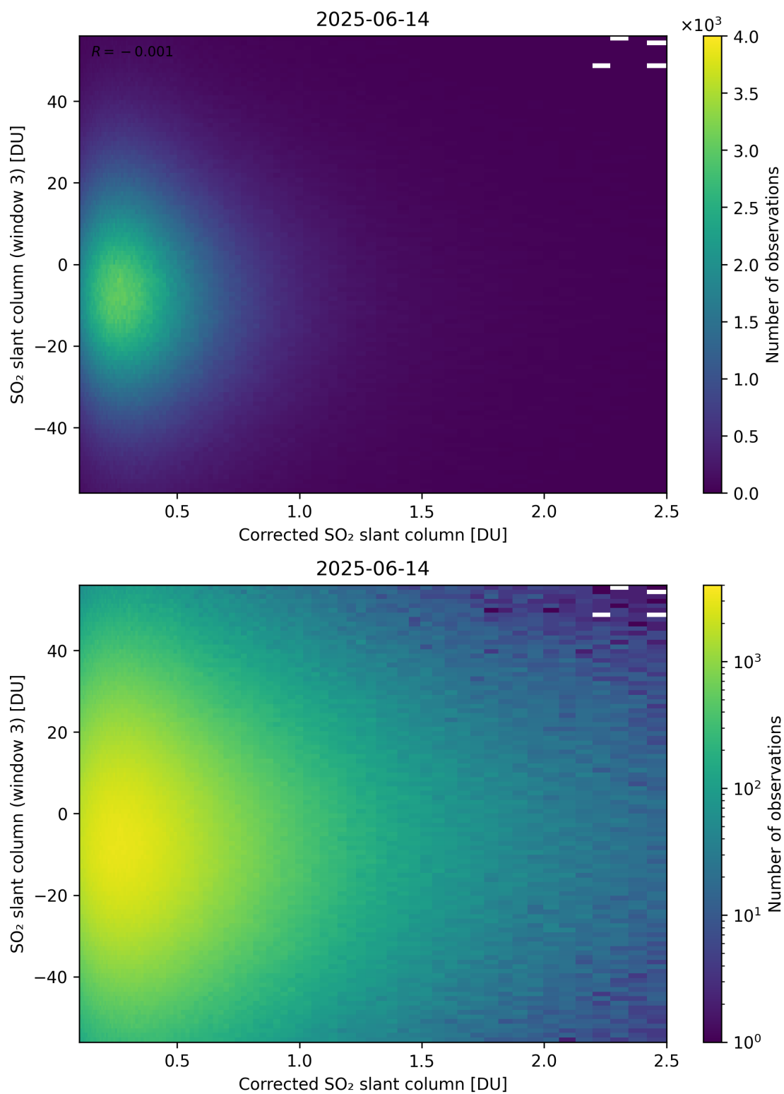
Figure 240: Scatter density plot of “Corrected SO 2 slant column” against “SO 2 slant column (window 3)” for 2025-06-13 to 2025-06-15.
