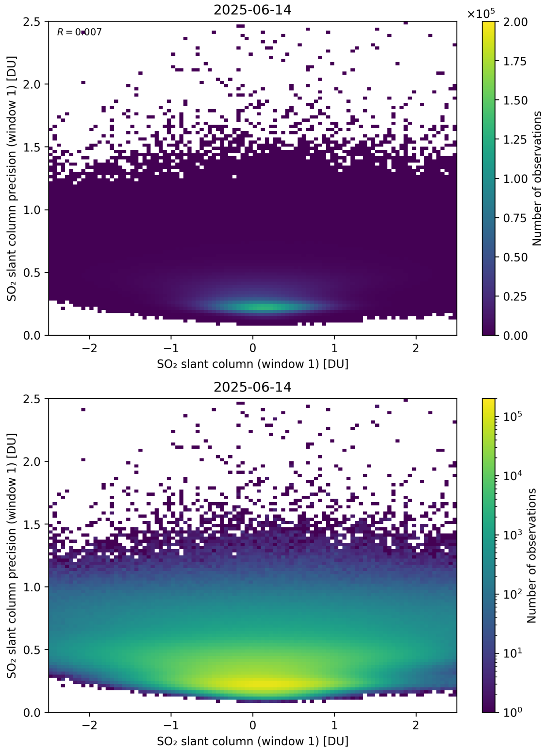
Figure 285: Scatter density plot of “SO 2 slant column (window 1)” against “SO 2 slant column precision (window 1)” for 2025-06-13 to 2025-06-15.
