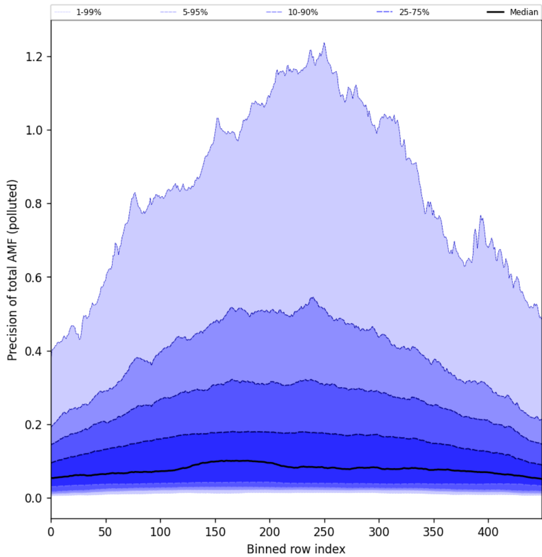
Figure 106: Along track statistics of “Precision of total AMF (polluted)” for 2025-06-13 to 2025-06-15
