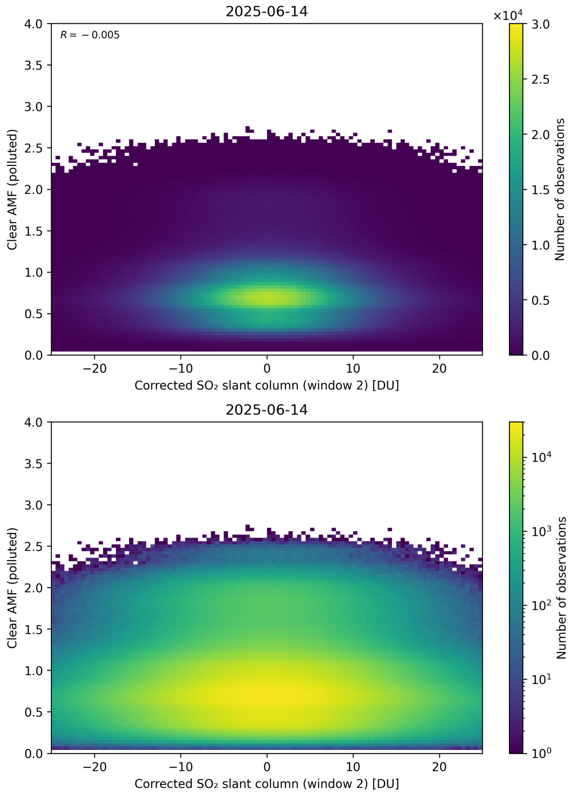
Figure 249: Scatter density plot of “Corrected SO 2 slant column (window 2)” against “Clear AMF (polluted)” for 2025-06-13 to 2025-06-15.
