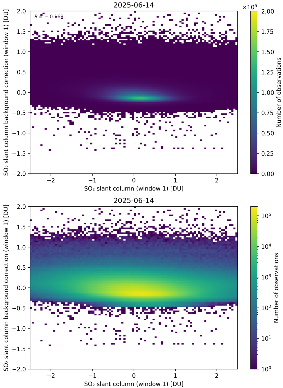
Figure 262: Scatter density plot of “SO 2 slant column (window 1)” against “SO 2 slant column background correction (window 1)” for 2025-06-13 to 2025-06-15.
