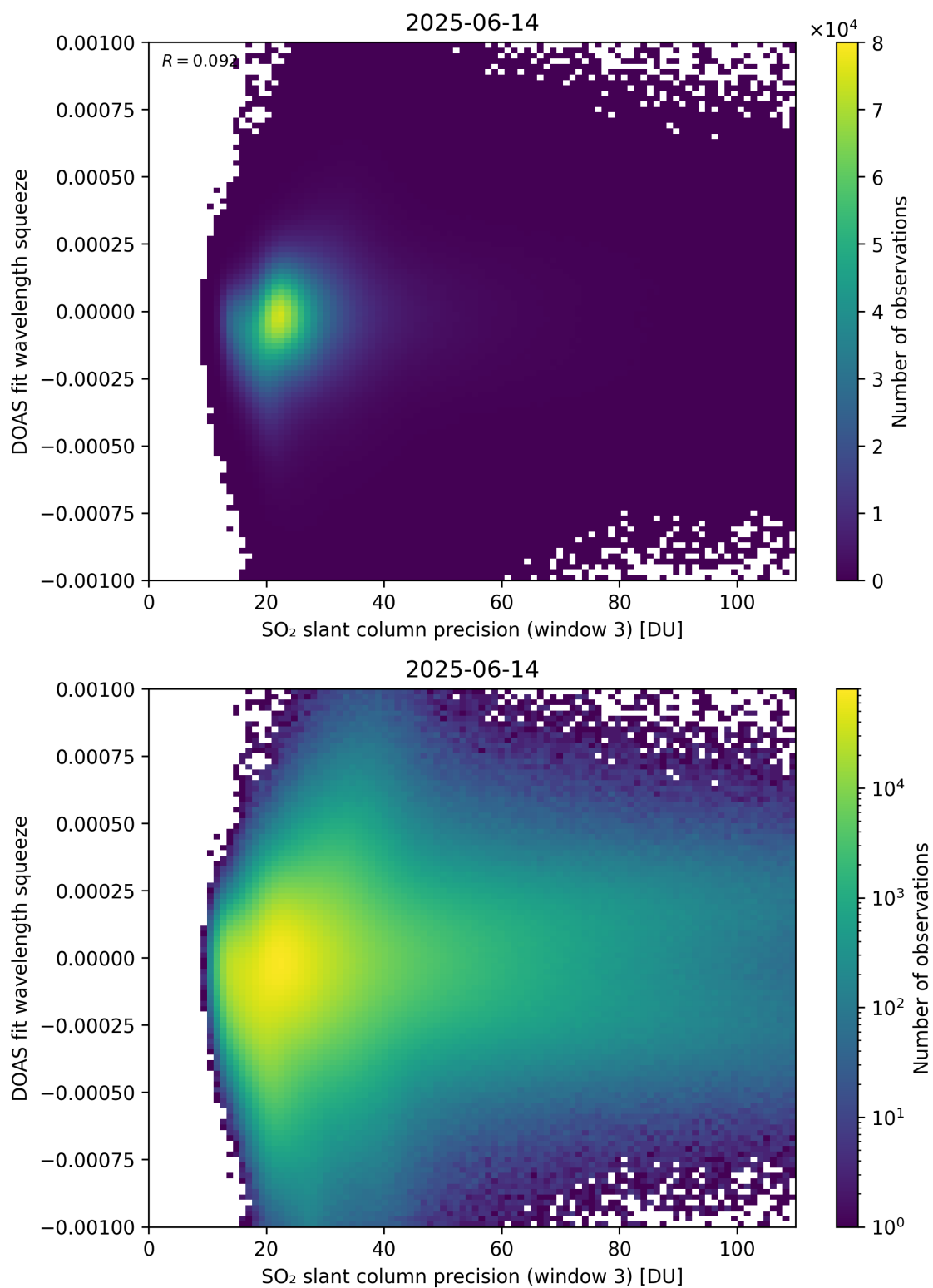
Figure 309: Scatter density plot of “SO 2 slant column precision (window 3)” against “DOAS fit wavelength squeeze” for 2025-06-13 to 2025-06-15.
