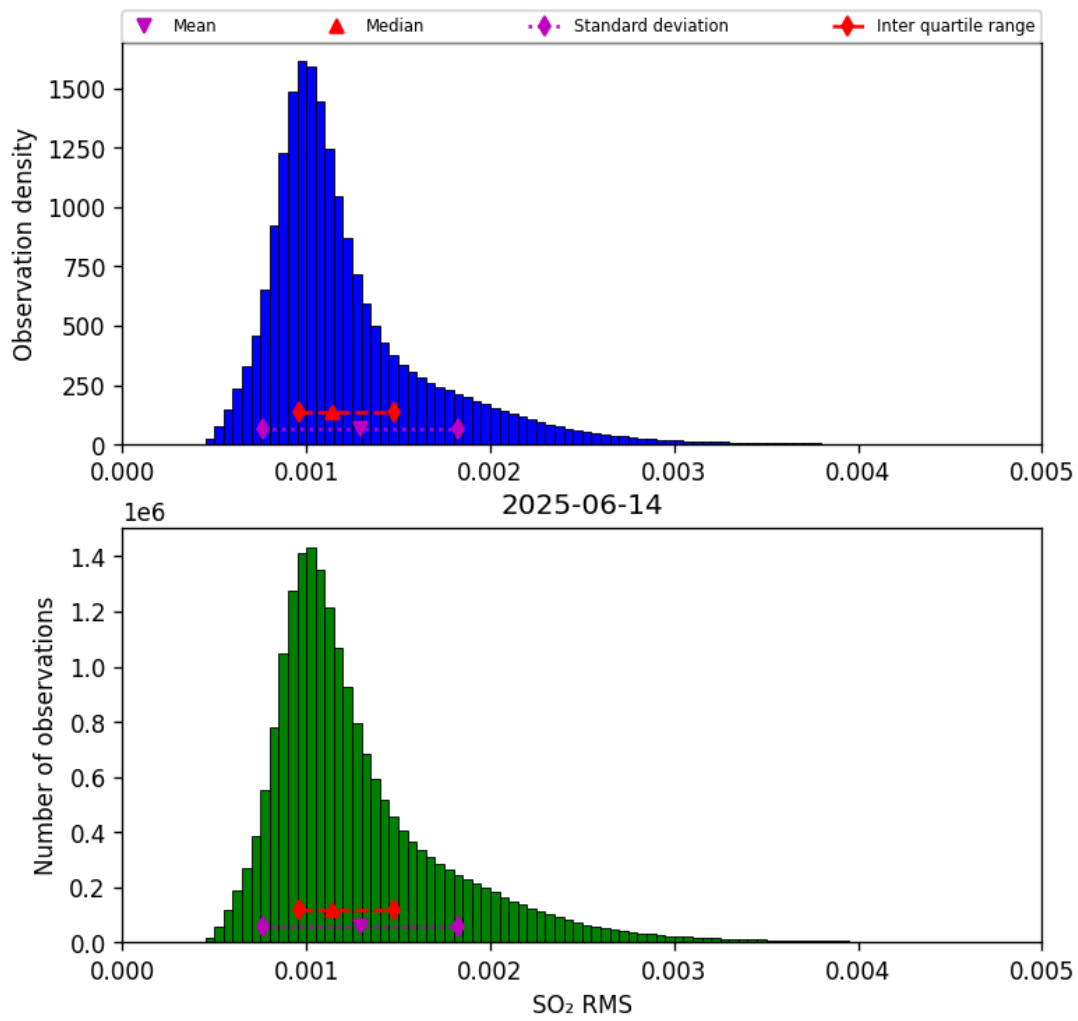
Figure 78: Histogram of “SO 2 RMS” for 2025-06-13 to 2025-06-15
