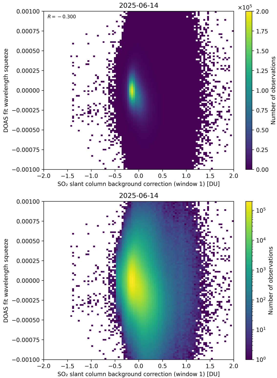
Figure 112: Scatter density plot of “SO 2 slant column background correction (window 1)” against “DOAS fit wavelength squeeze” for 2025-06-13 to 2025-06-15.
