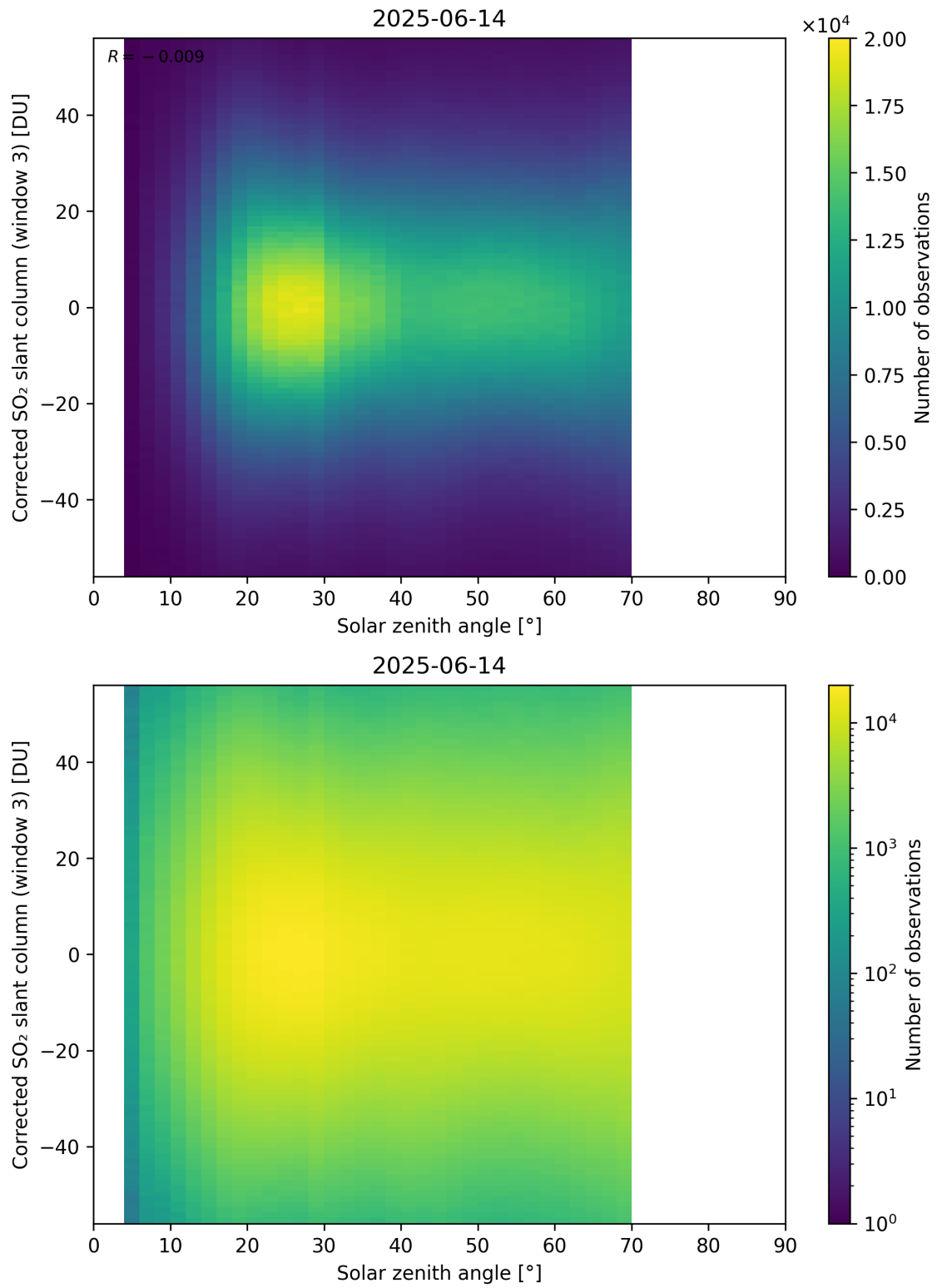
Figure 183: Scatter density plot of “Solar zenith angle” against “Corrected SO 2 slant column (window 3)” for 2025-06-13 to 2025-06-15.
