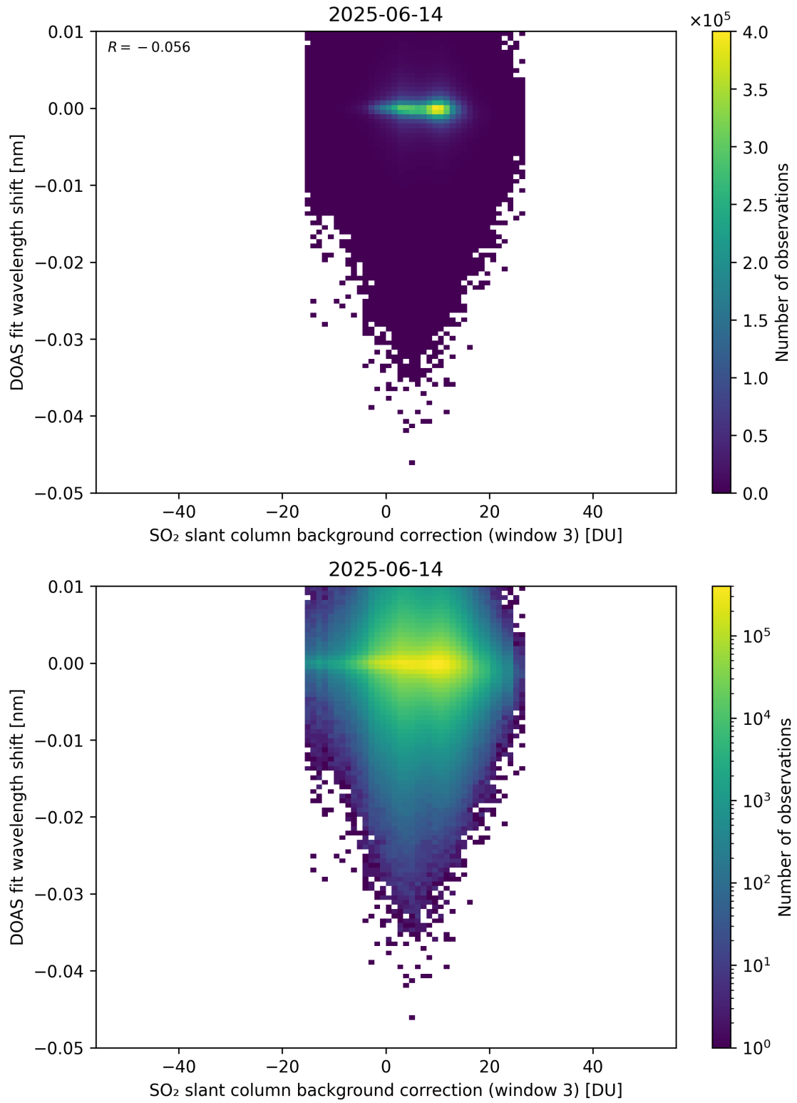
Figure 132: Scatter density plot of “SO 2 slant column background correction (window 3)” against “DOAS fit wavelength shift” for 2025-06-13 to 2025-06-15.
