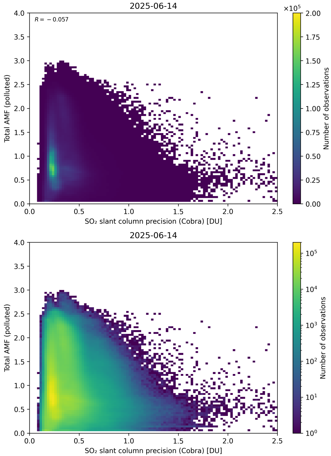
Figure 213: Scatter density plot of “SO 2 slant column precision (Cobra)” against “Total AMF (polluted)” for 2025-06-13 to 2025-06-15.
