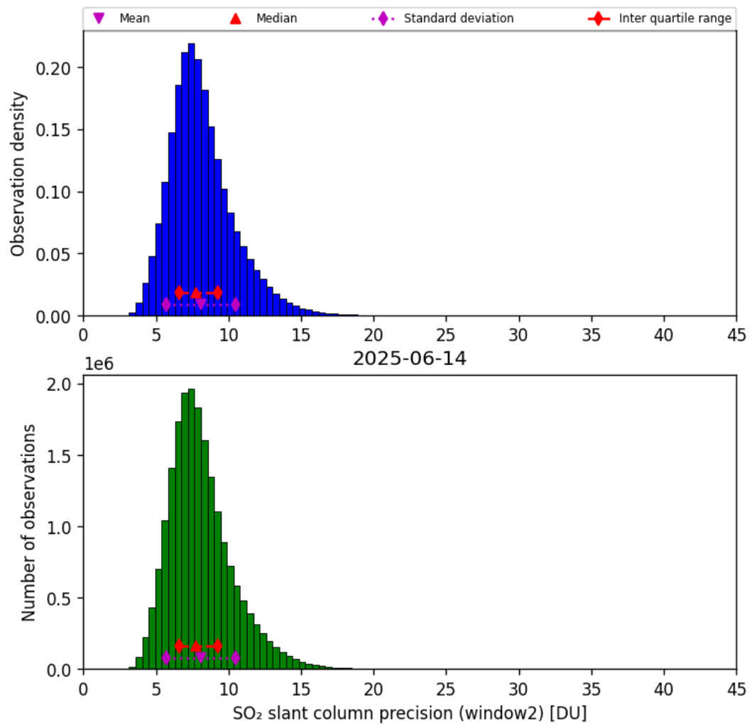
Figure 68: Histogram of “SO 2 slant column precision (window2)” for 2025-06-13 to 2025-06-15
