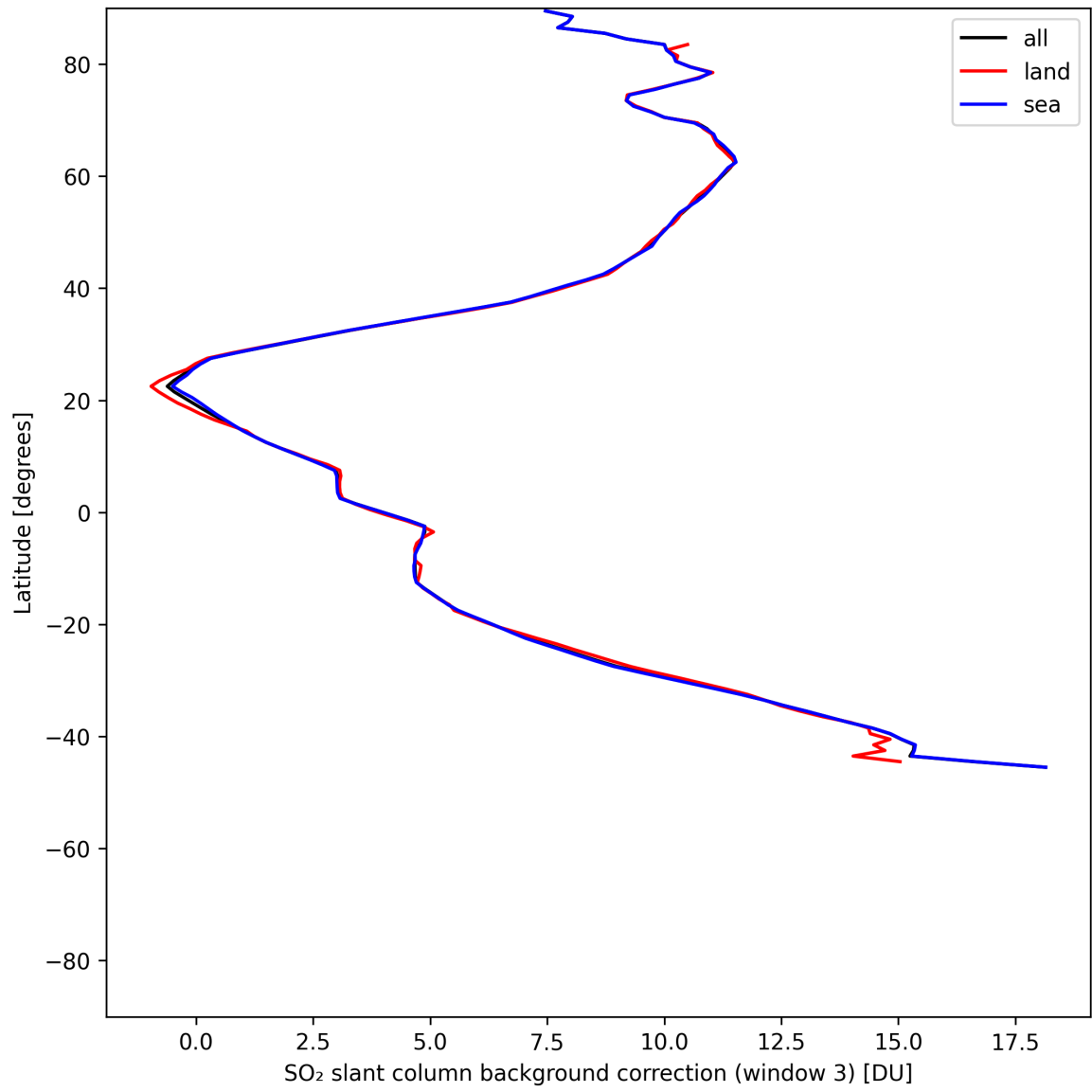
Figure 48: Zonal average of “SO 2 slant column background correction (window 3)” for 2025-06-13 to 2025-06-15.
