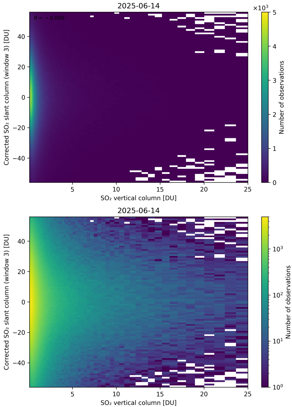
Figure 353: Scatter density plot of “SO 2 vertical column” against “Corrected SO 2 slant column (window 3)” for 2025-06-13 to 2025-06-15.
