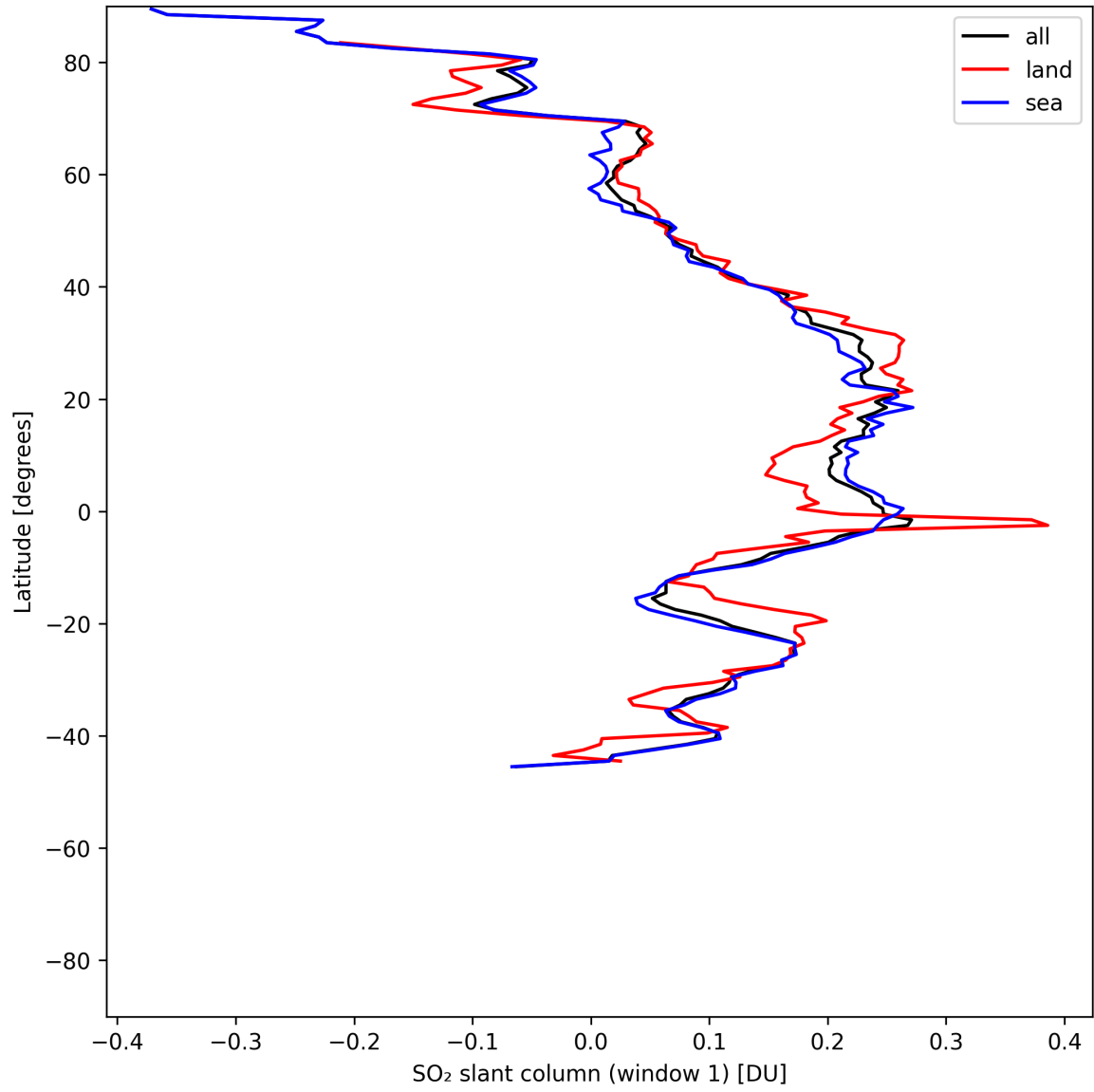
Figure 37: Zonal average of “SO 2 slant column (window 1)” for 2025-06-13 to 2025-06-15.
