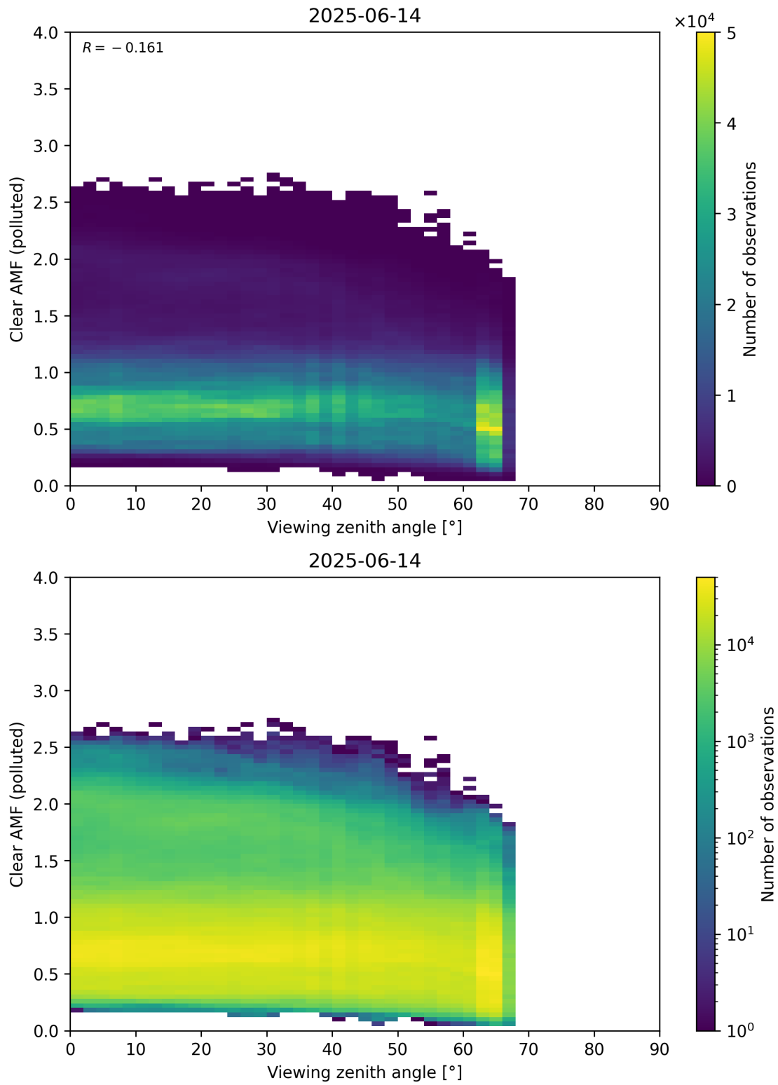
Figure 370: Scatter density plot of “Viewing zenith angle” against “Clear AMF (polluted)” for 2025-06-13 to 2025-06-15.
