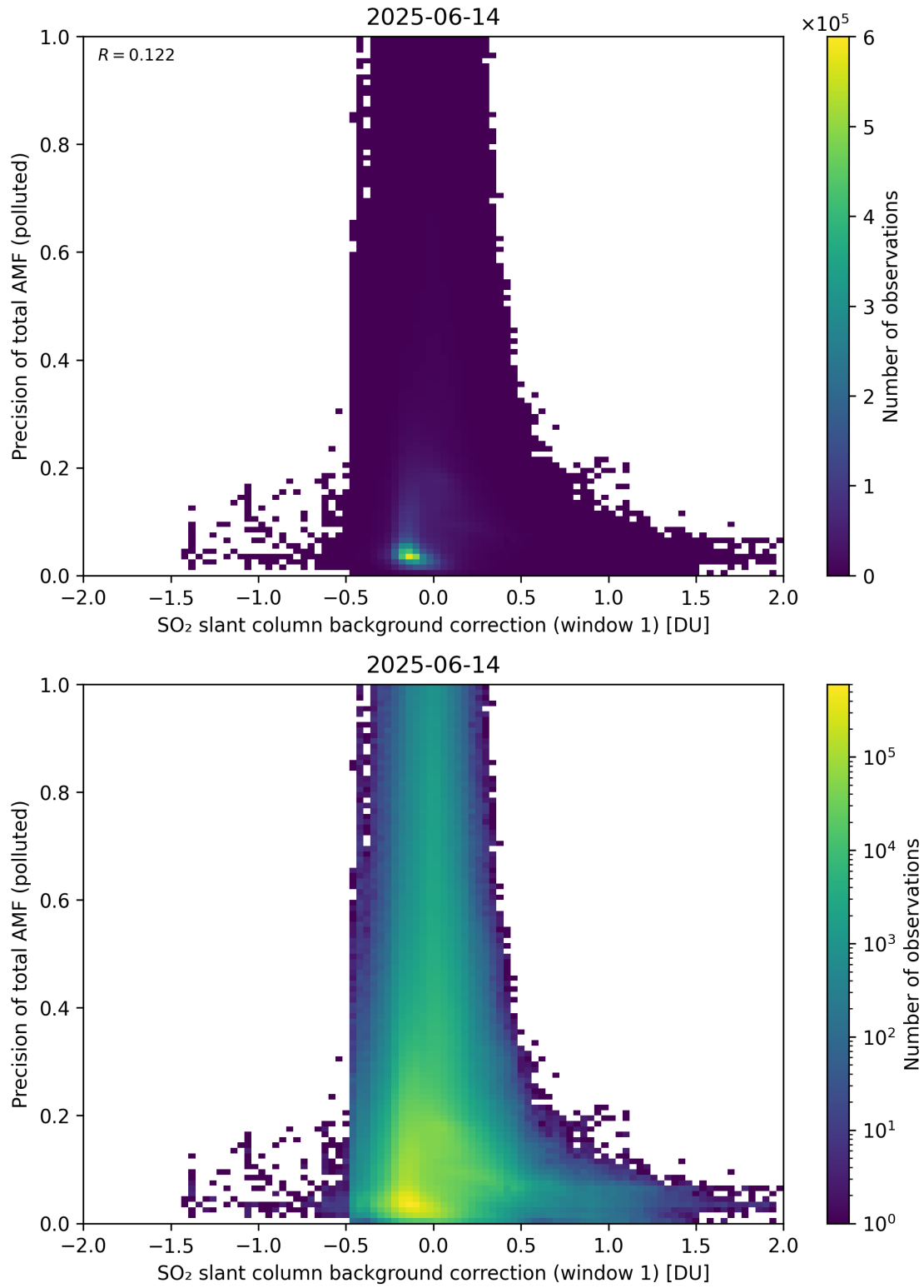
Figure 121: Scatter density plot of “SO 2 slant column background correction (window 1)” against “Precision of total AMF (polluted)” for 2025-06-13 to 2025-06-15.
