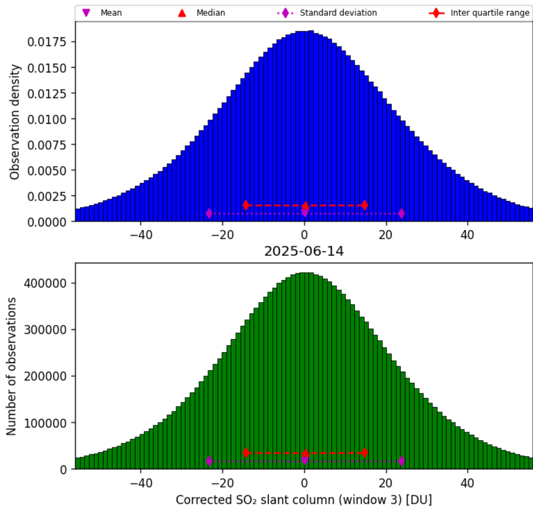
Figure 73: Histogram of “Corrected SO 2 slant column (window 3)” for 2025-06-13 to 2025-06-15
