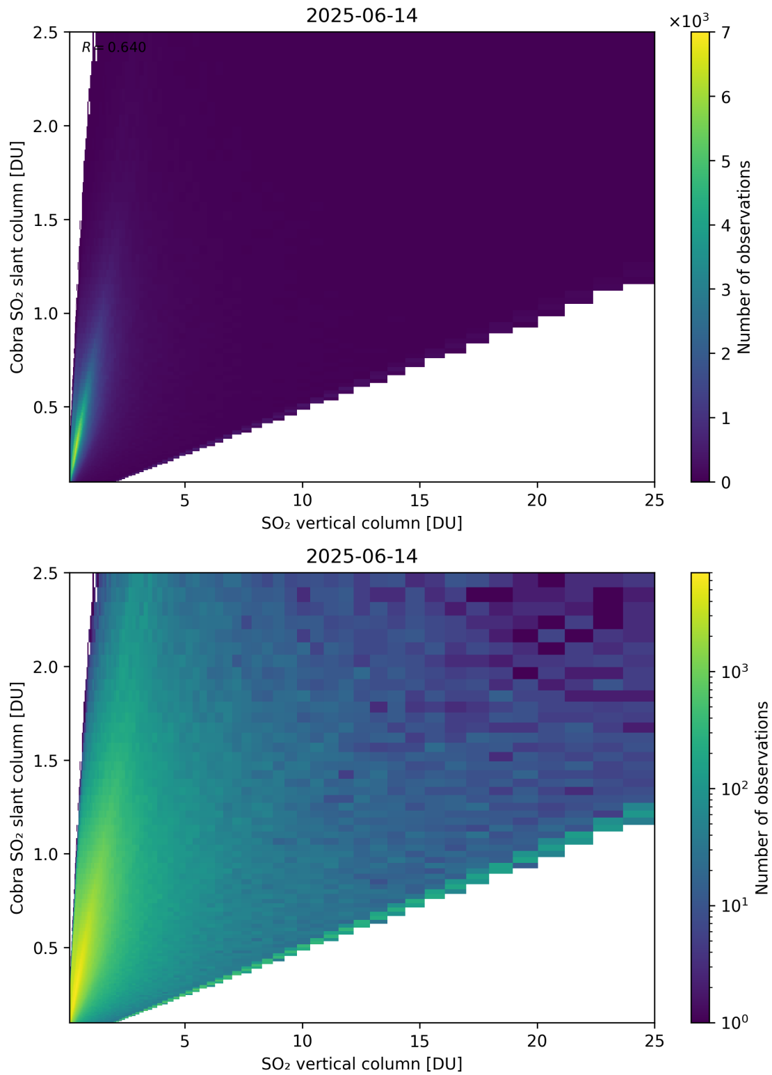
Figure 349: Scatter density plot of “SO 2 vertical column” against “Cobra SO 2 slant column” for 2025-06-13 to 2025-06-15.
