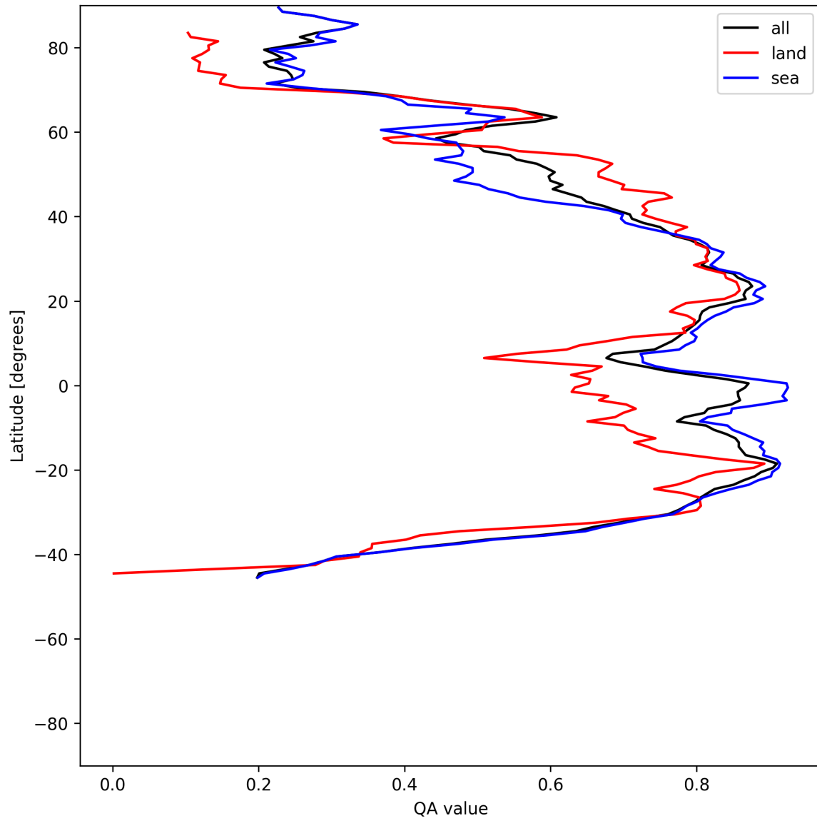
Figure 31: Zonal average of “QA value” for 2025-06-13 to 2025-06-15.
