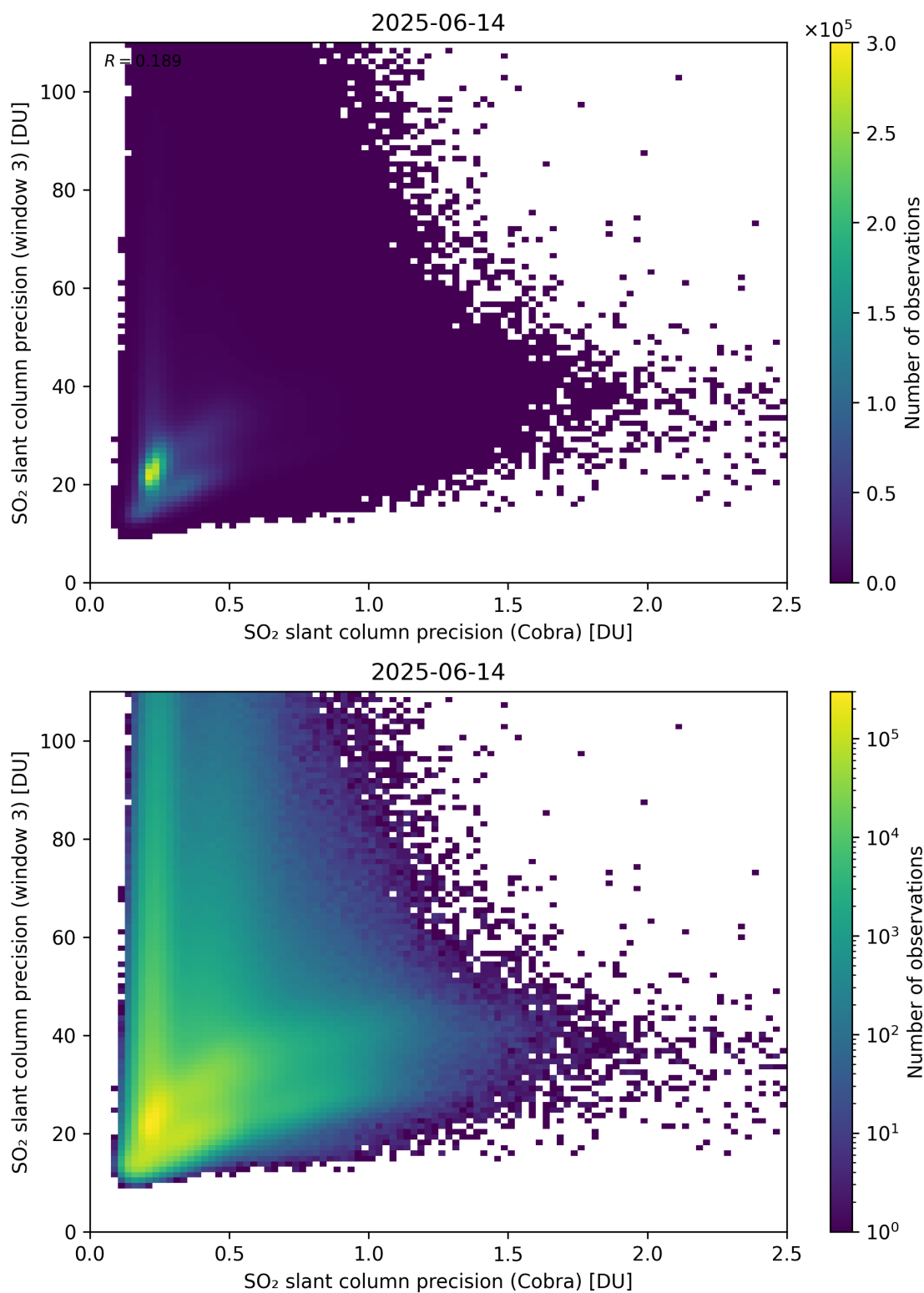
Figure 212: Scatter density plot of “SO 2 slant column precision (Cobra)” against “SO 2 slant column precision (window 3)” for 2025-06-13 to 2025-06-15.
