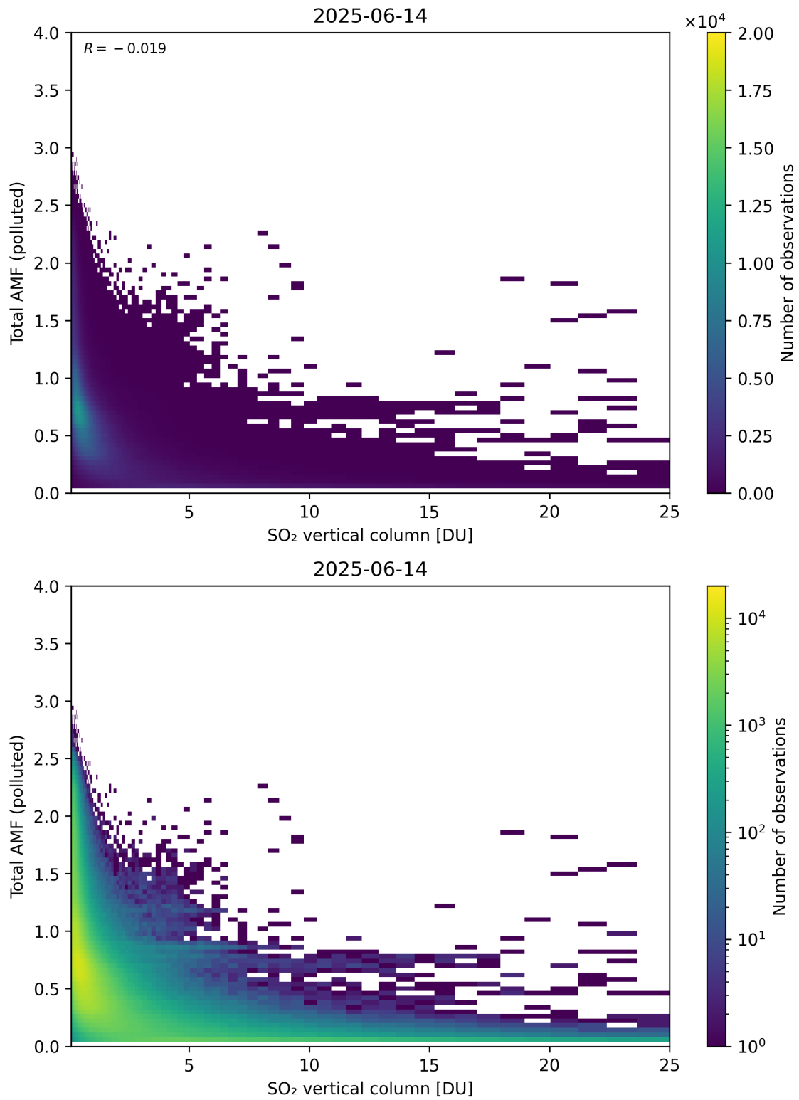
Figure 359: Scatter density plot of “SO 2 vertical column” against “Total AMF (polluted)” for 2025-06-13 to 2025-06-15.
