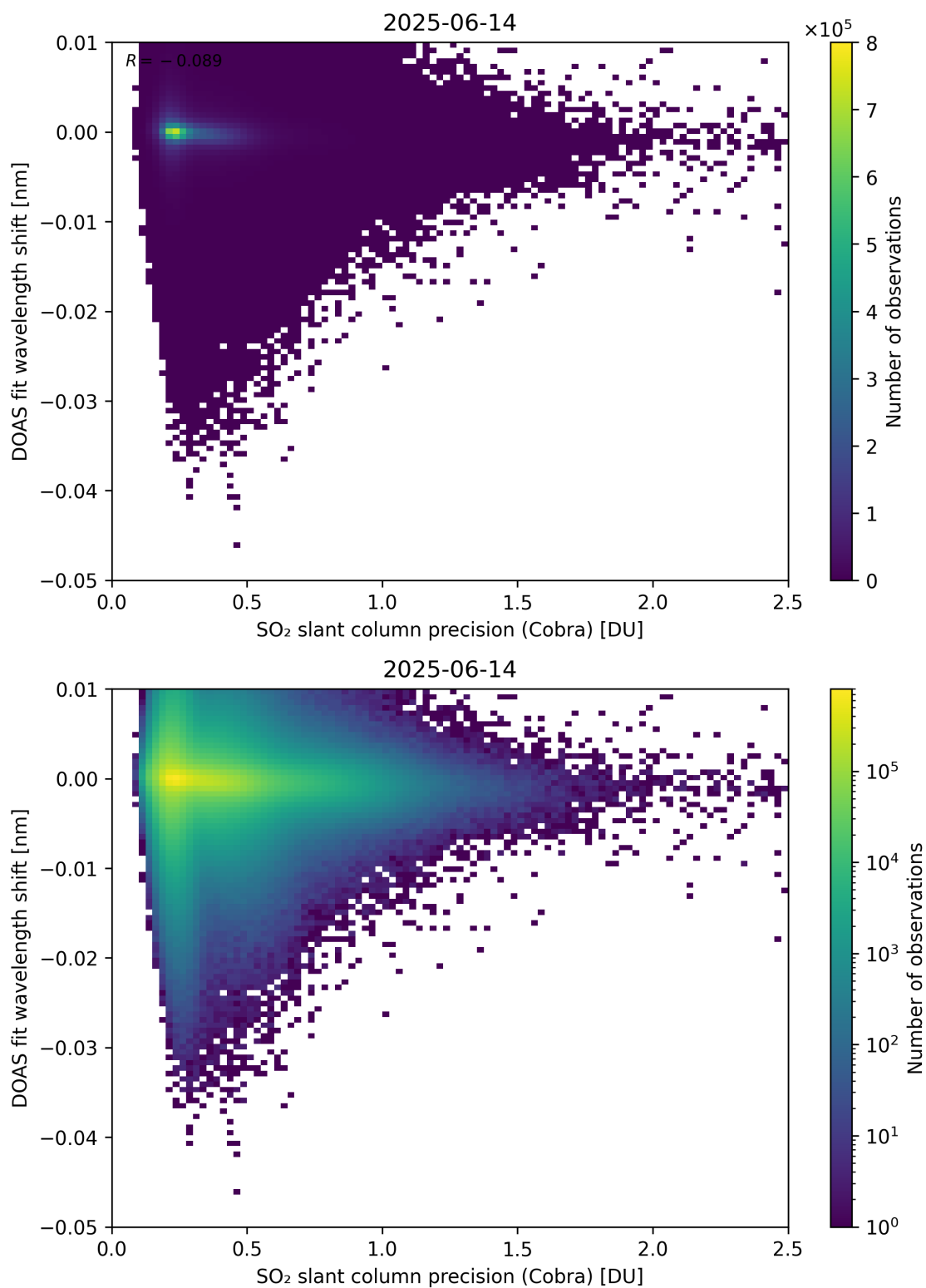
Figure 202: Scatter density plot of “SO 2 slant column precision (Cobra)” against “DOAS fit wavelength shift” for 2025-06-13 to 2025-06-15.
