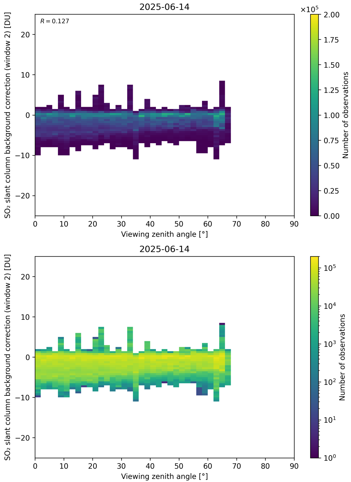
Figure 363: Scatter density plot of “Viewing zenith angle” against “SO 2 slant column background correction (window 2)” for 2025-06-13 to 2025-06-15.
