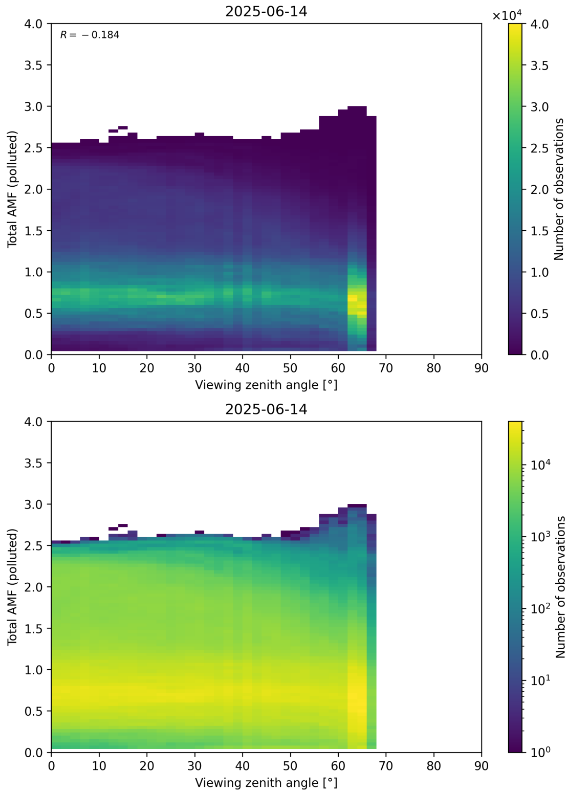
Figure 381: Scatter density plot of “Viewing zenith angle” against “Total AMF (polluted)” for 2025-06-13 to 2025-06-15.
