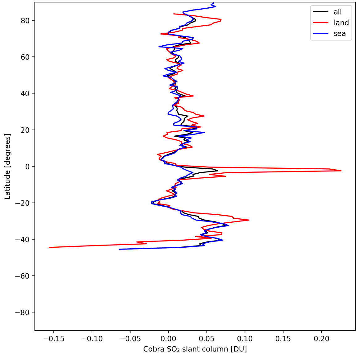
Figure 35: Zonal average of “Cobra SO 2 slant column” for 2025-06-13 to 2025-06-15.
