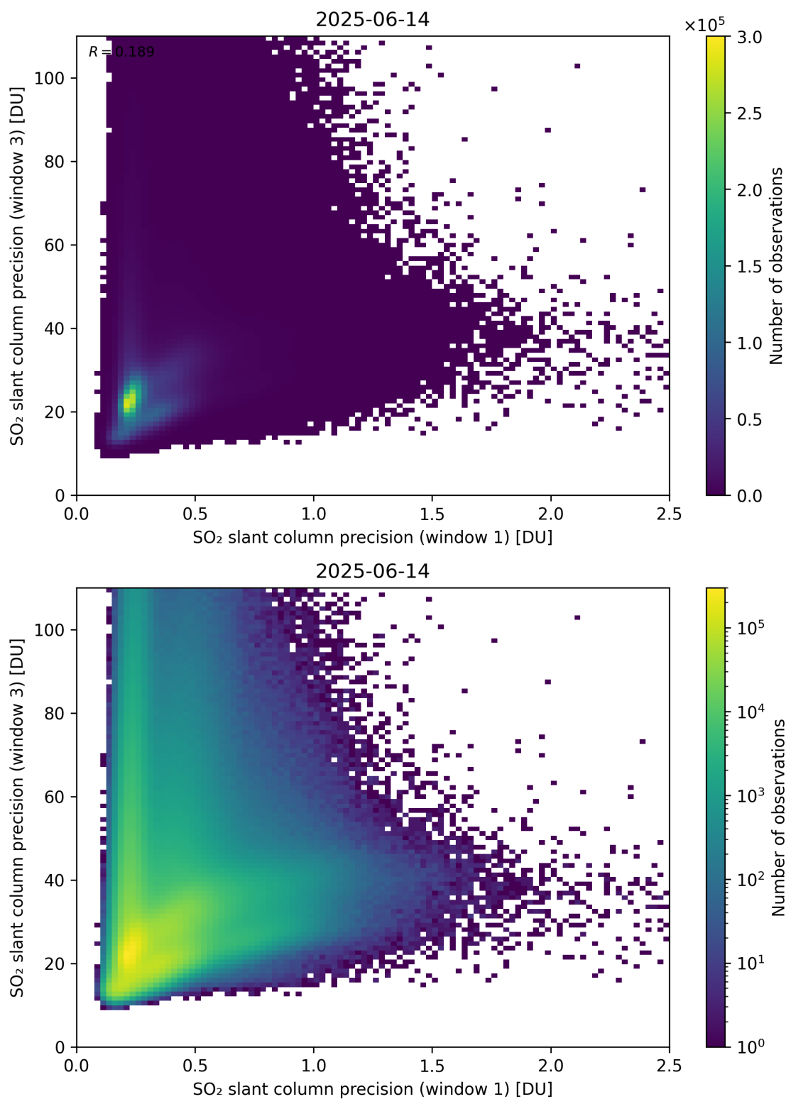
Figure 279: Scatter density plot of “SO 2 slant column precision (window 1)” against “SO 2 slant column precision (window 3)” for 2025-06-13 to 2025-06-15.
