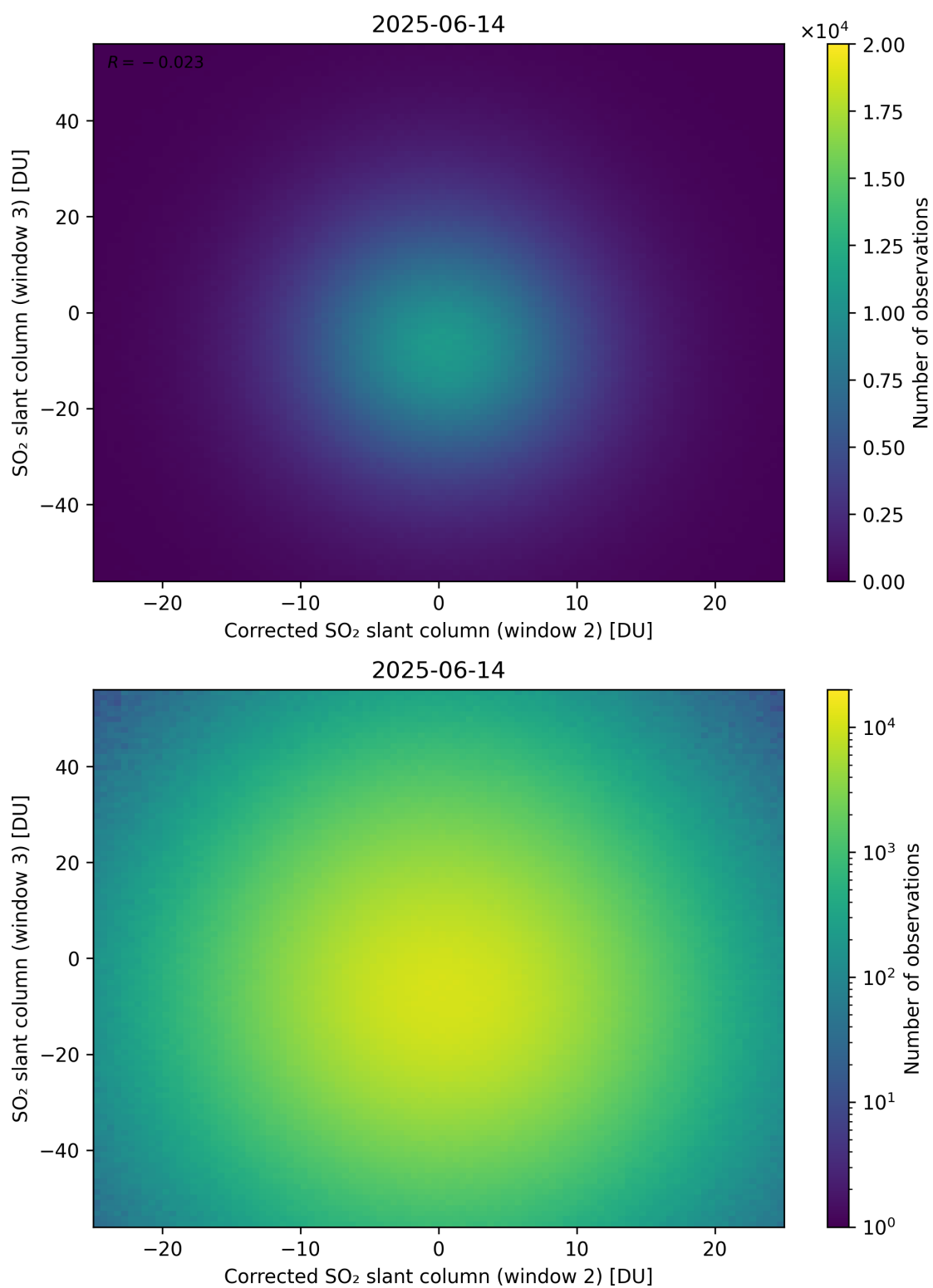
Figure 251: Scatter density plot of “Corrected SO 2 slant column (window 2)” against “SO 2 slant column (window 3)” for 2025-06-13 to 2025-06-15.
