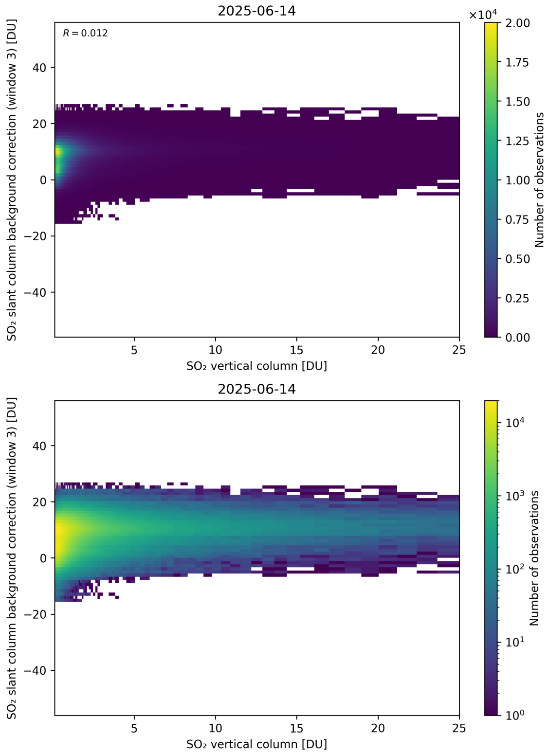
Figure 325: Scatter density plot of “SO 2 vertical column” against “SO 2 slant column background correction (window 3)” for 2025-06-13 to 2025-06-15.
