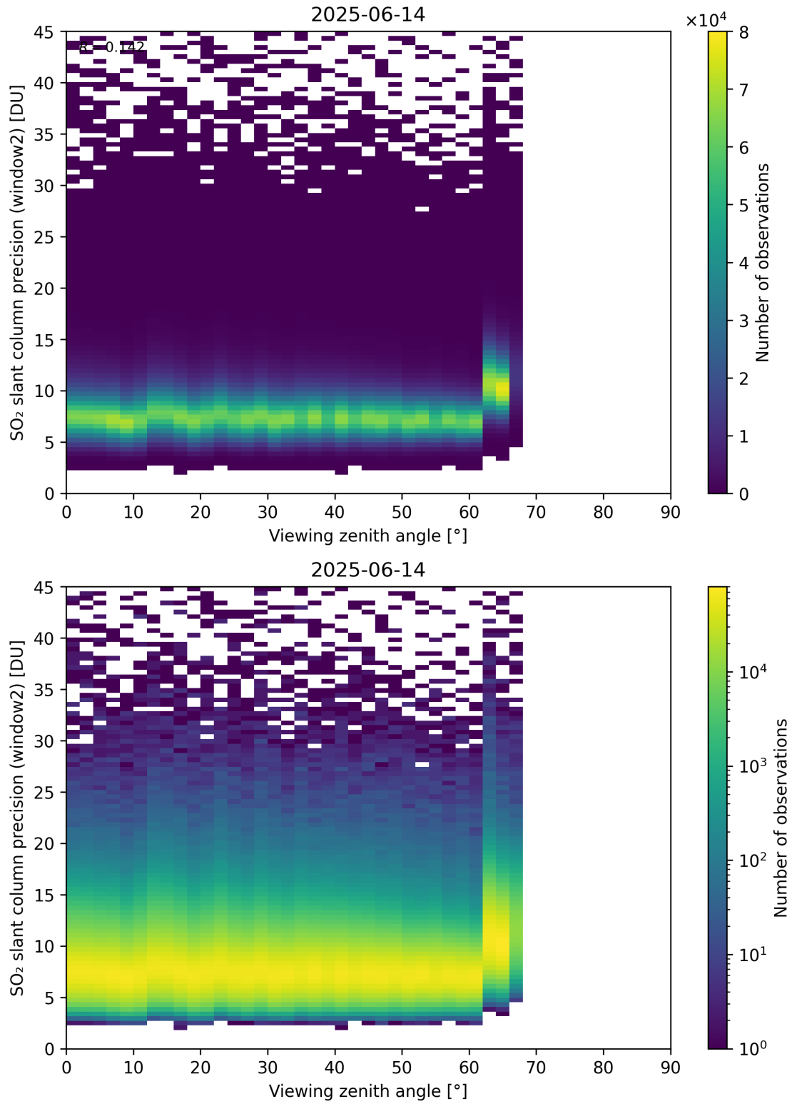
Figure 378: Scatter density plot of “Viewing zenith angle” against “SO 2 slant column precision (window2)” for 2025-06-13 to 2025-06-15.
