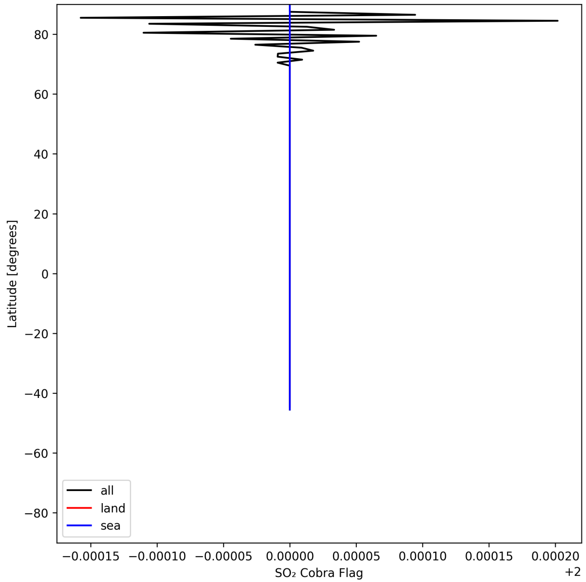
Figure 49: Zonal average of "SO 2 Cobra Flag" for 2025-06-13 to 2025-06-15.
