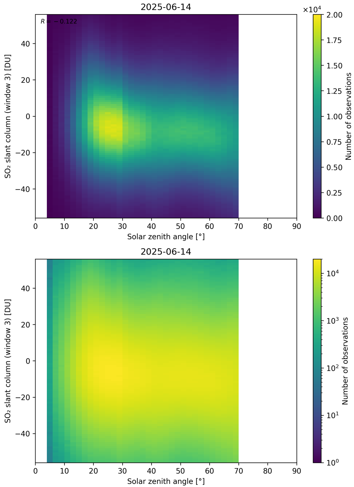
Figure 187: Scatter density plot of “Solar zenith angle” against “SO 2 slant column (window 3)” for 2025-06-13 to 2025-06-15.
