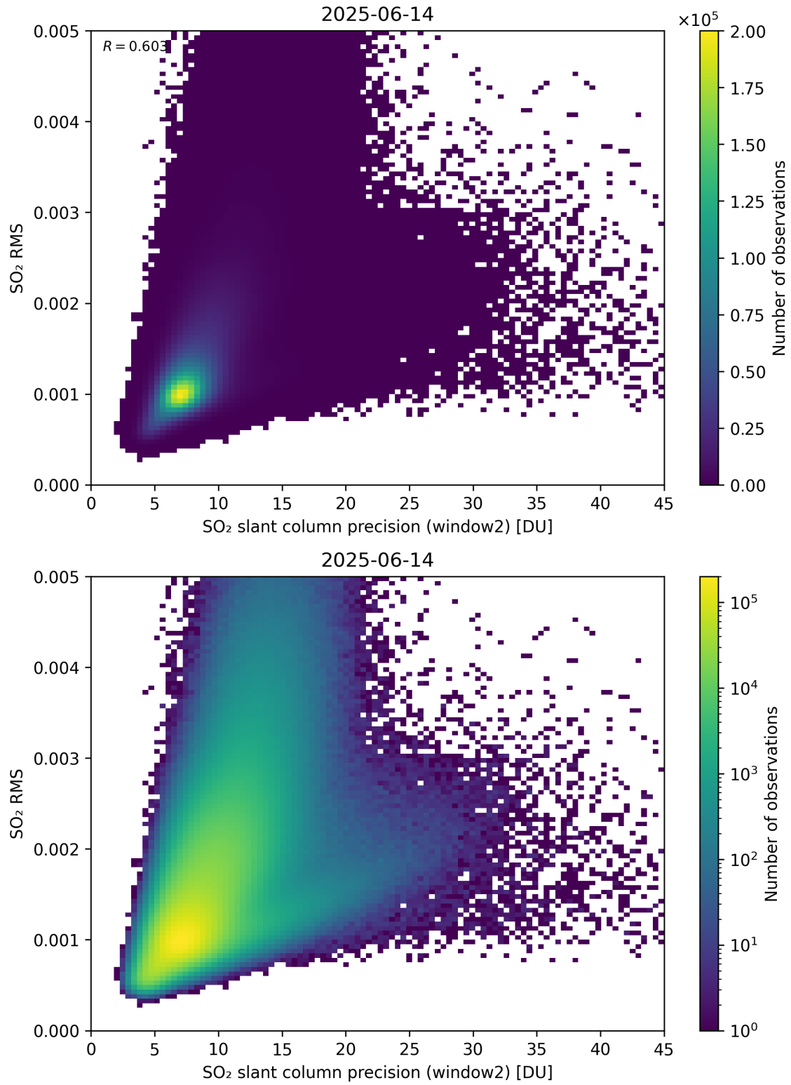
Figure 295: Scatter density plot of “SO 2 slant column precision (window2)” against “SO 2 RMS” for 2025-06-13 to 2025-06-15.
