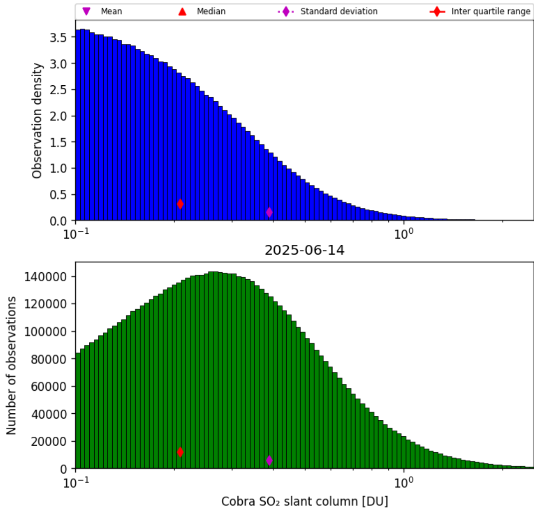
Figure 61: Histogram of “Cobra SO 2 slant column” for 2025-06-13 to 2025-06-15
