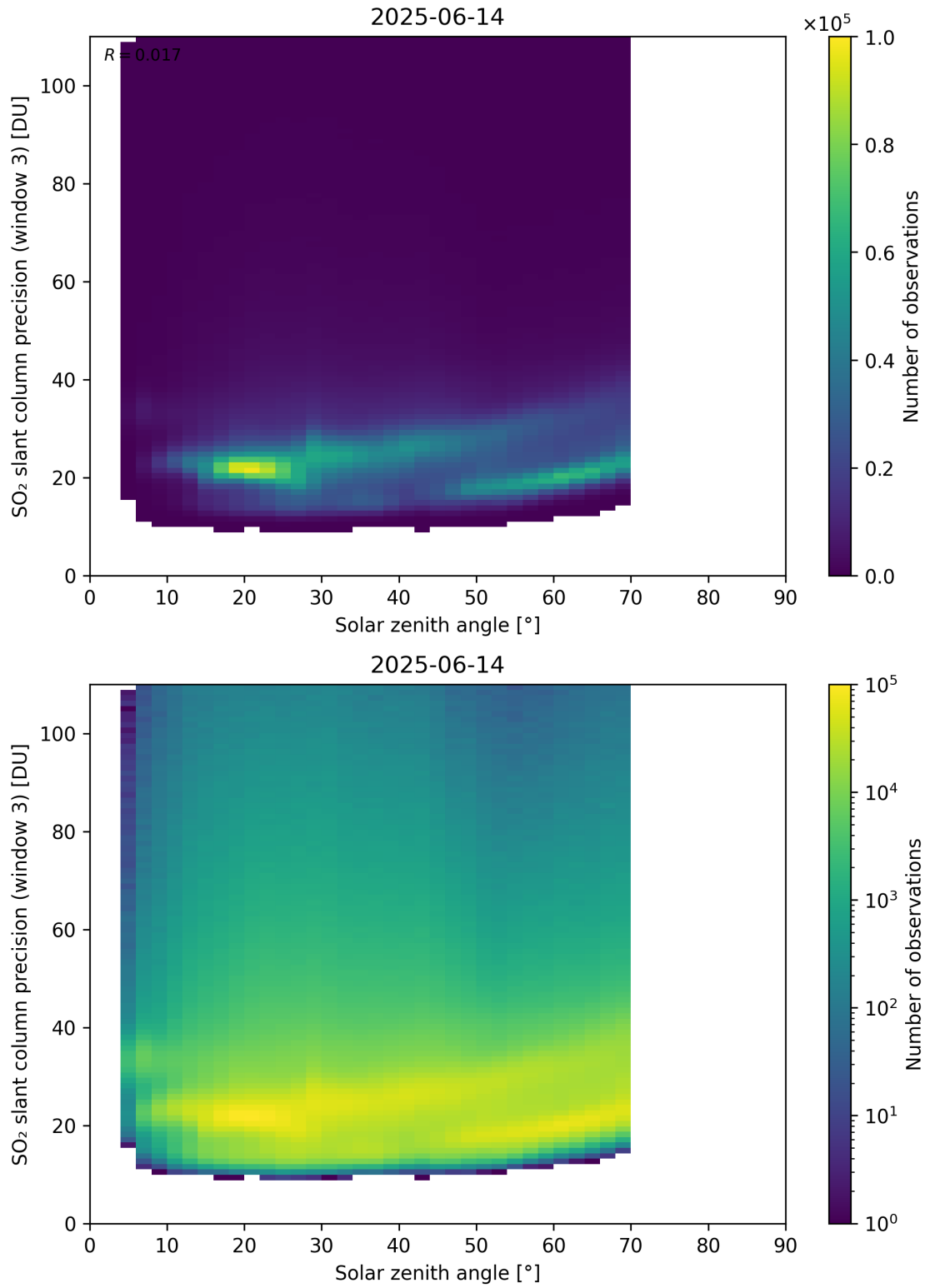
Figure 188: Scatter density plot of “Solar zenith angle” against “SO 2 slant column precision (window 3)” for 2025-06-13 to 2025-06-15.
