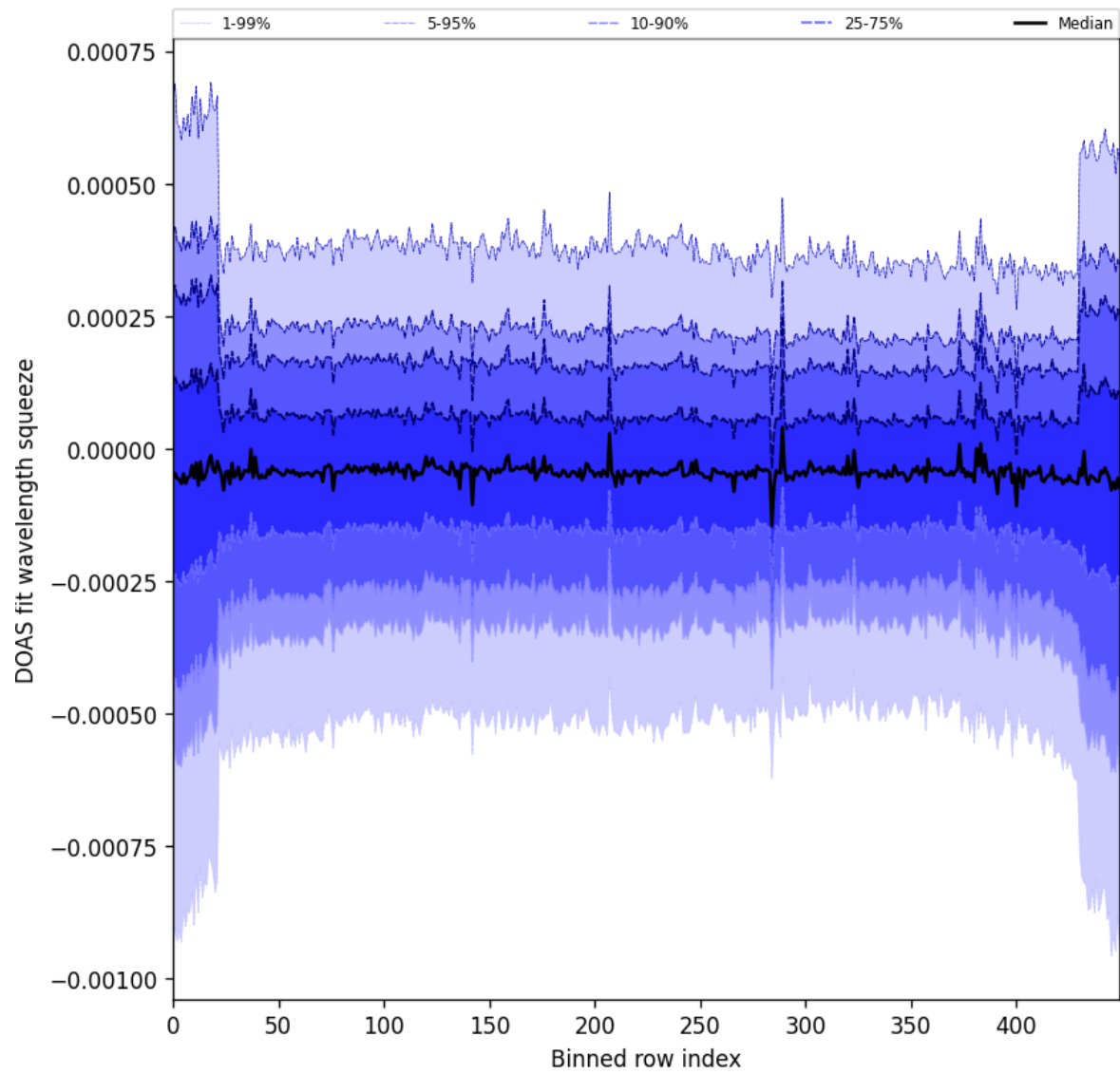
Figure 103: Along track statistics of “DOAS fit wavelength squeeze” for 2025-06-13 to 2025-06-15
