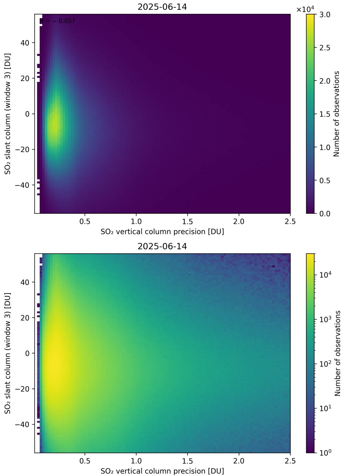
Figure 344: Scatter density plot of “SO 2 vertical column precision” against “SO 2 slant column (window 3)” for 2025-06-13 to 2025-06-15.
