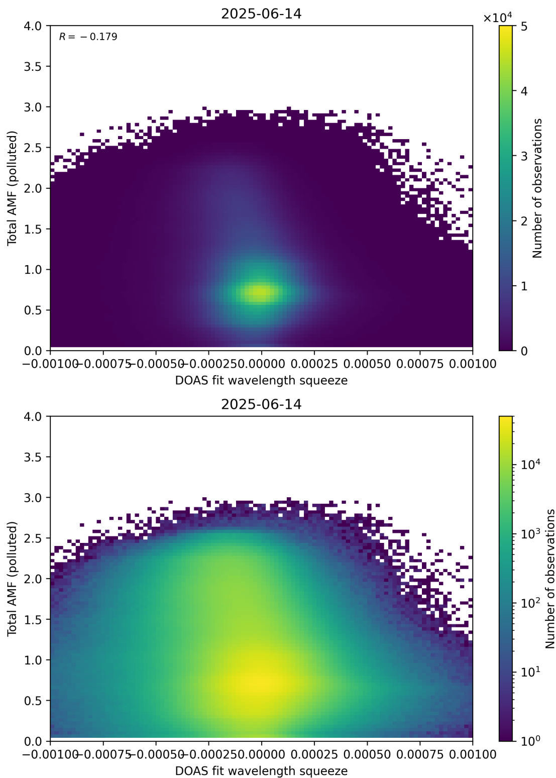
Figure 145: Scatter density plot of “DOAS fit wavelength squeeze” against “Total AMF (polluted)” for 2025-06-13 to 2025-06-15.
