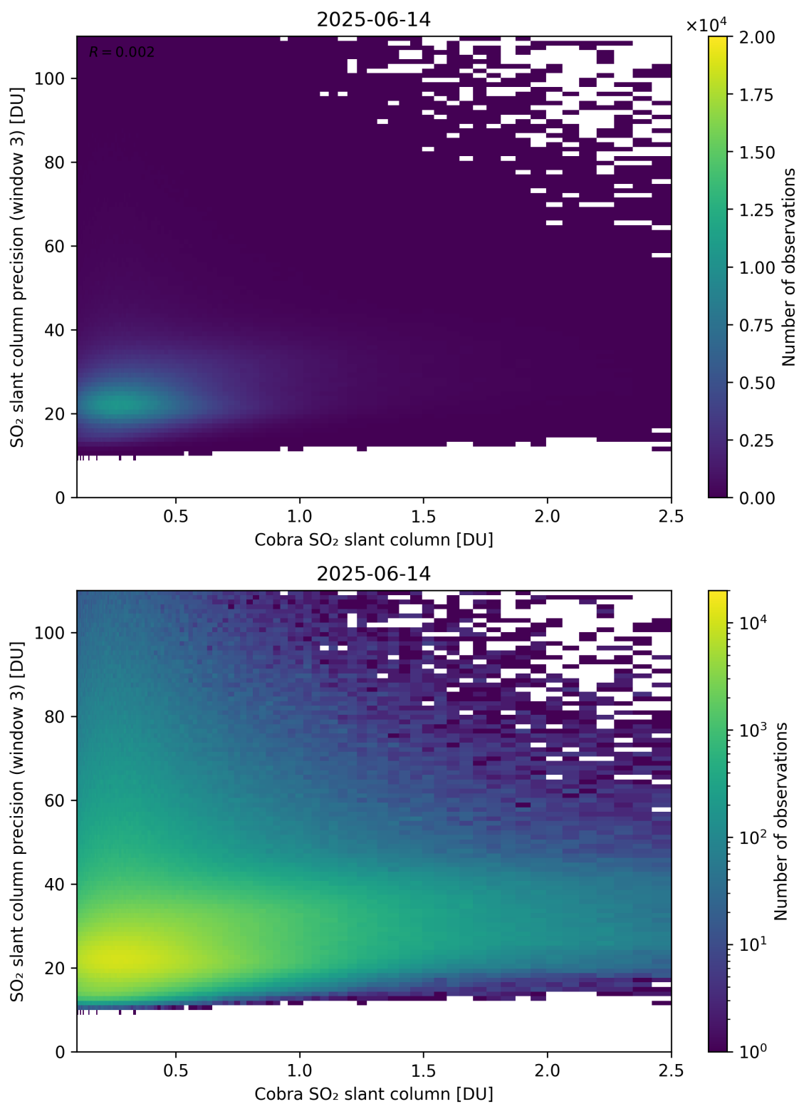
Figure 223: Scatter density plot of “Cobra SO 2 slant column” against “SO 2 slant column precision (window 3)” for 2025-06-13 to 2025-06-15.
