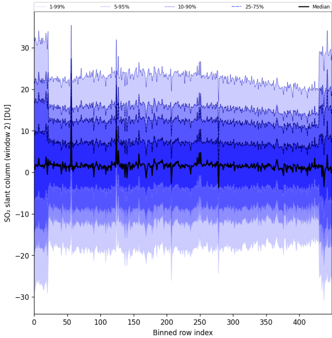
Figure 93: Along track statistics of “SO 2 slant column (window 2)” for 2025-06-13 to 2025-06-15
