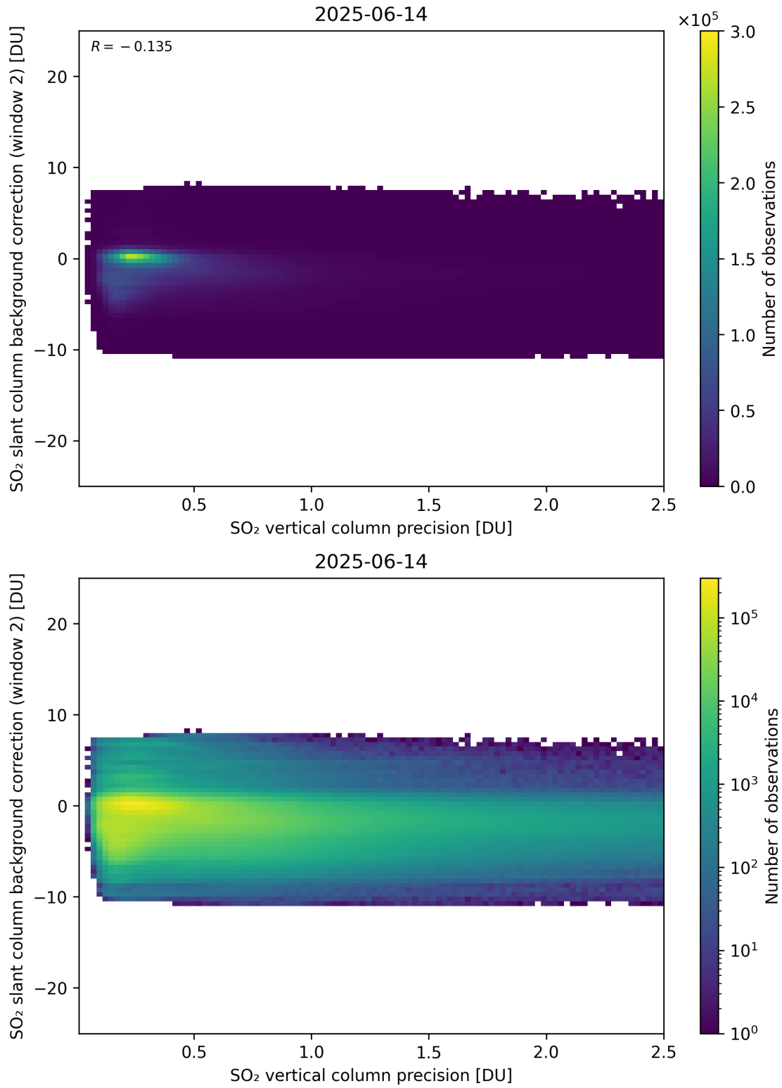
Figure 330: Scatter density plot of “SO 2 vertical column precision” against “SO 2 slant column background correction (window 2)” for 2025-06-13 to 2025-06-15.
