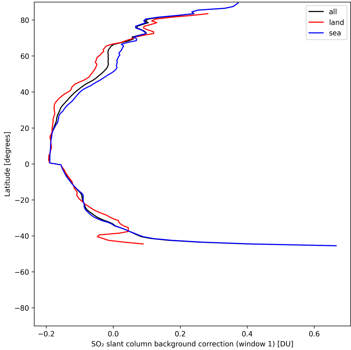
Figure 40: Zonal average of “SO 2 slant column background correction (window 1)” for 2025-06-13 to 2025-06-15.
