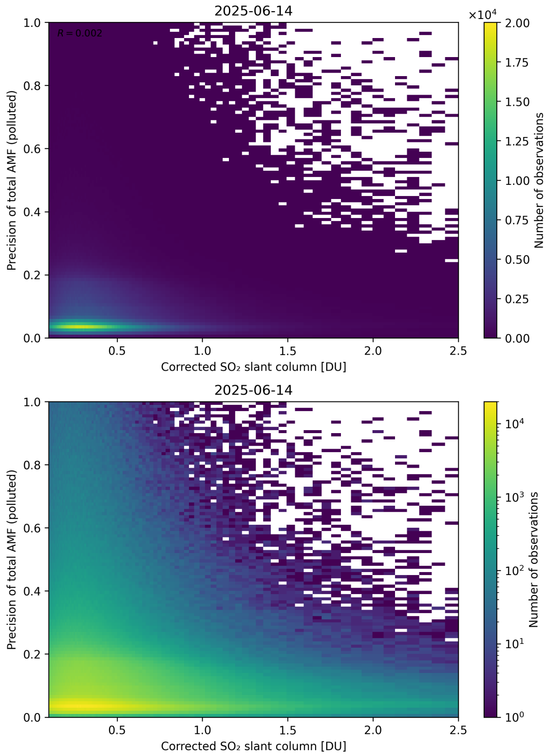
Figure 243: Scatter density plot of “Corrected SO 2 slant column” against “Precision of total AMF (polluted)” for 2025-06-13 to 2025-06-15.
