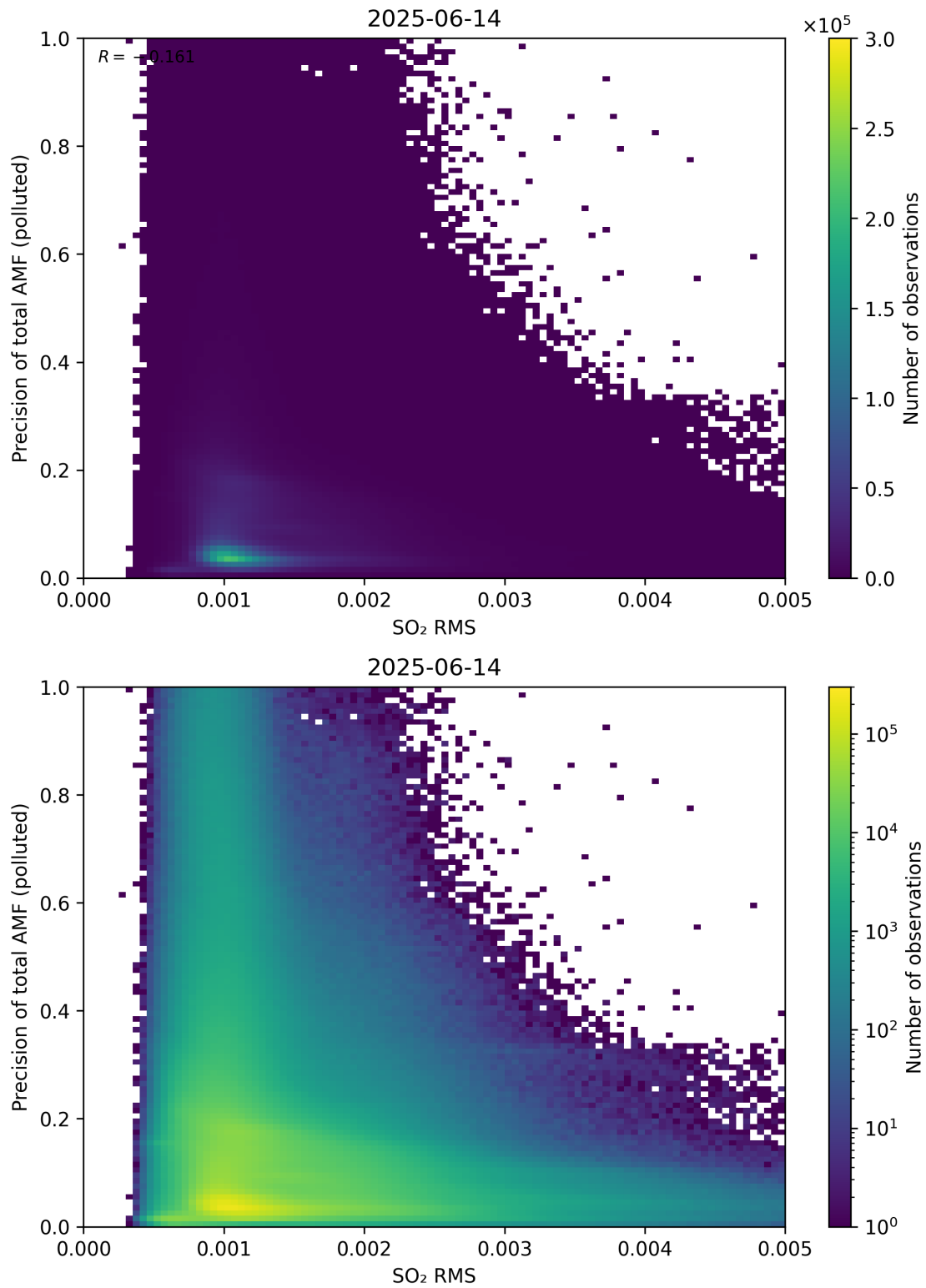
Figure 149: Scatter density plot of “SO 2 RMS” against “Precision of total AMF (polluted)” for 2025-06-13 to 2025-06-15.
