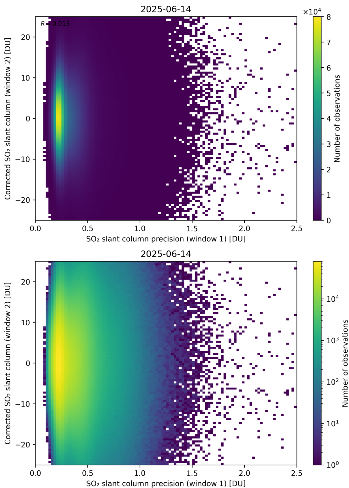
Figure 275: Scatter density plot of “SO 2 slant column precision (window 1)” against “Corrected SO 2 slant column (window 2)” for 2025-06-13 to 2025-06-15.
