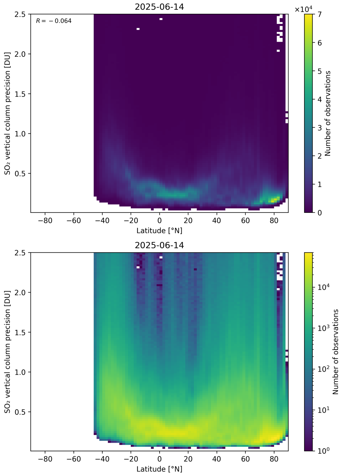
Figure 170: Scatter density plot of “Latitude” against “SO 2 vertical column precision” for 2025-06-13 to 2025-06-15.
