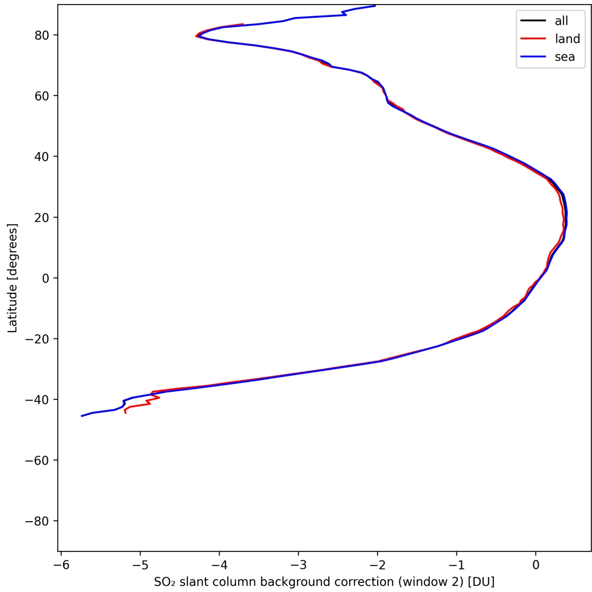
Figure 44: Zonal average of “SO 2 slant column background correction (window 2)” for 2025-06-13 to 2025-06-15.
