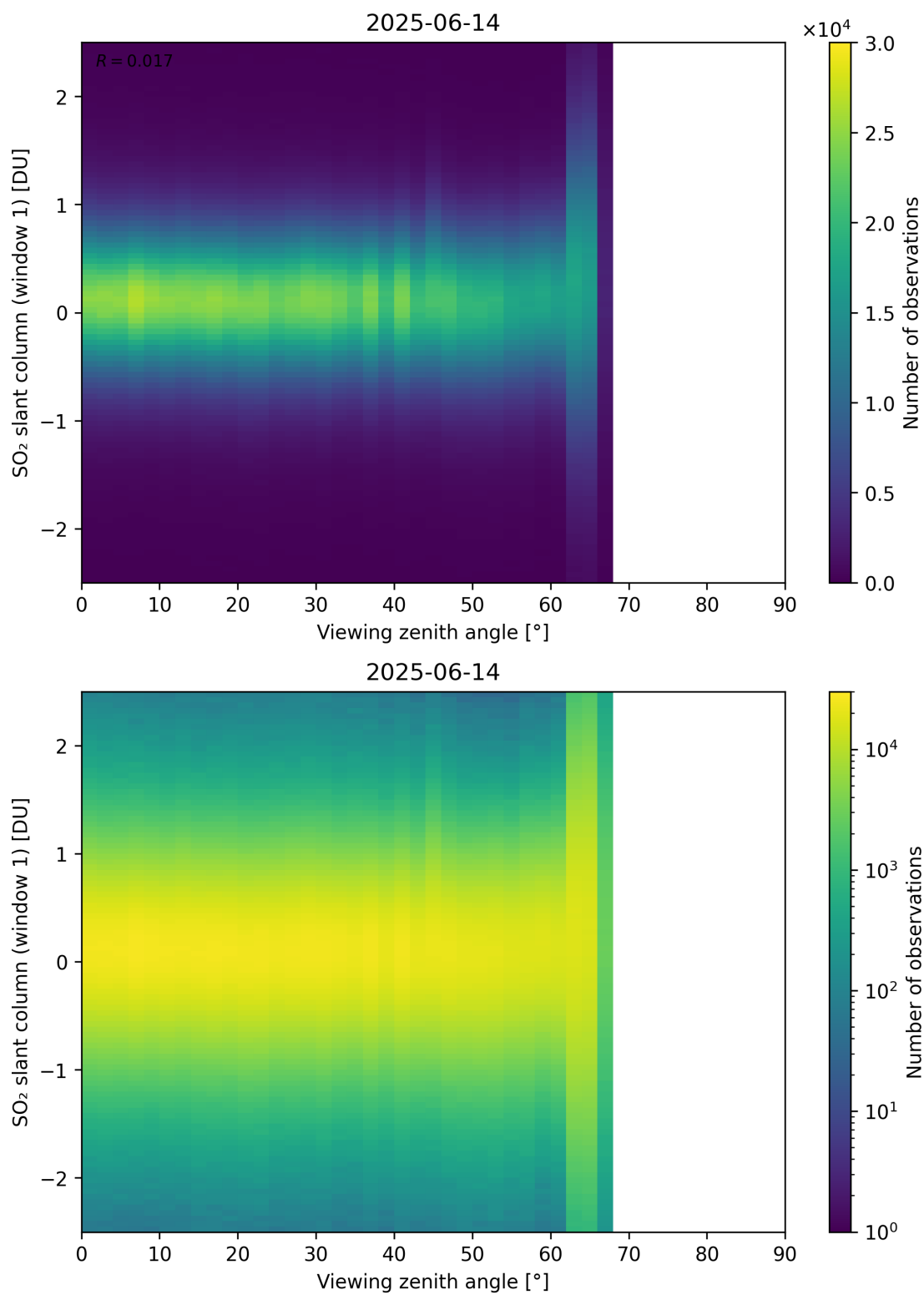
Figure 376: Scatter density plot of “Viewing zenith angle” against “SO 2 slant column (window 1)” for 2025-06-13 to 2025-06-15.
