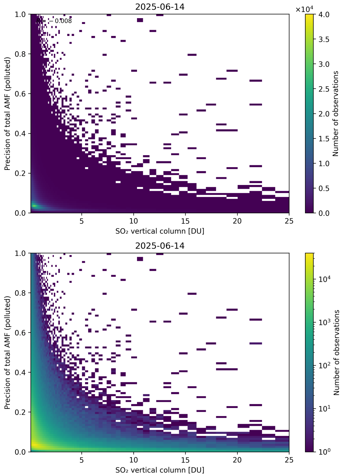
Figure 360: Scatter density plot of “SO 2 vertical column” against “Precision of total AMF (polluted)” for 2025-06-13 to 2025-06-15.
