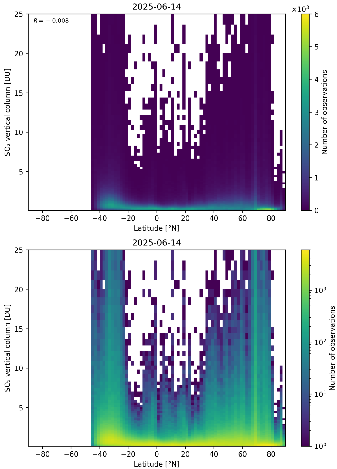
Figure 169: Scatter density plot of “Latitude” against “SO 2 vertical column” for 2025-06-13 to 2025-06-15.
