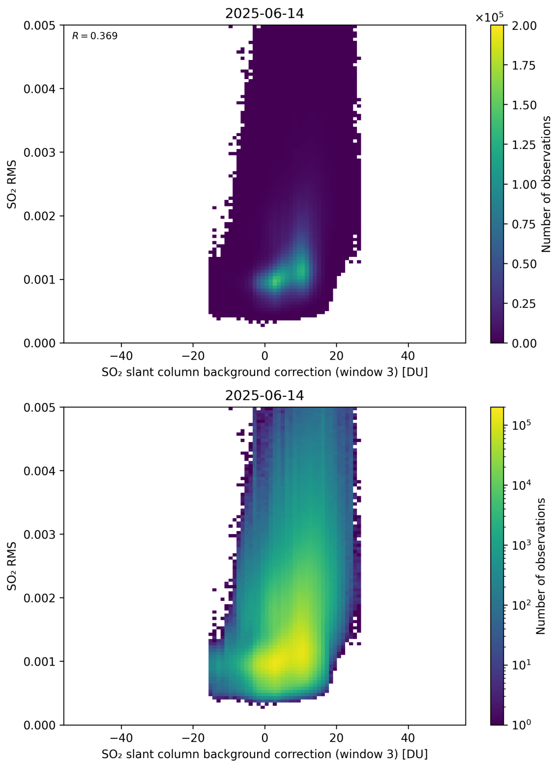
Figure 134: Scatter density plot of “SO 2 slant column background correction (window 3)” against “SO 2 RMS” for 2025-06-13 to 2025-06-15.
