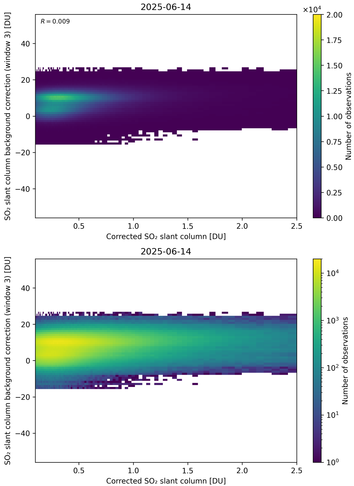
Figure 228: Scatter density plot of “Corrected SO 2 slant column” against “SO 2 slant column background correction (window 3)” for 2025-06-13 to 2025-06-15.
