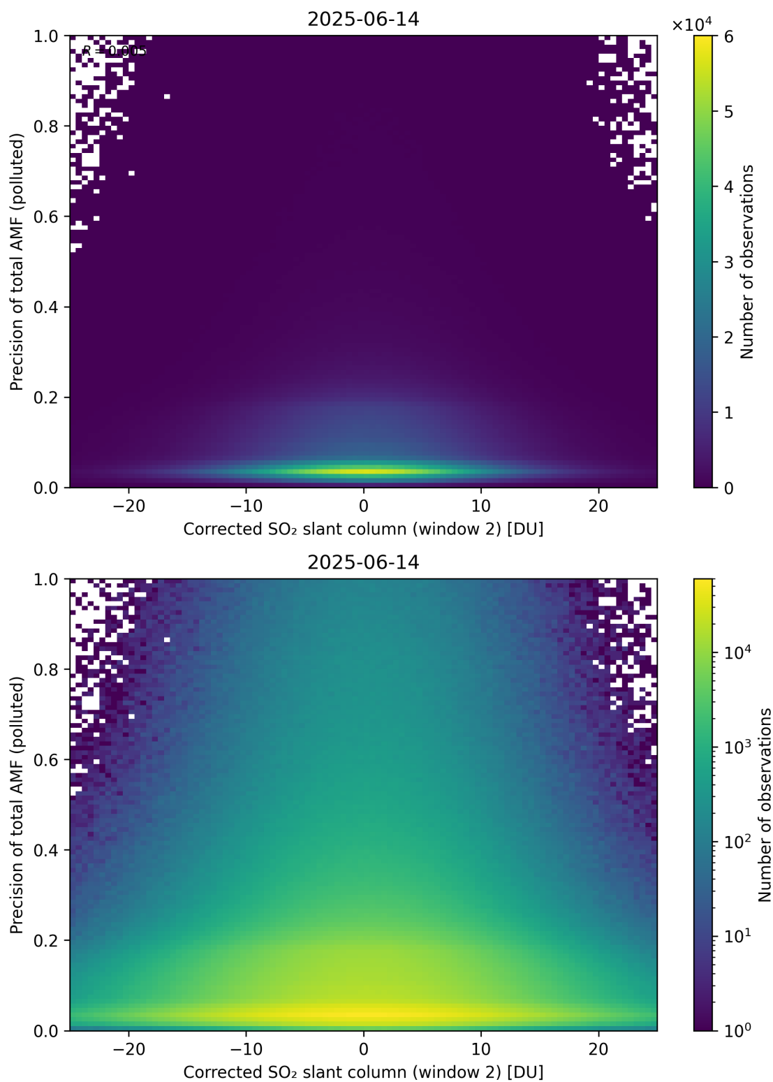
Figure 254: Scatter density plot of “Corrected SO 2 slant column (window 2)” against “Precision of total AMF (polluted)” for 2025-06-13 to 2025-06-15.
