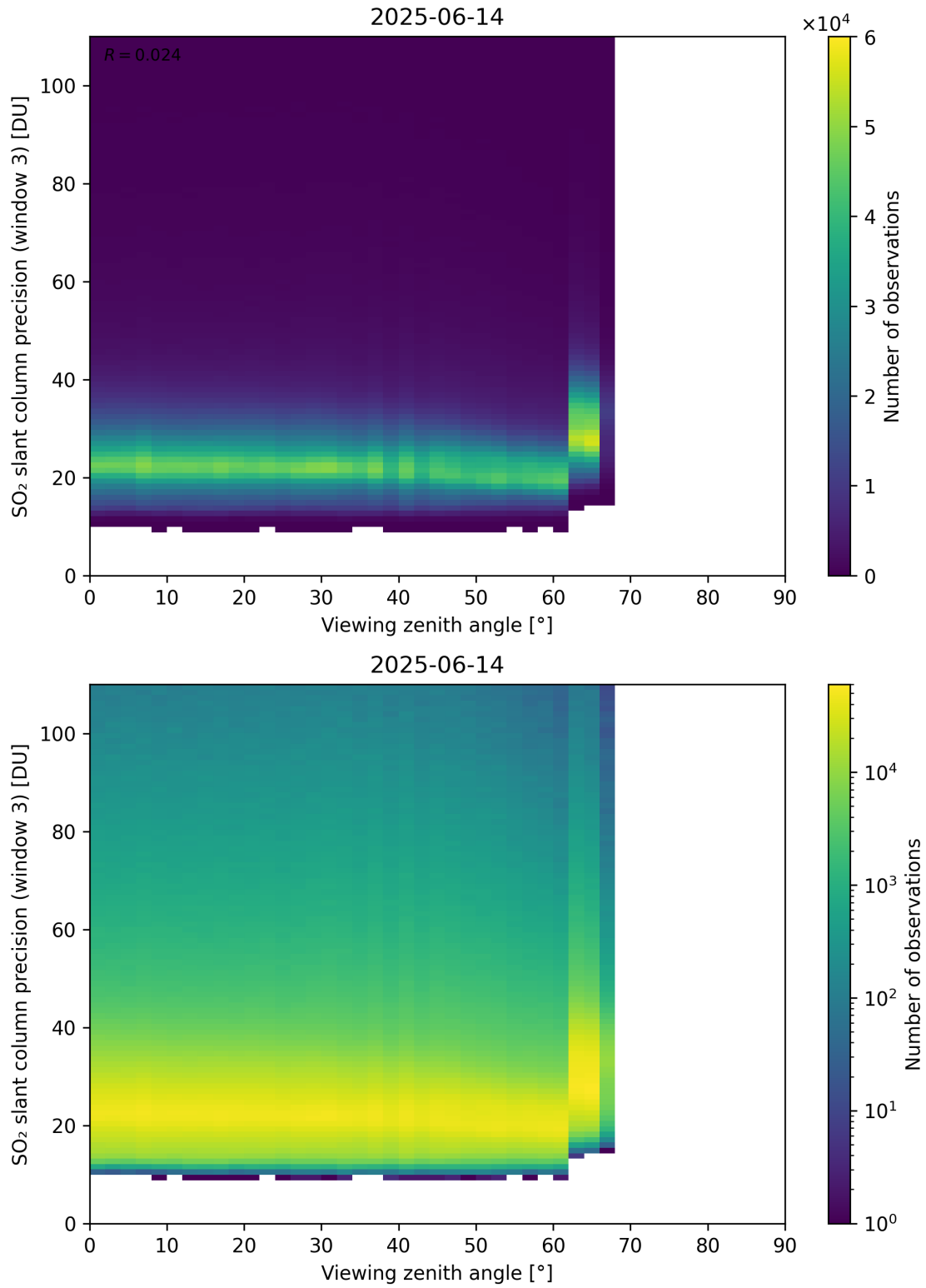
Figure 380: Scatter density plot of “Viewing zenith angle” against “SO 2 slant column precision (window 3)” for 2025-06-13 to 2025-06-15.
