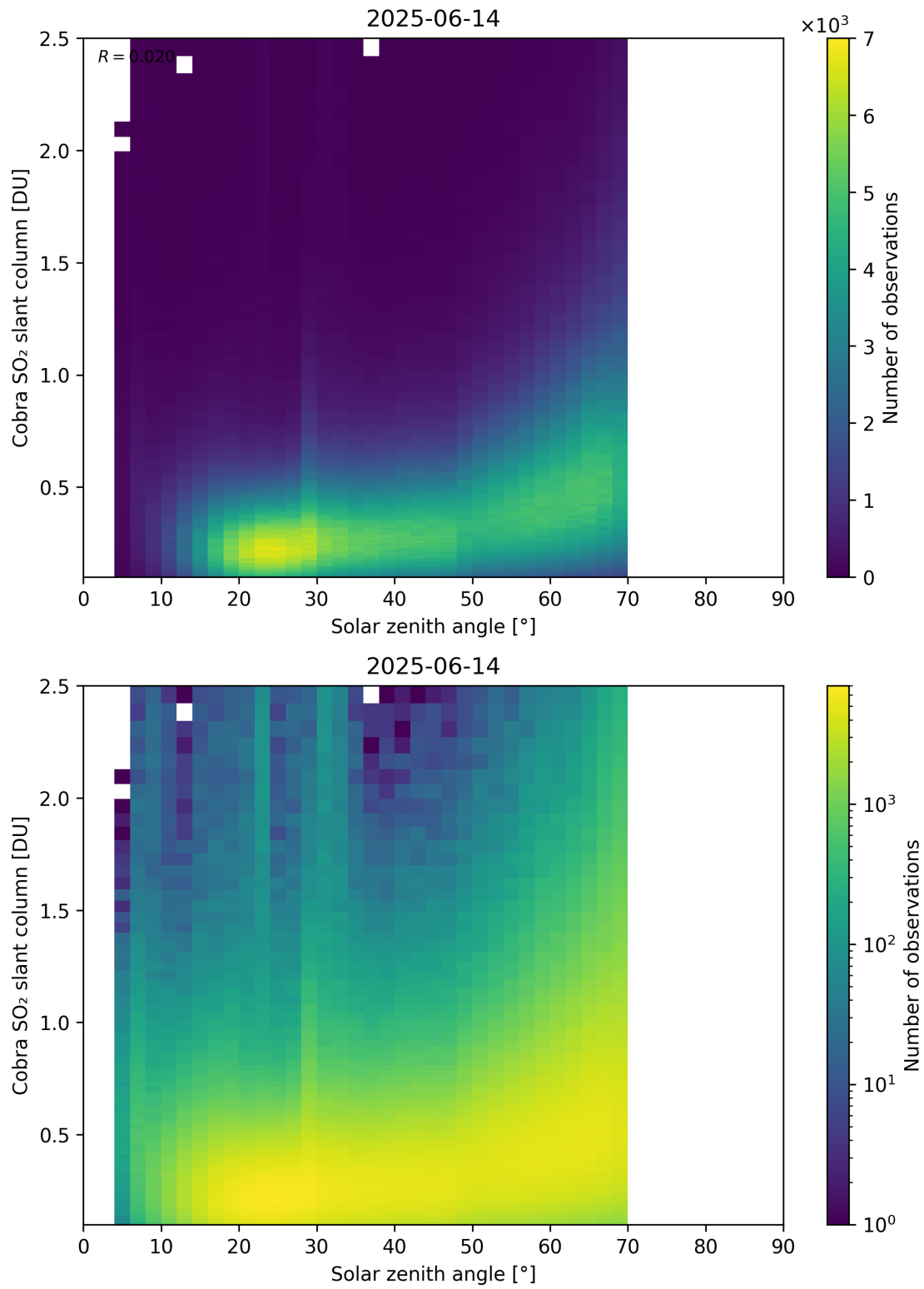
Figure 179: Scatter density plot of “Solar zenith angle” against “Cobra SO 2 slant column” for 2025-06-13 to 2025-06-15.
