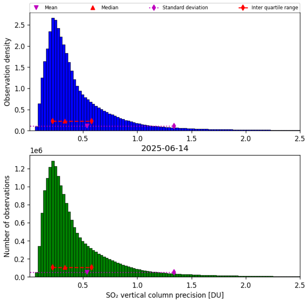
Figure 59: Histogram of “SO 2 vertical column precision” for 2025-06-13 to 2025-06-15
