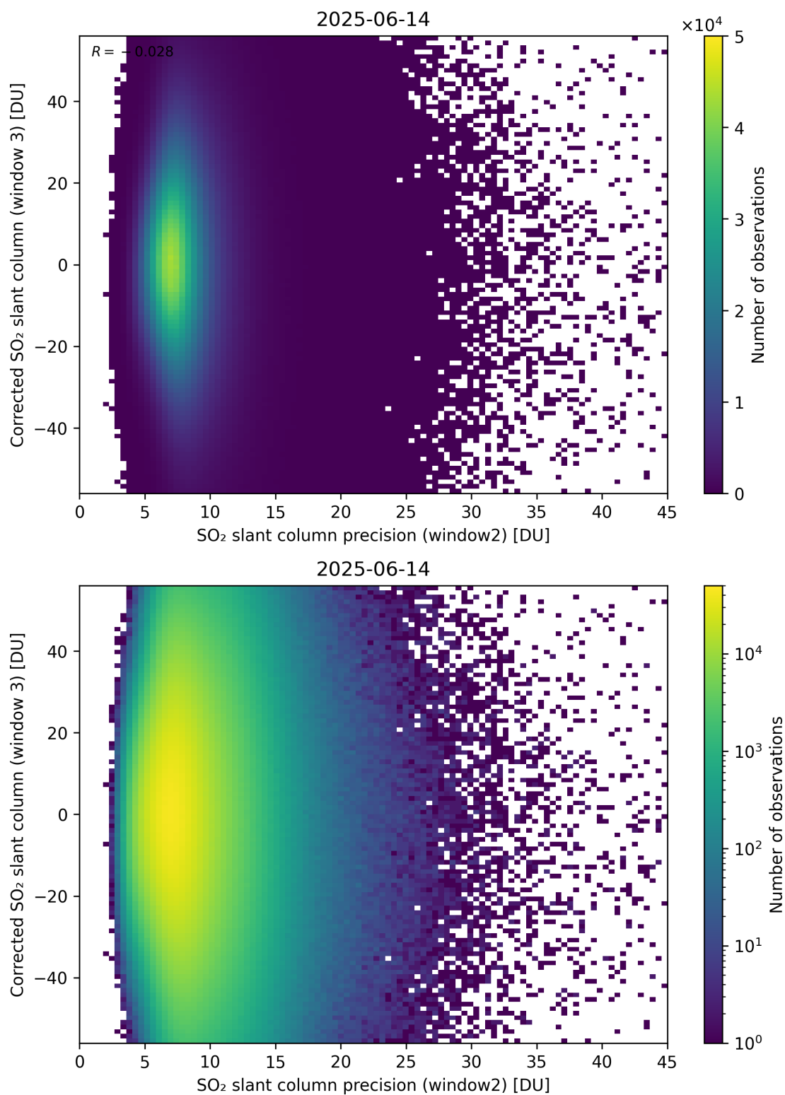
Figure 298: Scatter density plot of “SO 2 slant column precision (window2)” against “Corrected SO 2 slant column (window 3)” for 2025-06-13 to 2025-06-15.
