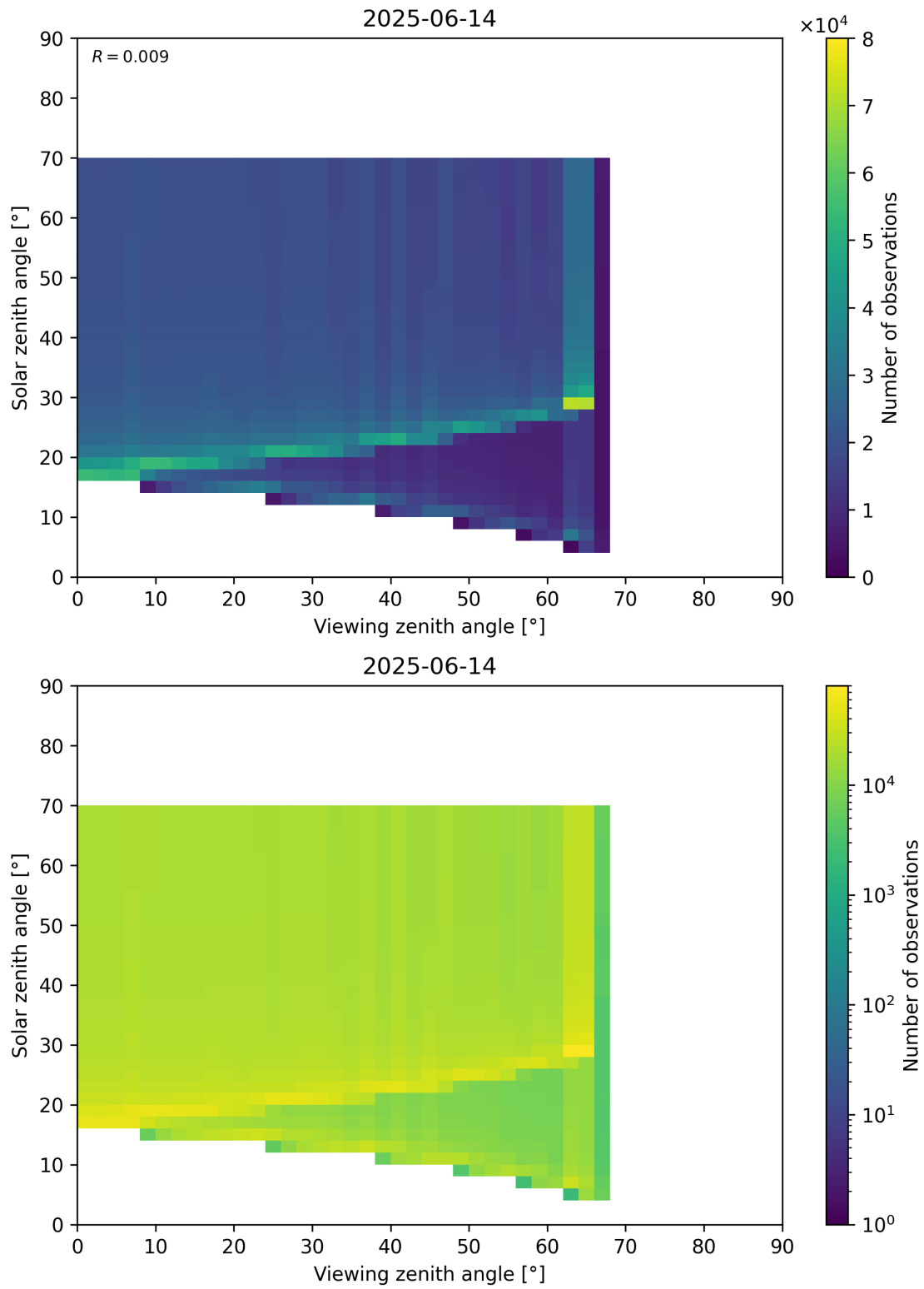
Figure 369: Scatter density plot of “Viewing zenith angle” against “Solar zenith angle” for 2025-06-13 to 2025-06-15.
