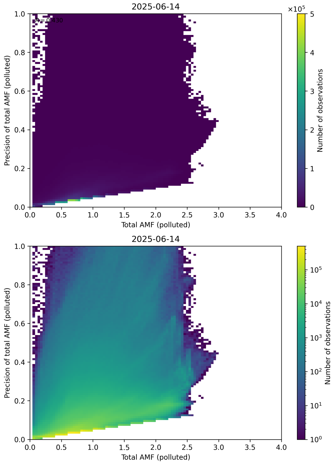
Figure 322: Scatter density plot of “Total AMF (polluted)” against “Precision of total AMF (polluted)” for 2025-06-13 to 2025-06-15.
