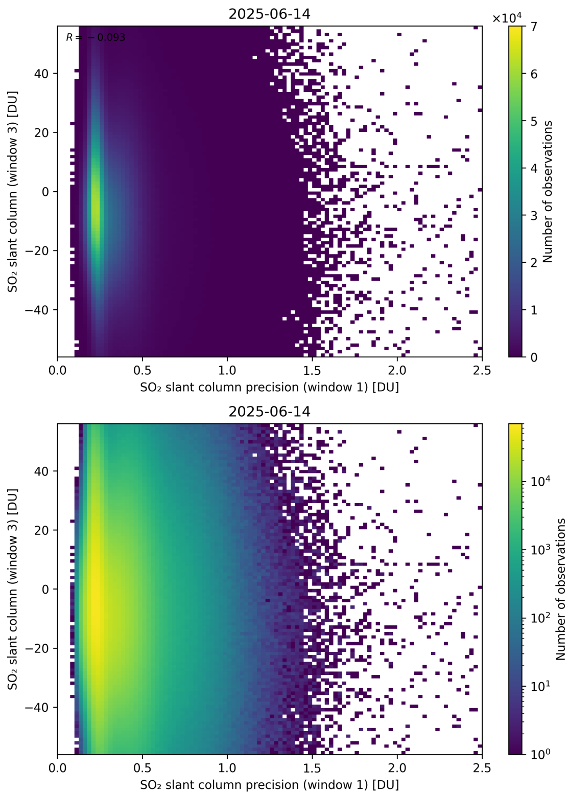
Figure 278: Scatter density plot of “SO 2 slant column precision (window 1)” against “SO 2 slant column (window 3)” for 2025-06-13 to 2025-06-15.
