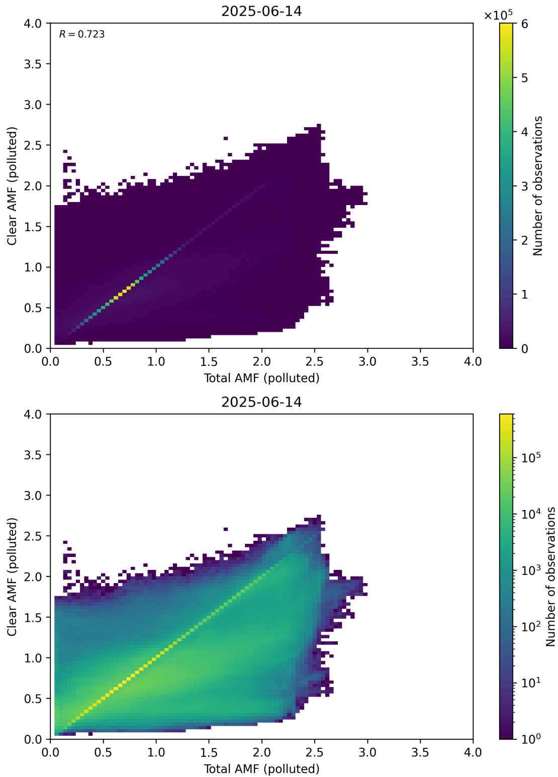
Figure 321: Scatter density plot of “Total AMF (polluted)” against “Clear AMF (polluted)” for 2025-06-13 to 2025-06-15.
