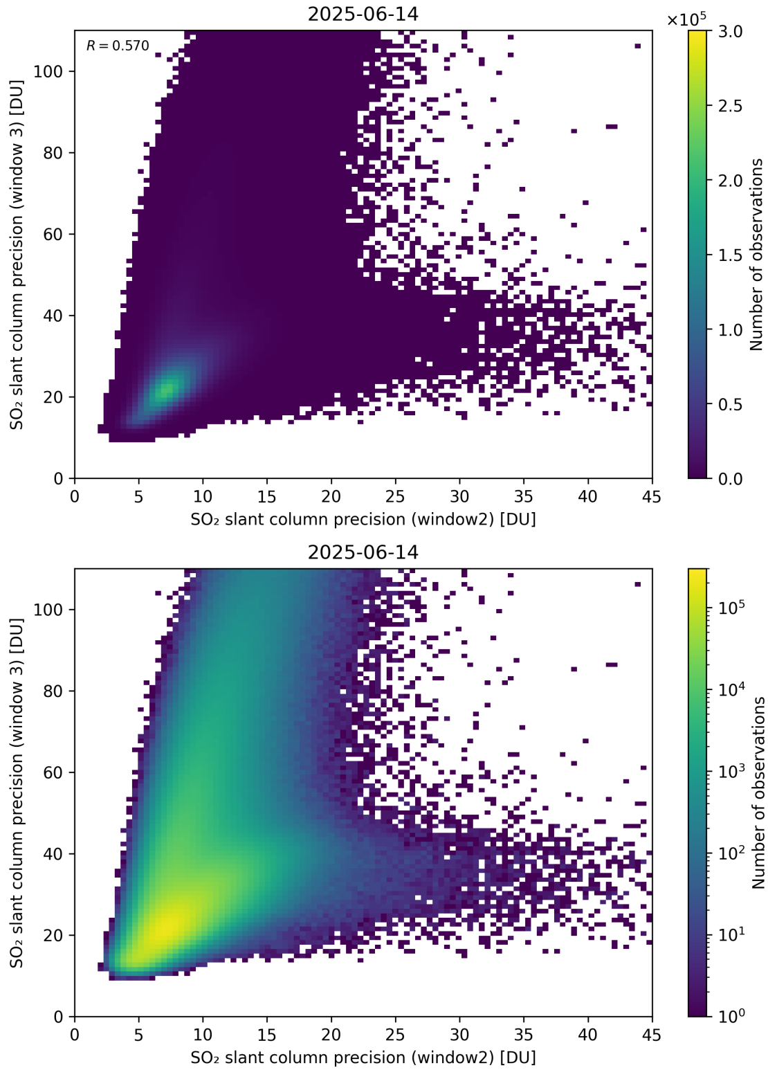
Figure 300: Scatter density plot of “SO 2 slant column precision (window2)” against “SO 2 slant column precision (window 3)” for 2025-06-13 to 2025-06-15.
