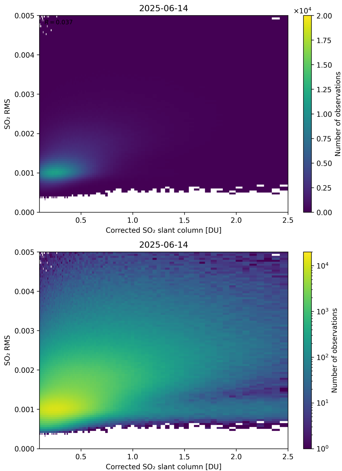
Figure 231: Scatter density plot of “Corrected SO 2 slant column” against “SO 2 RMS” for 2025-06-13 to 2025-06-15.
