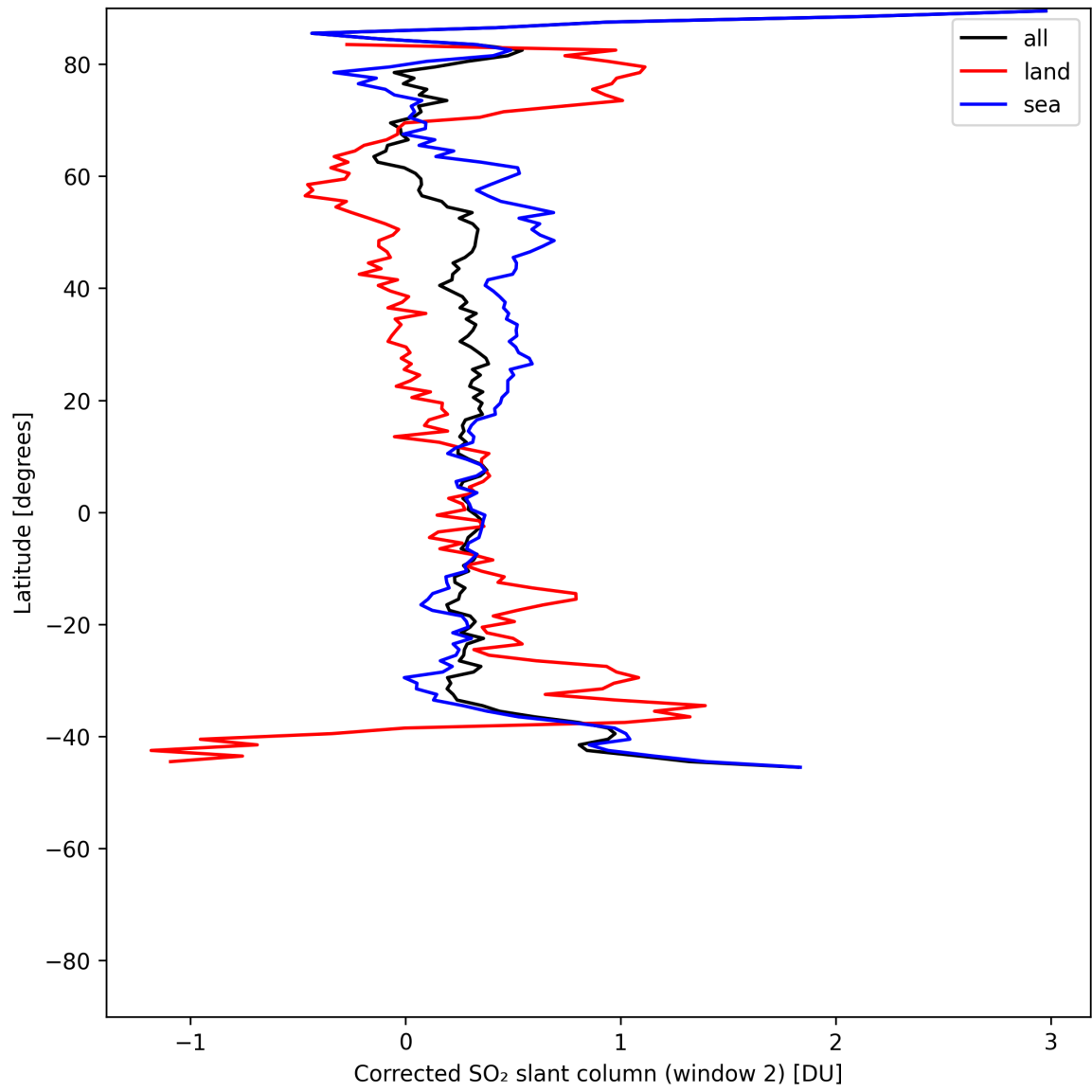
Figure 43: Zonal average of “Corrected SO 2 slant column (window 2)” for 2025-06-13 to 2025-06-15.
