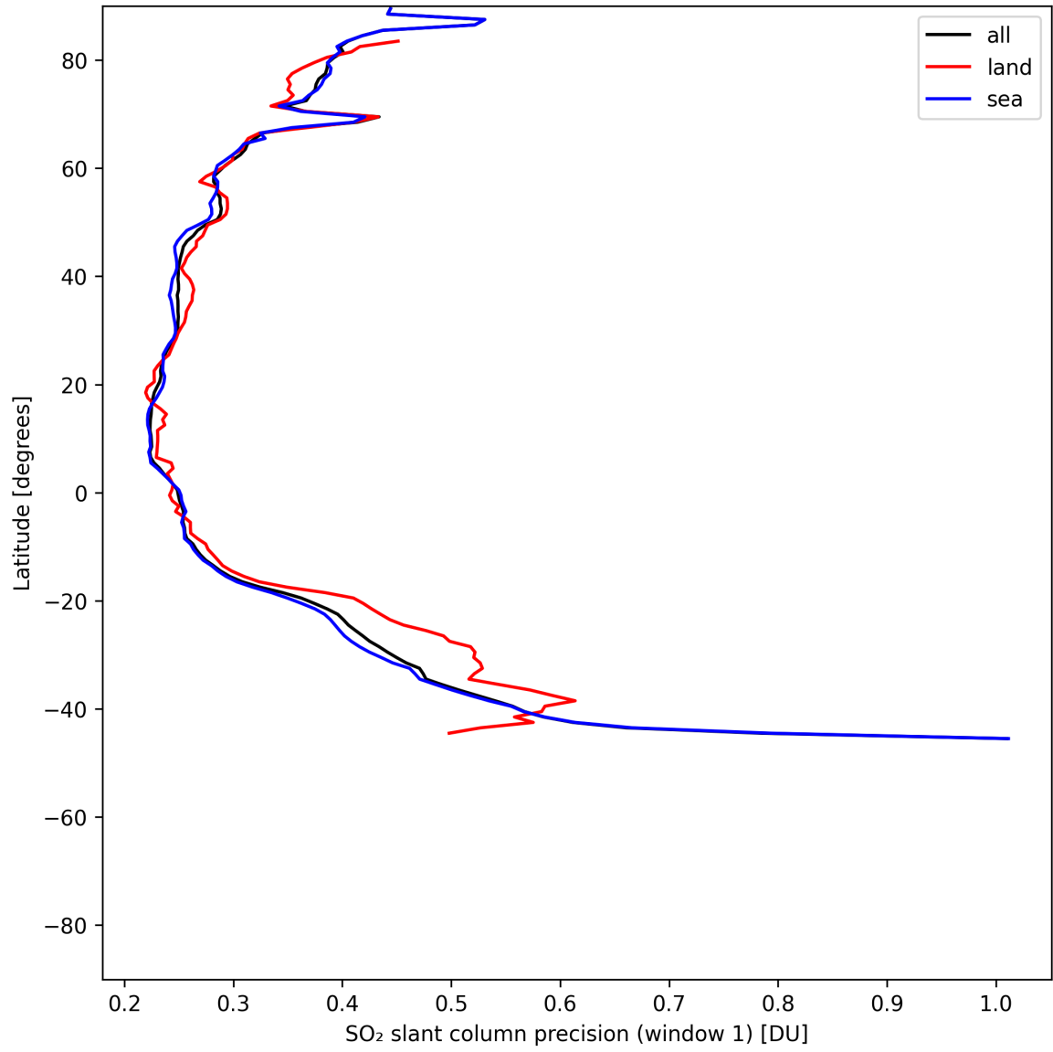
Figure 38: Zonal average of “SO 2 slant column precision (window 1)” for 2025-06-13 to 2025-06-15.
