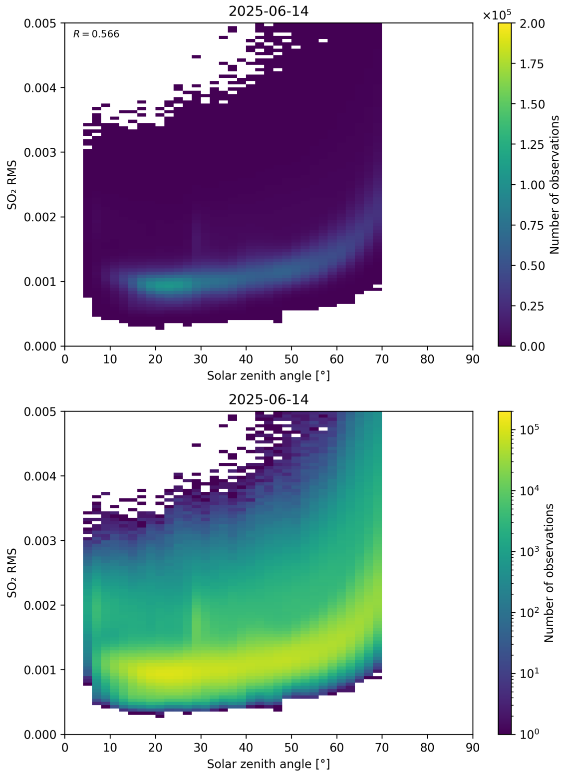
Figure 176: Scatter density plot of “Solar zenith angle” against “SO 2 RMS” for 2025-06-13 to 2025-06-15.
