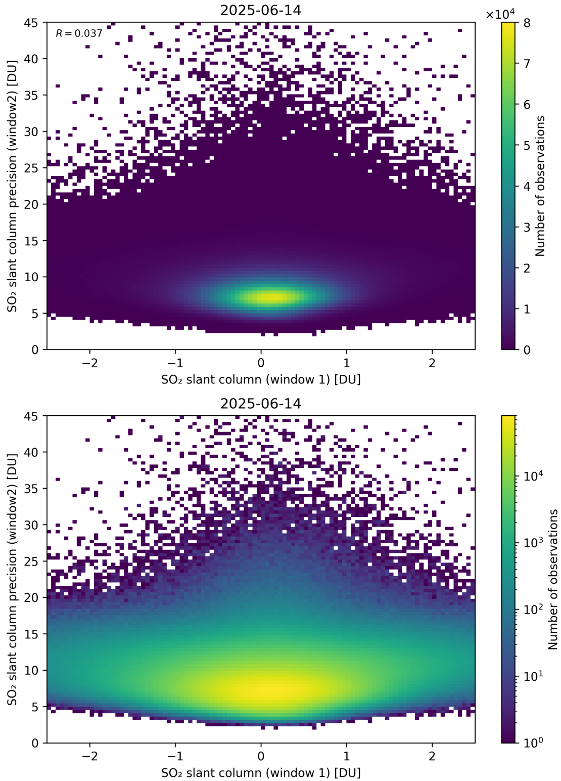
Figure 286: Scatter density plot of “SO 2 slant column (window 1)” against “SO 2 slant column precision (window2)” for 2025-06-13 to 2025-06-15.
