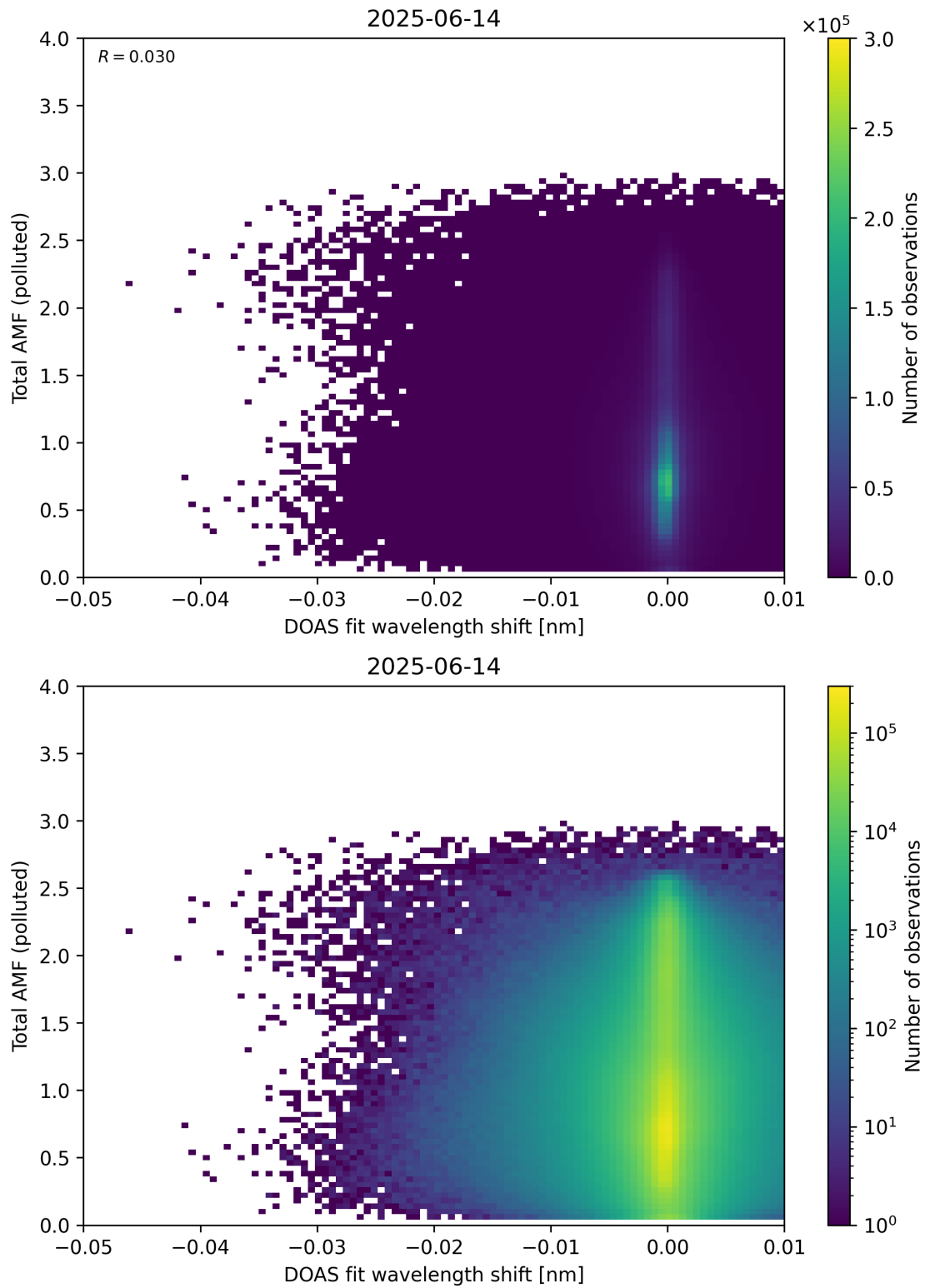
Figure 141: Scatter density plot of “DOAS fit wavelength shift” against “Total AMF (polluted)” for 2025-06-13 to 2025-06-15.
