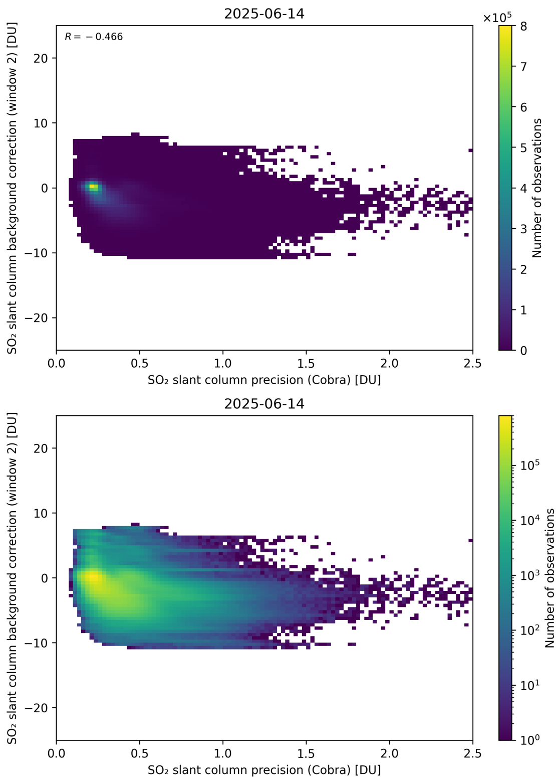
Figure 200: Scatter density plot of “SO 2 slant column precision (Cobra)” against “SO 2 slant column background correction (window 2)” for 2025-06-13 to 2025-06-15.
