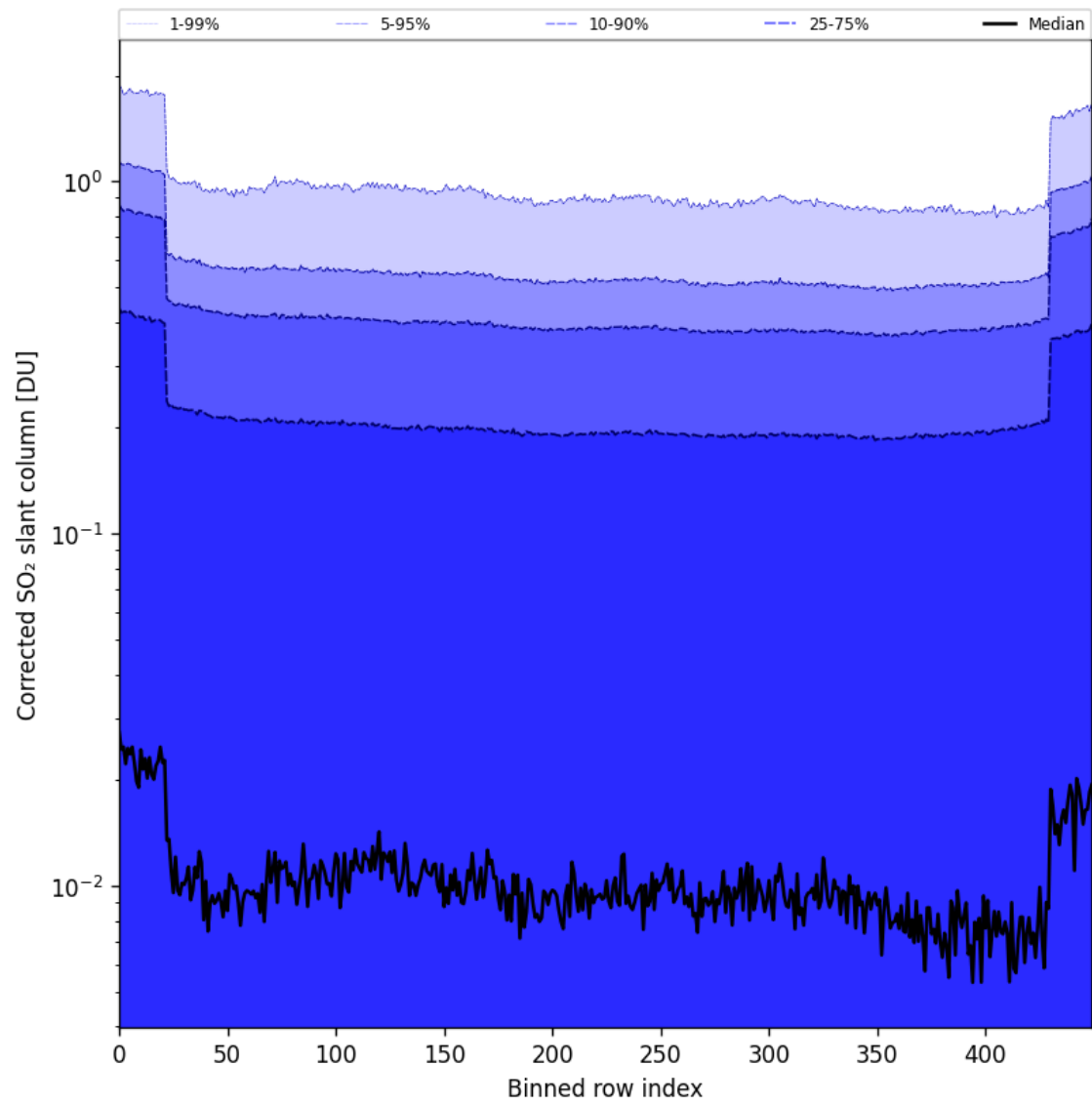
Figure 86: Along track statistics of "Corrected SO 2 slant column" for 2025-06-13 to 2025-06-15
