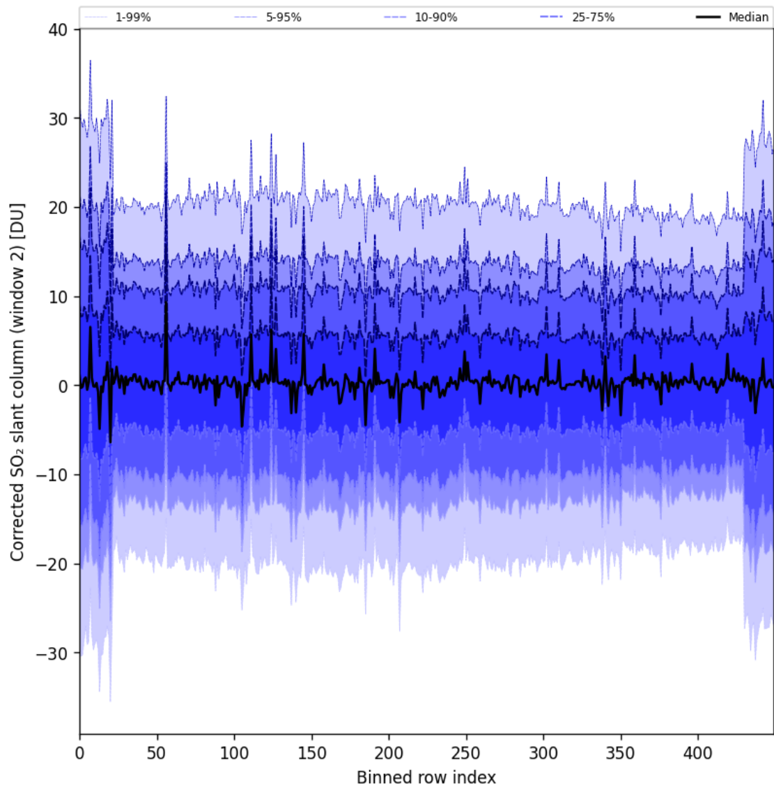
Figure 95: Along track statistics of “Corrected SO 2 slant column (window 2)” for 2025-06-13 to 2025-06-15
