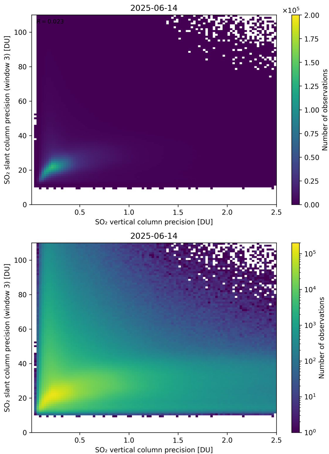
Figure 345: Scatter density plot of “SO 2 vertical column precision” against “SO 2 slant column precision (window 3)” for 2025-06-13 to 2025-06-15.
