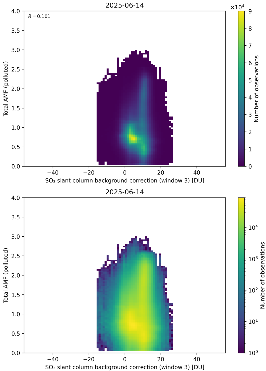
Figure 136: Scatter density plot of “SO 2 slant column background correction (window 3)” against “Total AMF (polluted)” for 2025-06-13 to 2025-06-15.
