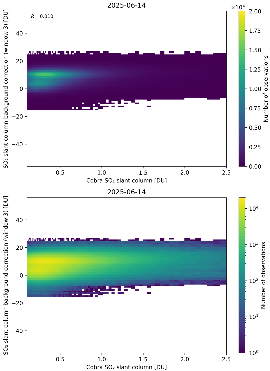
Figure 195: Scatter density plot of “Cobra SO 2 slant column” against “SO 2 slant column background correction (window 3)” for 2025-06-13 to 2025-06-15.
