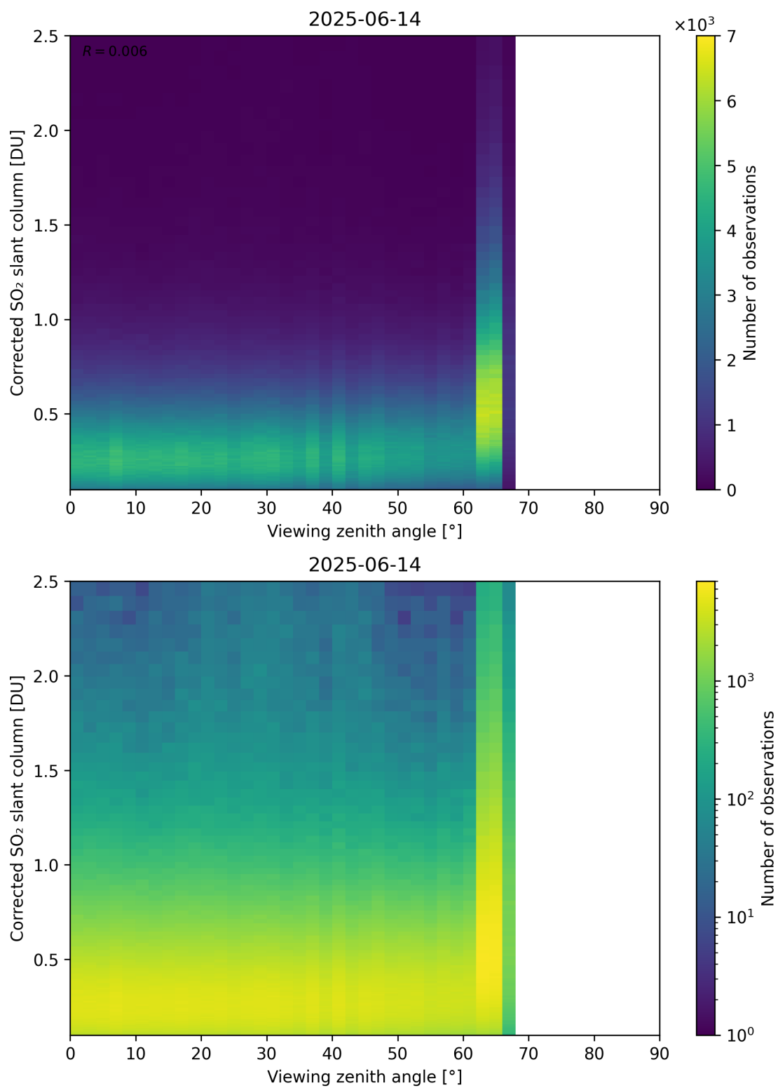
Figure 373: Scatter density plot of “Viewing zenith angle” against “Corrected SO 2 slant column” for 2025-06-13 to 2025-06-15.
