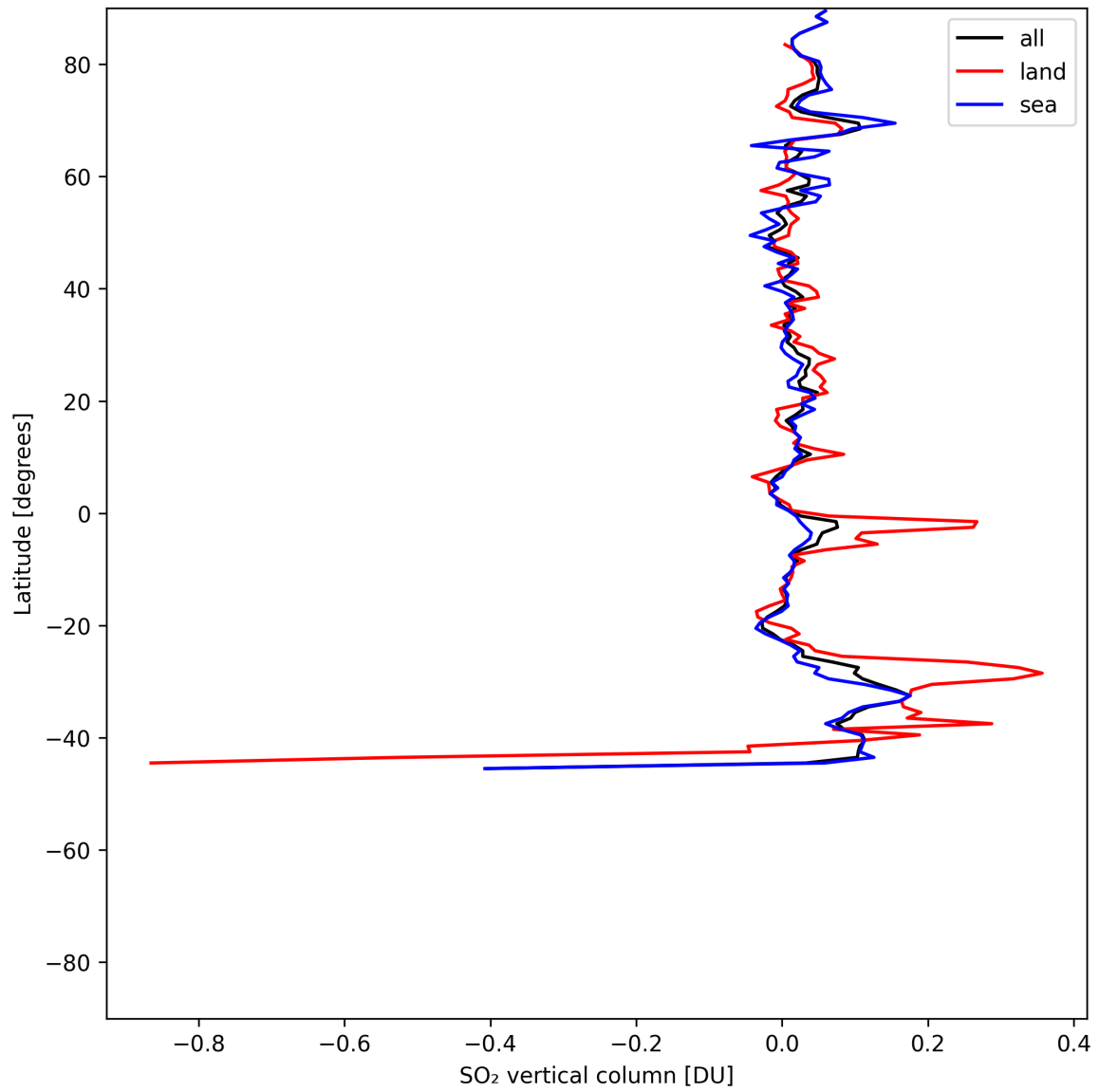
Figure 32: Zonal average of “SO 2 vertical column” for 2025-06-13 to 2025-06-15.
