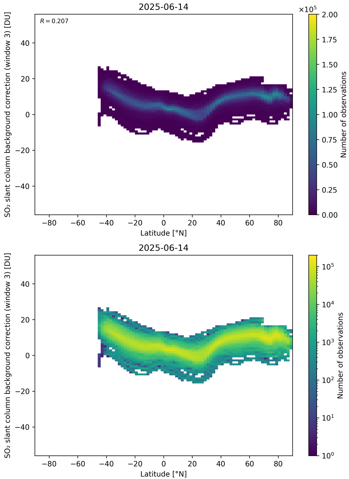
Figure 152: Scatter density plot of “Latitude” against “SO 2 slant column background correction (window 3)” for 2025-06-13 to 2025-06-15.
