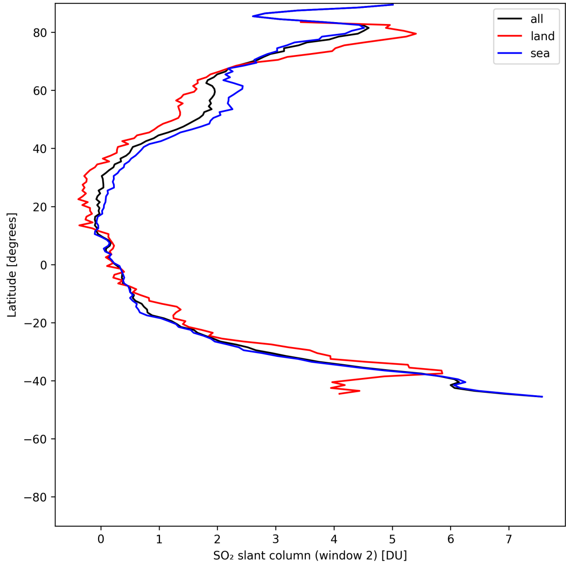
Figure 41: Zonal average of “SO 2 slant column (window 2)” for 2025-06-13 to 2025-06-15.
