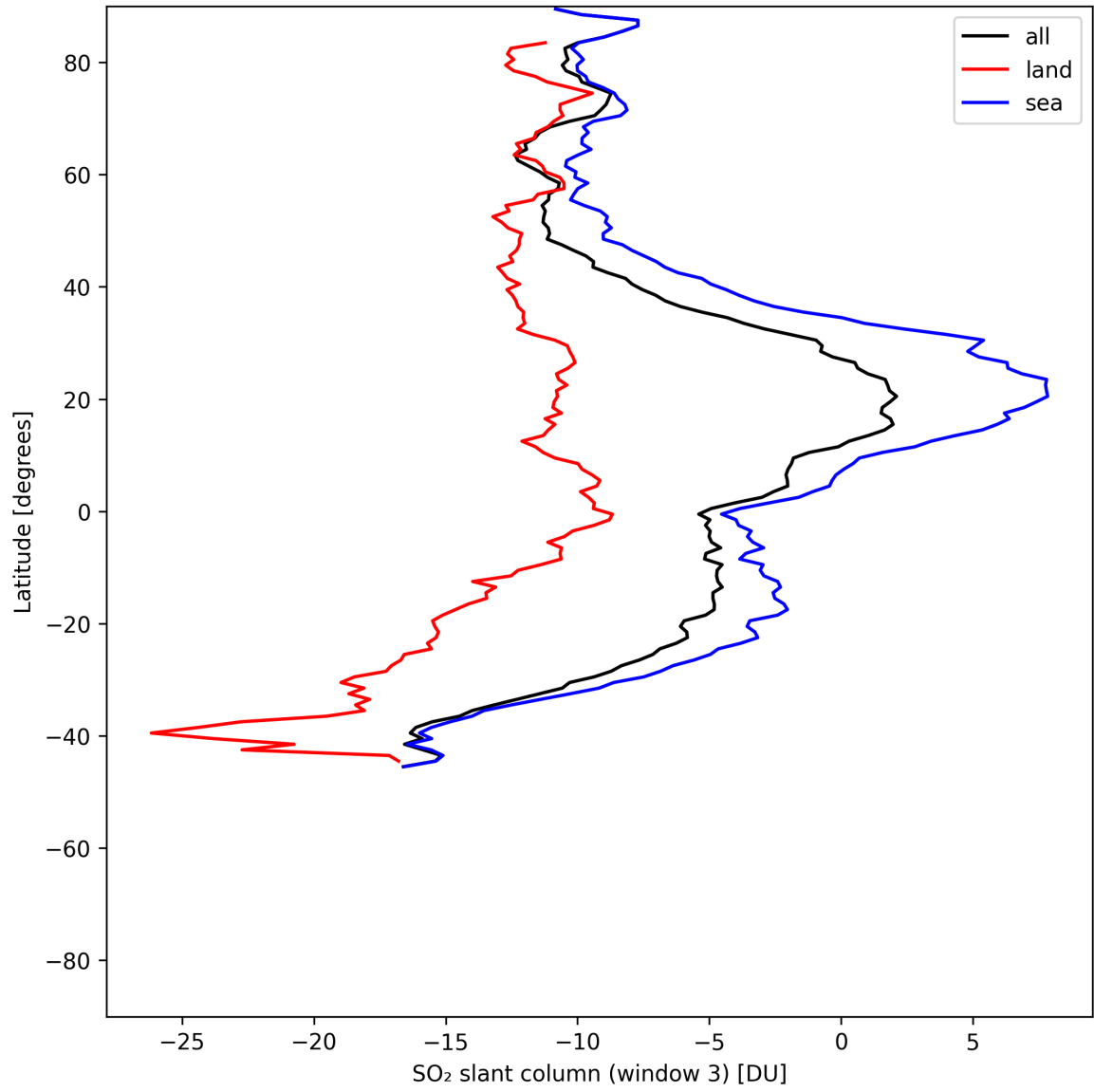
Figure 45: Zonal average of “SO 2 slant column (window 3)” for 2025-06-13 to 2025-06-15.
