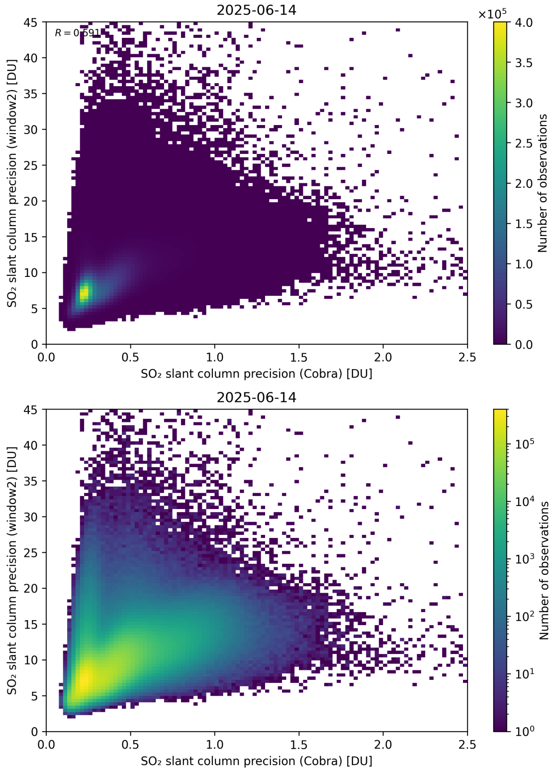
Figure 210: Scatter density plot of “SO 2 slant column precision (Cobra)” against “SO 2 slant column precision (window2)” for 2025-06-13 to 2025-06-15.
