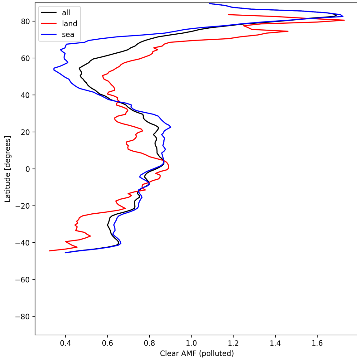
Figure 55: Zonal average of “Clear AMF (polluted)” for 2025-06-13 to 2025-06-15.
