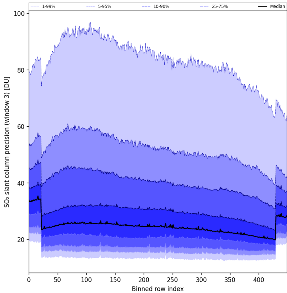
Figure 98: Along track statistics of “SO 2 slant column precision (window 3)” for 2025-06-13 to 2025-06-15
