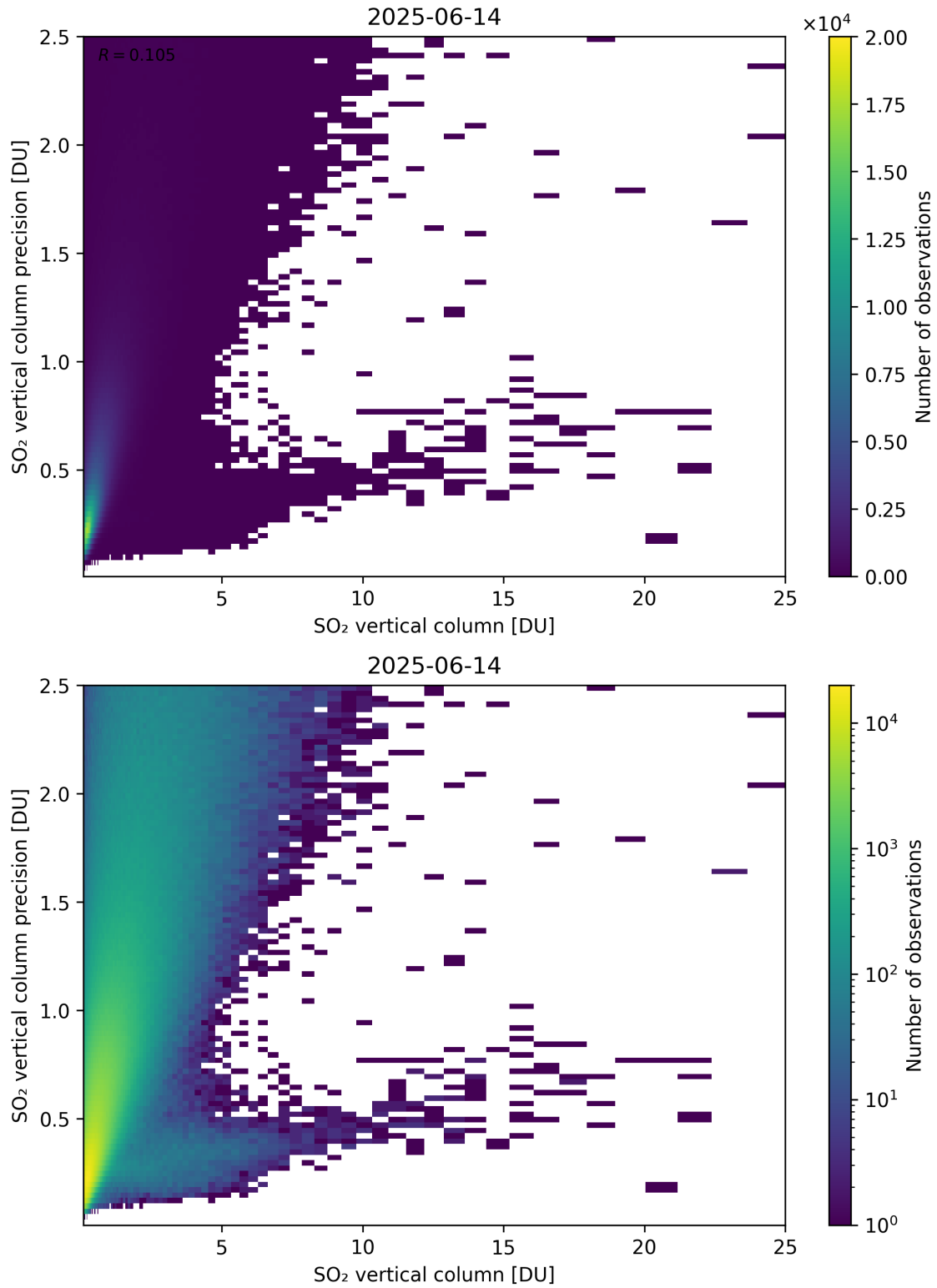
Figure 361: Scatter density plot of “SO 2 vertical column” against “SO 2 vertical column precision” for 2025-06-13 to 2025-06-15.
