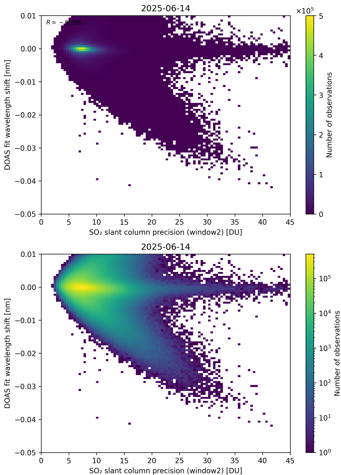
Figure 293: Scatter density plot of “SO 2 slant column precision (window2)” against “DOAS fit wavelength shift” for 2025-06-13 to 2025-06-15.
