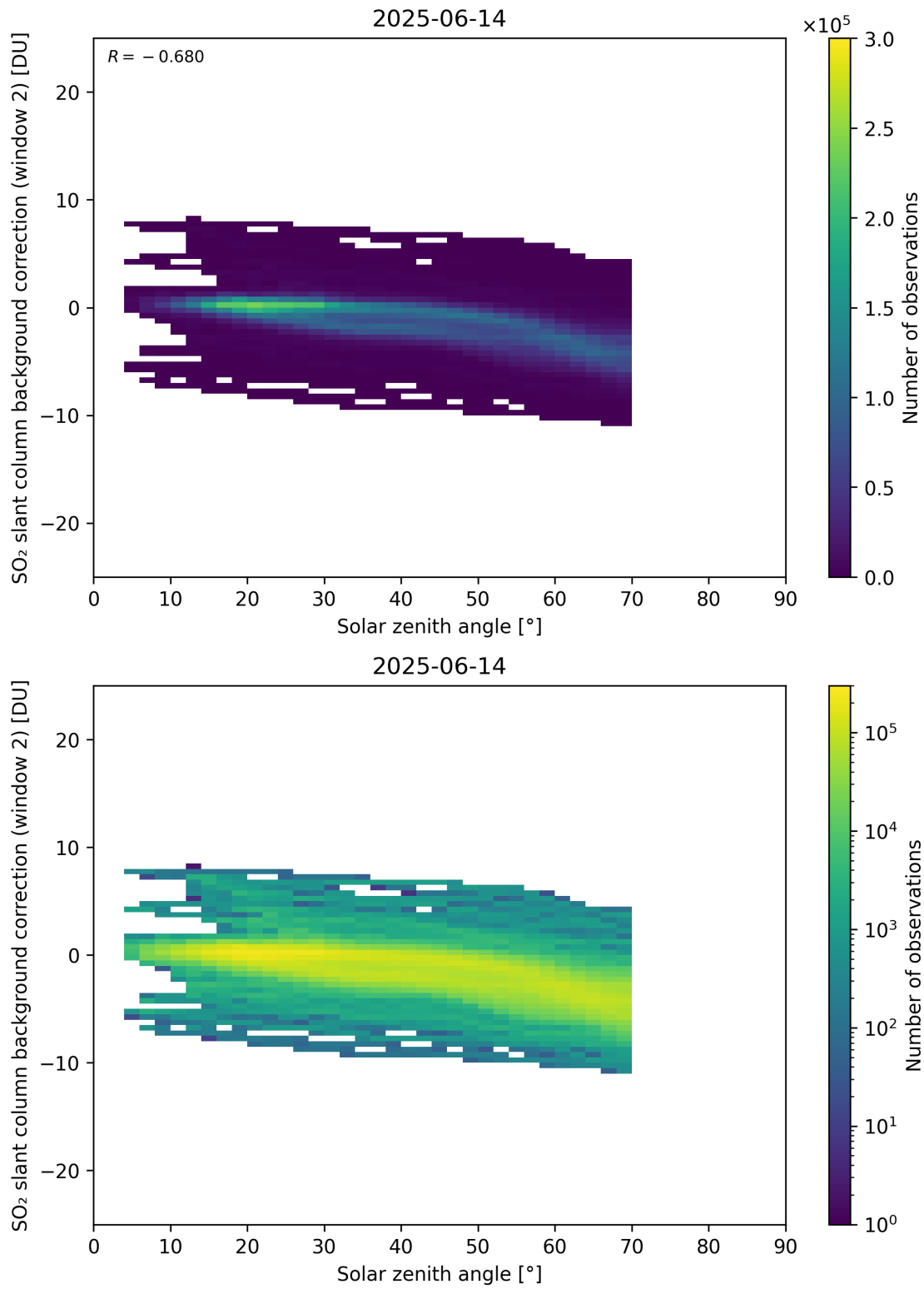
Figure 172: Scatter density plot of “Solar zenith angle” against “SO 2 slant column background correction (window 2)” for 2025-06-13 to 2025-06-15.
