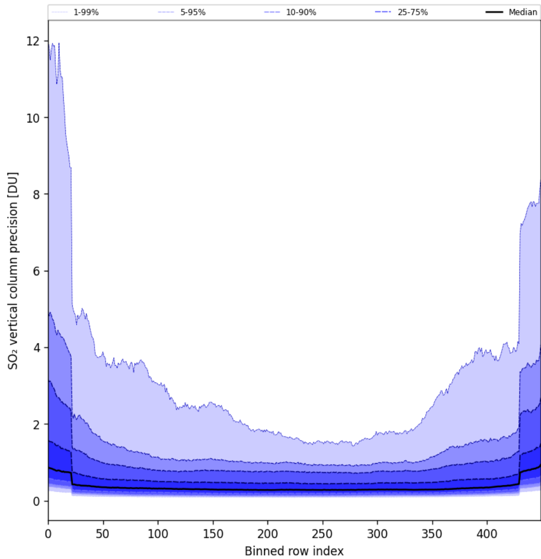
Figure 85: Along track statistics of “SO 2 vertical column precision” for 2025-06-13 to 2025-06-15
