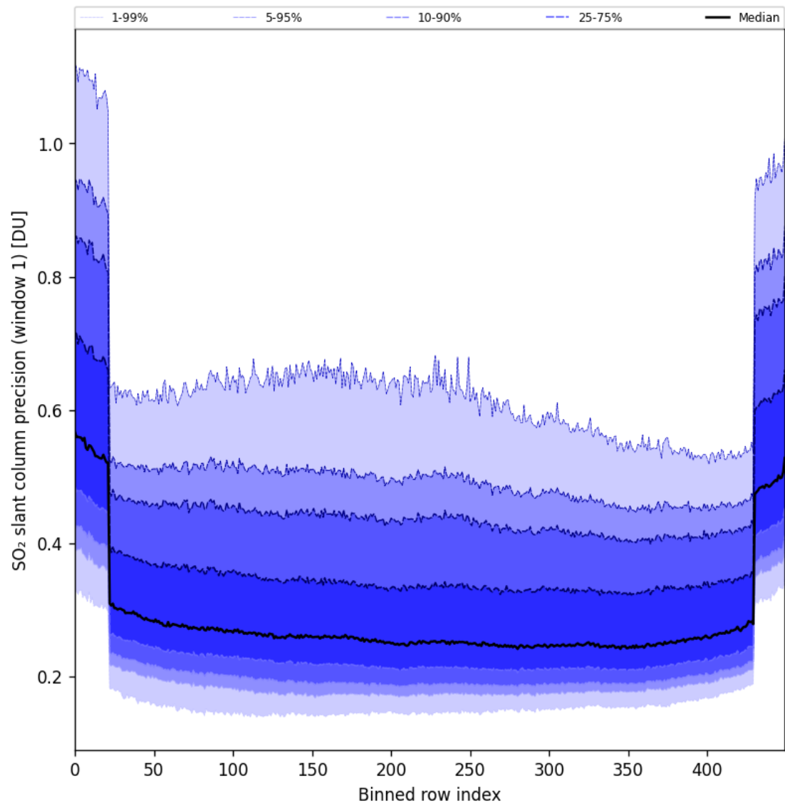
Figure 90: Along track statistics of “SO 2 slant column precision (window 1)” for 2025-06-13 to 2025-06-15
