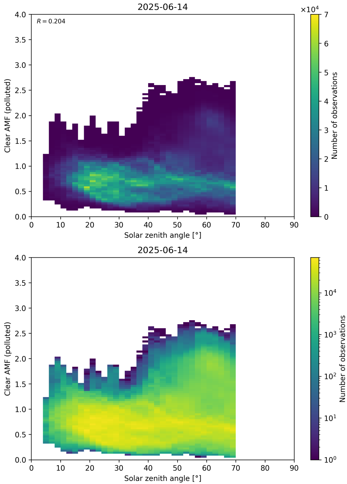
Figure 178: Scatter density plot of “Solar zenith angle” against “Clear AMF (polluted)” for 2025-06-13 to 2025-06-15.
