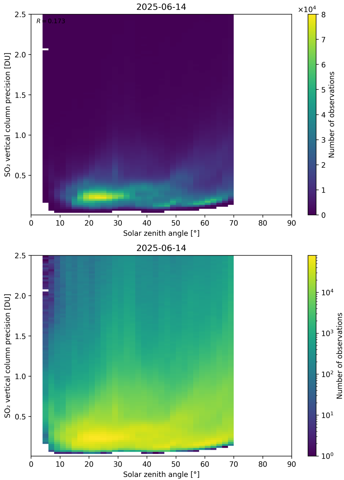
Figure 192: Scatter density plot of “Solar zenith angle” against “SO 2 vertical column precision” for 2025-06-13 to 2025-06-15.
