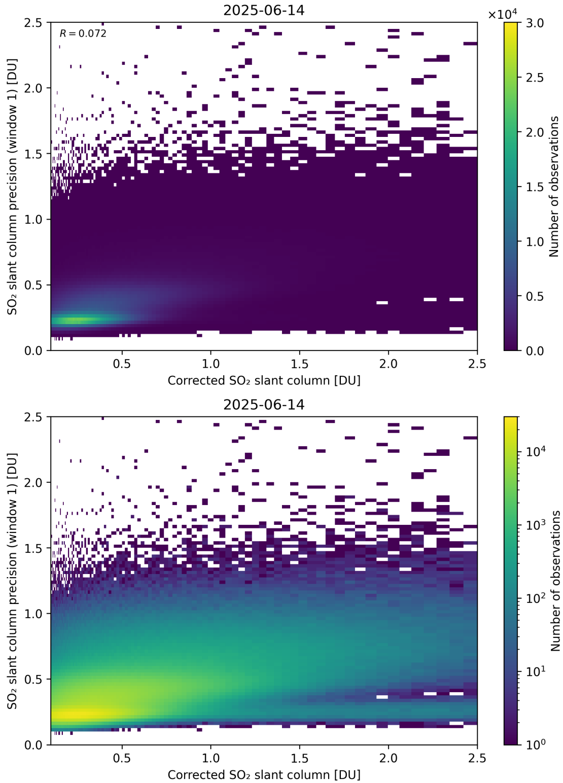
Figure 238: Scatter density plot of “Corrected SO 2 slant column” against “SO 2 slant column precision (window 1)” for 2025-06-13 to 2025-06-15.
