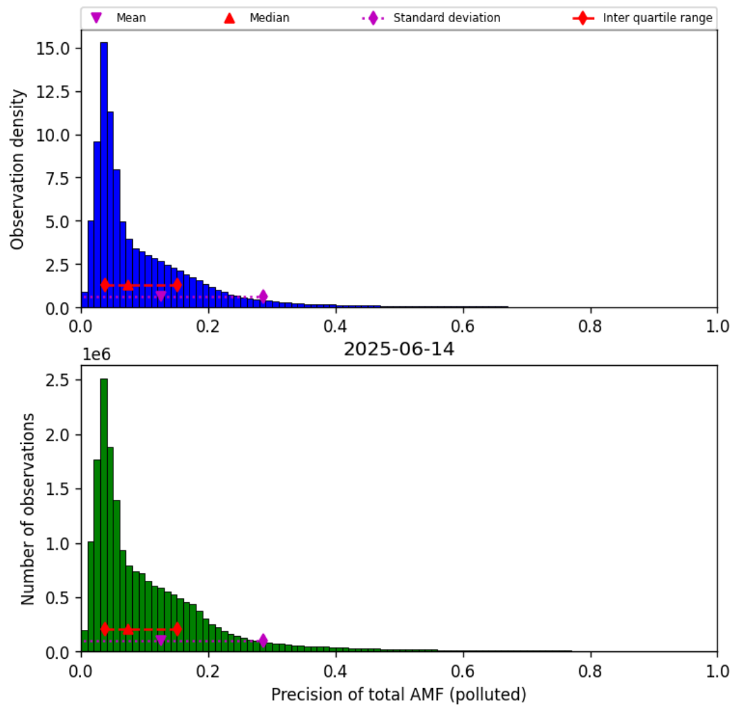
Figure 80: Histogram of “Precision of total AMF (polluted)” for 2025-06-13 to 2025-06-15
