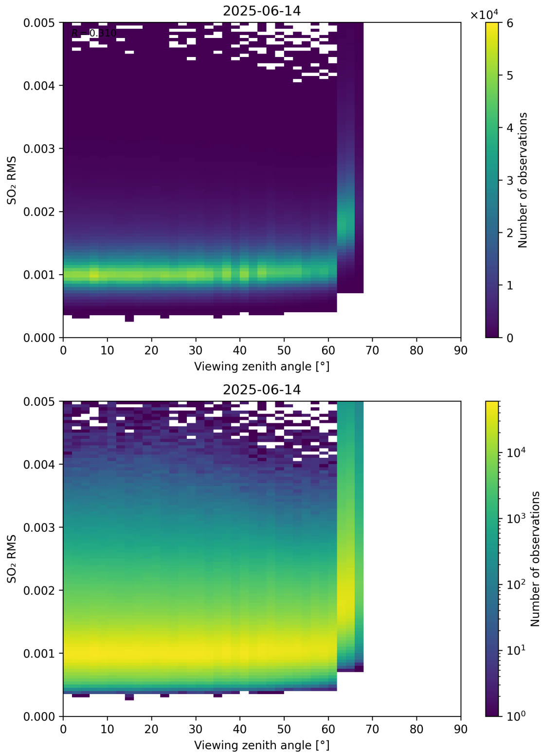
Figure 367: Scatter density plot of “Viewing zenith angle” against “SO 2 RMS” for 2025-06-13 to 2025-06-15.
