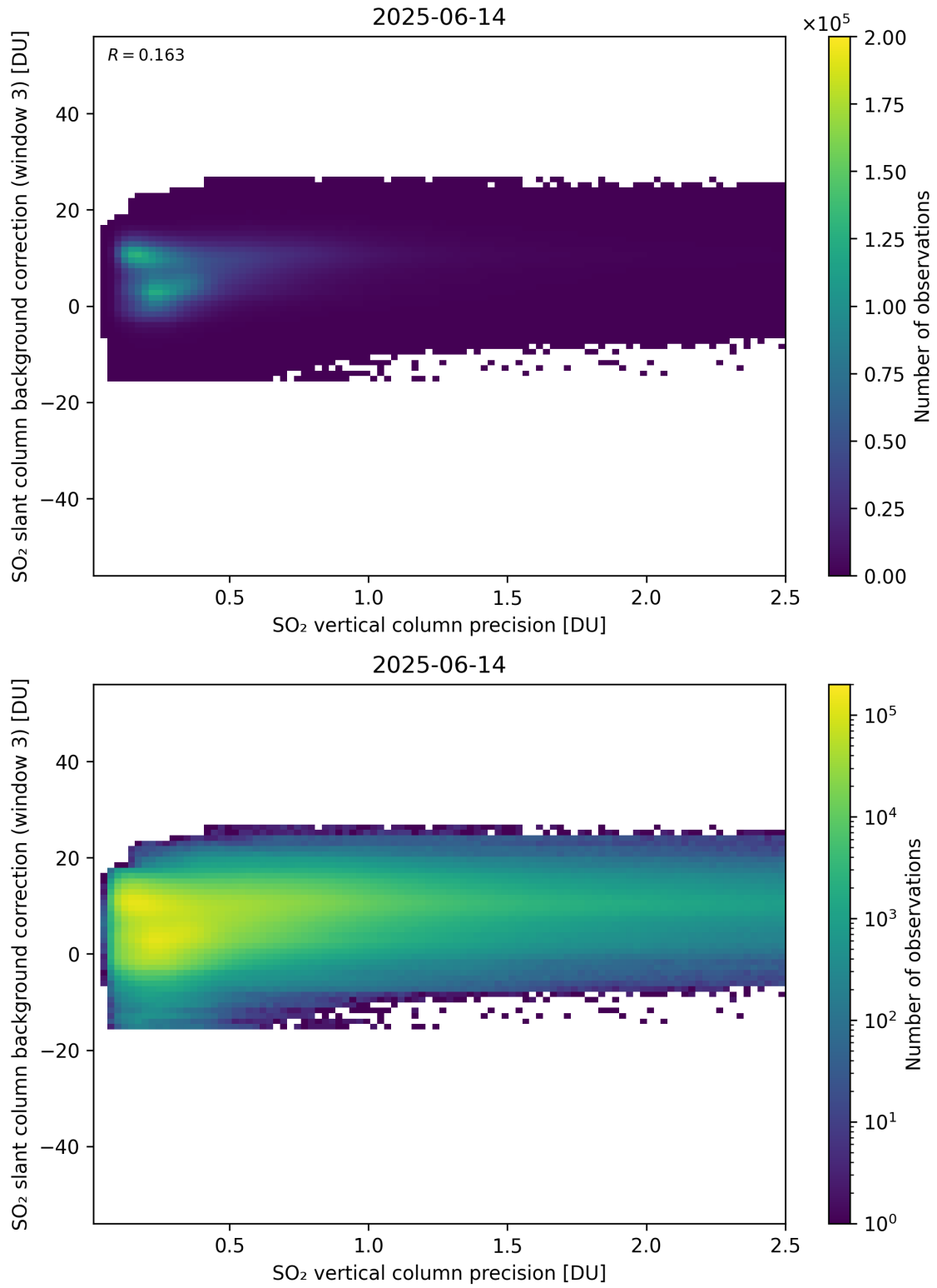
Figure 331: Scatter density plot of “SO 2 vertical column precision” against “SO 2 slant column background correction (window 3)” for 2025-06-13 to 2025-06-15.
