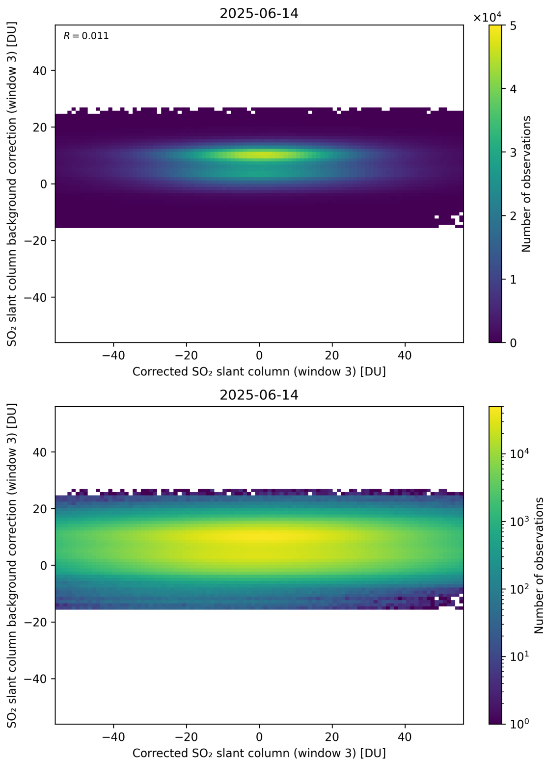
Figure 255: Scatter density plot of “Corrected SO 2 slant column (window 3)” against “SO 2 slant column background correction (window 3)” for 2025-06-13 to 2025-06-15.
