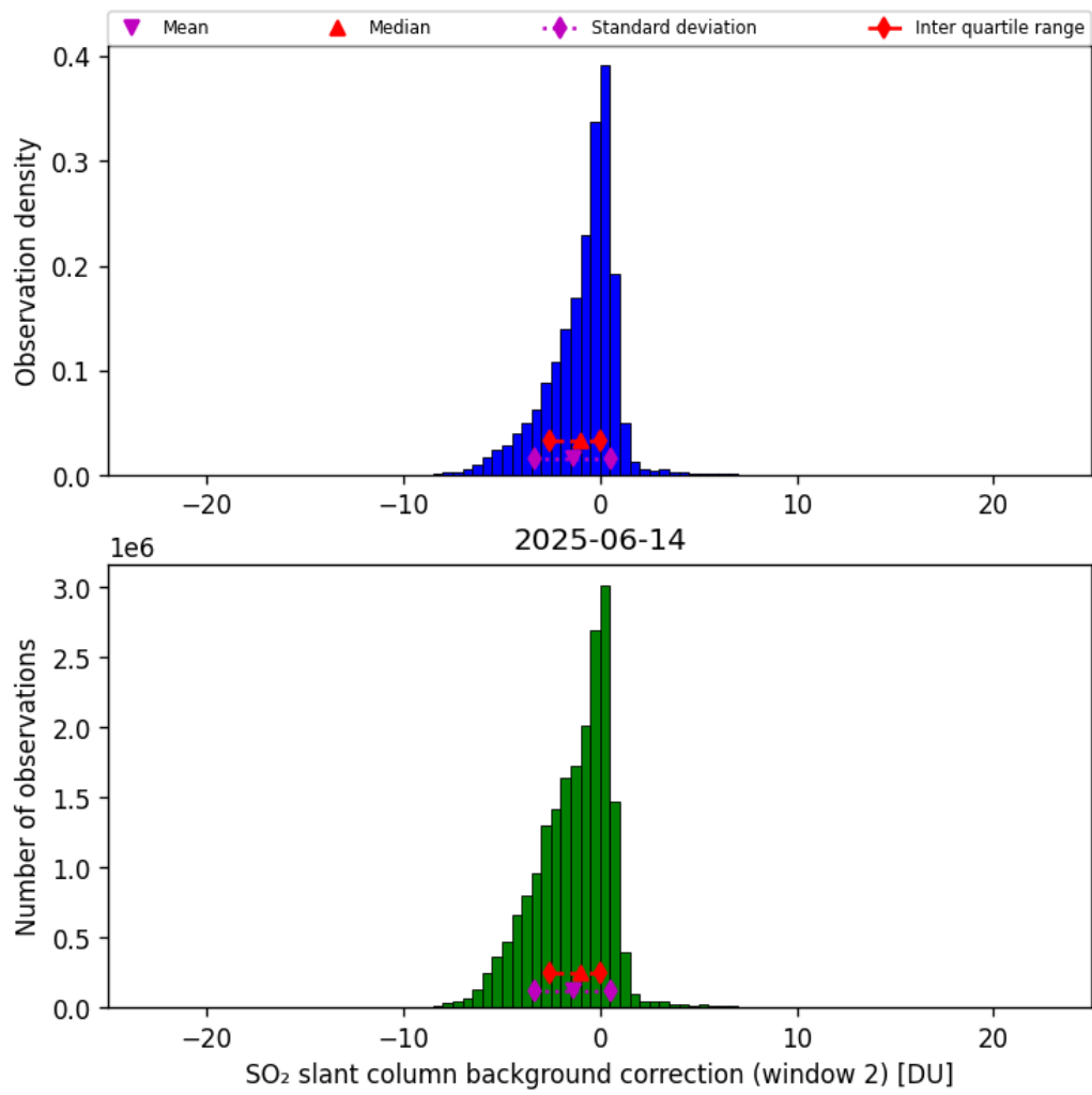
Figure 70: Histogram of “SO 2 slant column background correction (window 2)” for 2025-06-13 to 2025-06-15
