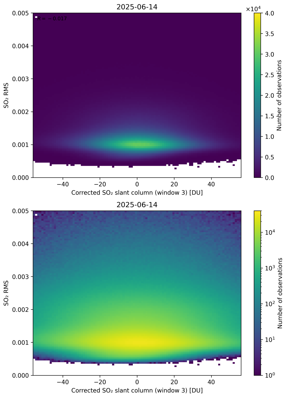
Figure 258: Scatter density plot of “Corrected SO 2 slant column (window 3)” against “SO 2 RMS” for 2025-06-13 to 2025-06-15.
