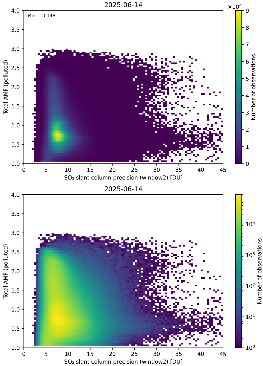
Figure 301: Scatter density plot of “SO 2 slant column precision (window2)” against “Total AMF (polluted)” for 2025-06-13 to 2025-06-15.
