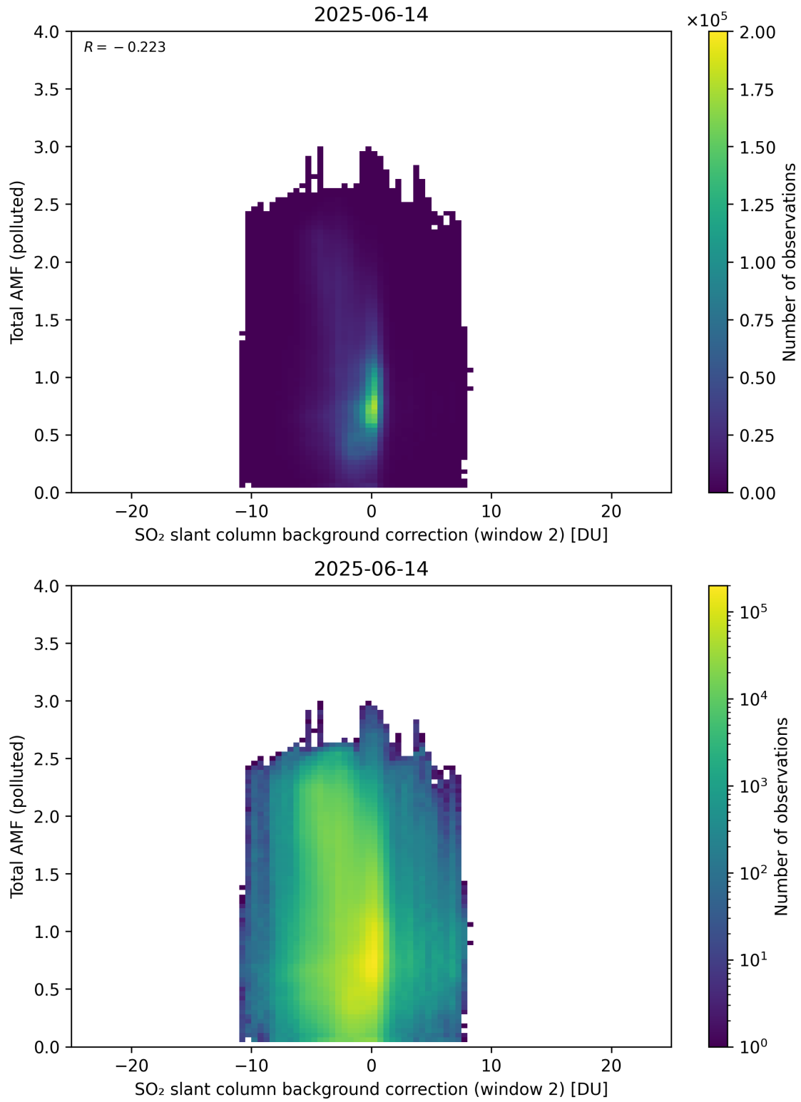
Figure 130: Scatter density plot of “SO 2 slant column background correction (window 2)” against “Total AMF (polluted)” for 2025-06-13 to 2025-06-15.
