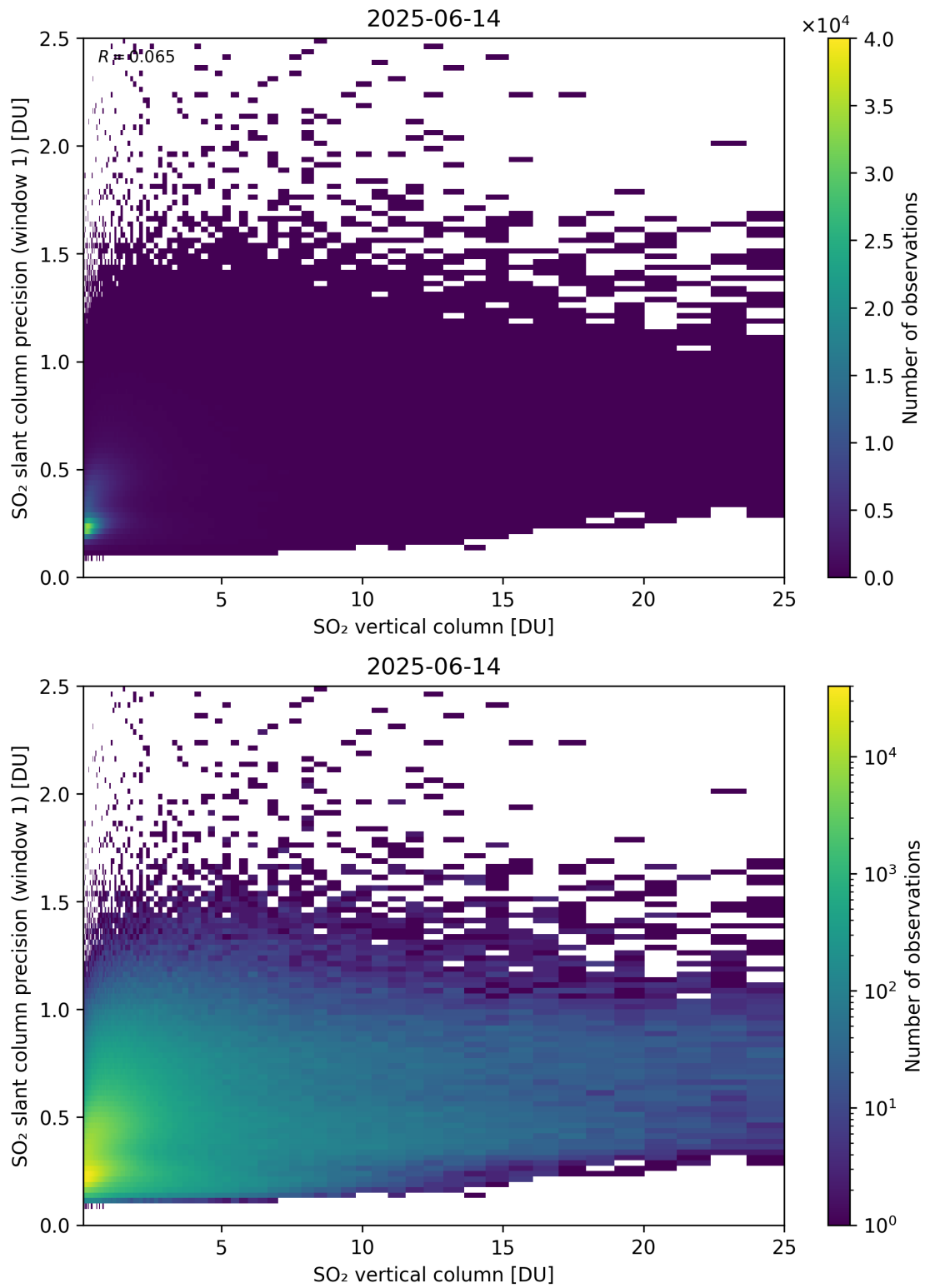
Figure 355: Scatter density plot of “SO 2 vertical column” against “SO 2 slant column precision (window 1)” for 2025-06-13 to 2025-06-15.
