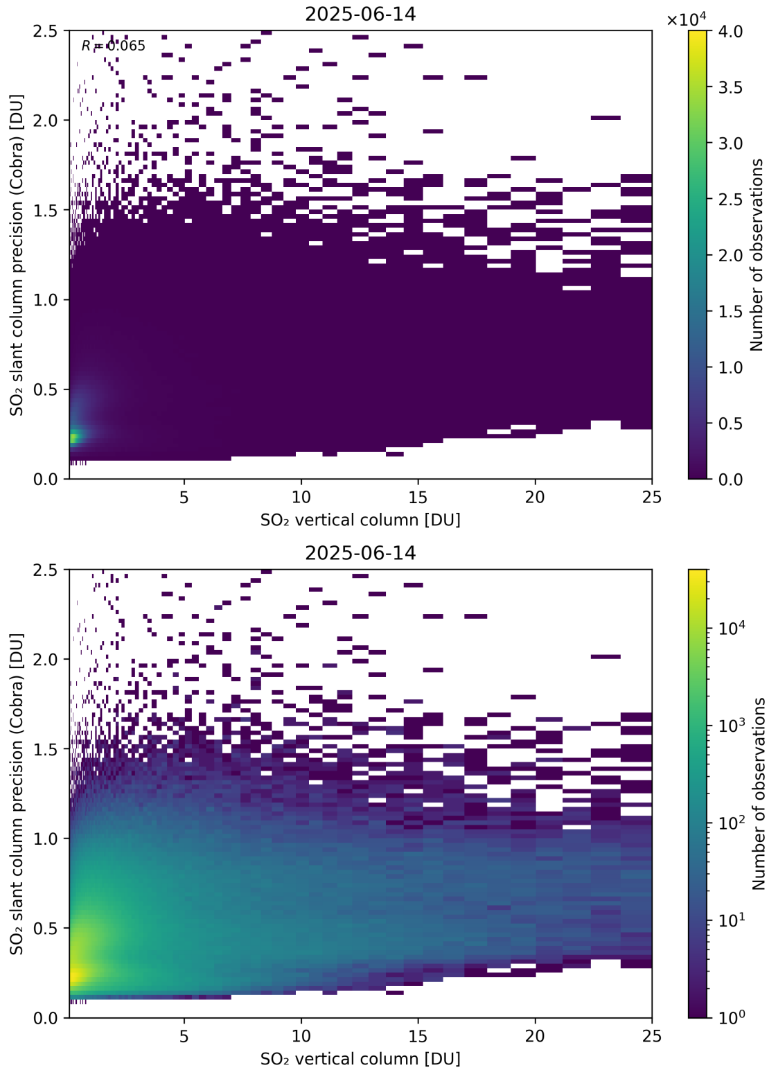
Figure 350: Scatter density plot of “SO 2 vertical column” against “SO 2 slant column precision (Cobra)” for 2025-06-13 to 2025-06-15.
