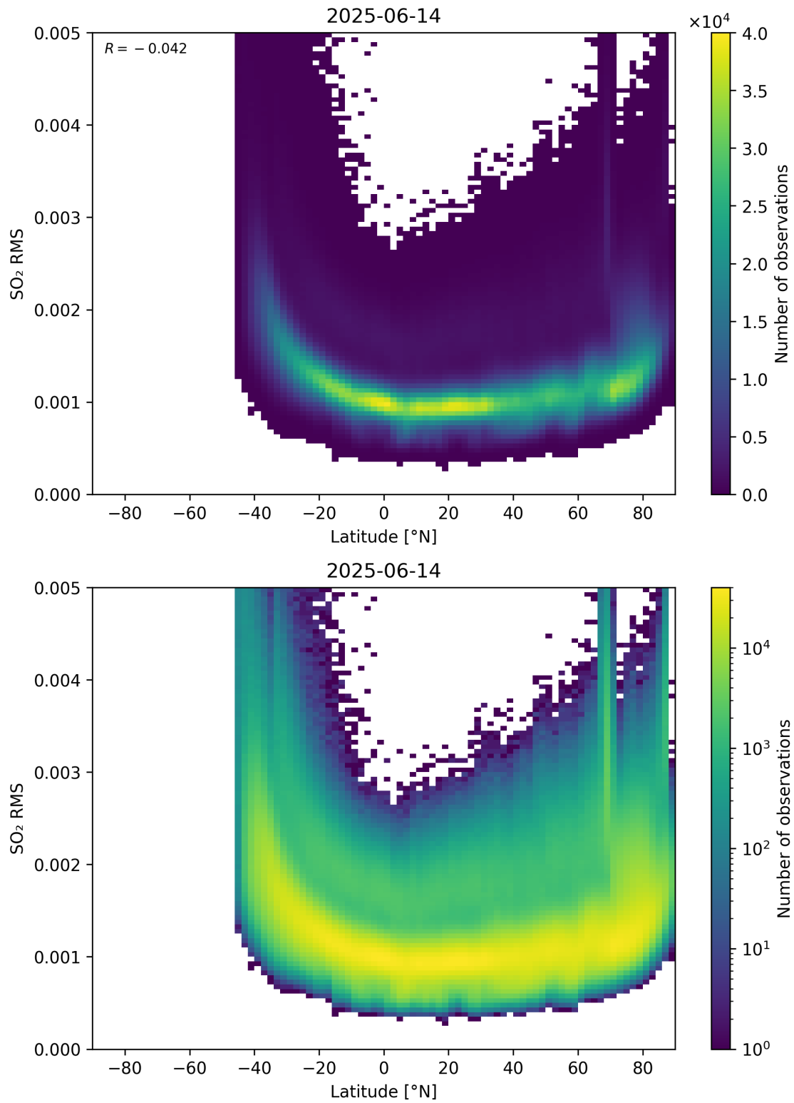
Figure 155: Scatter density plot of “Latitude” against “SO 2 RMS” for 2025-06-13 to 2025-06-15.
