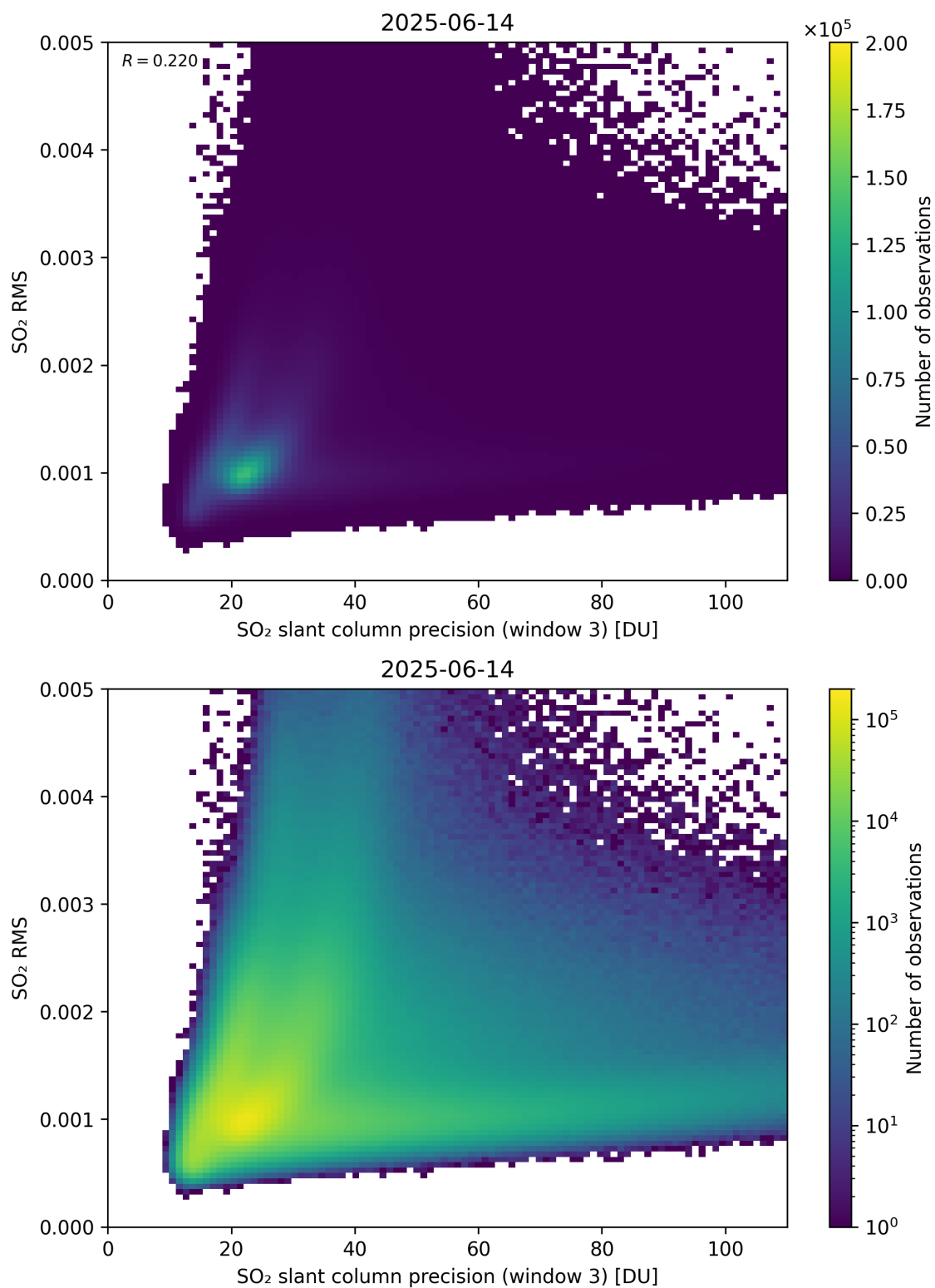
Figure 310: Scatter density plot of “SO 2 slant column precision (window 3)” against “SO 2 RMS” for 2025-06-13 to 2025-06-15.
