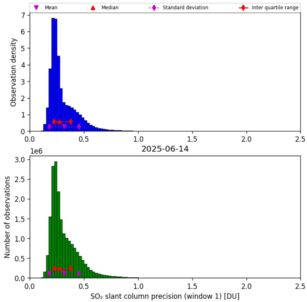
Figure 64: Histogram of “SO 2 slant column precision (window 1)” for 2025-06-13 to 2025-06-15
