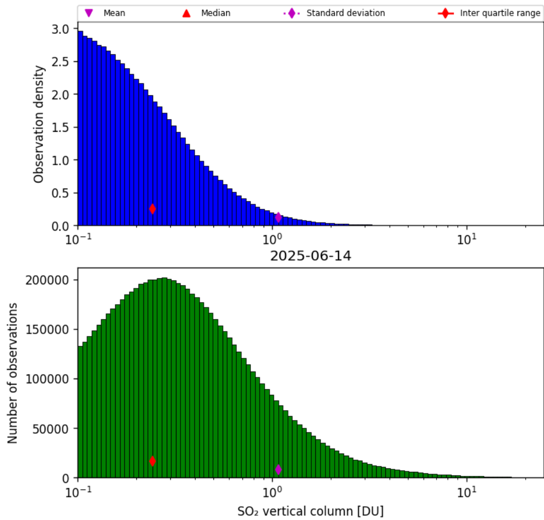
Figure 58: Histogram of “SO 2 vertical column” for 2025-06-13 to 2025-06-15
