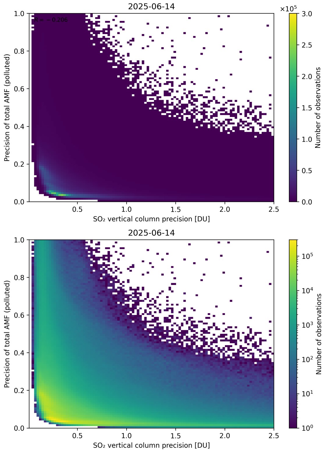
Figure 347: Scatter density plot of “SO 2 vertical column precision” against “Precision of total AMF (polluted)” for 2025-06-13 to 2025-06-15.
