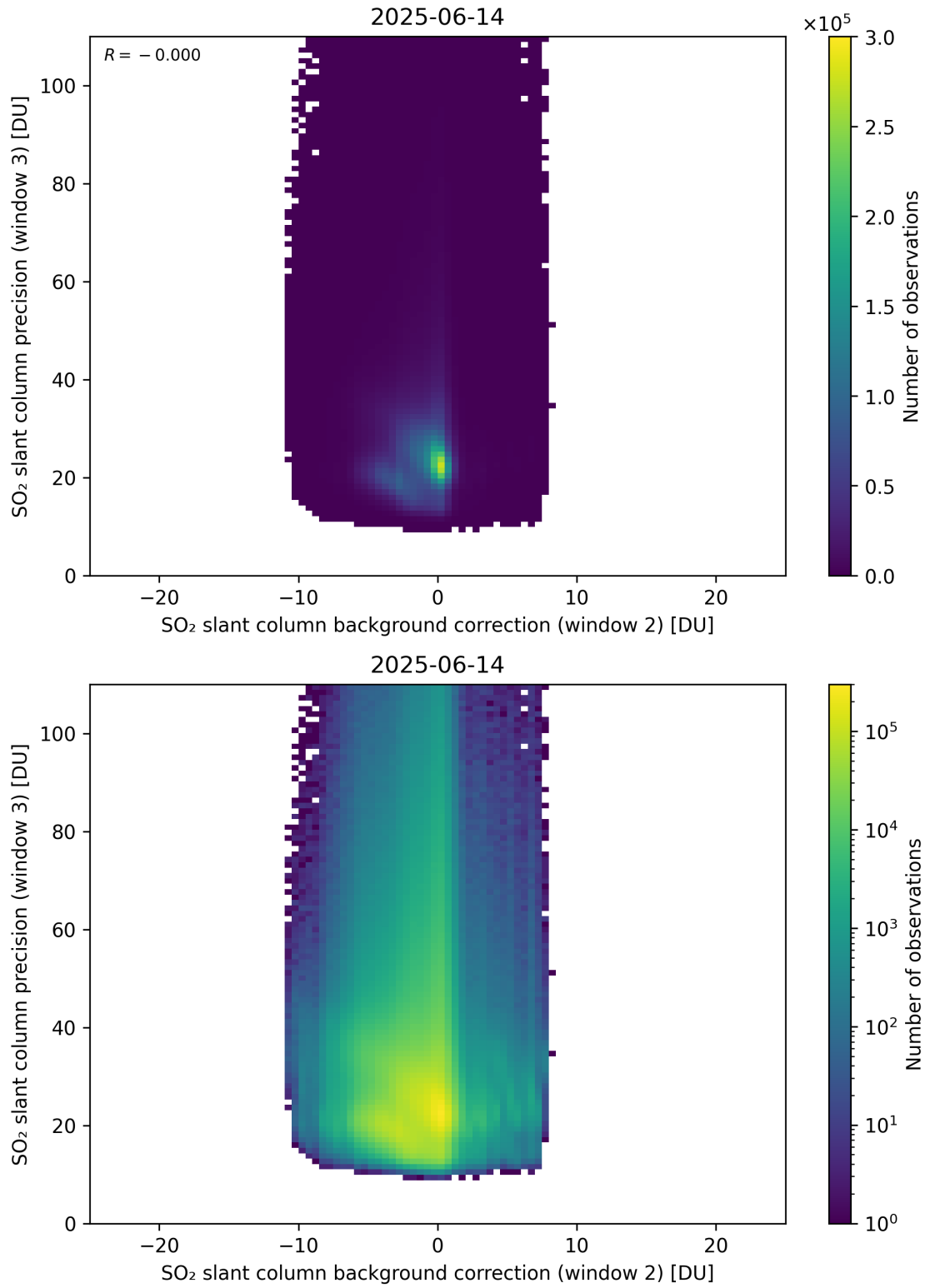
Figure 129: Scatter density plot of “SO 2 slant column background correction (window 2)” against “SO 2 slant column precision (window 3)” for 2025-06-13 to 2025-06-15.
