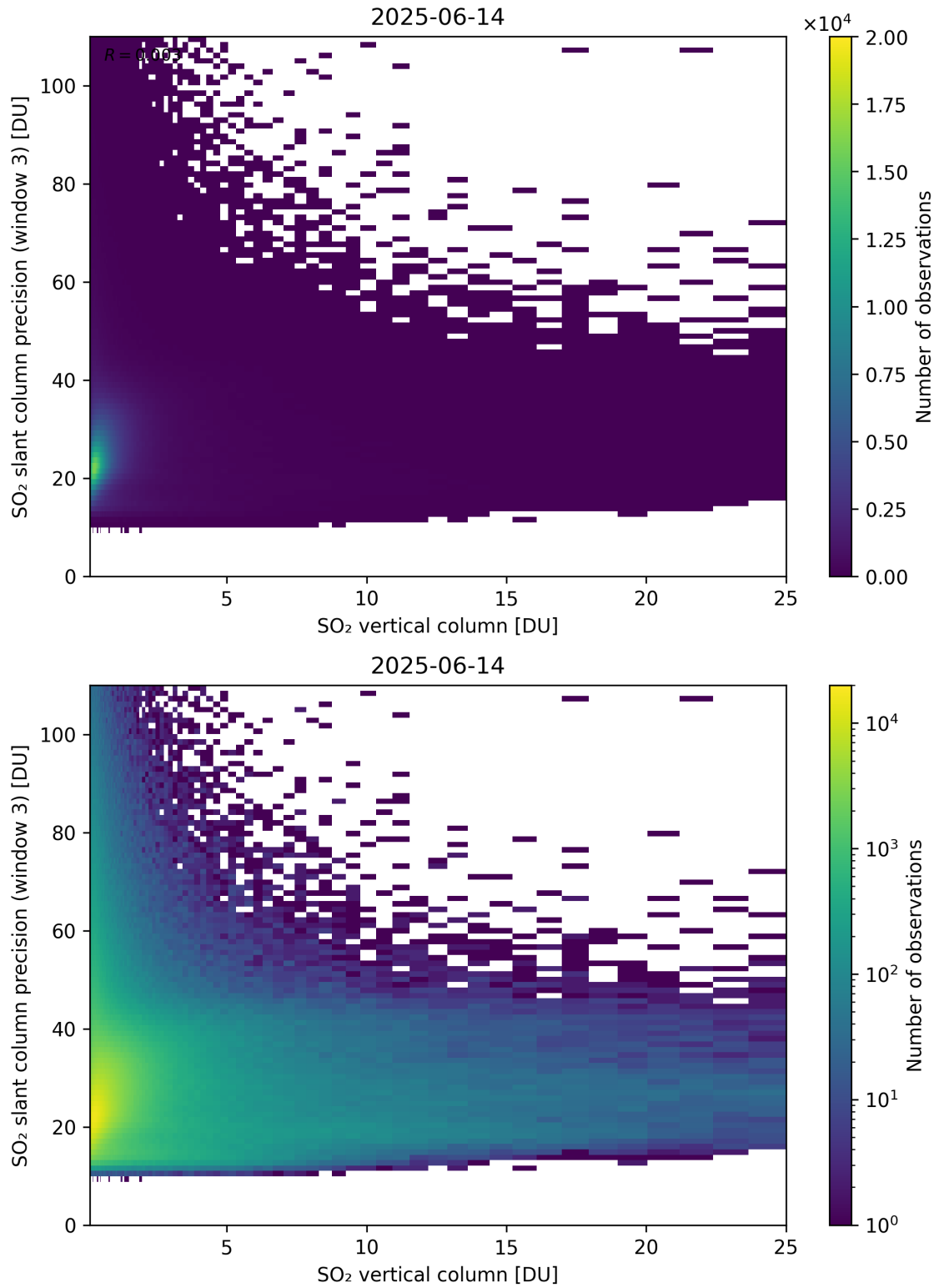
Figure 358: Scatter density plot of “SO 2 vertical column” against “SO 2 slant column precision (window 3)” for 2025-06-13 to 2025-06-15.
