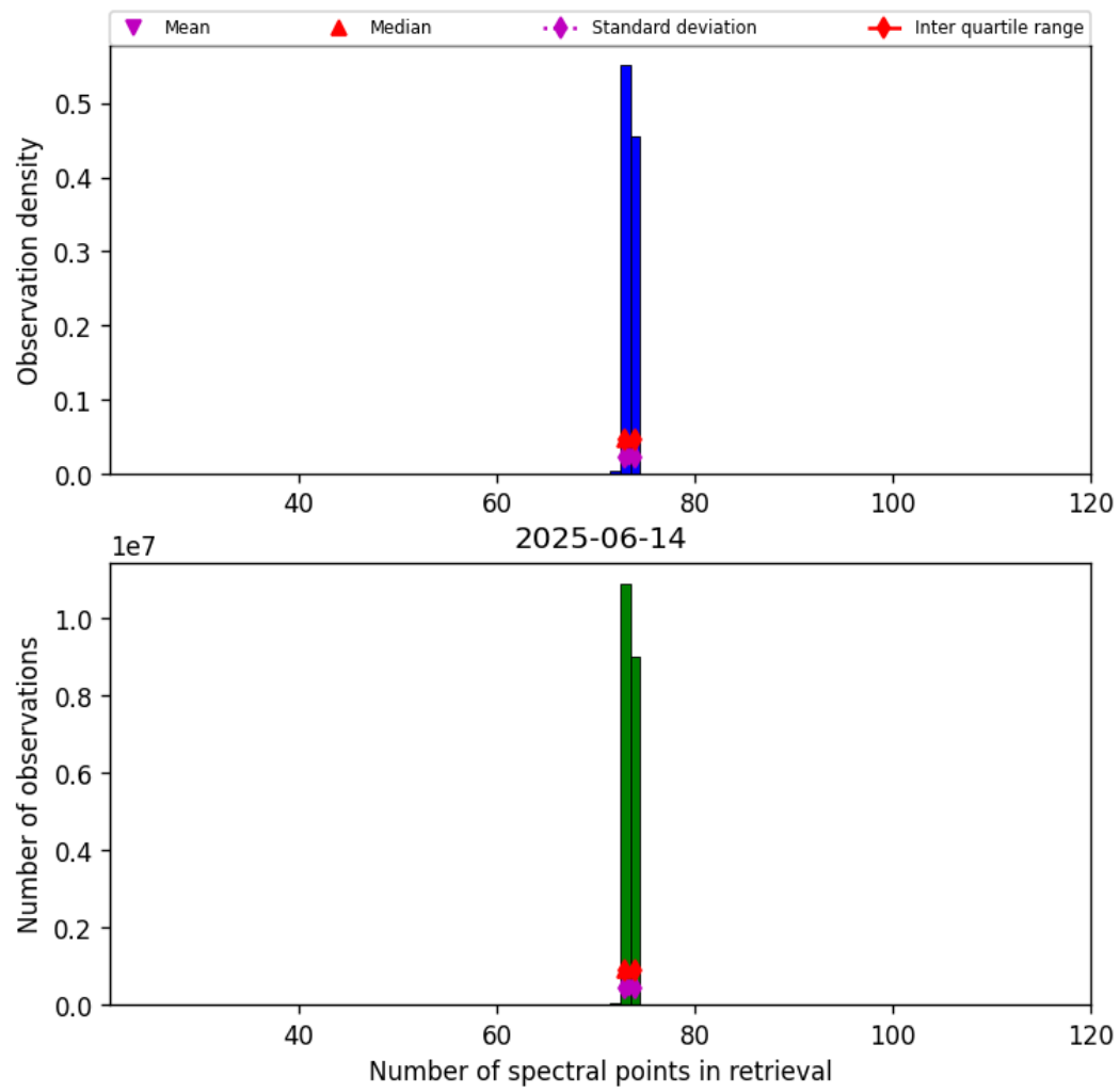
Figure 82: Histogram of “Number of spectral points in retrieval” for 2025-06-13 to 2025-06-15
