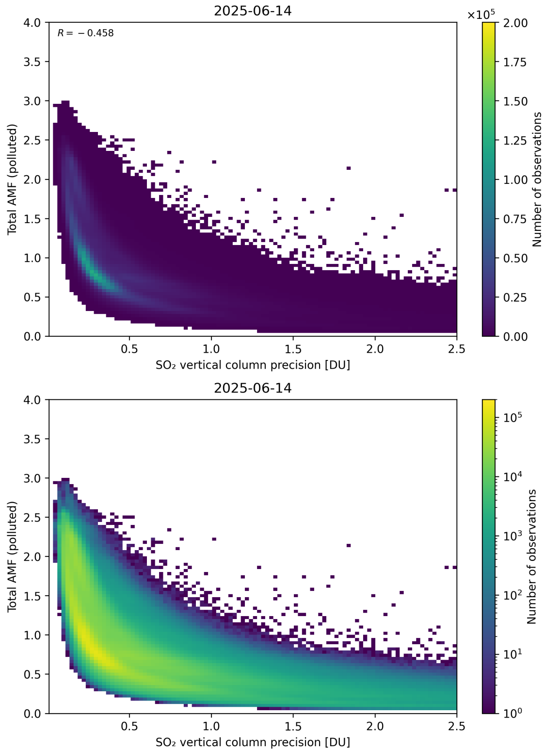
Figure 346: Scatter density plot of “SO 2 vertical column precision” against “Total AMF (polluted)” for 2025-06-13 to 2025-06-15.
