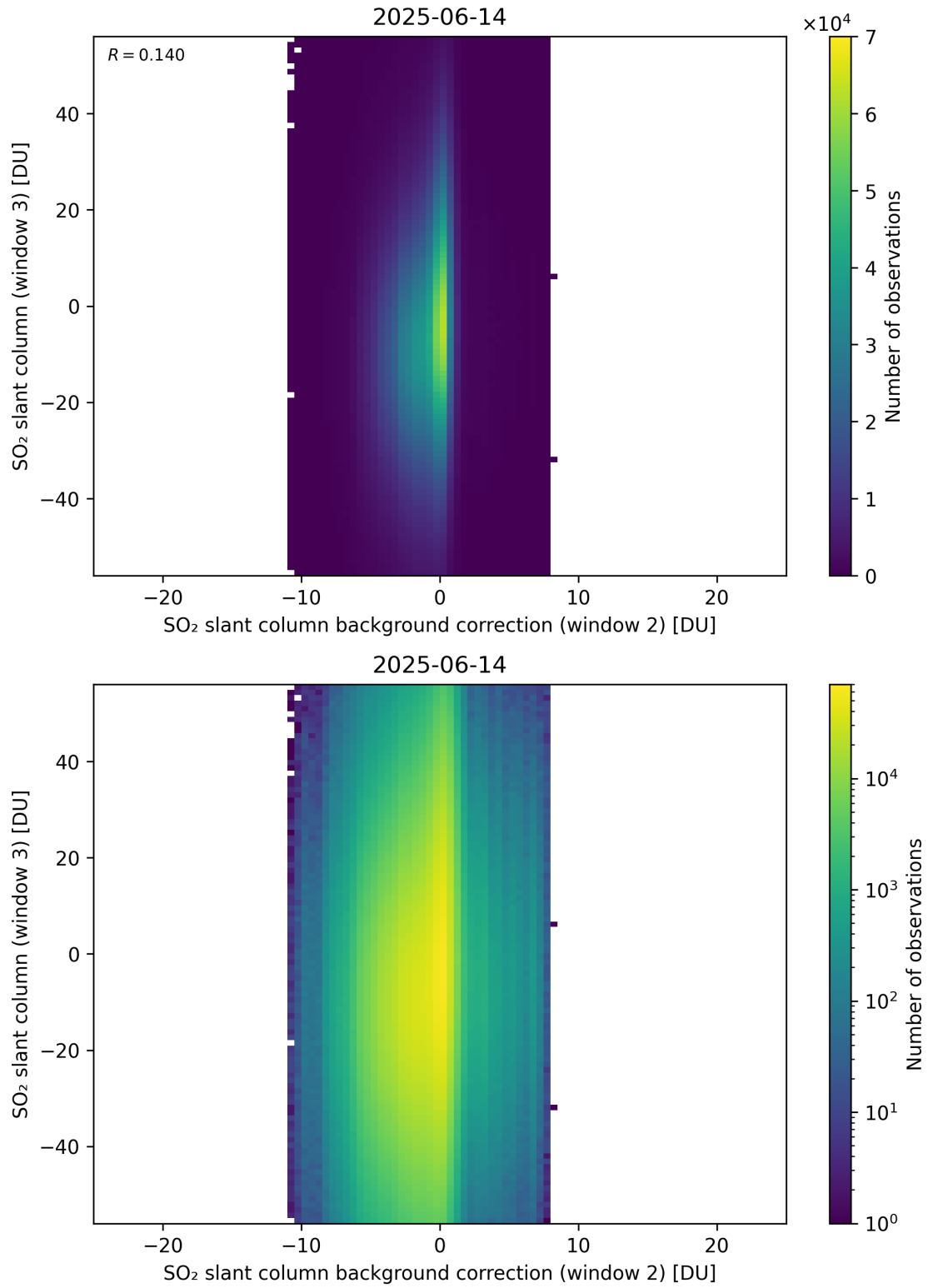
Figure 128: Scatter density plot of “SO 2 slant column background correction (window 2)” against “SO 2 slant column (window 3)” for 2025-06-13 to 2025-06-15.
