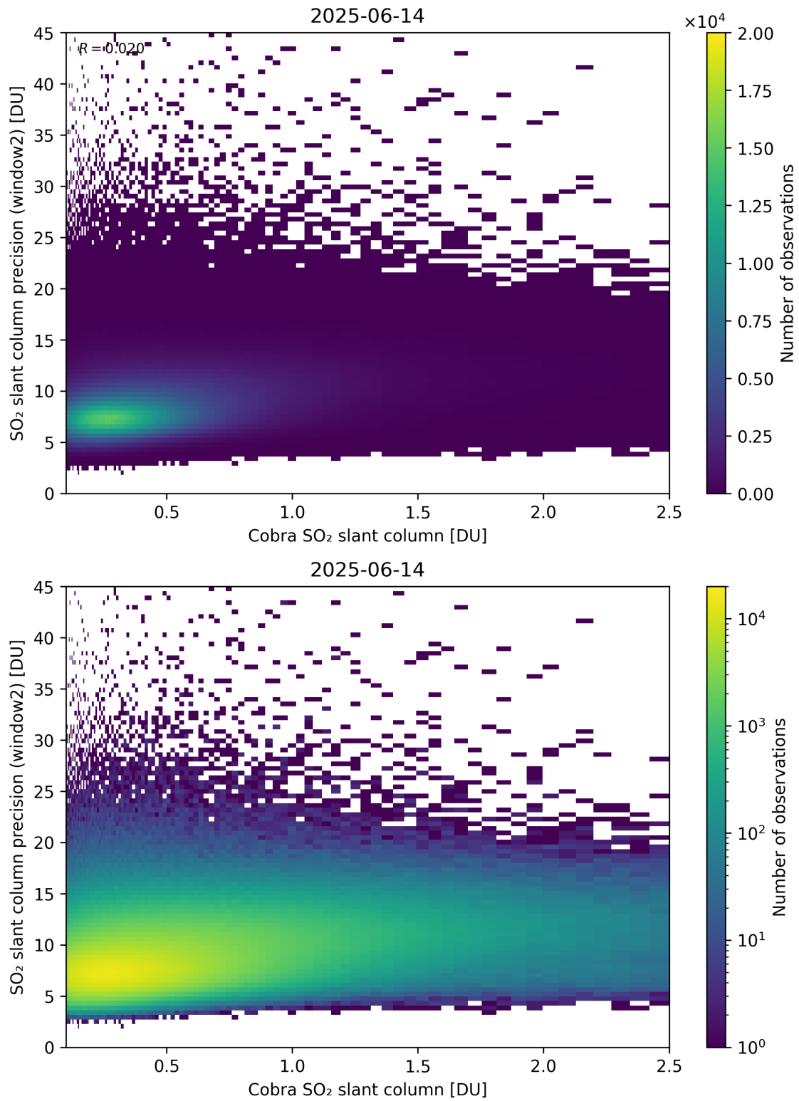
Figure 221: Scatter density plot of “Cobra SO 2 slant column” against “SO 2 slant column precision (window2)” for 2025-06-13 to 2025-06-15.
