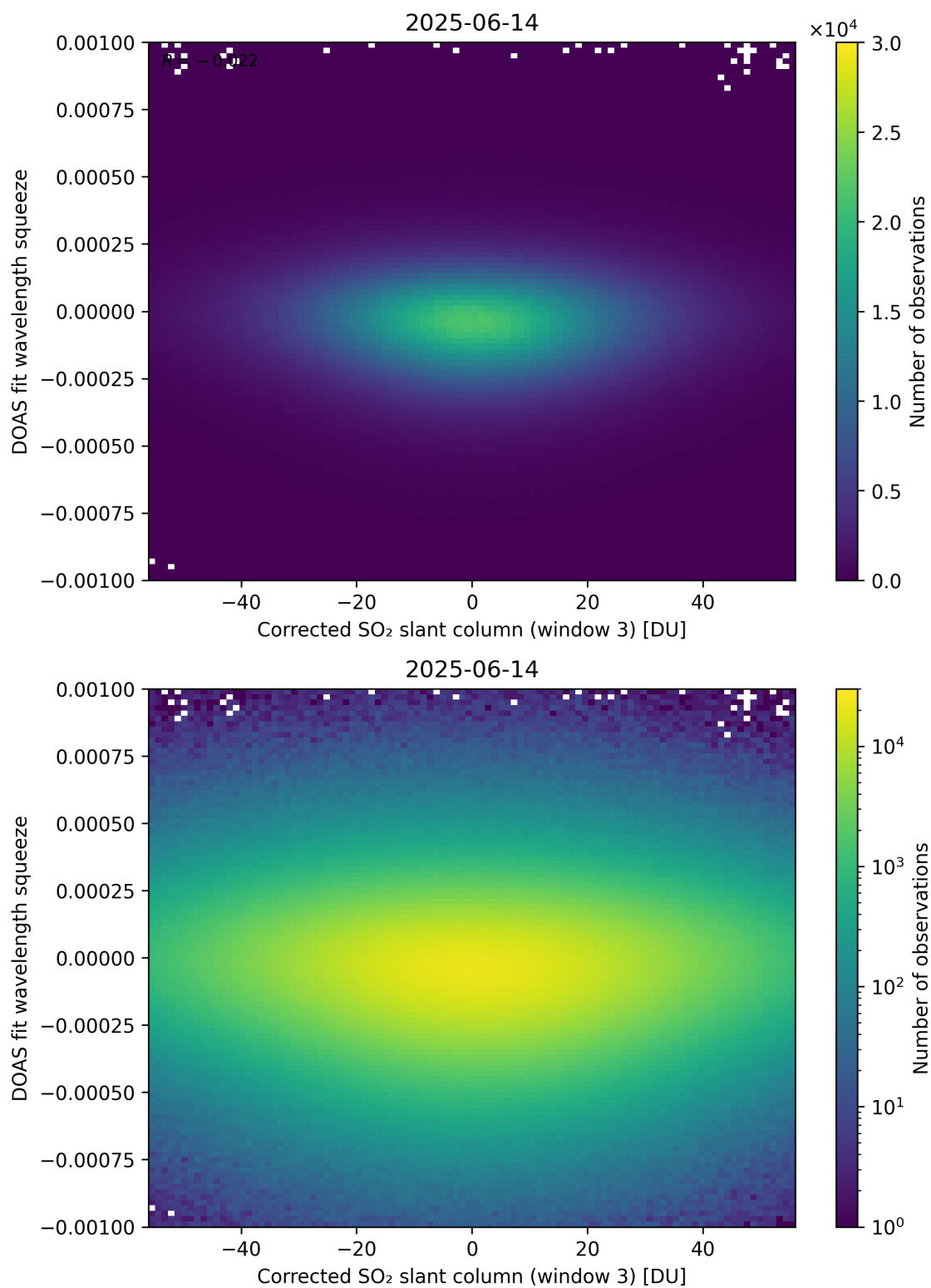
Figure 257: Scatter density plot of “Corrected SO 2 slant column (window 3)” against “DOAS fit wavelength squeeze” for 2025-06-13 to 2025-06-15.
