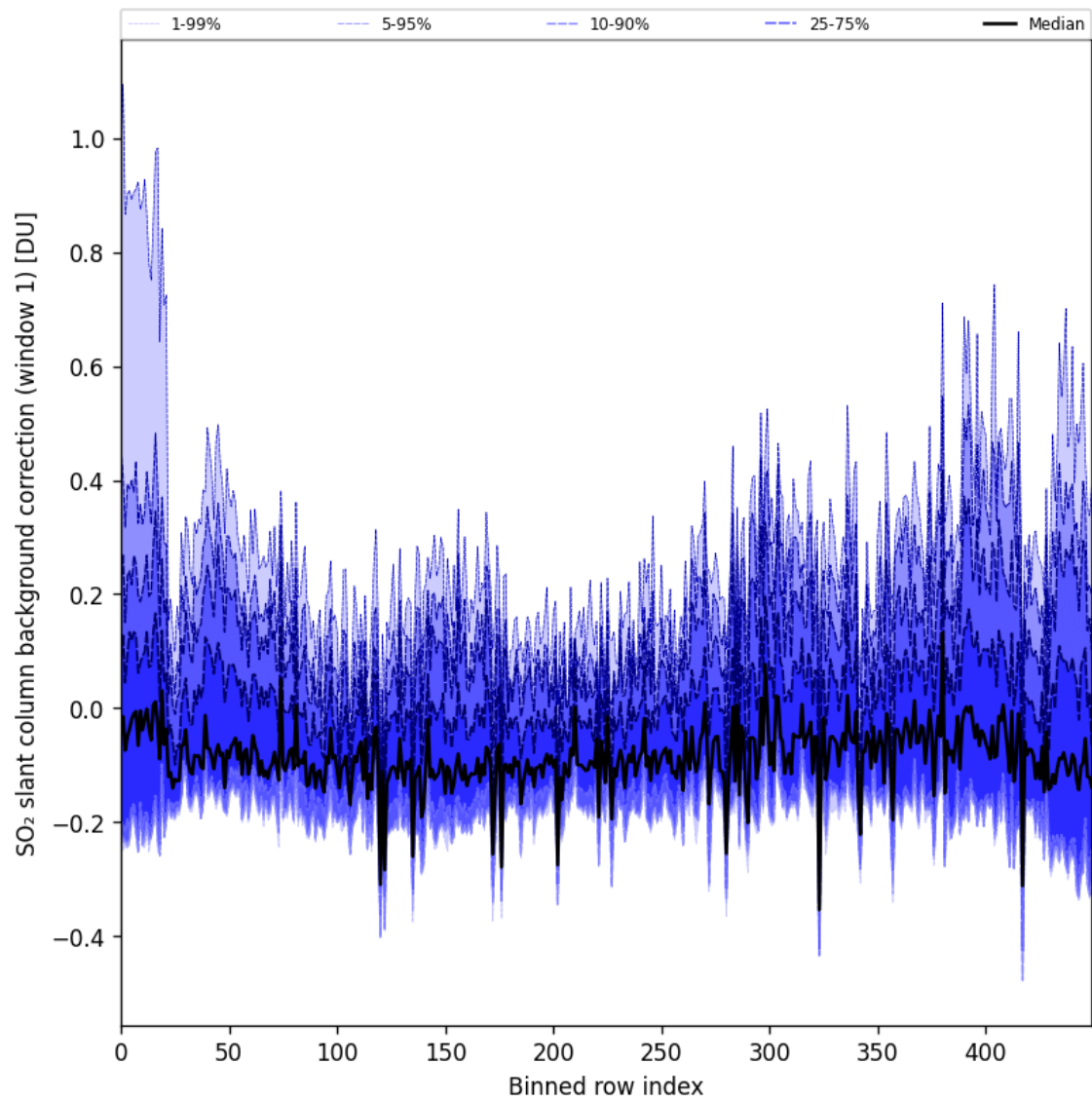
Figure 92: Along track statistics of “SO 2 slant column background correction (window 1)” for 2025-06-13 to 2025-06-15
