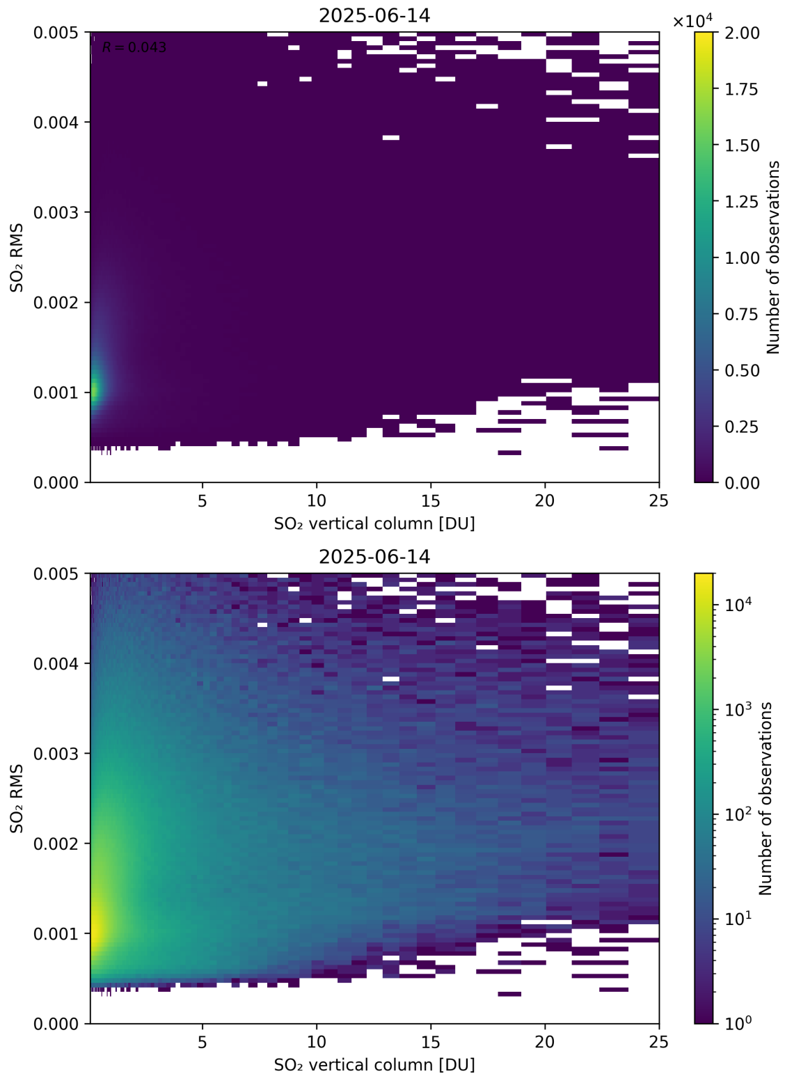
Figure 328: Scatter density plot of “SO 2 vertical column” against “SO 2 RMS” for 2025-06-13 to 2025-06-15.
