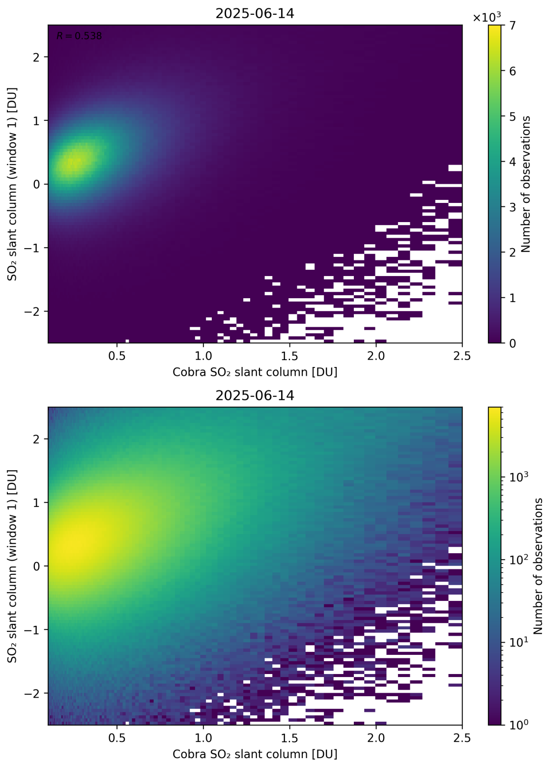
Figure 219: Scatter density plot of “Cobra SO 2 slant column” against “SO 2 slant column (window 1)” for 2025-06-13 to 2025-06-15.
