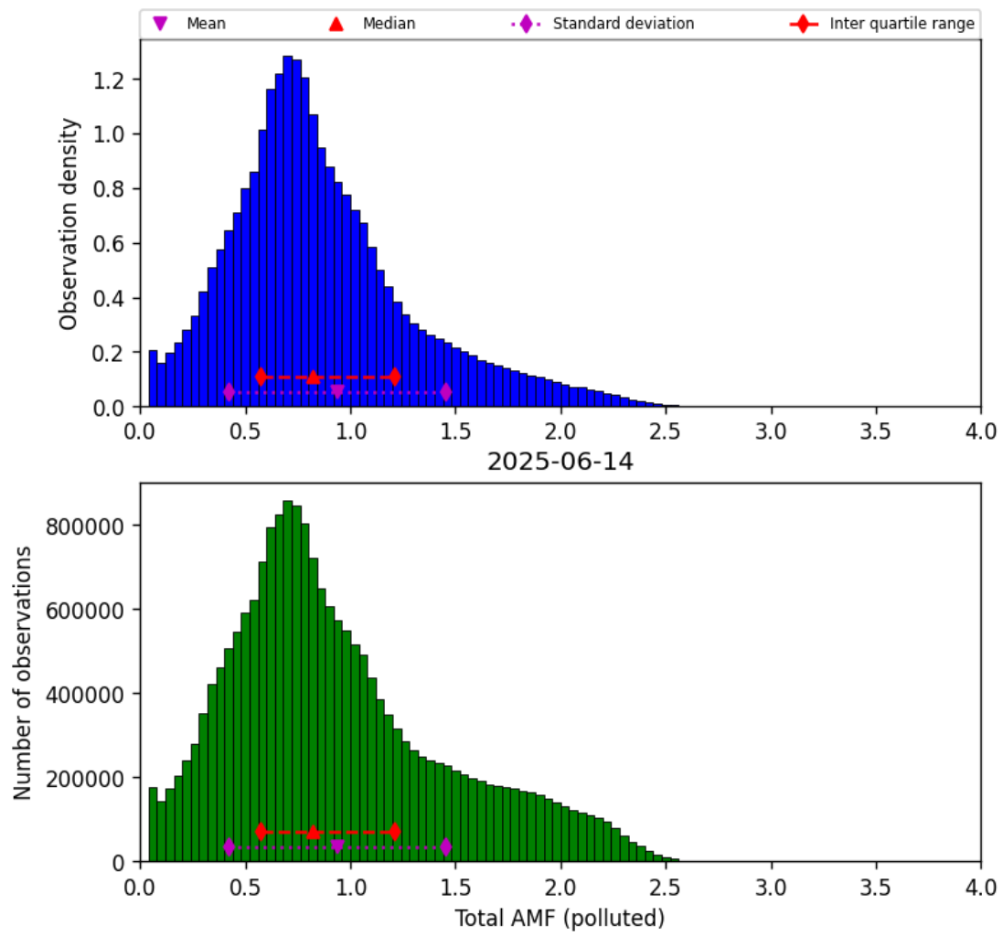
Figure 79: Histogram of “Total AMF (polluted)” for 2025-06-13 to 2025-06-15
