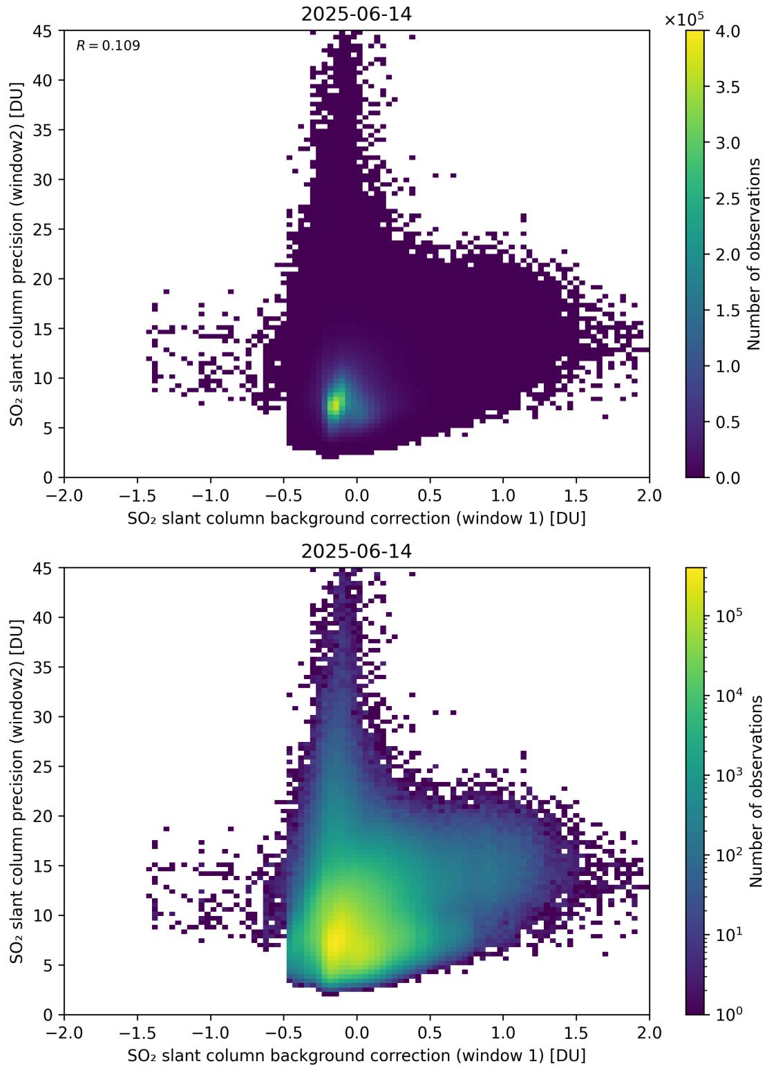
Figure 117: Scatter density plot of “SO 2 slant column background correction (window 1)” against “SO 2 slant column precision (window2)” for 2025-06-13 to 2025-06-15.
