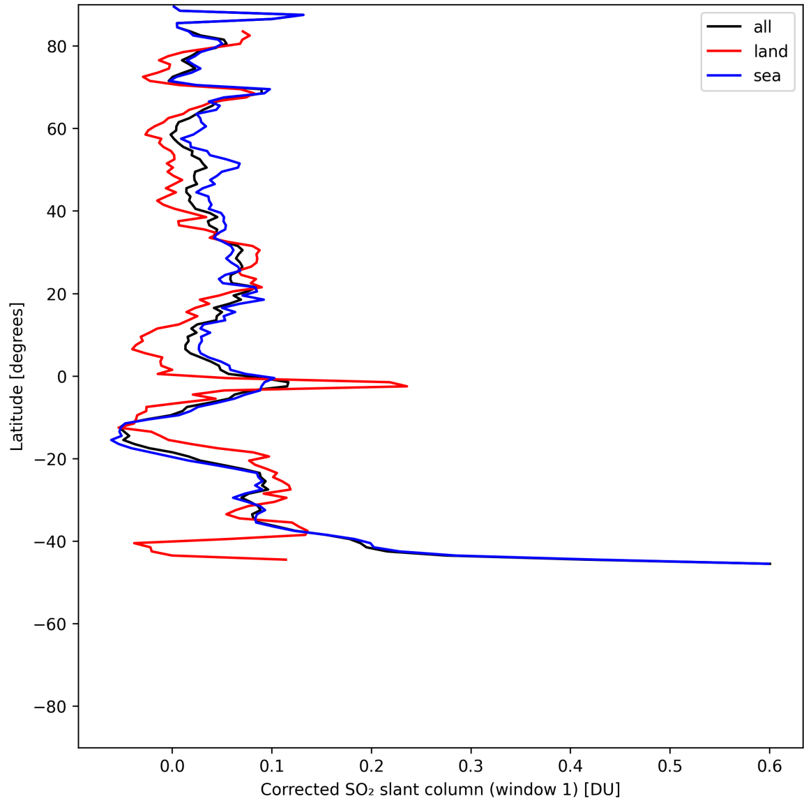
Figure 39: Zonal average of “Corrected SO 2 slant column (window 1)” for 2025-06-13 to 2025-06-15.
