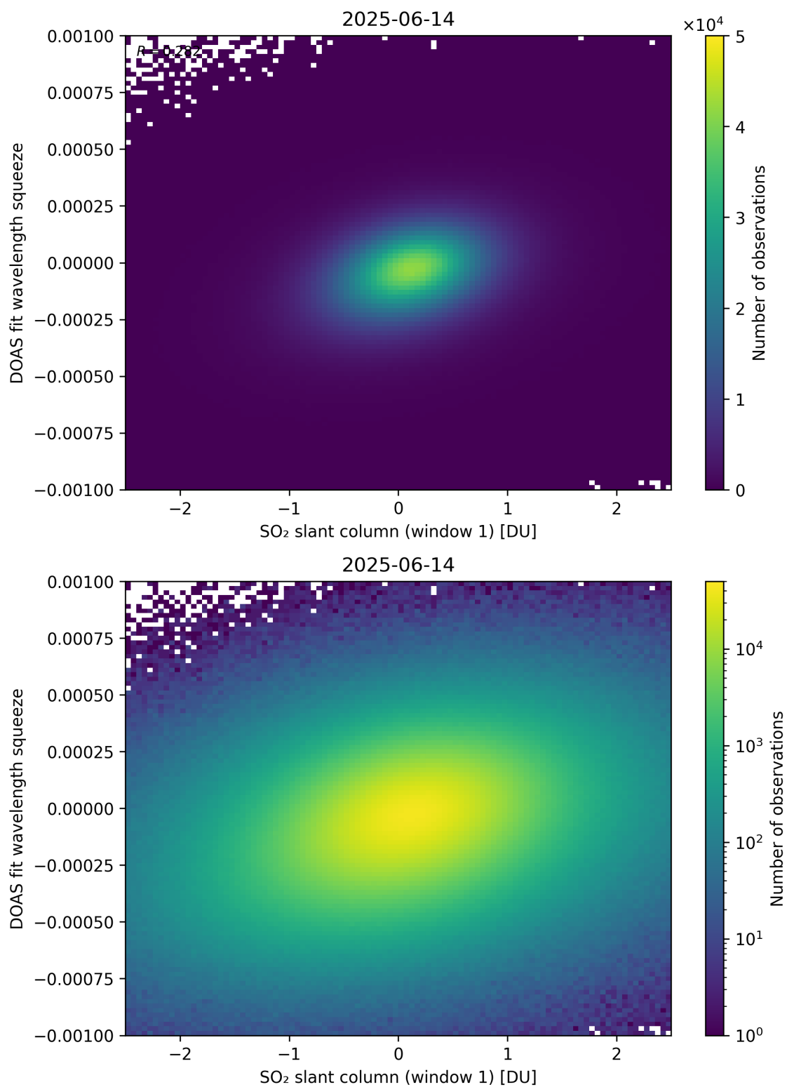
Figure 266: Scatter density plot of “SO 2 slant column (window 1)” against “DOAS fit wavelength squeeze” for 2025-06-13 to 2025-06-15.
