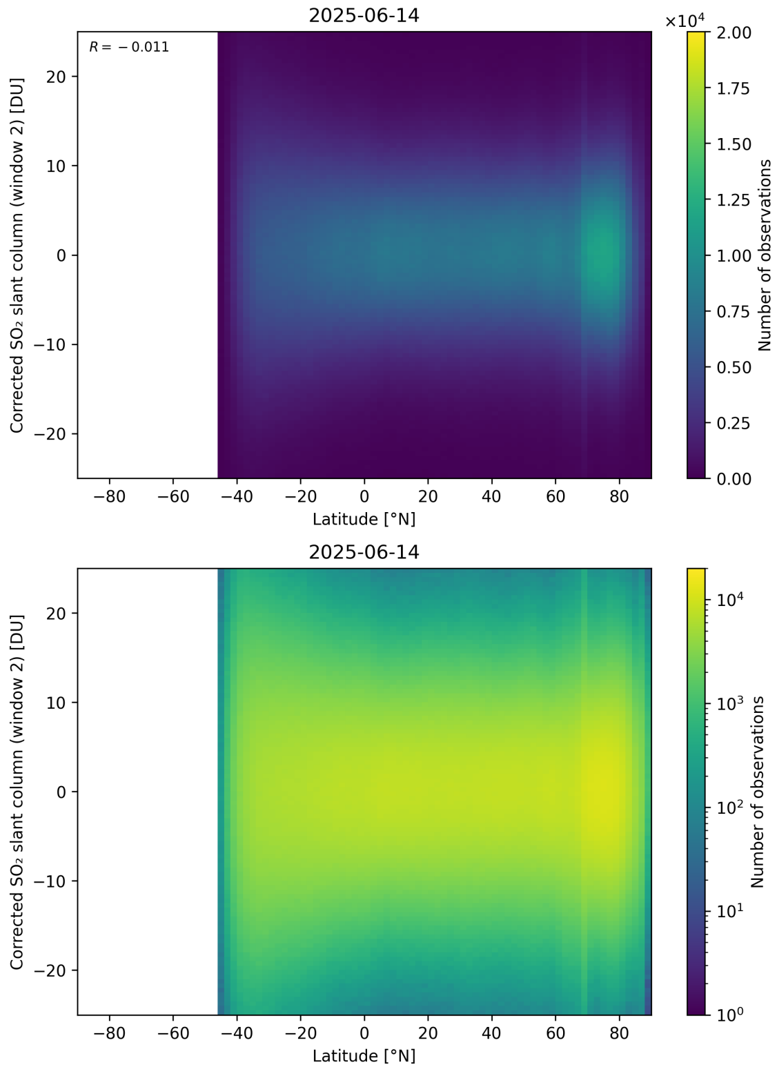
Figure 160: Scatter density plot of “Latitude” against “Corrected SO 2 slant column (window 2)” for 2025-06-13 to 2025-06-15.
