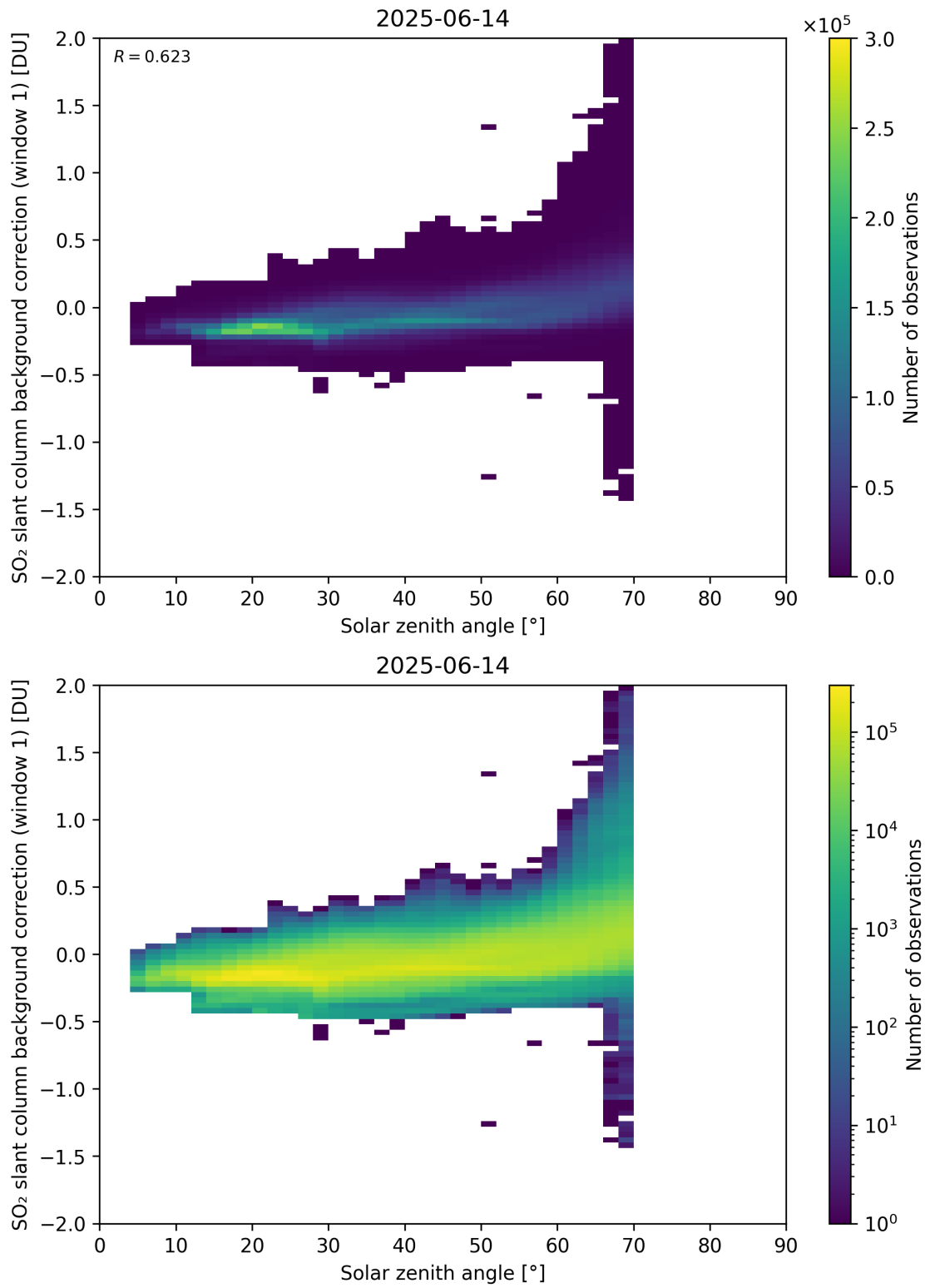
Figure 171: Scatter density plot of “Solar zenith angle” against “SO 2 slant column background correction (window 1)” for 2025-06-13 to 2025-06-15.
