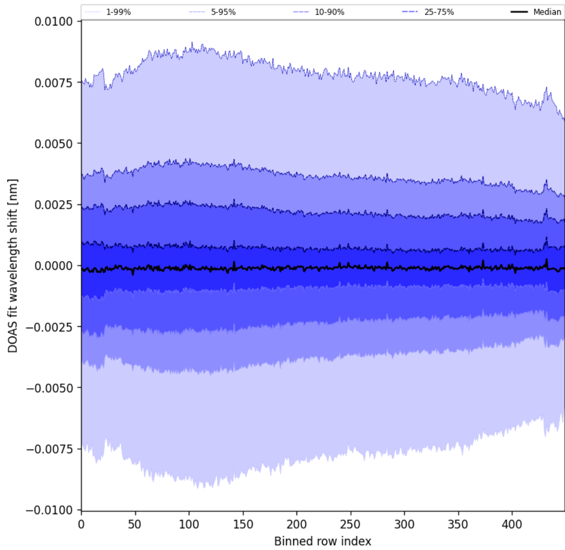
Figure 102: Along track statistics of “DOAS fit wavelength shift” for 2025-06-13 to 2025-06-15
