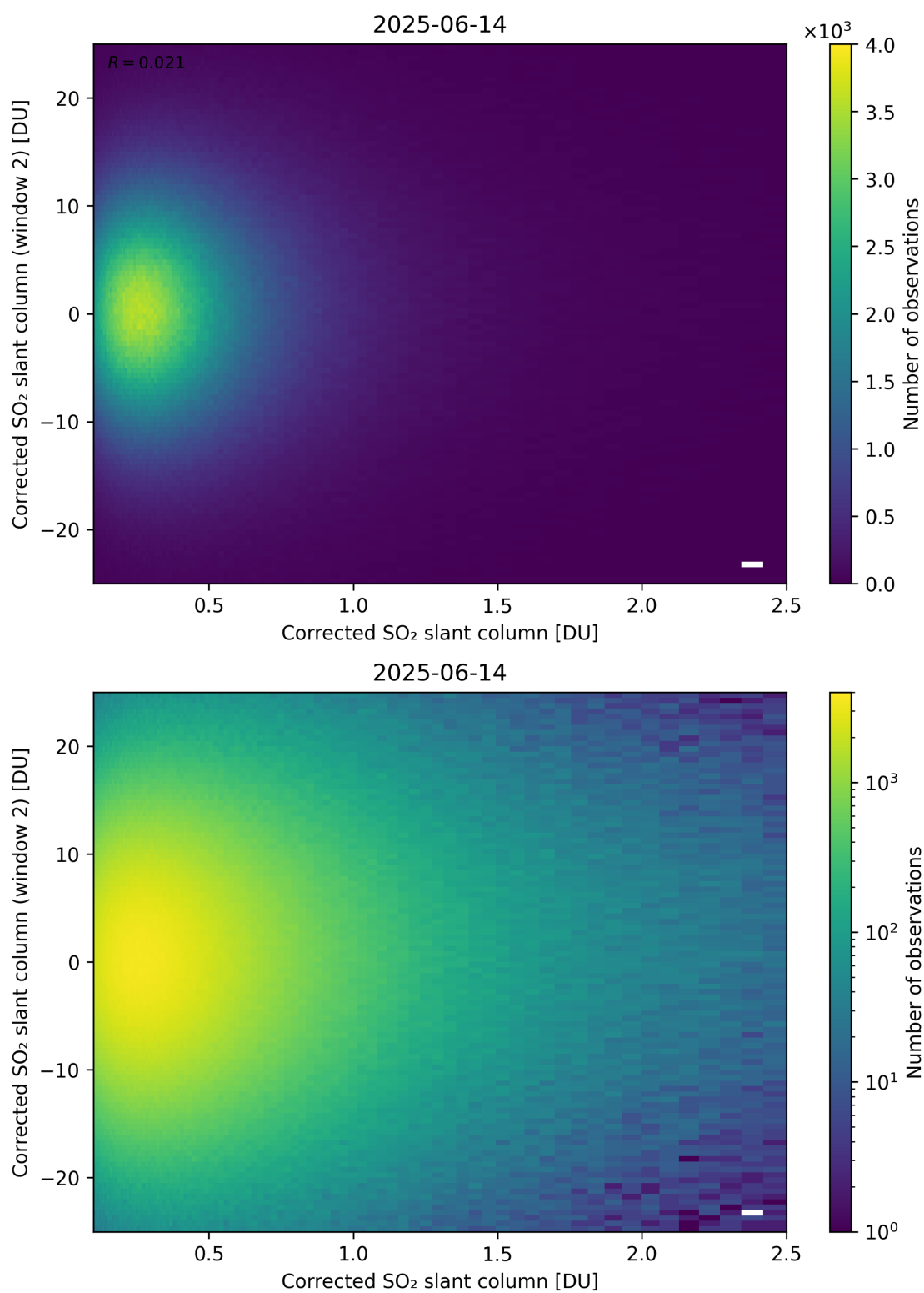
Figure 235: Scatter density plot of “Corrected SO 2 slant column” against “Corrected SO 2 slant column (window 2)” for 2025-06-13 to 2025-06-15.
