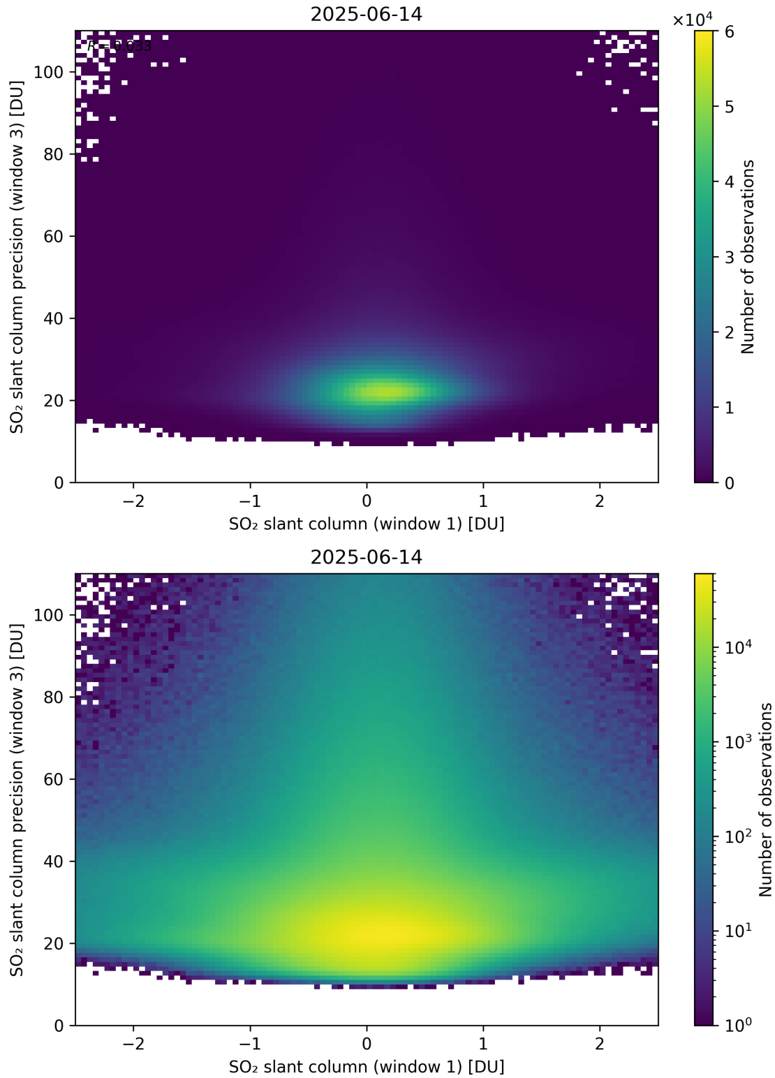
Figure 288: Scatter density plot of “SO 2 slant column (window 1)” against “SO 2 slant column precision (window 3)” for 2025-06-13 to 2025-06-15.
