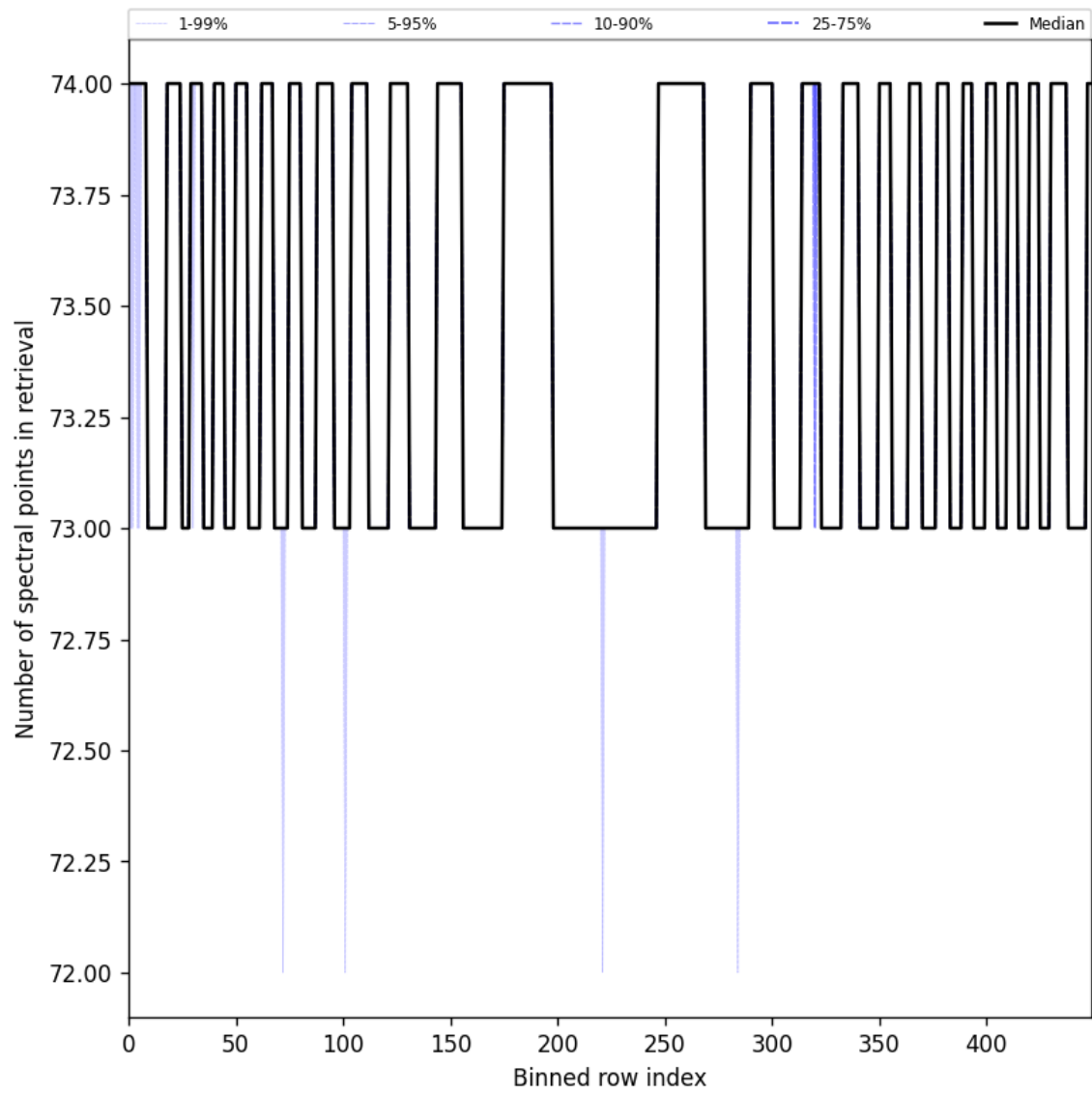
Figure 108: Along track statistics of “Number of spectral points in retrieval” for 2025-06-13 to 2025-06-15
