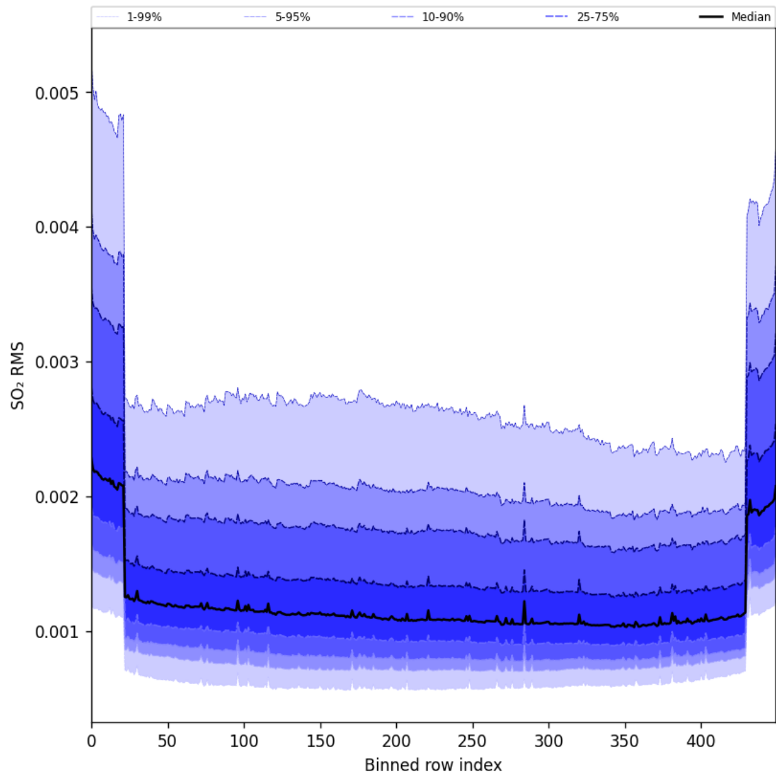
Figure 104: Along track statistics of “SO 2 RMS” for 2025-06-13 to 2025-06-15
