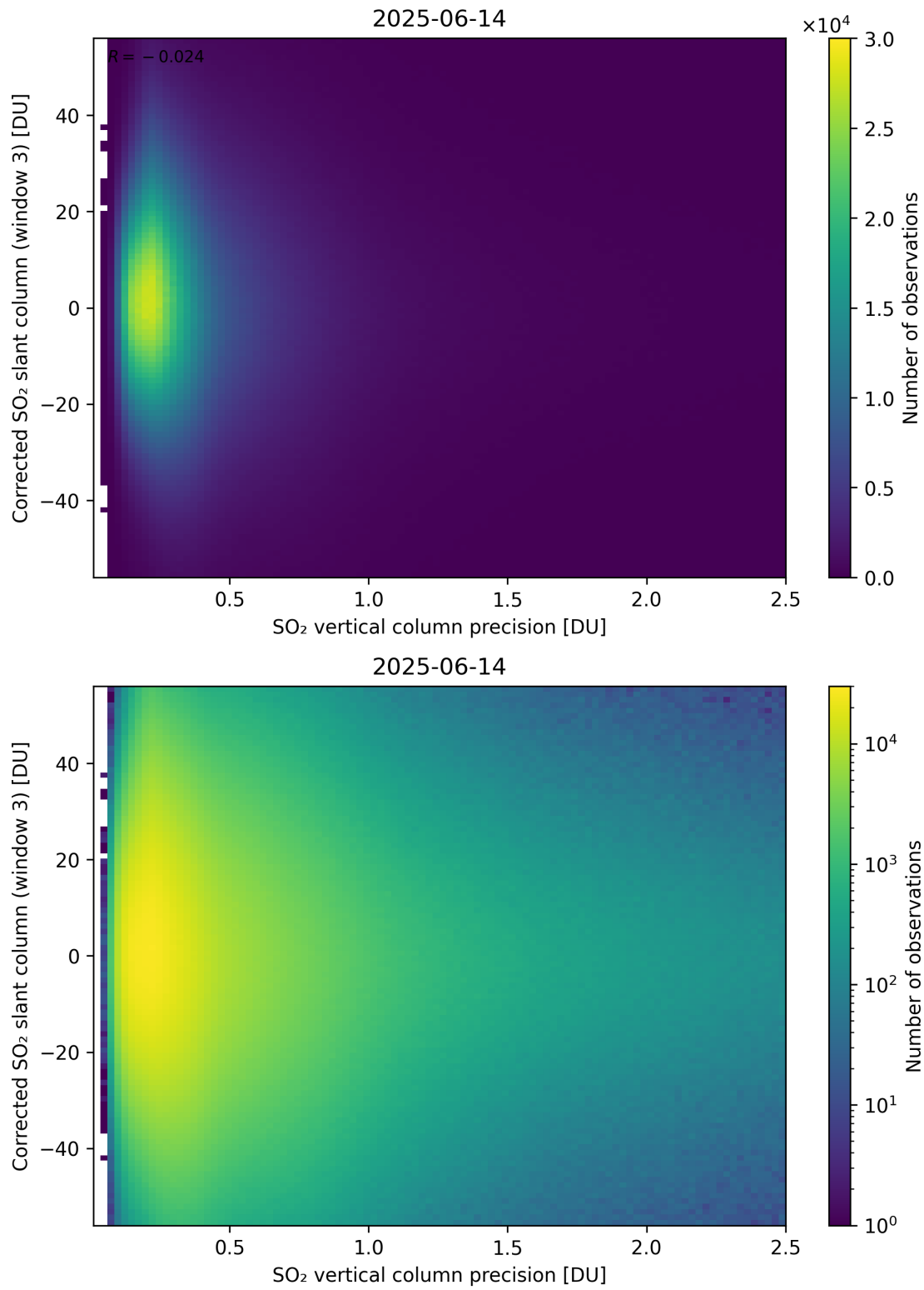
Figure 340: Scatter density plot of “SO 2 vertical column precision” against “Corrected SO 2 slant column (window 3)” for 2025-06-13 to 2025-06-15.
