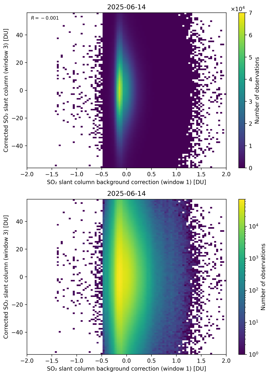
Figure 116: Scatter density plot of “SO 2 slant column background correction (window 1)” against “Corrected SO 2 slant column (window 3)” for 2025-06-13 to 2025-06-15.
