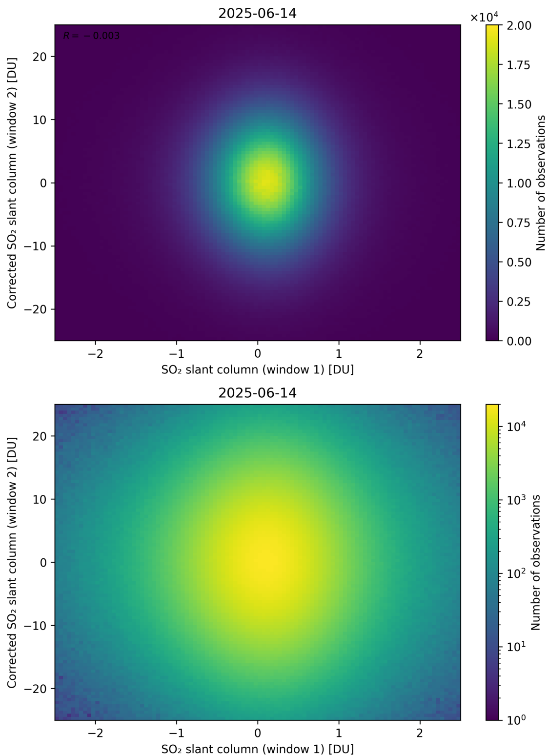
Figure 283: Scatter density plot of “SO 2 slant column (window 1)” against “Corrected SO 2 slant column (window 2)” for 2025-06-13 to 2025-06-15.
