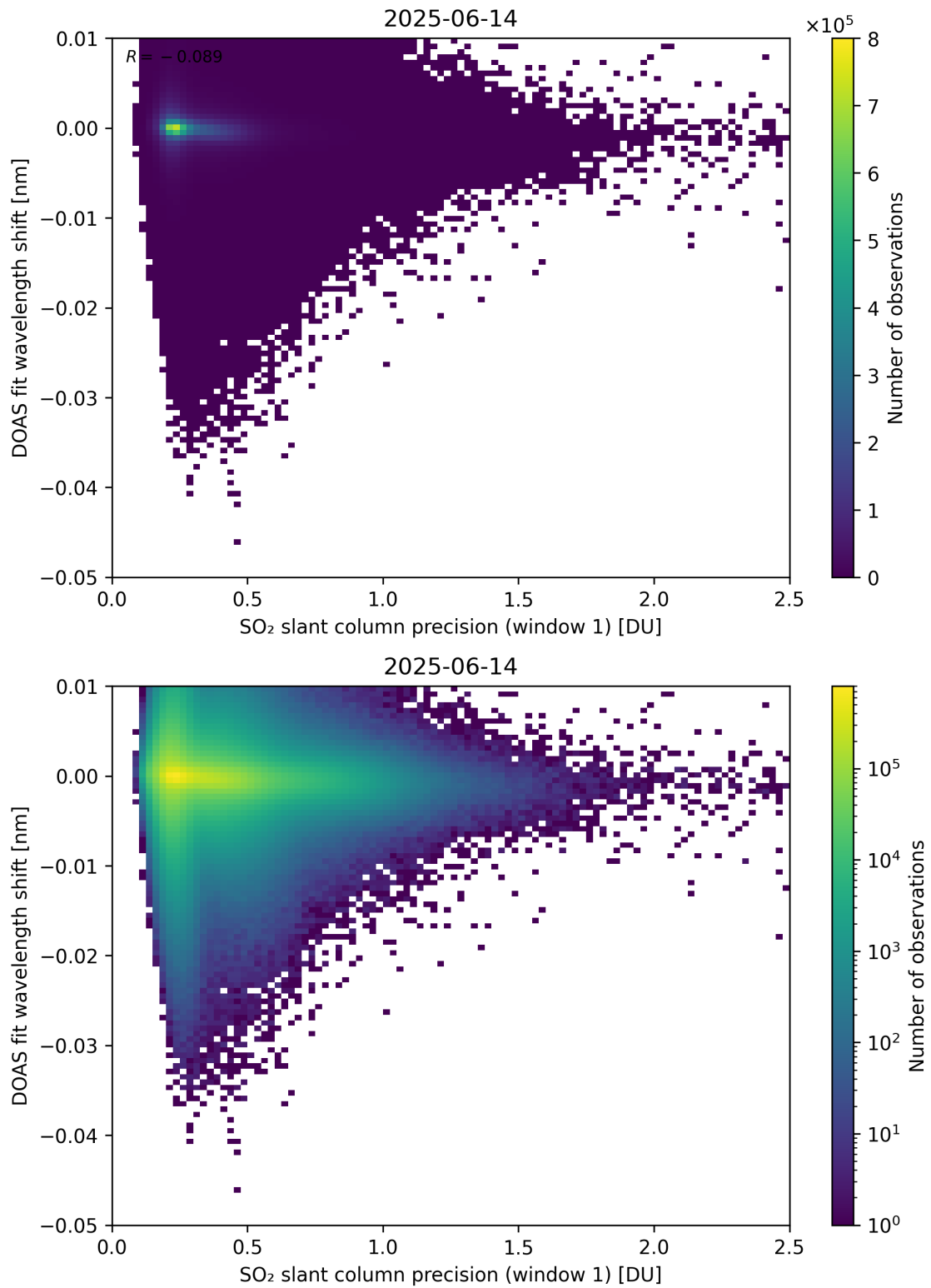
Figure 271: Scatter density plot of “SO 2 slant column precision (window 1)” against “DOAS fit wavelength shift” for 2025-06-13 to 2025-06-15.
