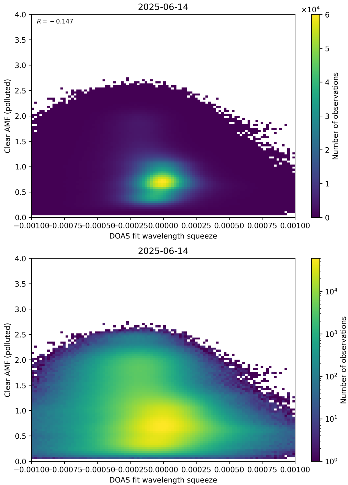
Figure 144: Scatter density plot of “DOAS fit wavelength squeeze” against “Clear AMF (polluted)” for 2025-06-13 to 2025-06-15.
