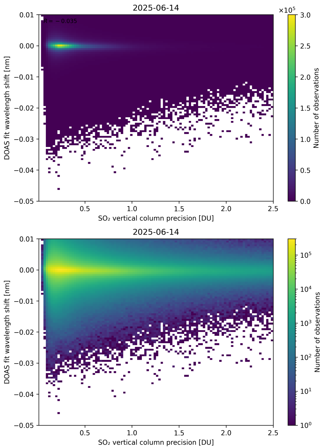
Figure 332: Scatter density plot of “SO 2 vertical column precision” against “DOAS fit wavelength shift” for 2025-06-13 to 2025-06-15.
