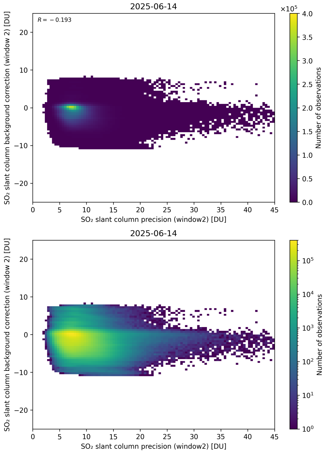
Figure 291: Scatter density plot of “SO 2 slant column precision (window2)” against “SO 2 slant column background correction (window 2)” for 2025-06-13 to 2025-06-15.
