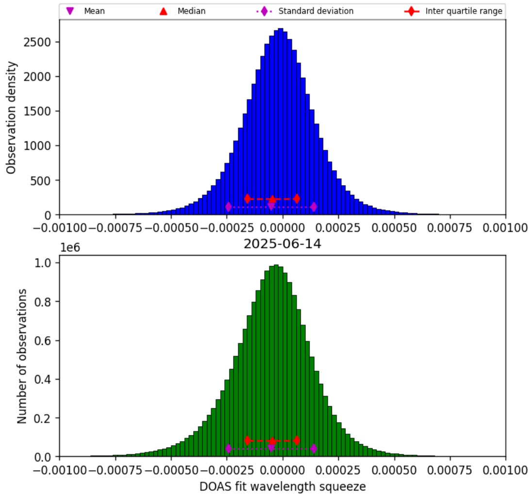
Figure 77: Histogram of “DOAS fit wavelength squeeze” for 2025-06-13 to 2025-06-15
