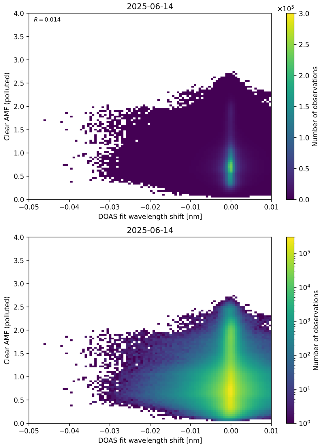
Figure 140: Scatter density plot of “DOAS fit wavelength shift” against “Clear AMF (polluted)” for 2025-06-13 to 2025-06-15.
