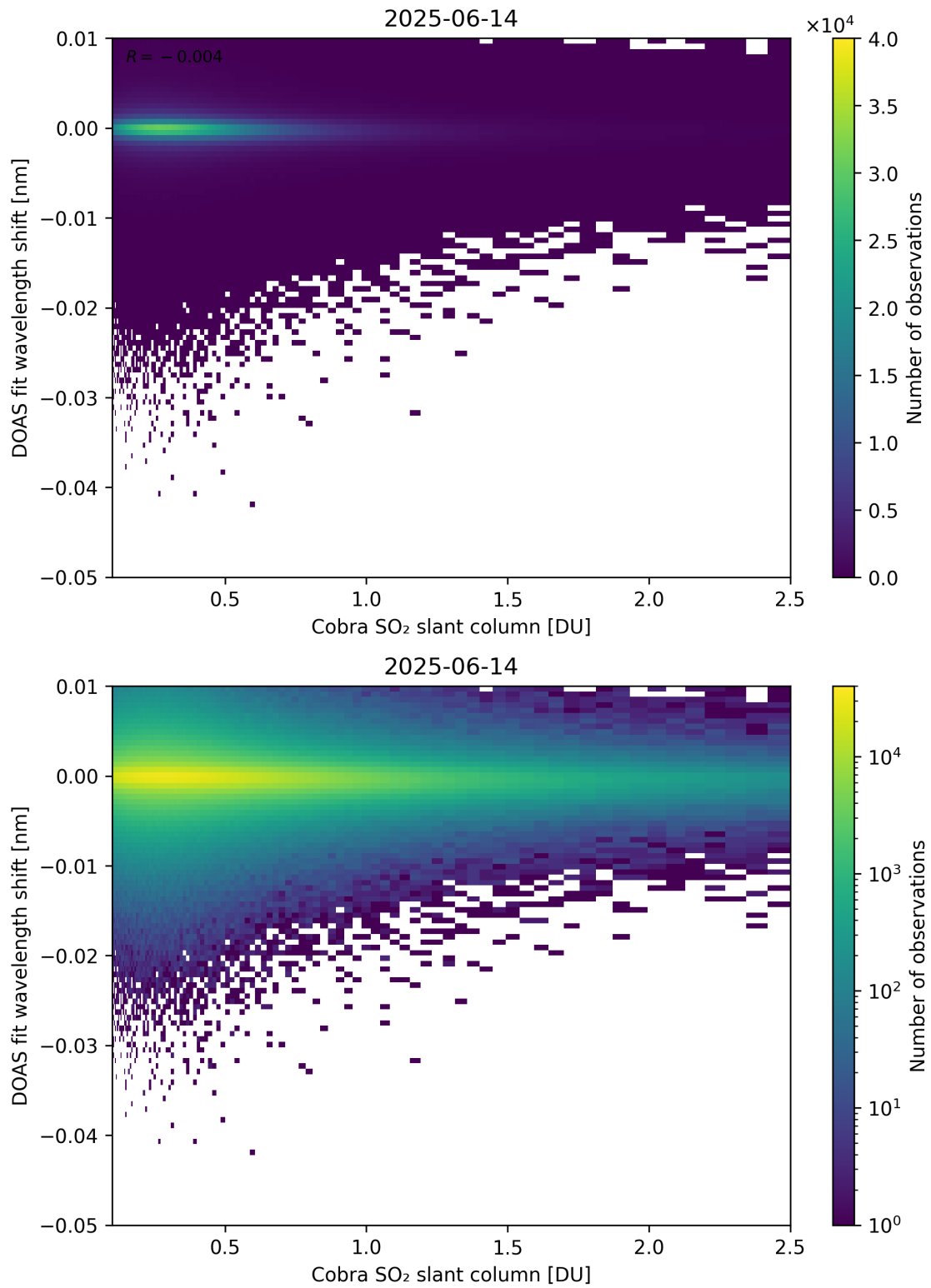
Figure 196: Scatter density plot of “Cobra SO 2 slant column” against “DOAS fit wavelength shift” for 2025-06-13 to 2025-06-15.
