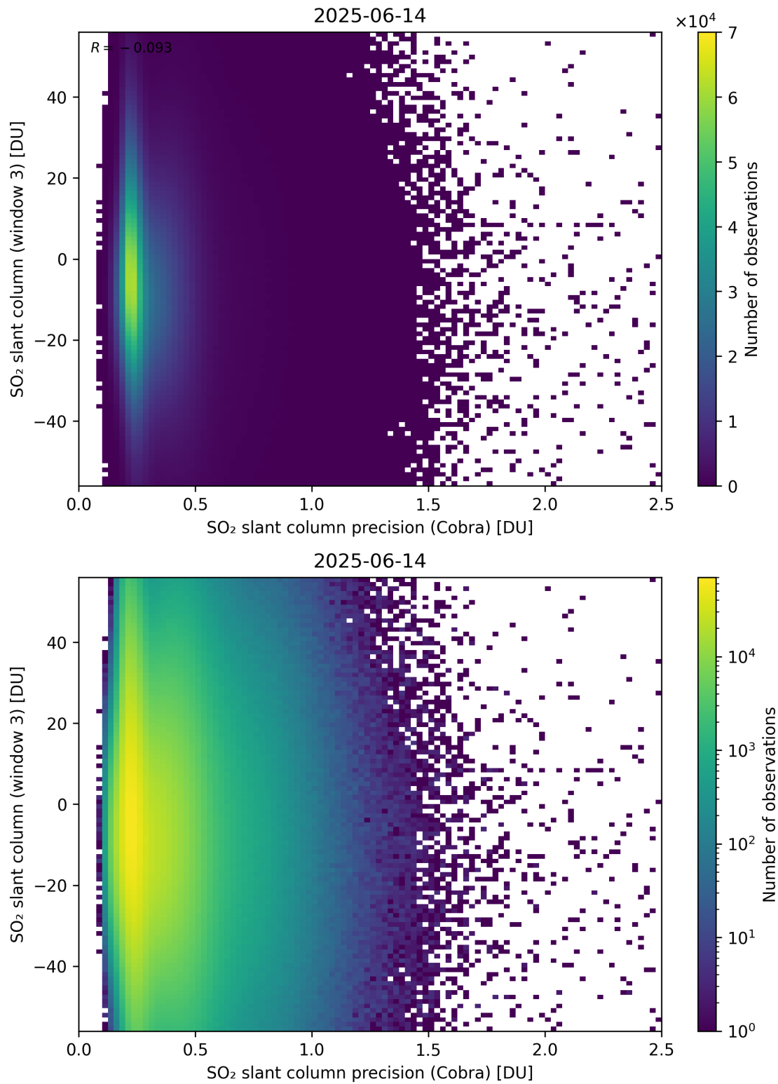
Figure 211: Scatter density plot of “SO 2 slant column precision (Cobra)” against “SO 2 slant column (window 3)” for 2025-06-13 to 2025-06-15.
