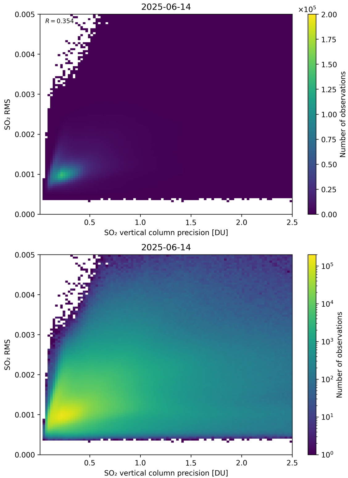
Figure 334: Scatter density plot of “SO 2 vertical column precision” against “SO 2 RMS” for 2025-06-13 to 2025-06-15.
