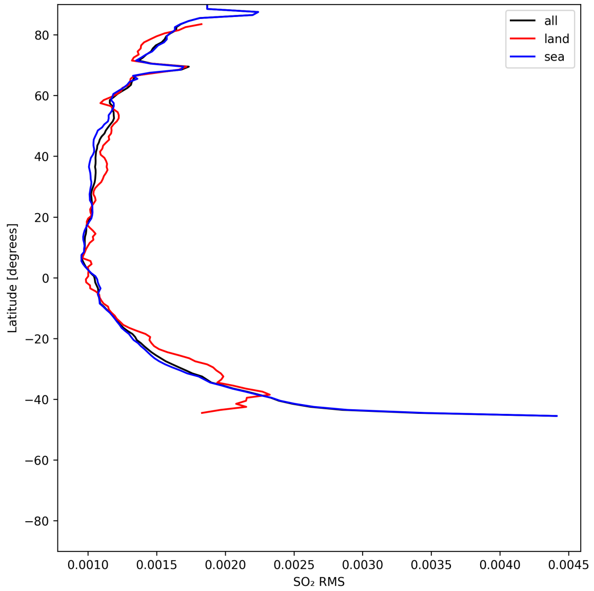
Figure 52: Zonal average of “SO 2 RMS” for 2025-06-13 to 2025-06-15.
