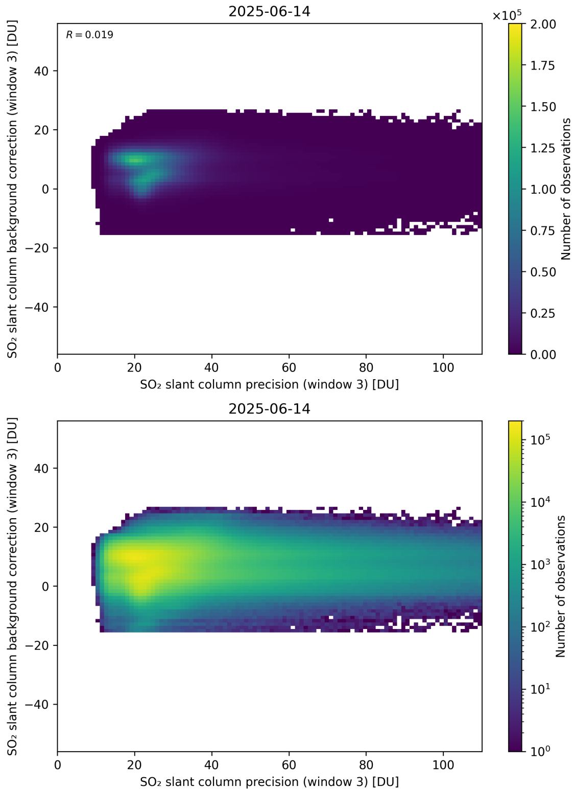
Figure 307: Scatter density plot of “SO 2 slant column precision (window 3)” against “SO 2 slant column background correction (window 3)” for 2025-06-13 to 2025-06-15.
