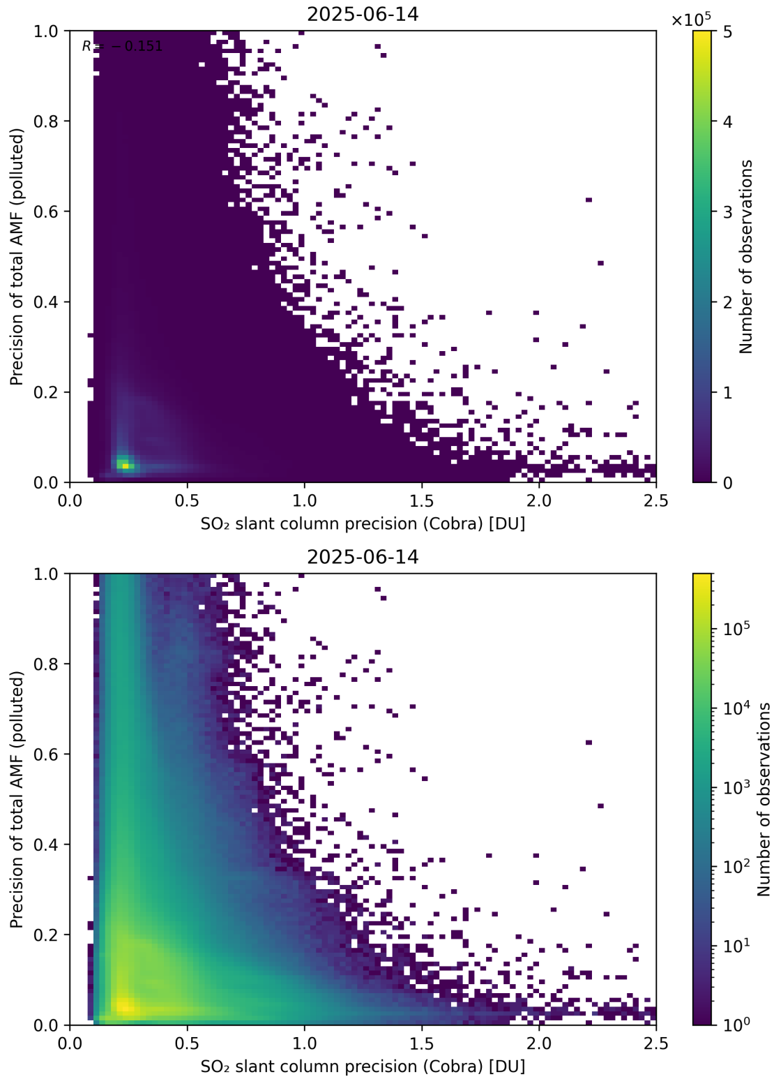
Figure 214: Scatter density plot of “SO 2 slant column precision (Cobra)” against “Precision of total AMF (polluted)” for 2025-06-13 to 2025-06-15.
