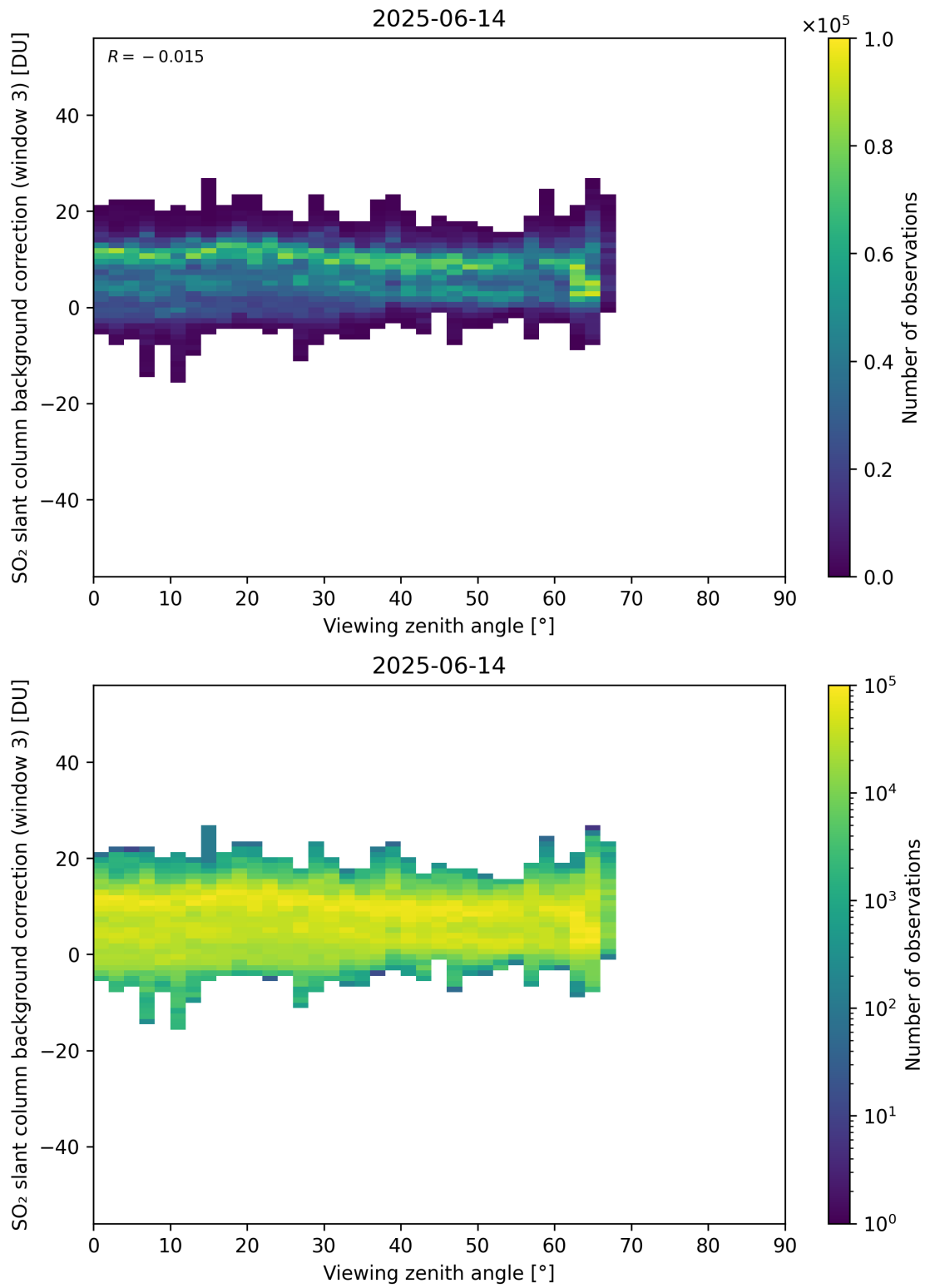
Figure 364: Scatter density plot of “Viewing zenith angle” against “SO 2 slant column background correction (window 3)” for 2025-06-13 to 2025-06-15.
