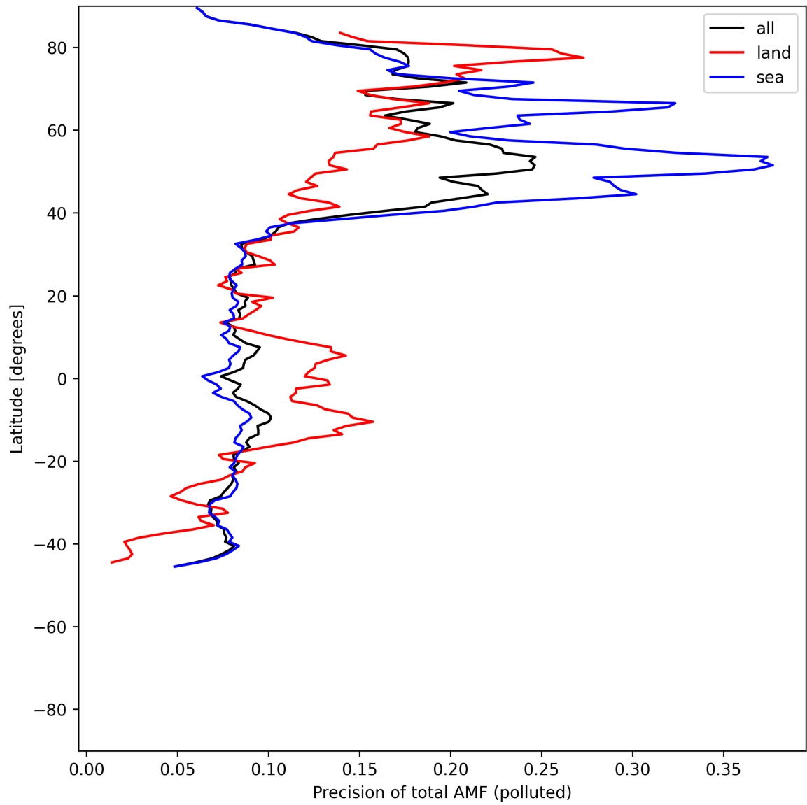
Figure 54: Zonal average of “Precision of total AMF (polluted)” for 2025-06-13 to 2025-06-15.
