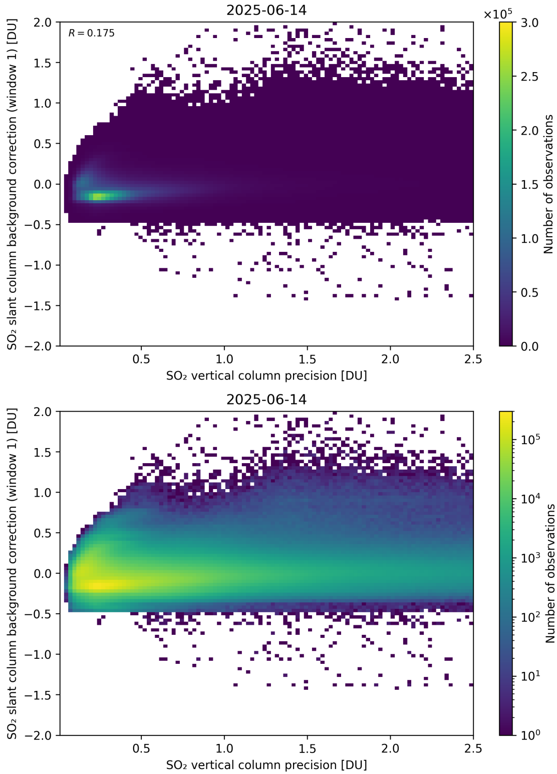
Figure 329: Scatter density plot of “SO 2 vertical column precision” against “SO 2 slant column background correction (window 1)” for 2025-06-13 to 2025-06-15.
