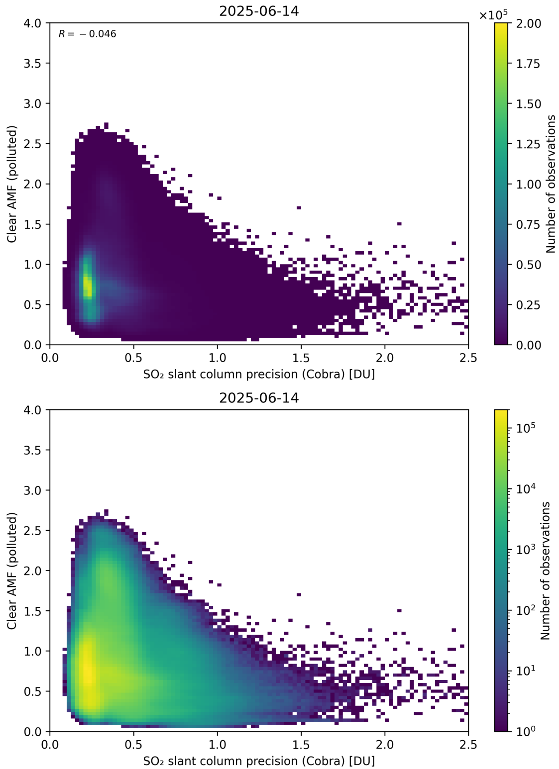
Figure 205: Scatter density plot of “SO 2 slant column precision (Cobra)” against “Clear AMF (polluted)” for 2025-06-13 to 2025-06-15.
