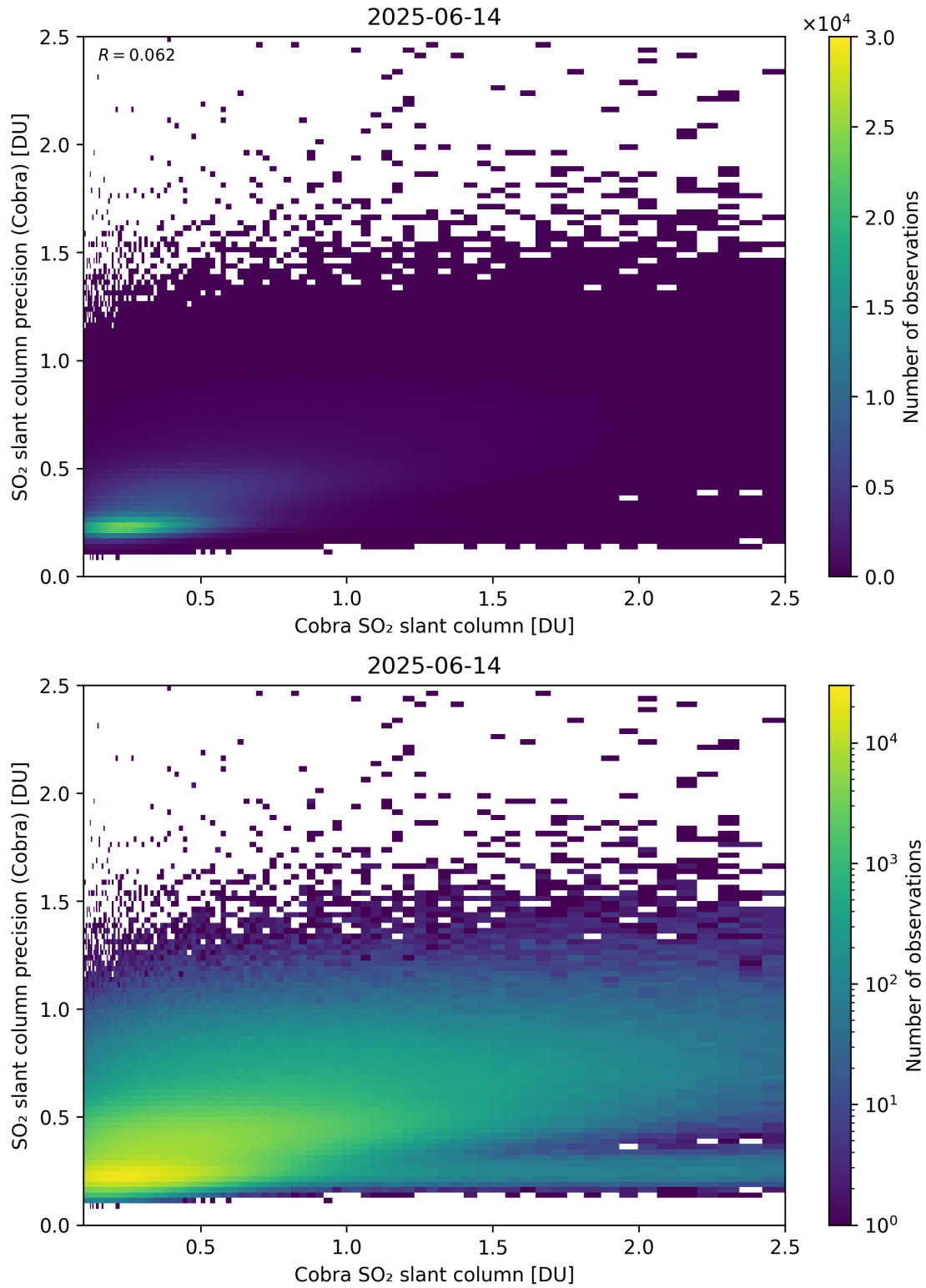
Figure 216: Scatter density plot of “Cobra SO 2 slant column” against “SO 2 slant column precision (Cobra)” for 2025-06-13 to 2025-06-15.
