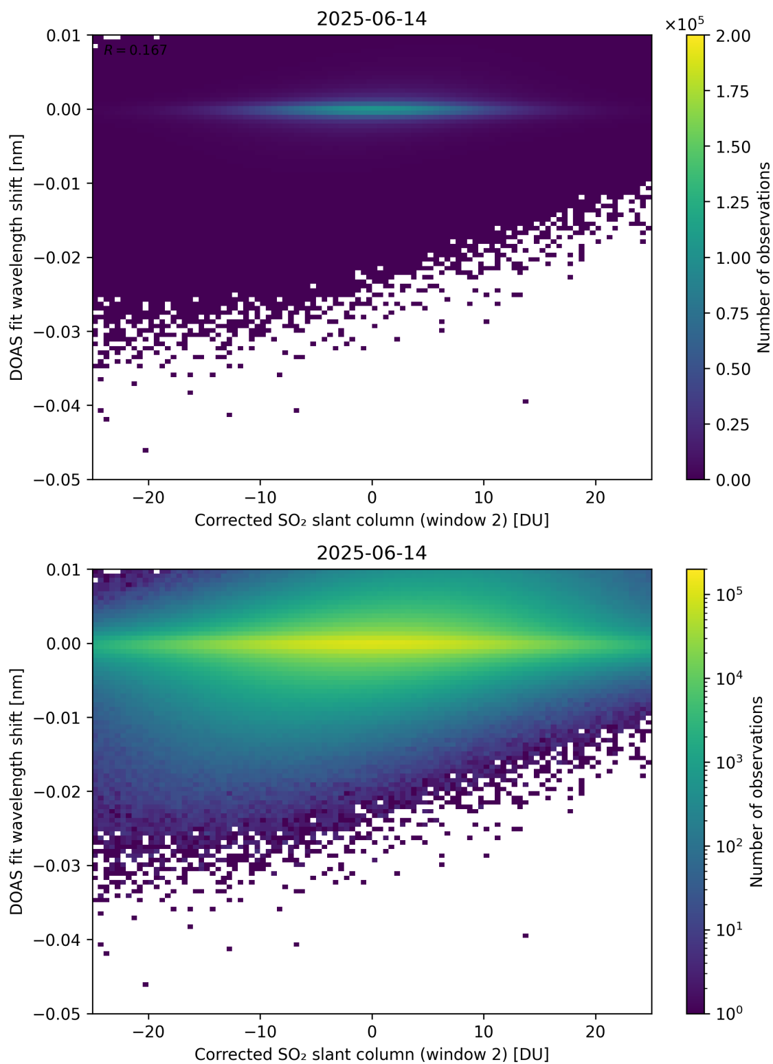
Figure 246: Scatter density plot of “Corrected SO 2 slant column (window 2)” against “DOAS fit wavelength shift” for 2025-06-13 to 2025-06-15.
