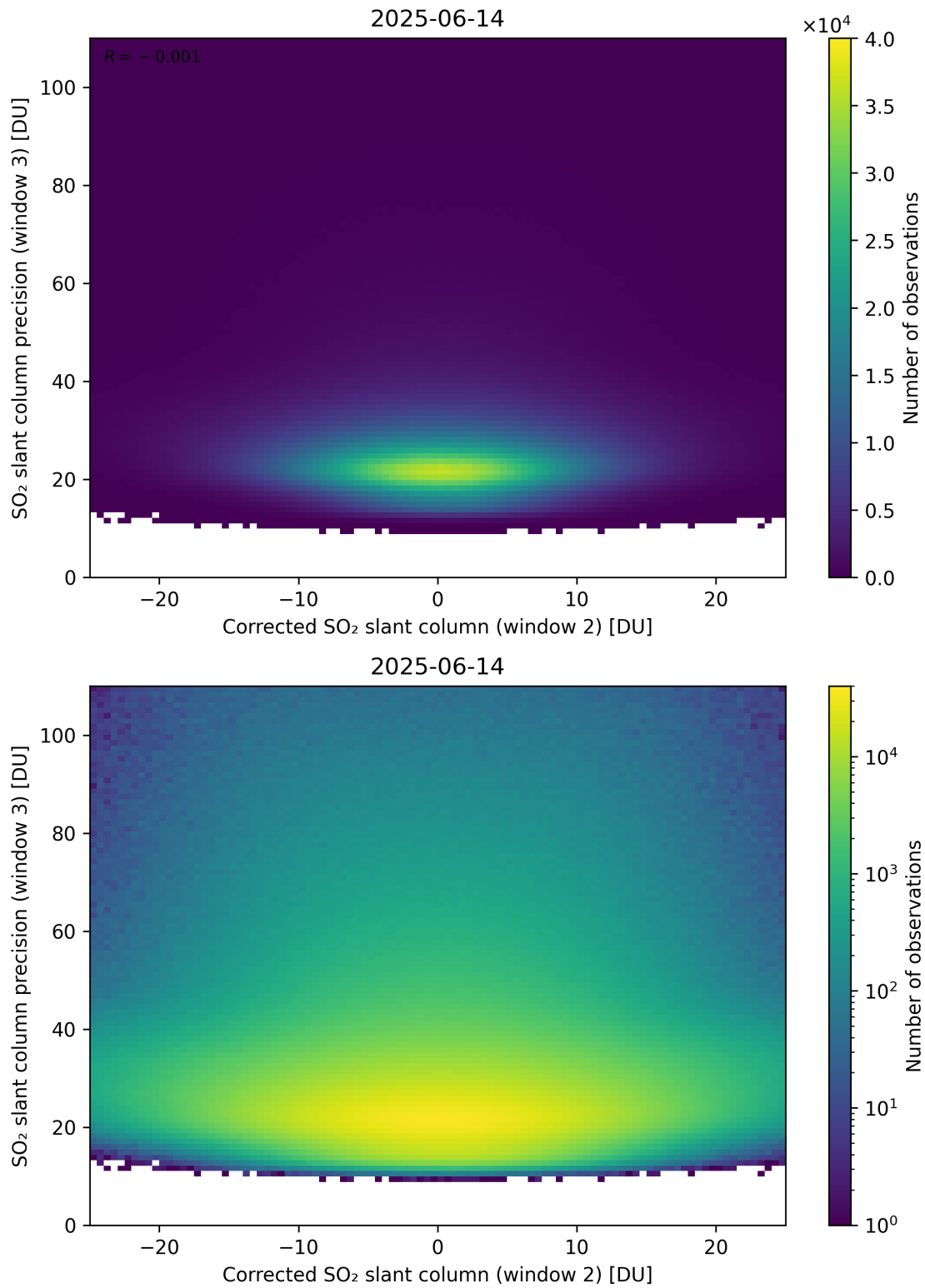
Figure 252: Scatter density plot of “Corrected SO 2 slant column (window 2)” against “SO 2 slant column precision (window 3)” for 2025-06-13 to 2025-06-15.
