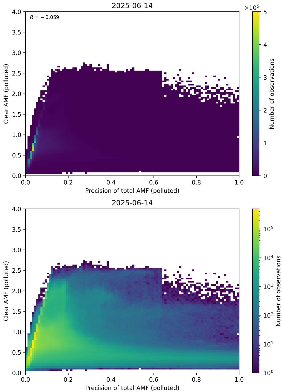
Figure 320: Scatter density plot of “Precision of total AMF (polluted)” against “Clear AMF (polluted)” for 2025-06-13 to 2025-06-15.
