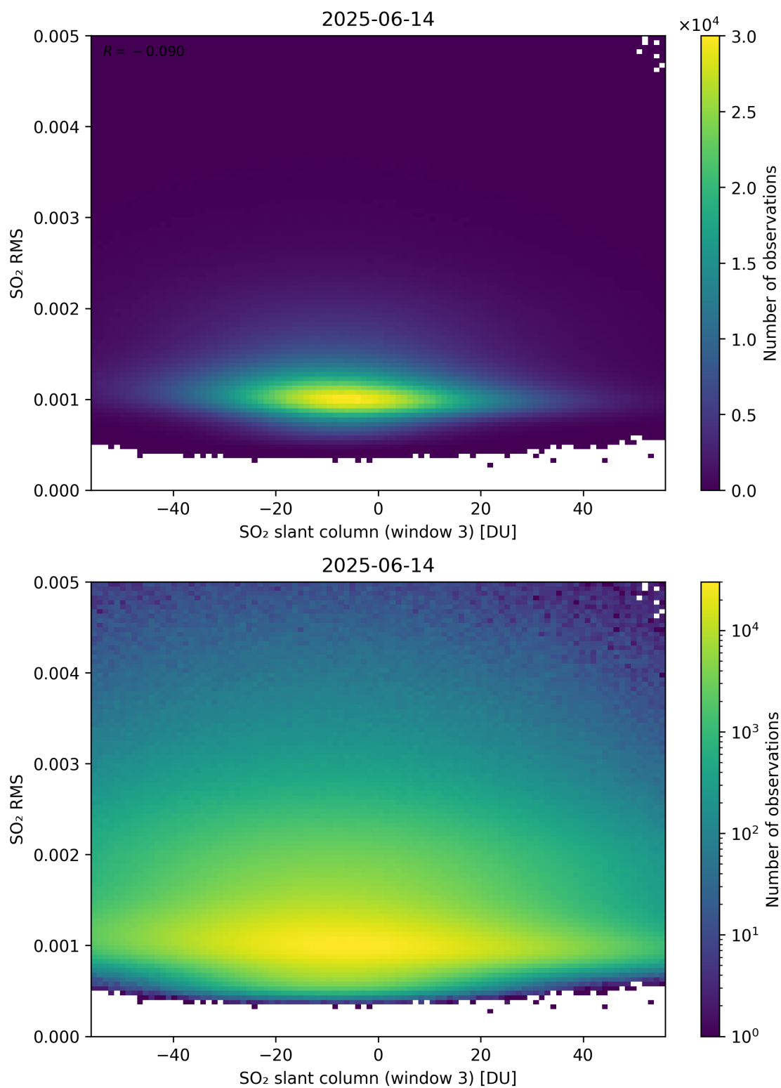
Figure 306: Scatter density plot of “SO 2 slant column (window 3)” against “SO 2 RMS” for 2025-06-13 to 2025-06-15.
