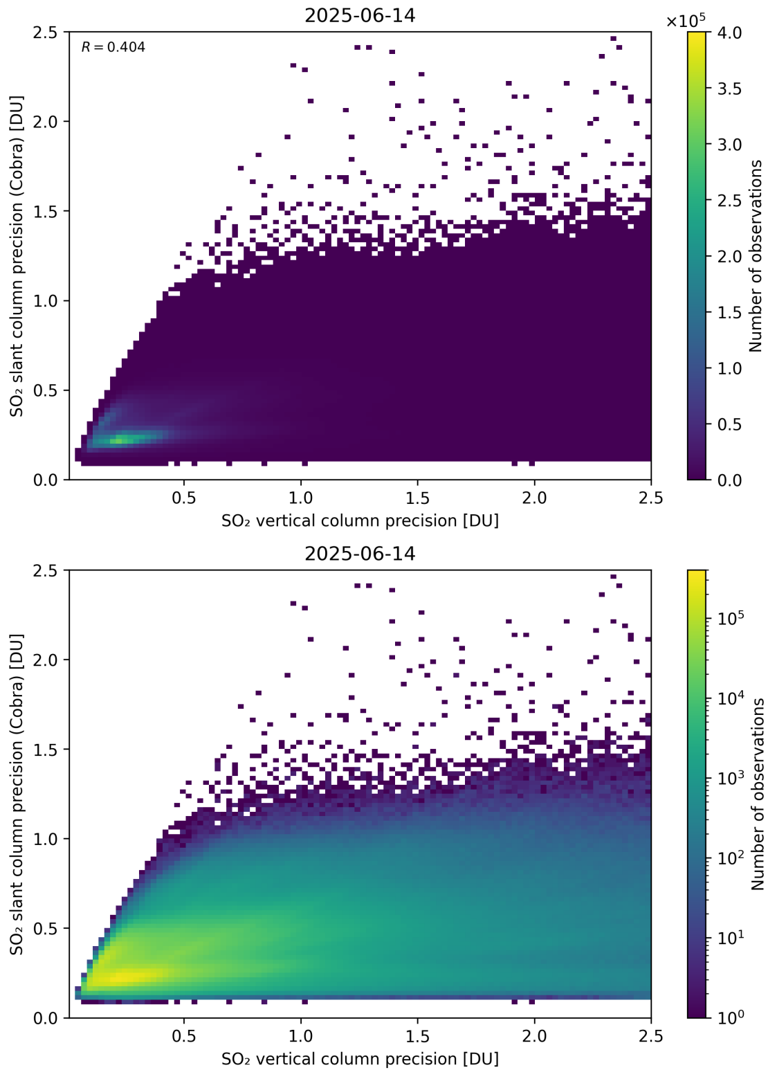
Figure 337: Scatter density plot of “SO 2 vertical column precision” against “SO 2 slant column precision (Cobra)” for 2025-06-13 to 2025-06-15.
