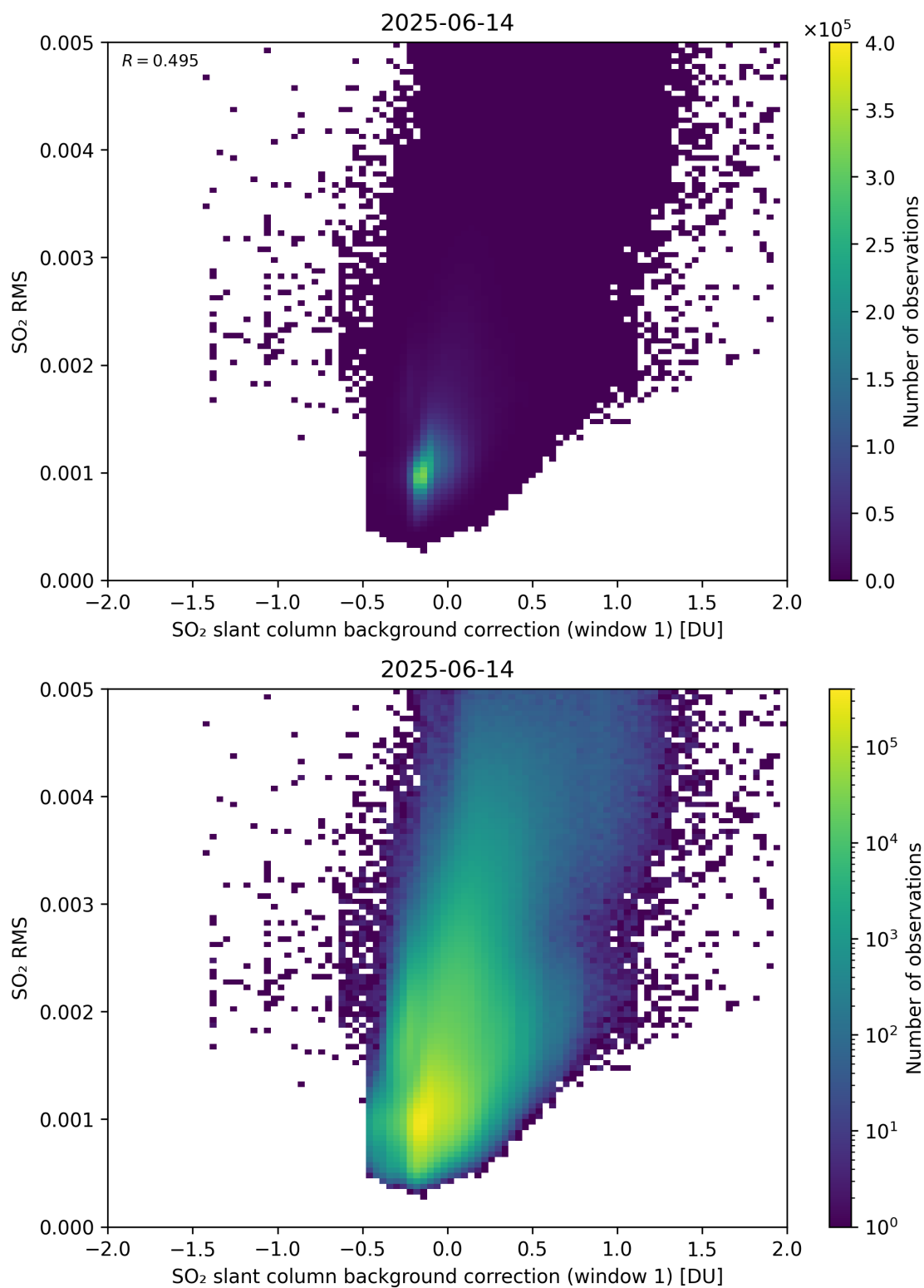
Figure 113: Scatter density plot of “SO 2 slant column background correction (window 1)” against “SO 2 RMS” for 2025-06-13 to 2025-06-15.
