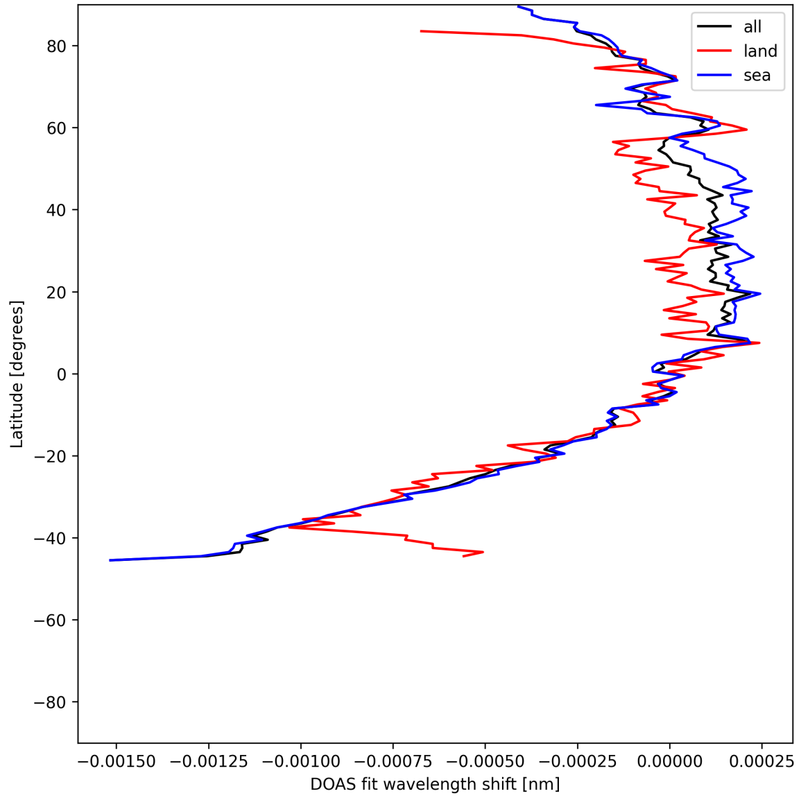
Figure 50: Zonal average of “DOAS fit wavelength shift” for 2025-06-13 to 2025-06-15.
