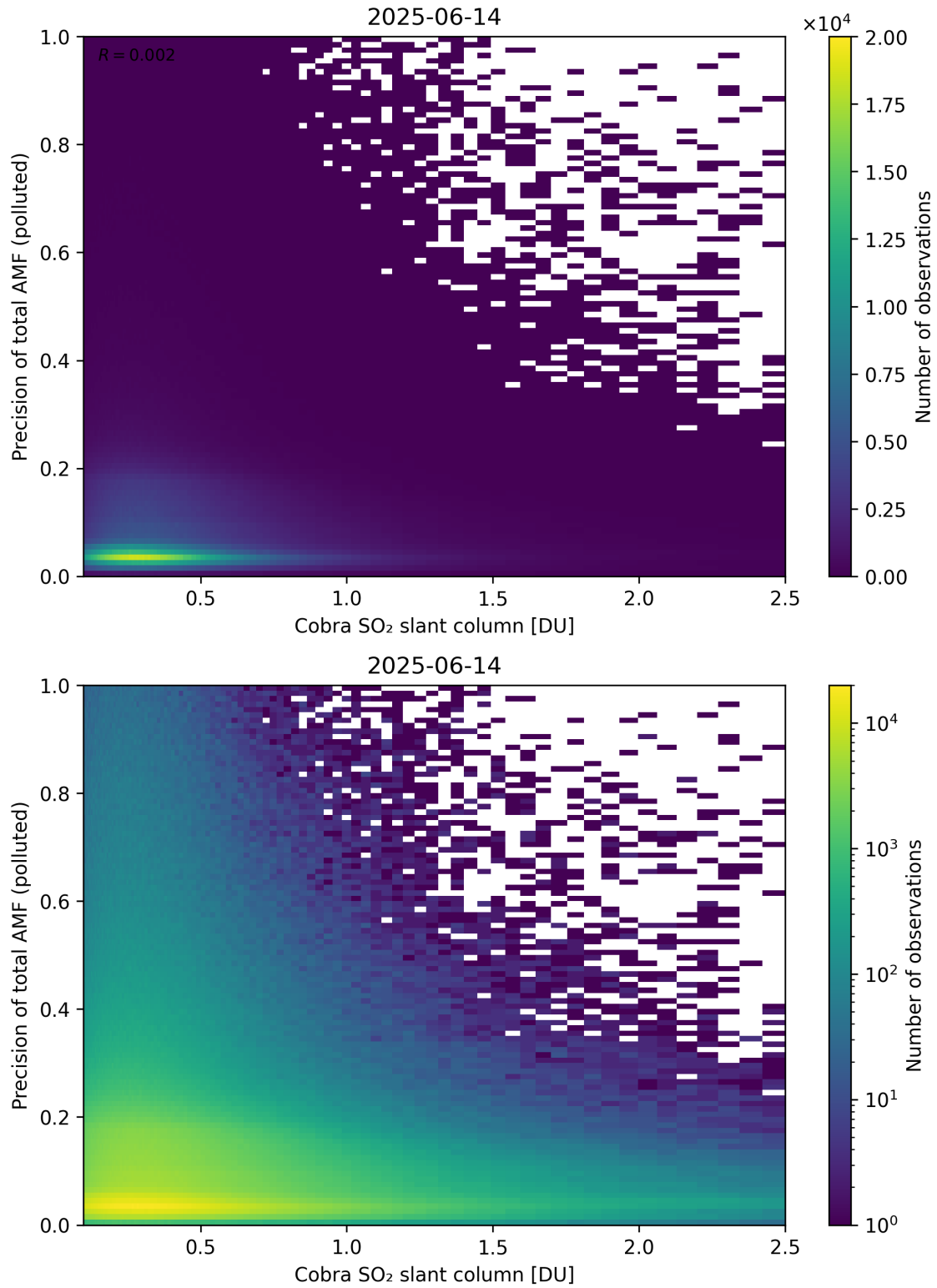
Figure 225: Scatter density plot of “Cobra SO 2 slant column” against “Precision of total AMF (polluted)” for 2025-06-13 to 2025-06-15.
