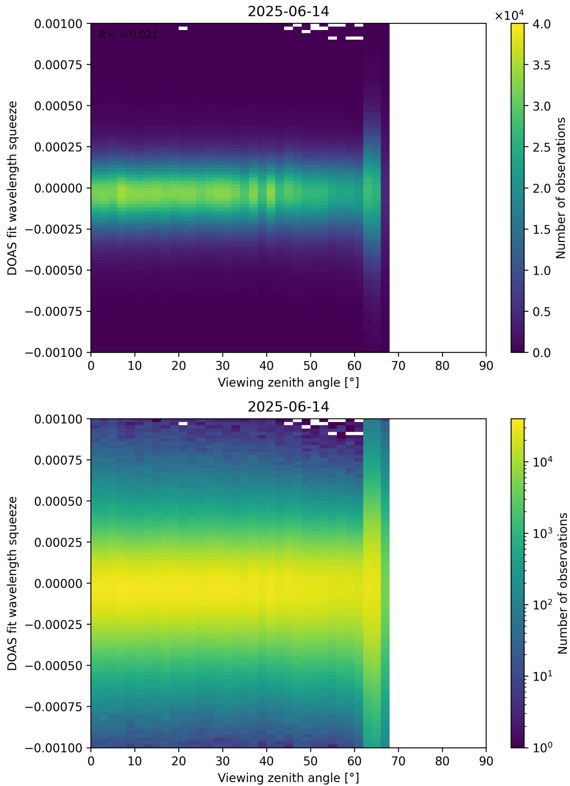
Figure 366: Scatter density plot of “Viewing zenith angle” against “DOAS fit wavelength squeeze” for 2025-06-13 to 2025-06-15.
