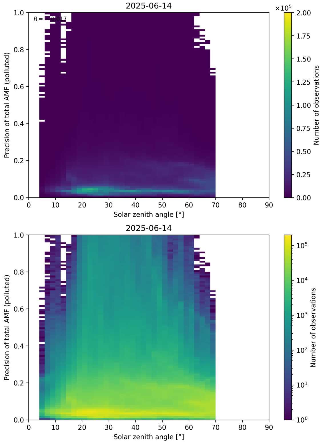
Figure 190: Scatter density plot of “Solar zenith angle” against “Precision of total AMF (polluted)” for 2025-06-13 to 2025-06-15.
