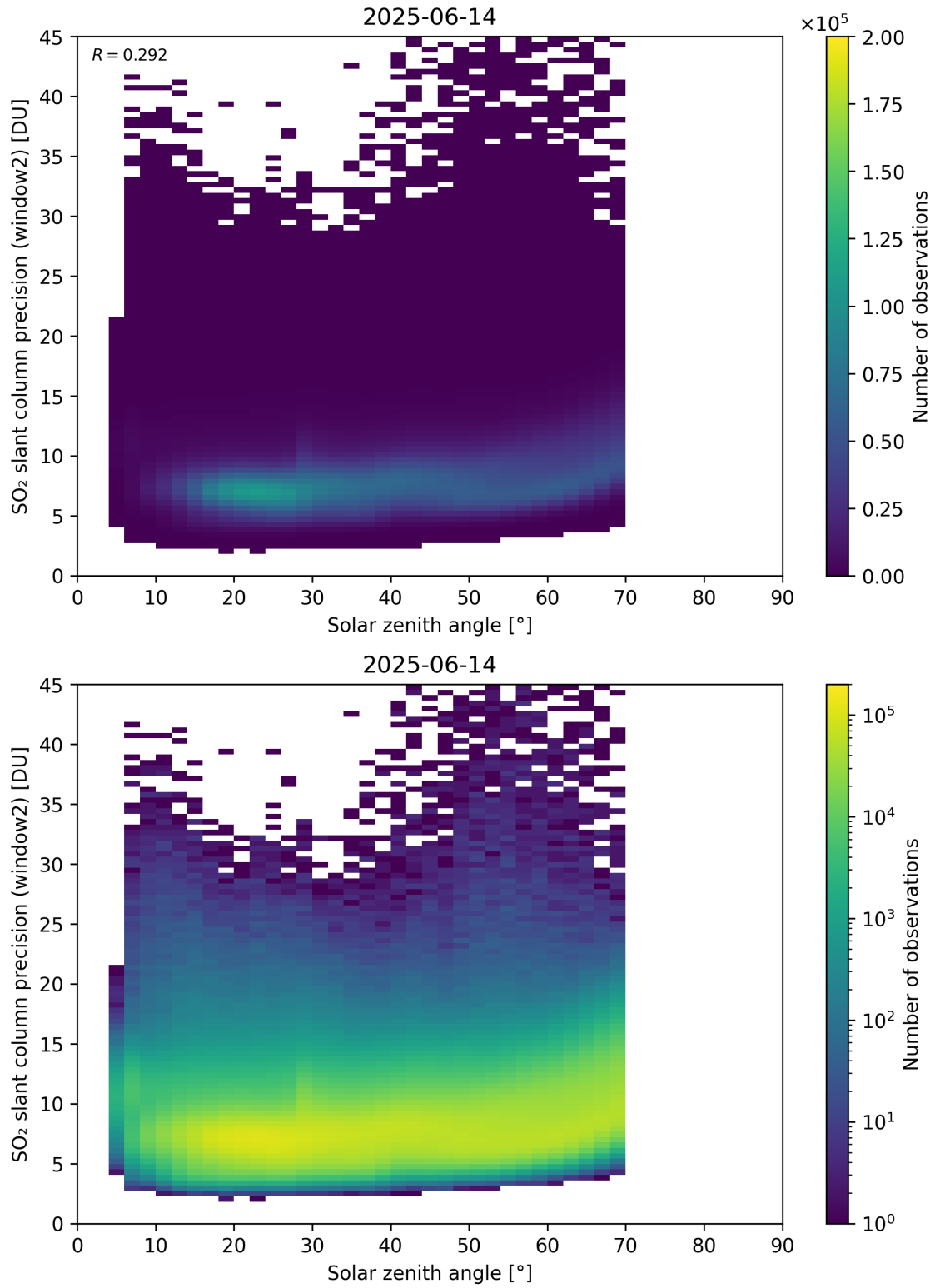
Figure 186: Scatter density plot of “Solar zenith angle” against “SO 2 slant column precision (window2)” for 2025-06-13 to 2025-06-15.
