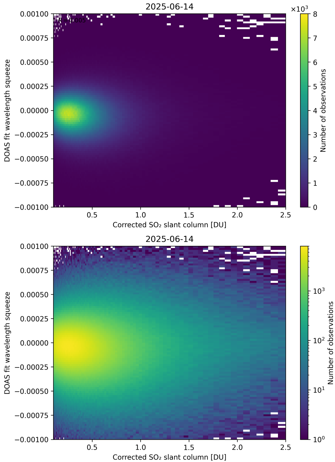
Figure 230: Scatter density plot of “Corrected SO 2 slant column” against “DOAS fit wavelength squeeze” for 2025-06-13 to 2025-06-15.
