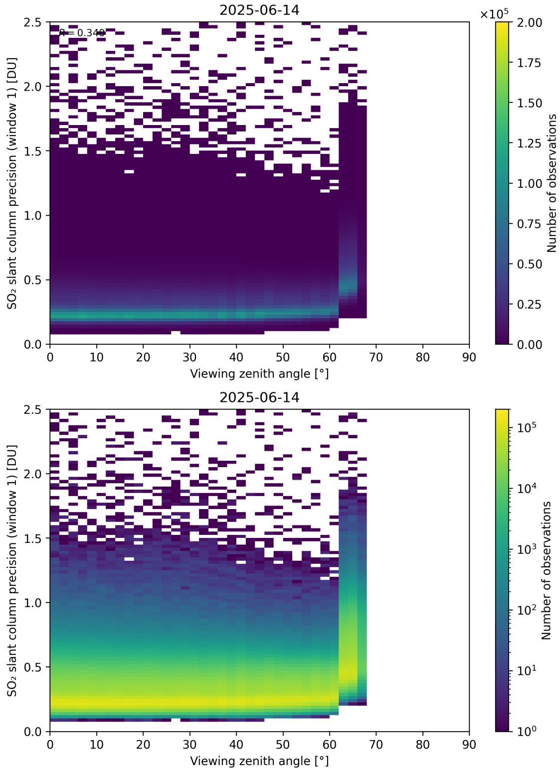
Figure 377: Scatter density plot of “Viewing zenith angle” against “SO 2 slant column precision (window 1)” for 2025-06-13 to 2025-06-15.
