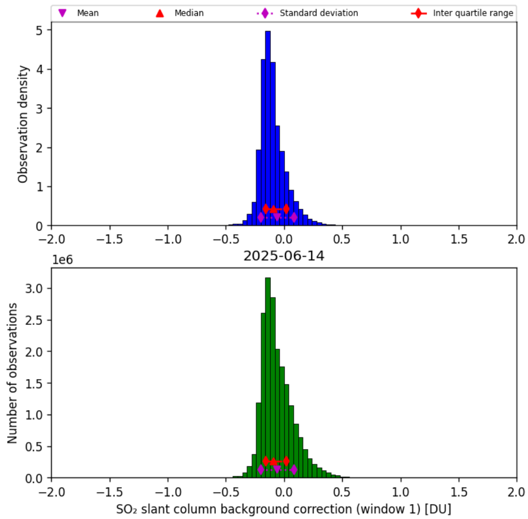
Figure 66: Histogram of “SO 2 slant column background correction (window 1)” for 2025-06-13 to 2025-06-15
