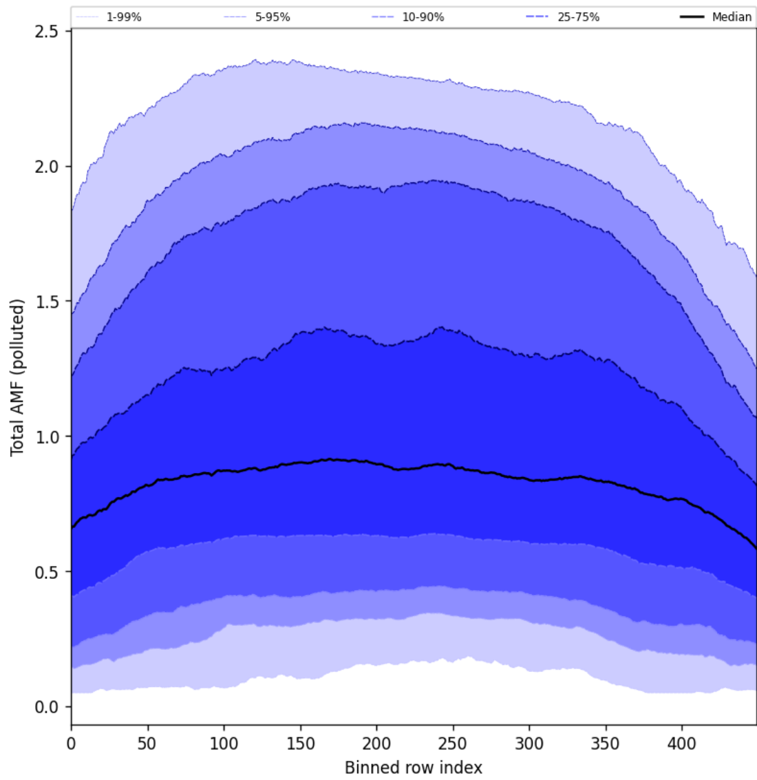
Figure 105: Along track statistics of “Total AMF (polluted)” for 2025-06-13 to 2025-06-15
