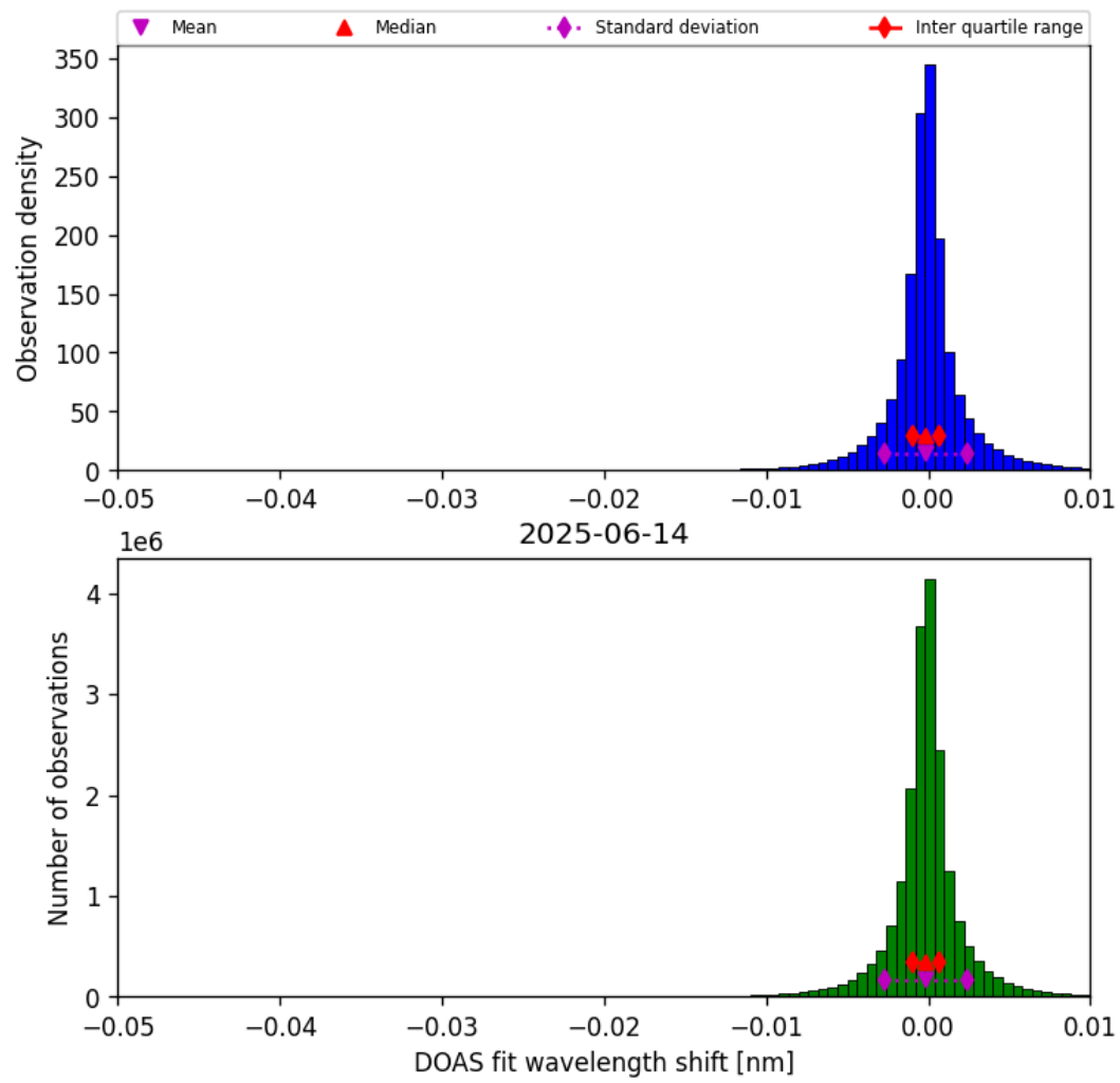
Figure 76: Histogram of “DOAS fit wavelength shift” for 2025-06-13 to 2025-06-15
