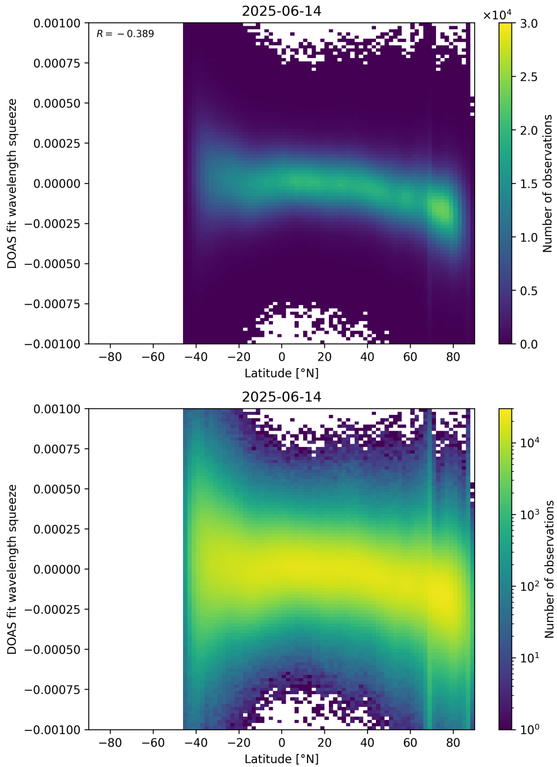
Figure 154: Scatter density plot of “Latitude” against “DOAS fit wavelength squeeze” for 2025-06-13 to 2025-06-15.
