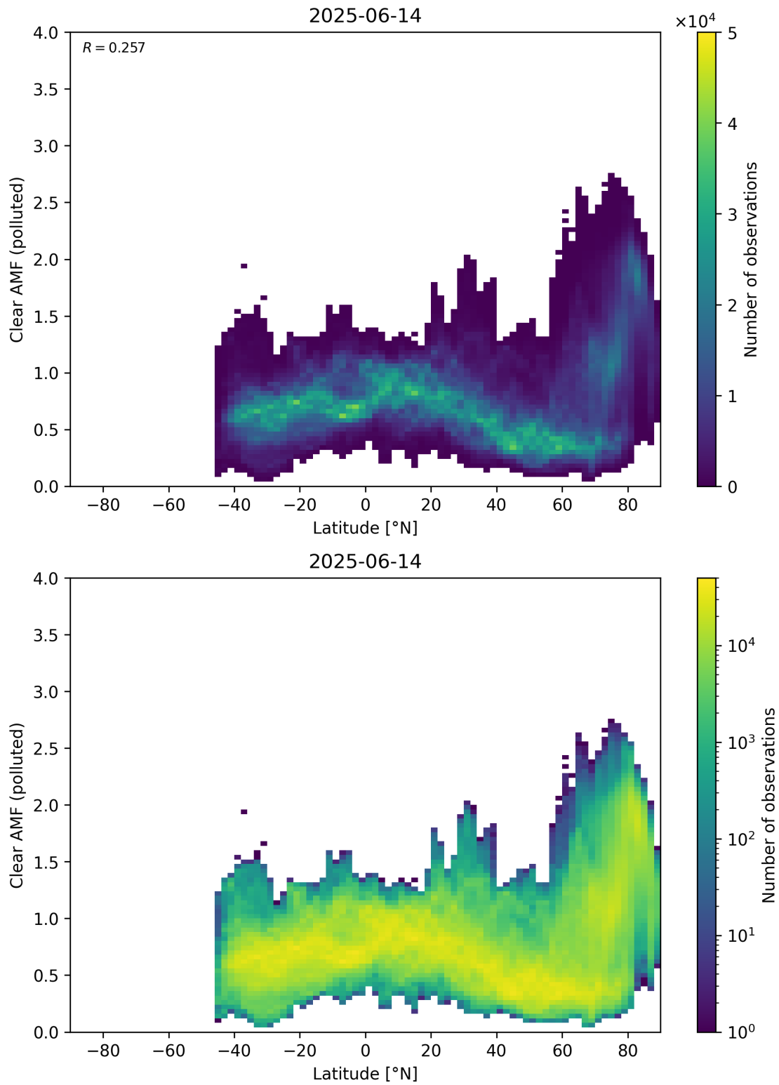
Figure 156: Scatter density plot of “Latitude” against “Clear AMF (polluted)” for 2025-06-13 to 2025-06-15.
