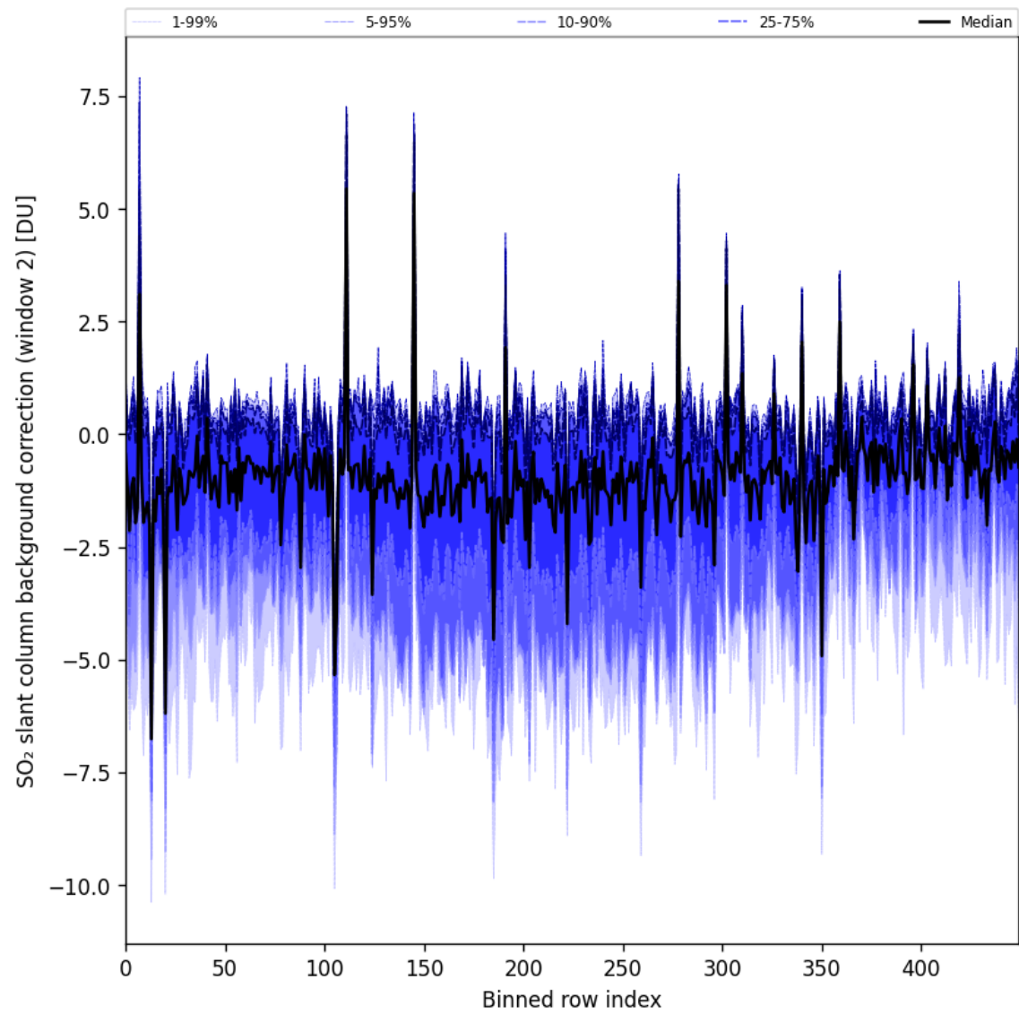
Figure 96: Along track statistics of “SO 2 slant column background correction (window 2)” for 2025-06-13 to 2025-06-15
