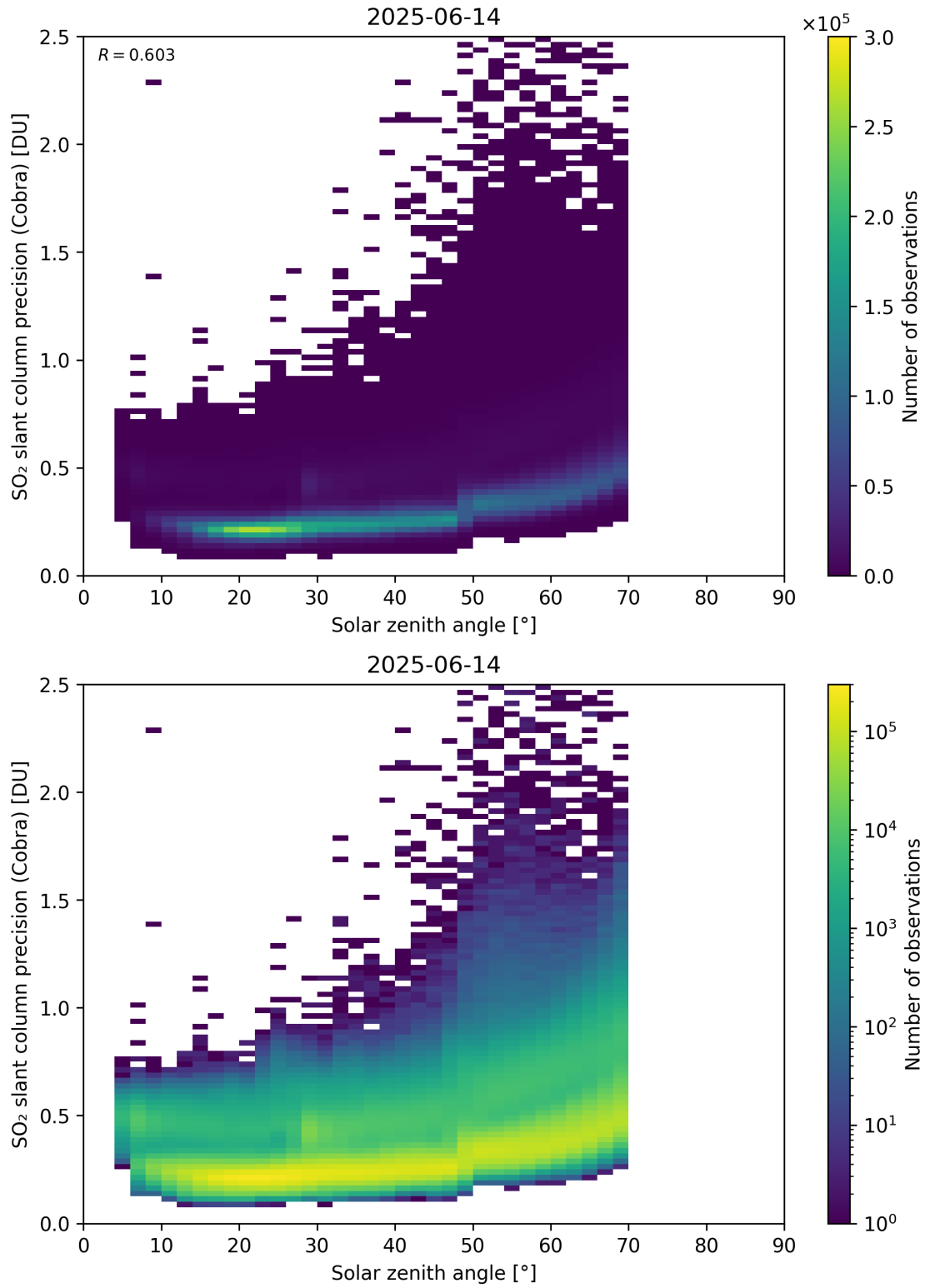
Figure 180: Scatter density plot of “Solar zenith angle” against “SO 2 slant column precision (Cobra)” for 2025-06-13 to 2025-06-15.
