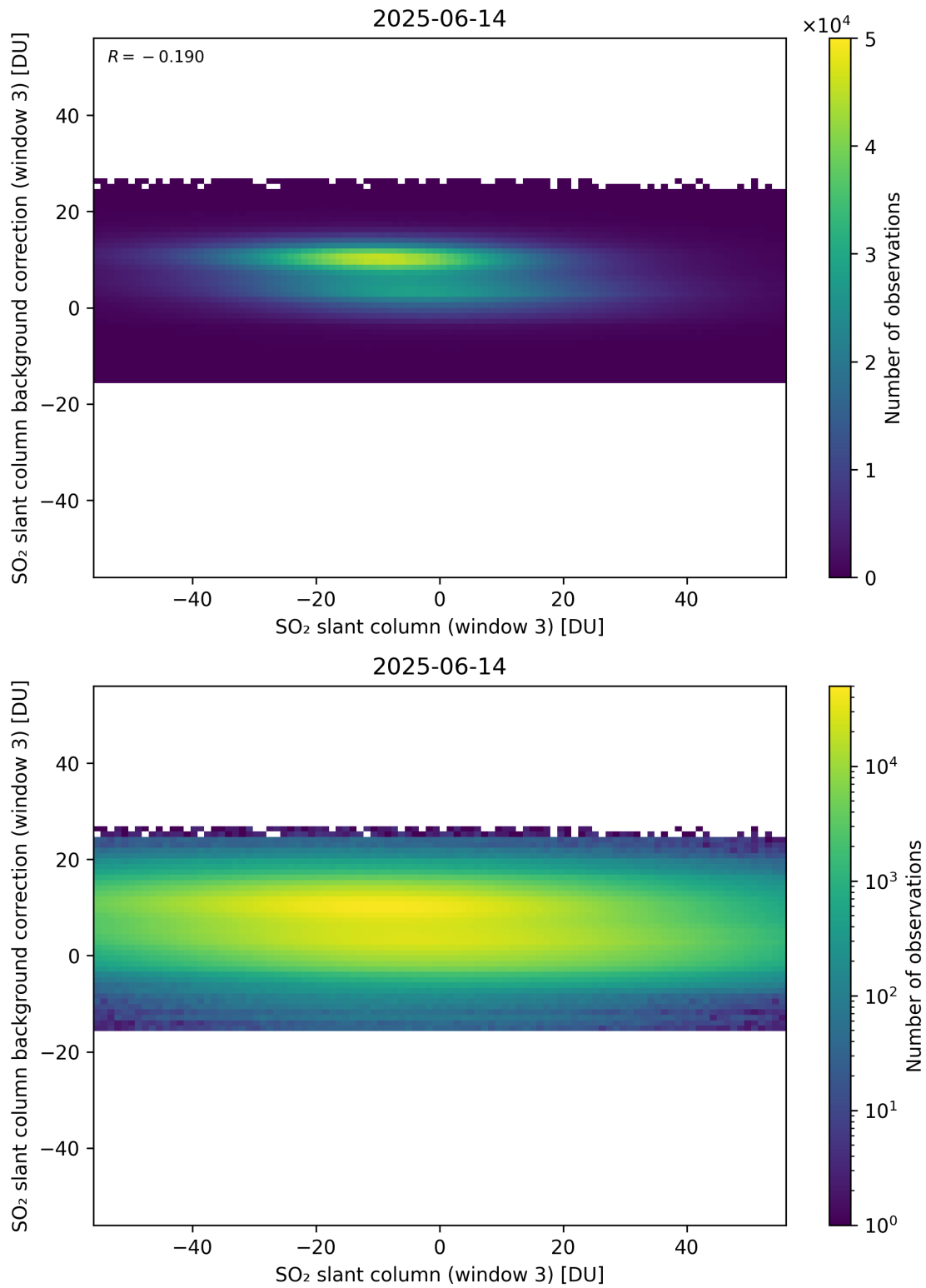
Figure 303: Scatter density plot of “SO 2 slant column (window 3)” against “SO 2 slant column background correction (window 3)” for 2025-06-13 to 2025-06-15.
