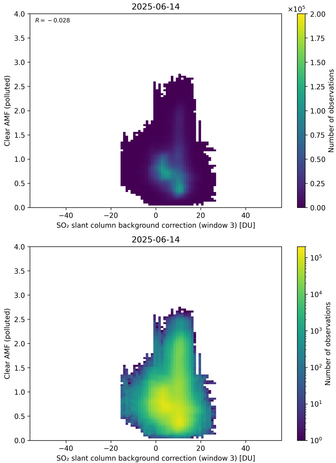
Figure 135: Scatter density plot of “SO 2 slant column background correction (window 3)” against “Clear AMF (polluted)” for 2025-06-13 to 2025-06-15.
