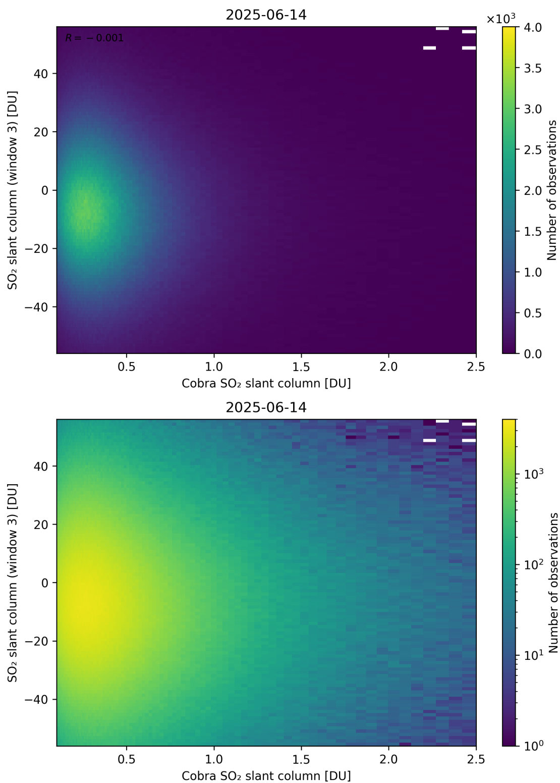
Figure 222: Scatter density plot of “Cobra SO 2 slant column” against “SO 2 slant column (window 3)” for 2025-06-13 to 2025-06-15.
