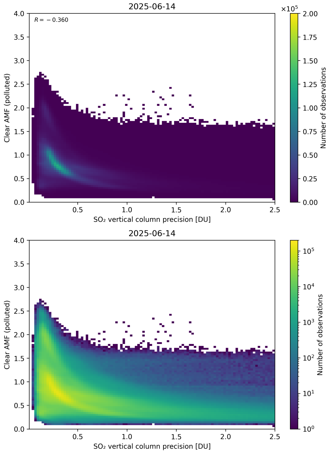
Figure 335: Scatter density plot of “SO 2 vertical column precision” against “Clear AMF (polluted)” for 2025-06-13 to 2025-06-15.
