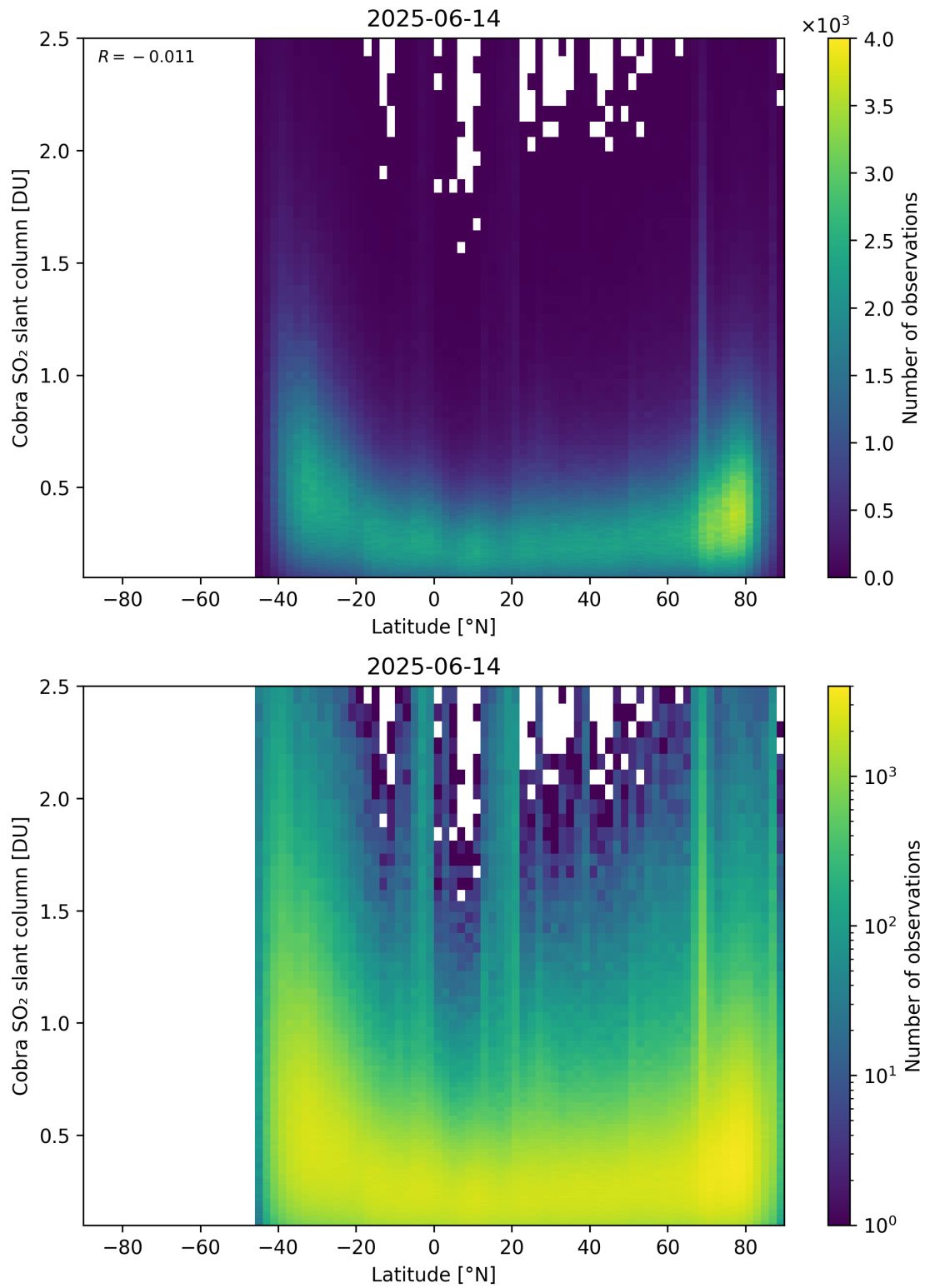
Figure 157: Scatter density plot of “Latitude” against “Cobra SO 2 slant column” for 2025-06-13 to 2025-06-15.
