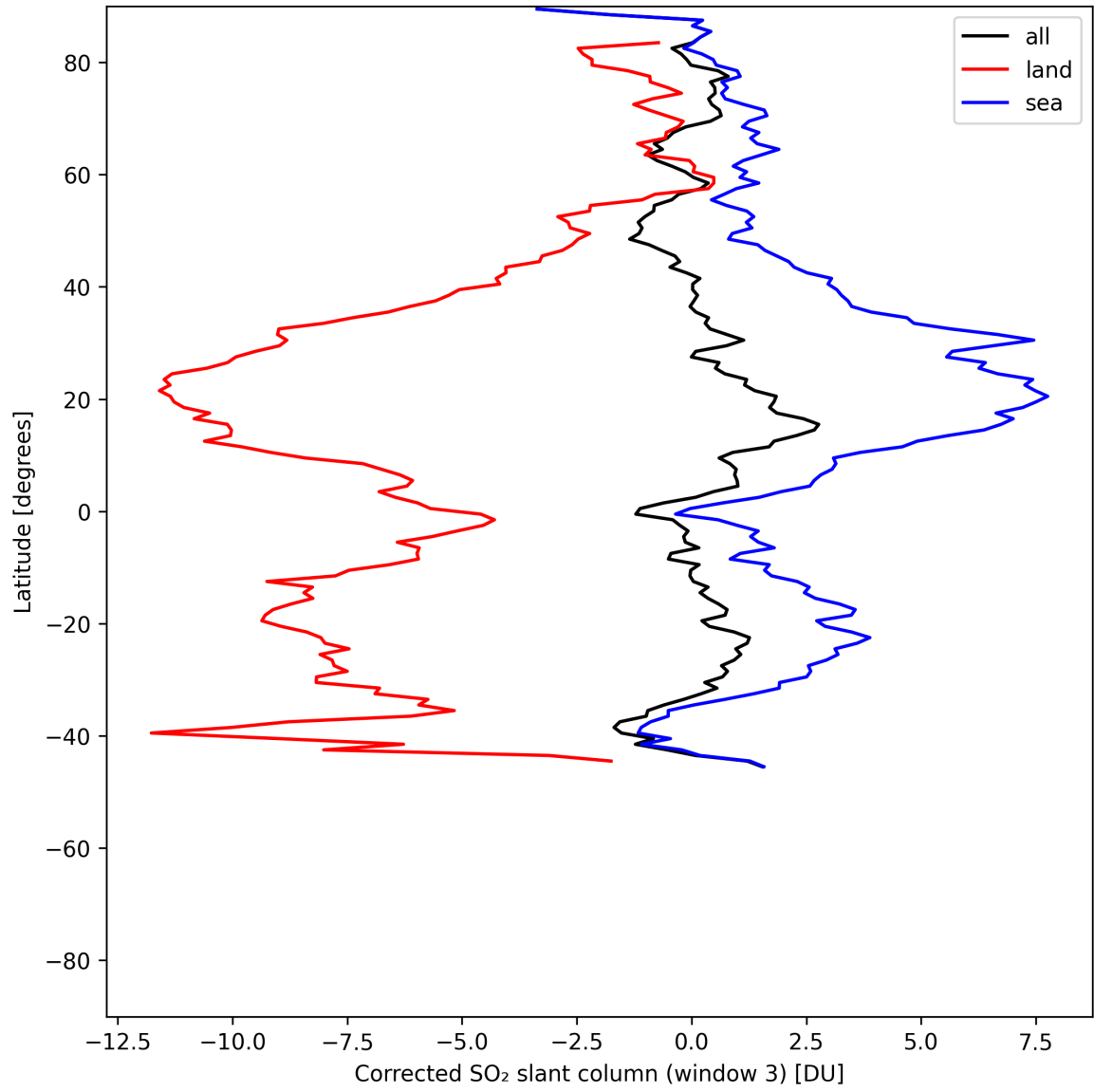
Figure 47: Zonal average of “Corrected SO 2 slant column (window 3)” for 2025-06-13 to 2025-06-15.
