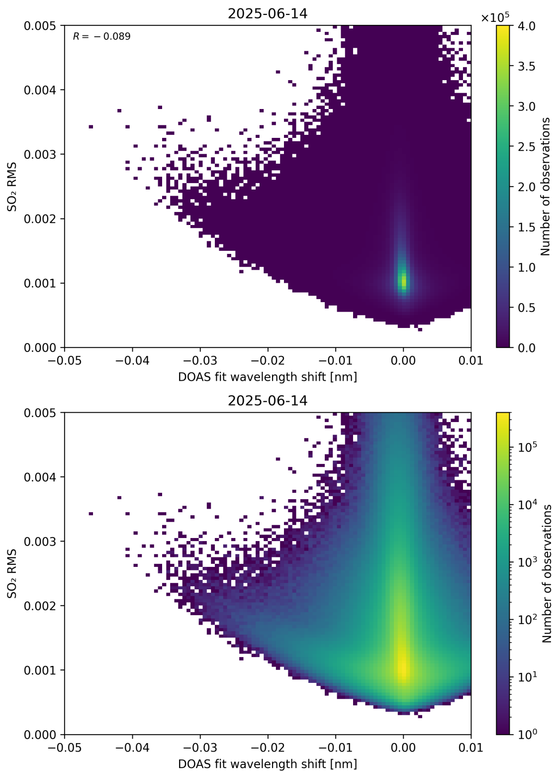
Figure 139: Scatter density plot of “DOAS fit wavelength shift” against “SO 2 RMS” for 2025-06-13 to 2025-06-15.
