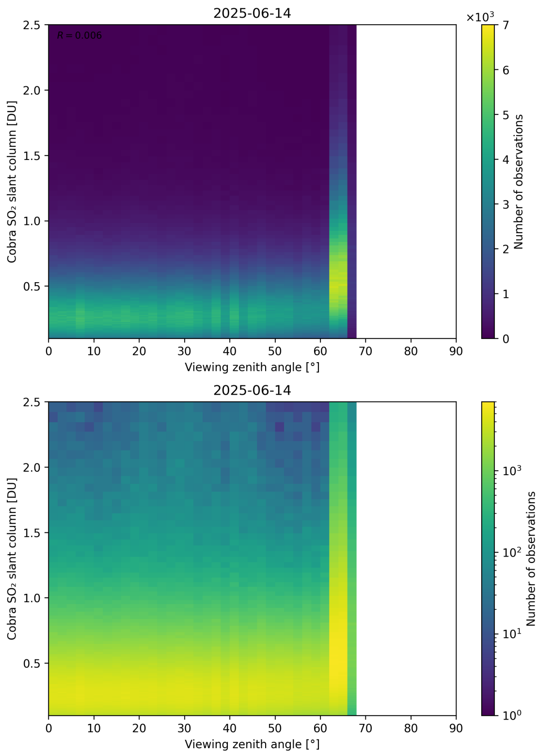
Figure 371: Scatter density plot of “Viewing zenith angle” against “Cobra SO 2 slant column” for 2025-06-13 to 2025-06-15.
