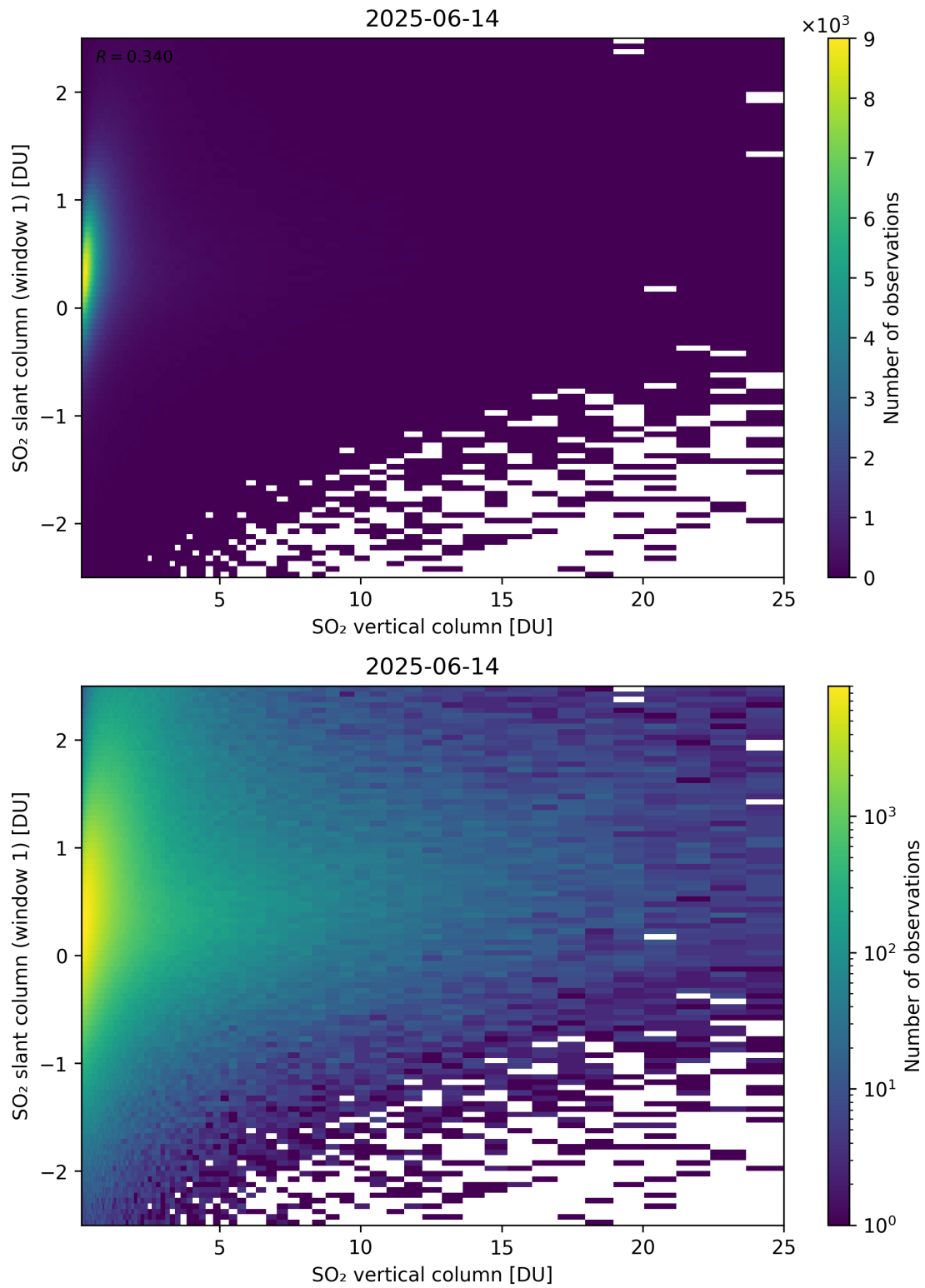
Figure 354: Scatter density plot of “SO 2 vertical column” against “SO 2 slant column (window 1)” for 2025-06-13 to 2025-06-15.
