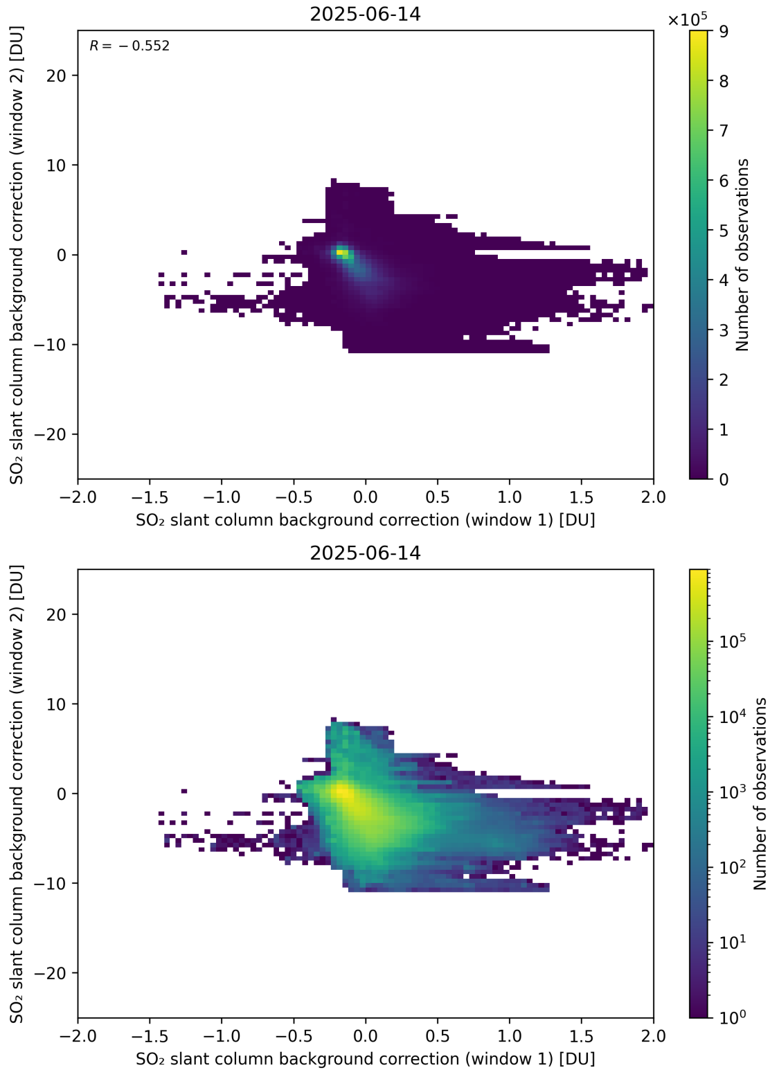
Figure 109: Scatter density plot of “SO 2 slant column background correction (window 1)” against “SO 2 slant column background correction (window 2)” for 2025-06-13 to 2025-06-15.
