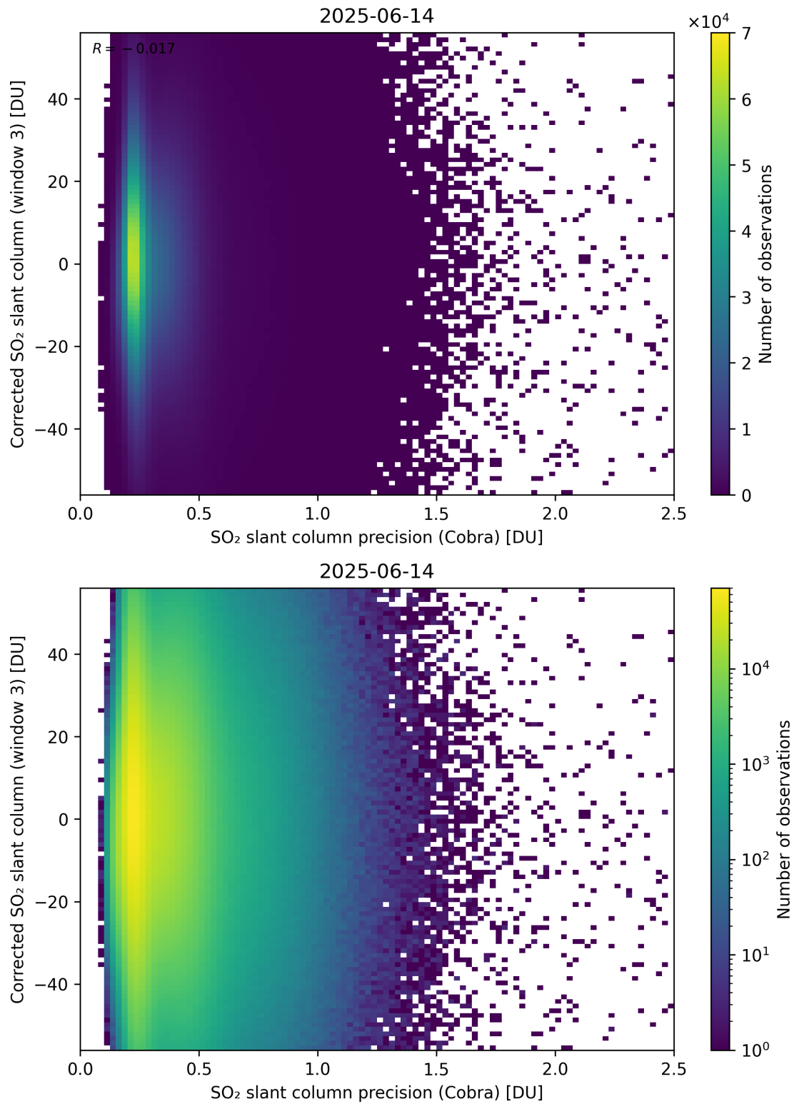
Figure 207: Scatter density plot of “SO 2 slant column precision (Cobra)” against “Corrected SO 2 slant column (window 3)” for 2025-06-13 to 2025-06-15.
