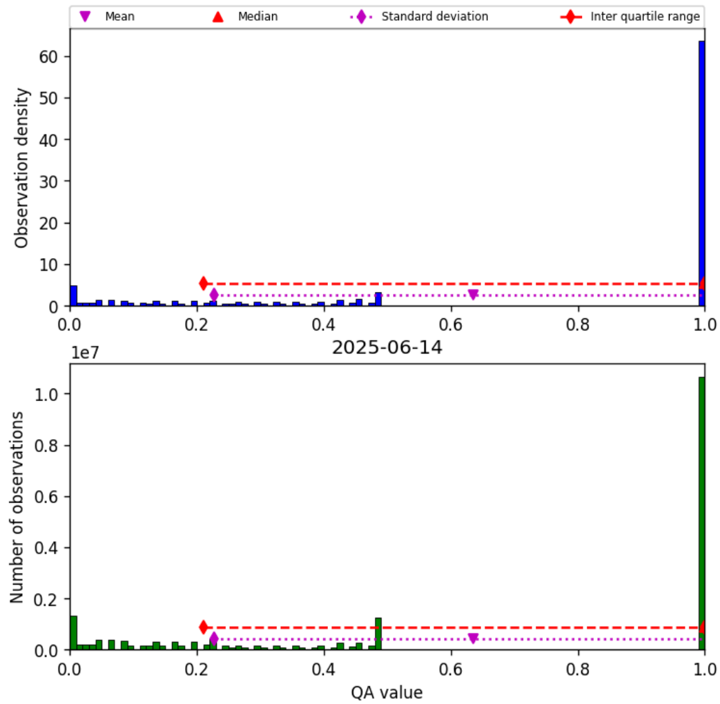
Figure 57: Histogram of “QA value” for 2025-06-13 to 2025-06-15
