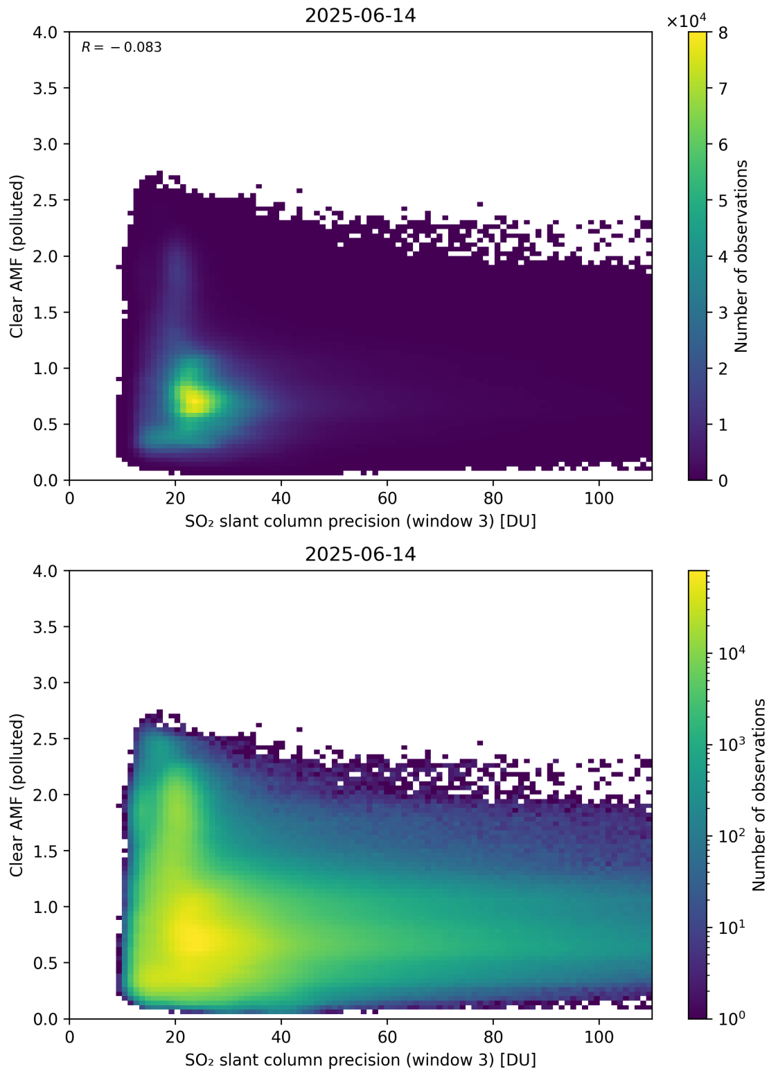
Figure 311: Scatter density plot of “SO 2 slant column precision (window 3)” against “Clear AMF (polluted)” for 2025-06-13 to 2025-06-15.
