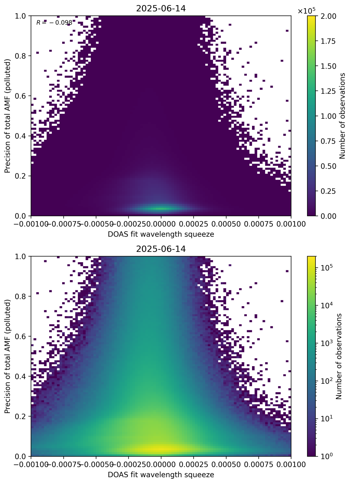
Figure 146: Scatter density plot of “DOAS fit wavelength squeeze” against “Precision of total AMF (polluted)” for 2025-06-13 to 2025-06-15.
