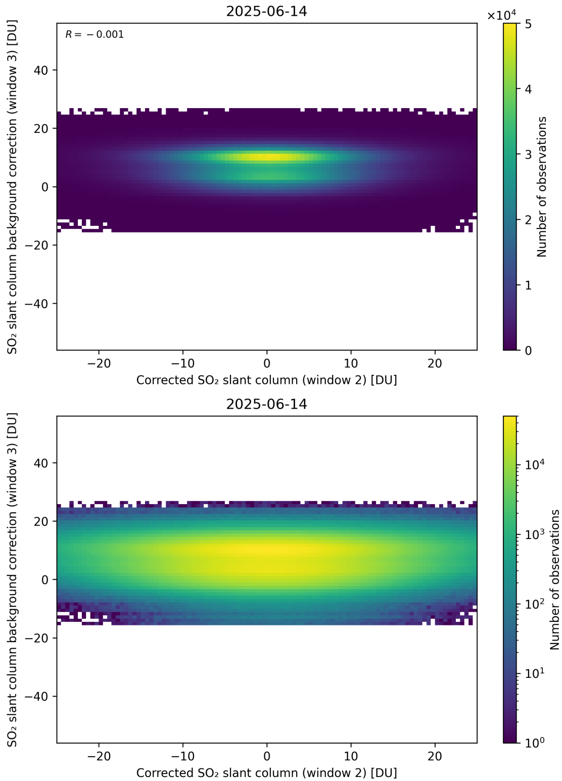
Figure 245: Scatter density plot of “Corrected SO 2 slant column (window 2)” against “SO 2 slant column background correction (window 3)” for 2025-06-13 to 2025-06-15.
