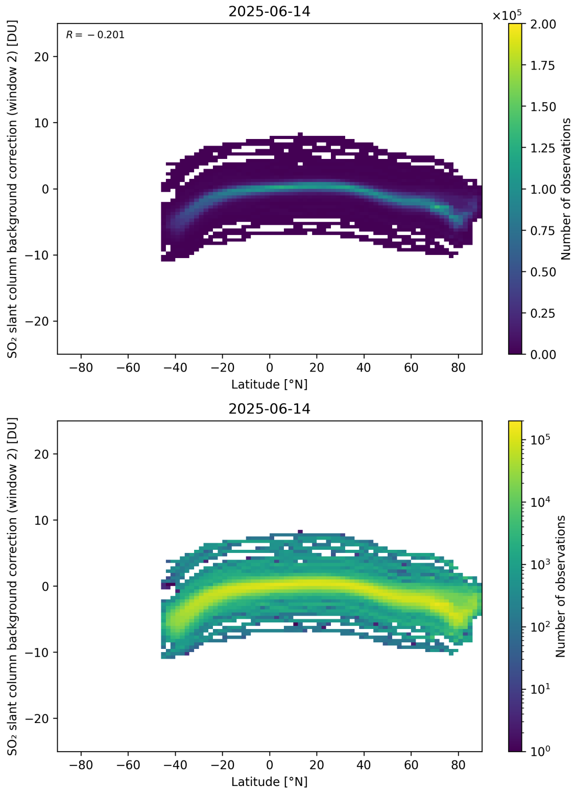
Figure 151: Scatter density plot of “Latitude” against “SO 2 slant column background correction (window 2)” for 2025-06-13 to 2025-06-15.
