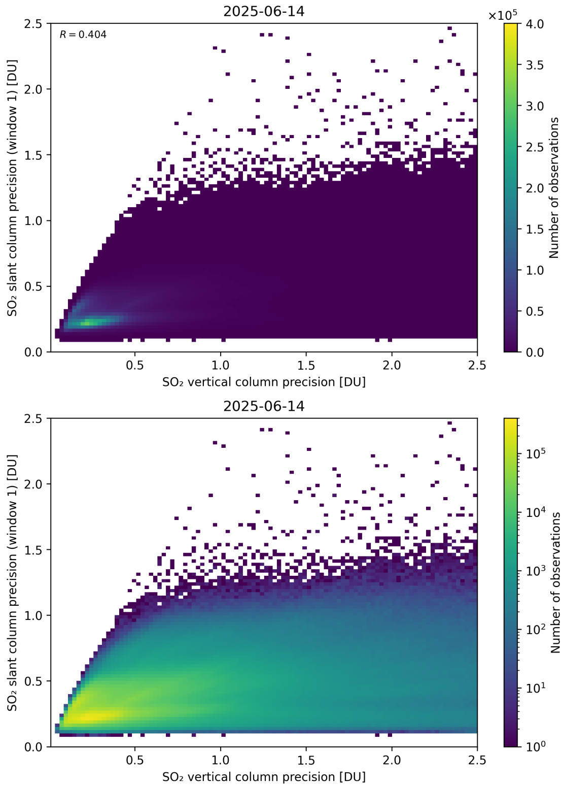
Figure 342: Scatter density plot of “SO 2 vertical column precision” against “SO 2 slant column precision (window 1)” for 2025-06-13 to 2025-06-15.
