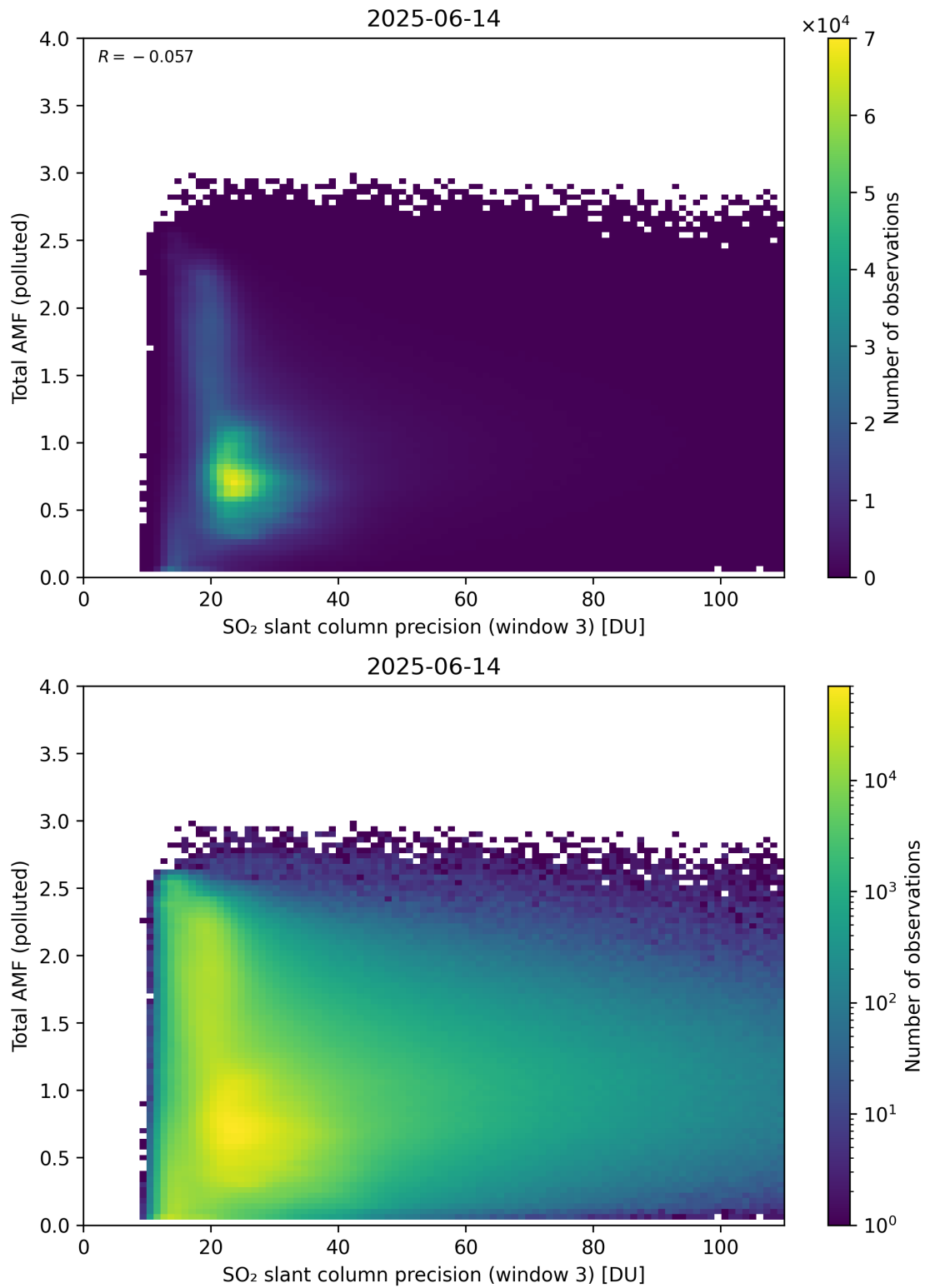
Figure 313: Scatter density plot of “SO 2 slant column precision (window 3)” against “Total AMF (polluted)” for 2025-06-13 to 2025-06-15.
