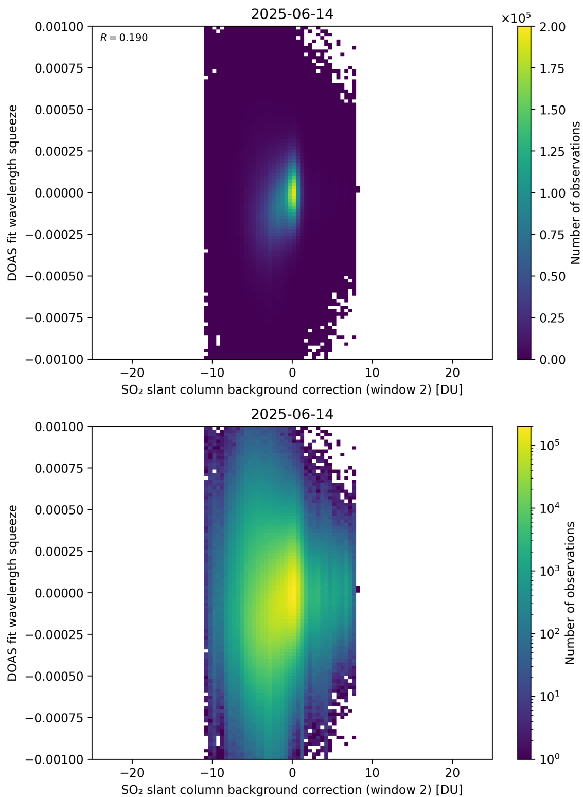
Figure 124: Scatter density plot of “SO 2 slant column background correction (window 2)” against “DOAS fit wavelength squeeze” for 2025-06-13 to 2025-06-15.
