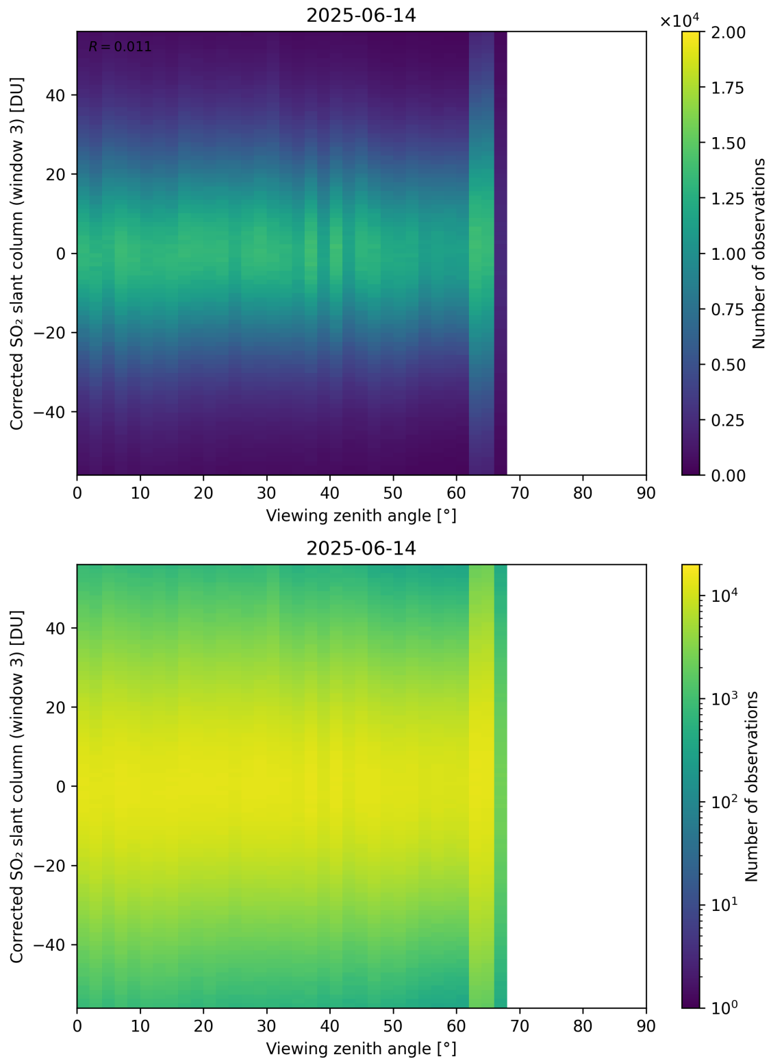
Figure 375: Scatter density plot of “Viewing zenith angle” against “Corrected SO 2 slant column (window 3)” for 2025-06-13 to 2025-06-15.
