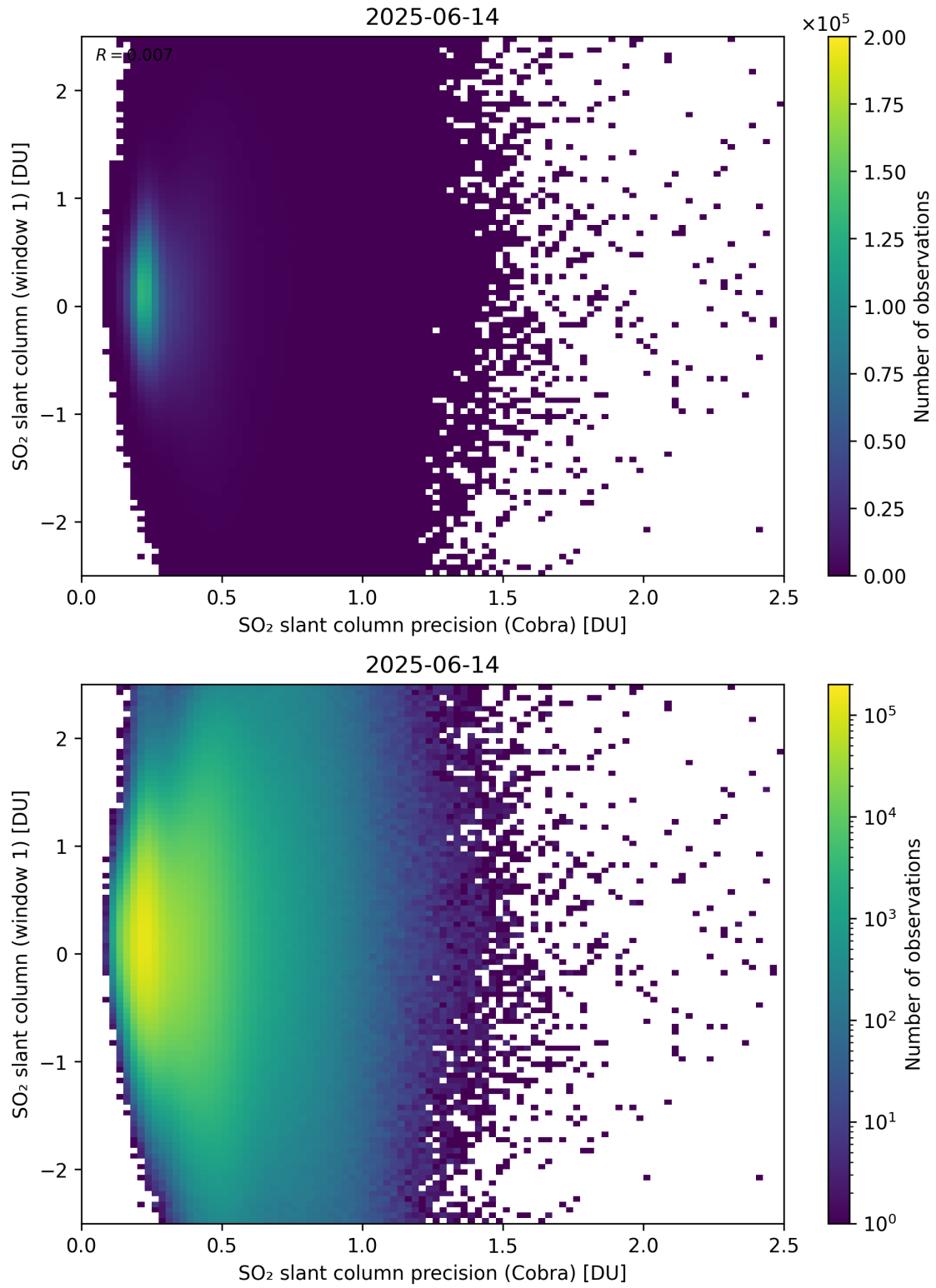
Figure 208: Scatter density plot of “SO 2 slant column precision (Cobra)” against “SO 2 slant column (window 1)” for 2025-06-13 to 2025-06-15.
