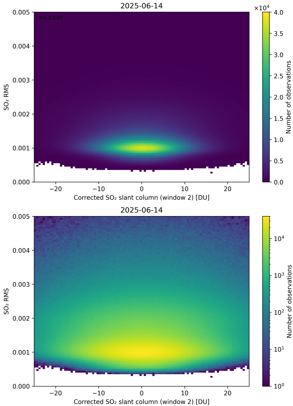
Figure 248: Scatter density plot of “Corrected SO 2 slant column (window 2)” against “SO 2 RMS” for 2025-06-13 to 2025-06-15.
