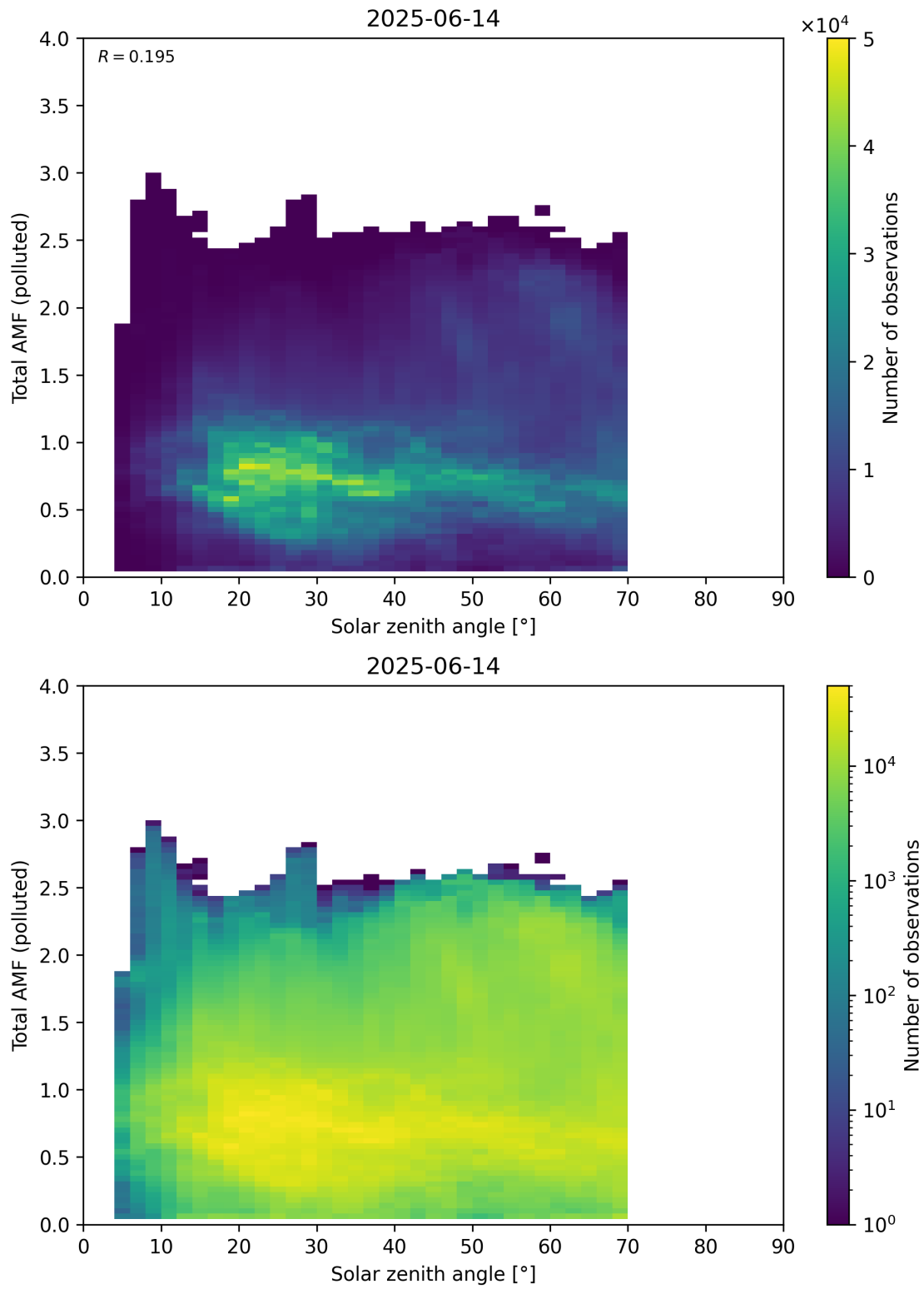
Figure 189: Scatter density plot of “Solar zenith angle” against “Total AMF (polluted)” for 2025-06-13 to 2025-06-15.
