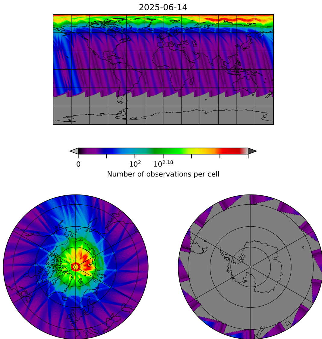
Figure 30: Map of the number of observations for 2025-06-13 to 2025-06-15
