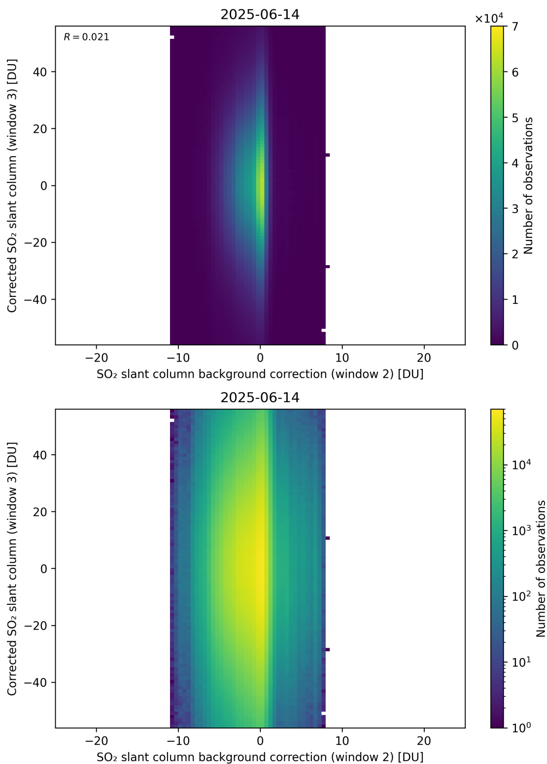
Figure 127: Scatter density plot of “SO 2 slant column background correction (window 2)” against “Corrected SO 2 slant column (window 3)” for 2025-06-13 to 2025-06-15.
