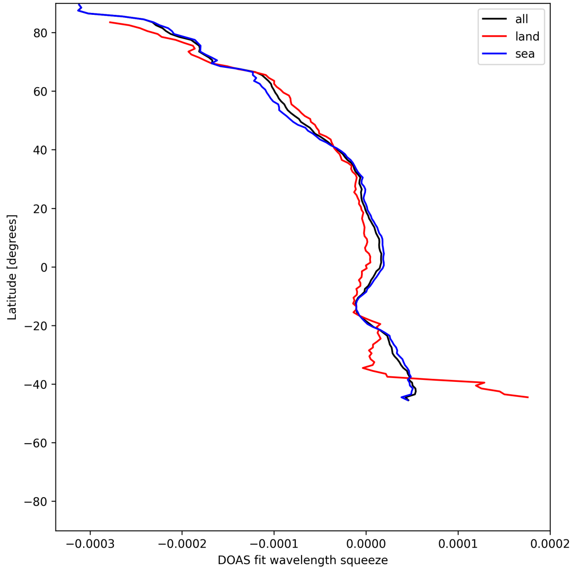
Figure 51: Zonal average of “DOAS fit wavelength squeeze” for 2025-06-13 to 2025-06-15.
