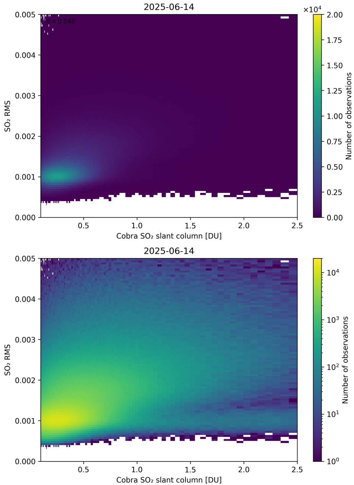
Figure 198: Scatter density plot of “Cobra SO 2 slant column” against “SO 2 RMS” for 2025-06-13 to 2025-06-15.
