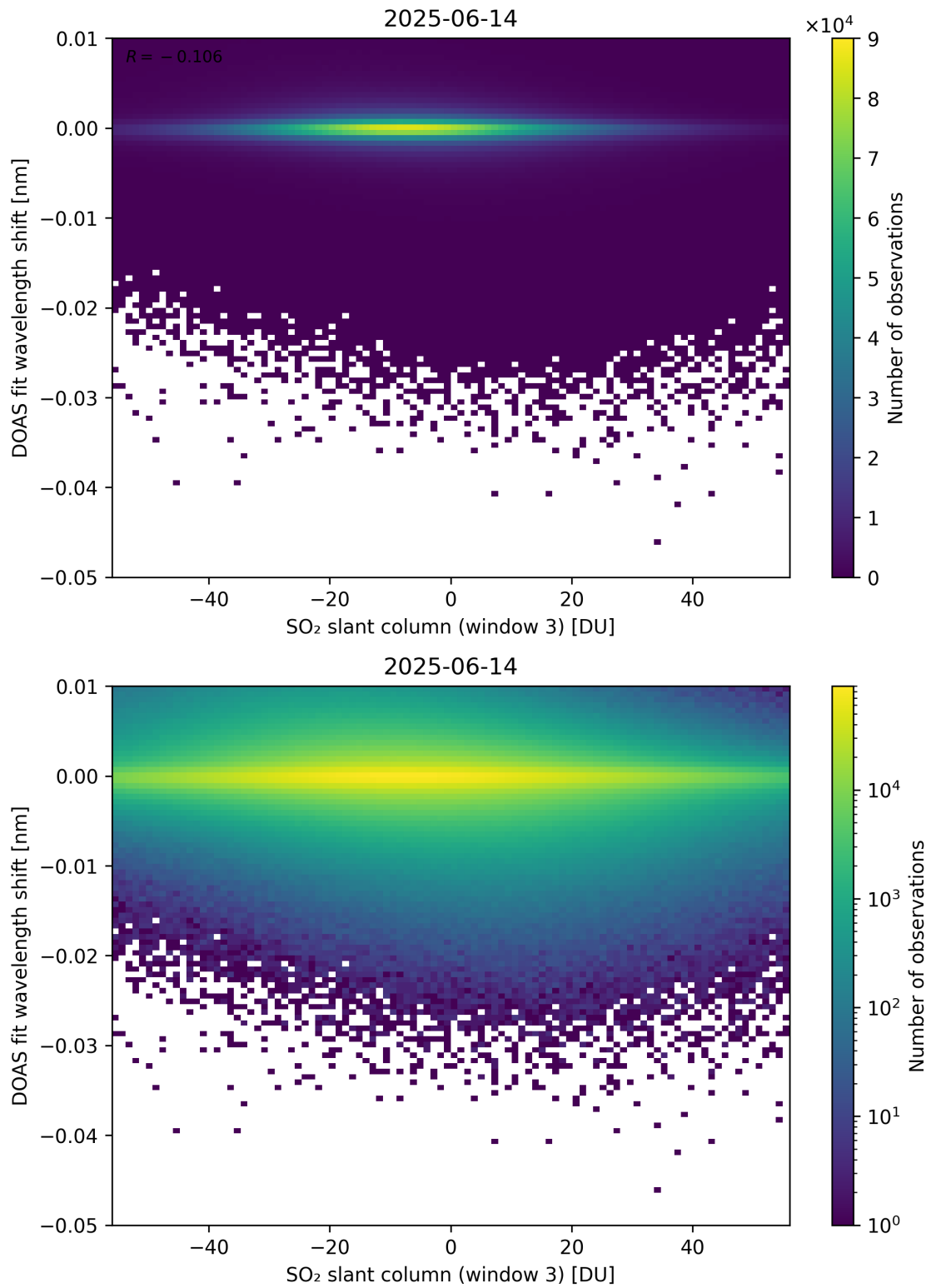
Figure 304: Scatter density plot of “SO 2 slant column (window 3)” against “DOAS fit wavelength shift” for 2025-06-13 to 2025-06-15.
