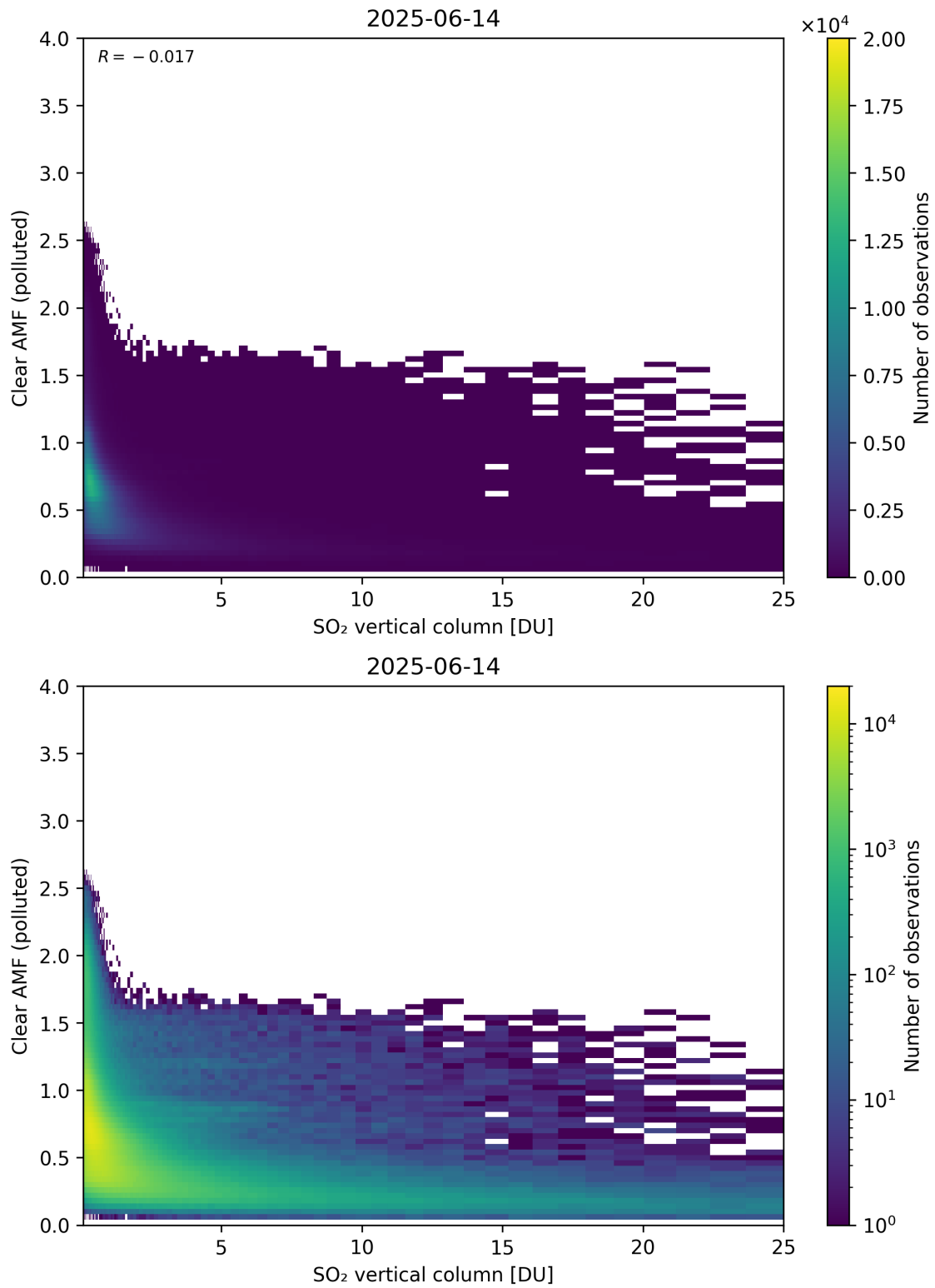
Figure 348: Scatter density plot of “SO 2 vertical column” against “Clear AMF (polluted)” for 2025-06-13 to 2025-06-15.
