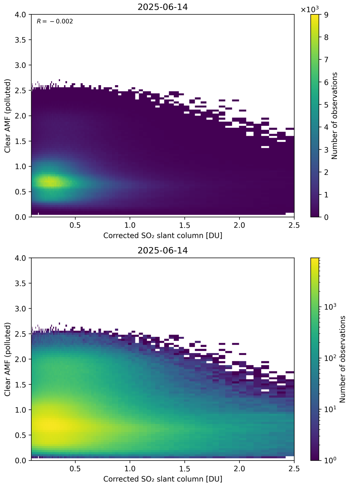
Figure 232: Scatter density plot of “Corrected SO 2 slant column” against “Clear AMF (polluted)” for 2025-06-13 to 2025-06-15.
