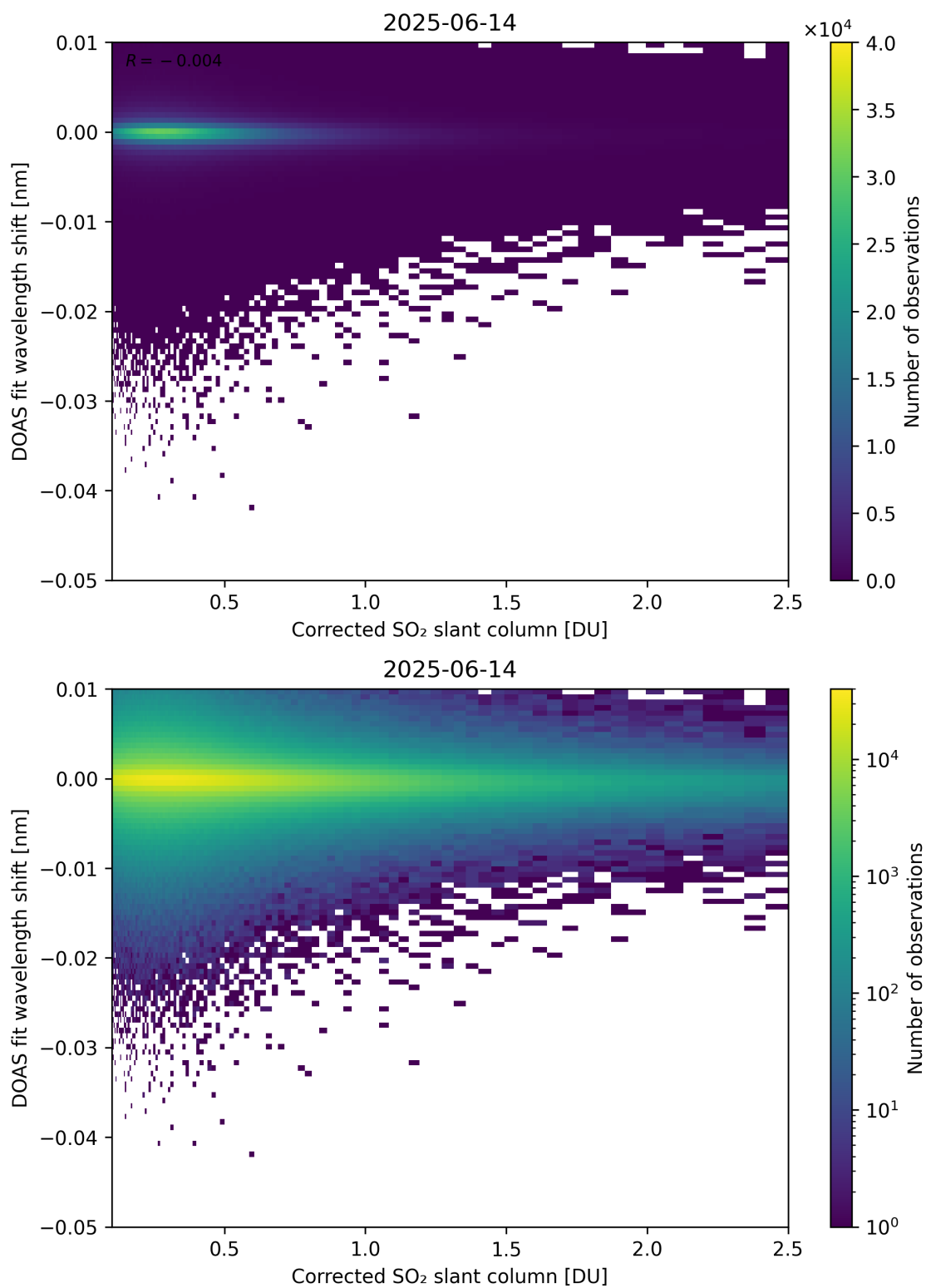
Figure 229: Scatter density plot of “Corrected SO 2 slant column” against “DOAS fit wavelength shift” for 2025-06-13 to 2025-06-15.
