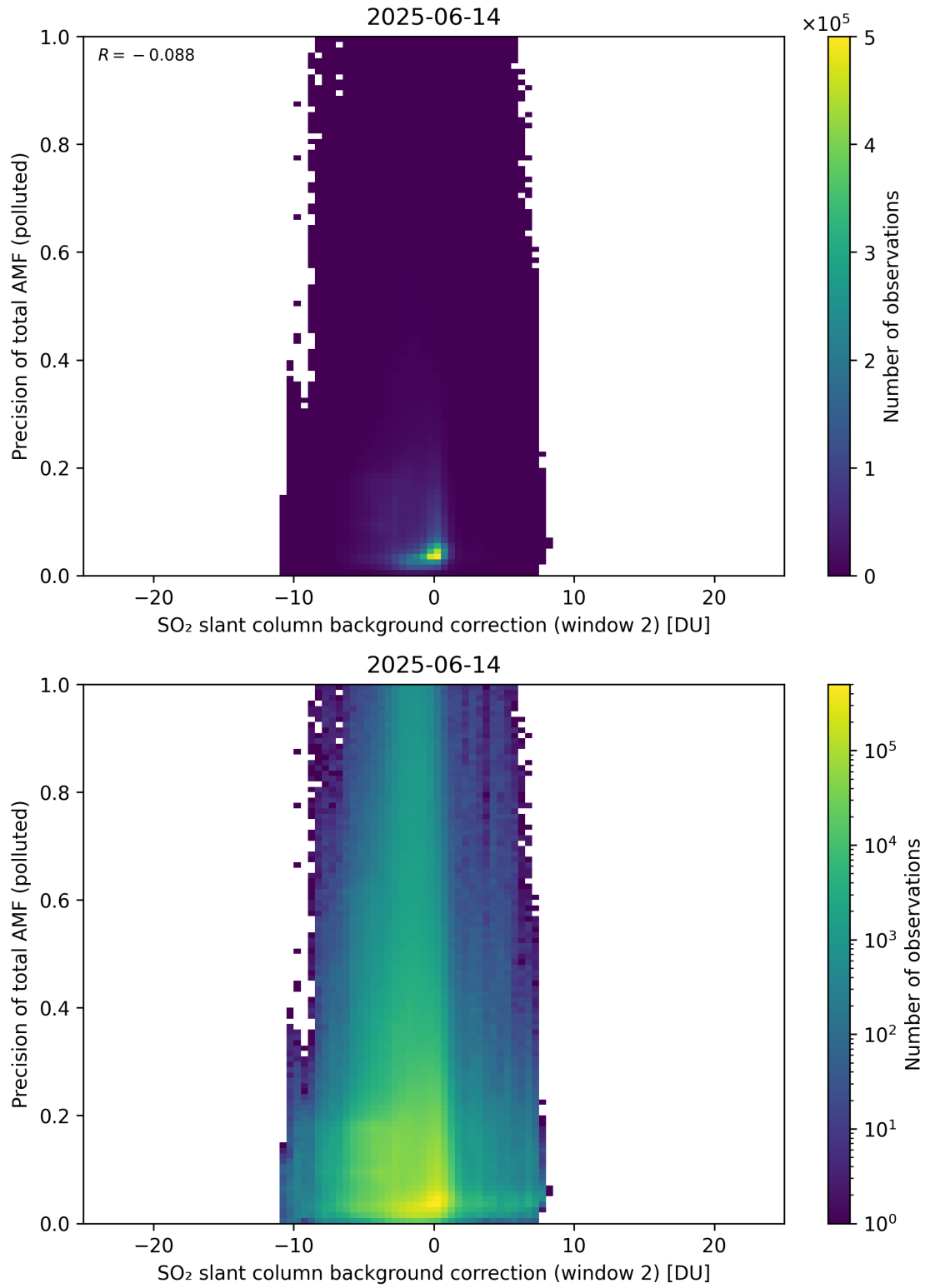
Figure 131: Scatter density plot of “SO 2 slant column background correction (window 2)” against “Precision of total AMF (polluted)” for 2025-06-13 to 2025-06-15.
