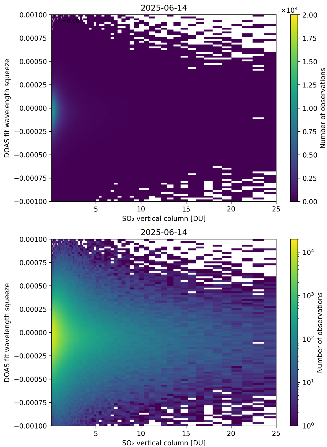
Figure 327: Scatter density plot of “SO 2 vertical column” against “DOAS fit wavelength squeeze” for 2025-06-13 to 2025-06-15.
