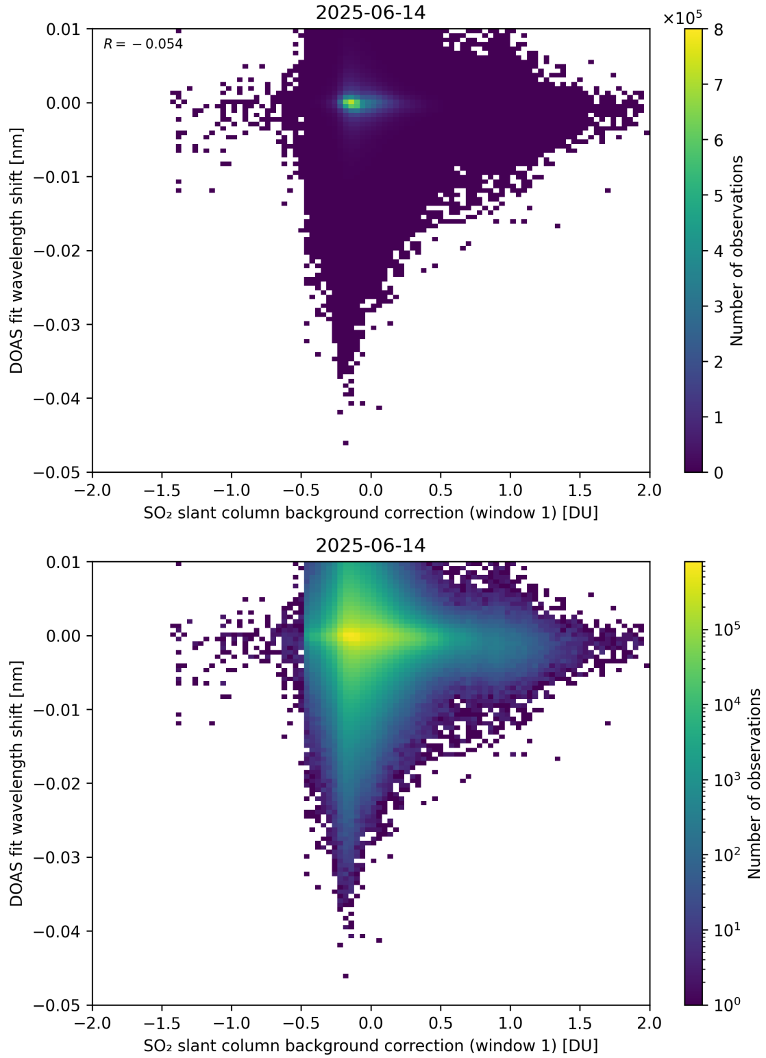
Figure 111: Scatter density plot of “SO 2 slant column background correction (window 1)” against “DOAS fit wavelength shift” for 2025-06-13 to 2025-06-15.
