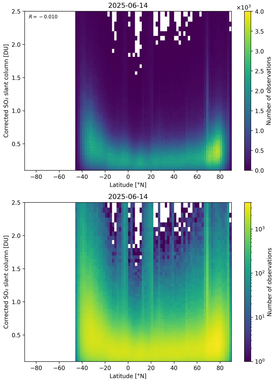
Figure 159: Scatter density plot of “Latitude” against “Corrected SO 2 slant column” for 2025-06-13 to 2025-06-15.
