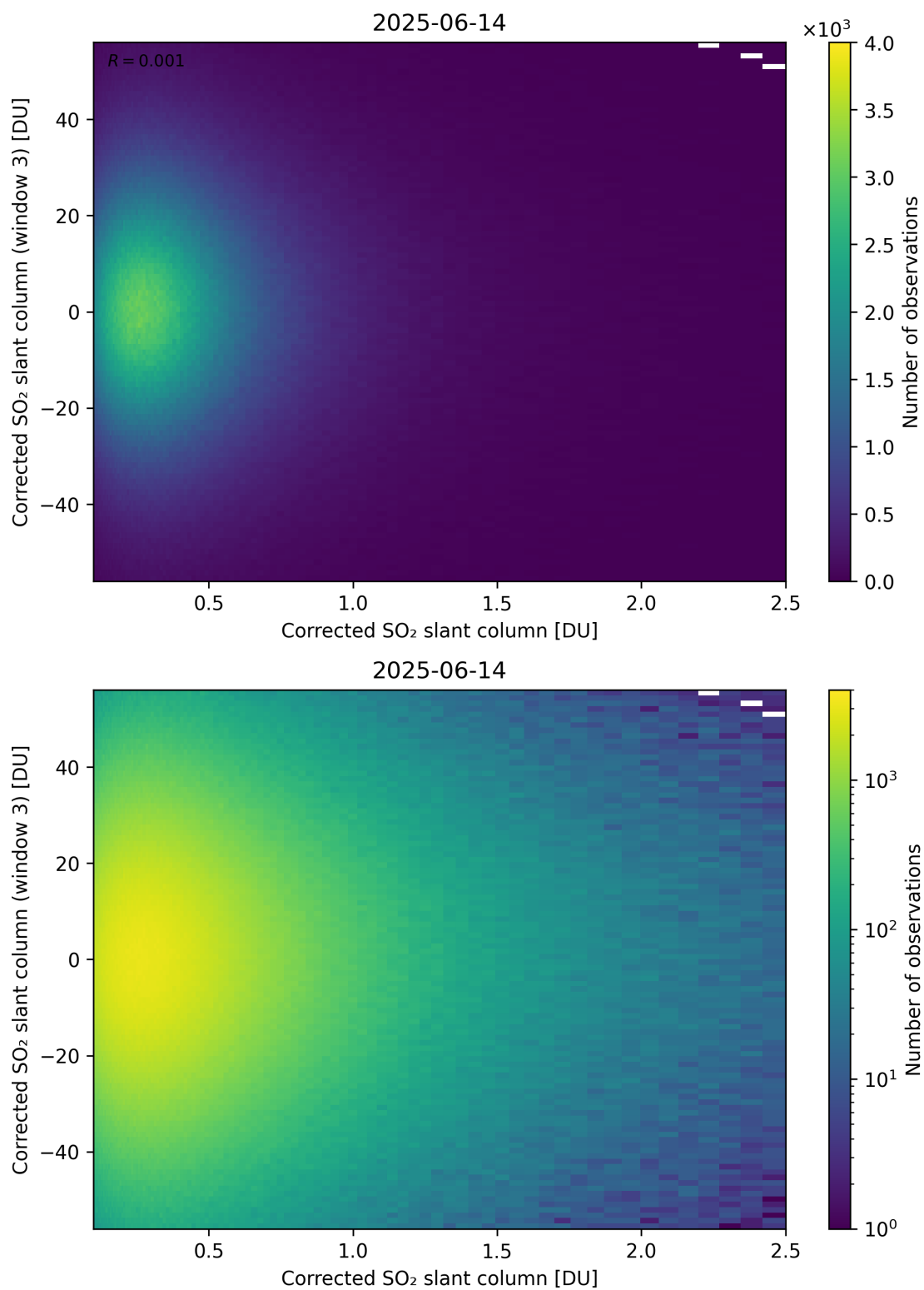
Figure 236: Scatter density plot of “Corrected SO 2 slant column” against “Corrected SO 2 slant column (window 3)” for 2025-06-13 to 2025-06-15.
