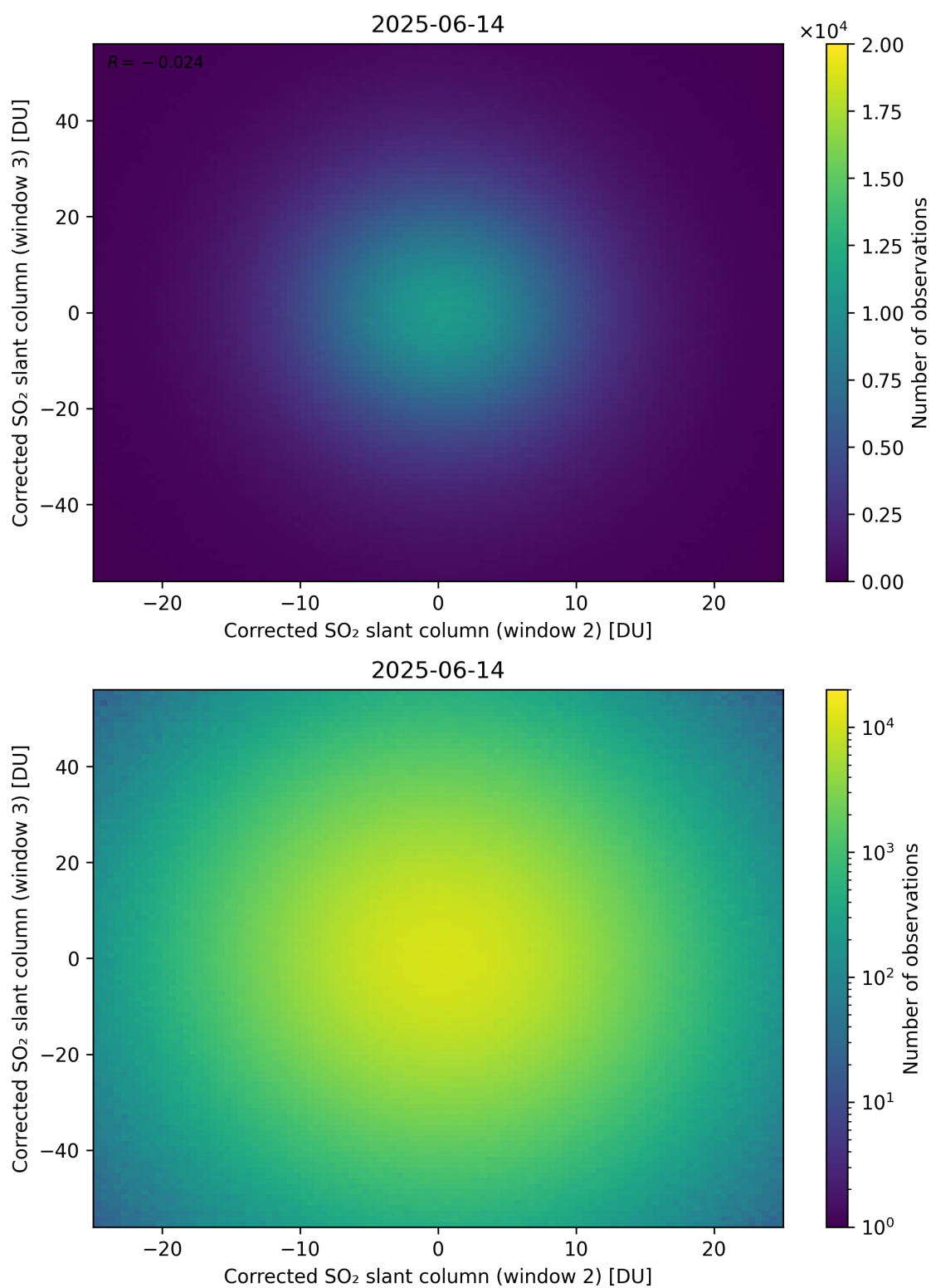
Figure 250: Scatter density plot of “Corrected SO 2 slant column (window 2)” against “Corrected SO 2 slant column (window 3)” for 2025-06-13 to 2025-06-15.
