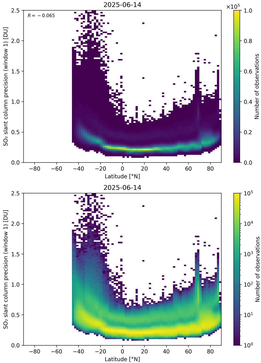
Figure 163: Scatter density plot of “Latitude” against “SO 2 slant column precision (window 1)” for 2025-06-13 to 2025-06-15.
