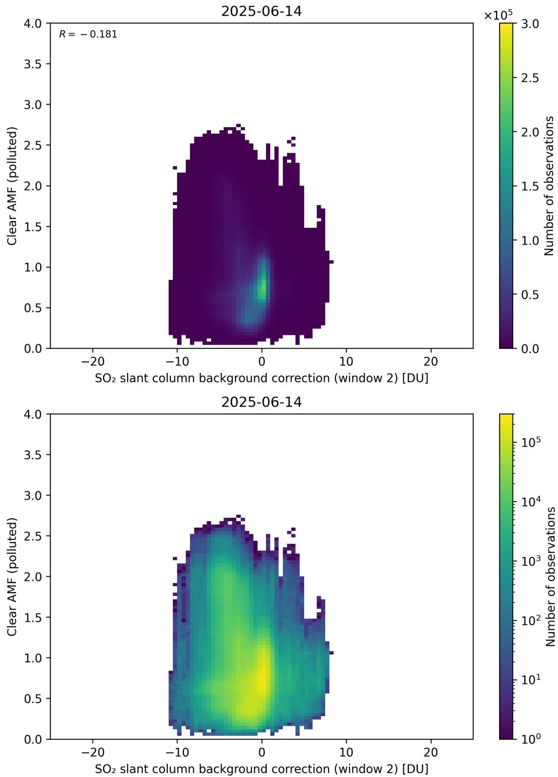
Figure 126: Scatter density plot of “SO 2 slant column background correction (window 2)” against “Clear AMF (polluted)” for 2025-06-13 to 2025-06-15.
