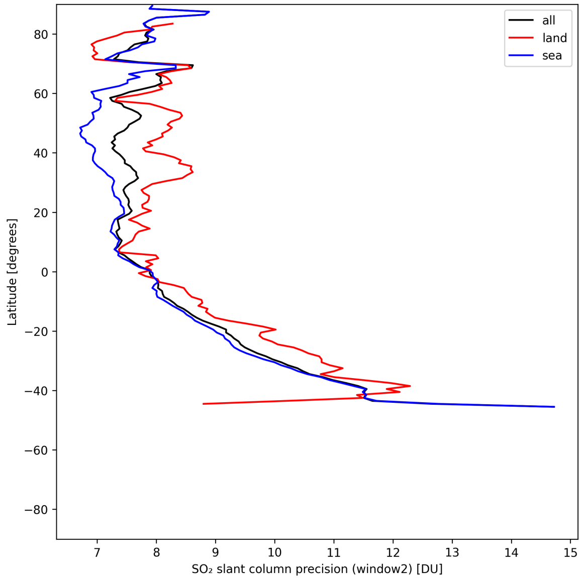
Figure 42: Zonal average of “SO 2 slant column precision (window2)” for 2025-06-13 to 2025-06-15.
