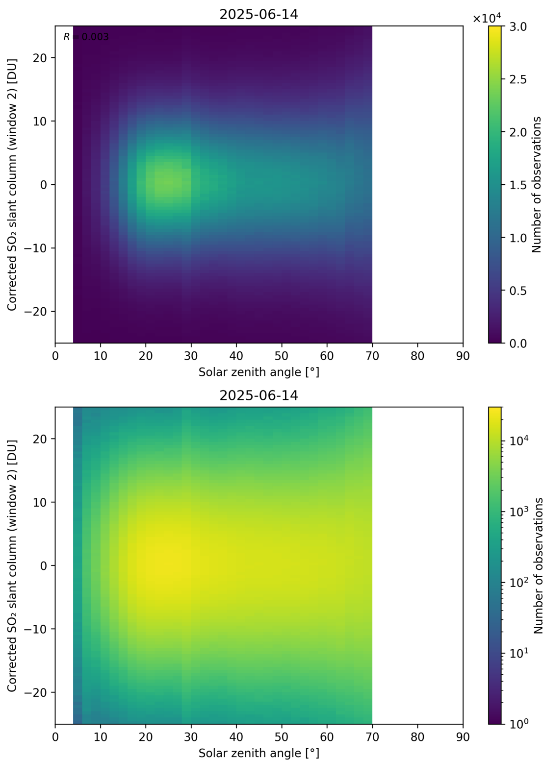
Figure 182: Scatter density plot of “Solar zenith angle” against “Corrected SO 2 slant column (window 2)” for 2025-06-13 to 2025-06-15.
