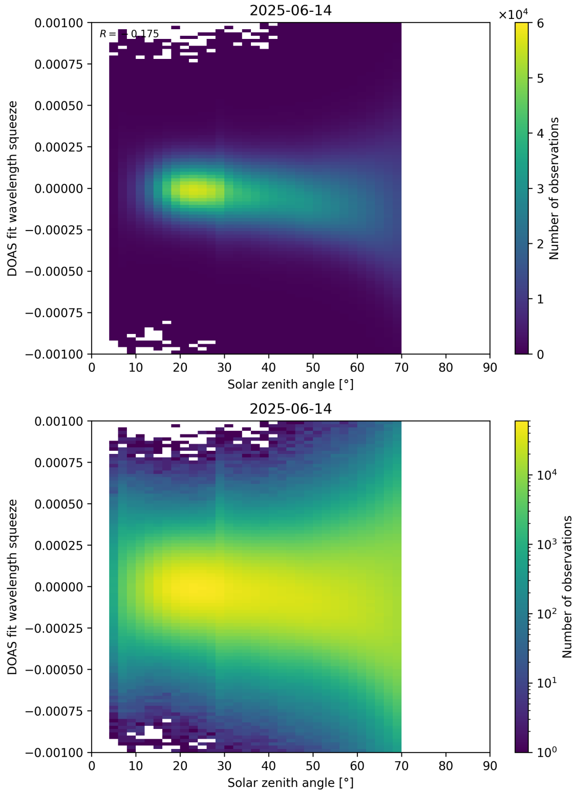
Figure 175: Scatter density plot of “Solar zenith angle” against “DOAS fit wavelength squeeze” for 2025-06-13 to 2025-06-15.
