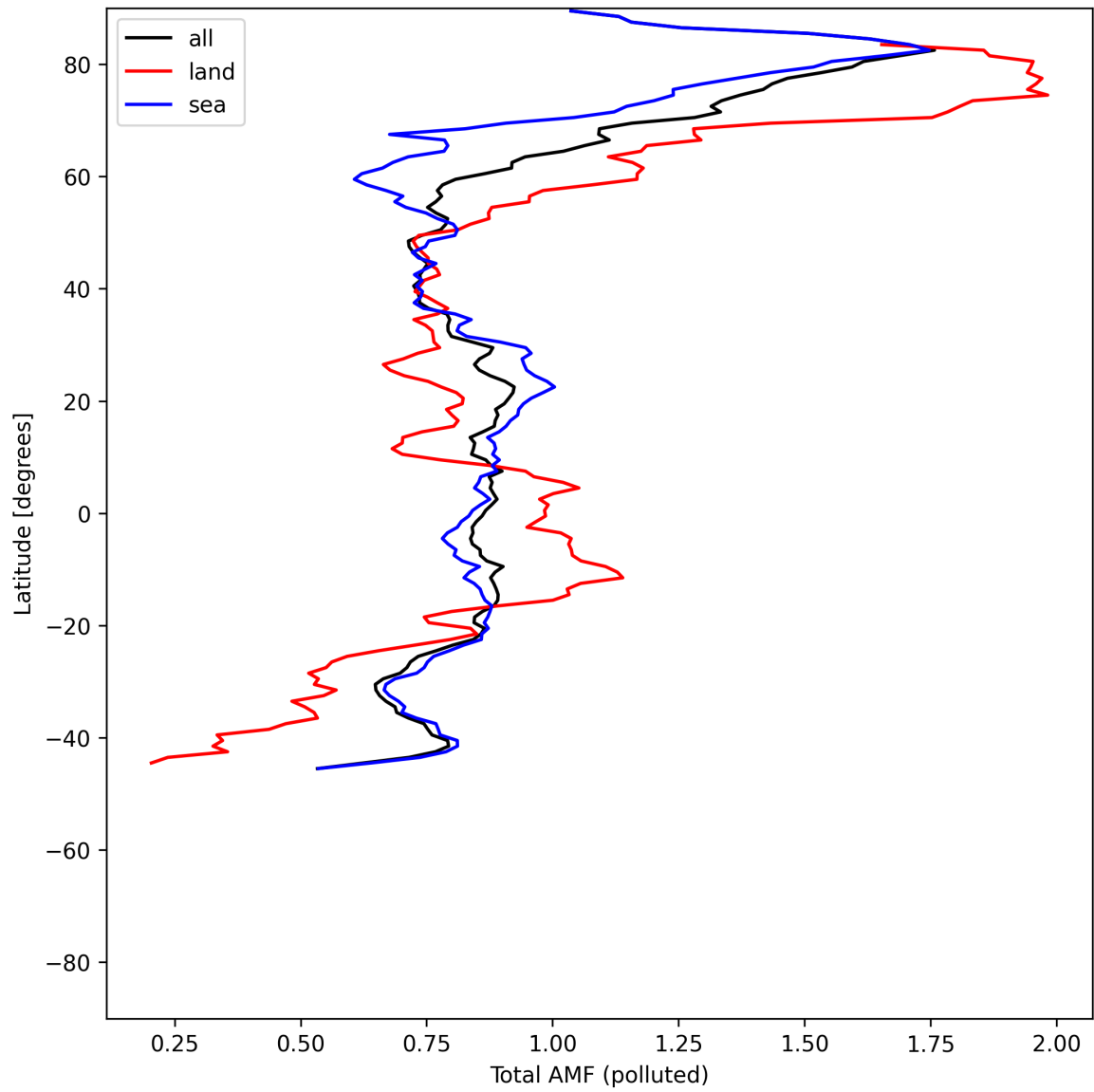
Figure 53: Zonal average of “Total AMF (polluted)” for 2025-06-13 to 2025-06-15.
