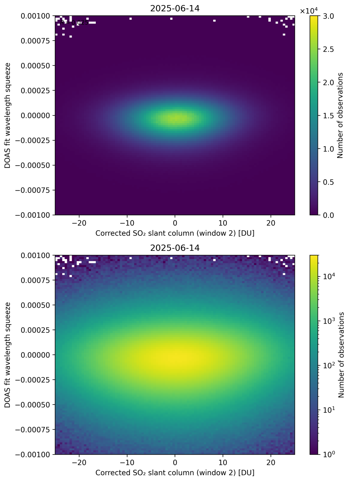
Figure 247: Scatter density plot of “Corrected SO 2 slant column (window 2)” against “DOAS fit wavelength squeeze” for 2025-06-13 to 2025-06-15.
