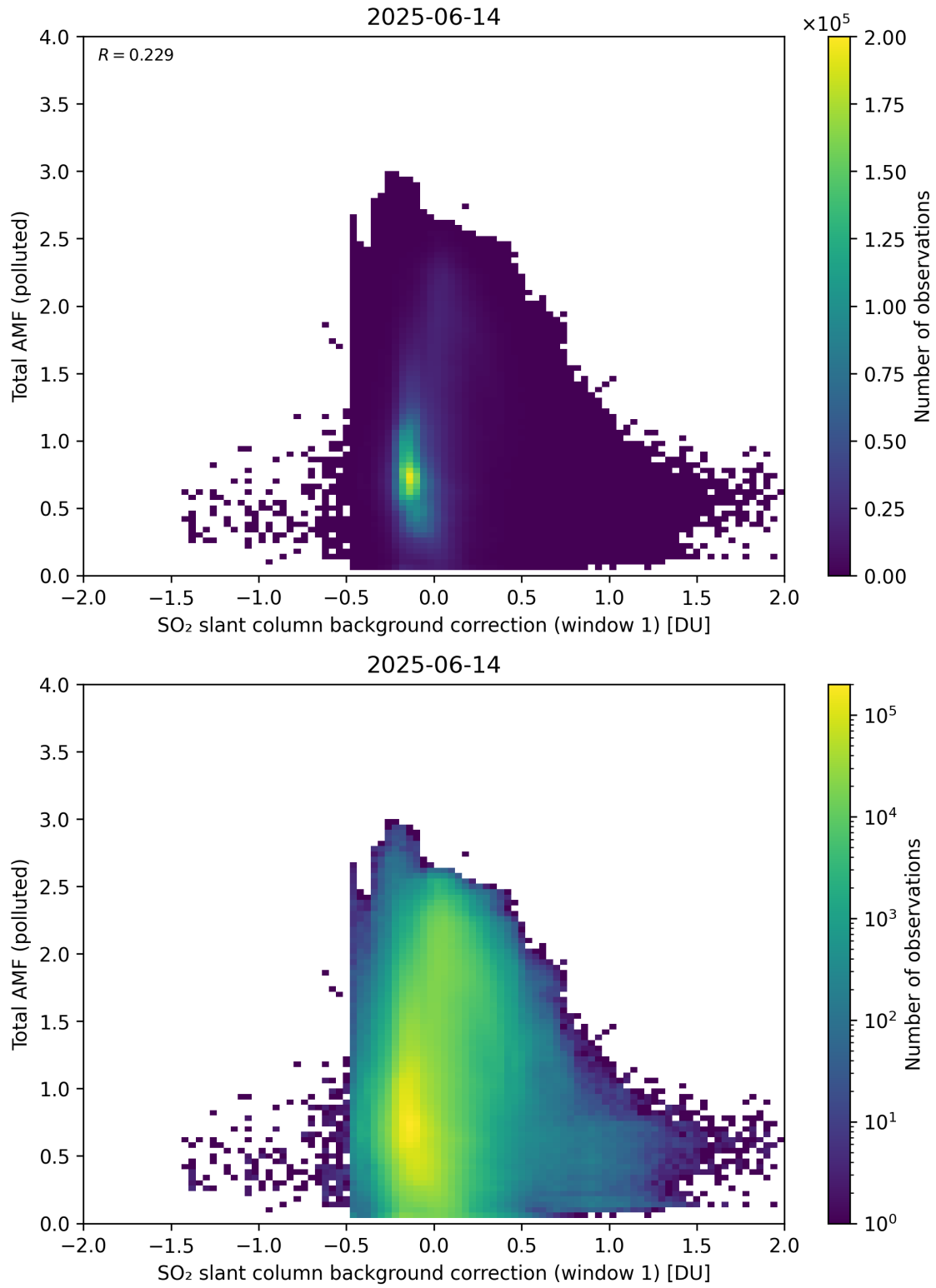
Figure 120: Scatter density plot of “SO 2 slant column background correction (window 1)” against “Total AMF (polluted)” for 2025-06-13 to 2025-06-15.
