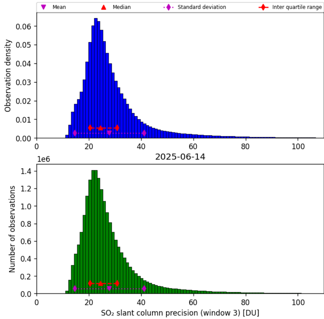
Figure 72: Histogram of “SO 2 slant column precision (window 3)” for 2025-06-13 to 2025-06-15
