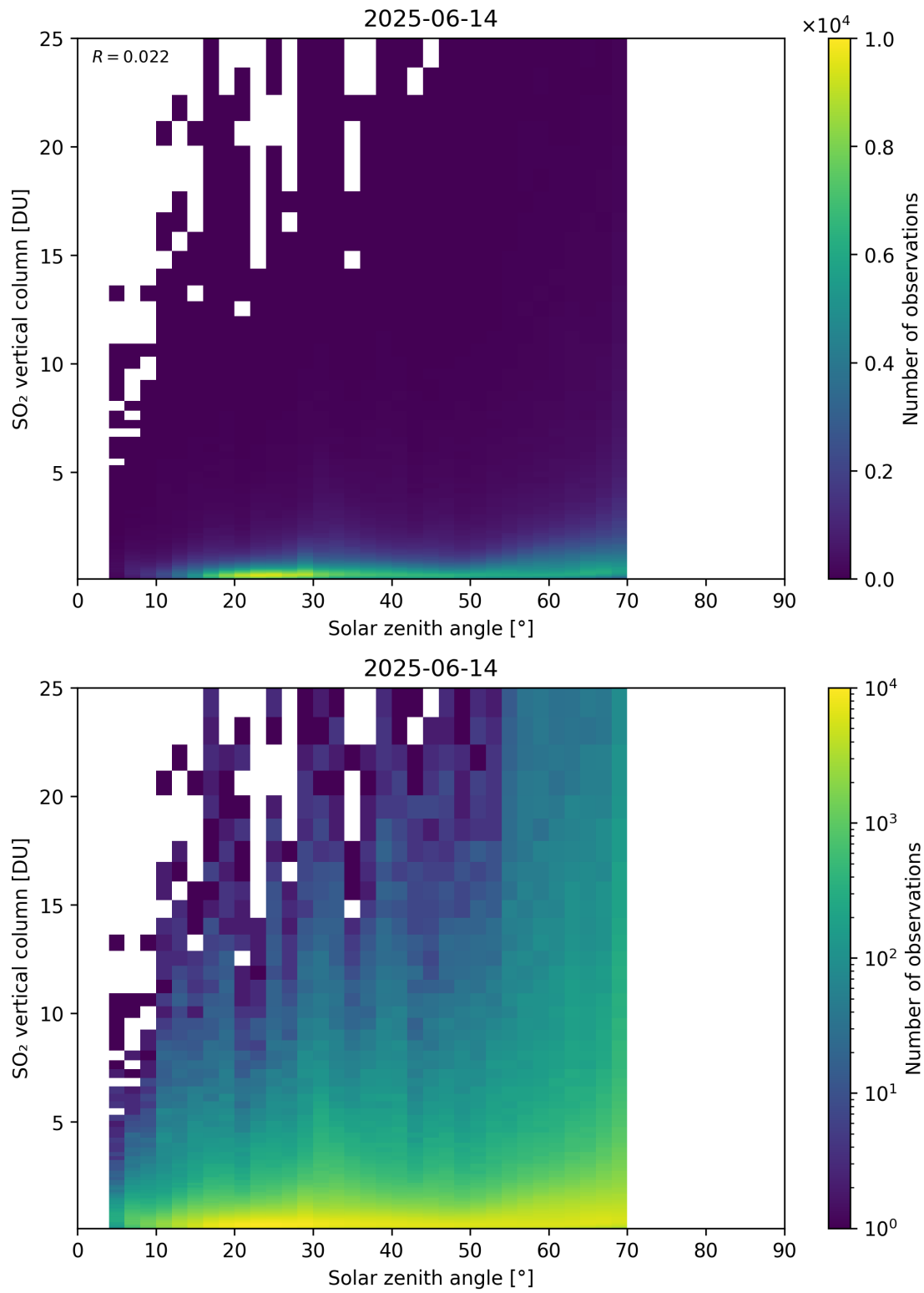
Figure 191: Scatter density plot of “Solar zenith angle” against “SO 2 vertical column” for 2025-06-13 to 2025-06-15.
