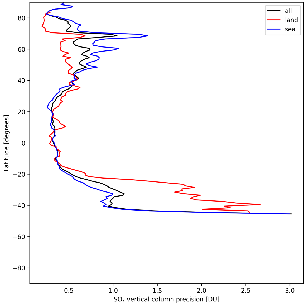
Figure 33: Zonal average of “SO 2 vertical column precision” for 2025-06-13 to 2025-06-15.
