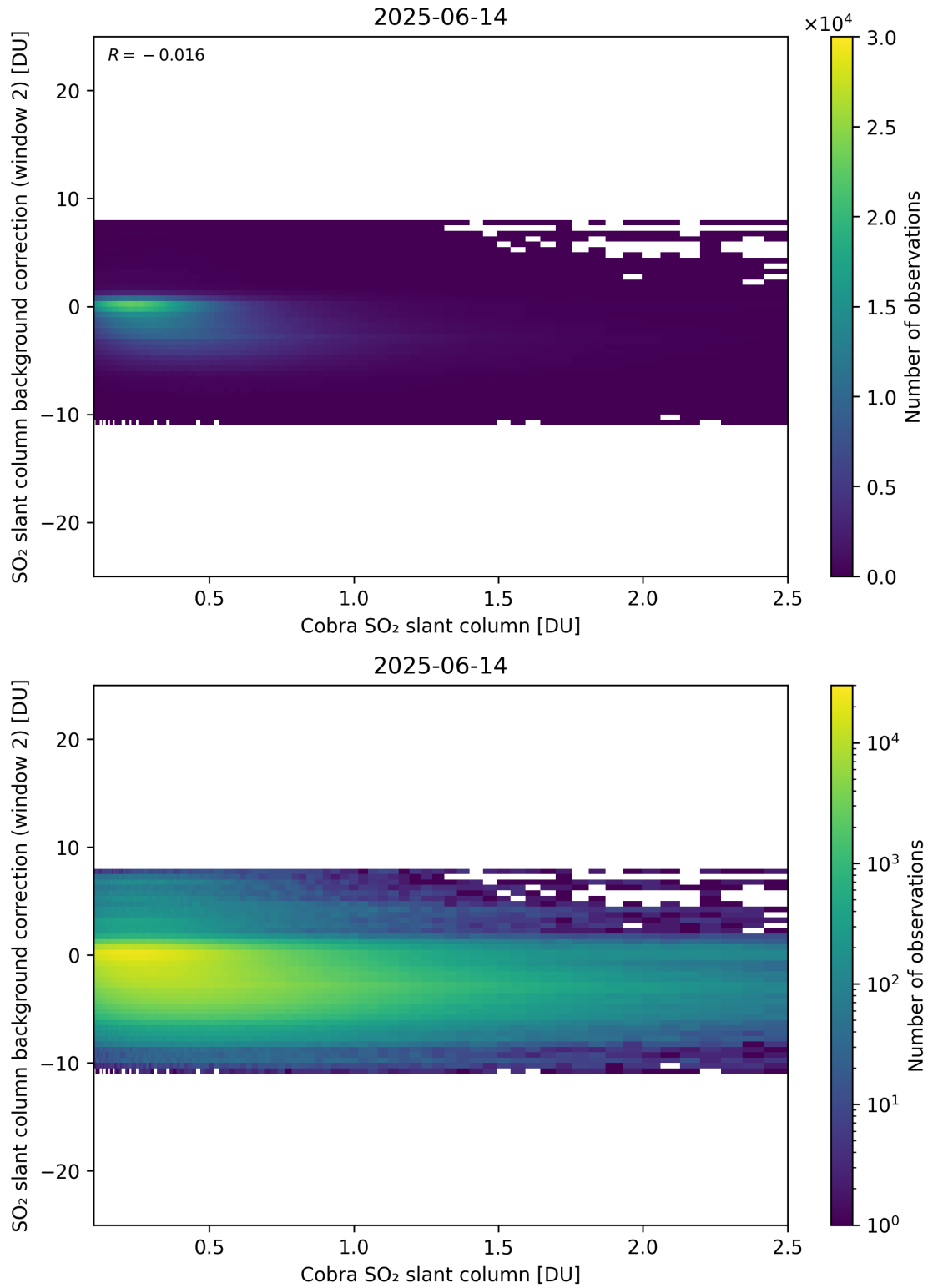
Figure 194: Scatter density plot of “Cobra SO 2 slant column” against “SO 2 slant column background correction (window 2)” for 2025-06-13 to 2025-06-15.
