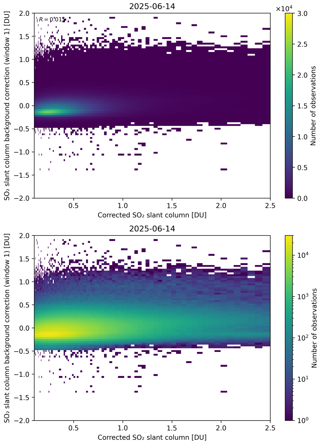
Figure 226: Scatter density plot of “Corrected SO 2 slant column” against “SO 2 slant column background correction (window 1)” for 2025-06-13 to 2025-06-15.
