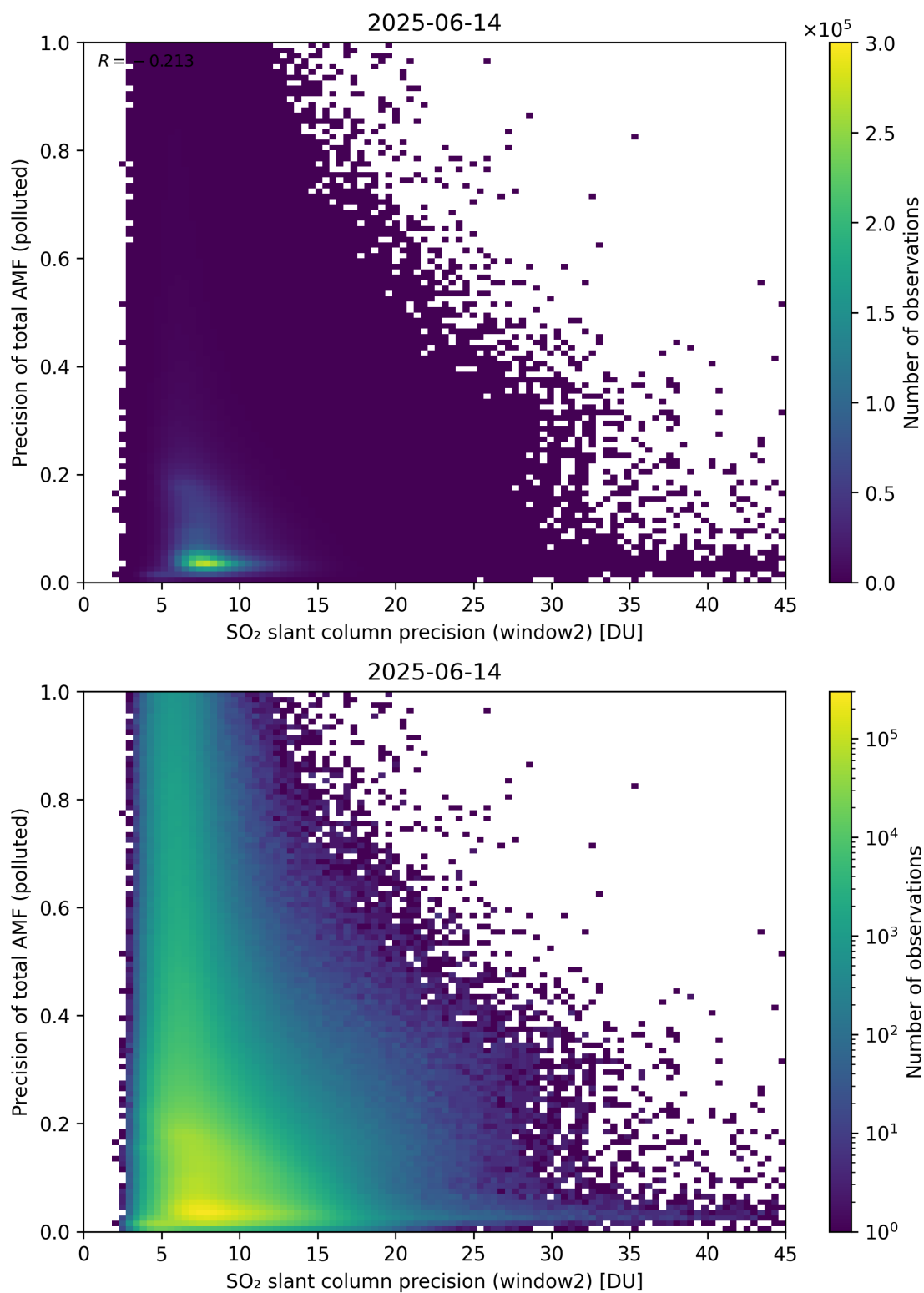
Figure 302: Scatter density plot of “SO 2 slant column precision (window2)” against “Precision of total AMF (polluted)” for 2025-06-13 to 2025-06-15.
