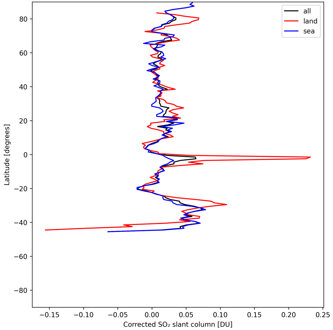
Figure 34: Zonal average of “Corrected SO 2 slant column” for 2025-06-13 to 2025-06-15.
