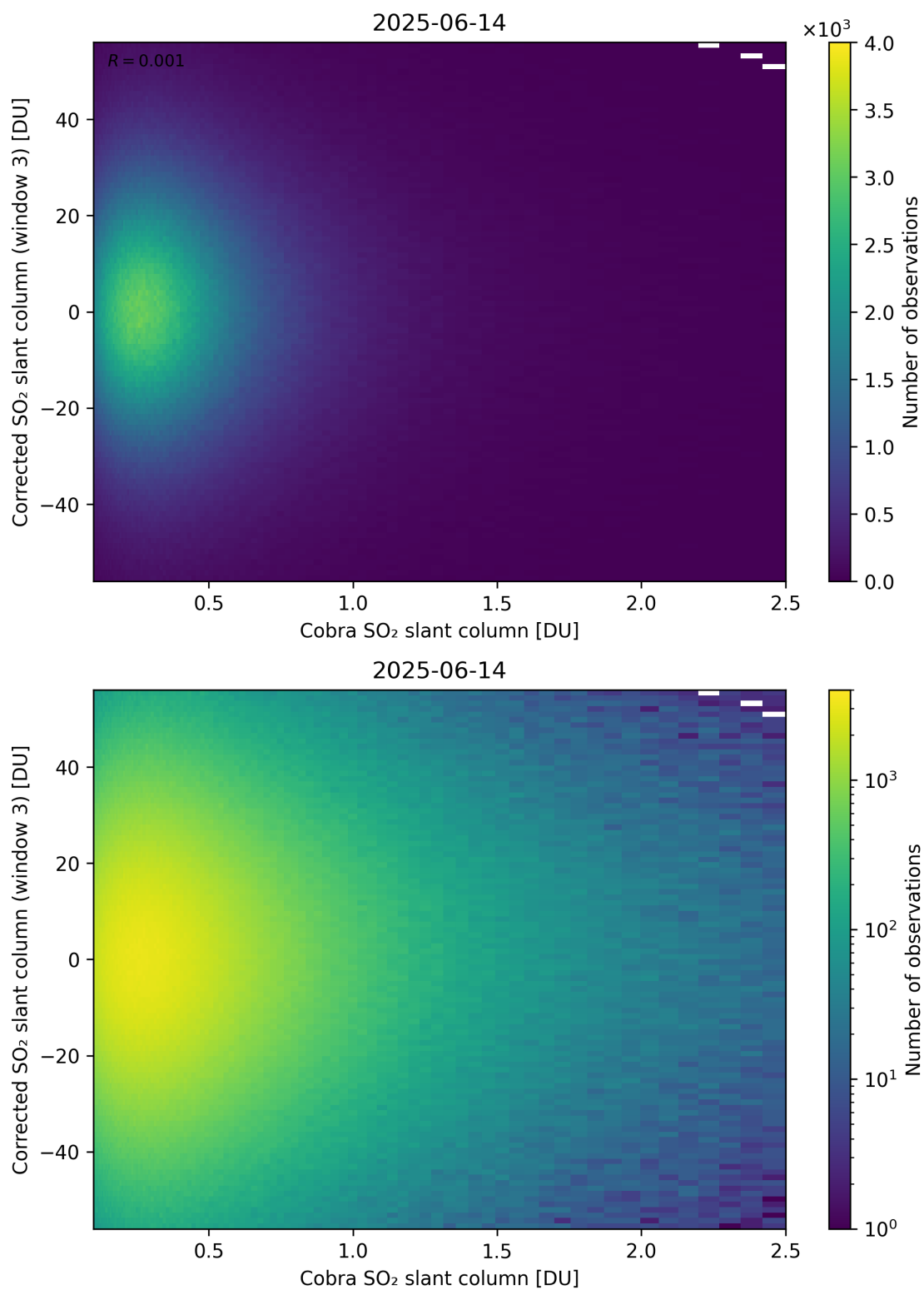
Figure 218: Scatter density plot of “Cobra SO 2 slant column” against “Corrected SO 2 slant column (window 3)” for 2025-06-13 to 2025-06-15.
