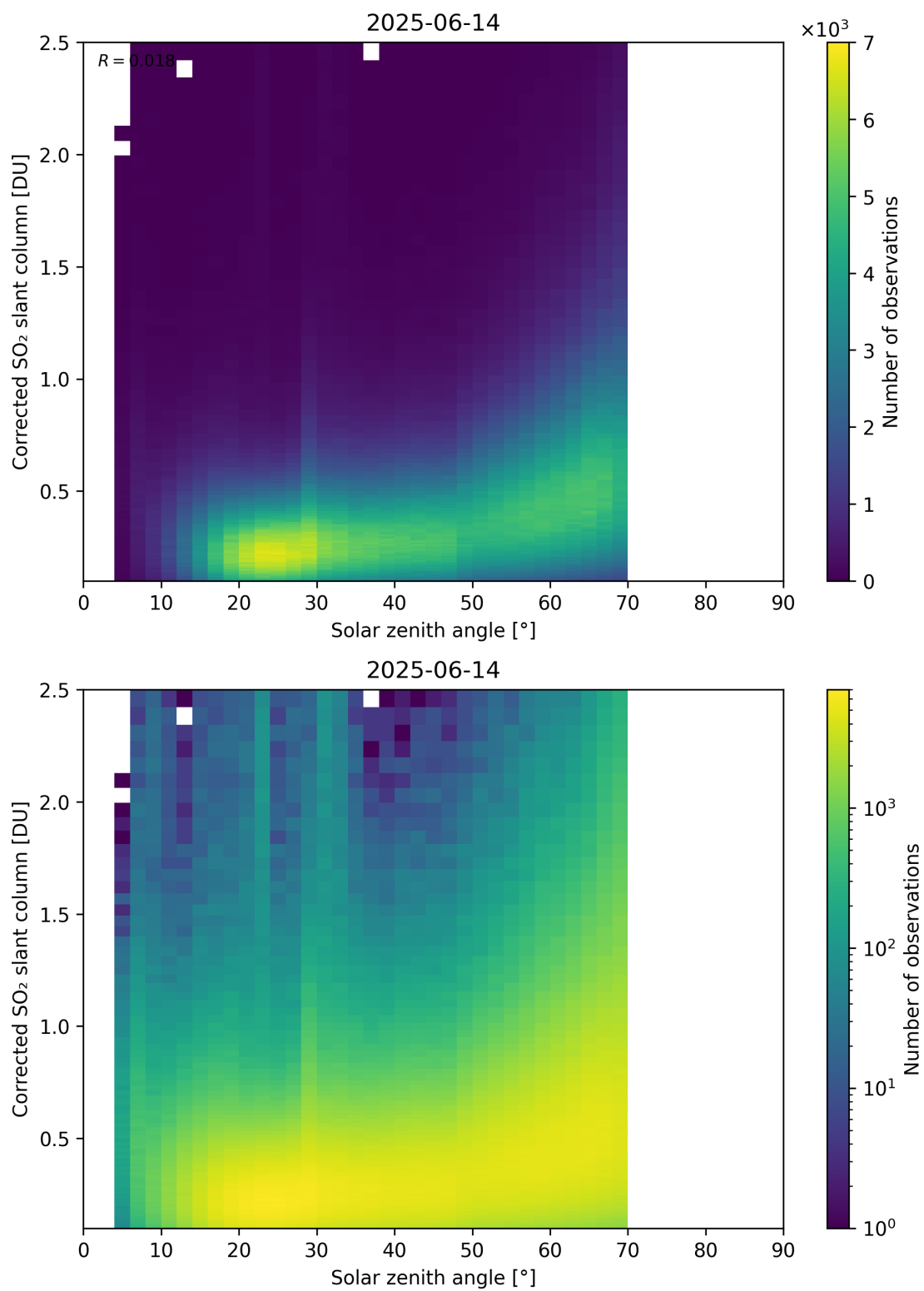
Figure 181: Scatter density plot of “Solar zenith angle” against “Corrected SO 2 slant column” for 2025-06-13 to 2025-06-15.
