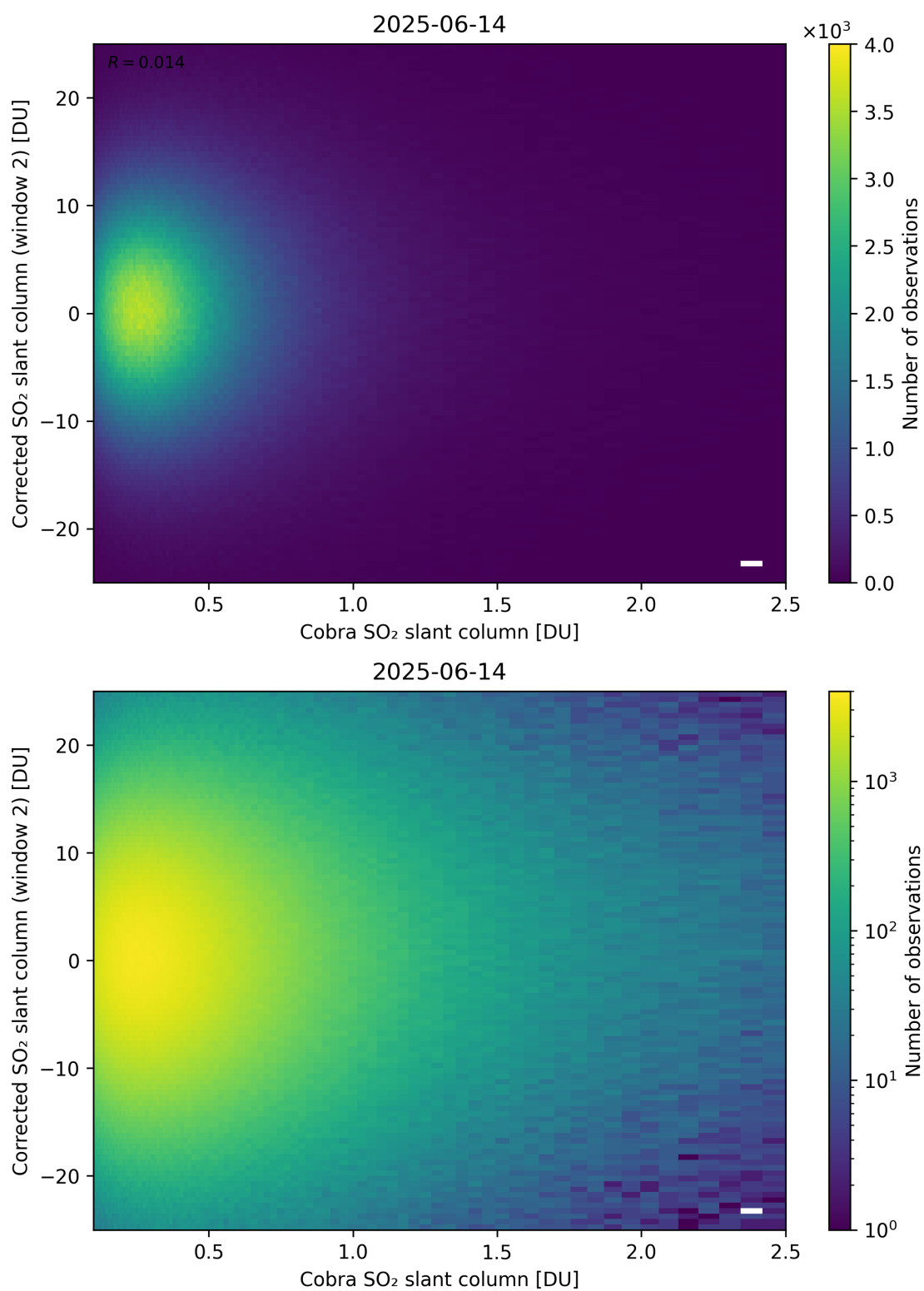
Figure 217: Scatter density plot of “Cobra SO 2 slant column” against “Corrected SO 2 slant column (window 2)” for 2025-06-13 to 2025-06-15.
