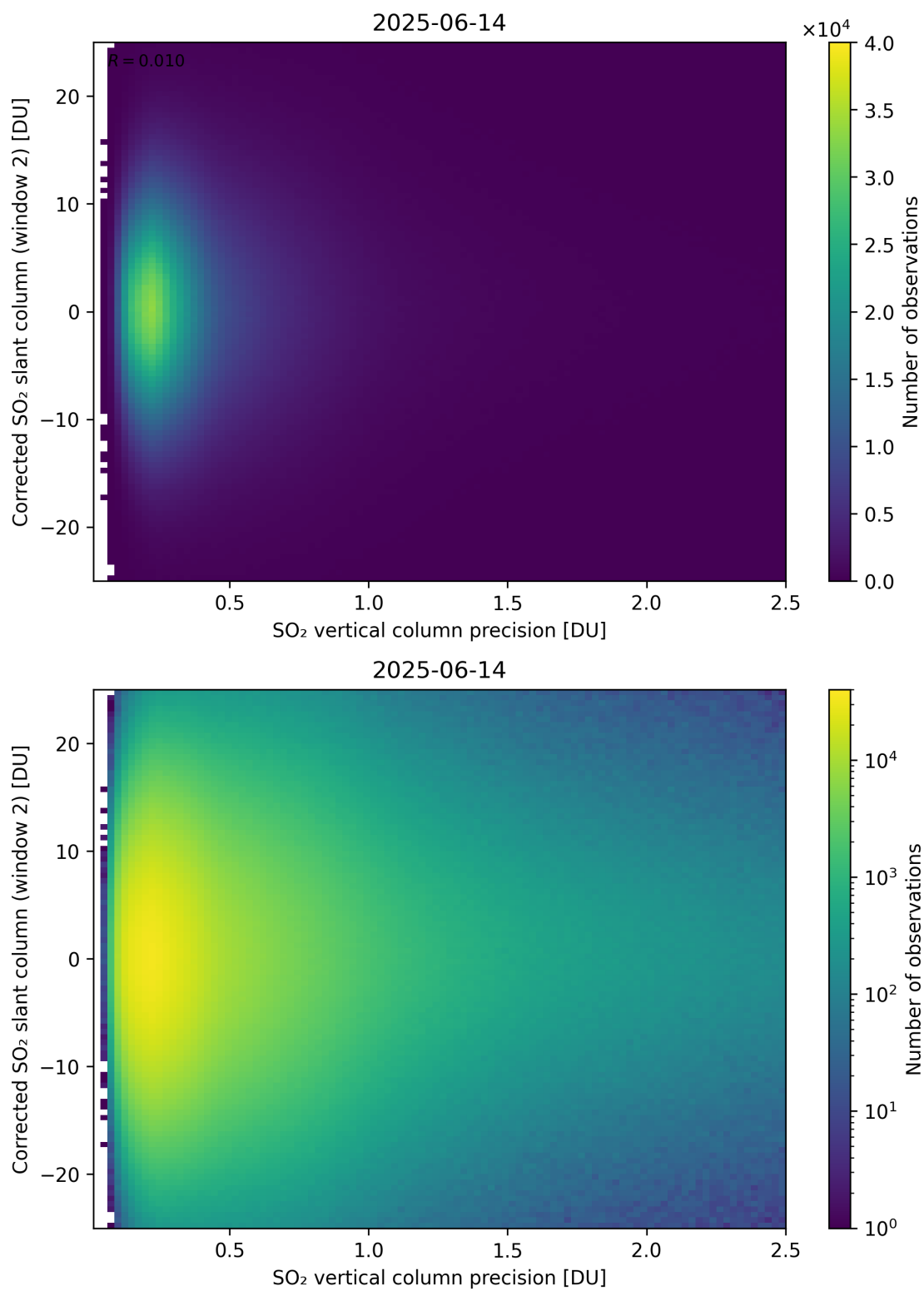
Figure 339: Scatter density plot of “SO 2 vertical column precision” against “Corrected SO 2 slant column (window 2)” for 2025-06-13 to 2025-06-15.
