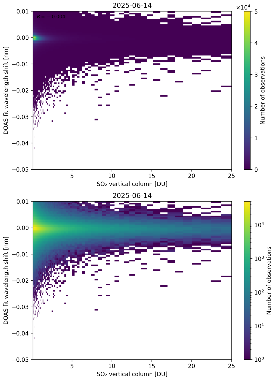
Figure 326: Scatter density plot of “SO 2 vertical column” against “DOAS fit wavelength shift” for 2025-06-13 to 2025-06-15.
