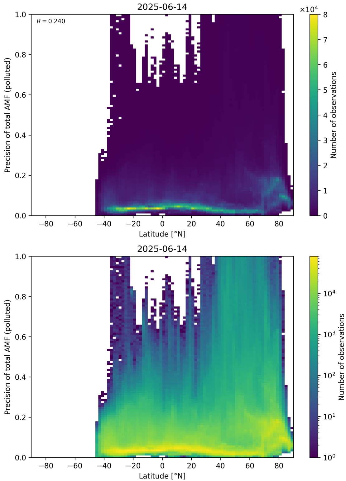
Figure 168: Scatter density plot of “Latitude” against “Precision of total AMF (polluted)” for 2025-06-13 to 2025-06-15.
