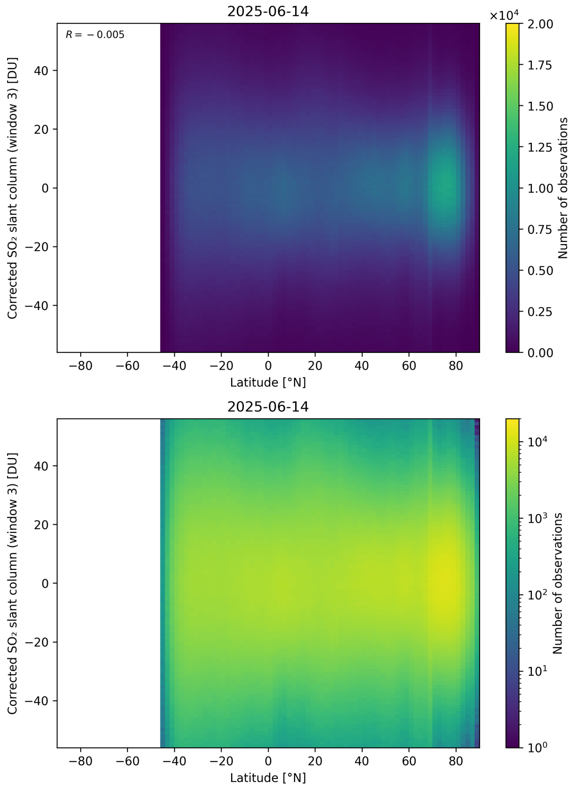
Figure 161: Scatter density plot of “Latitude” against “Corrected SO 2 slant column (window 3)” for 2025-06-13 to 2025-06-15.
