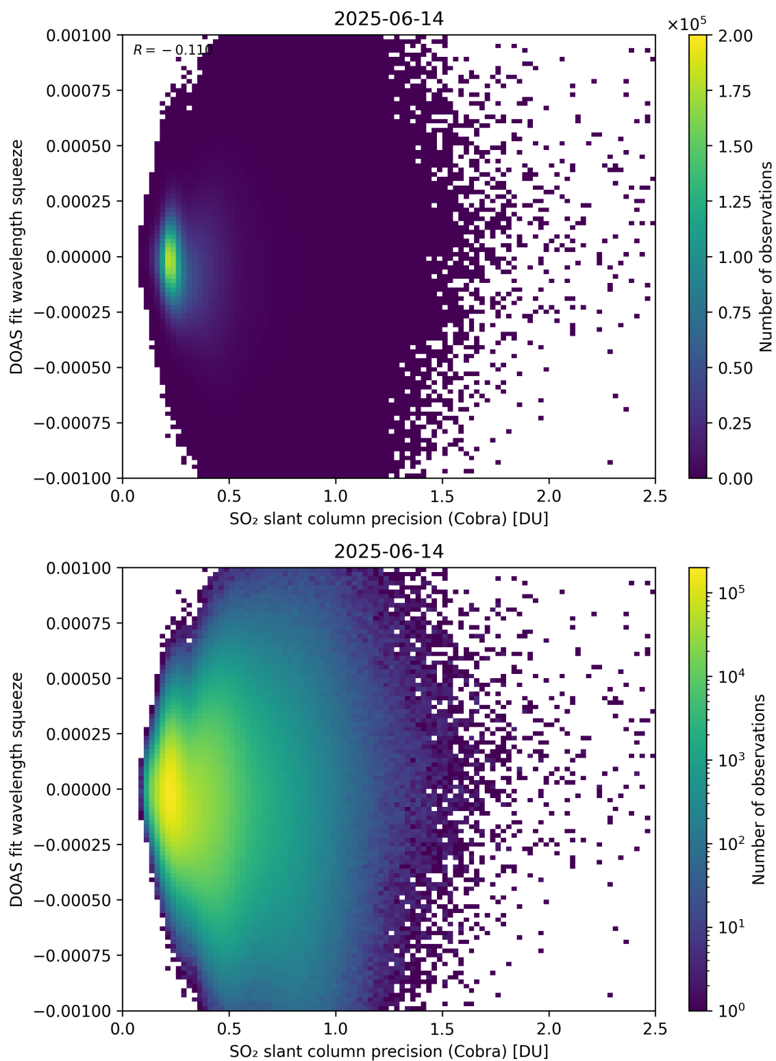
Figure 203: Scatter density plot of “SO 2 slant column precision (Cobra)” against “DOAS fit wavelength squeeze” for 2025-06-13 to 2025-06-15.
