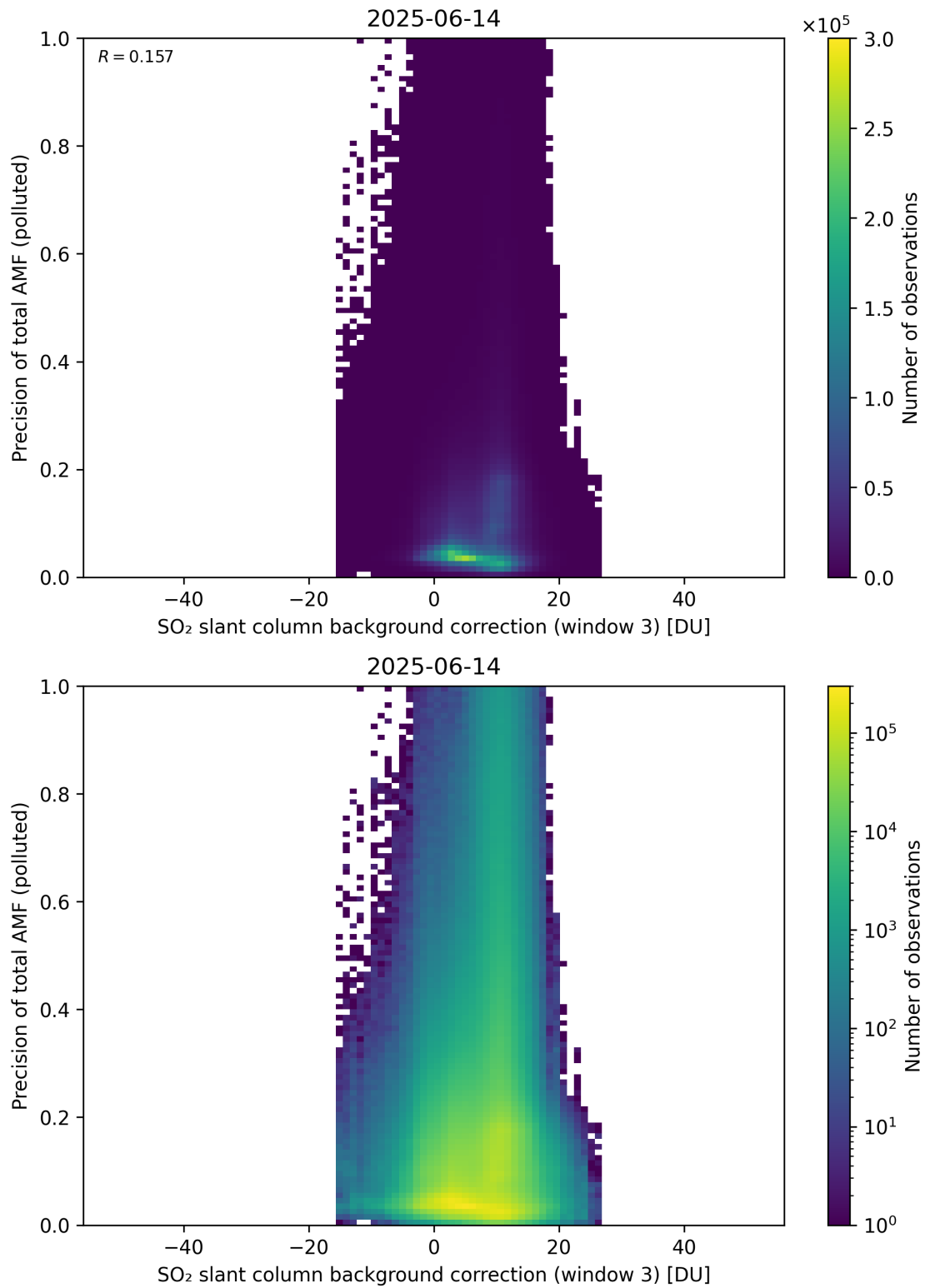
Figure 137: Scatter density plot of “SO 2 slant column background correction (window 3)” against “Precision of total AMF (polluted)” for 2025-06-13 to 2025-06-15.
