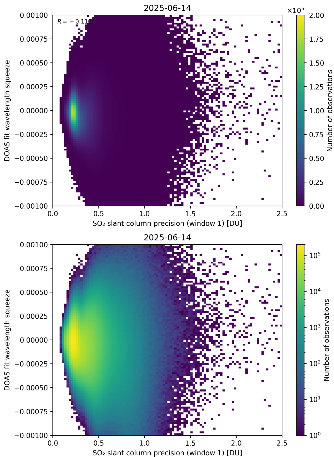
Figure 272: Scatter density plot of “SO 2 slant column precision (window 1)” against “DOAS fit wavelength squeeze” for 2025-06-13 to 2025-06-15.
