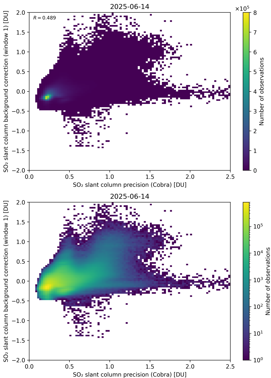
Figure 199: Scatter density plot of “SO 2 slant column precision (Cobra)” against “SO 2 slant column background correction (window 1)” for 2025-06-13 to 2025-06-15.
