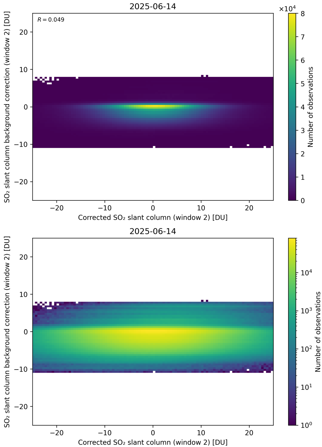
Figure 244: Scatter density plot of “Corrected SO 2 slant column (window 2)” against “SO 2 slant column background correction (window 2)” for 2025-06-13 to 2025-06-15.
