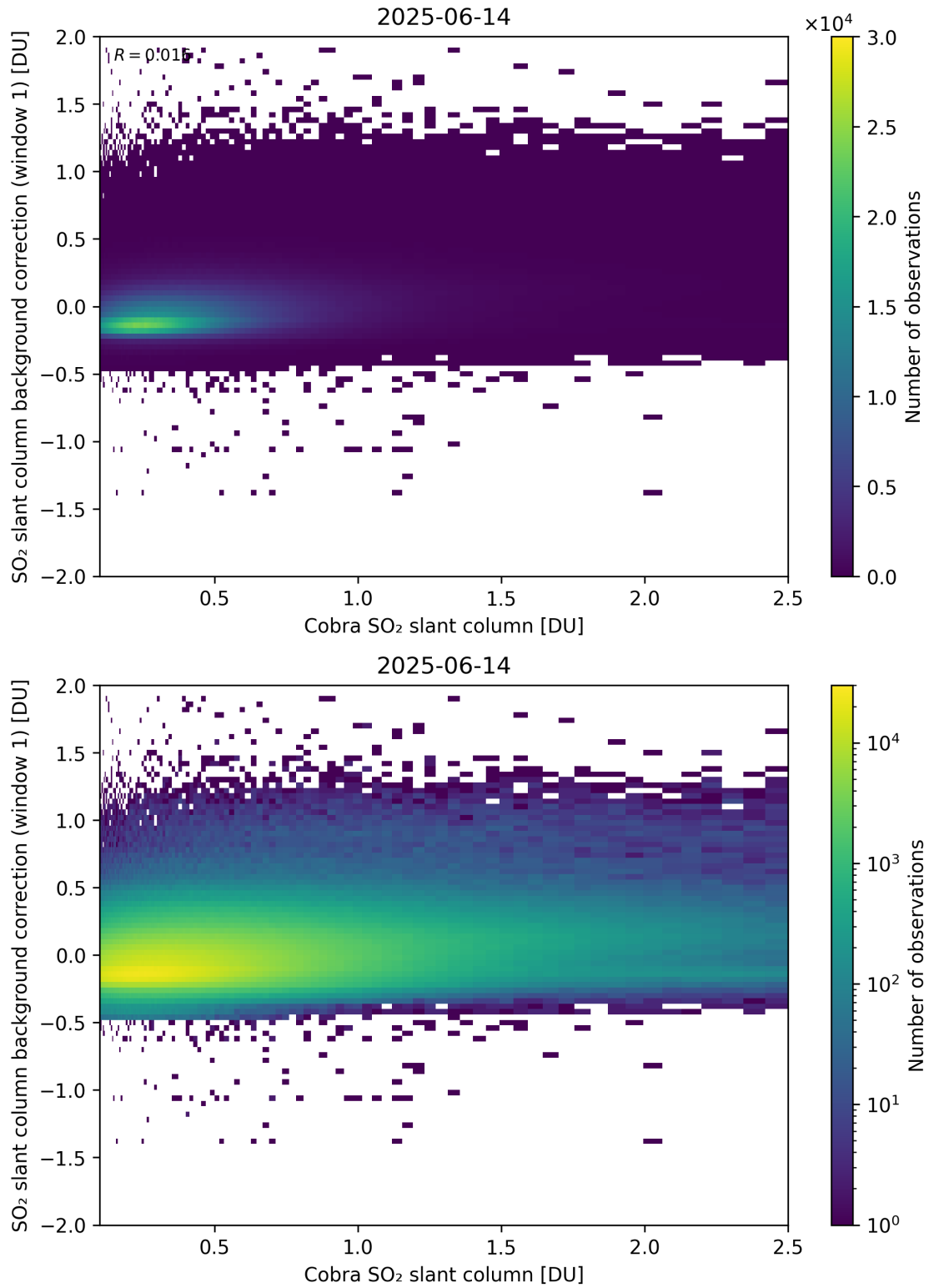
Figure 193: Scatter density plot of “Cobra SO 2 slant column” against “SO 2 slant column background correction (window 1)” for 2025-06-13 to 2025-06-15.
