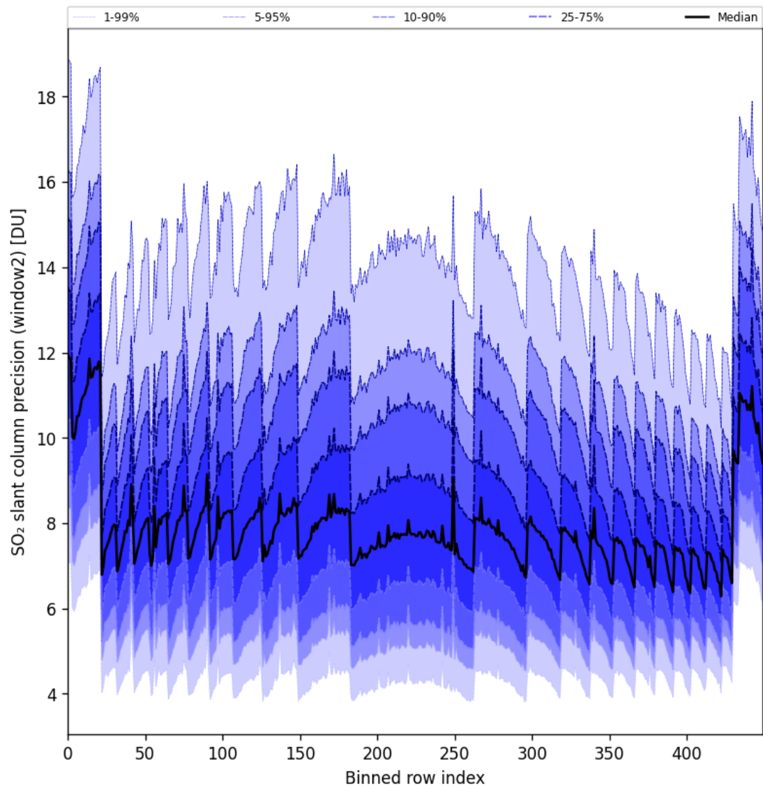
Figure 94: Along track statistics of “SO 2 slant column precision (window2)” for 2025-06-13 to 2025-06-15
