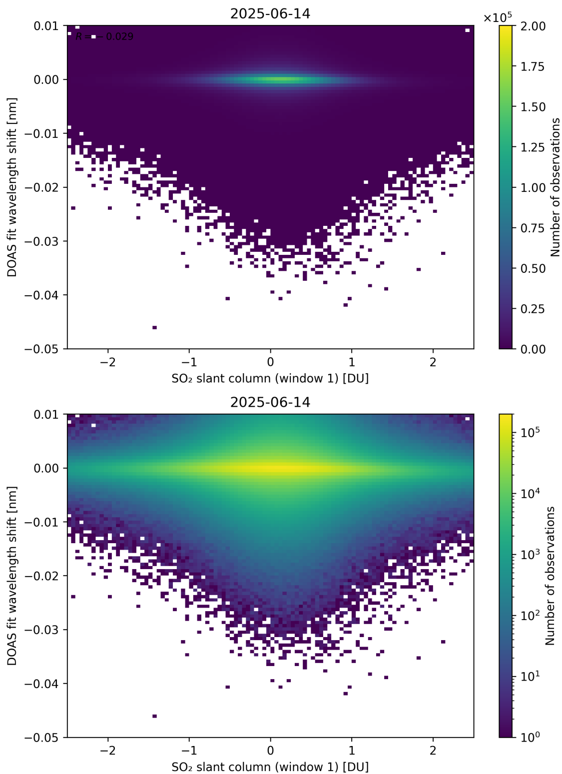
Figure 265: Scatter density plot of “SO 2 slant column (window 1)” against “DOAS fit wavelength shift” for 2025-06-13 to 2025-06-15.
