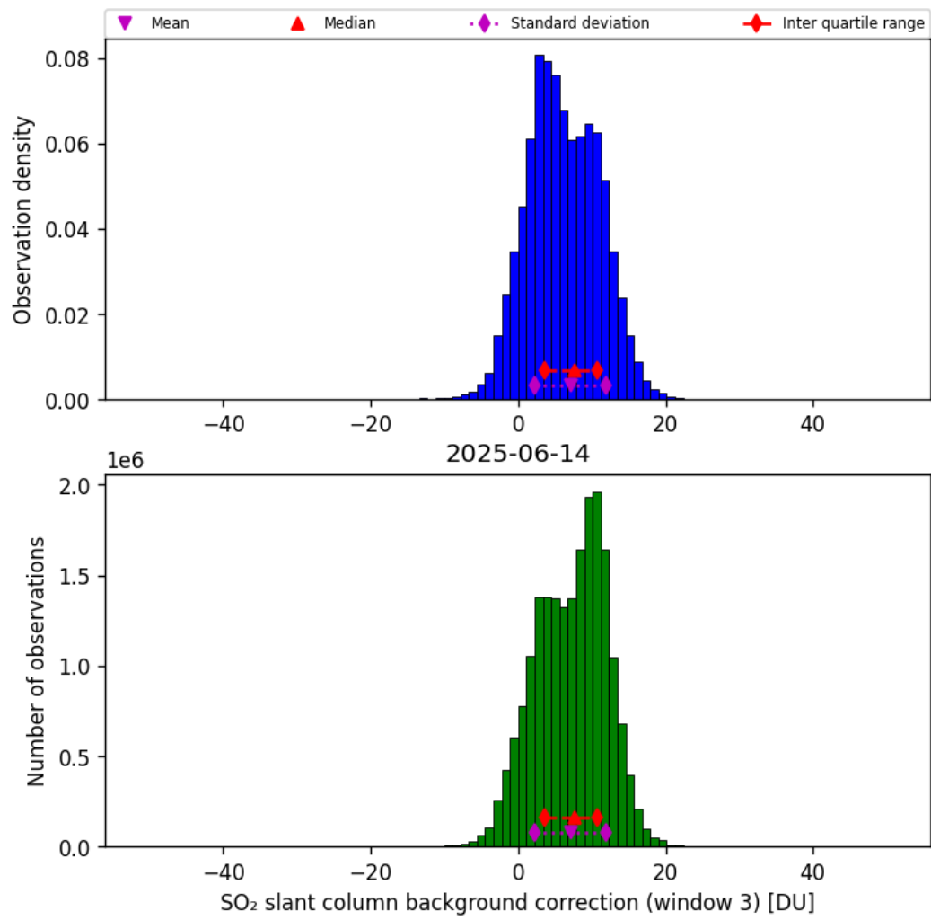
Figure 74: Histogram of “SO 2 slant column background correction (window 3)” for 2025-06-13 to 2025-06-15
