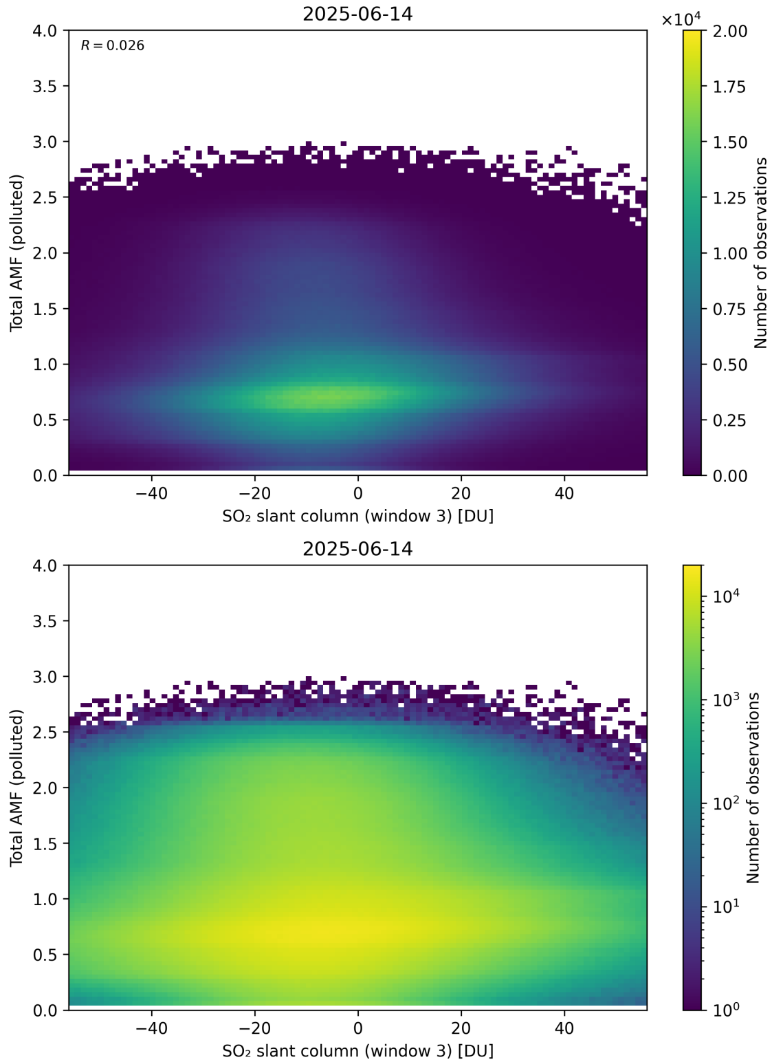
Figure 318: Scatter density plot of “SO 2 slant column (window 3)” against “Total AMF (polluted)” for 2025-06-13 to 2025-06-15.
