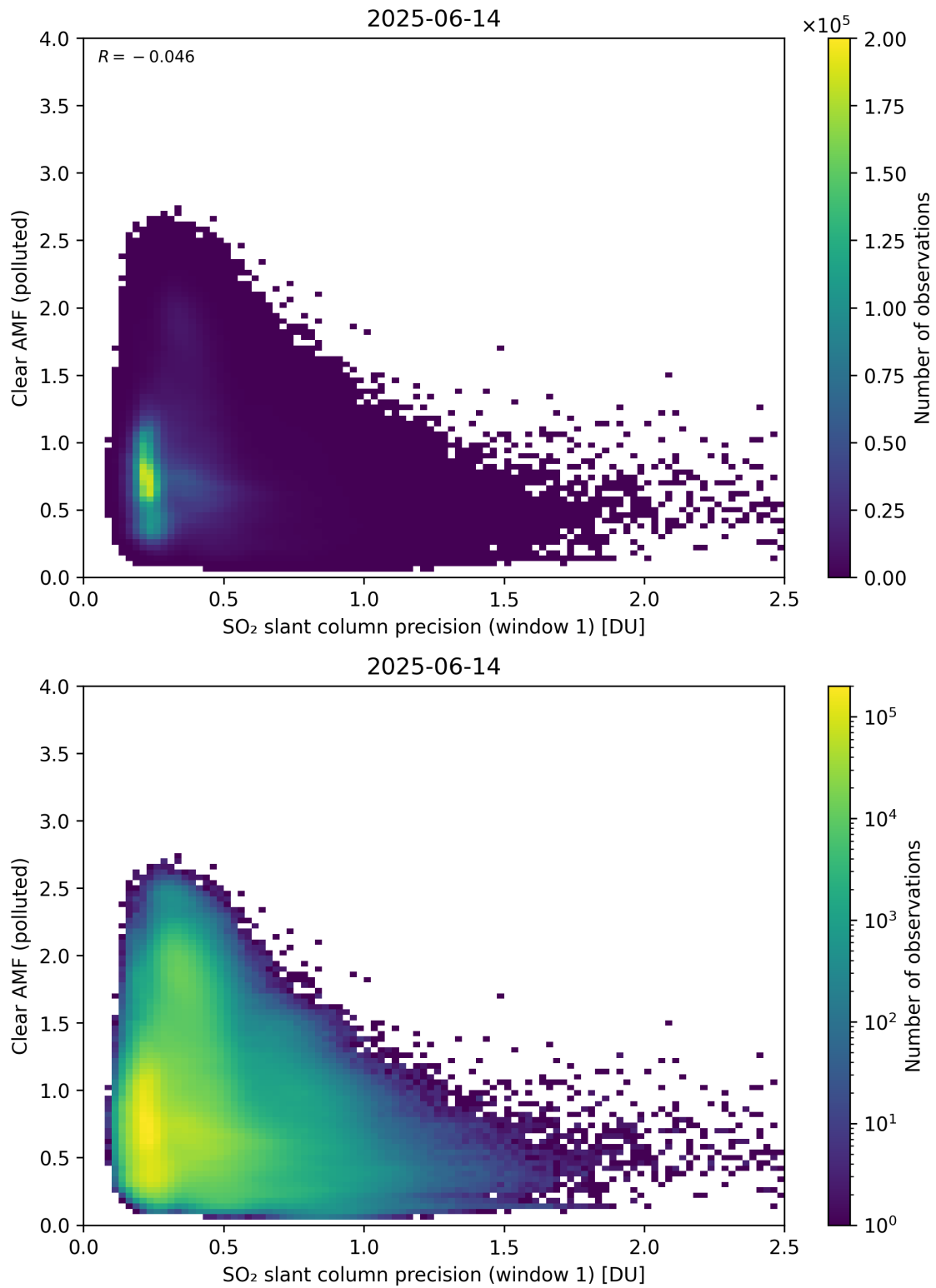
Figure 274: Scatter density plot of “SO 2 slant column precision (window 1)” against “Clear AMF (polluted)” for 2025-06-13 to 2025-06-15.
