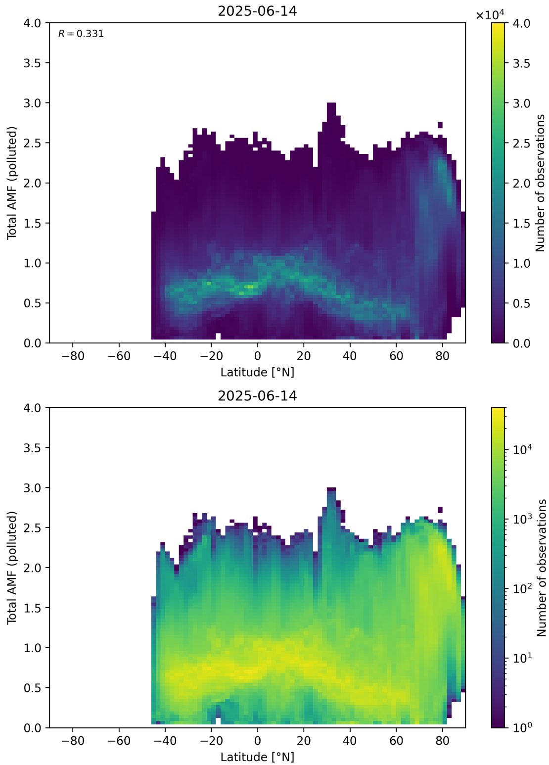
Figure 167: Scatter density plot of “Latitude” against “Total AMF (polluted)” for 2025-06-13 to 2025-06-15.
