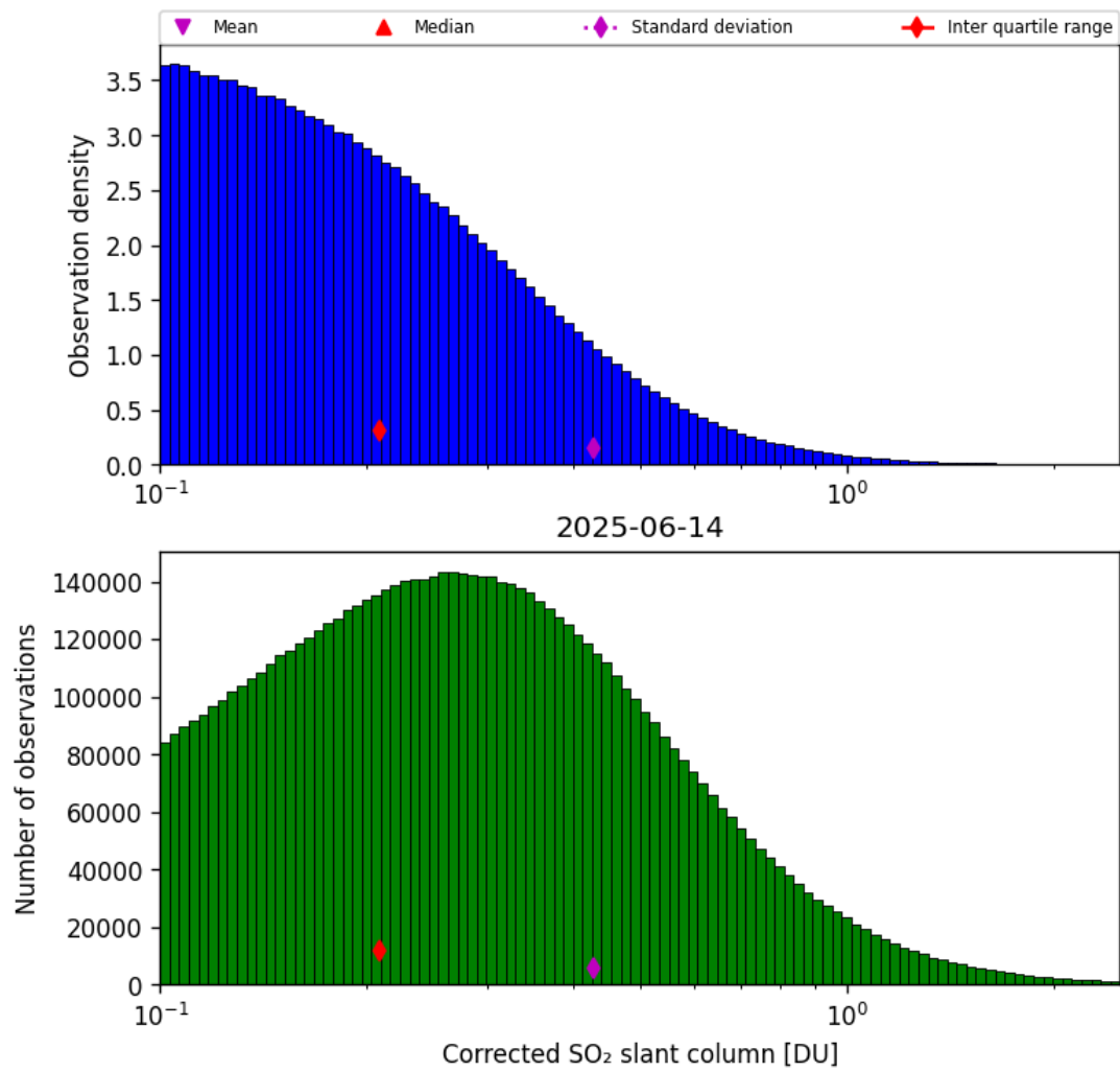
Figure 60: Histogram of “Corrected SO 2 slant column” for 2025-06-13 to 2025-06-15
