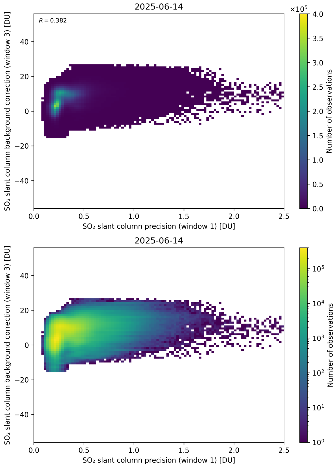
Figure 270: Scatter density plot of “SO 2 slant column precision (window 1)” against “SO 2 slant column background correction (window 3)” for 2025-06-13 to 2025-06-15.
