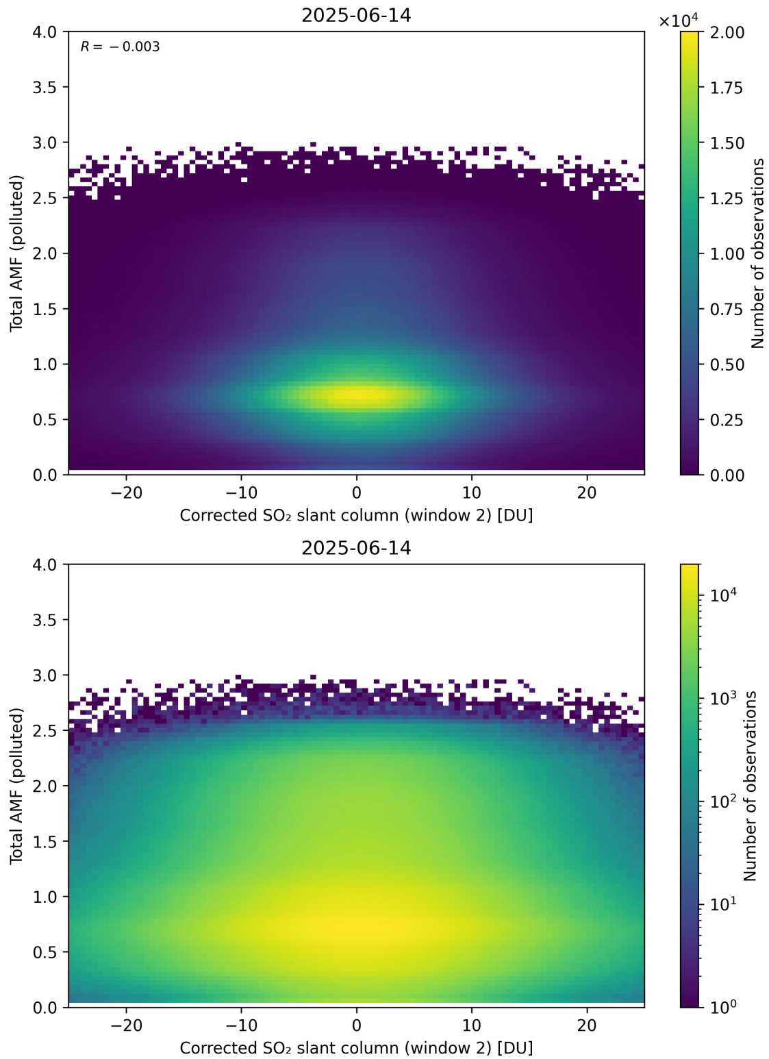
Figure 253: Scatter density plot of “Corrected SO 2 slant column (window 2)” against “Total AMF (polluted)” for 2025-06-13 to 2025-06-15.
