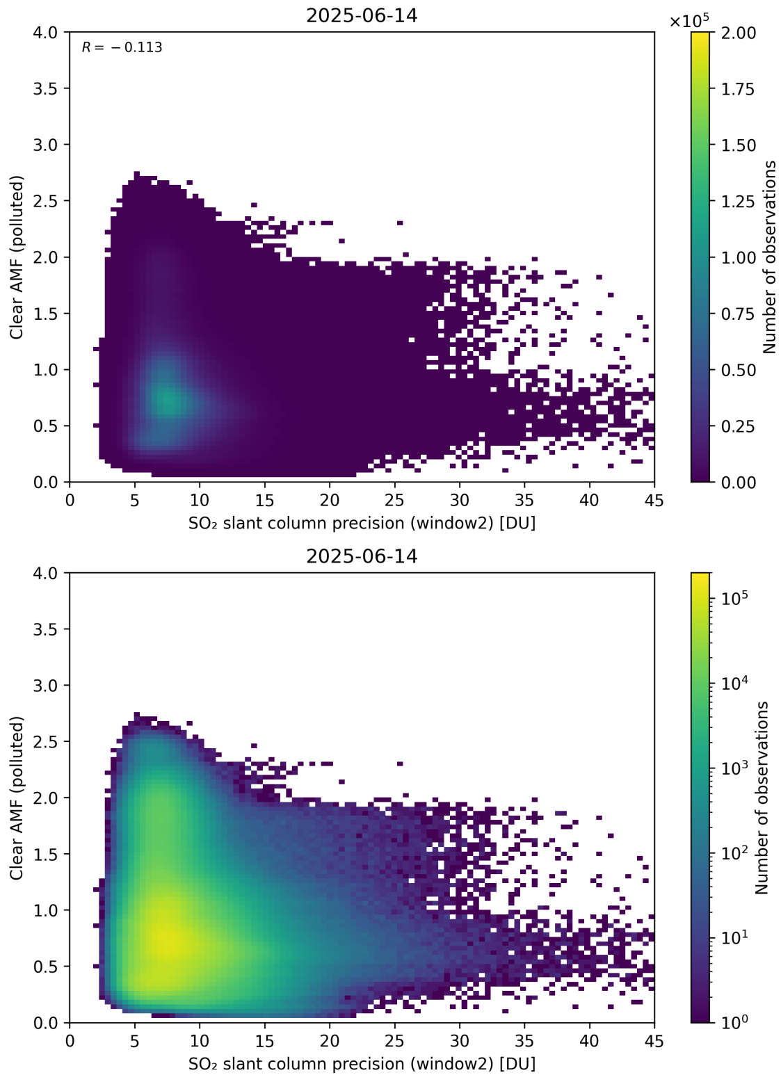
Figure 296: Scatter density plot of “SO 2 slant column precision (window2)” against “Clear AMF (polluted)” for 2025-06-13 to 2025-06-15.
