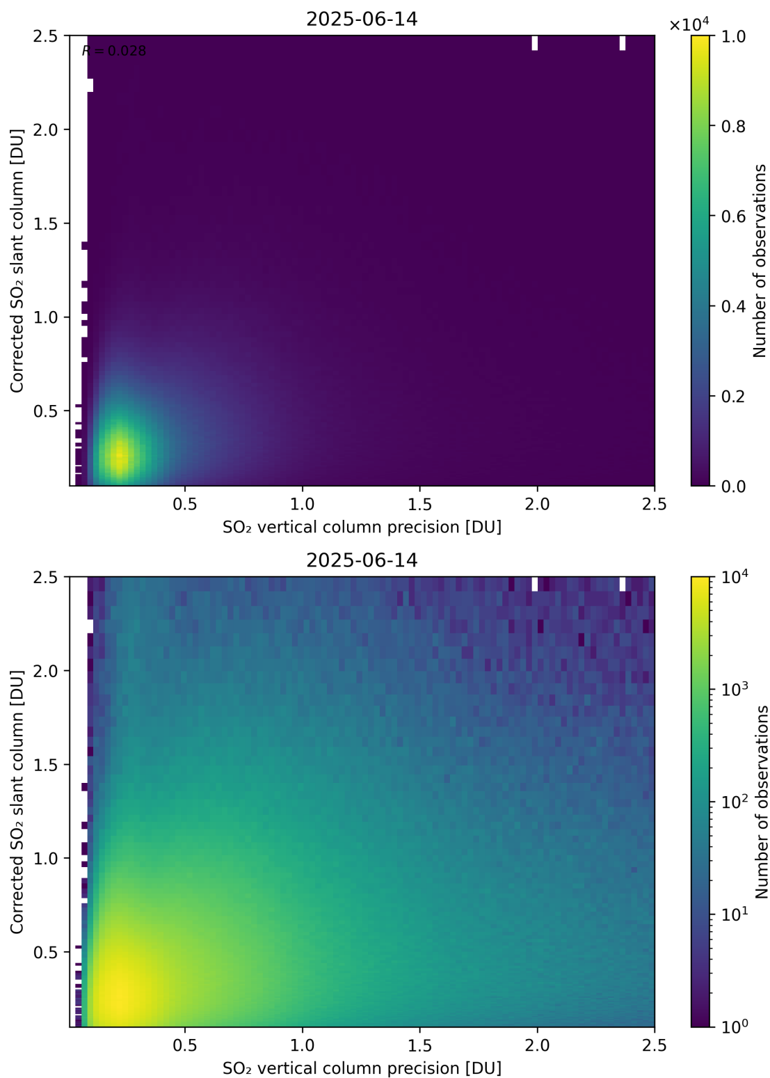
Figure 338: Scatter density plot of “SO 2 vertical column precision” against “Corrected SO 2 slant column” for 2025-06-13 to 2025-06-15.
