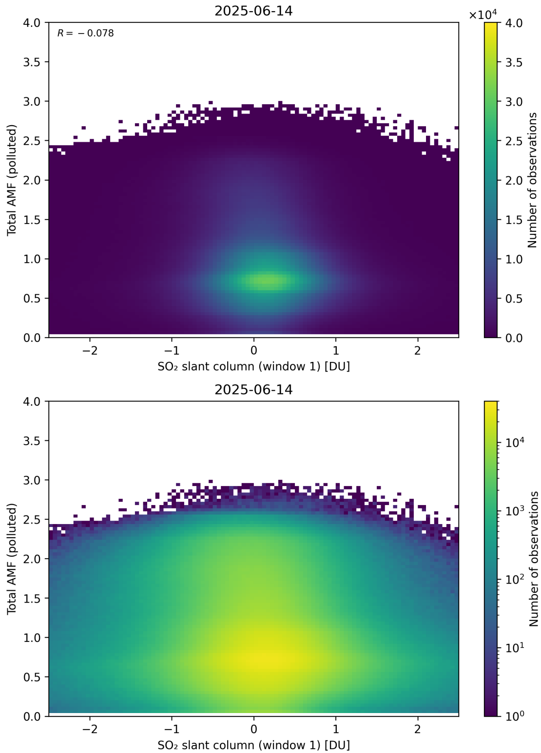
Figure 289: Scatter density plot of “SO 2 slant column (window 1)” against “Total AMF (polluted)” for 2025-06-13 to 2025-06-15.
