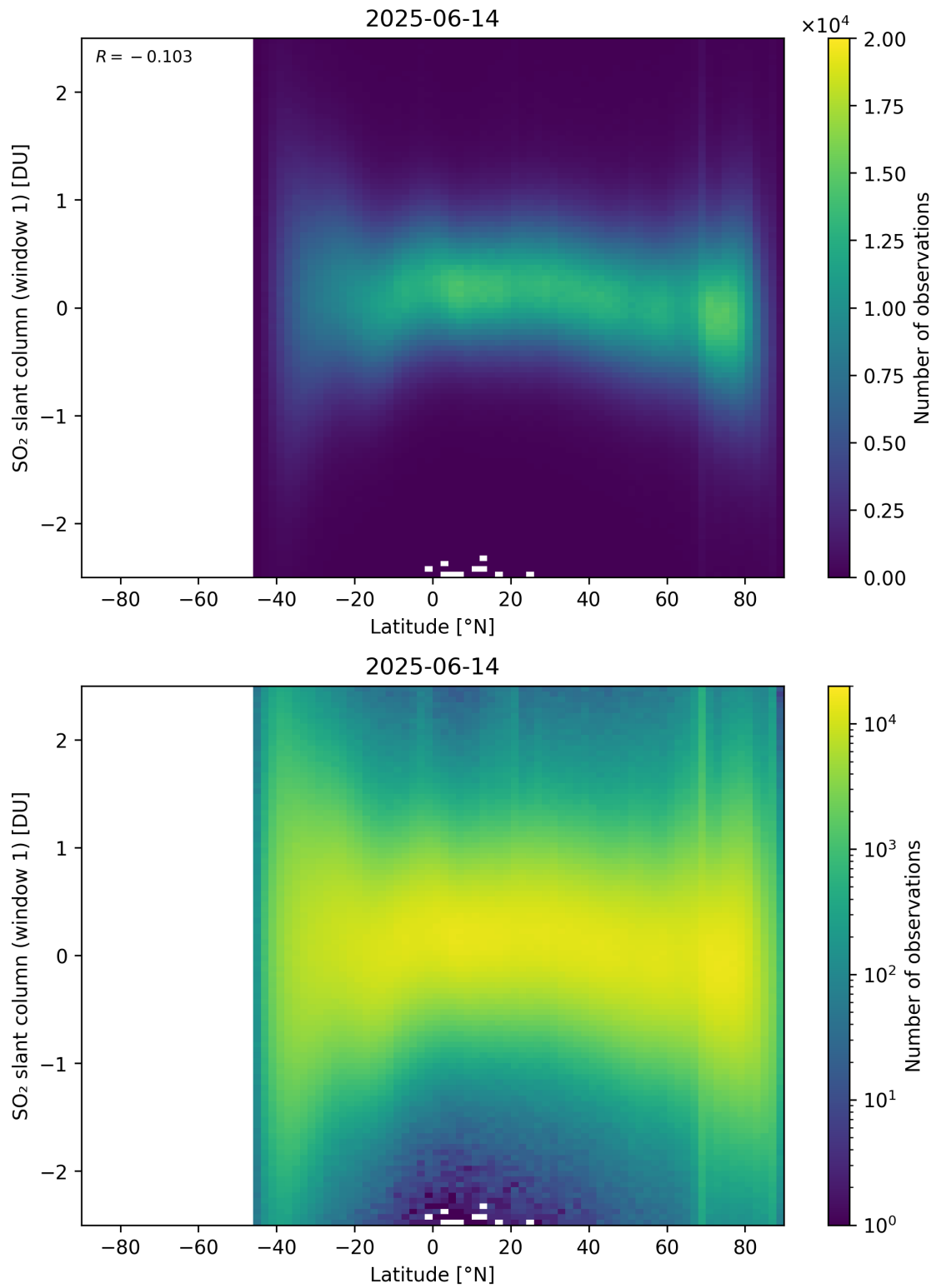
Figure 162: Scatter density plot of “Latitude” against “SO 2 slant column (window 1)” for 2025-06-13 to 2025-06-15.
