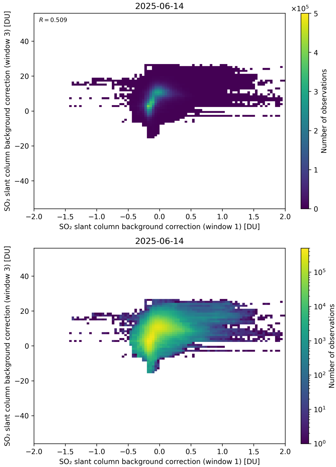
Figure 110: Scatter density plot of “SO 2 slant column background correction (window 1)” against “SO 2 slant column background correction (window 3)” for 2025-06-13 to 2025-06-15.
