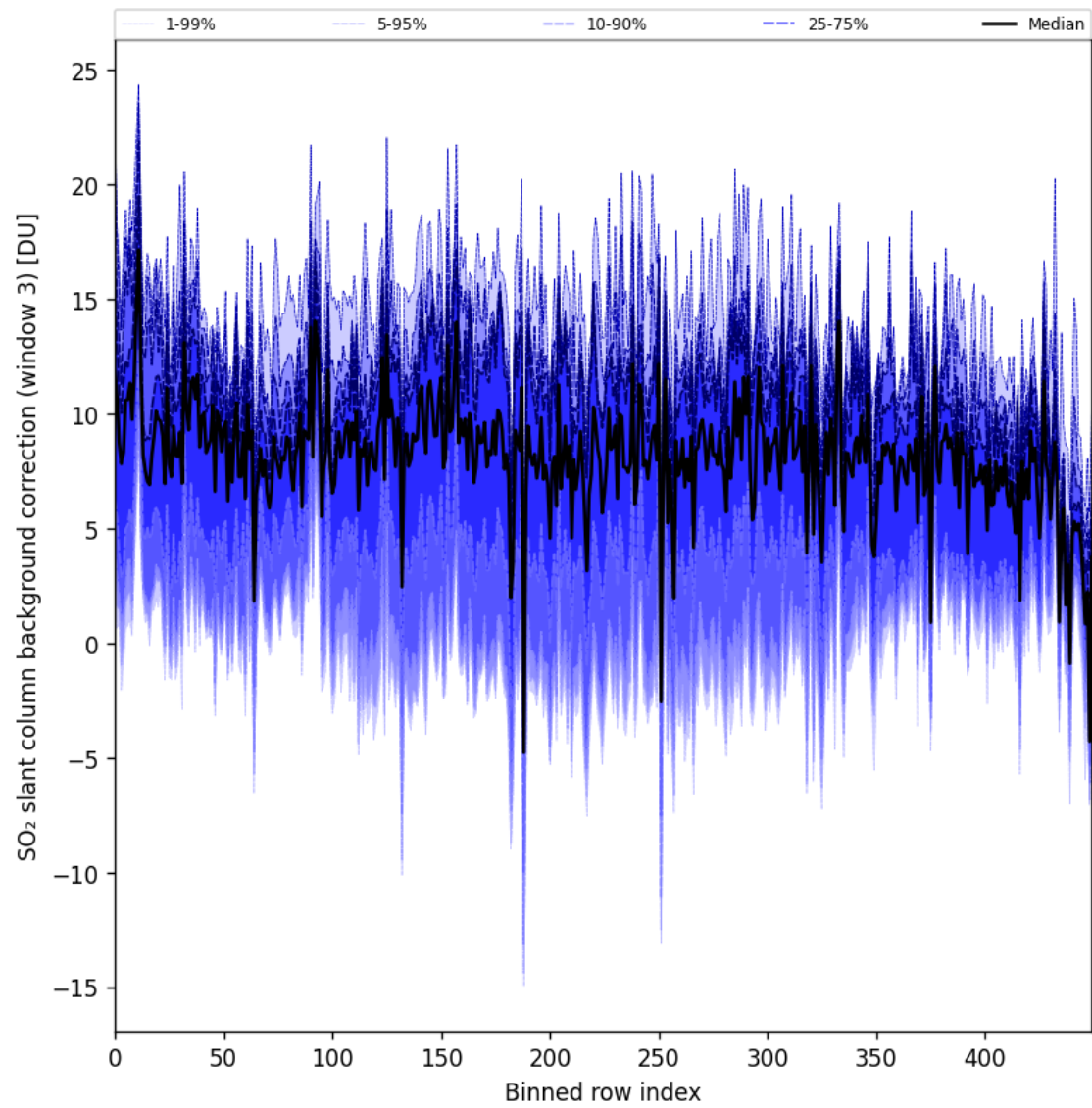
Figure 100: Along track statistics of “SO 2 slant column background correction (window 3)” for 2025-06-13 to 2025-06-15
