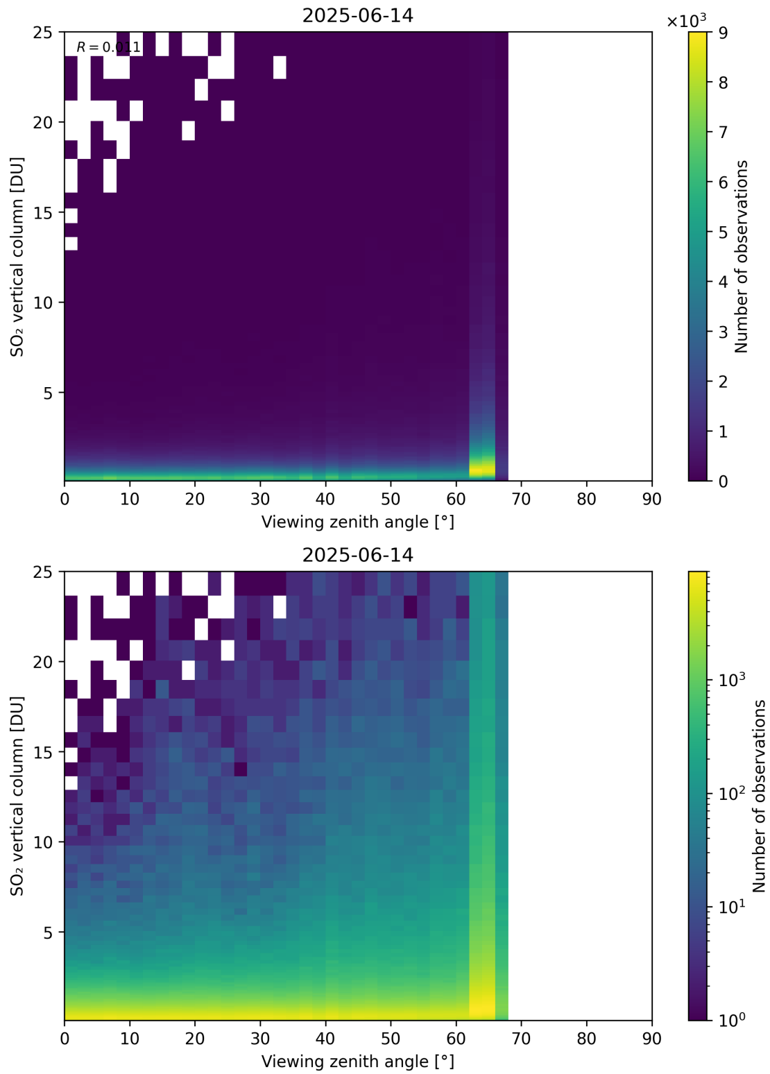
Figure 383: Scatter density plot of “Viewing zenith angle” against “SO 2 vertical column” for 2025-06-13 to 2025-06-15.
