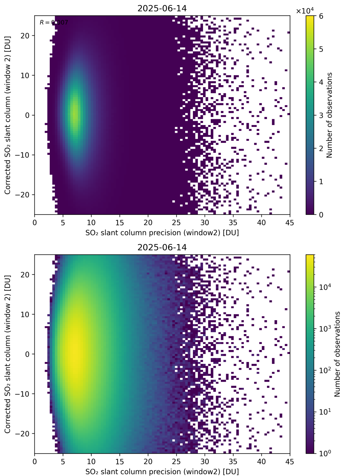
Figure 297: Scatter density plot of “SO 2 slant column precision (window2)” against “Corrected SO 2 slant column (window 2)” for 2025-06-13 to 2025-06-15.
