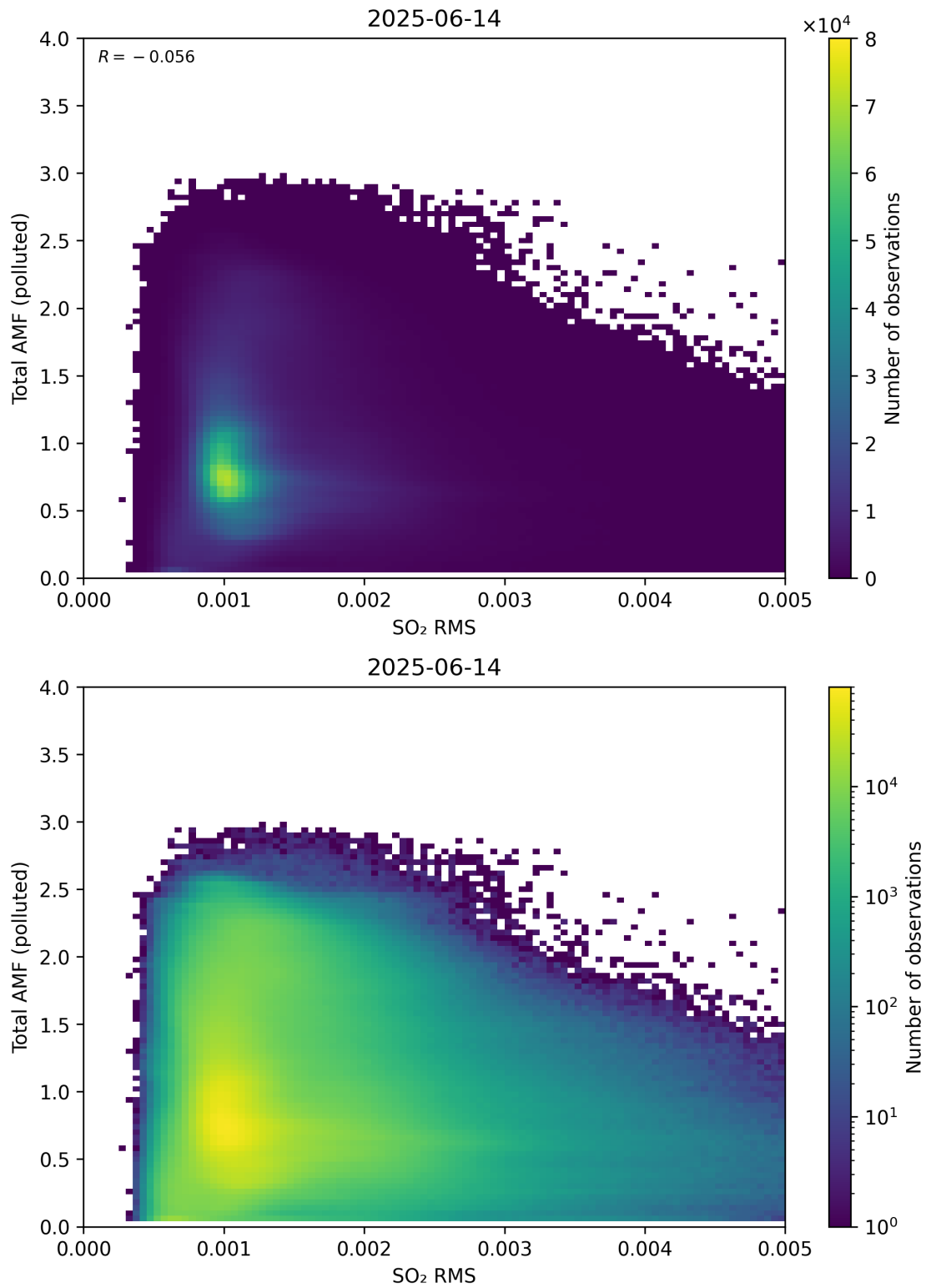
Figure 148: Scatter density plot of “SO 2 RMS” against “Total AMF (polluted)” for 2025-06-13 to 2025-06-15.
