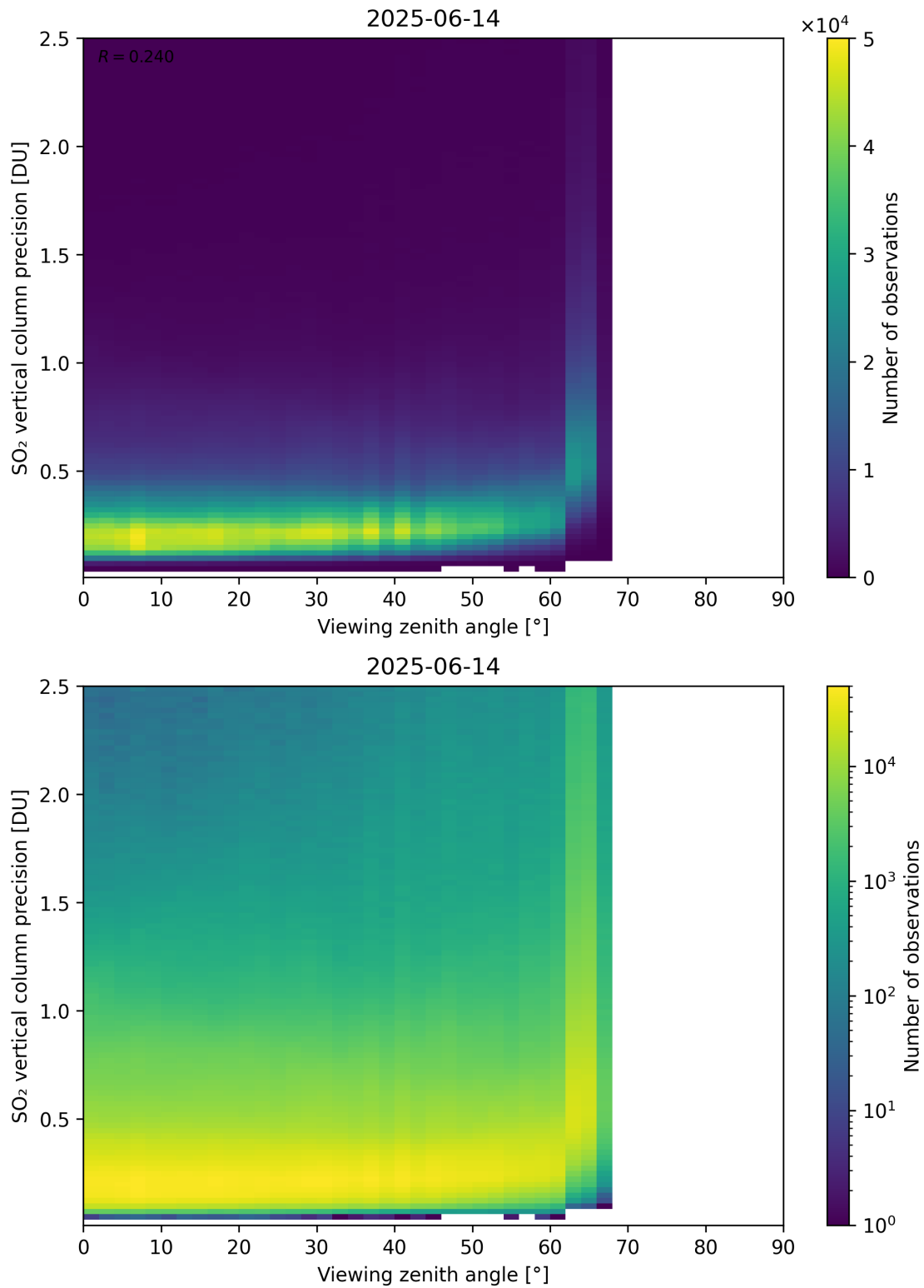
Figure 384: Scatter density plot of “Viewing zenith angle” against “SO 2 vertical column precision” for 2025-06-13 to 2025-06-15.
