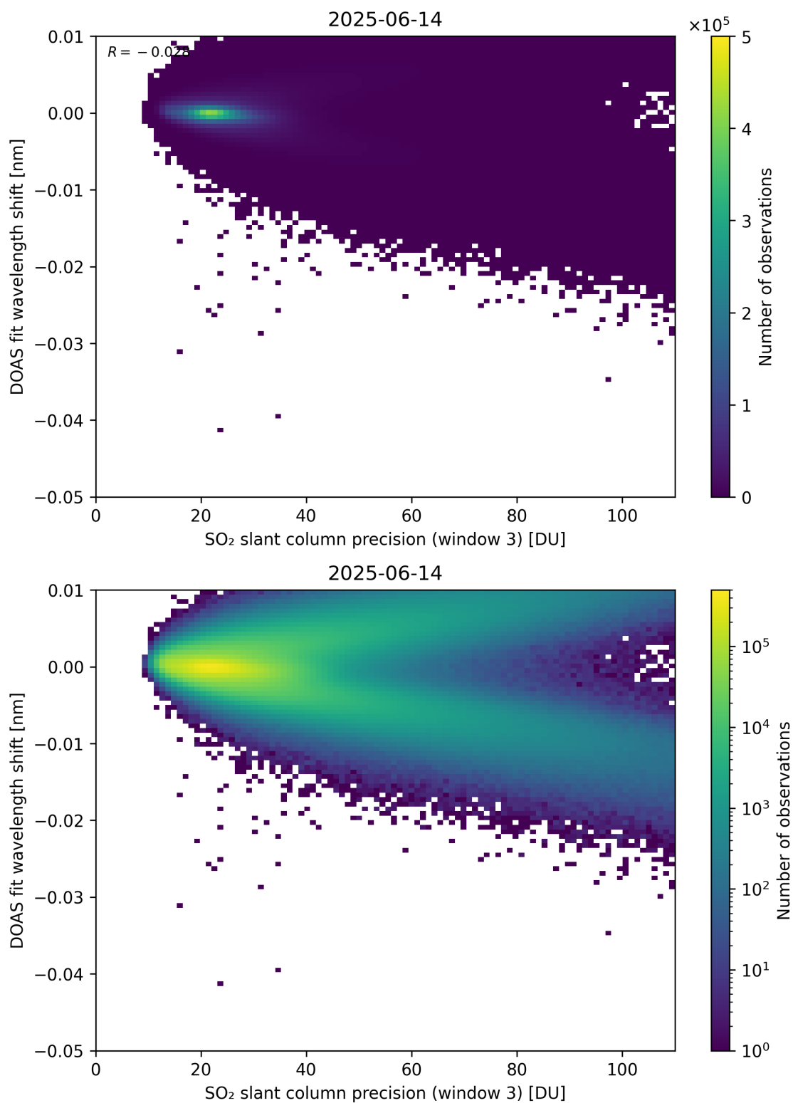
Figure 308: Scatter density plot of “SO 2 slant column precision (window 3)” against “DOAS fit wavelength shift” for 2025-06-13 to 2025-06-15.
