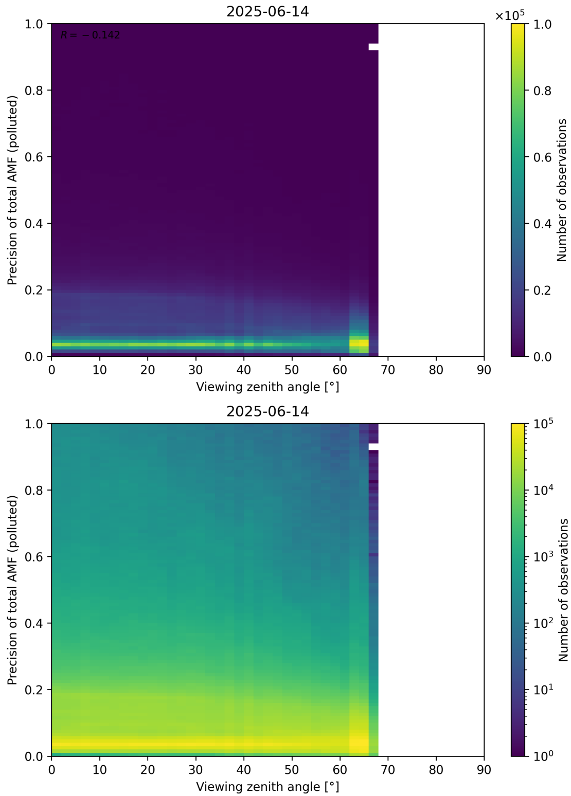
Figure 382: Scatter density plot of “Viewing zenith angle” against “Precision of total AMF (polluted)” for 2025-06-13 to 2025-06-15.
