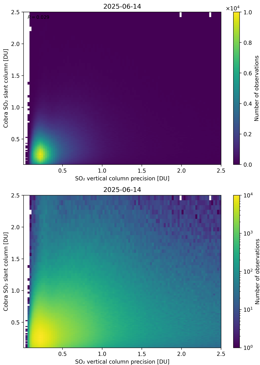
Figure 336: Scatter density plot of “SO 2 vertical column precision” against “Cobra SO 2 slant column” for 2025-06-13 to 2025-06-15.
