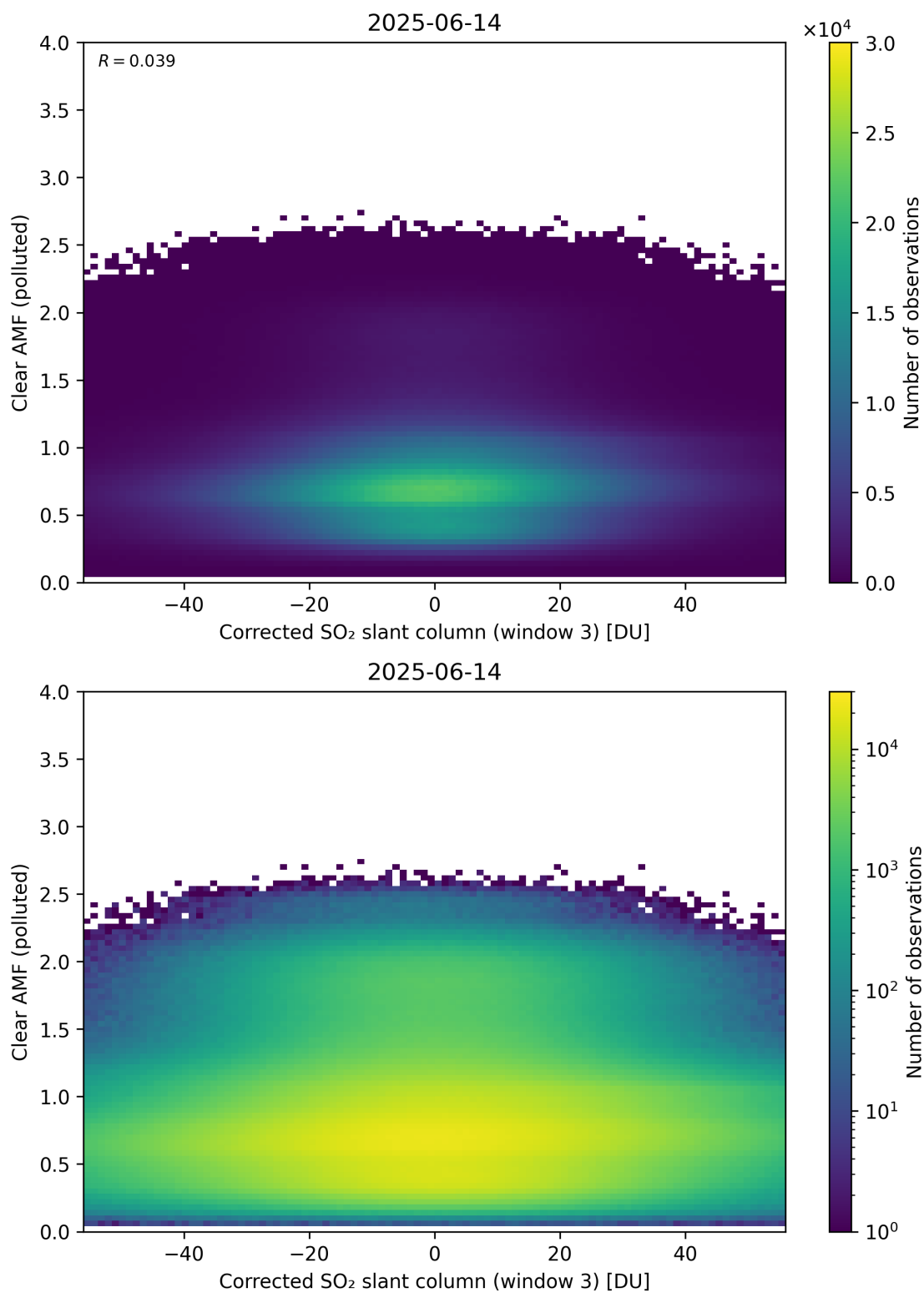
Figure 259: Scatter density plot of “Corrected SO 2 slant column (window 3)” against “Clear AMF (polluted)” for 2025-06-13 to 2025-06-15.
