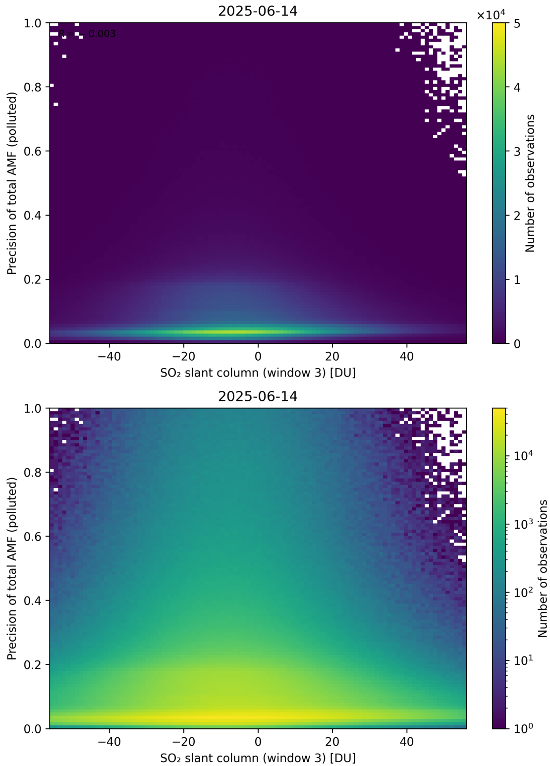
Figure 319: Scatter density plot of “SO 2 slant column (window 3)” against “Precision of total AMF (polluted)” for 2025-06-13 to 2025-06-15.
