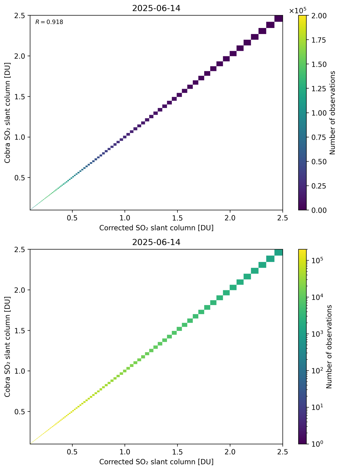
Figure 233: Scatter density plot of “Corrected SO 2 slant column” against “Cobra SO 2 slant column” for 2025-06-13 to 2025-06-15.
