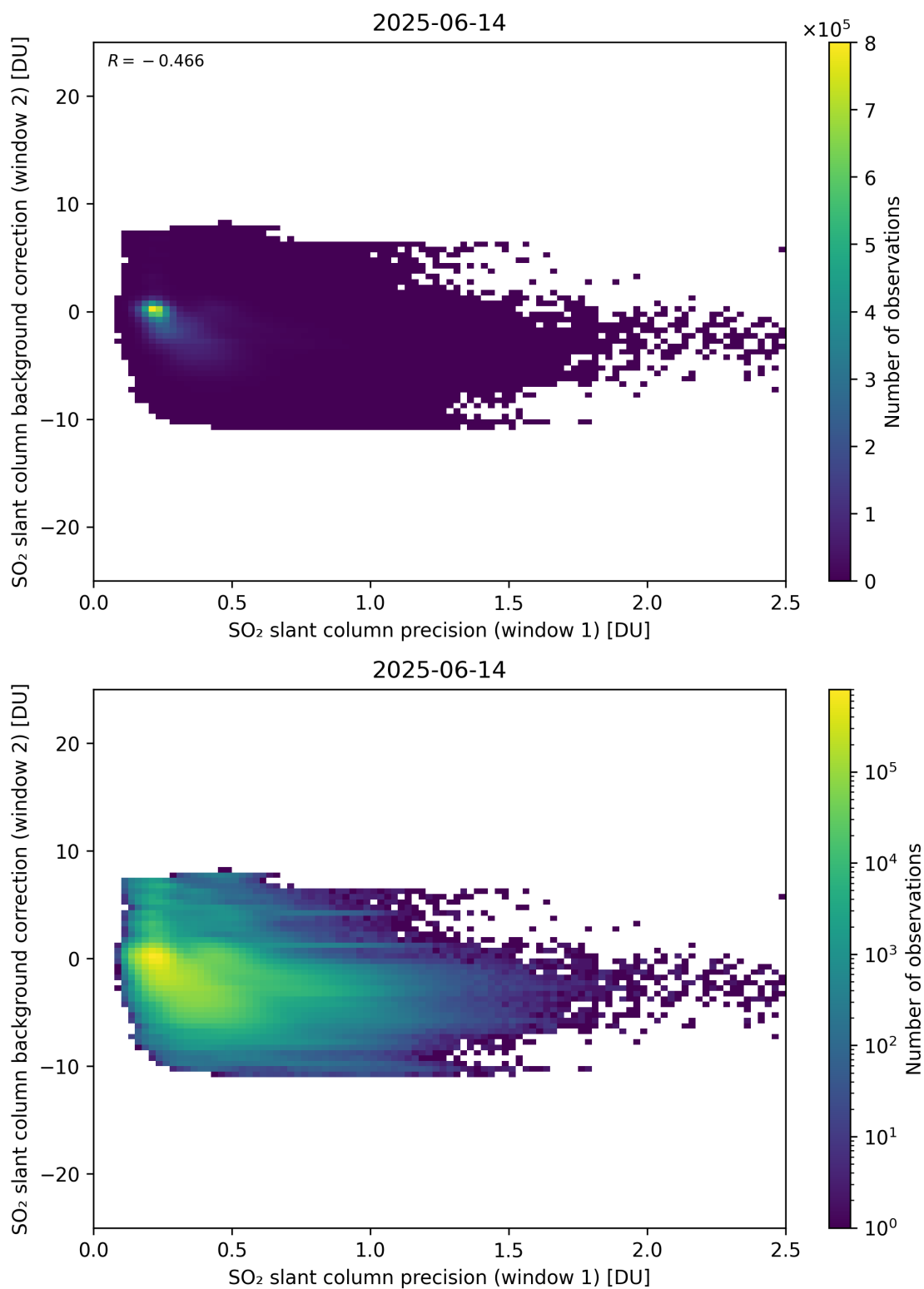
Figure 269: Scatter density plot of “SO 2 slant column precision (window 1)” against “SO 2 slant column background correction (window 2)” for 2025-06-13 to 2025-06-15.
