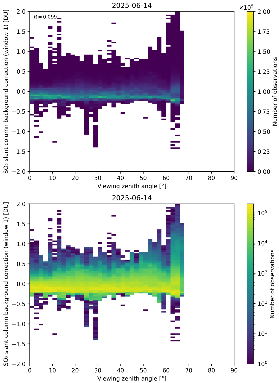
Figure 362: Scatter density plot of “Viewing zenith angle” against “SO 2 slant column background correction (window 1)” for 2025-06-13 to 2025-06-15.
