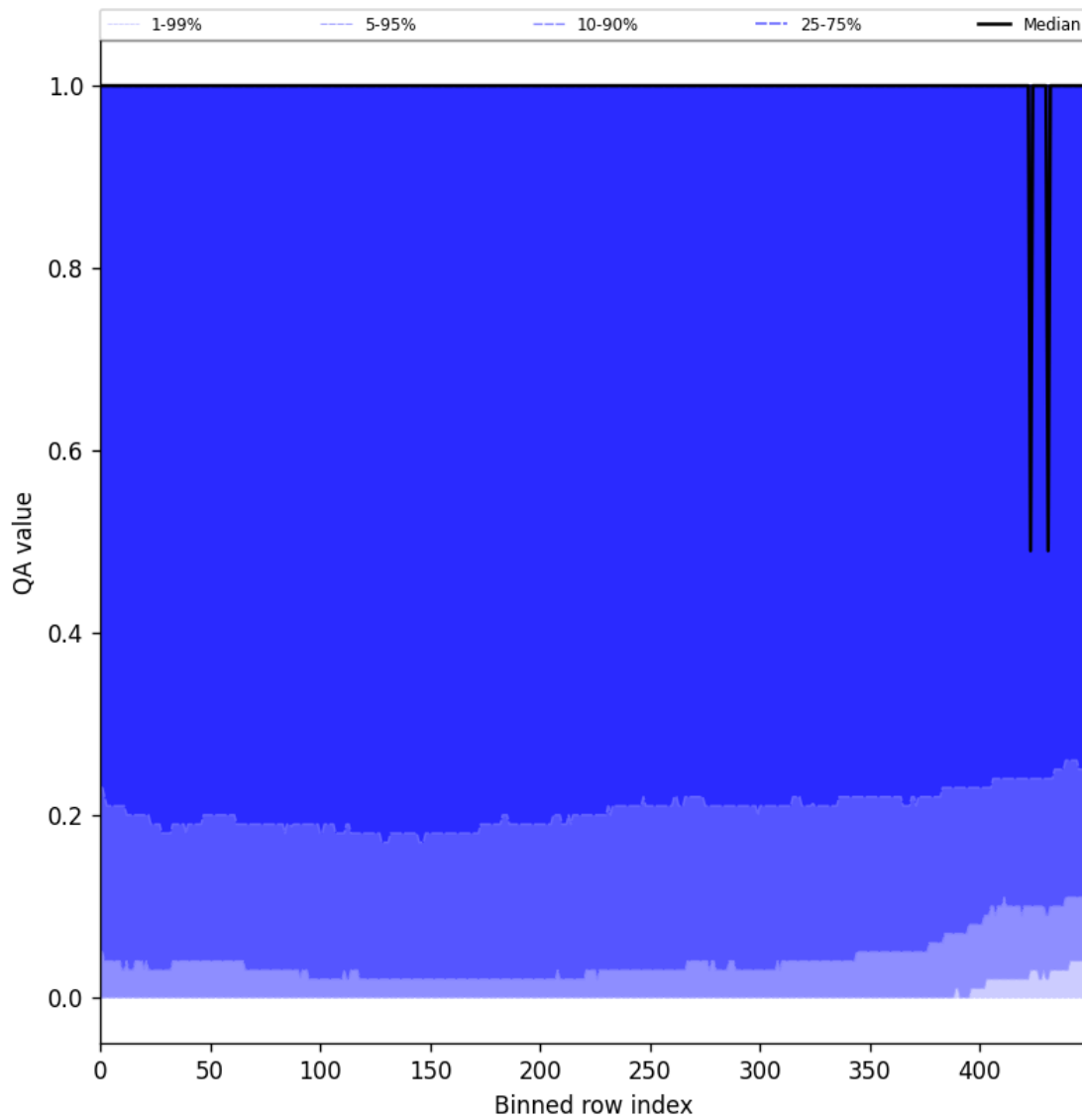
Figure 83: Along track statistics of “QA value” for 2025-06-13 to 2025-06-15
