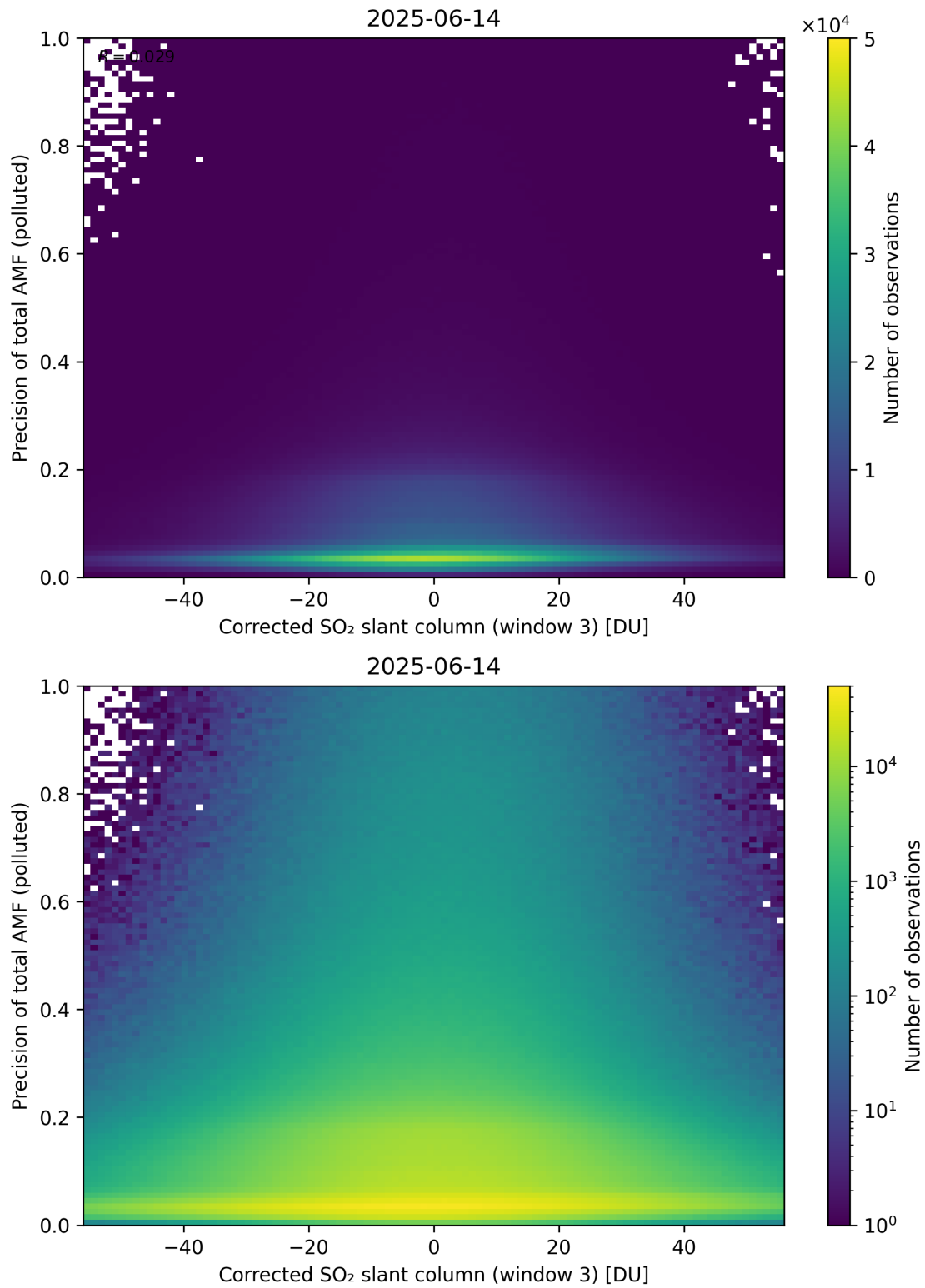
Figure 261: Scatter density plot of “Corrected SO 2 slant column (window 3)” against “Precision of total AMF (polluted)” for 2025-06-13 to 2025-06-15.
