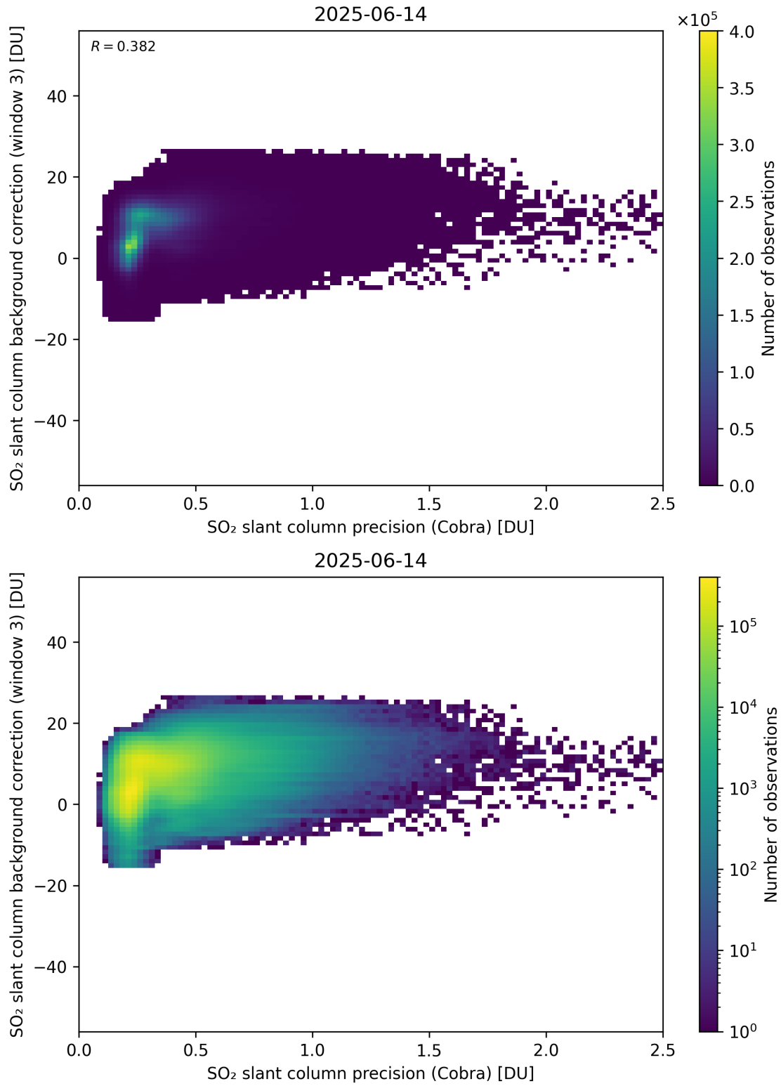
Figure 201: Scatter density plot of “SO 2 slant column precision (Cobra)” against “SO 2 slant column background correction (window 3)” for 2025-06-13 to 2025-06-15.
