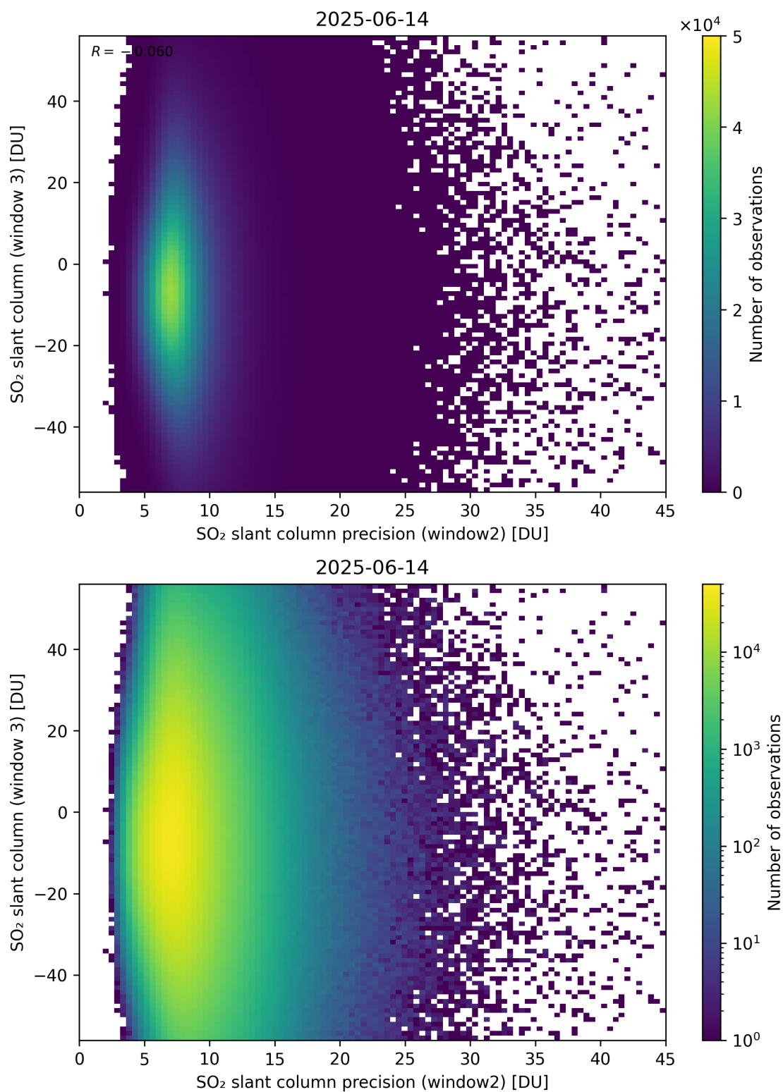
Figure 299: Scatter density plot of “SO 2 slant column precision (window2)” against “SO 2 slant column (window 3)” for 2025-06-13 to 2025-06-15.
