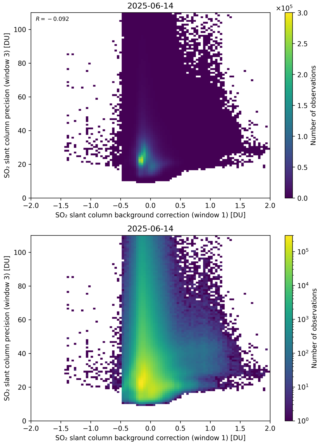
Figure 119: Scatter density plot of “SO 2 slant column background correction (window 1)” against “SO 2 slant column precision (window 3)” for 2025-06-13 to 2025-06-15.
