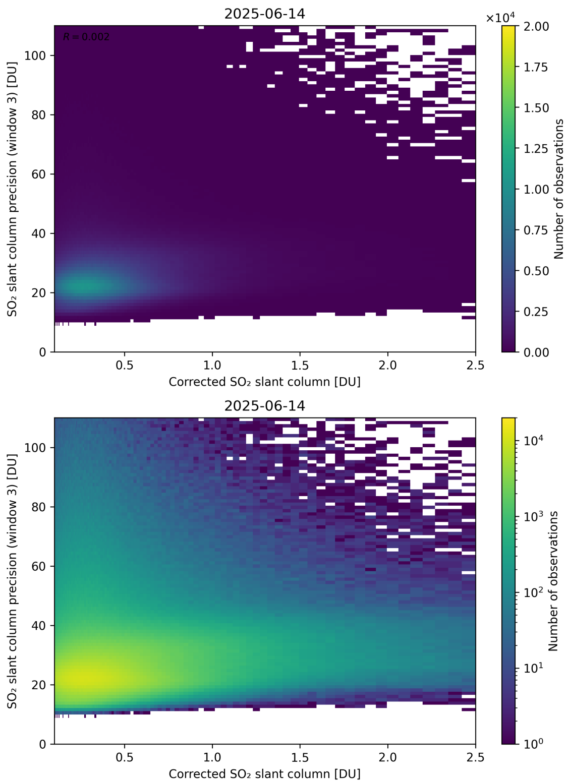
Figure 241: Scatter density plot of “Corrected SO 2 slant column” against “SO 2 slant column precision (window 3)” for 2025-06-13 to 2025-06-15.
