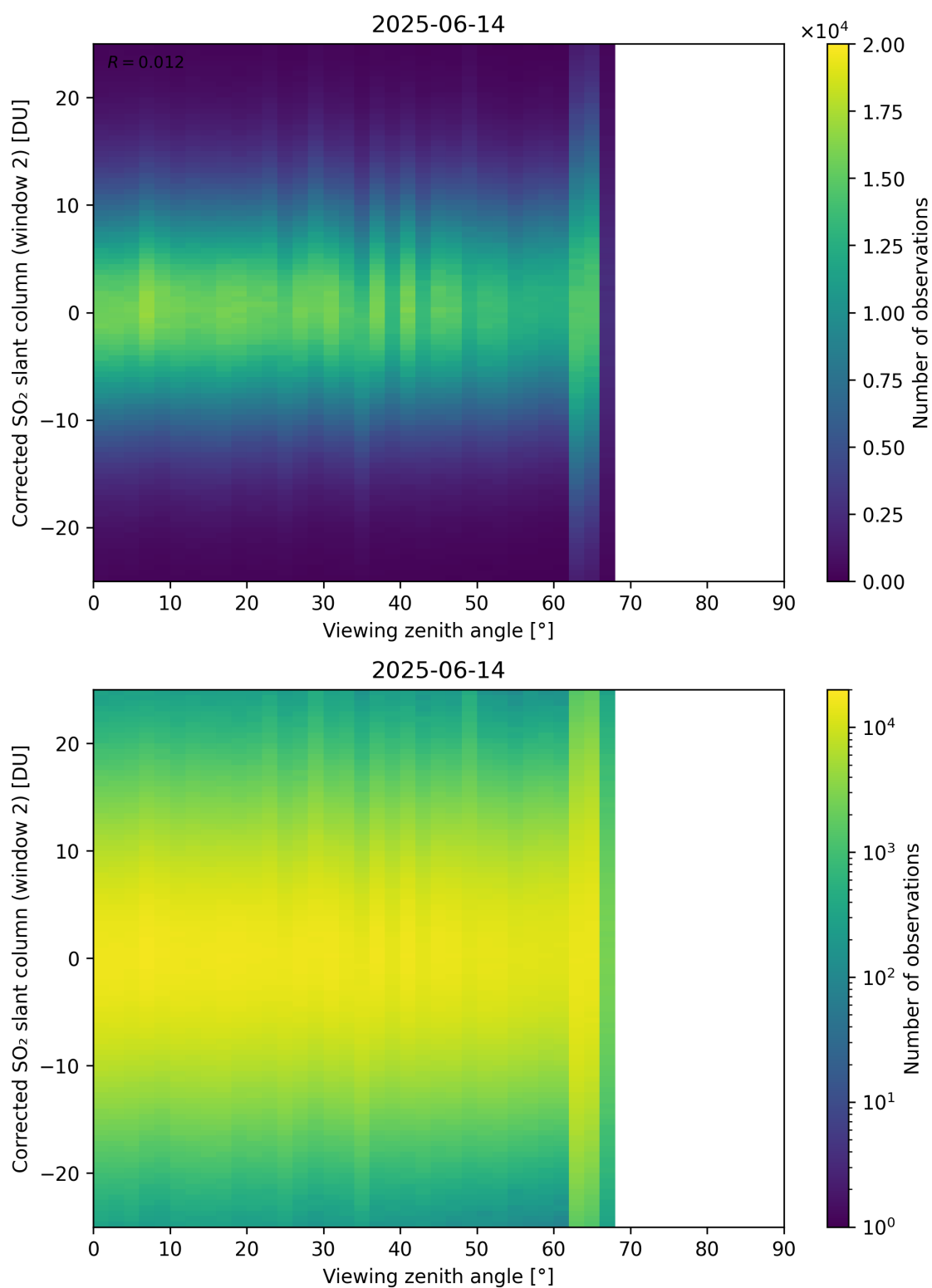
Figure 374: Scatter density plot of “Viewing zenith angle” against “Corrected SO 2 slant column (window 2)” for 2025-06-13 to 2025-06-15.
