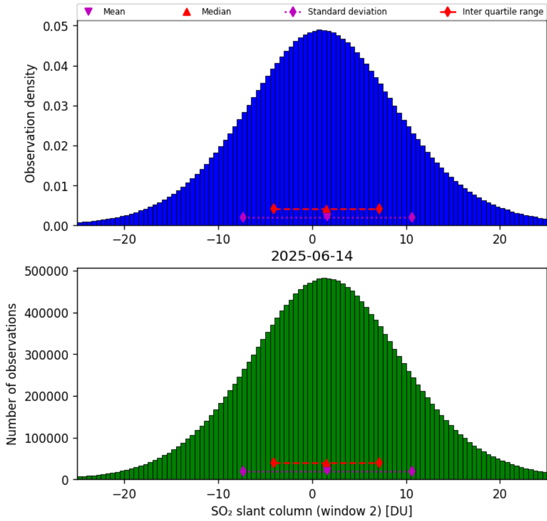
Figure 67: Histogram of “SO 2 slant column (window 2)” for 2025-06-13 to 2025-06-15
