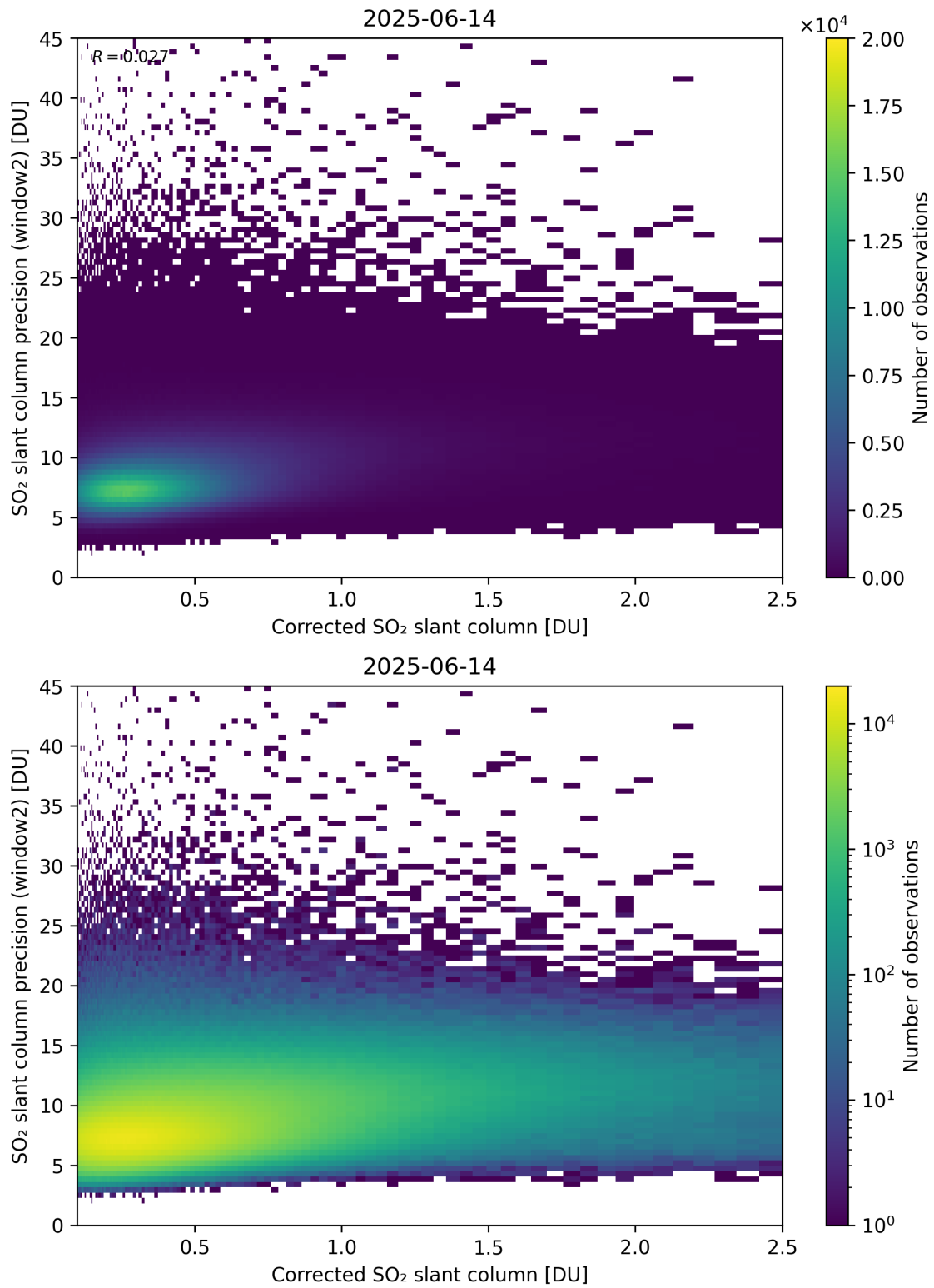
Figure 239: Scatter density plot of “Corrected SO 2 slant column” against “SO 2 slant column precision (window2)” for 2025-06-13 to 2025-06-15.
