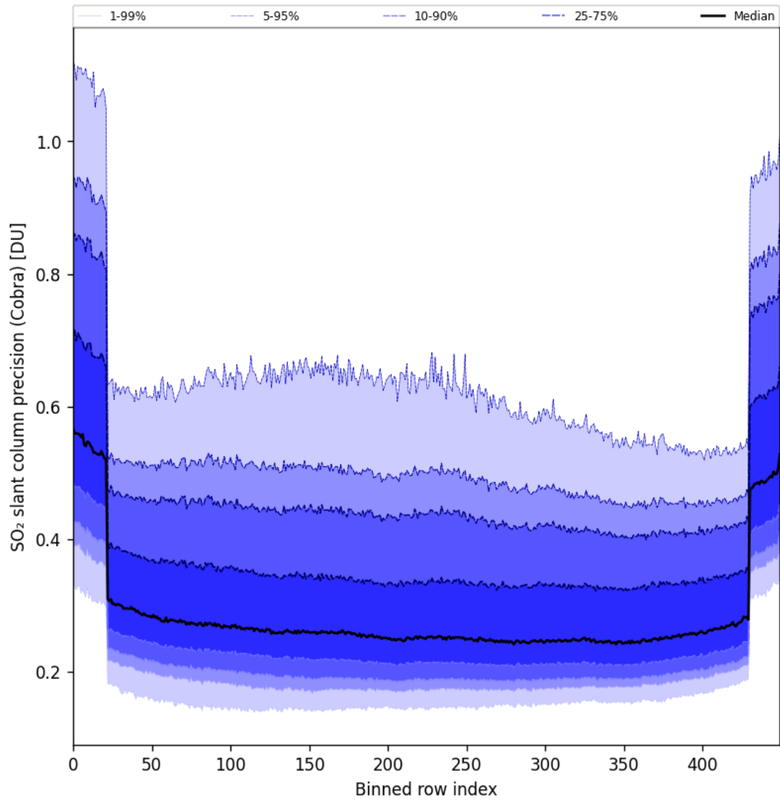
Figure 88: Along track statistics of “SO 2 slant column precision (Cobra)” for 2025-06-13 to 2025-06-15
