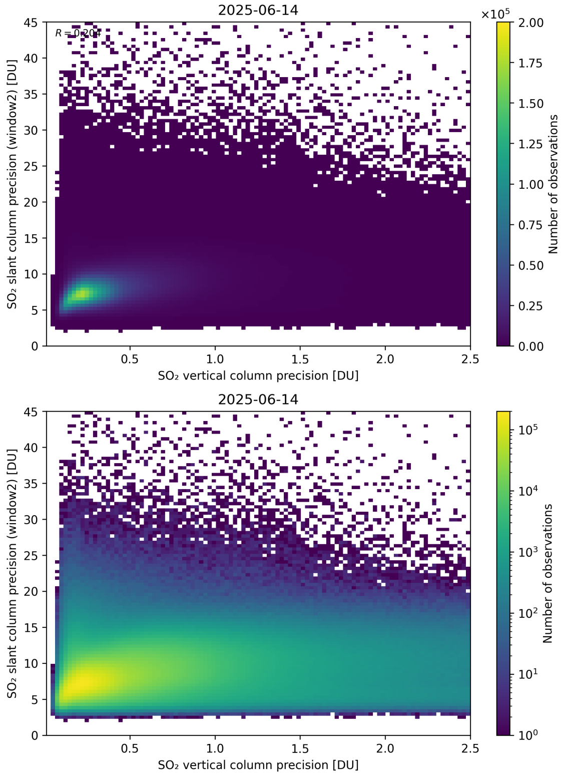
Figure 343: Scatter density plot of “SO 2 vertical column precision” against “SO 2 slant column precision (window2)” for 2025-06-13 to 2025-06-15.
