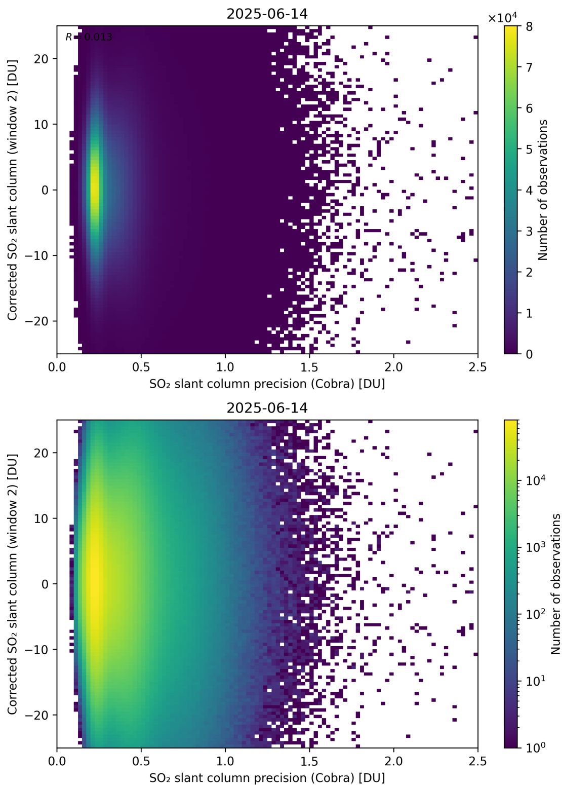
Figure 206: Scatter density plot of “SO 2 slant column precision (Cobra)” against “Corrected SO 2 slant column (window 2)” for 2025-06-13 to 2025-06-15.
