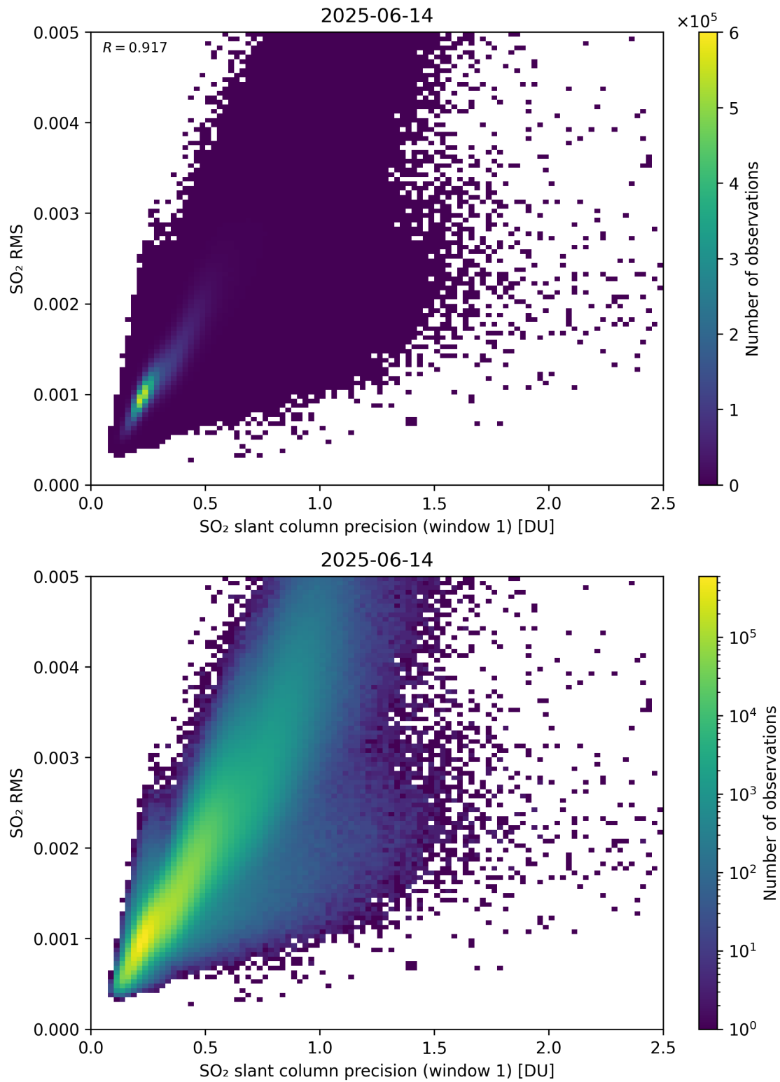
Figure 273: Scatter density plot of “SO 2 slant column precision (window 1)” against “SO 2 RMS” for 2025-06-13 to 2025-06-15.
