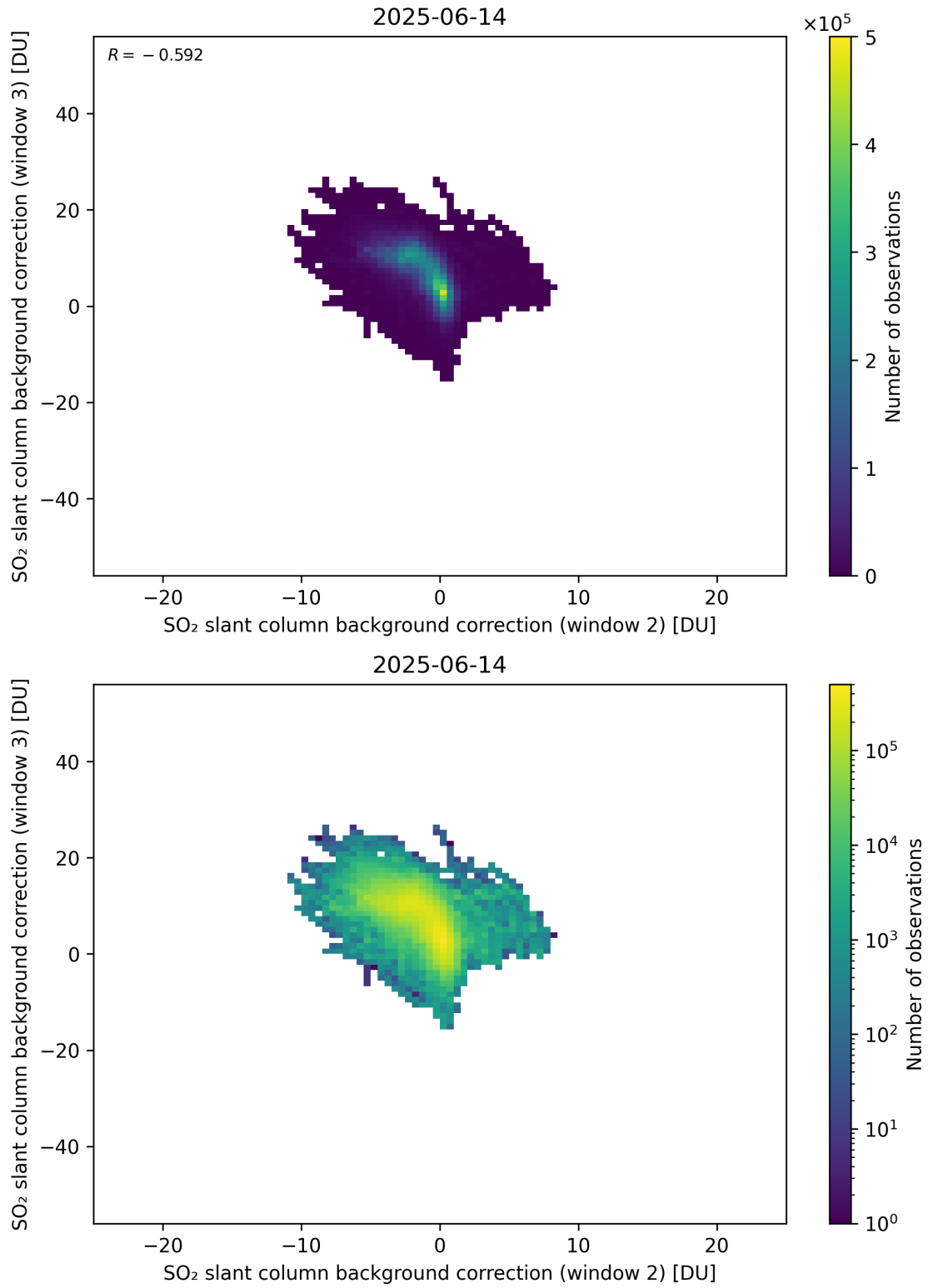
Figure 122: Scatter density plot of “SO 2 slant column background correction (window 2)” against “SO 2 slant column background correction (window 3)” for 2025-06-13 to 2025-06-15.
