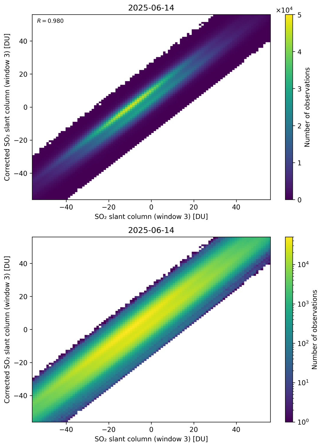
Figure 316: Scatter density plot of “SO 2 slant column (window 3)” against “Corrected SO 2 slant column (window 3)” for 2025-06-13 to 2025-06-15.
