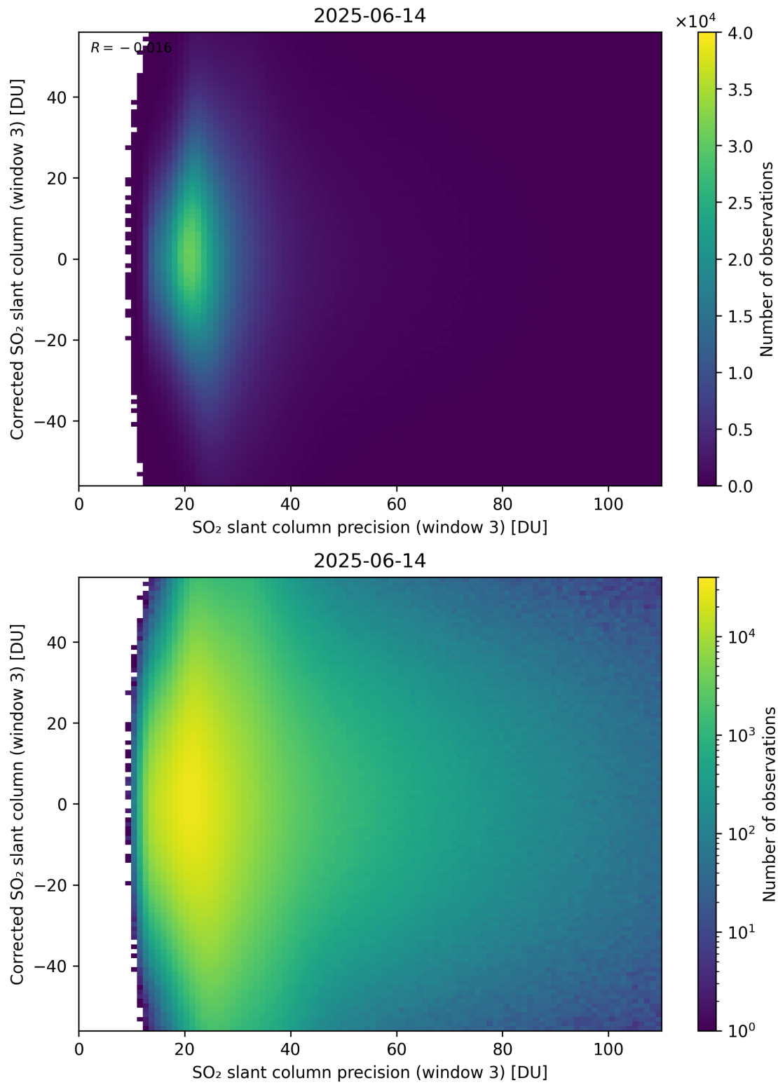
Figure 312: Scatter density plot of “SO 2 slant column precision (window 3)” against “Corrected SO 2 slant column (window 3)” for 2025-06-13 to 2025-06-15.
