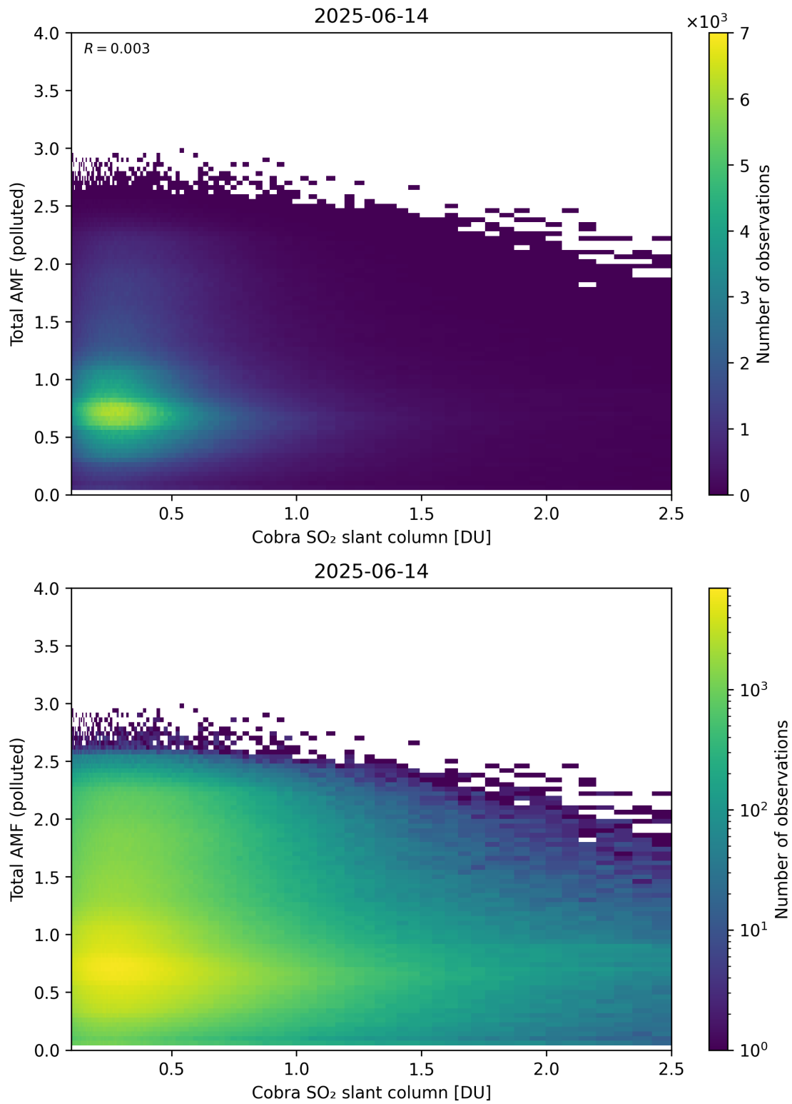
Figure 224: Scatter density plot of “Cobra SO 2 slant column” against “Total AMF (polluted)” for 2025-06-13 to 2025-06-15.
