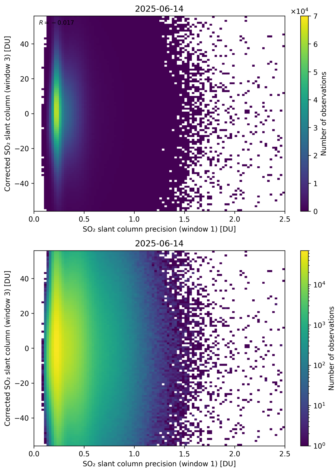
Figure 276: Scatter density plot of “SO 2 slant column precision (window 1)” against “Corrected SO 2 slant column (window 3)” for 2025-06-13 to 2025-06-15.
