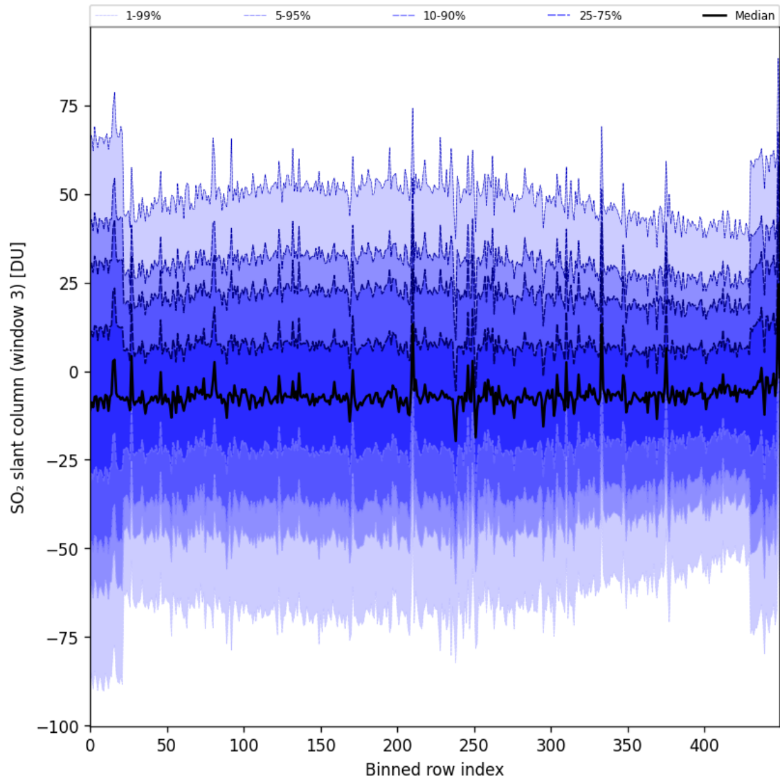
Figure 97: Along track statistics of “SO 2 slant column (window 3)” for 2025-06-13 to 2025-06-15
