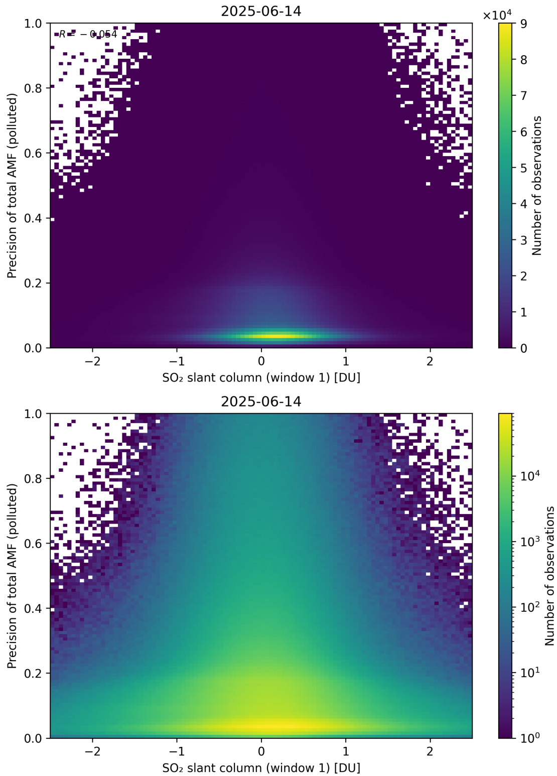
Figure 290: Scatter density plot of “SO 2 slant column (window 1)” against “Precision of total AMF (polluted)” for 2025-06-13 to 2025-06-15.
