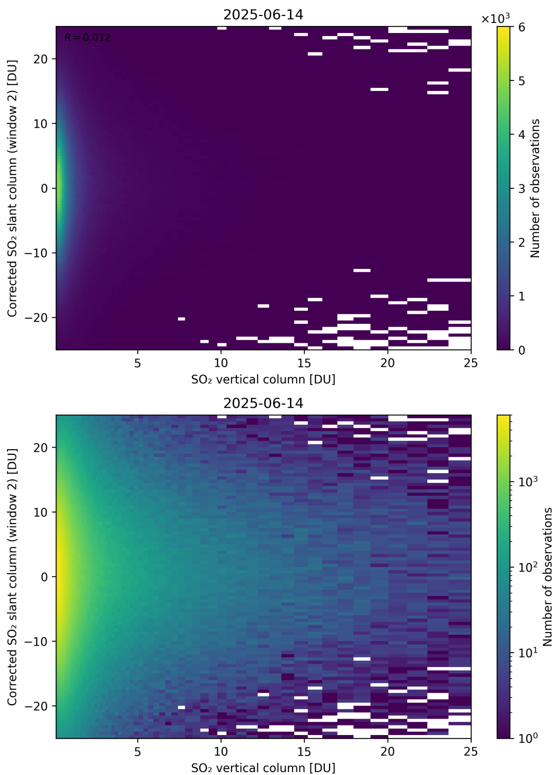
Figure 352: Scatter density plot of “SO 2 vertical column” against “Corrected SO 2 slant column (window 2)” for 2025-06-13 to 2025-06-15.
