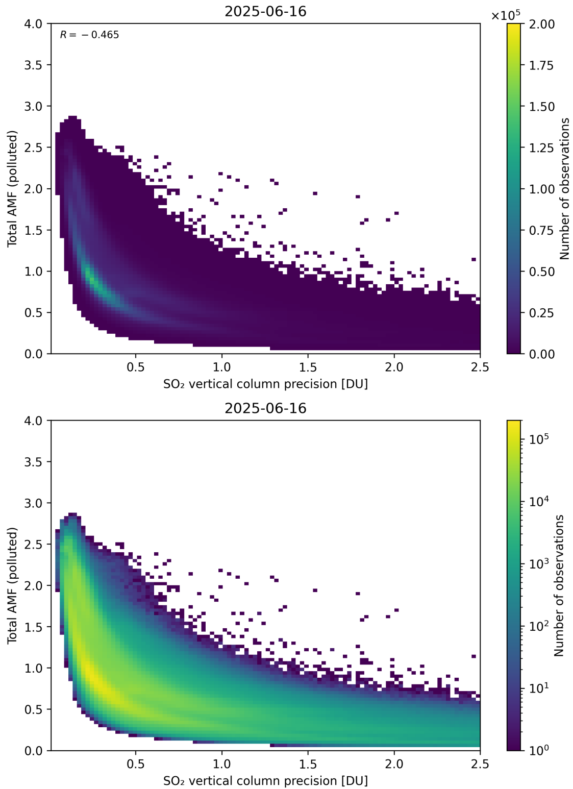
Figure 346: Scatter density plot of “SO 2 vertical column precision” against “Total AMF (polluted)” for 2025-06-16 to 2025-06-17.
