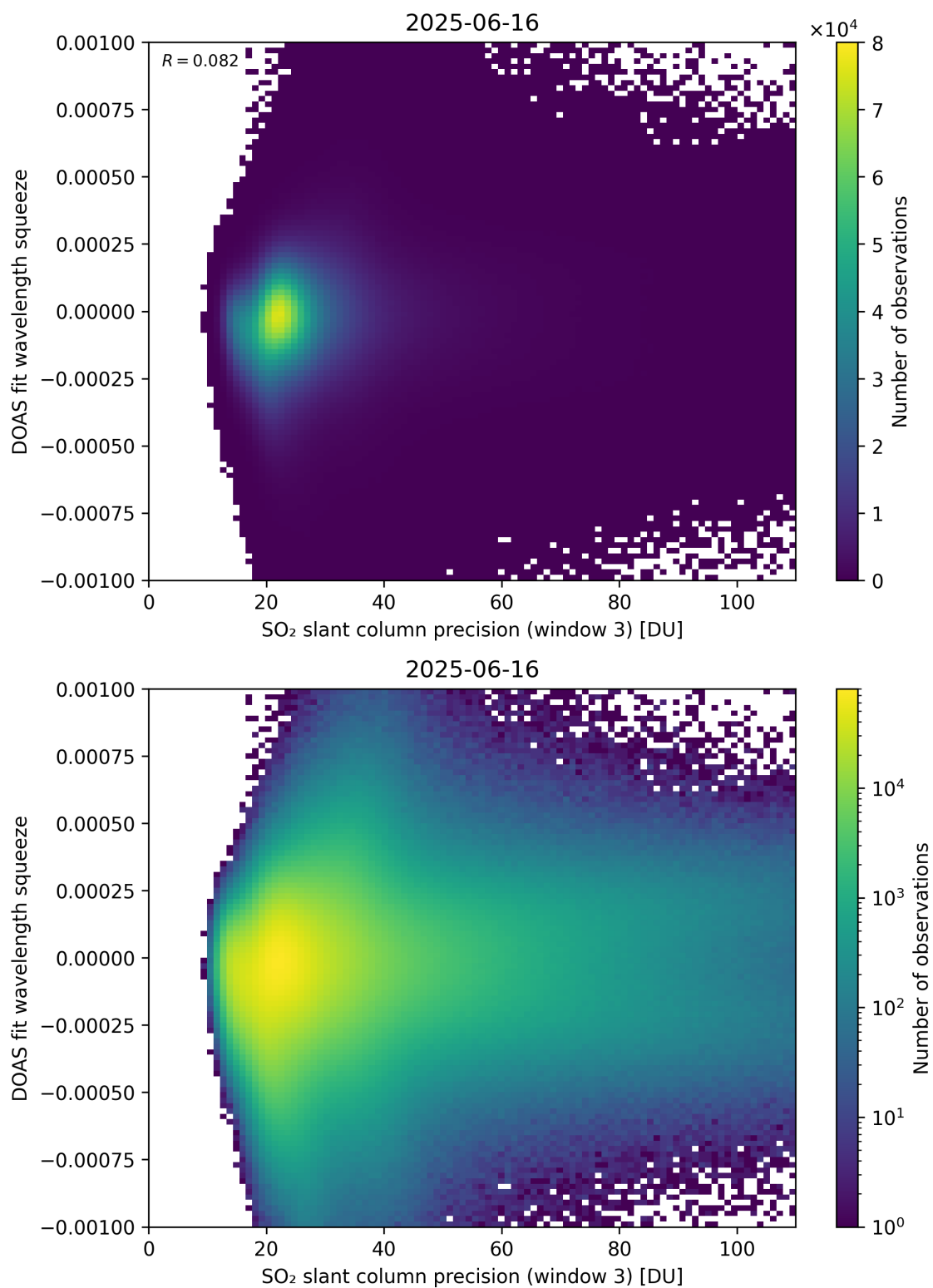
Figure 309: Scatter density plot of “SO 2 slant column precision (window 3)” against “DOAS fit wavelength squeeze” for 2025-06-16 to 2025-06-17.
