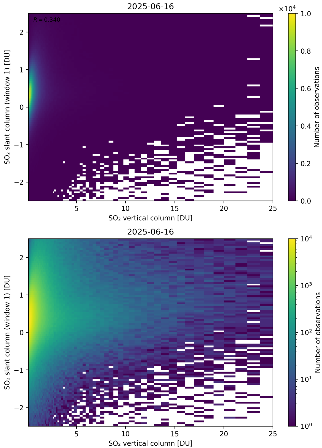
Figure 354: Scatter density plot of “SO 2 vertical column” against “SO 2 slant column (window 1)” for 2025-06-16 to 2025-06-17.
