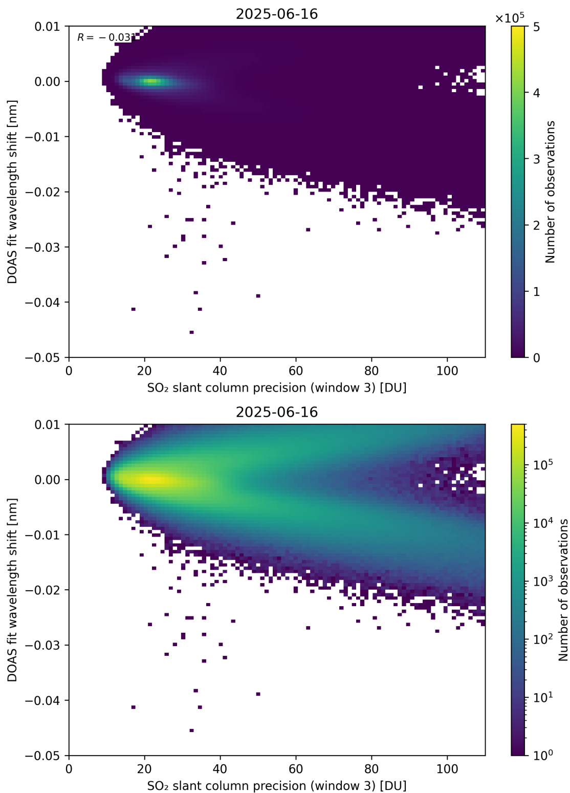
Figure 308: Scatter density plot of “SO 2 slant column precision (window 3)” against “DOAS fit wavelength shift” for 2025-06-16 to 2025-06-17.
