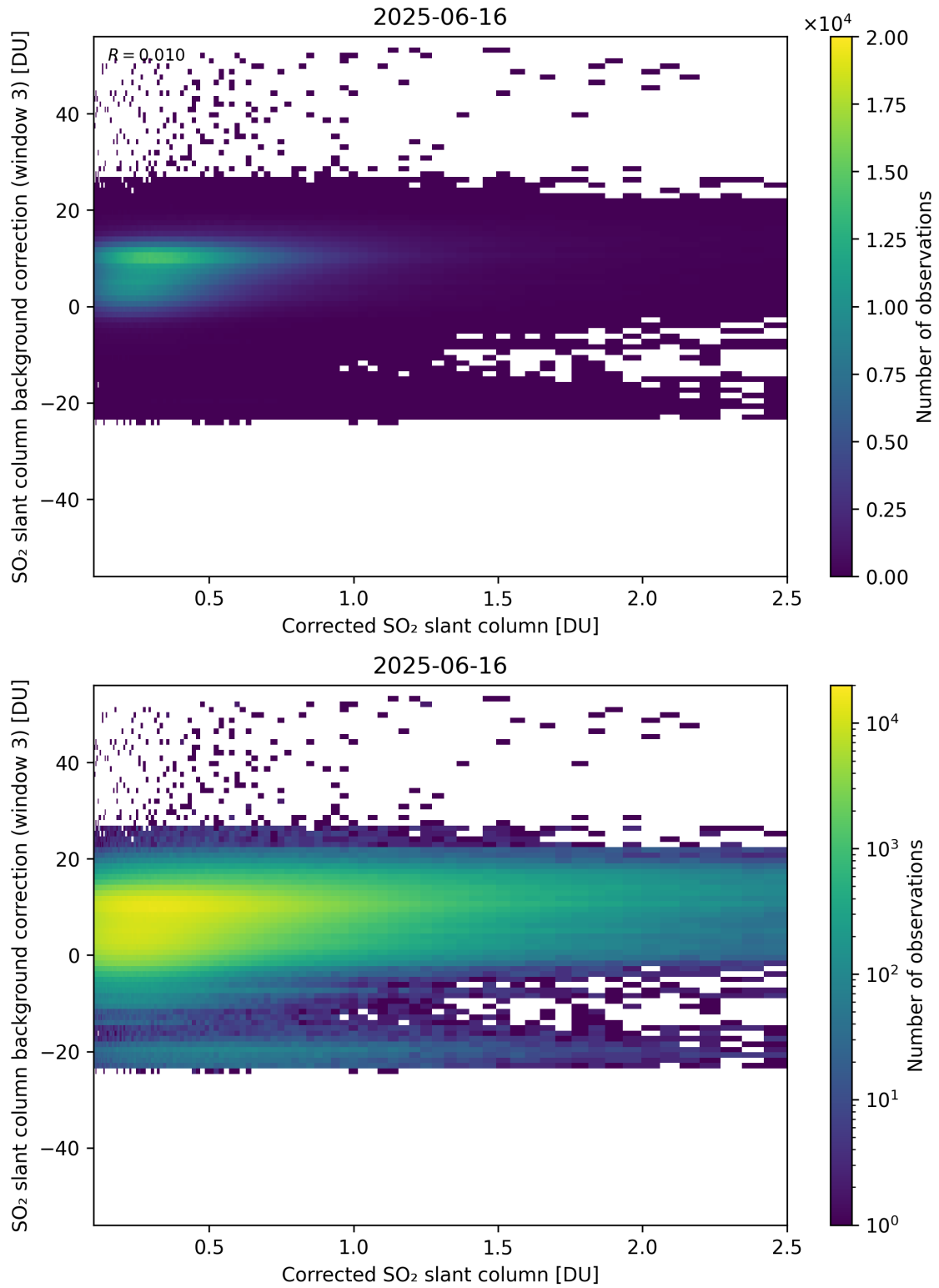
Figure 228: Scatter density plot of “Corrected SO 2 slant column” against “SO 2 slant column background correction (window 3)” for 2025-06-16 to 2025-06-17.
