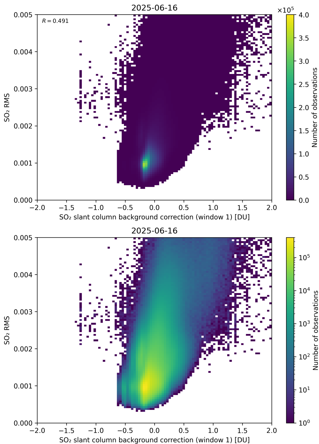
Figure 113: Scatter density plot of “SO 2 slant column background correction (window 1)” against “SO 2 RMS” for 2025-06-16 to 2025-06-17.
