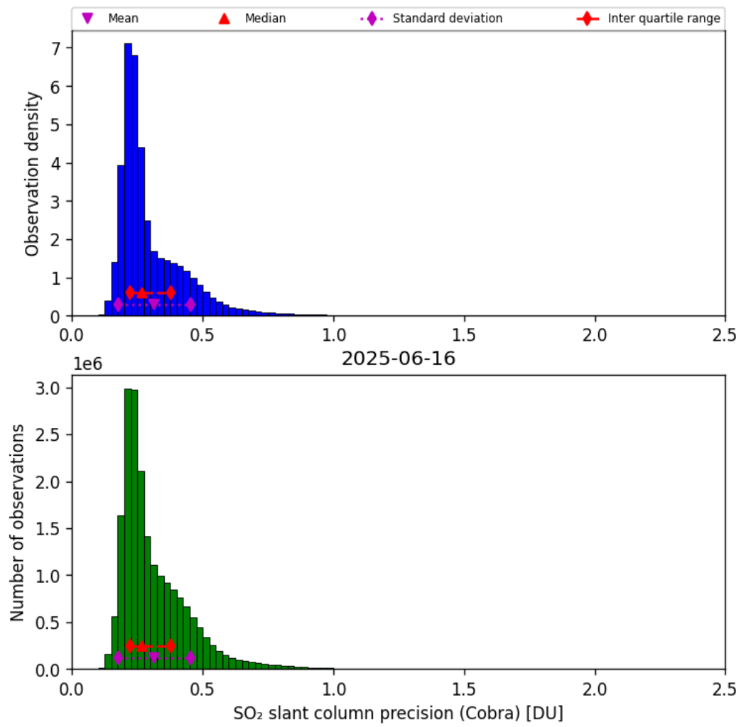
Figure 62: Histogram of “SO 2 slant column precision (Cobra)” for 2025-06-16 to 2025-06-17
