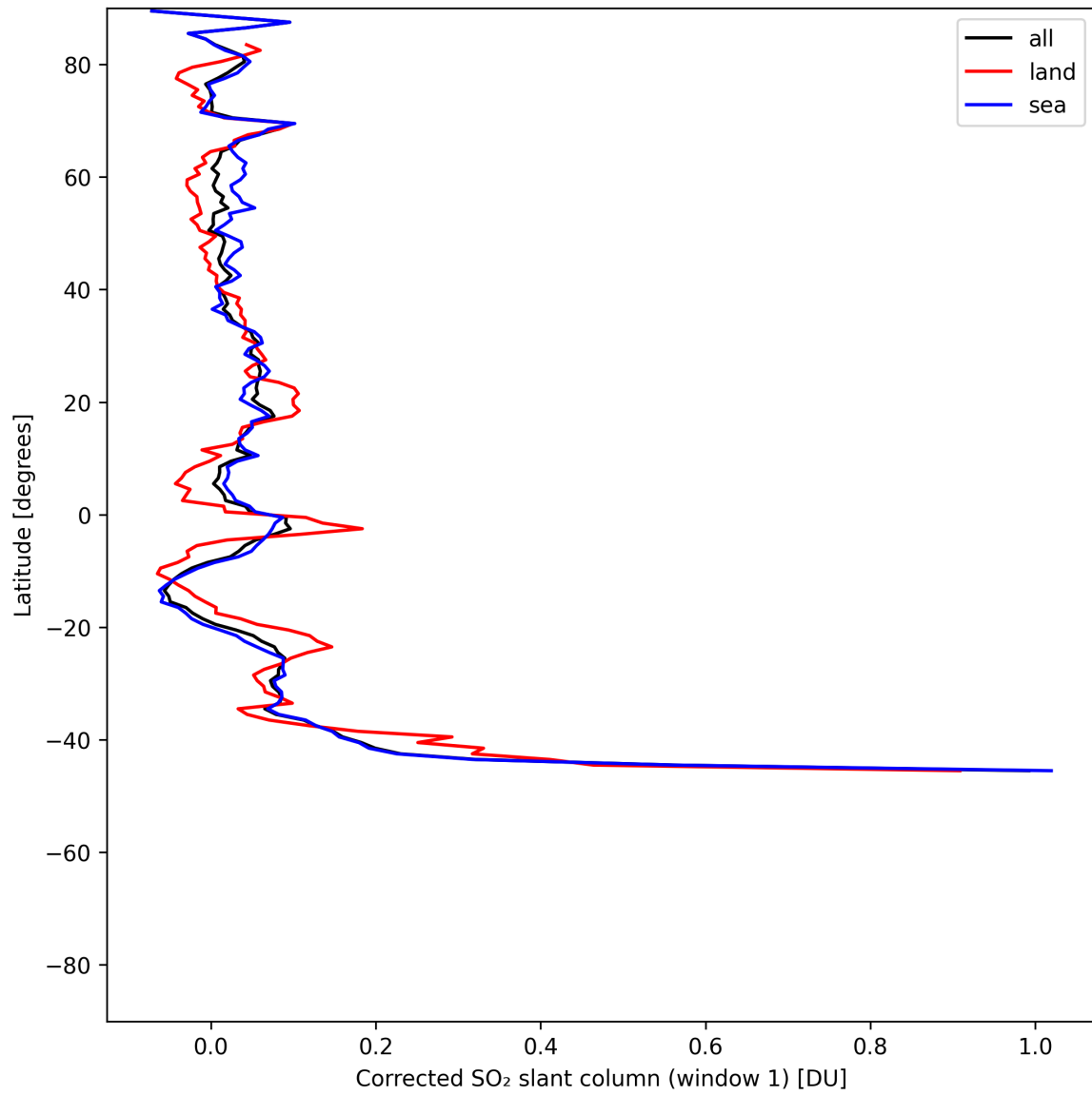
Figure 39: Zonal average of “Corrected SO 2 slant column (window 1)” for 2025-06-16 to 2025-06-17.
