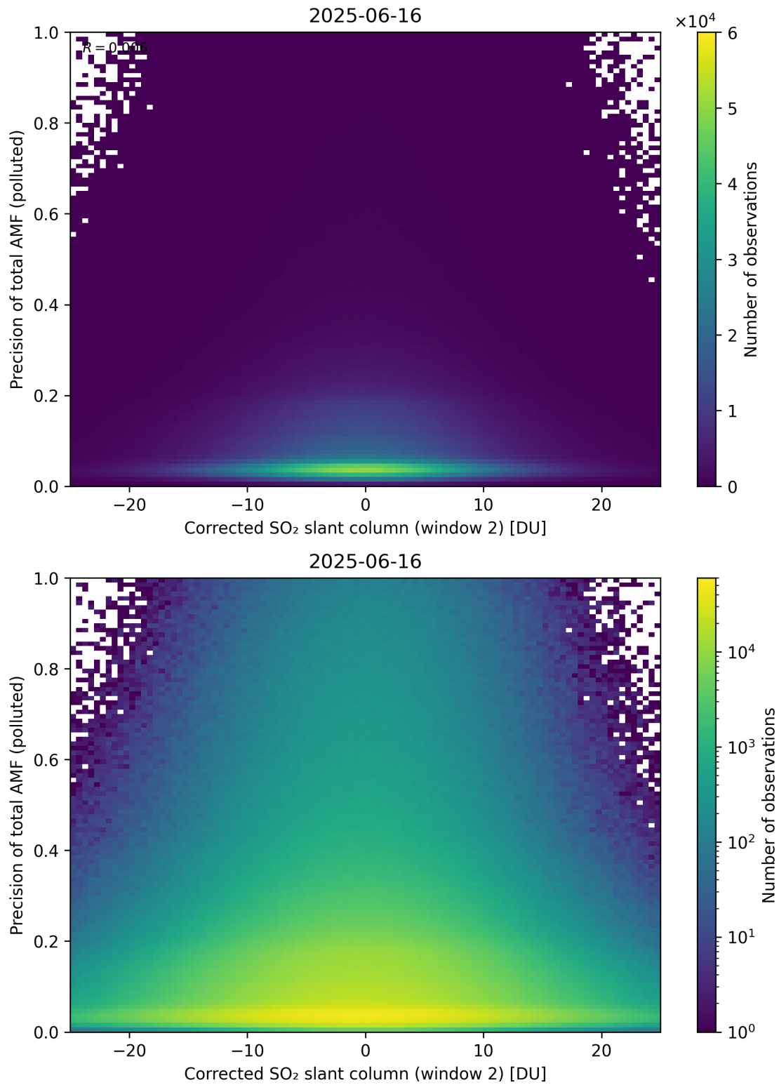
Figure 254: Scatter density plot of “Corrected SO 2 slant column (window 2)” against “Precision of total AMF (polluted)” for 2025-06-16 to 2025-06-17.
