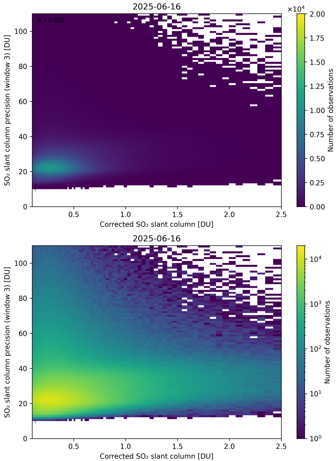
Figure 241: Scatter density plot of “Corrected SO 2 slant column” against “SO 2 slant column precision (window 3)” for 2025-06-16 to 2025-06-17.
