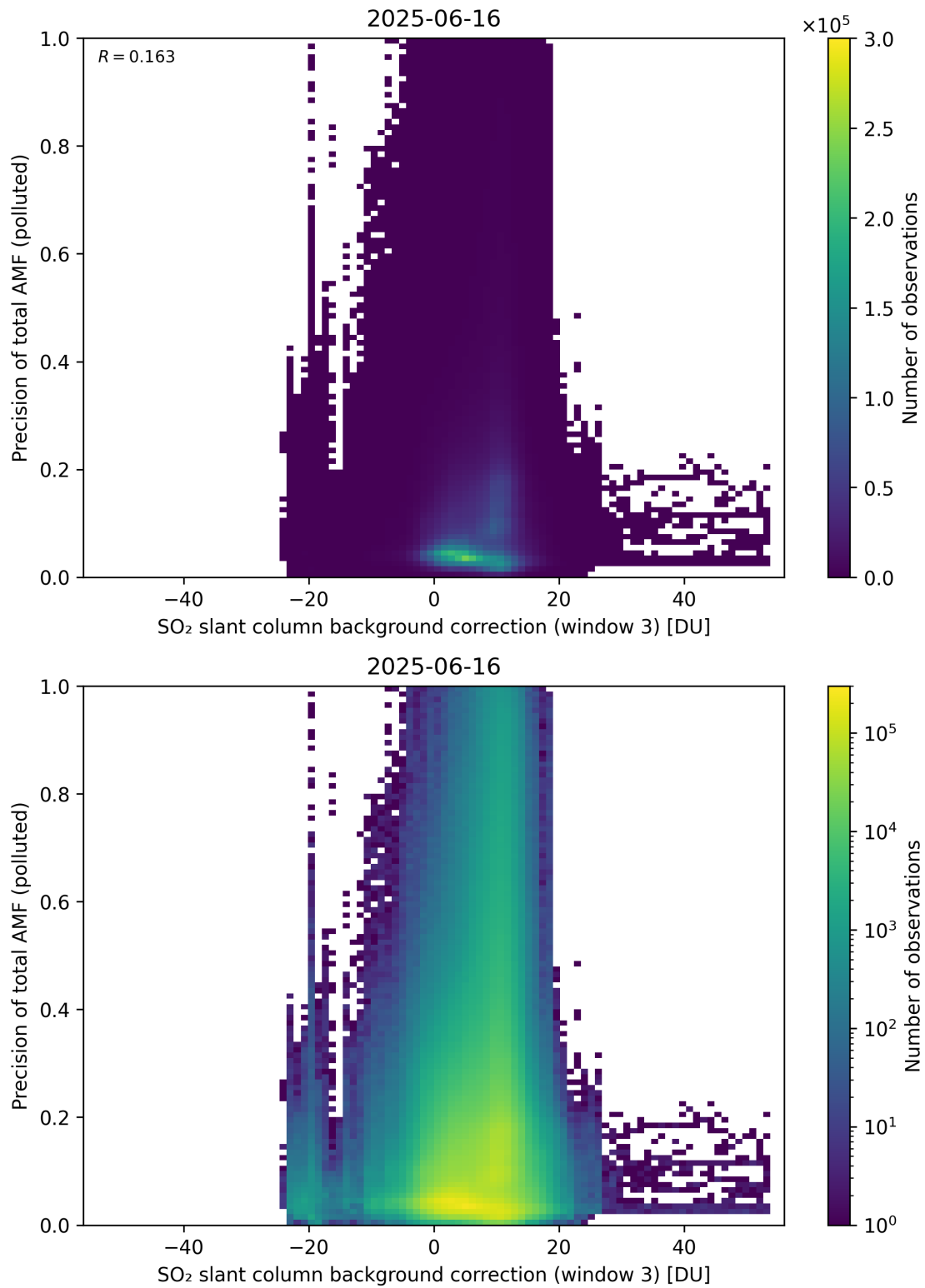
Figure 137: Scatter density plot of “SO 2 slant column background correction (window 3)” against “Precision of total AMF (polluted)” for 2025-06-16 to 2025-06-17.
