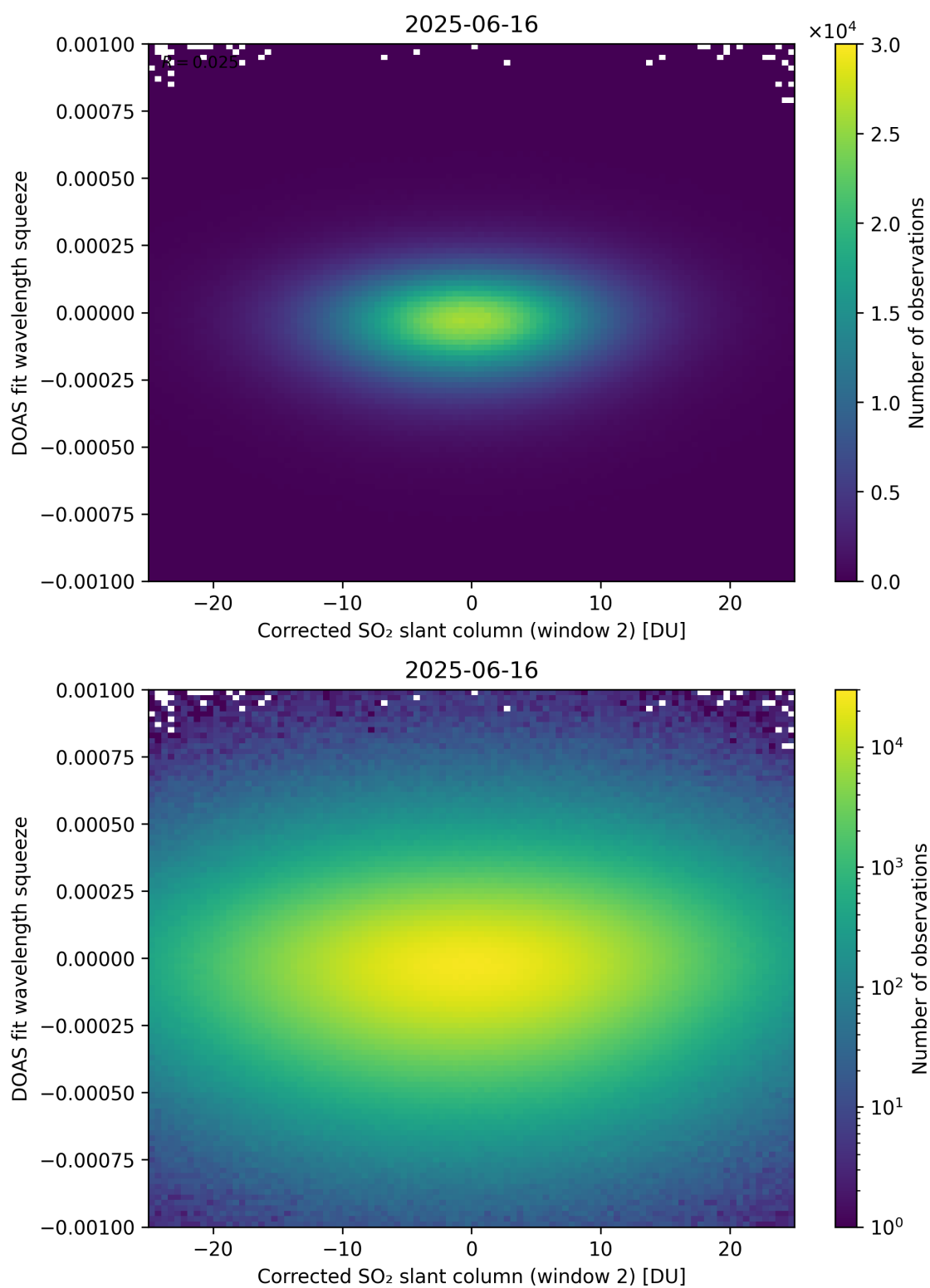
Figure 247: Scatter density plot of “Corrected SO 2 slant column (window 2)” against “DOAS fit wavelength squeeze” for 2025-06-16 to 2025-06-17.
