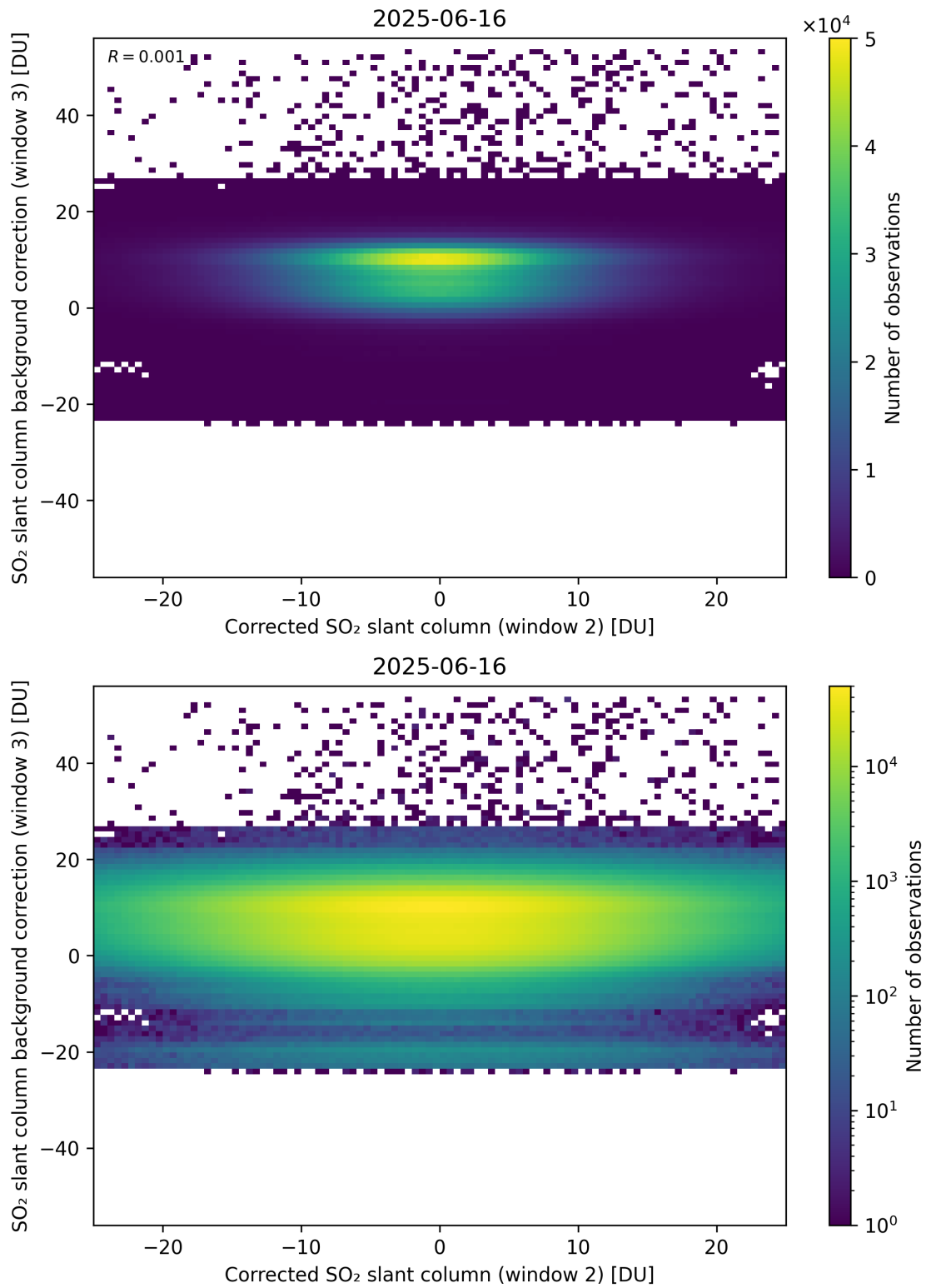
Figure 245: Scatter density plot of “Corrected SO 2 slant column (window 2)” against “SO 2 slant column background correction (window 3)” for 2025-06-16 to 2025-06-17.
