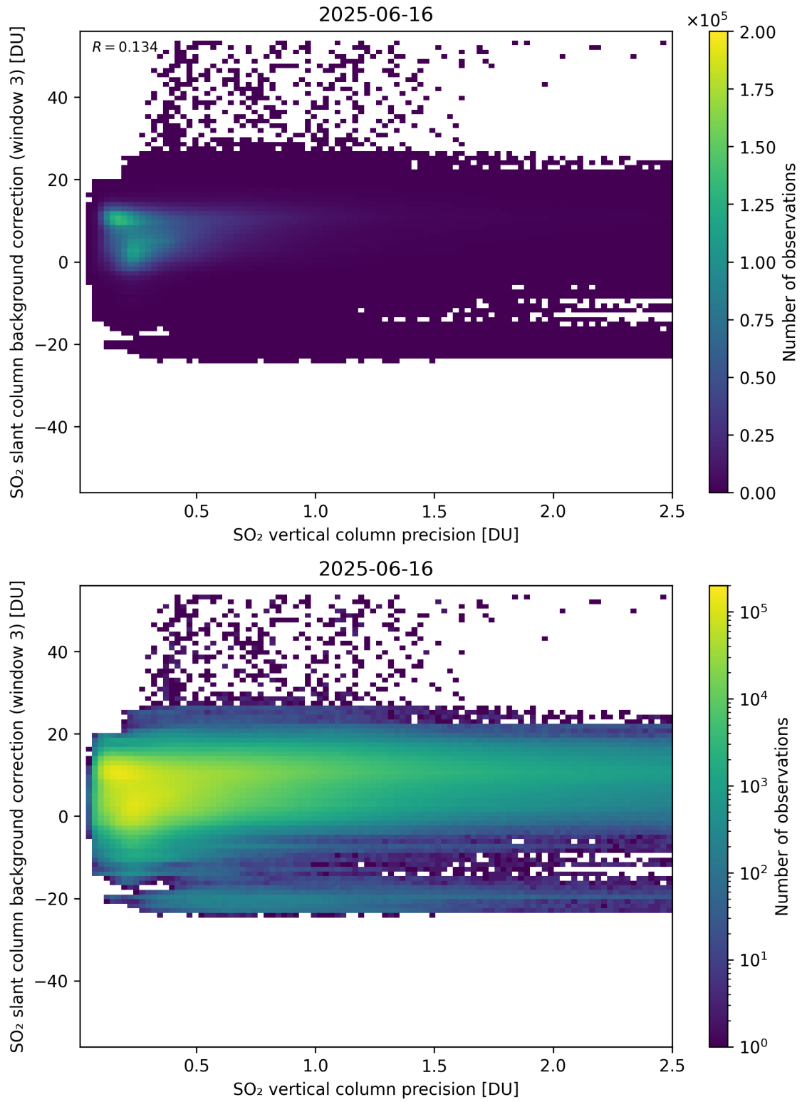
Figure 331: Scatter density plot of “SO 2 vertical column precision” against “SO 2 slant column background correction (window 3)” for 2025-06-16 to 2025-06-17.
