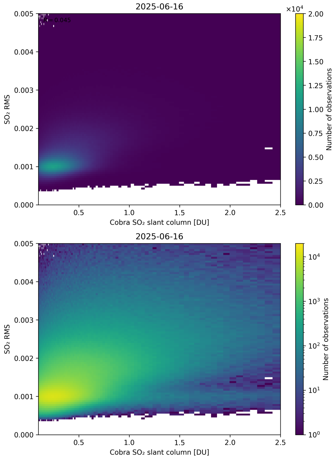
Figure 198: Scatter density plot of “Cobra SO 2 slant column” against “SO 2 RMS” for 2025-06-16 to 2025-06-17.
