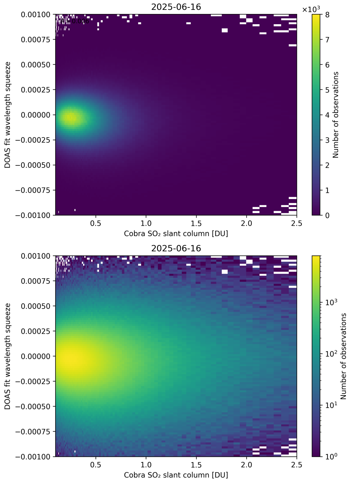
Figure 197: Scatter density plot of “Cobra SO 2 slant column” against “DOAS fit wavelength squeeze” for 2025-06-16 to 2025-06-17.
