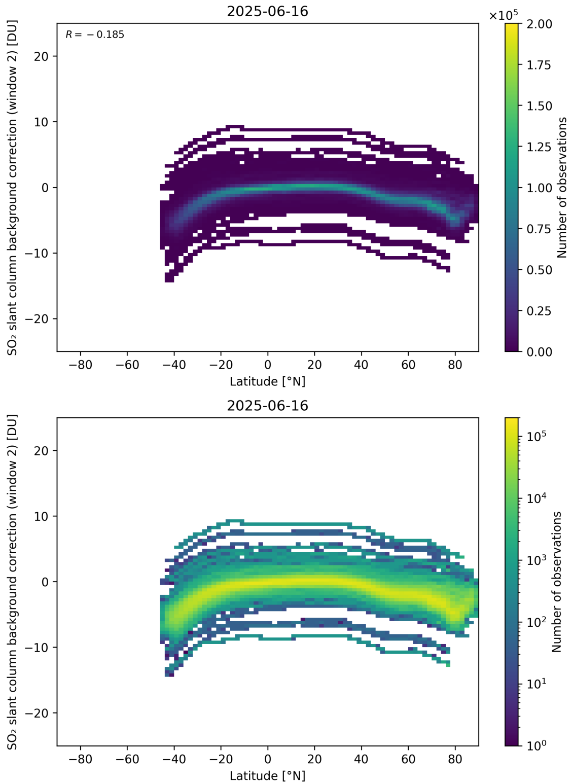
Figure 151: Scatter density plot of “Latitude” against “SO 2 slant column background correction (window 2)” for 2025-06-16 to 2025-06-17.
