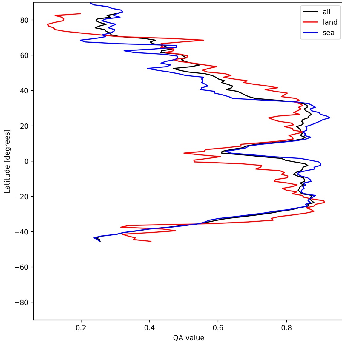
Figure 31: Zonal average of “QA value” for 2025-06-16 to 2025-06-17.
