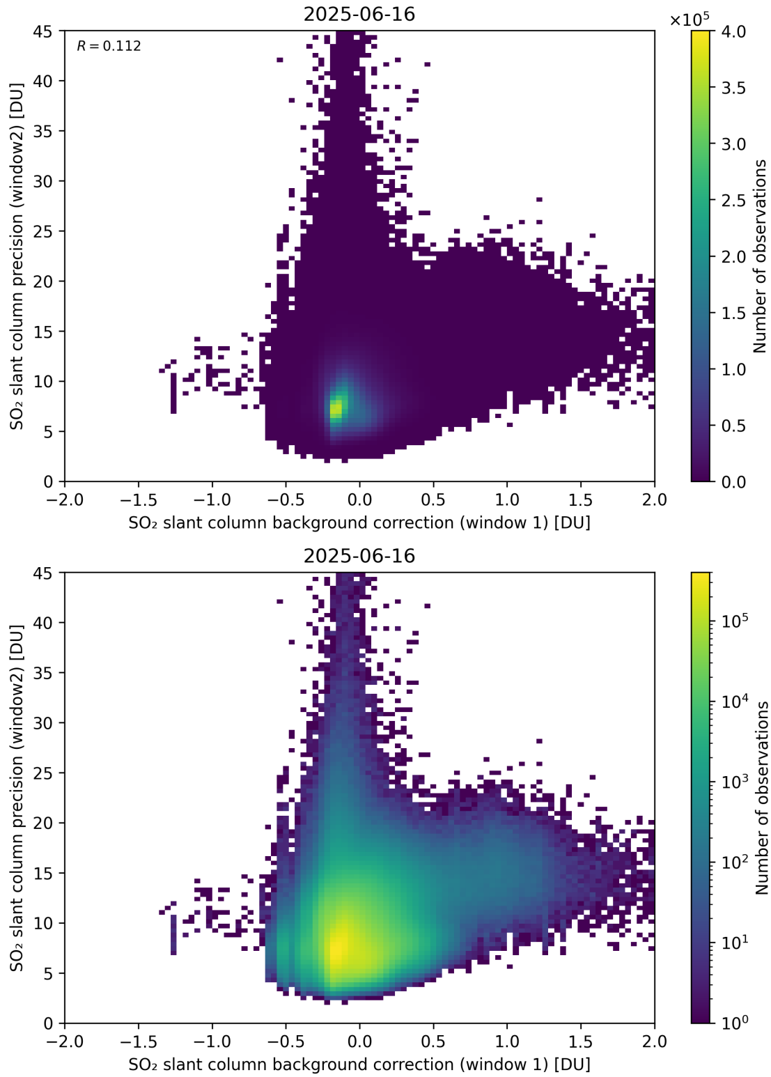
Figure 117: Scatter density plot of “SO 2 slant column background correction (window 1)” against “SO 2 slant column precision (window2)” for 2025-06-16 to 2025-06-17.
