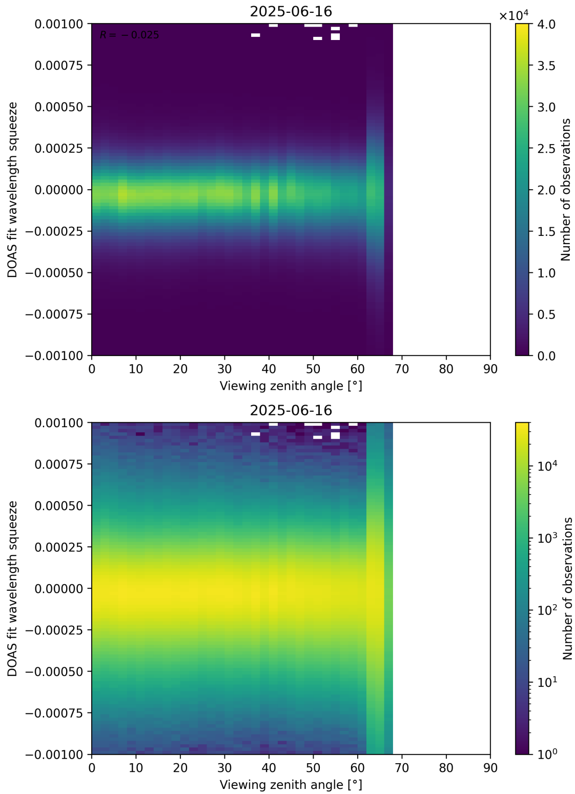
Figure 366: Scatter density plot of “Viewing zenith angle” against “DOAS fit wavelength squeeze” for 2025-06-16 to 2025-06-17.
