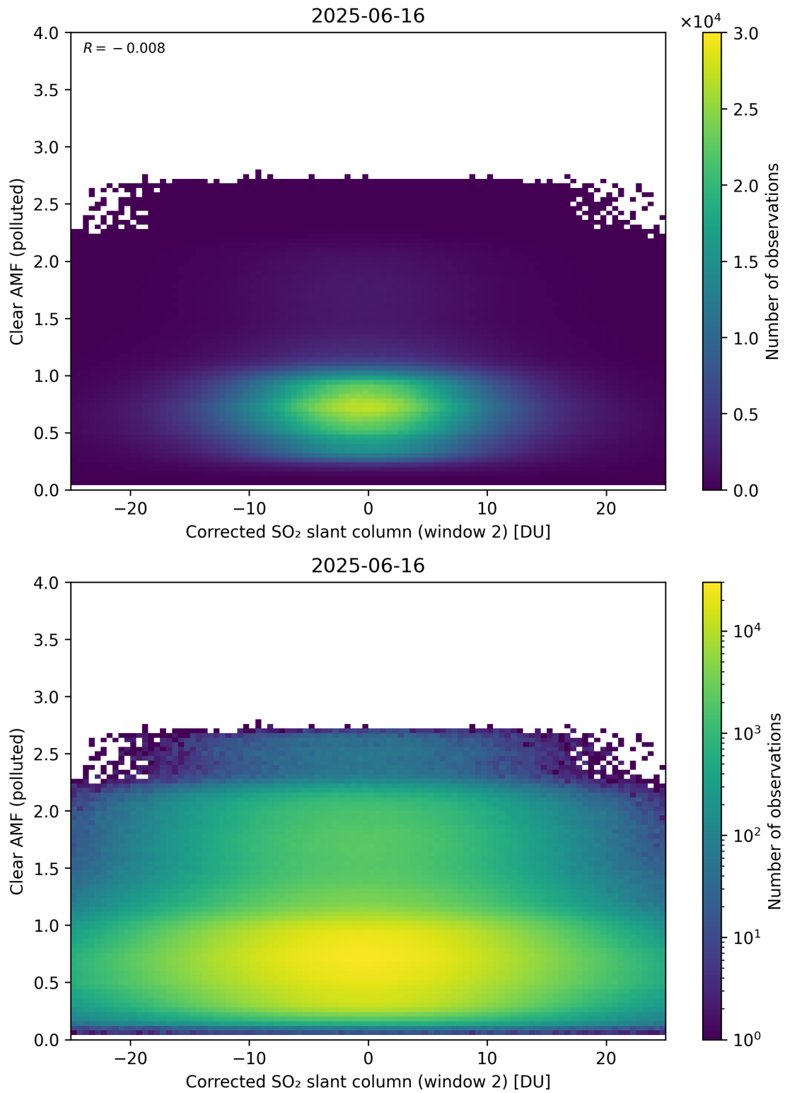
Figure 249: Scatter density plot of “Corrected SO 2 slant column (window 2)” against “Clear AMF (polluted)” for 2025-06-16 to 2025-06-17.
