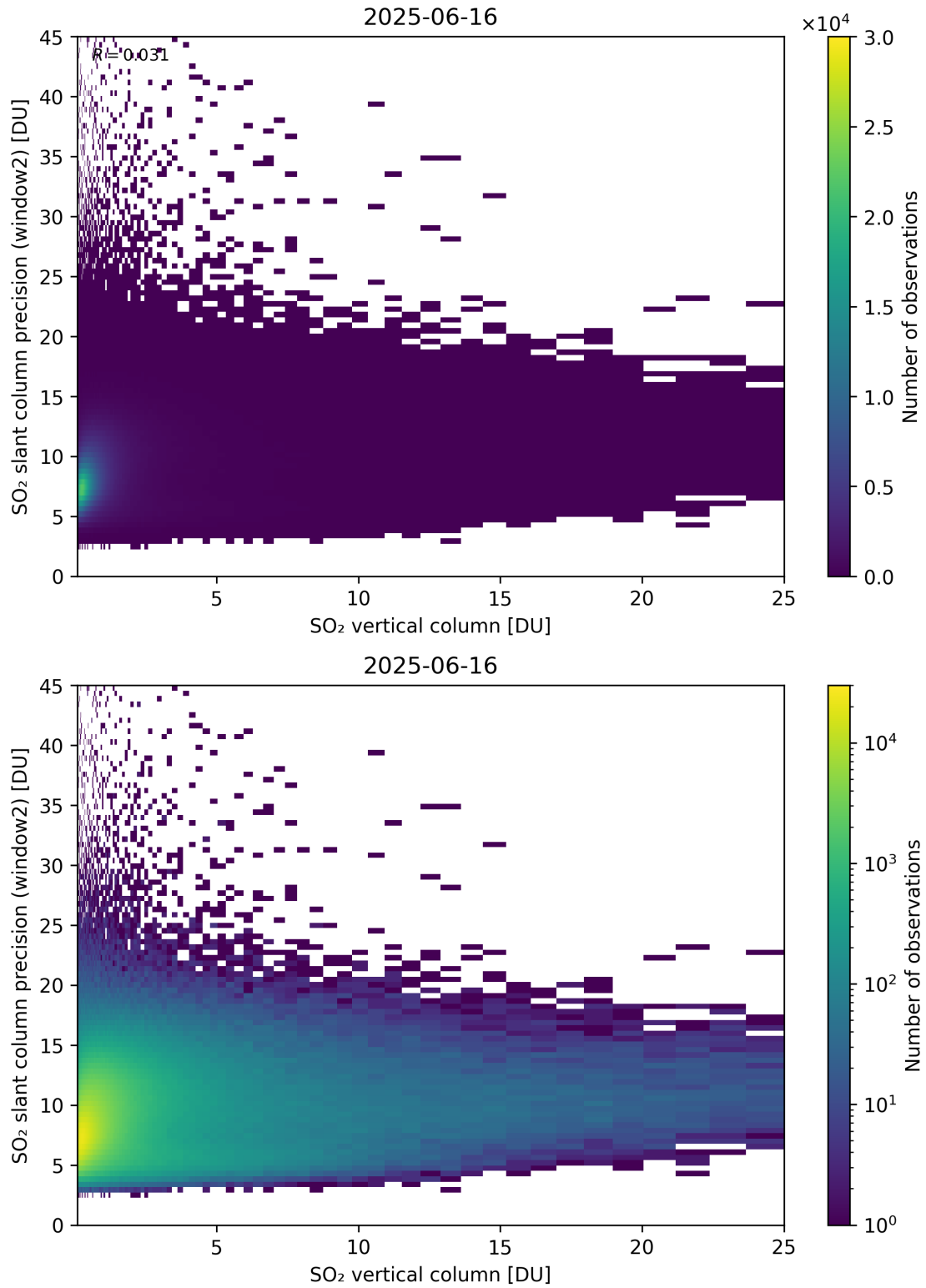
Figure 356: Scatter density plot of “SO 2 vertical column” against “SO 2 slant column precision (window2)” for 2025-06-16 to 2025-06-17.
