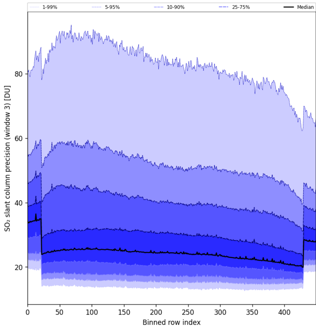
Figure 98: Along track statistics of “SO 2 slant column precision (window 3)” for 2025-06-16 to 2025-06-17
