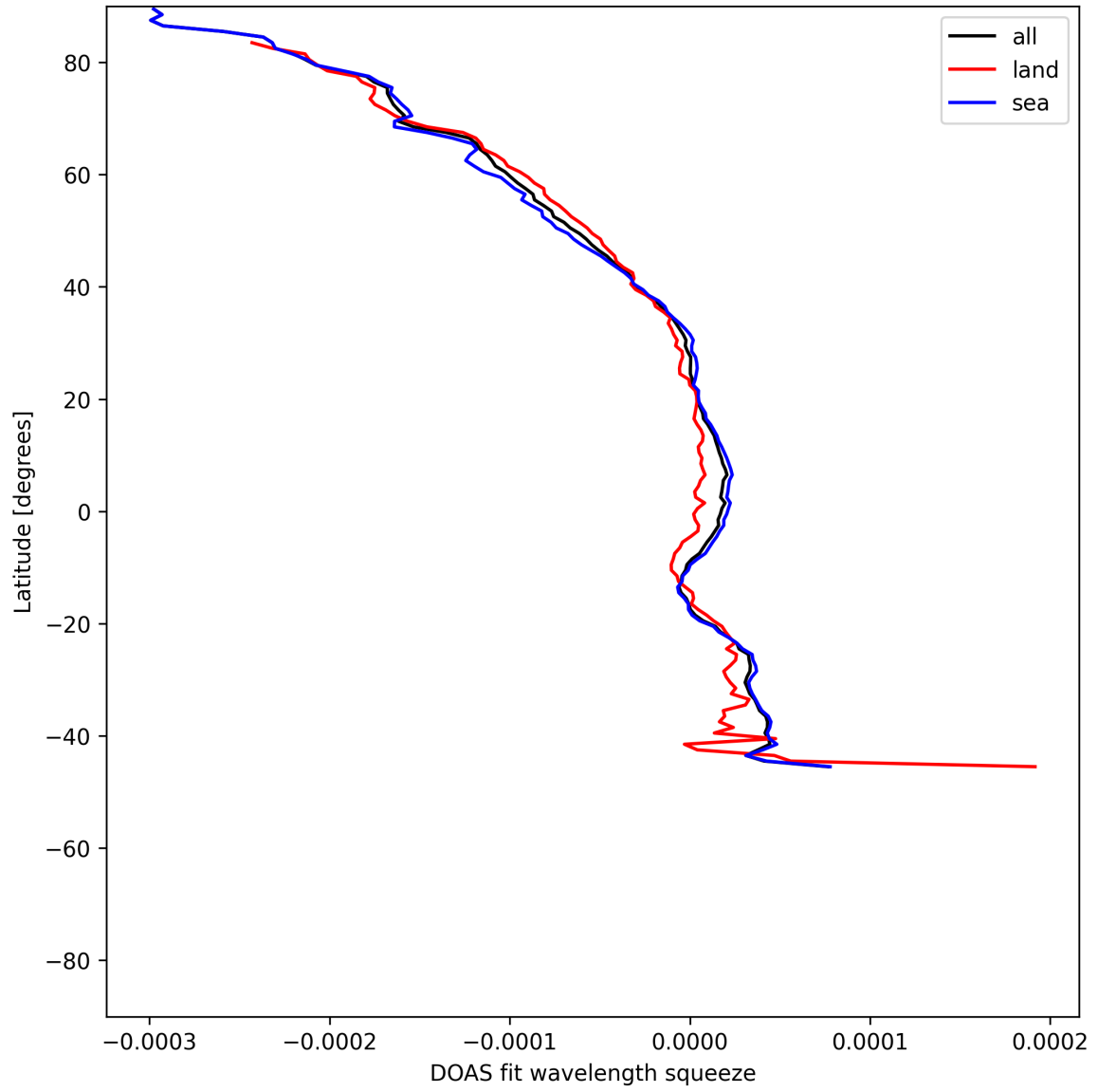
Figure 51: Zonal average of “DOAS fit wavelength squeeze” for 2025-06-16 to 2025-06-17.
