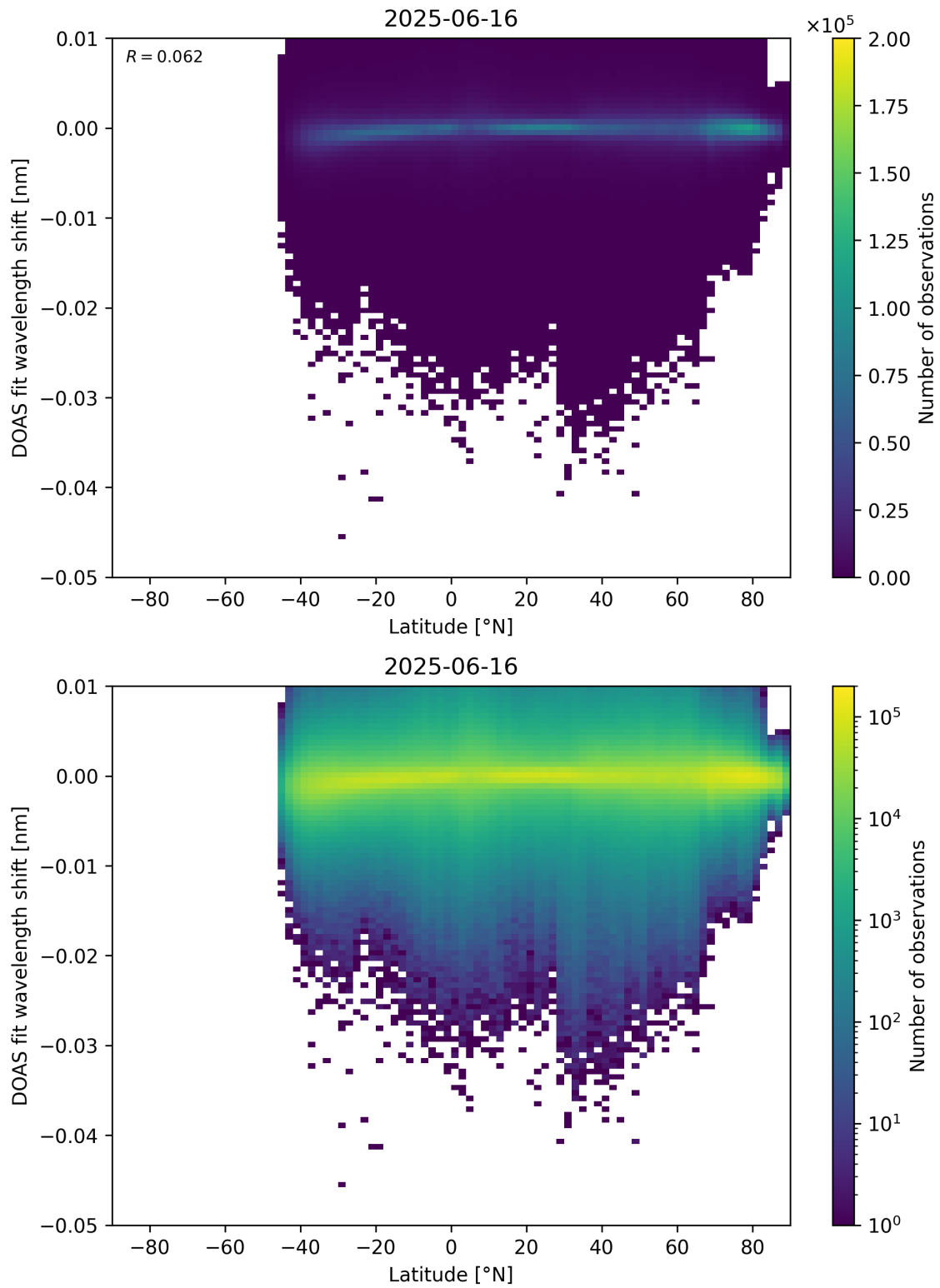
Figure 153: Scatter density plot of “Latitude” against “DOAS fit wavelength shift” for 2025-06-16 to 2025-06-17.
