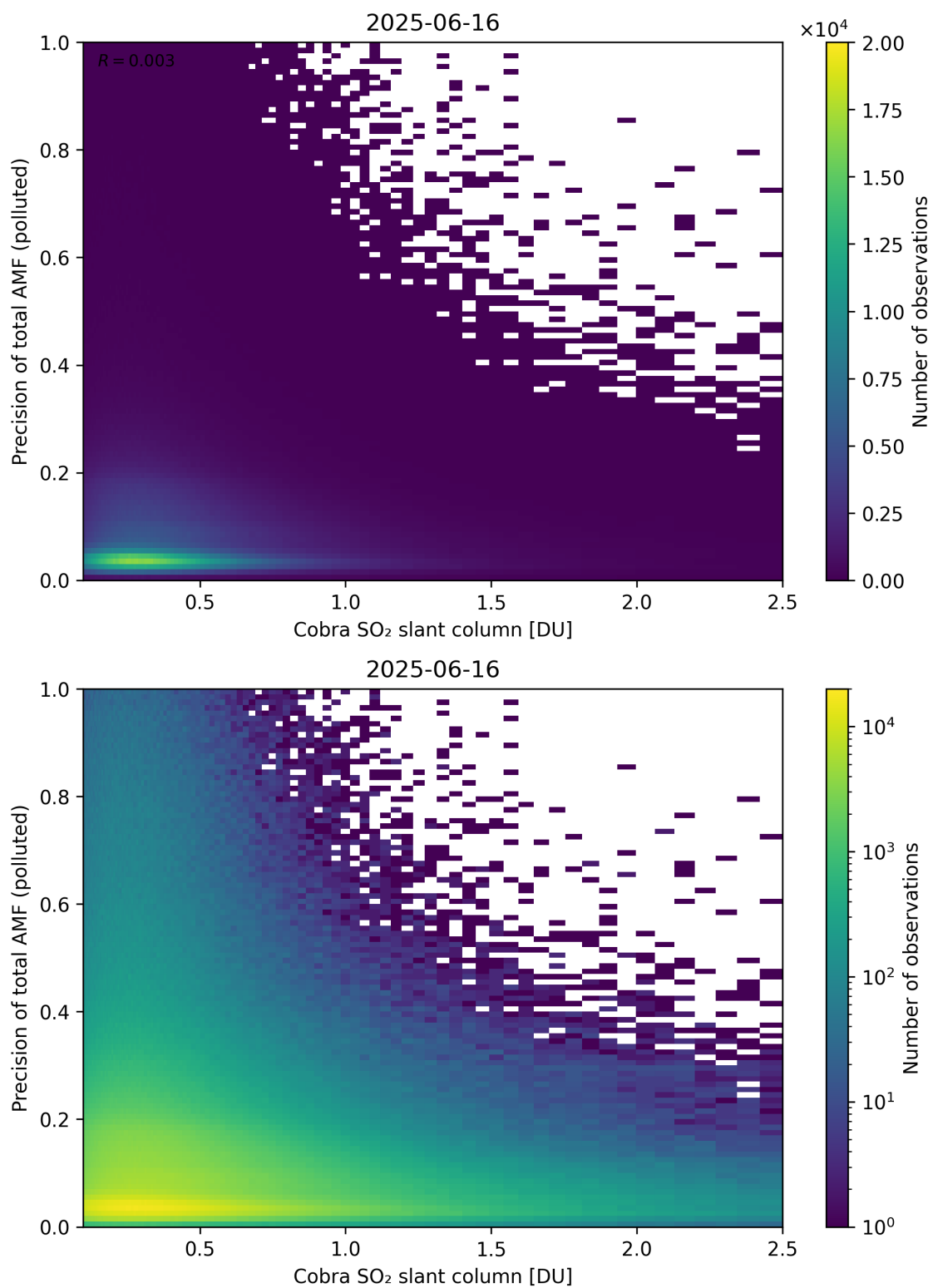
Figure 225: Scatter density plot of “Cobra SO 2 slant column” against “Precision of total AMF (polluted)” for 2025-06-16 to 2025-06-17.
