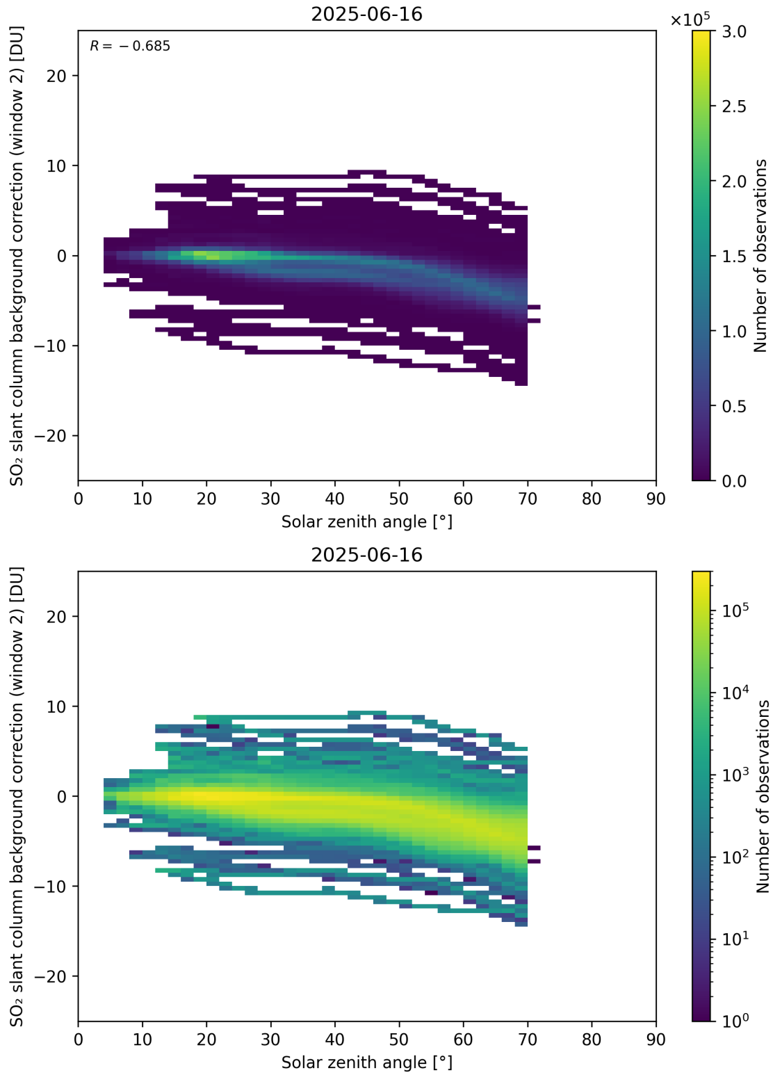
Figure 172: Scatter density plot of “Solar zenith angle” against “SO 2 slant column background correction (window 2)” for 2025-06-16 to 2025-06-17.
