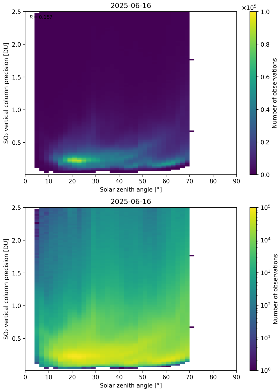
Figure 192: Scatter density plot of “Solar zenith angle” against “SO 2 vertical column precision” for 2025-06-16 to 2025-06-17.
