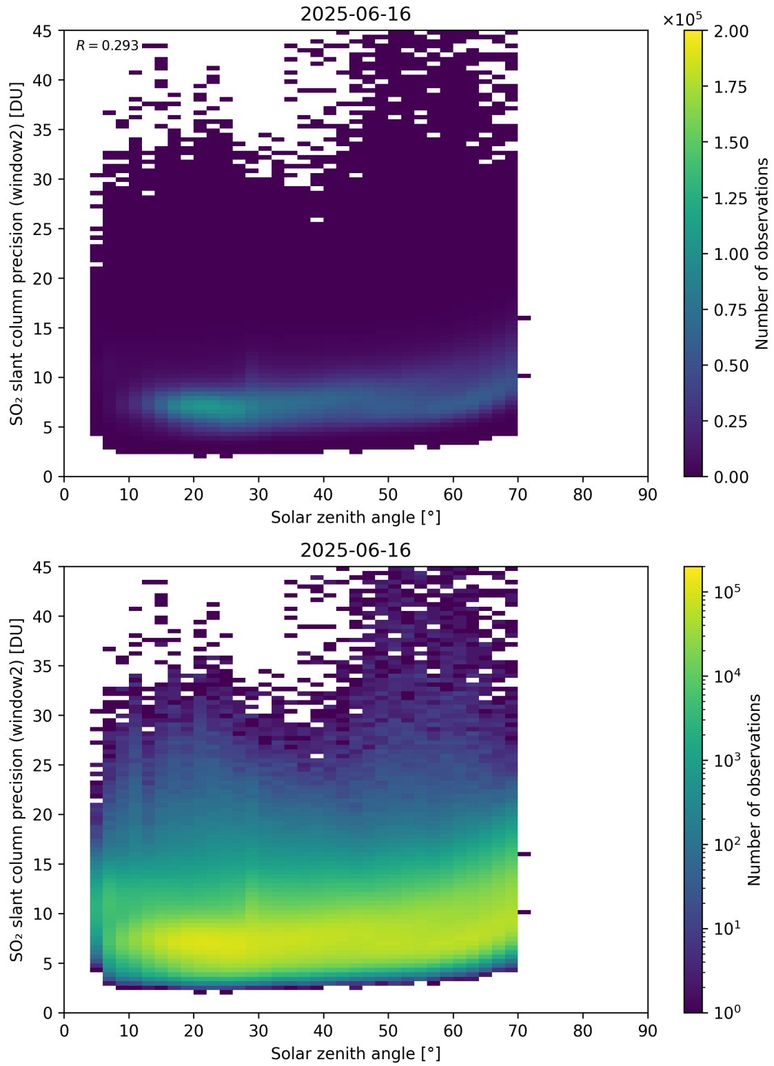
Figure 186: Scatter density plot of “Solar zenith angle” against “SO 2 slant column precision (window2)” for 2025-06-16 to 2025-06-17.
