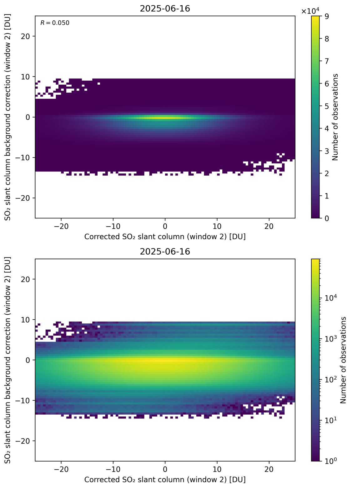
Figure 244: Scatter density plot of “Corrected SO 2 slant column (window 2)” against “SO 2 slant column background correction (window 2)” for 2025-06-16 to 2025-06-17.
