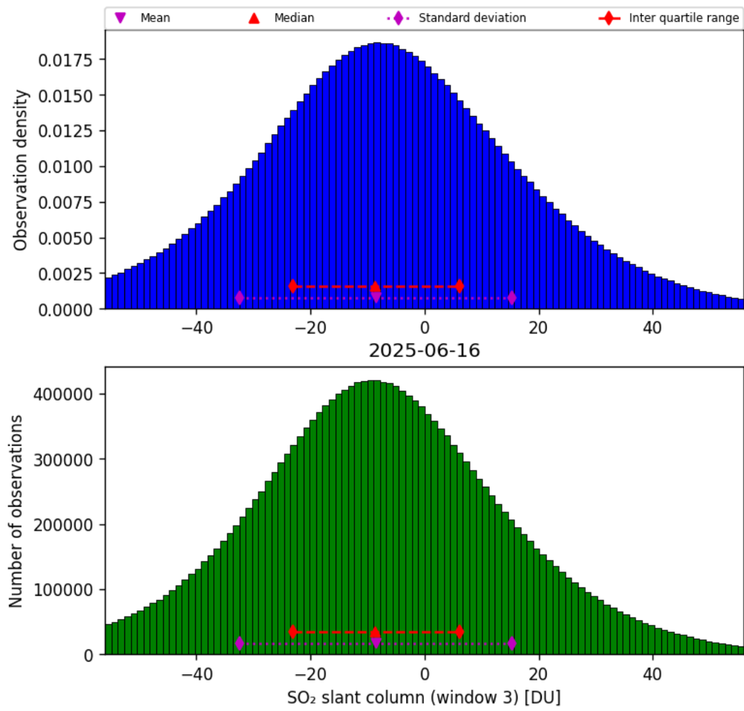
Figure 71: Histogram of “SO 2 slant column (window 3)” for 2025-06-16 to 2025-06-17
