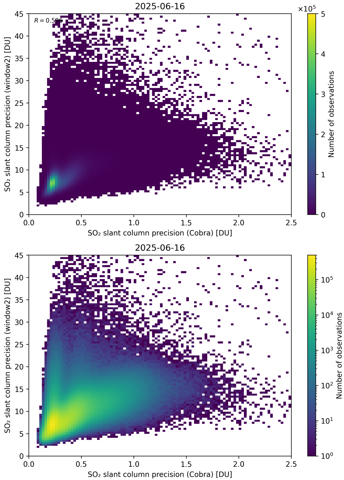
Figure 210: Scatter density plot of “SO 2 slant column precision (Cobra)” against “SO 2 slant column precision (window2)” for 2025-06-16 to 2025-06-17.
