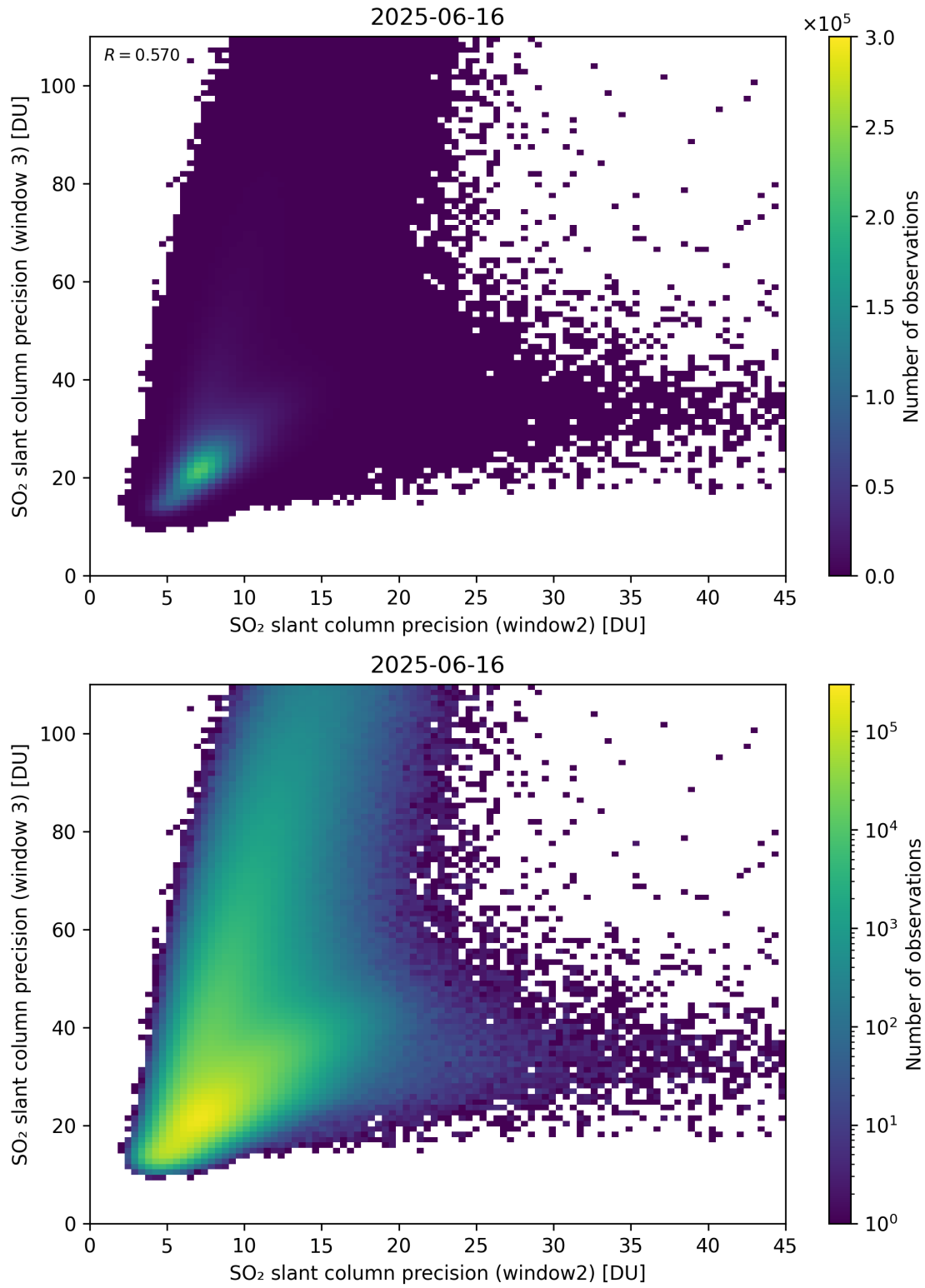
Figure 300: Scatter density plot of “SO 2 slant column precision (window2)” against “SO 2 slant column precision (window 3)” for 2025-06-16 to 2025-06-17.
