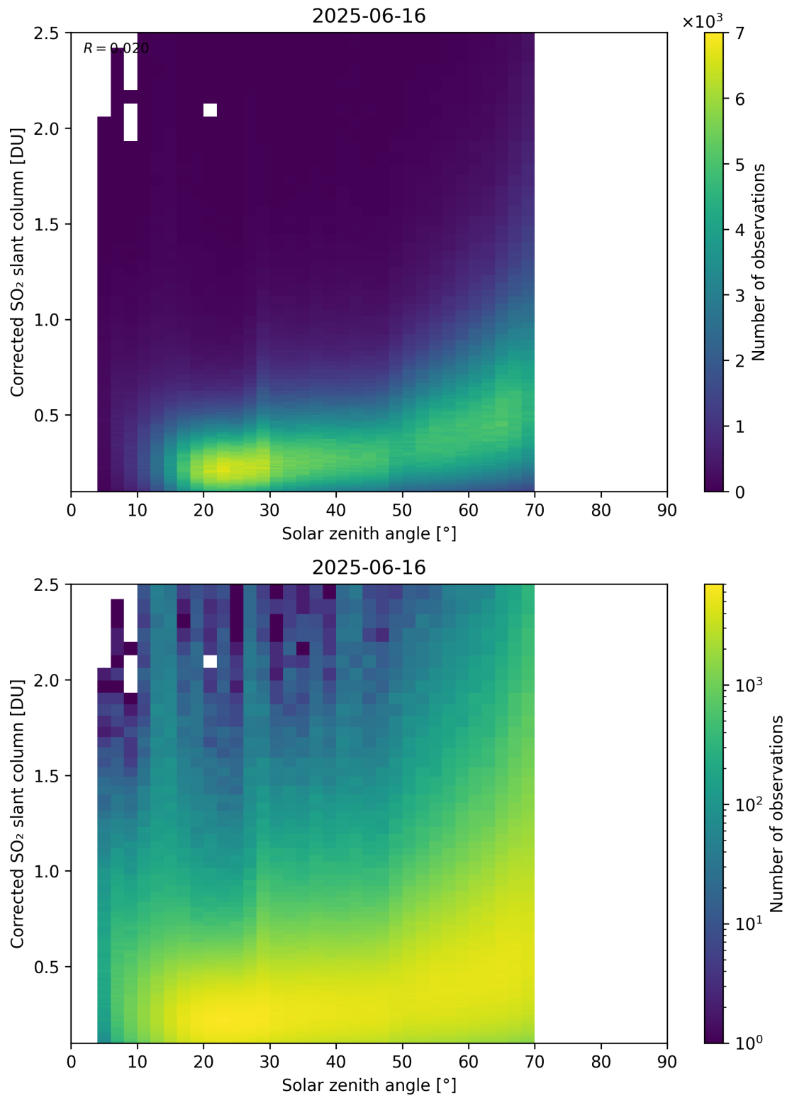
Figure 181: Scatter density plot of “Solar zenith angle” against “Corrected SO 2 slant column” for 2025-06-16 to 2025-06-17.
