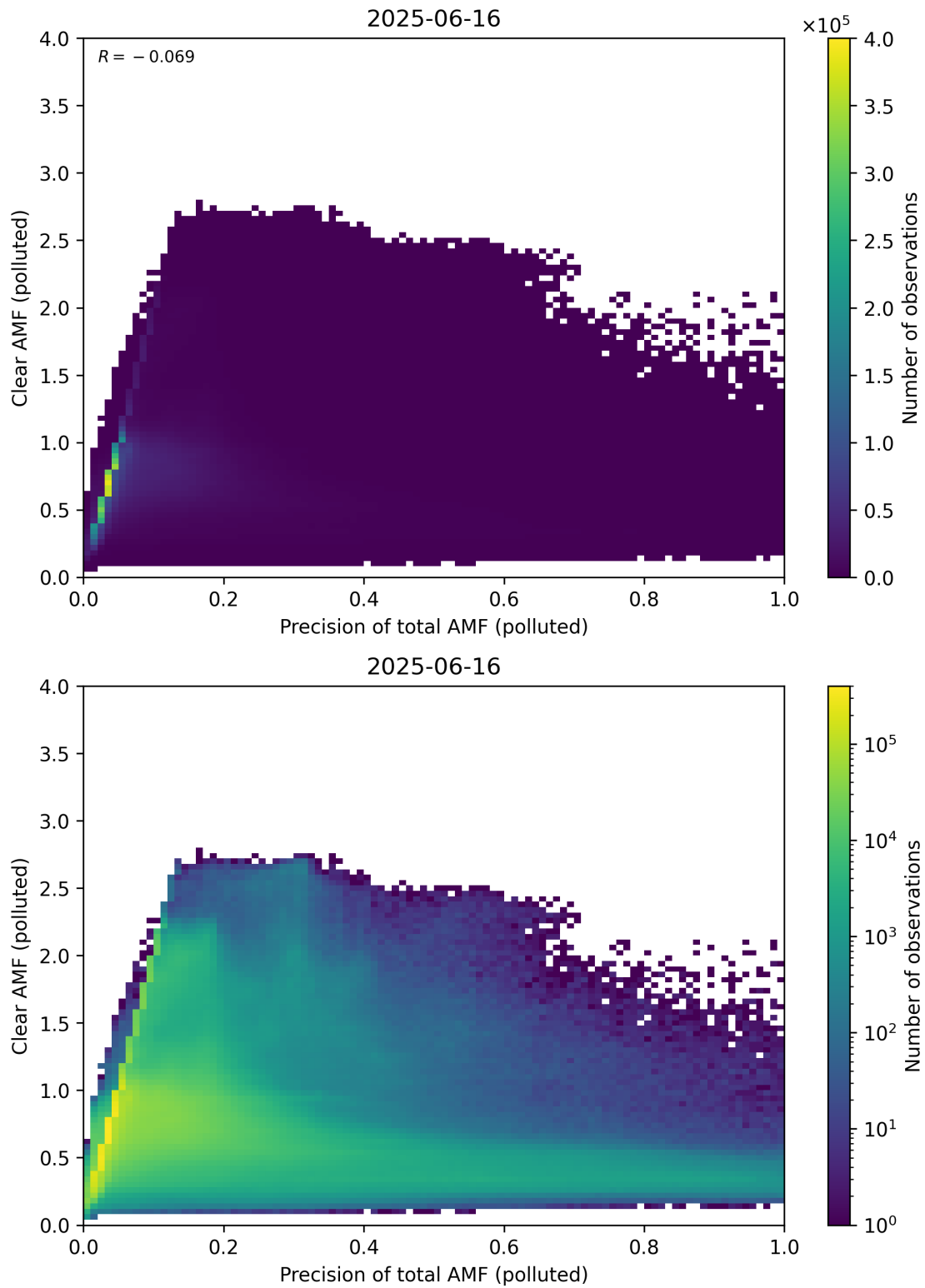
Figure 320: Scatter density plot of “Precision of total AMF (polluted)” against “Clear AMF (polluted)” for 2025-06-16 to 2025-06-17.
