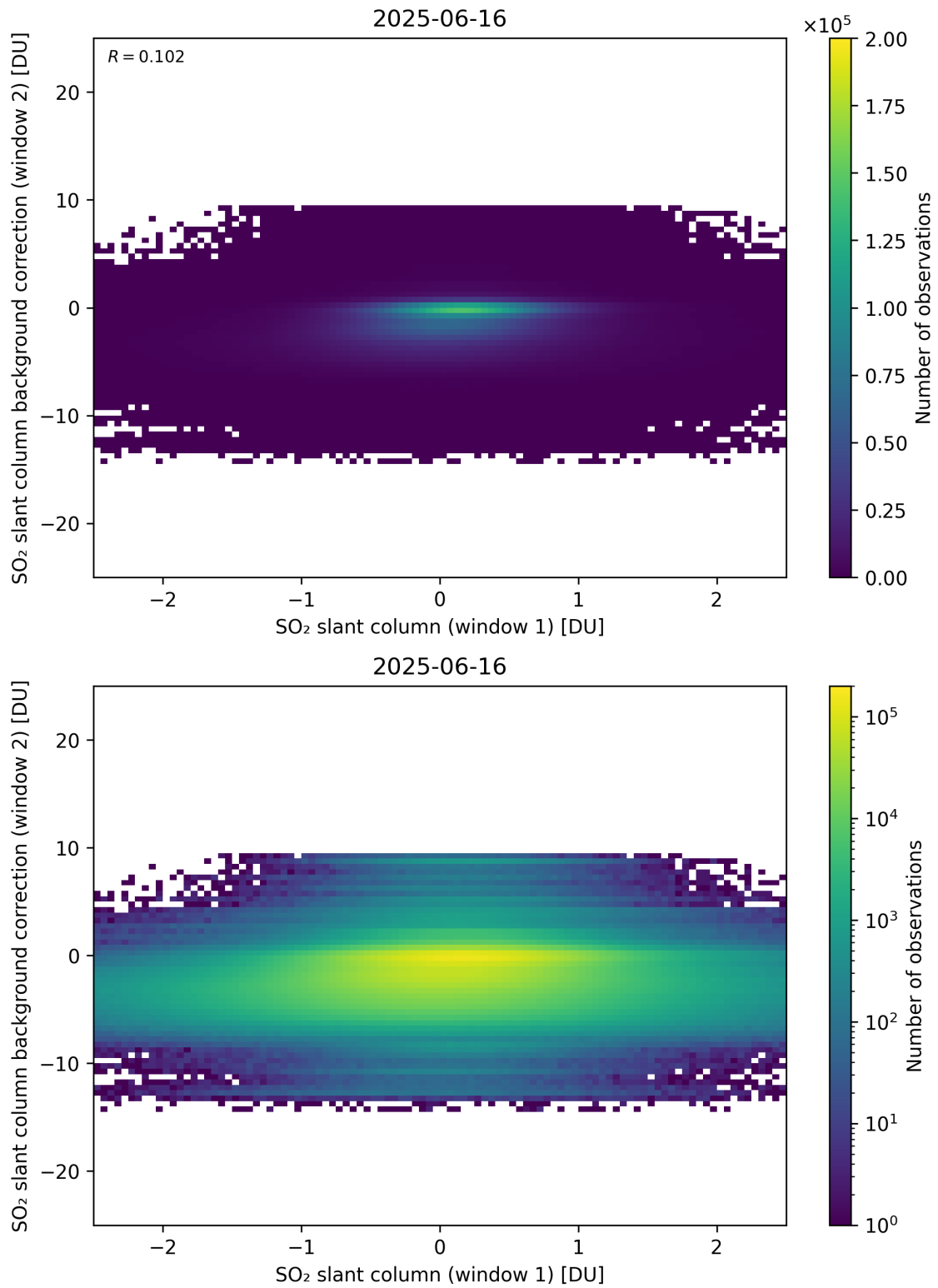
Figure 263: Scatter density plot of “SO 2 slant column (window 1)” against “SO 2 slant column background correction (window 2)” for 2025-06-16 to 2025-06-17.
