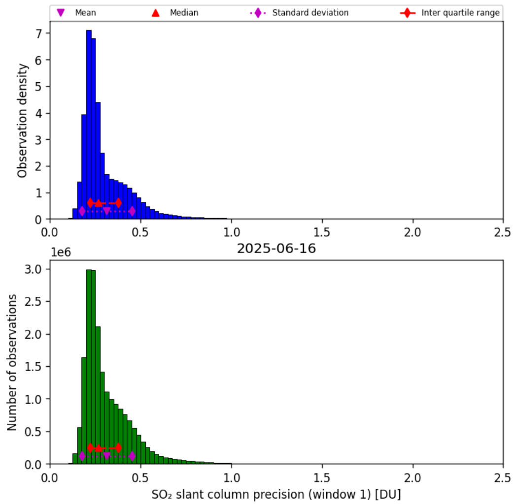
Figure 64: Histogram of “SO 2 slant column precision (window 1)” for 2025-06-16 to 2025-06-17
