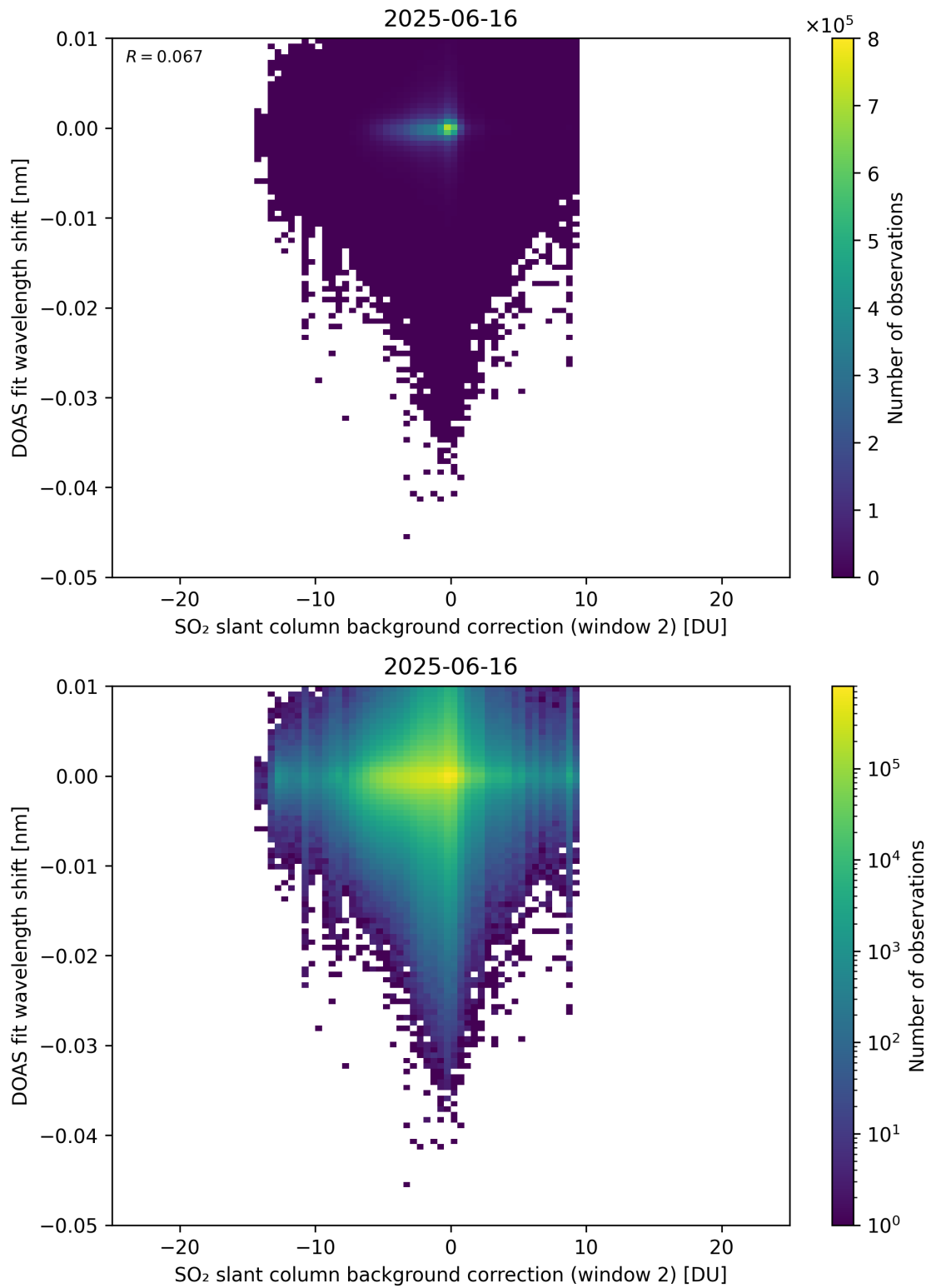
Figure 123: Scatter density plot of “SO 2 slant column background correction (window 2)” against “DOAS fit wavelength shift” for 2025-06-16 to 2025-06-17.
