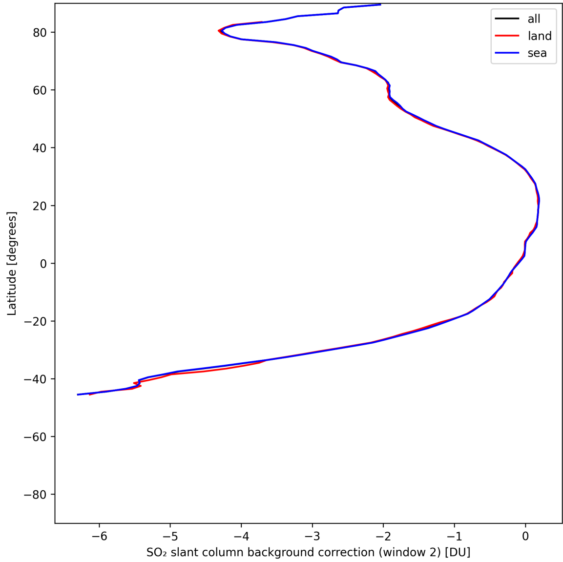
Figure 44: Zonal average of “SO 2 slant column background correction (window 2)” for 2025-06-16 to 2025-06-17.
