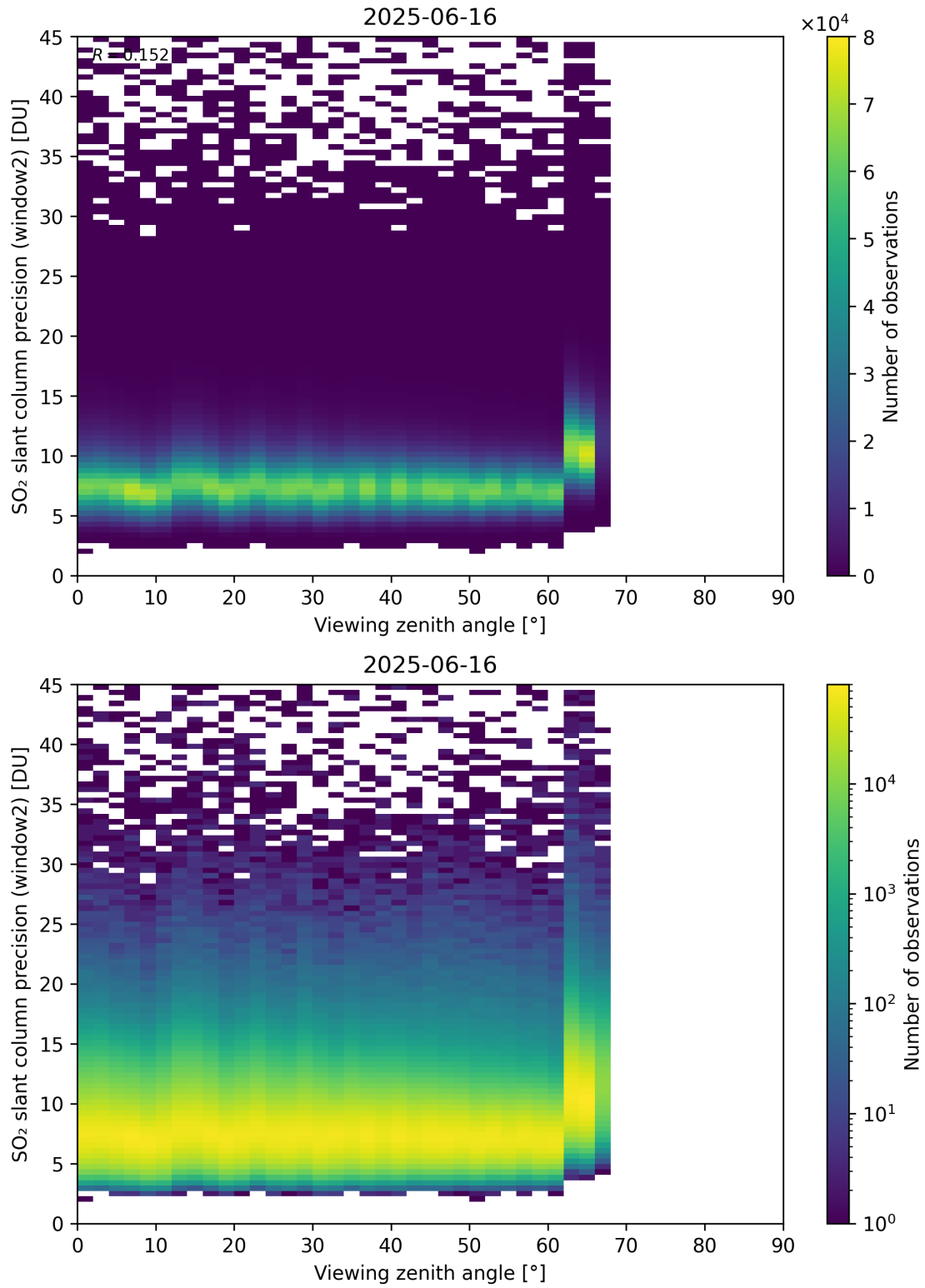
Figure 378: Scatter density plot of “Viewing zenith angle” against “SO 2 slant column precision (window2)” for 2025-06-16 to 2025-06-17.
