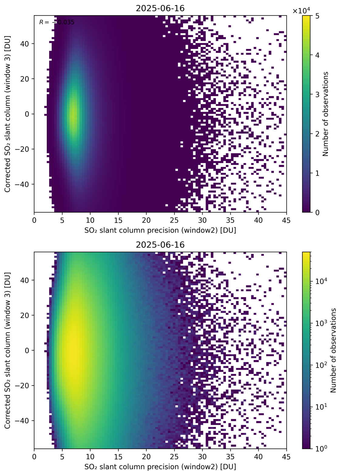
Figure 298: Scatter density plot of “SO 2 slant column precision (window2)” against “Corrected SO 2 slant column (window 3)” for 2025-06-16 to 2025-06-17.
