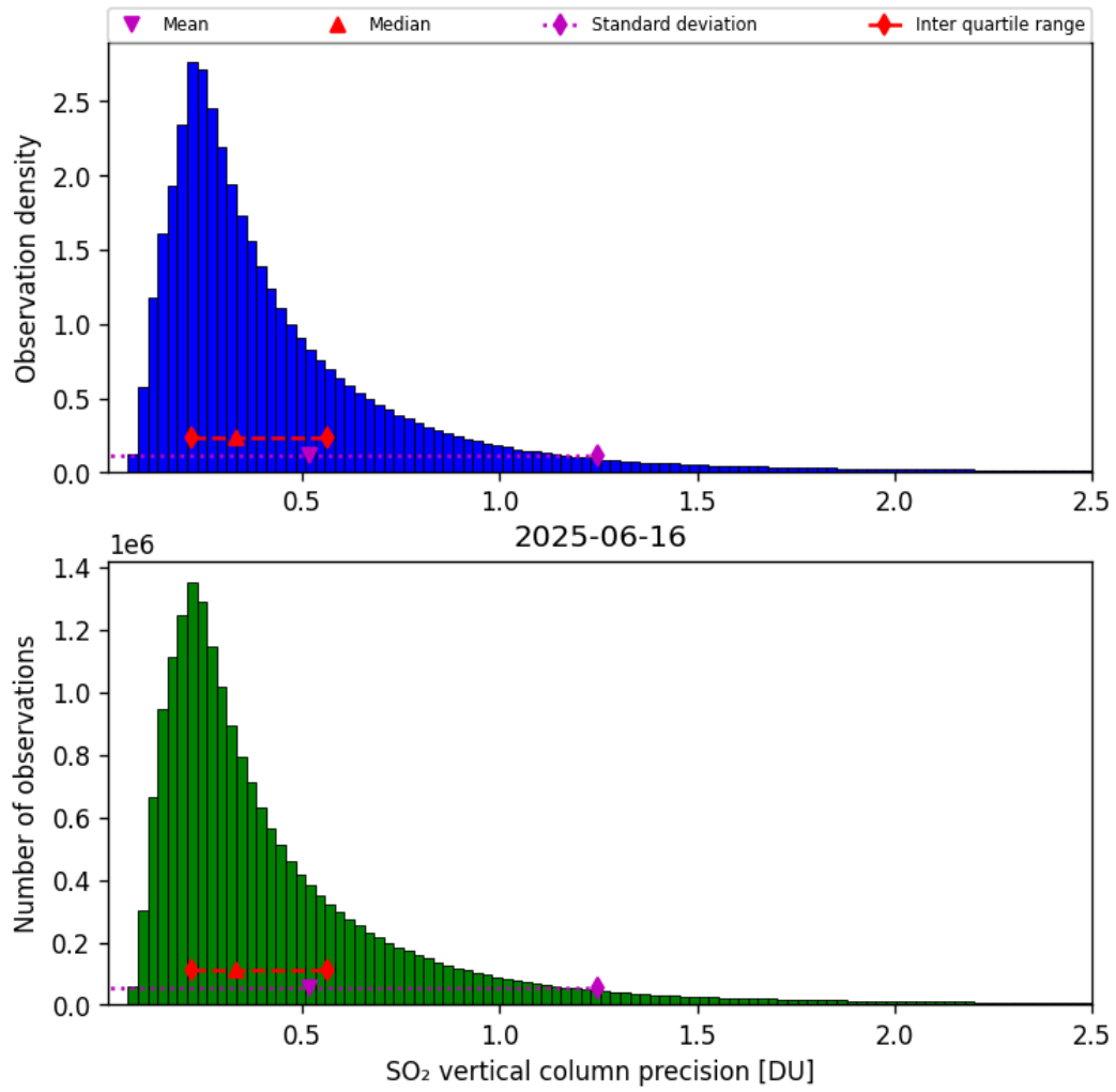
Figure 59: Histogram of “SO 2 vertical column precision” for 2025-06-16 to 2025-06-17
