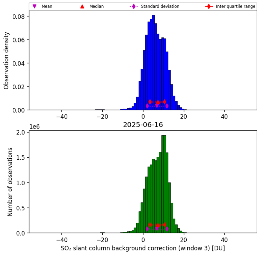
Figure 74: Histogram of “SO 2 slant column background correction (window 3)” for 2025-06-16 to 2025-06-17
