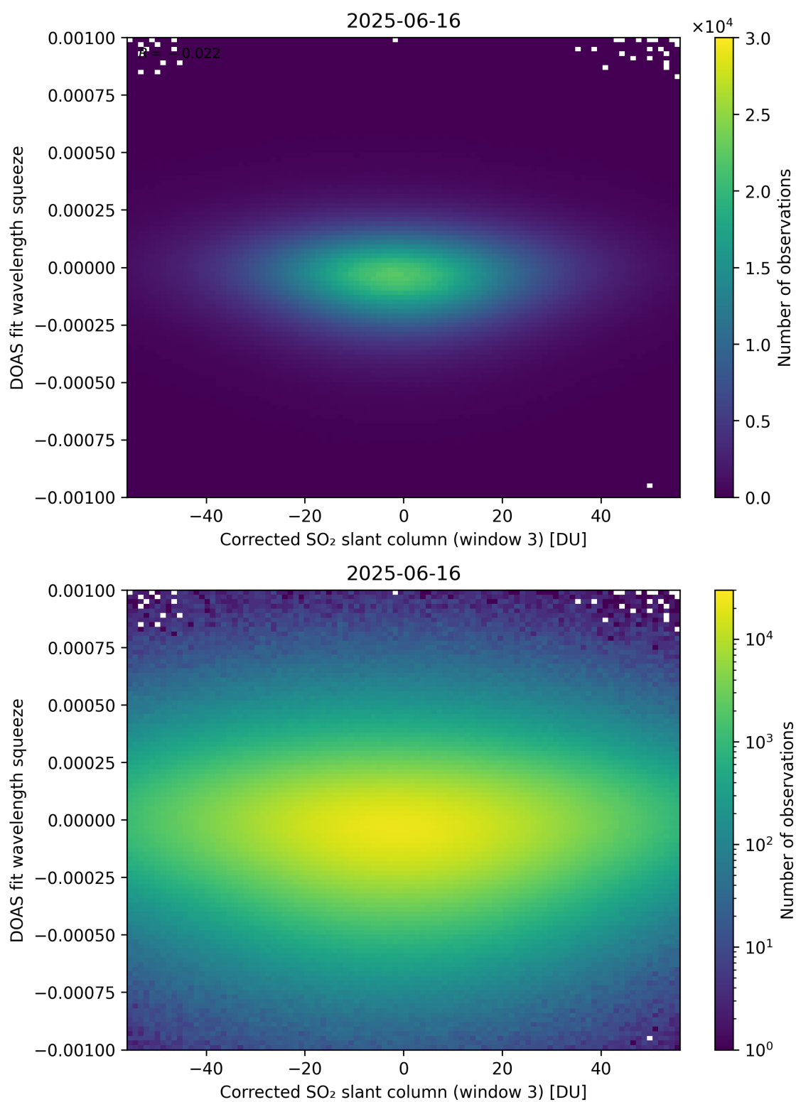
Figure 257: Scatter density plot of “Corrected SO 2 slant column (window 3)” against “DOAS fit wavelength squeeze” for 2025-06-16 to 2025-06-17.
