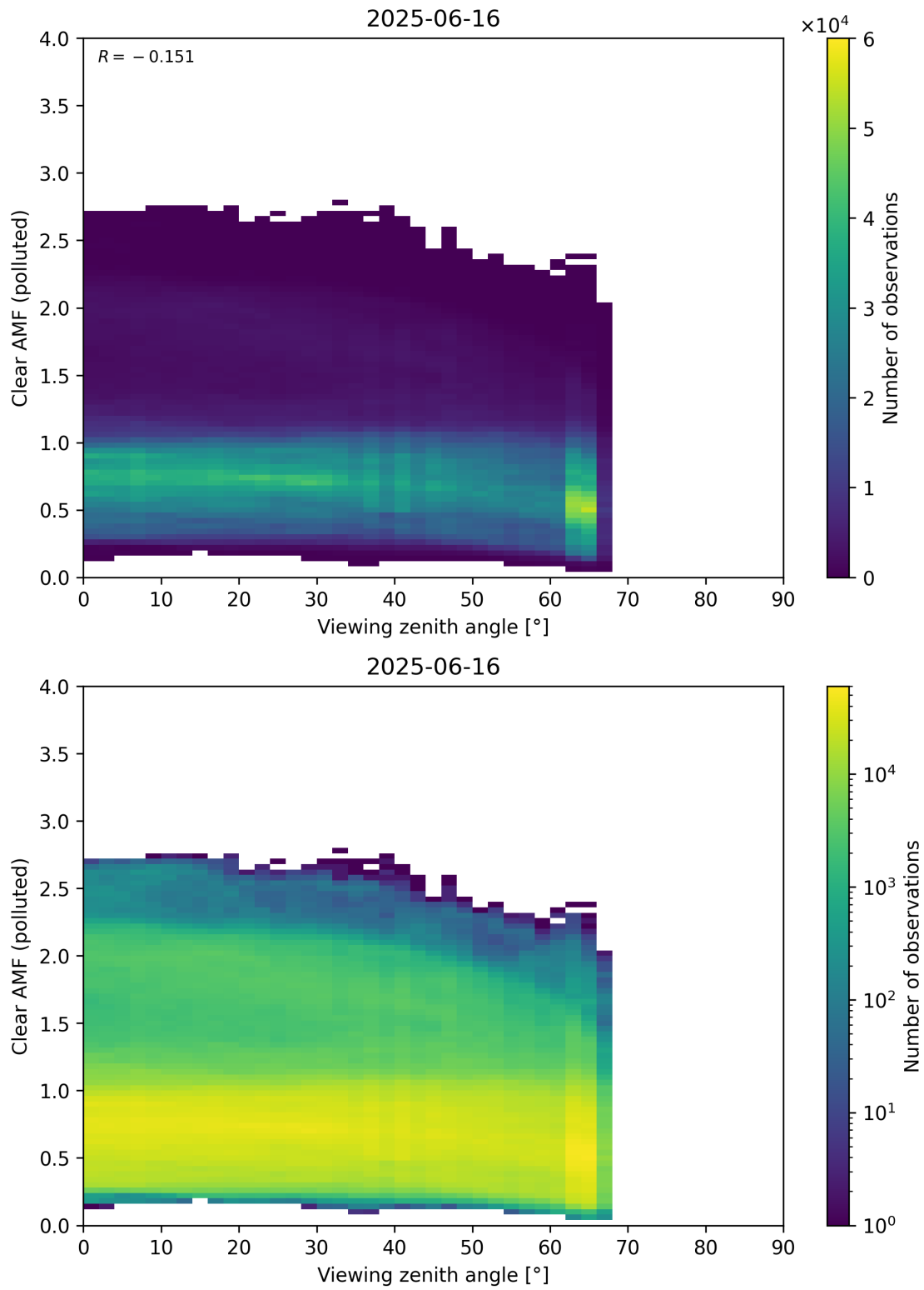
Figure 370: Scatter density plot of “Viewing zenith angle” against “Clear AMF (polluted)” for 2025-06-16 to 2025-06-17.
