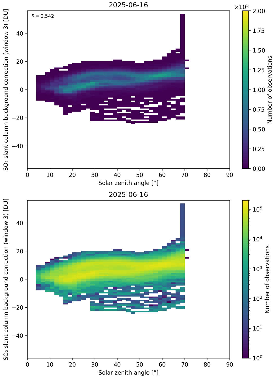
Figure 173: Scatter density plot of “Solar zenith angle” against “SO 2 slant column background correction (window 3)” for 2025-06-16 to 2025-06-17.
