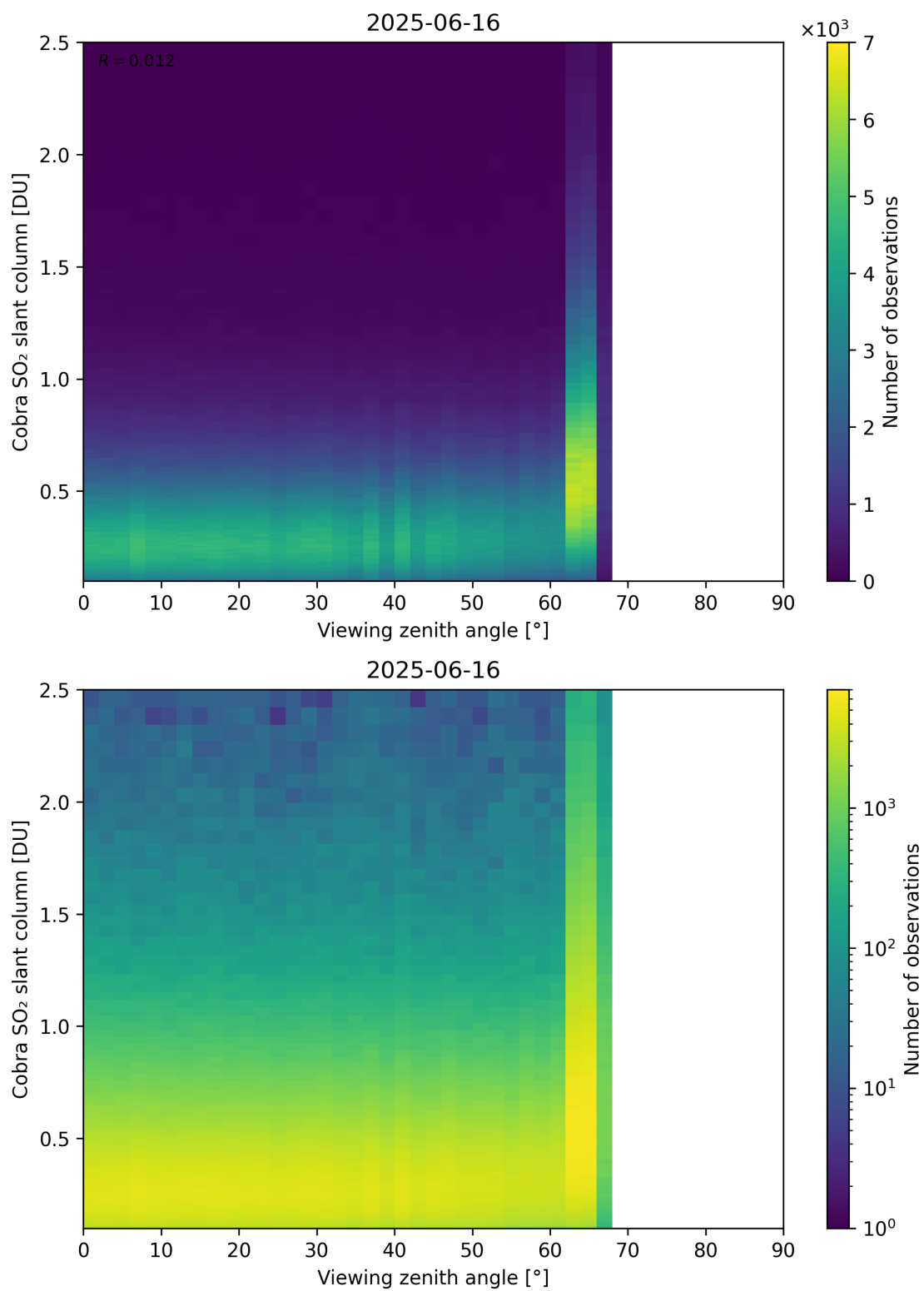
Figure 371: Scatter density plot of “Viewing zenith angle” against “Cobra SO 2 slant column” for 2025-06-16 to 2025-06-17.
