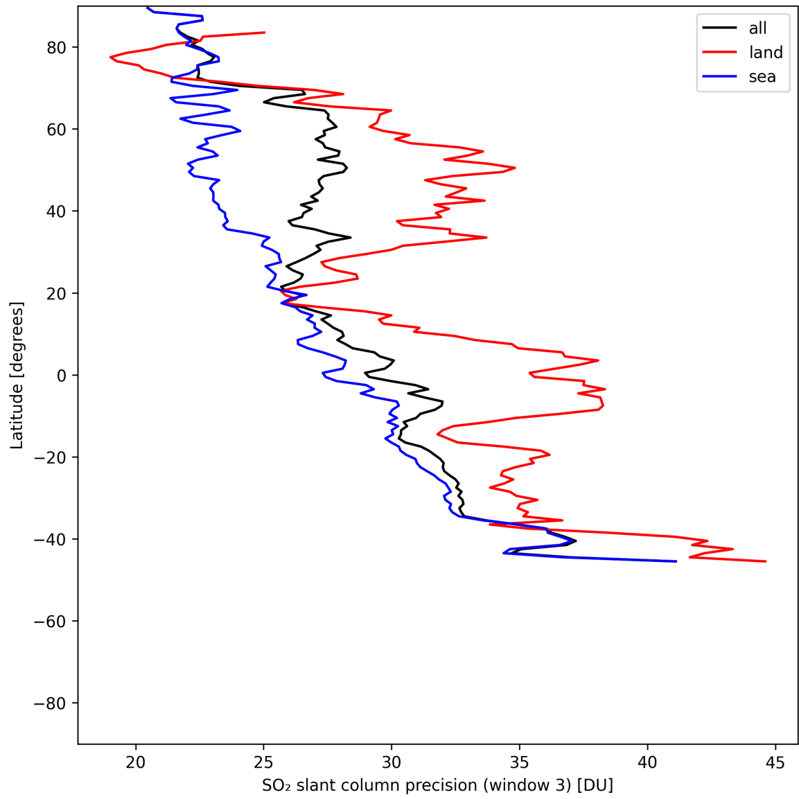
Figure 46: Zonal average of “SO 2 slant column precision (window 3)” for 2025-06-16 to 2025-06-17.
