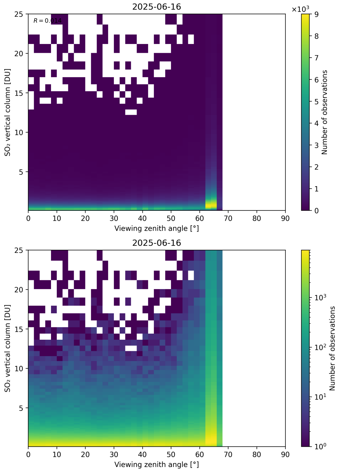
Figure 383: Scatter density plot of “Viewing zenith angle” against “SO 2 vertical column” for 2025-06-16 to 2025-06-17.
