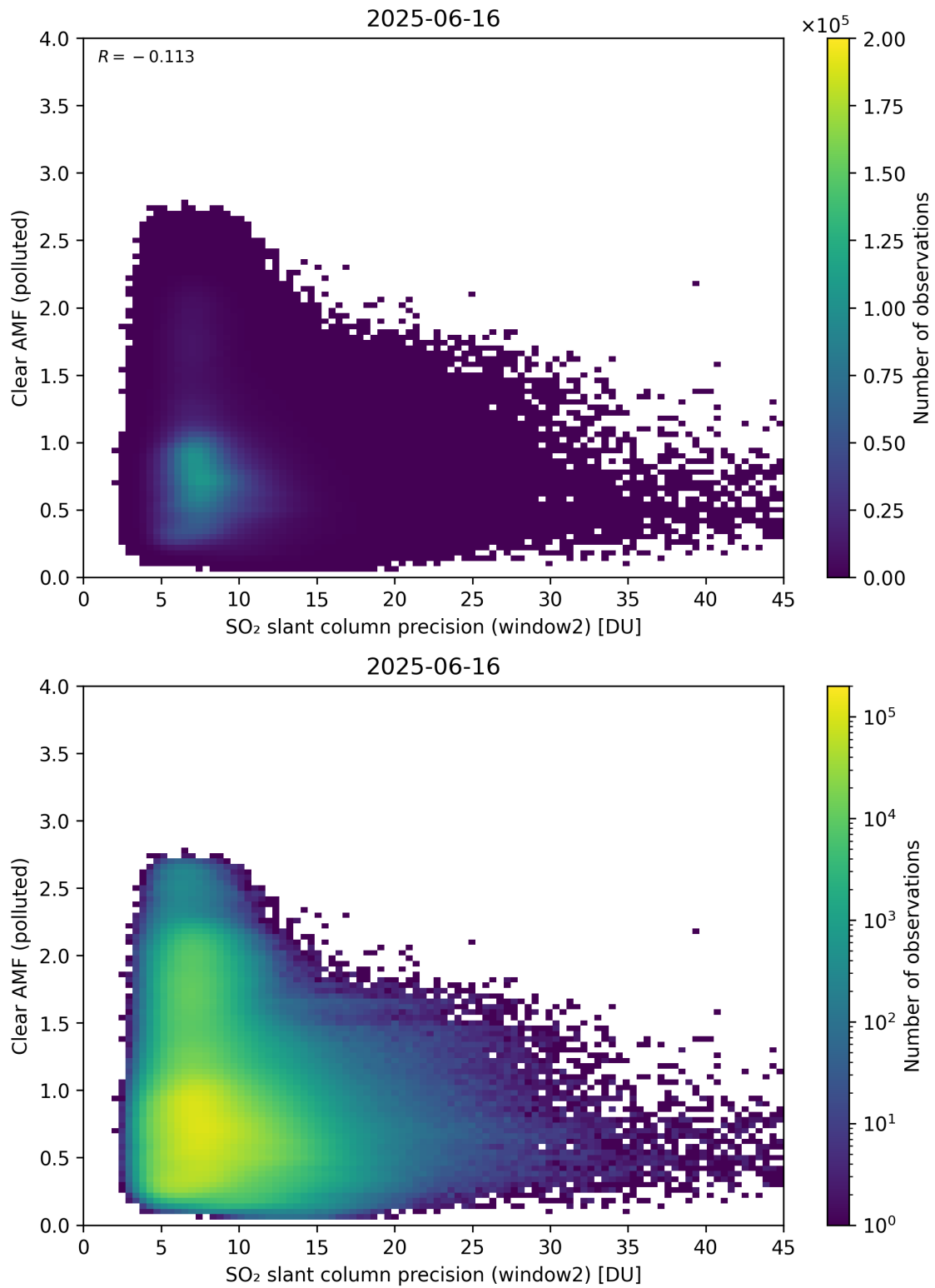
Figure 296: Scatter density plot of “SO 2 slant column precision (window2)” against “Clear AMF (polluted)” for 2025-06-16 to 2025-06-17.
