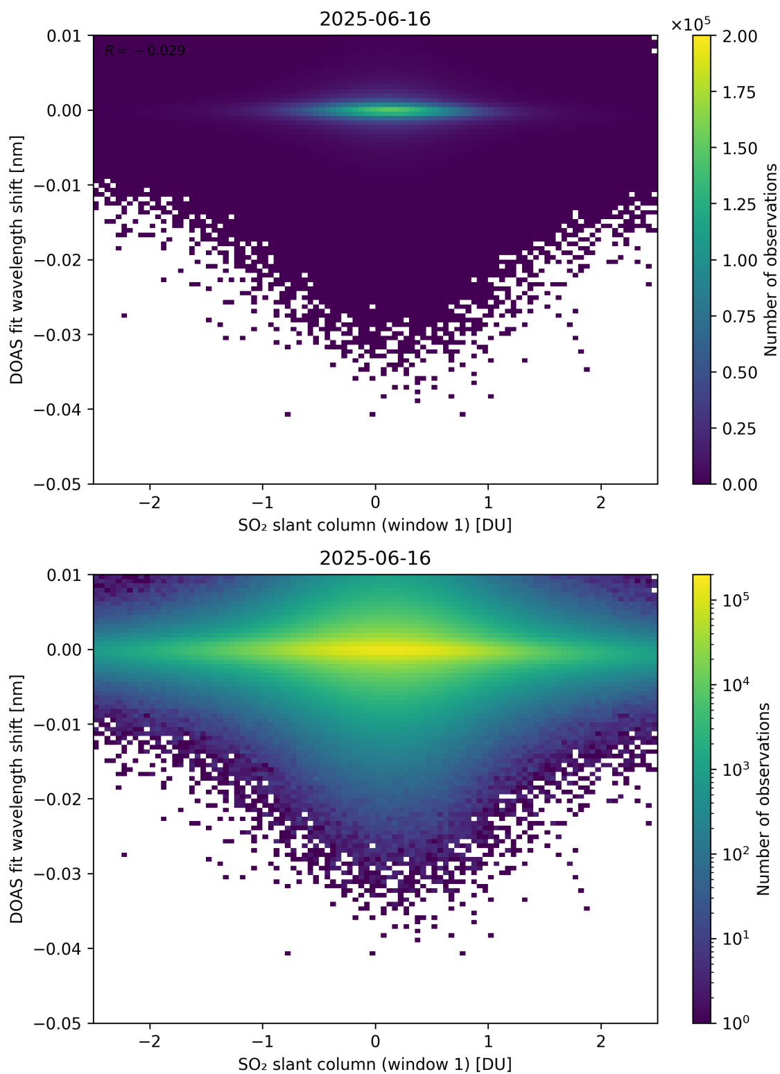
Figure 265: Scatter density plot of “SO 2 slant column (window 1)” against “DOAS fit wavelength shift” for 2025-06-16 to 2025-06-17.
