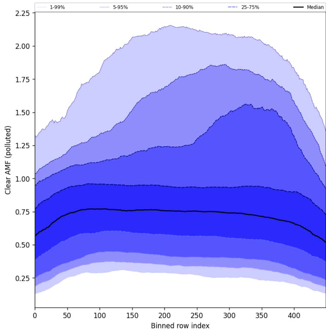
Figure 107: Along track statistics of “Clear AMF (polluted)” for 2025-06-16 to 2025-06-17
