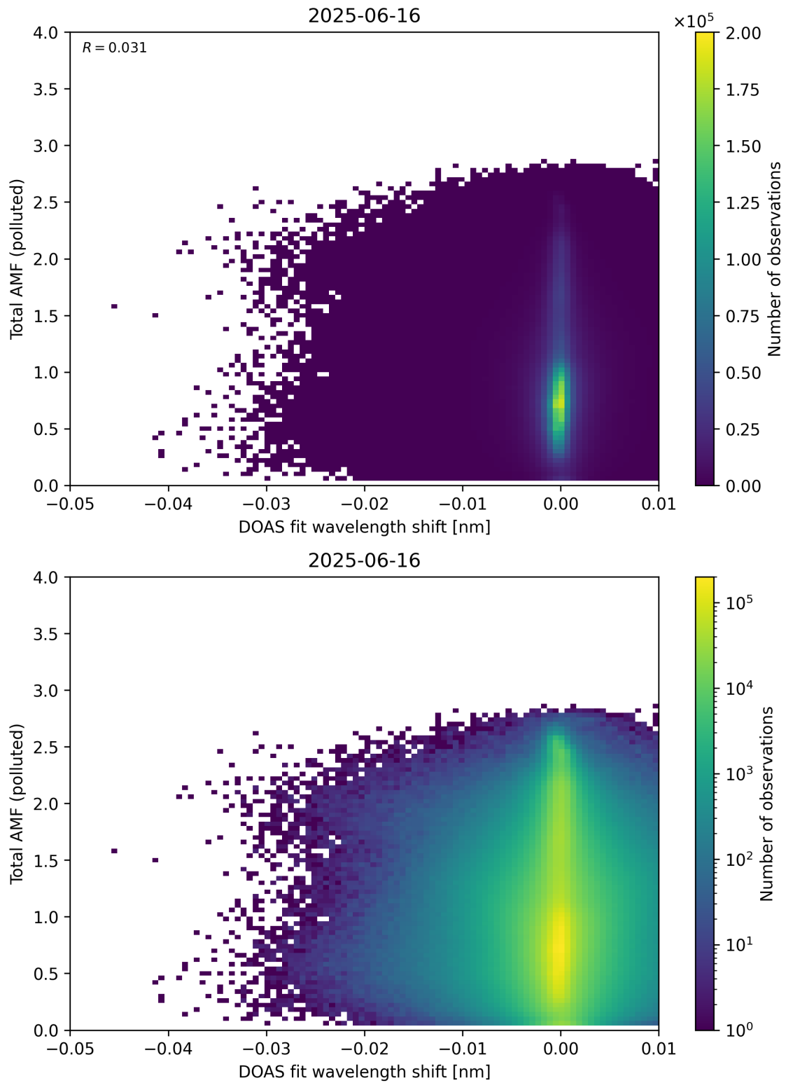
Figure 141: Scatter density plot of “DOAS fit wavelength shift” against “Total AMF (polluted)” for 2025-06-16 to 2025-06-17.
