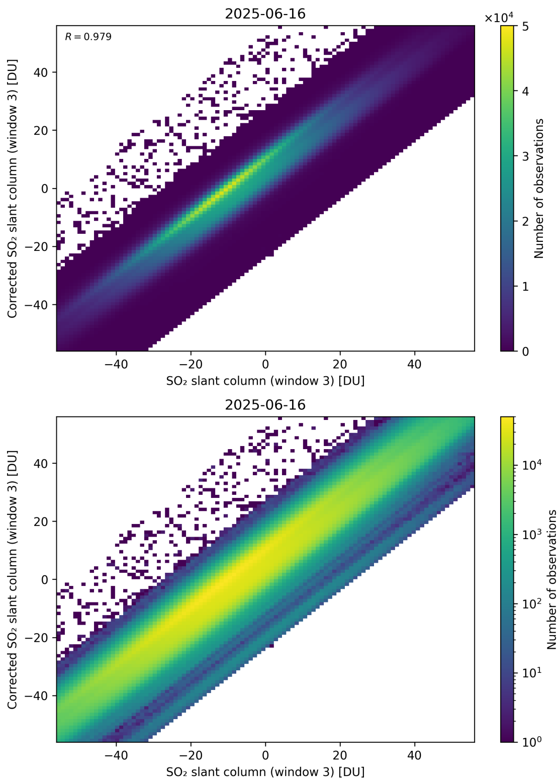
Figure 316: Scatter density plot of “SO 2 slant column (window 3)” against “Corrected SO 2 slant column (window 3)” for 2025-06-16 to 2025-06-17.
