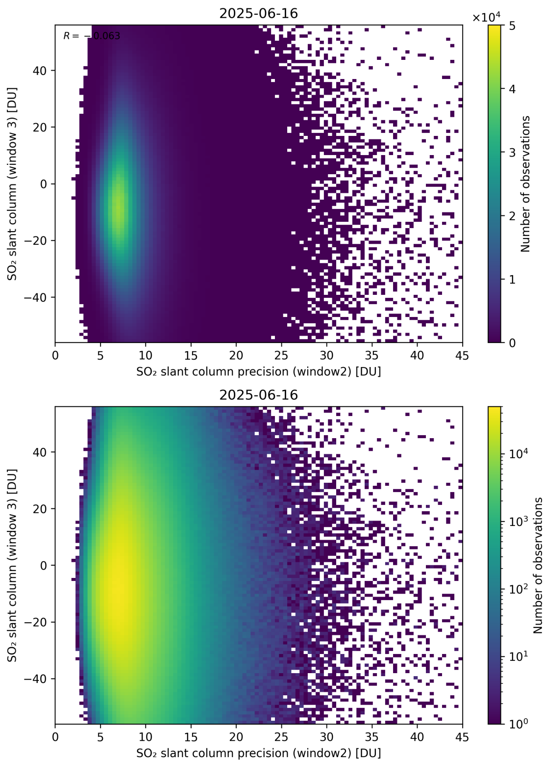
Figure 299: Scatter density plot of “SO 2 slant column precision (window2)” against “SO 2 slant column (window 3)” for 2025-06-16 to 2025-06-17.
