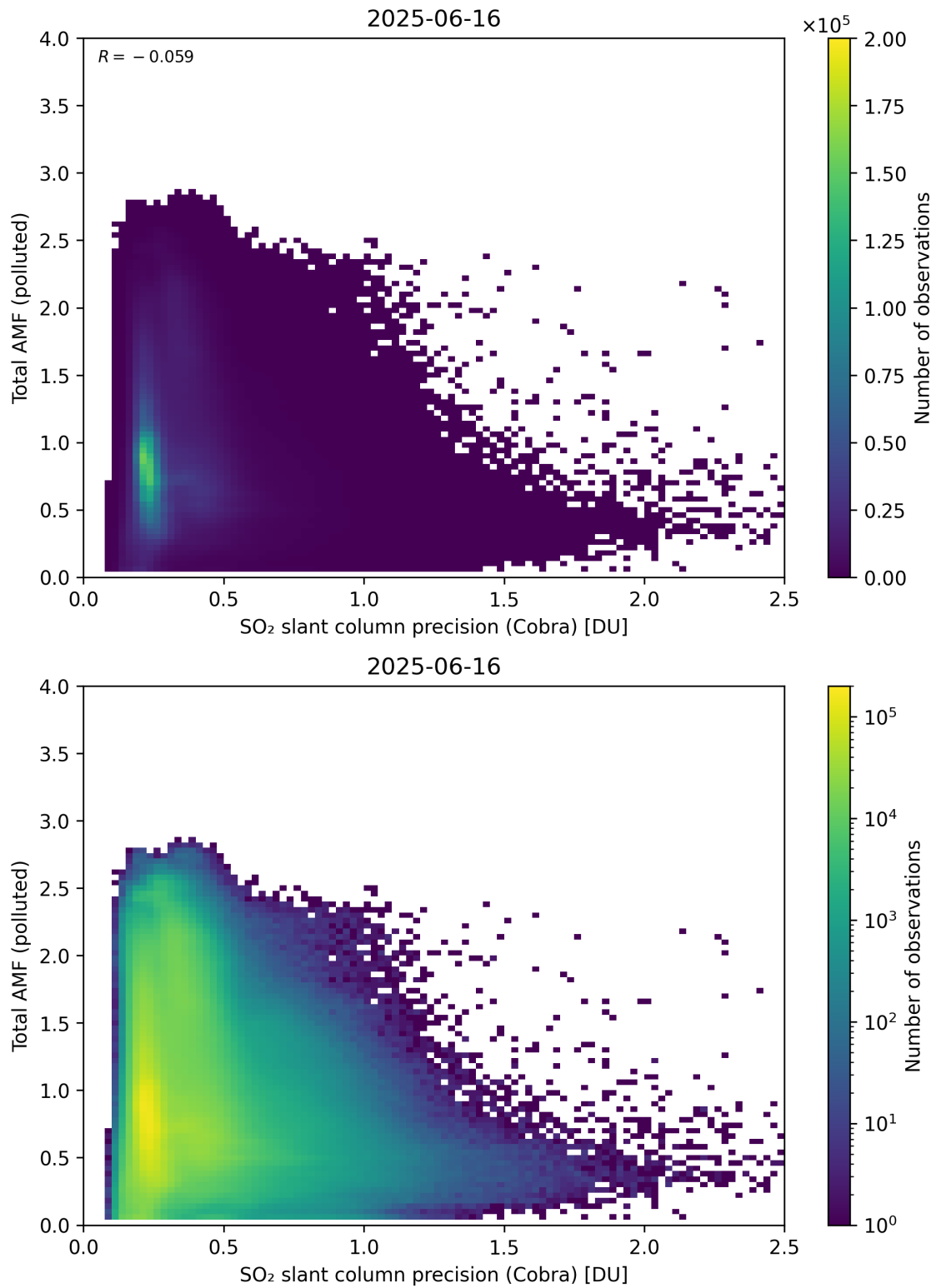
Figure 213: Scatter density plot of “SO 2 slant column precision (Cobra)” against “Total AMF (polluted)” for 2025-06-16 to 2025-06-17.
