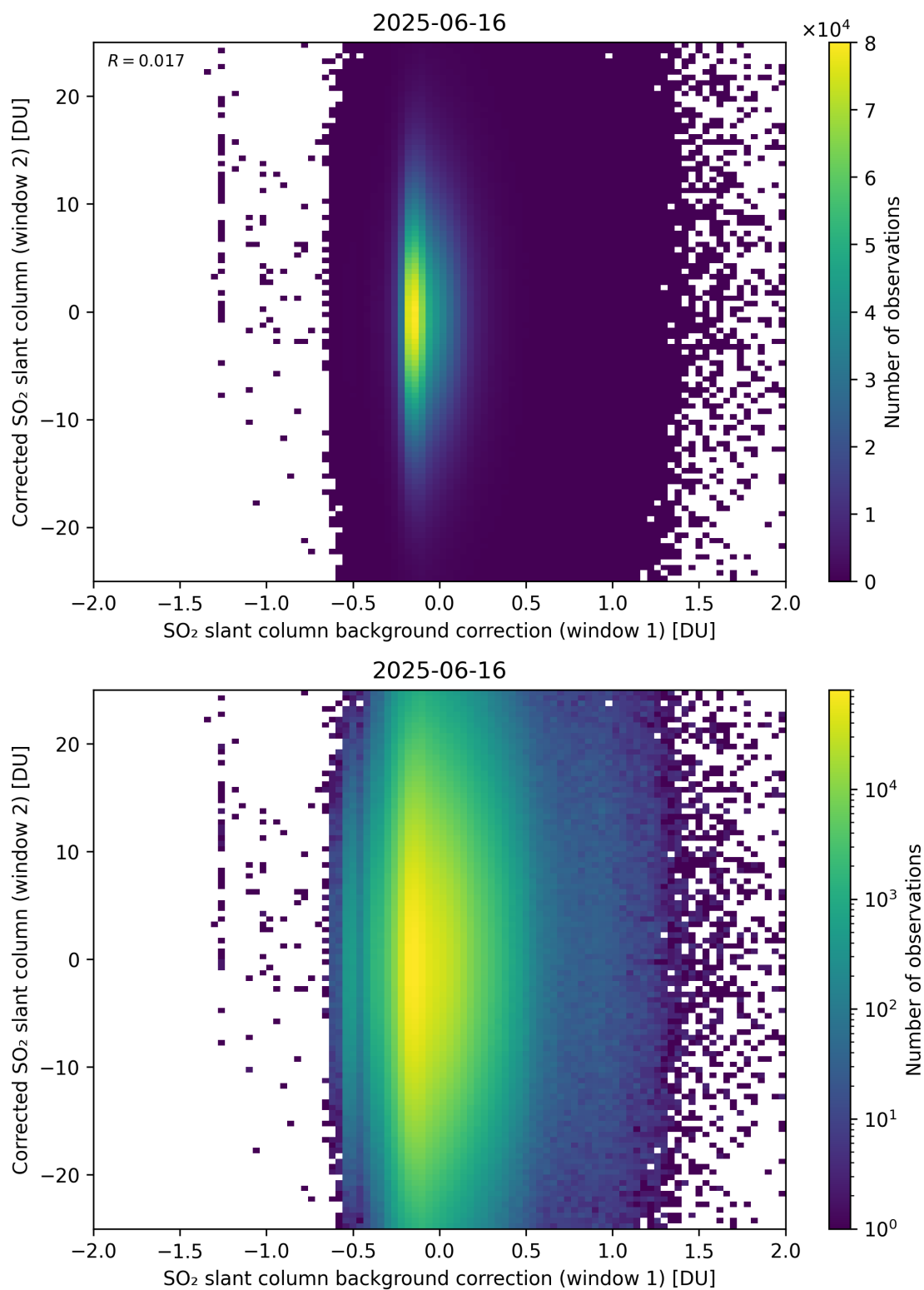
Figure 115: Scatter density plot of “SO 2 slant column background correction (window 1)” against “Corrected SO 2 slant column (window 2)” for 2025-06-16 to 2025-06-17.
