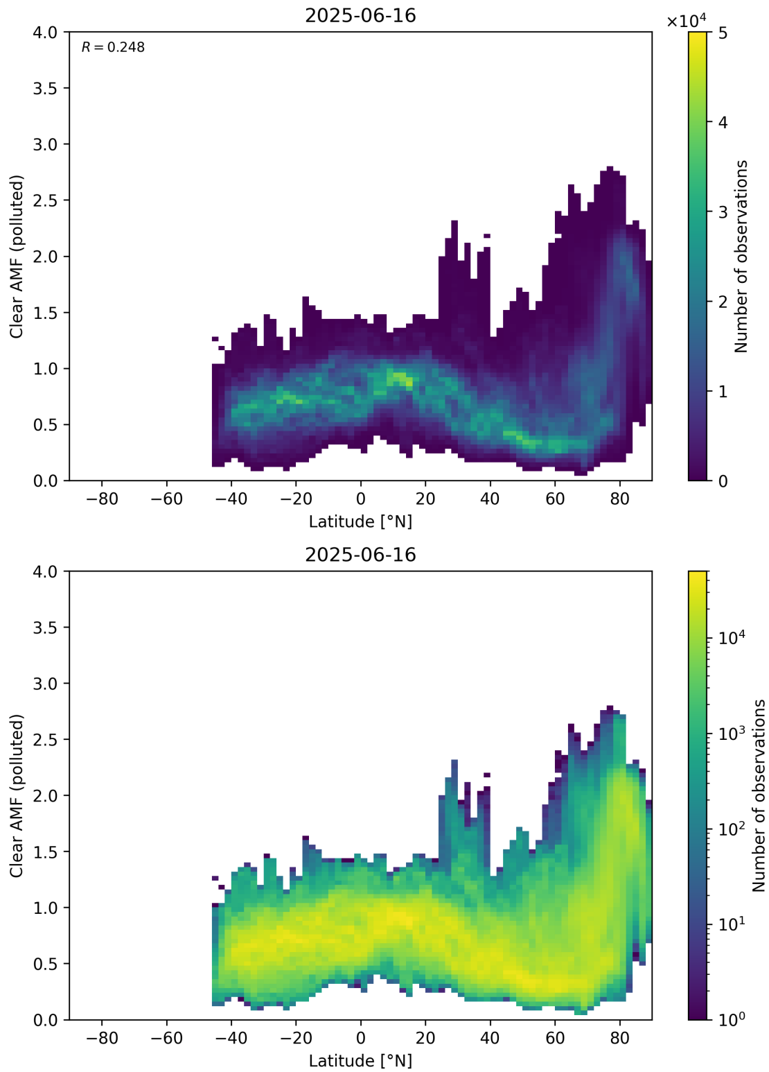
Figure 156: Scatter density plot of “Latitude” against “Clear AMF (polluted)” for 2025-06-16 to 2025-06-17.
