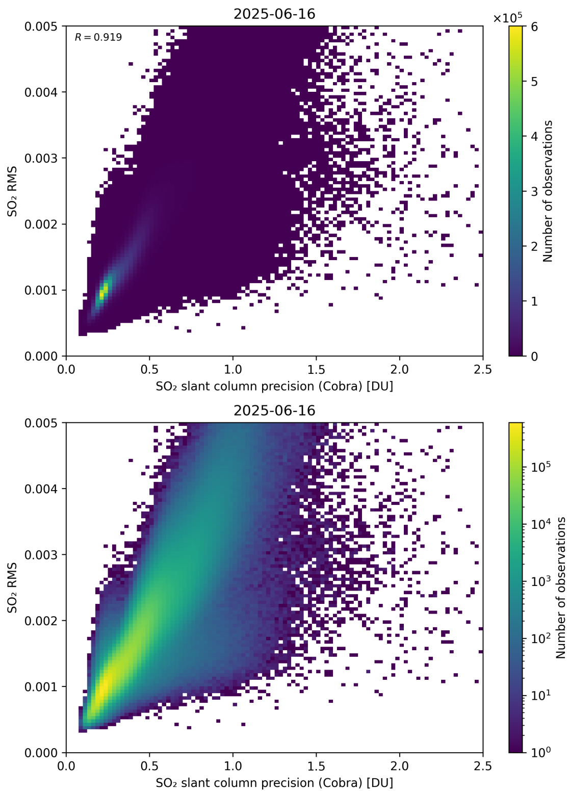
Figure 204: Scatter density plot of “SO 2 slant column precision (Cobra)” against “SO 2 RMS” for 2025-06-16 to 2025-06-17.
