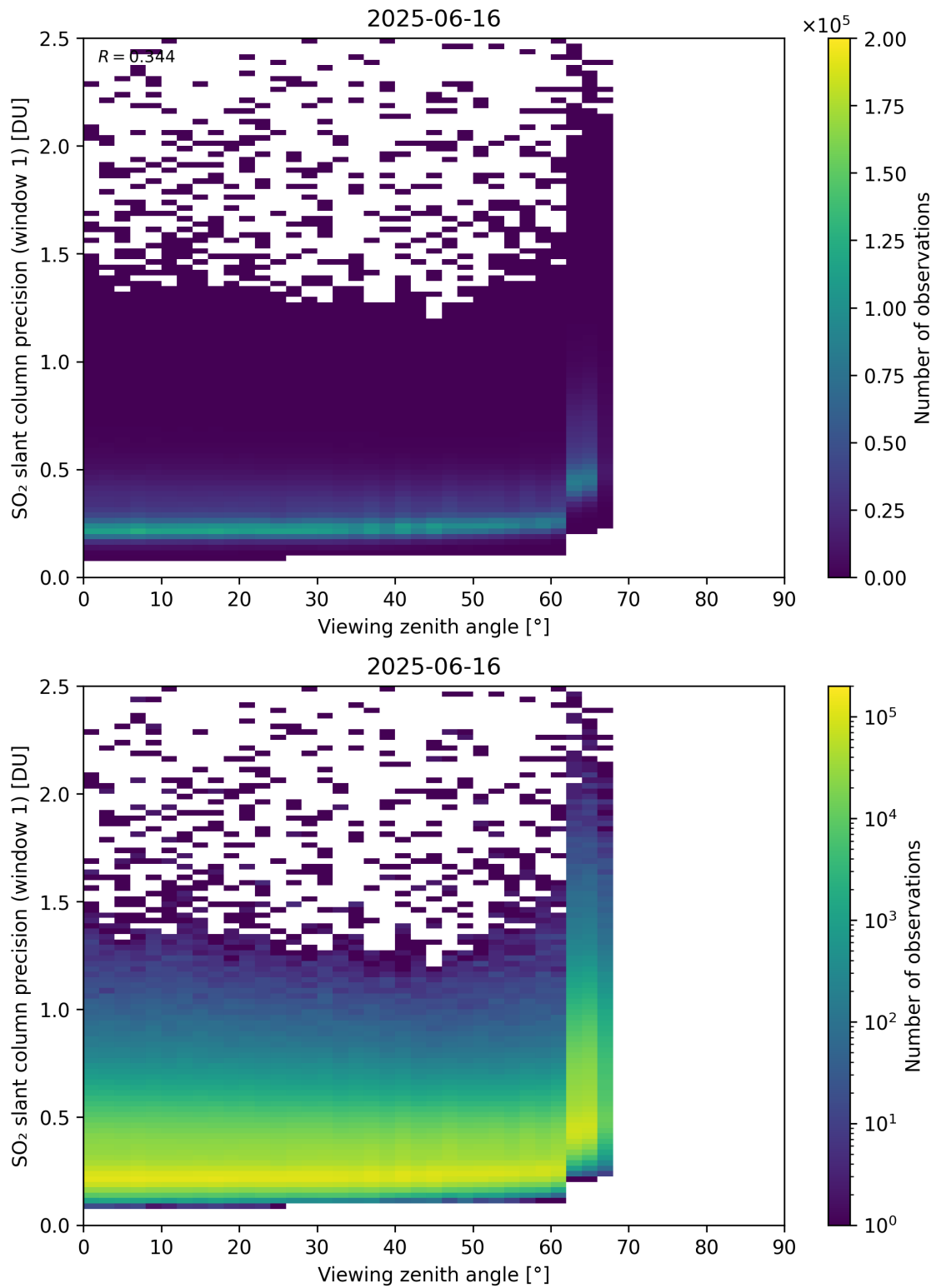
Figure 377: Scatter density plot of “Viewing zenith angle” against “SO 2 slant column precision (window 1)” for 2025-06-16 to 2025-06-17.
