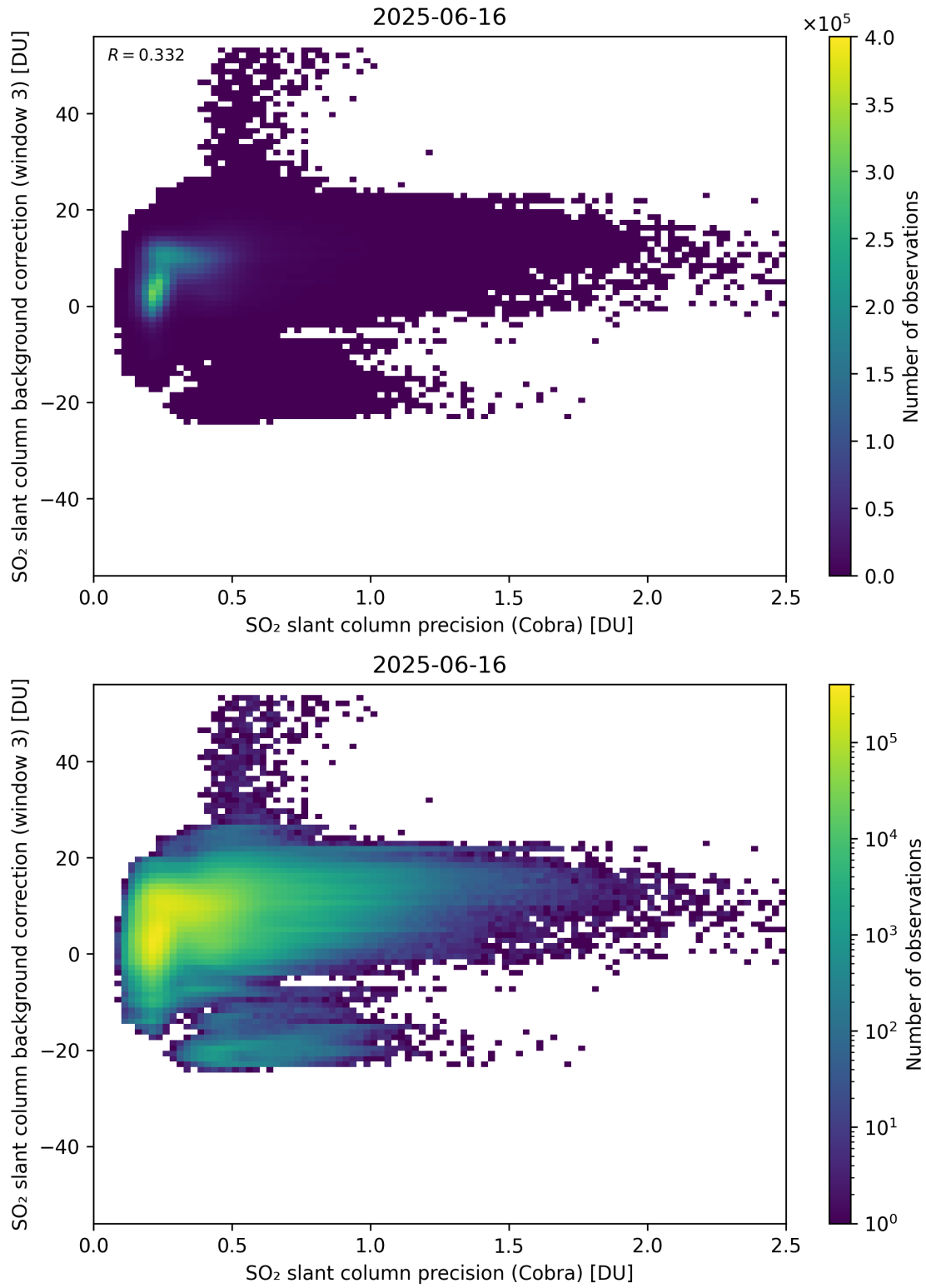
Figure 201: Scatter density plot of “SO 2 slant column precision (Cobra)” against “SO 2 slant column background correction (window 3)” for 2025-06-16 to 2025-06-17.
