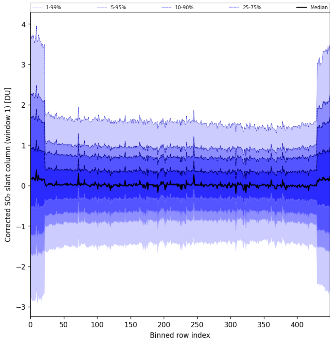
Figure 91: Along track statistics of “Corrected SO 2 slant column (window 1)” for 2025-06-16 to 2025-06-17
