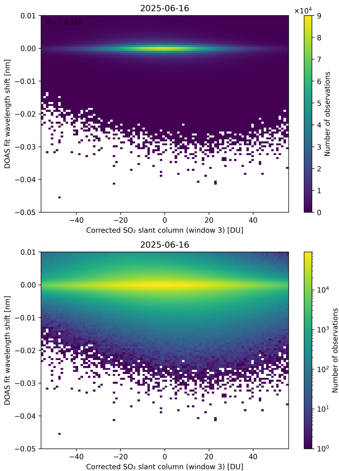
Figure 256: Scatter density plot of “Corrected SO 2 slant column (window 3)” against “DOAS fit wavelength shift” for 2025-06-16 to 2025-06-17.
