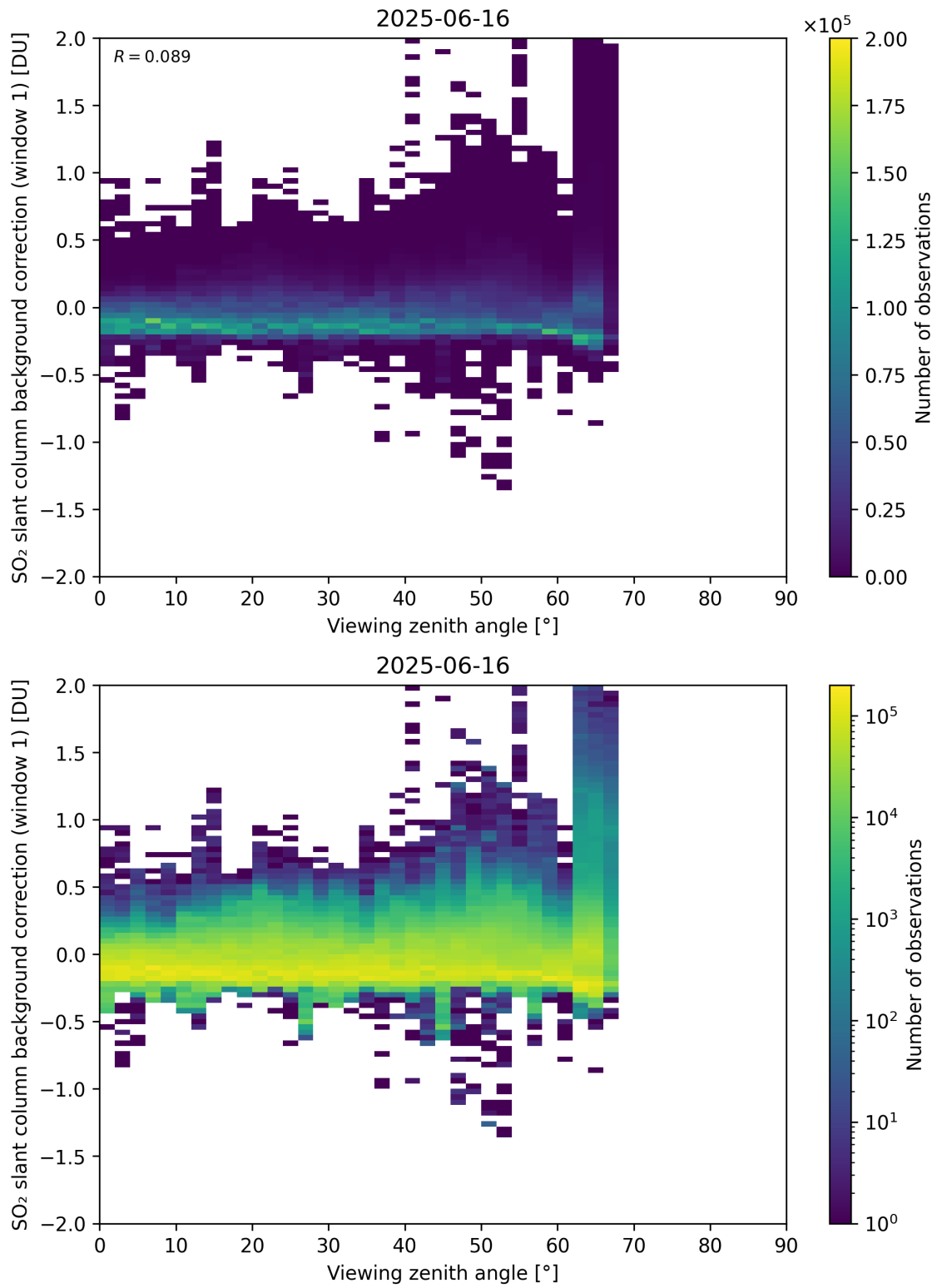
Figure 362: Scatter density plot of “Viewing zenith angle” against “SO 2 slant column background correction (window 1)” for 2025-06-16 to 2025-06-17.
