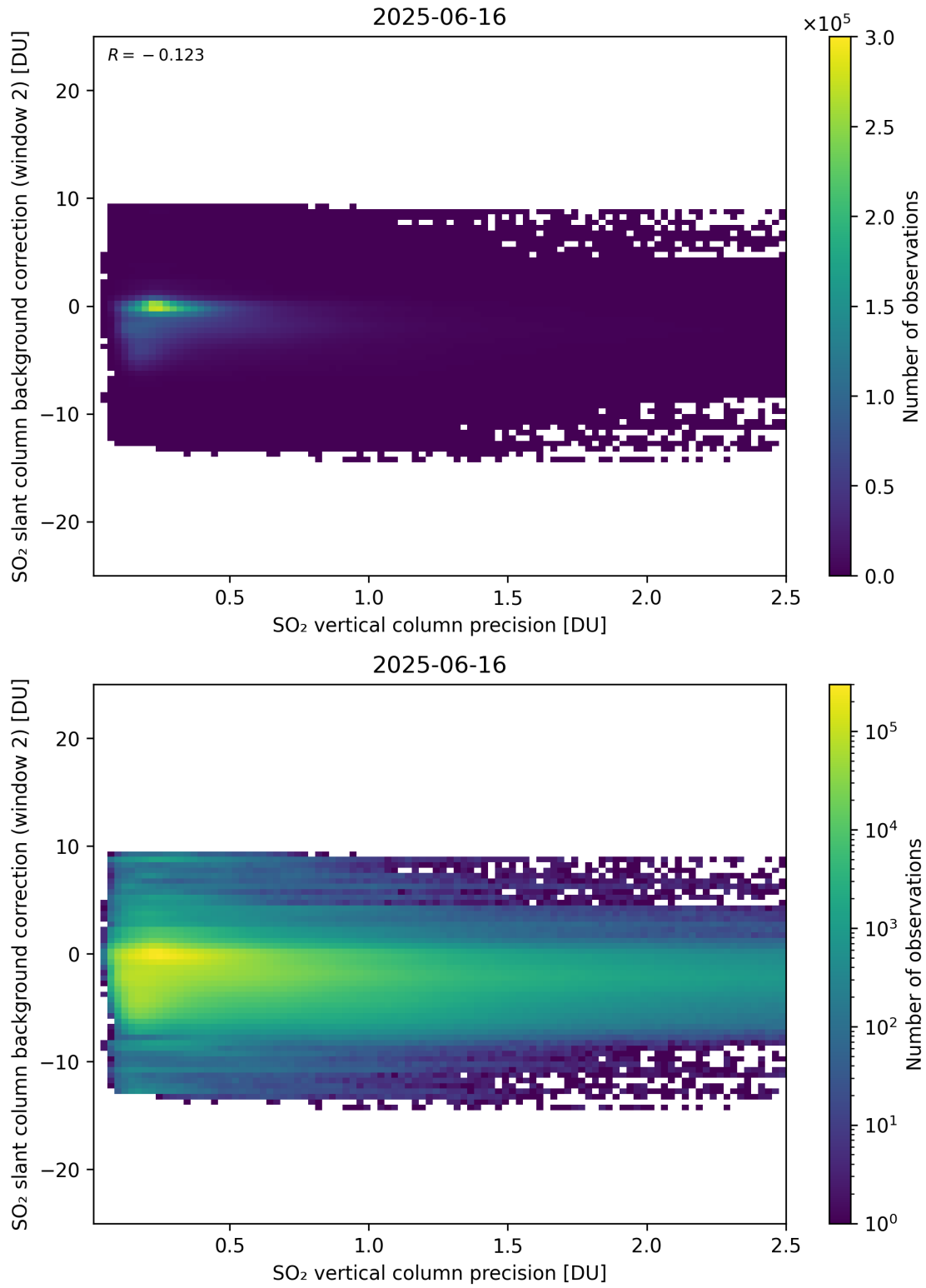
Figure 330: Scatter density plot of “SO 2 vertical column precision” against “SO 2 slant column background correction (window 2)” for 2025-06-16 to 2025-06-17.
