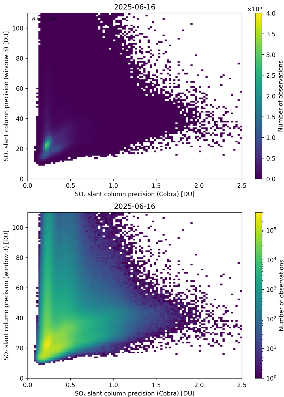
Figure 212: Scatter density plot of “SO 2 slant column precision (Cobra)” against “SO 2 slant column precision (window 3)” for 2025-06-16 to 2025-06-17.
