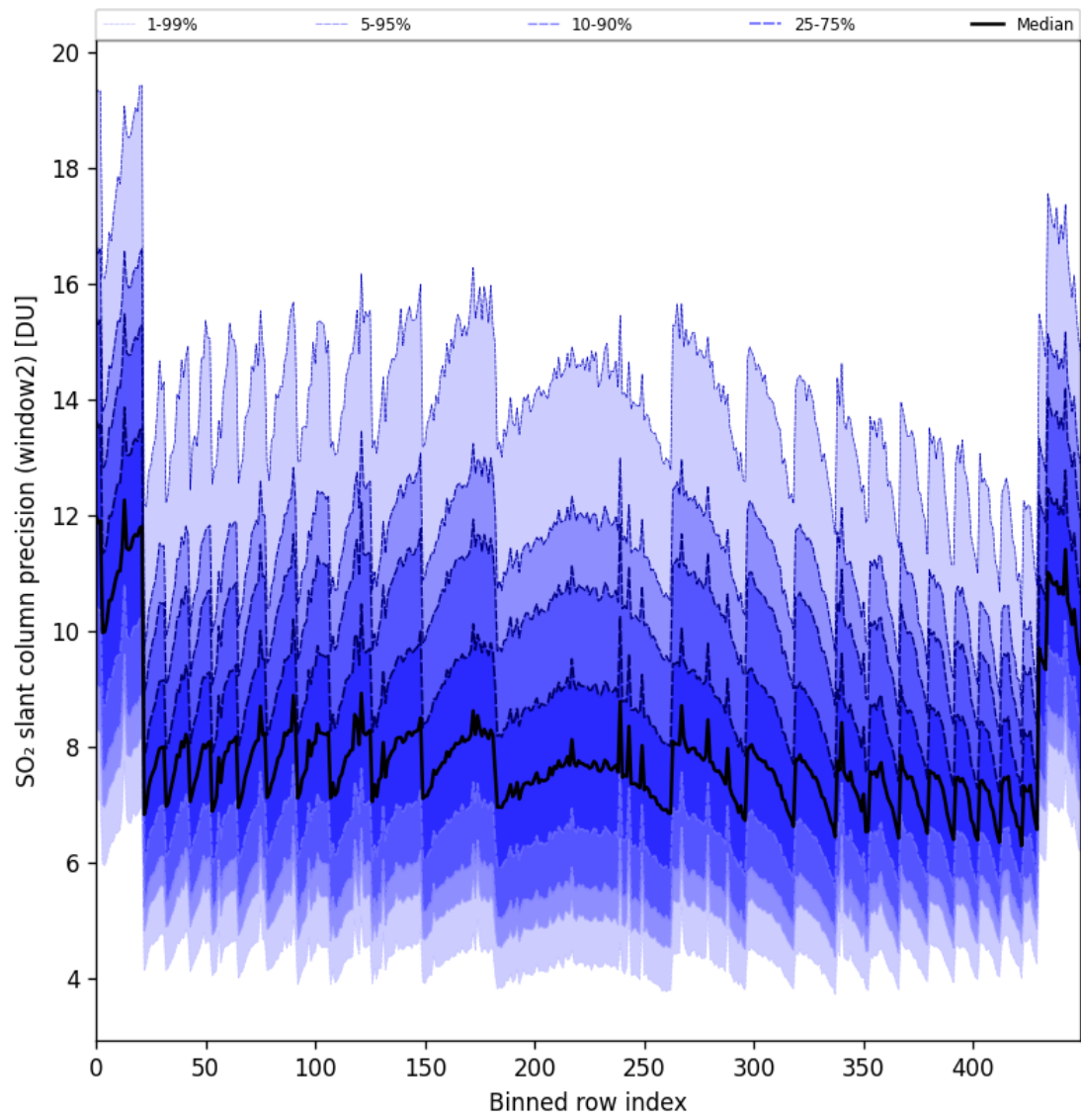
Figure 94: Along track statistics of “SO 2 slant column precision (window2)” for 2025-06-16 to 2025-06-17
