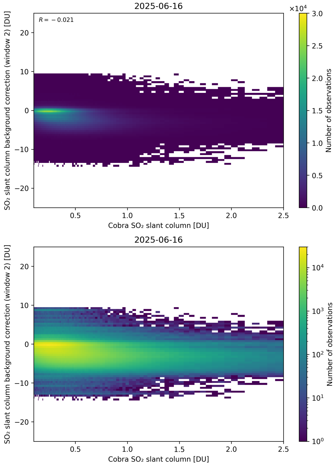
Figure 194: Scatter density plot of “Cobra SO 2 slant column” against “SO 2 slant column background correction (window 2)” for 2025-06-16 to 2025-06-17.
