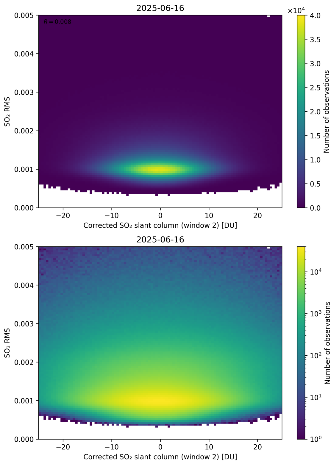
Figure 248: Scatter density plot of “Corrected SO 2 slant column (window 2)” against “SO 2 RMS” for 2025-06-16 to 2025-06-17.
