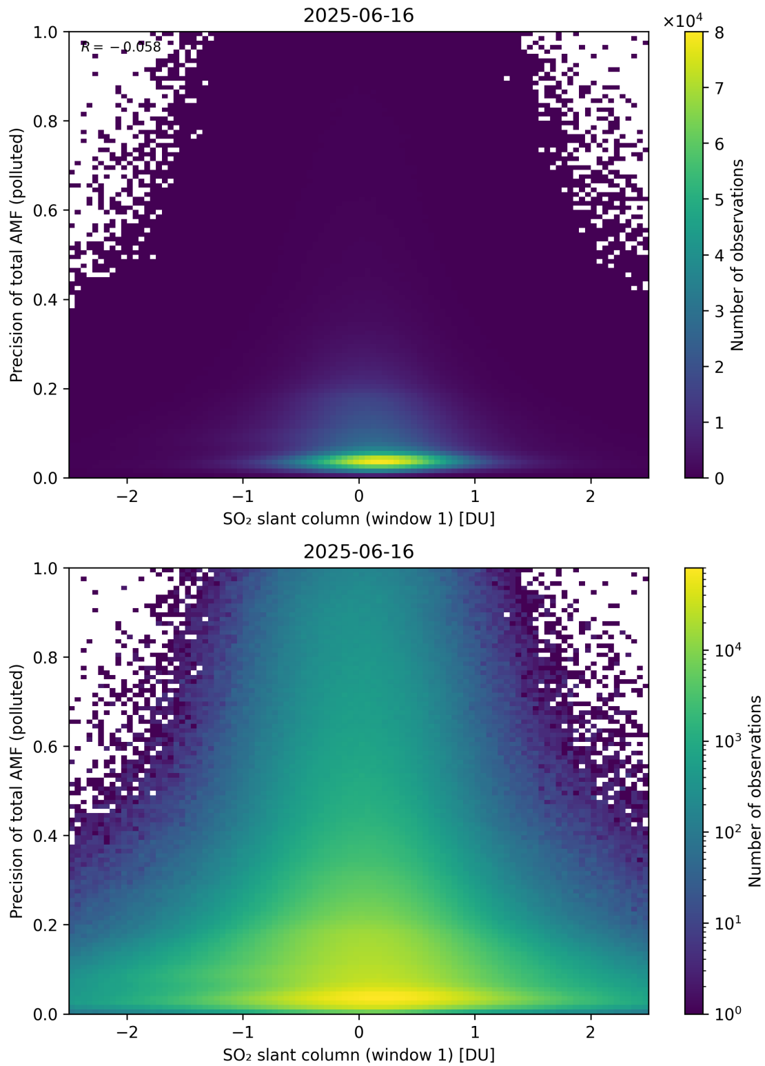
Figure 290: Scatter density plot of “SO 2 slant column (window 1)” against “Precision of total AMF (polluted)” for 2025-06-16 to 2025-06-17.
