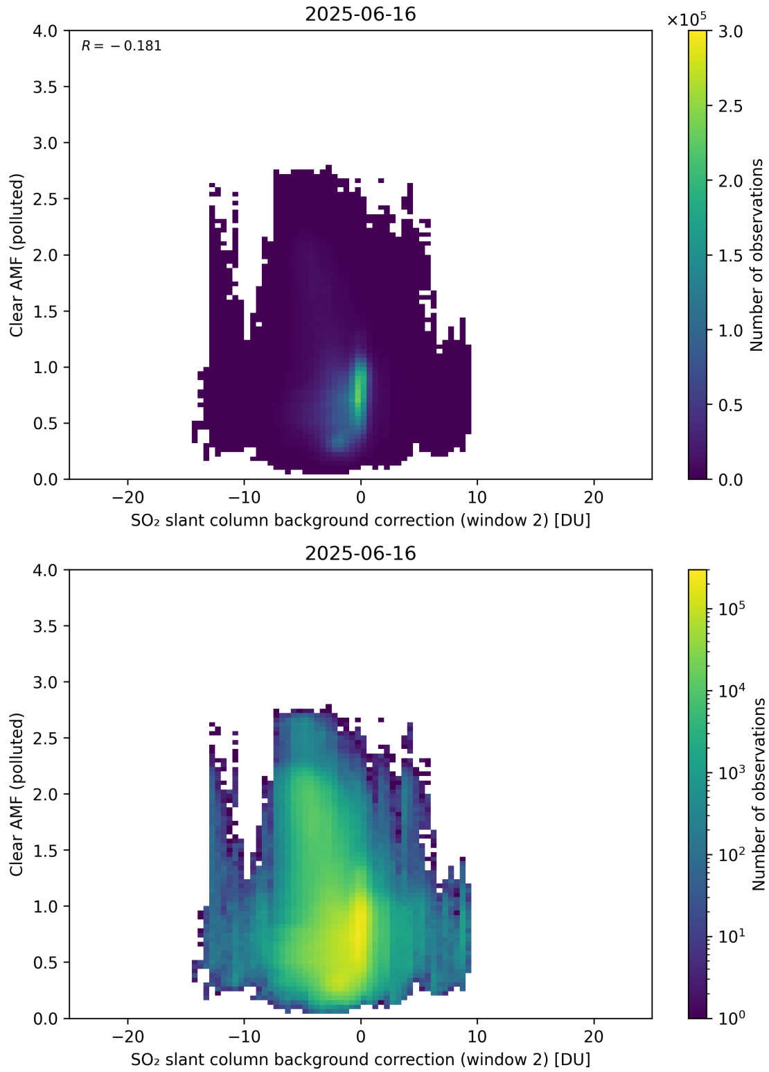
Figure 126: Scatter density plot of “SO 2 slant column background correction (window 2)” against “Clear AMF (polluted)” for 2025-06-16 to 2025-06-17.
