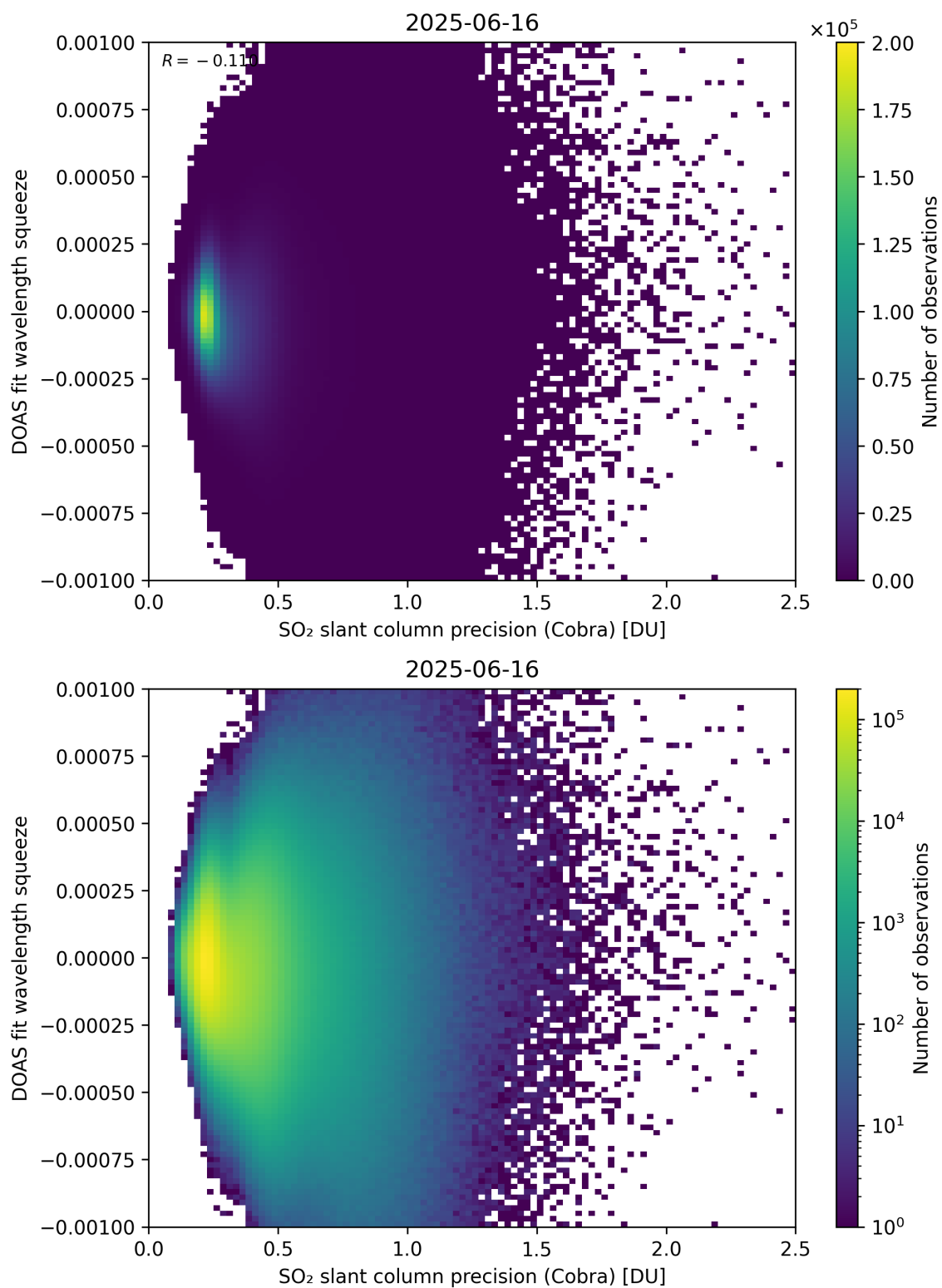
Figure 203: Scatter density plot of “SO 2 slant column precision (Cobra)” against “DOAS fit wavelength squeeze” for 2025-06-16 to 2025-06-17.
