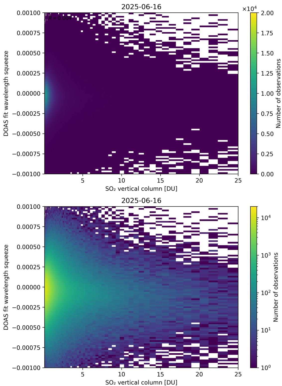
Figure 327: Scatter density plot of “SO 2 vertical column” against “DOAS fit wavelength squeeze” for 2025-06-16 to 2025-06-17.
