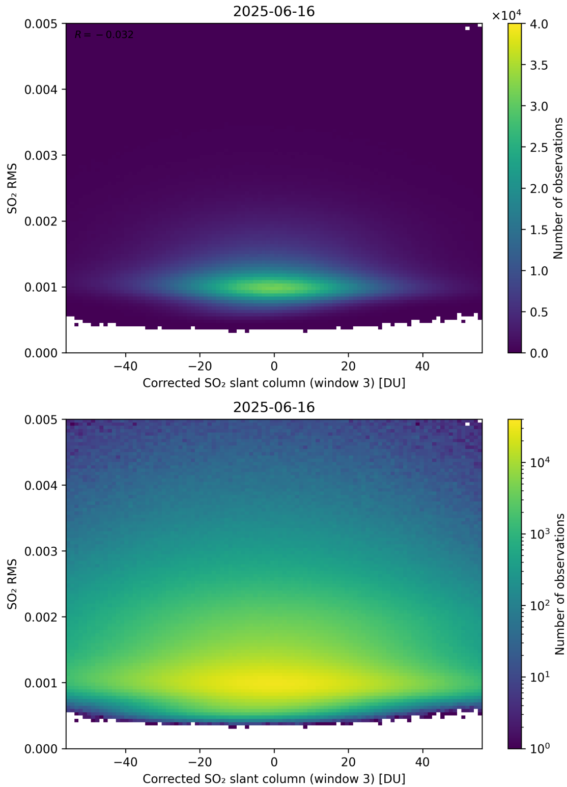
Figure 258: Scatter density plot of “Corrected SO 2 slant column (window 3)” against “SO 2 RMS” for 2025-06-16 to 2025-06-17.
