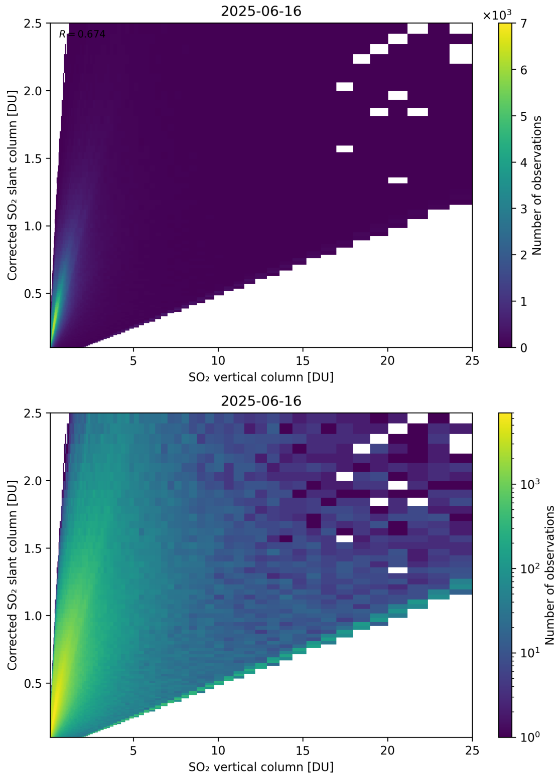
Figure 351: Scatter density plot of “SO 2 vertical column” against “Corrected SO 2 slant column” for 2025-06-16 to 2025-06-17.
