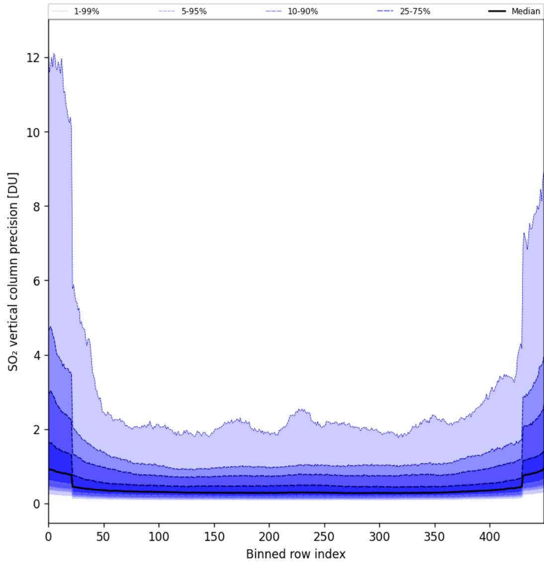
Figure 85: Along track statistics of “SO 2 vertical column precision” for 2025-06-16 to 2025-06-17
