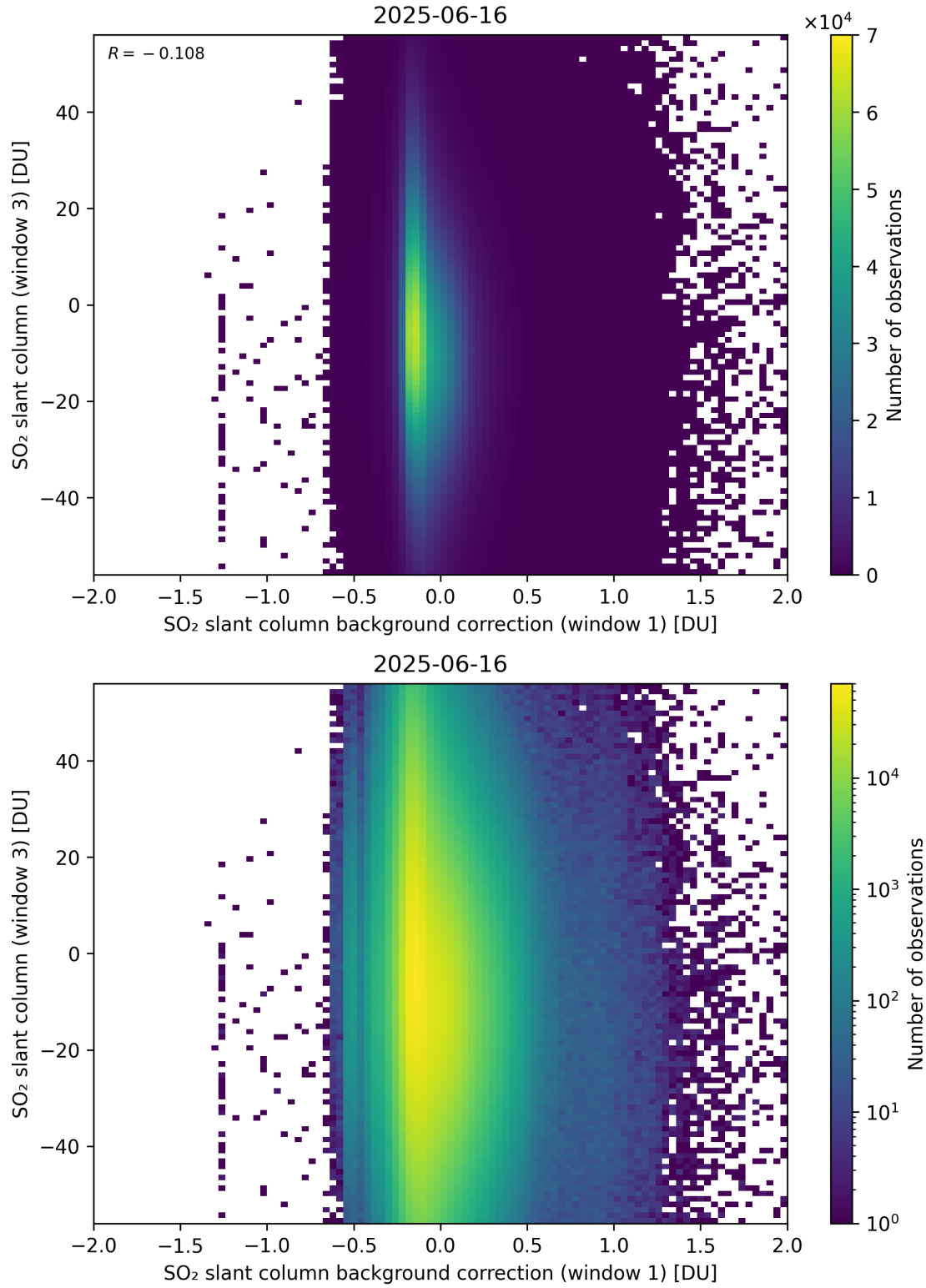
Figure 118: Scatter density plot of “SO 2 slant column background correction (window 1)” against “SO 2 slant column (window 3)” for 2025-06-16 to 2025-06-17.
