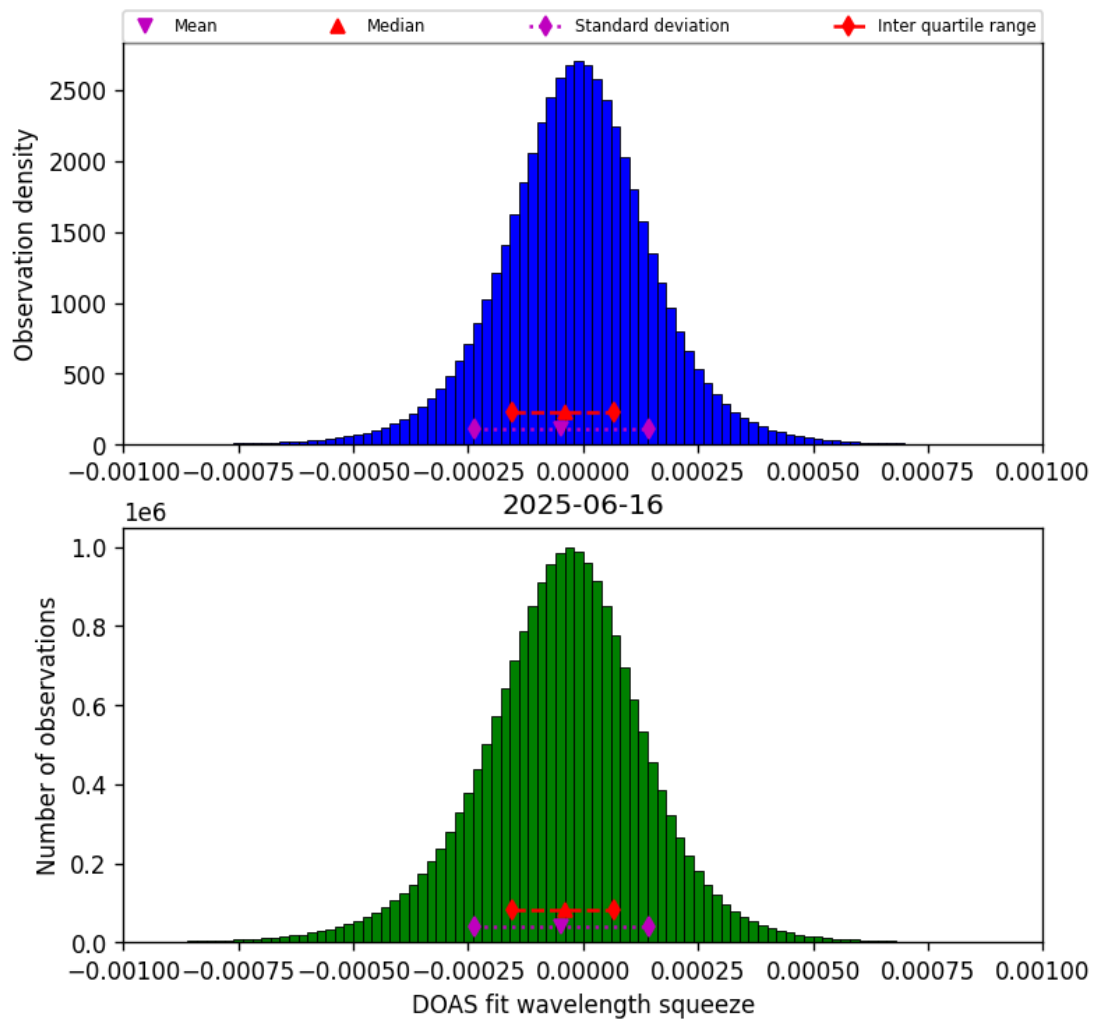
Figure 77: Histogram of “DOAS fit wavelength squeeze” for 2025-06-16 to 2025-06-17
