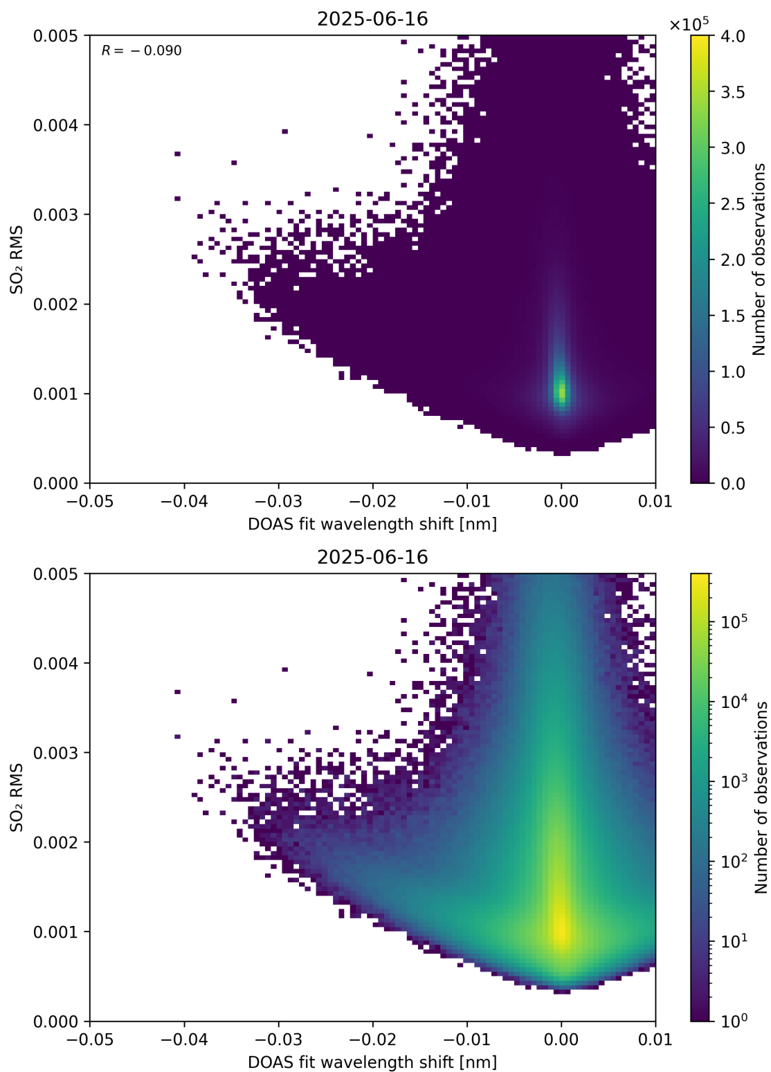
Figure 139: Scatter density plot of “DOAS fit wavelength shift” against “SO 2 RMS” for 2025-06-16 to 2025-06-17.
