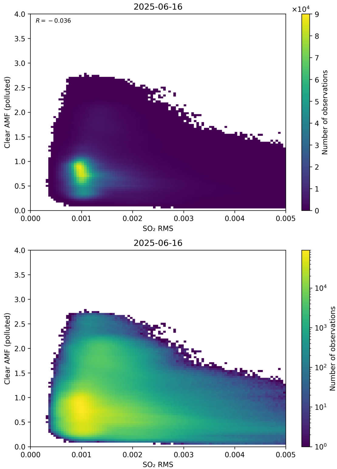
Figure 147: Scatter density plot of “SO 2 RMS” against “Clear AMF (polluted)” for 2025-06-16 to 2025-06-17.
