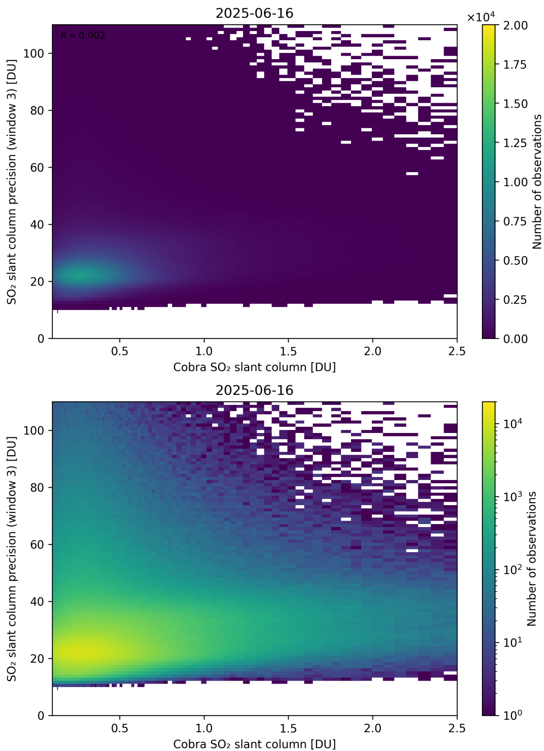
Figure 223: Scatter density plot of “Cobra SO 2 slant column” against “SO 2 slant column precision (window 3)” for 2025-06-16 to 2025-06-17.
