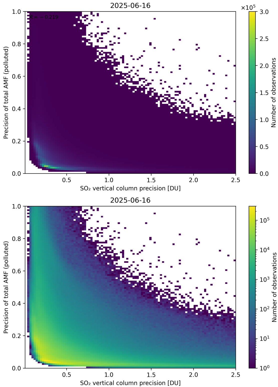
Figure 347: Scatter density plot of “SO 2 vertical column precision” against “Precision of total AMF (polluted)” for 2025-06-16 to 2025-06-17.
