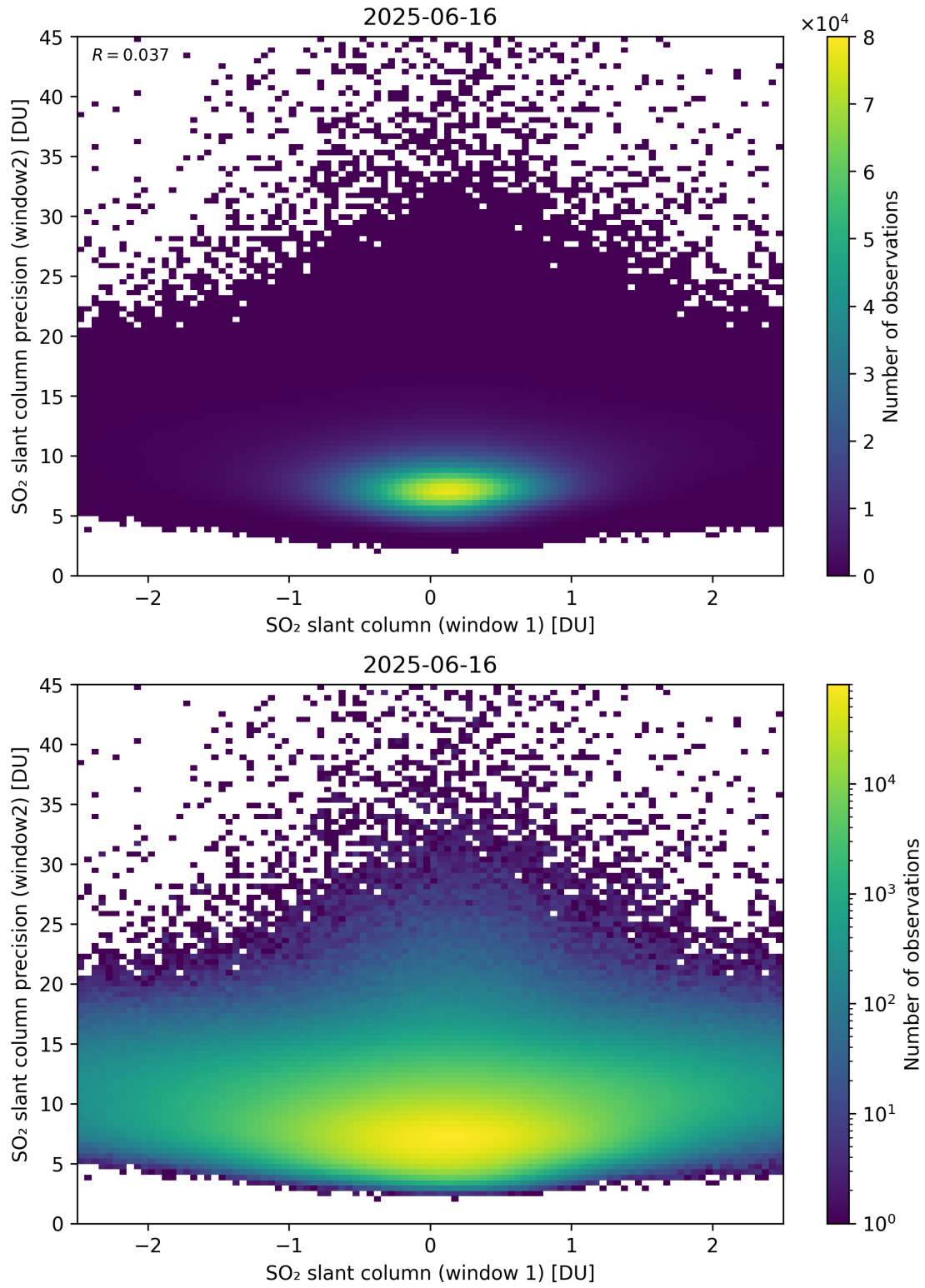
Figure 286: Scatter density plot of “SO 2 slant column (window 1)” against “SO 2 slant column precision (window2)” for 2025-06-16 to 2025-06-17.
