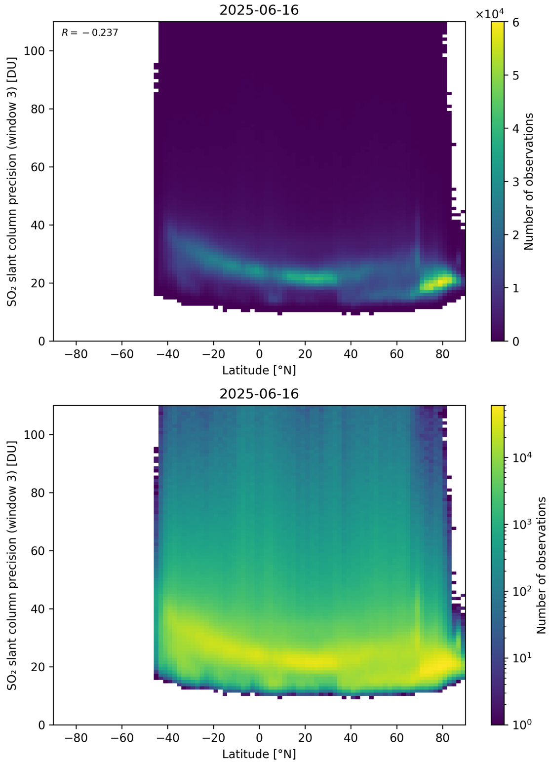
Figure 166: Scatter density plot of “Latitude” against “SO 2 slant column precision (window 3)” for 2025-06-16 to 2025-06-17.
