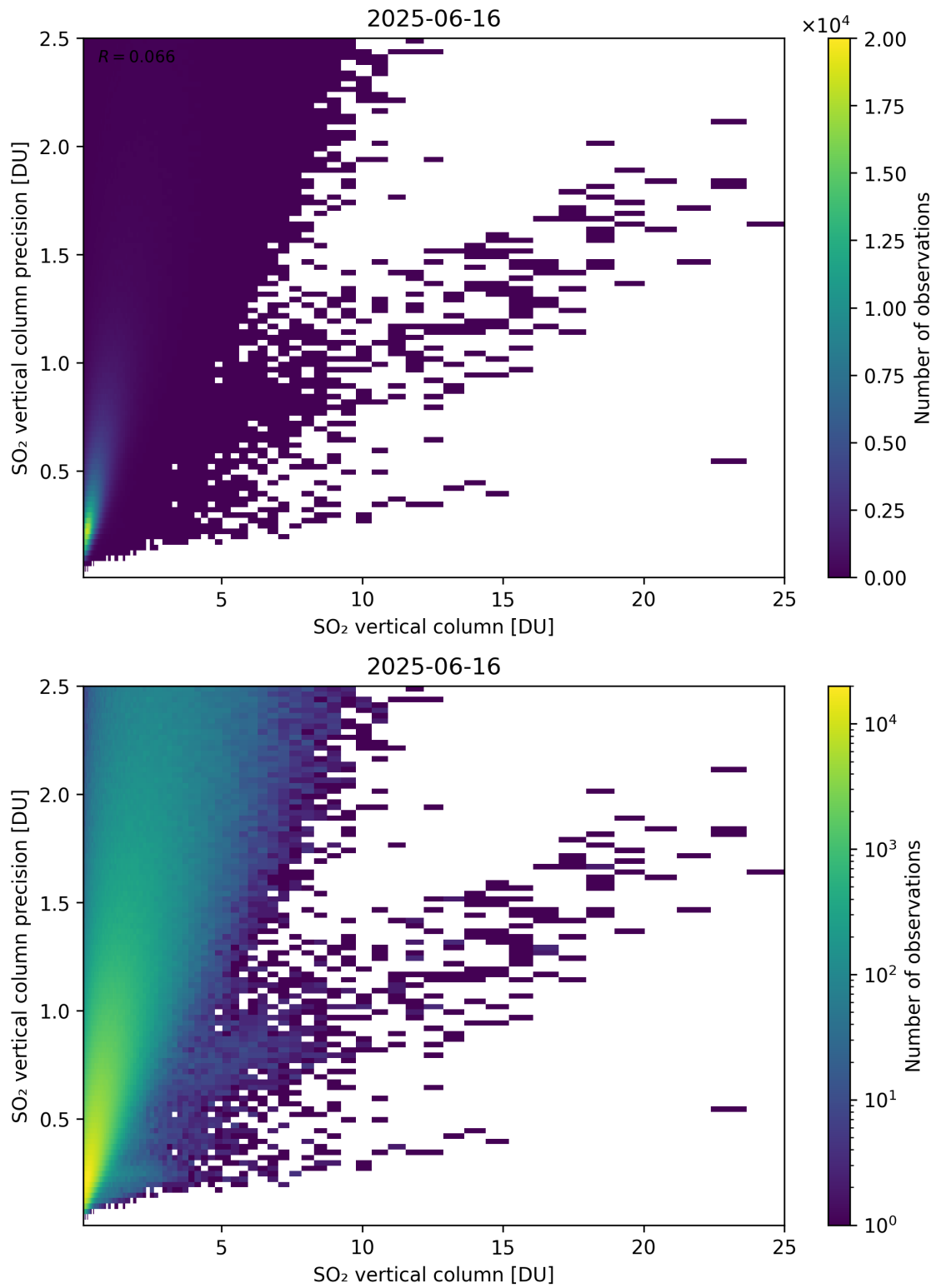
Figure 361: Scatter density plot of “SO 2 vertical column” against “SO 2 vertical column precision” for 2025-06-16 to 2025-06-17.
