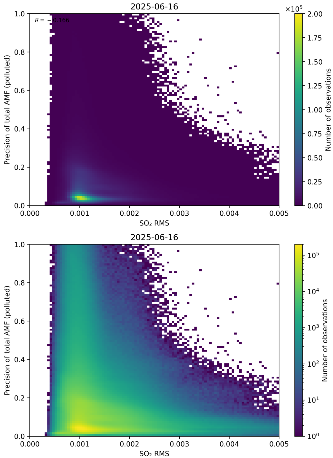
Figure 149: Scatter density plot of “SO 2 RMS” against “Precision of total AMF (polluted)” for 2025-06-16 to 2025-06-17.
