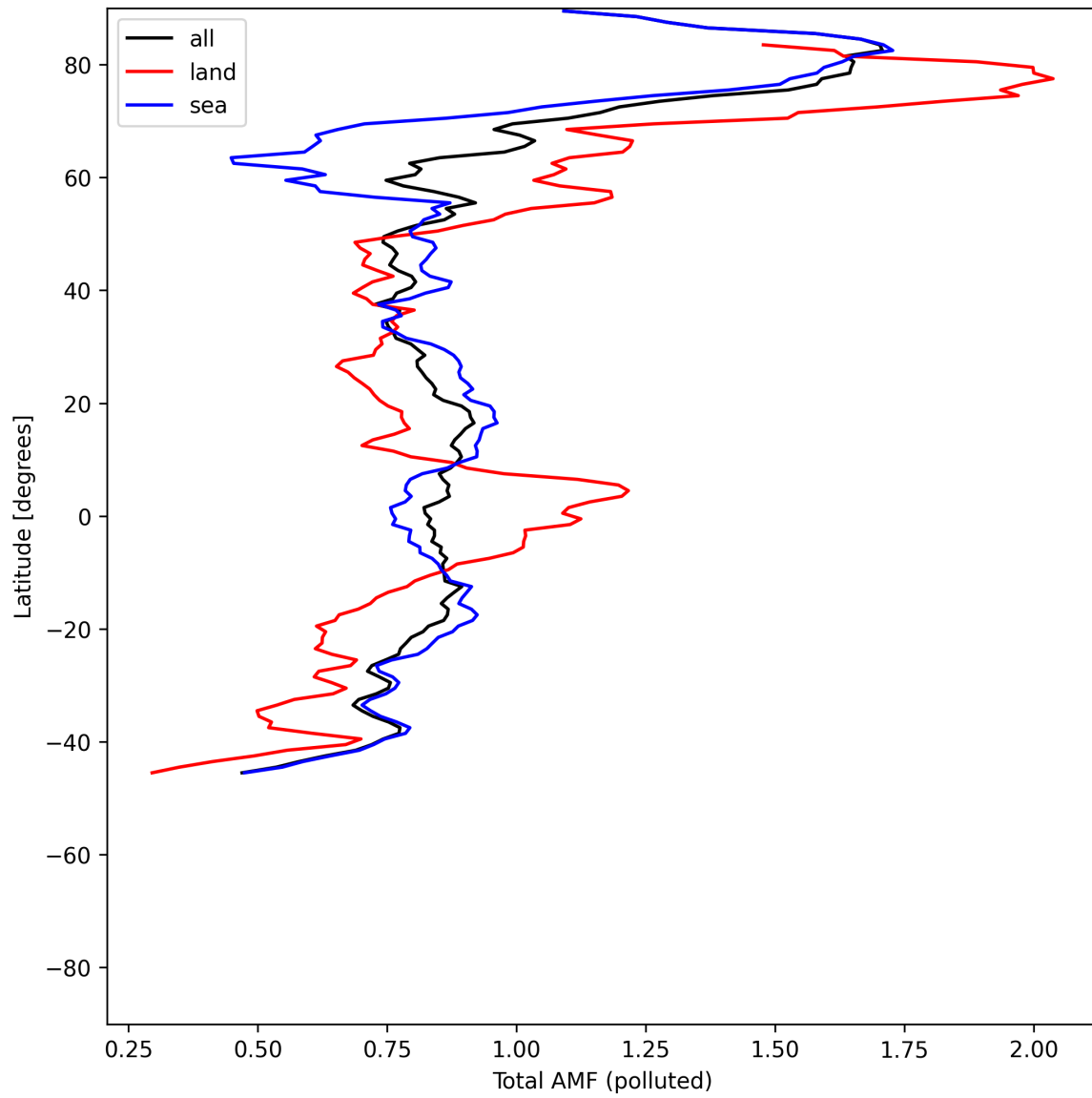
Figure 53: Zonal average of “Total AMF (polluted)” for 2025-06-16 to 2025-06-17.
