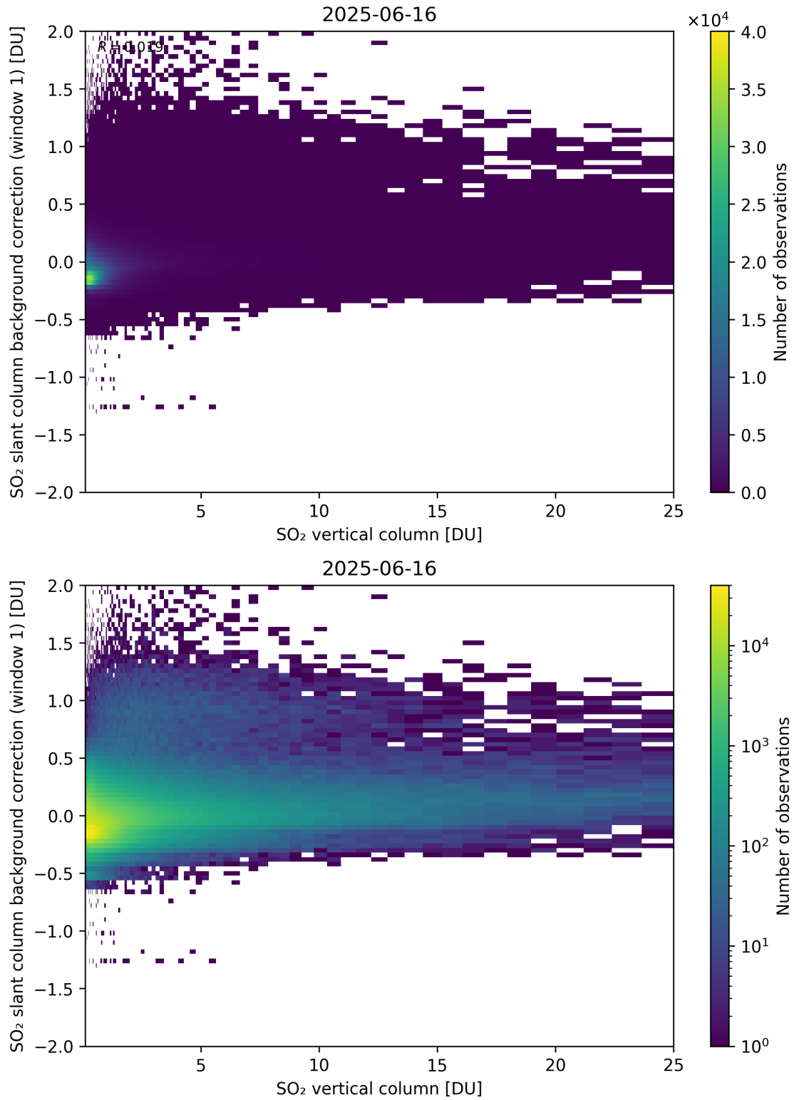
Figure 323: Scatter density plot of “SO 2 vertical column” against “SO 2 slant column background correction (window 1)” for 2025-06-16 to 2025-06-17.
