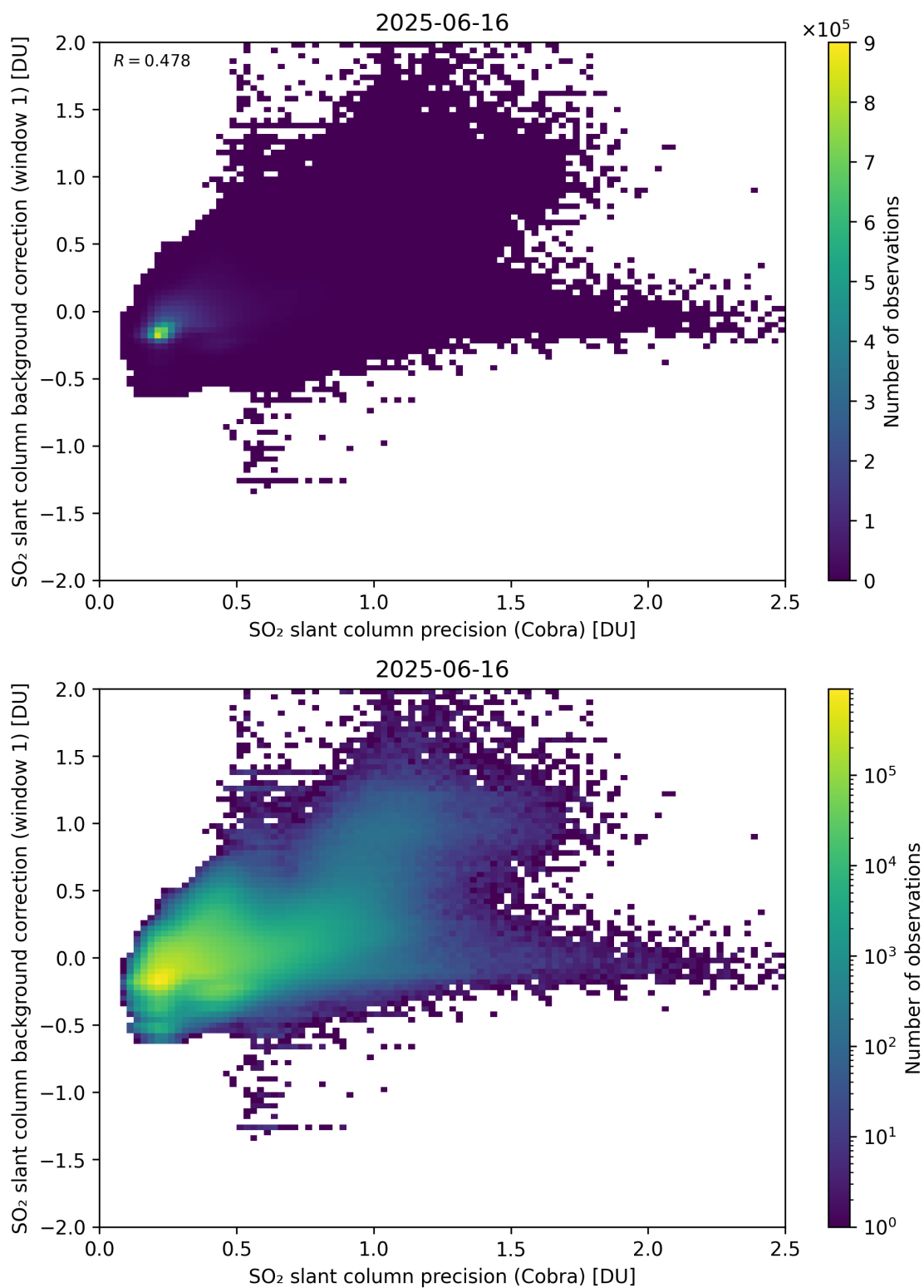
Figure 199: Scatter density plot of “SO 2 slant column precision (Cobra)” against “SO 2 slant column background correction (window 1)” for 2025-06-16 to 2025-06-17.
