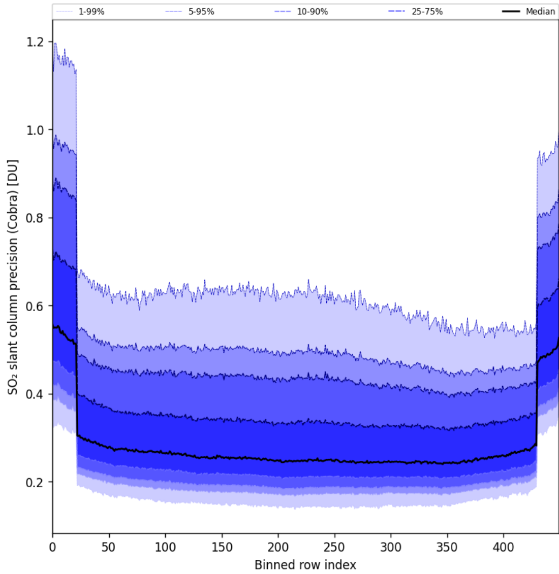
Figure 88: Along track statistics of “SO 2 slant column precision (Cobra)” for 2025-06-16 to 2025-06-17
