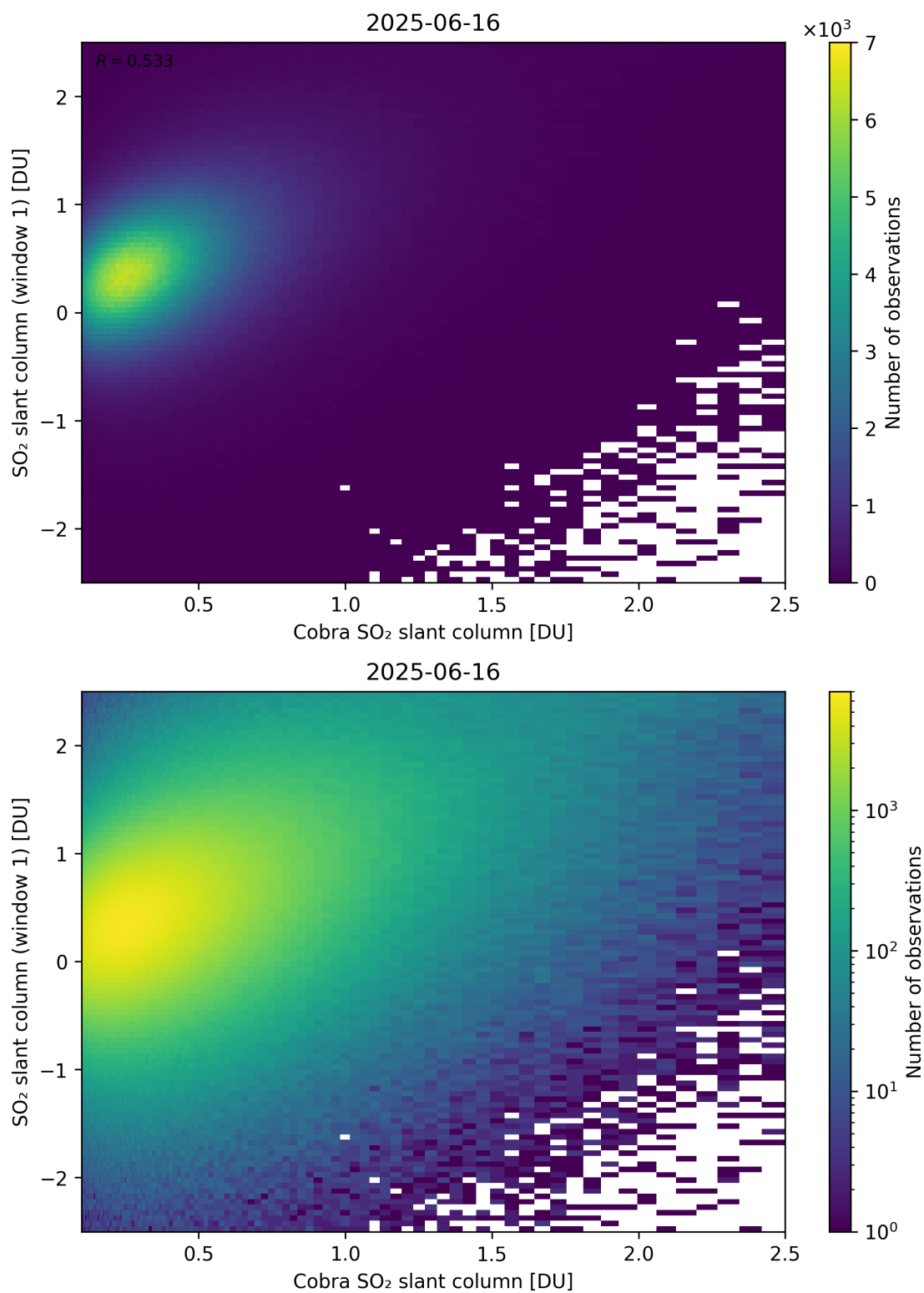
Figure 219: Scatter density plot of “Cobra SO 2 slant column” against “SO 2 slant column (window 1)” for 2025-06-16 to 2025-06-17.
