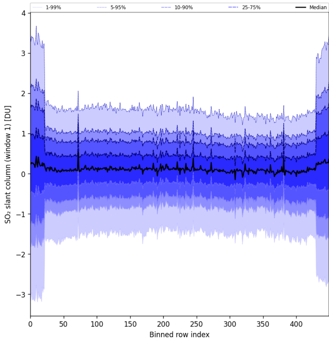
Figure 89: Along track statistics of “SO 2 slant column (window 1)” for 2025-06-16 to 2025-06-17
