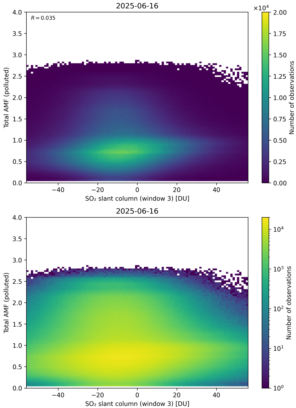
Figure 318: Scatter density plot of “SO 2 slant column (window 3)” against “Total AMF (polluted)” for 2025-06-16 to 2025-06-17.
