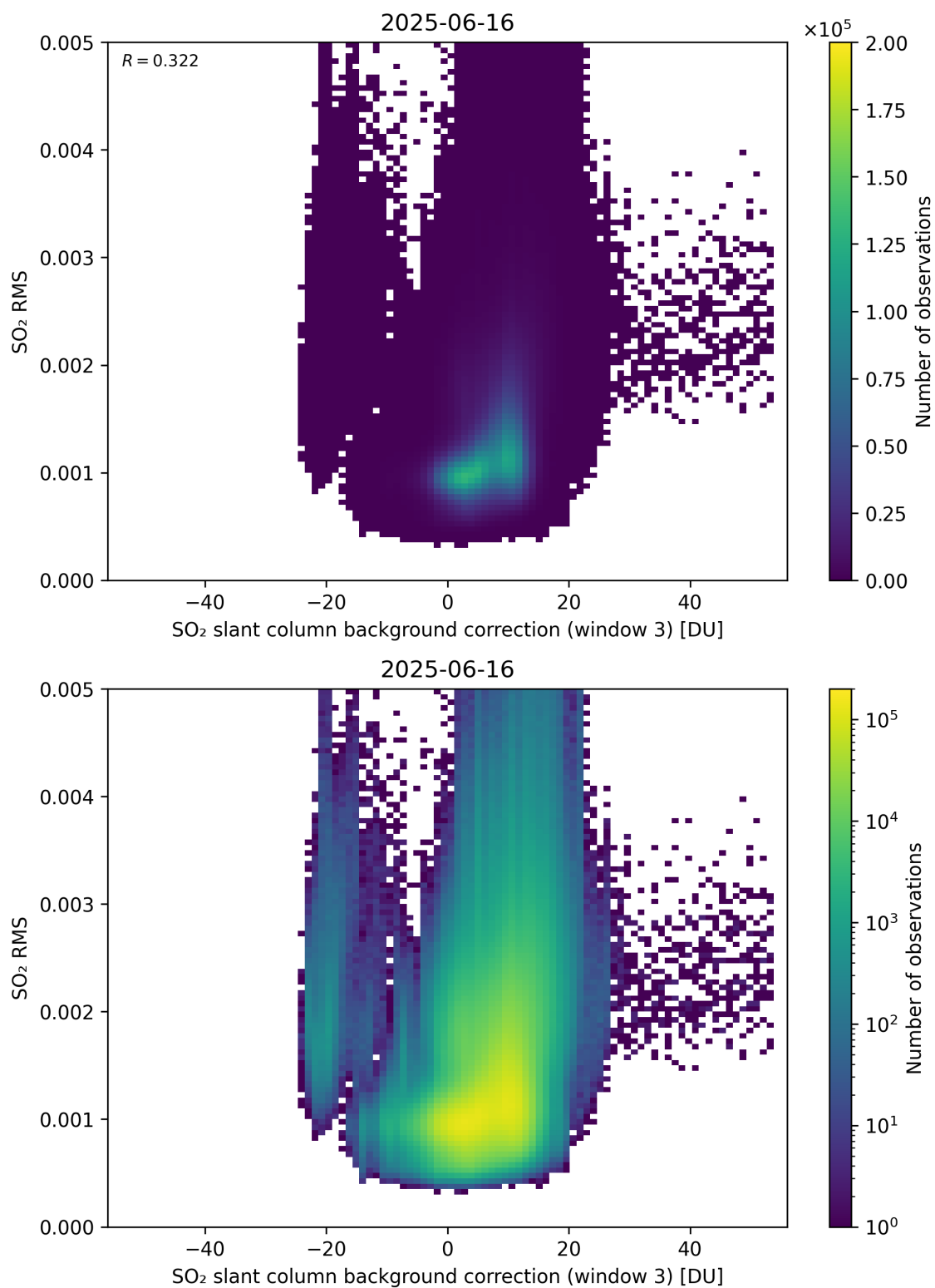
Figure 134: Scatter density plot of “SO 2 slant column background correction (window 3)” against “SO 2 RMS” for 2025-06-16 to 2025-06-17.
