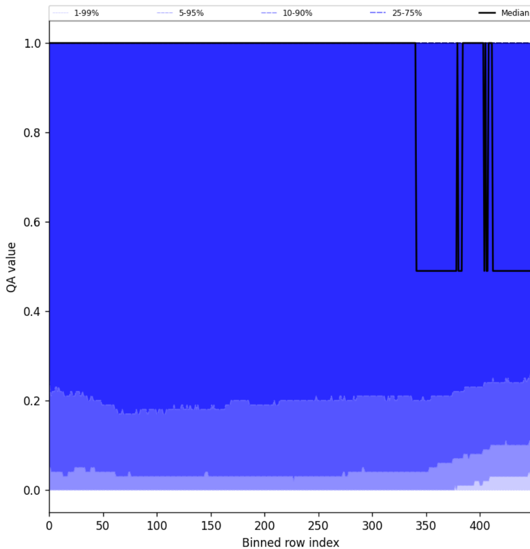
Figure 83: Along track statistics of “QA value” for 2025-06-16 to 2025-06-17
