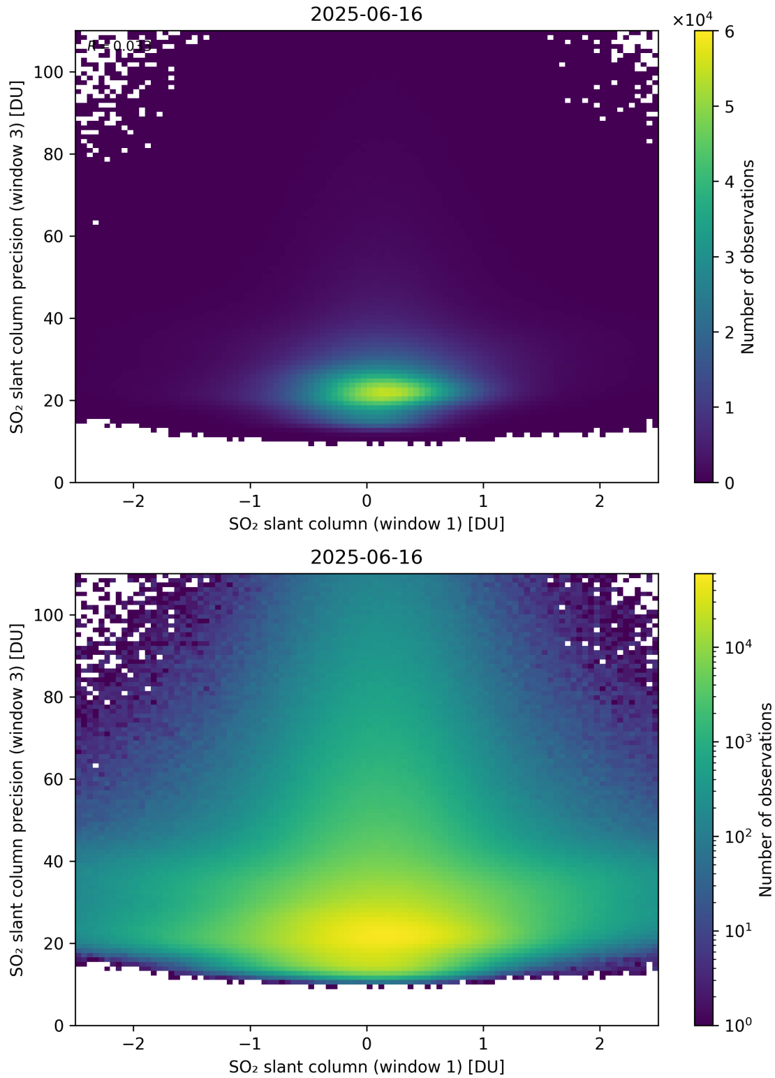
Figure 288: Scatter density plot of “SO 2 slant column (window 1)” against “SO 2 slant column precision (window 3)” for 2025-06-16 to 2025-06-17.
