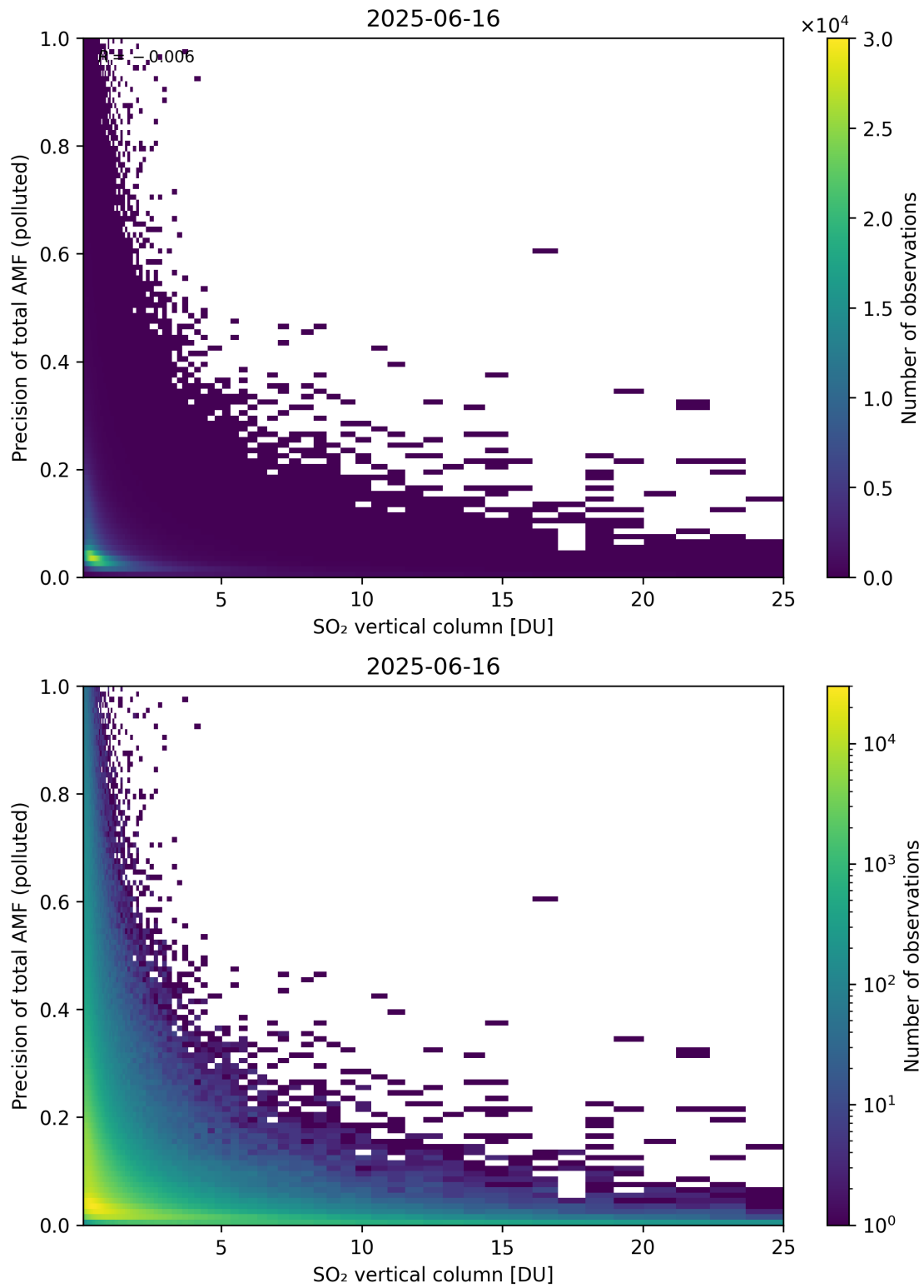
Figure 360: Scatter density plot of “SO 2 vertical column” against “Precision of total AMF (polluted)” for 2025-06-16 to 2025-06-17.
