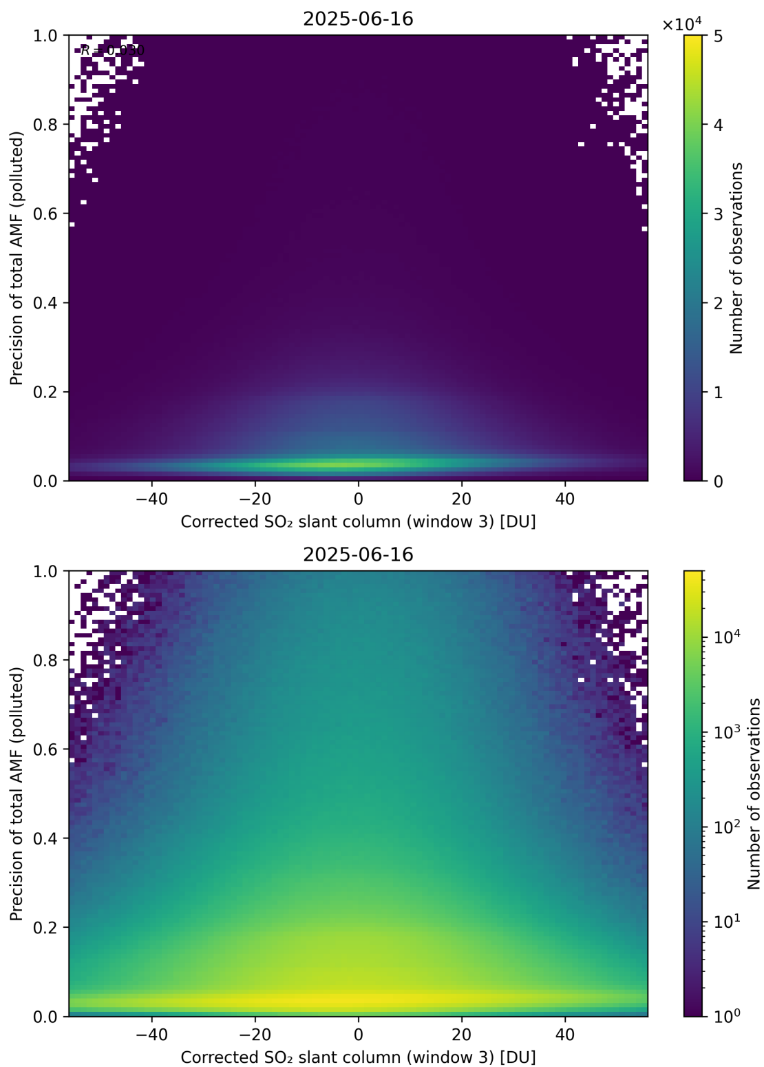
Figure 261: Scatter density plot of “Corrected SO 2 slant column (window 3)” against “Precision of total AMF (polluted)” for 2025-06-16 to 2025-06-17.
