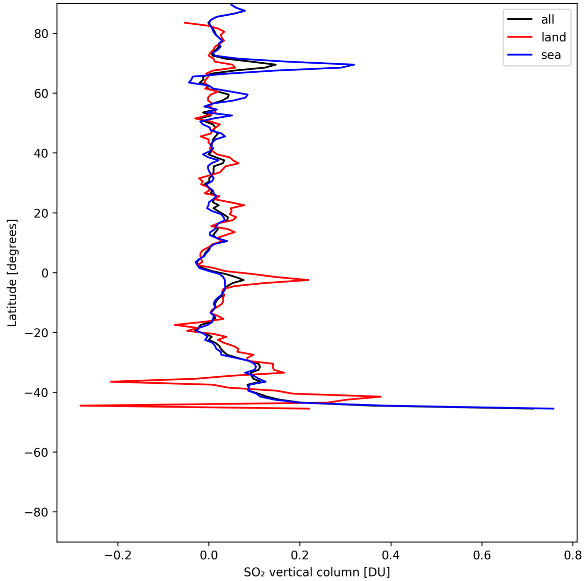
Figure 32: Zonal average of “SO 2 vertical column” for 2025-06-16 to 2025-06-17.
