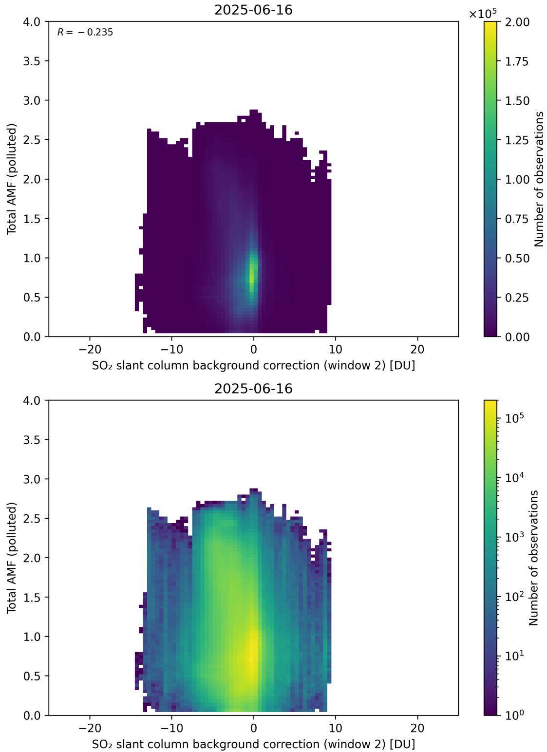
Figure 130: Scatter density plot of “SO 2 slant column background correction (window 2)” against “Total AMF (polluted)” for 2025-06-16 to 2025-06-17.
