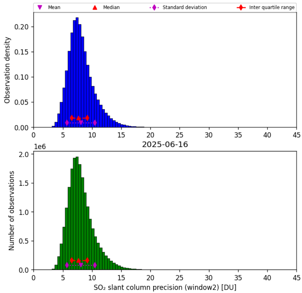
Figure 68: Histogram of “SO 2 slant column precision (window2)” for 2025-06-16 to 2025-06-17
