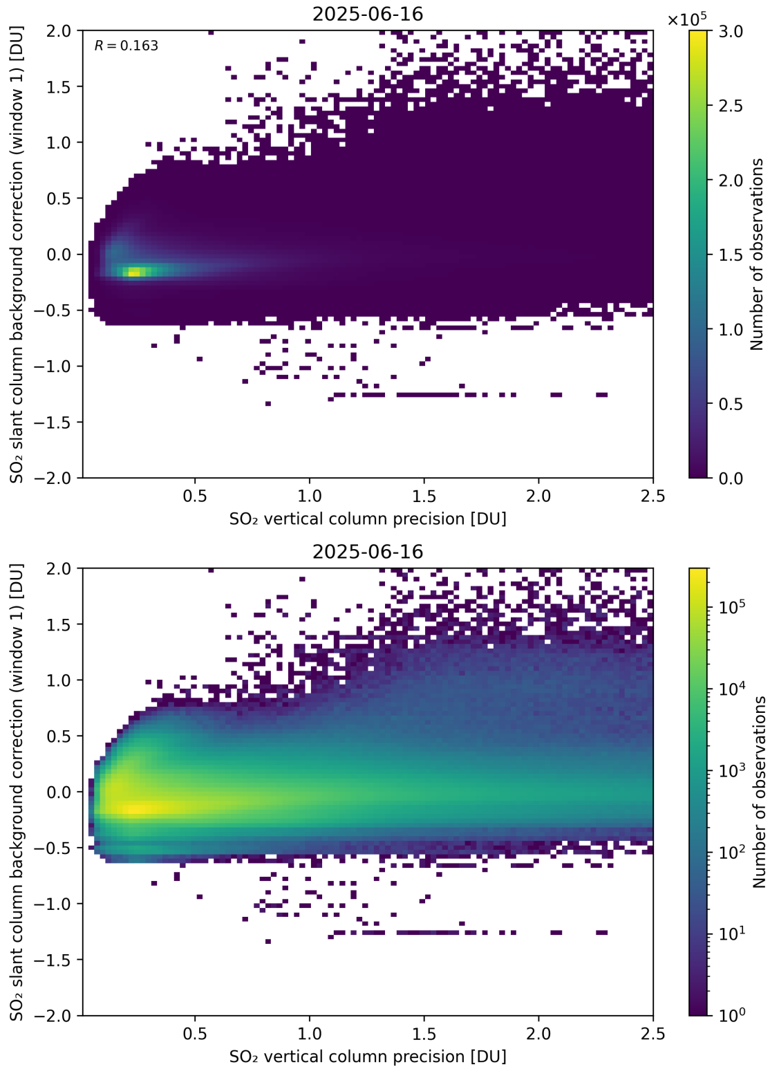
Figure 329: Scatter density plot of “SO 2 vertical column precision” against “SO 2 slant column background correction (window 1)” for 2025-06-16 to 2025-06-17.
