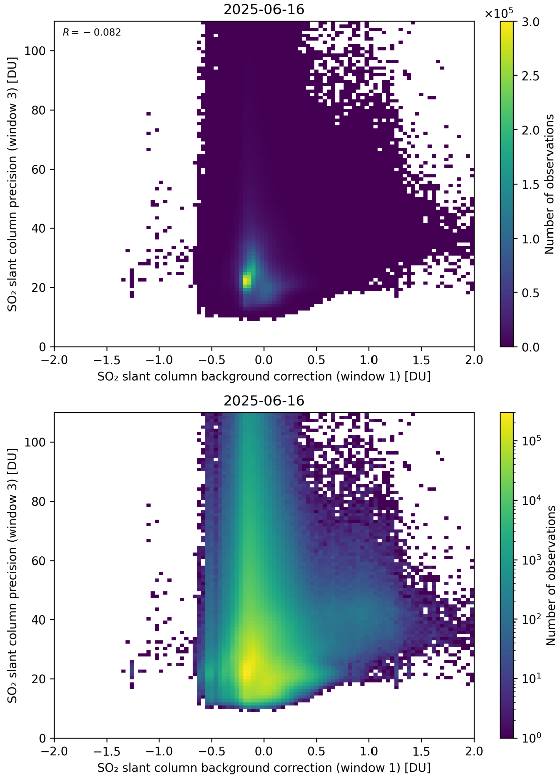
Figure 119: Scatter density plot of “SO 2 slant column background correction (window 1)” against “SO 2 slant column precision (window 3)” for 2025-06-16 to 2025-06-17.
