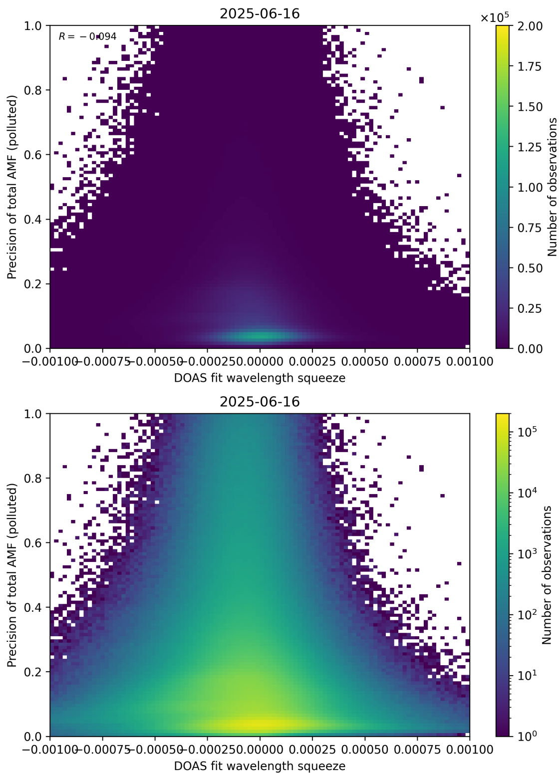
Figure 146: Scatter density plot of “DOAS fit wavelength squeeze” against “Precision of total AMF (polluted)” for 2025-06-16 to 2025-06-17.
