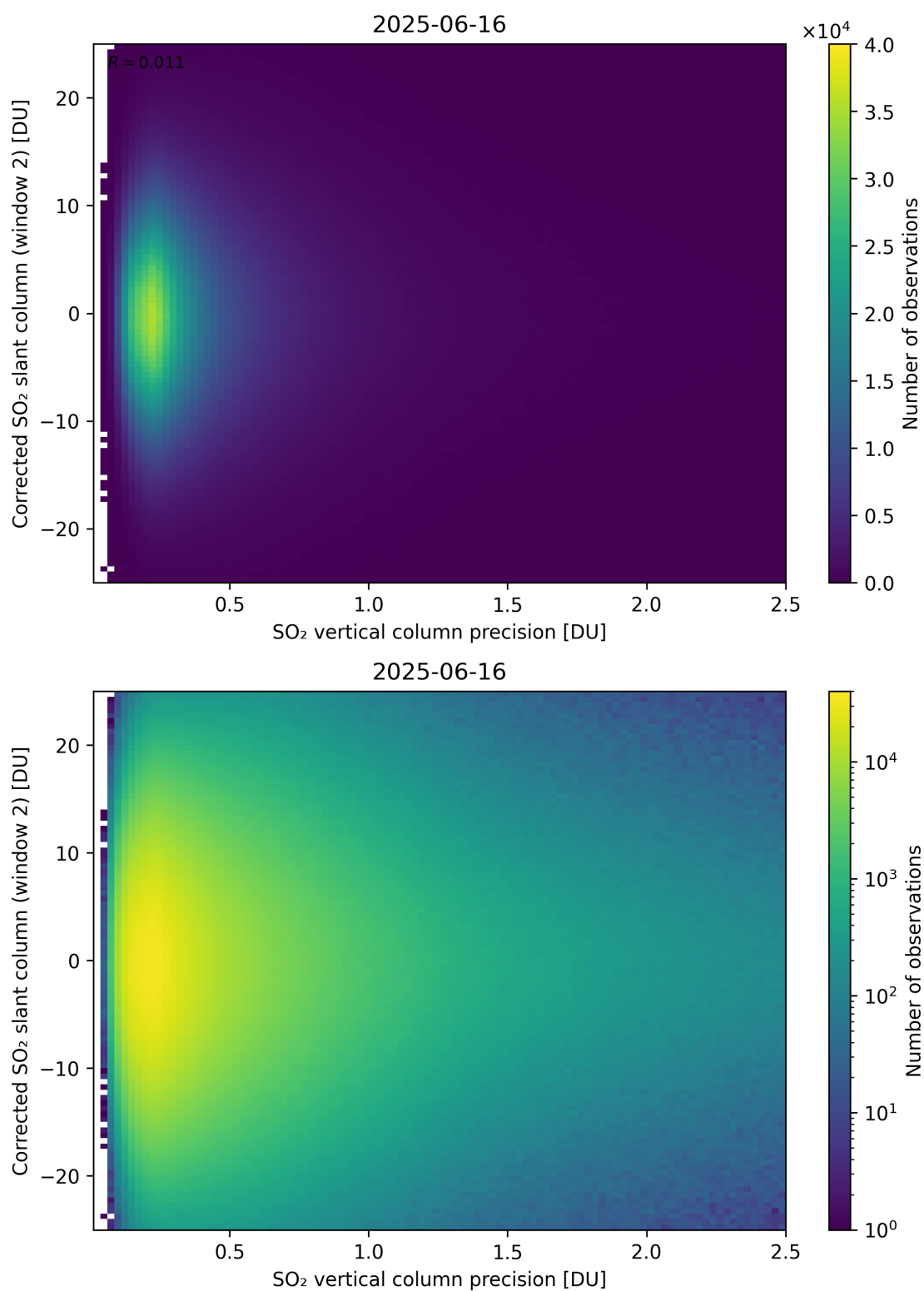
Figure 339: Scatter density plot of “SO 2 vertical column precision” against “Corrected SO 2 slant column (window 2)” for 2025-06-16 to 2025-06-17.
