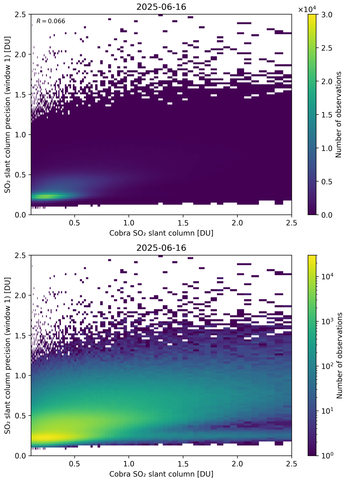
Figure 220: Scatter density plot of “Cobra SO 2 slant column” against “SO 2 slant column precision (window 1)” for 2025-06-16 to 2025-06-17.
