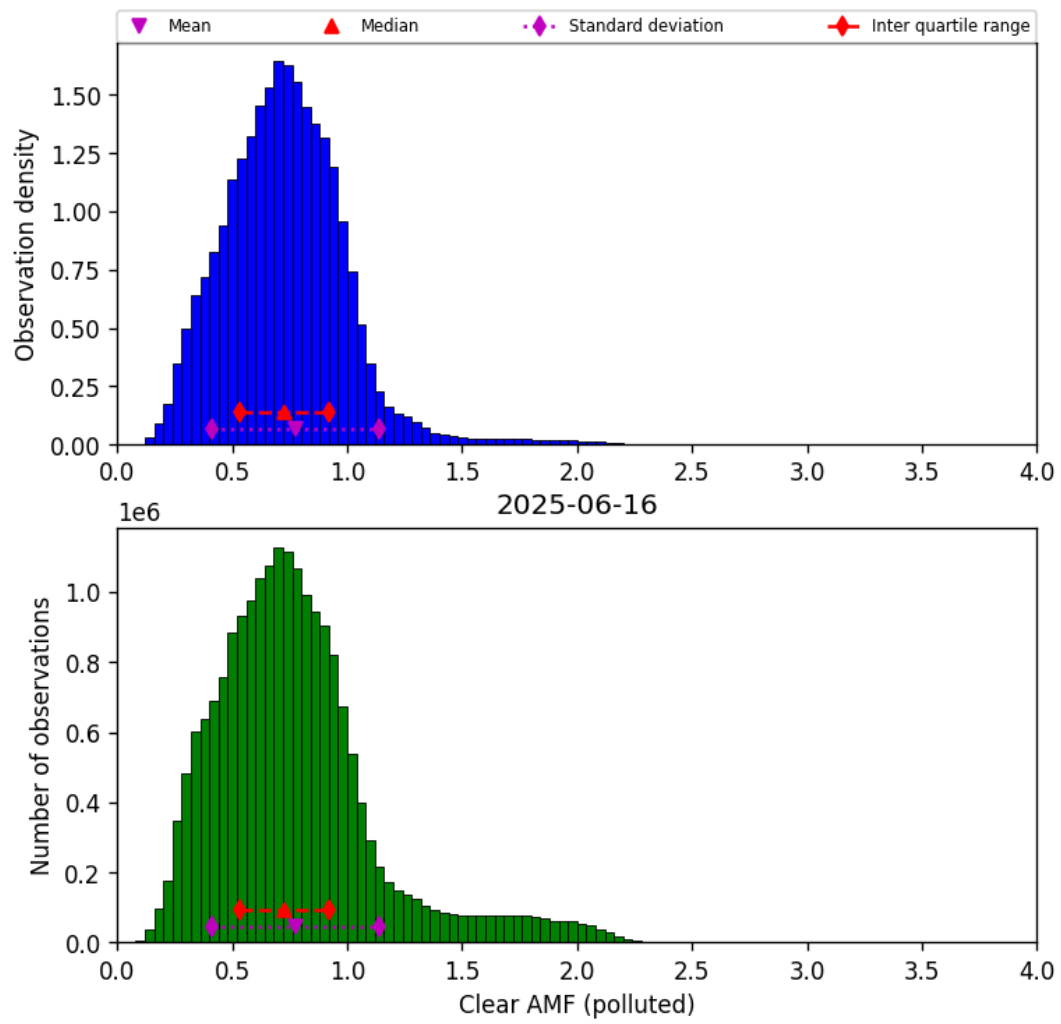
Figure 81: Histogram of “Clear AMF (polluted)” for 2025-06-16 to 2025-06-17
