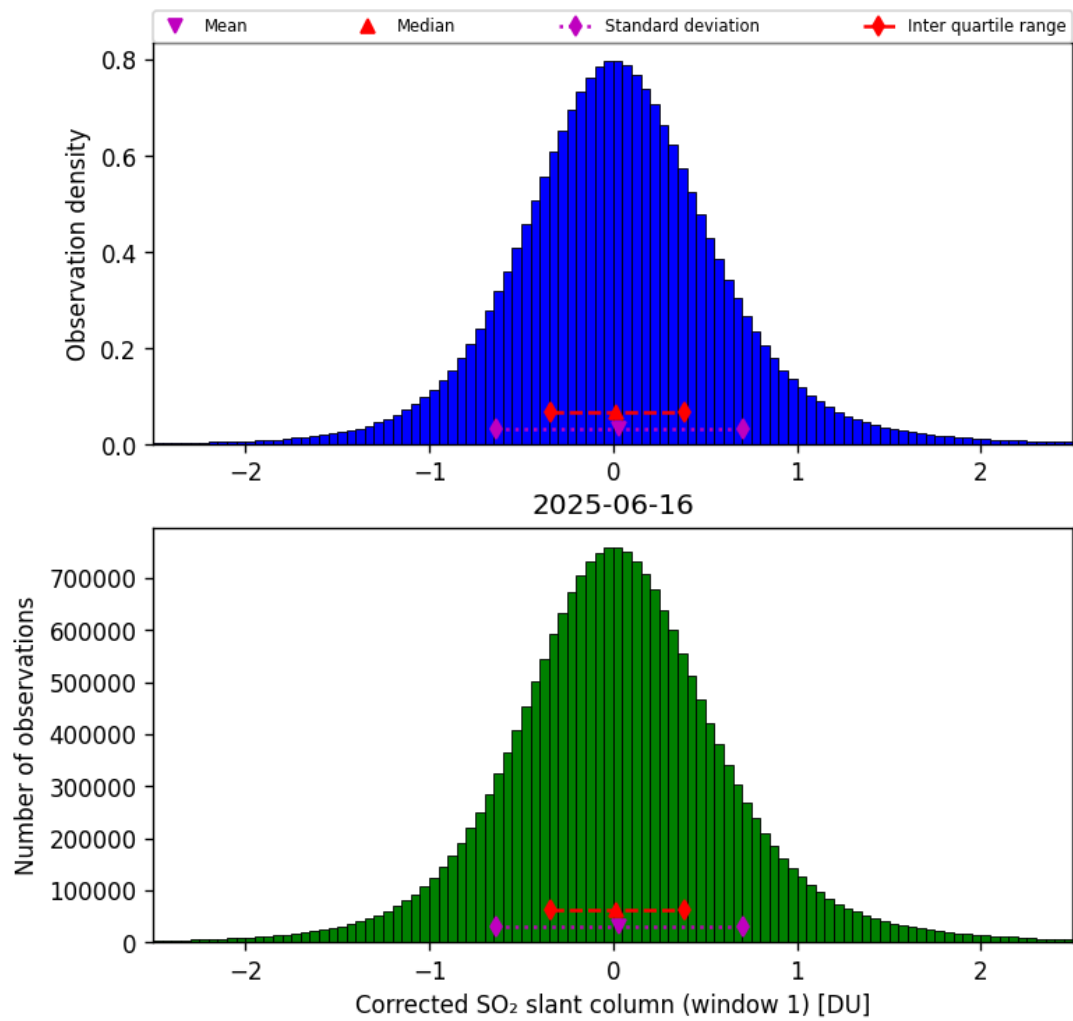
Figure 65: Histogram of “Corrected SO 2 slant column (window 1)” for 2025-06-16 to 2025-06-17
