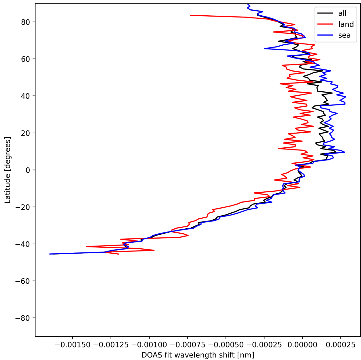
Figure 50: Zonal average of “DOAS fit wavelength shift” for 2025-06-16 to 2025-06-17.
