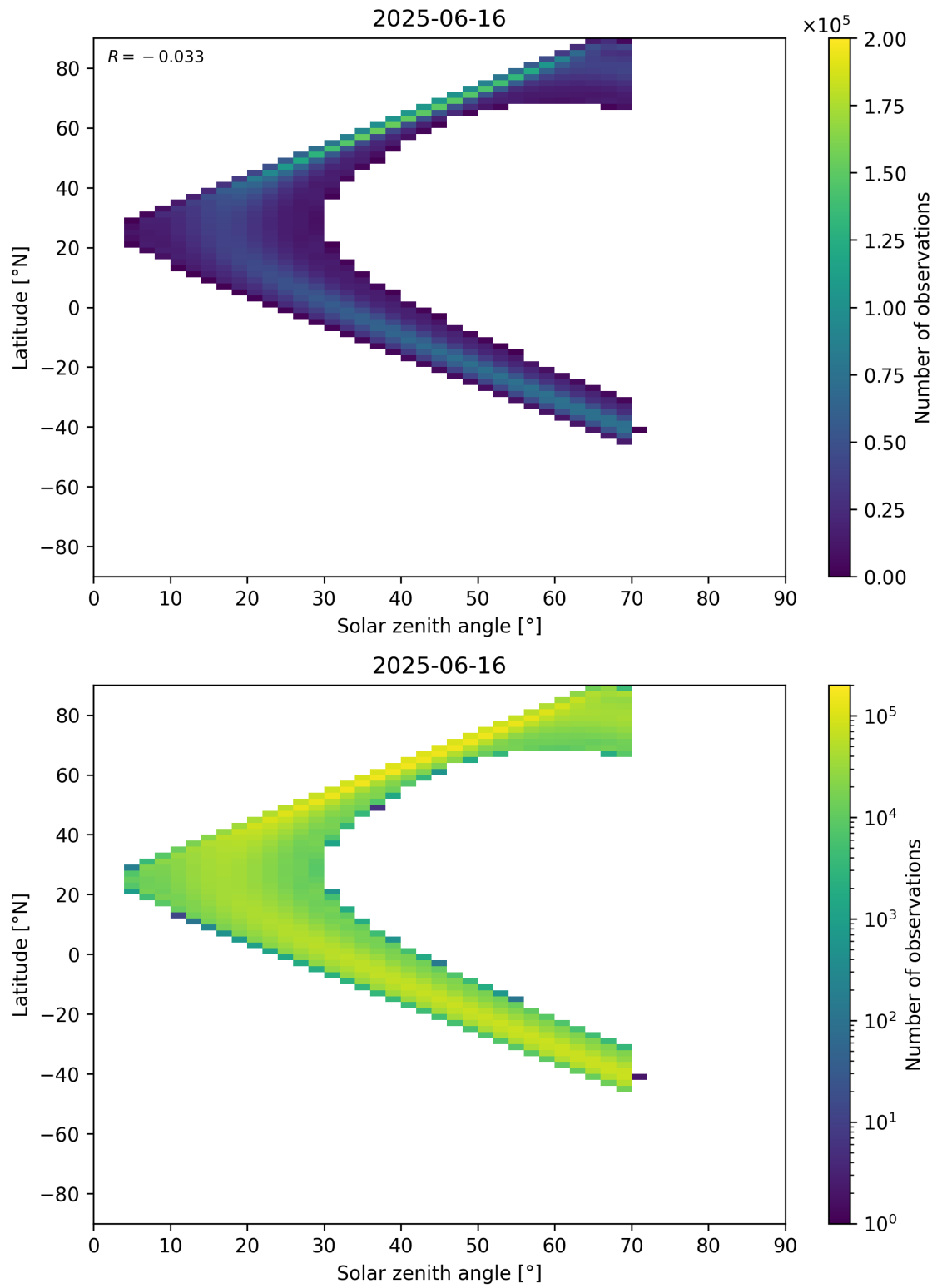
Figure 177: Scatter density plot of “Solar zenith angle” against “Latitude” for 2025-06-16 to 2025-06-17.
