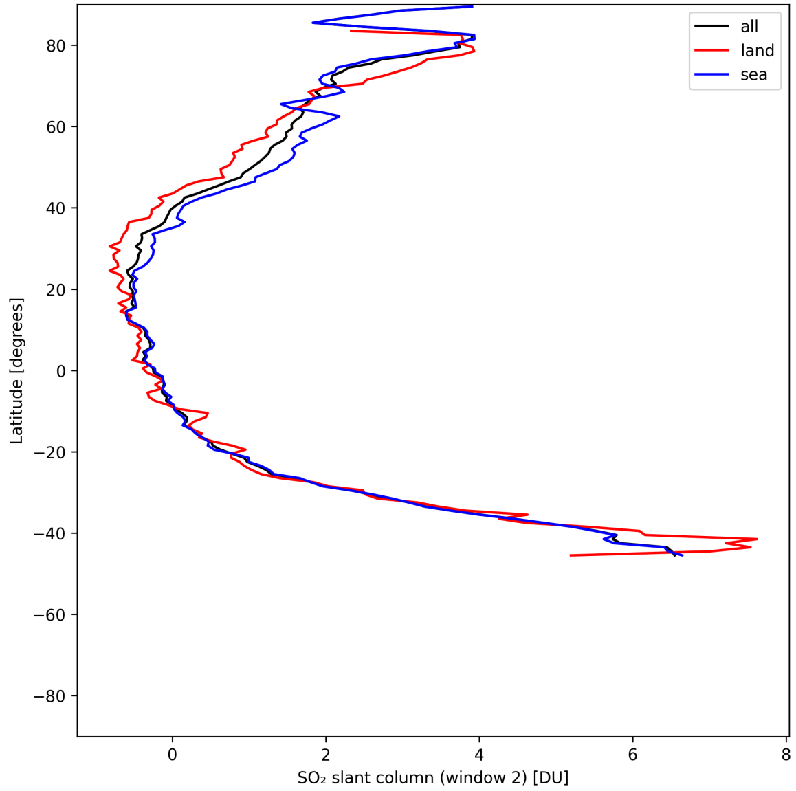
Figure 41: Zonal average of “SO 2 slant column (window 2)” for 2025-06-16 to 2025-06-17.
