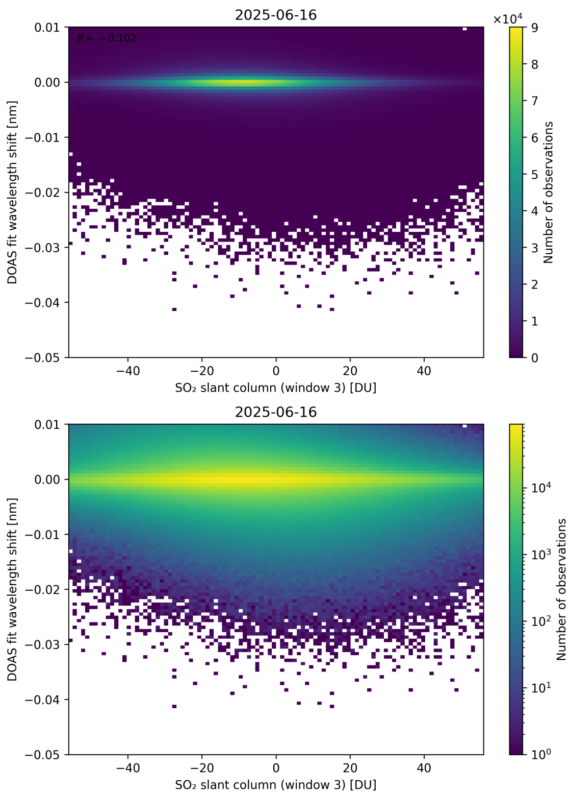
Figure 304: Scatter density plot of “SO 2 slant column (window 3)” against “DOAS fit wavelength shift” for 2025-06-16 to 2025-06-17.
