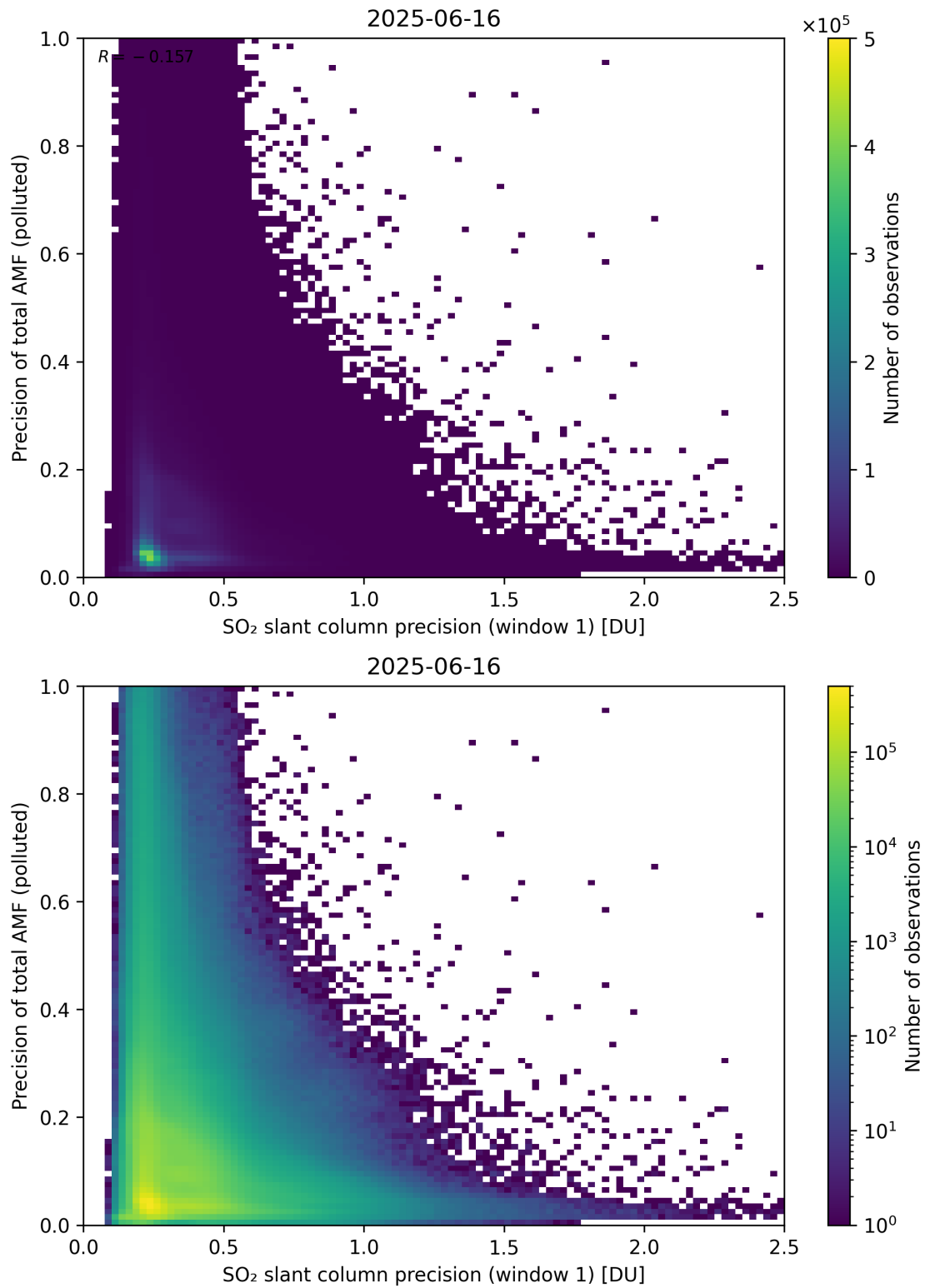
Figure 281: Scatter density plot of “SO 2 slant column precision (window 1)” against “Precision of total AMF (polluted)” for 2025-06-16 to 2025-06-17.
