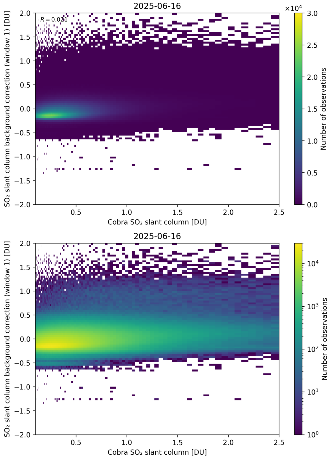
Figure 193: Scatter density plot of “Cobra SO 2 slant column” against “SO 2 slant column background correction (window 1)” for 2025-06-16 to 2025-06-17.
