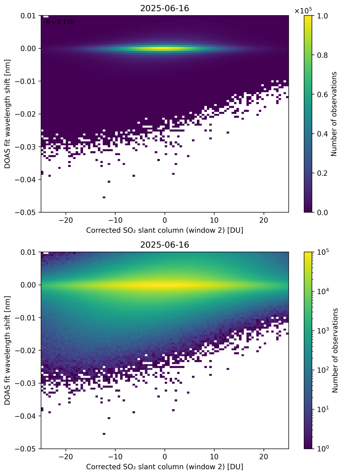
Figure 246: Scatter density plot of “Corrected SO 2 slant column (window 2)” against “DOAS fit wavelength shift” for 2025-06-16 to 2025-06-17.
