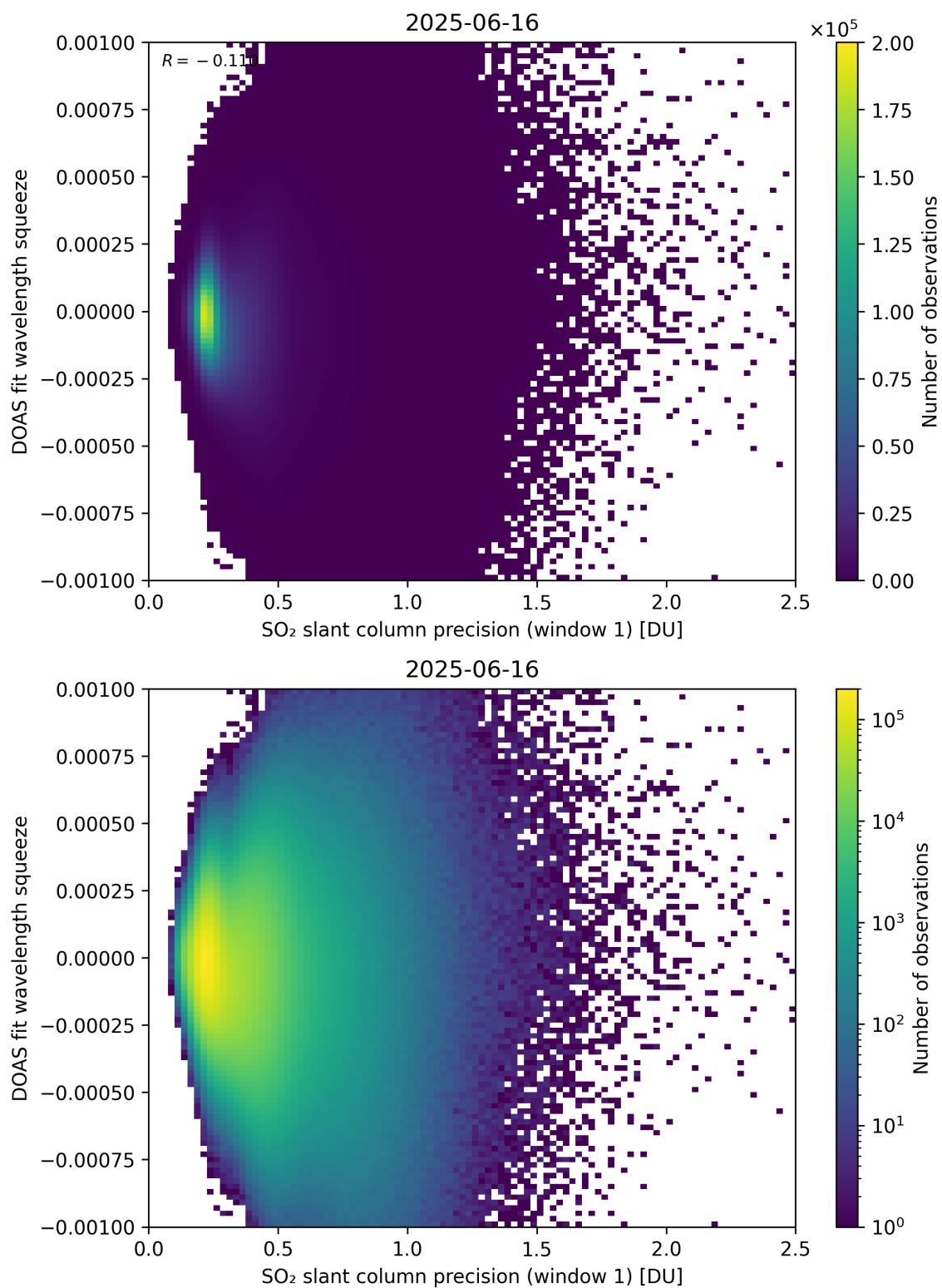
Figure 272: Scatter density plot of “SO 2 slant column precision (window 1)” against “DOAS fit wavelength squeeze” for 2025-06-16 to 2025-06-17.
