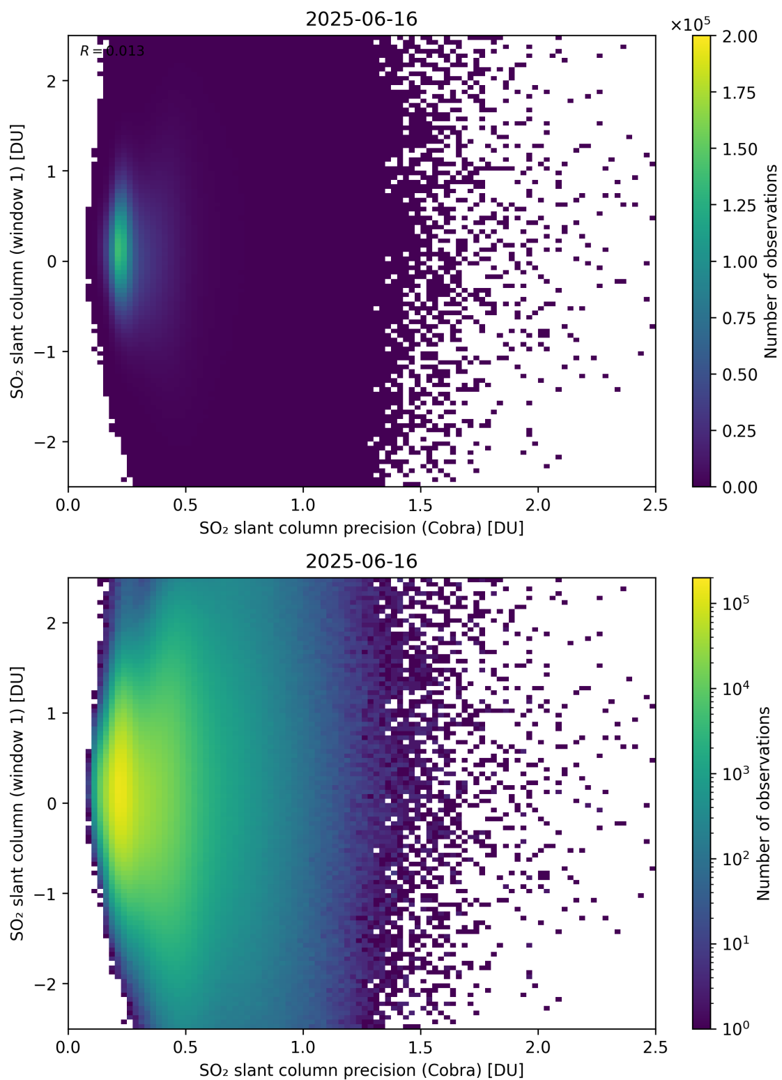
Figure 208: Scatter density plot of “SO 2 slant column precision (Cobra)” against “SO 2 slant column (window 1)” for 2025-06-16 to 2025-06-17.
