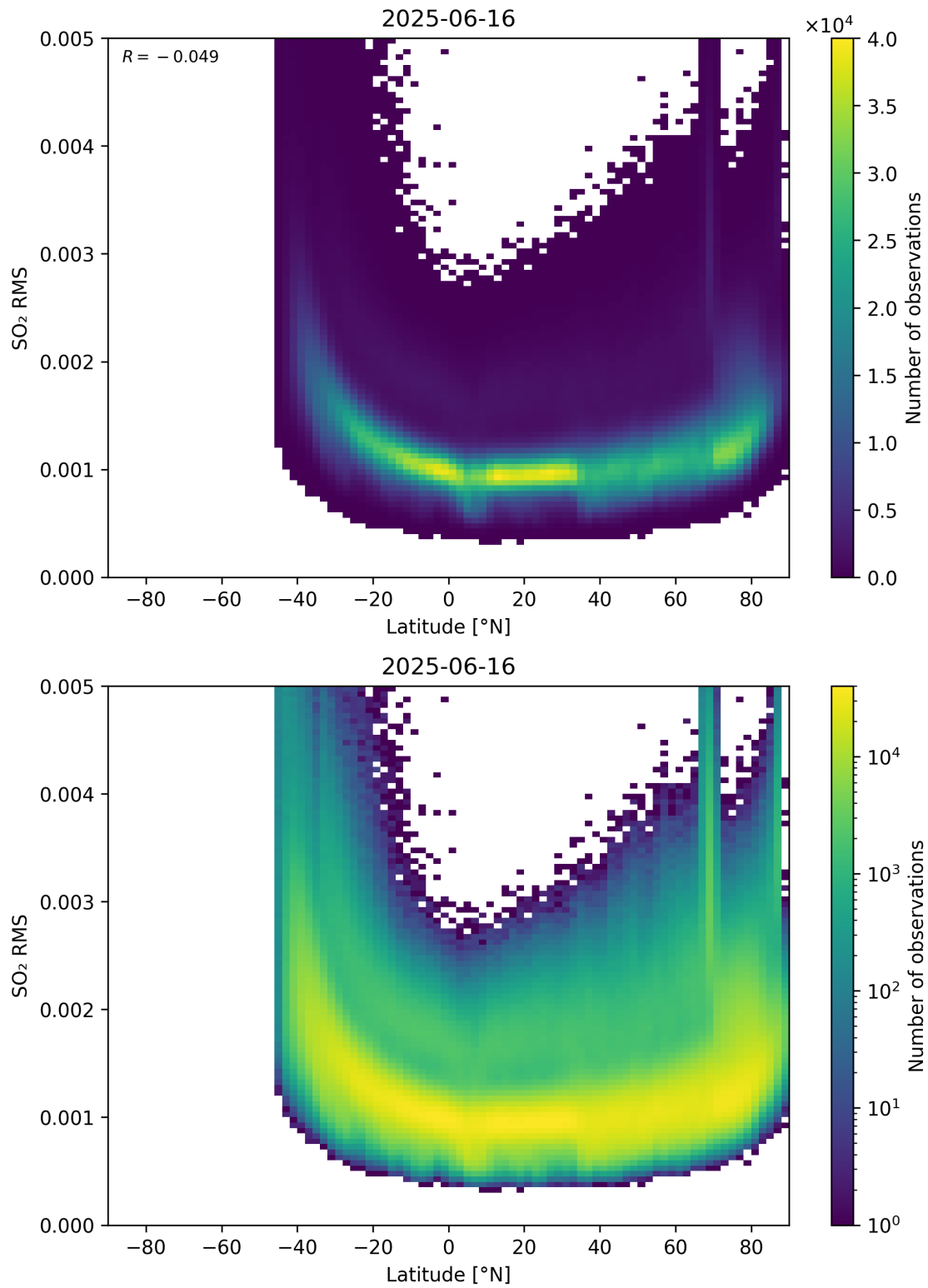
Figure 155: Scatter density plot of “Latitude” against “SO 2 RMS” for 2025-06-16 to 2025-06-17.
