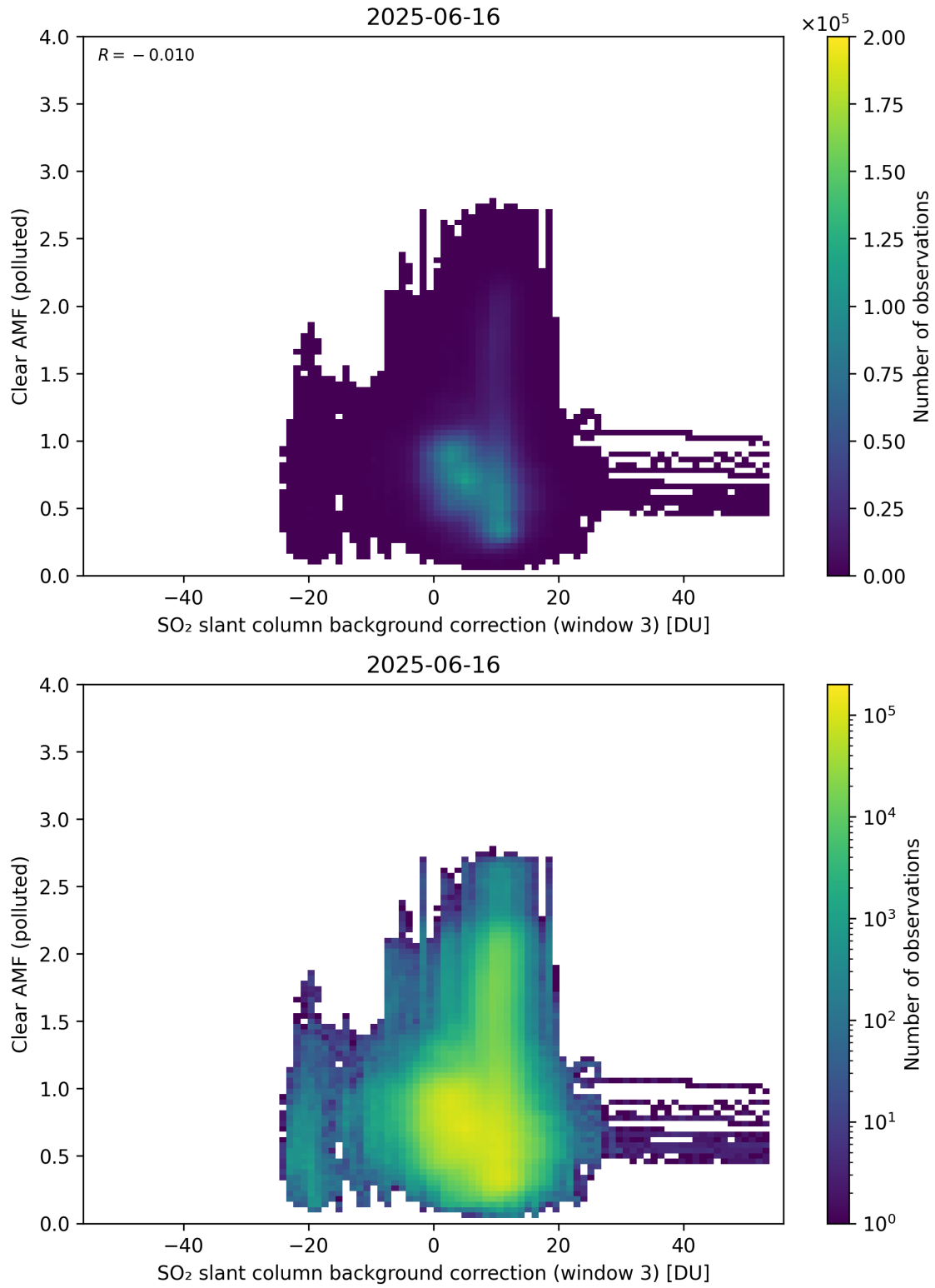
Figure 135: Scatter density plot of “SO 2 slant column background correction (window 3)” against “Clear AMF (polluted)” for 2025-06-16 to 2025-06-17.
