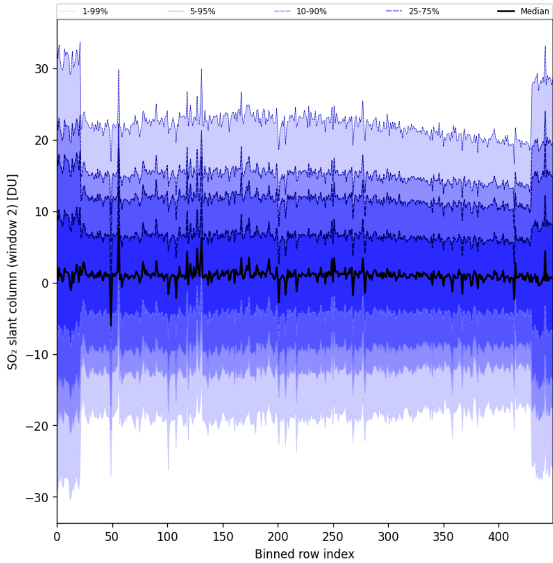
Figure 93: Along track statistics of “SO 2 slant column (window 2)” for 2025-06-16 to 2025-06-17
