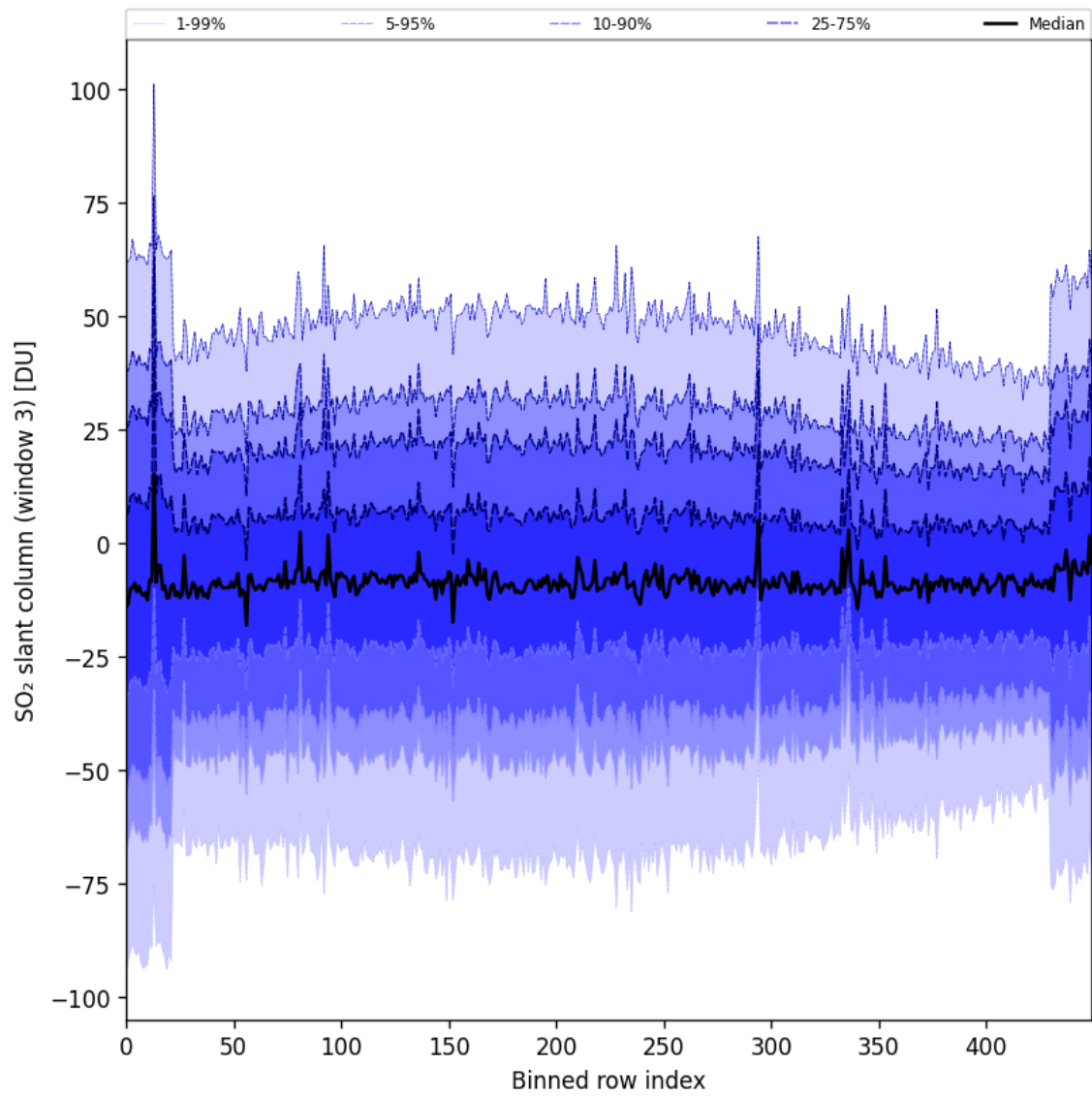
Figure 97: Along track statistics of “SO 2 slant column (window 3)” for 2025-06-16 to 2025-06-17
