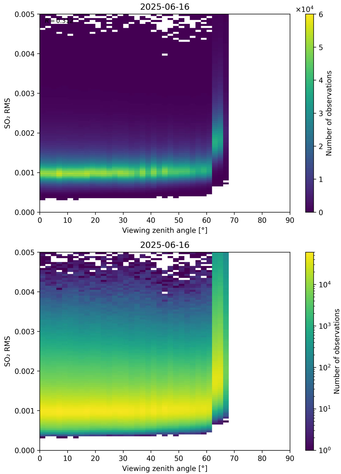
Figure 367: Scatter density plot of “Viewing zenith angle” against “SO 2 RMS” for 2025-06-16 to 2025-06-17.
