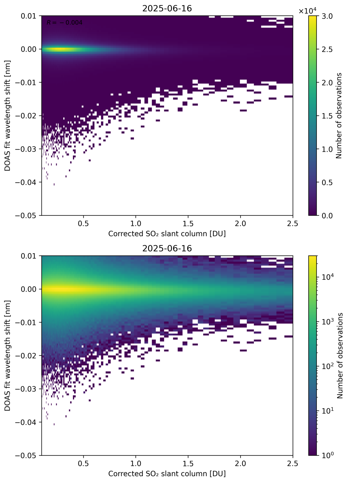
Figure 229: Scatter density plot of “Corrected SO 2 slant column” against “DOAS fit wavelength shift” for 2025-06-16 to 2025-06-17.
