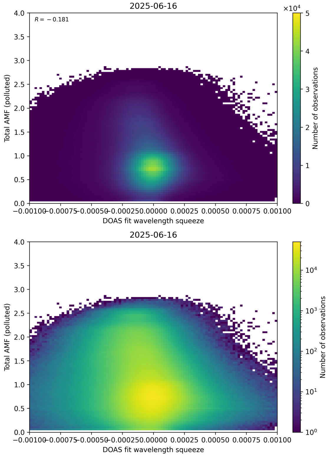
Figure 145: Scatter density plot of “DOAS fit wavelength squeeze” against “Total AMF (polluted)” for 2025-06-16 to 2025-06-17.
