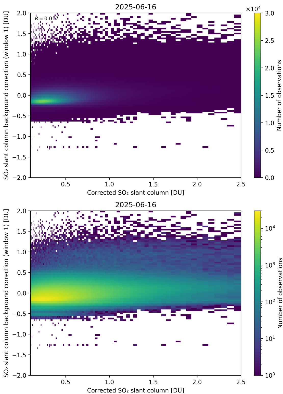
Figure 226: Scatter density plot of “Corrected SO 2 slant column” against “SO 2 slant column background correction (window 1)” for 2025-06-16 to 2025-06-17.
