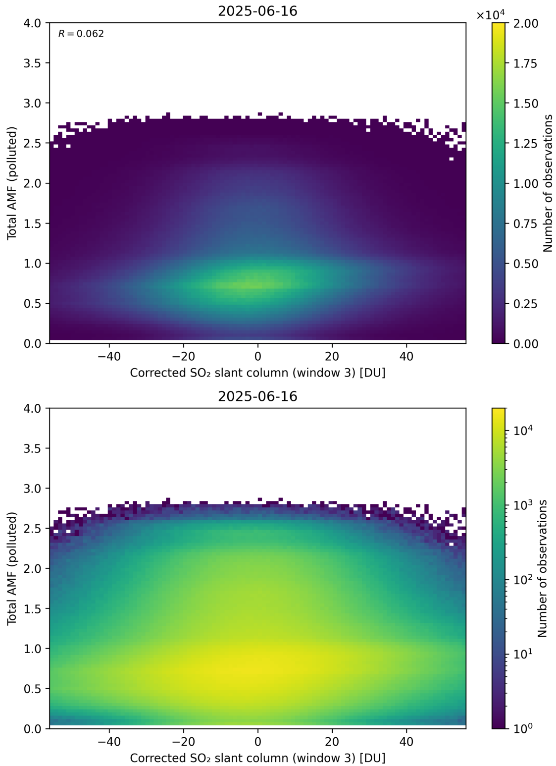
Figure 260: Scatter density plot of “Corrected SO 2 slant column (window 3)” against “Total AMF (polluted)” for 2025-06-16 to 2025-06-17.
