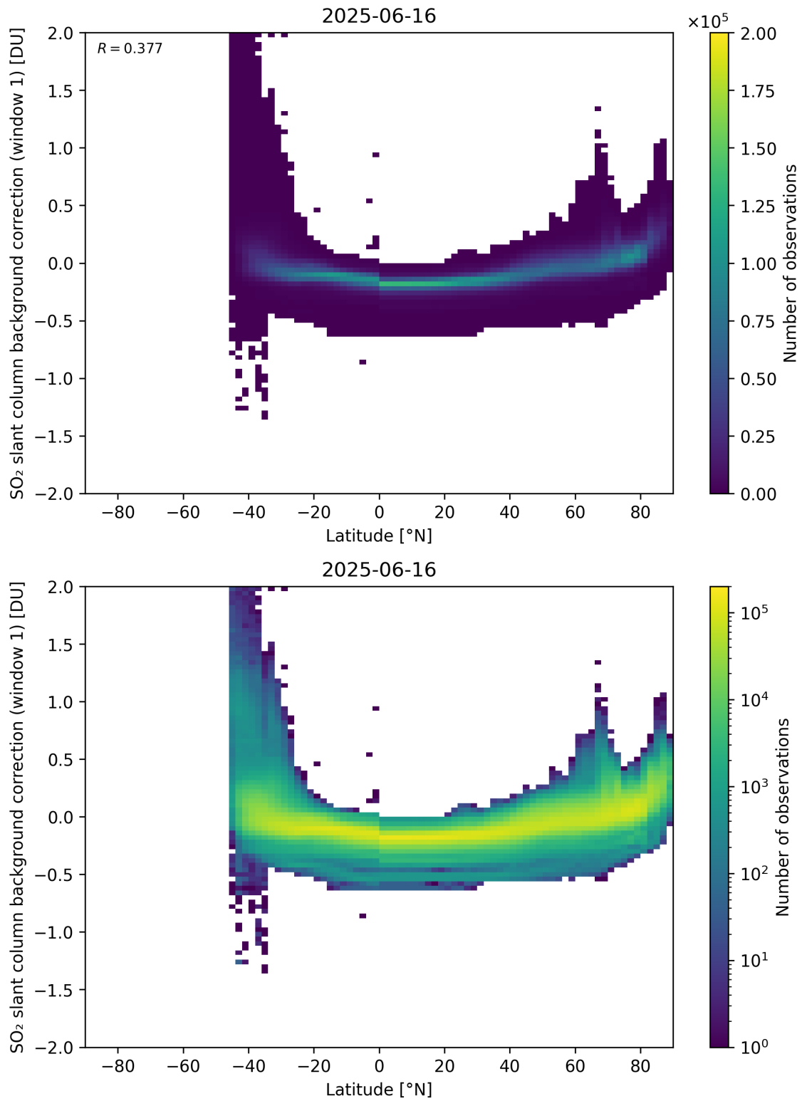
Figure 150: Scatter density plot of “Latitude” against “SO 2 slant column background correction (window 1)” for 2025-06-16 to 2025-06-17.
