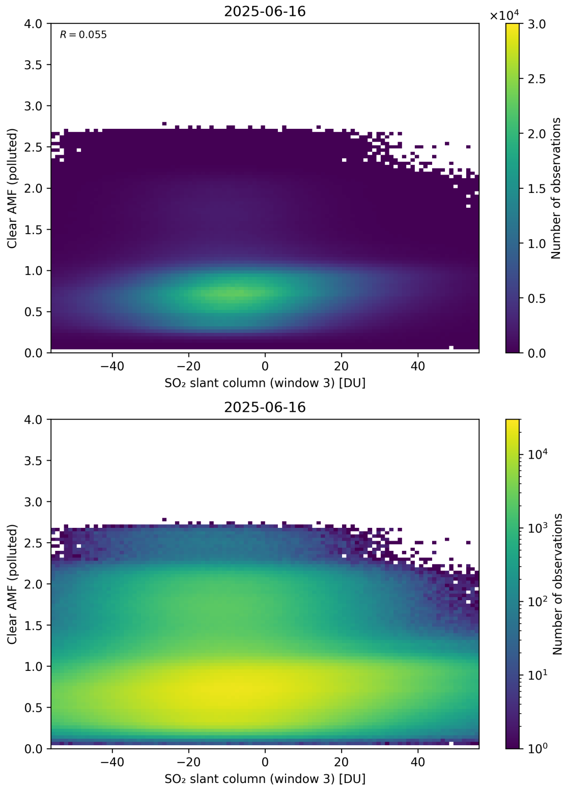
Figure 315: Scatter density plot of “SO 2 slant column (window 3)” against “Clear AMF (polluted)” for 2025-06-16 to 2025-06-17.
