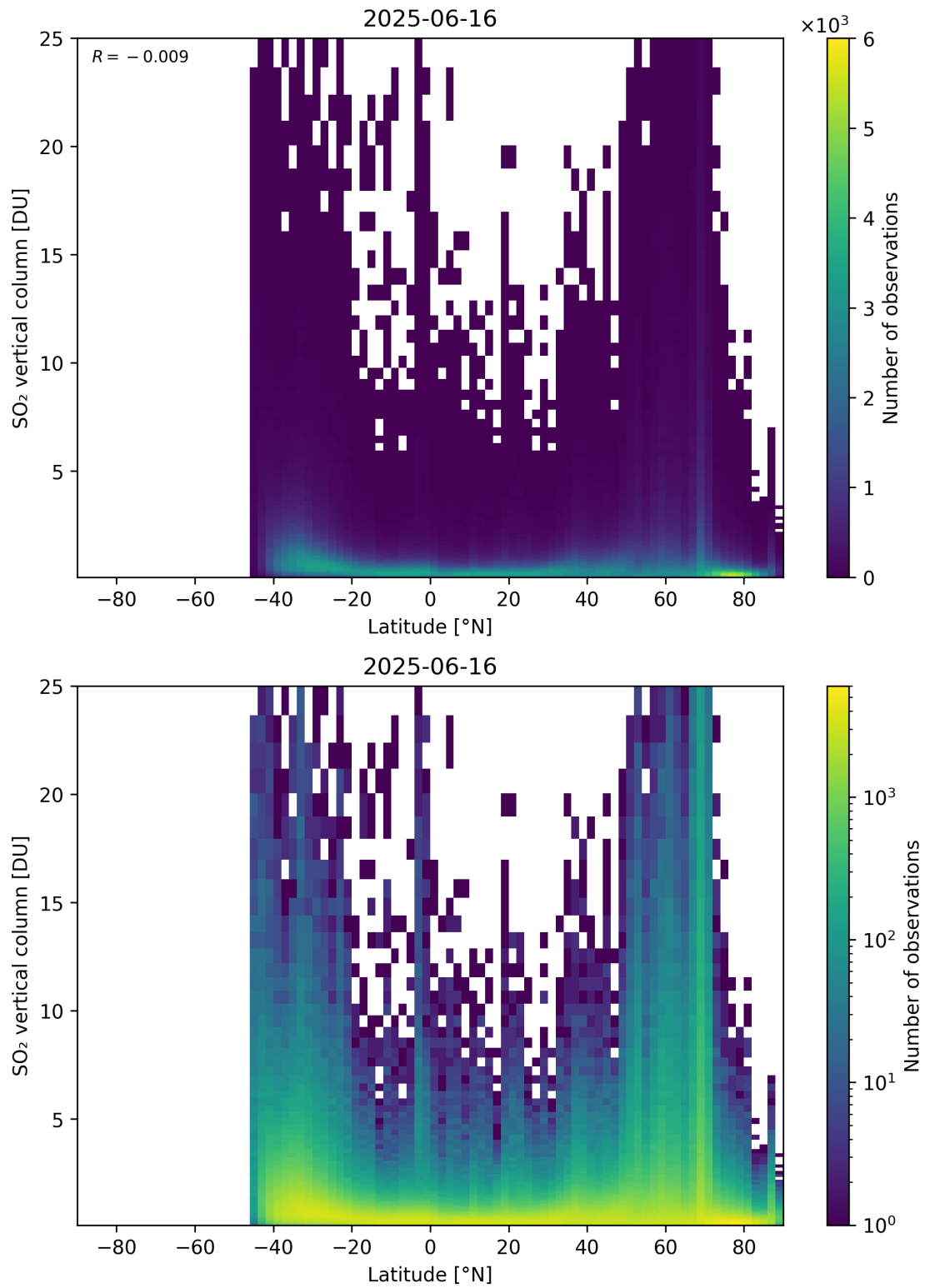
Figure 169: Scatter density plot of “Latitude” against “SO 2 vertical column” for 2025-06-16 to 2025-06-17.
