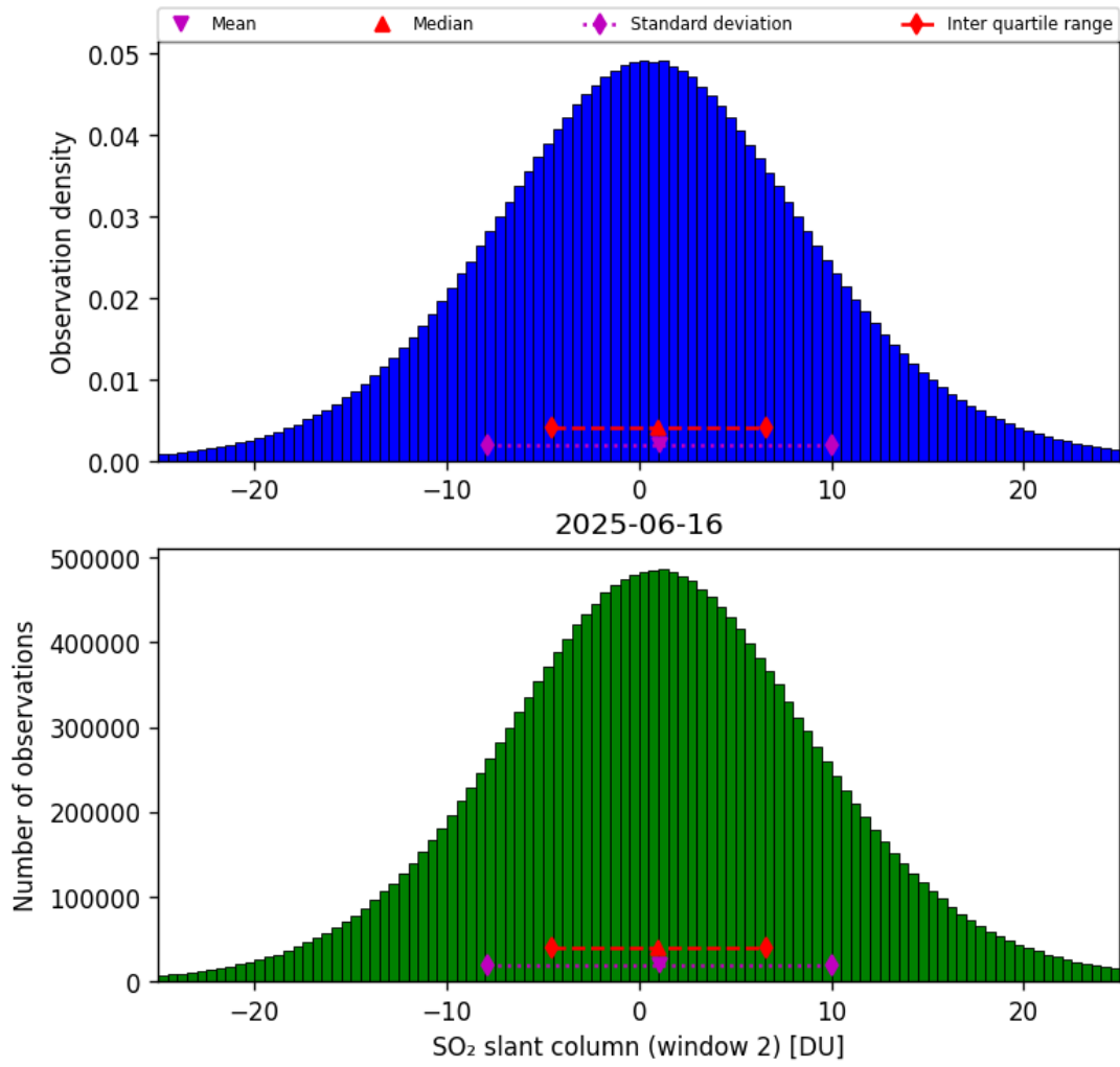
Figure 67: Histogram of “SO 2 slant column (window 2)” for 2025-06-16 to 2025-06-17
