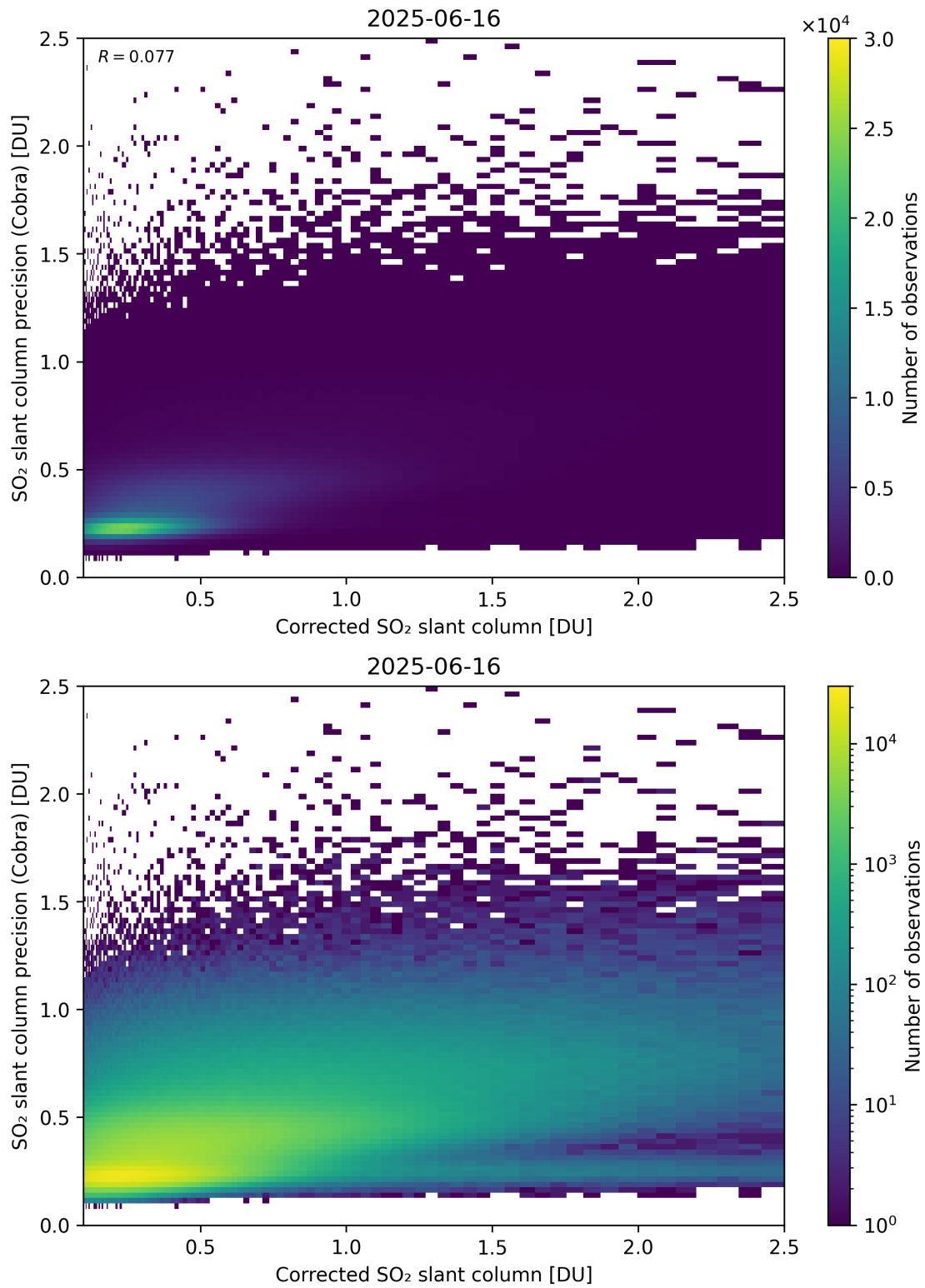
Figure 234: Scatter density plot of “Corrected SO 2 slant column” against “SO 2 slant column precision (Cobra)” for 2025-06-16 to 2025-06-17.
