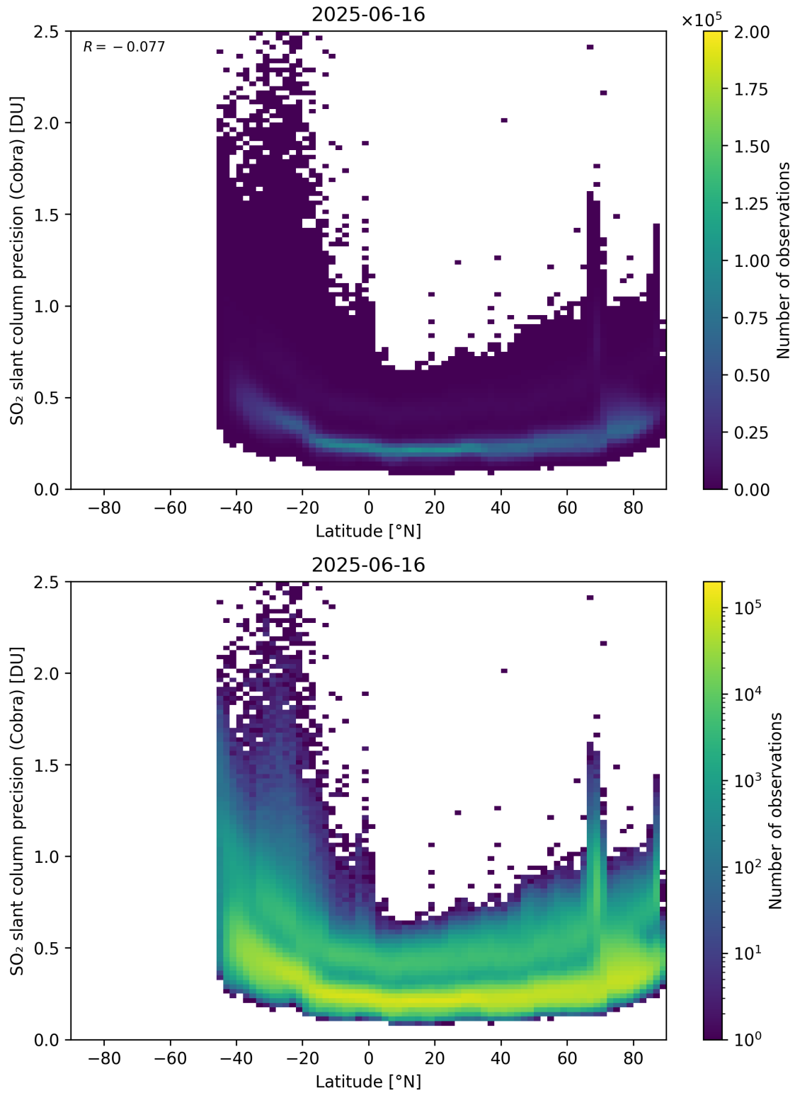
Figure 158: Scatter density plot of “Latitude” against “SO 2 slant column precision (Cobra)” for 2025-06-16 to 2025-06-17.
