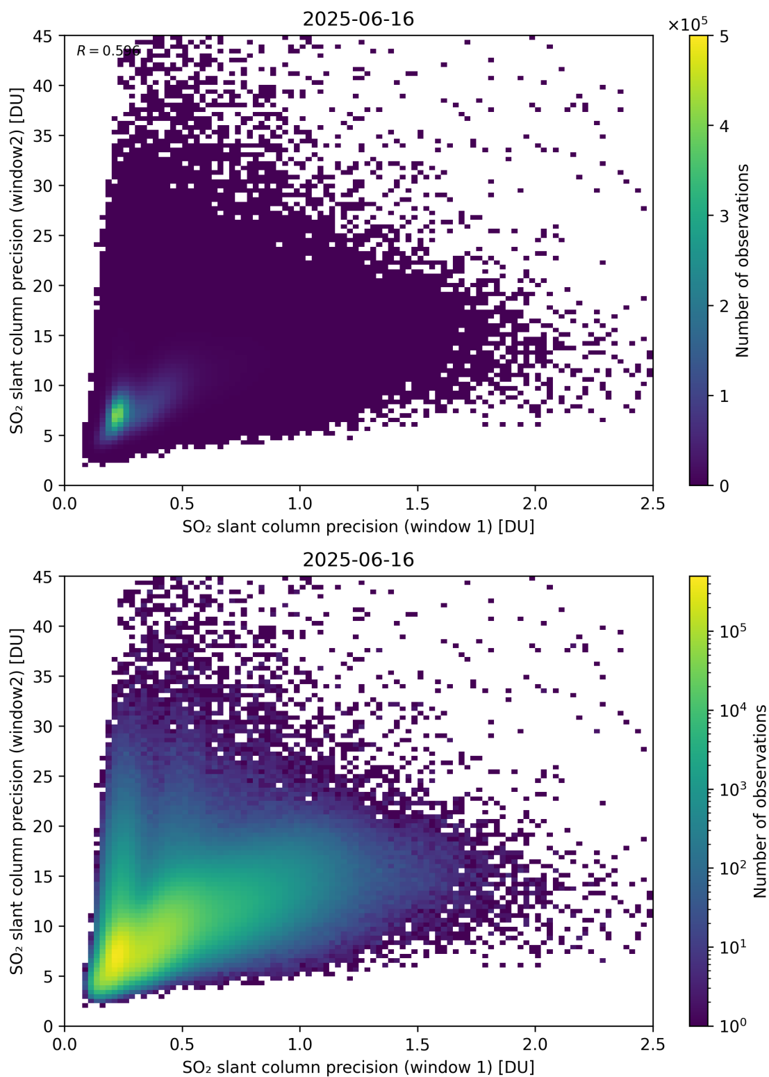
Figure 277: Scatter density plot of “SO 2 slant column precision (window 1)” against “SO 2 slant column precision (window2)” for 2025-06-16 to 2025-06-17.
