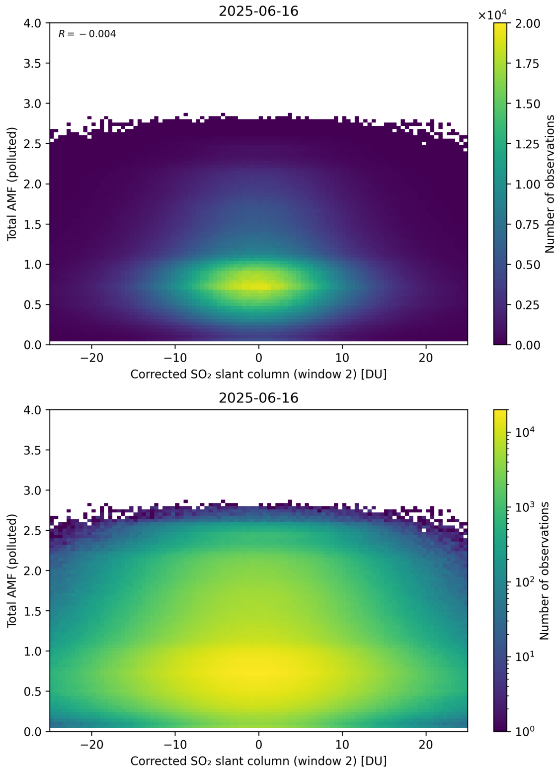
Figure 253: Scatter density plot of “Corrected SO 2 slant column (window 2)” against “Total AMF (polluted)” for 2025-06-16 to 2025-06-17.
