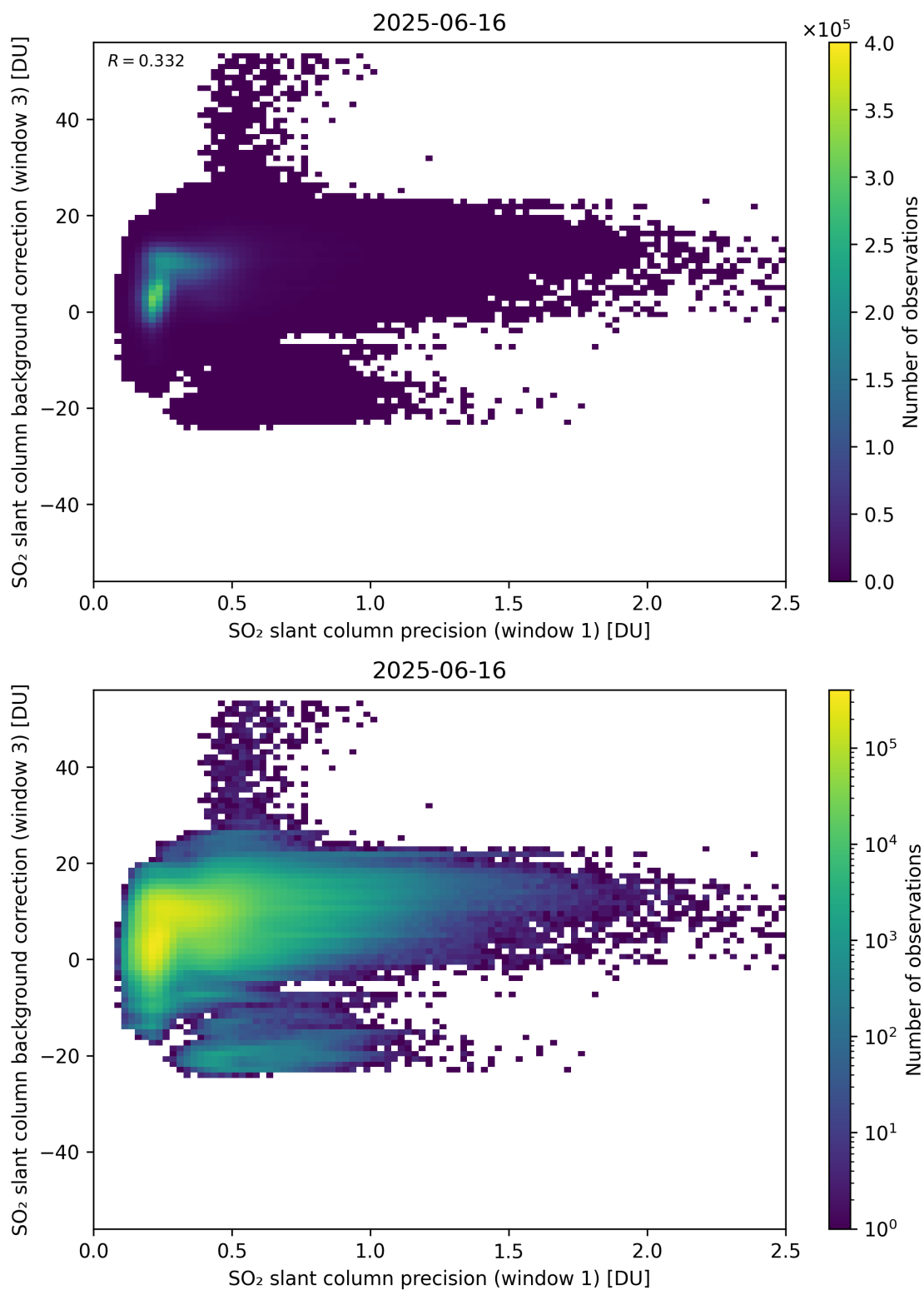
Figure 270: Scatter density plot of “SO 2 slant column precision (window 1)” against “SO 2 slant column background correction (window 3)” for 2025-06-16 to 2025-06-17.
