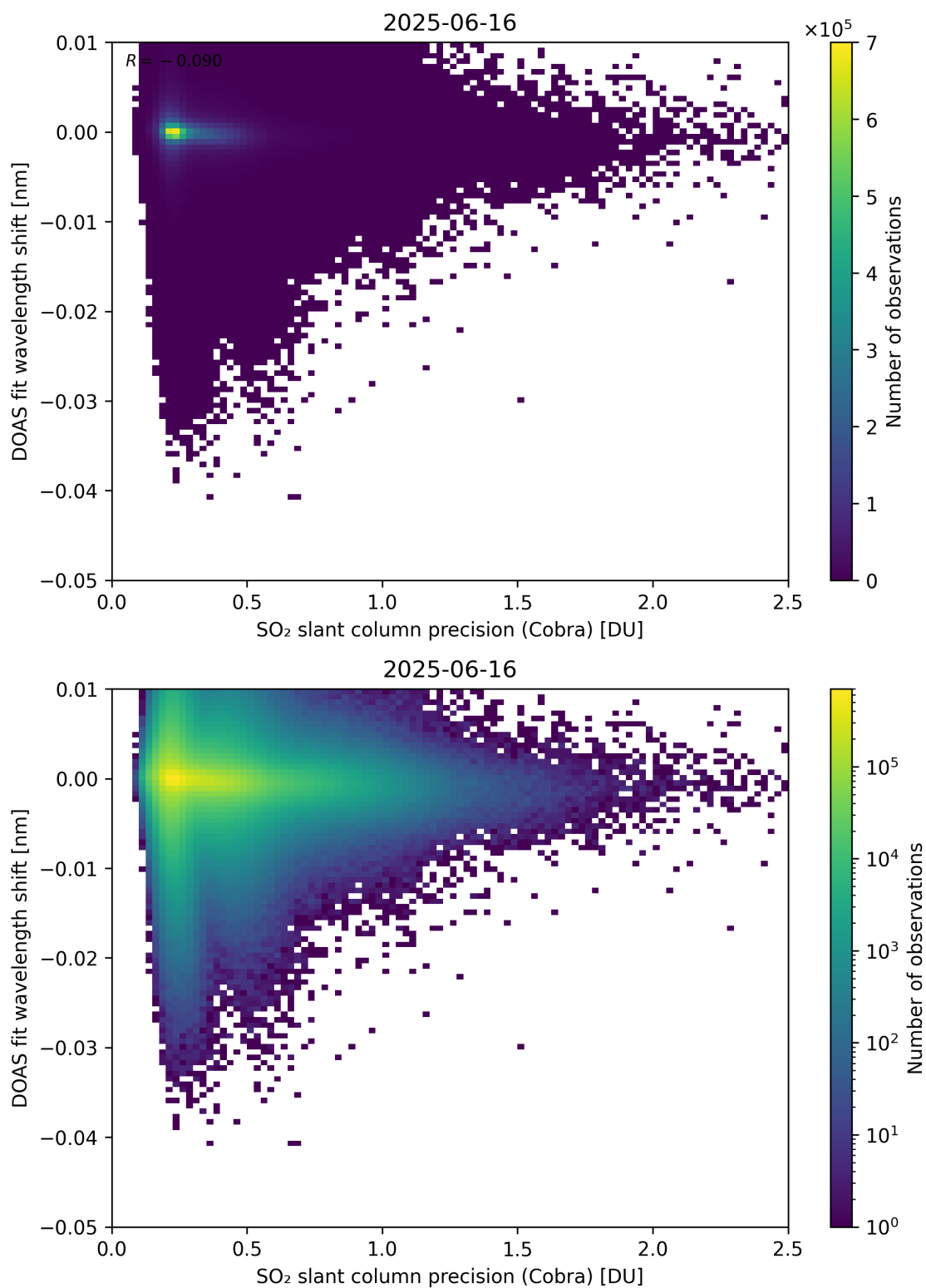
Figure 202: Scatter density plot of “SO 2 slant column precision (Cobra)” against “DOAS fit wavelength shift” for 2025-06-16 to 2025-06-17.
