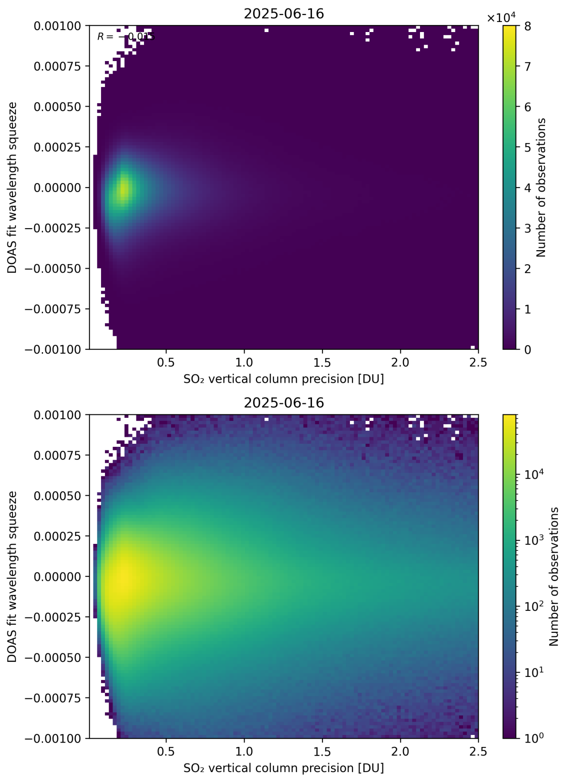
Figure 333: Scatter density plot of “SO 2 vertical column precision” against “DOAS fit wavelength squeeze” for 2025-06-16 to 2025-06-17.
