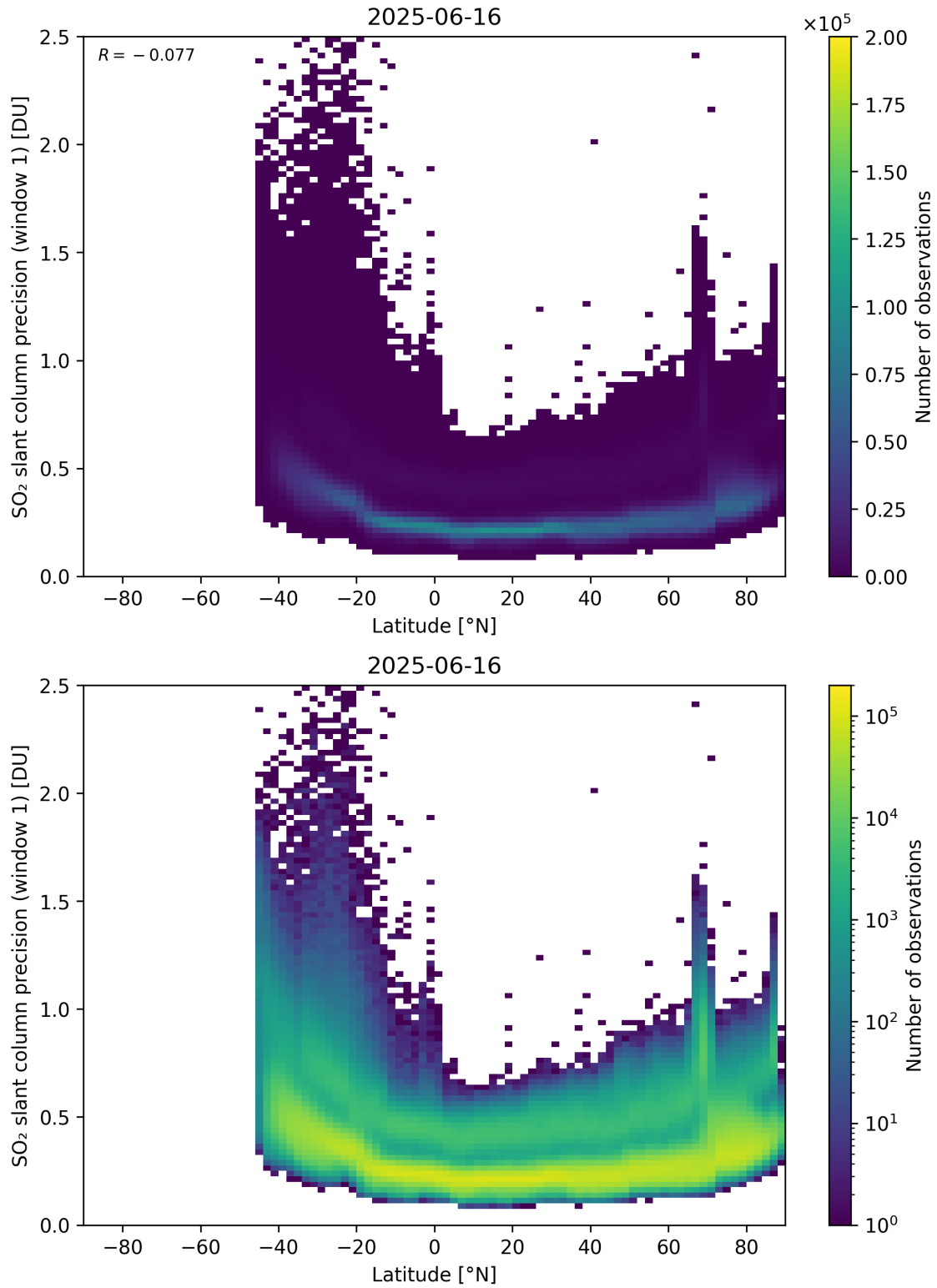
Figure 163: Scatter density plot of “Latitude” against “SO 2 slant column precision (window 1)” for 2025-06-16 to 2025-06-17.
