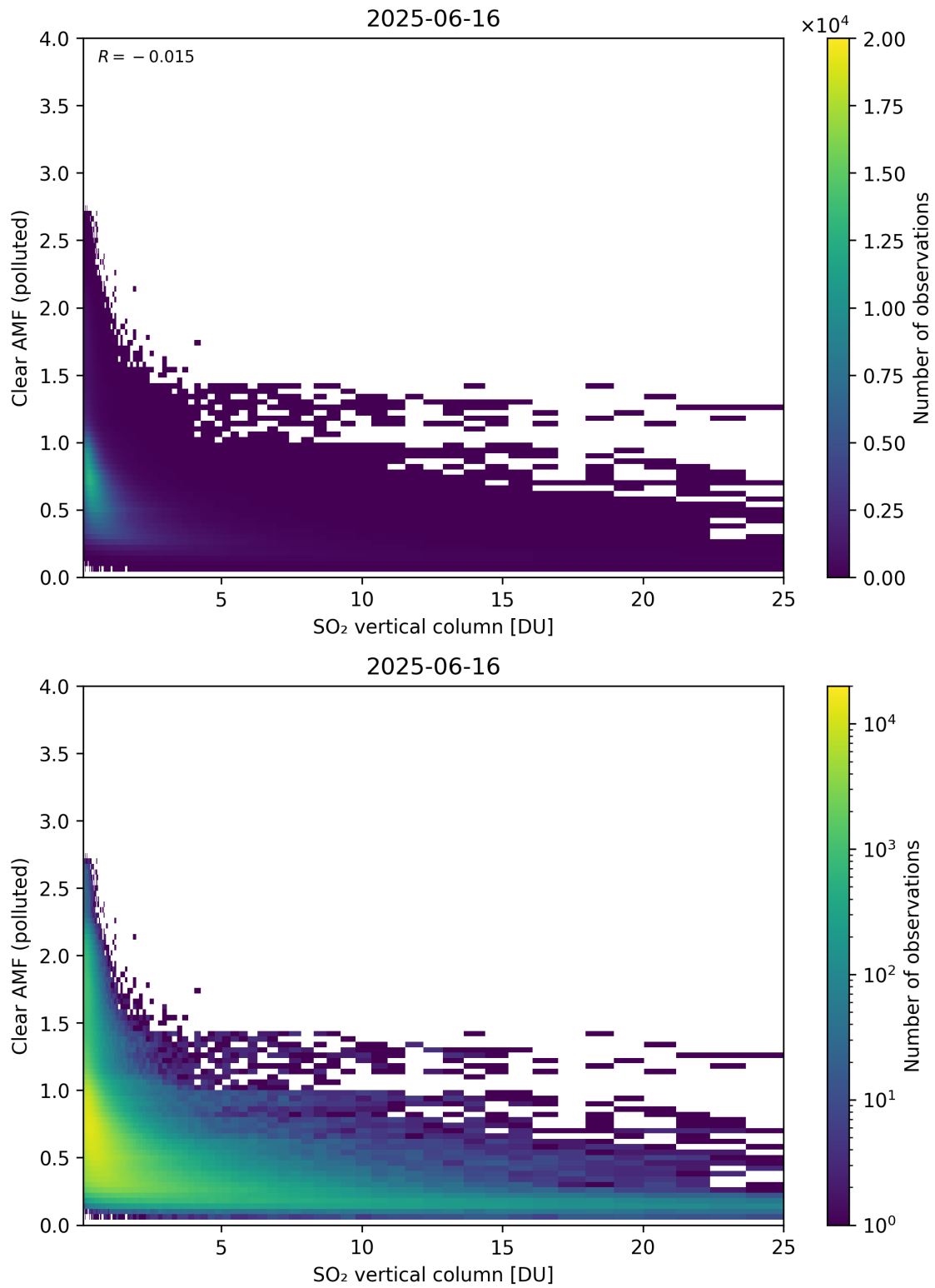
Figure 348: Scatter density plot of “SO 2 vertical column” against “Clear AMF (polluted)” for 2025-06-16 to 2025-06-17.
