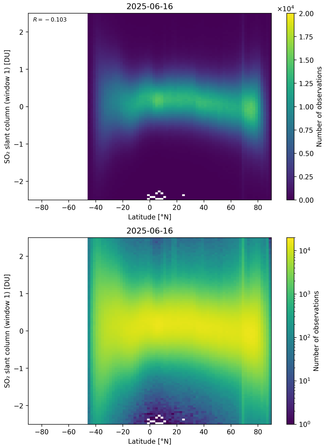
Figure 162: Scatter density plot of “Latitude” against “SO 2 slant column (window 1)” for 2025-06-16 to 2025-06-17.
