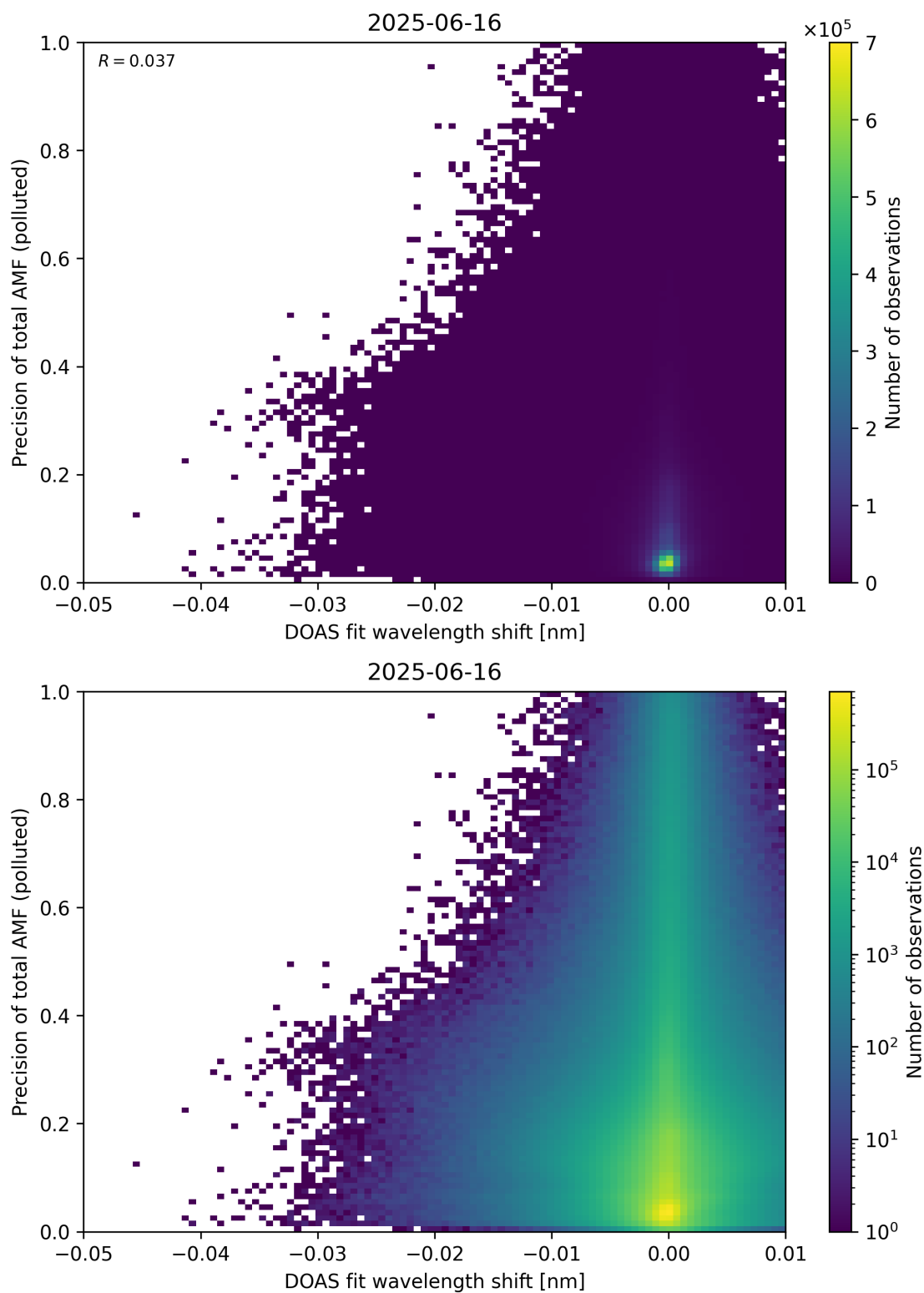
Figure 142: Scatter density plot of “DOAS fit wavelength shift” against “Precision of total AMF (polluted)” for 2025-06-16 to 2025-06-17.
