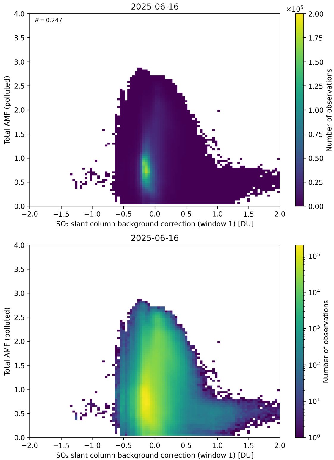
Figure 120: Scatter density plot of “SO 2 slant column background correction (window 1)” against “Total AMF (polluted)” for 2025-06-16 to 2025-06-17.
