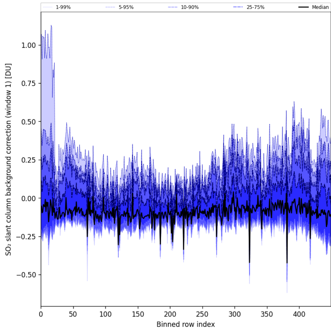
Figure 92: Along track statistics of “SO 2 slant column background correction (window 1)” for 2025-06-16 to 2025-06-17
