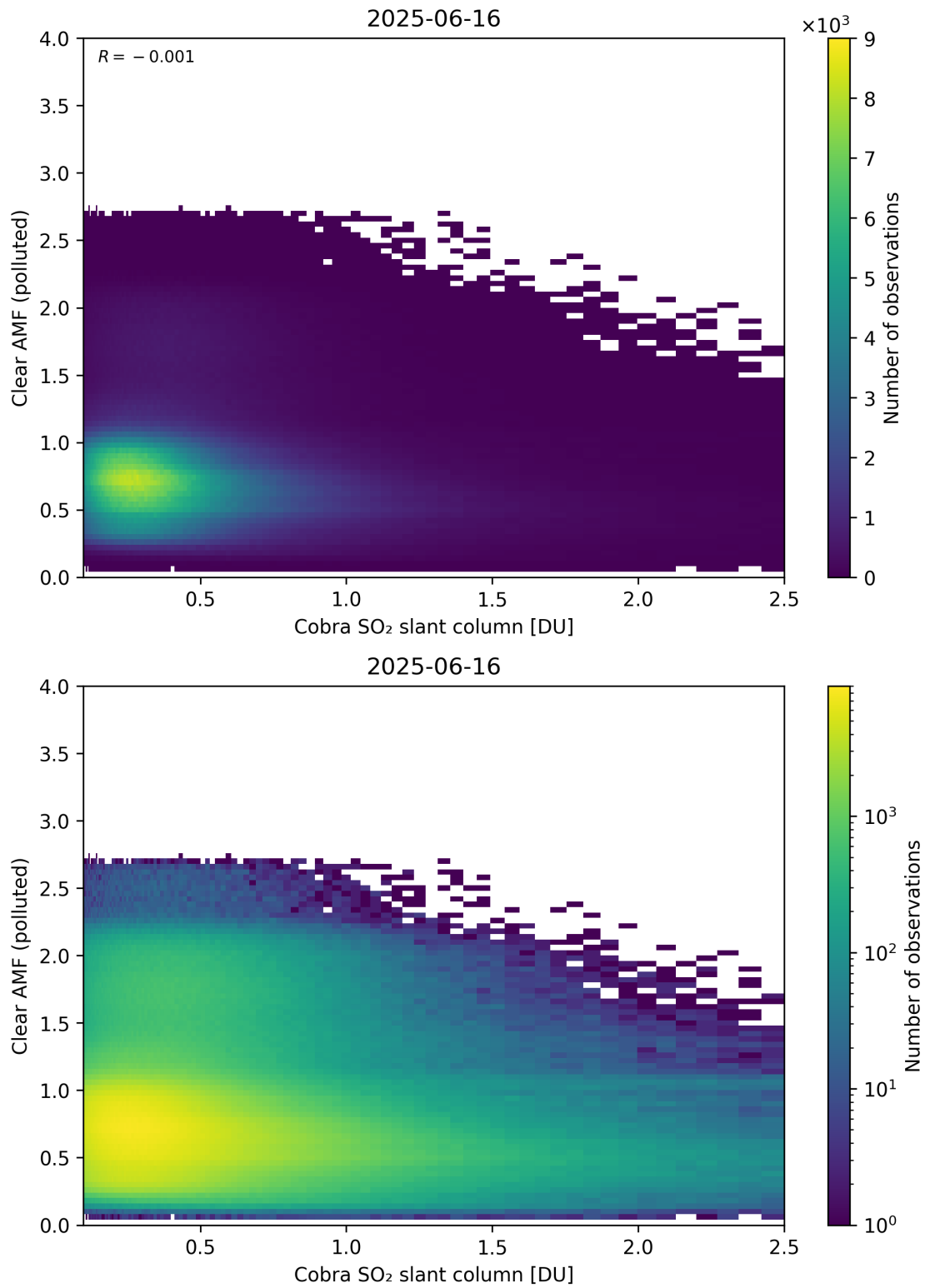
Figure 215: Scatter density plot of “Cobra SO 2 slant column” against “Clear AMF (polluted)” for 2025-06-16 to 2025-06-17.
