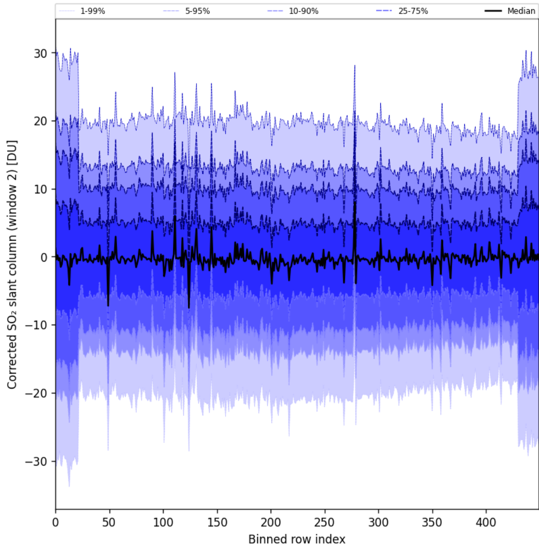
Figure 95: Along track statistics of “Corrected SO 2 slant column (window 2)” for 2025-06-16 to 2025-06-17
