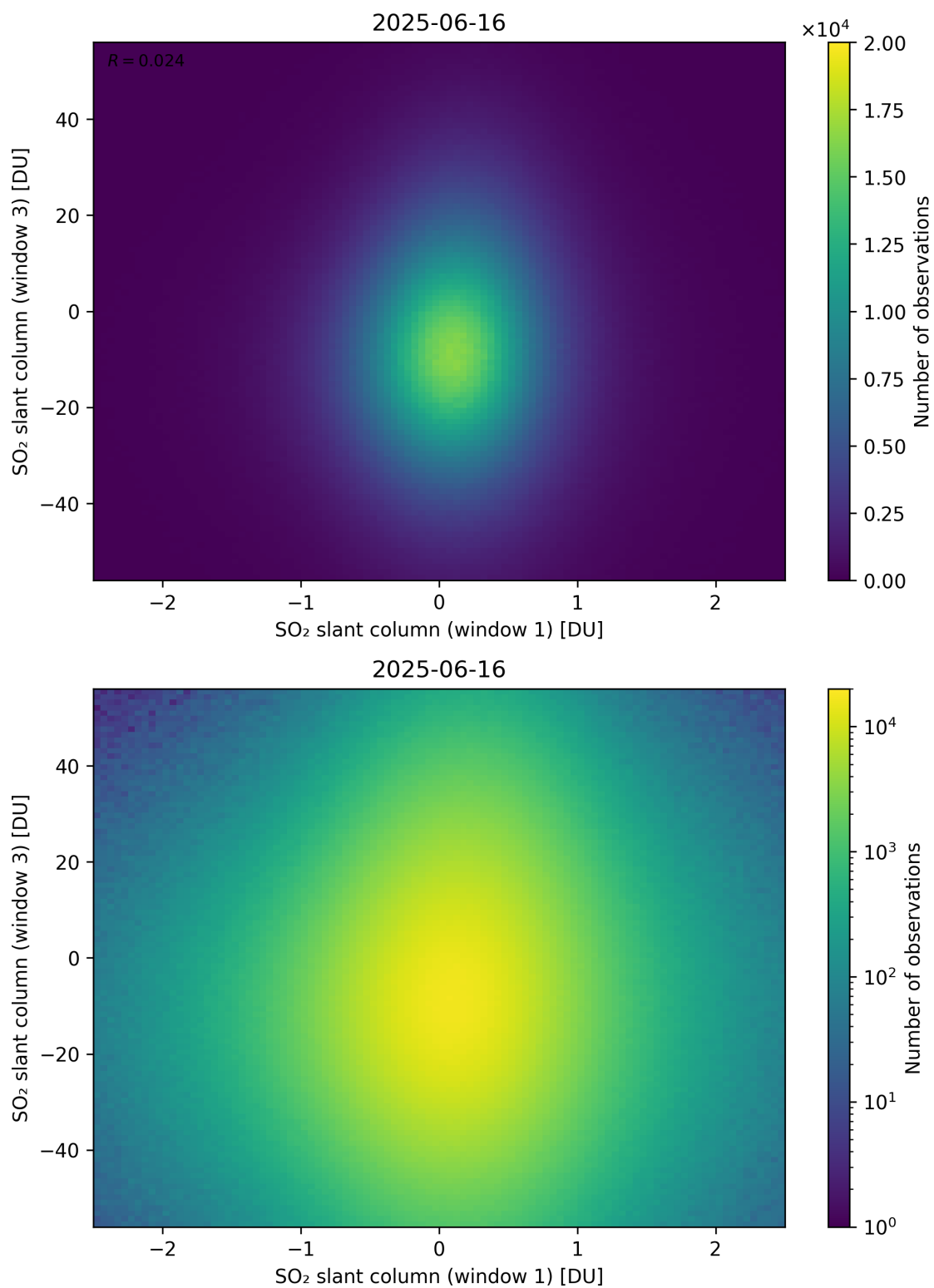
Figure 287: Scatter density plot of “SO 2 slant column (window 1)” against “SO 2 slant column (window 3)” for 2025-06-16 to 2025-06-17.
