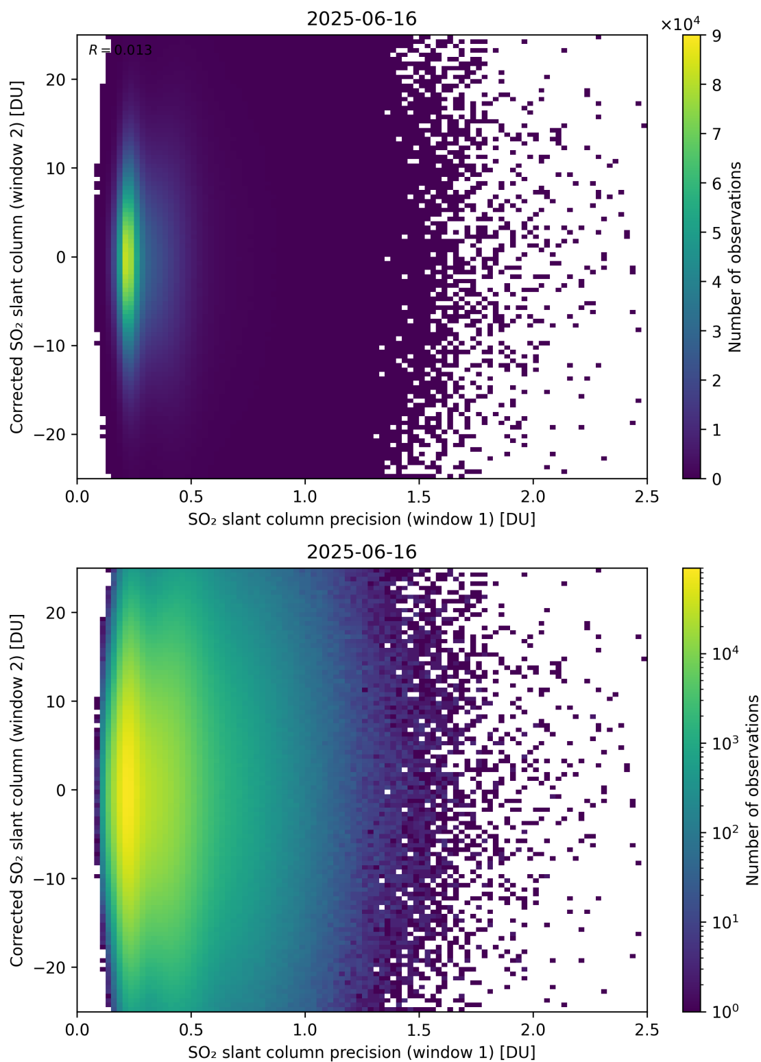
Figure 275: Scatter density plot of “SO 2 slant column precision (window 1)” against “Corrected SO 2 slant column (window 2)” for 2025-06-16 to 2025-06-17.
