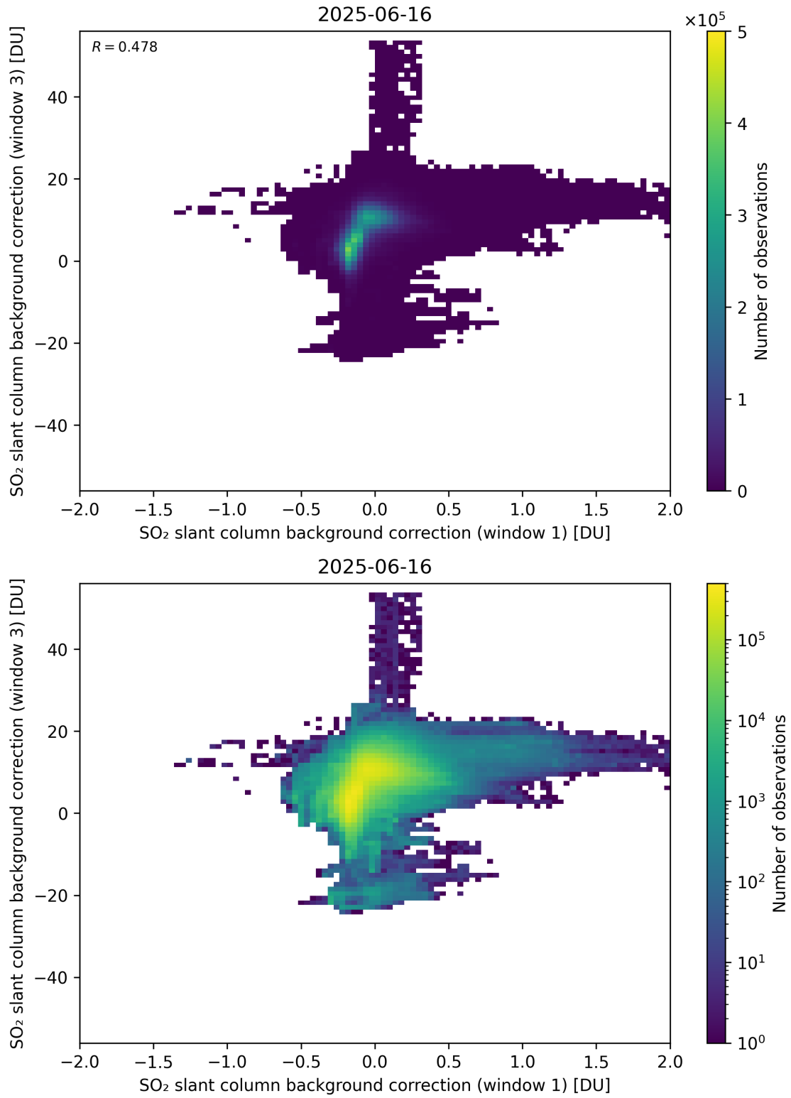
Figure 110: Scatter density plot of “SO 2 slant column background correction (window 1)” against “SO 2 slant column background correction (window 3)” for 2025-06-16 to 2025-06-17.
