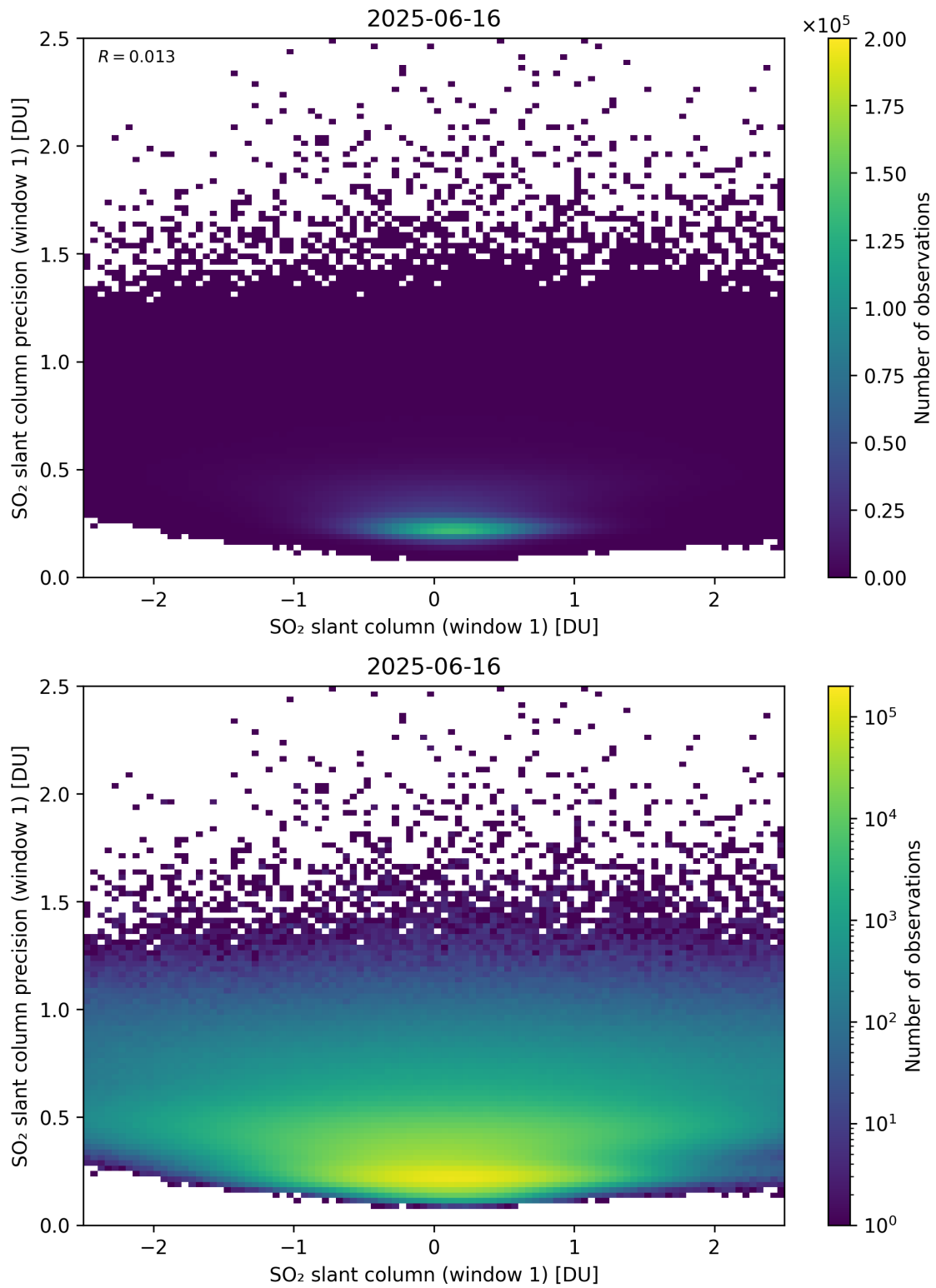
Figure 285: Scatter density plot of “SO 2 slant column (window 1)” against “SO 2 slant column precision (window 1)” for 2025-06-16 to 2025-06-17.
