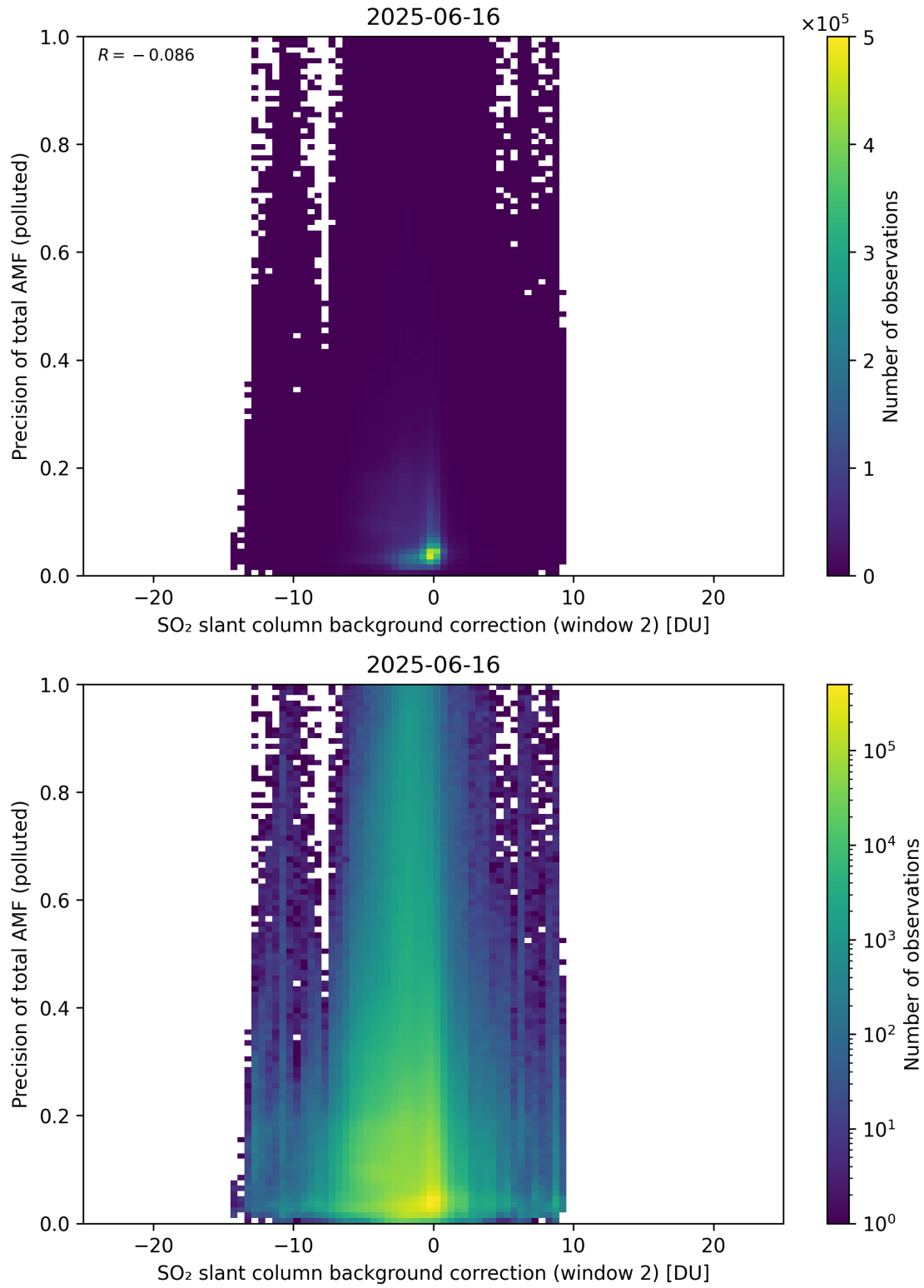
Figure 131: Scatter density plot of “SO 2 slant column background correction (window 2)” against “Precision of total AMF (polluted)” for 2025-06-16 to 2025-06-17.
