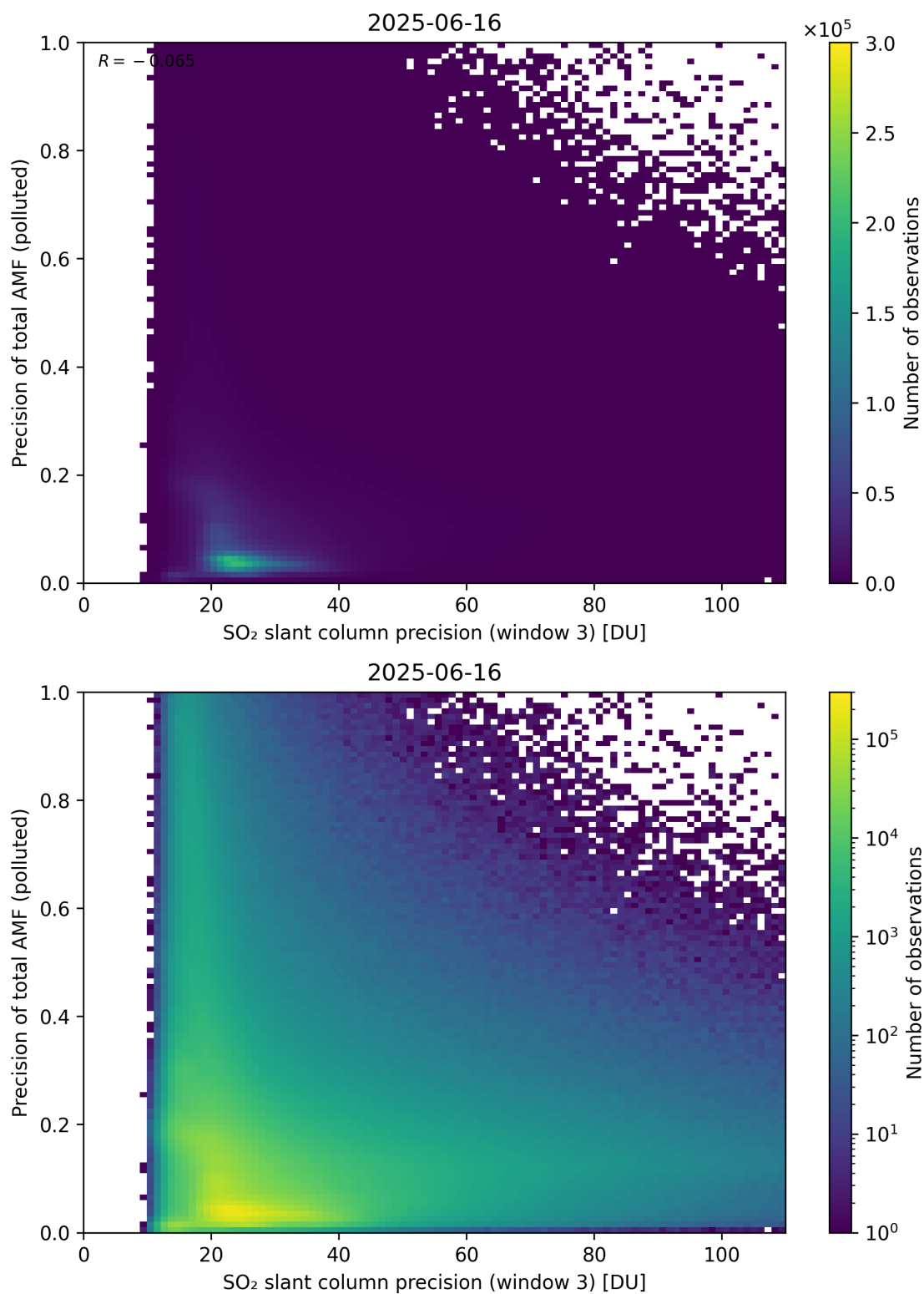
Figure 314: Scatter density plot of “SO 2 slant column precision (window 3)” against “Precision of total AMF (polluted)” for 2025-06-16 to 2025-06-17.
