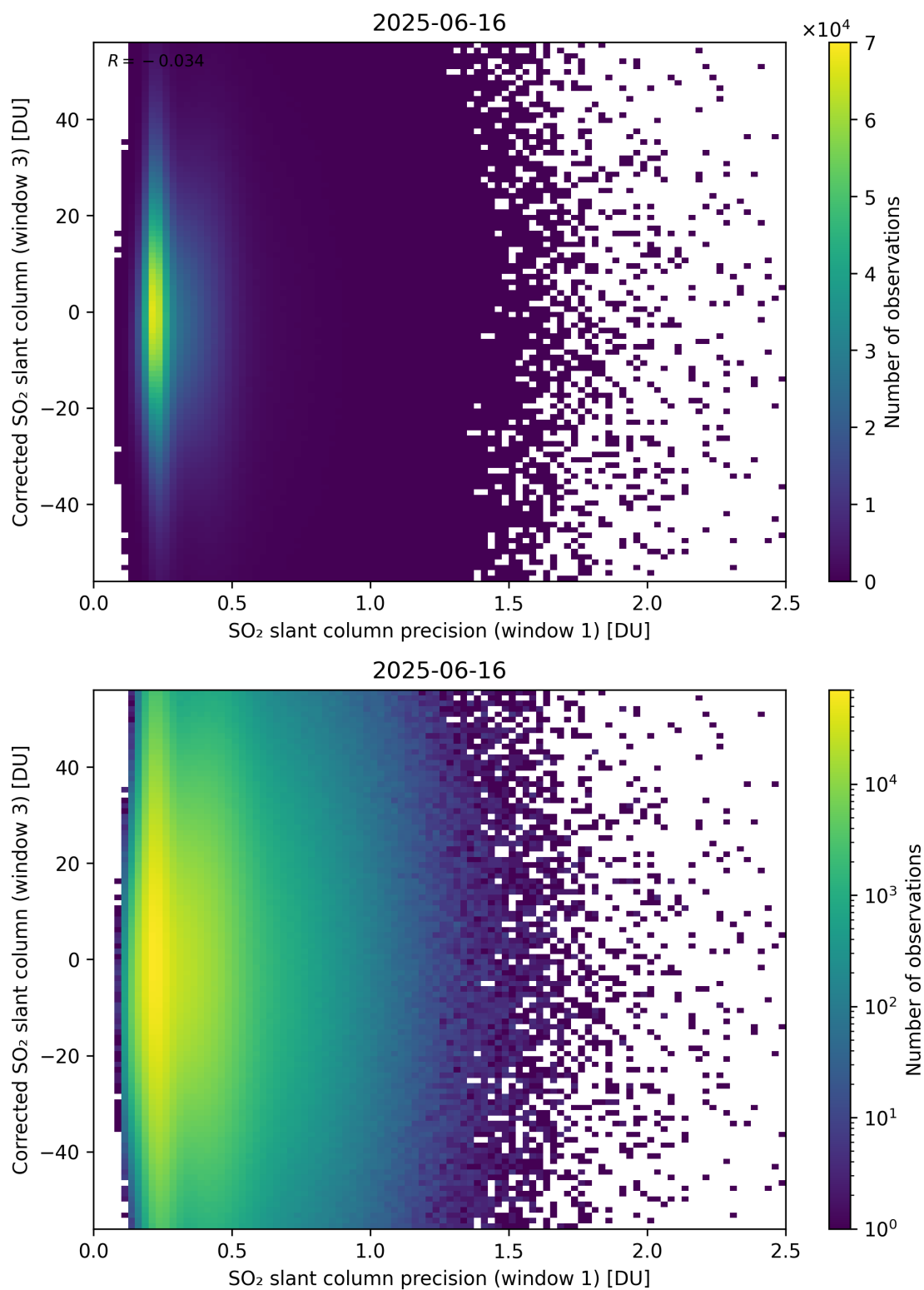
Figure 276: Scatter density plot of “SO 2 slant column precision (window 1)” against “Corrected SO 2 slant column (window 3)” for 2025-06-16 to 2025-06-17.
