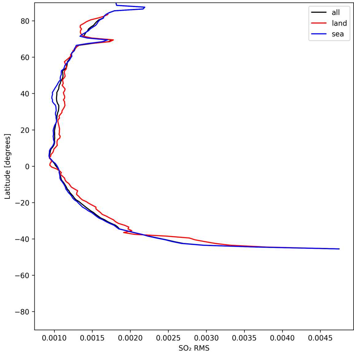
Figure 52: Zonal average of “SO 2 RMS” for 2025-06-16 to 2025-06-17.
