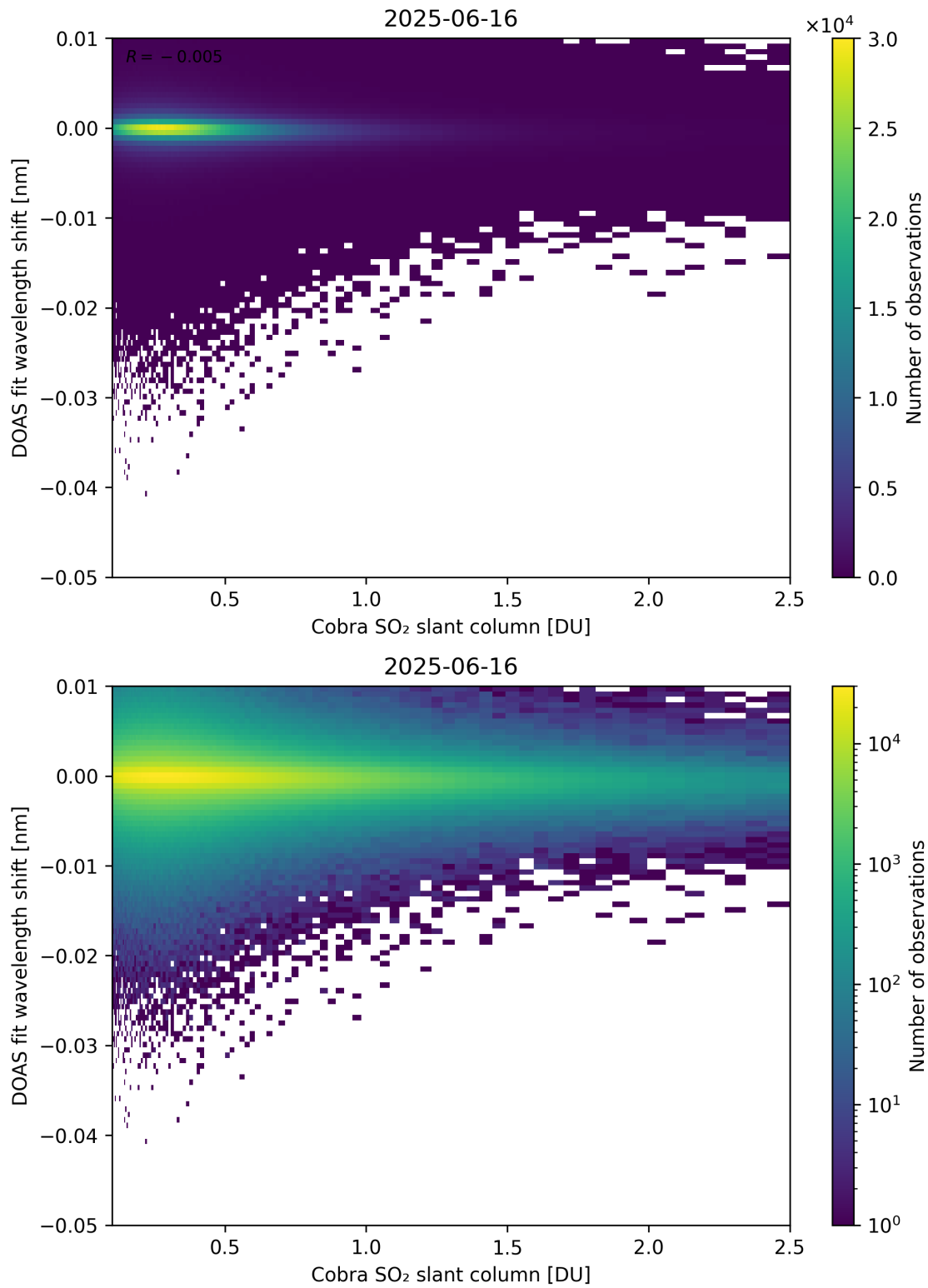
Figure 196: Scatter density plot of “Cobra SO 2 slant column” against “DOAS fit wavelength shift” for 2025-06-16 to 2025-06-17.
