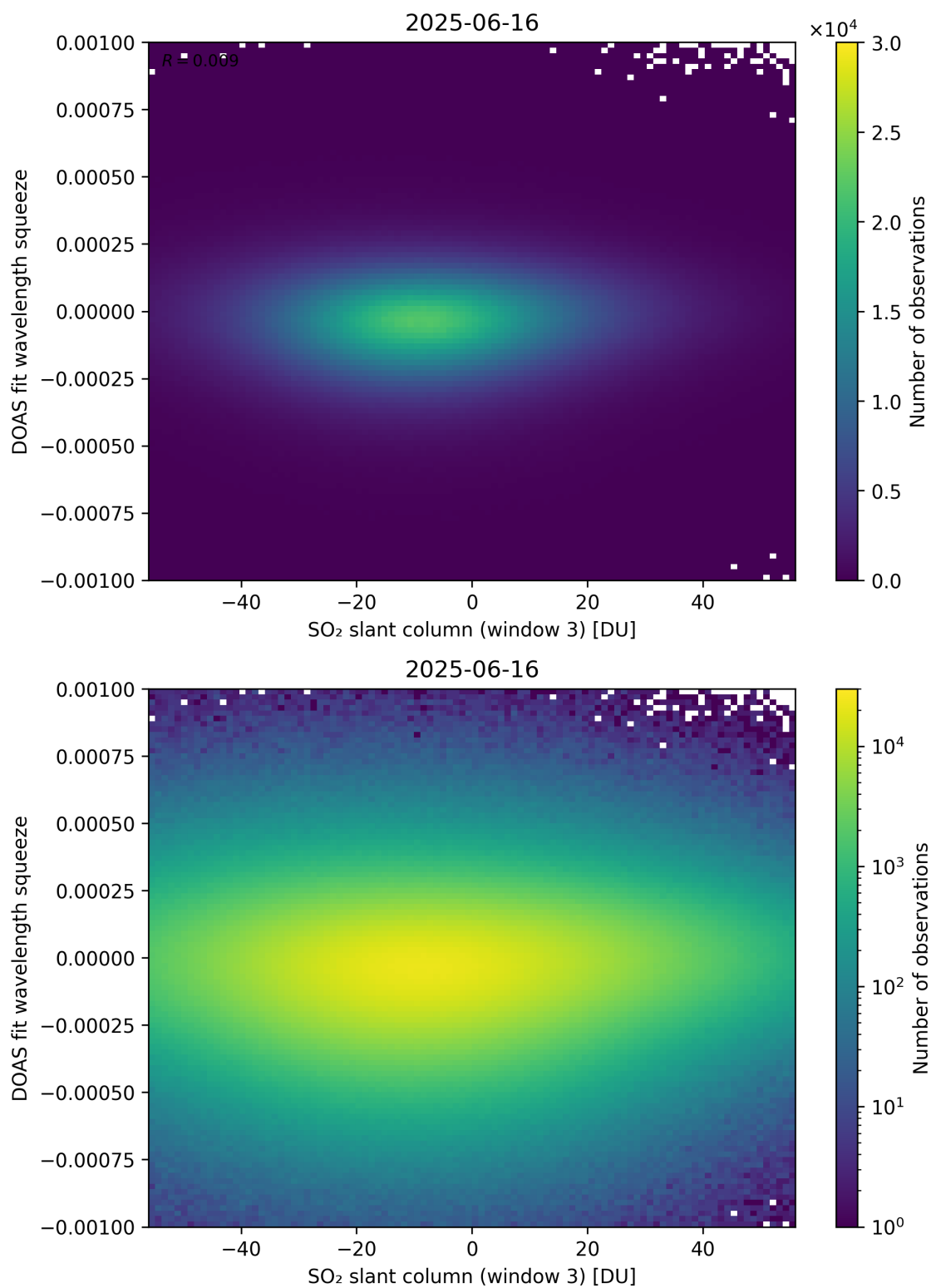
Figure 305: Scatter density plot of “SO 2 slant column (window 3)” against “DOAS fit wavelength squeeze” for 2025-06-16 to 2025-06-17.
