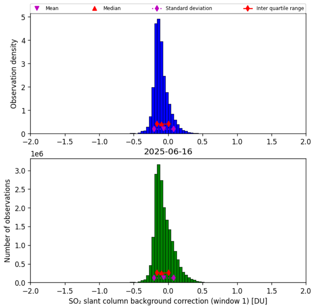
Figure 66: Histogram of “SO 2 slant column background correction (window 1)” for 2025-06-16 to 2025-06-17
