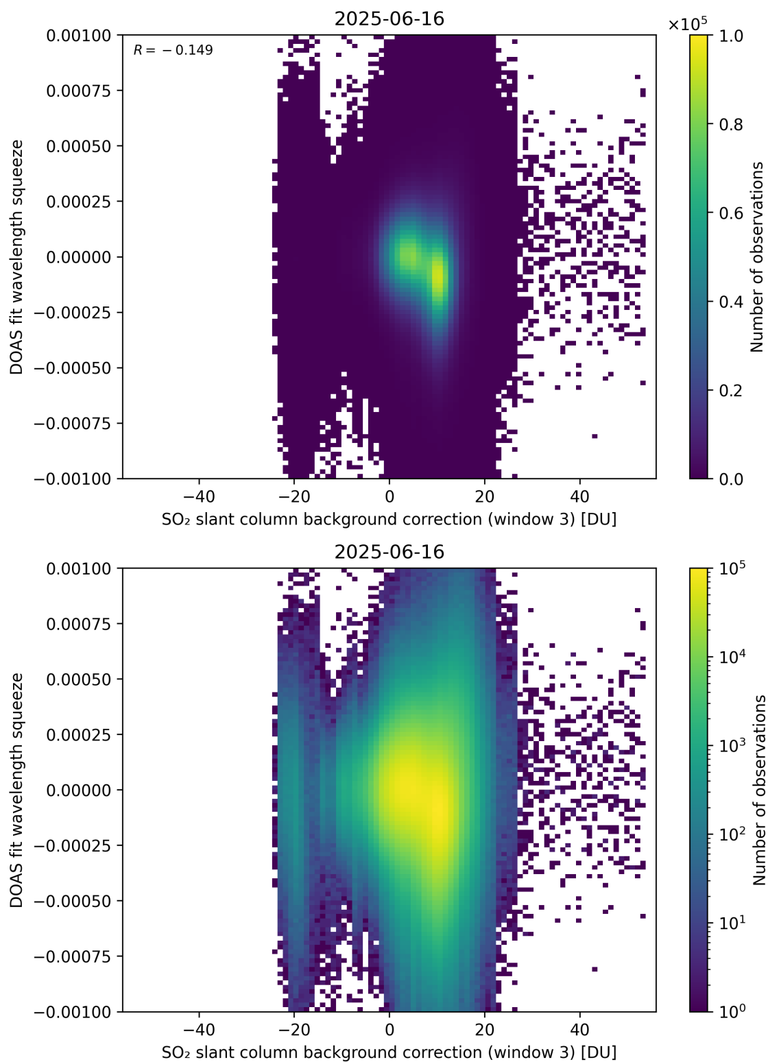
Figure 133: Scatter density plot of “SO 2 slant column background correction (window 3)” against “DOAS fit wavelength squeeze” for 2025-06-16 to 2025-06-17.
