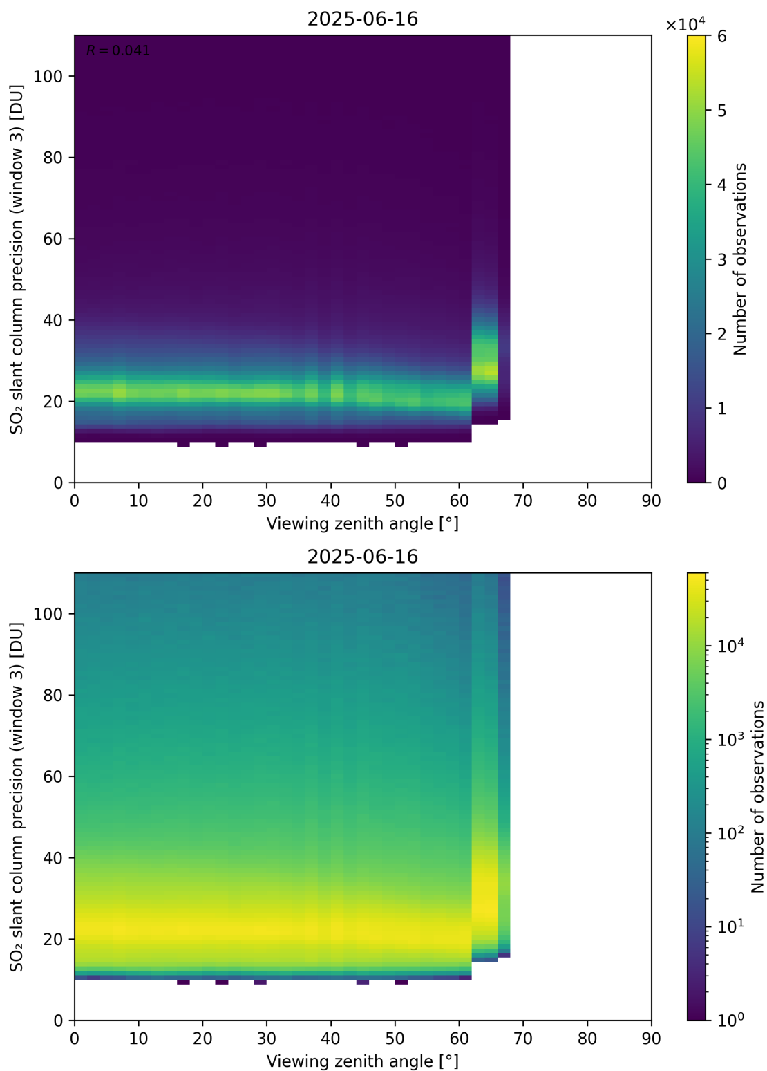
Figure 380: Scatter density plot of “Viewing zenith angle” against “SO 2 slant column precision (window 3)” for 2025-06-16 to 2025-06-17.
