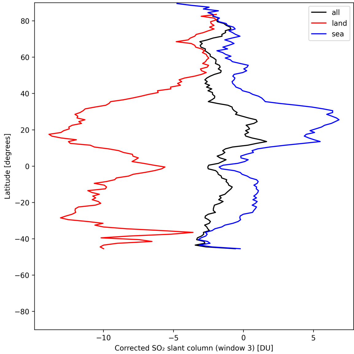
Figure 47: Zonal average of “Corrected SO 2 slant column (window 3)” for 2025-06-16 to 2025-06-17.
