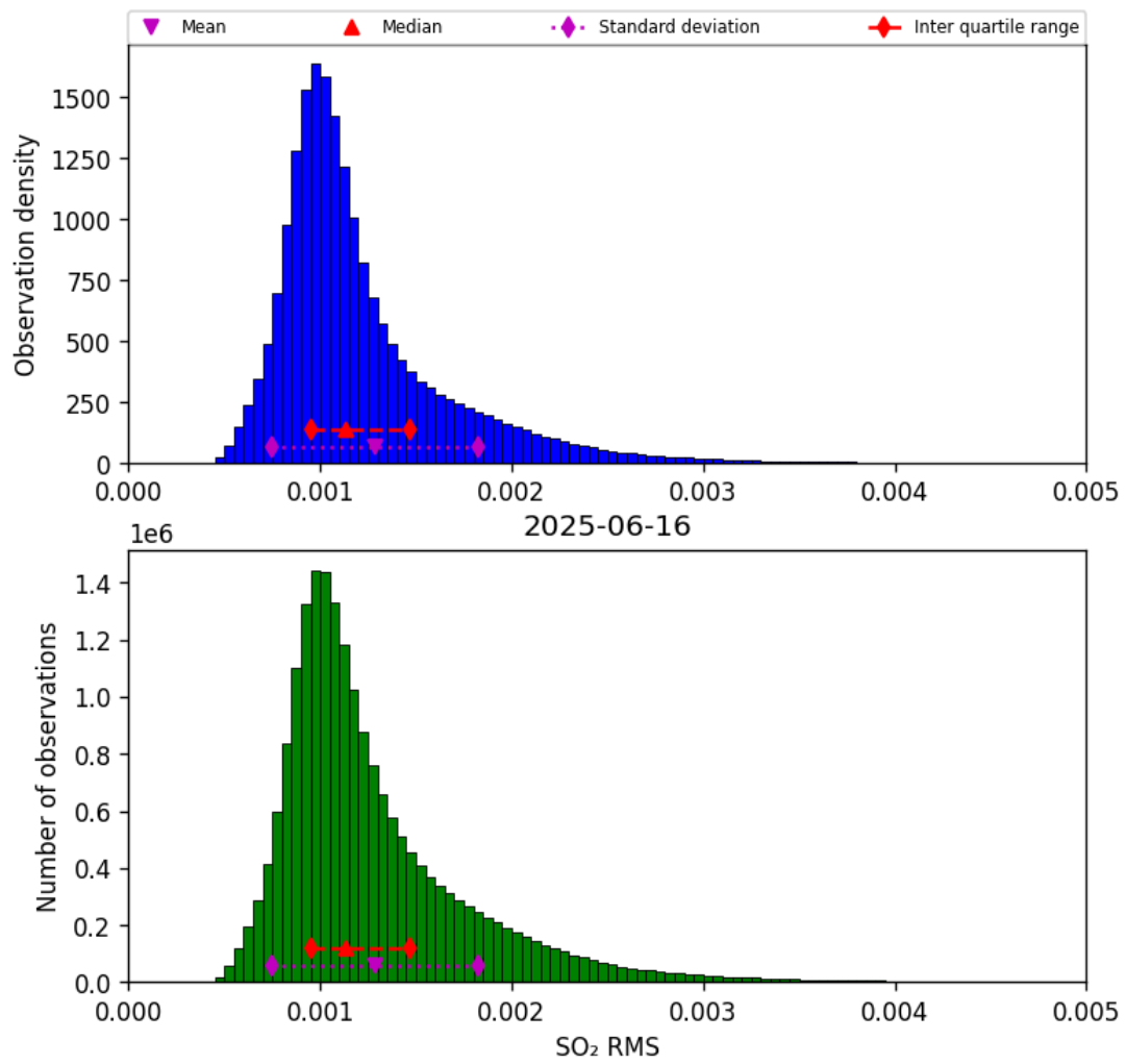
Figure 78: Histogram of “SO 2 RMS” for 2025-06-16 to 2025-06-17
