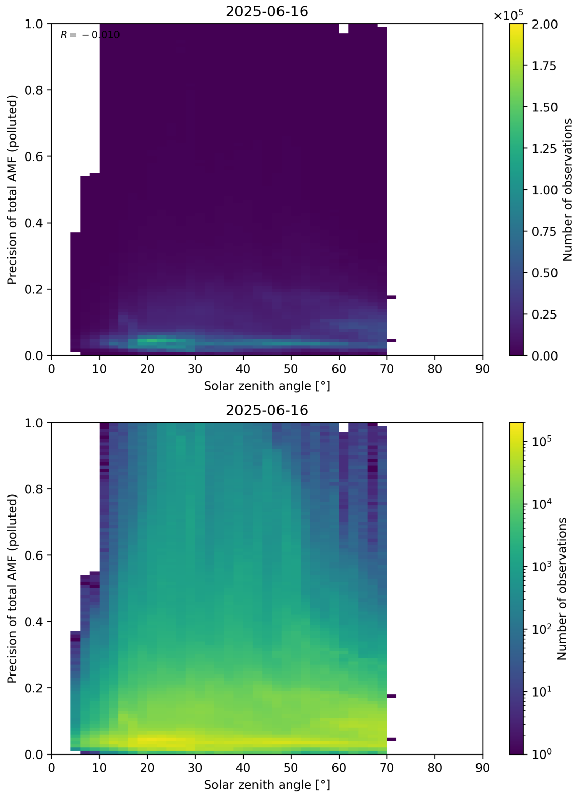
Figure 190: Scatter density plot of “Solar zenith angle” against “Precision of total AMF (polluted)” for 2025-06-16 to 2025-06-17.
