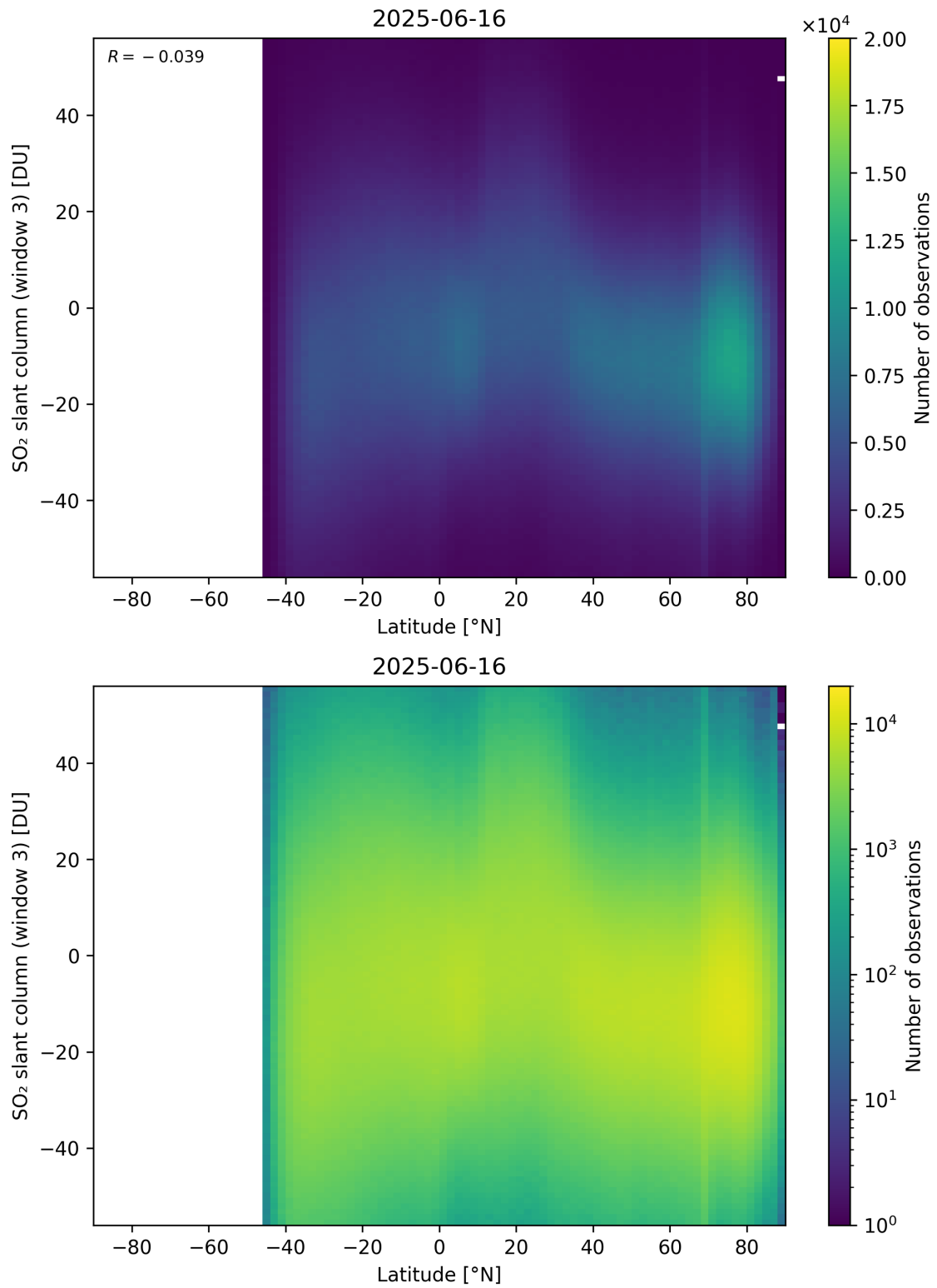
Figure 165: Scatter density plot of “Latitude” against “SO 2 slant column (window 3)” for 2025-06-16 to 2025-06-17.
