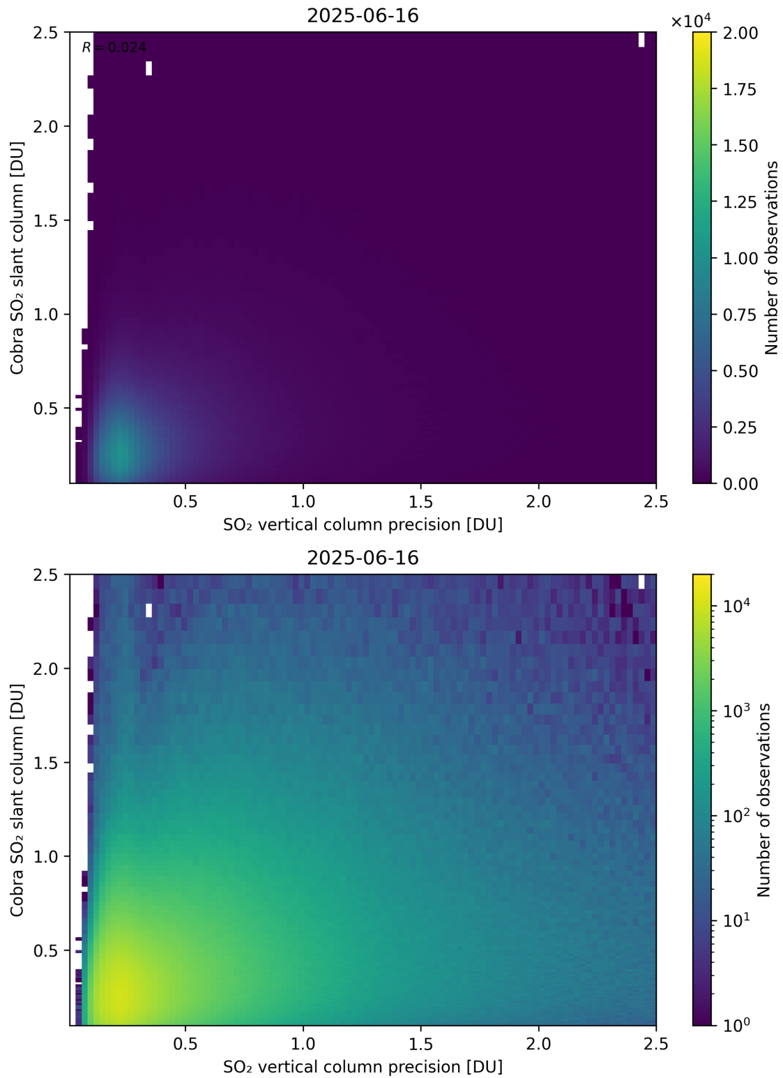
Figure 336: Scatter density plot of “SO 2 vertical column precision” against “Cobra SO 2 slant column” for 2025-06-16 to 2025-06-17.
