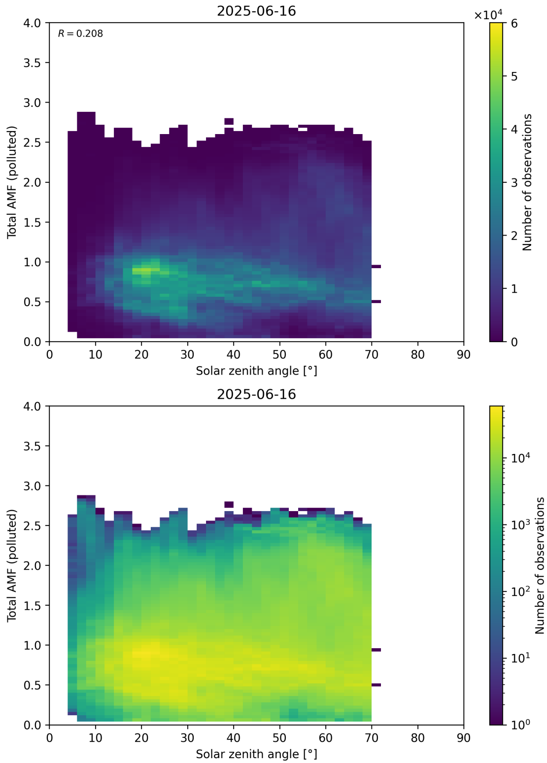
Figure 189: Scatter density plot of “Solar zenith angle” against “Total AMF (polluted)” for 2025-06-16 to 2025-06-17.
