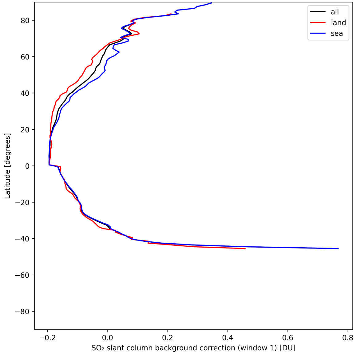
Figure 40: Zonal average of “SO 2 slant column background correction (window 1)” for 2025-06-16 to 2025-06-17.
