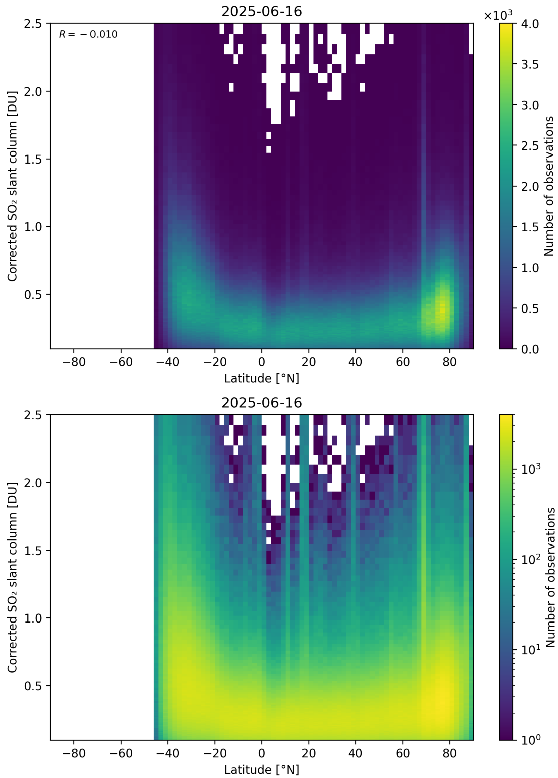
Figure 159: Scatter density plot of “Latitude” against “Corrected SO 2 slant column” for 2025-06-16 to 2025-06-17.
