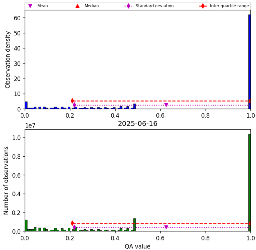
Figure 57: Histogram of “QA value” for 2025-06-16 to 2025-06-17
