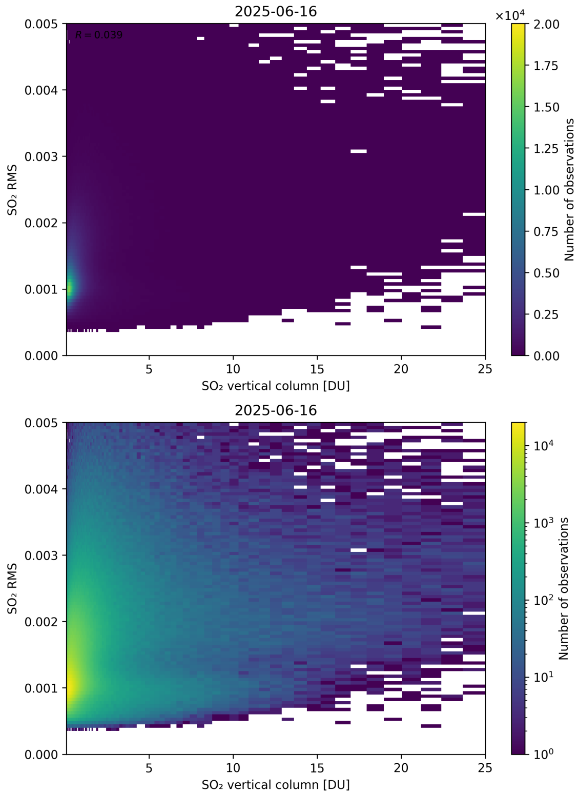
Figure 328: Scatter density plot of “SO 2 vertical column” against “SO 2 RMS” for 2025-06-16 to 2025-06-17.
