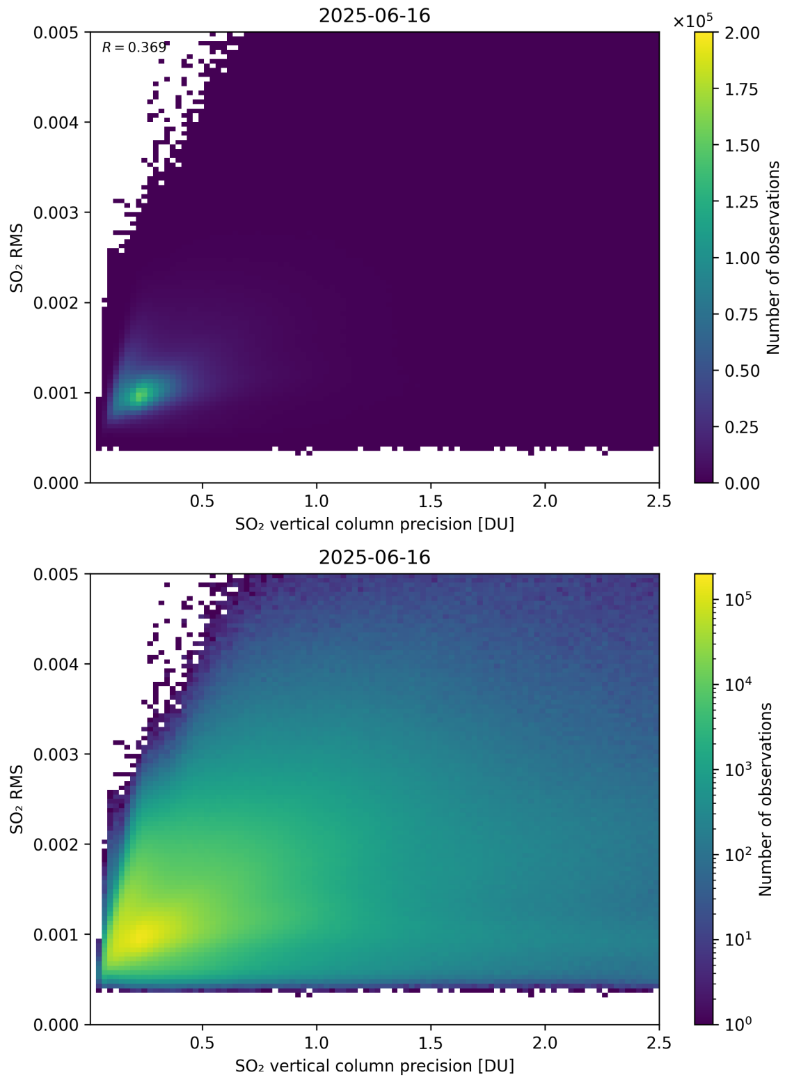
Figure 334: Scatter density plot of “SO 2 vertical column precision” against “SO 2 RMS” for 2025-06-16 to 2025-06-17.
