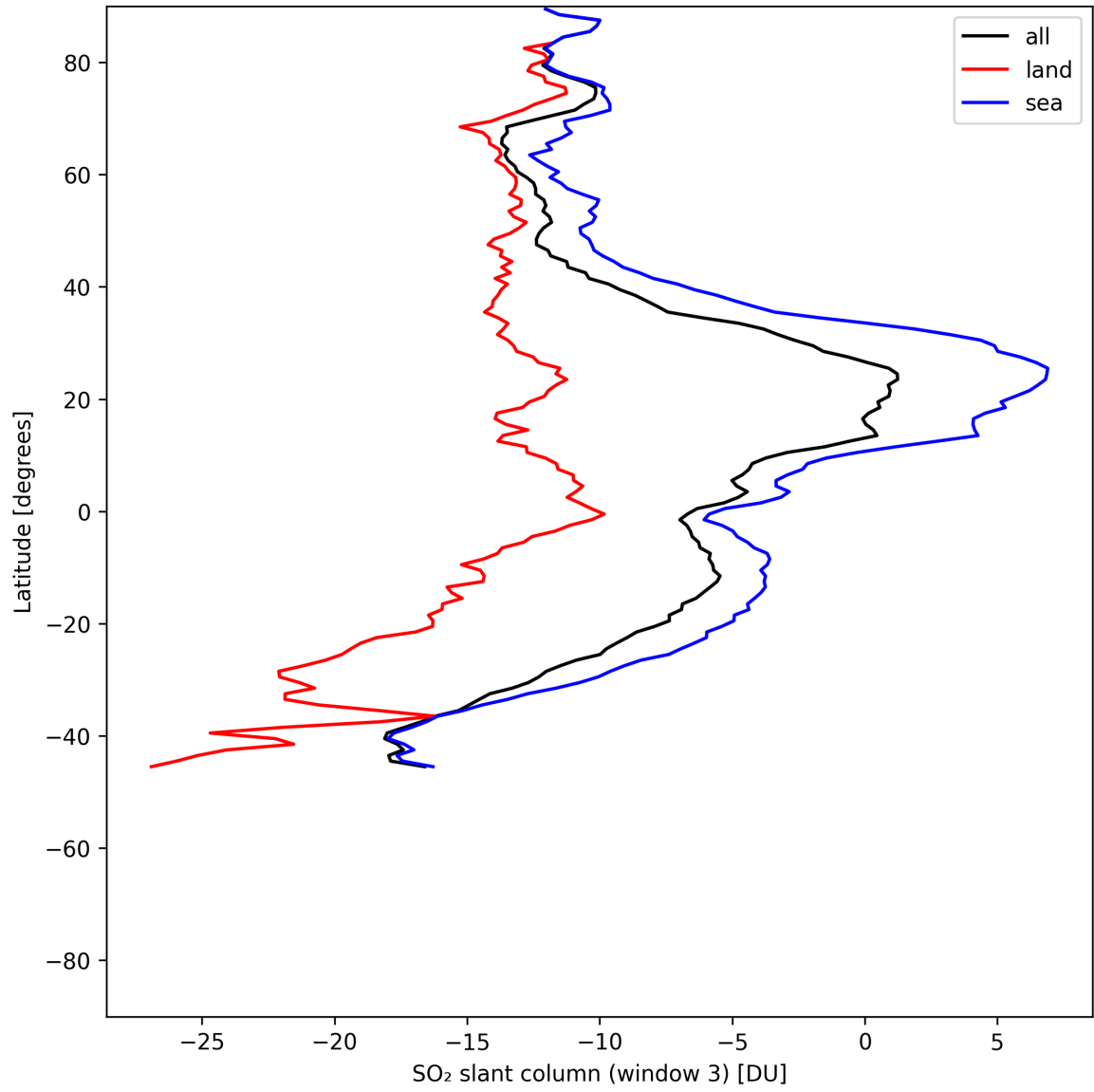
Figure 45: Zonal average of “SO 2 slant column (window 3)” for 2025-06-16 to 2025-06-17.
