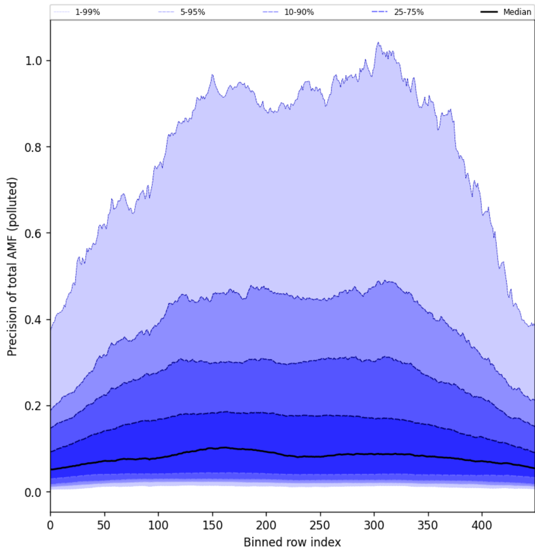
Figure 106: Along track statistics of “Precision of total AMF (polluted)” for 2025-06-16 to 2025-06-17
