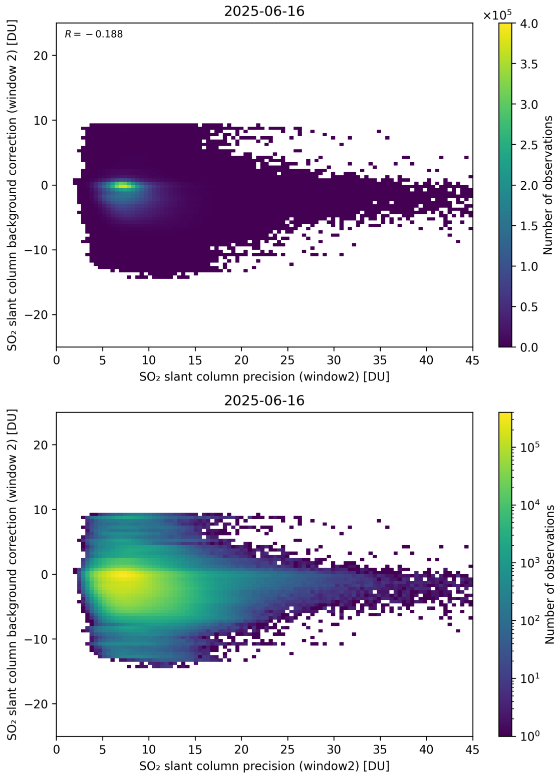
Figure 291: Scatter density plot of “SO 2 slant column precision (window2)” against “SO 2 slant column background correction (window 2)” for 2025-06-16 to 2025-06-17.
