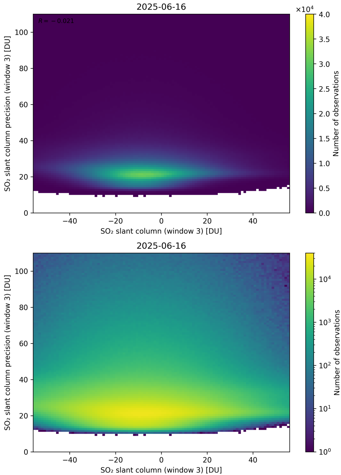
Figure 317: Scatter density plot of “SO 2 slant column (window 3)” against “SO 2 slant column precision (window 3)” for 2025-06-16 to 2025-06-17.
