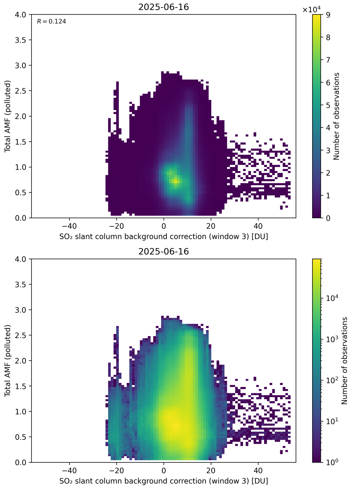
Figure 136: Scatter density plot of “SO 2 slant column background correction (window 3)” against “Total AMF (polluted)” for 2025-06-16 to 2025-06-17.
