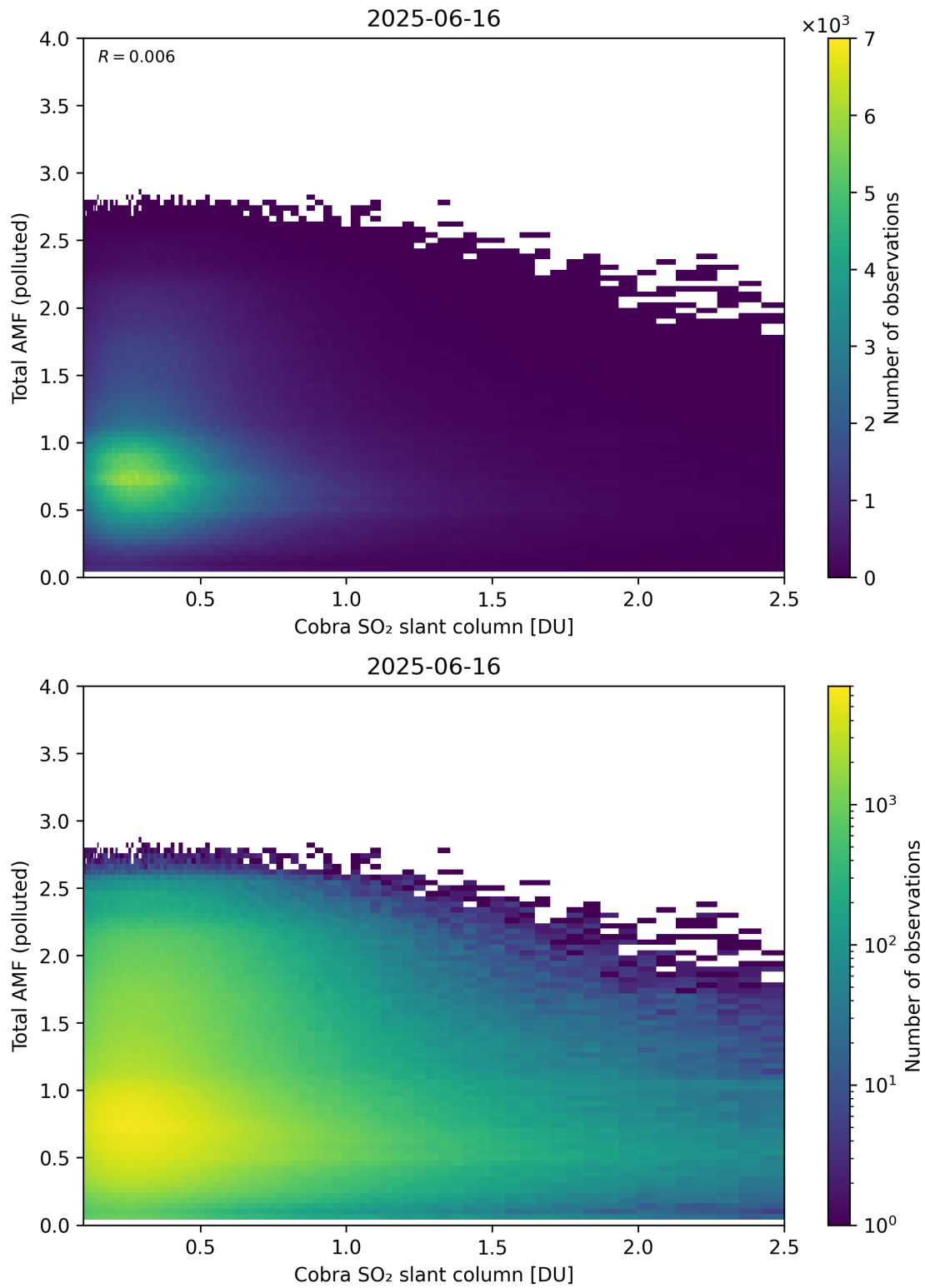
Figure 224: Scatter density plot of “Cobra SO 2 slant column” against “Total AMF (polluted)” for 2025-06-16 to 2025-06-17.
