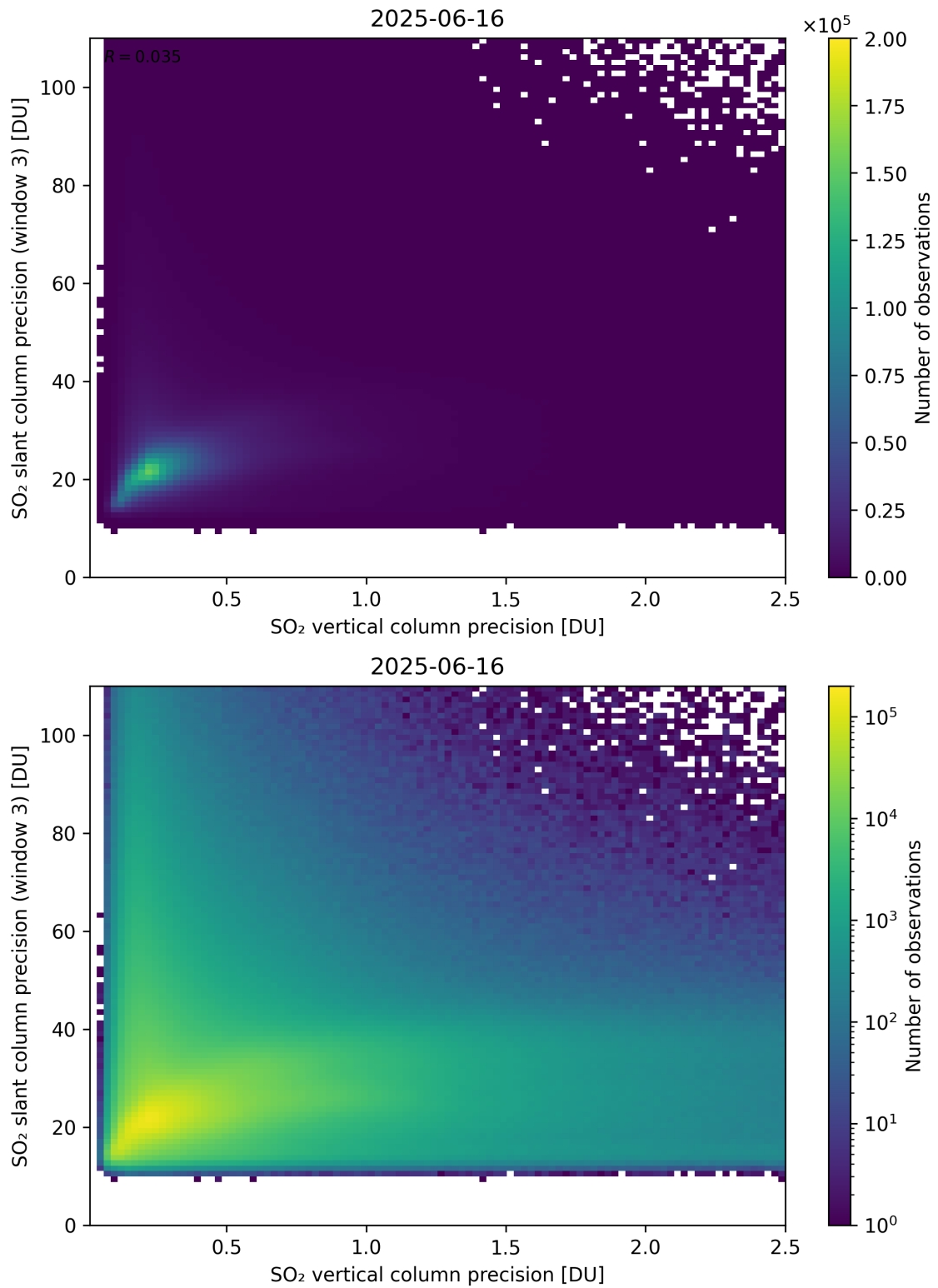
Figure 345: Scatter density plot of “SO 2 vertical column precision” against “SO 2 slant column precision (window 3)” for 2025-06-16 to 2025-06-17.
