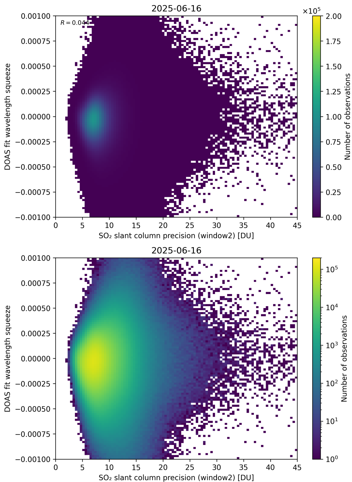
Figure 294: Scatter density plot of “SO 2 slant column precision (window2)” against “DOAS fit wavelength squeeze” for 2025-06-16 to 2025-06-17.
