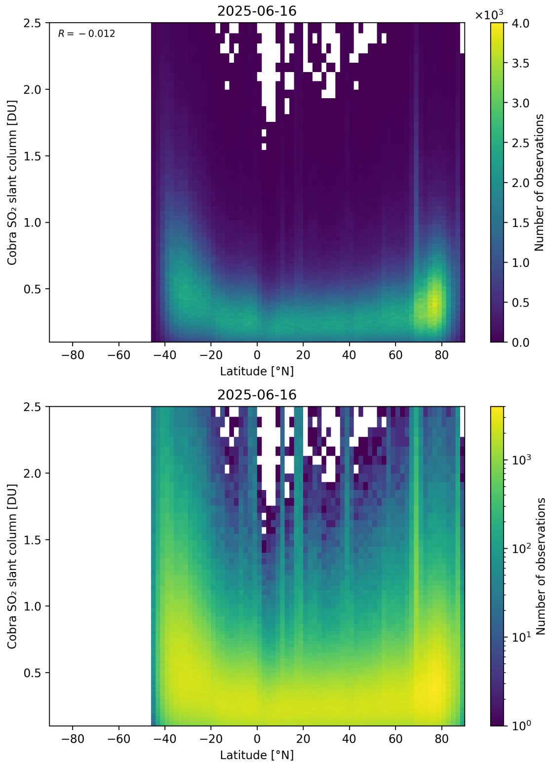
Figure 157: Scatter density plot of “Latitude” against “Cobra SO 2 slant column” for 2025-06-16 to 2025-06-17.
