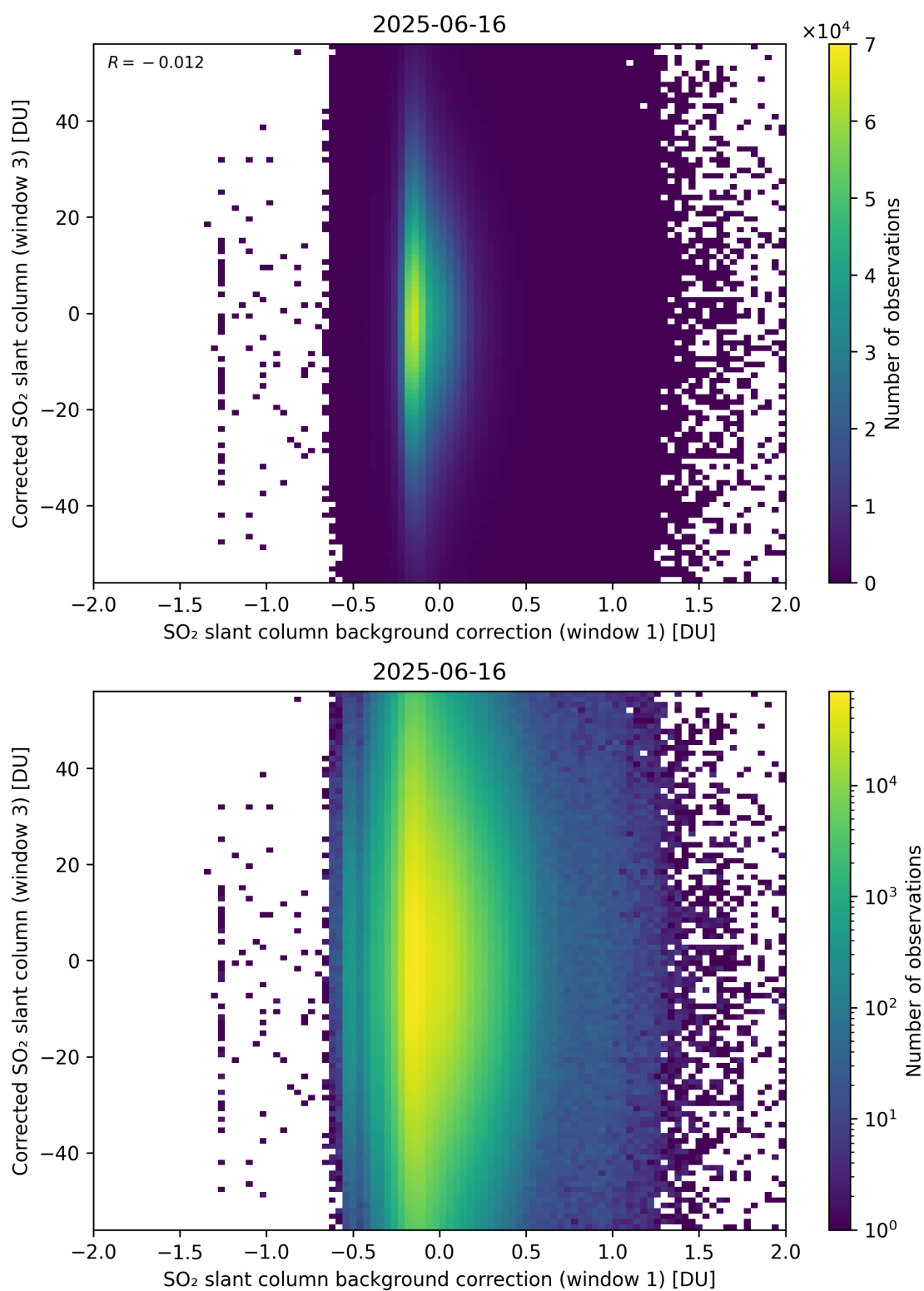
Figure 116: Scatter density plot of “SO 2 slant column background correction (window 1)” against “Corrected SO 2 slant column (window 3)” for 2025-06-16 to 2025-06-17.
