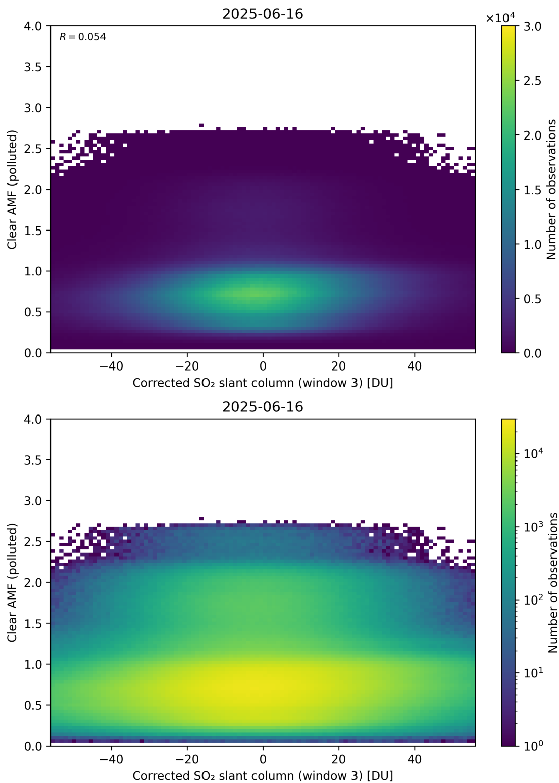
Figure 259: Scatter density plot of “Corrected SO 2 slant column (window 3)” against “Clear AMF (polluted)” for 2025-06-16 to 2025-06-17.
