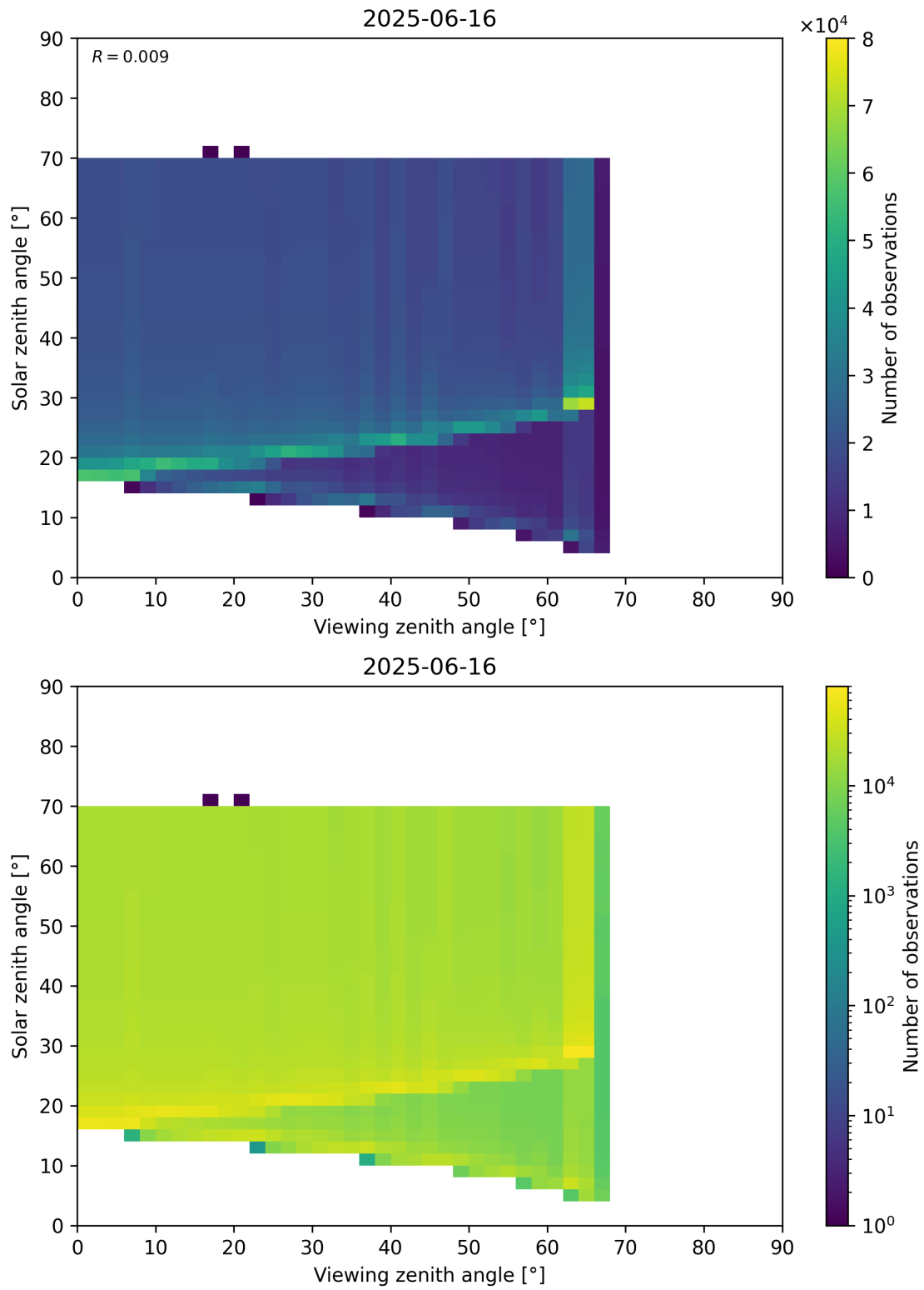
Figure 369: Scatter density plot of “Viewing zenith angle” against “Solar zenith angle” for 2025-06-16 to 2025-06-17.
