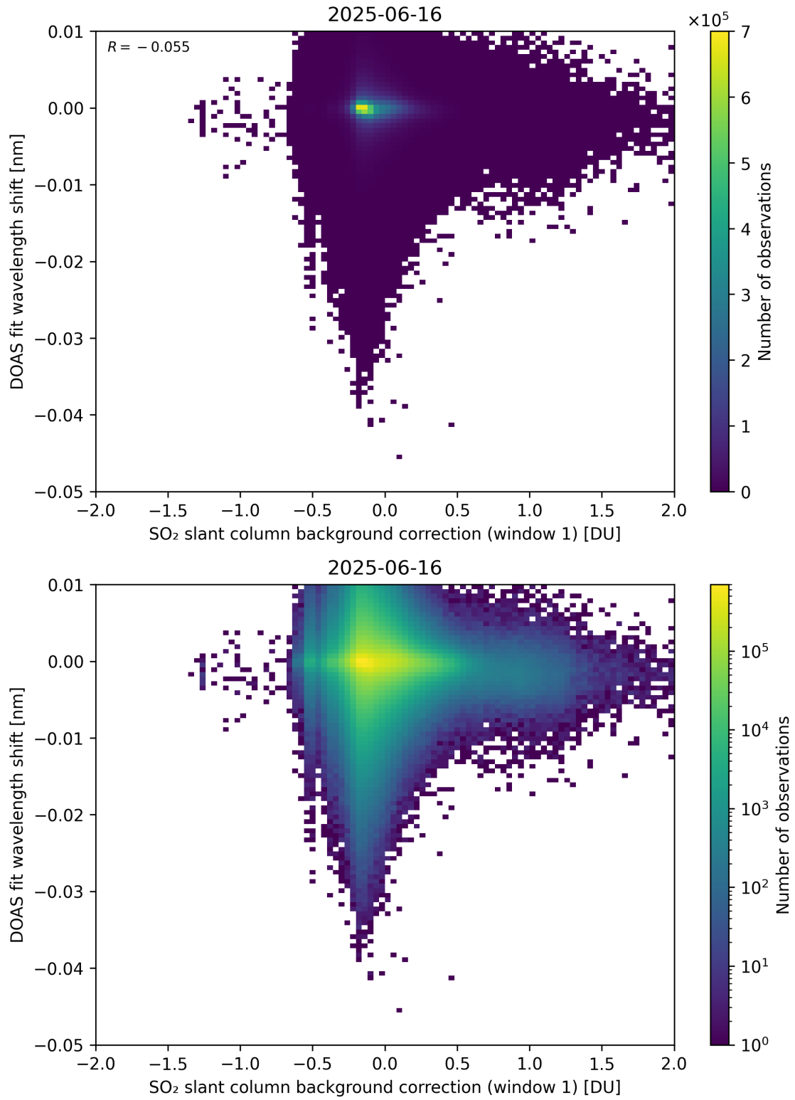
Figure 111: Scatter density plot of “SO 2 slant column background correction (window 1)” against “DOAS fit wavelength shift” for 2025-06-16 to 2025-06-17.
