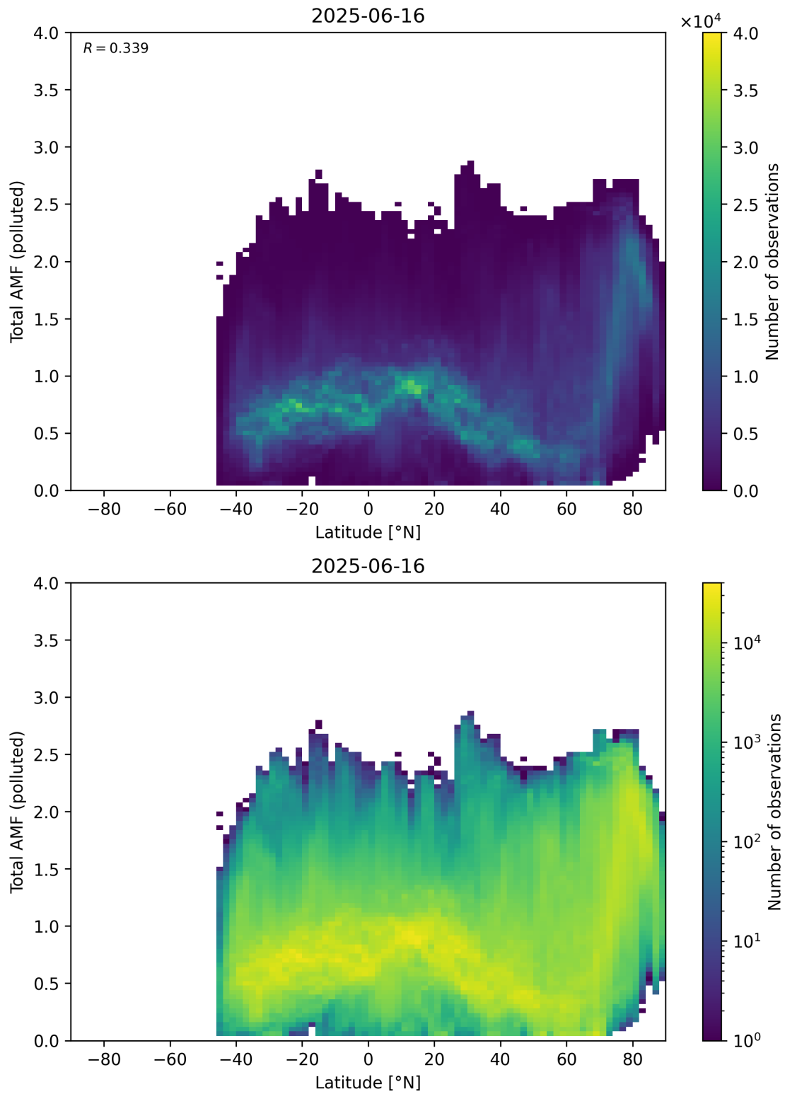
Figure 167: Scatter density plot of “Latitude” against “Total AMF (polluted)” for 2025-06-16 to 2025-06-17.
