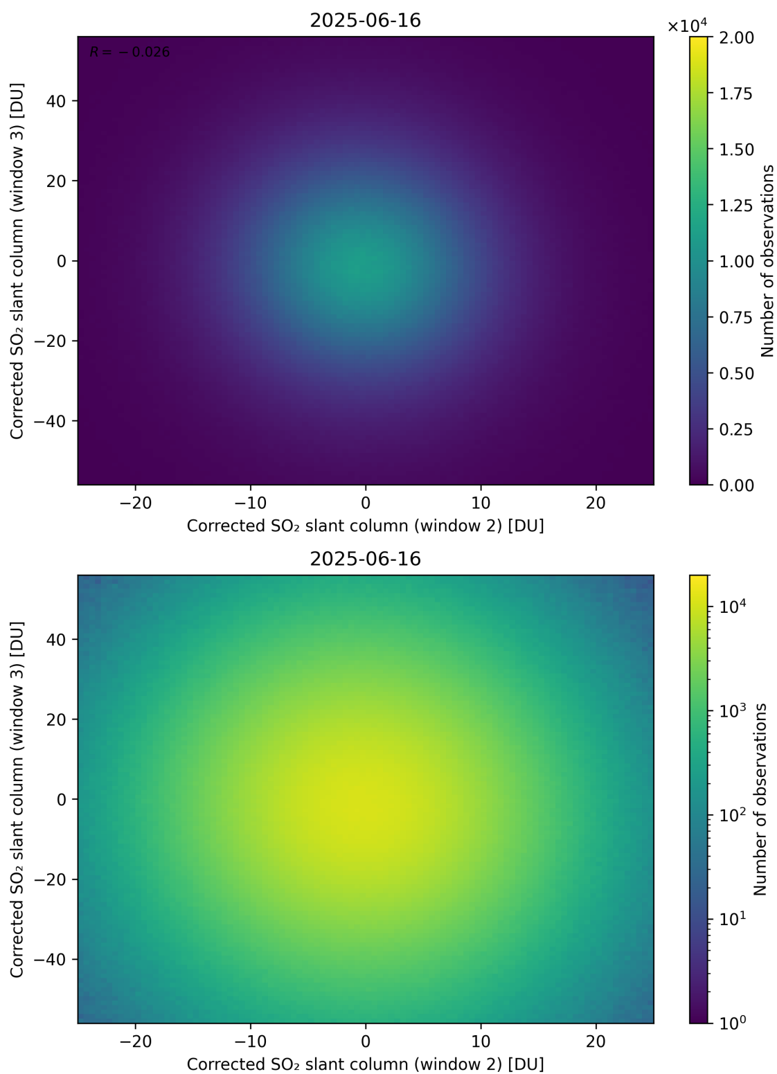
Figure 250: Scatter density plot of “Corrected SO 2 slant column (window 2)” against “Corrected SO 2 slant column (window 3)” for 2025-06-16 to 2025-06-17.
