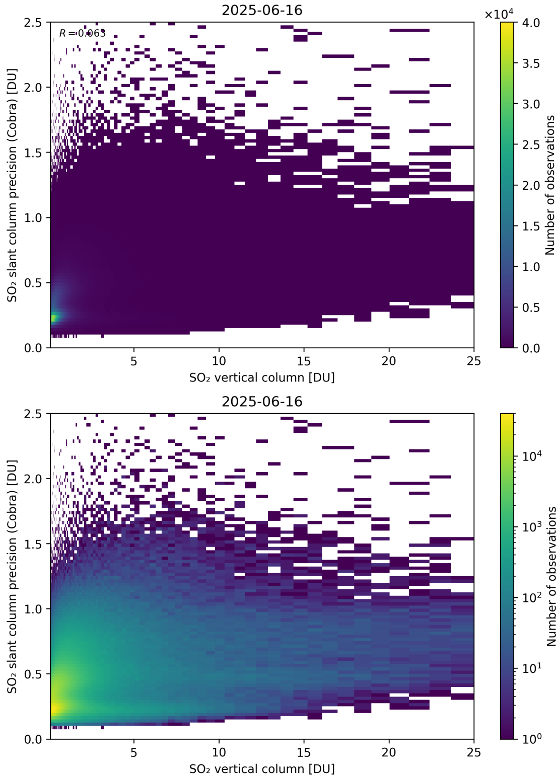
Figure 350: Scatter density plot of “SO 2 vertical column” against “SO 2 slant column precision (Cobra)” for 2025-06-16 to 2025-06-17.
