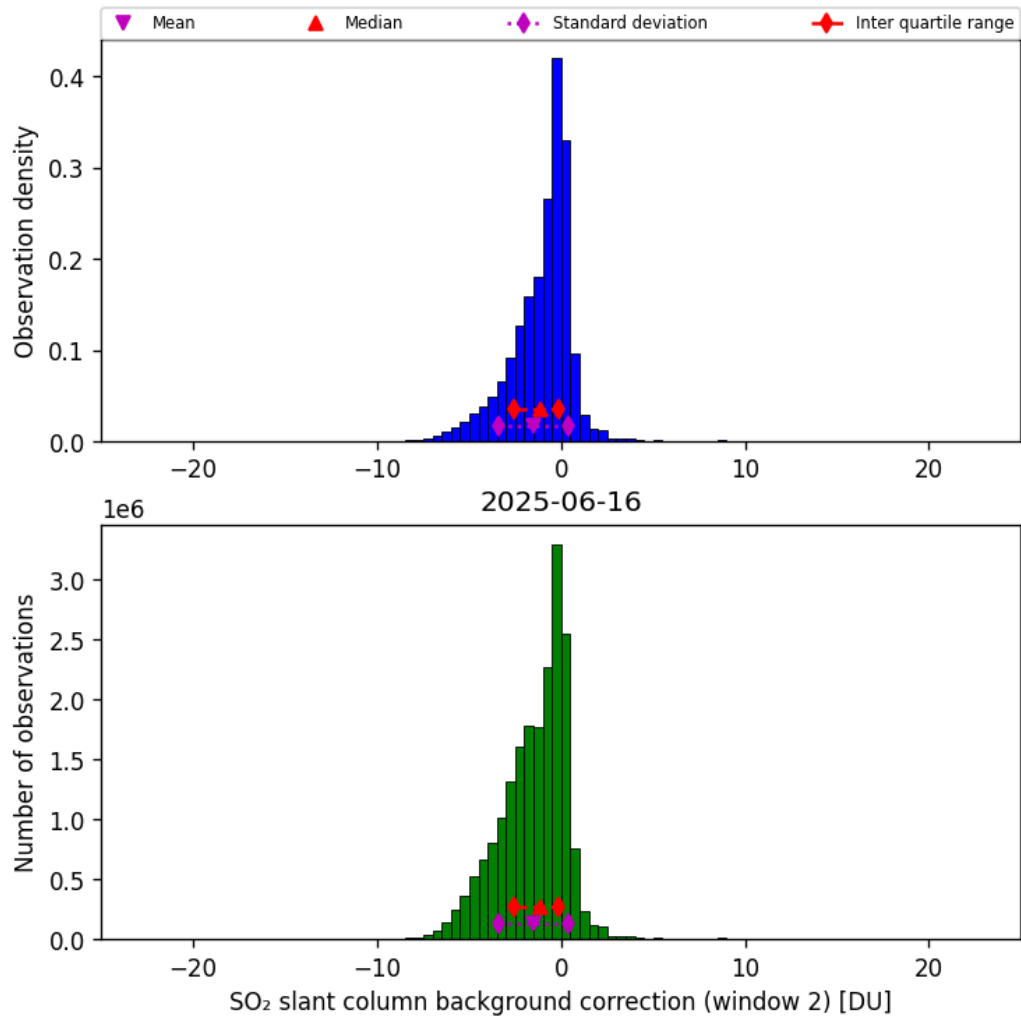
Figure 70: Histogram of “SO 2 slant column background correction (window 2)” for 2025-06-16 to 2025-06-17
