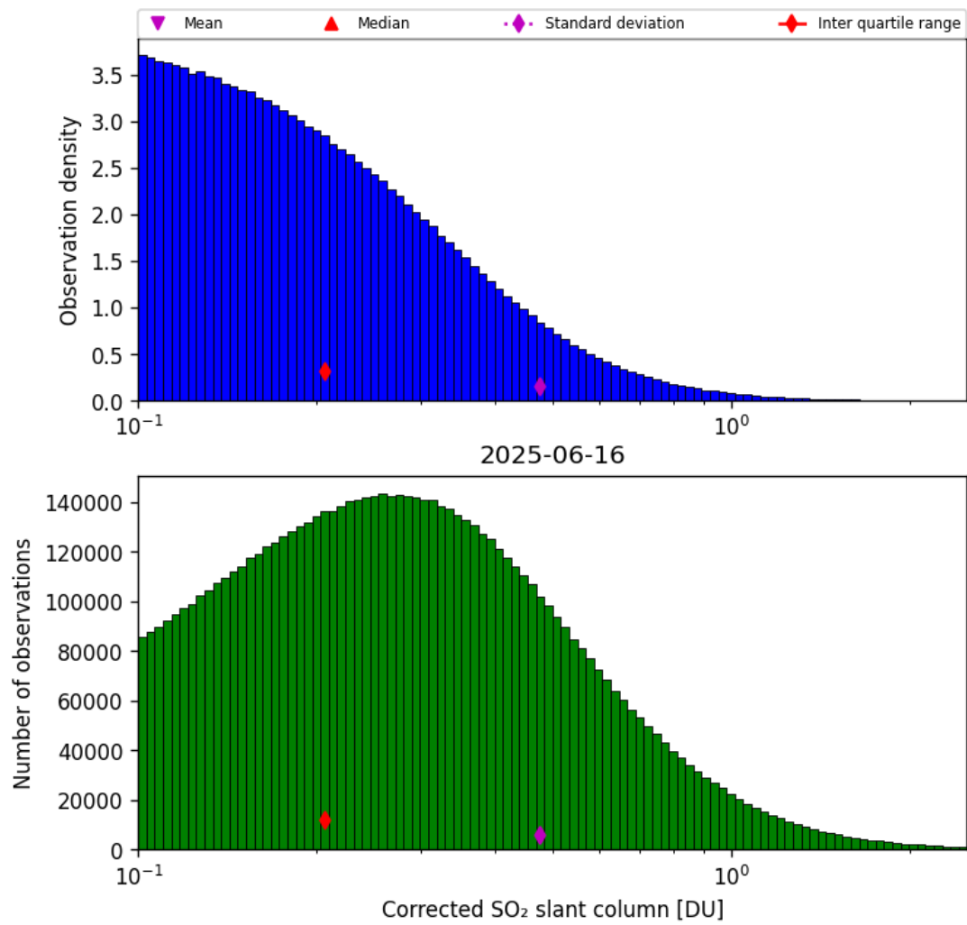
Figure 60: Histogram of “Corrected SO 2 slant column” for 2025-06-16 to 2025-06-17
