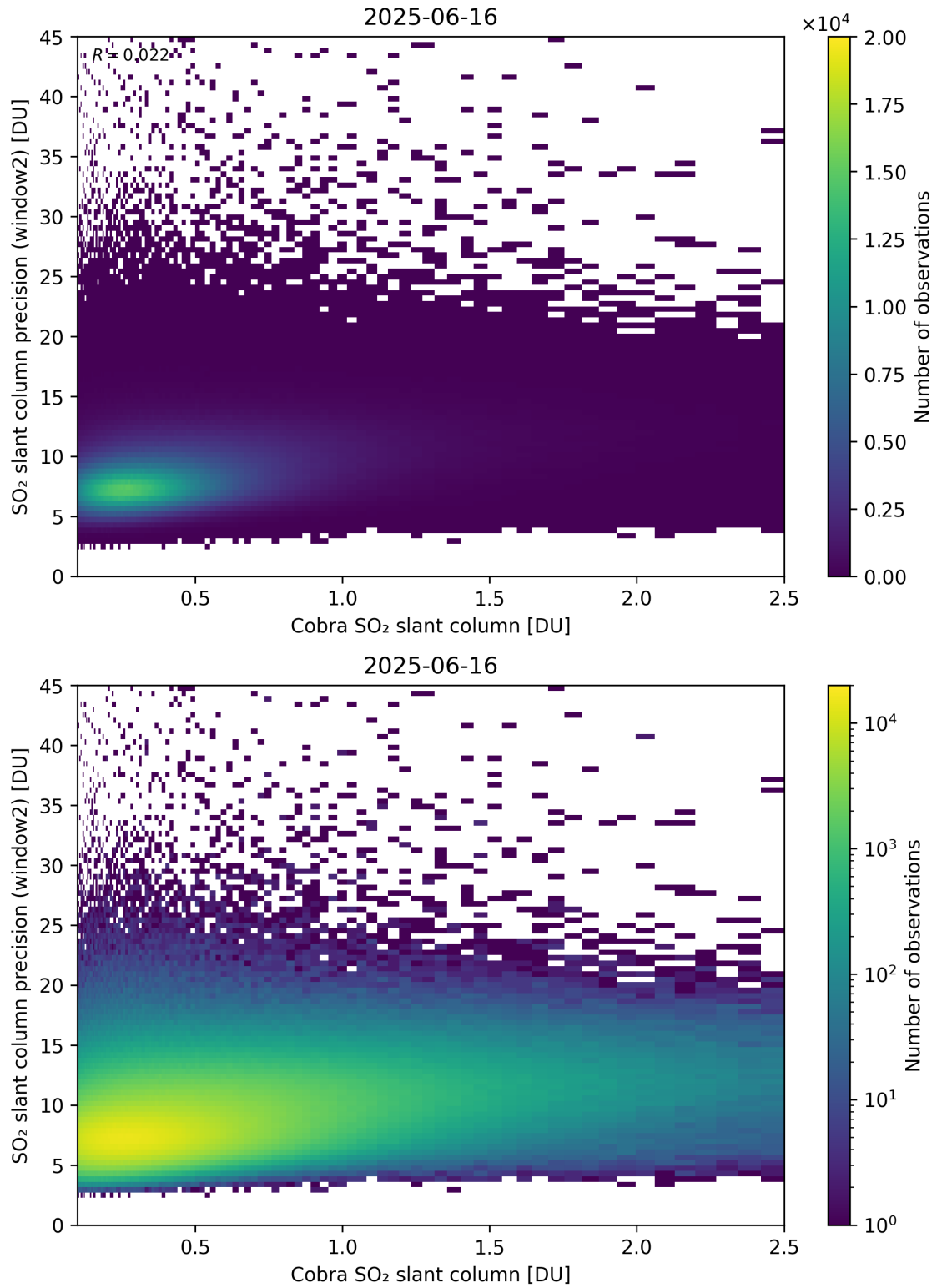
Figure 221: Scatter density plot of “Cobra SO 2 slant column” against “SO 2 slant column precision (window2)” for 2025-06-16 to 2025-06-17.
