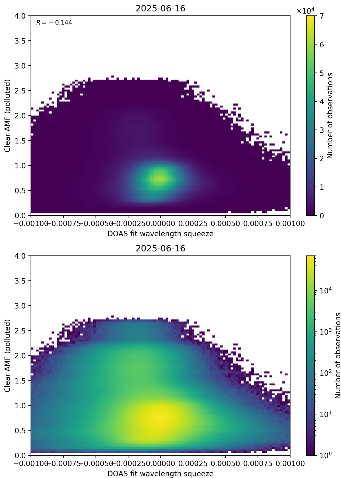
Figure 144: Scatter density plot of “DOAS fit wavelength squeeze” against “Clear AMF (polluted)” for 2025-06-16 to 2025-06-17.
