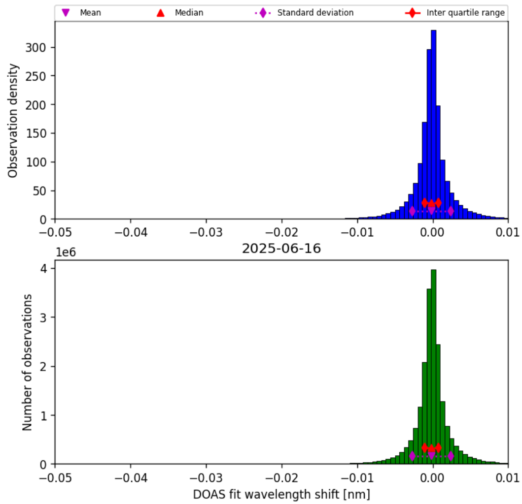
Figure 76: Histogram of “DOAS fit wavelength shift” for 2025-06-16 to 2025-06-17
