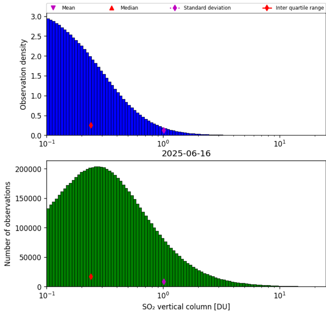
Figure 58: Histogram of “SO 2 vertical column” for 2025-06-16 to 2025-06-17
