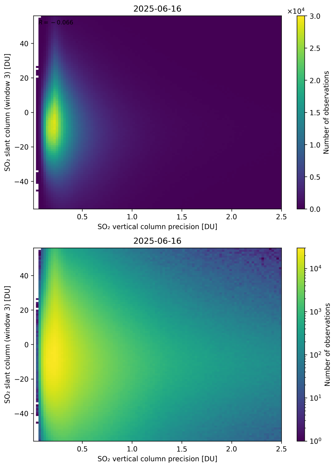
Figure 344: Scatter density plot of “SO 2 vertical column precision” against “SO 2 slant column (window 3)” for 2025-06-16 to 2025-06-17.
