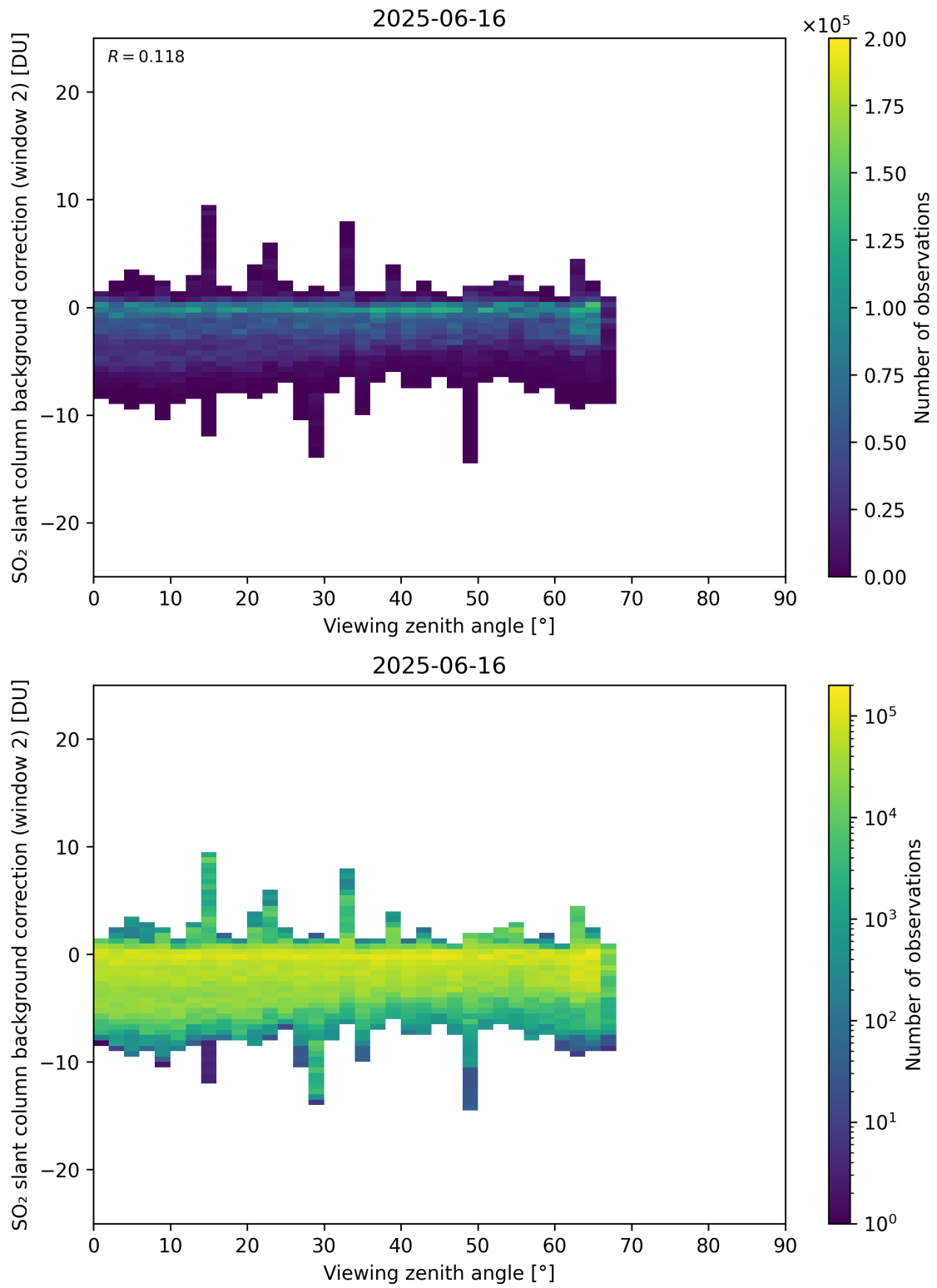
Figure 363: Scatter density plot of “Viewing zenith angle” against “SO 2 slant column background correction (window 2)” for 2025-06-16 to 2025-06-17.
