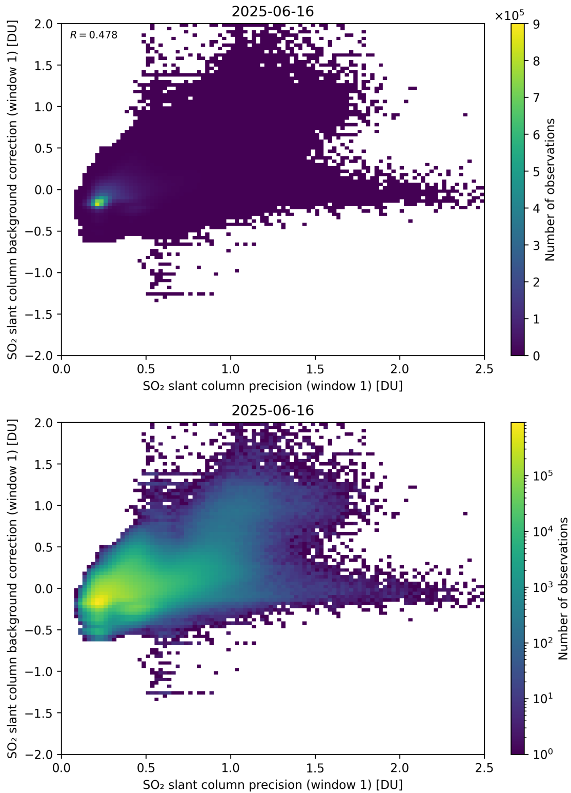
Figure 268: Scatter density plot of “SO 2 slant column precision (window 1)” against “SO 2 slant column background correction (window 1)” for 2025-06-16 to 2025-06-17.
