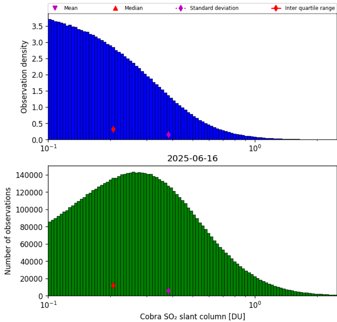
Figure 61: Histogram of “Cobra SO 2 slant column” for 2025-06-16 to 2025-06-17
