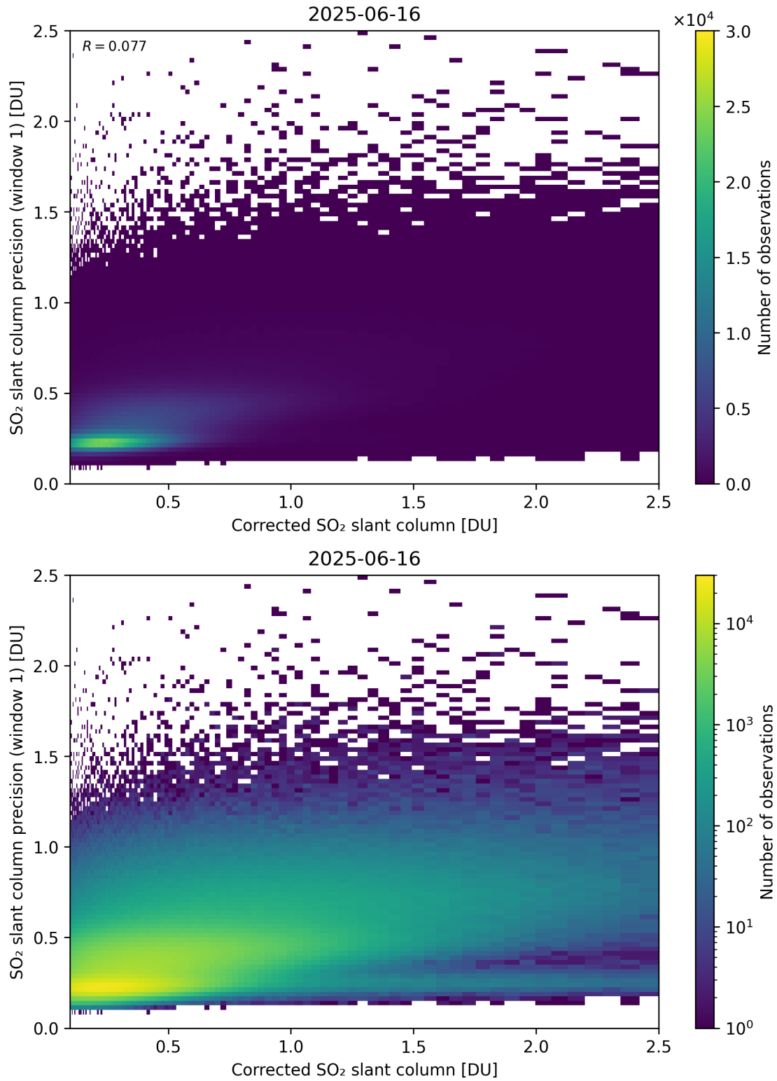
Figure 238: Scatter density plot of “Corrected SO 2 slant column” against “SO 2 slant column precision (window 1)” for 2025-06-16 to 2025-06-17.
