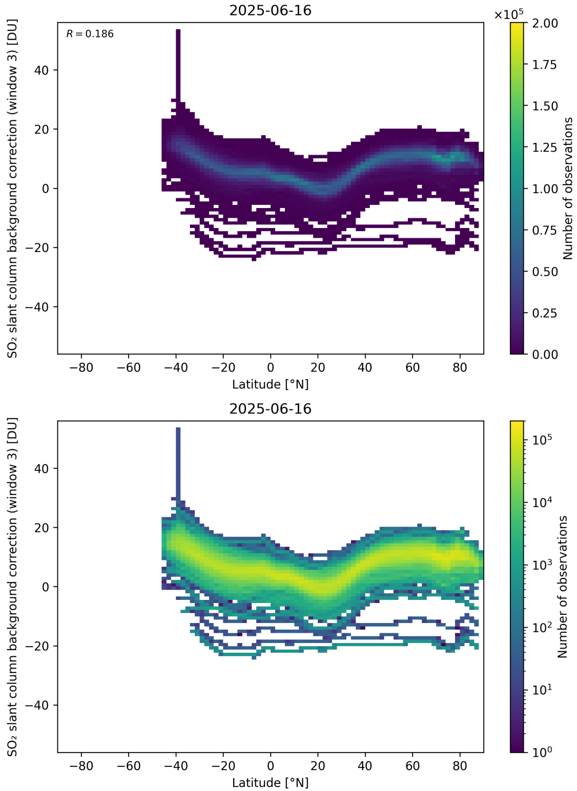
Figure 152: Scatter density plot of “Latitude” against “SO 2 slant column background correction (window 3)” for 2025-06-16 to 2025-06-17.
