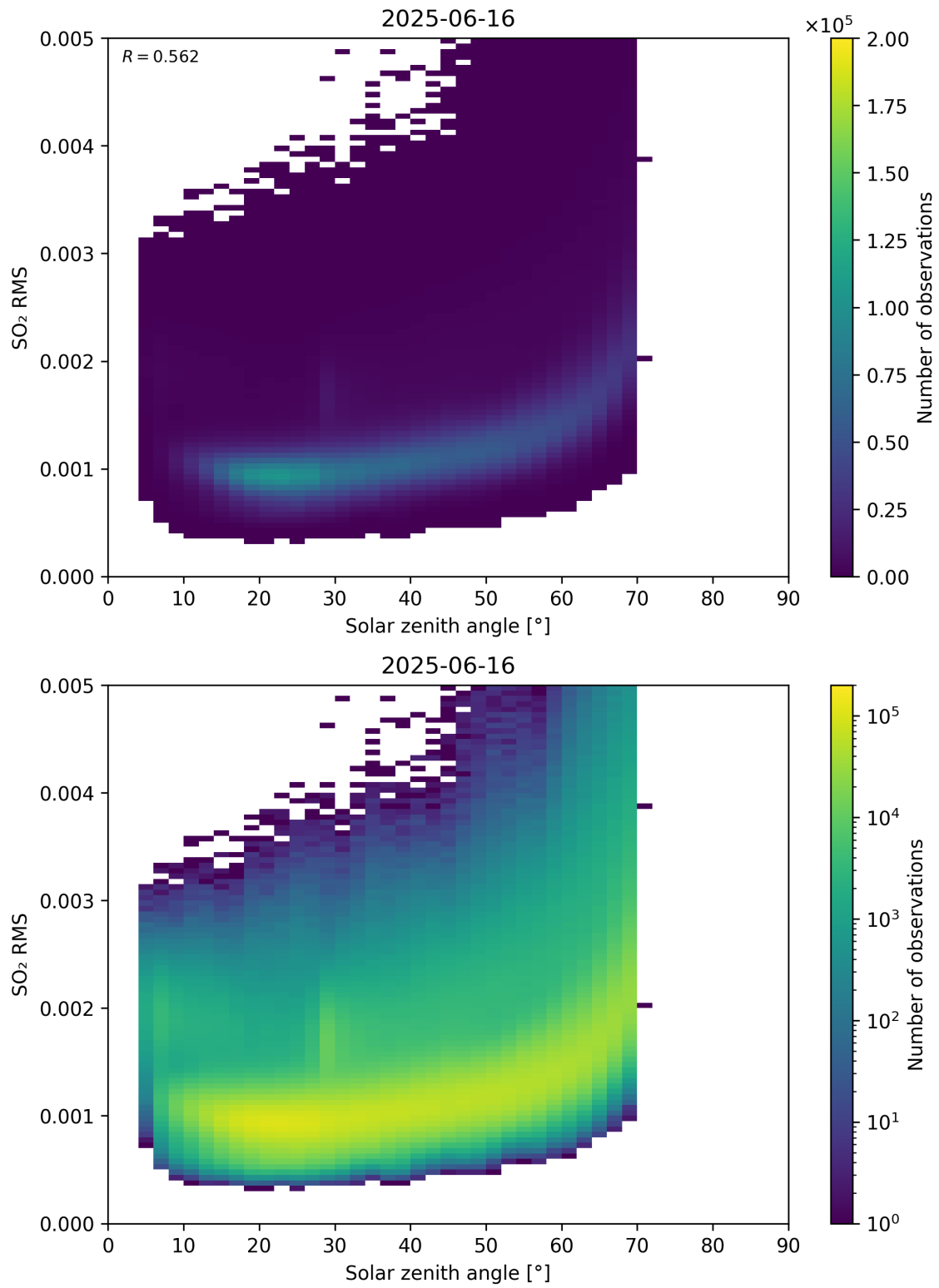
Figure 176: Scatter density plot of “Solar zenith angle” against “SO 2 RMS” for 2025-06-16 to 2025-06-17.
