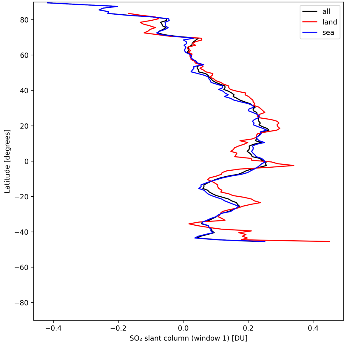
Figure 37: Zonal average of “SO 2 slant column (window 1)” for 2025-06-16 to 2025-06-17.
