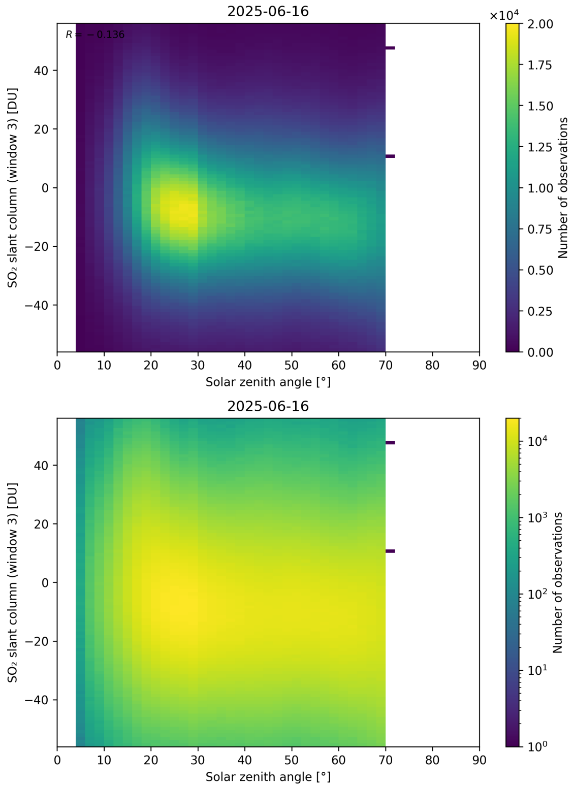
Figure 187: Scatter density plot of “Solar zenith angle” against “SO 2 slant column (window 3)” for 2025-06-16 to 2025-06-17.
