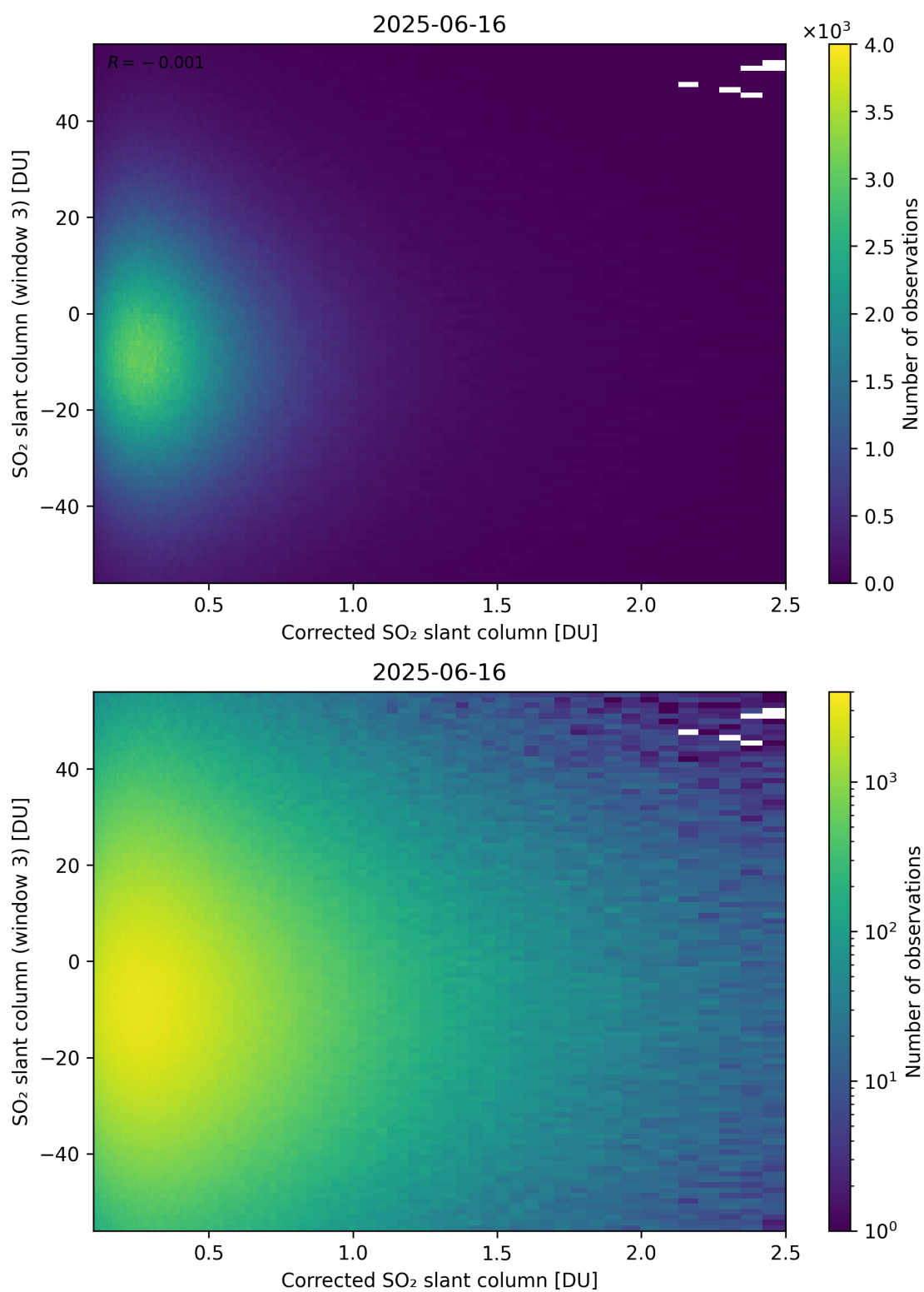
Figure 240: Scatter density plot of “Corrected SO 2 slant column” against “SO 2 slant column (window 3)” for 2025-06-16 to 2025-06-17.
