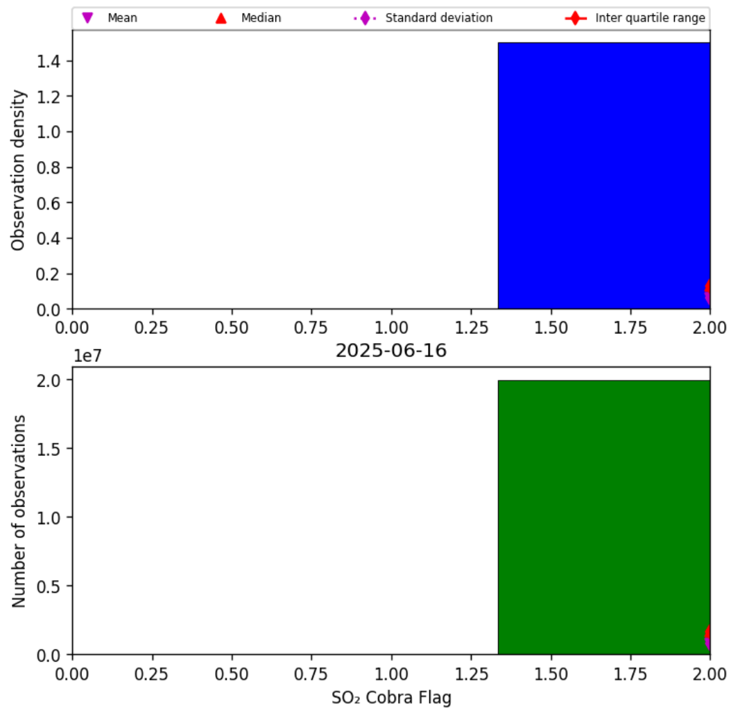
Figure 75: Histogram of “SO 2 Cobra Flag” for 2025-06-16 to 2025-06-17
