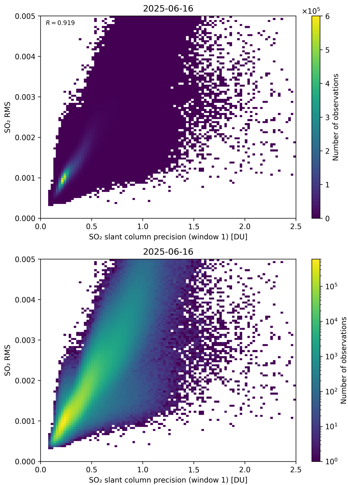
Figure 273: Scatter density plot of “SO 2 slant column precision (window 1)” against “SO 2 RMS” for 2025-06-16 to 2025-06-17.
