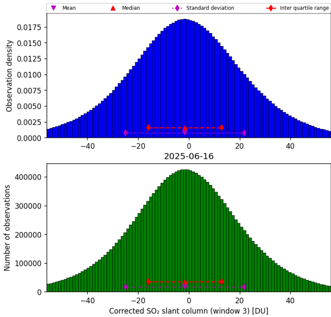
Figure 73: Histogram of “Corrected SO 2 slant column (window 3)” for 2025-06-16 to 2025-06-17
