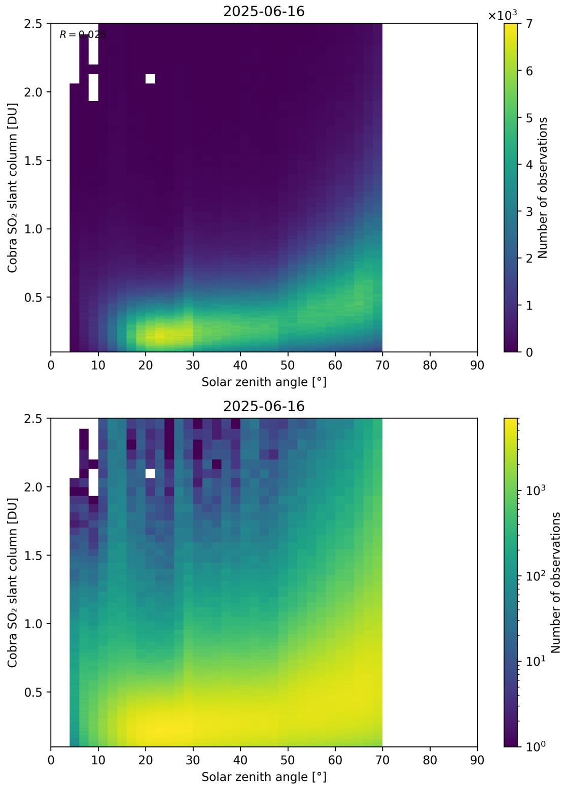
Figure 179: Scatter density plot of “Solar zenith angle” against “Cobra SO 2 slant column” for 2025-06-16 to 2025-06-17.
