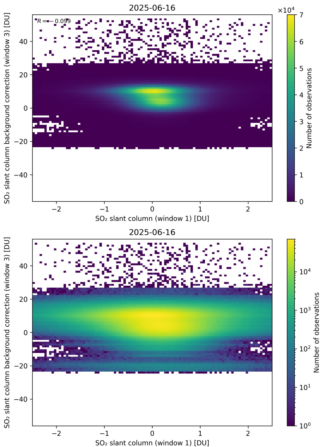
Figure 264: Scatter density plot of “SO 2 slant column (window 1)” against “SO 2 slant column background correction (window 3)” for 2025-06-16 to 2025-06-17.
