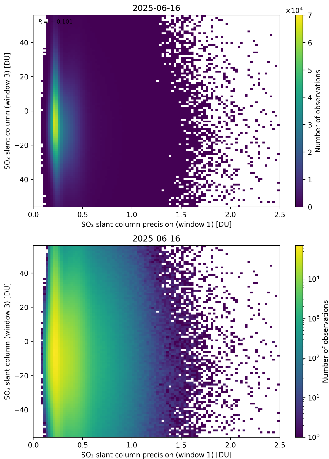
Figure 278: Scatter density plot of “SO 2 slant column precision (window 1)” against “SO 2 slant column (window 3)” for 2025-06-16 to 2025-06-17.
