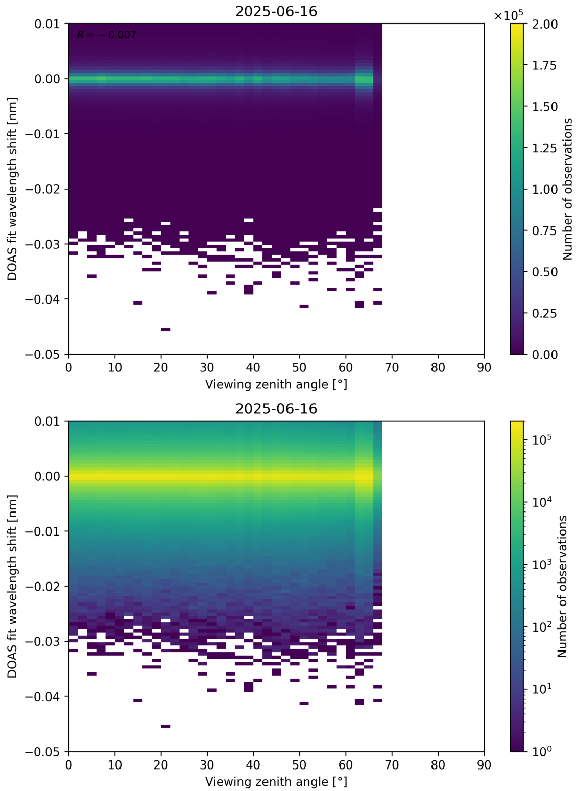
Figure 365: Scatter density plot of “Viewing zenith angle” against “DOAS fit wavelength shift” for 2025-06-16 to 2025-06-17.
