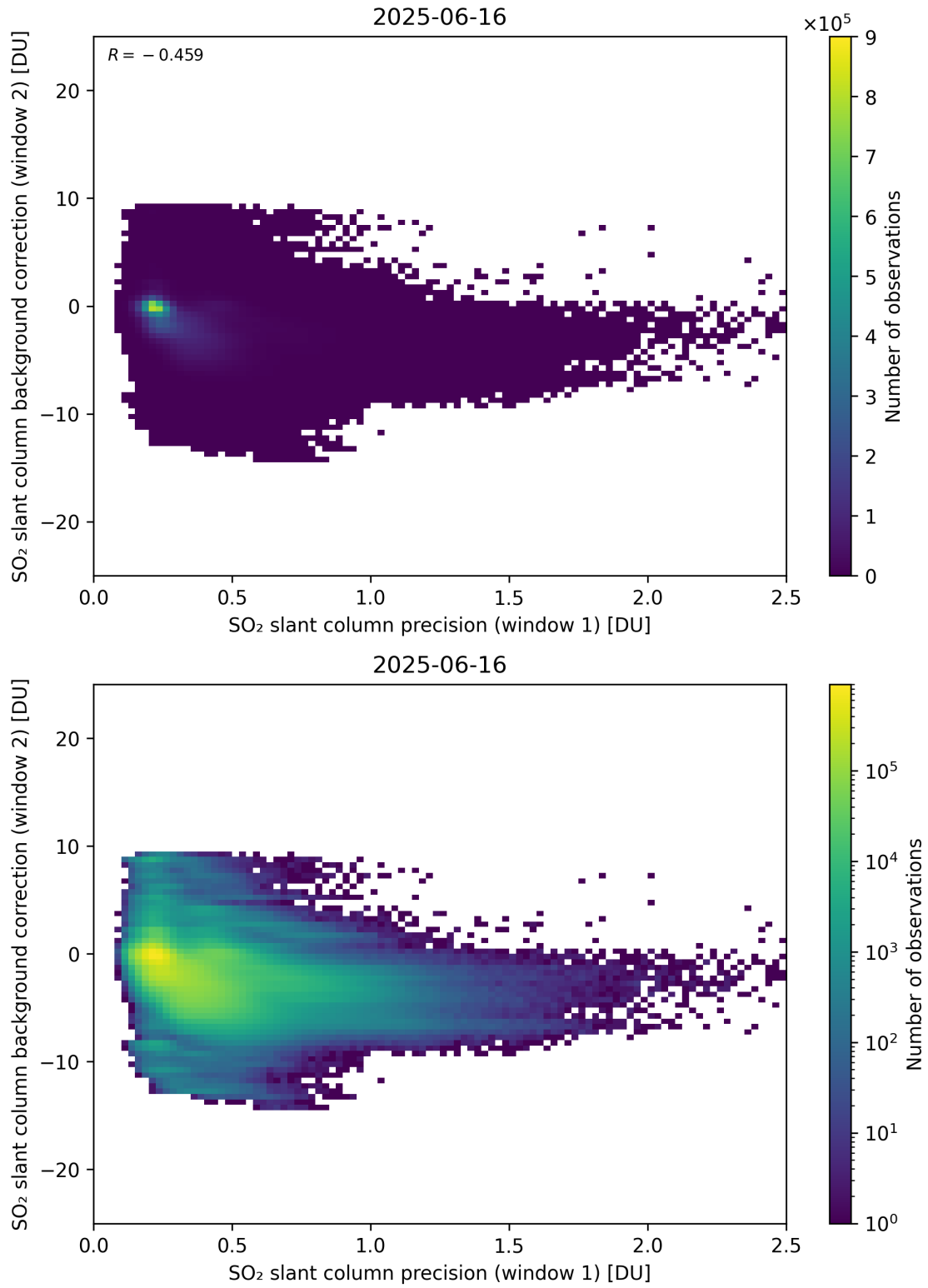
Figure 269: Scatter density plot of “SO 2 slant column precision (window 1)” against “SO 2 slant column background correction (window 2)” for 2025-06-16 to 2025-06-17.
