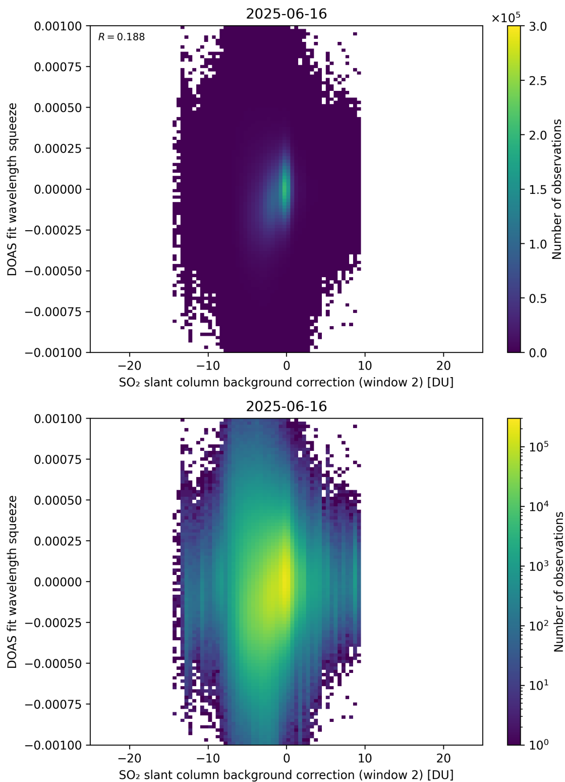
Figure 124: Scatter density plot of “SO 2 slant column background correction (window 2)” against “DOAS fit wavelength squeeze” for 2025-06-16 to 2025-06-17.
