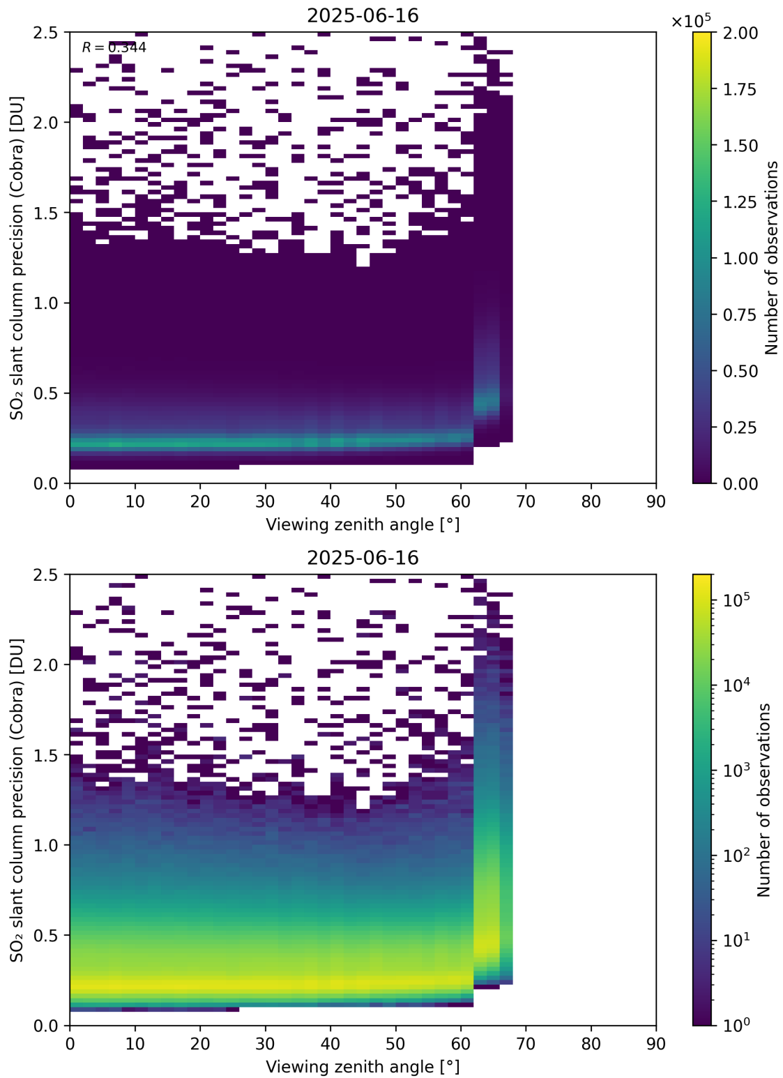
Figure 372: Scatter density plot of “Viewing zenith angle” against “SO 2 slant column precision (Cobra)” for 2025-06-16 to 2025-06-17.
