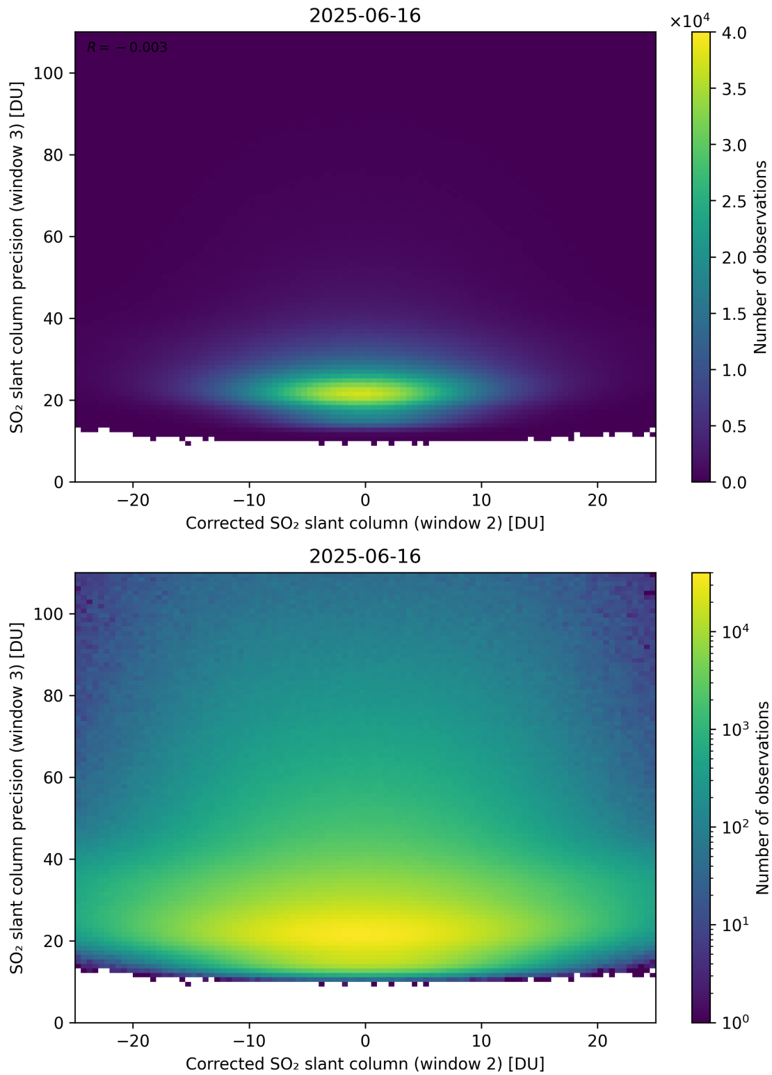
Figure 252: Scatter density plot of “Corrected SO 2 slant column (window 2)” against “SO 2 slant column precision (window 3)” for 2025-06-16 to 2025-06-17.
