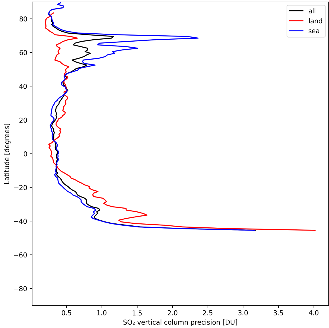
Figure 33: Zonal average of “SO 2 vertical column precision” for 2025-06-16 to 2025-06-17.
