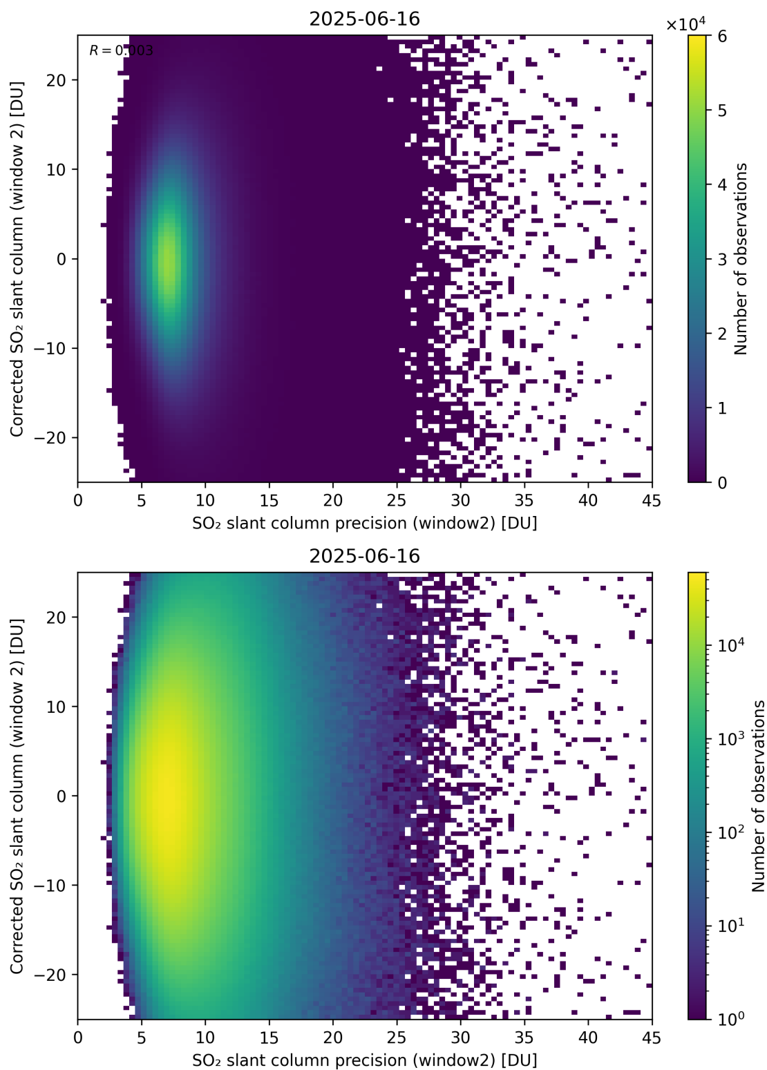
Figure 297: Scatter density plot of “SO 2 slant column precision (window2)” against “Corrected SO 2 slant column (window 2)” for 2025-06-16 to 2025-06-17.
