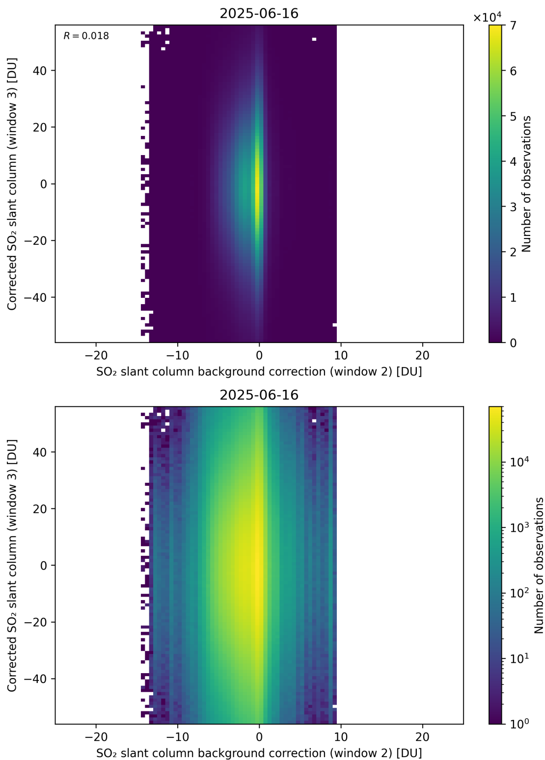
Figure 127: Scatter density plot of “SO 2 slant column background correction (window 2)” against “Corrected SO 2 slant column (window 3)” for 2025-06-16 to 2025-06-17.
