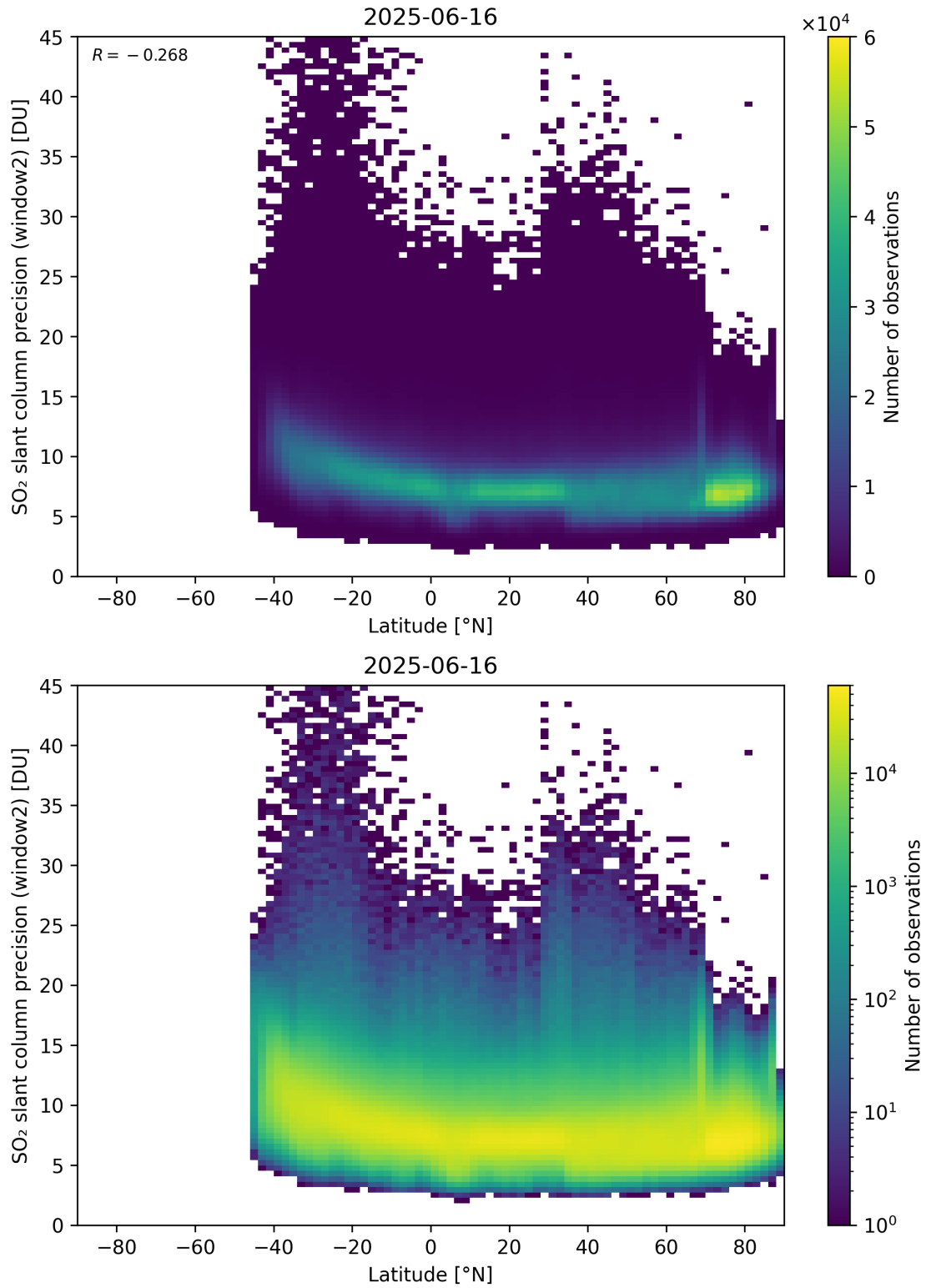
Figure 164: Scatter density plot of “Latitude” against “SO 2 slant column precision (window2)” for 2025-06-16 to 2025-06-17.
