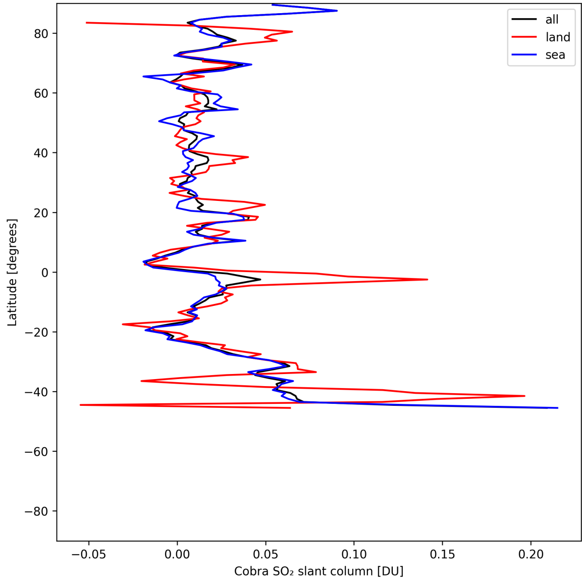
Figure 35: Zonal average of “Cobra SO 2 slant column” for 2025-06-16 to 2025-06-17.
