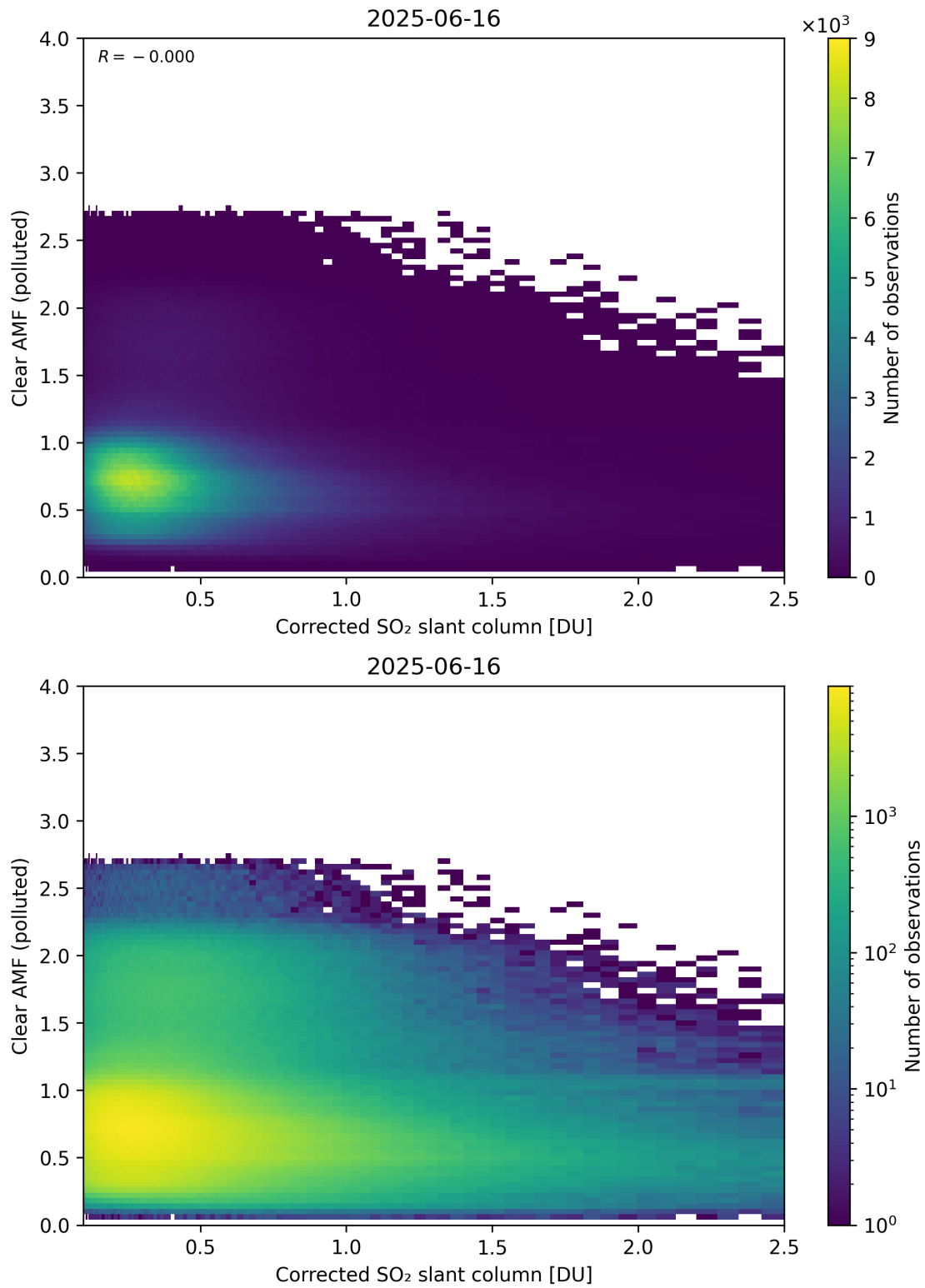
Figure 232: Scatter density plot of “Corrected SO 2 slant column” against “Clear AMF (polluted)” for 2025-06-16 to 2025-06-17.
