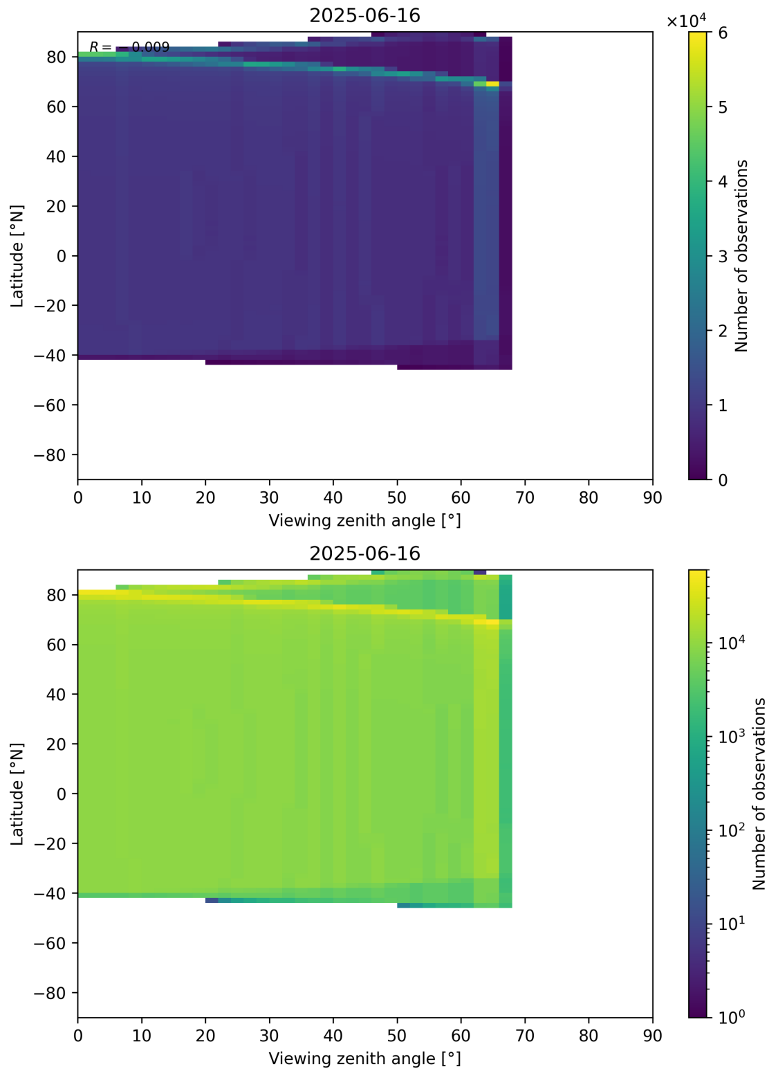
Figure 368: Scatter density plot of “Viewing zenith angle” against “Latitude” for 2025-06-16 to 2025-06-17.
