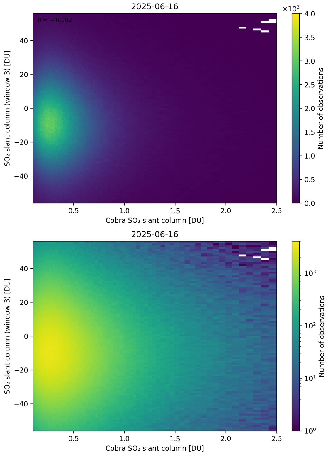
Figure 222: Scatter density plot of “Cobra SO 2 slant column” against “SO 2 slant column (window 3)” for 2025-06-16 to 2025-06-17.
