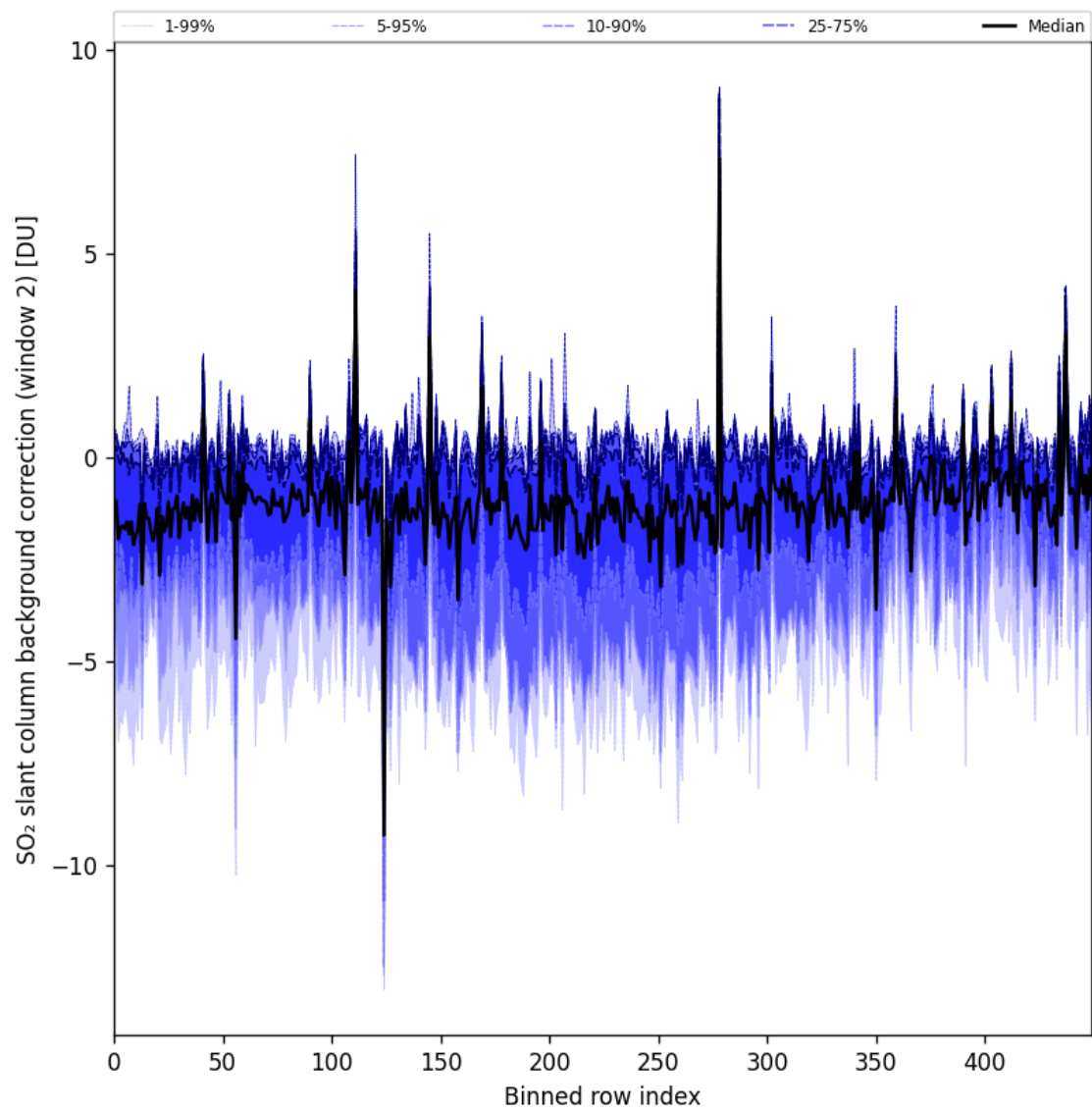
Figure 96: Along track statistics of “SO 2 slant column background correction (window 2)” for 2025-06-16 to 2025-06-17
