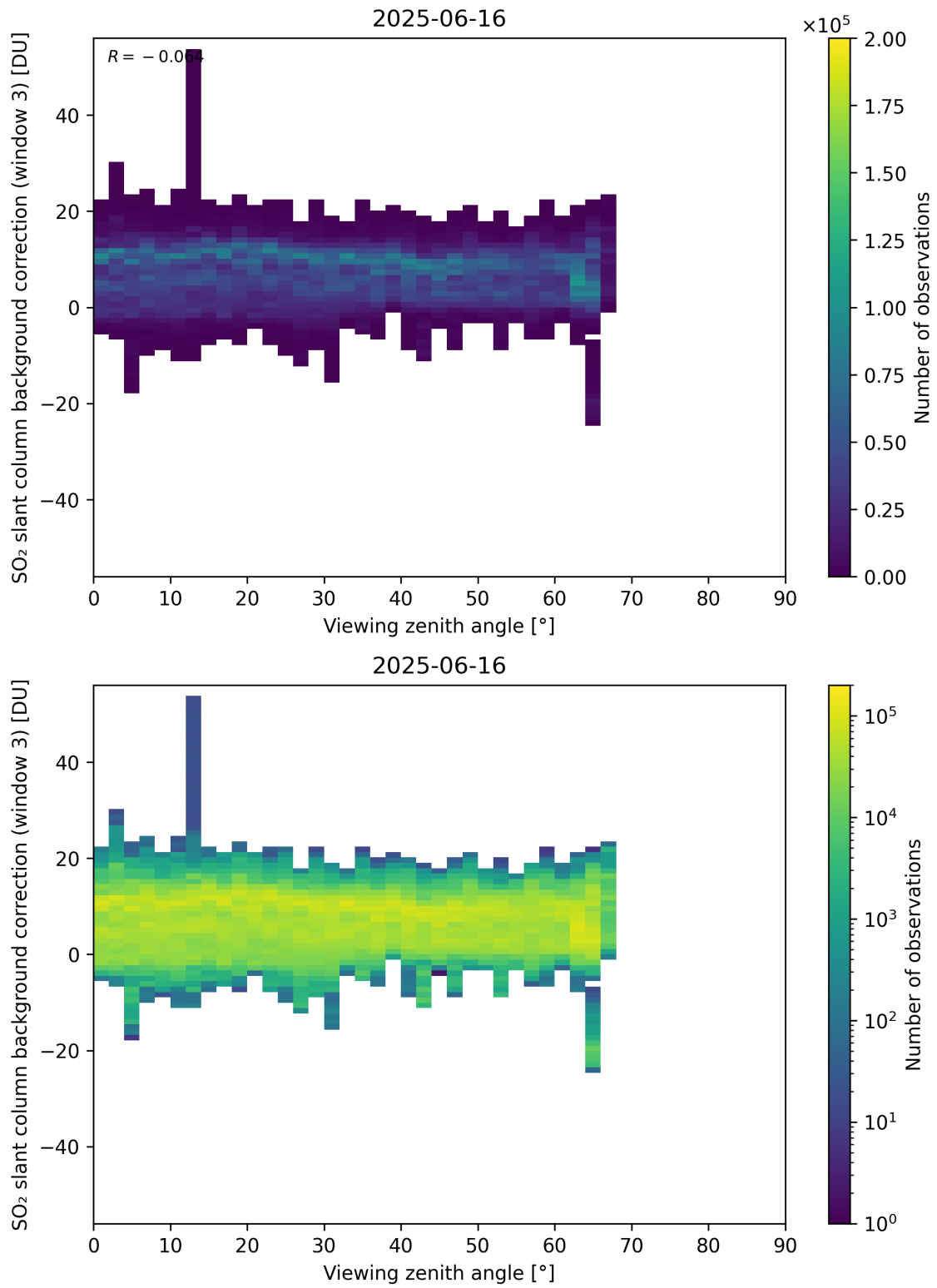
Figure 364: Scatter density plot of “Viewing zenith angle” against “SO 2 slant column background correction (window 3)” for 2025-06-16 to 2025-06-17.
