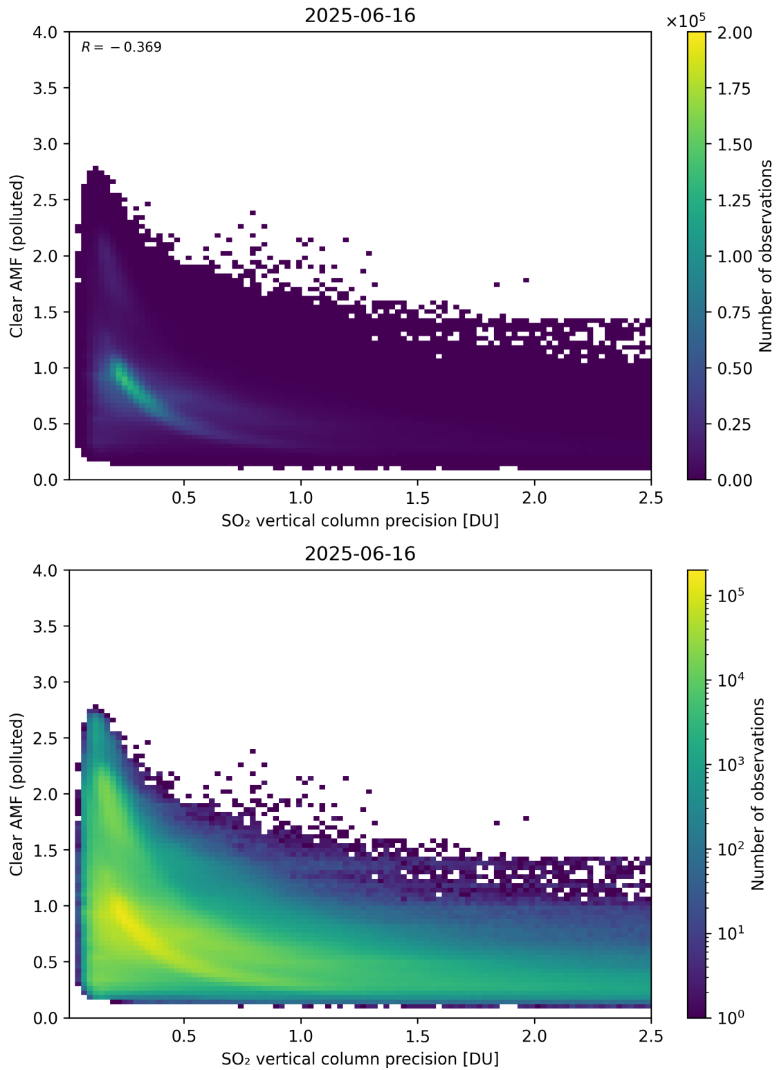
Figure 335: Scatter density plot of “SO 2 vertical column precision” against “Clear AMF (polluted)” for 2025-06-16 to 2025-06-17.
