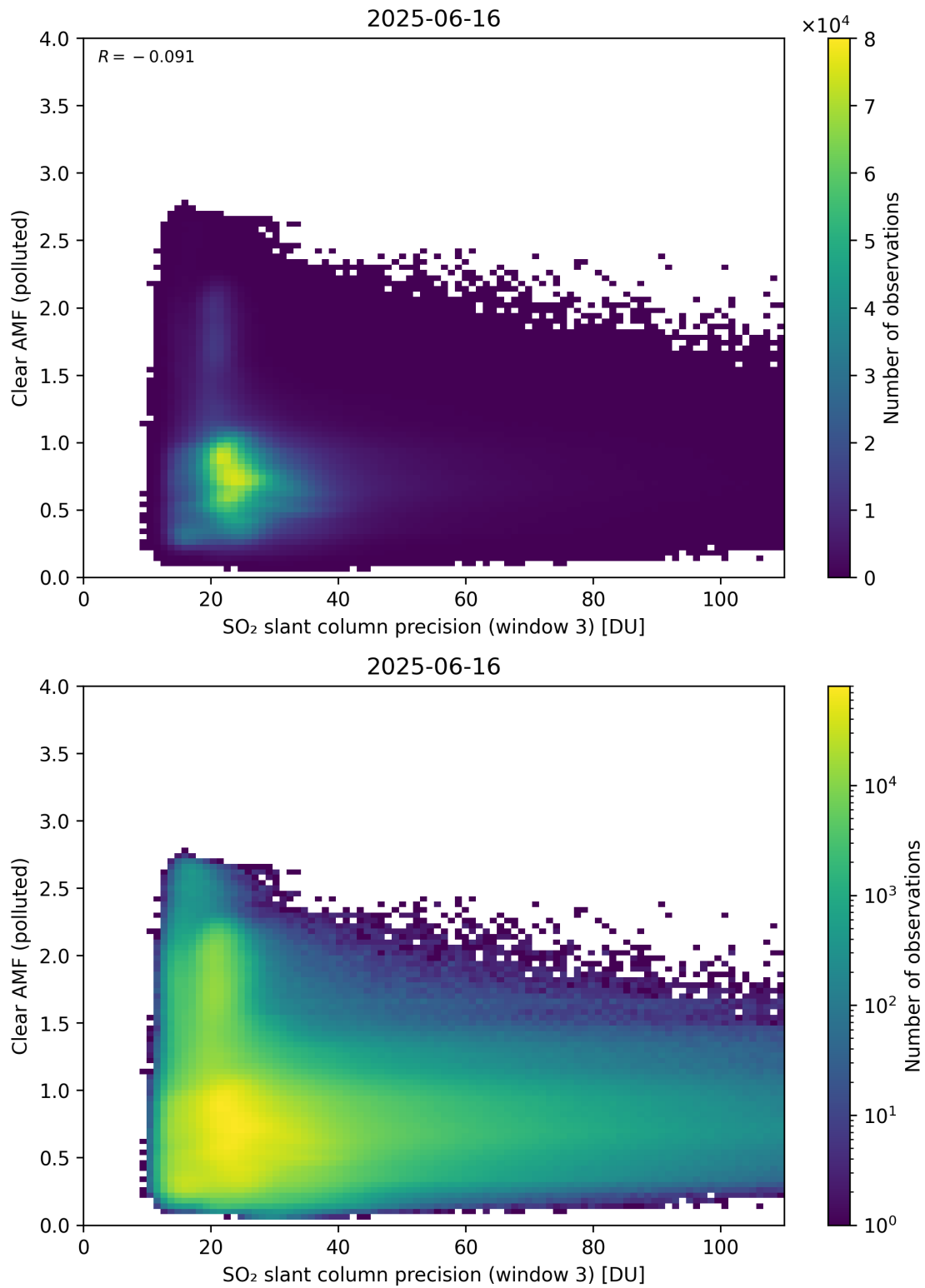
Figure 311: Scatter density plot of “SO 2 slant column precision (window 3)” against “Clear AMF (polluted)” for 2025-06-16 to 2025-06-17.
