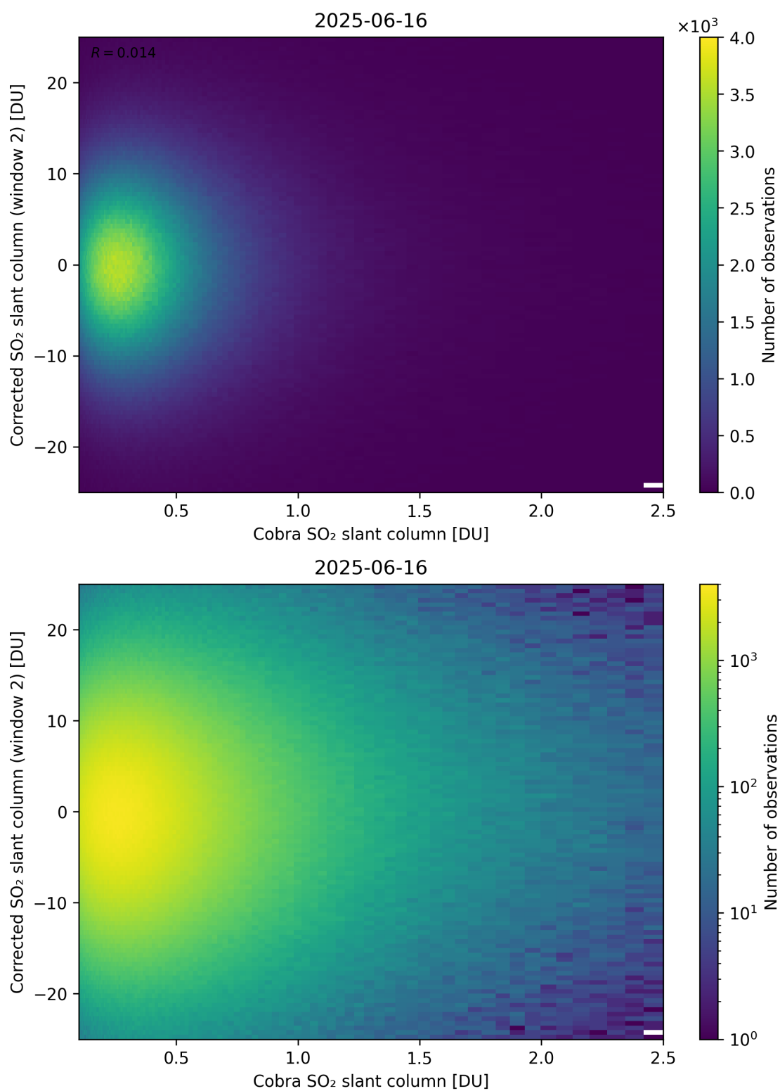
Figure 217: Scatter density plot of “Cobra SO 2 slant column” against “Corrected SO 2 slant column (window 2)” for 2025-06-16 to 2025-06-17.
