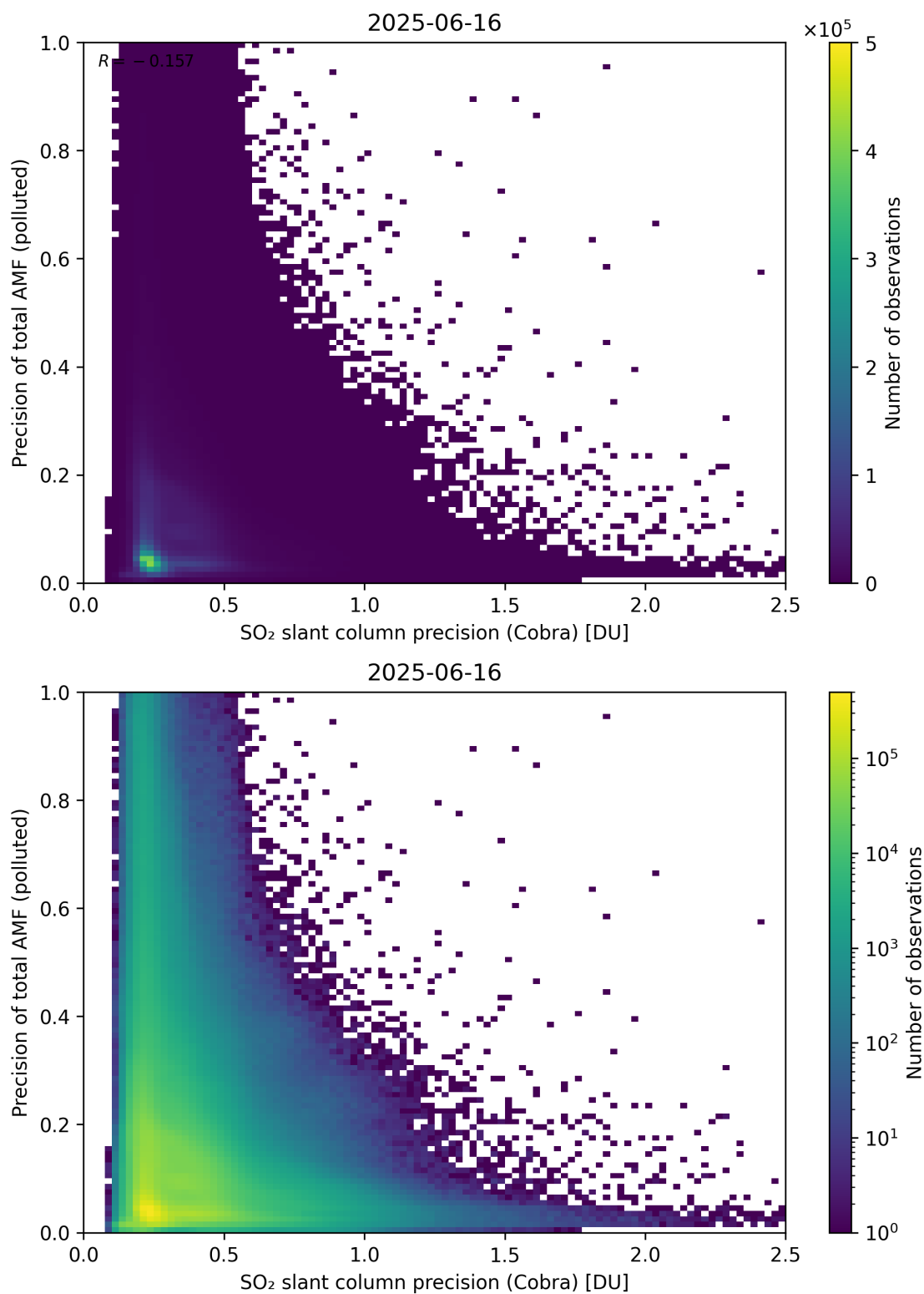
Figure 214: Scatter density plot of “SO 2 slant column precision (Cobra)” against “Precision of total AMF (polluted)” for 2025-06-16 to 2025-06-17.
