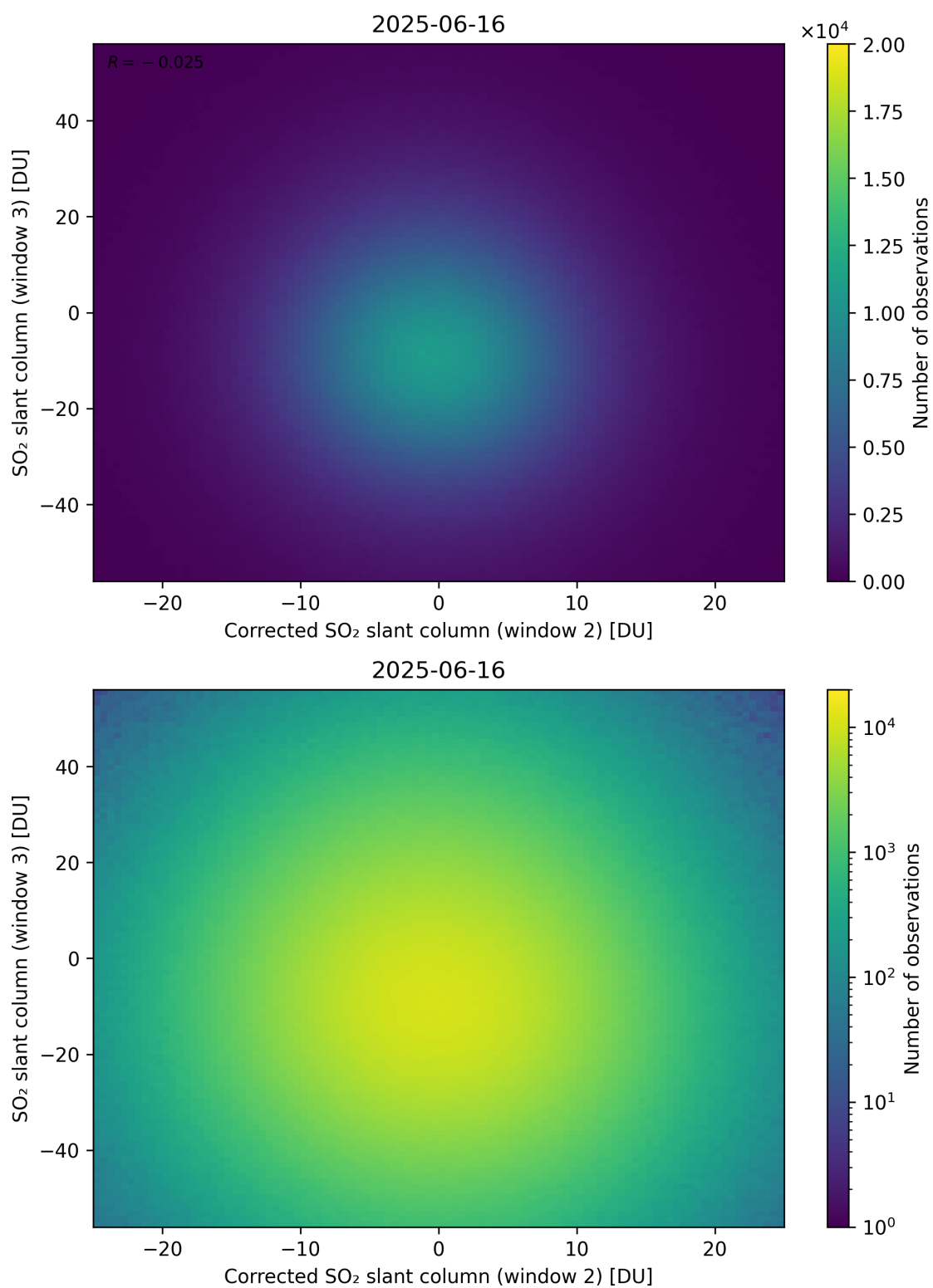
Figure 251: Scatter density plot of “Corrected SO 2 slant column (window 2)” against “SO 2 slant column (window 3)” for 2025-06-16 to 2025-06-17.
