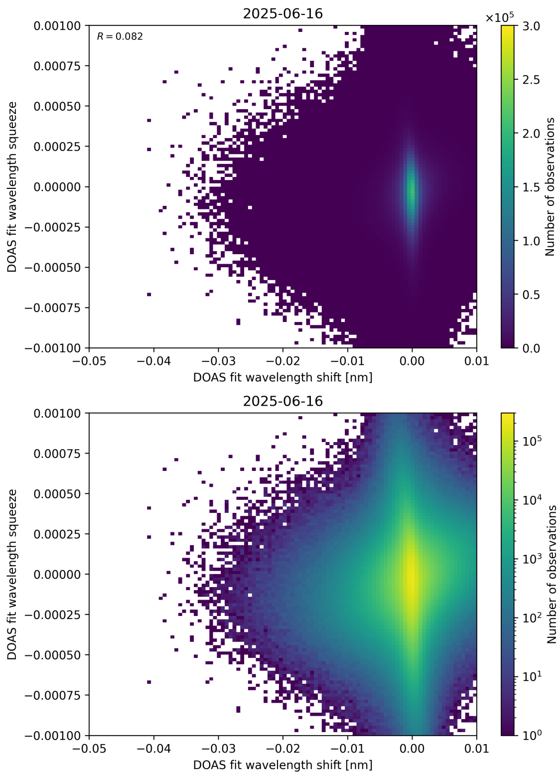
Figure 138: Scatter density plot of “DOAS fit wavelength shift” against “DOAS fit wavelength squeeze” for 2025-06-16 to 2025-06-17.
