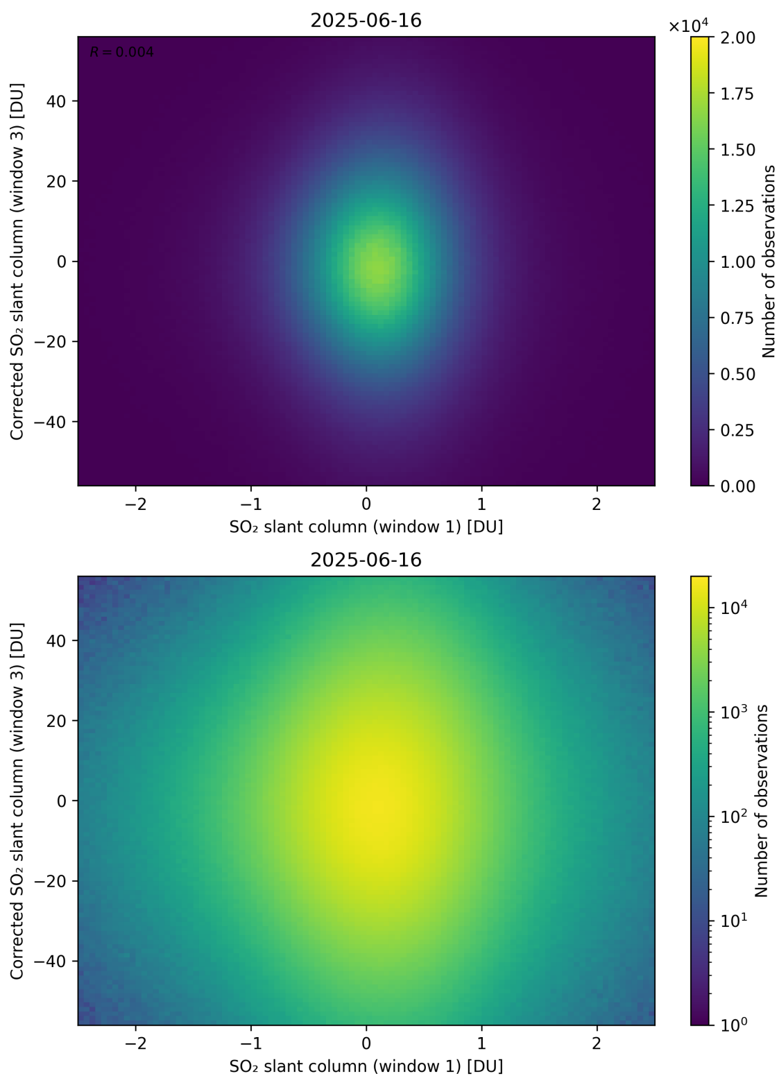
Figure 284: Scatter density plot of “SO 2 slant column (window 1)” against “Corrected SO 2 slant column (window 3)” for 2025-06-16 to 2025-06-17.
