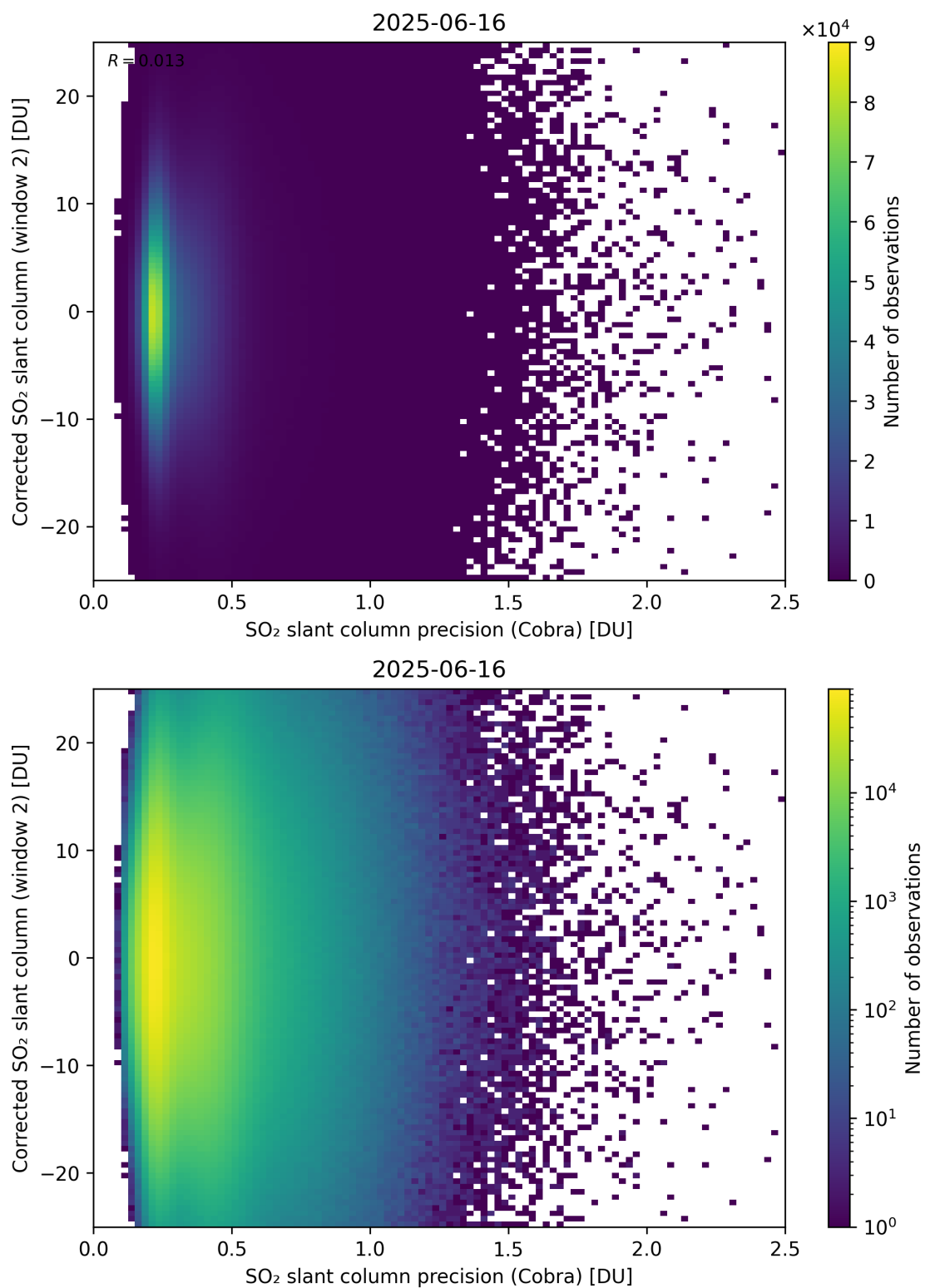
Figure 206: Scatter density plot of “SO 2 slant column precision (Cobra)” against “Corrected SO 2 slant column (window 2)” for 2025-06-16 to 2025-06-17.
