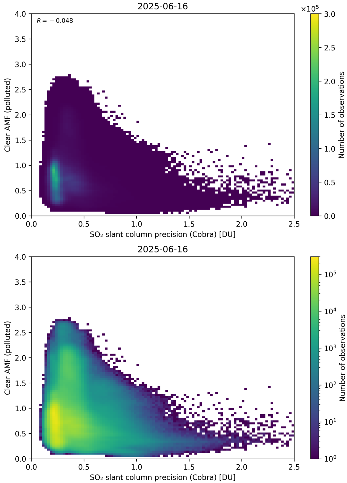
Figure 205: Scatter density plot of “SO 2 slant column precision (Cobra)” against “Clear AMF (polluted)” for 2025-06-16 to 2025-06-17.
