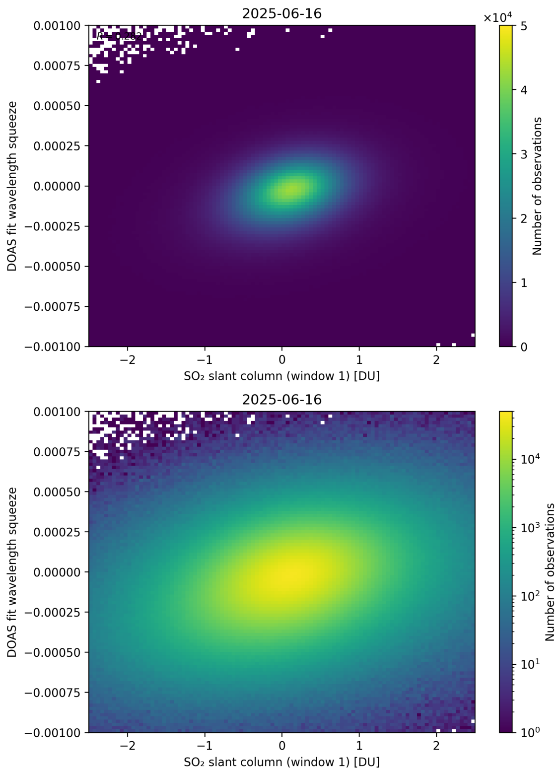
Figure 266: Scatter density plot of “SO 2 slant column (window 1)” against “DOAS fit wavelength squeeze” for 2025-06-16 to 2025-06-17.
