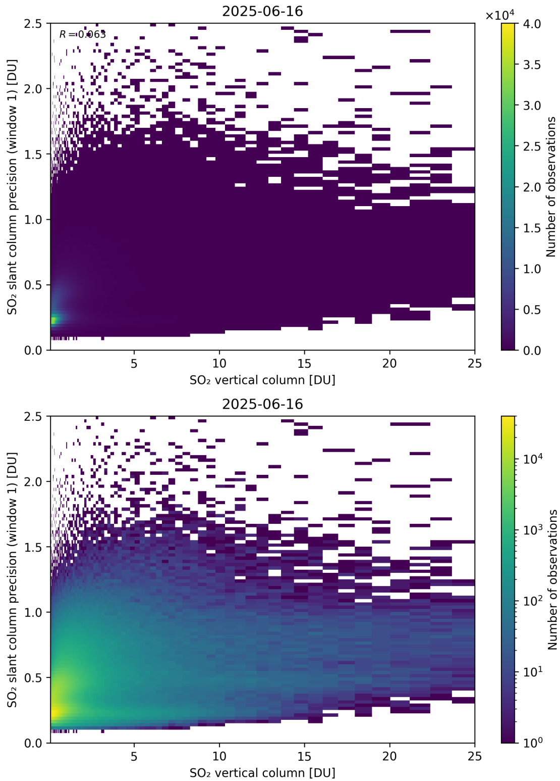
Figure 355: Scatter density plot of “SO 2 vertical column” against “SO 2 slant column precision (window 1)” for 2025-06-16 to 2025-06-17.
