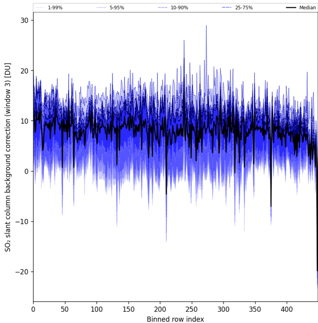
Figure 100: Along track statistics of “SO 2 slant column background correction (window 3)” for 2025-06-16 to 2025-06-17
