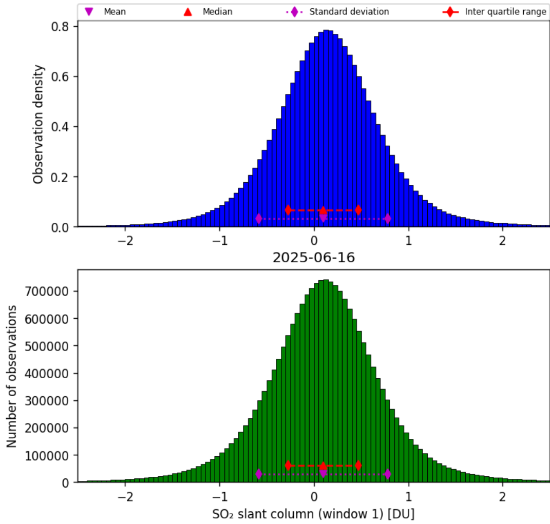
Figure 63: Histogram of “SO 2 slant column (window 1)” for 2025-06-16 to 2025-06-17
