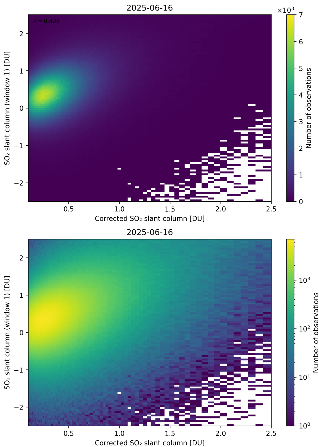
Figure 237: Scatter density plot of “Corrected SO 2 slant column” against “SO 2 slant column (window 1)” for 2025-06-16 to 2025-06-17.
