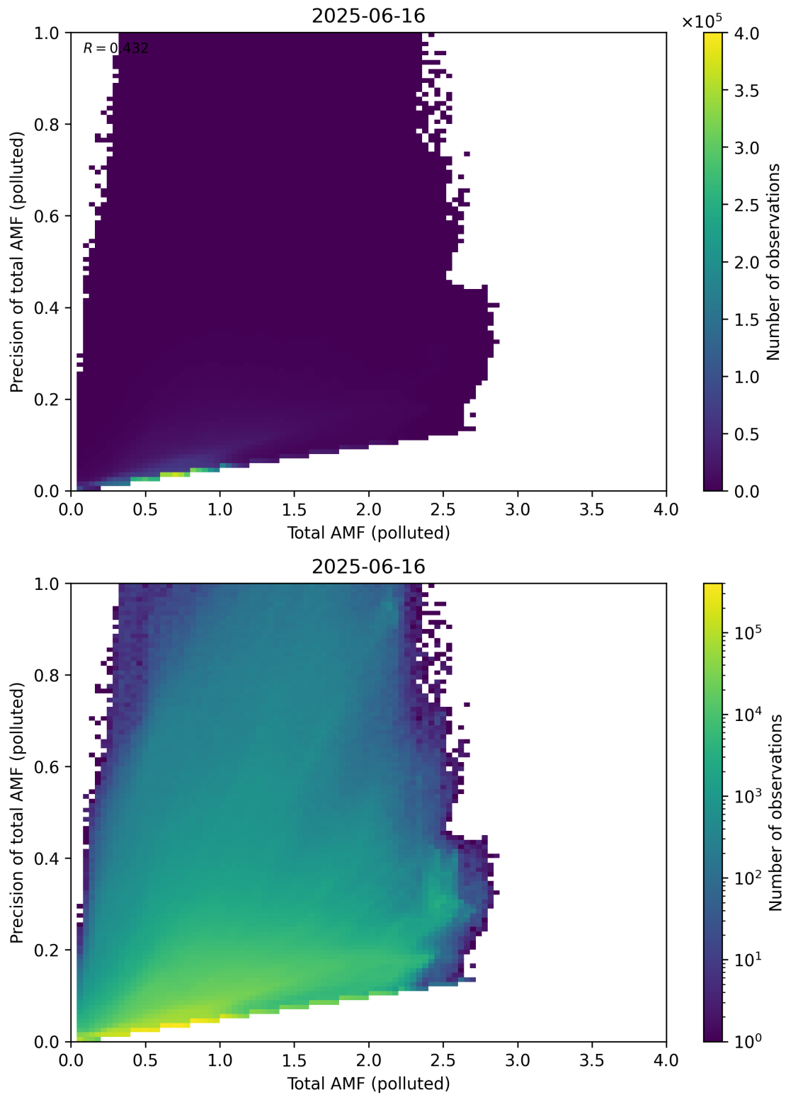
Figure 322: Scatter density plot of “Total AMF (polluted)” against “Precision of total AMF (polluted)” for 2025-06-16 to 2025-06-17.
