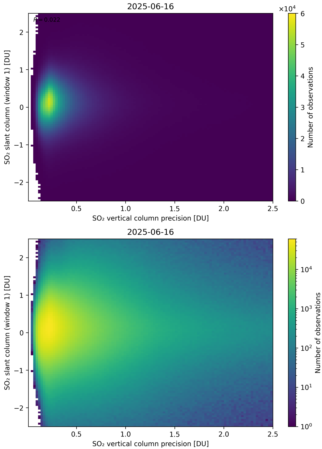
Figure 341: Scatter density plot of “SO 2 vertical column precision” against “SO 2 slant column (window 1)” for 2025-06-16 to 2025-06-17.
