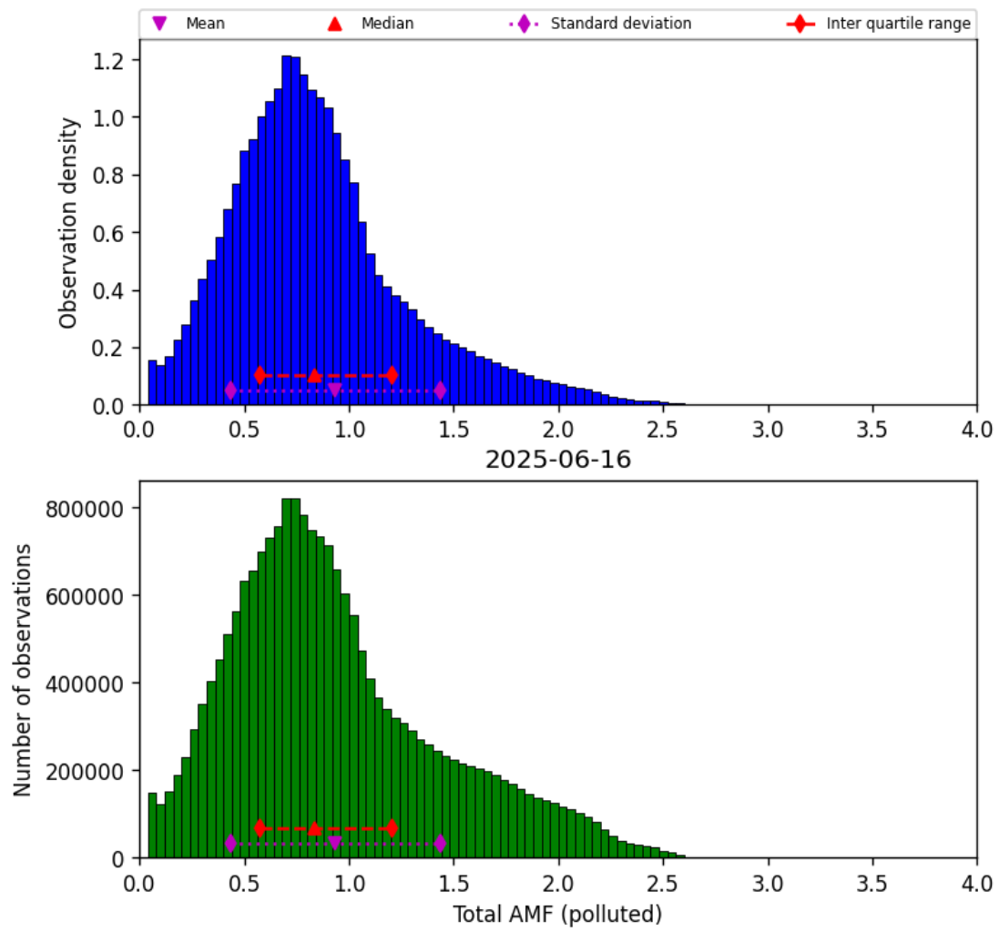
Figure 79: Histogram of “Total AMF (polluted)” for 2025-06-16 to 2025-06-17
