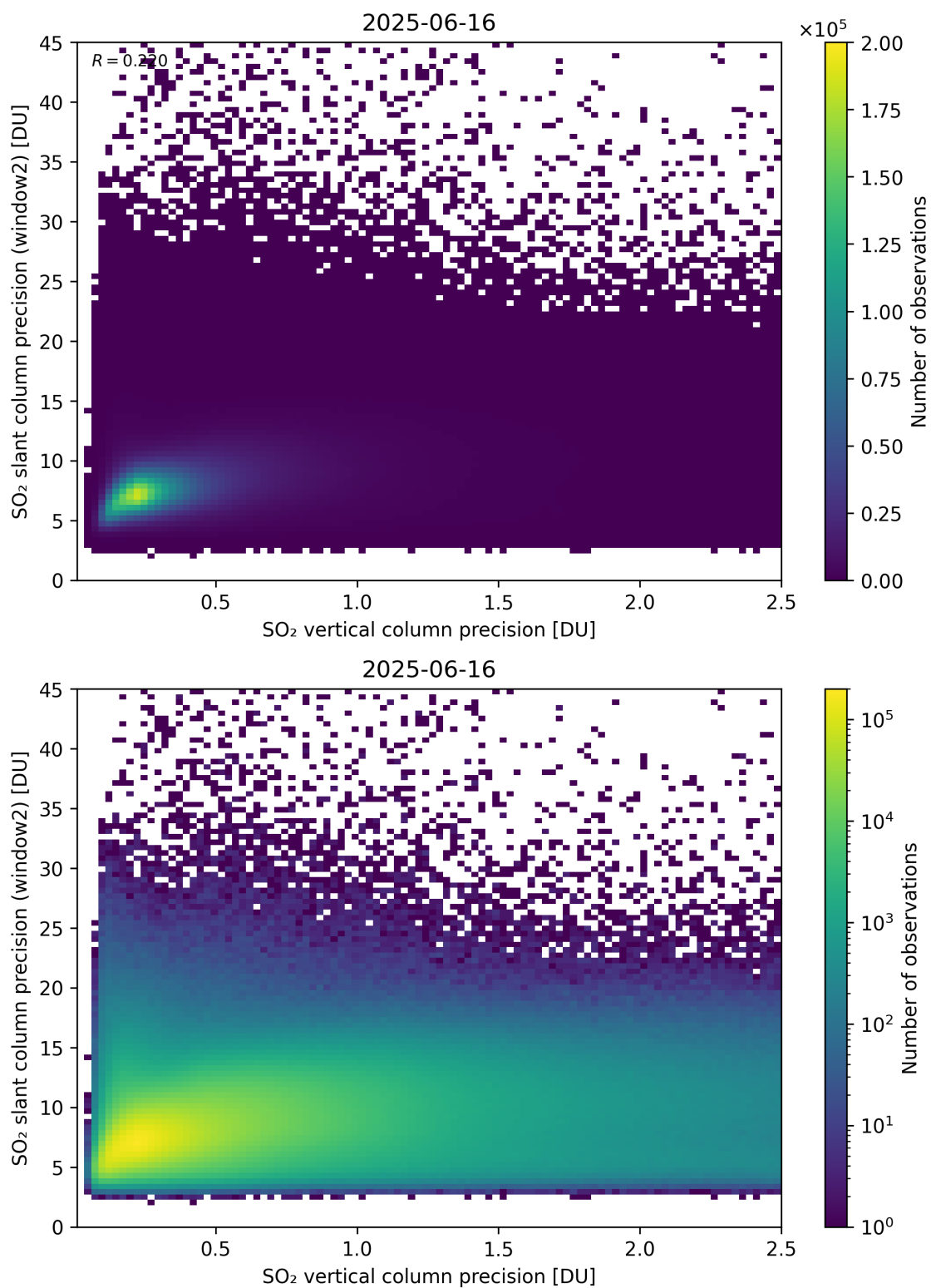
Figure 343: Scatter density plot of “SO 2 vertical column precision” against “SO 2 slant column precision (window2)” for 2025-06-16 to 2025-06-17.
