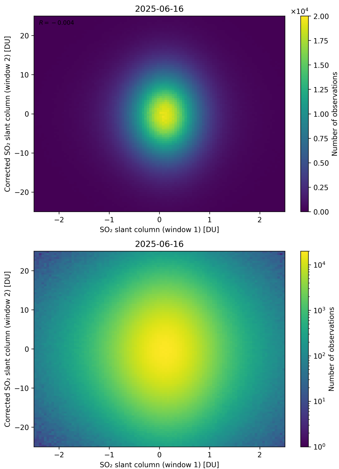
Figure 283: Scatter density plot of “SO 2 slant column (window 1)” against “Corrected SO 2 slant column (window 2)” for 2025-06-16 to 2025-06-17.
