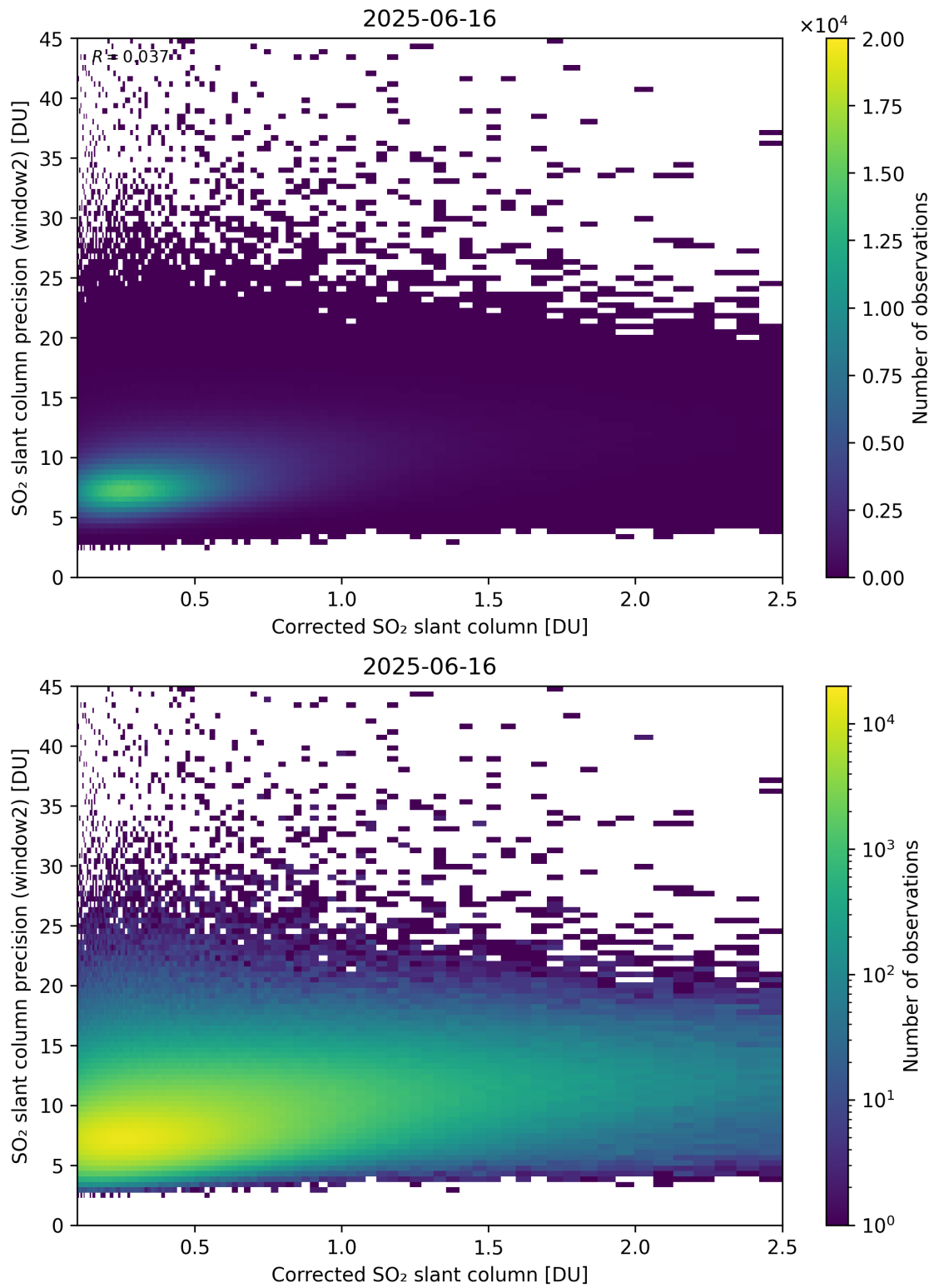
Figure 239: Scatter density plot of “Corrected SO 2 slant column” against “SO 2 slant column precision (window2)” for 2025-06-16 to 2025-06-17.
