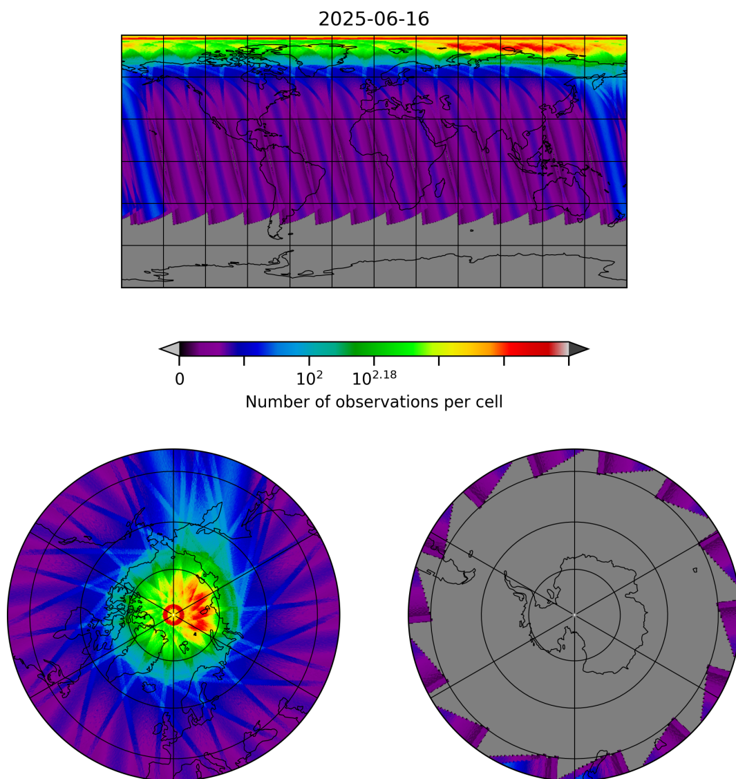
Figure 30: Map of the number of observations for 2025-06-16 to 2025-06-17
