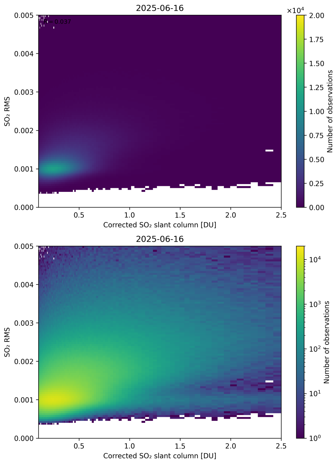
Figure 231: Scatter density plot of “Corrected SO 2 slant column” against “SO 2 RMS” for 2025-06-16 to 2025-06-17.
