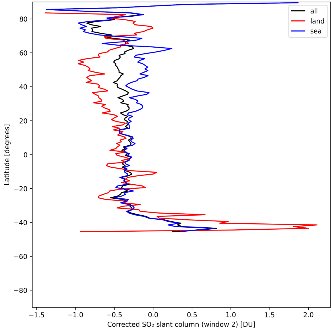
Figure 43: Zonal average of “Corrected SO 2 slant column (window 2)” for 2025-06-16 to 2025-06-17.
