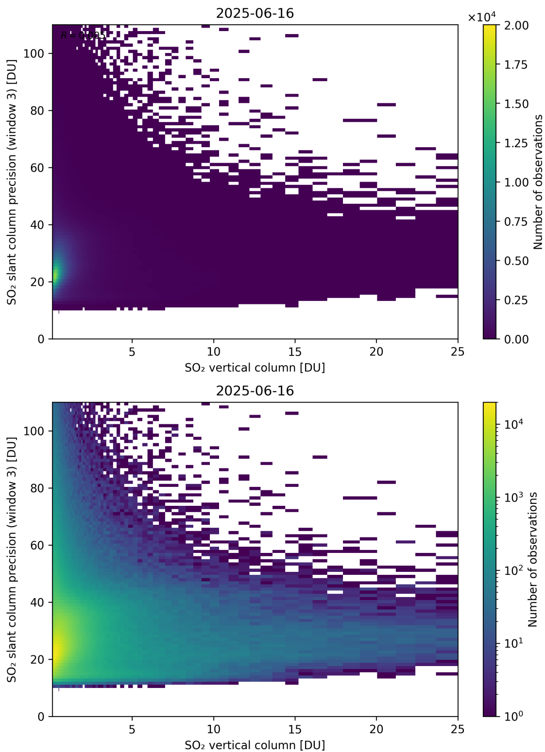
Figure 358: Scatter density plot of “SO 2 vertical column” against “SO 2 slant column precision (window 3)” for 2025-06-16 to 2025-06-17.
