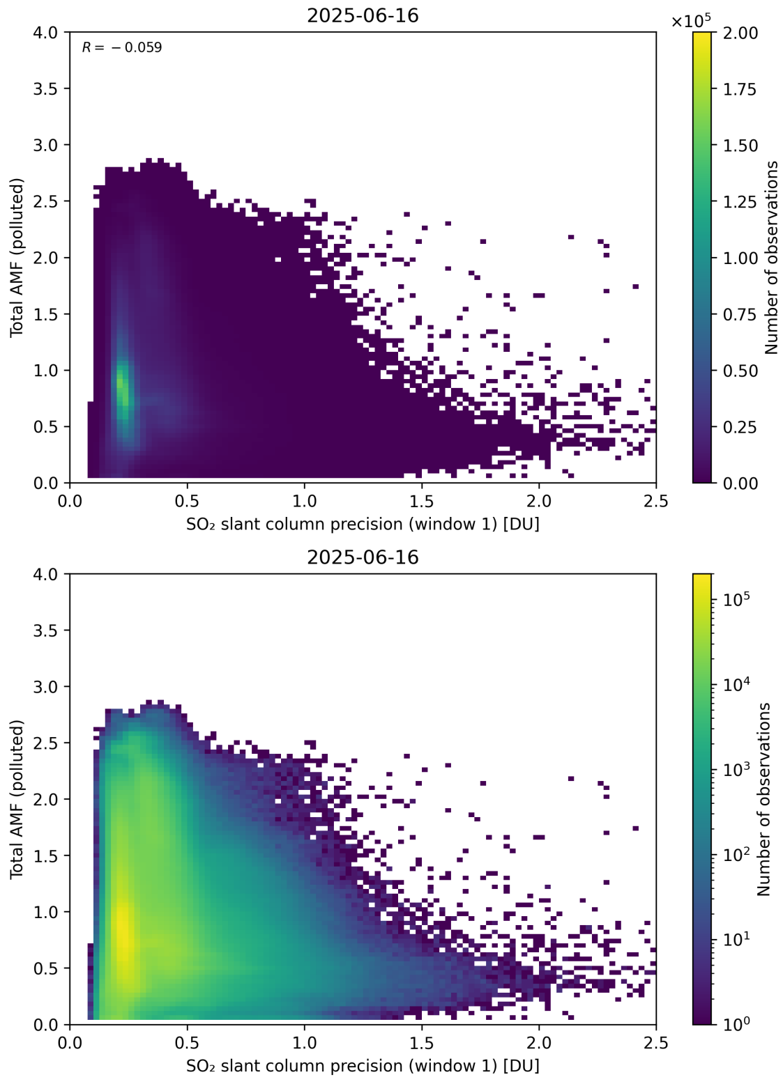
Figure 280: Scatter density plot of “SO 2 slant column precision (window 1)” against “Total AMF (polluted)” for 2025-06-16 to 2025-06-17.
