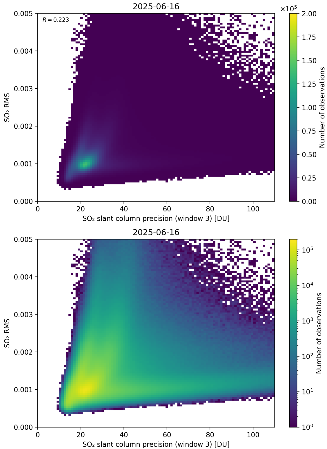
Figure 310: Scatter density plot of “SO 2 slant column precision (window 3)” against “SO 2 RMS” for 2025-06-16 to 2025-06-17.
