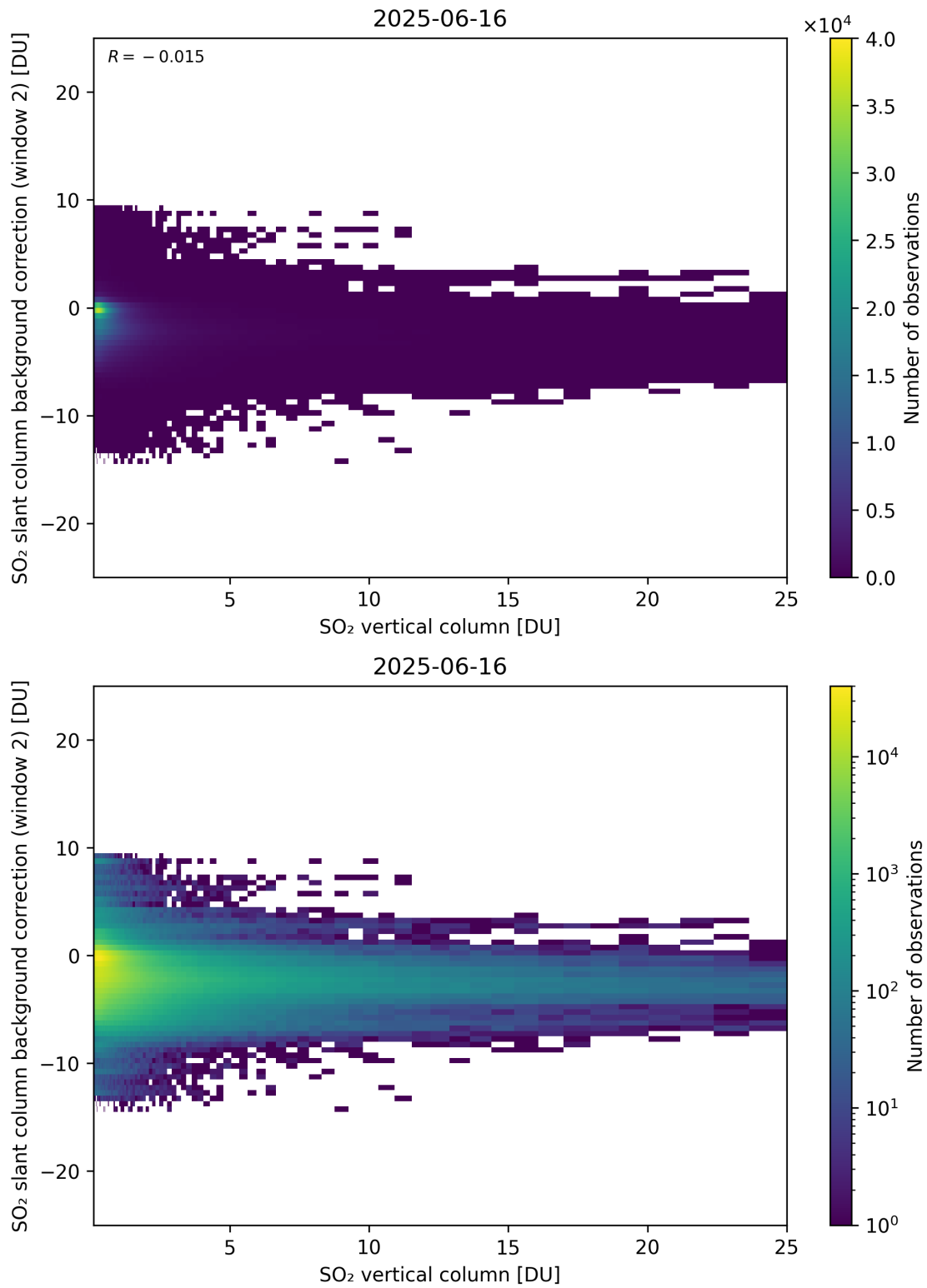
Figure 324: Scatter density plot of “SO 2 vertical column” against “SO 2 slant column background correction (window 2)” for 2025-06-16 to 2025-06-17.
