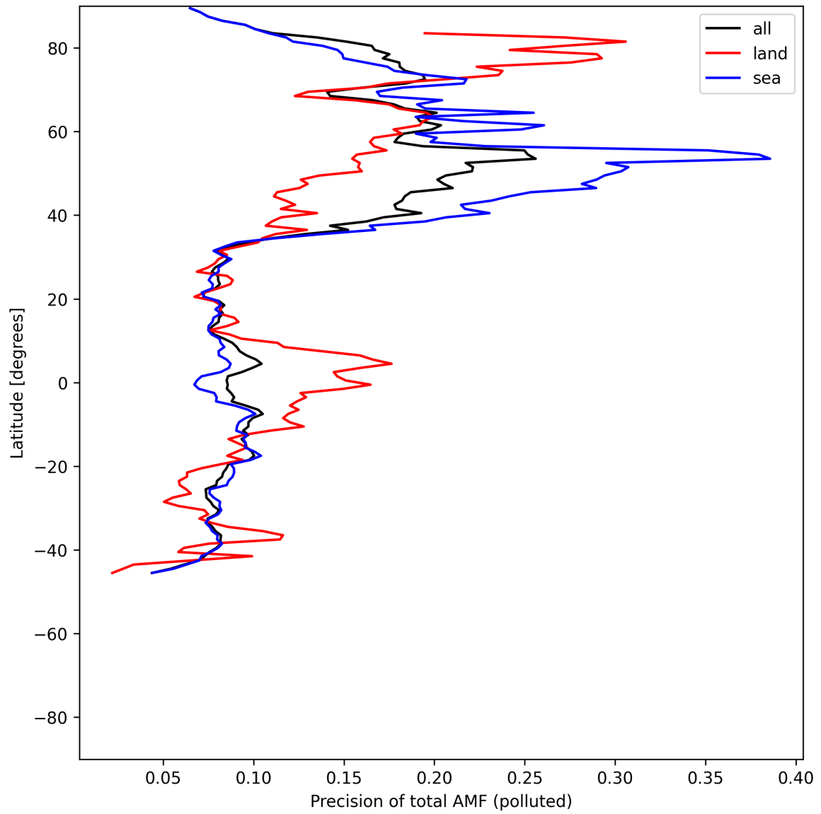
Figure 54: Zonal average of “Precision of total AMF (polluted)” for 2025-06-16 to 2025-06-17.
