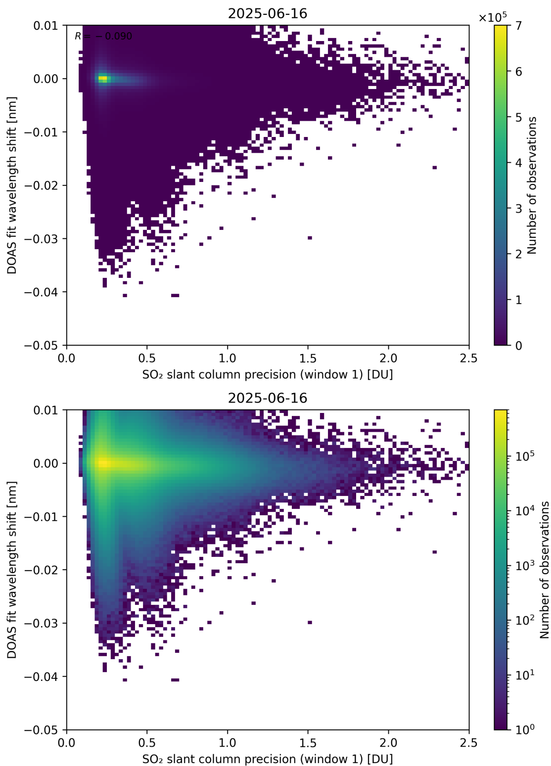
Figure 271: Scatter density plot of “SO 2 slant column precision (window 1)” against “DOAS fit wavelength shift” for 2025-06-16 to 2025-06-17.
