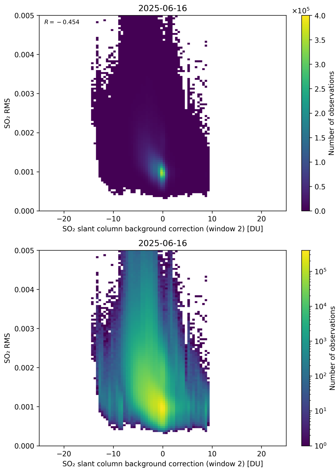
Figure 125: Scatter density plot of “SO 2 slant column background correction (window 2)” against “SO 2 RMS” for 2025-06-16 to 2025-06-17.
