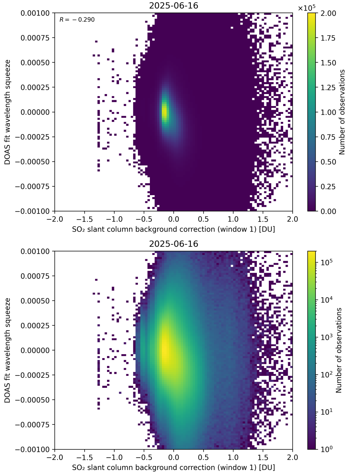
Figure 112: Scatter density plot of “SO 2 slant column background correction (window 1)” against “DOAS fit wavelength squeeze” for 2025-06-16 to 2025-06-17.
