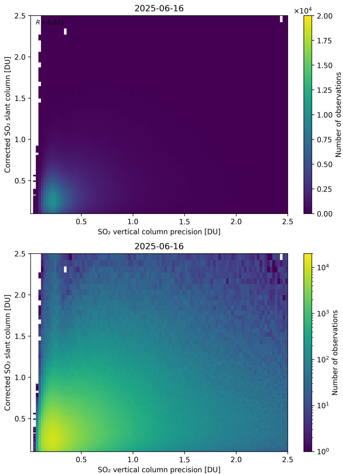
Figure 338: Scatter density plot of “SO 2 vertical column precision” against “Corrected SO 2 slant column” for 2025-06-16 to 2025-06-17.
