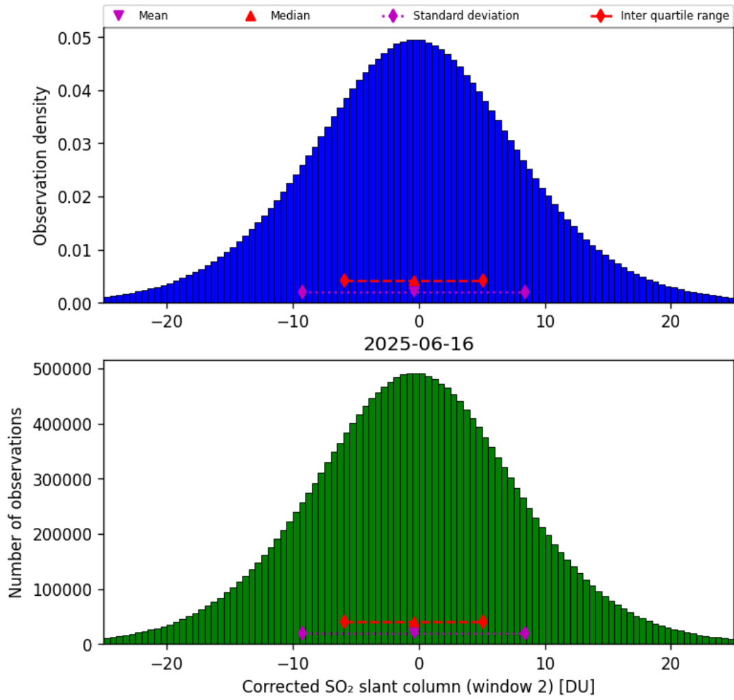
Figure 69: Histogram of “Corrected SO 2 slant column (window 2)” for 2025-06-16 to 2025-06-17
