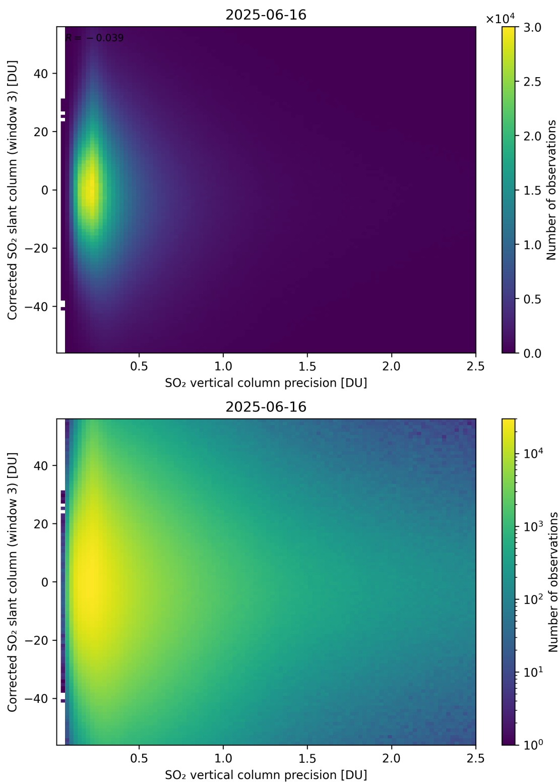
Figure 340: Scatter density plot of “SO 2 vertical column precision” against “Corrected SO 2 slant column (window 3)” for 2025-06-16 to 2025-06-17.
