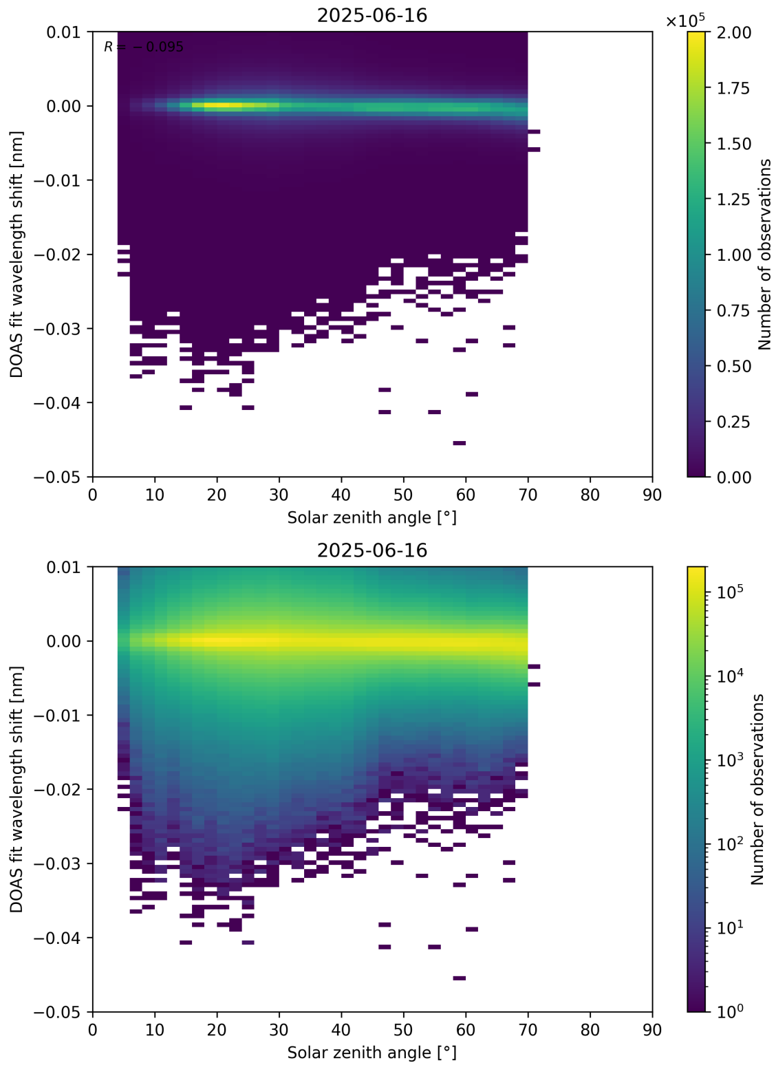
Figure 174: Scatter density plot of “Solar zenith angle” against “DOAS fit wavelength shift” for 2025-06-16 to 2025-06-17.
