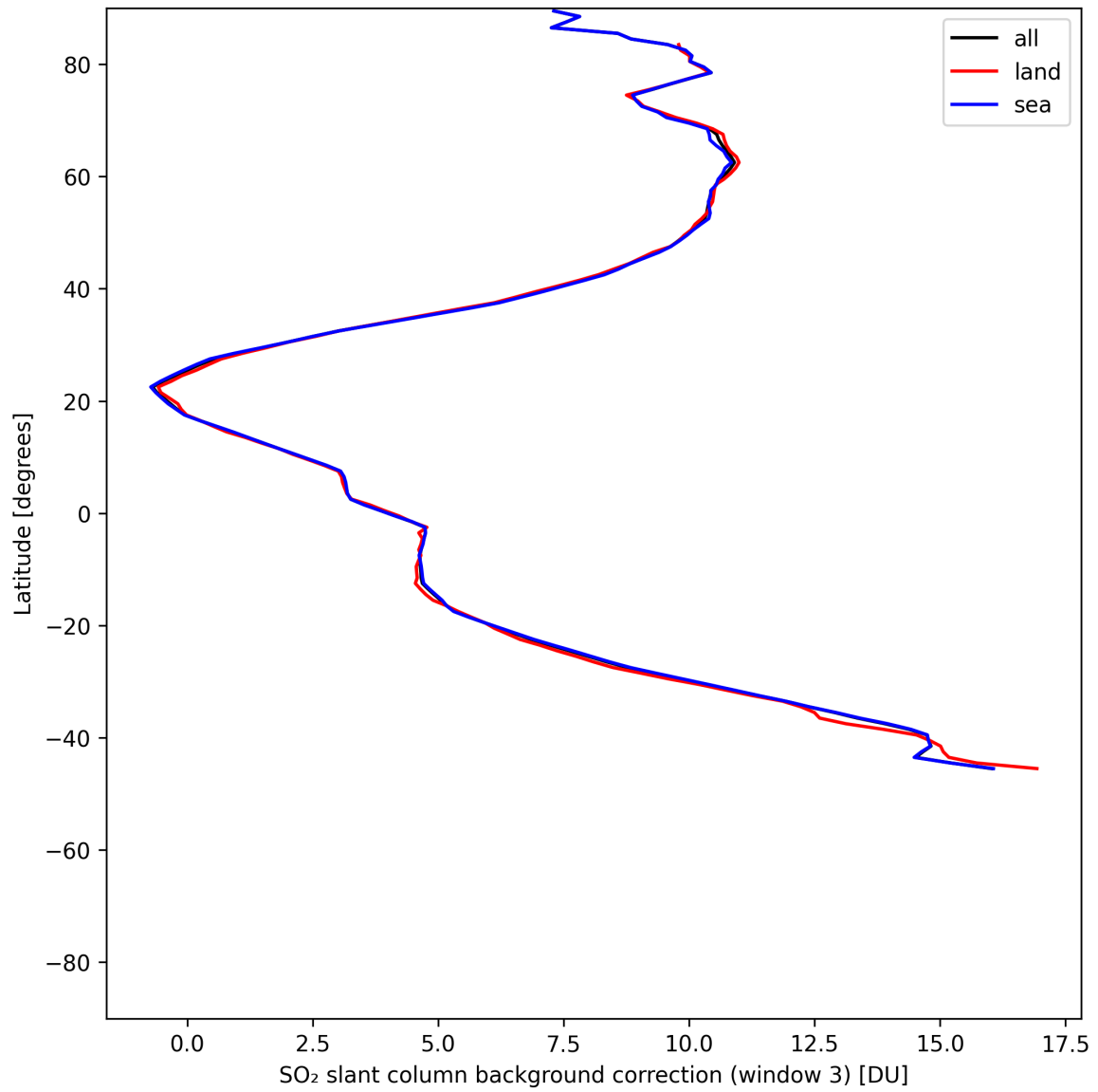
Figure 48: Zonal average of “SO 2 slant column background correction (window 3)” for 2025-06-16 to 2025-06-17.
