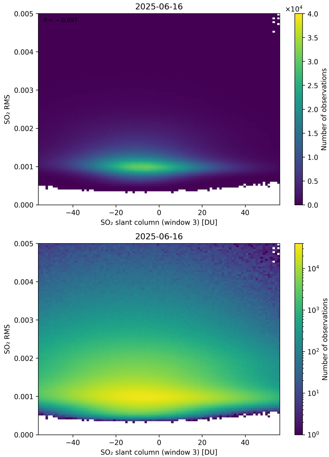
Figure 306: Scatter density plot of “SO 2 slant column (window 3)” against “SO 2 RMS” for 2025-06-16 to 2025-06-17.
