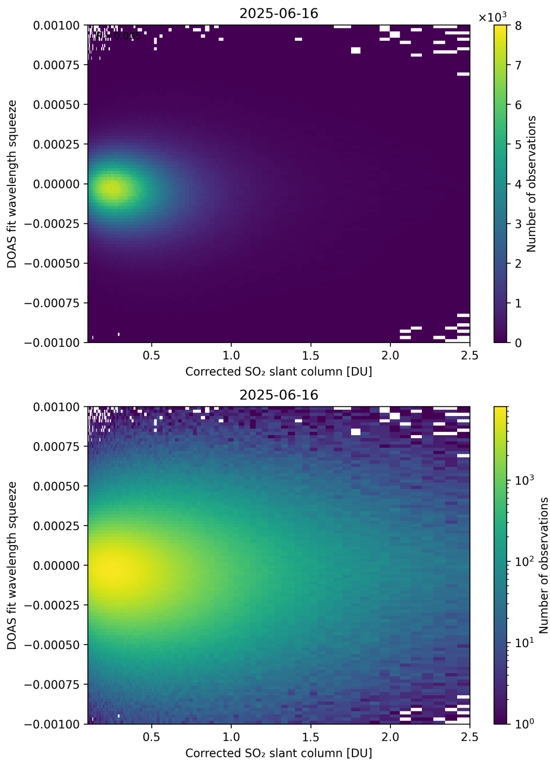
Figure 230: Scatter density plot of “Corrected SO 2 slant column” against “DOAS fit wavelength squeeze” for 2025-06-16 to 2025-06-17.
