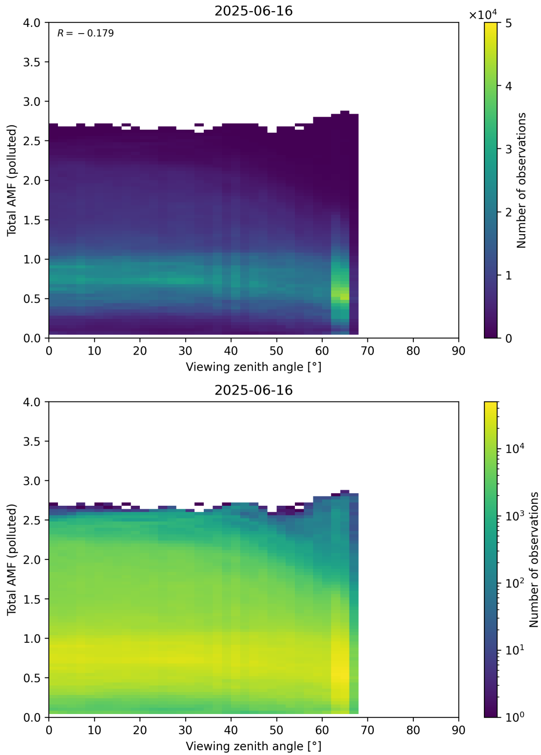
Figure 381: Scatter density plot of “Viewing zenith angle” against “Total AMF (polluted)” for 2025-06-16 to 2025-06-17.
