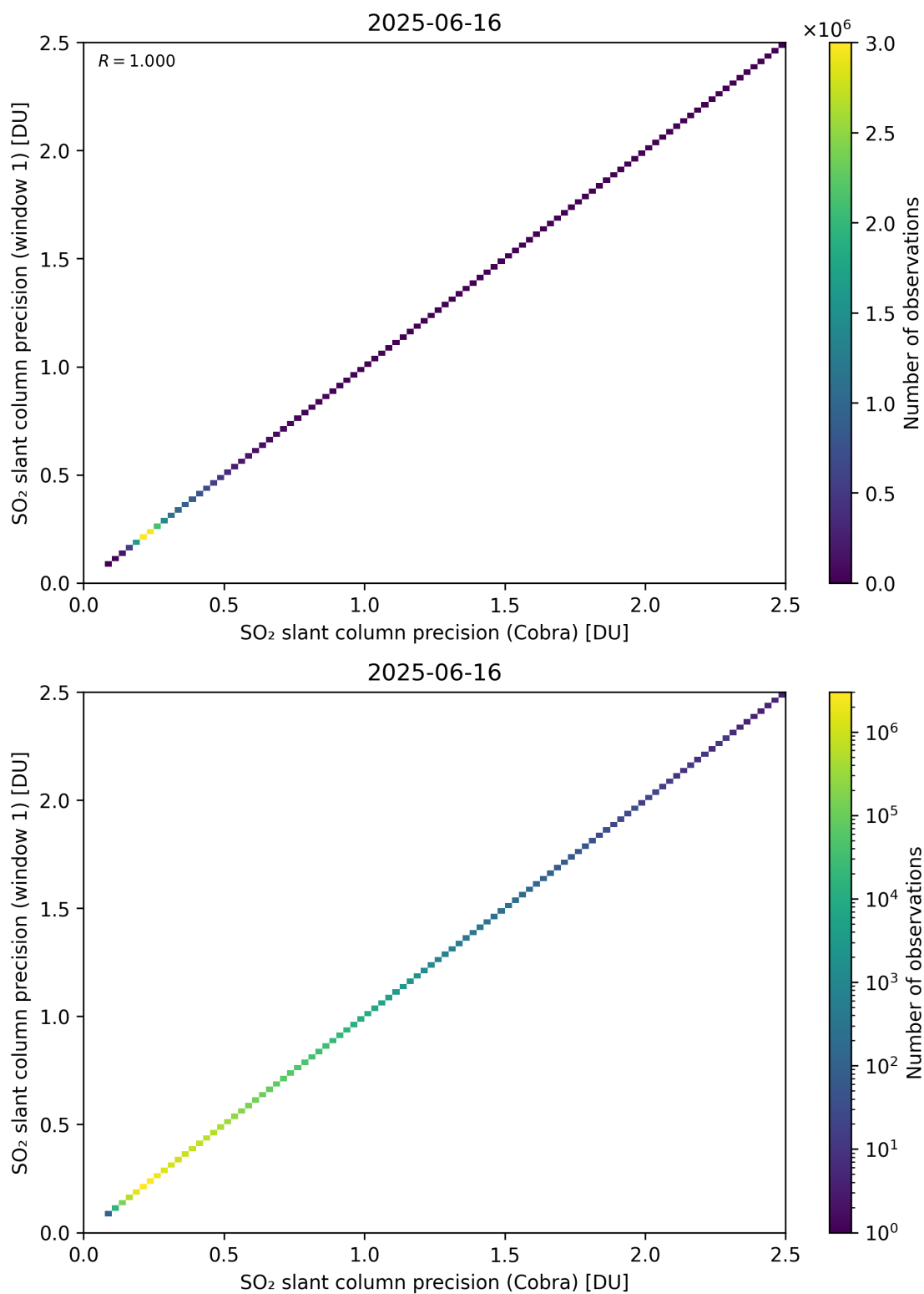
Figure 209: Scatter density plot of “SO 2 slant column precision (Cobra)” against “SO 2 slant column precision (window 1)” for 2025-06-16 to 2025-06-17.
