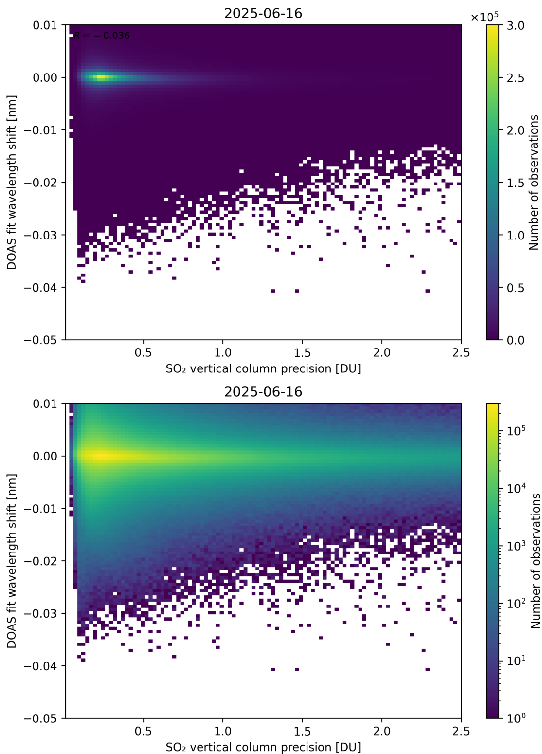
Figure 332: Scatter density plot of “SO 2 vertical column precision” against “DOAS fit wavelength shift” for 2025-06-16 to 2025-06-17.
