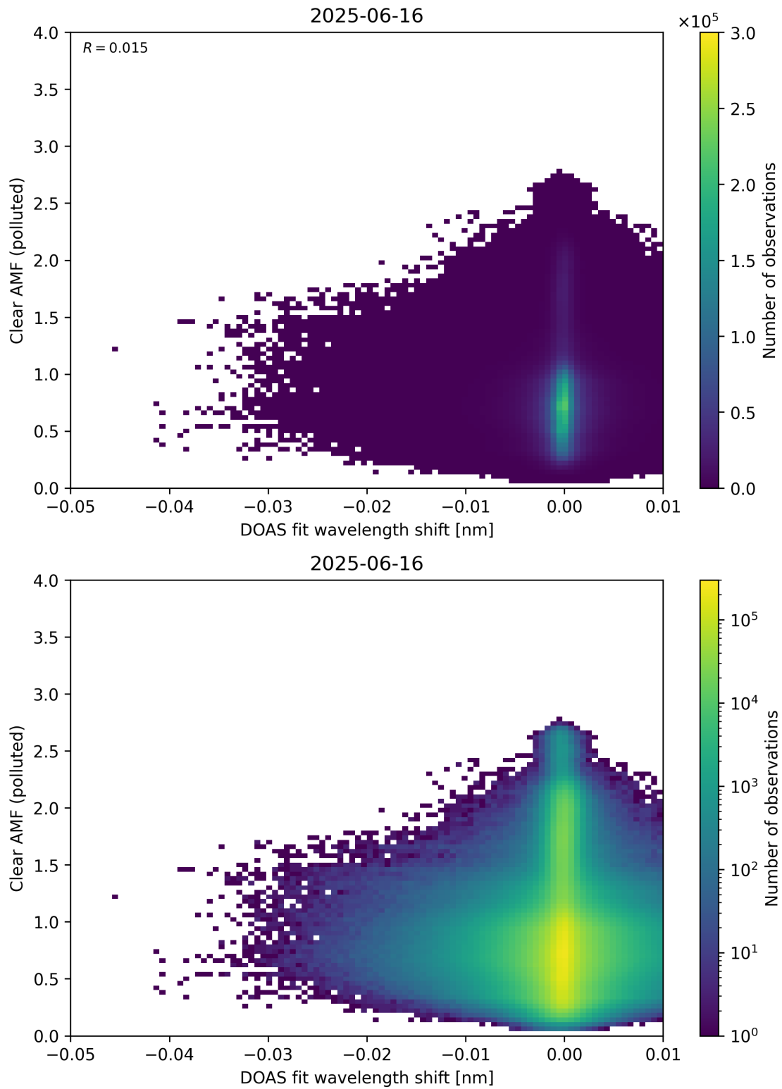
Figure 140: Scatter density plot of “DOAS fit wavelength shift” against “Clear AMF (polluted)” for 2025-06-16 to 2025-06-17.
