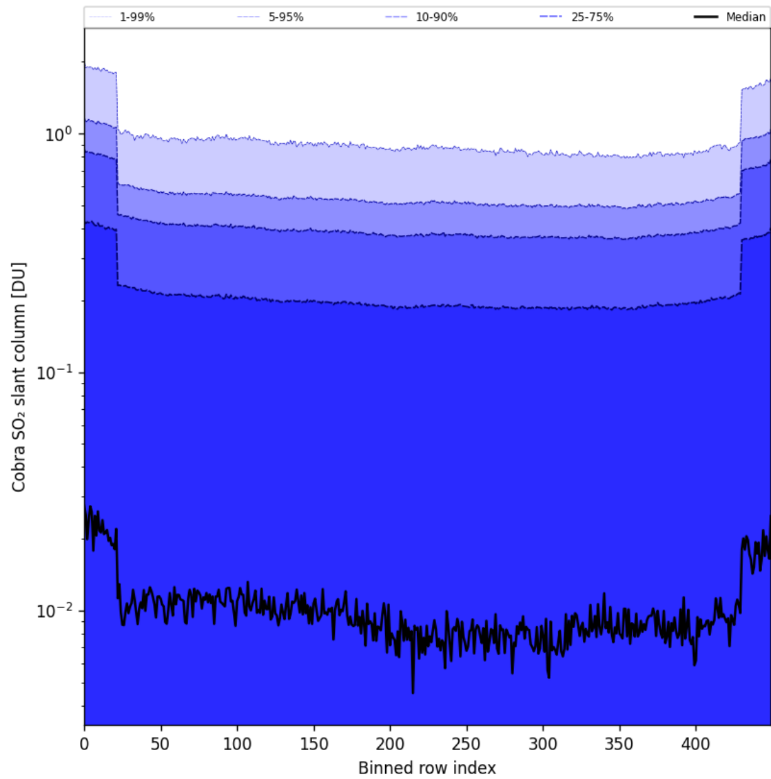
Figure 87: Along track statistics of “Cobra SO 2 slant column” for 2025-06-16 to 2025-06-17
