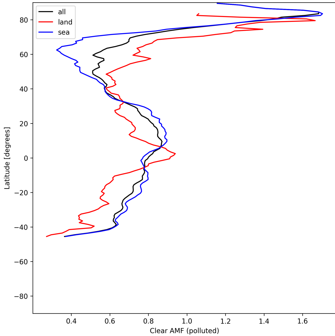
Figure 55: Zonal average of “Clear AMF (polluted)” for 2025-06-16 to 2025-06-17.
