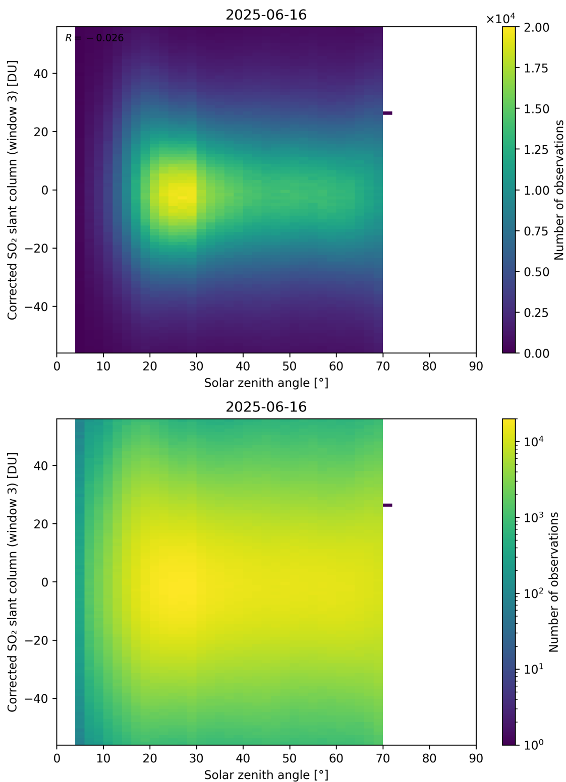
Figure 183: Scatter density plot of “Solar zenith angle” against “Corrected SO 2 slant column (window 3)” for 2025-06-16 to 2025-06-17.
