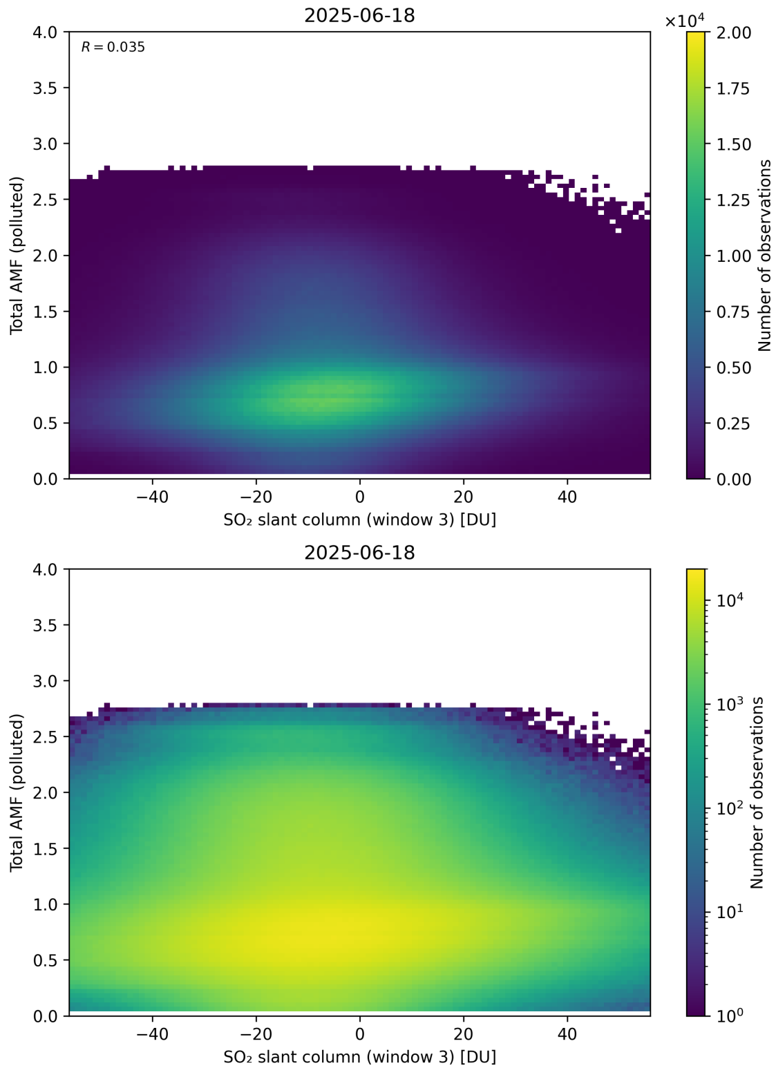
Figure 318: Scatter density plot of “SO 2 slant column (window 3)” against “Total AMF (polluted)” for 2025-06-17 to 2025-06-19.
