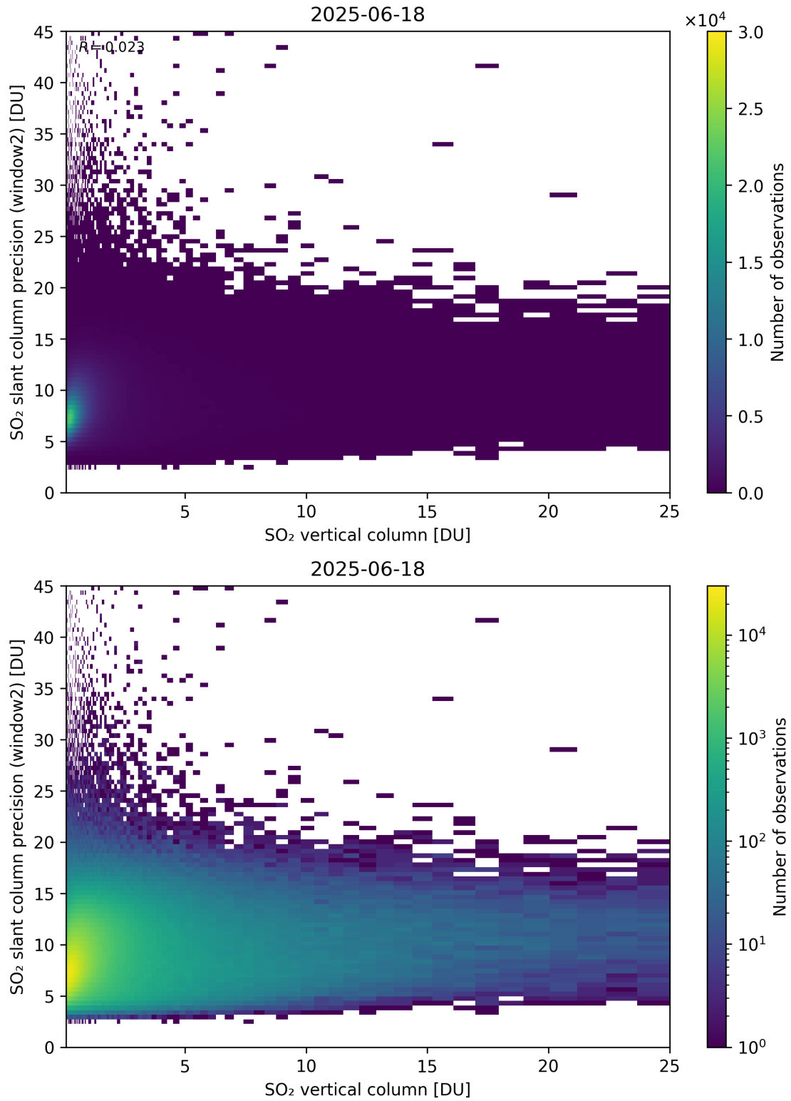
Figure 356: Scatter density plot of “SO 2 vertical column” against “SO 2 slant column precision (window2)” for 2025-06-17 to 2025-06-19.
