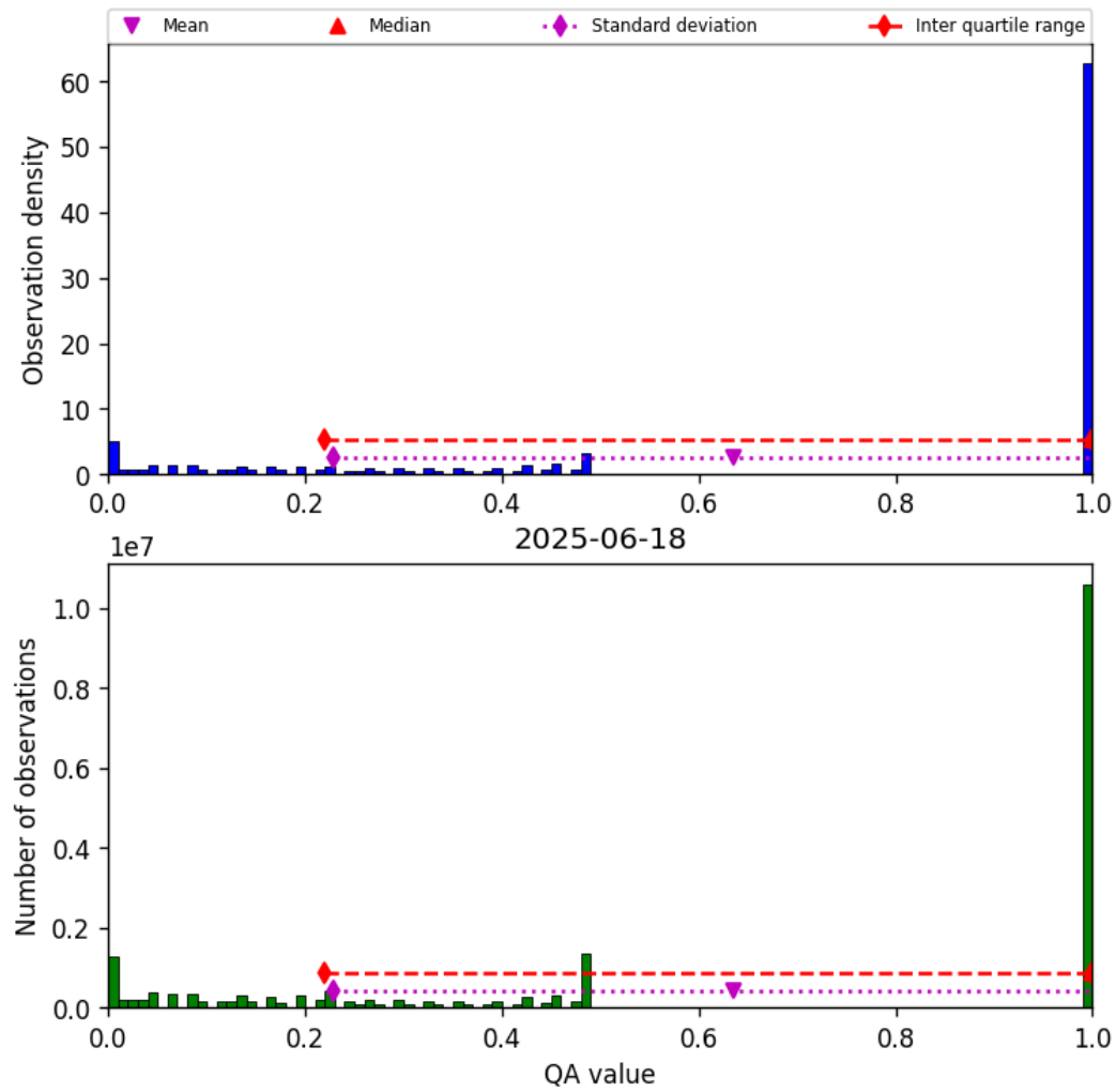
Figure 57: Histogram of “QA value” for 2025-06-17 to 2025-06-19
