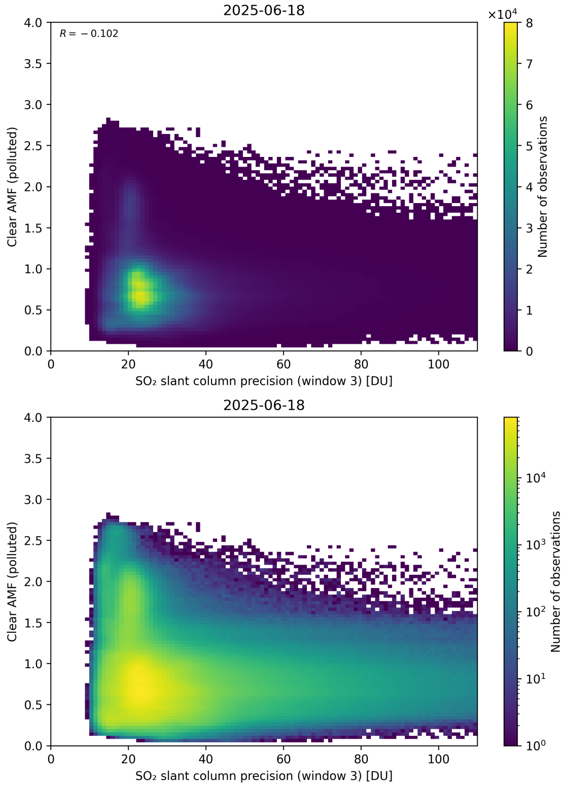
Figure 311: Scatter density plot of “SO 2 slant column precision (window 3)” against “Clear AMF (polluted)” for 2025-06-17 to 2025-06-19.
