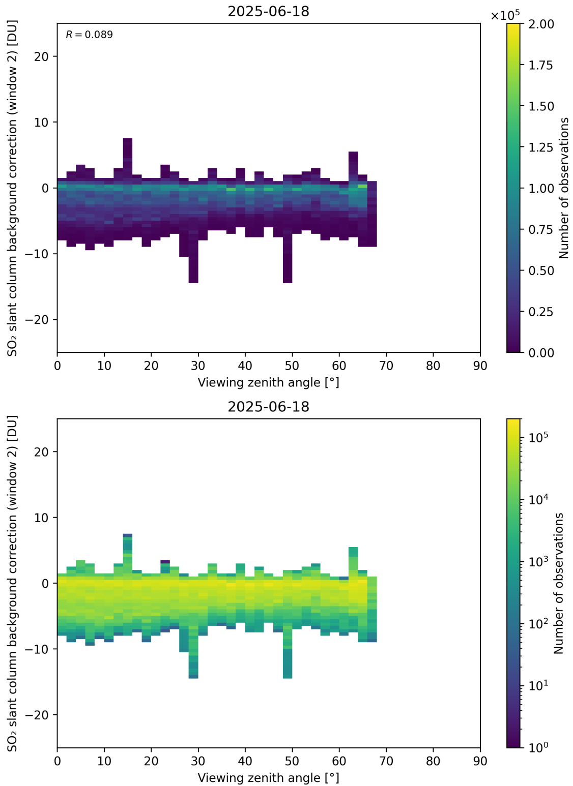
Figure 363: Scatter density plot of “Viewing zenith angle” against “SO 2 slant column background correction (window 2)” for 2025-06-17 to 2025-06-19.
