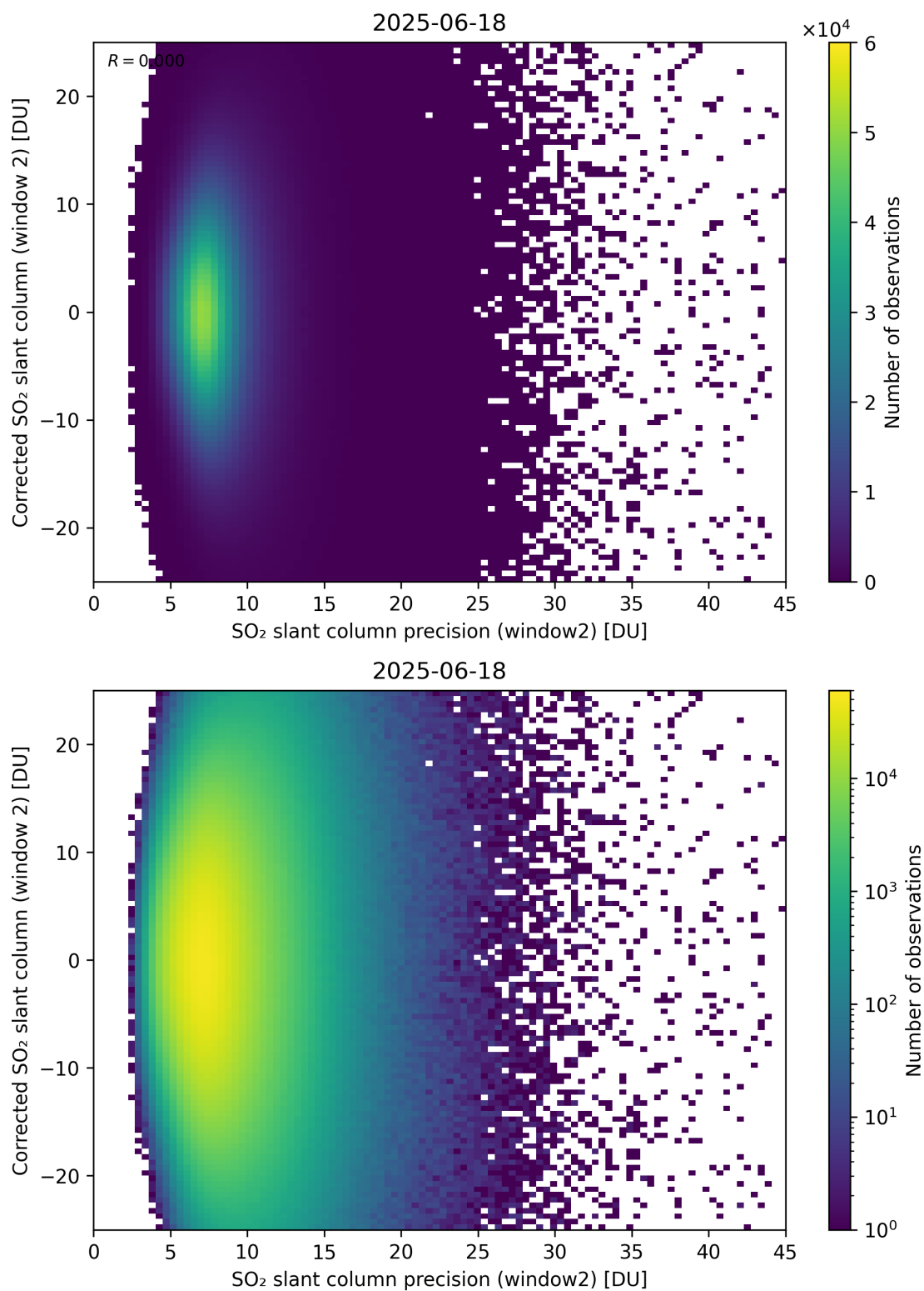
Figure 297: Scatter density plot of “SO 2 slant column precision (window2)” against “Corrected SO 2 slant column (window 2)” for 2025-06-17 to 2025-06-19.
