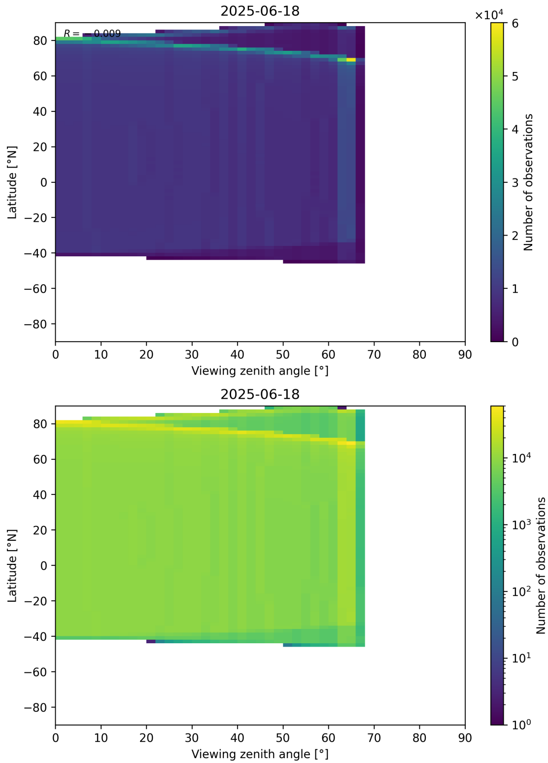
Figure 368: Scatter density plot of “Viewing zenith angle” against “Latitude” for 2025-06-17 to 2025-06-19.
