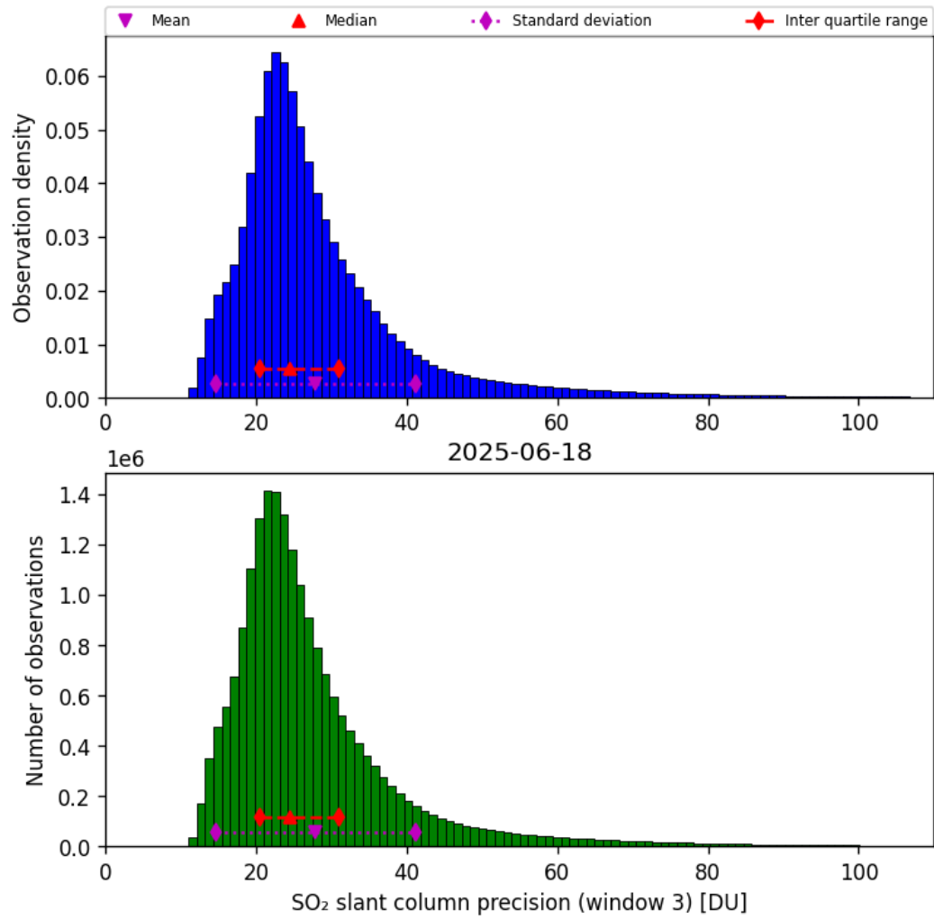
Figure 72: Histogram of “SO 2 slant column precision (window 3)” for 2025-06-17 to 2025-06-19
