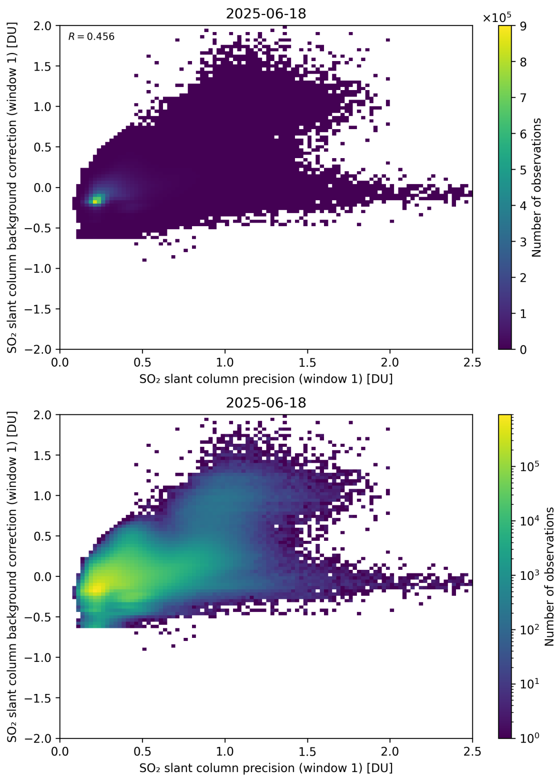
Figure 268: Scatter density plot of “SO 2 slant column precision (window 1)” against “SO 2 slant column background correction (window 1)” for 2025-06-17 to 2025-06-19.
