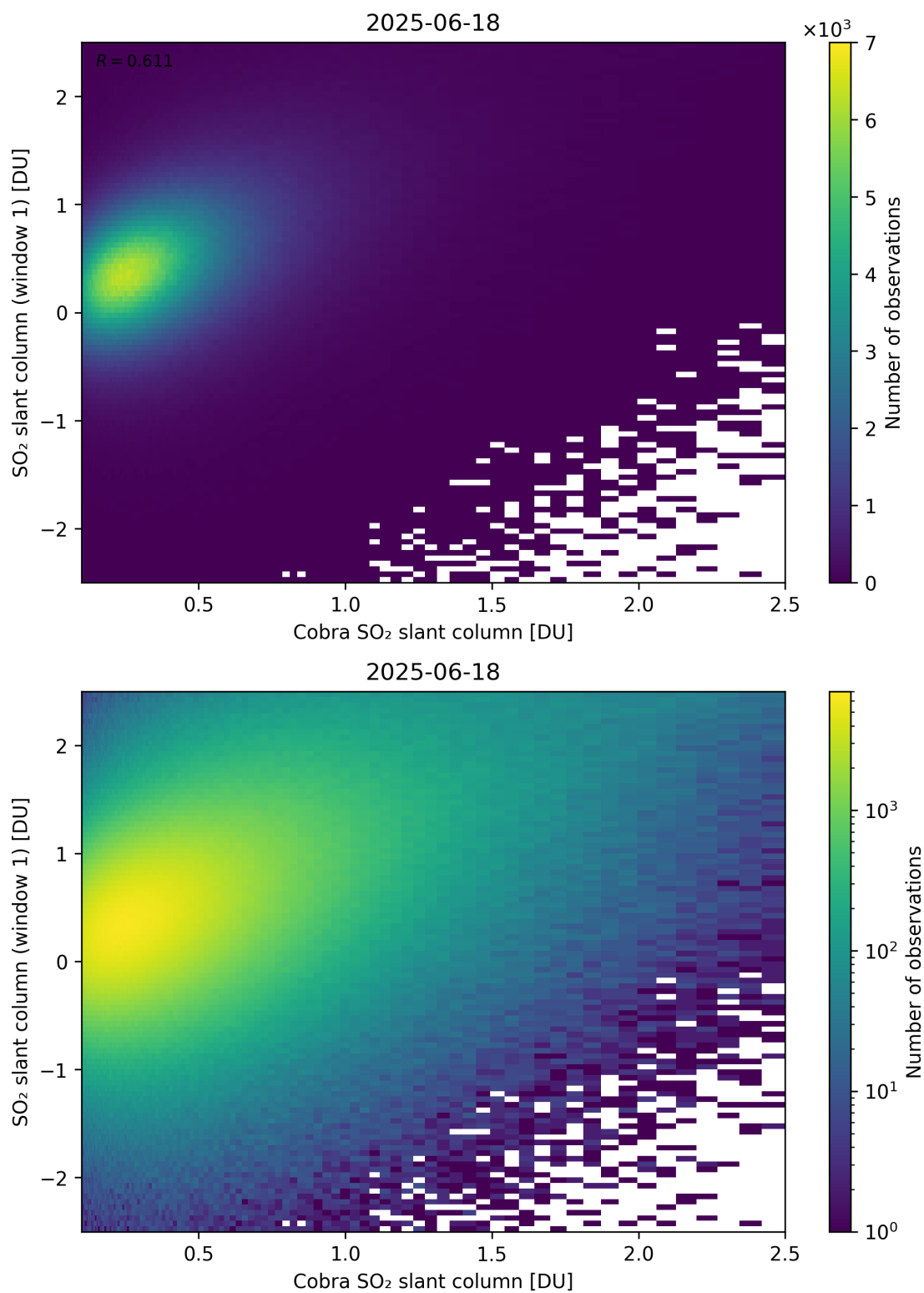
Figure 219: Scatter density plot of “Cobra SO 2 slant column” against “SO 2 slant column (window 1)” for 2025-06-17 to 2025-06-19.
