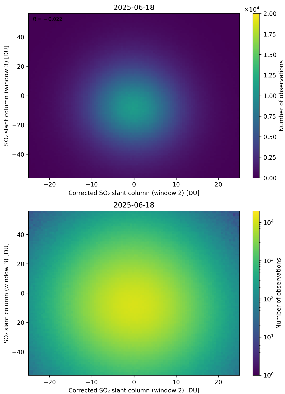
Figure 251: Scatter density plot of “Corrected SO 2 slant column (window 2)” against “SO 2 slant column (window 3)” for 2025-06-17 to 2025-06-19.
