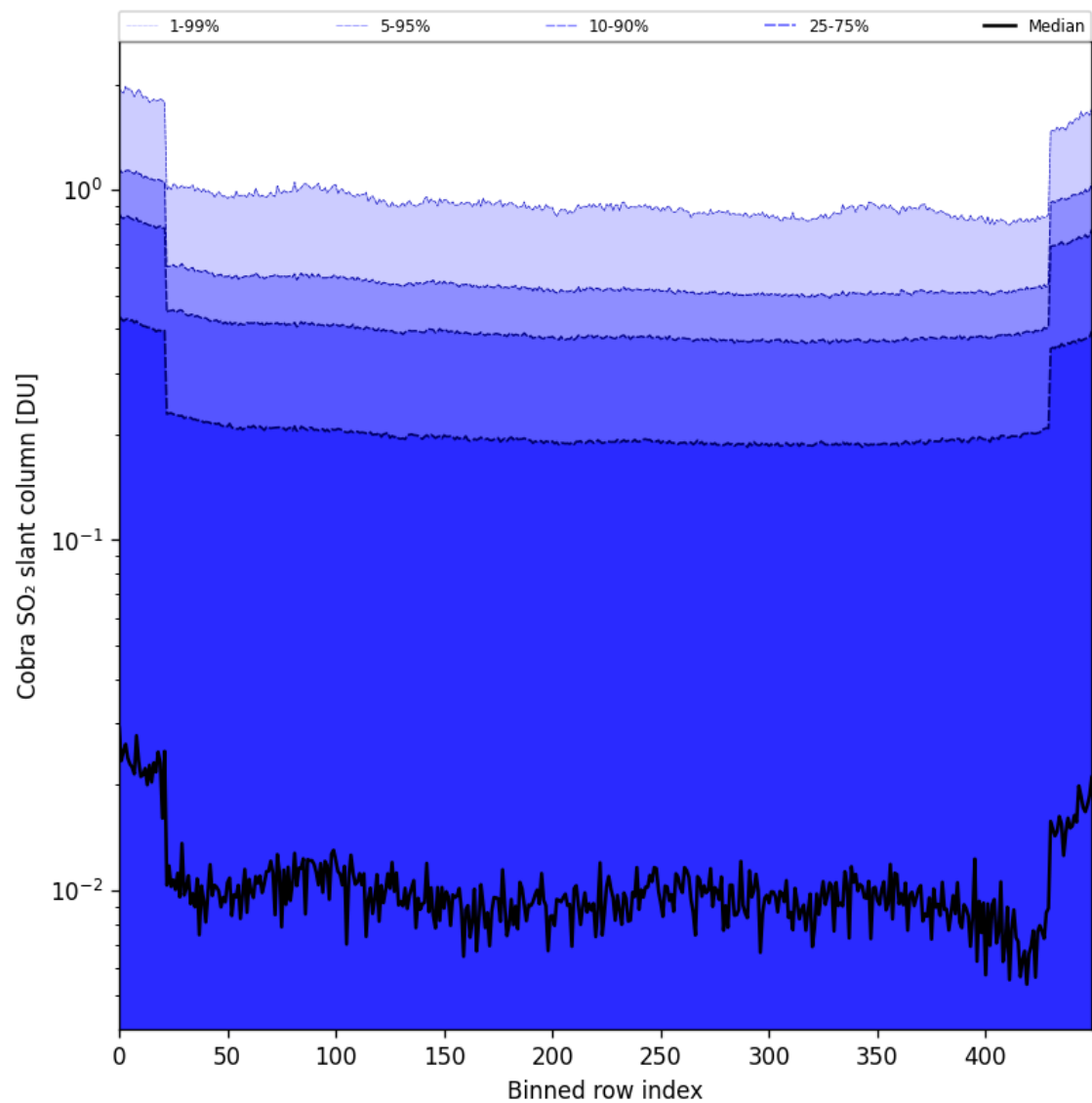
Figure 87: Along track statistics of “Cobra SO 2 slant column” for 2025-06-17 to 2025-06-19
