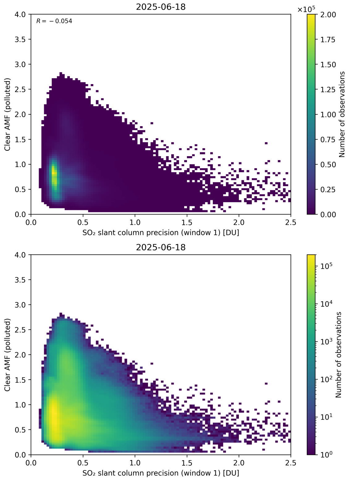
Figure 274: Scatter density plot of “SO 2 slant column precision (window 1)” against “Clear AMF (polluted)” for 2025-06-17 to 2025-06-19.
