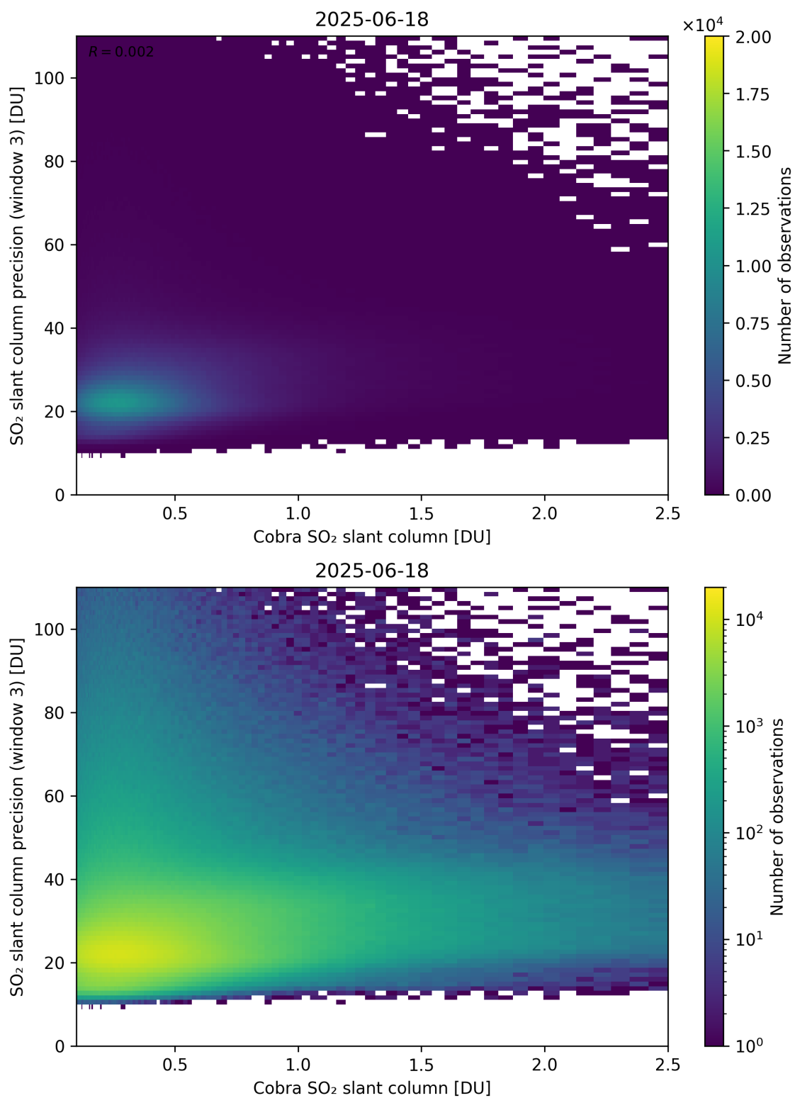
Figure 223: Scatter density plot of “Cobra SO 2 slant column” against “SO 2 slant column precision (window 3)” for 2025-06-17 to 2025-06-19.
