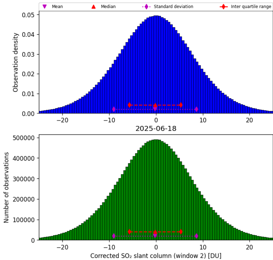
Figure 69: Histogram of “Corrected SO 2 slant column (window 2)” for 2025-06-17 to 2025-06-19
