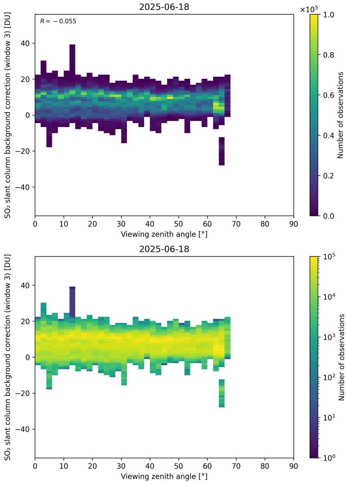
Figure 364: Scatter density plot of “Viewing zenith angle” against “SO 2 slant column background correction (window 3)” for 2025-06-17 to 2025-06-19.
