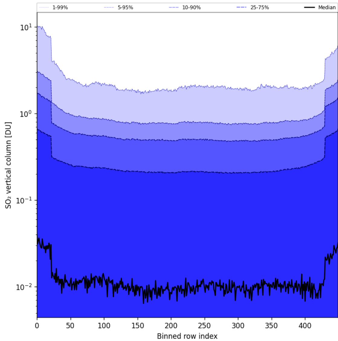
Figure 84: Along track statistics of “SO 2 vertical column” for 2025-06-17 to 2025-06-19
