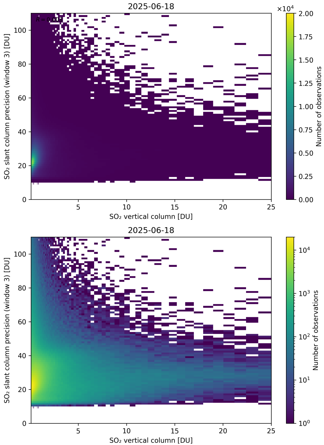
Figure 358: Scatter density plot of “SO 2 vertical column” against “SO 2 slant column precision (window 3)” for 2025-06-17 to 2025-06-19.
