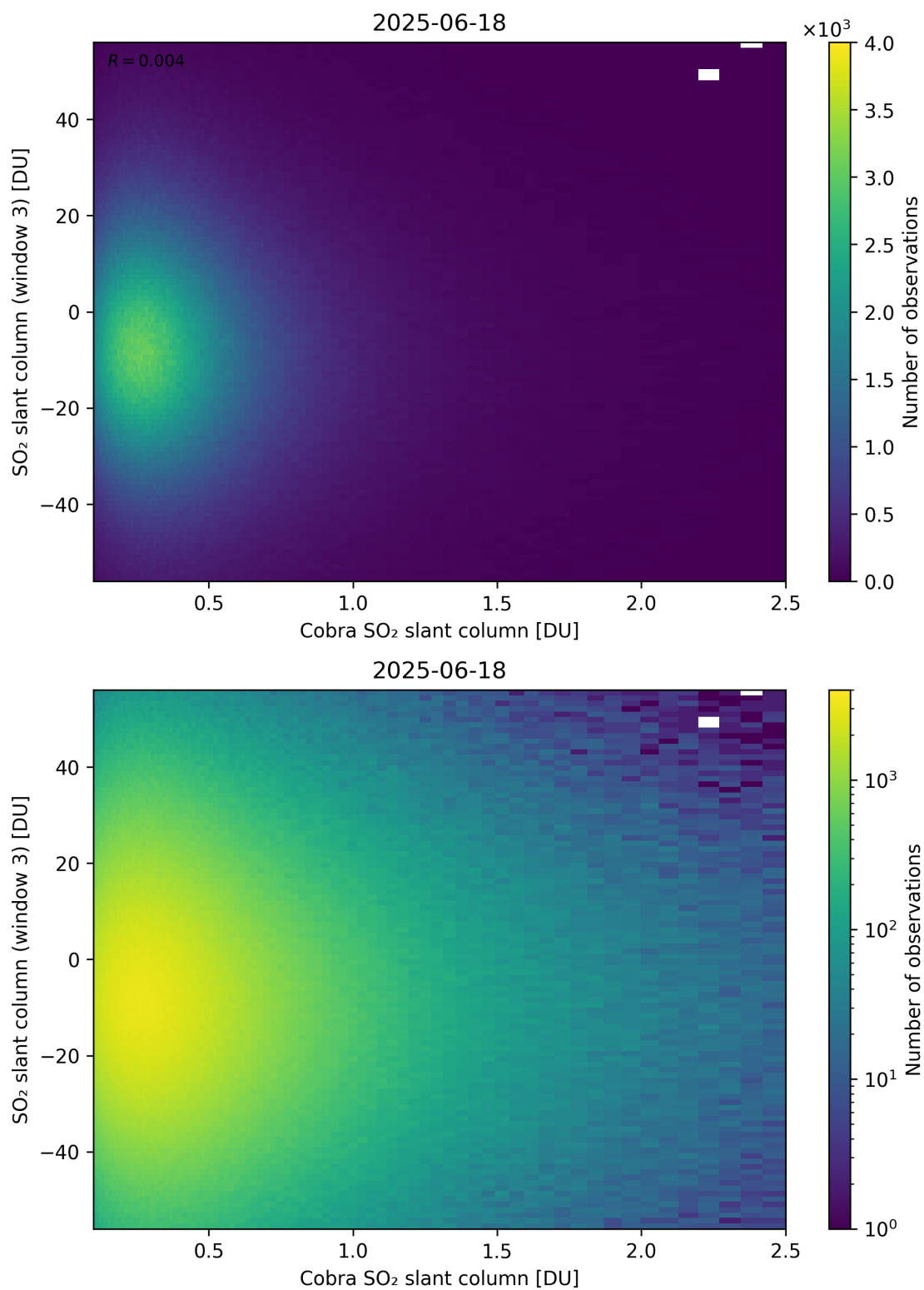
Figure 222: Scatter density plot of “Cobra SO 2 slant column” against “SO 2 slant column (window 3)” for 2025-06-17 to 2025-06-19.
