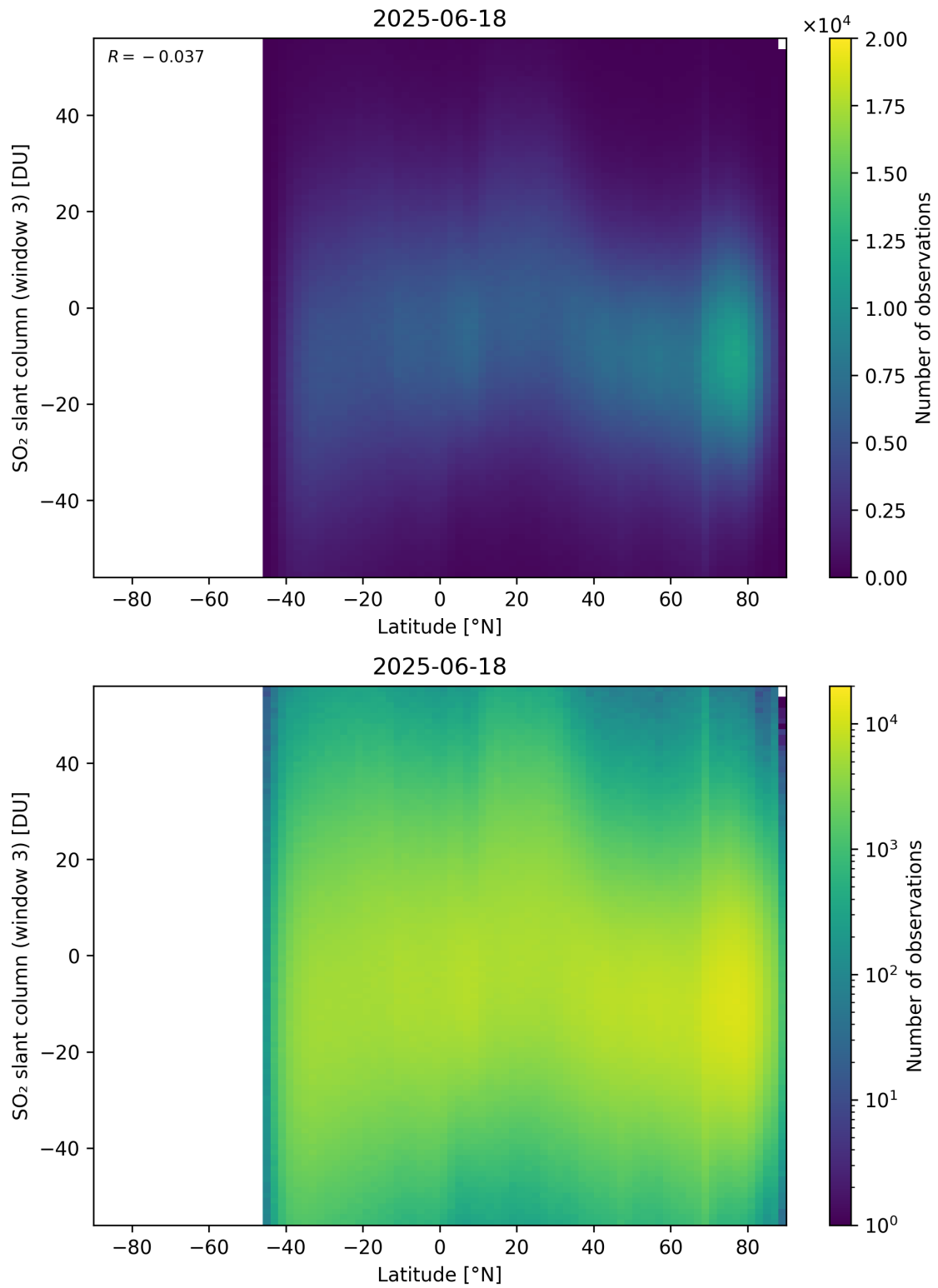
Figure 165: Scatter density plot of “Latitude” against “SO 2 slant column (window 3)” for 2025-06-17 to 2025-06-19.
