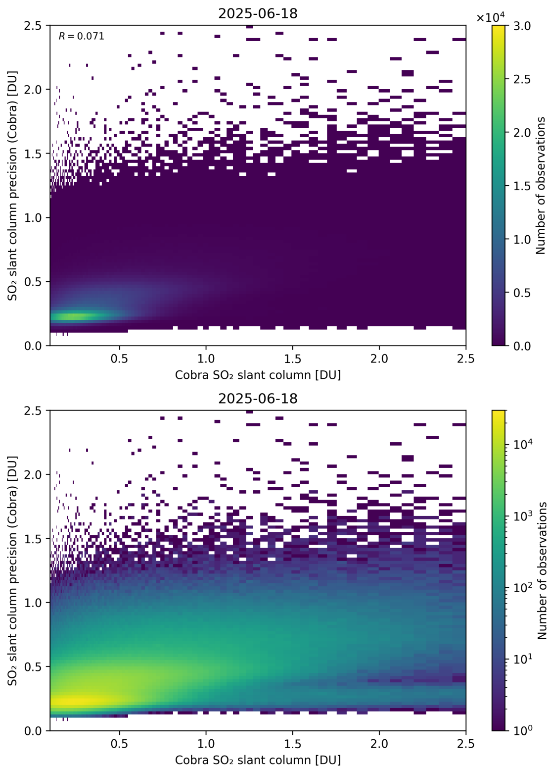
Figure 216: Scatter density plot of “Cobra SO 2 slant column” against “SO 2 slant column precision (Cobra)” for 2025-06-17 to 2025-06-19.
