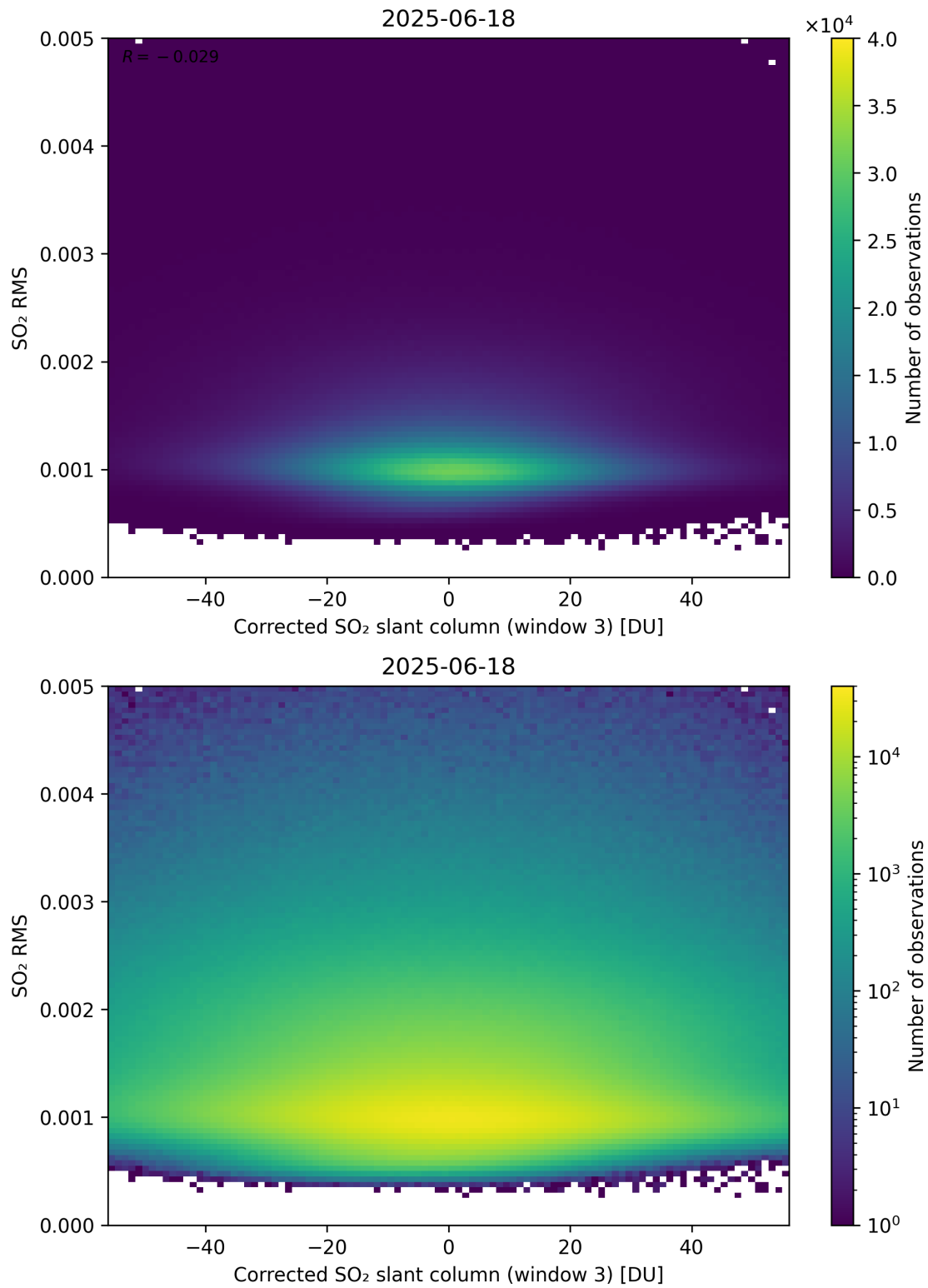
Figure 258: Scatter density plot of “Corrected SO 2 slant column (window 3)” against “SO 2 RMS” for 2025-06-17 to 2025-06-19.
