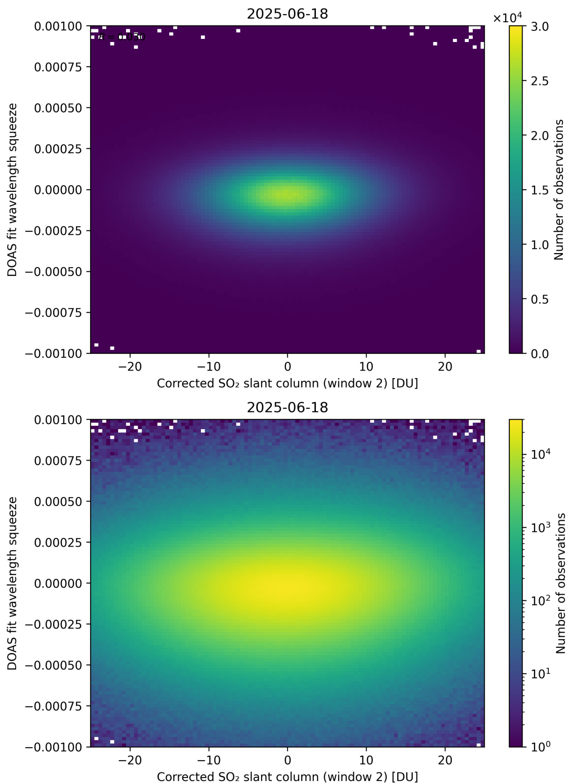
Figure 247: Scatter density plot of “Corrected SO 2 slant column (window 2)” against “DOAS fit wavelength squeeze” for 2025-06-17 to 2025-06-19.
