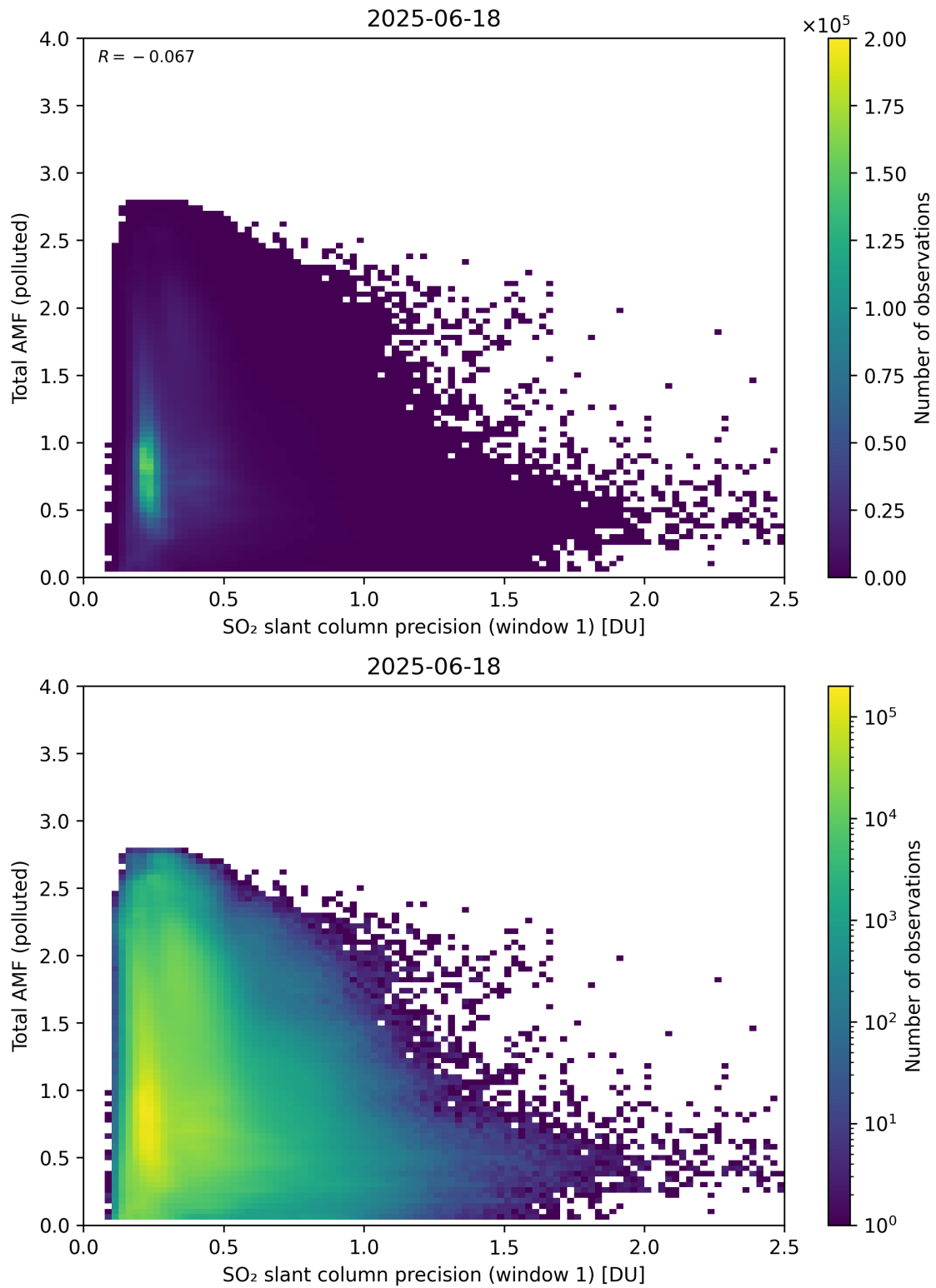
Figure 280: Scatter density plot of “SO 2 slant column precision (window 1)” against “Total AMF (polluted)” for 2025-06-17 to 2025-06-19.
