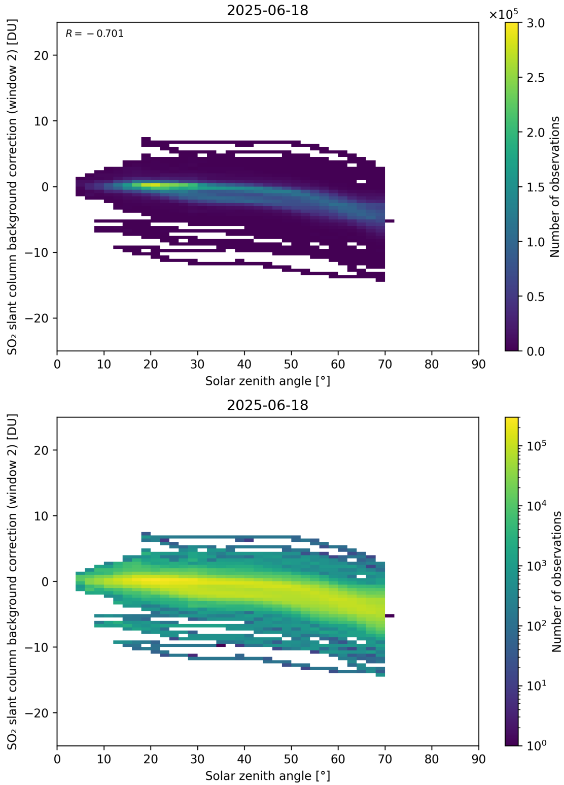
Figure 172: Scatter density plot of “Solar zenith angle” against “SO 2 slant column background correction (window 2)” for 2025-06-17 to 2025-06-19.
