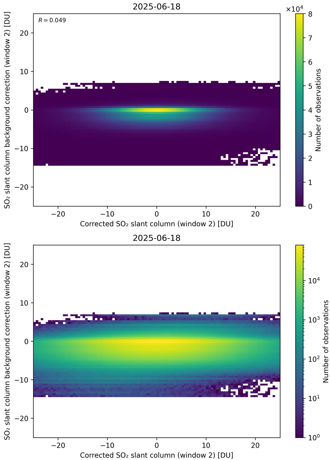
Figure 244: Scatter density plot of “Corrected SO 2 slant column (window 2)” against “SO 2 slant column background correction (window 2)” for 2025-06-17 to 2025-06-19.
