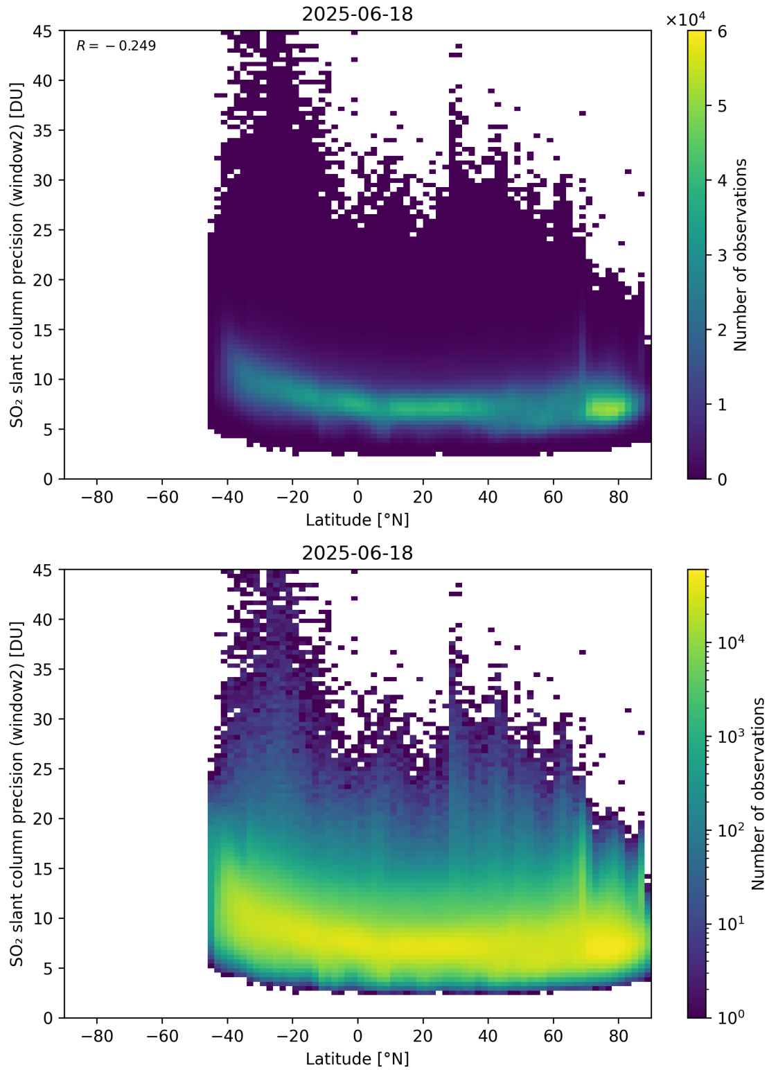
Figure 164: Scatter density plot of “Latitude” against “SO 2 slant column precision (window2)” for 2025-06-17 to 2025-06-19.
