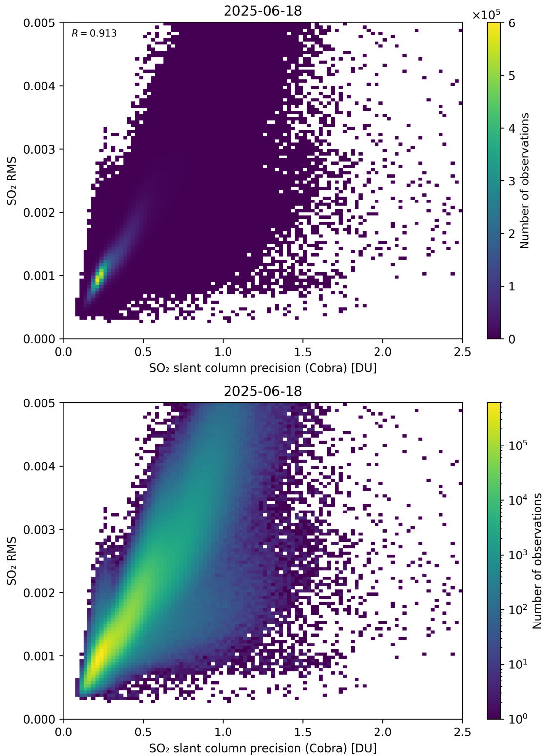
Figure 204: Scatter density plot of “SO 2 slant column precision (Cobra)” against “SO 2 RMS” for 2025-06-17 to 2025-06-19.
