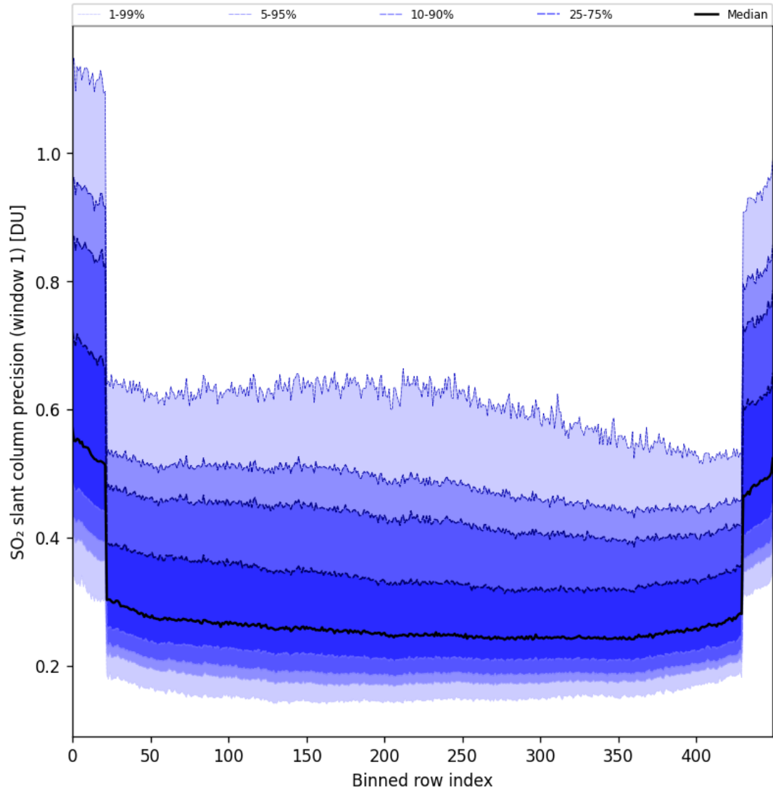
Figure 90: Along track statistics of “SO 2 slant column precision (window 1)” for 2025-06-17 to 2025-06-19
