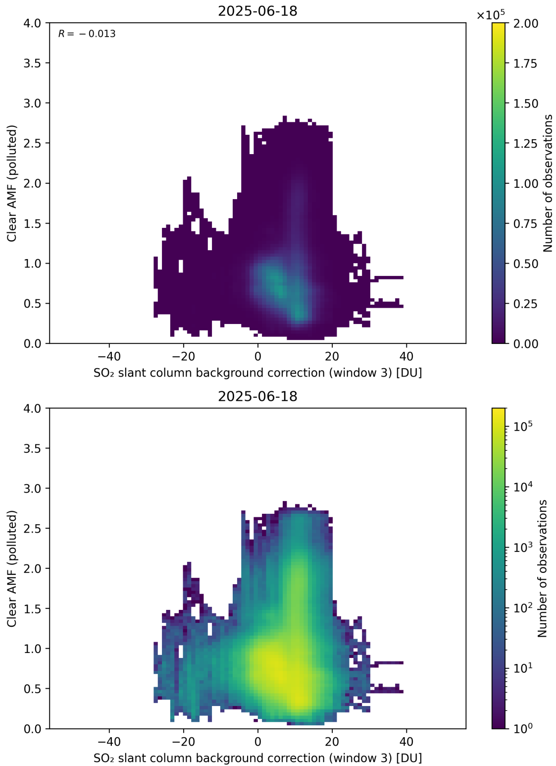
Figure 135: Scatter density plot of “SO 2 slant column background correction (window 3)” against “Clear AMF (polluted)” for 2025-06-17 to 2025-06-19.
