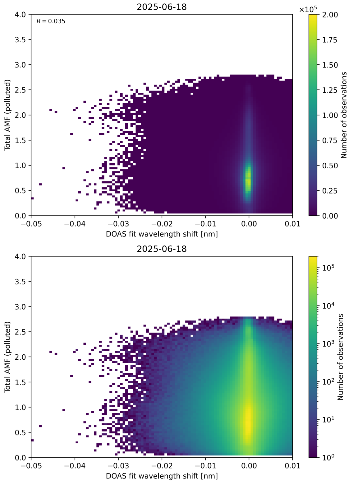
Figure 141: Scatter density plot of “DOAS fit wavelength shift” against “Total AMF (polluted)” for 2025-06-17 to 2025-06-19.
