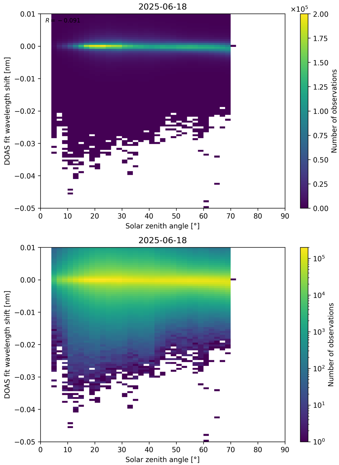
Figure 174: Scatter density plot of “Solar zenith angle” against “DOAS fit wavelength shift” for 2025-06-17 to 2025-06-19.
