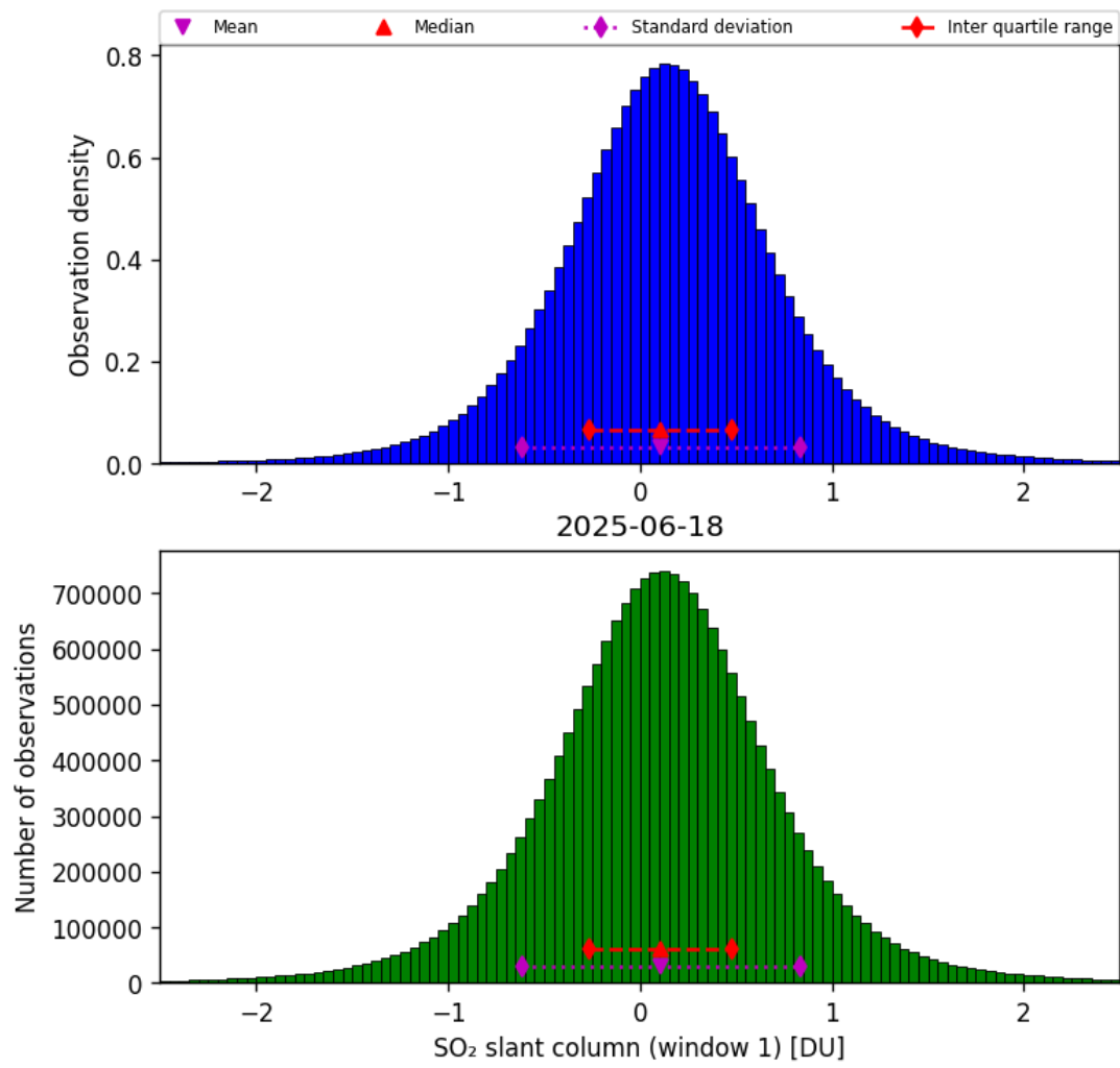
Figure 63: Histogram of “SO 2 slant column (window 1)” for 2025-06-17 to 2025-06-19
