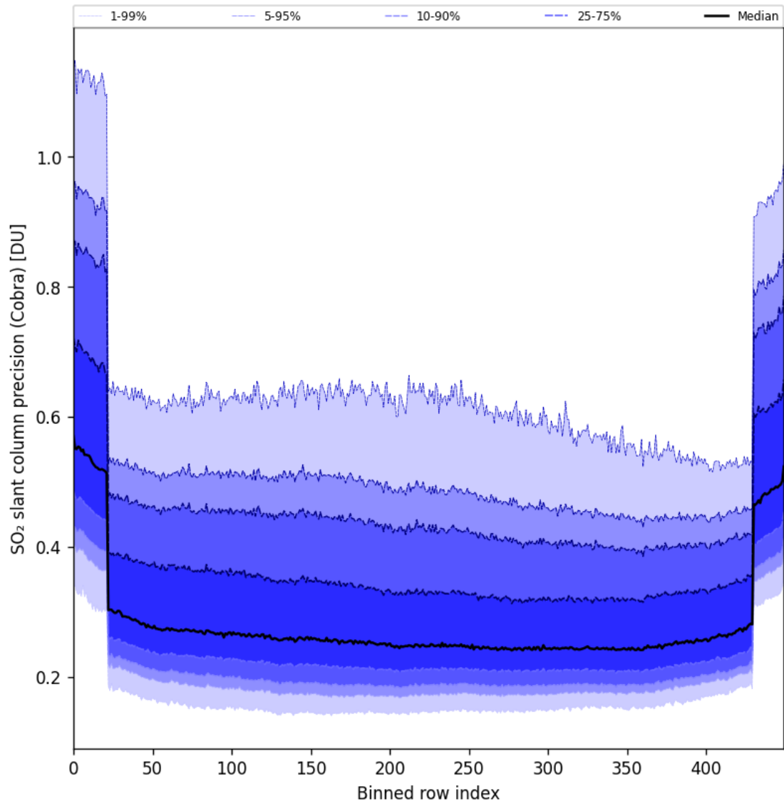
Figure 88: Along track statistics of “SO 2 slant column precision (Cobra)” for 2025-06-17 to 2025-06-19
