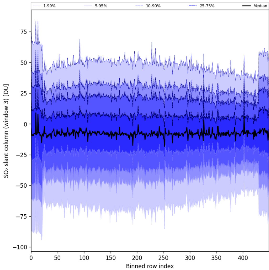
Figure 97: Along track statistics of “SO 2 slant column (window 3)” for 2025-06-17 to 2025-06-19
