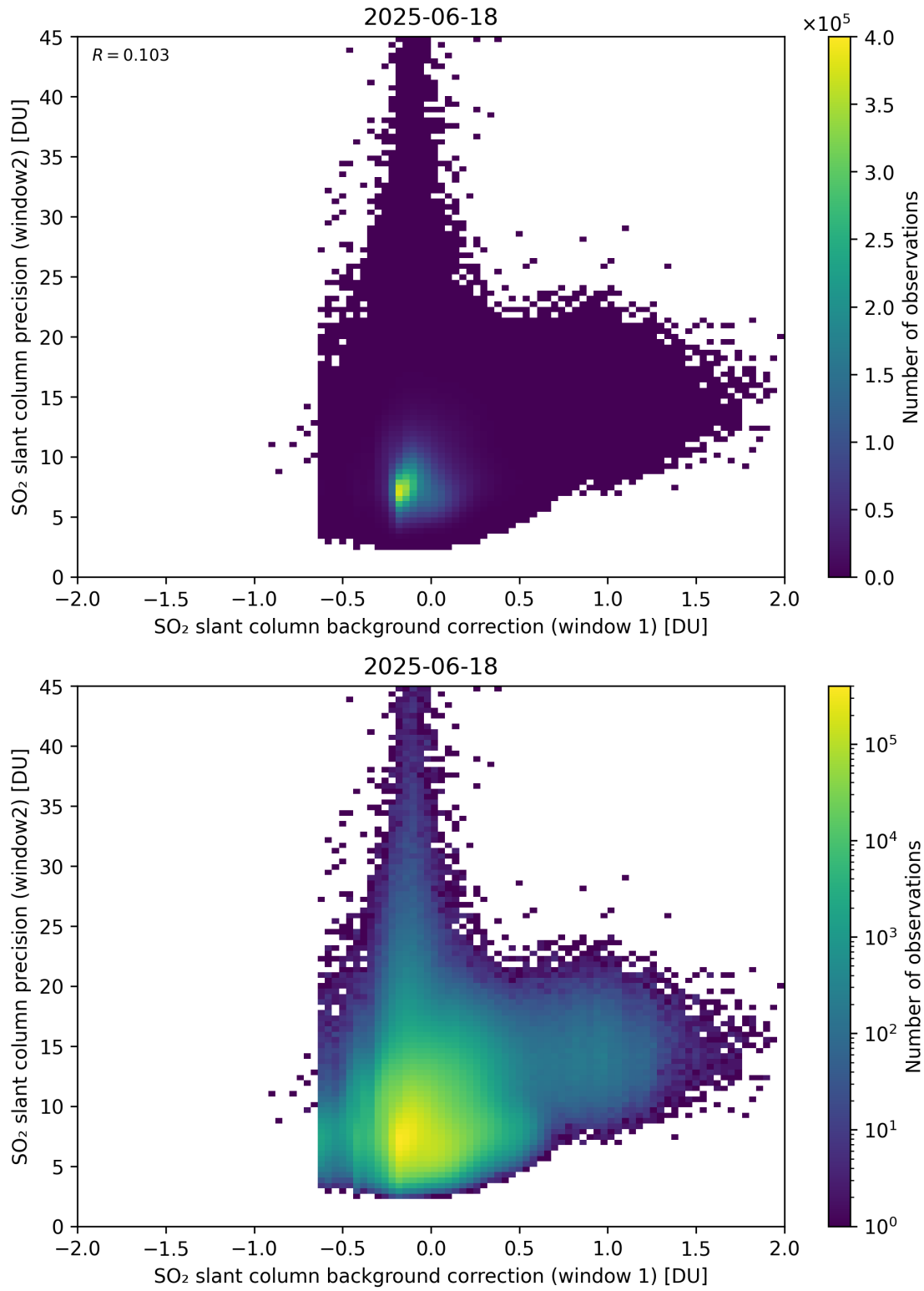
Figure 117: Scatter density plot of “SO 2 slant column background correction (window 1)” against “SO 2 slant column precision (window2)” for 2025-06-17 to 2025-06-19.
