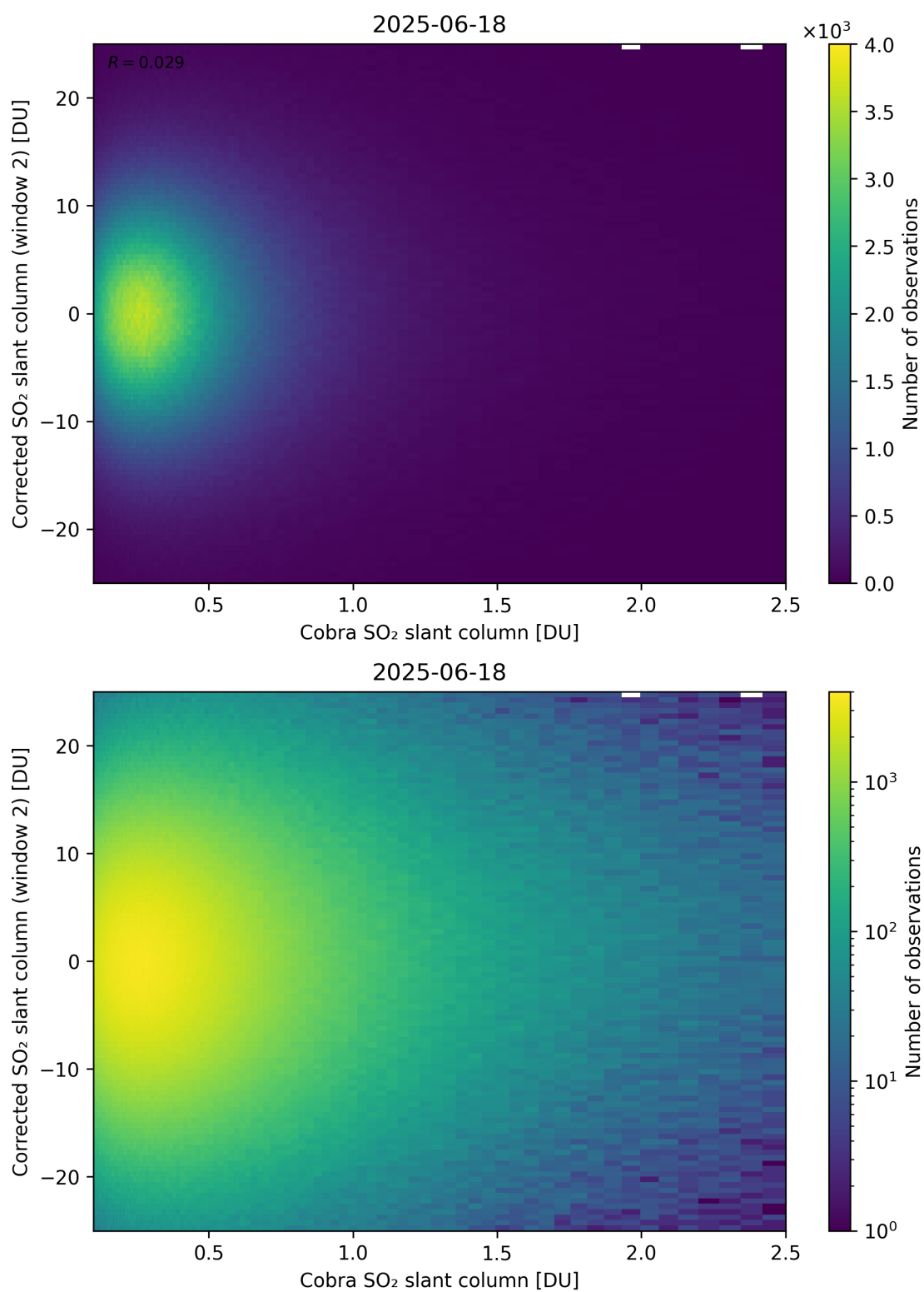
Figure 217: Scatter density plot of “Cobra SO 2 slant column” against “Corrected SO 2 slant column (window 2)” for 2025-06-17 to 2025-06-19.
