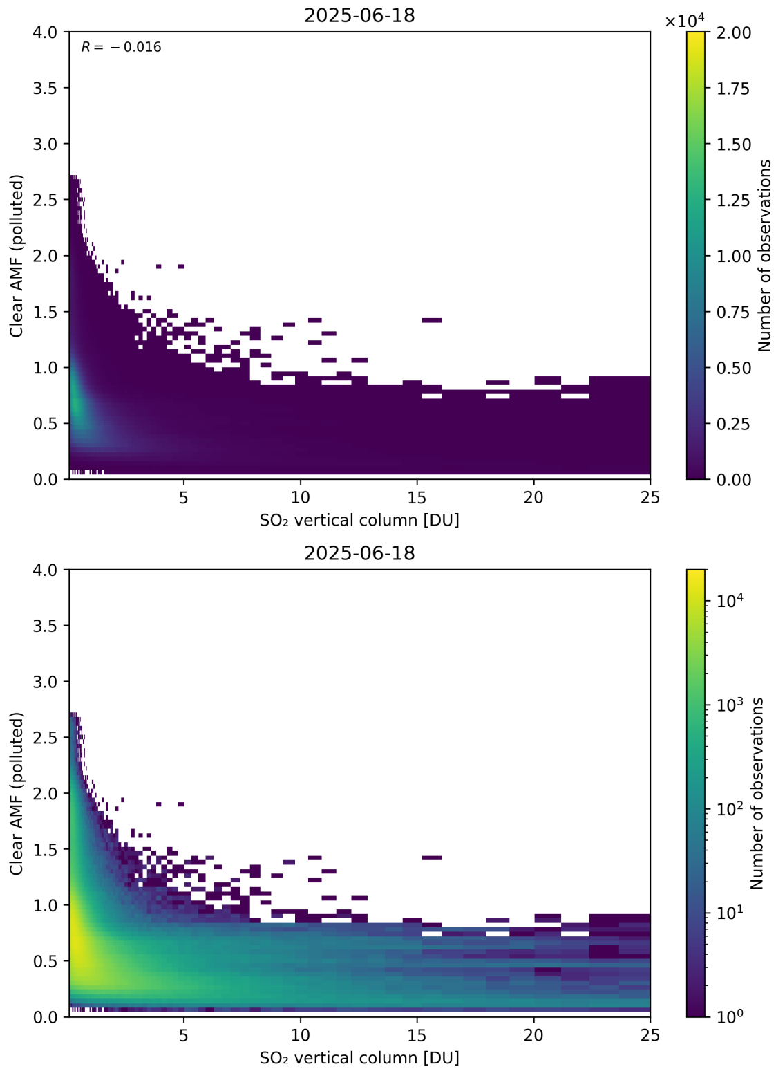
Figure 348: Scatter density plot of “SO 2 vertical column” against “Clear AMF (polluted)” for 2025-06-17 to 2025-06-19.
