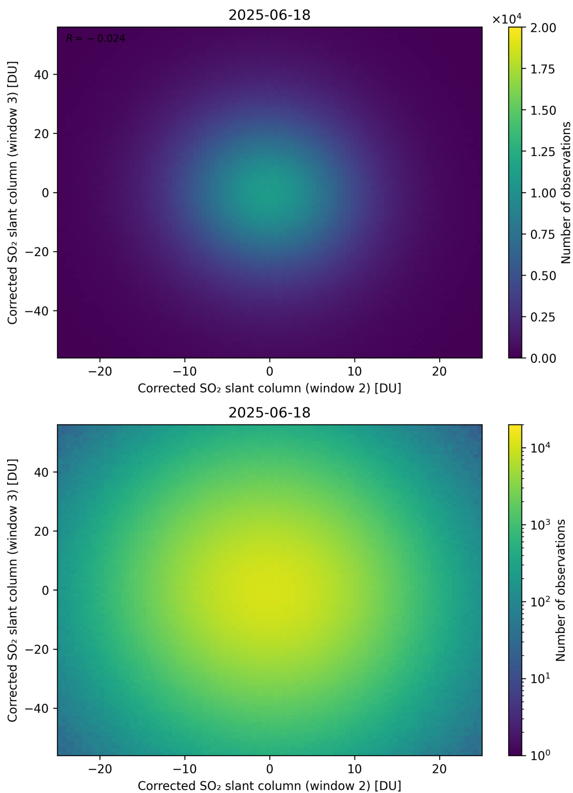
Figure 250: Scatter density plot of “Corrected SO 2 slant column (window 2)” against “Corrected SO 2 slant column (window 3)” for 2025-06-17 to 2025-06-19.
