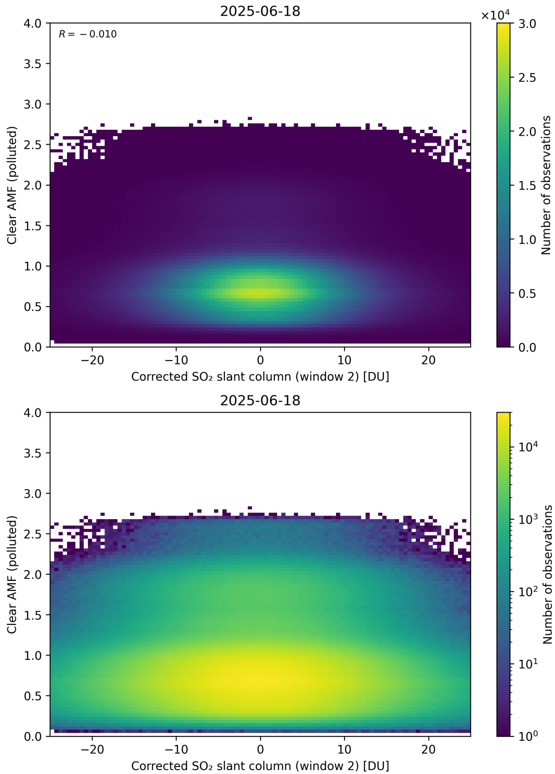
Figure 249: Scatter density plot of “Corrected SO 2 slant column (window 2)” against “Clear AMF (polluted)” for 2025-06-17 to 2025-06-19.
