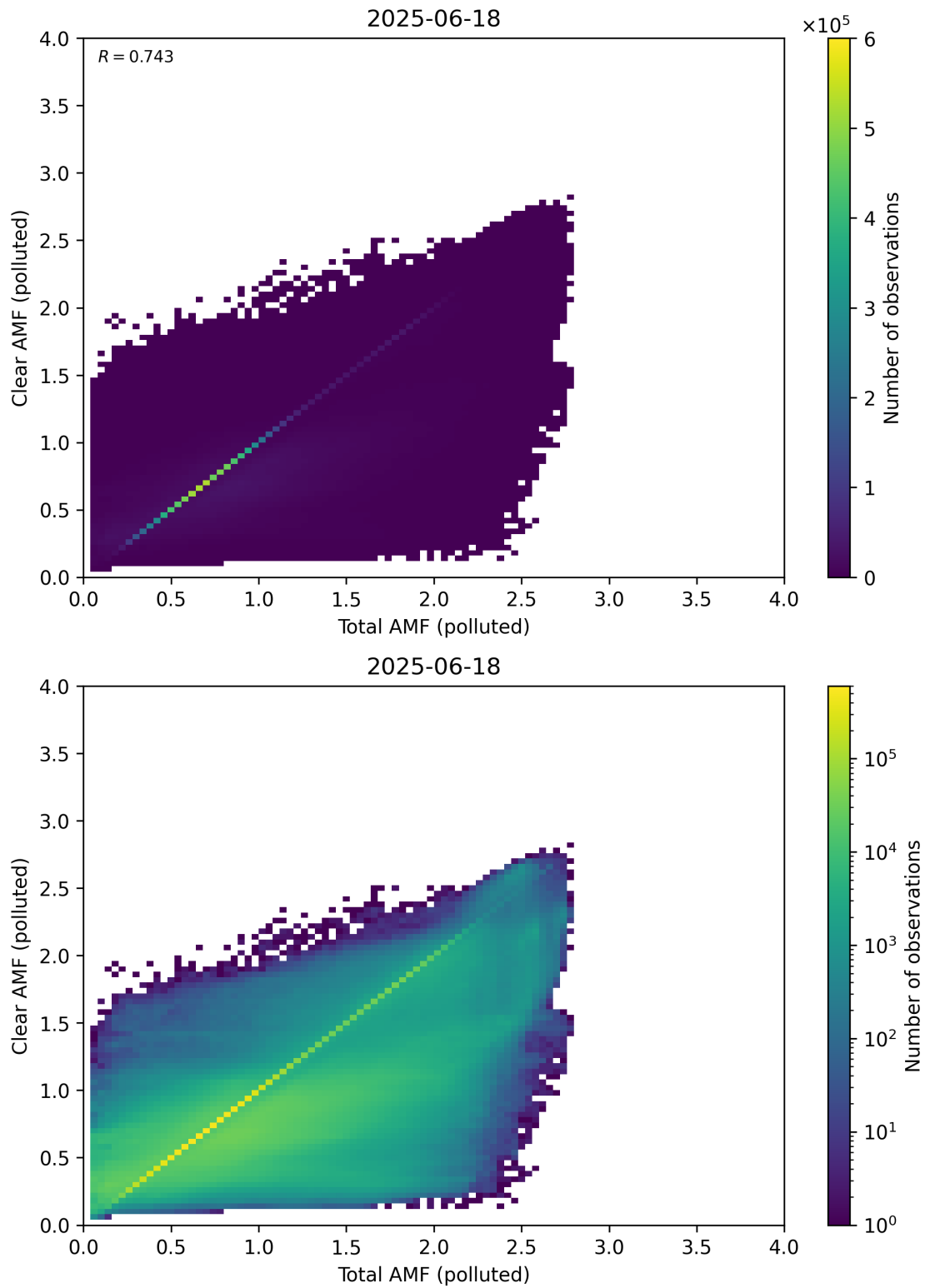
Figure 321: Scatter density plot of “Total AMF (polluted)” against “Clear AMF (polluted)” for 2025-06-17 to 2025-06-19.
