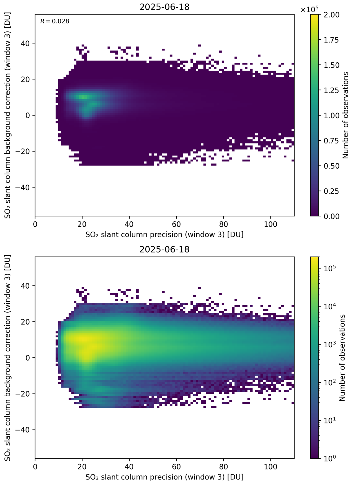
Figure 307: Scatter density plot of “SO 2 slant column precision (window 3)” against “SO 2 slant column background correction (window 3)” for 2025-06-17 to 2025-06-19.
