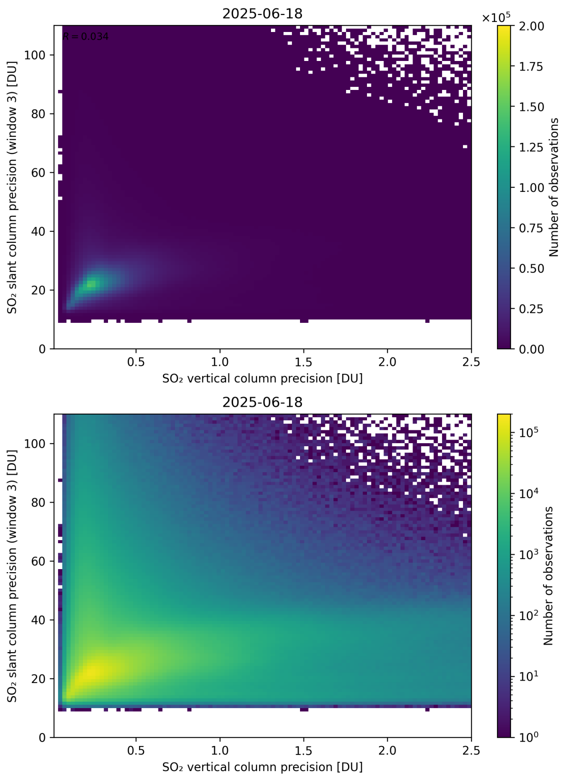
Figure 345: Scatter density plot of “SO 2 vertical column precision” against “SO 2 slant column precision (window 3)” for 2025-06-17 to 2025-06-19.
