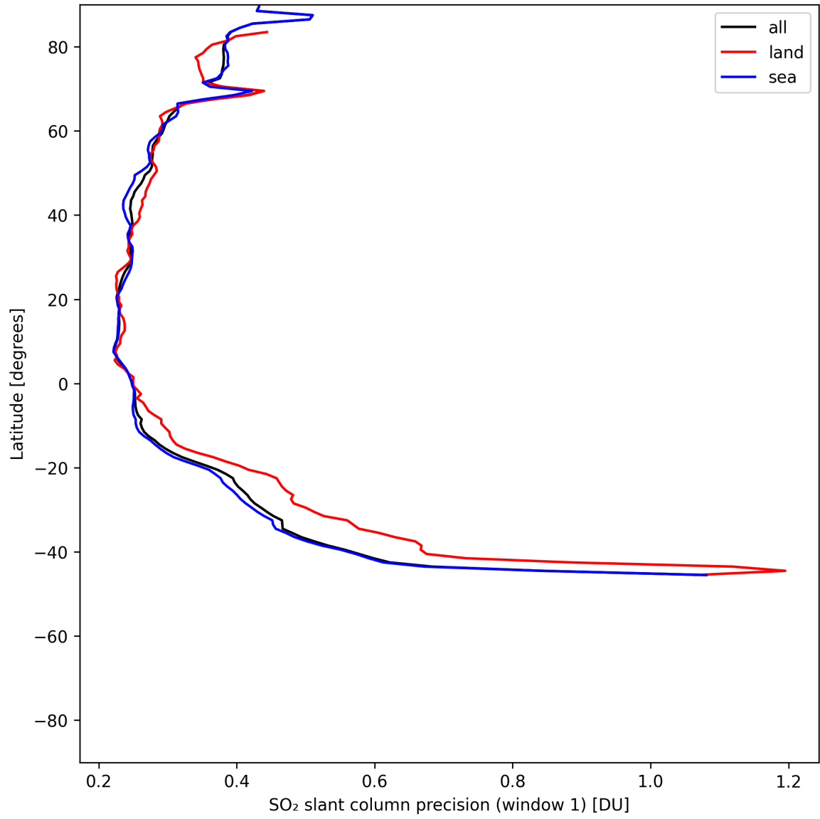
Figure 38: Zonal average of “SO 2 slant column precision (window 1)” for 2025-06-17 to 2025-06-19.
