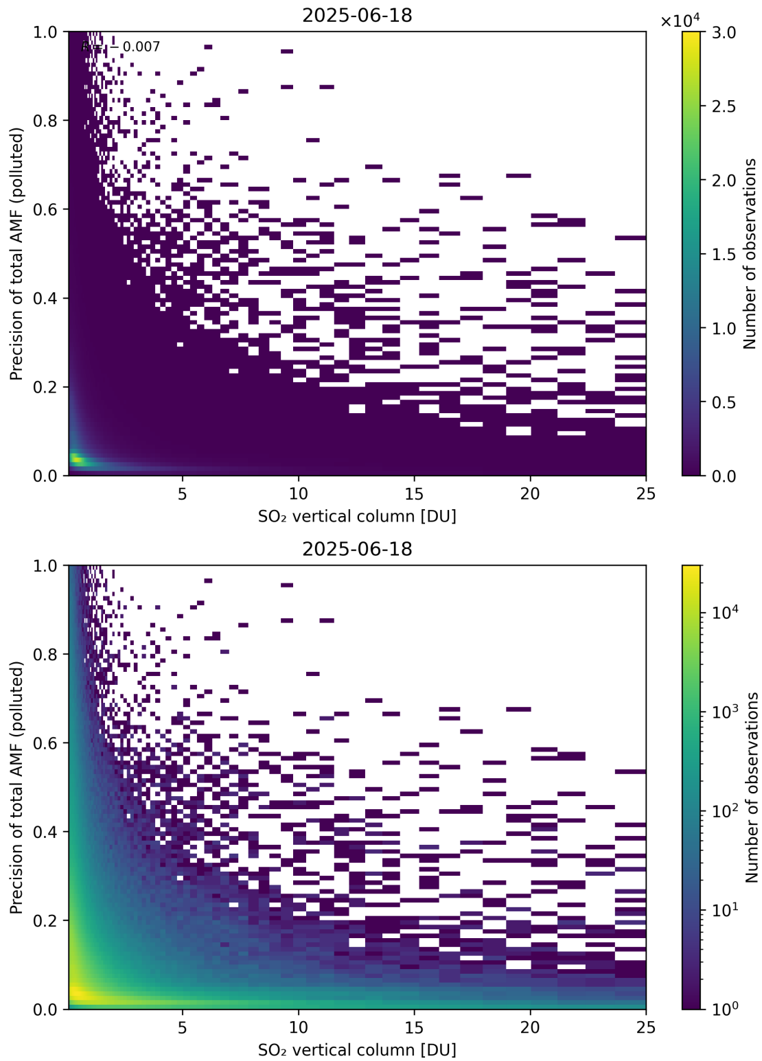
Figure 360: Scatter density plot of “SO 2 vertical column” against “Precision of total AMF (polluted)” for 2025-06-17 to 2025-06-19.
