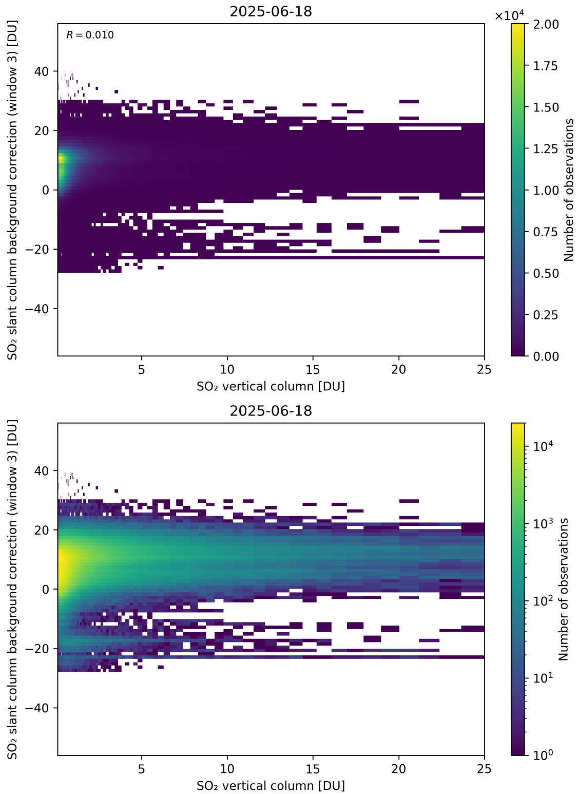
Figure 325: Scatter density plot of “SO 2 vertical column” against “SO 2 slant column background correction (window 3)” for 2025-06-17 to 2025-06-19.
