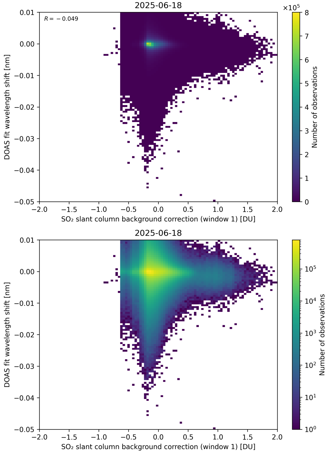
Figure 111: Scatter density plot of “SO 2 slant column background correction (window 1)” against “DOAS fit wavelength shift” for 2025-06-17 to 2025-06-19.
