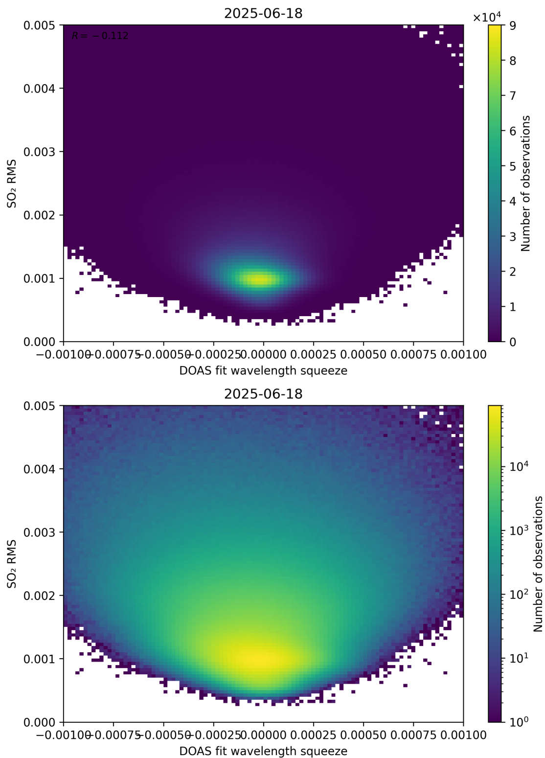
Figure 143: Scatter density plot of “DOAS fit wavelength squeeze” against “SO 2 RMS” for 2025-06-17 to 2025-06-19.
