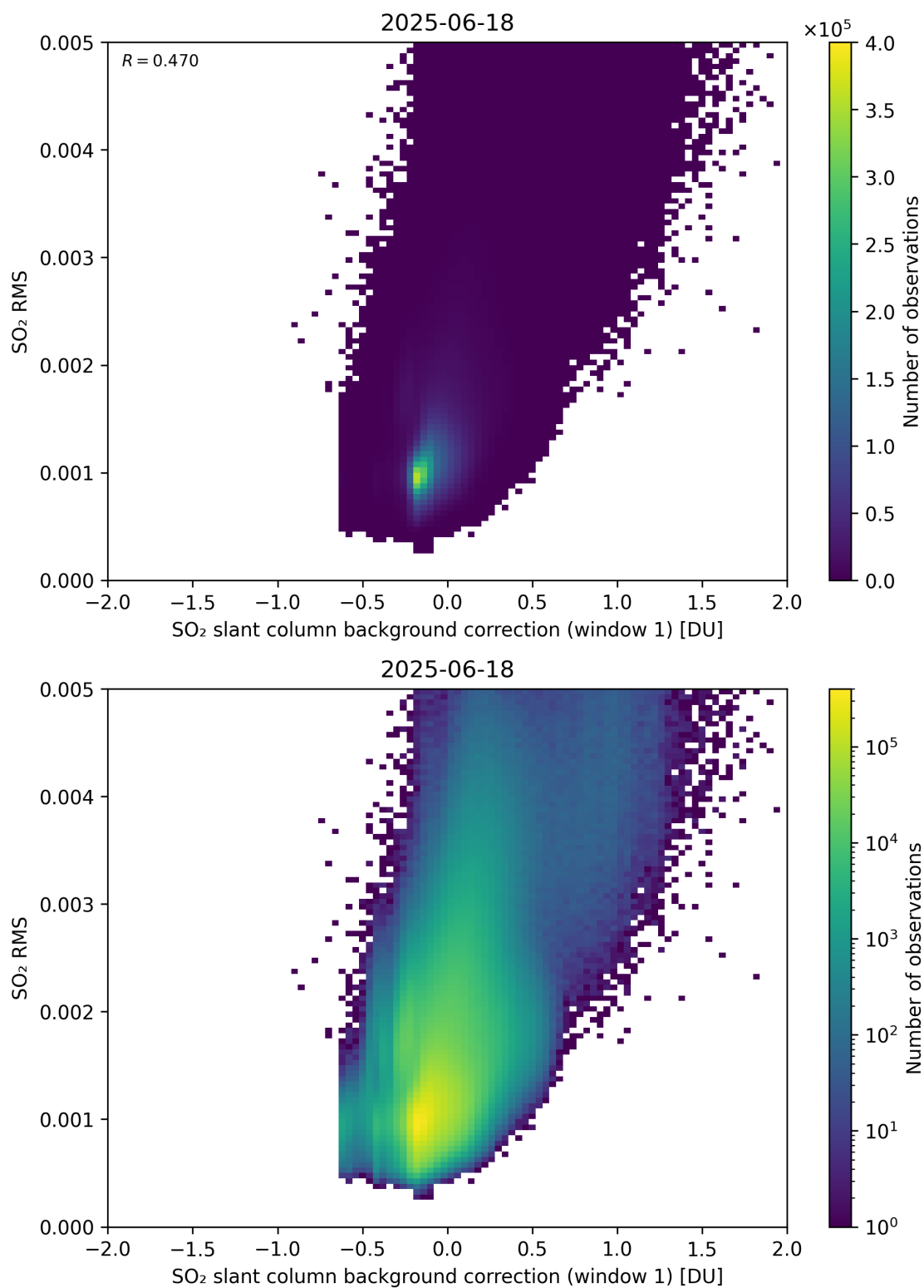
Figure 113: Scatter density plot of “SO 2 slant column background correction (window 1)” against “SO 2 RMS” for 2025-06-17 to 2025-06-19.
