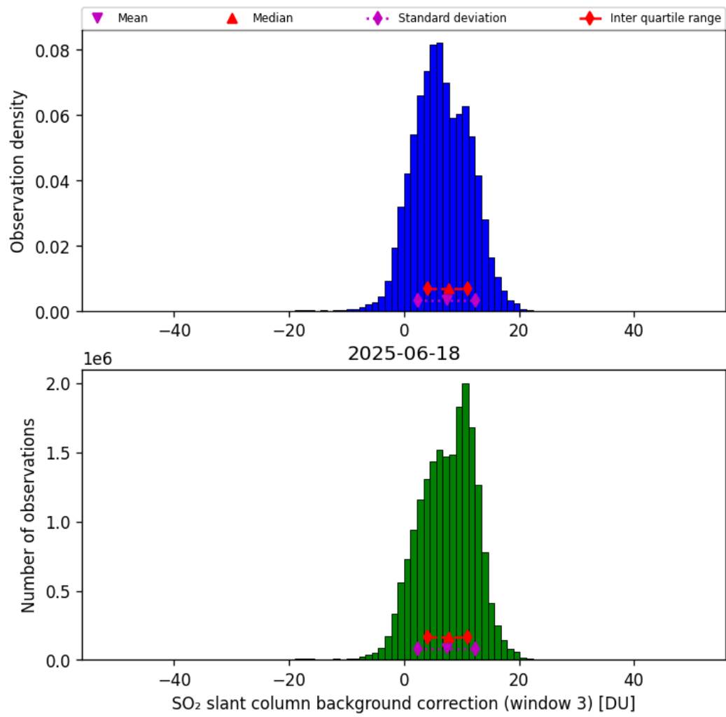
Figure 74: Histogram of “SO 2 slant column background correction (window 3)” for 2025-06-17 to 2025-06-19
