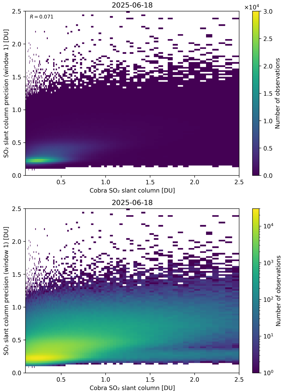
Figure 220: Scatter density plot of “Cobra SO 2 slant column” against “SO 2 slant column precision (window 1)” for 2025-06-17 to 2025-06-19.
