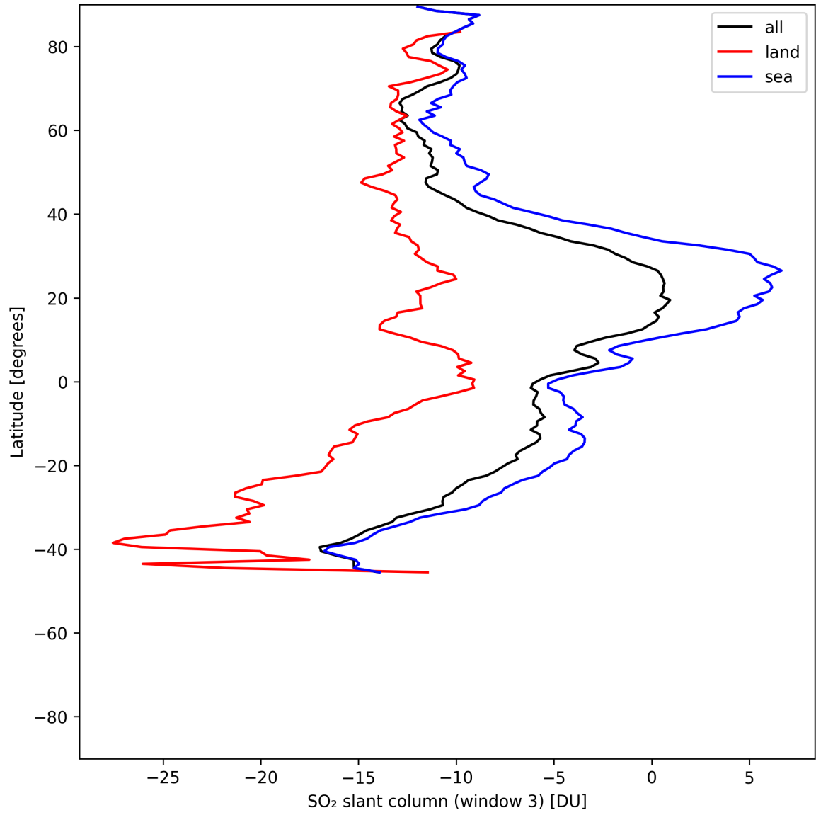
Figure 45: Zonal average of “SO 2 slant column (window 3)” for 2025-06-17 to 2025-06-19.
