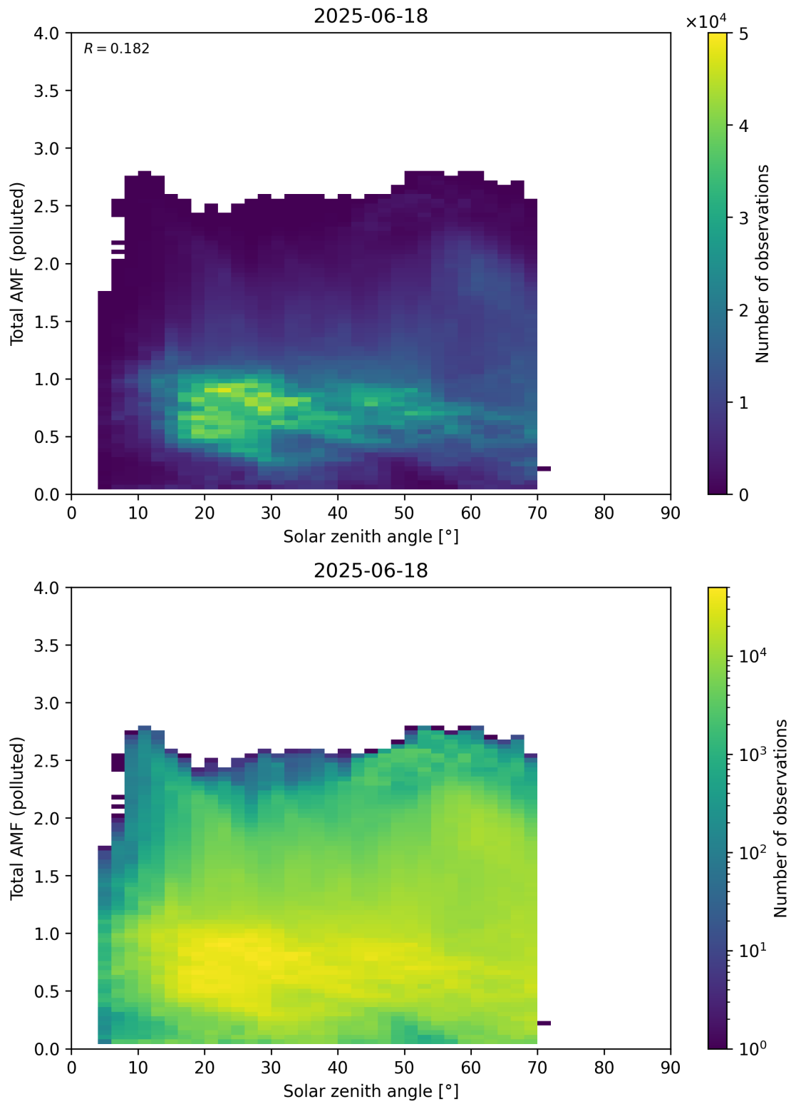
Figure 189: Scatter density plot of “Solar zenith angle” against “Total AMF (polluted)” for 2025-06-17 to 2025-06-19.
