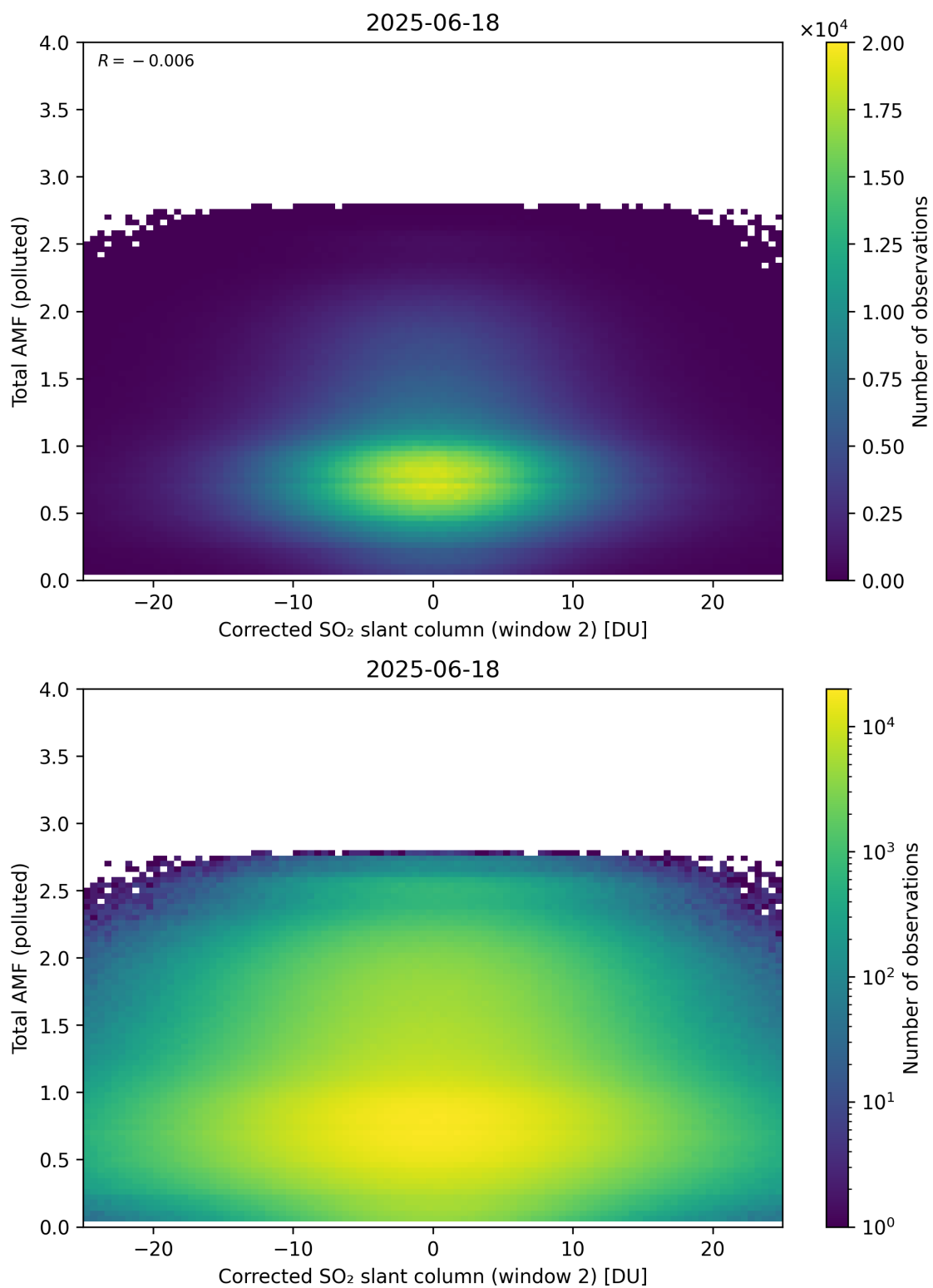
Figure 253: Scatter density plot of “Corrected SO 2 slant column (window 2)” against “Total AMF (polluted)” for 2025-06-17 to 2025-06-19.
