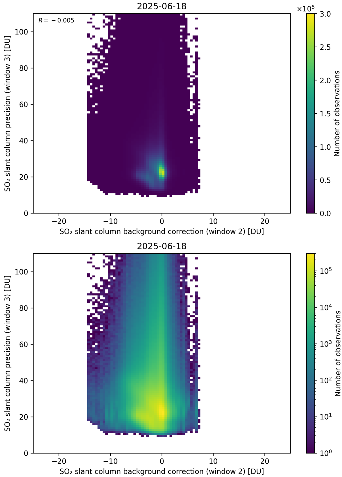
Figure 129: Scatter density plot of “SO 2 slant column background correction (window 2)” against “SO 2 slant column precision (window 3)” for 2025-06-17 to 2025-06-19.
