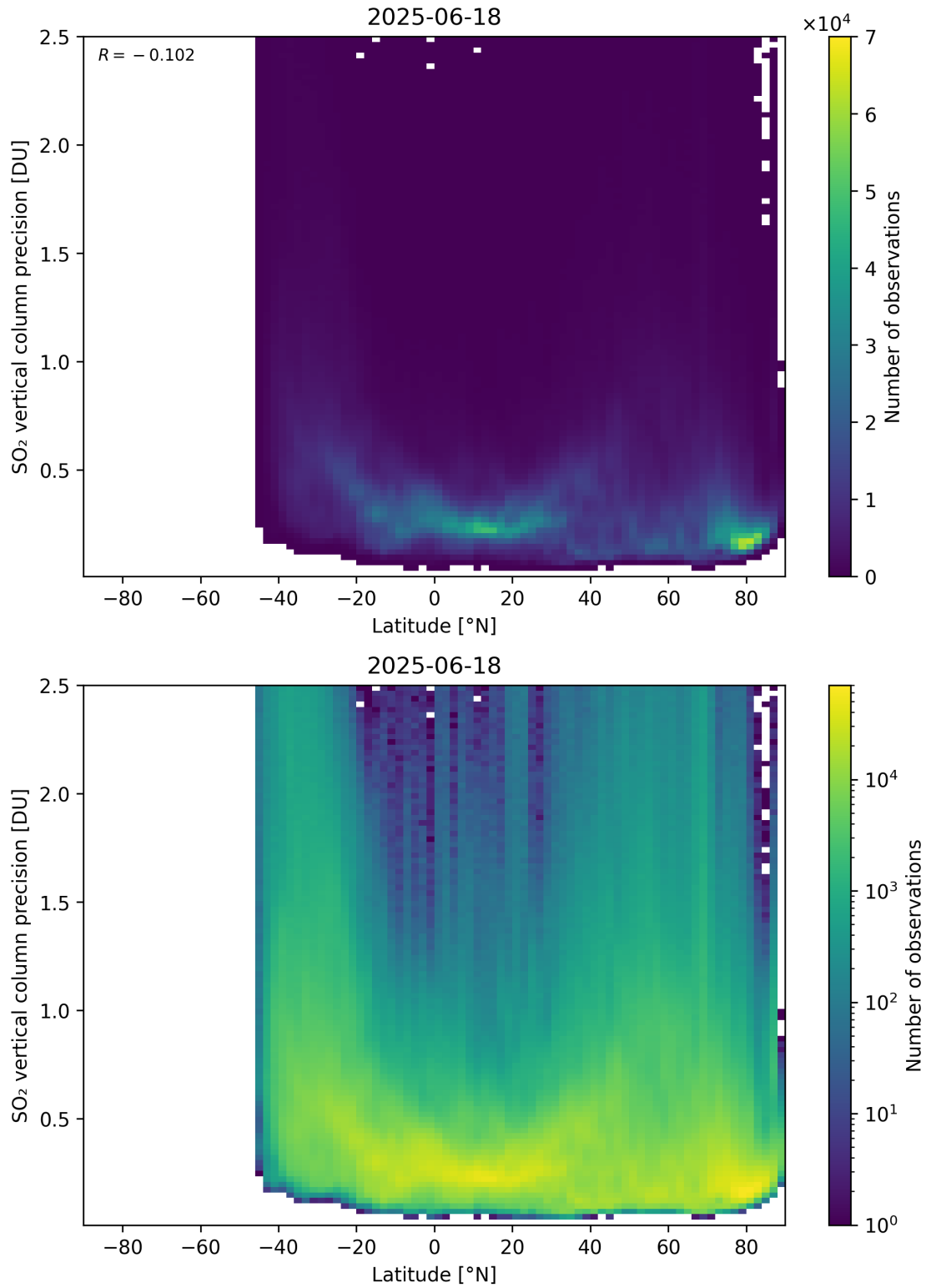
Figure 170: Scatter density plot of “Latitude” against “SO 2 vertical column precision” for 2025-06-17 to 2025-06-19.
