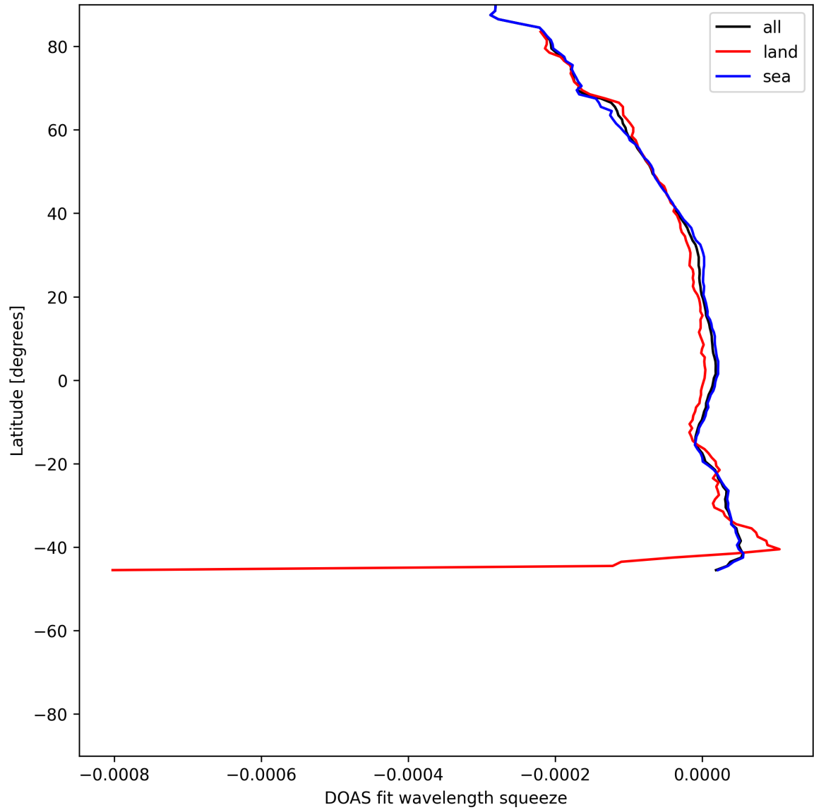
Figure 51: Zonal average of “DOAS fit wavelength squeeze” for 2025-06-17 to 2025-06-19.
