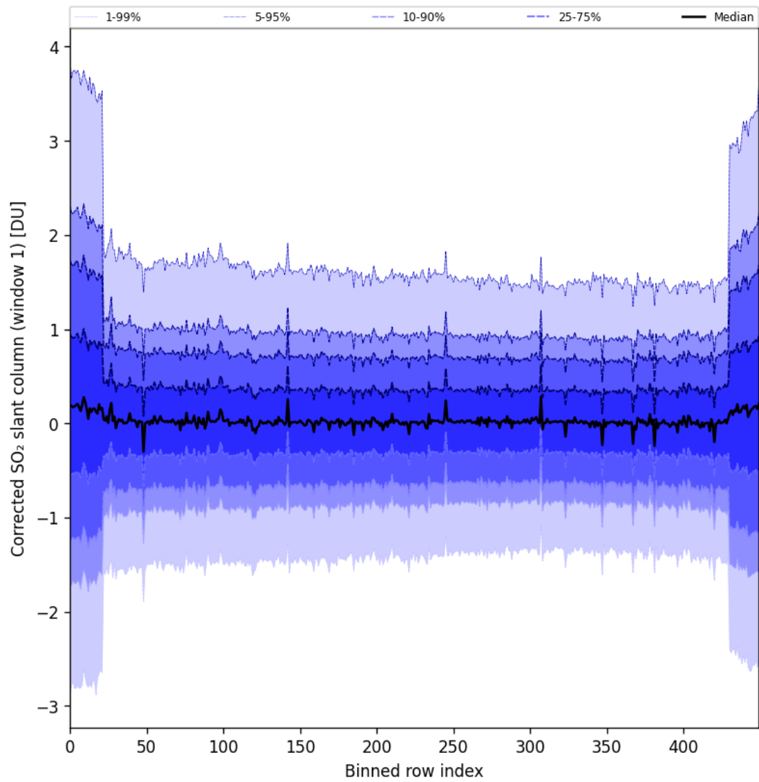
Figure 91: Along track statistics of “Corrected SO 2 slant column (window 1)” for 2025-06-17 to 2025-06-19
