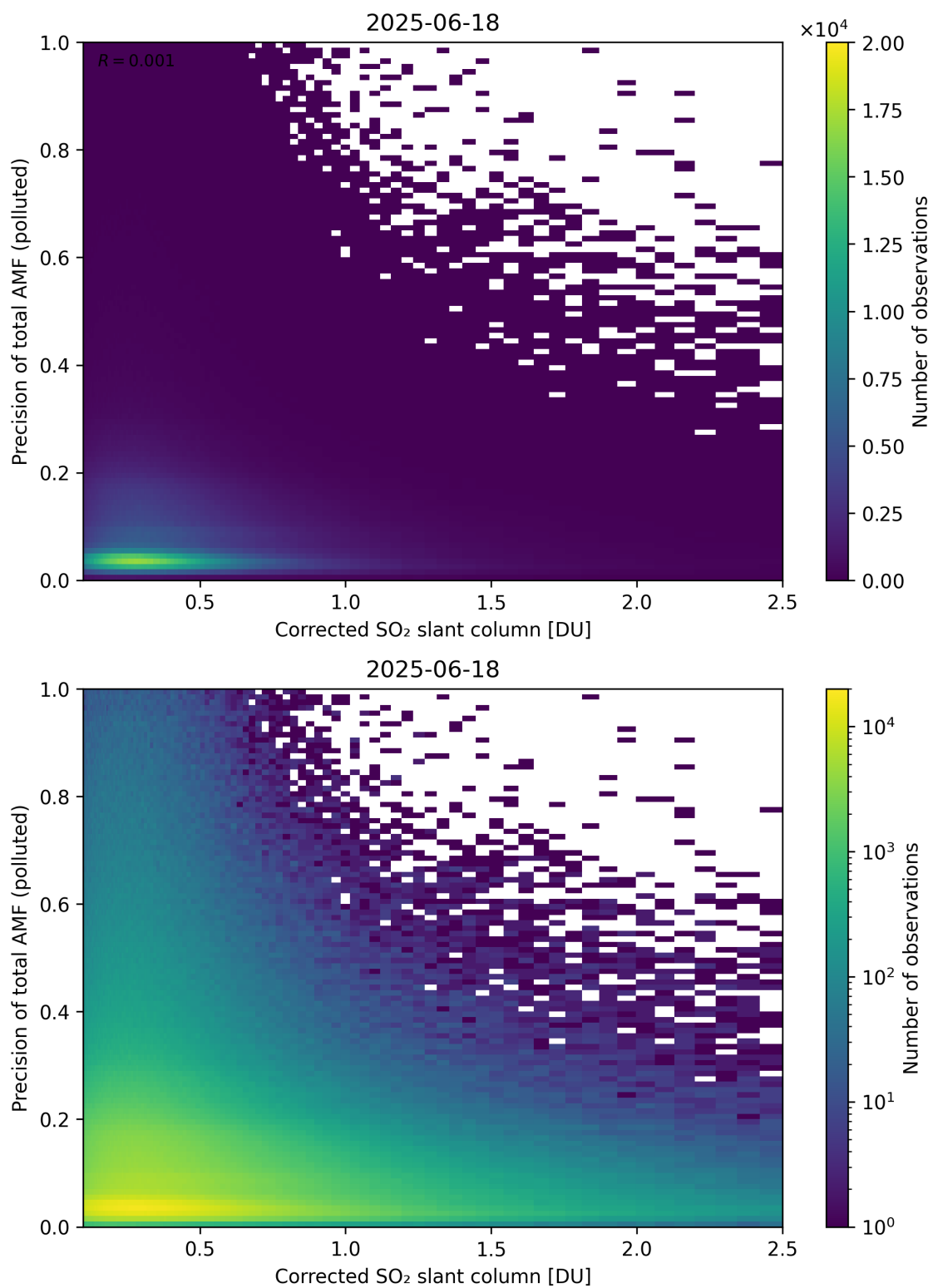
Figure 243: Scatter density plot of “Corrected SO 2 slant column” against “Precision of total AMF (polluted)” for 2025-06-17 to 2025-06-19.
