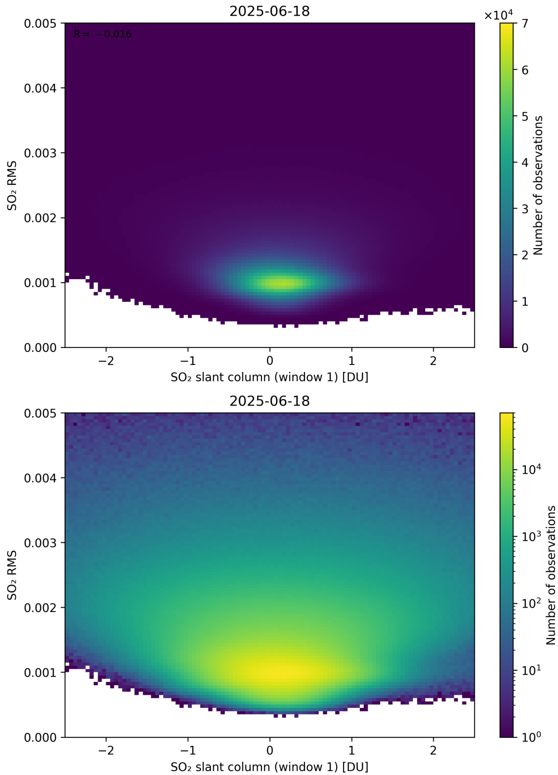
Figure 267: Scatter density plot of “SO 2 slant column (window 1)” against “SO 2 RMS” for 2025-06-17 to 2025-06-19.
