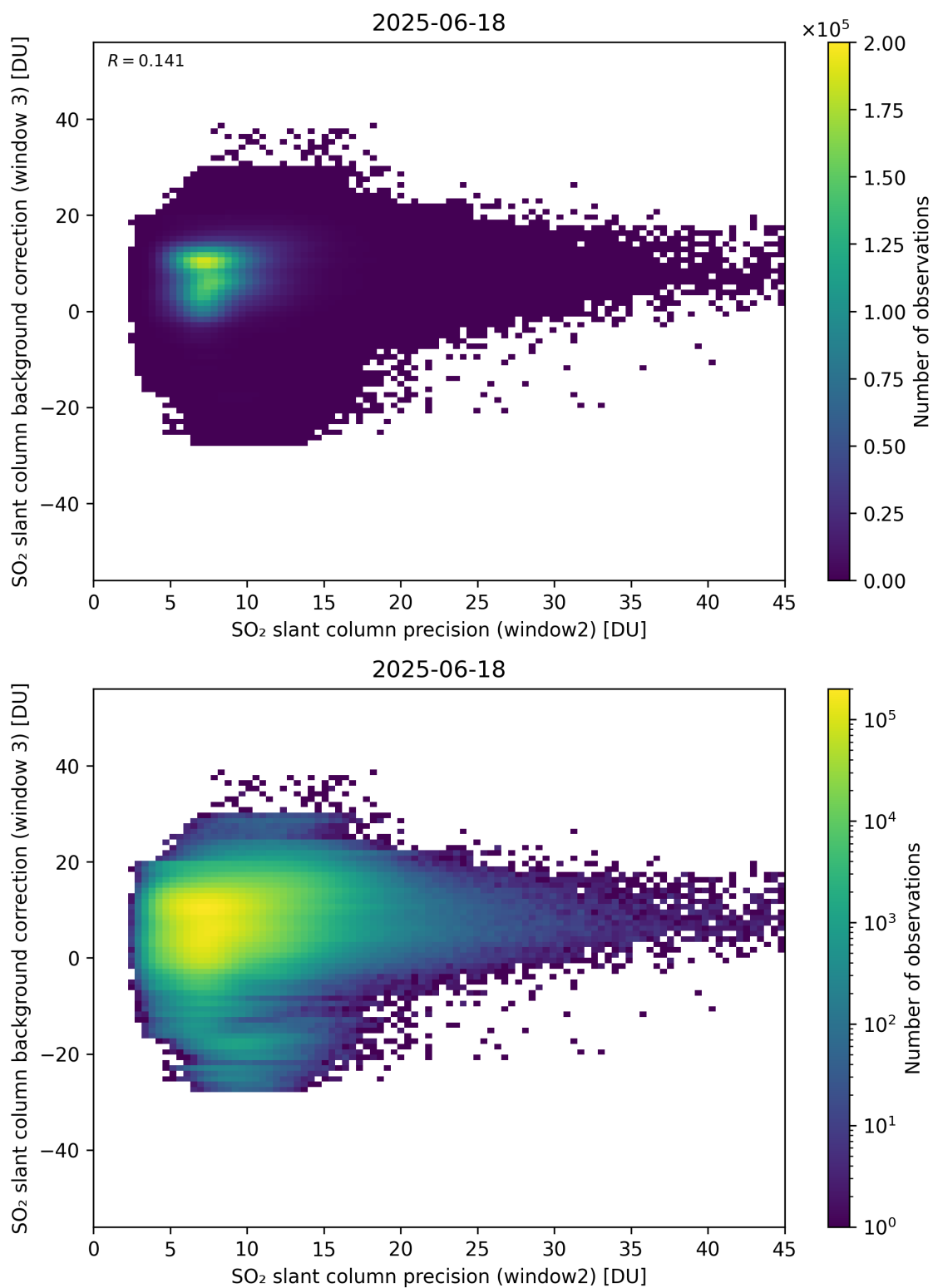
Figure 292: Scatter density plot of “SO 2 slant column precision (window2)” against “SO 2 slant column background correction (window 3)” for 2025-06-17 to 2025-06-19.
