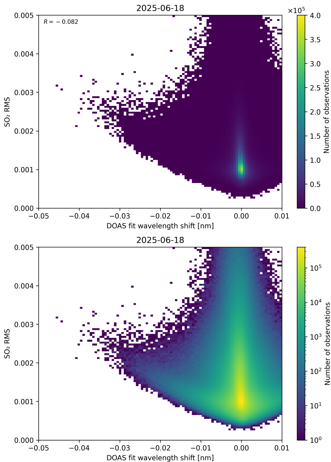
Figure 139: Scatter density plot of “DOAS fit wavelength shift” against “SO 2 RMS” for 2025-06-17 to 2025-06-19.
