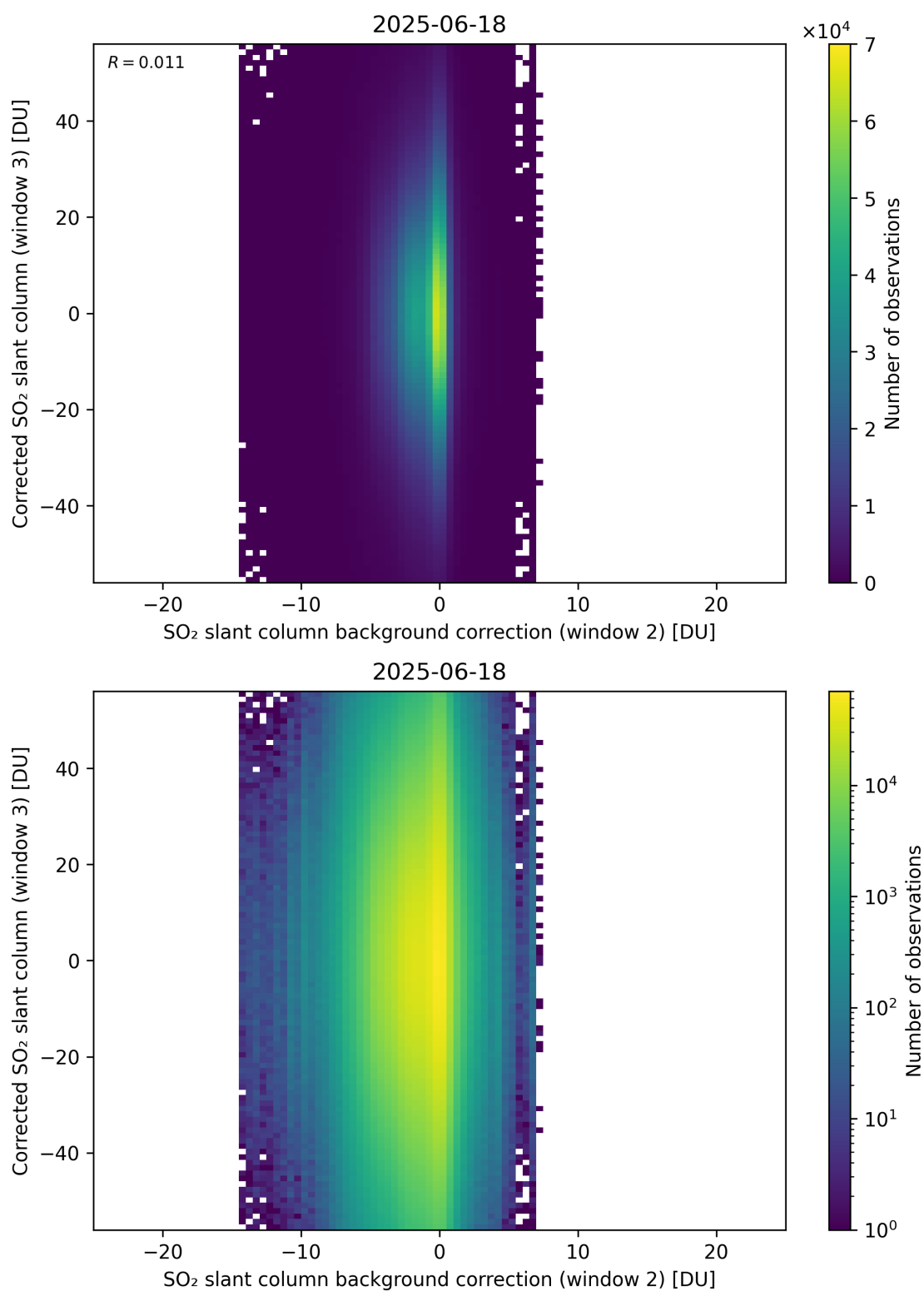
Figure 127: Scatter density plot of “SO 2 slant column background correction (window 2)” against “Corrected SO 2 slant column (window 3)” for 2025-06-17 to 2025-06-19.
