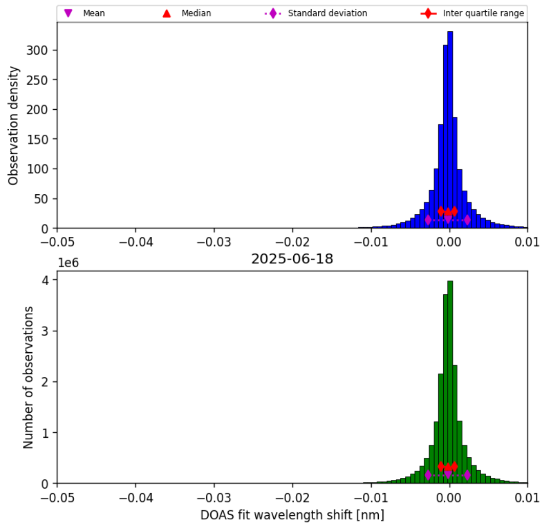
Figure 76: Histogram of “DOAS fit wavelength shift” for 2025-06-17 to 2025-06-19
