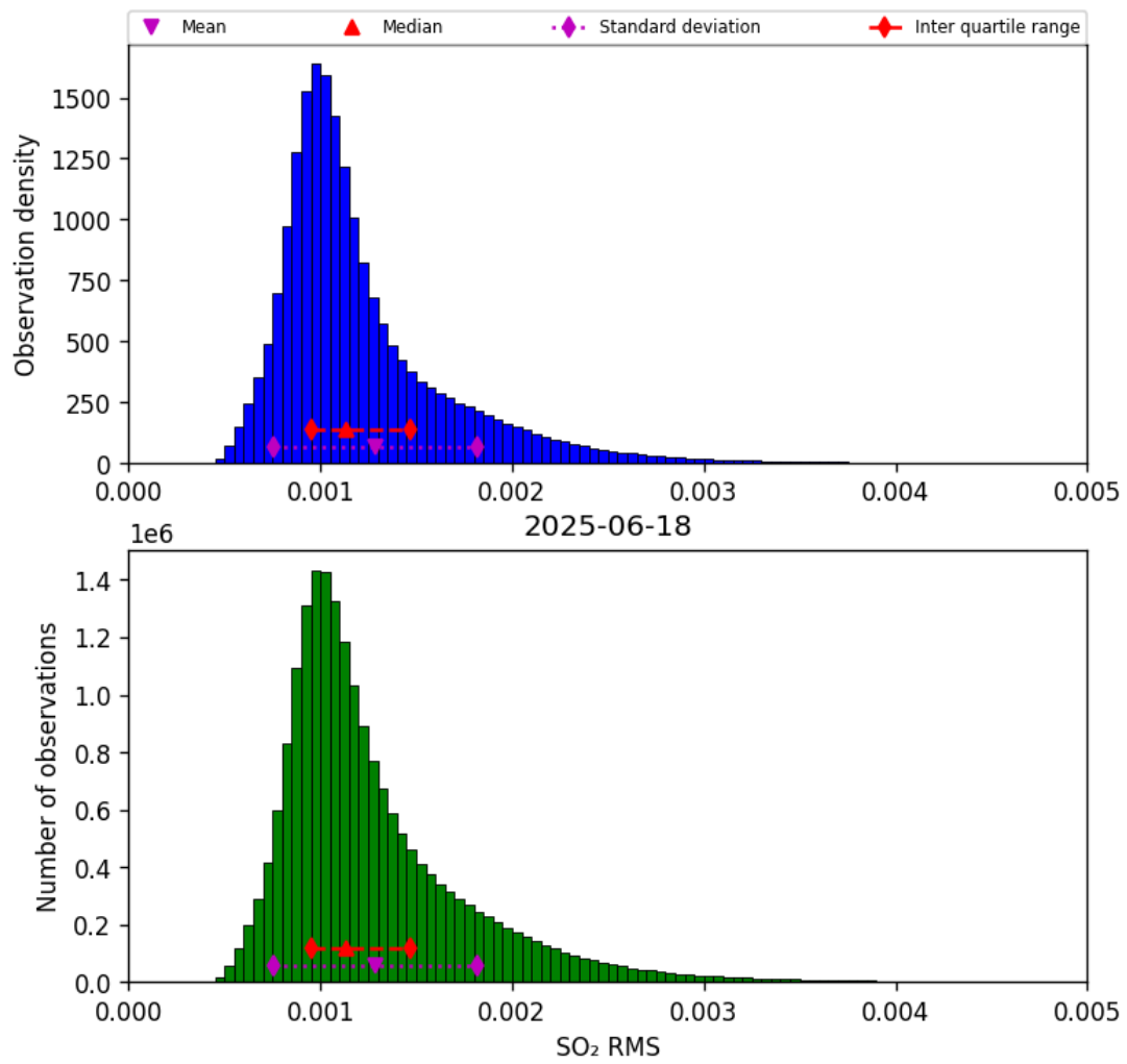
Figure 78: Histogram of “SO 2 RMS” for 2025-06-17 to 2025-06-19
