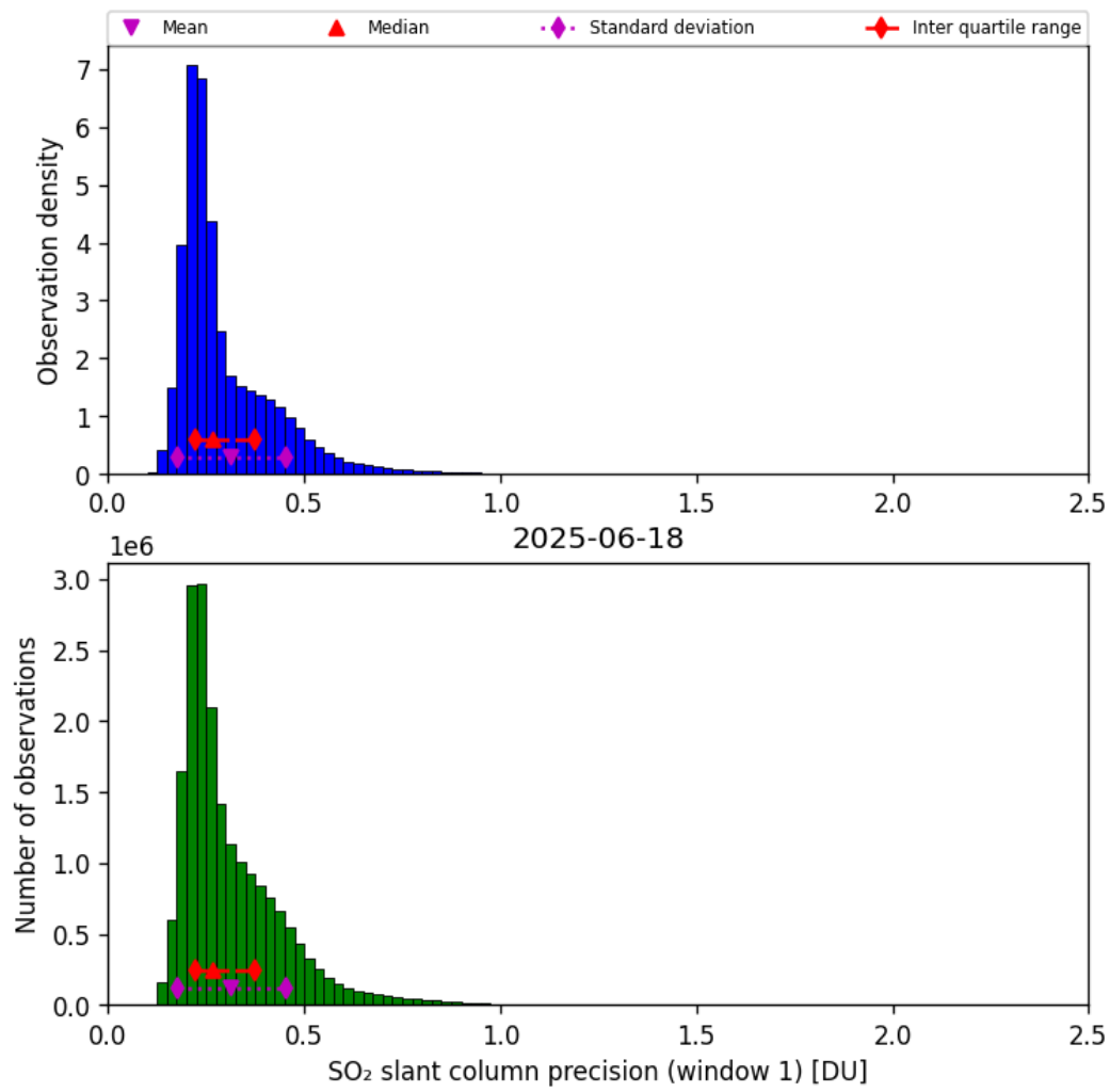
Figure 64: Histogram of “SO 2 slant column precision (window 1)” for 2025-06-17 to 2025-06-19
