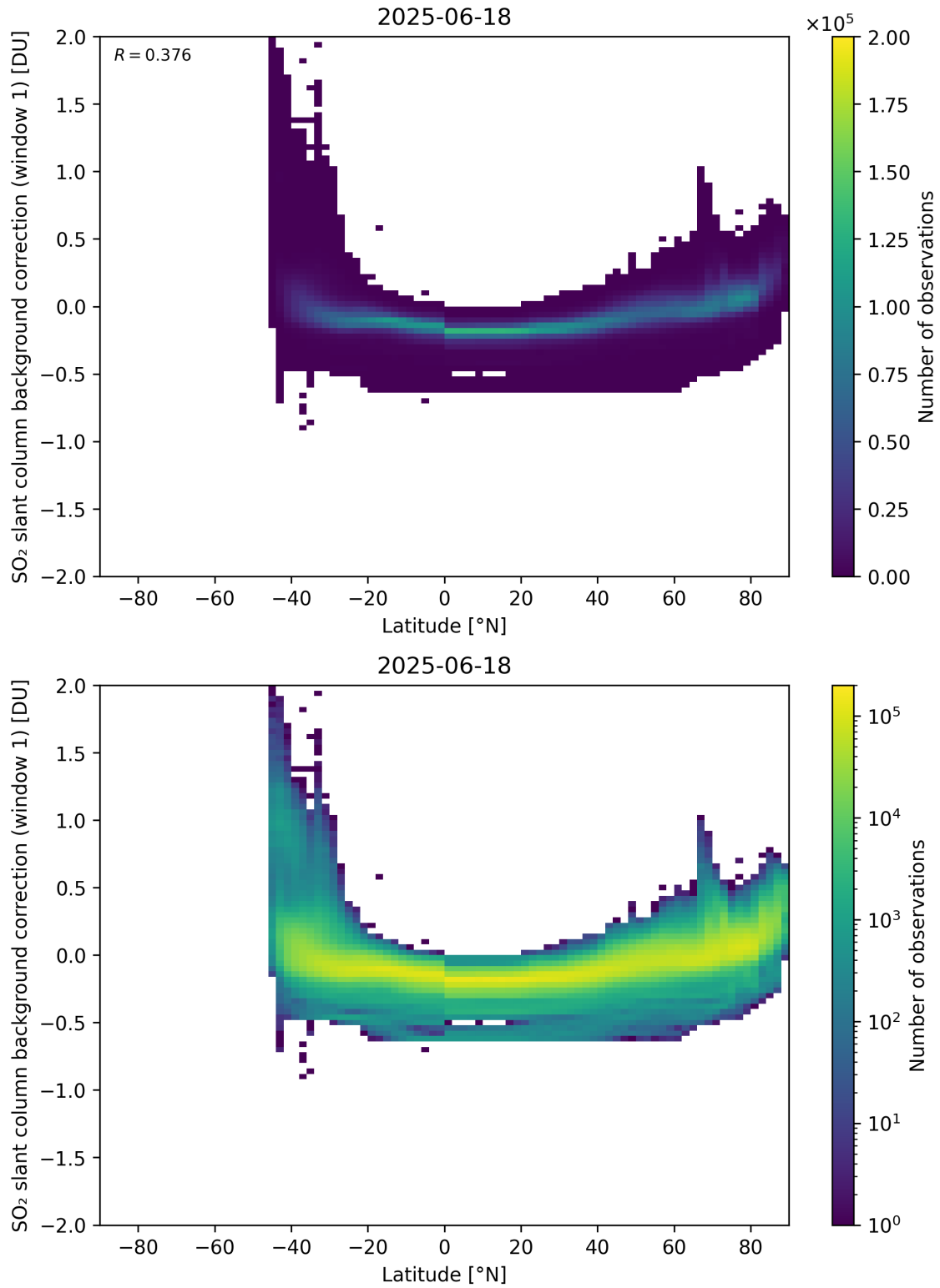
Figure 150: Scatter density plot of “Latitude” against “SO 2 slant column background correction (window 1)” for 2025-06-17 to 2025-06-19.
