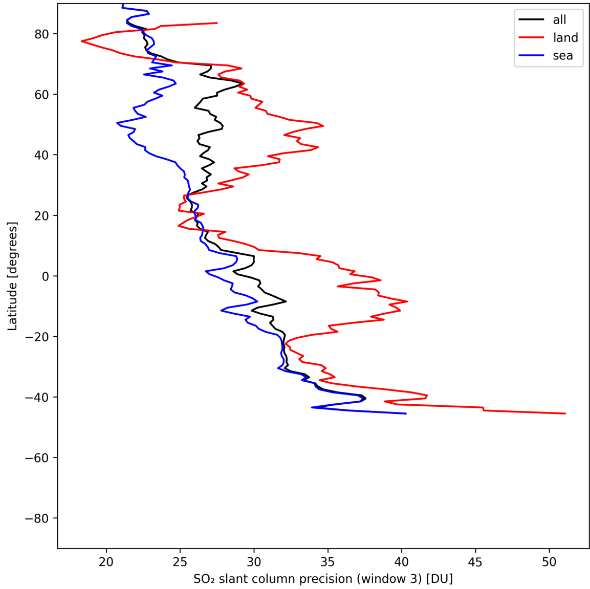
Figure 46: Zonal average of “SO 2 slant column precision (window 3)” for 2025-06-17 to 2025-06-19.
