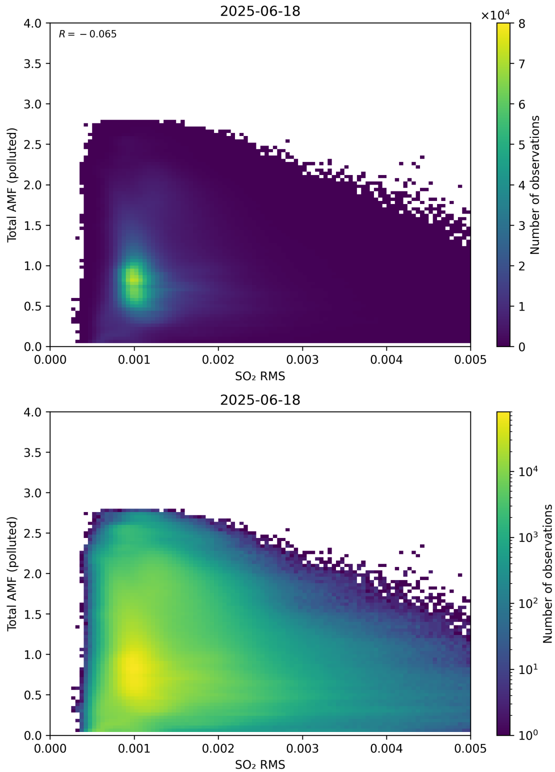
Figure 148: Scatter density plot of “SO 2 RMS” against “Total AMF (polluted)” for 2025-06-17 to 2025-06-19.
