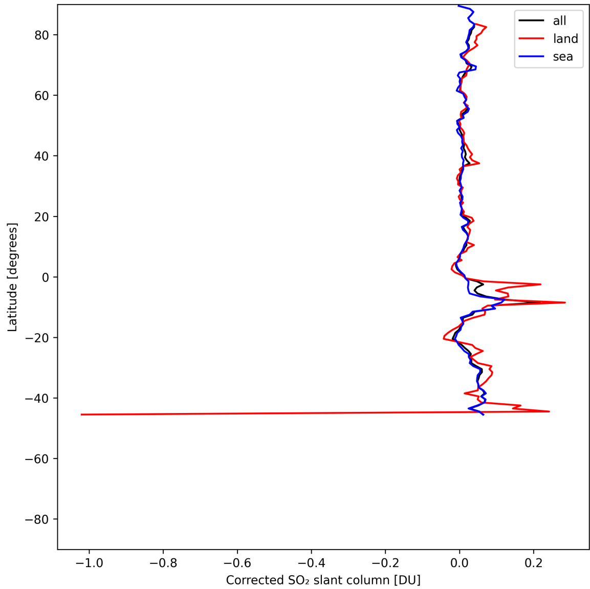
Figure 34: Zonal average of “Corrected SO 2 slant column” for 2025-06-17 to 2025-06-19.
