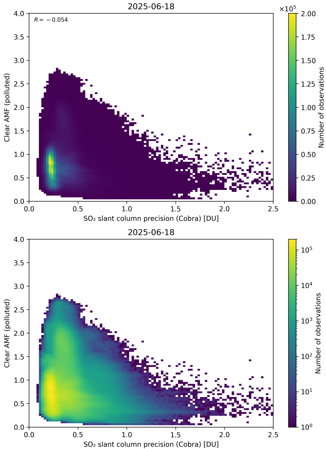
Figure 205: Scatter density plot of “SO 2 slant column precision (Cobra)” against “Clear AMF (polluted)” for 2025-06-17 to 2025-06-19.
