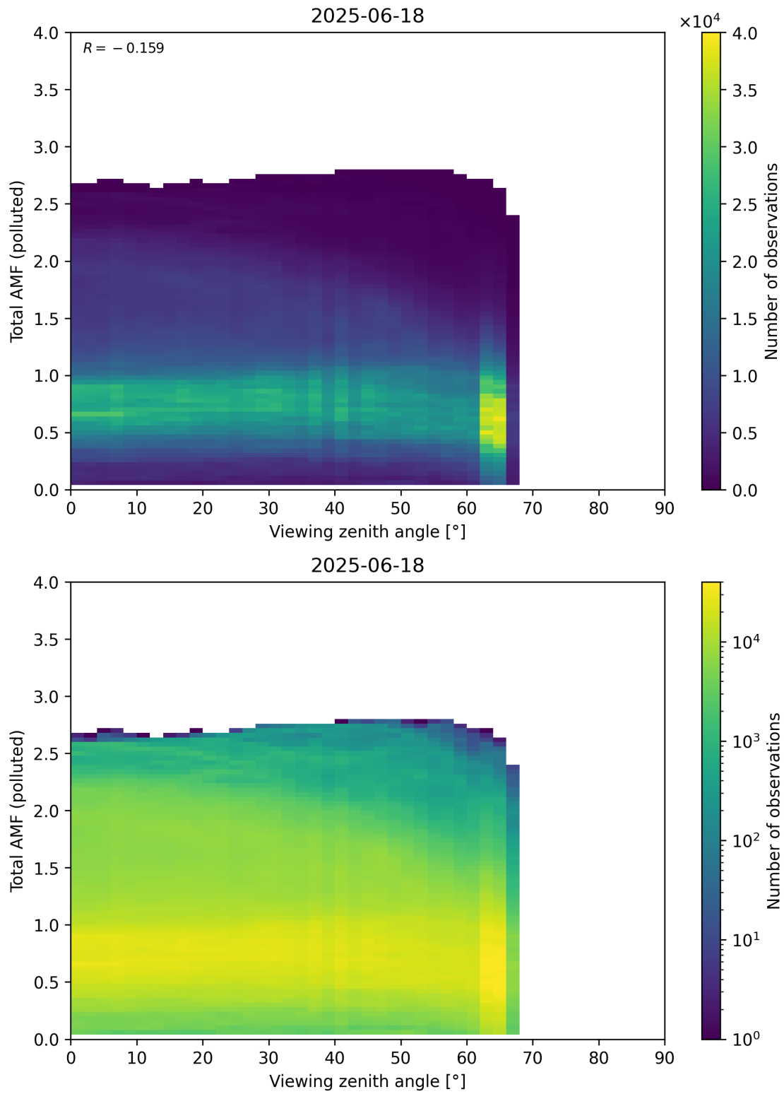
Figure 381: Scatter density plot of “Viewing zenith angle” against “Total AMF (polluted)” for 2025-06-17 to 2025-06-19.
