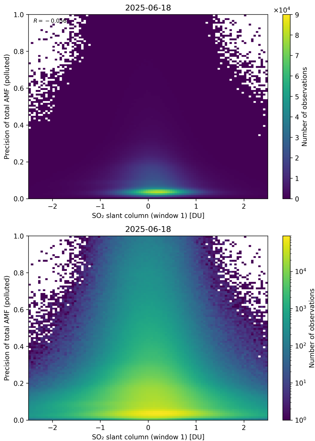
Figure 290: Scatter density plot of “SO 2 slant column (window 1)” against “Precision of total AMF (polluted)” for 2025-06-17 to 2025-06-19.
