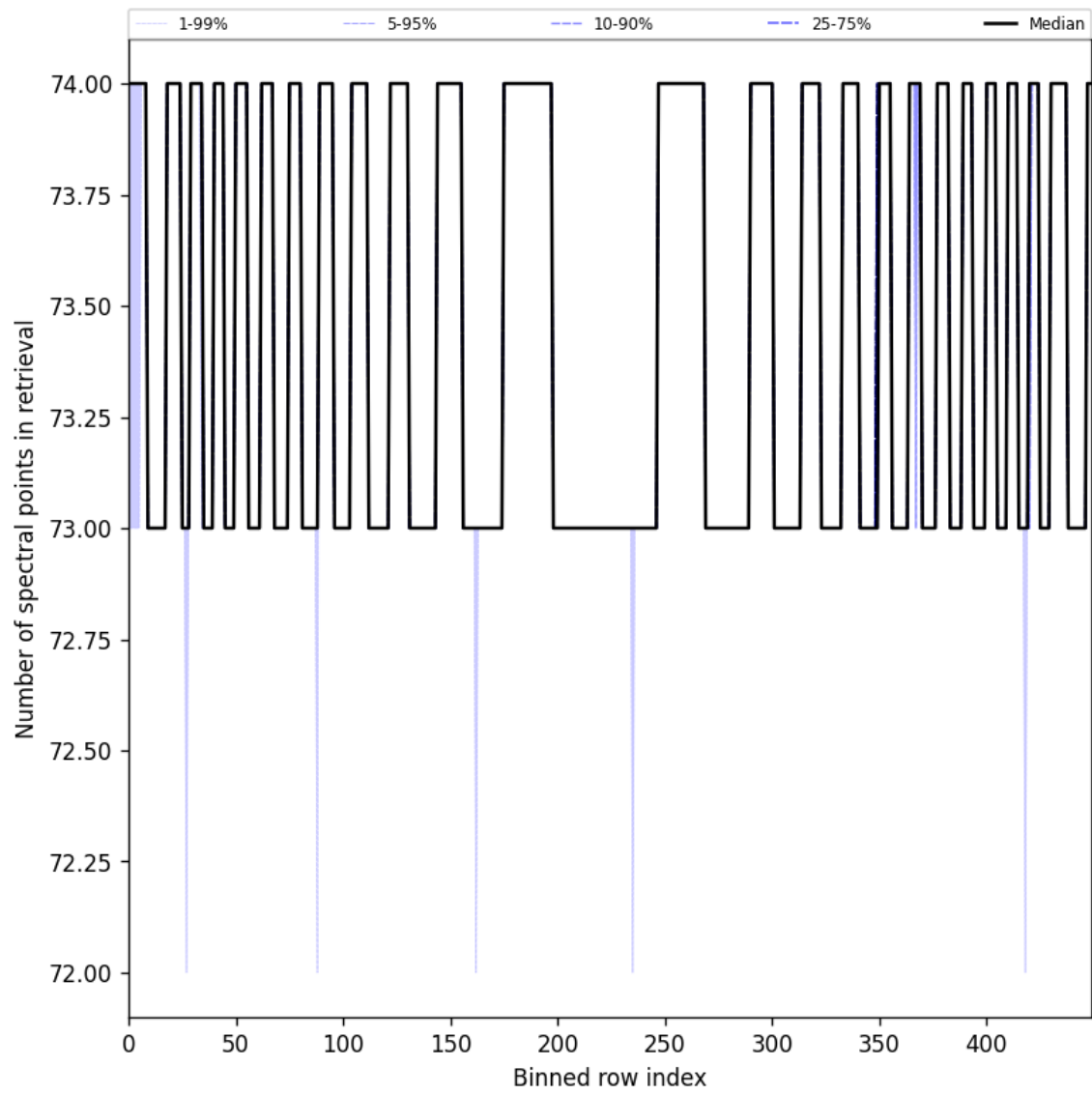
Figure 108: Along track statistics of “Number of spectral points in retrieval” for 2025-06-17 to 2025-06-19
