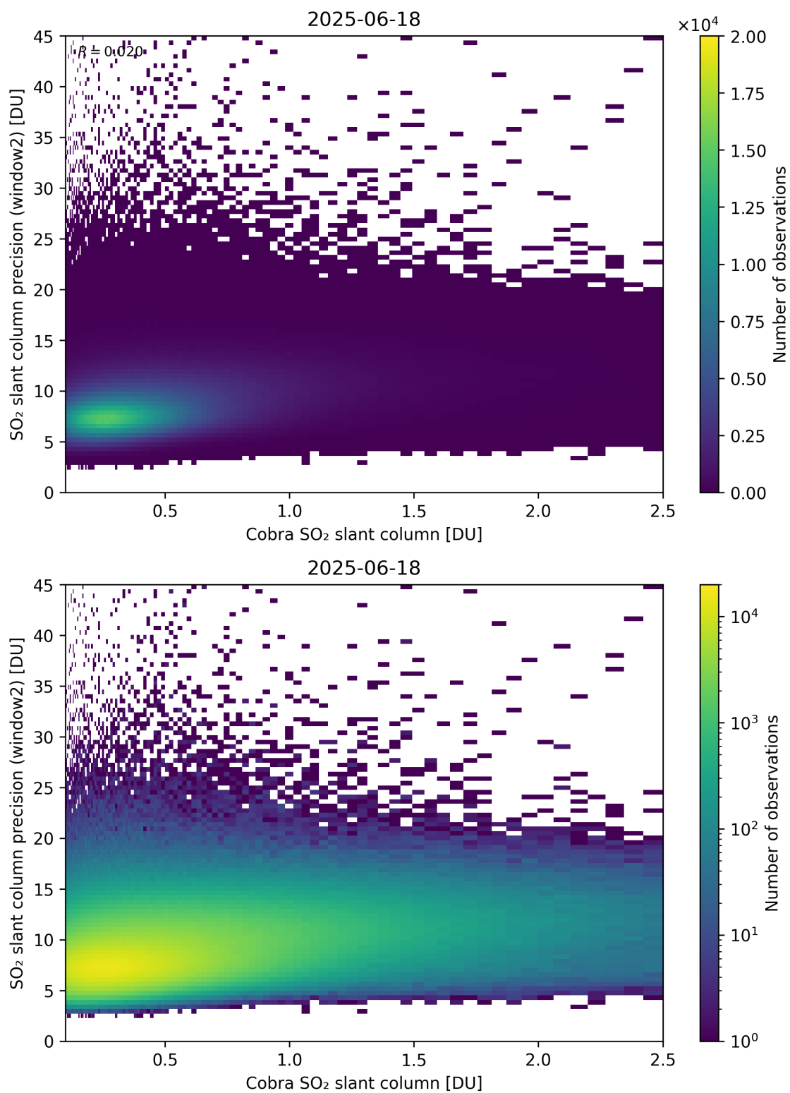
Figure 221: Scatter density plot of “Cobra SO 2 slant column” against “SO 2 slant column precision (window2)” for 2025-06-17 to 2025-06-19.
