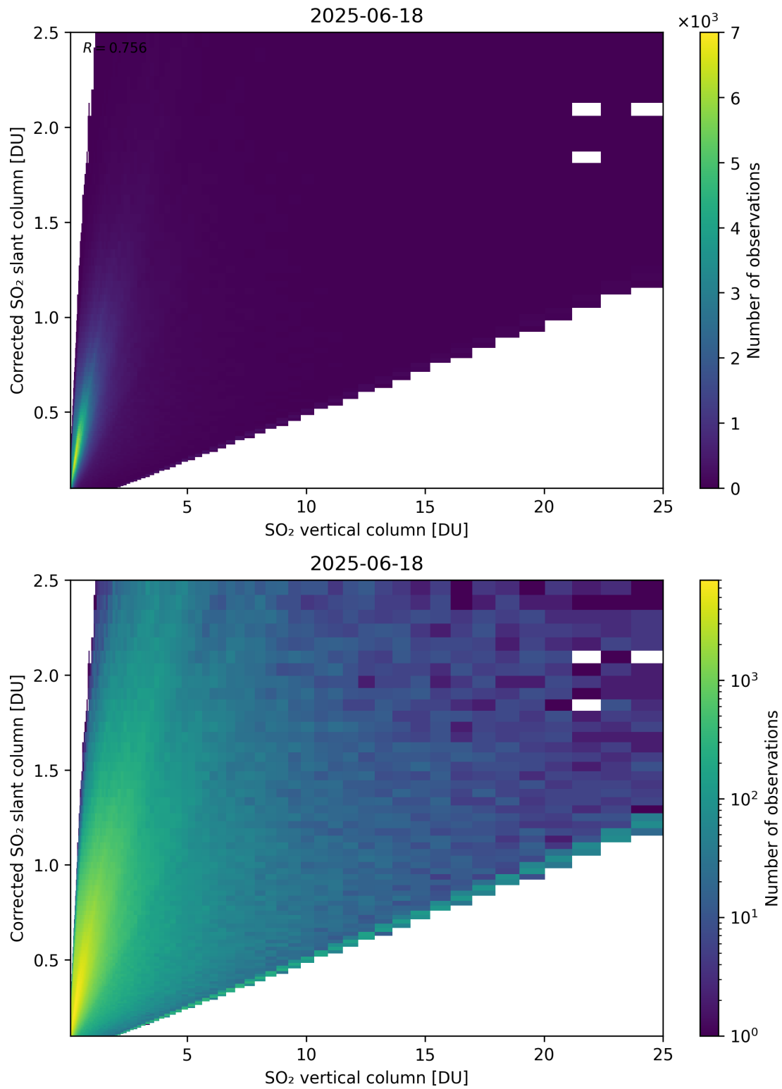
Figure 351: Scatter density plot of “SO 2 vertical column” against “Corrected SO 2 slant column” for 2025-06-17 to 2025-06-19.
