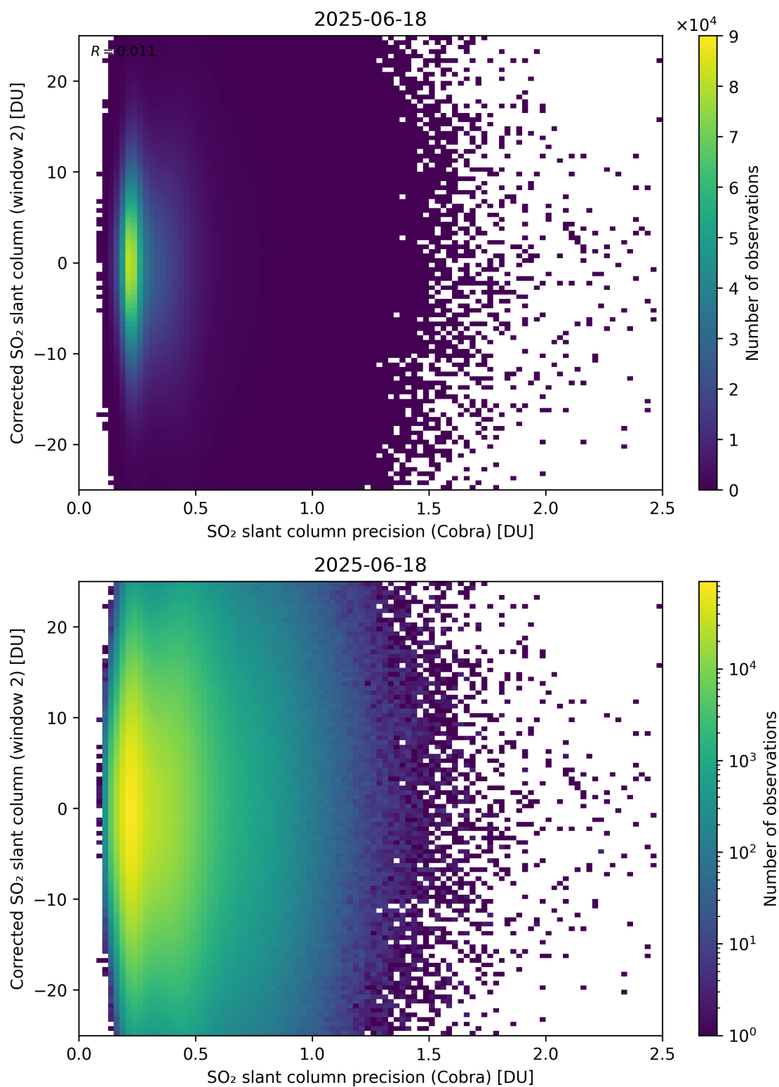
Figure 206: Scatter density plot of “SO 2 slant column precision (Cobra)” against “Corrected SO 2 slant column (window 2)” for 2025-06-17 to 2025-06-19.
