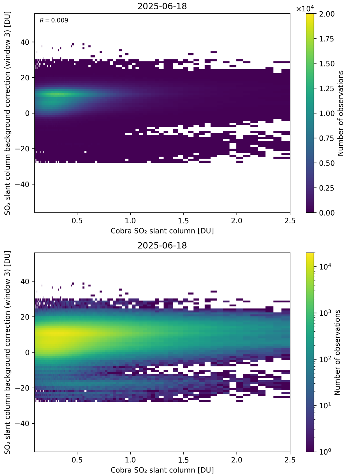
Figure 195: Scatter density plot of “Cobra SO 2 slant column” against “SO 2 slant column background correction (window 3)” for 2025-06-17 to 2025-06-19.
