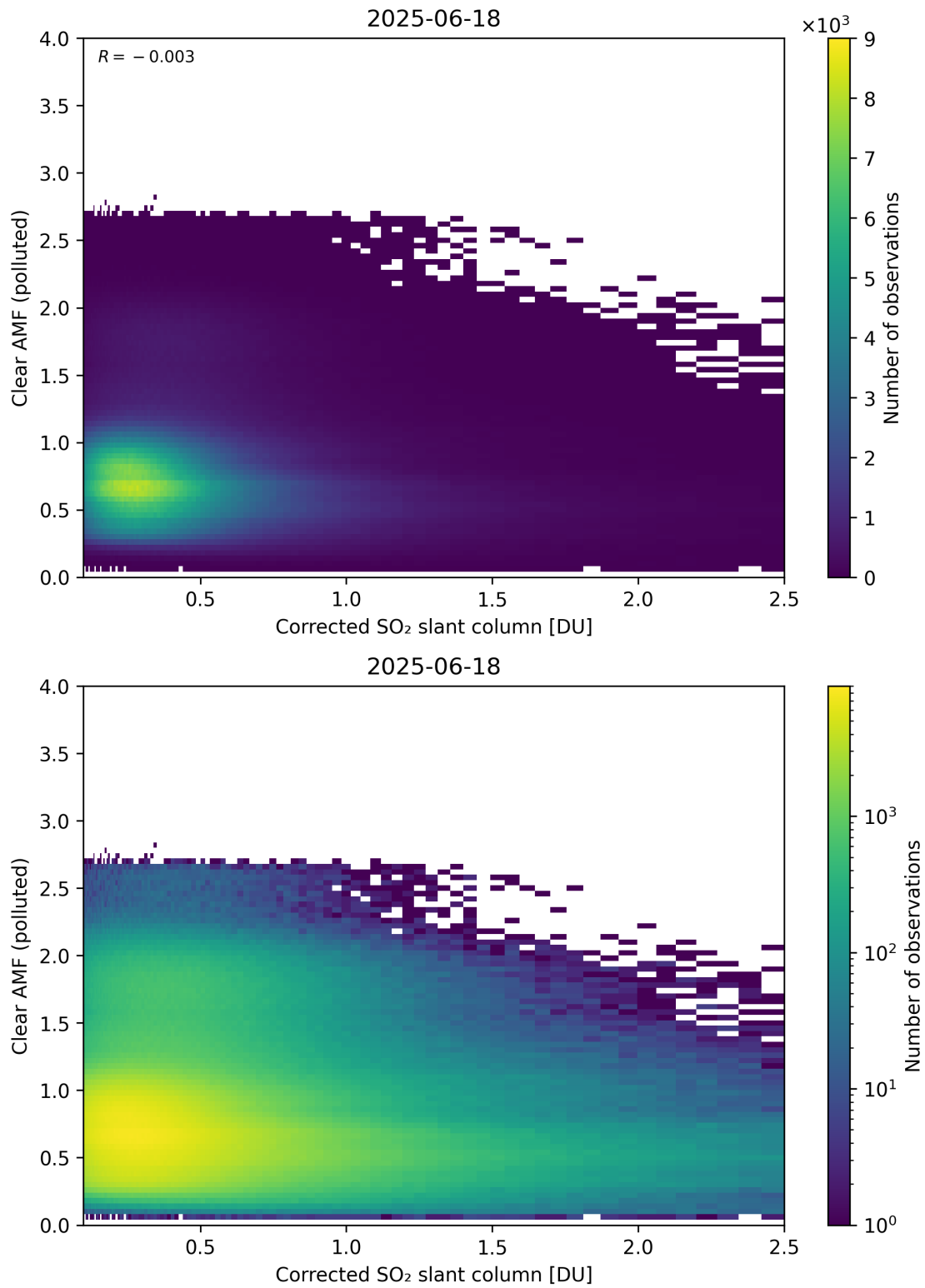
Figure 232: Scatter density plot of “Corrected SO 2 slant column” against “Clear AMF (polluted)” for 2025-06-17 to 2025-06-19.
