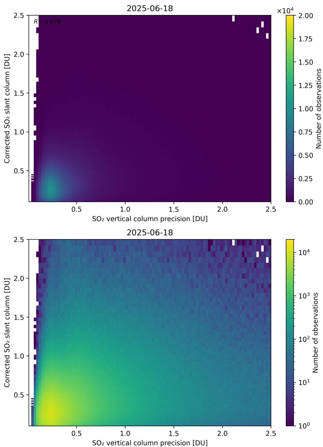
Figure 338: Scatter density plot of “SO 2 vertical column precision” against “Corrected SO 2 slant column” for 2025-06-17 to 2025-06-19.
