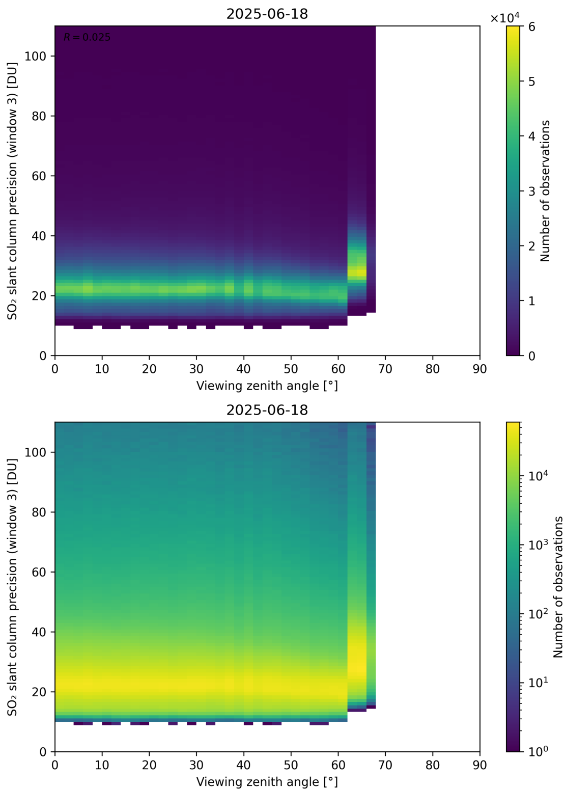
Figure 380: Scatter density plot of “Viewing zenith angle” against “SO 2 slant column precision (window 3)” for 2025-06-17 to 2025-06-19.
