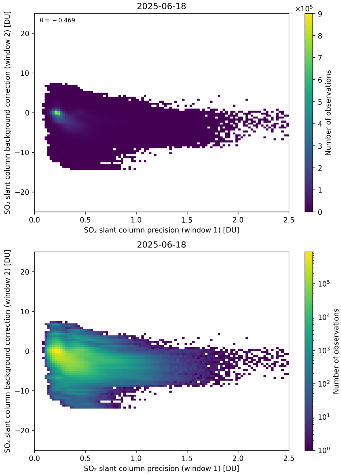
Figure 269: Scatter density plot of “SO 2 slant column precision (window 1)” against “SO 2 slant column background correction (window 2)” for 2025-06-17 to 2025-06-19.
