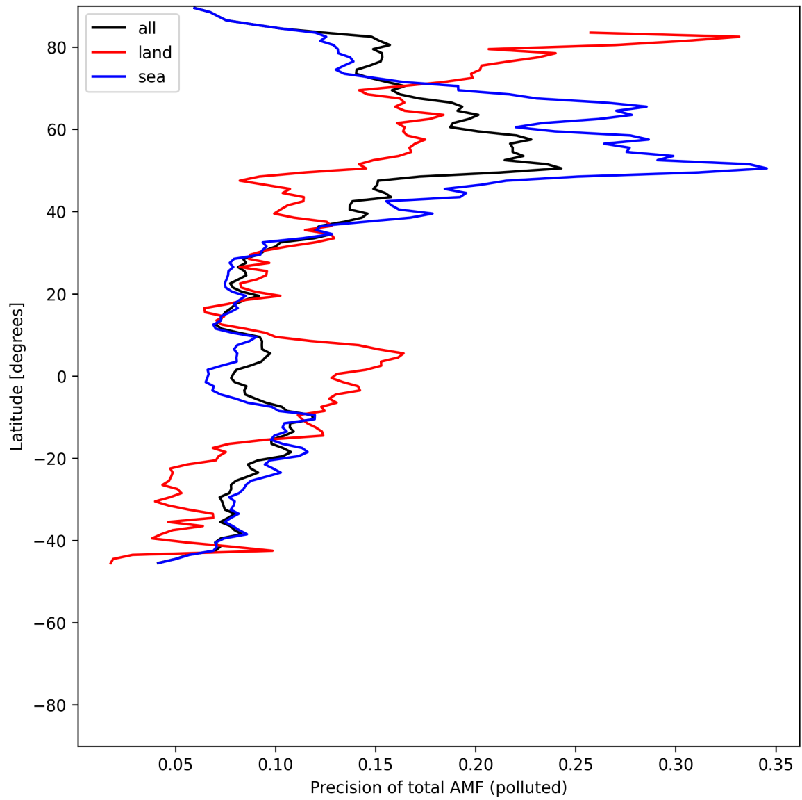
Figure 54: Zonal average of “Precision of total AMF (polluted)” for 2025-06-17 to 2025-06-19.
