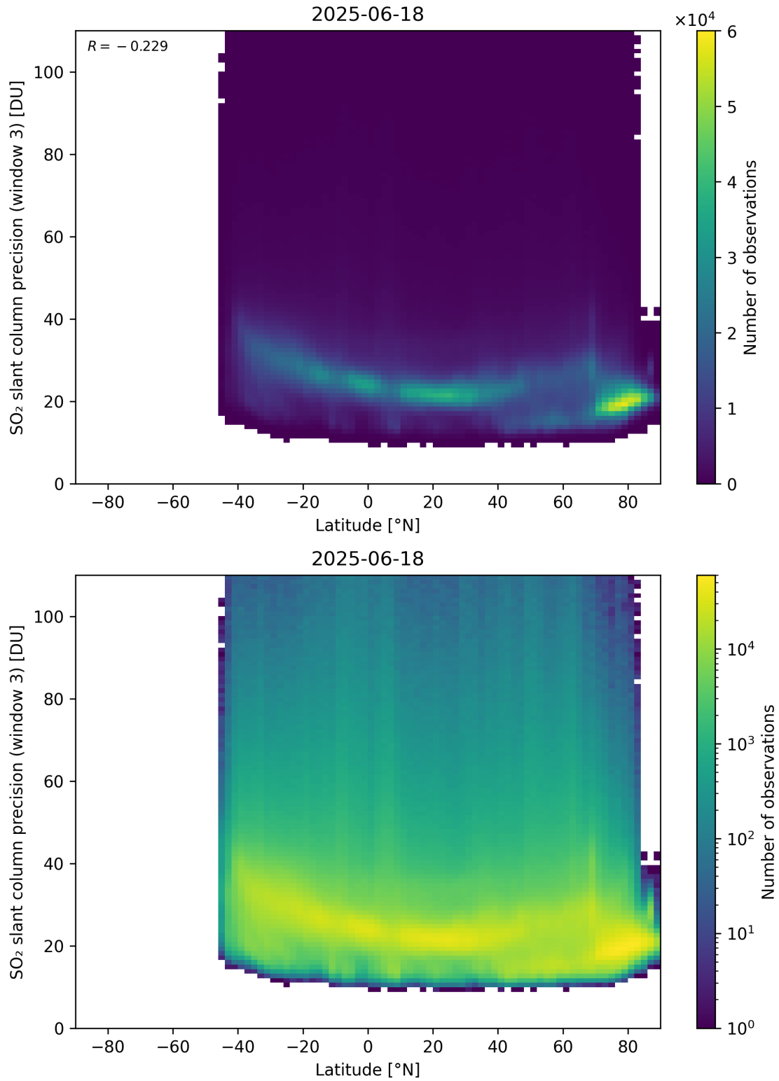
Figure 166: Scatter density plot of “Latitude” against “SO 2 slant column precision (window 3)” for 2025-06-17 to 2025-06-19.
