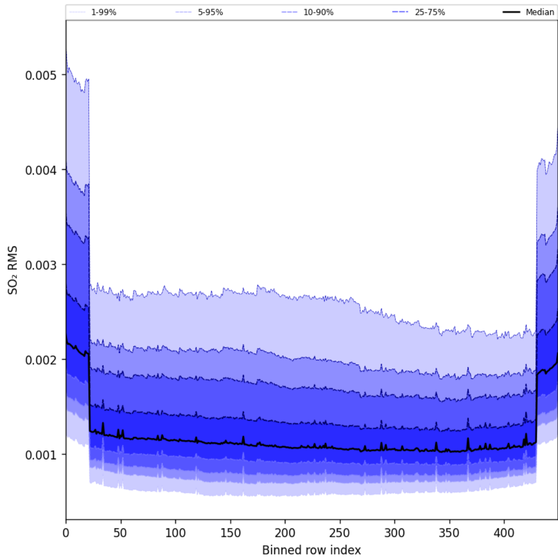
Figure 104: Along track statistics of “SO 2 RMS” for 2025-06-17 to 2025-06-19
