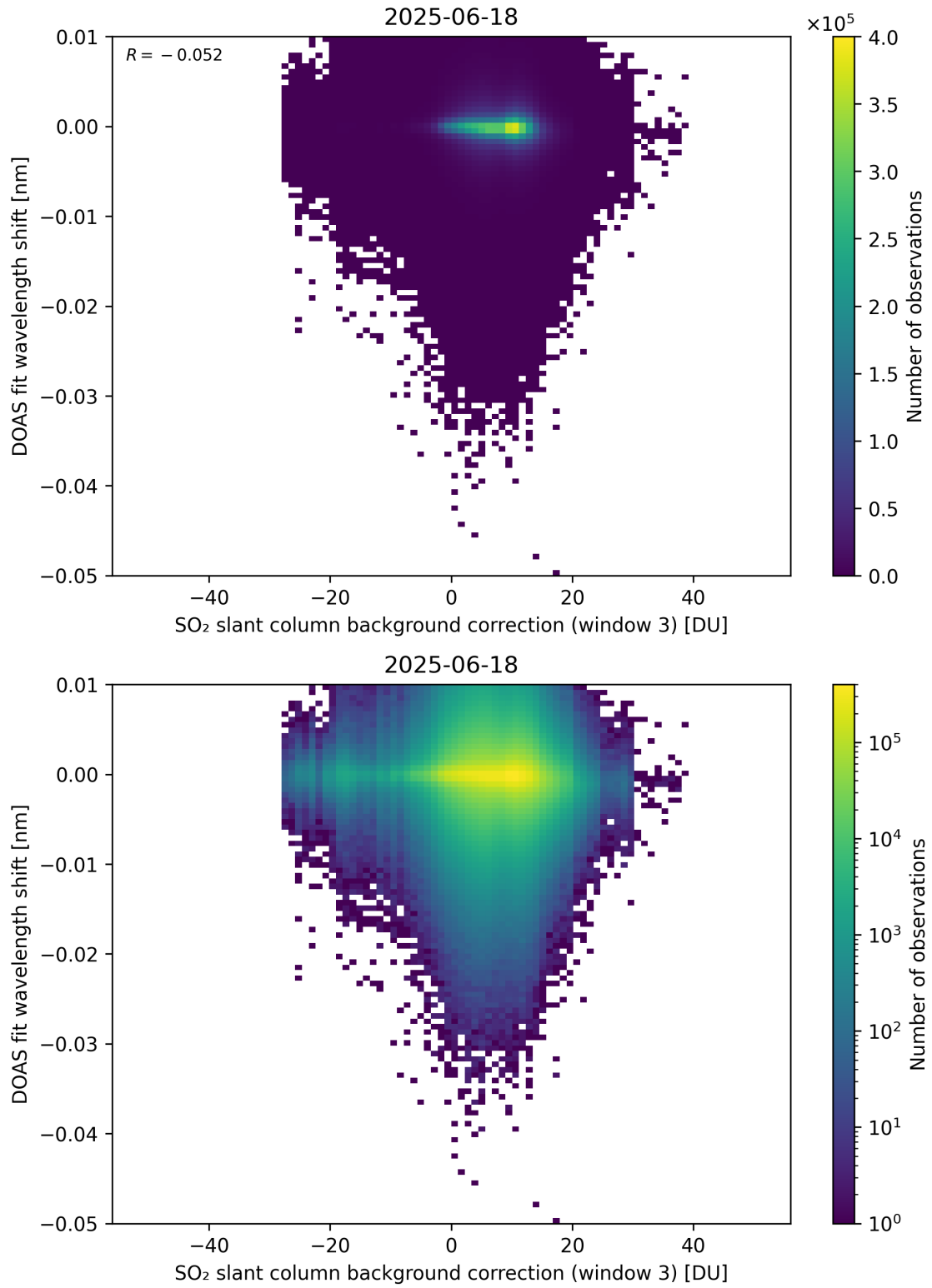
Figure 132: Scatter density plot of “SO 2 slant column background correction (window 3)” against “DOAS fit wavelength shift” for 2025-06-17 to 2025-06-19.
