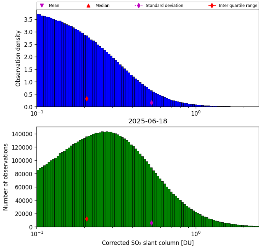
Figure 60: Histogram of "Corrected SO 2 slant column" for 2025-06-17 to 2025-06-19
