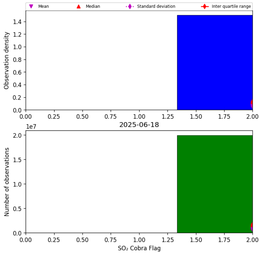
Figure 75: Histogram of “SO 2 Cobra Flag” for 2025-06-17 to 2025-06-19
