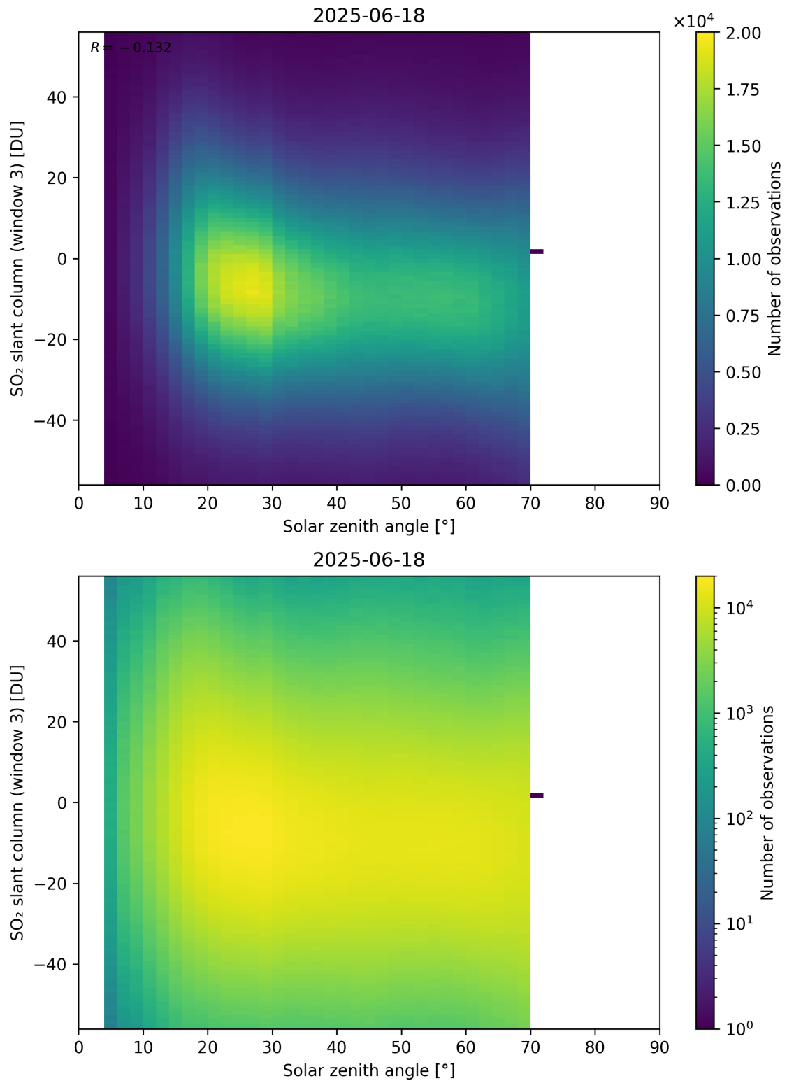
Figure 187: Scatter density plot of “Solar zenith angle” against “SO 2 slant column (window 3)” for 2025-06-17 to 2025-06-19.
