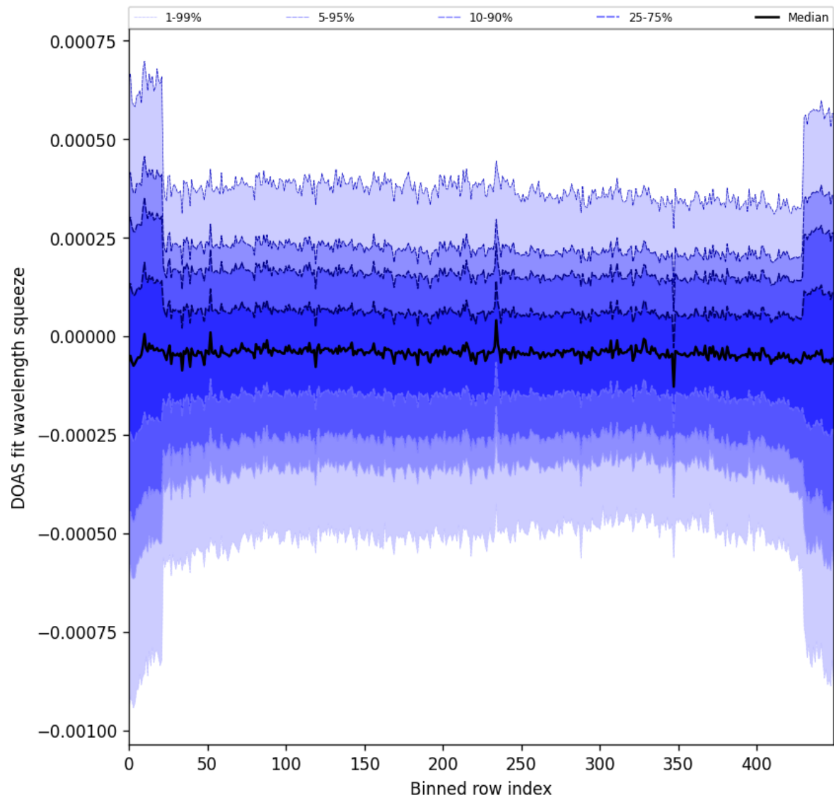
Figure 103: Along track statistics of “DOAS fit wavelength squeeze” for 2025-06-17 to 2025-06-19
