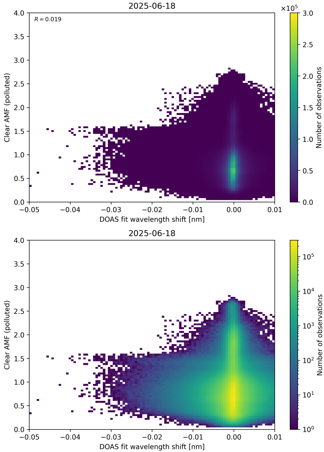
Figure 140: Scatter density plot of “DOAS fit wavelength shift” against “Clear AMF (polluted)” for 2025-06-17 to 2025-06-19.
