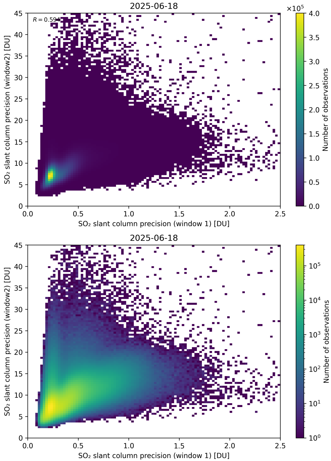
Figure 277: Scatter density plot of “SO 2 slant column precision (window 1)” against “SO 2 slant column precision (window2)” for 2025-06-17 to 2025-06-19.
