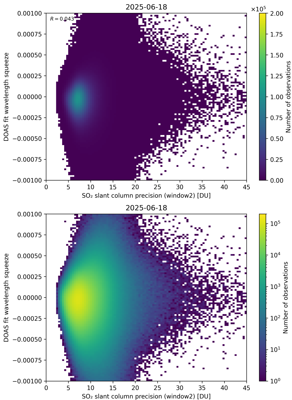
Figure 294: Scatter density plot of “SO 2 slant column precision (window2)” against “DOAS fit wavelength squeeze” for 2025-06-17 to 2025-06-19.
