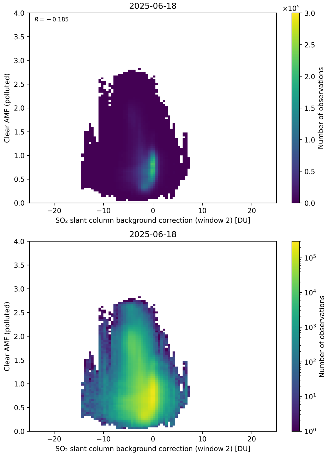
Figure 126: Scatter density plot of “SO 2 slant column background correction (window 2)” against “Clear AMF (polluted)” for 2025-06-17 to 2025-06-19.
