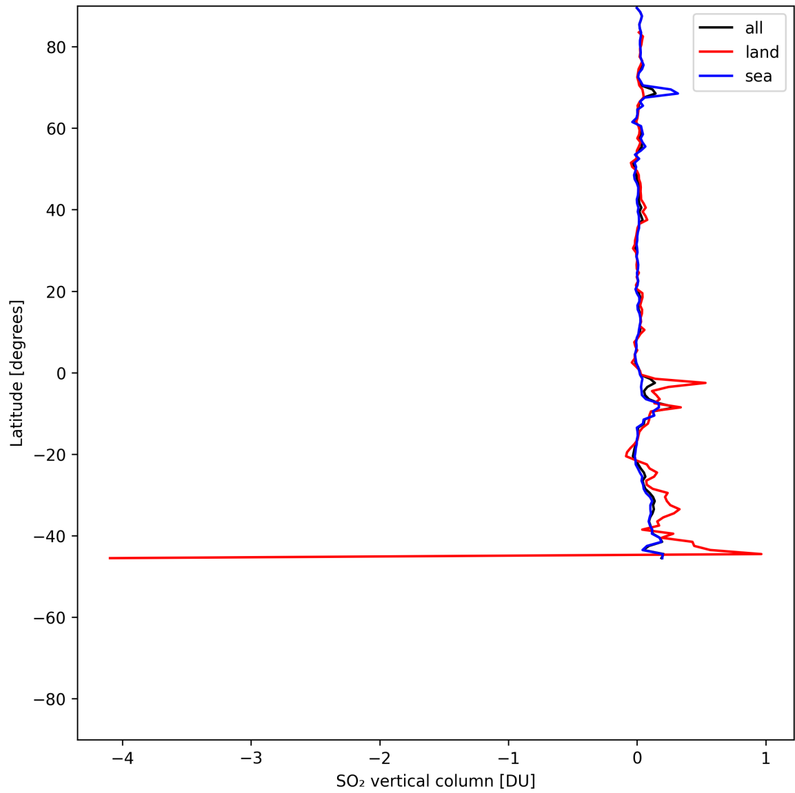
Figure 32: Zonal average of “SO 2 vertical column” for 2025-06-17 to 2025-06-19.
