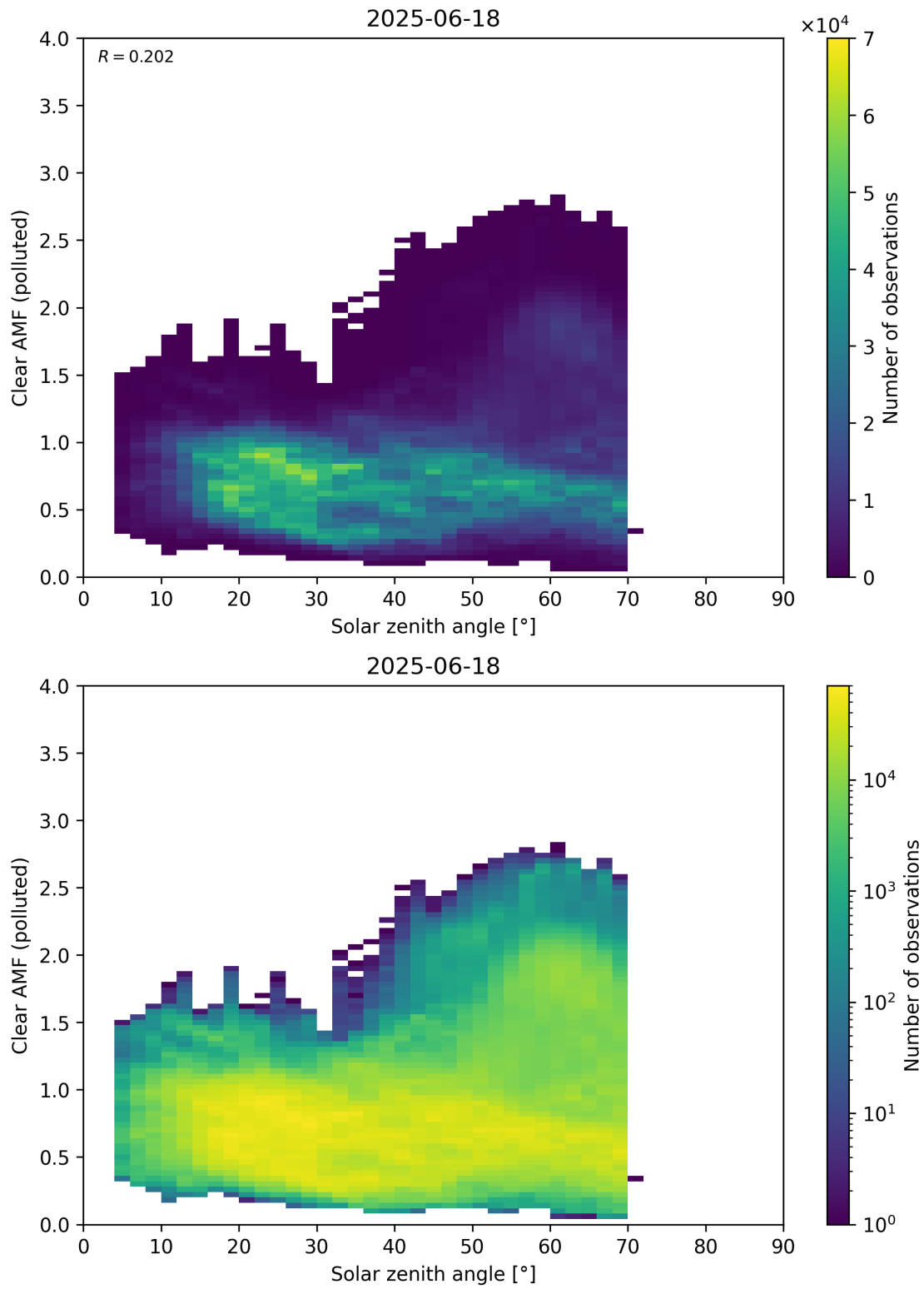
Figure 178: Scatter density plot of “Solar zenith angle” against “Clear AMF (polluted)” for 2025-06-17 to 2025-06-19.
