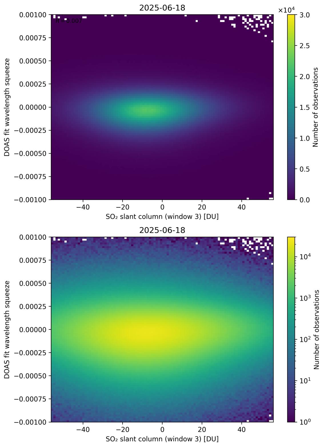
Figure 305: Scatter density plot of “SO 2 slant column (window 3)” against “DOAS fit wavelength squeeze” for 2025-06-17 to 2025-06-19.
