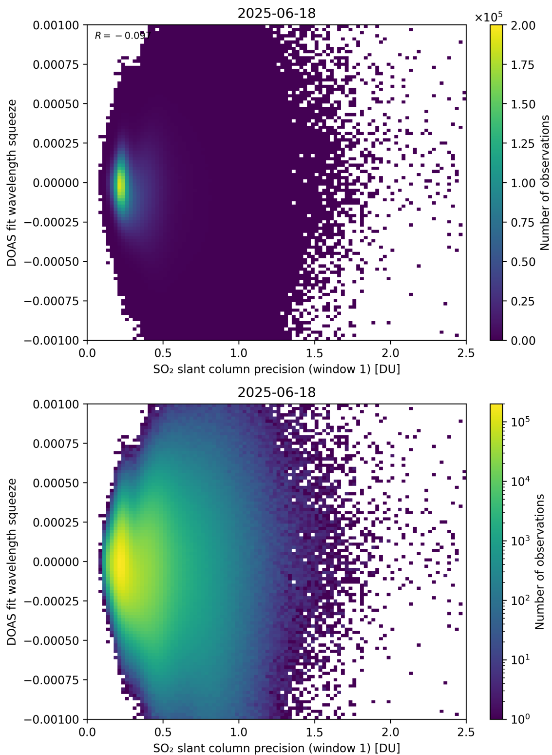
Figure 272: Scatter density plot of “SO 2 slant column precision (window 1)” against “DOAS fit wavelength squeeze” for 2025-06-17 to 2025-06-19.
