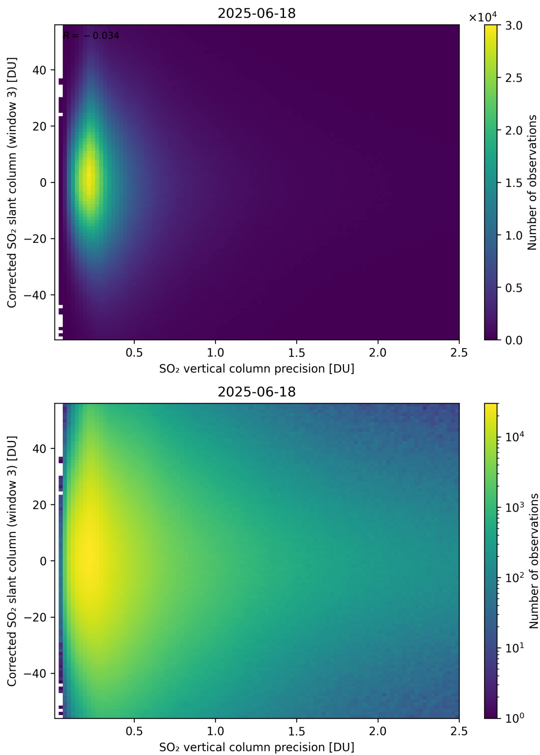
Figure 340: Scatter density plot of “SO 2 vertical column precision” against “Corrected SO 2 slant column (window 3)” for 2025-06-17 to 2025-06-19.
