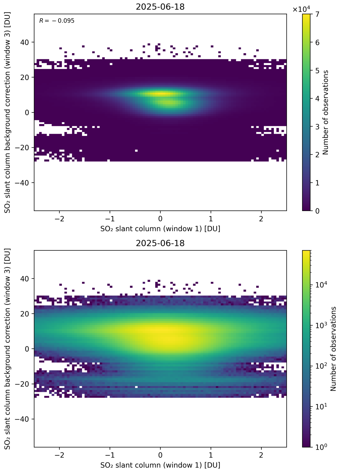
Figure 264: Scatter density plot of “SO 2 slant column (window 1)” against “SO 2 slant column background correction (window 3)” for 2025-06-17 to 2025-06-19.
