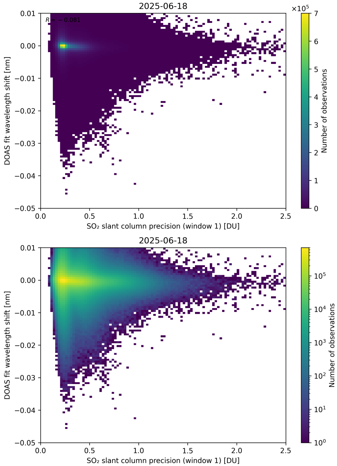
Figure 271: Scatter density plot of “SO 2 slant column precision (window 1)” against “DOAS fit wavelength shift” for 2025-06-17 to 2025-06-19.
