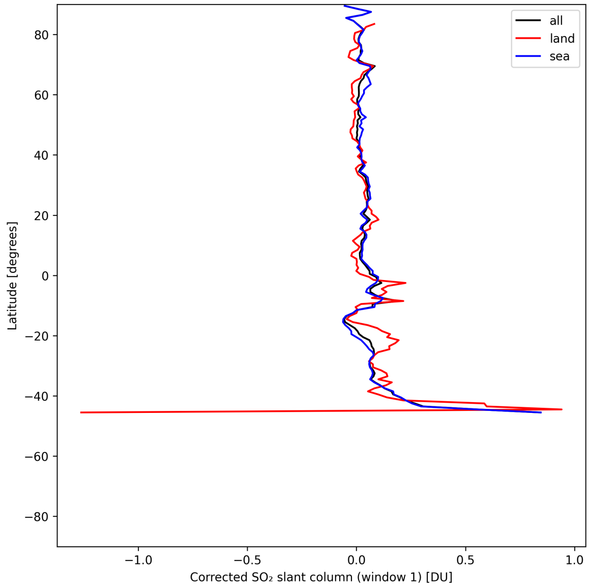
Figure 39: Zonal average of “Corrected SO 2 slant column (window 1)” for 2025-06-17 to 2025-06-19.
