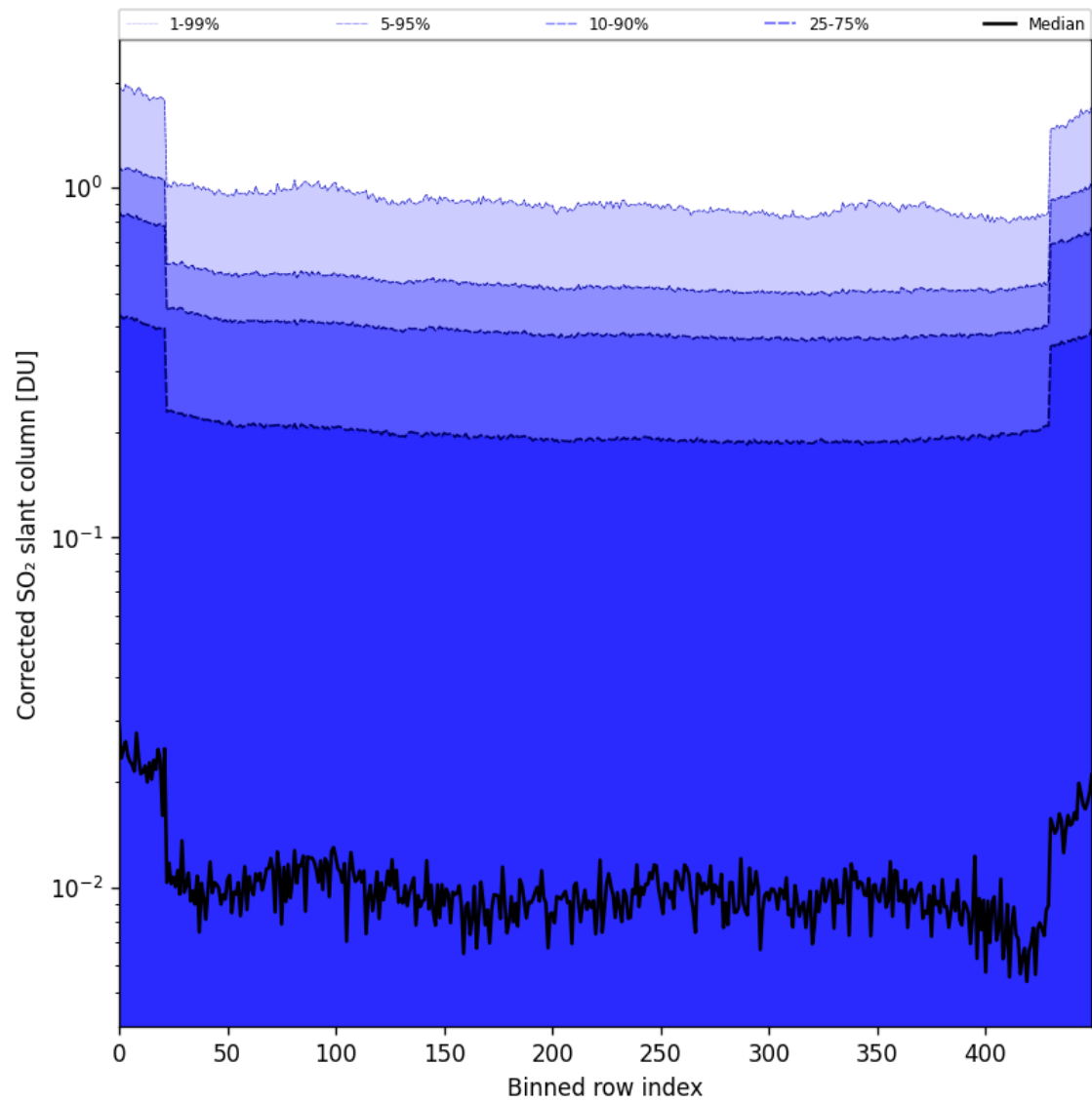
Figure 86: Along track statistics of "Corrected SO 2 slant column" for 2025-06-17 to 2025-06-19
