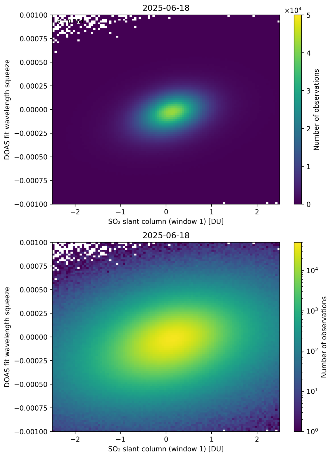
Figure 266: Scatter density plot of “SO 2 slant column (window 1)” against “DOAS fit wavelength squeeze” for 2025-06-17 to 2025-06-19.
