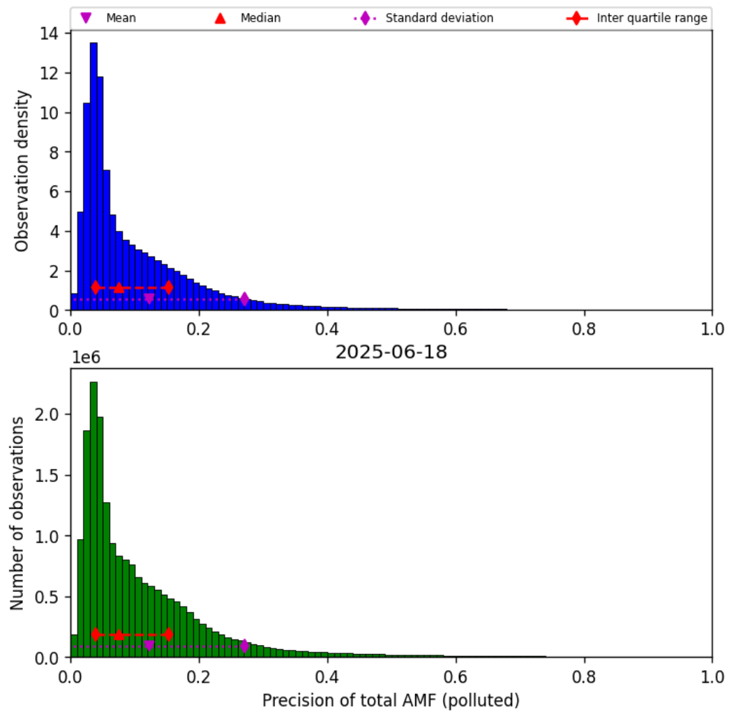
Figure 80: Histogram of “Precision of total AMF (polluted)” for 2025-06-17 to 2025-06-19
