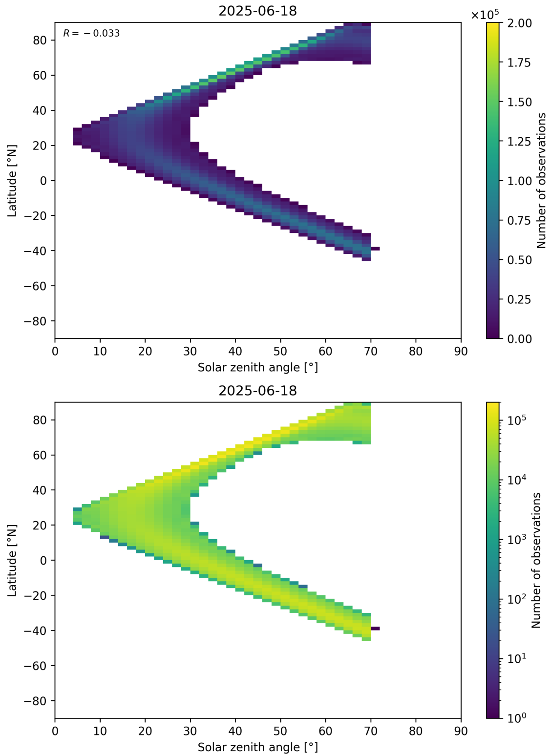
Figure 177: Scatter density plot of “Solar zenith angle” against “Latitude” for 2025-06-17 to 2025-06-19.
