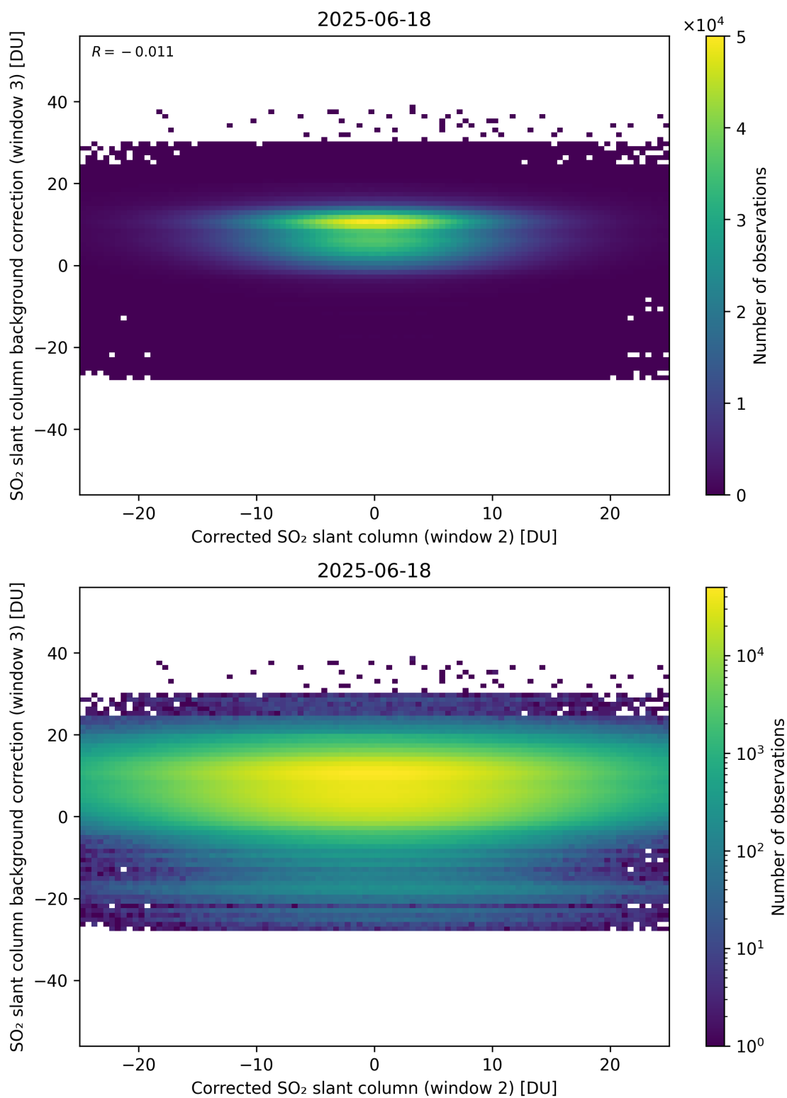
Figure 245: Scatter density plot of “Corrected SO 2 slant column (window 2)” against “SO 2 slant column background correction (window 3)” for 2025-06-17 to 2025-06-19.
