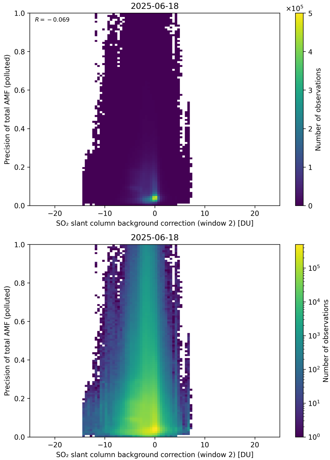
Figure 131: Scatter density plot of “SO 2 slant column background correction (window 2)” against “Precision of total AMF (polluted)” for 2025-06-17 to 2025-06-19.
