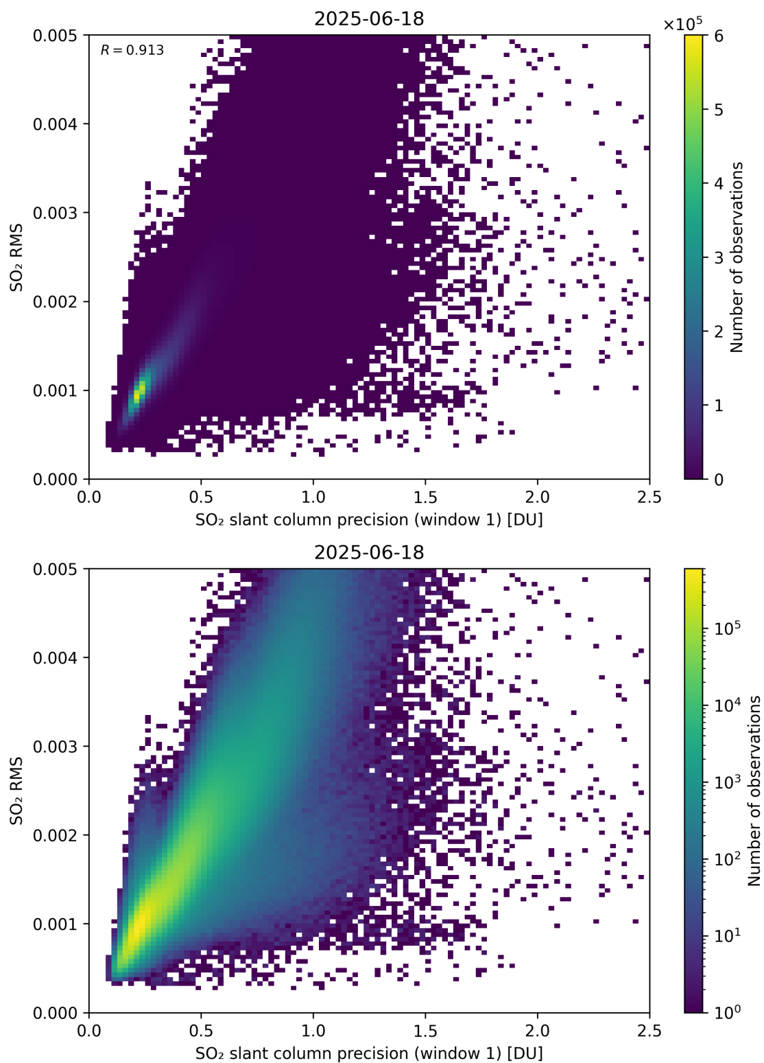
Figure 273: Scatter density plot of “SO 2 slant column precision (window 1)” against “SO 2 RMS” for 2025-06-17 to 2025-06-19.
