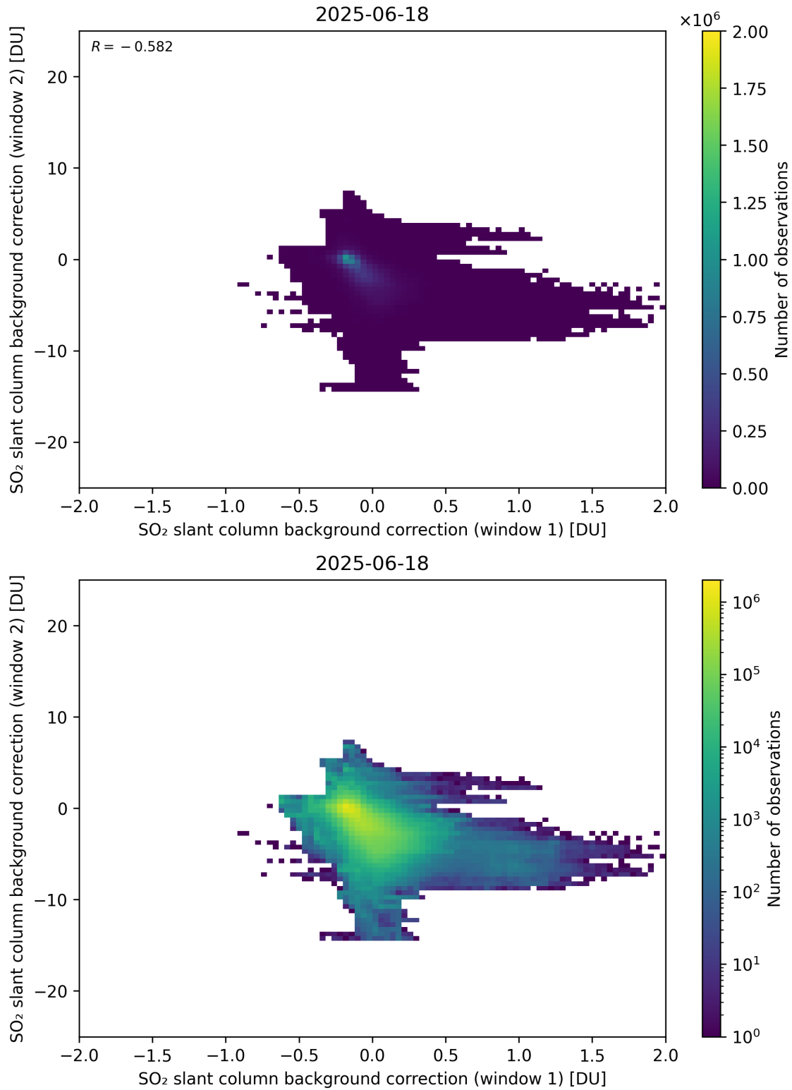
Figure 109: Scatter density plot of “SO 2 slant column background correction (window 1)” against “SO 2 slant column background correction (window 2)” for 2025-06-17 to 2025-06-19.
