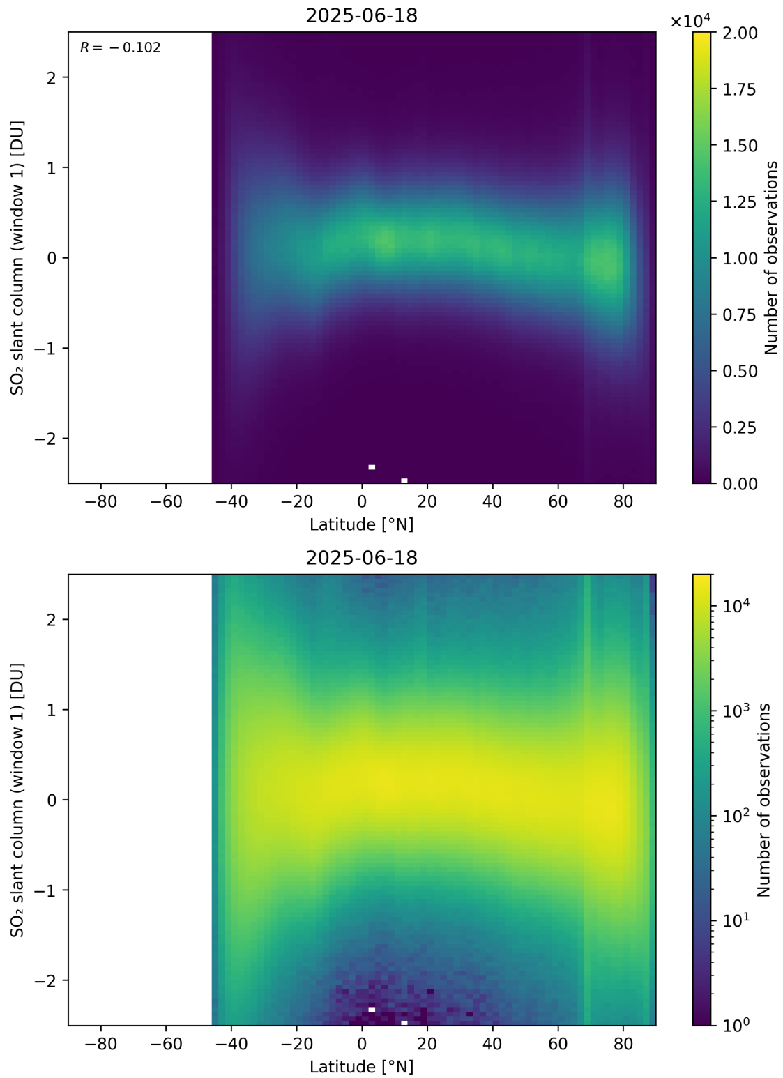
Figure 162: Scatter density plot of “Latitude” against “SO 2 slant column (window 1)” for 2025-06-17 to 2025-06-19.
