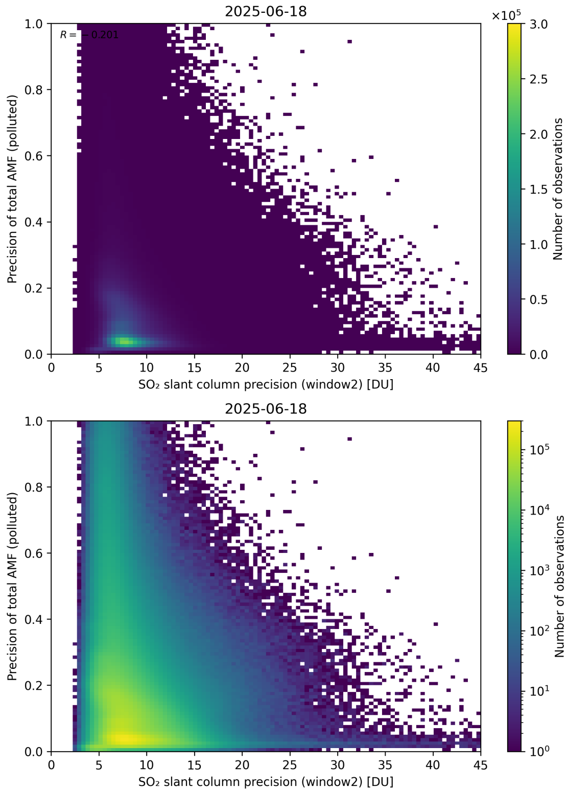
Figure 302: Scatter density plot of “SO 2 slant column precision (window2)” against “Precision of total AMF (polluted)” for 2025-06-17 to 2025-06-19.
