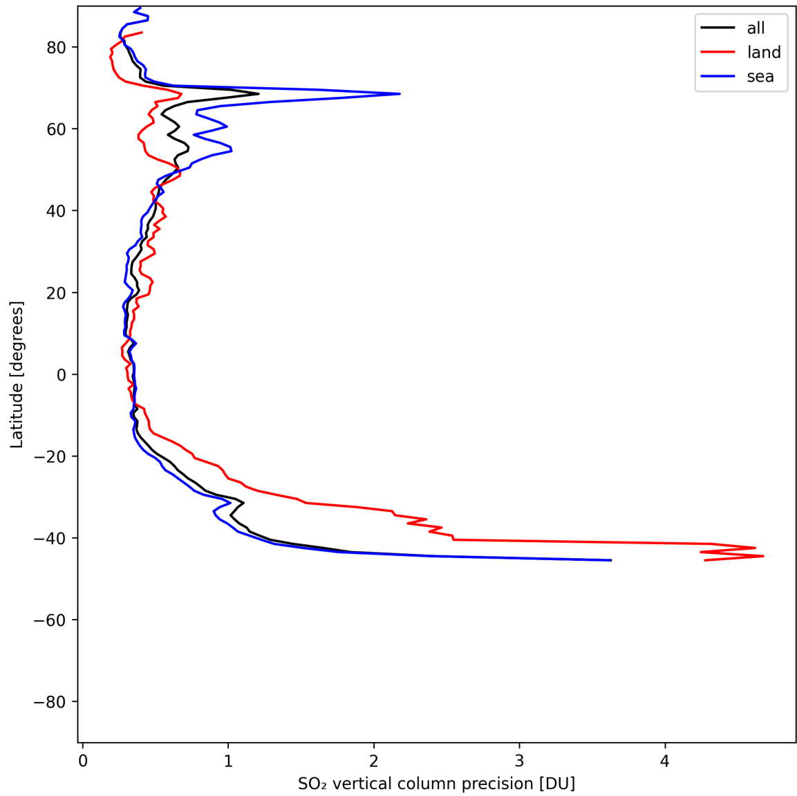
Figure 33: Zonal average of “SO 2 vertical column precision” for 2025-06-17 to 2025-06-19.
