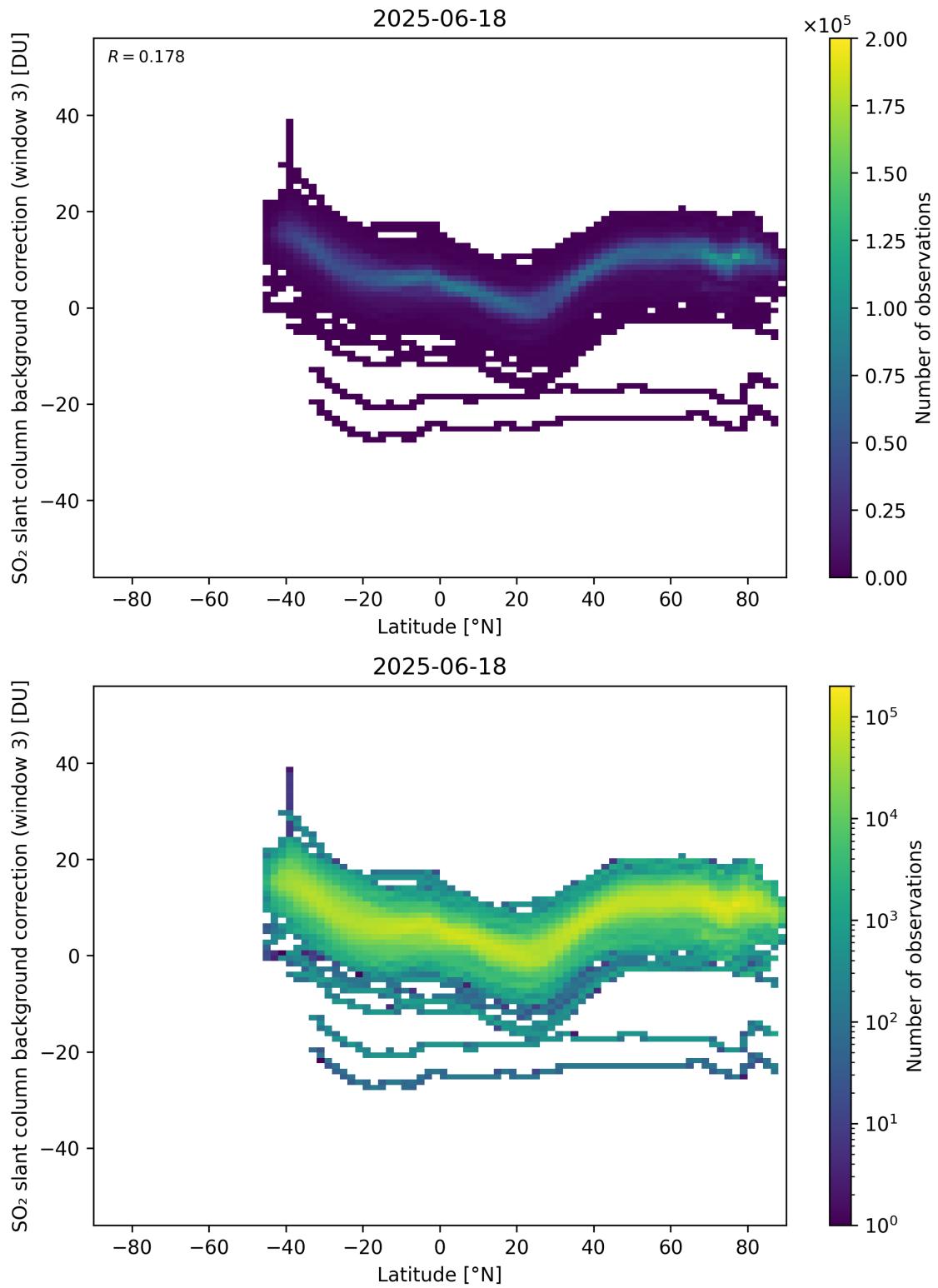
Figure 152: Scatter density plot of “Latitude” against “SO 2 slant column background correction (window 3)” for 2025-06-17 to 2025-06-19.
