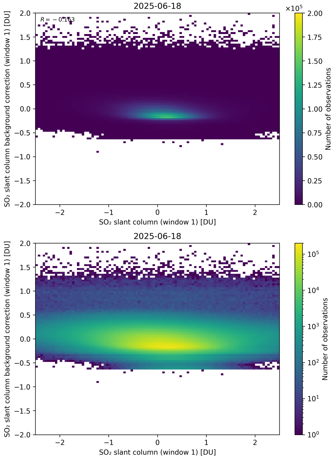
Figure 262: Scatter density plot of “SO 2 slant column (window 1)” against “SO 2 slant column background correction (window 1)” for 2025-06-17 to 2025-06-19.
