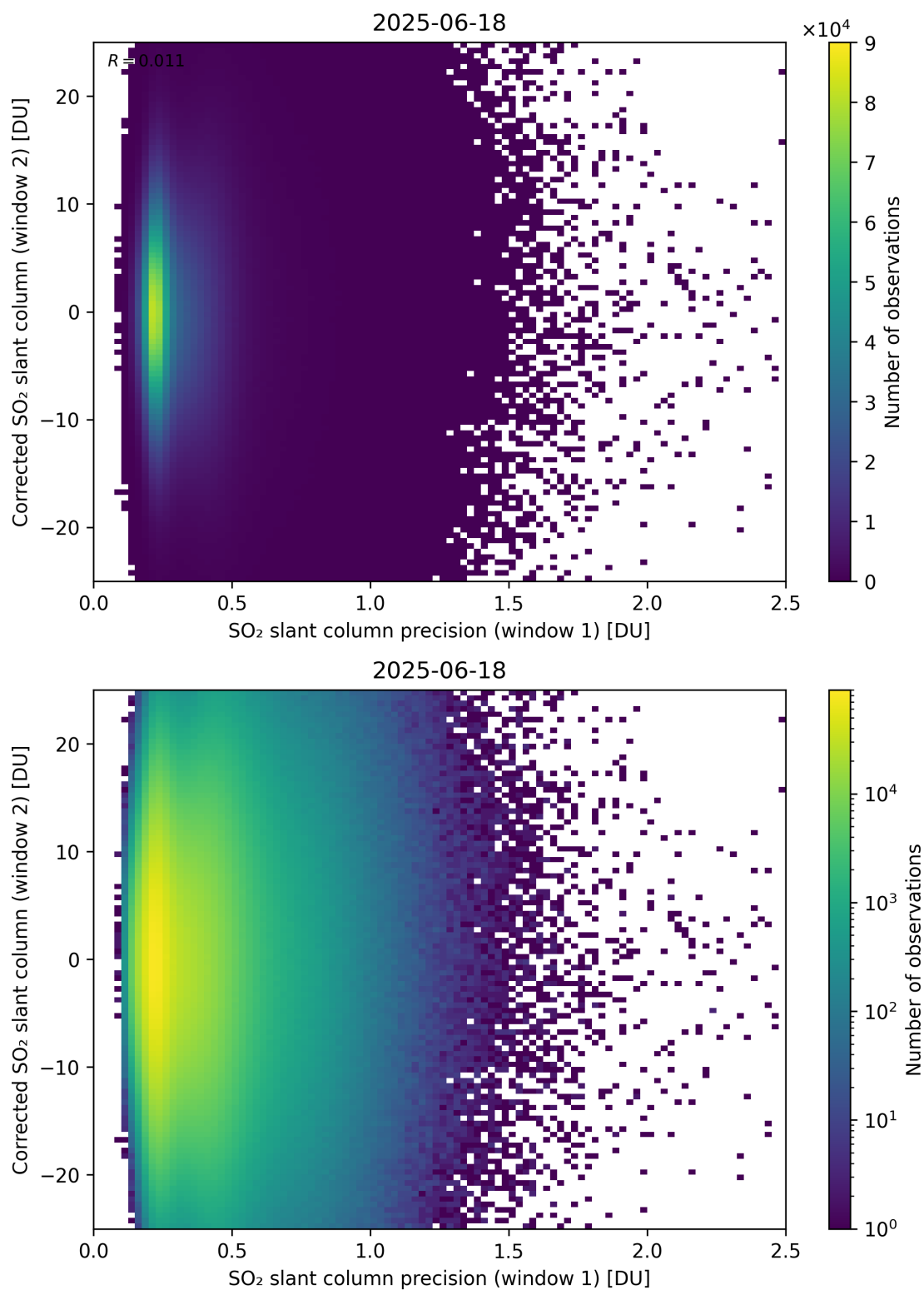
Figure 275: Scatter density plot of “SO 2 slant column precision (window 1)” against “Corrected SO 2 slant column (window 2)” for 2025-06-17 to 2025-06-19.
