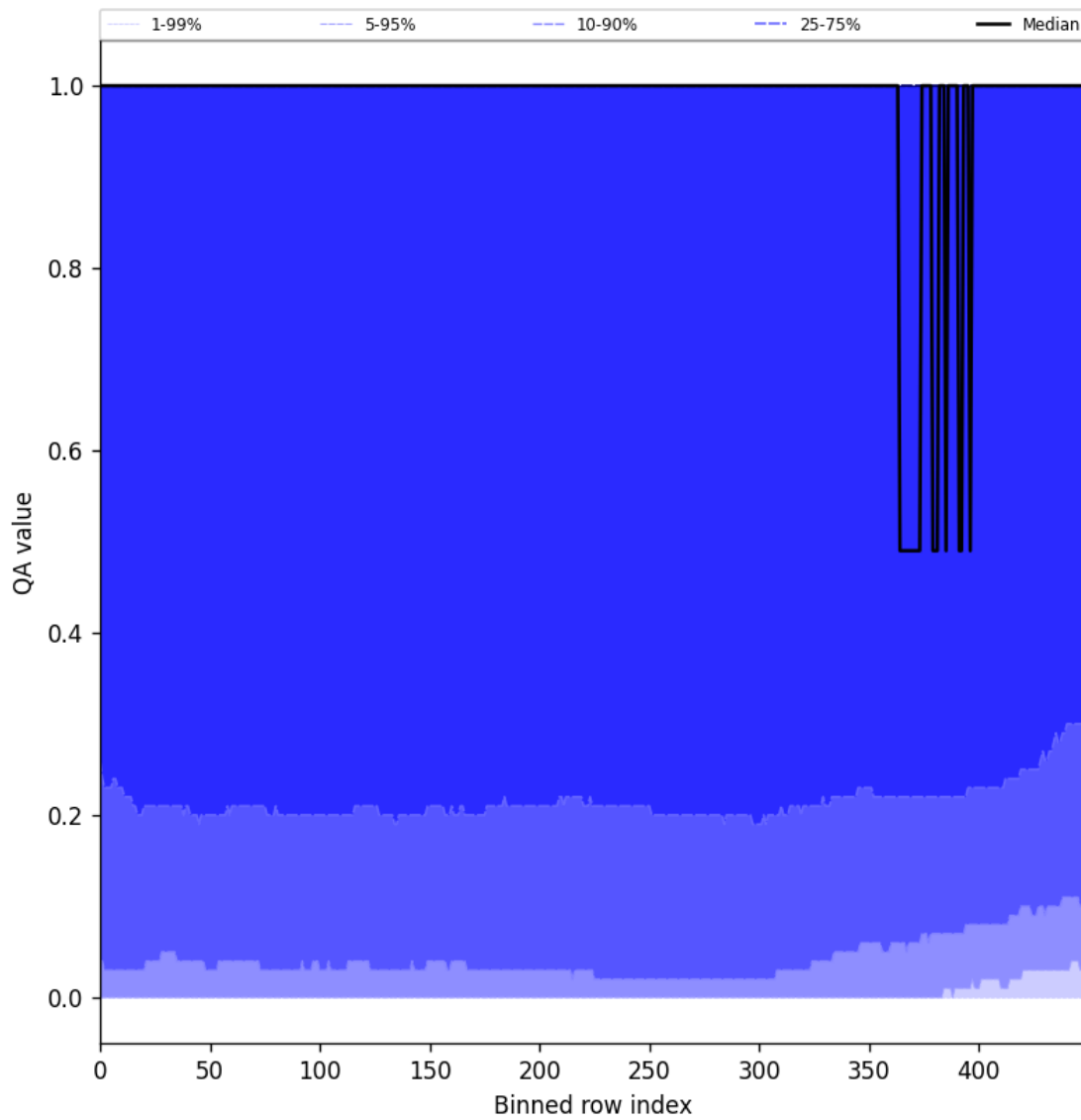
Figure 83: Along track statistics of “QA value” for 2025-06-17 to 2025-06-19
