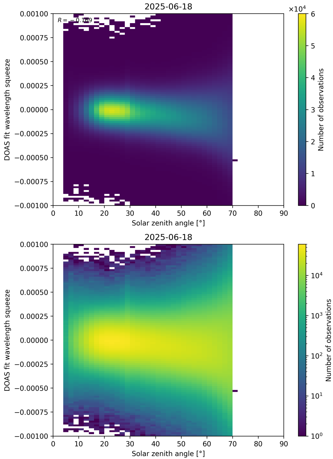
Figure 175: Scatter density plot of “Solar zenith angle” against “DOAS fit wavelength squeeze” for 2025-06-17 to 2025-06-19.
