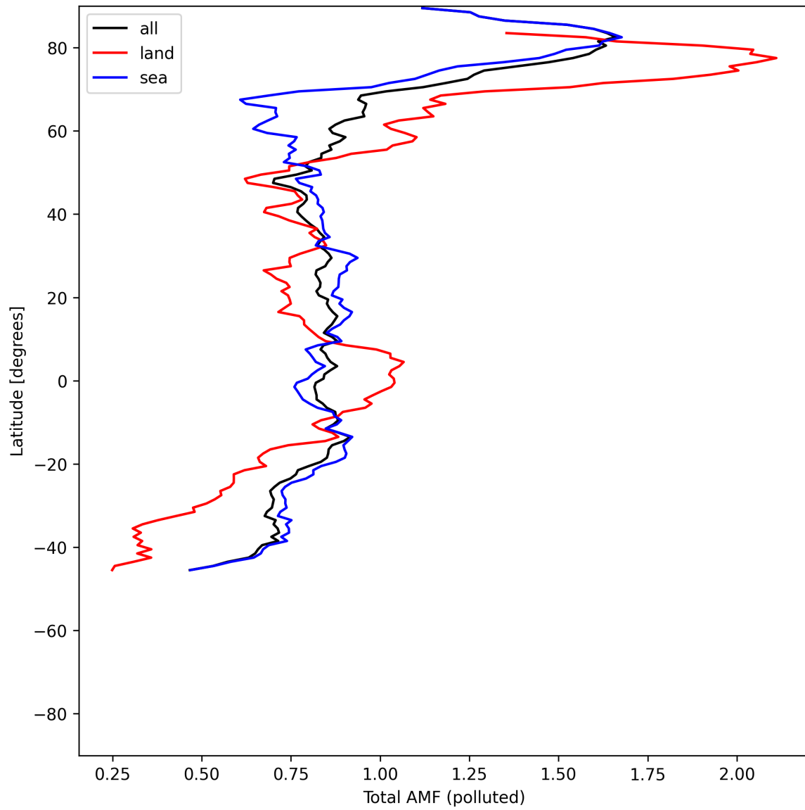
Figure 53: Zonal average of “Total AMF (polluted)” for 2025-06-17 to 2025-06-19.
