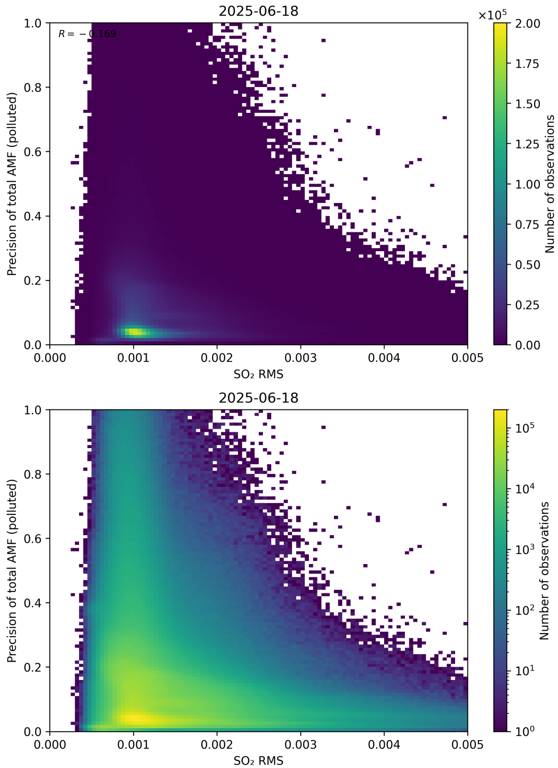
Figure 149: Scatter density plot of “SO 2 RMS” against “Precision of total AMF (polluted)” for 2025-06-17 to 2025-06-19.
