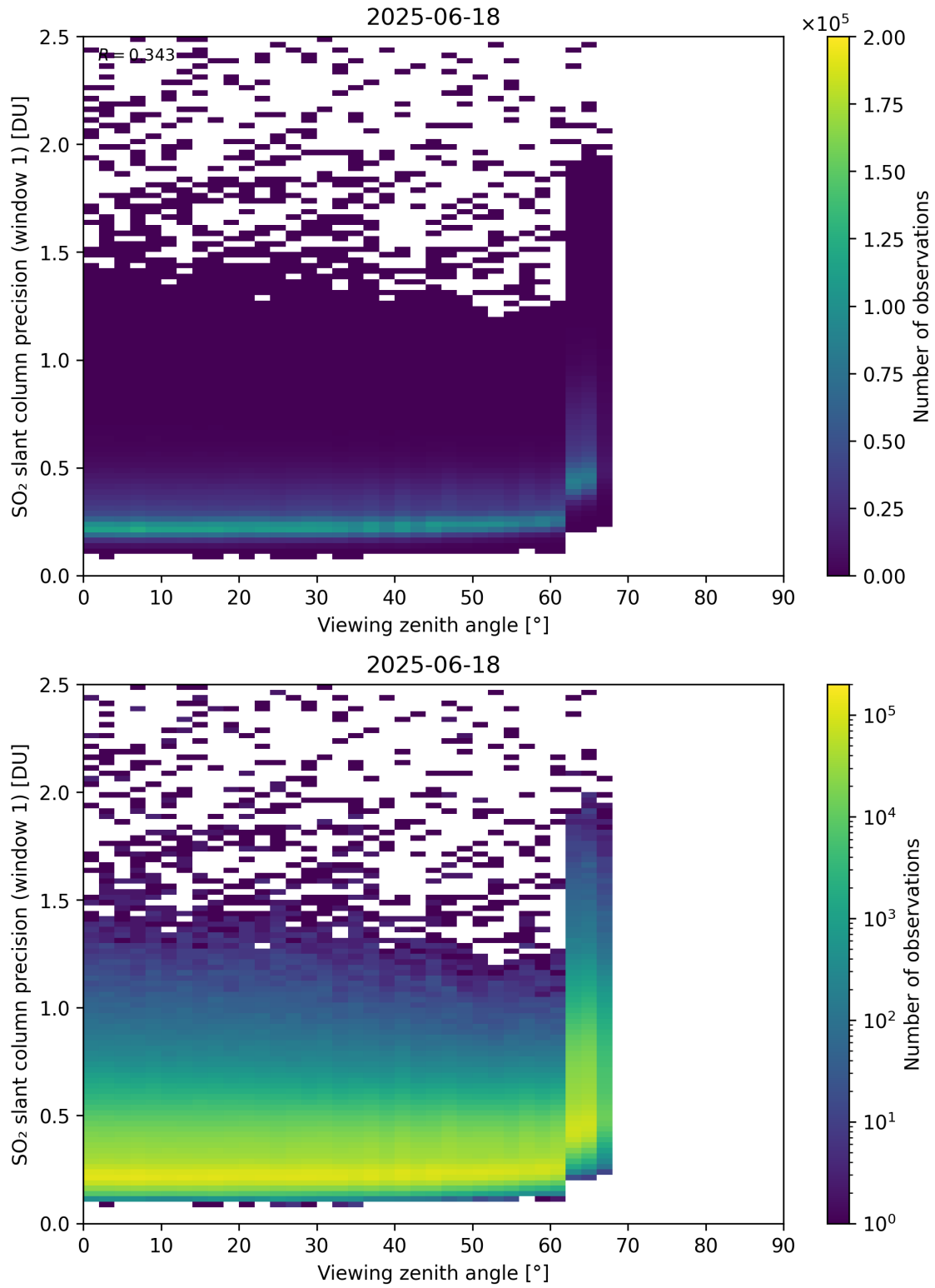
Figure 377: Scatter density plot of “Viewing zenith angle” against “SO 2 slant column precision (window 1)” for 2025-06-17 to 2025-06-19.
