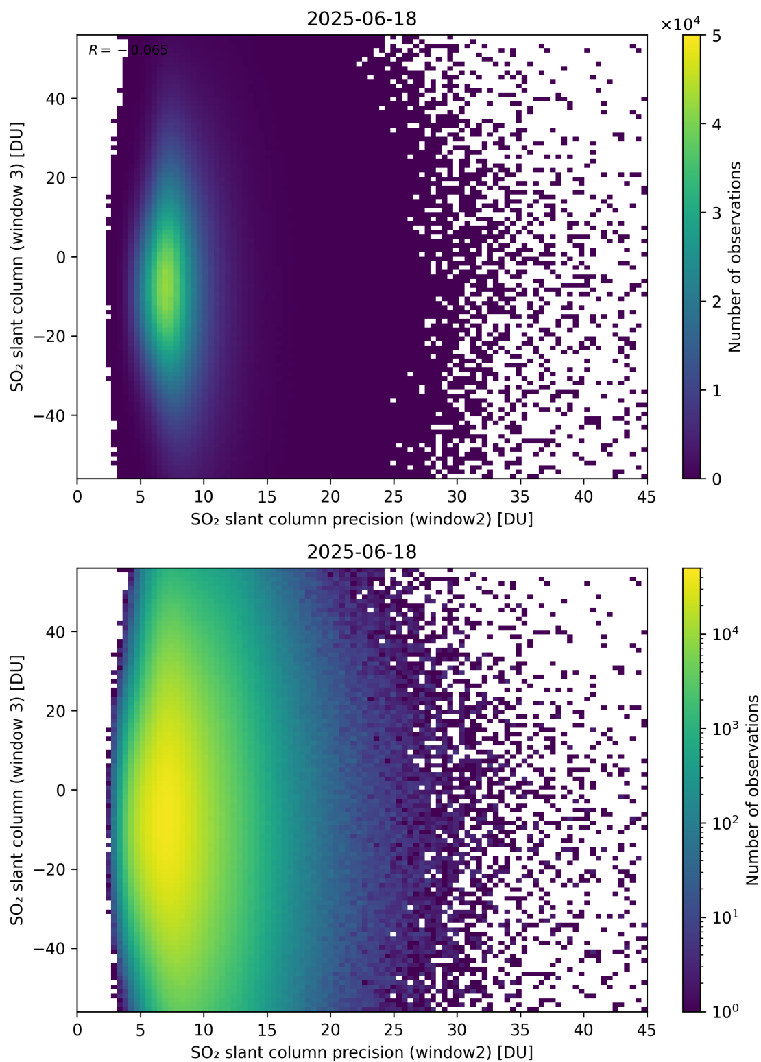
Figure 299: Scatter density plot of “SO 2 slant column precision (window2)” against “SO 2 slant column (window 3)” for 2025-06-17 to 2025-06-19.
