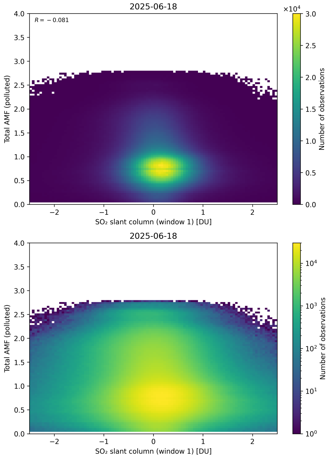
Figure 289: Scatter density plot of “SO 2 slant column (window 1)” against “Total AMF (polluted)” for 2025-06-17 to 2025-06-19.
