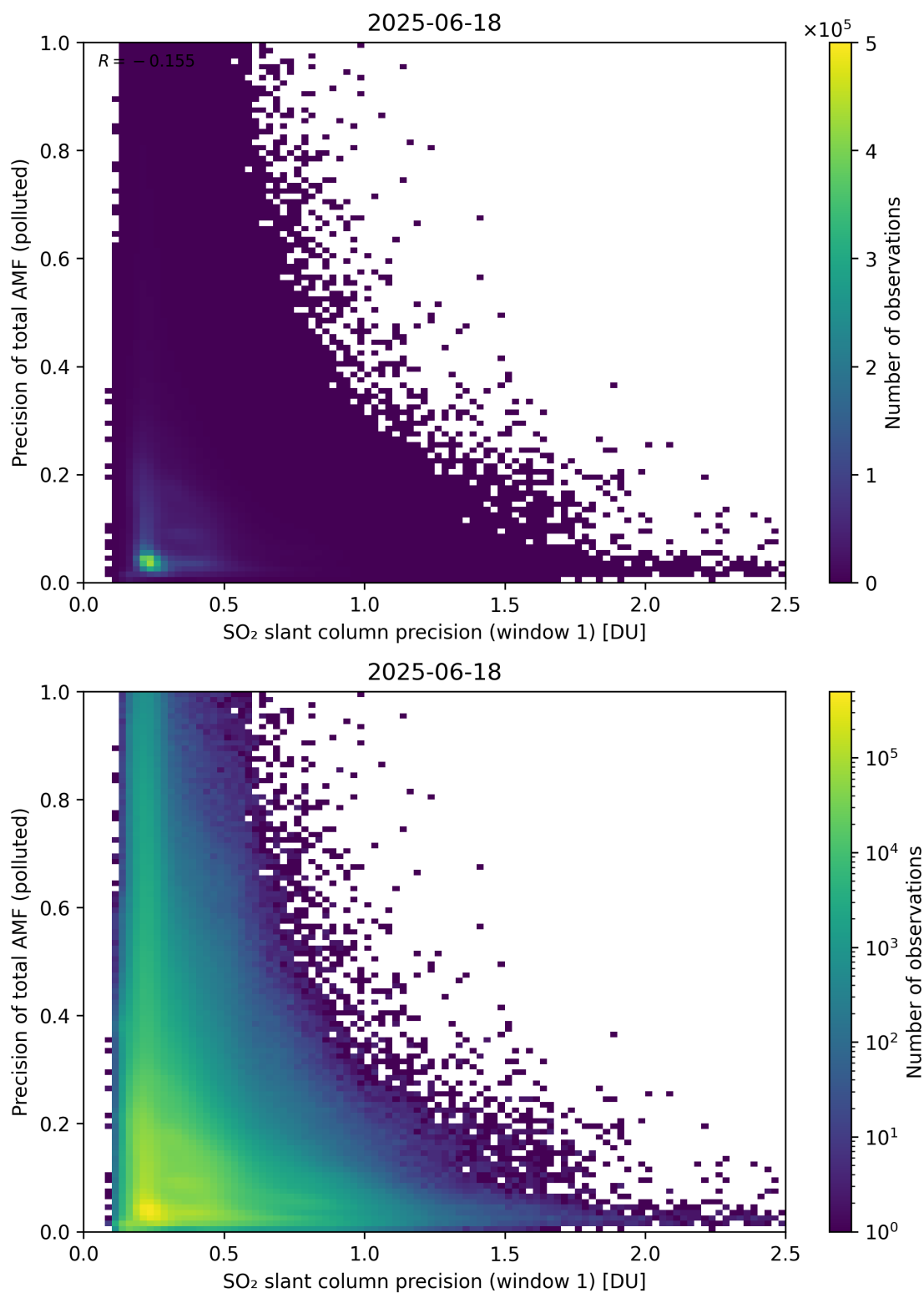
Figure 281: Scatter density plot of “SO 2 slant column precision (window 1)” against “Precision of total AMF (polluted)” for 2025-06-17 to 2025-06-19.
