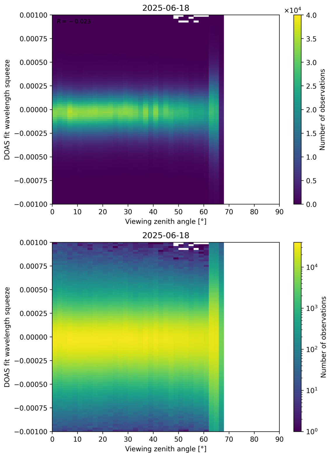
Figure 366: Scatter density plot of “Viewing zenith angle” against “DOAS fit wavelength squeeze” for 2025-06-17 to 2025-06-19.
