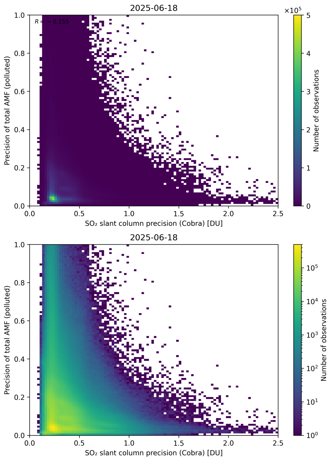
Figure 214: Scatter density plot of “SO 2 slant column precision (Cobra)” against “Precision of total AMF (polluted)” for 2025-06-17 to 2025-06-19.
