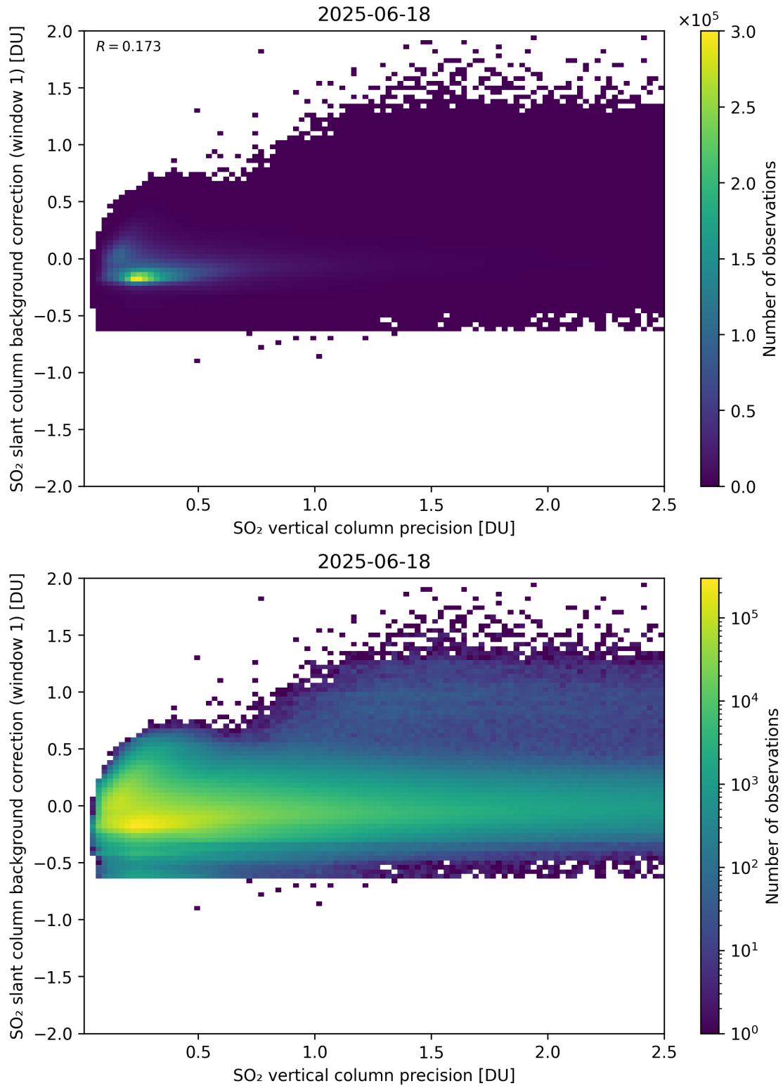
Figure 329: Scatter density plot of “SO 2 vertical column precision” against “SO 2 slant column background correction (window 1)” for 2025-06-17 to 2025-06-19.
