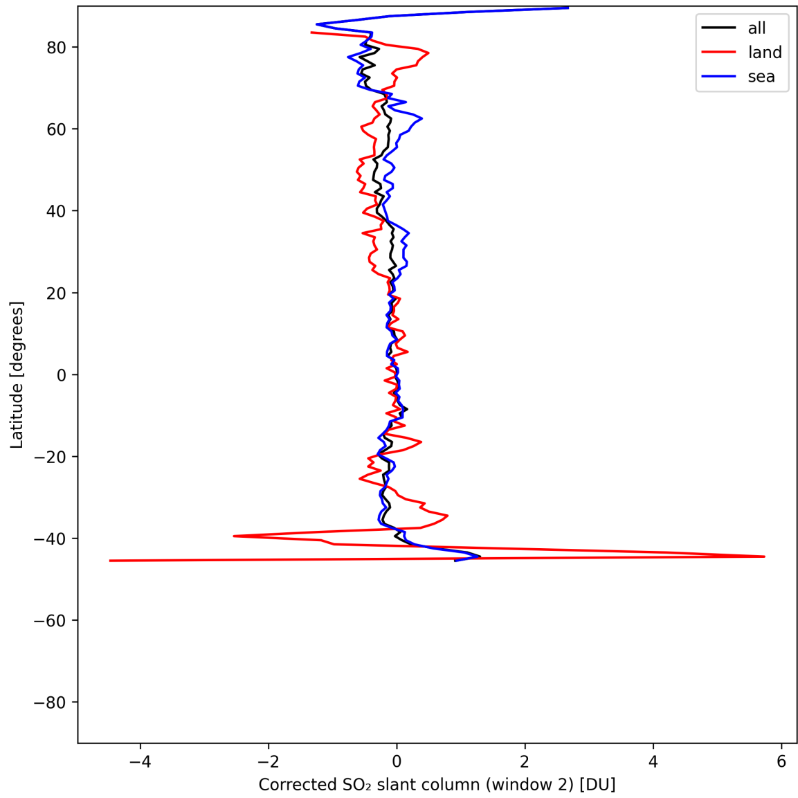
Figure 43: Zonal average of "Corrected SO 2 slant column (window 2)" for 2025-06-17 to 2025-06-19.
