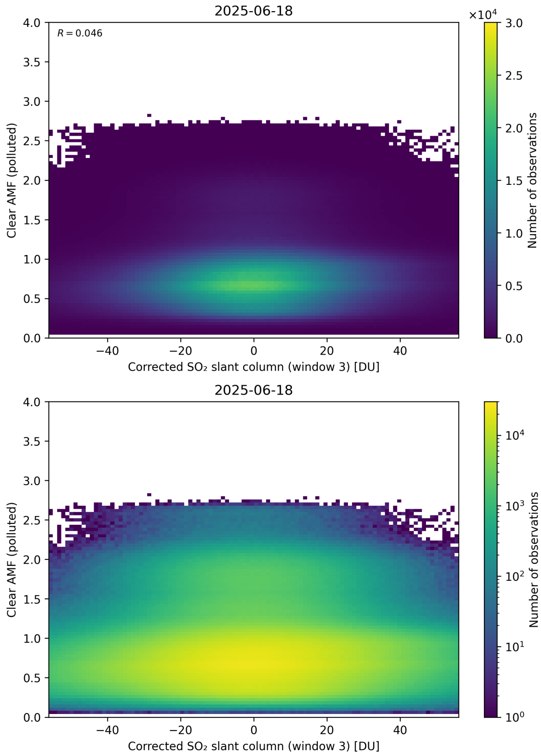
Figure 259: Scatter density plot of “Corrected SO 2 slant column (window 3)” against “Clear AMF (polluted)” for 2025-06-17 to 2025-06-19.
