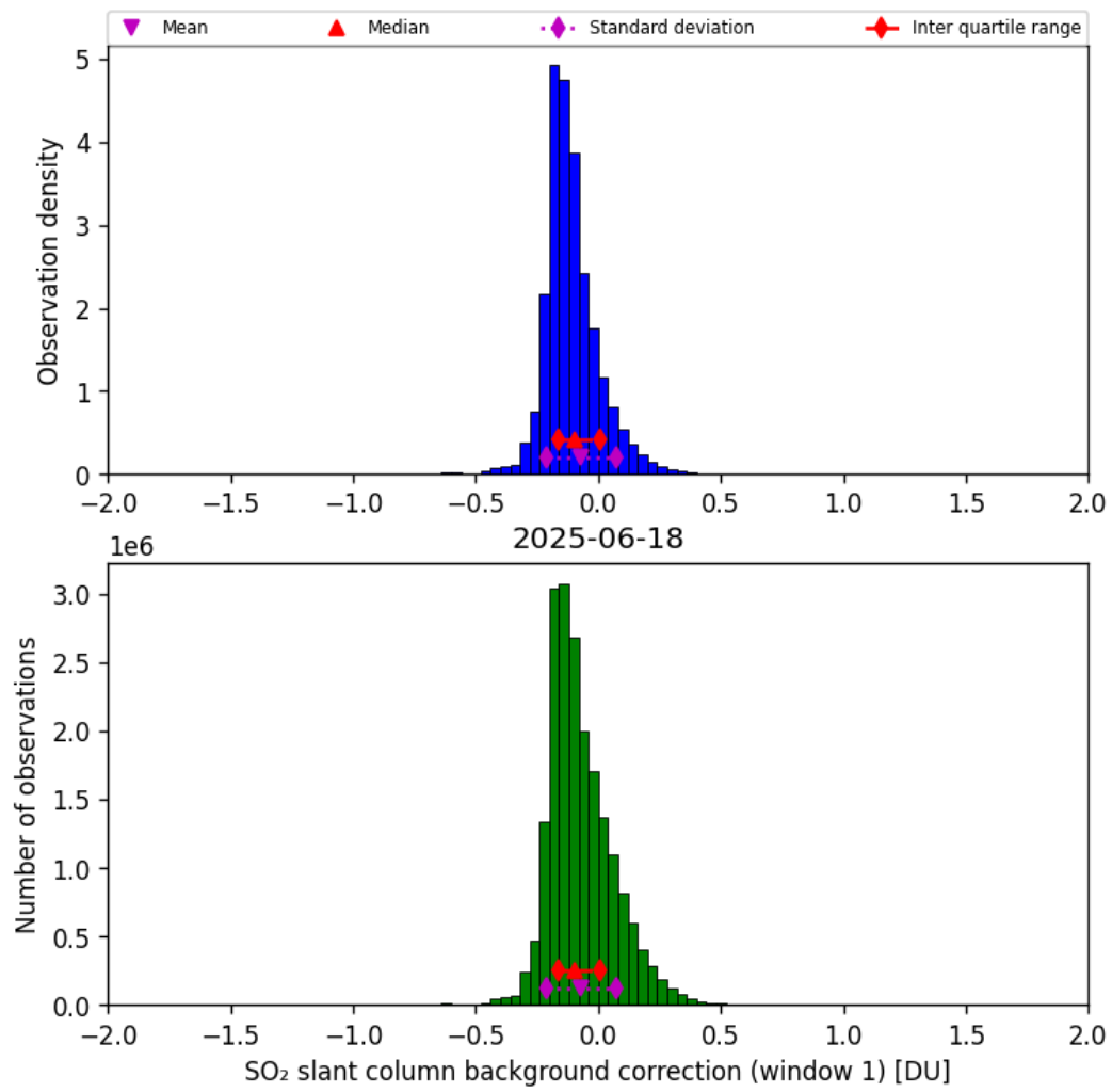
Figure 66: Histogram of “SO 2 slant column background correction (window 1)” for 2025-06-17 to 2025-06-19
