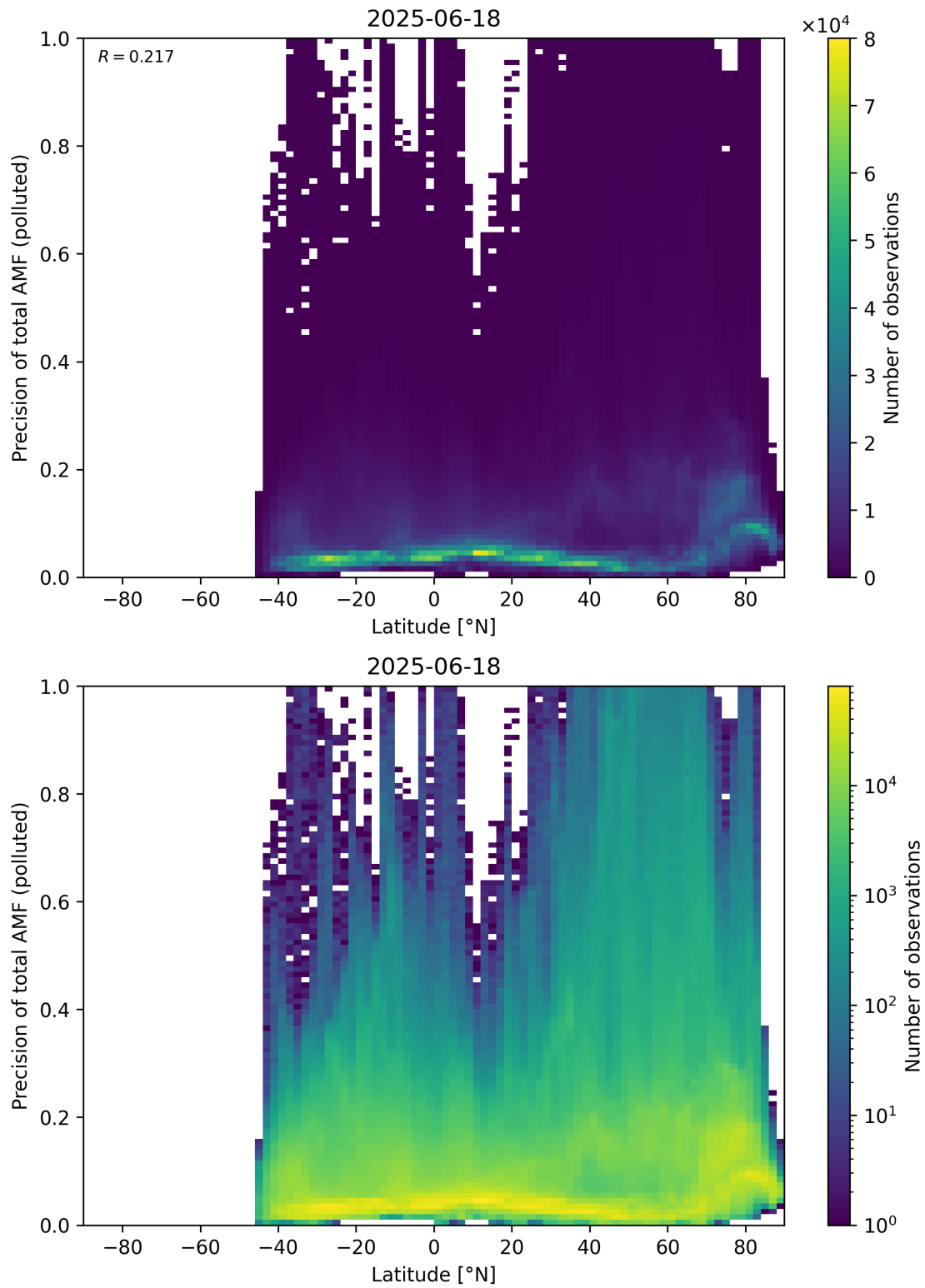
Figure 168: Scatter density plot of “Latitude” against “Precision of total AMF (polluted)” for 2025-06-17 to 2025-06-19.
