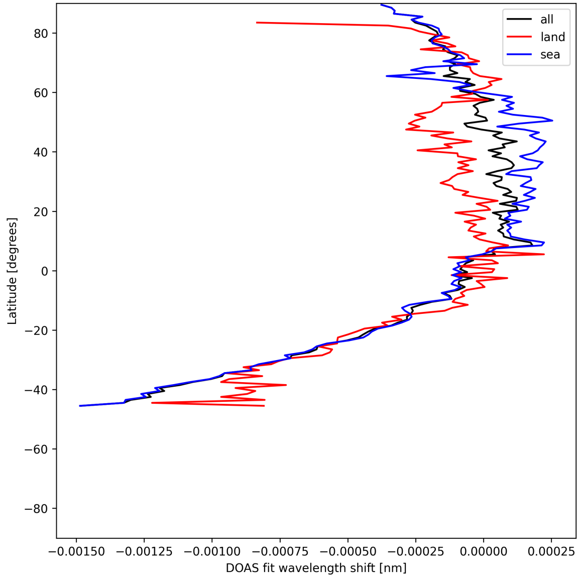
Figure 50: Zonal average of “DOAS fit wavelength shift” for 2025-06-17 to 2025-06-19.
