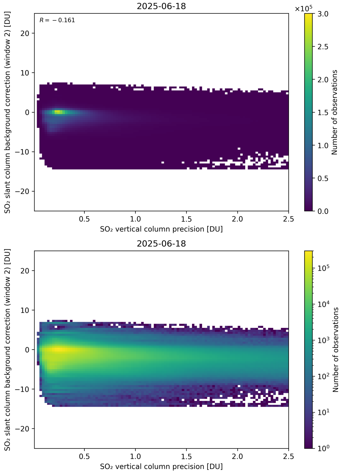
Figure 330: Scatter density plot of “SO 2 vertical column precision” against “SO 2 slant column background correction (window 2)” for 2025-06-17 to 2025-06-19.
