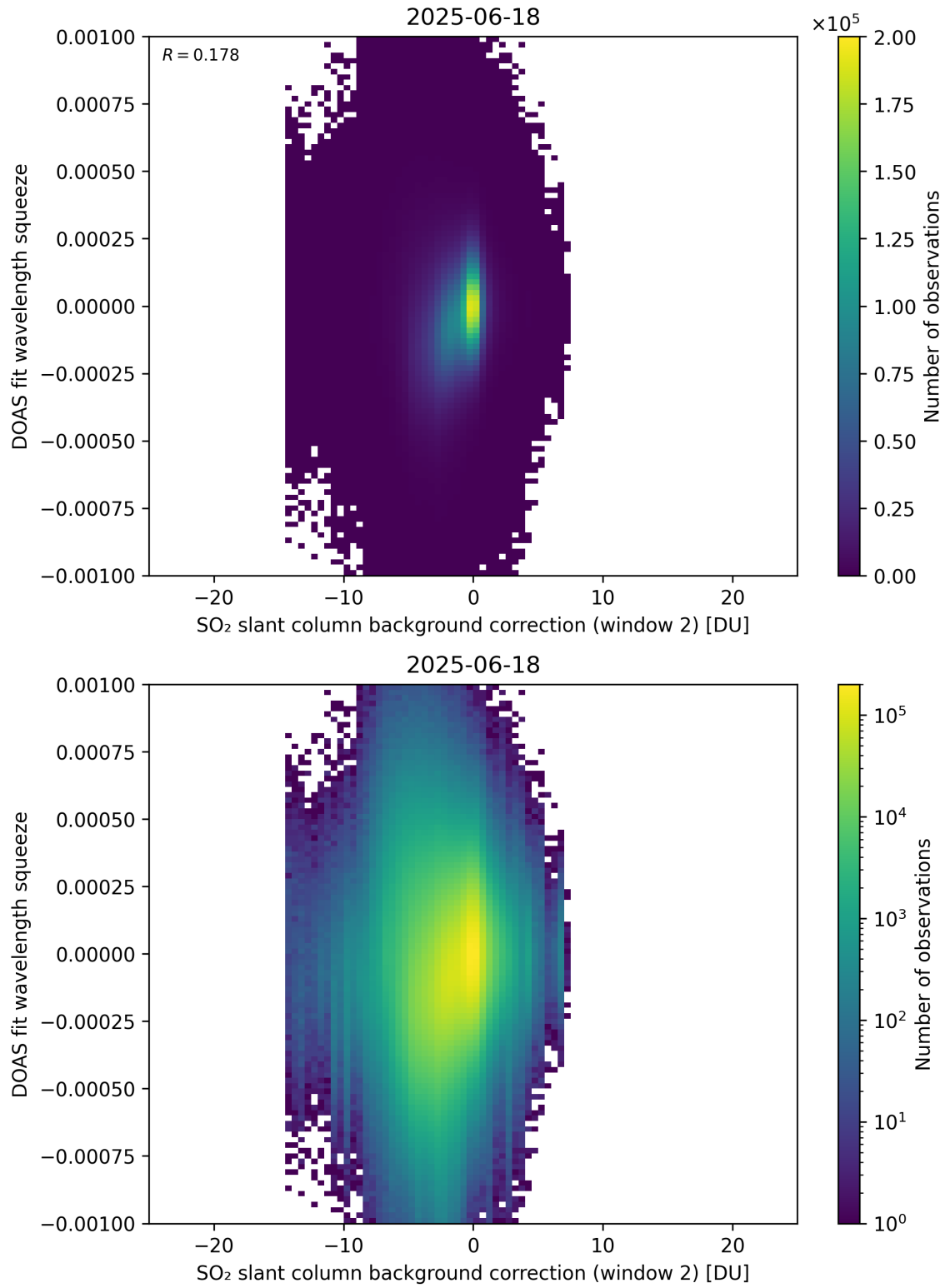
Figure 124: Scatter density plot of “SO 2 slant column background correction (window 2)” against “DOAS fit wavelength squeeze” for 2025-06-17 to 2025-06-19.
