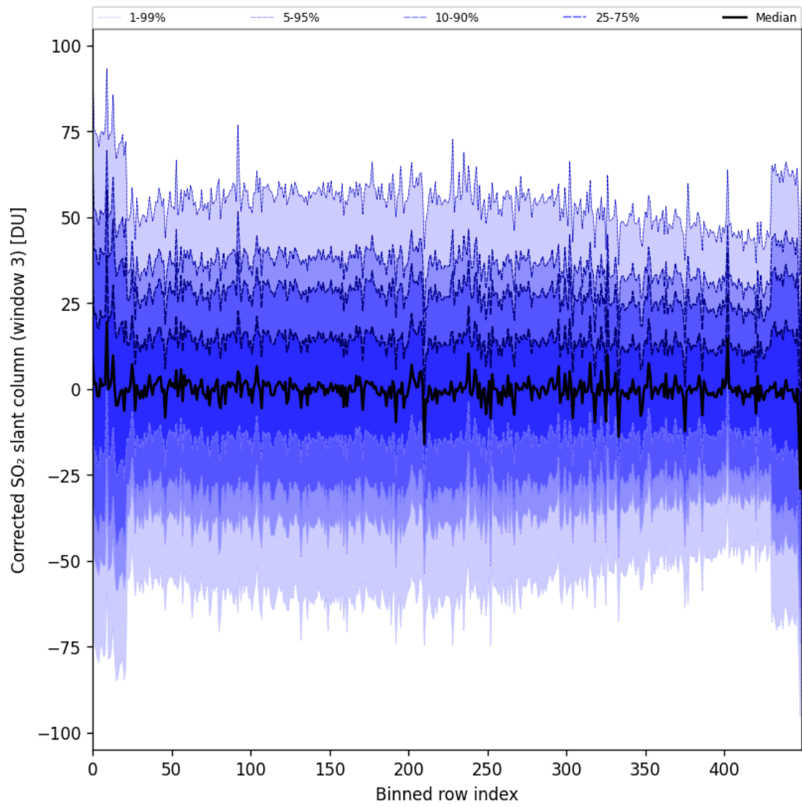
Figure 99: Along track statistics of “Corrected SO 2 slant column (window 3)” for 2025-06-17 to 2025-06-19
