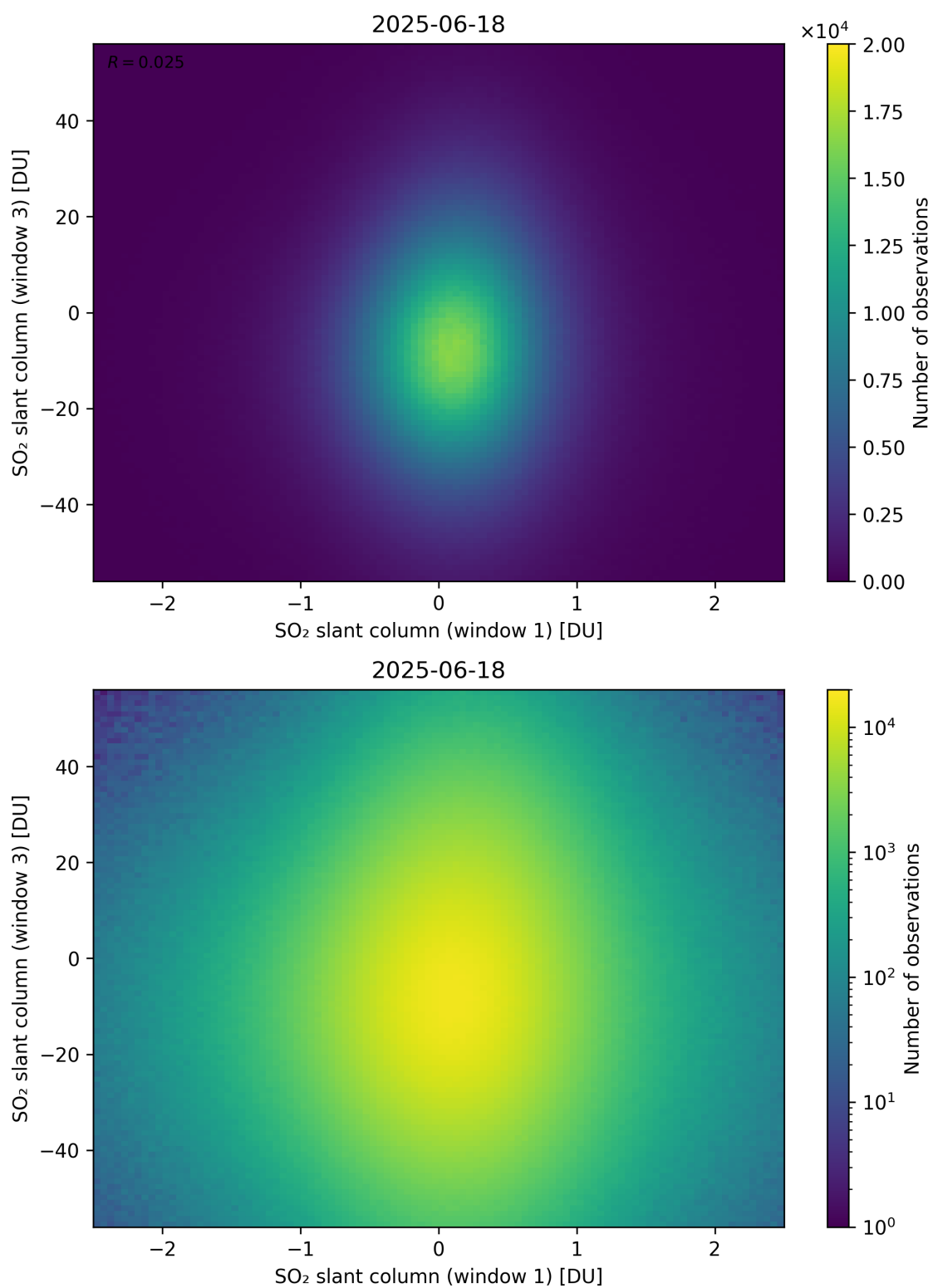
Figure 287: Scatter density plot of “SO 2 slant column (window 1)” against “SO 2 slant column (window 3)” for 2025-06-17 to 2025-06-19.
