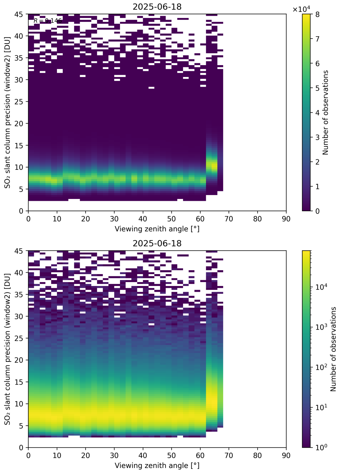
Figure 378: Scatter density plot of “Viewing zenith angle” against “SO 2 slant column precision (window2)” for 2025-06-17 to 2025-06-19.
