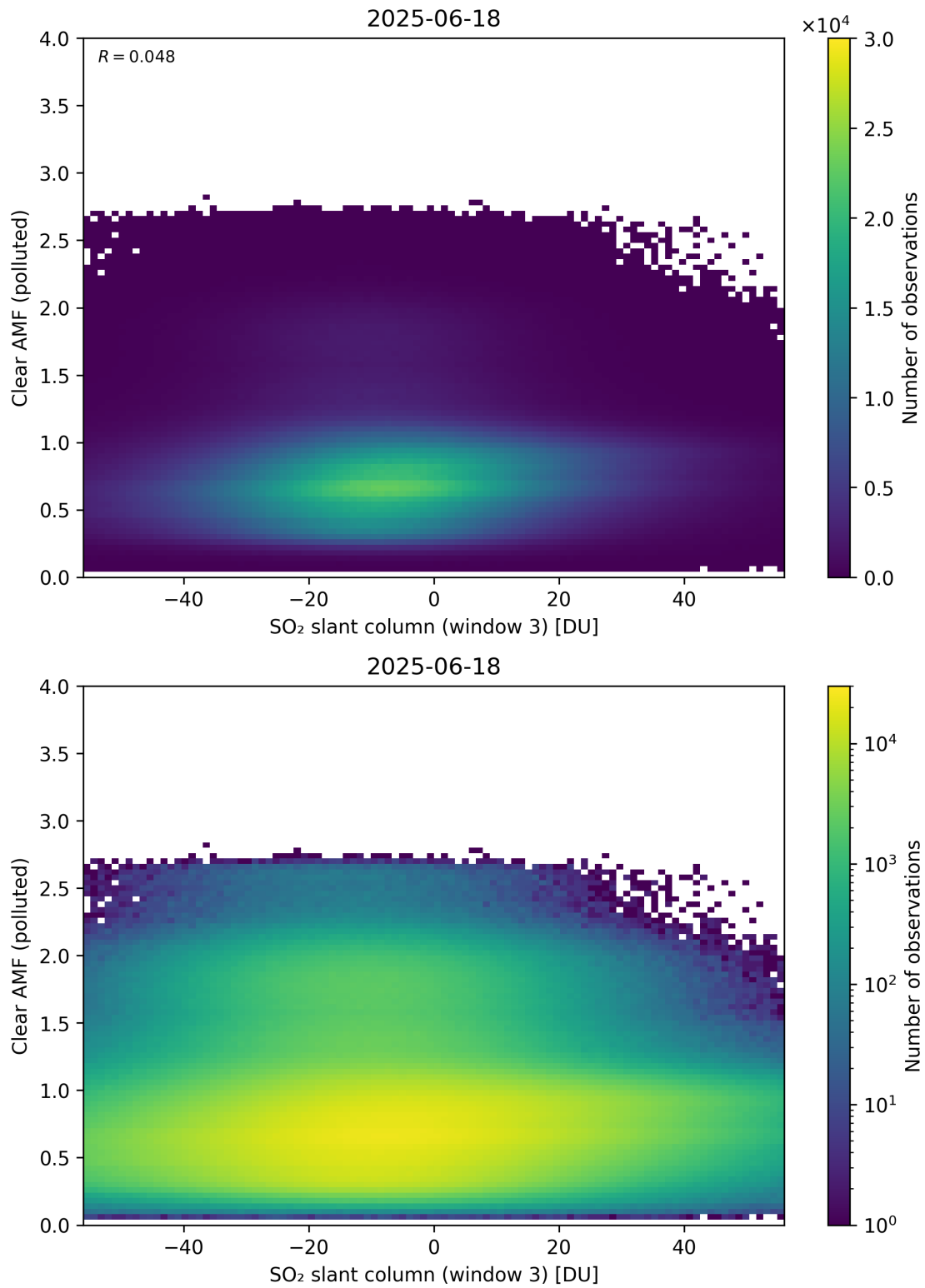
Figure 315: Scatter density plot of “SO 2 slant column (window 3)” against “Clear AMF (polluted)” for 2025-06-17 to 2025-06-19.
