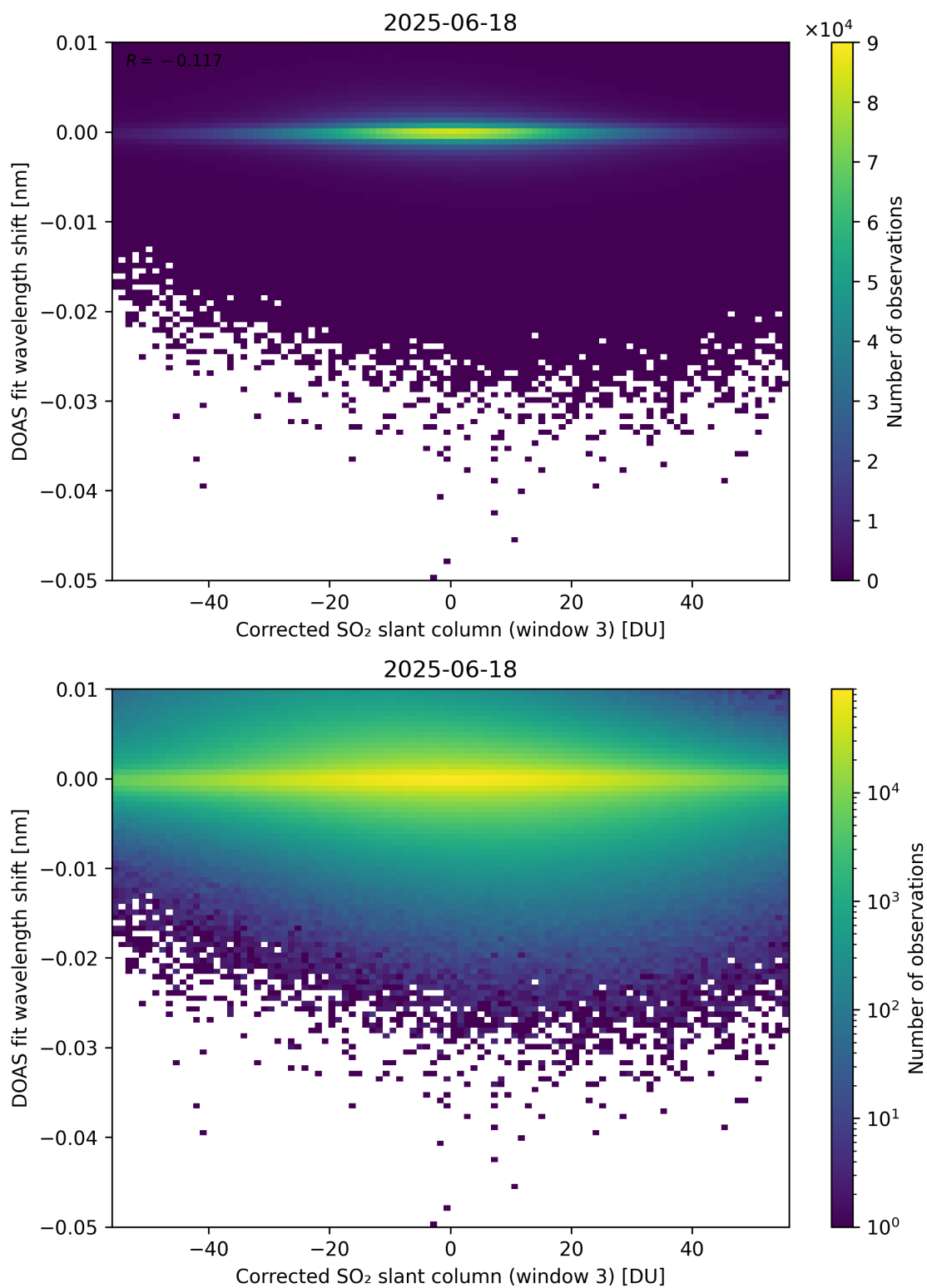
Figure 256: Scatter density plot of “Corrected SO 2 slant column (window 3)” against “DOAS fit wavelength shift” for 2025-06-17 to 2025-06-19.
