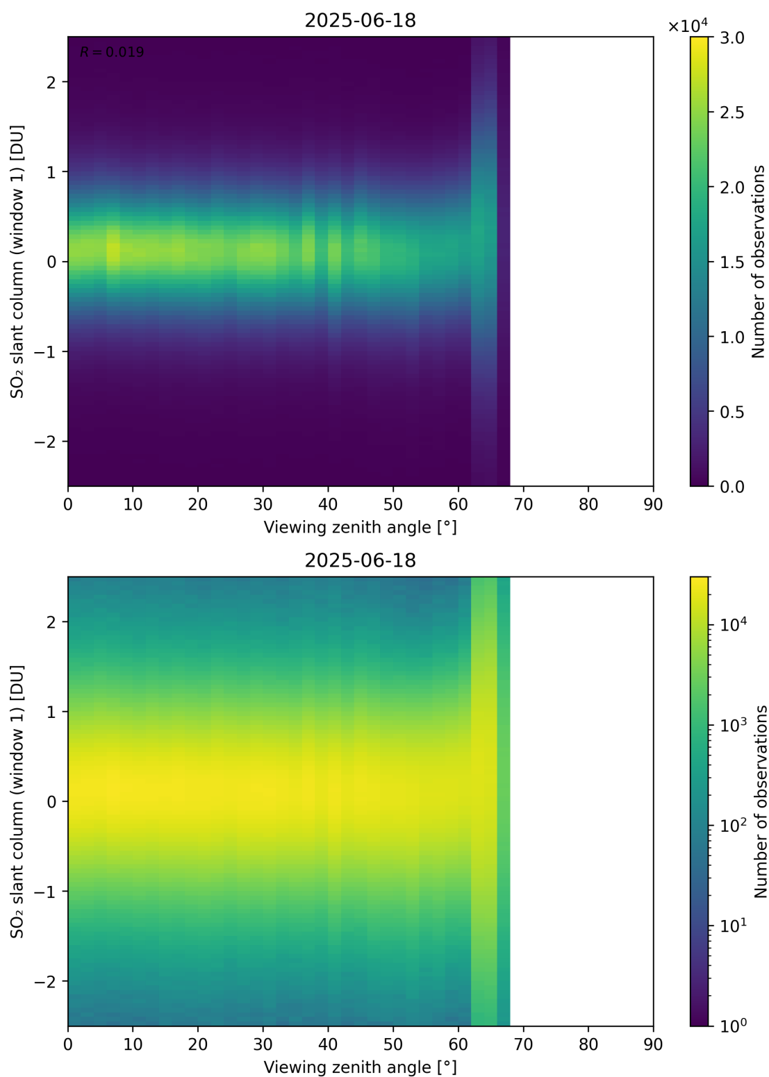
Figure 376: Scatter density plot of “Viewing zenith angle” against “SO 2 slant column (window 1)” for 2025-06-17 to 2025-06-19.
