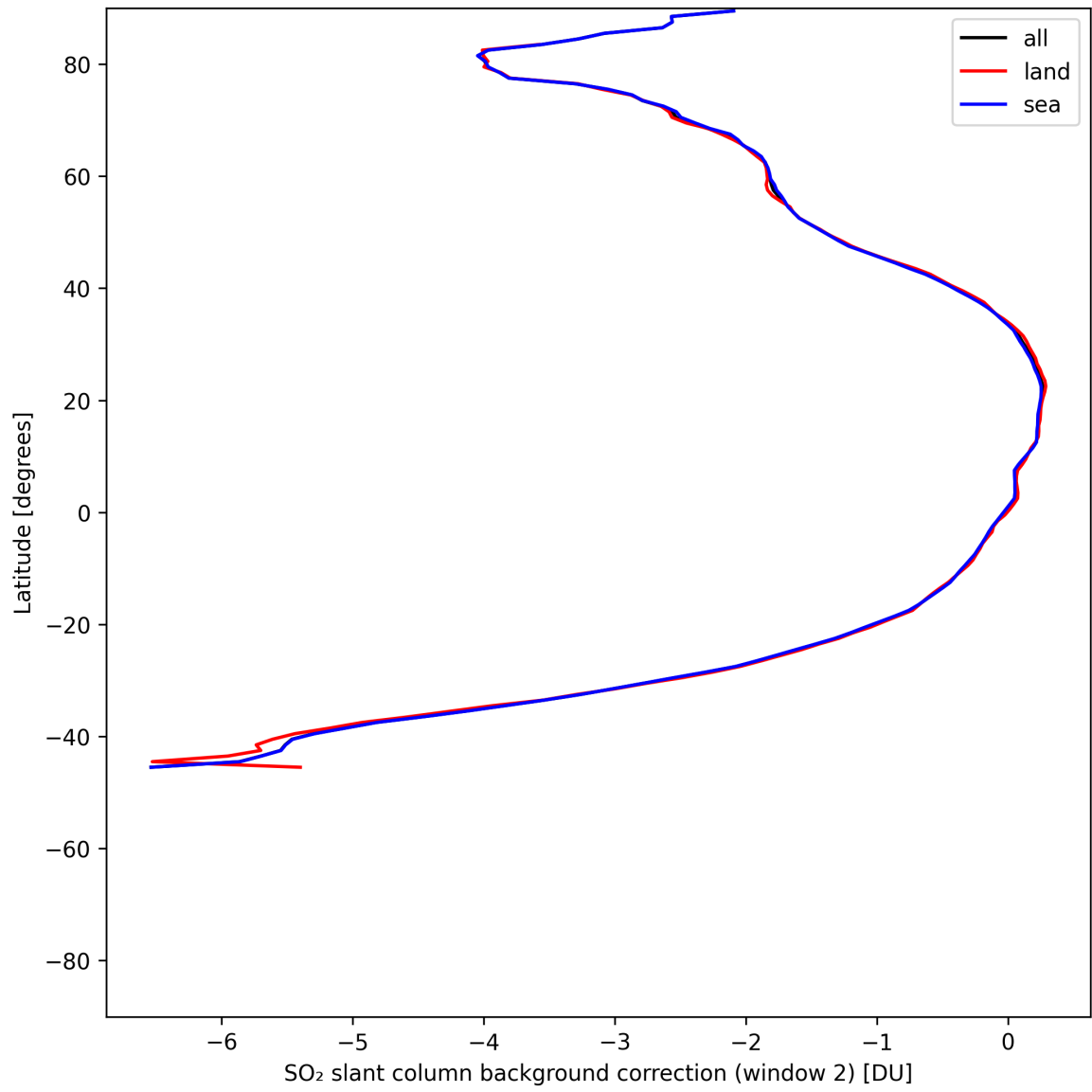
Figure 44: Zonal average of “SO 2 slant column background correction (window 2)” for 2025-06-17 to 2025-06-19.
