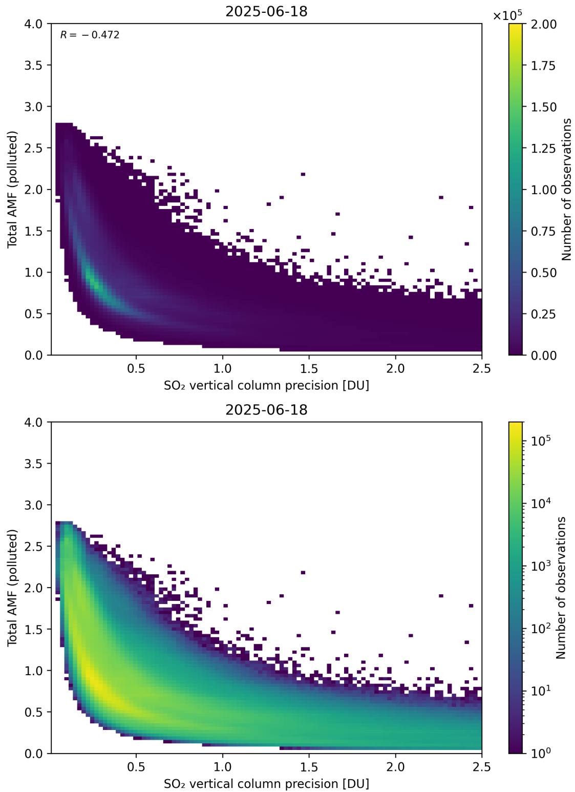
Figure 346: Scatter density plot of “SO 2 vertical column precision” against “Total AMF (polluted)” for 2025-06-17 to 2025-06-19.
