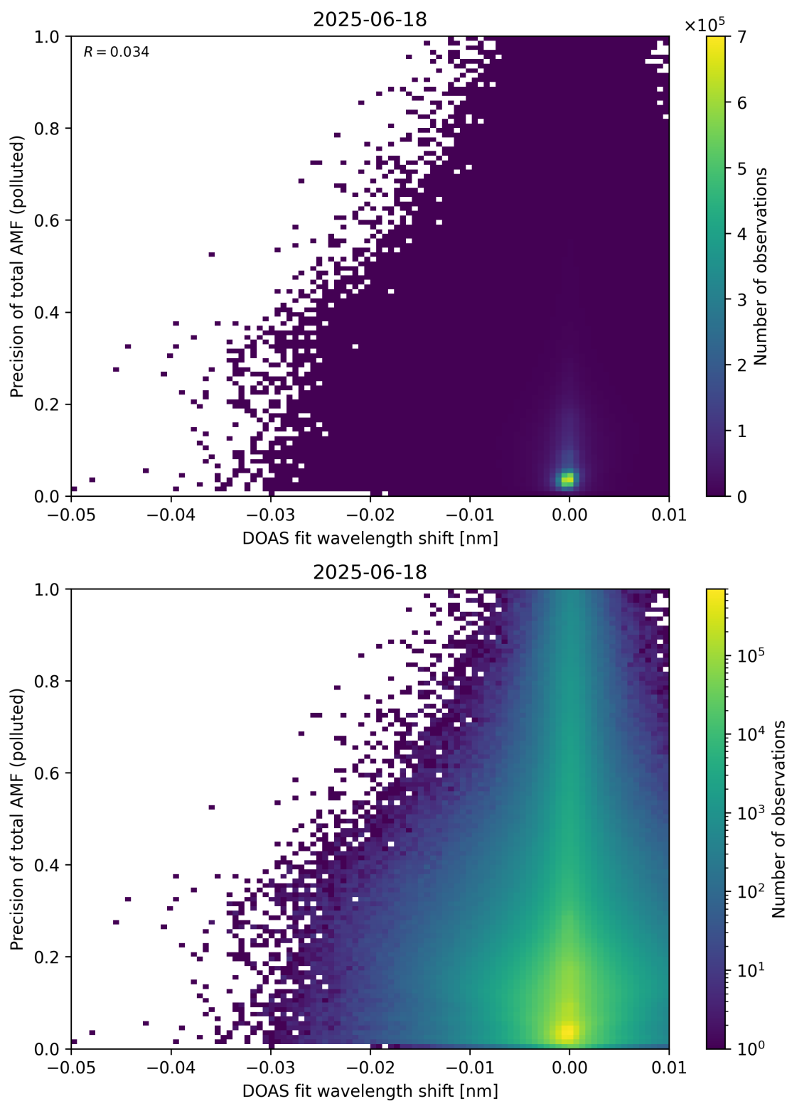
Figure 142: Scatter density plot of “DOAS fit wavelength shift” against “Precision of total AMF (polluted)” for 2025-06-17 to 2025-06-19.
