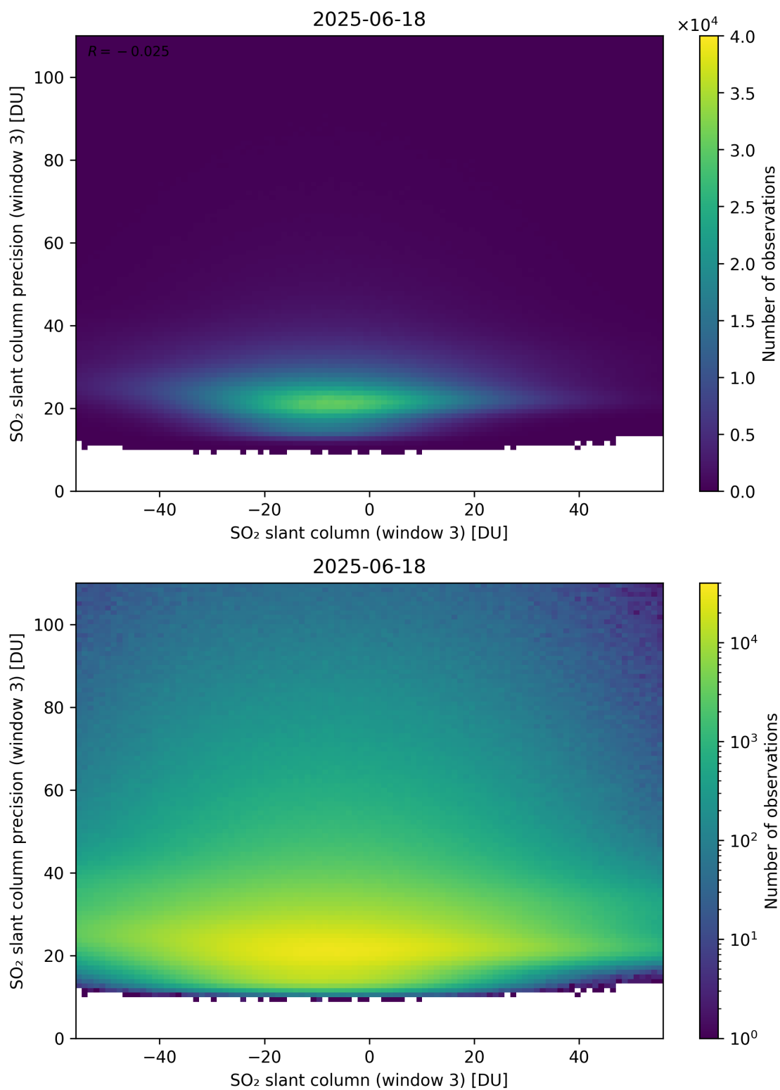
Figure 317: Scatter density plot of “SO 2 slant column (window 3)” against “SO 2 slant column precision (window 3)” for 2025-06-17 to 2025-06-19.
