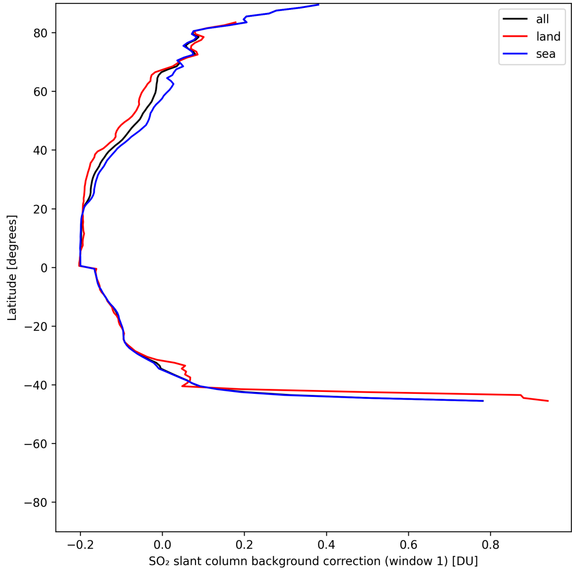
Figure 40: Zonal average of “SO 2 slant column background correction (window 1)” for 2025-06-17 to 2025-06-19.
