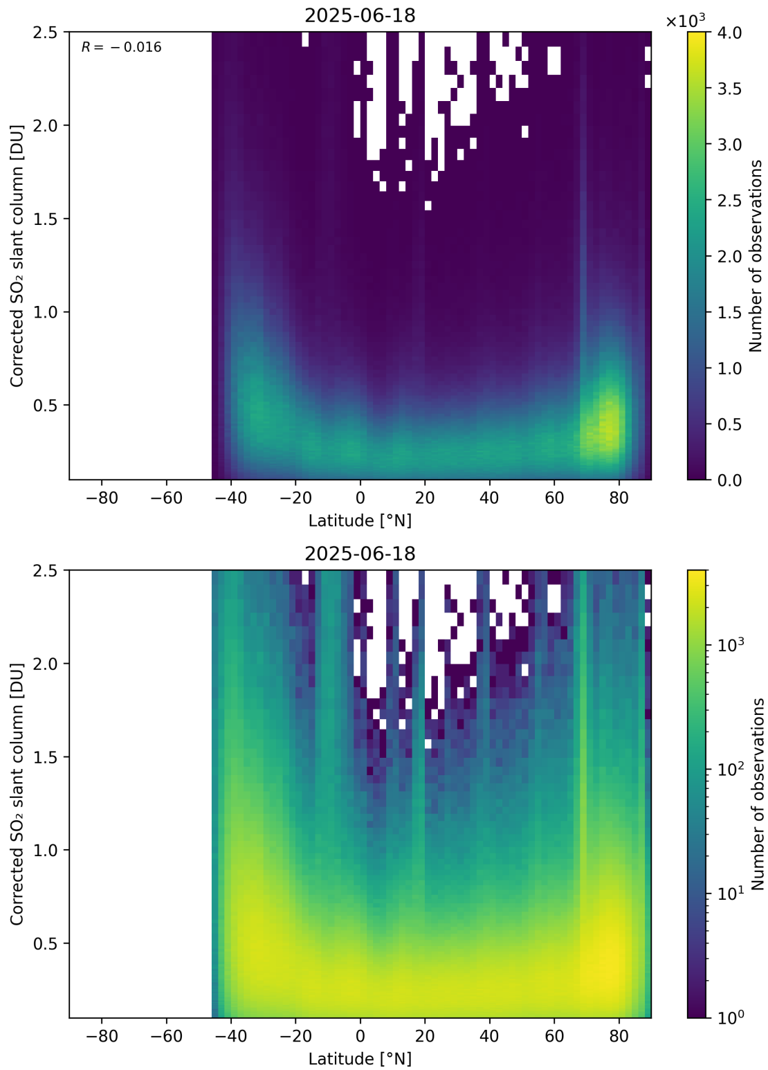
Figure 159: Scatter density plot of “Latitude” against “Corrected SO 2 slant column” for 2025-06-17 to 2025-06-19.
