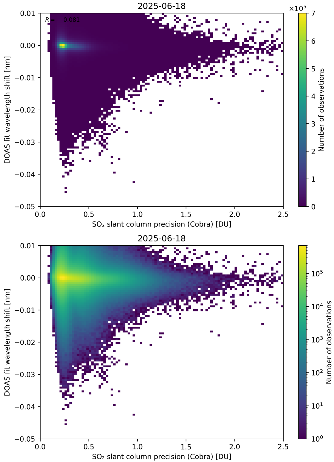
Figure 202: Scatter density plot of “SO 2 slant column precision (Cobra)” against “DOAS fit wavelength shift” for 2025-06-17 to 2025-06-19.
