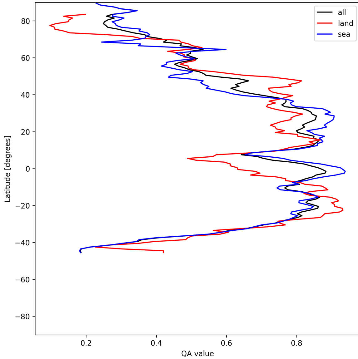
Figure 31: Zonal average of “QA value” for 2025-06-17 to 2025-06-19.
