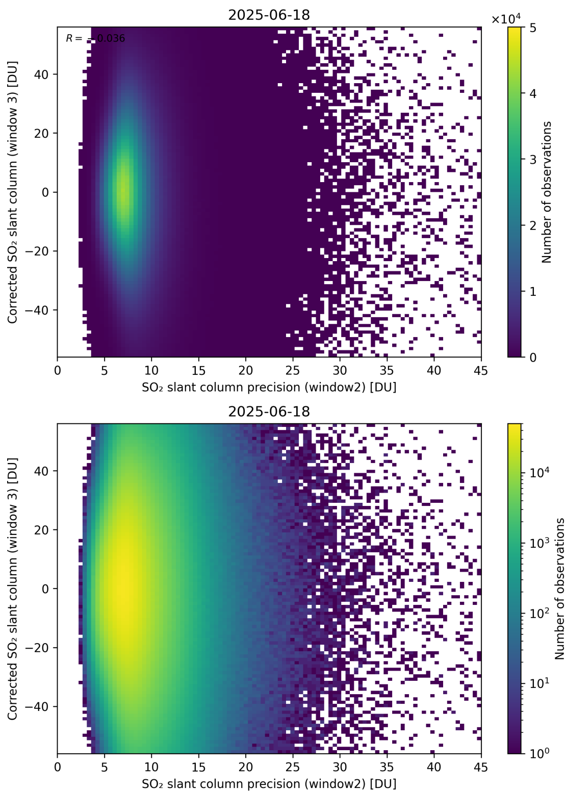
Figure 298: Scatter density plot of “SO 2 slant column precision (window2)” against “Corrected SO 2 slant column (window 3)” for 2025-06-17 to 2025-06-19.
