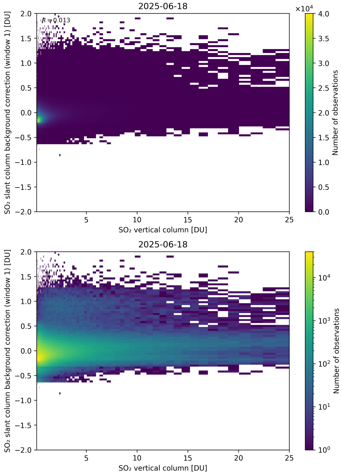
Figure 323: Scatter density plot of “SO 2 vertical column” against “SO 2 slant column background correction (window 1)” for 2025-06-17 to 2025-06-19.
