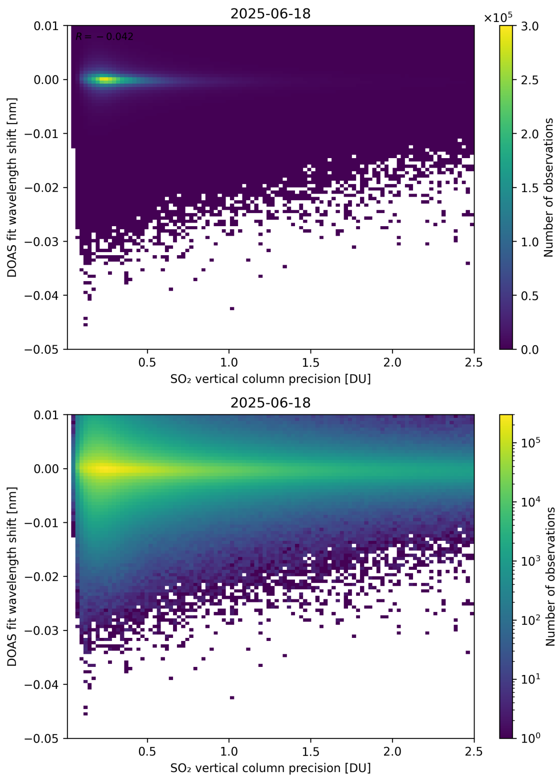
Figure 332: Scatter density plot of “SO 2 vertical column precision” against “DOAS fit wavelength shift” for 2025-06-17 to 2025-06-19.
