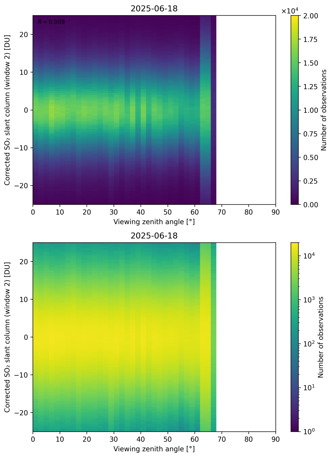
Figure 374: Scatter density plot of “Viewing zenith angle” against “Corrected SO 2 slant column (window 2)” for 2025-06-17 to 2025-06-19.
