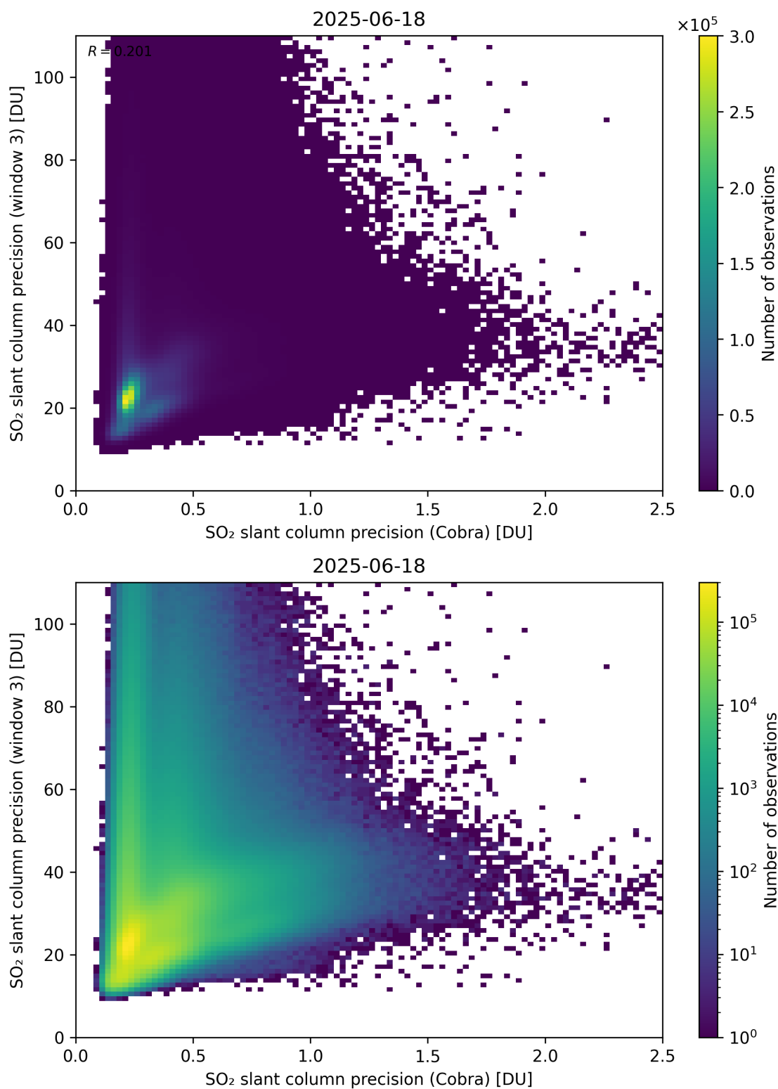
Figure 212: Scatter density plot of “SO 2 slant column precision (Cobra)” against “SO 2 slant column precision (window 3)” for 2025-06-17 to 2025-06-19.
