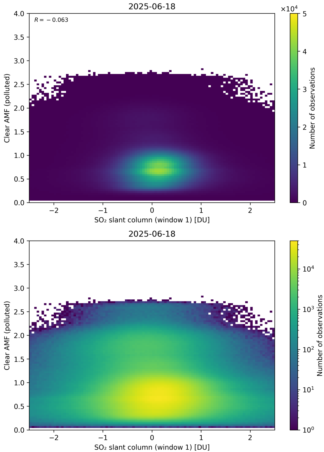
Figure 282: Scatter density plot of “SO 2 slant column (window 1)” against “Clear AMF (polluted)” for 2025-06-17 to 2025-06-19.
