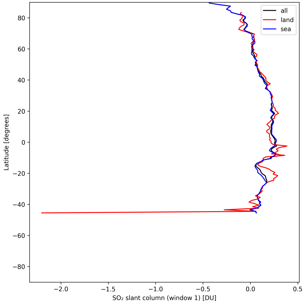
Figure 37: Zonal average of “SO 2 slant column (window 1)” for 2025-06-17 to 2025-06-19.
