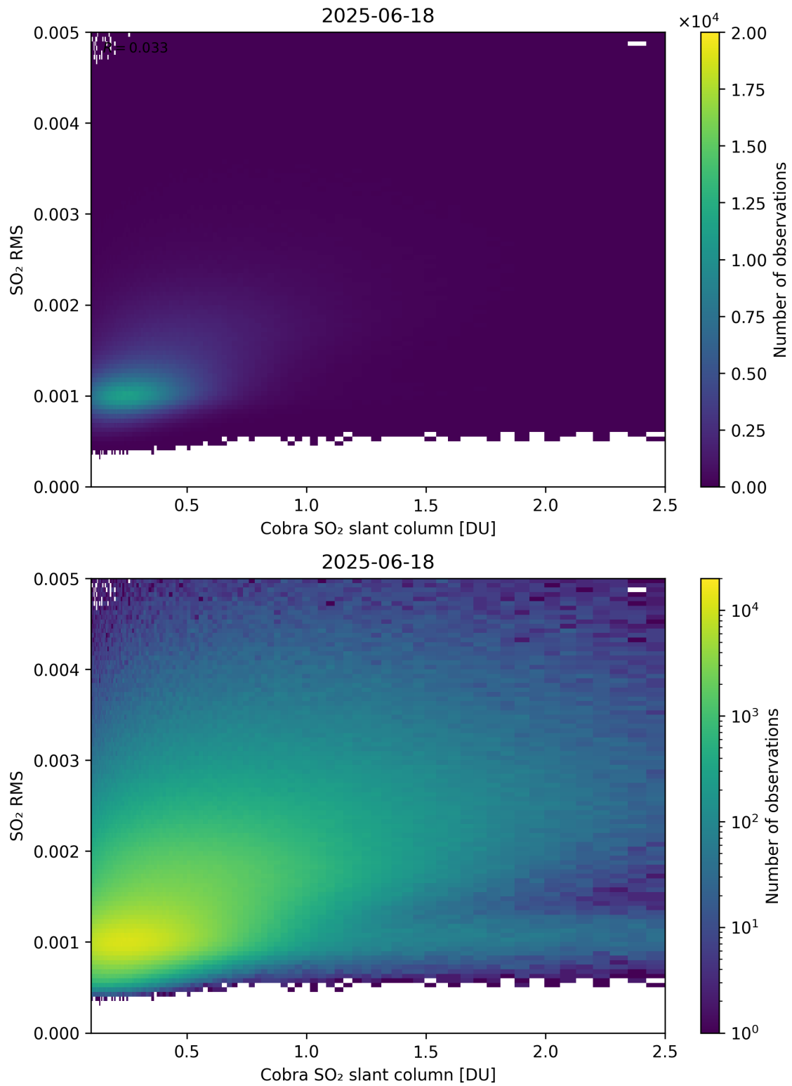
Figure 198: Scatter density plot of “Cobra SO 2 slant column” against “SO 2 RMS” for 2025-06-17 to 2025-06-19.
