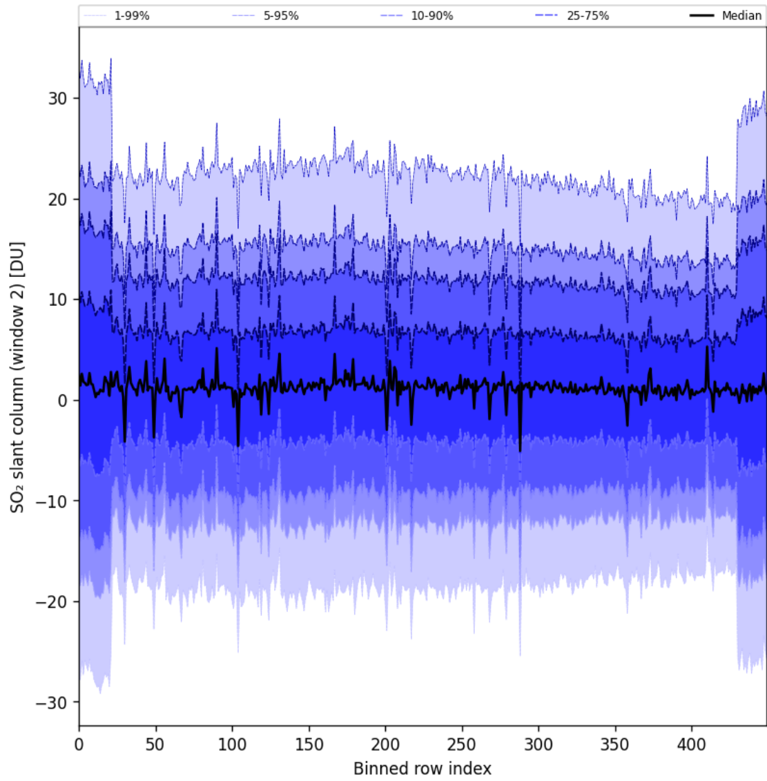
Figure 93: Along track statistics of “SO 2 slant column (window 2)” for 2025-06-17 to 2025-06-19
