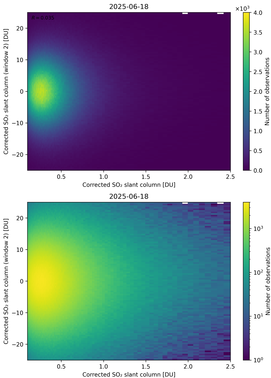
Figure 235: Scatter density plot of “Corrected SO 2 slant column” against “Corrected SO 2 slant column (window 2)” for 2025-06-17 to 2025-06-19.
