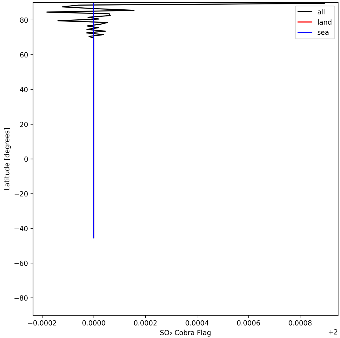
Figure 49: Zonal average of "SO 2 Cobra Flag" for 2025-06-17 to 2025-06-19.
