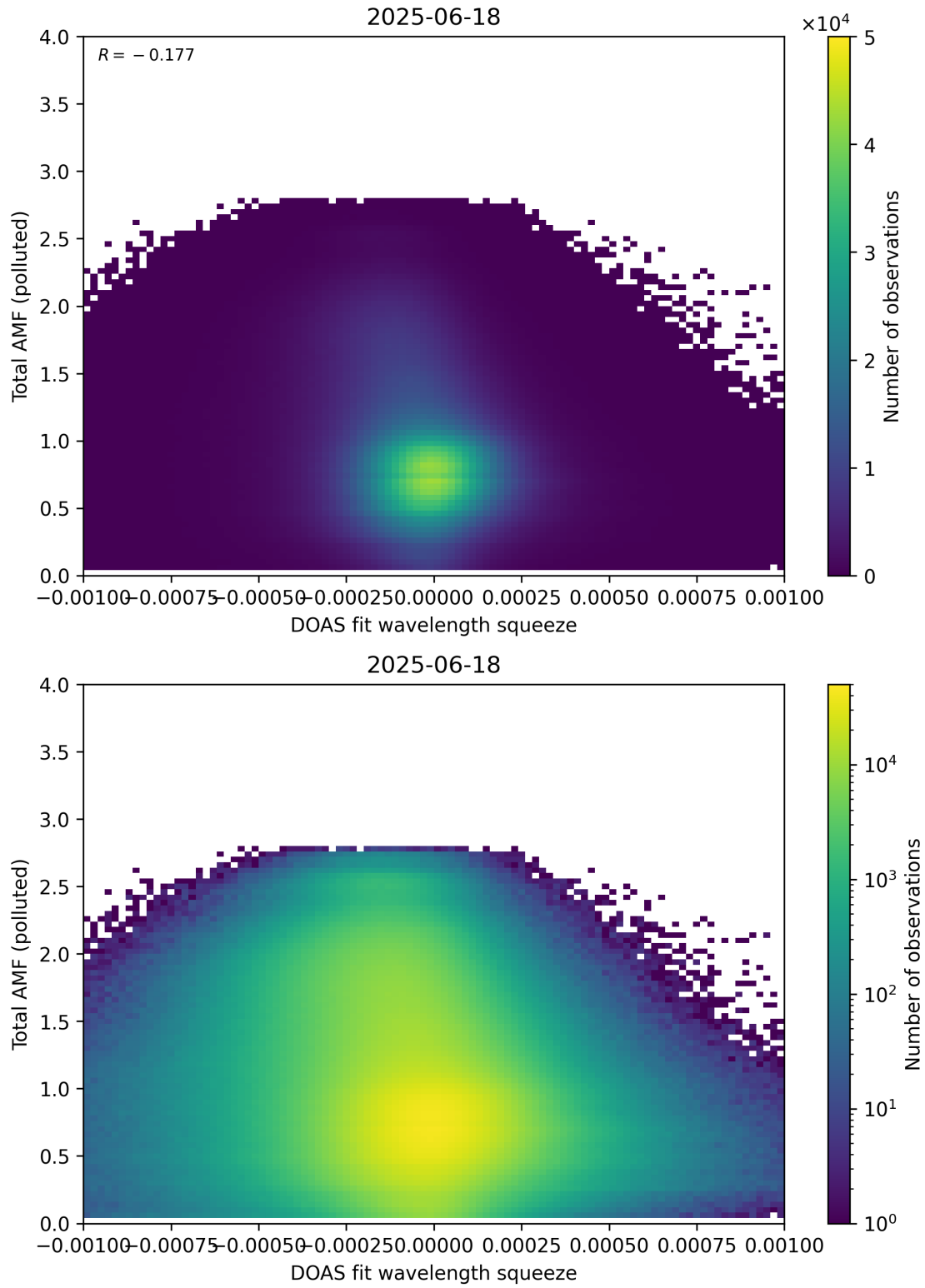
Figure 145: Scatter density plot of “DOAS fit wavelength squeeze” against “Total AMF (polluted)” for 2025-06-17 to 2025-06-19.
