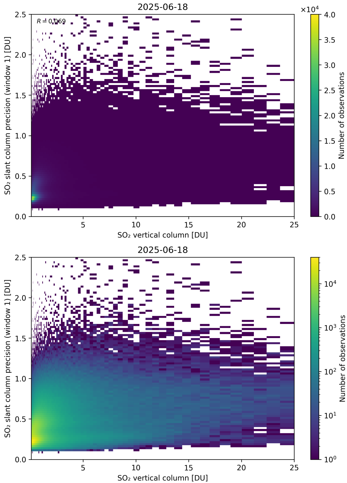
Figure 355: Scatter density plot of “SO 2 vertical column” against “SO 2 slant column precision (window 1)” for 2025-06-17 to 2025-06-19.
