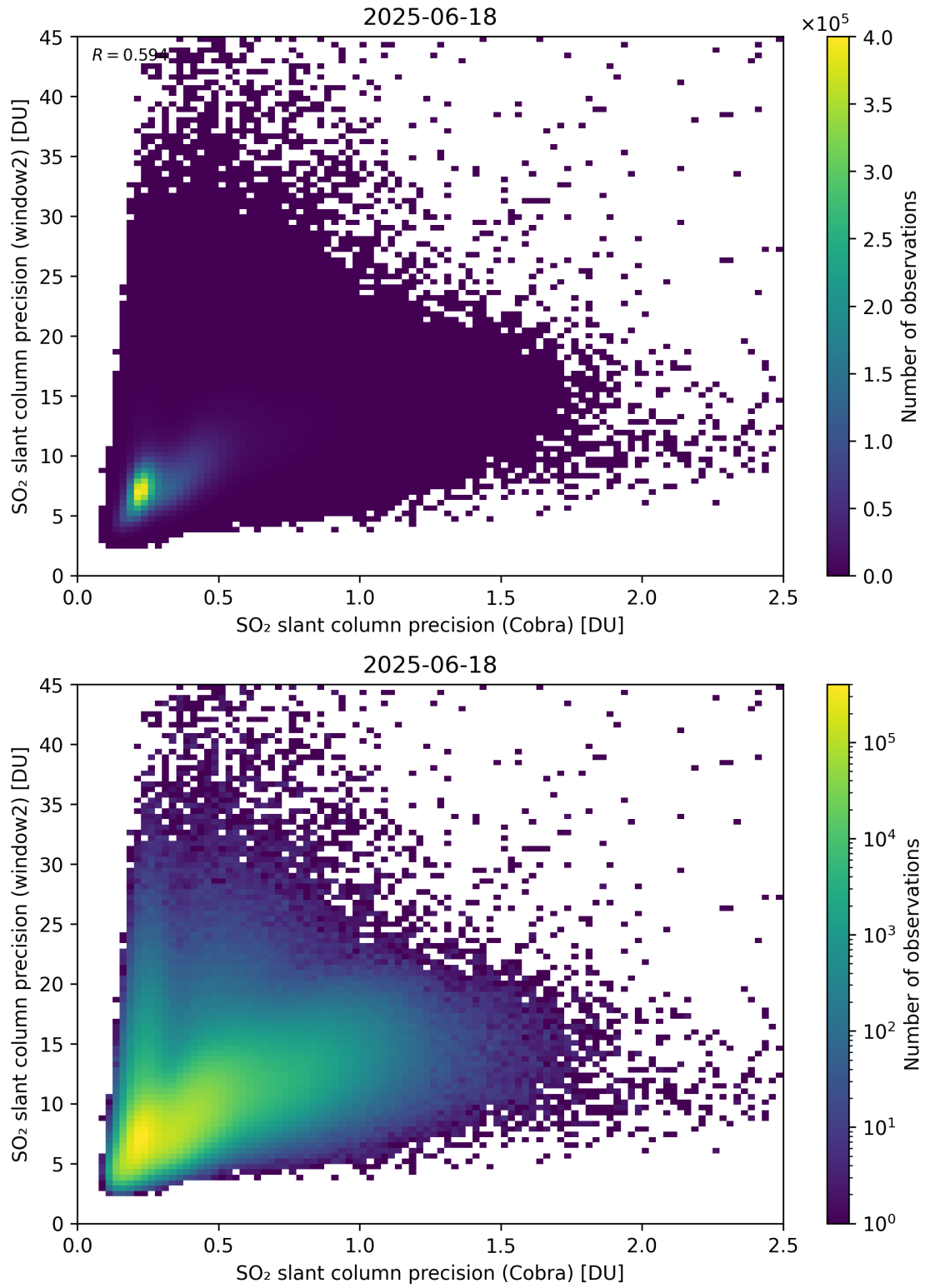
Figure 210: Scatter density plot of “SO 2 slant column precision (Cobra)” against “SO 2 slant column precision (window2)” for 2025-06-17 to 2025-06-19.
