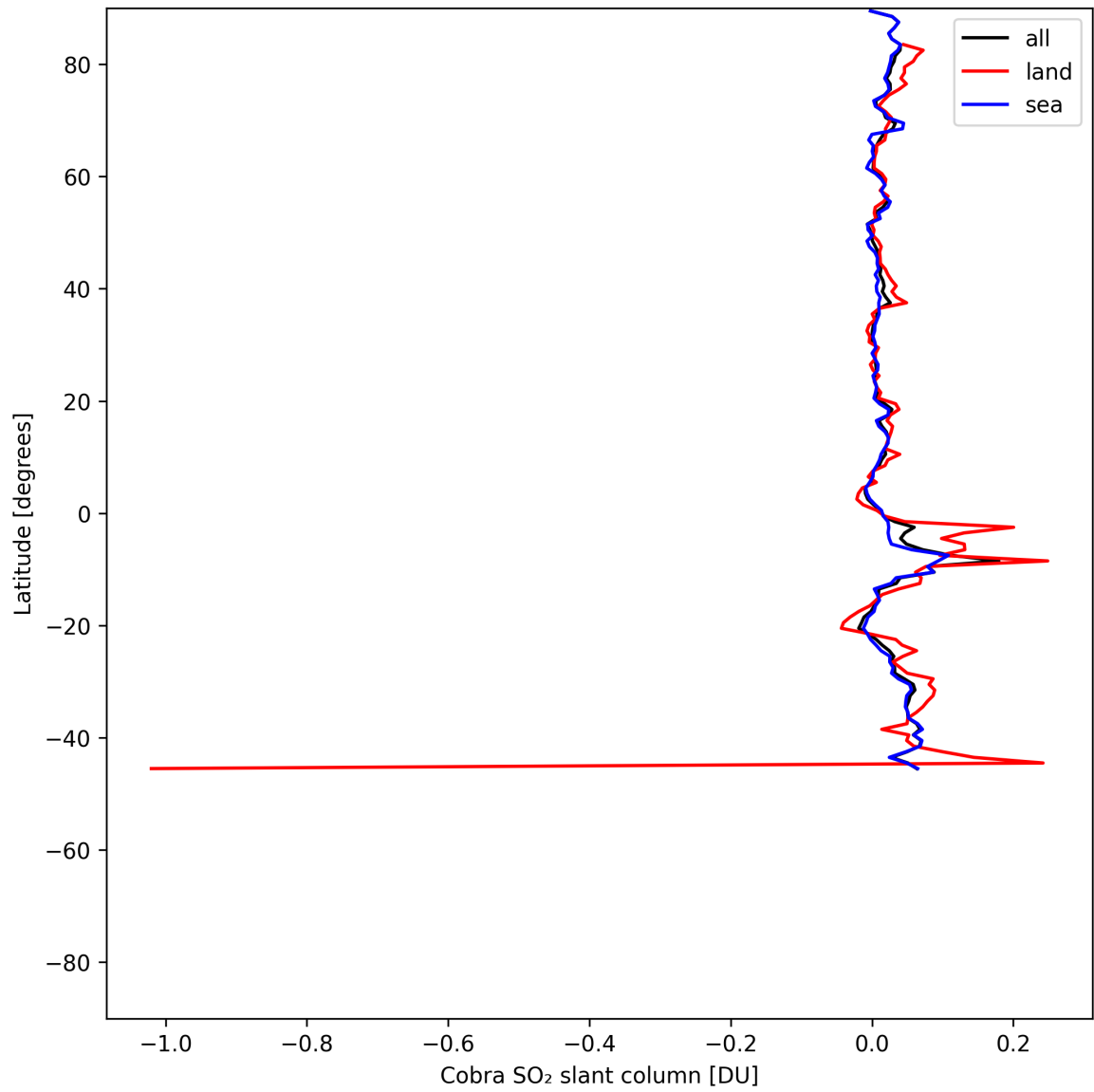
Figure 35: Zonal average of “Cobra SO 2 slant column” for 2025-06-17 to 2025-06-19.
