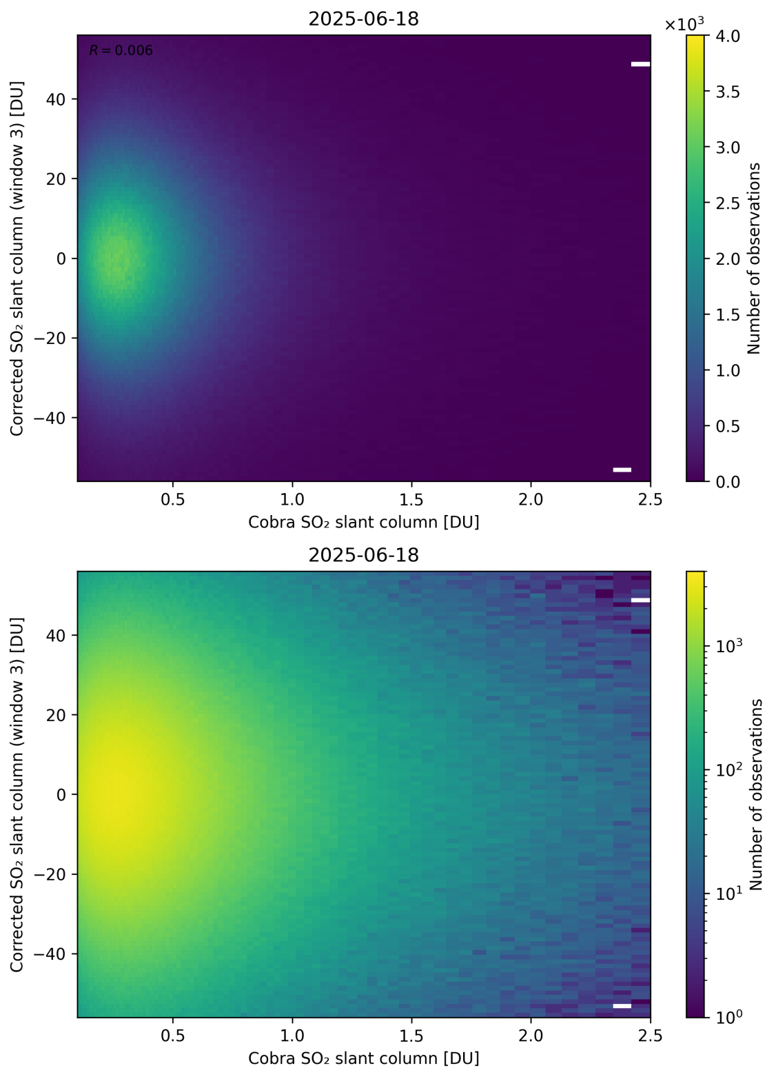
Figure 218: Scatter density plot of “Cobra SO 2 slant column” against “Corrected SO 2 slant column (window 3)” for 2025-06-17 to 2025-06-19.
