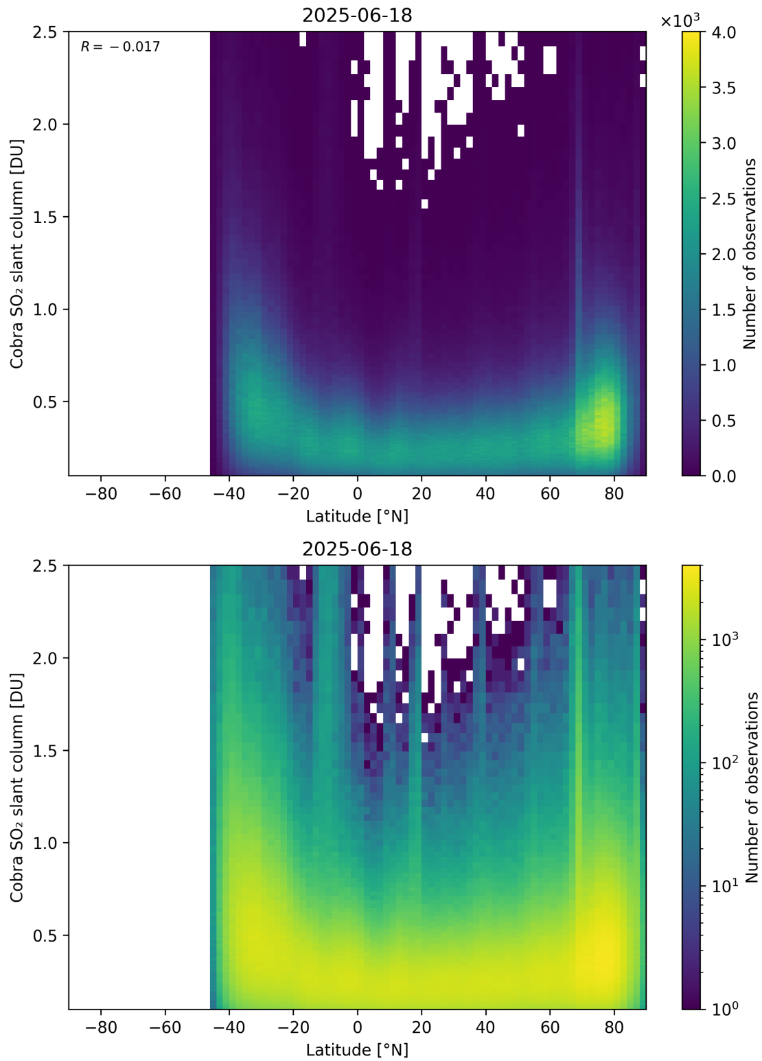
Figure 157: Scatter density plot of “Latitude” against “Cobra SO 2 slant column” for 2025-06-17 to 2025-06-19.
