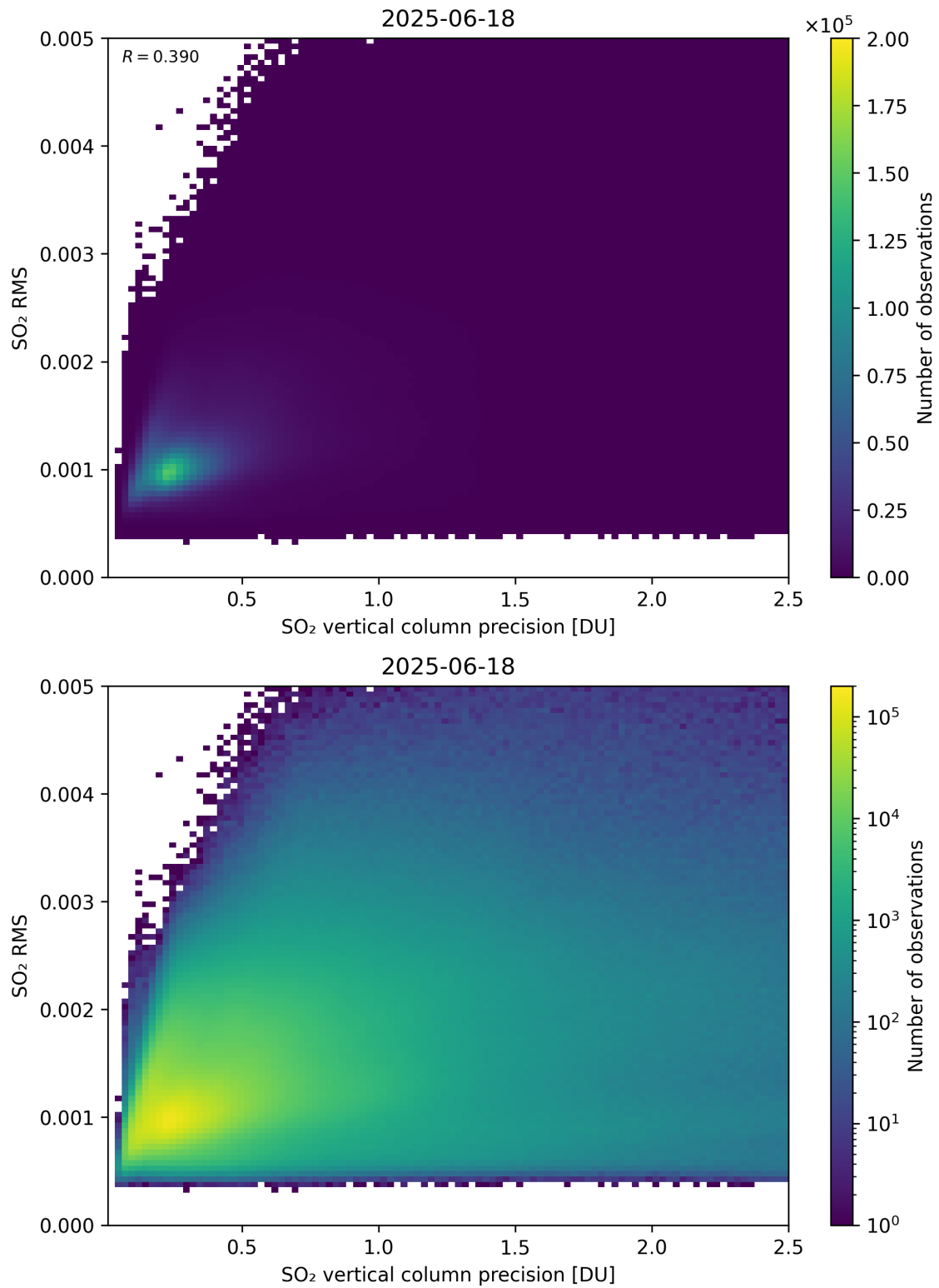
Figure 334: Scatter density plot of “SO 2 vertical column precision” against “SO 2 RMS” for 2025-06-17 to 2025-06-19.
