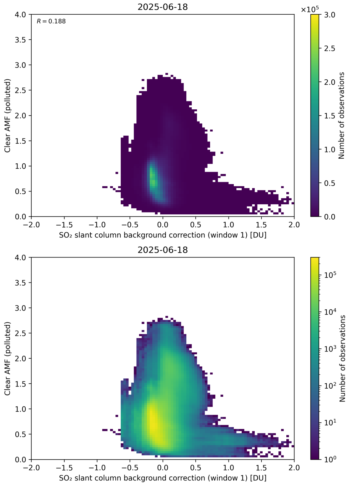
Figure 114: Scatter density plot of “SO 2 slant column background correction (window 1)” against “Clear AMF (polluted)” for 2025-06-17 to 2025-06-19.
