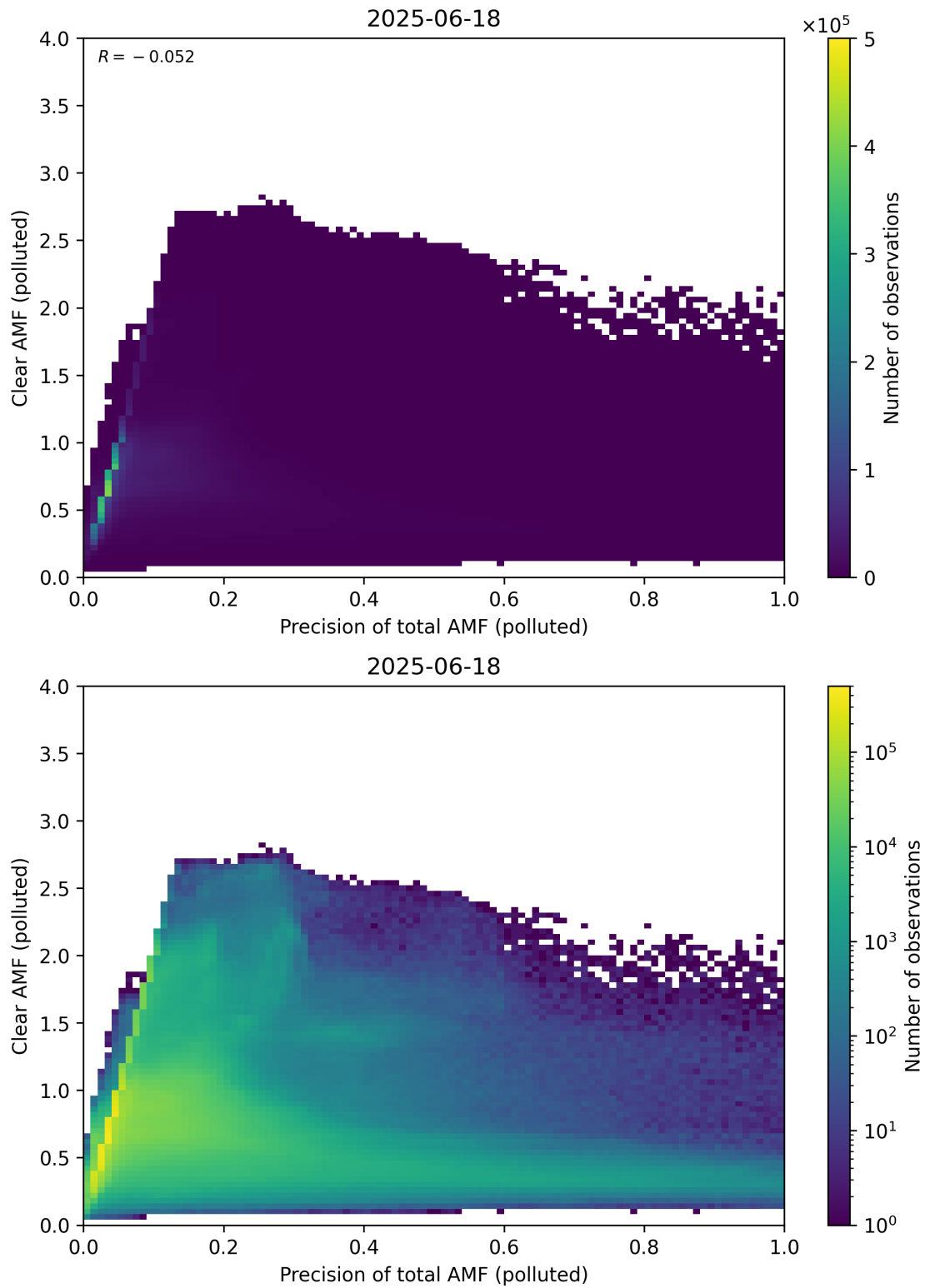
Figure 320: Scatter density plot of “Precision of total AMF (polluted)” against “Clear AMF (polluted)” for 2025-06-17 to 2025-06-19.
