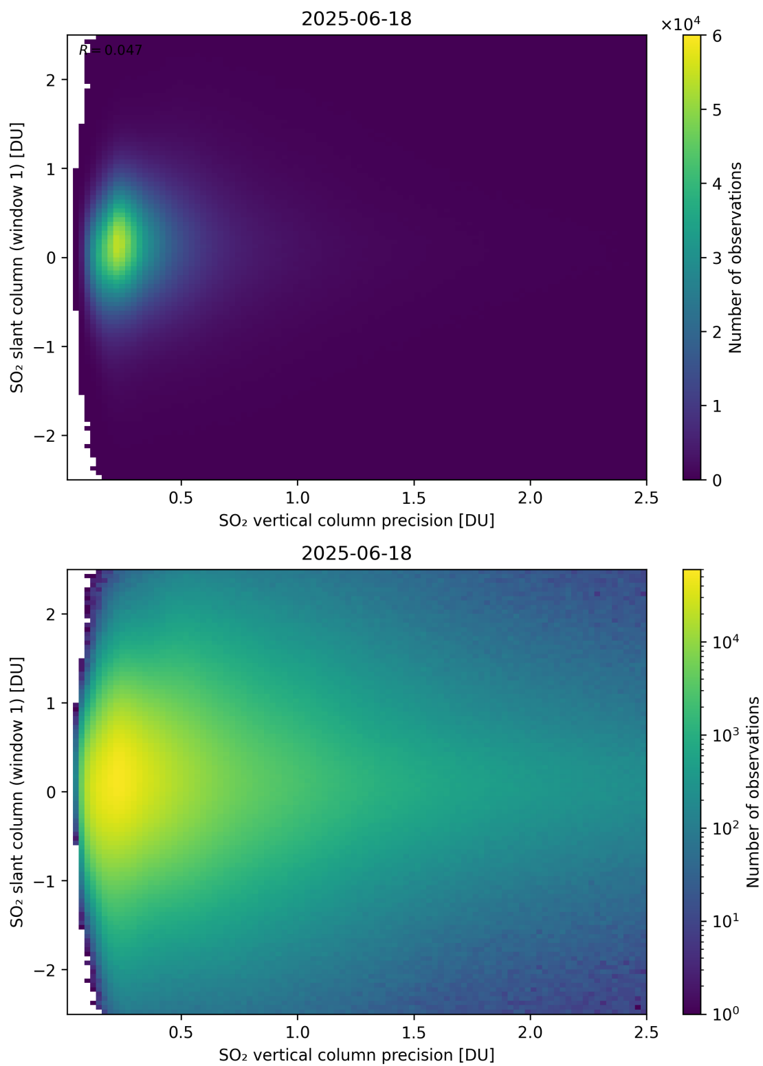
Figure 341: Scatter density plot of “SO 2 vertical column precision” against “SO 2 slant column (window 1)” for 2025-06-17 to 2025-06-19.
