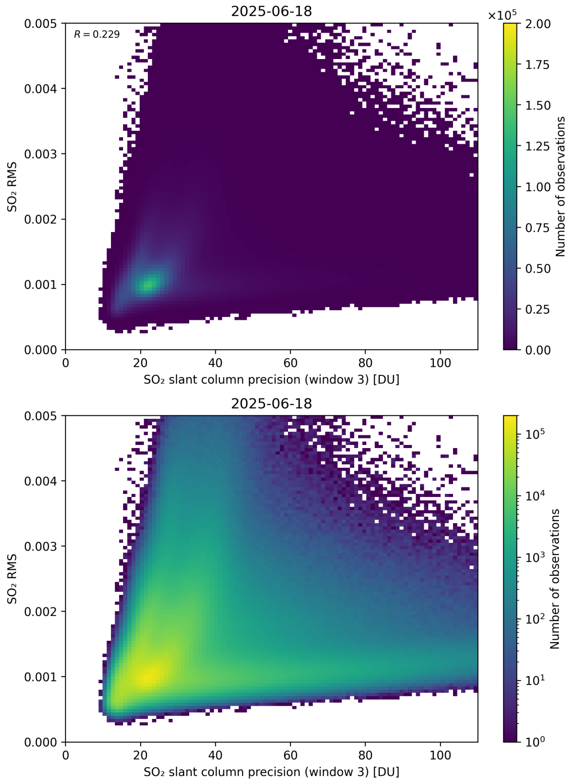
Figure 310: Scatter density plot of “SO 2 slant column precision (window 3)” against “SO 2 RMS” for 2025-06-17 to 2025-06-19.
