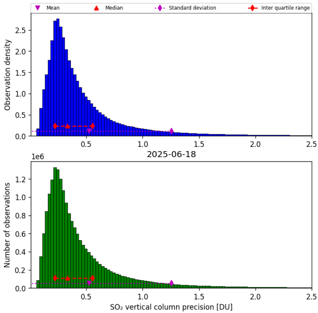
Figure 59: Histogram of “SO 2 vertical column precision” for 2025-06-17 to 2025-06-19
