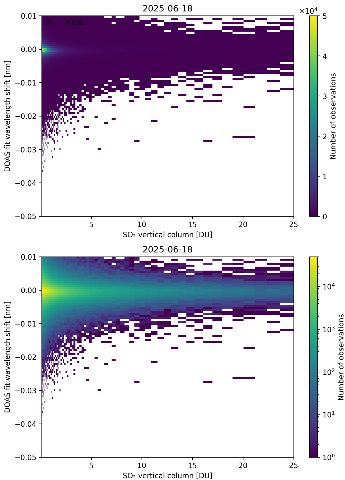
Figure 326: Scatter density plot of “SO 2 vertical column” against “DOAS fit wavelength shift” for 2025-06-17 to 2025-06-19.
