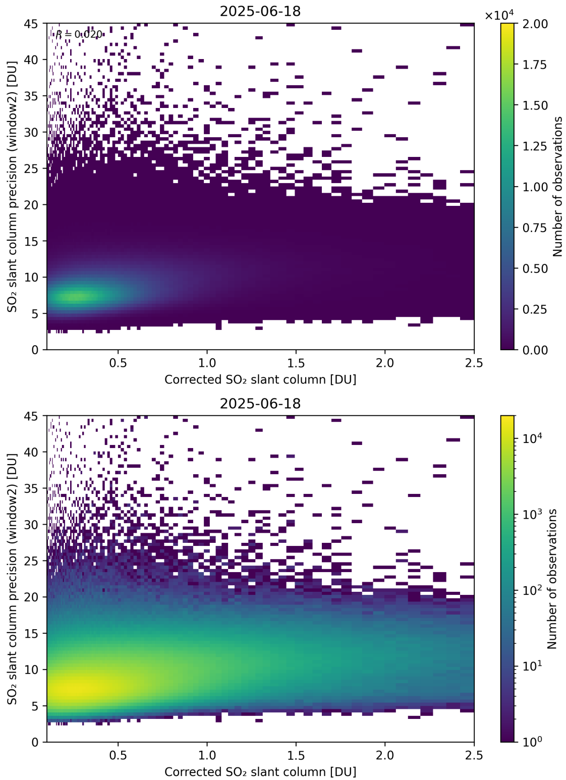
Figure 239: Scatter density plot of “Corrected SO 2 slant column” against “SO 2 slant column precision (window2)” for 2025-06-17 to 2025-06-19.
