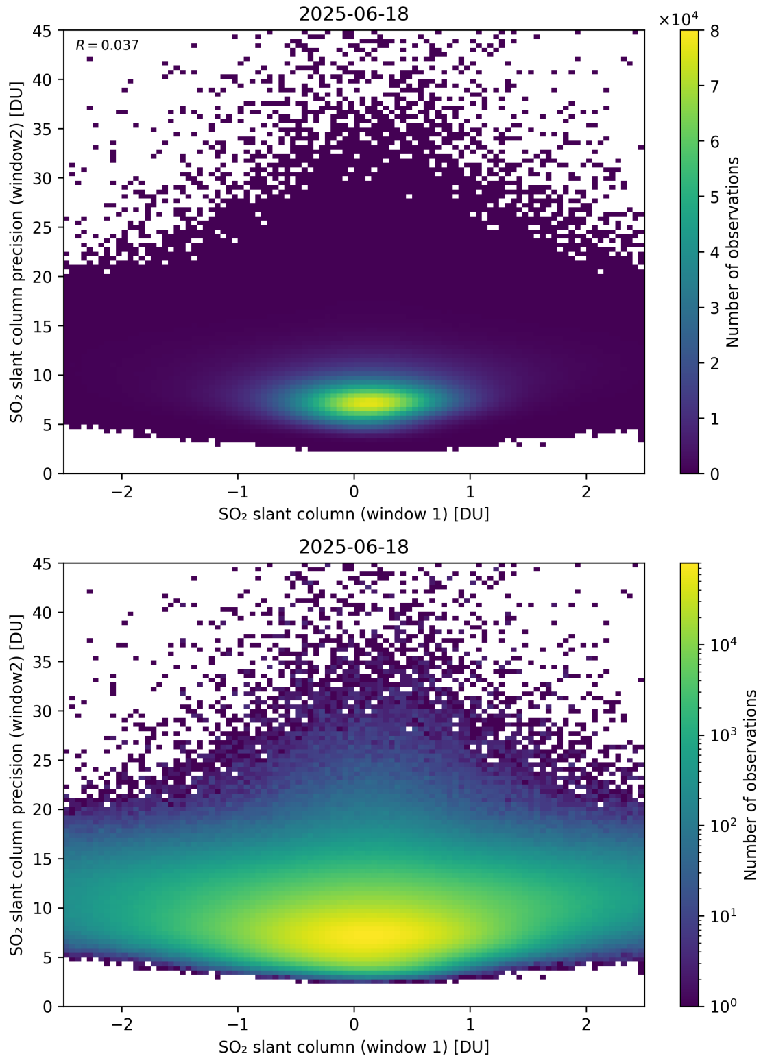
Figure 286: Scatter density plot of “SO 2 slant column (window 1)” against “SO 2 slant column precision (window2)” for 2025-06-17 to 2025-06-19.
