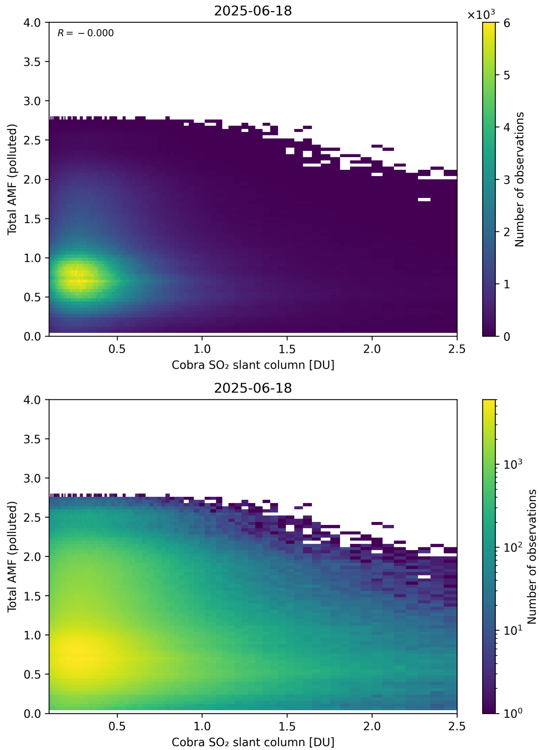
Figure 224: Scatter density plot of “Cobra SO 2 slant column” against “Total AMF (polluted)” for 2025-06-17 to 2025-06-19.
