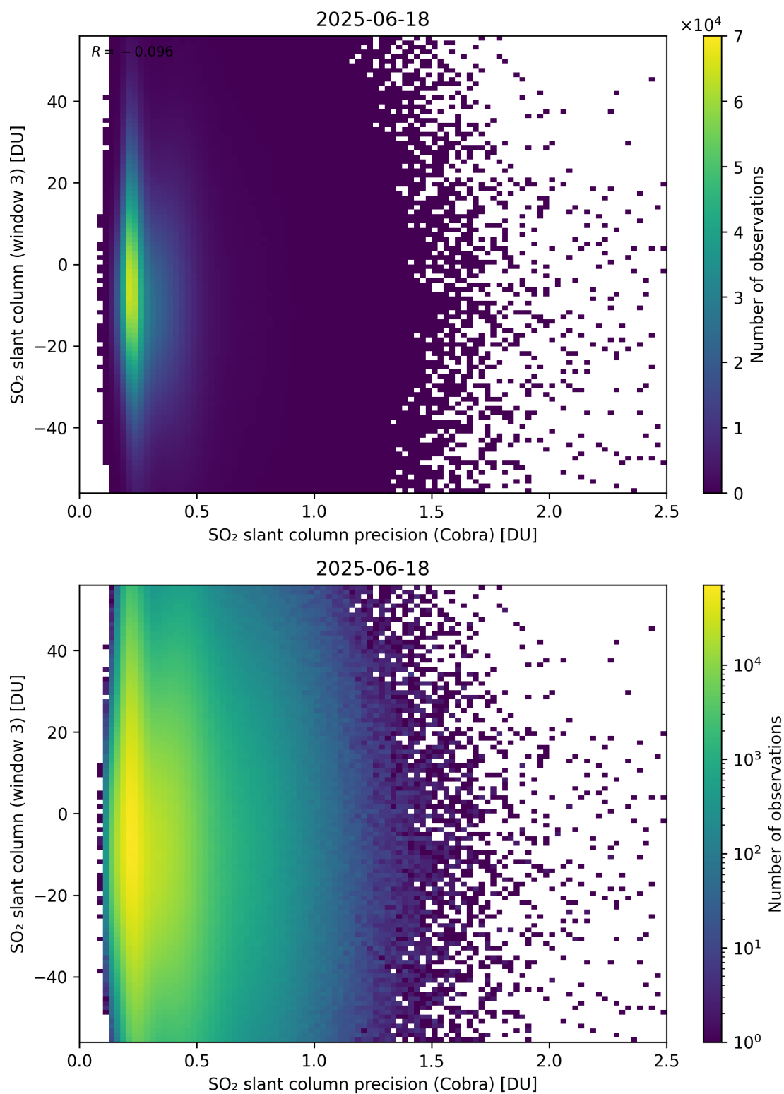
Figure 211: Scatter density plot of “SO 2 slant column precision (Cobra)” against “SO 2 slant column (window 3)” for 2025-06-17 to 2025-06-19.
