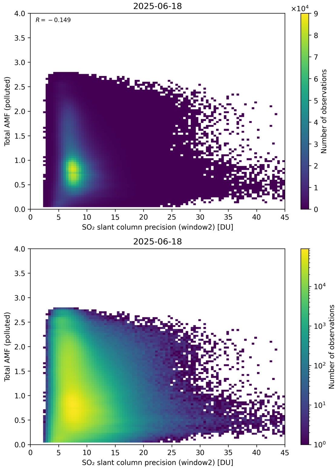
Figure 301: Scatter density plot of “SO 2 slant column precision (window2)” against “Total AMF (polluted)” for 2025-06-17 to 2025-06-19.
