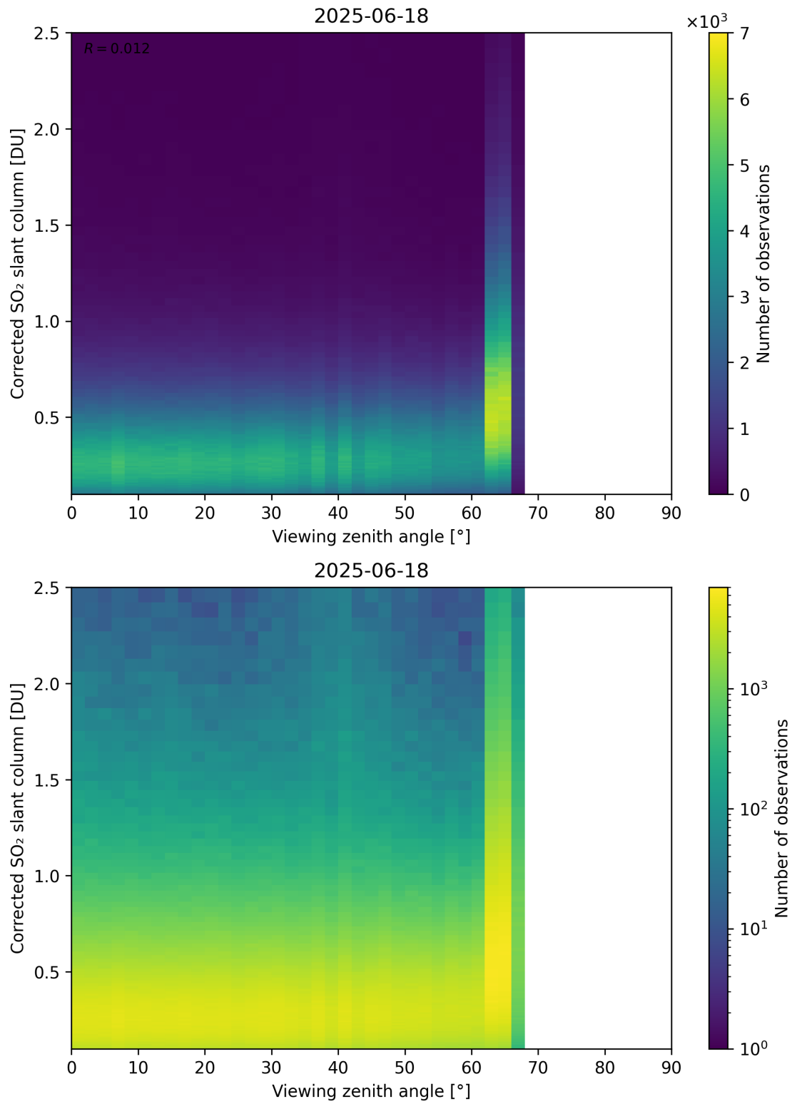
Figure 373: Scatter density plot of “Viewing zenith angle” against “Corrected SO 2 slant column” for 2025-06-17 to 2025-06-19.
