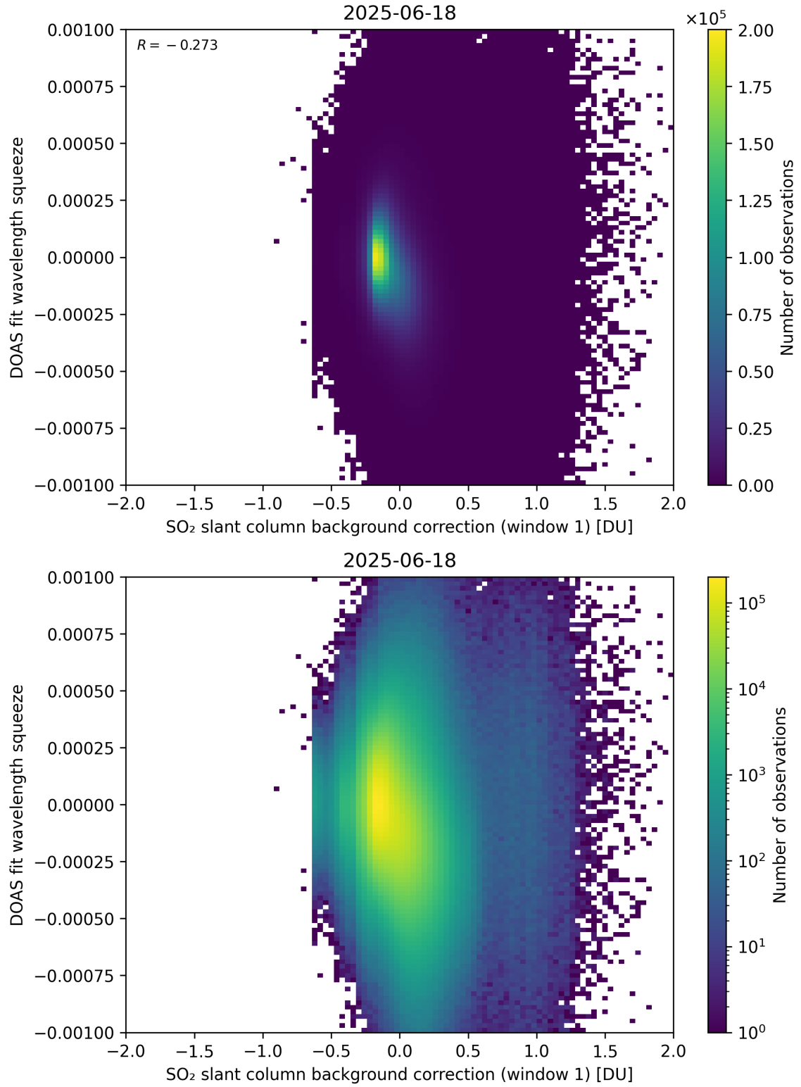
Figure 112: Scatter density plot of “SO 2 slant column background correction (window 1)” against “DOAS fit wavelength squeeze” for 2025-06-17 to 2025-06-19.
