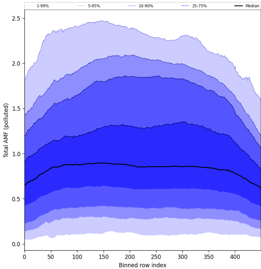
Figure 105: Along track statistics of “Total AMF (polluted)” for 2025-06-17 to 2025-06-19
