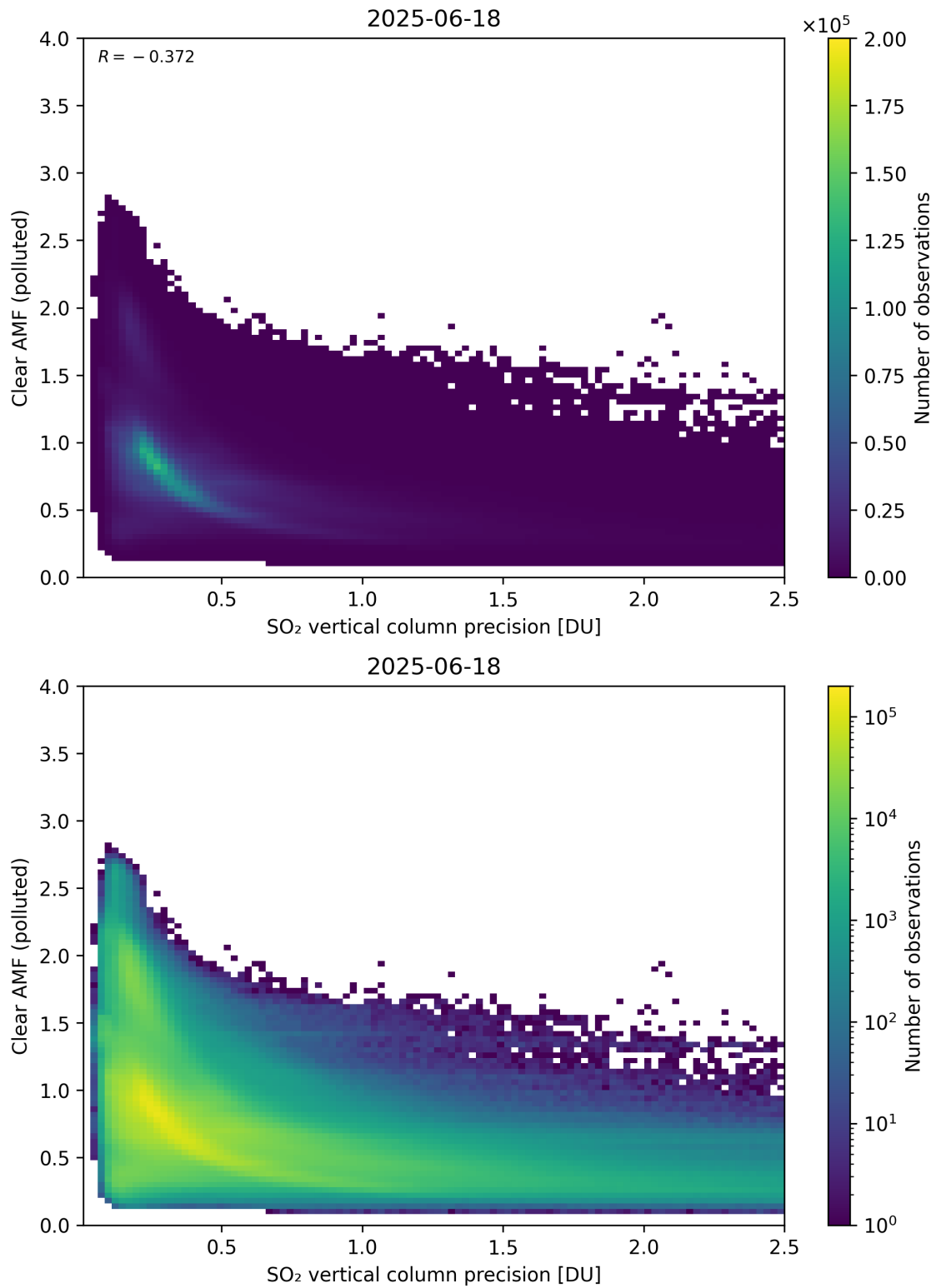
Figure 335: Scatter density plot of “SO 2 vertical column precision” against “Clear AMF (polluted)” for 2025-06-17 to 2025-06-19.
