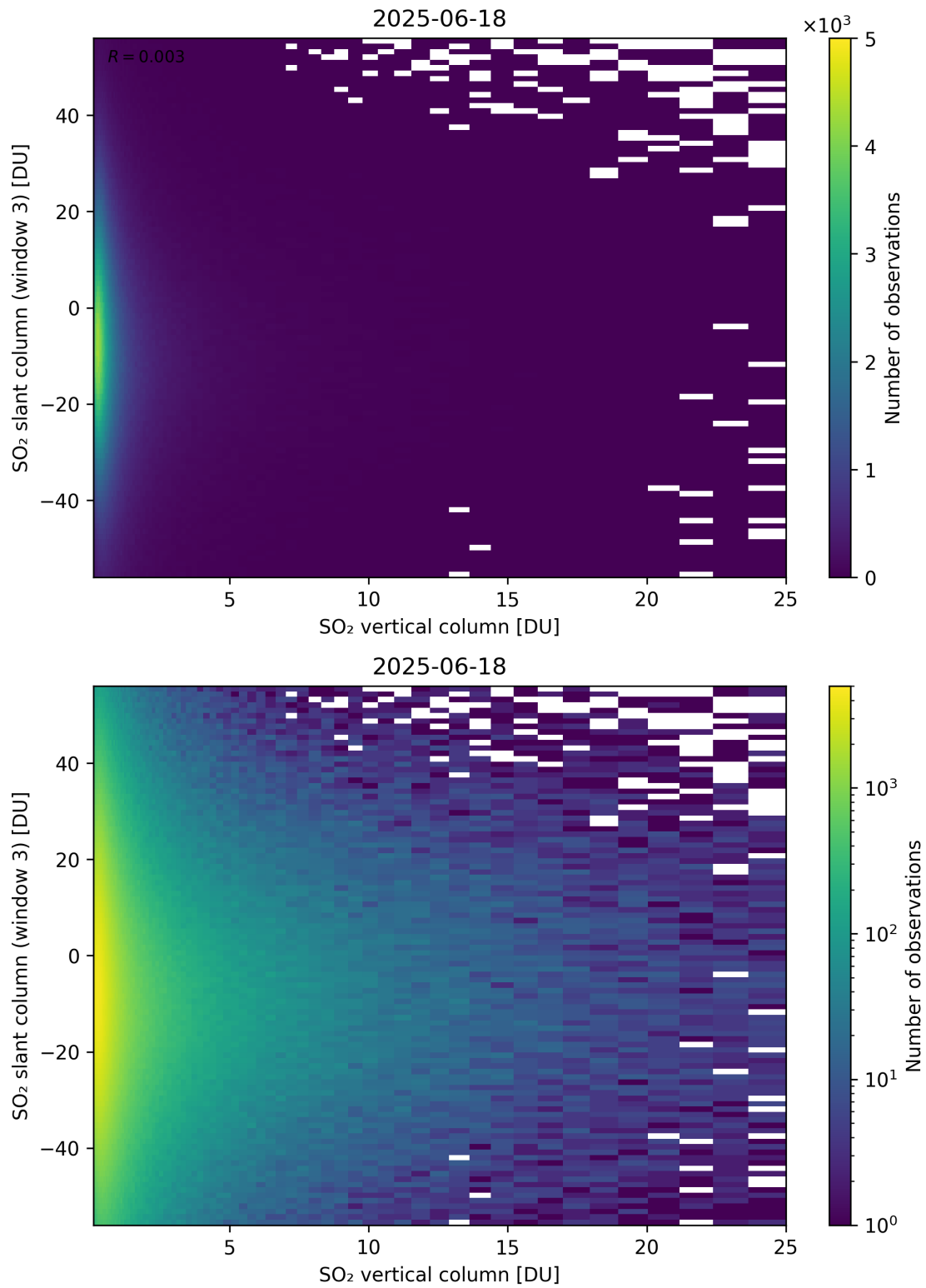
Figure 357: Scatter density plot of “SO 2 vertical column” against “SO 2 slant column (window 3)” for 2025-06-17 to 2025-06-19.
