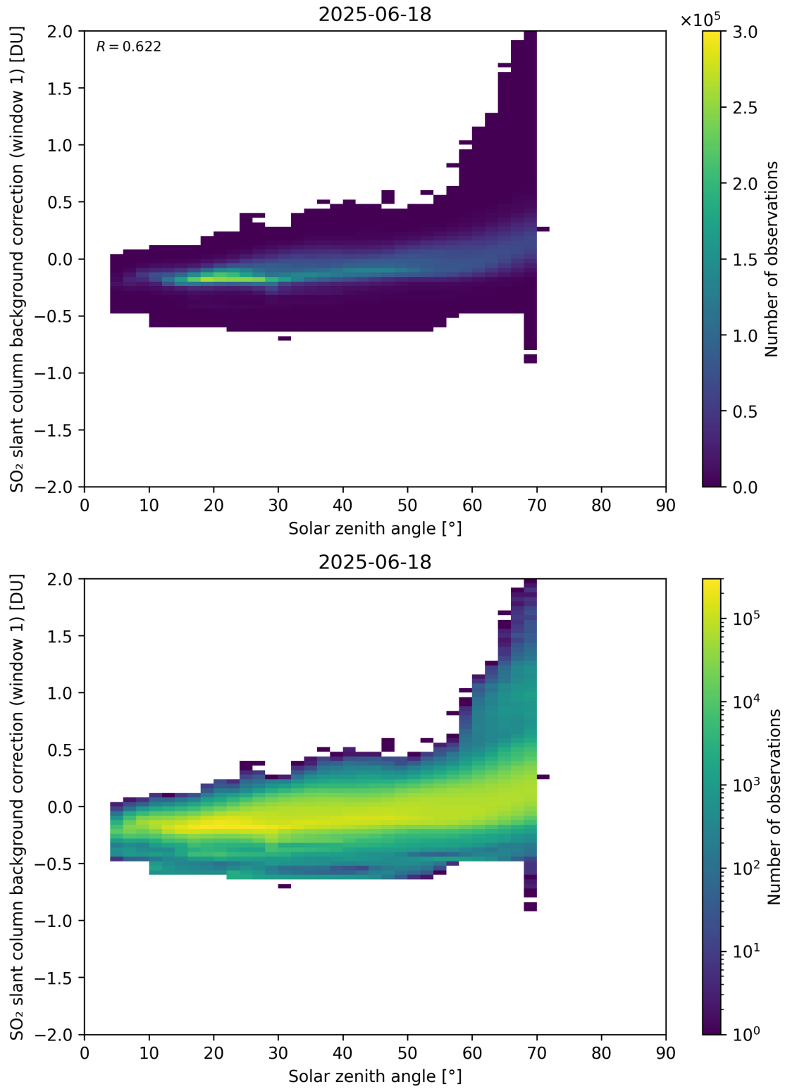
Figure 171: Scatter density plot of “Solar zenith angle” against “SO 2 slant column background correction (window 1)” for 2025-06-17 to 2025-06-19.
