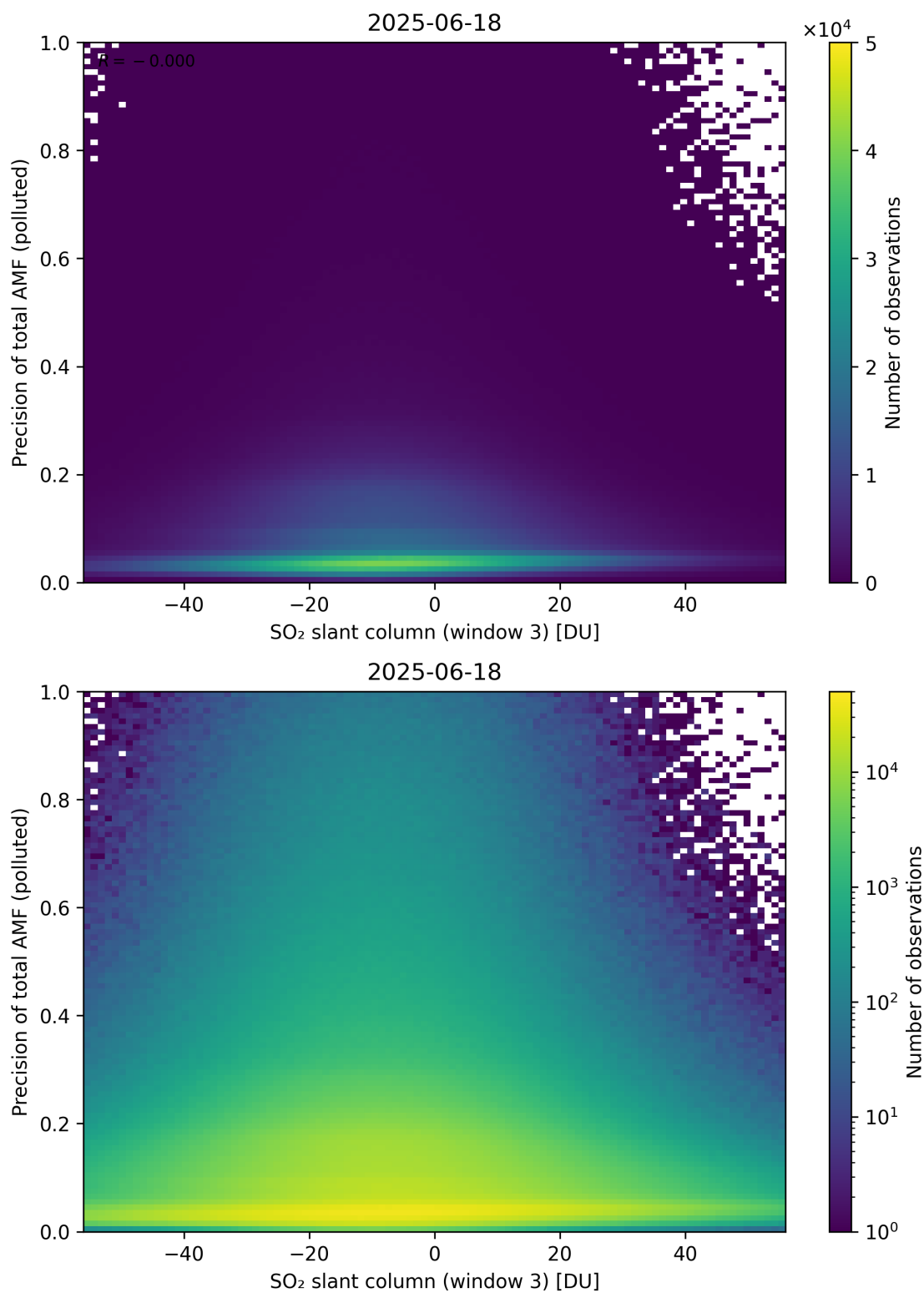
Figure 319: Scatter density plot of “SO 2 slant column (window 3)” against “Precision of total AMF (polluted)” for 2025-06-17 to 2025-06-19.
