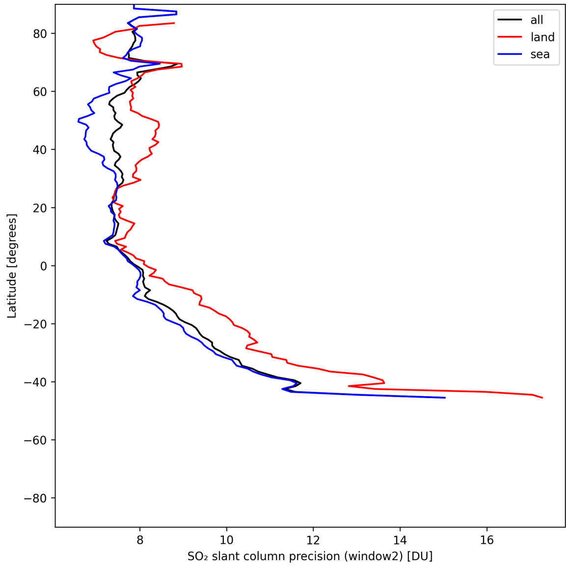
Figure 42: Zonal average of “SO 2 slant column precision (window2)” for 2025-06-17 to 2025-06-19.
