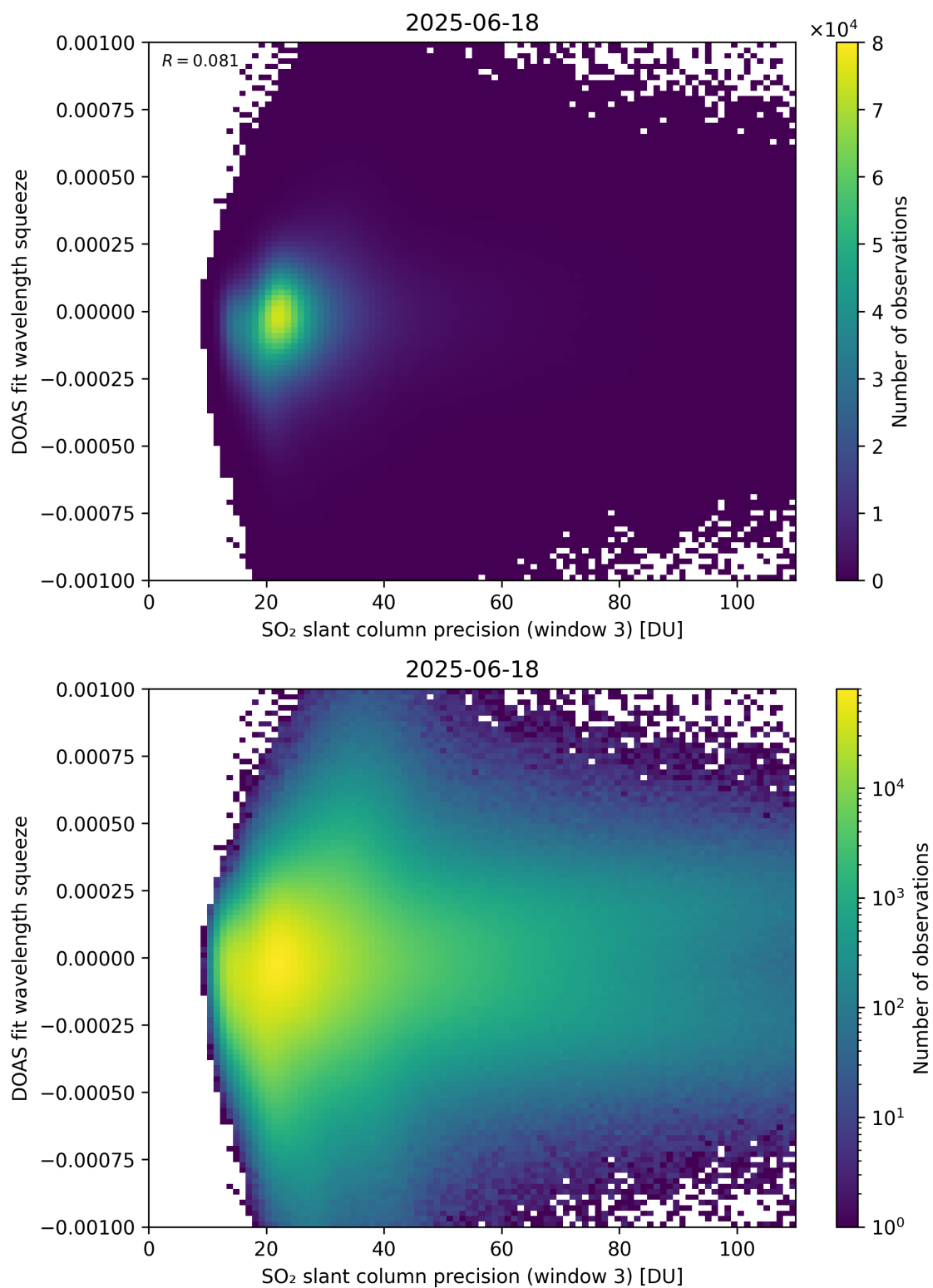
Figure 309: Scatter density plot of “SO 2 slant column precision (window 3)” against “DOAS fit wavelength squeeze” for 2025-06-17 to 2025-06-19.
