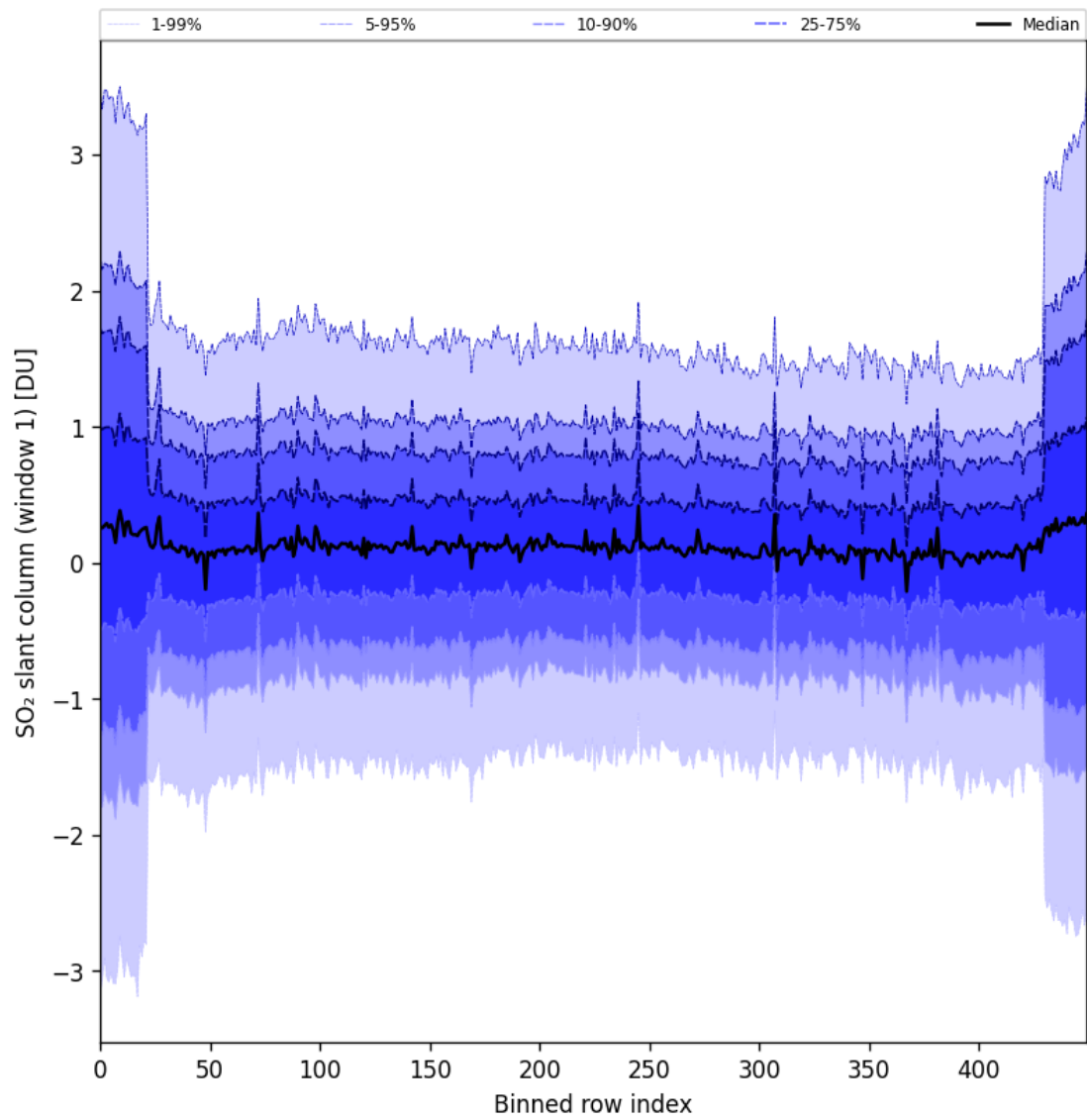
Figure 89: Along track statistics of “SO 2 slant column (window 1)” for 2025-06-17 to 2025-06-19
