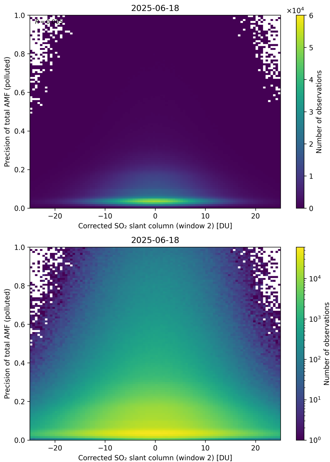
Figure 254: Scatter density plot of “Corrected SO 2 slant column (window 2)” against “Precision of total AMF (polluted)” for 2025-06-17 to 2025-06-19.
