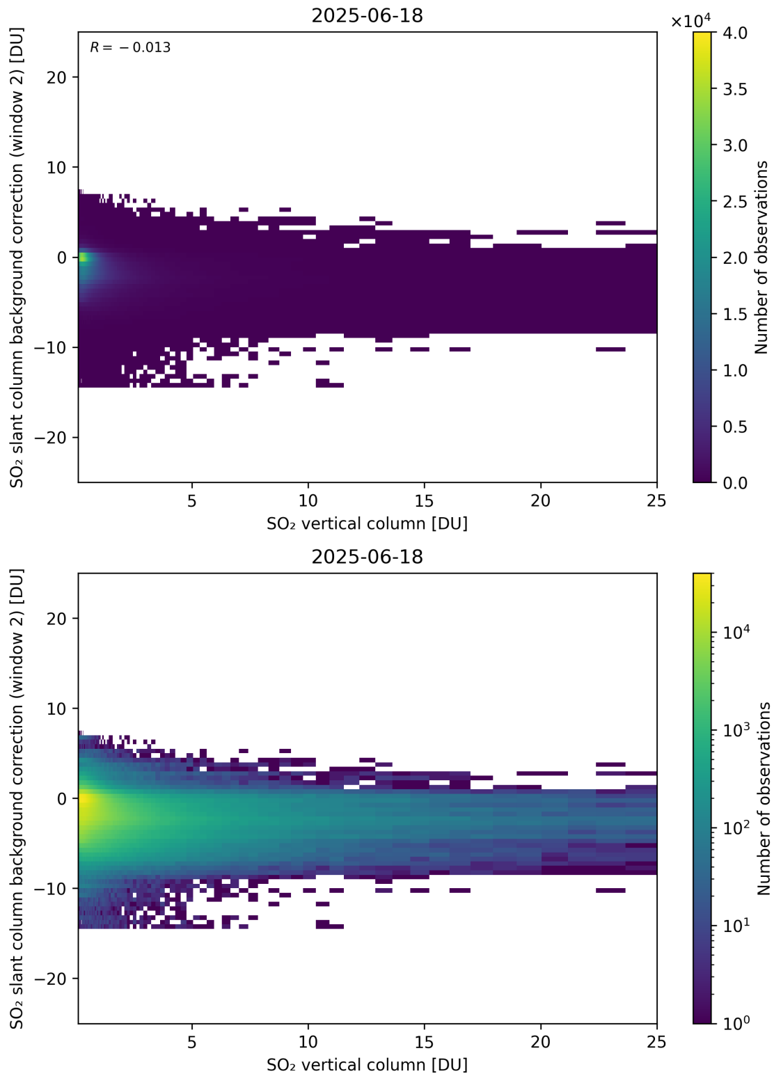
Figure 324: Scatter density plot of “SO 2 vertical column” against “SO 2 slant column background correction (window 2)” for 2025-06-17 to 2025-06-19.
