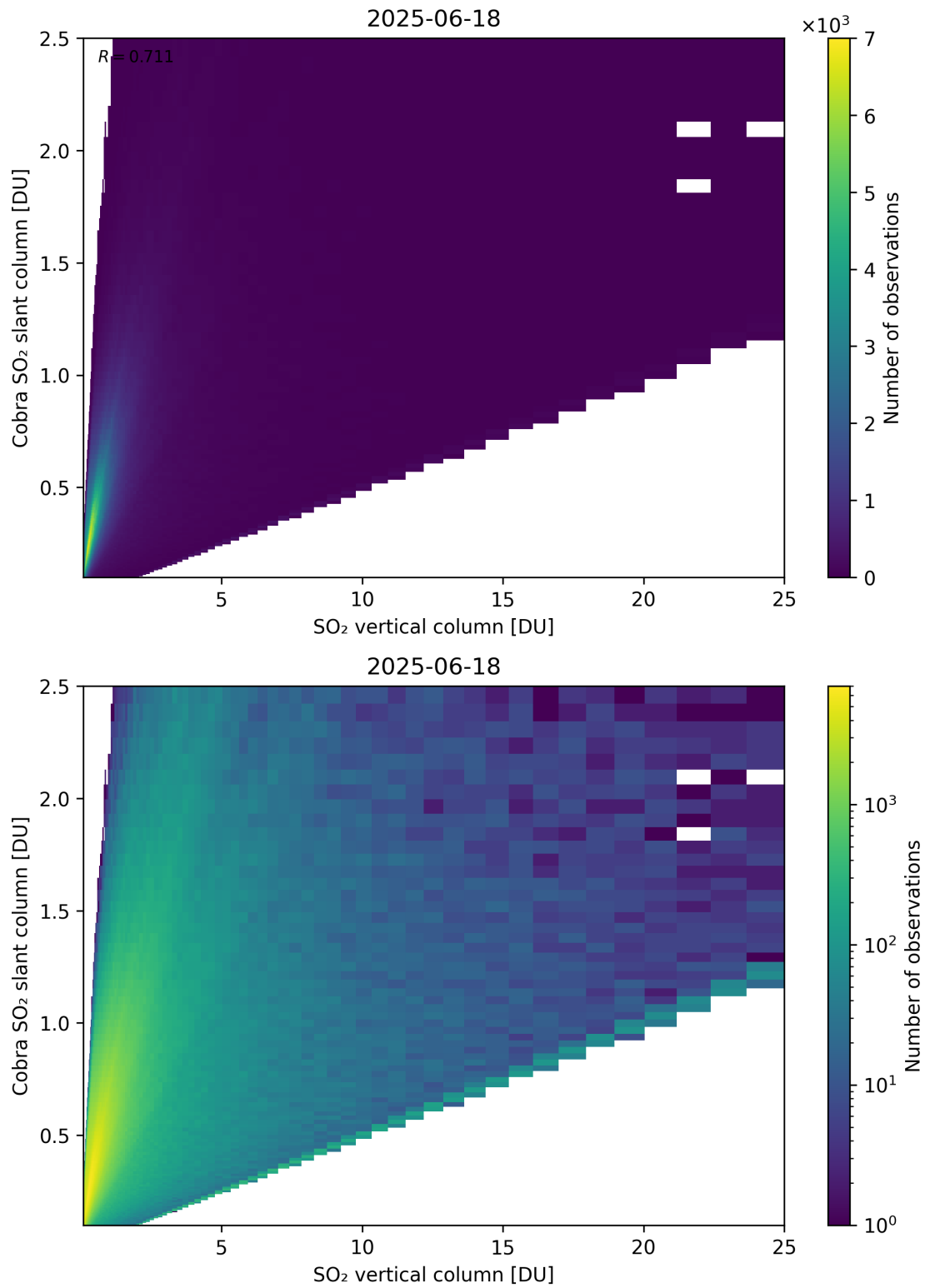
Figure 349: Scatter density plot of “SO 2 vertical column” against “Cobra SO 2 slant column” for 2025-06-17 to 2025-06-19.
