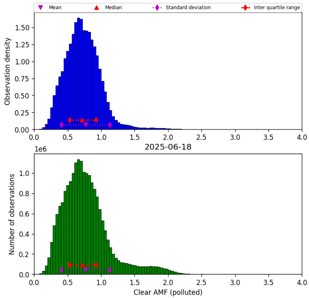
Figure 81: Histogram of “Clear AMF (polluted)” for 2025-06-17 to 2025-06-19
