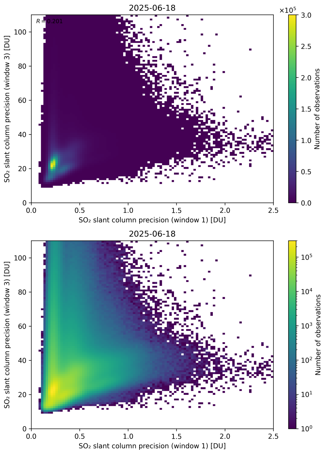
Figure 279: Scatter density plot of “SO 2 slant column precision (window 1)” against “SO 2 slant column precision (window 3)” for 2025-06-17 to 2025-06-19.
