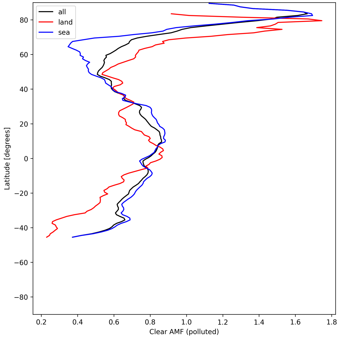
Figure 55: Zonal average of “Clear AMF (polluted)” for 2025-06-17 to 2025-06-19.
