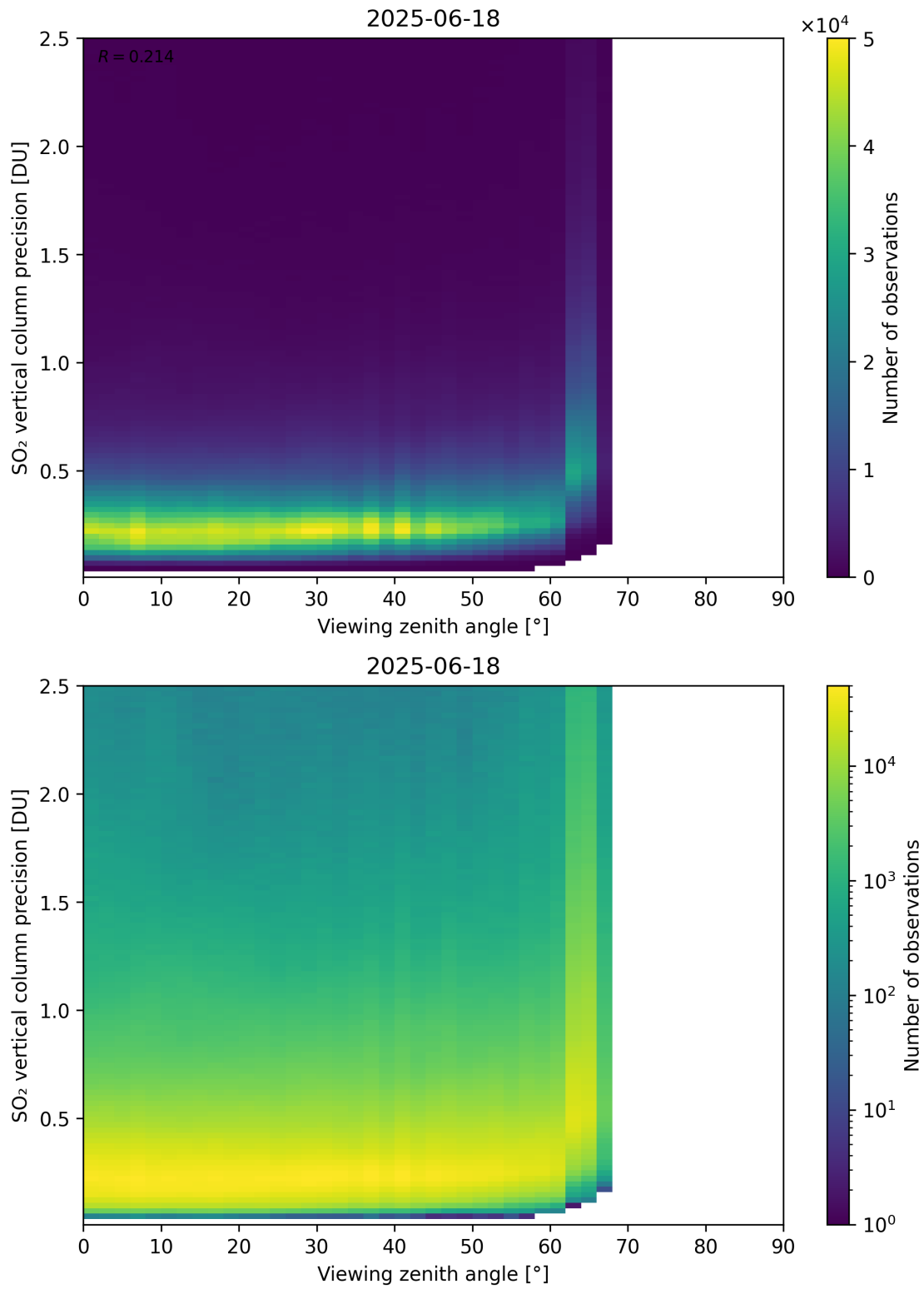
Figure 384: Scatter density plot of “Viewing zenith angle” against “SO 2 vertical column precision” for 2025-06-17 to 2025-06-19.
