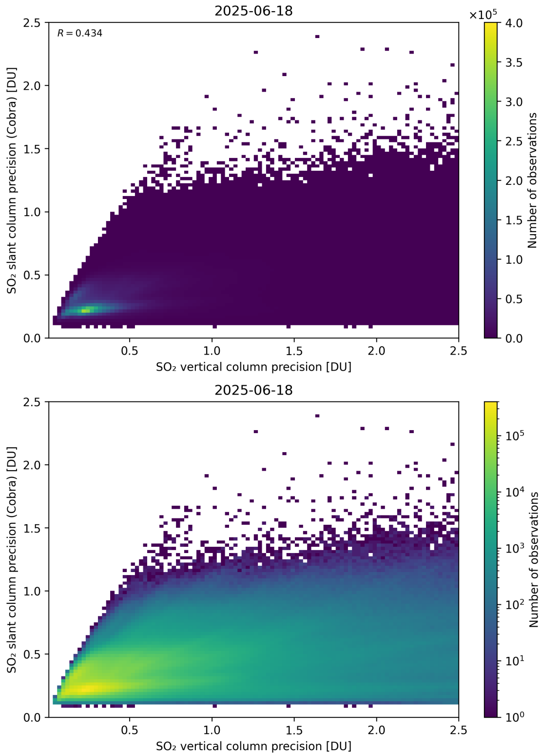
Figure 337: Scatter density plot of “SO 2 vertical column precision” against “SO 2 slant column precision (Cobra)” for 2025-06-17 to 2025-06-19.
