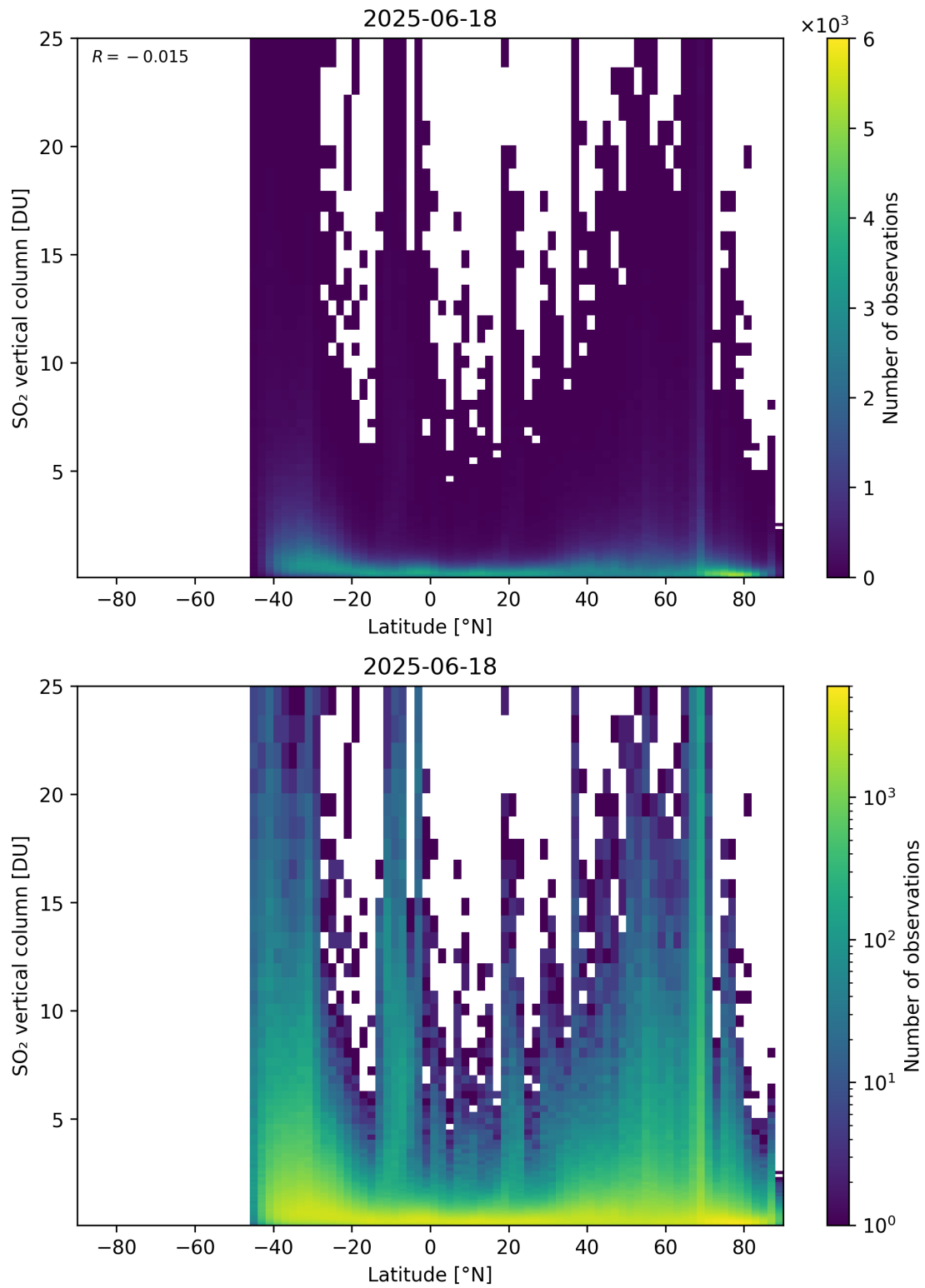
Figure 169: Scatter density plot of “Latitude” against “SO 2 vertical column” for 2025-06-17 to 2025-06-19.
