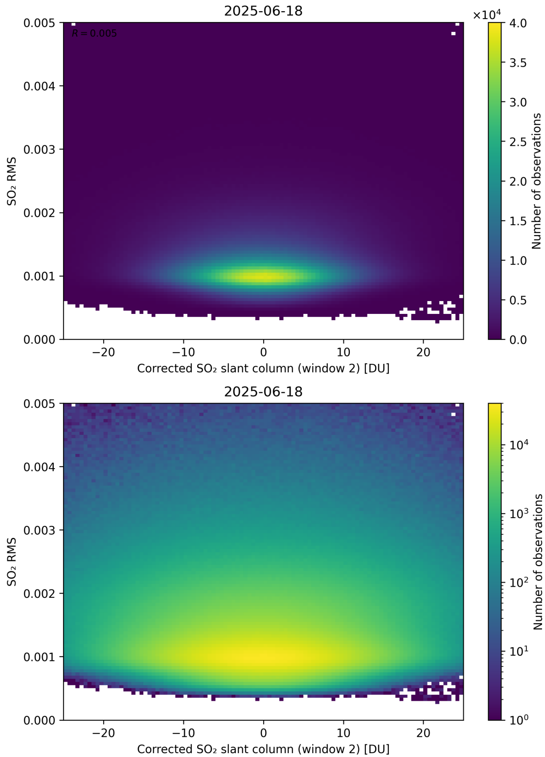
Figure 248: Scatter density plot of “Corrected SO 2 slant column (window 2)” against “SO 2 RMS” for 2025-06-17 to 2025-06-19.
