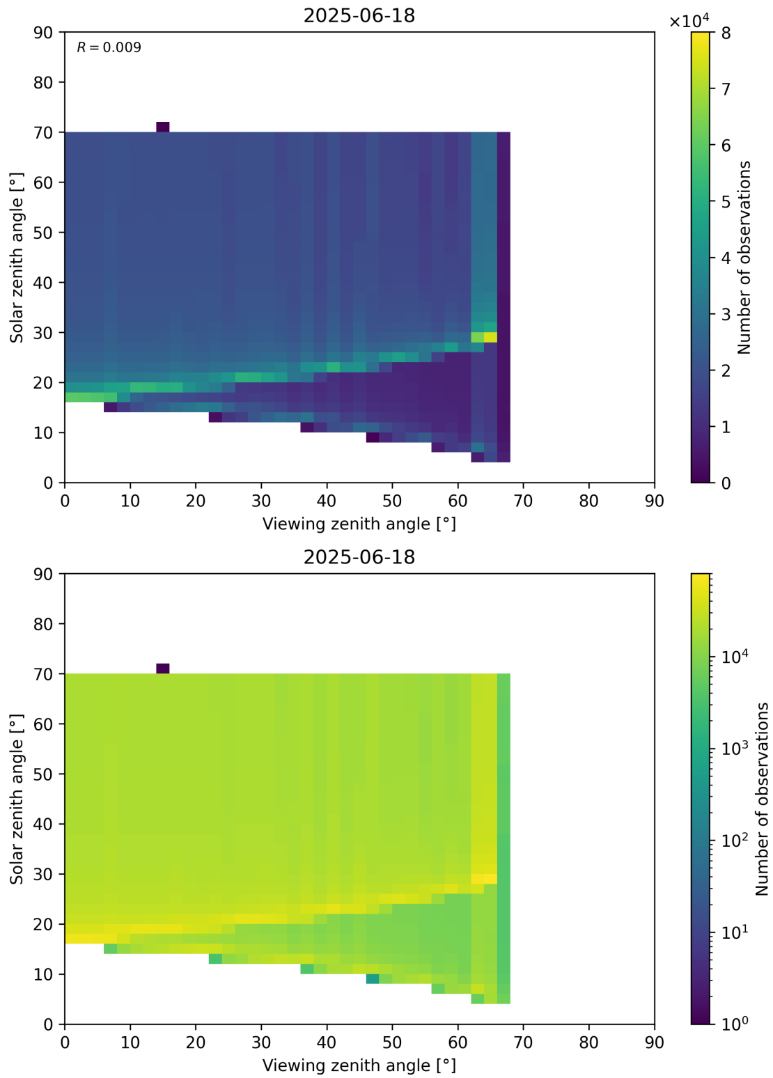
Figure 369: Scatter density plot of “Viewing zenith angle” against “Solar zenith angle” for 2025-06-17 to 2025-06-19.
