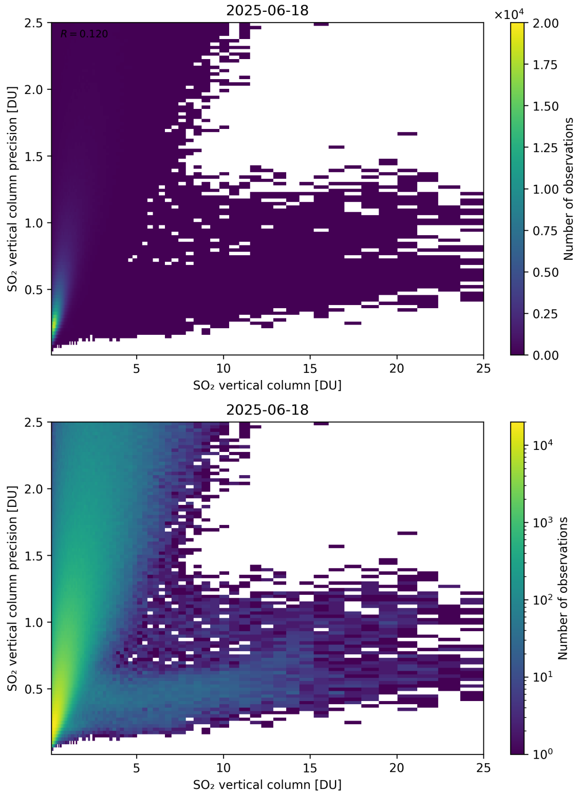
Figure 361: Scatter density plot of “SO 2 vertical column” against “SO 2 vertical column precision” for 2025-06-17 to 2025-06-19.
