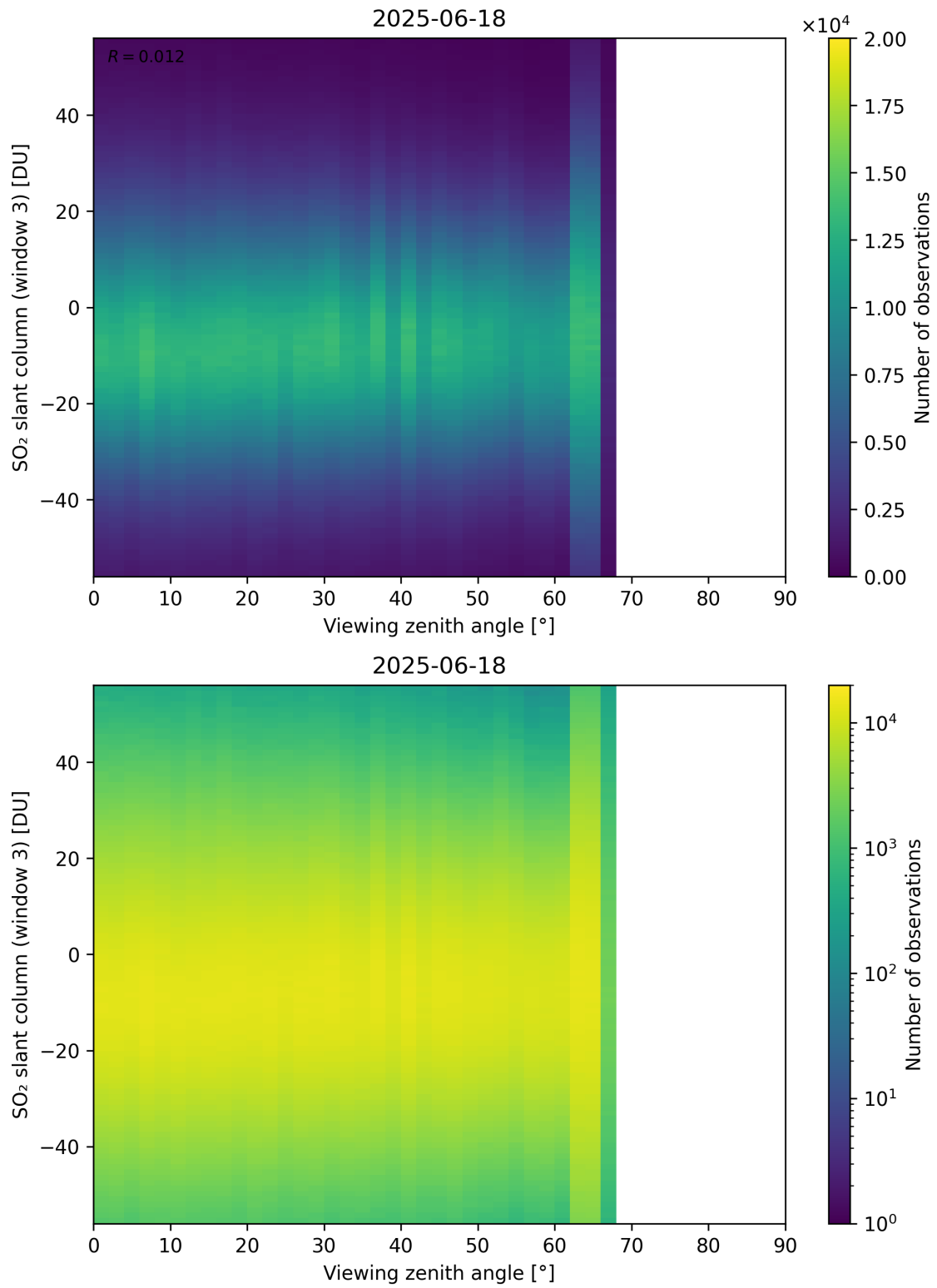
Figure 379: Scatter density plot of “Viewing zenith angle” against “SO 2 slant column (window 3)” for 2025-06-17 to 2025-06-19.
