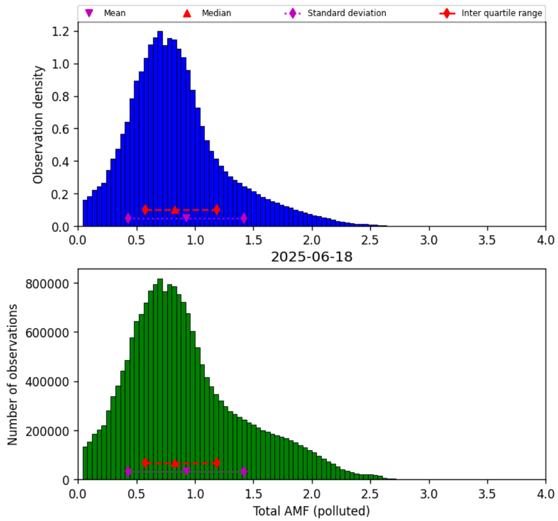
Figure 79: Histogram of “Total AMF (polluted)” for 2025-06-17 to 2025-06-19
