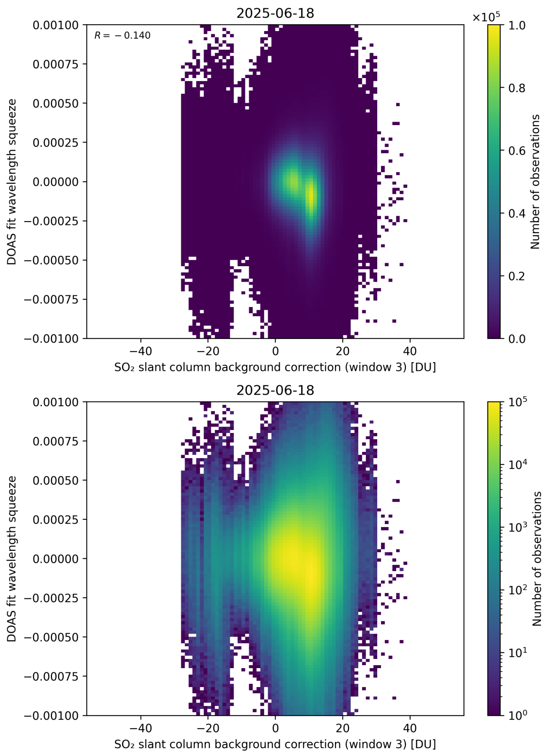
Figure 133: Scatter density plot of “SO 2 slant column background correction (window 3)” against “DOAS fit wavelength squeeze” for 2025-06-17 to 2025-06-19.
