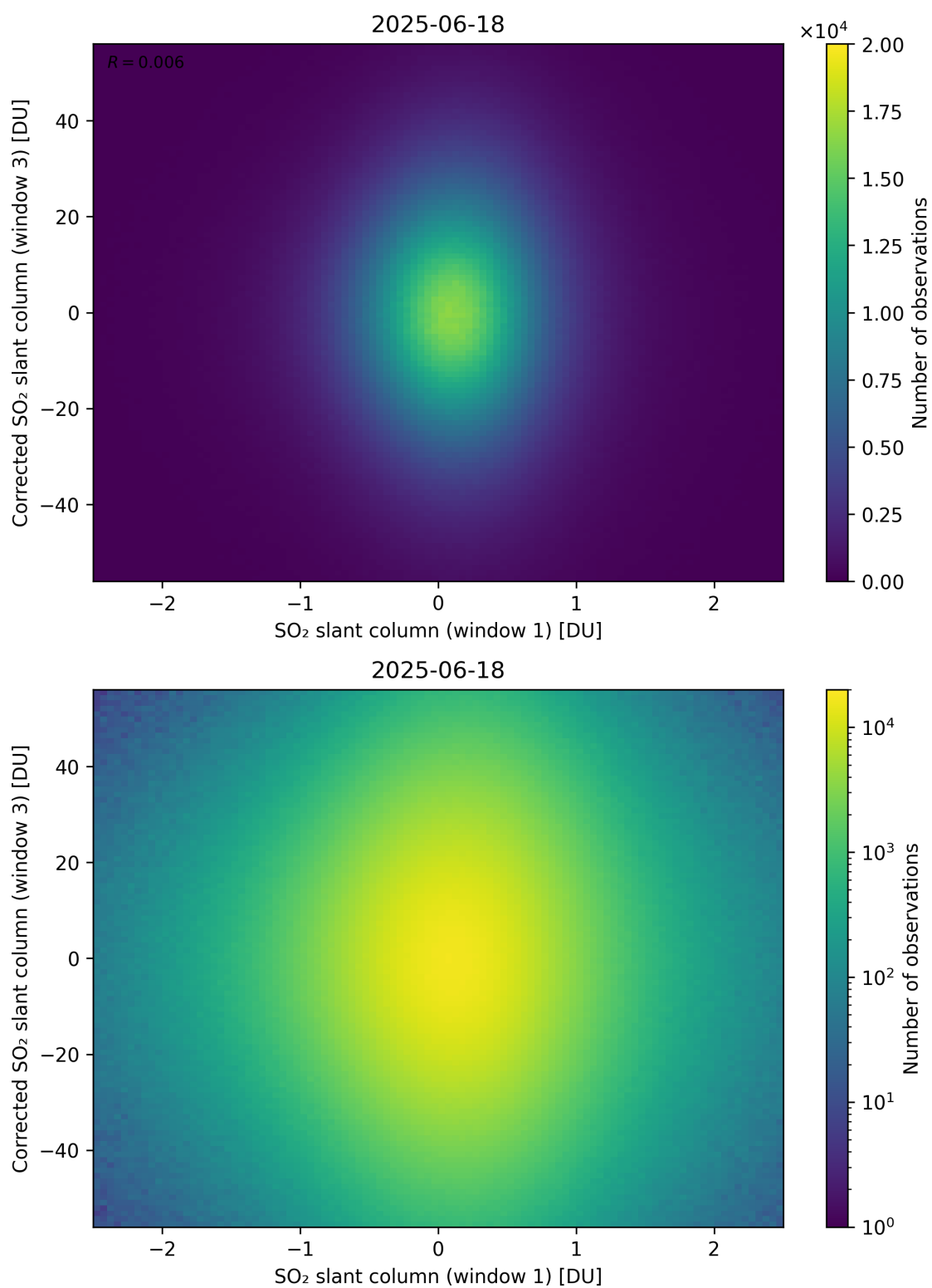
Figure 284: Scatter density plot of “SO 2 slant column (window 1)” against “Corrected SO 2 slant column (window 3)” for 2025-06-17 to 2025-06-19.
