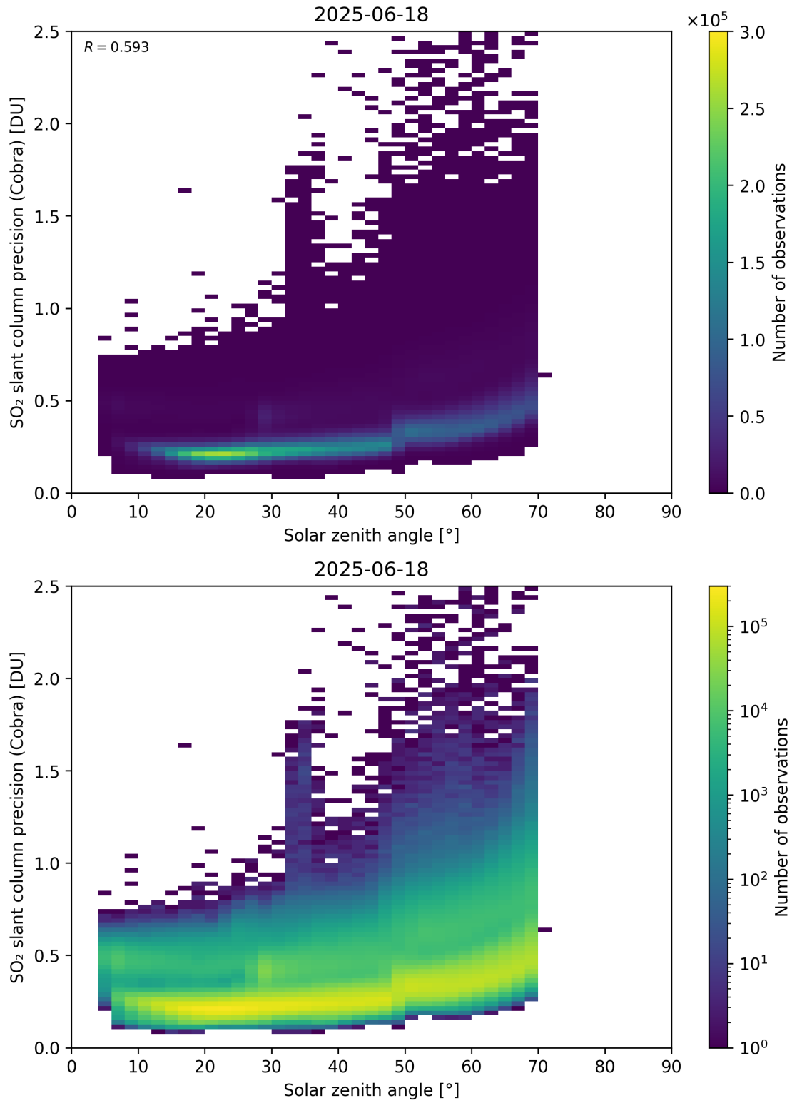
Figure 180: Scatter density plot of “Solar zenith angle” against “SO 2 slant column precision (Cobra)” for 2025-06-17 to 2025-06-19.
