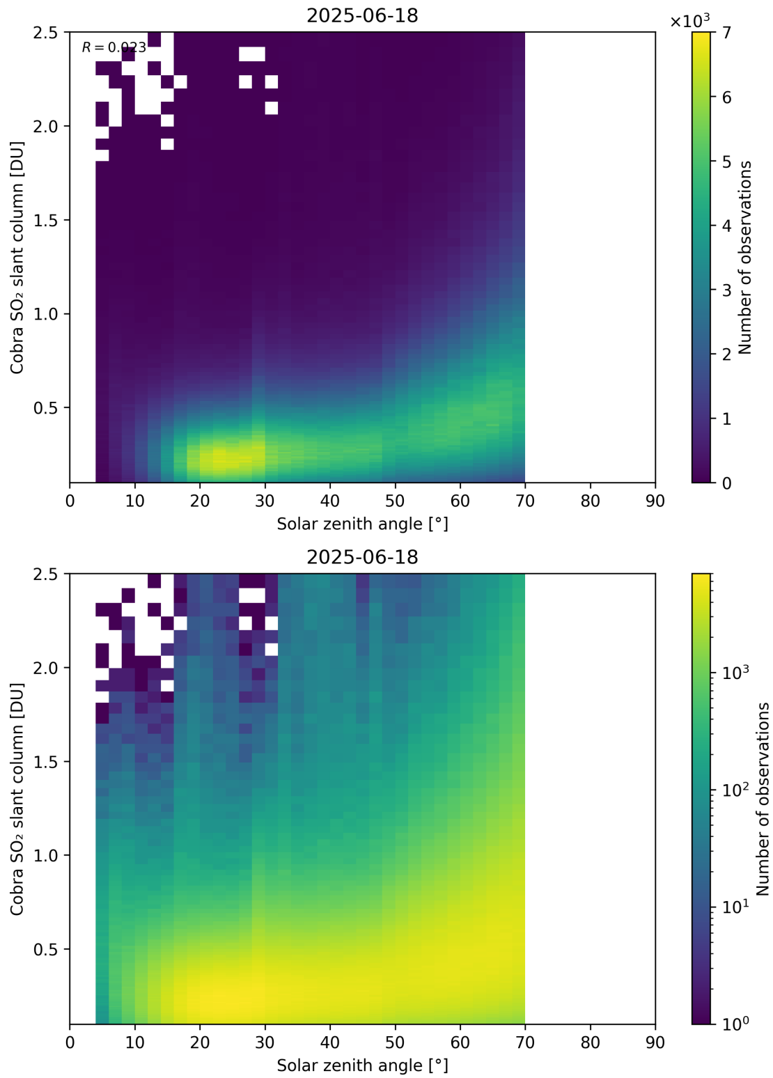
Figure 179: Scatter density plot of “Solar zenith angle” against “Cobra SO 2 slant column” for 2025-06-17 to 2025-06-19.
