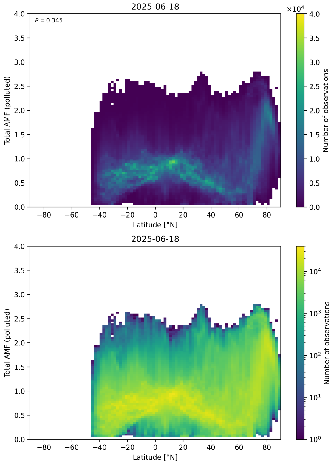
Figure 167: Scatter density plot of “Latitude” against “Total AMF (polluted)” for 2025-06-17 to 2025-06-19.
