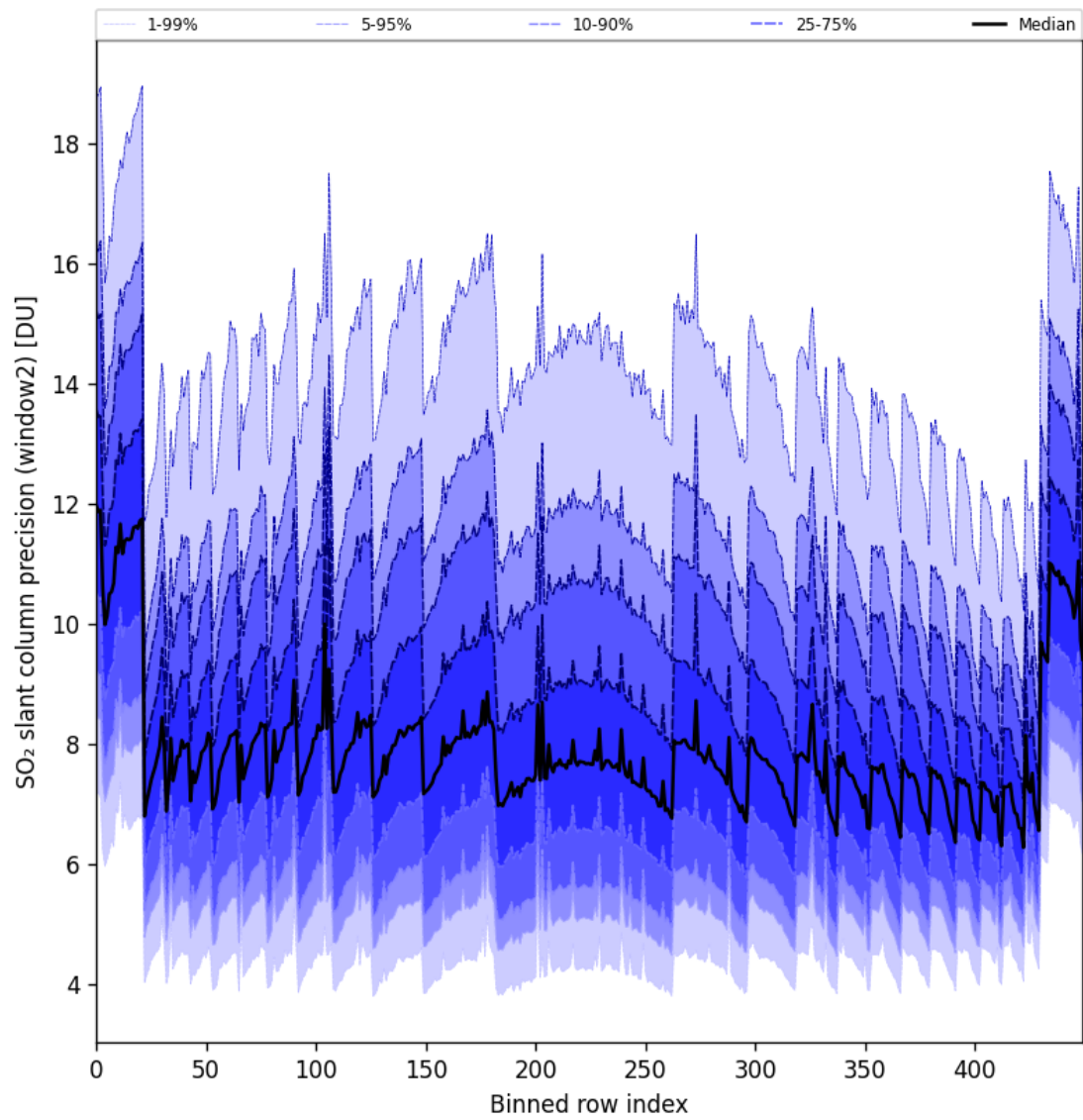
Figure 94: Along track statistics of “SO 2 slant column precision (window2)” for 2025-06-17 to 2025-06-19
