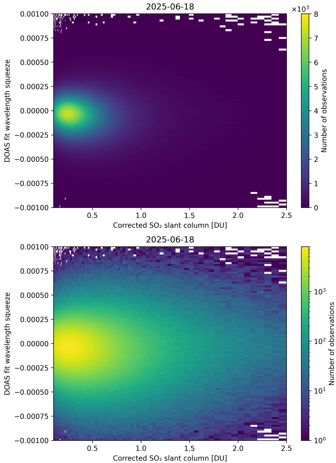
Figure 230: Scatter density plot of “Corrected SO 2 slant column” against “DOAS fit wavelength squeeze” for 2025-06-17 to 2025-06-19.
