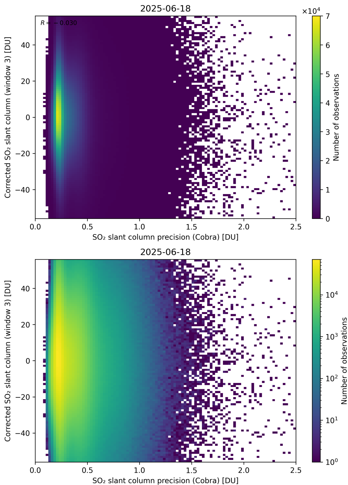
Figure 207: Scatter density plot of “SO 2 slant column precision (Cobra)” against “Corrected SO 2 slant column (window 3)” for 2025-06-17 to 2025-06-19.
