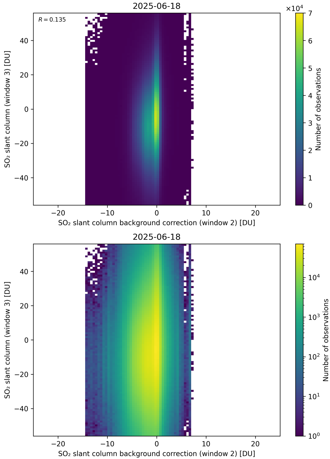
Figure 128: Scatter density plot of “SO 2 slant column background correction (window 2)” against “SO 2 slant column (window 3)” for 2025-06-17 to 2025-06-19.
