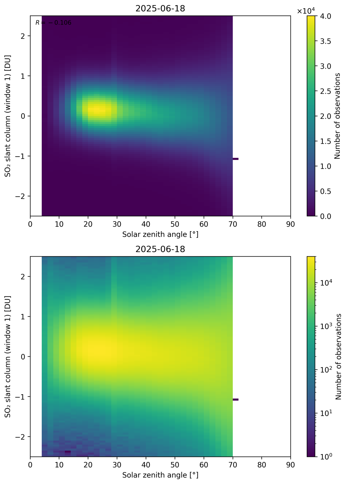
Figure 184: Scatter density plot of “Solar zenith angle” against “SO 2 slant column (window 1)” for 2025-06-17 to 2025-06-19.
