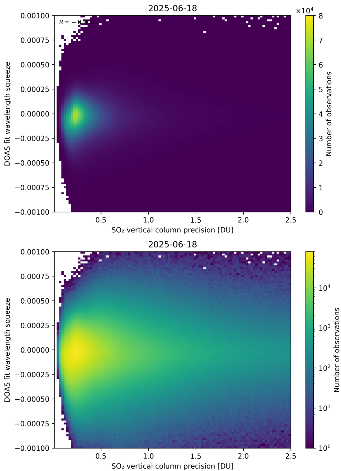
Figure 333: Scatter density plot of “SO 2 vertical column precision” against “DOAS fit wavelength squeeze” for 2025-06-17 to 2025-06-19.
