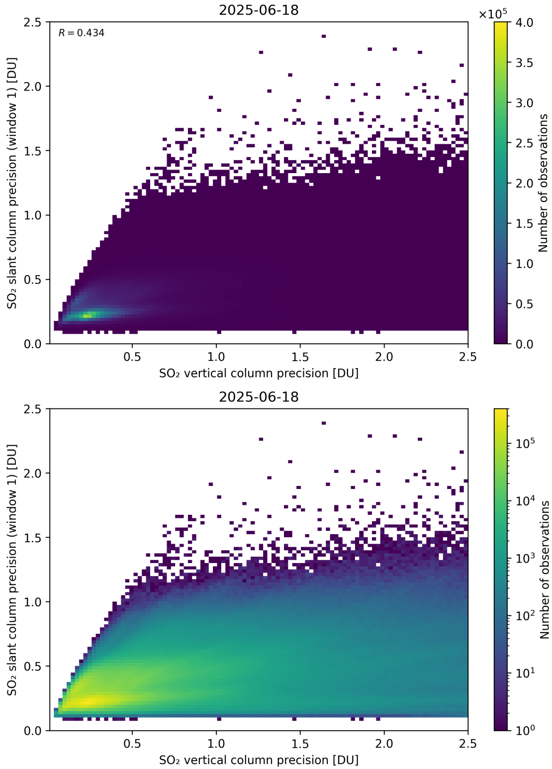
Figure 342: Scatter density plot of “SO 2 vertical column precision” against “SO 2 slant column precision (window 1)” for 2025-06-17 to 2025-06-19.
