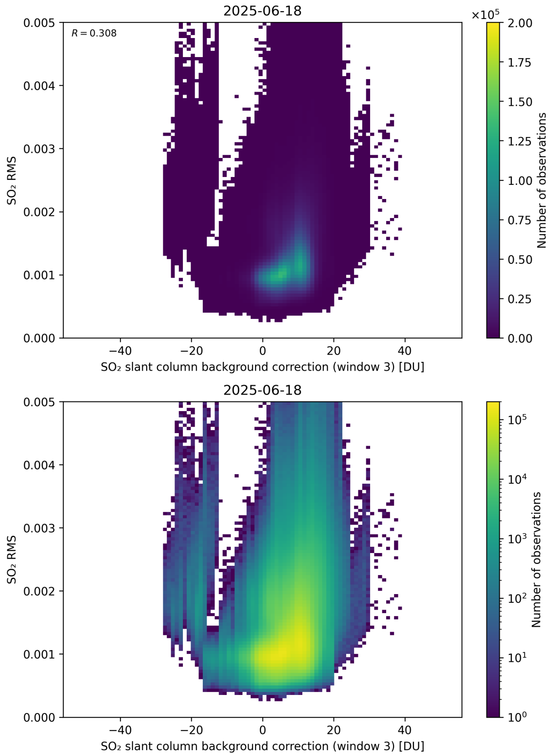
Figure 134: Scatter density plot of “SO 2 slant column background correction (window 3)” against “SO 2 RMS” for 2025-06-17 to 2025-06-19.
