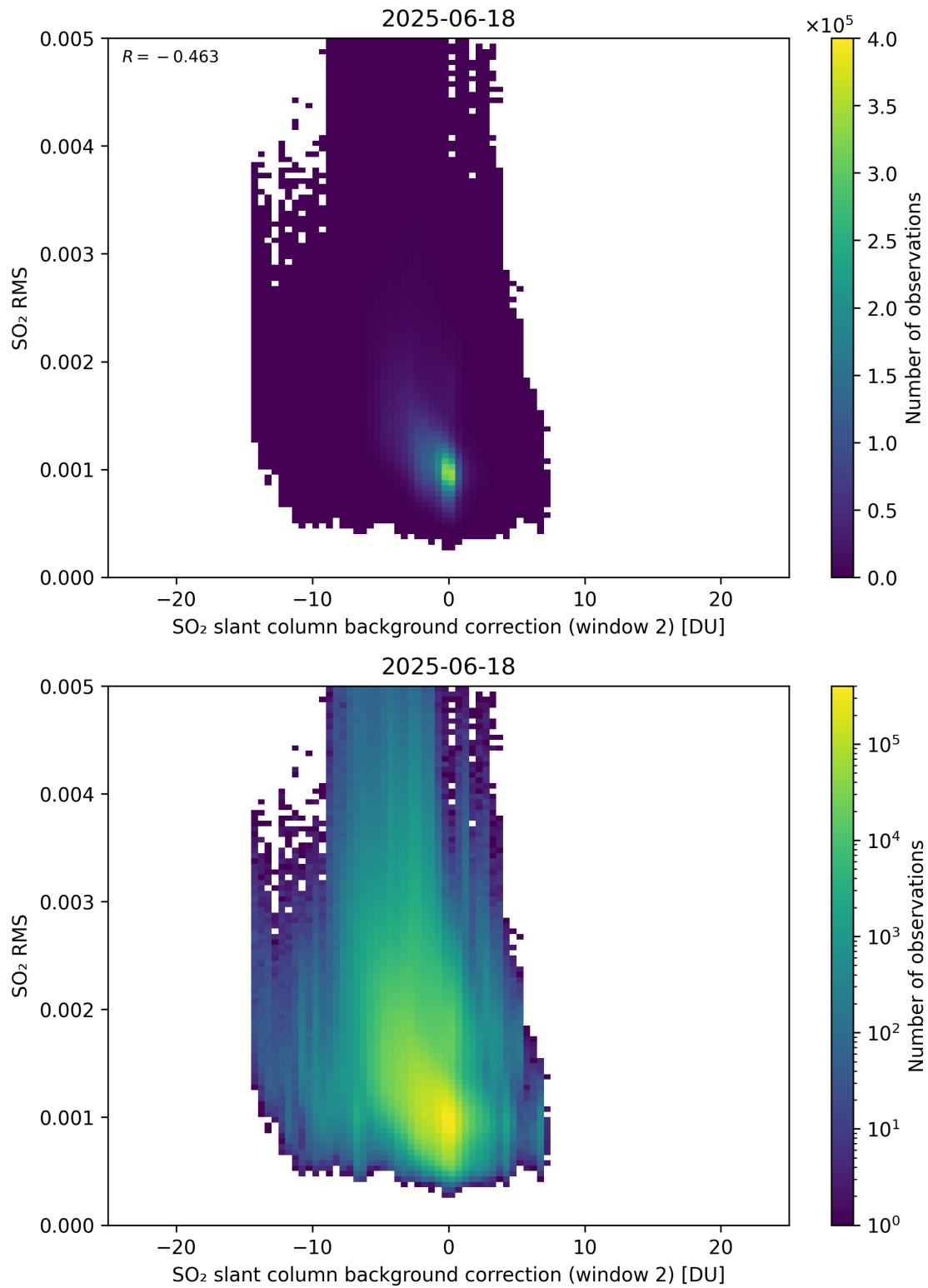
Figure 125: Scatter density plot of “SO 2 slant column background correction (window 2)” against “SO 2 RMS” for 2025-06-17 to 2025-06-19.
