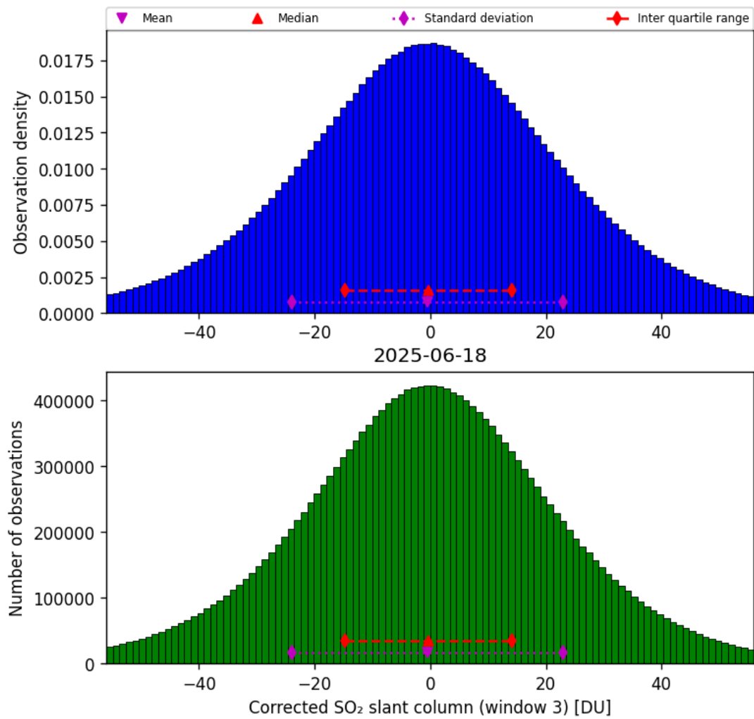
Figure 73: Histogram of “Corrected SO 2 slant column (window 3)” for 2025-06-17 to 2025-06-19
