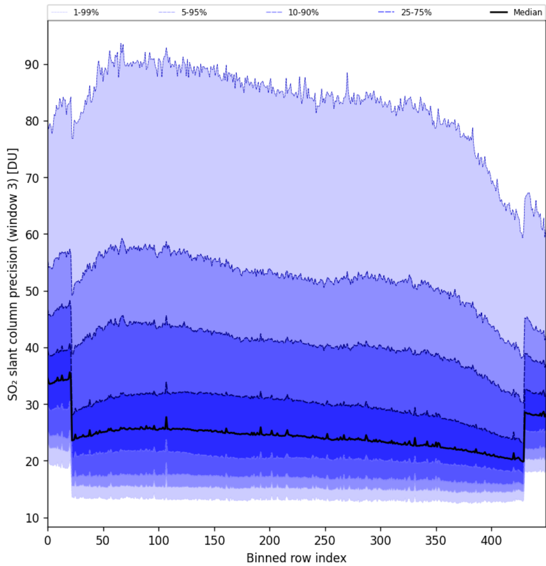
Figure 98: Along track statistics of “SO 2 slant column precision (window 3)” for 2025-06-17 to 2025-06-19
