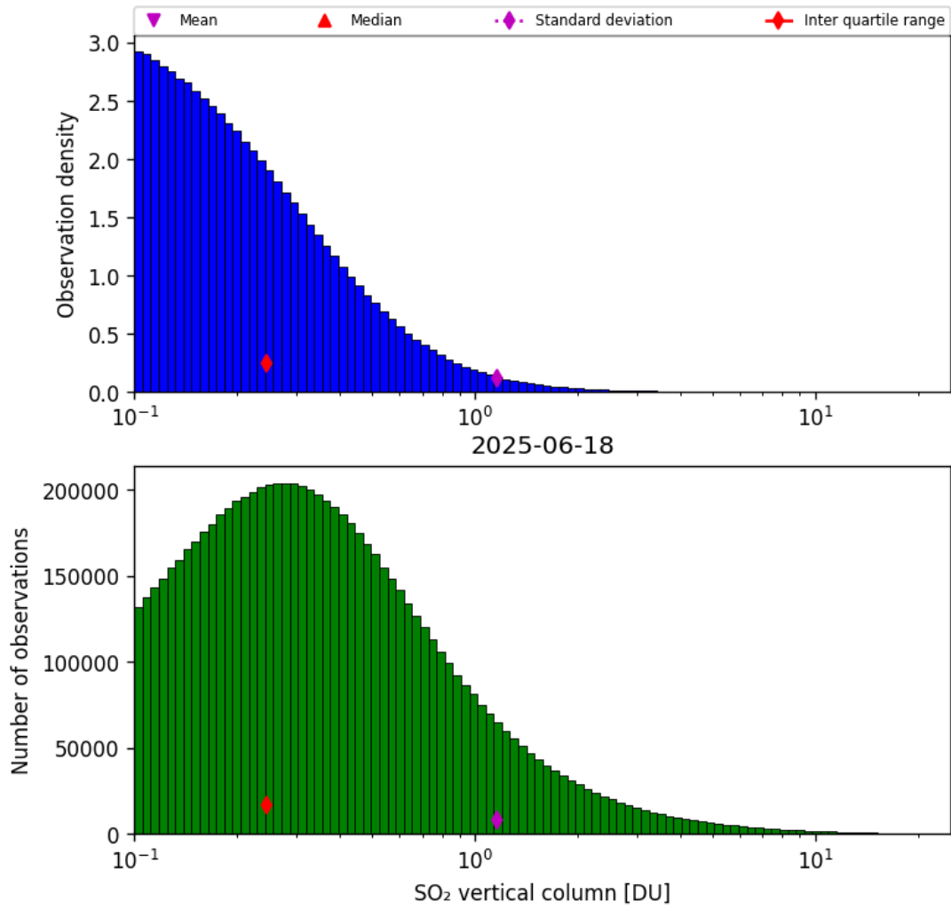
Figure 58: Histogram of “SO 2 vertical column” for 2025-06-17 to 2025-06-19
