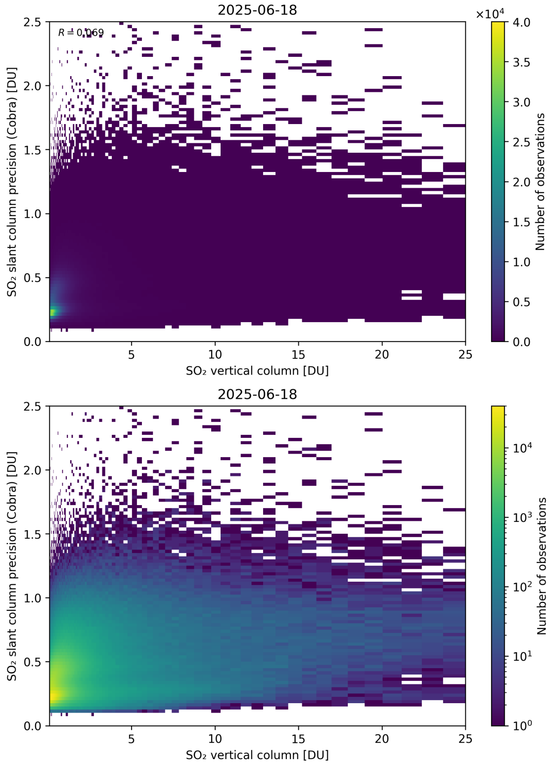
Figure 350: Scatter density plot of “SO 2 vertical column” against “SO 2 slant column precision (Cobra)” for 2025-06-17 to 2025-06-19.
