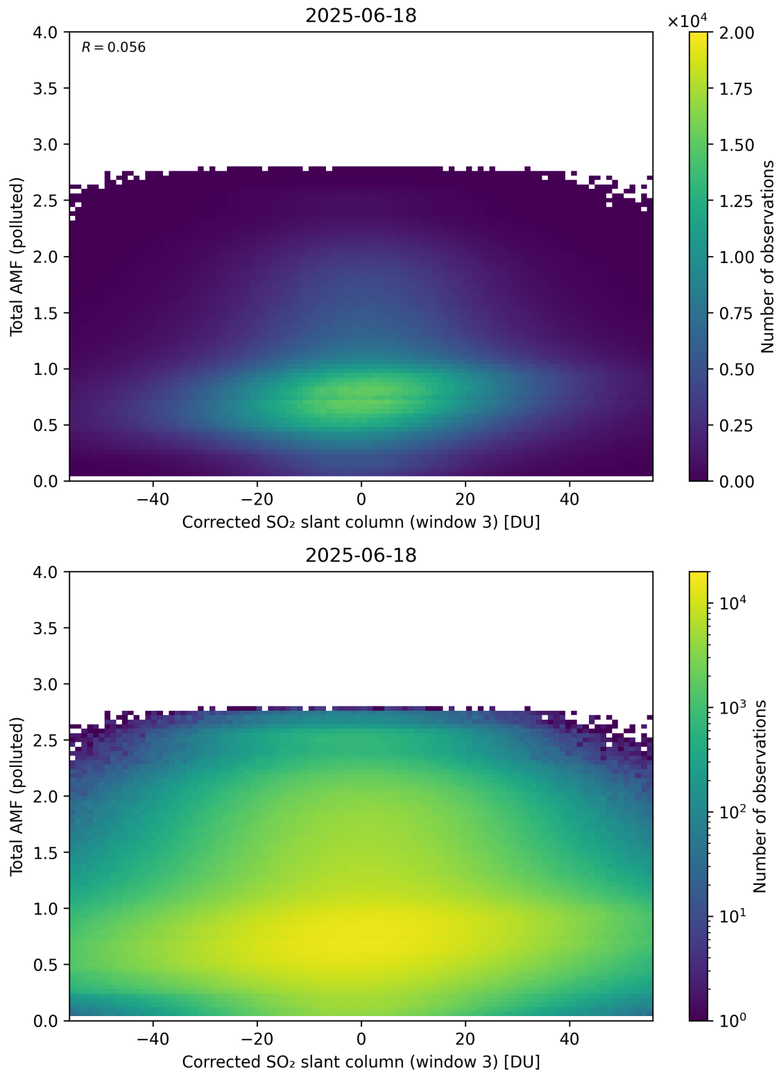
Figure 260: Scatter density plot of “Corrected SO 2 slant column (window 3)” against “Total AMF (polluted)” for 2025-06-17 to 2025-06-19.
