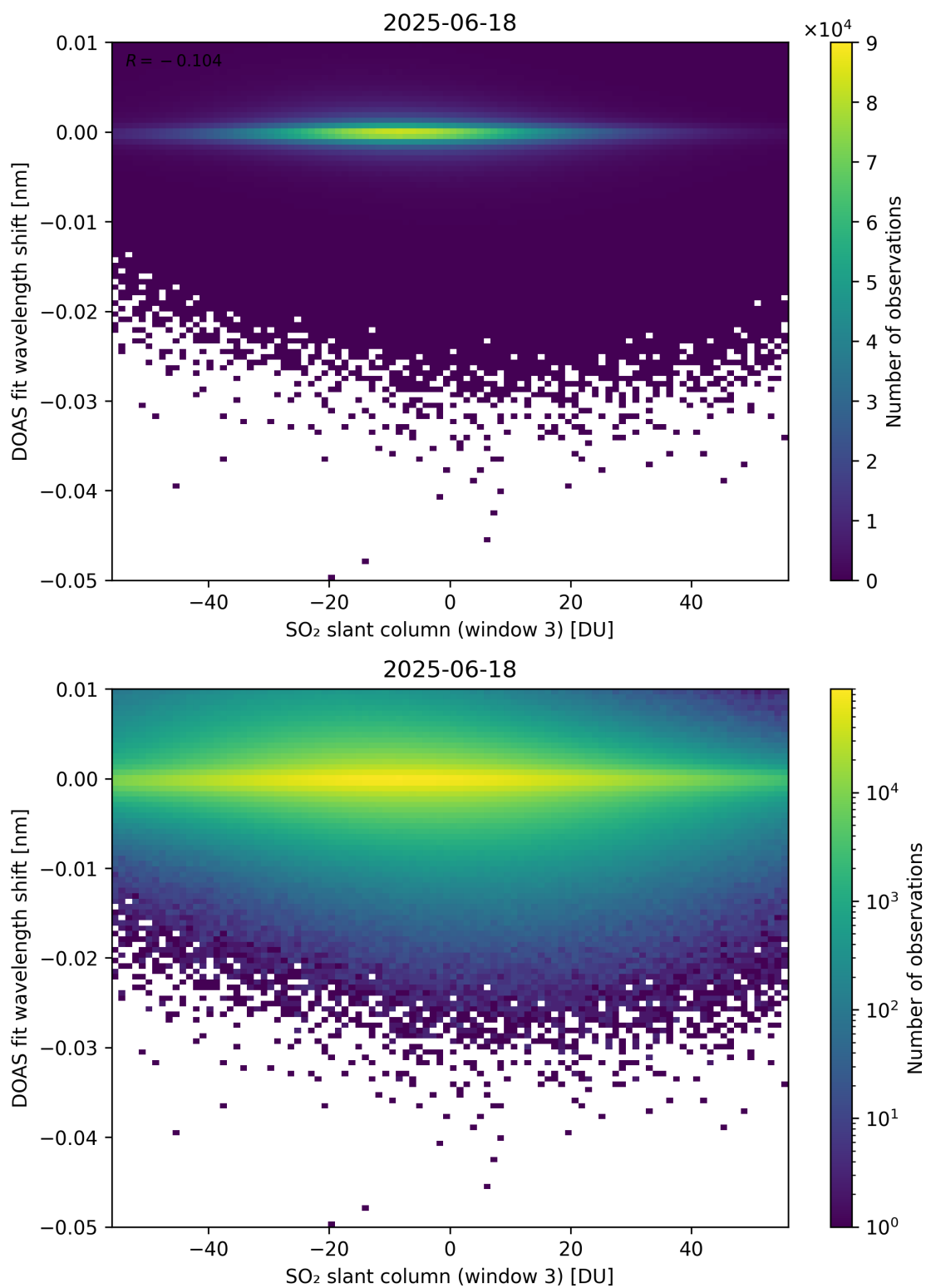
Figure 304: Scatter density plot of “SO 2 slant column (window 3)” against “DOAS fit wavelength shift” for 2025-06-17 to 2025-06-19.
