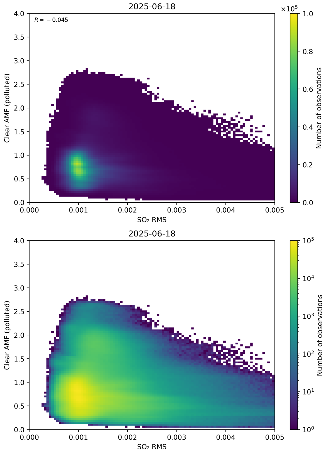
Figure 147: Scatter density plot of “SO 2 RMS” against “Clear AMF (polluted)” for 2025-06-17 to 2025-06-19.
