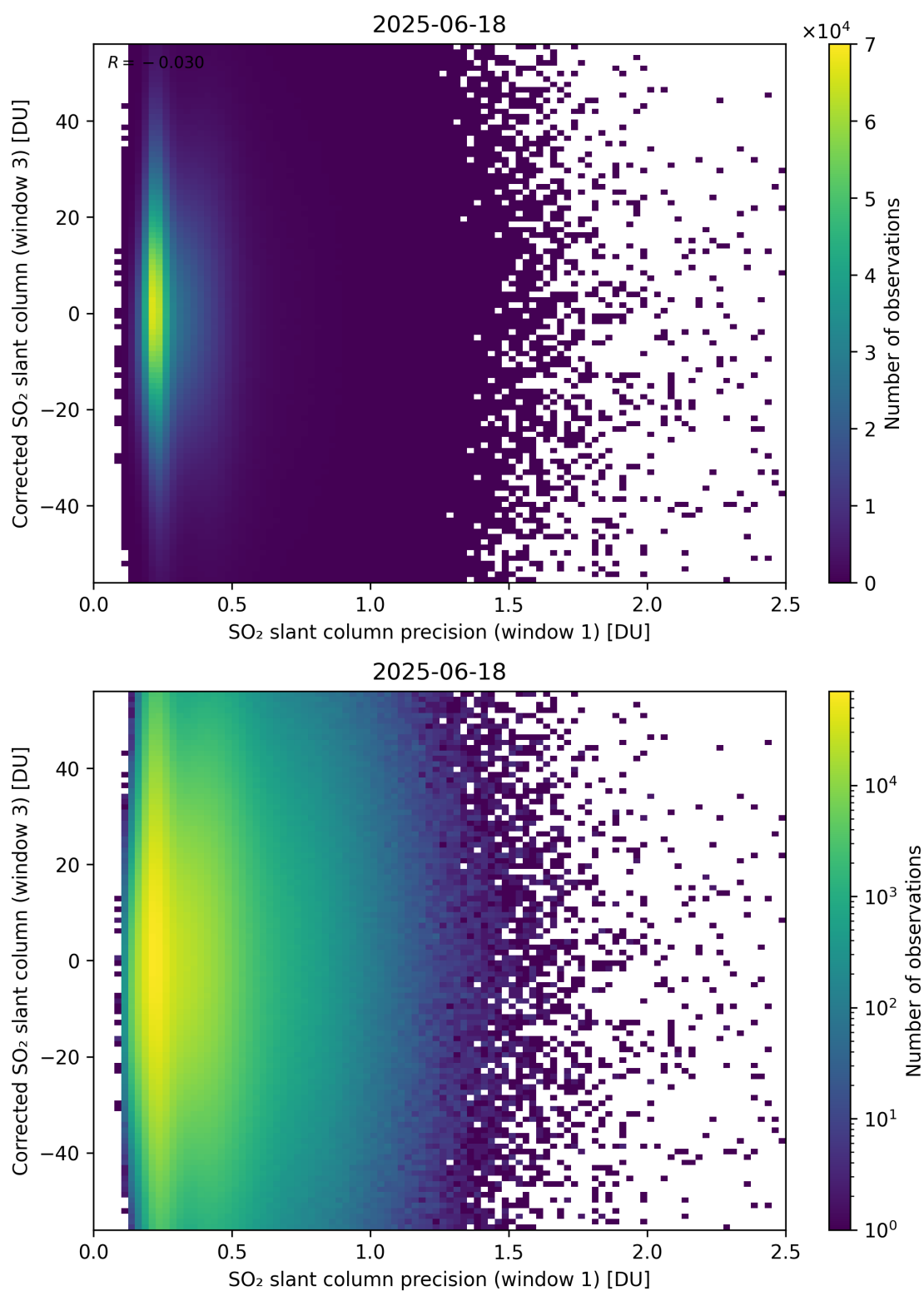
Figure 276: Scatter density plot of “SO 2 slant column precision (window 1)” against “Corrected SO 2 slant column (window 3)” for 2025-06-17 to 2025-06-19.
