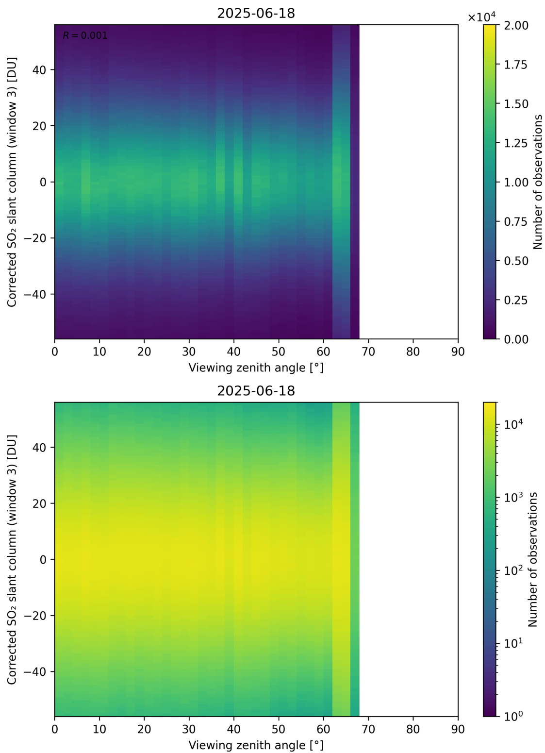
Figure 375: Scatter density plot of “Viewing zenith angle” against “Corrected SO 2 slant column (window 3)” for 2025-06-17 to 2025-06-19.
