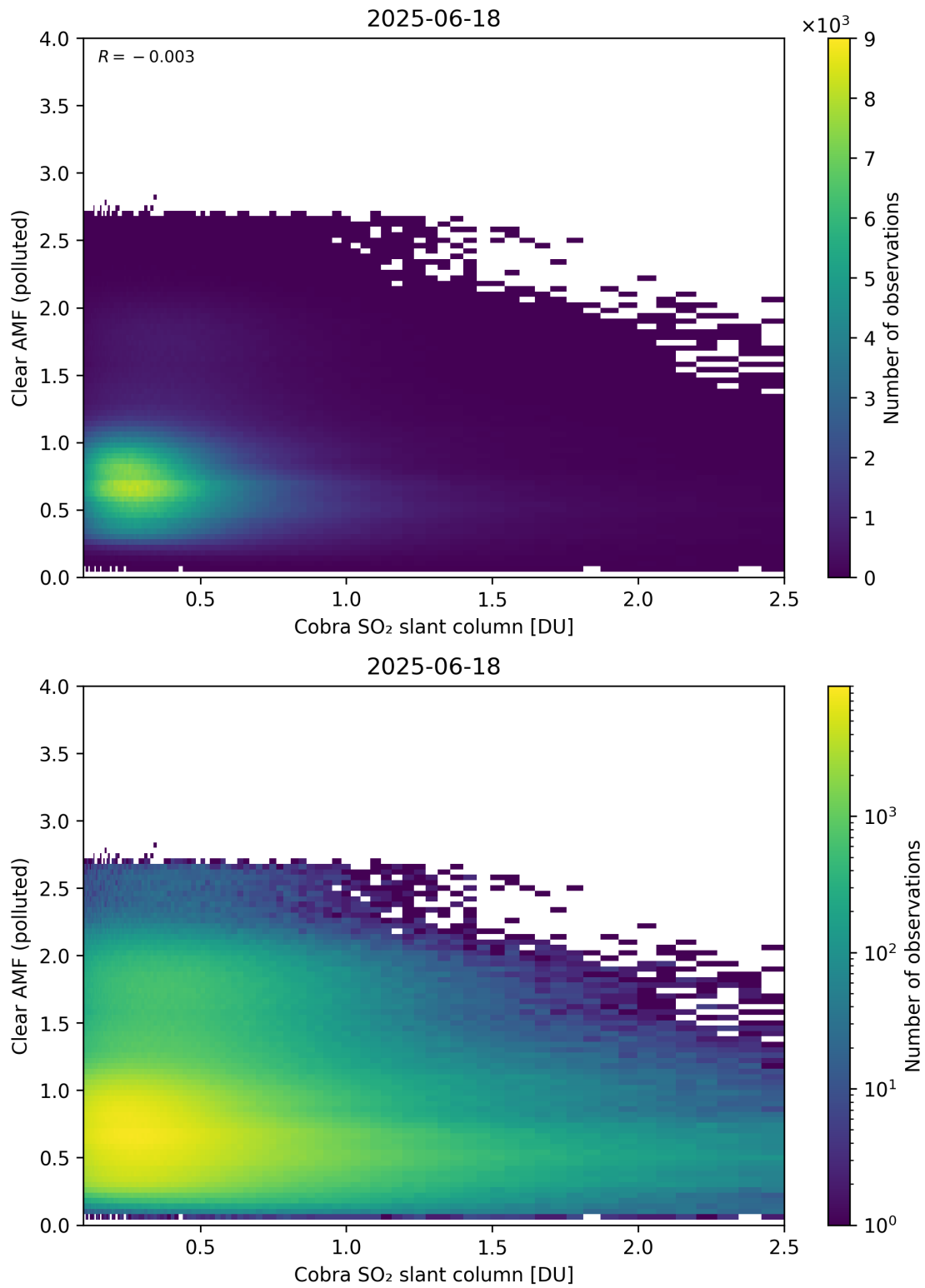
Figure 215: Scatter density plot of “Cobra SO 2 slant column” against “Clear AMF (polluted)” for 2025-06-17 to 2025-06-19.
