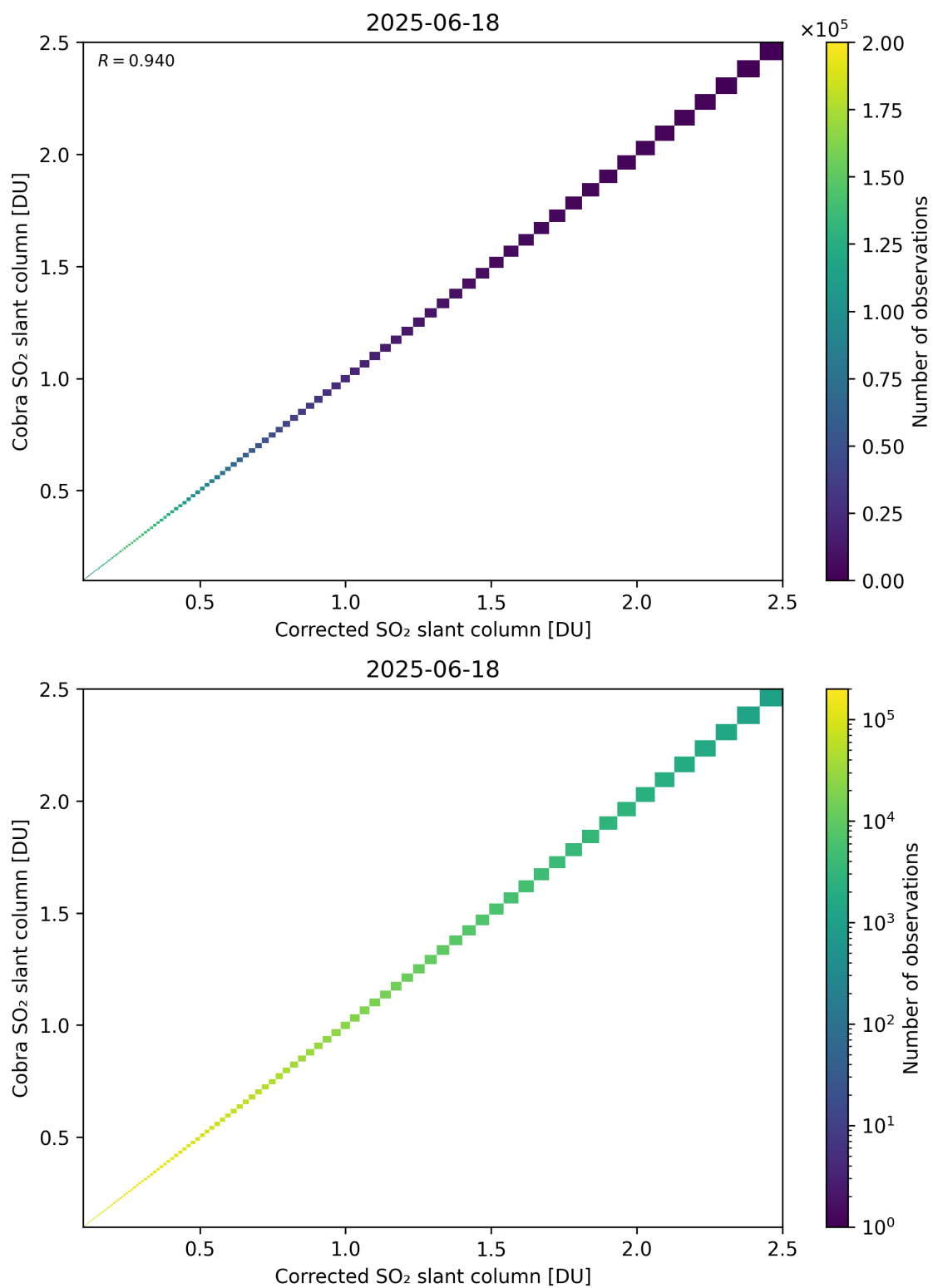
Figure 233: Scatter density plot of “Corrected SO 2 slant column” against “Cobra SO 2 slant column” for 2025-06-17 to 2025-06-19.
