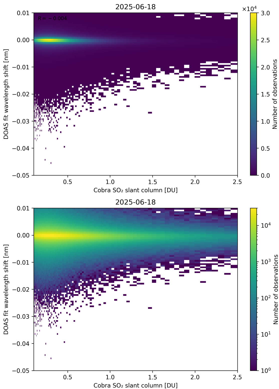
Figure 196: Scatter density plot of “Cobra SO 2 slant column” against “DOAS fit wavelength shift” for 2025-06-17 to 2025-06-19.
