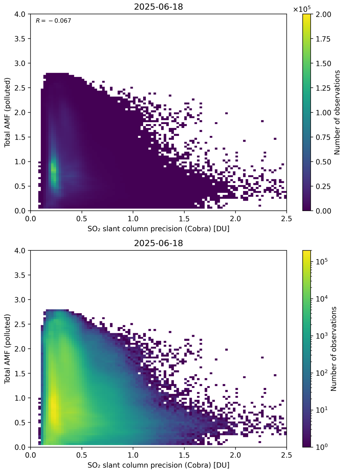
Figure 213: Scatter density plot of “SO 2 slant column precision (Cobra)” against “Total AMF (polluted)” for 2025-06-17 to 2025-06-19.
