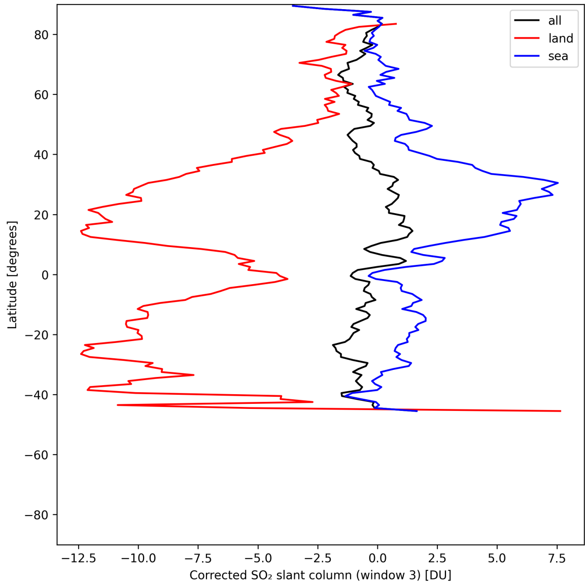
Figure 47: Zonal average of “Corrected SO 2 slant column (window 3)” for 2025-06-17 to 2025-06-19.
