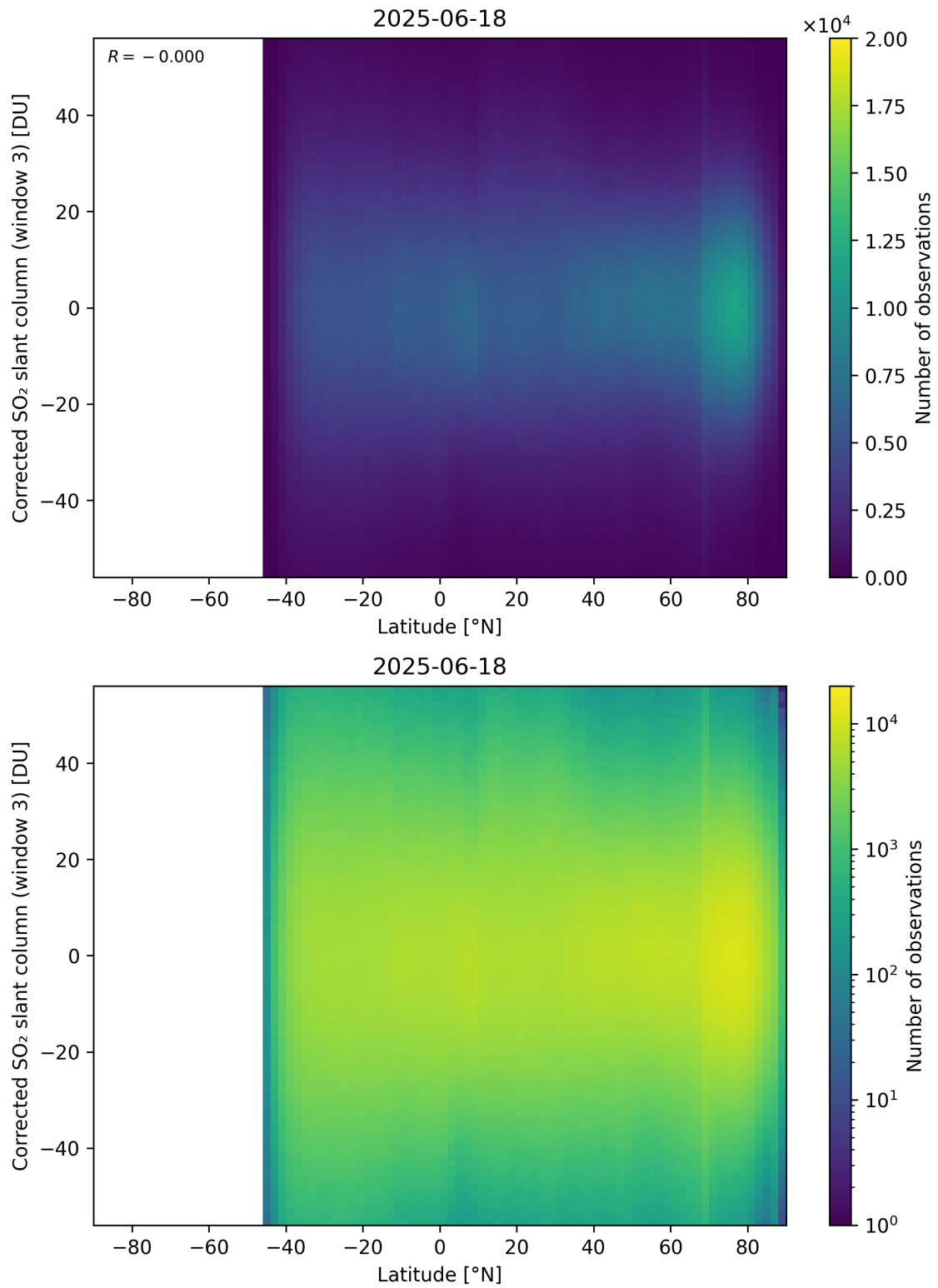
Figure 161: Scatter density plot of “Latitude” against “Corrected SO 2 slant column (window 3)” for 2025-06-17 to 2025-06-19.
