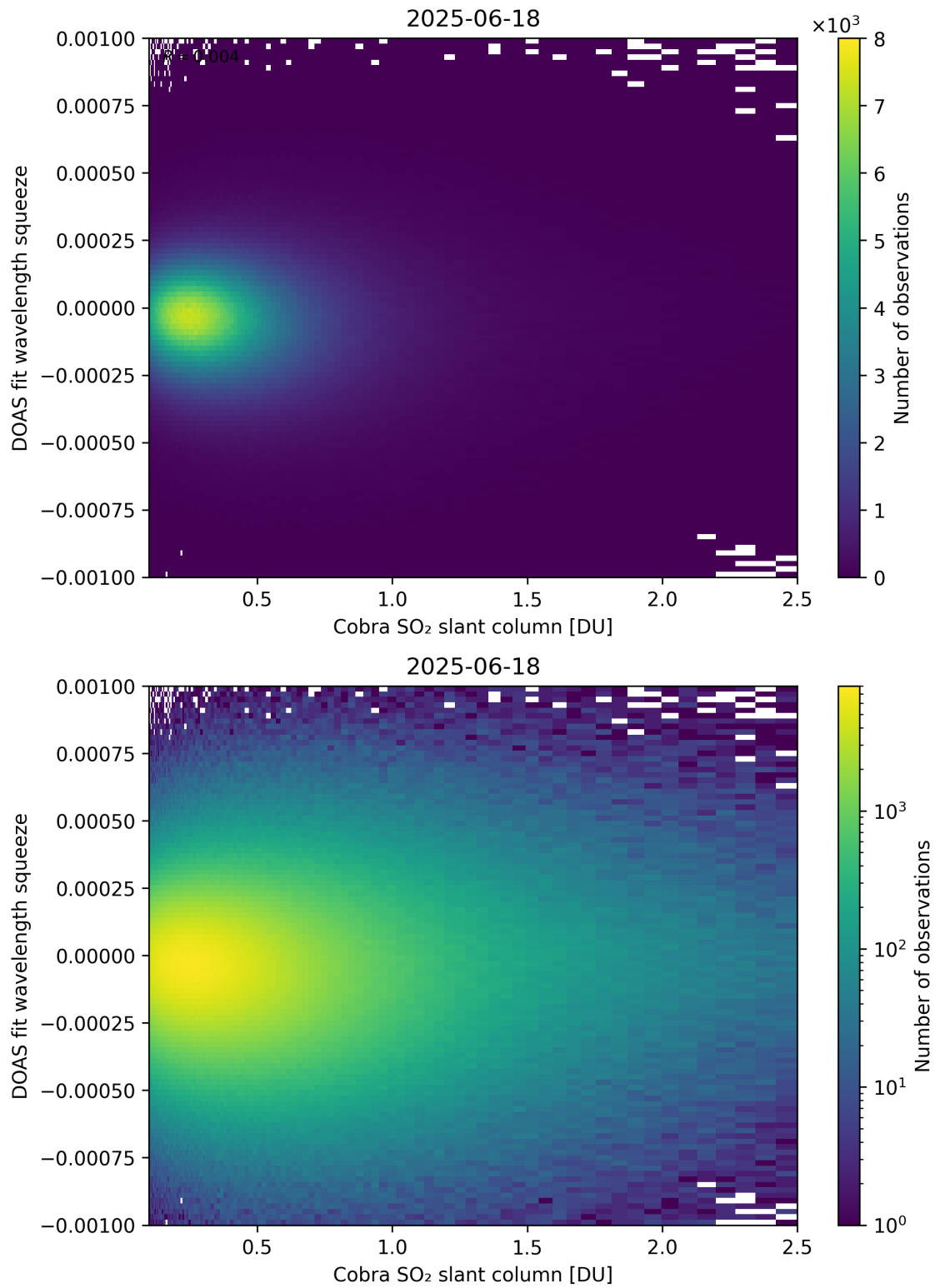
Figure 197: Scatter density plot of “Cobra SO 2 slant column” against “DOAS fit wavelength squeeze” for 2025-06-17 to 2025-06-19.
