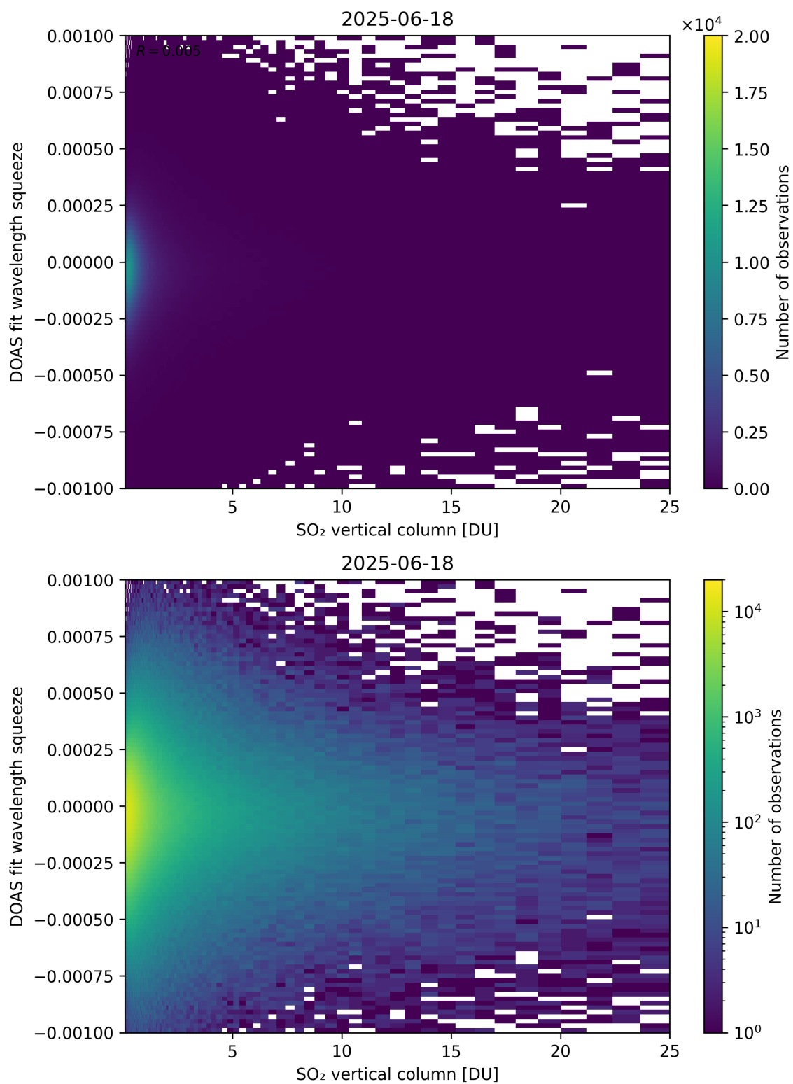
Figure 327: Scatter density plot of “SO 2 vertical column” against “DOAS fit wavelength squeeze” for 2025-06-17 to 2025-06-19.
