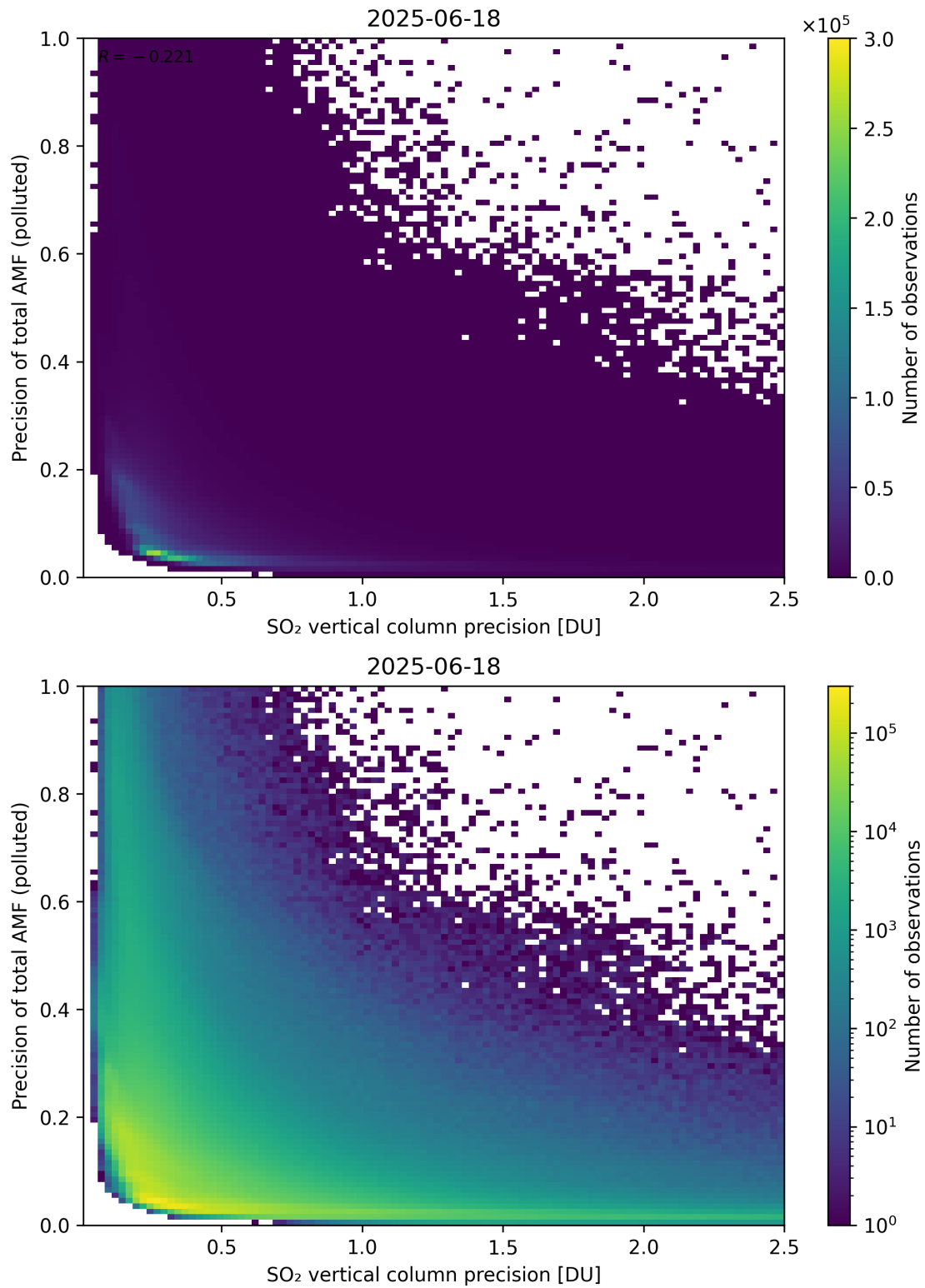
Figure 347: Scatter density plot of “SO 2 vertical column precision” against “Precision of total AMF (polluted)” for 2025-06-17 to 2025-06-19.
