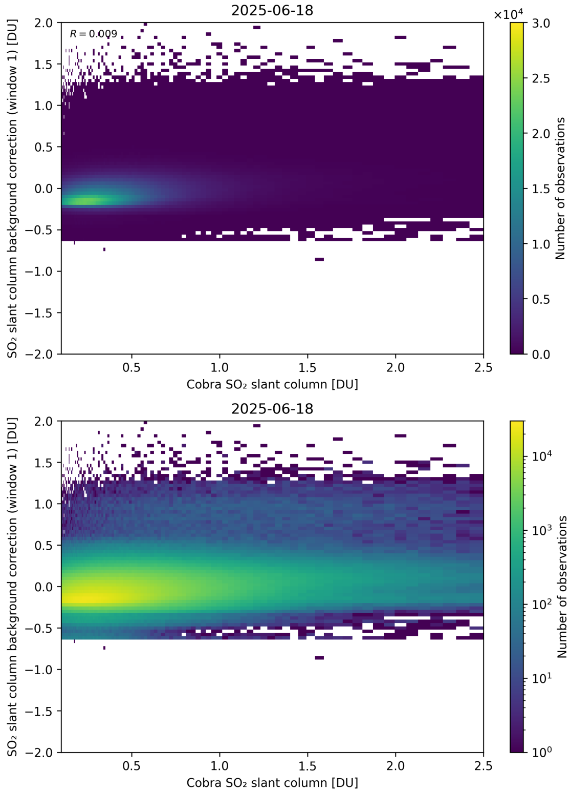
Figure 193: Scatter density plot of “Cobra SO 2 slant column” against “SO 2 slant column background correction (window 1)” for 2025-06-17 to 2025-06-19.
