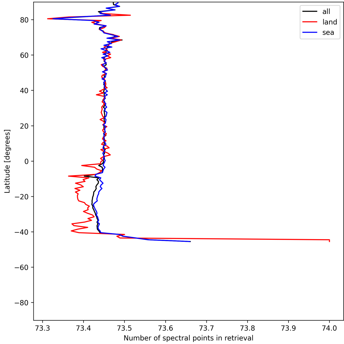
Figure 56: Zonal average of “Number of spectral points in retrieval” for 2025-06-17 to 2025-06-19.
