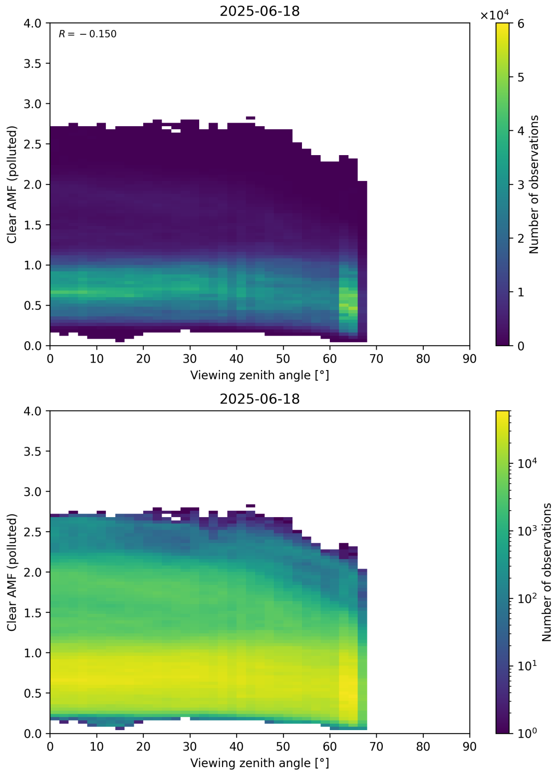
Figure 370: Scatter density plot of “Viewing zenith angle” against “Clear AMF (polluted)” for 2025-06-17 to 2025-06-19.
