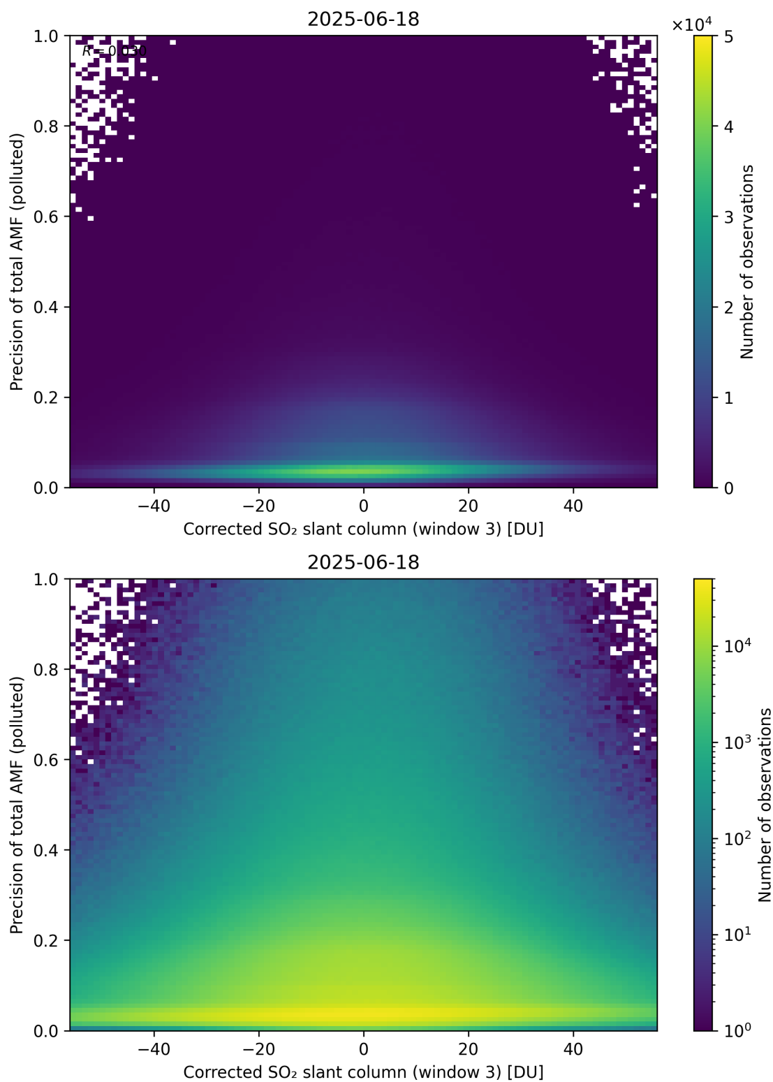
Figure 261: Scatter density plot of “Corrected SO 2 slant column (window 3)” against “Precision of total AMF (polluted)” for 2025-06-17 to 2025-06-19.
