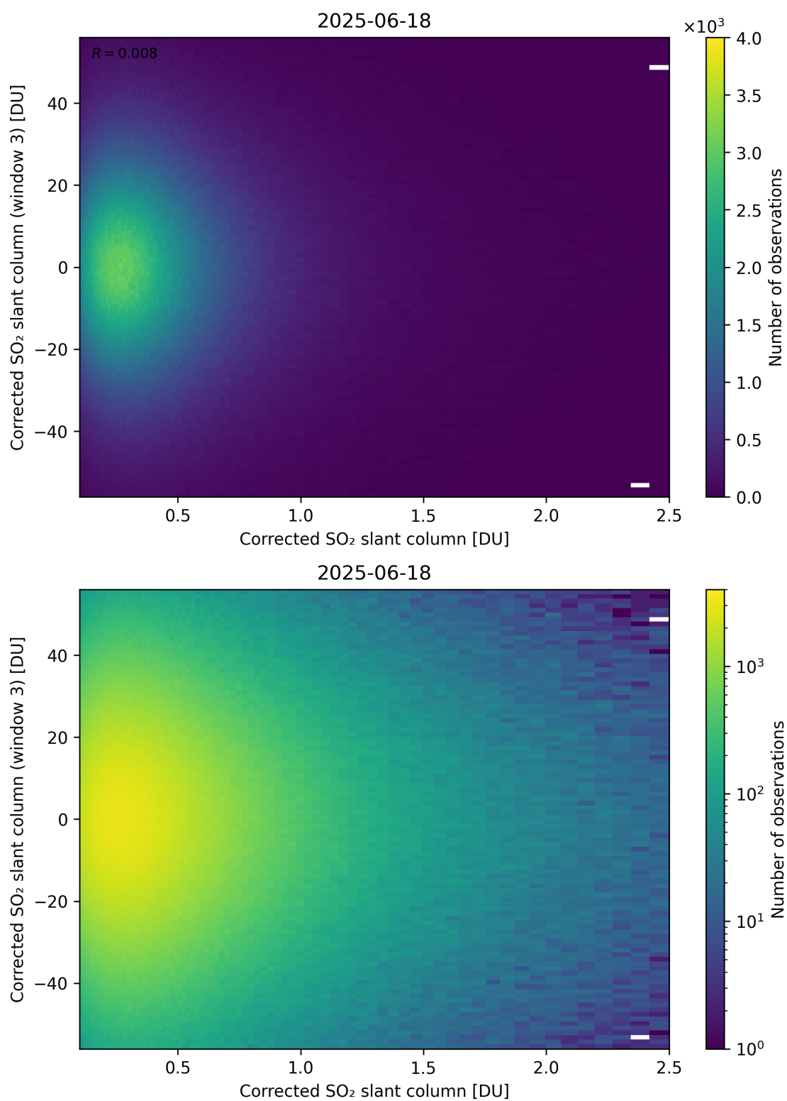
Figure 236: Scatter density plot of “Corrected SO 2 slant column” against “Corrected SO 2 slant column (window 3)” for 2025-06-17 to 2025-06-19.
