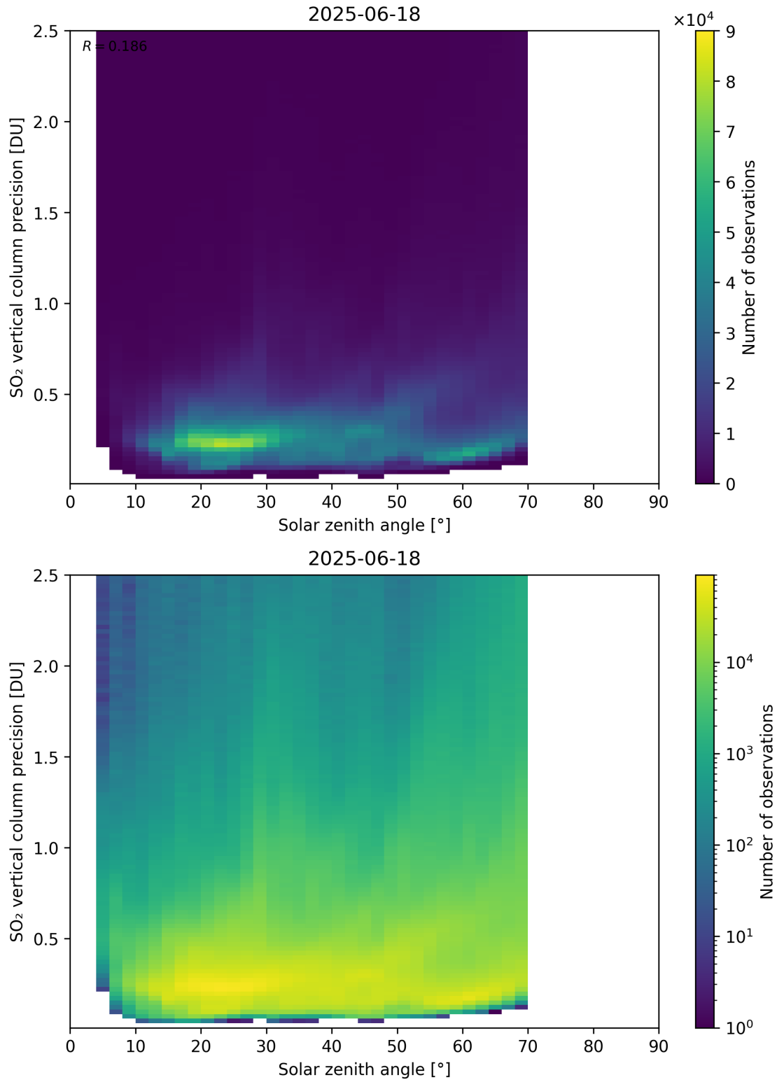
Figure 192: Scatter density plot of “Solar zenith angle” against “SO 2 vertical column precision” for 2025-06-17 to 2025-06-19.
