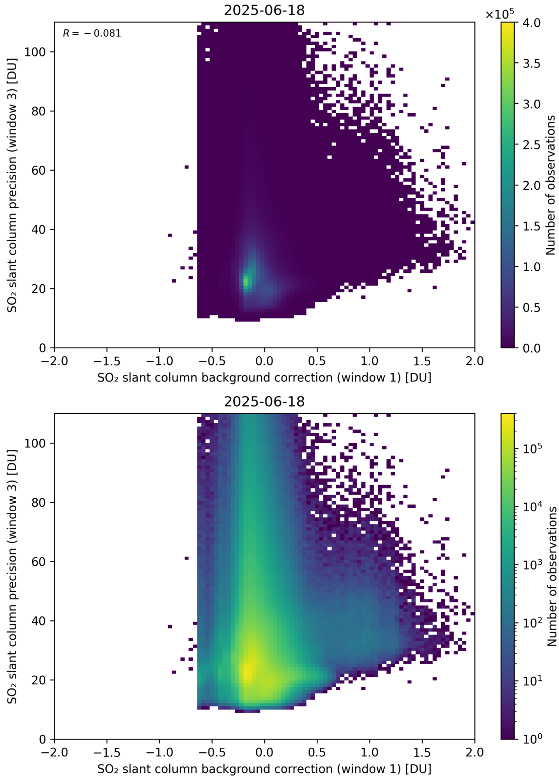
Figure 119: Scatter density plot of “SO 2 slant column background correction (window 1)” against “SO 2 slant column precision (window 3)” for 2025-06-17 to 2025-06-19.
