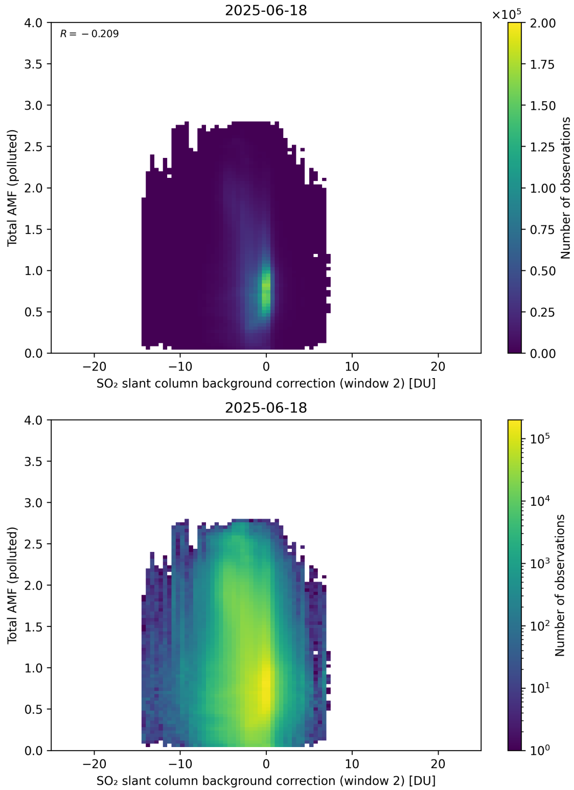
Figure 130: Scatter density plot of “SO 2 slant column background correction (window 2)” against “Total AMF (polluted)” for 2025-06-17 to 2025-06-19.
