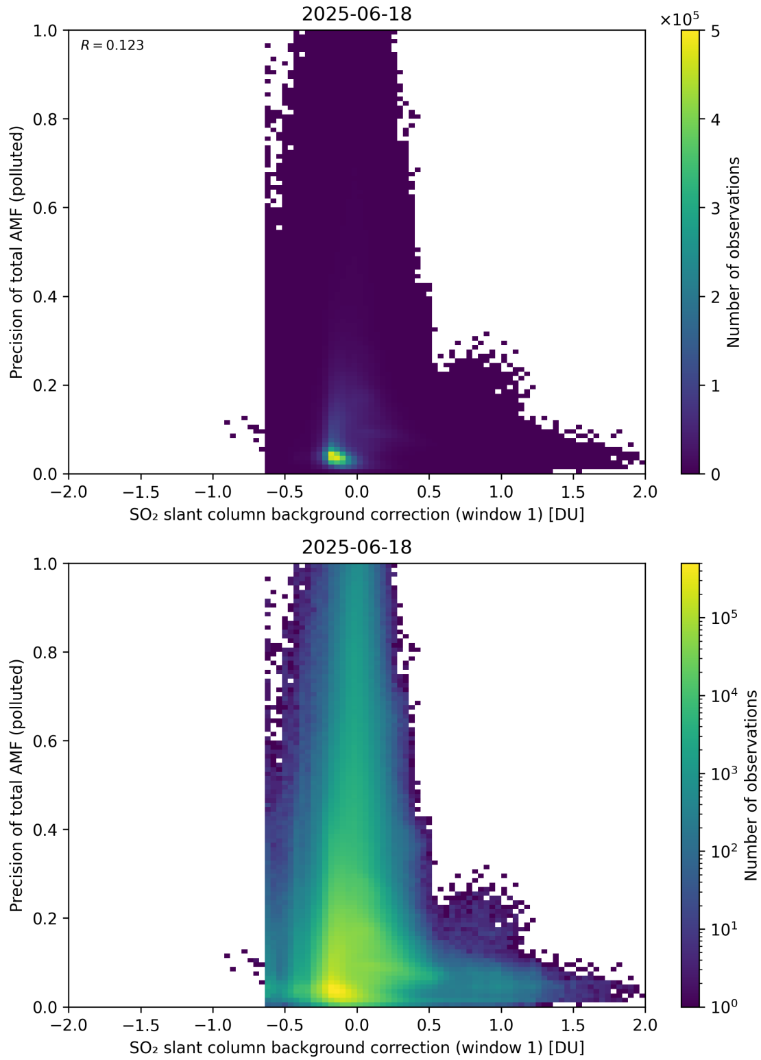
Figure 121: Scatter density plot of “SO 2 slant column background correction (window 1)” against “Precision of total AMF (polluted)” for 2025-06-17 to 2025-06-19.
