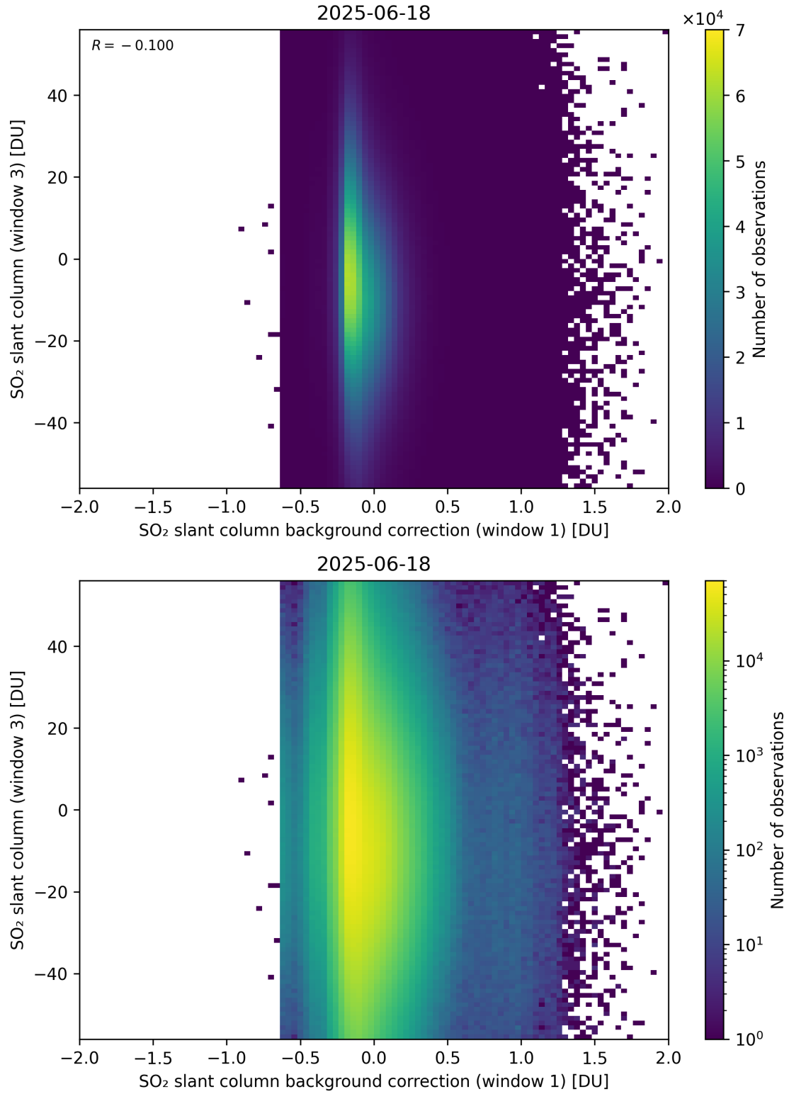
Figure 118: Scatter density plot of “SO 2 slant column background correction (window 1)” against “SO 2 slant column (window 3)” for 2025-06-17 to 2025-06-19.
