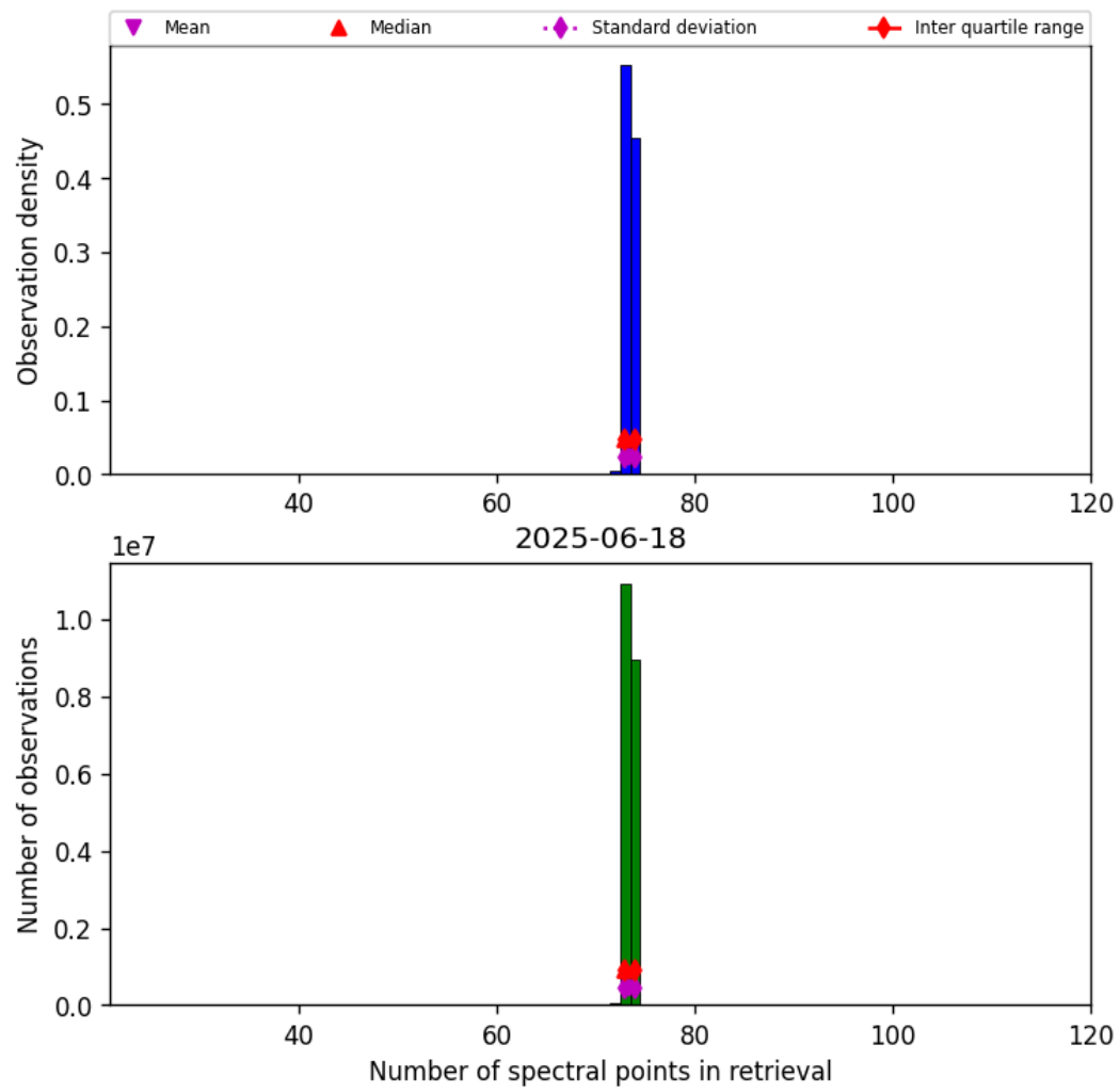
Figure 82: Histogram of “Number of spectral points in retrieval” for 2025-06-17 to 2025-06-19
