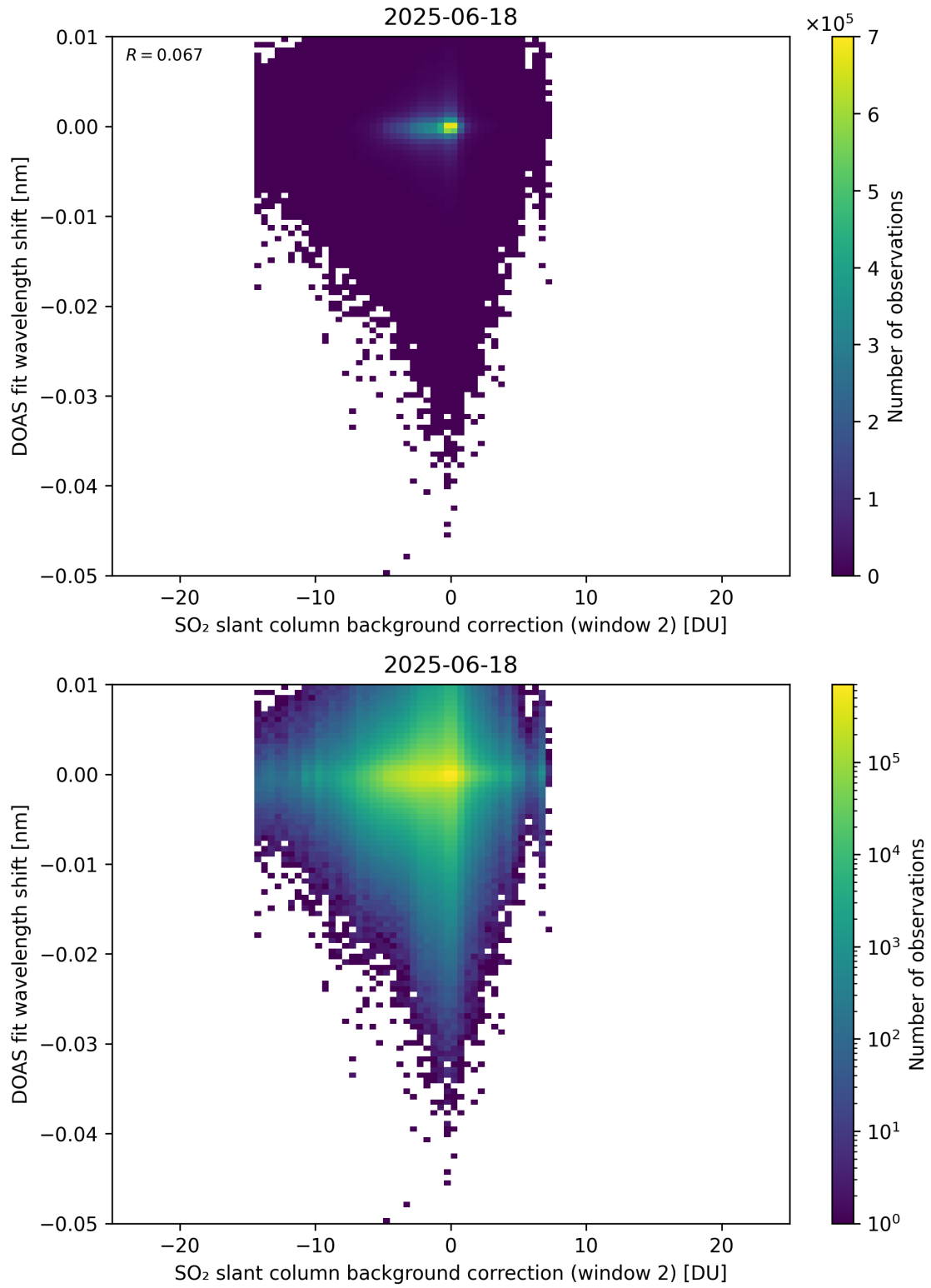
Figure 123: Scatter density plot of “SO 2 slant column background correction (window 2)” against “DOAS fit wavelength shift” for 2025-06-17 to 2025-06-19.
