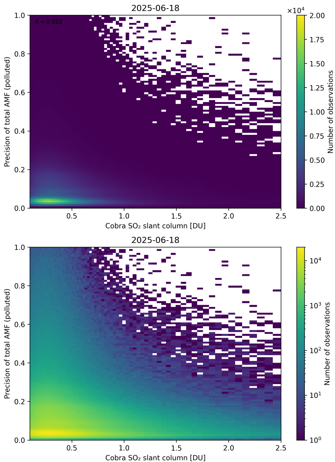
Figure 225: Scatter density plot of “Cobra SO 2 slant column” against “Precision of total AMF (polluted)” for 2025-06-17 to 2025-06-19.
