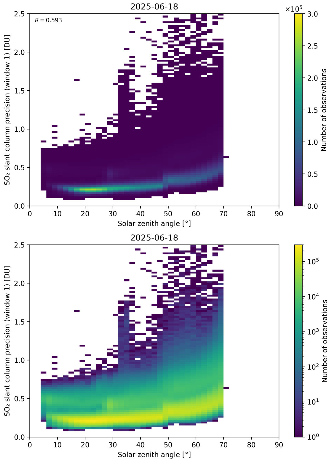
Figure 185: Scatter density plot of “Solar zenith angle” against “SO 2 slant column precision (window 1)” for 2025-06-17 to 2025-06-19.
