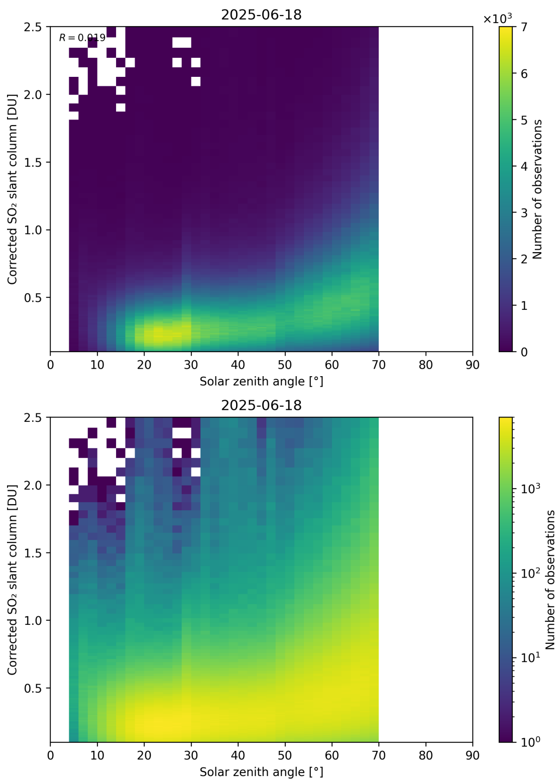
Figure 181: Scatter density plot of “Solar zenith angle” against “Corrected SO 2 slant column” for 2025-06-17 to 2025-06-19.
