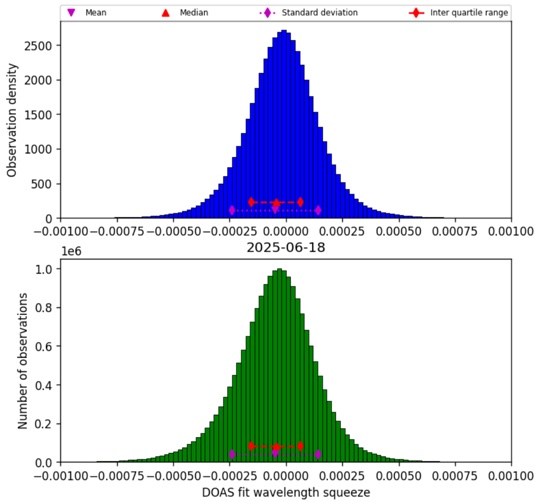
Figure 77: Histogram of “DOAS fit wavelength squeeze” for 2025-06-17 to 2025-06-19
