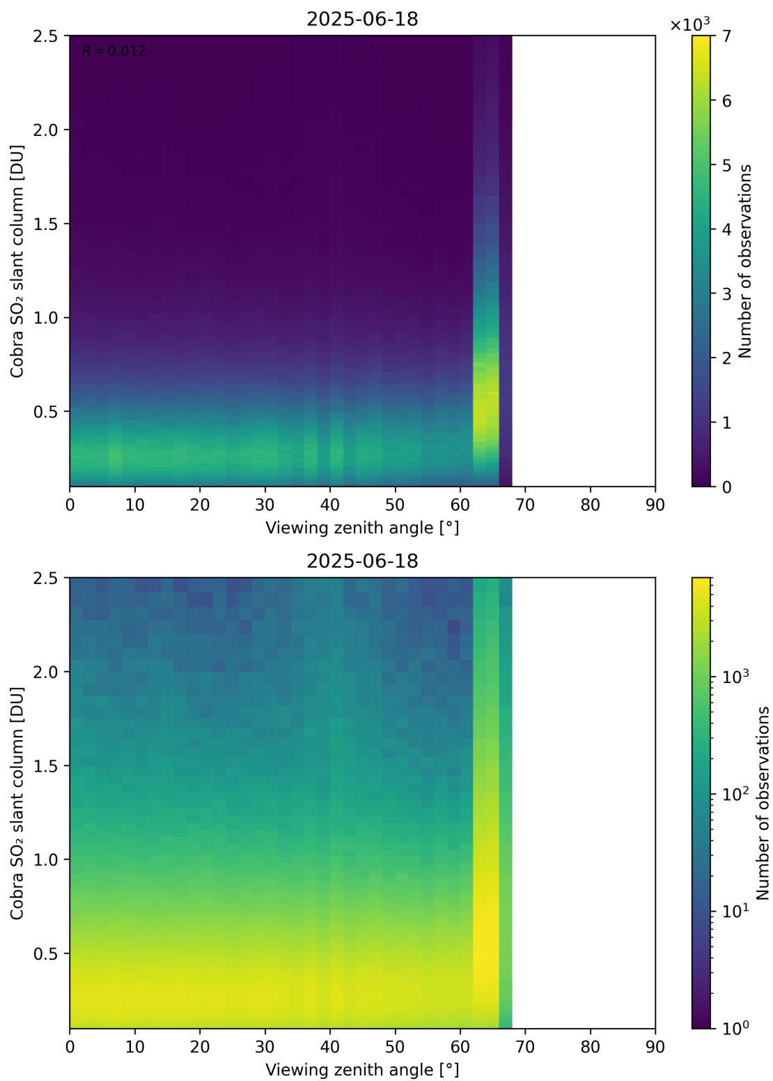
Figure 371: Scatter density plot of “Viewing zenith angle” against “Cobra SO 2 slant column” for 2025-06-17 to 2025-06-19.
