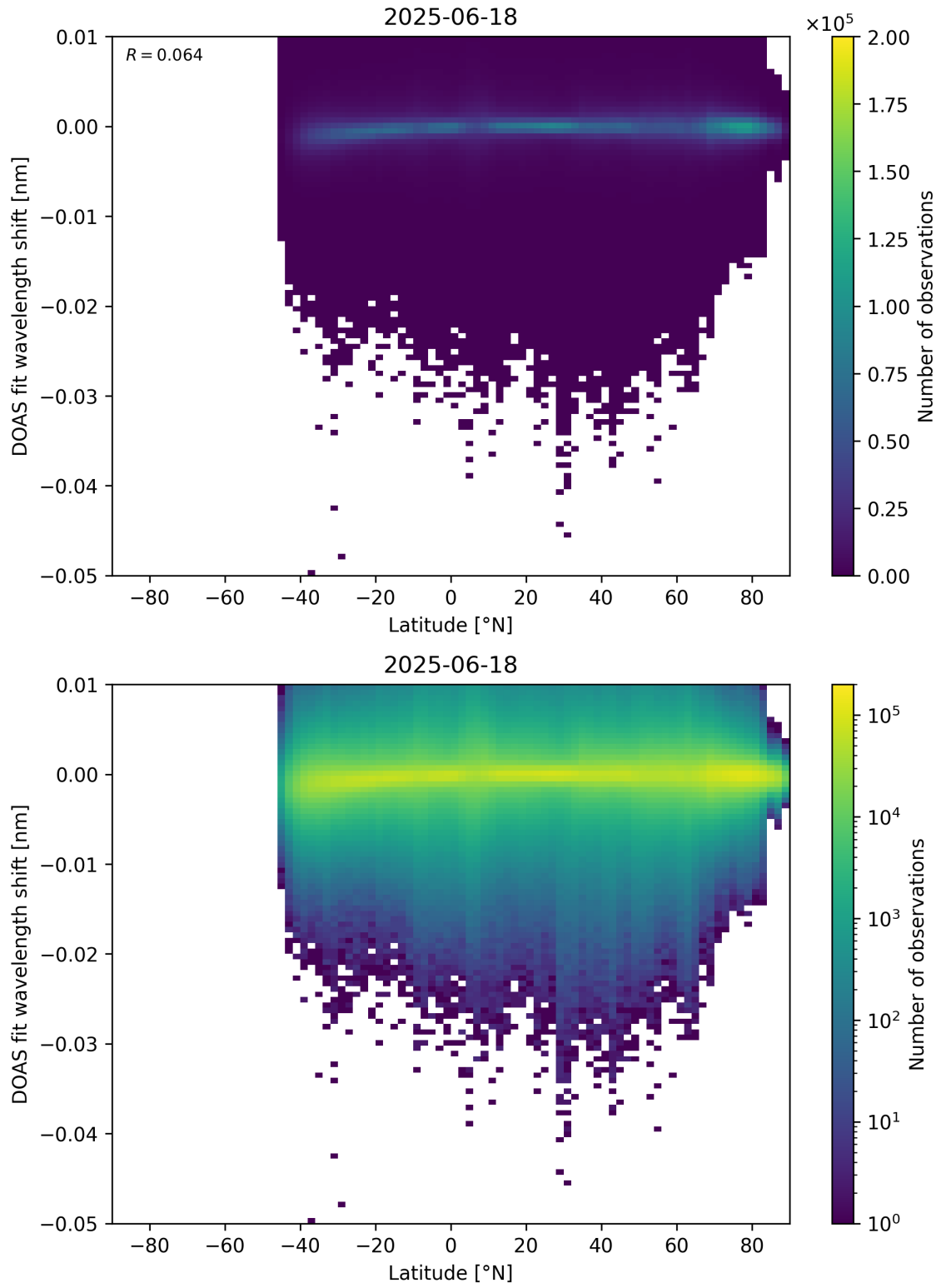
Figure 153: Scatter density plot of “Latitude” against “DOAS fit wavelength shift” for 2025-06-17 to 2025-06-19.
