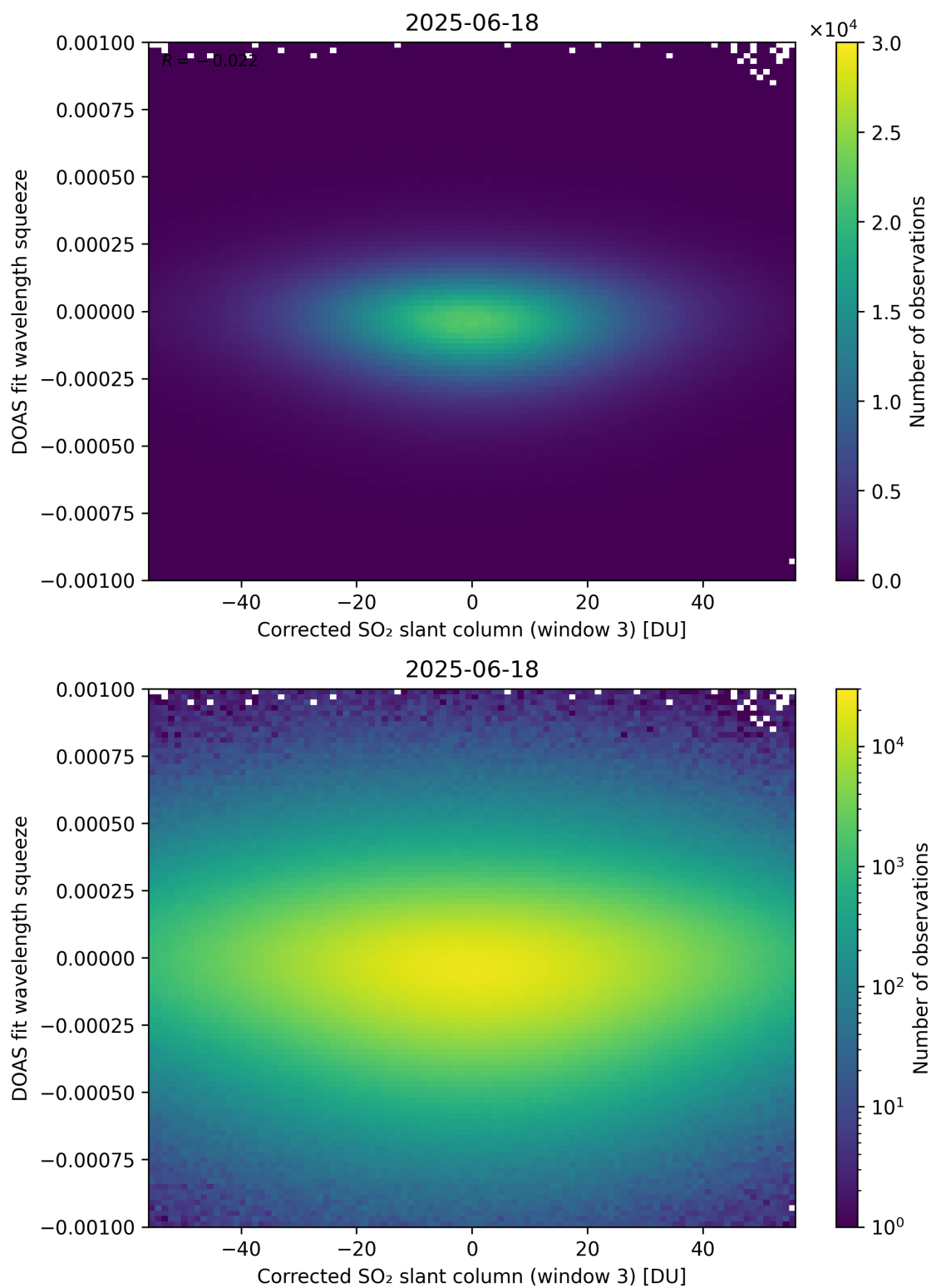
Figure 257: Scatter density plot of “Corrected SO 2 slant column (window 3)” against “DOAS fit wavelength squeeze” for 2025-06-17 to 2025-06-19.
