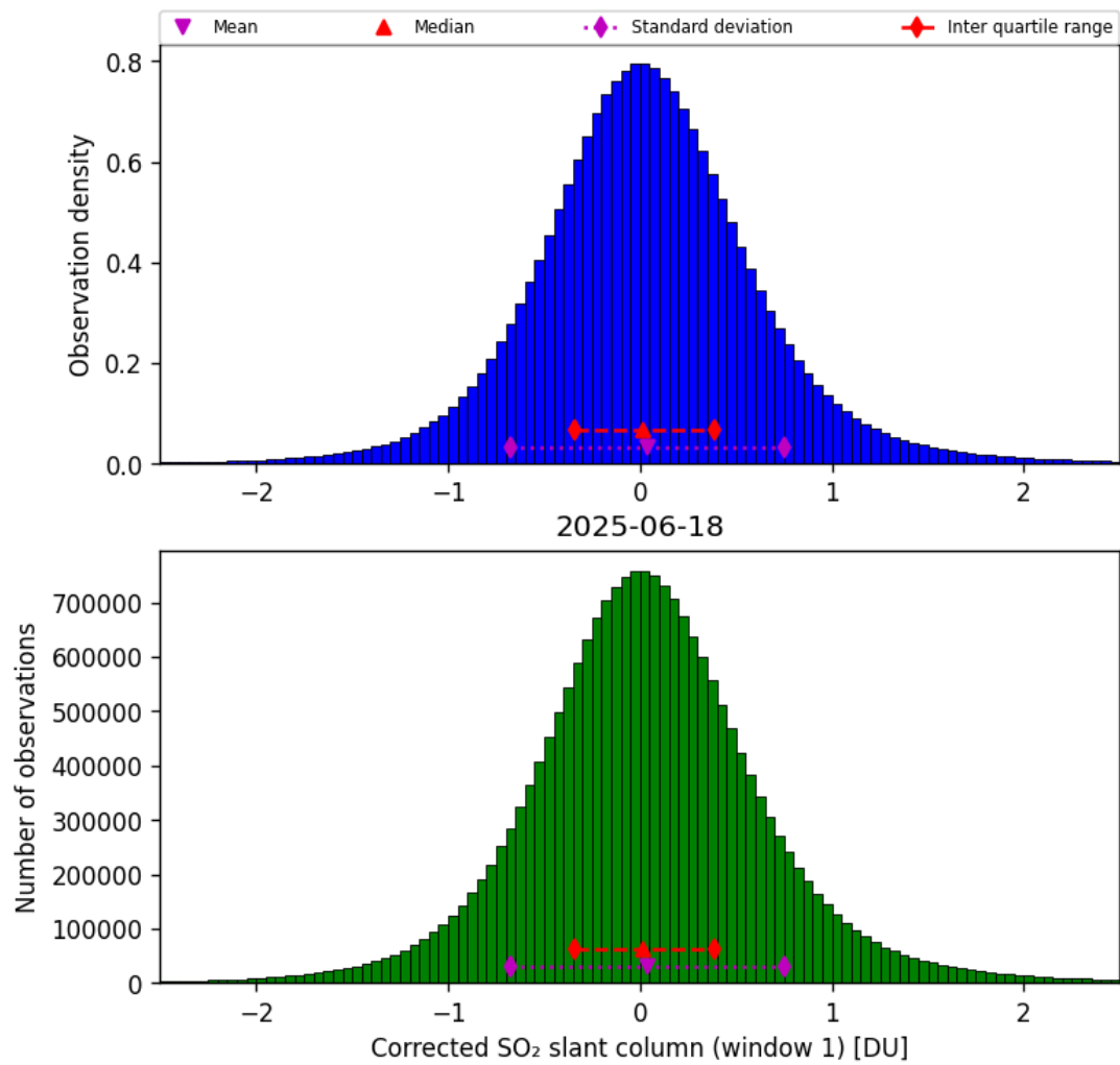
Figure 65: Histogram of “Corrected SO 2 slant column (window 1)” for 2025-06-17 to 2025-06-19
