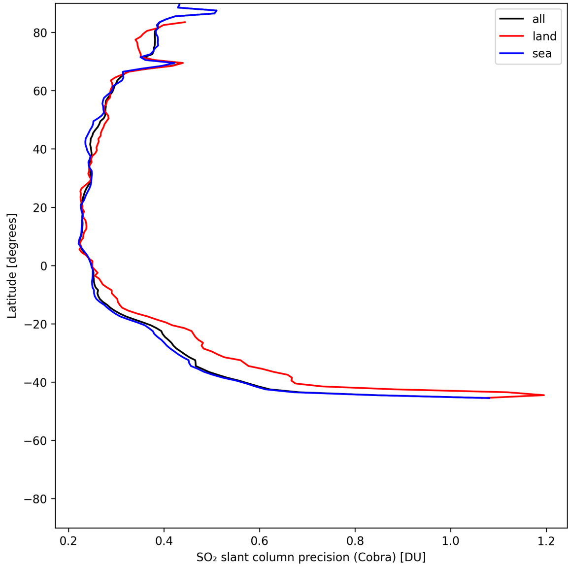
Figure 36: Zonal average of “SO 2 slant column precision (Cobra)” for 2025-06-17 to 2025-06-19.
