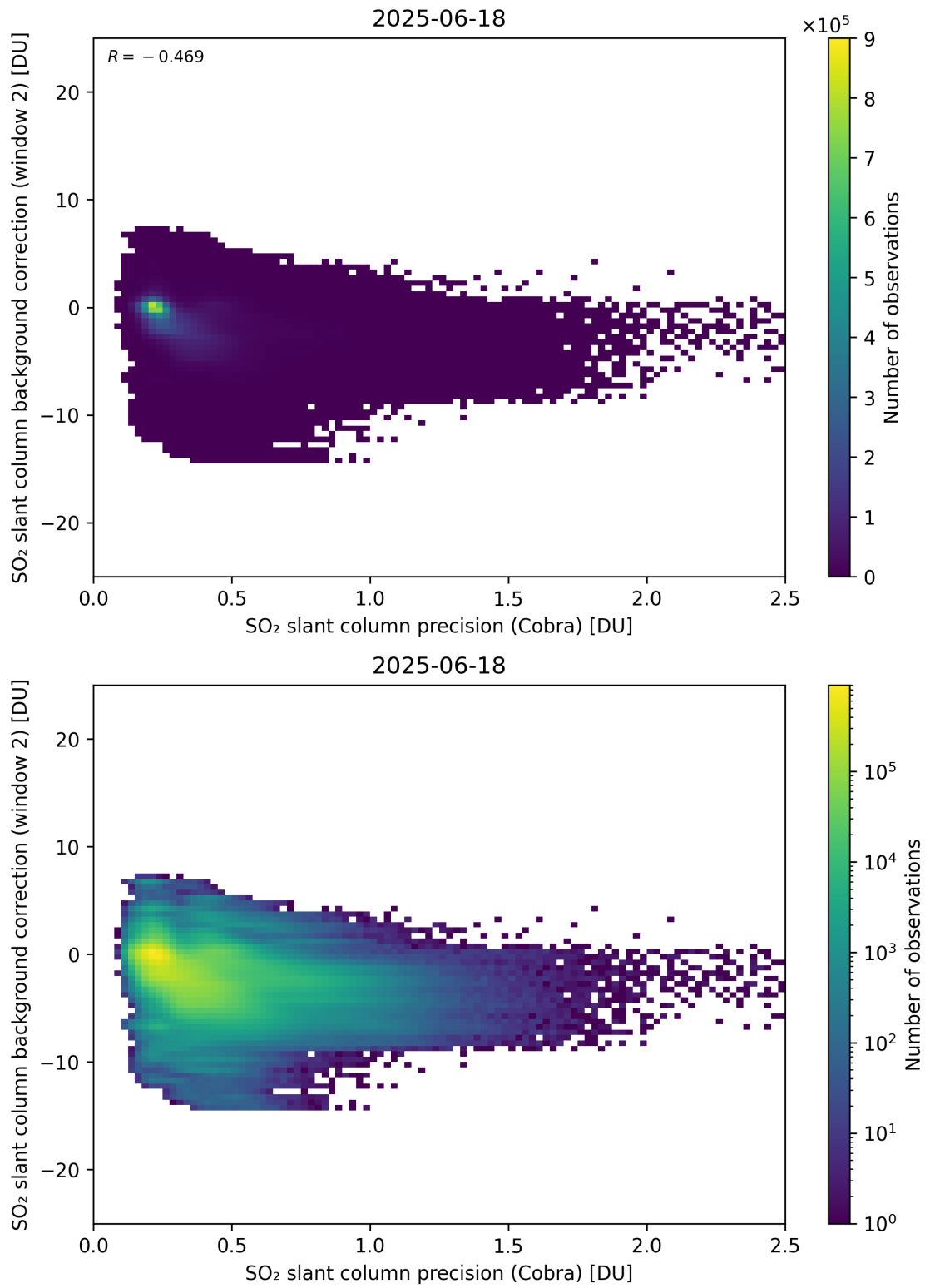
Figure 200: Scatter density plot of “SO 2 slant column precision (Cobra)” against “SO 2 slant column background correction (window 2)” for 2025-06-17 to 2025-06-19.
