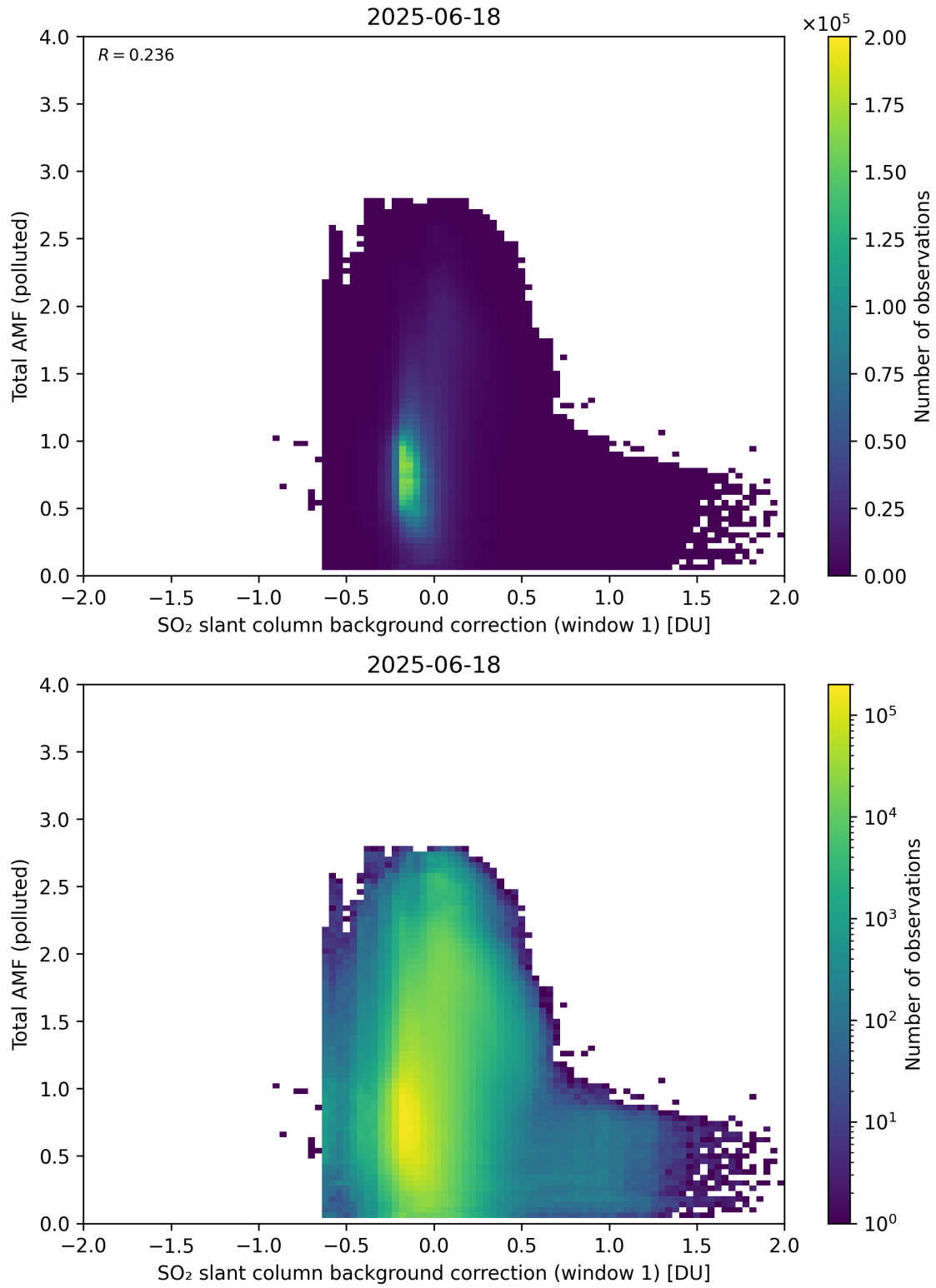
Figure 120: Scatter density plot of “SO 2 slant column background correction (window 1)” against “Total AMF (polluted)” for 2025-06-17 to 2025-06-19.
