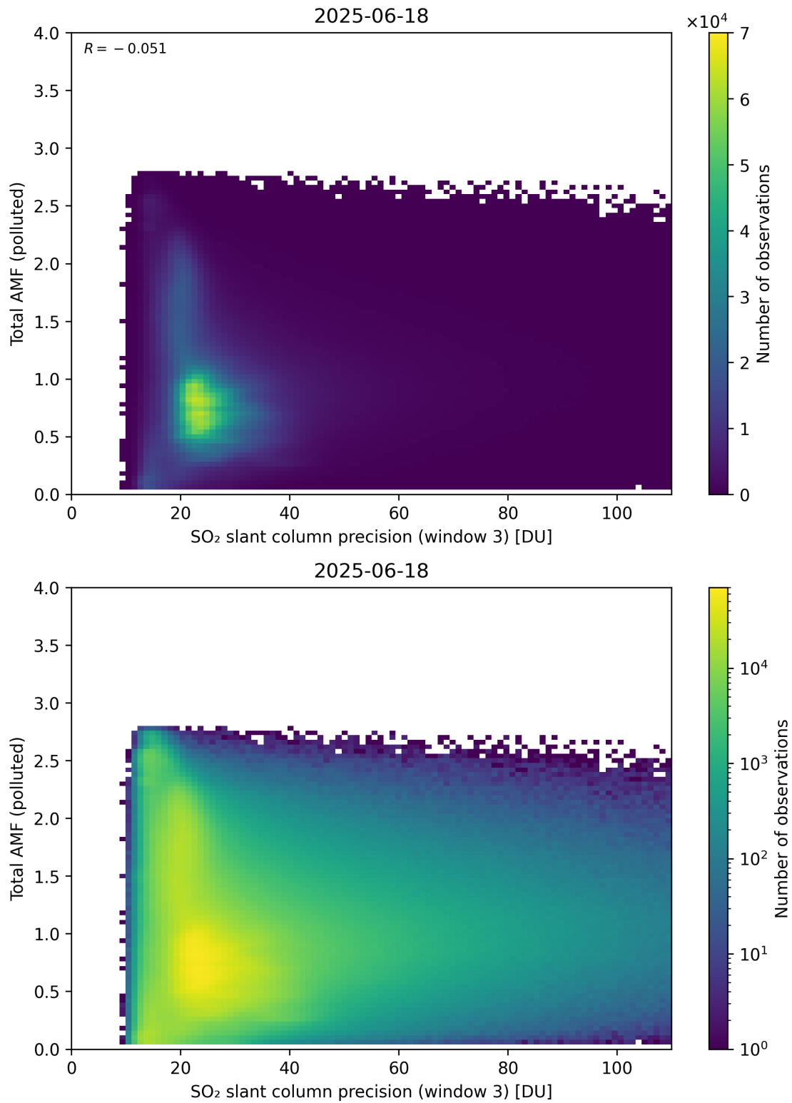
Figure 313: Scatter density plot of “SO 2 slant column precision (window 3)” against “Total AMF (polluted)” for 2025-06-17 to 2025-06-19.
