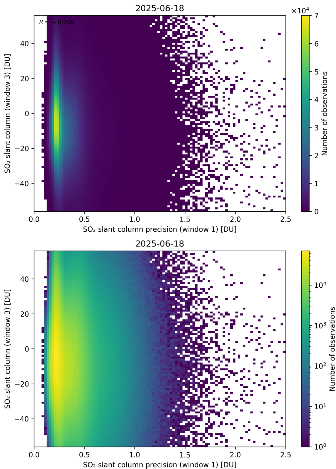
Figure 278: Scatter density plot of “SO 2 slant column precision (window 1)” against “SO 2 slant column (window 3)” for 2025-06-17 to 2025-06-19.
