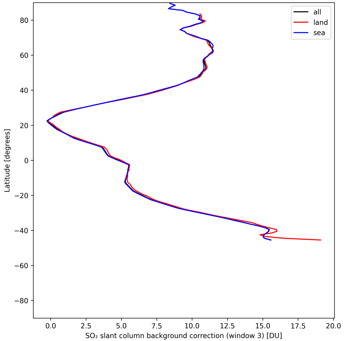
Figure 48: Zonal average of “SO 2 slant column background correction (window 3)” for 2025-06-17 to 2025-06-19.
