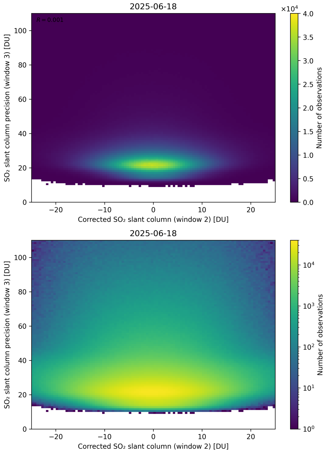
Figure 252: Scatter density plot of “Corrected SO 2 slant column (window 2)” against “SO 2 slant column precision (window 3)” for 2025-06-17 to 2025-06-19.
