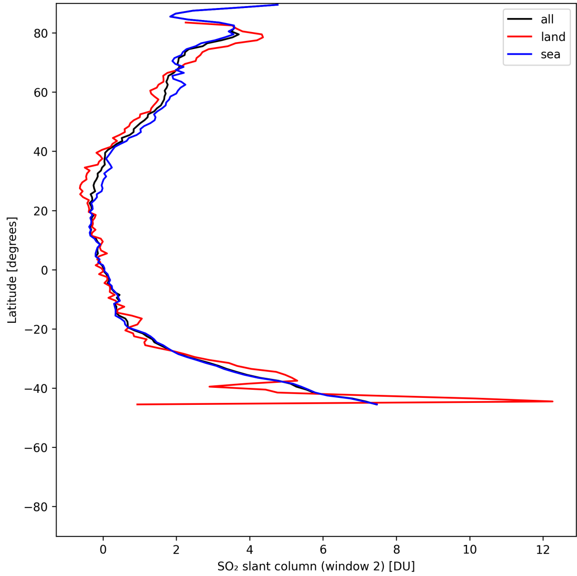
Figure 41: Zonal average of “SO 2 slant column (window 2)” for 2025-06-17 to 2025-06-19.
