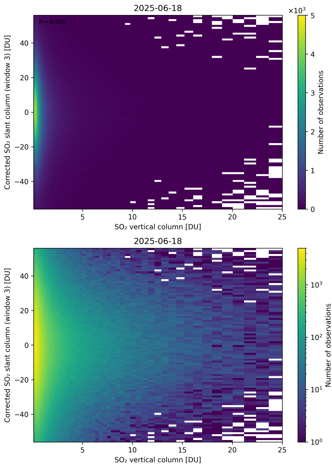
Figure 353: Scatter density plot of “SO 2 vertical column” against “Corrected SO 2 slant column (window 3)” for 2025-06-17 to 2025-06-19.
