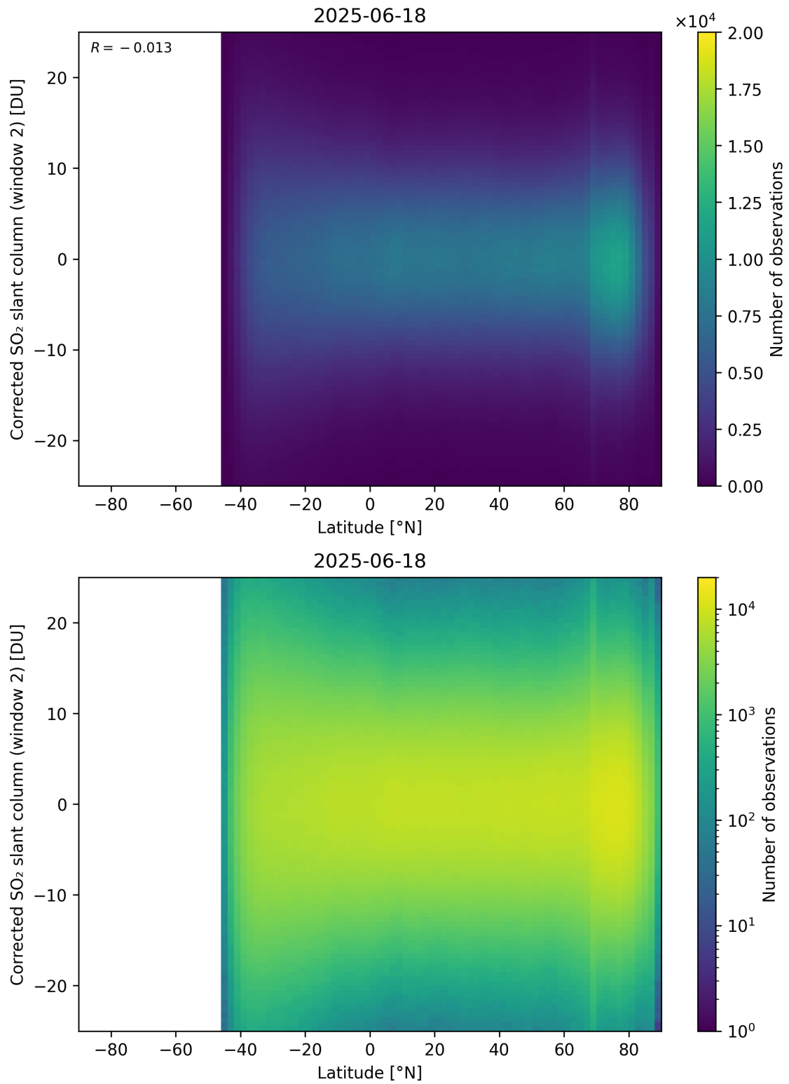
Figure 160: Scatter density plot of “Latitude” against “Corrected SO 2 slant column (window 2)” for 2025-06-17 to 2025-06-19.
