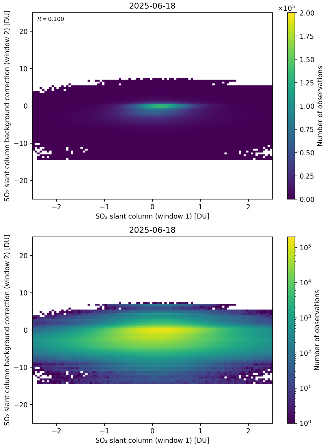
Figure 263: Scatter density plot of “SO 2 slant column (window 1)” against “SO 2 slant column background correction (window 2)” for 2025-06-17 to 2025-06-19.
