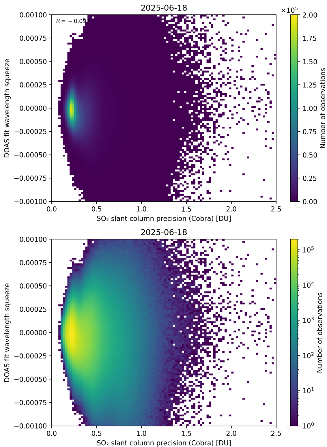
Figure 203: Scatter density plot of “SO 2 slant column precision (Cobra)” against “DOAS fit wavelength squeeze” for 2025-06-17 to 2025-06-19.
