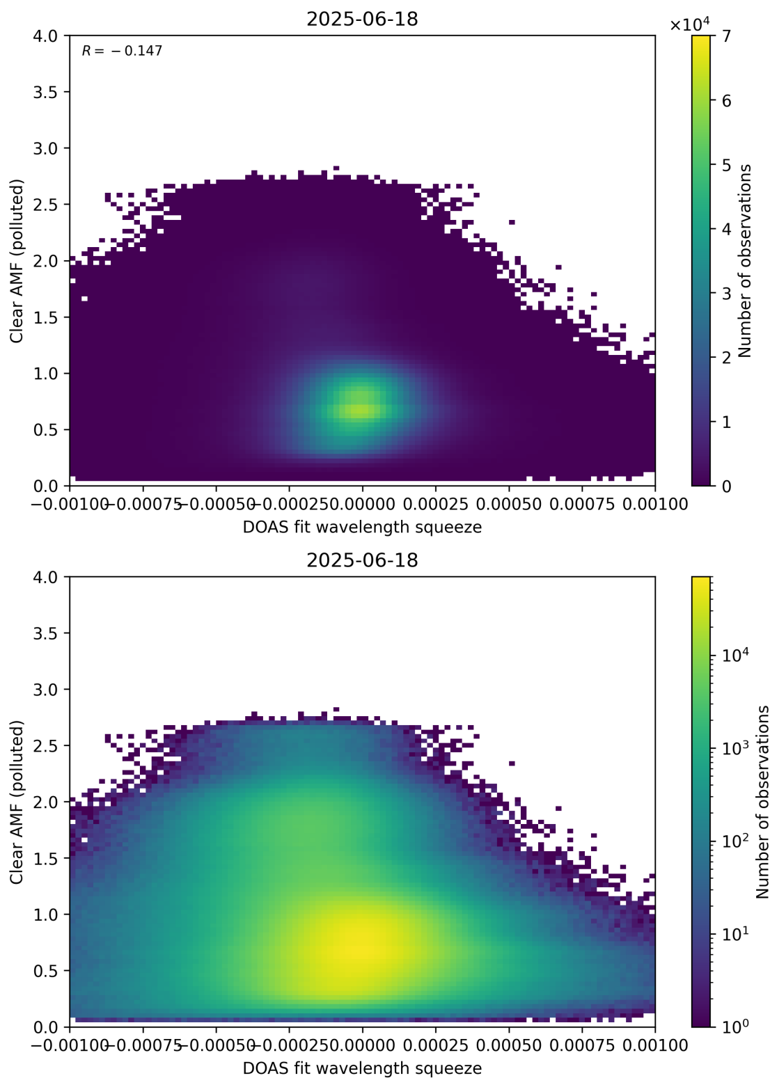
Figure 144: Scatter density plot of “DOAS fit wavelength squeeze” against “Clear AMF (polluted)” for 2025-06-17 to 2025-06-19.
