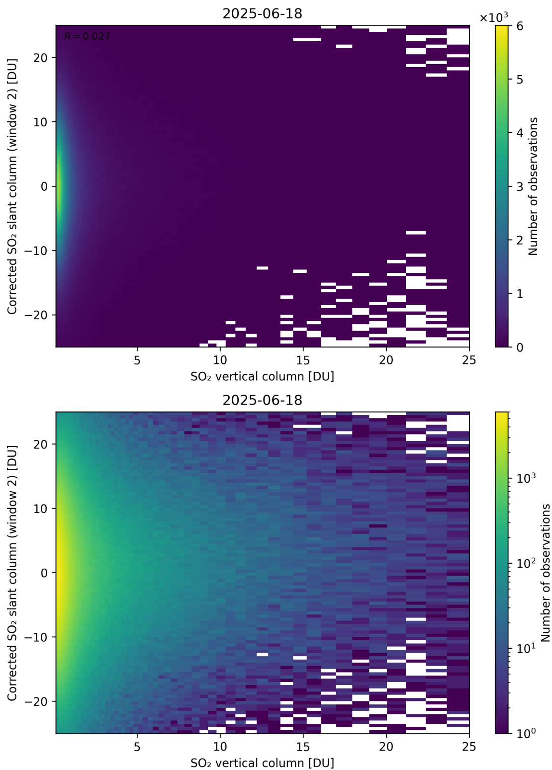
Figure 352: Scatter density plot of “SO 2 vertical column” against “Corrected SO 2 slant column (window 2)” for 2025-06-17 to 2025-06-19.
