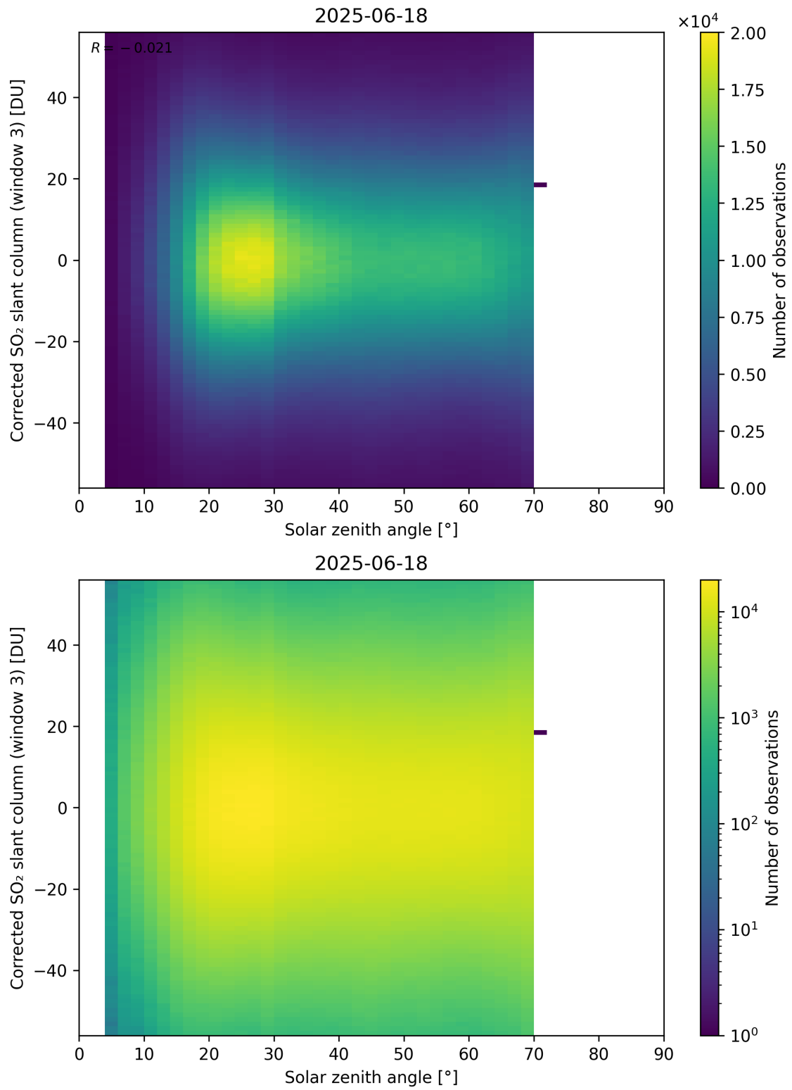
Figure 183: Scatter density plot of “Solar zenith angle” against “Corrected SO 2 slant column (window 3)” for 2025-06-17 to 2025-06-19.
