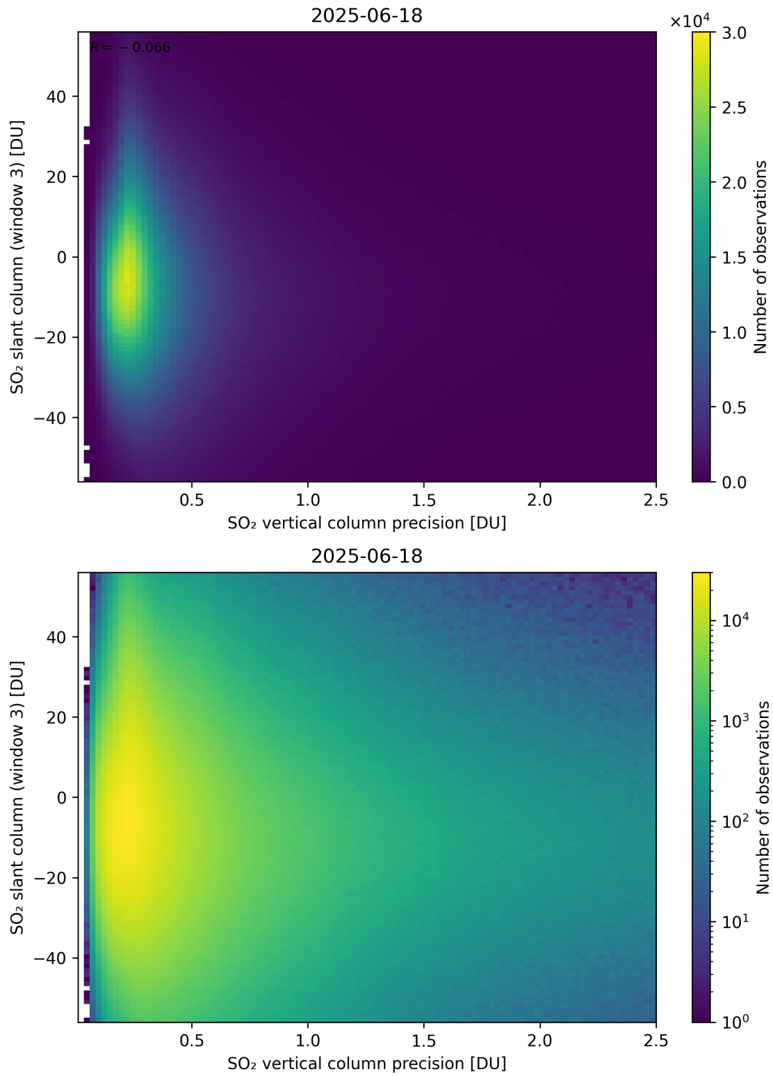
Figure 344: Scatter density plot of “SO 2 vertical column precision” against “SO 2 slant column (window 3)” for 2025-06-17 to 2025-06-19.
