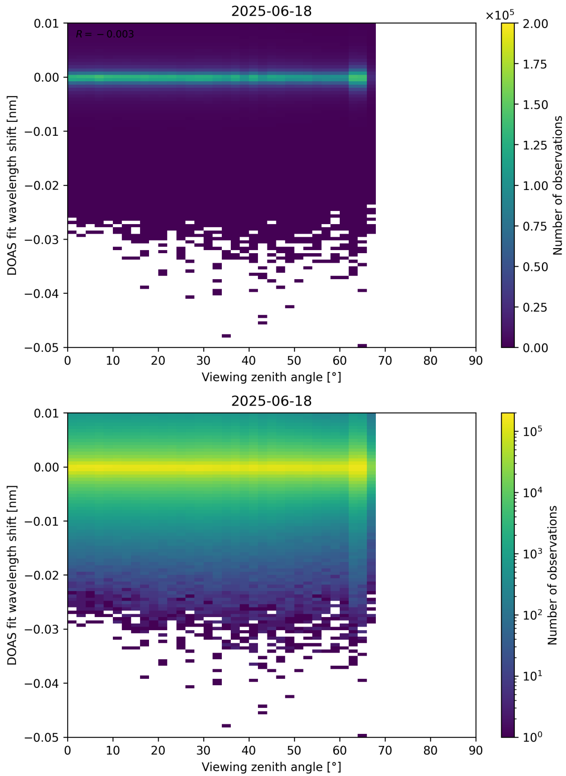
Figure 365: Scatter density plot of “Viewing zenith angle” against “DOAS fit wavelength shift” for 2025-06-17 to 2025-06-19.
