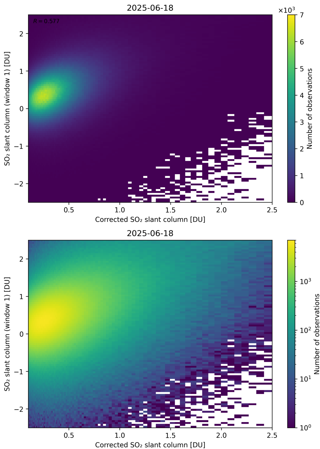
Figure 237: Scatter density plot of “Corrected SO 2 slant column” against “SO 2 slant column (window 1)” for 2025-06-17 to 2025-06-19.
