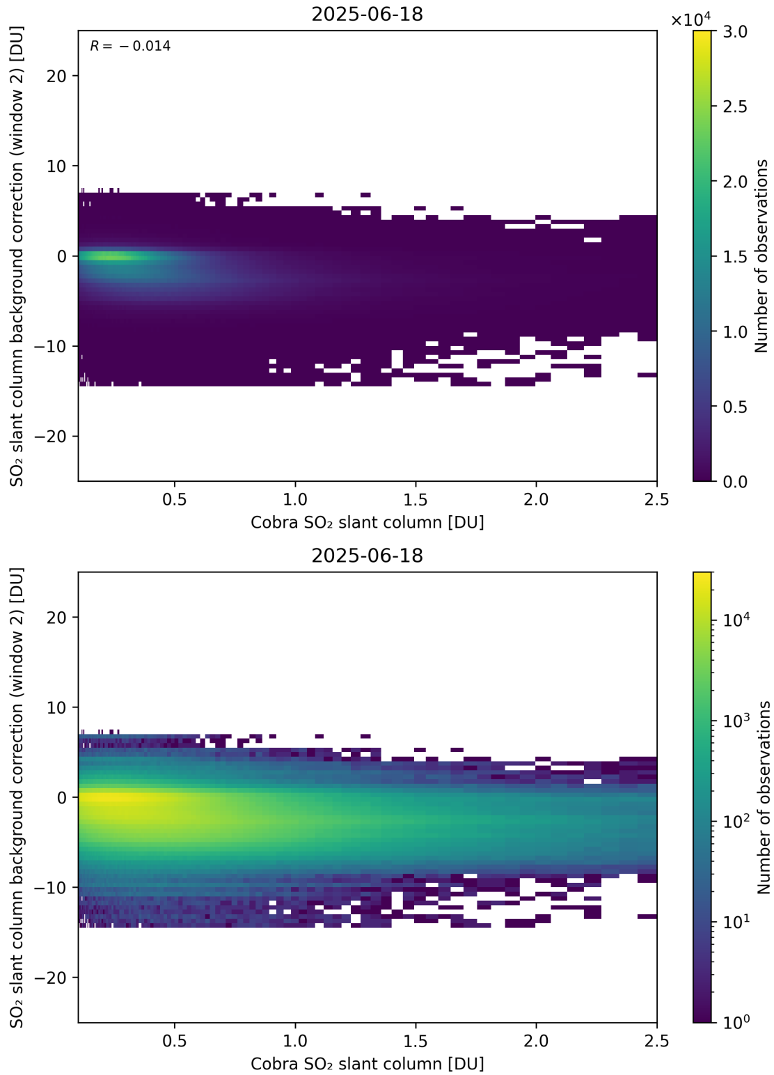
Figure 194: Scatter density plot of “Cobra SO 2 slant column” against “SO 2 slant column background correction (window 2)” for 2025-06-17 to 2025-06-19.
