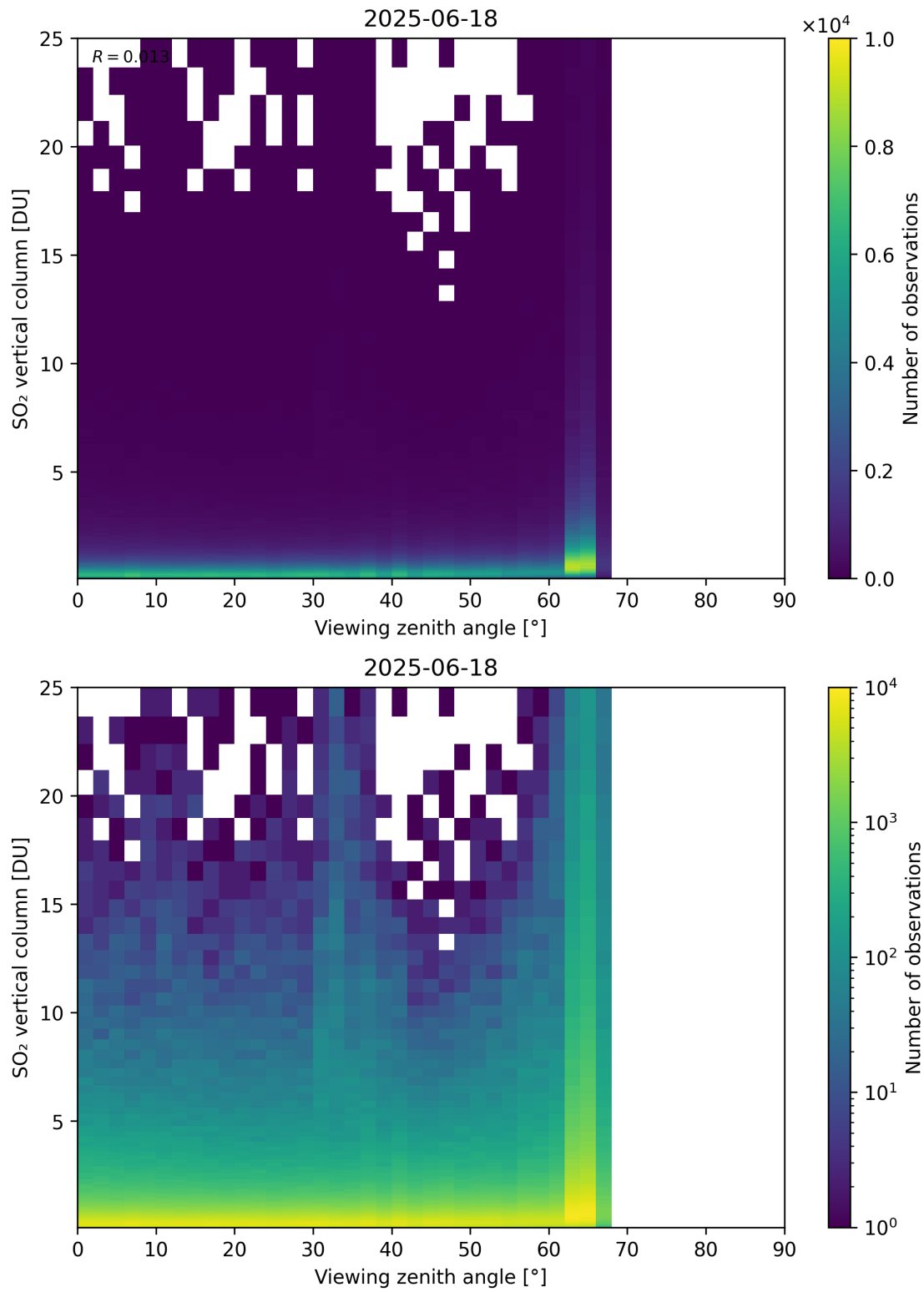
Figure 383: Scatter density plot of “Viewing zenith angle” against “SO 2 vertical column” for 2025-06-17 to 2025-06-19.
