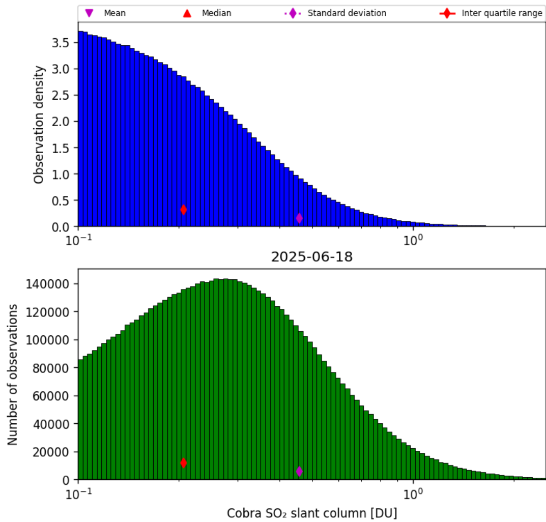
Figure 61: Histogram of “Cobra SO 2 slant column” for 2025-06-17 to 2025-06-19
