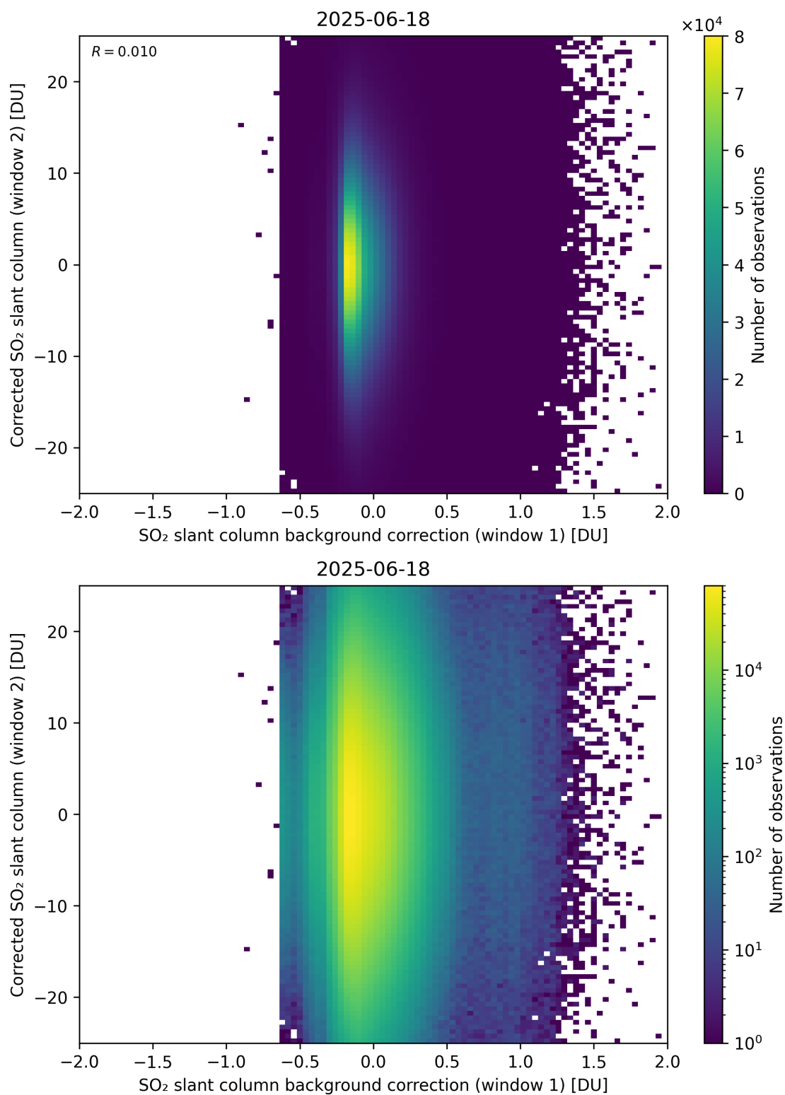
Figure 115: Scatter density plot of “SO 2 slant column background correction (window 1)” against “Corrected SO 2 slant column (window 2)” for 2025-06-17 to 2025-06-19.
