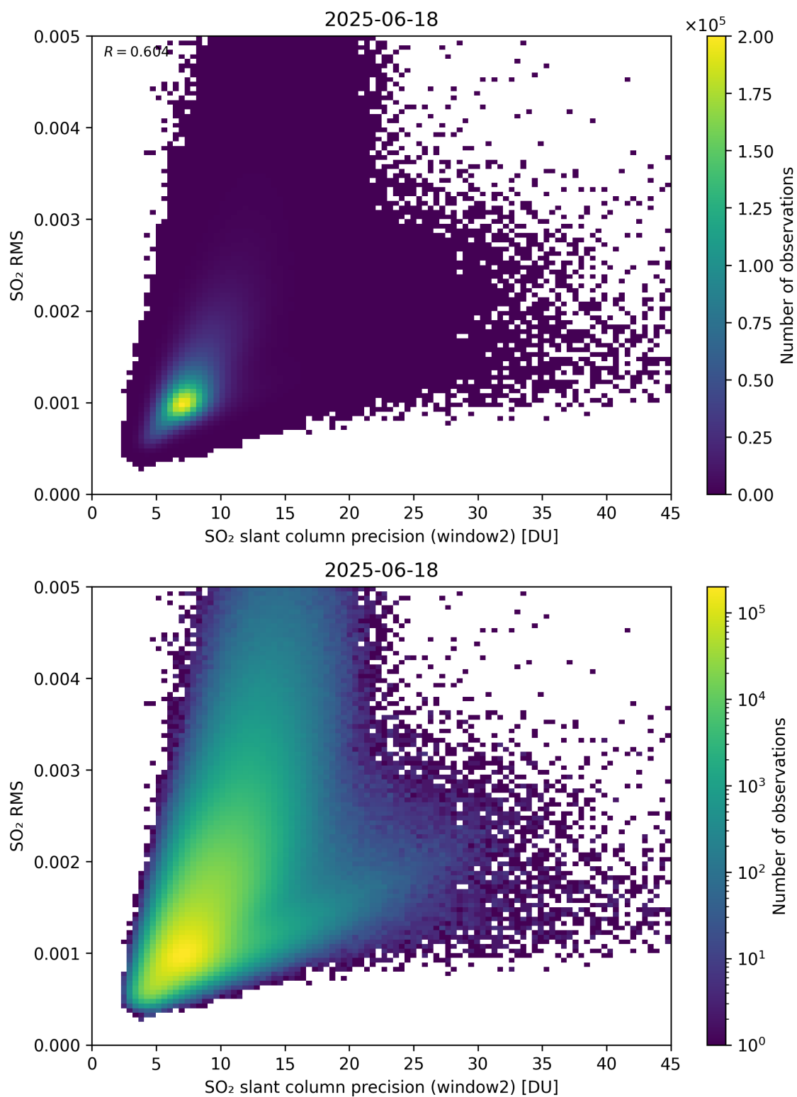
Figure 295: Scatter density plot of “SO 2 slant column precision (window2)” against “SO 2 RMS” for 2025-06-17 to 2025-06-19.
