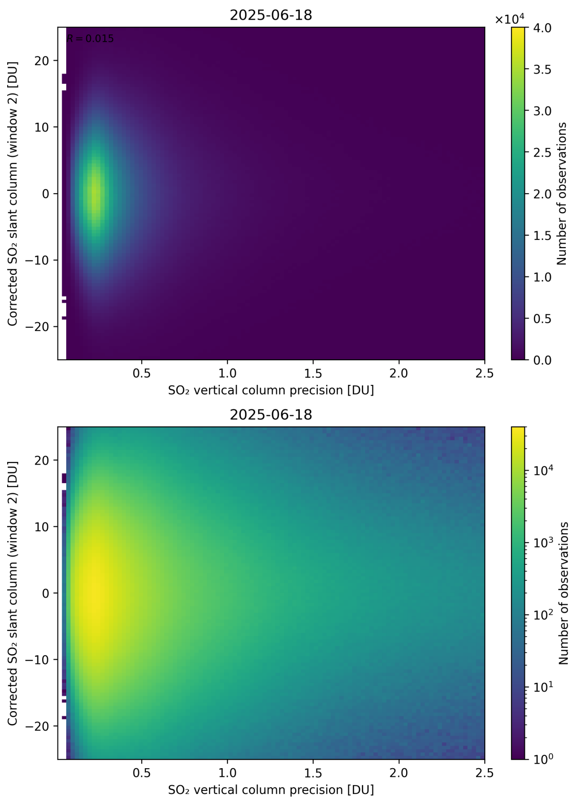
Figure 339: Scatter density plot of “SO 2 vertical column precision” against “Corrected SO 2 slant column (window 2)” for 2025-06-17 to 2025-06-19.
