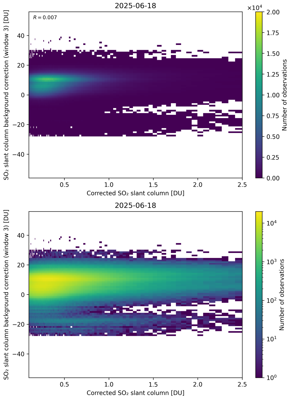
Figure 228: Scatter density plot of “Corrected SO 2 slant column” against “SO 2 slant column background correction (window 3)” for 2025-06-17 to 2025-06-19.
