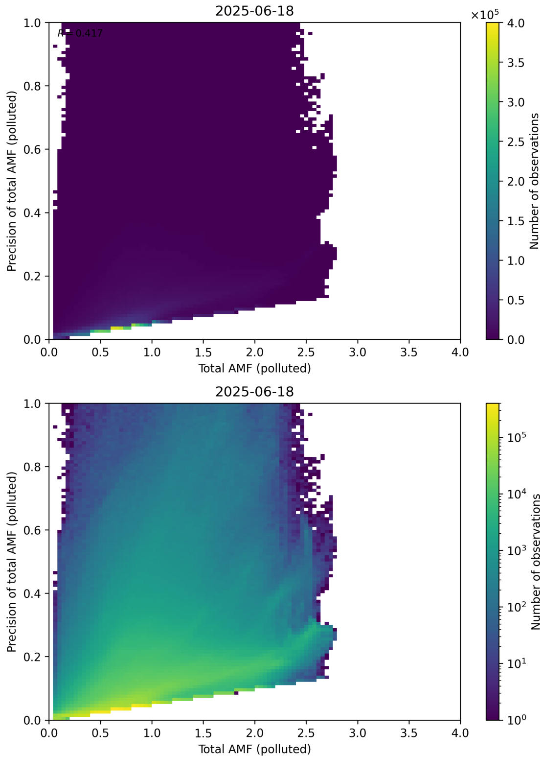
Figure 322: Scatter density plot of “Total AMF (polluted)” against “Precision of total AMF (polluted)” for 2025-06-17 to 2025-06-19.
