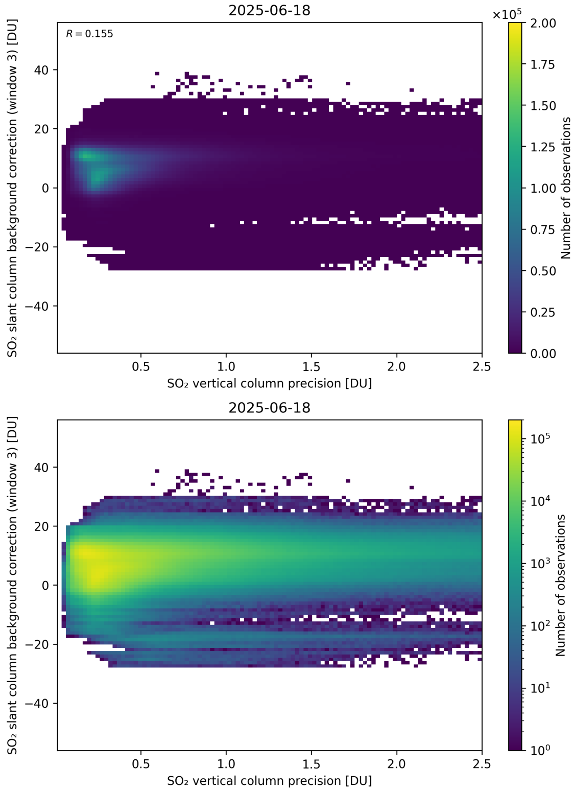
Figure 331: Scatter density plot of “SO 2 vertical column precision” against “SO 2 slant column background correction (window 3)” for 2025-06-17 to 2025-06-19.
