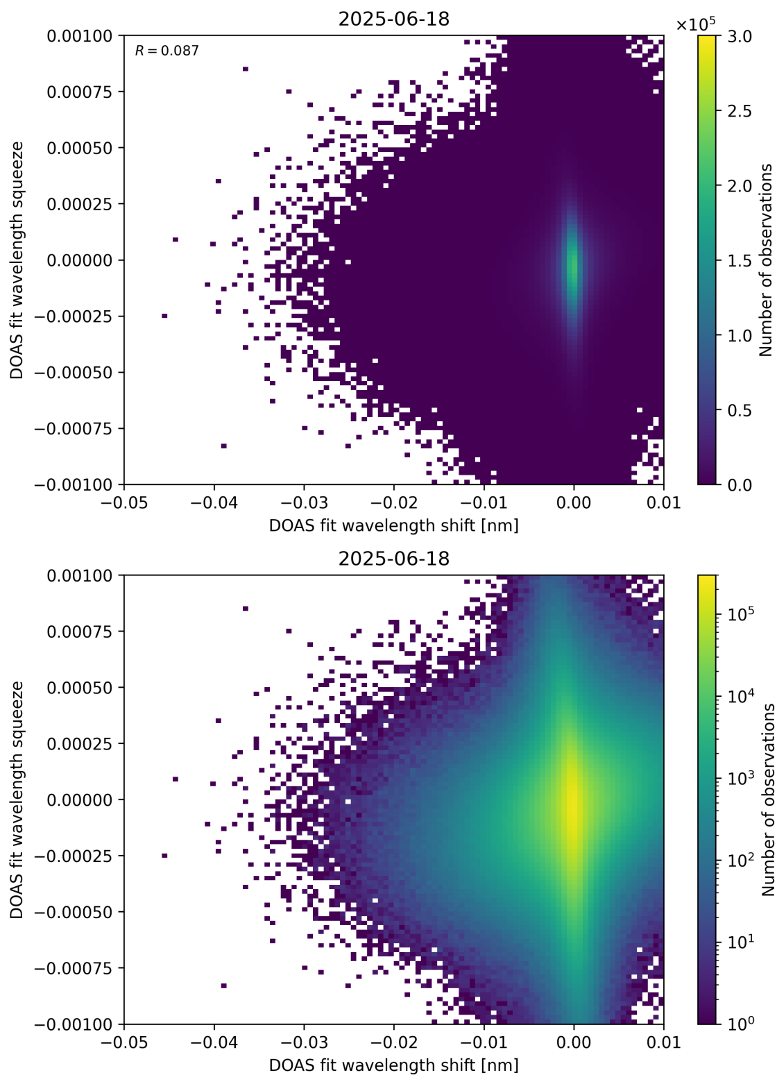
Figure 138: Scatter density plot of “DOAS fit wavelength shift” against “DOAS fit wavelength squeeze” for 2025-06-17 to 2025-06-19.
