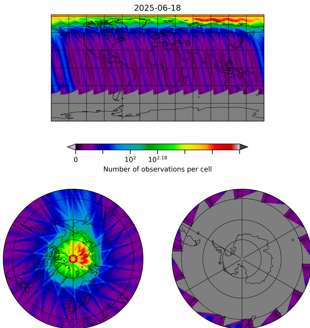
Figure 30: Map of the number of observations for 2025-06-17 to 2025-06-19
