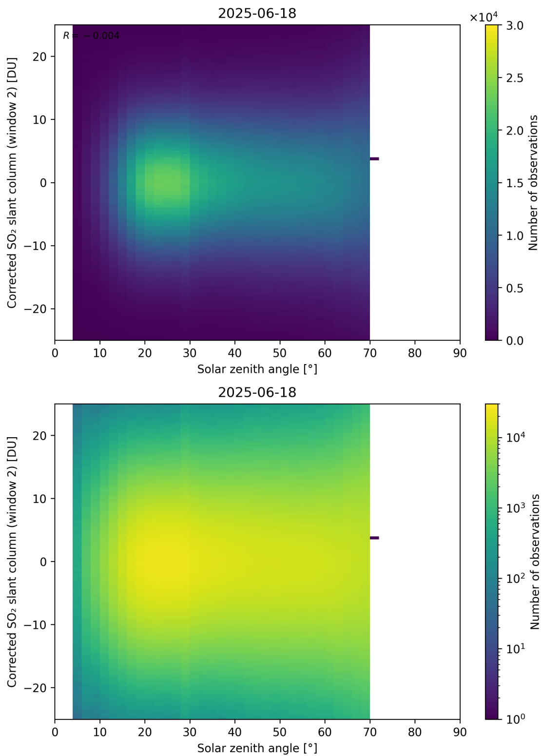
Figure 182: Scatter density plot of “Solar zenith angle” against “Corrected SO 2 slant column (window 2)” for 2025-06-17 to 2025-06-19.
