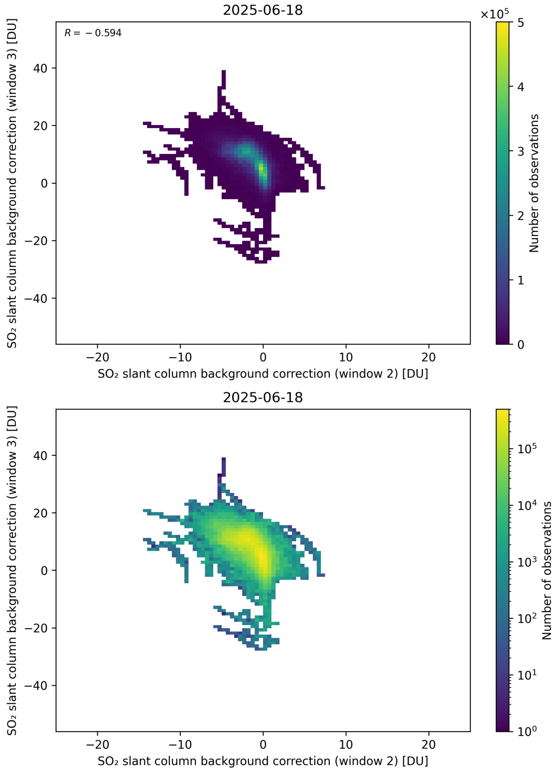
Figure 122: Scatter density plot of “SO 2 slant column background correction (window 2)” against “SO 2 slant column background correction (window 3)” for 2025-06-17 to 2025-06-19.
