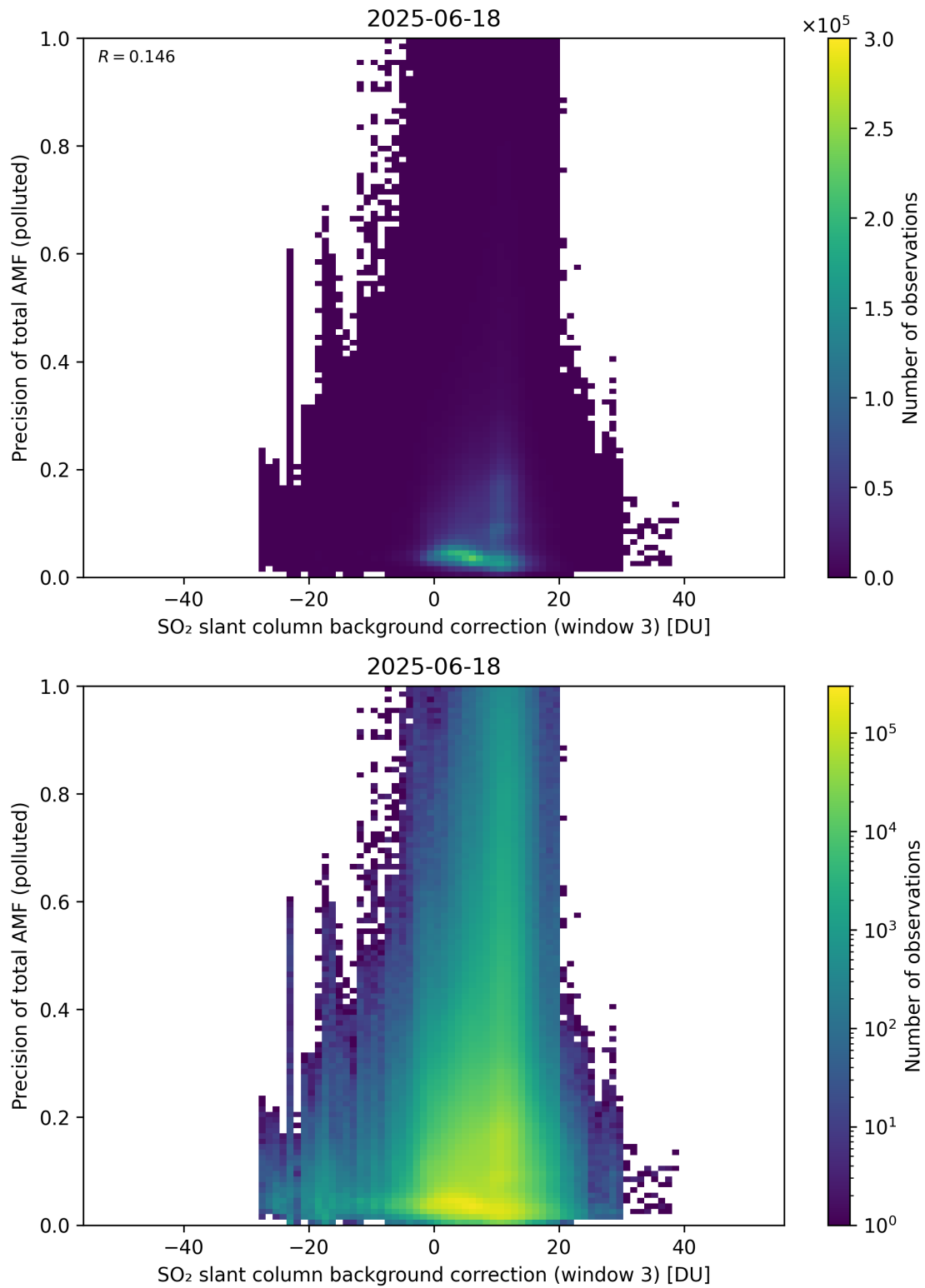
Figure 137: Scatter density plot of “SO 2 slant column background correction (window 3)” against “Precision of total AMF (polluted)” for 2025-06-17 to 2025-06-19.
