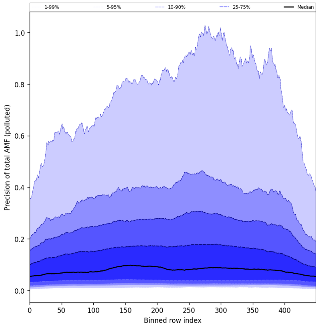
Figure 106: Along track statistics of “Precision of total AMF (polluted)” for 2025-06-17 to 2025-06-19
