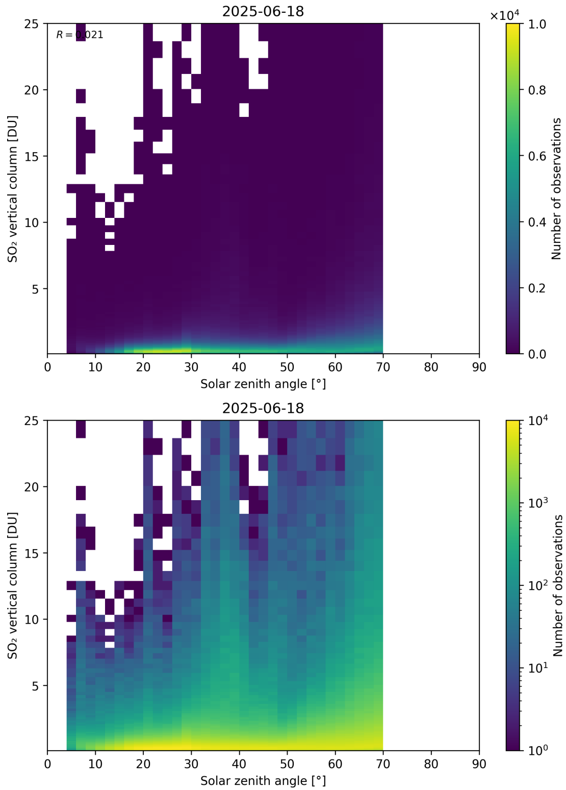
Figure 191: Scatter density plot of “Solar zenith angle” against “SO 2 vertical column” for 2025-06-17 to 2025-06-19.
