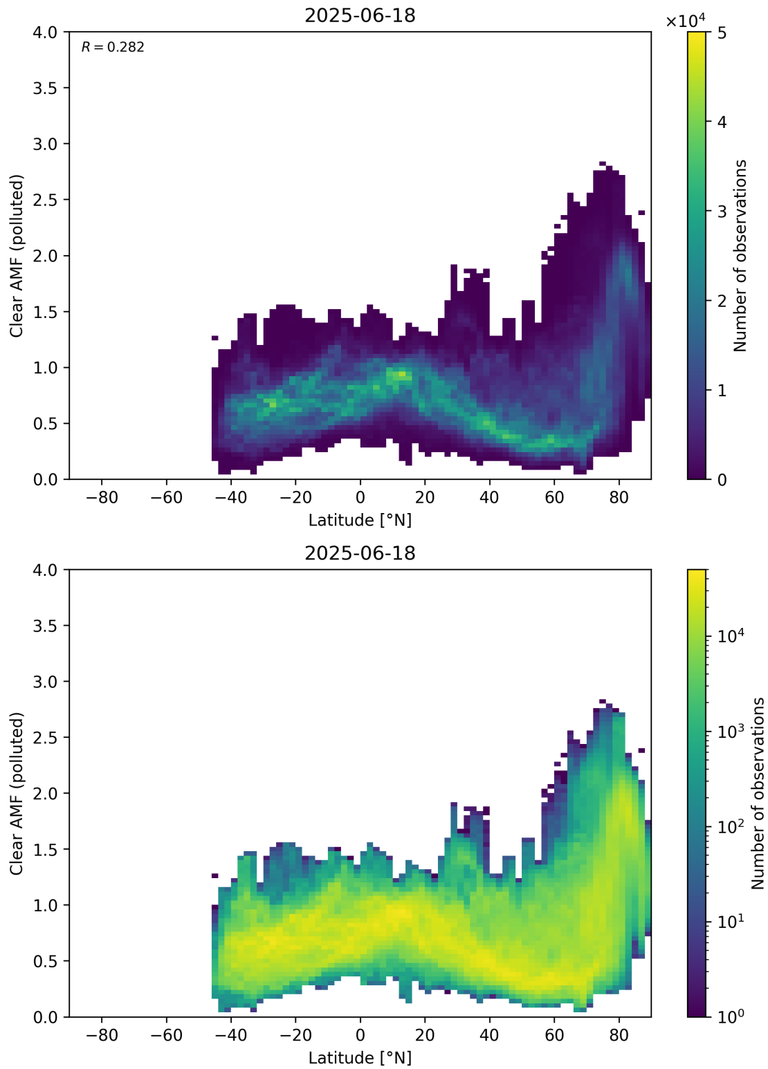
Figure 156: Scatter density plot of “Latitude” against “Clear AMF (polluted)” for 2025-06-17 to 2025-06-19.
