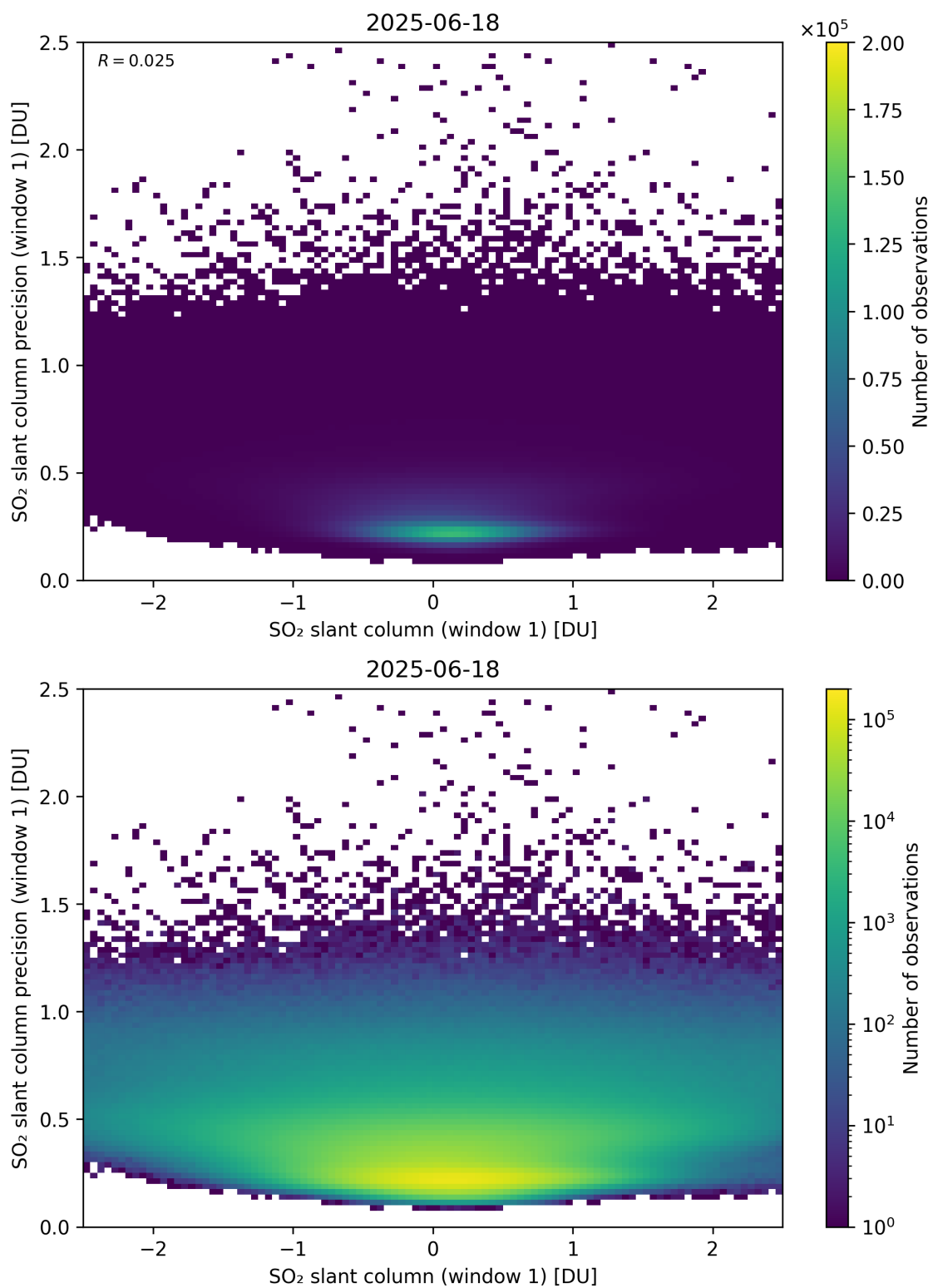
Figure 285: Scatter density plot of “SO 2 slant column (window 1)” against “SO 2 slant column precision (window 1)” for 2025-06-17 to 2025-06-19.
