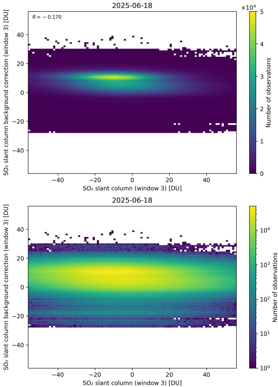
Figure 303: Scatter density plot of “SO 2 slant column (window 3)” against “SO 2 slant column background correction (window 3)” for 2025-06-17 to 2025-06-19.
