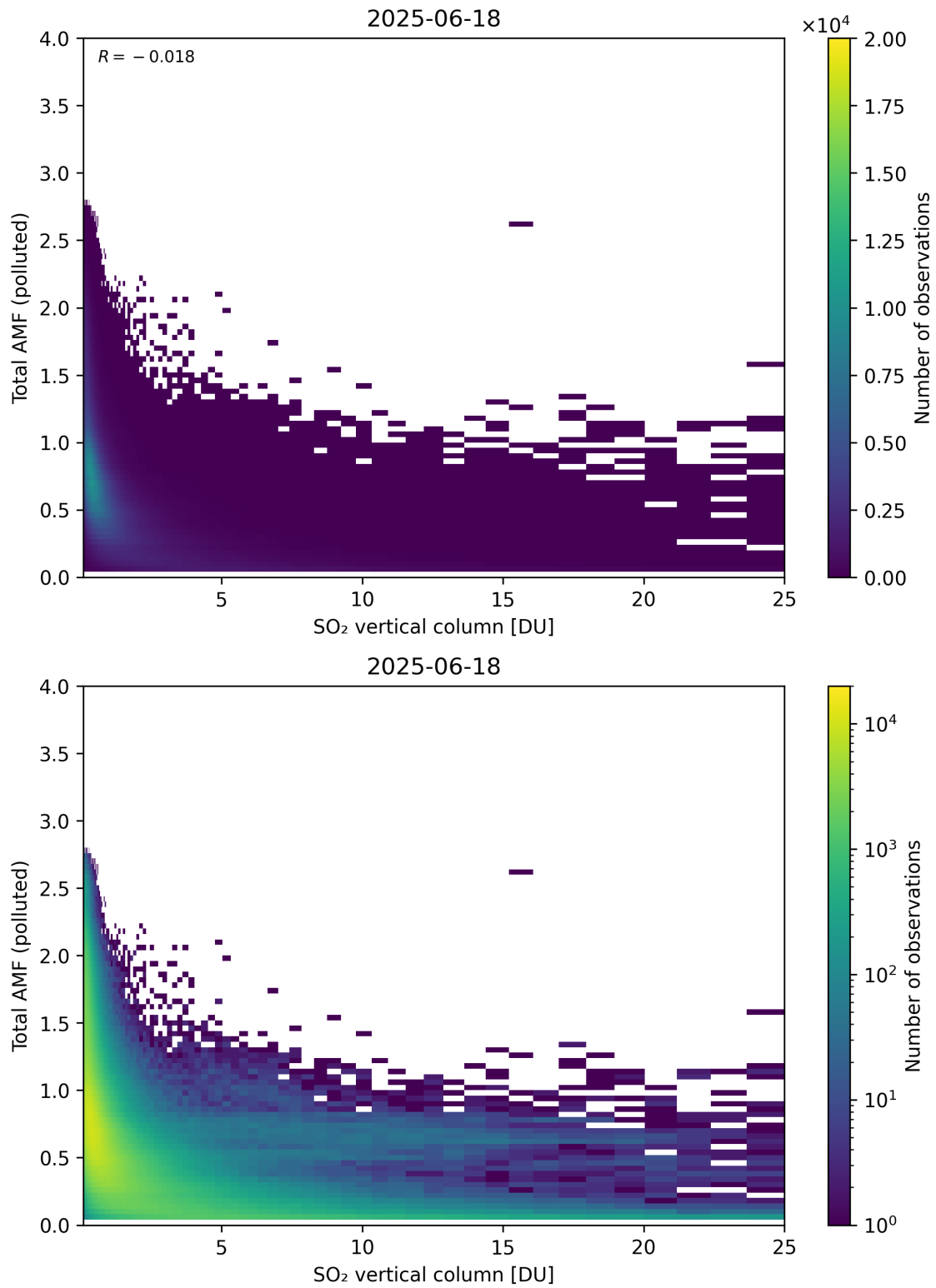
Figure 359: Scatter density plot of “SO 2 vertical column” against “Total AMF (polluted)” for 2025-06-17 to 2025-06-19.
