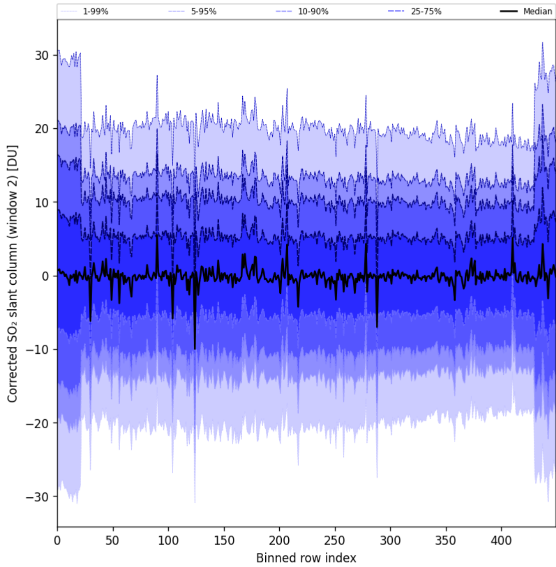
Figure 95: Along track statistics of “Corrected SO 2 slant column (window 2)” for 2025-06-17 to 2025-06-19
