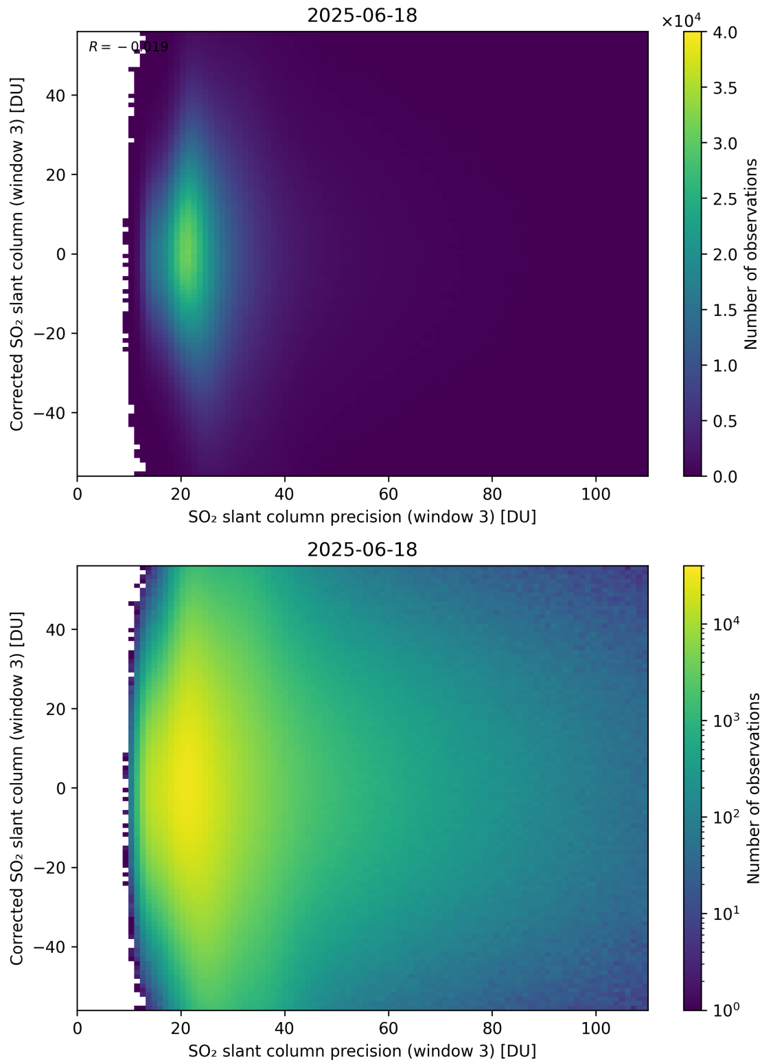
Figure 312: Scatter density plot of “SO 2 slant column precision (window 3)” against “Corrected SO 2 slant column (window 3)” for 2025-06-17 to 2025-06-19.
