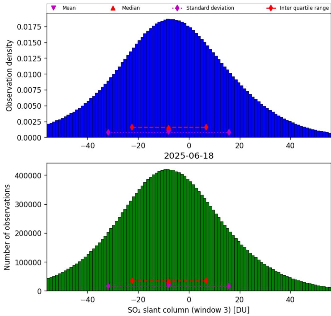
Figure 71: Histogram of “SO 2 slant column (window 3)” for 2025-06-17 to 2025-06-19
