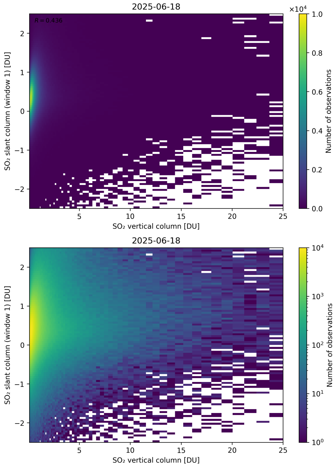
Figure 354: Scatter density plot of “SO 2 vertical column” against “SO 2 slant column (window 1)” for 2025-06-17 to 2025-06-19.
