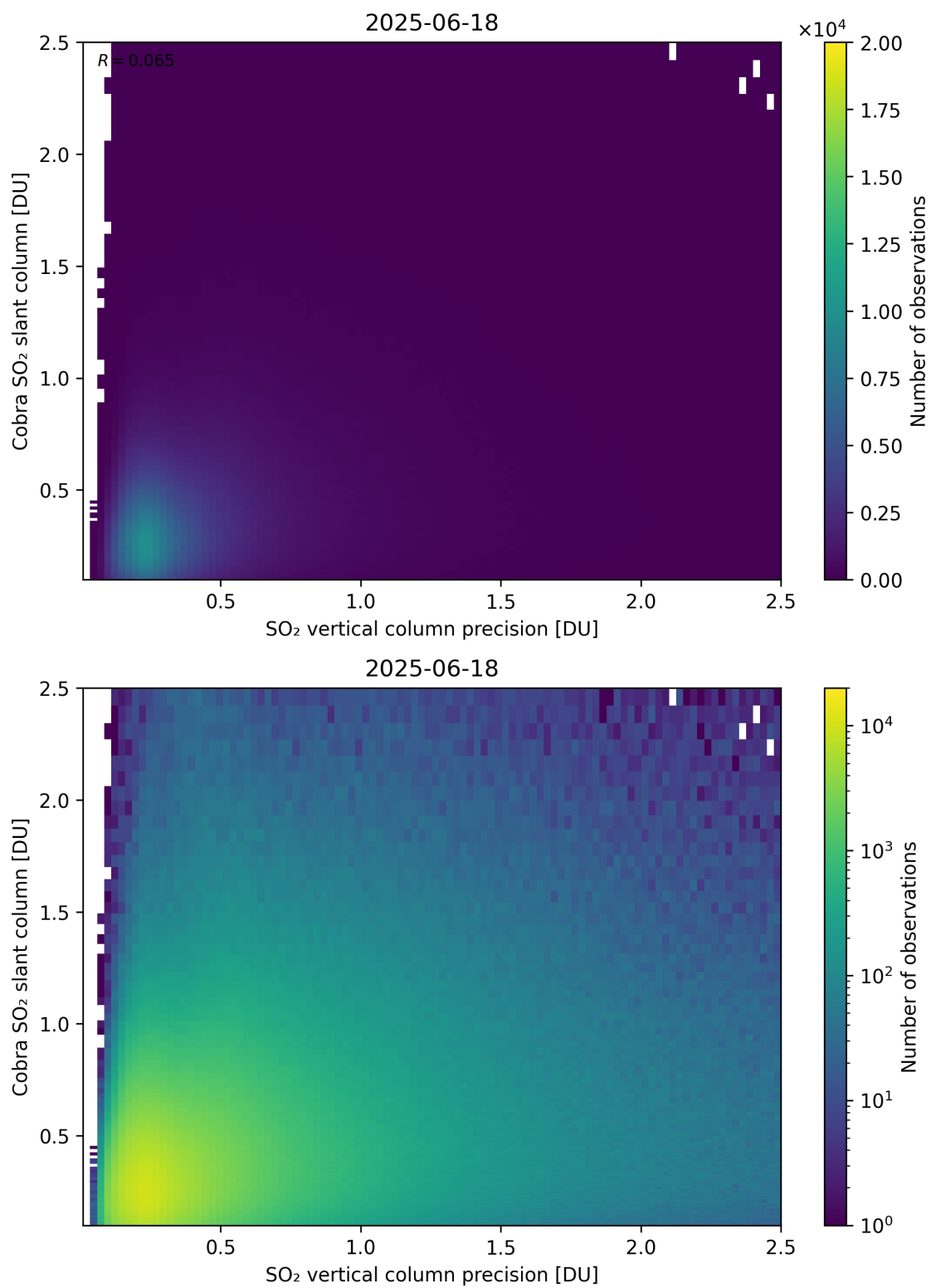
Figure 336: Scatter density plot of “SO 2 vertical column precision” against “Cobra SO 2 slant column” for 2025-06-17 to 2025-06-19.
