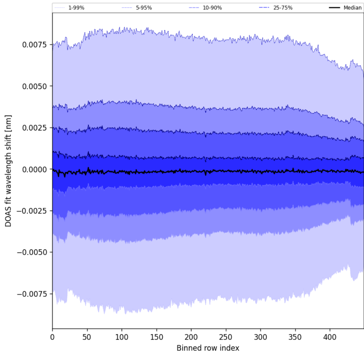
Figure 102: Along track statistics of “DOAS fit wavelength shift” for 2025-06-17 to 2025-06-19
