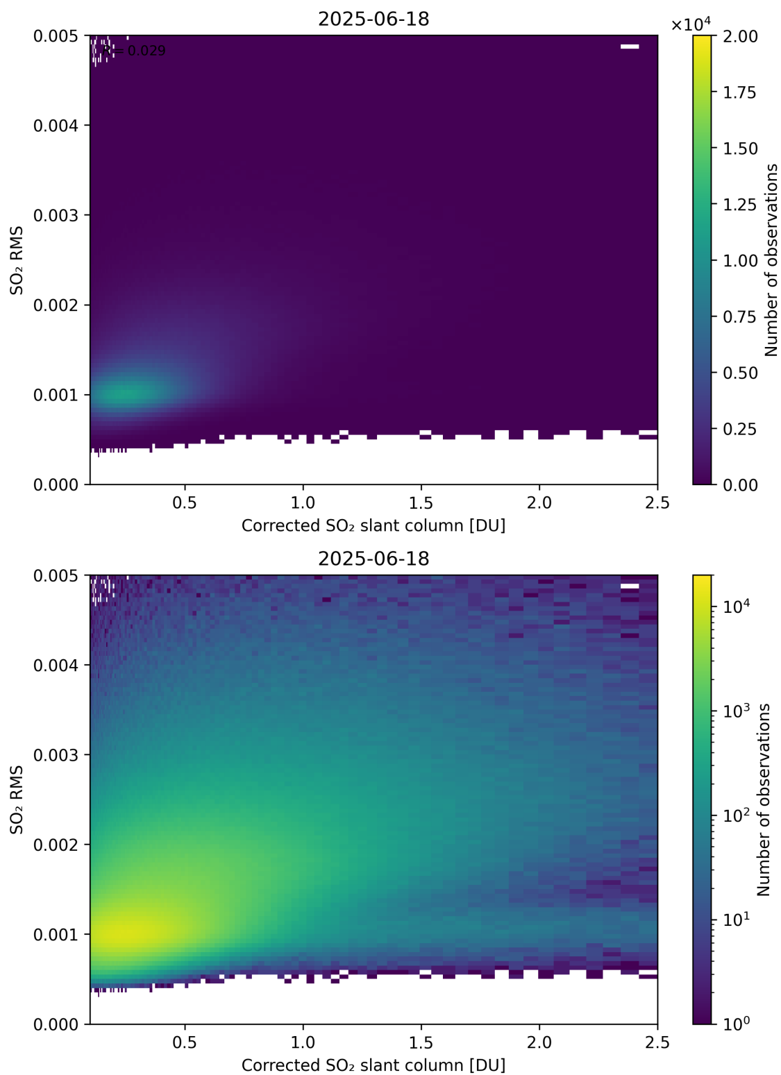
Figure 231: Scatter density plot of “Corrected SO 2 slant column” against “SO 2 RMS” for 2025-06-17 to 2025-06-19.
