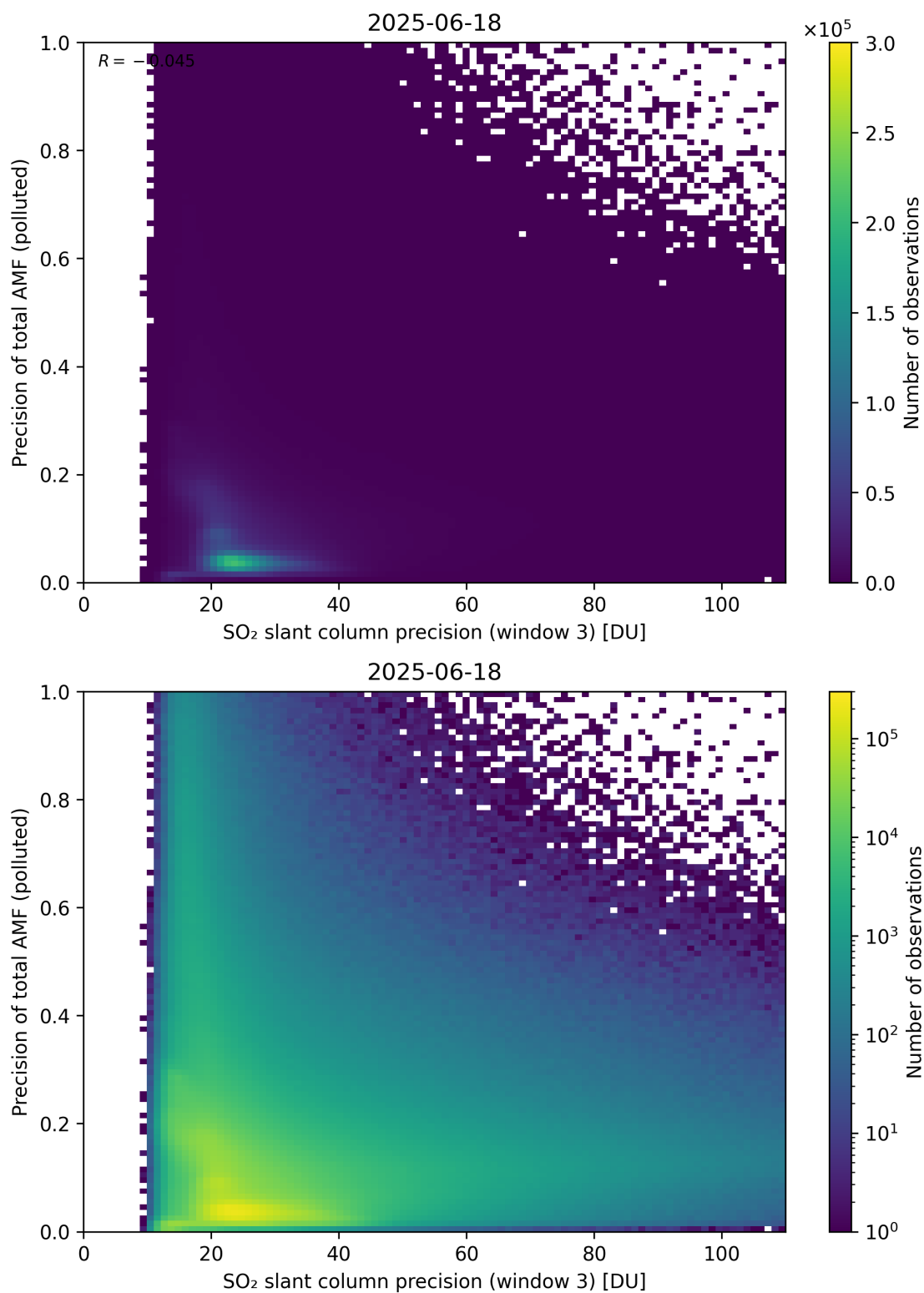
Figure 314: Scatter density plot of “SO 2 slant column precision (window 3)” against “Precision of total AMF (polluted)” for 2025-06-17 to 2025-06-19.
