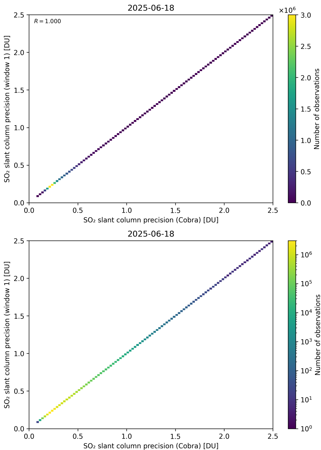
Figure 209: Scatter density plot of “SO 2 slant column precision (Cobra)” against “SO 2 slant column precision (window 1)” for 2025-06-17 to 2025-06-19.
