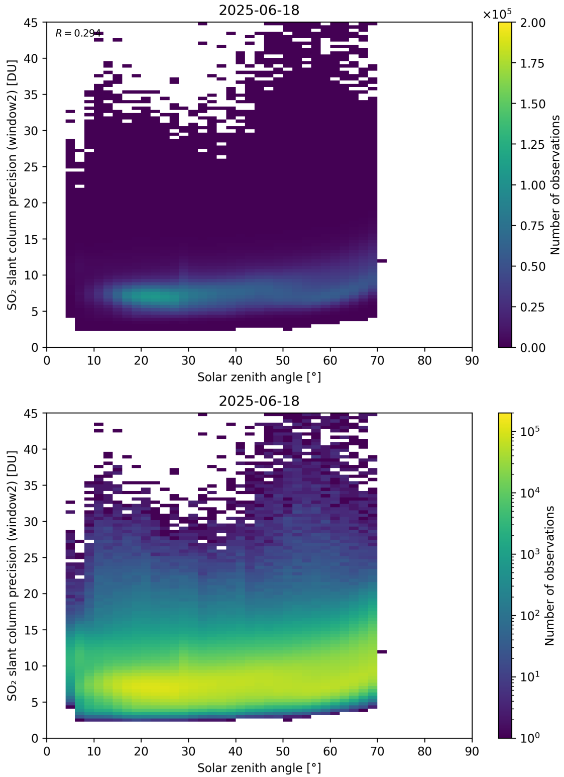
Figure 186: Scatter density plot of “Solar zenith angle” against “SO 2 slant column precision (window2)” for 2025-06-17 to 2025-06-19.
