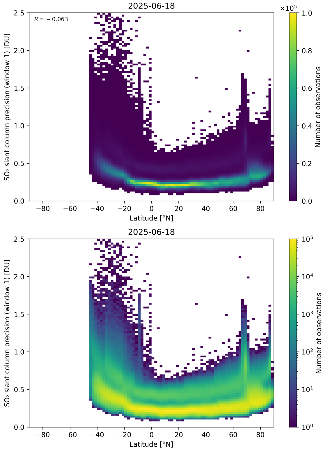
Figure 163: Scatter density plot of “Latitude” against “SO 2 slant column precision (window 1)” for 2025-06-17 to 2025-06-19.
