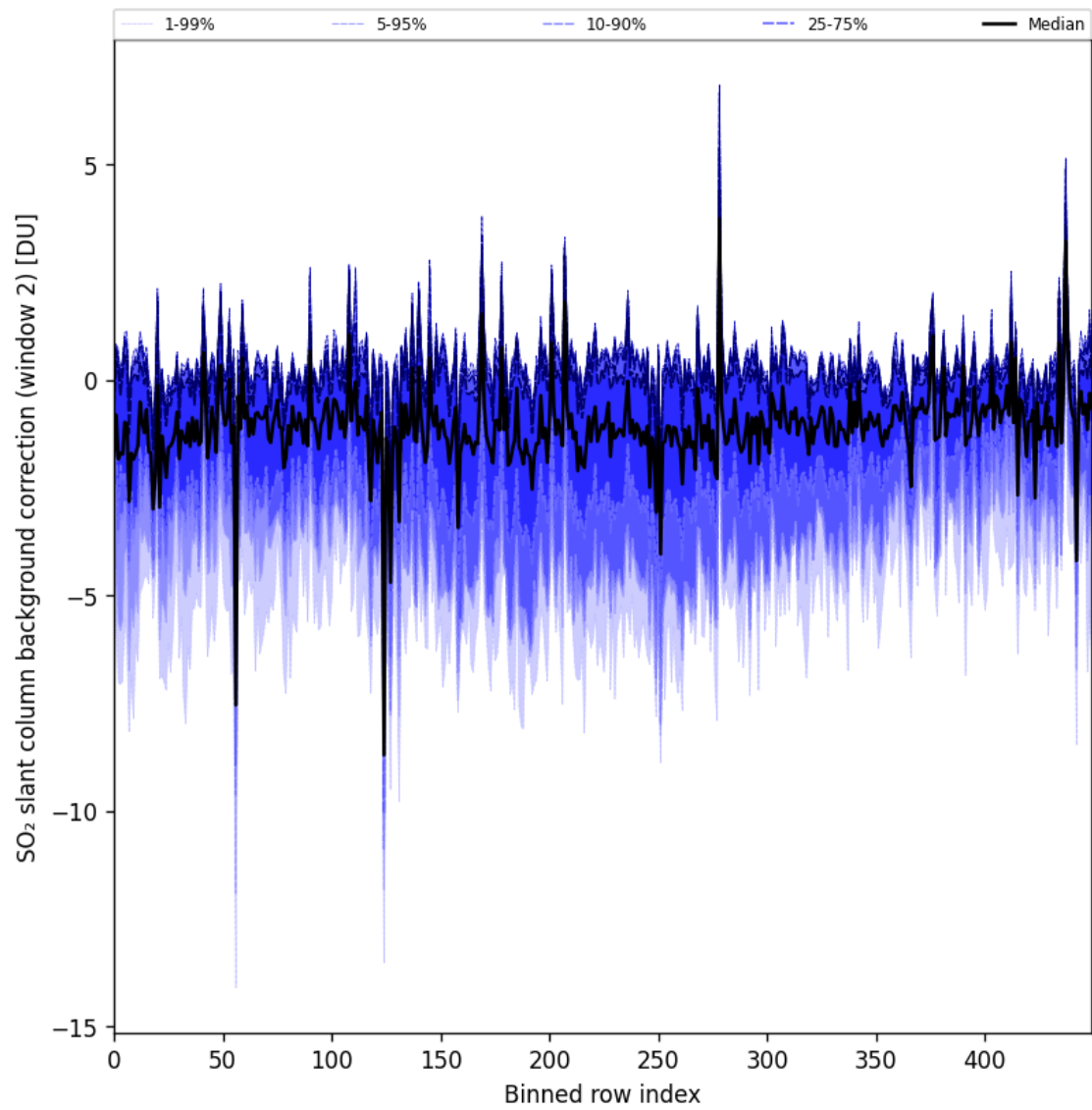
Figure 96: Along track statistics of “SO 2 slant column background correction (window 2)” for 2025-06-17 to 2025-06-19
