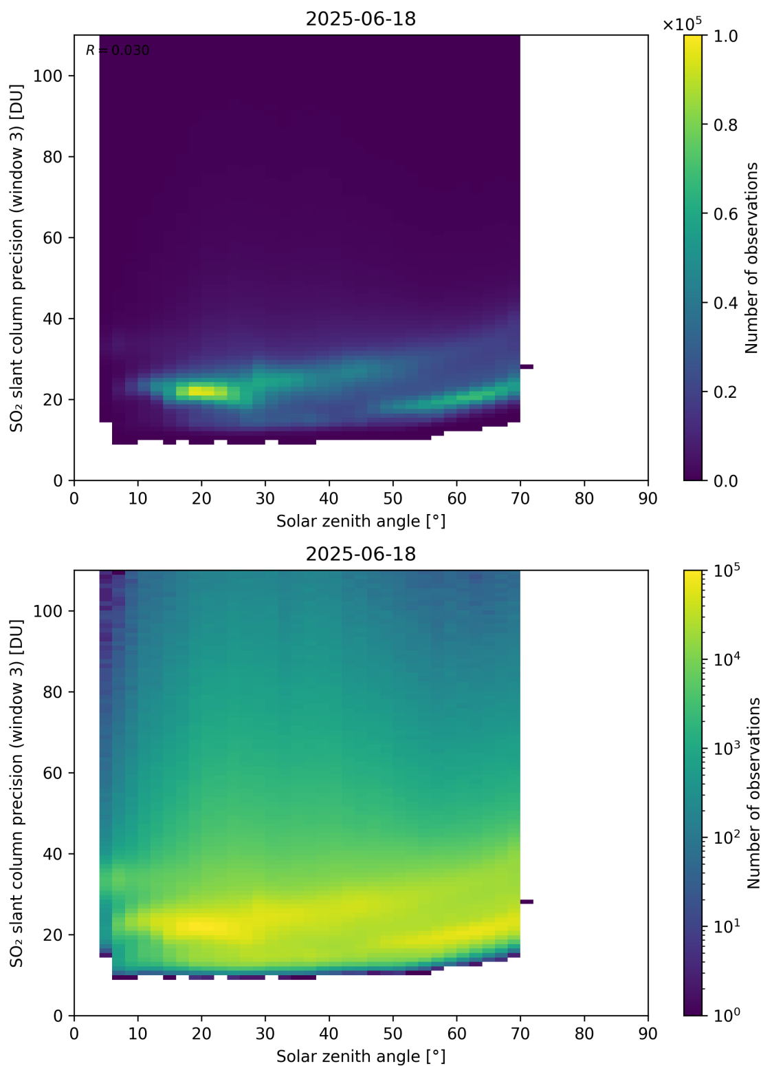
Figure 188: Scatter density plot of “Solar zenith angle” against “SO 2 slant column precision (window 3)” for 2025-06-17 to 2025-06-19.
