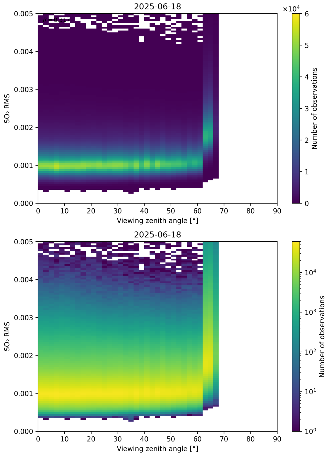
Figure 367: Scatter density plot of “Viewing zenith angle” against “SO 2 RMS” for 2025-06-17 to 2025-06-19.
