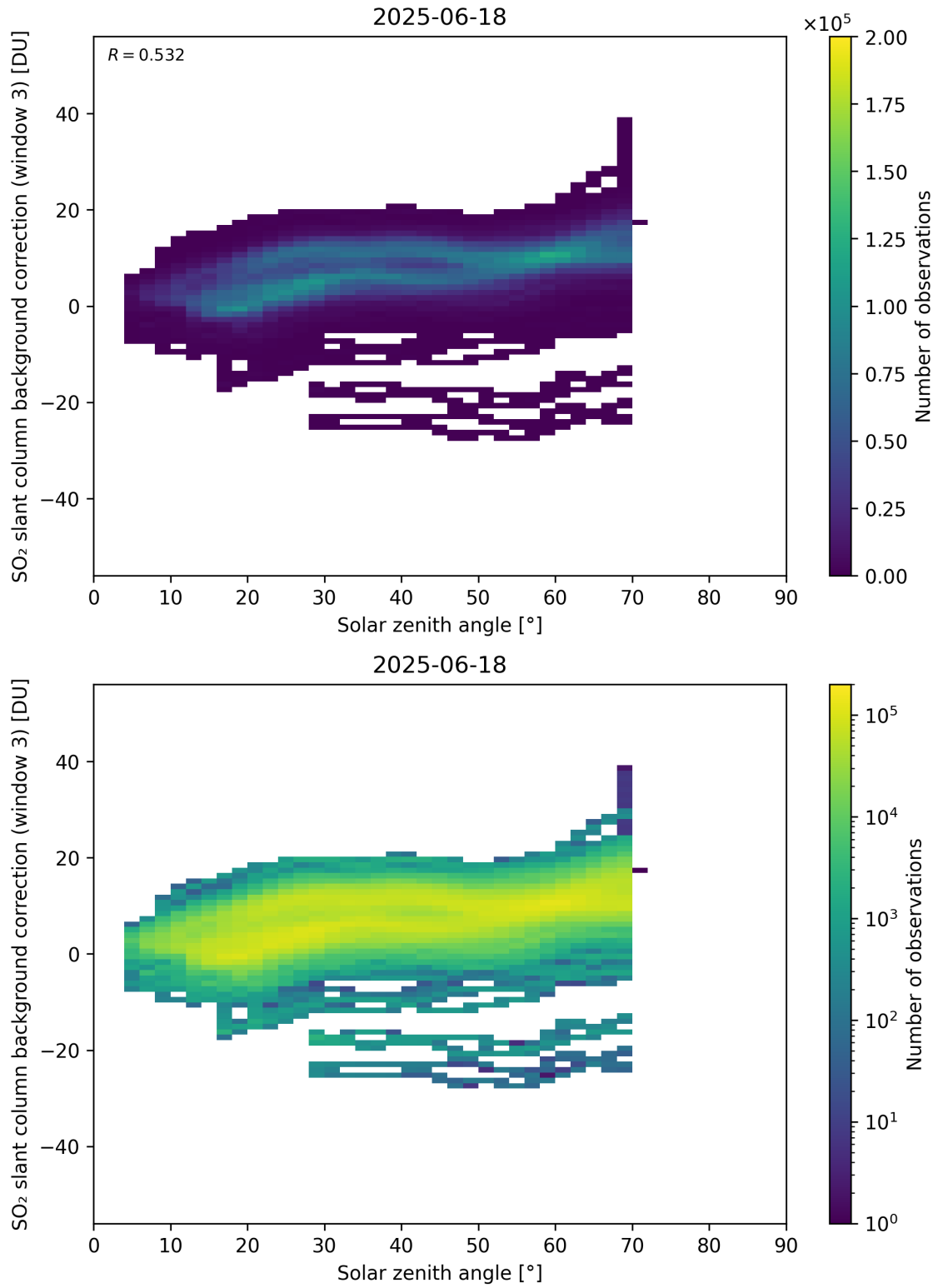
Figure 173: Scatter density plot of “Solar zenith angle” against “SO 2 slant column background correction (window 3)” for 2025-06-17 to 2025-06-19.
