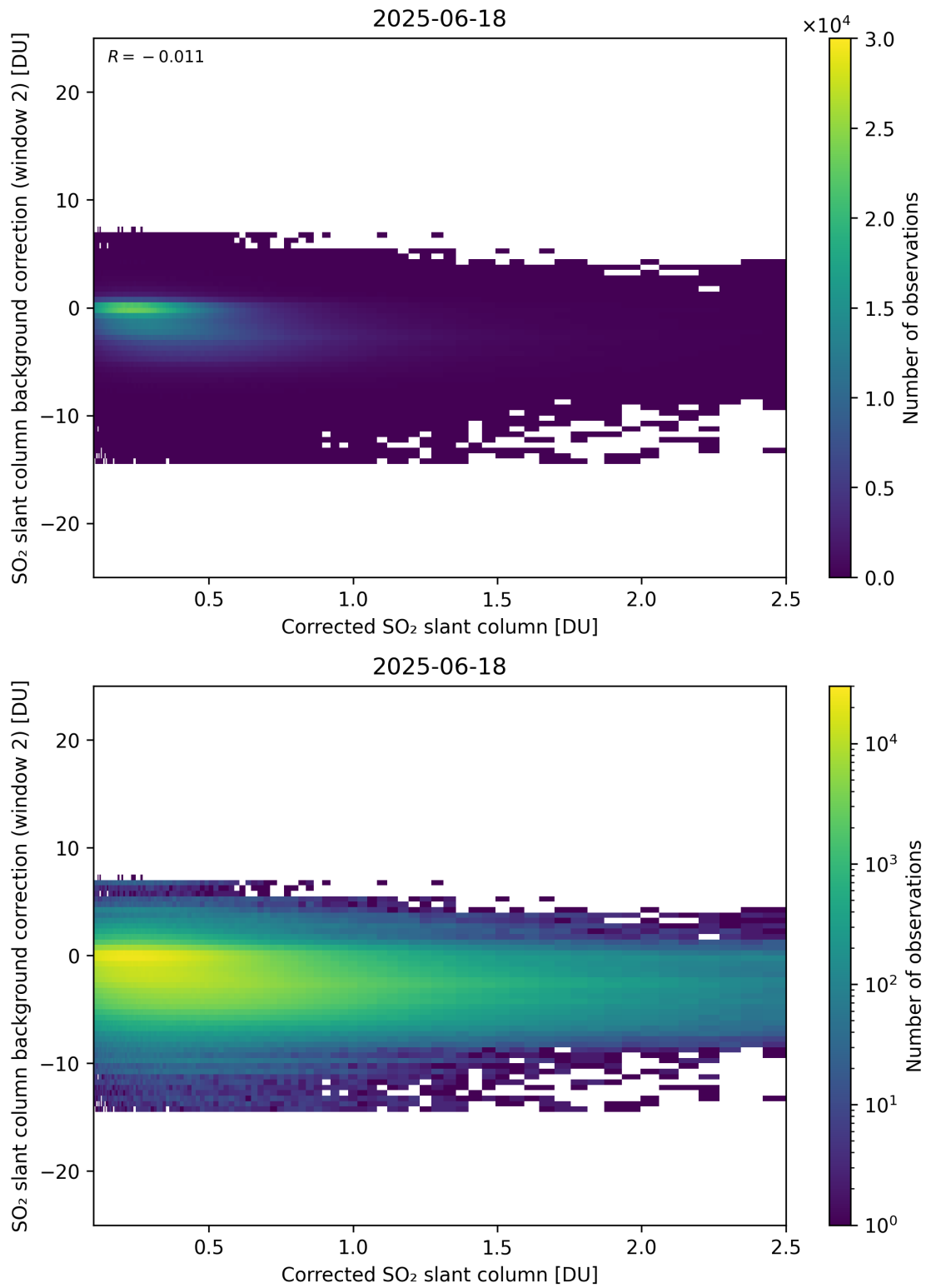
Figure 227: Scatter density plot of “Corrected SO 2 slant column” against “SO 2 slant column background correction (window 2)” for 2025-06-17 to 2025-06-19.
