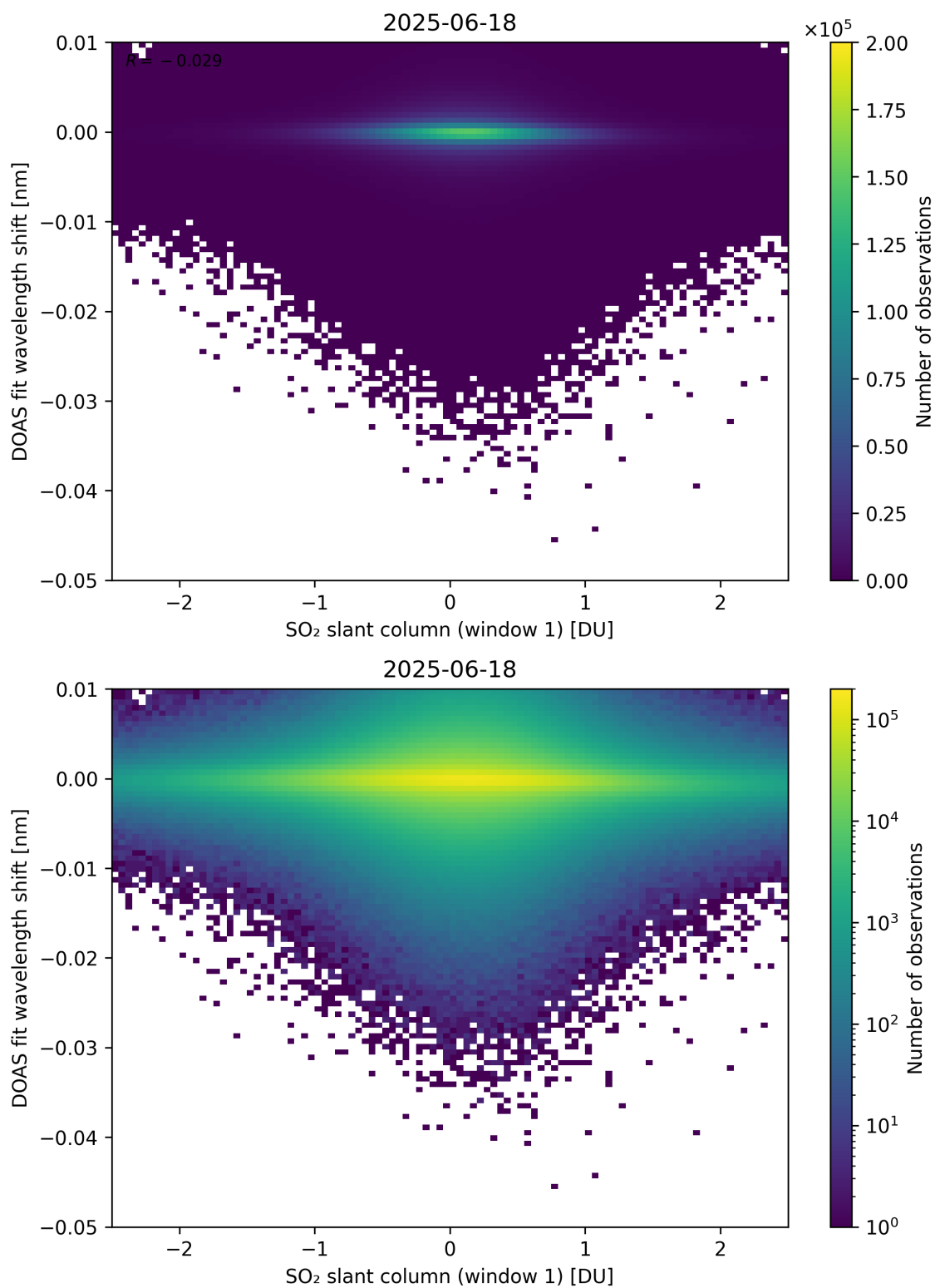
Figure 265: Scatter density plot of “SO 2 slant column (window 1)” against “DOAS fit wavelength shift” for 2025-06-17 to 2025-06-19.
