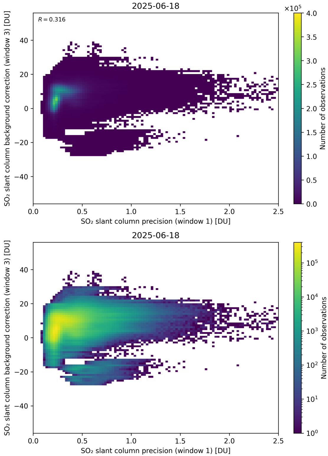
Figure 270: Scatter density plot of “SO 2 slant column precision (window 1)” against “SO 2 slant column background correction (window 3)” for 2025-06-17 to 2025-06-19.
