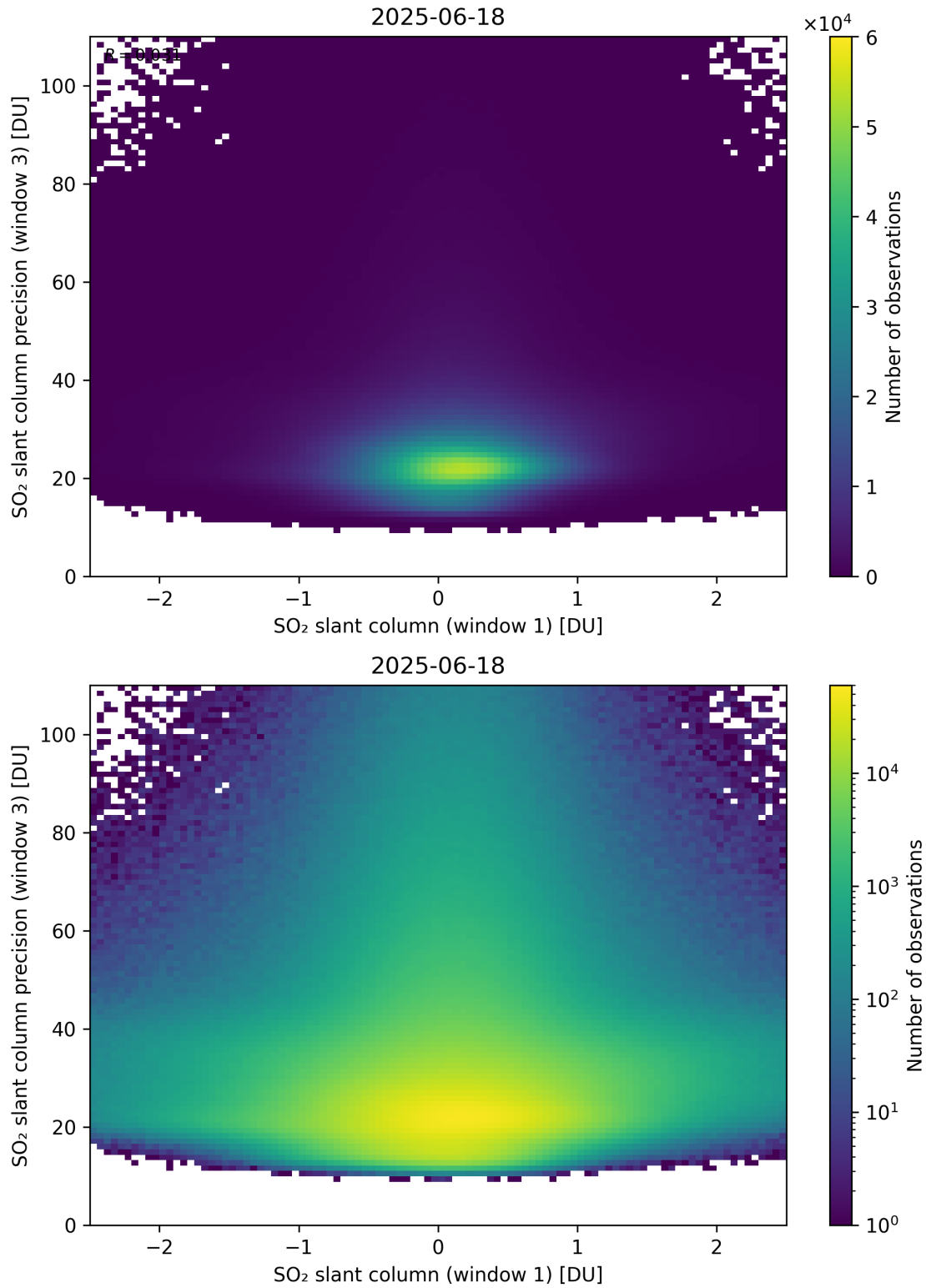
Figure 288: Scatter density plot of “SO 2 slant column (window 1)” against “SO 2 slant column precision (window 3)” for 2025-06-17 to 2025-06-19.
