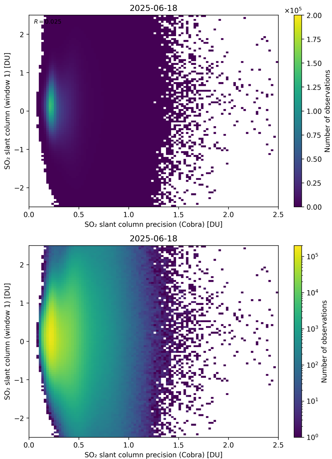
Figure 208: Scatter density plot of “SO 2 slant column precision (Cobra)” against “SO 2 slant column (window 1)” for 2025-06-17 to 2025-06-19.
