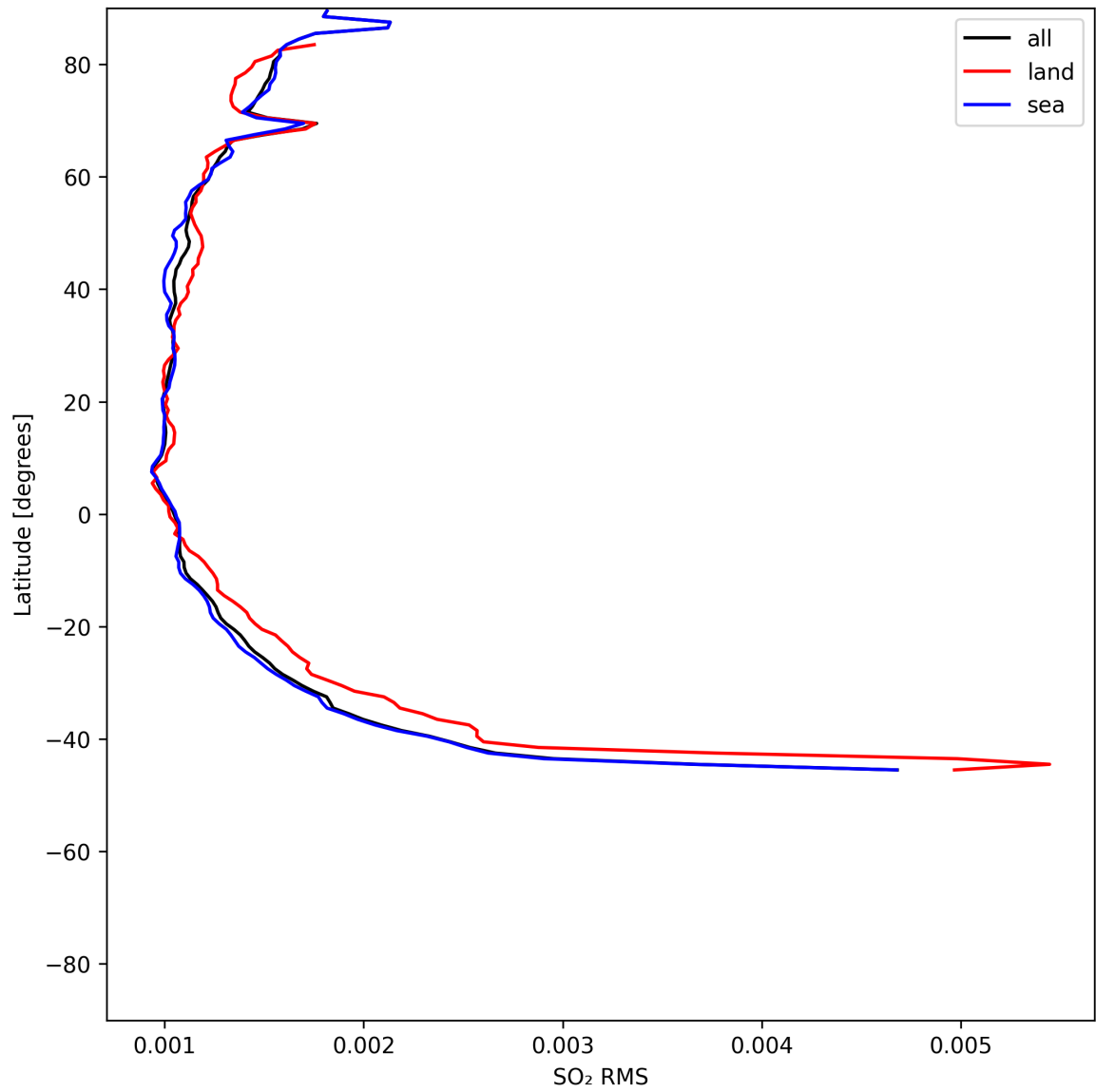
Figure 52: Zonal average of “SO 2 RMS” for 2025-06-17 to 2025-06-19.
