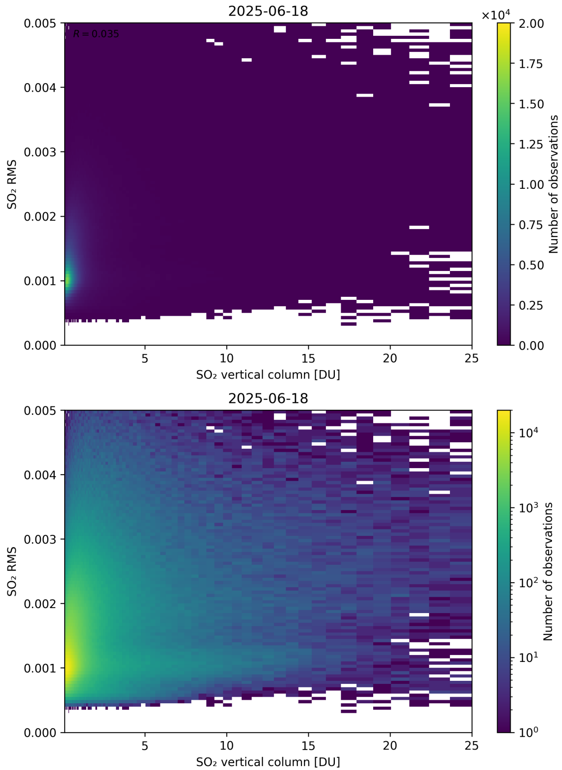
Figure 328: Scatter density plot of “SO 2 vertical column” against “SO 2 RMS” for 2025-06-17 to 2025-06-19.
