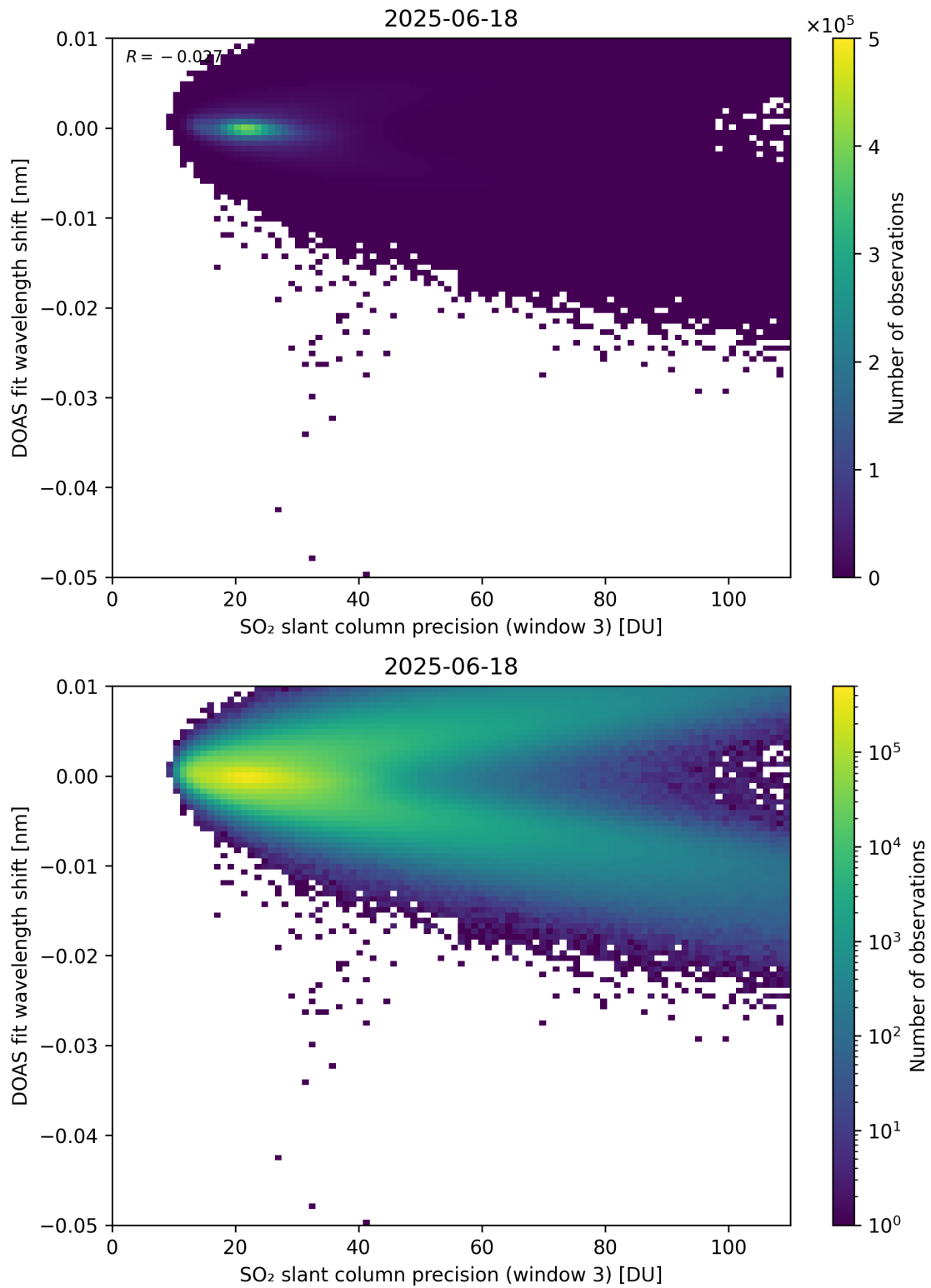
Figure 308: Scatter density plot of “SO 2 slant column precision (window 3)” against “DOAS fit wavelength shift” for 2025-06-17 to 2025-06-19.
