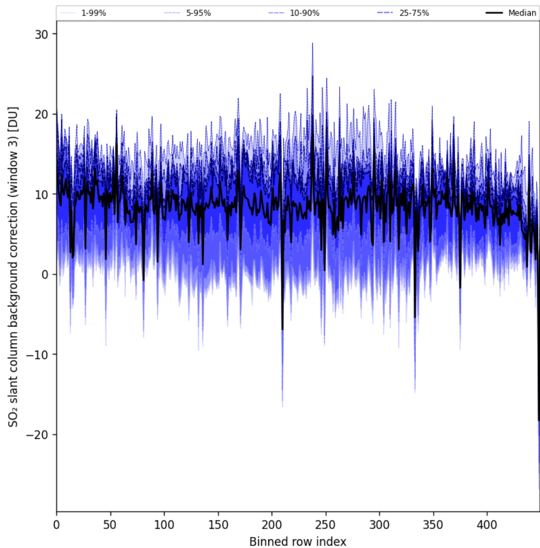
Figure 100: Along track statistics of “SO 2 slant column background correction (window 3)” for 2025-06-17 to 2025-06-19
