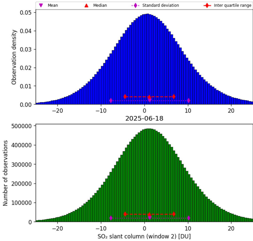
Figure 67: Histogram of “SO 2 slant column (window 2)” for 2025-06-17 to 2025-06-19
