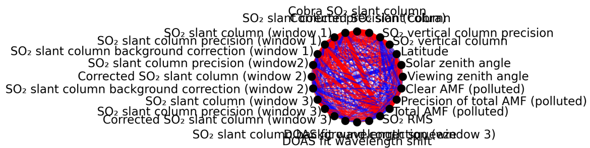
Figure 1: Map of correlation graph for 2025-06-17 to 2025-06-19.
