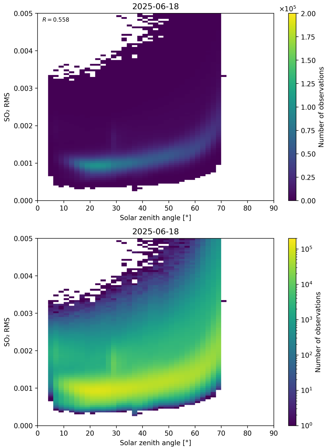
Figure 176: Scatter density plot of “Solar zenith angle” against “SO 2 RMS” for 2025-06-17 to 2025-06-19.
