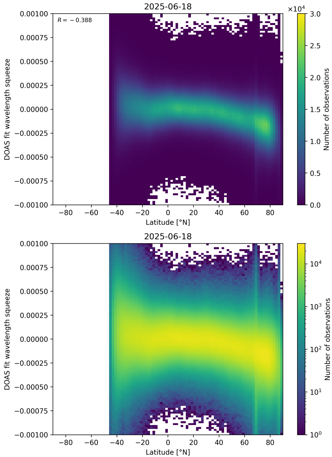
Figure 154: Scatter density plot of “Latitude” against “DOAS fit wavelength squeeze” for 2025-06-17 to 2025-06-19.
