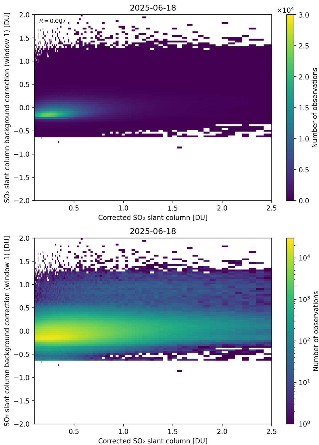
Figure 226: Scatter density plot of “Corrected SO 2 slant column” against “SO 2 slant column background correction (window 1)” for 2025-06-17 to 2025-06-19.
