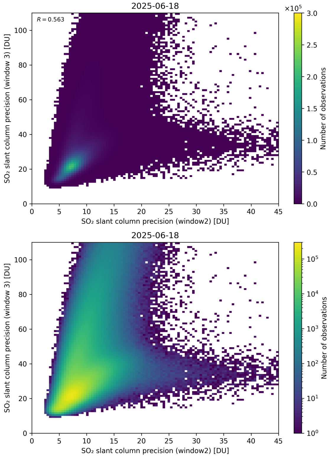
Figure 300: Scatter density plot of “SO 2 slant column precision (window2)” against “SO 2 slant column precision (window 3)” for 2025-06-17 to 2025-06-19.
