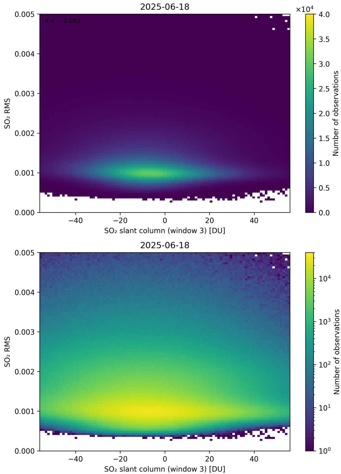
Figure 306: Scatter density plot of “SO 2 slant column (window 3)” against “SO 2 RMS” for 2025-06-17 to 2025-06-19.
