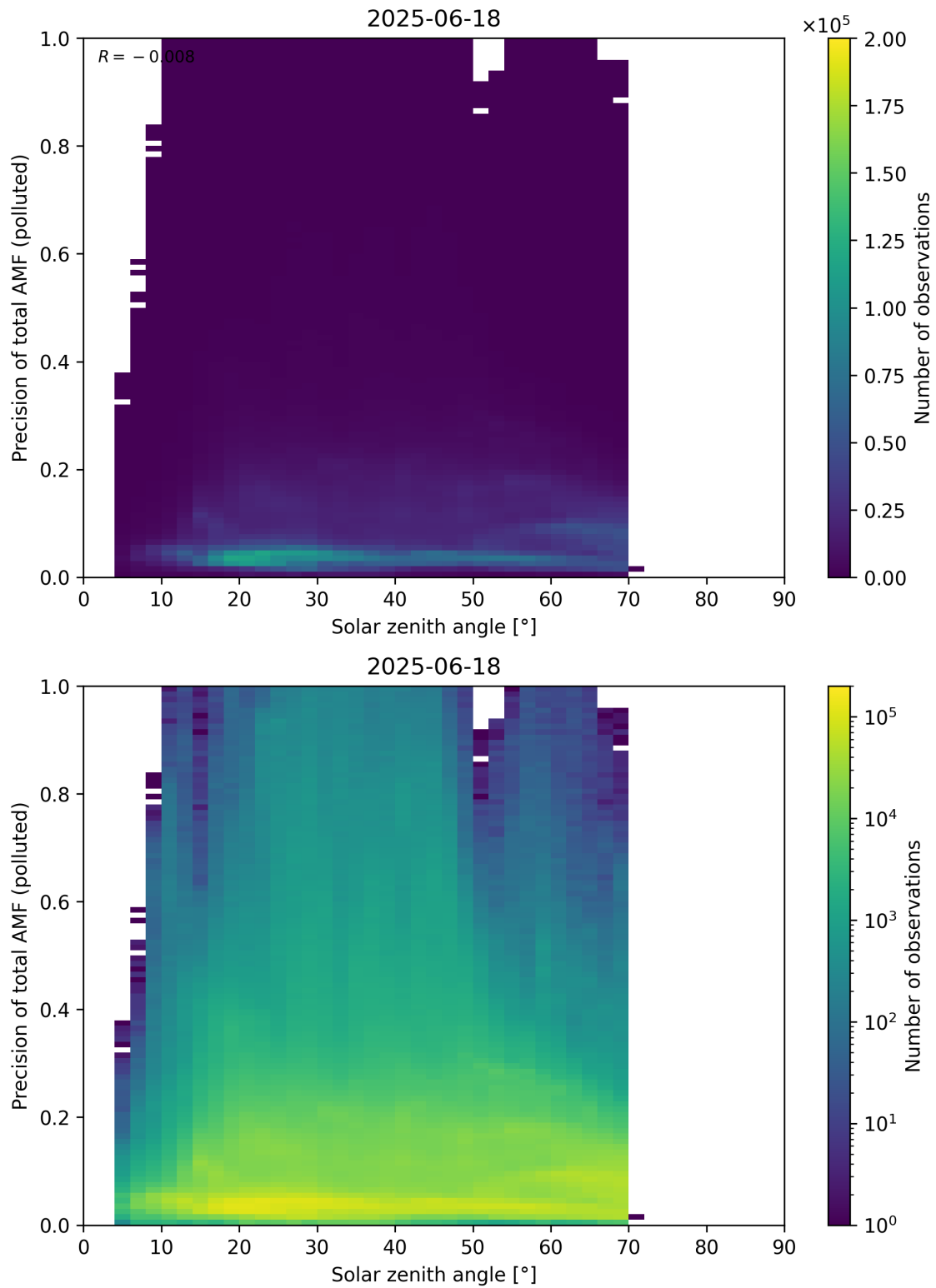
Figure 190: Scatter density plot of “Solar zenith angle” against “Precision of total AMF (polluted)” for 2025-06-17 to 2025-06-19.
