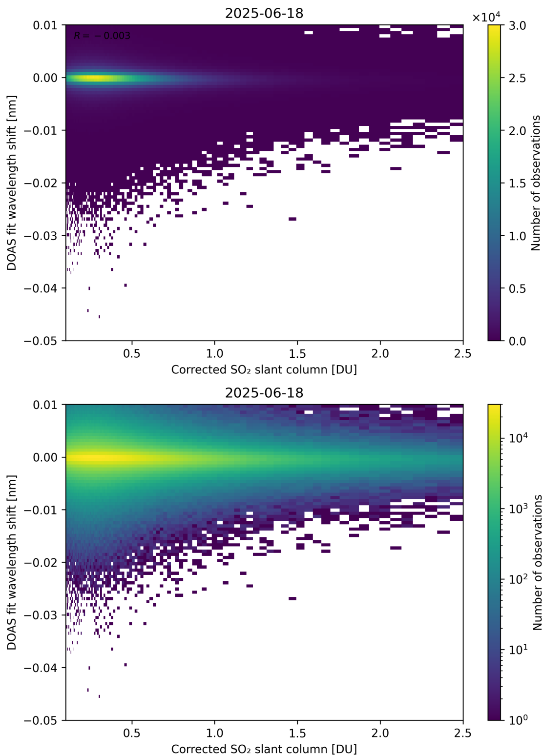
Figure 229: Scatter density plot of “Corrected SO 2 slant column” against “DOAS fit wavelength shift” for 2025-06-17 to 2025-06-19.
