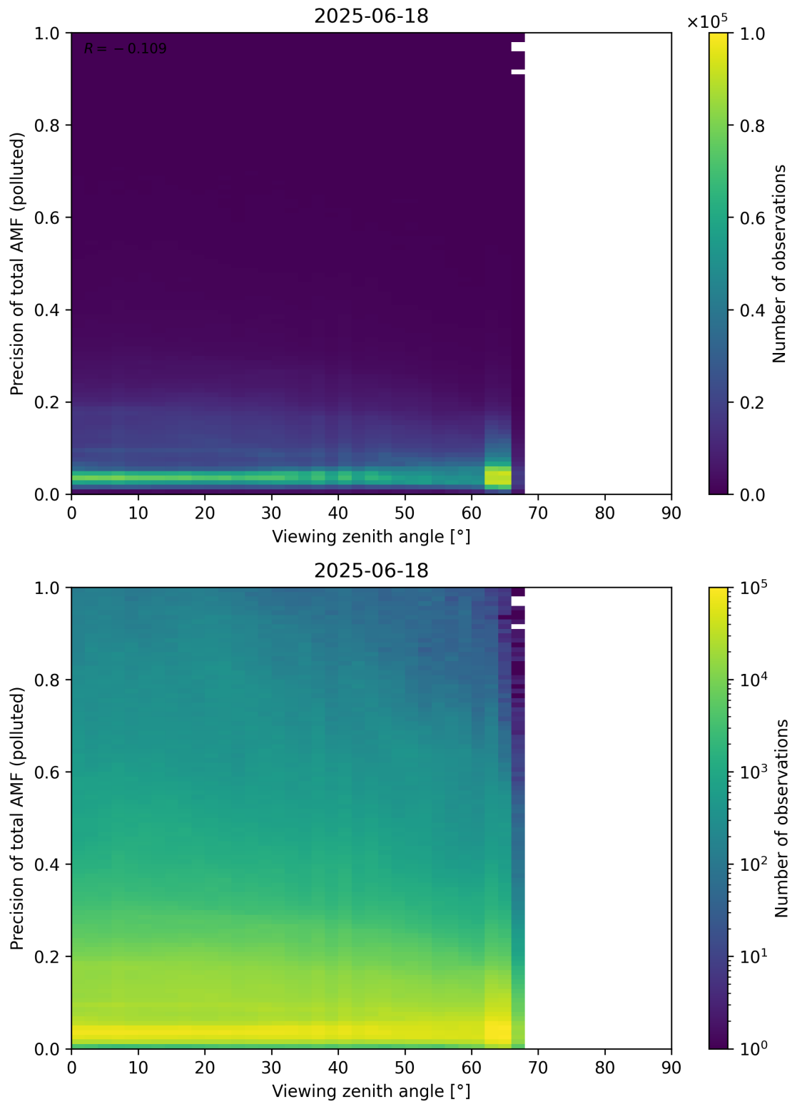
Figure 382: Scatter density plot of “Viewing zenith angle” against “Precision of total AMF (polluted)” for 2025-06-17 to 2025-06-19.
