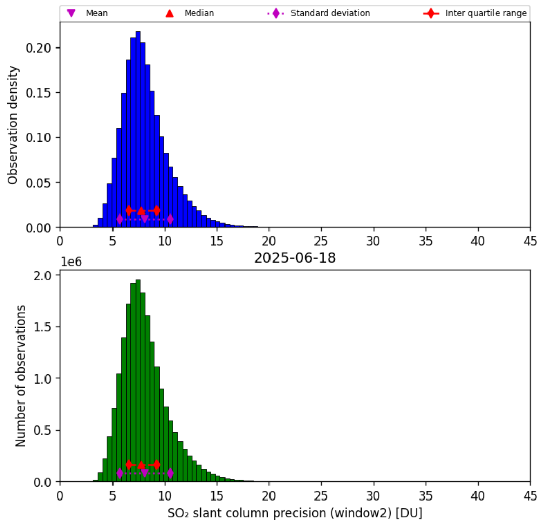
Figure 68: Histogram of “SO 2 slant column precision (window2)” for 2025-06-17 to 2025-06-19
