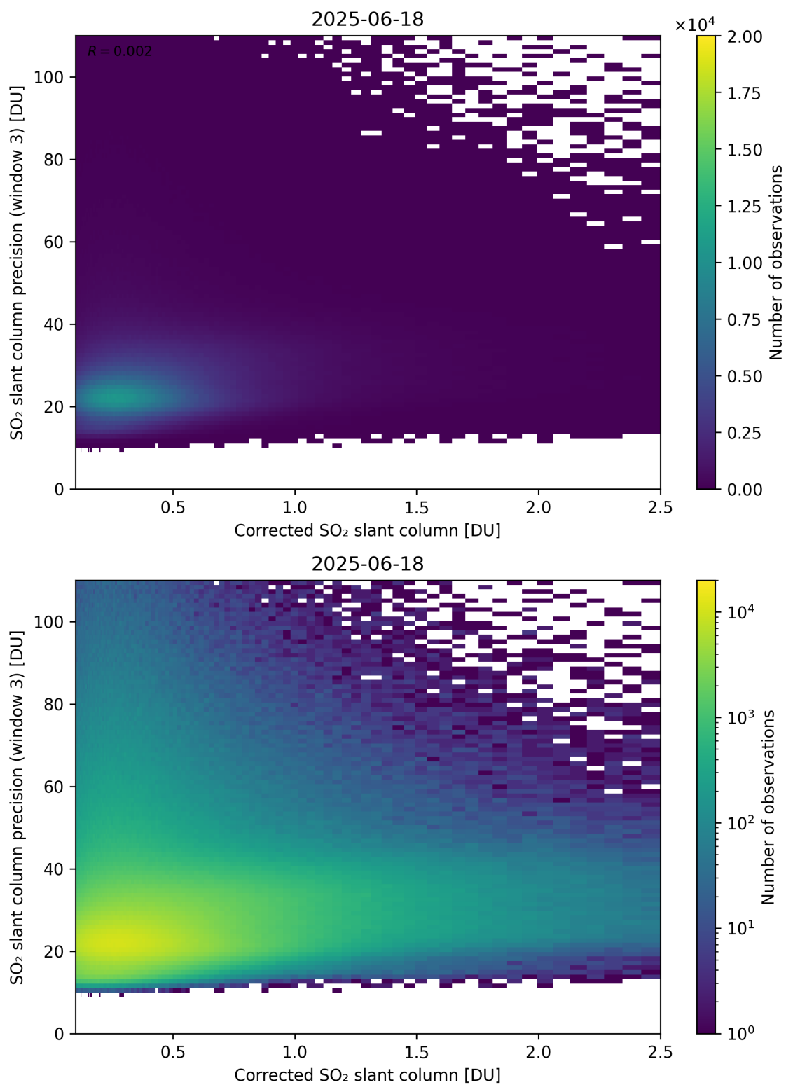
Figure 241: Scatter density plot of “Corrected SO 2 slant column” against “SO 2 slant column precision (window 3)” for 2025-06-17 to 2025-06-19.
