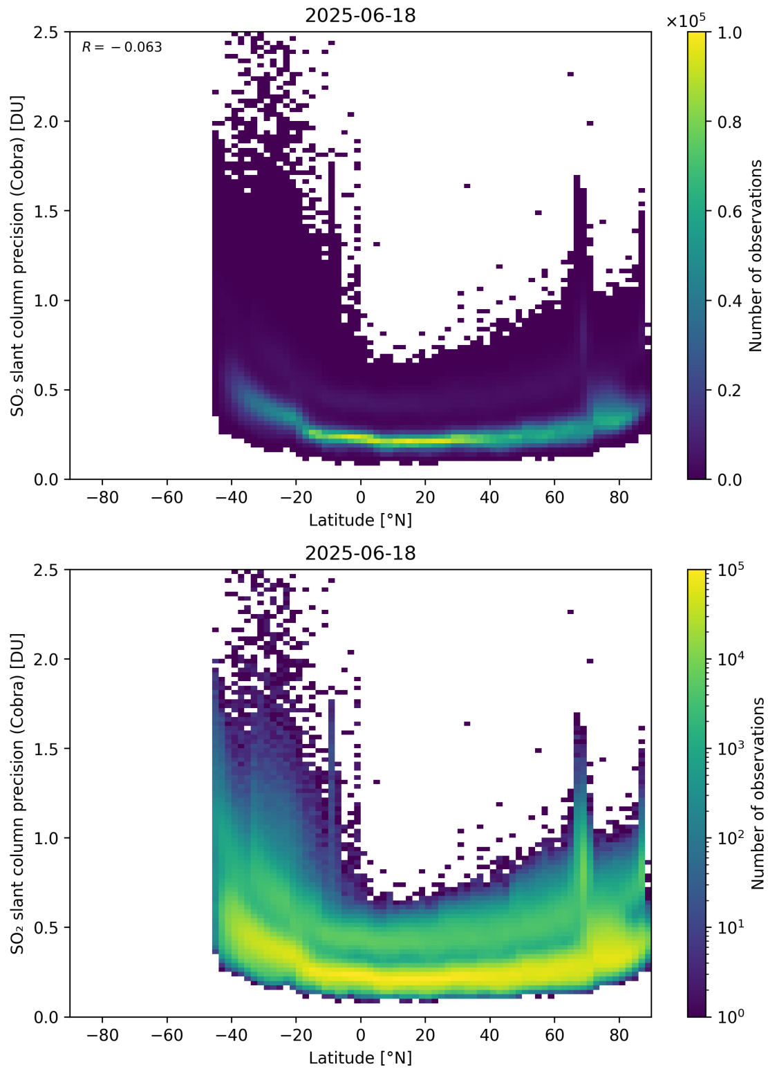
Figure 158: Scatter density plot of “Latitude” against “SO 2 slant column precision (Cobra)” for 2025-06-17 to 2025-06-19.
