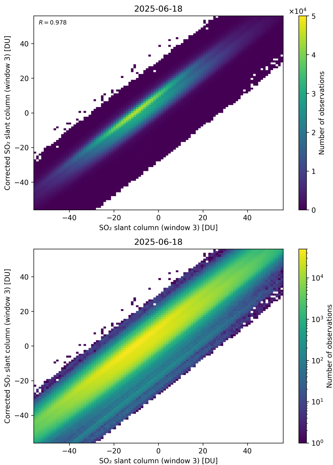
Figure 316: Scatter density plot of “SO 2 slant column (window 3)” against “Corrected SO 2 slant column (window 3)” for 2025-06-17 to 2025-06-19.
