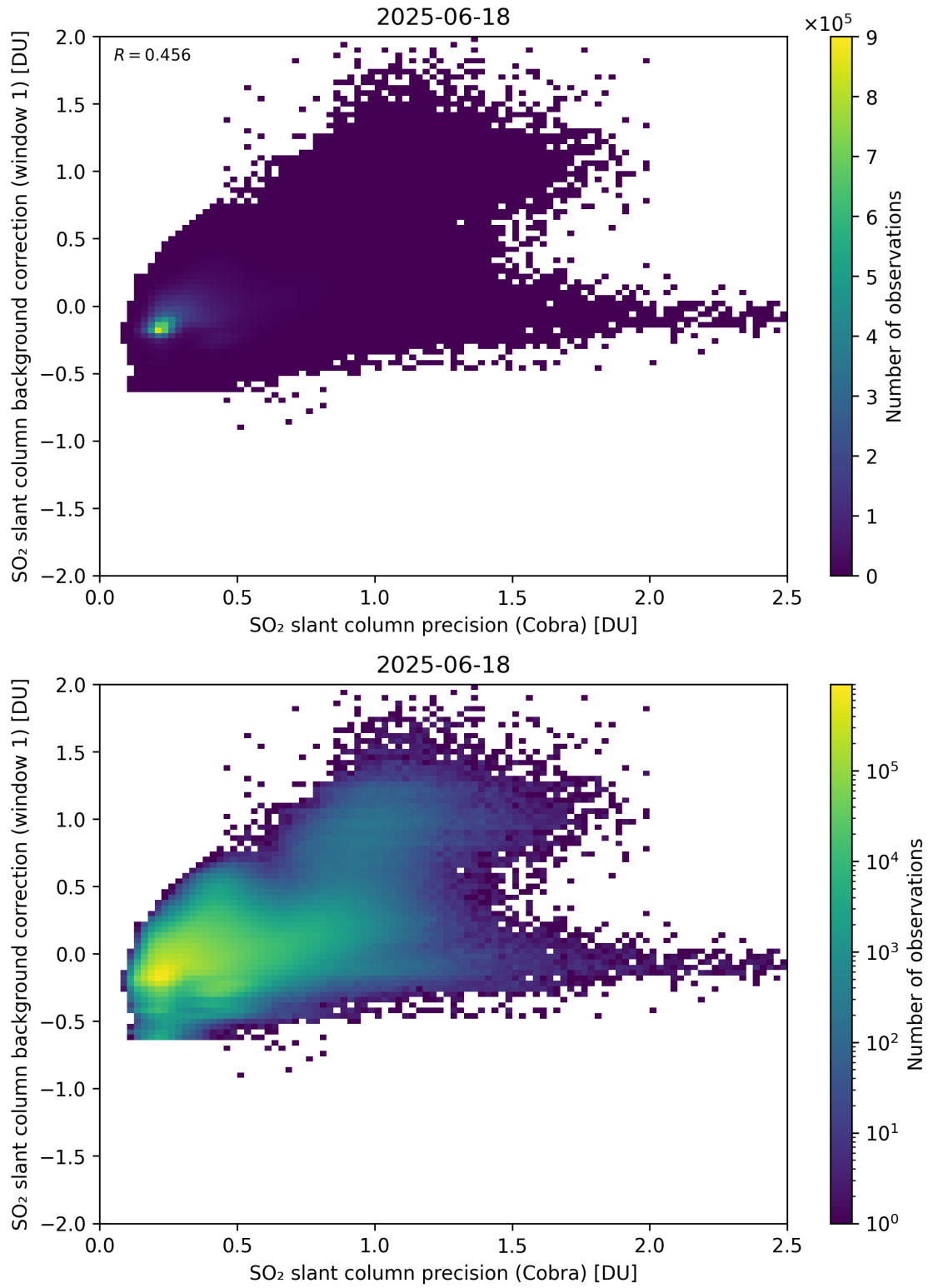
Figure 199: Scatter density plot of “SO 2 slant column precision (Cobra)” against “SO 2 slant column background correction (window 1)” for 2025-06-17 to 2025-06-19.
