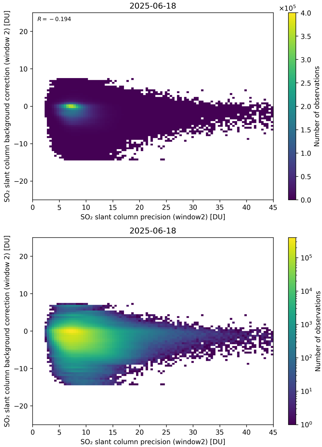
Figure 291: Scatter density plot of “SO 2 slant column precision (window2)” against “SO 2 slant column background correction (window 2)” for 2025-06-17 to 2025-06-19.
