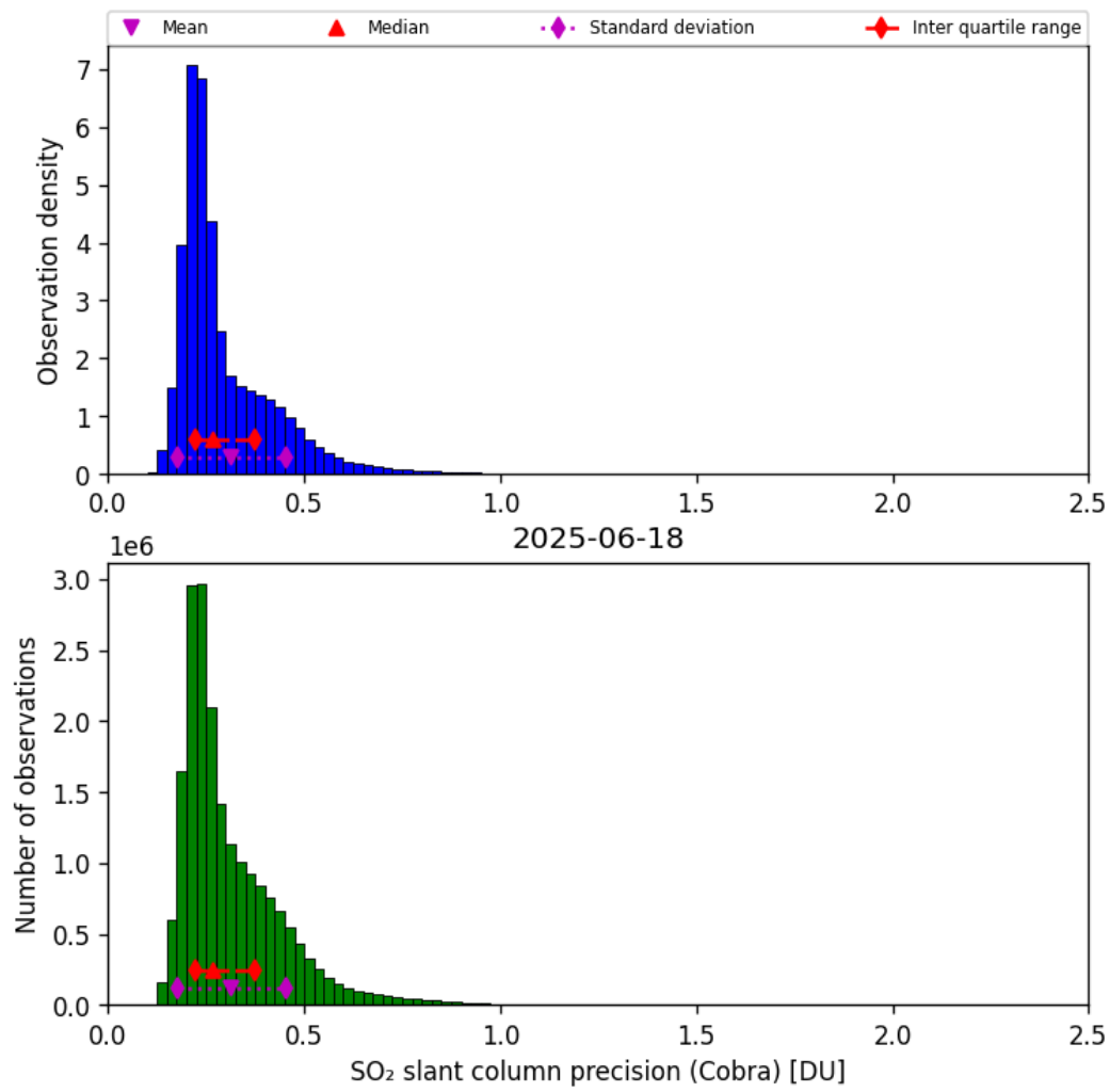
Figure 62: Histogram of “SO 2 slant column precision (Cobra)” for 2025-06-17 to 2025-06-19
