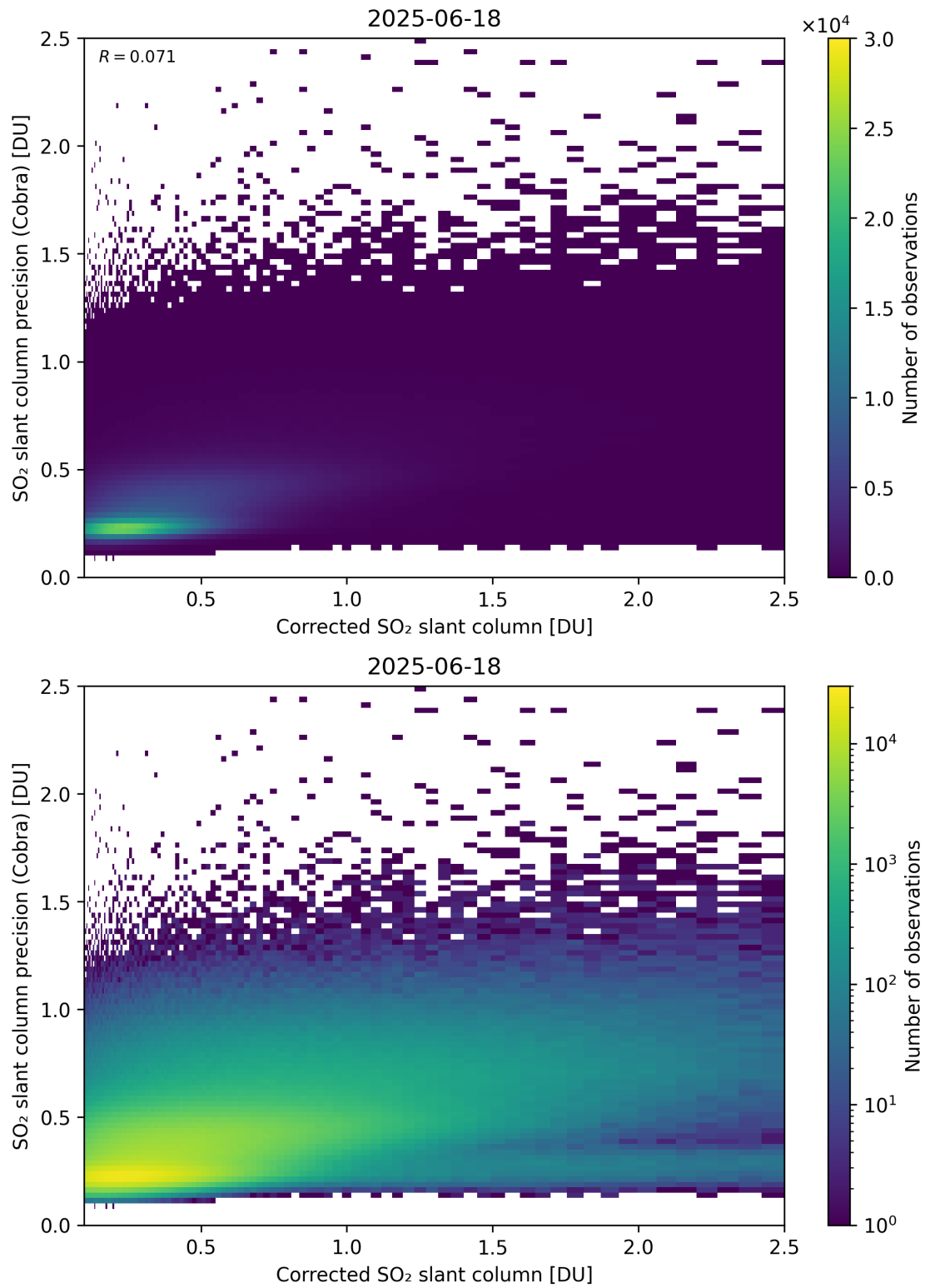
Figure 234: Scatter density plot of “Corrected SO 2 slant column” against “SO 2 slant column precision (Cobra)” for 2025-06-17 to 2025-06-19.
