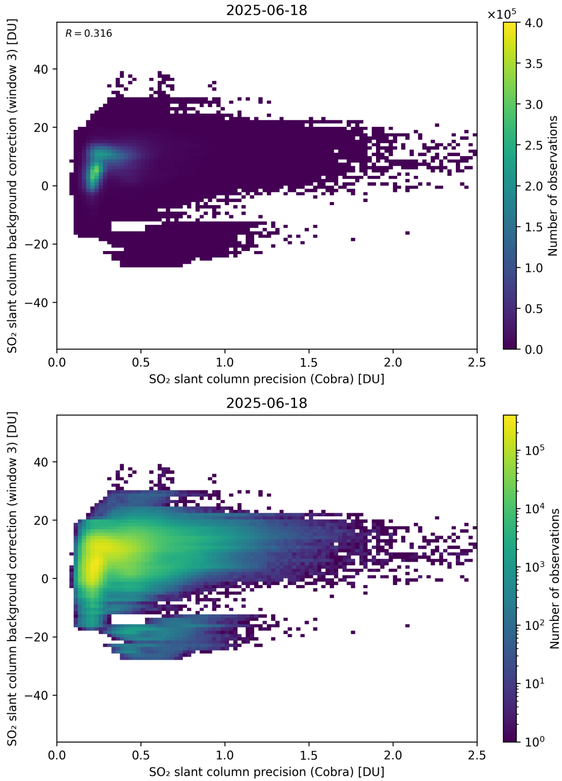
Figure 201: Scatter density plot of “SO 2 slant column precision (Cobra)” against “SO 2 slant column background correction (window 3)” for 2025-06-17 to 2025-06-19.
