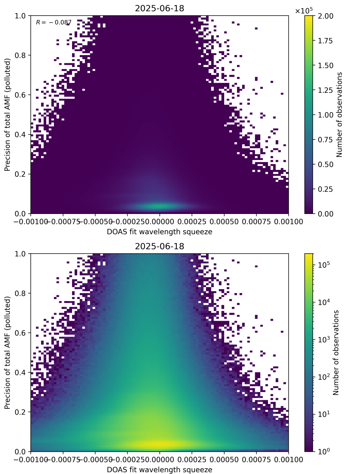
Figure 146: Scatter density plot of “DOAS fit wavelength squeeze” against “Precision of total AMF (polluted)” for 2025-06-17 to 2025-06-19.
