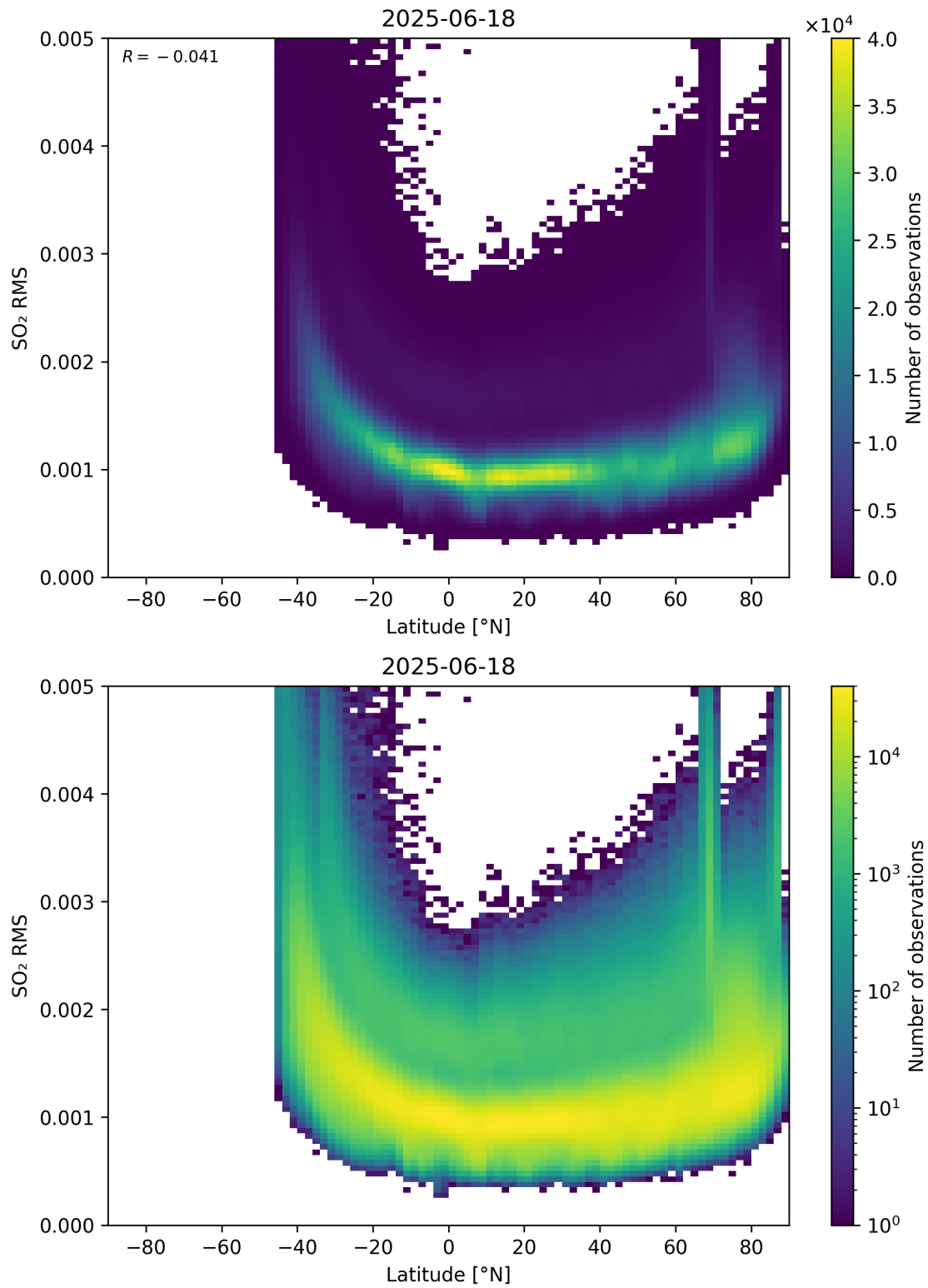
Figure 155: Scatter density plot of “Latitude” against “SO 2 RMS” for 2025-06-17 to 2025-06-19.
