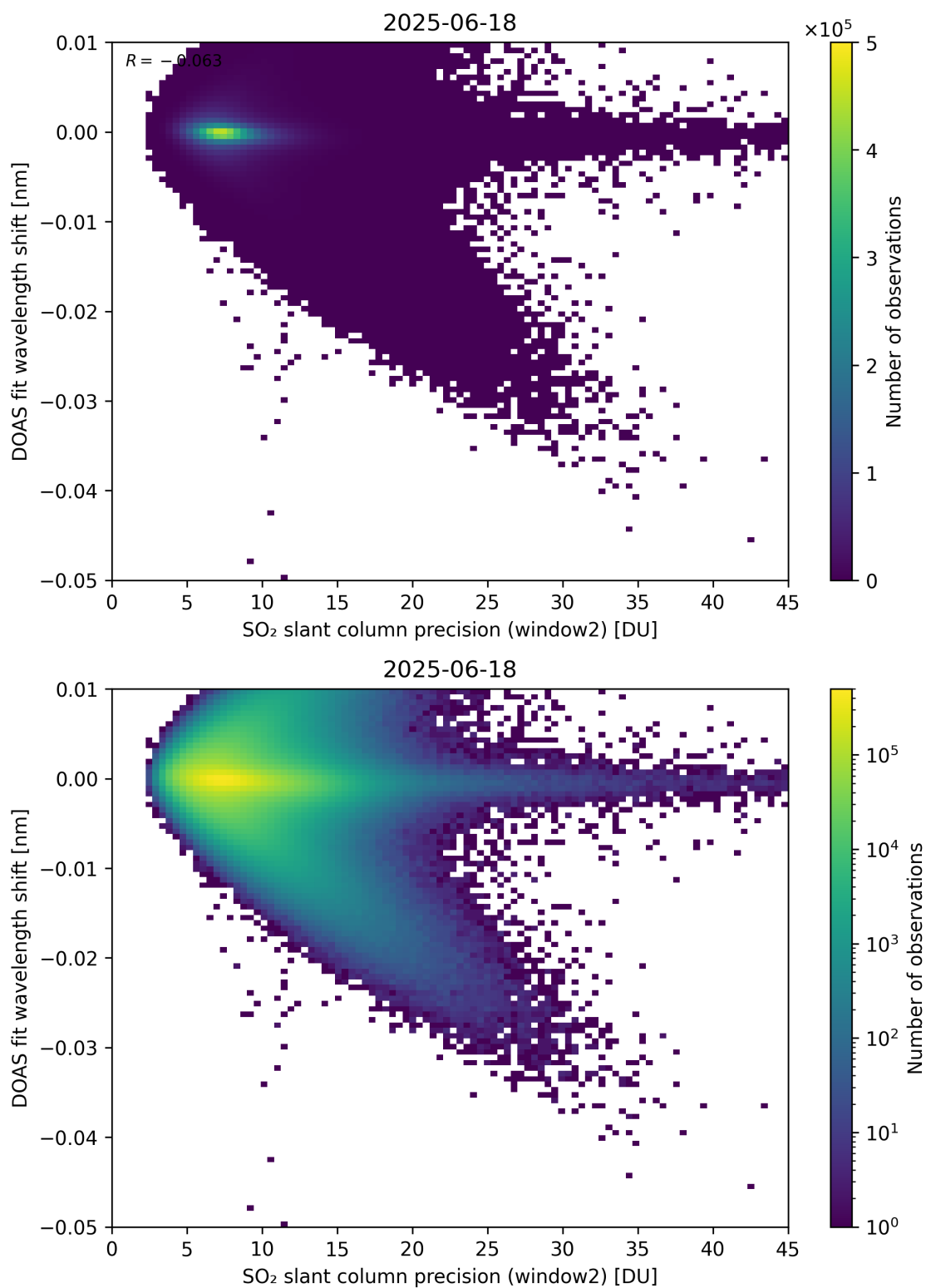
Figure 293: Scatter density plot of “SO 2 slant column precision (window2)” against “DOAS fit wavelength shift” for 2025-06-17 to 2025-06-19.
