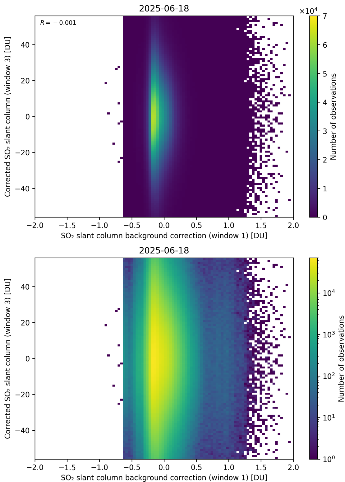
Figure 116: Scatter density plot of “SO 2 slant column background correction (window 1)” against “Corrected SO 2 slant column (window 3)” for 2025-06-17 to 2025-06-19.
