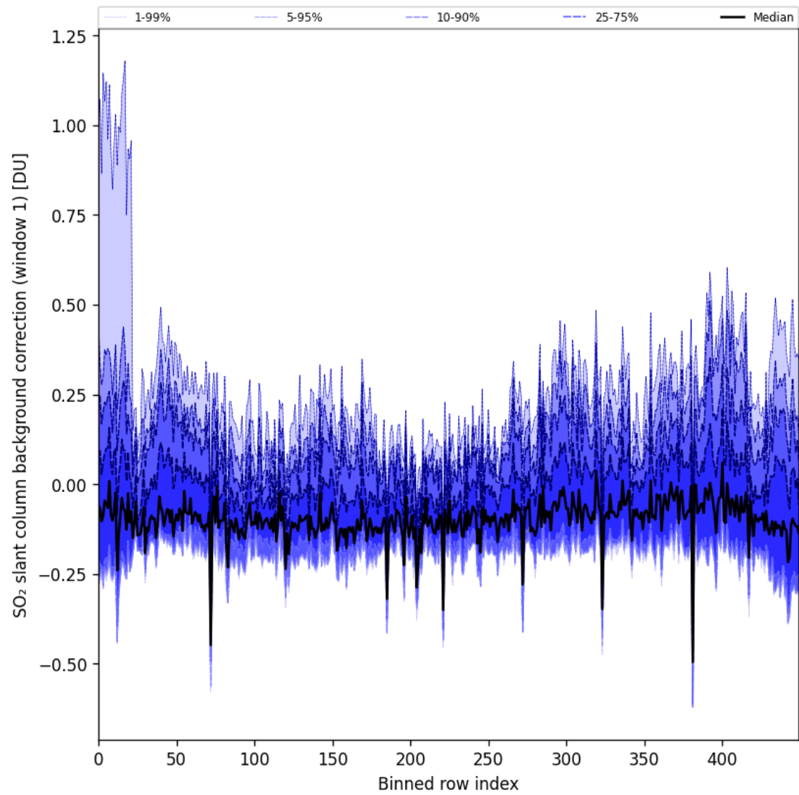
Figure 92: Along track statistics of “SO 2 slant column background correction (window 1)” for 2025-06-17 to 2025-06-19
