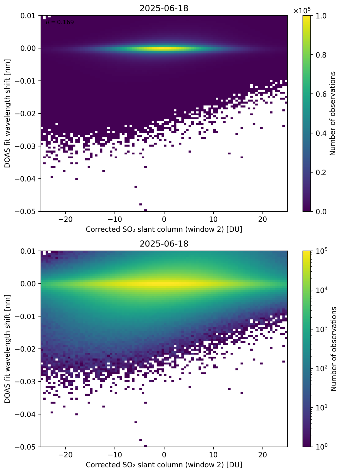
Figure 246: Scatter density plot of “Corrected SO 2 slant column (window 2)” against “DOAS fit wavelength shift” for 2025-06-17 to 2025-06-19.
