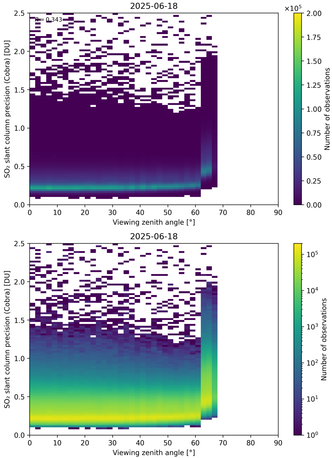
Figure 372: Scatter density plot of “Viewing zenith angle” against “SO 2 slant column precision (Cobra)” for 2025-06-17 to 2025-06-19.
