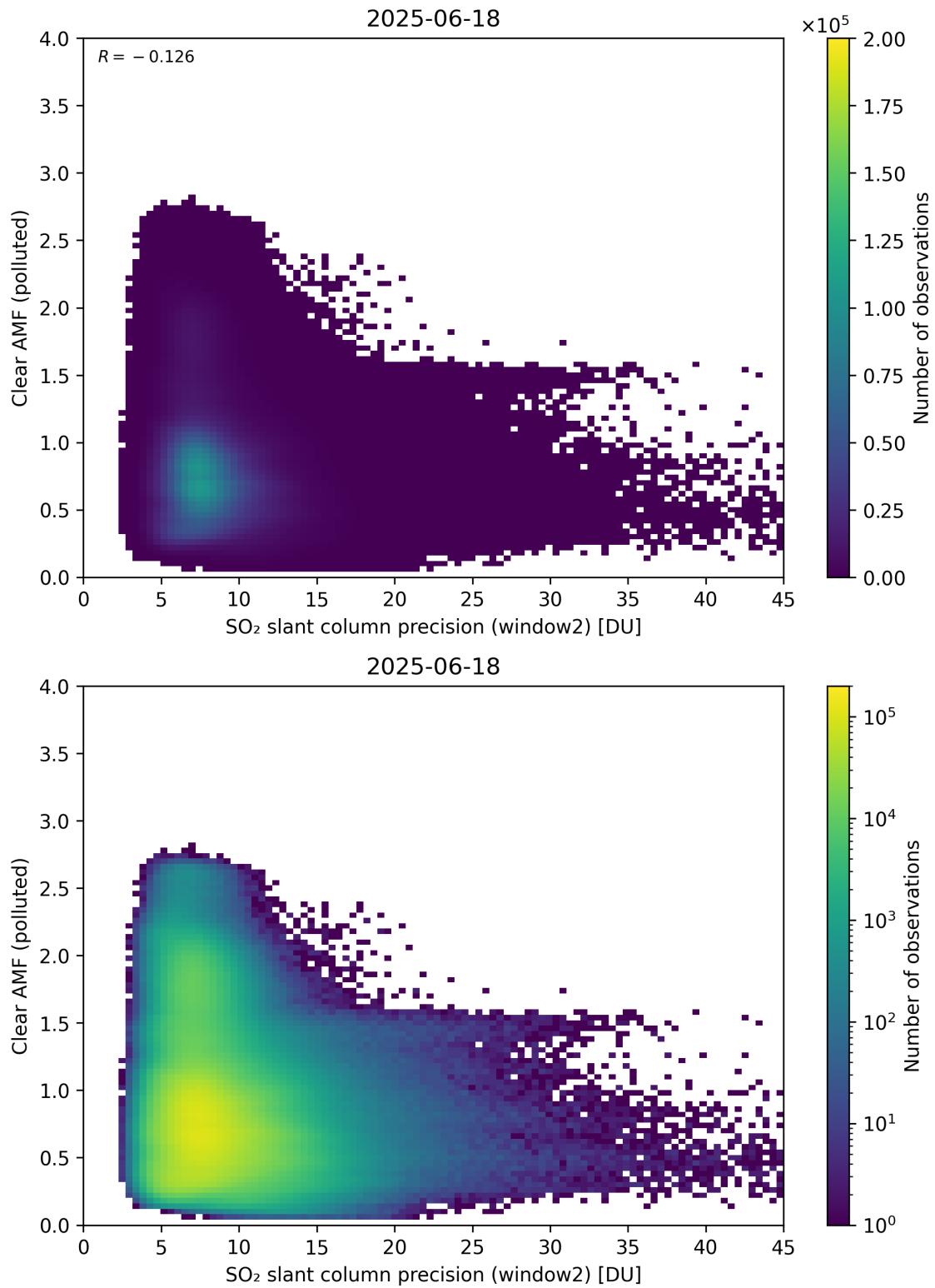
Figure 296: Scatter density plot of “SO 2 slant column precision (window2)” against “Clear AMF (polluted)” for 2025-06-17 to 2025-06-19.
