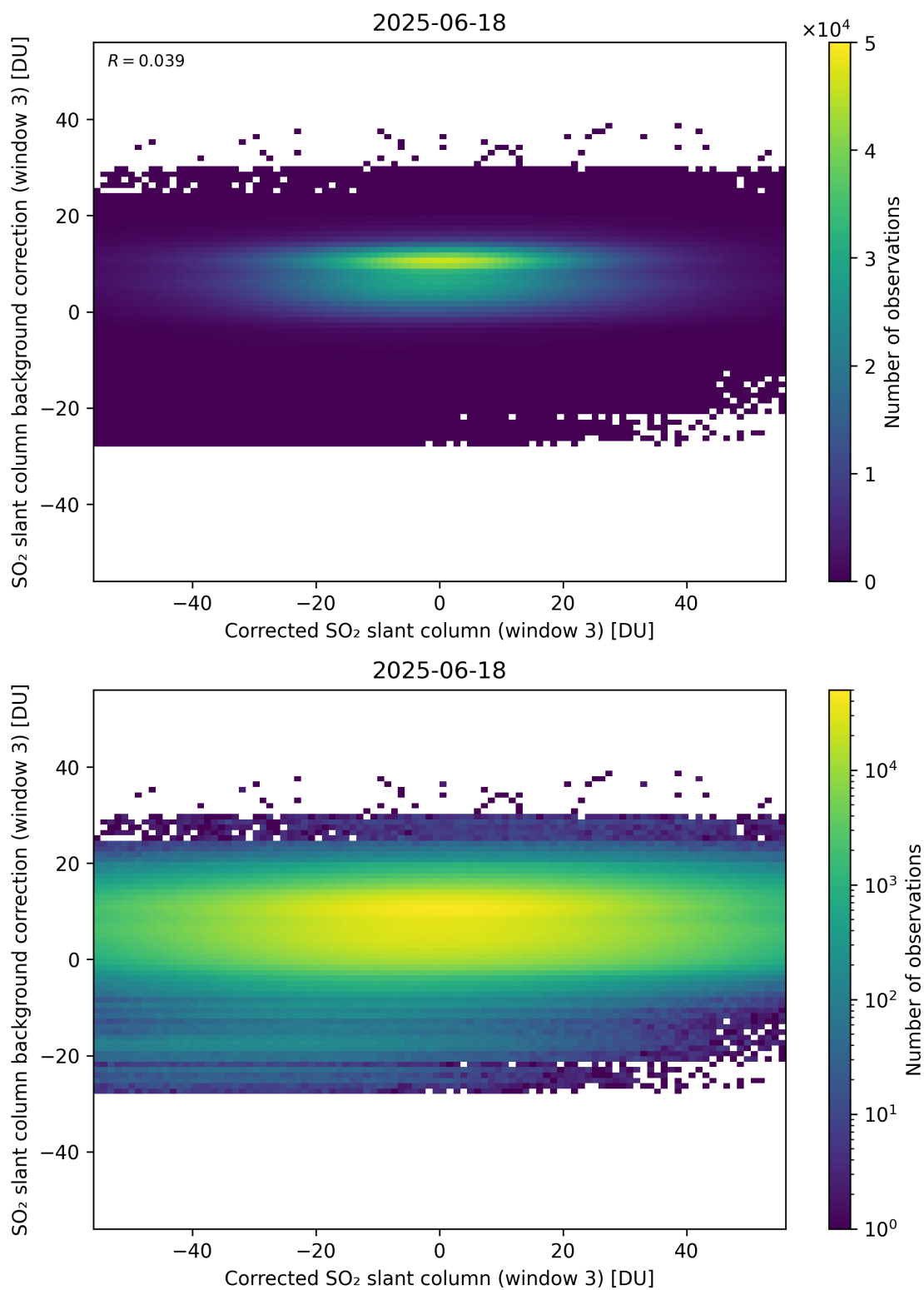
Figure 255: Scatter density plot of “Corrected SO 2 slant column (window 3)” against “SO 2 slant column background correction (window 3)” for 2025-06-17 to 2025-06-19.
