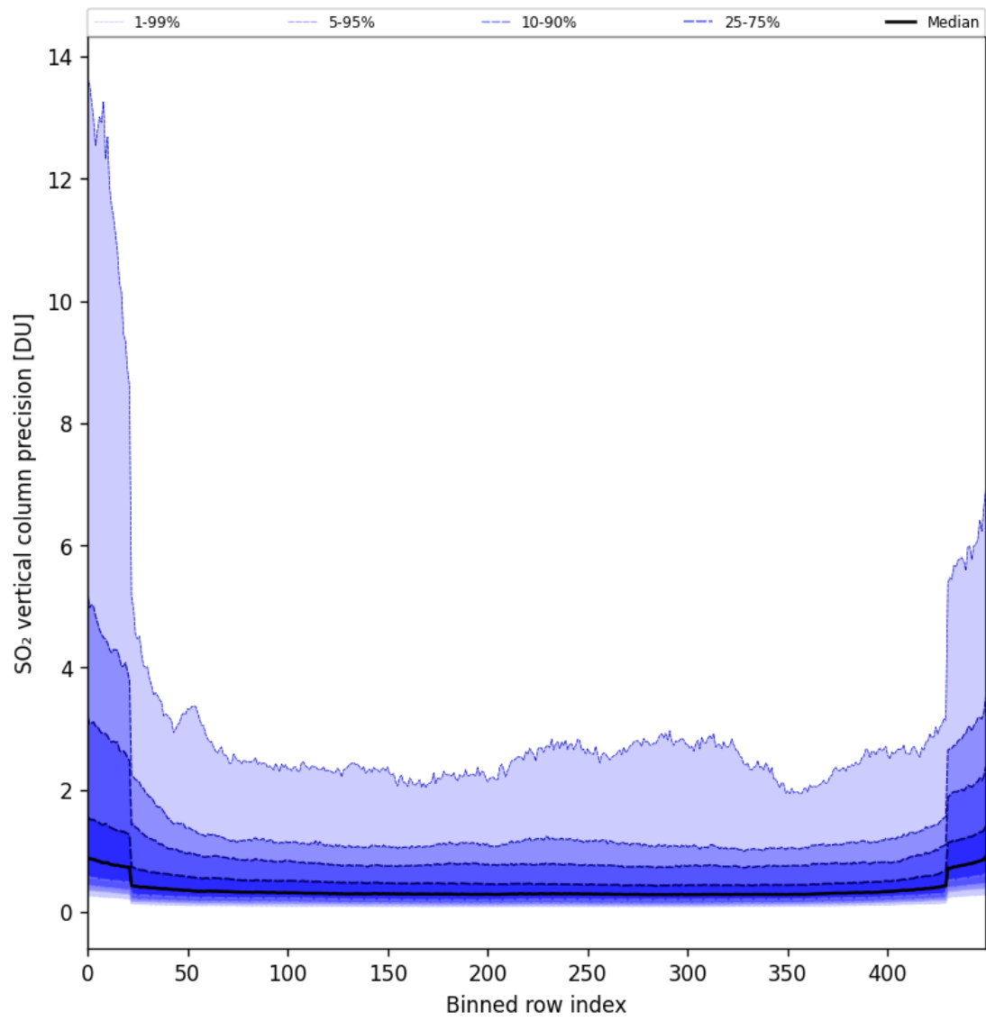
Figure 85: Along track statistics of “SO 2 vertical column precision” for 2025-06-17 to 2025-06-19
