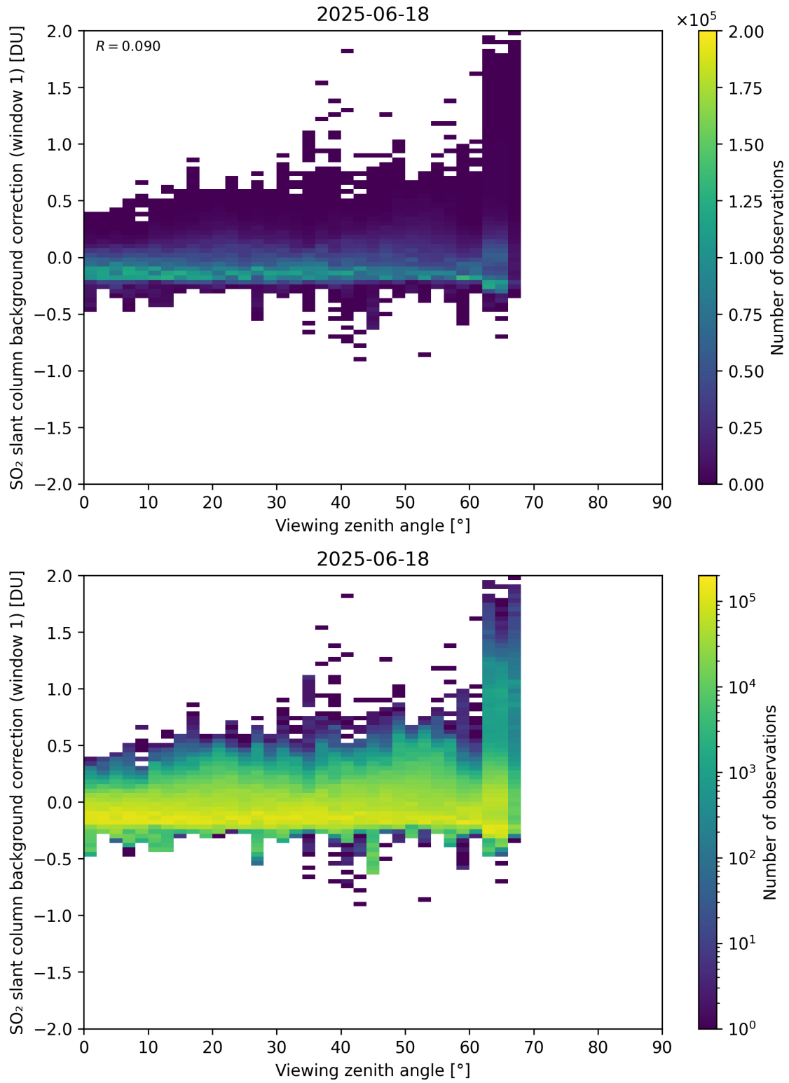
Figure 362: Scatter density plot of “Viewing zenith angle” against “SO 2 slant column background correction (window 1)” for 2025-06-17 to 2025-06-19.
