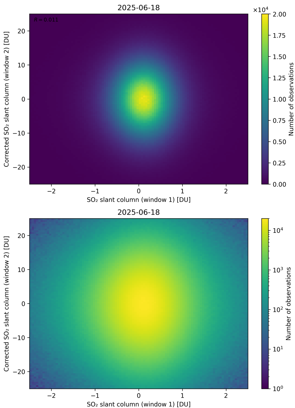
Figure 283: Scatter density plot of “SO 2 slant column (window 1)” against “Corrected SO 2 slant column (window 2)” for 2025-06-17 to 2025-06-19.
