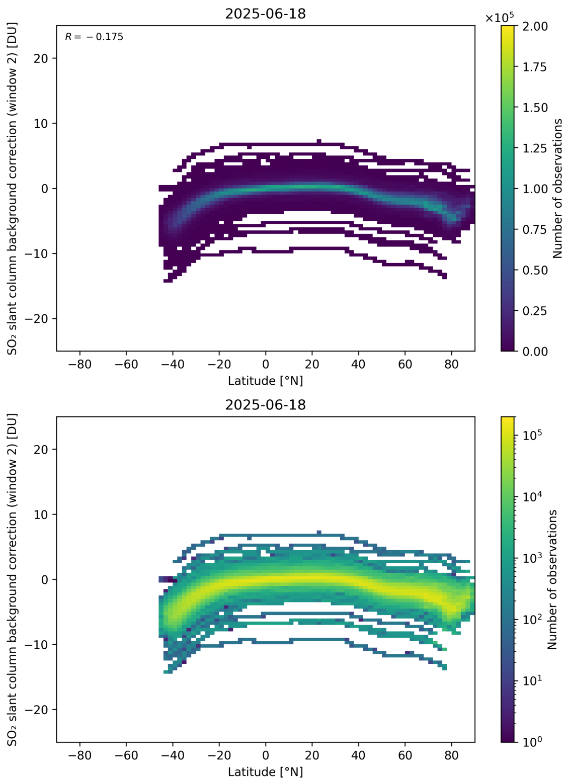
Figure 151: Scatter density plot of “Latitude” against “SO 2 slant column background correction (window 2)” for 2025-06-17 to 2025-06-19.
