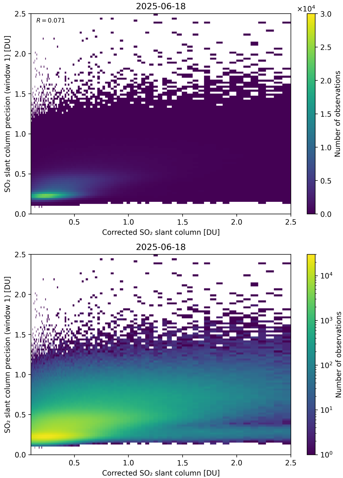
Figure 238: Scatter density plot of “Corrected SO 2 slant column” against “SO 2 slant column precision (window 1)” for 2025-06-17 to 2025-06-19.
