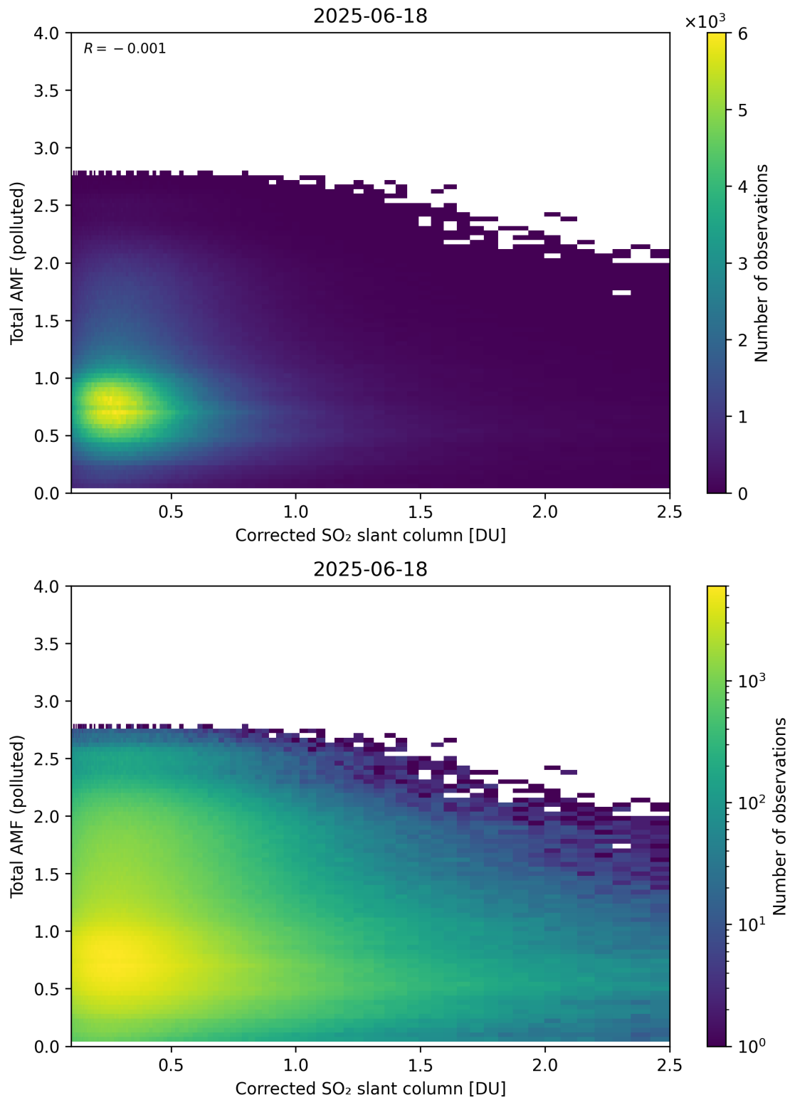
Figure 242: Scatter density plot of “Corrected SO 2 slant column” against “Total AMF (polluted)” for 2025-06-17 to 2025-06-19.
