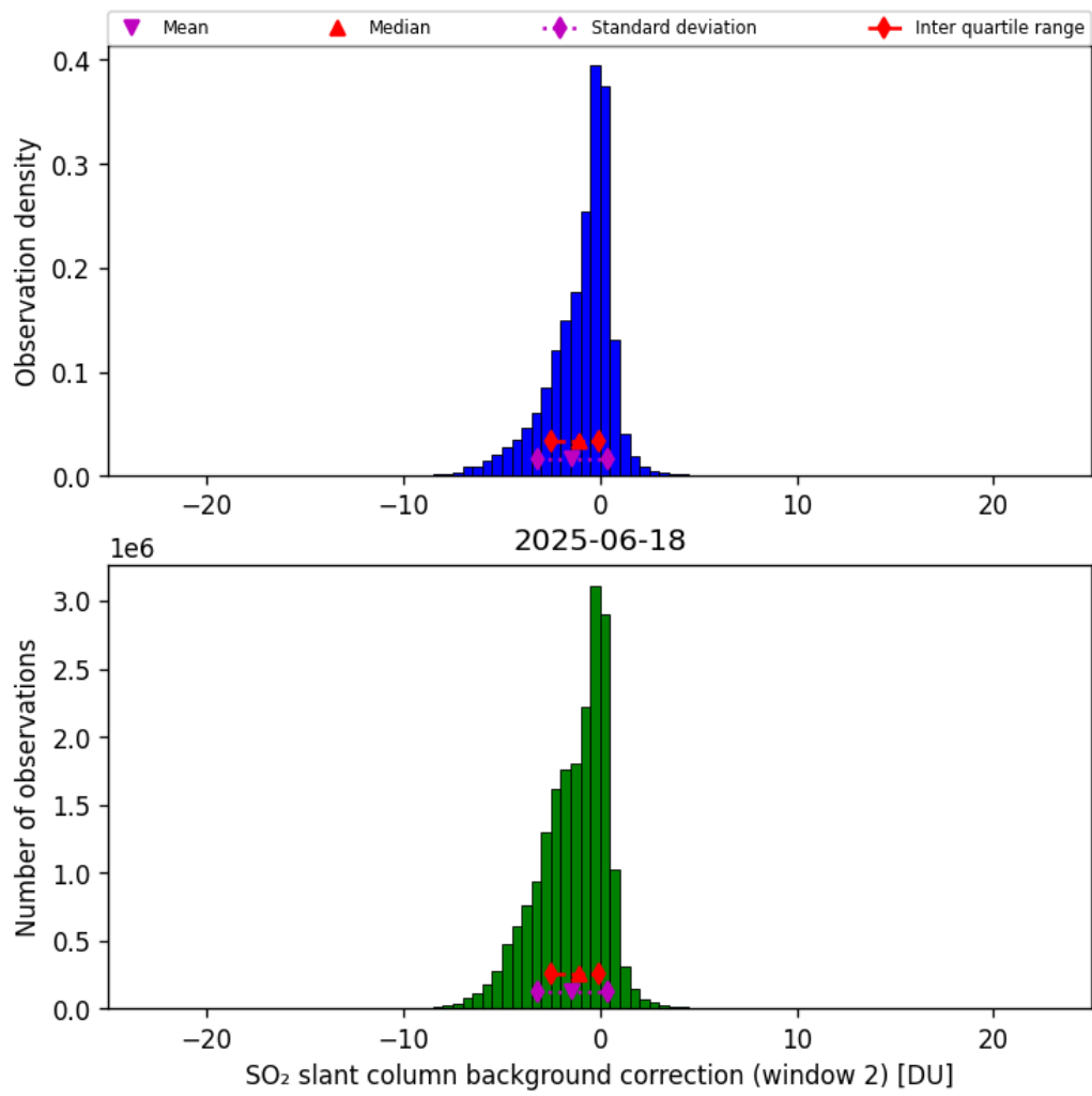
Figure 70: Histogram of “SO 2 slant column background correction (window 2)” for 2025-06-17 to 2025-06-19
