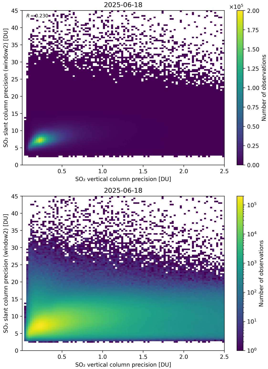
Figure 343: Scatter density plot of “SO 2 vertical column precision” against “SO 2 slant column precision (window2)” for 2025-06-17 to 2025-06-19.
