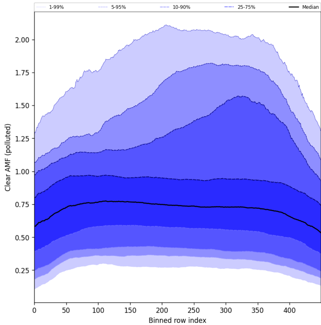
Figure 107: Along track statistics of “Clear AMF (polluted)” for 2025-06-17 to 2025-06-19
