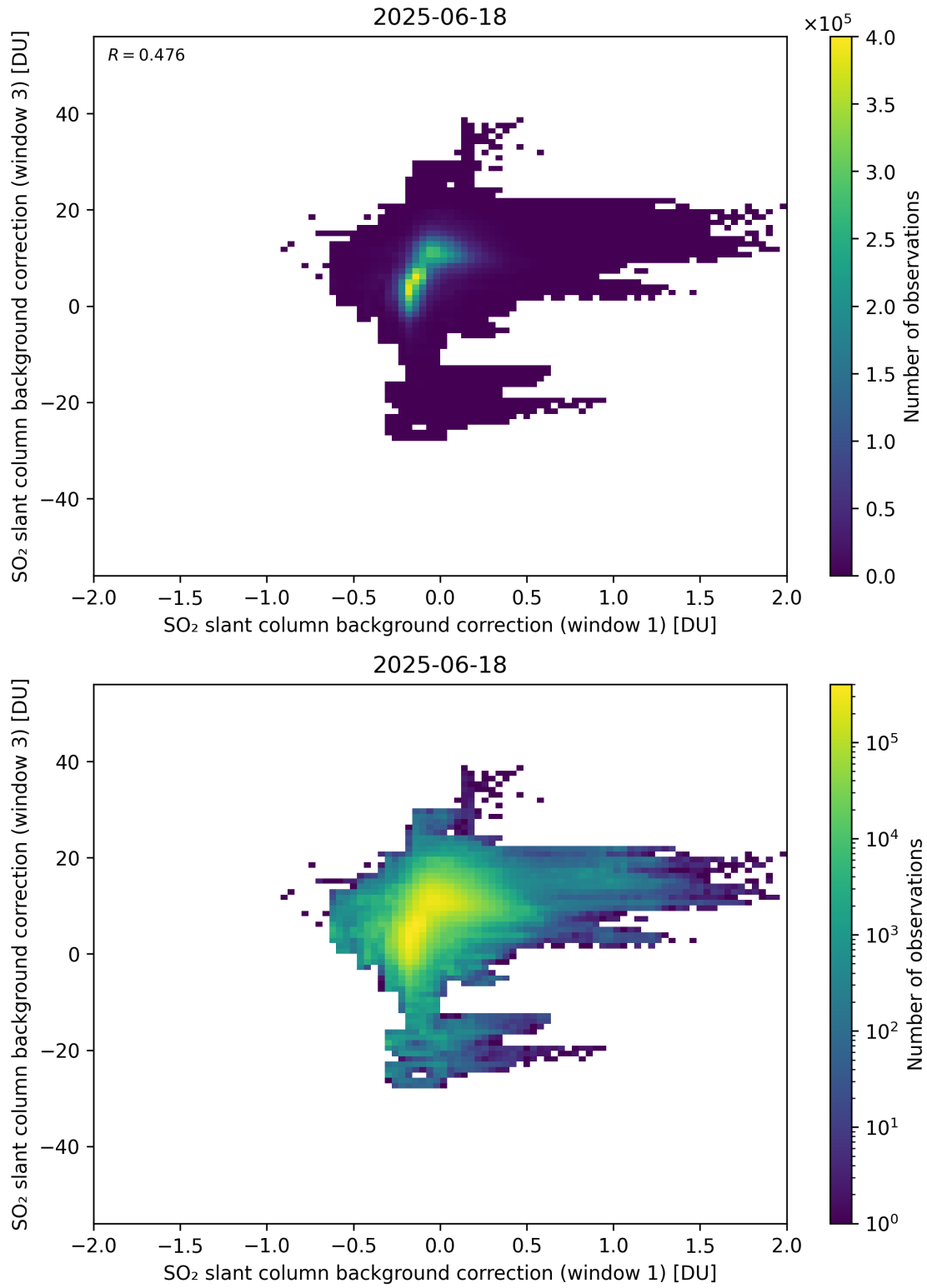
Figure 110: Scatter density plot of “SO 2 slant column background correction (window 1)” against “SO 2 slant column background correction (window 3)” for 2025-06-17 to 2025-06-19.
