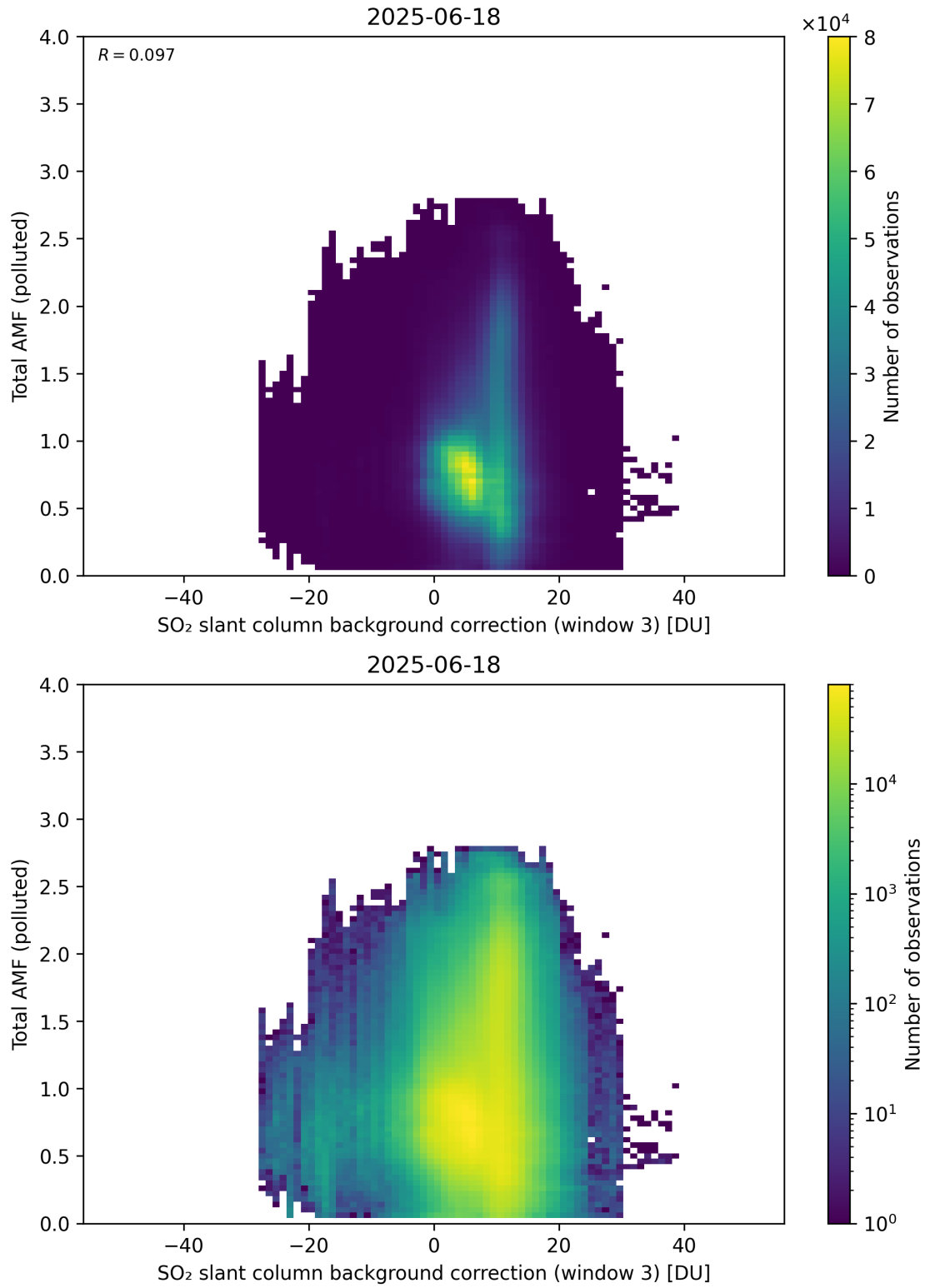
Figure 136: Scatter density plot of “SO 2 slant column background correction (window 3)” against “Total AMF (polluted)” for 2025-06-17 to 2025-06-19.
