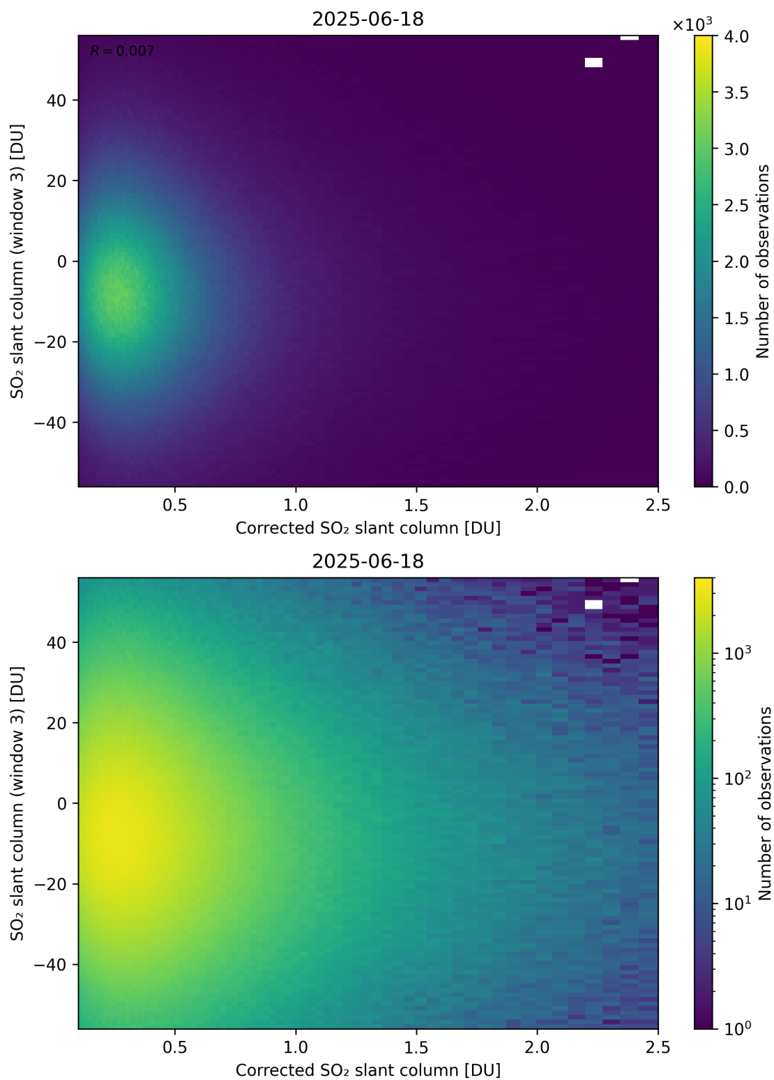
Figure 240: Scatter density plot of “Corrected SO 2 slant column” against “SO 2 slant column (window 3)” for 2025-06-17 to 2025-06-19.
