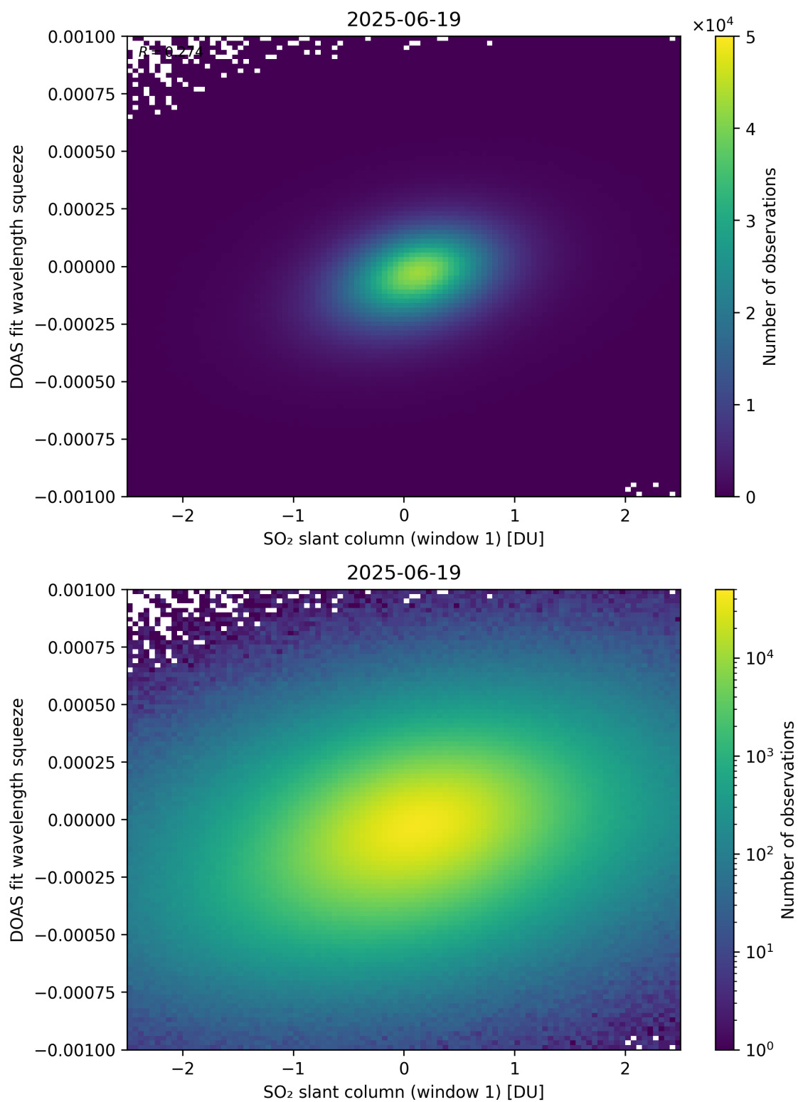
Figure 266: Scatter density plot of “SO 2 slant column (window 1)” against “DOAS fit wavelength squeeze” for 2025-06-18 to 2025-06-20.
