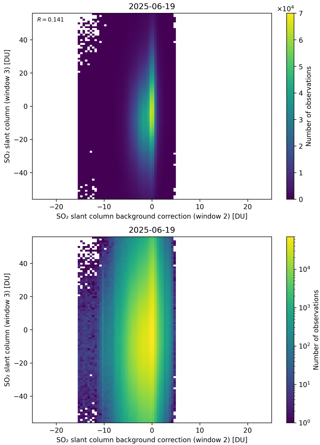
Figure 128: Scatter density plot of “SO 2 slant column background correction (window 2)” against “SO 2 slant column (window 3)” for 2025-06-18 to 2025-06-20.
