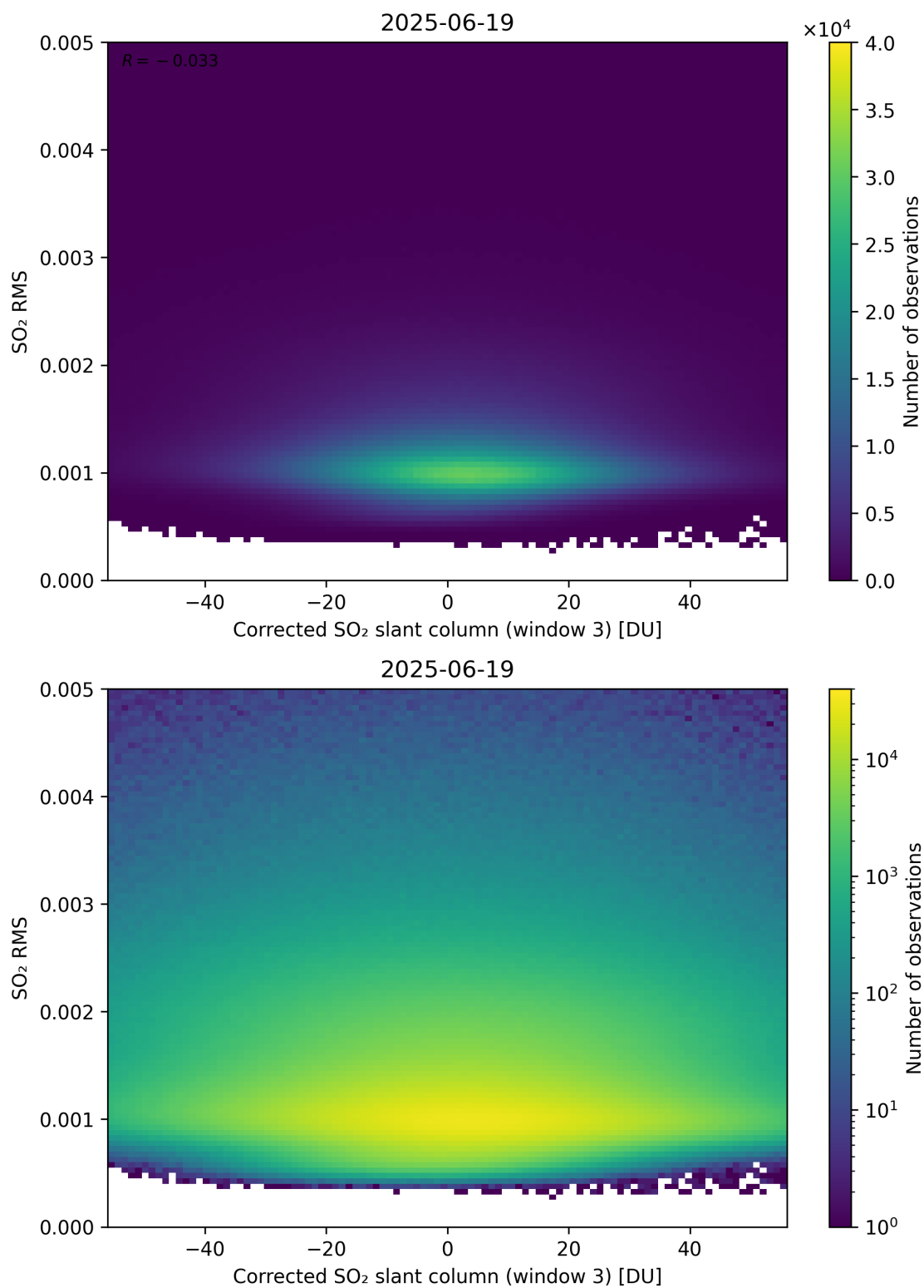
Figure 258: Scatter density plot of “Corrected SO 2 slant column (window 3)” against “SO 2 RMS” for 2025-06-18 to 2025-06-20.
