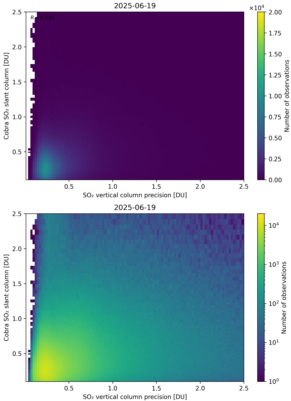
Figure 336: Scatter density plot of “SO 2 vertical column precision” against “Cobra SO 2 slant column” for 2025-06-18 to 2025-06-20.
