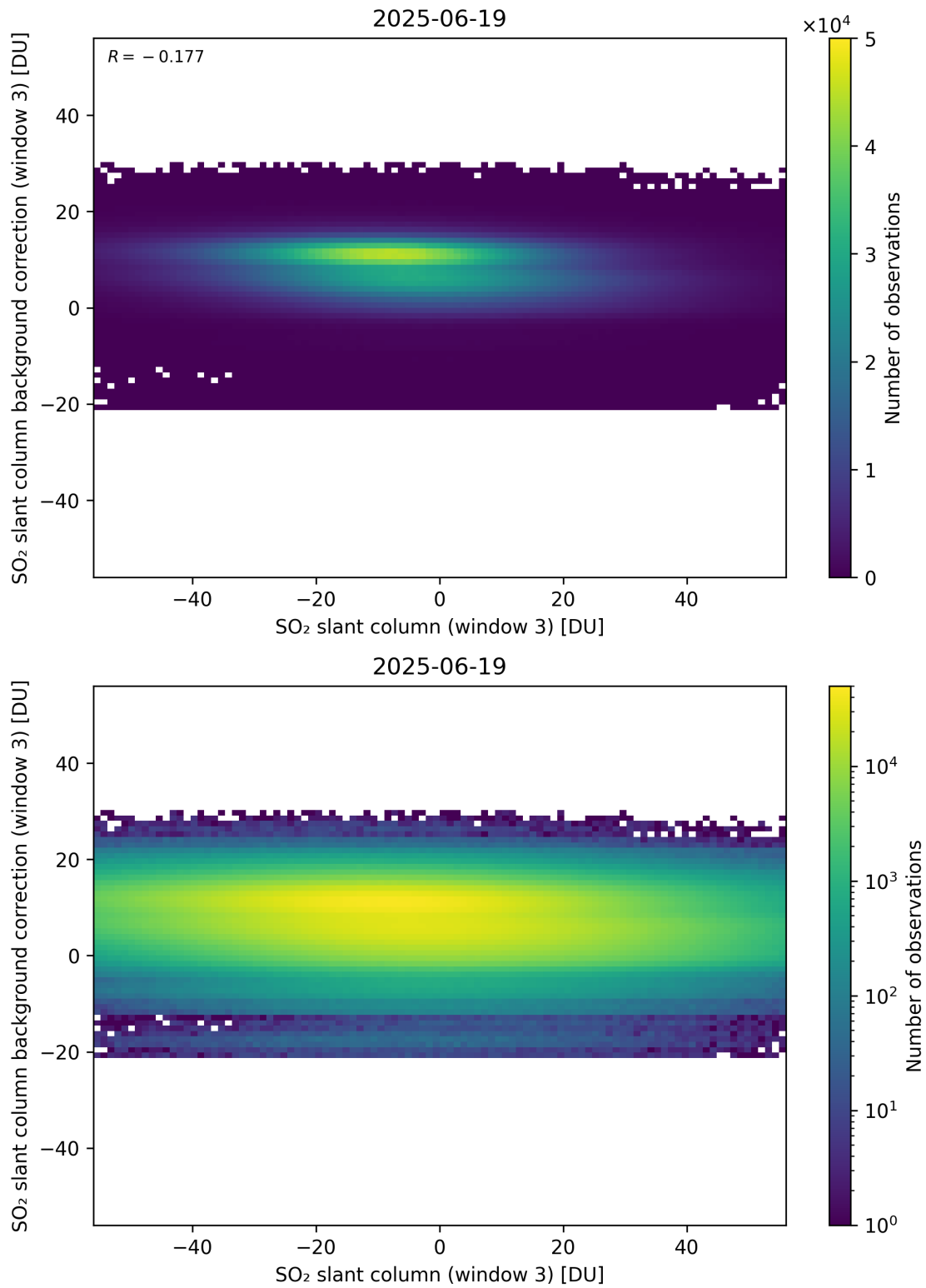
Figure 303: Scatter density plot of “SO 2 slant column (window 3)” against “SO 2 slant column background correction (window 3)” for 2025-06-18 to 2025-06-20.
