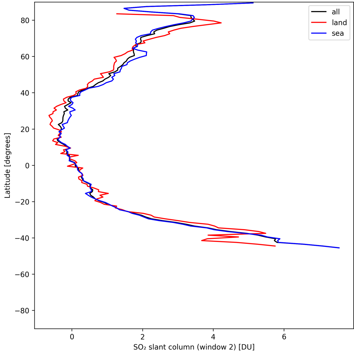
Figure 41: Zonal average of “SO 2 slant column (window 2)” for 2025-06-18 to 2025-06-20.
