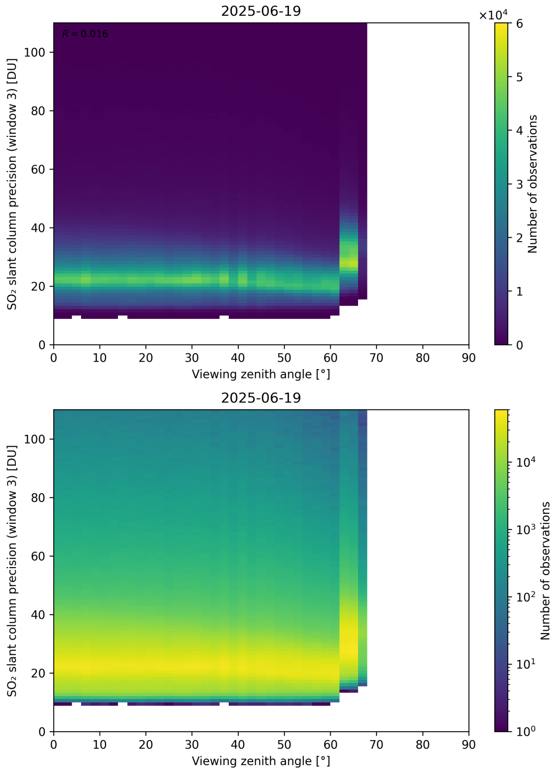
Figure 380: Scatter density plot of “Viewing zenith angle” against “SO 2 slant column precision (window 3)” for 2025-06-18 to 2025-06-20.
