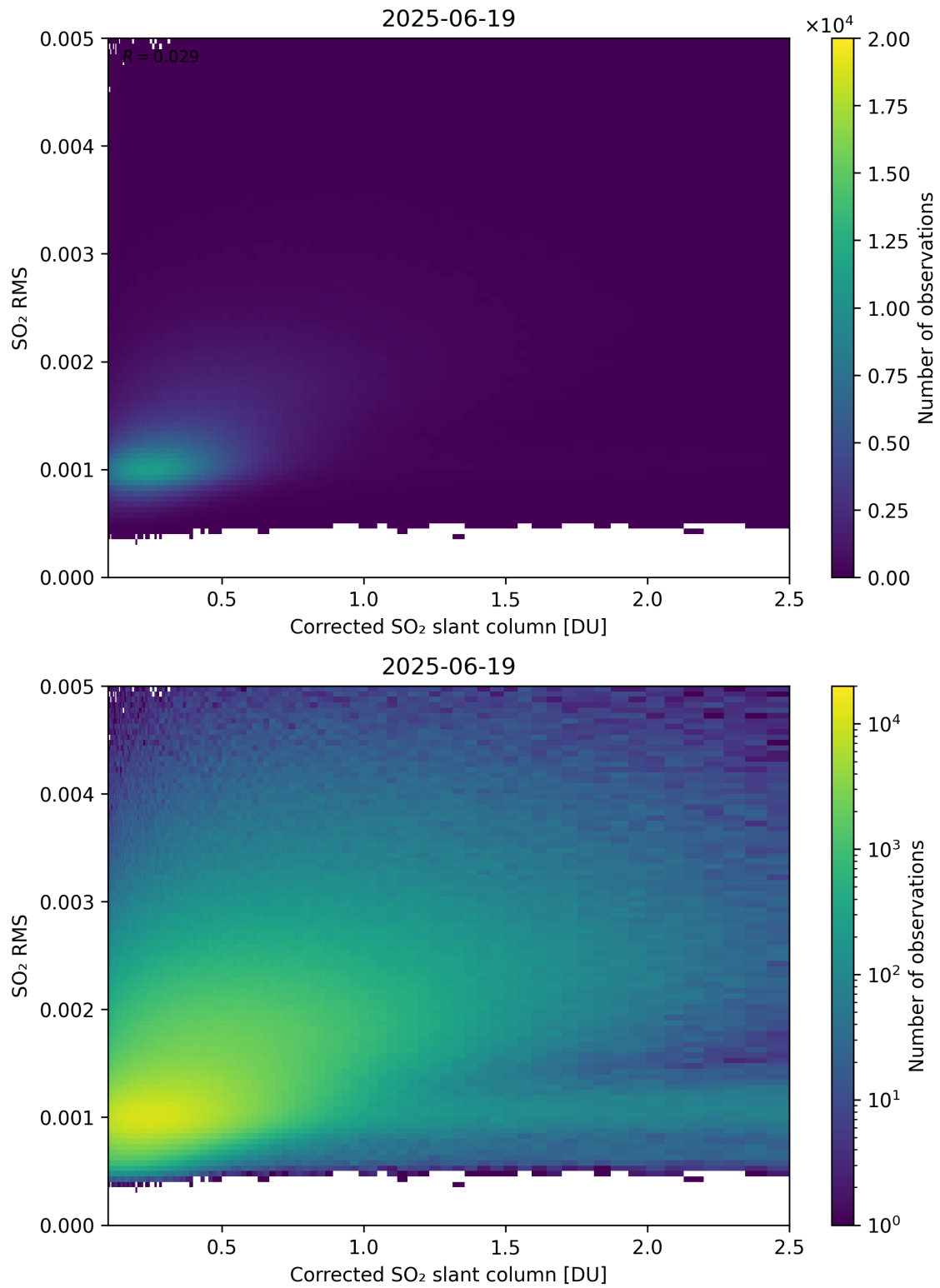
Figure 231: Scatter density plot of “Corrected SO 2 slant column” against “SO 2 RMS” for 2025-06-18 to 2025-06-20.
