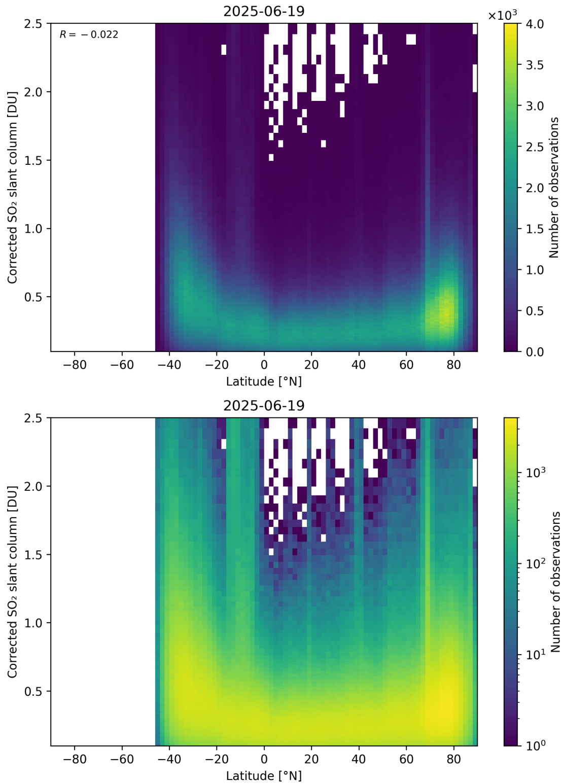
Figure 159: Scatter density plot of “Latitude” against “Corrected SO 2 slant column” for 2025-06-18 to 2025-06-20.
