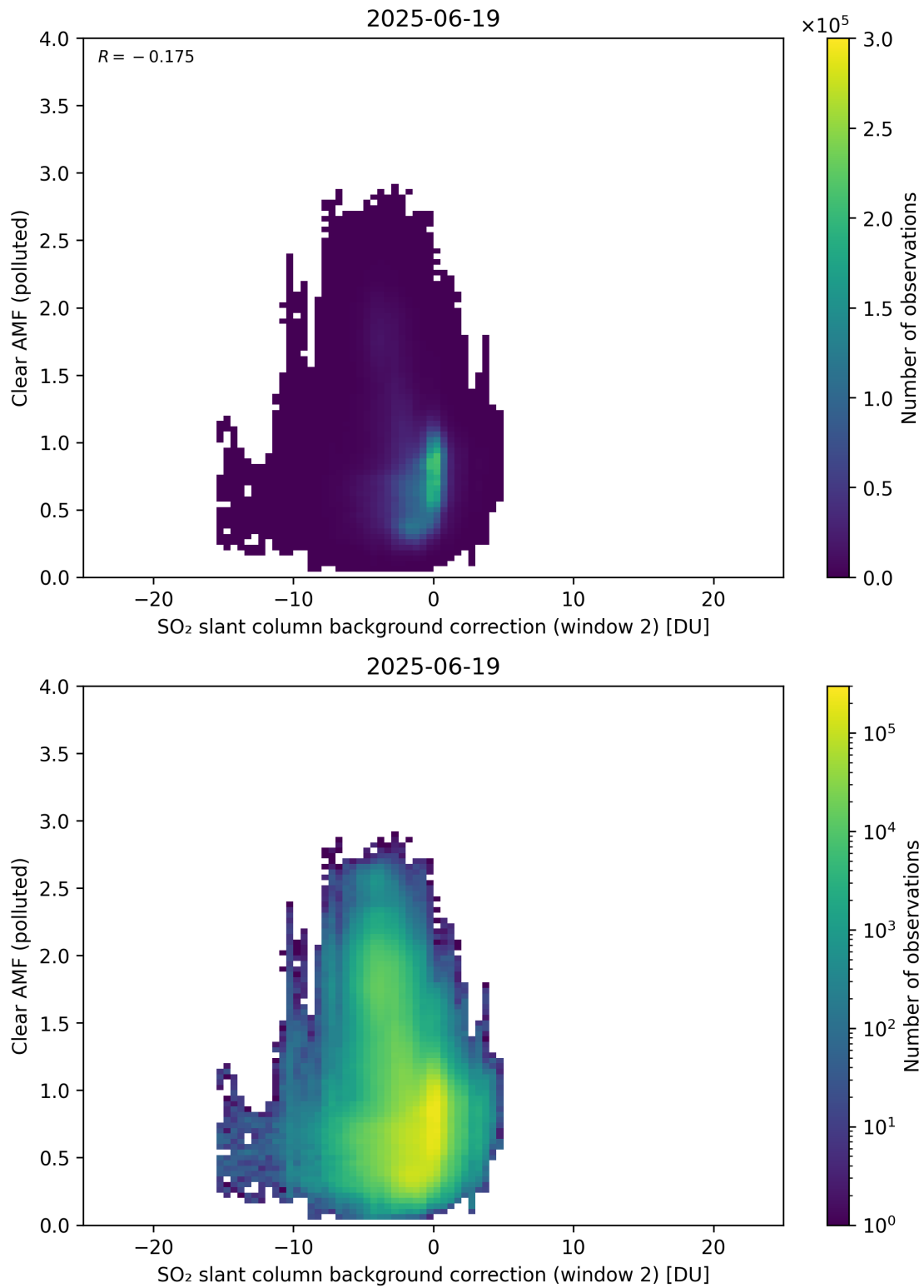
Figure 126: Scatter density plot of “SO 2 slant column background correction (window 2)” against “Clear AMF (polluted)” for 2025-06-18 to 2025-06-20.
