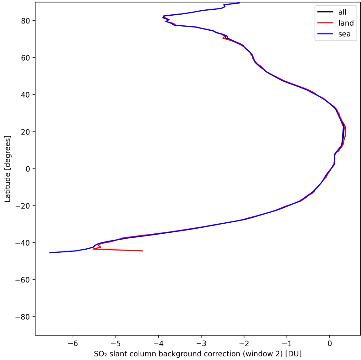
Figure 44: Zonal average of “SO 2 slant column background correction (window 2)” for 2025-06-18 to 2025-06-20.
