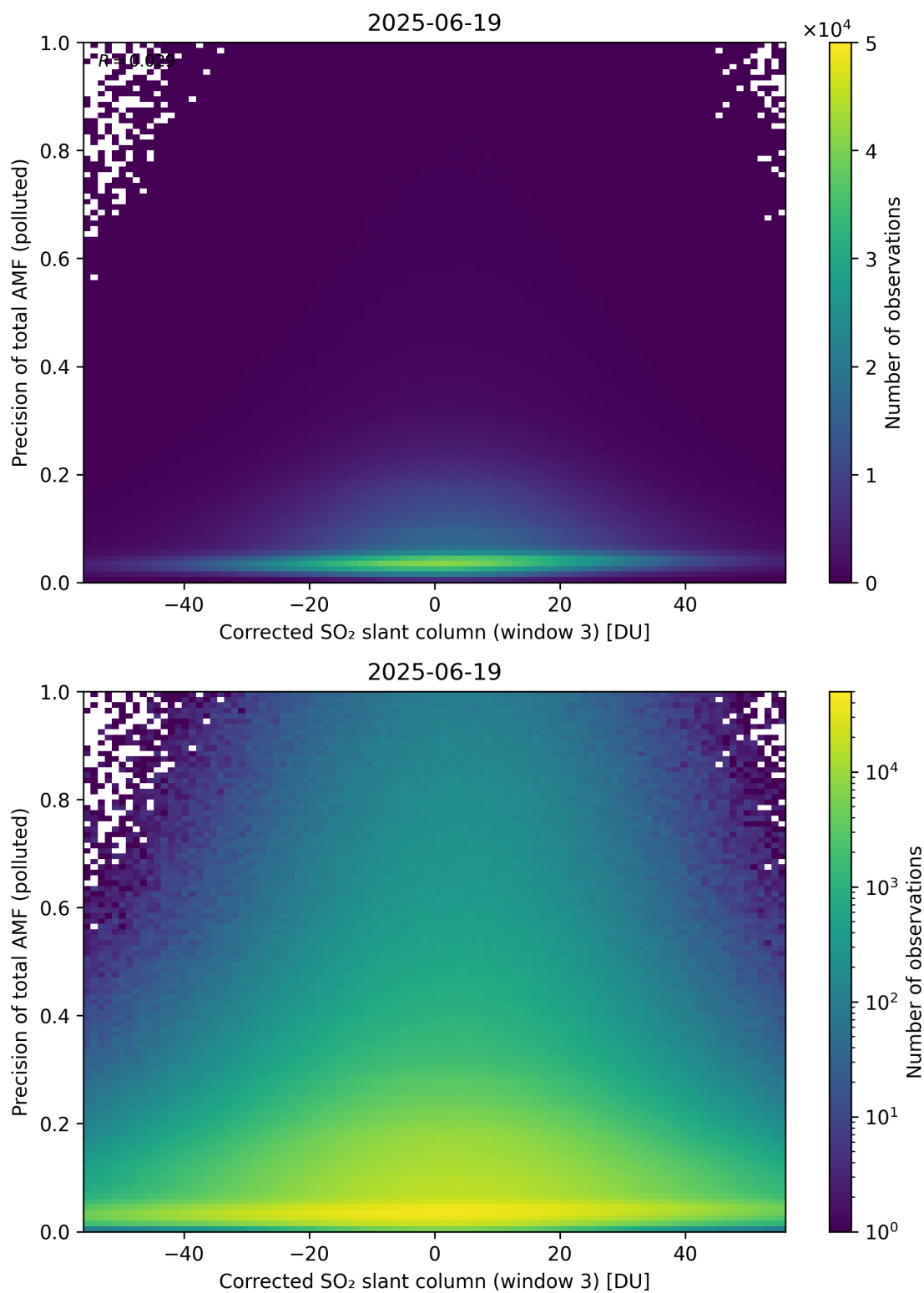
Figure 261: Scatter density plot of “Corrected SO 2 slant column (window 3)” against “Precision of total AMF (polluted)” for 2025-06-18 to 2025-06-20.
