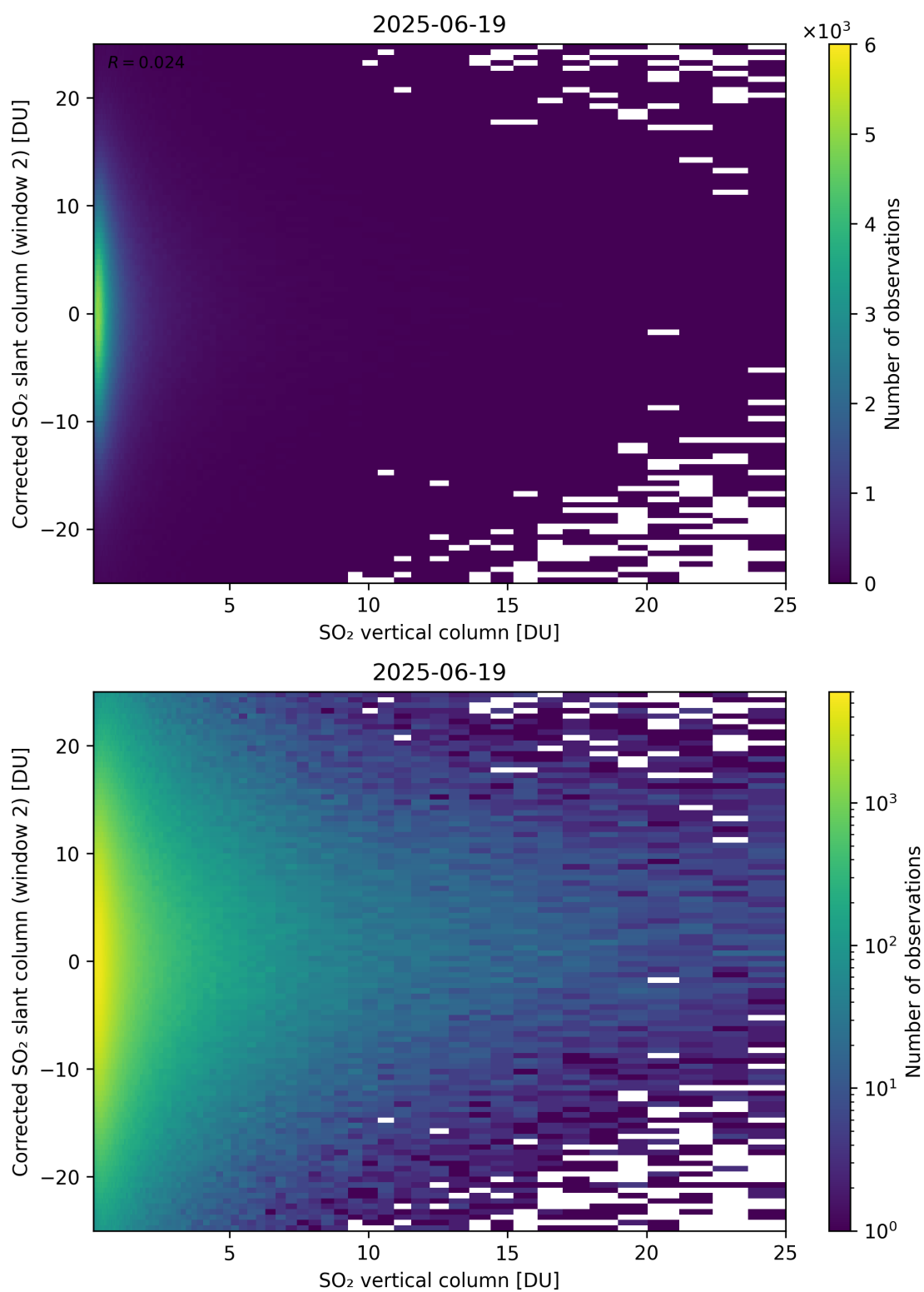
Figure 352: Scatter density plot of “SO 2 vertical column” against “Corrected SO 2 slant column (window 2)” for 2025-06-18 to 2025-06-20.
