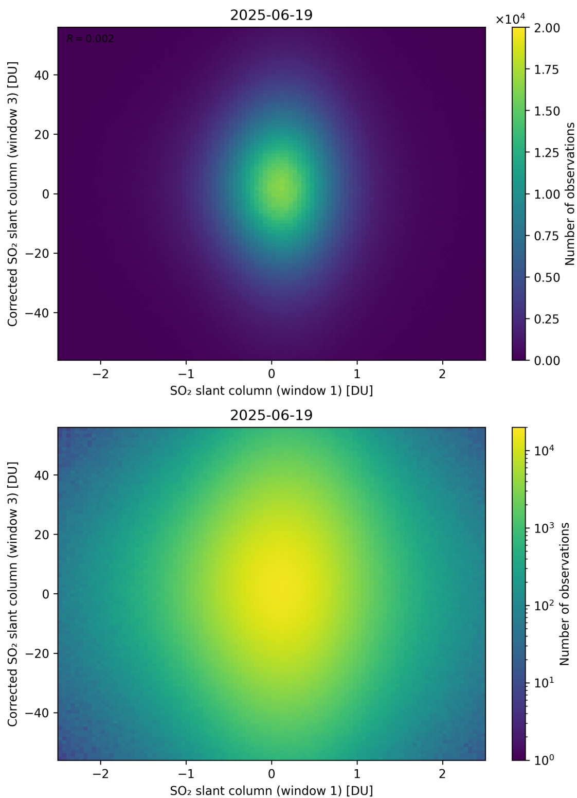
Figure 284: Scatter density plot of “SO 2 slant column (window 1)” against “Corrected SO 2 slant column (window 3)” for 2025-06-18 to 2025-06-20.
