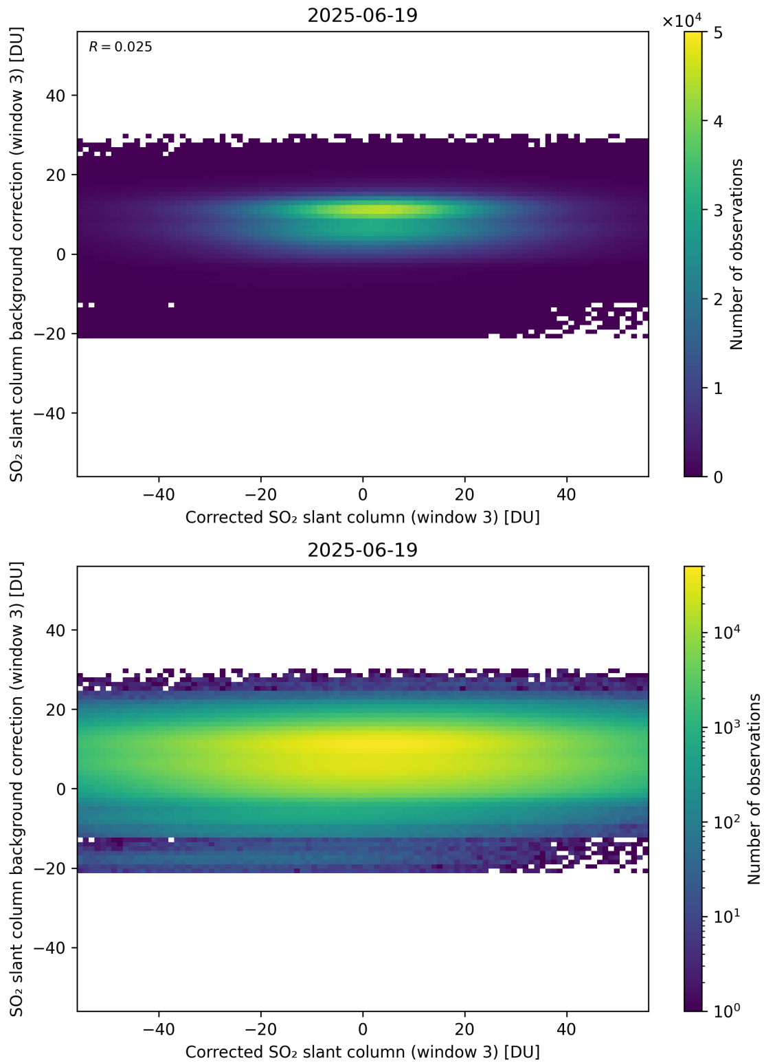
Figure 255: Scatter density plot of “Corrected SO 2 slant column (window 3)” against “SO 2 slant column background correction (window 3)” for 2025-06-18 to 2025-06-20.
