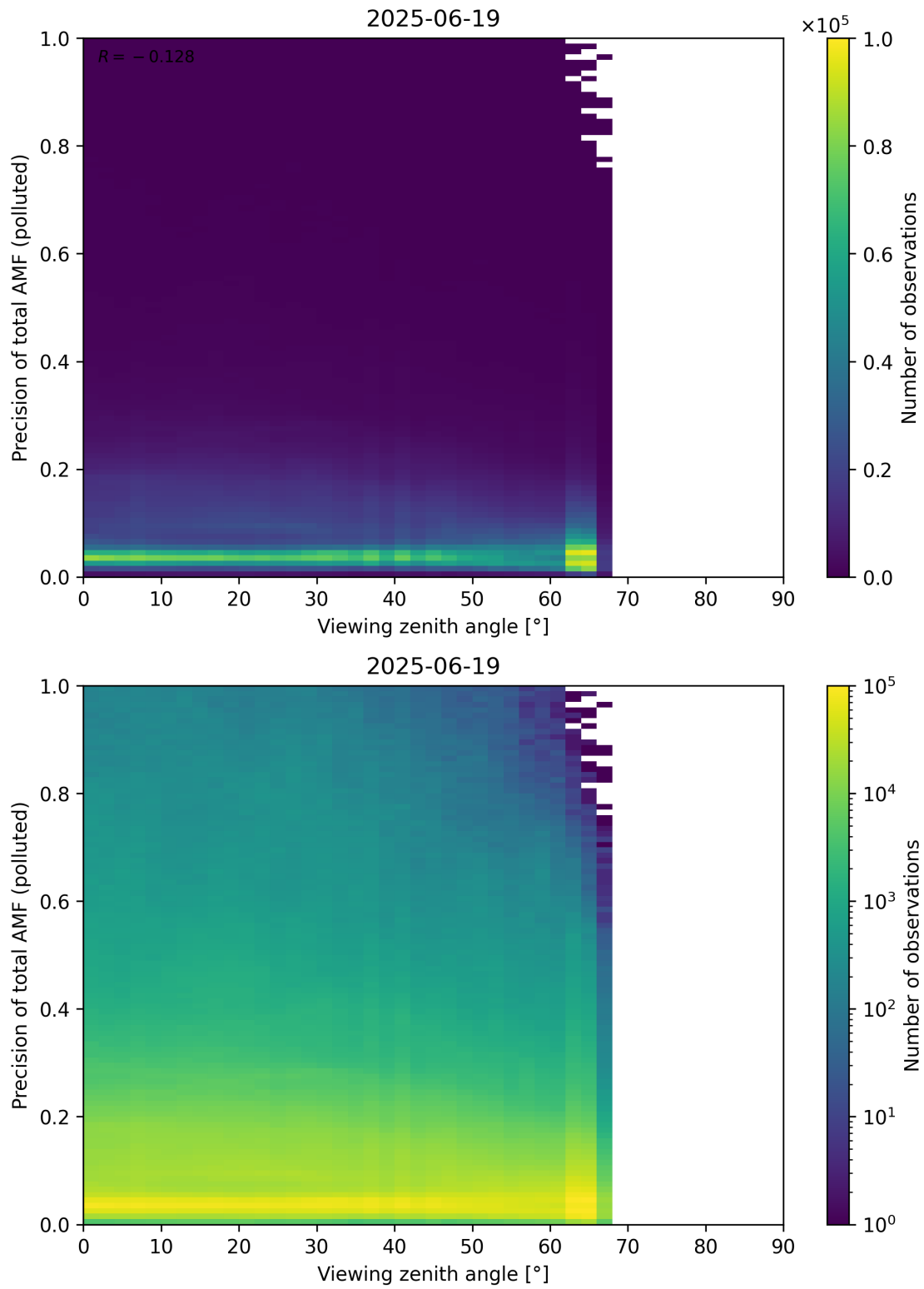
Figure 382: Scatter density plot of “Viewing zenith angle” against “Precision of total AMF (polluted)” for 2025-06-18 to 2025-06-20.
