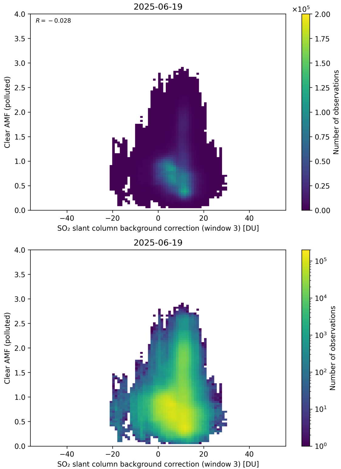
Figure 135: Scatter density plot of “SO 2 slant column background correction (window 3)” against “Clear AMF (polluted)” for 2025-06-18 to 2025-06-20.
