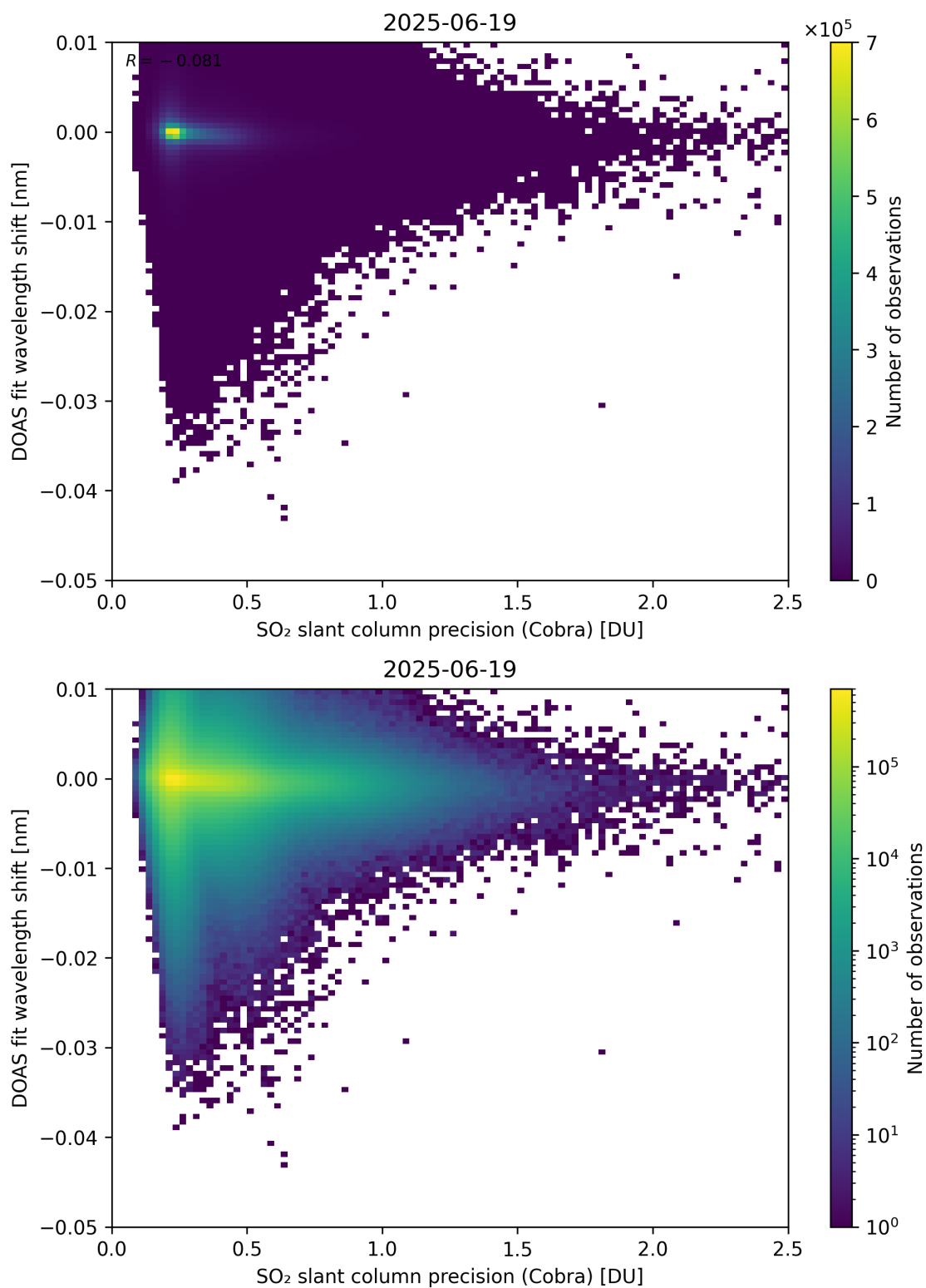
Figure 202: Scatter density plot of “SO 2 slant column precision (Cobra)” against “DOAS fit wavelength shift” for 2025-06-18 to 2025-06-20.
