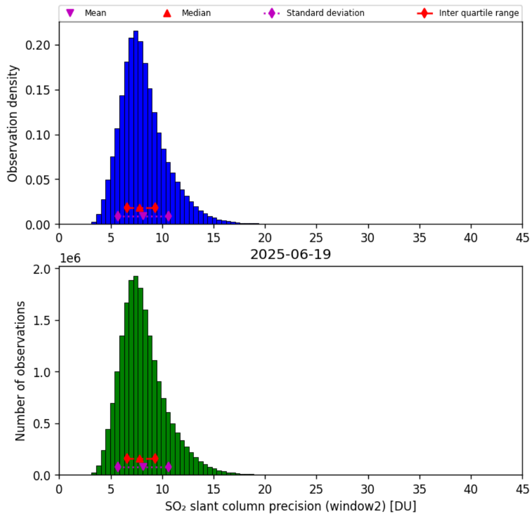
Figure 68: Histogram of “SO 2 slant column precision (window2)” for 2025-06-18 to 2025-06-20
