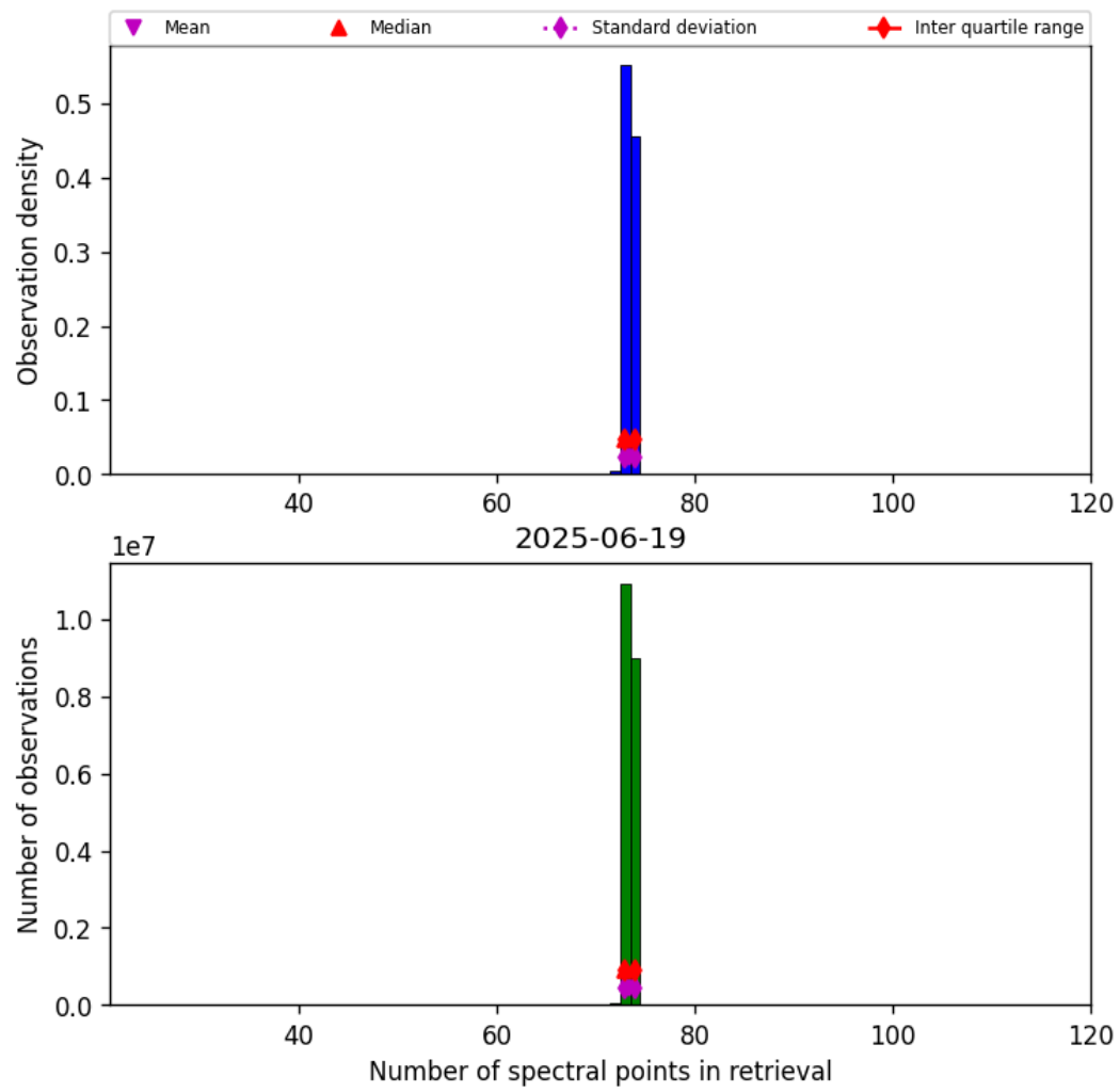
Figure 82: Histogram of “Number of spectral points in retrieval” for 2025-06-18 to 2025-06-20
