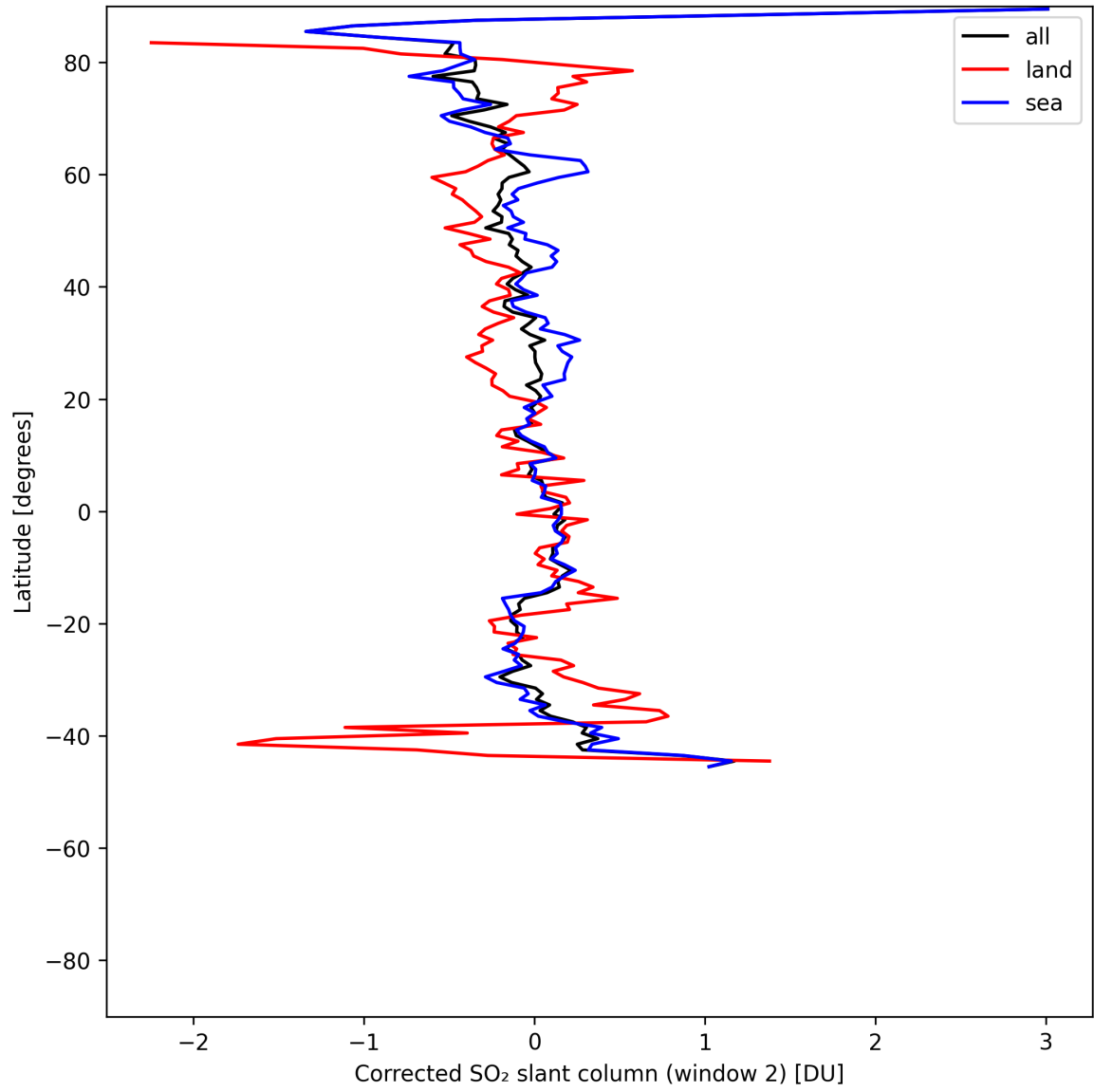
Figure 43: Zonal average of “Corrected SO 2 slant column (window 2)” for 2025-06-18 to 2025-06-20.
