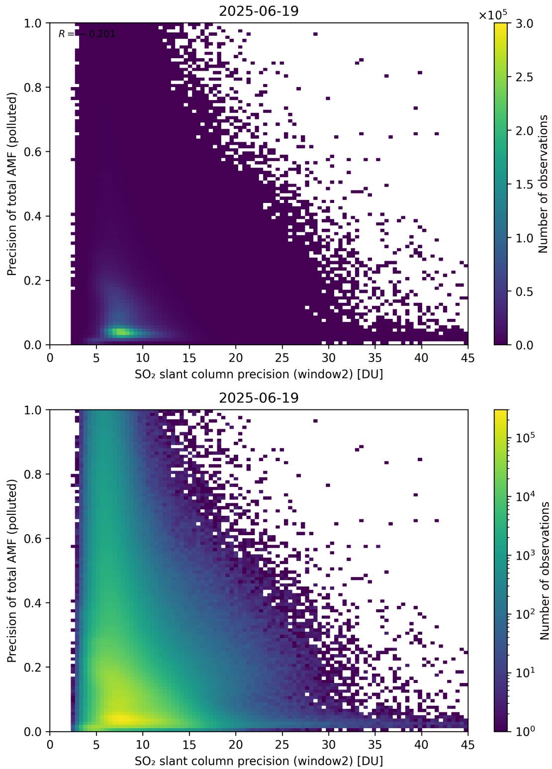
Figure 302: Scatter density plot of “SO 2 slant column precision (window2)” against “Precision of total AMF (polluted)” for 2025-06-18 to 2025-06-20.
