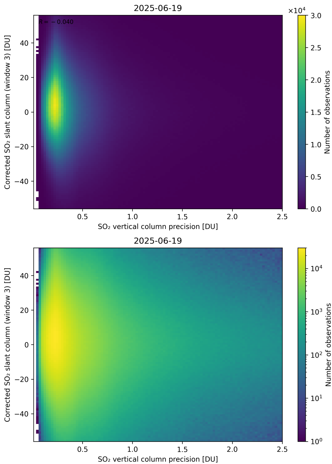
Figure 340: Scatter density plot of “SO 2 vertical column precision” against “Corrected SO 2 slant column (window 3)” for 2025-06-18 to 2025-06-20.
