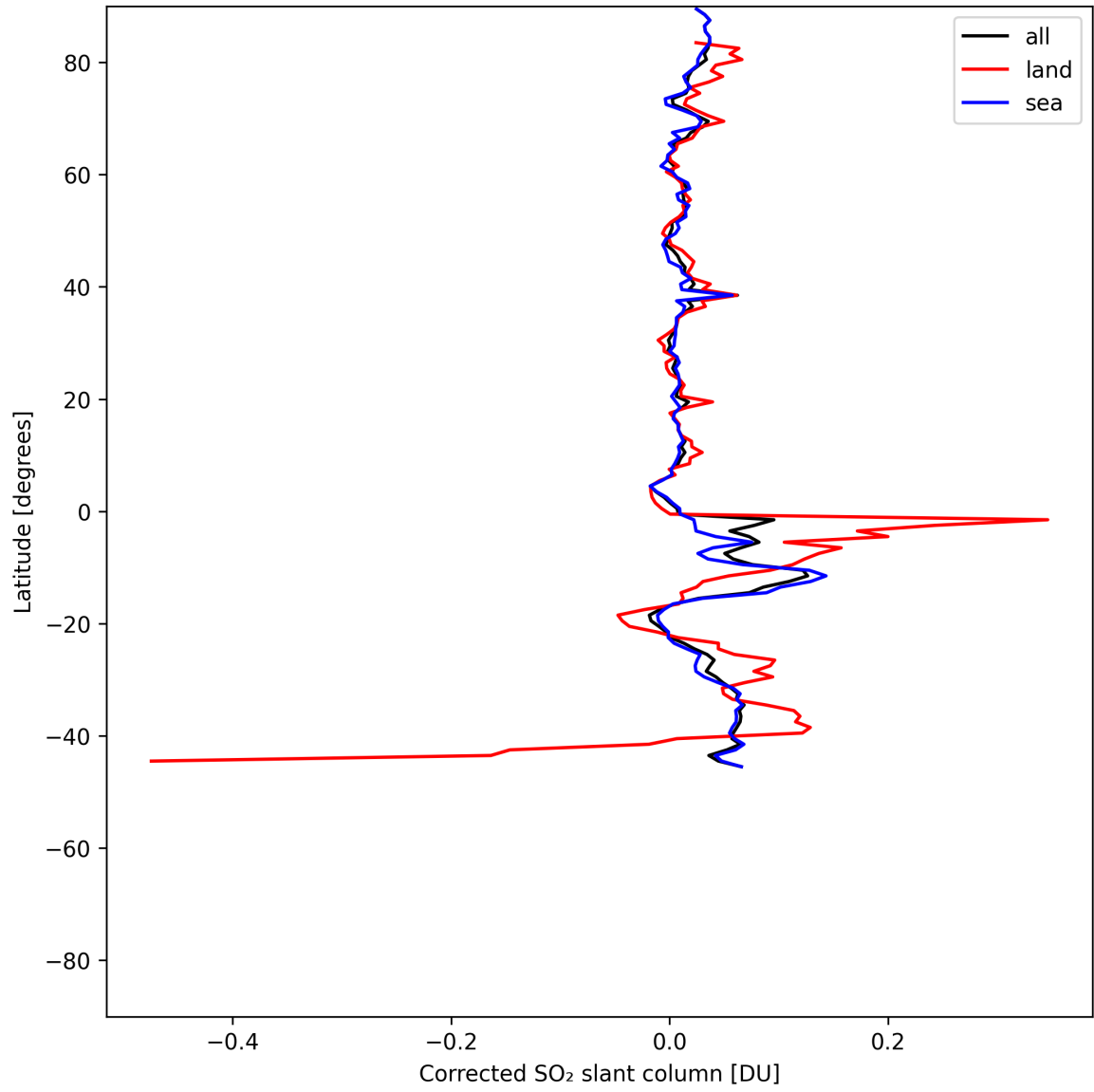
Figure 34: Zonal average of “Corrected SO 2 slant column” for 2025-06-18 to 2025-06-20.
