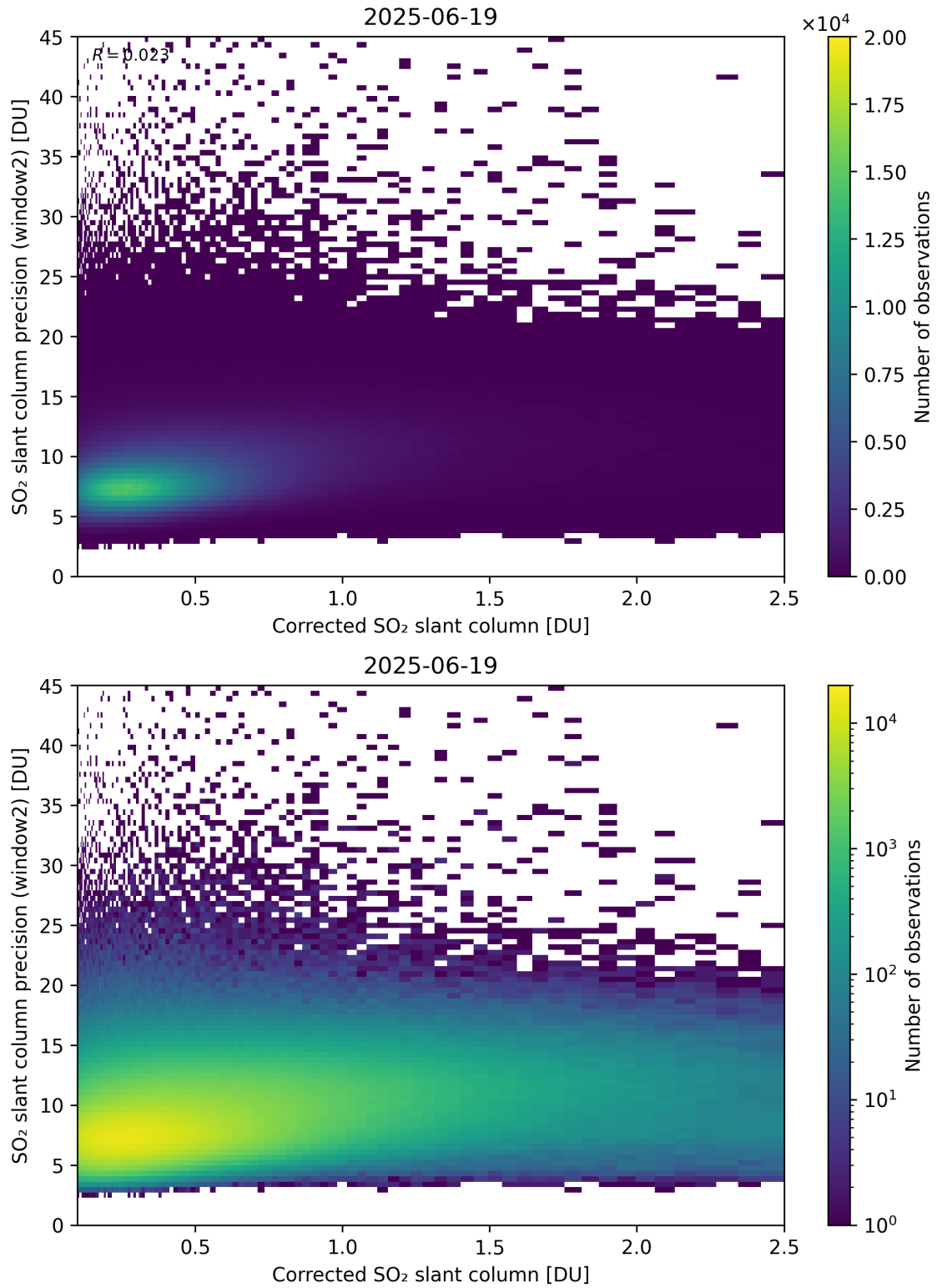
Figure 239: Scatter density plot of “Corrected SO 2 slant column” against “SO 2 slant column precision (window2)” for 2025-06-18 to 2025-06-20.
