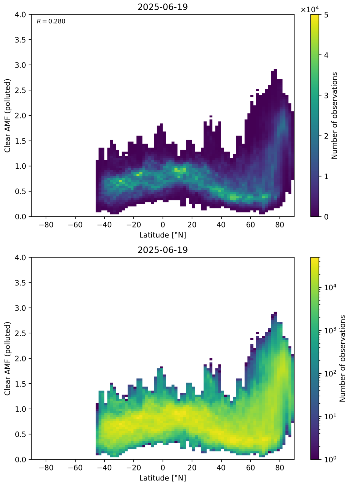
Figure 156: Scatter density plot of “Latitude” against “Clear AMF (polluted)” for 2025-06-18 to 2025-06-20.
