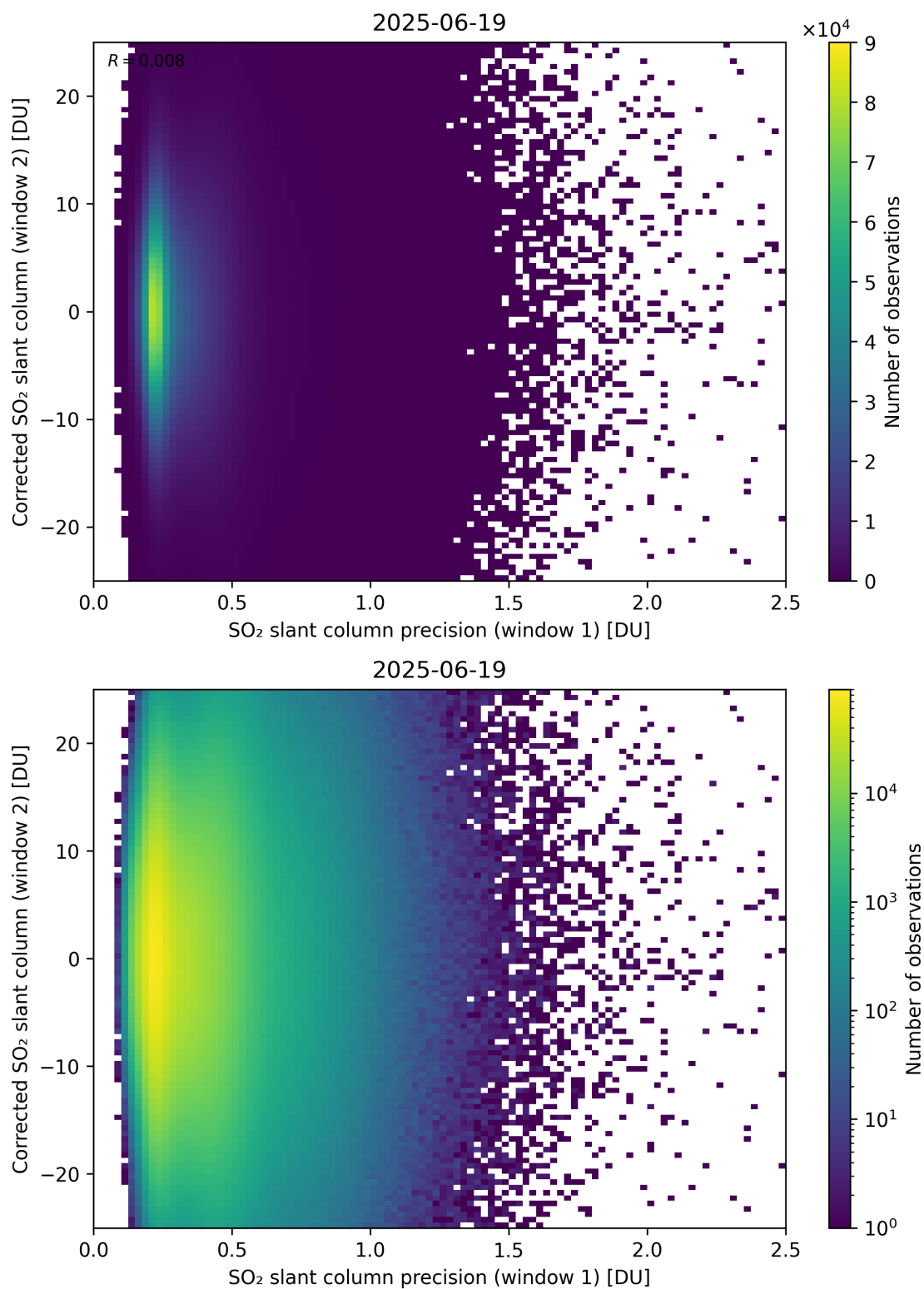
Figure 275: Scatter density plot of “SO 2 slant column precision (window 1)” against “Corrected SO 2 slant column (window 2)” for 2025-06-18 to 2025-06-20.
