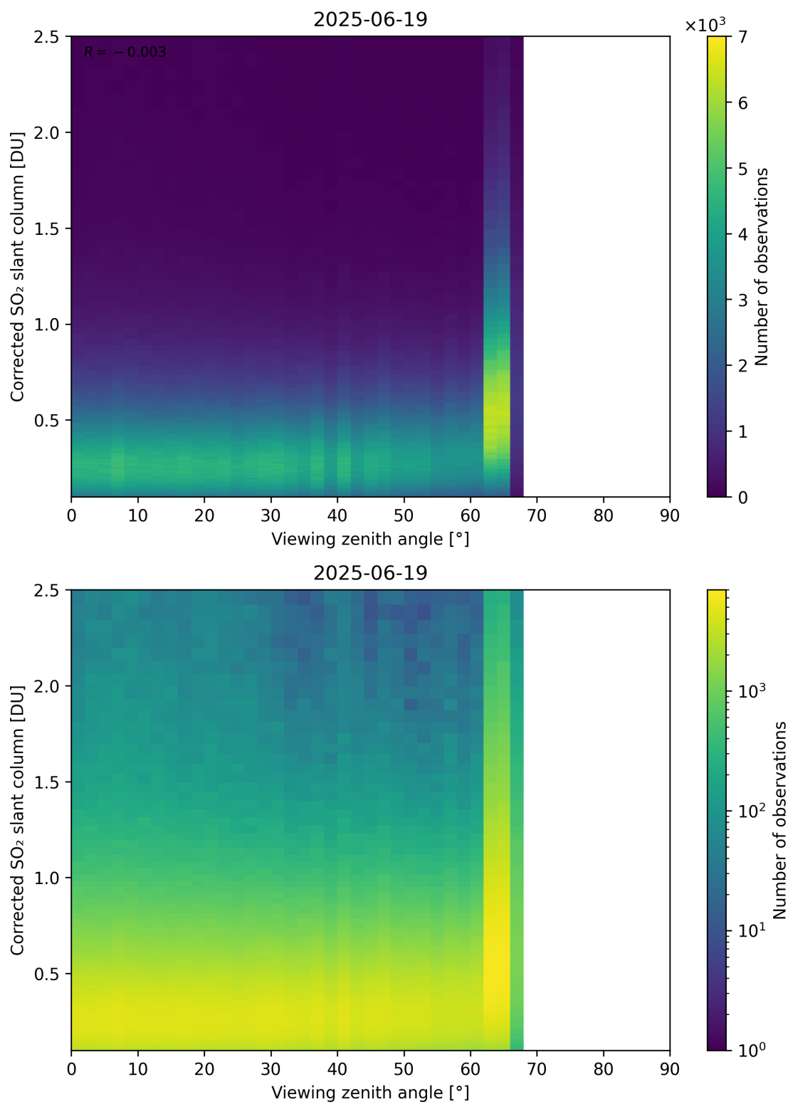
Figure 373: Scatter density plot of “Viewing zenith angle” against “Corrected SO 2 slant column” for 2025-06-18 to 2025-06-20.
