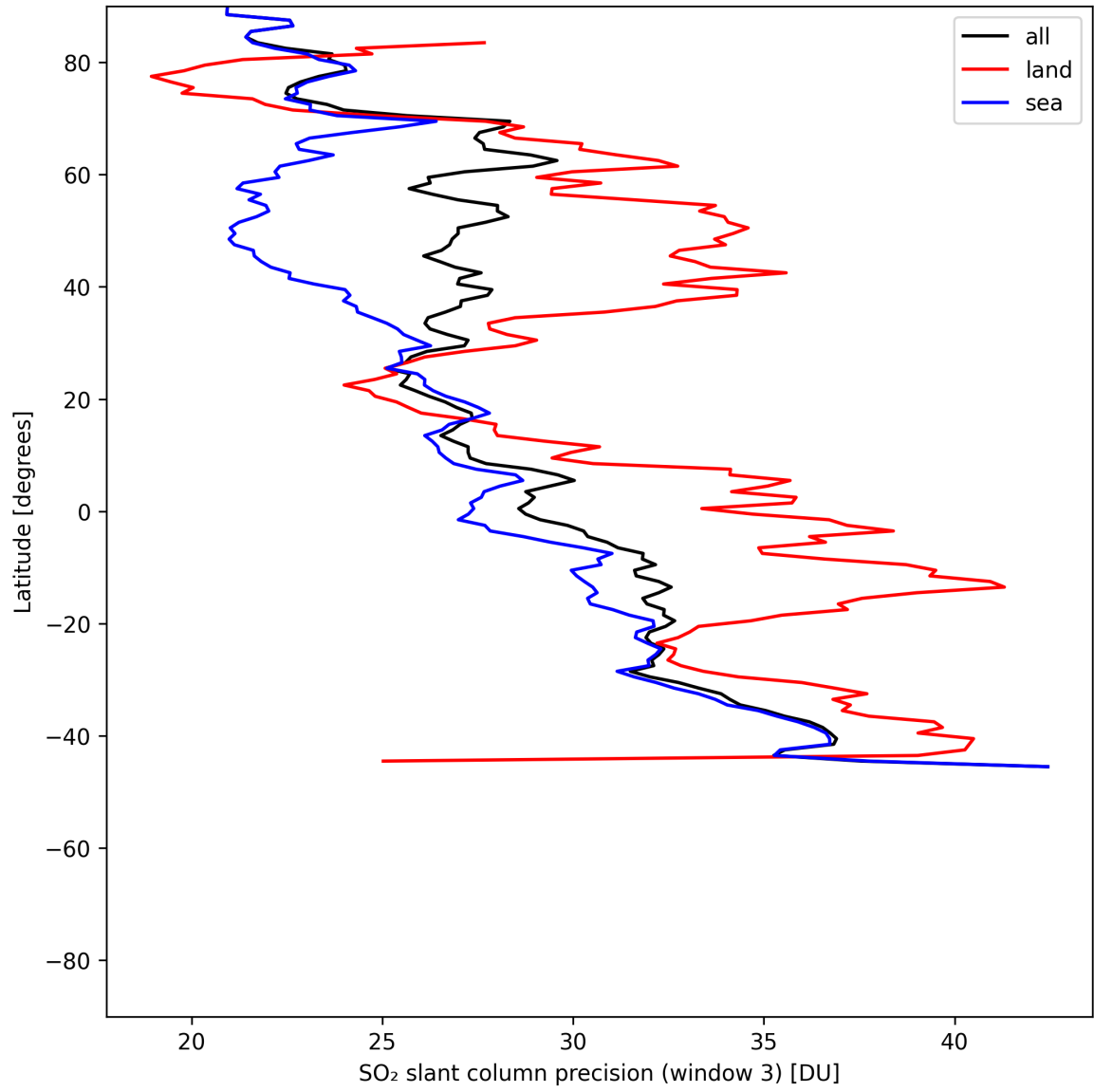
Figure 46: Zonal average of “SO 2 slant column precision (window 3)” for 2025-06-18 to 2025-06-20.
