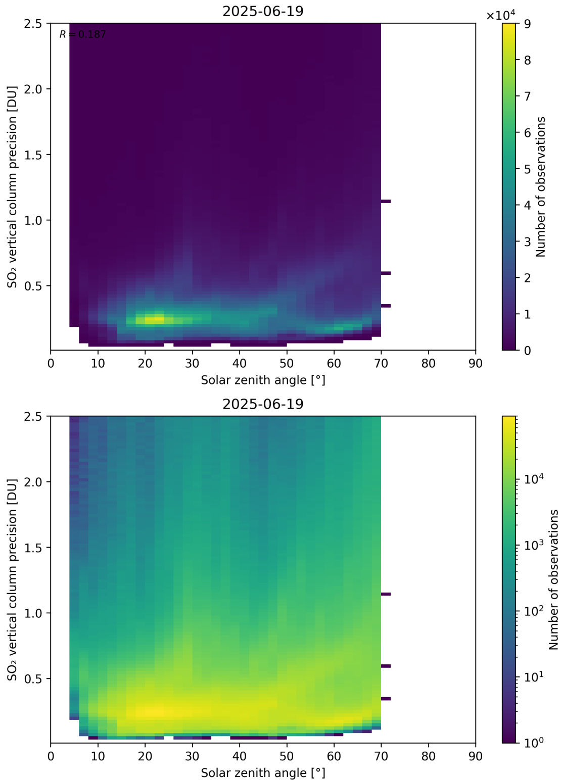
Figure 192: Scatter density plot of “Solar zenith angle” against “SO 2 vertical column precision” for 2025-06-18 to 2025-06-20.
