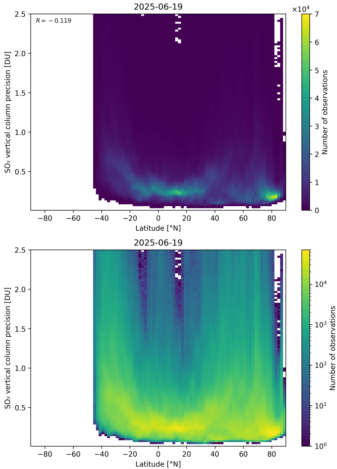
Figure 170: Scatter density plot of “Latitude” against “SO 2 vertical column precision” for 2025-06-18 to 2025-06-20.
