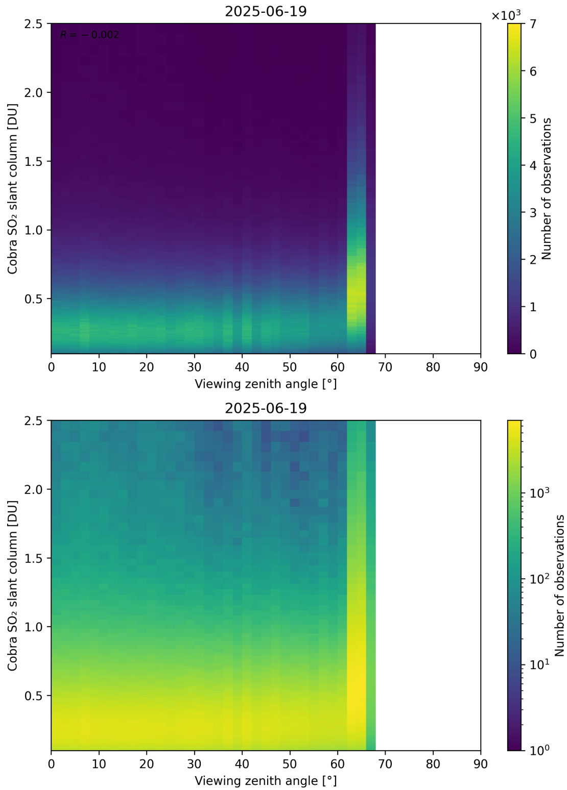
Figure 371: Scatter density plot of “Viewing zenith angle” against “Cobra SO 2 slant column” for 2025-06-18 to 2025-06-20.
