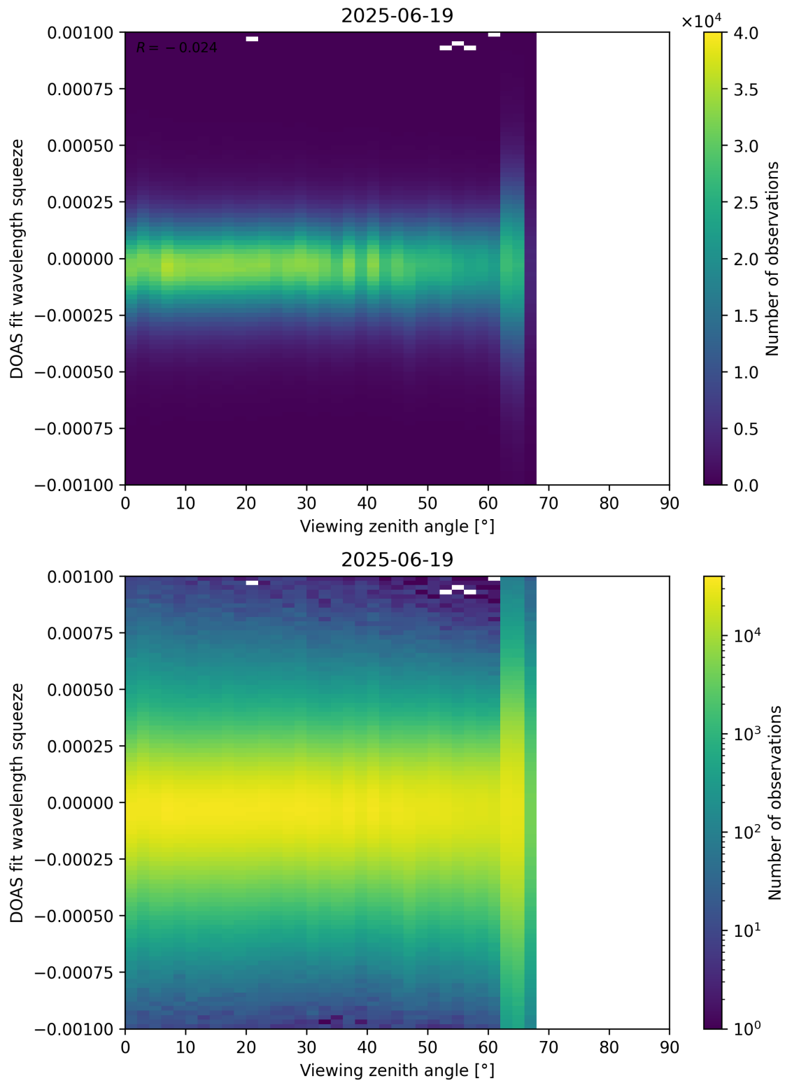
Figure 366: Scatter density plot of “Viewing zenith angle” against “DOAS fit wavelength squeeze” for 2025-06-18 to 2025-06-20.
