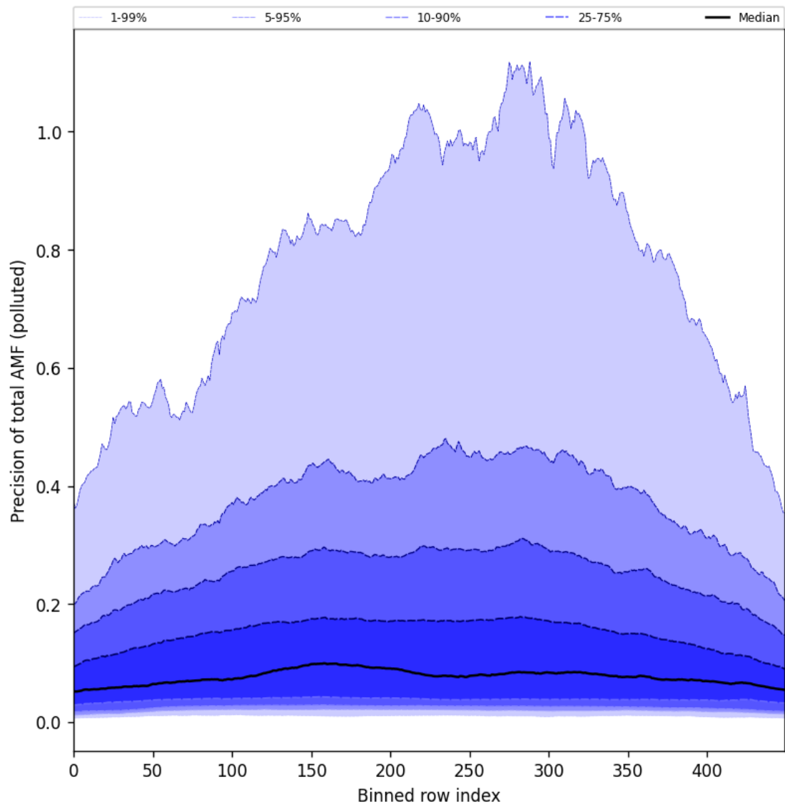
Figure 106: Along track statistics of “Precision of total AMF (polluted)” for 2025-06-18 to 2025-06-20
