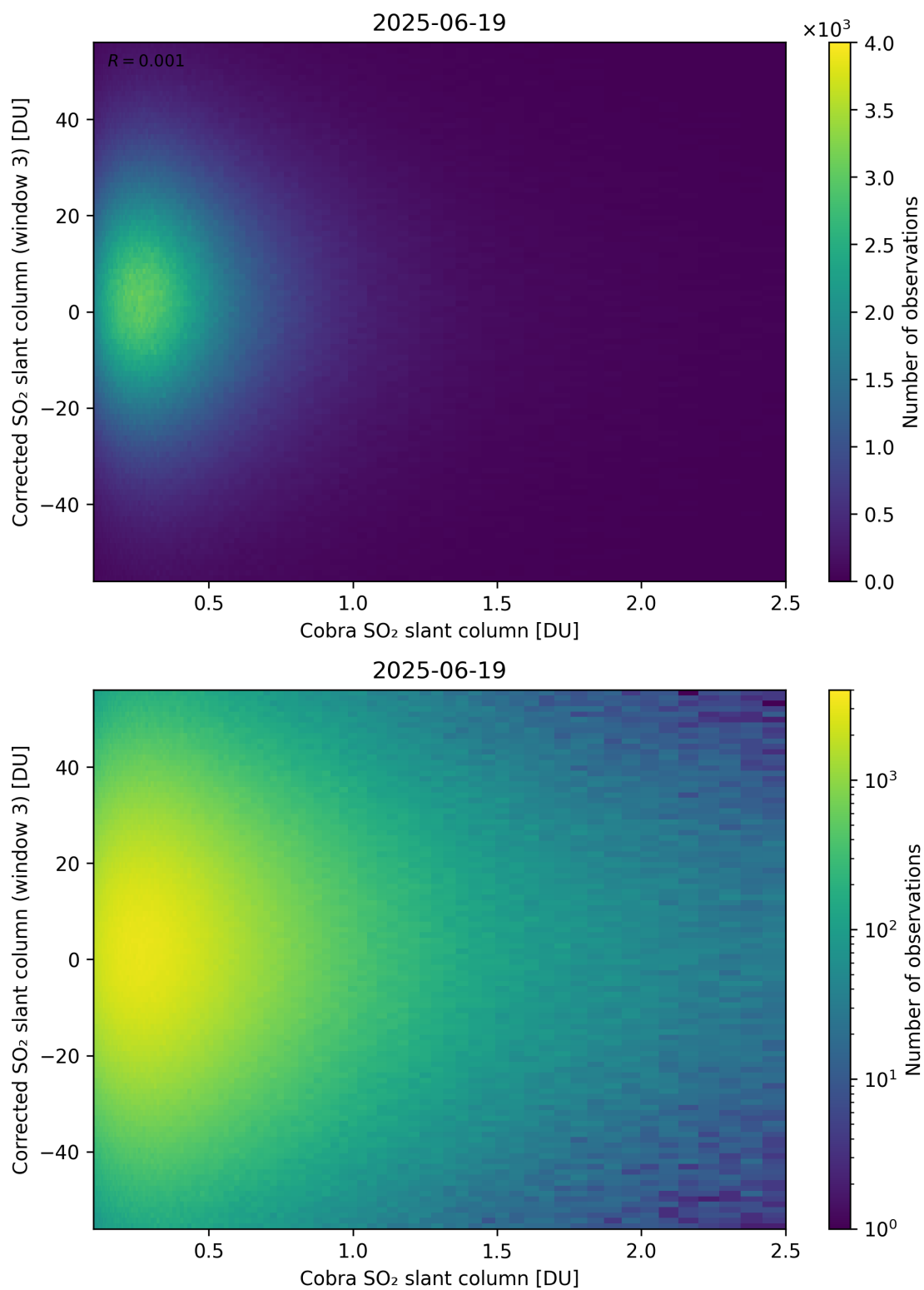
Figure 218: Scatter density plot of “Cobra SO 2 slant column” against “Corrected SO 2 slant column (window 3)” for 2025-06-18 to 2025-06-20.
