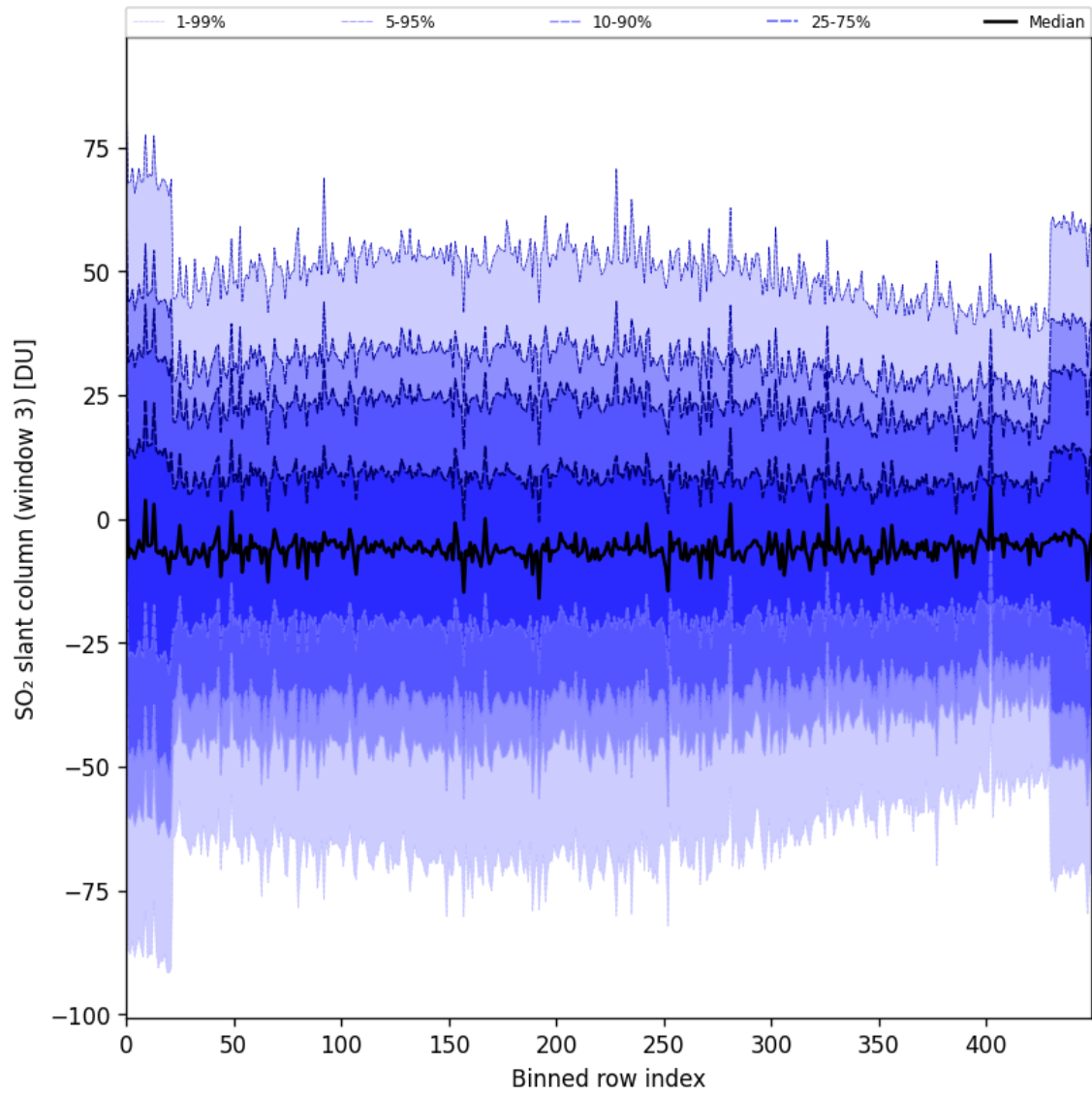
Figure 97: Along track statistics of “SO 2 slant column (window 3)” for 2025-06-18 to 2025-06-20
