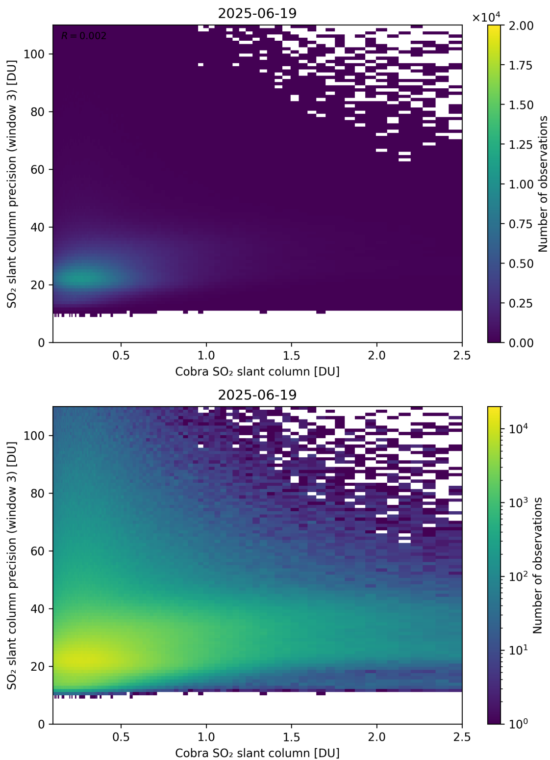
Figure 223: Scatter density plot of “Cobra SO 2 slant column” against “SO 2 slant column precision (window 3)” for 2025-06-18 to 2025-06-20.
