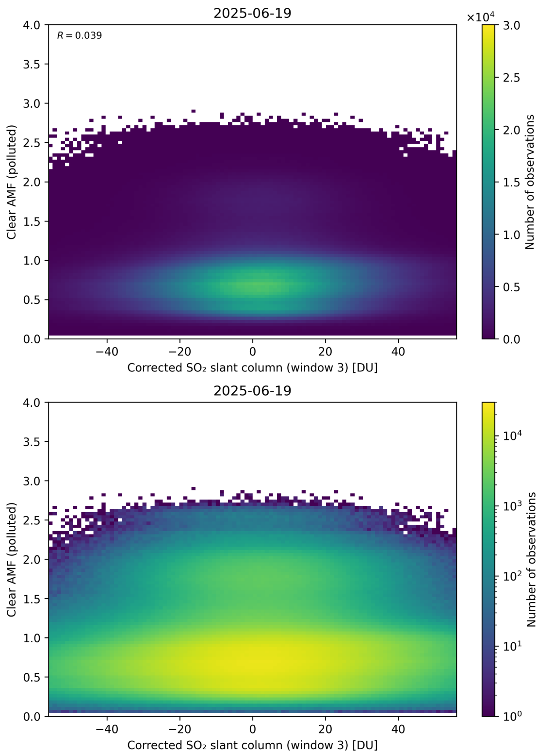
Figure 259: Scatter density plot of “Corrected SO 2 slant column (window 3)” against “Clear AMF (polluted)” for 2025-06-18 to 2025-06-20.
