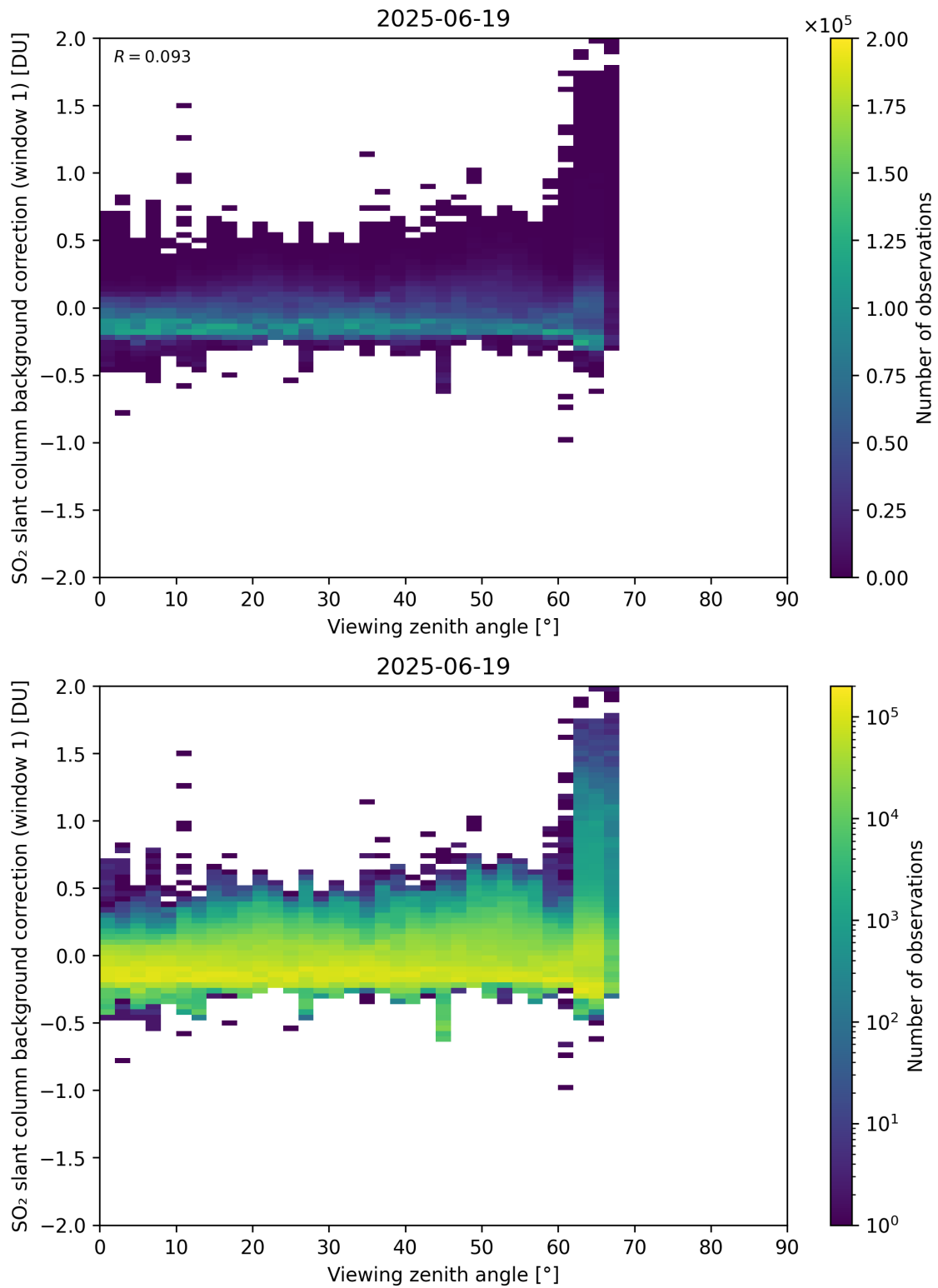
Figure 362: Scatter density plot of “Viewing zenith angle” against “SO 2 slant column background correction (window 1)” for 2025-06-18 to 2025-06-20.
