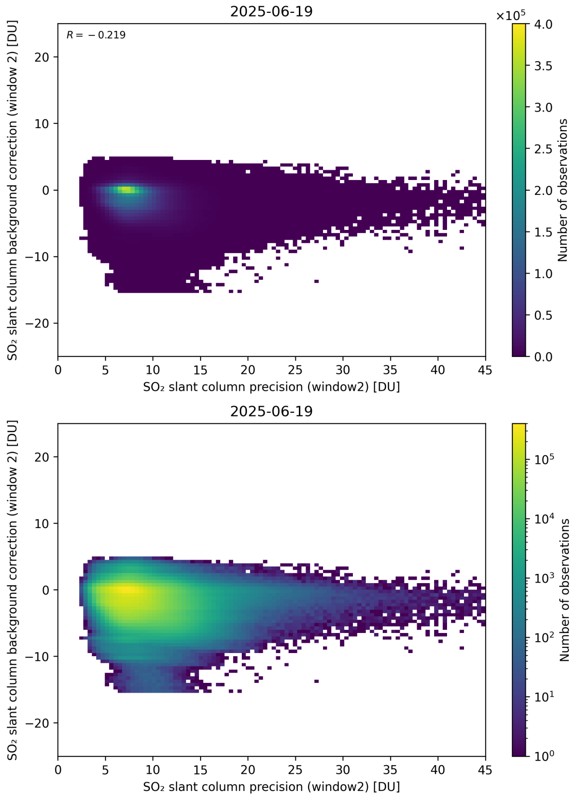
Figure 291: Scatter density plot of “SO 2 slant column precision (window2)” against “SO 2 slant column background correction (window 2)” for 2025-06-18 to 2025-06-20.
