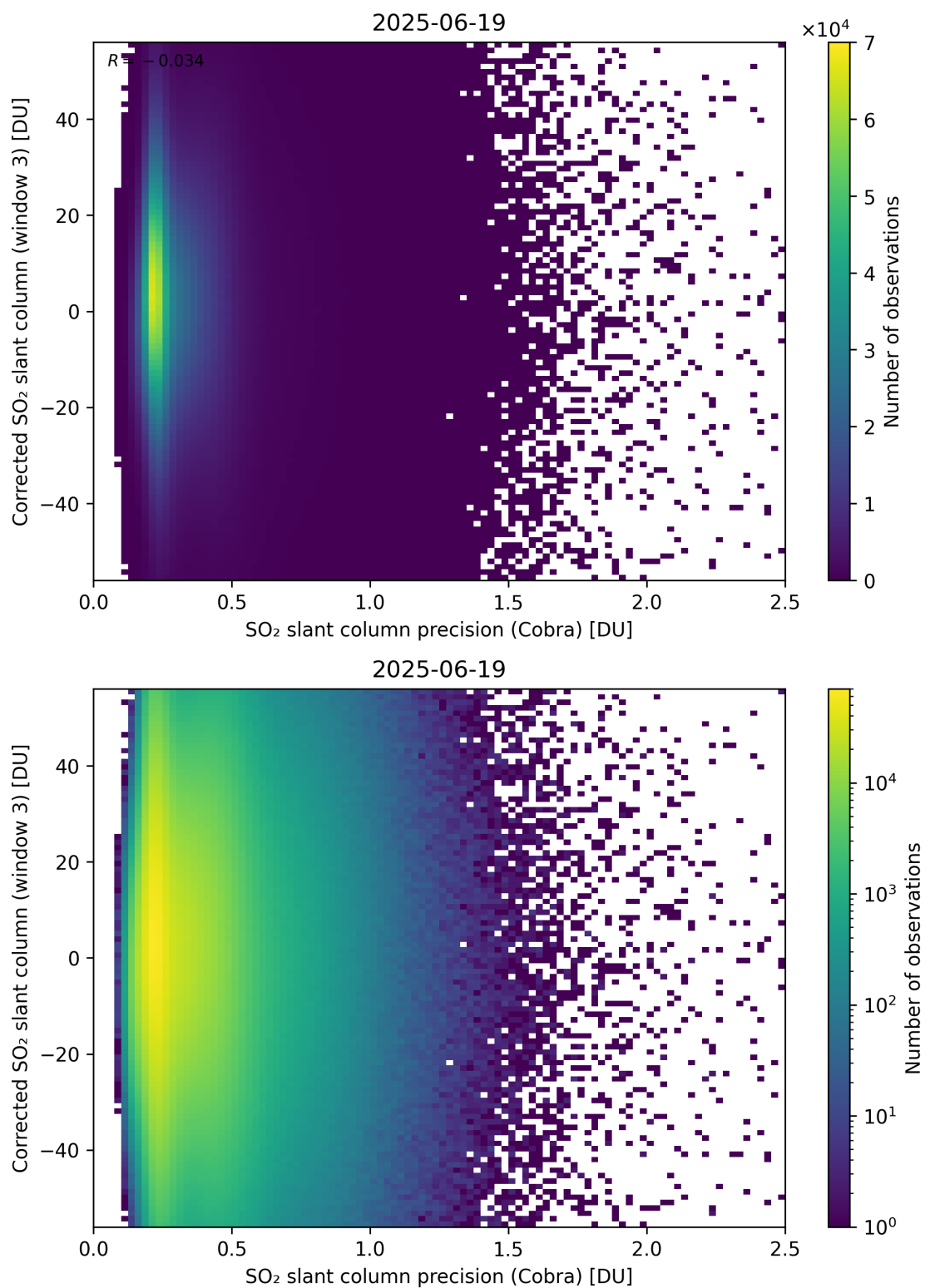
Figure 207: Scatter density plot of “SO 2 slant column precision (Cobra)” against “Corrected SO 2 slant column (window 3)” for 2025-06-18 to 2025-06-20.
