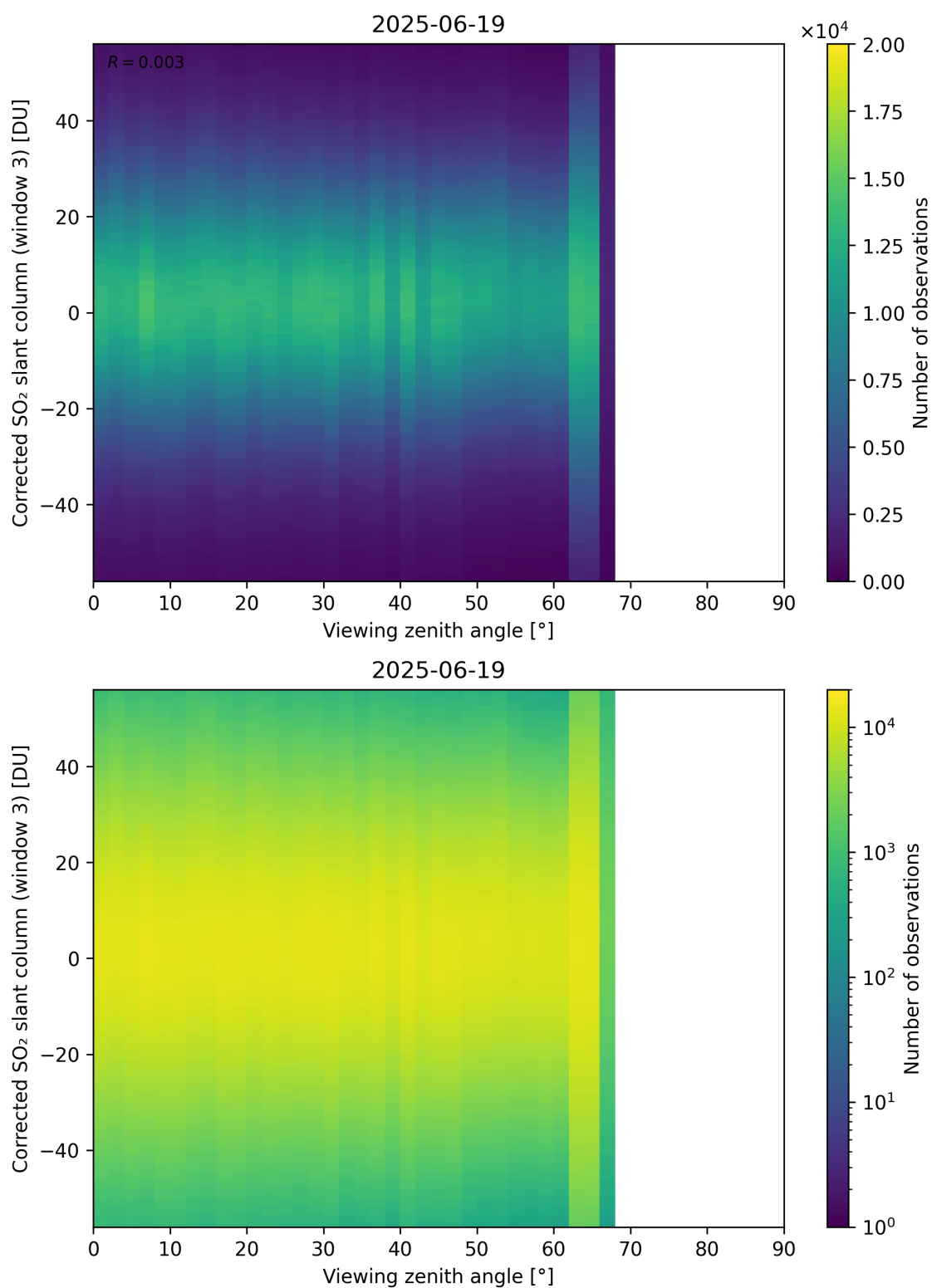
Figure 375: Scatter density plot of “Viewing zenith angle” against “Corrected SO 2 slant column (window 3)” for 2025-06-18 to 2025-06-20.
