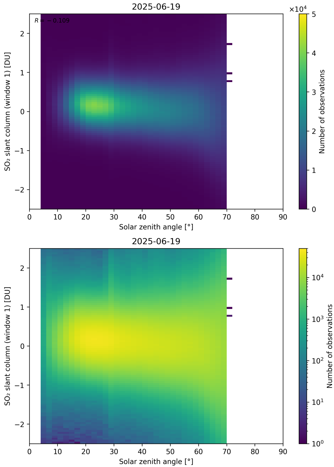
Figure 184: Scatter density plot of “Solar zenith angle” against “SO 2 slant column (window 1)” for 2025-06-18 to 2025-06-20.
