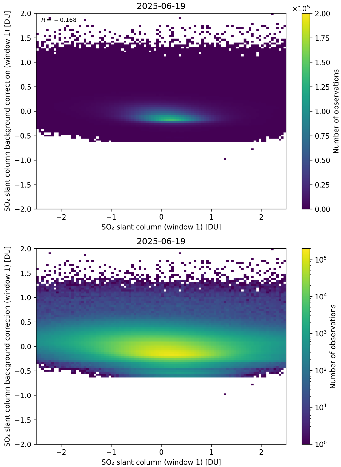
Figure 262: Scatter density plot of “SO 2 slant column (window 1)” against “SO 2 slant column background correction (window 1)” for 2025-06-18 to 2025-06-20.
