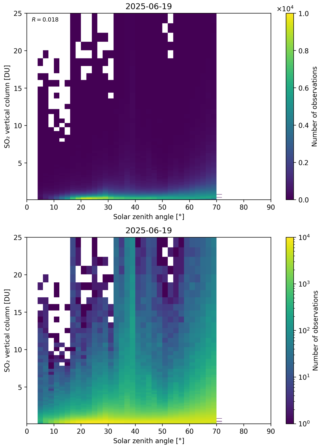
Figure 191: Scatter density plot of “Solar zenith angle” against “SO 2 vertical column” for 2025-06-18 to 2025-06-20.
