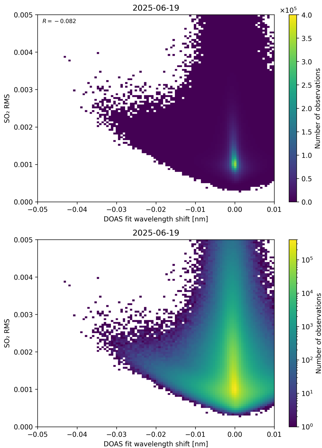
Figure 139: Scatter density plot of “DOAS fit wavelength shift” against “SO 2 RMS” for 2025-06-18 to 2025-06-20.
