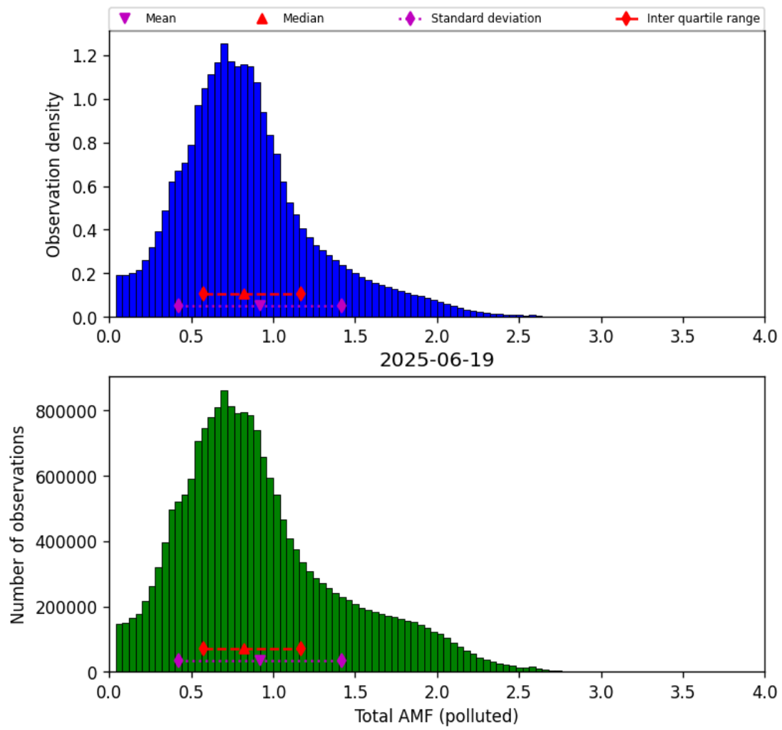
Figure 79: Histogram of “Total AMF (polluted)” for 2025-06-18 to 2025-06-20
