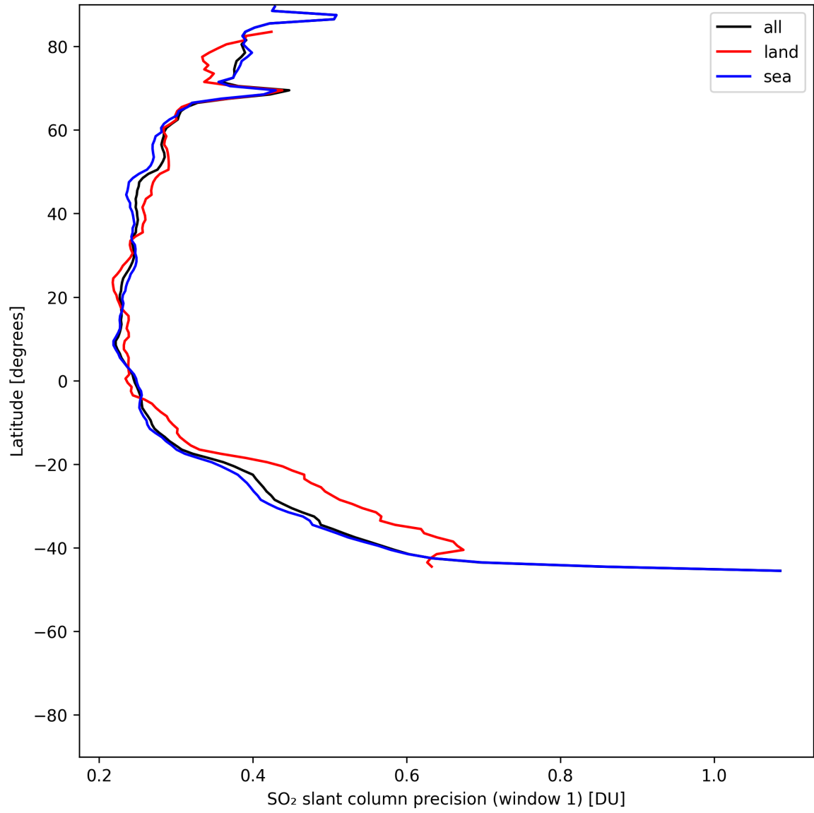
Figure 38: Zonal average of “SO 2 slant column precision (window 1)” for 2025-06-18 to 2025-06-20.
