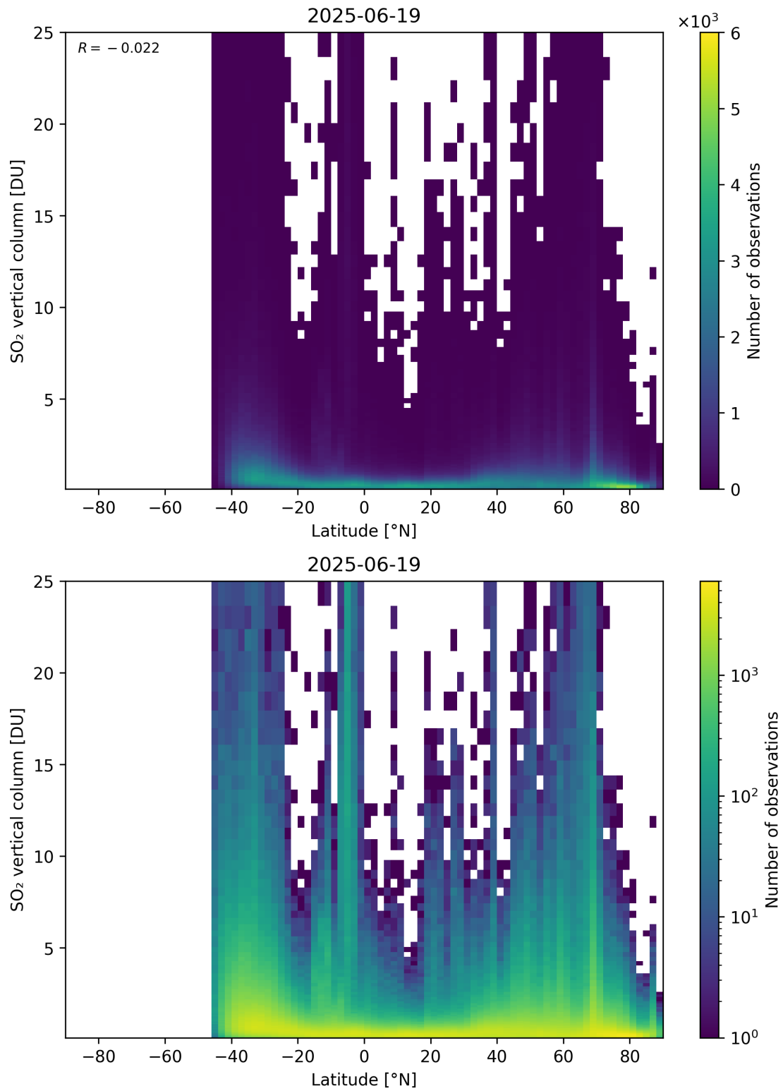
Figure 169: Scatter density plot of “Latitude” against “SO 2 vertical column” for 2025-06-18 to 2025-06-20.
