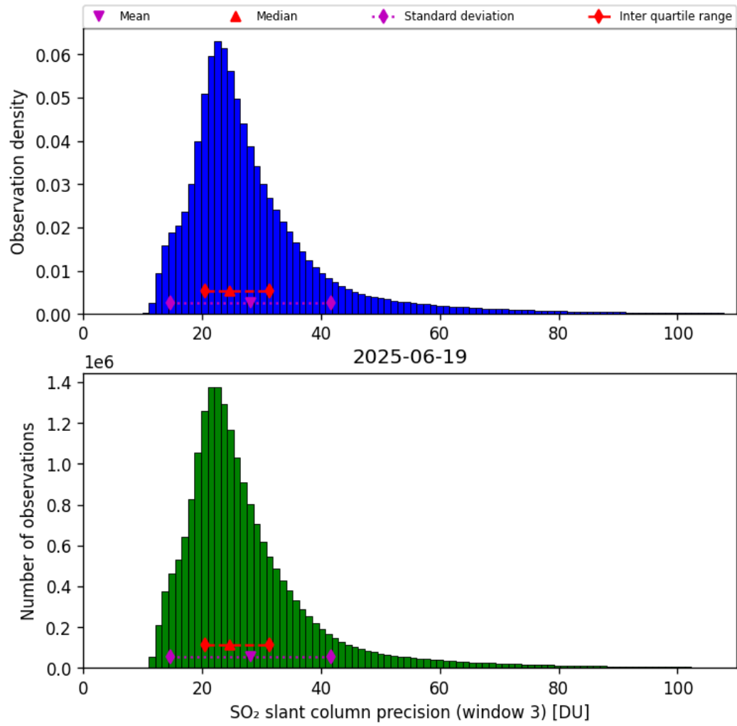
Figure 72: Histogram of “SO 2 slant column precision (window 3)” for 2025-06-18 to 2025-06-20
