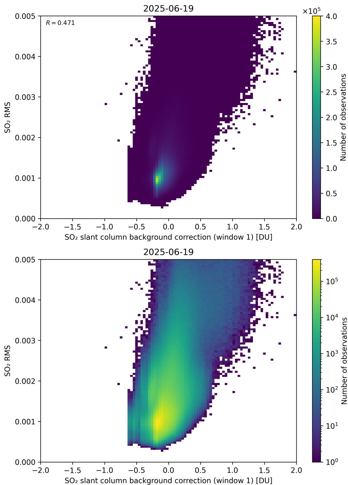
Figure 113: Scatter density plot of “SO 2 slant column background correction (window 1)” against “SO 2 RMS” for 2025-06-18 to 2025-06-20.
