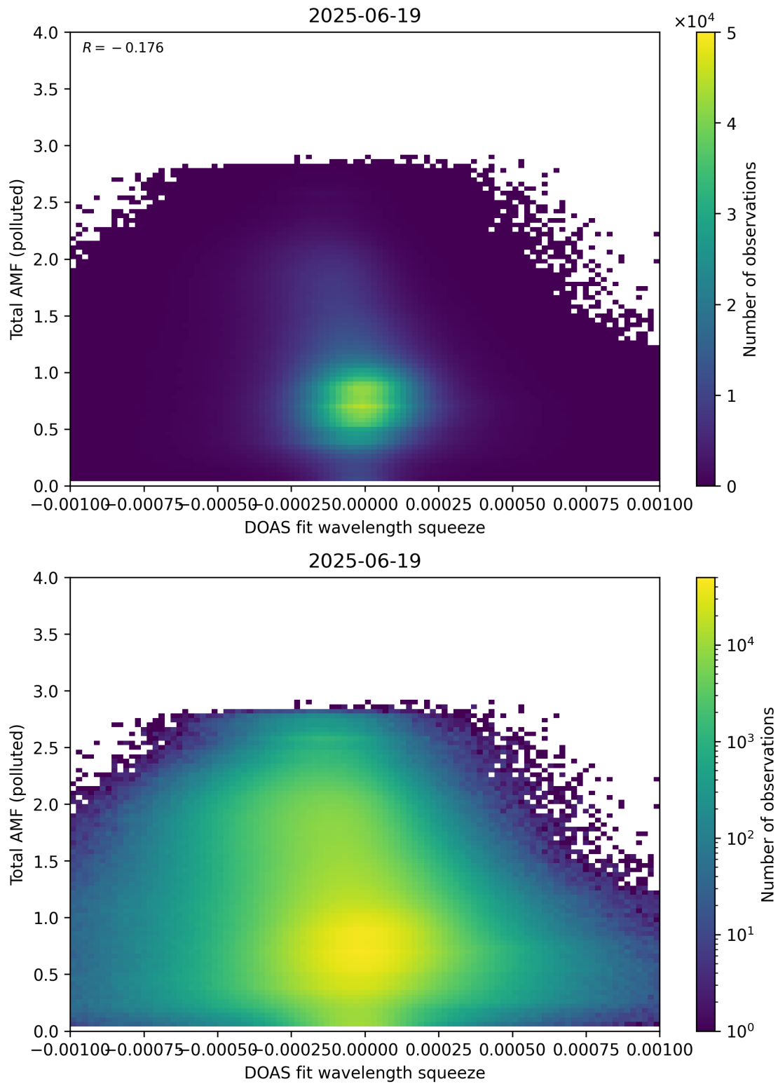
Figure 145: Scatter density plot of “DOAS fit wavelength squeeze” against “Total AMF (polluted)” for 2025-06-18 to 2025-06-20.
