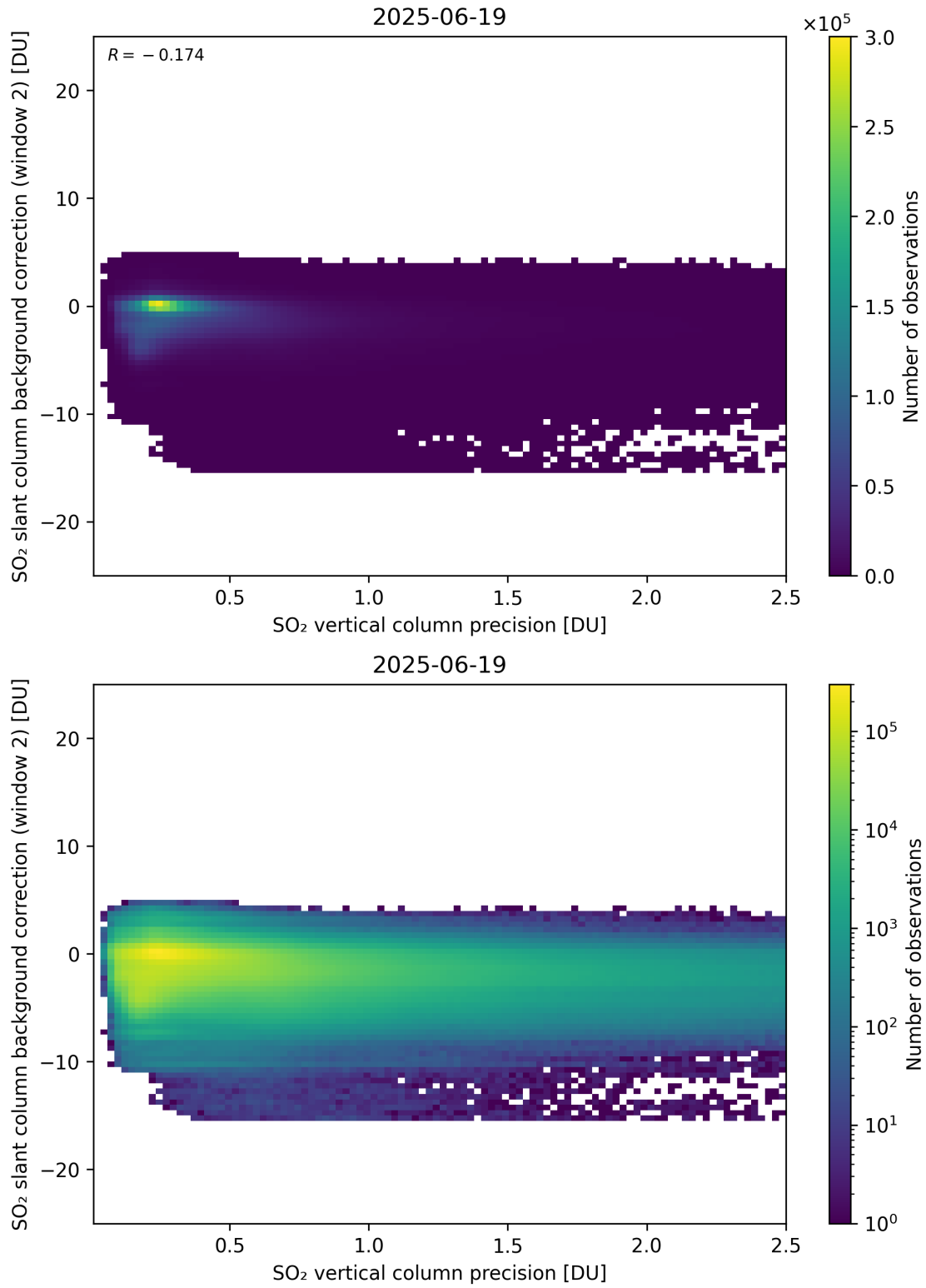
Figure 330: Scatter density plot of “SO 2 vertical column precision” against “SO 2 slant column background correction (window 2)” for 2025-06-18 to 2025-06-20.
