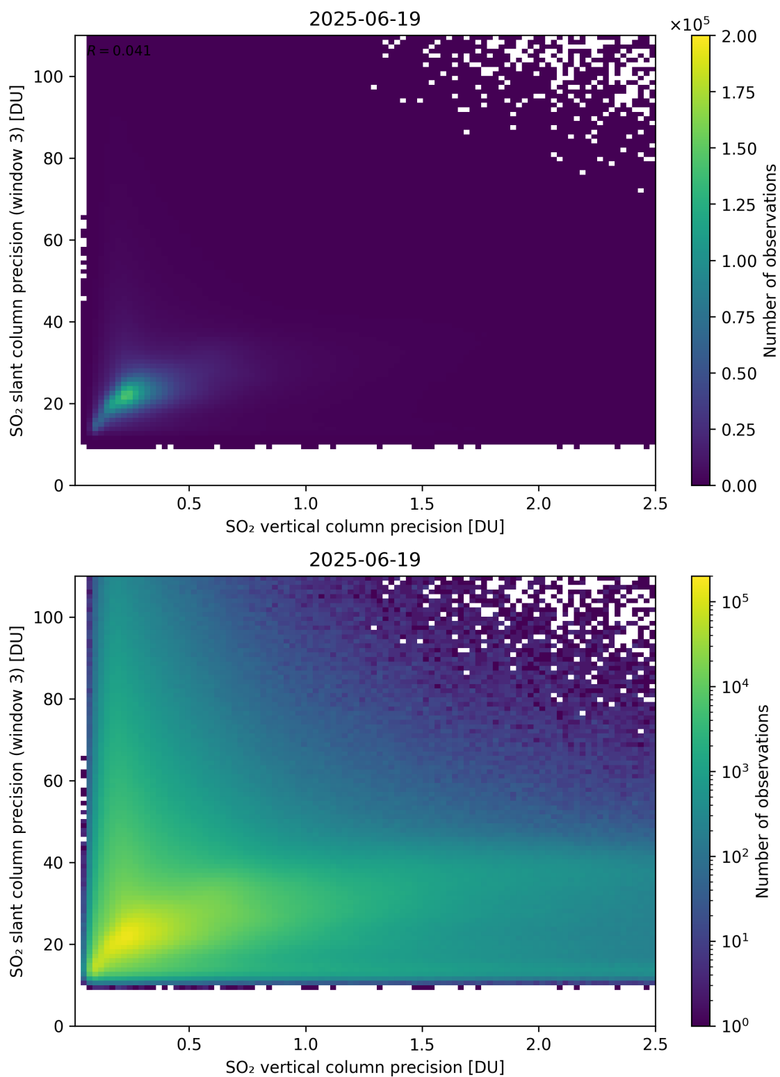
Figure 345: Scatter density plot of “SO 2 vertical column precision” against “SO 2 slant column precision (window 3)” for 2025-06-18 to 2025-06-20.
