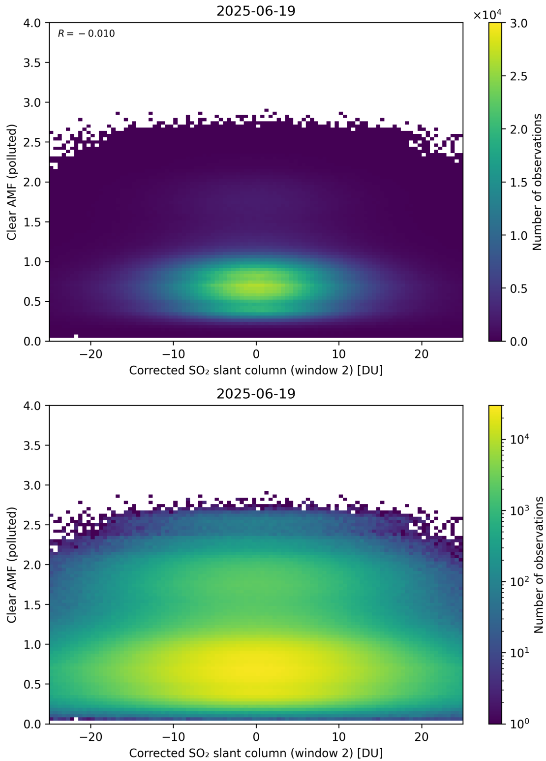
Figure 249: Scatter density plot of “Corrected SO 2 slant column (window 2)” against “Clear AMF (polluted)” for 2025-06-18 to 2025-06-20.
