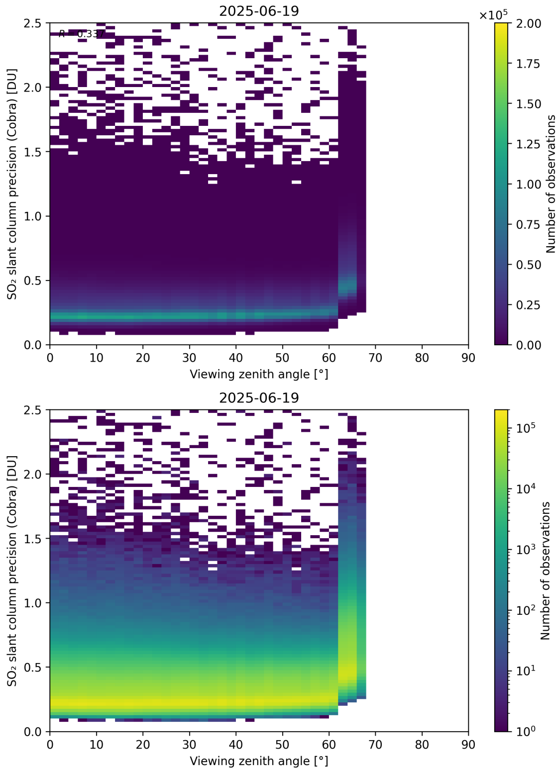
Figure 372: Scatter density plot of “Viewing zenith angle” against “SO 2 slant column precision (Cobra)” for 2025-06-18 to 2025-06-20.
