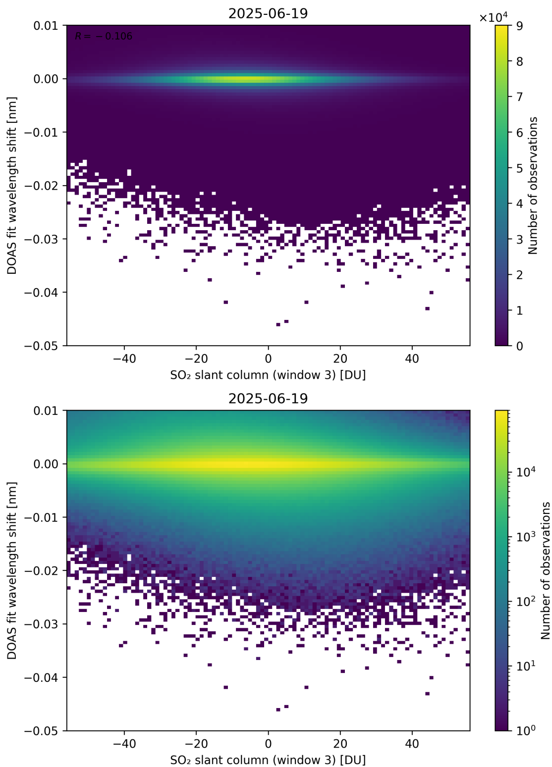
Figure 304: Scatter density plot of “SO 2 slant column (window 3)” against “DOAS fit wavelength shift” for 2025-06-18 to 2025-06-20.
