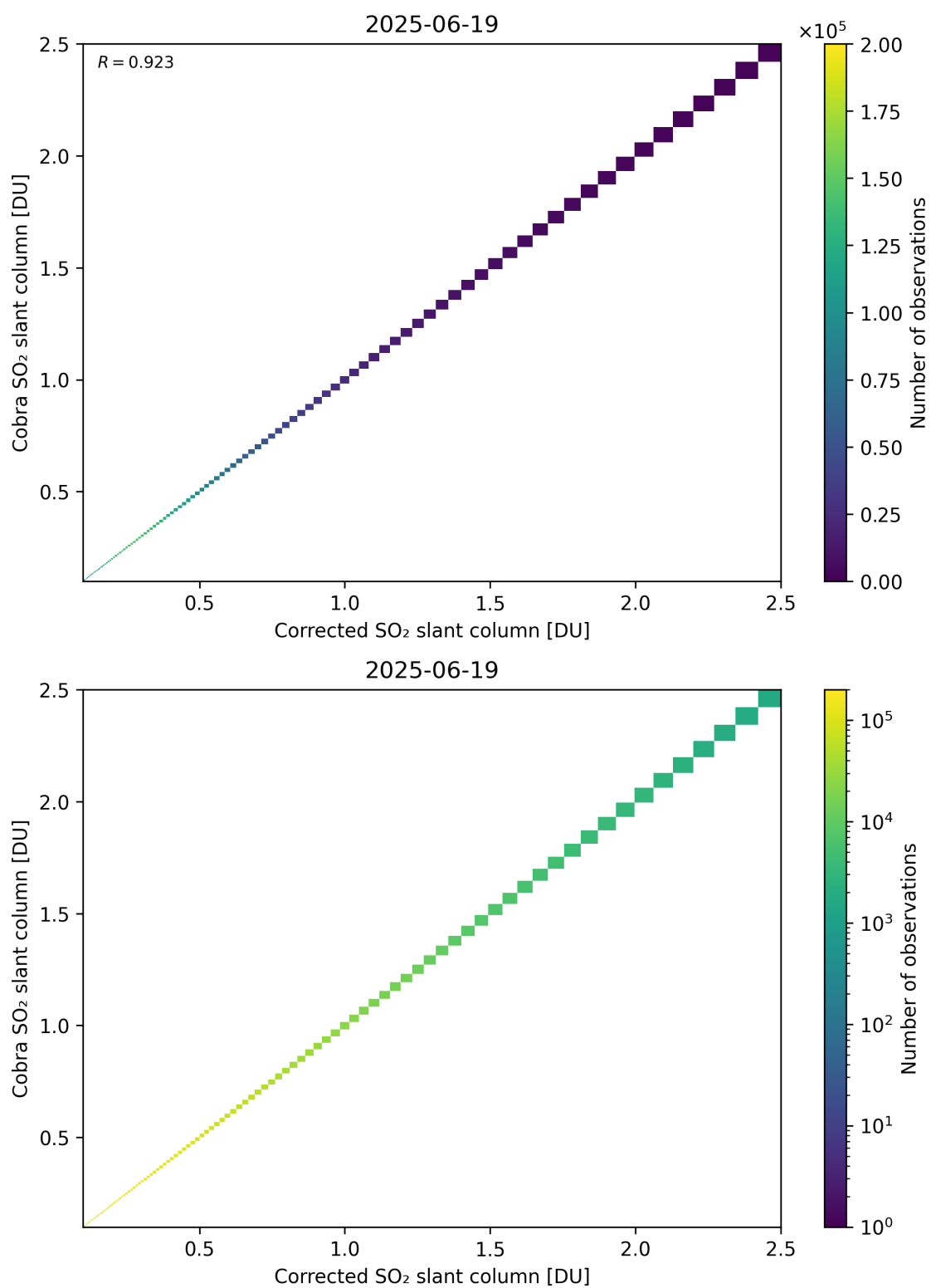
Figure 233: Scatter density plot of “Corrected SO 2 slant column” against “Cobra SO 2 slant column” for 2025-06-18 to 2025-06-20.
