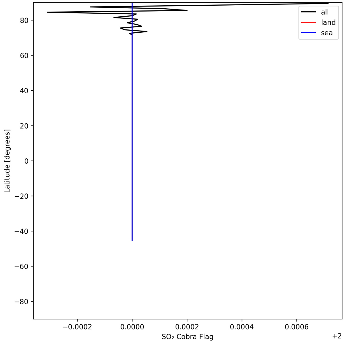
Figure 49: Zonal average of "SO 2 Cobra Flag" for 2025-06-18 to 2025-06-20.
