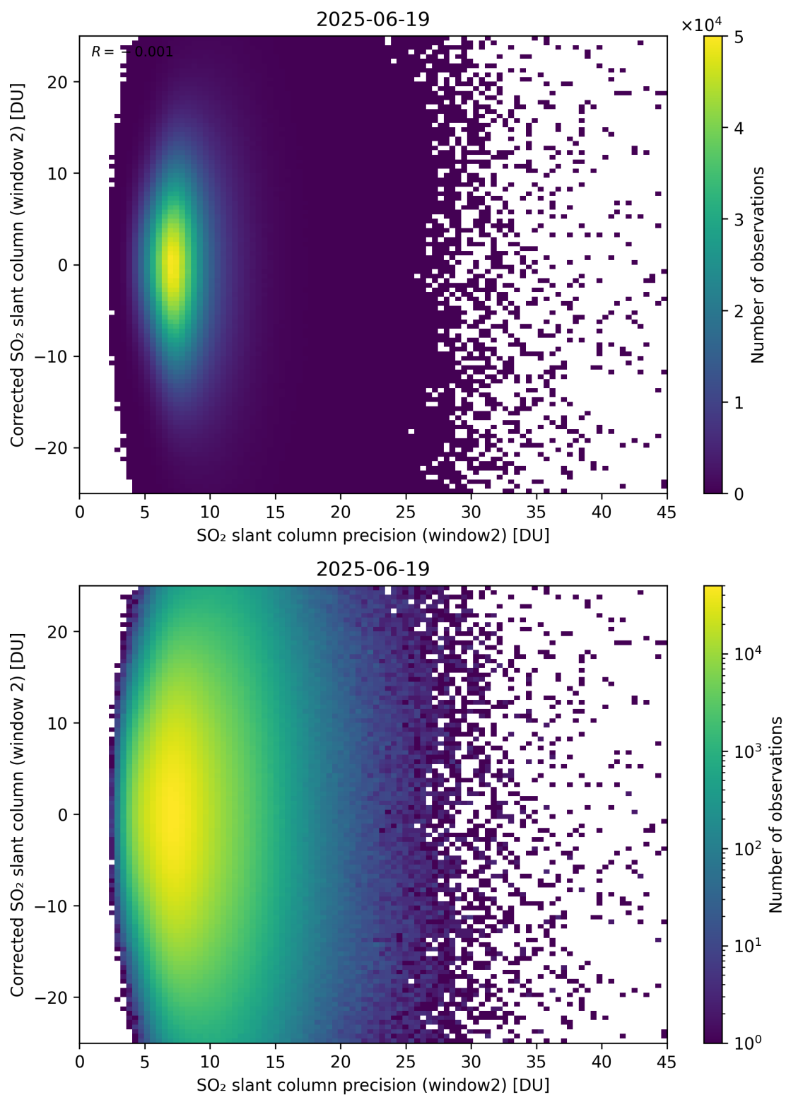
Figure 297: Scatter density plot of “SO 2 slant column precision (window2)” against “Corrected SO 2 slant column (window 2)” for 2025-06-18 to 2025-06-20.
