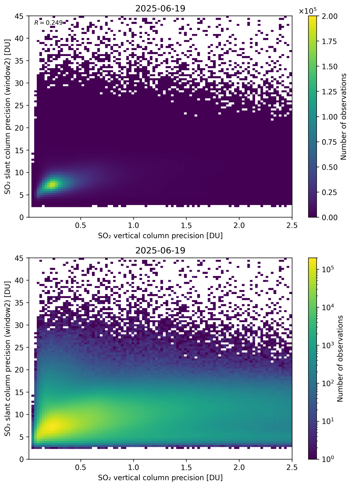
Figure 343: Scatter density plot of “SO 2 vertical column precision” against “SO 2 slant column precision (window2)” for 2025-06-18 to 2025-06-20.
