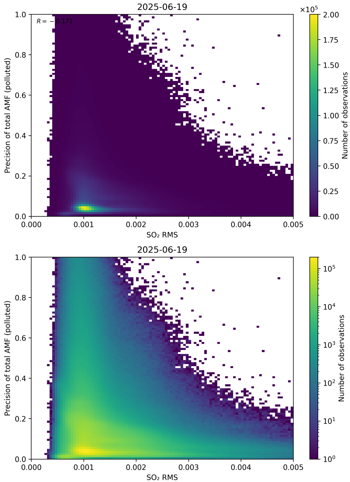
Figure 149: Scatter density plot of “SO 2 RMS” against “Precision of total AMF (polluted)” for 2025-06-18 to 2025-06-20.
