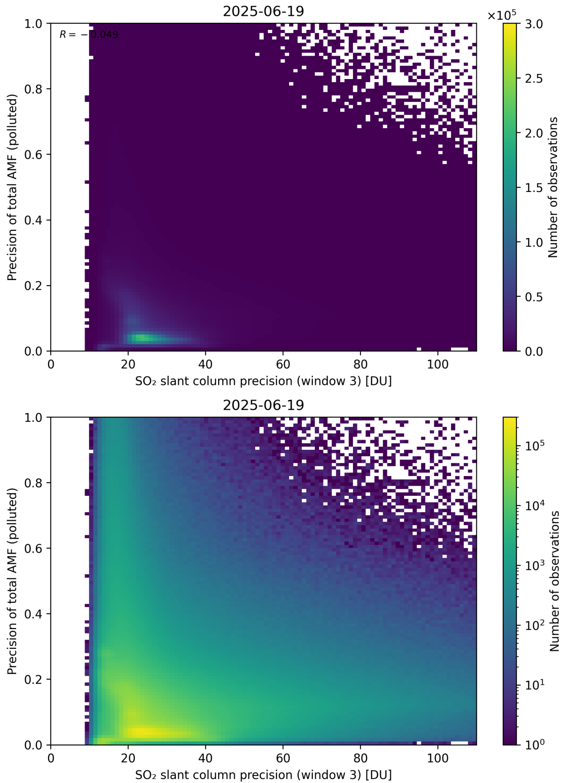
Figure 314: Scatter density plot of “SO 2 slant column precision (window 3)” against “Precision of total AMF (polluted)” for 2025-06-18 to 2025-06-20.
