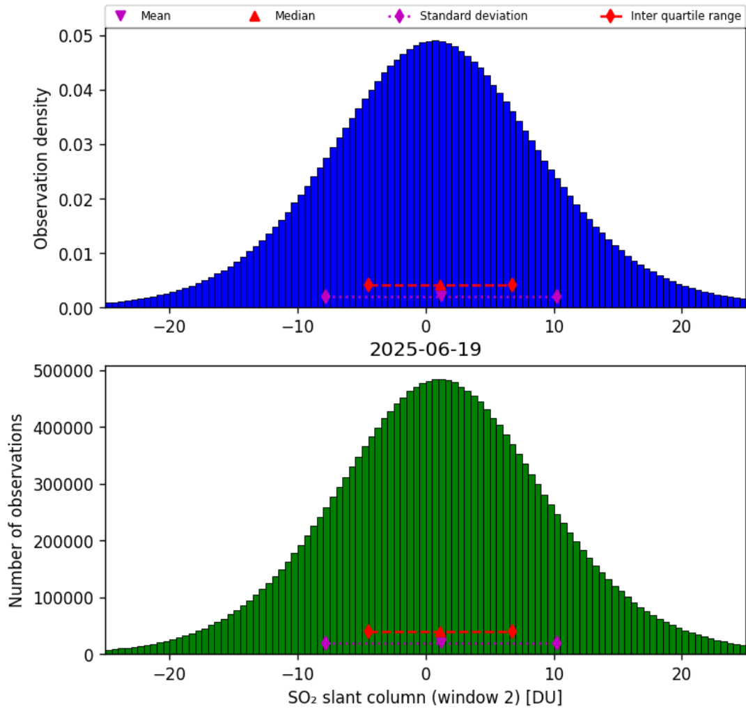
Figure 67: Histogram of “SO 2 slant column (window 2)” for 2025-06-18 to 2025-06-20
