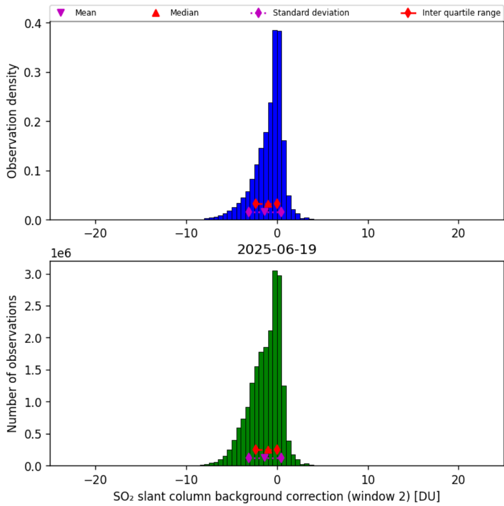
Figure 70: Histogram of “SO 2 slant column background correction (window 2)” for 2025-06-18 to 2025-06-20
