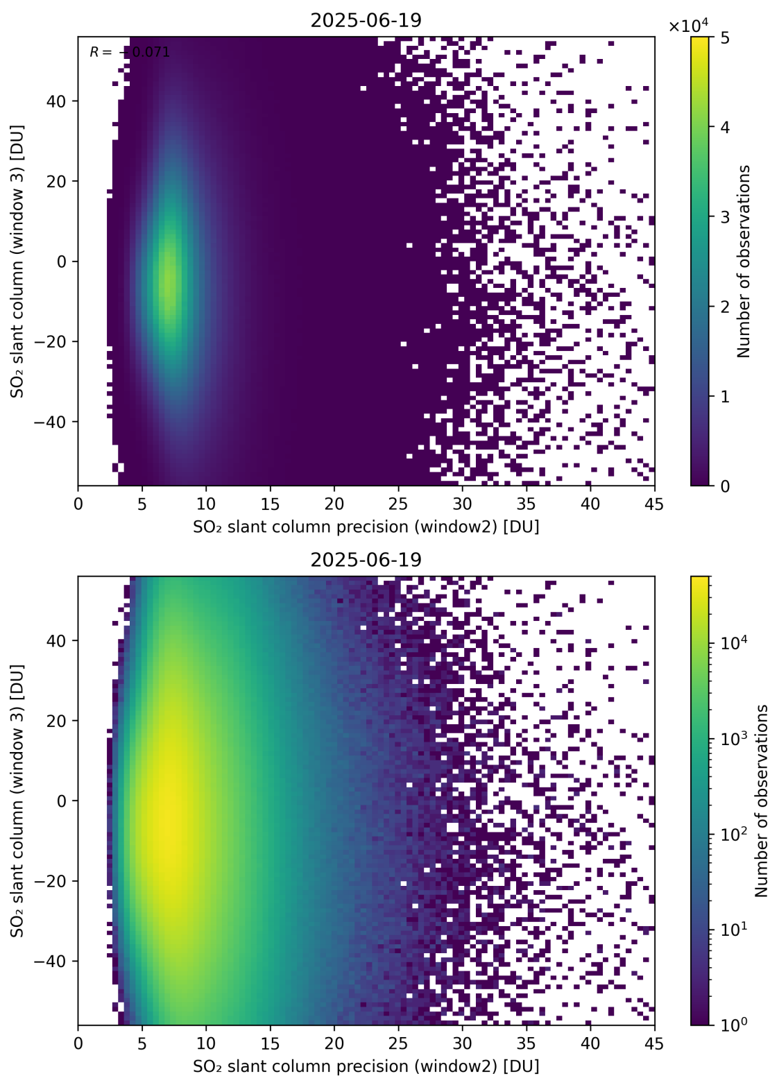
Figure 299: Scatter density plot of “SO 2 slant column precision (window2)” against “SO 2 slant column (window 3)” for 2025-06-18 to 2025-06-20.
