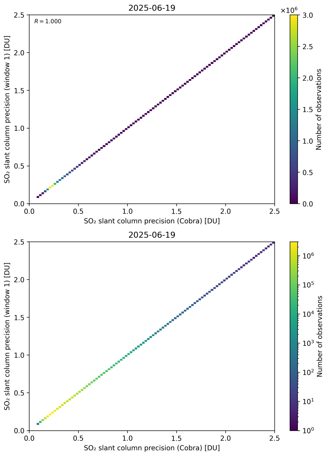
Figure 209: Scatter density plot of “SO 2 slant column precision (Cobra)” against “SO 2 slant column precision (window 1)” for 2025-06-18 to 2025-06-20.
