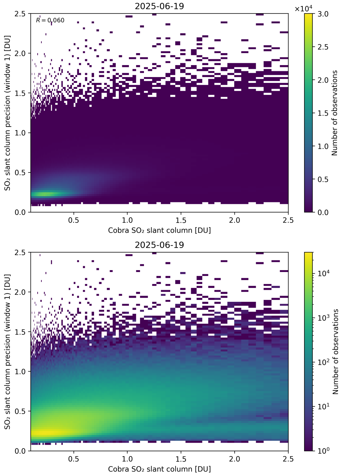
Figure 220: Scatter density plot of “Cobra SO 2 slant column” against “SO 2 slant column precision (window 1)” for 2025-06-18 to 2025-06-20.
