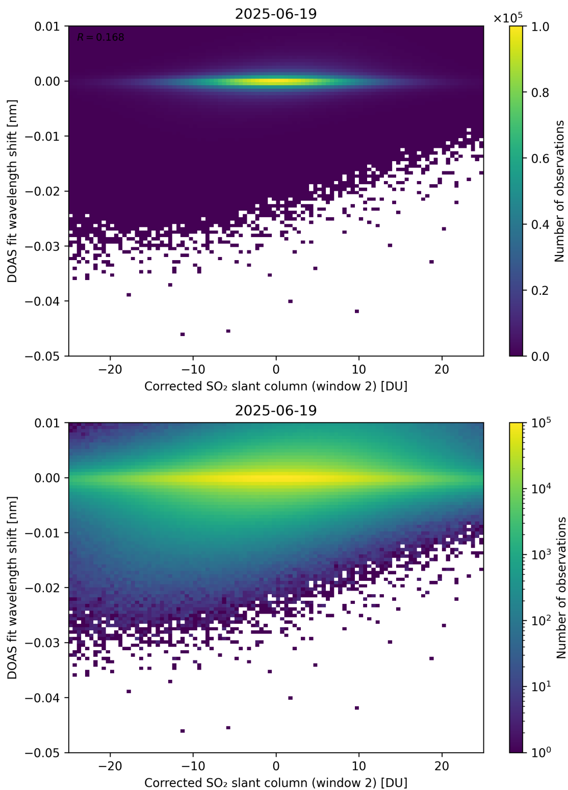
Figure 246: Scatter density plot of “Corrected SO 2 slant column (window 2)” against “DOAS fit wavelength shift” for 2025-06-18 to 2025-06-20.
