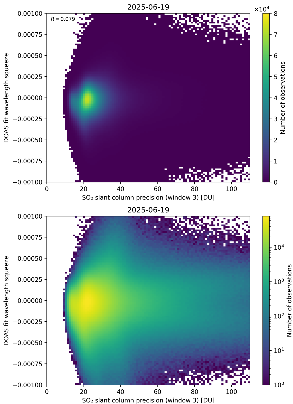
Figure 309: Scatter density plot of “SO 2 slant column precision (window 3)” against “DOAS fit wavelength squeeze” for 2025-06-18 to 2025-06-20.
