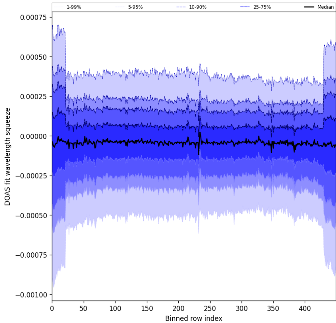
Figure 103: Along track statistics of “DOAS fit wavelength squeeze” for 2025-06-18 to 2025-06-20
