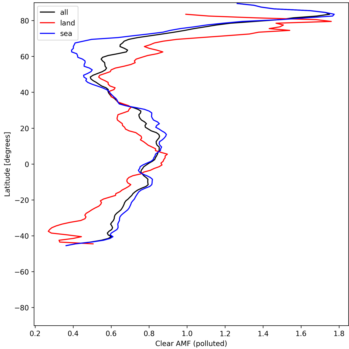
Figure 55: Zonal average of “Clear AMF (polluted)” for 2025-06-18 to 2025-06-20.
