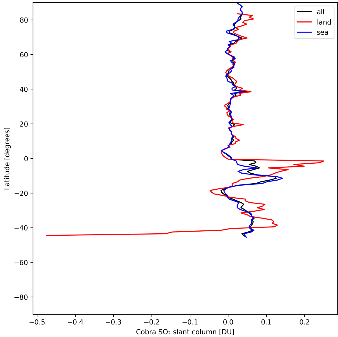
Figure 35: Zonal average of “Cobra SO 2 slant column” for 2025-06-18 to 2025-06-20.
