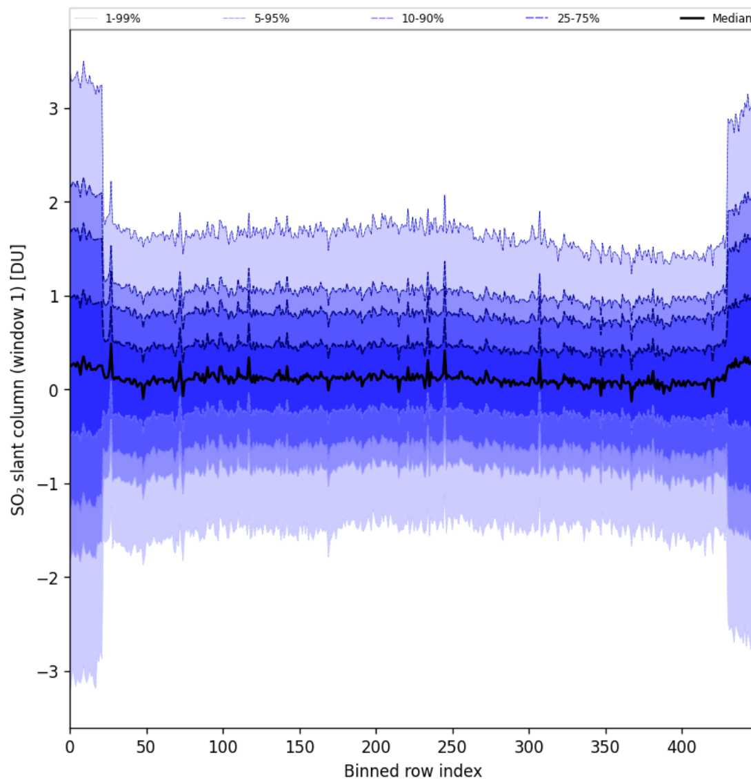
Figure 89: Along track statistics of “SO 2 slant column (window 1)” for 2025-06-18 to 2025-06-20
