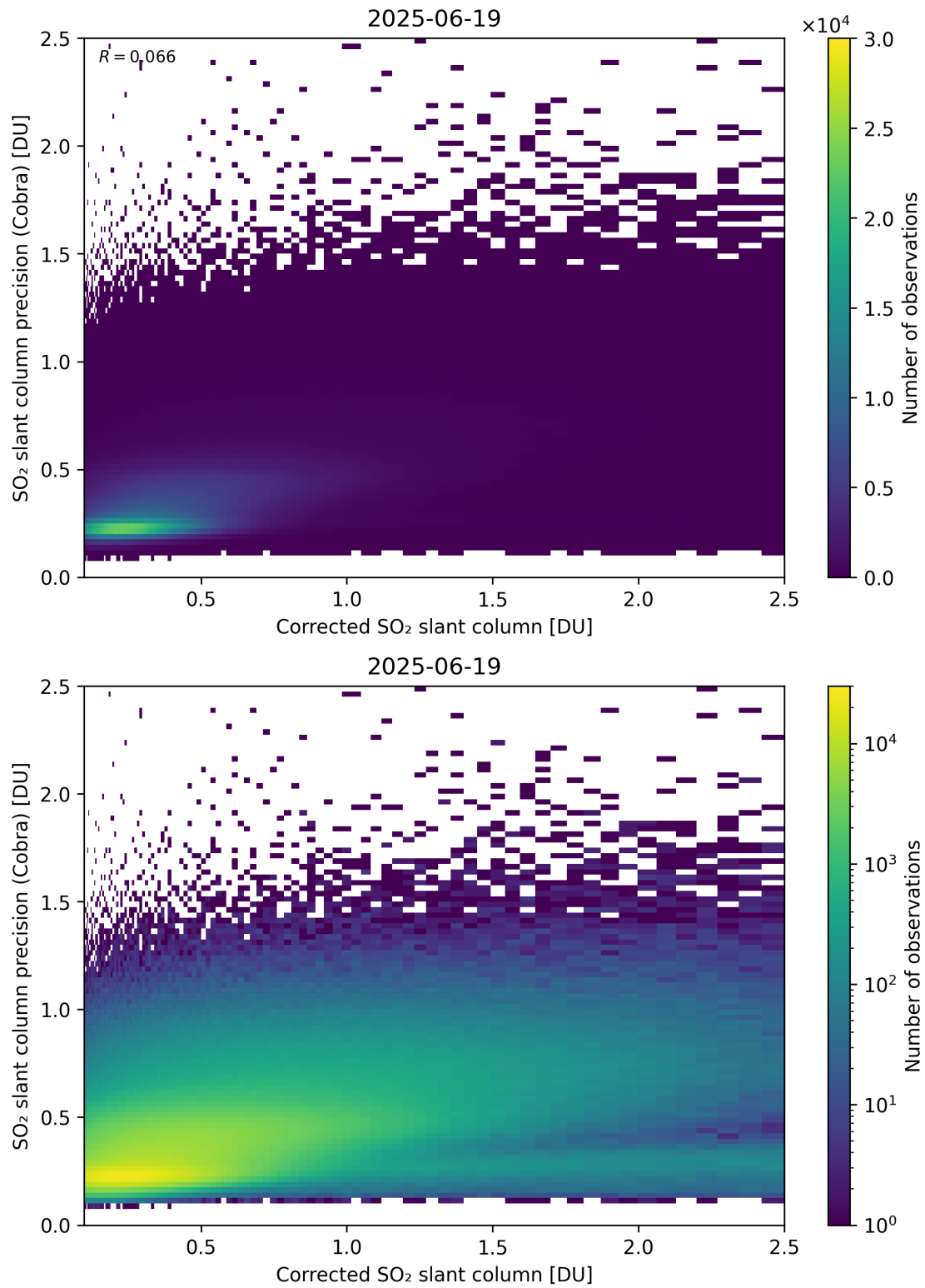
Figure 234: Scatter density plot of “Corrected SO 2 slant column” against “SO 2 slant column precision (Cobra)” for 2025-06-18 to 2025-06-20.
