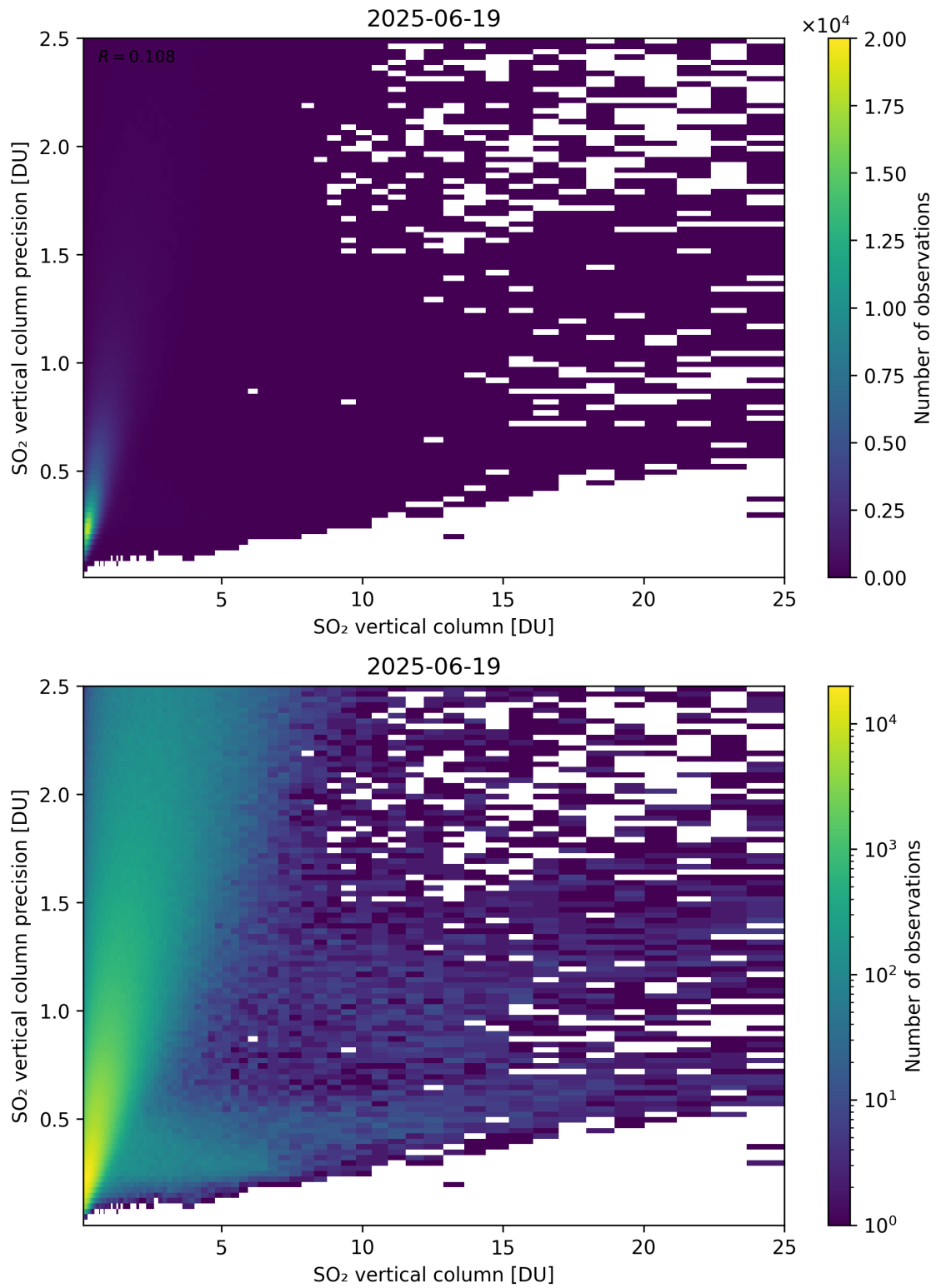
Figure 361: Scatter density plot of “SO 2 vertical column” against “SO 2 vertical column precision” for 2025-06-18 to 2025-06-20.
