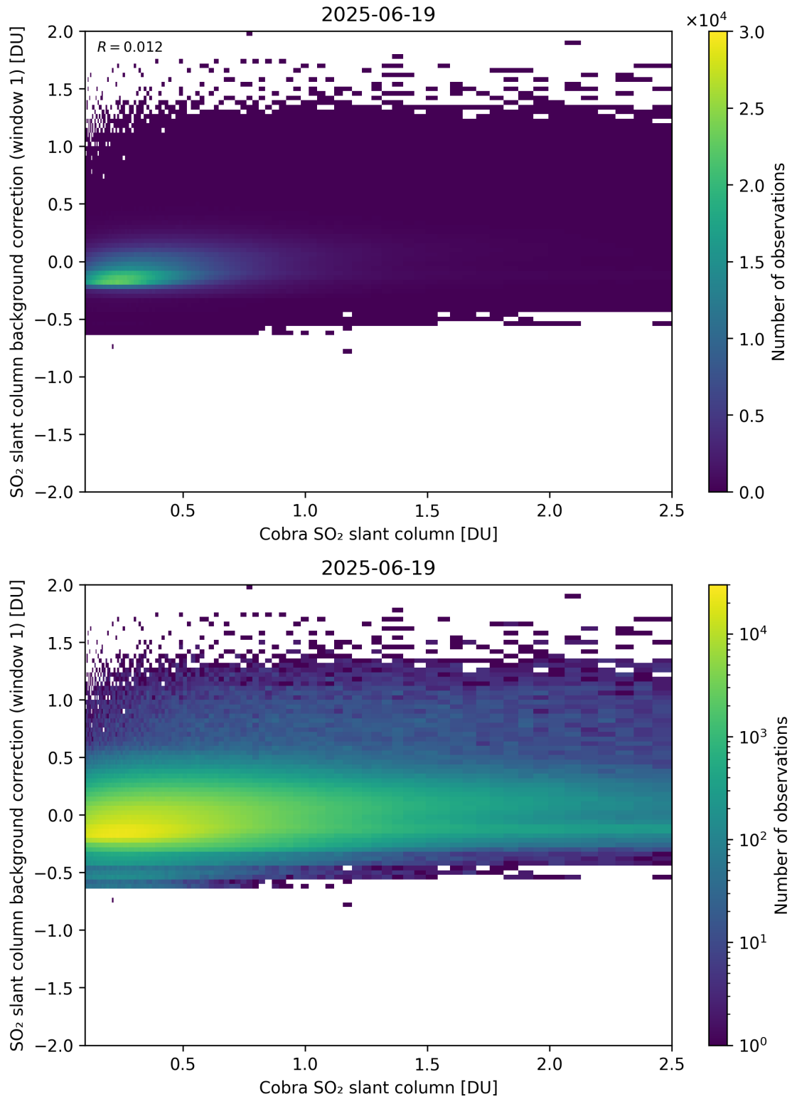
Figure 193: Scatter density plot of “Cobra SO 2 slant column” against “SO 2 slant column background correction (window 1)” for 2025-06-18 to 2025-06-20.
