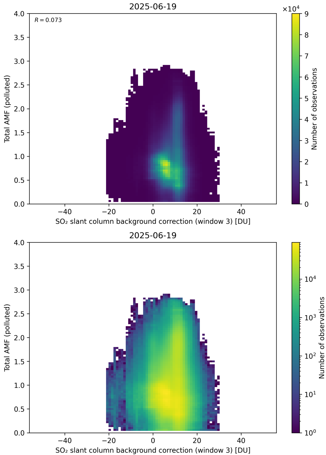
Figure 136: Scatter density plot of “SO 2 slant column background correction (window 3)” against “Total AMF (polluted)” for 2025-06-18 to 2025-06-20.
