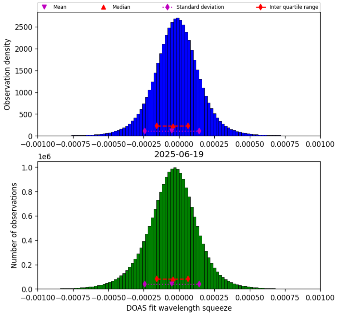
Figure 77: Histogram of “DOAS fit wavelength squeeze” for 2025-06-18 to 2025-06-20
