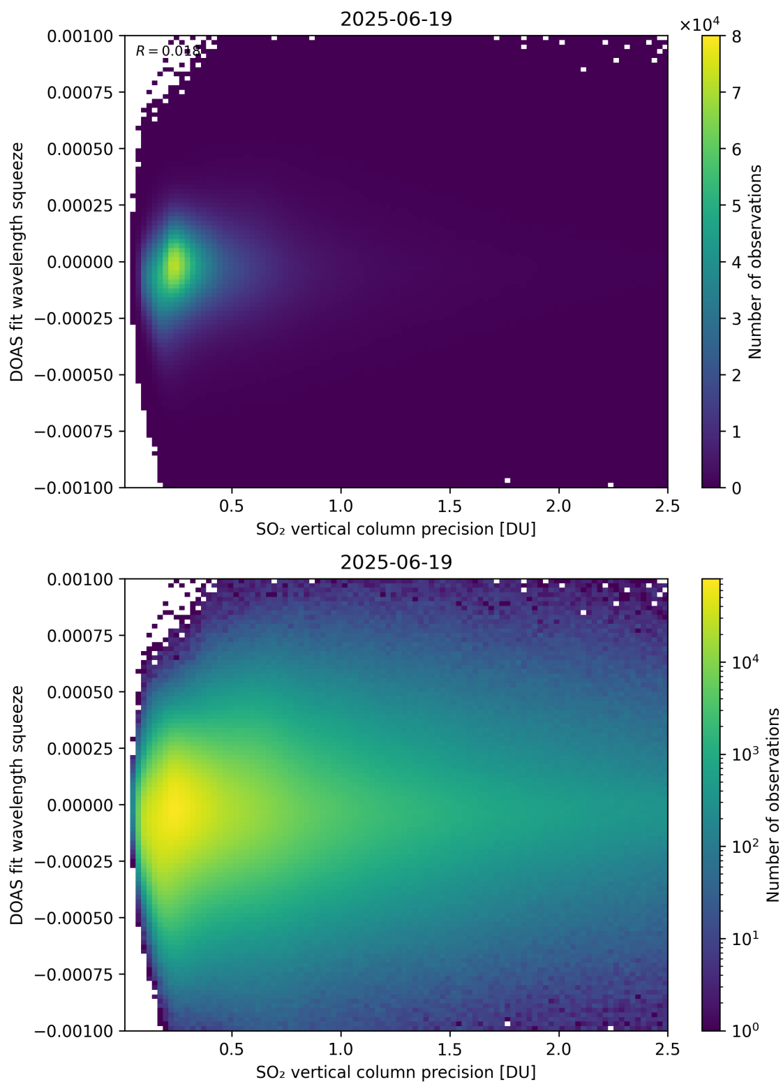
Figure 333: Scatter density plot of “SO 2 vertical column precision” against “DOAS fit wavelength squeeze” for 2025-06-18 to 2025-06-20.
