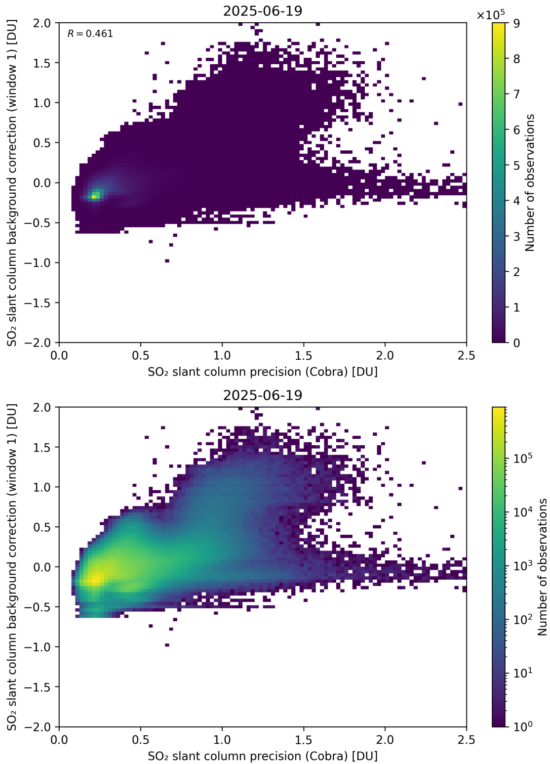
Figure 199: Scatter density plot of “SO 2 slant column precision (Cobra)” against “SO 2 slant column background correction (window 1)” for 2025-06-18 to 2025-06-20.
