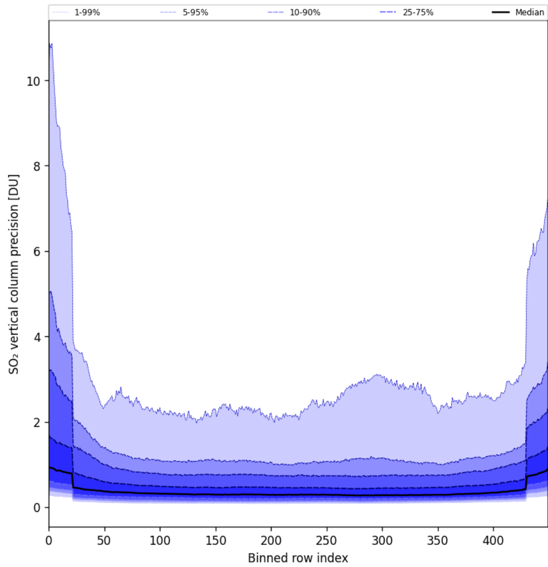
Figure 85: Along track statistics of “SO 2 vertical column precision” for 2025-06-18 to 2025-06-20
