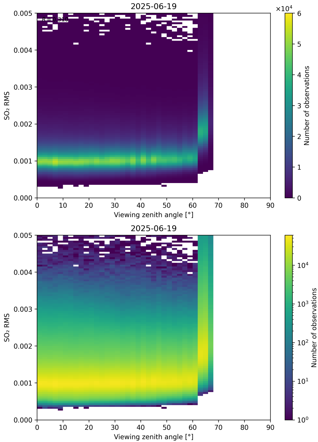
Figure 367: Scatter density plot of “Viewing zenith angle” against “SO 2 RMS” for 2025-06-18 to 2025-06-20.
