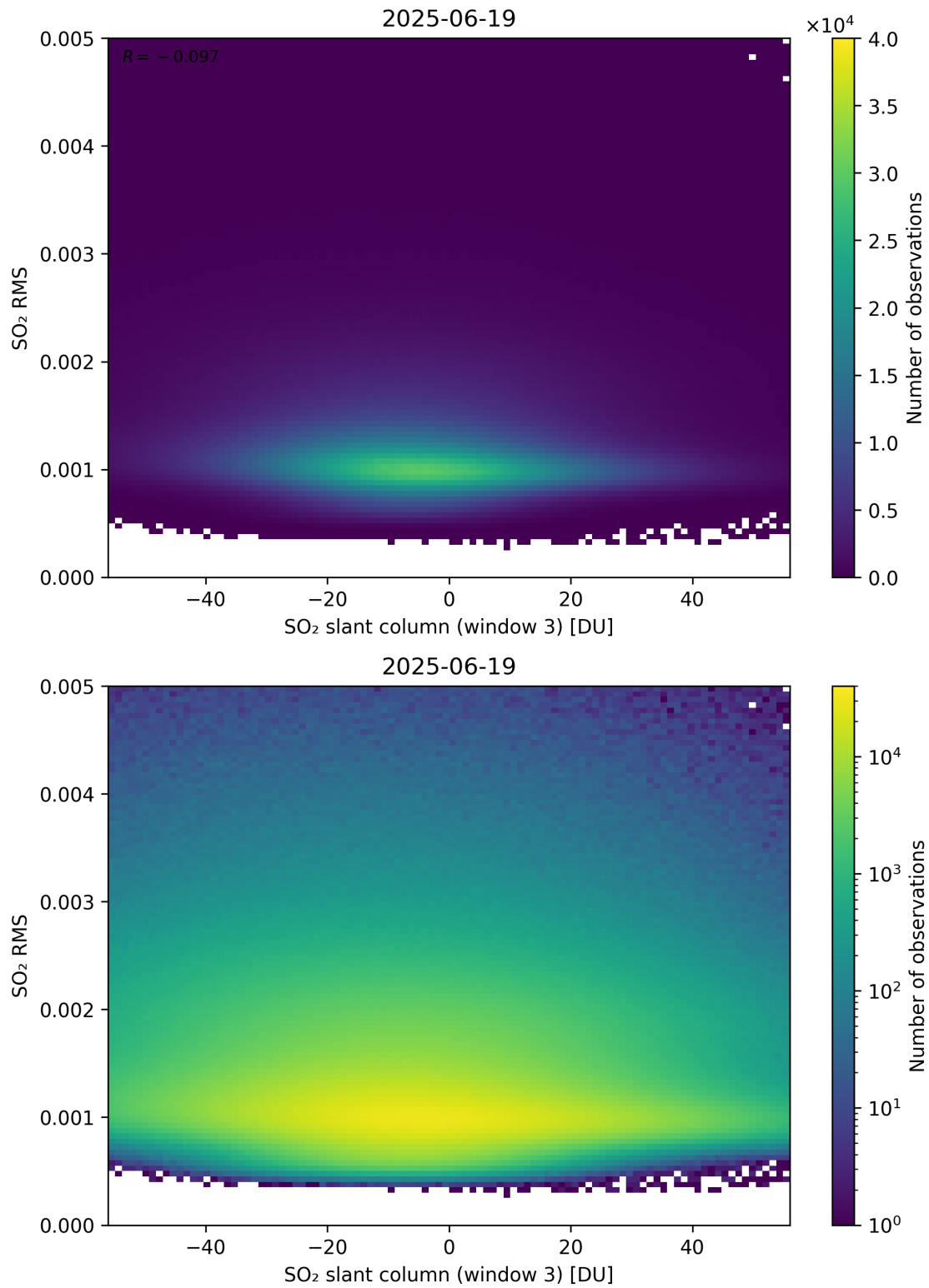
Figure 306: Scatter density plot of “SO 2 slant column (window 3)” against “SO 2 RMS” for 2025-06-18 to 2025-06-20.
