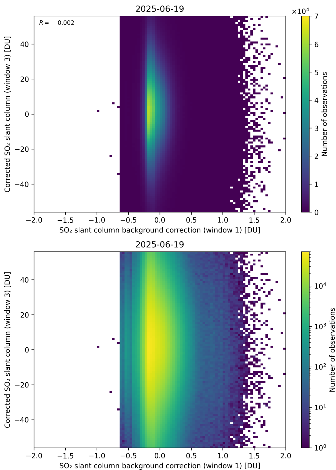
Figure 116: Scatter density plot of “SO 2 slant column background correction (window 1)” against “Corrected SO 2 slant column (window 3)” for 2025-06-18 to 2025-06-20.
