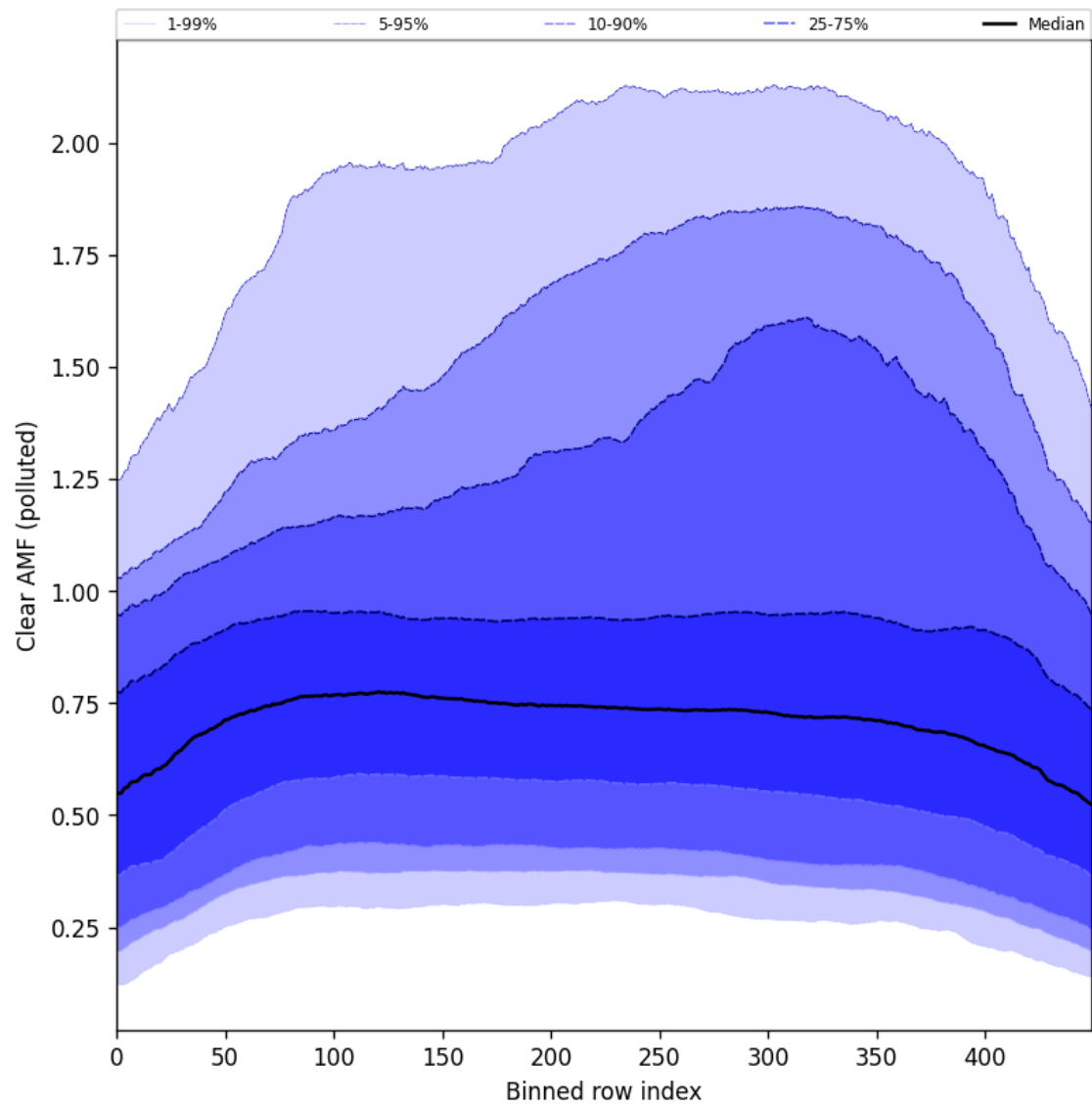
Figure 107: Along track statistics of “Clear AMF (polluted)” for 2025-06-18 to 2025-06-20
