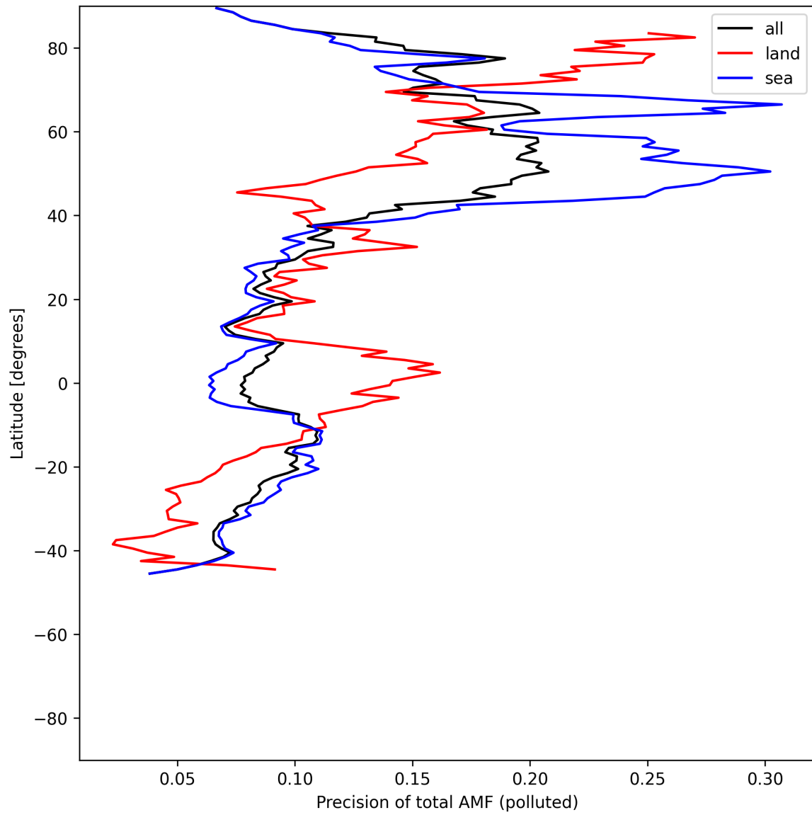
Figure 54: Zonal average of “Precision of total AMF (polluted)” for 2025-06-18 to 2025-06-20.
