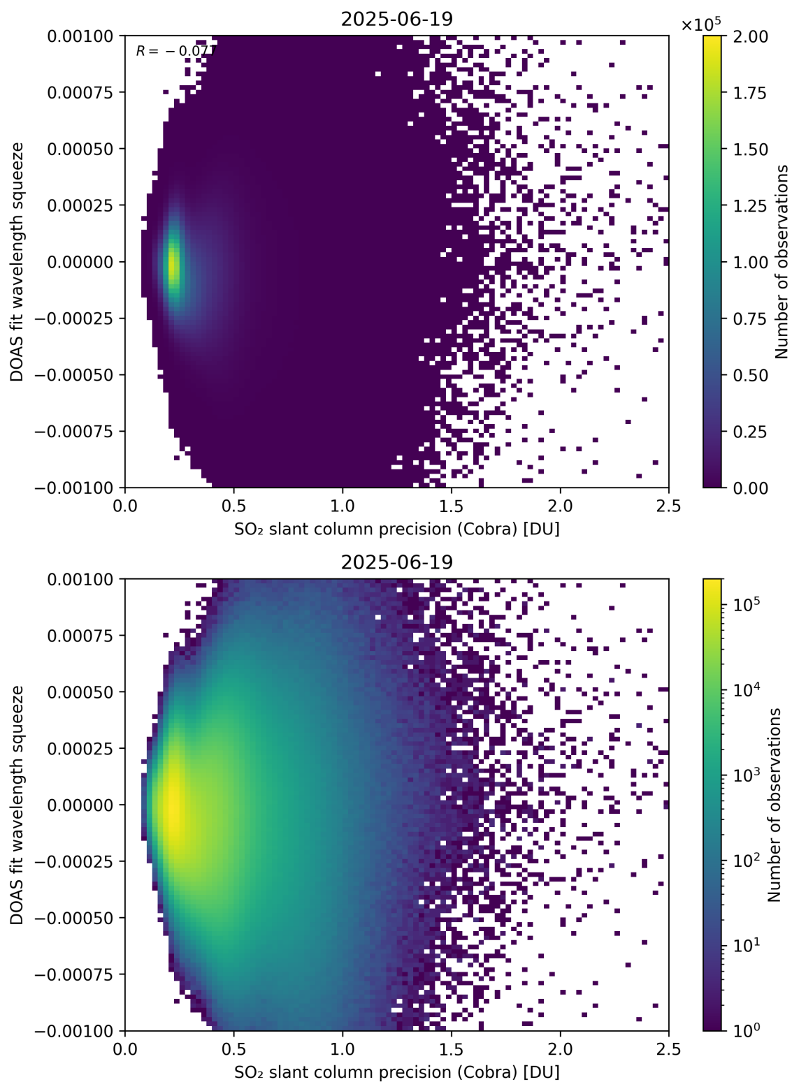
Figure 203: Scatter density plot of “SO 2 slant column precision (Cobra)” against “DOAS fit wavelength squeeze” for 2025-06-18 to 2025-06-20.
