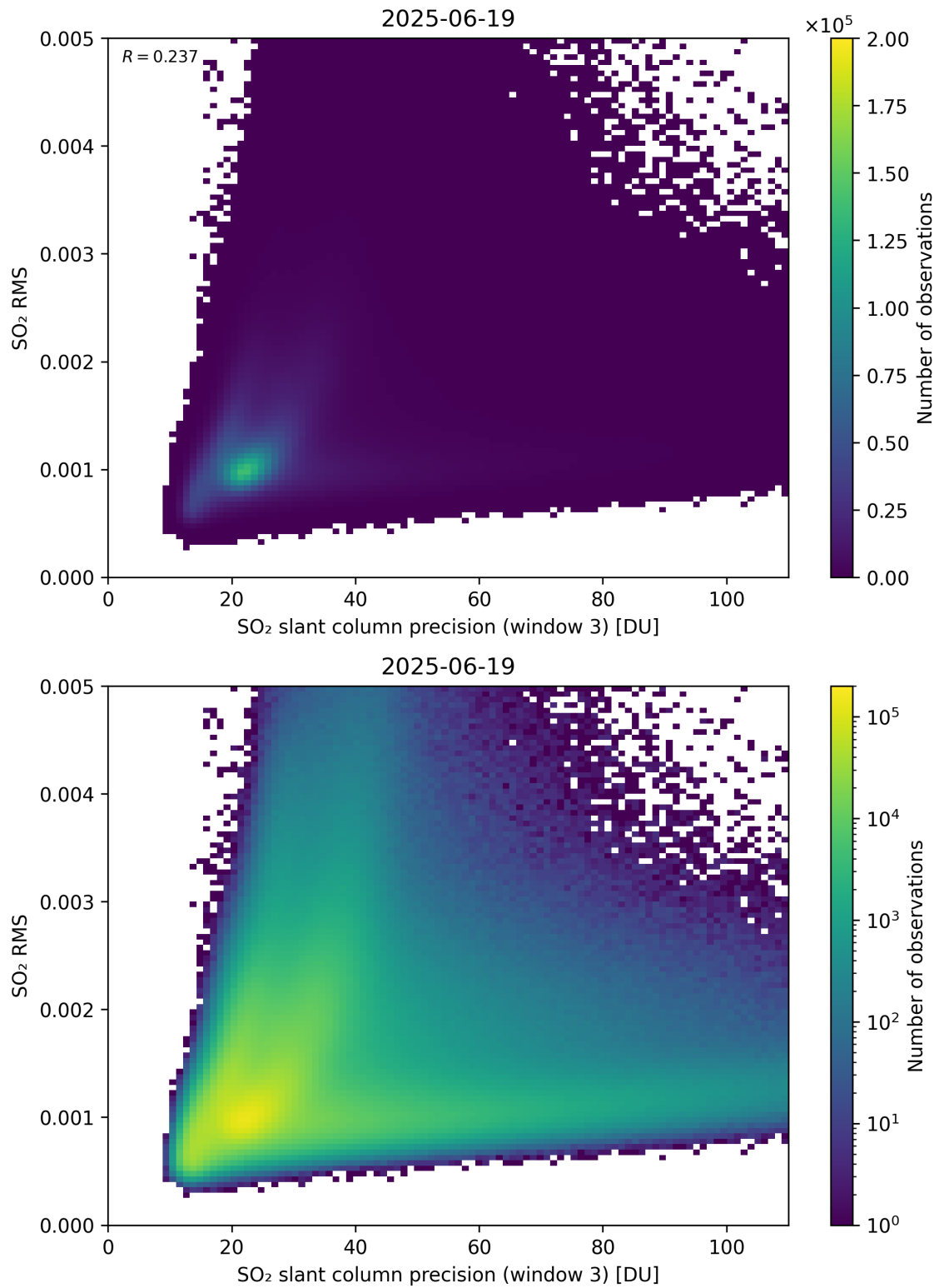
Figure 310: Scatter density plot of “SO 2 slant column precision (window 3)” against “SO 2 RMS” for 2025-06-18 to 2025-06-20.
