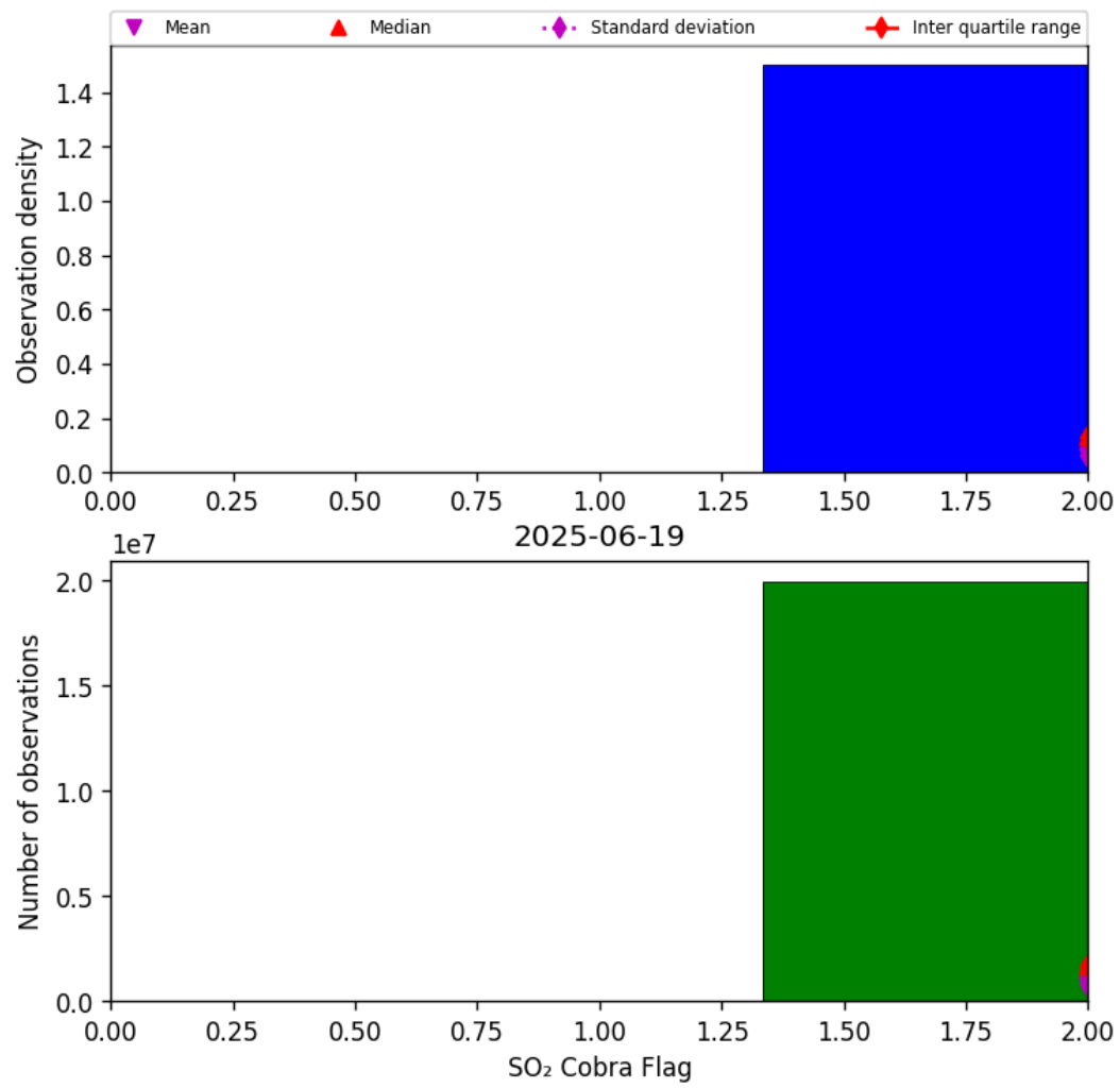
Figure 75: Histogram of “SO 2 Cobra Flag” for 2025-06-18 to 2025-06-20
