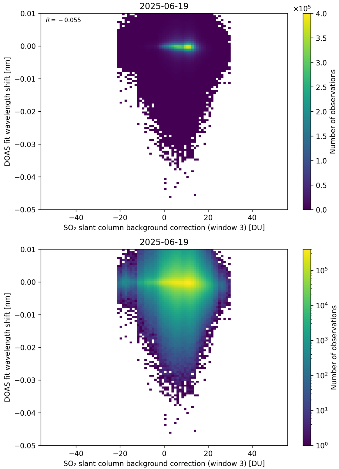
Figure 132: Scatter density plot of “SO 2 slant column background correction (window 3)” against “DOAS fit wavelength shift” for 2025-06-18 to 2025-06-20.
