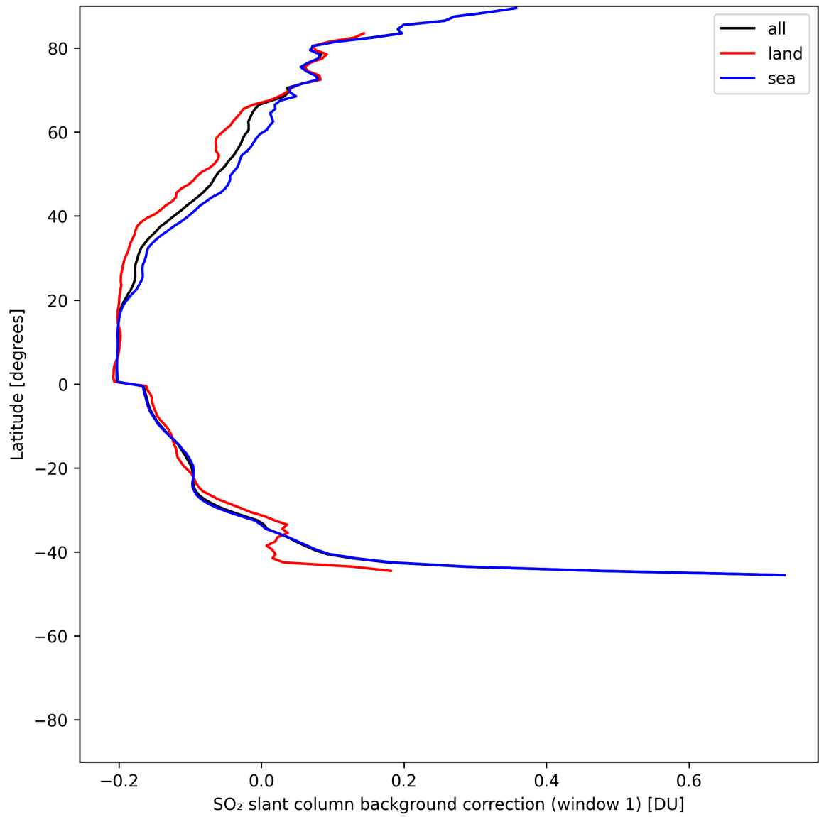
Figure 40: Zonal average of “SO 2 slant column background correction (window 1)” for 2025-06-18 to 2025-06-20.
