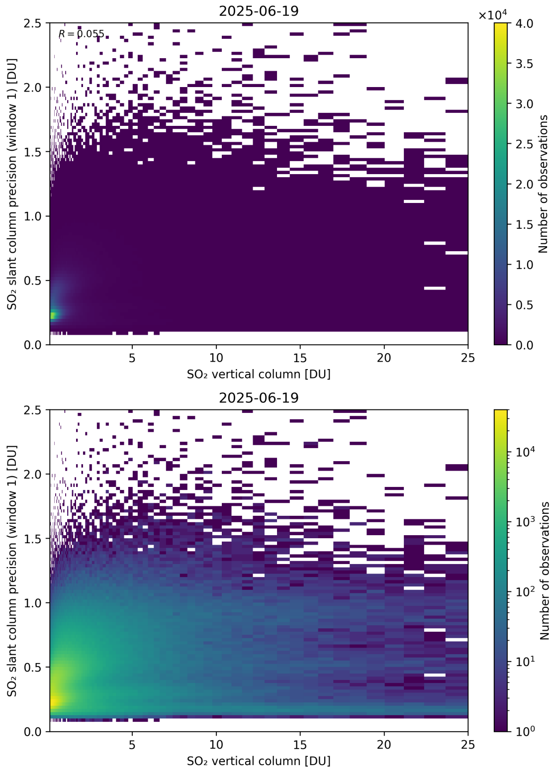
Figure 355: Scatter density plot of “SO 2 vertical column” against “SO 2 slant column precision (window 1)” for 2025-06-18 to 2025-06-20.
