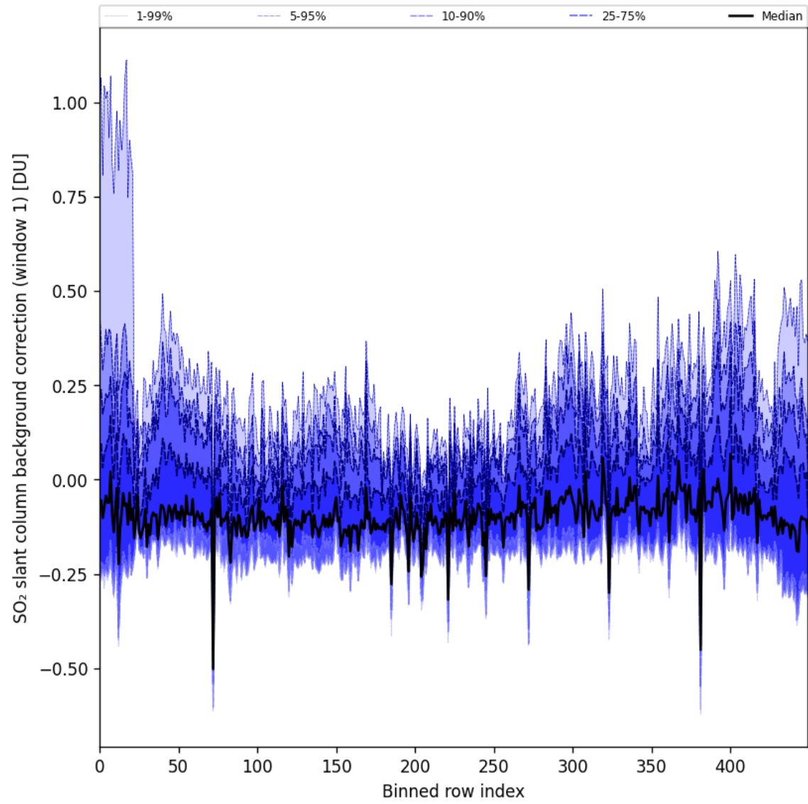
Figure 92: Along track statistics of “SO 2 slant column background correction (window 1)” for 2025-06-18 to 2025-06-20
