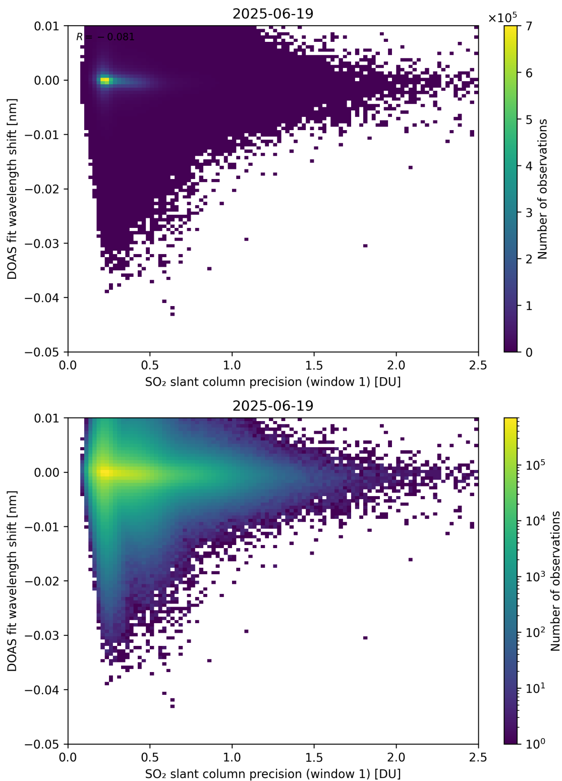
Figure 271: Scatter density plot of “SO 2 slant column precision (window 1)” against “DOAS fit wavelength shift” for 2025-06-18 to 2025-06-20.
