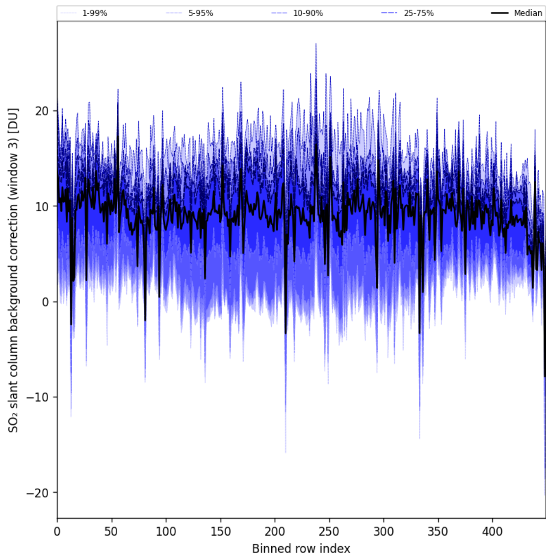
Figure 100: Along track statistics of "SO 2 slant column background correction (window 3)" for 2025-06-18 to 2025-06-20
