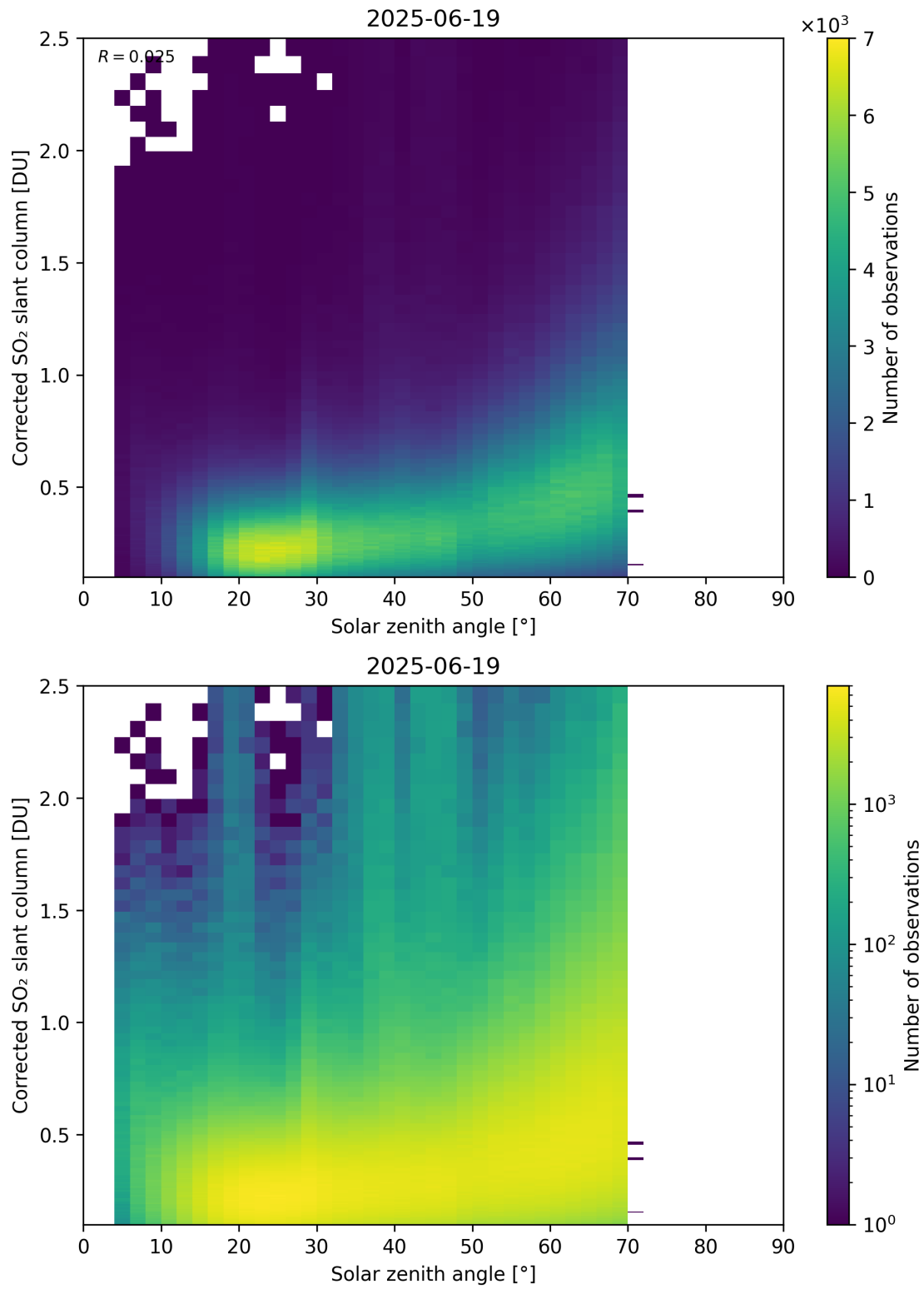
Figure 181: Scatter density plot of “Solar zenith angle” against “Corrected SO 2 slant column” for 2025-06-18 to 2025-06-20.
