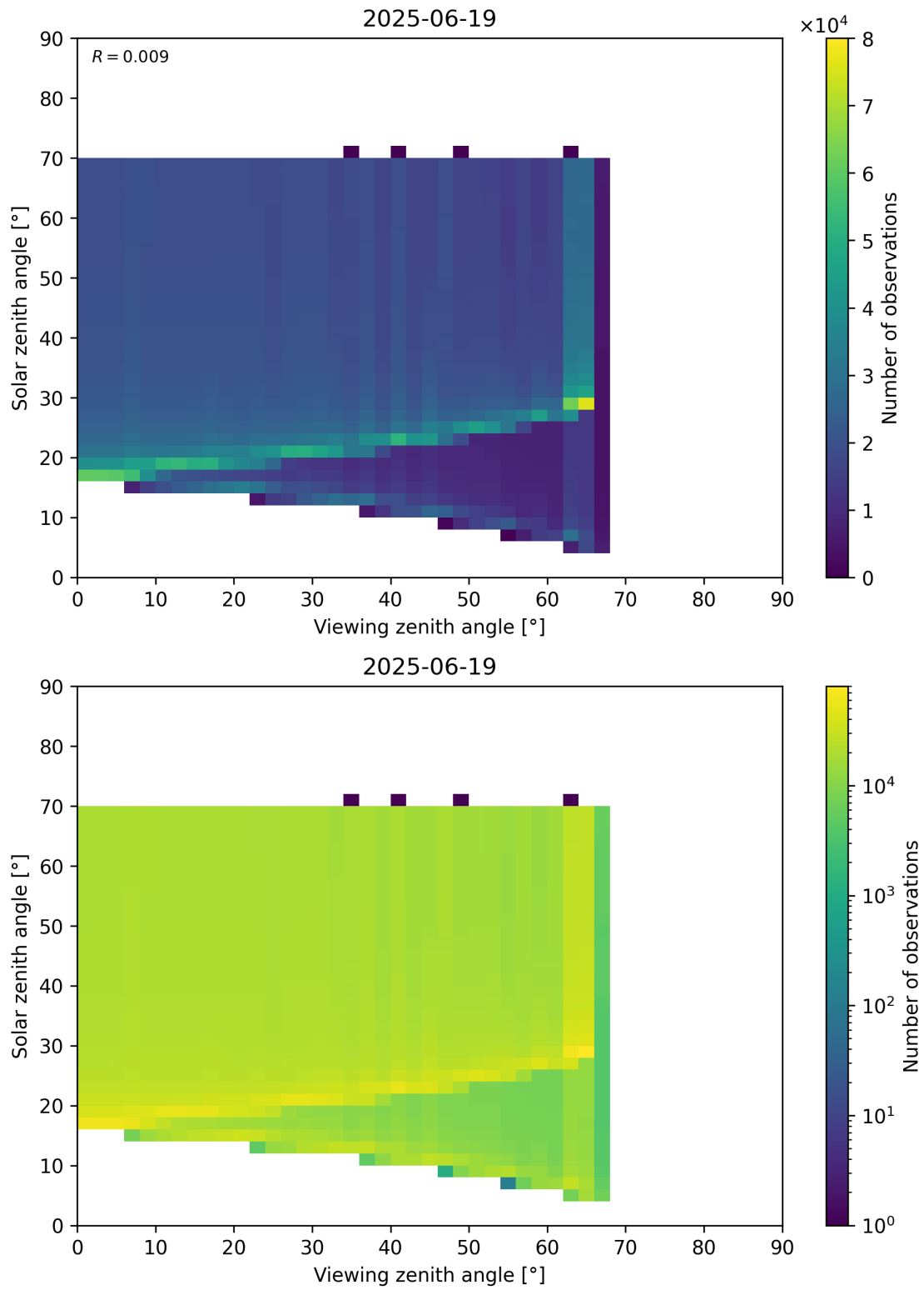
Figure 369: Scatter density plot of “Viewing zenith angle” against “Solar zenith angle” for 2025-06-18 to 2025-06-20.
