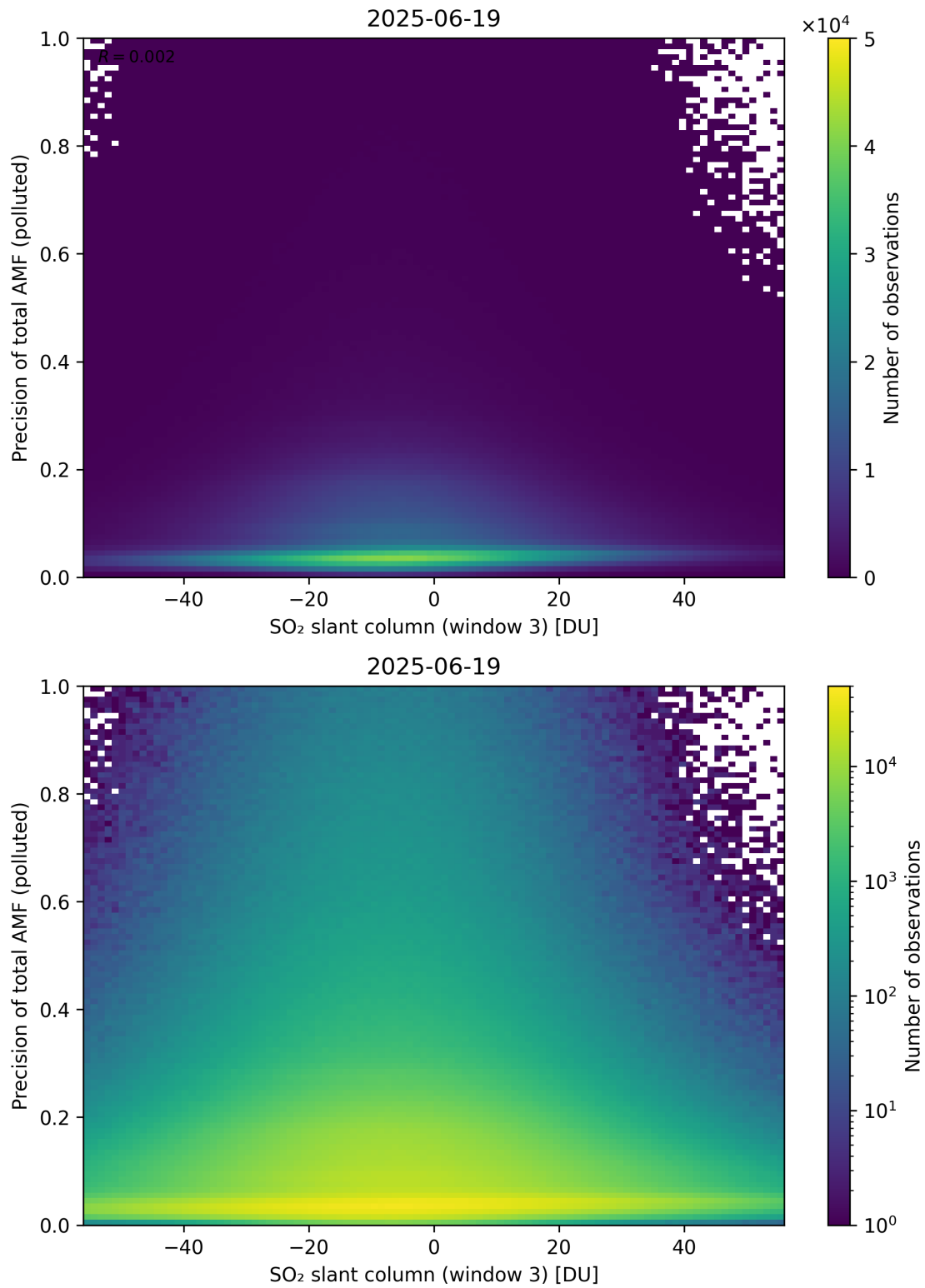
Figure 319: Scatter density plot of “SO 2 slant column (window 3)” against “Precision of total AMF (polluted)” for 2025-06-18 to 2025-06-20.
