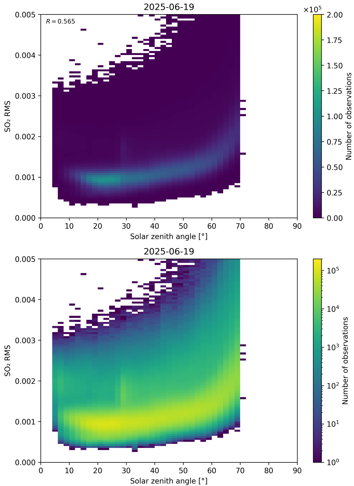
Figure 176: Scatter density plot of “Solar zenith angle” against “SO 2 RMS” for 2025-06-18 to 2025-06-20.
