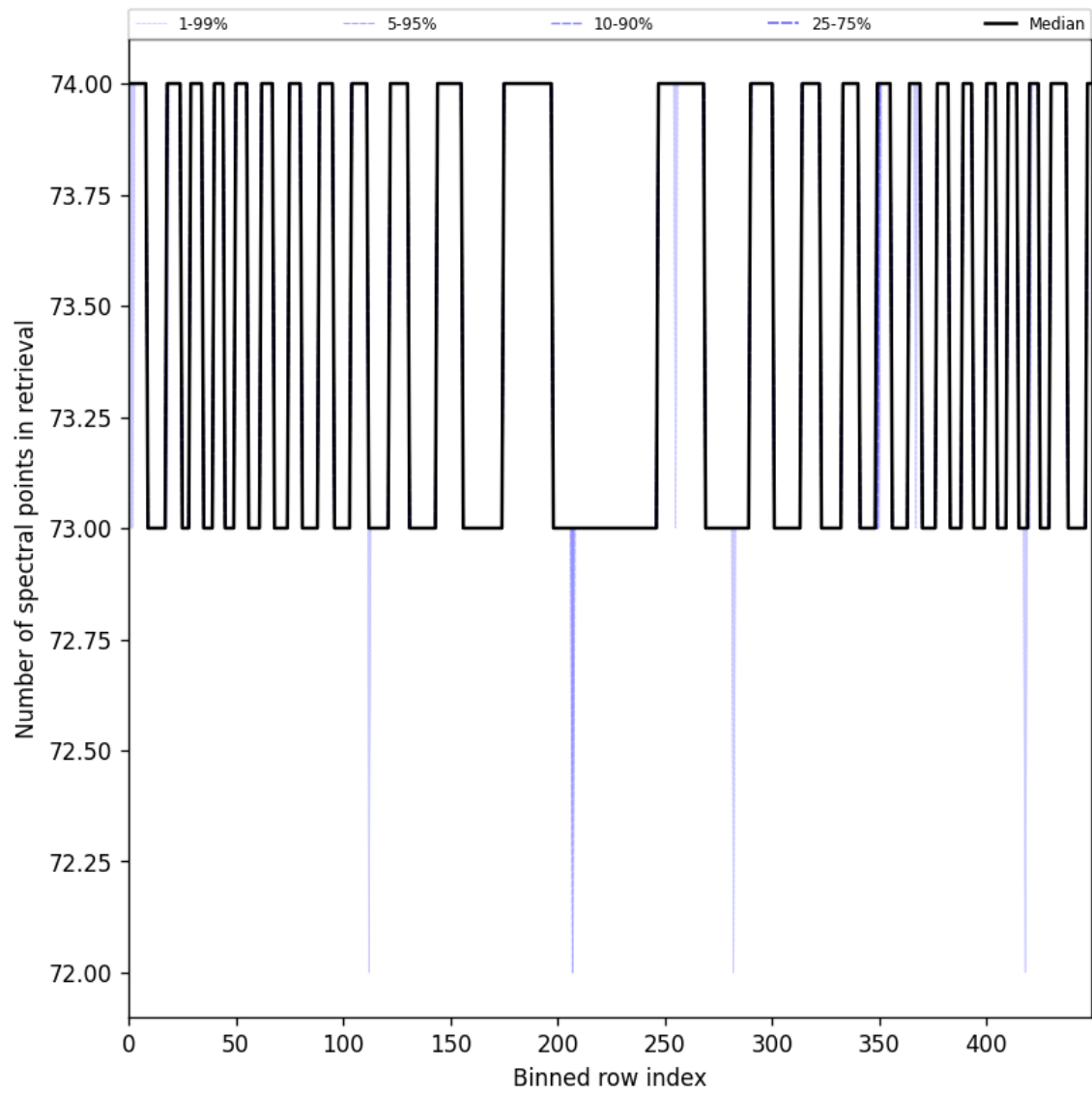
Figure 108: Along track statistics of “Number of spectral points in retrieval” for 2025-06-18 to 2025-06-20
