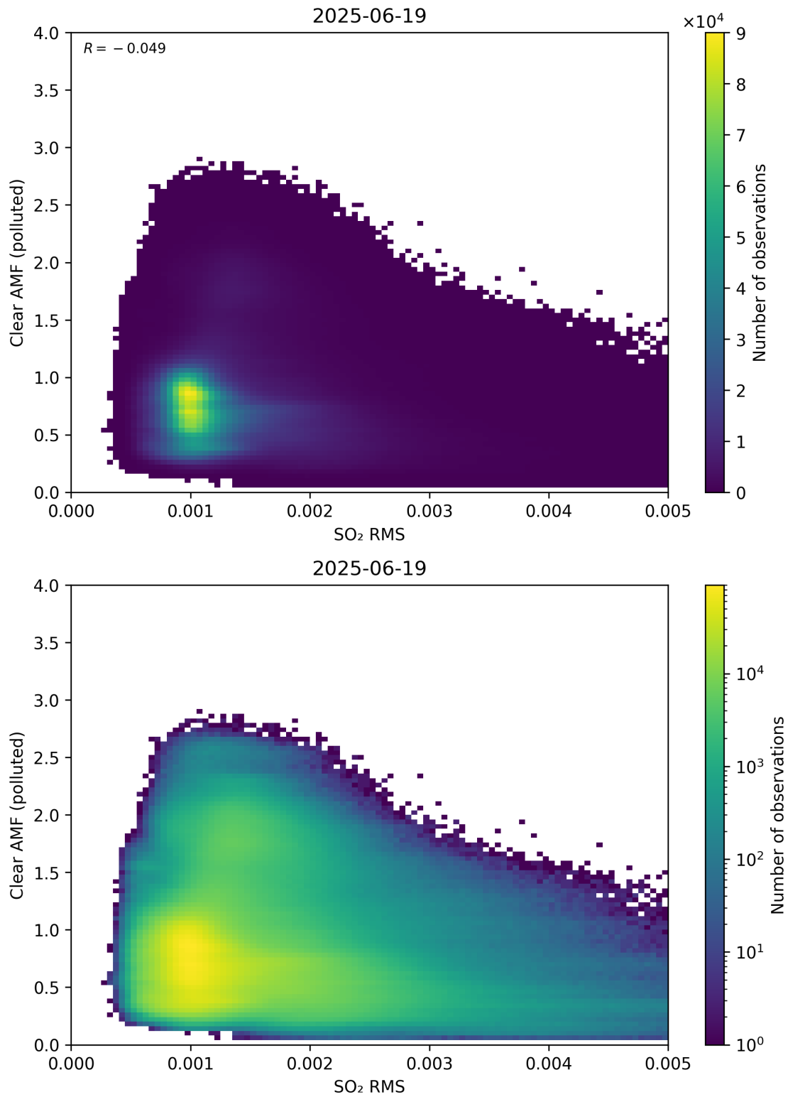
Figure 147: Scatter density plot of “SO 2 RMS” against “Clear AMF (polluted)” for 2025-06-18 to 2025-06-20.
