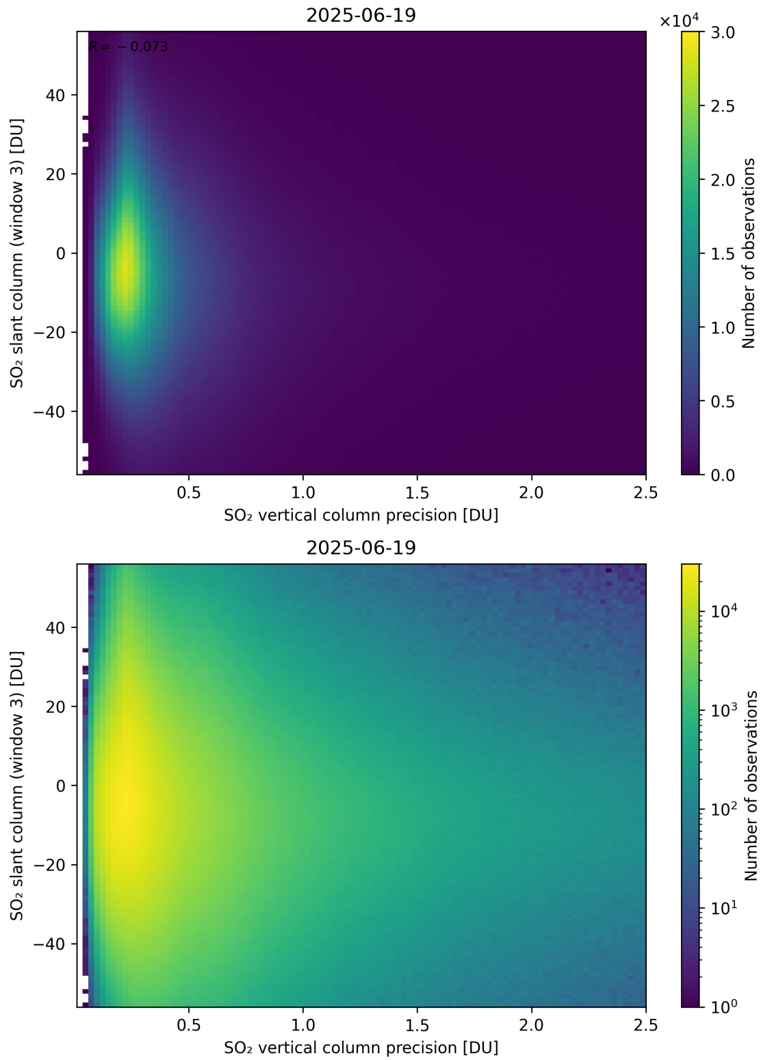
Figure 344: Scatter density plot of “SO 2 vertical column precision” against “SO 2 slant column (window 3)” for 2025-06-18 to 2025-06-20.
