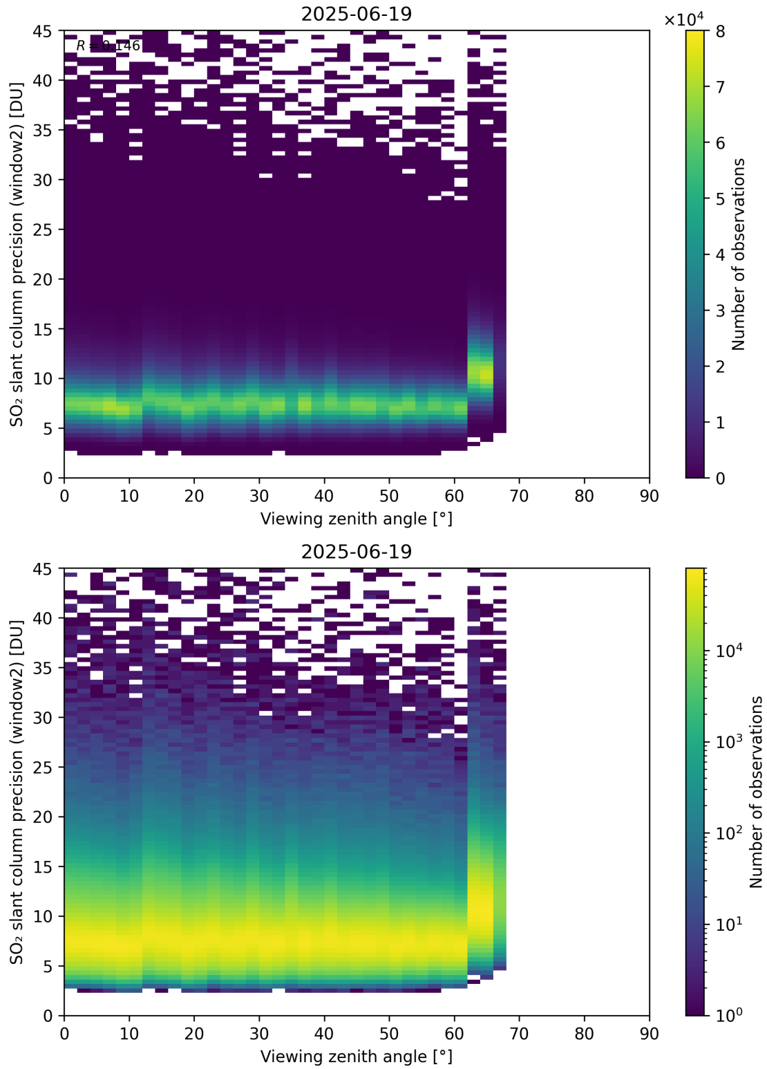
Figure 378: Scatter density plot of “Viewing zenith angle” against “SO 2 slant column precision (window2)” for 2025-06-18 to 2025-06-20.
