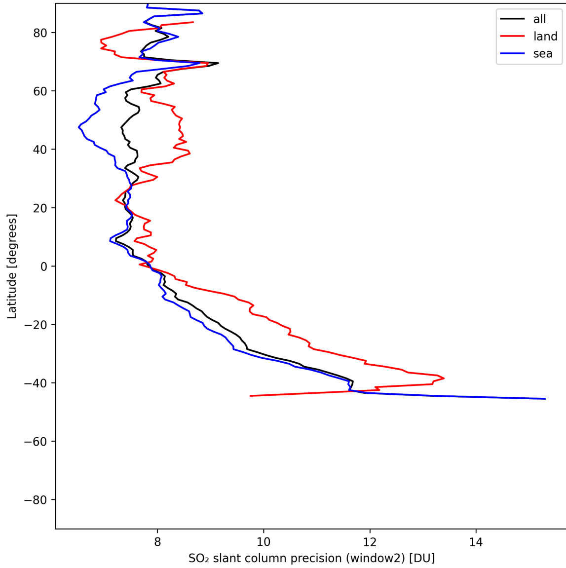
Figure 42: Zonal average of “SO 2 slant column precision (window2)” for 2025-06-18 to 2025-06-20.
