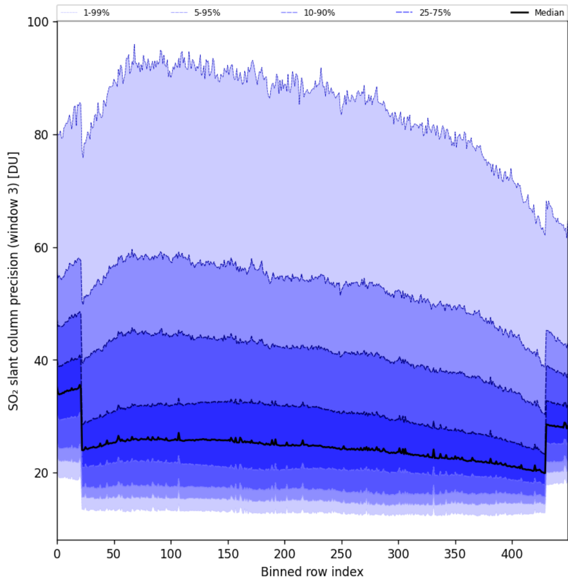
Figure 98: Along track statistics of “SO 2 slant column precision (window 3)” for 2025-06-18 to 2025-06-20
