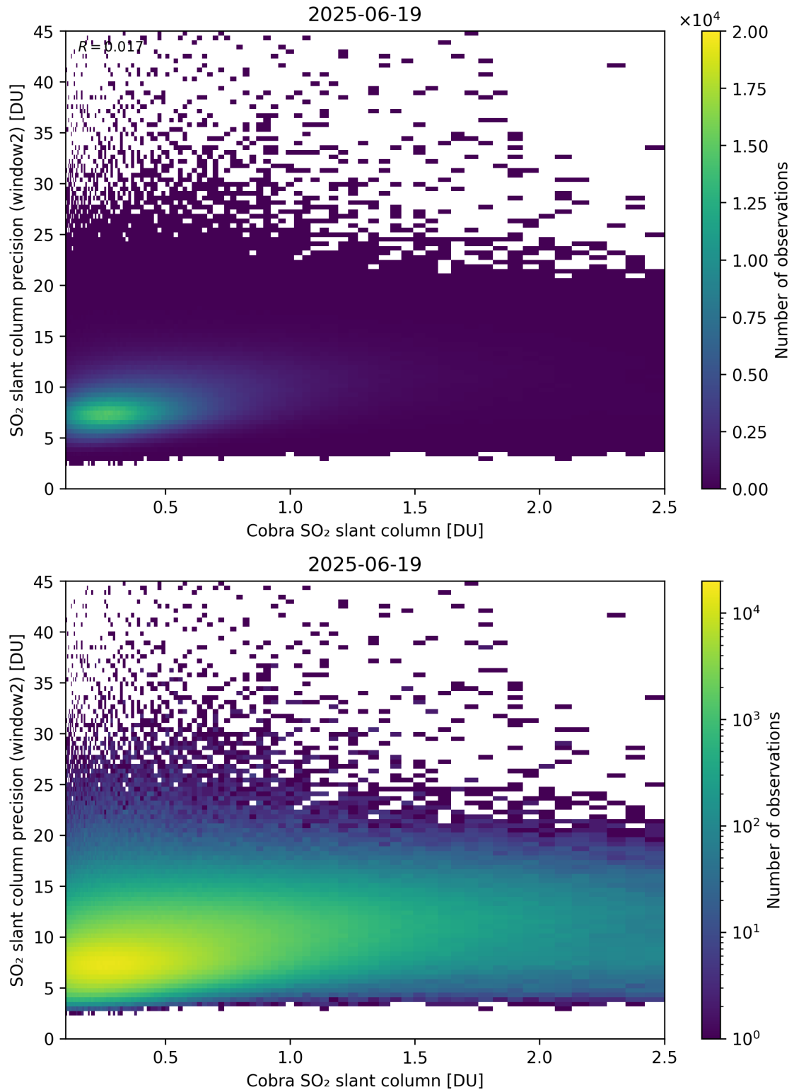
Figure 221: Scatter density plot of “Cobra SO 2 slant column” against “SO 2 slant column precision (window2)” for 2025-06-18 to 2025-06-20.
