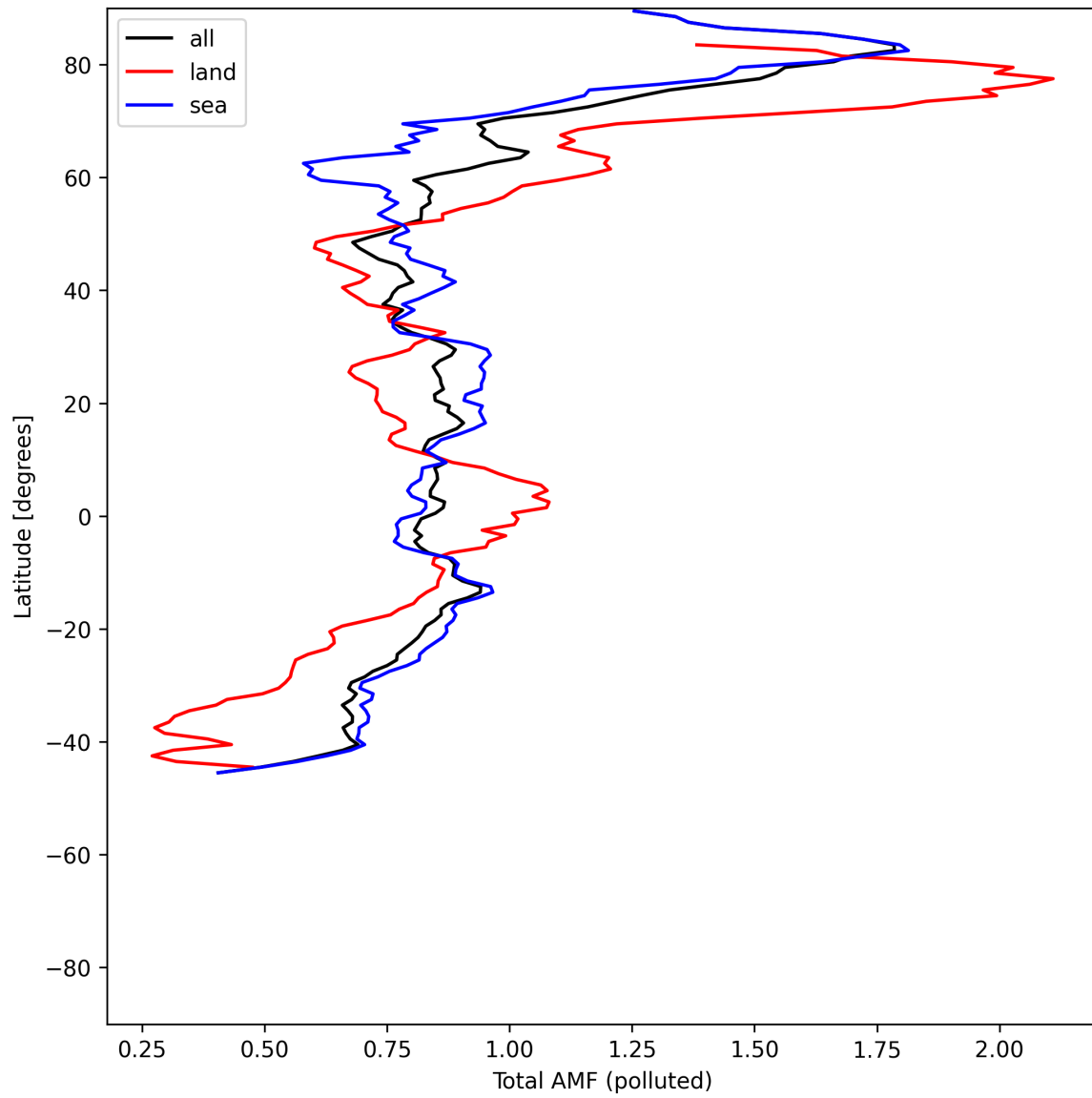
Figure 53: Zonal average of “Total AMF (polluted)” for 2025-06-18 to 2025-06-20.
