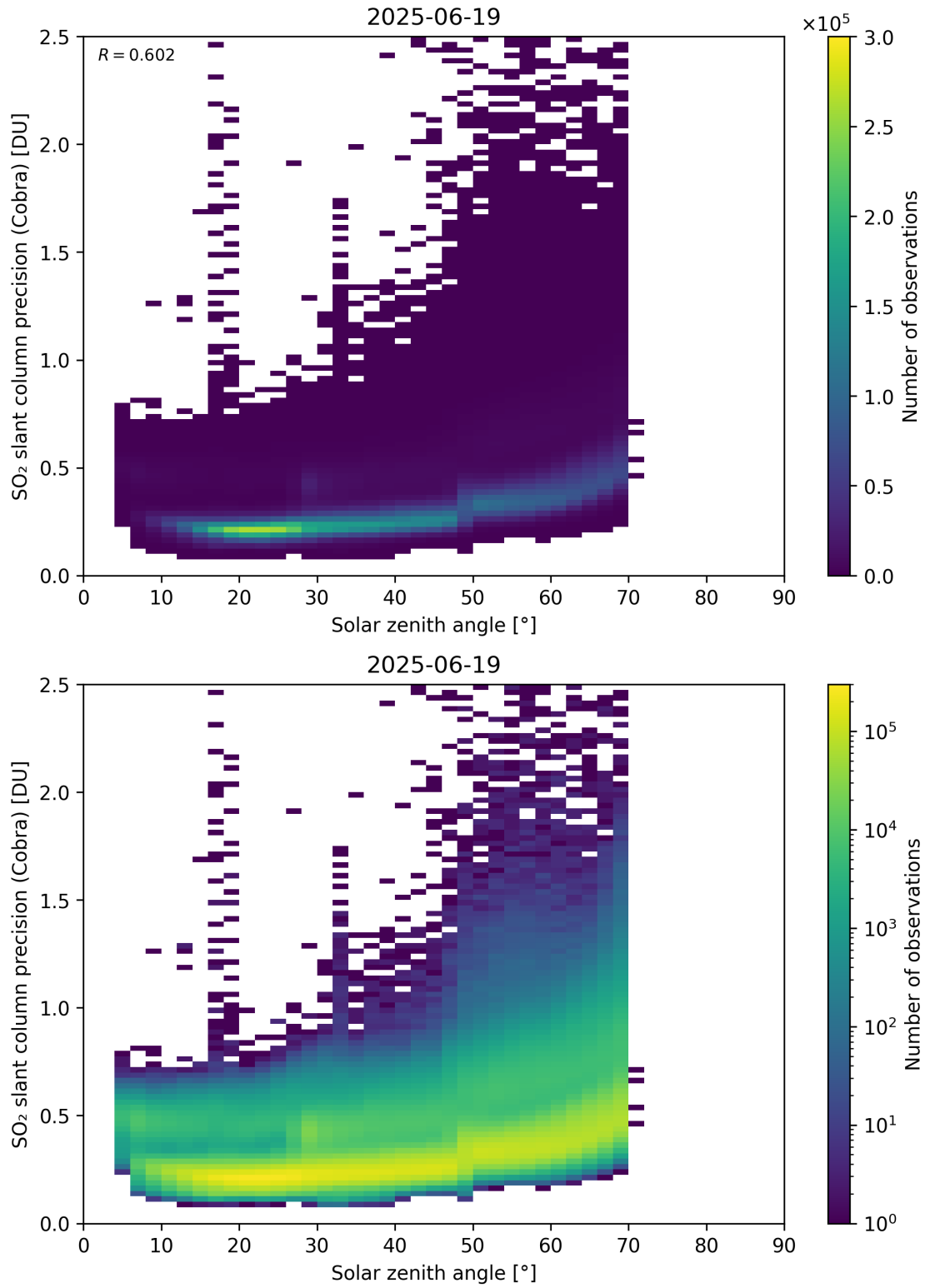
Figure 180: Scatter density plot of “Solar zenith angle” against “SO 2 slant column precision (Cobra)” for 2025-06-18 to 2025-06-20.
