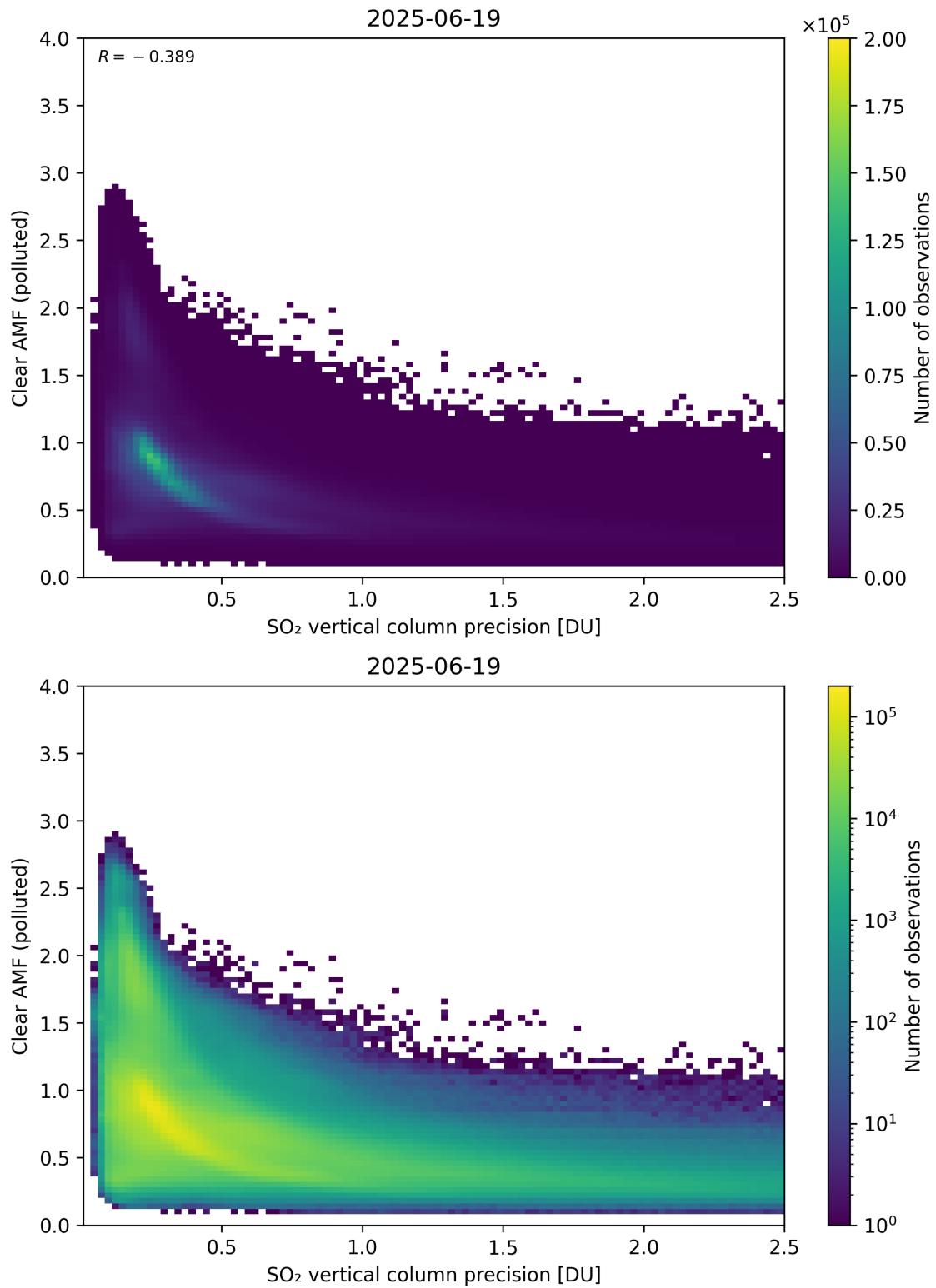
Figure 335: Scatter density plot of “SO 2 vertical column precision” against “Clear AMF (polluted)” for 2025-06-18 to 2025-06-20.
