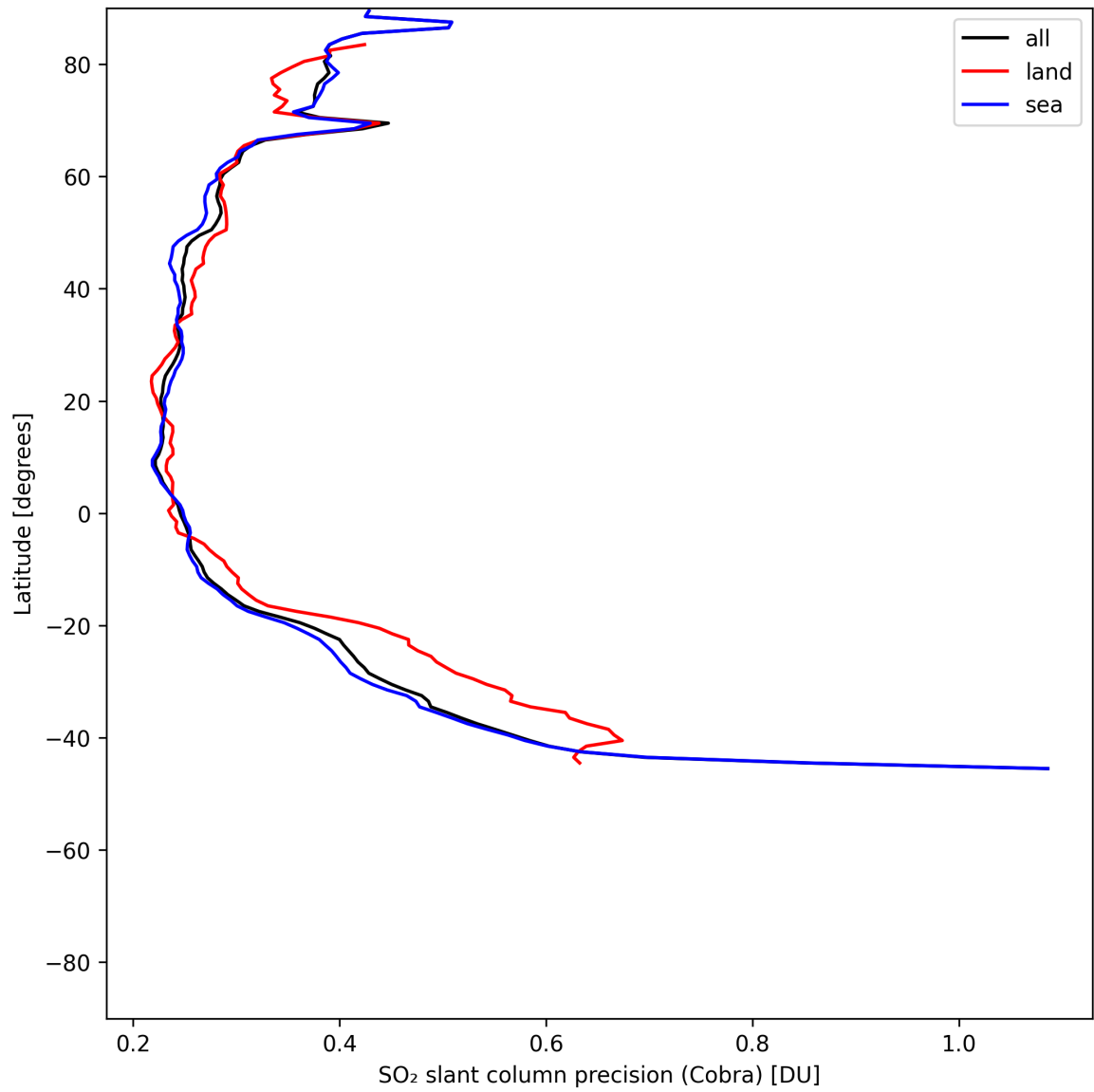
Figure 36: Zonal average of “SO 2 slant column precision (Cobra)” for 2025-06-18 to 2025-06-20.
