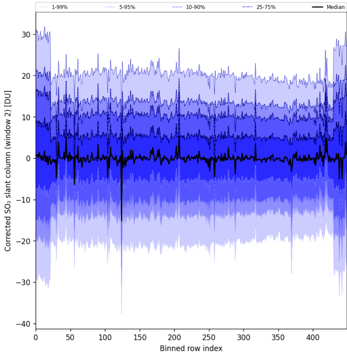
Figure 95: Along track statistics of “Corrected SO 2 slant column (window 2)” for 2025-06-18 to 2025-06-20
