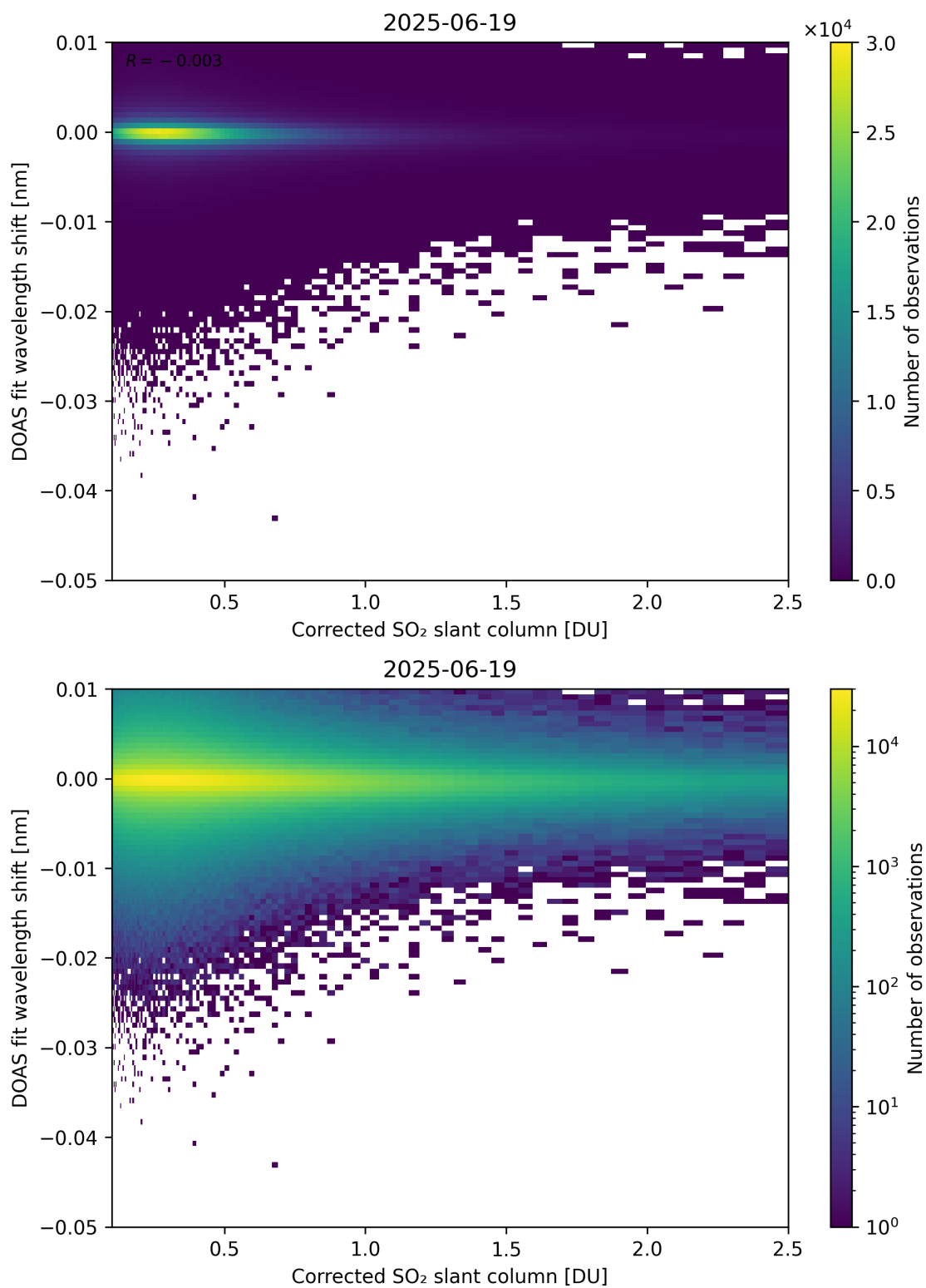
Figure 229: Scatter density plot of “Corrected SO 2 slant column” against “DOAS fit wavelength shift” for 2025-06-18 to 2025-06-20.
