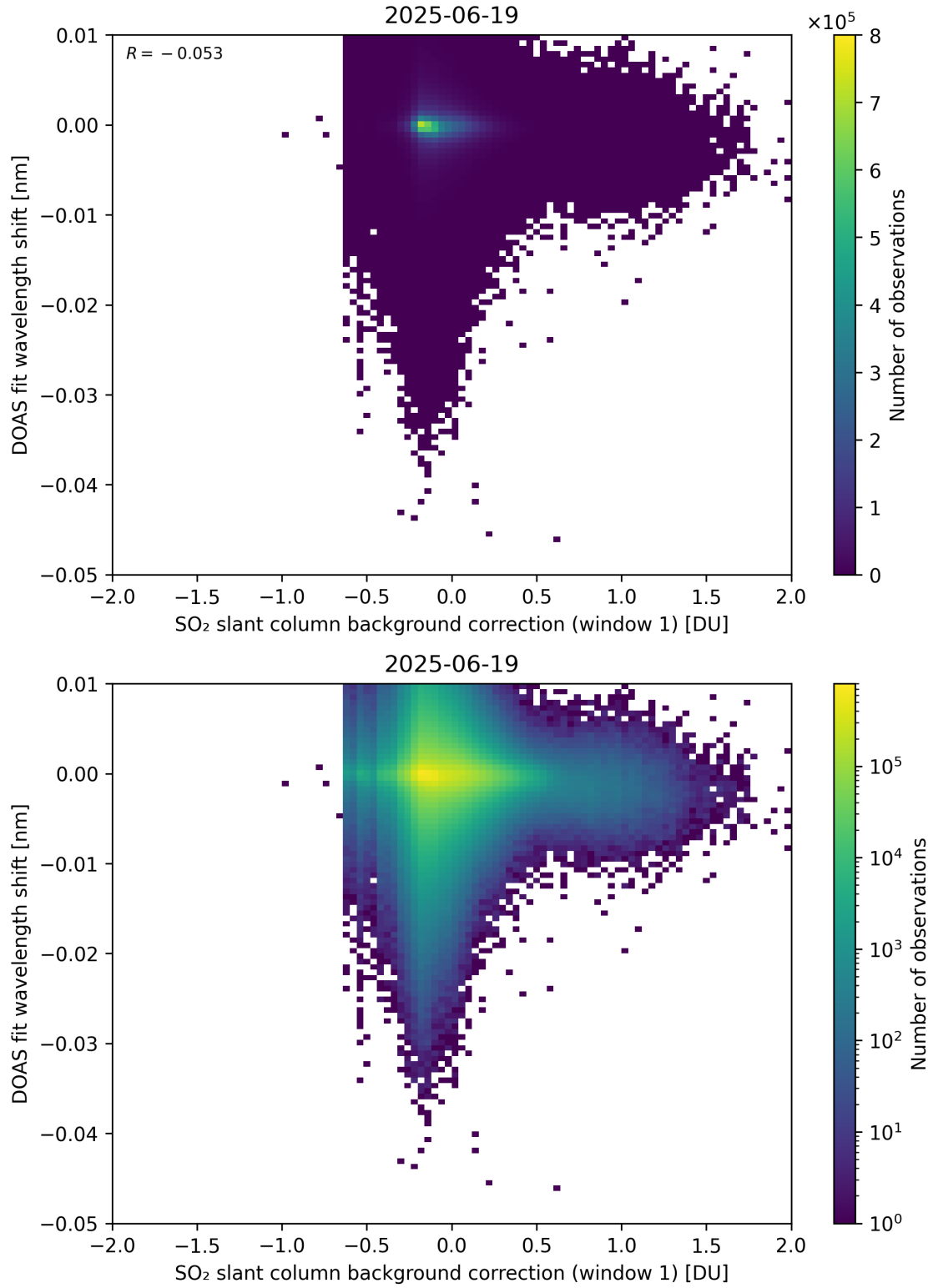
Figure 111: Scatter density plot of “SO 2 slant column background correction (window 1)” against “DOAS fit wavelength shift” for 2025-06-18 to 2025-06-20.
