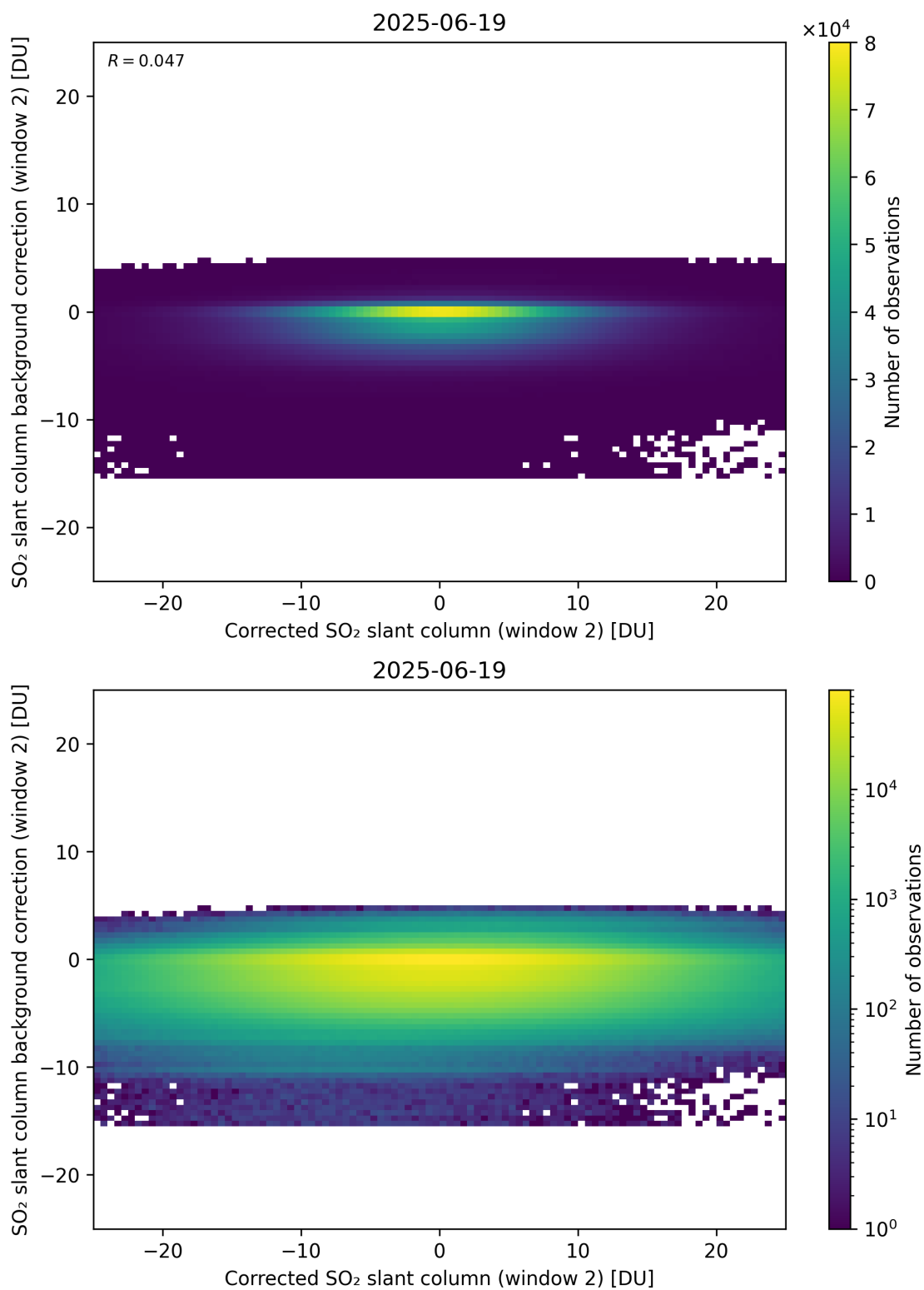
Figure 244: Scatter density plot of “Corrected SO 2 slant column (window 2)” against “SO 2 slant column background correction (window 2)” for 2025-06-18 to 2025-06-20.
