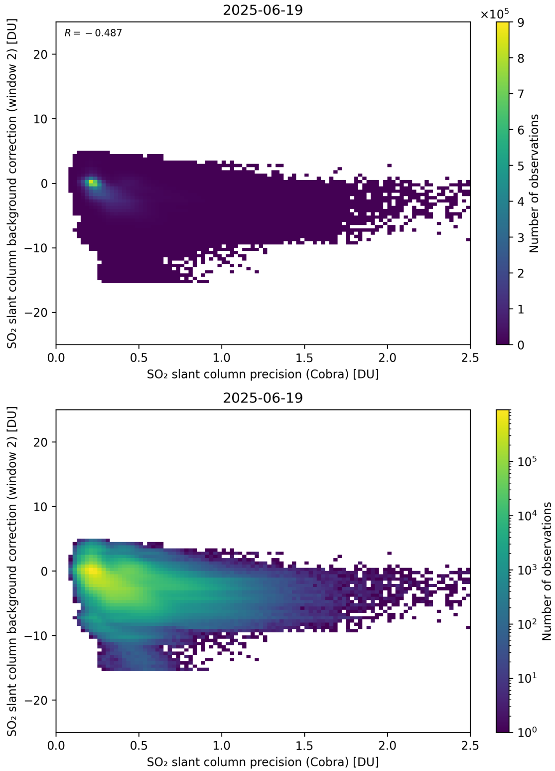
Figure 200: Scatter density plot of “SO 2 slant column precision (Cobra)” against “SO 2 slant column background correction (window 2)” for 2025-06-18 to 2025-06-20.
