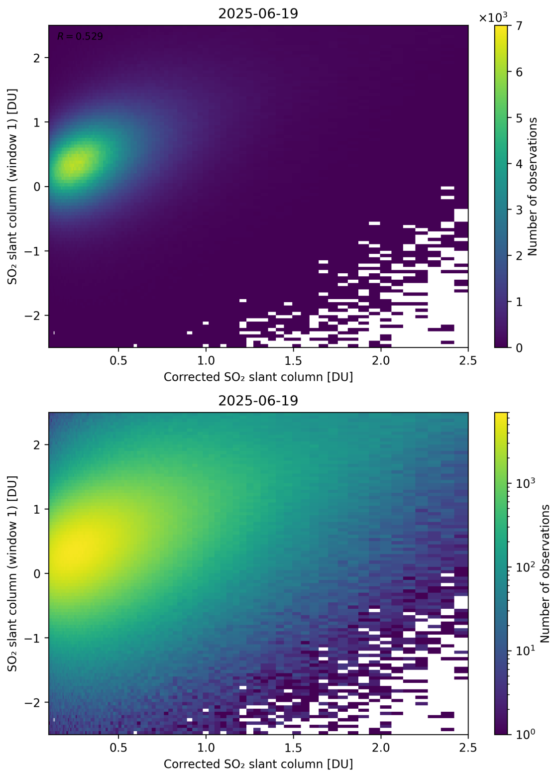
Figure 237: Scatter density plot of “Corrected SO 2 slant column” against “SO 2 slant column (window 1)” for 2025-06-18 to 2025-06-20.
