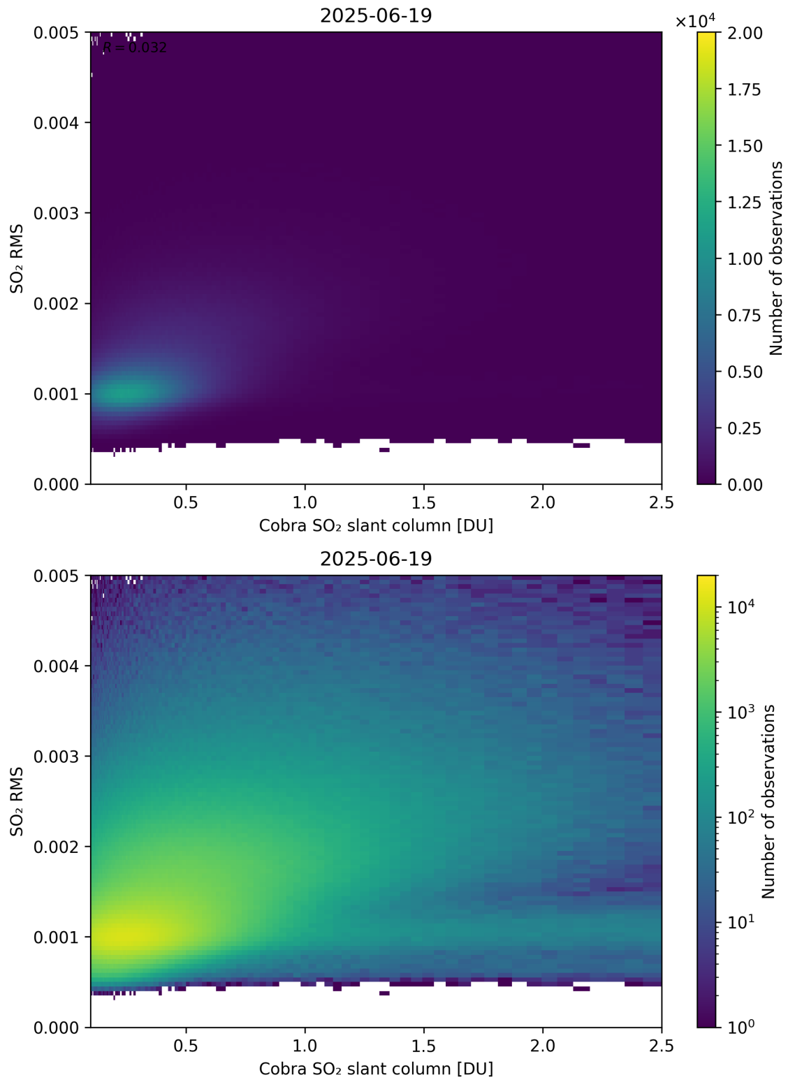
Figure 198: Scatter density plot of “Cobra SO 2 slant column” against “SO 2 RMS” for 2025-06-18 to 2025-06-20.
