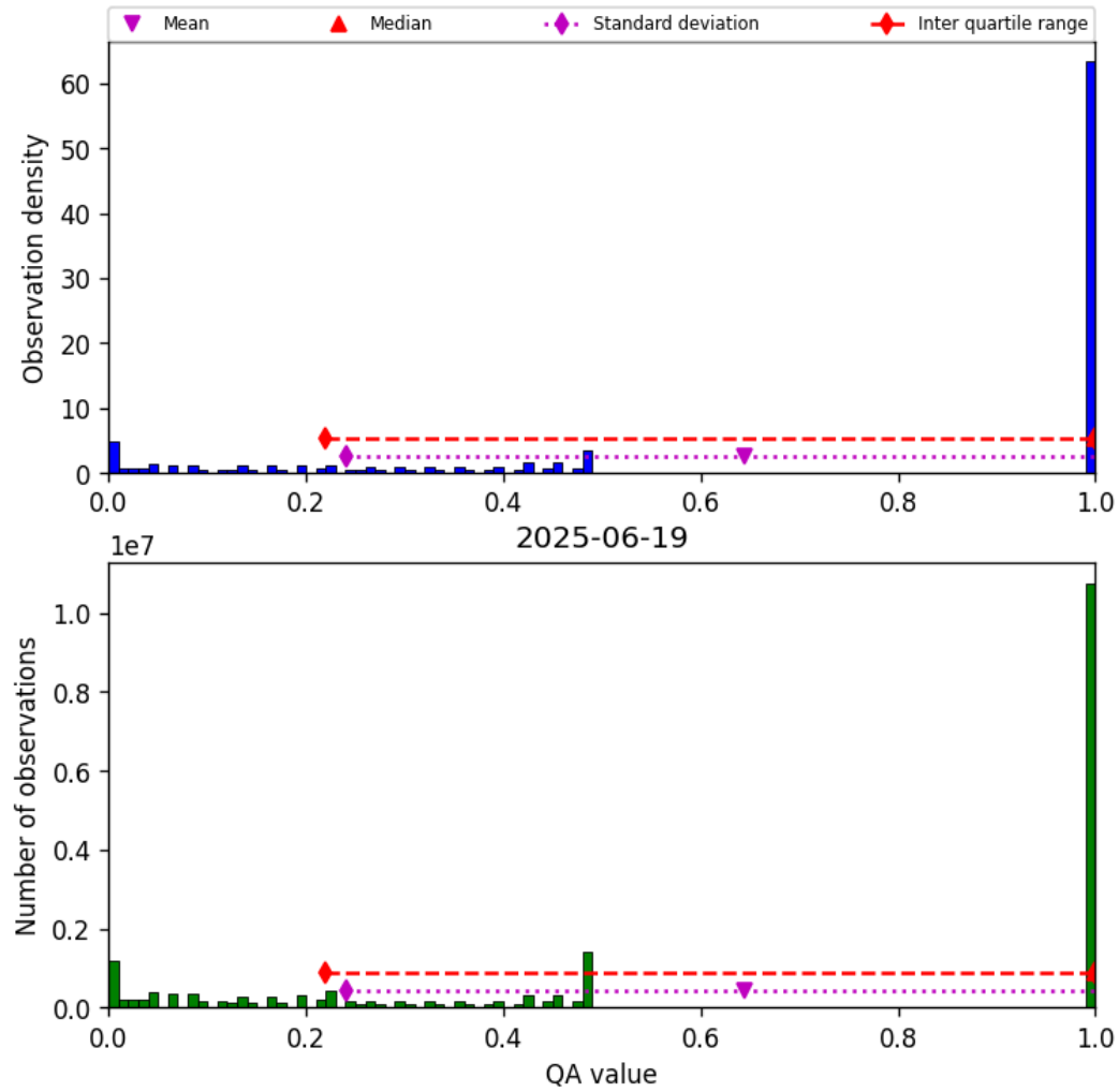
Figure 57: Histogram of “QA value” for 2025-06-18 to 2025-06-20
