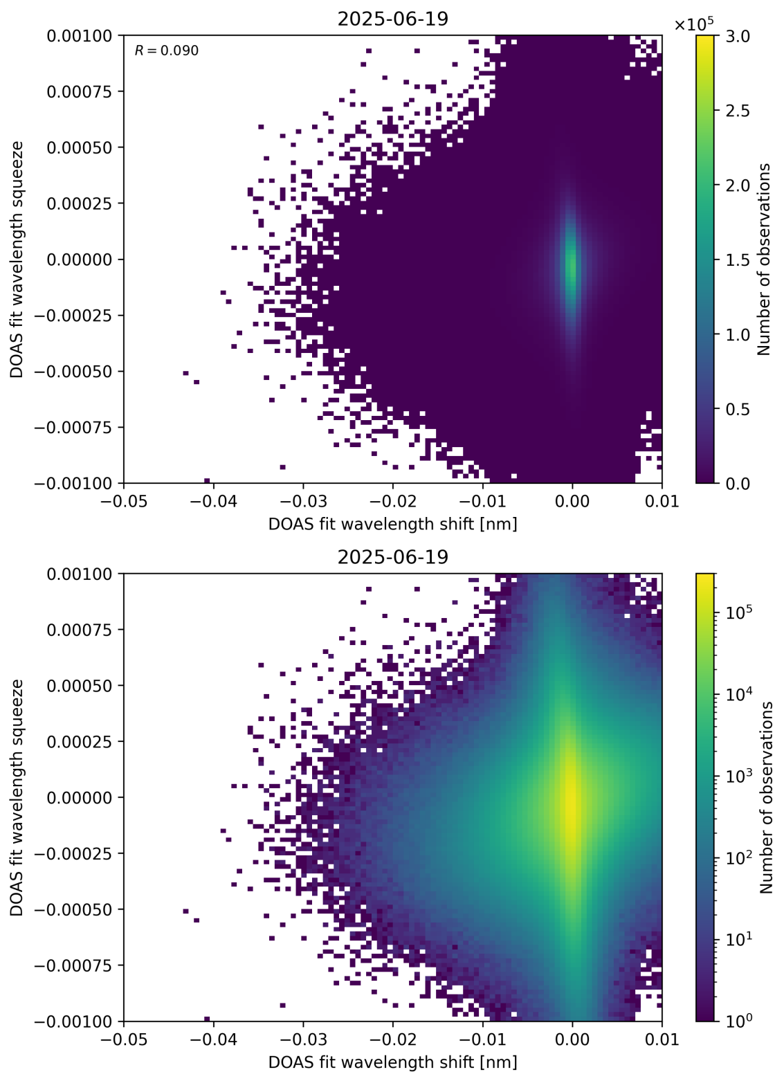
Figure 138: Scatter density plot of “DOAS fit wavelength shift” against “DOAS fit wavelength squeeze” for 2025-06-18 to 2025-06-20.
