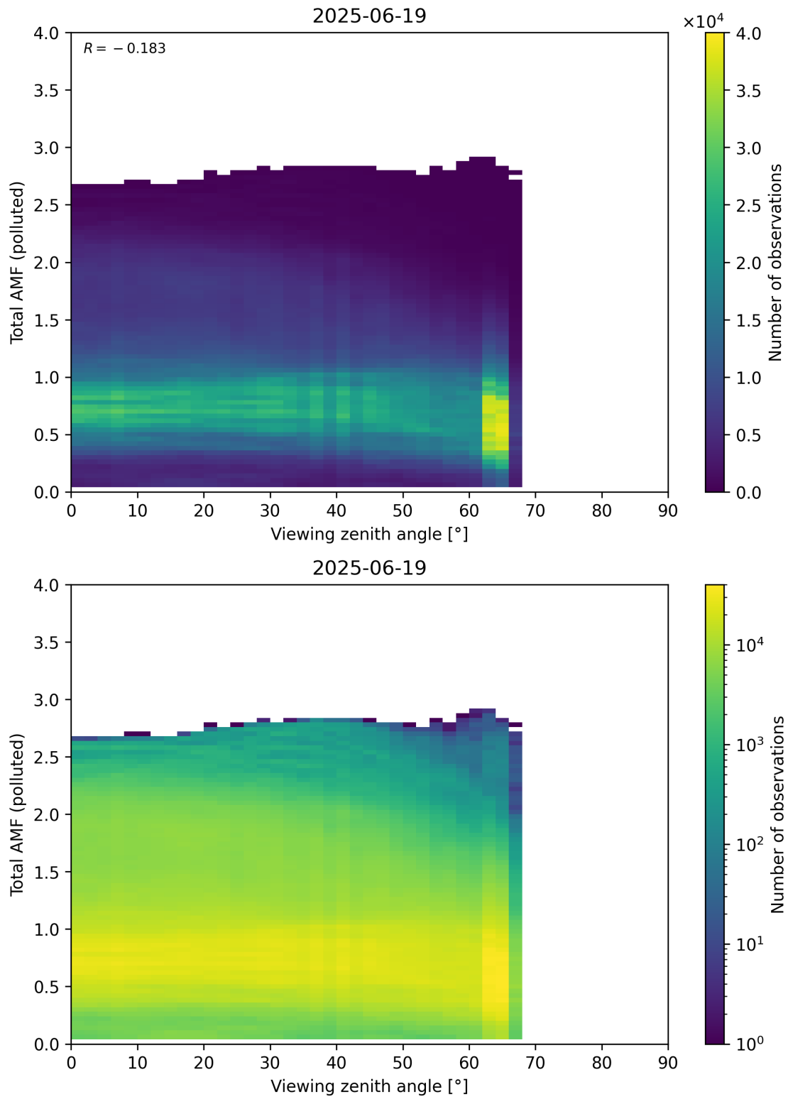
Figure 381: Scatter density plot of “Viewing zenith angle” against “Total AMF (polluted)” for 2025-06-18 to 2025-06-20.
