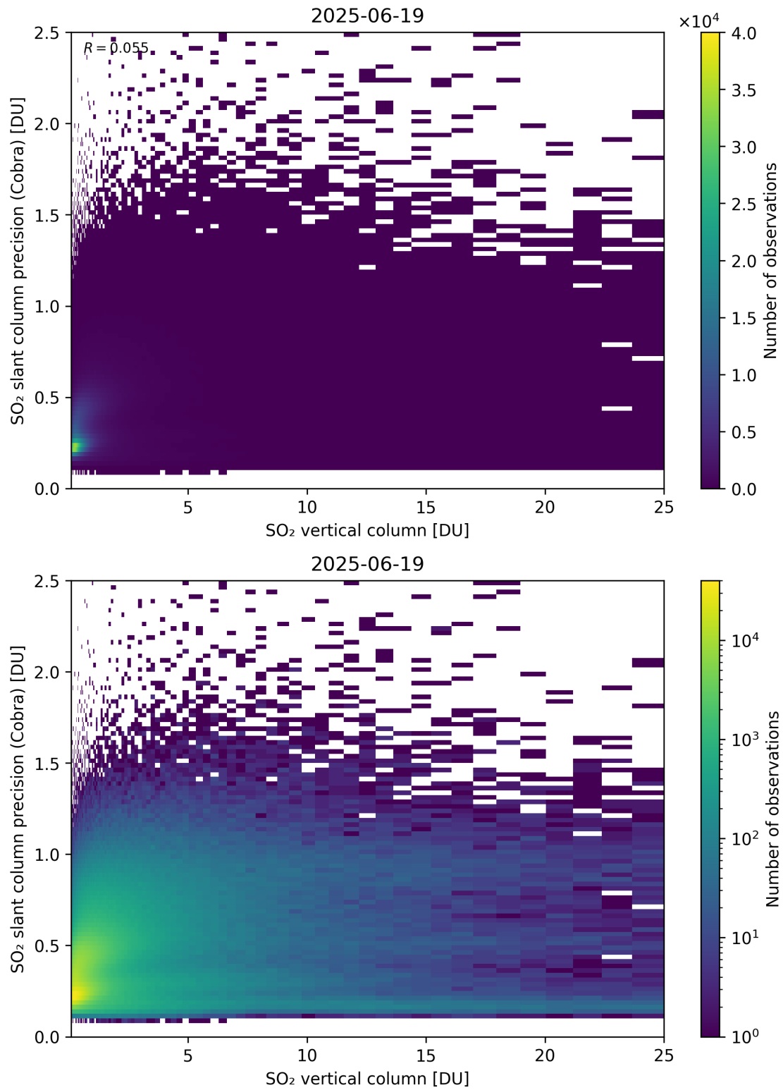
Figure 350: Scatter density plot of “SO 2 vertical column” against “SO 2 slant column precision (Cobra)” for 2025-06-18 to 2025-06-20.
