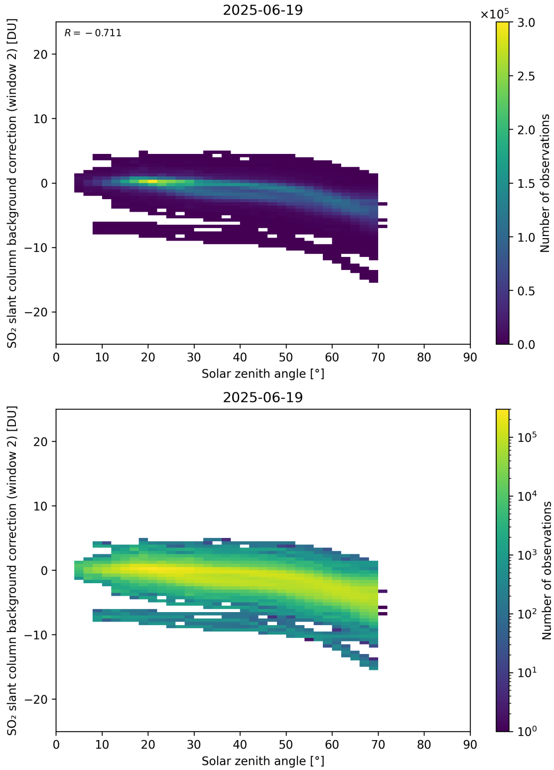
Figure 172: Scatter density plot of “Solar zenith angle” against “SO 2 slant column background correction (window 2)” for 2025-06-18 to 2025-06-20.
