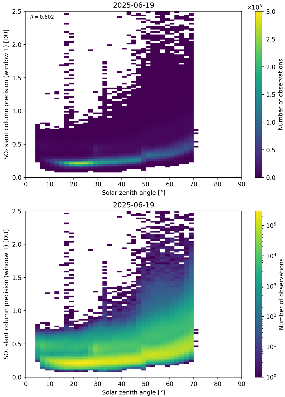
Figure 185: Scatter density plot of “Solar zenith angle” against “SO 2 slant column precision (window 1)” for 2025-06-18 to 2025-06-20.
