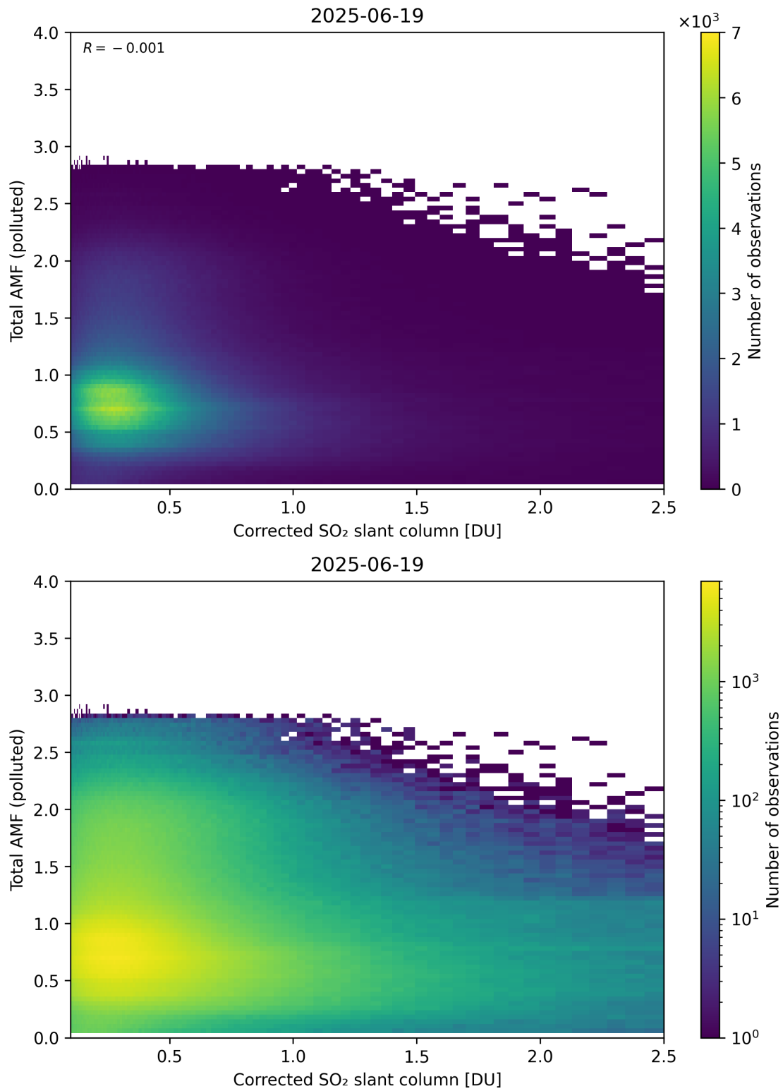
Figure 242: Scatter density plot of “Corrected SO 2 slant column” against “Total AMF (polluted)” for 2025-06-18 to 2025-06-20.
