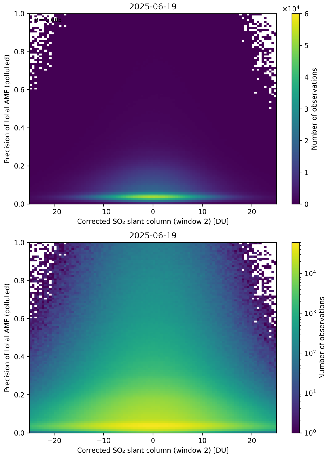
Figure 254: Scatter density plot of “Corrected SO 2 slant column (window 2)” against “Precision of total AMF (polluted)” for 2025-06-18 to 2025-06-20.
