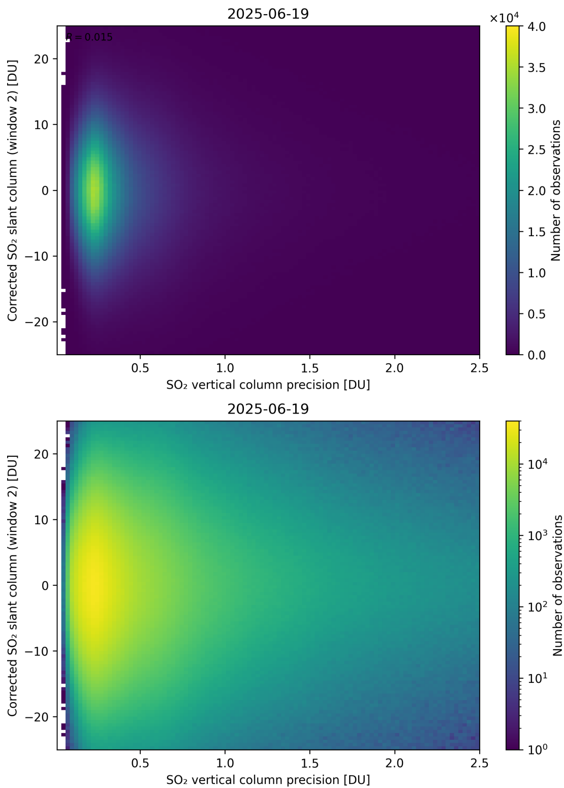
Figure 339: Scatter density plot of “SO 2 vertical column precision” against “Corrected SO 2 slant column (window 2)” for 2025-06-18 to 2025-06-20.
