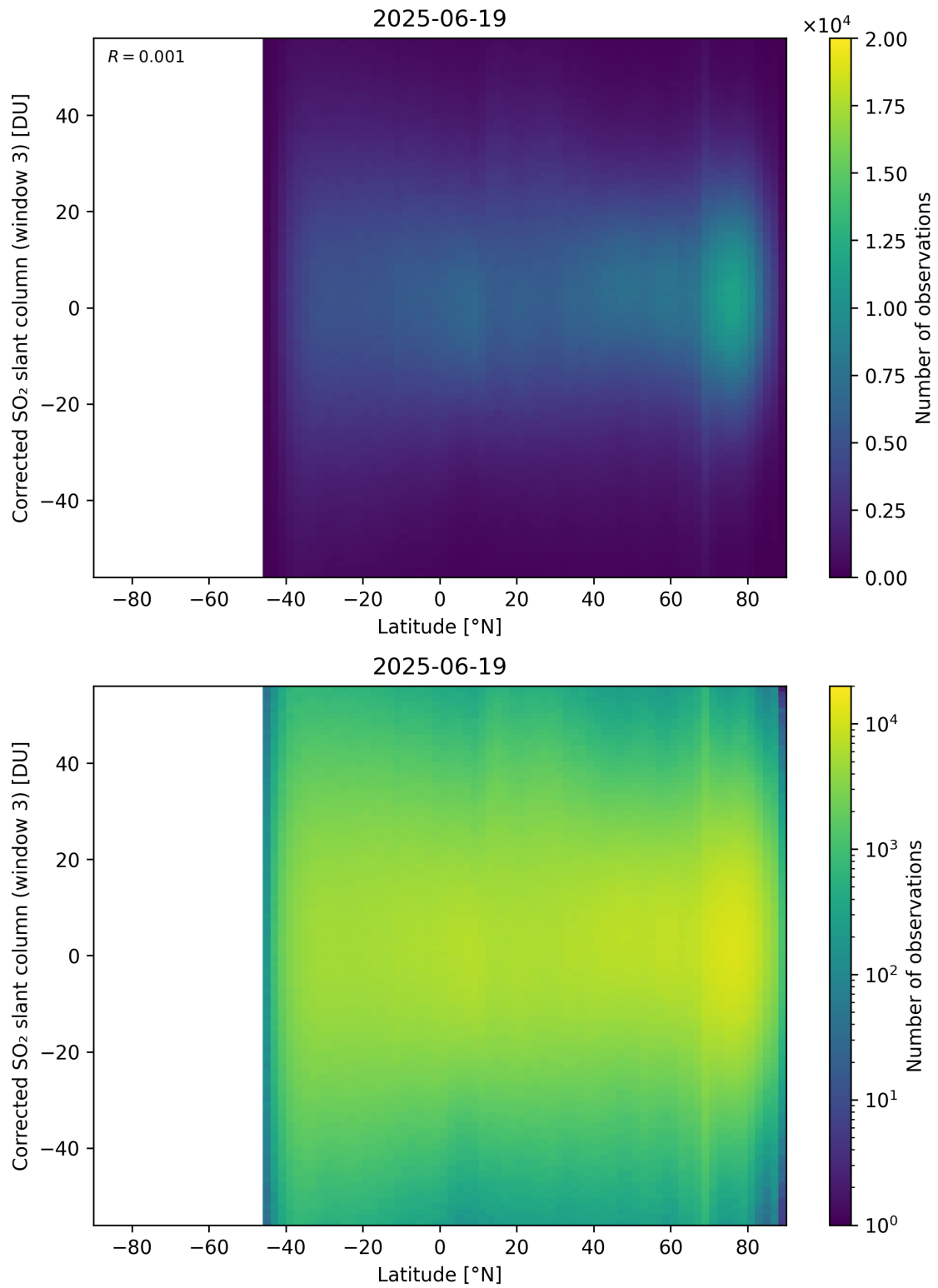
Figure 161: Scatter density plot of “Latitude” against “Corrected SO 2 slant column (window 3)” for 2025-06-18 to 2025-06-20.
