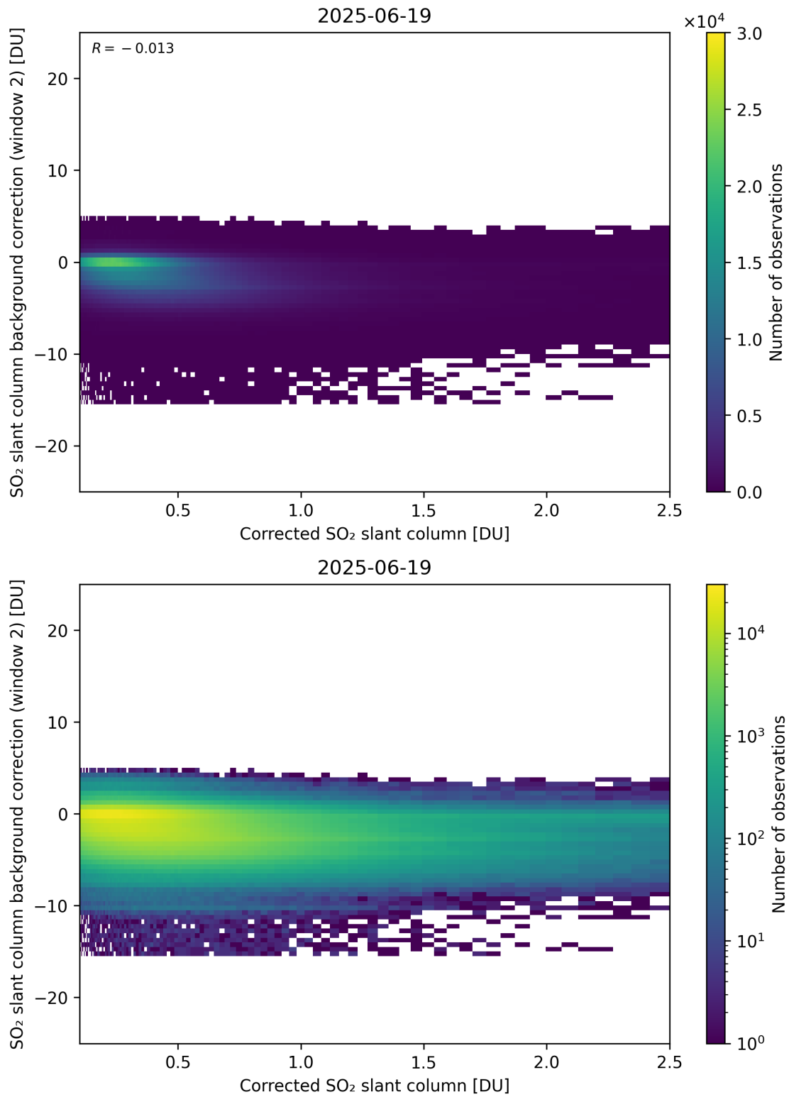
Figure 227: Scatter density plot of “Corrected SO 2 slant column” against “SO 2 slant column background correction (window 2)” for 2025-06-18 to 2025-06-20.
