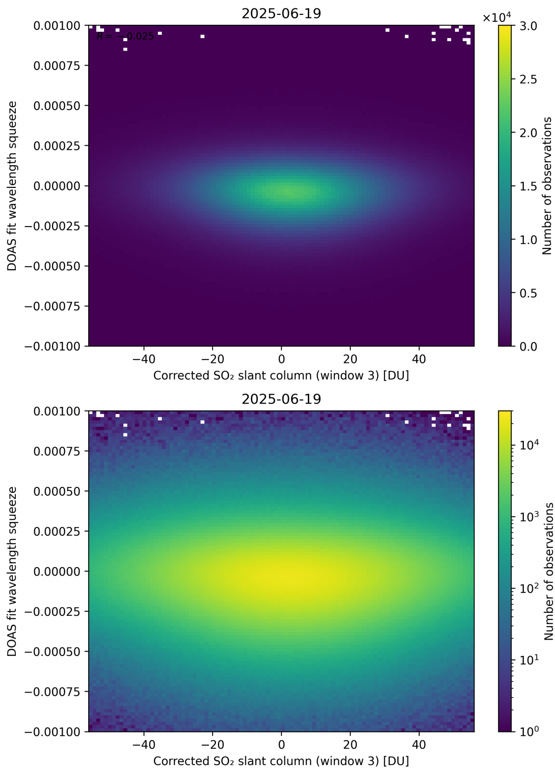
Figure 257: Scatter density plot of “Corrected SO 2 slant column (window 3)” against “DOAS fit wavelength squeeze” for 2025-06-18 to 2025-06-20.
