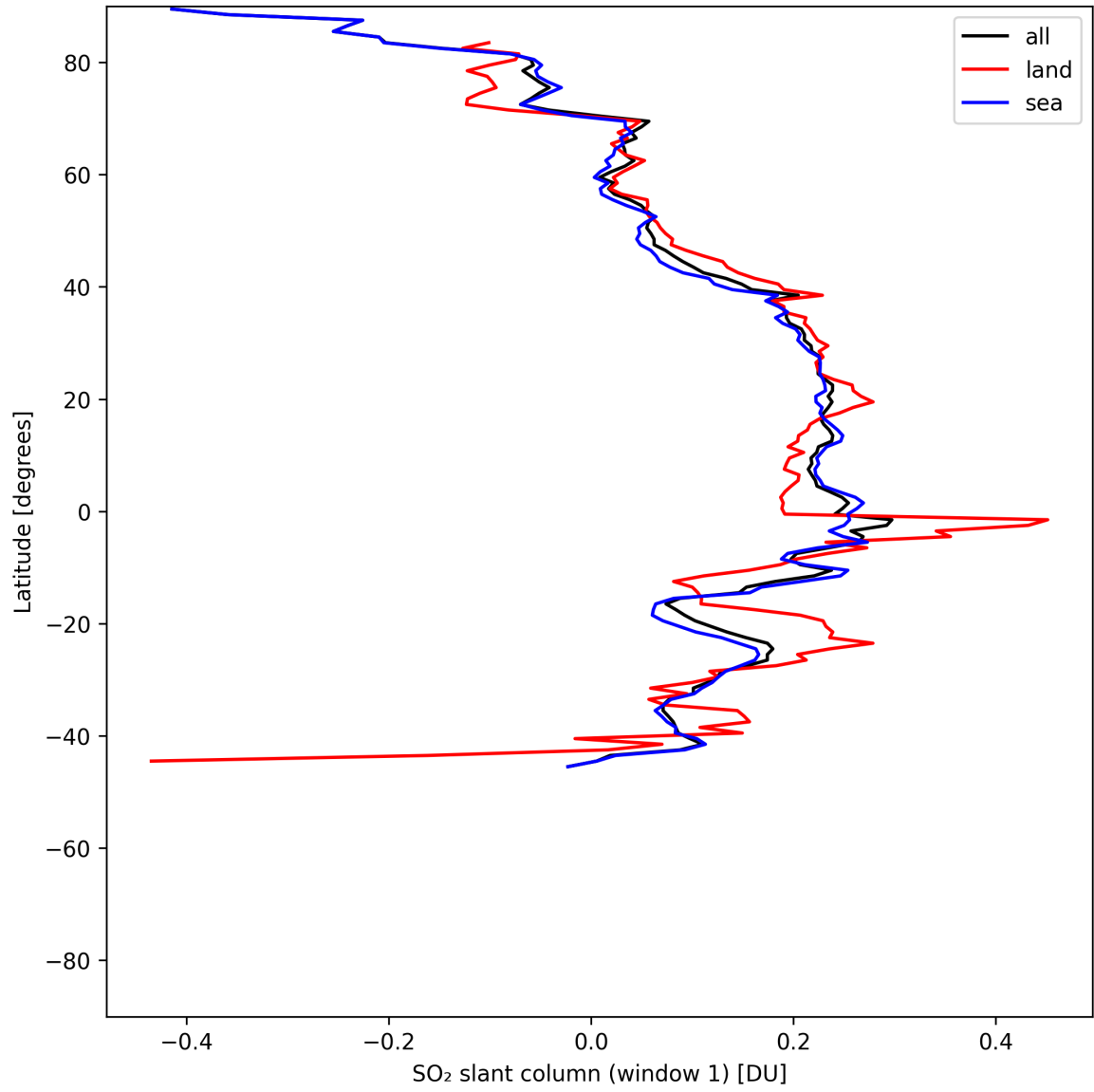
Figure 37: Zonal average of “SO 2 slant column (window 1)” for 2025-06-18 to 2025-06-20.
