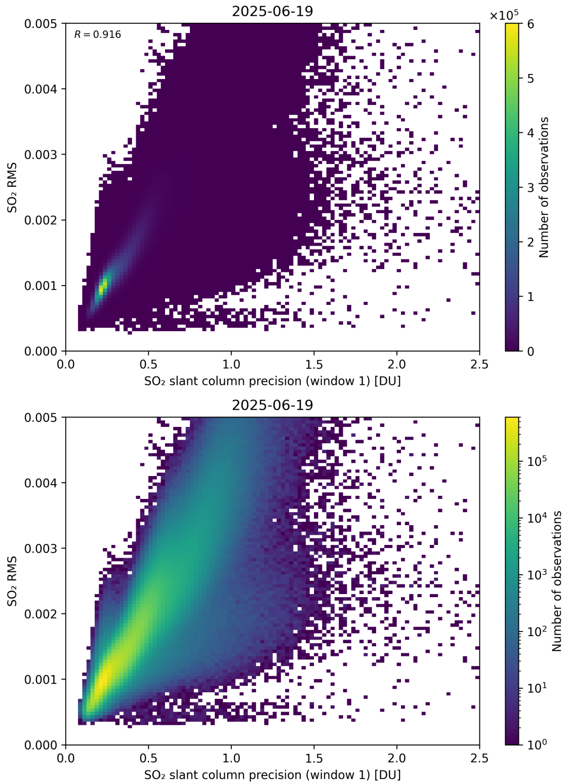
Figure 273: Scatter density plot of “SO 2 slant column precision (window 1)” against “SO 2 RMS” for 2025-06-18 to 2025-06-20.
