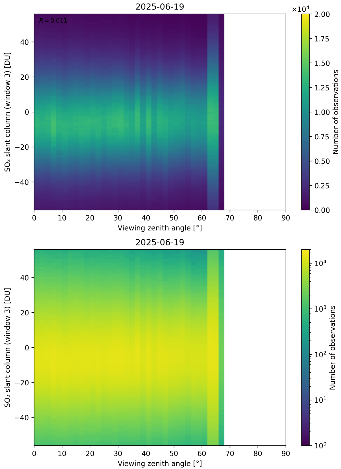
Figure 379: Scatter density plot of “Viewing zenith angle” against “SO 2 slant column (window 3)” for 2025-06-18 to 2025-06-20.
