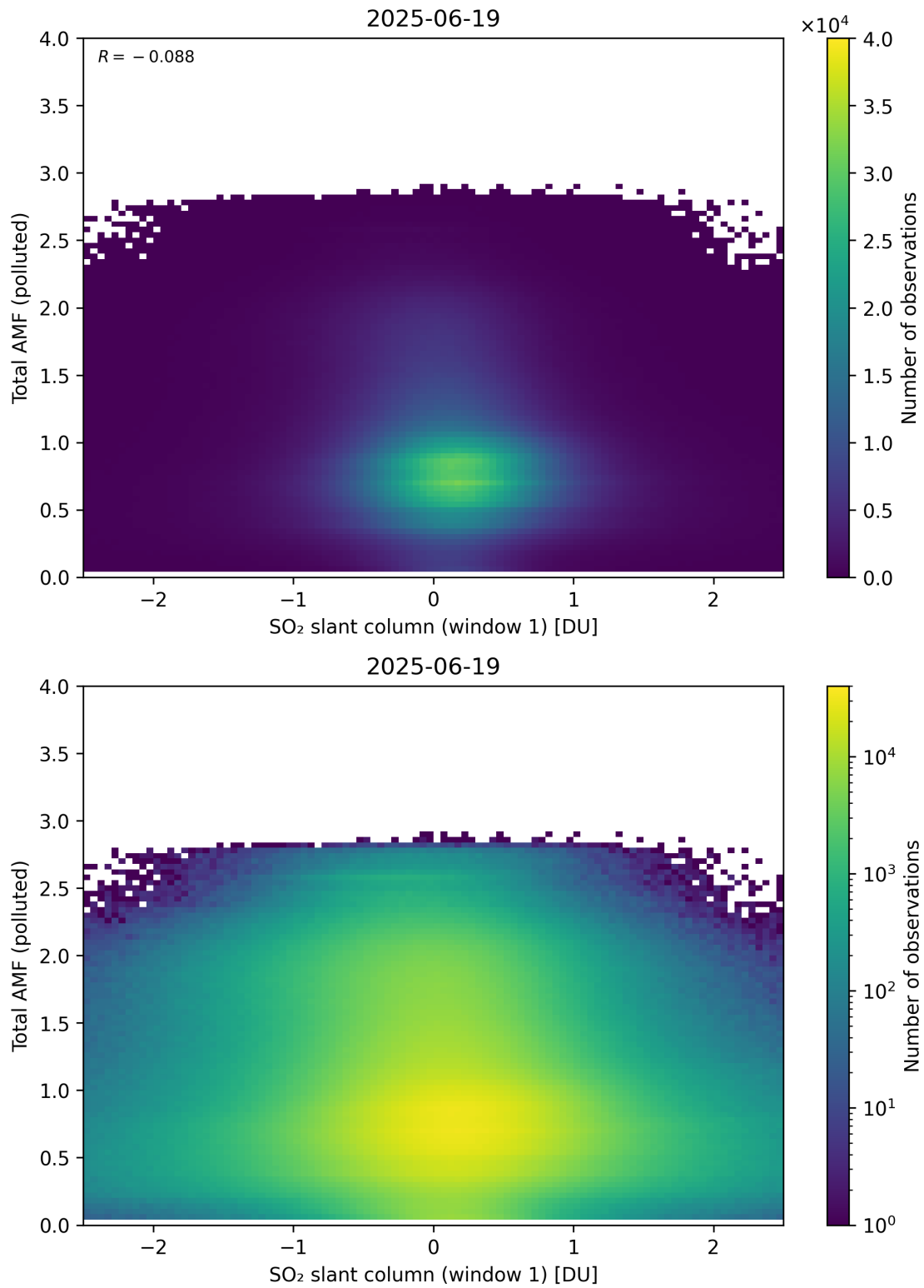
Figure 289: Scatter density plot of “SO 2 slant column (window 1)” against “Total AMF (polluted)” for 2025-06-18 to 2025-06-20.
