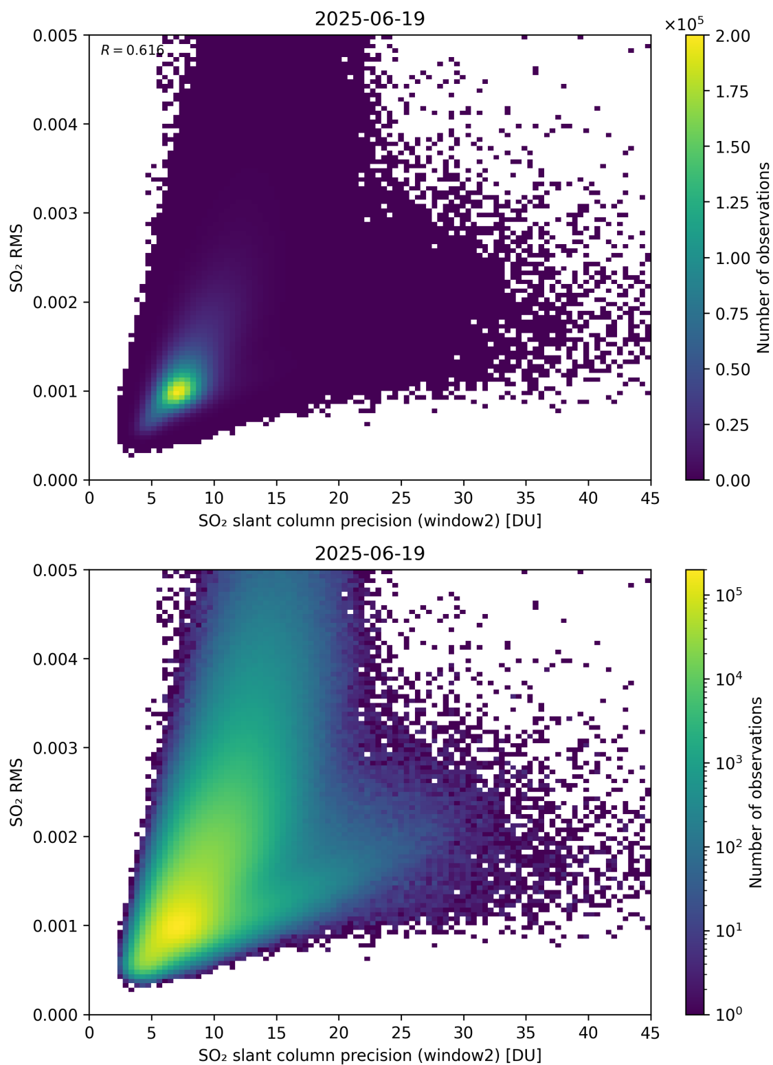
Figure 295: Scatter density plot of “SO 2 slant column precision (window2)” against “SO 2 RMS” for 2025-06-18 to 2025-06-20.
