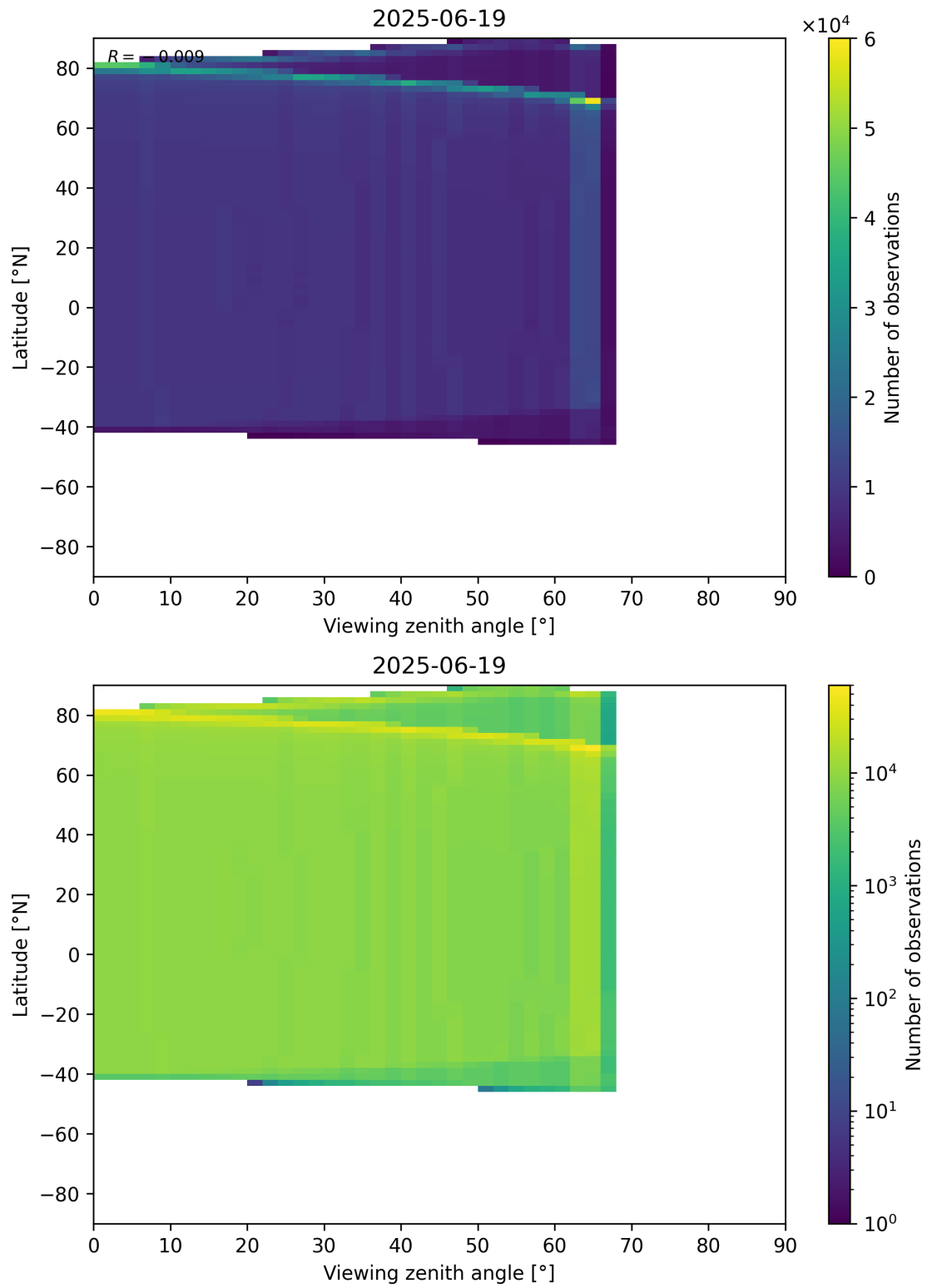
Figure 368: Scatter density plot of “Viewing zenith angle” against “Latitude” for 2025-06-18 to 2025-06-20.
