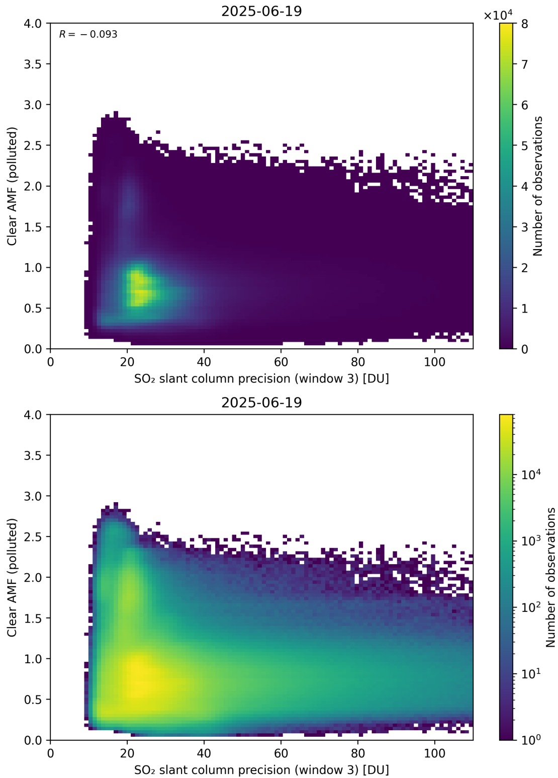
Figure 311: Scatter density plot of “SO 2 slant column precision (window 3)” against “Clear AMF (polluted)” for 2025-06-18 to 2025-06-20.
