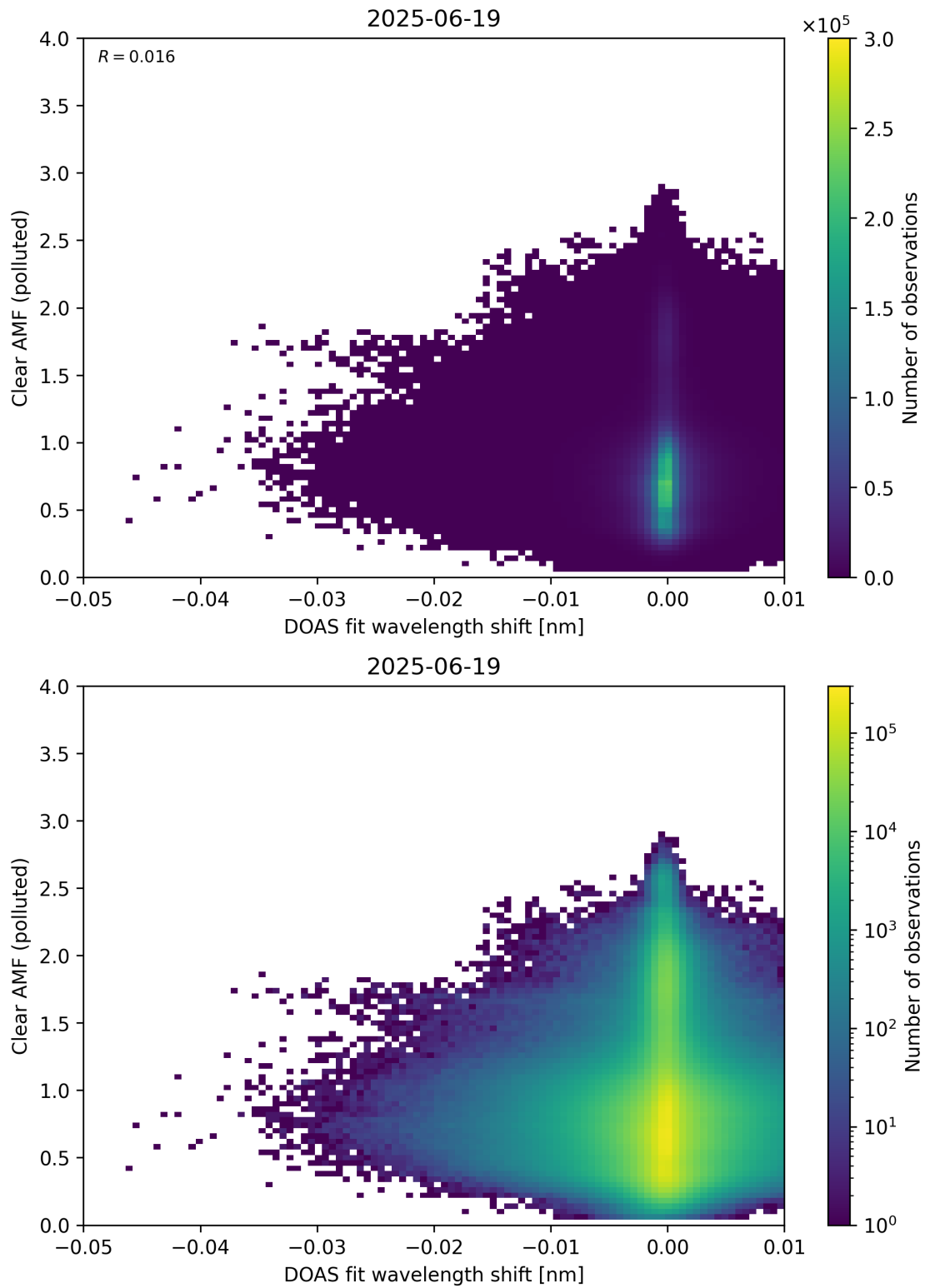
Figure 140: Scatter density plot of “DOAS fit wavelength shift” against “Clear AMF (polluted)” for 2025-06-18 to 2025-06-20.
