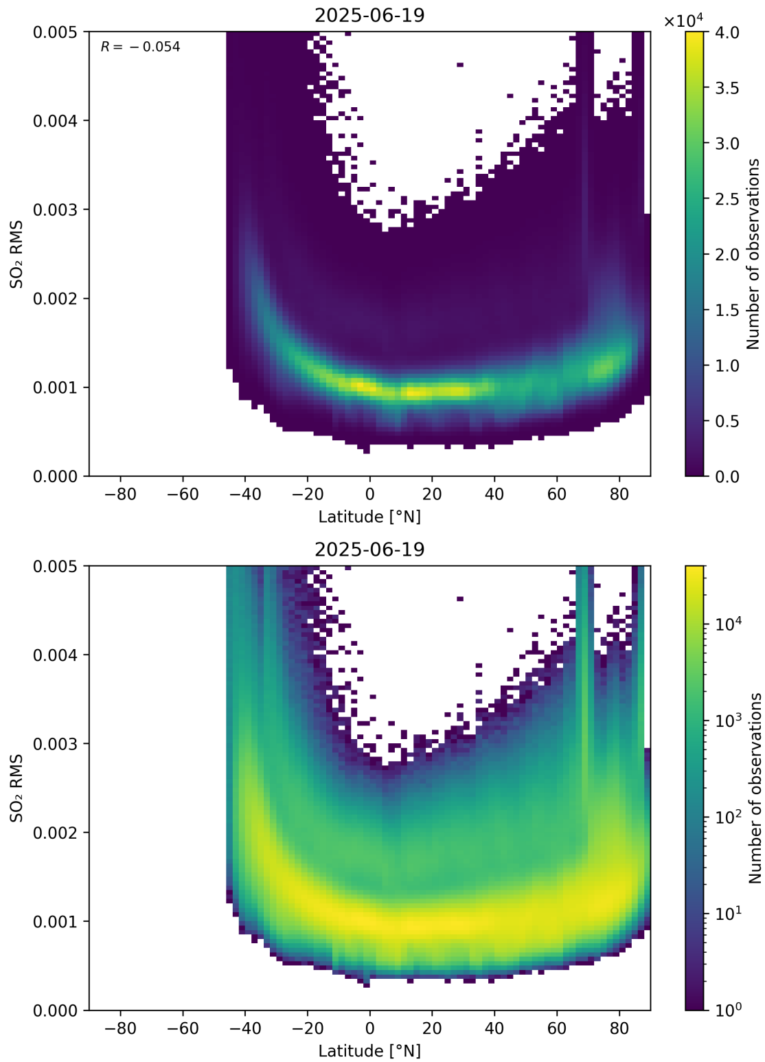
Figure 155: Scatter density plot of “Latitude” against “SO 2 RMS” for 2025-06-18 to 2025-06-20.
