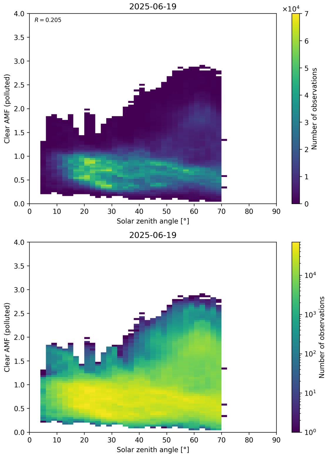
Figure 178: Scatter density plot of “Solar zenith angle” against “Clear AMF (polluted)” for 2025-06-18 to 2025-06-20.
