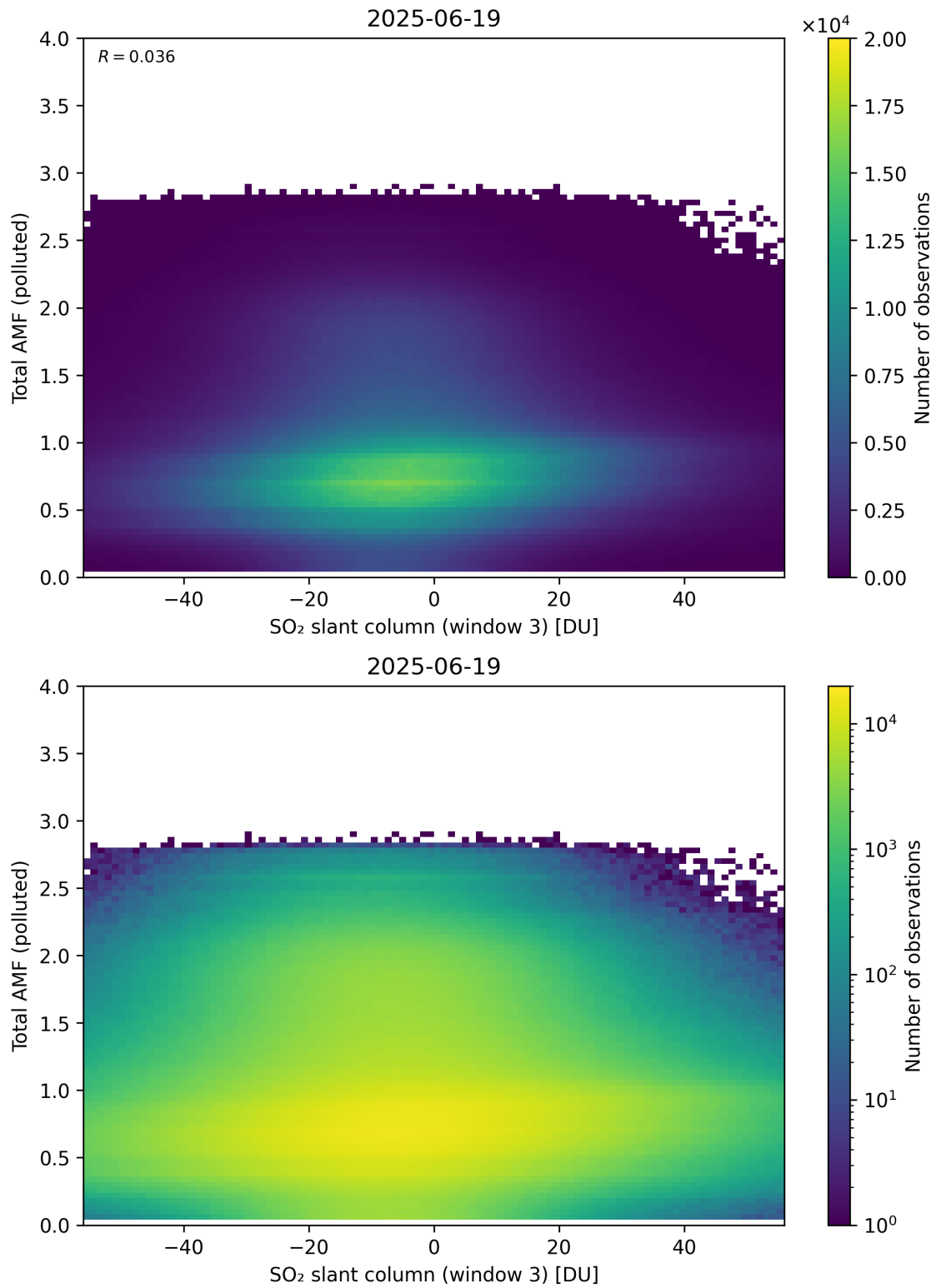
Figure 318: Scatter density plot of “SO 2 slant column (window 3)” against “Total AMF (polluted)” for 2025-06-18 to 2025-06-20.
