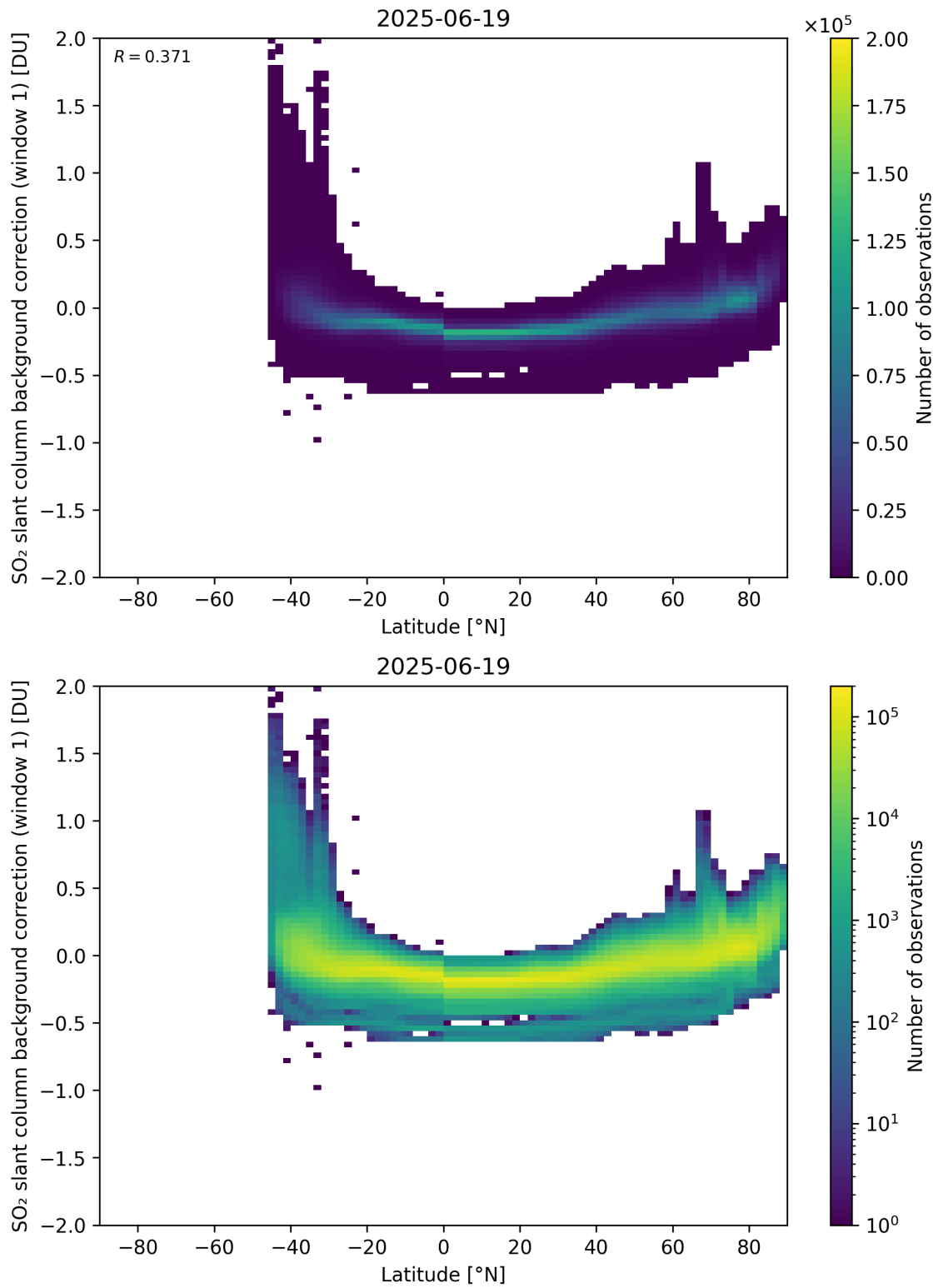
Figure 150: Scatter density plot of “Latitude” against “SO 2 slant column background correction (window 1)” for 2025-06-18 to 2025-06-20.
