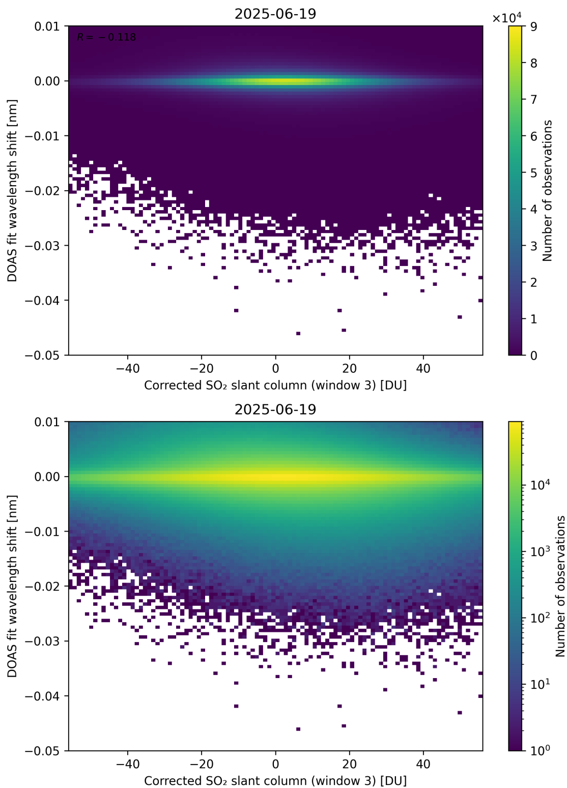
Figure 256: Scatter density plot of “Corrected SO 2 slant column (window 3)” against “DOAS fit wavelength shift” for 2025-06-18 to 2025-06-20.
