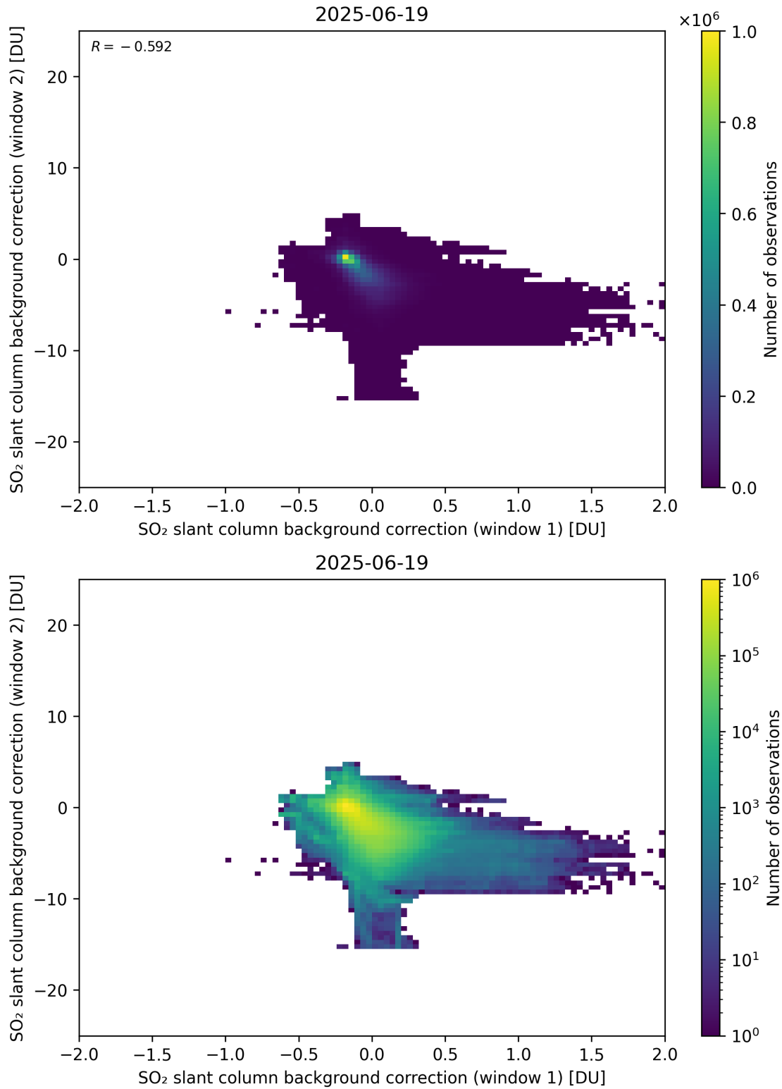
Figure 109: Scatter density plot of “SO 2 slant column background correction (window 1)” against “SO 2 slant column background correction (window 2)” for 2025-06-18 to 2025-06-20.
