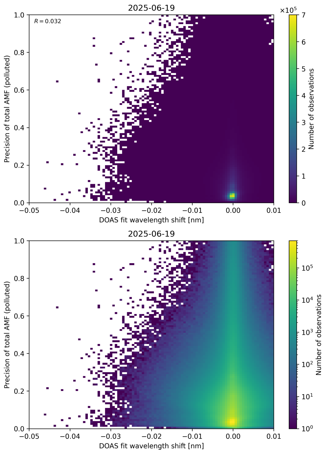
Figure 142: Scatter density plot of “DOAS fit wavelength shift” against “Precision of total AMF (polluted)” for 2025-06-18 to 2025-06-20.
