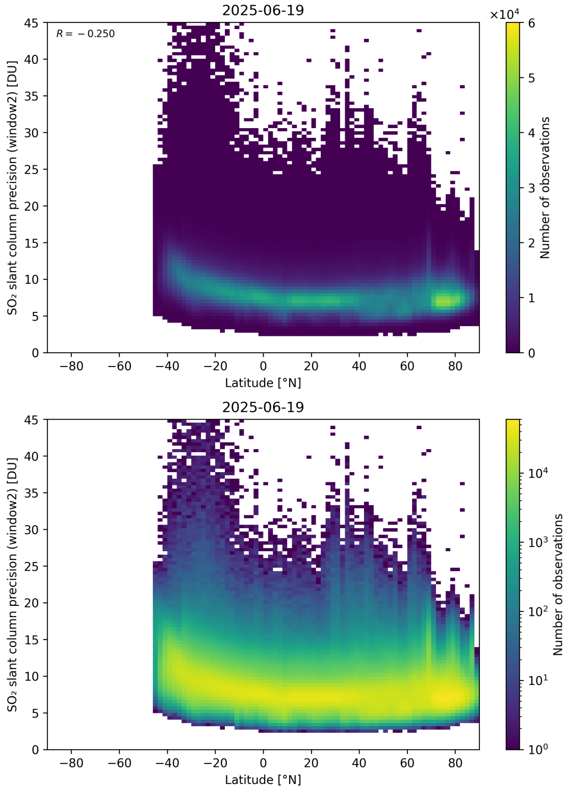
Figure 164: Scatter density plot of “Latitude” against “SO 2 slant column precision (window2)” for 2025-06-18 to 2025-06-20.
