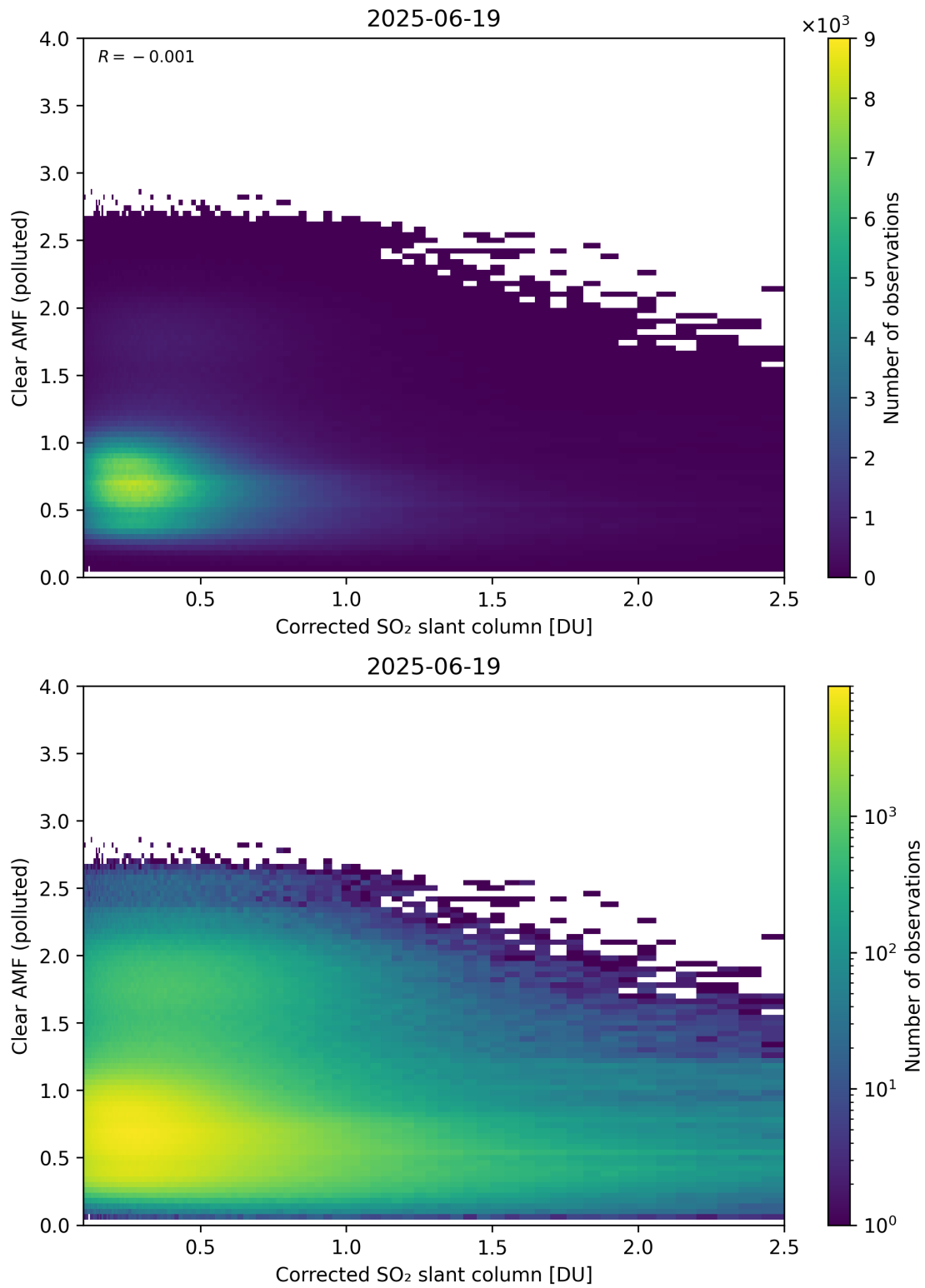
Figure 232: Scatter density plot of “Corrected SO 2 slant column” against “Clear AMF (polluted)” for 2025-06-18 to 2025-06-20.
