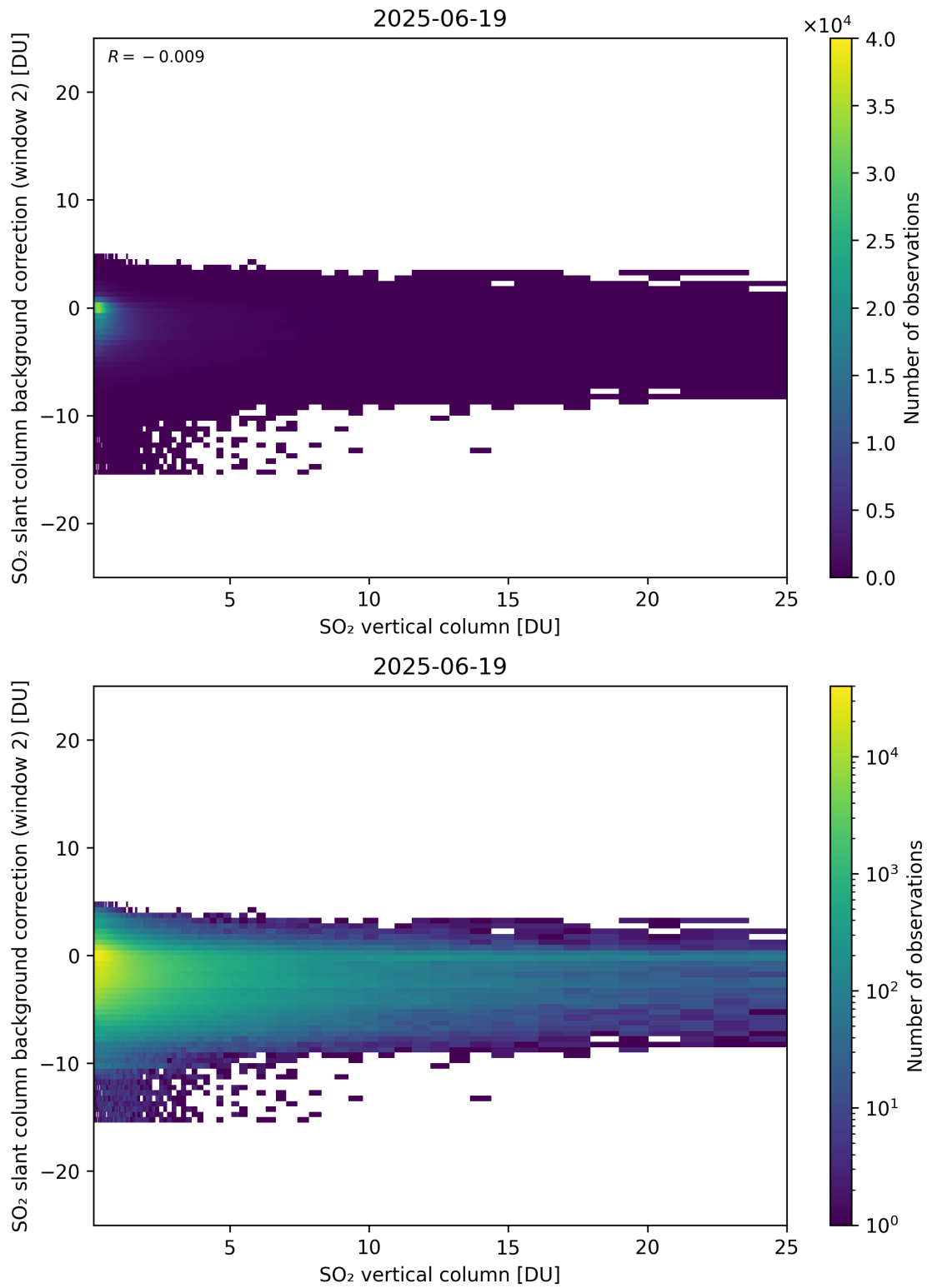
Figure 324: Scatter density plot of “SO 2 vertical column” against “SO 2 slant column background correction (window 2)” for 2025-06-18 to 2025-06-20.
