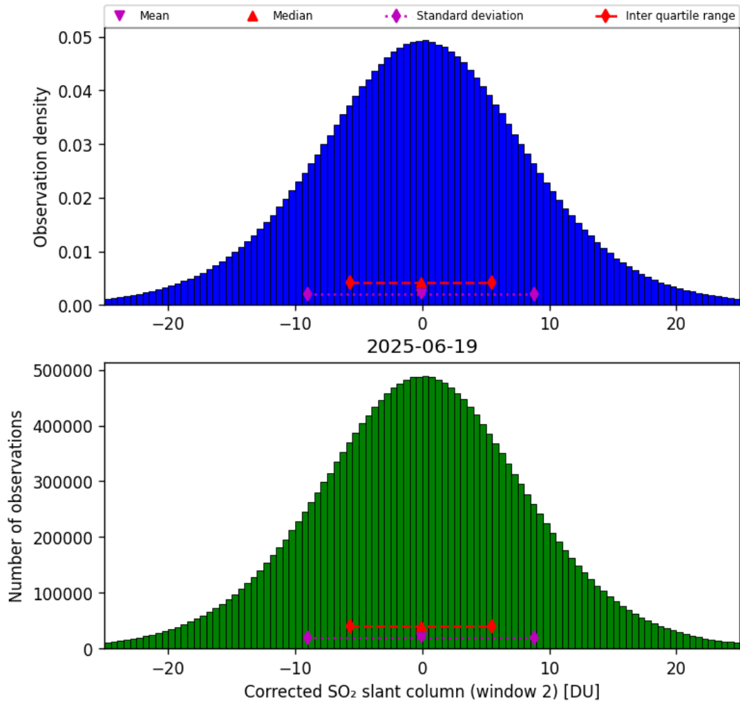
Figure 69: Histogram of “Corrected SO 2 slant column (window 2)” for 2025-06-18 to 2025-06-20
