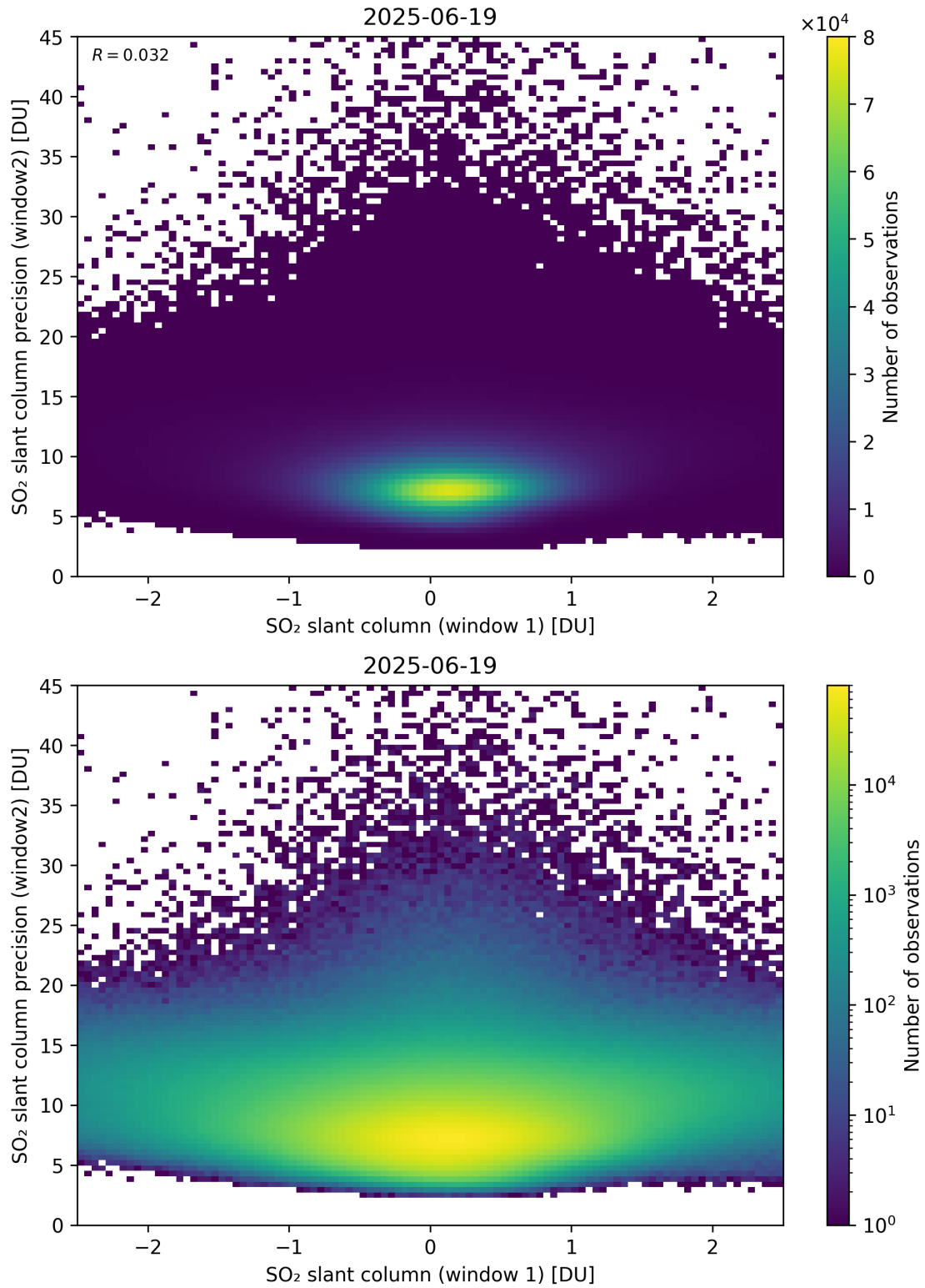
Figure 286: Scatter density plot of “SO 2 slant column (window 1)” against “SO 2 slant column precision (window2)” for 2025-06-18 to 2025-06-20.
