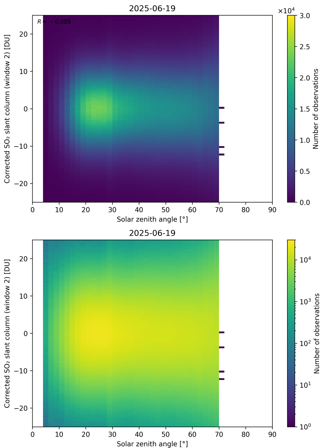
Figure 182: Scatter density plot of “Solar zenith angle” against “Corrected SO 2 slant column (window 2)” for 2025-06-18 to 2025-06-20.
