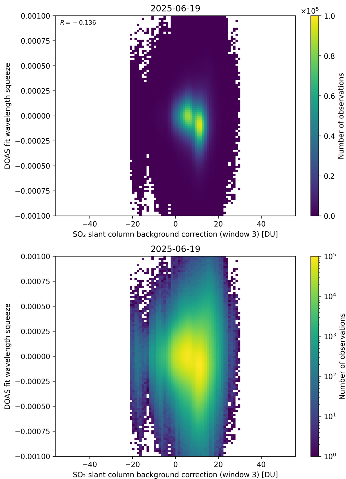
Figure 133: Scatter density plot of “SO 2 slant column background correction (window 3)” against “DOAS fit wavelength squeeze” for 2025-06-18 to 2025-06-20.
