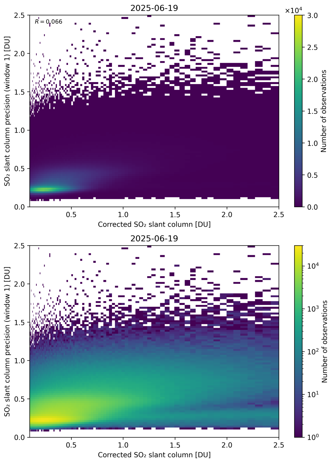
Figure 238: Scatter density plot of “Corrected SO 2 slant column” against “SO 2 slant column precision (window 1)” for 2025-06-18 to 2025-06-20.
