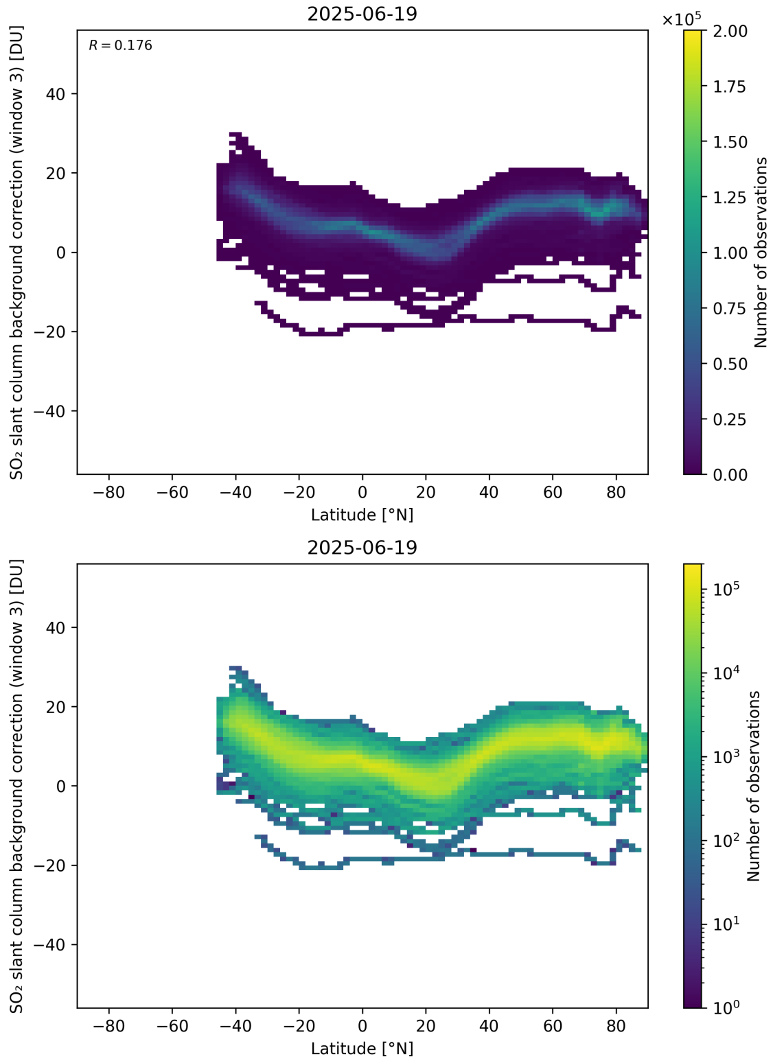
Figure 152: Scatter density plot of “Latitude” against “SO 2 slant column background correction (window 3)” for 2025-06-18 to 2025-06-20.
