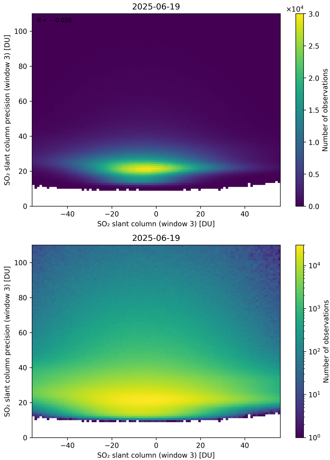
Figure 317: Scatter density plot of “SO 2 slant column (window 3)” against “SO 2 slant column precision (window 3)” for 2025-06-18 to 2025-06-20.
