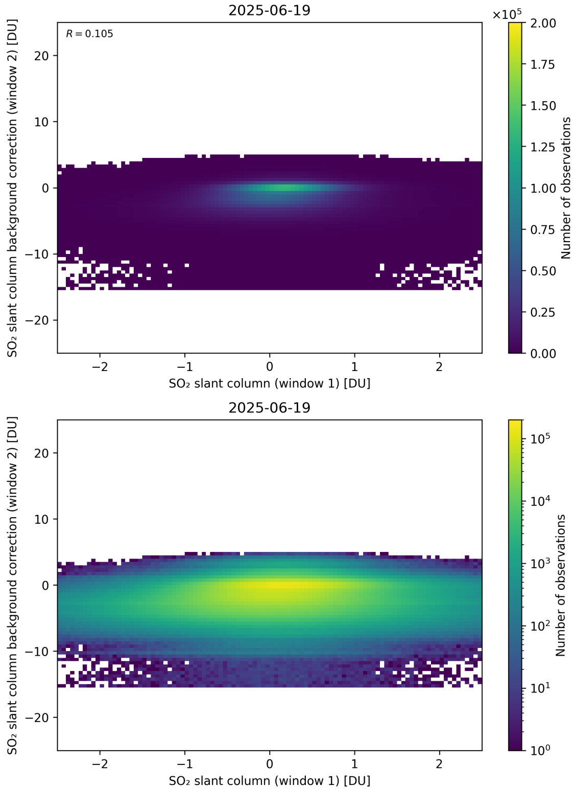
Figure 263: Scatter density plot of “SO 2 slant column (window 1)” against “SO 2 slant column background correction (window 2)” for 2025-06-18 to 2025-06-20.
