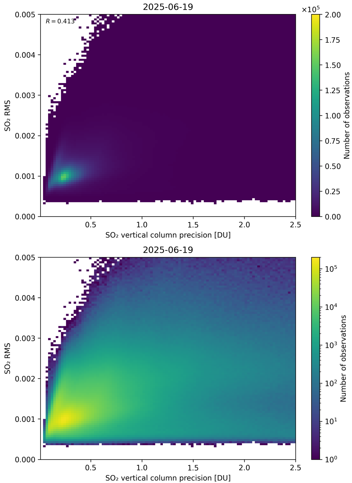
Figure 334: Scatter density plot of “SO 2 vertical column precision” against “SO 2 RMS” for 2025-06-18 to 2025-06-20.
