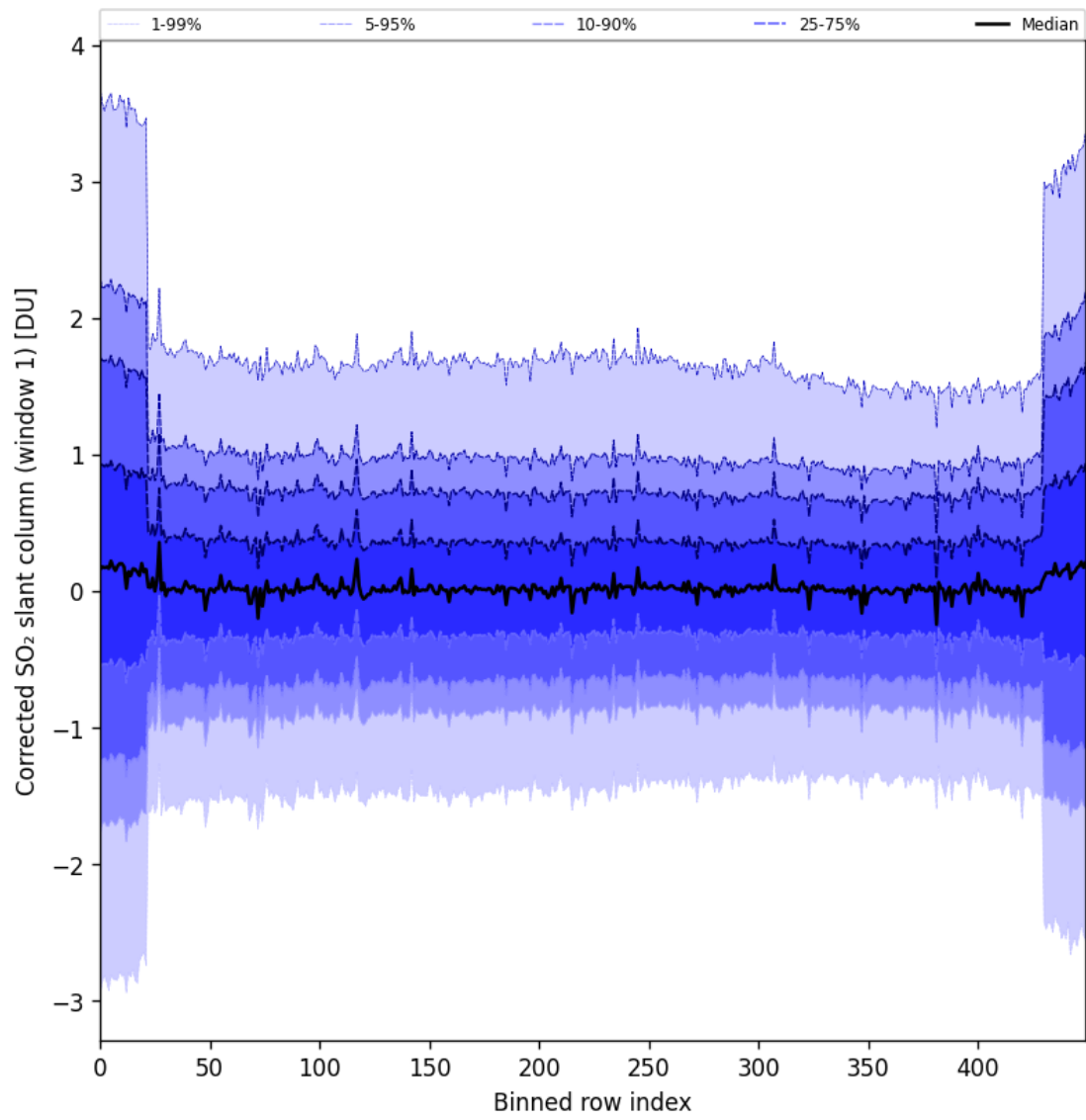
Figure 91: Along track statistics of “Corrected SO 2 slant column (window 1)” for 2025-06-18 to 2025-06-20
