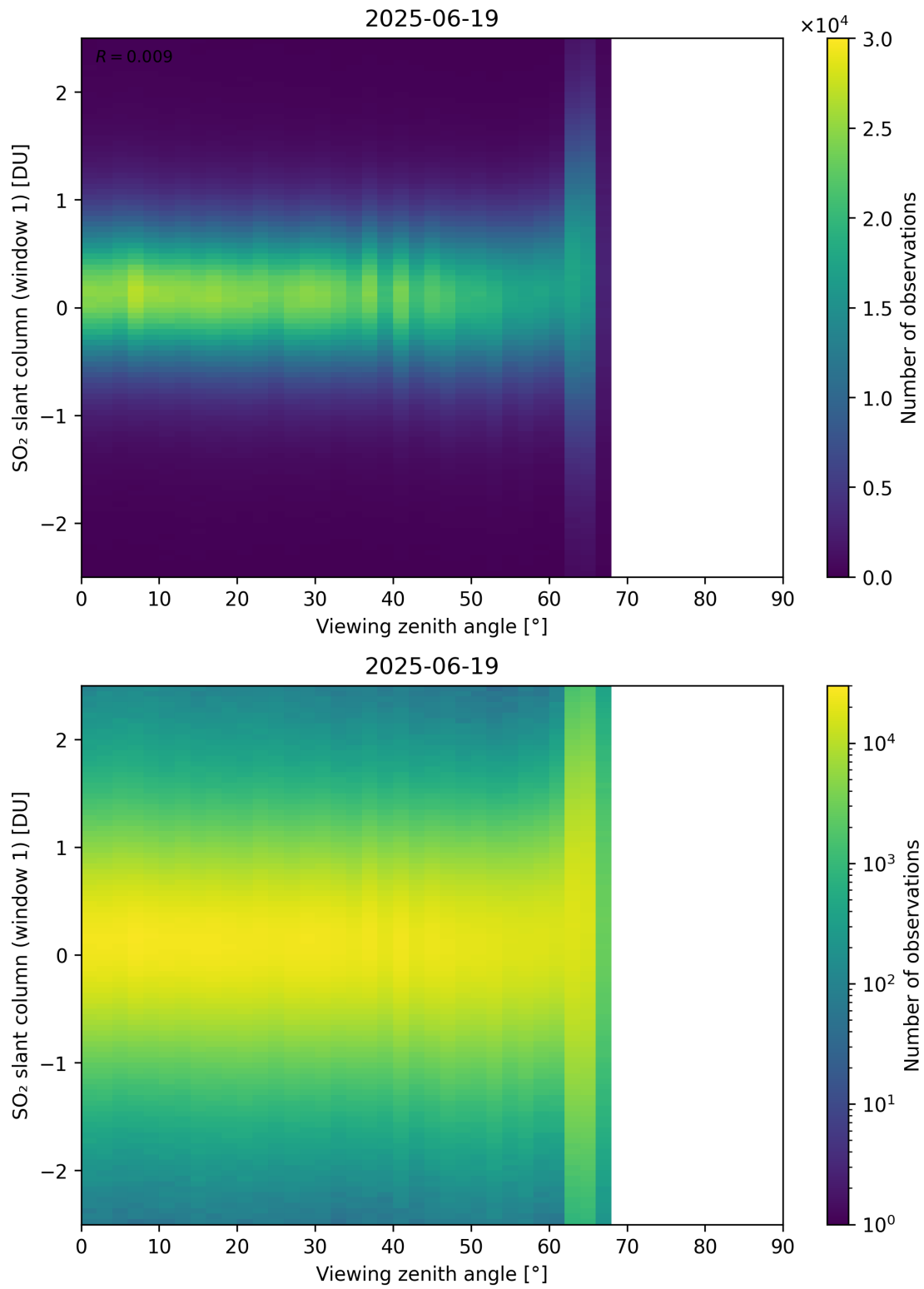
Figure 376: Scatter density plot of “Viewing zenith angle” against “SO 2 slant column (window 1)” for 2025-06-18 to 2025-06-20.
