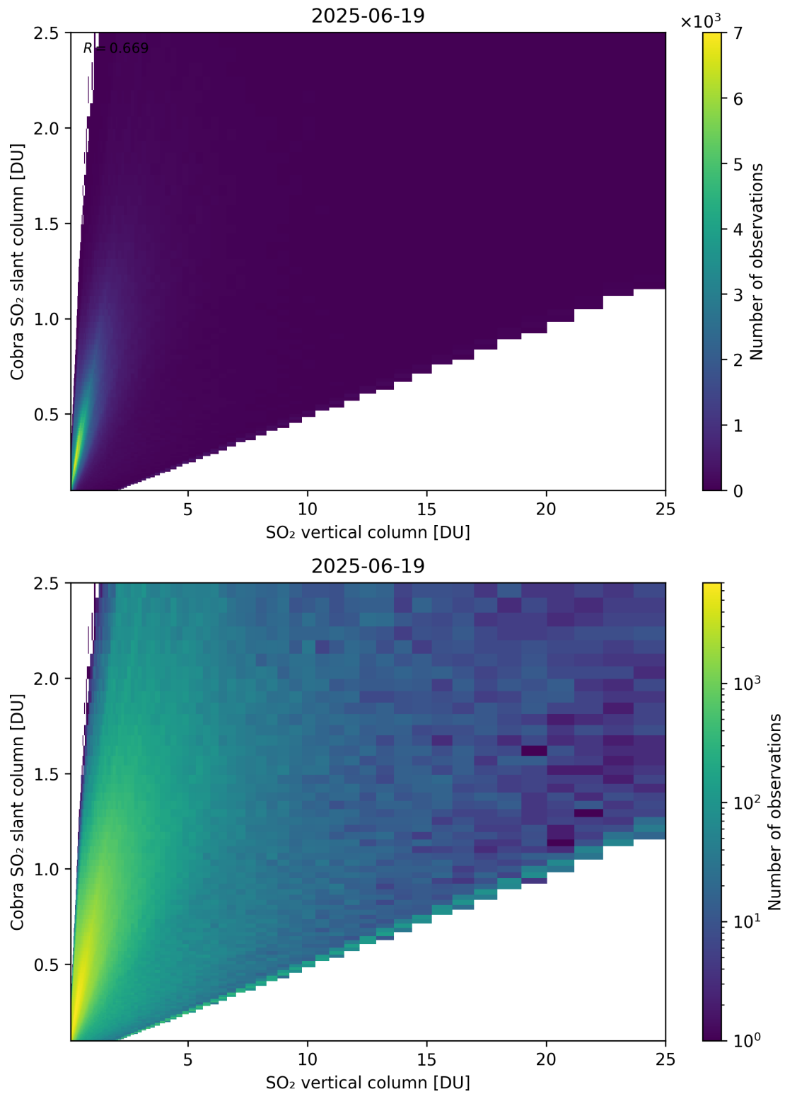
Figure 349: Scatter density plot of “SO 2 vertical column” against “Cobra SO 2 slant column” for 2025-06-18 to 2025-06-20.
