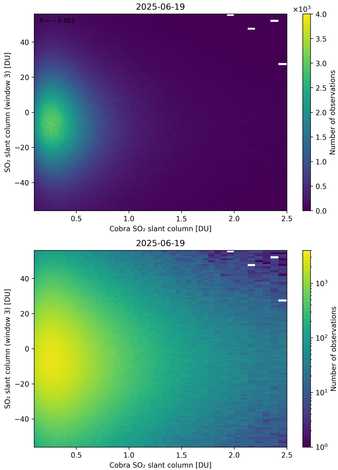
Figure 222: Scatter density plot of “Cobra SO 2 slant column” against “SO 2 slant column (window 3)” for 2025-06-18 to 2025-06-20.
