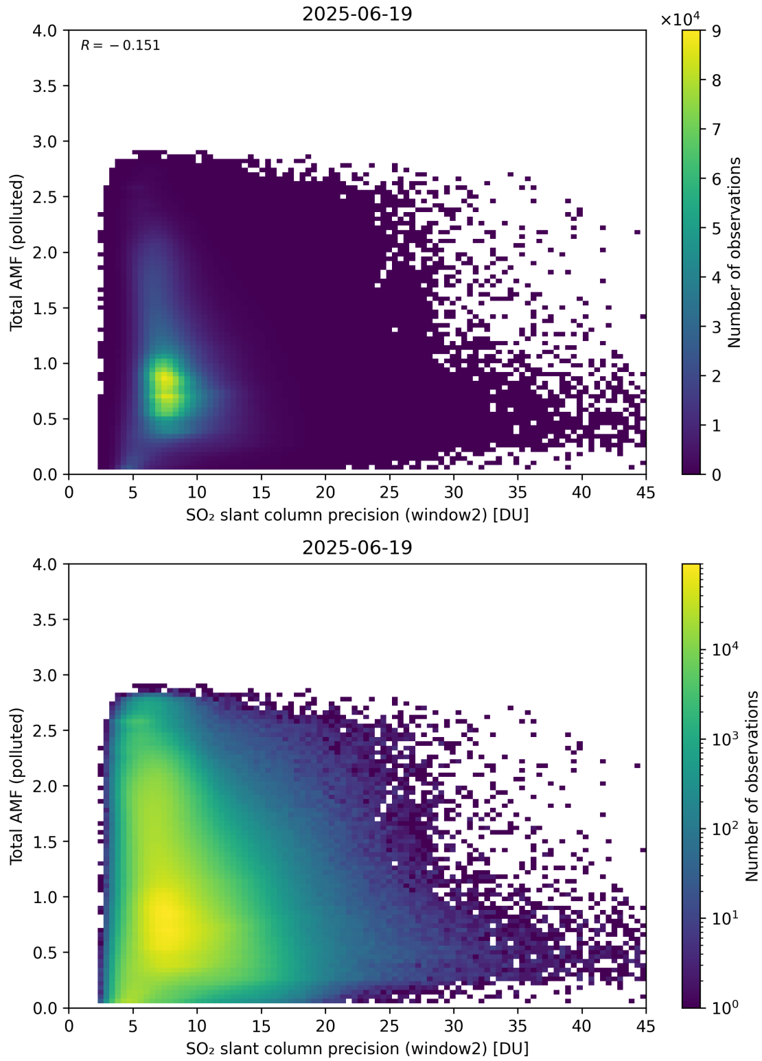
Figure 301: Scatter density plot of “SO 2 slant column precision (window2)” against “Total AMF (polluted)” for 2025-06-18 to 2025-06-20.
