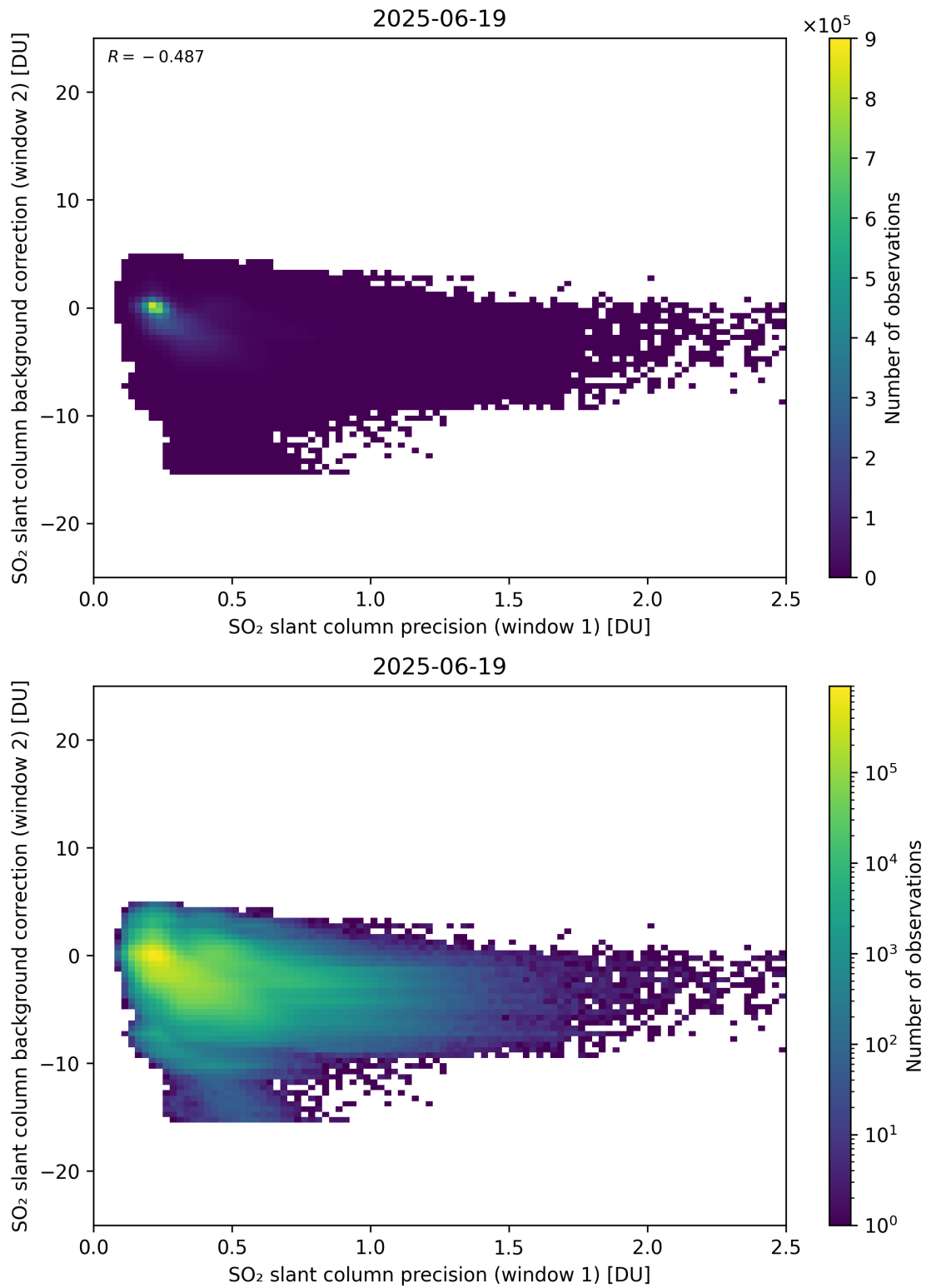
Figure 269: Scatter density plot of “SO 2 slant column precision (window 1)” against “SO 2 slant column background correction (window 2)” for 2025-06-18 to 2025-06-20.
