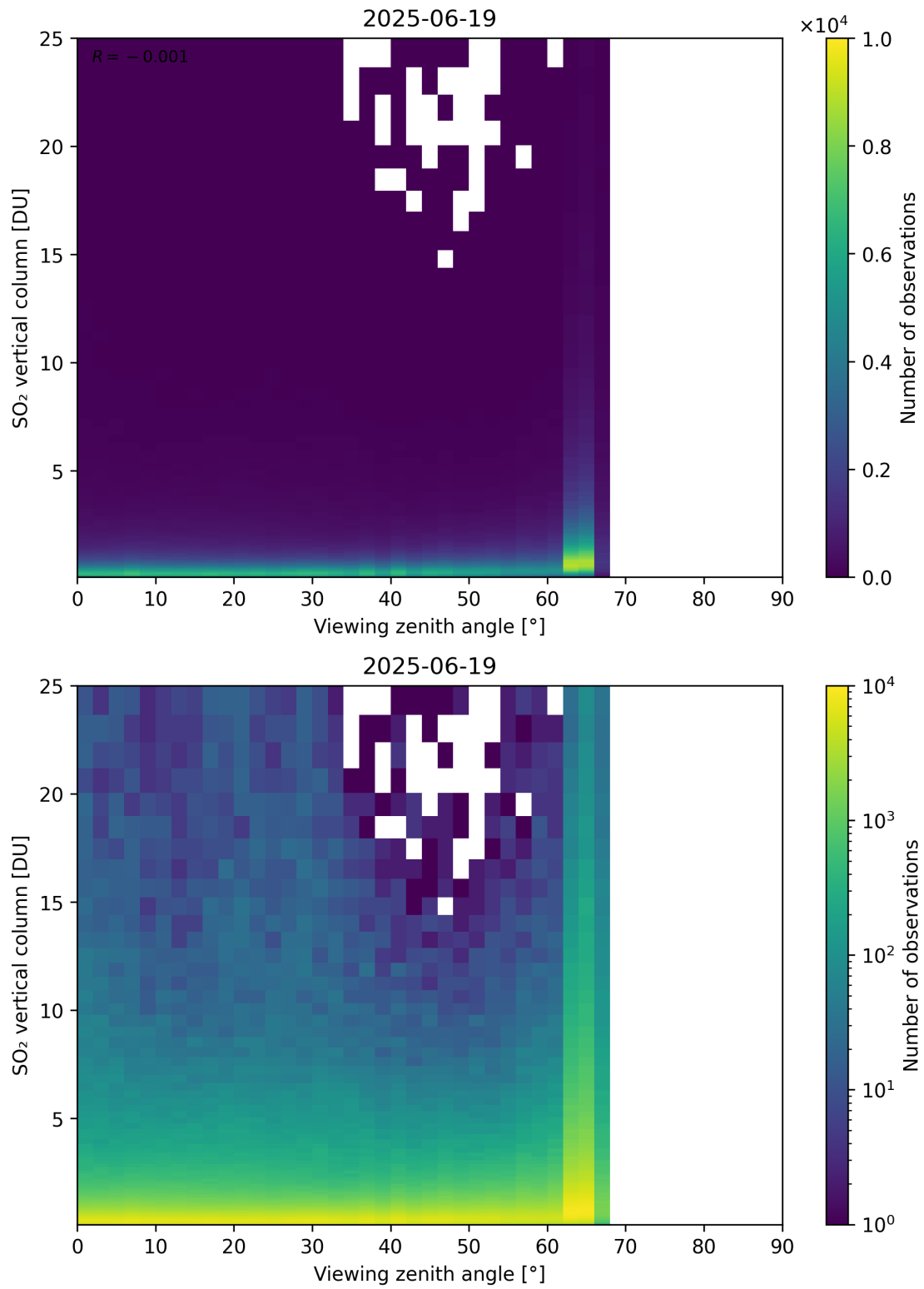
Figure 383: Scatter density plot of “Viewing zenith angle” against “SO 2 vertical column” for 2025-06-18 to 2025-06-20.
