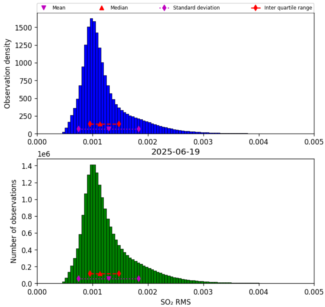
Figure 78: Histogram of “SO 2 RMS” for 2025-06-18 to 2025-06-20
