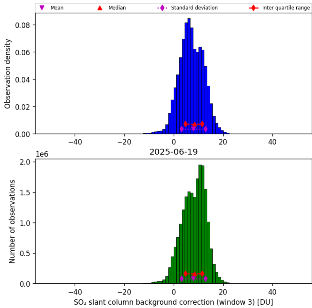
Figure 74: Histogram of “SO 2 slant column background correction (window 3)” for 2025-06-18 to 2025-06-20
