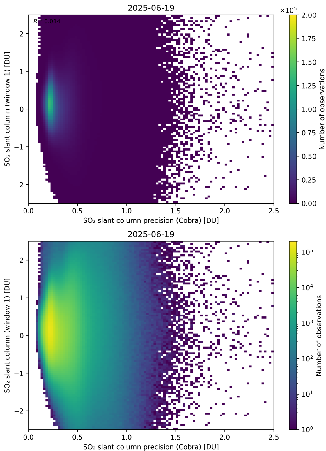
Figure 208: Scatter density plot of “SO 2 slant column precision (Cobra)” against “SO 2 slant column (window 1)” for 2025-06-18 to 2025-06-20.
