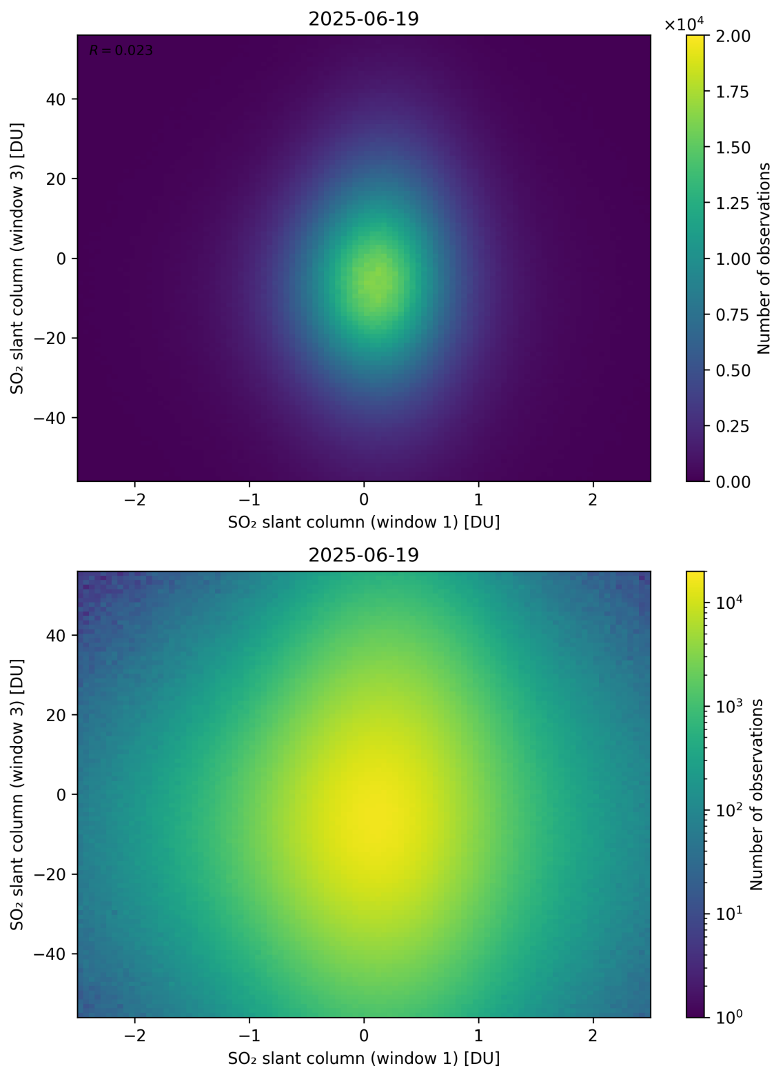
Figure 287: Scatter density plot of “SO 2 slant column (window 1)” against “SO 2 slant column (window 3)” for 2025-06-18 to 2025-06-20.
