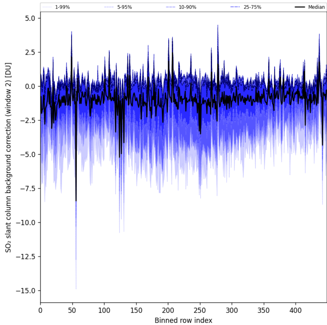
Figure 96: Along track statistics of “SO 2 slant column background correction (window 2)” for 2025-06-18 to 2025-06-20
