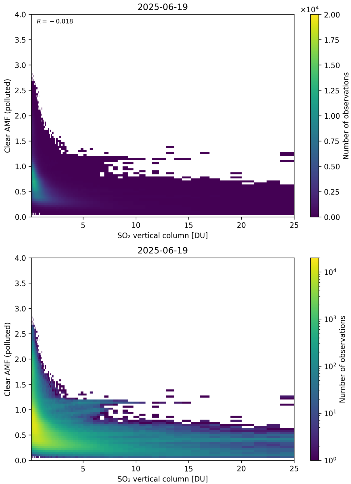
Figure 348: Scatter density plot of “SO 2 vertical column” against “Clear AMF (polluted)” for 2025-06-18 to 2025-06-20.
