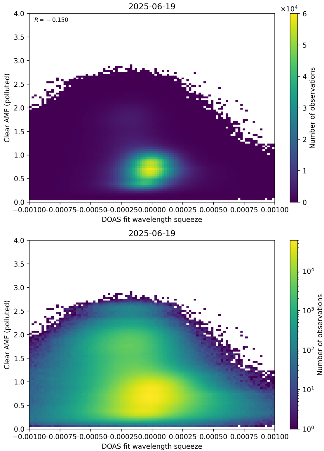
Figure 144: Scatter density plot of “DOAS fit wavelength squeeze” against “Clear AMF (polluted)” for 2025-06-18 to 2025-06-20.
