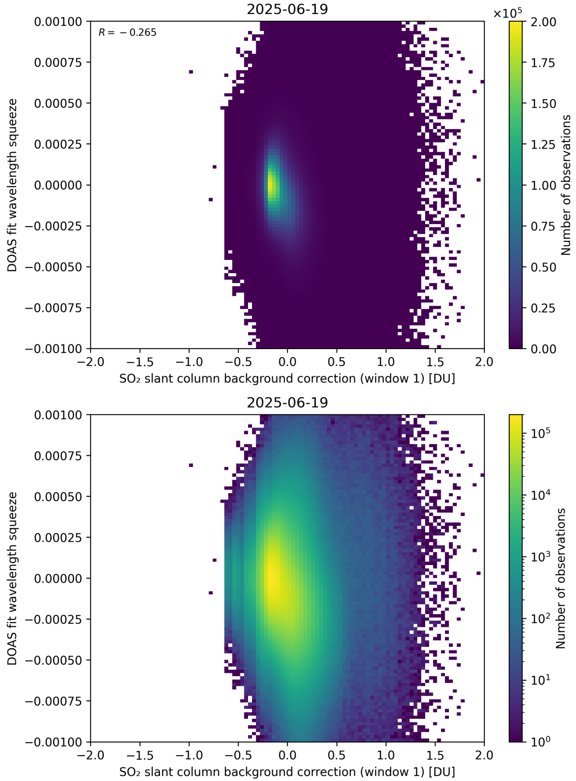
Figure 112: Scatter density plot of “SO 2 slant column background correction (window 1)” against “DOAS fit wavelength squeeze” for 2025-06-18 to 2025-06-20.
