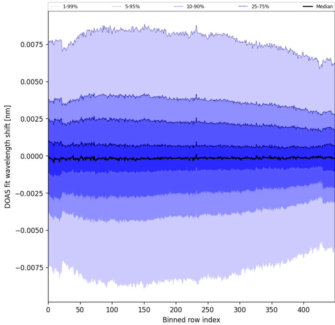
Figure 102: Along track statistics of “DOAS fit wavelength shift” for 2025-06-18 to 2025-06-20
