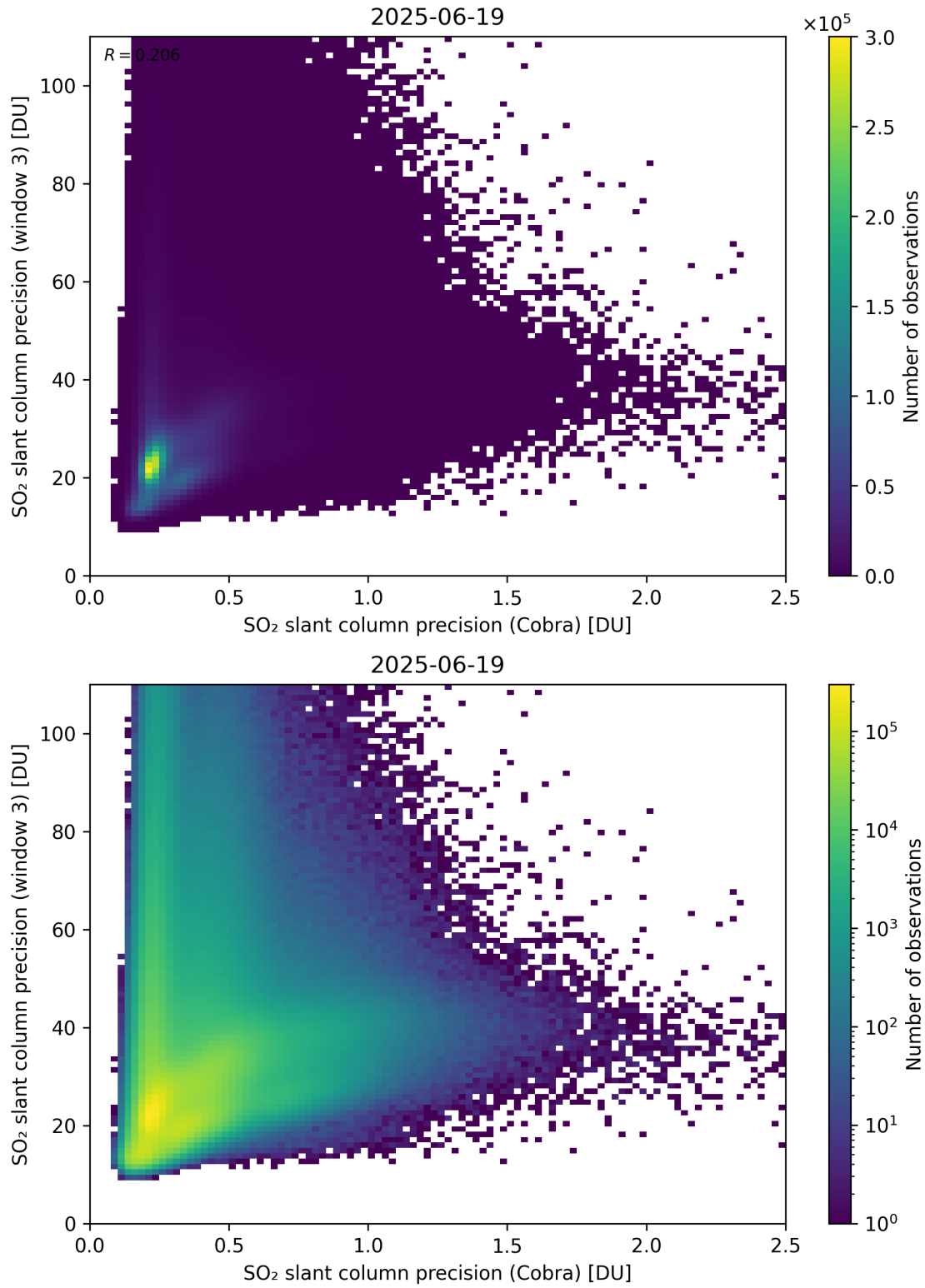
Figure 212: Scatter density plot of “SO 2 slant column precision (Cobra)” against “SO 2 slant column precision (window 3)” for 2025-06-18 to 2025-06-20.
