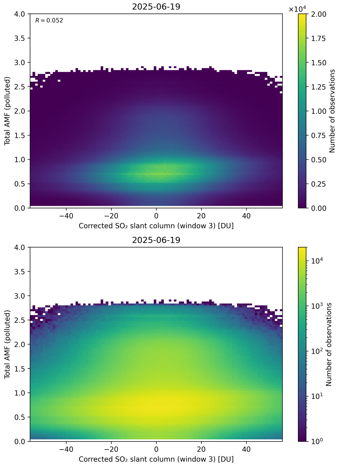
Figure 260: Scatter density plot of “Corrected SO 2 slant column (window 3)” against “Total AMF (polluted)” for 2025-06-18 to 2025-06-20.
