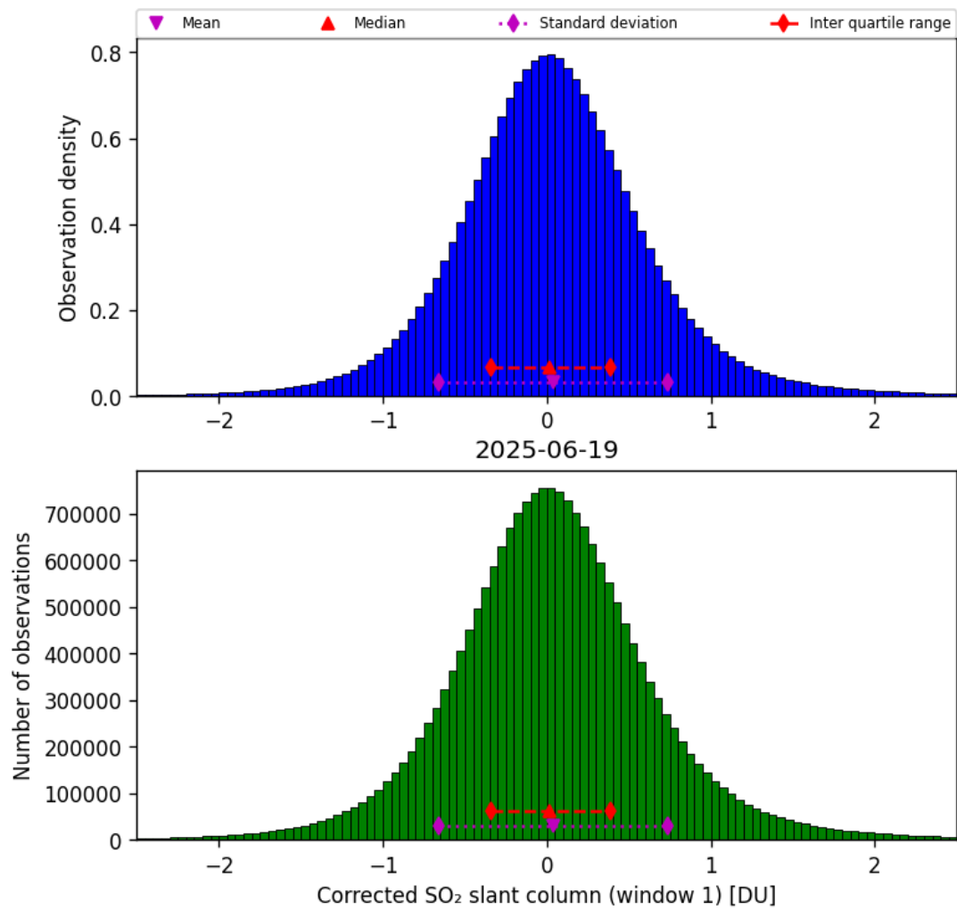
Figure 65: Histogram of “Corrected SO 2 slant column (window 1)” for 2025-06-18 to 2025-06-20
