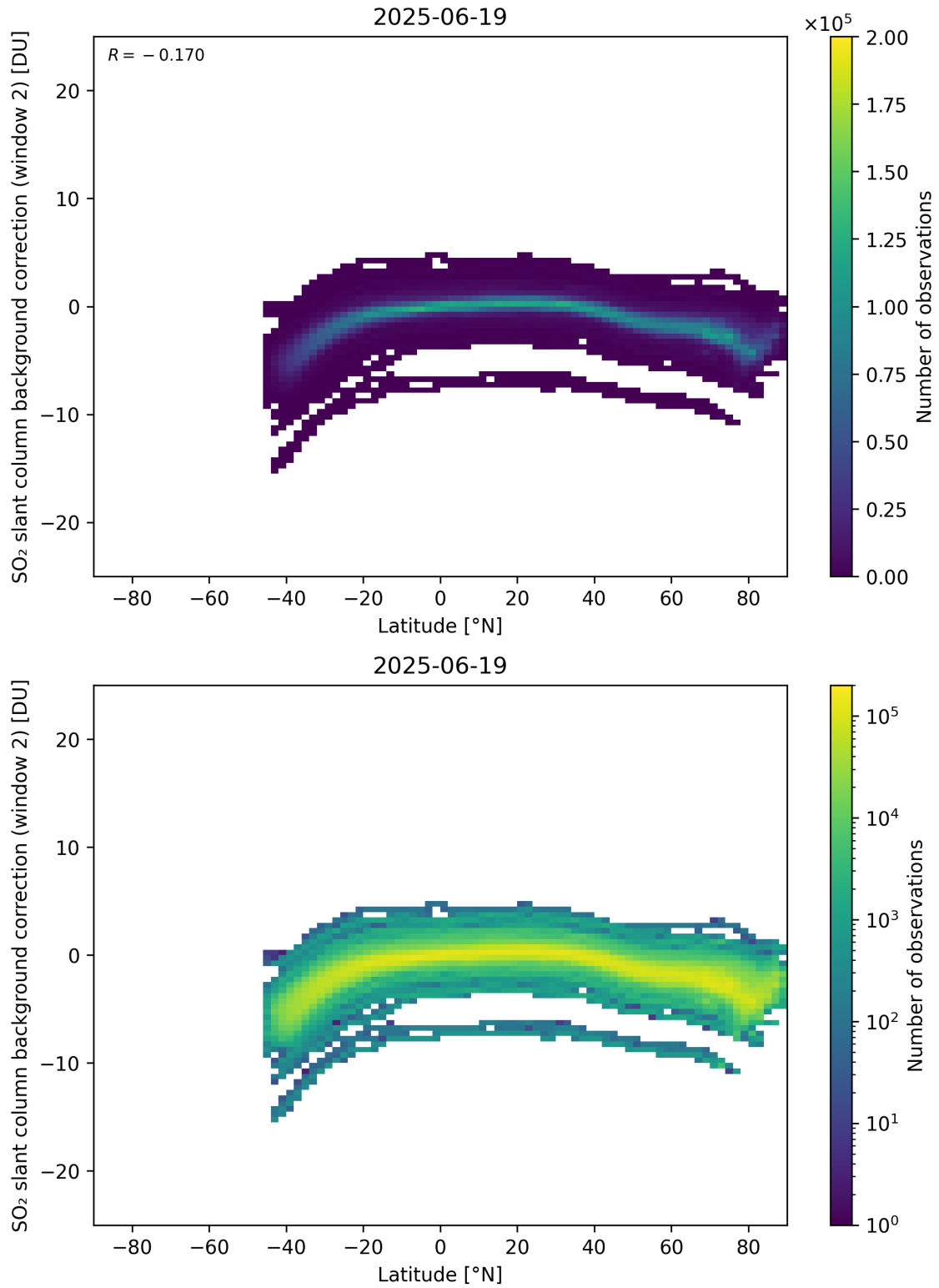
Figure 151: Scatter density plot of “Latitude” against “SO 2 slant column background correction (window 2)” for 2025-06-18 to 2025-06-20.
