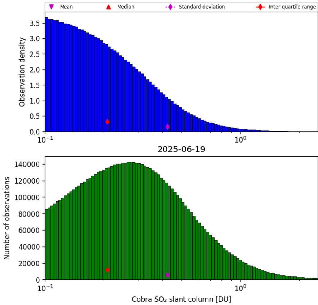
Figure 61: Histogram of “Cobra SO 2 slant column” for 2025-06-18 to 2025-06-20
