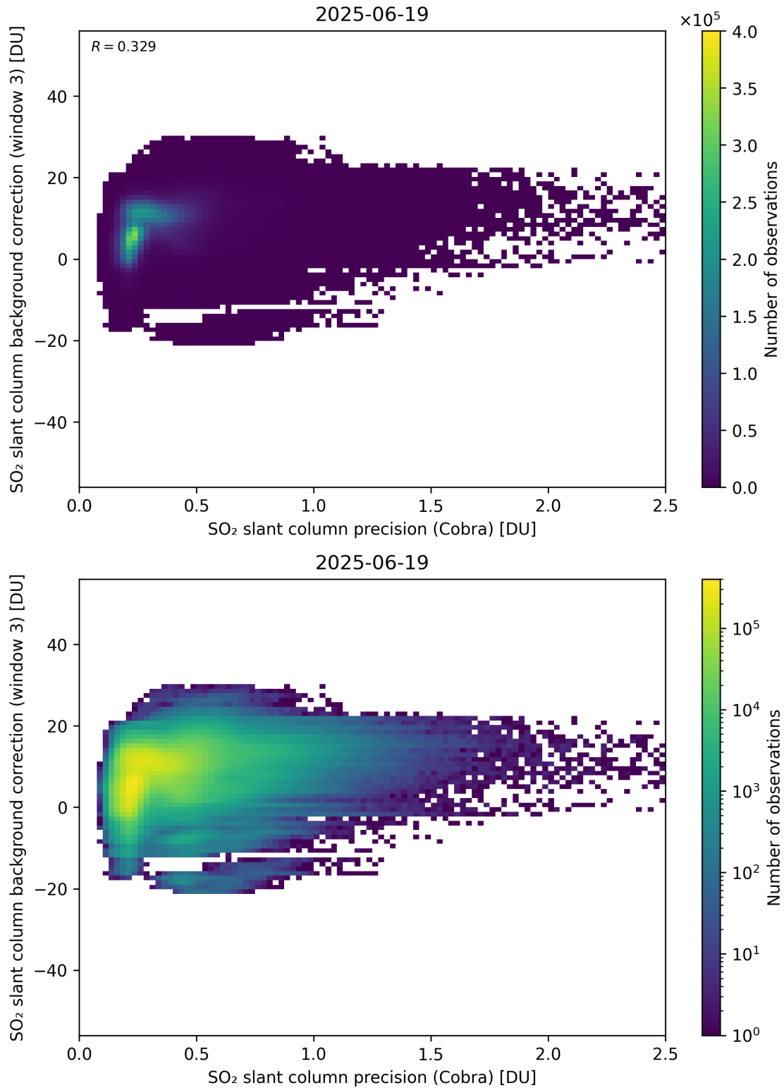
Figure 201: Scatter density plot of “SO 2 slant column precision (Cobra)” against “SO 2 slant column background correction (window 3)” for 2025-06-18 to 2025-06-20.
