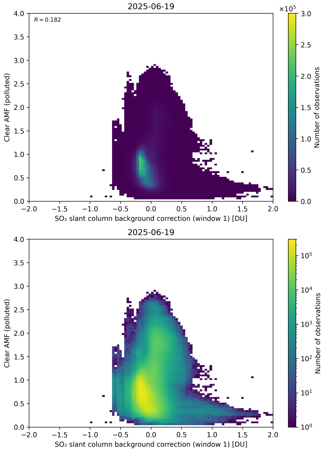
Figure 114: Scatter density plot of “SO 2 slant column background correction (window 1)” against “Clear AMF (polluted)” for 2025-06-18 to 2025-06-20.
