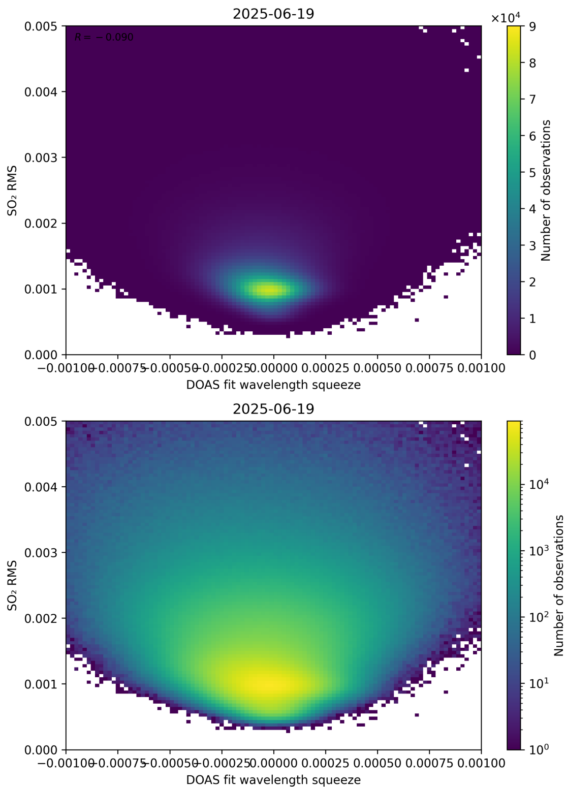
Figure 143: Scatter density plot of “DOAS fit wavelength squeeze” against “SO 2 RMS” for 2025-06-18 to 2025-06-20.
