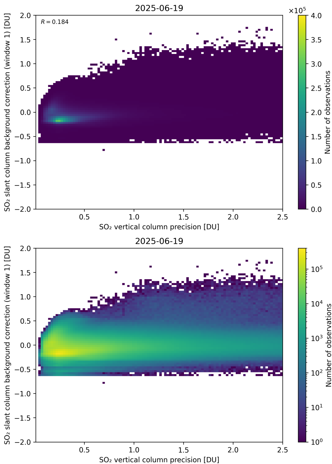
Figure 329: Scatter density plot of “SO 2 vertical column precision” against “SO 2 slant column background correction (window 1)” for 2025-06-18 to 2025-06-20.
