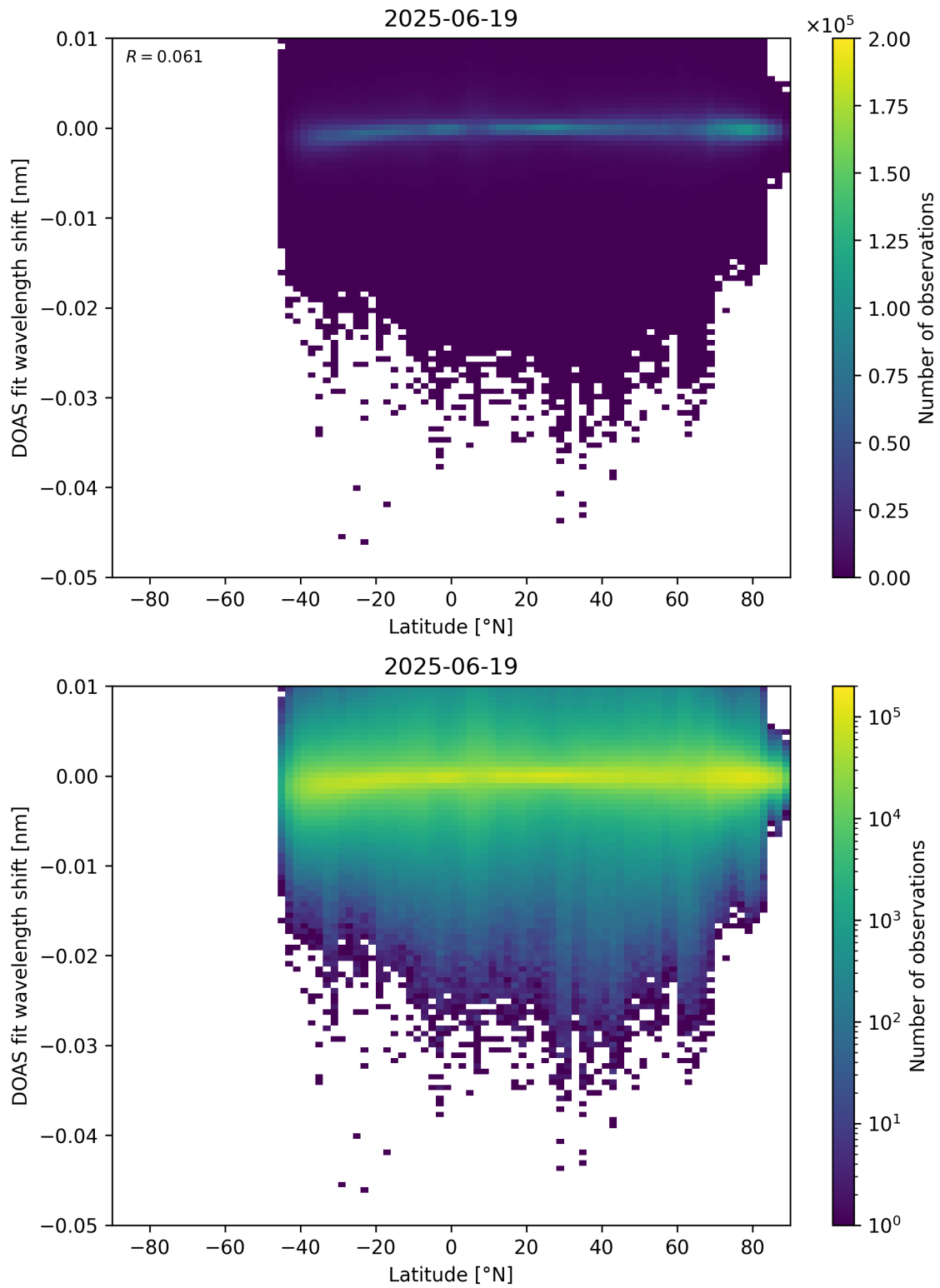
Figure 153: Scatter density plot of “Latitude” against “DOAS fit wavelength shift” for 2025-06-18 to 2025-06-20.
