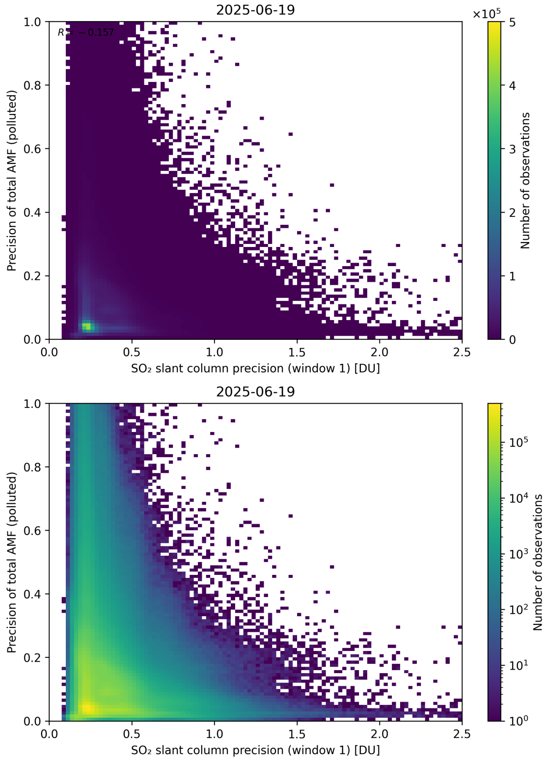
Figure 281: Scatter density plot of “SO 2 slant column precision (window 1)” against “Precision of total AMF (polluted)” for 2025-06-18 to 2025-06-20.
