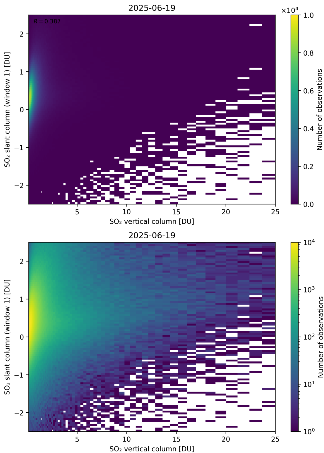
Figure 354: Scatter density plot of “SO 2 vertical column” against “SO 2 slant column (window 1)” for 2025-06-18 to 2025-06-20.
