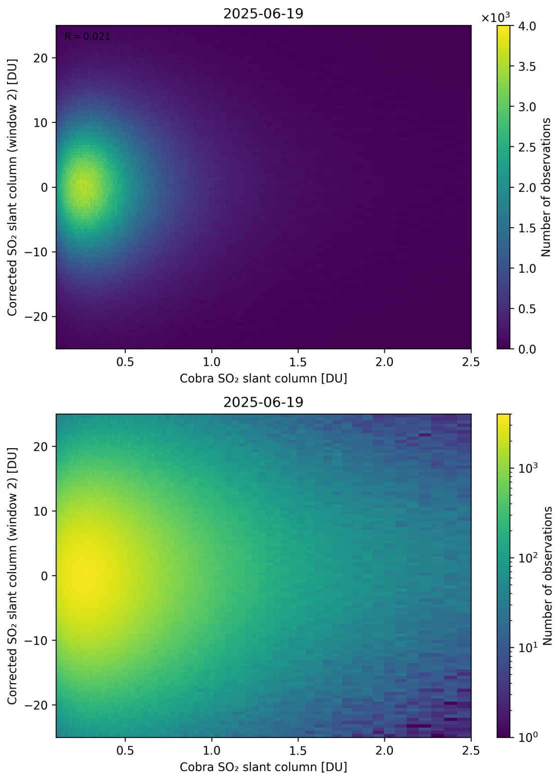
Figure 217: Scatter density plot of “Cobra SO 2 slant column” against “Corrected SO 2 slant column (window 2)” for 2025-06-18 to 2025-06-20.
