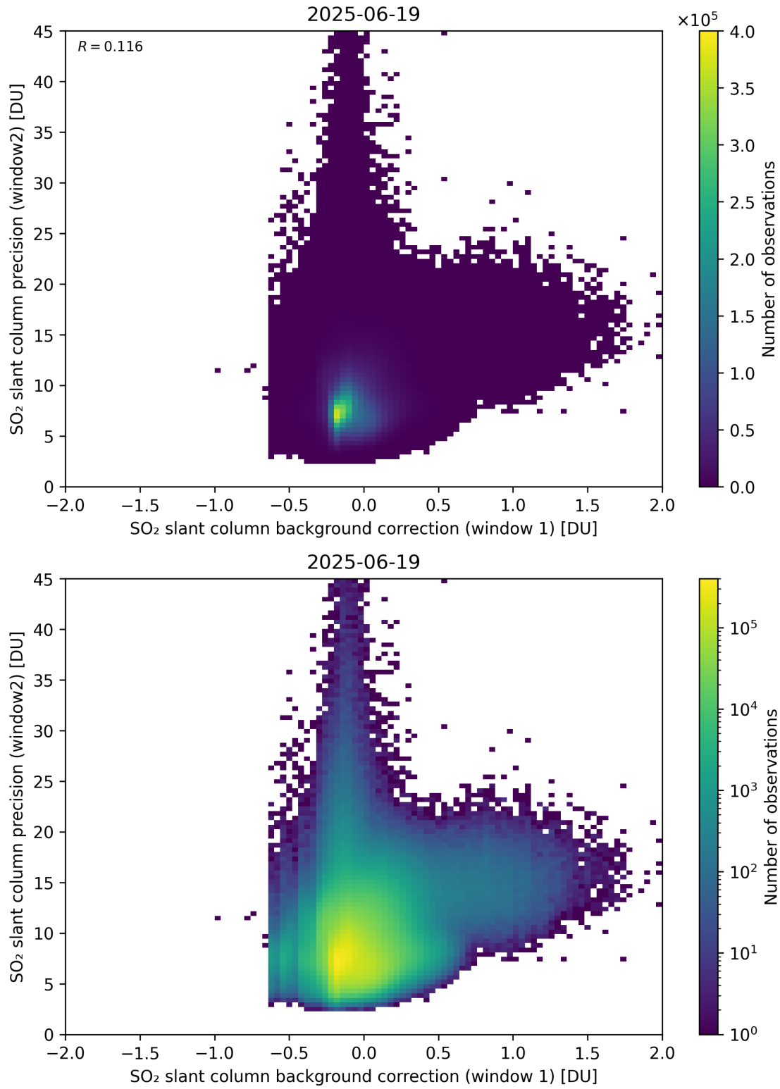
Figure 117: Scatter density plot of “SO 2 slant column background correction (window 1)” against “SO 2 slant column precision (window2)” for 2025-06-18 to 2025-06-20.
