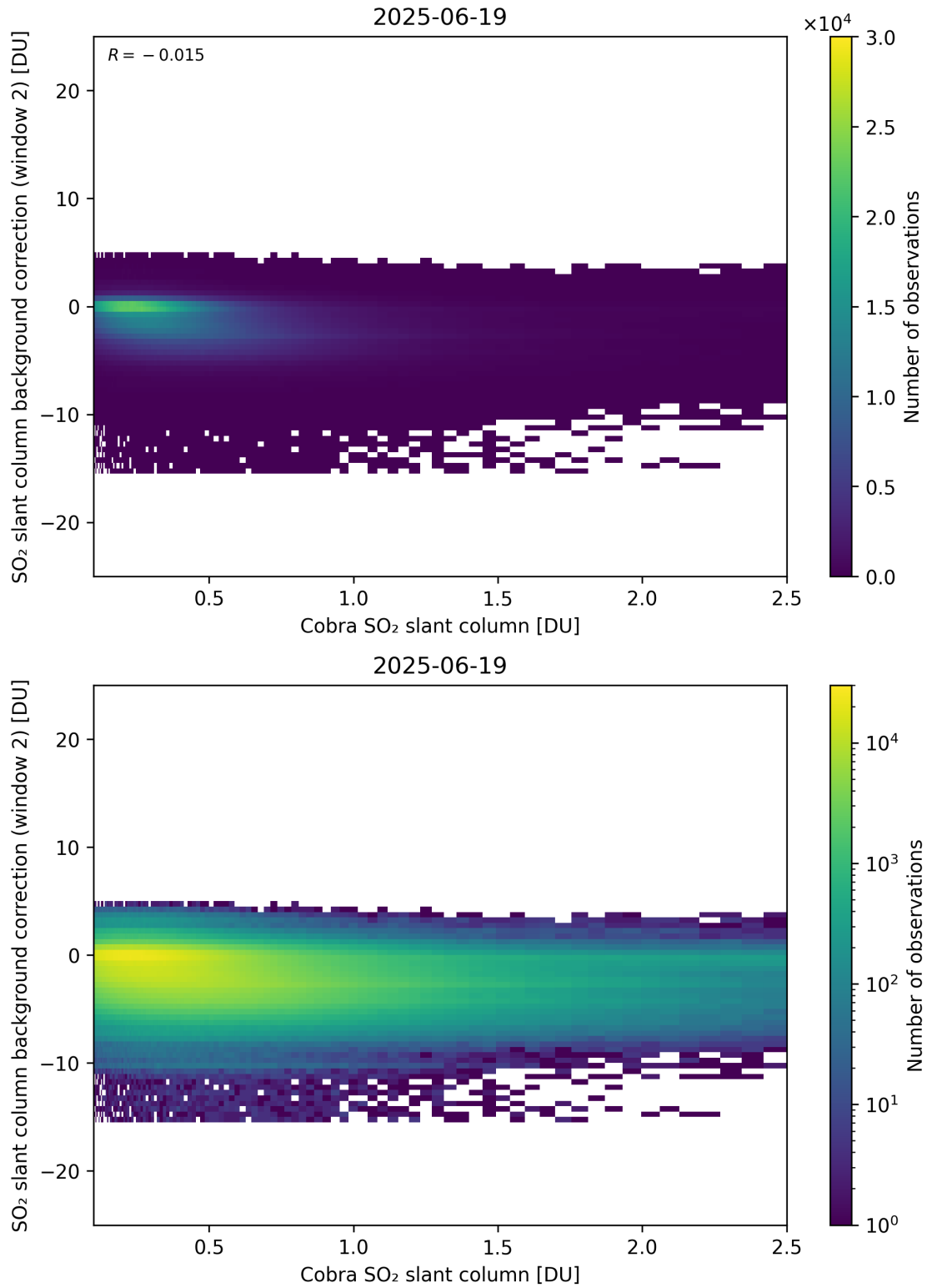
Figure 194: Scatter density plot of “Cobra SO 2 slant column” against “SO 2 slant column background correction (window 2)” for 2025-06-18 to 2025-06-20.
