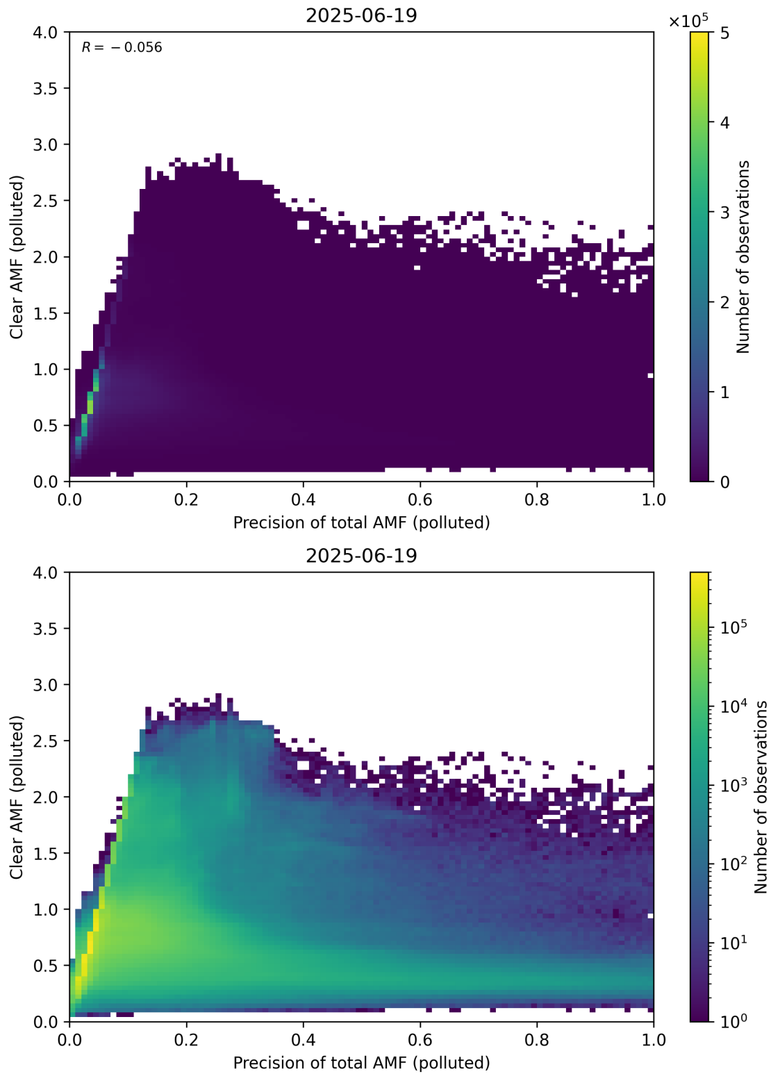
Figure 320: Scatter density plot of “Precision of total AMF (polluted)” against “Clear AMF (polluted)” for 2025-06-18 to 2025-06-20.
