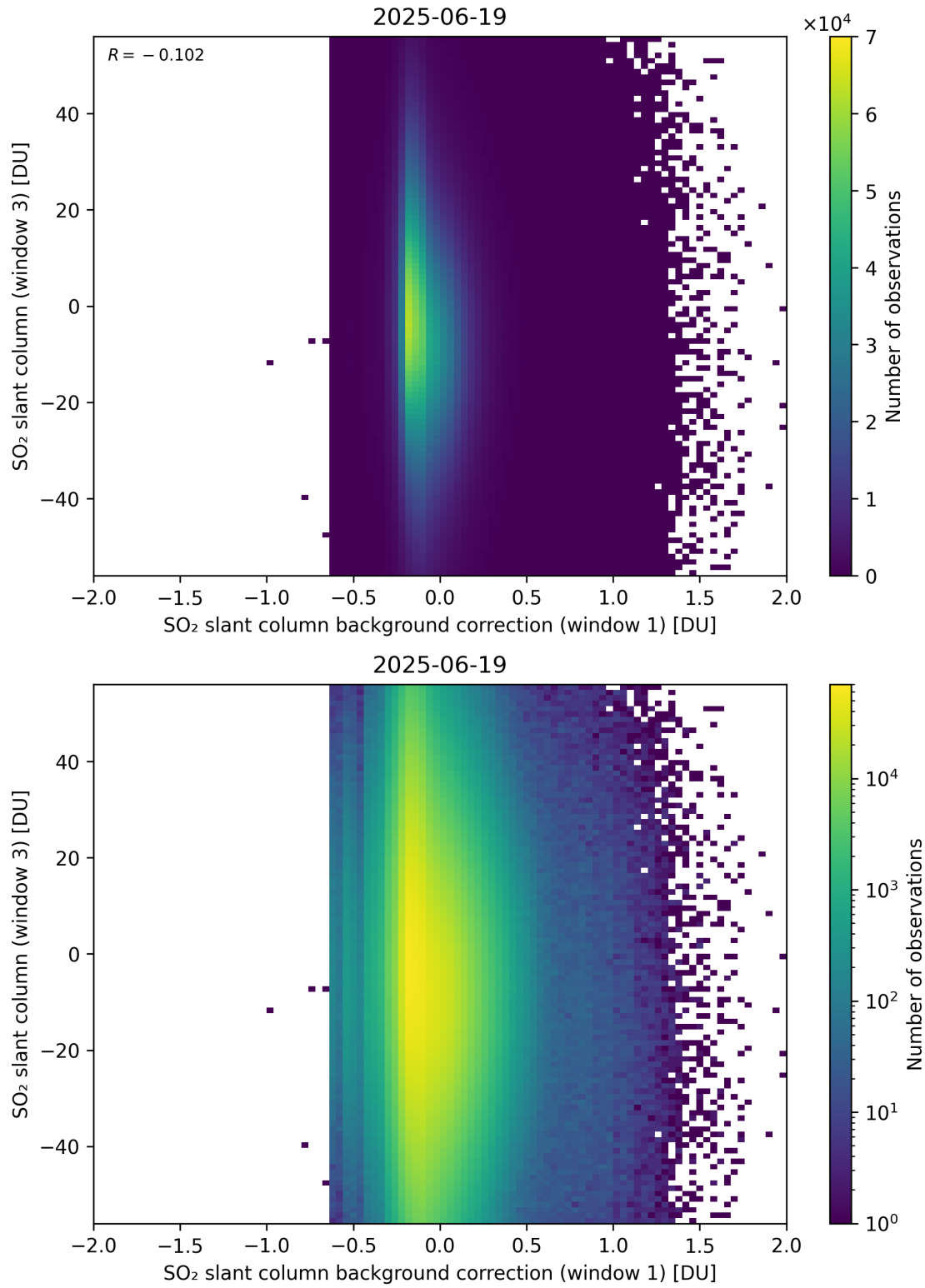
Figure 118: Scatter density plot of “SO 2 slant column background correction (window 1)” against “SO 2 slant column (window 3)” for 2025-06-18 to 2025-06-20.
