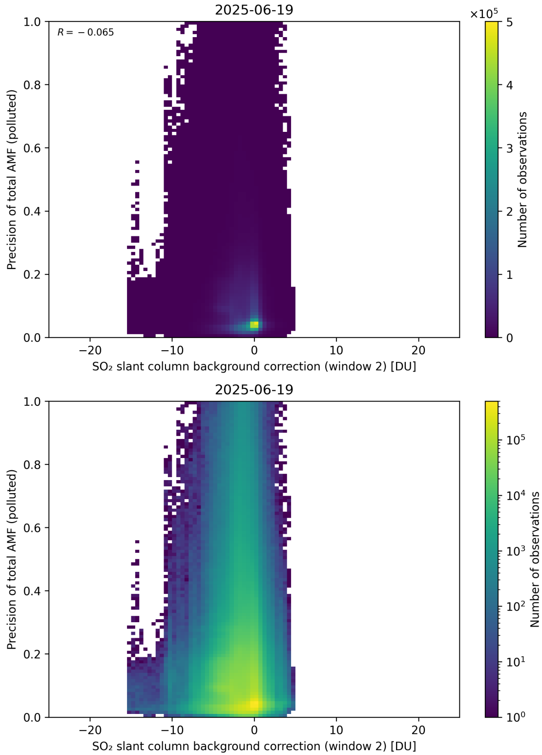
Figure 131: Scatter density plot of “SO 2 slant column background correction (window 2)” against “Precision of total AMF (polluted)” for 2025-06-18 to 2025-06-20.
