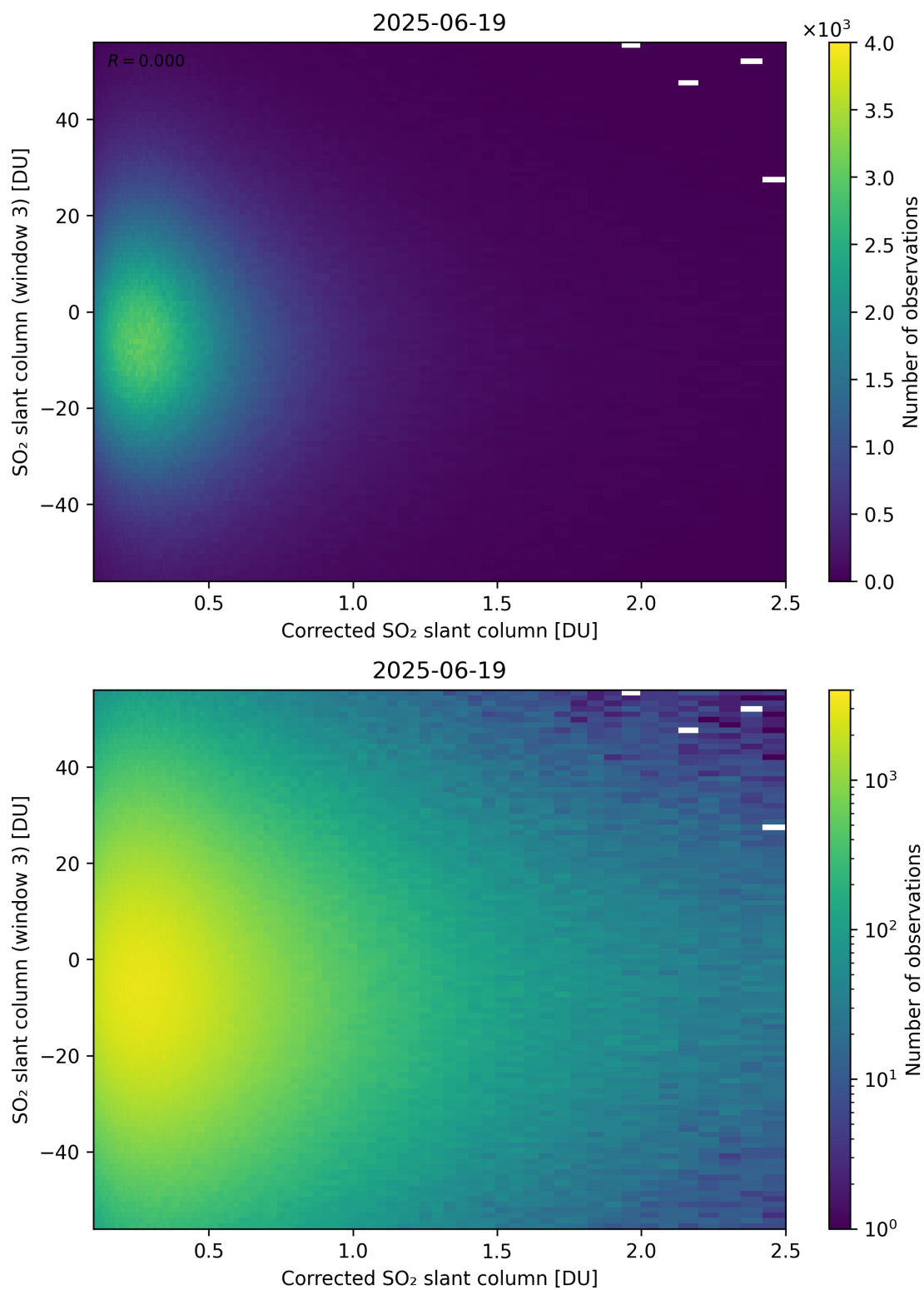
Figure 240: Scatter density plot of “Corrected SO 2 slant column” against “SO 2 slant column (window 3)” for 2025-06-18 to 2025-06-20.
