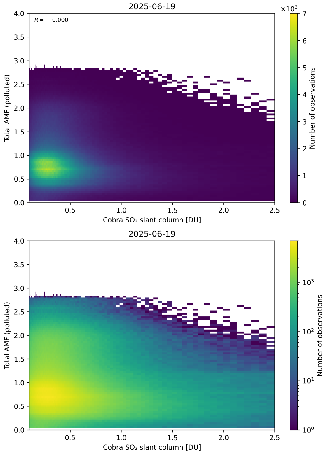
Figure 224: Scatter density plot of “Cobra SO 2 slant column” against “Total AMF (polluted)” for 2025-06-18 to 2025-06-20.
