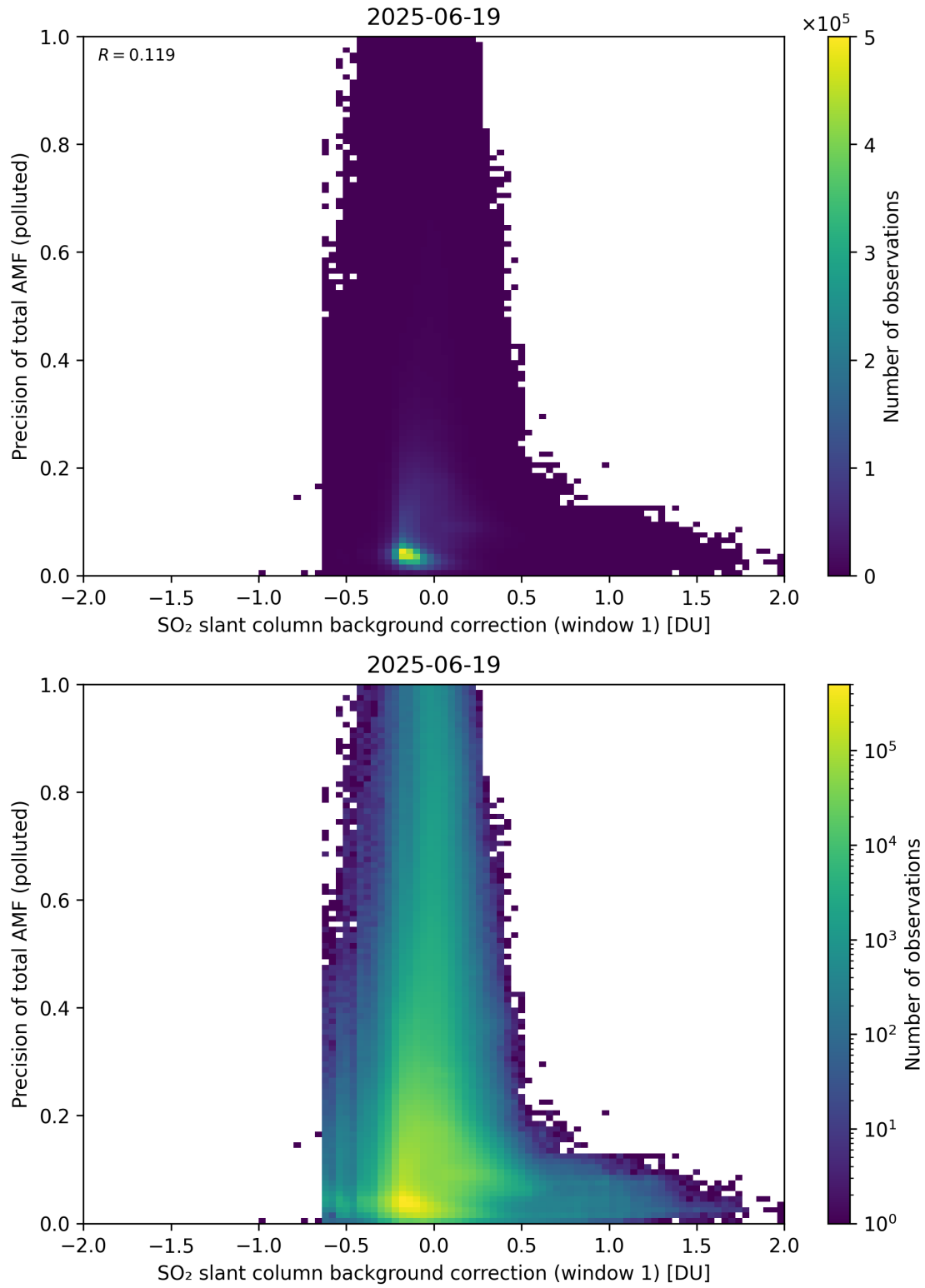
Figure 121: Scatter density plot of “SO 2 slant column background correction (window 1)” against “Precision of total AMF (polluted)” for 2025-06-18 to 2025-06-20.
