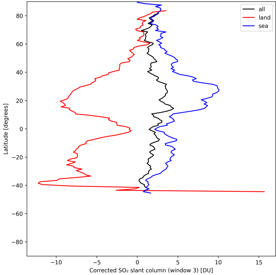
Figure 47: Zonal average of “Corrected SO 2 slant column (window 3)” for 2025-06-18 to 2025-06-20.
