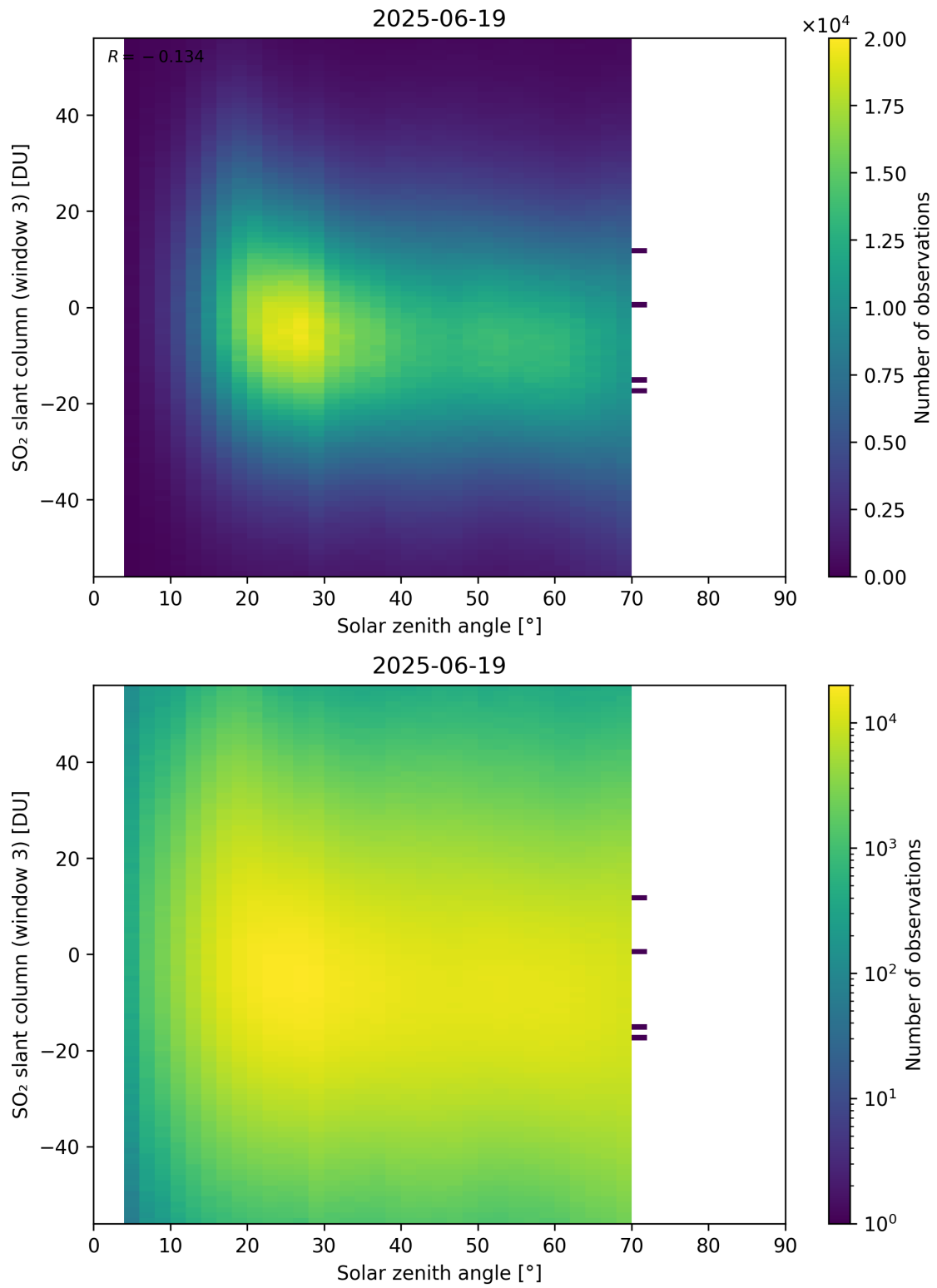
Figure 187: Scatter density plot of “Solar zenith angle” against “SO 2 slant column (window 3)” for 2025-06-18 to 2025-06-20.
