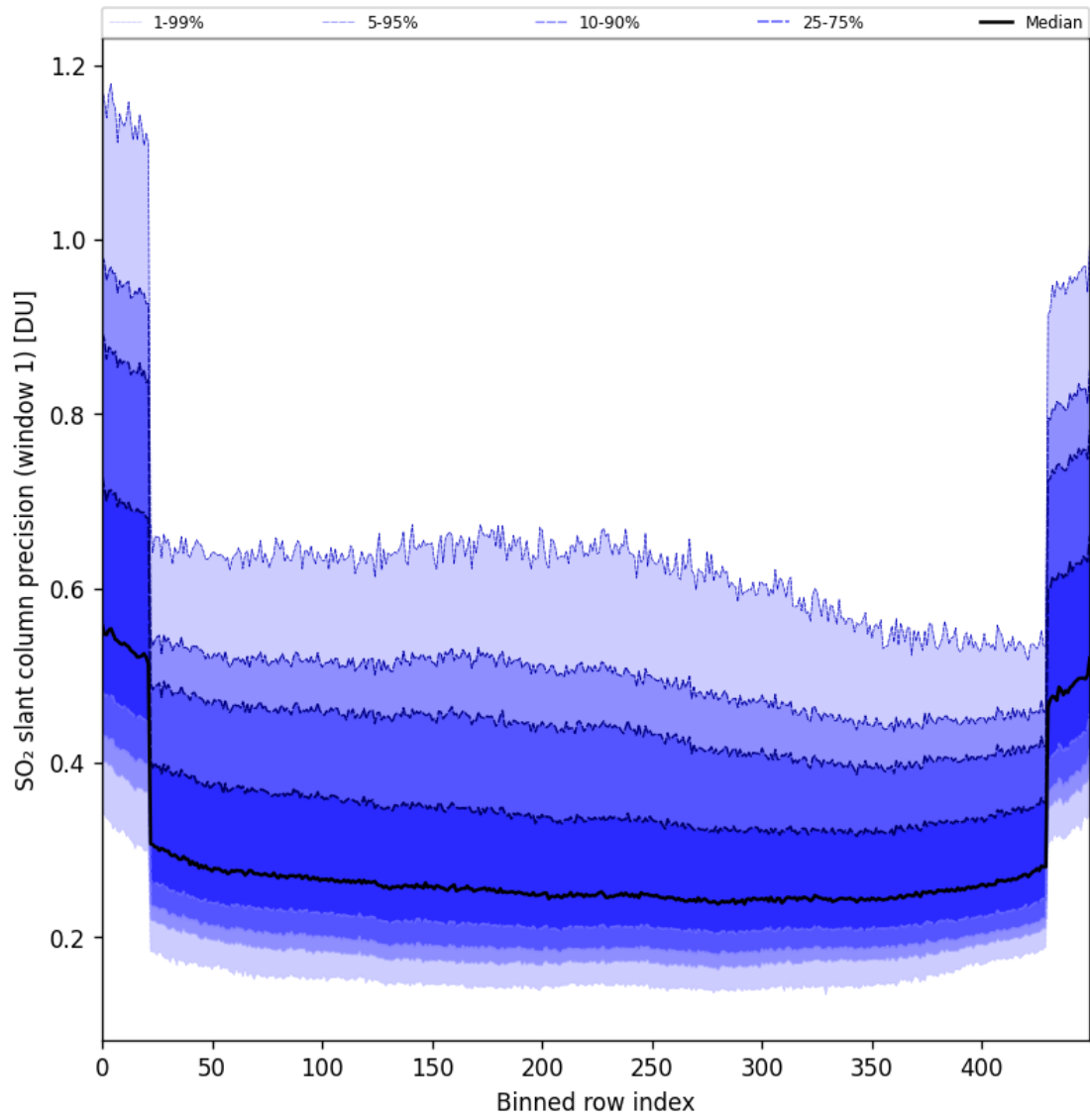
Figure 90: Along track statistics of “SO 2 slant column precision (window 1)” for 2025-06-18 to 2025-06-20
