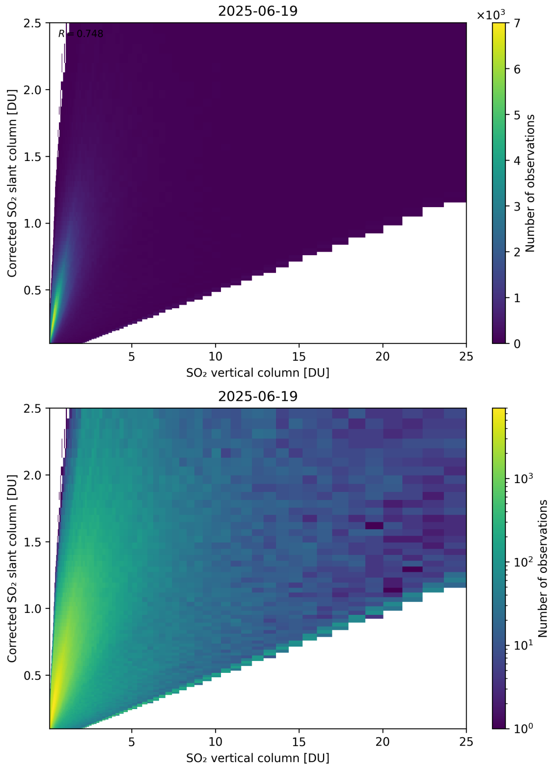
Figure 351: Scatter density plot of “SO 2 vertical column” against “Corrected SO 2 slant column” for 2025-06-18 to 2025-06-20.
