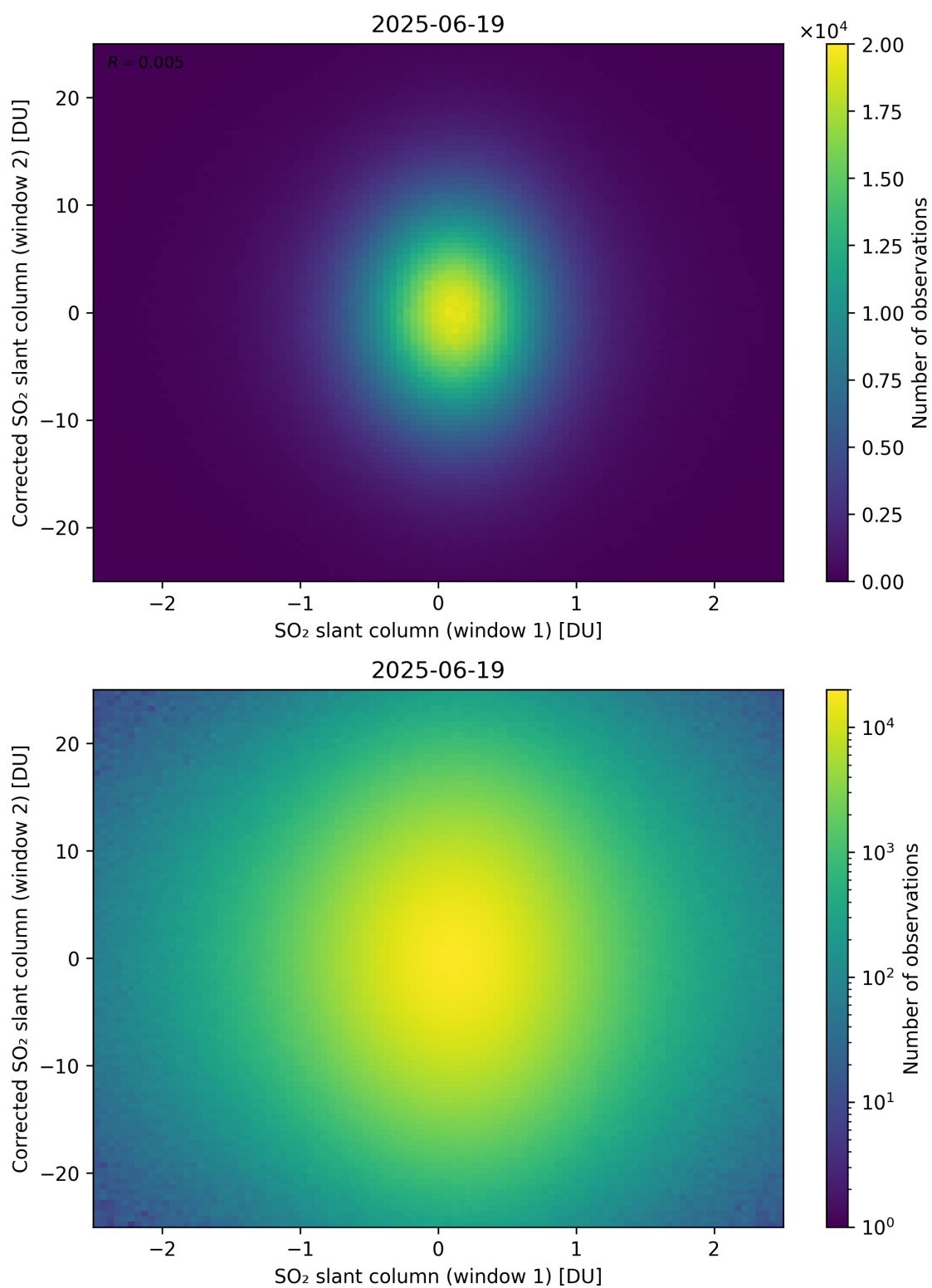
Figure 283: Scatter density plot of “SO 2 slant column (window 1)” against “Corrected SO 2 slant column (window 2)” for 2025-06-18 to 2025-06-20.
