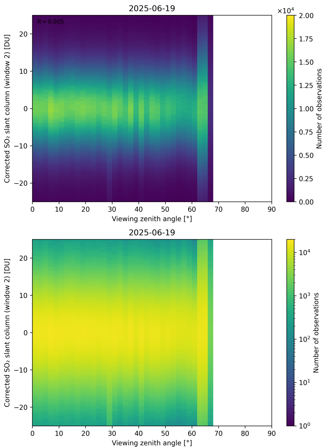
Figure 374: Scatter density plot of “Viewing zenith angle” against “Corrected SO 2 slant column (window 2)” for 2025-06-18 to 2025-06-20.
