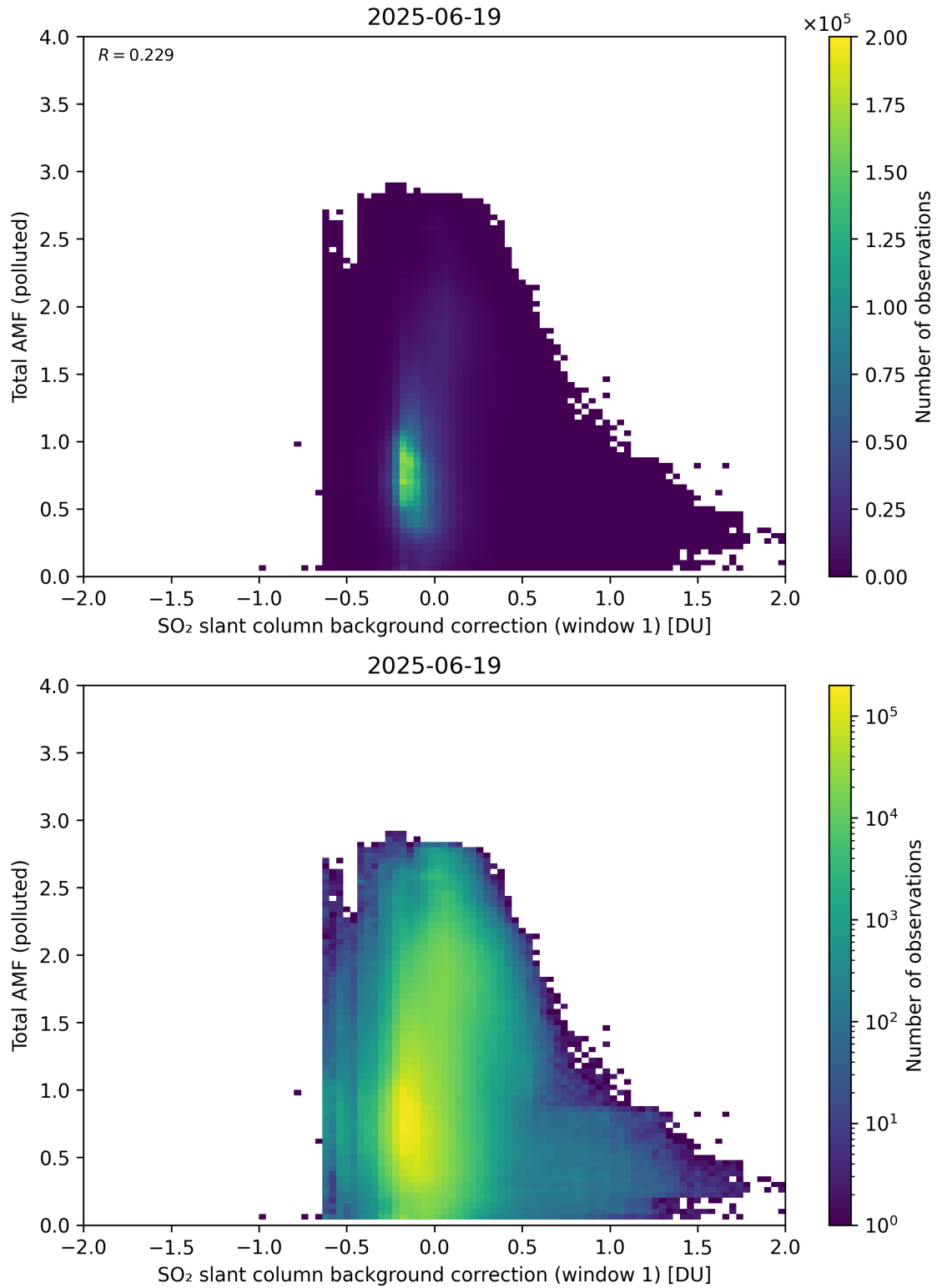
Figure 120: Scatter density plot of “SO 2 slant column background correction (window 1)” against “Total AMF (polluted)” for 2025-06-18 to 2025-06-20.
