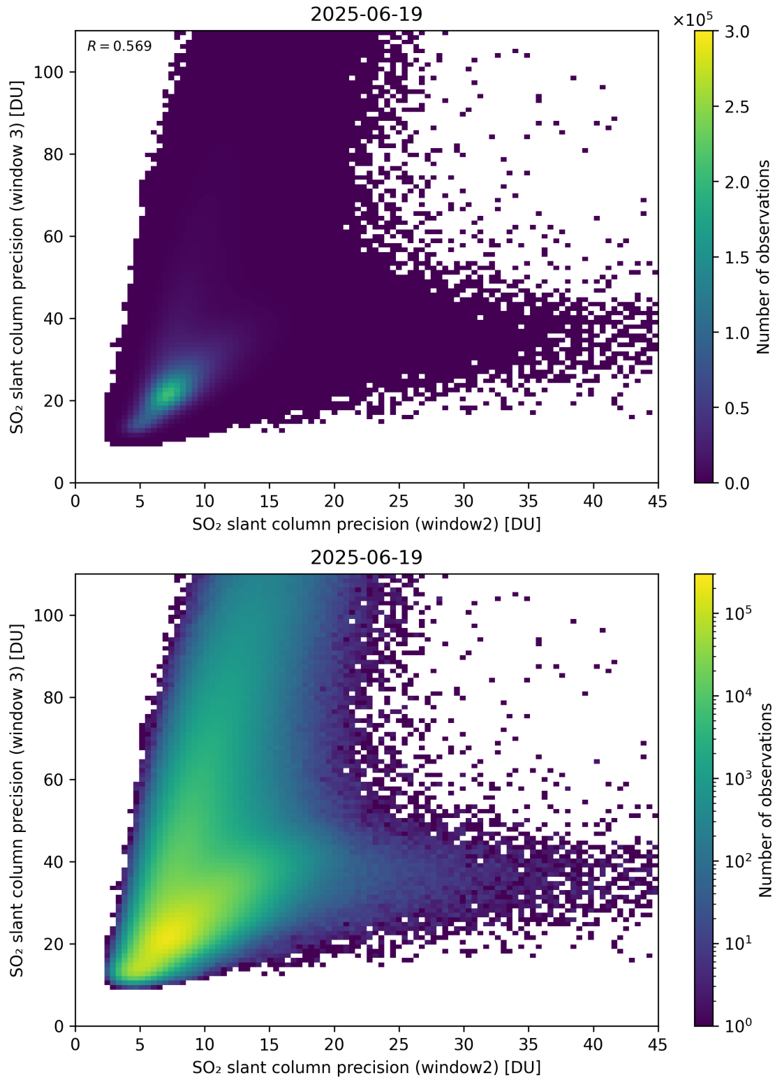
Figure 300: Scatter density plot of “SO 2 slant column precision (window2)” against “SO 2 slant column precision (window 3)” for 2025-06-18 to 2025-06-20.
