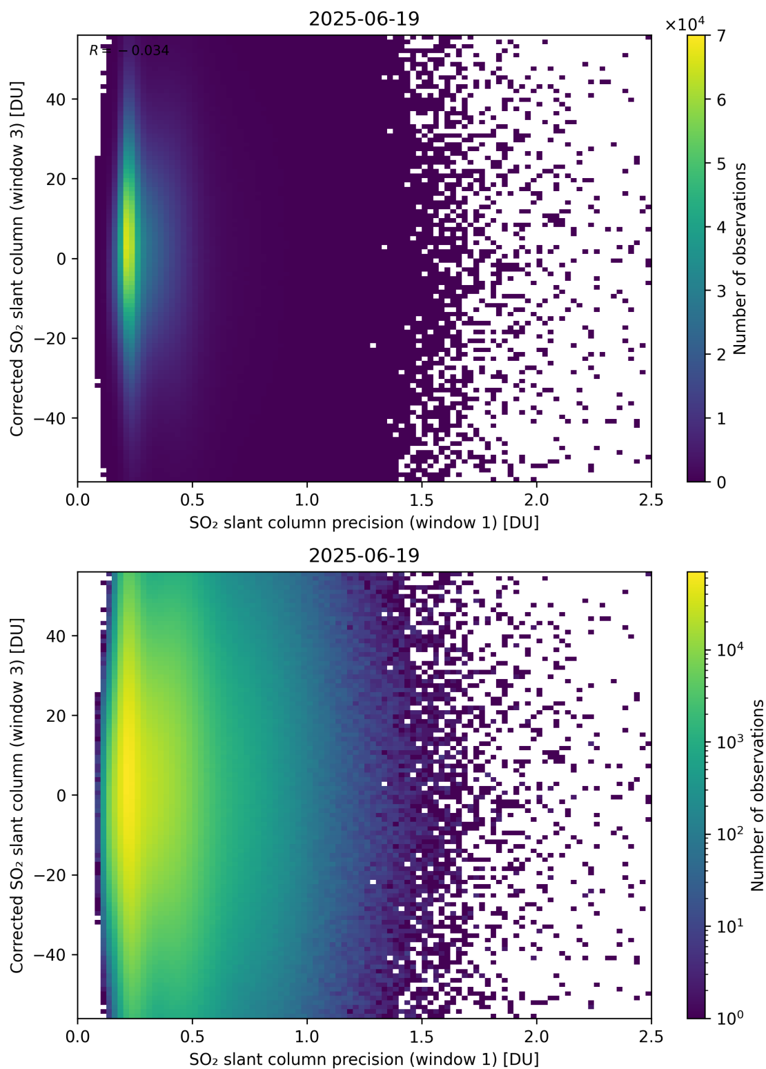
Figure 276: Scatter density plot of “SO 2 slant column precision (window 1)” against “Corrected SO 2 slant column (window 3)” for 2025-06-18 to 2025-06-20.
