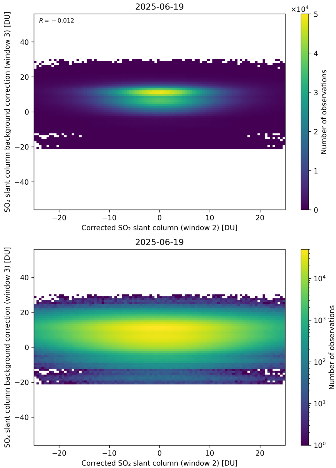
Figure 245: Scatter density plot of “Corrected SO 2 slant column (window 2)” against “SO 2 slant column background correction (window 3)” for 2025-06-18 to 2025-06-20.
