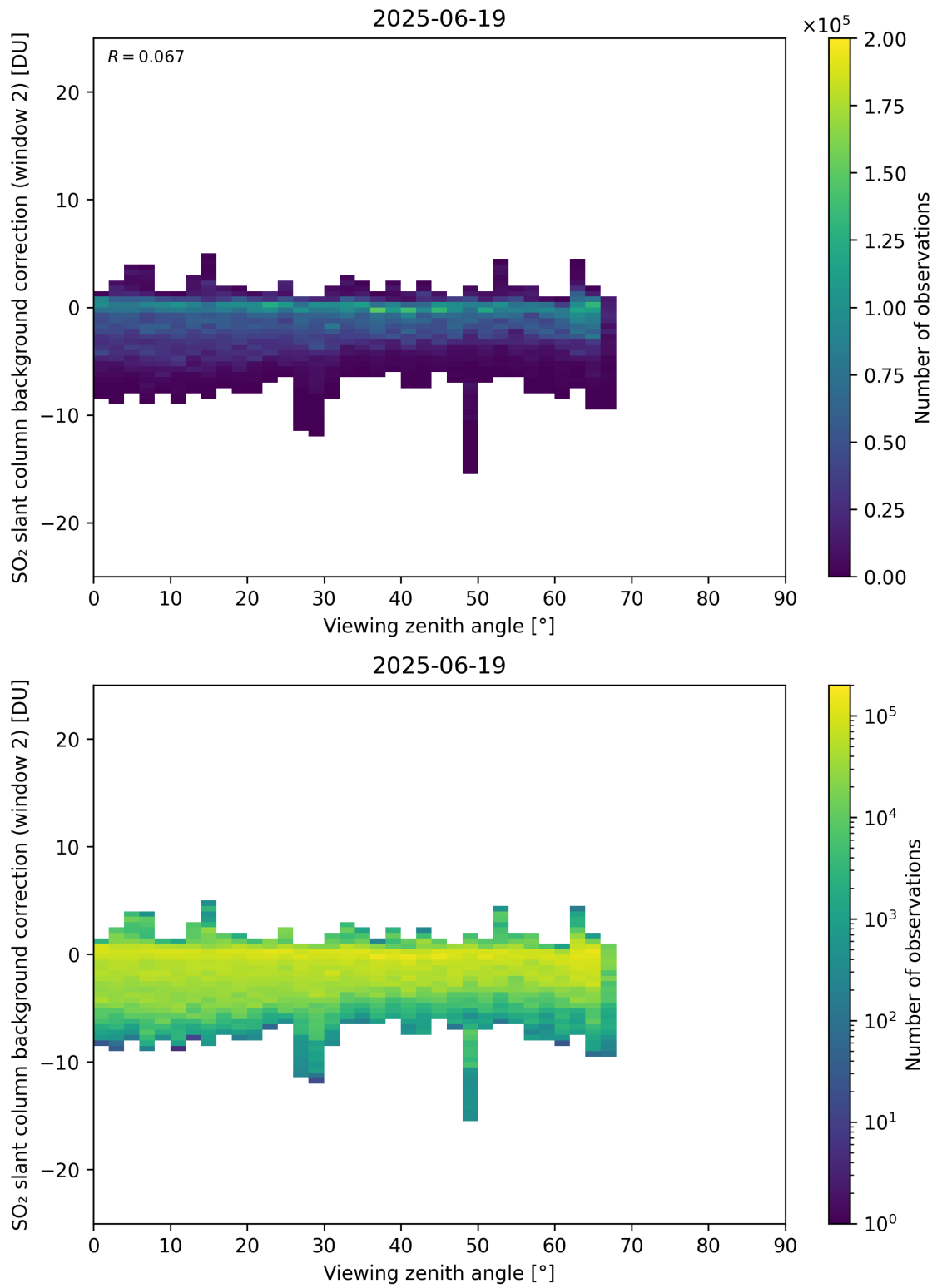
Figure 363: Scatter density plot of “Viewing zenith angle” against “SO 2 slant column background correction (window 2)” for 2025-06-18 to 2025-06-20.
