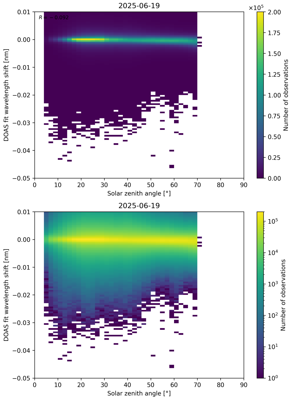
Figure 174: Scatter density plot of “Solar zenith angle” against “DOAS fit wavelength shift” for 2025-06-18 to 2025-06-20.
