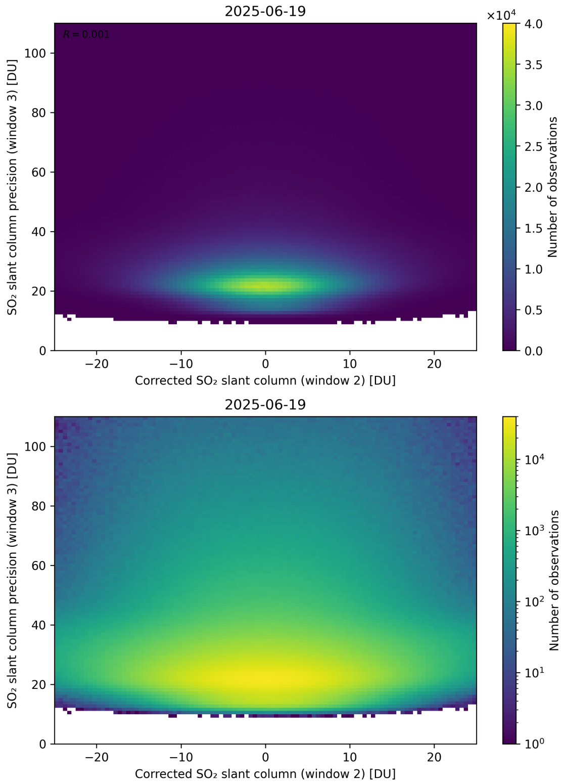
Figure 252: Scatter density plot of “Corrected SO 2 slant column (window 2)” against “SO 2 slant column precision (window 3)” for 2025-06-18 to 2025-06-20.
