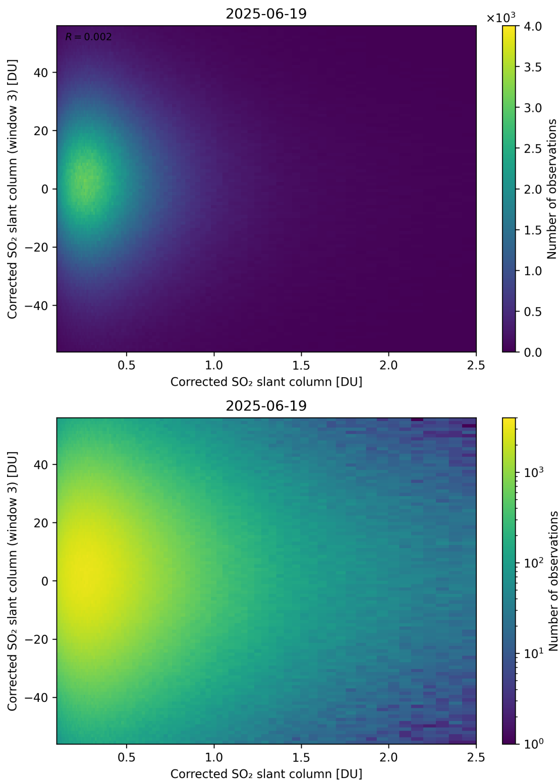
Figure 236: Scatter density plot of “Corrected SO 2 slant column” against “Corrected SO 2 slant column (window 3)” for 2025-06-18 to 2025-06-20.
