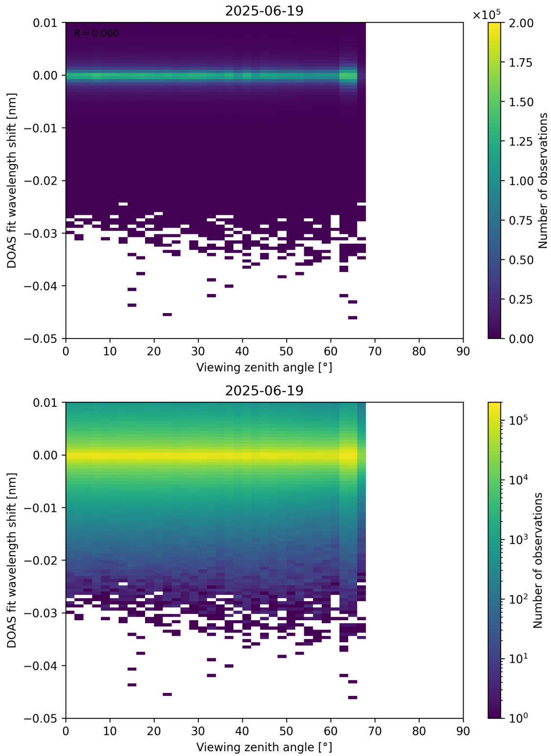
Figure 365: Scatter density plot of “Viewing zenith angle” against “DOAS fit wavelength shift” for 2025-06-18 to 2025-06-20.
