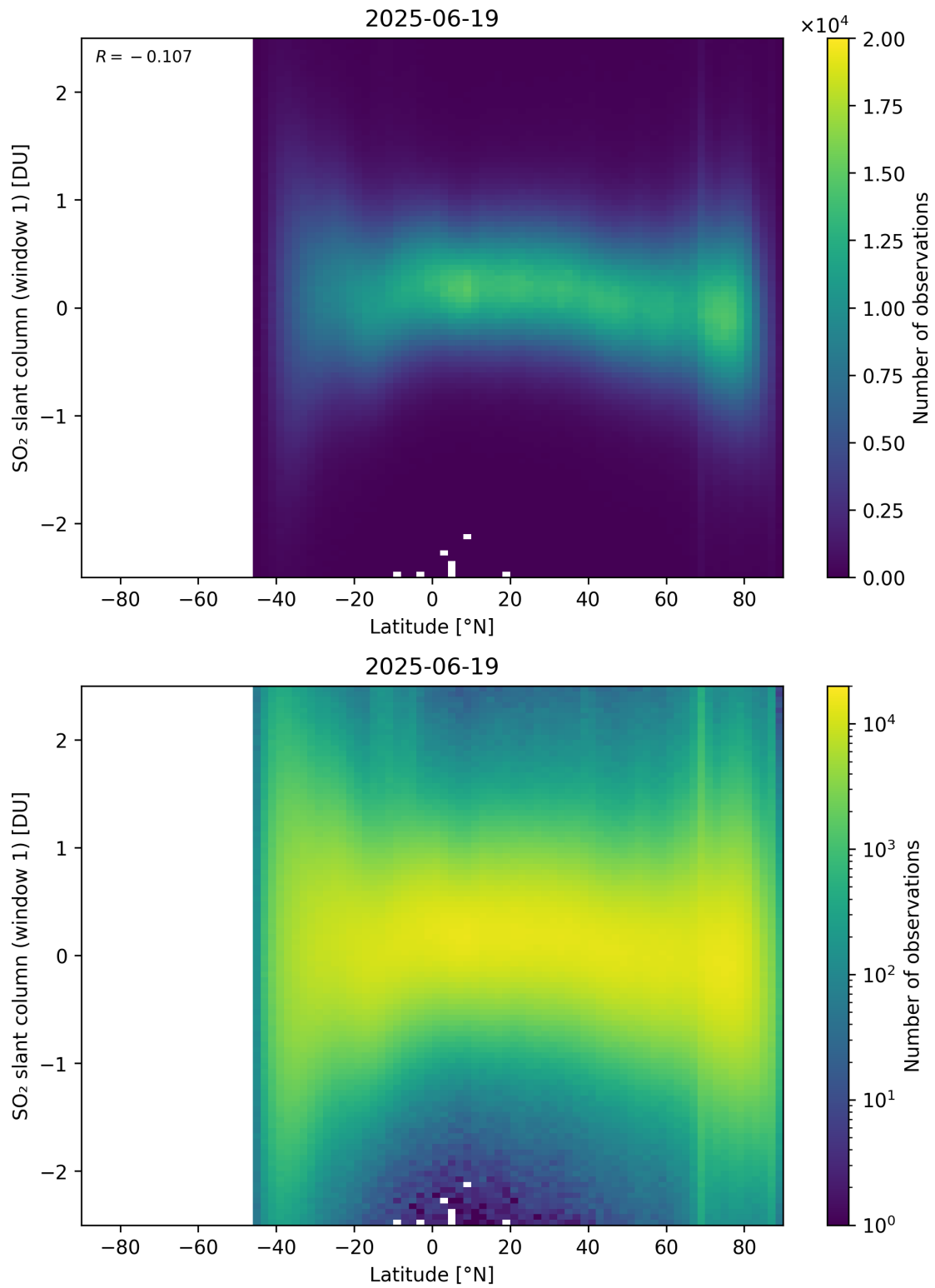
Figure 162: Scatter density plot of “Latitude” against “SO 2 slant column (window 1)” for 2025-06-18 to 2025-06-20.
