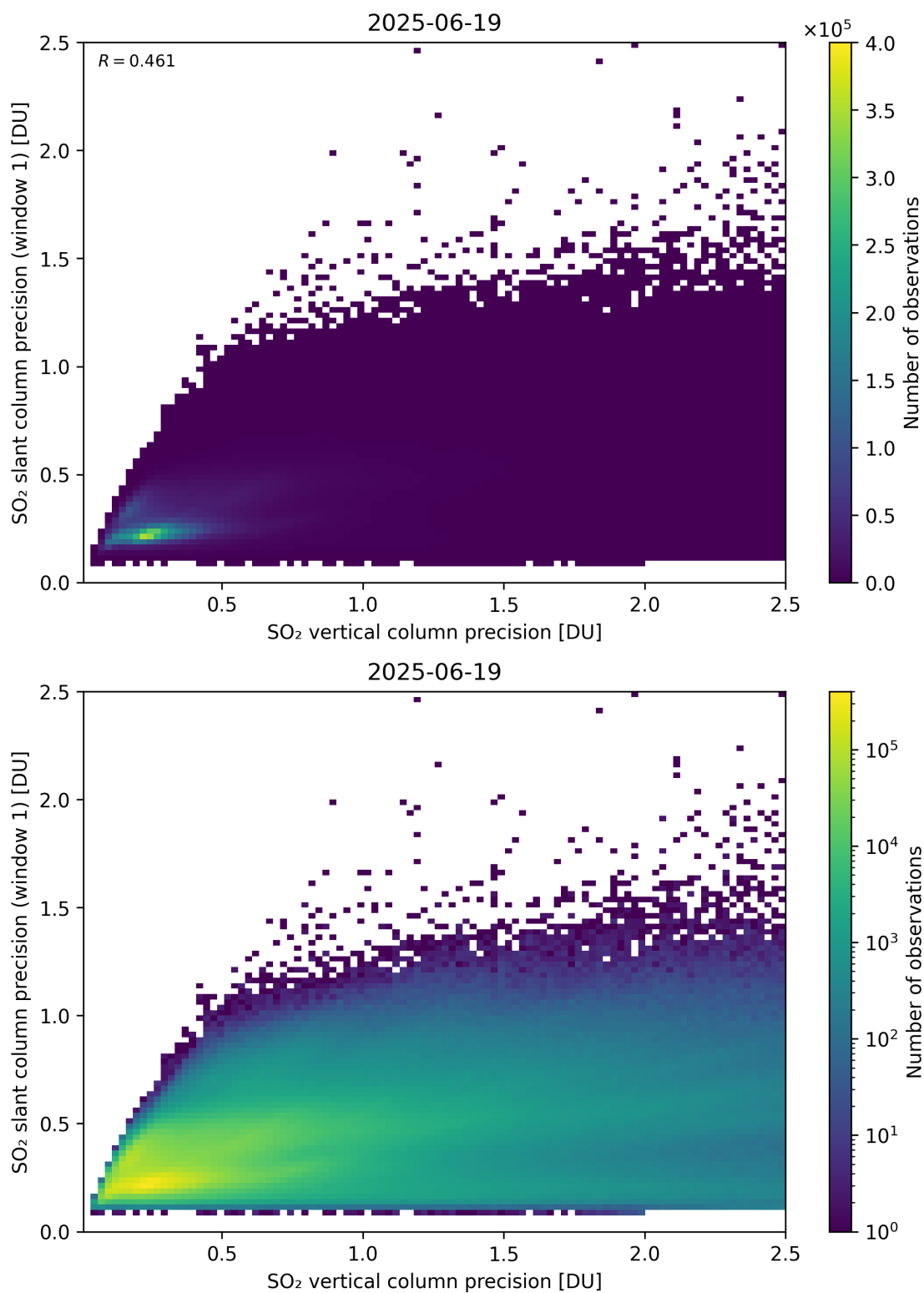
Figure 342: Scatter density plot of “SO 2 vertical column precision” against “SO 2 slant column precision (window 1)” for 2025-06-18 to 2025-06-20.
