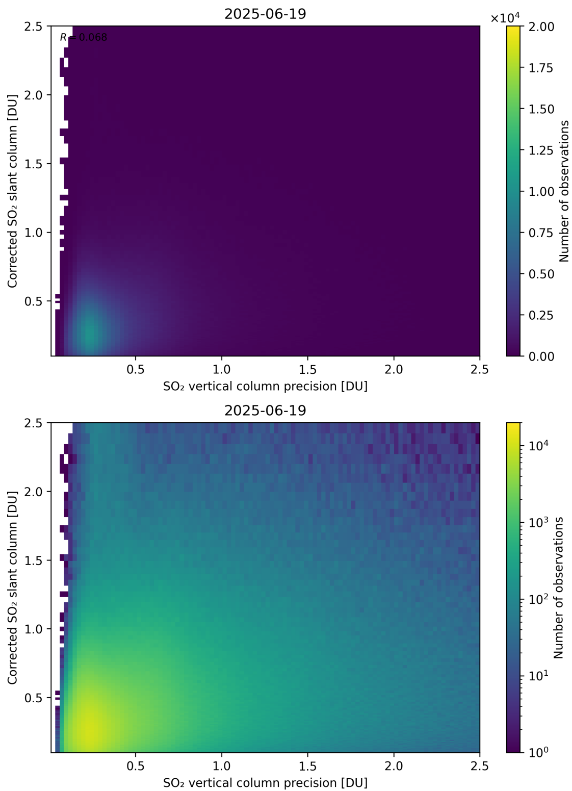
Figure 338: Scatter density plot of “SO 2 vertical column precision” against “Corrected SO 2 slant column” for 2025-06-18 to 2025-06-20.
