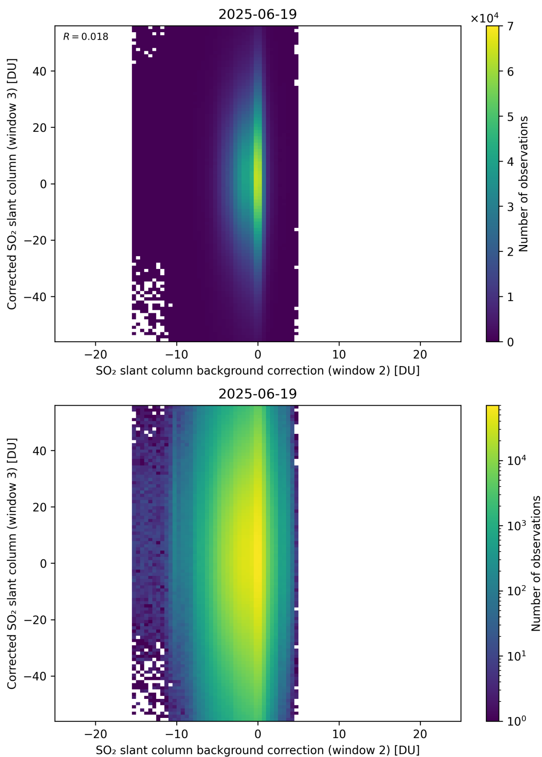
Figure 127: Scatter density plot of “SO 2 slant column background correction (window 2)” against “Corrected SO 2 slant column (window 3)” for 2025-06-18 to 2025-06-20.
