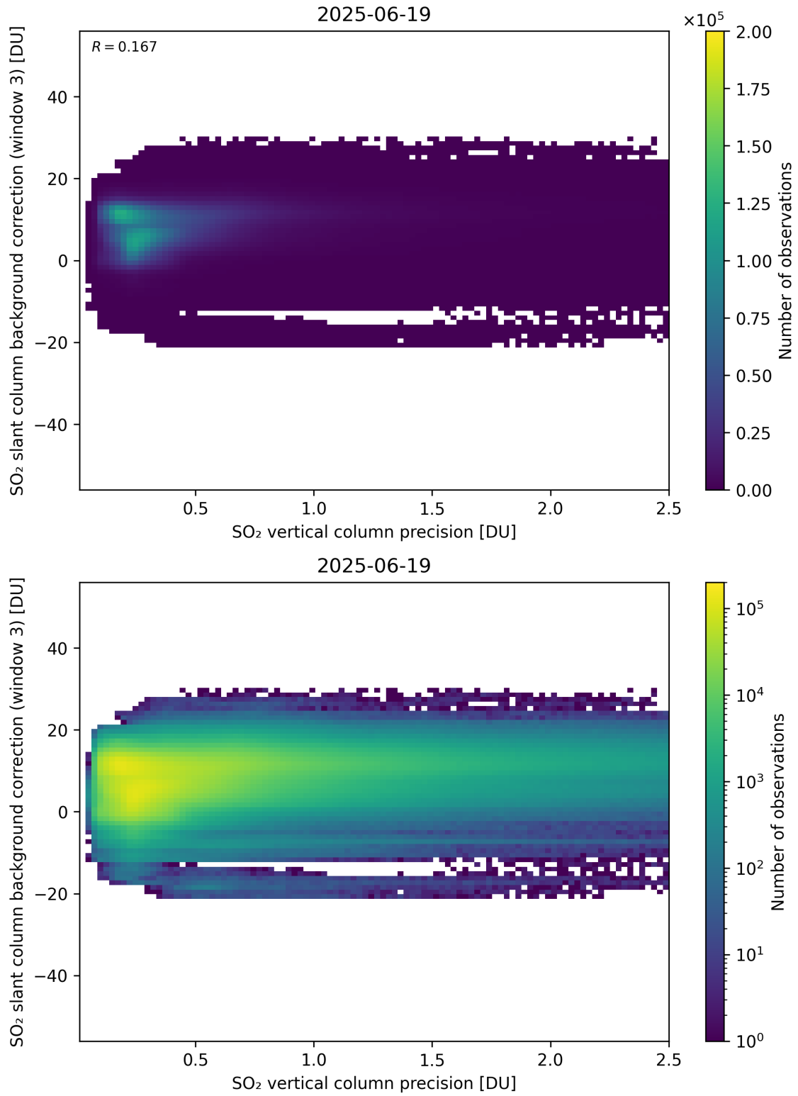
Figure 331: Scatter density plot of “SO 2 vertical column precision” against “SO 2 slant column background correction (window 3)” for 2025-06-18 to 2025-06-20.
