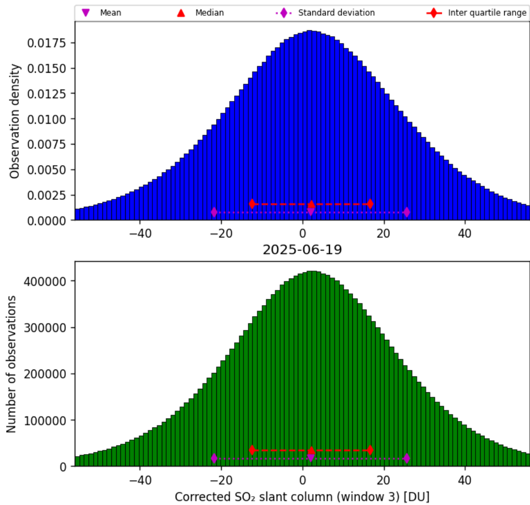
Figure 73: Histogram of “Corrected SO 2 slant column (window 3)” for 2025-06-18 to 2025-06-20
