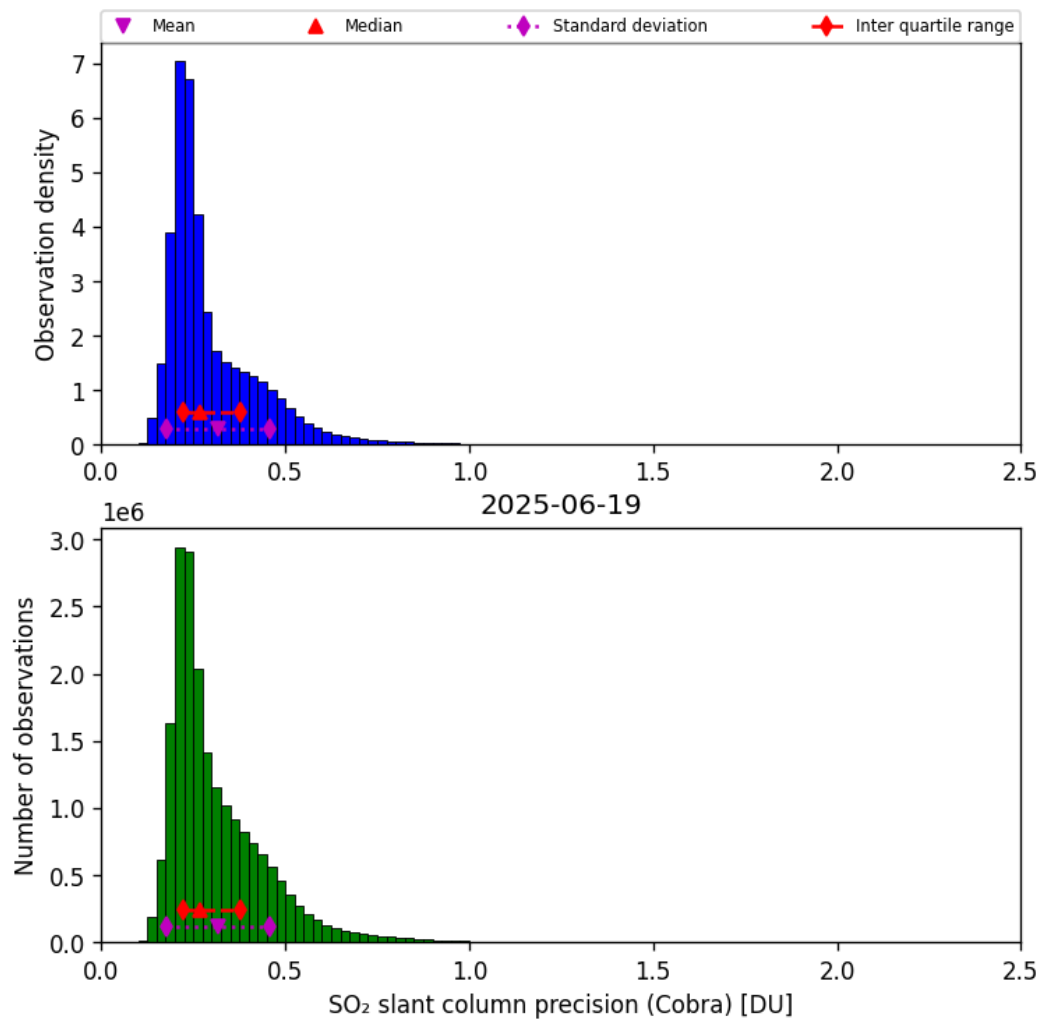
Figure 62: Histogram of “SO 2 slant column precision (Cobra)” for 2025-06-18 to 2025-06-20
