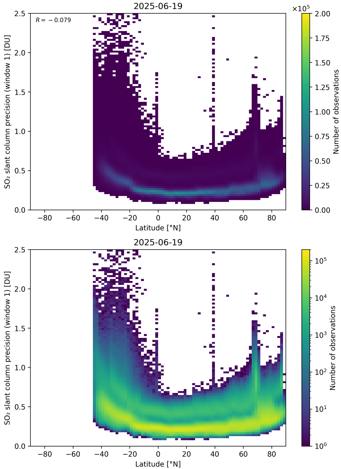
Figure 163: Scatter density plot of “Latitude” against “SO 2 slant column precision (window 1)” for 2025-06-18 to 2025-06-20.
