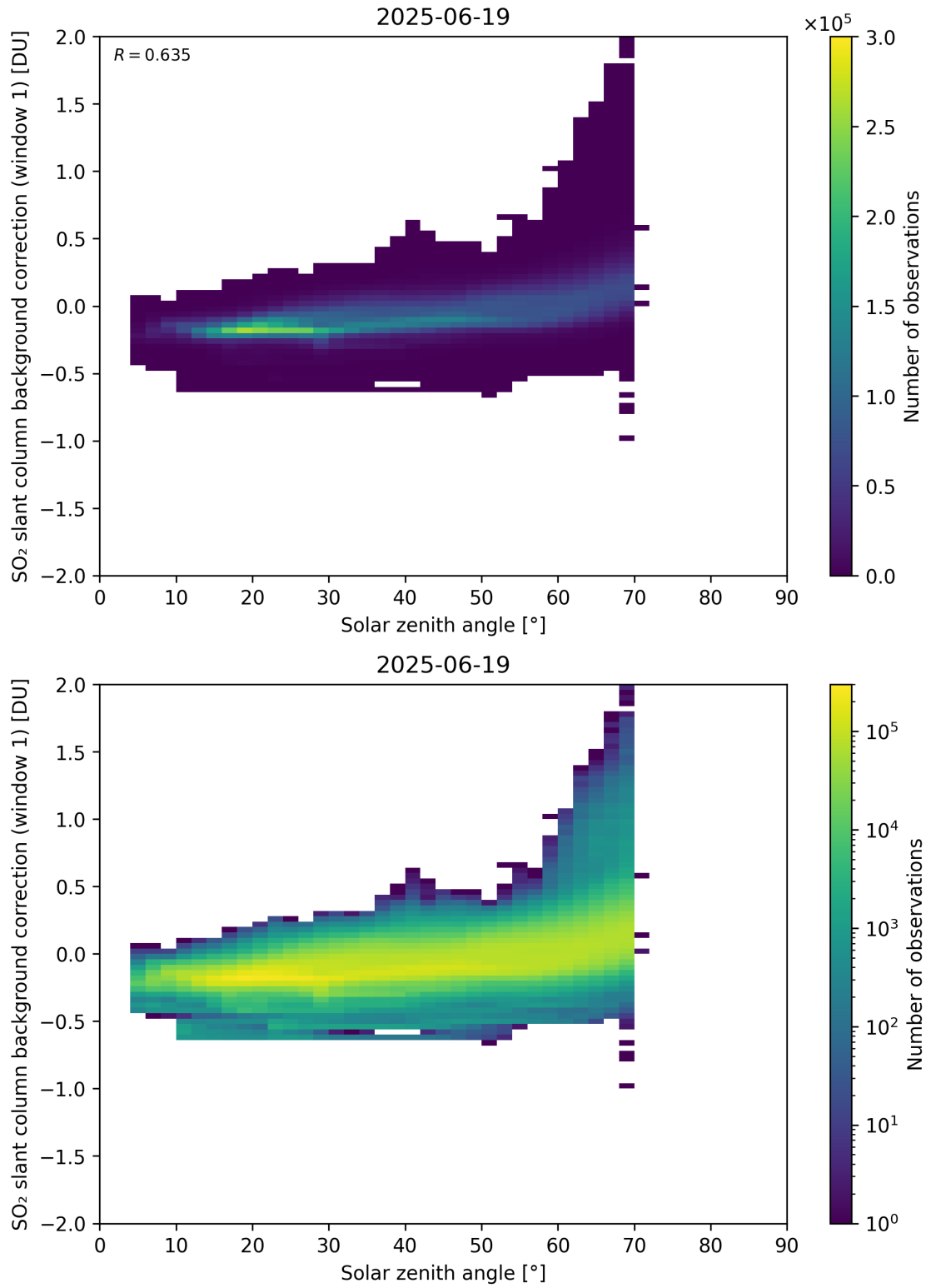
Figure 171: Scatter density plot of “Solar zenith angle” against “SO 2 slant column background correction (window 1)” for 2025-06-18 to 2025-06-20.
