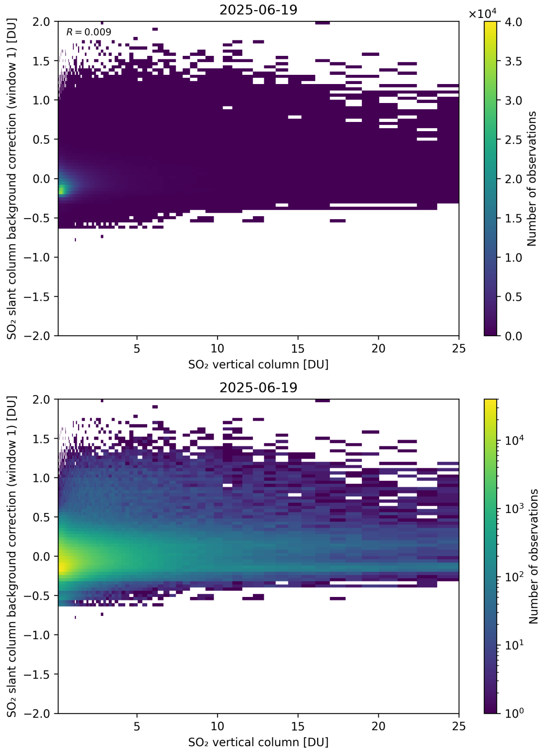
Figure 323: Scatter density plot of “SO 2 vertical column” against “SO 2 slant column background correction (window 1)” for 2025-06-18 to 2025-06-20.
