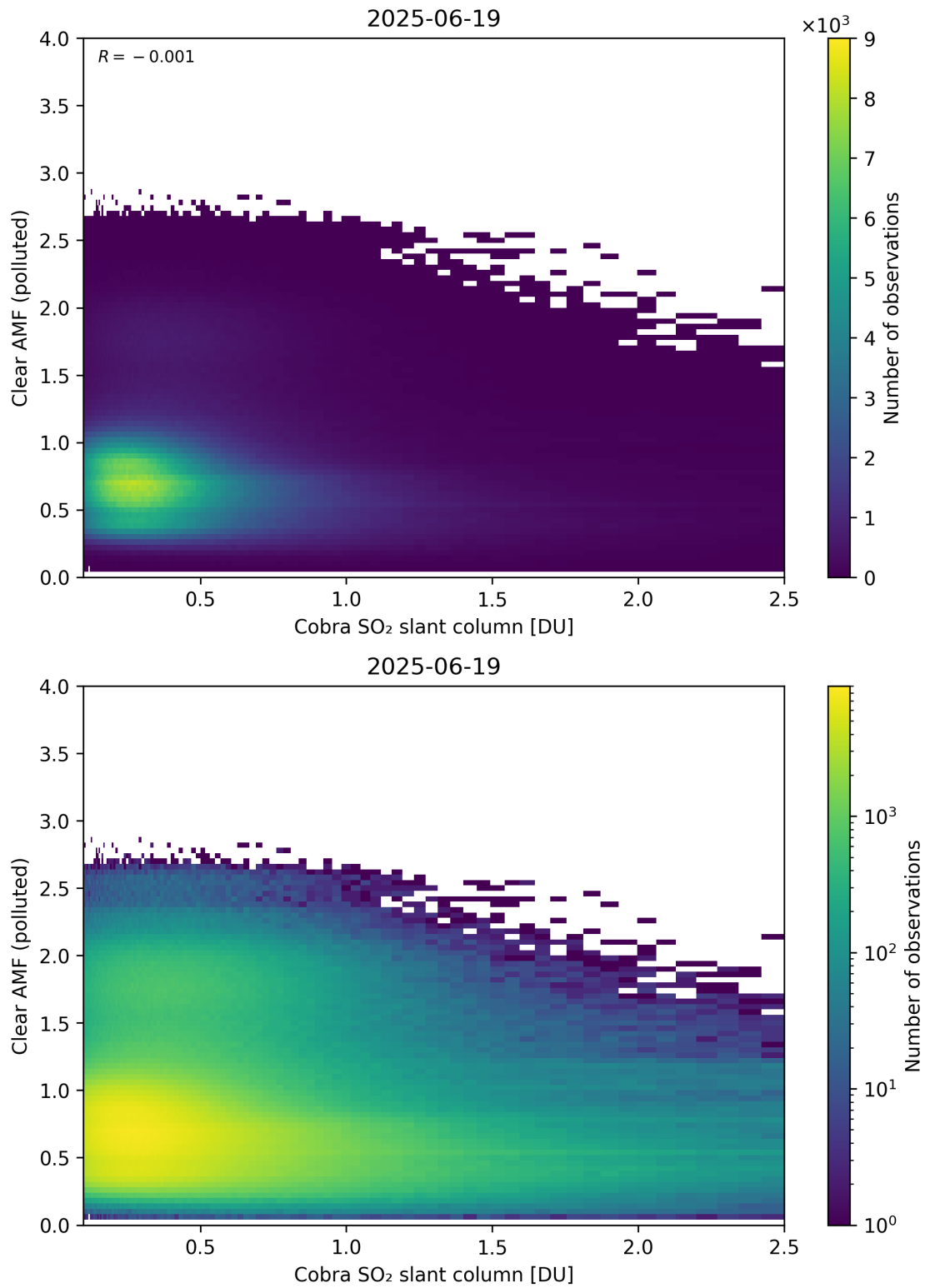
Figure 215: Scatter density plot of “Cobra SO 2 slant column” against “Clear AMF (polluted)” for 2025-06-18 to 2025-06-20.
