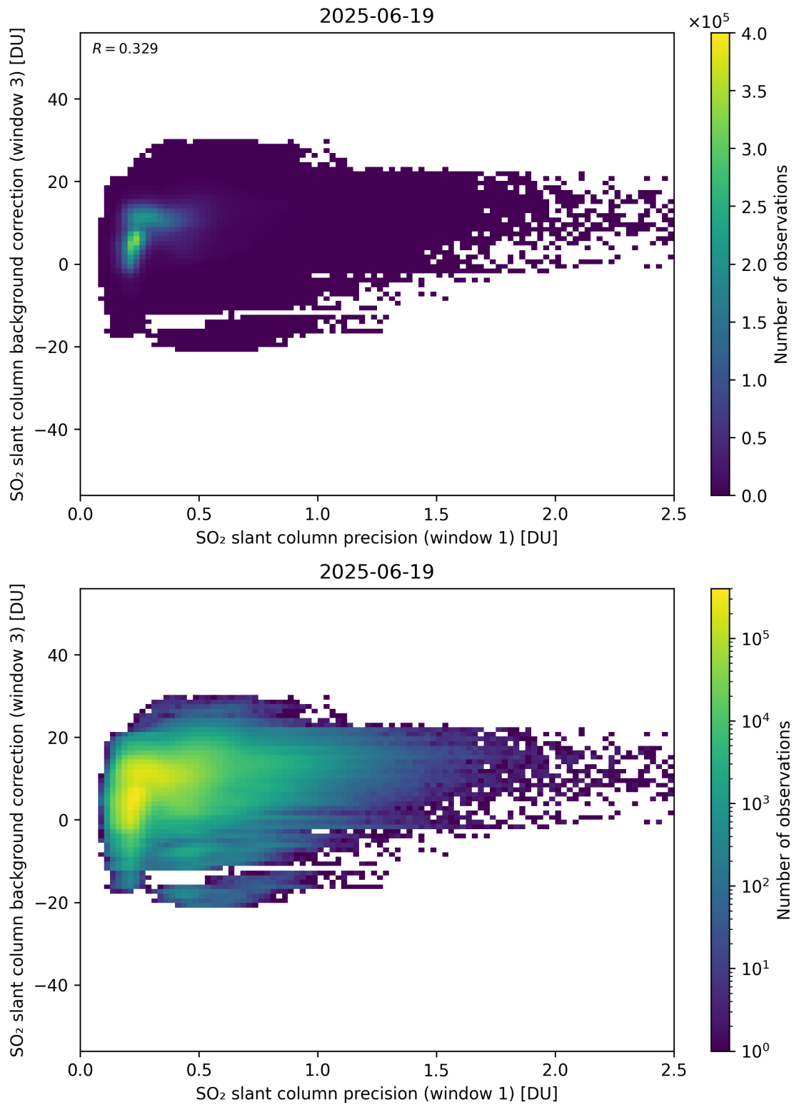
Figure 270: Scatter density plot of “SO 2 slant column precision (window 1)” against “SO 2 slant column background correction (window 3)” for 2025-06-18 to 2025-06-20.
