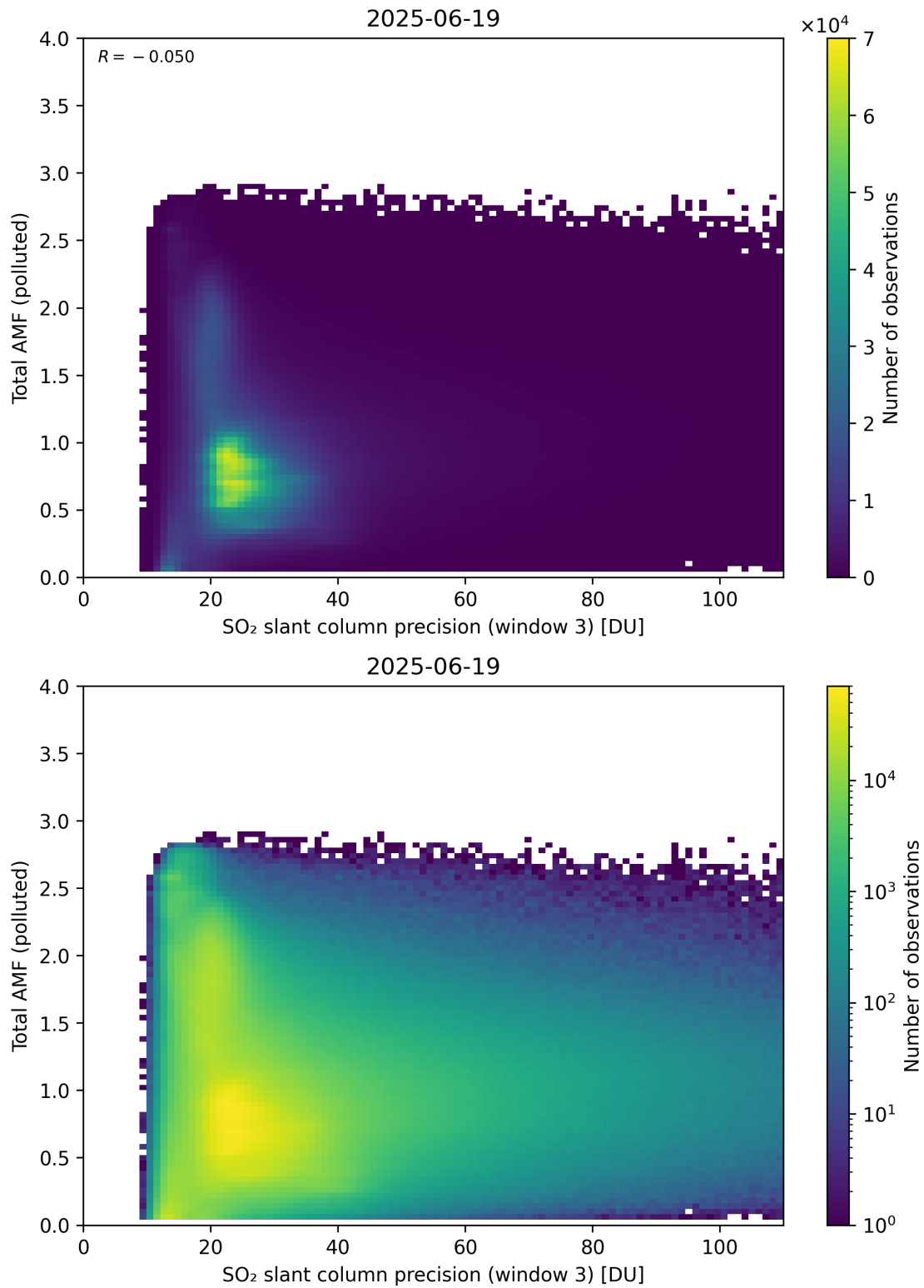
Figure 313: Scatter density plot of “SO 2 slant column precision (window 3)” against “Total AMF (polluted)” for 2025-06-18 to 2025-06-20.
