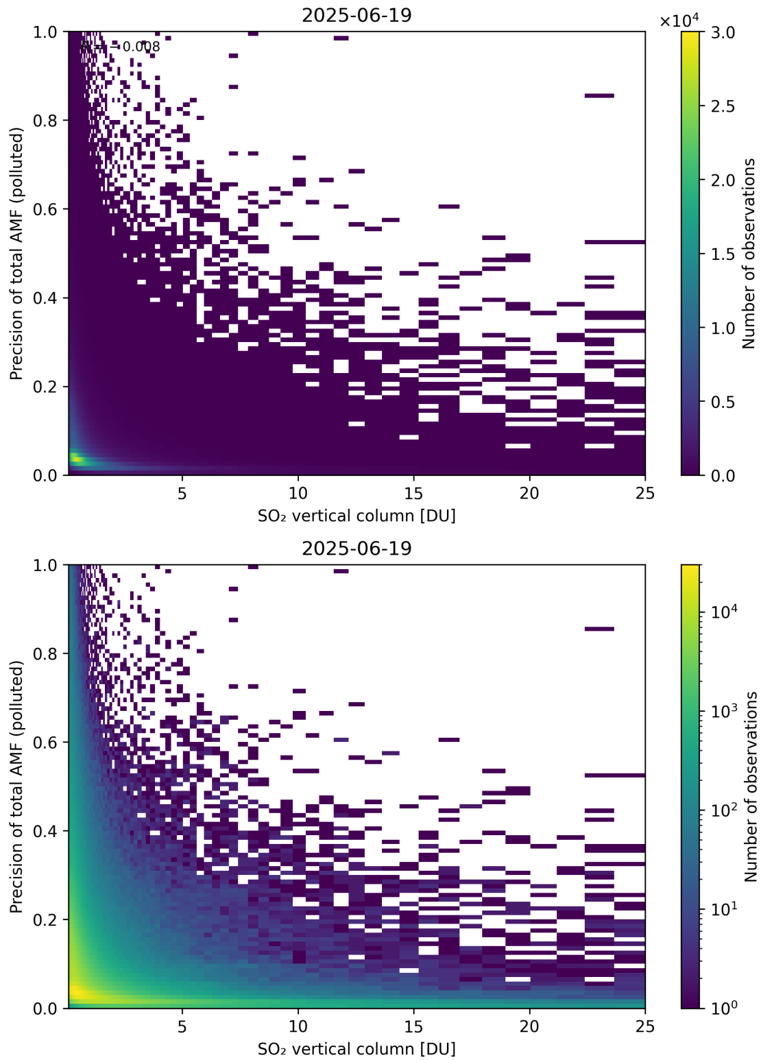
Figure 360: Scatter density plot of “SO 2 vertical column” against “Precision of total AMF (polluted)” for 2025-06-18 to 2025-06-20.
