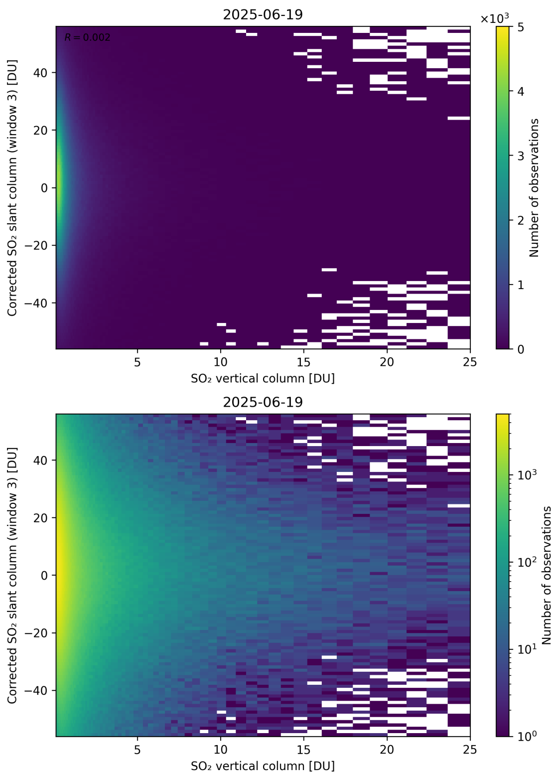
Figure 353: Scatter density plot of “SO 2 vertical column” against “Corrected SO 2 slant column (window 3)” for 2025-06-18 to 2025-06-20.
