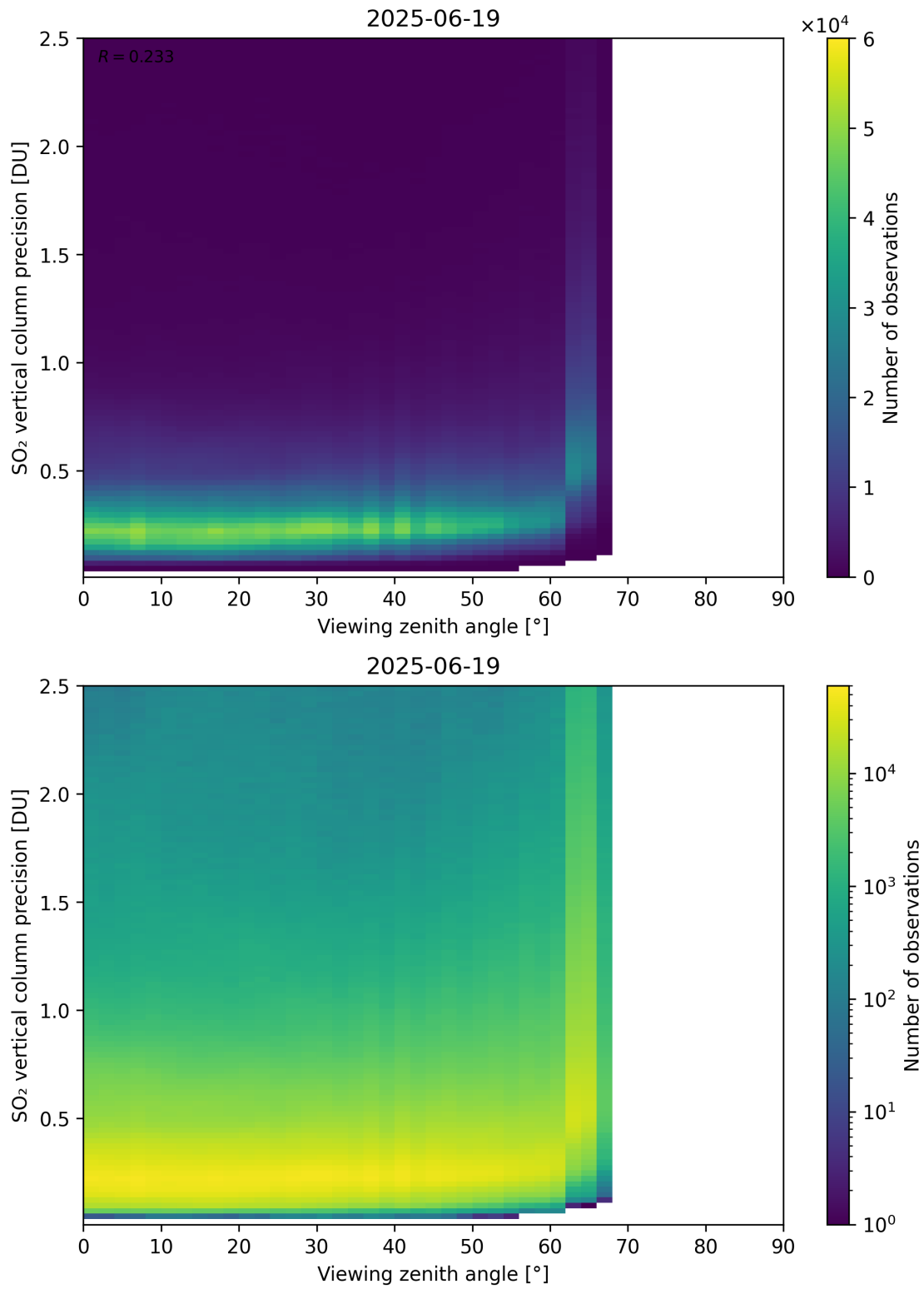
Figure 384: Scatter density plot of “Viewing zenith angle” against “SO 2 vertical column precision” for 2025-06-18 to 2025-06-20.
