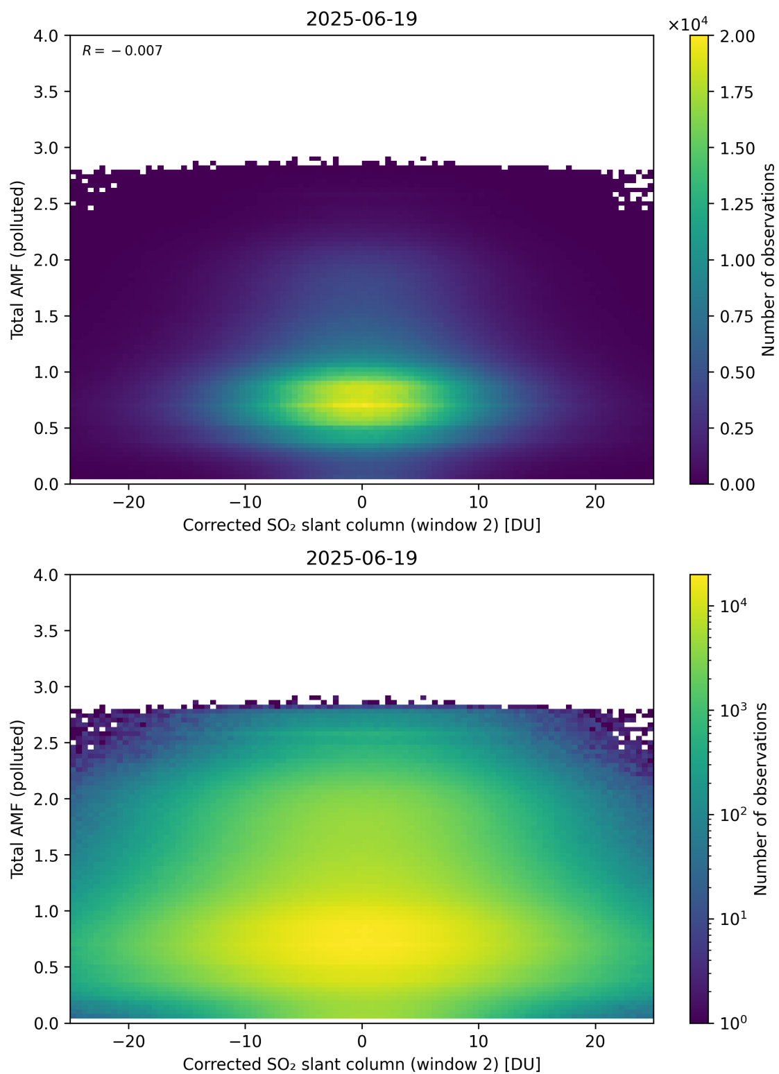
Figure 253: Scatter density plot of “Corrected SO 2 slant column (window 2)” against “Total AMF (polluted)” for 2025-06-18 to 2025-06-20.
