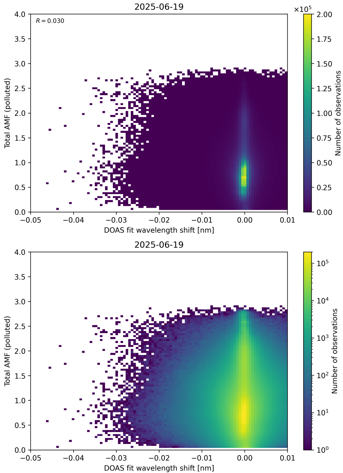
Figure 141: Scatter density plot of “DOAS fit wavelength shift” against “Total AMF (polluted)” for 2025-06-18 to 2025-06-20.
