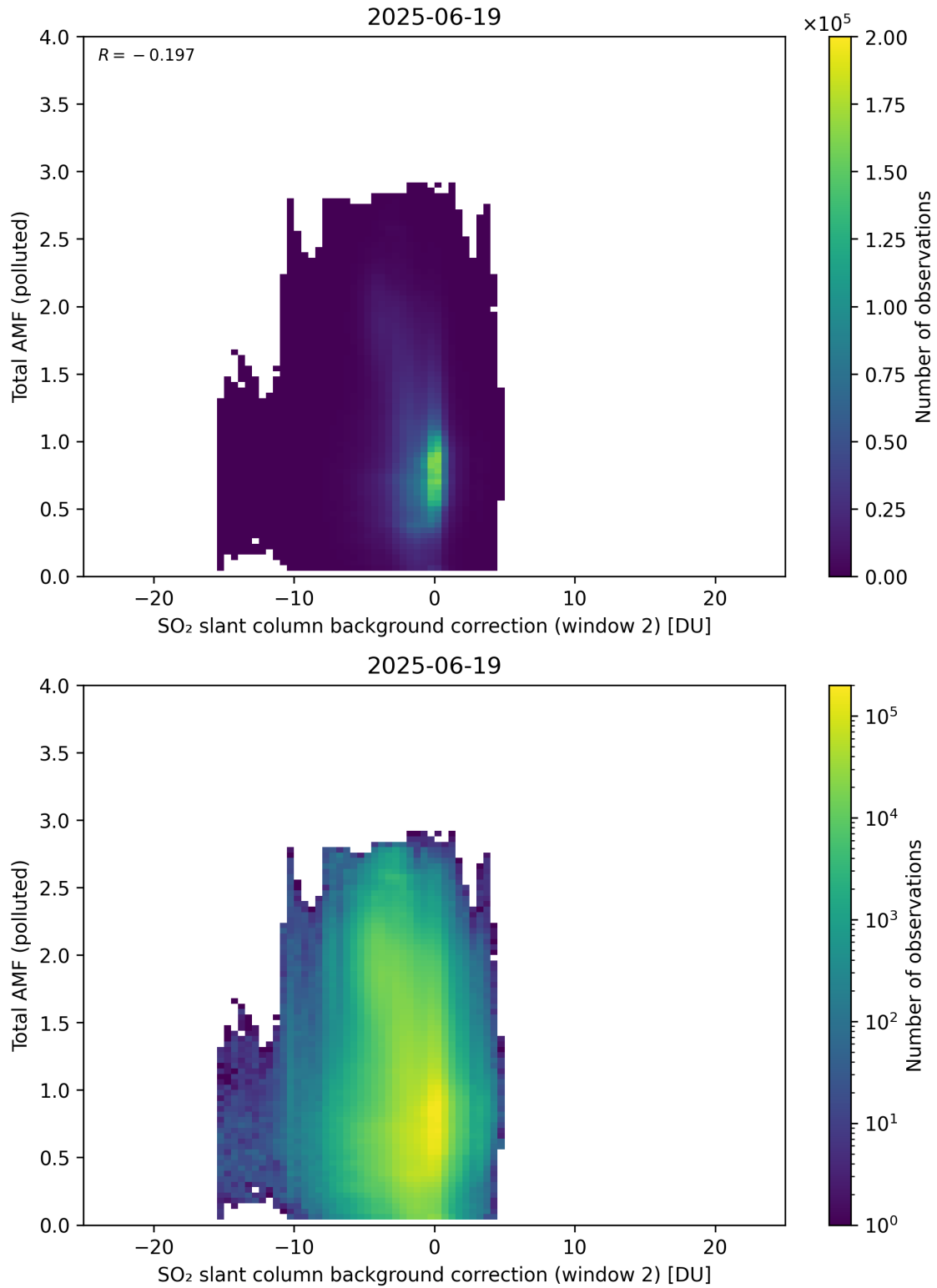
Figure 130: Scatter density plot of “SO 2 slant column background correction (window 2)” against “Total AMF (polluted)” for 2025-06-18 to 2025-06-20.
