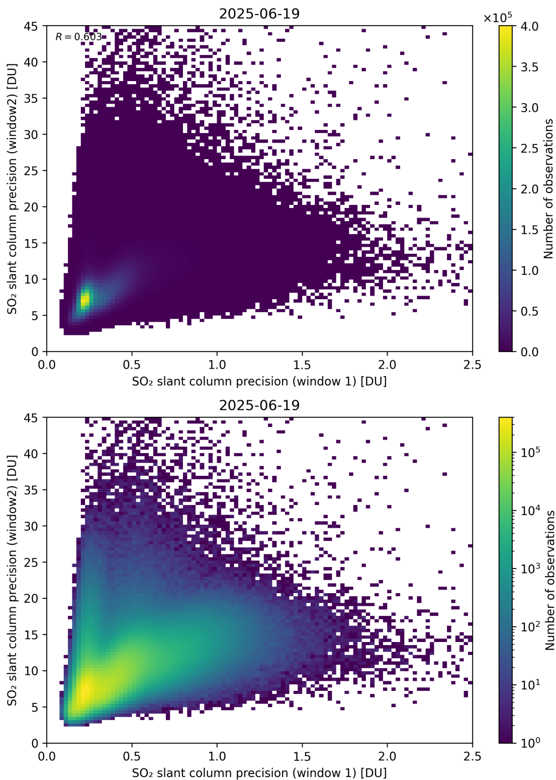
Figure 277: Scatter density plot of “SO 2 slant column precision (window 1)” against “SO 2 slant column precision (window2)” for 2025-06-18 to 2025-06-20.
