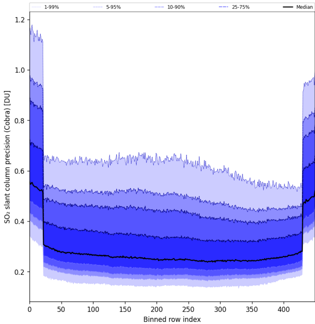
Figure 88: Along track statistics of “SO 2 slant column precision (Cobra)” for 2025-06-18 to 2025-06-20
