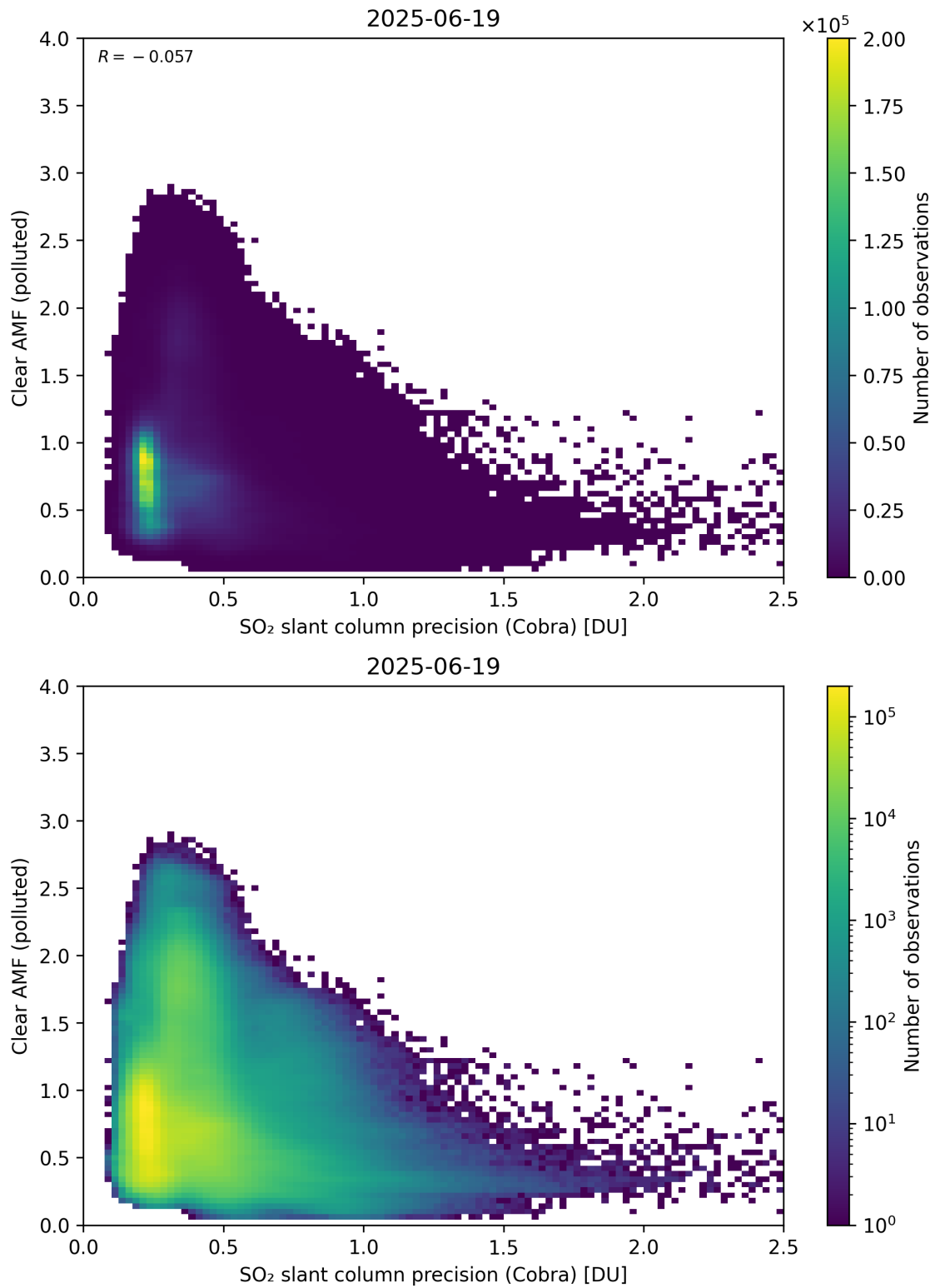
Figure 205: Scatter density plot of “SO 2 slant column precision (Cobra)” against “Clear AMF (polluted)” for 2025-06-18 to 2025-06-20.
