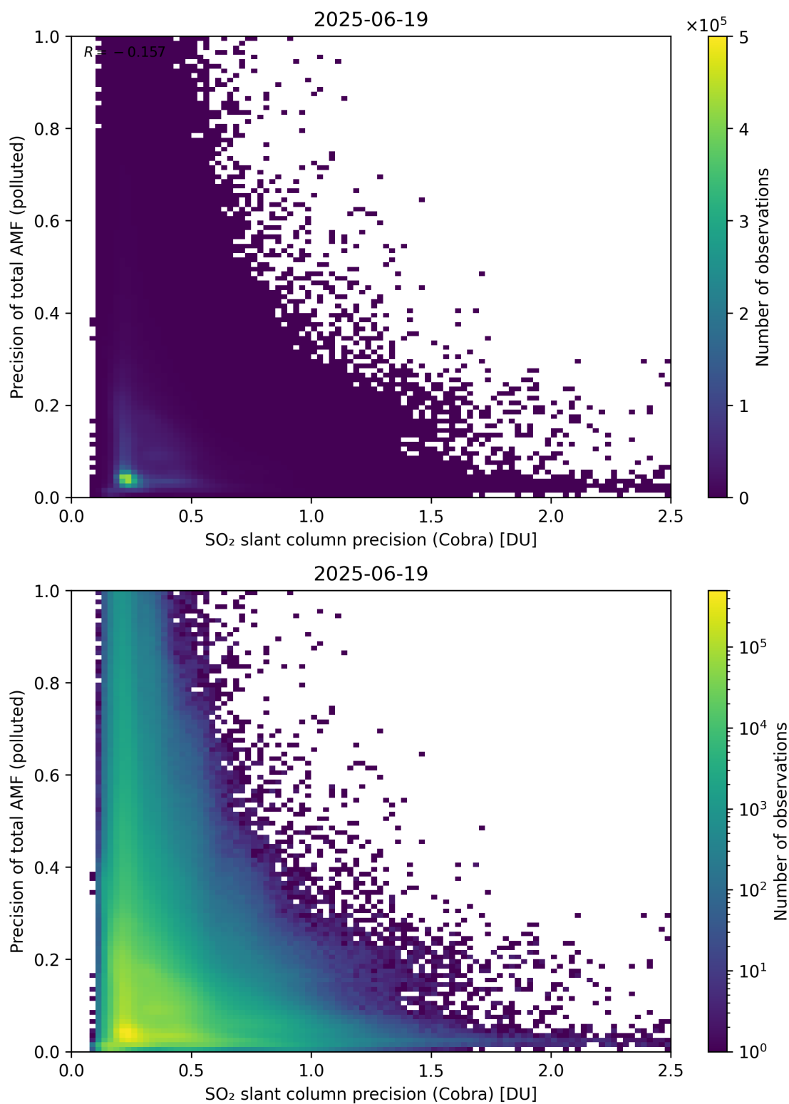
Figure 214: Scatter density plot of “SO 2 slant column precision (Cobra)” against “Precision of total AMF (polluted)” for 2025-06-18 to 2025-06-20.
