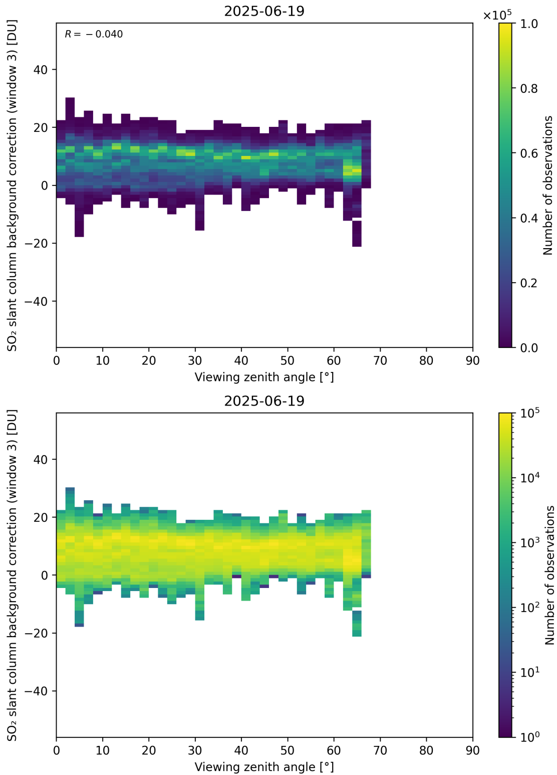
Figure 364: Scatter density plot of “Viewing zenith angle” against “SO 2 slant column background correction (window 3)” for 2025-06-18 to 2025-06-20.
