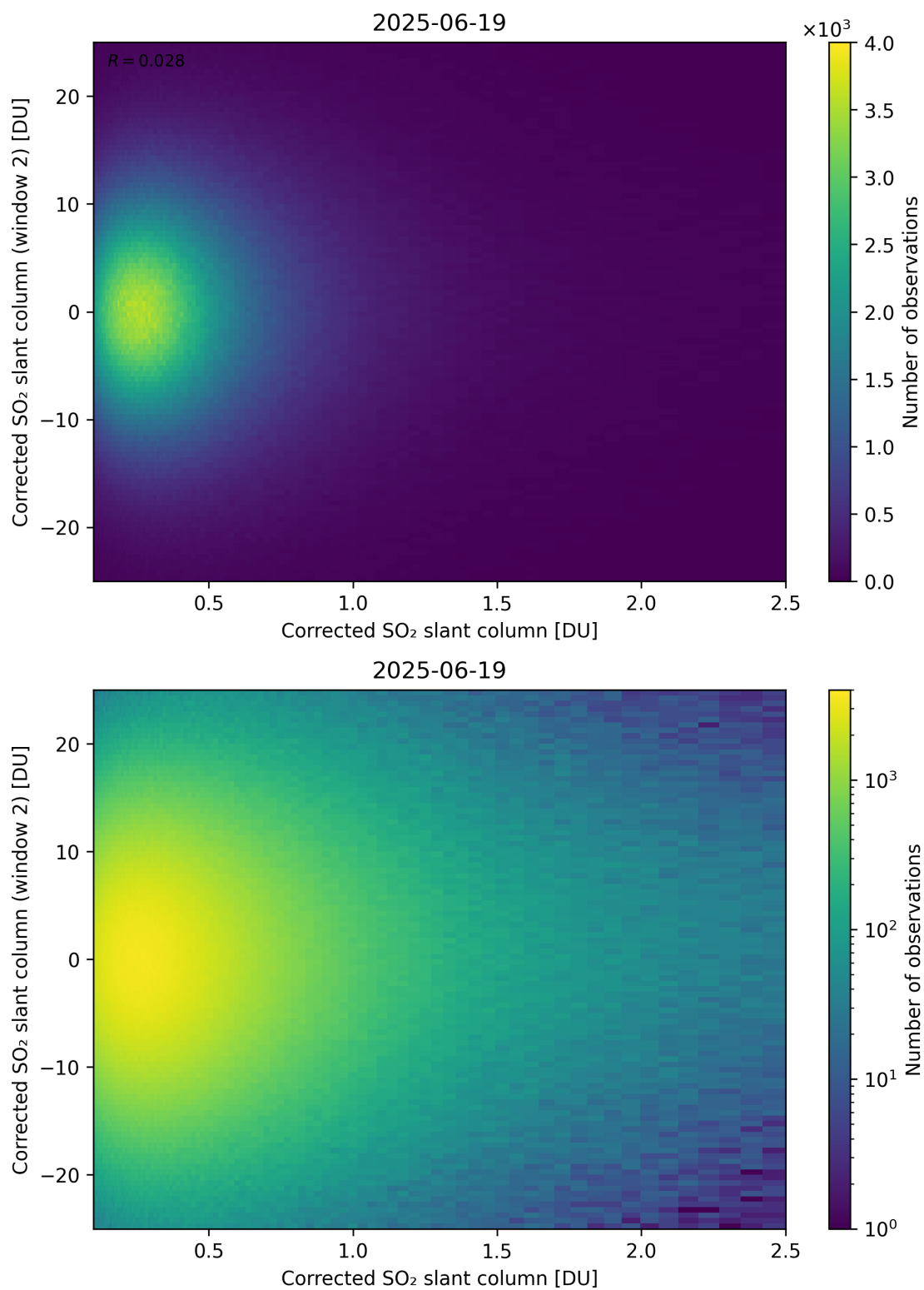
Figure 235: Scatter density plot of “Corrected SO 2 slant column” against “Corrected SO 2 slant column (window 2)” for 2025-06-18 to 2025-06-20.
