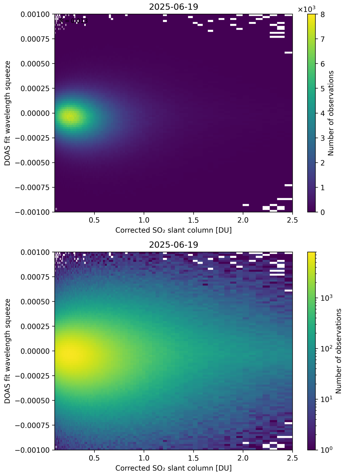
Figure 230: Scatter density plot of “Corrected SO 2 slant column” against “DOAS fit wavelength squeeze” for 2025-06-18 to 2025-06-20.
