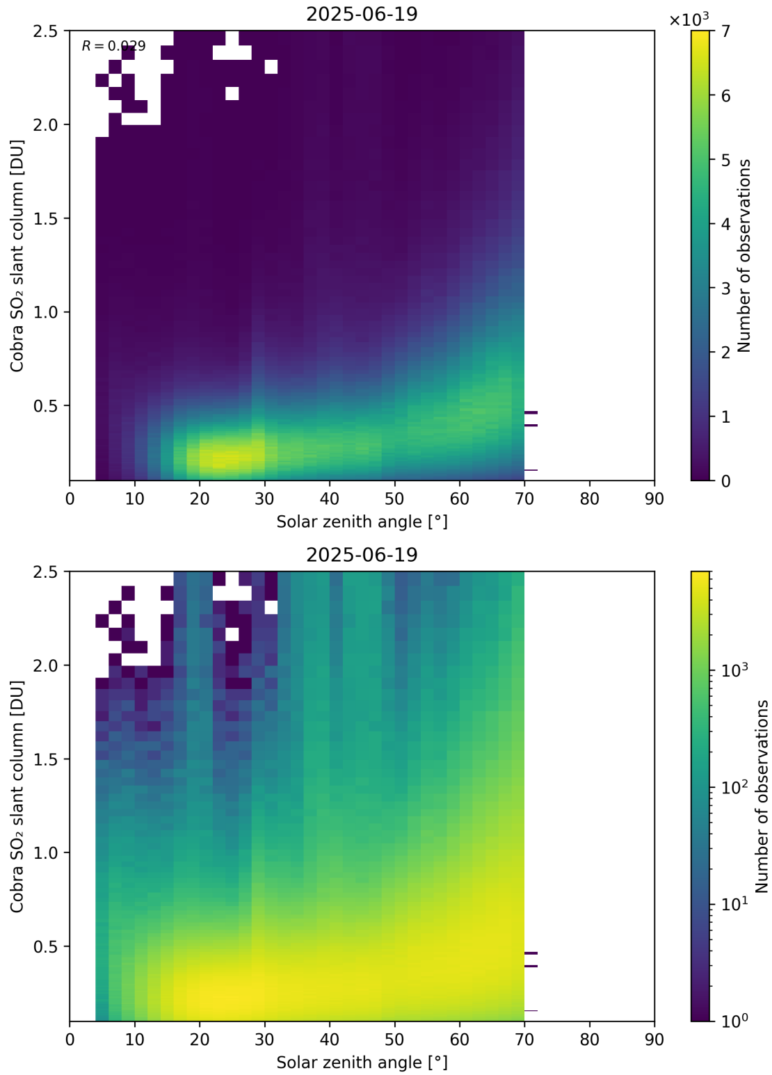
Figure 179: Scatter density plot of “Solar zenith angle” against “Cobra SO 2 slant column” for 2025-06-18 to 2025-06-20.
