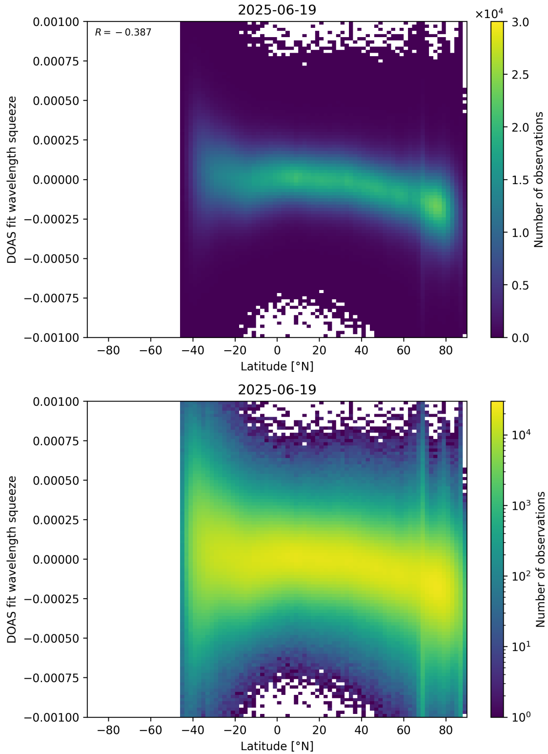
Figure 154: Scatter density plot of “Latitude” against “DOAS fit wavelength squeeze” for 2025-06-18 to 2025-06-20.
