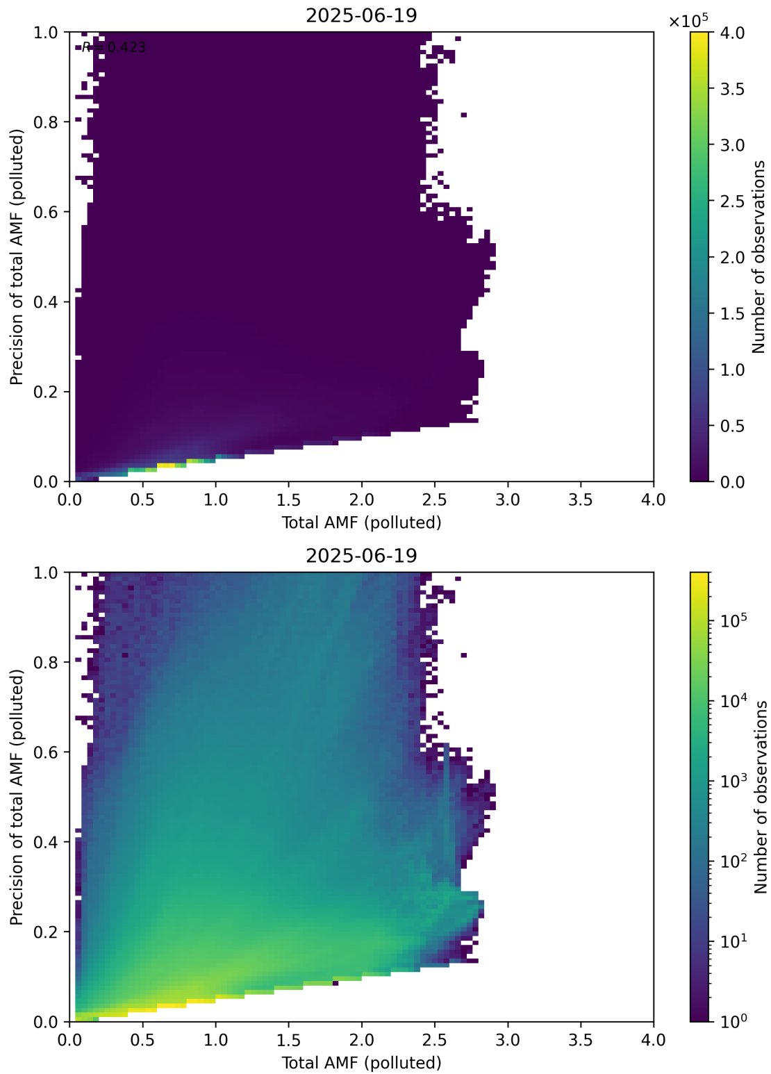
Figure 322: Scatter density plot of “Total AMF (polluted)” against “Precision of total AMF (polluted)” for 2025-06-18 to 2025-06-20.
