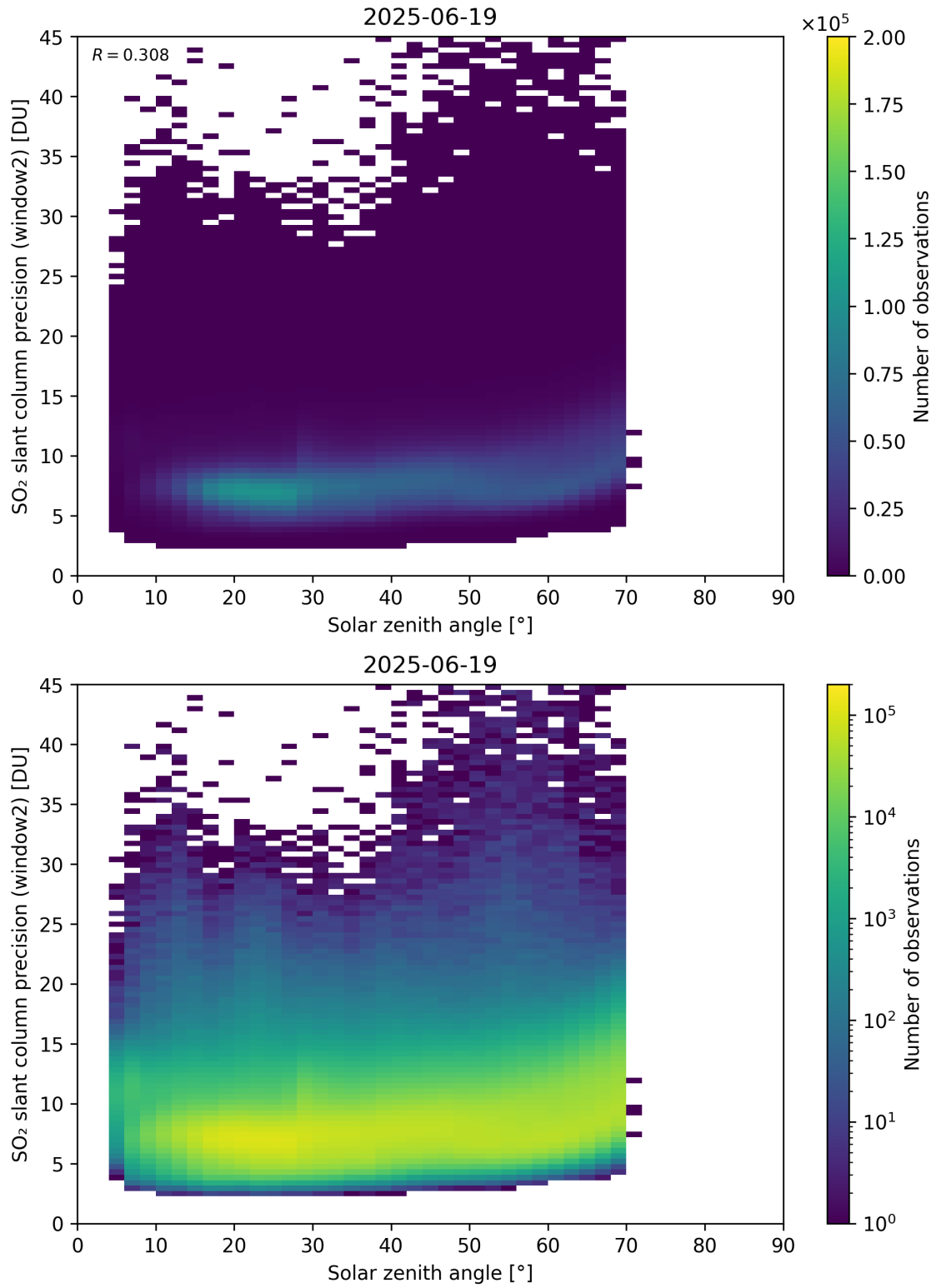
Figure 186: Scatter density plot of “Solar zenith angle” against “SO 2 slant column precision (window2)” for 2025-06-18 to 2025-06-20.
