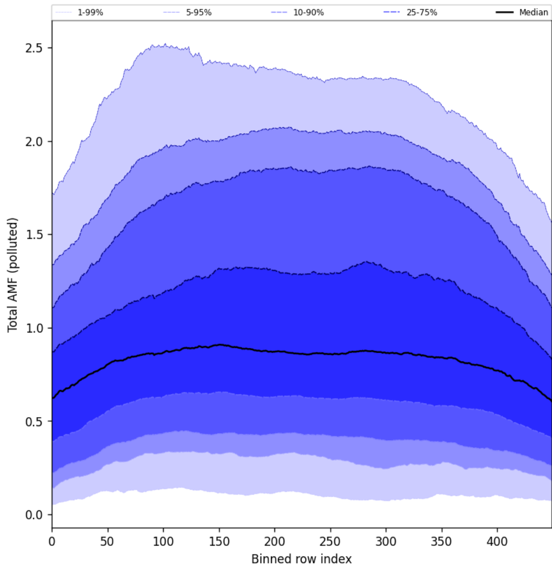
Figure 105: Along track statistics of “Total AMF (polluted)” for 2025-06-18 to 2025-06-20
