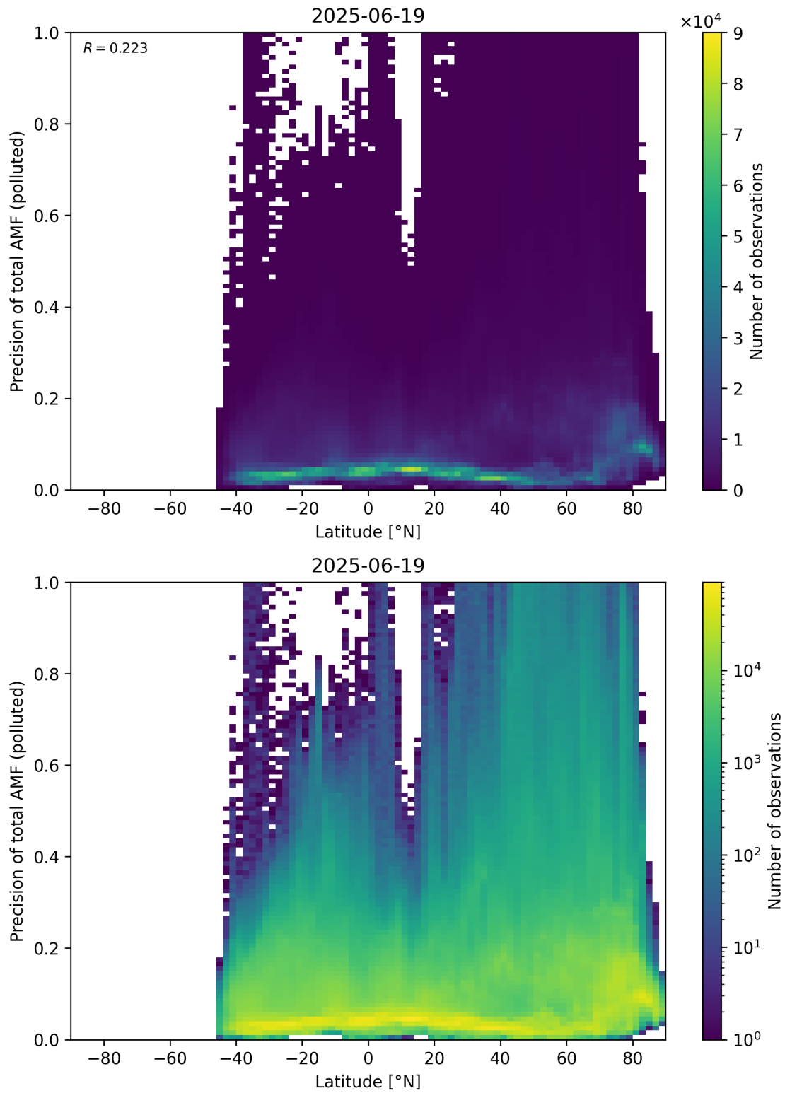
Figure 168: Scatter density plot of “Latitude” against “Precision of total AMF (polluted)” for 2025-06-18 to 2025-06-20.
