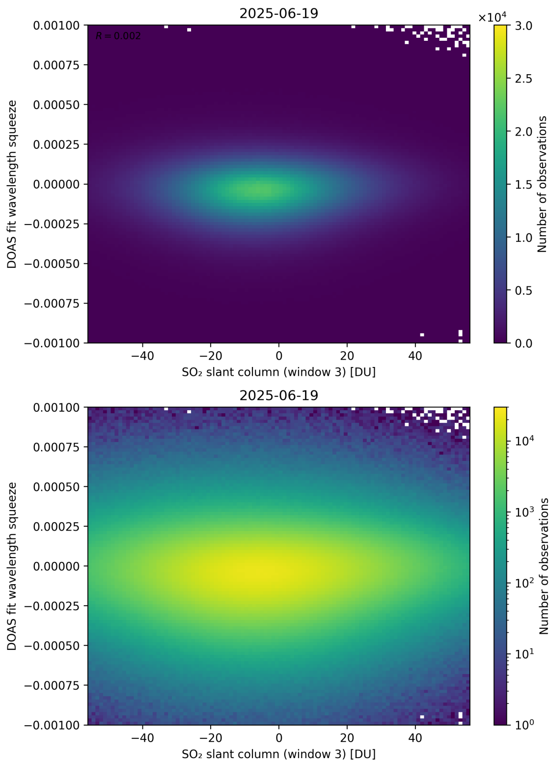
Figure 305: Scatter density plot of “SO 2 slant column (window 3)” against “DOAS fit wavelength squeeze” for 2025-06-18 to 2025-06-20.
