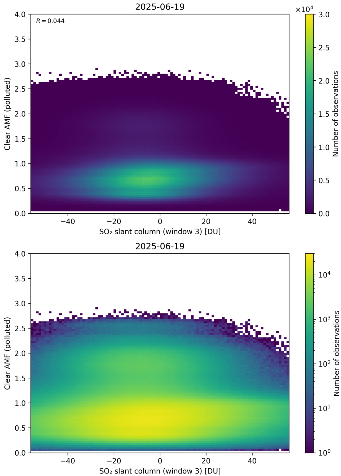
Figure 315: Scatter density plot of “SO 2 slant column (window 3)” against “Clear AMF (polluted)” for 2025-06-18 to 2025-06-20.
