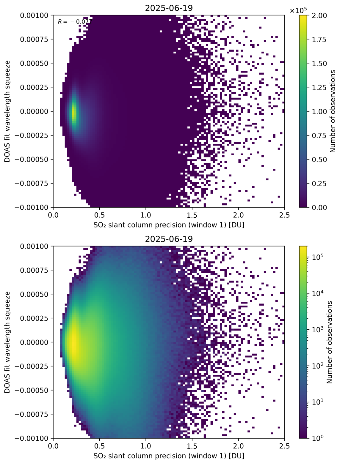
Figure 272: Scatter density plot of “SO 2 slant column precision (window 1)” against “DOAS fit wavelength squeeze” for 2025-06-18 to 2025-06-20.
