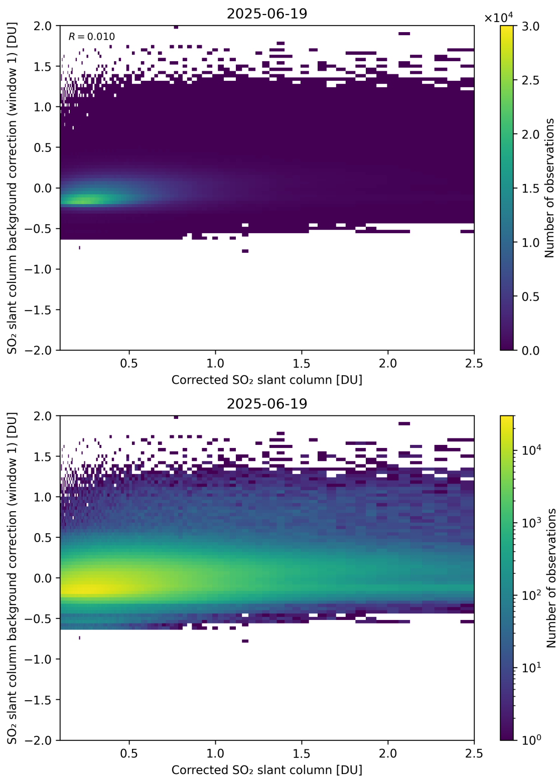
Figure 226: Scatter density plot of “Corrected SO 2 slant column” against “SO 2 slant column background correction (window 1)” for 2025-06-18 to 2025-06-20.
