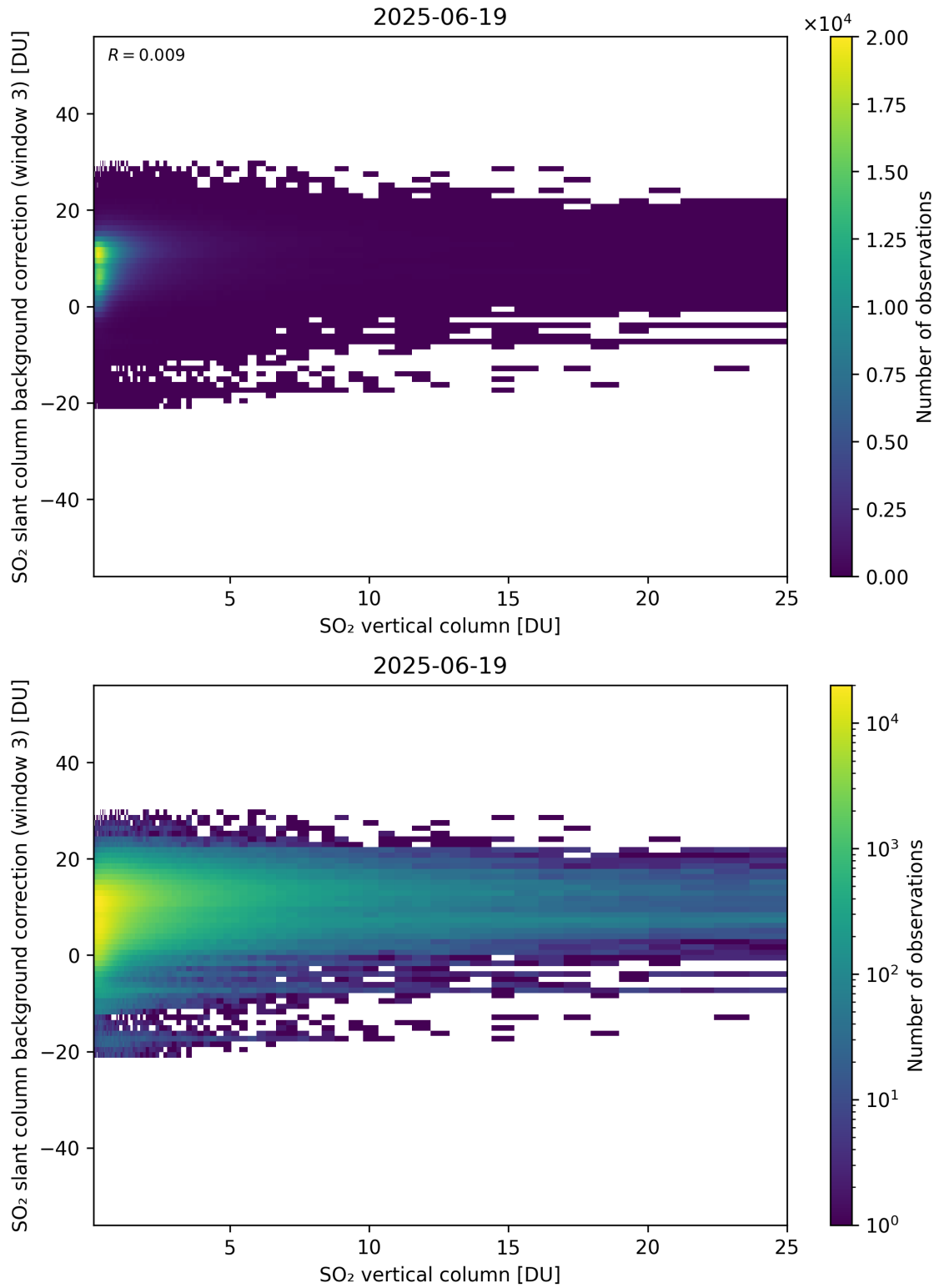
Figure 325: Scatter density plot of “SO 2 vertical column” against “SO 2 slant column background correction (window 3)” for 2025-06-18 to 2025-06-20.
