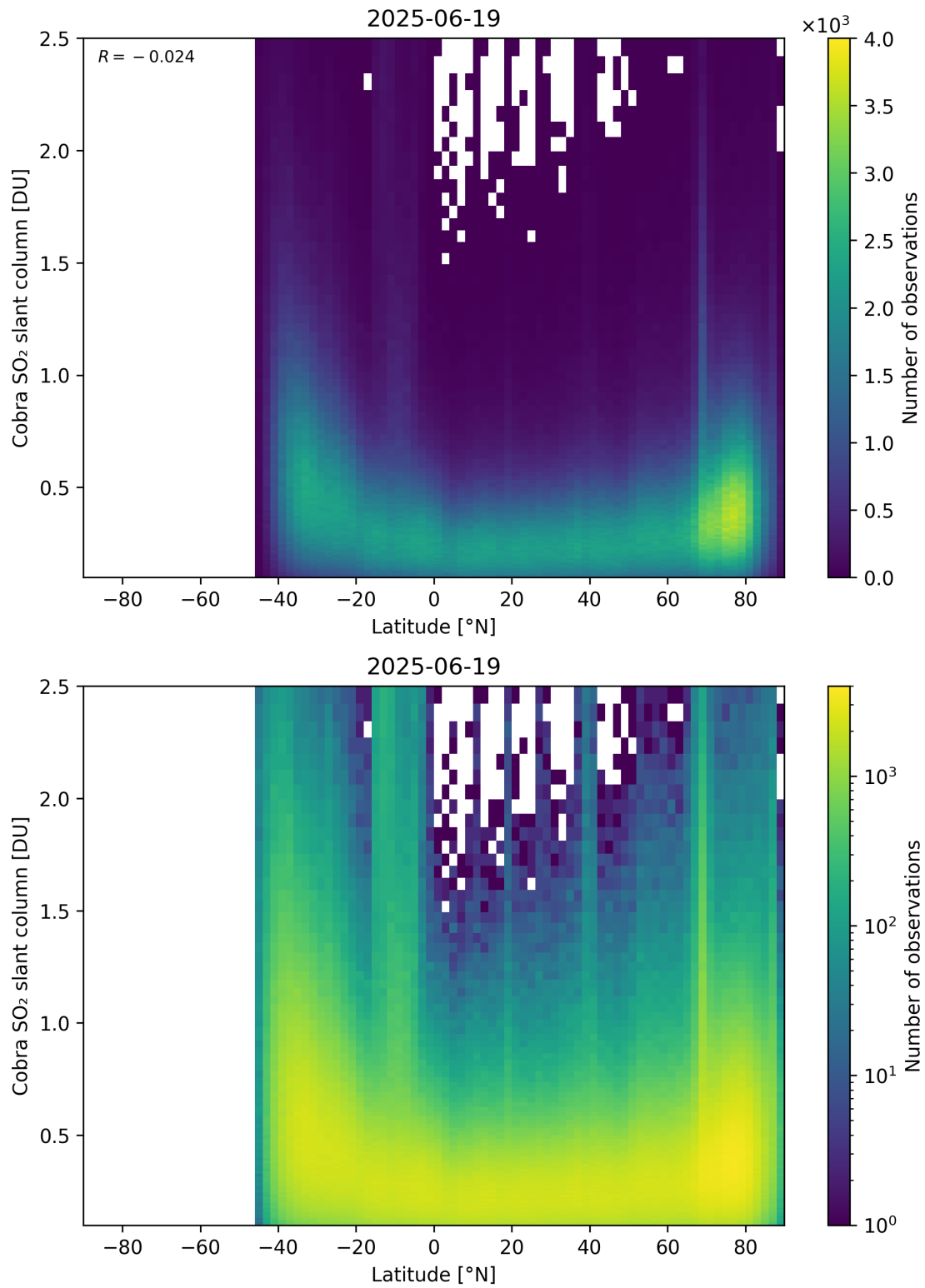
Figure 157: Scatter density plot of “Latitude” against “Cobra SO 2 slant column” for 2025-06-18 to 2025-06-20.
