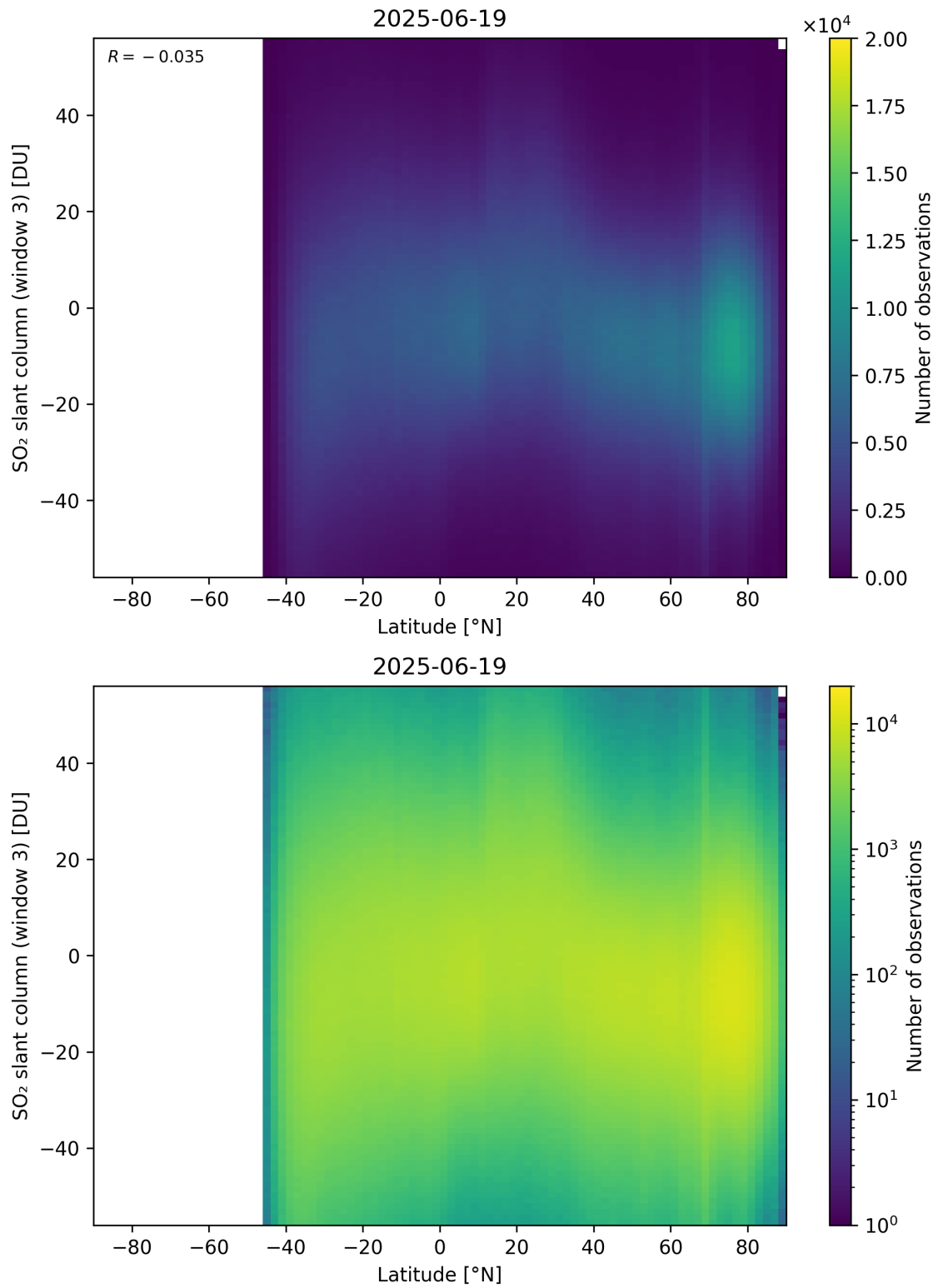
Figure 165: Scatter density plot of “Latitude” against “SO 2 slant column (window 3)” for 2025-06-18 to 2025-06-20.
