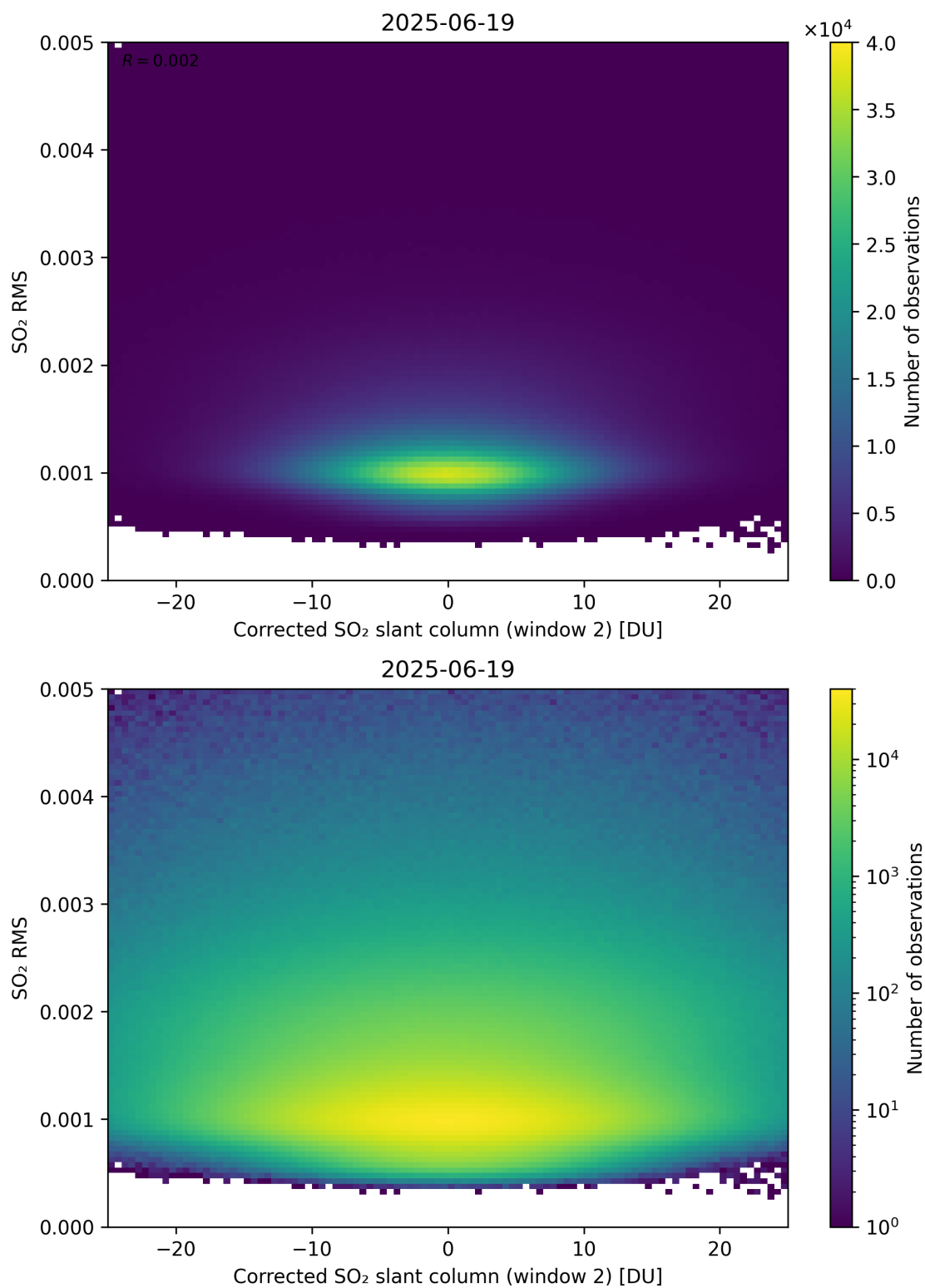
Figure 248: Scatter density plot of “Corrected SO 2 slant column (window 2)” against “SO 2 RMS” for 2025-06-18 to 2025-06-20.
