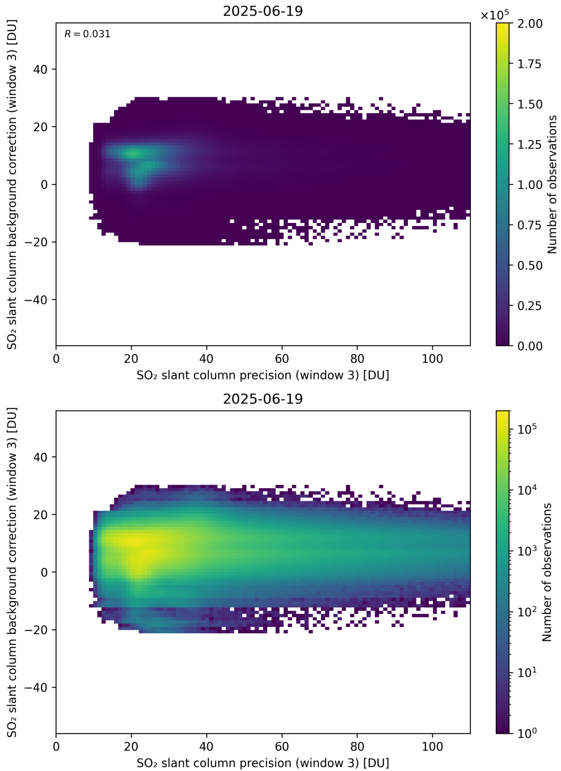
Figure 307: Scatter density plot of “SO 2 slant column precision (window 3)” against “SO 2 slant column background correction (window 3)” for 2025-06-18 to 2025-06-20.
