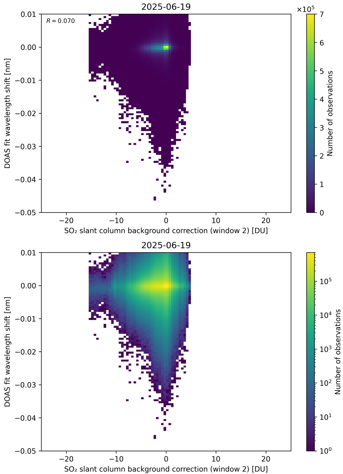
Figure 123: Scatter density plot of “SO 2 slant column background correction (window 2)” against “DOAS fit wavelength shift” for 2025-06-18 to 2025-06-20.
