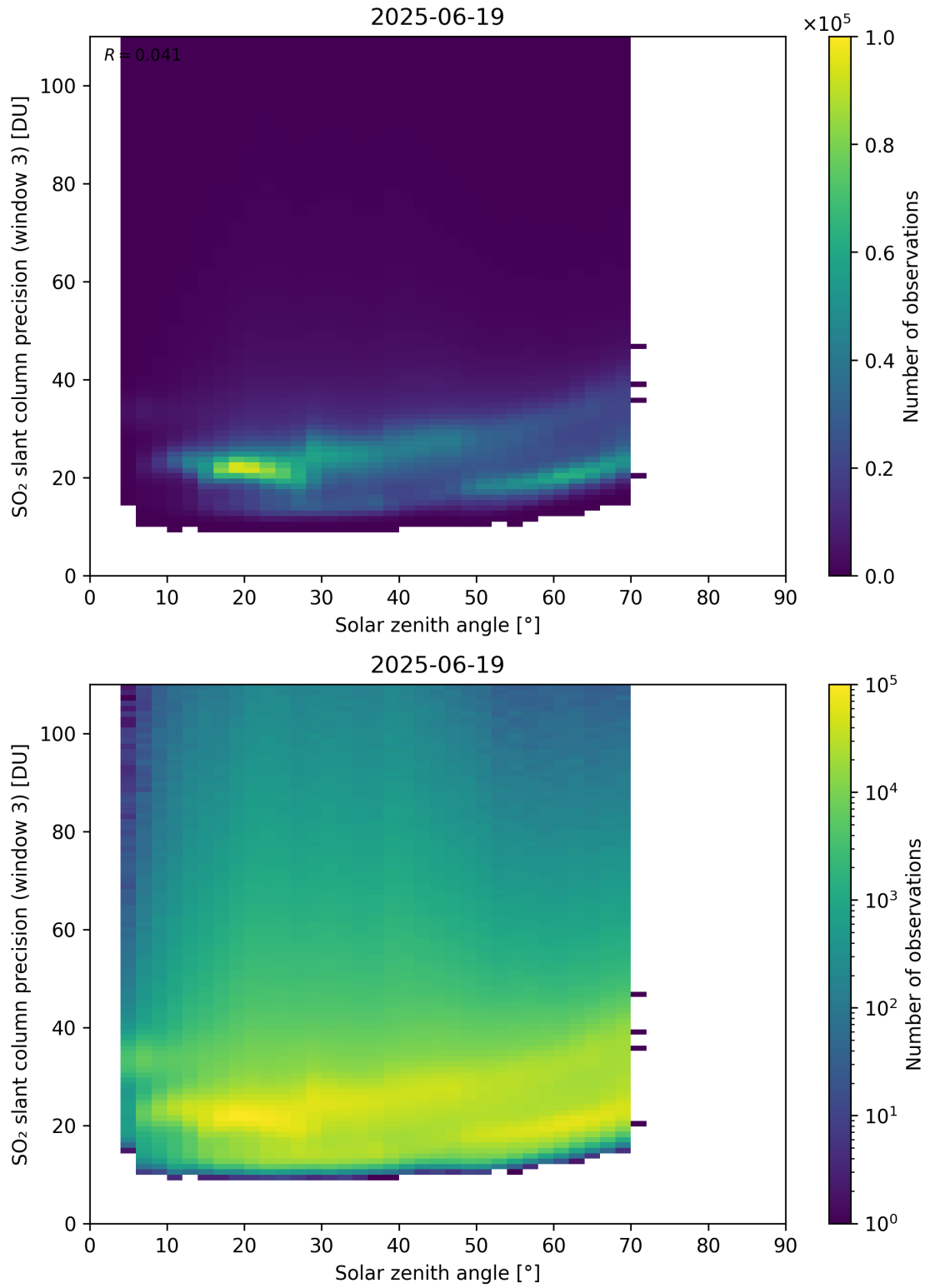
Figure 188: Scatter density plot of “Solar zenith angle” against “SO 2 slant column precision (window 3)” for 2025-06-18 to 2025-06-20.
