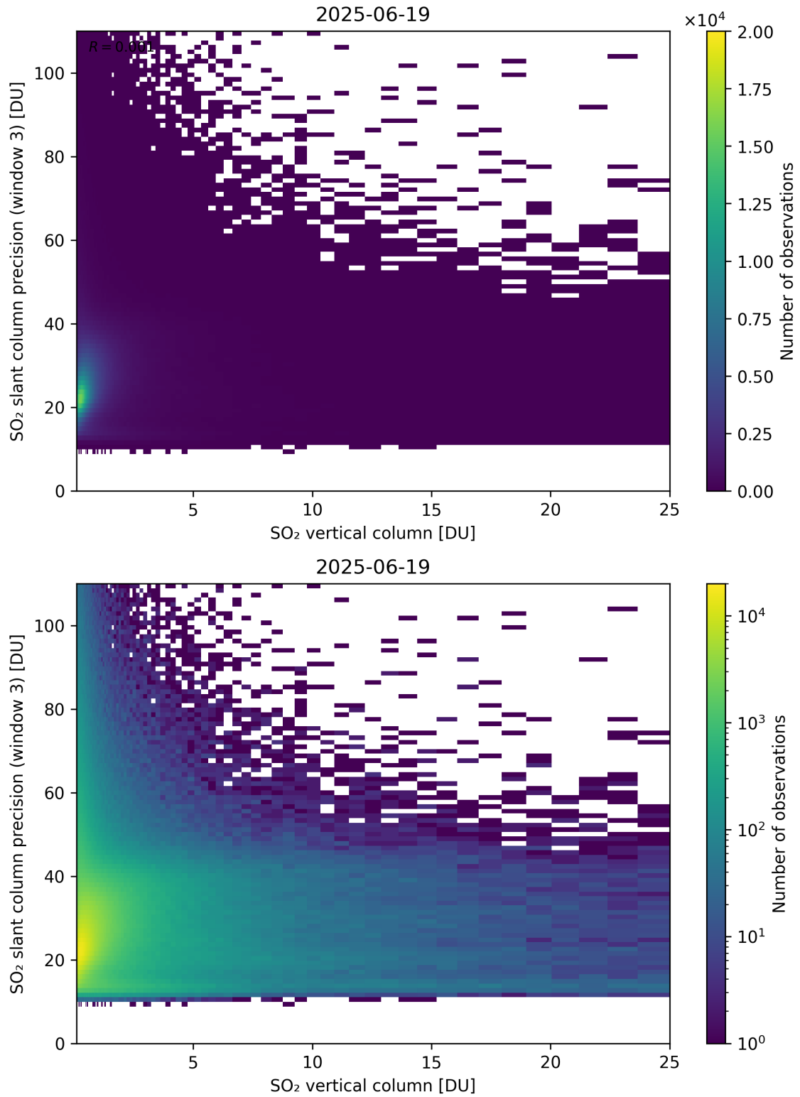
Figure 358: Scatter density plot of “SO 2 vertical column” against “SO 2 slant column precision (window 3)” for 2025-06-18 to 2025-06-20.
