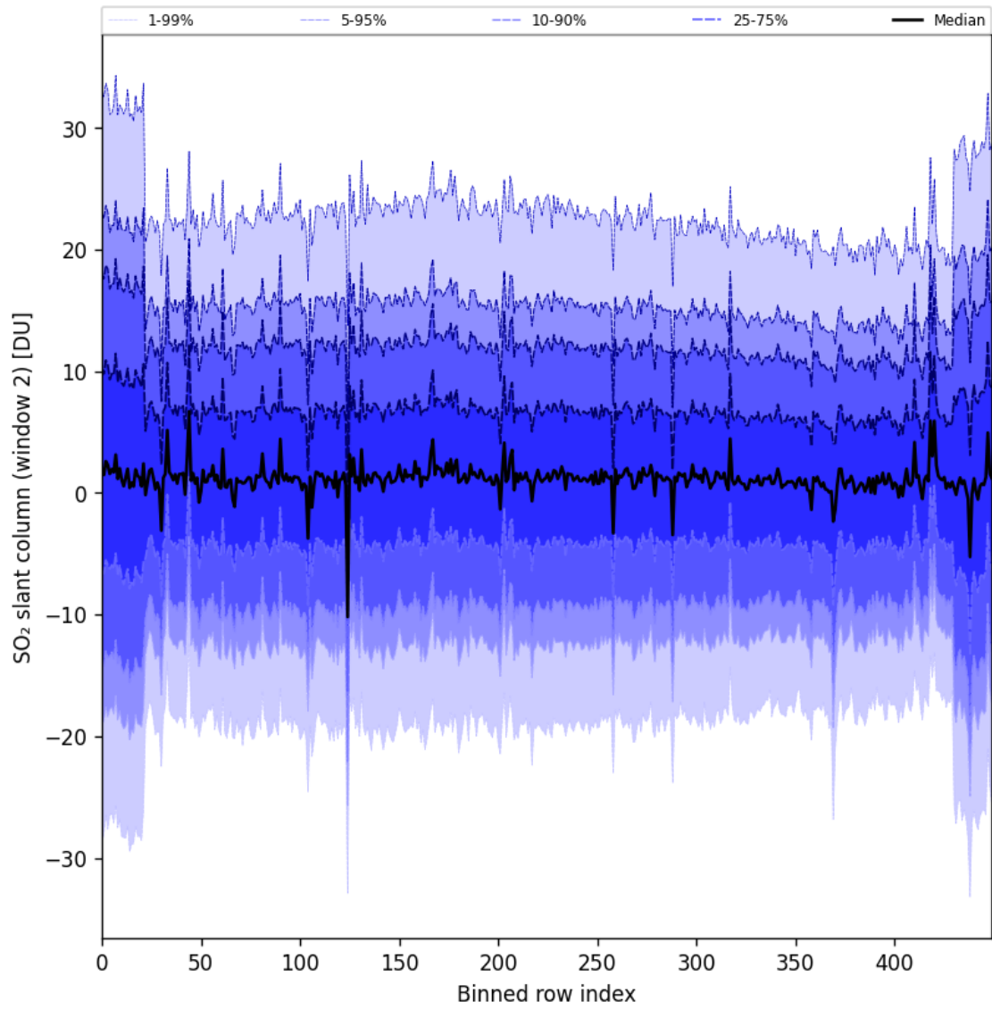
Figure 93: Along track statistics of “SO 2 slant column (window 2)” for 2025-06-18 to 2025-06-20
