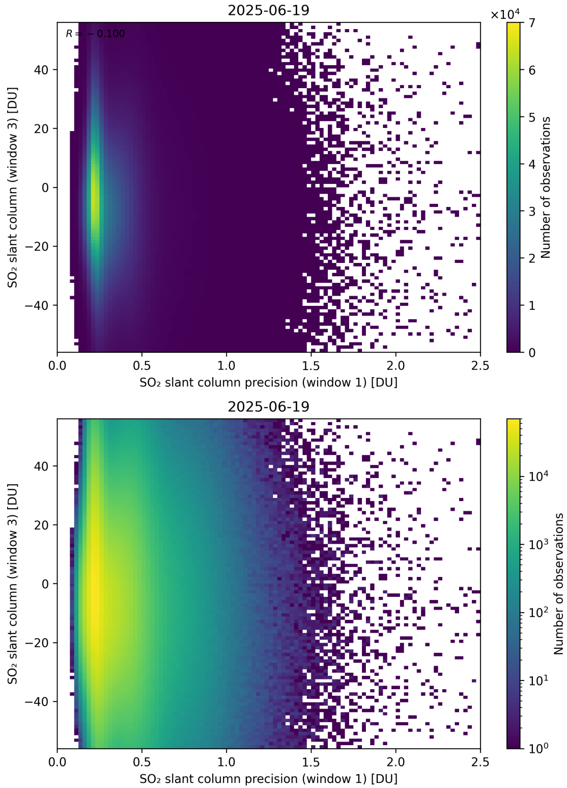
Figure 278: Scatter density plot of “SO 2 slant column precision (window 1)” against “SO 2 slant column (window 3)” for 2025-06-18 to 2025-06-20.
