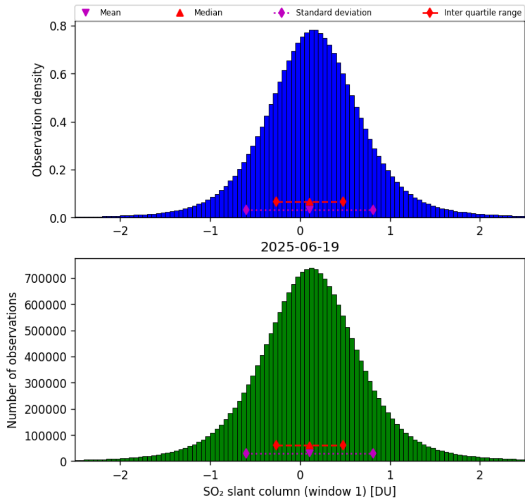
Figure 63: Histogram of “SO 2 slant column (window 1)” for 2025-06-18 to 2025-06-20
