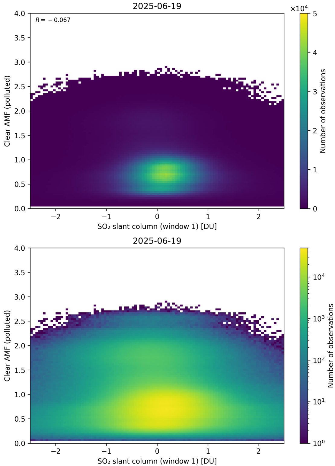
Figure 282: Scatter density plot of “SO 2 slant column (window 1)” against “Clear AMF (polluted)” for 2025-06-18 to 2025-06-20.
