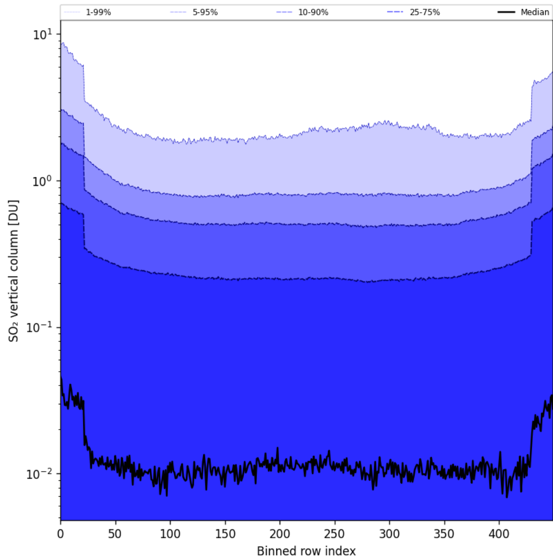
Figure 84: Along track statistics of “SO 2 vertical column” for 2025-06-18 to 2025-06-20
