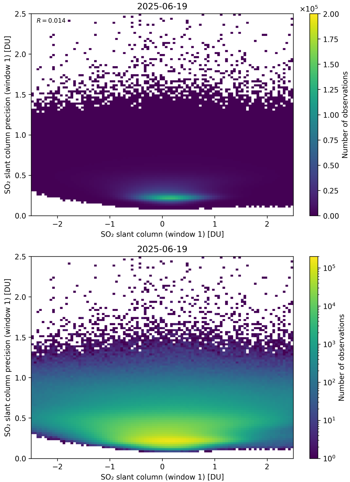
Figure 285: Scatter density plot of “SO 2 slant column (window 1)” against “SO 2 slant column precision (window 1)” for 2025-06-18 to 2025-06-20.
