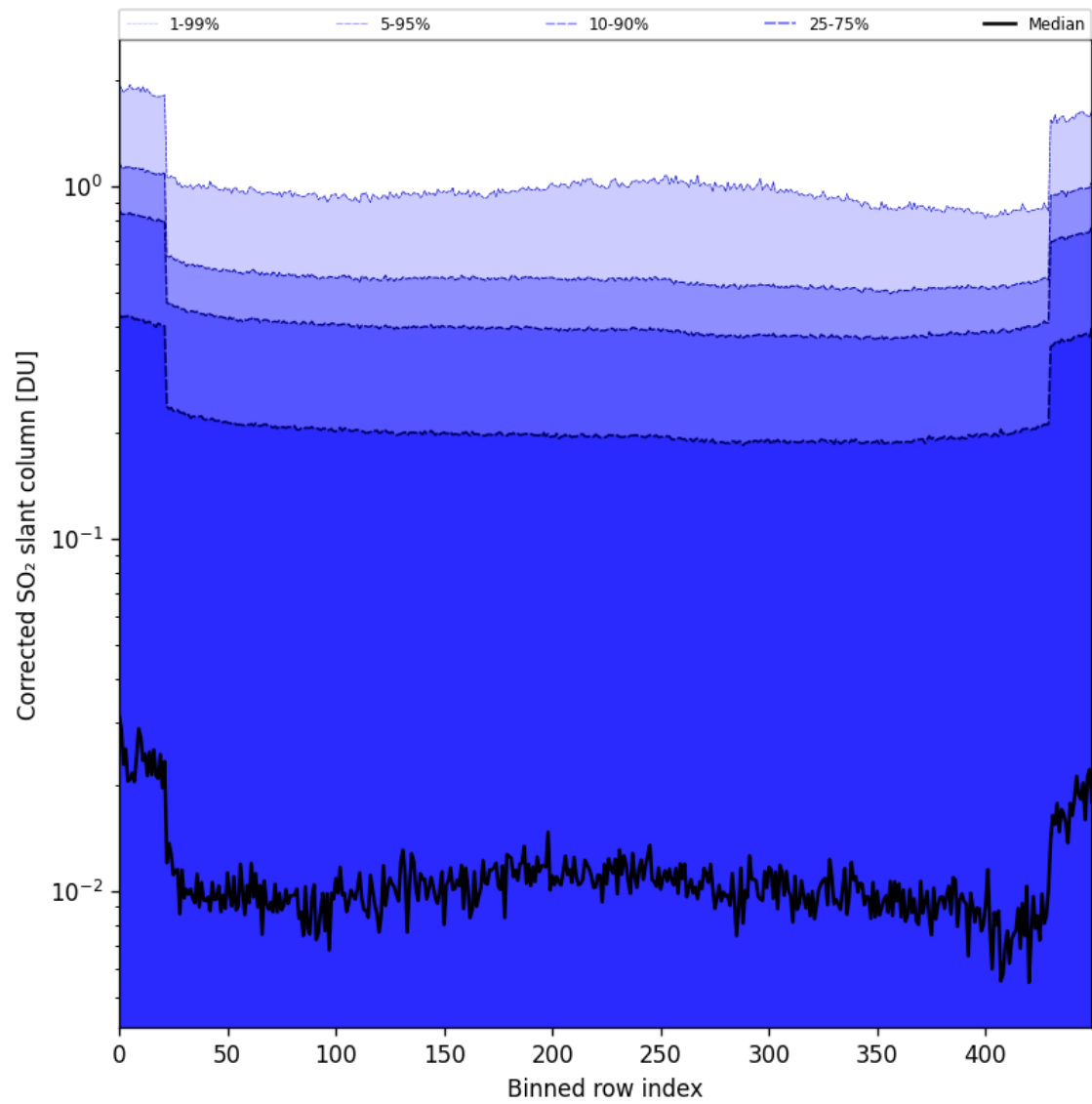
Figure 86: Along track statistics of “Corrected SO 2 slant column” for 2025-06-18 to 2025-06-20
