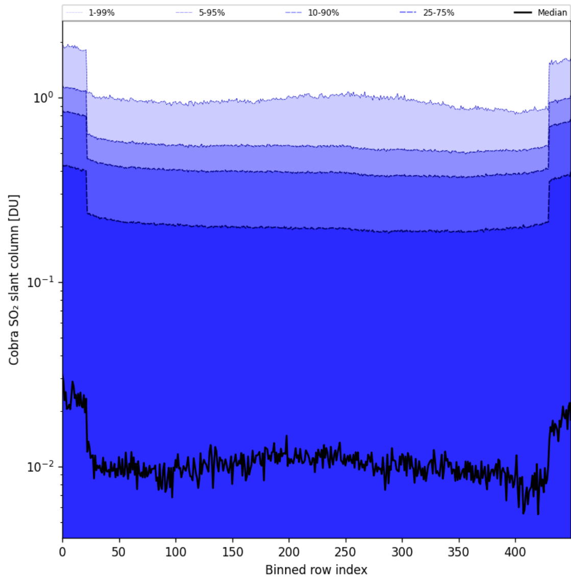
Figure 87: Along track statistics of “Cobra SO 2 slant column” for 2025-06-18 to 2025-06-20
