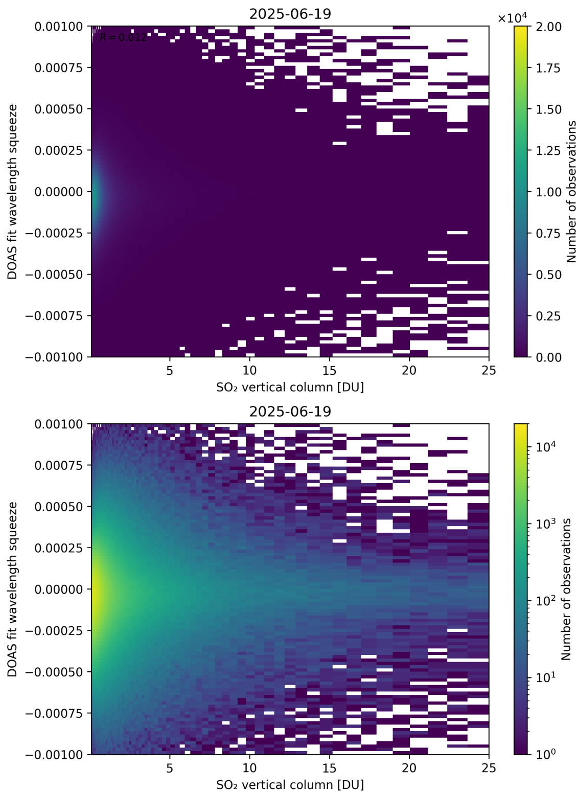
Figure 327: Scatter density plot of “SO 2 vertical column” against “DOAS fit wavelength squeeze” for 2025-06-18 to 2025-06-20.
