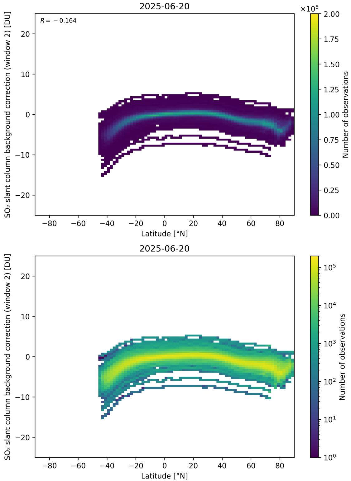
Figure 151: Scatter density plot of “Latitude” against “SO 2 slant column background correction (window 2)” for 2025-06-19 to 2025-06-21.
