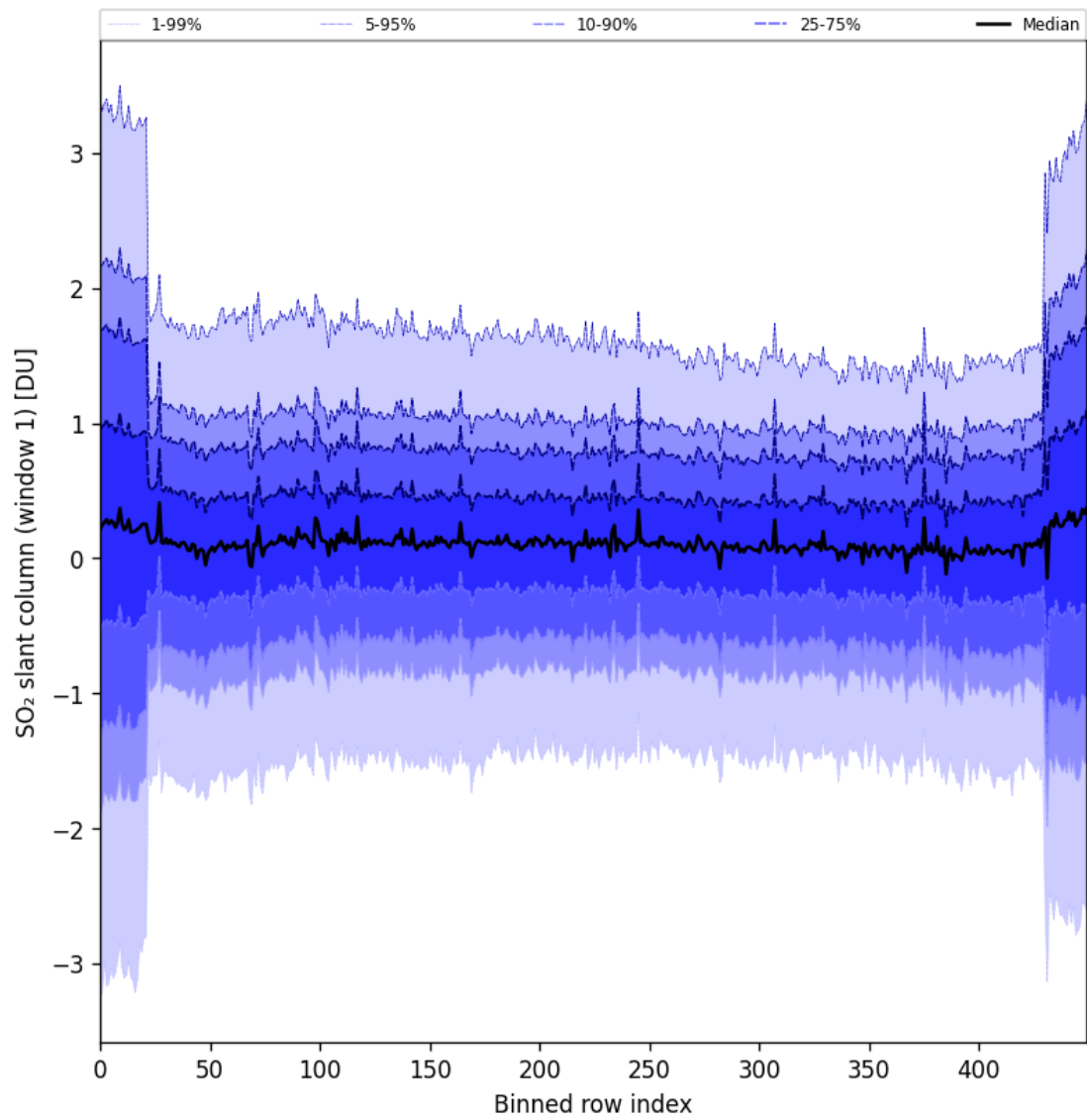
Figure 89: Along track statistics of “SO 2 slant column (window 1)” for 2025-06-19 to 2025-06-21
