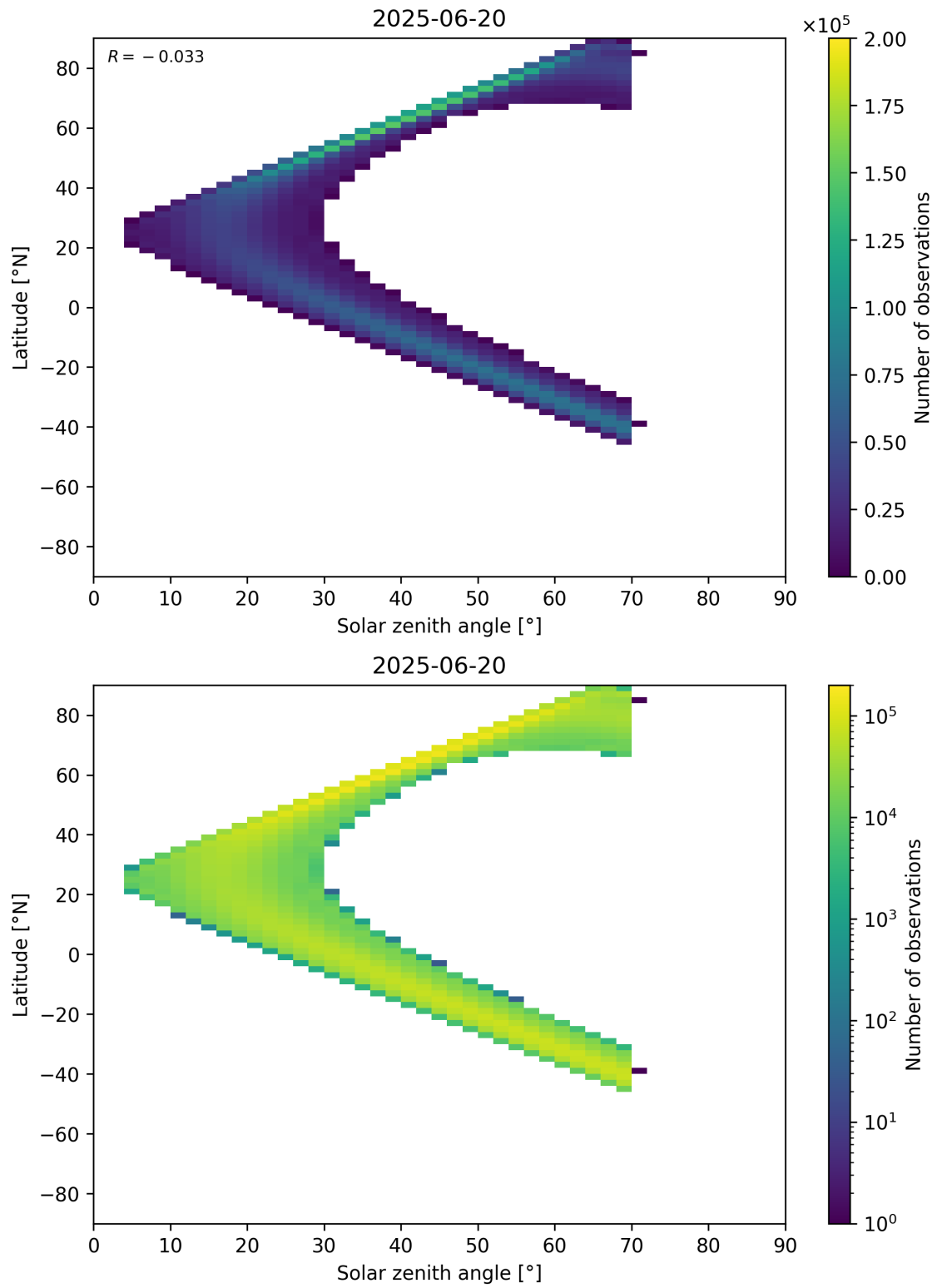
Figure 177: Scatter density plot of “Solar zenith angle” against “Latitude” for 2025-06-19 to 2025-06-21.
