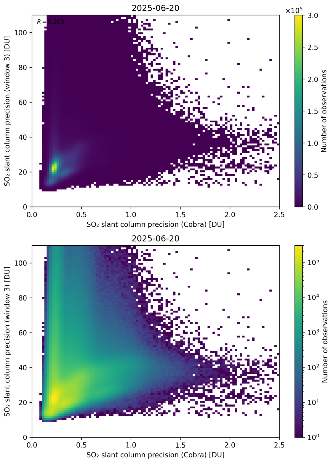
Figure 212: Scatter density plot of “SO 2 slant column precision (Cobra)” against “SO 2 slant column precision (window 3)” for 2025-06-19 to 2025-06-21.
