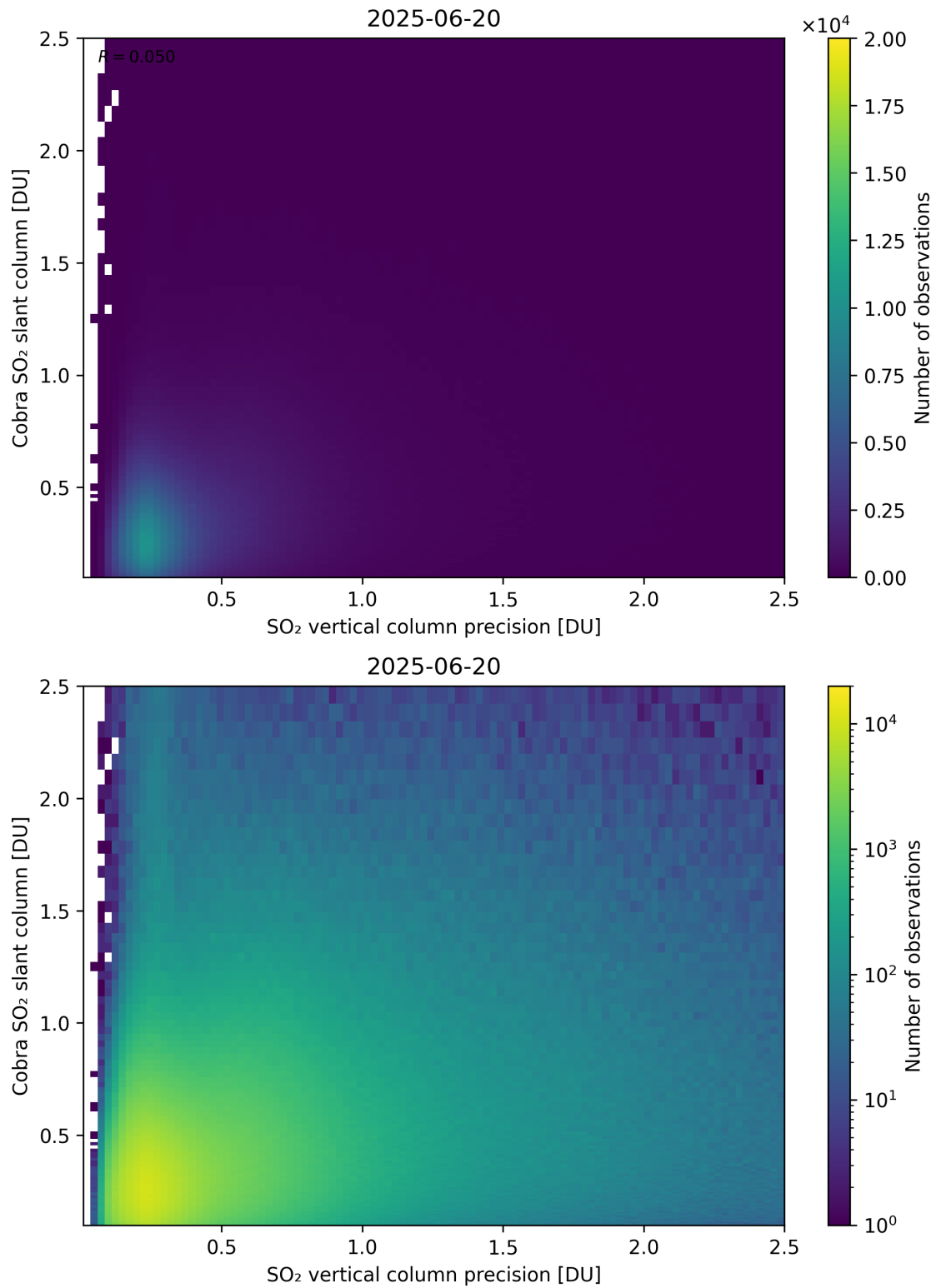
Figure 336: Scatter density plot of “SO 2 vertical column precision” against “Cobra SO 2 slant column” for 2025-06-19 to 2025-06-21.
