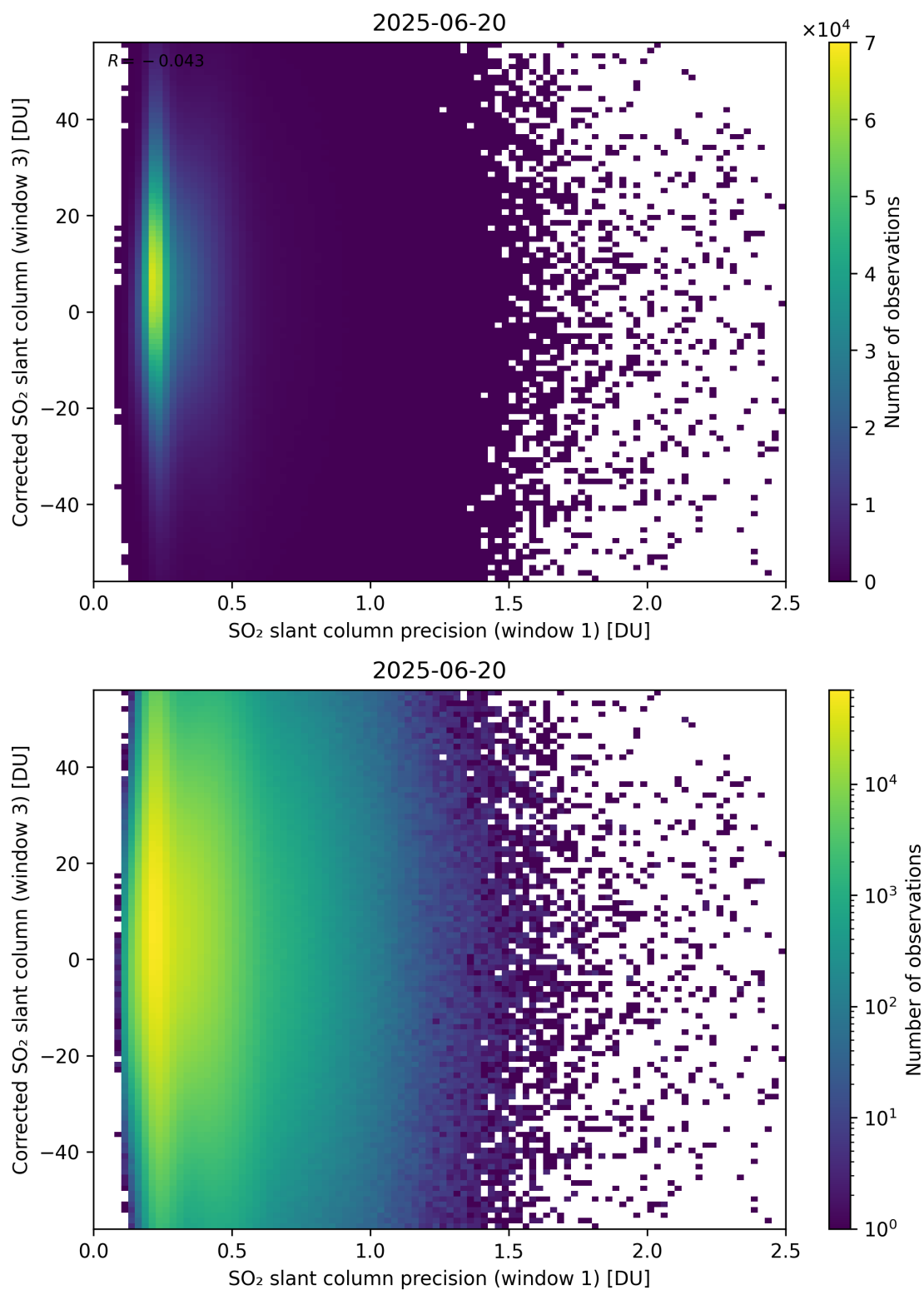
Figure 276: Scatter density plot of “SO 2 slant column precision (window 1)” against “Corrected SO 2 slant column (window 3)” for 2025-06-19 to 2025-06-21.
