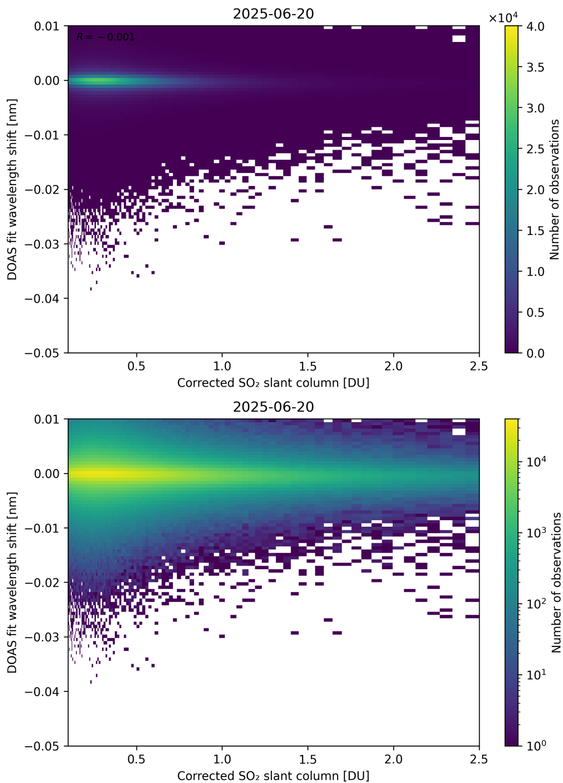
Figure 229: Scatter density plot of “Corrected SO 2 slant column” against “DOAS fit wavelength shift” for 2025-06-19 to 2025-06-21.
