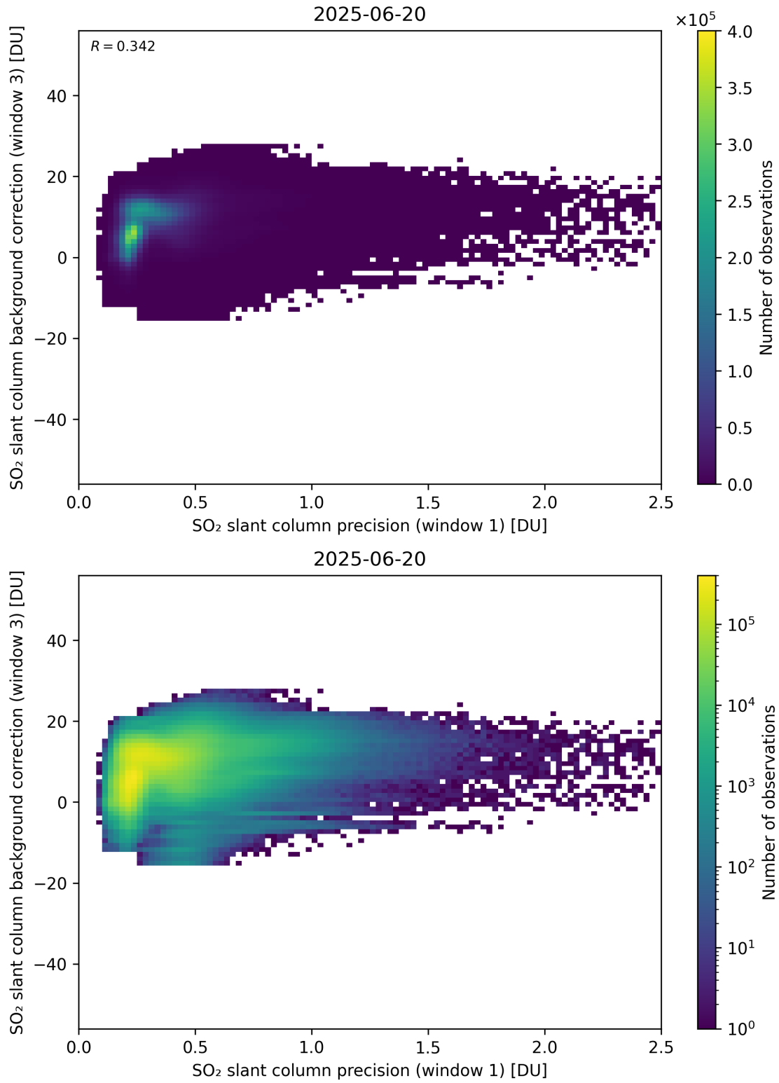
Figure 270: Scatter density plot of “SO 2 slant column precision (window 1)” against “SO 2 slant column background correction (window 3)” for 2025-06-19 to 2025-06-21.
