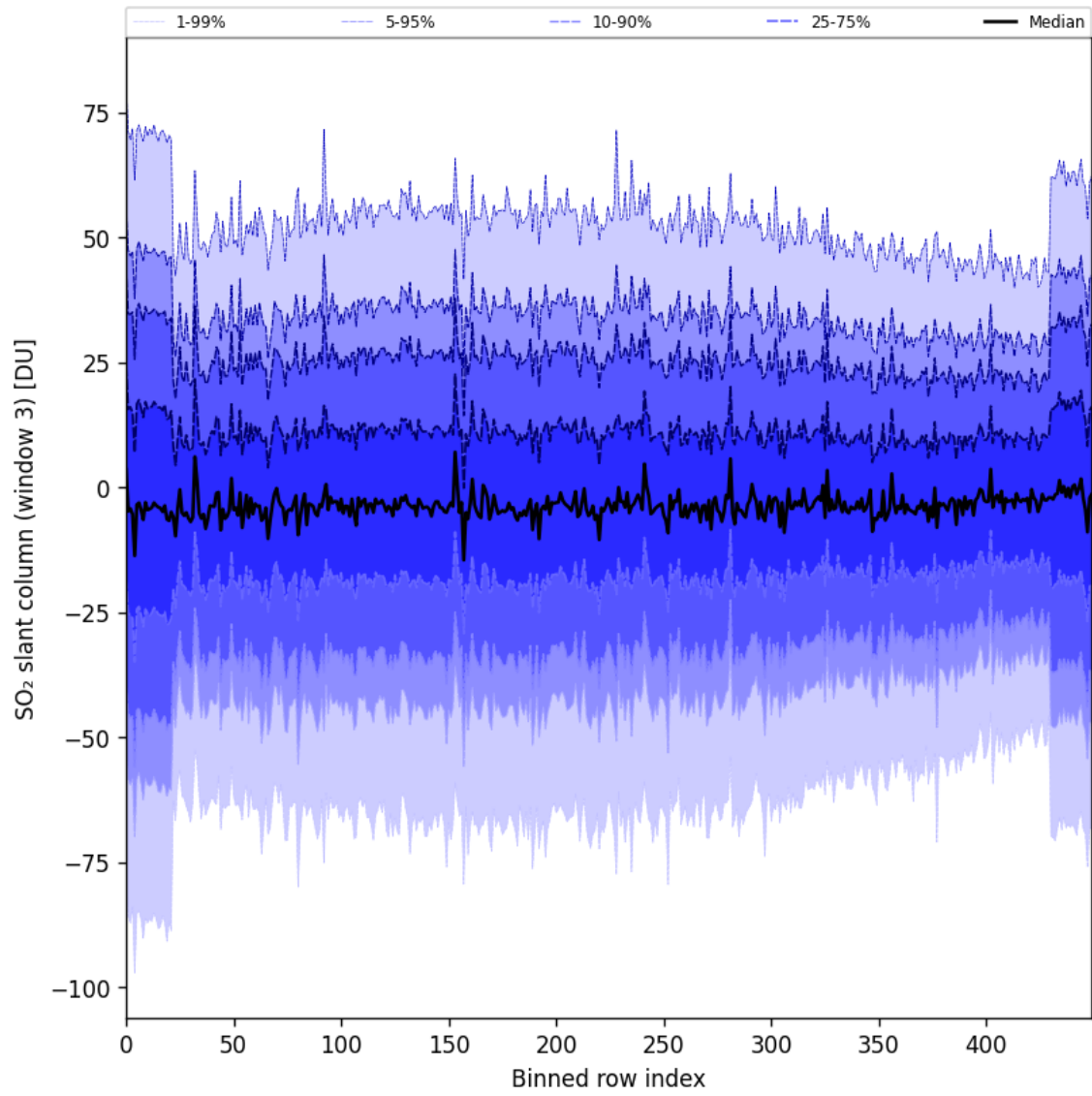
Figure 97: Along track statistics of “SO 2 slant column (window 3)” for 2025-06-19 to 2025-06-21
