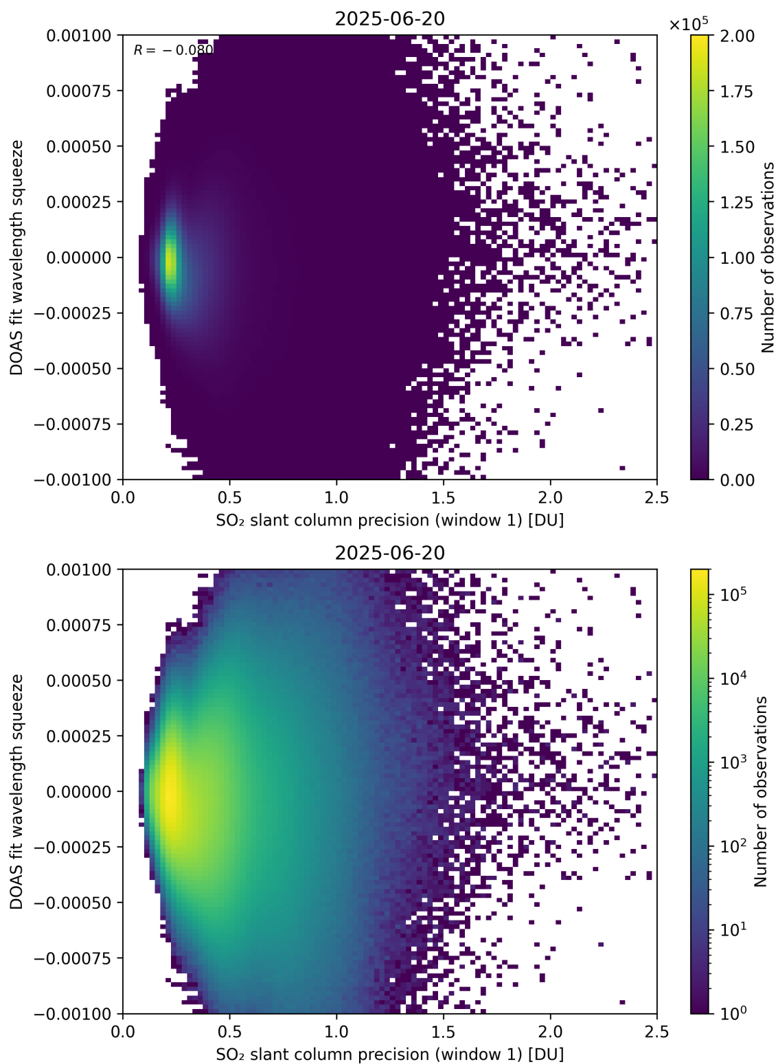
Figure 272: Scatter density plot of “SO 2 slant column precision (window 1)” against “DOAS fit wavelength squeeze” for 2025-06-19 to 2025-06-21.
