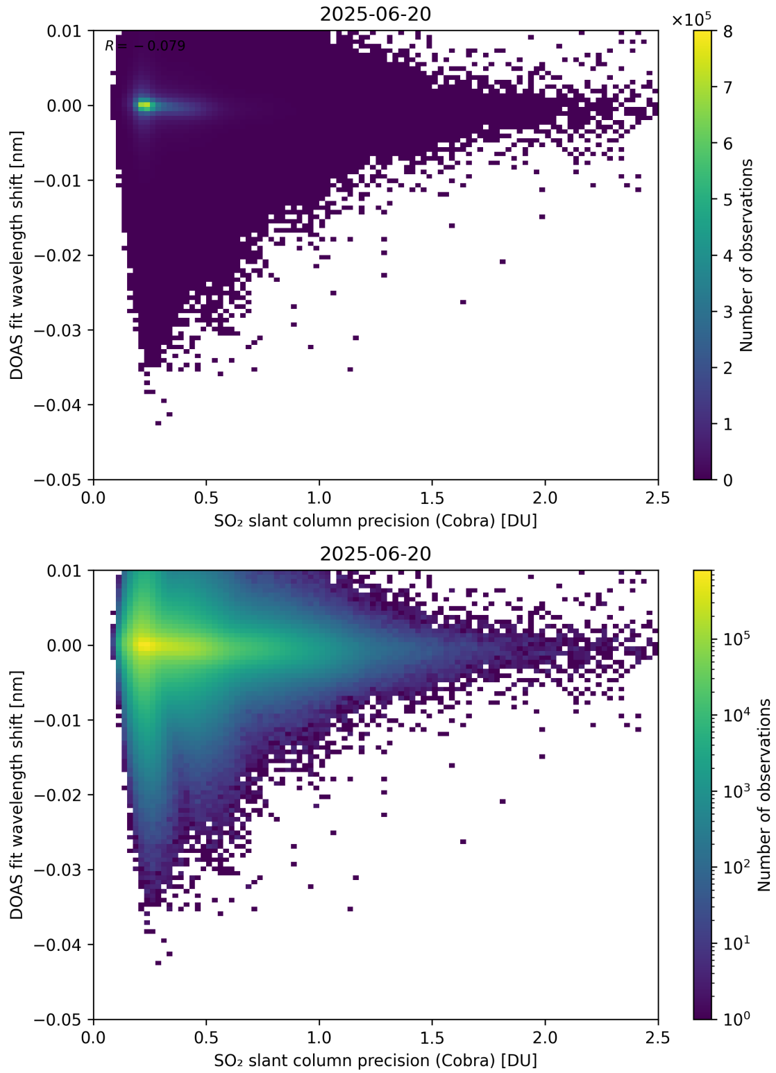
Figure 202: Scatter density plot of “SO 2 slant column precision (Cobra)” against “DOAS fit wavelength shift” for 2025-06-19 to 2025-06-21.
