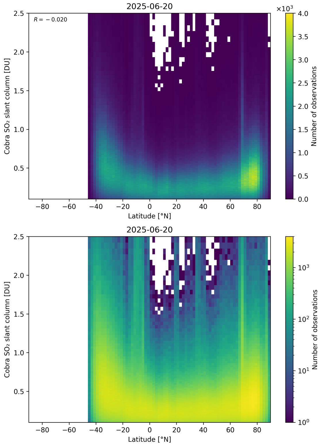
Figure 157: Scatter density plot of “Latitude” against “Cobra SO 2 slant column” for 2025-06-19 to 2025-06-21.
