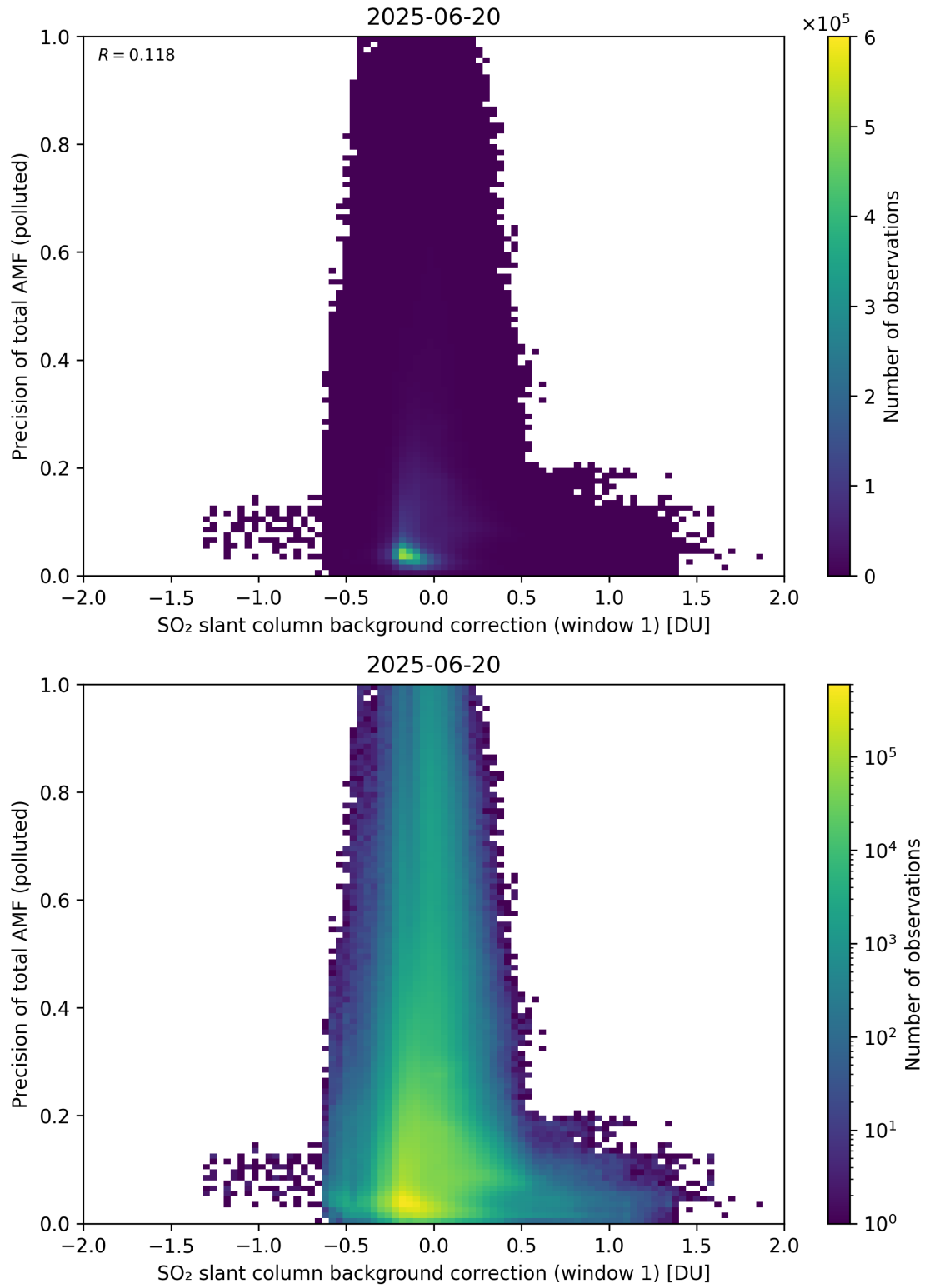
Figure 121: Scatter density plot of “SO 2 slant column background correction (window 1)” against “Precision of total AMF (polluted)” for 2025-06-19 to 2025-06-21.
