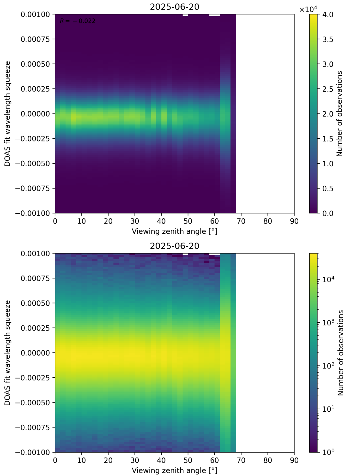
Figure 366: Scatter density plot of “Viewing zenith angle” against “DOAS fit wavelength squeeze” for 2025-06-19 to 2025-06-21.
