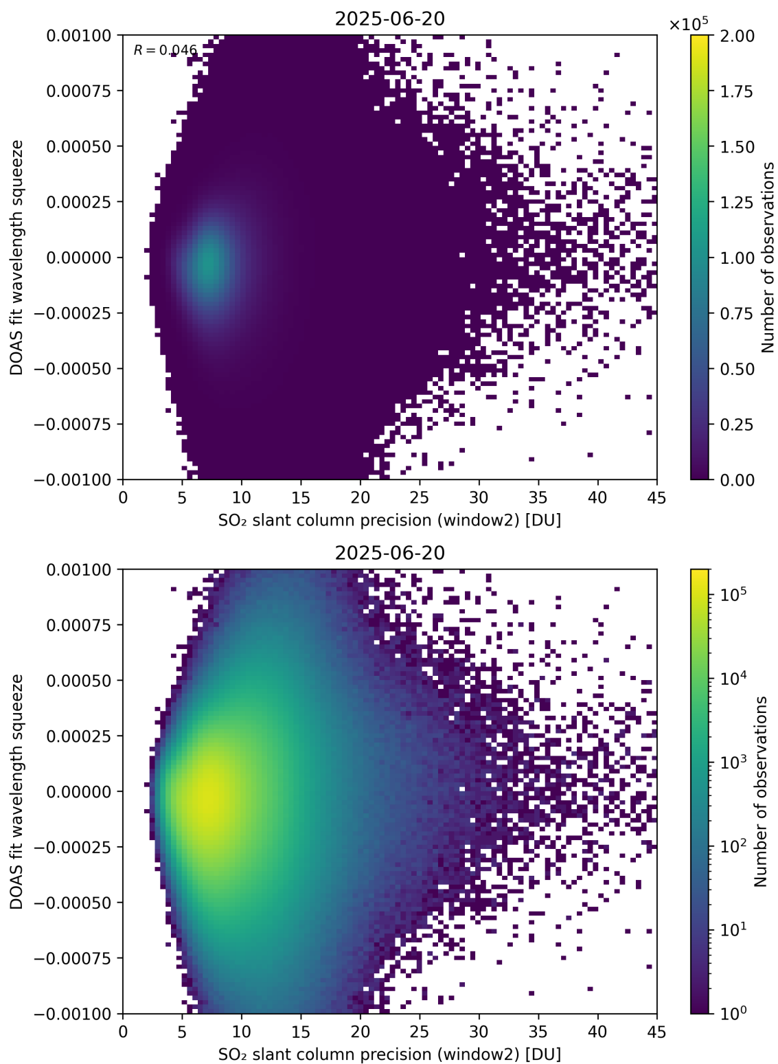
Figure 294: Scatter density plot of “SO 2 slant column precision (window2)” against “DOAS fit wavelength squeeze” for 2025-06-19 to 2025-06-21.
