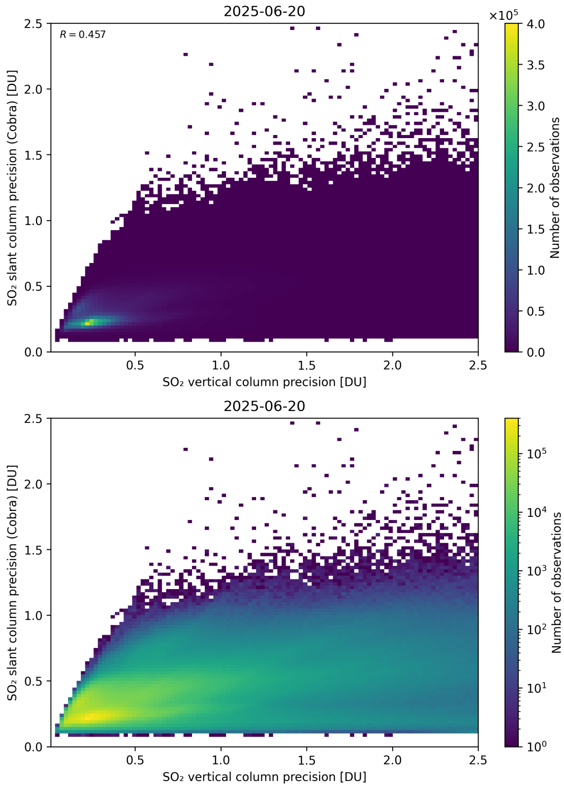
Figure 337: Scatter density plot of “SO 2 vertical column precision” against “SO 2 slant column precision (Cobra)” for 2025-06-19 to 2025-06-21.
