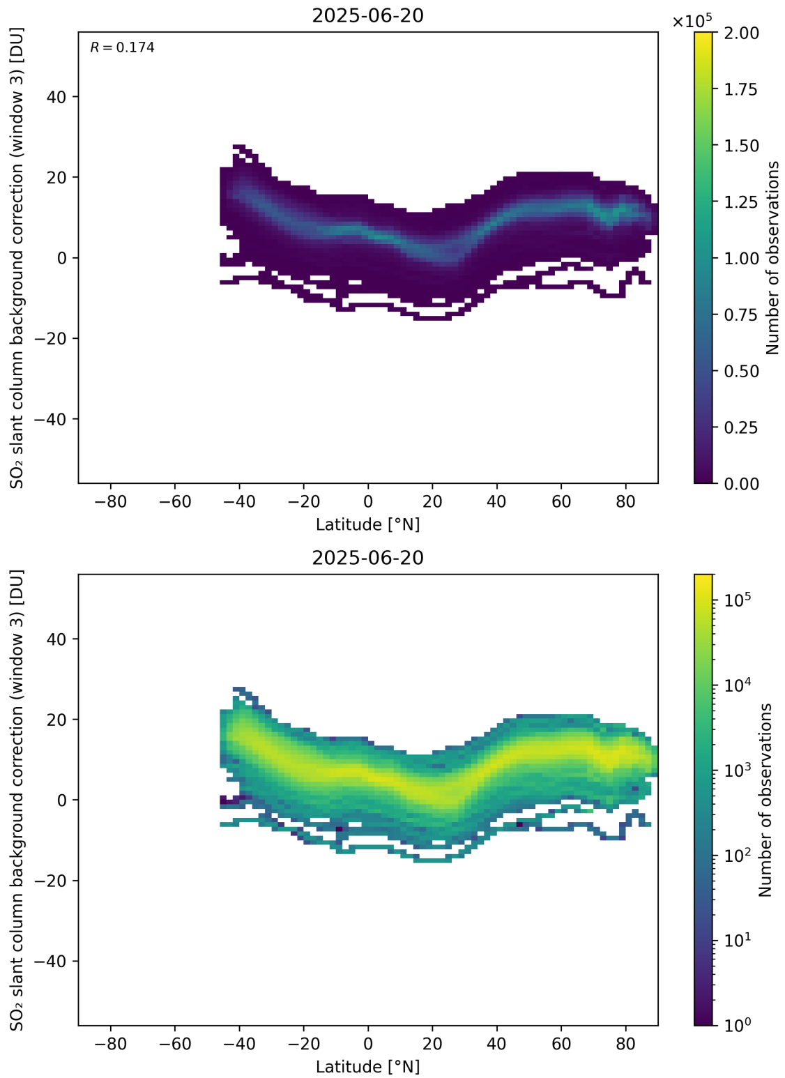
Figure 152: Scatter density plot of “Latitude” against “SO 2 slant column background correction (window 3)” for 2025-06-19 to 2025-06-21.
