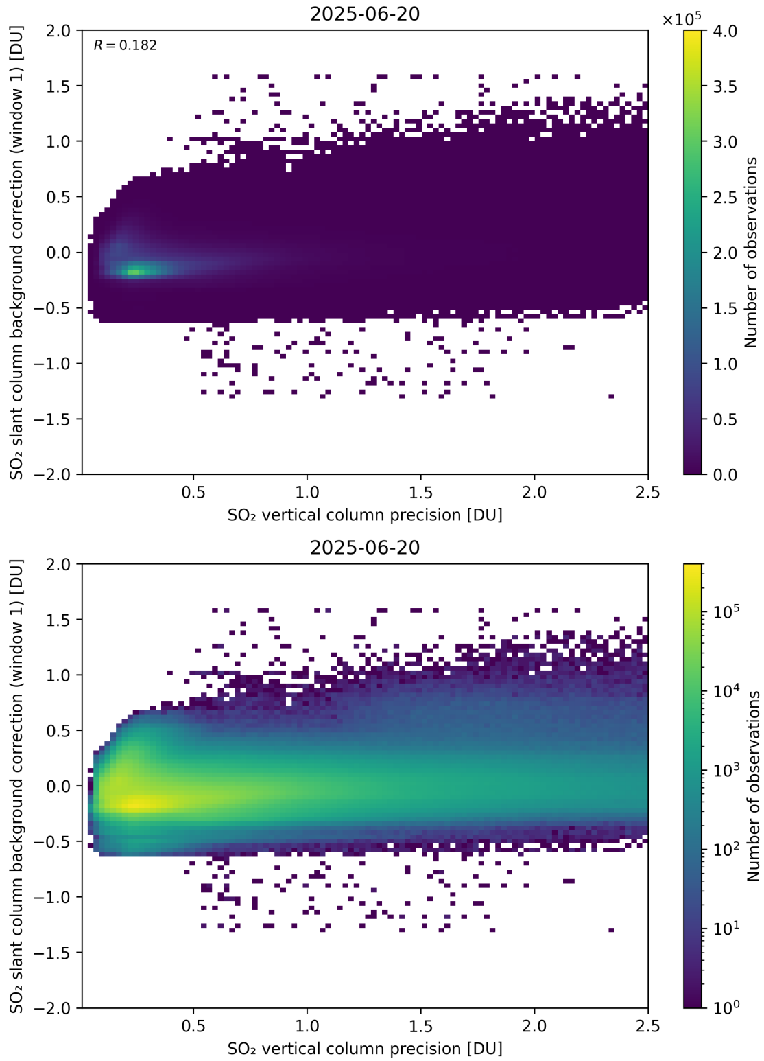
Figure 329: Scatter density plot of “SO 2 vertical column precision” against “SO 2 slant column background correction (window 1)” for 2025-06-19 to 2025-06-21.
