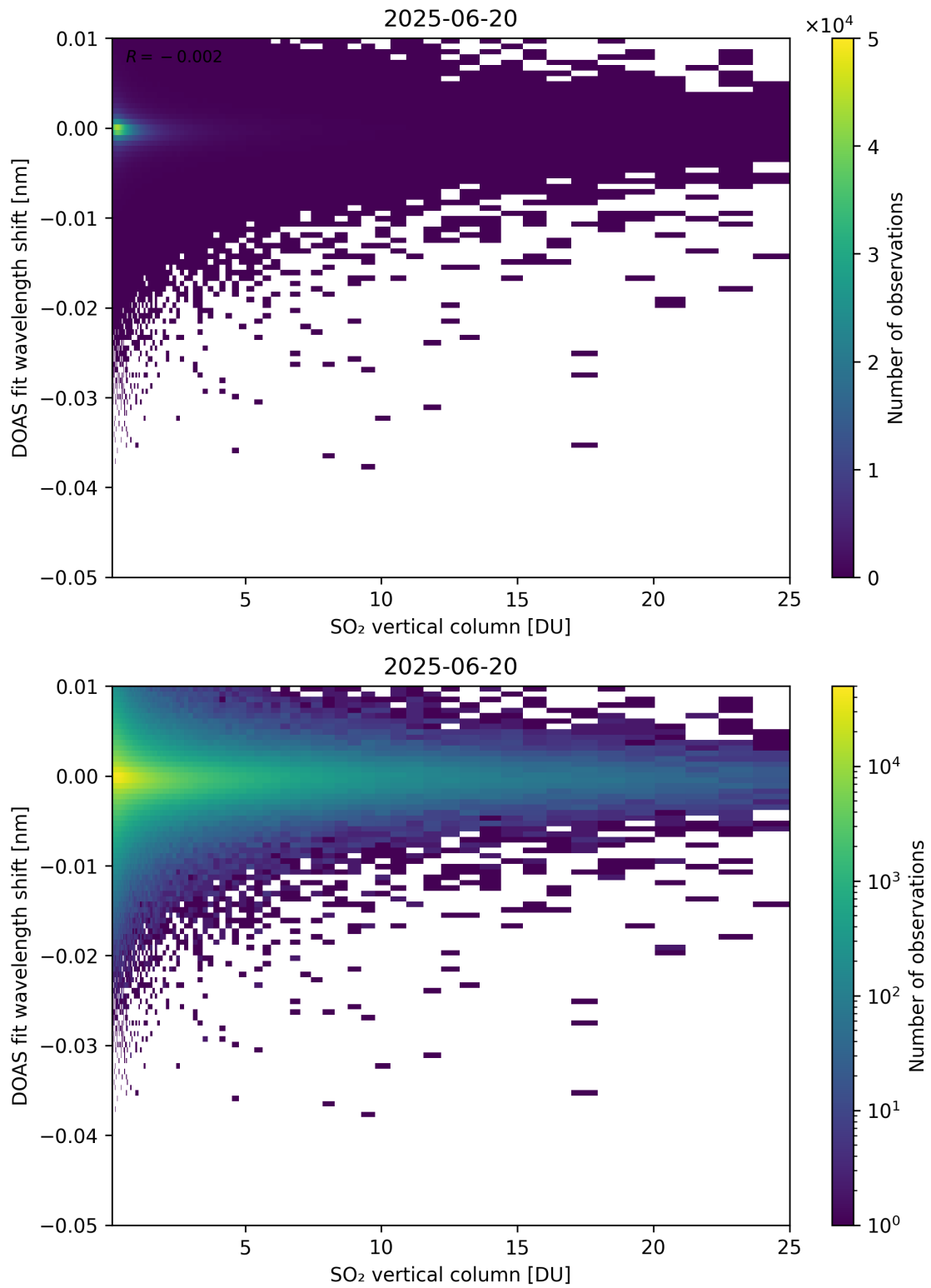
Figure 326: Scatter density plot of “SO 2 vertical column” against “DOAS fit wavelength shift” for 2025-06-19 to 2025-06-21.
