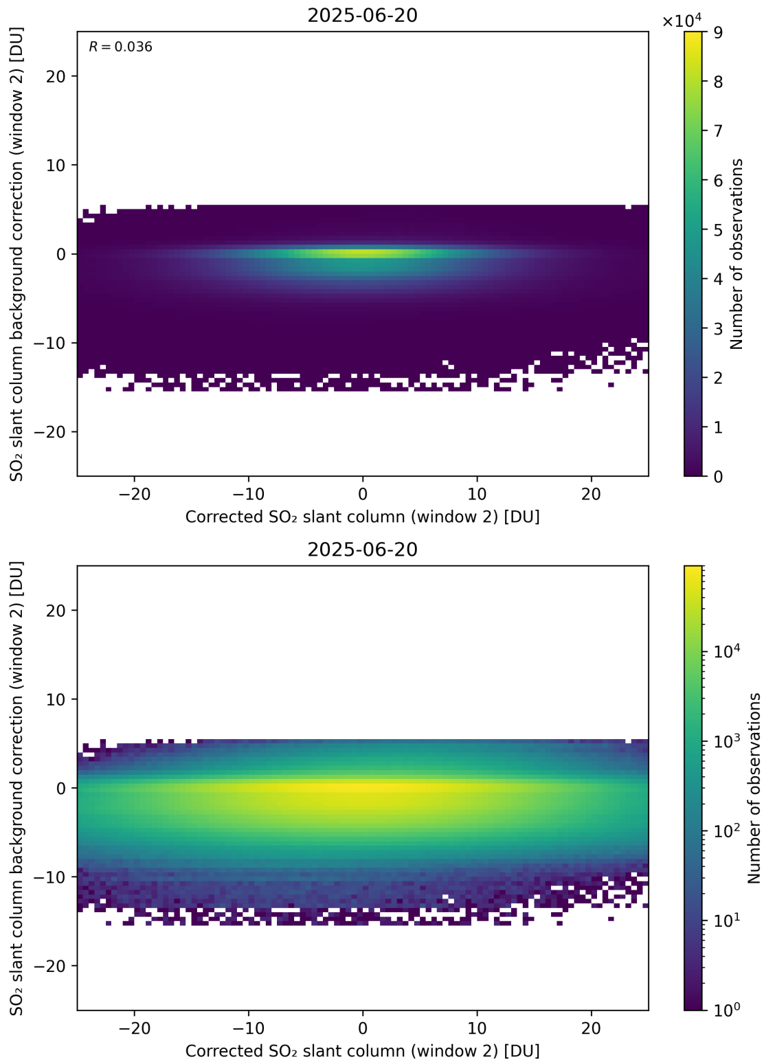
Figure 244: Scatter density plot of “Corrected SO 2 slant column (window 2)” against “SO 2 slant column background correction (window 2)” for 2025-06-19 to 2025-06-21.
