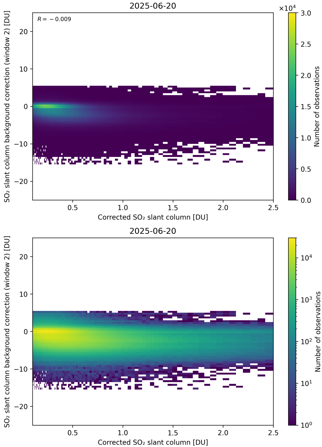
Figure 227: Scatter density plot of “Corrected SO 2 slant column” against “SO 2 slant column background correction (window 2)” for 2025-06-19 to 2025-06-21.
