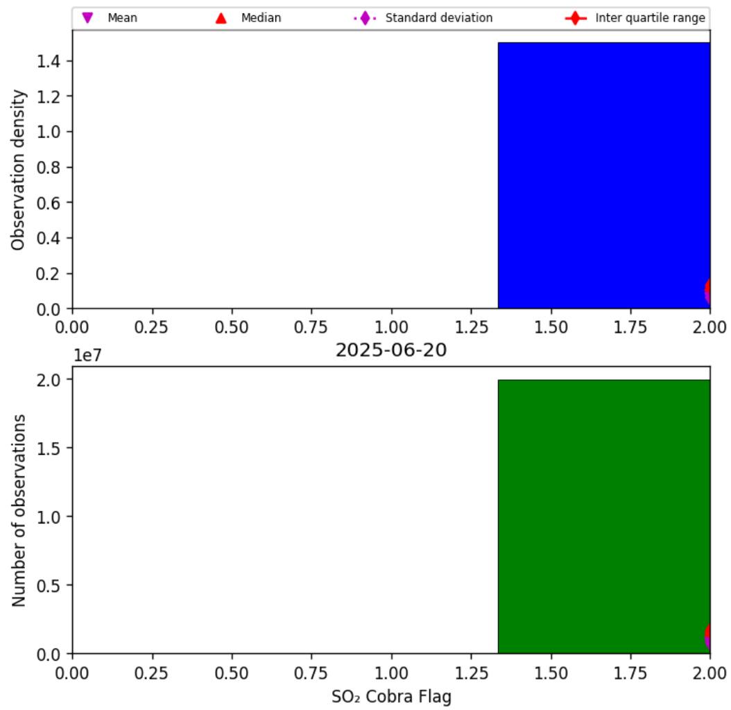
Figure 75: Histogram of “SO 2 Cobra Flag” for 2025-06-19 to 2025-06-21
