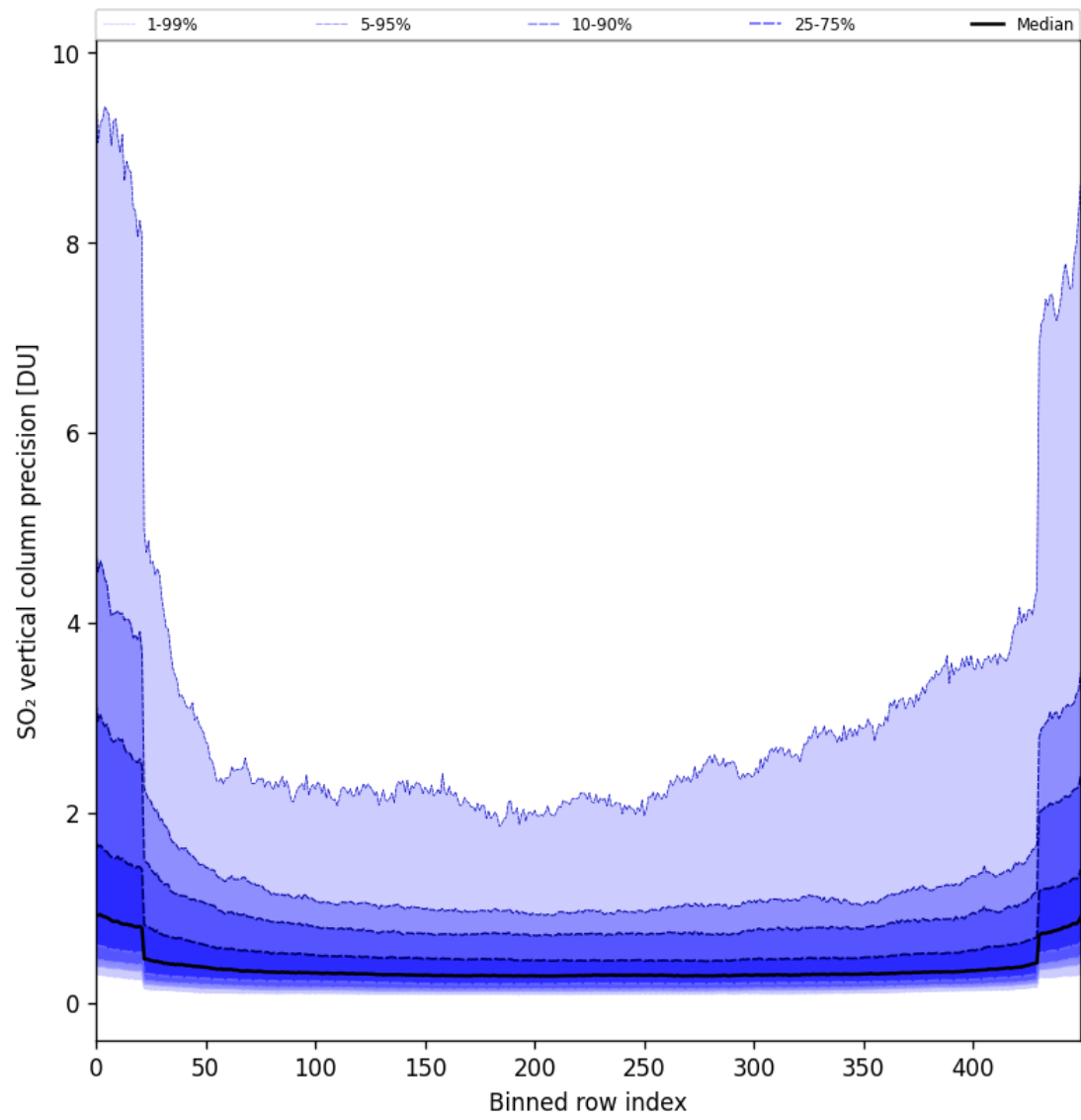
Figure 85: Along track statistics of “SO 2 vertical column precision” for 2025-06-19 to 2025-06-21
