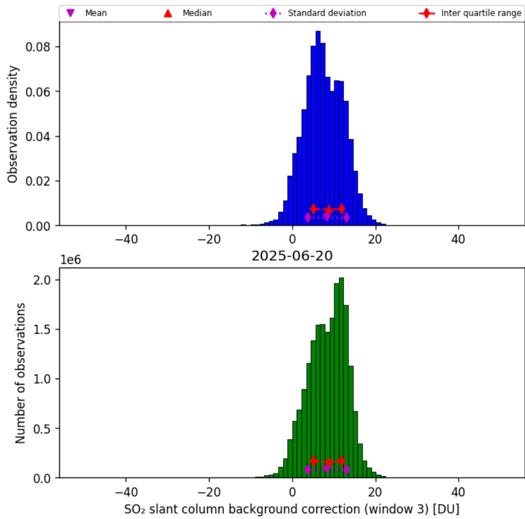
Figure 74: Histogram of “SO 2 slant column background correction (window 3)” for 2025-06-19 to 2025-06-21
