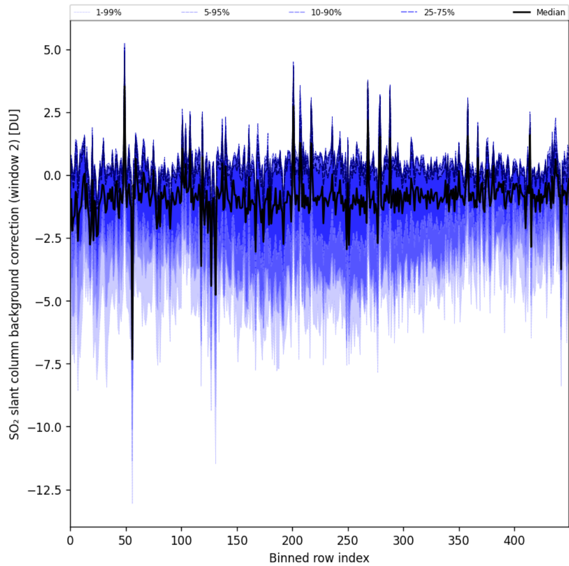
Figure 96: Along track statistics of “SO 2 slant column background correction (window 2)” for 2025-06-19 to 2025-06-21
