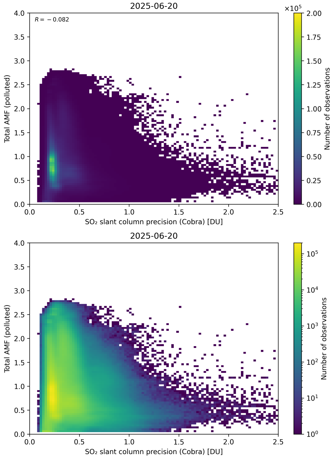
Figure 213: Scatter density plot of “SO 2 slant column precision (Cobra)” against “Total AMF (polluted)” for 2025-06-19 to 2025-06-21.
