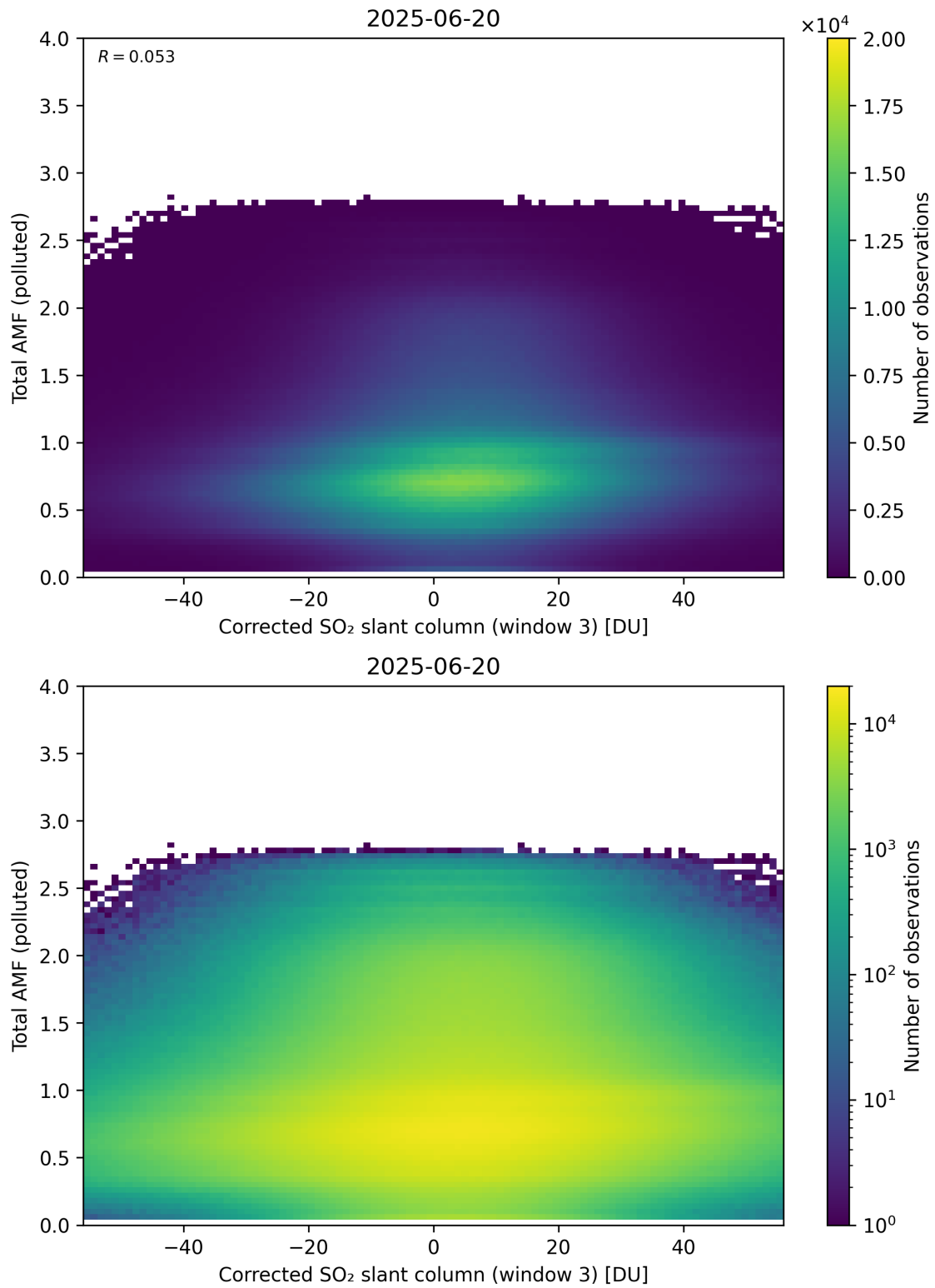
Figure 260: Scatter density plot of “Corrected SO 2 slant column (window 3)” against “Total AMF (polluted)” for 2025-06-19 to 2025-06-21.
