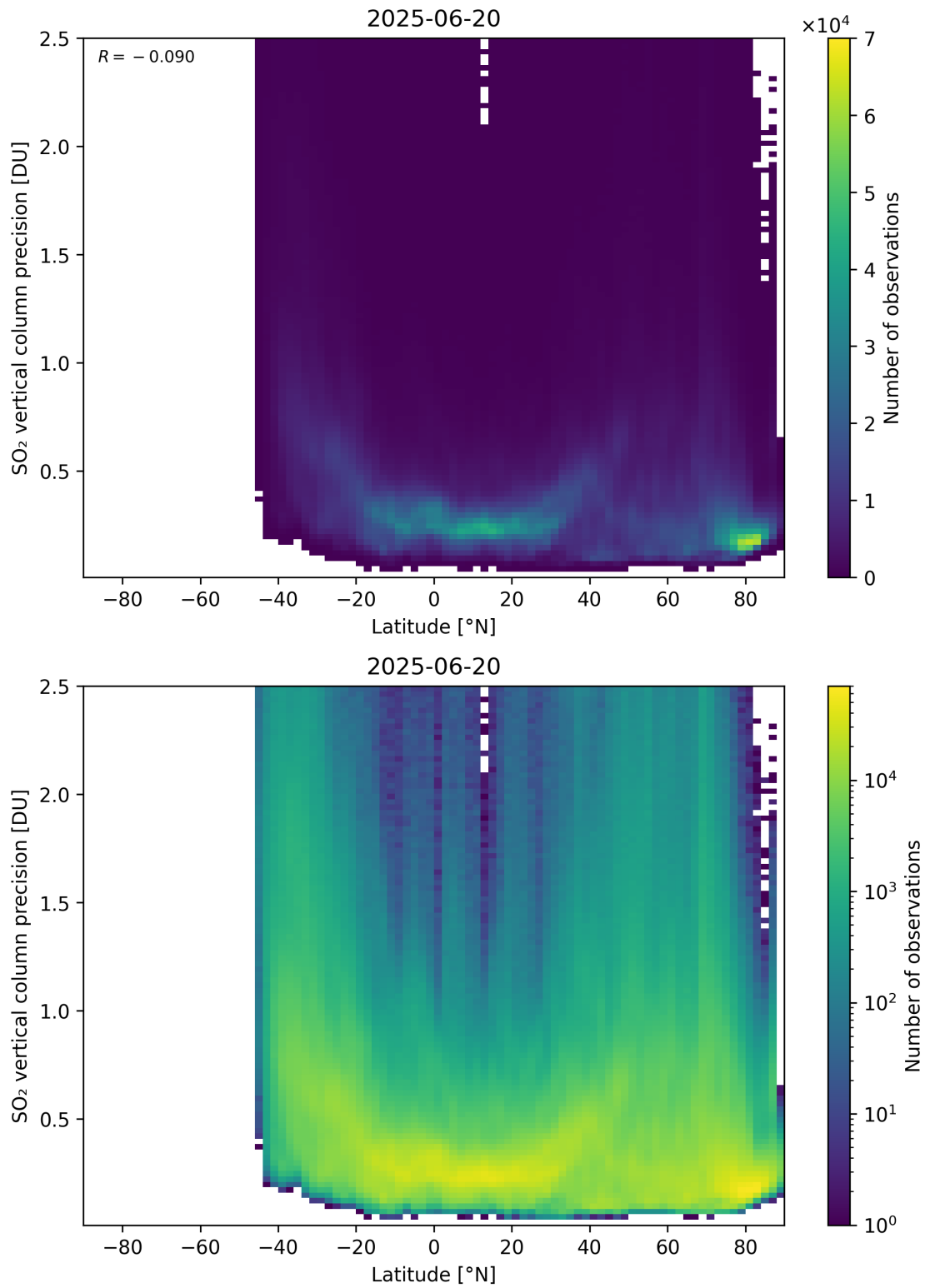
Figure 170: Scatter density plot of “Latitude” against “SO 2 vertical column precision” for 2025-06-19 to 2025-06-21.
