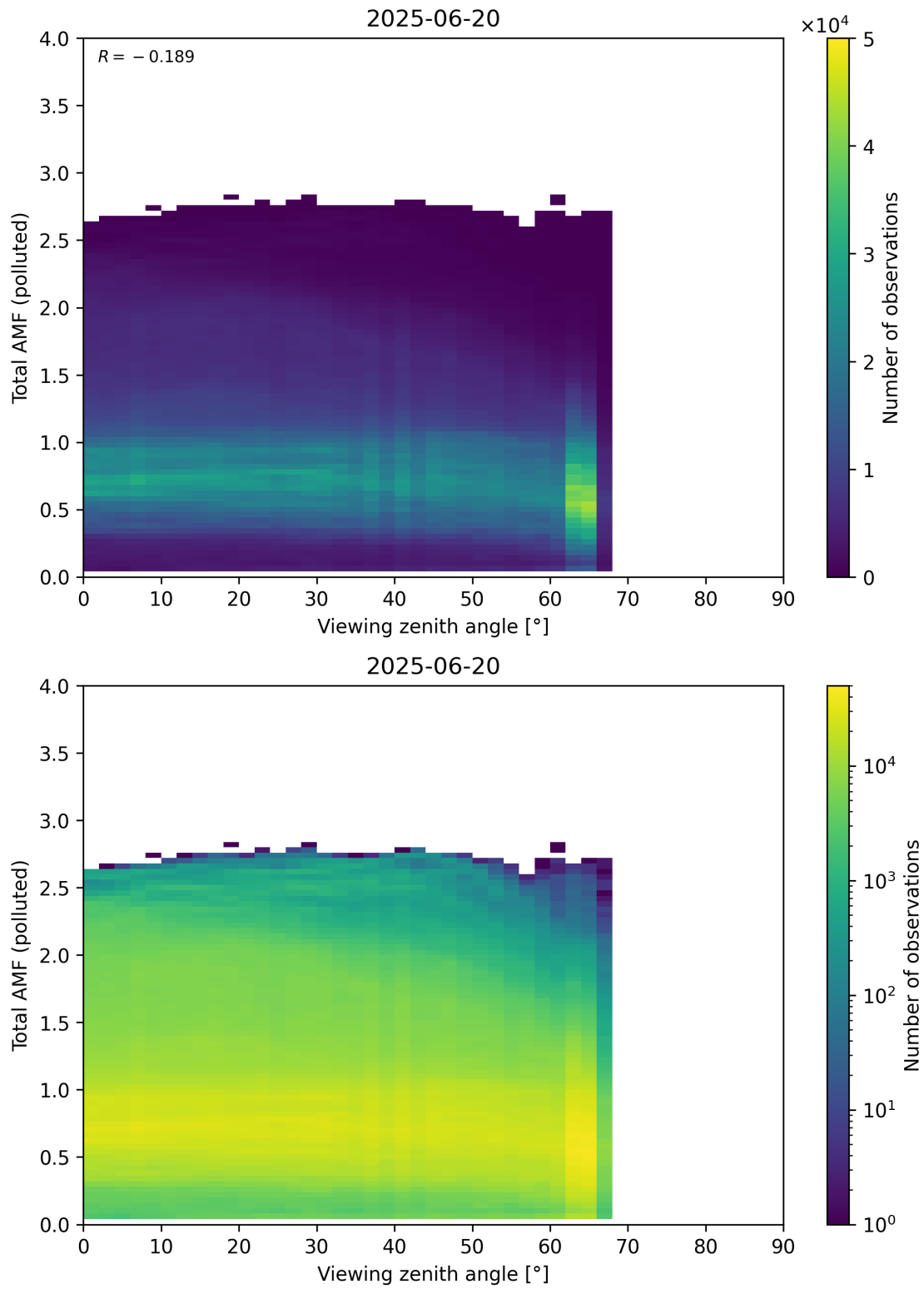
Figure 381: Scatter density plot of “Viewing zenith angle” against “Total AMF (polluted)” for 2025-06-19 to 2025-06-21.
