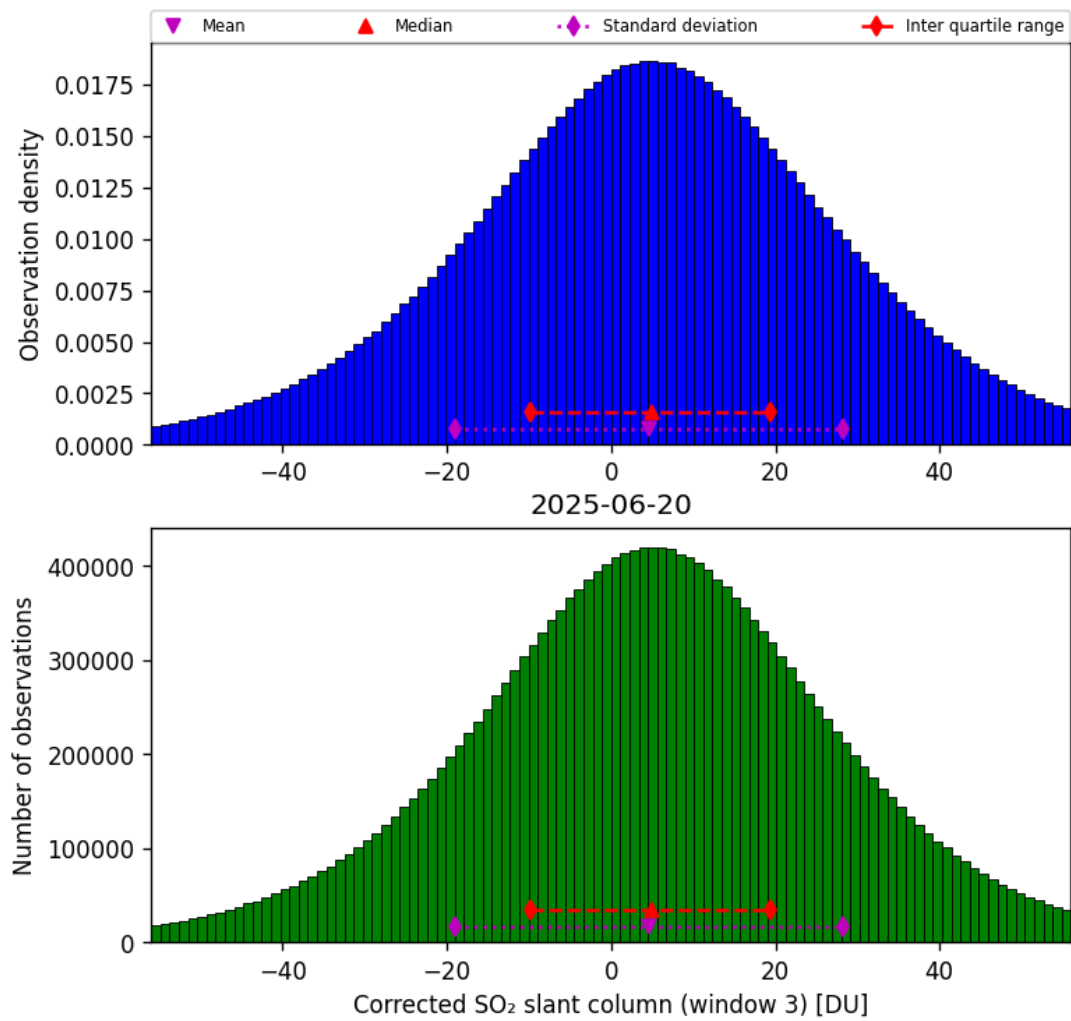
Figure 73: Histogram of “Corrected SO 2 slant column (window 3)” for 2025-06-19 to 2025-06-21
