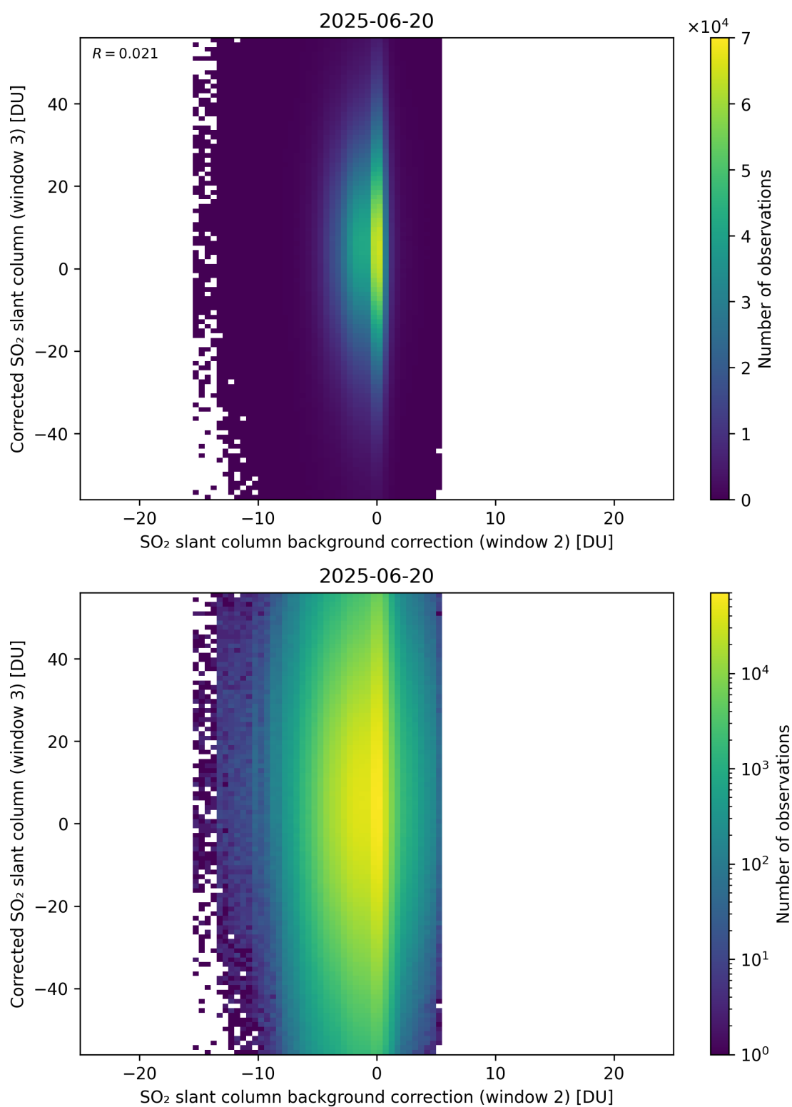
Figure 127: Scatter density plot of “SO 2 slant column background correction (window 2)” against “Corrected SO 2 slant column (window 3)” for 2025-06-19 to 2025-06-21.
