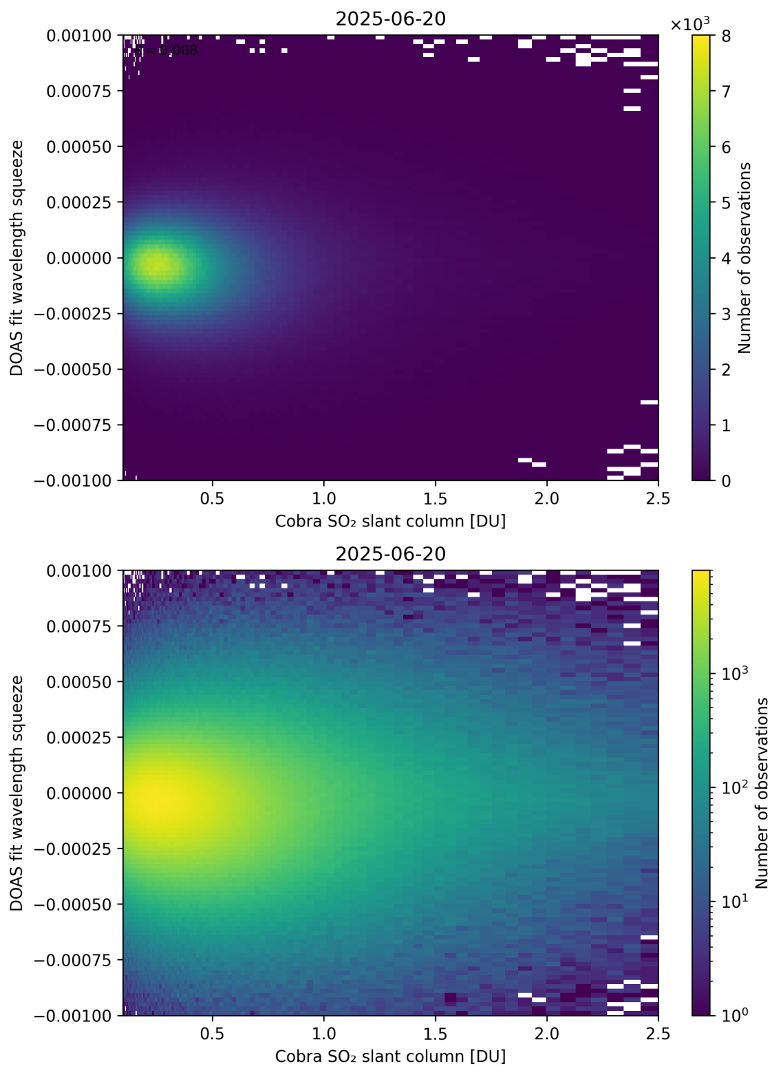
Figure 197: Scatter density plot of “Cobra SO 2 slant column” against “DOAS fit wavelength squeeze” for 2025-06-19 to 2025-06-21.
