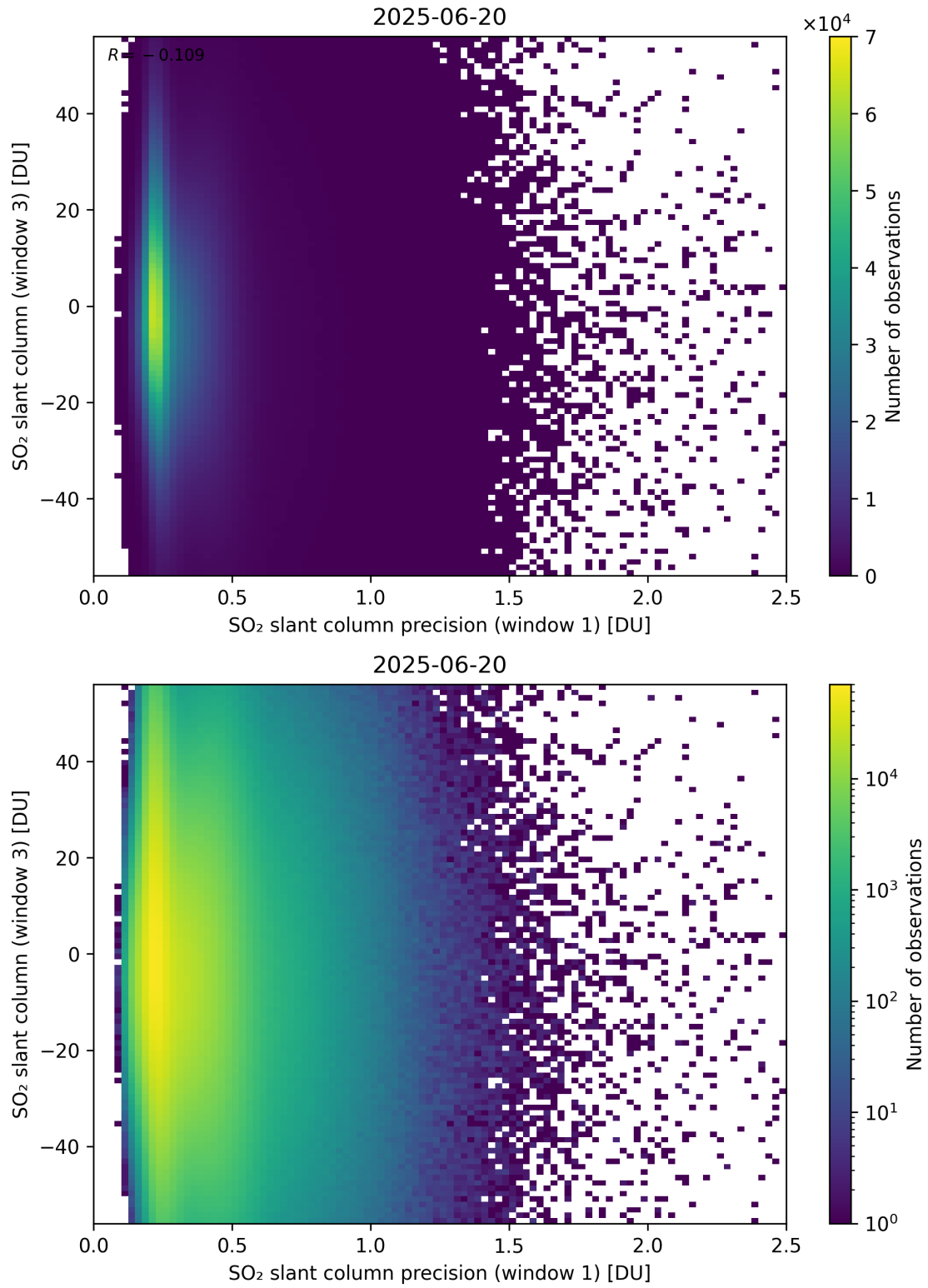
Figure 278: Scatter density plot of “SO 2 slant column precision (window 1)” against “SO 2 slant column (window 3)” for 2025-06-19 to 2025-06-21.
