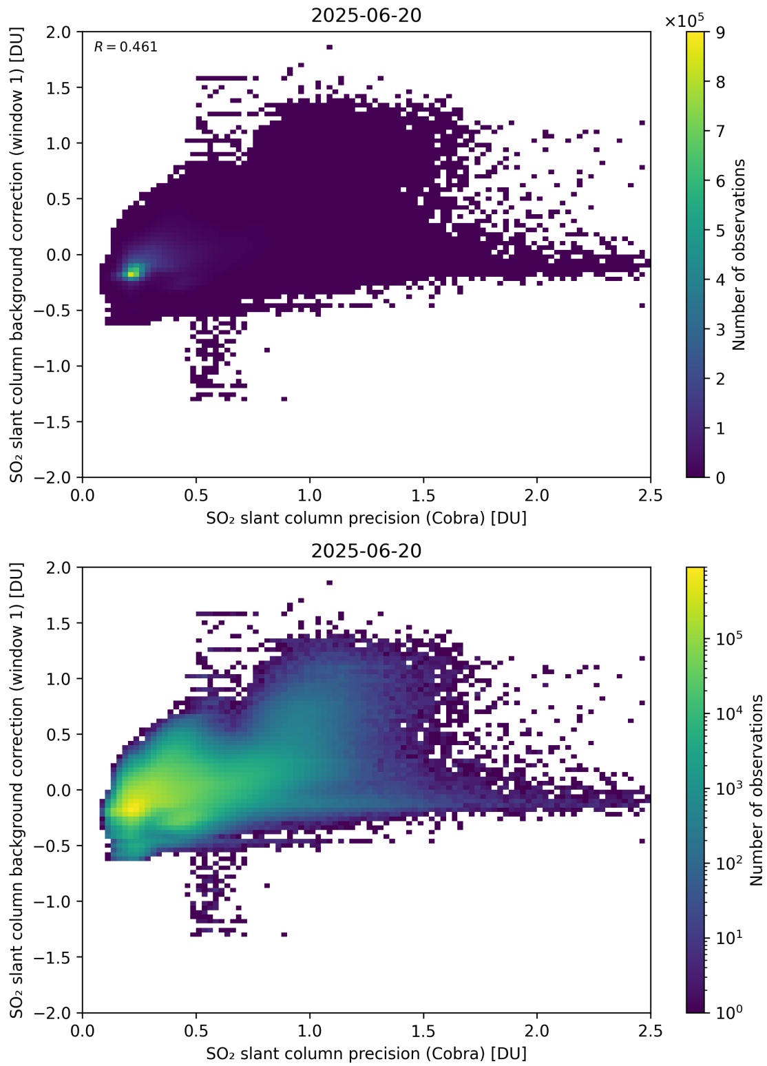
Figure 199: Scatter density plot of “SO 2 slant column precision (Cobra)” against “SO 2 slant column background correction (window 1)” for 2025-06-19 to 2025-06-21.
