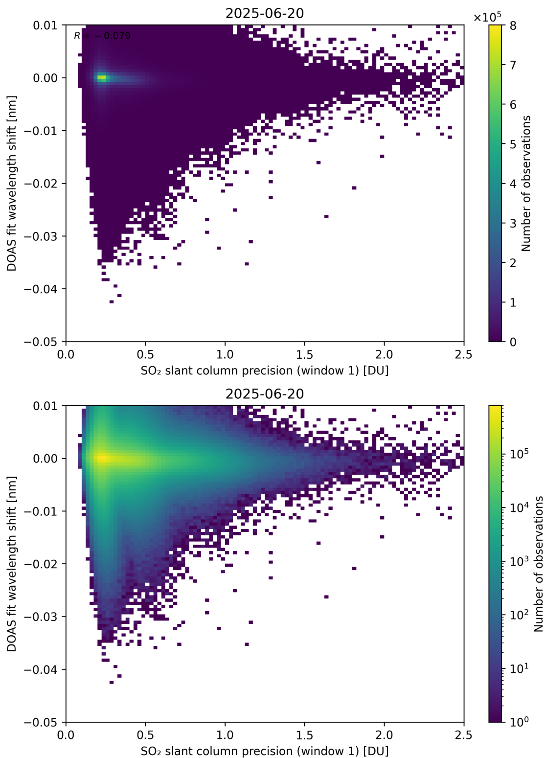
Figure 271: Scatter density plot of “SO 2 slant column precision (window 1)” against “DOAS fit wavelength shift” for 2025-06-19 to 2025-06-21.
