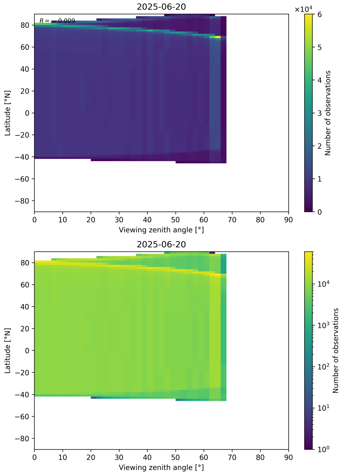
Figure 368: Scatter density plot of “Viewing zenith angle” against “Latitude” for 2025-06-19 to 2025-06-21.
