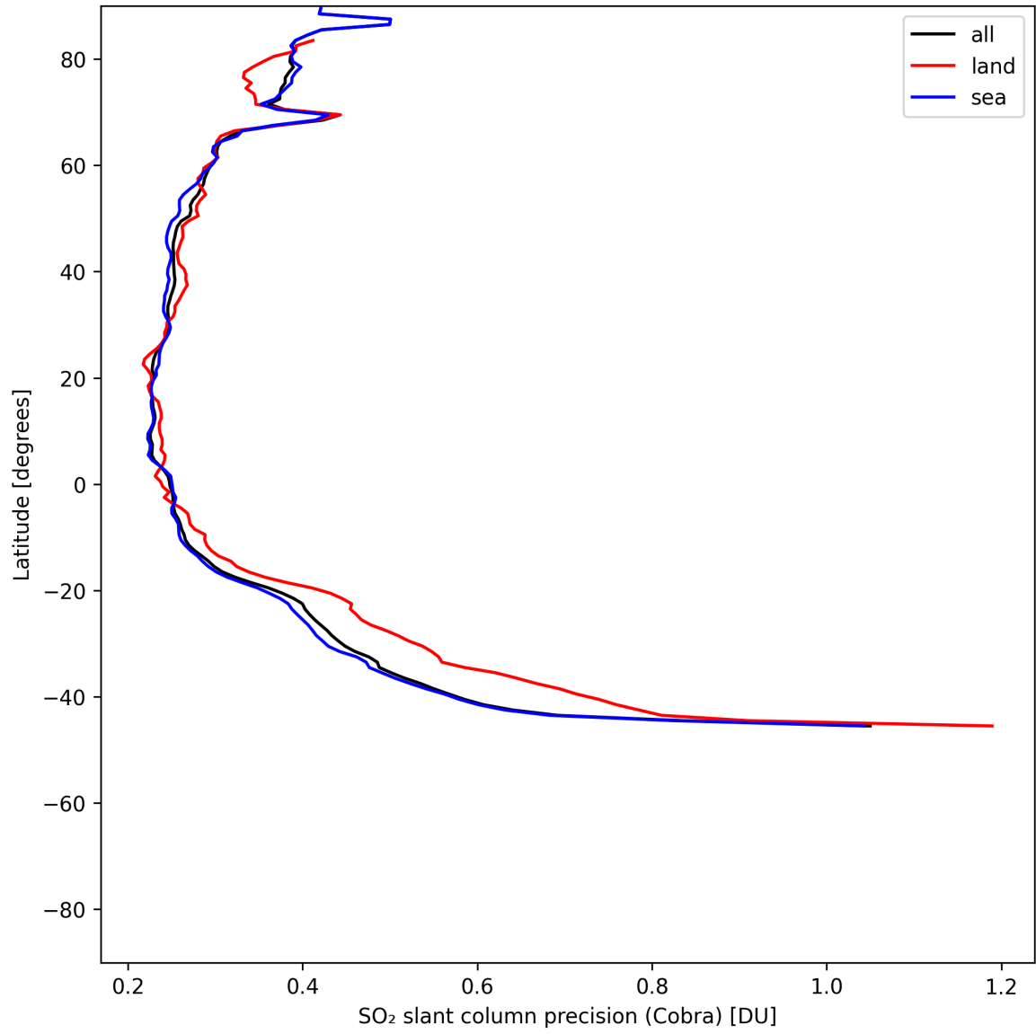
Figure 36: Zonal average of “SO 2 slant column precision (Cobra)” for 2025-06-19 to 2025-06-21.
