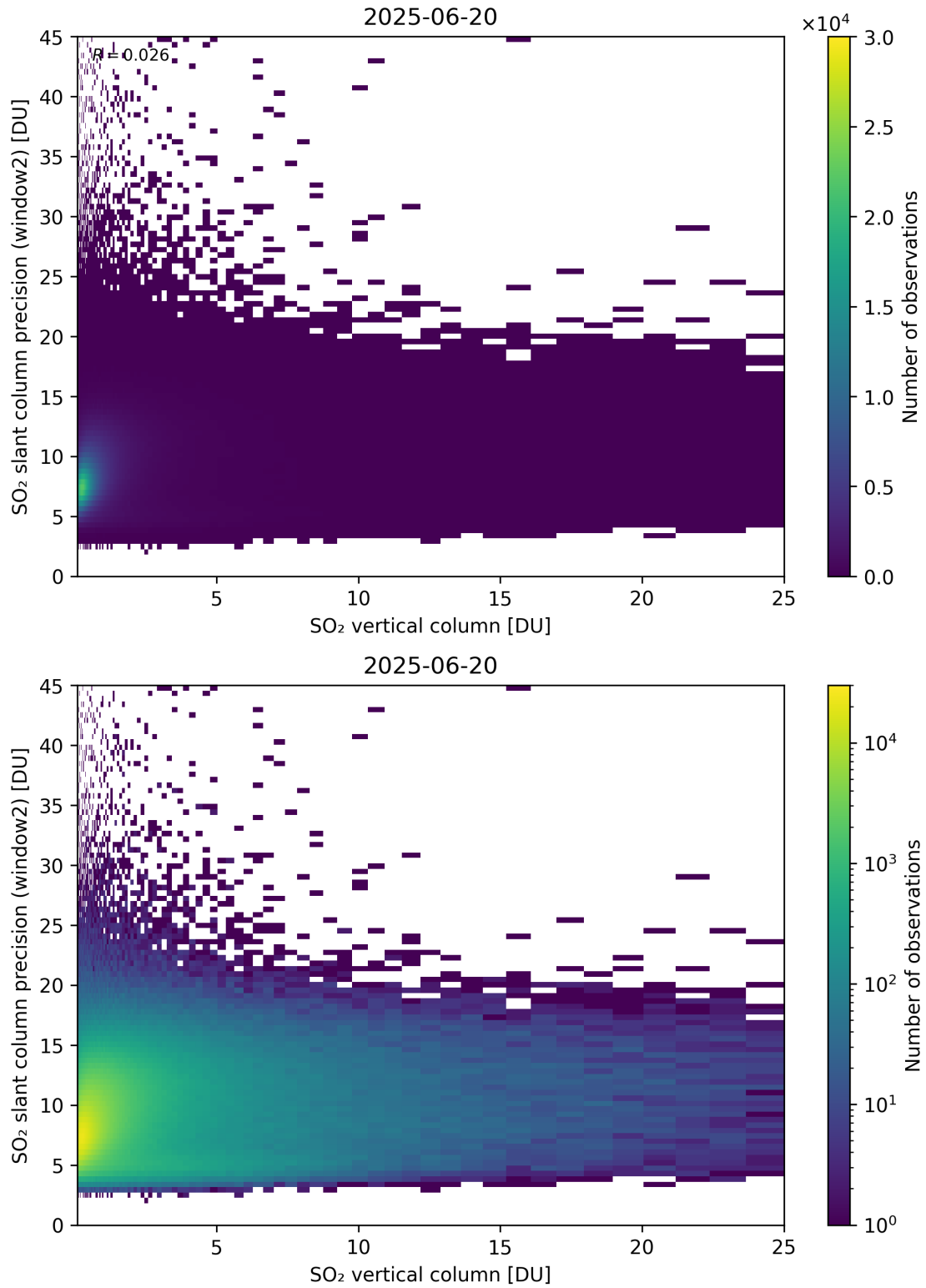
Figure 356: Scatter density plot of “SO 2 vertical column” against “SO 2 slant column precision (window2)” for 2025-06-19 to 2025-06-21.
