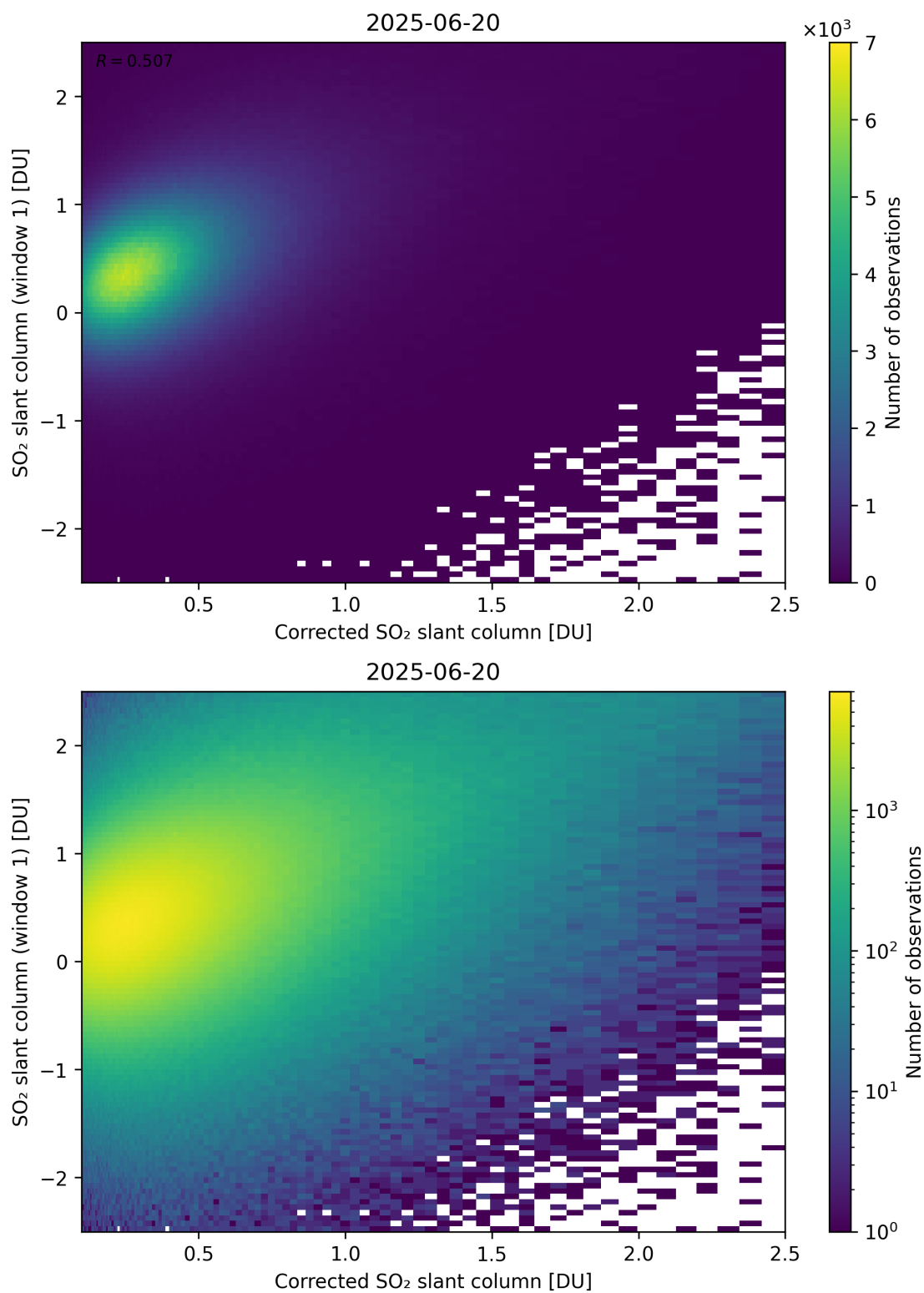
Figure 237: Scatter density plot of “Corrected SO 2 slant column” against “SO 2 slant column (window 1)” for 2025-06-19 to 2025-06-21.
