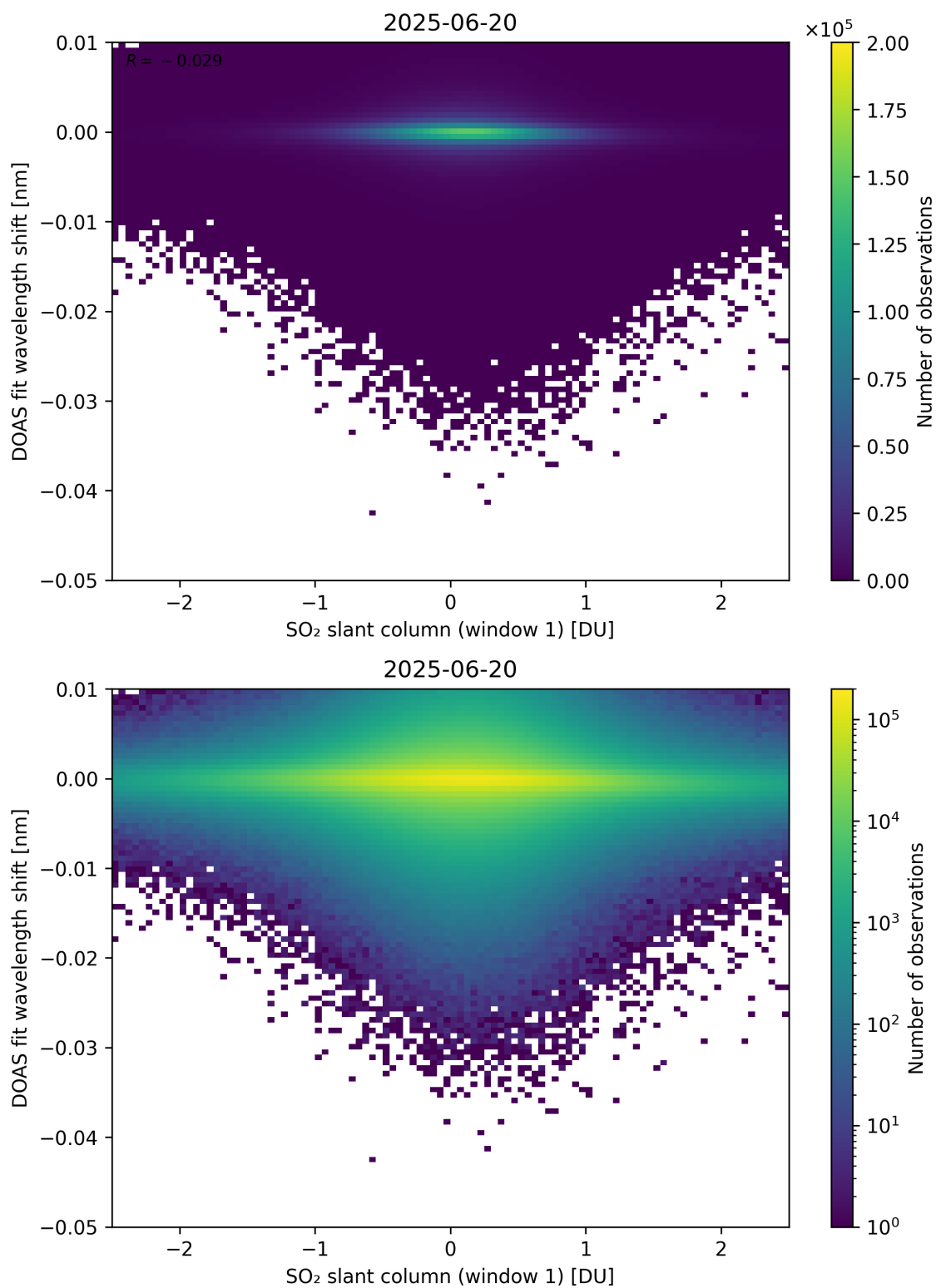
Figure 265: Scatter density plot of “SO 2 slant column (window 1)” against “DOAS fit wavelength shift” for 2025-06-19 to 2025-06-21.
