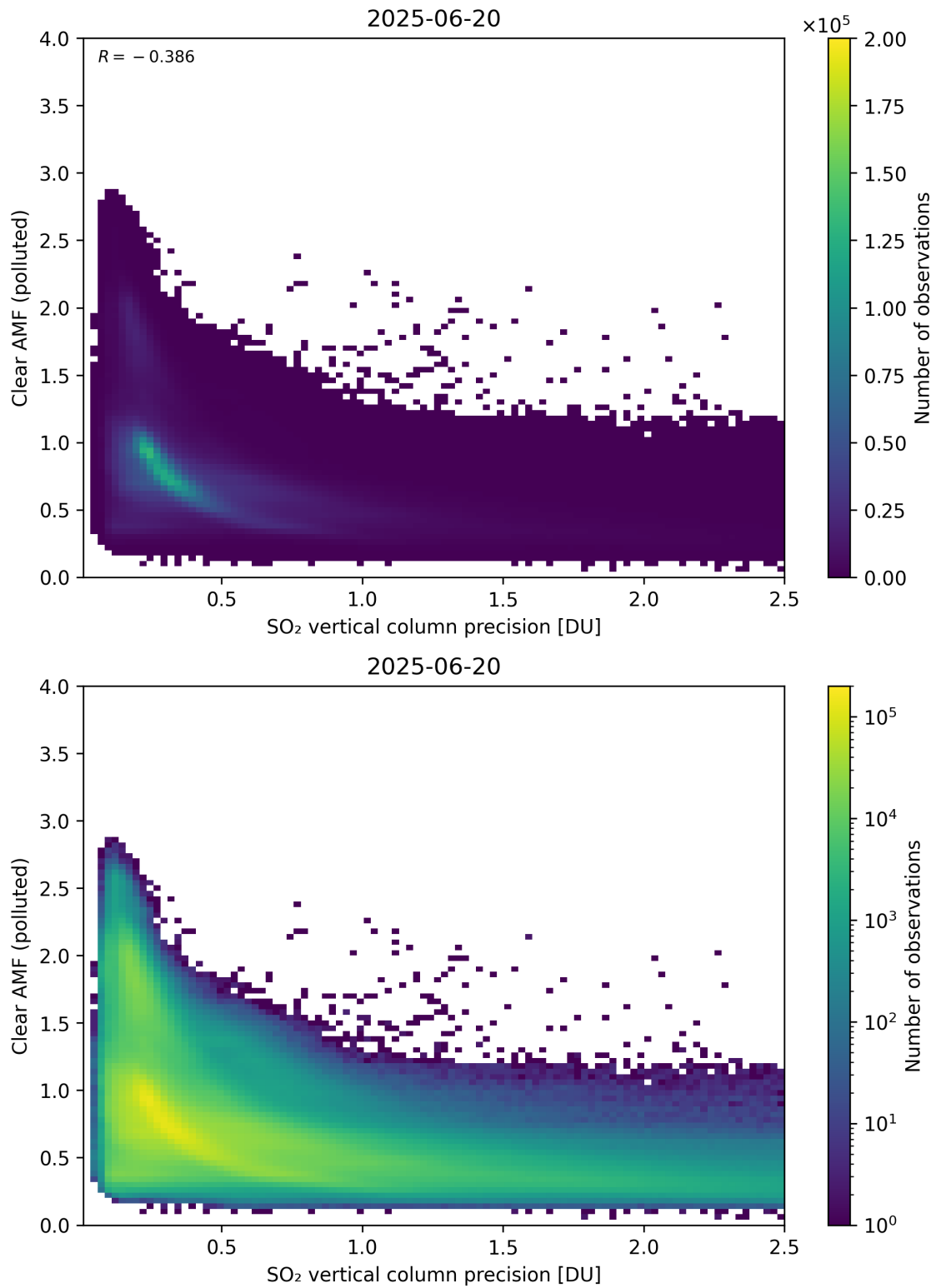
Figure 335: Scatter density plot of “SO 2 vertical column precision” against “Clear AMF (polluted)” for 2025-06-19 to 2025-06-21.
