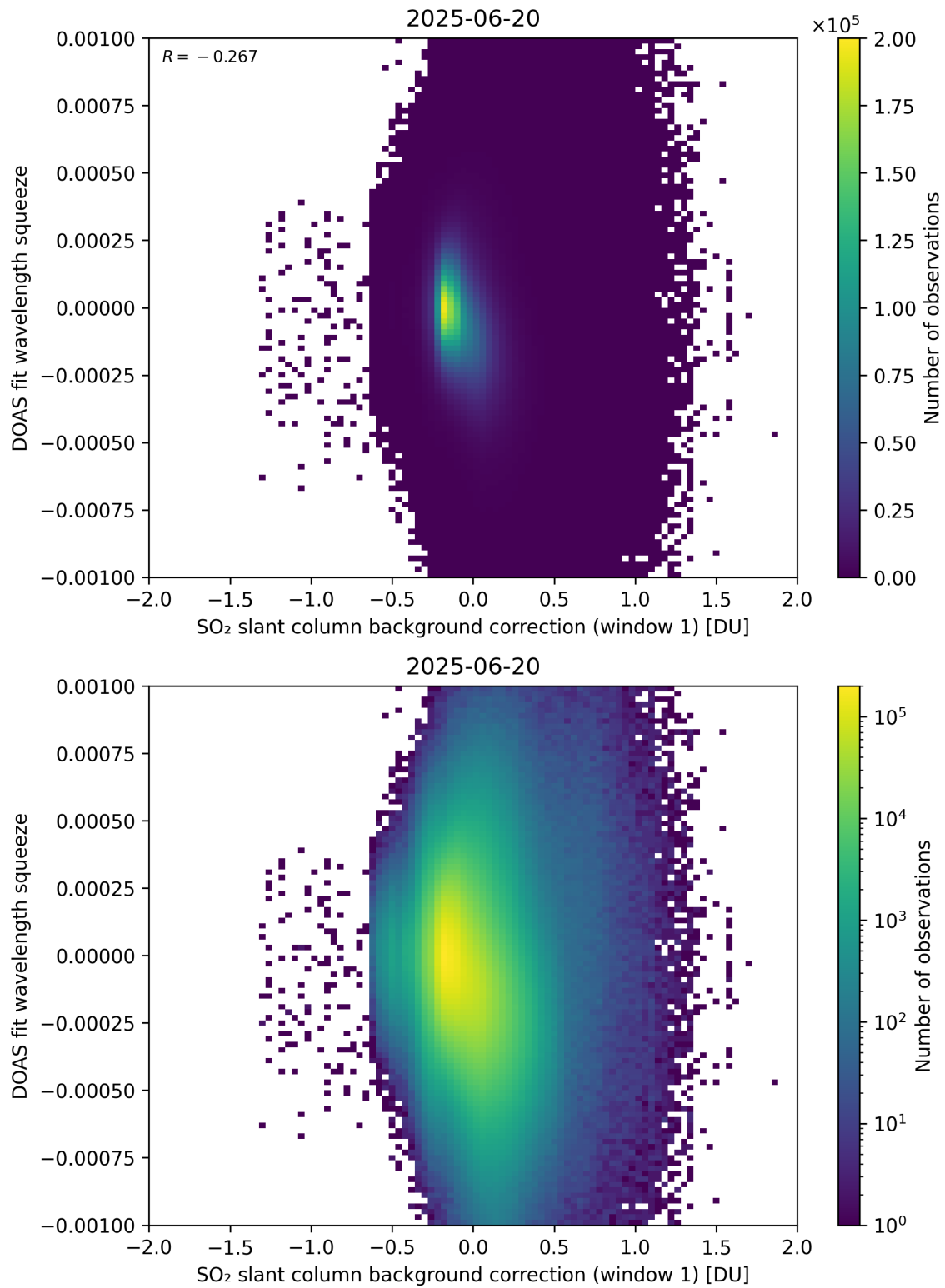
Figure 112: Scatter density plot of “SO 2 slant column background correction (window 1)” against “DOAS fit wavelength squeeze” for 2025-06-19 to 2025-06-21.
