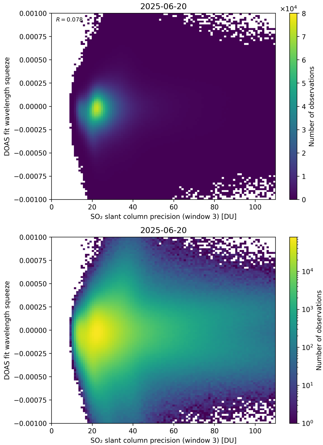
Figure 309: Scatter density plot of “SO 2 slant column precision (window 3)” against “DOAS fit wavelength squeeze” for 2025-06-19 to 2025-06-21.
