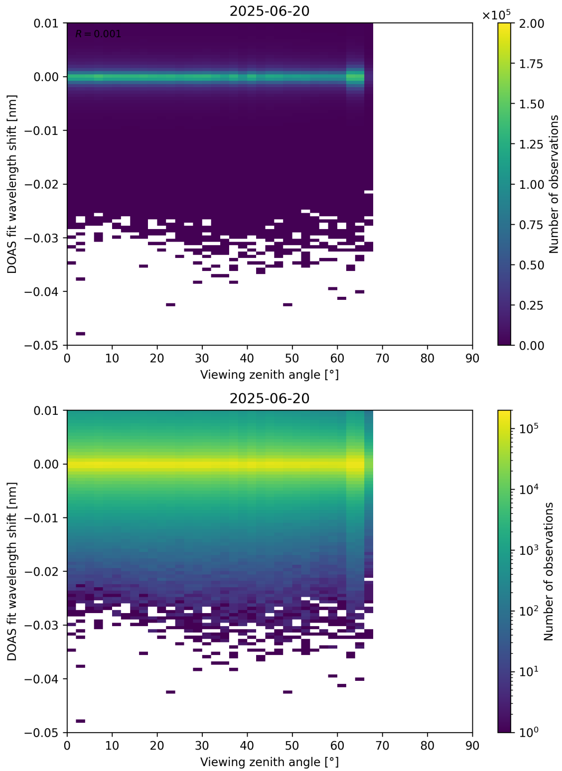
Figure 365: Scatter density plot of “Viewing zenith angle” against “DOAS fit wavelength shift” for 2025-06-19 to 2025-06-21.
