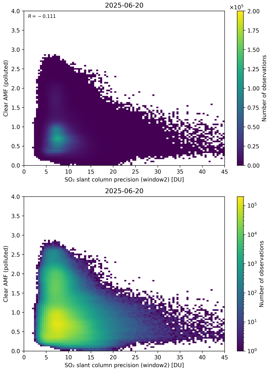
Figure 296: Scatter density plot of “SO 2 slant column precision (window2)” against “Clear AMF (polluted)” for 2025-06-19 to 2025-06-21.
