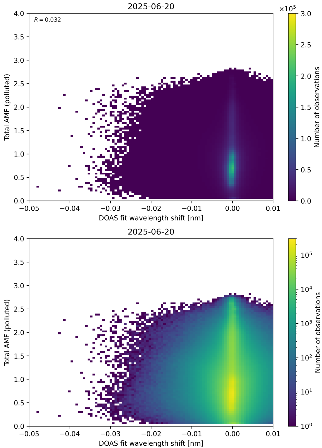
Figure 141: Scatter density plot of “DOAS fit wavelength shift” against “Total AMF (polluted)” for 2025-06-19 to 2025-06-21.
