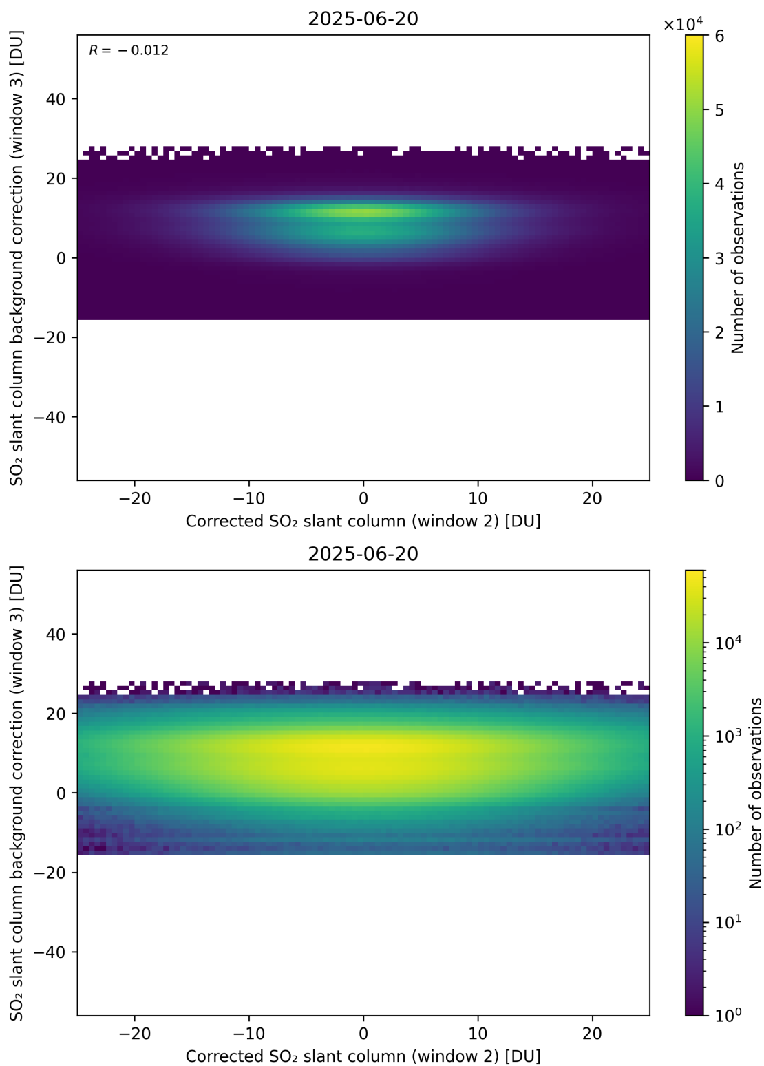
Figure 245: Scatter density plot of “Corrected SO 2 slant column (window 2)” against “SO 2 slant column background correction (window 3)” for 2025-06-19 to 2025-06-21.
