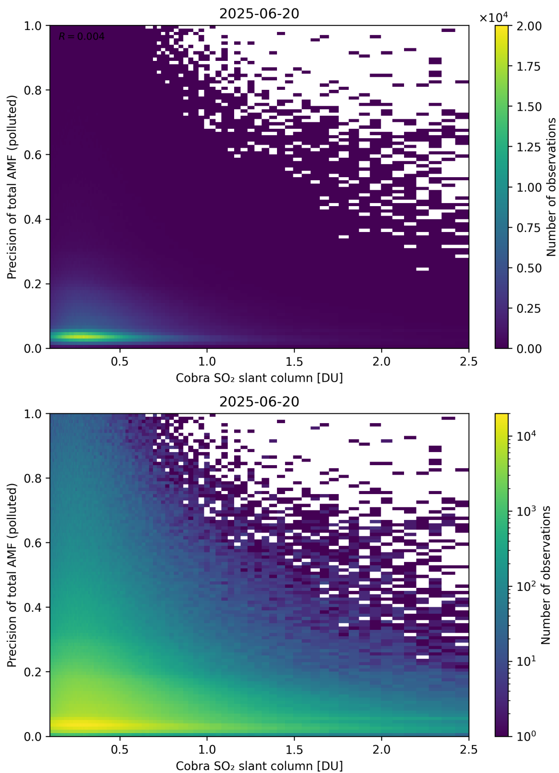
Figure 225: Scatter density plot of “Cobra SO 2 slant column” against “Precision of total AMF (polluted)” for 2025-06-19 to 2025-06-21.
