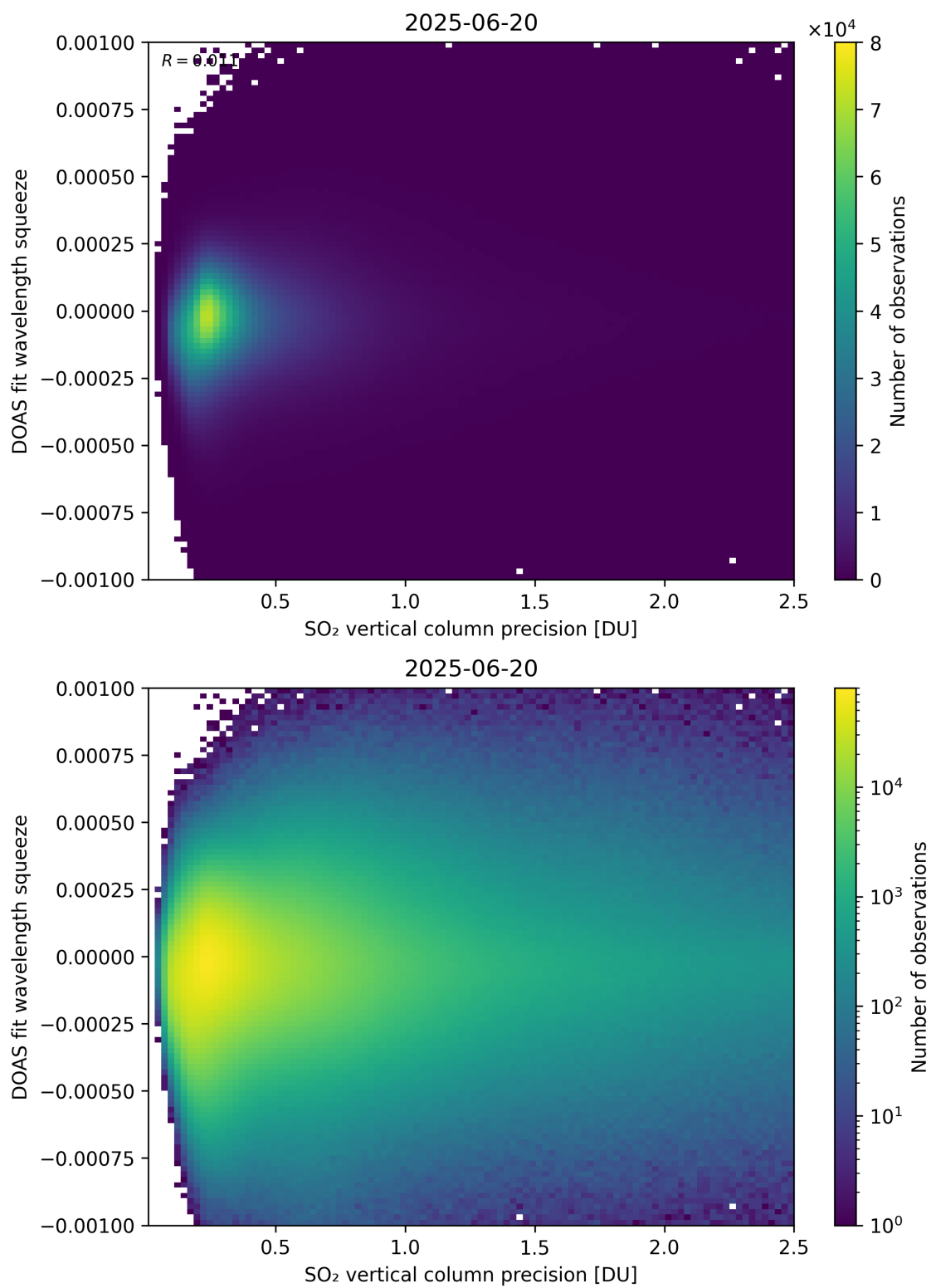
Figure 333: Scatter density plot of “SO 2 vertical column precision” against “DOAS fit wavelength squeeze” for 2025-06-19 to 2025-06-21.
