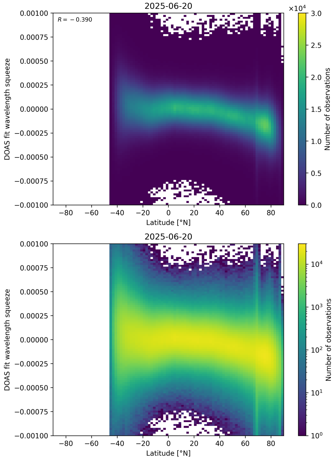
Figure 154: Scatter density plot of “Latitude” against “DOAS fit wavelength squeeze” for 2025-06-19 to 2025-06-21.
