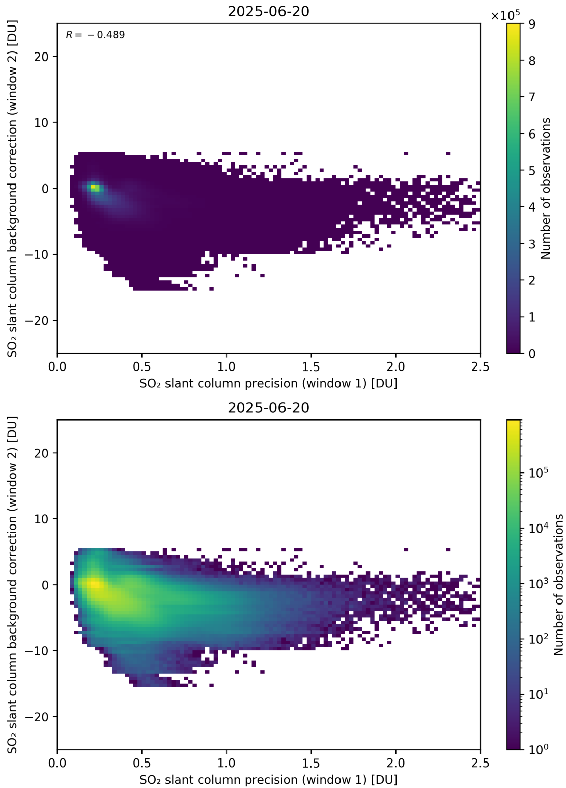
Figure 269: Scatter density plot of “SO 2 slant column precision (window 1)” against “SO 2 slant column background correction (window 2)” for 2025-06-19 to 2025-06-21.
