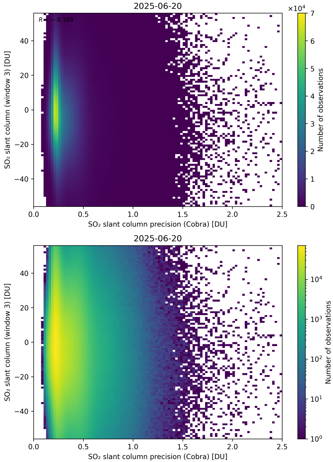
Figure 211: Scatter density plot of “SO 2 slant column precision (Cobra)” against “SO 2 slant column (window 3)” for 2025-06-19 to 2025-06-21.
