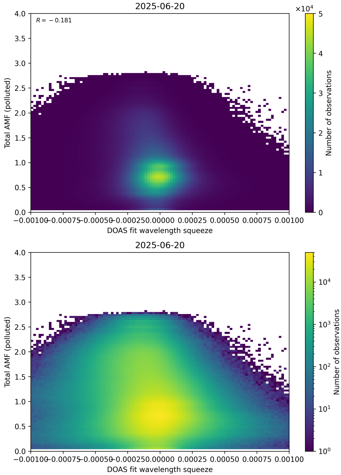
Figure 145: Scatter density plot of “DOAS fit wavelength squeeze” against “Total AMF (polluted)” for 2025-06-19 to 2025-06-21.
