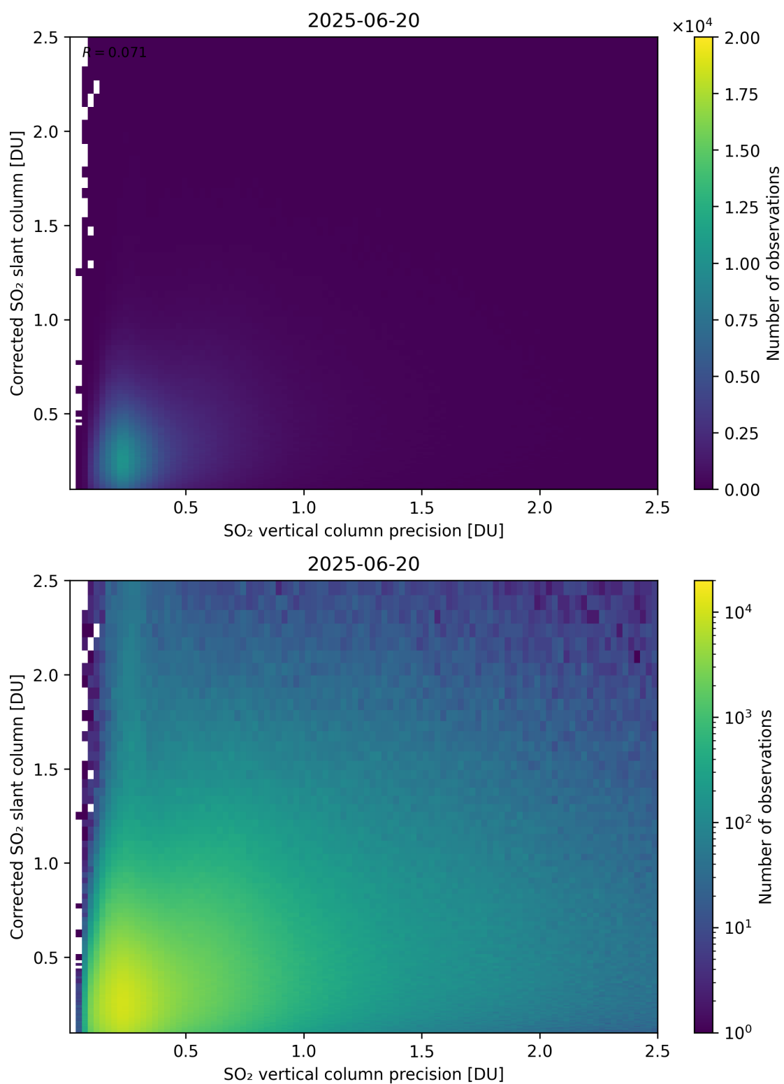
Figure 338: Scatter density plot of “SO 2 vertical column precision” against “Corrected SO 2 slant column” for 2025-06-19 to 2025-06-21.
