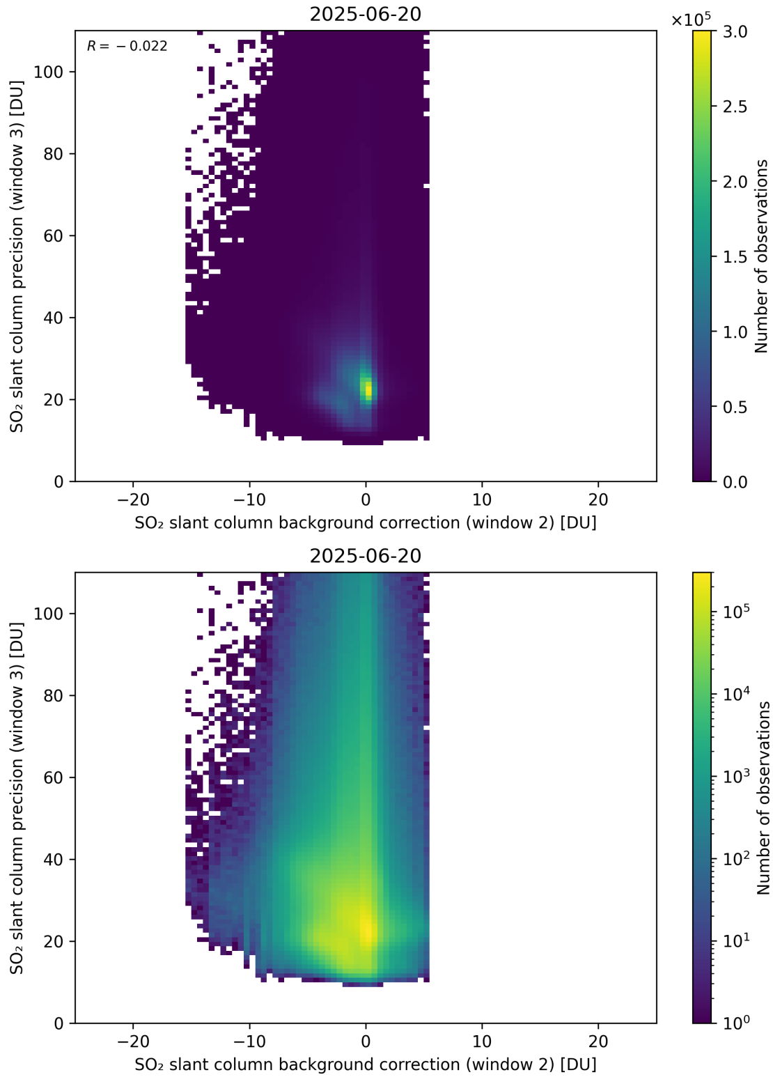
Figure 129: Scatter density plot of “SO 2 slant column background correction (window 2)” against “SO 2 slant column precision (window 3)” for 2025-06-19 to 2025-06-21.
