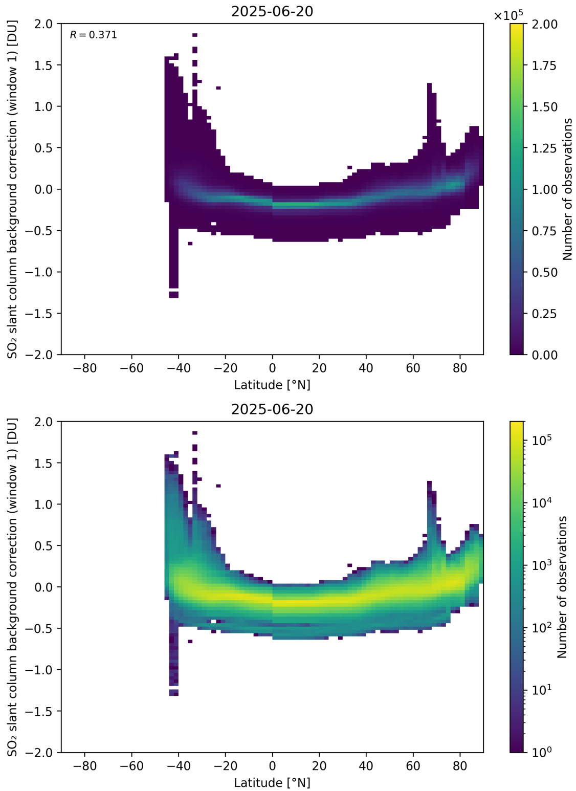
Figure 150: Scatter density plot of “Latitude” against “SO 2 slant column background correction (window 1)” for 2025-06-19 to 2025-06-21.
