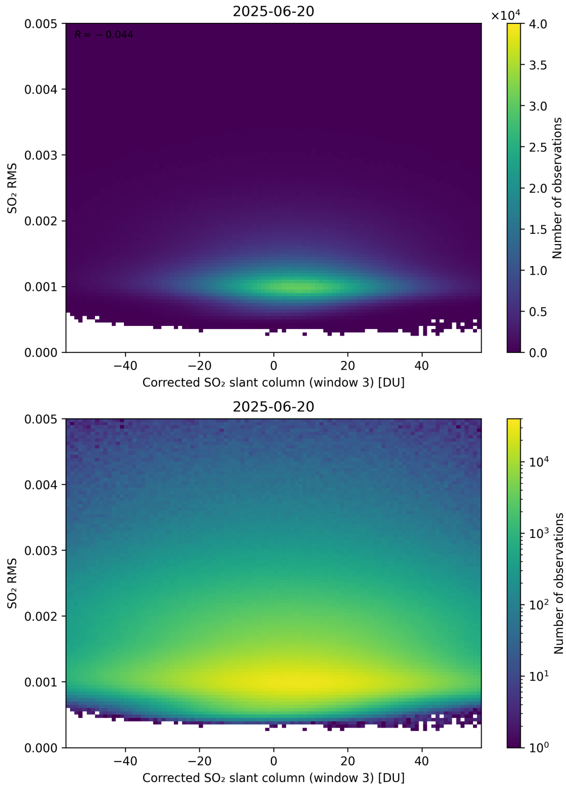
Figure 258: Scatter density plot of “Corrected SO 2 slant column (window 3)” against “SO 2 RMS” for 2025-06-19 to 2025-06-21.
