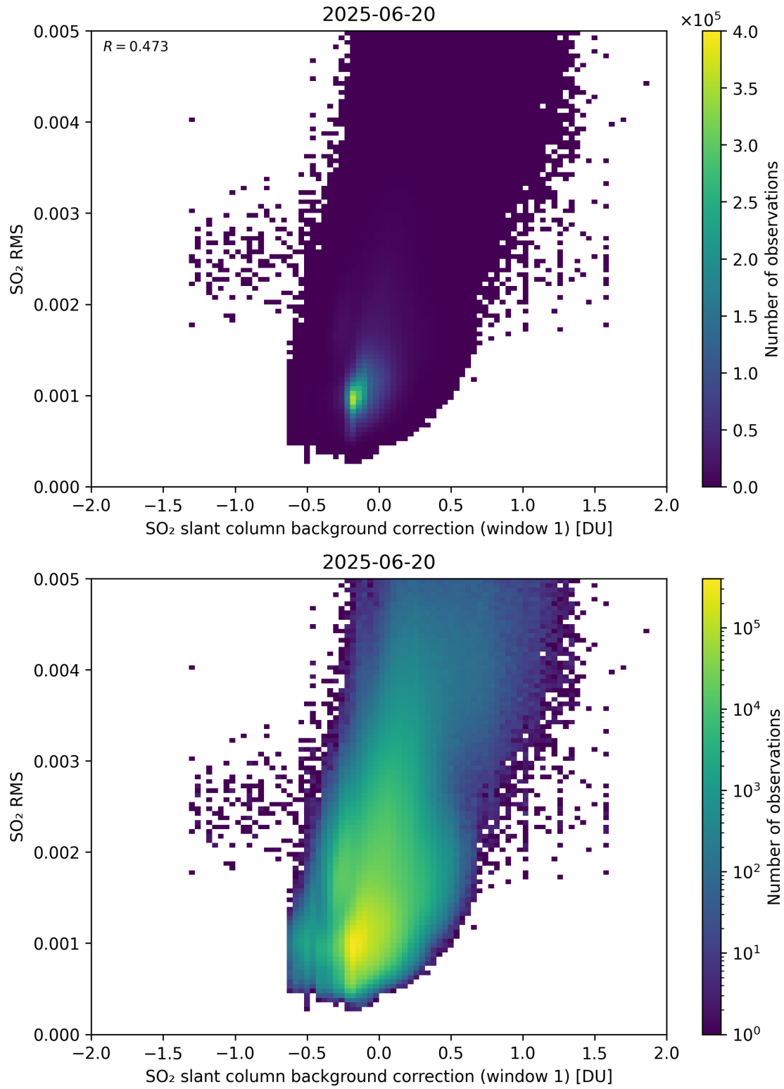
Figure 113: Scatter density plot of “SO 2 slant column background correction (window 1)” against “SO 2 RMS” for 2025-06-19 to 2025-06-21.
