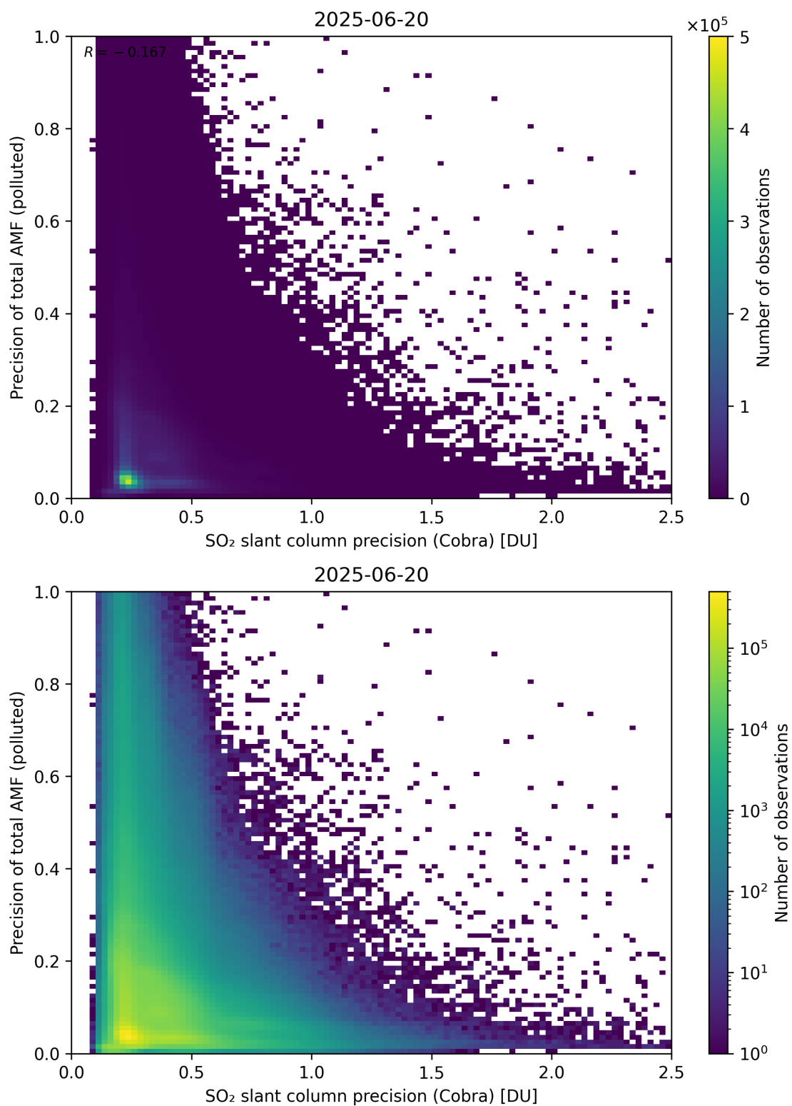
Figure 214: Scatter density plot of “SO 2 slant column precision (Cobra)” against “Precision of total AMF (polluted)” for 2025-06-19 to 2025-06-21.
