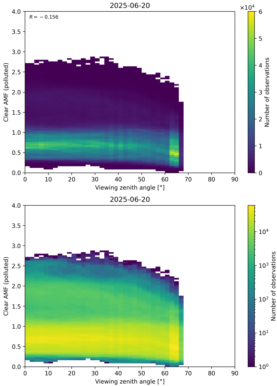
Figure 370: Scatter density plot of “Viewing zenith angle” against “Clear AMF (polluted)” for 2025-06-19 to 2025-06-21.
