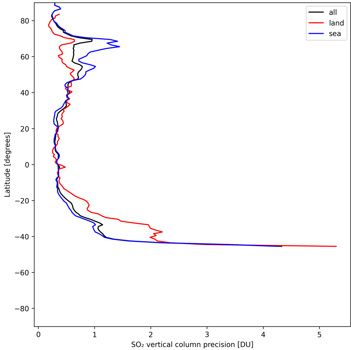
Figure 33: Zonal average of “SO 2 vertical column precision” for 2025-06-19 to 2025-06-21.
