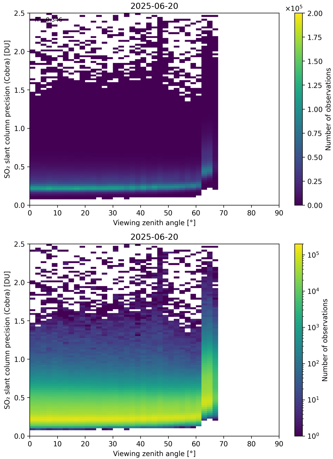
Figure 372: Scatter density plot of “Viewing zenith angle” against “SO 2 slant column precision (Cobra)” for 2025-06-19 to 2025-06-21.
