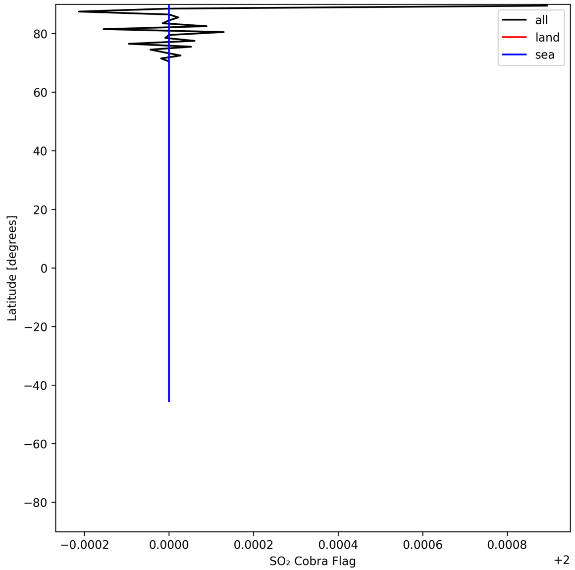
Figure 49: Zonal average of "SO 2 Cobra Flag" for 2025-06-19 to 2025-06-21.
