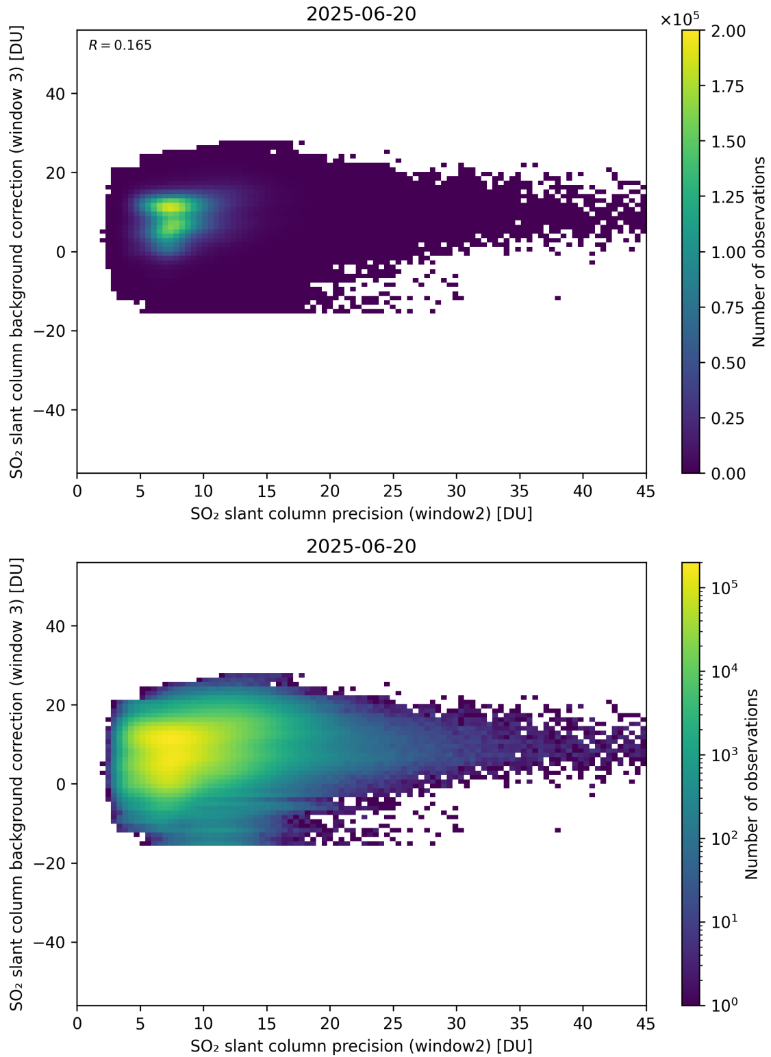
Figure 292: Scatter density plot of “SO 2 slant column precision (window2)” against “SO 2 slant column background correction (window 3)” for 2025-06-19 to 2025-06-21.
