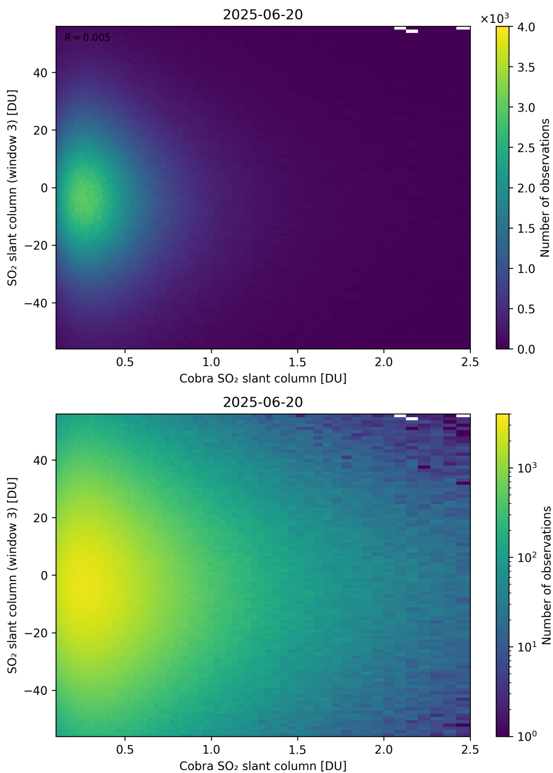
Figure 222: Scatter density plot of “Cobra SO 2 slant column” against “SO 2 slant column (window 3)” for 2025-06-19 to 2025-06-21.
