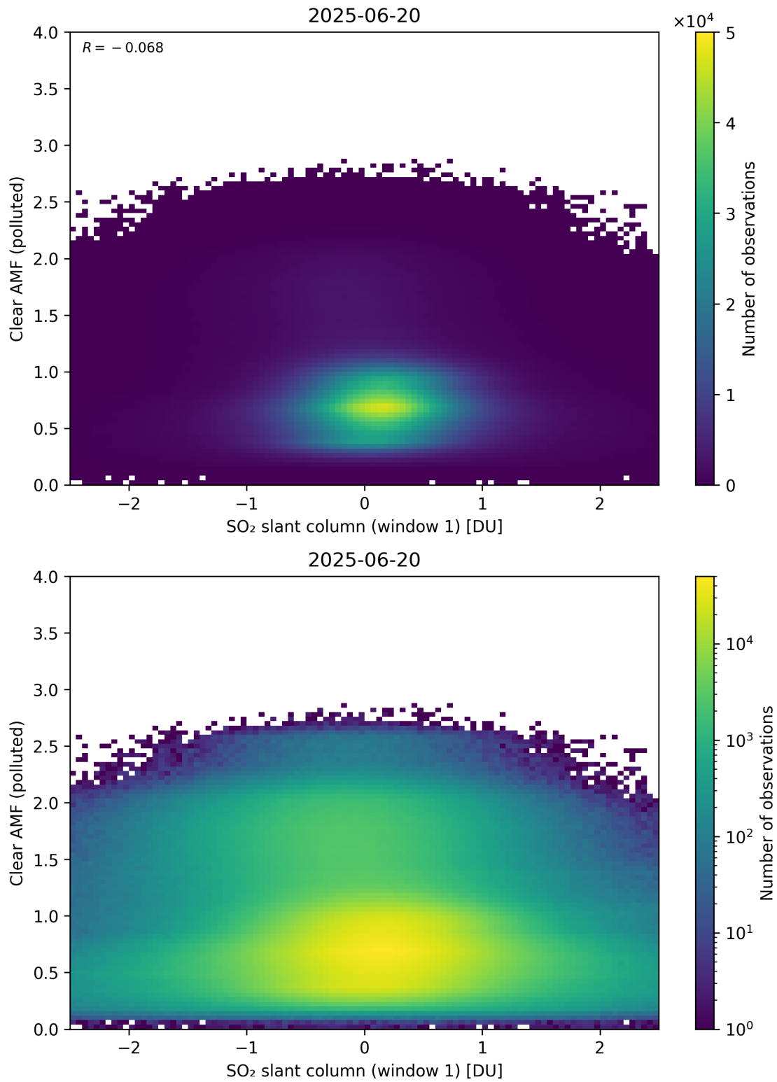
Figure 282: Scatter density plot of “SO 2 slant column (window 1)” against “Clear AMF (polluted)” for 2025-06-19 to 2025-06-21.
