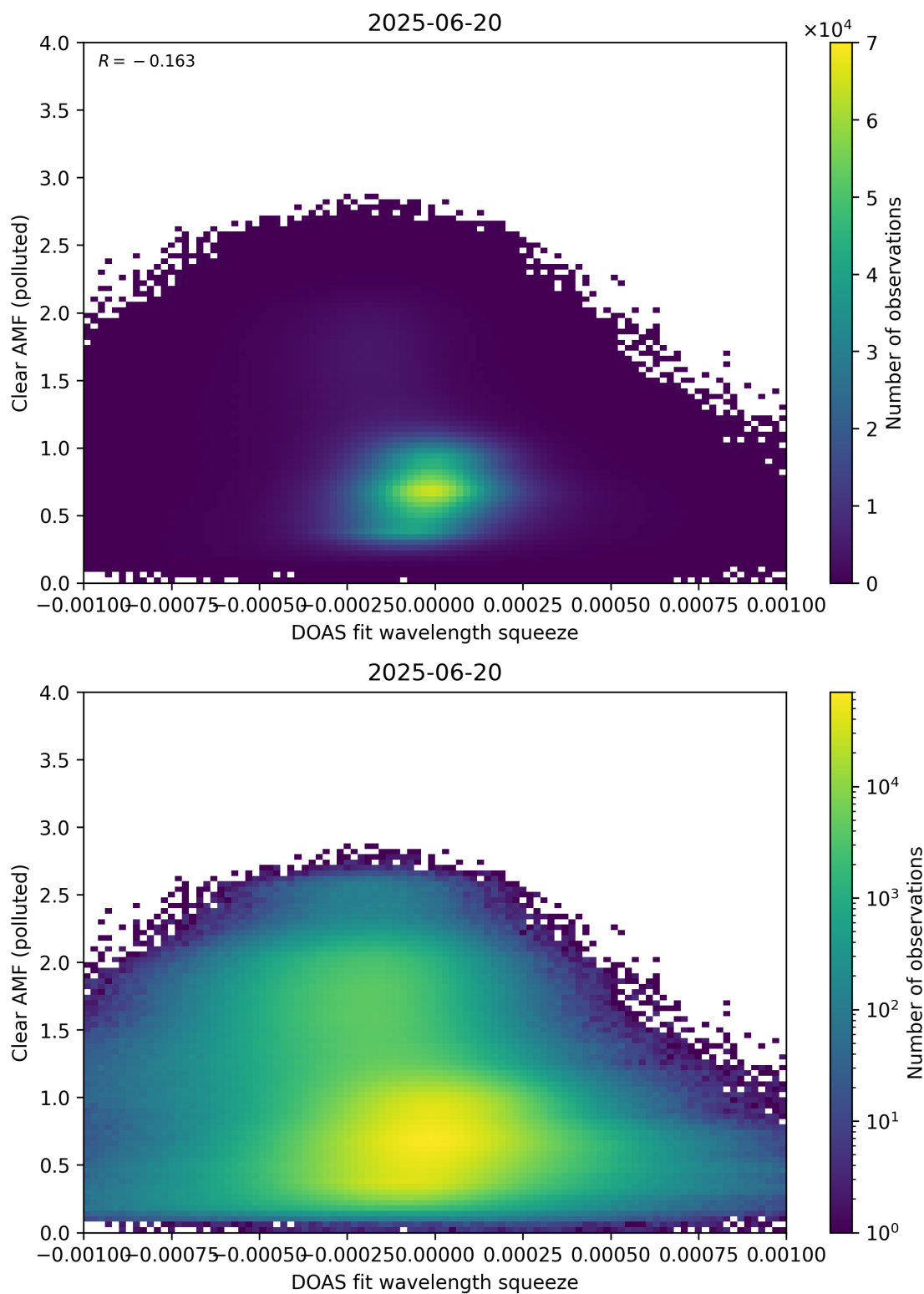
Figure 144: Scatter density plot of “DOAS fit wavelength squeeze” against “Clear AMF (polluted)” for 2025-06-19 to 2025-06-21.
