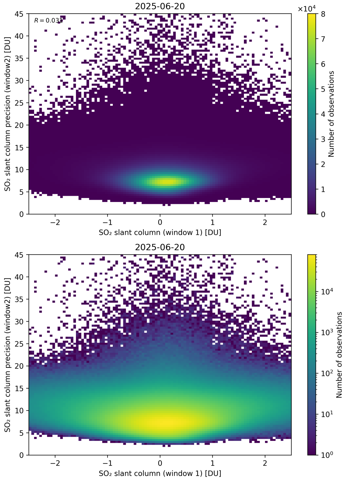
Figure 286: Scatter density plot of “SO 2 slant column (window 1)” against “SO 2 slant column precision (window2)” for 2025-06-19 to 2025-06-21.
