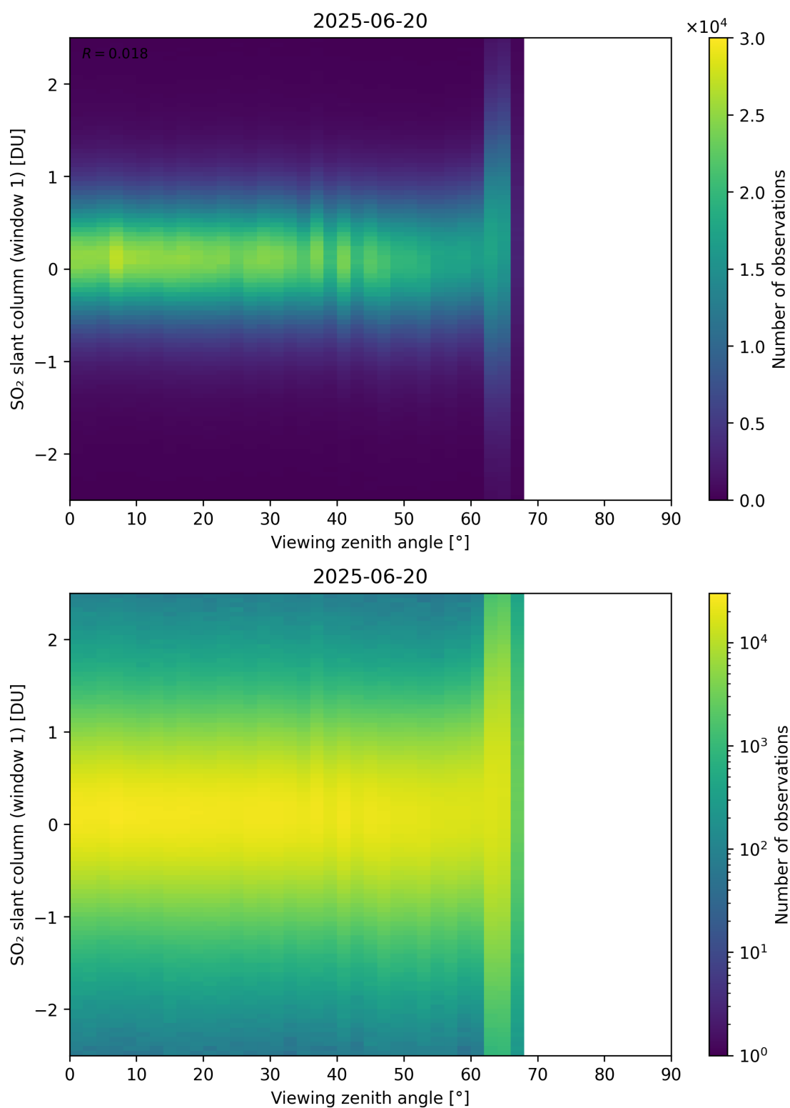
Figure 376: Scatter density plot of “Viewing zenith angle” against “SO 2 slant column (window 1)” for 2025-06-19 to 2025-06-21.
