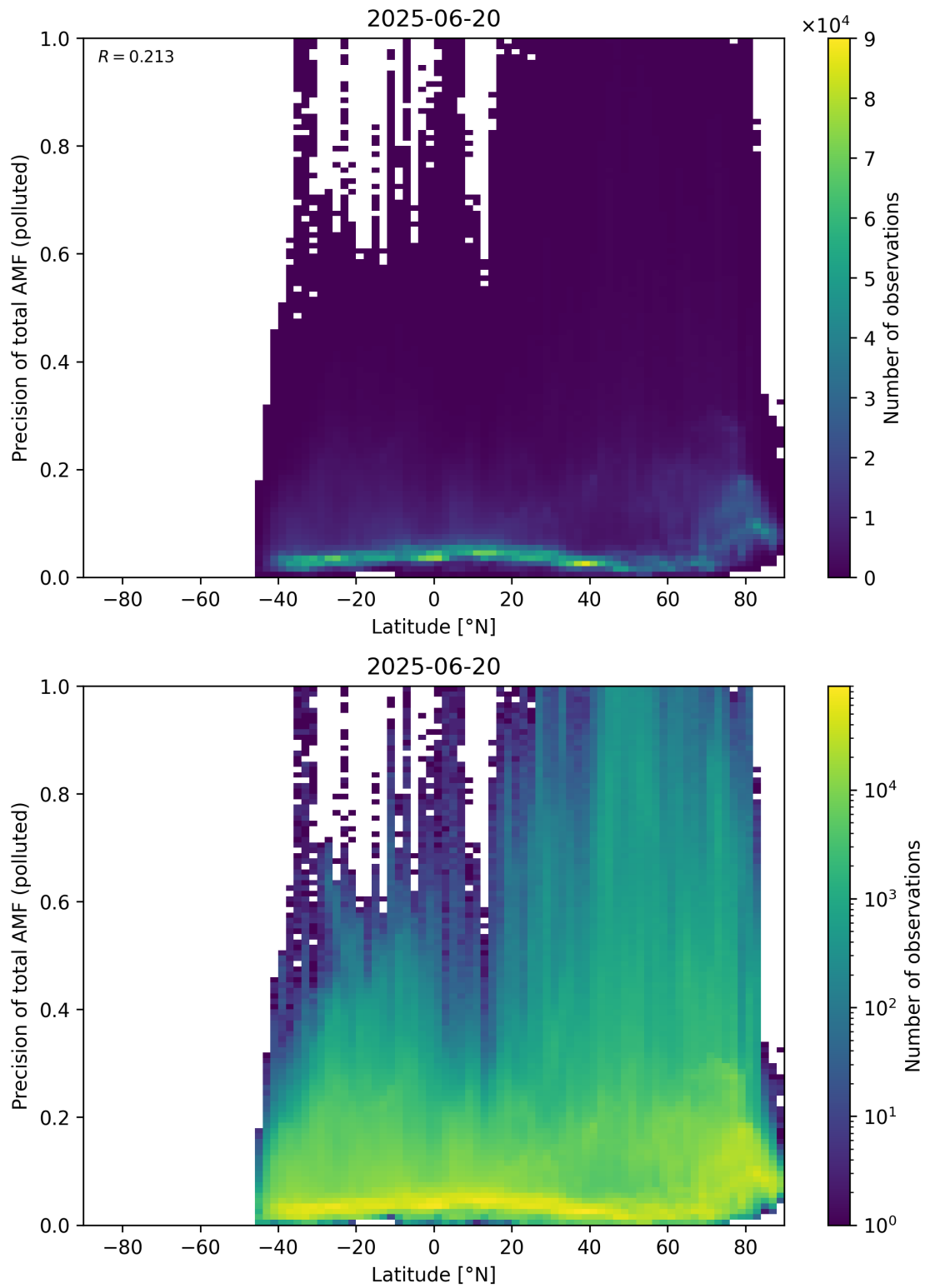
Figure 168: Scatter density plot of “Latitude” against “Precision of total AMF (polluted)” for 2025-06-19 to 2025-06-21.
