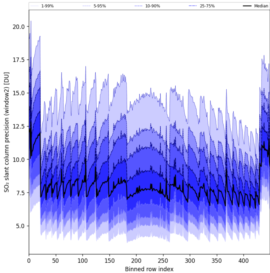
Figure 94: Along track statistics of “SO 2 slant column precision (window2)” for 2025-06-19 to 2025-06-21
