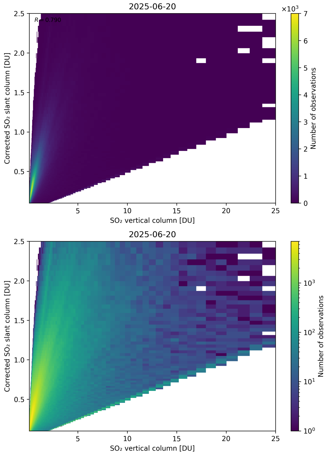
Figure 351: Scatter density plot of “SO 2 vertical column” against “Corrected SO 2 slant column” for 2025-06-19 to 2025-06-21.
