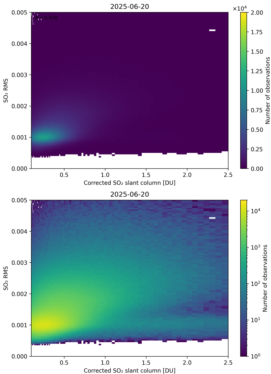
Figure 231: Scatter density plot of “Corrected SO 2 slant column” against “SO 2 RMS” for 2025-06-19 to 2025-06-21.
