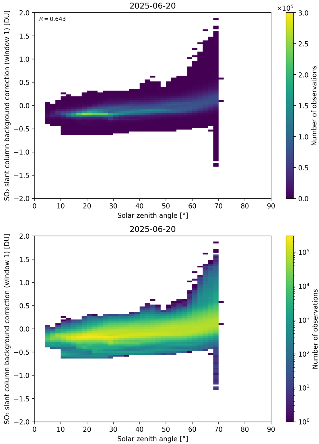
Figure 171: Scatter density plot of “Solar zenith angle” against “SO 2 slant column background correction (window 1)” for 2025-06-19 to 2025-06-21.
