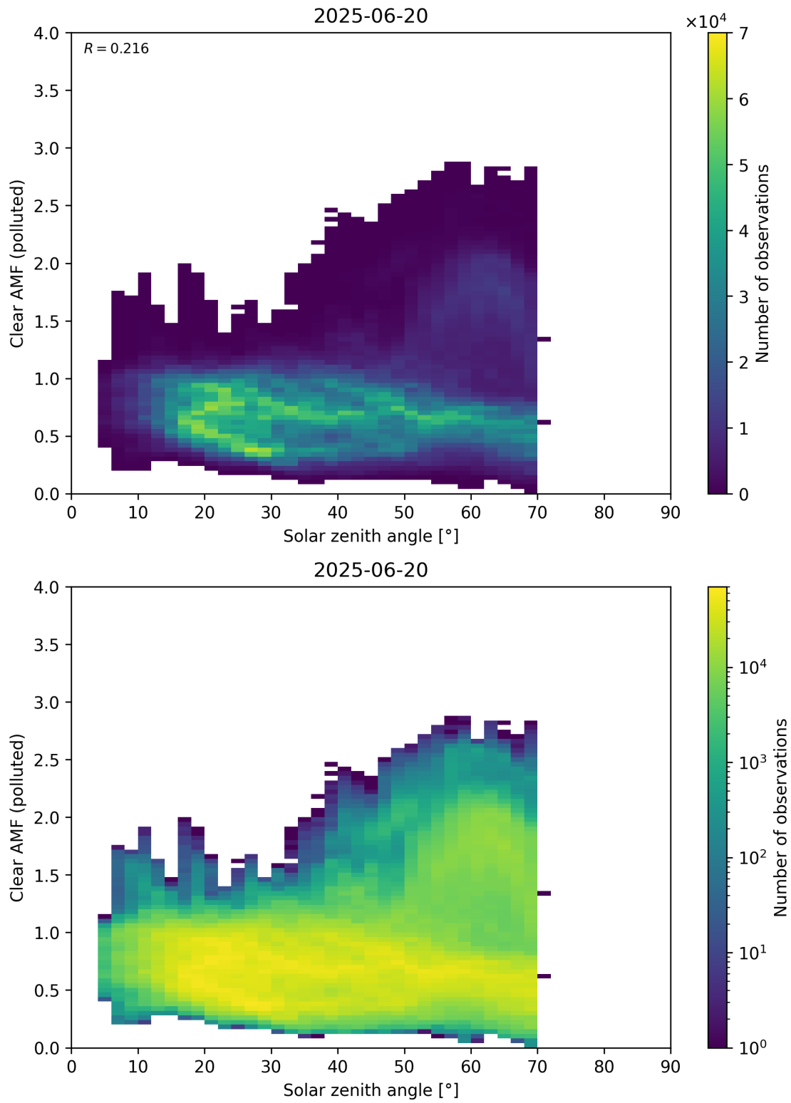
Figure 178: Scatter density plot of “Solar zenith angle” against “Clear AMF (polluted)” for 2025-06-19 to 2025-06-21.
