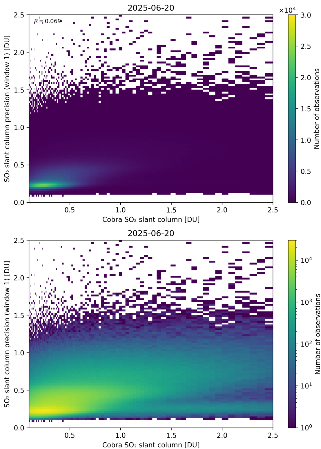
Figure 220: Scatter density plot of “Cobra SO 2 slant column” against “SO 2 slant column precision (window 1)” for 2025-06-19 to 2025-06-21.
