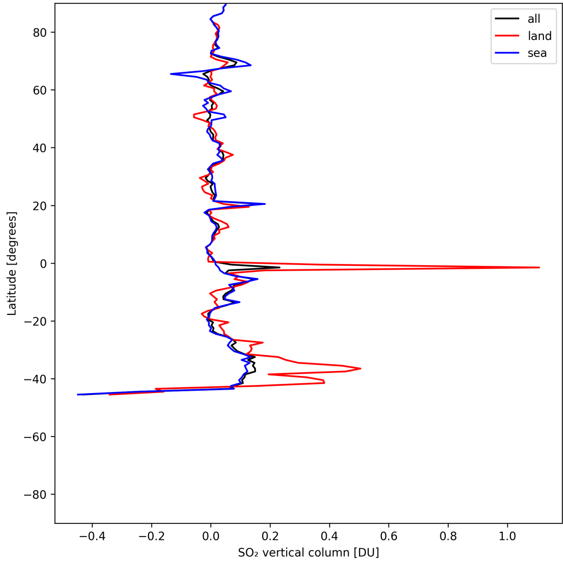
Figure 32: Zonal average of “SO 2 vertical column” for 2025-06-19 to 2025-06-21.
