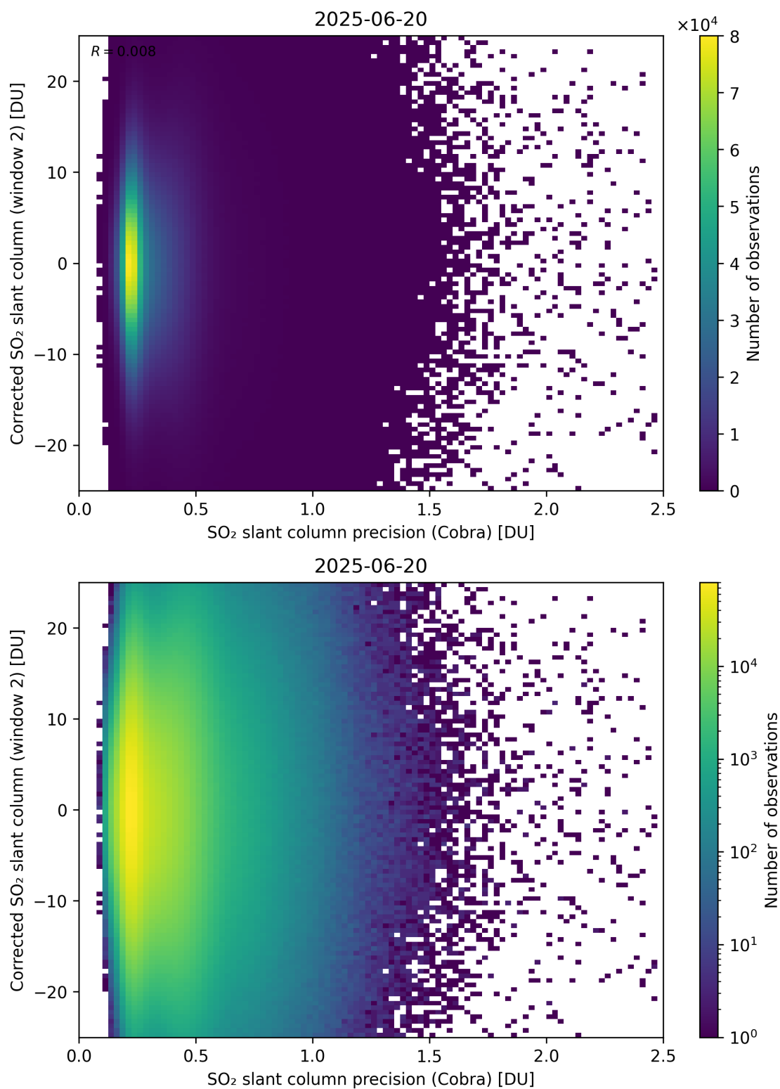
Figure 206: Scatter density plot of “SO 2 slant column precision (Cobra)” against “Corrected SO 2 slant column (window 2)” for 2025-06-19 to 2025-06-21.
