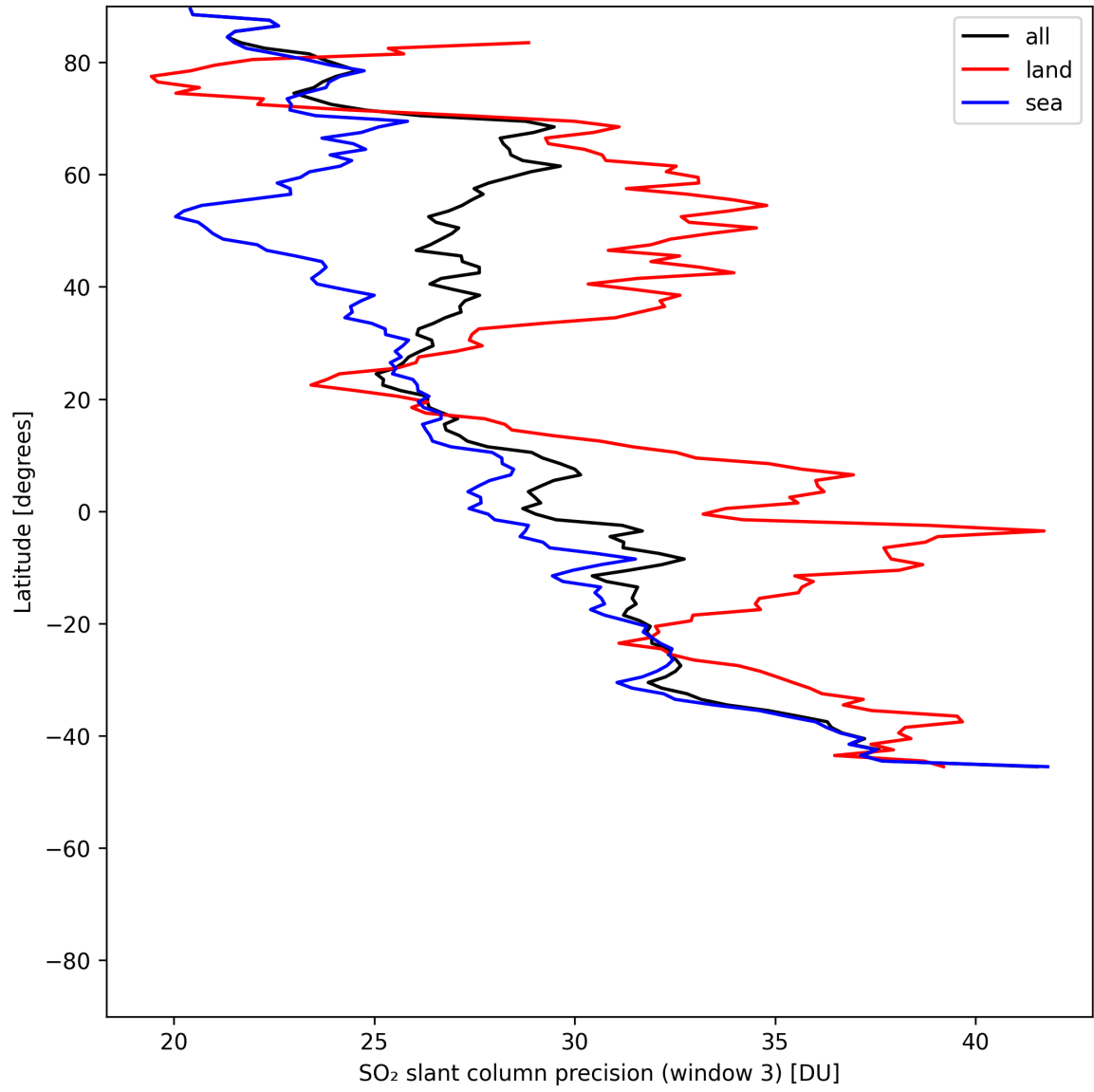
Figure 46: Zonal average of “SO 2 slant column precision (window 3)” for 2025-06-19 to 2025-06-21.
