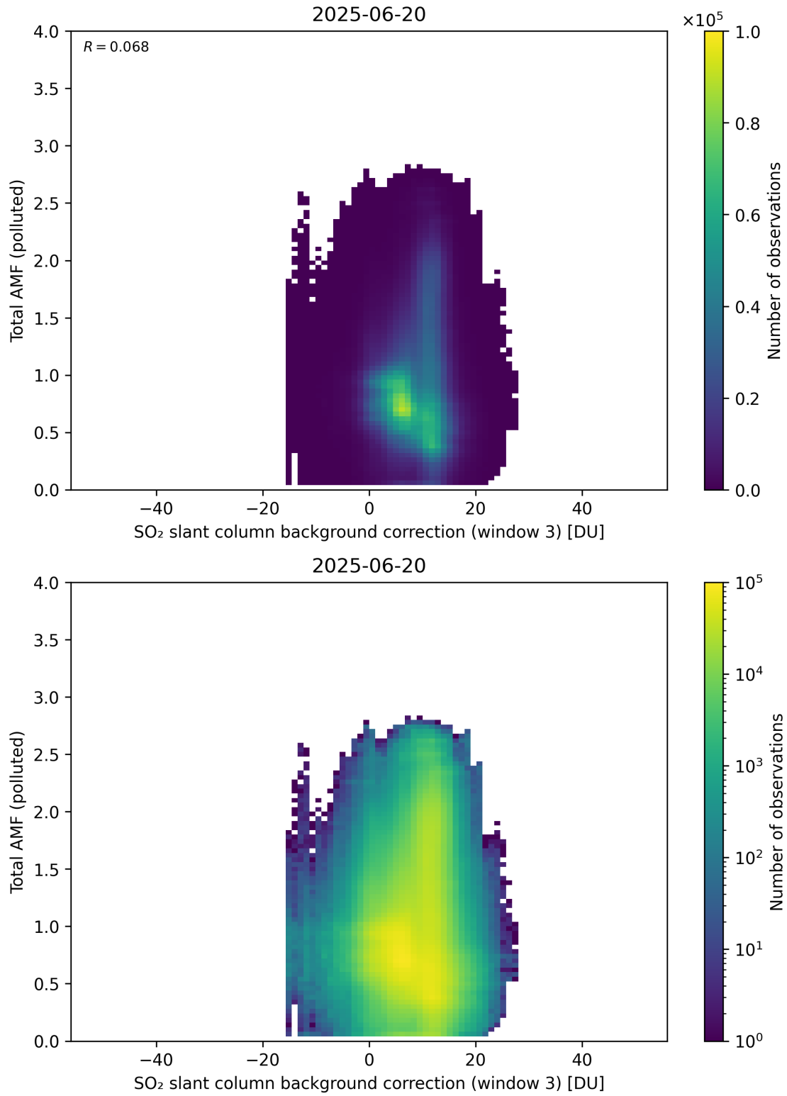
Figure 136: Scatter density plot of “SO 2 slant column background correction (window 3)” against “Total AMF (polluted)” for 2025-06-19 to 2025-06-21.
