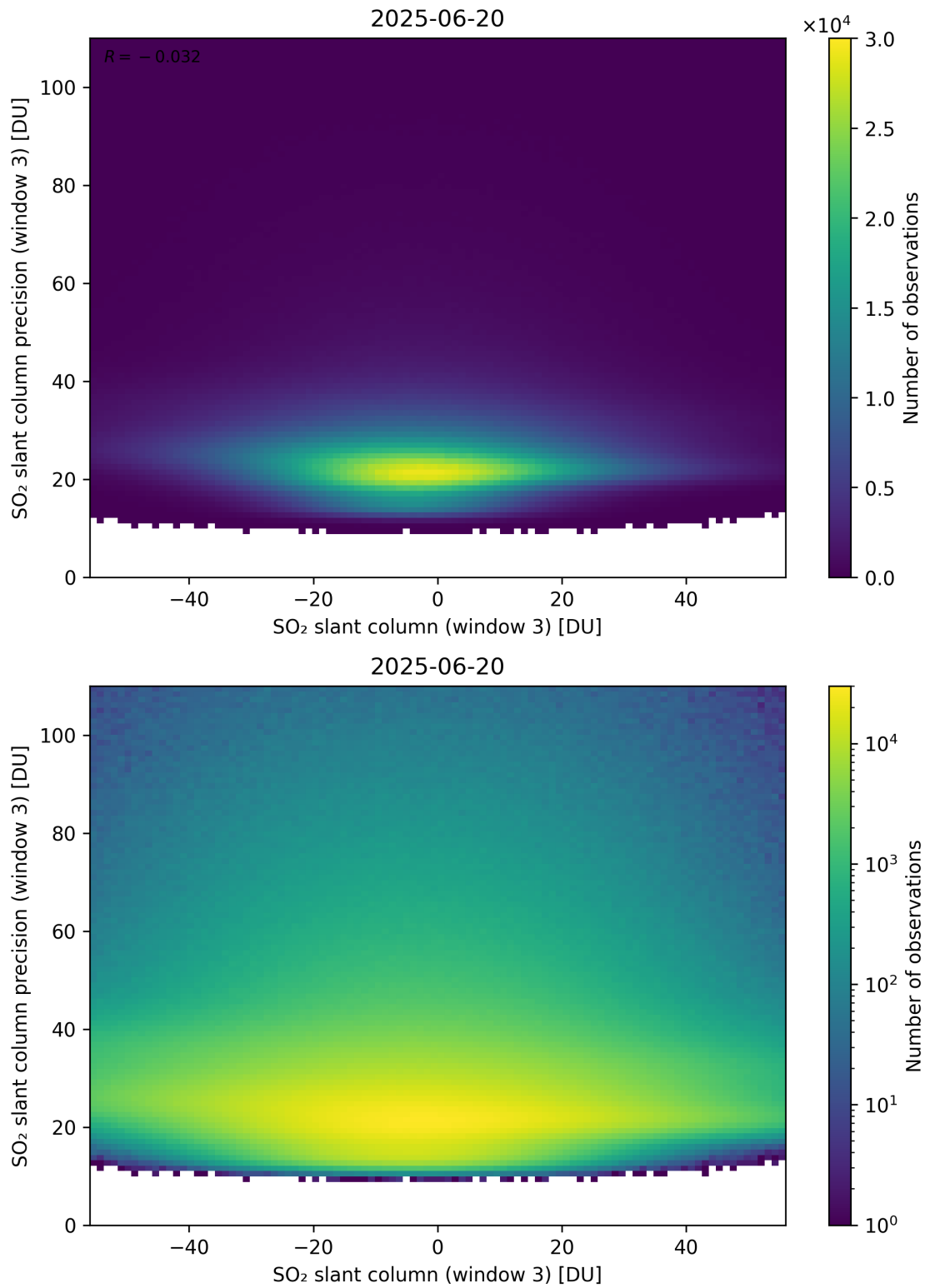
Figure 317: Scatter density plot of “SO 2 slant column (window 3)” against “SO 2 slant column precision (window 3)” for 2025-06-19 to 2025-06-21.
