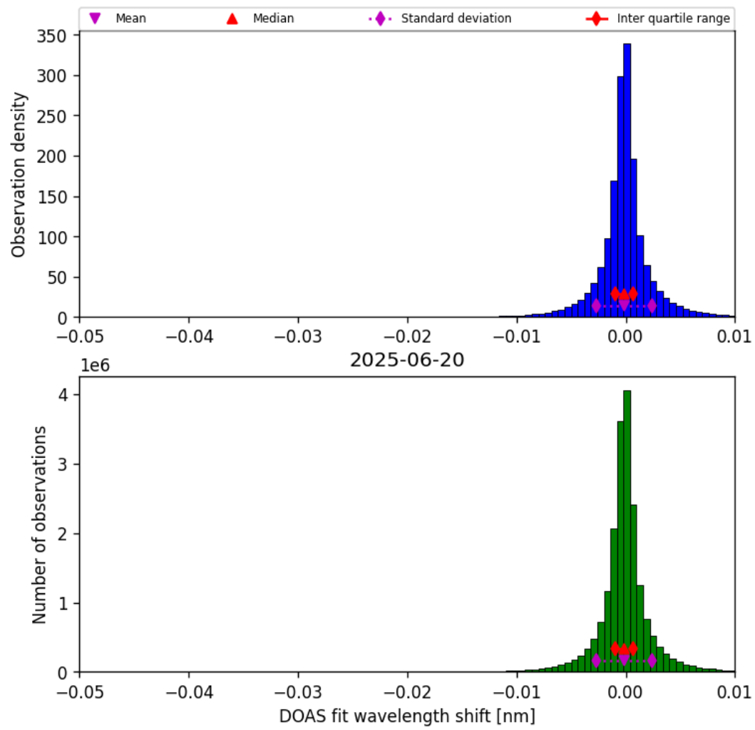
Figure 76: Histogram of “DOAS fit wavelength shift” for 2025-06-19 to 2025-06-21
