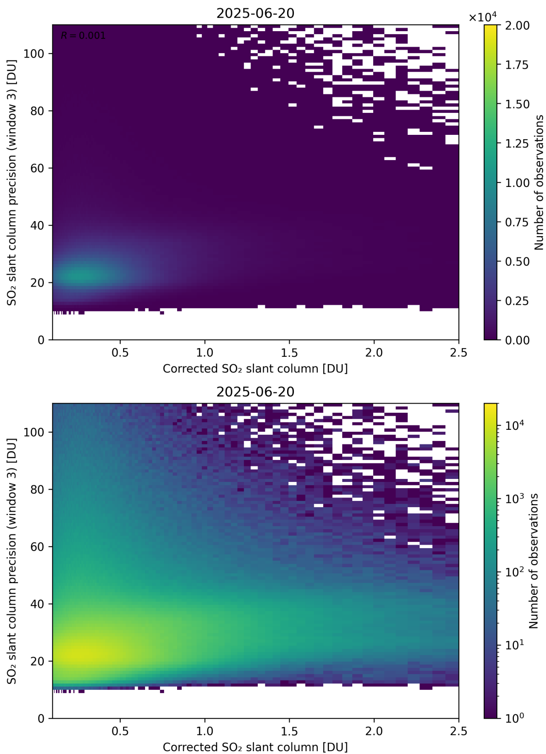
Figure 241: Scatter density plot of “Corrected SO 2 slant column” against “SO 2 slant column precision (window 3)” for 2025-06-19 to 2025-06-21.
