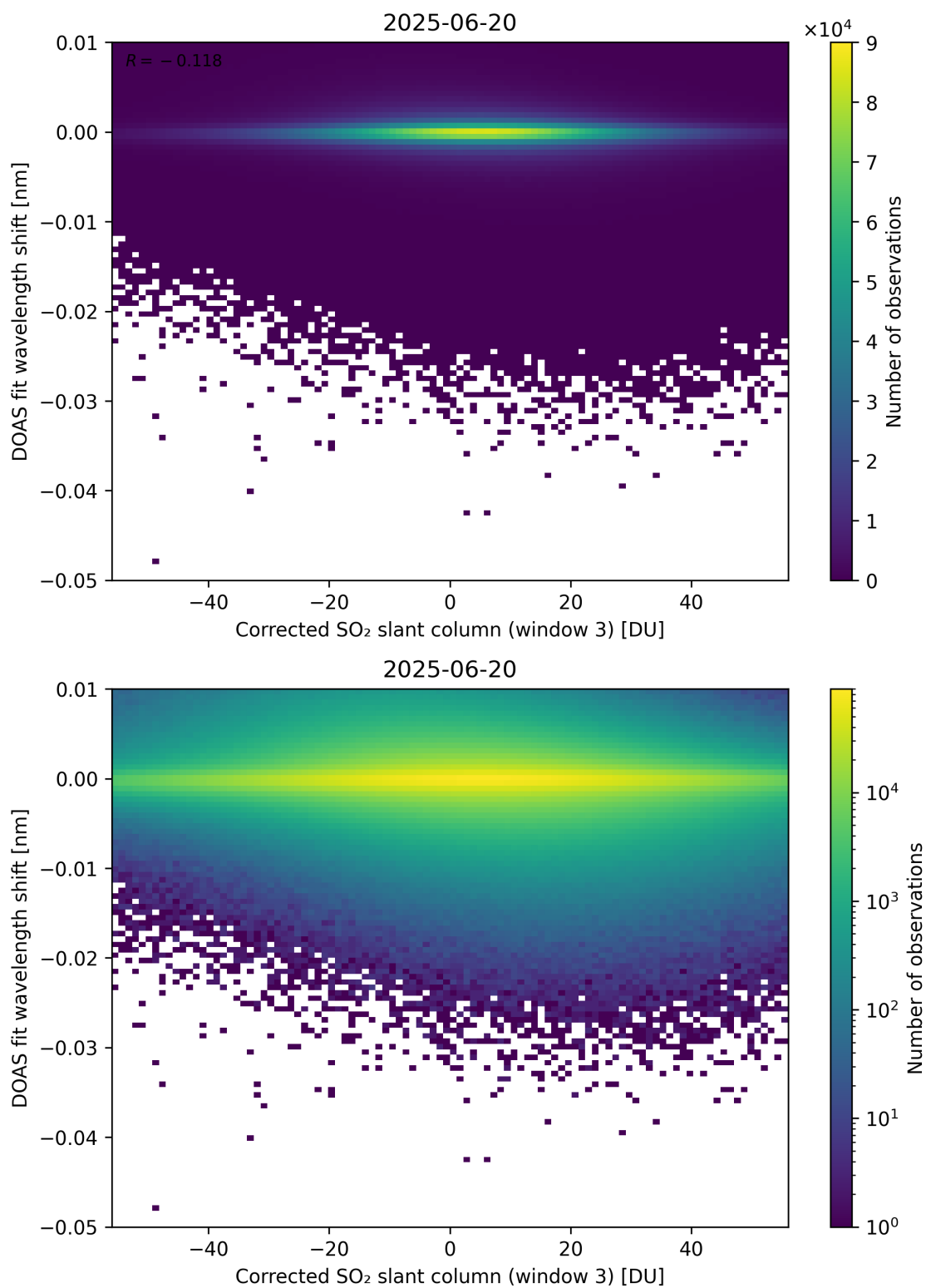
Figure 256: Scatter density plot of “Corrected SO 2 slant column (window 3)” against “DOAS fit wavelength shift” for 2025-06-19 to 2025-06-21.
