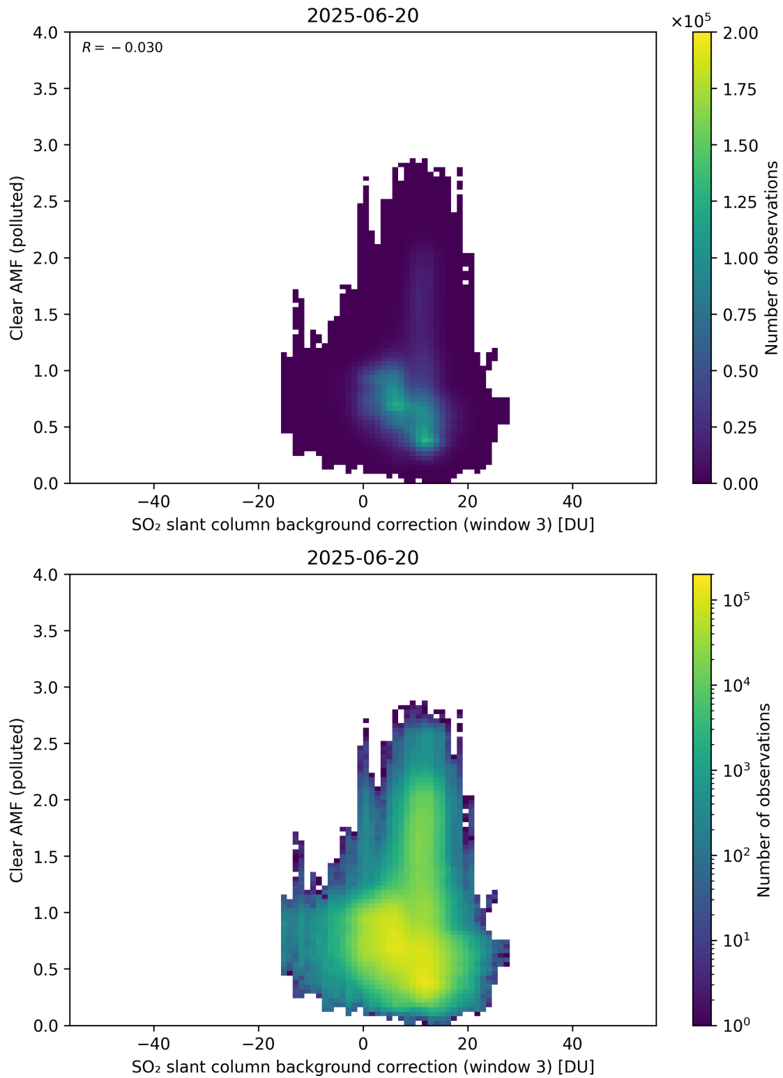
Figure 135: Scatter density plot of “SO 2 slant column background correction (window 3)” against “Clear AMF (polluted)” for 2025-06-19 to 2025-06-21.
