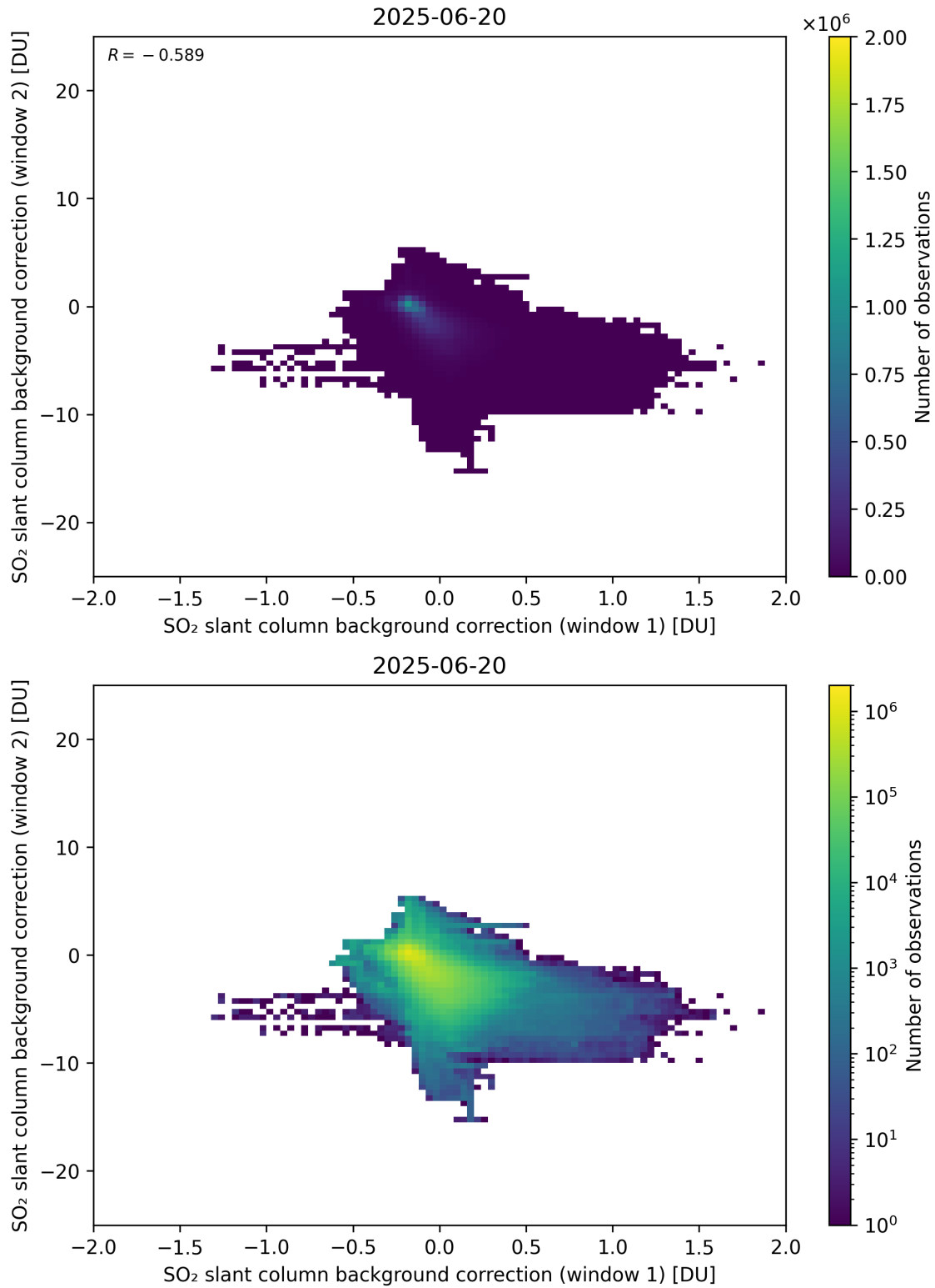
Figure 109: Scatter density plot of “SO 2 slant column background correction (window 1)” against “SO 2 slant column background correction (window 2)” for 2025-06-19 to 2025-06-21.
