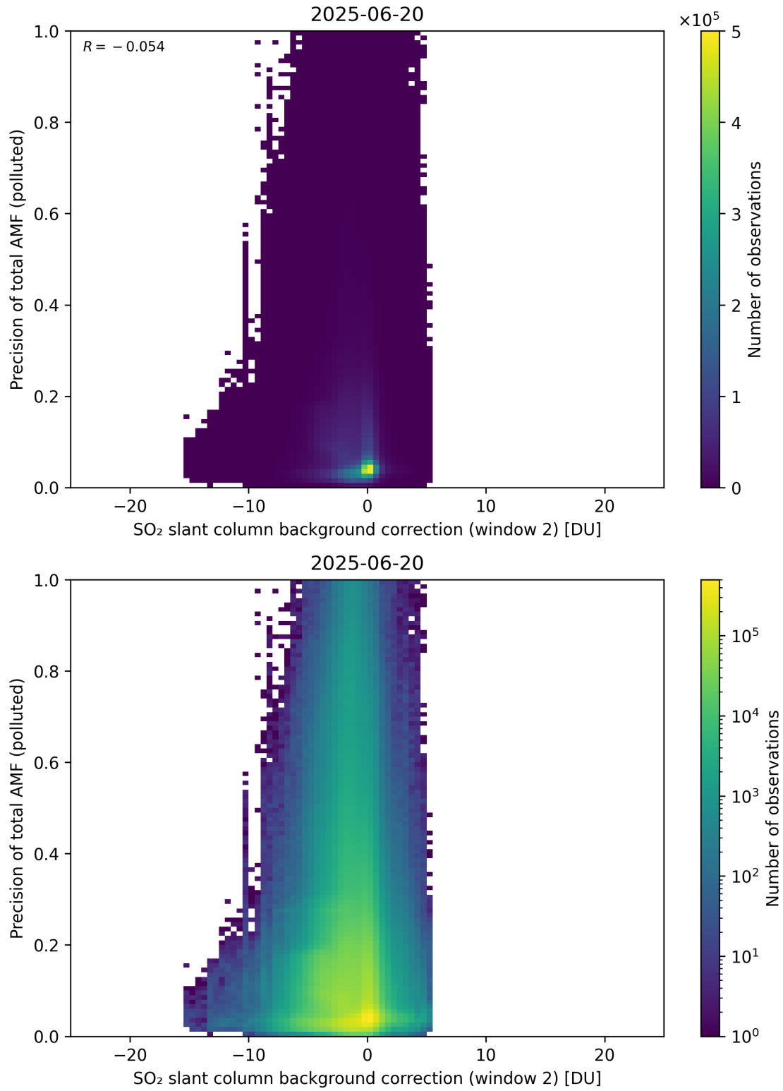
Figure 131: Scatter density plot of “SO 2 slant column background correction (window 2)” against “Precision of total AMF (polluted)” for 2025-06-19 to 2025-06-21.
