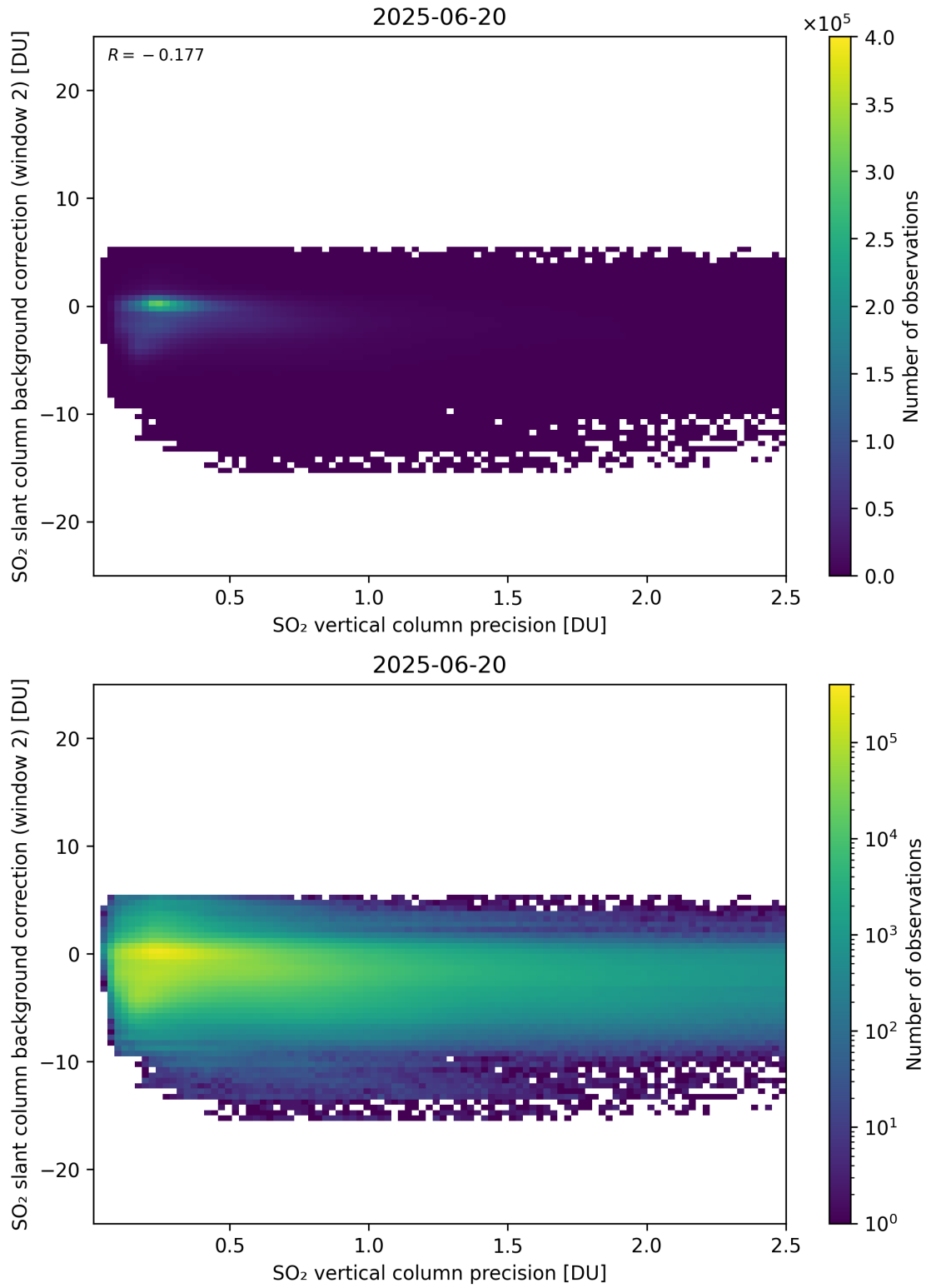
Figure 330: Scatter density plot of “SO 2 vertical column precision” against “SO 2 slant column background correction (window 2)” for 2025-06-19 to 2025-06-21.
