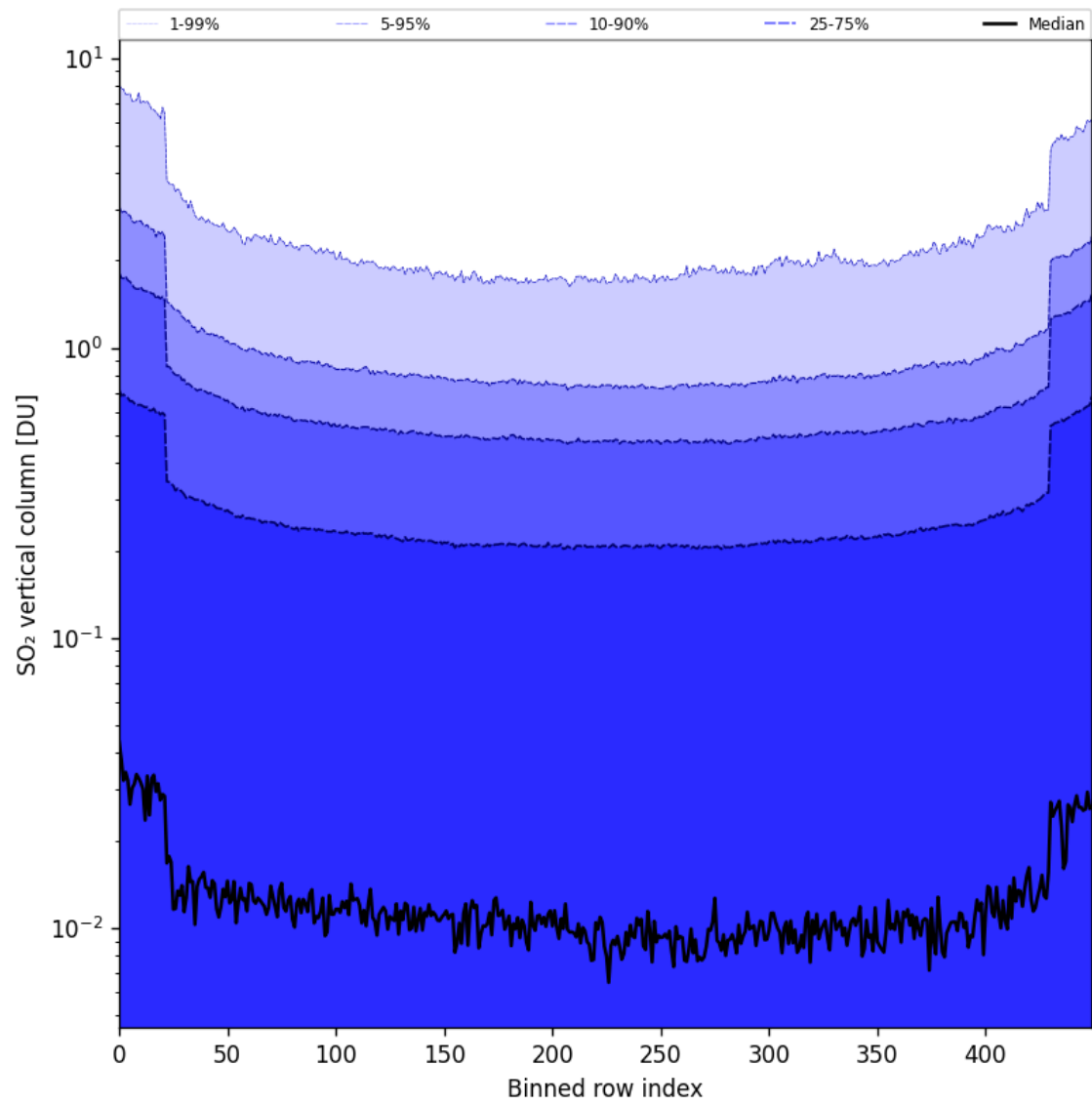
Figure 84: Along track statistics of “SO 2 vertical column” for 2025-06-19 to 2025-06-21
