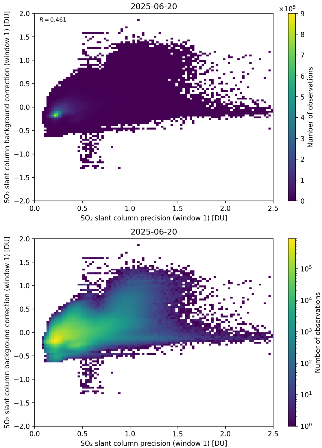
Figure 268: Scatter density plot of “SO 2 slant column precision (window 1)” against “SO 2 slant column background correction (window 1)” for 2025-06-19 to 2025-06-21.
