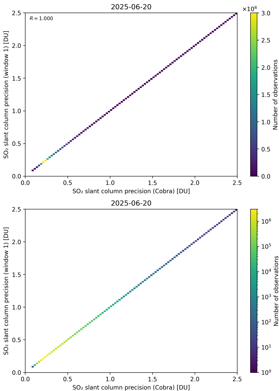
Figure 209: Scatter density plot of “SO 2 slant column precision (Cobra)” against “SO 2 slant column precision (window 1)” for 2025-06-19 to 2025-06-21.
