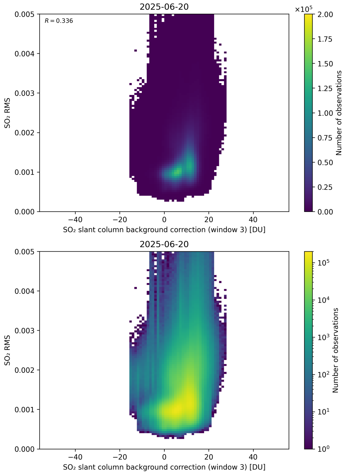
Figure 134: Scatter density plot of “SO 2 slant column background correction (window 3)” against “SO 2 RMS” for 2025-06-19 to 2025-06-21.
