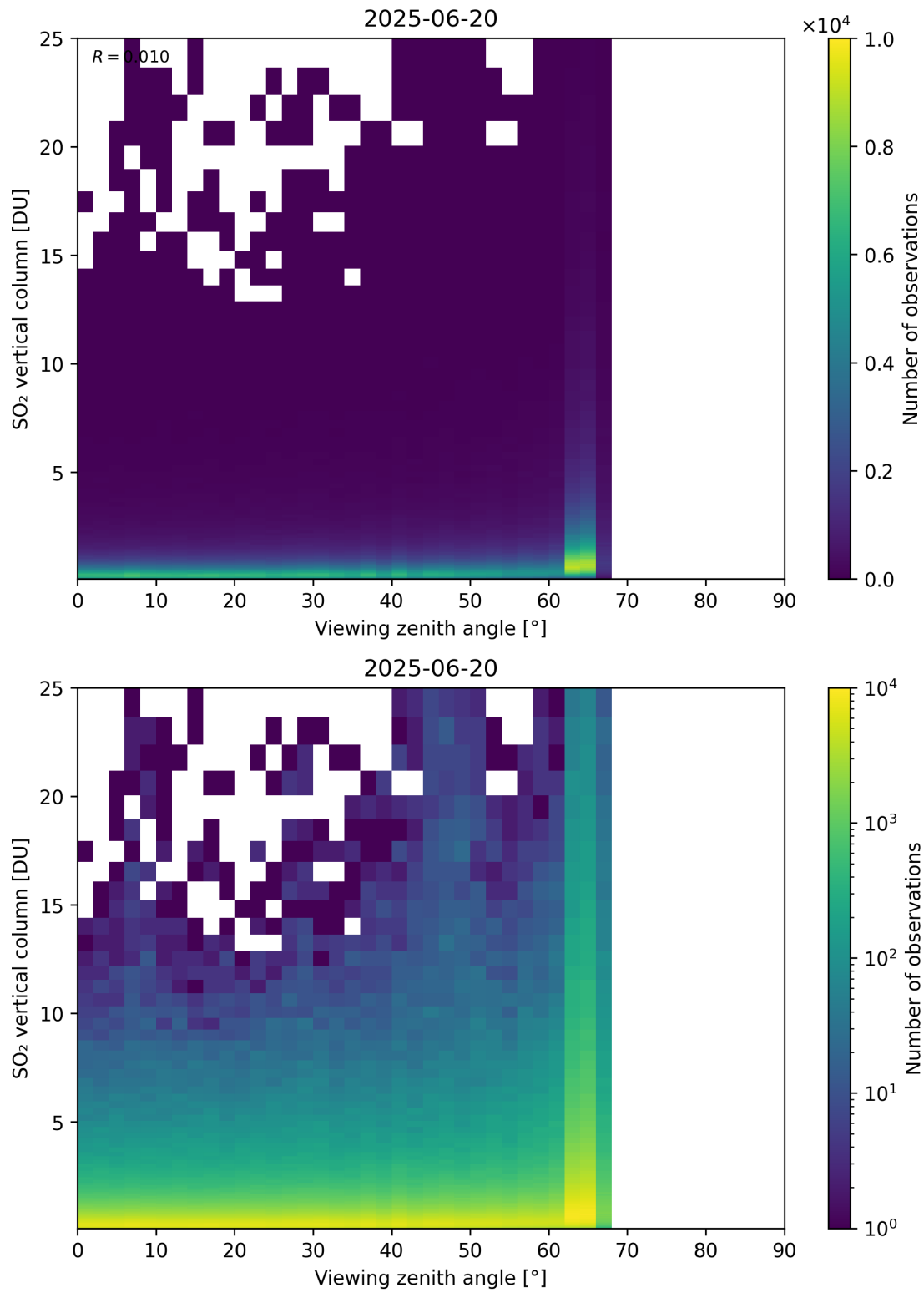
Figure 383: Scatter density plot of “Viewing zenith angle” against “SO 2 vertical column” for 2025-06-19 to 2025-06-21.
