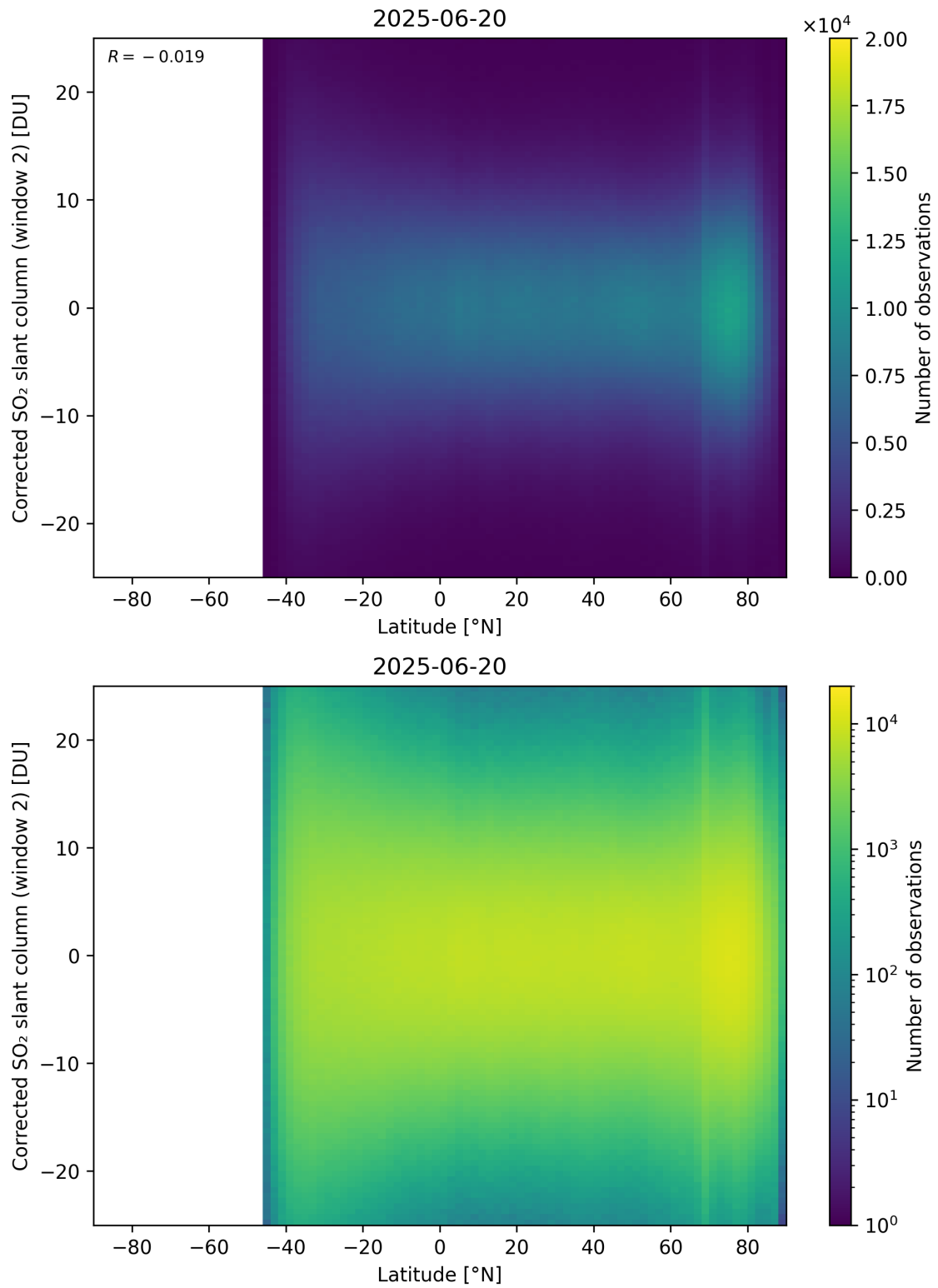
Figure 160: Scatter density plot of “Latitude” against “Corrected SO 2 slant column (window 2)” for 2025-06-19 to 2025-06-21.
