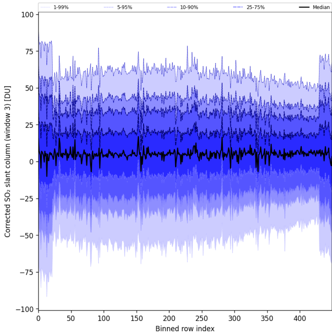
Figure 99: Along track statistics of “Corrected SO 2 slant column (window 3)” for 2025-06-19 to 2025-06-21
