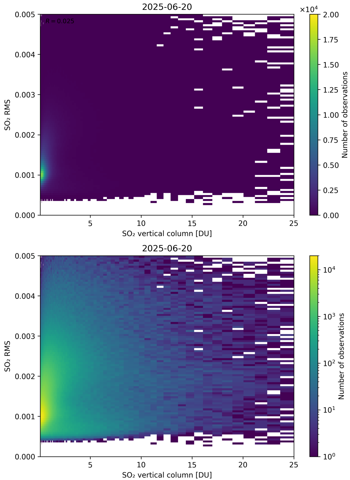
Figure 328: Scatter density plot of “SO 2 vertical column” against “SO 2 RMS” for 2025-06-19 to 2025-06-21.
