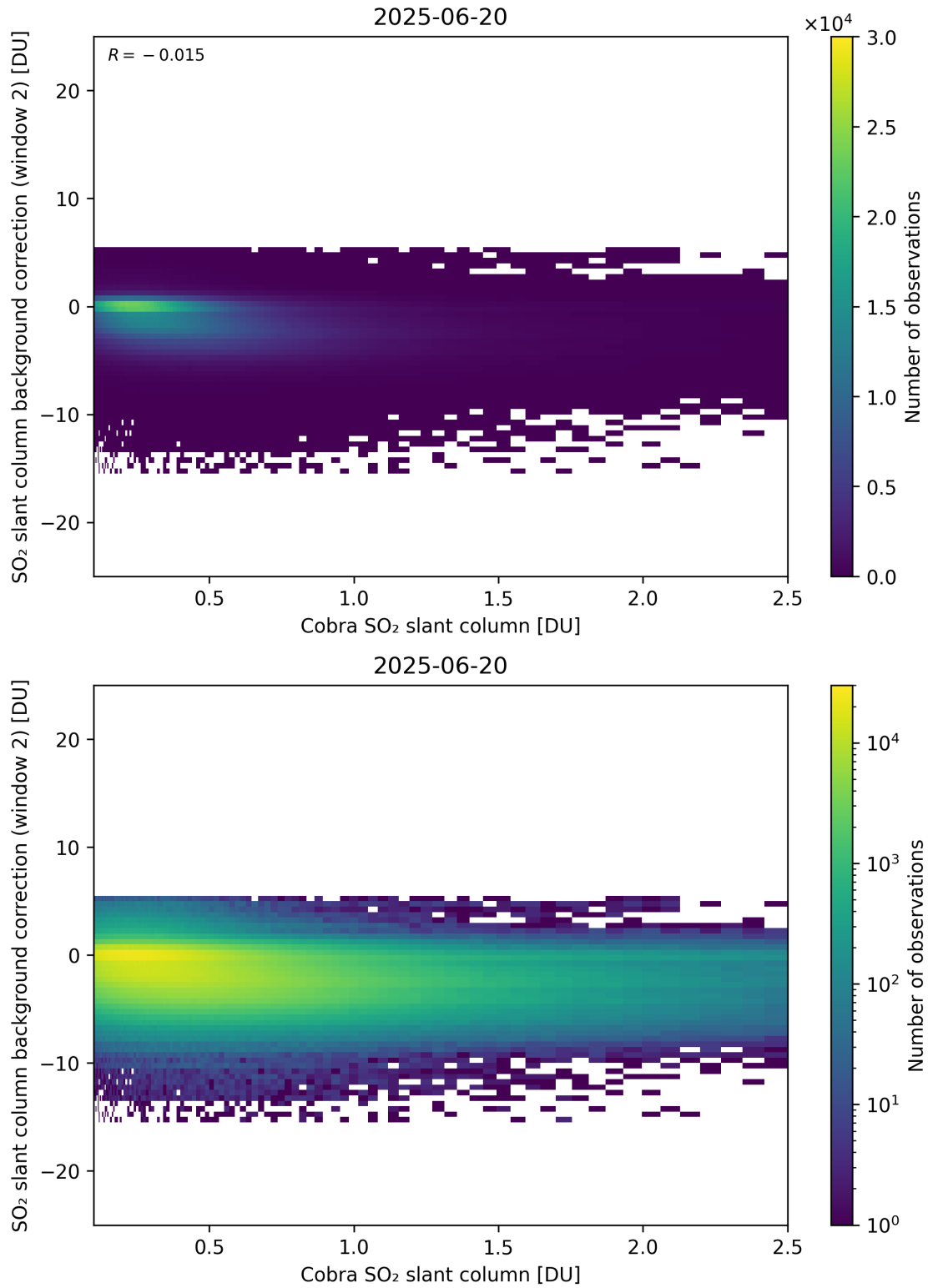
Figure 194: Scatter density plot of “Cobra SO 2 slant column” against “SO 2 slant column background correction (window 2)” for 2025-06-19 to 2025-06-21.
