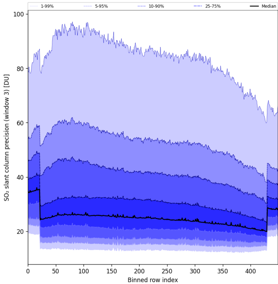
Figure 98: Along track statistics of “SO 2 slant column precision (window 3)” for 2025-06-19 to 2025-06-21
