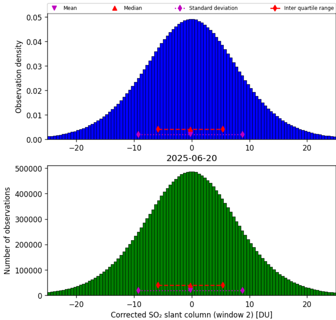
Figure 69: Histogram of “Corrected SO 2 slant column (window 2)” for 2025-06-19 to 2025-06-21
