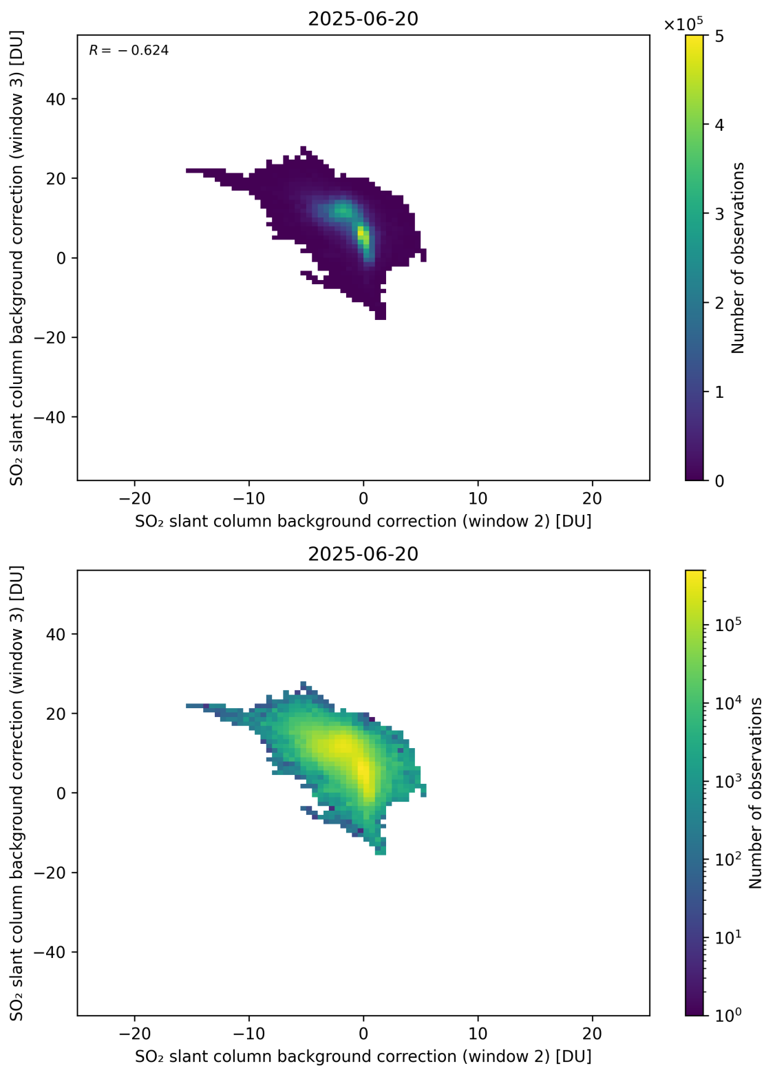
Figure 122: Scatter density plot of “SO 2 slant column background correction (window 2)” against “SO 2 slant column background correction (window 3)” for 2025-06-19 to 2025-06-21.
