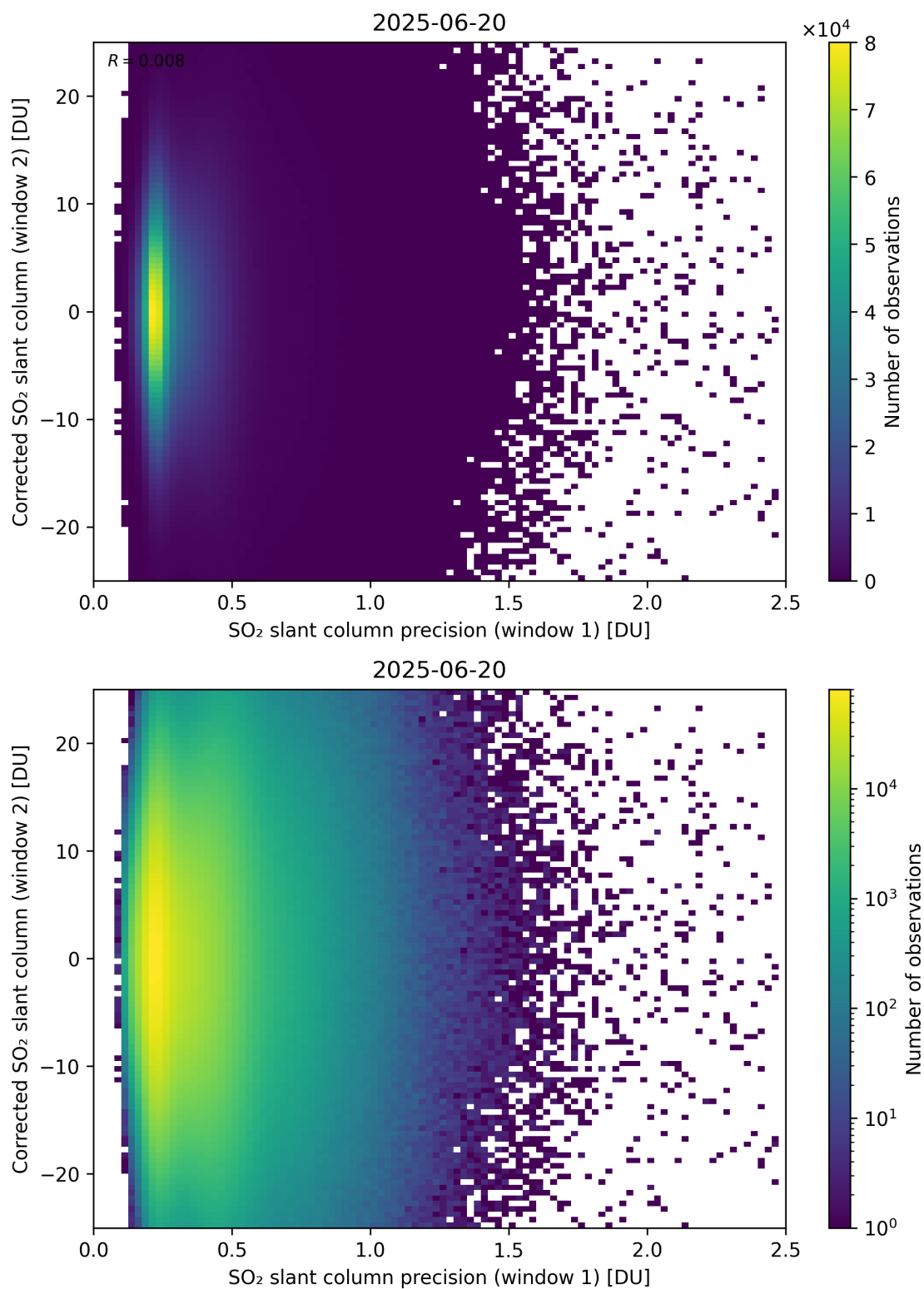
Figure 275: Scatter density plot of “SO 2 slant column precision (window 1)” against “Corrected SO 2 slant column (window 2)” for 2025-06-19 to 2025-06-21.
