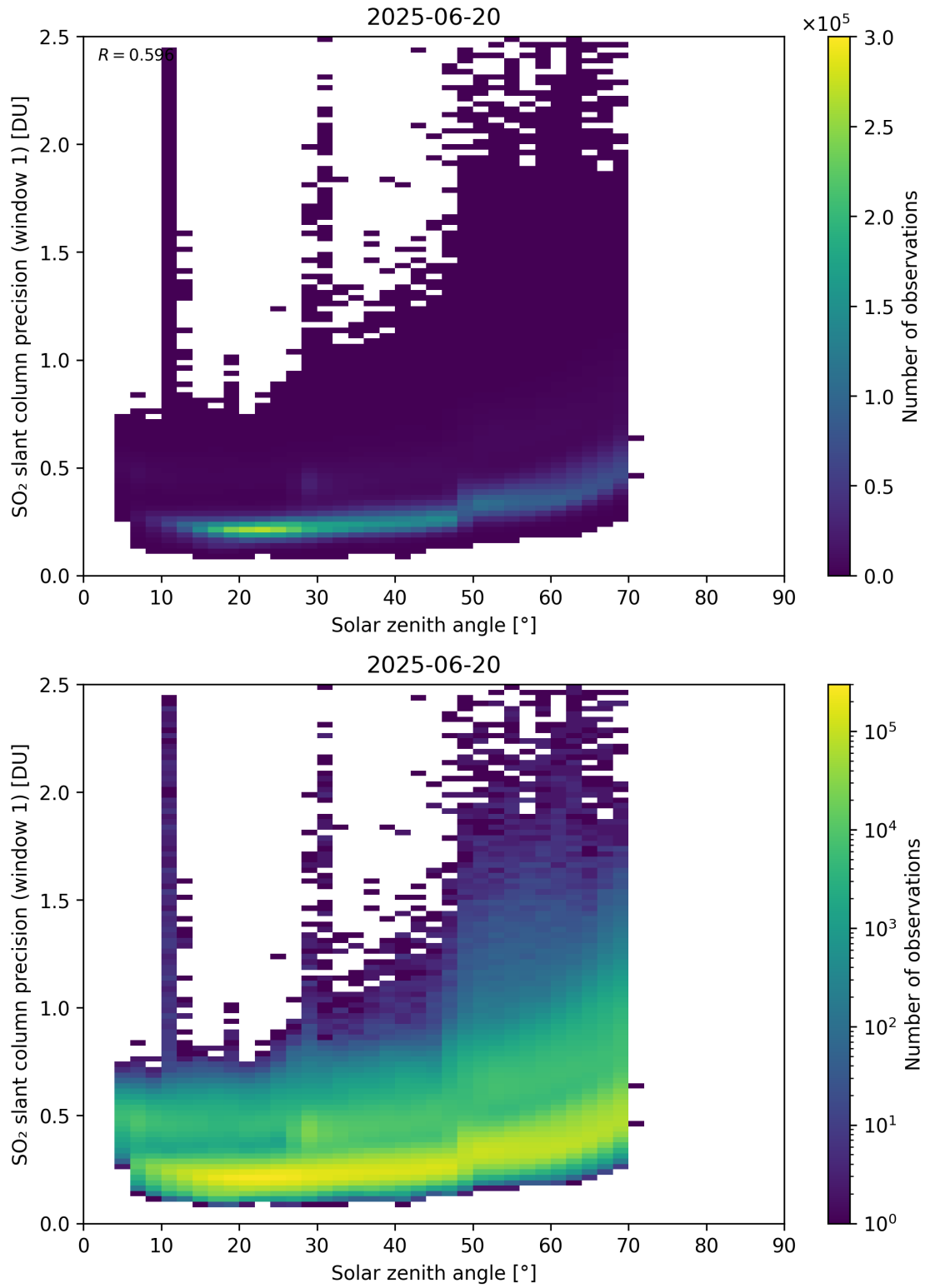
Figure 185: Scatter density plot of “Solar zenith angle” against “SO 2 slant column precision (window 1)” for 2025-06-19 to 2025-06-21.
