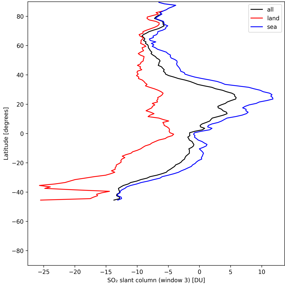
Figure 45: Zonal average of “SO 2 slant column (window 3)” for 2025-06-19 to 2025-06-21.
