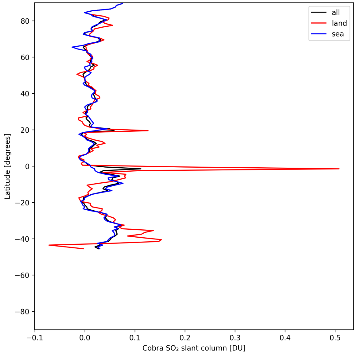
Figure 35: Zonal average of “Cobra SO 2 slant column” for 2025-06-19 to 2025-06-21.
