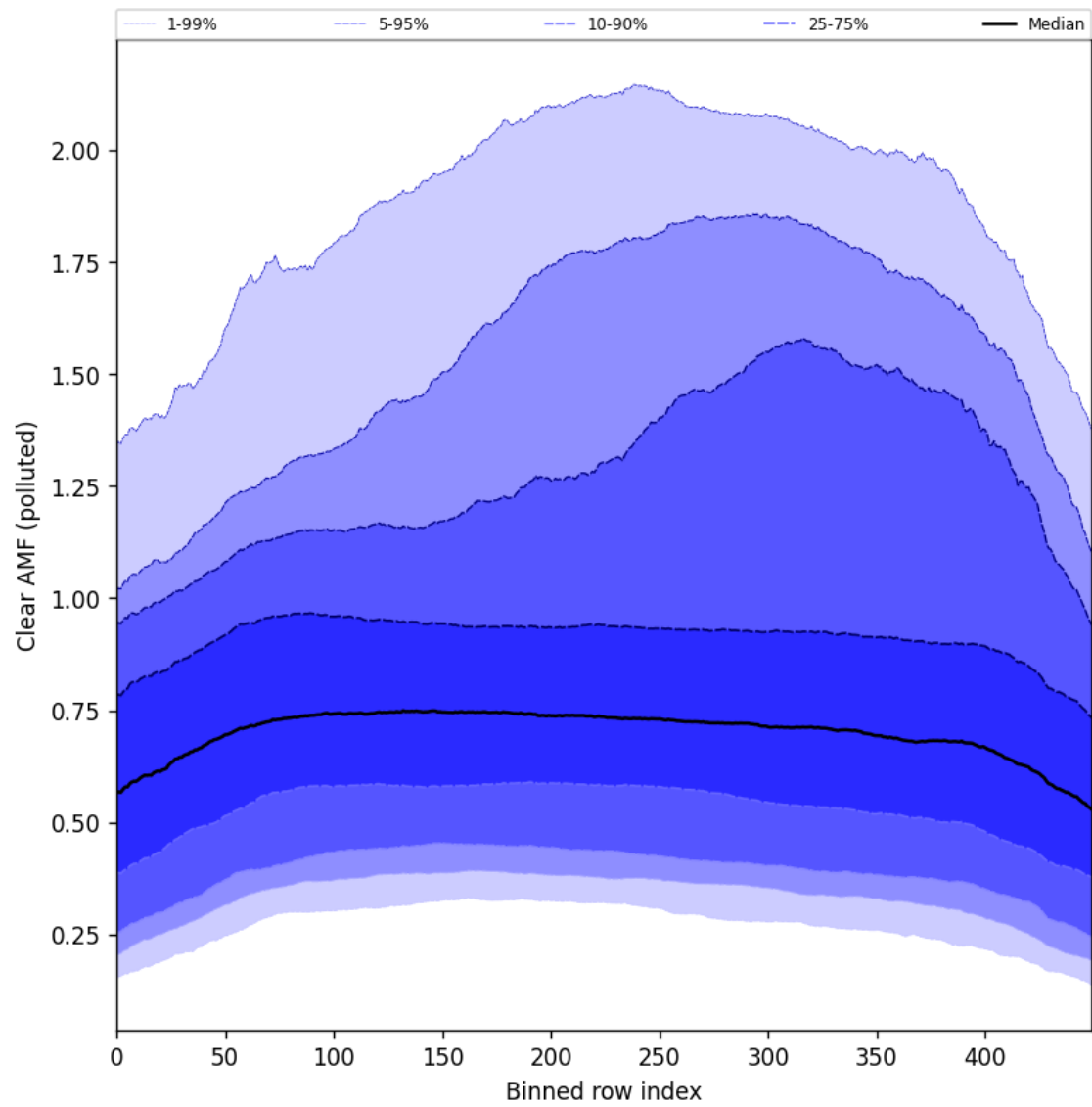
Figure 107: Along track statistics of “Clear AMF (polluted)” for 2025-06-19 to 2025-06-21
