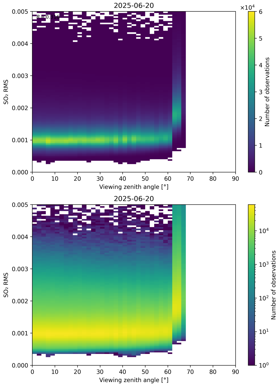
Figure 367: Scatter density plot of “Viewing zenith angle” against “SO 2 RMS” for 2025-06-19 to 2025-06-21.
