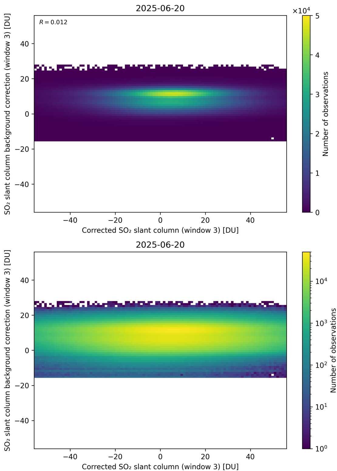
Figure 255: Scatter density plot of “Corrected SO 2 slant column (window 3)” against “SO 2 slant column background correction (window 3)” for 2025-06-19 to 2025-06-21.
