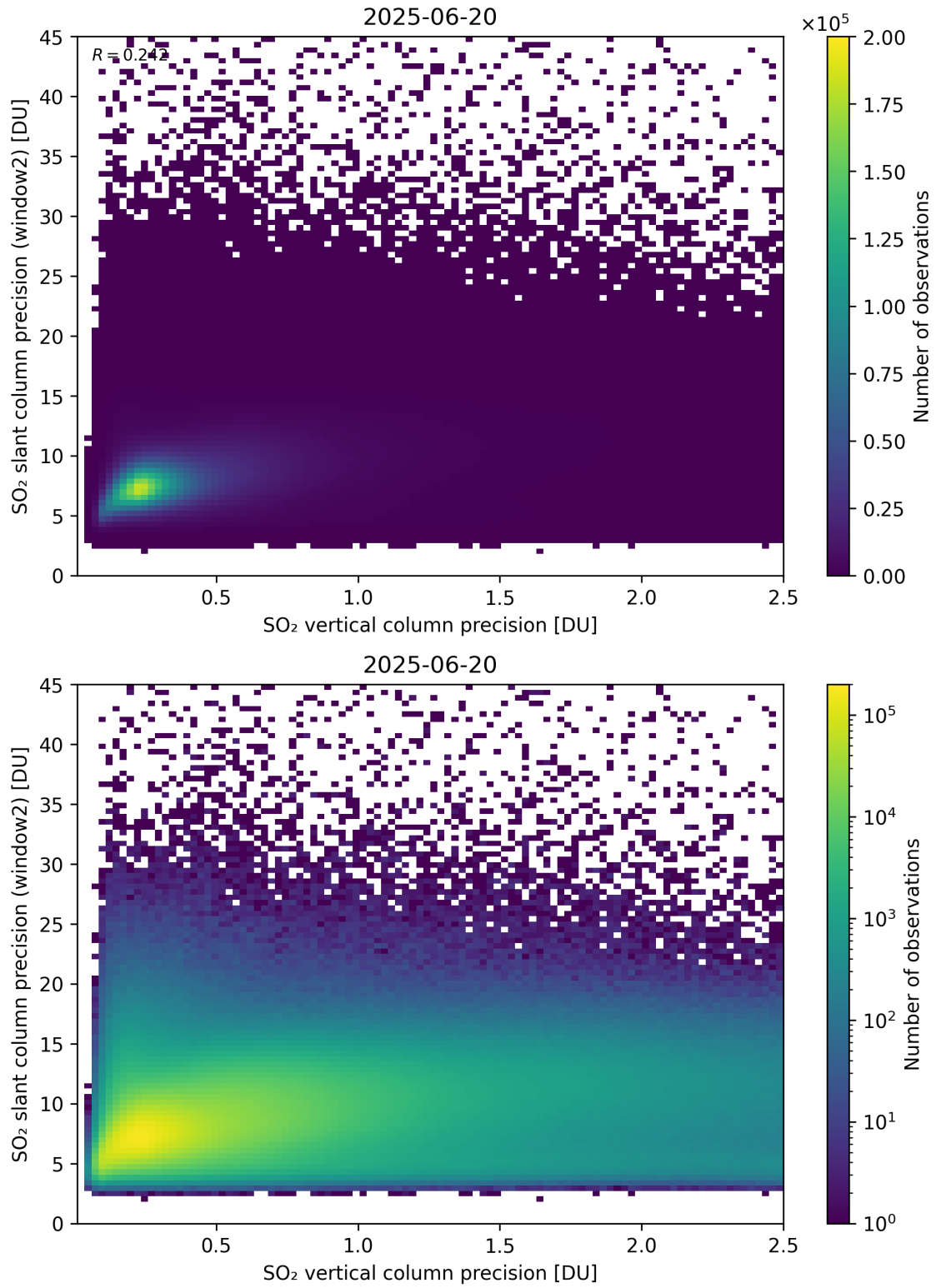
Figure 343: Scatter density plot of “SO 2 vertical column precision” against “SO 2 slant column precision (window2)” for 2025-06-19 to 2025-06-21.
