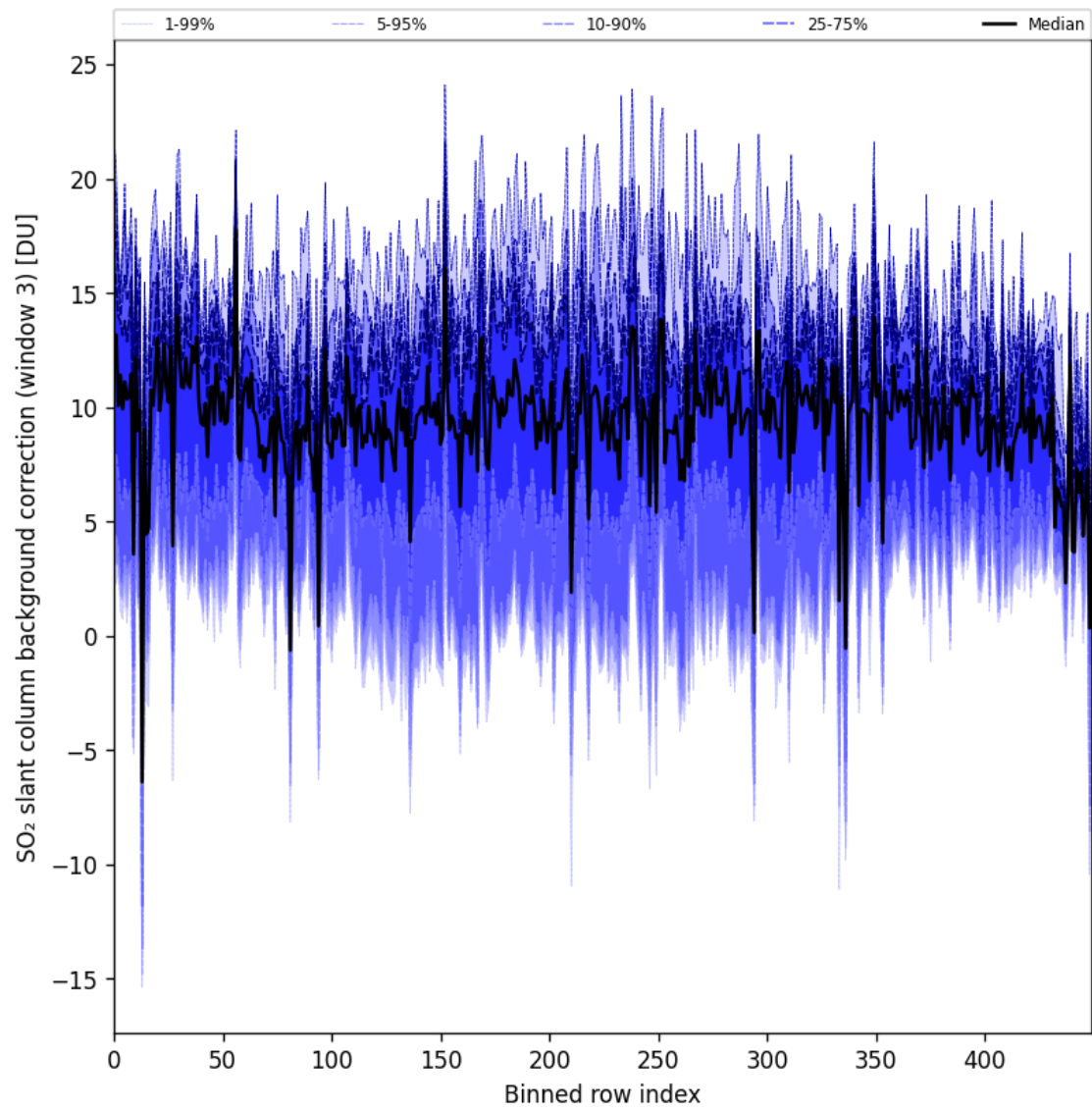
Figure 100: Along track statistics of “SO 2 slant column background correction (window 3)” for 2025-06-19 to 2025-06-21
