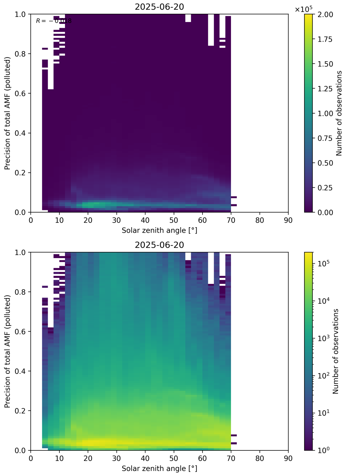
Figure 190: Scatter density plot of “Solar zenith angle” against “Precision of total AMF (polluted)” for 2025-06-19 to 2025-06-21.
