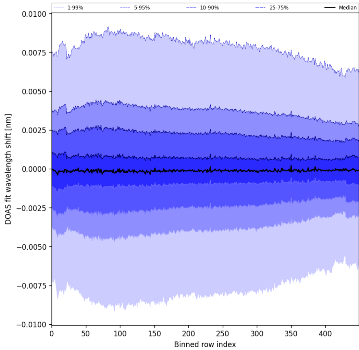
Figure 102: Along track statistics of “DOAS fit wavelength shift” for 2025-06-19 to 2025-06-21
