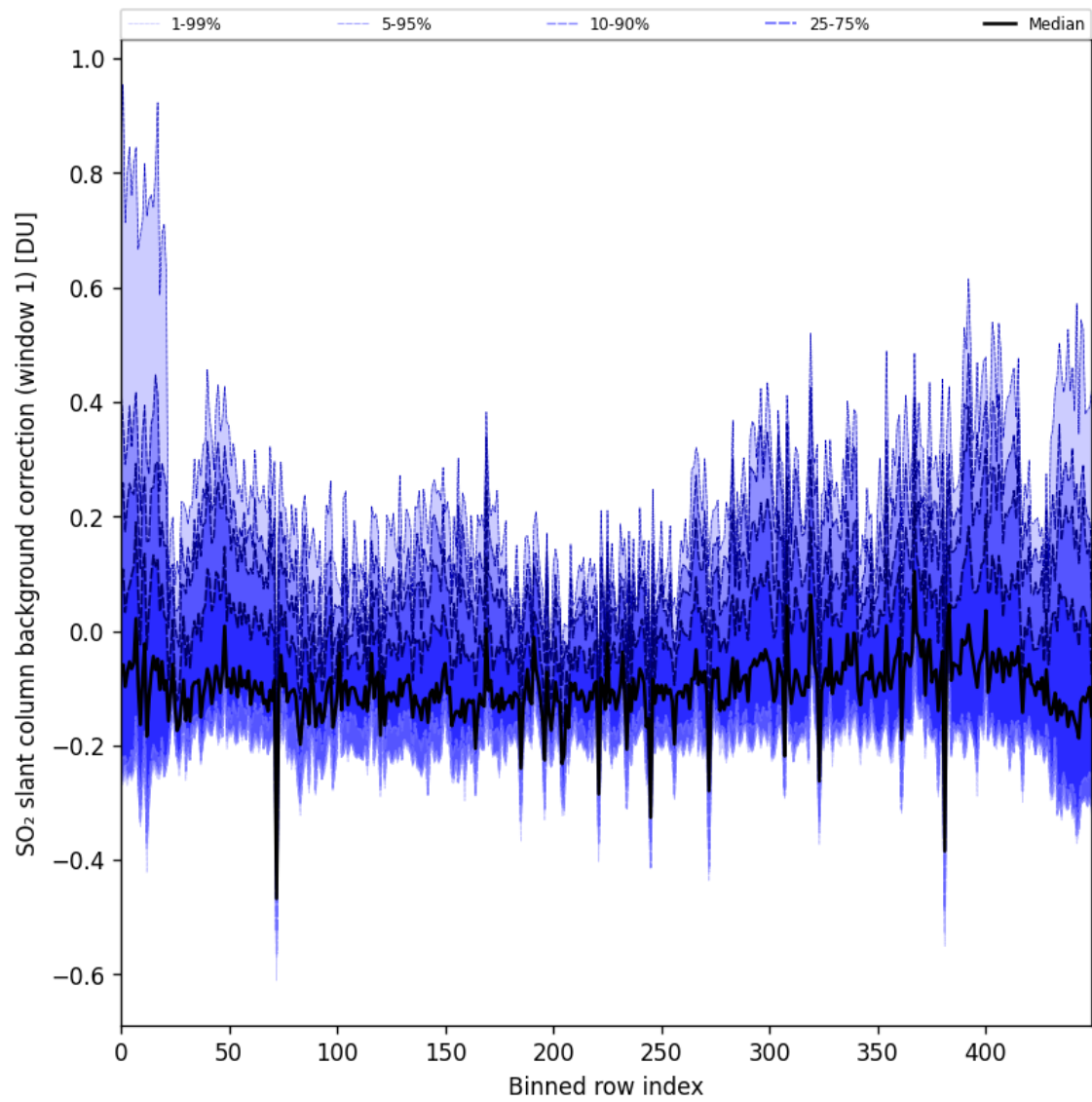
Figure 92: Along track statistics of “SO 2 slant column background correction (window 1)” for 2025-06-19 to 2025-06-21
