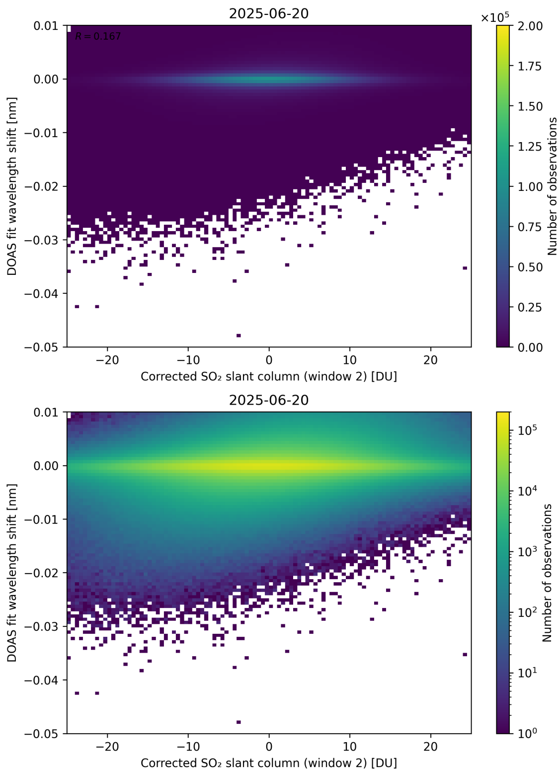
Figure 246: Scatter density plot of “Corrected SO 2 slant column (window 2)” against “DOAS fit wavelength shift” for 2025-06-19 to 2025-06-21.
