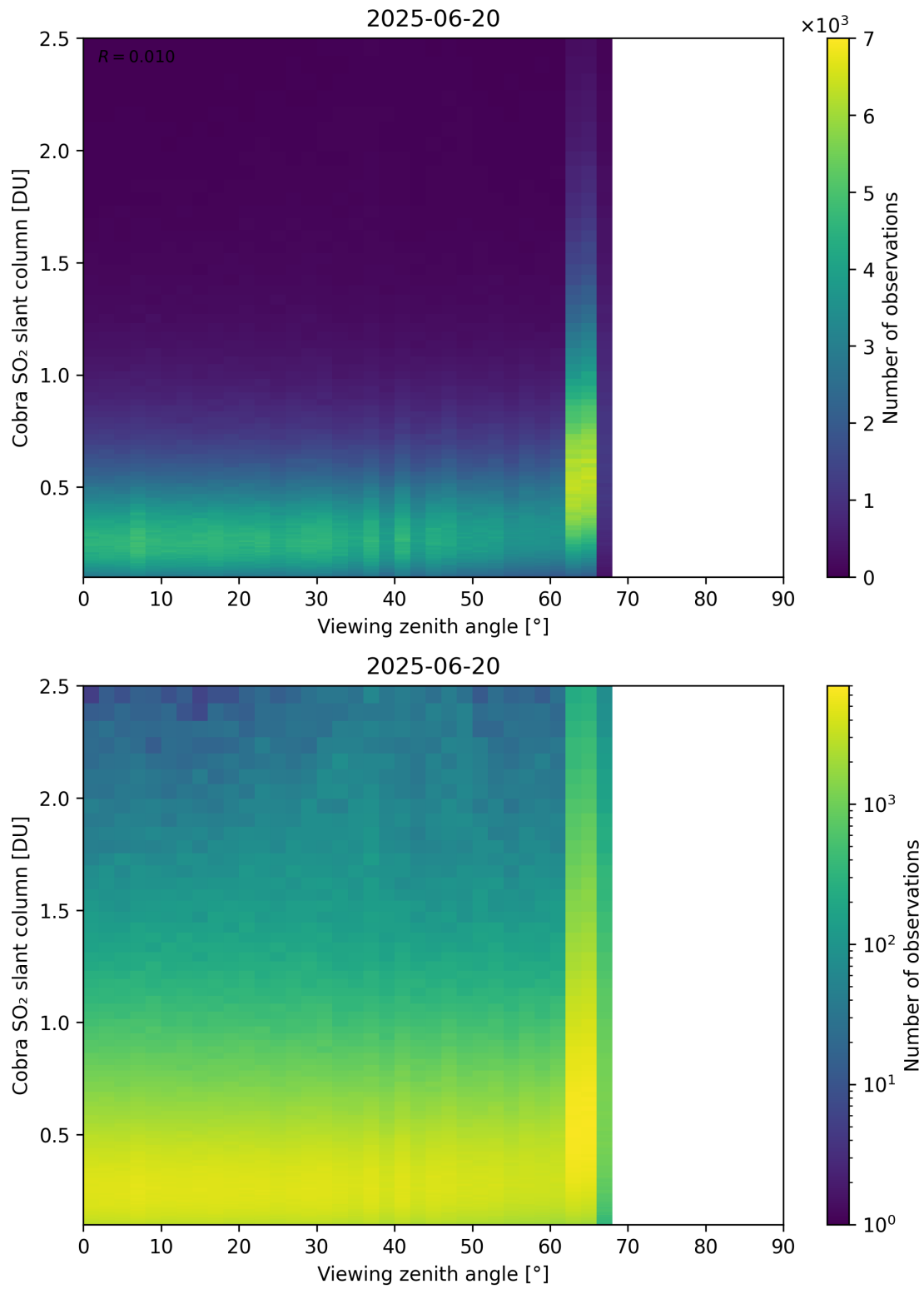
Figure 371: Scatter density plot of “Viewing zenith angle” against “Cobra SO 2 slant column” for 2025-06-19 to 2025-06-21.
