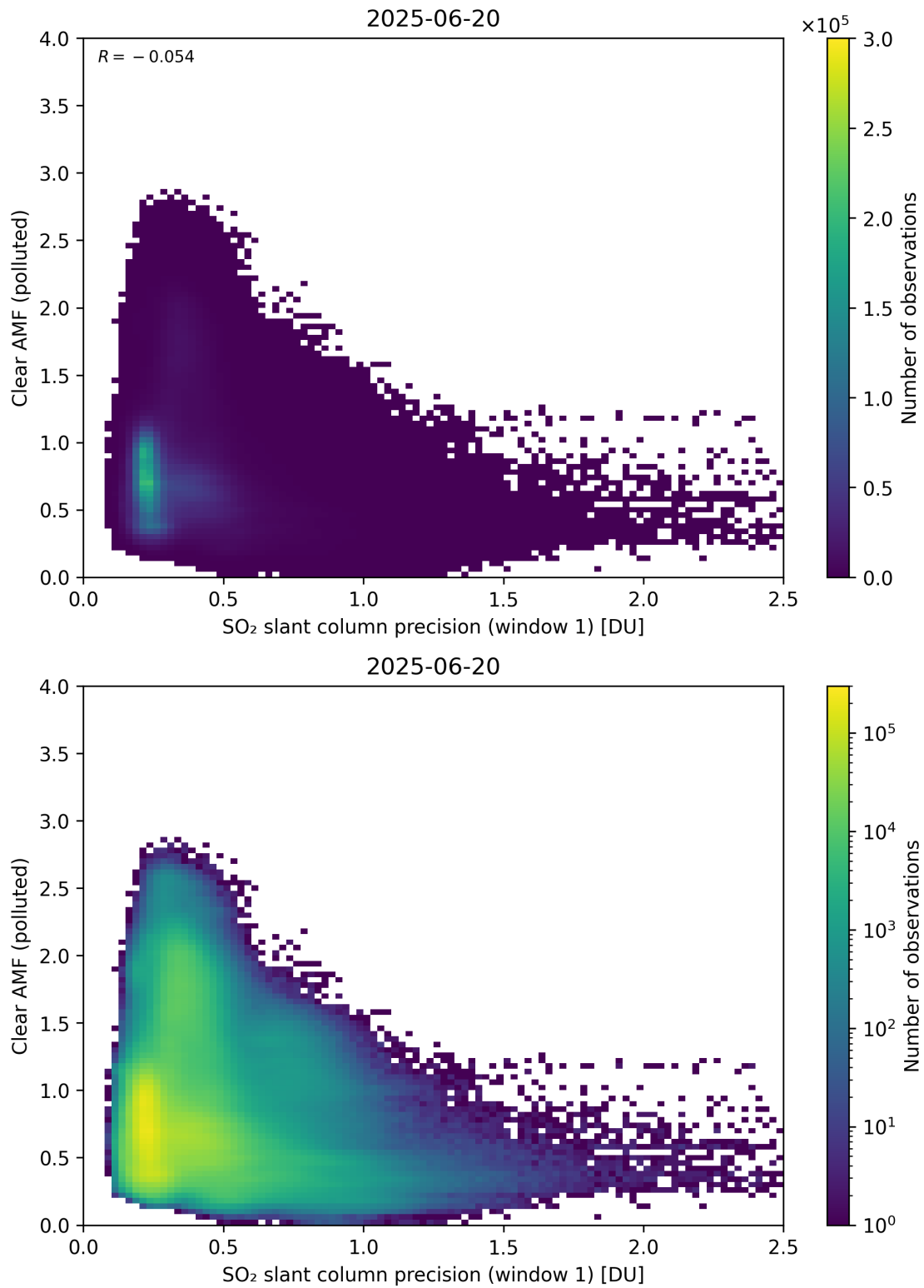
Figure 274: Scatter density plot of “SO 2 slant column precision (window 1)” against “Clear AMF (polluted)” for 2025-06-19 to 2025-06-21.
