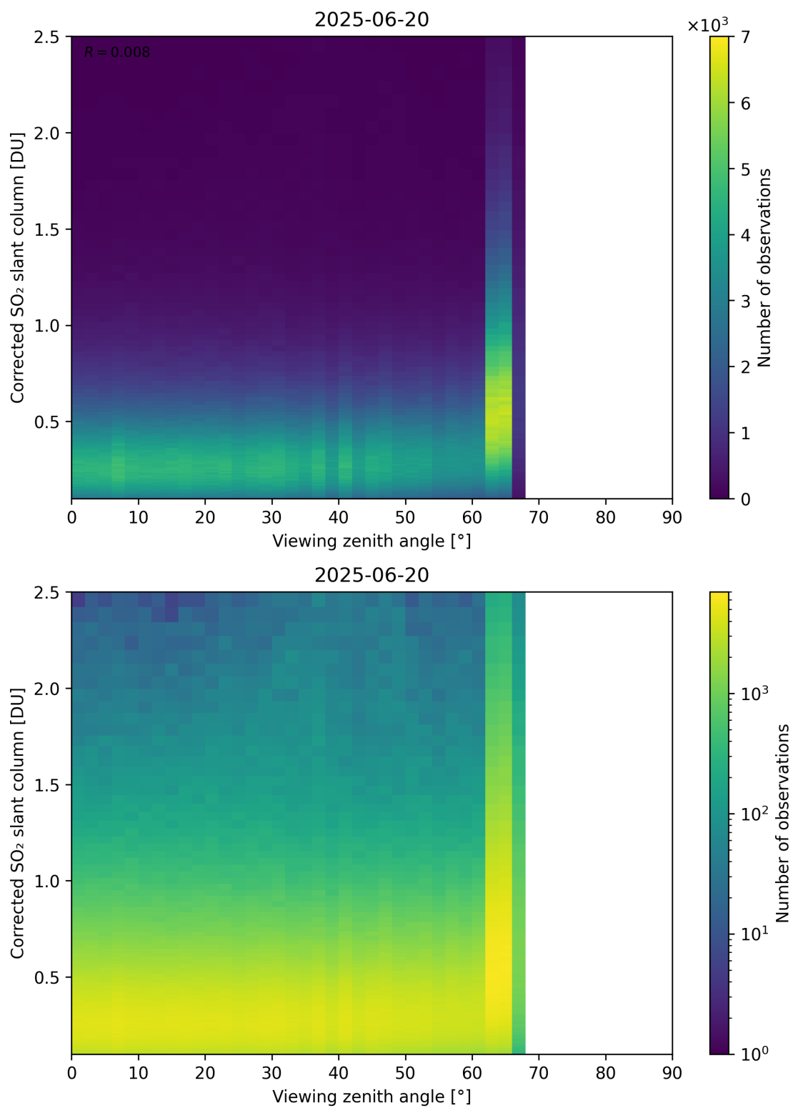
Figure 373: Scatter density plot of “Viewing zenith angle” against “Corrected SO 2 slant column” for 2025-06-19 to 2025-06-21.
