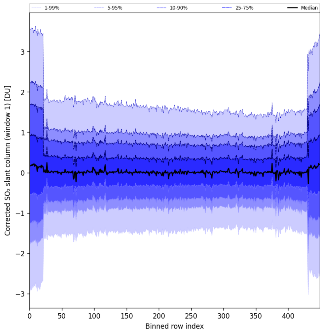
Figure 91: Along track statistics of “Corrected SO 2 slant column (window 1)” for 2025-06-19 to 2025-06-21
