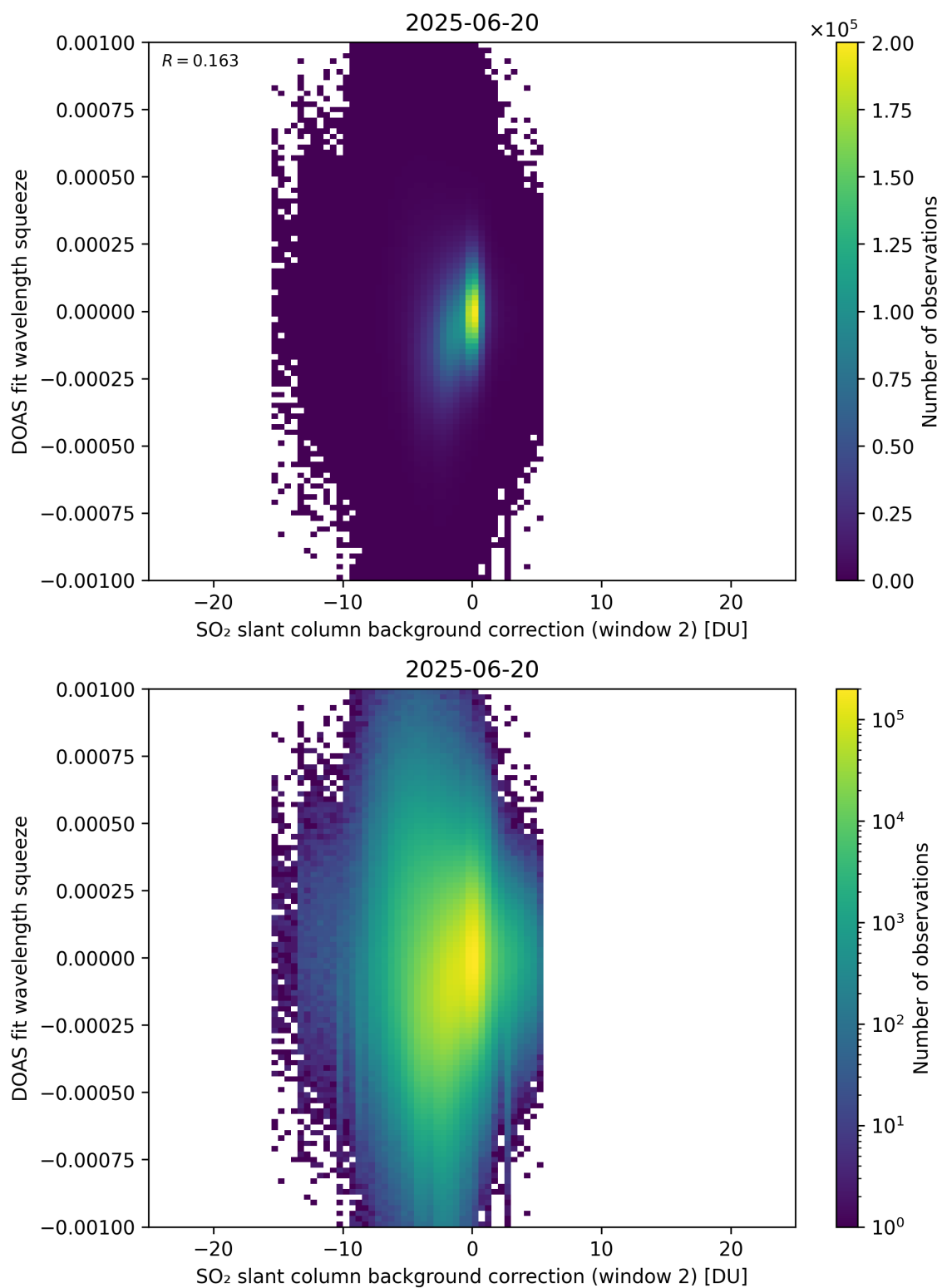
Figure 124: Scatter density plot of “SO 2 slant column background correction (window 2)” against “DOAS fit wavelength squeeze” for 2025-06-19 to 2025-06-21.
