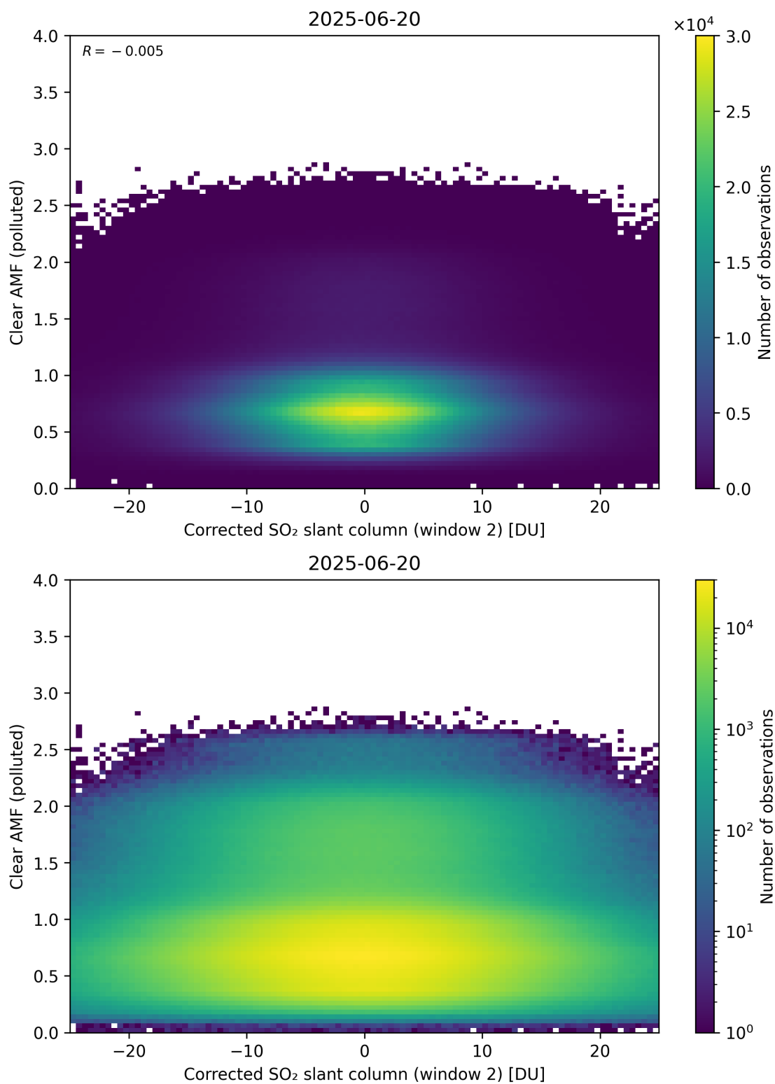
Figure 249: Scatter density plot of “Corrected SO 2 slant column (window 2)” against “Clear AMF (polluted)” for 2025-06-19 to 2025-06-21.
