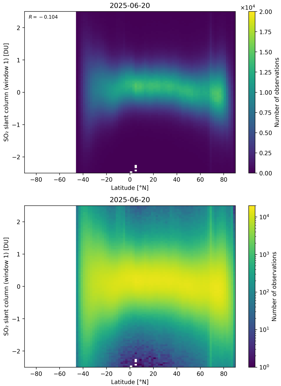
Figure 162: Scatter density plot of “Latitude” against “SO 2 slant column (window 1)” for 2025-06-19 to 2025-06-21.
