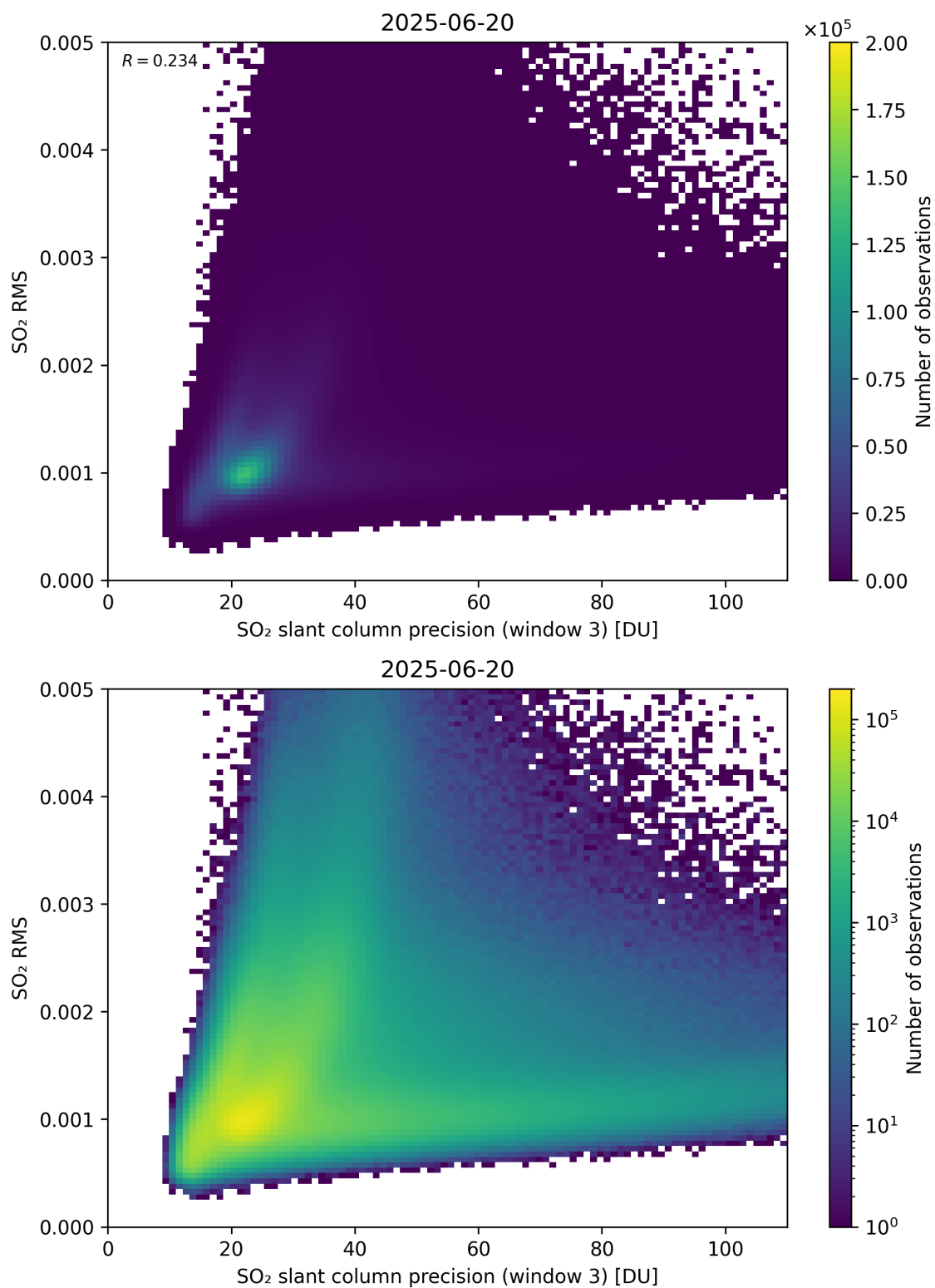
Figure 310: Scatter density plot of “SO 2 slant column precision (window 3)” against “SO 2 RMS” for 2025-06-19 to 2025-06-21.
