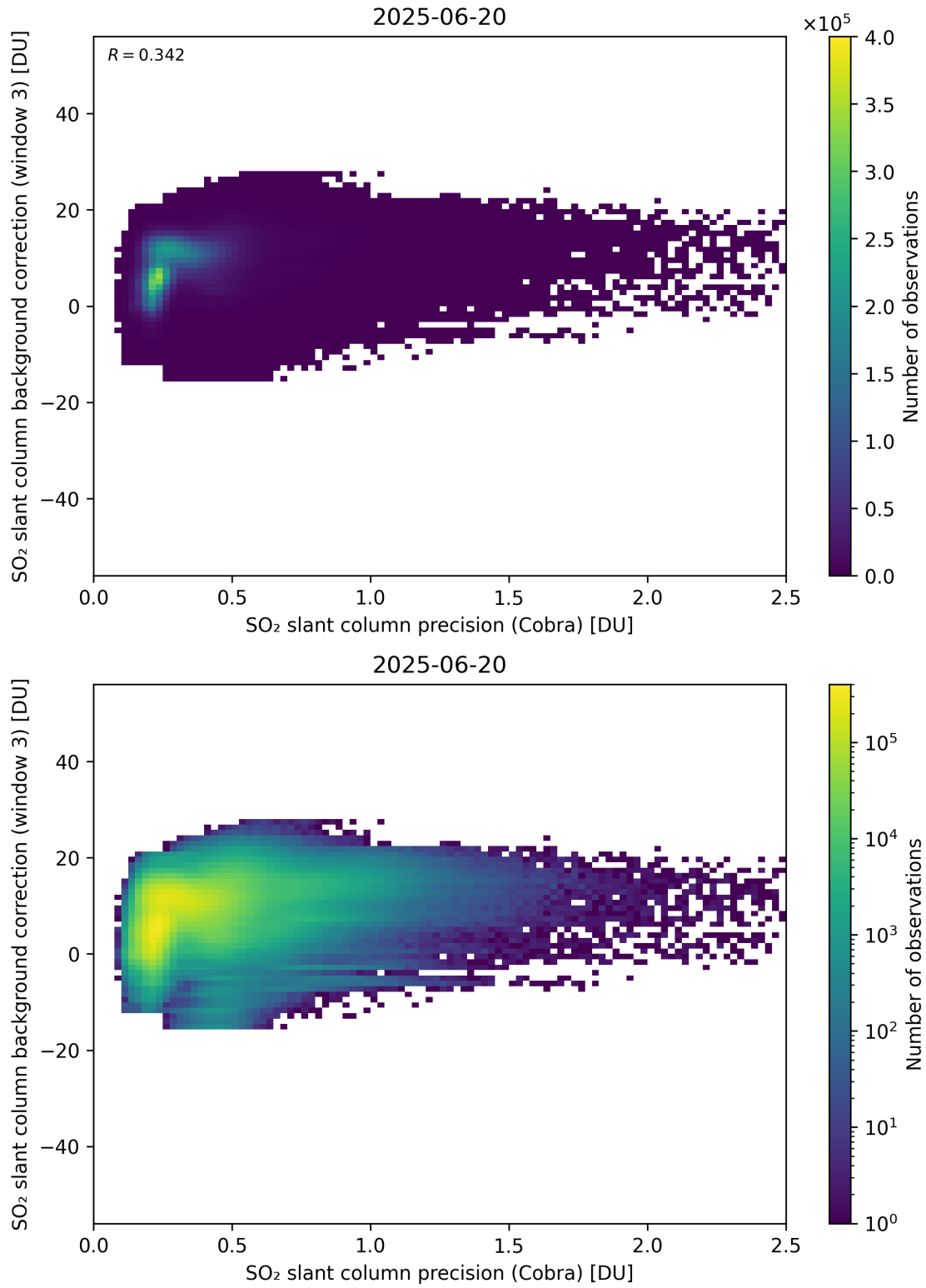
Figure 201: Scatter density plot of “SO 2 slant column precision (Cobra)” against “SO 2 slant column background correction (window 3)” for 2025-06-19 to 2025-06-21.
