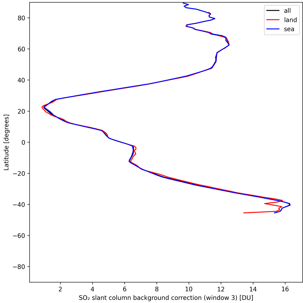
Figure 48: Zonal average of “SO 2 slant column background correction (window 3)” for 2025-06-19 to 2025-06-21.
