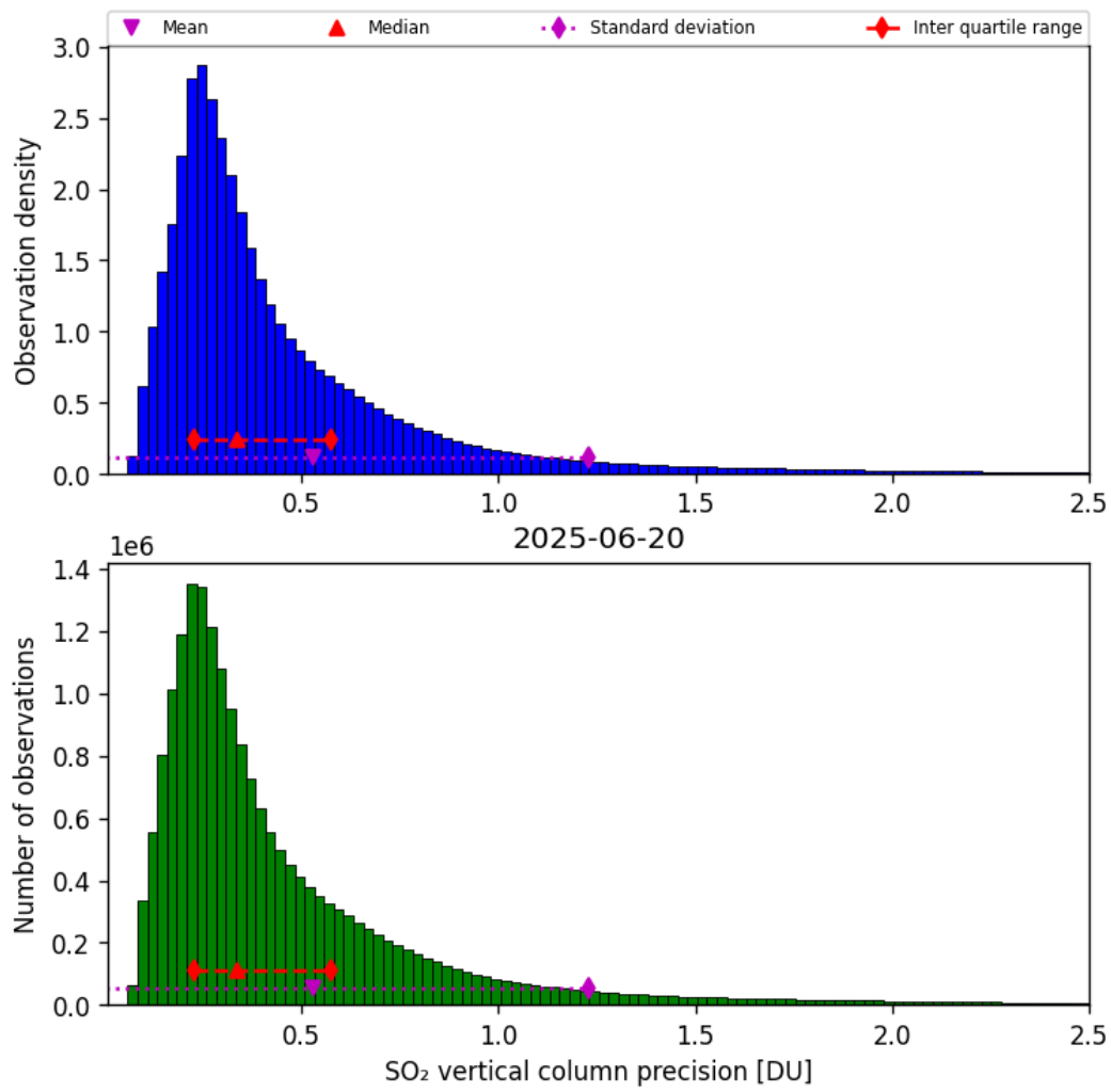
Figure 59: Histogram of “SO 2 vertical column precision” for 2025-06-19 to 2025-06-21
