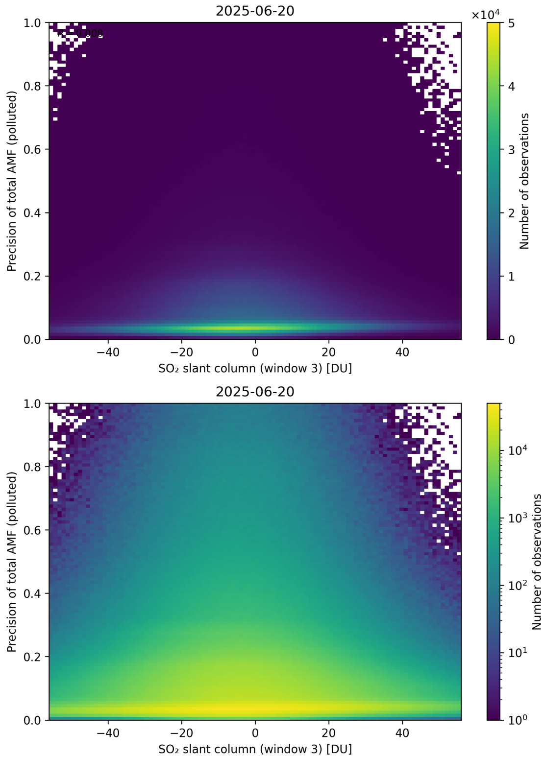
Figure 319: Scatter density plot of “SO 2 slant column (window 3)” against “Precision of total AMF (polluted)” for 2025-06-19 to 2025-06-21.
