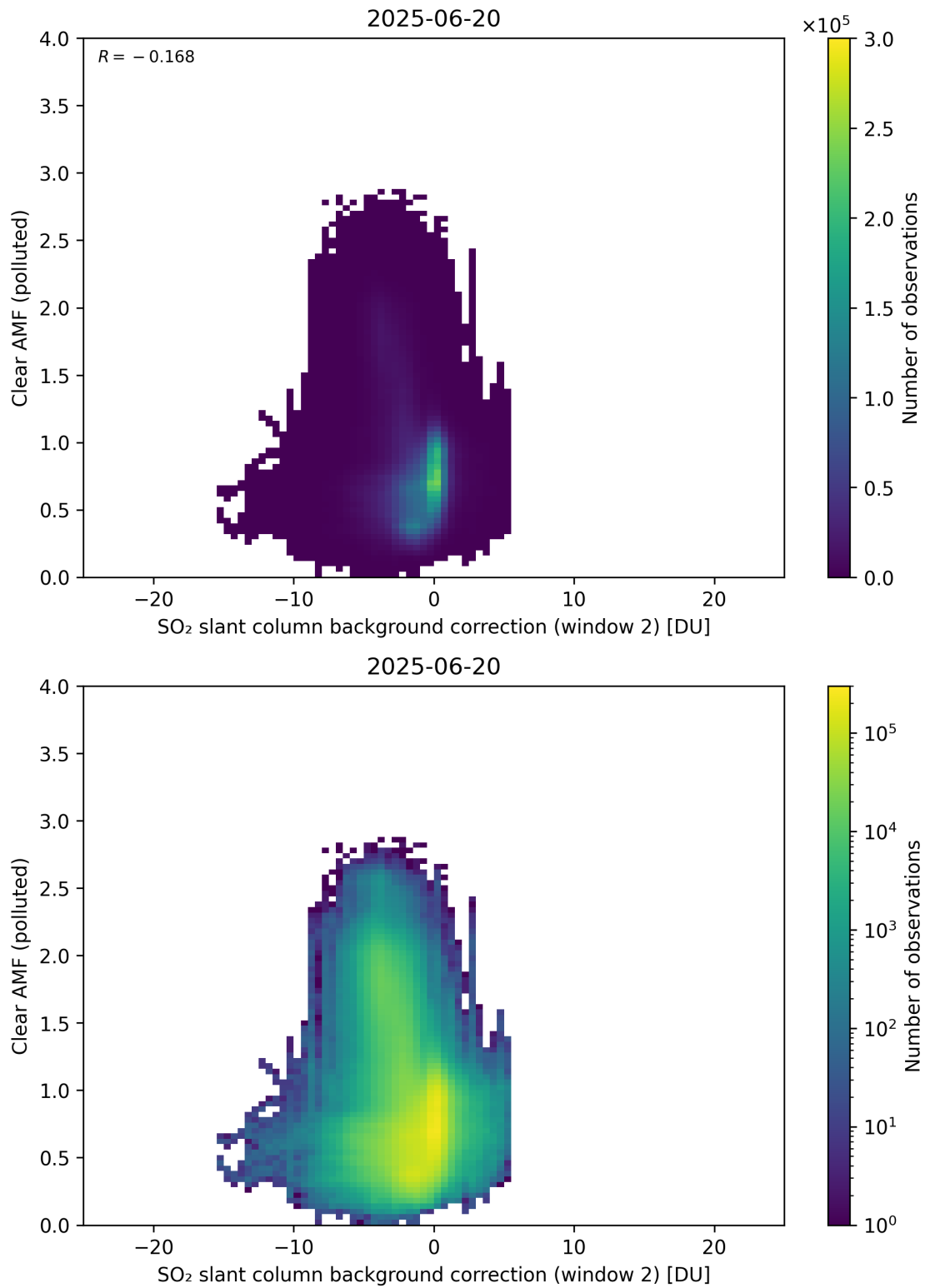
Figure 126: Scatter density plot of “SO 2 slant column background correction (window 2)” against “Clear AMF (polluted)” for 2025-06-19 to 2025-06-21.
