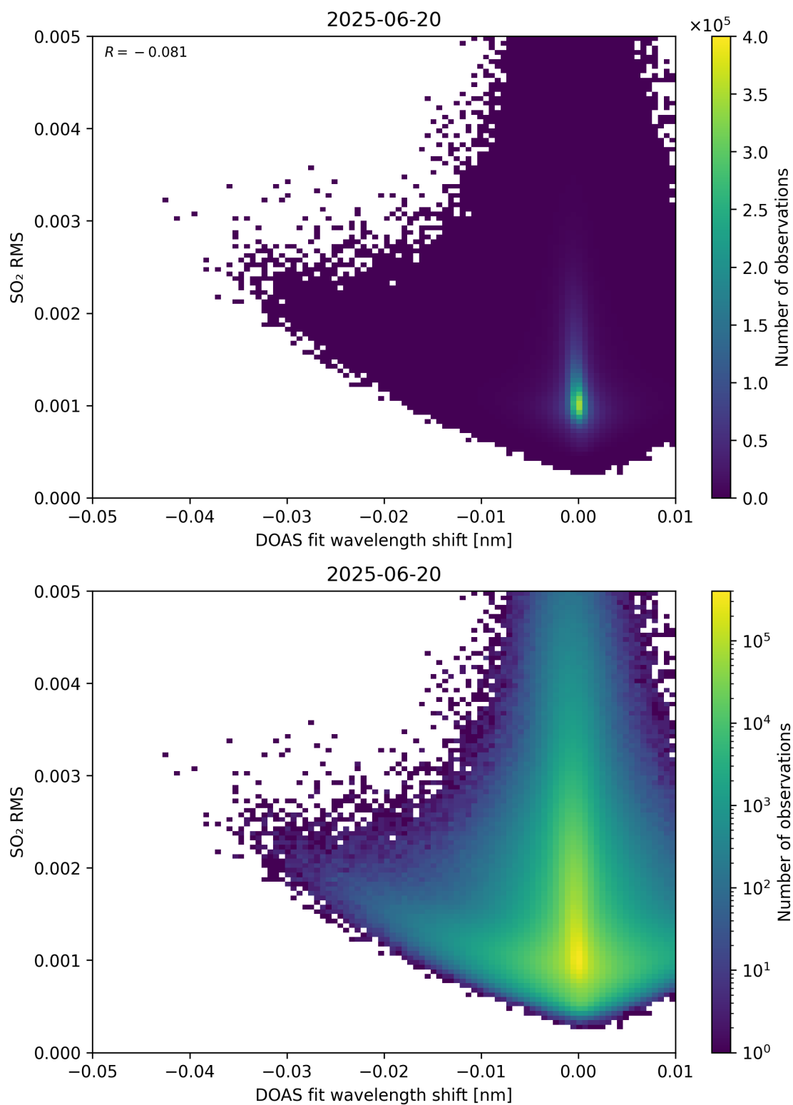
Figure 139: Scatter density plot of “DOAS fit wavelength shift” against “SO 2 RMS” for 2025-06-19 to 2025-06-21.
