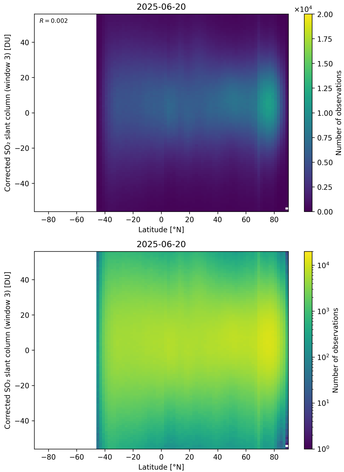
Figure 161: Scatter density plot of “Latitude” against “Corrected SO 2 slant column (window 3)” for 2025-06-19 to 2025-06-21.
