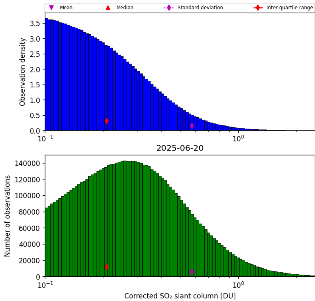
Figure 60: Histogram of “Corrected SO 2 slant column” for 2025-06-19 to 2025-06-21
