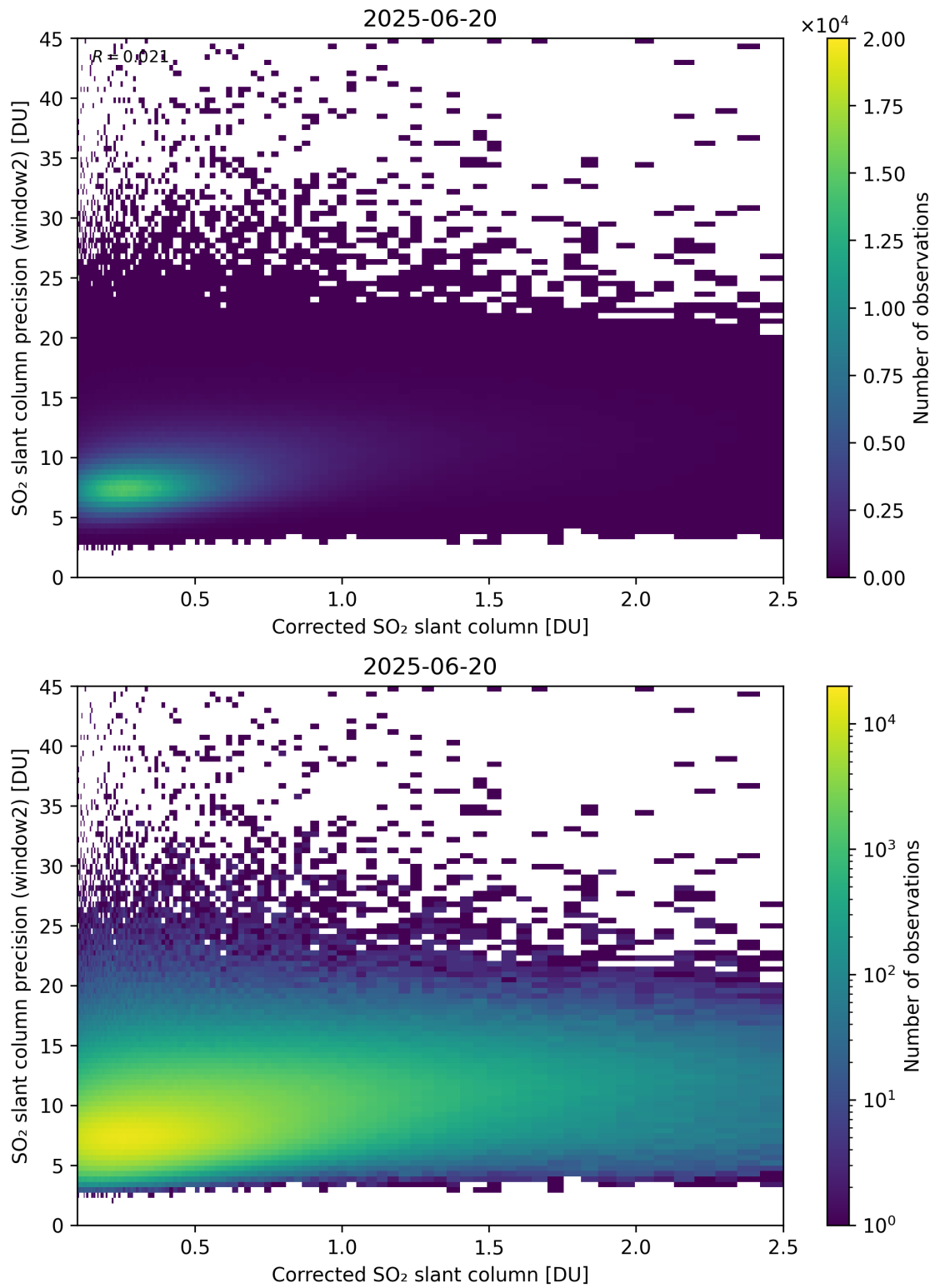
Figure 239: Scatter density plot of “Corrected SO 2 slant column” against “SO 2 slant column precision (window2)” for 2025-06-19 to 2025-06-21.
