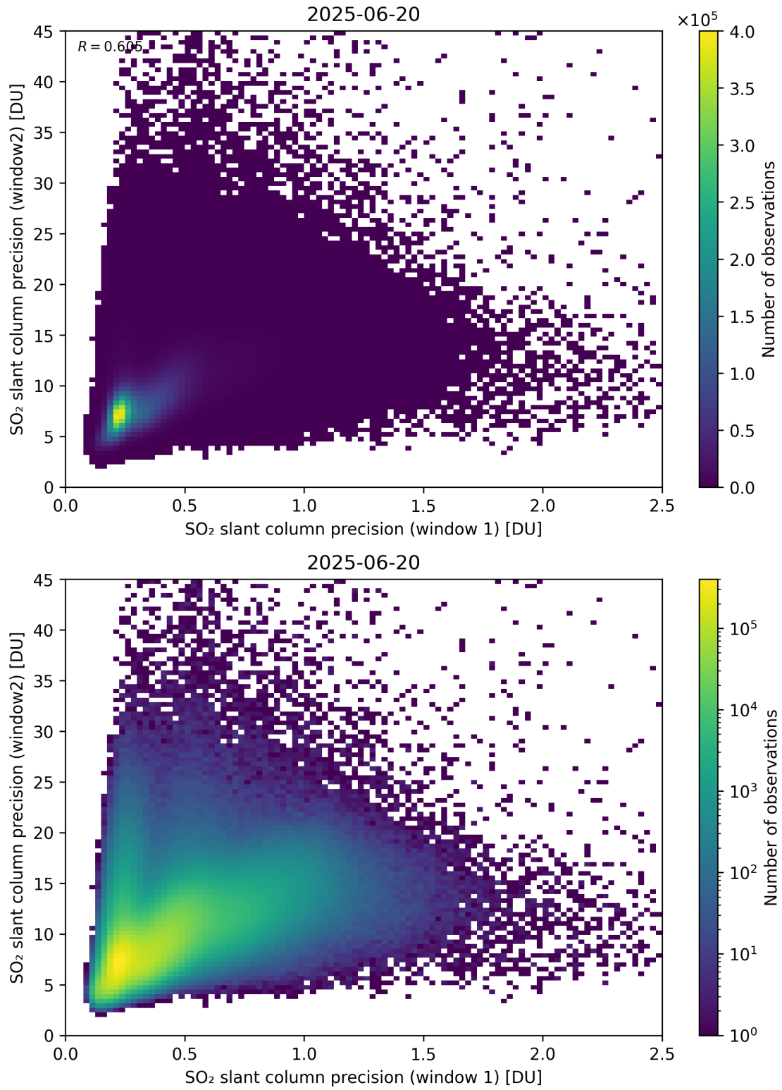
Figure 277: Scatter density plot of “SO 2 slant column precision (window 1)” against “SO 2 slant column precision (window2)” for 2025-06-19 to 2025-06-21.
