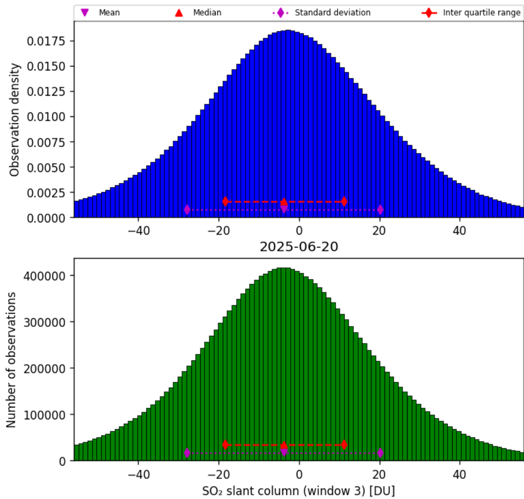
Figure 71: Histogram of “SO 2 slant column (window 3)” for 2025-06-19 to 2025-06-21
