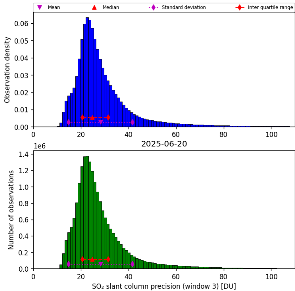
Figure 72: Histogram of “SO 2 slant column precision (window 3)” for 2025-06-19 to 2025-06-21
