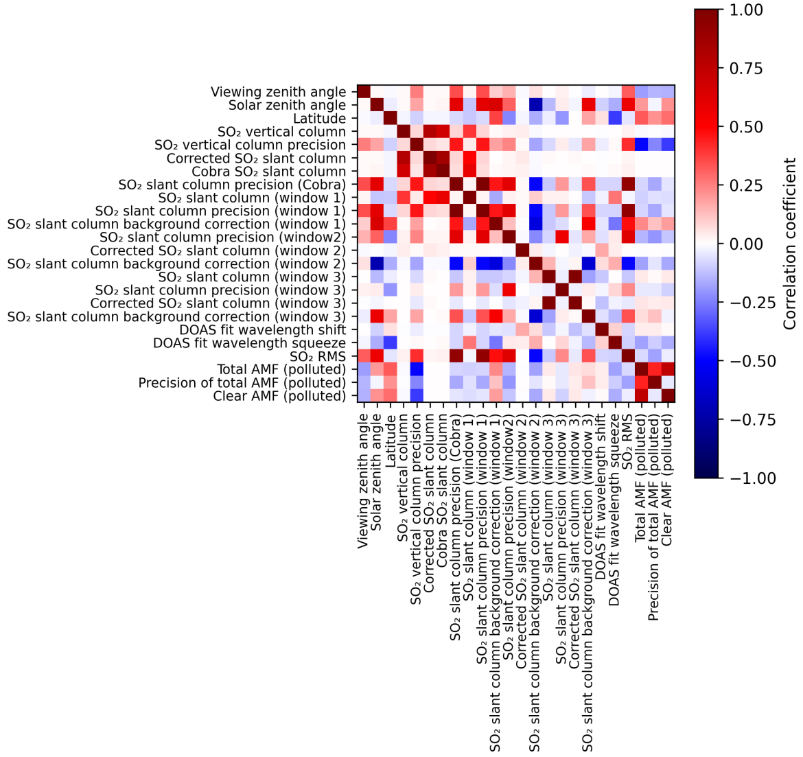
Figure 2: Map of correlation matrix for 2025-06-19 to 2025-06-21.
