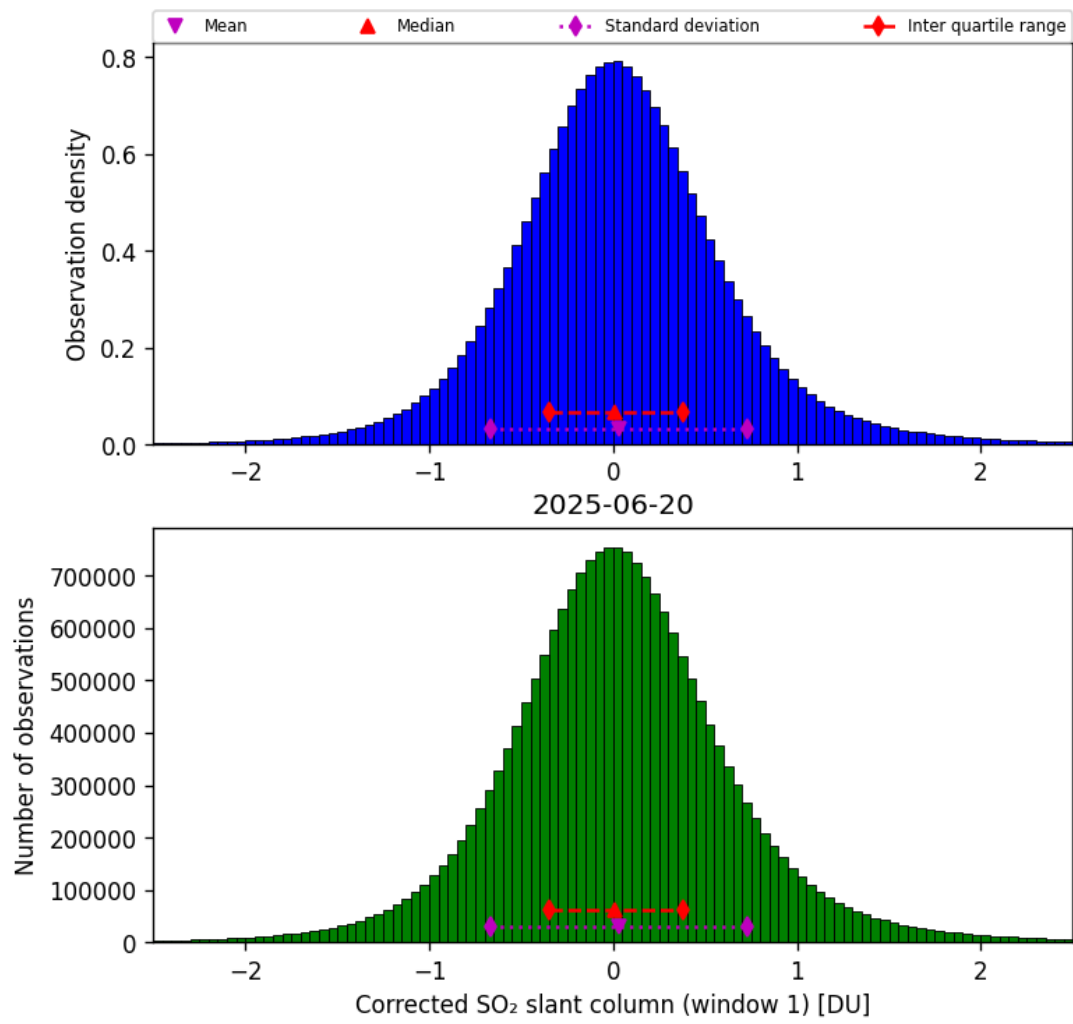
Figure 65: Histogram of “Corrected SO 2 slant column (window 1)” for 2025-06-19 to 2025-06-21
