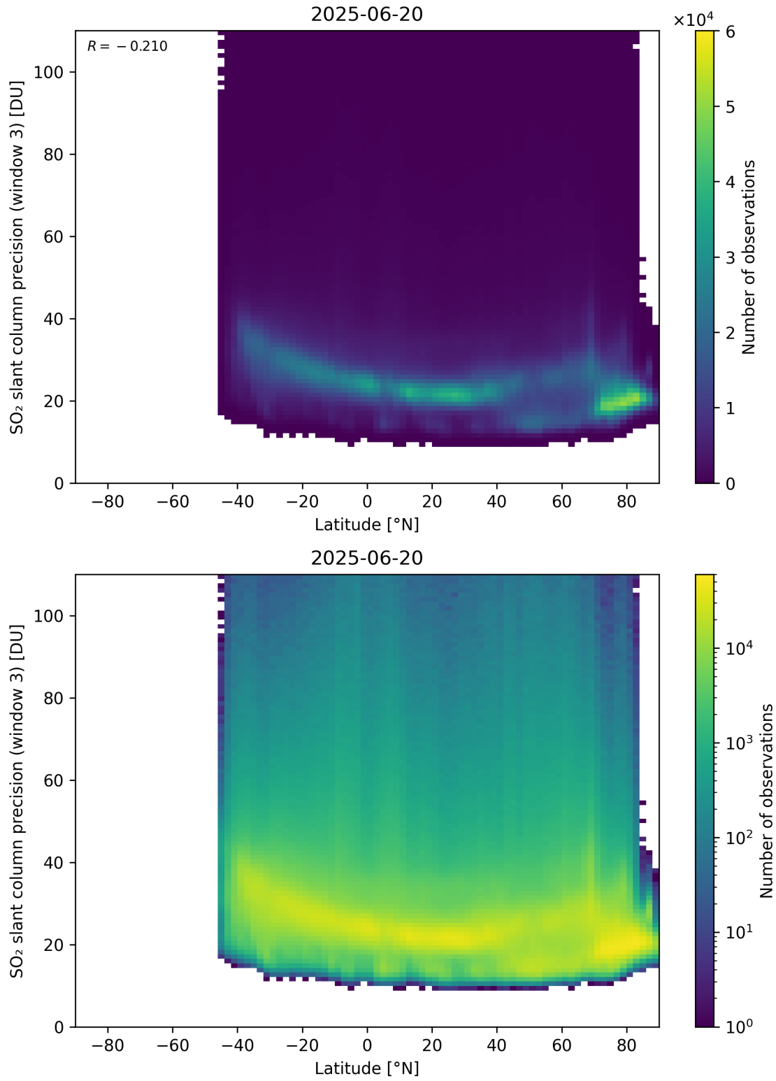
Figure 166: Scatter density plot of “Latitude” against “SO 2 slant column precision (window 3)” for 2025-06-19 to 2025-06-21.
