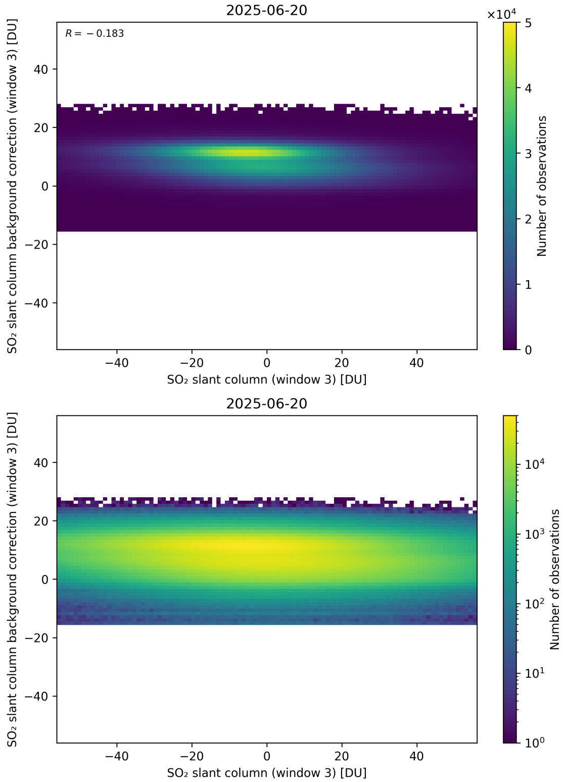
Figure 303: Scatter density plot of “SO 2 slant column (window 3)” against “SO 2 slant column background correction (window 3)” for 2025-06-19 to 2025-06-21.
