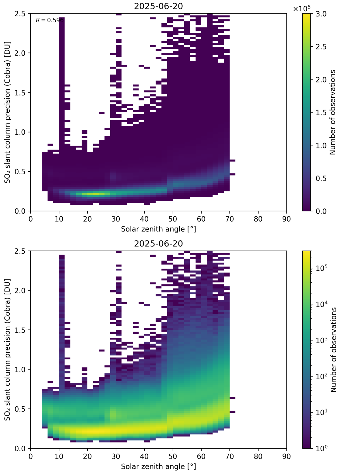
Figure 180: Scatter density plot of “Solar zenith angle” against “SO 2 slant column precision (Cobra)” for 2025-06-19 to 2025-06-21.
