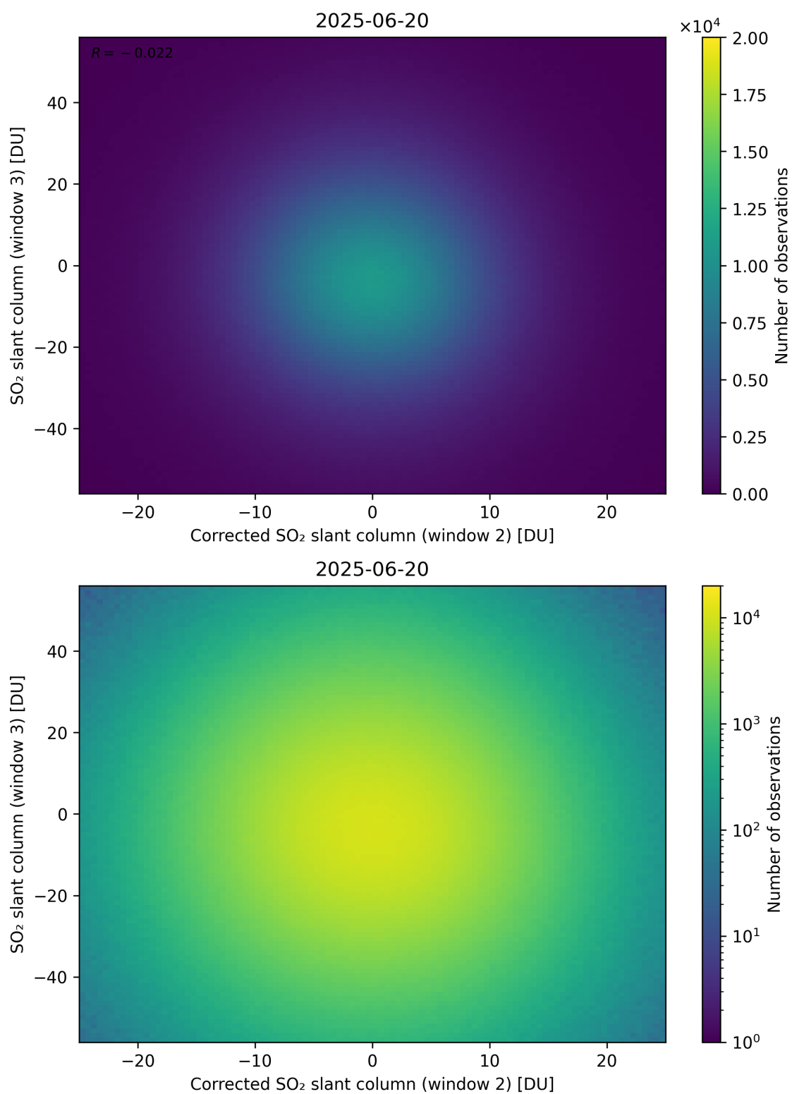
Figure 251: Scatter density plot of “Corrected SO 2 slant column (window 2)” against “SO 2 slant column (window 3)” for 2025-06-19 to 2025-06-21.
