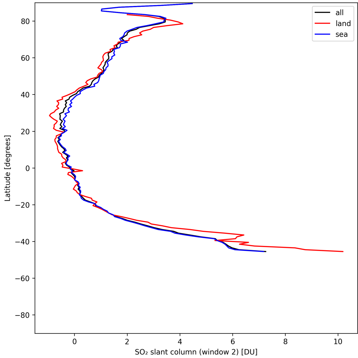
Figure 41: Zonal average of “SO 2 slant column (window 2)” for 2025-06-19 to 2025-06-21.
