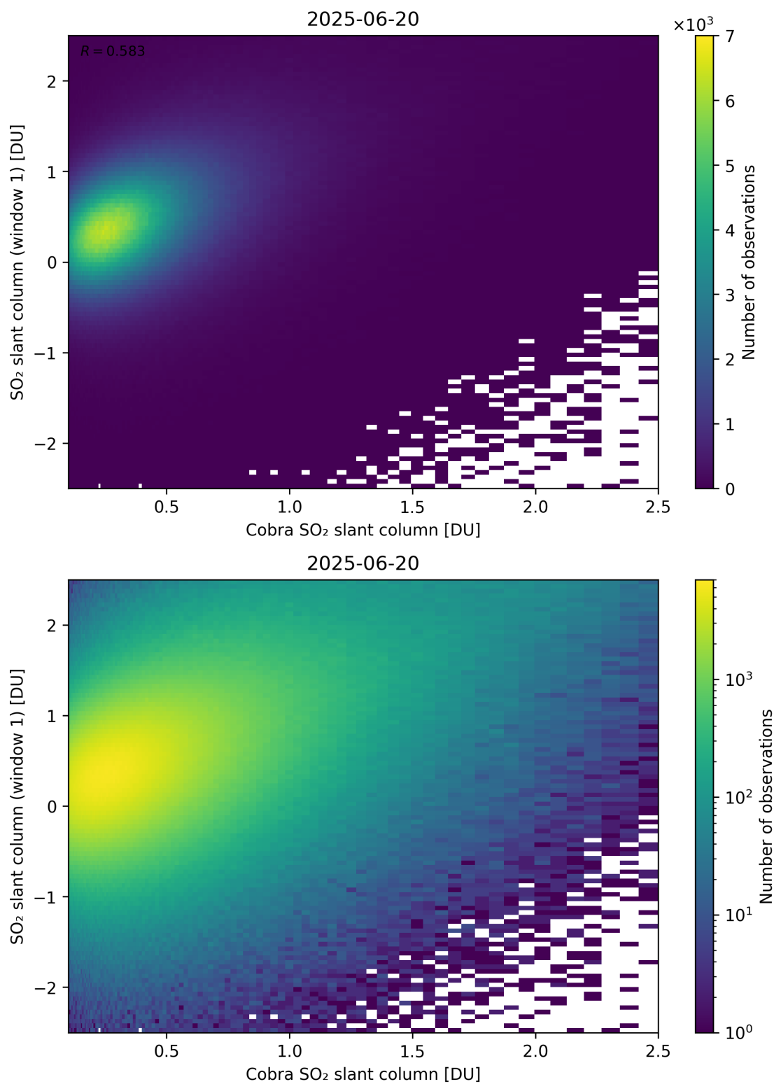
Figure 219: Scatter density plot of “Cobra SO 2 slant column” against “SO 2 slant column (window 1)” for 2025-06-19 to 2025-06-21.
