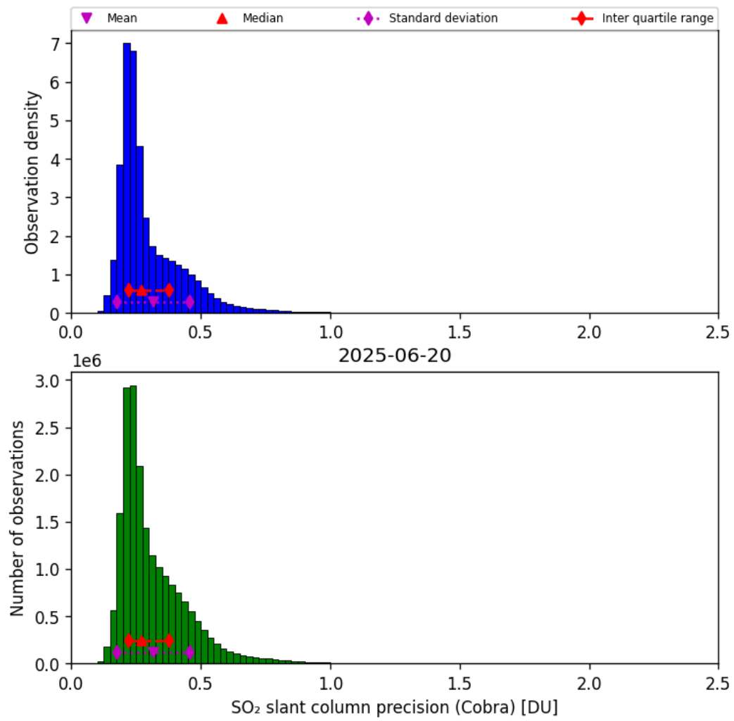
Figure 62: Histogram of “SO 2 slant column precision (Cobra)” for 2025-06-19 to 2025-06-21
