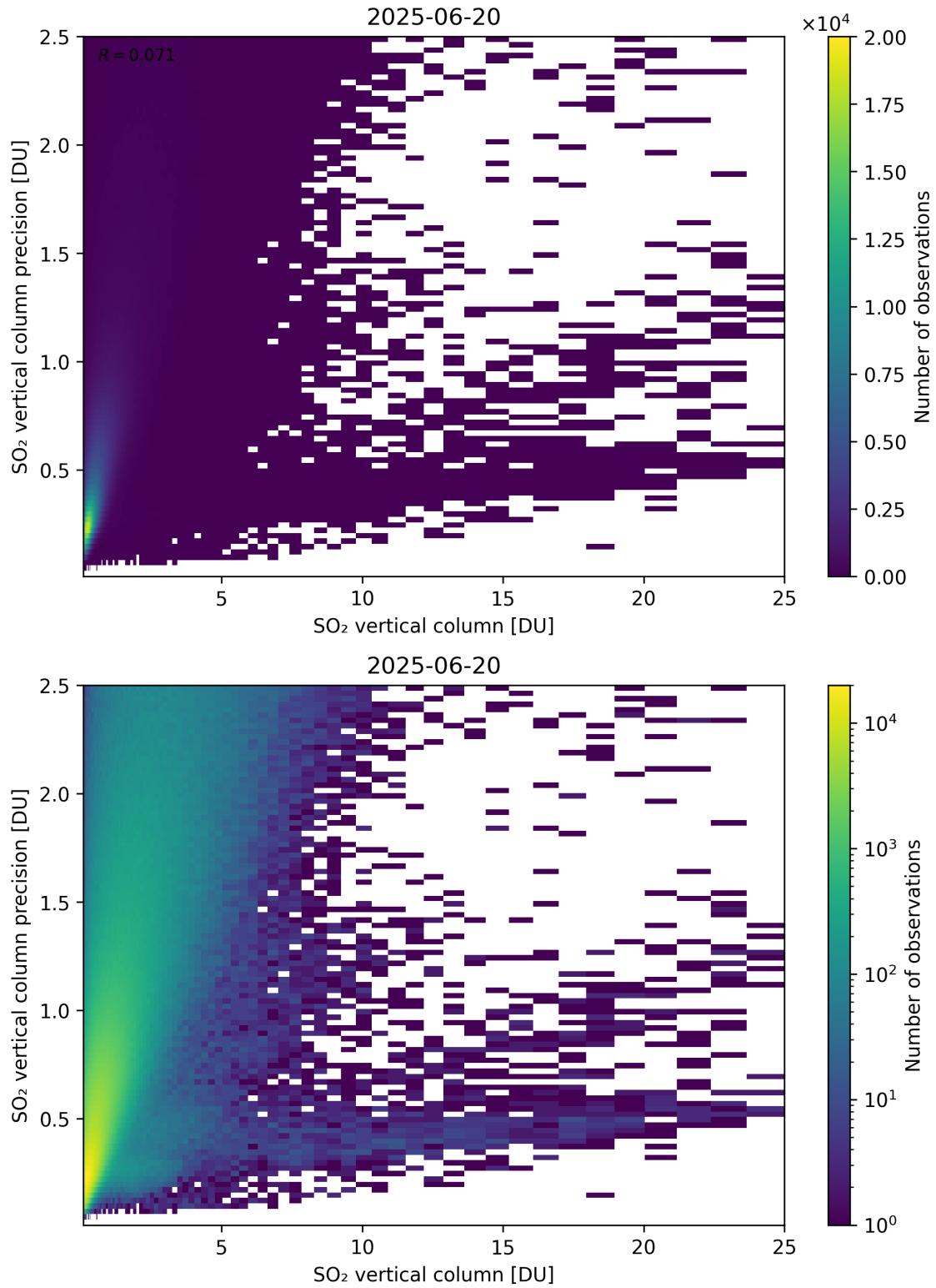
Figure 361: Scatter density plot of “SO 2 vertical column” against “SO 2 vertical column precision” for 2025-06-19 to 2025-06-21.
