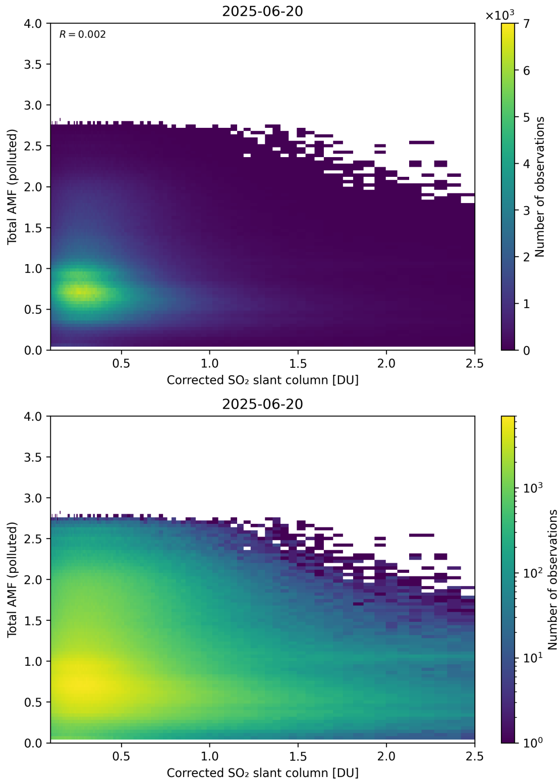
Figure 242: Scatter density plot of “Corrected SO 2 slant column” against “Total AMF (polluted)” for 2025-06-19 to 2025-06-21.
