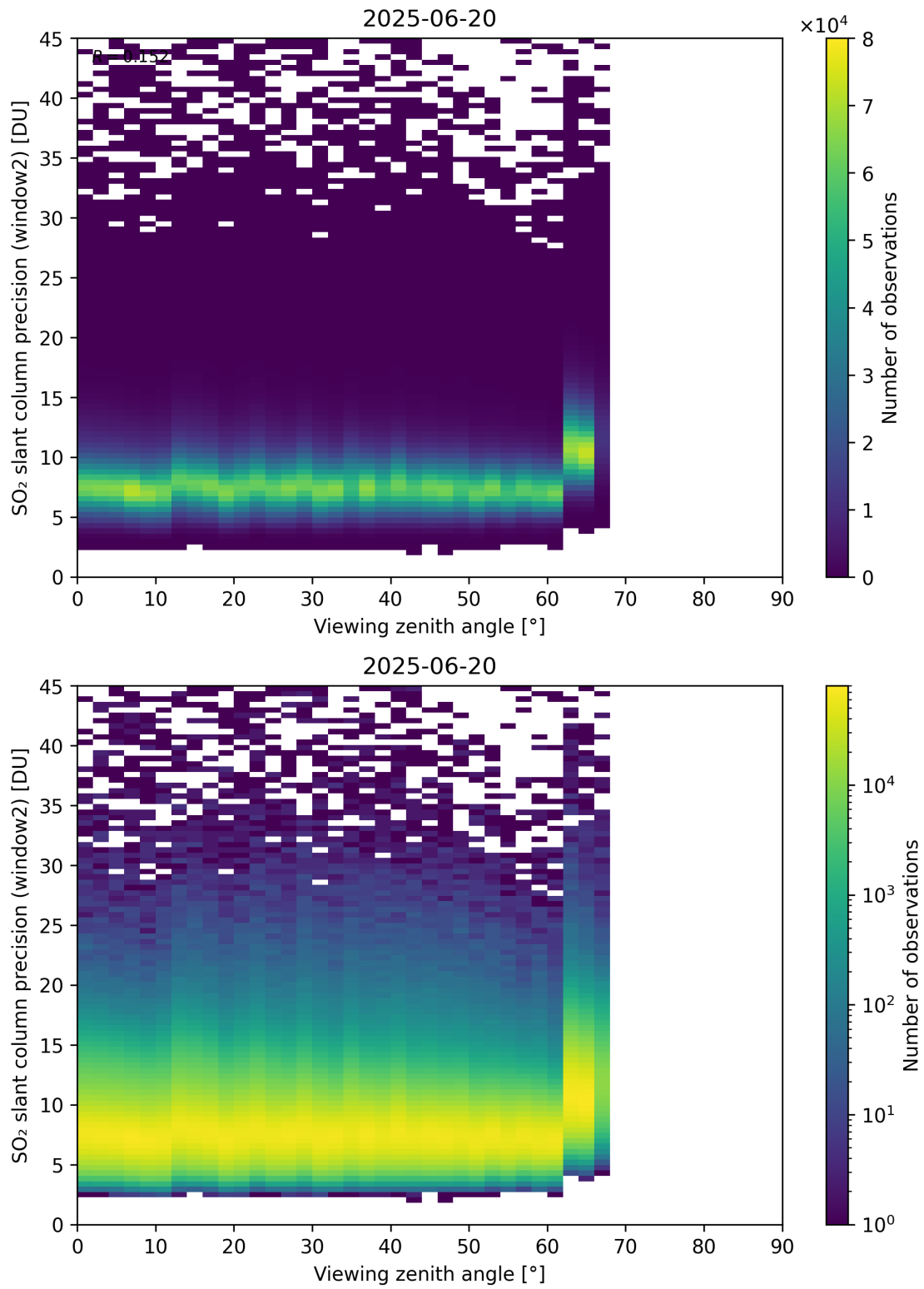
Figure 378: Scatter density plot of “Viewing zenith angle” against “SO 2 slant column precision (window2)” for 2025-06-19 to 2025-06-21.
