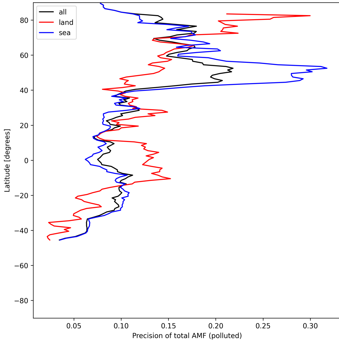
Figure 54: Zonal average of “Precision of total AMF (polluted)” for 2025-06-19 to 2025-06-21.
