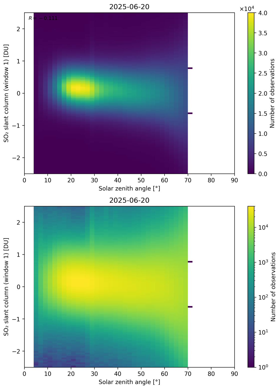
Figure 184: Scatter density plot of “Solar zenith angle” against “SO 2 slant column (window 1)” for 2025-06-19 to 2025-06-21.
