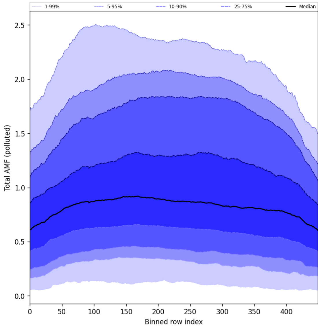
Figure 105: Along track statistics of “Total AMF (polluted)” for 2025-06-19 to 2025-06-21
