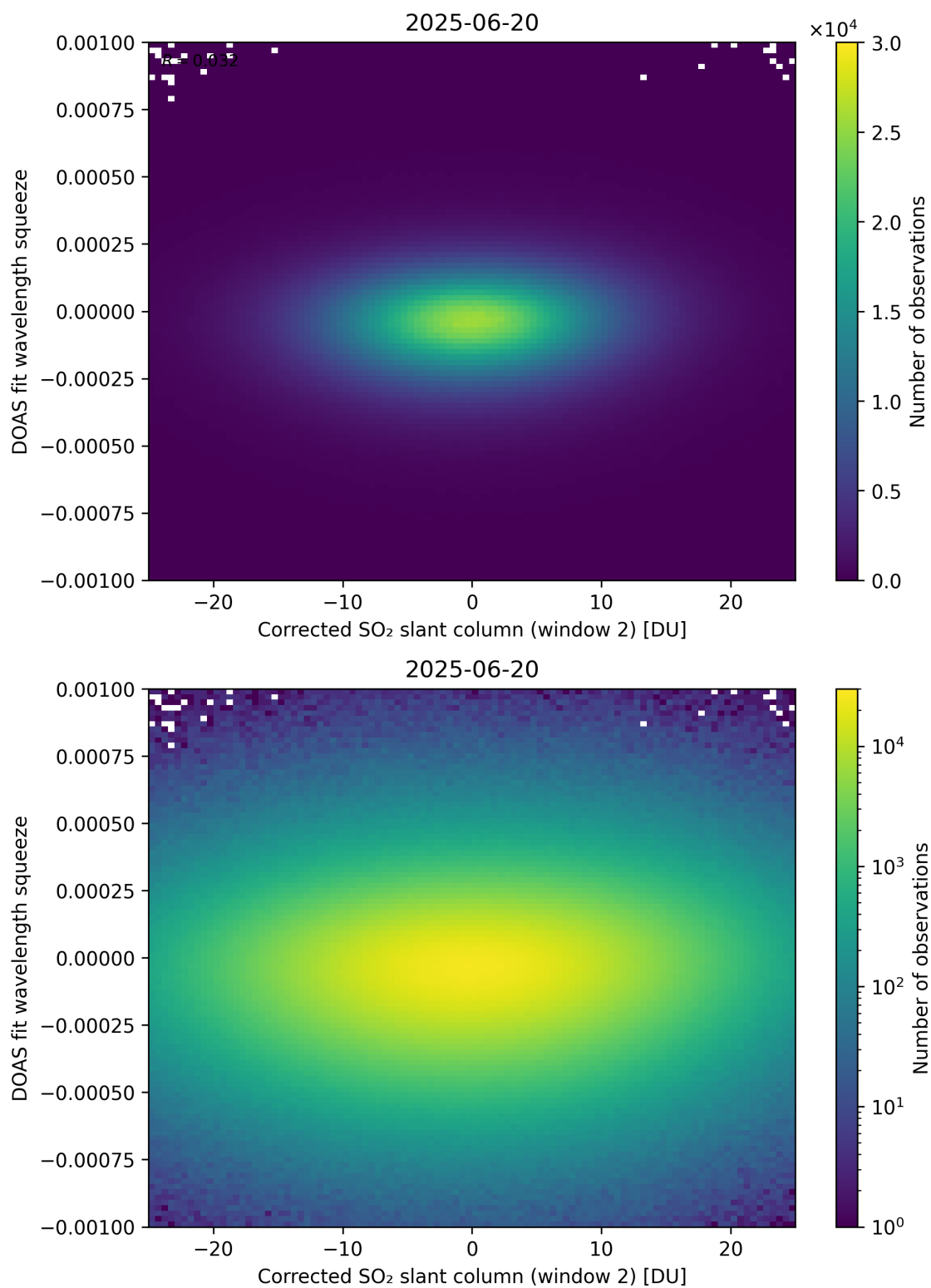
Figure 247: Scatter density plot of “Corrected SO 2 slant column (window 2)” against “DOAS fit wavelength squeeze” for 2025-06-19 to 2025-06-21.
