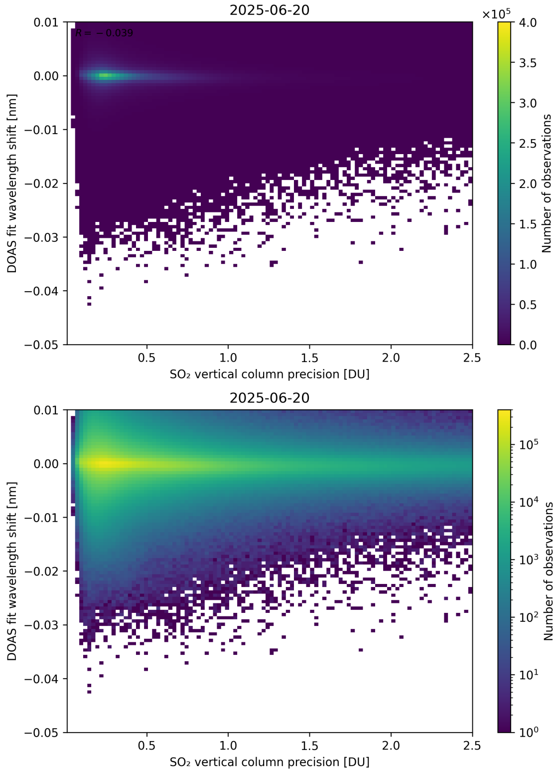
Figure 332: Scatter density plot of “SO 2 vertical column precision” against “DOAS fit wavelength shift” for 2025-06-19 to 2025-06-21.
