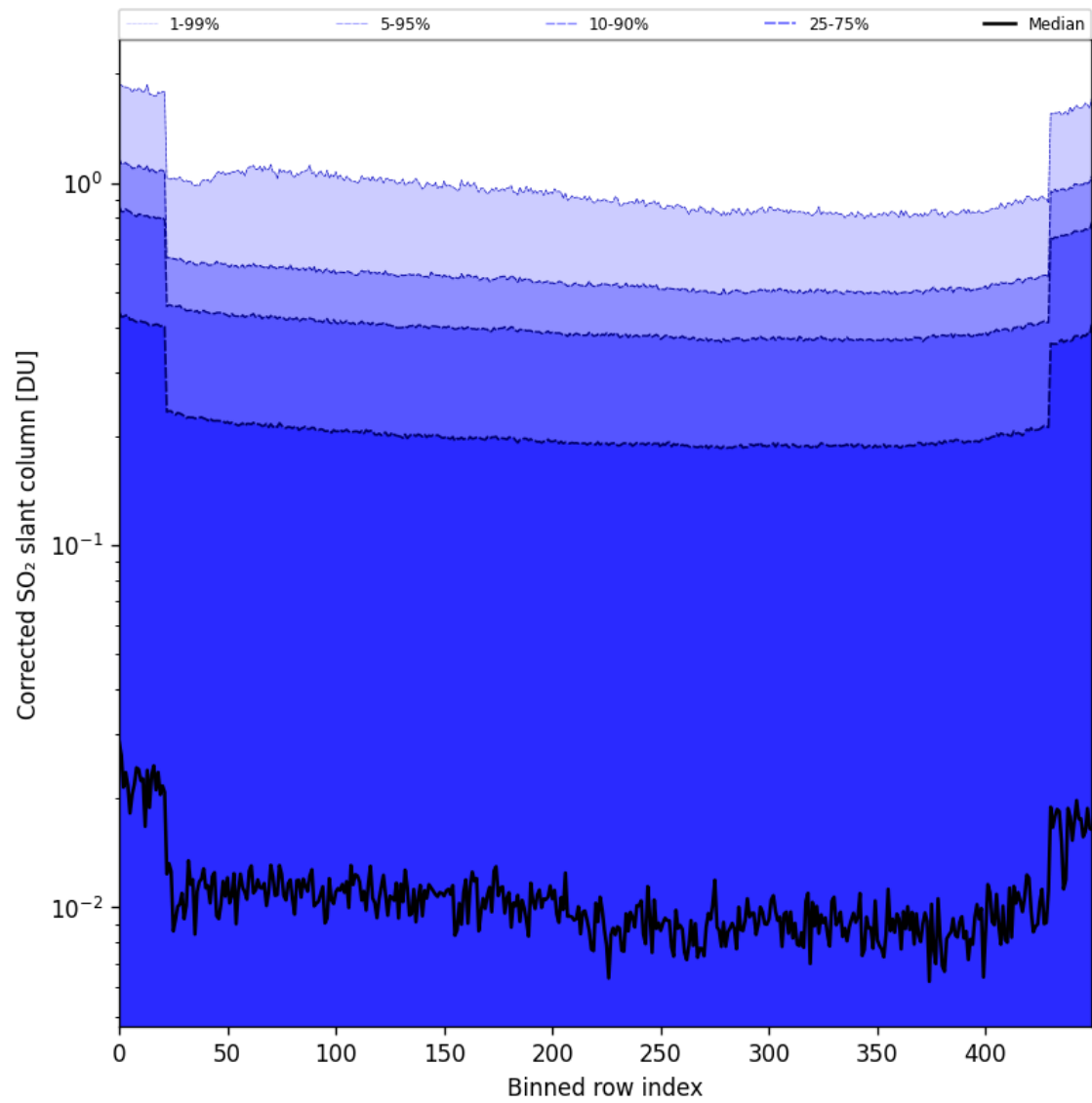
Figure 86: Along track statistics of “Corrected SO 2 slant column” for 2025-06-19 to 2025-06-21
