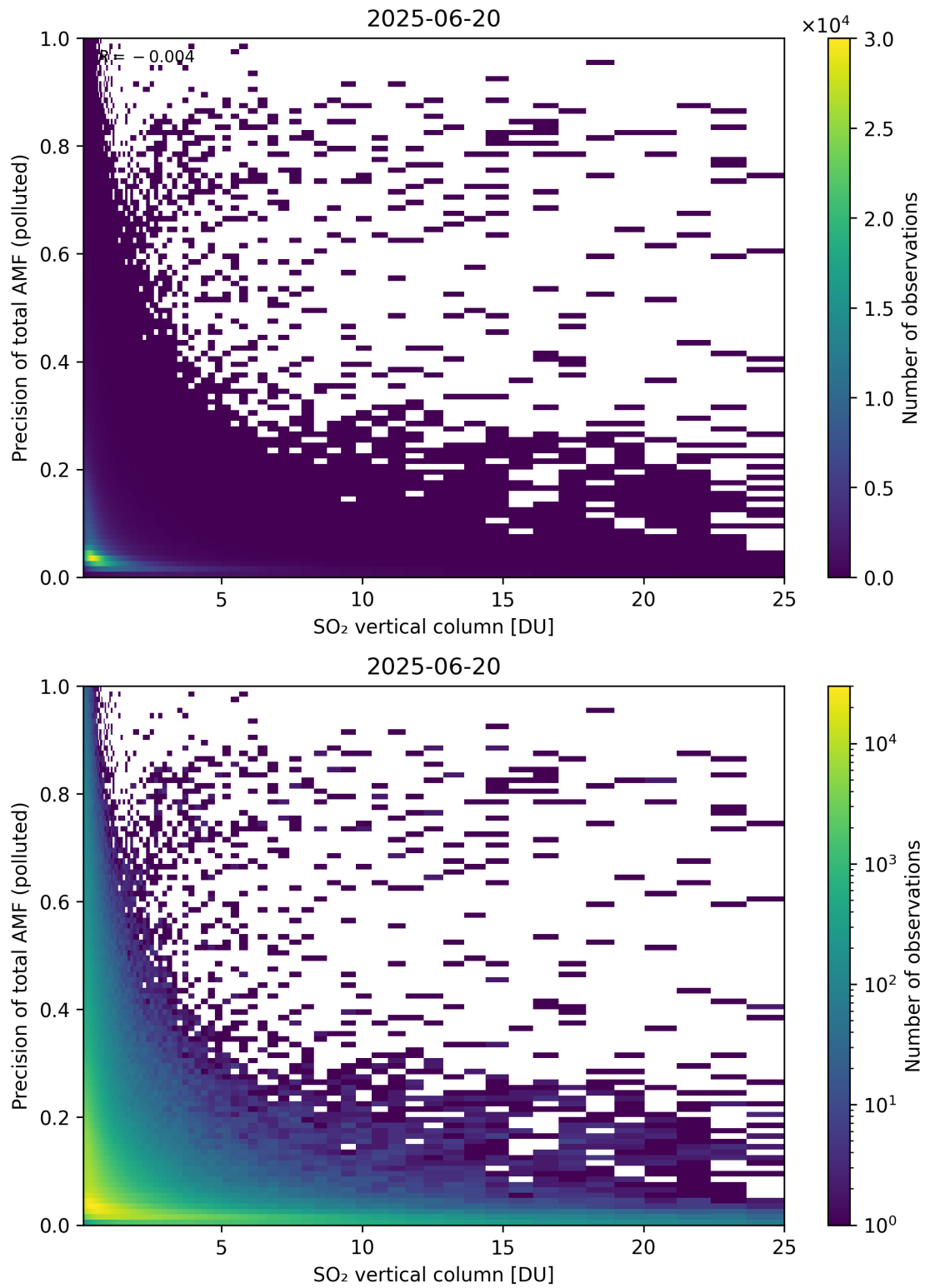
Figure 360: Scatter density plot of “SO 2 vertical column” against “Precision of total AMF (polluted)” for 2025-06-19 to 2025-06-21.
