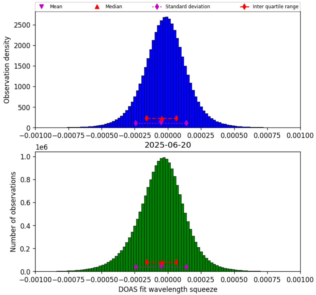
Figure 77: Histogram of “DOAS fit wavelength squeeze” for 2025-06-19 to 2025-06-21
