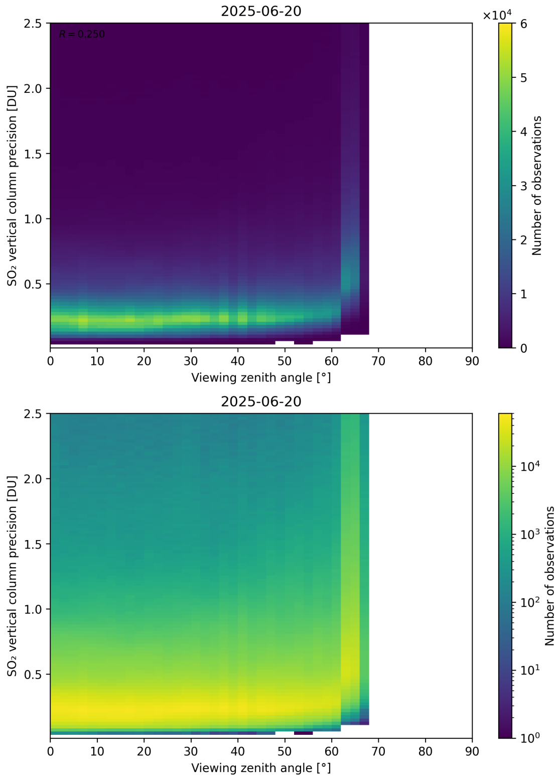
Figure 384: Scatter density plot of “Viewing zenith angle” against “SO 2 vertical column precision” for 2025-06-19 to 2025-06-21.
