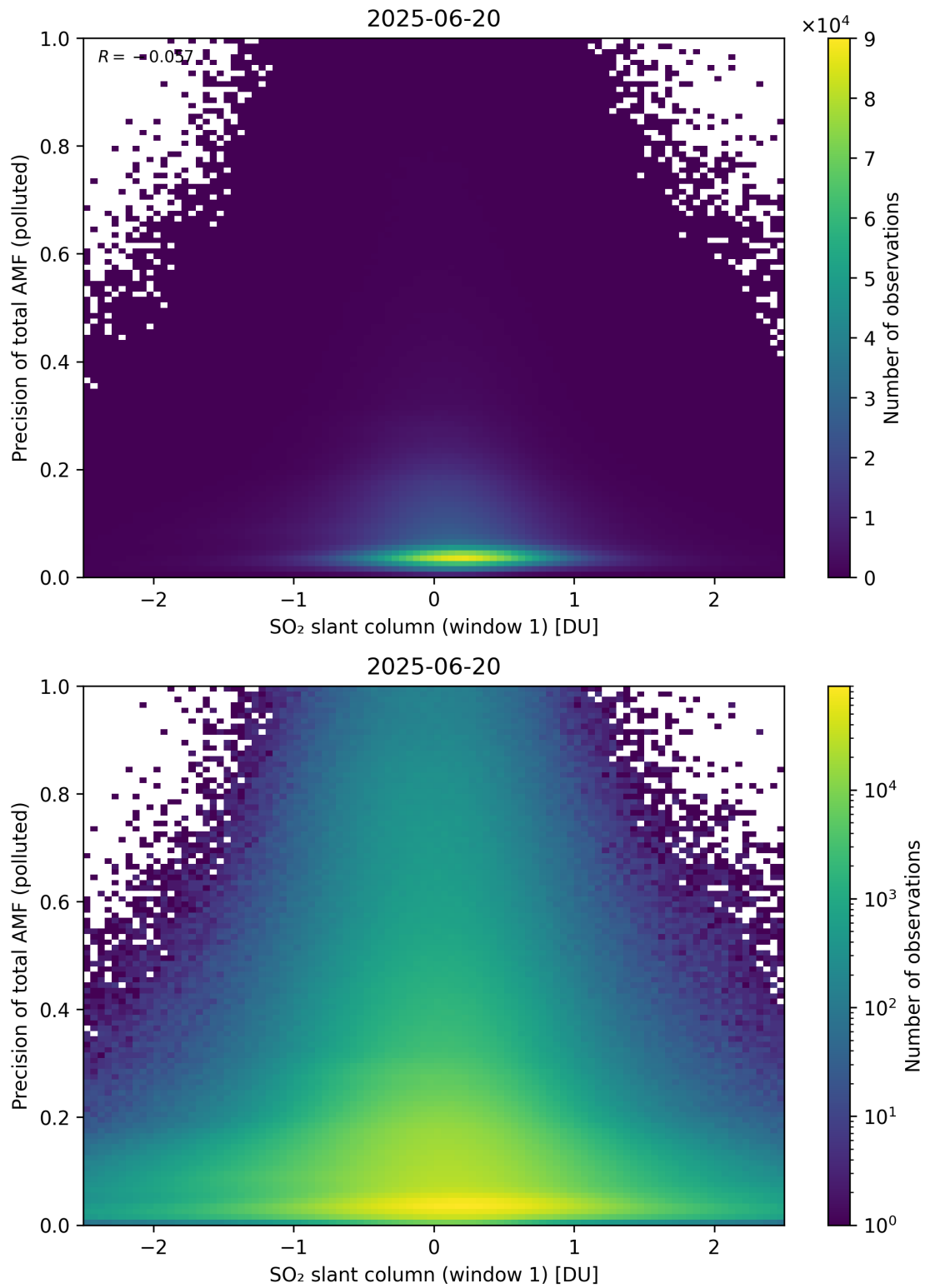
Figure 290: Scatter density plot of “SO 2 slant column (window 1)” against “Precision of total AMF (polluted)” for 2025-06-19 to 2025-06-21.
