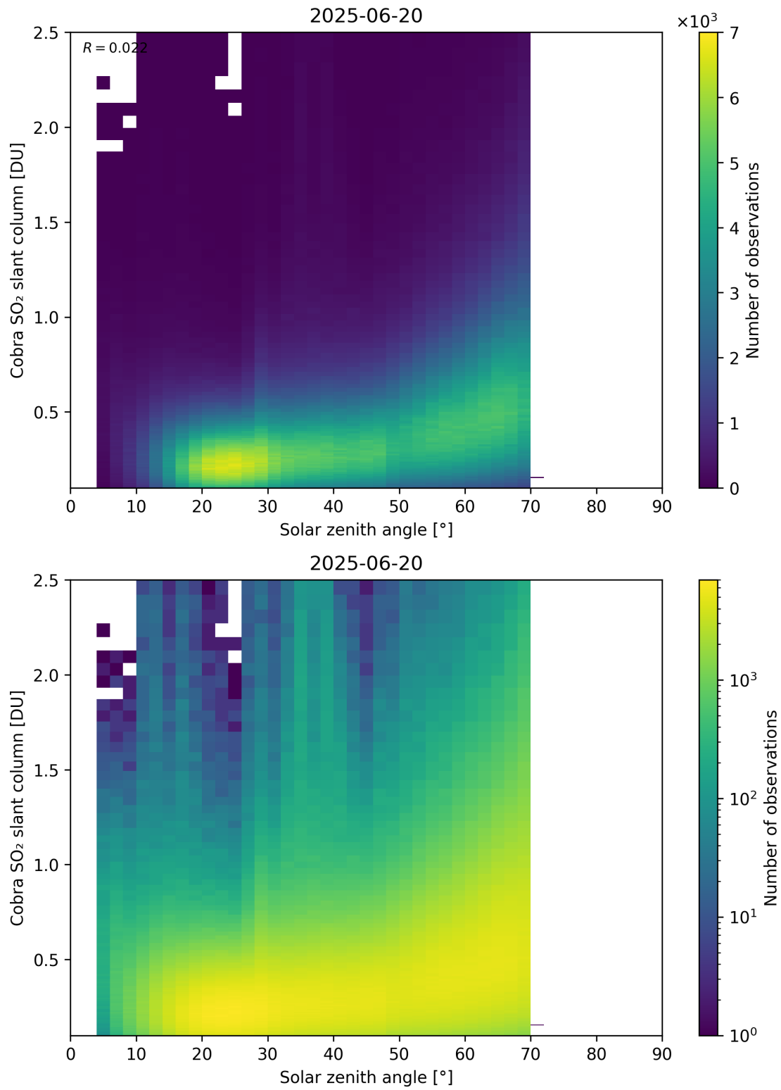
Figure 179: Scatter density plot of “Solar zenith angle” against “Cobra SO 2 slant column” for 2025-06-19 to 2025-06-21.
