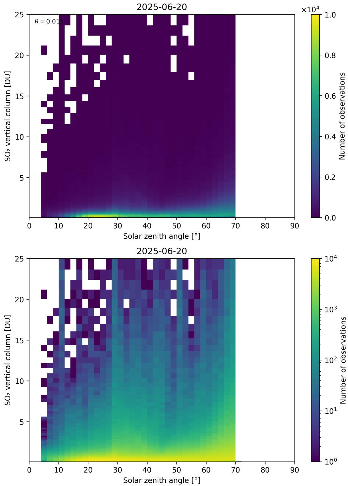
Figure 191: Scatter density plot of “Solar zenith angle” against “SO 2 vertical column” for 2025-06-19 to 2025-06-21.
