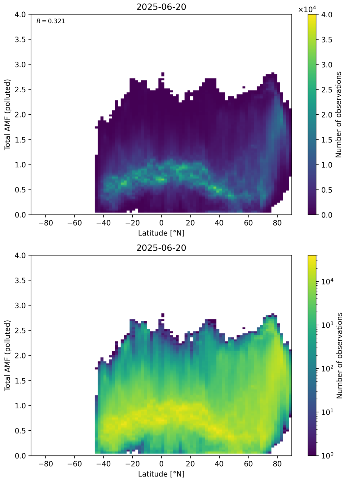
Figure 167: Scatter density plot of “Latitude” against “Total AMF (polluted)” for 2025-06-19 to 2025-06-21.
