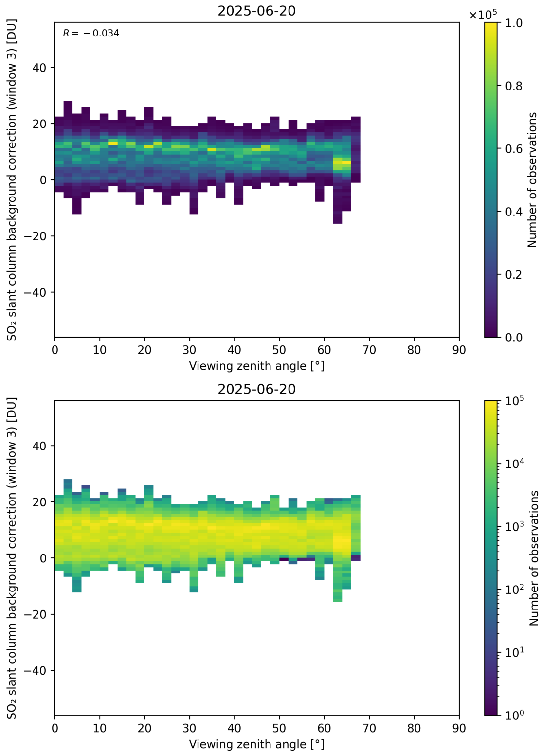
Figure 364: Scatter density plot of “Viewing zenith angle” against “SO 2 slant column background correction (window 3)” for 2025-06-19 to 2025-06-21.
