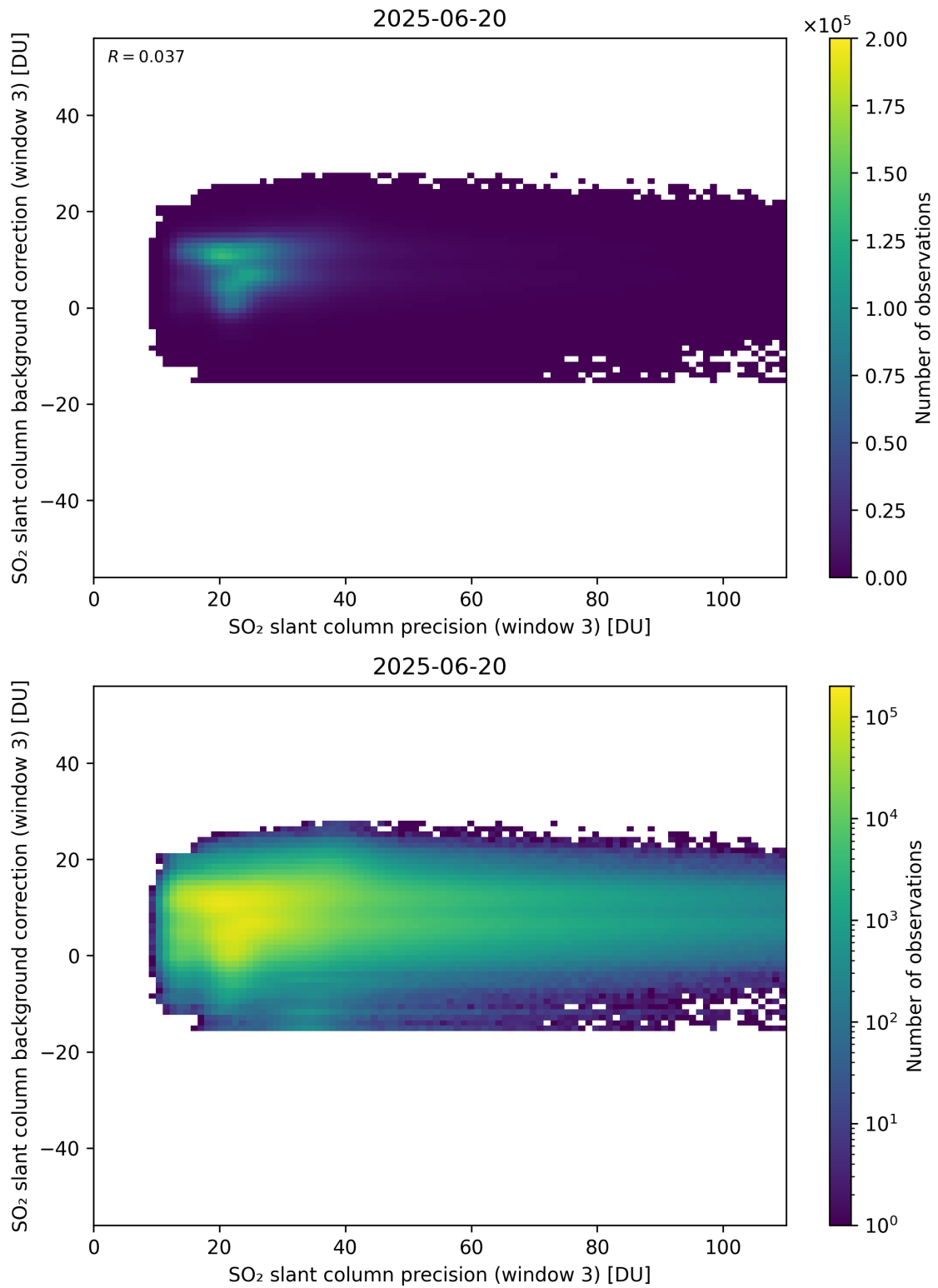
Figure 307: Scatter density plot of “SO 2 slant column precision (window 3)” against “SO 2 slant column background correction (window 3)” for 2025-06-19 to 2025-06-21.
