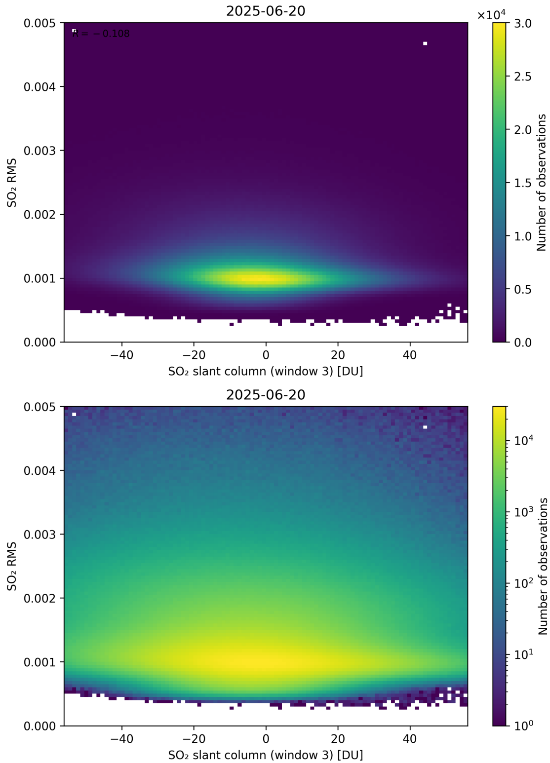
Figure 306: Scatter density plot of “SO 2 slant column (window 3)” against “SO 2 RMS” for 2025-06-19 to 2025-06-21.
