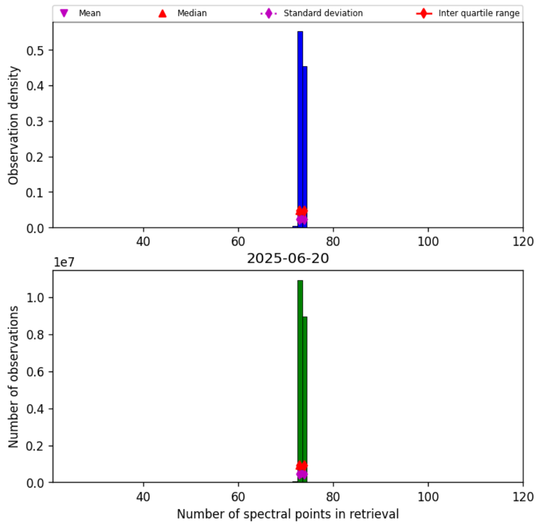
Figure 82: Histogram of “Number of spectral points in retrieval” for 2025-06-19 to 2025-06-21
