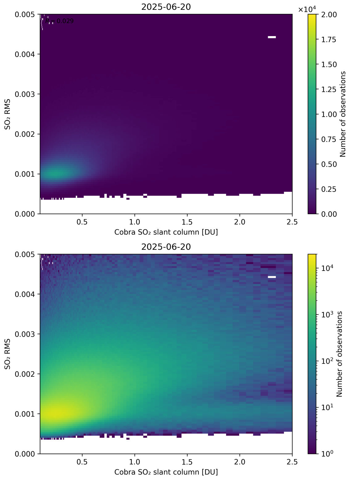
Figure 198: Scatter density plot of “Cobra SO 2 slant column” against “SO 2 RMS” for 2025-06-19 to 2025-06-21.
