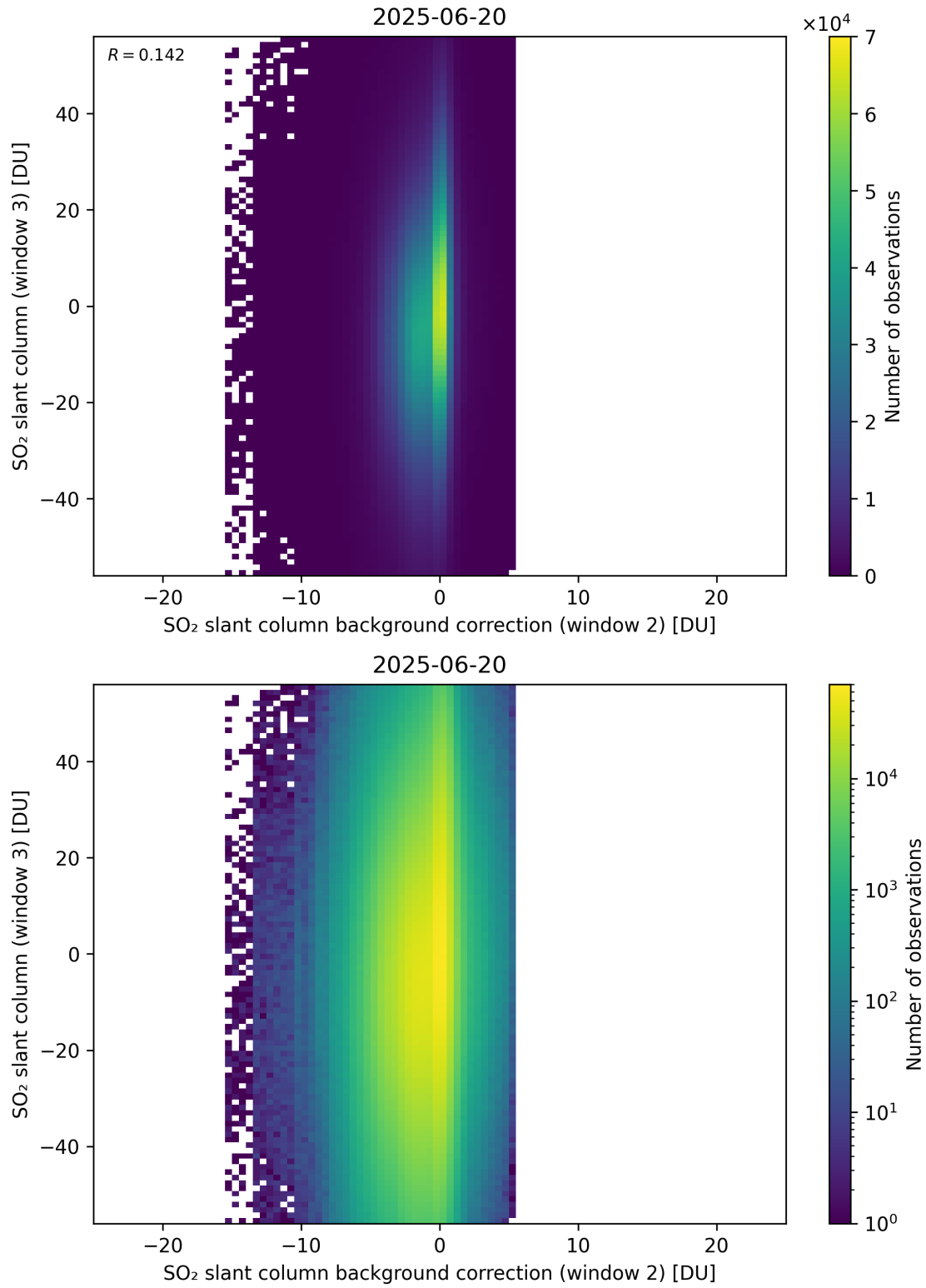
Figure 128: Scatter density plot of “SO 2 slant column background correction (window 2)” against “SO 2 slant column (window 3)” for 2025-06-19 to 2025-06-21.
