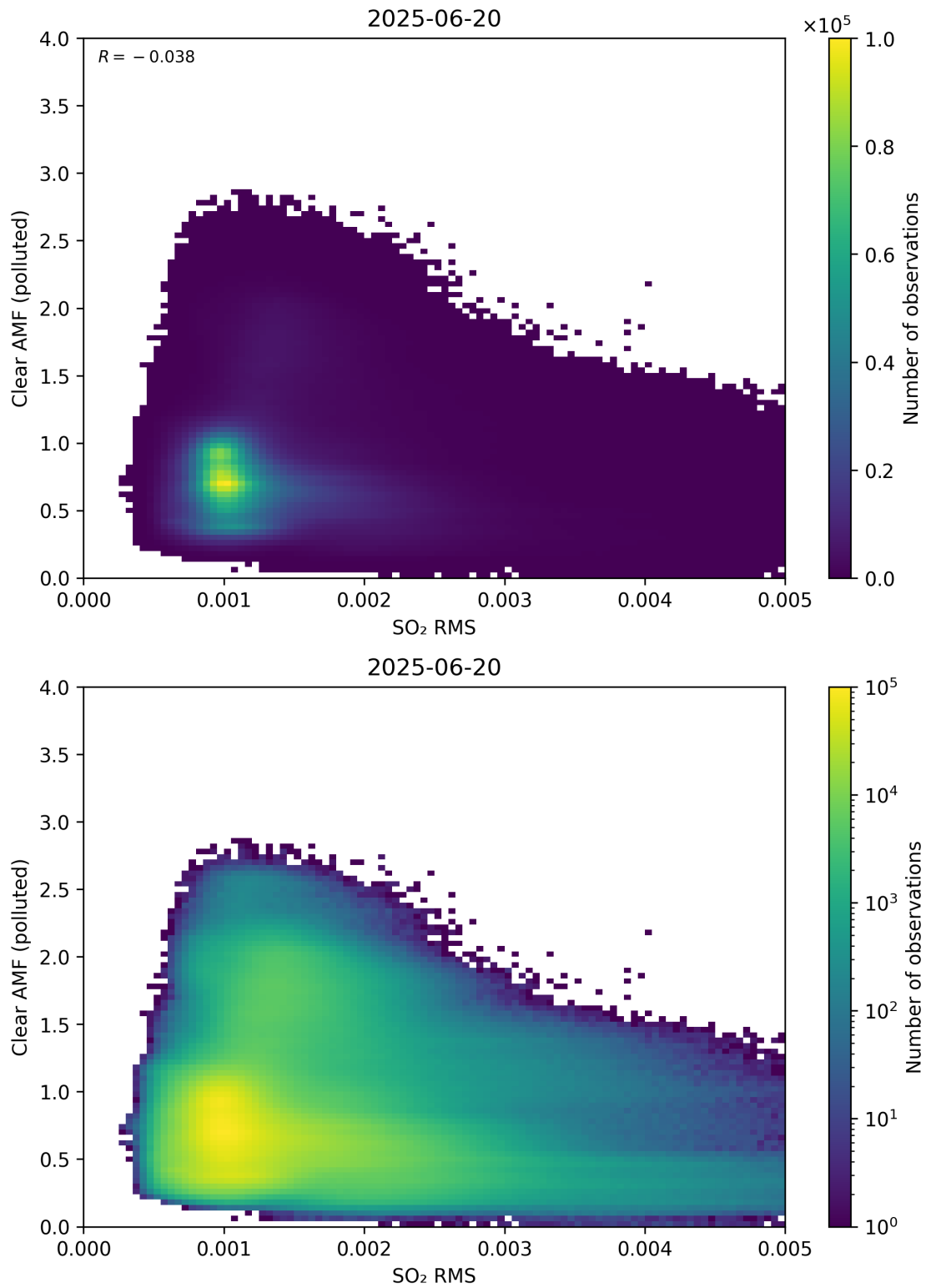
Figure 147: Scatter density plot of “SO 2 RMS” against “Clear AMF (polluted)” for 2025-06-19 to 2025-06-21.
