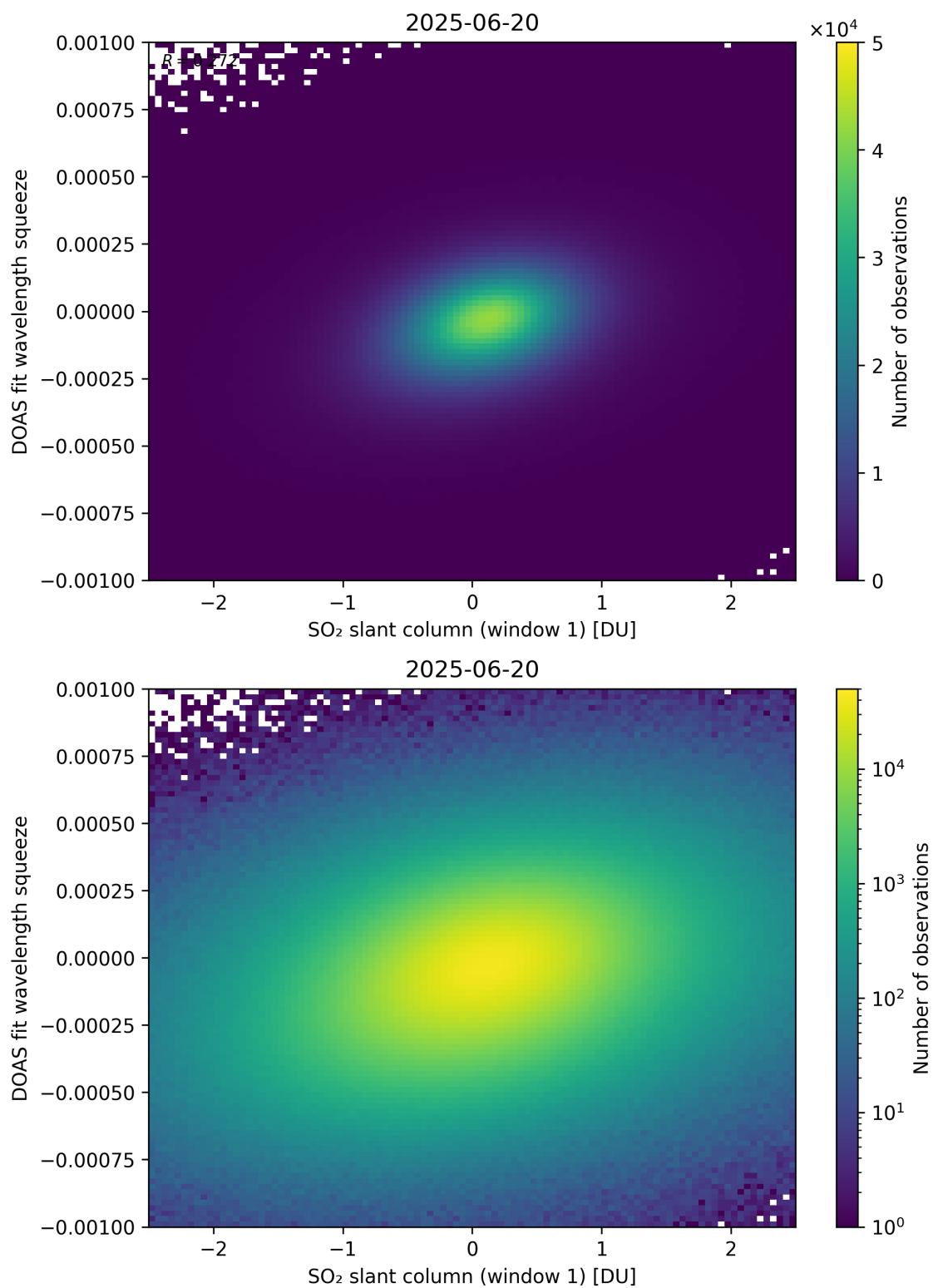
Figure 266: Scatter density plot of “SO 2 slant column (window 1)” against “DOAS fit wavelength squeeze” for 2025-06-19 to 2025-06-21.
