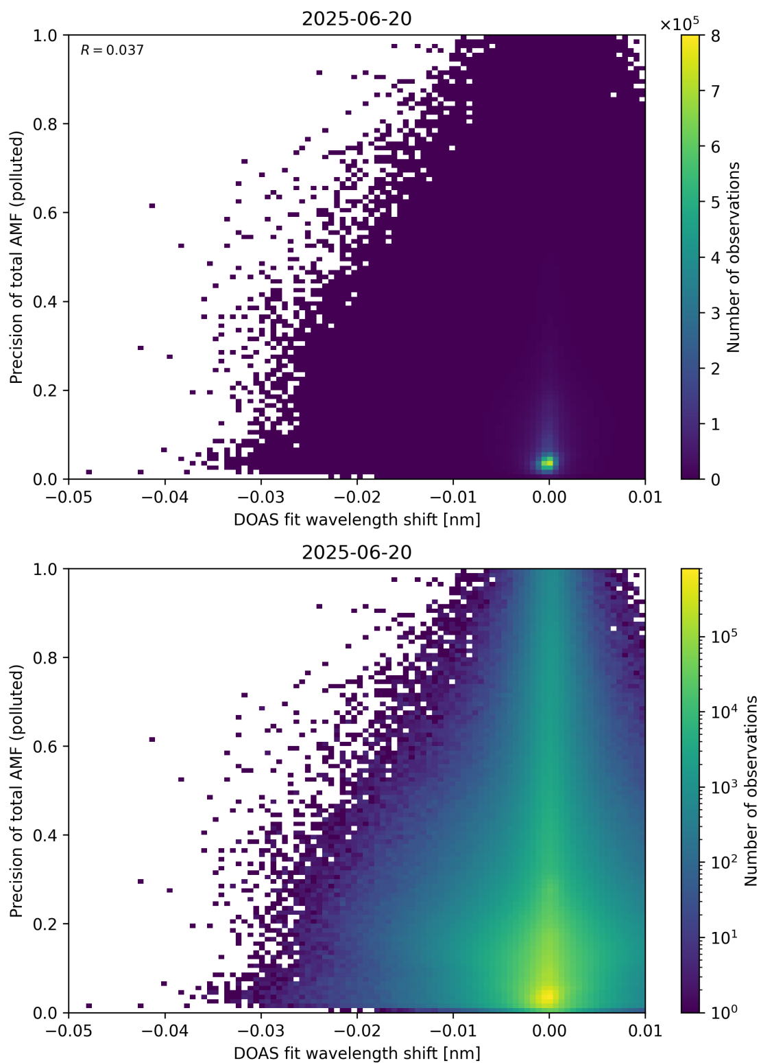
Figure 142: Scatter density plot of “DOAS fit wavelength shift” against “Precision of total AMF (polluted)” for 2025-06-19 to 2025-06-21.
