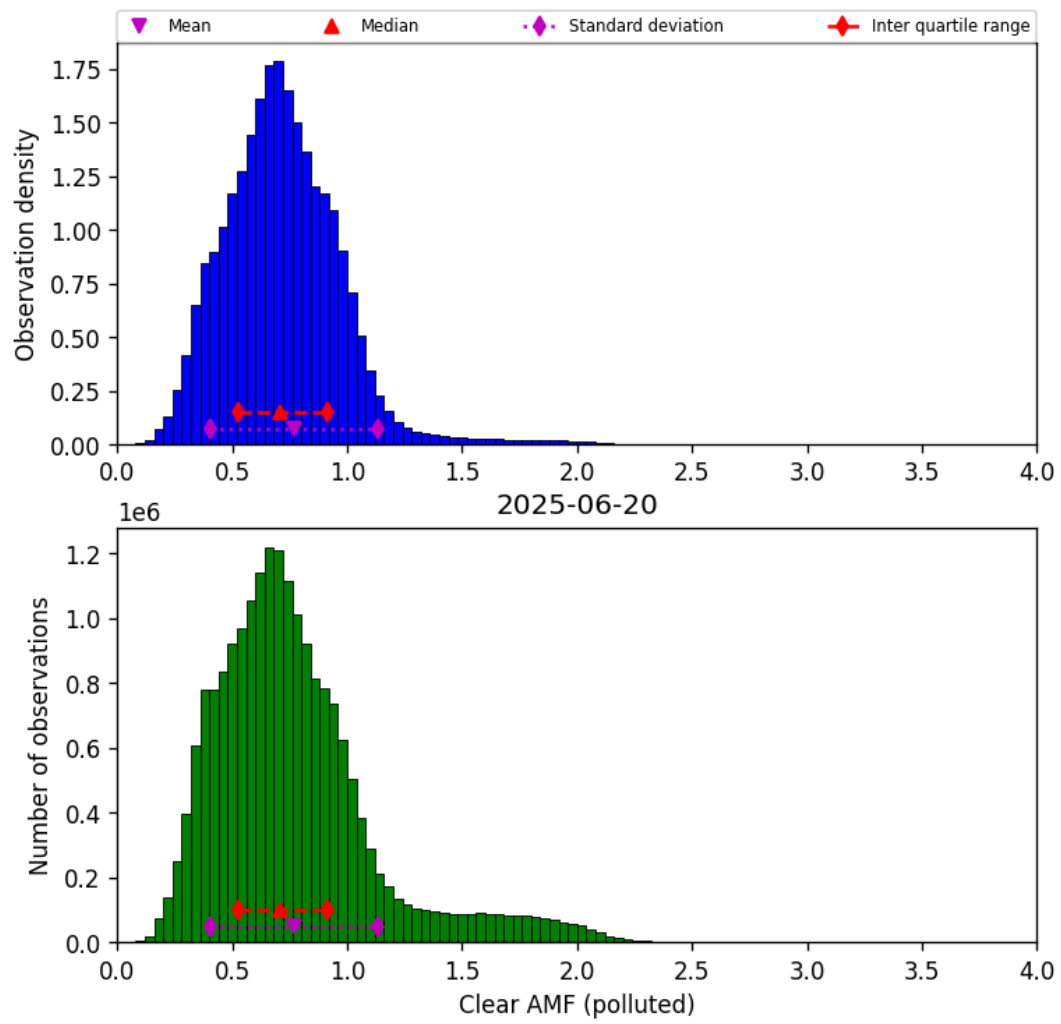
Figure 81: Histogram of “Clear AMF (polluted)” for 2025-06-19 to 2025-06-21
