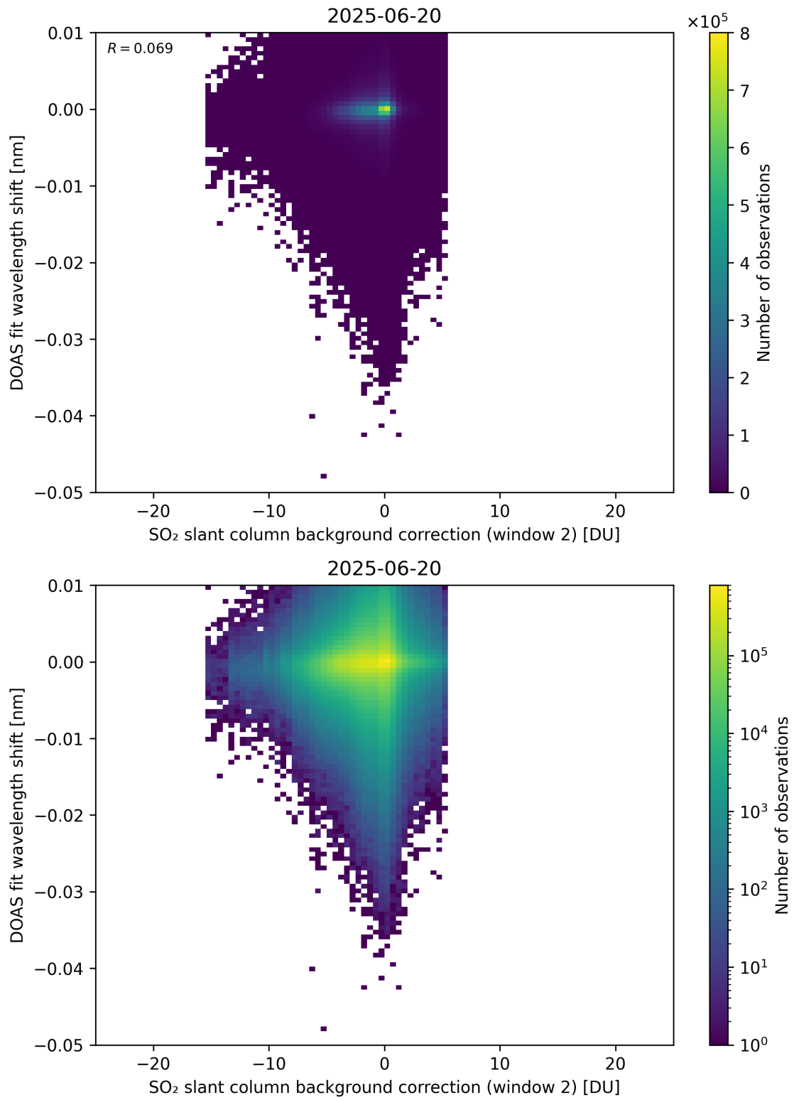
Figure 123: Scatter density plot of “SO 2 slant column background correction (window 2)” against “DOAS fit wavelength shift” for 2025-06-19 to 2025-06-21.
