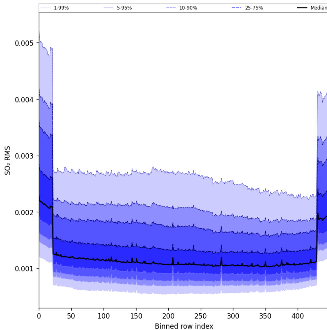
Figure 104: Along track statistics of “SO 2 RMS” for 2025-06-19 to 2025-06-21
