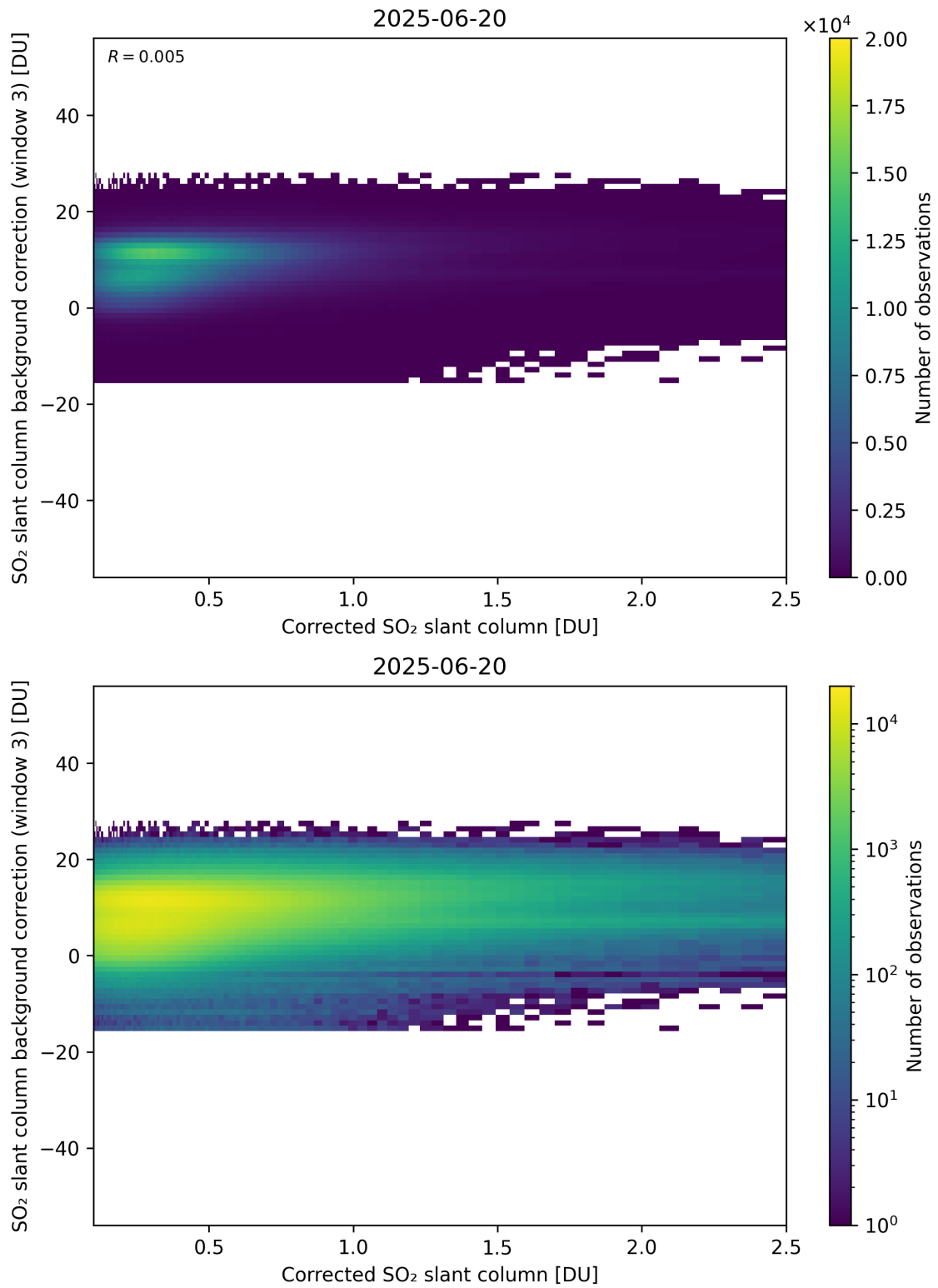
Figure 228: Scatter density plot of “Corrected SO 2 slant column” against “SO 2 slant column background correction (window 3)” for 2025-06-19 to 2025-06-21.
