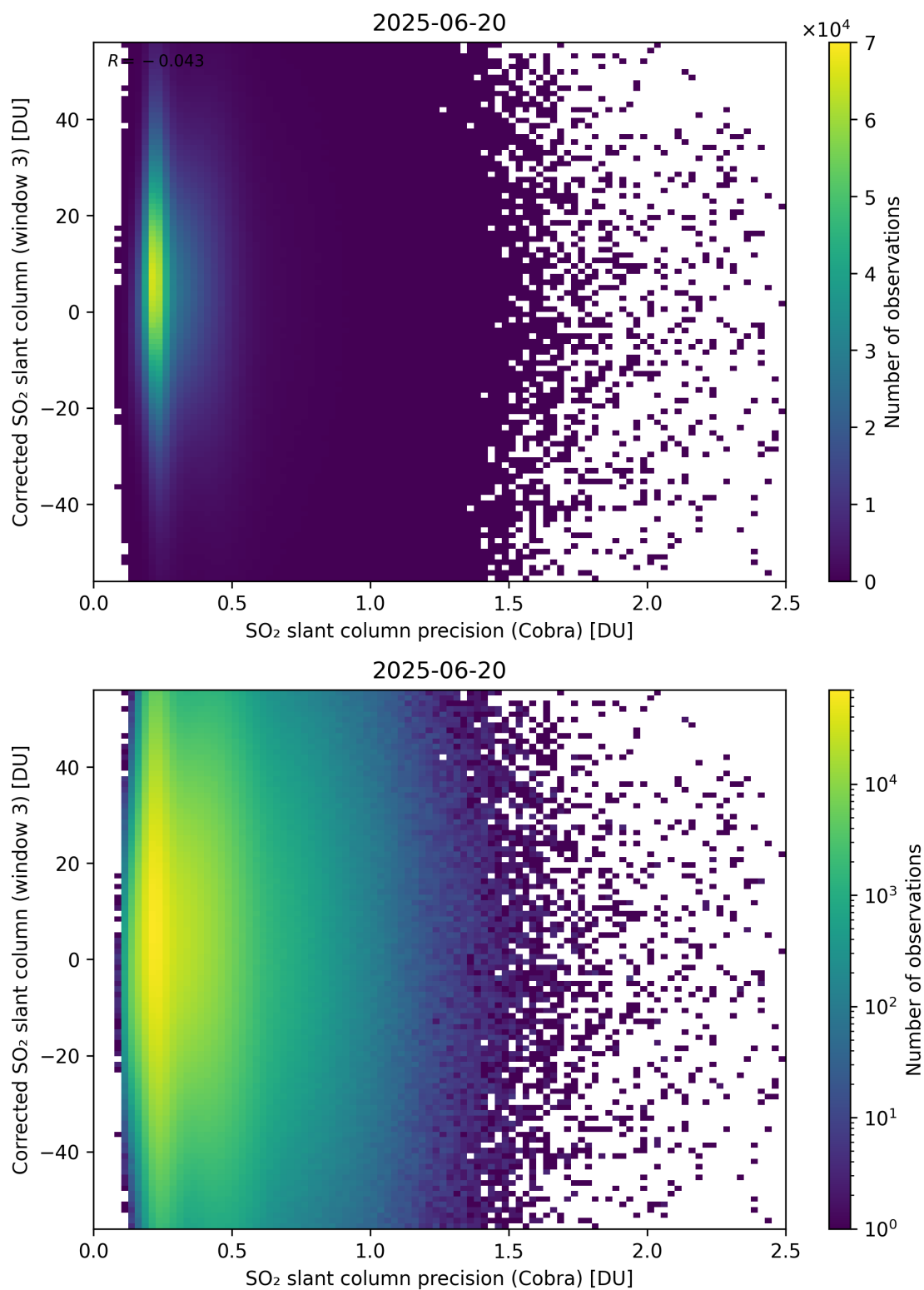
Figure 207: Scatter density plot of “SO 2 slant column precision (Cobra)” against “Corrected SO 2 slant column (window 3)” for 2025-06-19 to 2025-06-21.
