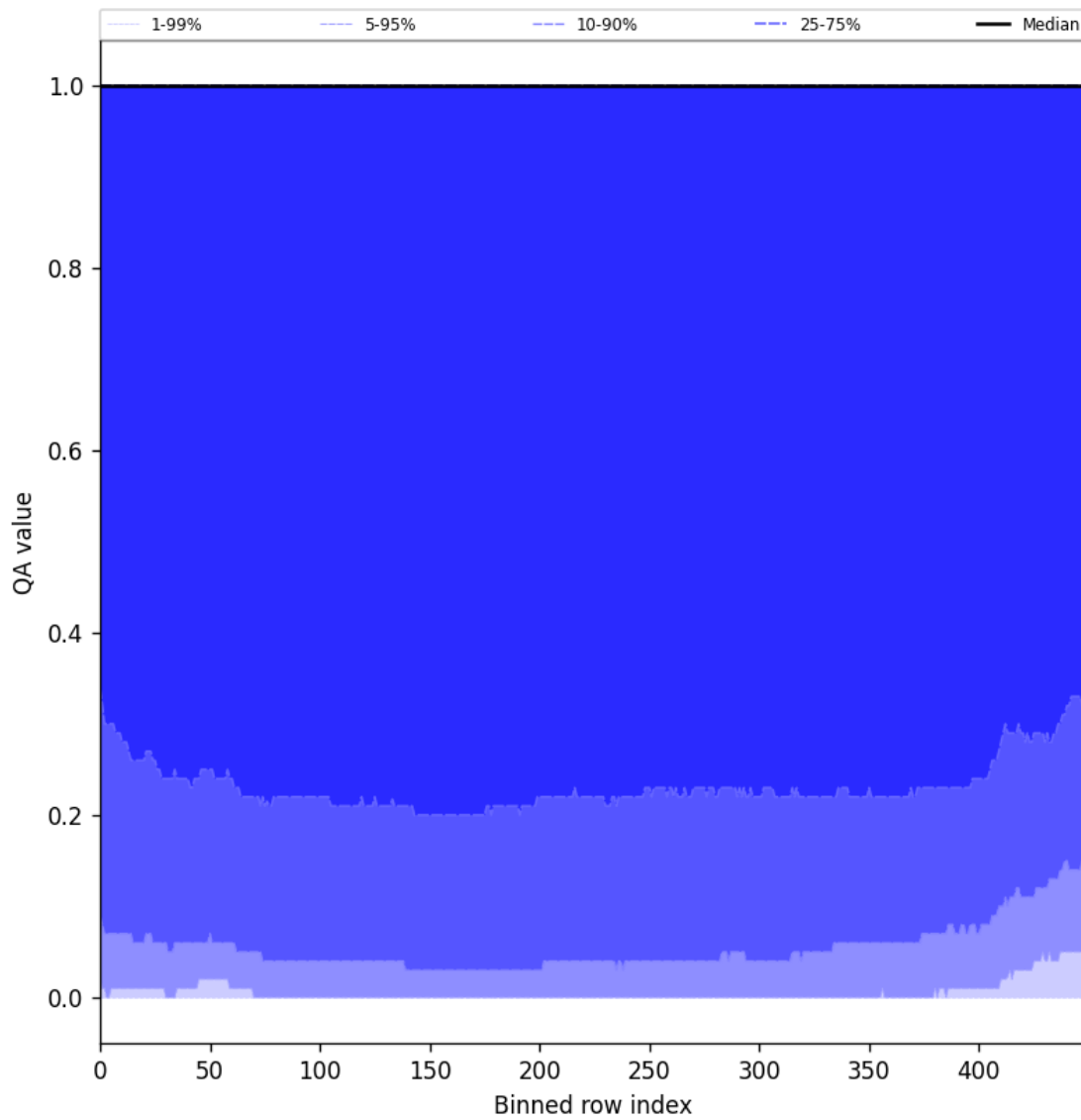
Figure 83: Along track statistics of “QA value” for 2025-06-19 to 2025-06-21
