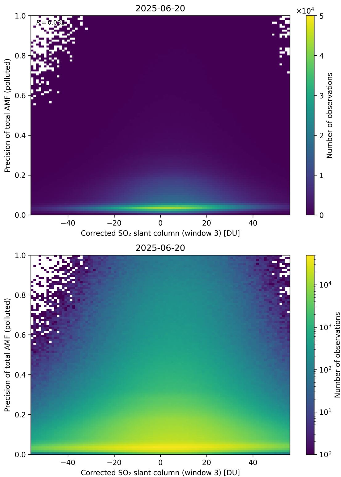
Figure 261: Scatter density plot of “Corrected SO 2 slant column (window 3)” against “Precision of total AMF (polluted)” for 2025-06-19 to 2025-06-21.
