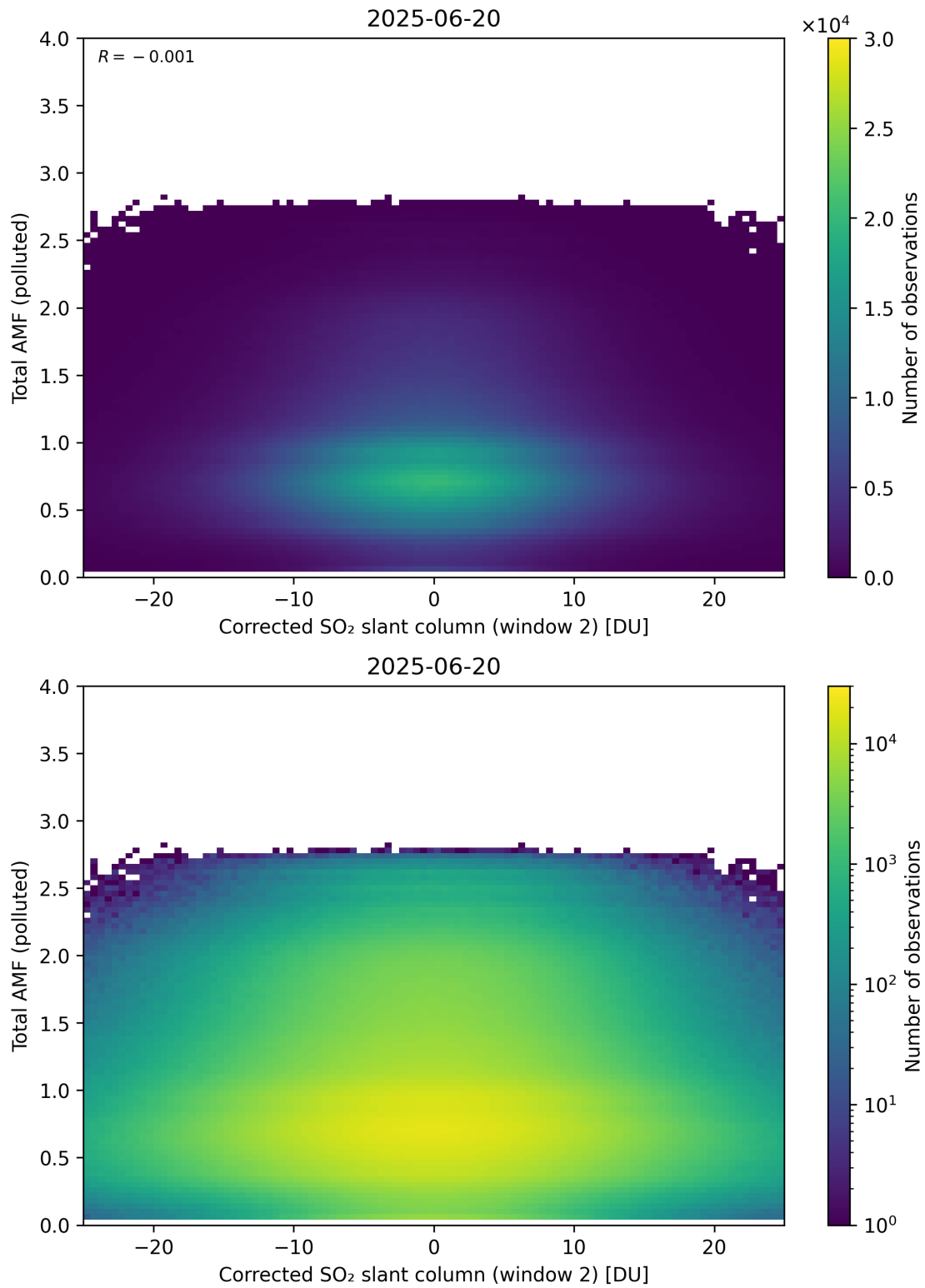
Figure 253: Scatter density plot of “Corrected SO 2 slant column (window 2)” against “Total AMF (polluted)” for 2025-06-19 to 2025-06-21.
