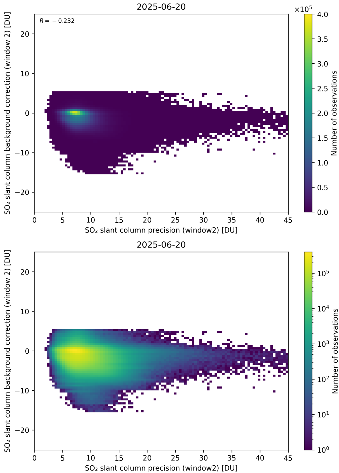
Figure 291: Scatter density plot of “SO 2 slant column precision (window2)” against “SO 2 slant column background correction (window 2)” for 2025-06-19 to 2025-06-21.
