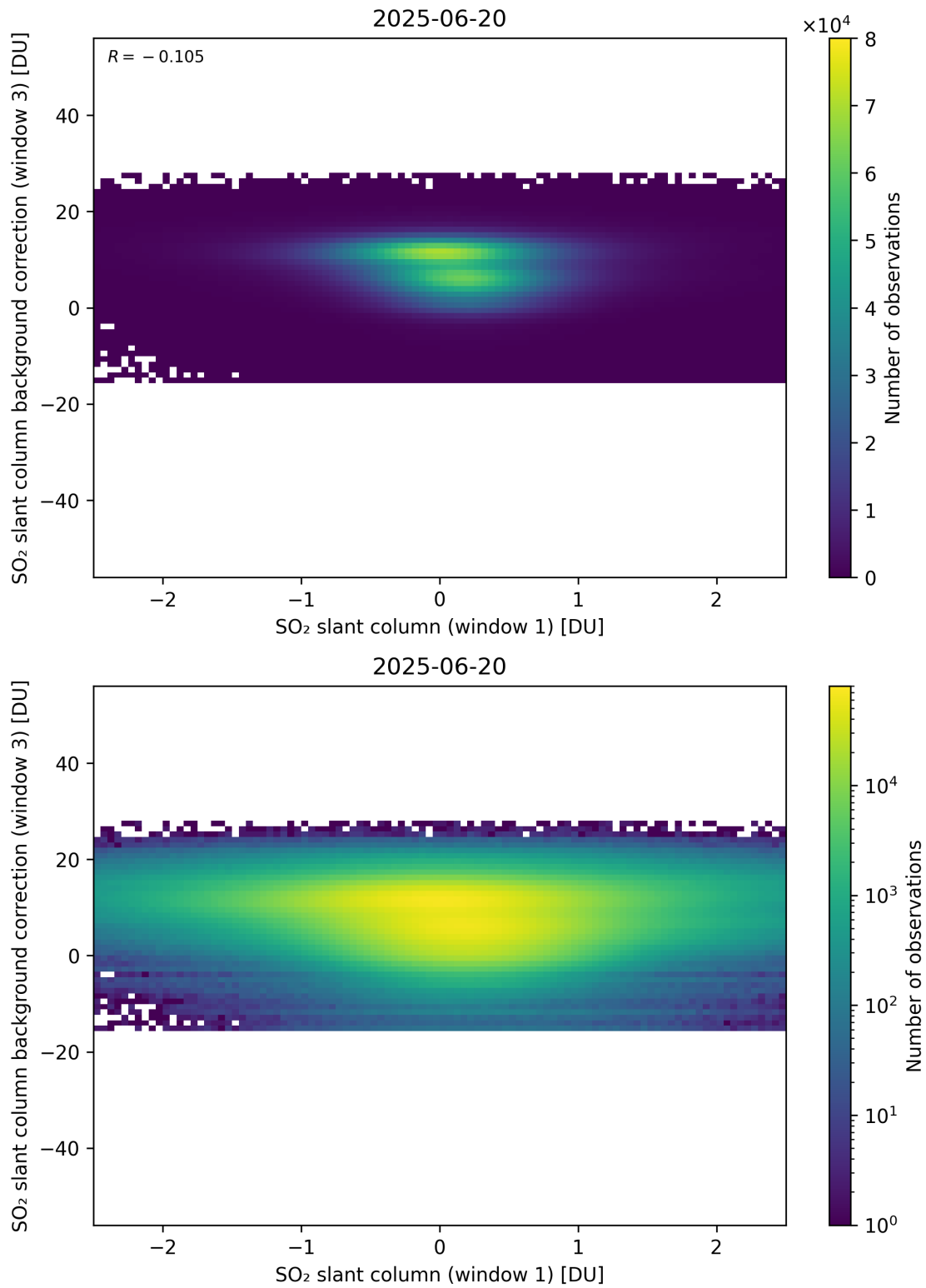
Figure 264: Scatter density plot of “SO 2 slant column (window 1)” against “SO 2 slant column background correction (window 3)” for 2025-06-19 to 2025-06-21.
