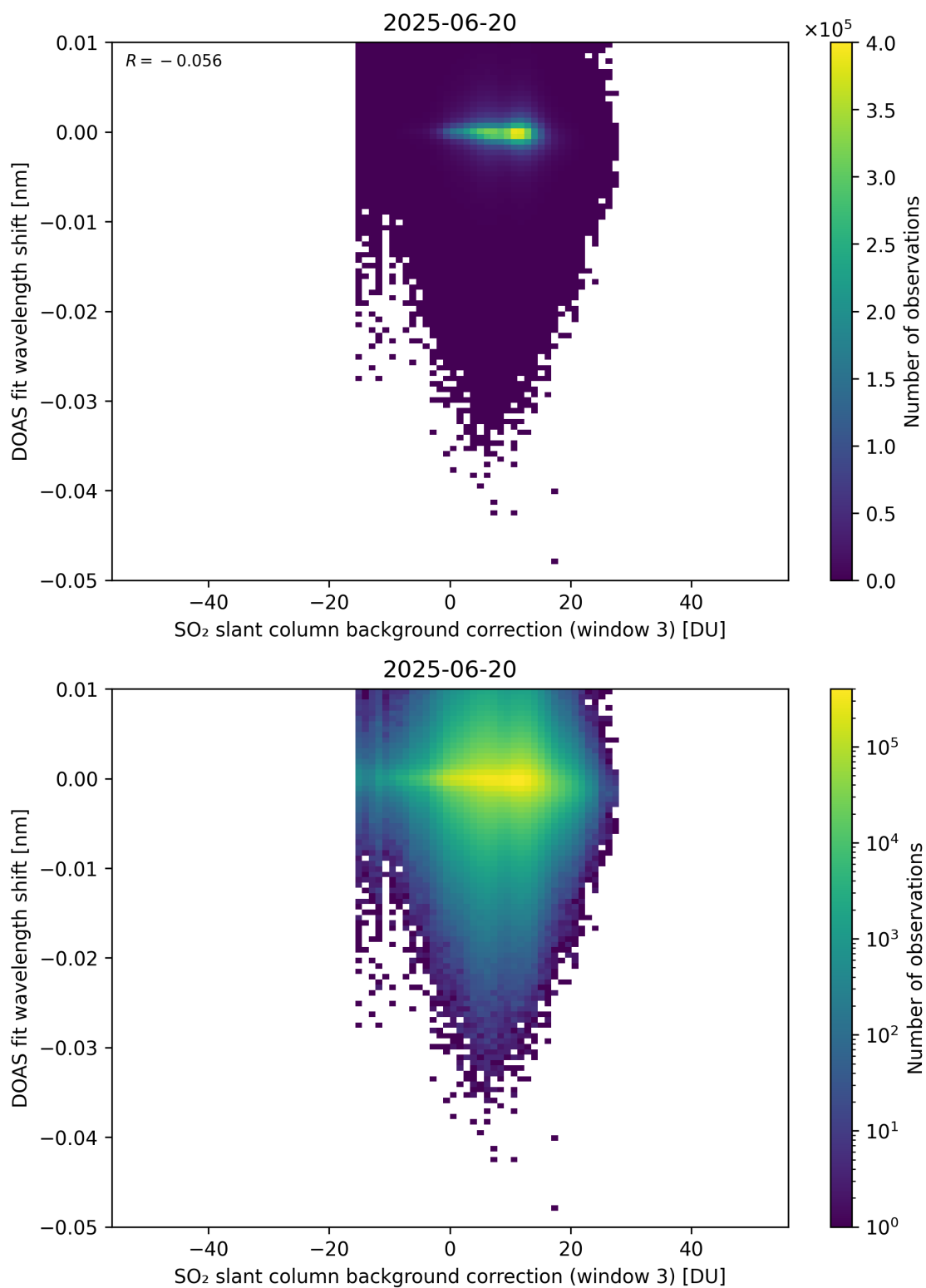
Figure 132: Scatter density plot of “SO 2 slant column background correction (window 3)” against “DOAS fit wavelength shift” for 2025-06-19 to 2025-06-21.
