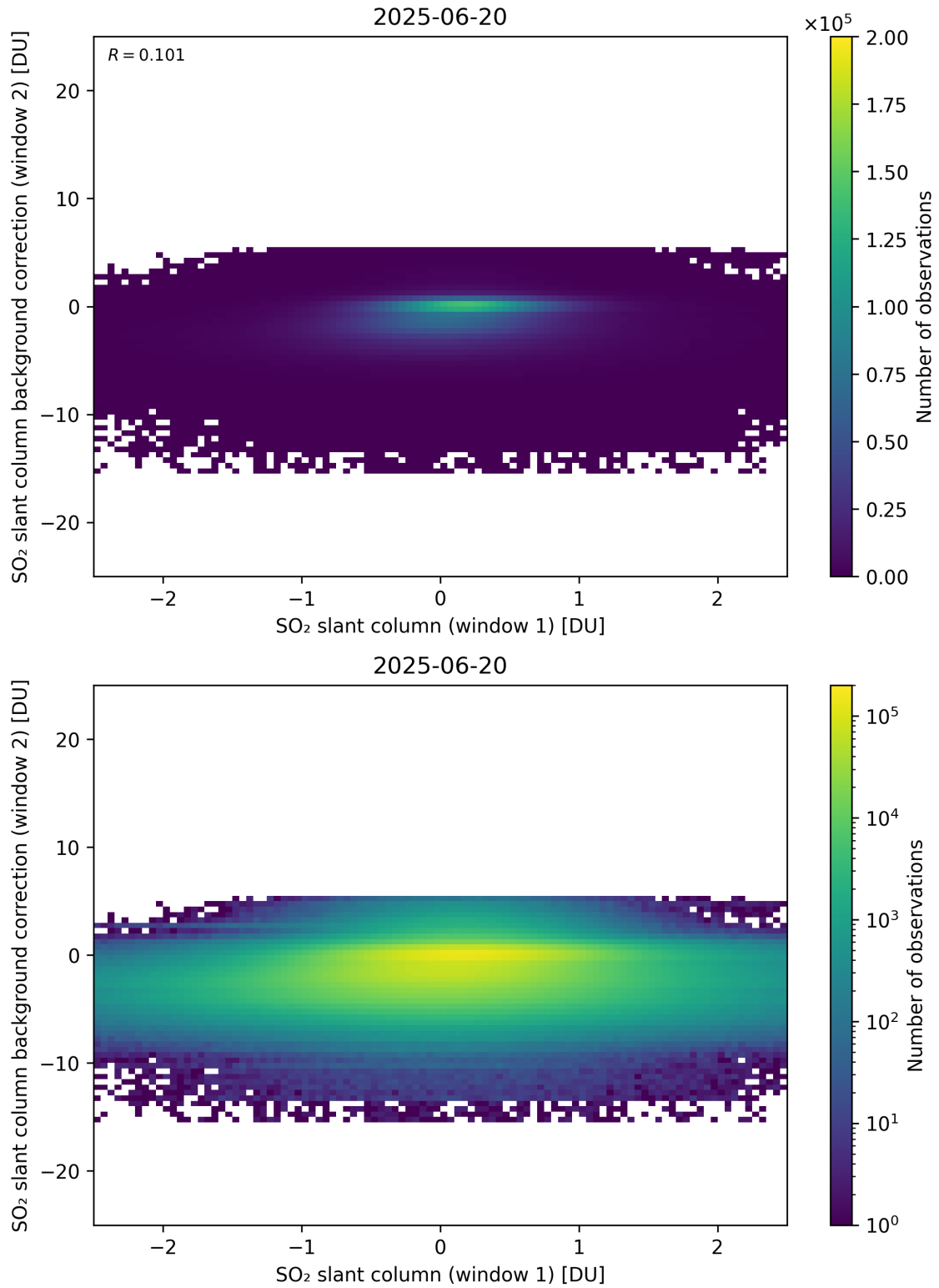
Figure 263: Scatter density plot of “SO 2 slant column (window 1)” against “SO 2 slant column background correction (window 2)” for 2025-06-19 to 2025-06-21.
