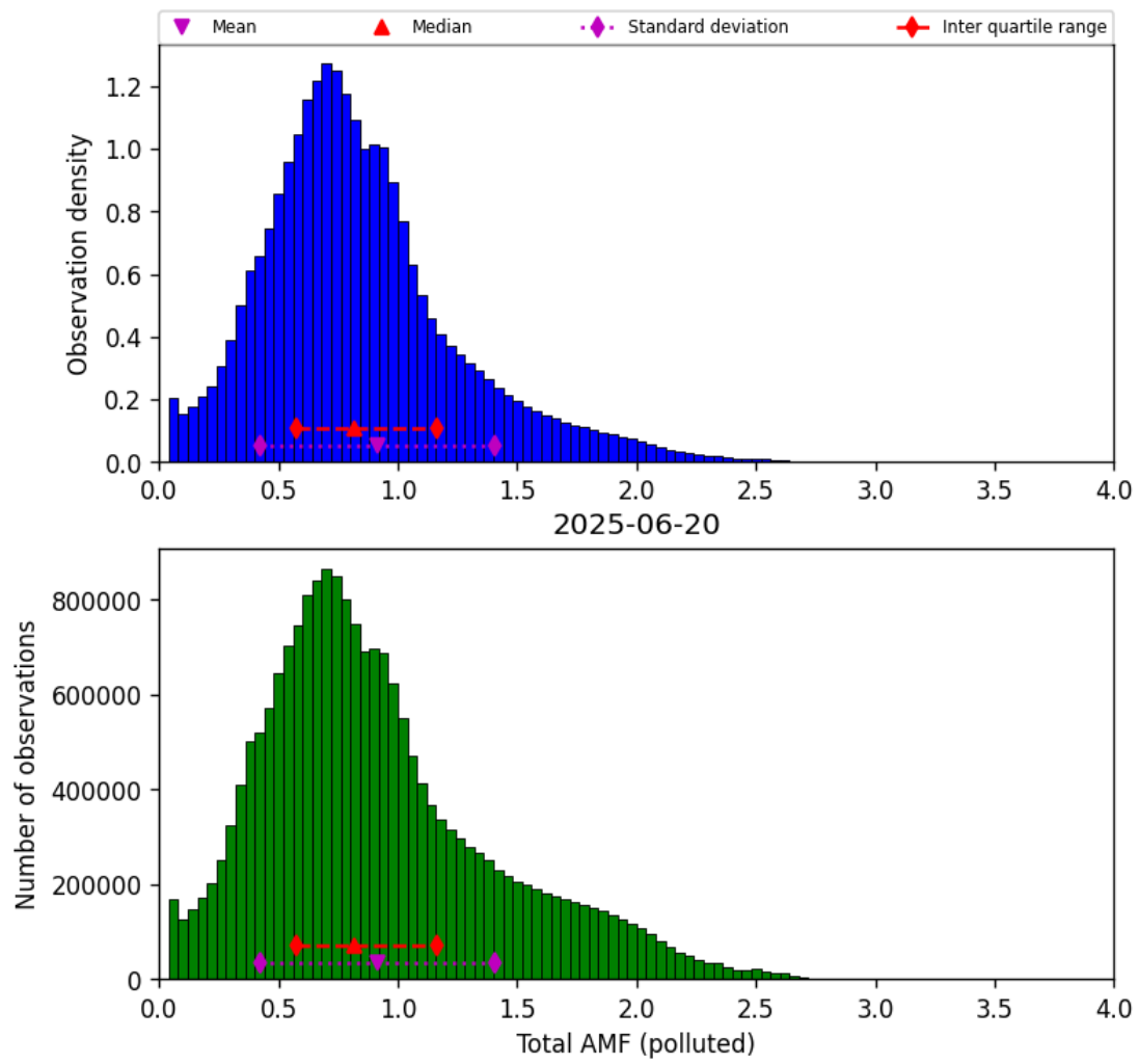
Figure 79: Histogram of “Total AMF (polluted)” for 2025-06-19 to 2025-06-21
