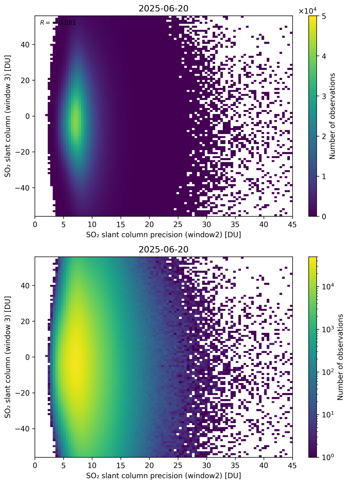
Figure 299: Scatter density plot of “SO 2 slant column precision (window2)” against “SO 2 slant column (window 3)” for 2025-06-19 to 2025-06-21.
