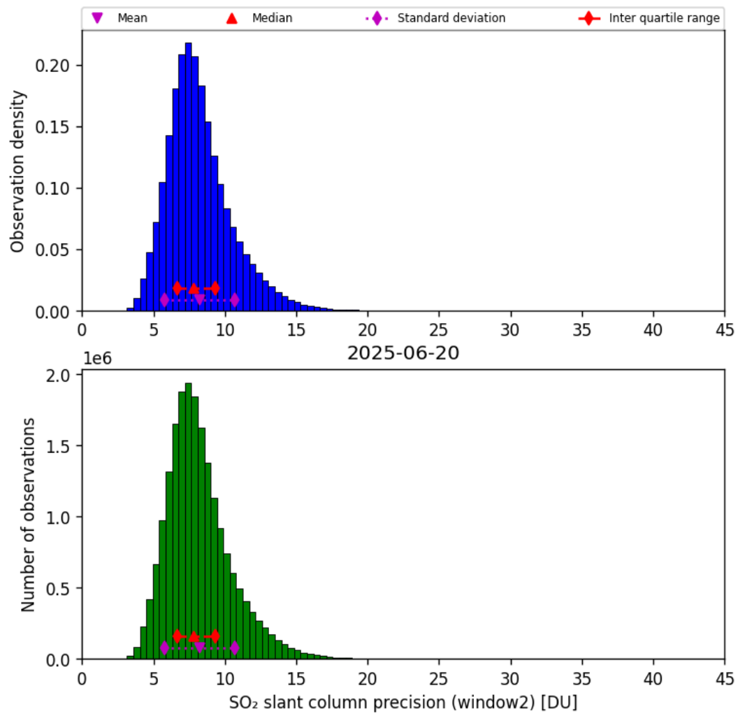
Figure 68: Histogram of “SO 2 slant column precision (window2)” for 2025-06-19 to 2025-06-21
