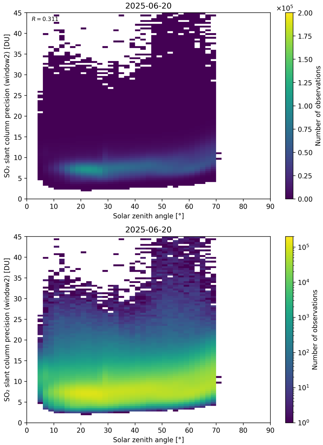
Figure 186: Scatter density plot of “Solar zenith angle” against “SO 2 slant column precision (window2)” for 2025-06-19 to 2025-06-21.
