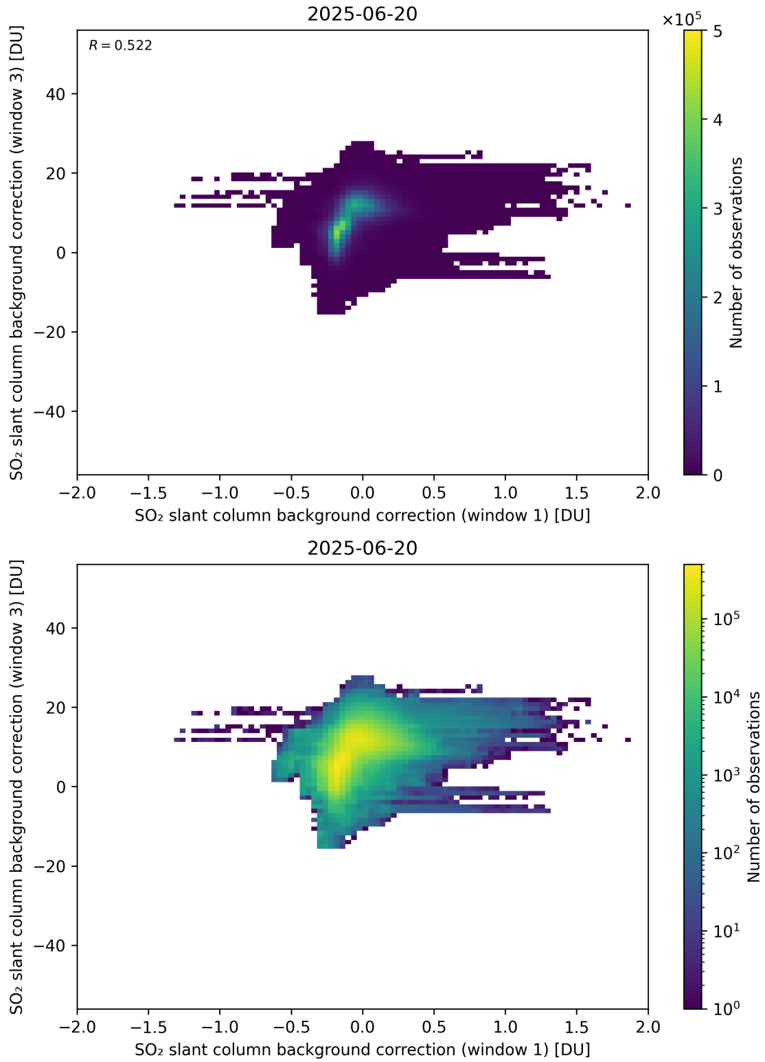
Figure 110: Scatter density plot of “SO 2 slant column background correction (window 1)” against “SO 2 slant column background correction (window 3)” for 2025-06-19 to 2025-06-21.
