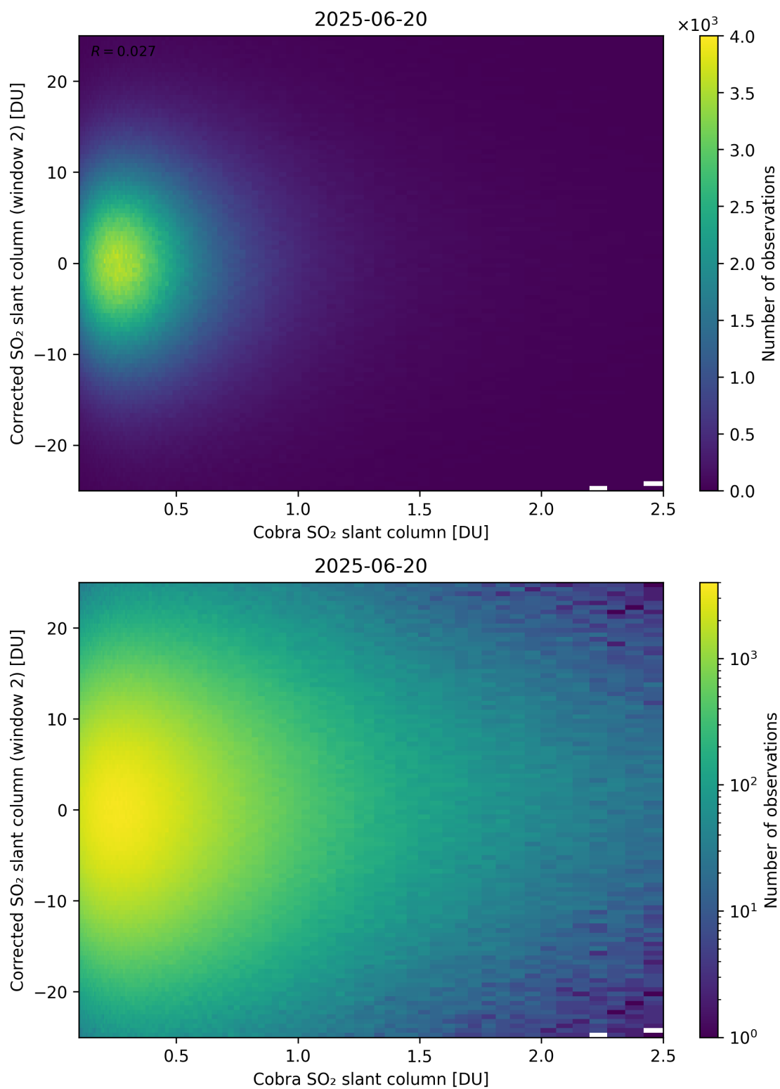
Figure 217: Scatter density plot of “Cobra SO 2 slant column” against “Corrected SO 2 slant column (window 2)” for 2025-06-19 to 2025-06-21.
