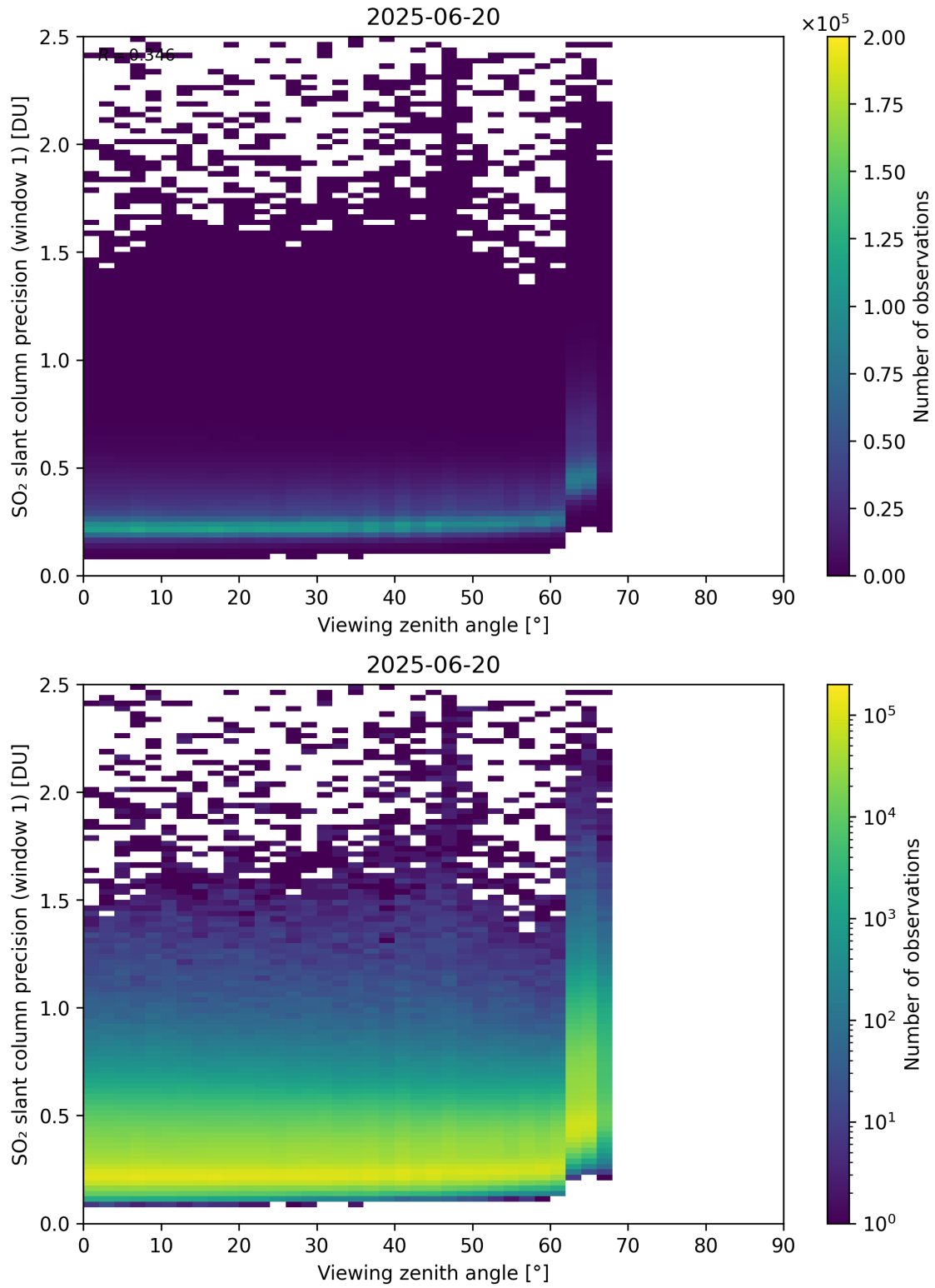
Figure 377: Scatter density plot of “Viewing zenith angle” against “SO 2 slant column precision (window 1)” for 2025-06-19 to 2025-06-21.
