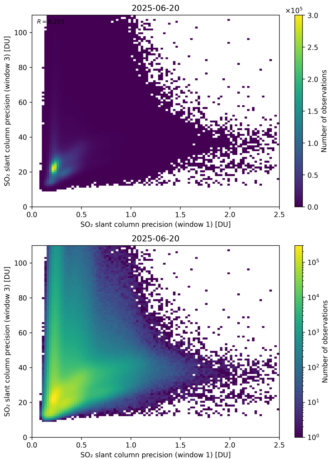
Figure 279: Scatter density plot of “SO 2 slant column precision (window 1)” against “SO 2 slant column precision (window 3)” for 2025-06-19 to 2025-06-21.
