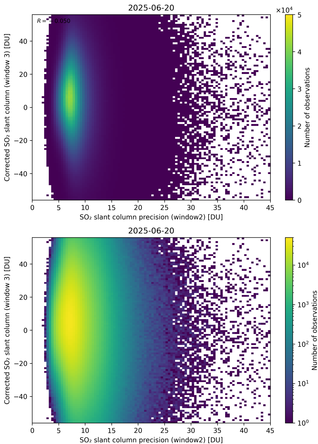
Figure 298: Scatter density plot of “SO 2 slant column precision (window2)” against “Corrected SO 2 slant column (window 3)” for 2025-06-19 to 2025-06-21.
