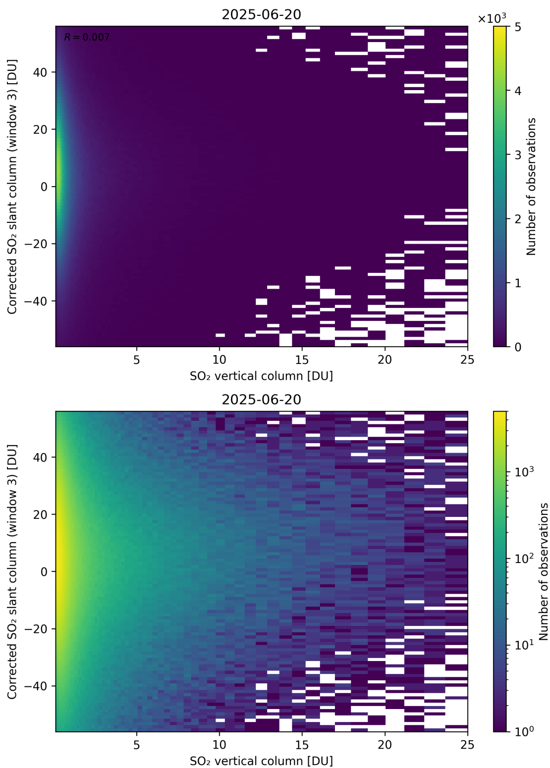
Figure 353: Scatter density plot of “SO 2 vertical column” against “Corrected SO 2 slant column (window 3)” for 2025-06-19 to 2025-06-21.
