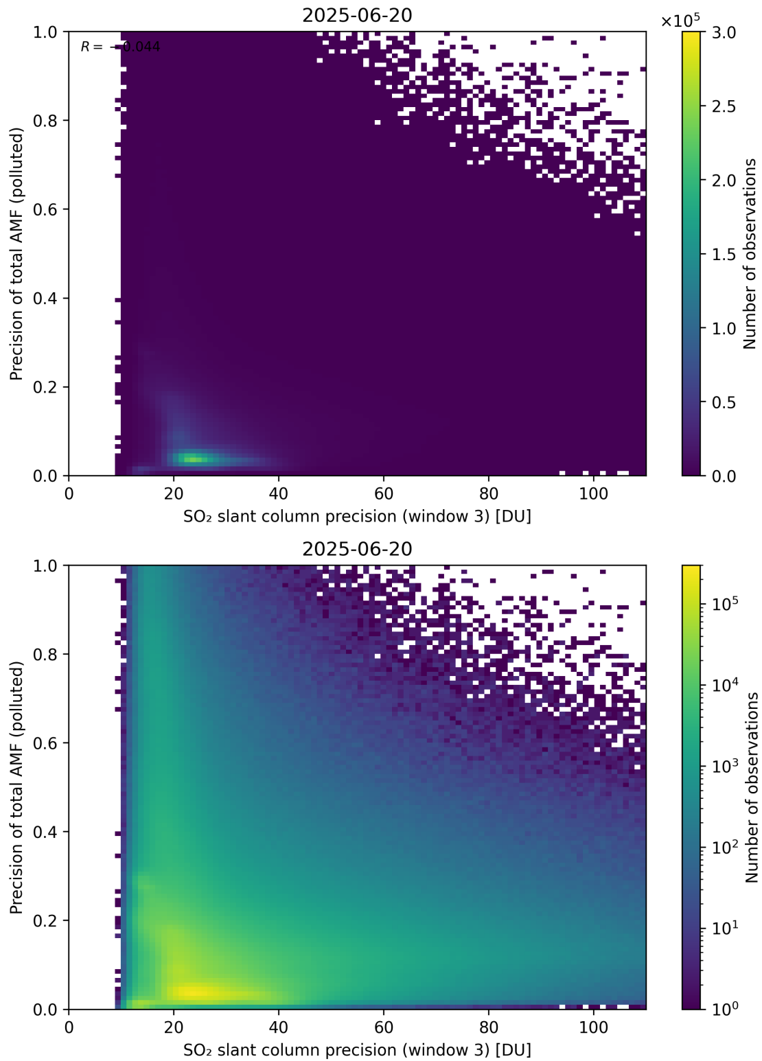
Figure 314: Scatter density plot of “SO 2 slant column precision (window 3)” against “Precision of total AMF (polluted)” for 2025-06-19 to 2025-06-21.
