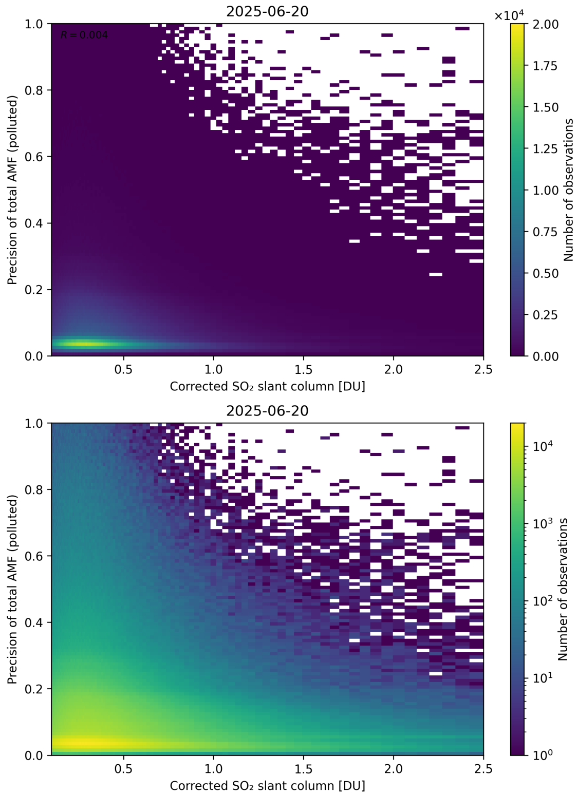
Figure 243: Scatter density plot of “Corrected SO 2 slant column” against “Precision of total AMF (polluted)” for 2025-06-19 to 2025-06-21.
