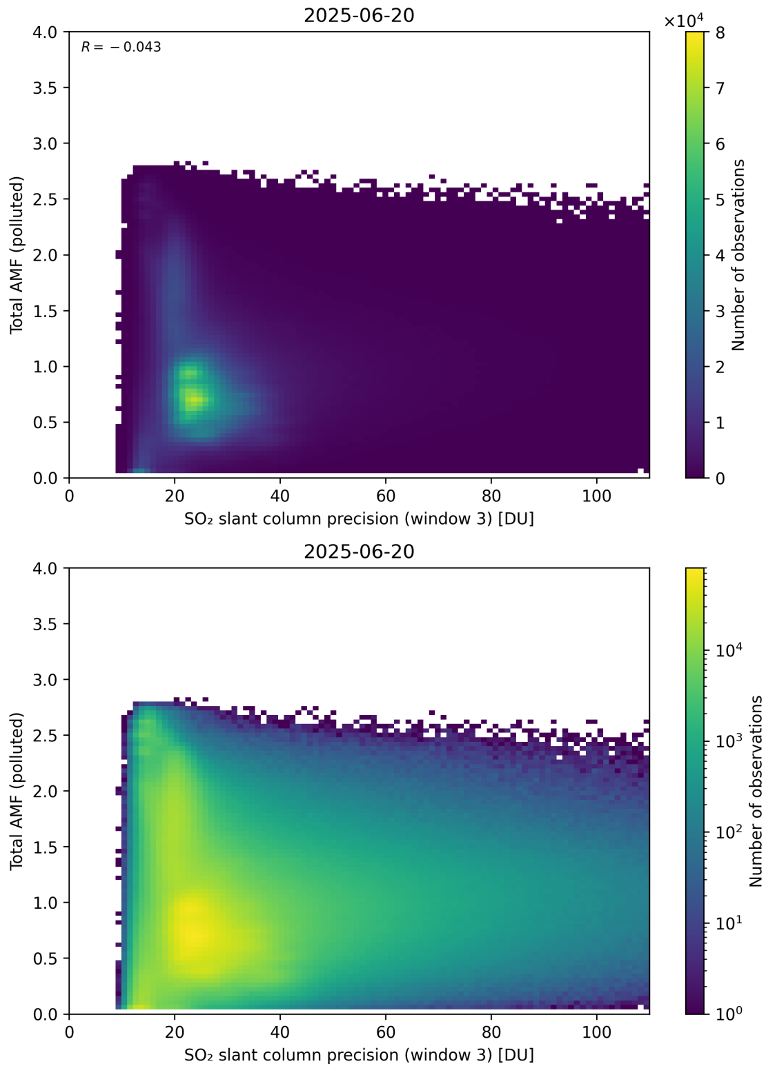
Figure 313: Scatter density plot of “SO 2 slant column precision (window 3)” against “Total AMF (polluted)” for 2025-06-19 to 2025-06-21.
