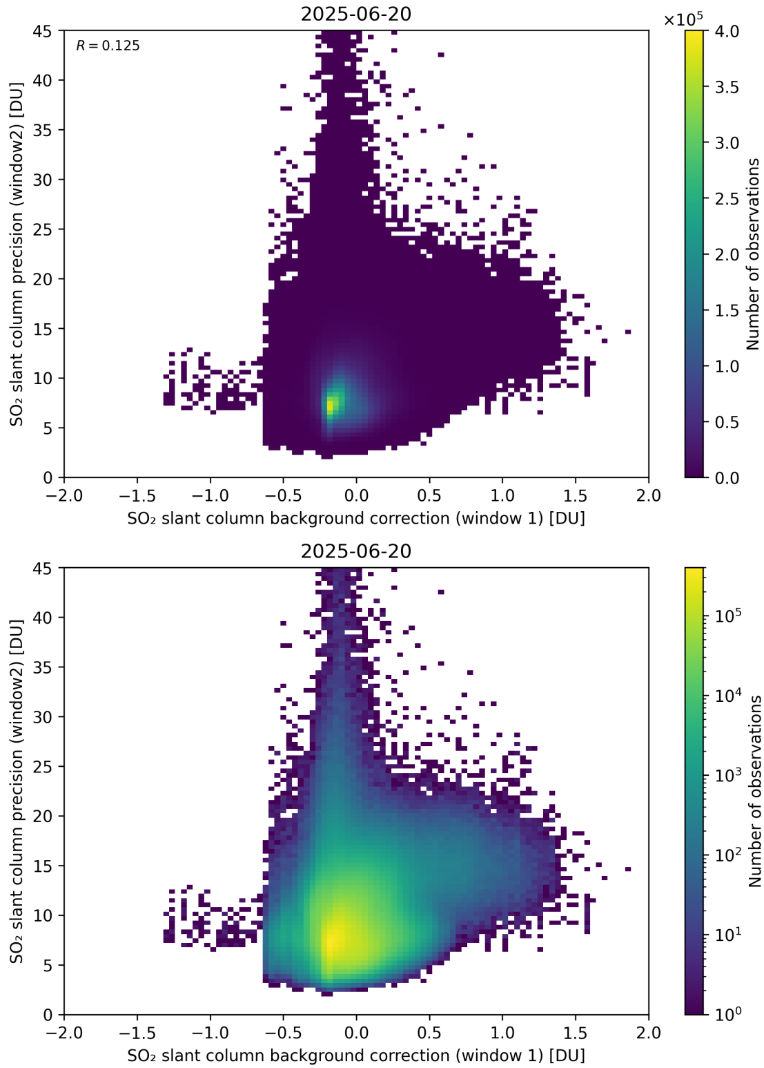
Figure 117: Scatter density plot of “SO 2 slant column background correction (window 1)” against “SO 2 slant column precision (window2)” for 2025-06-19 to 2025-06-21.
