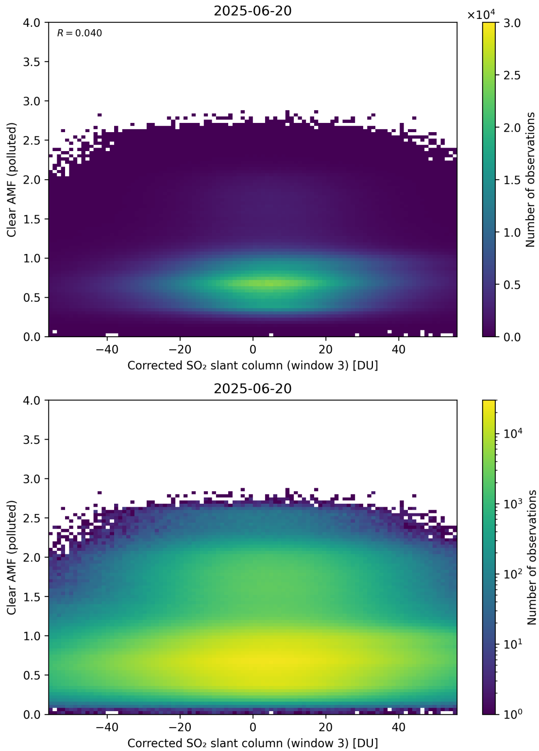
Figure 259: Scatter density plot of “Corrected SO 2 slant column (window 3)” against “Clear AMF (polluted)” for 2025-06-19 to 2025-06-21.
