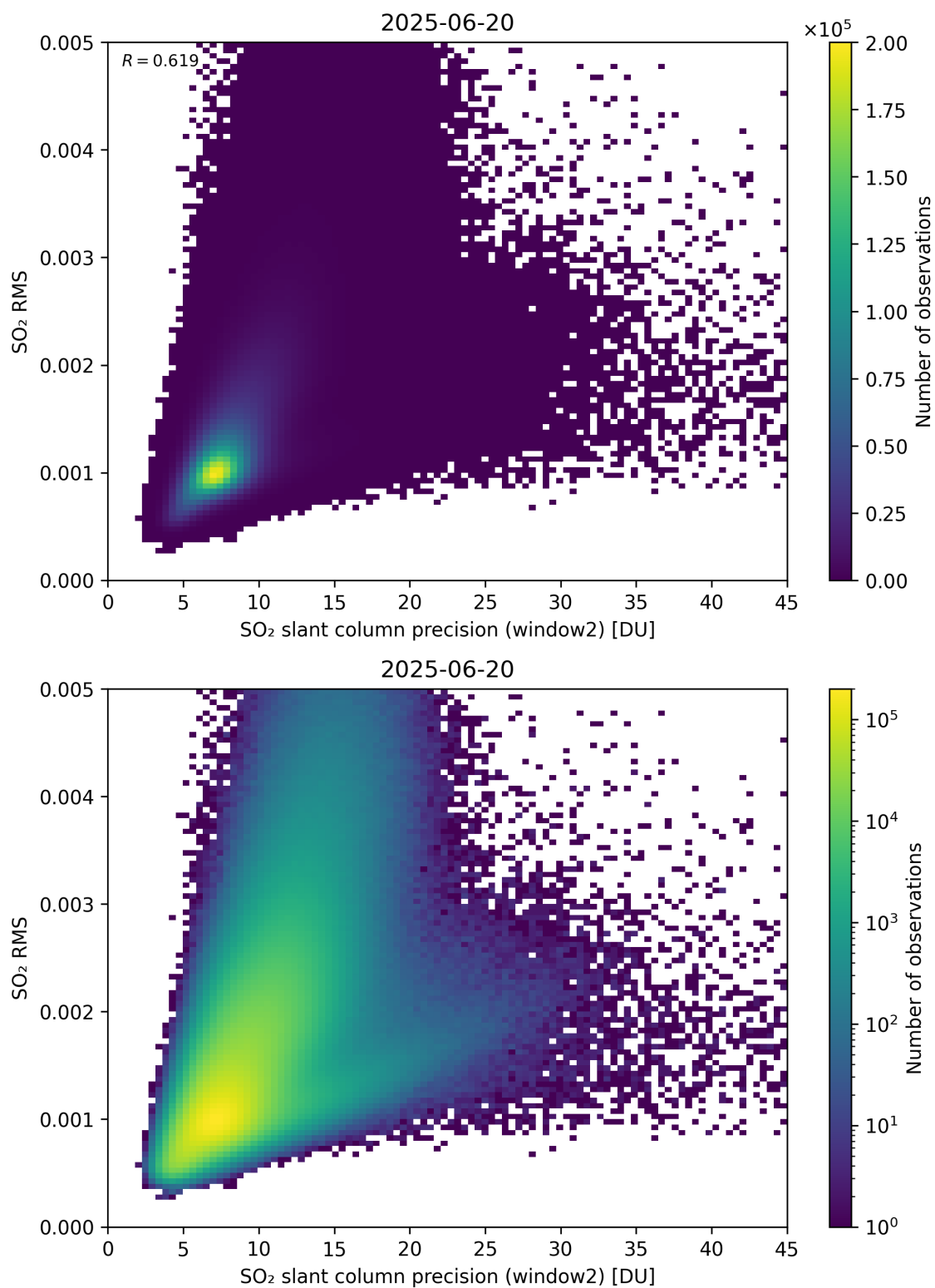
Figure 295: Scatter density plot of “SO 2 slant column precision (window2)” against “SO 2 RMS” for 2025-06-19 to 2025-06-21.
