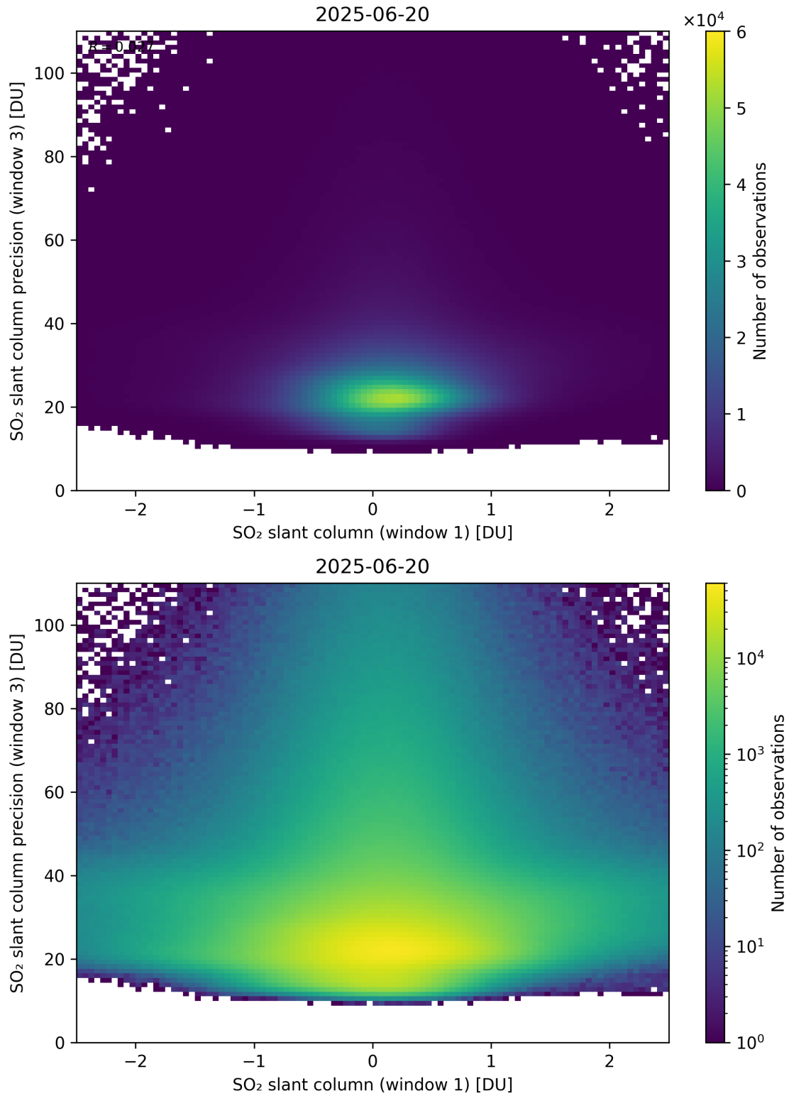
Figure 288: Scatter density plot of “SO 2 slant column (window 1)” against “SO 2 slant column precision (window 3)” for 2025-06-19 to 2025-06-21.
