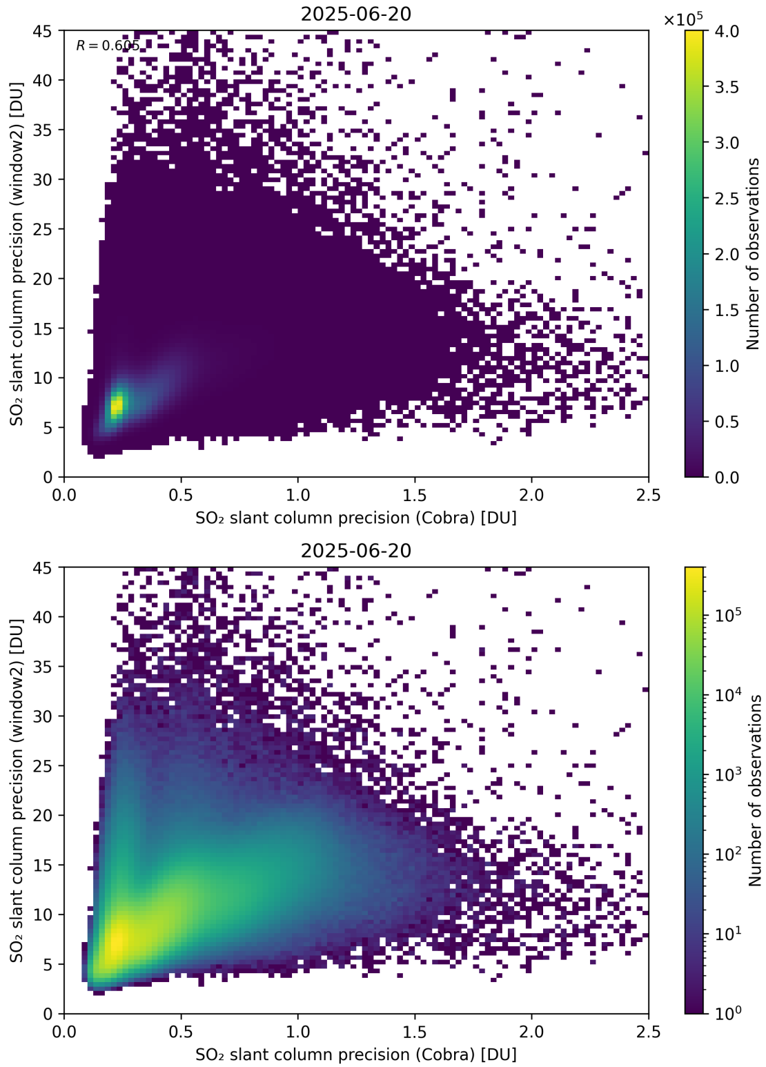
Figure 210: Scatter density plot of “SO 2 slant column precision (Cobra)” against “SO 2 slant column precision (window2)” for 2025-06-19 to 2025-06-21.
