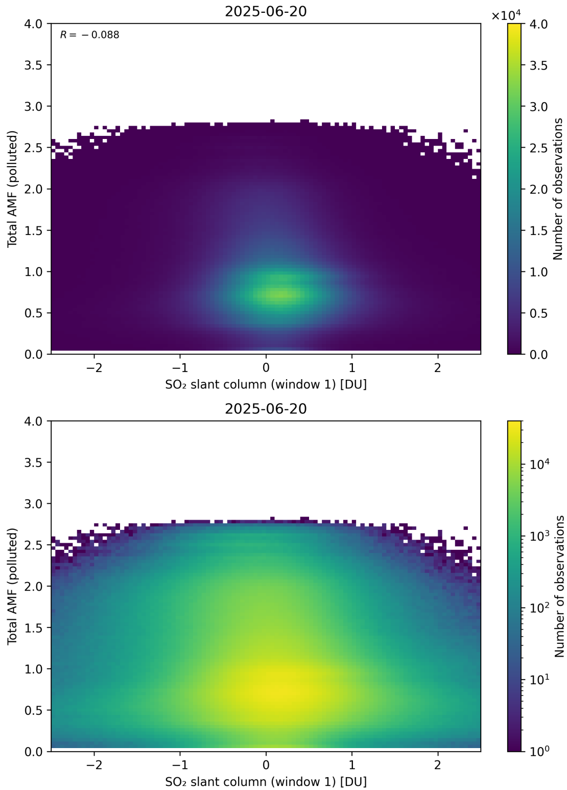
Figure 289: Scatter density plot of “SO 2 slant column (window 1)” against “Total AMF (polluted)” for 2025-06-19 to 2025-06-21.
