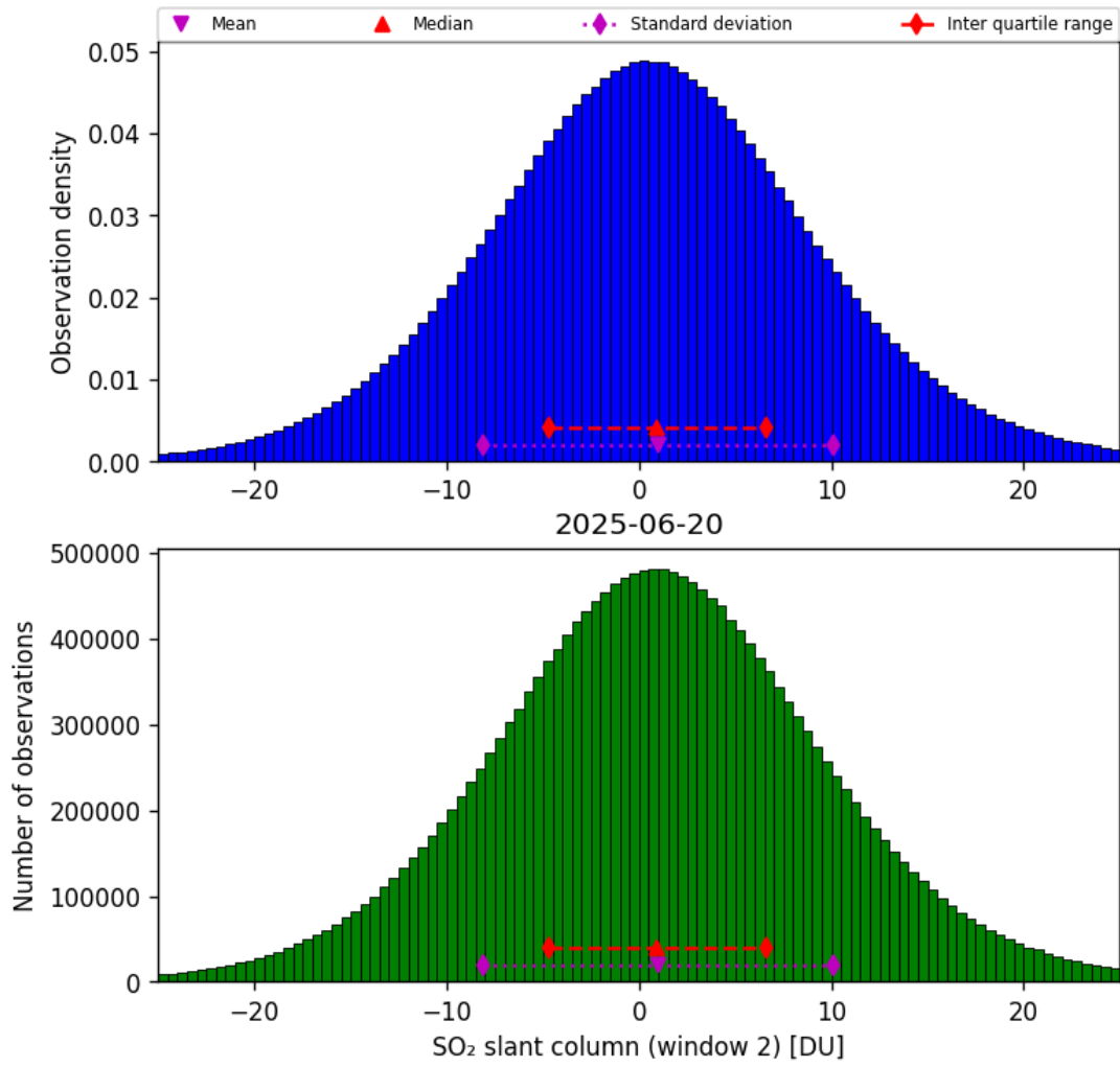
Figure 67: Histogram of “SO 2 slant column (window 2)” for 2025-06-19 to 2025-06-21
