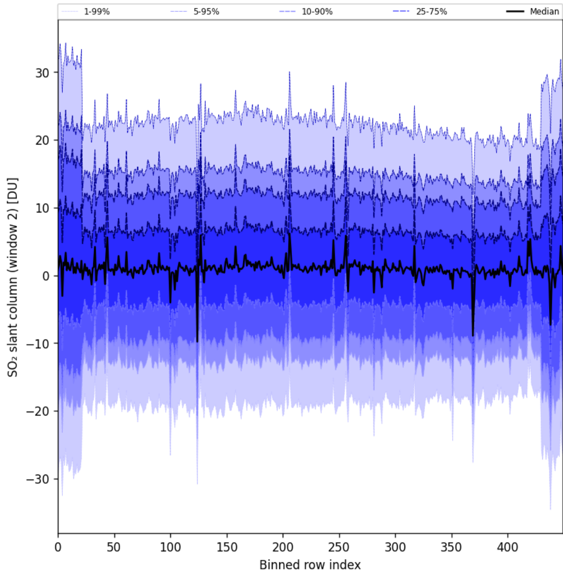
Figure 93: Along track statistics of “SO 2 slant column (window 2)” for 2025-06-19 to 2025-06-21
