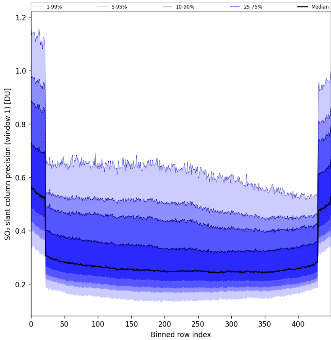
Figure 90: Along track statistics of “SO 2 slant column precision (window 1)” for 2025-06-19 to 2025-06-21
