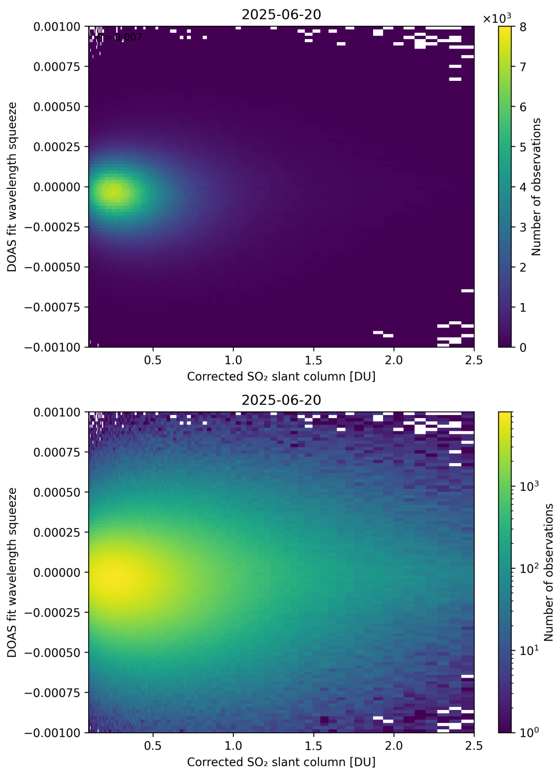
Figure 230: Scatter density plot of “Corrected SO 2 slant column” against “DOAS fit wavelength squeeze” for 2025-06-19 to 2025-06-21.
