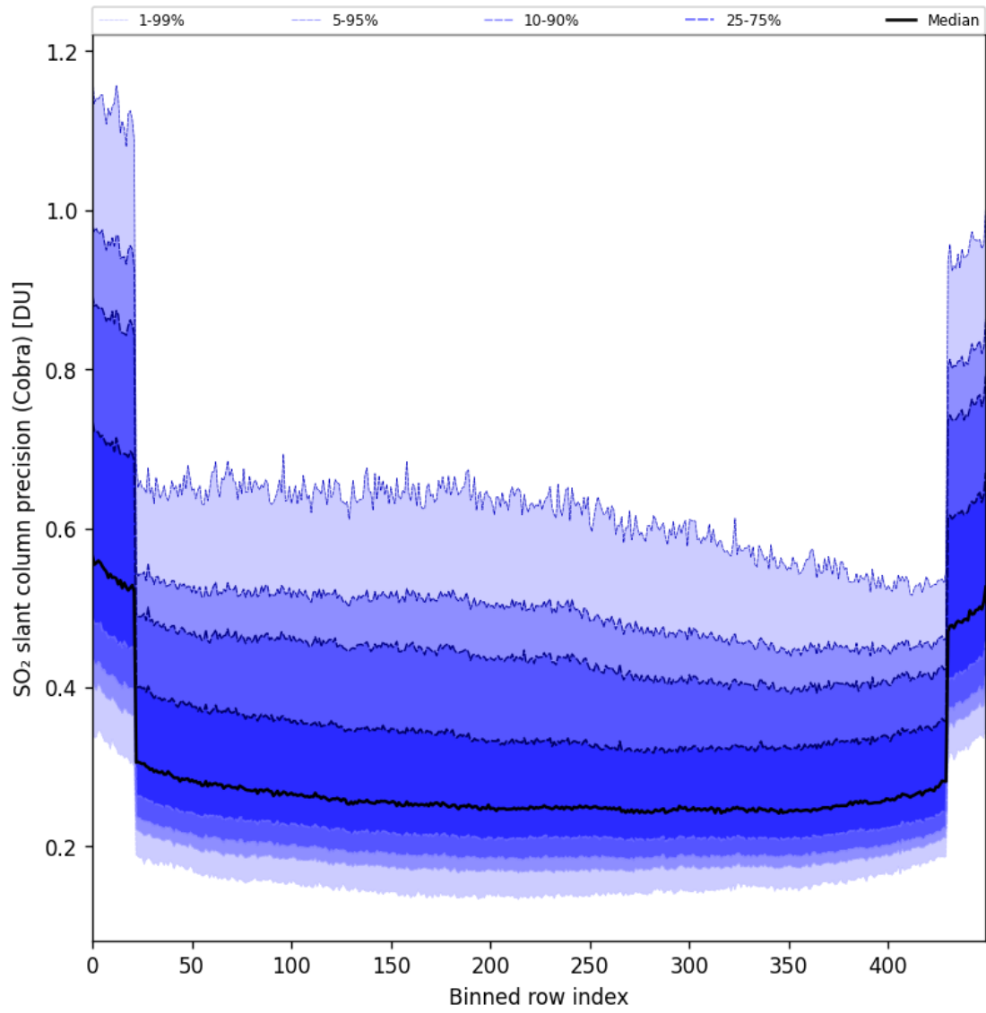
Figure 88: Along track statistics of “SO 2 slant column precision (Cobra)” for 2025-06-19 to 2025-06-21
