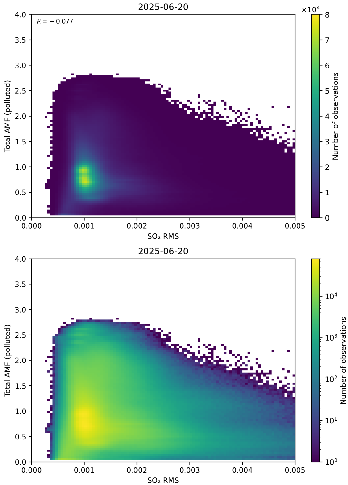
Figure 148: Scatter density plot of “SO 2 RMS” against “Total AMF (polluted)” for 2025-06-19 to 2025-06-21.
