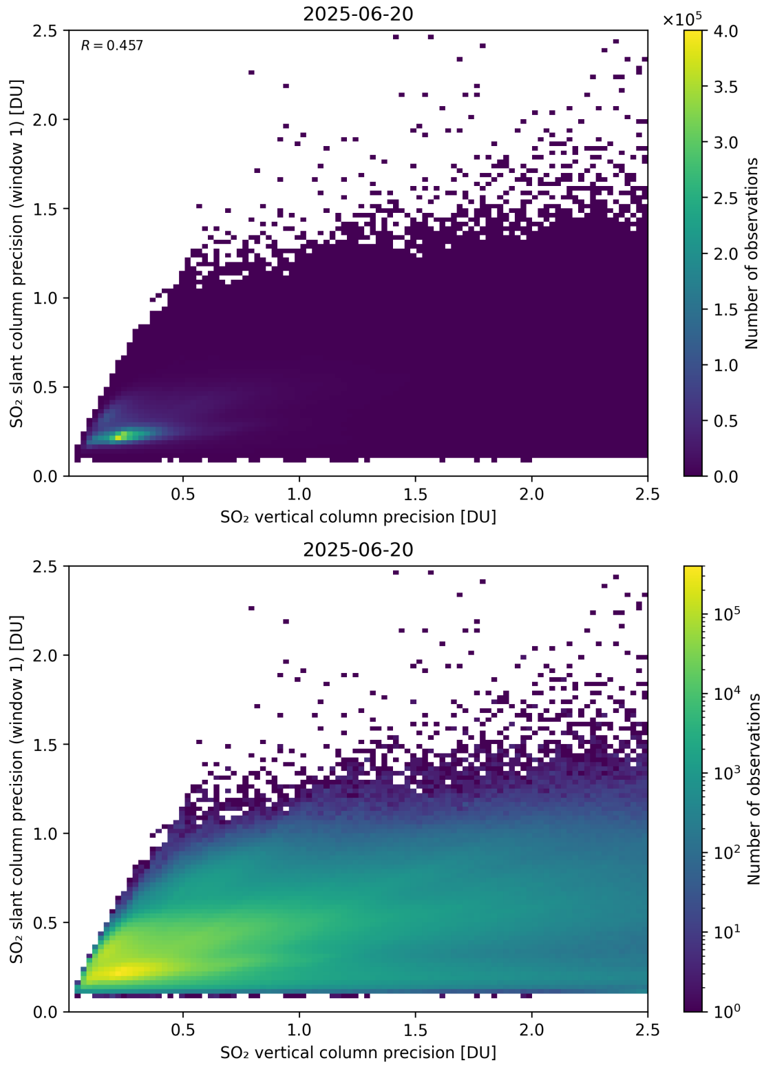
Figure 342: Scatter density plot of “SO 2 vertical column precision” against “SO 2 slant column precision (window 1)” for 2025-06-19 to 2025-06-21.
