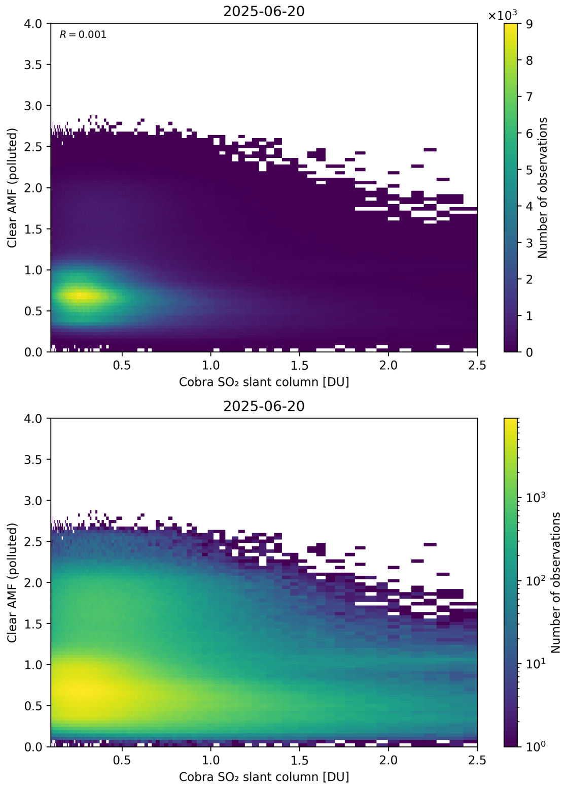
Figure 215: Scatter density plot of “Cobra SO 2 slant column” against “Clear AMF (polluted)” for 2025-06-19 to 2025-06-21.
