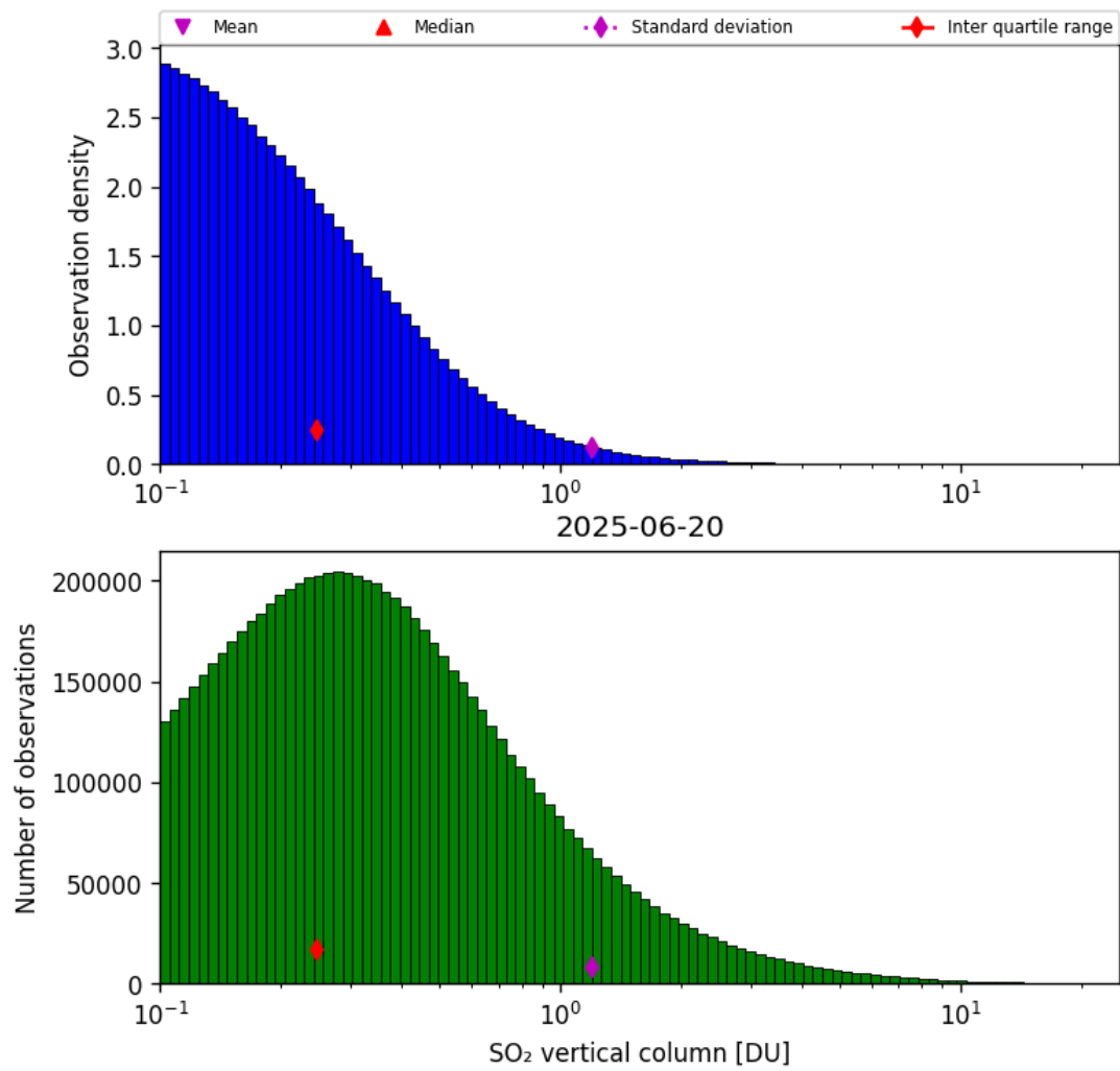
Figure 58: Histogram of “SO 2 vertical column” for 2025-06-19 to 2025-06-21
