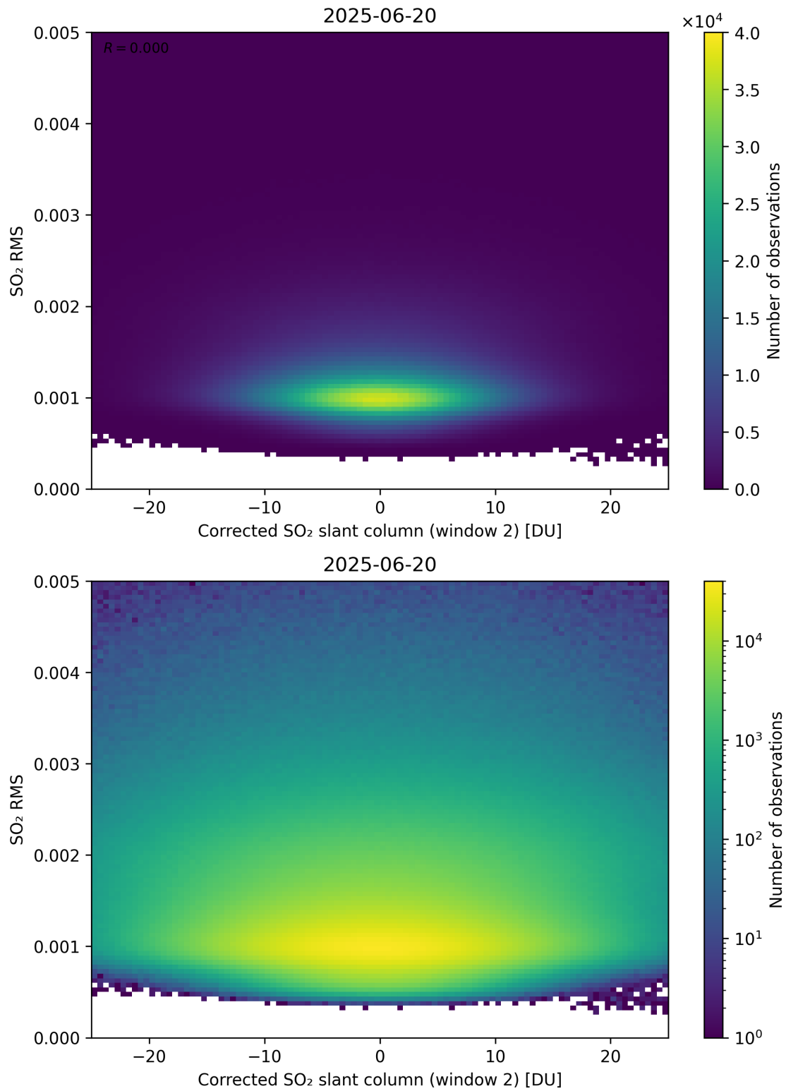
Figure 248: Scatter density plot of “Corrected SO 2 slant column (window 2)” against “SO 2 RMS” for 2025-06-19 to 2025-06-21.
