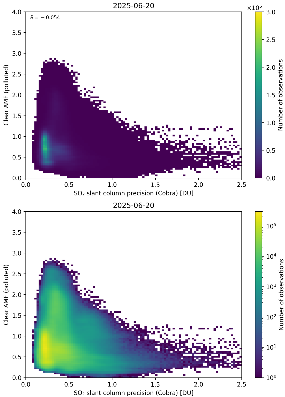
Figure 205: Scatter density plot of “SO 2 slant column precision (Cobra)” against “Clear AMF (polluted)” for 2025-06-19 to 2025-06-21.
