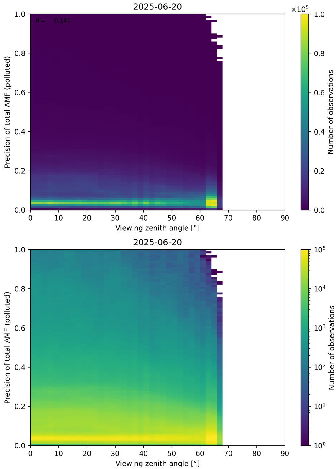
Figure 382: Scatter density plot of “Viewing zenith angle” against “Precision of total AMF (polluted)” for 2025-06-19 to 2025-06-21.
