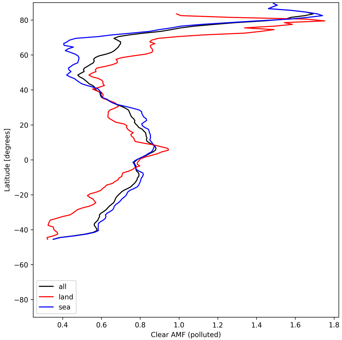
Figure 55: Zonal average of “Clear AMF (polluted)” for 2025-06-19 to 2025-06-21.
