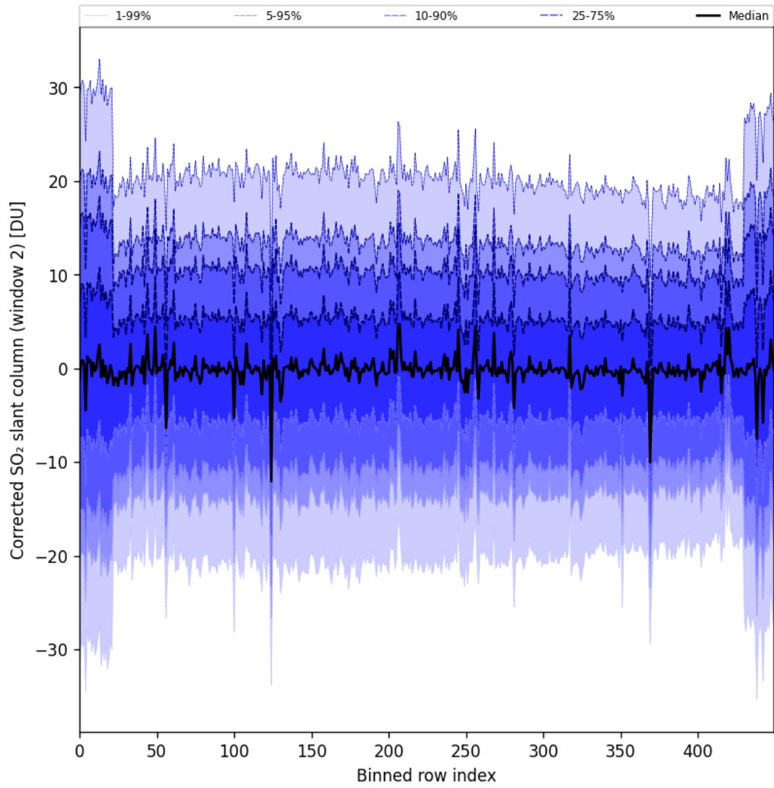
Figure 95: Along track statistics of “Corrected SO 2 slant column (window 2)” for 2025-06-19 to 2025-06-21
