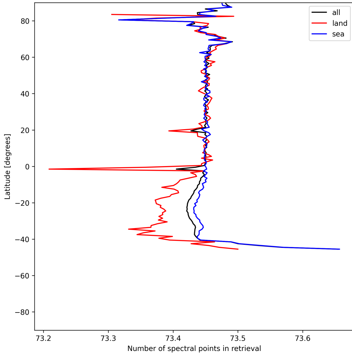
Figure 56: Zonal average of “Number of spectral points in retrieval” for 2025-06-19 to 2025-06-21.
