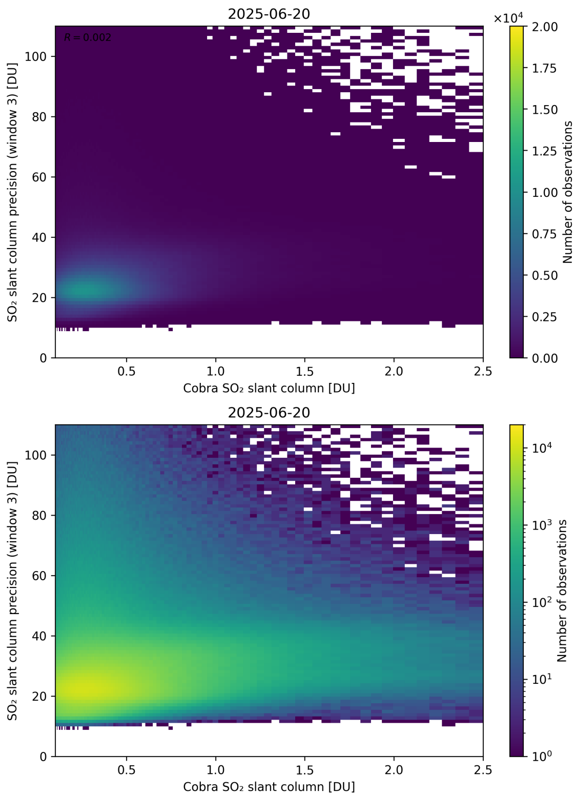
Figure 223: Scatter density plot of “Cobra SO 2 slant column” against “SO 2 slant column precision (window 3)” for 2025-06-19 to 2025-06-21.
