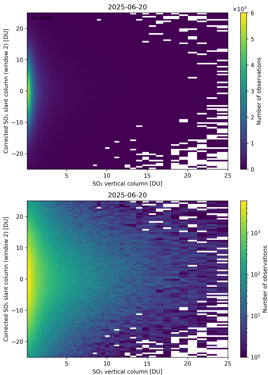
Figure 352: Scatter density plot of “SO 2 vertical column” against “Corrected SO 2 slant column (window 2)” for 2025-06-19 to 2025-06-21.
