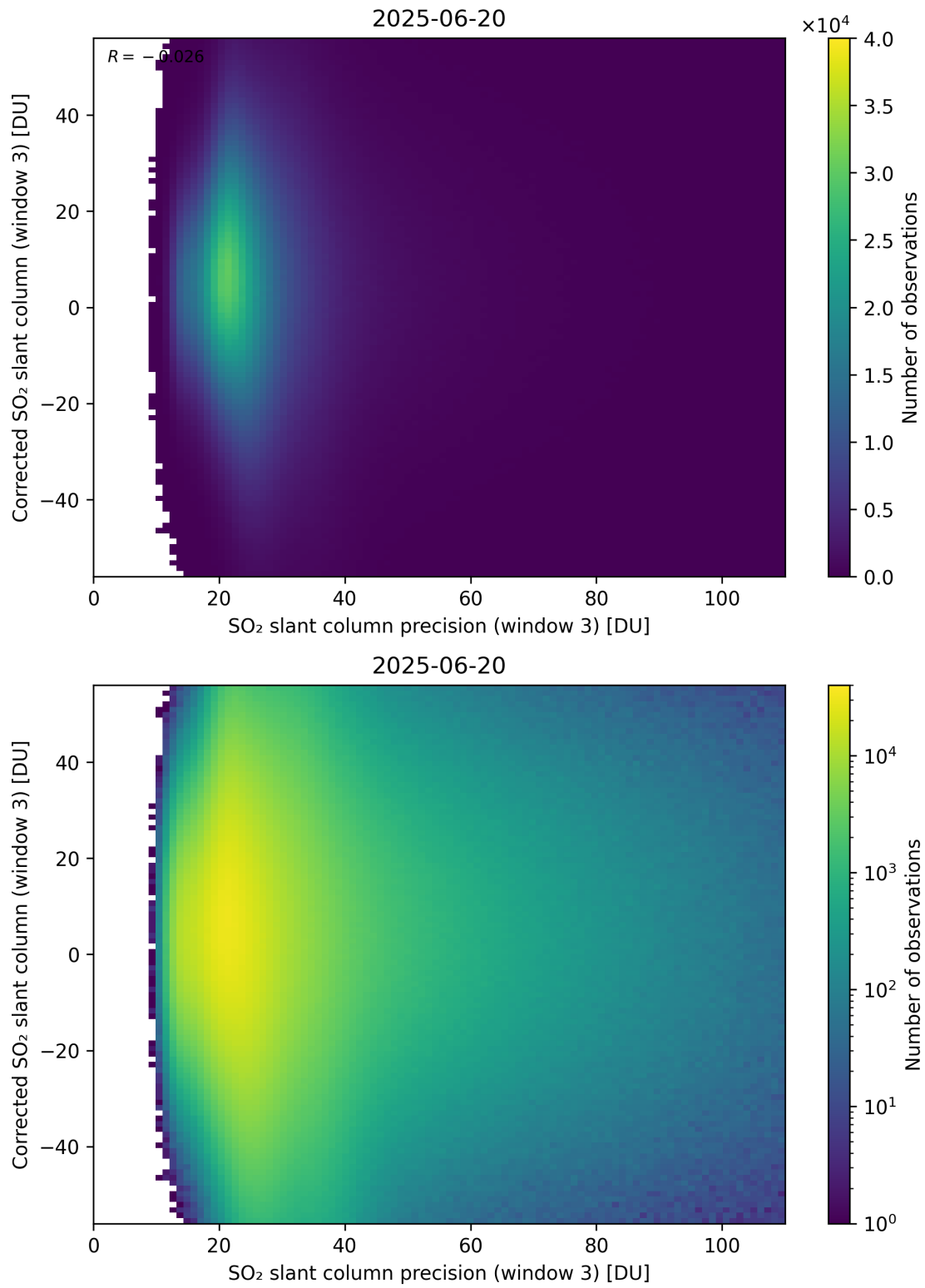
Figure 312: Scatter density plot of “SO 2 slant column precision (window 3)” against “Corrected SO 2 slant column (window 3)” for 2025-06-19 to 2025-06-21.
