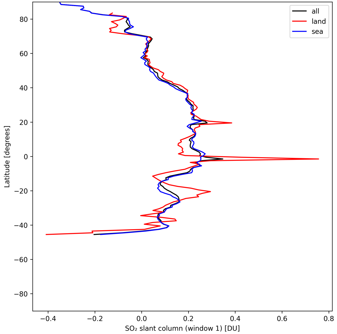
Figure 37: Zonal average of “SO 2 slant column (window 1)” for 2025-06-19 to 2025-06-21.
