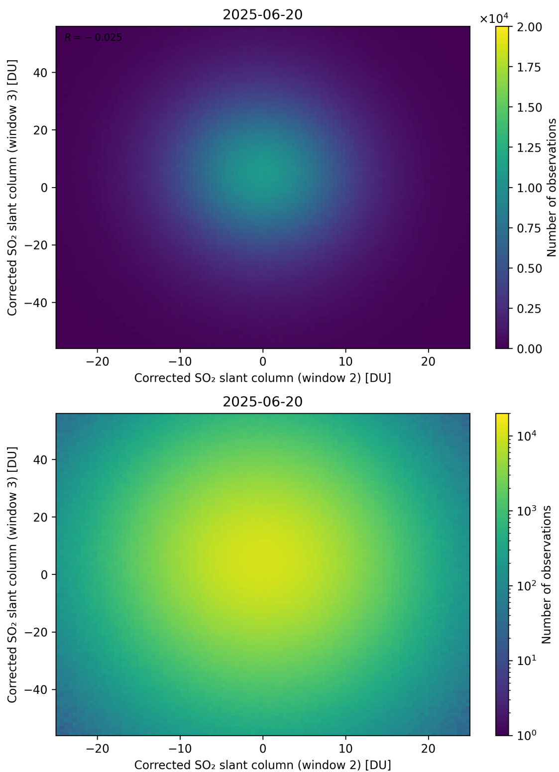
Figure 250: Scatter density plot of “Corrected SO 2 slant column (window 2)” against “Corrected SO 2 slant column (window 3)” for 2025-06-19 to 2025-06-21.
