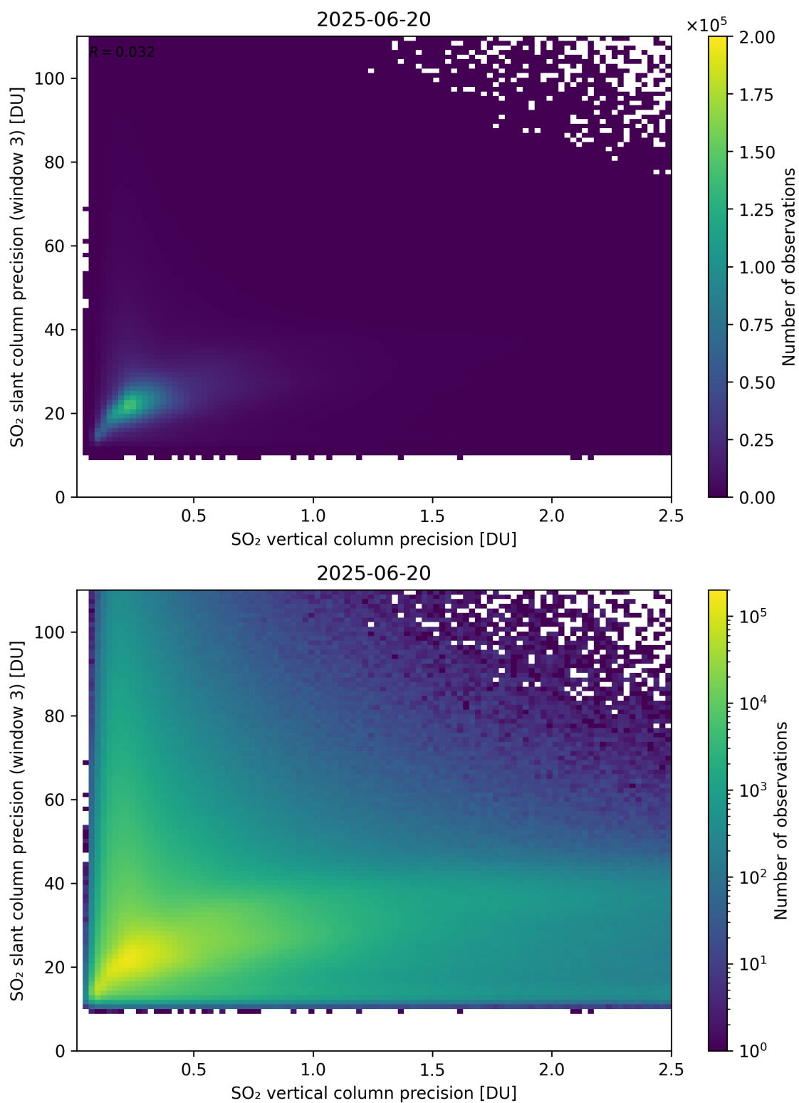
Figure 345: Scatter density plot of “SO 2 vertical column precision” against “SO 2 slant column precision (window 3)” for 2025-06-19 to 2025-06-21.
