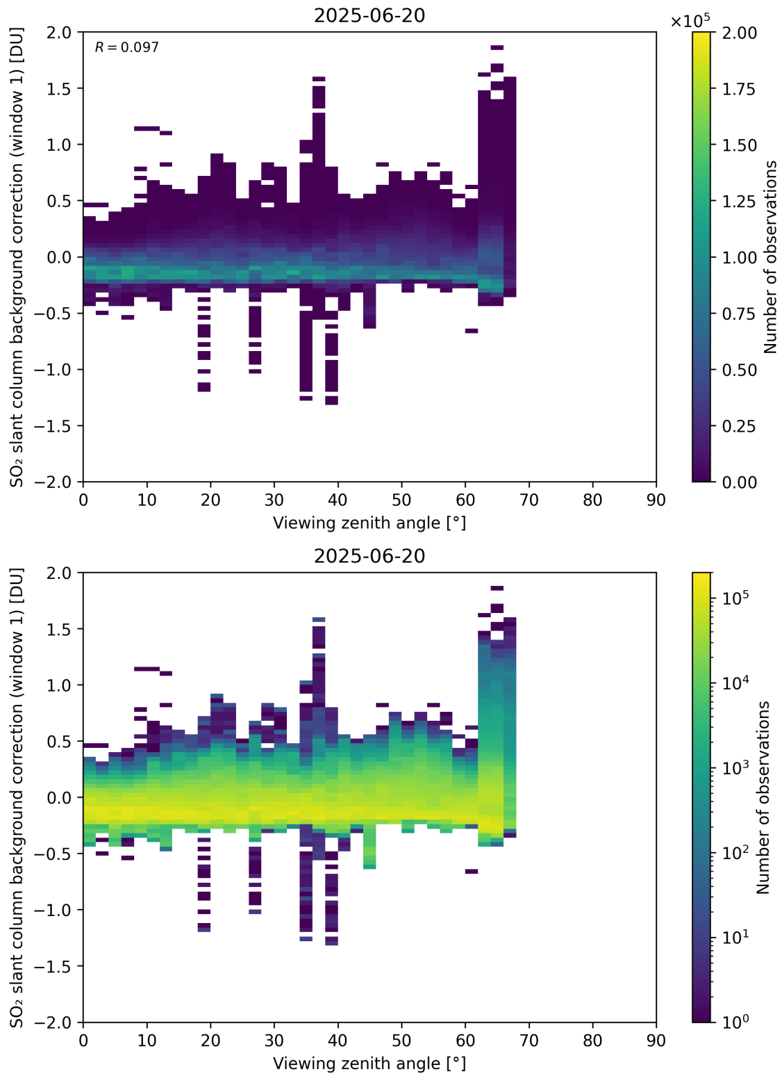
Figure 362: Scatter density plot of “Viewing zenith angle” against “SO 2 slant column background correction (window 1)” for 2025-06-19 to 2025-06-21.
