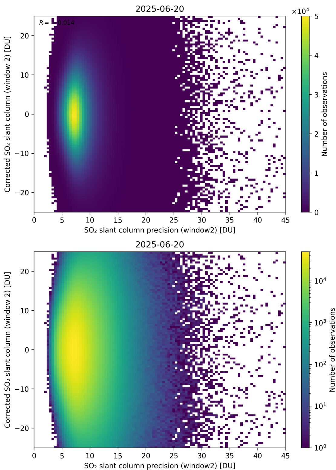
Figure 297: Scatter density plot of “SO 2 slant column precision (window2)” against “Corrected SO 2 slant column (window 2)” for 2025-06-19 to 2025-06-21.
