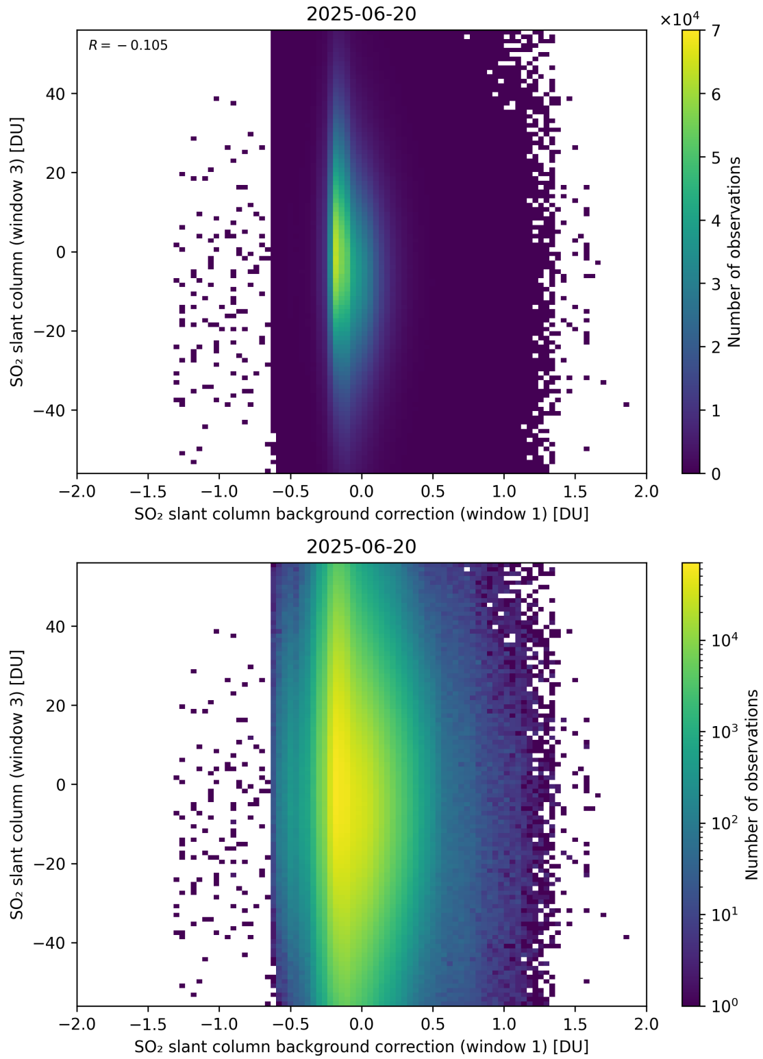
Figure 118: Scatter density plot of “SO 2 slant column background correction (window 1)” against “SO 2 slant column (window 3)” for 2025-06-19 to 2025-06-21.
