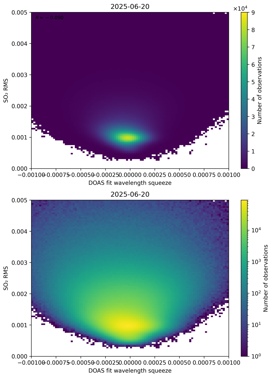
Figure 143: Scatter density plot of “DOAS fit wavelength squeeze” against “SO 2 RMS” for 2025-06-19 to 2025-06-21.
