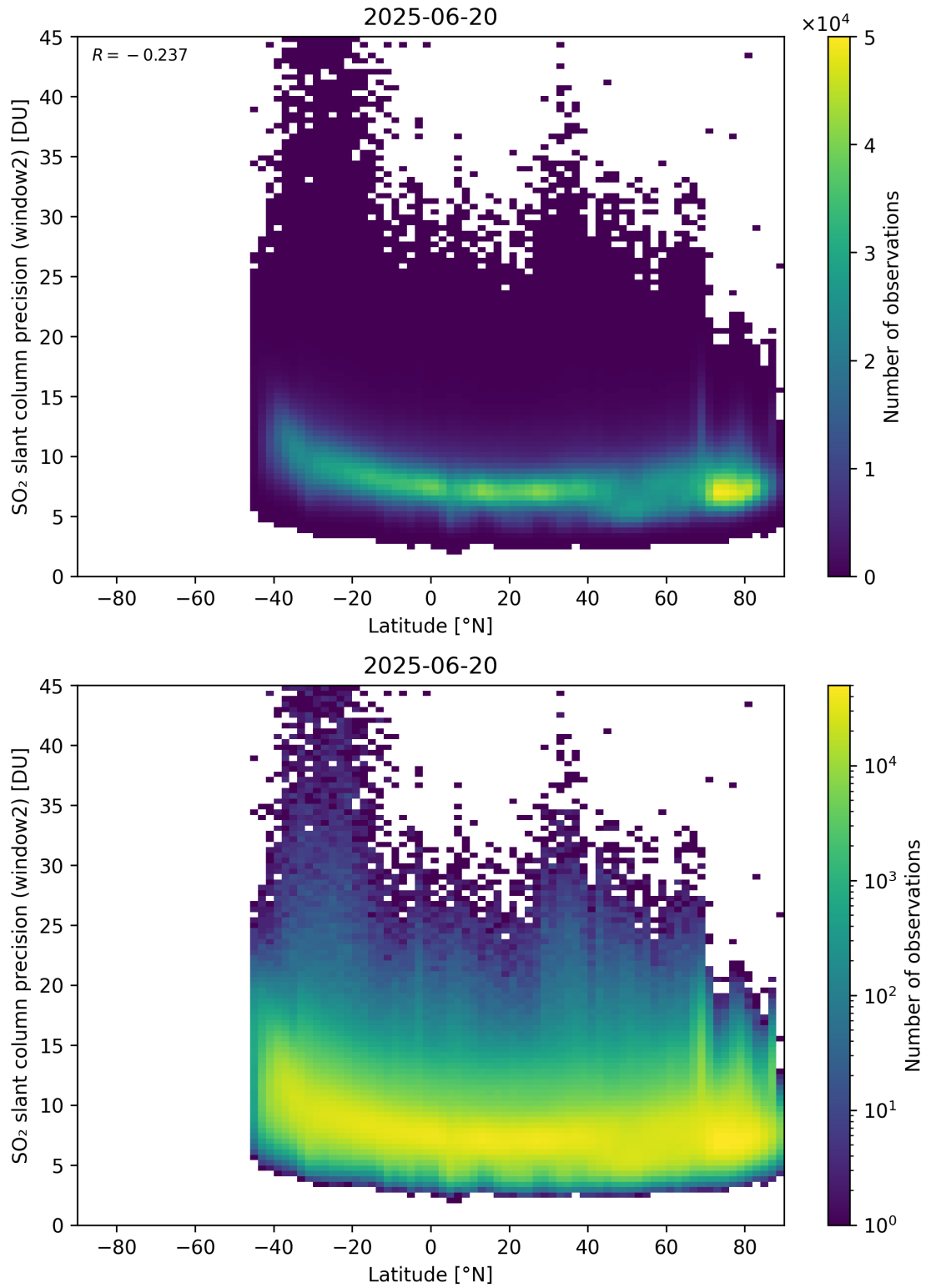
Figure 164: Scatter density plot of “Latitude” against “SO 2 slant column precision (window2)” for 2025-06-19 to 2025-06-21.
