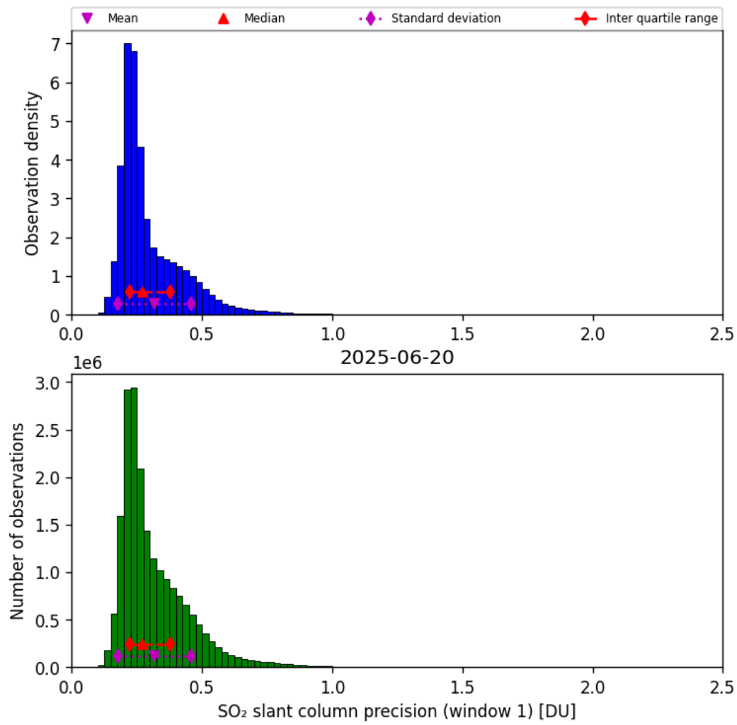
Figure 64: Histogram of “SO 2 slant column precision (window 1)” for 2025-06-19 to 2025-06-21
