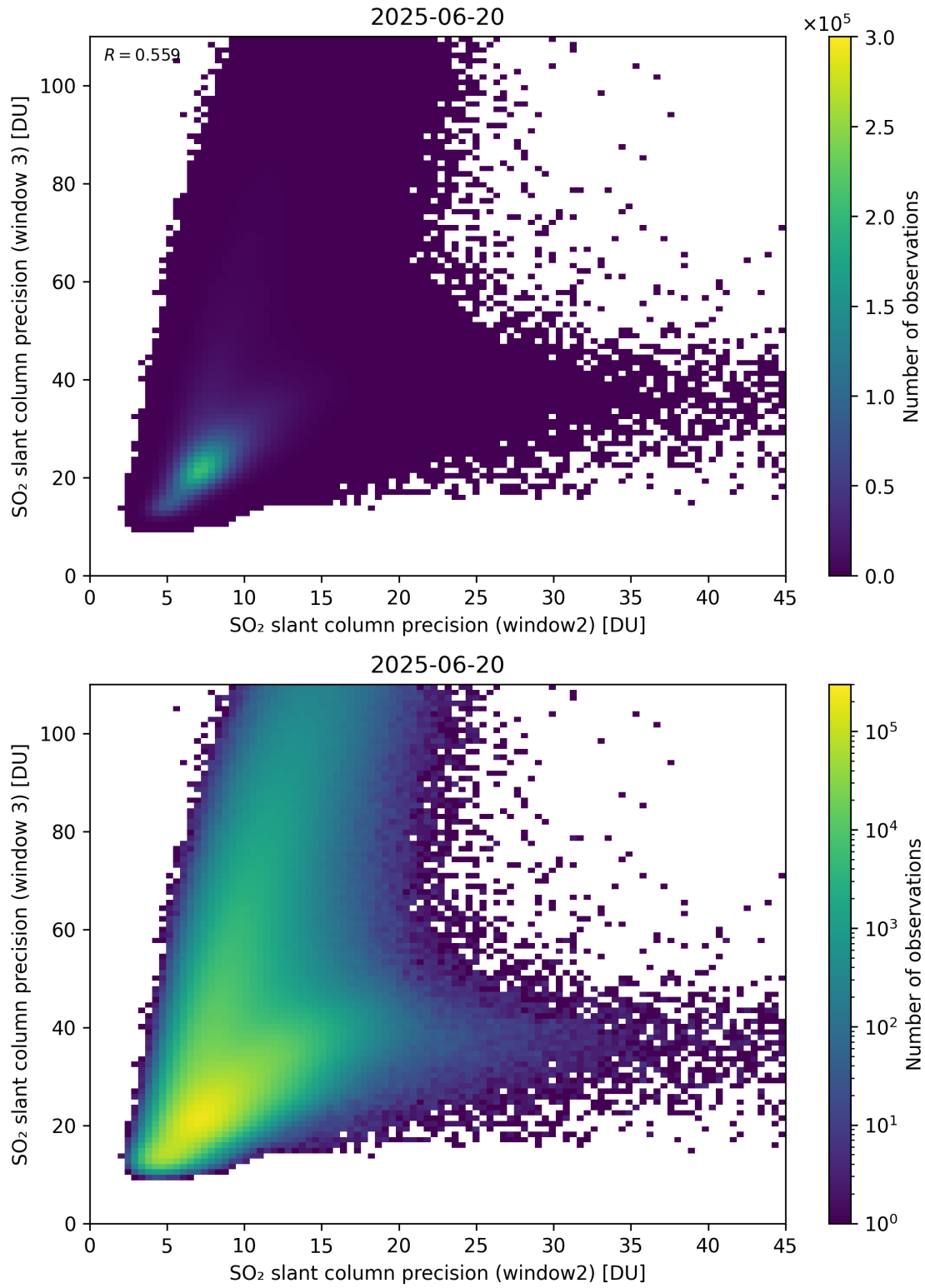
Figure 300: Scatter density plot of “SO 2 slant column precision (window2)” against “SO 2 slant column precision (window 3)” for 2025-06-19 to 2025-06-21.
