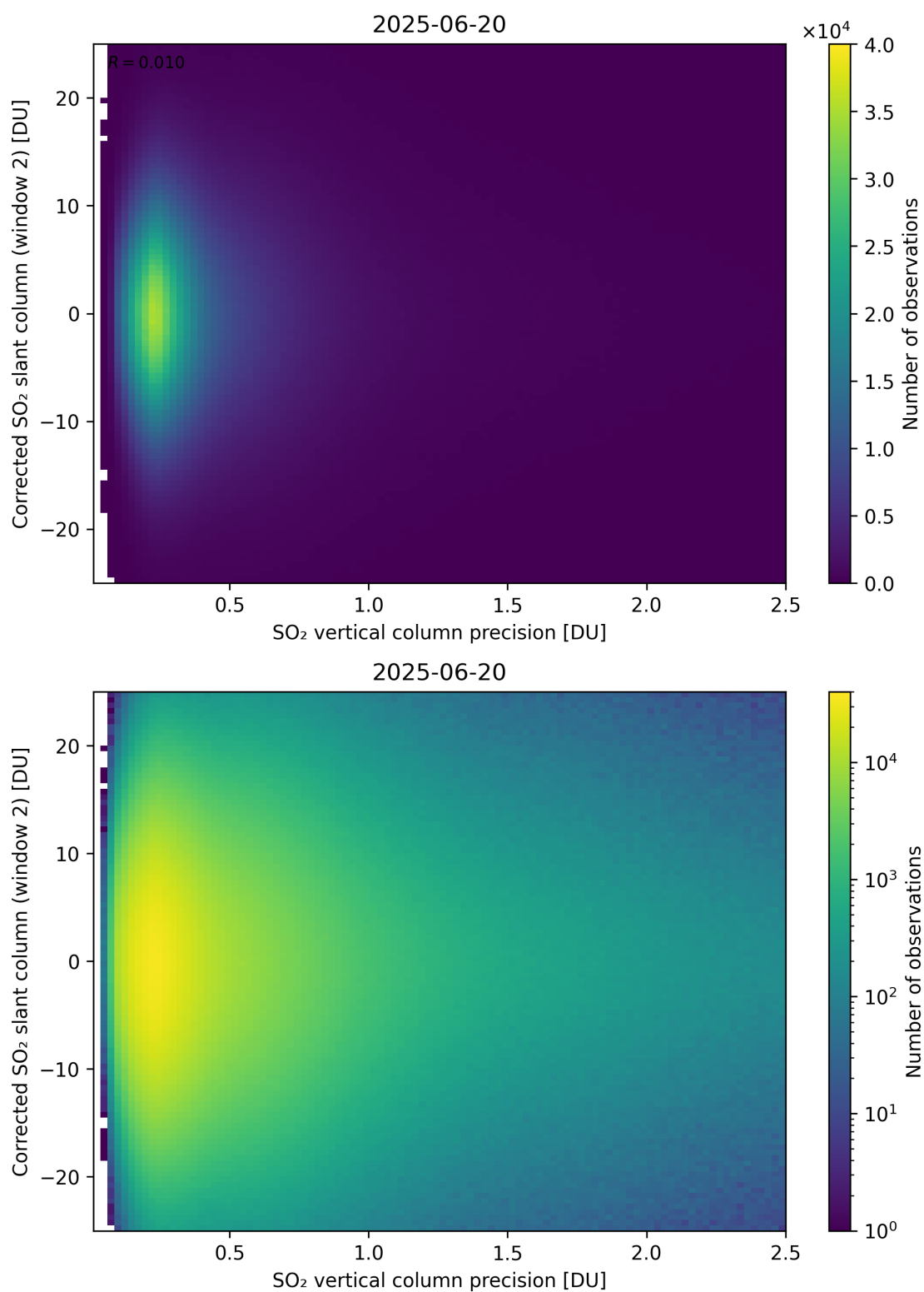
Figure 339: Scatter density plot of “SO 2 vertical column precision” against “Corrected SO 2 slant column (window 2)” for 2025-06-19 to 2025-06-21.
