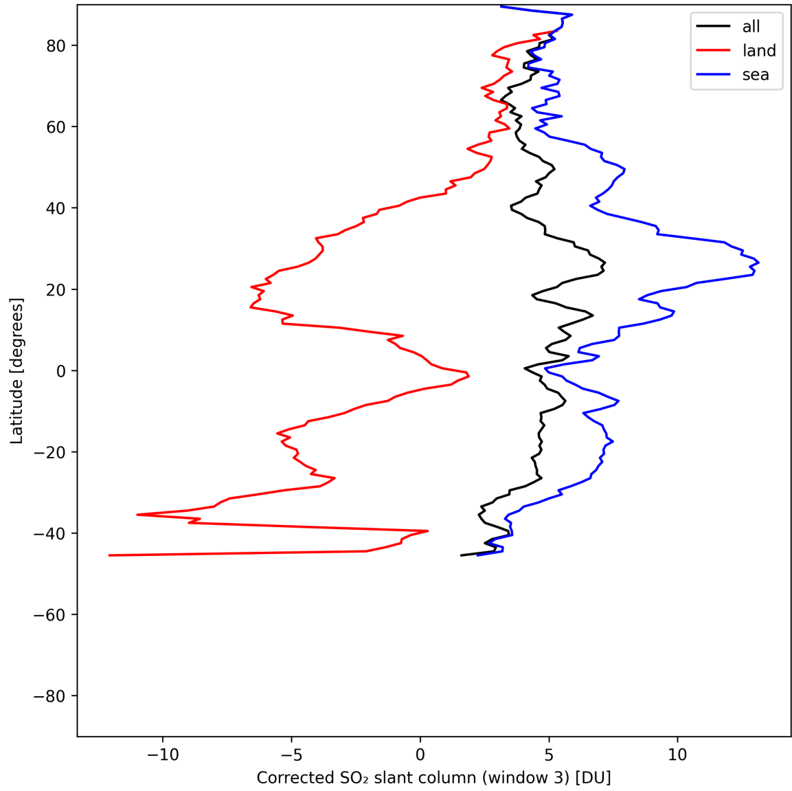
Figure 47: Zonal average of "Corrected SO 2 slant column (window 3)" for 2025-06-19 to 2025-06-21.
