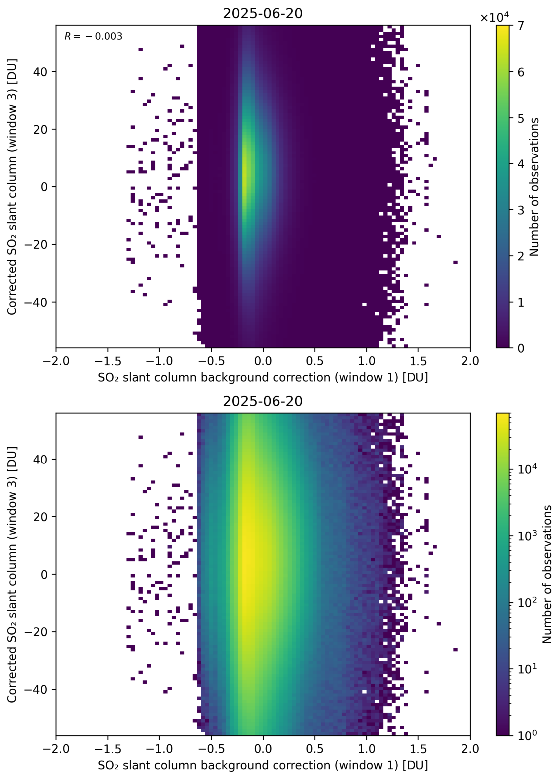
Figure 116: Scatter density plot of “SO 2 slant column background correction (window 1)” against “Corrected SO 2 slant column (window 3)” for 2025-06-19 to 2025-06-21.
