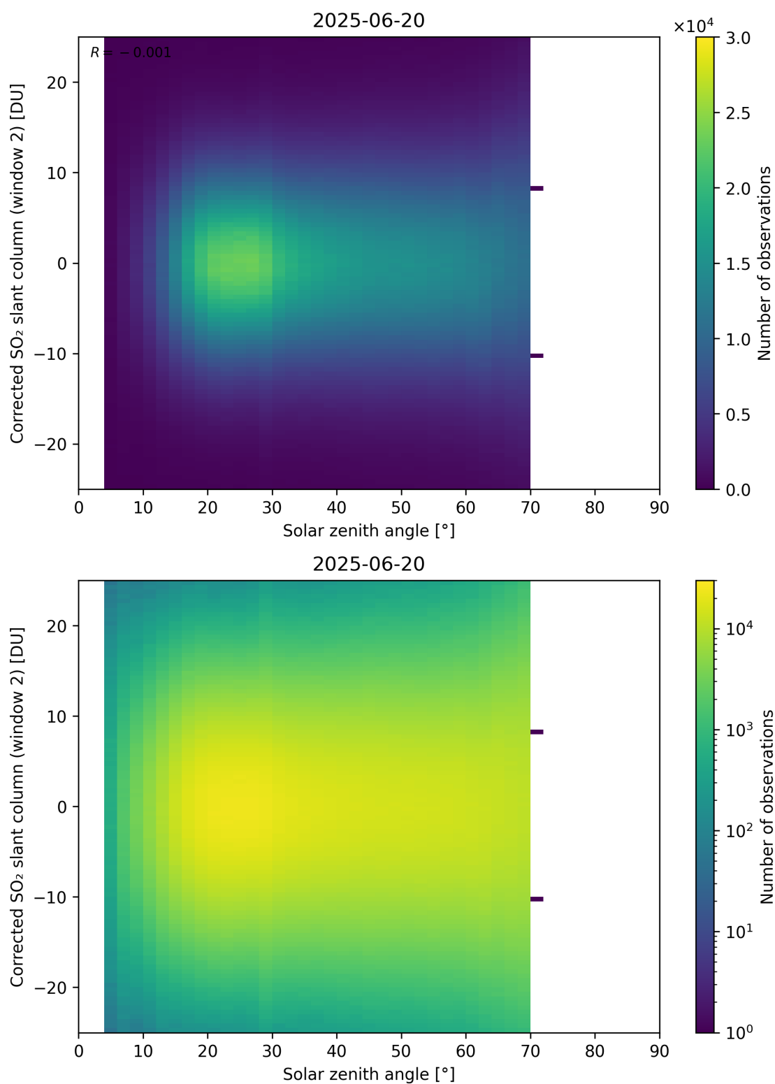
Figure 182: Scatter density plot of “Solar zenith angle” against “Corrected SO 2 slant column (window 2)” for 2025-06-19 to 2025-06-21.
