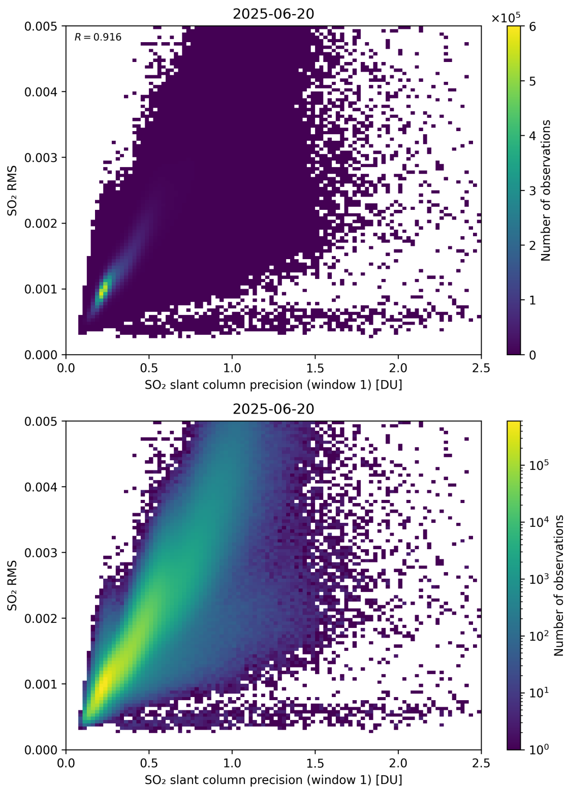
Figure 273: Scatter density plot of “SO 2 slant column precision (window 1)” against “SO 2 RMS” for 2025-06-19 to 2025-06-21.
