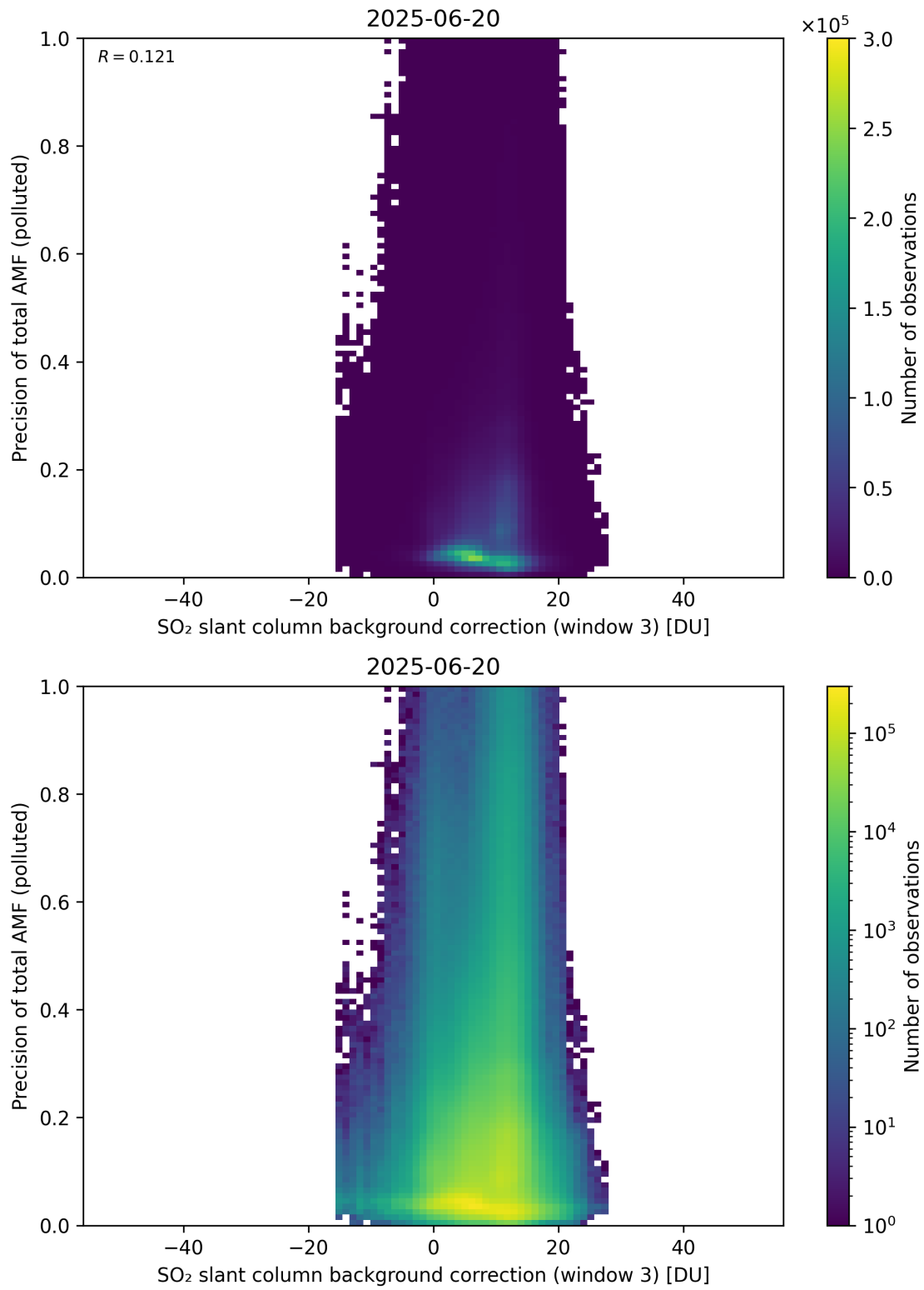
Figure 137: Scatter density plot of “SO 2 slant column background correction (window 3)” against “Precision of total AMF (polluted)” for 2025-06-19 to 2025-06-21.
