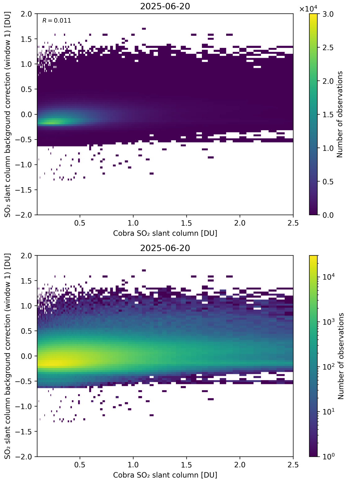
Figure 193: Scatter density plot of “Cobra SO 2 slant column” against “SO 2 slant column background correction (window 1)” for 2025-06-19 to 2025-06-21.
