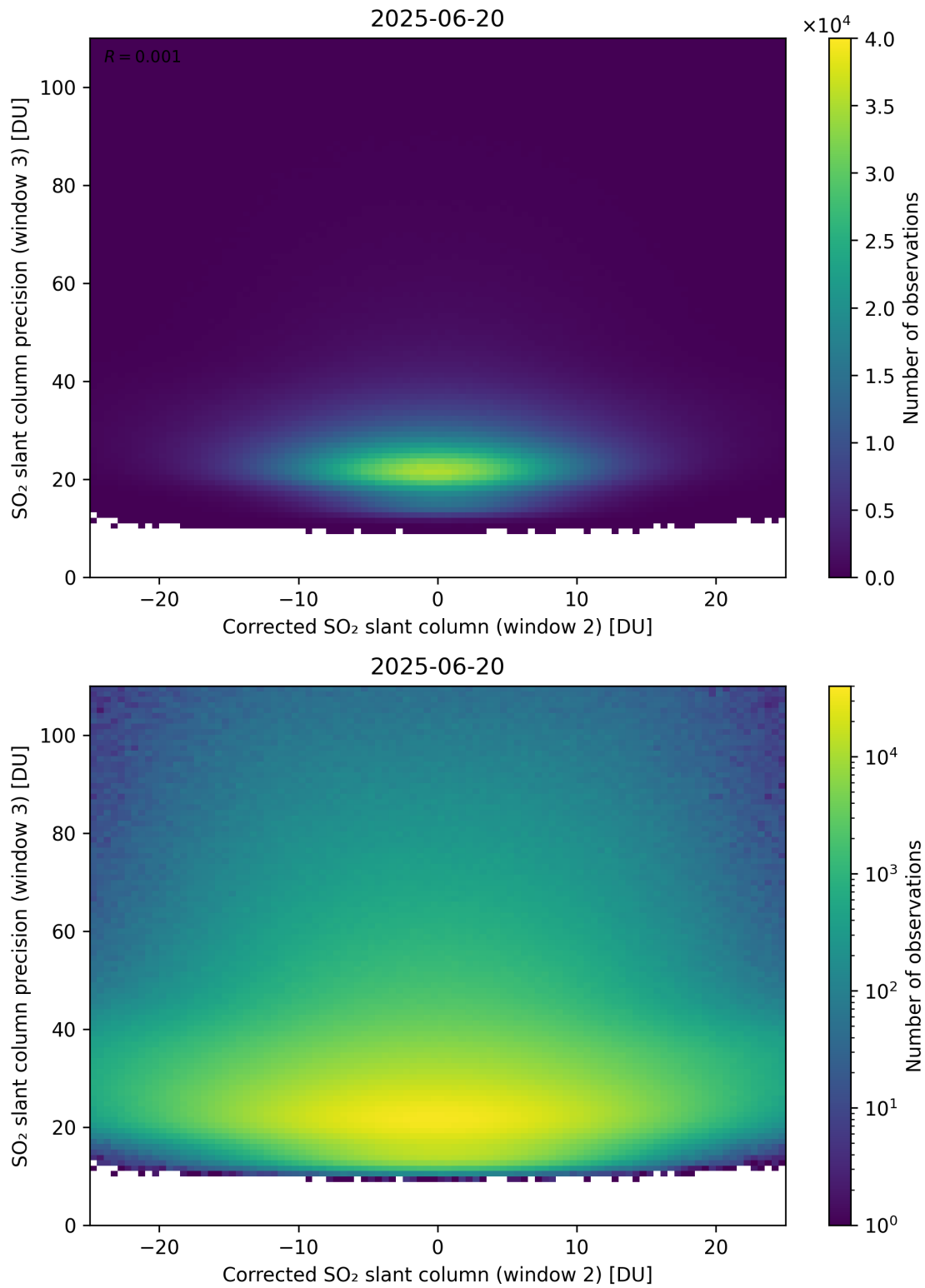
Figure 252: Scatter density plot of “Corrected SO 2 slant column (window 2)” against “SO 2 slant column precision (window 3)” for 2025-06-19 to 2025-06-21.
