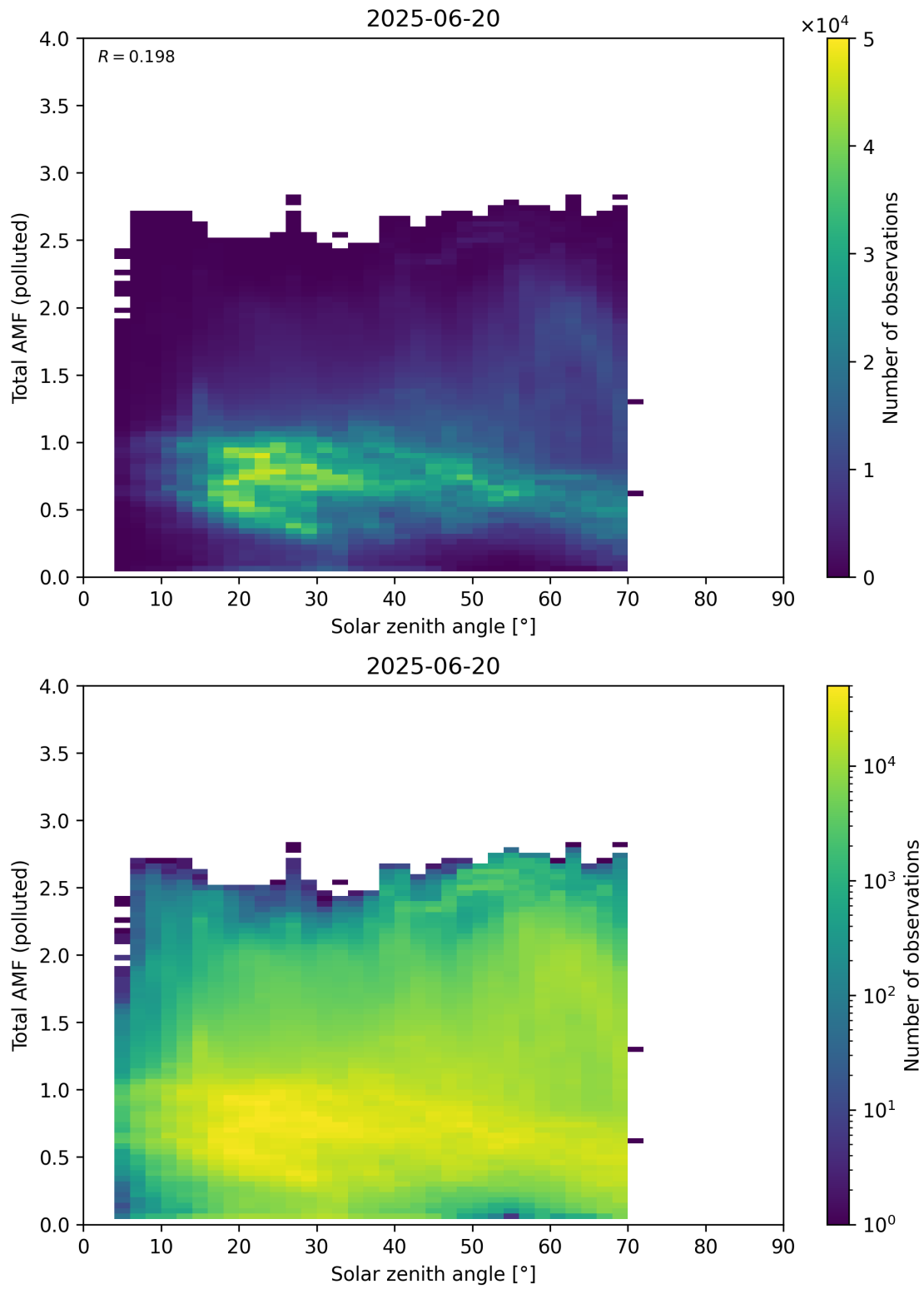
Figure 189: Scatter density plot of “Solar zenith angle” against “Total AMF (polluted)” for 2025-06-19 to 2025-06-21.
