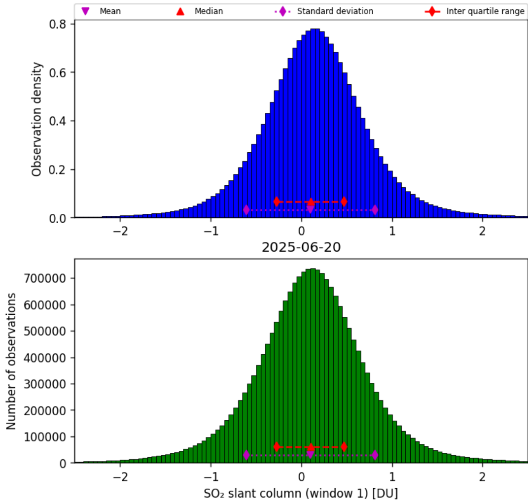
Figure 63: Histogram of “SO 2 slant column (window 1)” for 2025-06-19 to 2025-06-21
