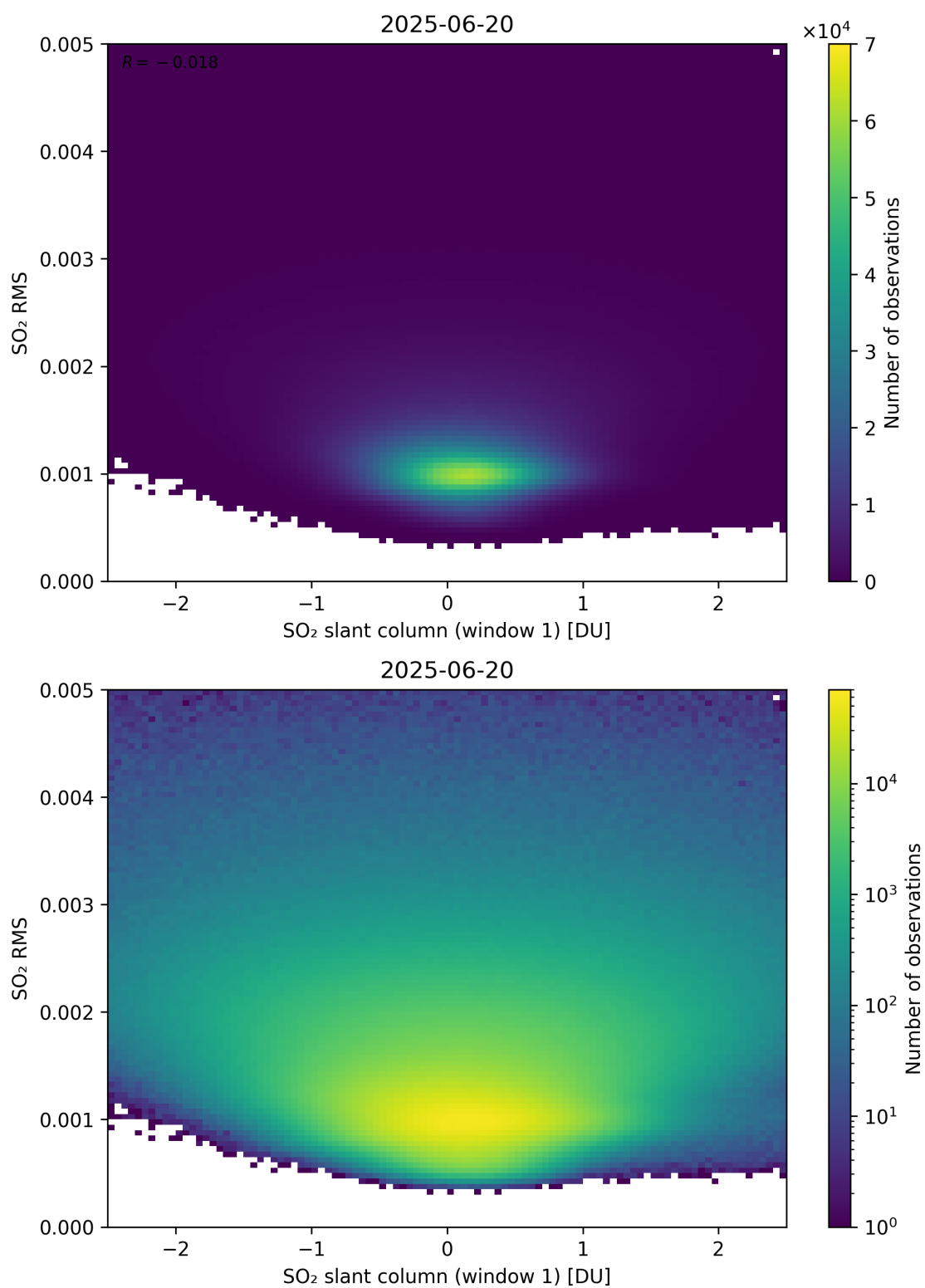
Figure 267: Scatter density plot of “SO 2 slant column (window 1)” against “SO 2 RMS” for 2025-06-19 to 2025-06-21.
