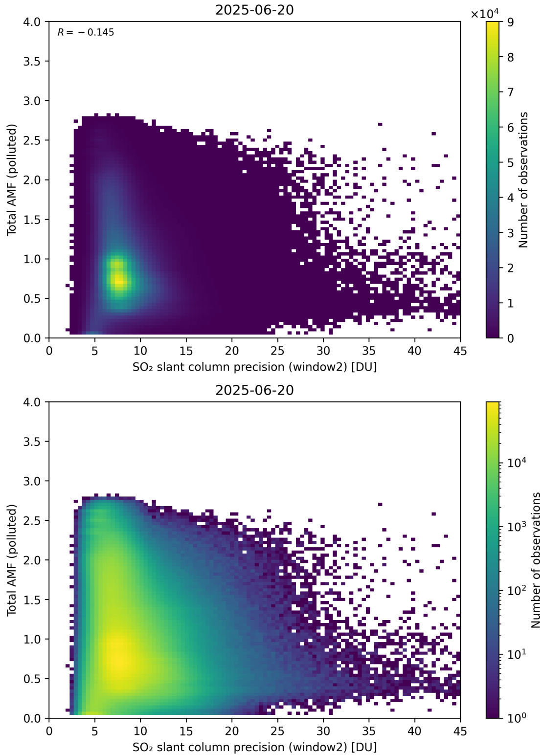
Figure 301: Scatter density plot of “SO 2 slant column precision (window2)” against “Total AMF (polluted)” for 2025-06-19 to 2025-06-21.
