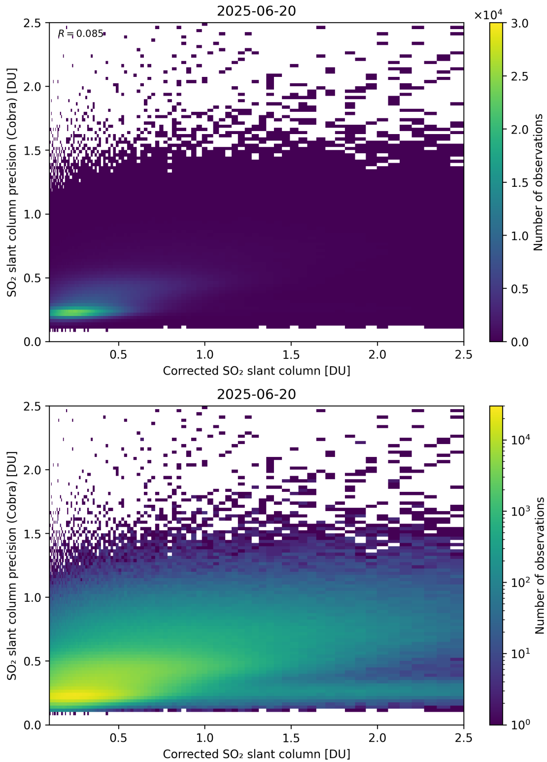
Figure 234: Scatter density plot of “Corrected SO 2 slant column” against “SO 2 slant column precision (Cobra)” for 2025-06-19 to 2025-06-21.
