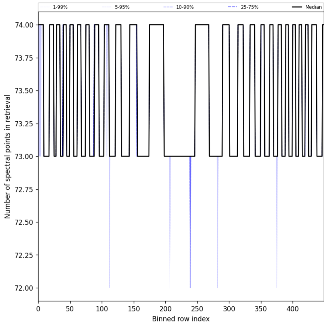
Figure 108: Along track statistics of “Number of spectral points in retrieval” for 2025-06-19 to 2025-06-21
