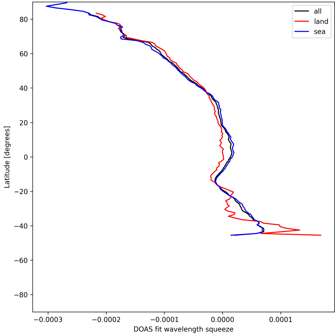
Figure 51: Zonal average of “DOAS fit wavelength squeeze” for 2025-06-19 to 2025-06-21.
