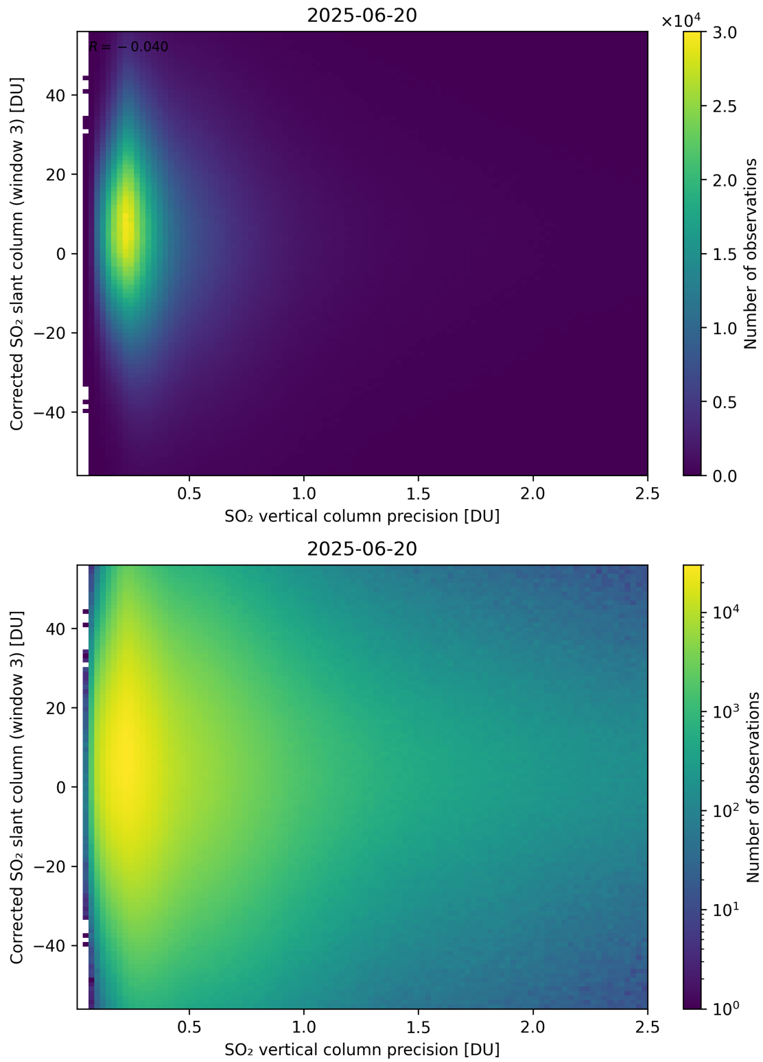
Figure 340: Scatter density plot of “SO 2 vertical column precision” against “Corrected SO 2 slant column (window 3)” for 2025-06-19 to 2025-06-21.
