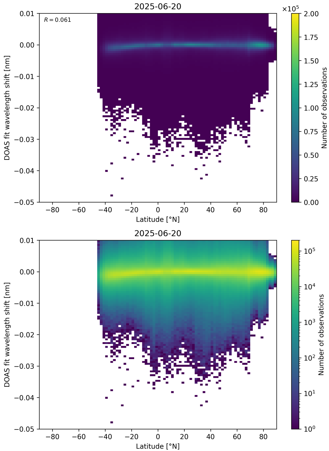
Figure 153: Scatter density plot of “Latitude” against “DOAS fit wavelength shift” for 2025-06-19 to 2025-06-21.
