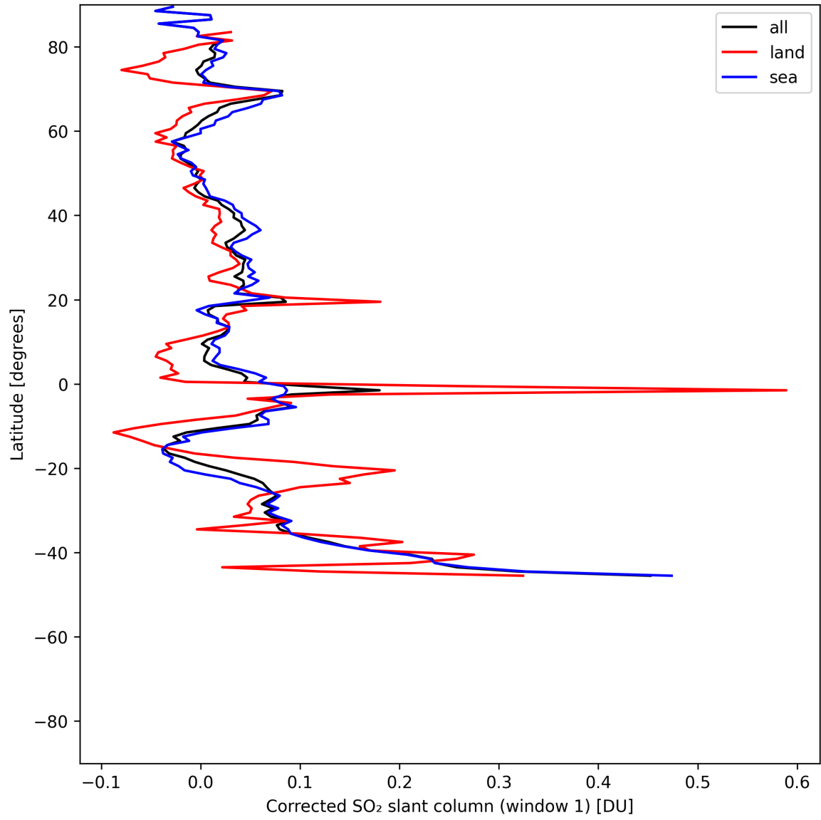
Figure 39: Zonal average of “Corrected SO 2 slant column (window 1)” for 2025-06-19 to 2025-06-21.
