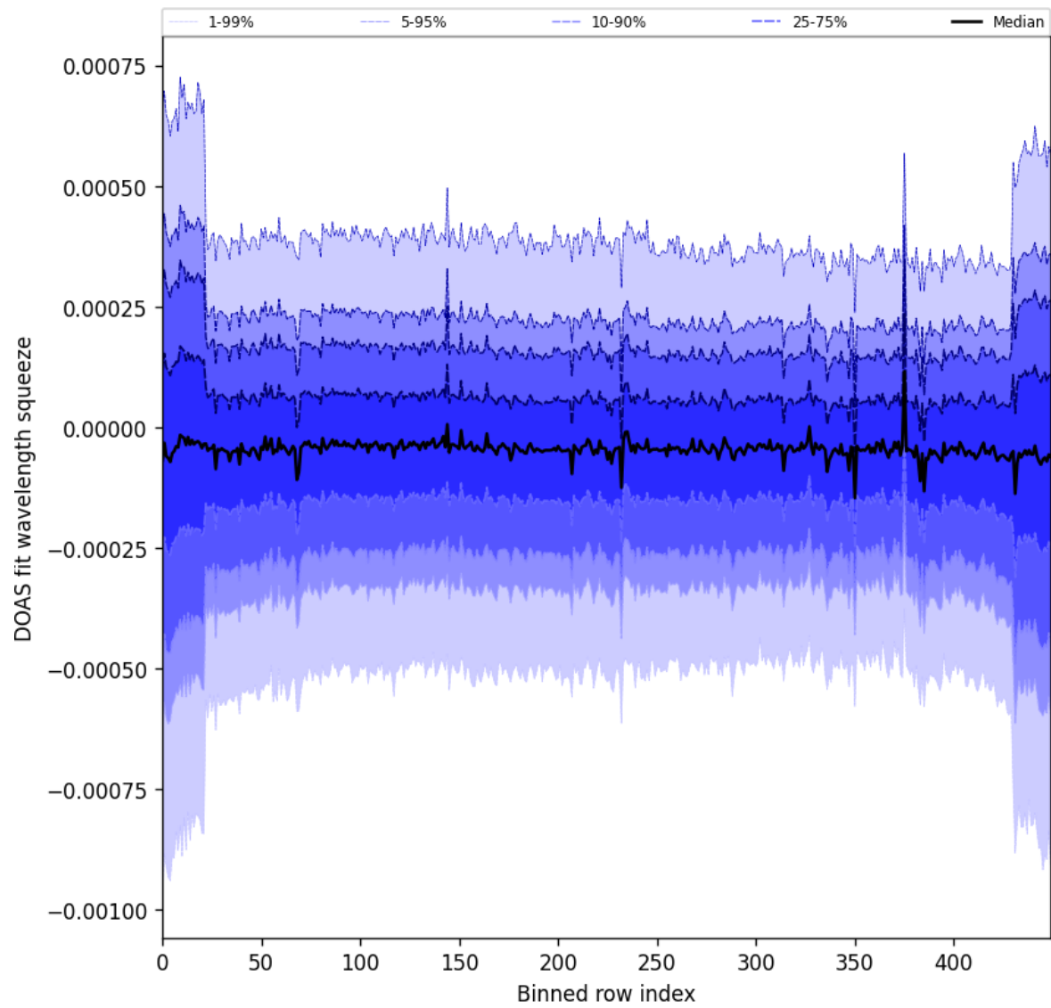
Figure 103: Along track statistics of “DOAS fit wavelength squeeze” for 2025-06-19 to 2025-06-21
