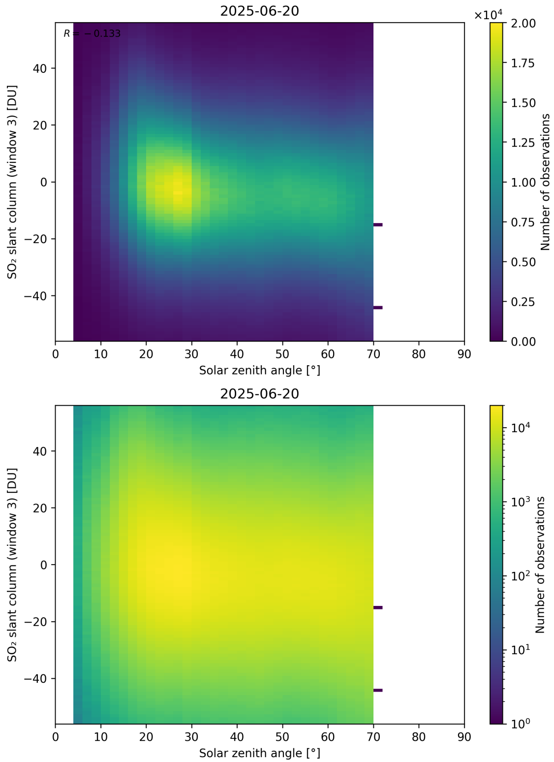
Figure 187: Scatter density plot of “Solar zenith angle” against “SO 2 slant column (window 3)” for 2025-06-19 to 2025-06-21.
