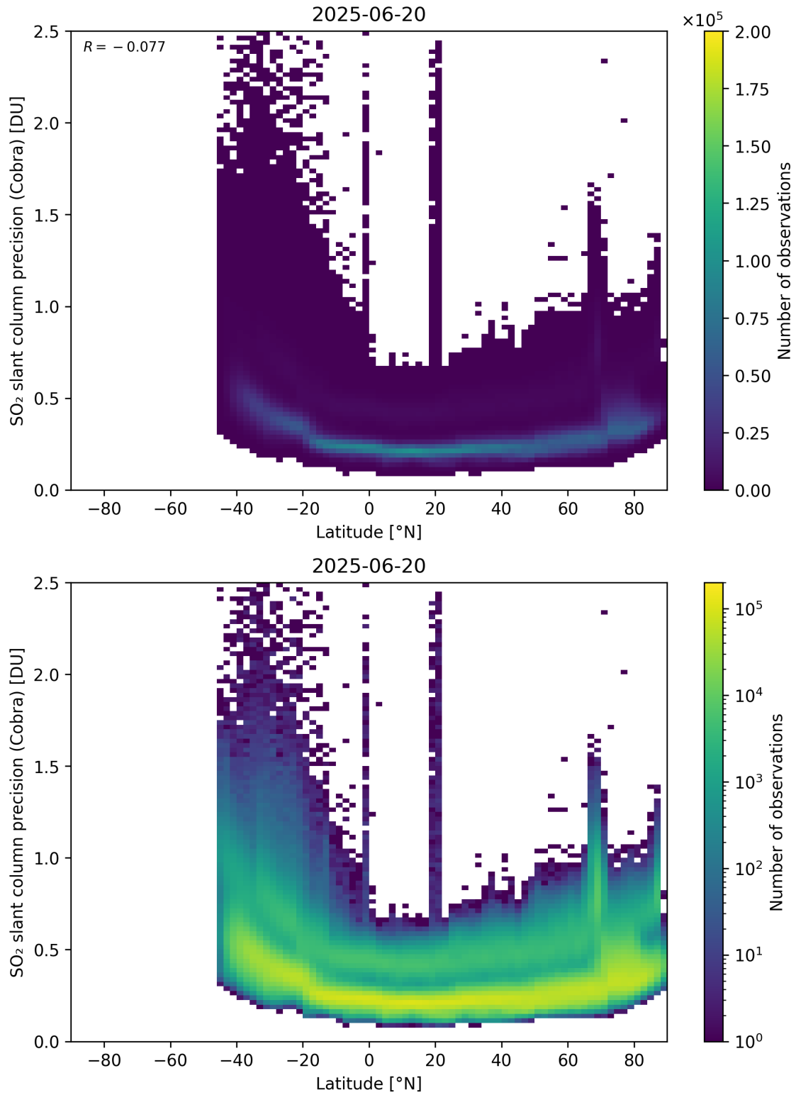
Figure 158: Scatter density plot of “Latitude” against “SO 2 slant column precision (Cobra)” for 2025-06-19 to 2025-06-21.
