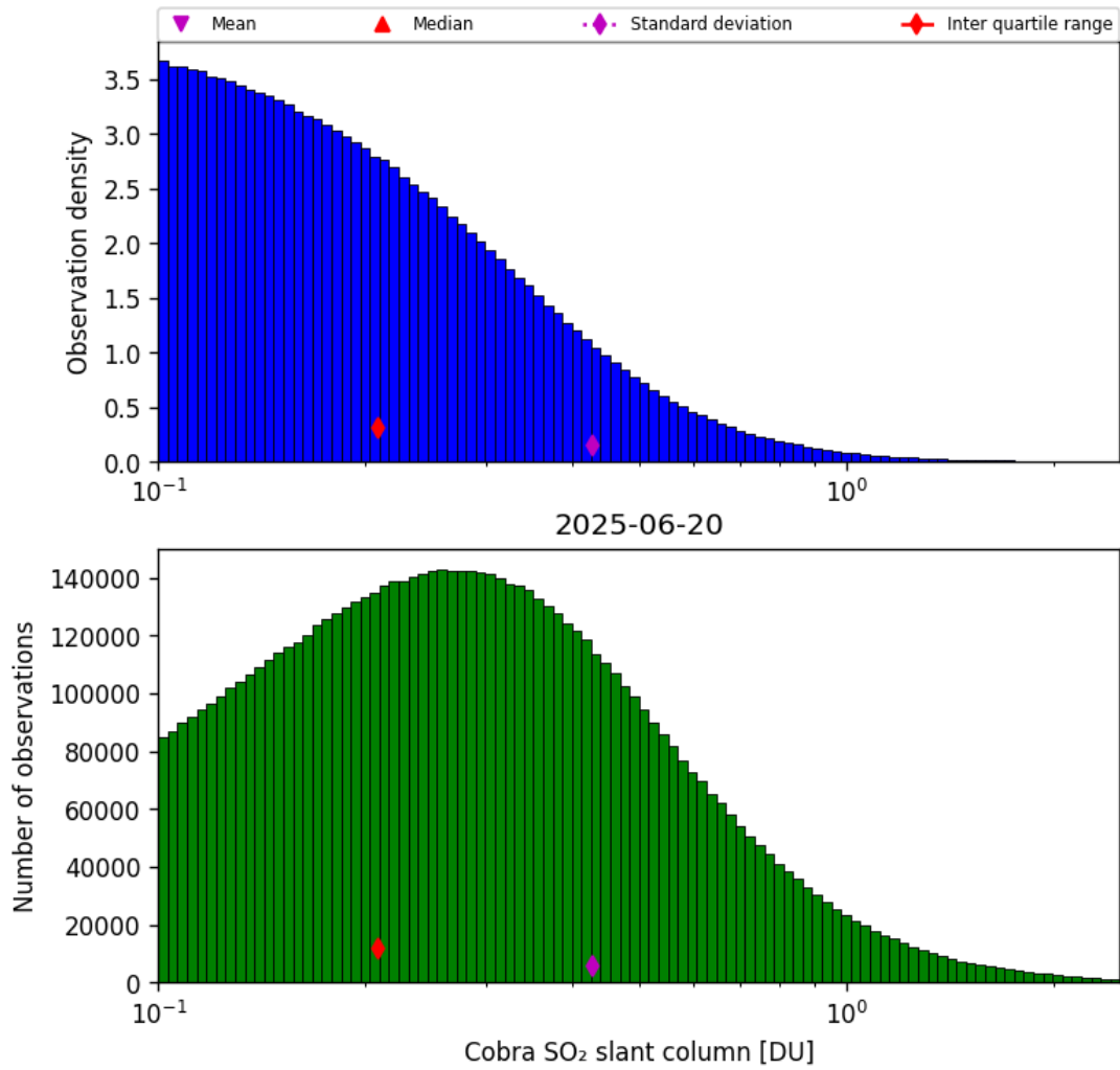
Figure 61: Histogram of “Cobra SO 2 slant column” for 2025-06-19 to 2025-06-21
