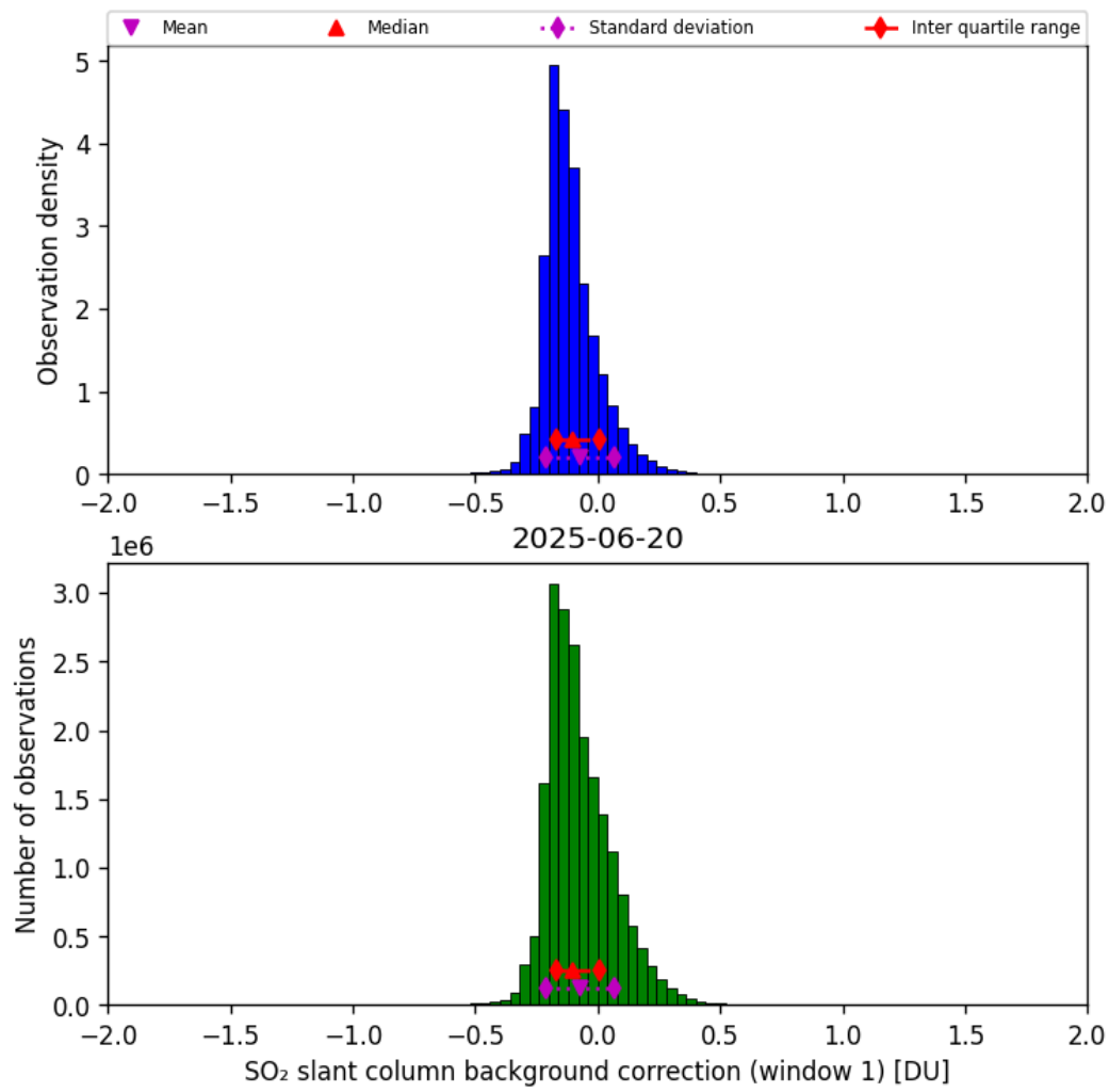
Figure 66: Histogram of “SO 2 slant column background correction (window 1)” for 2025-06-19 to 2025-06-21
