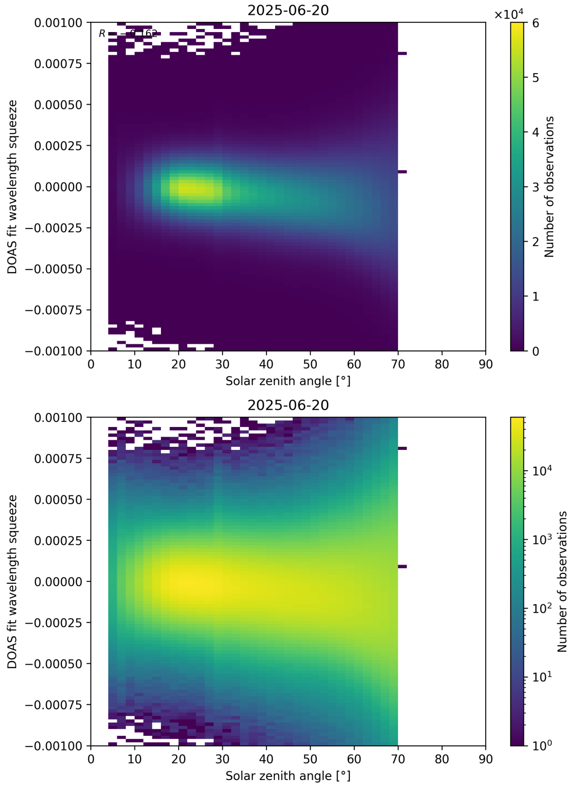
Figure 175: Scatter density plot of “Solar zenith angle” against “DOAS fit wavelength squeeze” for 2025-06-19 to 2025-06-21.
