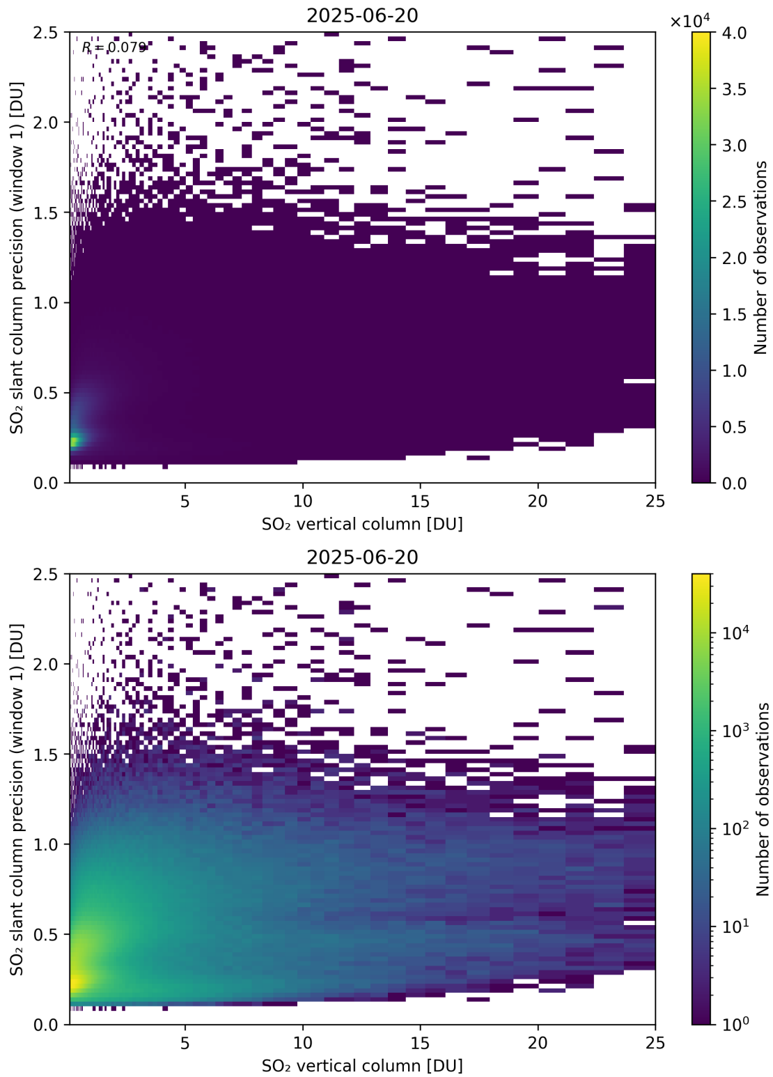
Figure 355: Scatter density plot of “SO 2 vertical column” against “SO 2 slant column precision (window 1)” for 2025-06-19 to 2025-06-21.
