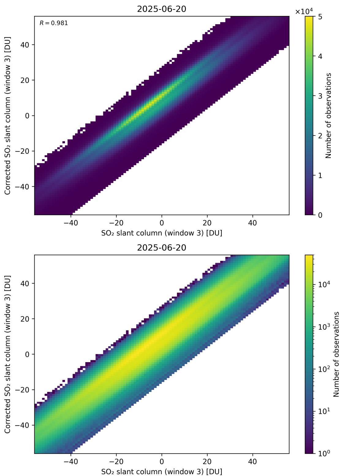
Figure 316: Scatter density plot of “SO 2 slant column (window 3)” against “Corrected SO 2 slant column (window 3)” for 2025-06-19 to 2025-06-21.
