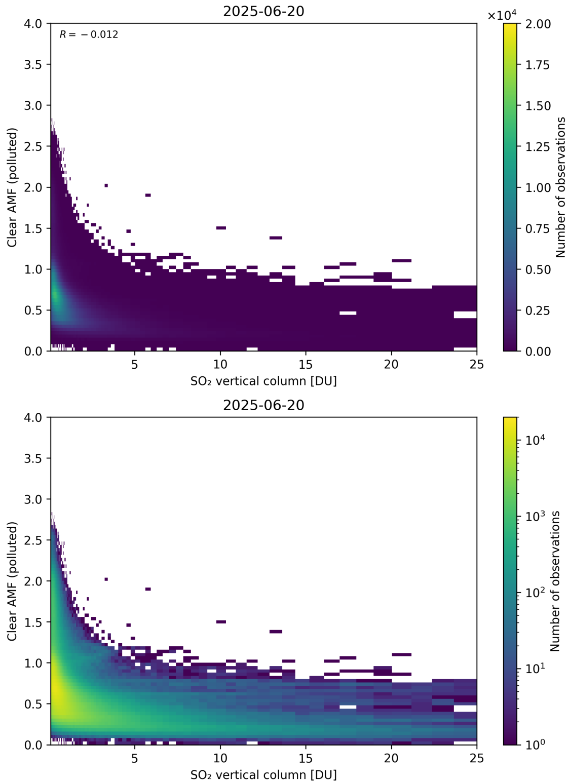
Figure 348: Scatter density plot of “SO 2 vertical column” against “Clear AMF (polluted)” for 2025-06-19 to 2025-06-21.
