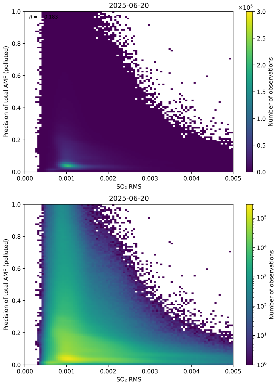
Figure 149: Scatter density plot of “SO 2 RMS” against “Precision of total AMF (polluted)” for 2025-06-19 to 2025-06-21.
