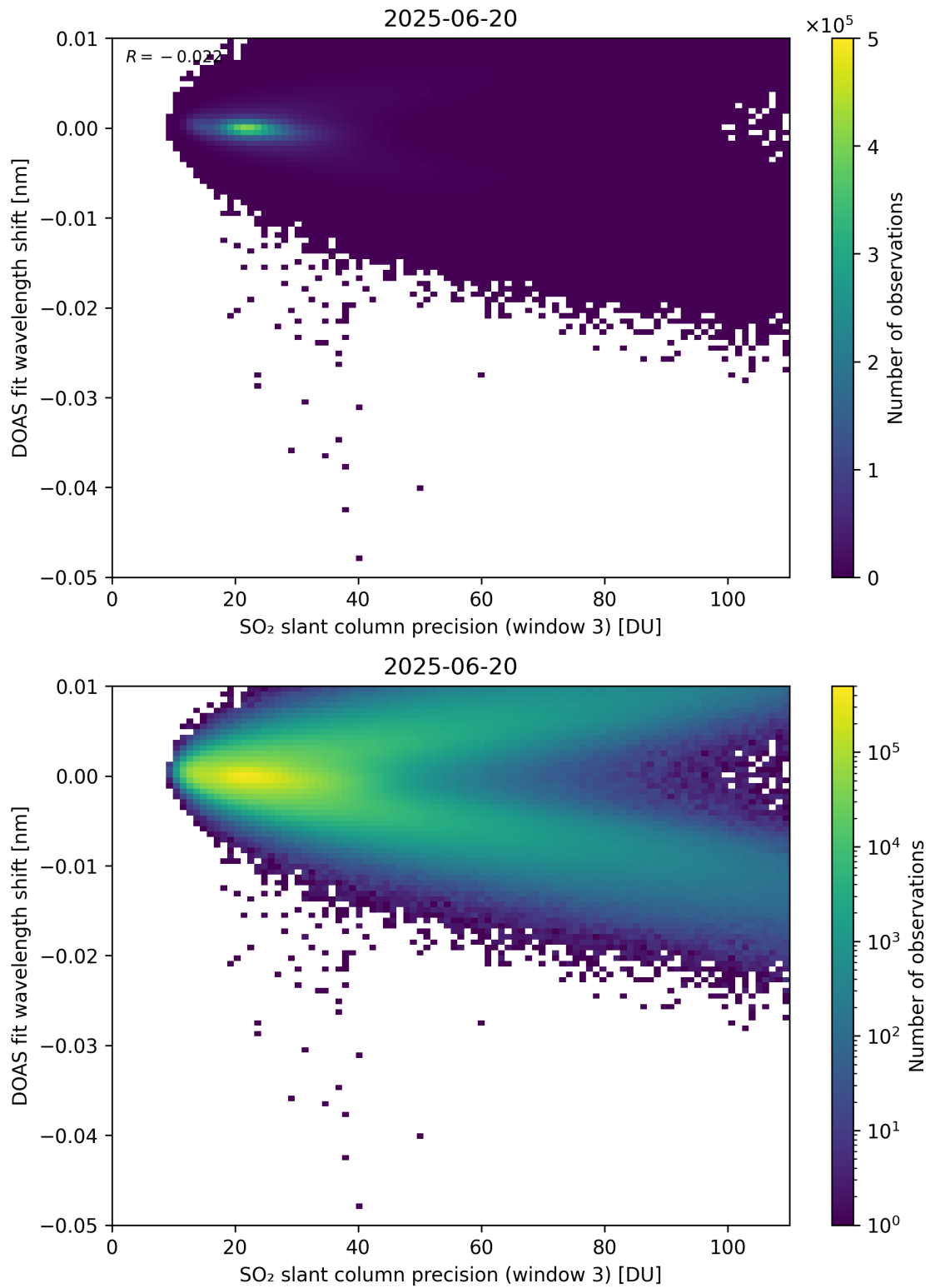
Figure 308: Scatter density plot of “SO 2 slant column precision (window 3)” against “DOAS fit wavelength shift” for 2025-06-19 to 2025-06-21.
