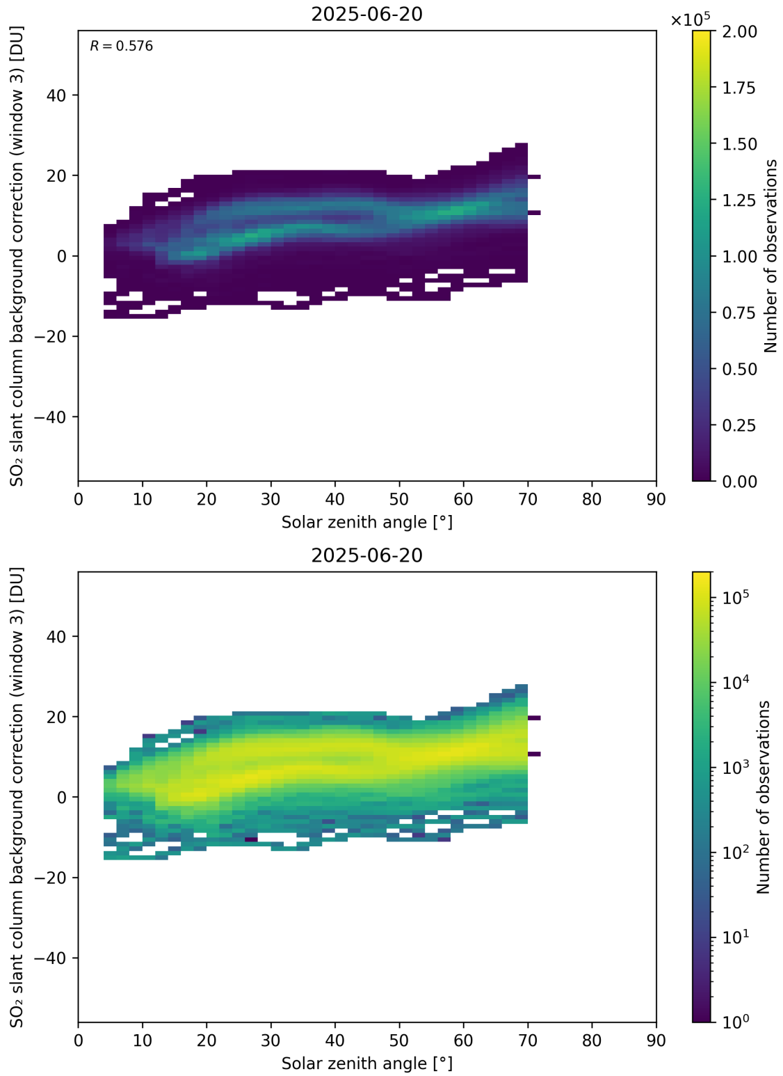
Figure 173: Scatter density plot of “Solar zenith angle” against “SO 2 slant column background correction (window 3)” for 2025-06-19 to 2025-06-21.
