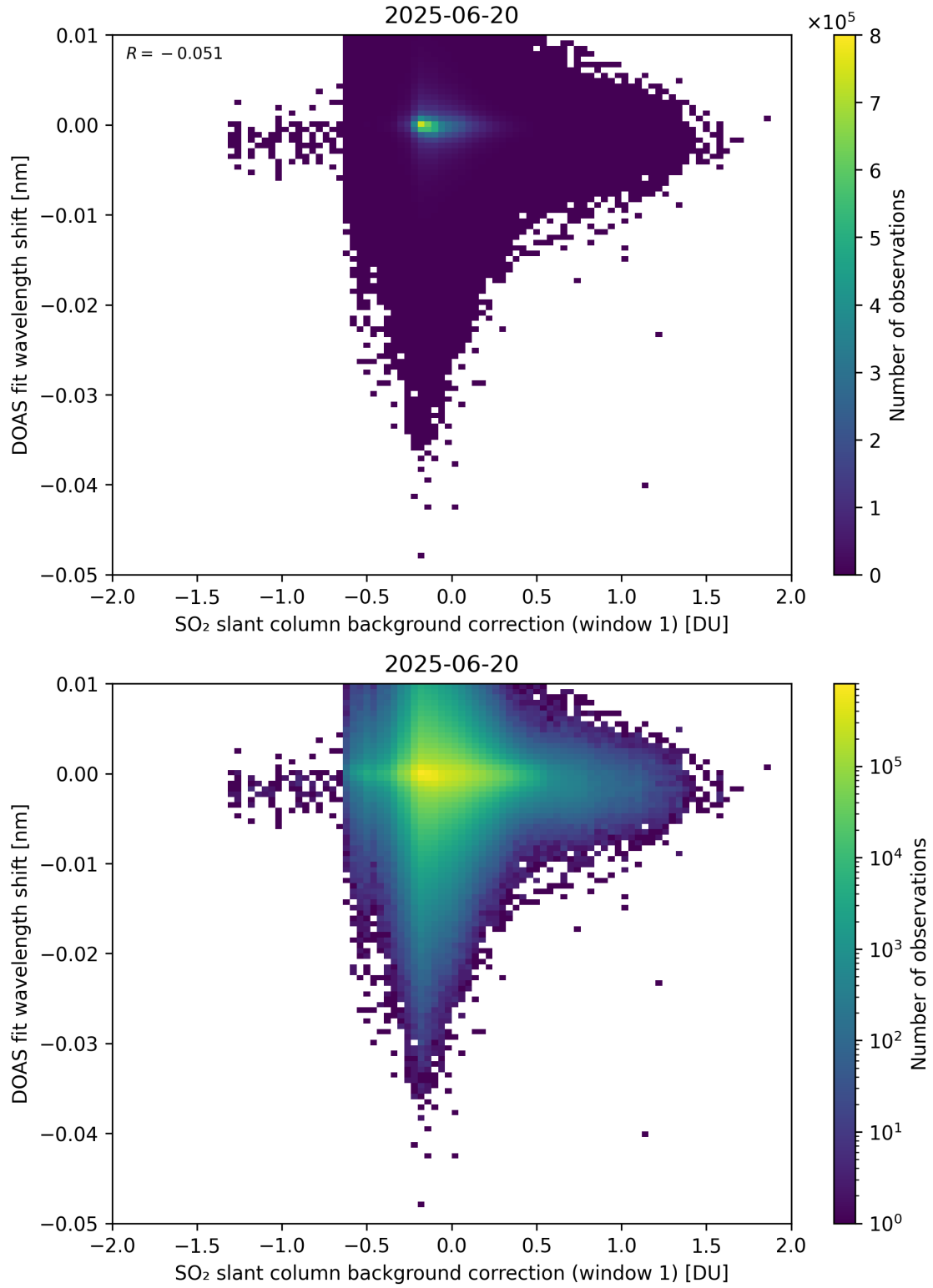
Figure 111: Scatter density plot of “SO 2 slant column background correction (window 1)” against “DOAS fit wavelength shift” for 2025-06-19 to 2025-06-21.
