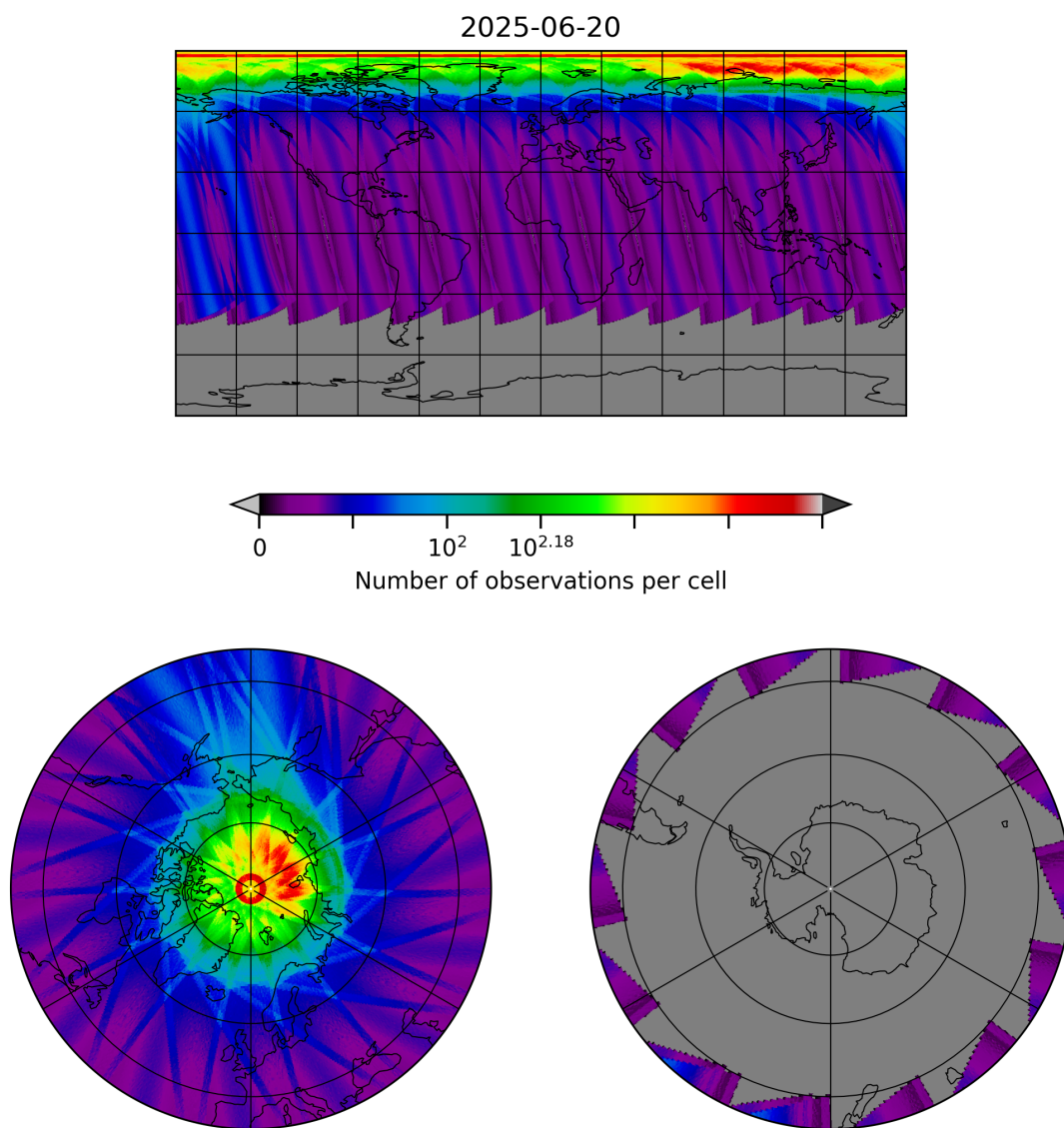
Figure 30: Map of the number of observations for 2025-06-19 to 2025-06-21
