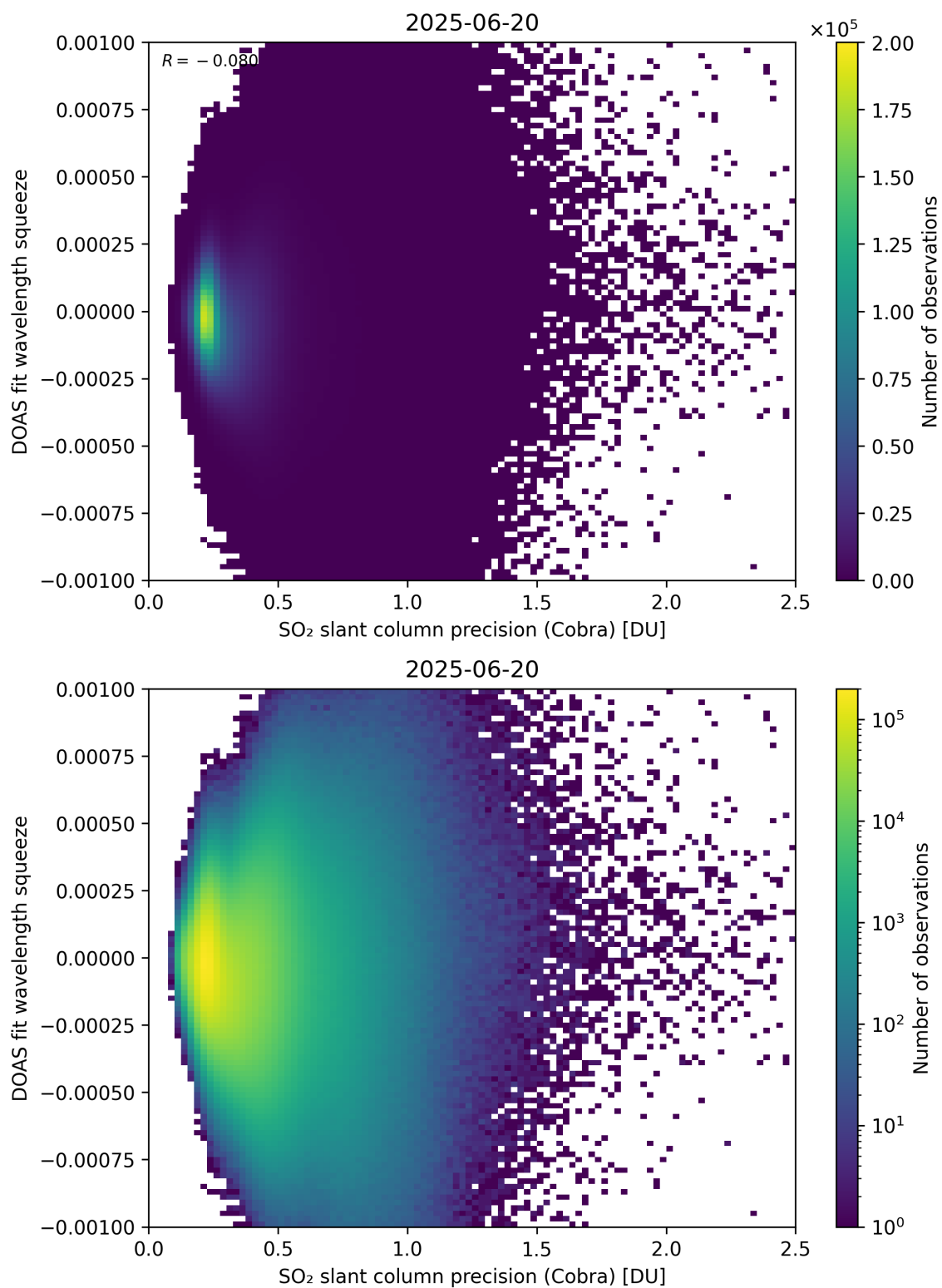
Figure 203: Scatter density plot of “SO 2 slant column precision (Cobra)” against “DOAS fit wavelength squeeze” for 2025-06-19 to 2025-06-21.
