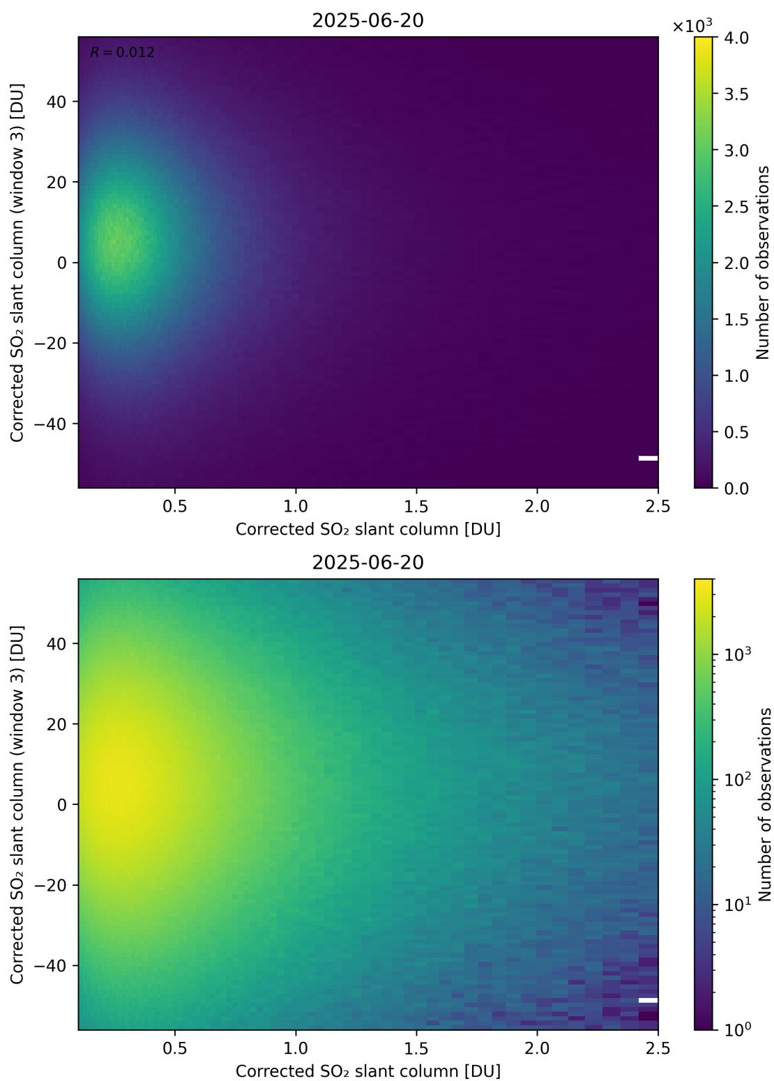
Figure 236: Scatter density plot of “Corrected SO 2 slant column” against “Corrected SO 2 slant column (window 3)” for 2025-06-19 to 2025-06-21.
