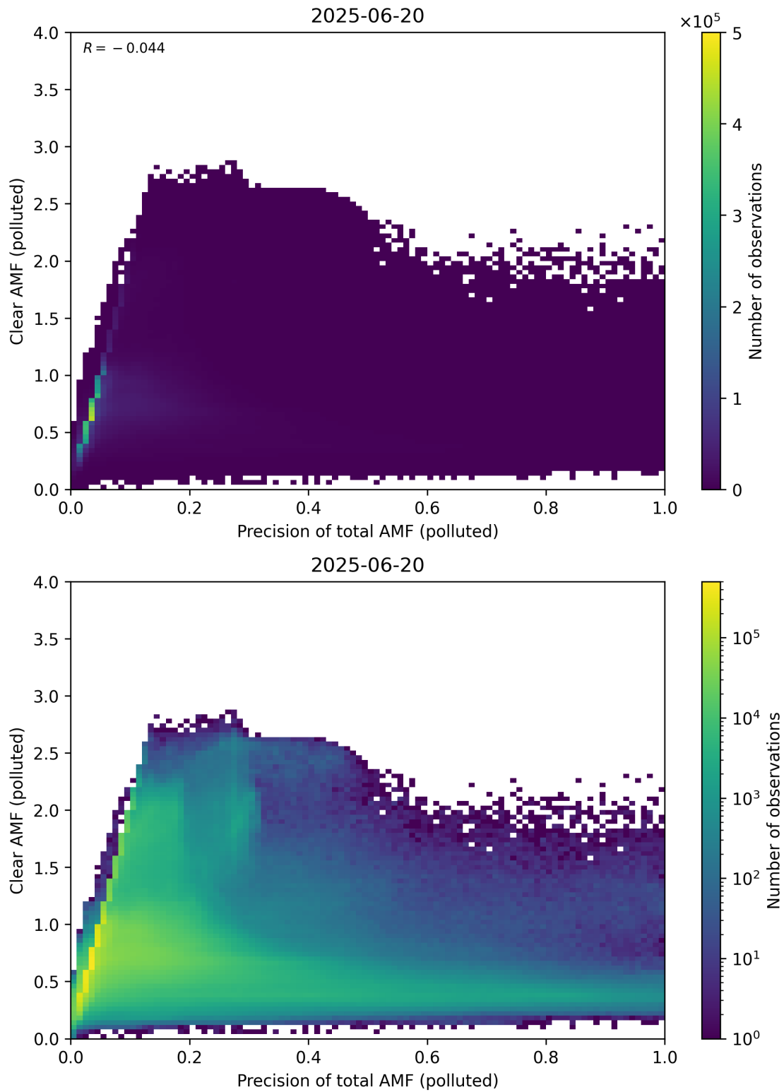
Figure 320: Scatter density plot of “Precision of total AMF (polluted)” against “Clear AMF (polluted)” for 2025-06-19 to 2025-06-21.
