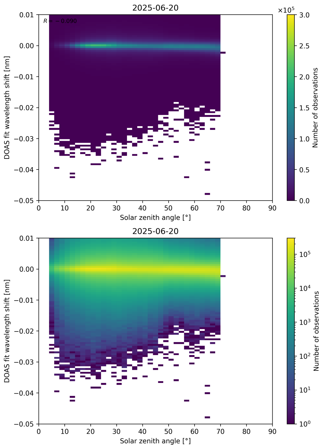
Figure 174: Scatter density plot of “Solar zenith angle” against “DOAS fit wavelength shift” for 2025-06-19 to 2025-06-21.
