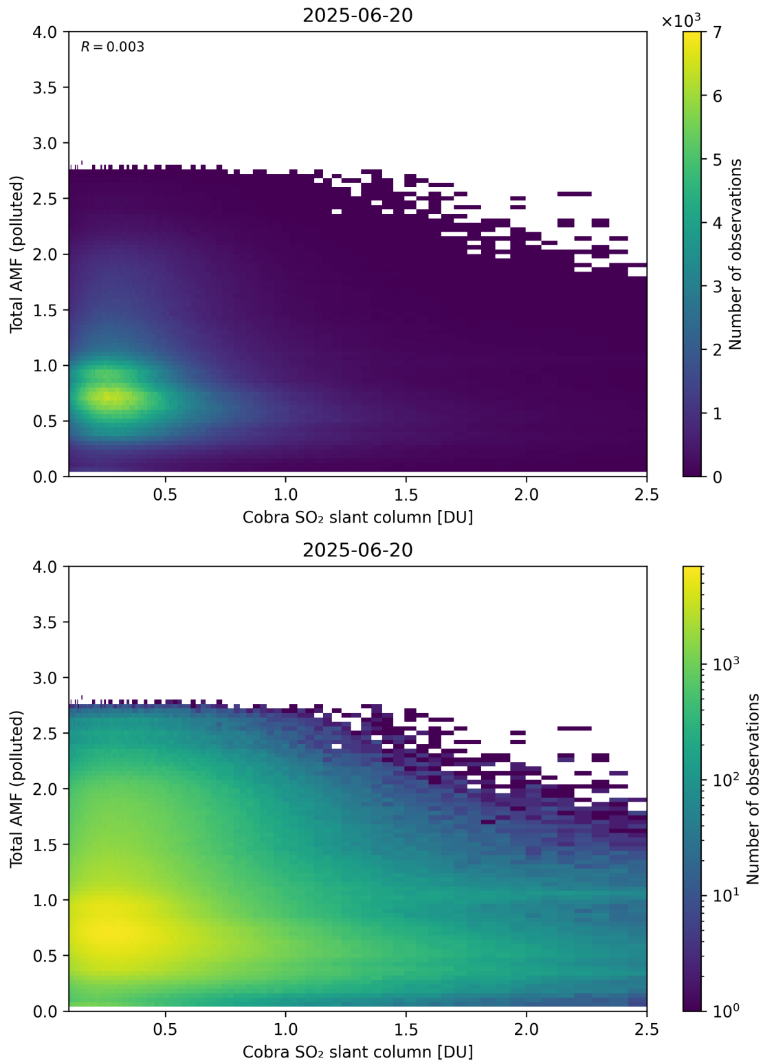
Figure 224: Scatter density plot of “Cobra SO 2 slant column” against “Total AMF (polluted)” for 2025-06-19 to 2025-06-21.
