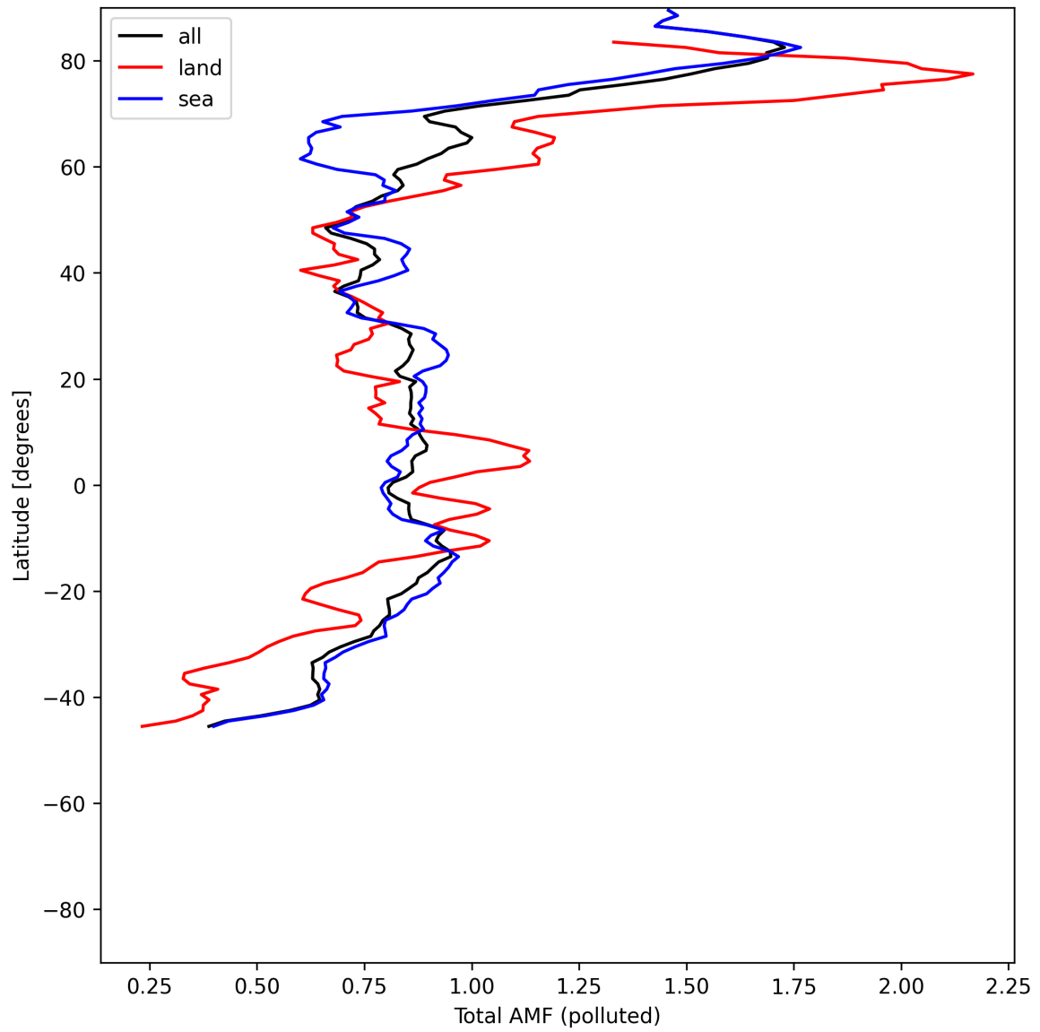
Figure 53: Zonal average of “Total AMF (polluted)” for 2025-06-19 to 2025-06-21.
