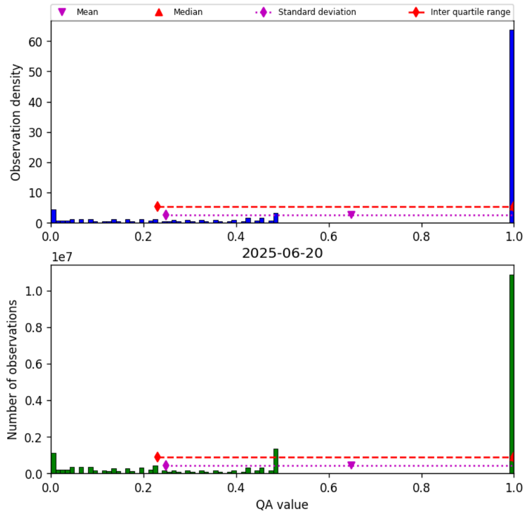
Figure 57: Histogram of “QA value” for 2025-06-19 to 2025-06-21
