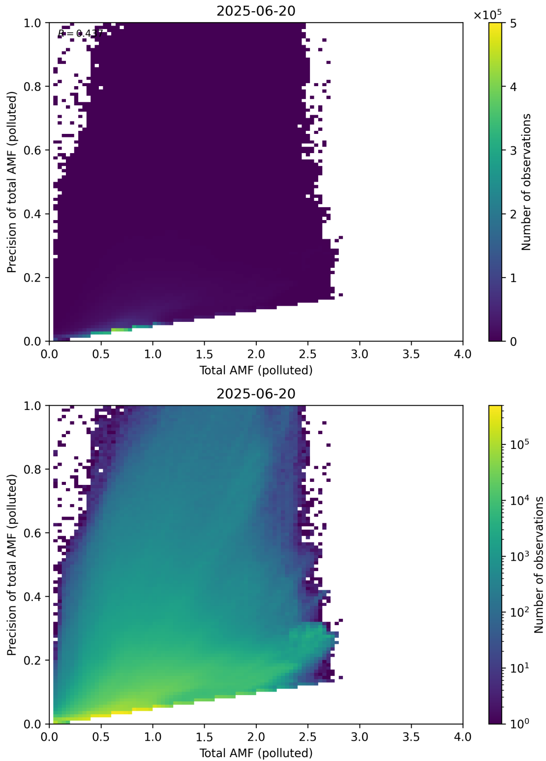
Figure 322: Scatter density plot of “Total AMF (polluted)” against “Precision of total AMF (polluted)” for 2025-06-19 to 2025-06-21.
