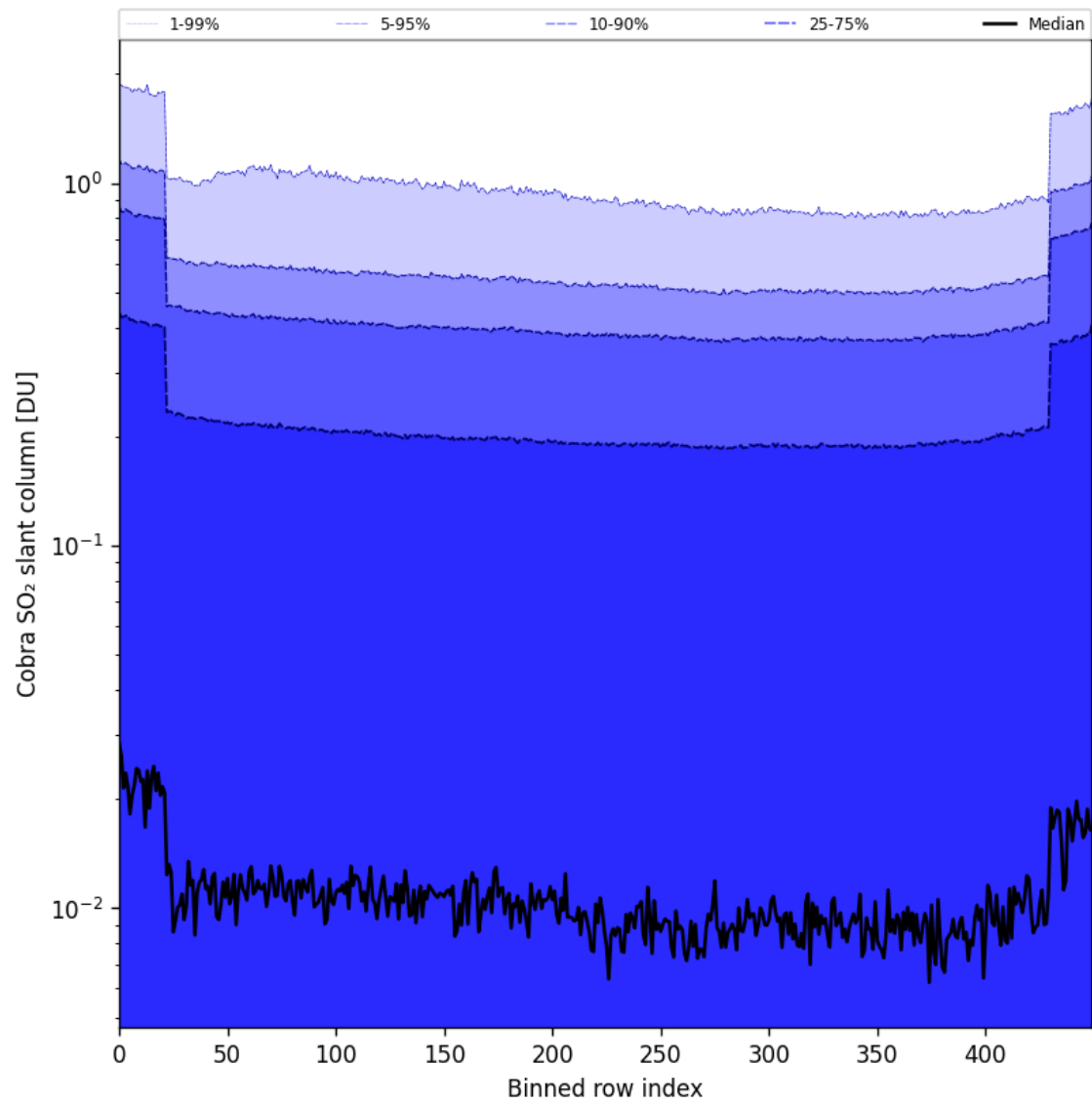
Figure 87: Along track statistics of "Cobra SO 2 slant column" for 2025-06-19 to 2025-06-21
