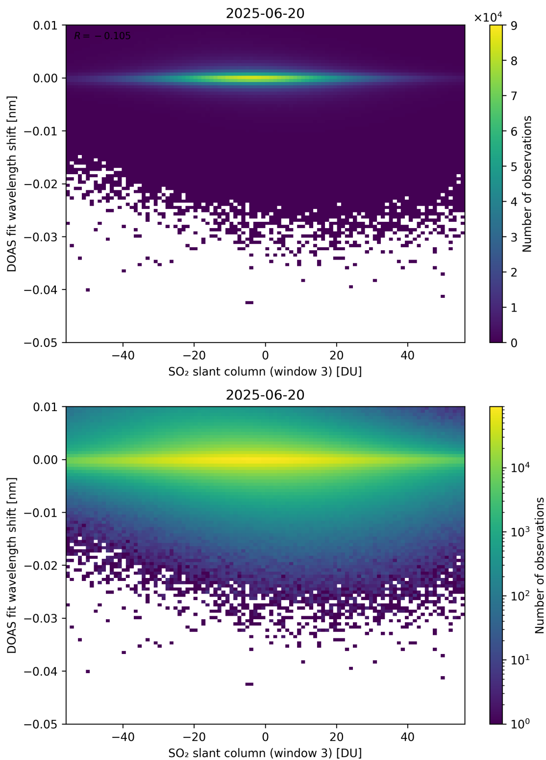
Figure 304: Scatter density plot of “SO 2 slant column (window 3)” against “DOAS fit wavelength shift” for 2025-06-19 to 2025-06-21.
