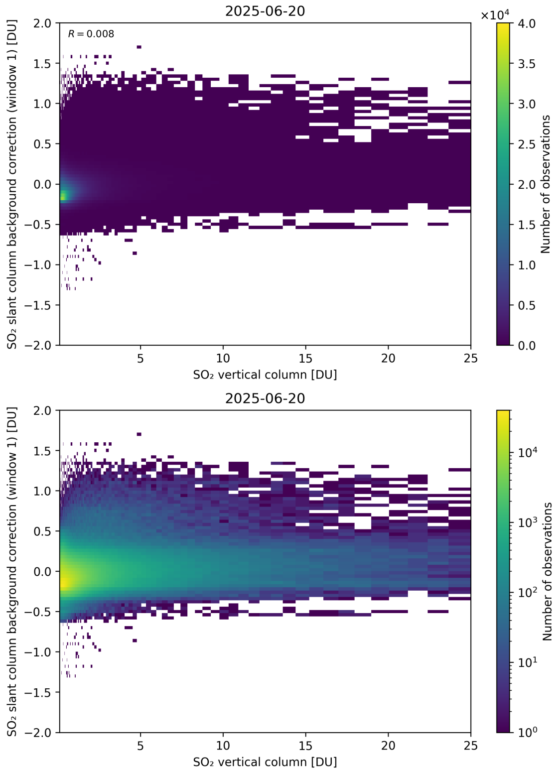
Figure 323: Scatter density plot of “SO 2 vertical column” against “SO 2 slant column background correction (window 1)” for 2025-06-19 to 2025-06-21.
