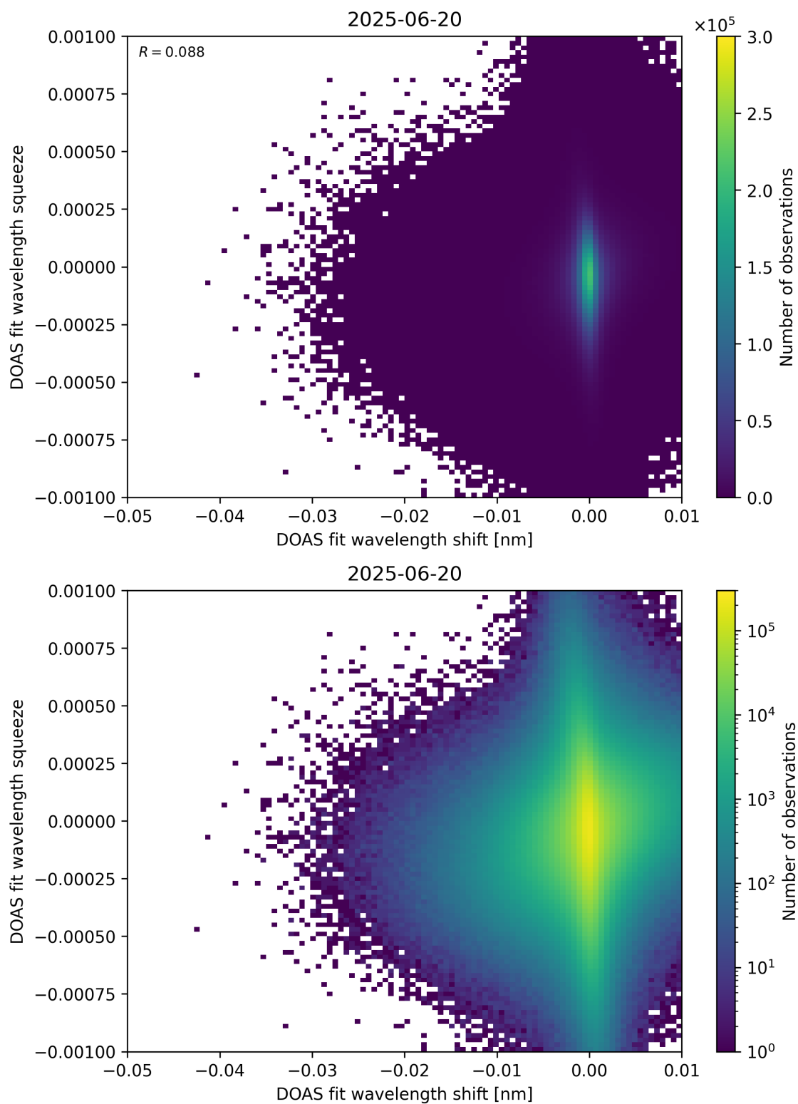
Figure 138: Scatter density plot of “DOAS fit wavelength shift” against “DOAS fit wavelength squeeze” for 2025-06-19 to 2025-06-21.
