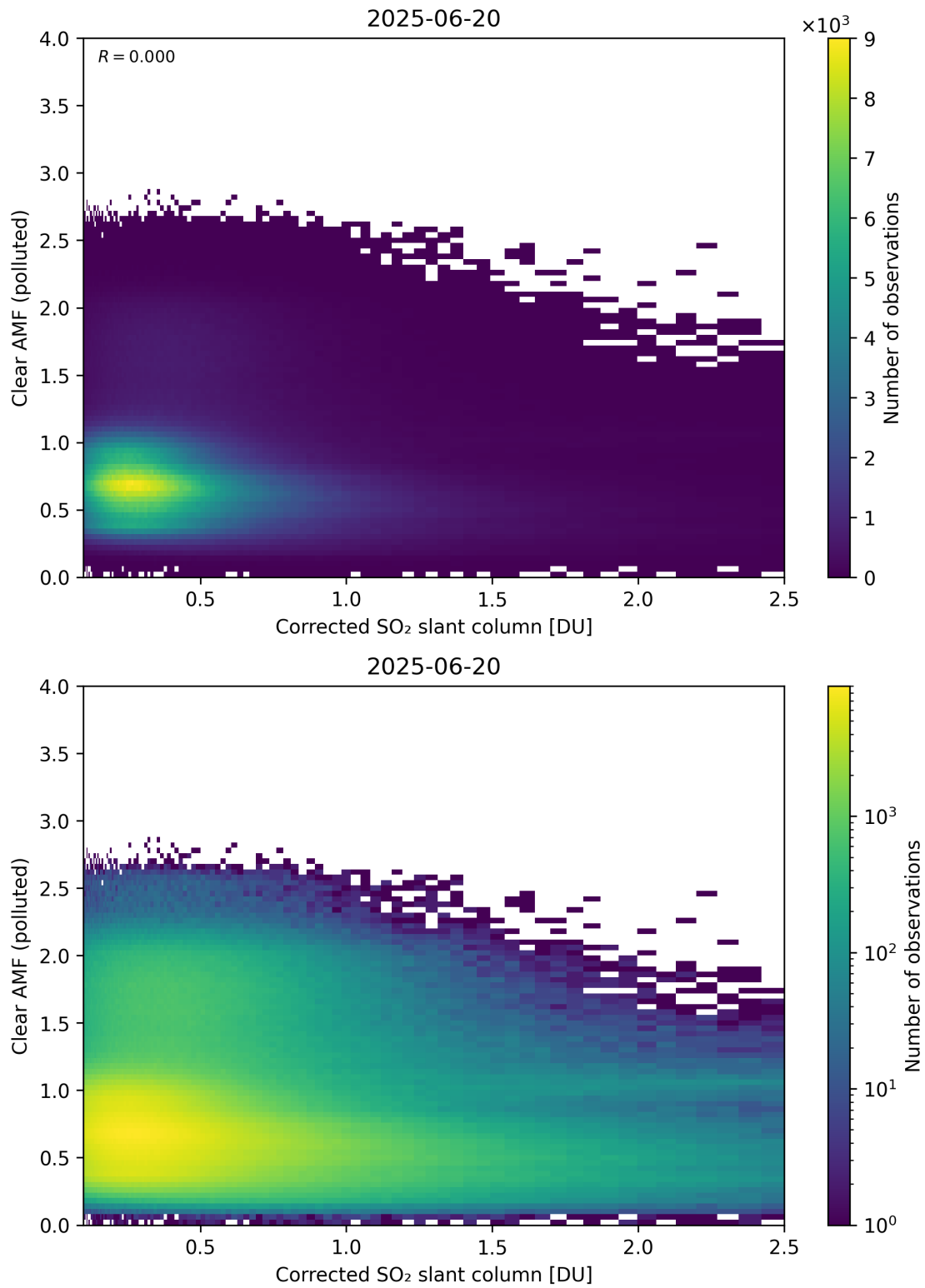
Figure 232: Scatter density plot of “Corrected SO 2 slant column” against “Clear AMF (polluted)” for 2025-06-19 to 2025-06-21.
