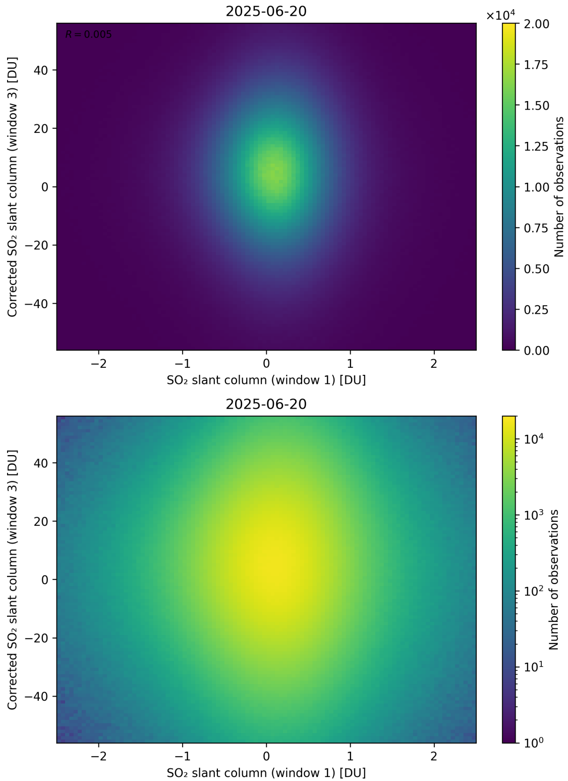
Figure 284: Scatter density plot of “SO 2 slant column (window 1)” against “Corrected SO 2 slant column (window 3)” for 2025-06-19 to 2025-06-21.
