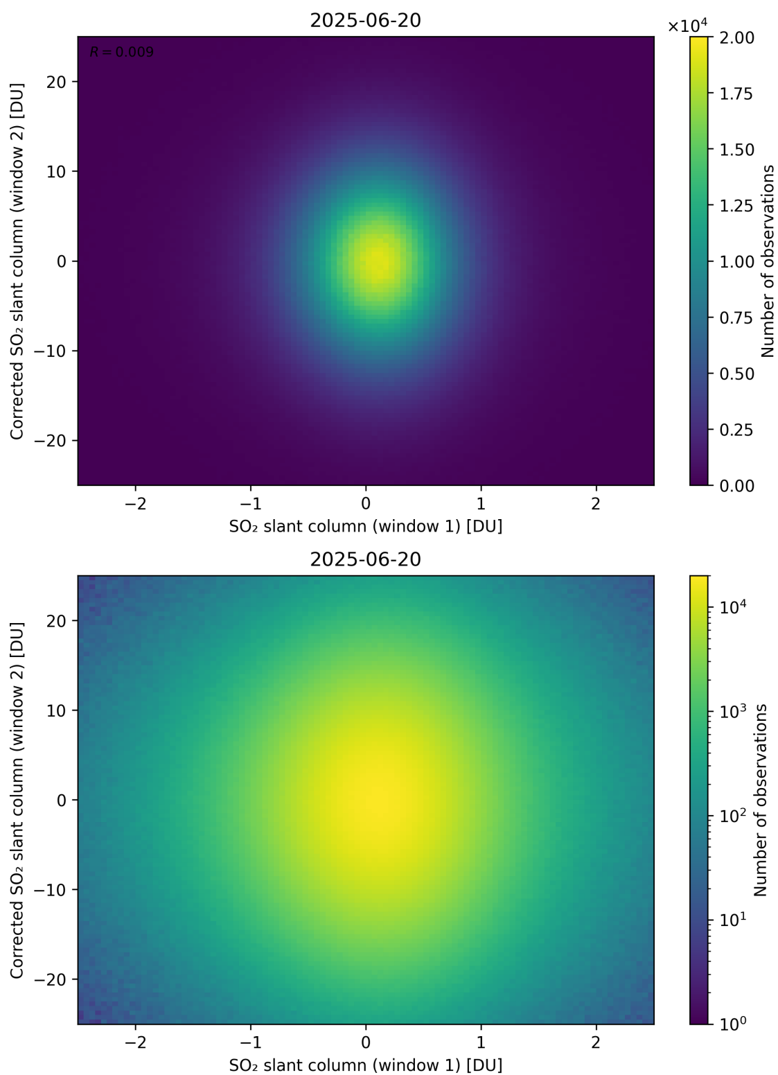
Figure 283: Scatter density plot of “SO 2 slant column (window 1)” against “Corrected SO 2 slant column (window 2)” for 2025-06-19 to 2025-06-21.
