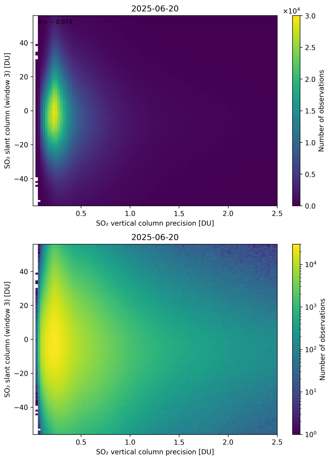
Figure 344: Scatter density plot of “SO 2 vertical column precision” against “SO 2 slant column (window 3)” for 2025-06-19 to 2025-06-21.
