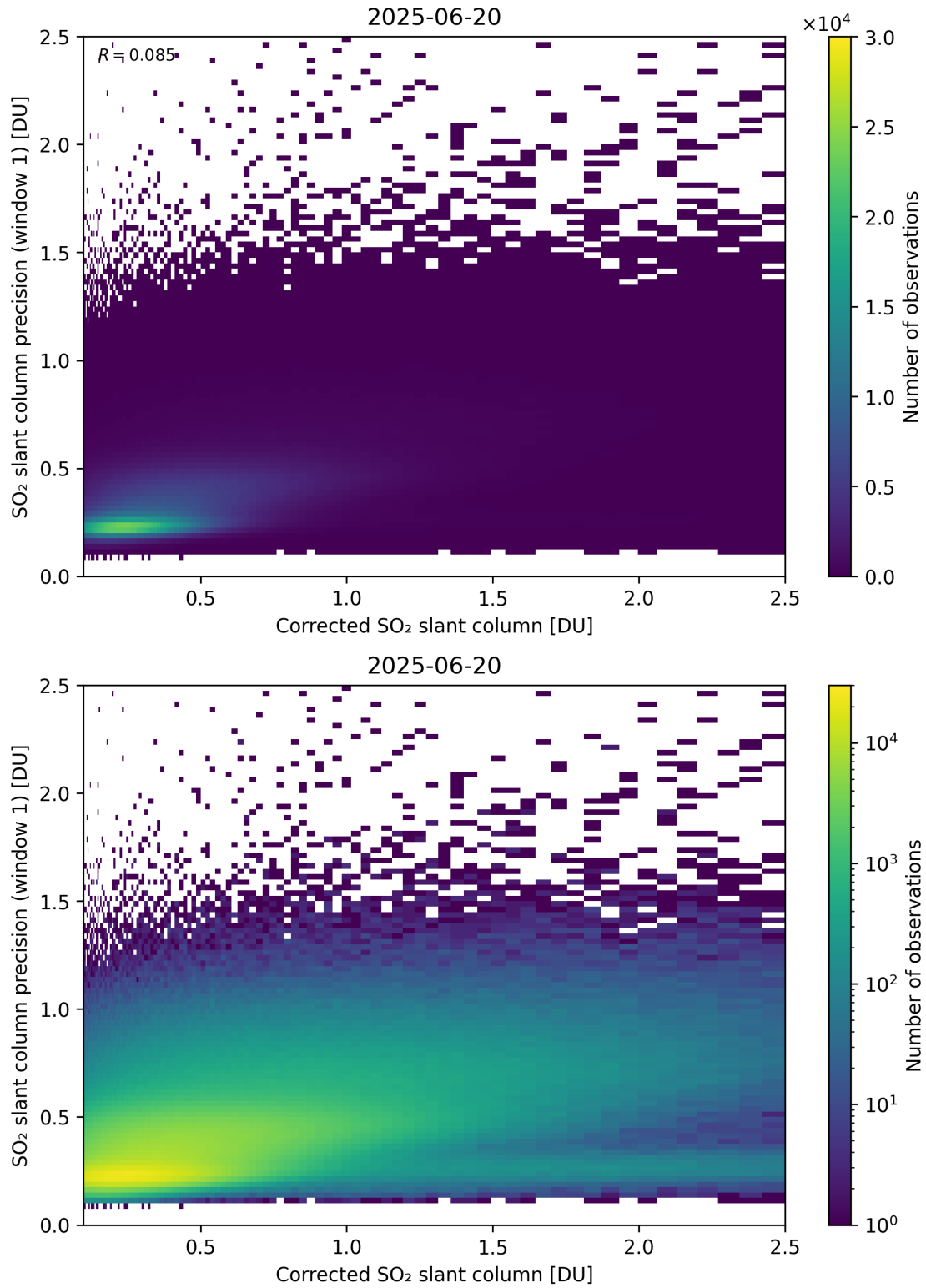
Figure 238: Scatter density plot of “Corrected SO 2 slant column” against “SO 2 slant column precision (window 1)” for 2025-06-19 to 2025-06-21.
