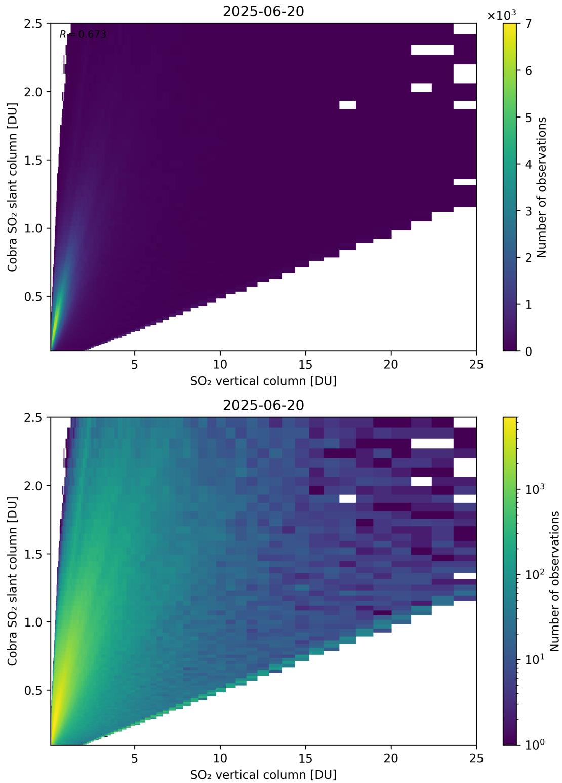
Figure 349: Scatter density plot of “SO 2 vertical column” against “Cobra SO 2 slant column” for 2025-06-19 to 2025-06-21.
