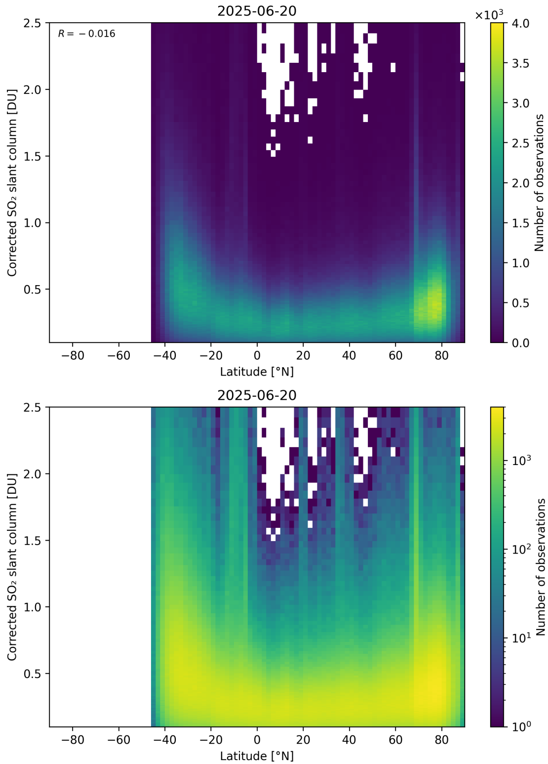
Figure 159: Scatter density plot of “Latitude” against “Corrected SO 2 slant column” for 2025-06-19 to 2025-06-21.
