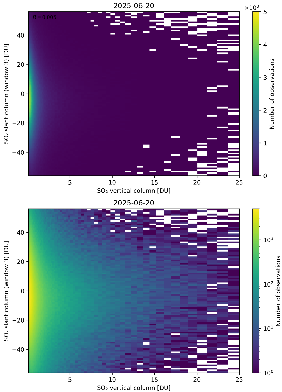
Figure 357: Scatter density plot of “SO 2 vertical column” against “SO 2 slant column (window 3)” for 2025-06-19 to 2025-06-21.
