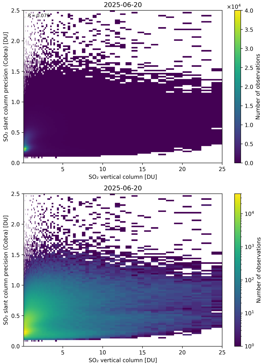
Figure 350: Scatter density plot of “SO 2 vertical column” against “SO 2 slant column precision (Cobra)” for 2025-06-19 to 2025-06-21.
