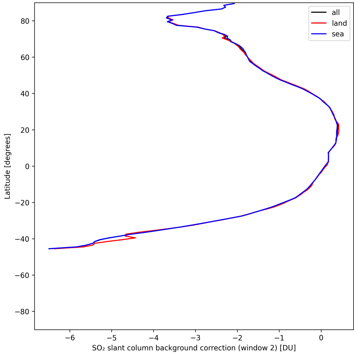
Figure 44: Zonal average of “SO 2 slant column background correction (window 2)” for 2025-06-19 to 2025-06-21.
