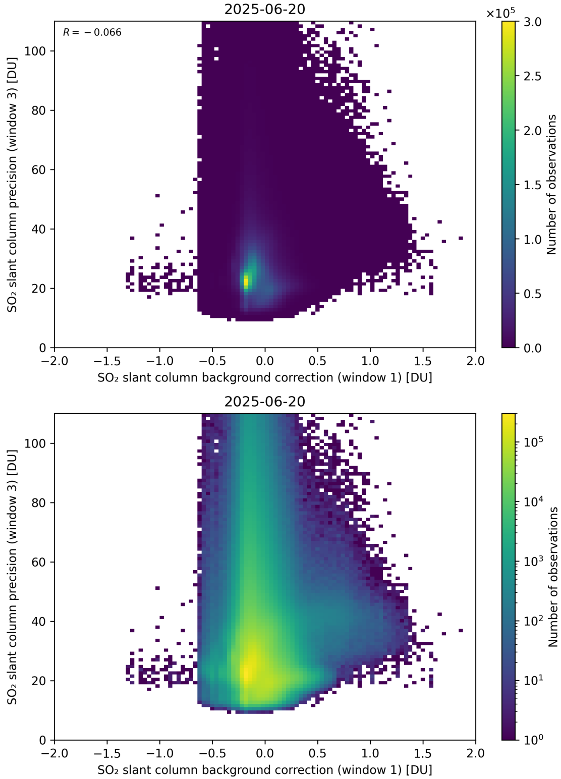
Figure 119: Scatter density plot of “SO 2 slant column background correction (window 1)” against “SO 2 slant column precision (window 3)” for 2025-06-19 to 2025-06-21.
