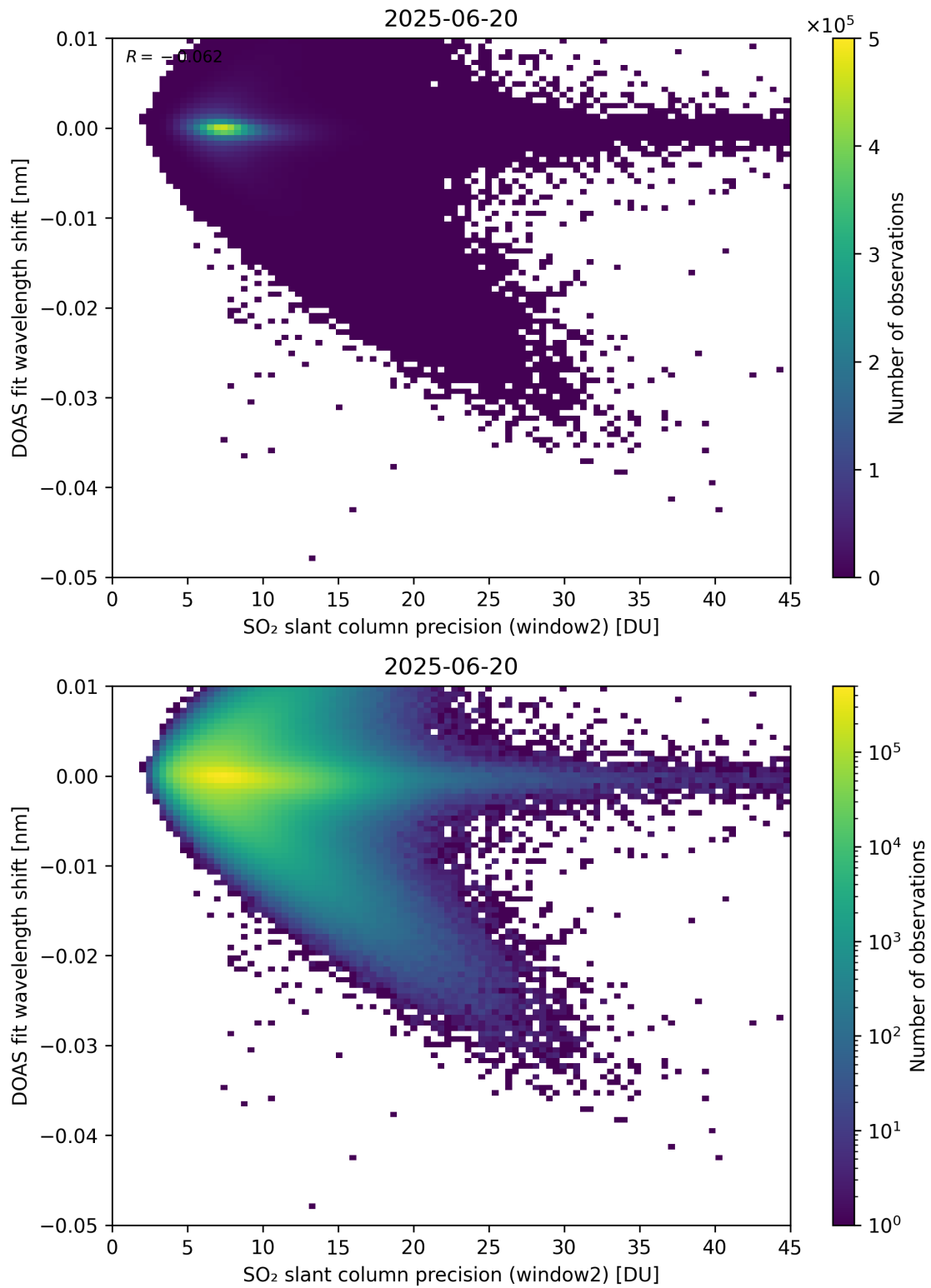
Figure 293: Scatter density plot of “SO 2 slant column precision (window2)” against “DOAS fit wavelength shift” for 2025-06-19 to 2025-06-21.
