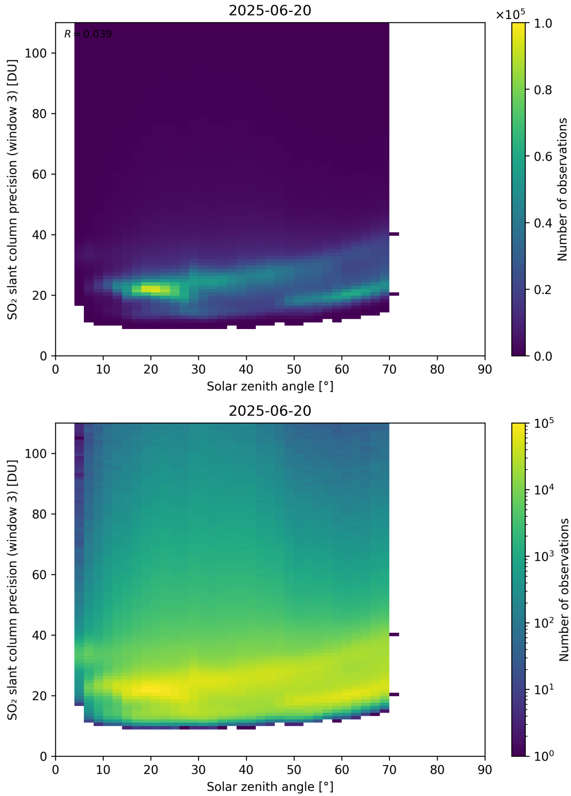
Figure 188: Scatter density plot of “Solar zenith angle” against “SO 2 slant column precision (window 3)” for 2025-06-19 to 2025-06-21.
