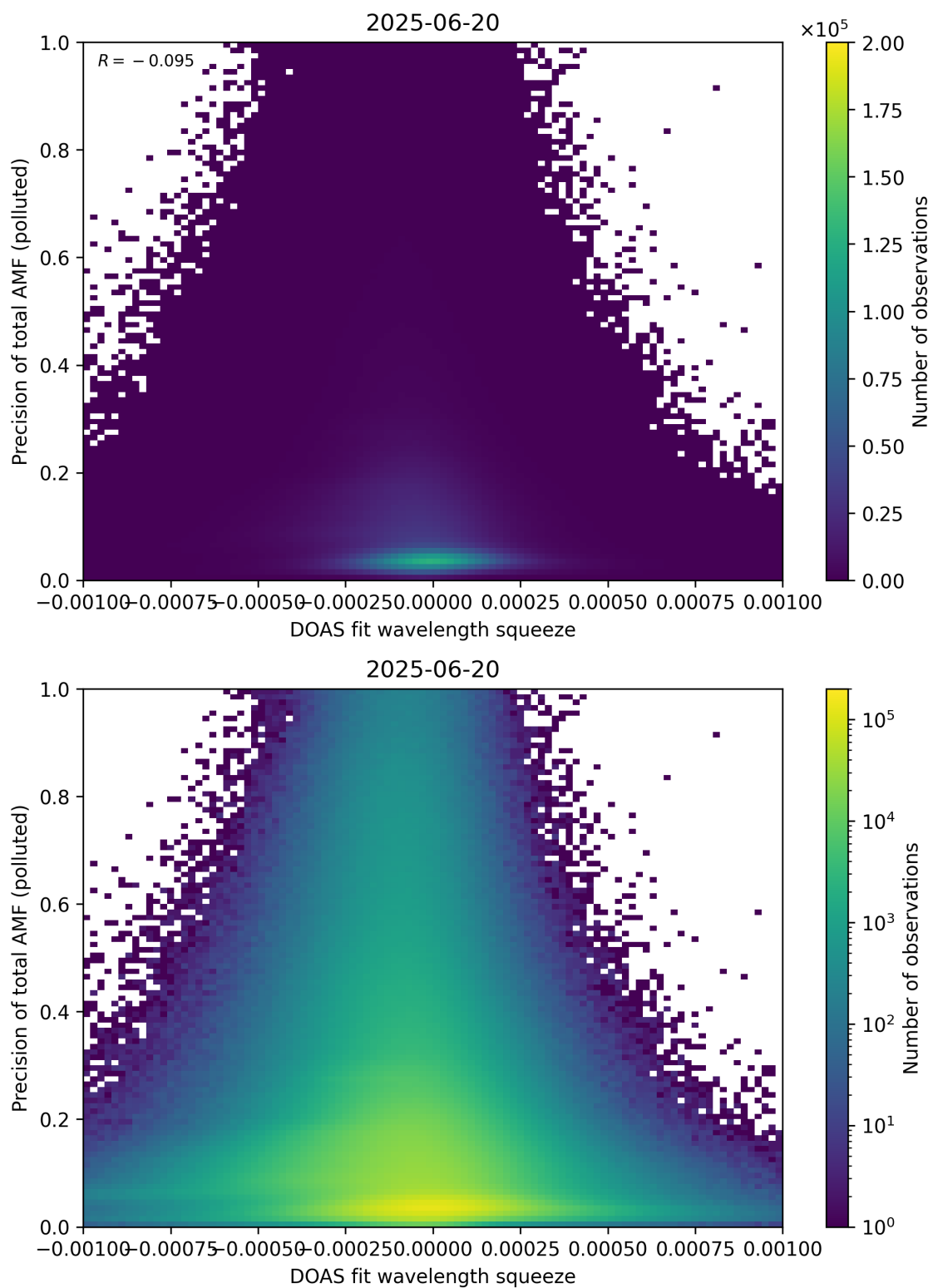
Figure 146: Scatter density plot of “DOAS fit wavelength squeeze” against “Precision of total AMF (polluted)” for 2025-06-19 to 2025-06-21.
