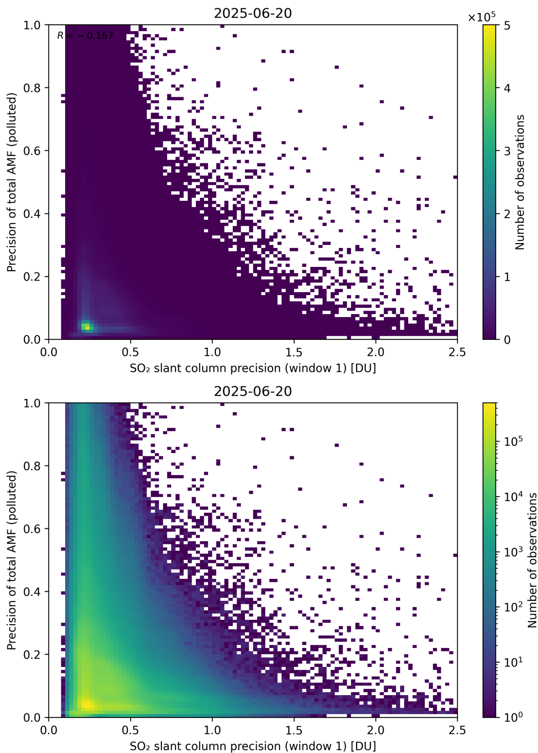
Figure 281: Scatter density plot of “SO 2 slant column precision (window 1)” against “Precision of total AMF (polluted)” for 2025-06-19 to 2025-06-21.
