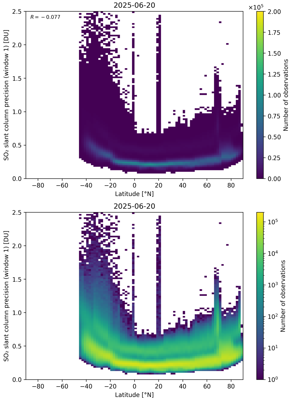
Figure 163: Scatter density plot of “Latitude” against “SO 2 slant column precision (window 1)” for 2025-06-19 to 2025-06-21.
