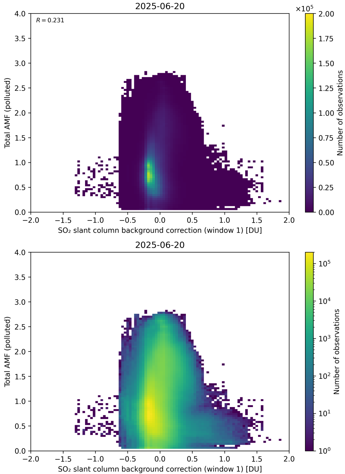
Figure 120: Scatter density plot of “SO 2 slant column background correction (window 1)” against “Total AMF (polluted)” for 2025-06-19 to 2025-06-21.
