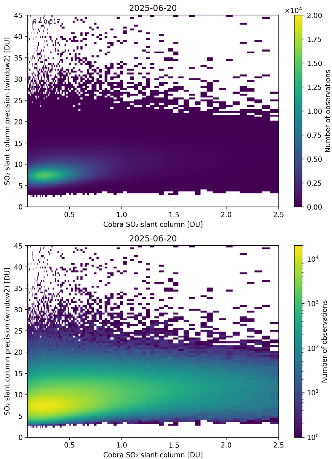
Figure 221: Scatter density plot of “Cobra SO 2 slant column” against “SO 2 slant column precision (window2)” for 2025-06-19 to 2025-06-21.
