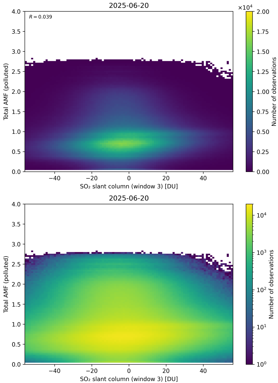
Figure 318: Scatter density plot of “SO 2 slant column (window 3)” against “Total AMF (polluted)” for 2025-06-19 to 2025-06-21.
