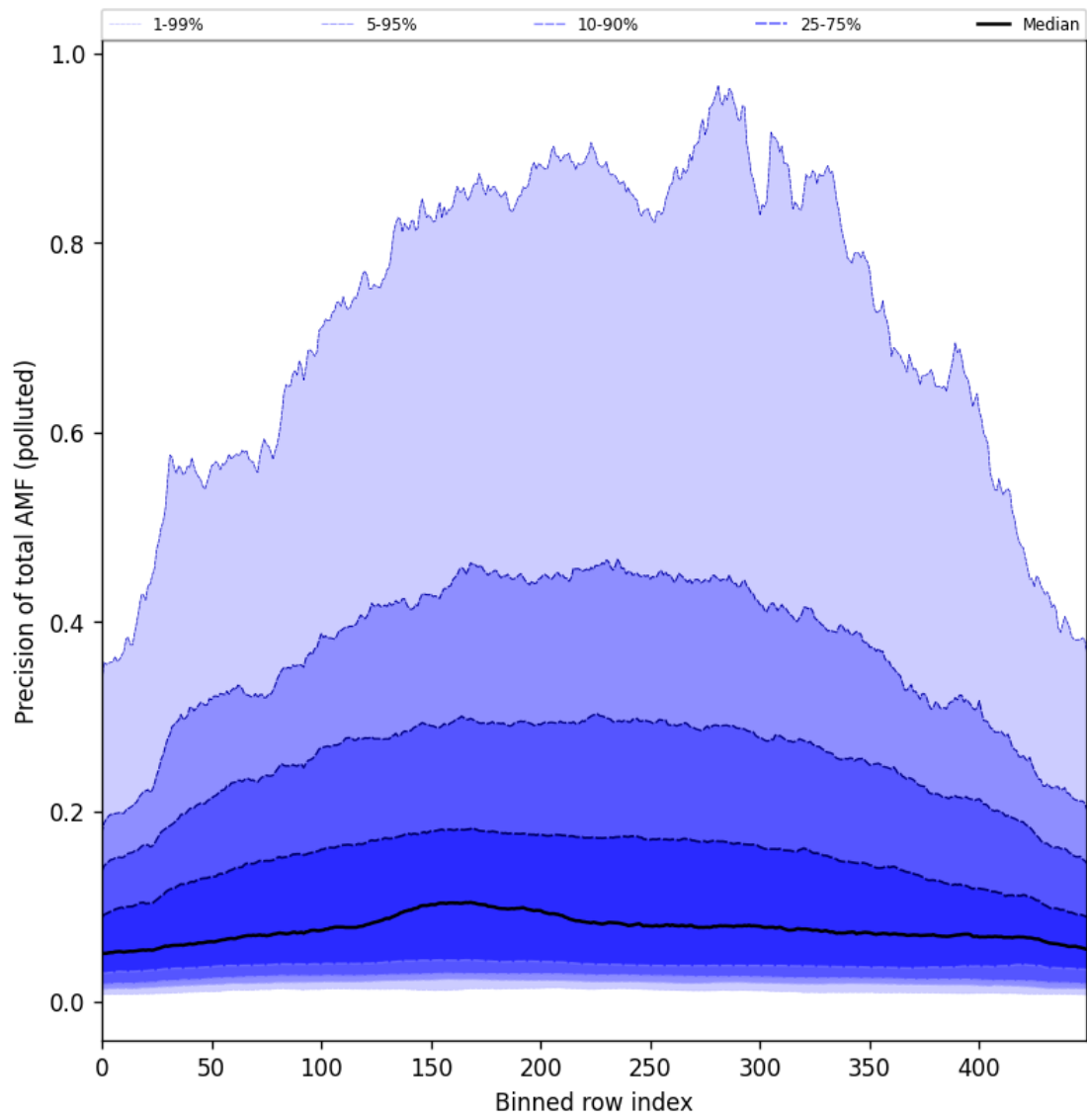
Figure 106: Along track statistics of “Precision of total AMF (polluted)” for 2025-06-19 to 2025-06-21
