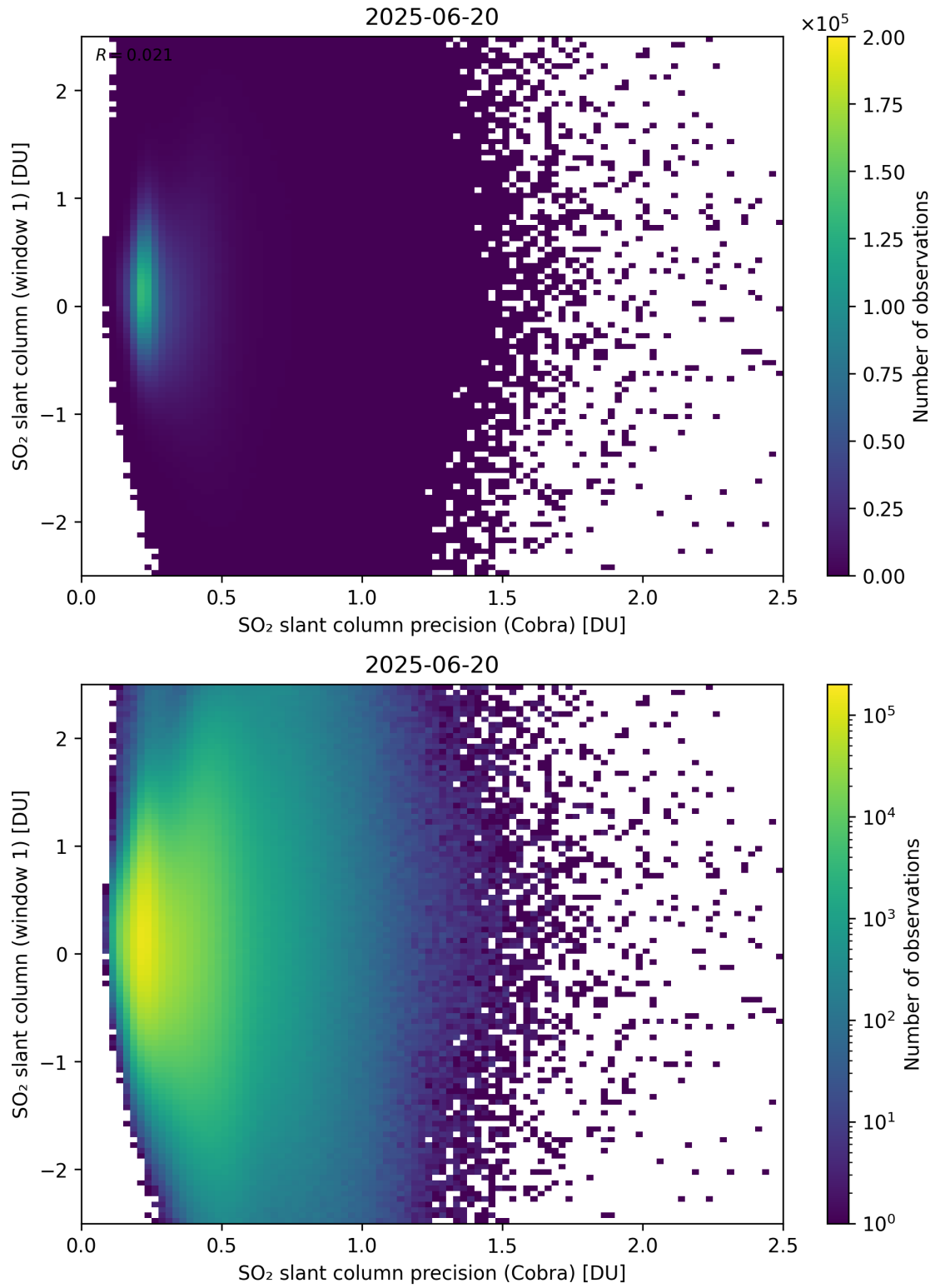
Figure 208: Scatter density plot of “SO 2 slant column precision (Cobra)” against “SO 2 slant column (window 1)” for 2025-06-19 to 2025-06-21.
