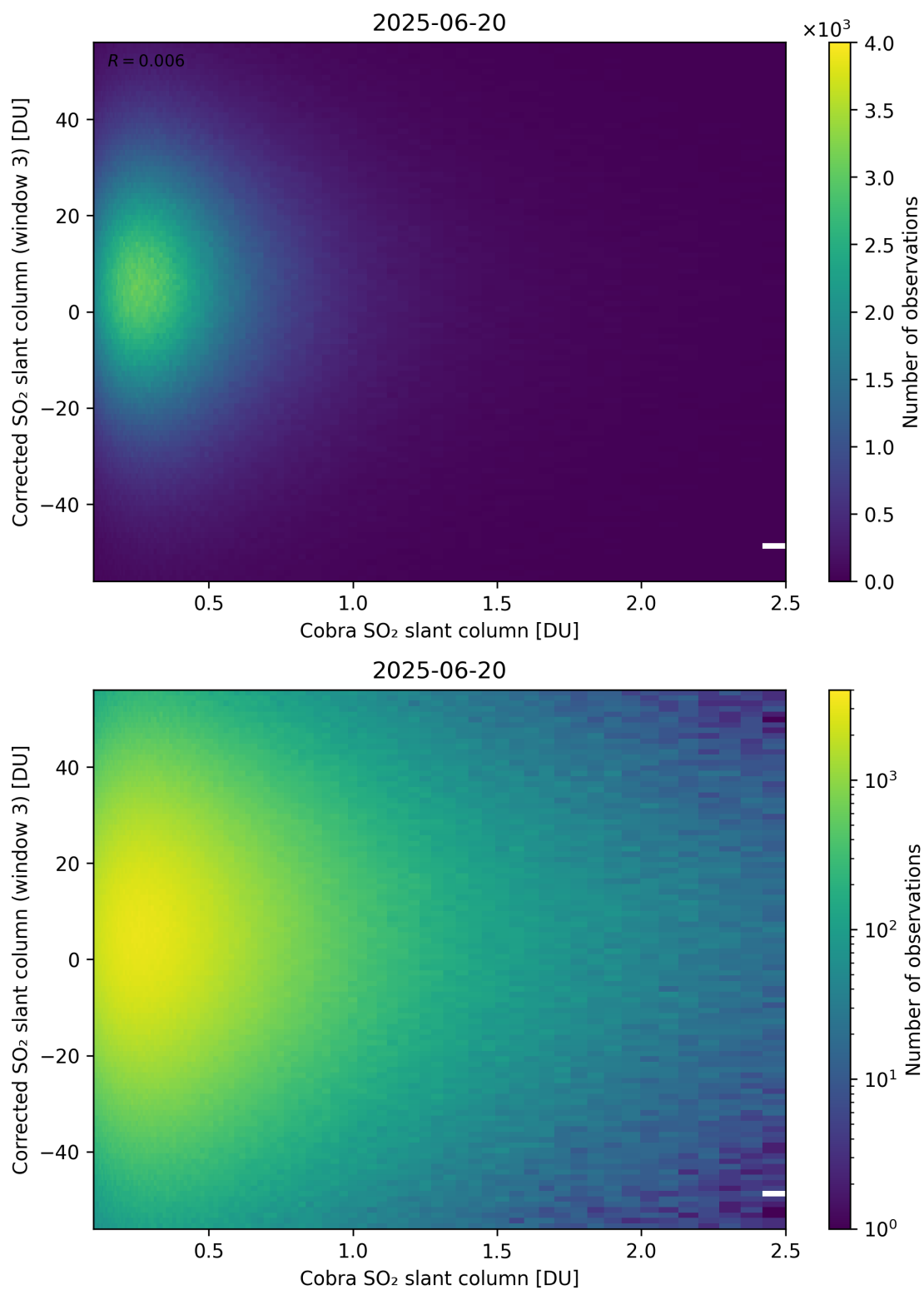
Figure 218: Scatter density plot of “Cobra SO 2 slant column” against “Corrected SO 2 slant column (window 3)” for 2025-06-19 to 2025-06-21.
