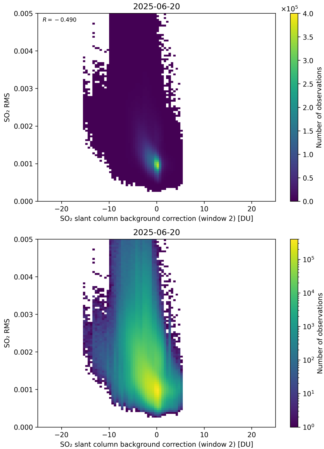
Figure 125: Scatter density plot of “SO 2 slant column background correction (window 2)” against “SO 2 RMS” for 2025-06-19 to 2025-06-21.
