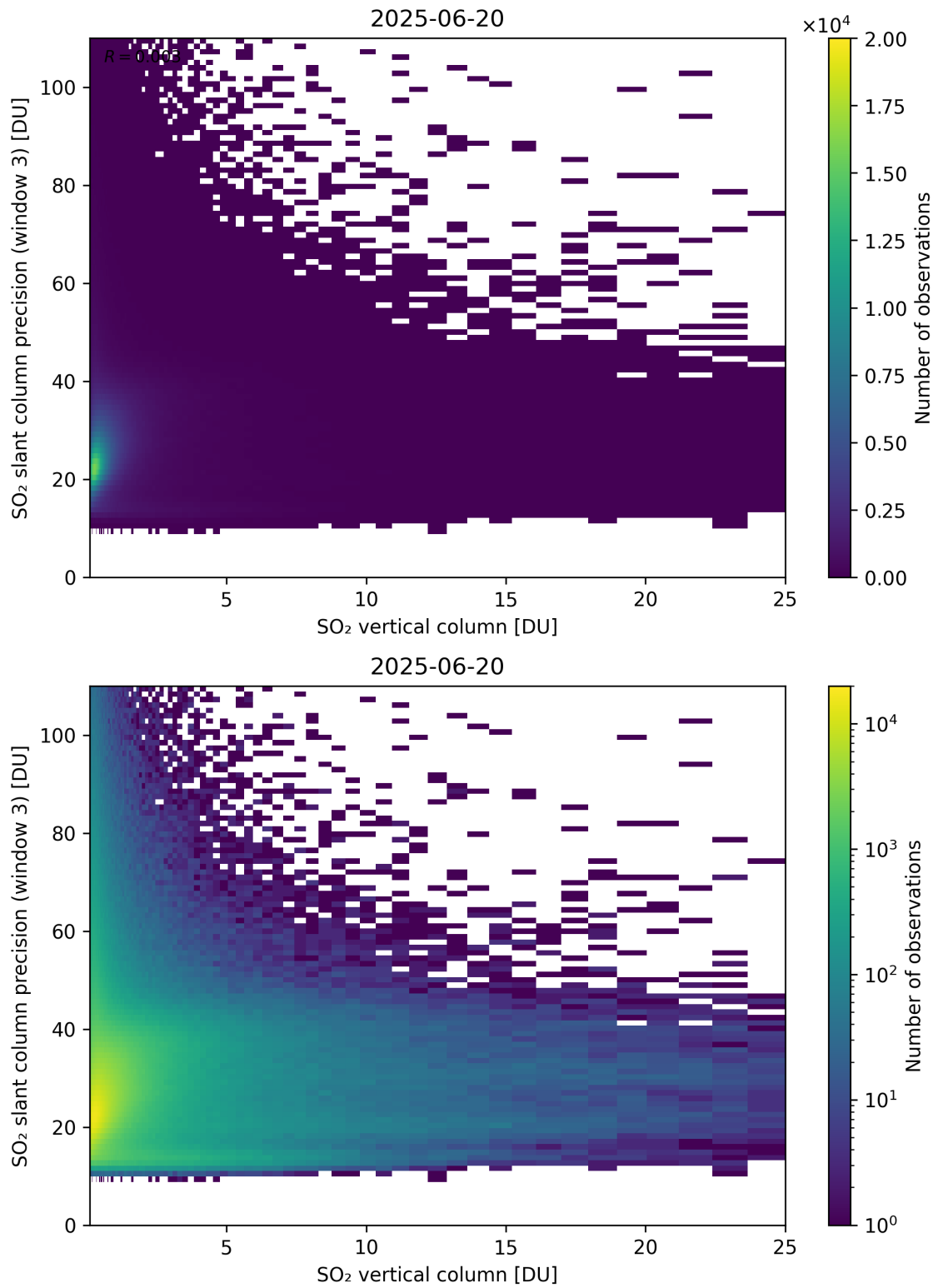
Figure 358: Scatter density plot of “SO 2 vertical column” against “SO 2 slant column precision (window 3)” for 2025-06-19 to 2025-06-21.
