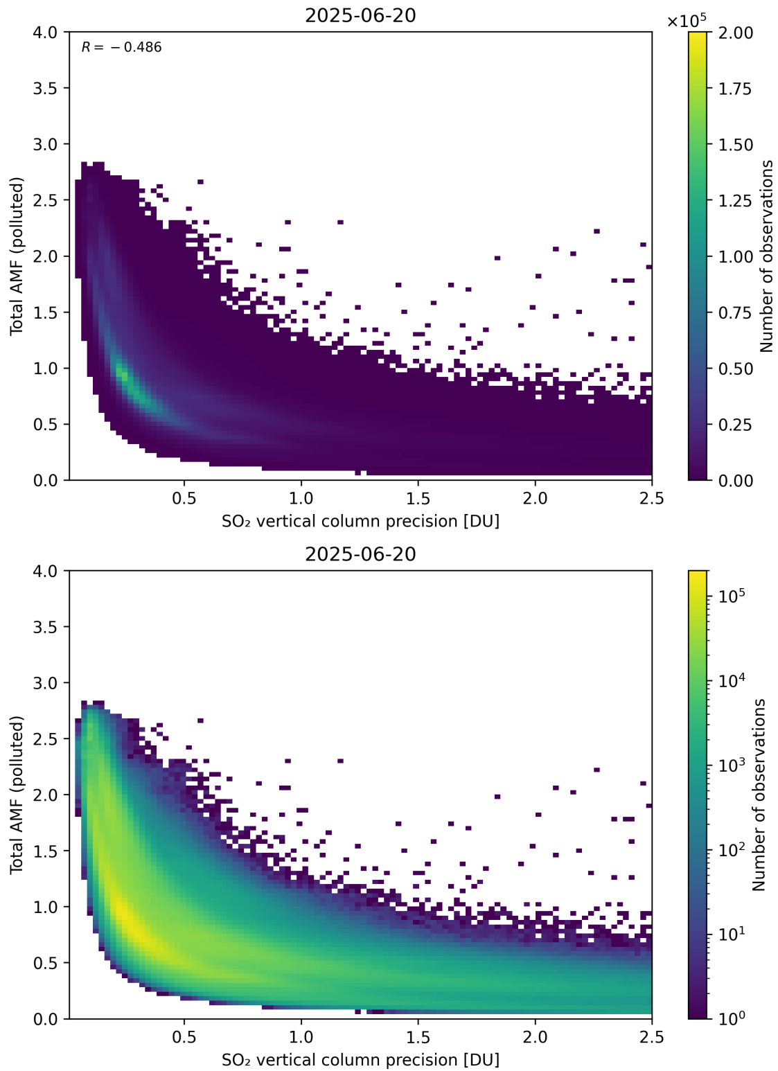
Figure 346: Scatter density plot of “SO 2 vertical column precision” against “Total AMF (polluted)” for 2025-06-19 to 2025-06-21.
