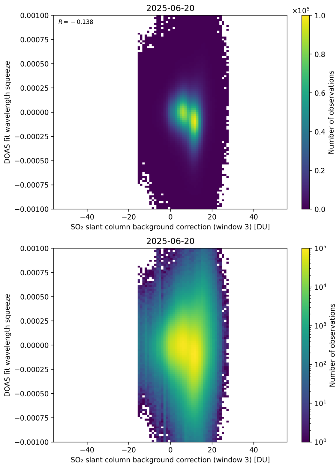
Figure 133: Scatter density plot of “SO 2 slant column background correction (window 3)” against “DOAS fit wavelength squeeze” for 2025-06-19 to 2025-06-21.
