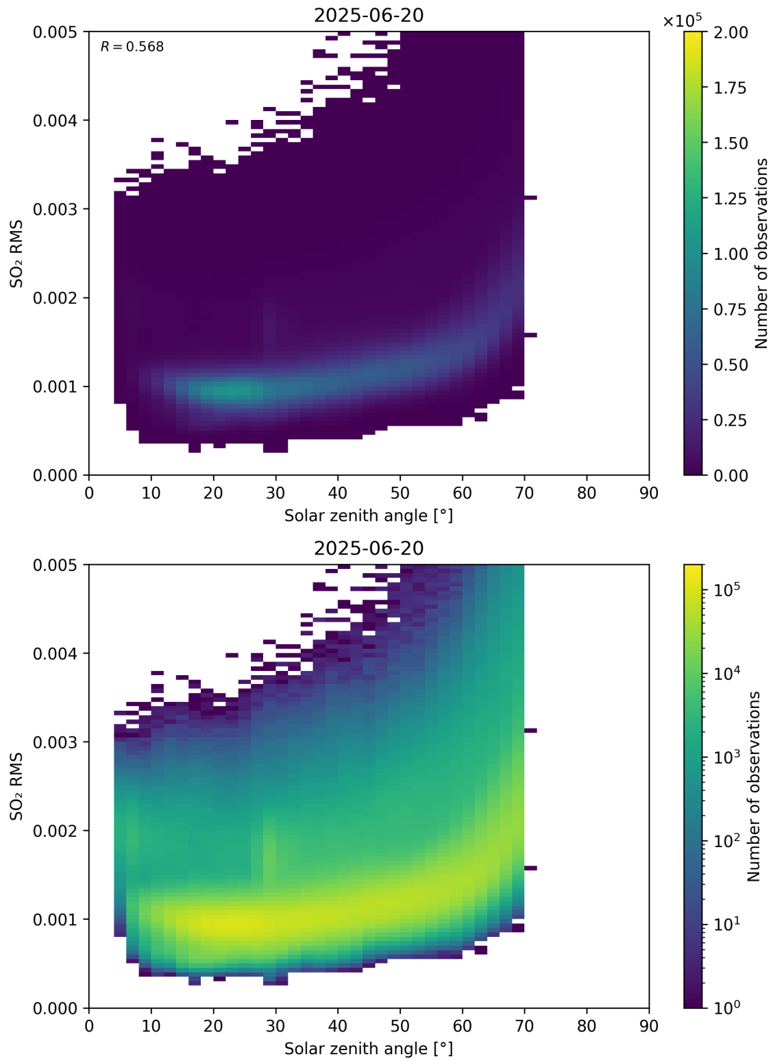
Figure 176: Scatter density plot of “Solar zenith angle” against “SO 2 RMS” for 2025-06-19 to 2025-06-21.
