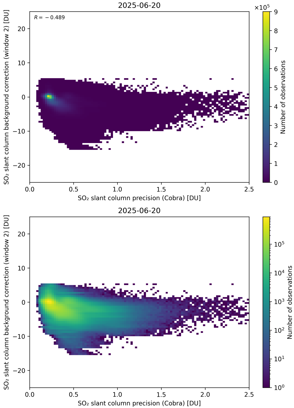
Figure 200: Scatter density plot of “SO 2 slant column precision (Cobra)” against “SO 2 slant column background correction (window 2)” for 2025-06-19 to 2025-06-21.
