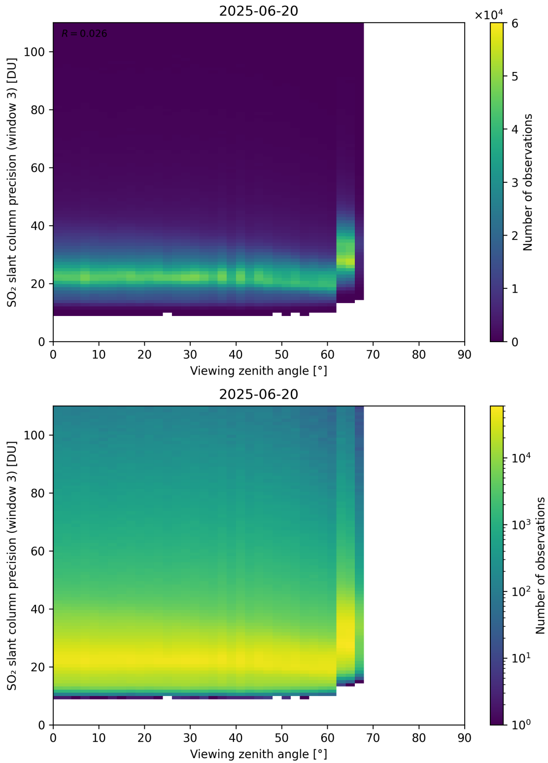
Figure 380: Scatter density plot of “Viewing zenith angle” against “SO 2 slant column precision (window 3)” for 2025-06-19 to 2025-06-21.
