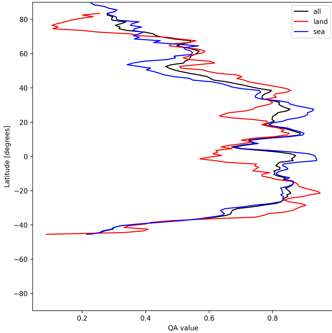
Figure 31: Zonal average of “QA value” for 2025-06-19 to 2025-06-21.
