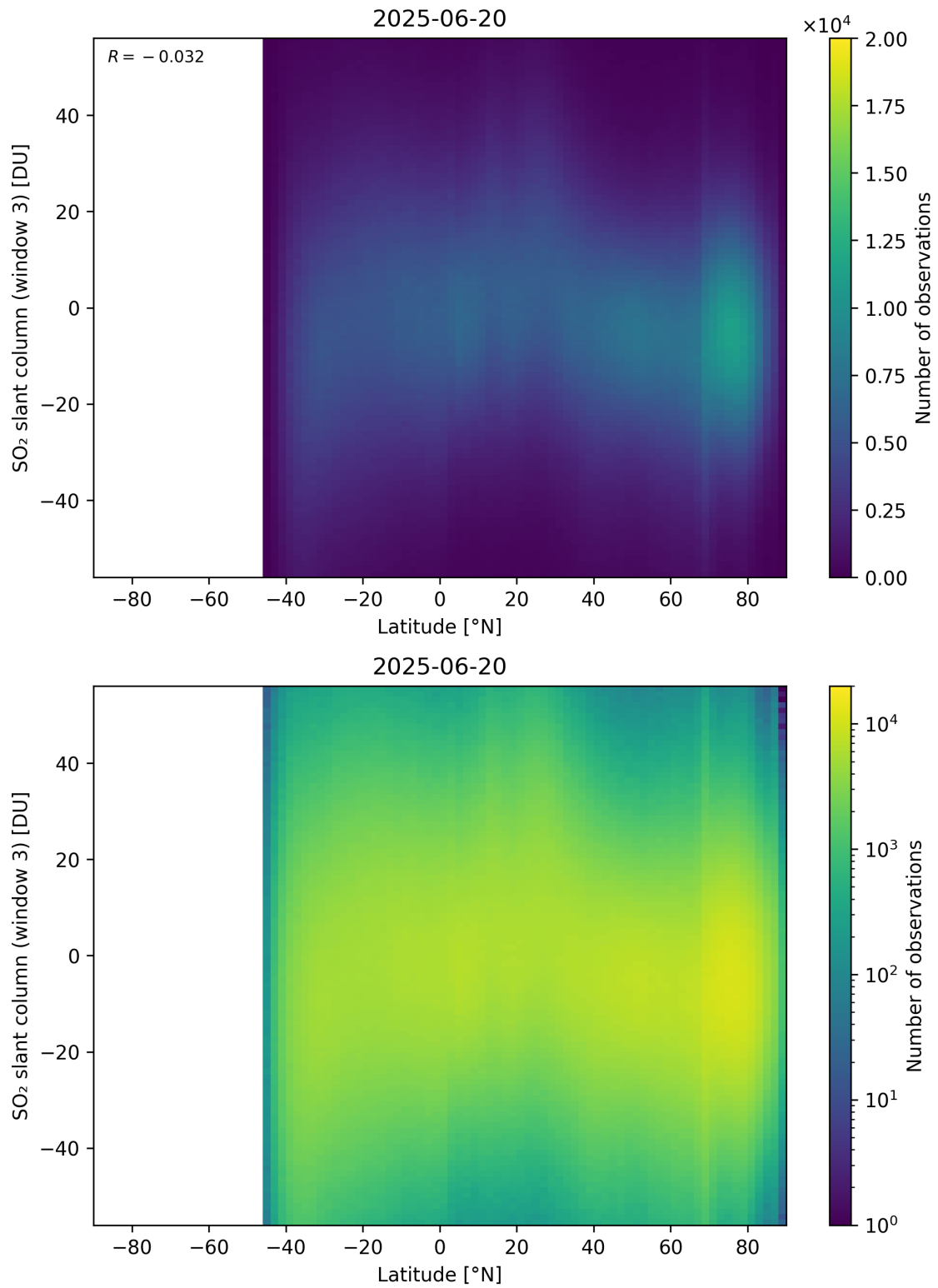
Figure 165: Scatter density plot of “Latitude” against “SO 2 slant column (window 3)” for 2025-06-19 to 2025-06-21.
