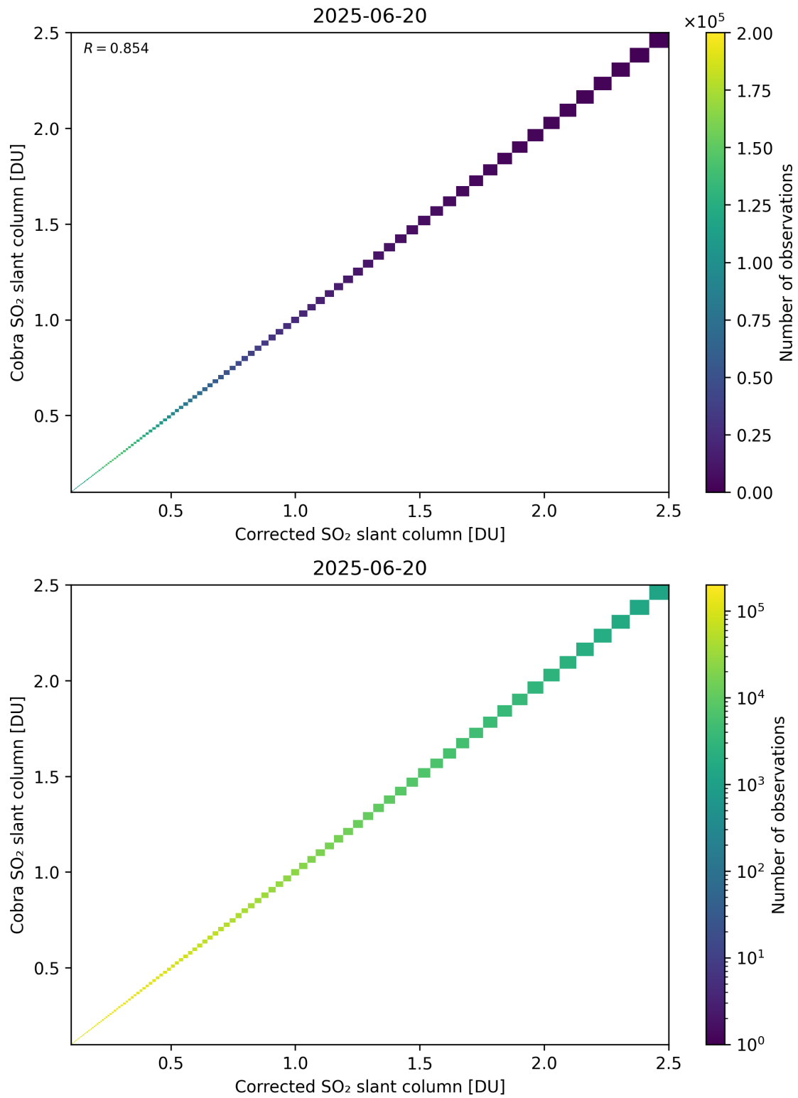
Figure 233: Scatter density plot of “Corrected SO 2 slant column” against “Cobra SO 2 slant column” for 2025-06-19 to 2025-06-21.
