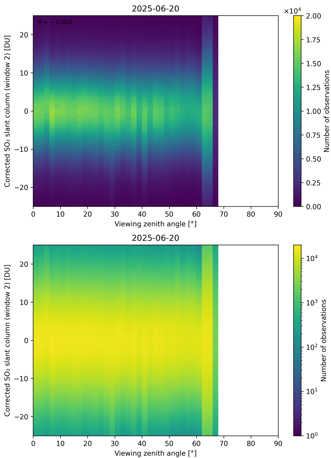
Figure 374: Scatter density plot of “Viewing zenith angle” against “Corrected SO 2 slant column (window 2)” for 2025-06-19 to 2025-06-21.
