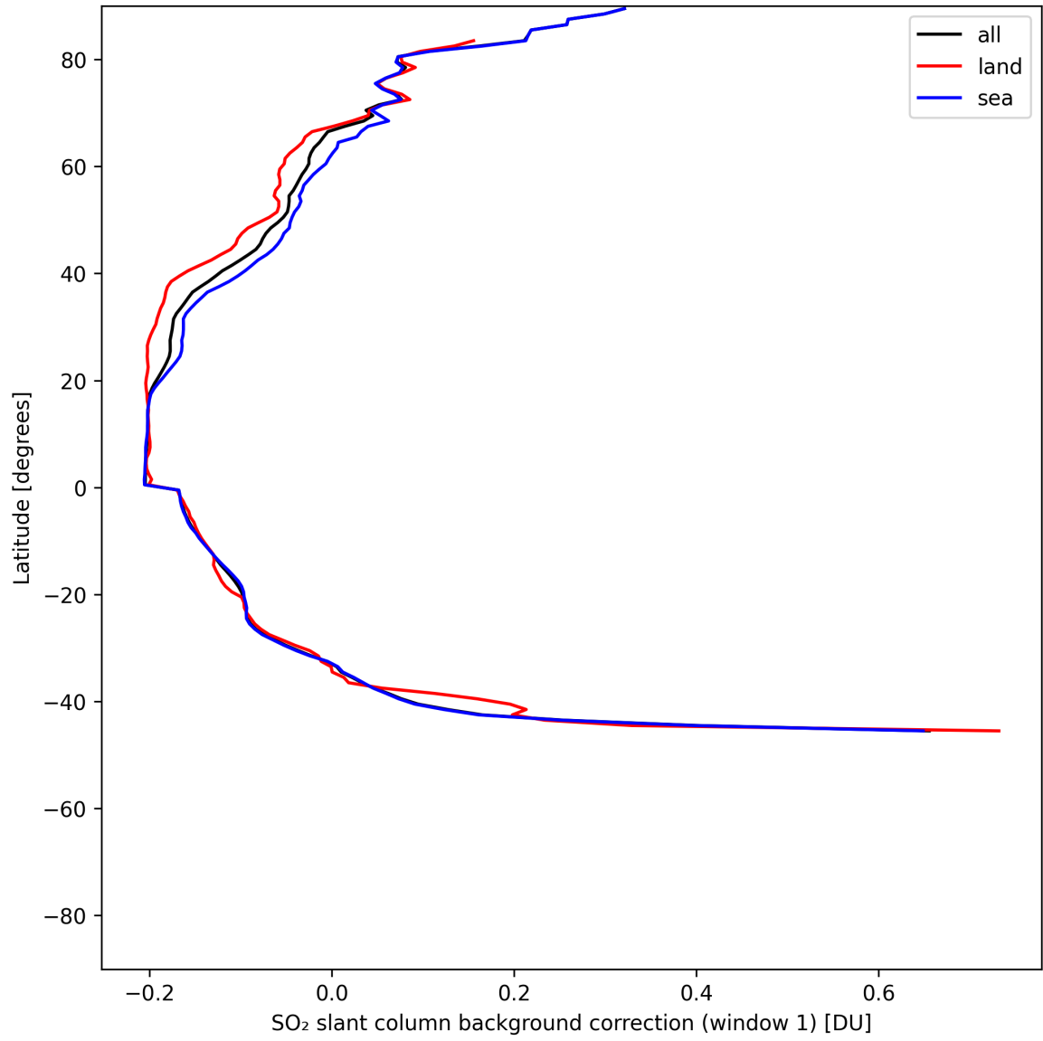
Figure 40: Zonal average of "SO 2 slant column background correction (window 1)" for 2025-06-19 to 2025-06-21.
