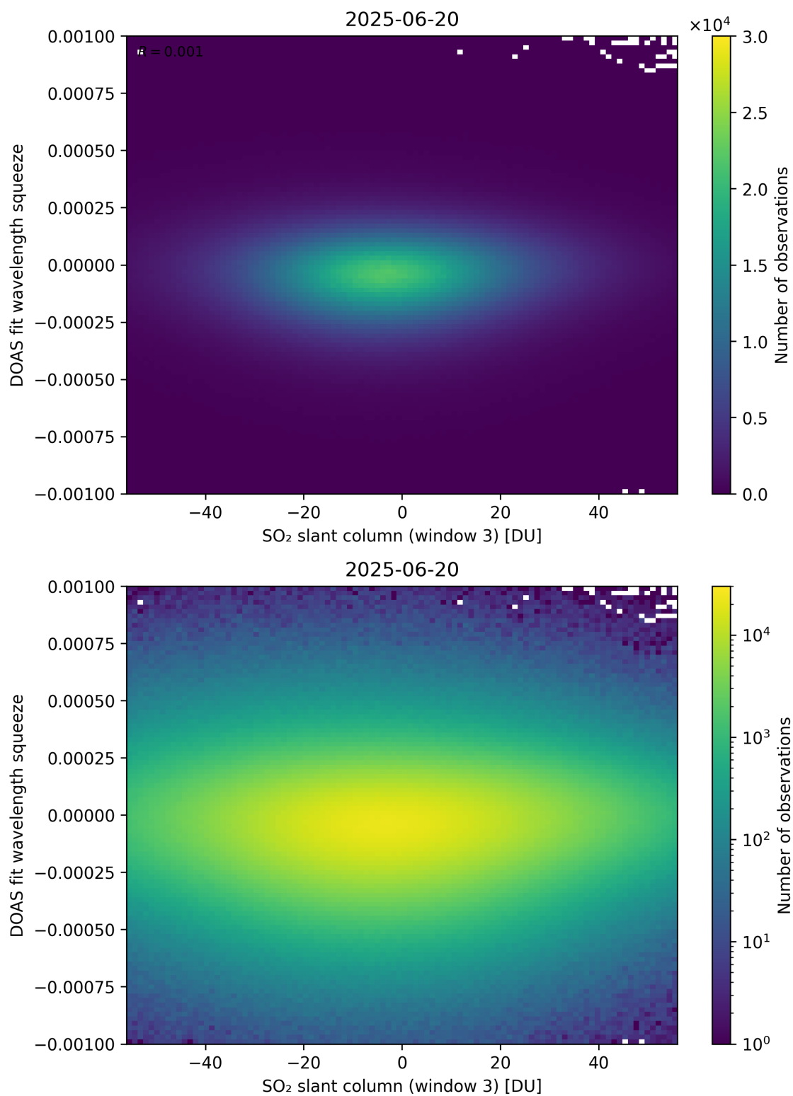
Figure 305: Scatter density plot of “SO 2 slant column (window 3)” against “DOAS fit wavelength squeeze” for 2025-06-19 to 2025-06-21.
