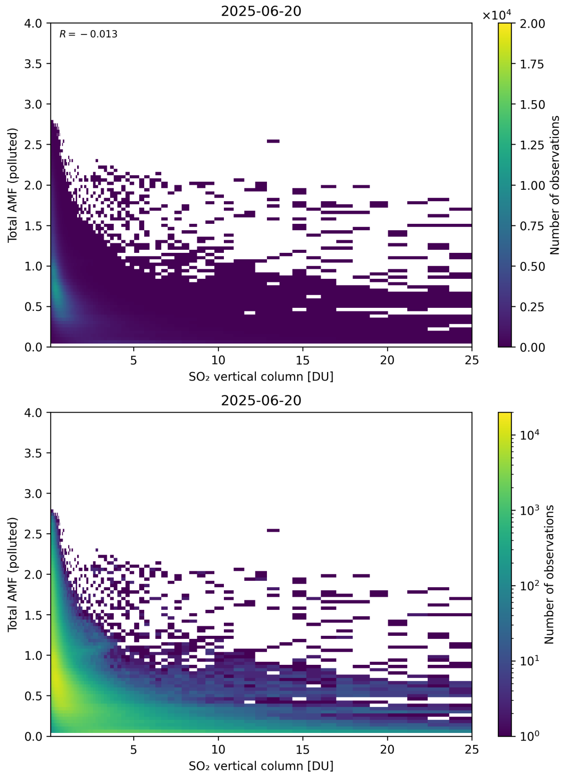
Figure 359: Scatter density plot of “SO 2 vertical column” against “Total AMF (polluted)” for 2025-06-19 to 2025-06-21.
