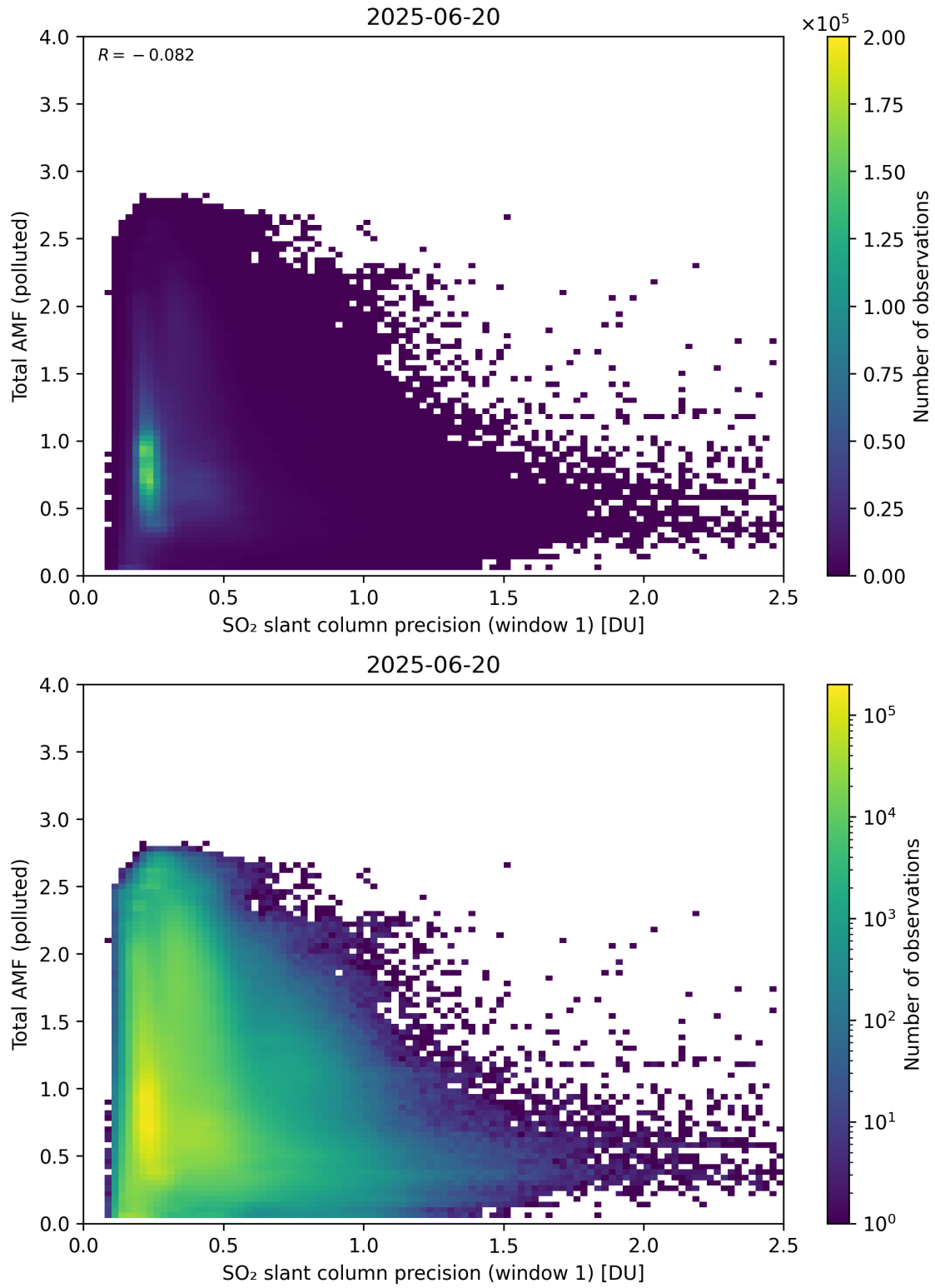
Figure 280: Scatter density plot of “SO 2 slant column precision (window 1)” against “Total AMF (polluted)” for 2025-06-19 to 2025-06-21.
