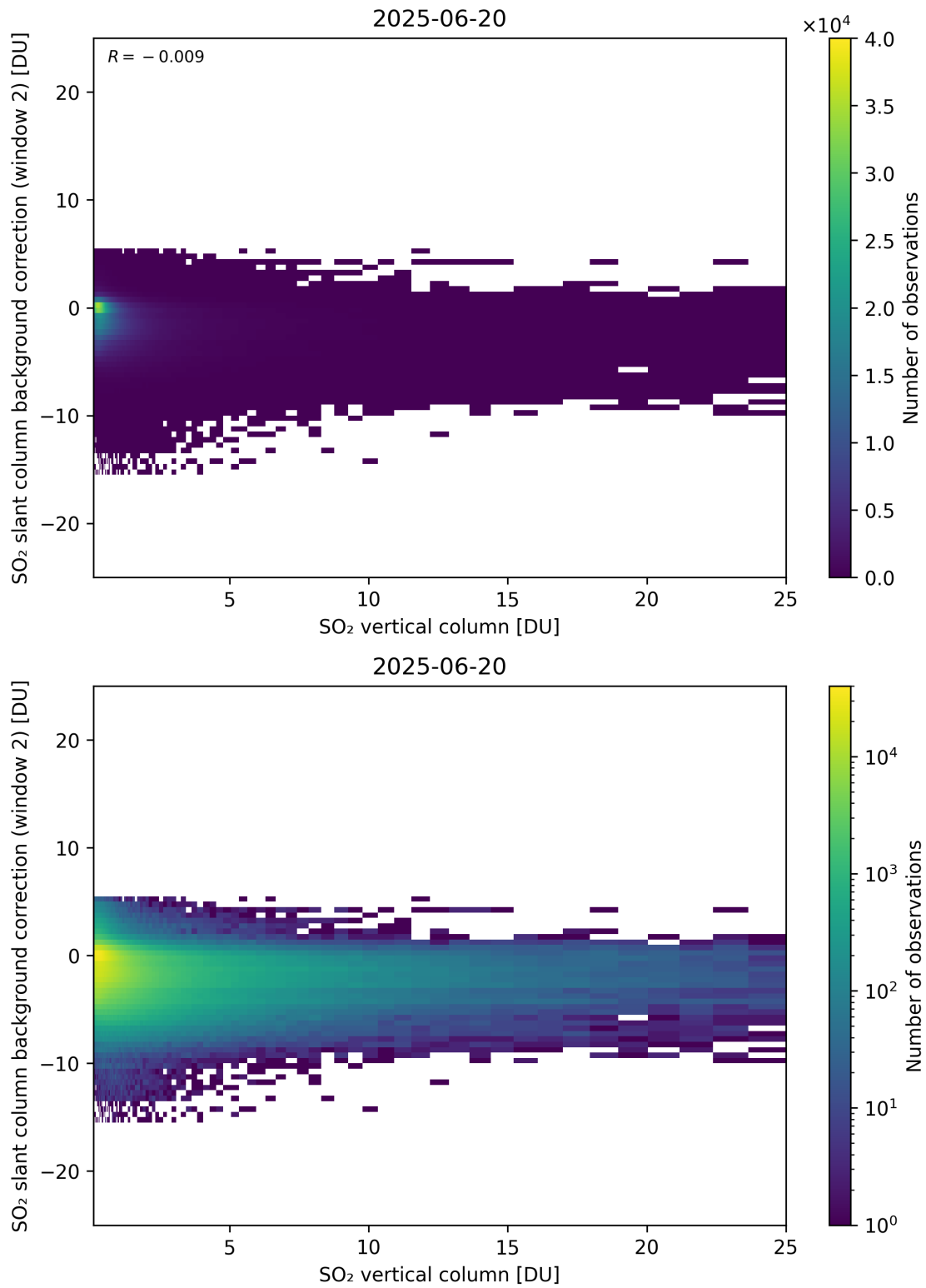
Figure 324: Scatter density plot of “SO 2 vertical column” against “SO 2 slant column background correction (window 2)” for 2025-06-19 to 2025-06-21.
