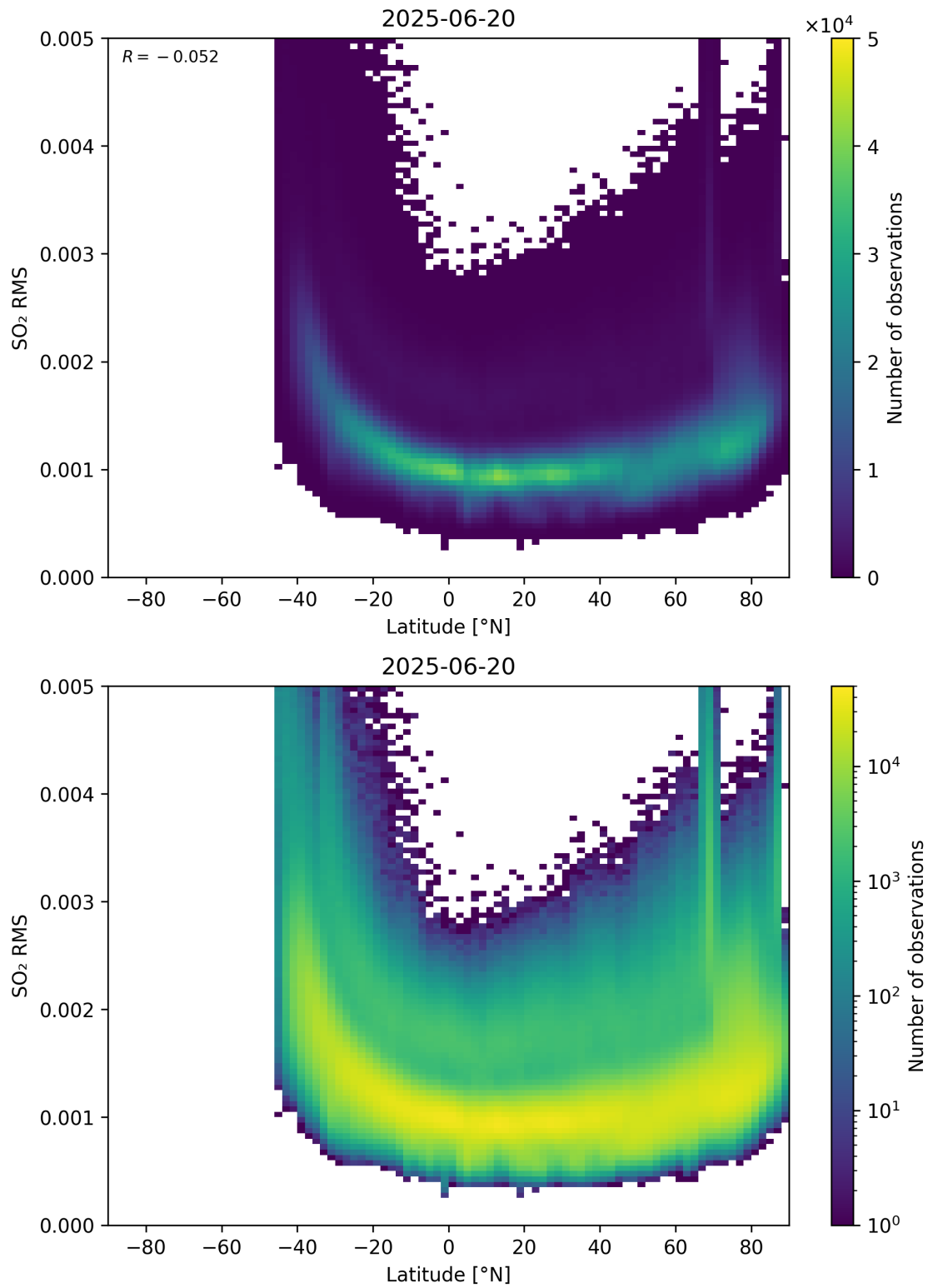
Figure 155: Scatter density plot of “Latitude” against “SO 2 RMS” for 2025-06-19 to 2025-06-21.
