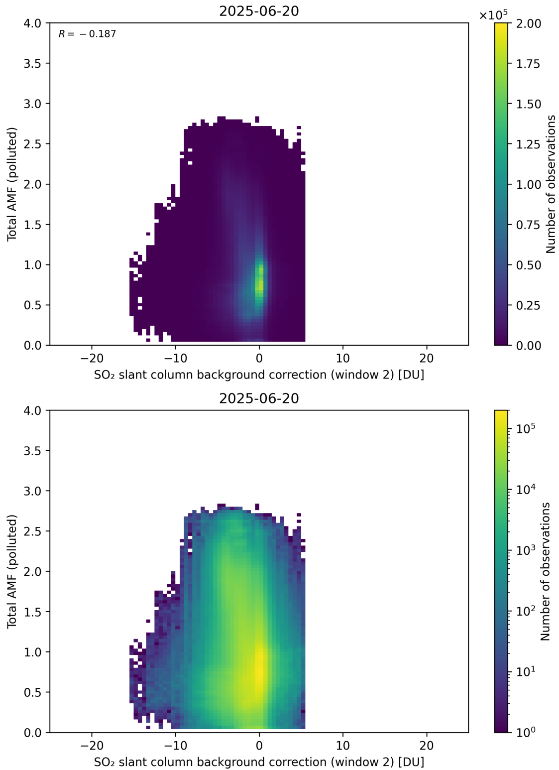
Figure 130: Scatter density plot of “SO 2 slant column background correction (window 2)” against “Total AMF (polluted)” for 2025-06-19 to 2025-06-21.
