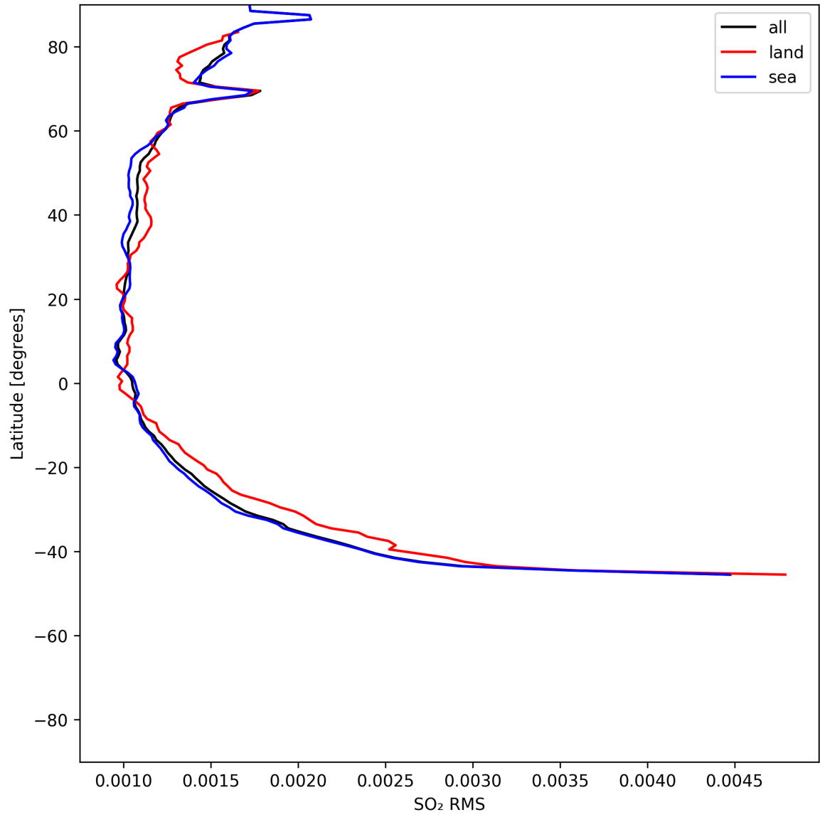
Figure 52: Zonal average of “SO 2 RMS” for 2025-06-19 to 2025-06-21.
