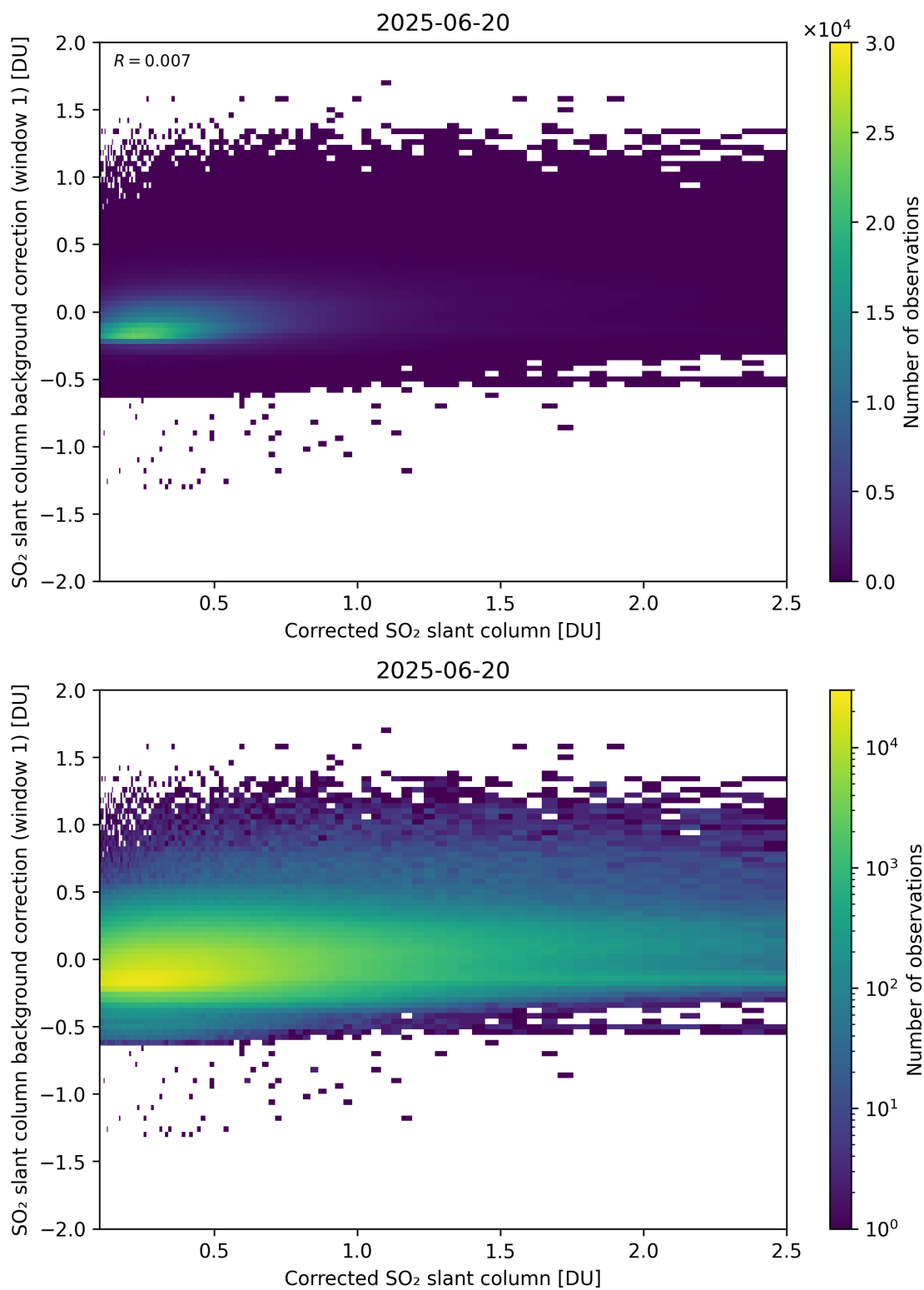
Figure 226: Scatter density plot of “Corrected SO 2 slant column” against “SO 2 slant column background correction (window 1)” for 2025-06-19 to 2025-06-21.
