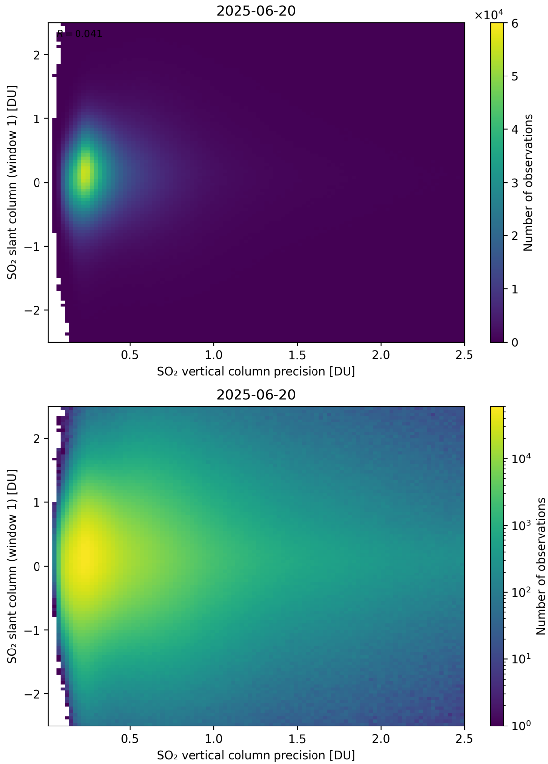
Figure 341: Scatter density plot of “SO 2 vertical column precision” against “SO 2 slant column (window 1)” for 2025-06-19 to 2025-06-21.
