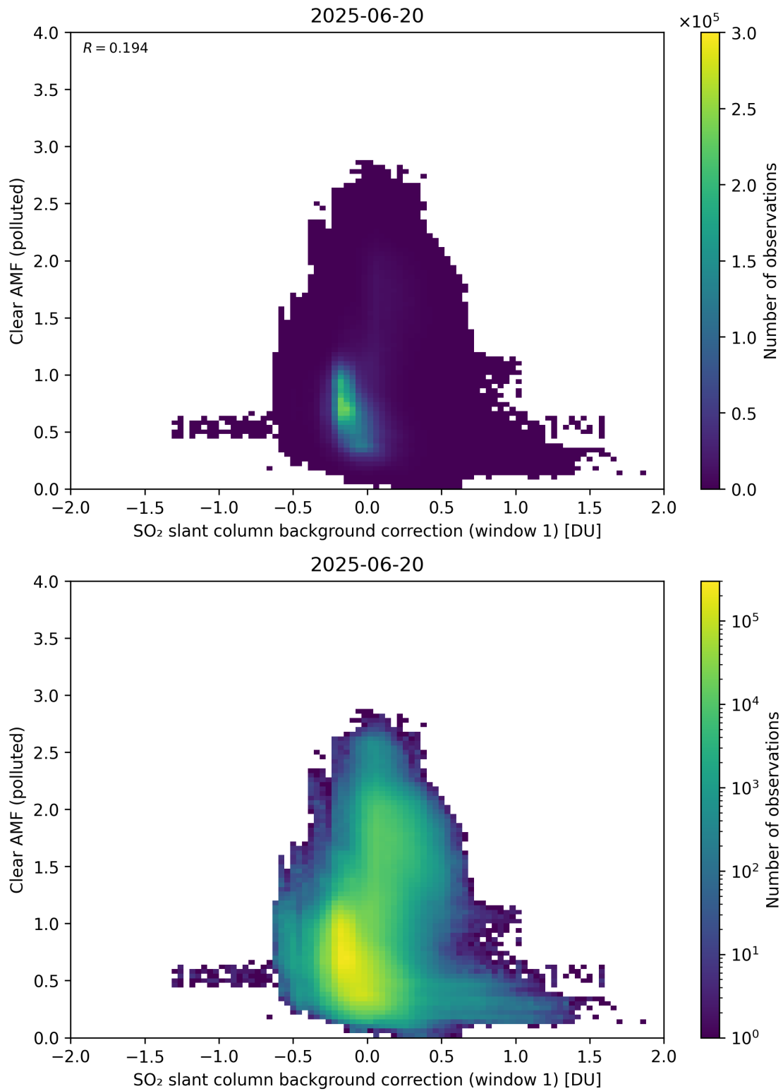
Figure 114: Scatter density plot of “SO 2 slant column background correction (window 1)” against “Clear AMF (polluted)” for 2025-06-19 to 2025-06-21.
