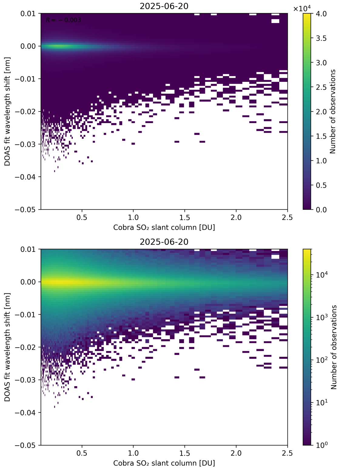
Figure 196: Scatter density plot of “Cobra SO 2 slant column” against “DOAS fit wavelength shift” for 2025-06-19 to 2025-06-21.
