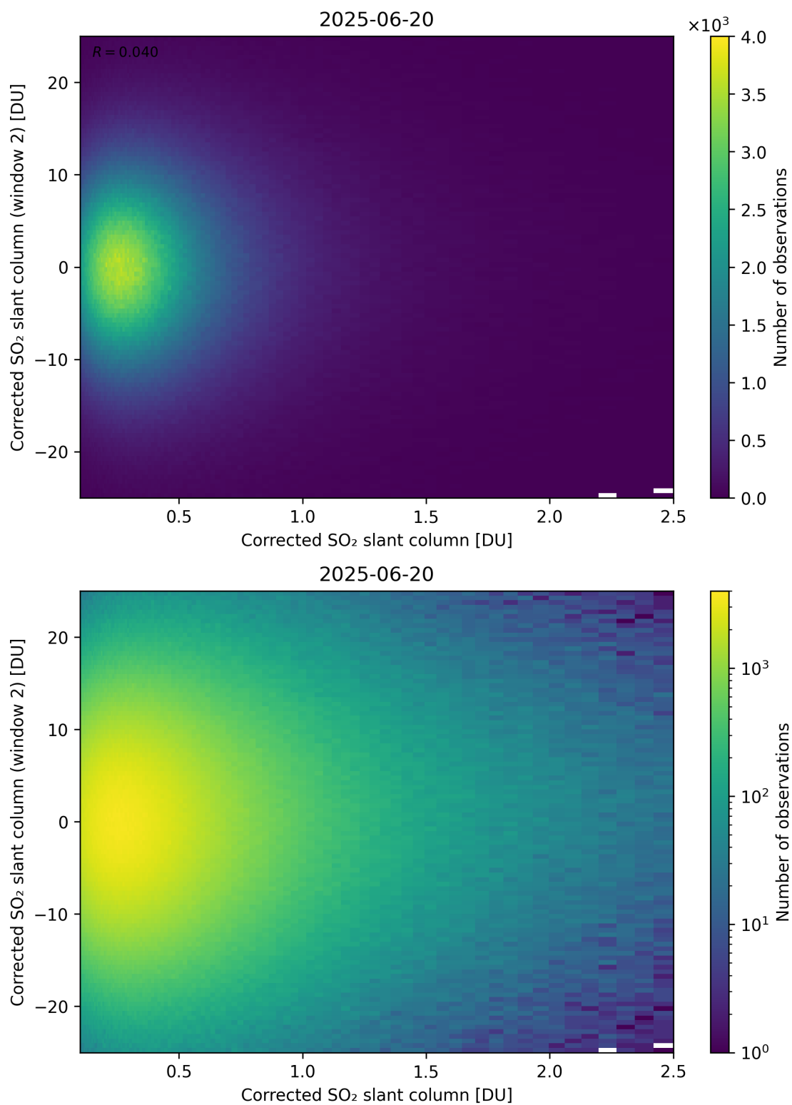
Figure 235: Scatter density plot of “Corrected SO 2 slant column” against “Corrected SO 2 slant column (window 2)” for 2025-06-19 to 2025-06-21.
