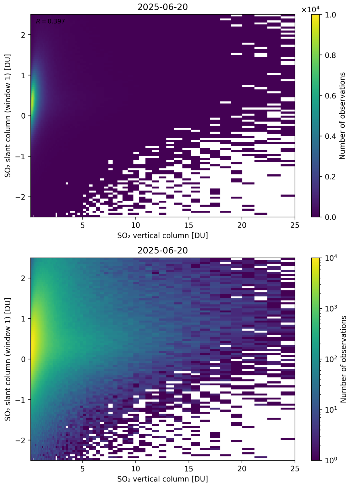
Figure 354: Scatter density plot of “SO 2 vertical column” against “SO 2 slant column (window 1)” for 2025-06-19 to 2025-06-21.
