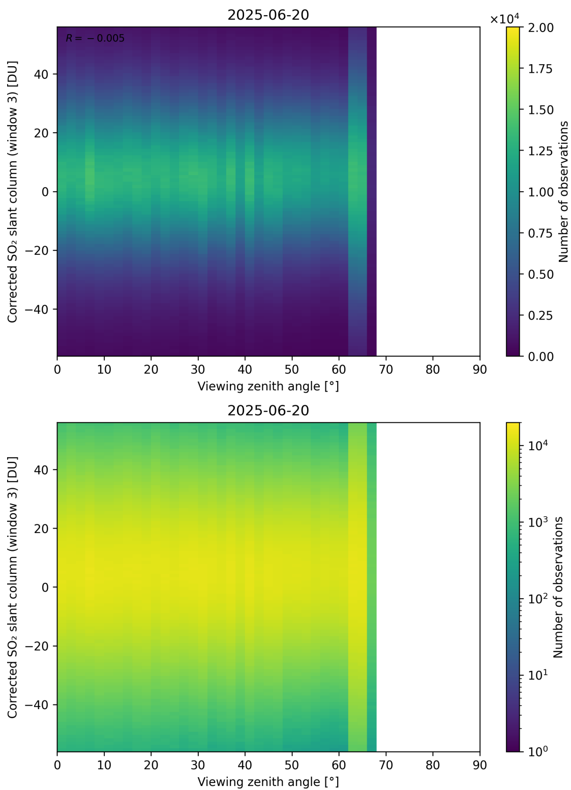
Figure 375: Scatter density plot of “Viewing zenith angle” against “Corrected SO 2 slant column (window 3)” for 2025-06-19 to 2025-06-21.
