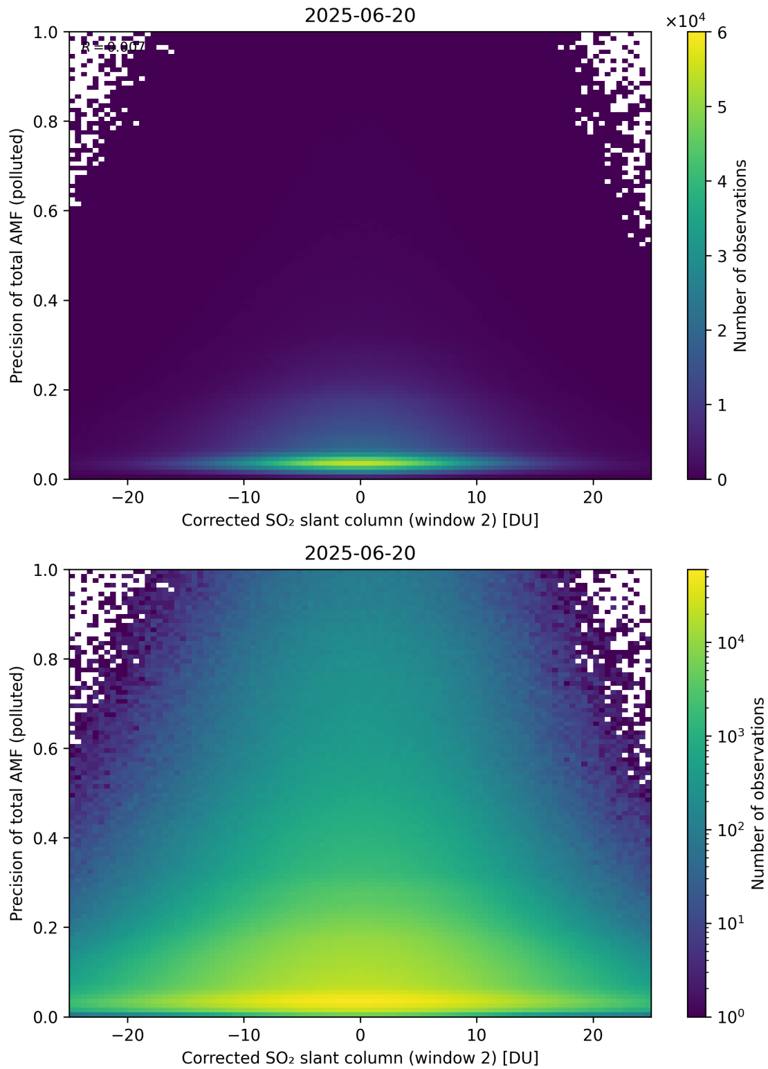
Figure 254: Scatter density plot of “Corrected SO 2 slant column (window 2)” against “Precision of total AMF (polluted)” for 2025-06-19 to 2025-06-21.
