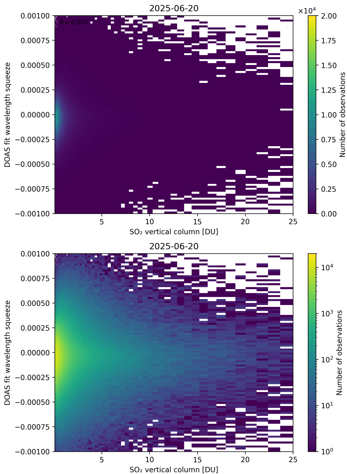
Figure 327: Scatter density plot of “SO 2 vertical column” against “DOAS fit wavelength squeeze” for 2025-06-19 to 2025-06-21.
