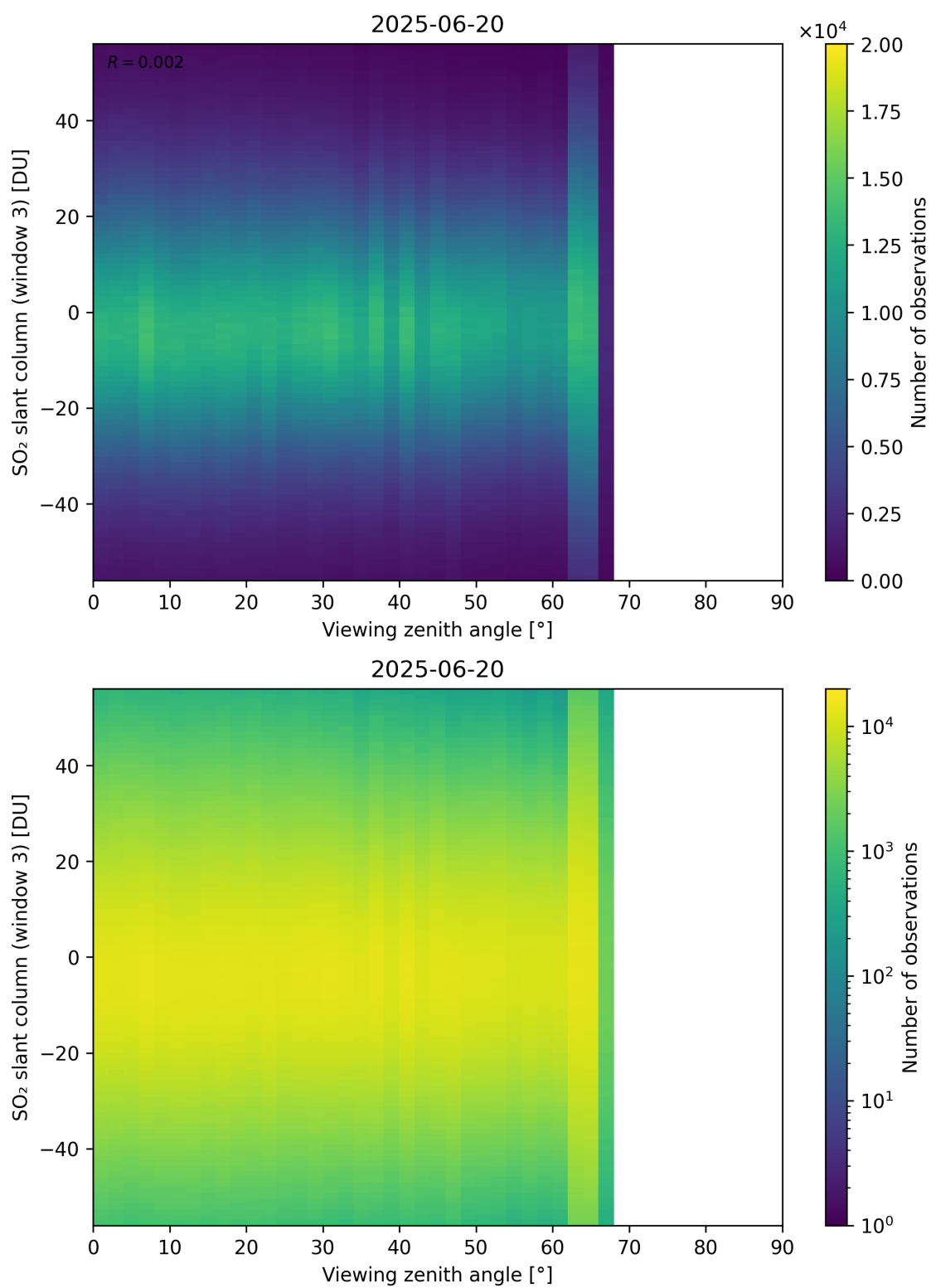
Figure 379: Scatter density plot of “Viewing zenith angle” against “SO 2 slant column (window 3)” for 2025-06-19 to 2025-06-21.
