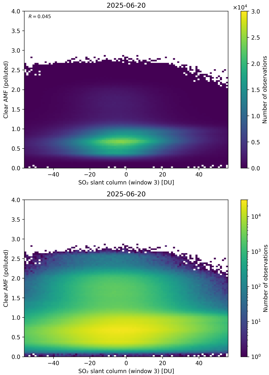
Figure 315: Scatter density plot of “SO 2 slant column (window 3)” against “Clear AMF (polluted)” for 2025-06-19 to 2025-06-21.
