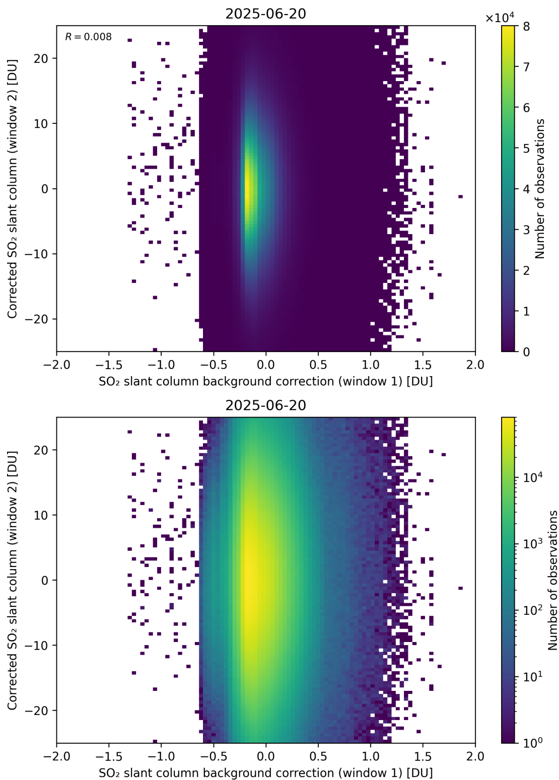
Figure 115: Scatter density plot of “SO 2 slant column background correction (window 1)” against “Corrected SO 2 slant column (window 2)” for 2025-06-19 to 2025-06-21.
