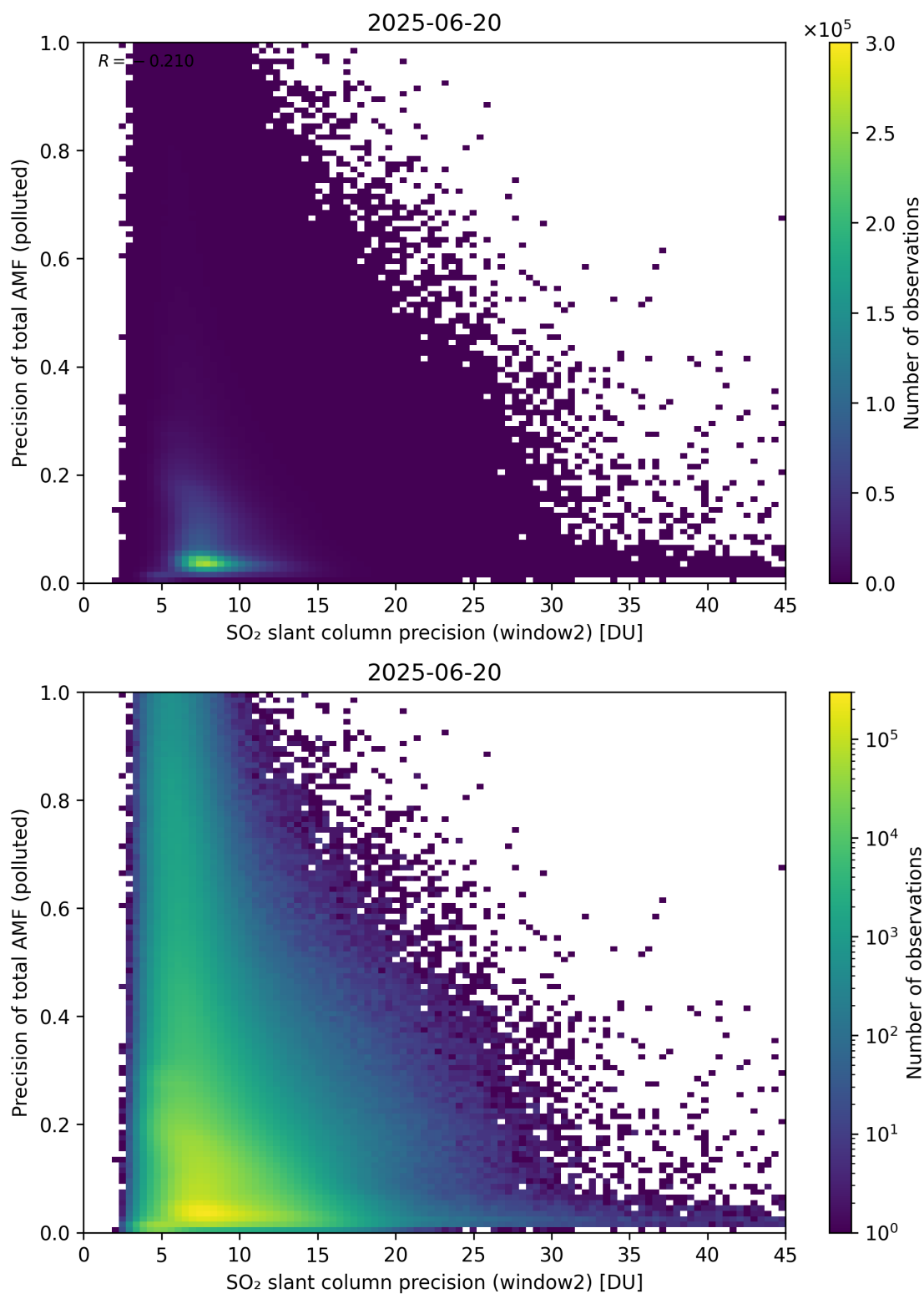
Figure 302: Scatter density plot of “SO 2 slant column precision (window2)” against “Precision of total AMF (polluted)” for 2025-06-19 to 2025-06-21.
