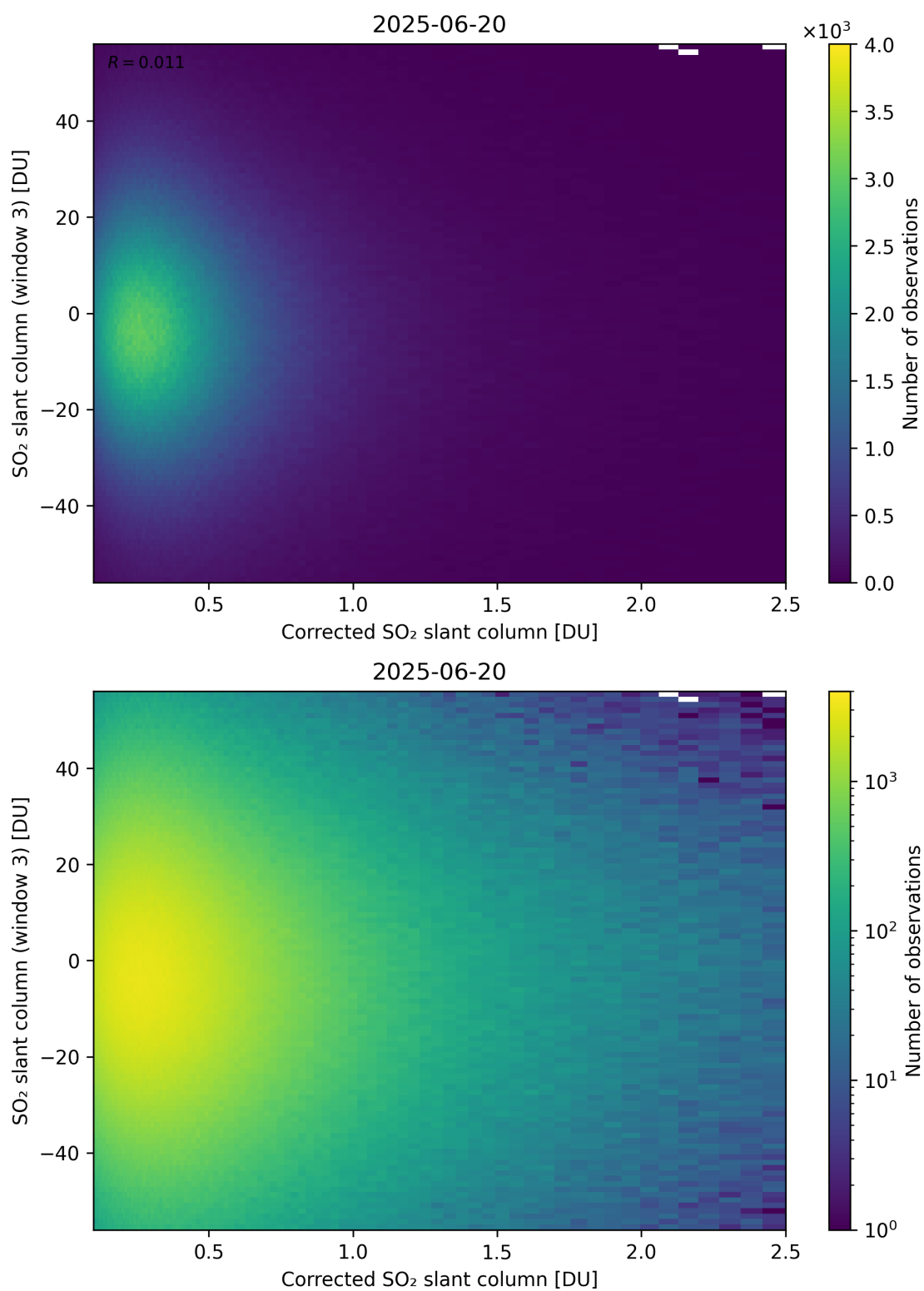
Figure 240: Scatter density plot of “Corrected SO 2 slant column” against “SO 2 slant column (window 3)” for 2025-06-19 to 2025-06-21.
