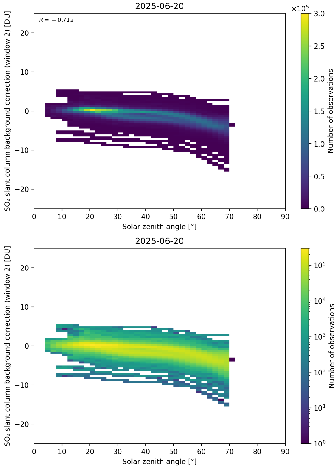
Figure 172: Scatter density plot of “Solar zenith angle” against “SO 2 slant column background correction (window 2)” for 2025-06-19 to 2025-06-21.
