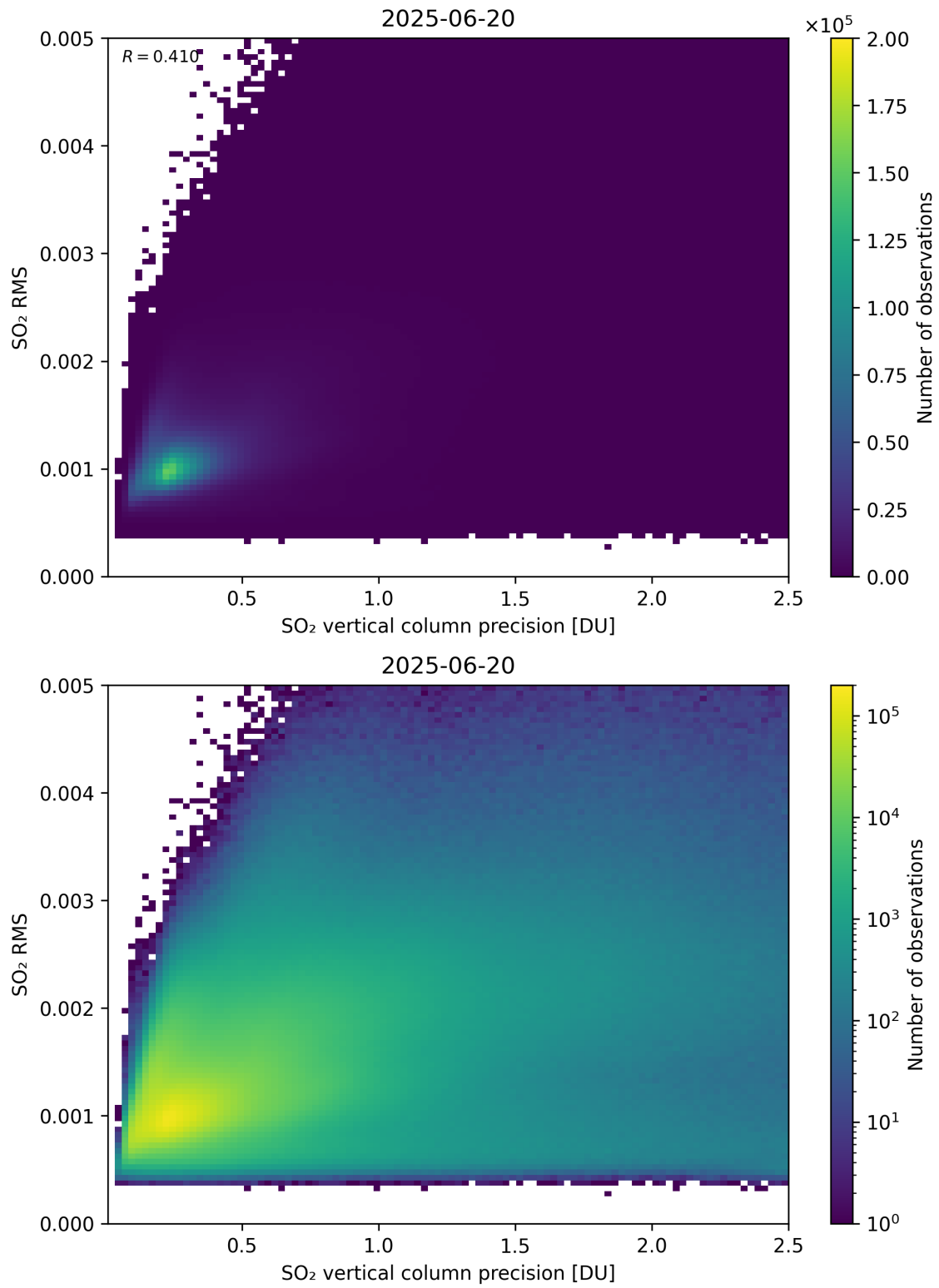
Figure 334: Scatter density plot of “SO 2 vertical column precision” against “SO 2 RMS” for 2025-06-19 to 2025-06-21.
