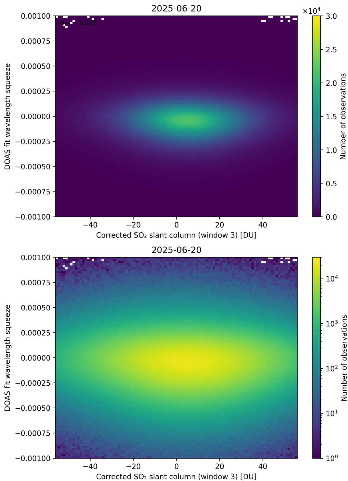
Figure 257: Scatter density plot of “Corrected SO 2 slant column (window 3)” against “DOAS fit wavelength squeeze” for 2025-06-19 to 2025-06-21.
