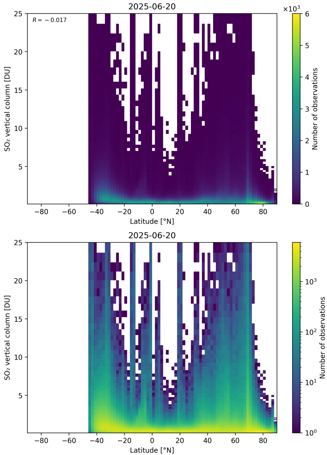
Figure 169: Scatter density plot of “Latitude” against “SO 2 vertical column” for 2025-06-19 to 2025-06-21.
