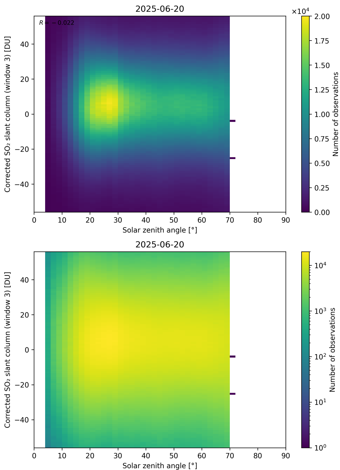
Figure 183: Scatter density plot of “Solar zenith angle” against “Corrected SO 2 slant column (window 3)” for 2025-06-19 to 2025-06-21.
