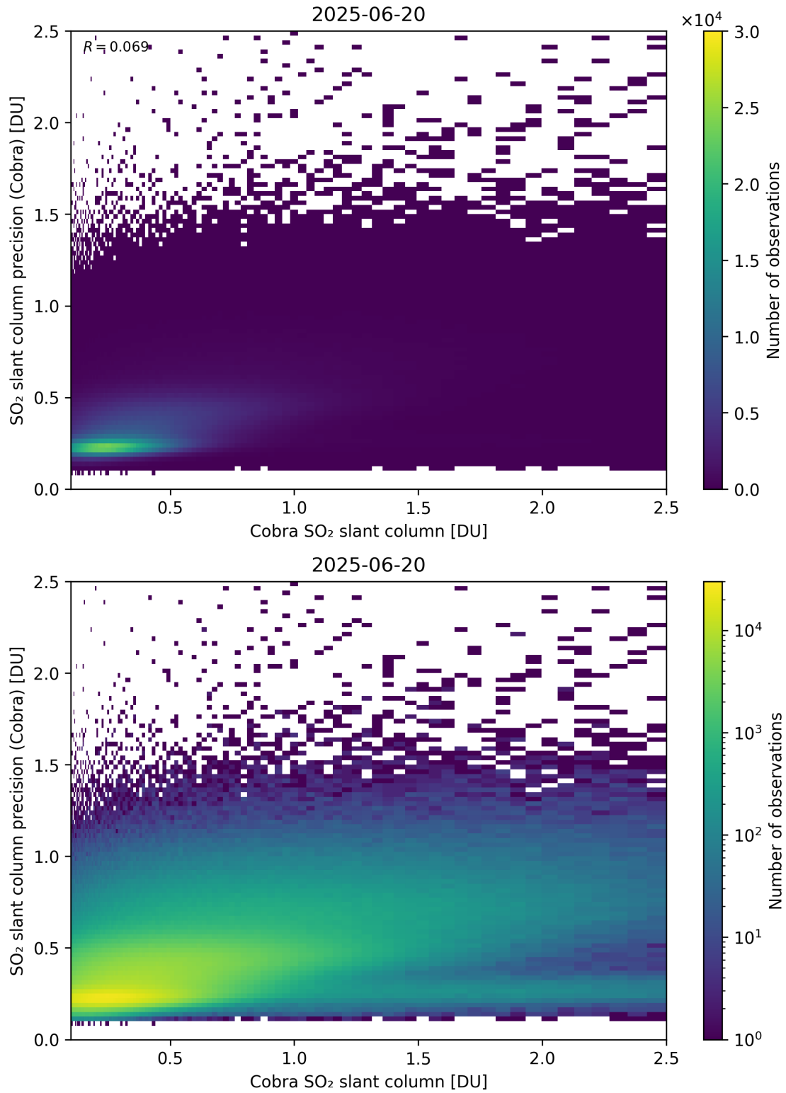
Figure 216: Scatter density plot of “Cobra SO 2 slant column” against “SO 2 slant column precision (Cobra)” for 2025-06-19 to 2025-06-21.
