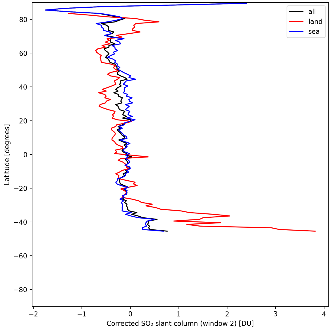
Figure 43: Zonal average of “Corrected SO 2 slant column (window 2)” for 2025-06-19 to 2025-06-21.
