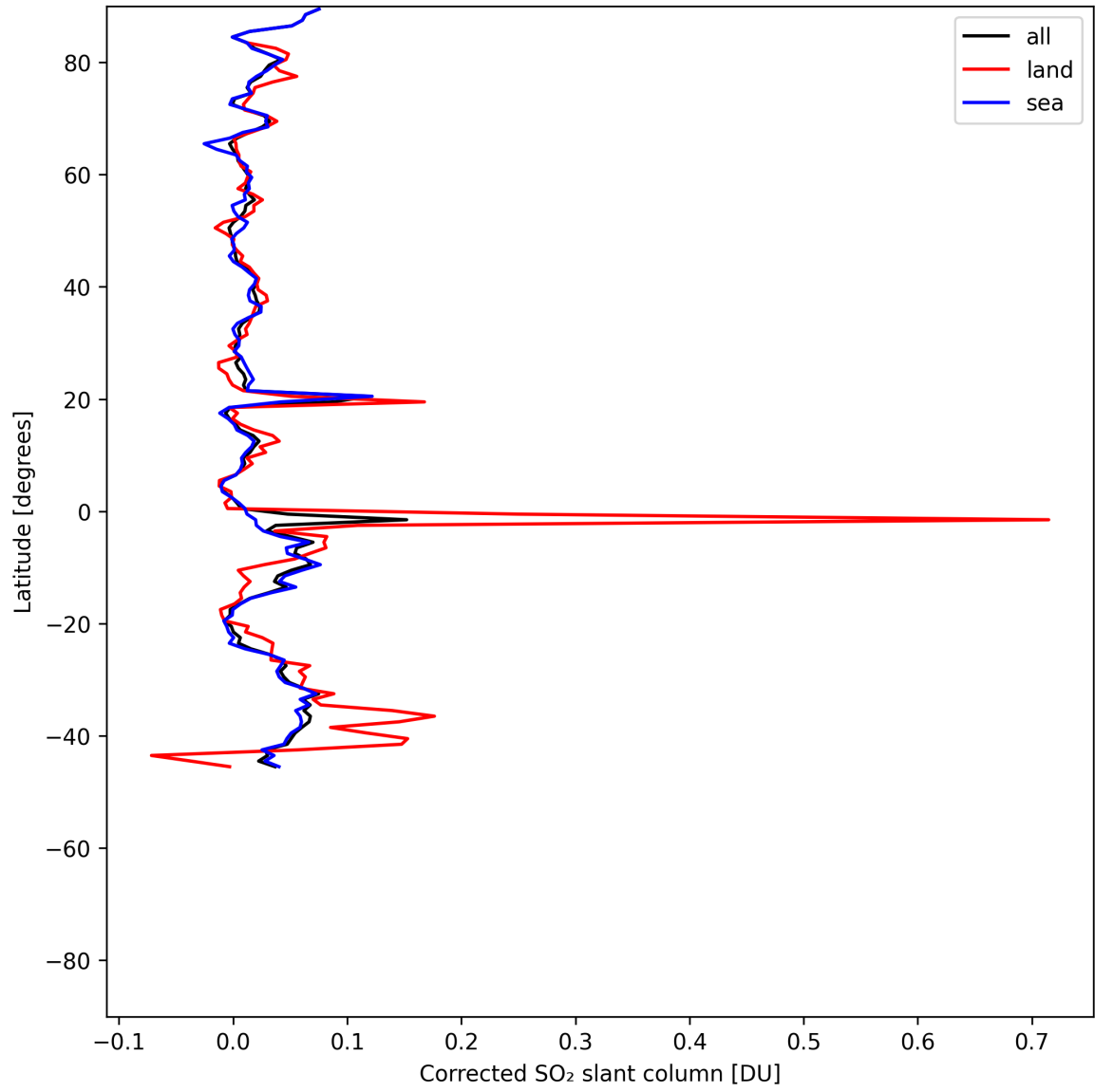
Figure 34: Zonal average of “Corrected SO 2 slant column” for 2025-06-19 to 2025-06-21.
