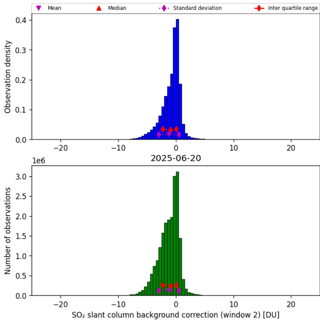
Figure 70: Histogram of “SO 2 slant column background correction (window 2)” for 2025-06-19 to 2025-06-21
