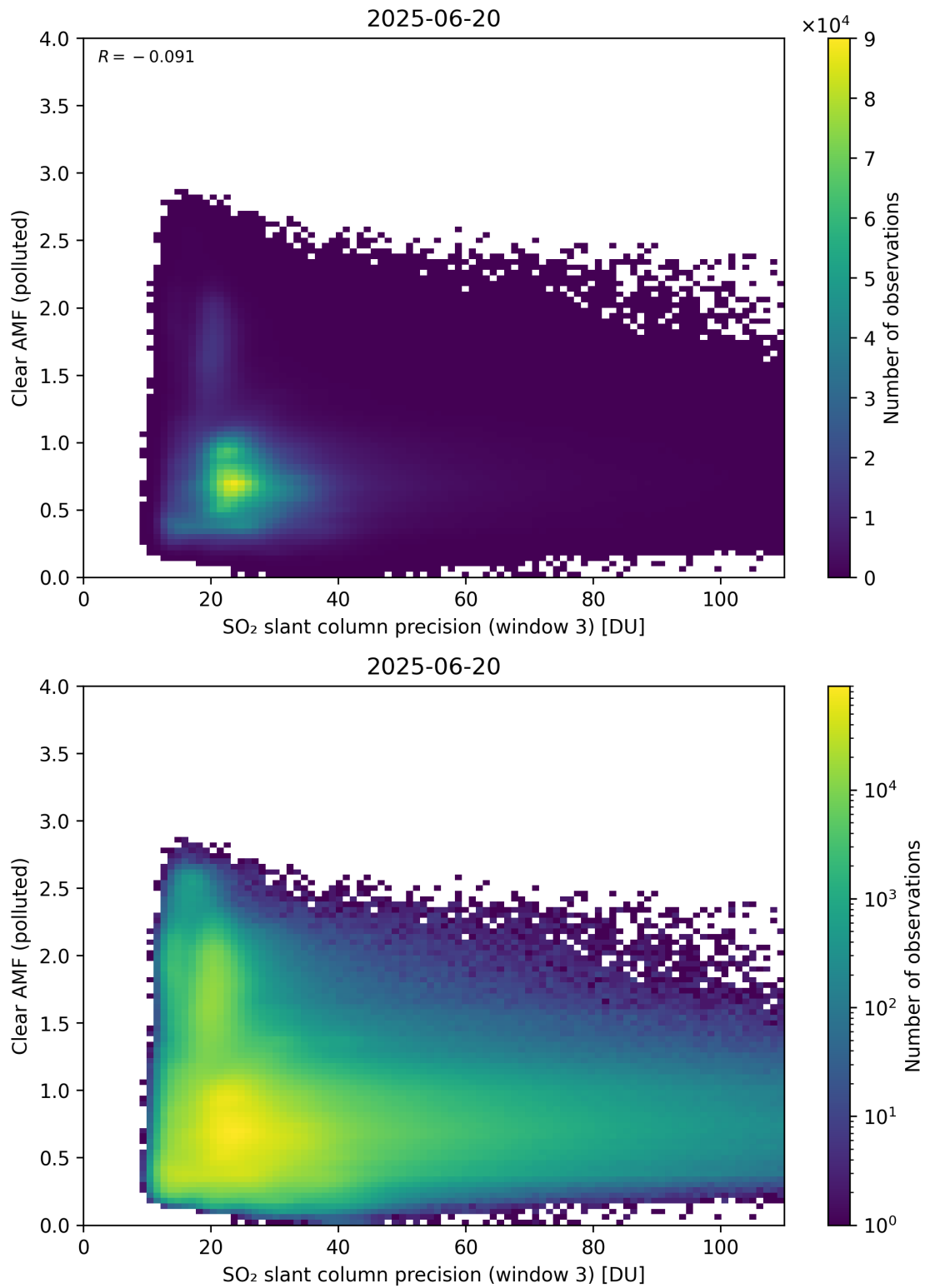
Figure 311: Scatter density plot of “SO 2 slant column precision (window 3)” against “Clear AMF (polluted)” for 2025-06-19 to 2025-06-21.
