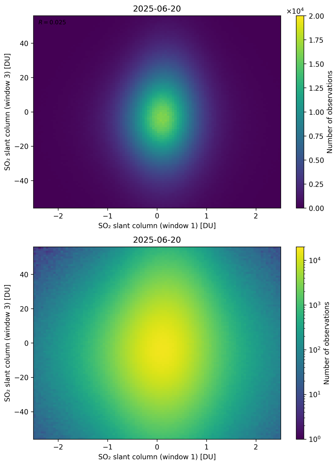
Figure 287: Scatter density plot of “SO 2 slant column (window 1)” against “SO 2 slant column (window 3)” for 2025-06-19 to 2025-06-21.
