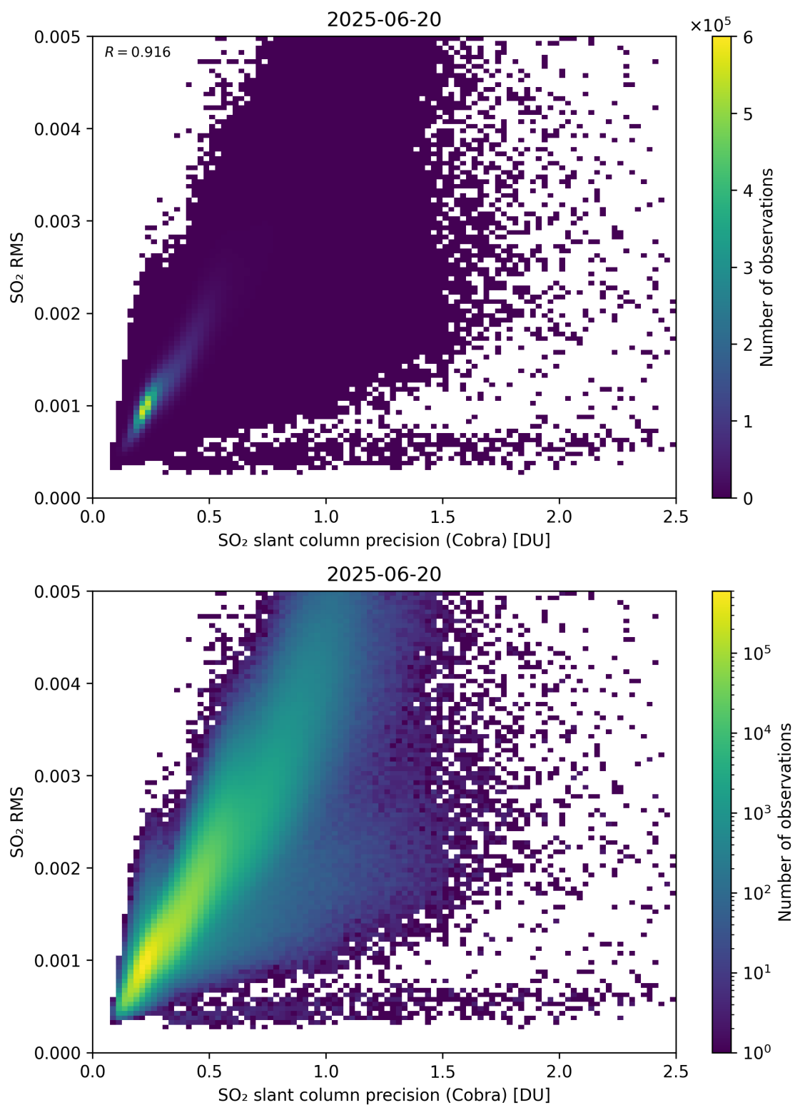
Figure 204: Scatter density plot of “SO 2 slant column precision (Cobra)” against “SO 2 RMS” for 2025-06-19 to 2025-06-21.
