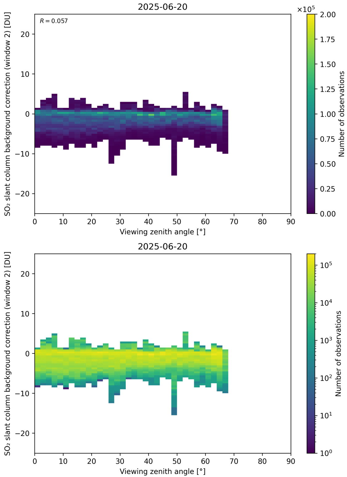
Figure 363: Scatter density plot of “Viewing zenith angle” against “SO 2 slant column background correction (window 2)” for 2025-06-19 to 2025-06-21.
