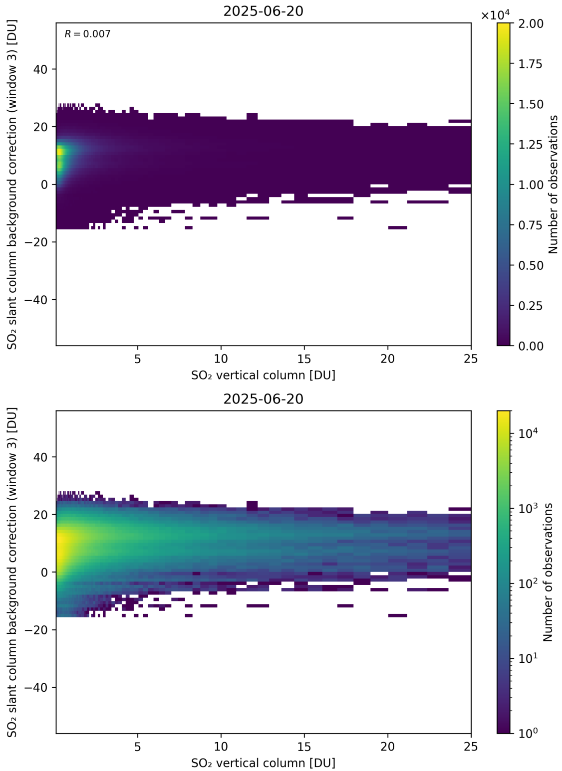
Figure 325: Scatter density plot of “SO 2 vertical column” against “SO 2 slant column background correction (window 3)” for 2025-06-19 to 2025-06-21.
