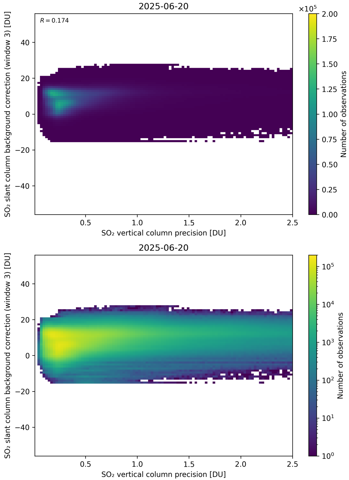
Figure 331: Scatter density plot of “SO 2 vertical column precision” against “SO 2 slant column background correction (window 3)” for 2025-06-19 to 2025-06-21.
