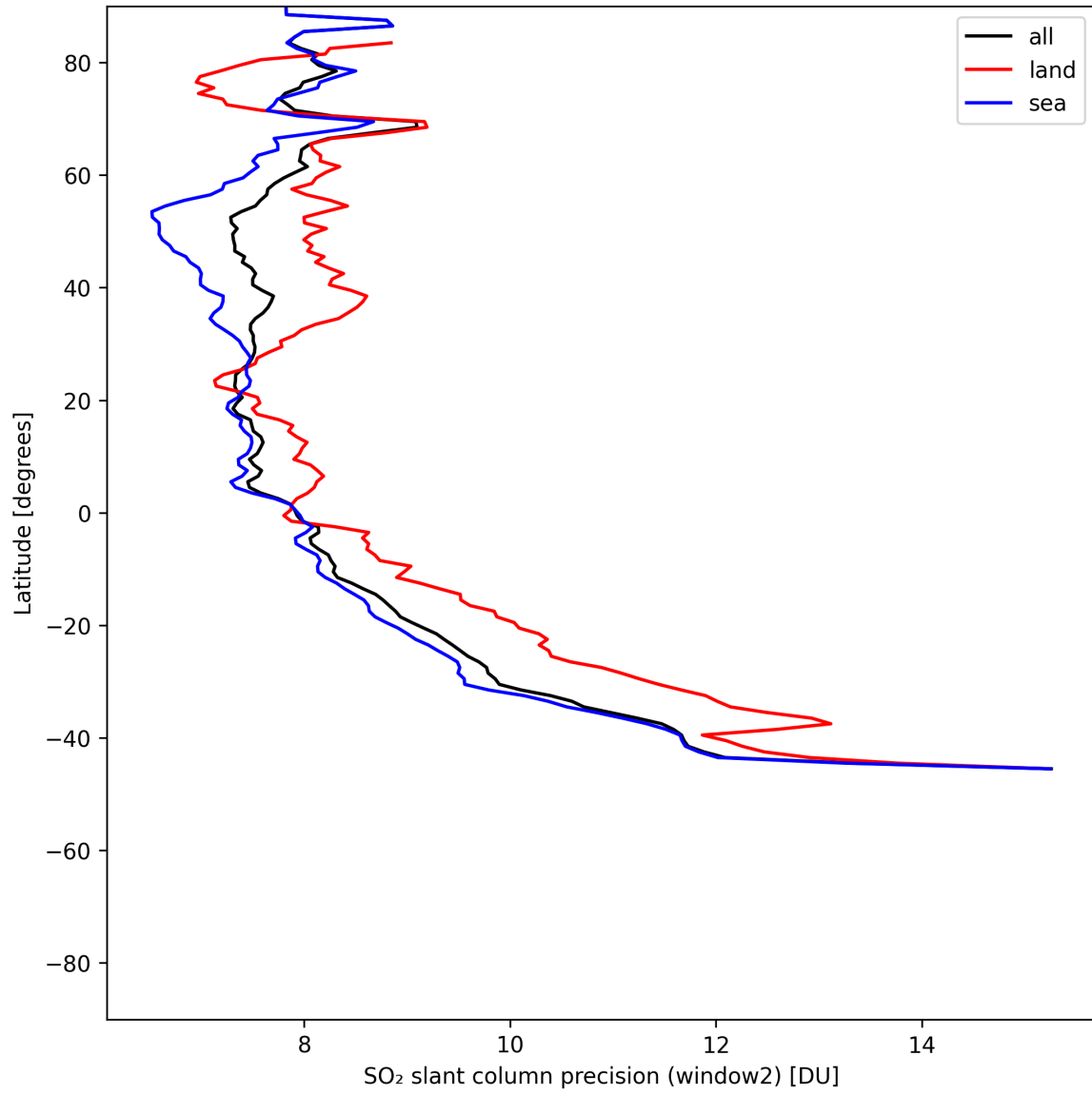
Figure 42: Zonal average of “SO 2 slant column precision (window2)” for 2025-06-19 to 2025-06-21.
