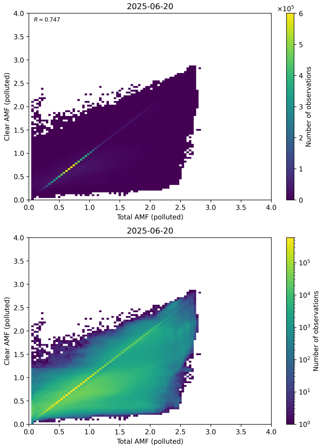
Figure 321: Scatter density plot of “Total AMF (polluted)” against “Clear AMF (polluted)” for 2025-06-19 to 2025-06-21.
