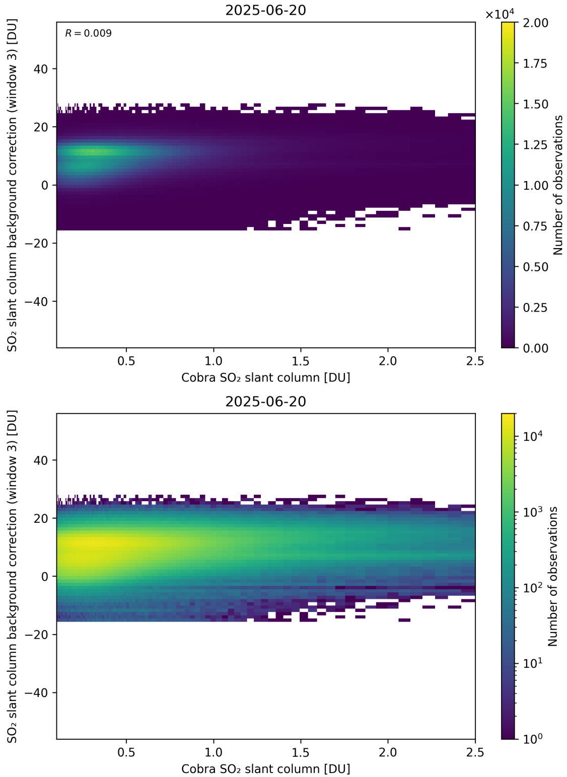
Figure 195: Scatter density plot of “Cobra SO 2 slant column” against “SO 2 slant column background correction (window 3)” for 2025-06-19 to 2025-06-21.
