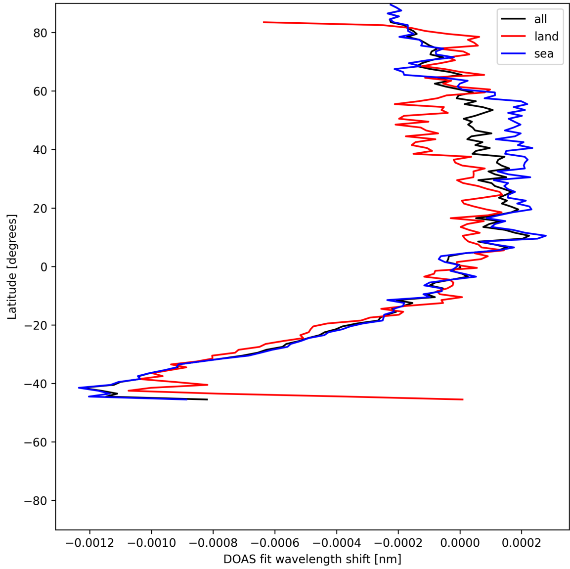
Figure 50: Zonal average of “DOAS fit wavelength shift” for 2025-06-19 to 2025-06-21.
