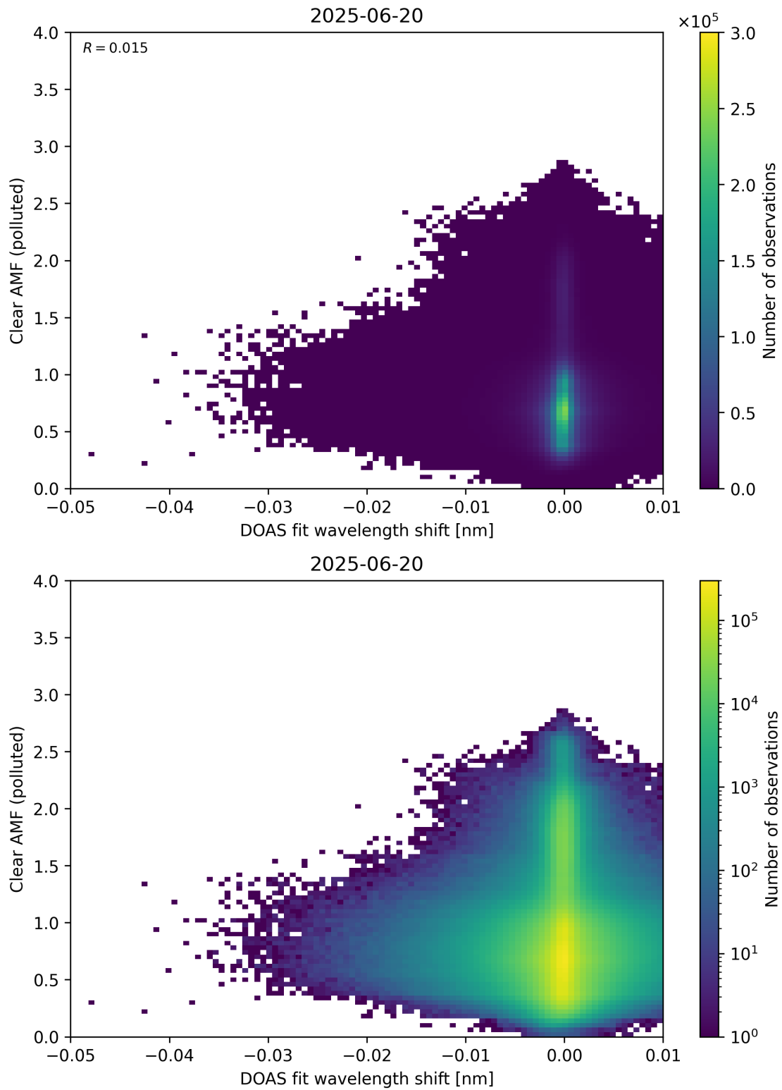
Figure 140: Scatter density plot of “DOAS fit wavelength shift” against “Clear AMF (polluted)” for 2025-06-19 to 2025-06-21.
