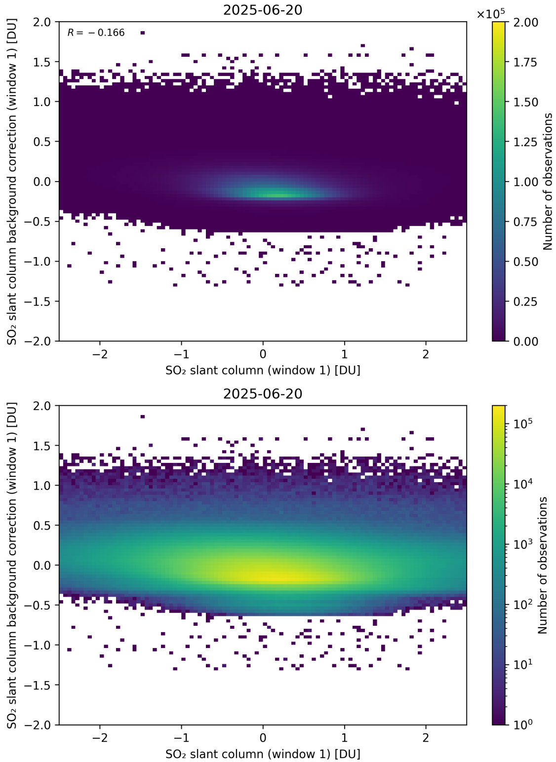
Figure 262: Scatter density plot of “SO 2 slant column (window 1)” against “SO 2 slant column background correction (window 1)” for 2025-06-19 to 2025-06-21.
