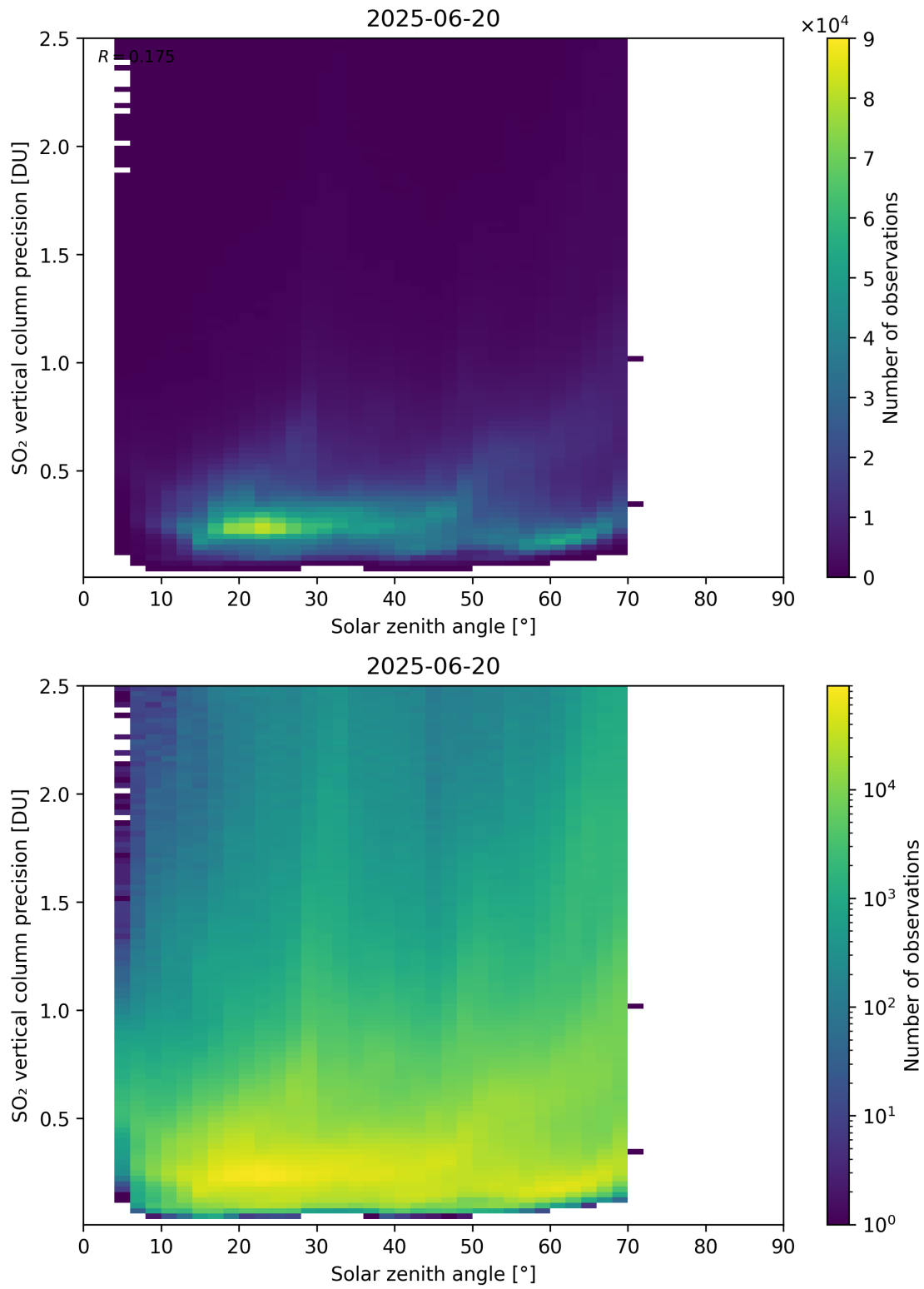
Figure 192: Scatter density plot of “Solar zenith angle” against “SO 2 vertical column precision” for 2025-06-19 to 2025-06-21.
