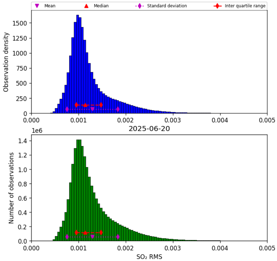
Figure 78: Histogram of “SO 2 RMS” for 2025-06-19 to 2025-06-21
