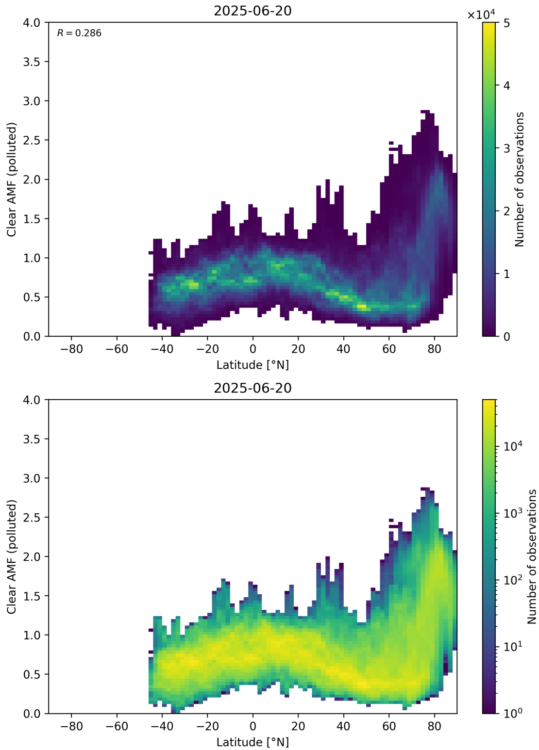
Figure 156: Scatter density plot of “Latitude” against “Clear AMF (polluted)” for 2025-06-19 to 2025-06-21.
