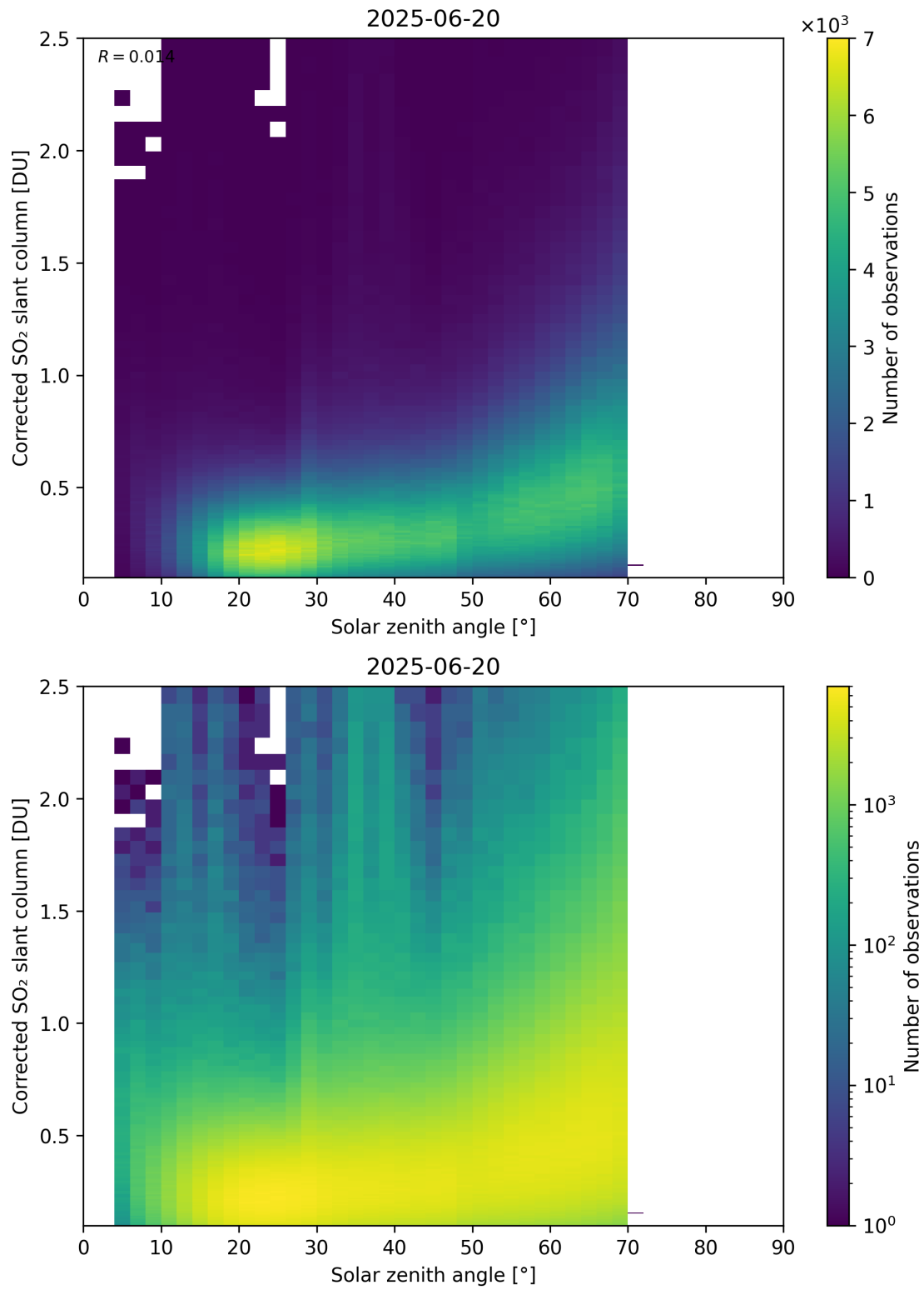
Figure 181: Scatter density plot of “Solar zenith angle” against “Corrected SO 2 slant column” for 2025-06-19 to 2025-06-21.
