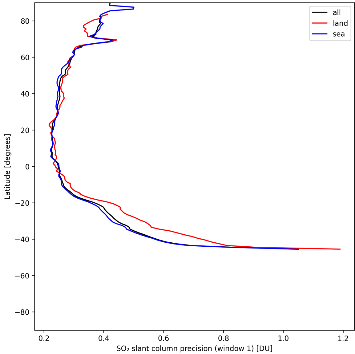
Figure 38: Zonal average of “SO 2 slant column precision (window 1)” for 2025-06-19 to 2025-06-21.
