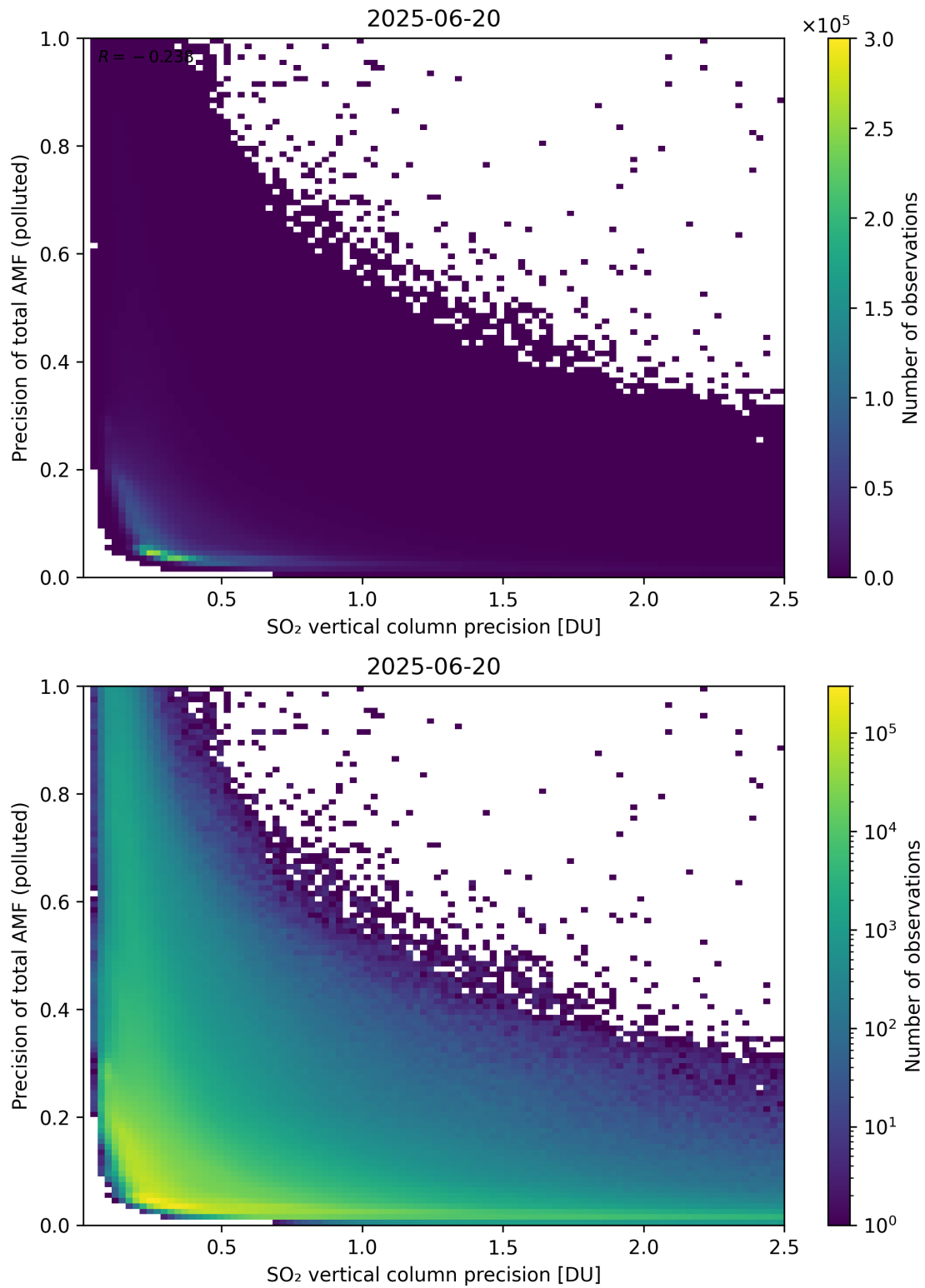
Figure 347: Scatter density plot of “SO 2 vertical column precision” against “Precision of total AMF (polluted)” for 2025-06-19 to 2025-06-21.
