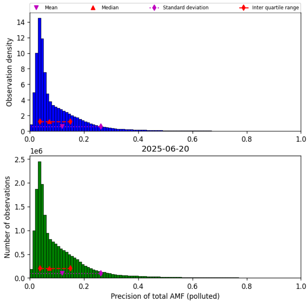
Figure 80: Histogram of “Precision of total AMF (polluted)” for 2025-06-19 to 2025-06-21
