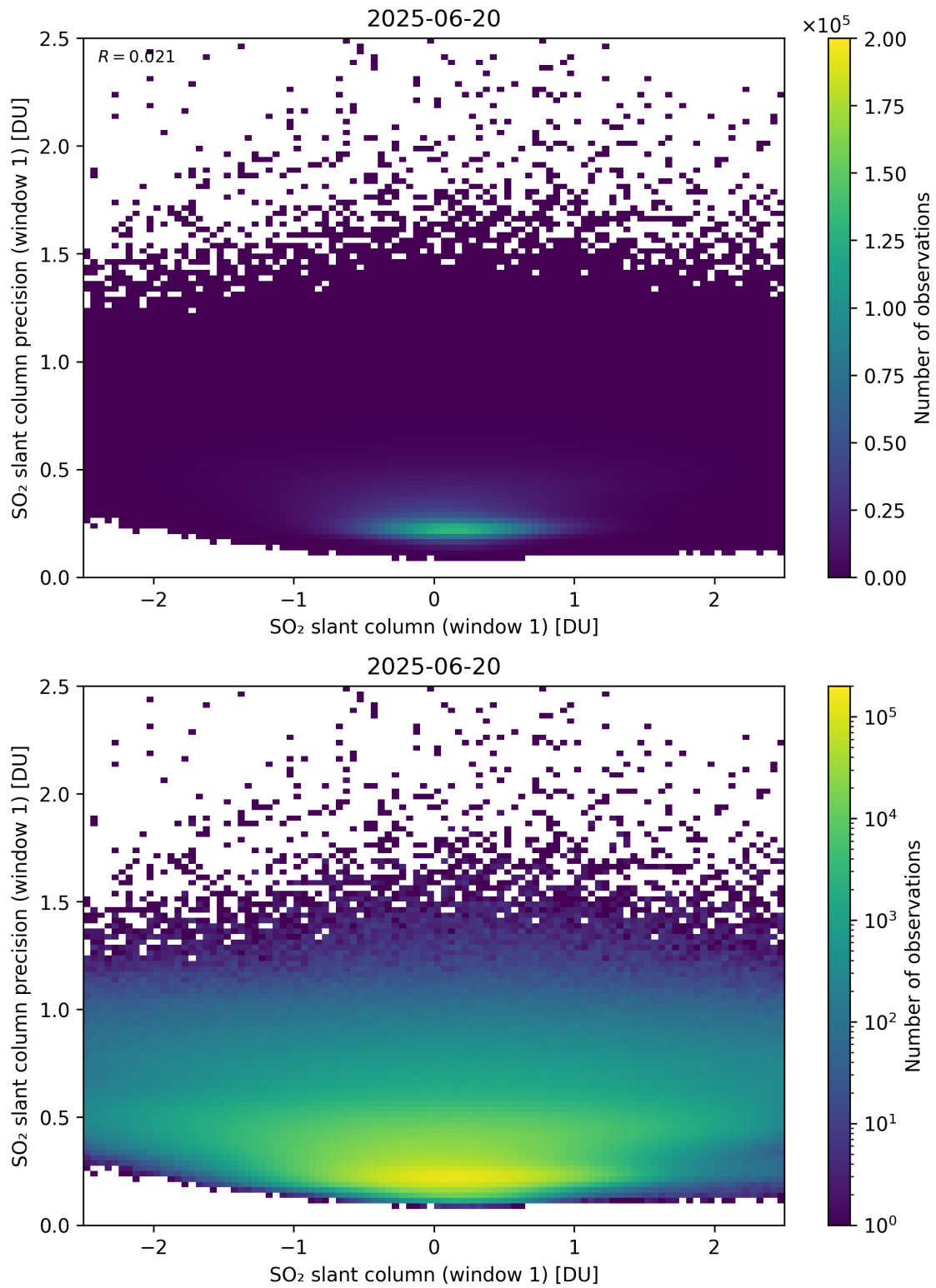
Figure 285: Scatter density plot of “SO 2 slant column (window 1)” against “SO 2 slant column precision (window 1)” for 2025-06-19 to 2025-06-21.
