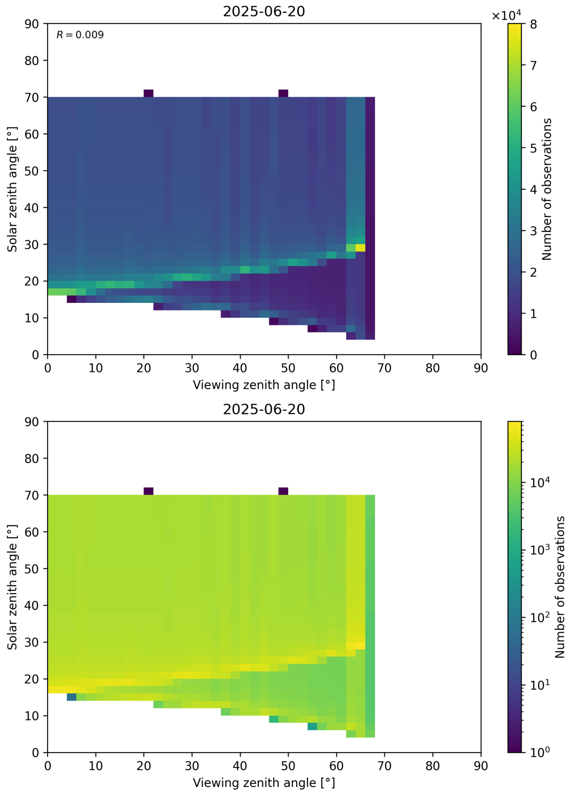
Figure 369: Scatter density plot of “Viewing zenith angle” against “Solar zenith angle” for 2025-06-19 to 2025-06-21.
