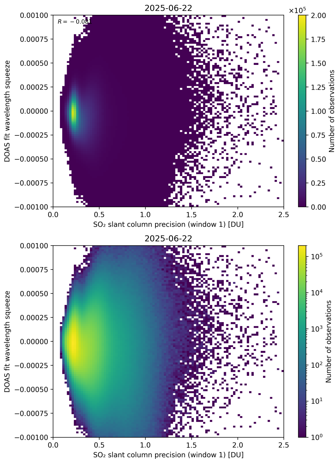
Figure 272: Scatter density plot of “SO 2 slant column precision (window 1)” against “DOAS fit wavelength squeeze” for 2025-06-22 to 2025-06-23.
