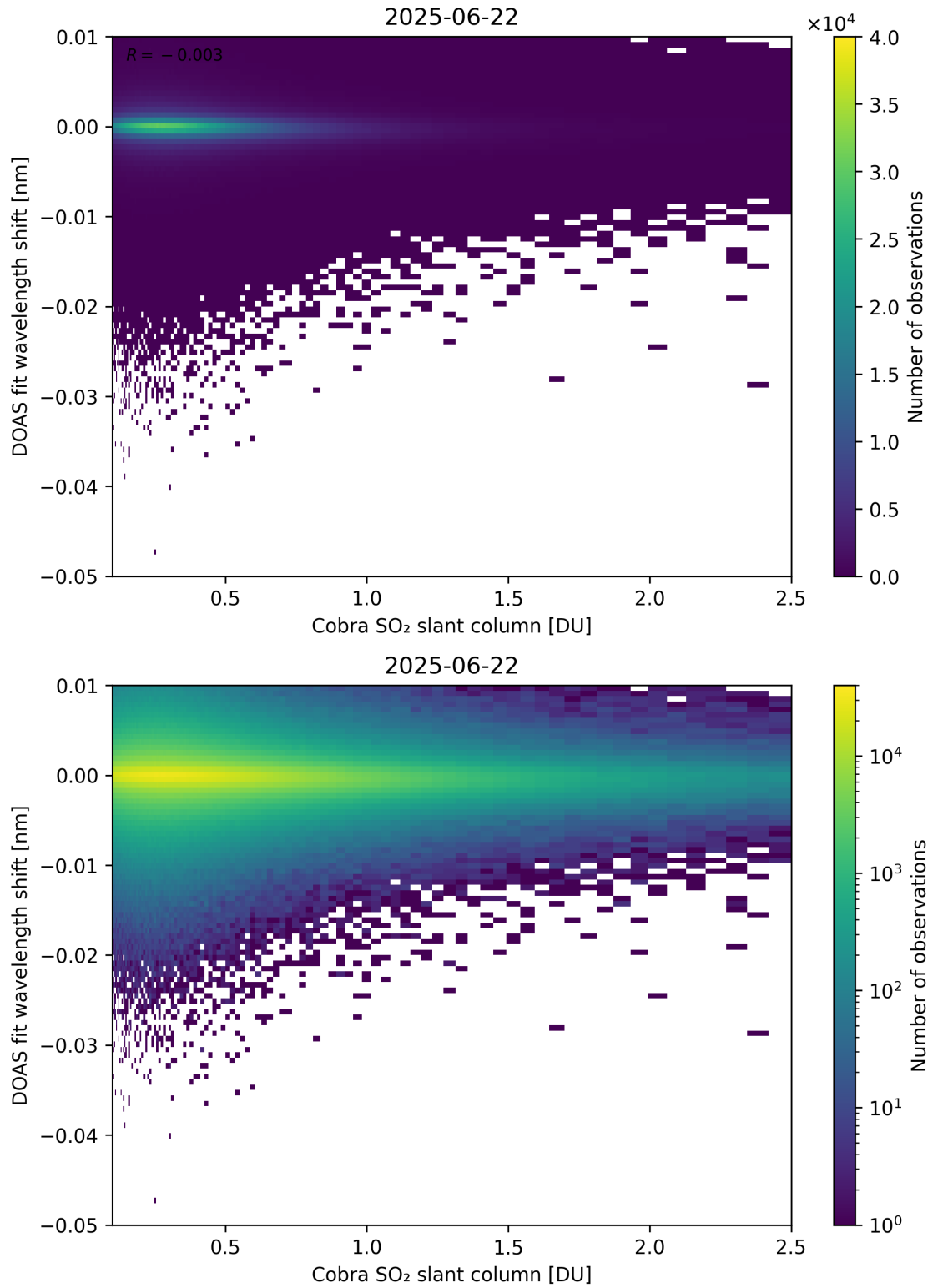
Figure 196: Scatter density plot of “Cobra SO 2 slant column” against “DOAS fit wavelength shift” for 2025-06-22 to 2025-06-23.
