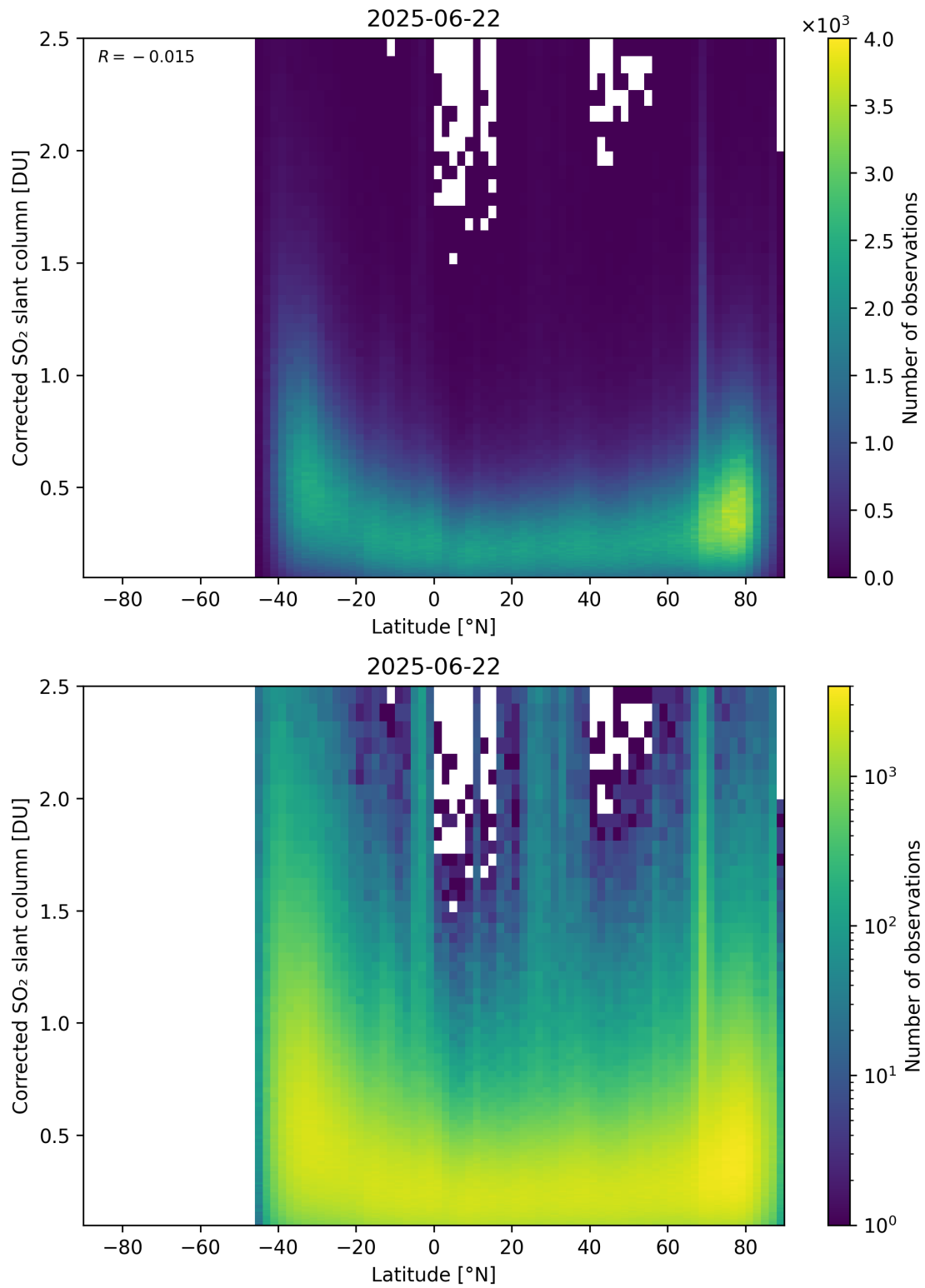
Figure 159: Scatter density plot of “Latitude” against “Corrected SO 2 slant column” for 2025-06-22 to 2025-06-23.
