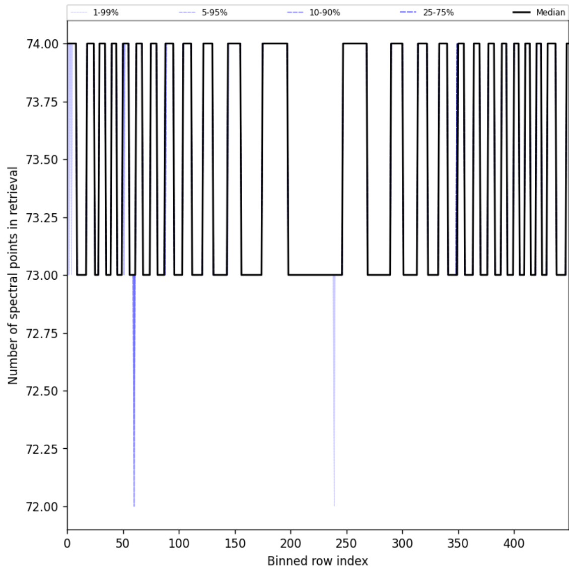
Figure 108: Along track statistics of “Number of spectral points in retrieval” for 2025-06-22 to 2025-06-23
