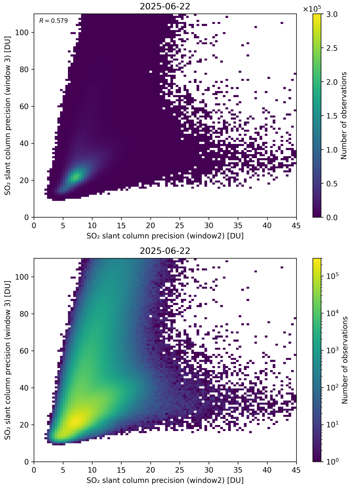
Figure 300: Scatter density plot of “SO 2 slant column precision (window2)” against “SO 2 slant column precision (window 3)” for 2025-06-22 to 2025-06-23.
