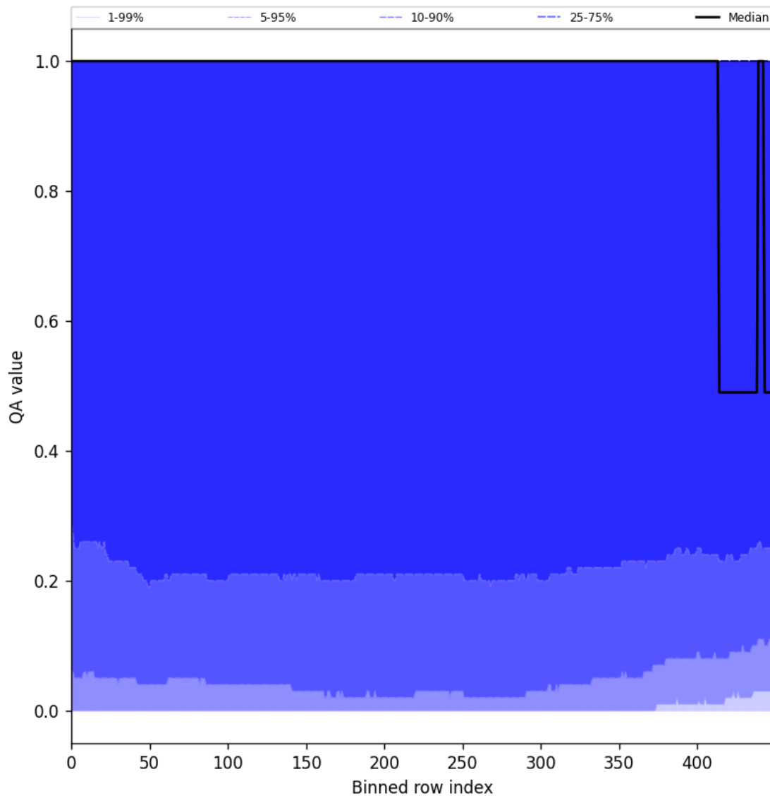
Figure 83: Along track statistics of “QA value” for 2025-06-22 to 2025-06-23
