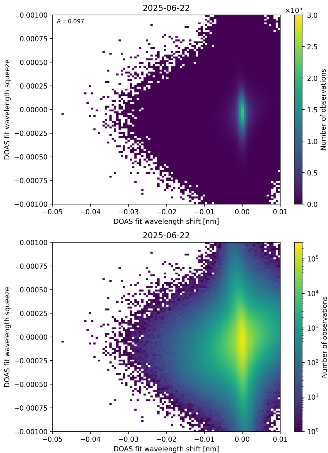
Figure 138: Scatter density plot of “DOAS fit wavelength shift” against “DOAS fit wavelength squeeze” for 2025-06-22 to 2025-06-23.
