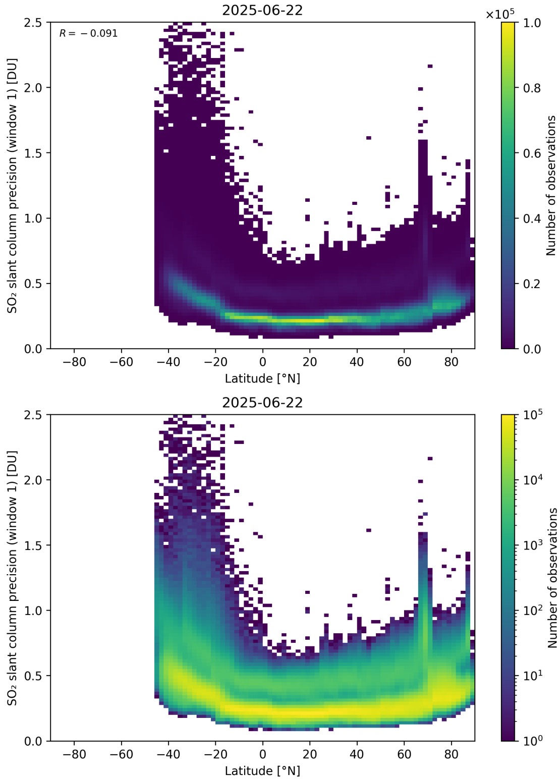
Figure 163: Scatter density plot of “Latitude” against “SO 2 slant column precision (window 1)” for 2025-06-22 to 2025-06-23.
