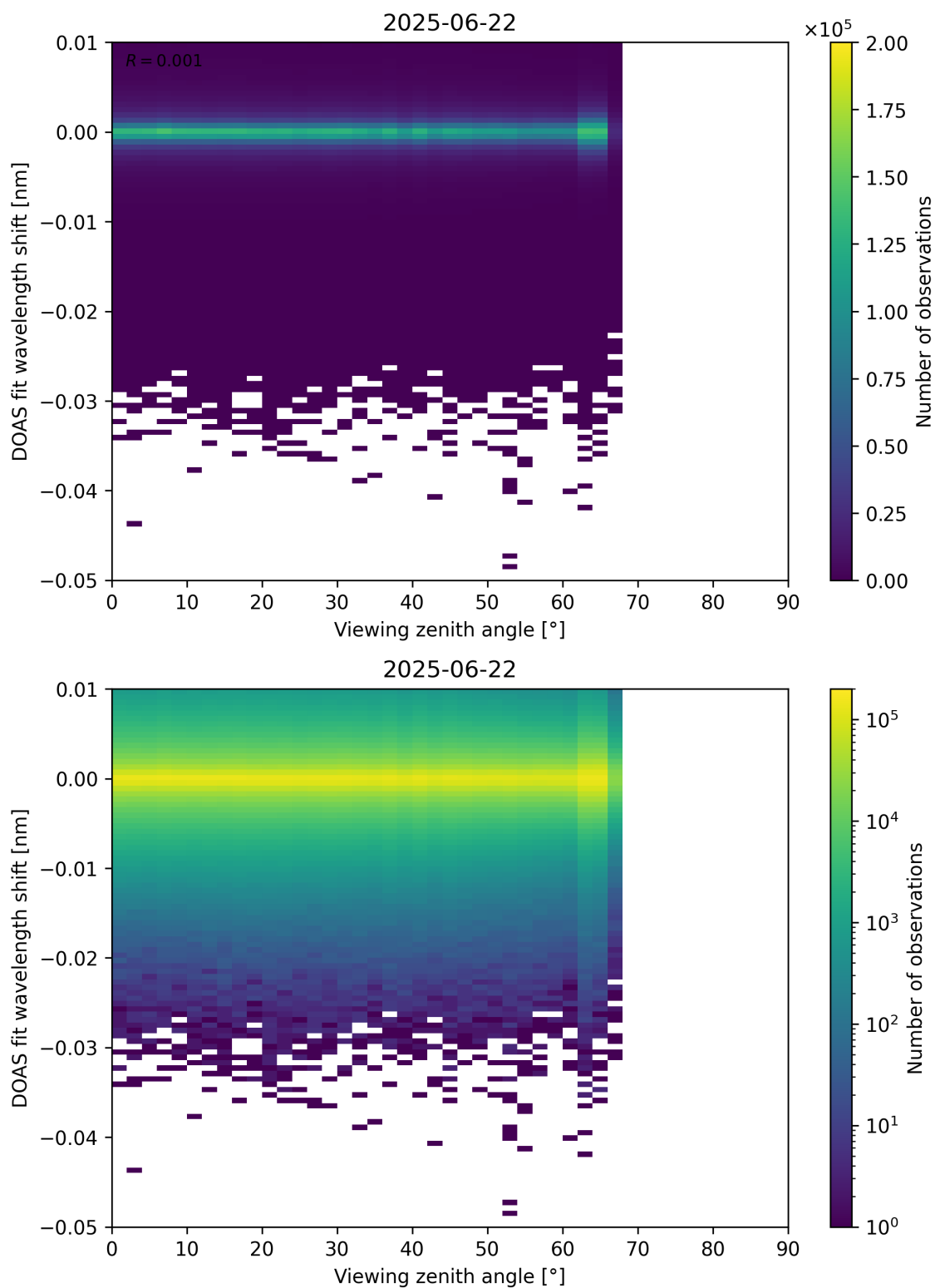
Figure 365: Scatter density plot of “Viewing zenith angle” against “DOAS fit wavelength shift” for 2025-06-22 to 2025-06-23.
