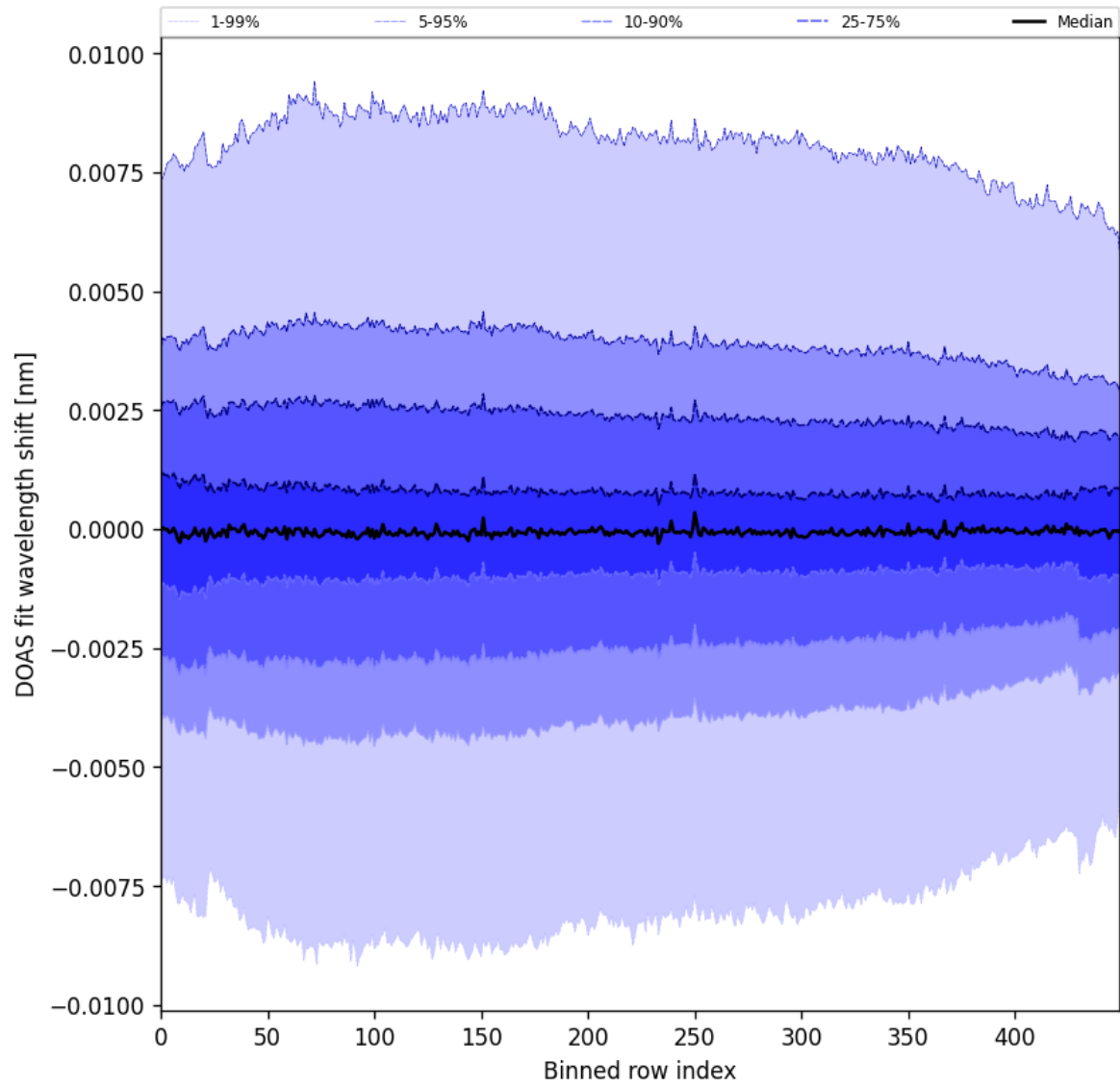
Figure 102: Along track statistics of “DOAS fit wavelength shift” for 2025-06-22 to 2025-06-23
