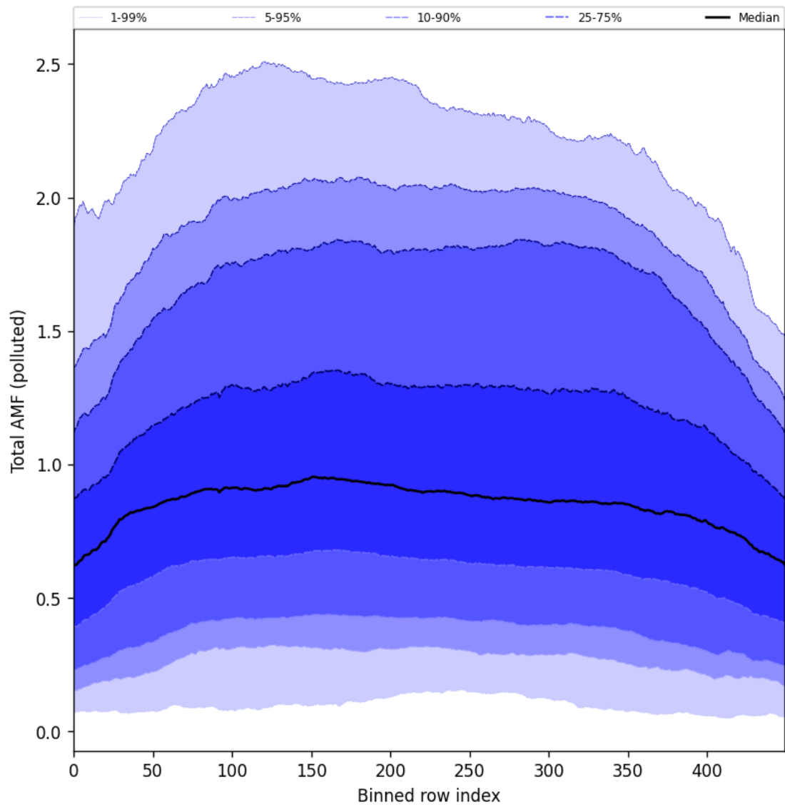
Figure 105: Along track statistics of “Total AMF (polluted)” for 2025-06-22 to 2025-06-23
