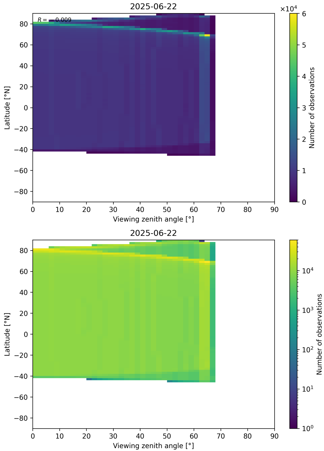
Figure 368: Scatter density plot of “Viewing zenith angle” against “Latitude” for 2025-06-22 to 2025-06-23.
