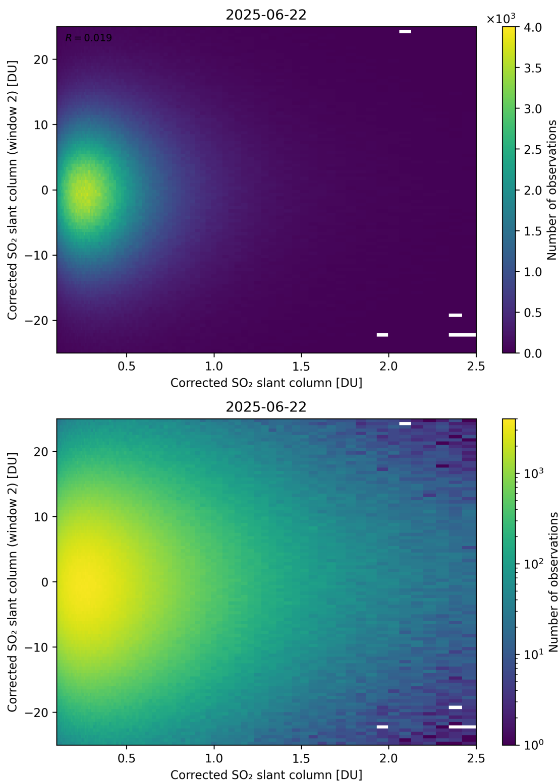
Figure 235: Scatter density plot of “Corrected SO 2 slant column” against “Corrected SO 2 slant column (window 2)” for 2025-06-22 to 2025-06-23.
