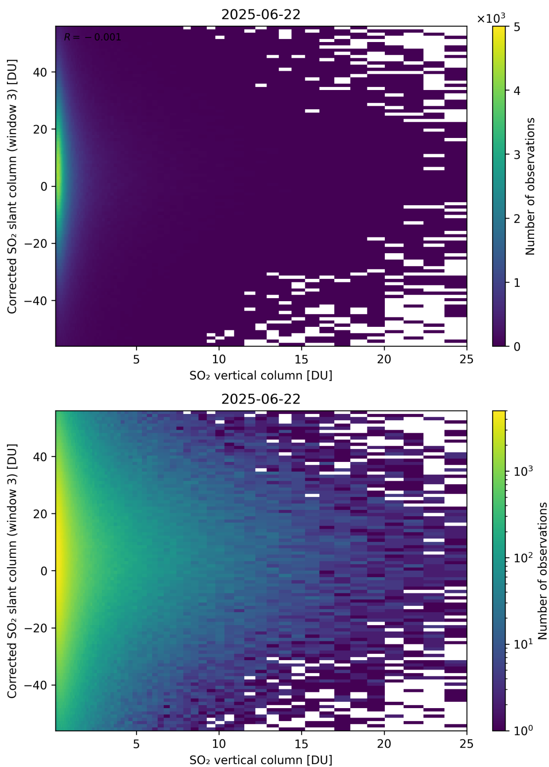
Figure 353: Scatter density plot of “SO 2 vertical column” against “Corrected SO 2 slant column (window 3)” for 2025-06-22 to 2025-06-23.
