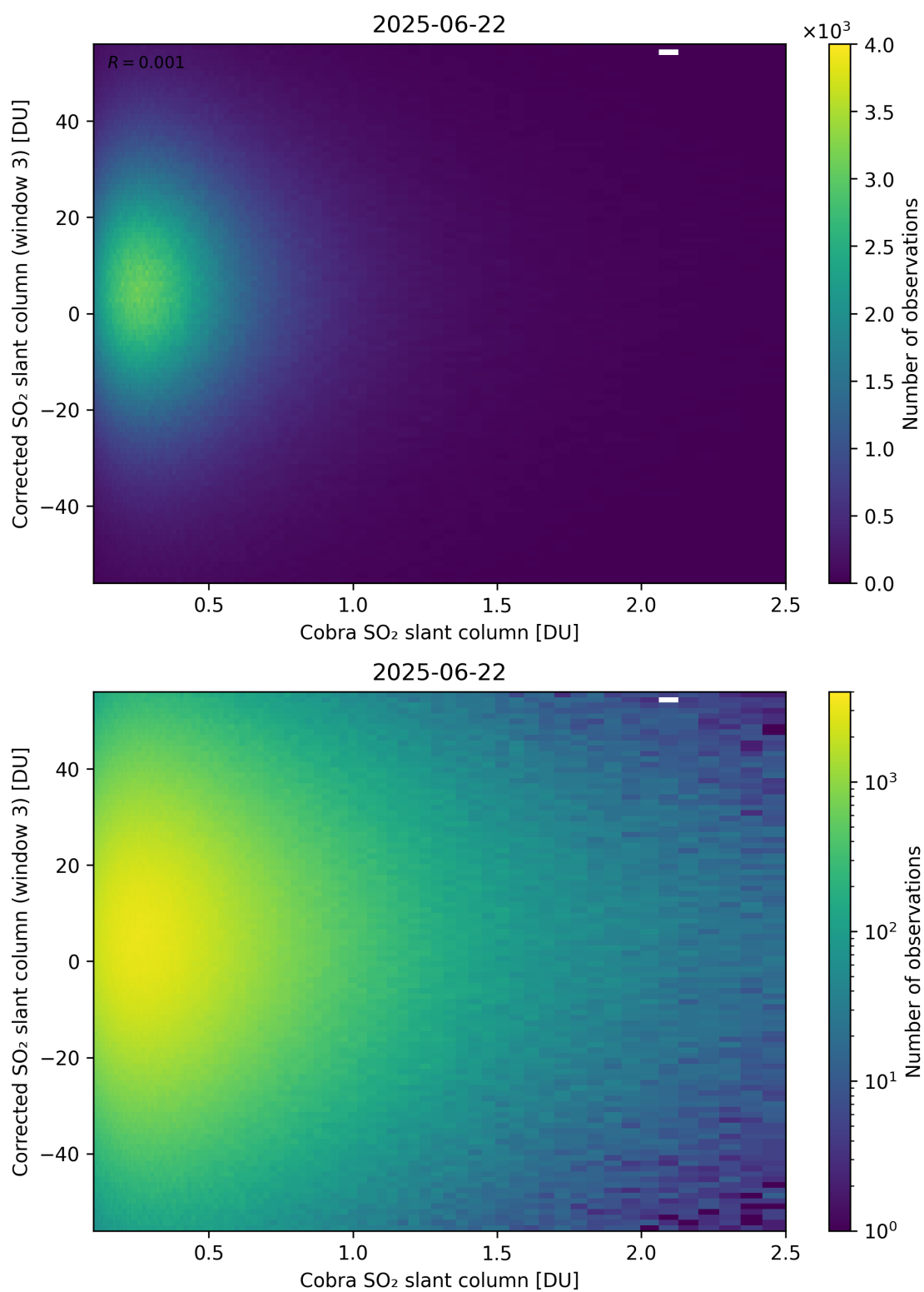
Figure 218: Scatter density plot of “Cobra SO 2 slant column” against “Corrected SO 2 slant column (window 3)” for 2025-06-22 to 2025-06-23.
