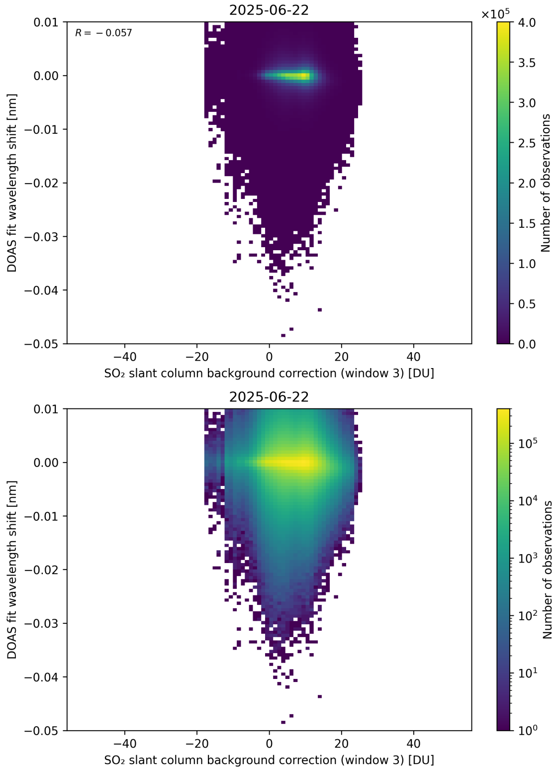
Figure 132: Scatter density plot of “SO 2 slant column background correction (window 3)” against “DOAS fit wavelength shift” for 2025-06-22 to 2025-06-23.
