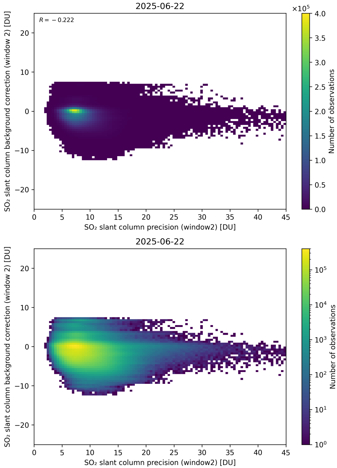
Figure 291: Scatter density plot of “SO 2 slant column precision (window2)” against “SO 2 slant column background correction (window 2)” for 2025-06-22 to 2025-06-23.
