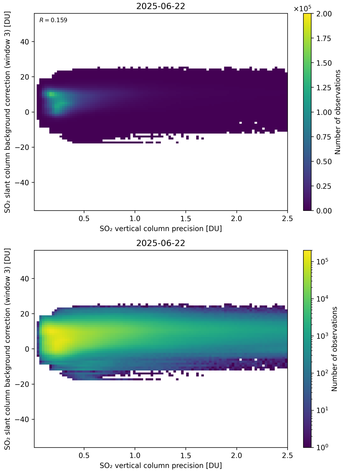
Figure 331: Scatter density plot of “SO 2 vertical column precision” against “SO 2 slant column background correction (window 3)” for 2025-06-22 to 2025-06-23.
