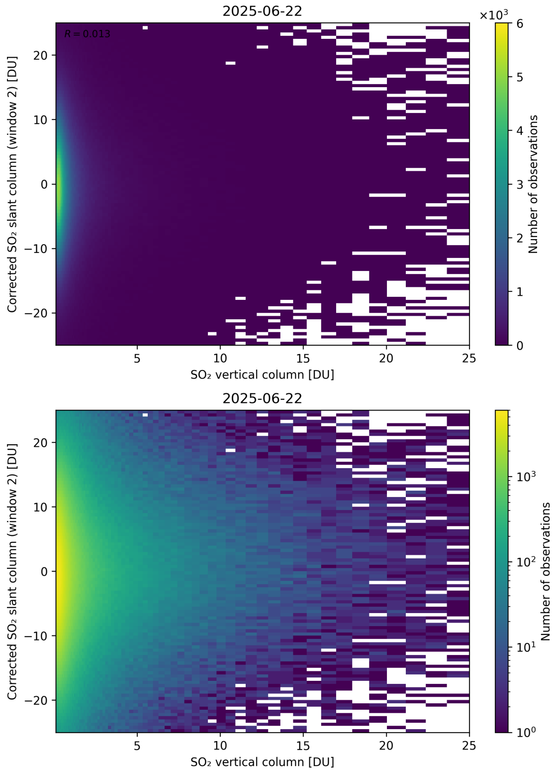
Figure 352: Scatter density plot of “SO 2 vertical column” against “Corrected SO 2 slant column (window 2)” for 2025-06-22 to 2025-06-23.
