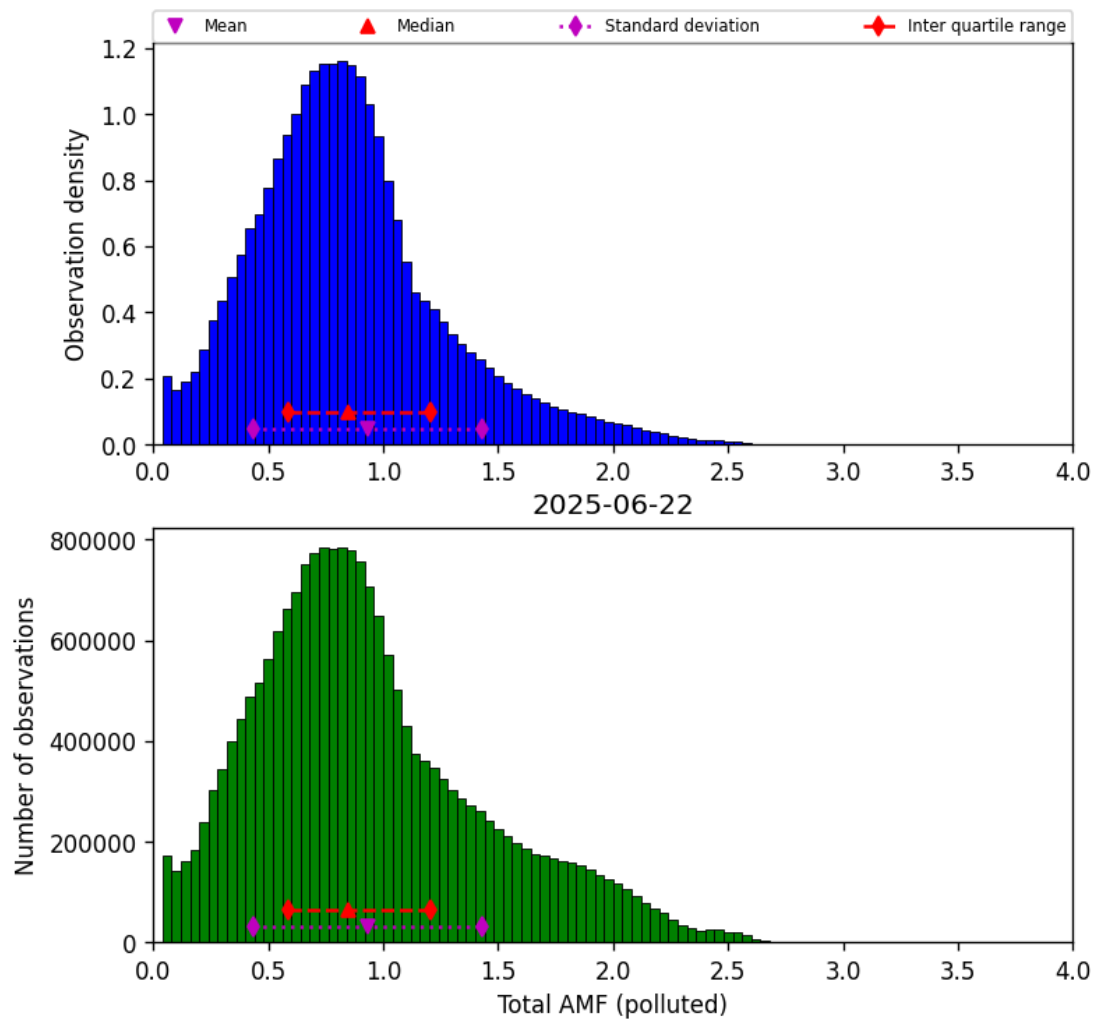
Figure 79: Histogram of “Total AMF (polluted)” for 2025-06-22 to 2025-06-23
