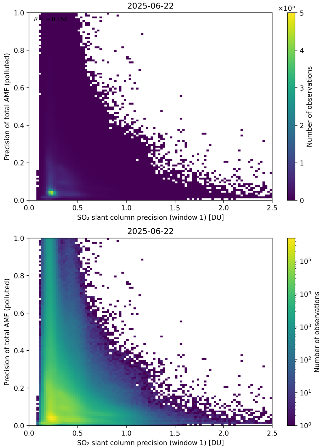
Figure 281: Scatter density plot of “SO 2 slant column precision (window 1)” against “Precision of total AMF (polluted)” for 2025-06-22 to 2025-06-23.
