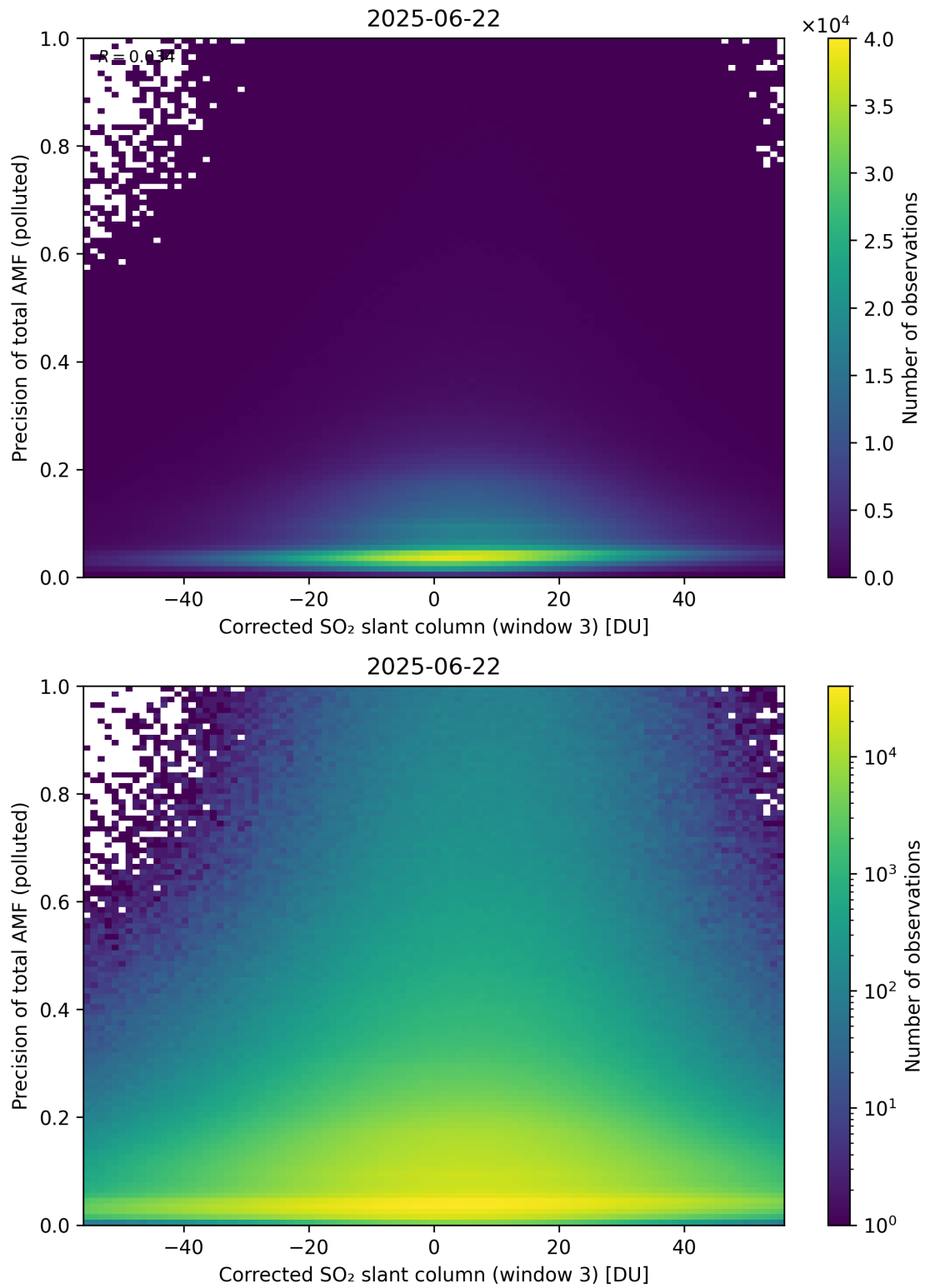
Figure 261: Scatter density plot of “Corrected SO 2 slant column (window 3)” against “Precision of total AMF (polluted)” for 2025-06-22 to 2025-06-23.
