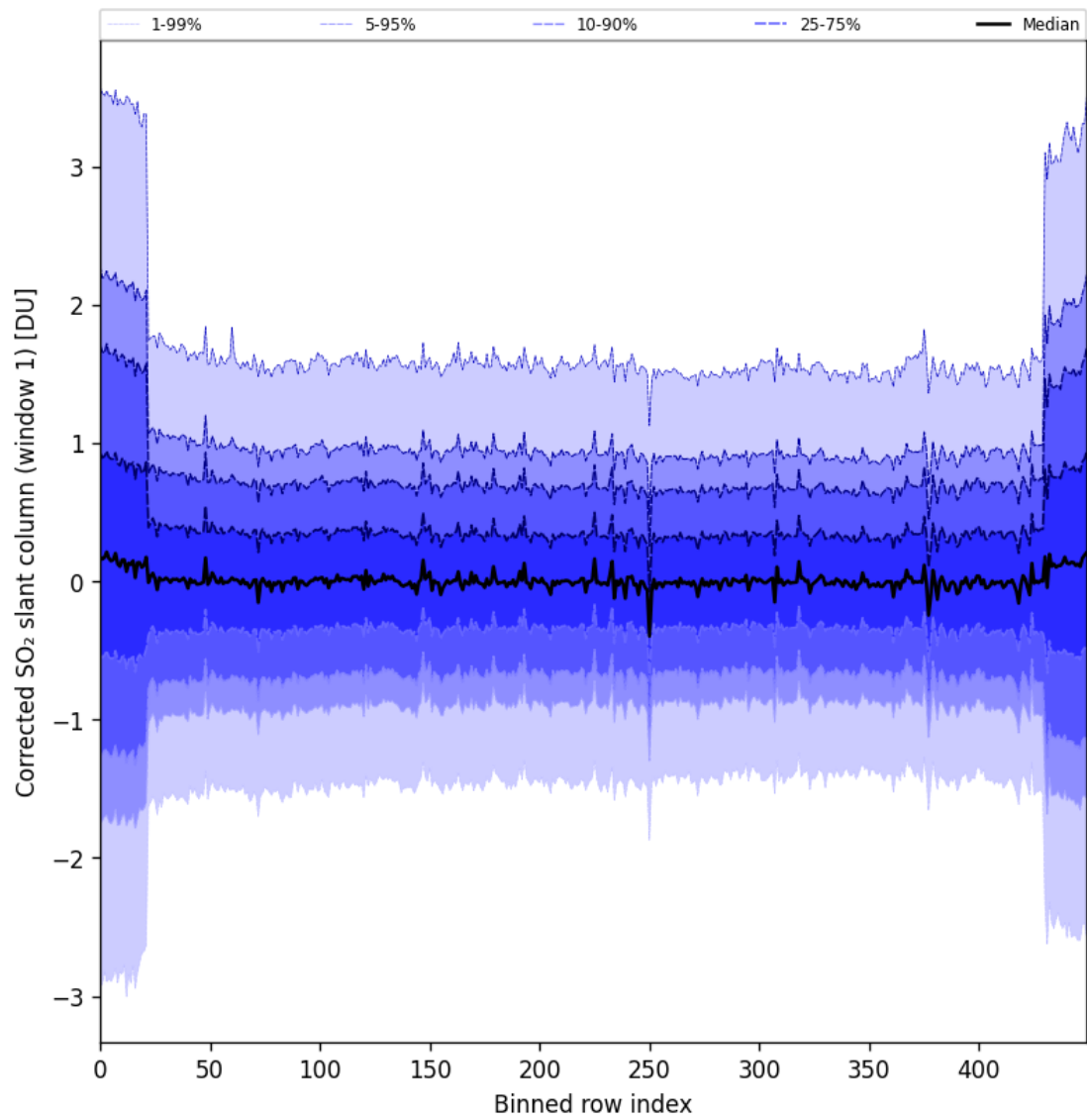
Figure 91: Along track statistics of “Corrected SO 2 slant column (window 1)” for 2025-06-22 to 2025-06-23
