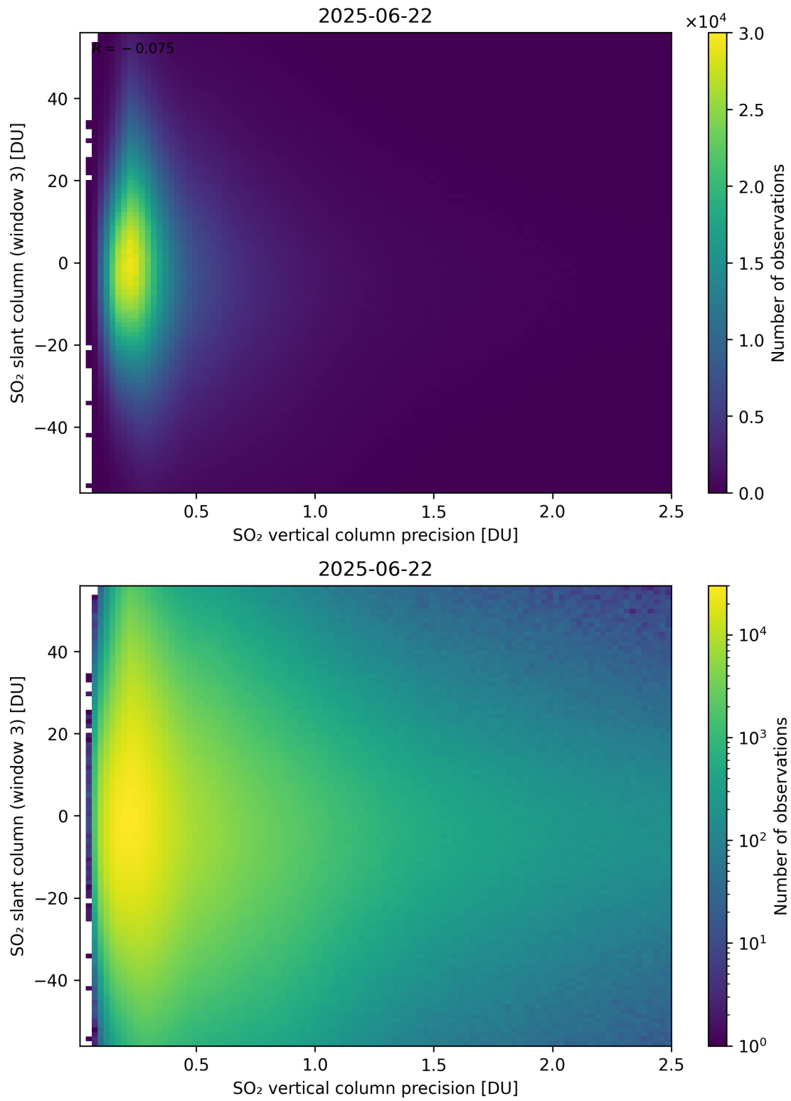
Figure 344: Scatter density plot of “SO 2 vertical column precision” against “SO 2 slant column (window 3)” for 2025-06-22 to 2025-06-23.
