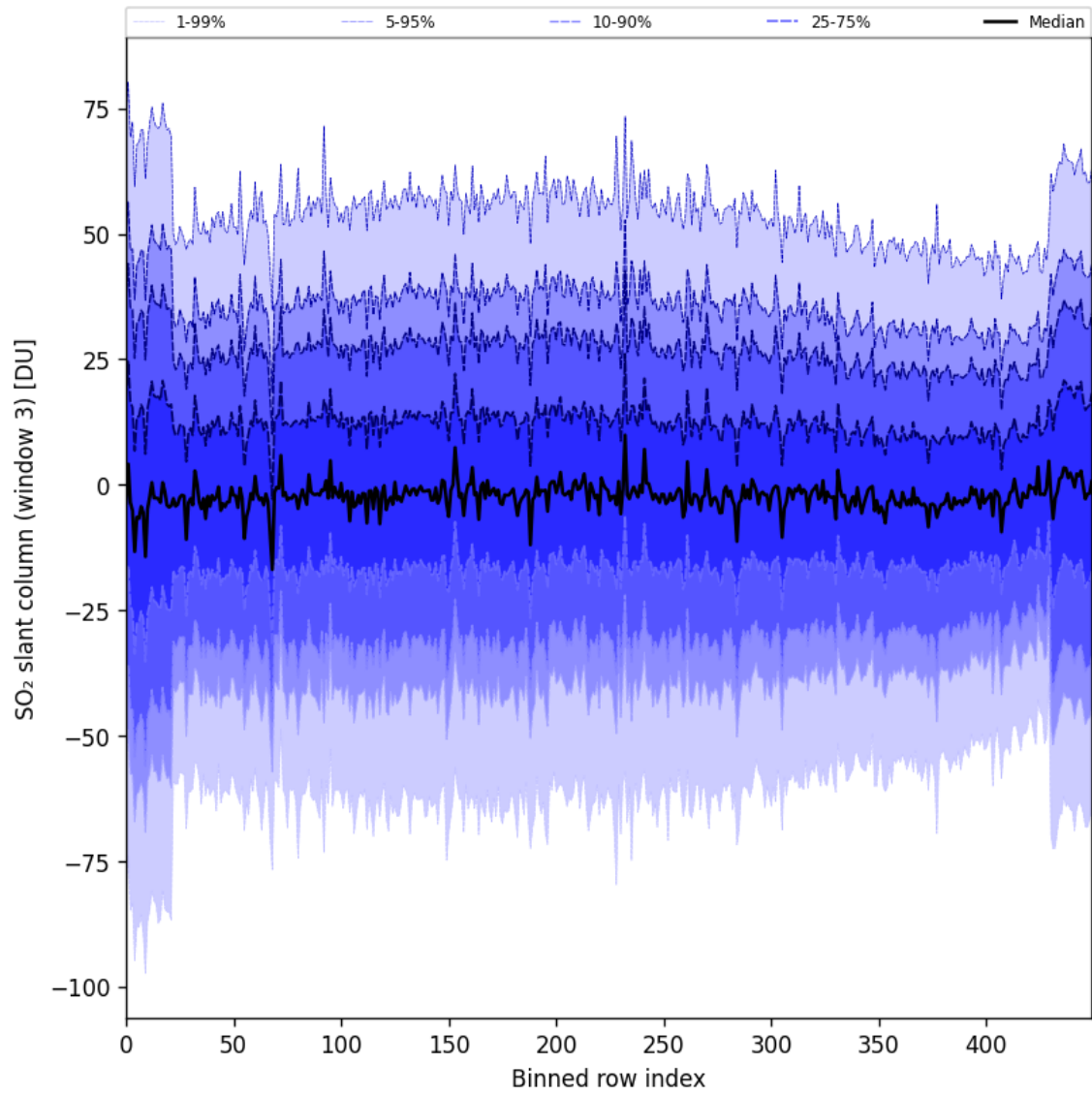
Figure 97: Along track statistics of “SO 2 slant column (window 3)” for 2025-06-22 to 2025-06-23
