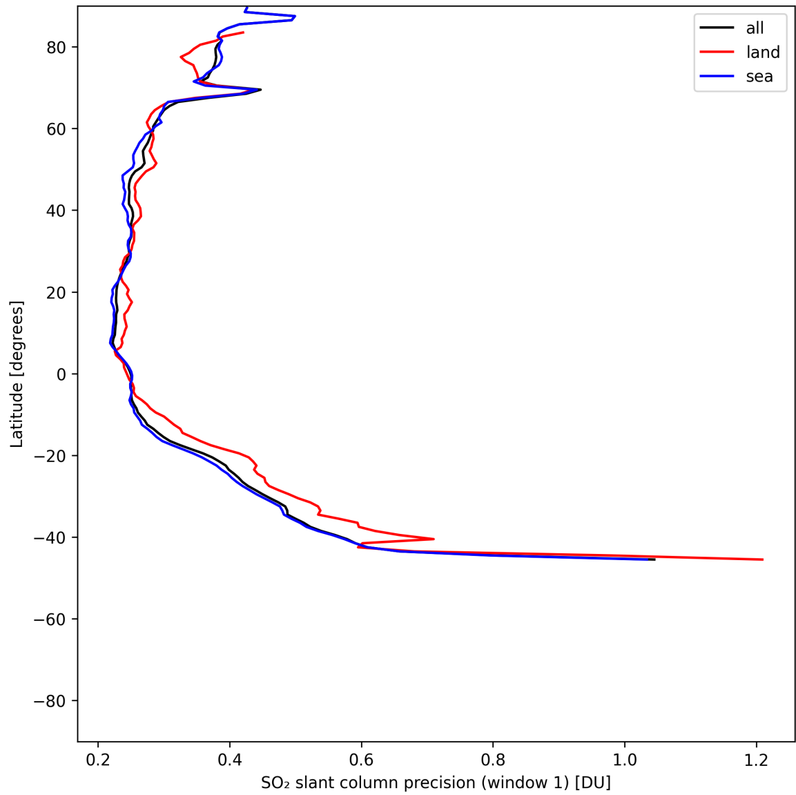
Figure 38: Zonal average of “SO 2 slant column precision (window 1)” for 2025-06-22 to 2025-06-23.
