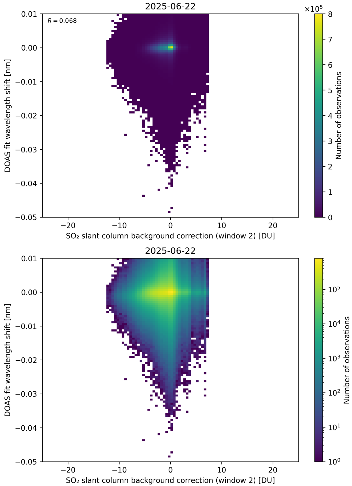
Figure 123: Scatter density plot of “SO 2 slant column background correction (window 2)” against “DOAS fit wavelength shift” for 2025-06-22 to 2025-06-23.
