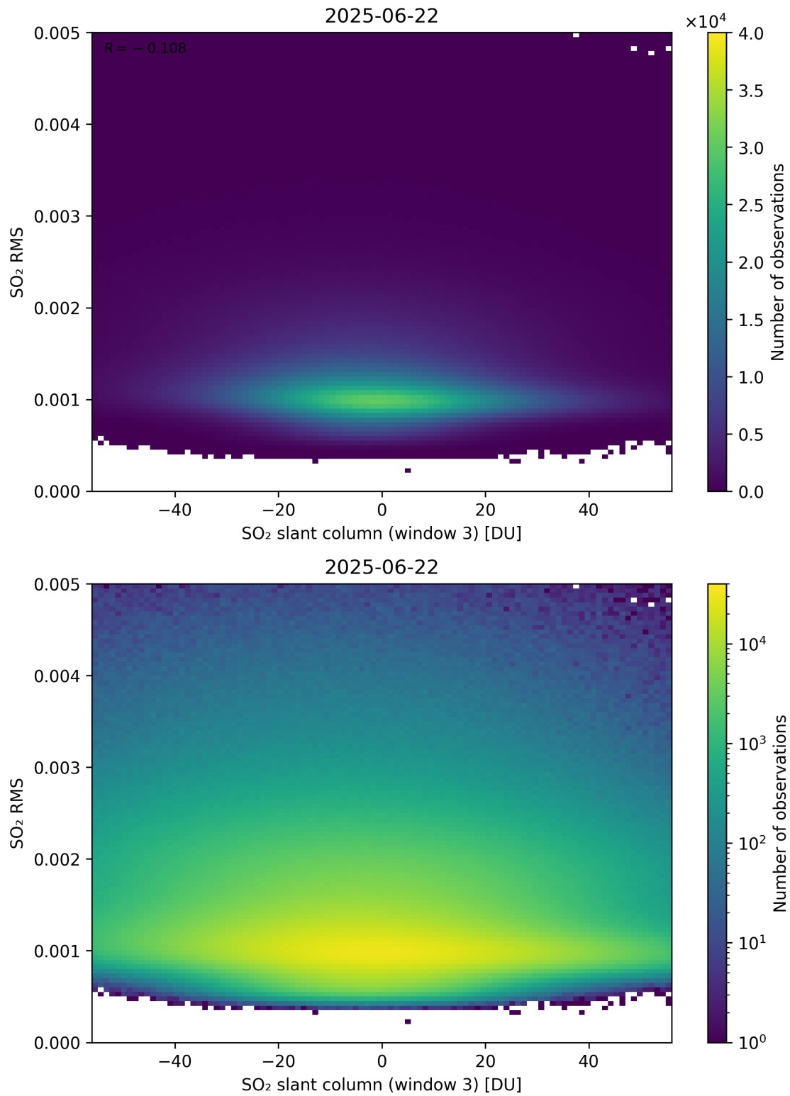
Figure 306: Scatter density plot of “SO 2 slant column (window 3)” against “SO 2 RMS” for 2025-06-22 to 2025-06-23.
