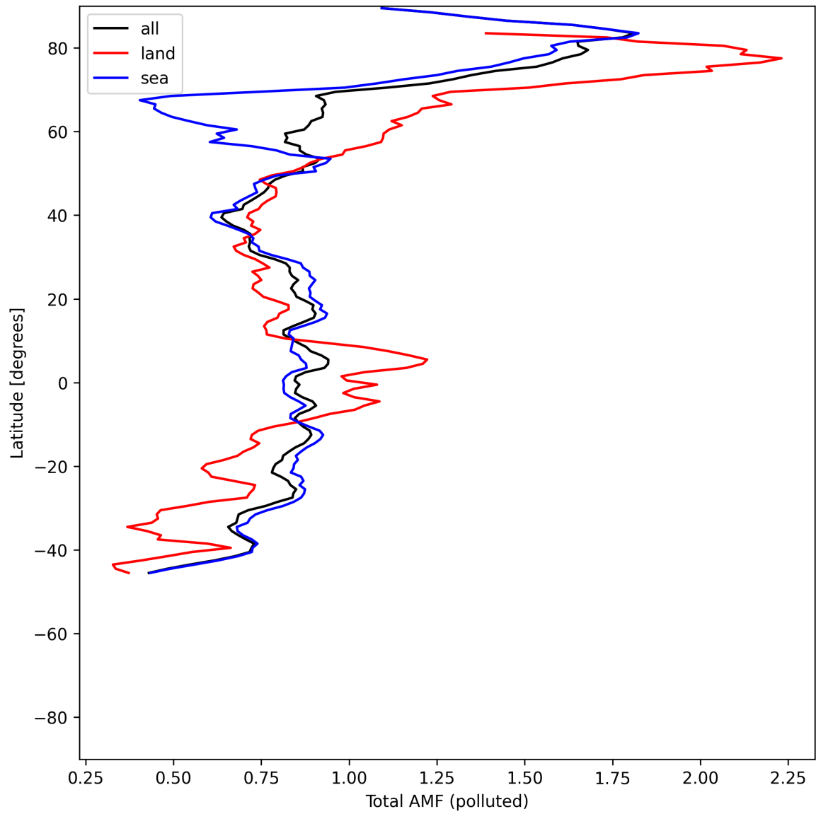
Figure 53: Zonal average of “Total AMF (polluted)” for 2025-06-22 to 2025-06-23.
