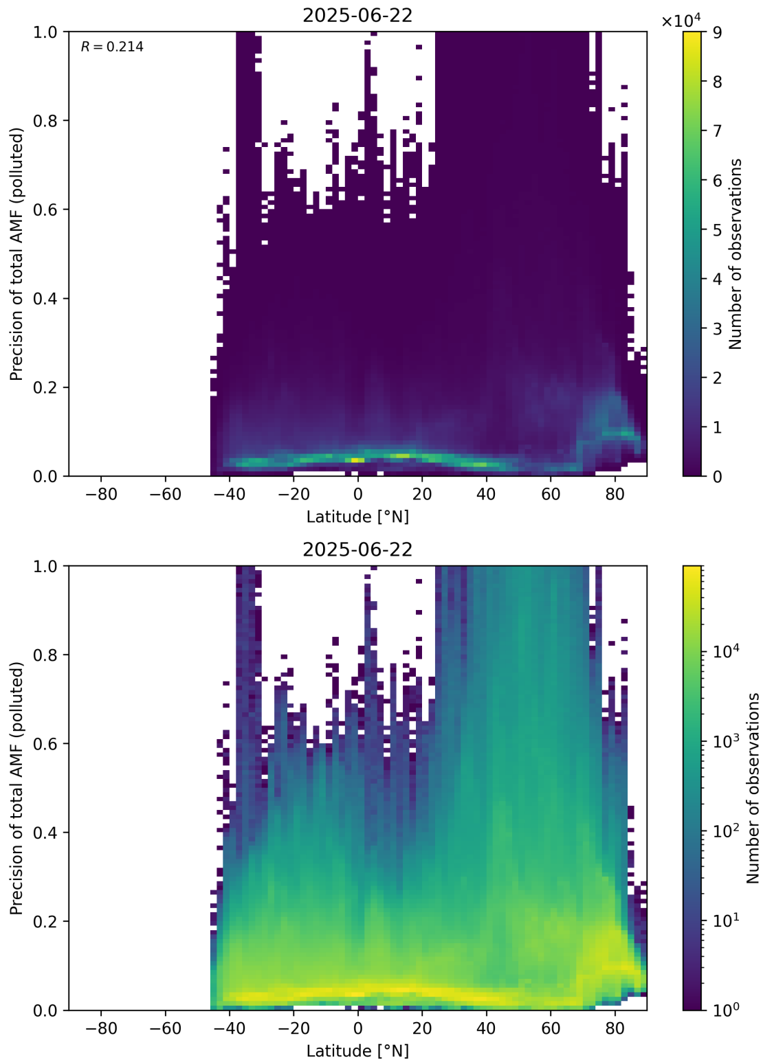
Figure 168: Scatter density plot of “Latitude” against “Precision of total AMF (polluted)” for 2025-06-22 to 2025-06-23.
