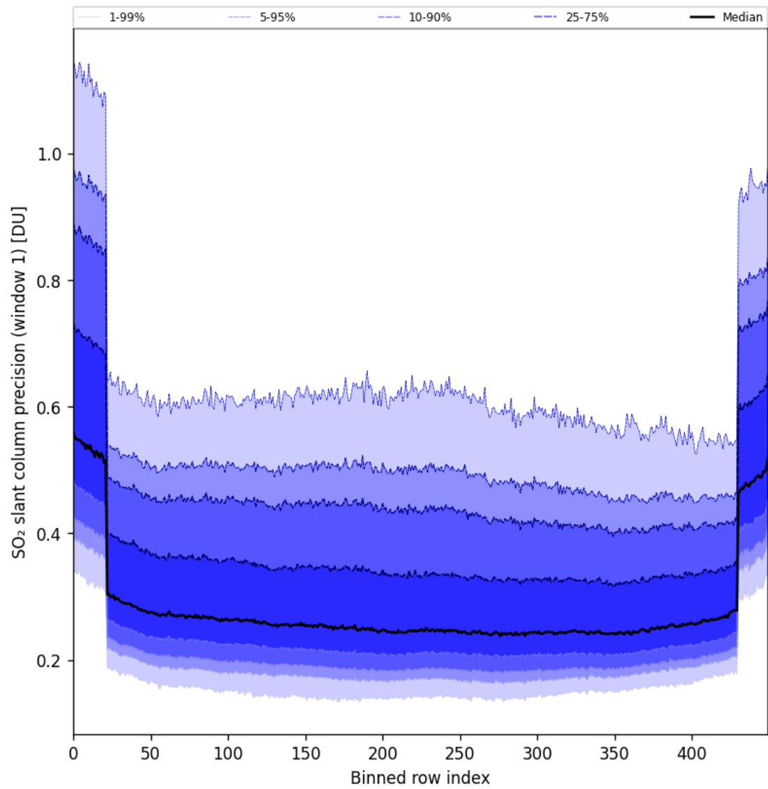
Figure 90: Along track statistics of “SO 2 slant column precision (window 1)” for 2025-06-22 to 2025-06-23
