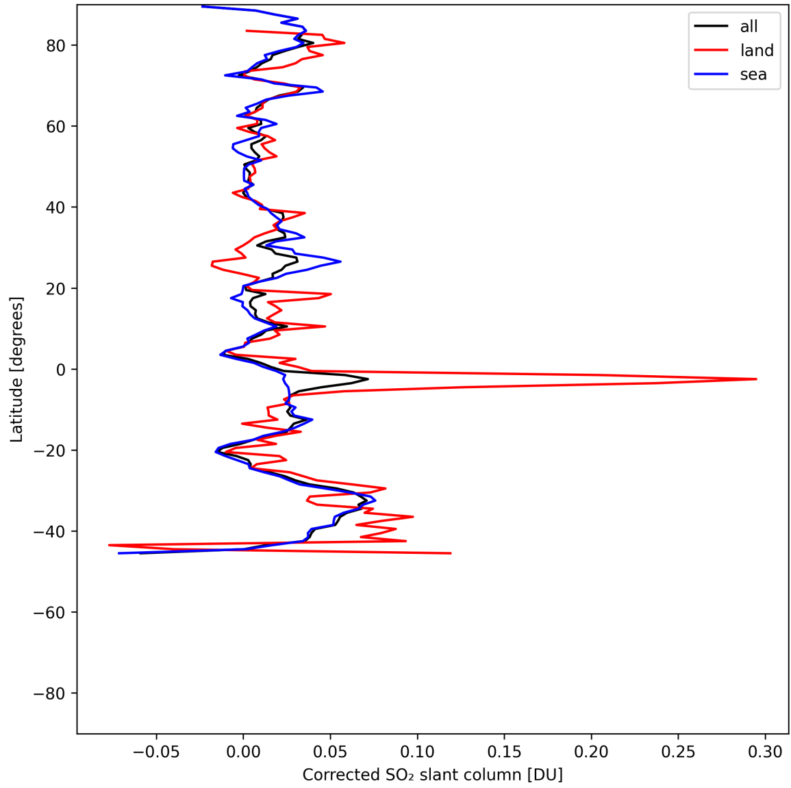
Figure 34: Zonal average of “Corrected SO 2 slant column” for 2025-06-22 to 2025-06-23.
