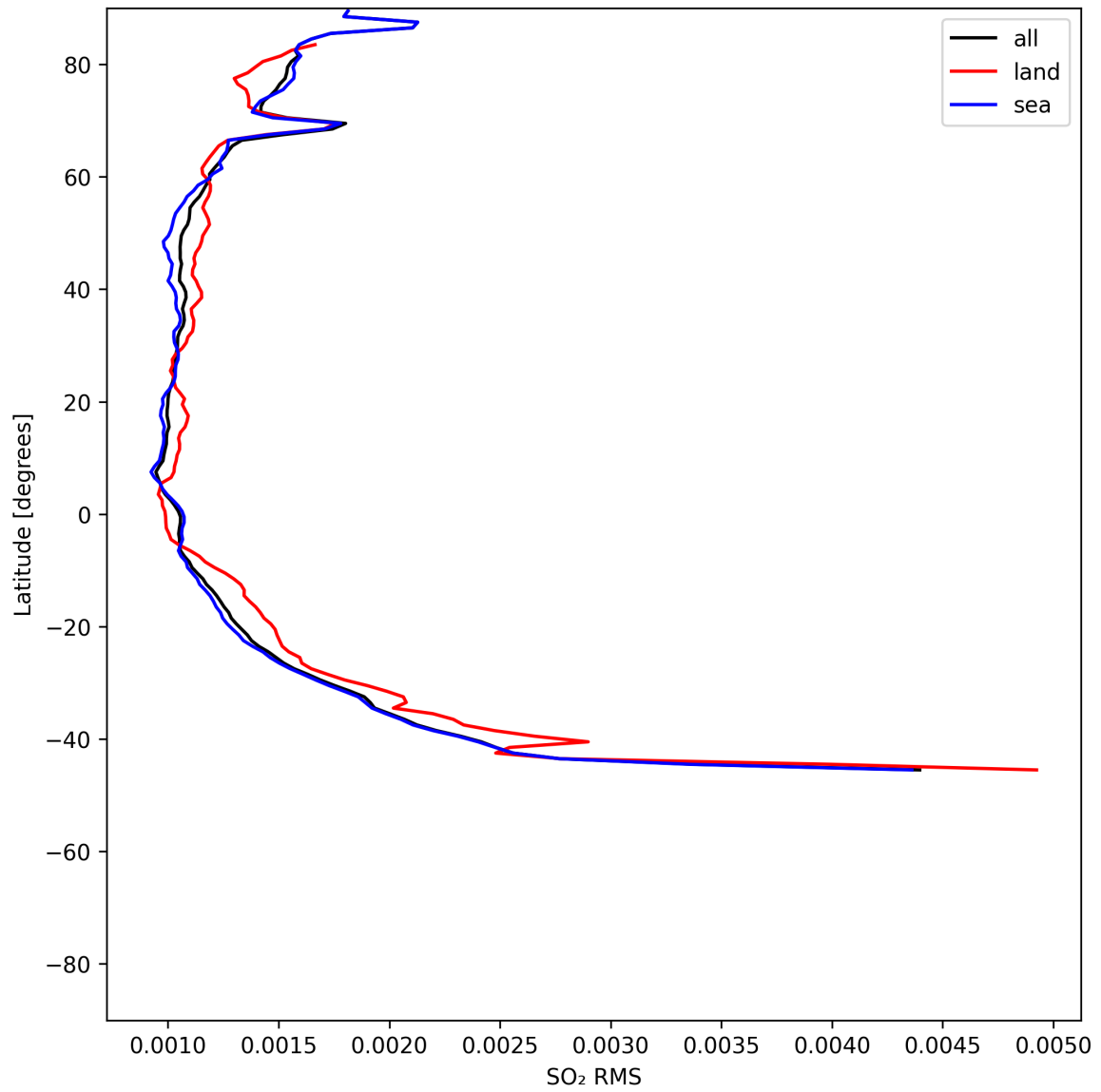
Figure 52: Zonal average of “SO 2 RMS” for 2025-06-22 to 2025-06-23.
