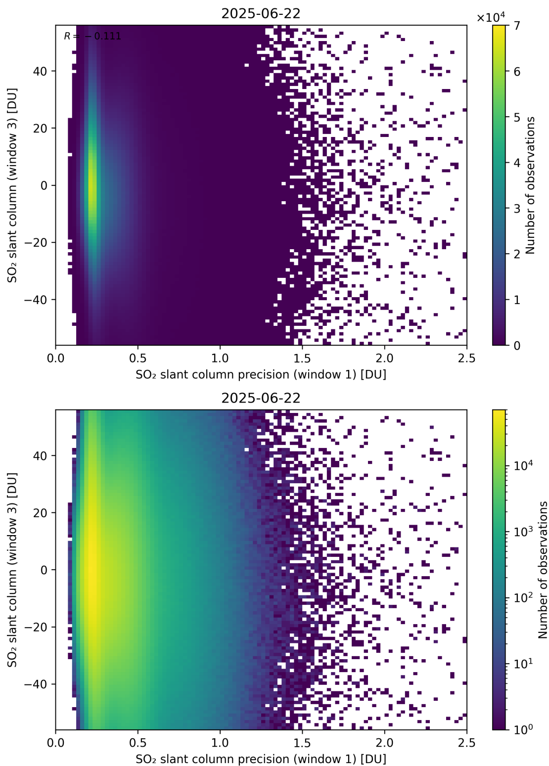
Figure 278: Scatter density plot of “SO 2 slant column precision (window 1)” against “SO 2 slant column (window 3)” for 2025-06-22 to 2025-06-23.
