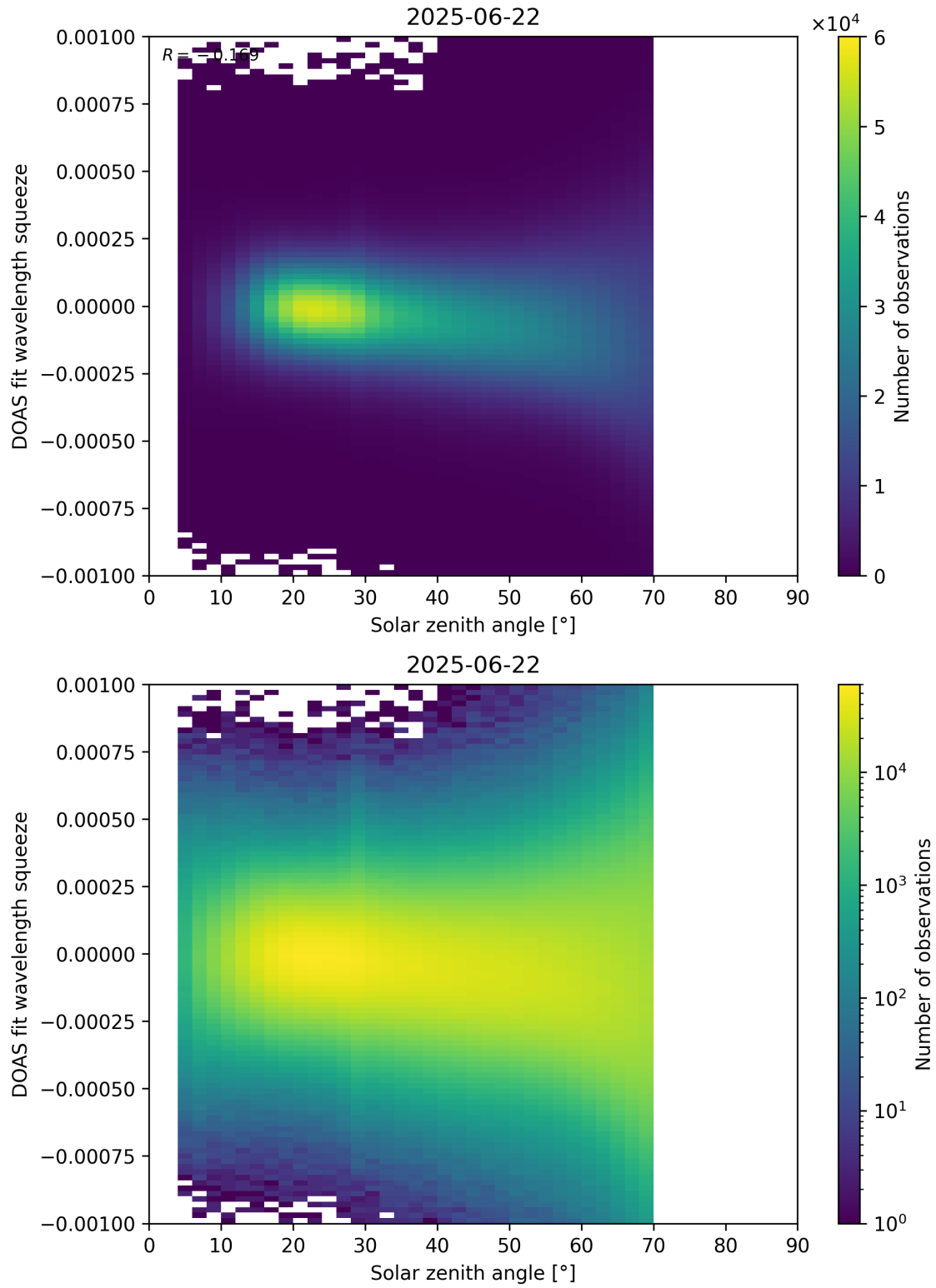
Figure 175: Scatter density plot of “Solar zenith angle” against “DOAS fit wavelength squeeze” for 2025-06-22 to 2025-06-23.
