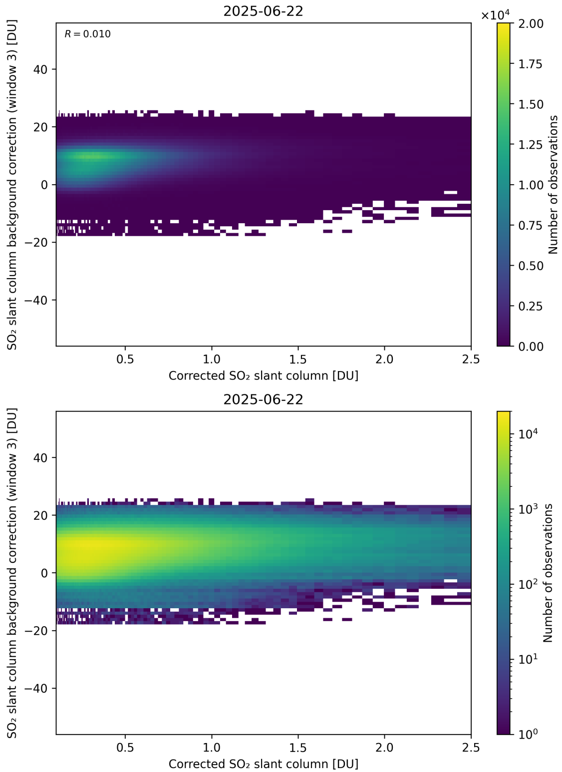
Figure 228: Scatter density plot of “Corrected SO 2 slant column” against “SO 2 slant column background correction (window 3)” for 2025-06-22 to 2025-06-23.
