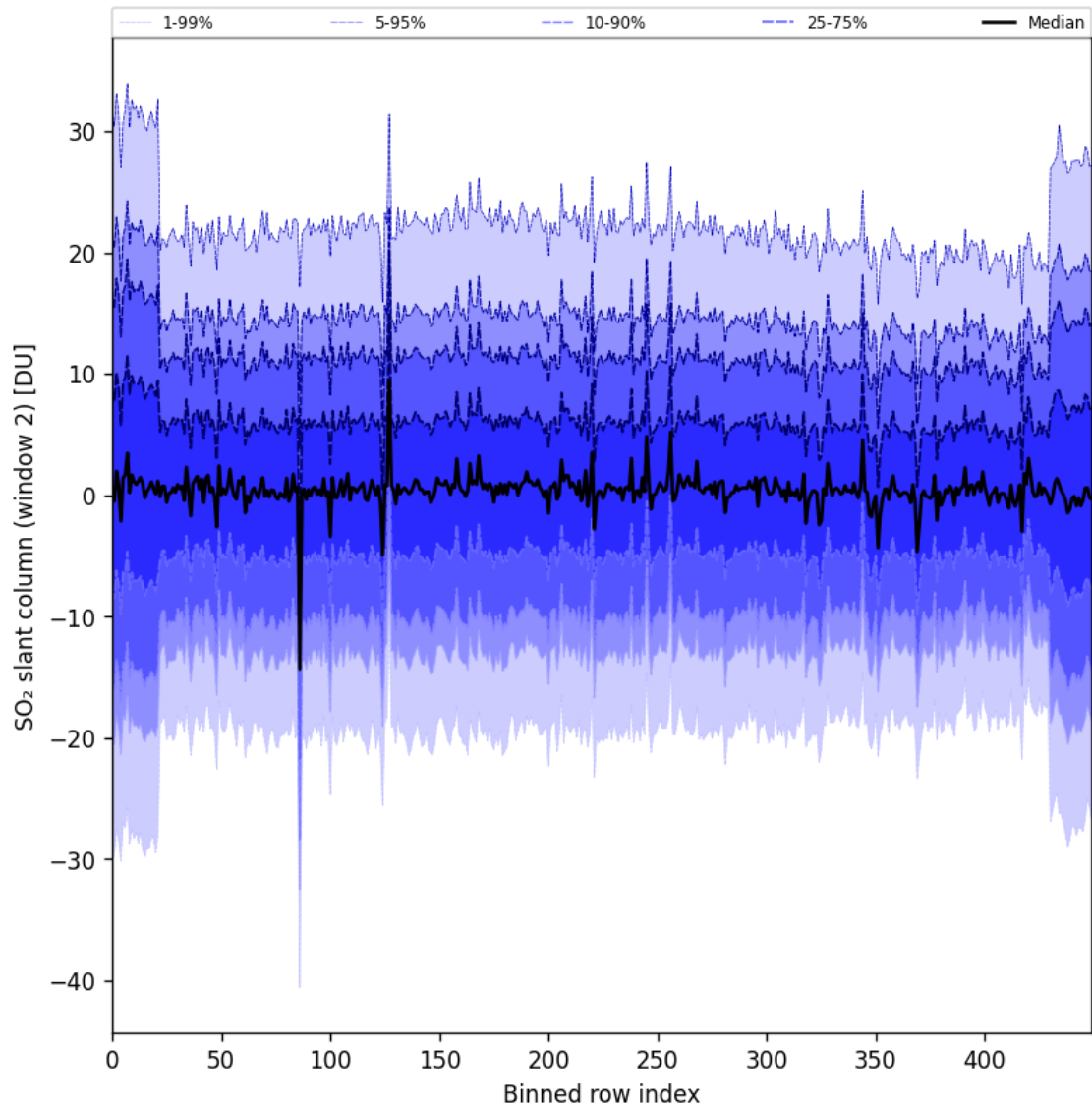
Figure 93: Along track statistics of “SO 2 slant column (window 2)” for 2025-06-22 to 2025-06-23
