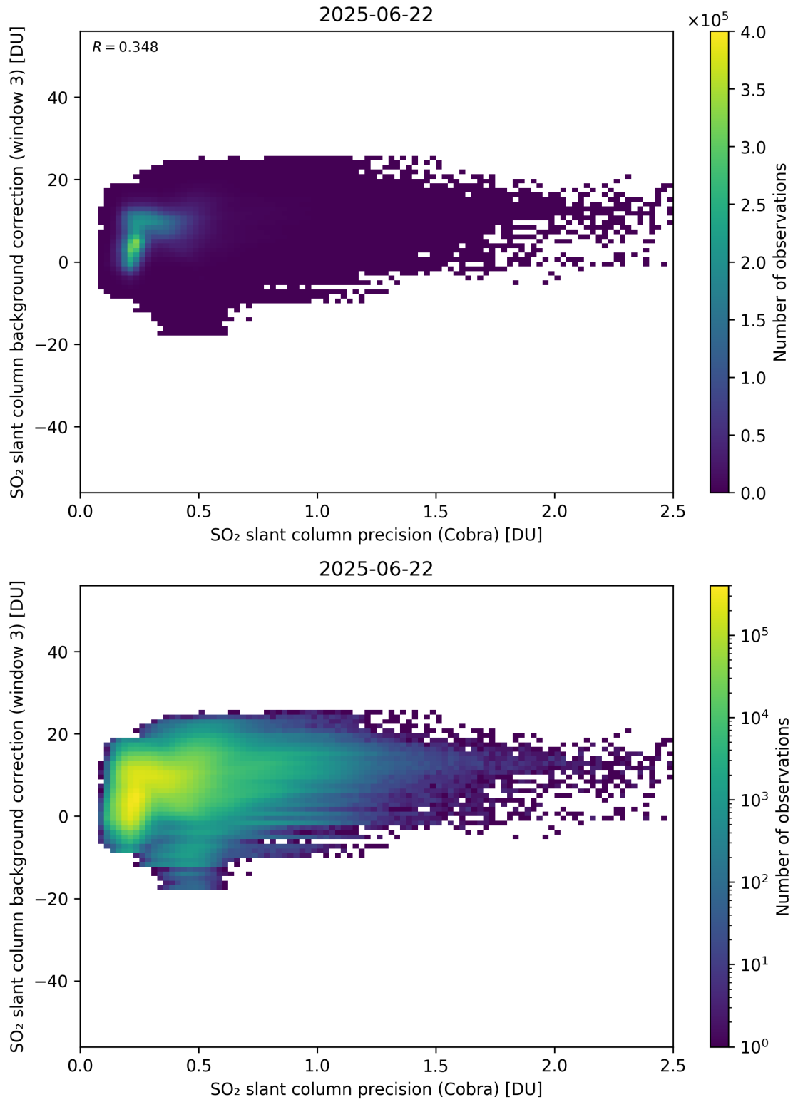
Figure 201: Scatter density plot of “SO 2 slant column precision (Cobra)” against “SO 2 slant column background correction (window 3)” for 2025-06-22 to 2025-06-23.
