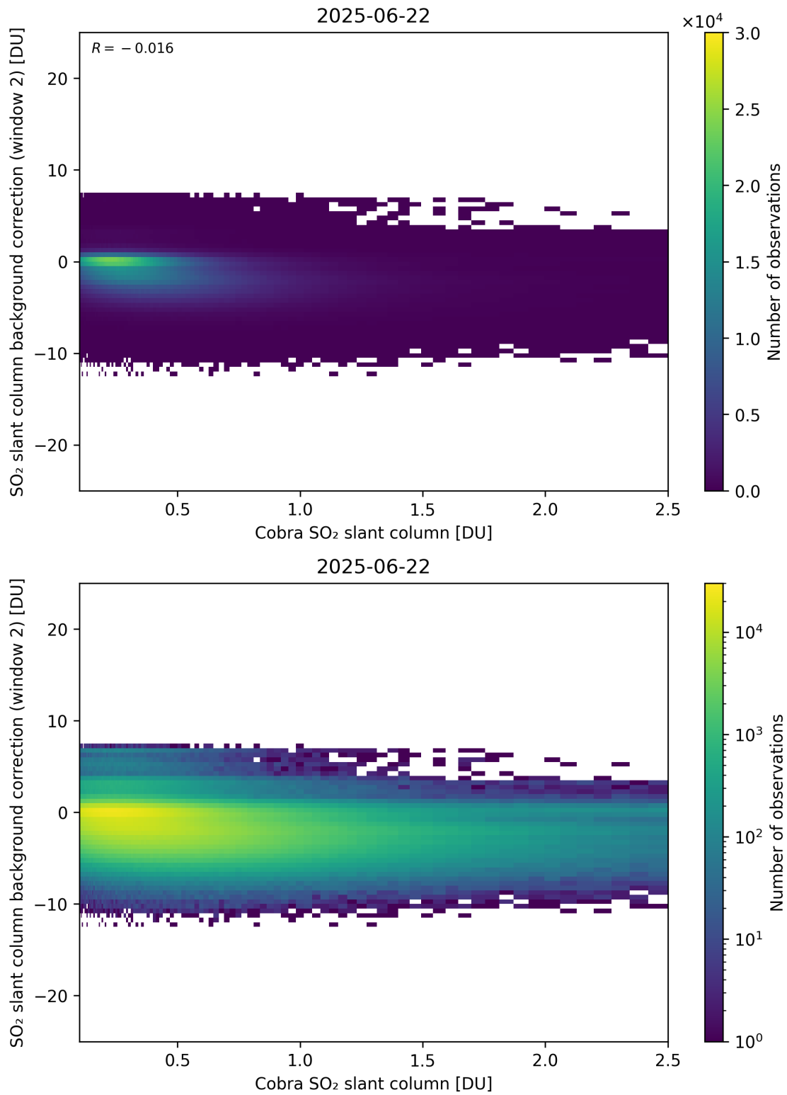
Figure 194: Scatter density plot of “Cobra SO 2 slant column” against “SO 2 slant column background correction (window 2)” for 2025-06-22 to 2025-06-23.
