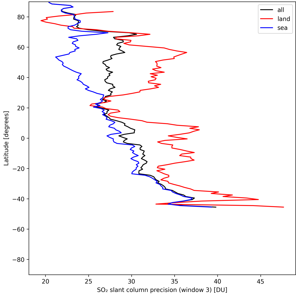
Figure 46: Zonal average of “SO 2 slant column precision (window 3)” for 2025-06-22 to 2025-06-23.
