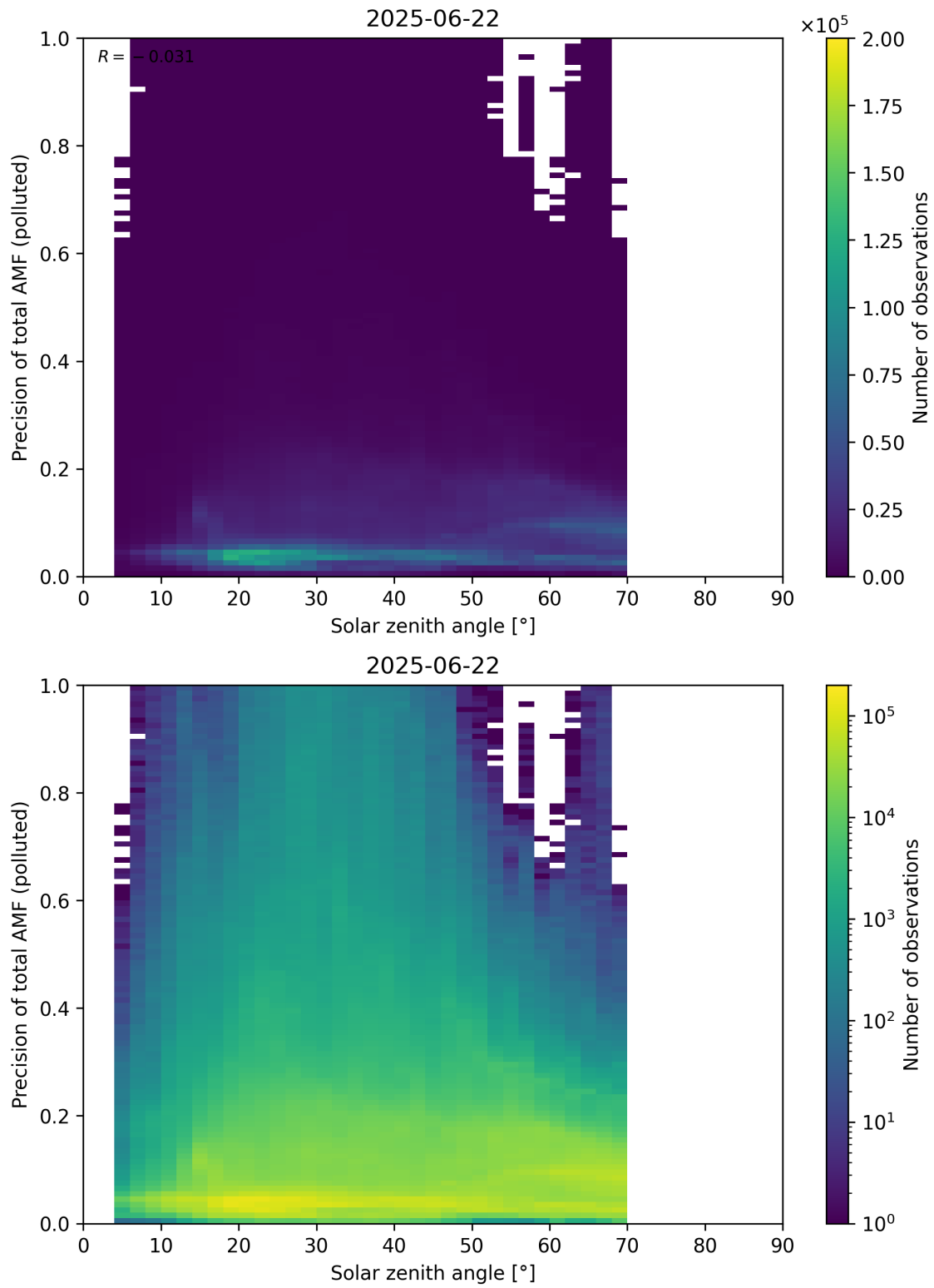
Figure 190: Scatter density plot of “Solar zenith angle” against “Precision of total AMF (polluted)” for 2025-06-22 to 2025-06-23.
