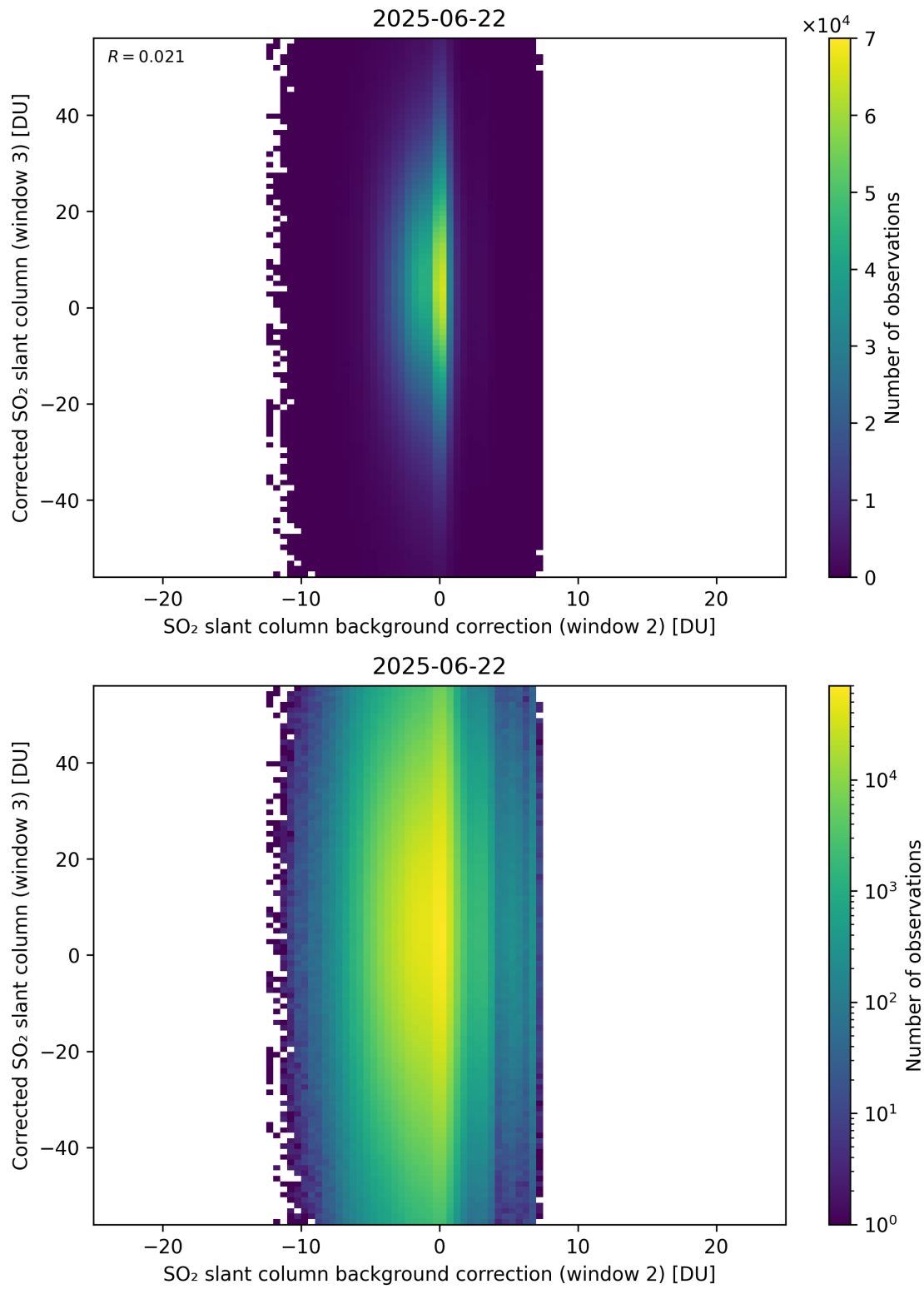
Figure 127: Scatter density plot of “SO 2 slant column background correction (window 2)” against “Corrected SO 2 slant column (window 3)” for 2025-06-22 to 2025-06-23.
