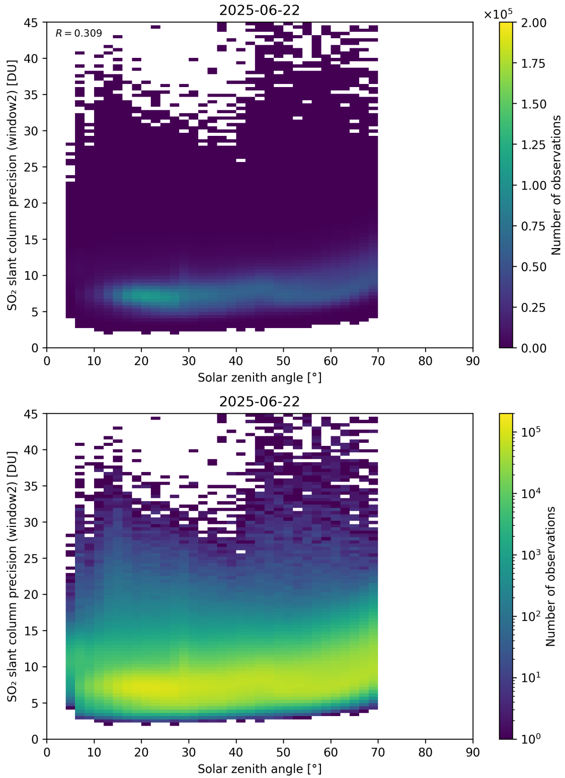
Figure 186: Scatter density plot of “Solar zenith angle” against “SO 2 slant column precision (window2)” for 2025-06-22 to 2025-06-23.
