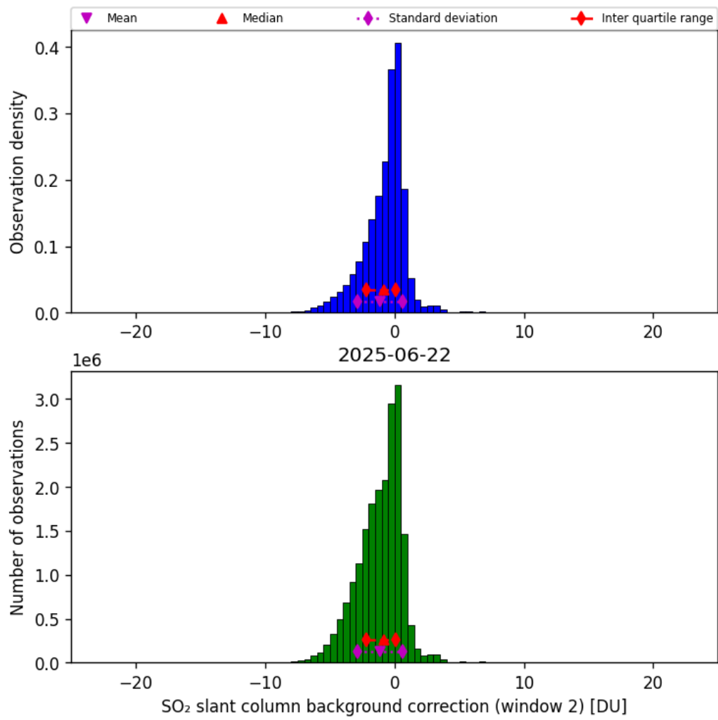
Figure 70: Histogram of “SO 2 slant column background correction (window 2)” for 2025-06-22 to 2025-06-23
