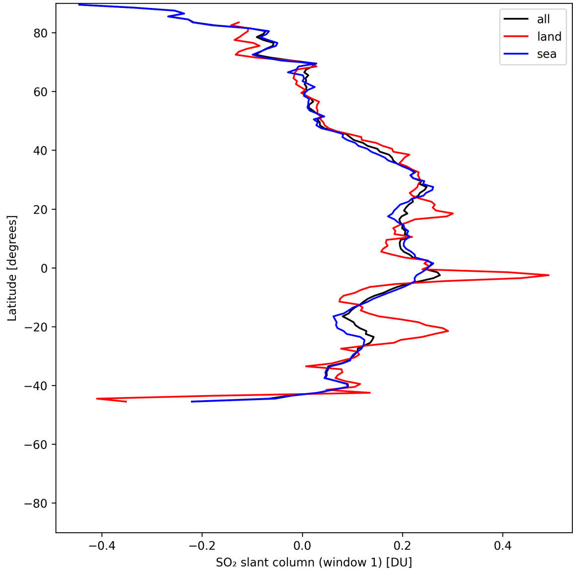
Figure 37: Zonal average of “SO 2 slant column (window 1)” for 2025-06-22 to 2025-06-23.
