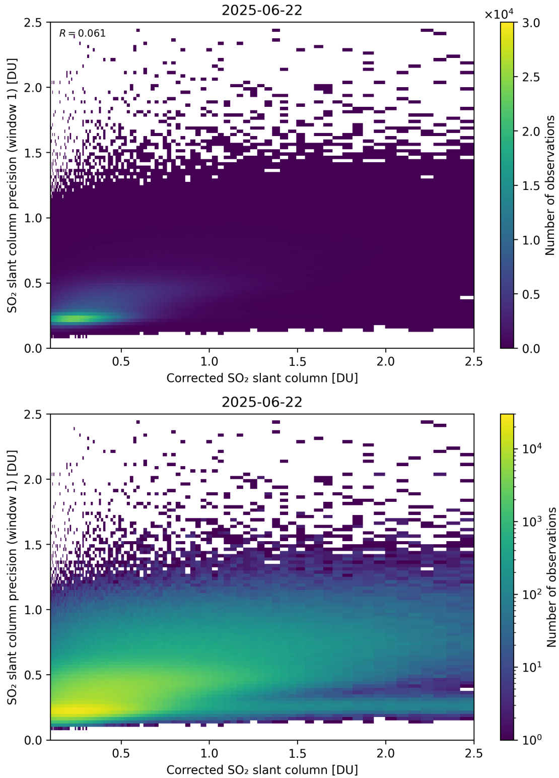
Figure 238: Scatter density plot of “Corrected SO 2 slant column” against “SO 2 slant column precision (window 1)” for 2025-06-22 to 2025-06-23.
