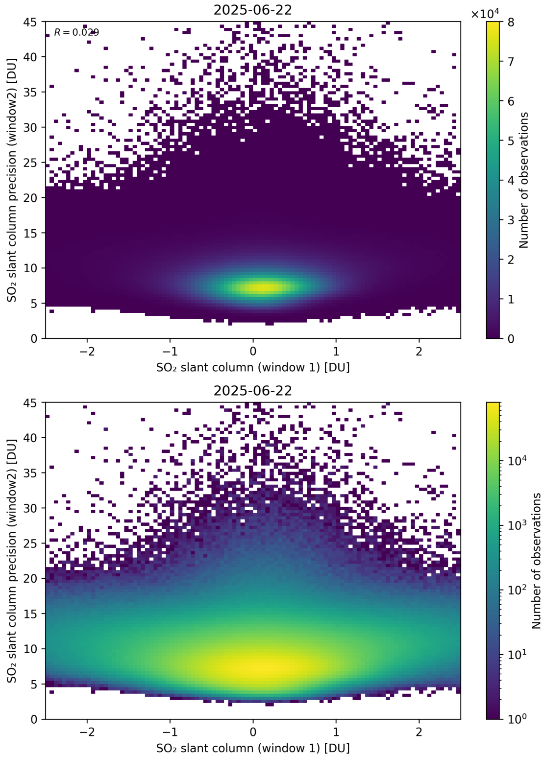
Figure 286: Scatter density plot of “SO 2 slant column (window 1)” against “SO 2 slant column precision (window2)” for 2025-06-22 to 2025-06-23.
