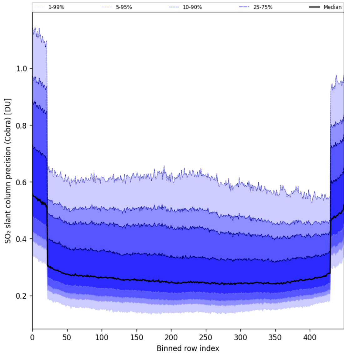
Figure 88: Along track statistics of “SO 2 slant column precision (Cobra)” for 2025-06-22 to 2025-06-23
