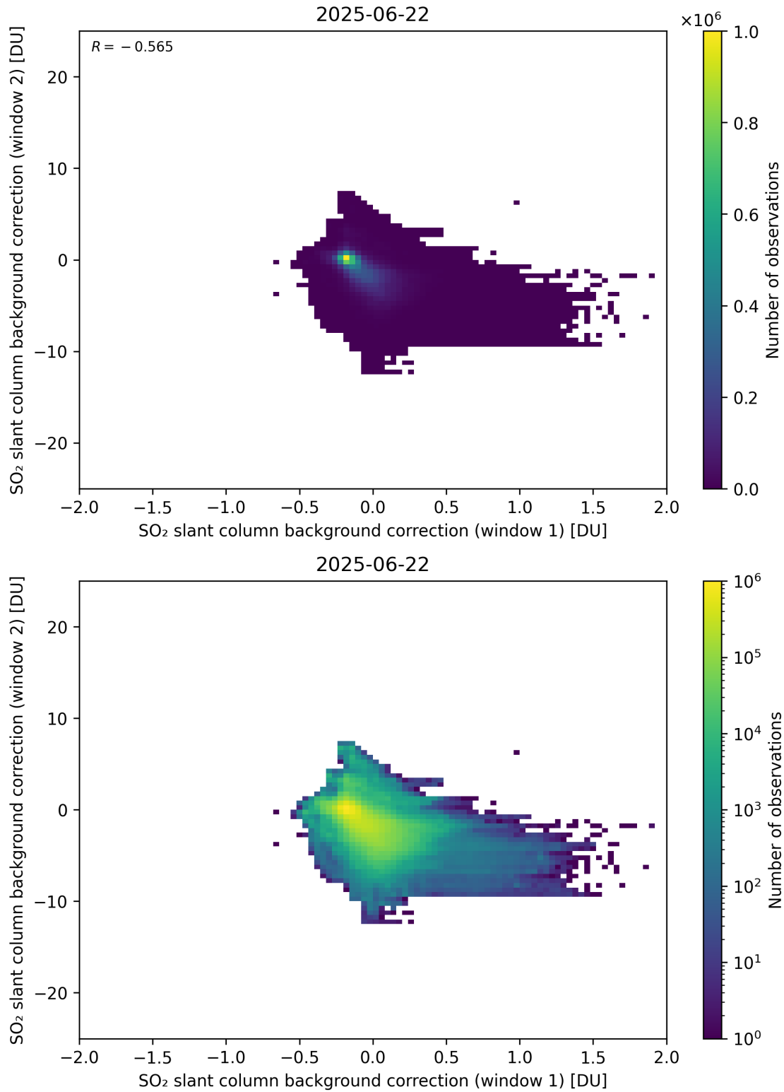
Figure 109: Scatter density plot of “SO 2 slant column background correction (window 1)” against “SO 2 slant column background correction (window 2)” for 2025-06-22 to 2025-06-23.
