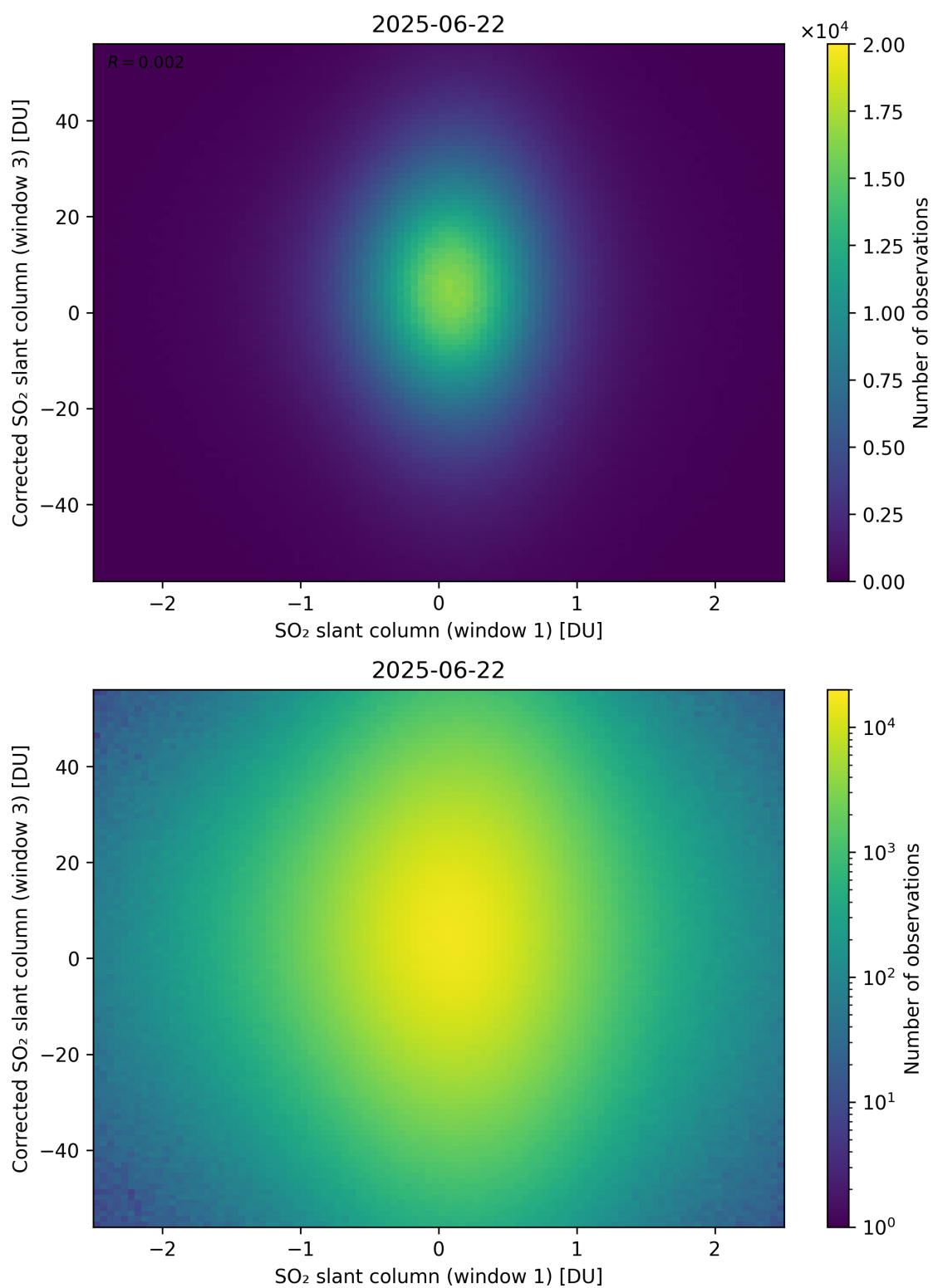
Figure 284: Scatter density plot of “SO 2 slant column (window 1)” against “Corrected SO 2 slant column (window 3)” for 2025-06-22 to 2025-06-23.
