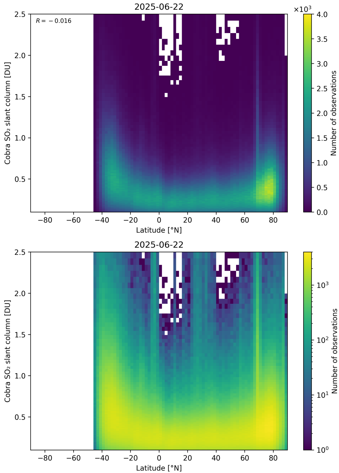
Figure 157: Scatter density plot of “Latitude” against “Cobra SO 2 slant column” for 2025-06-22 to 2025-06-23.
