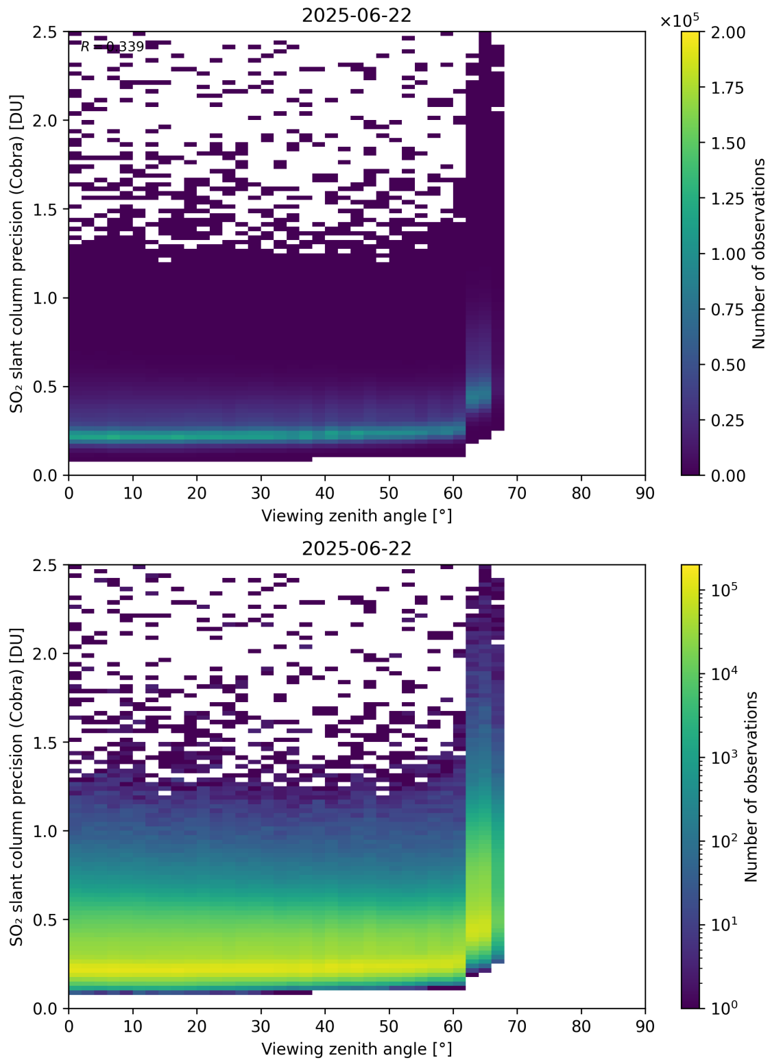
Figure 372: Scatter density plot of “Viewing zenith angle” against “SO 2 slant column precision (Cobra)” for 2025-06-22 to 2025-06-23.
