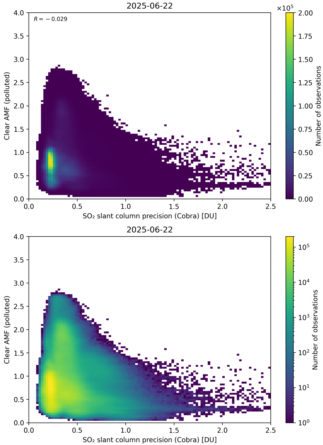
Figure 205: Scatter density plot of “SO 2 slant column precision (Cobra)” against “Clear AMF (polluted)” for 2025-06-22 to 2025-06-23.
