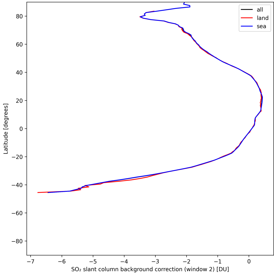
Figure 44: Zonal average of “SO 2 slant column background correction (window 2)” for 2025-06-22 to 2025-06-23.
