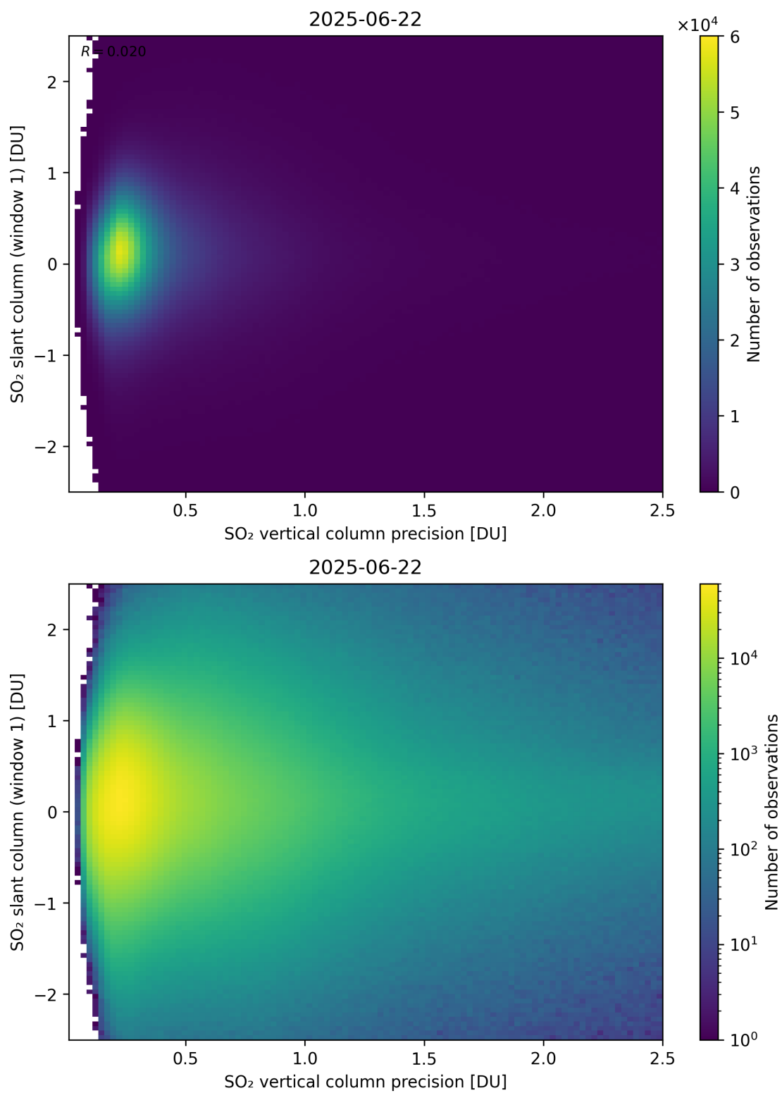
Figure 341: Scatter density plot of “SO 2 vertical column precision” against “SO 2 slant column (window 1)” for 2025-06-22 to 2025-06-23.
