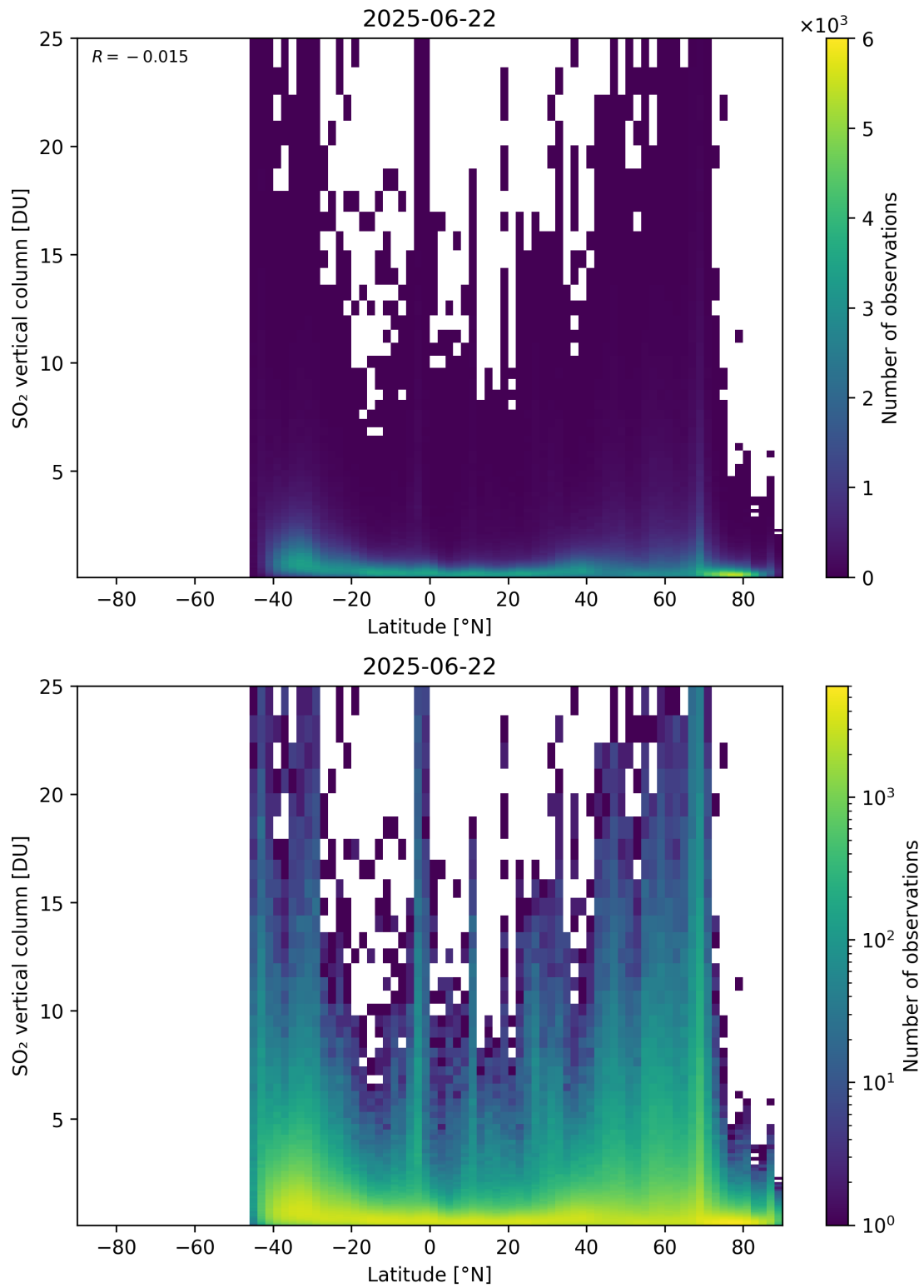
Figure 169: Scatter density plot of “Latitude” against “SO 2 vertical column” for 2025-06-22 to 2025-06-23.
