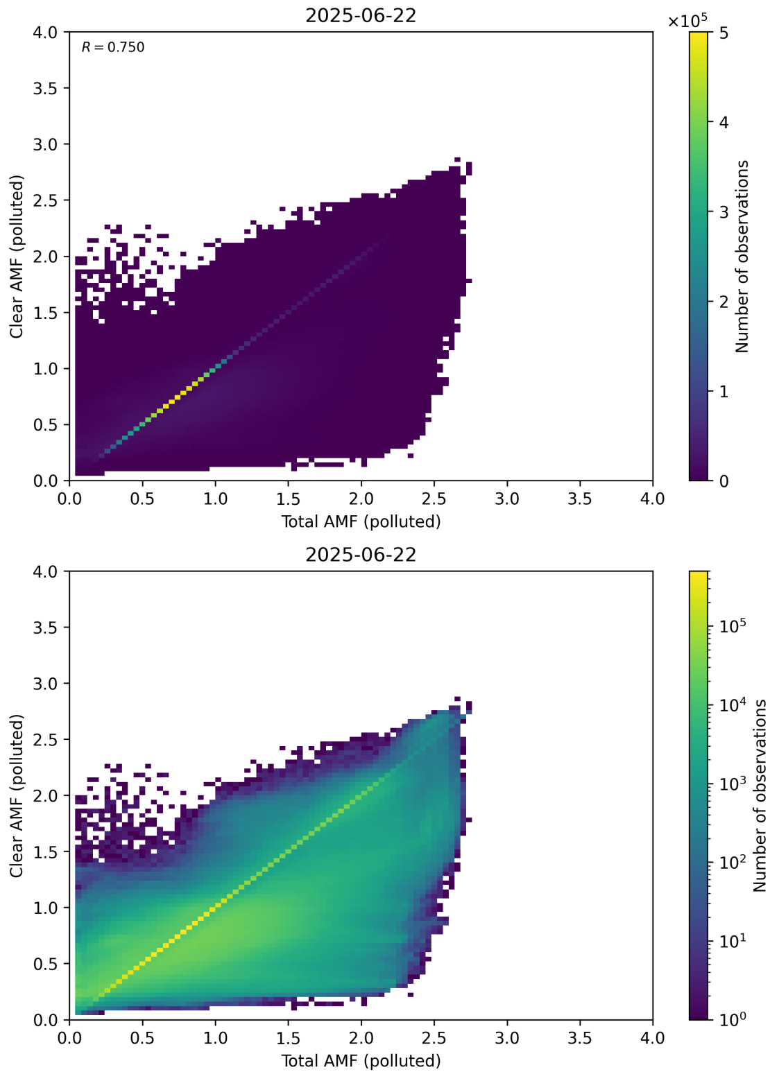
Figure 321: Scatter density plot of “Total AMF (polluted)” against “Clear AMF (polluted)” for 2025-06-22 to 2025-06-23.
