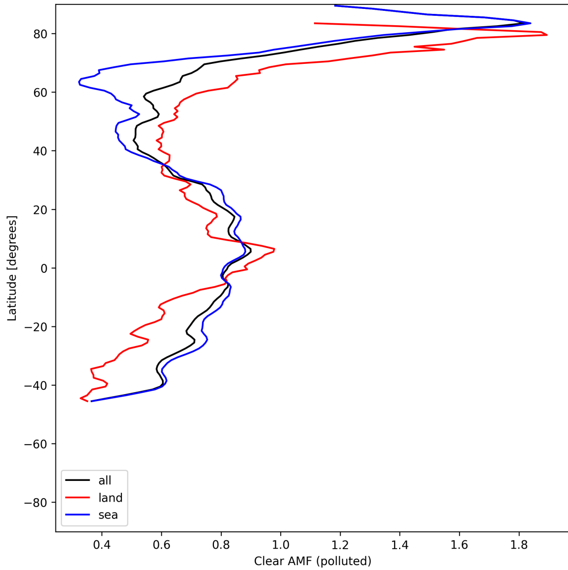
Figure 55: Zonal average of “Clear AMF (polluted)” for 2025-06-22 to 2025-06-23.
