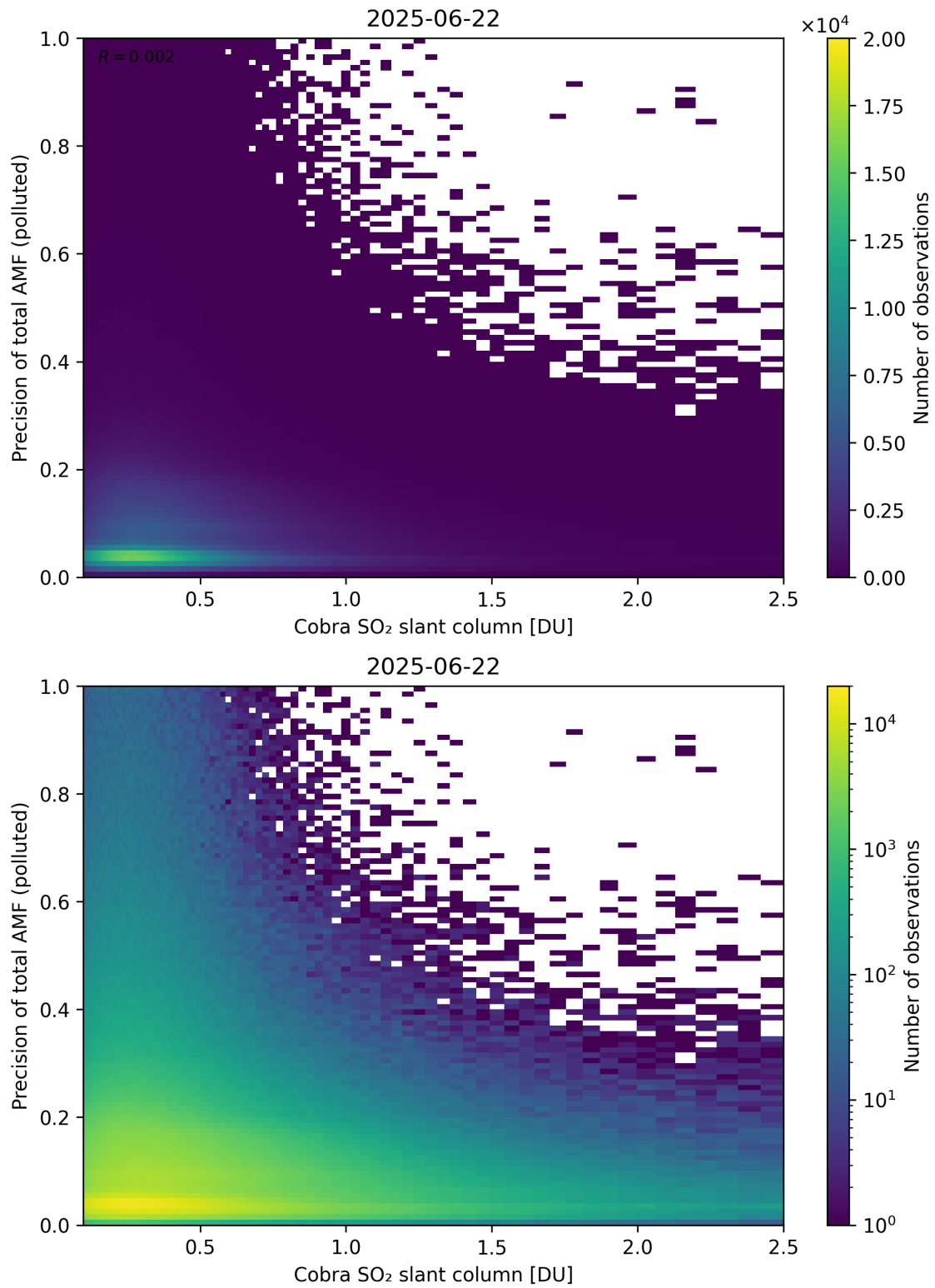
Figure 225: Scatter density plot of “Cobra SO 2 slant column” against “Precision of total AMF (polluted)” for 2025-06-22 to 2025-06-23.
