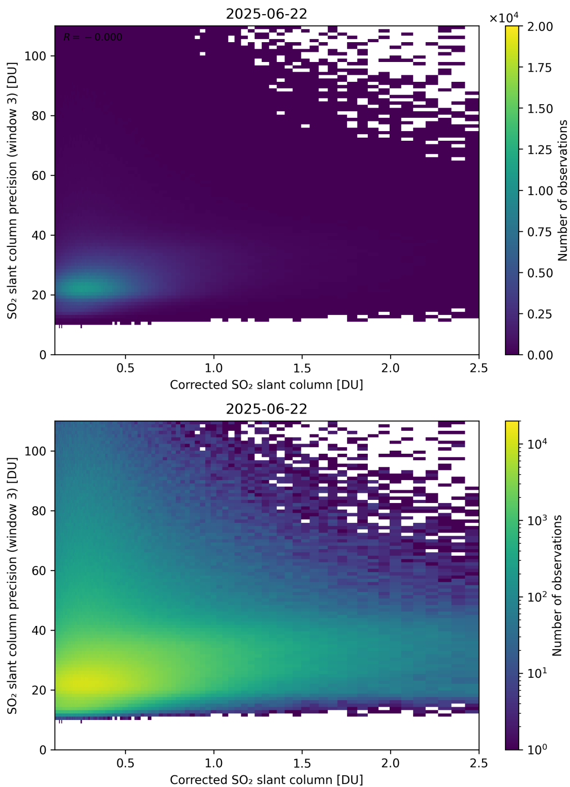
Figure 241: Scatter density plot of “Corrected SO 2 slant column” against “SO 2 slant column precision (window 3)” for 2025-06-22 to 2025-06-23.
