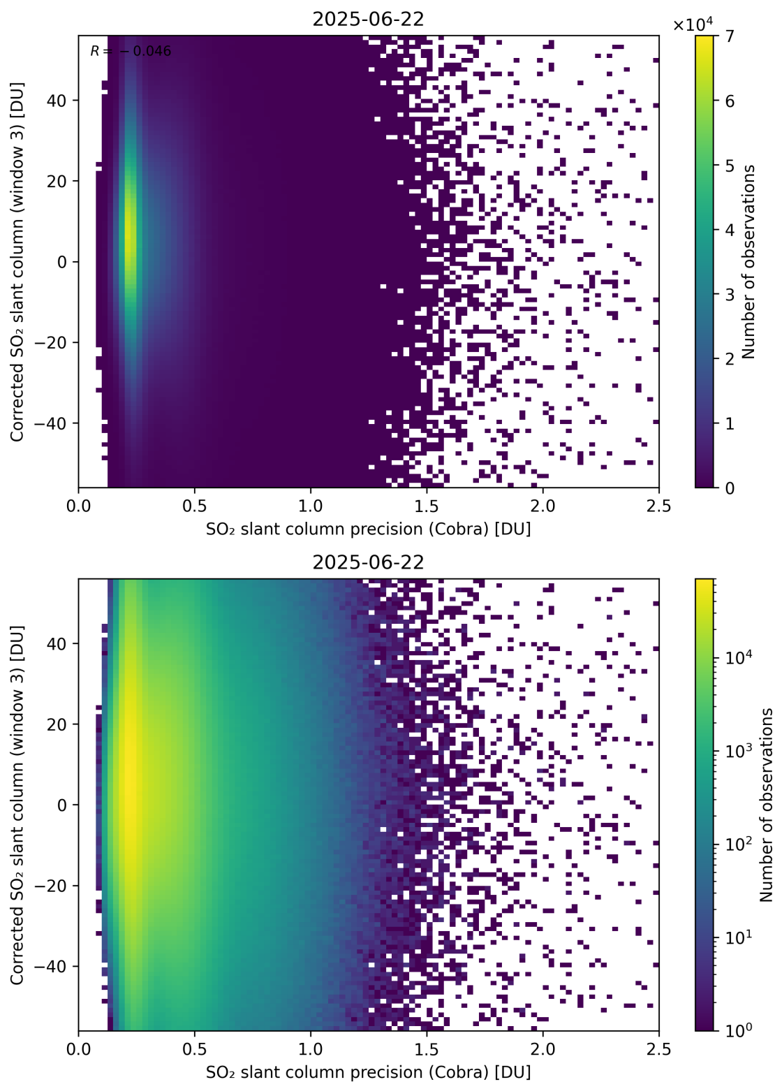
Figure 207: Scatter density plot of “SO 2 slant column precision (Cobra)” against “Corrected SO 2 slant column (window 3)” for 2025-06-22 to 2025-06-23.
