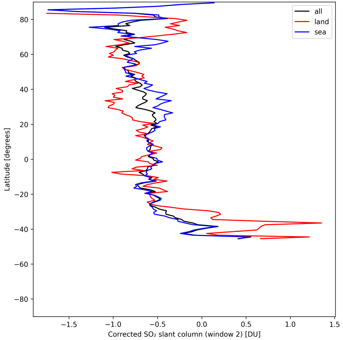
Figure 43: Zonal average of “Corrected SO 2 slant column (window 2)” for 2025-06-22 to 2025-06-23.
