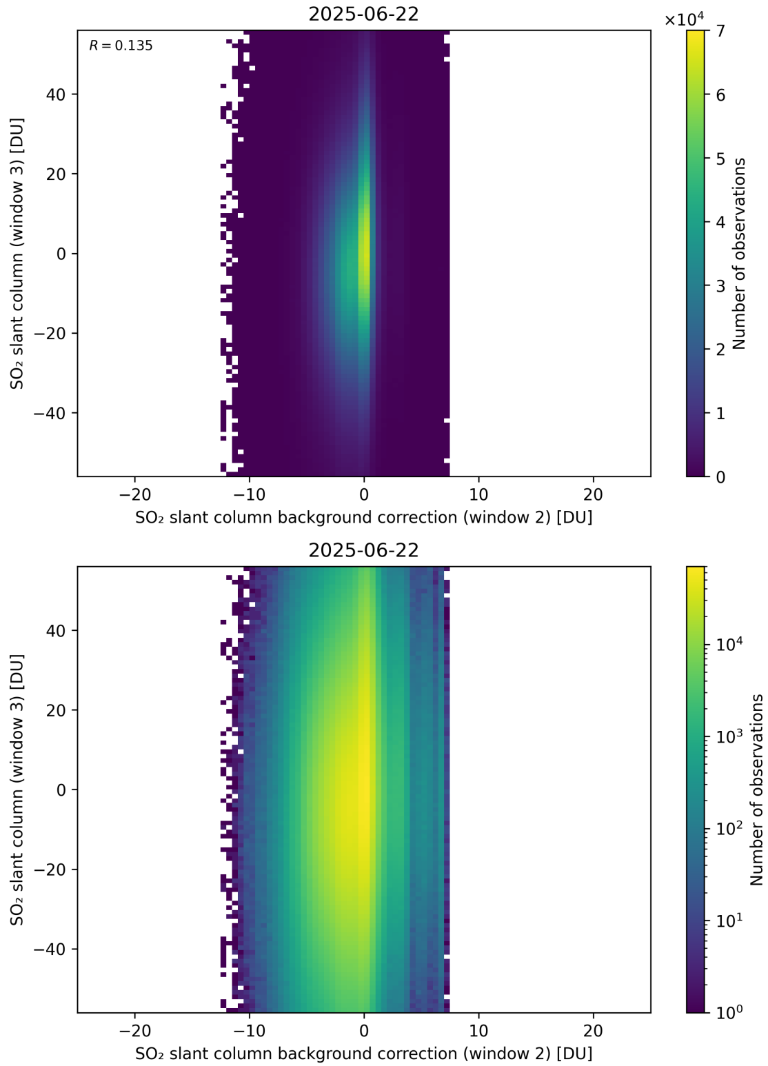
Figure 128: Scatter density plot of “SO 2 slant column background correction (window 2)” against “SO 2 slant column (window 3)” for 2025-06-22 to 2025-06-23.
