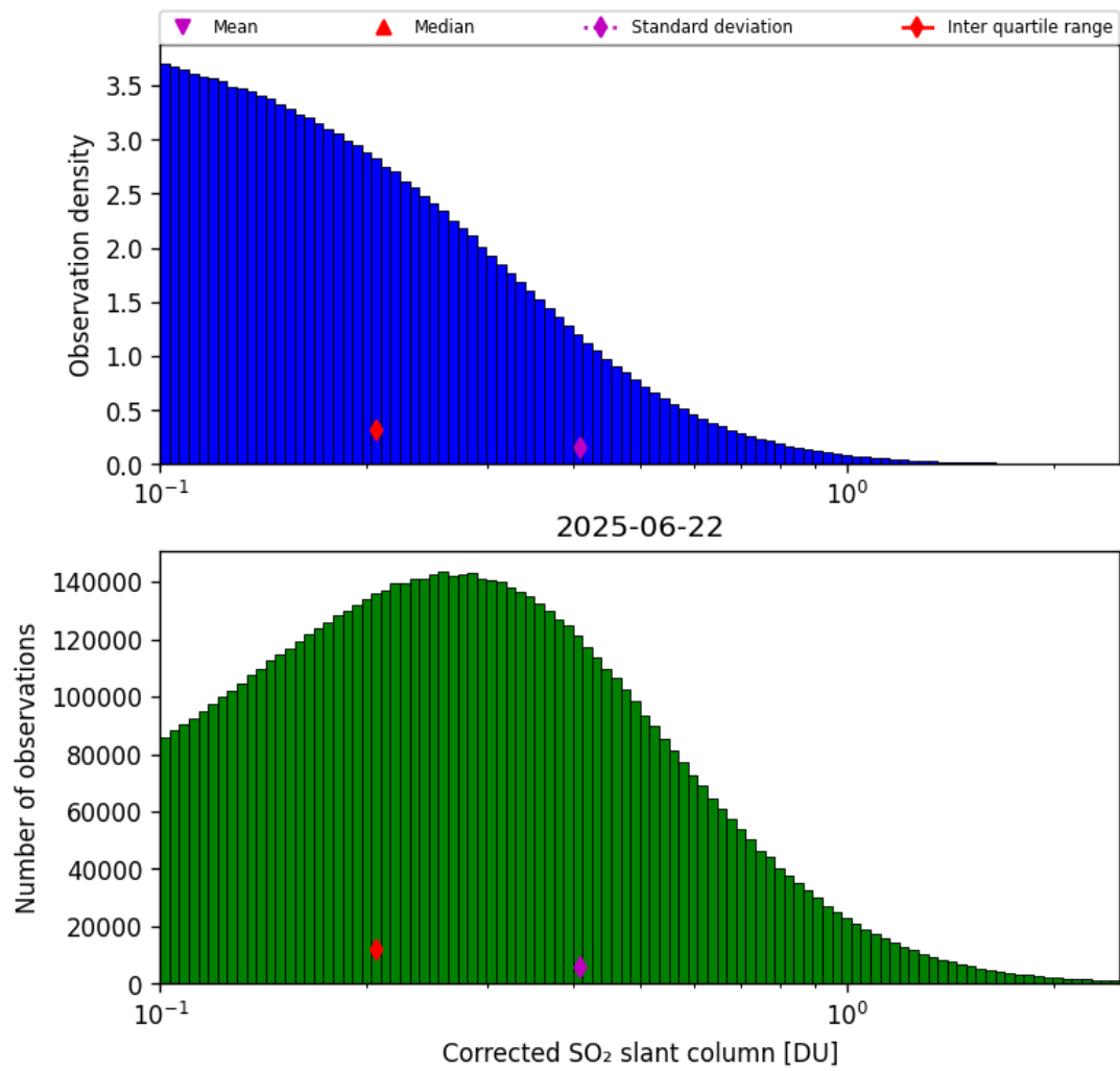
Figure 60: Histogram of "Corrected SO 2 slant column" for 2025-06-22 to 2025-06-23
