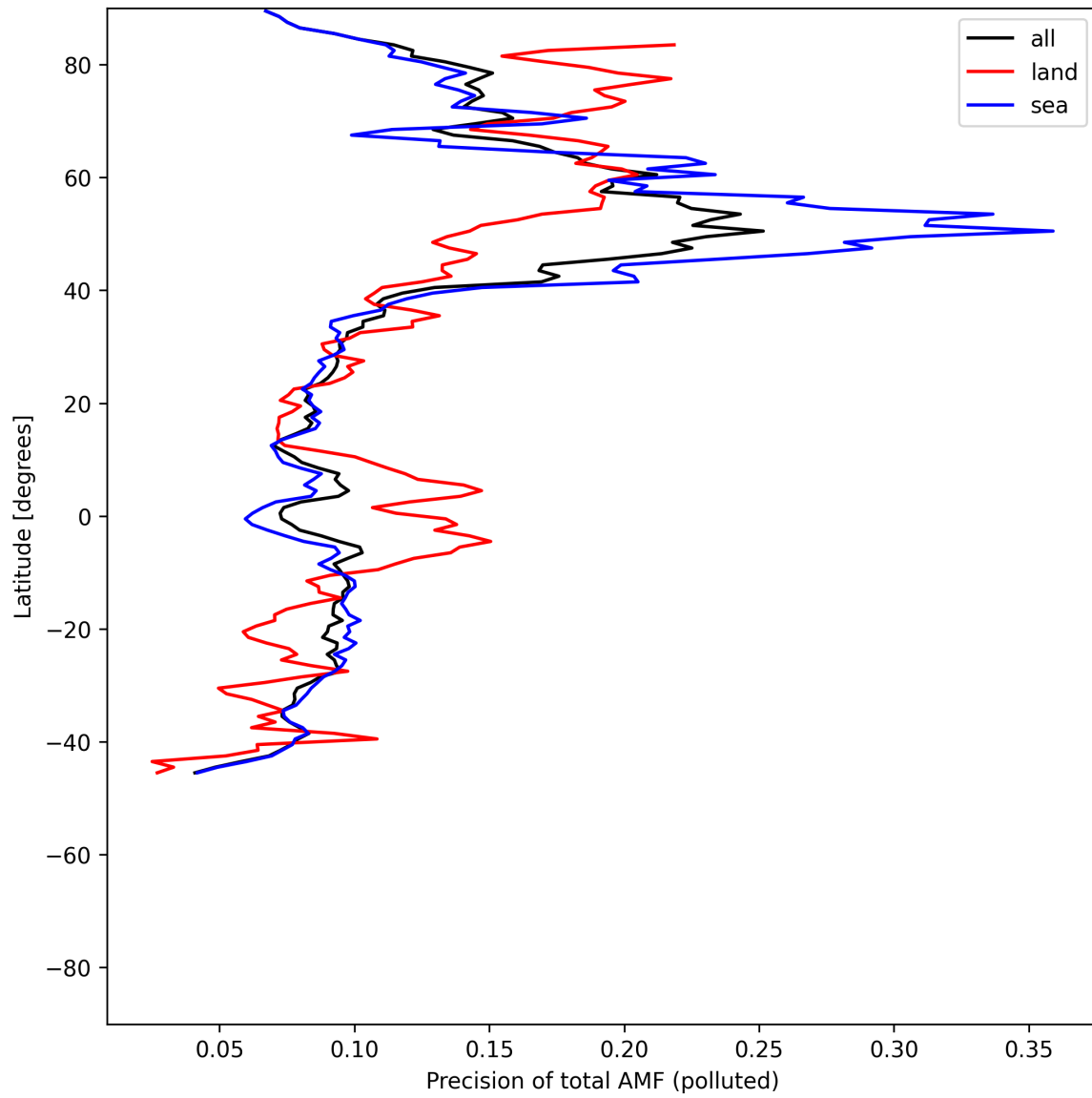
Figure 54: Zonal average of “Precision of total AMF (polluted)” for 2025-06-22 to 2025-06-23.
