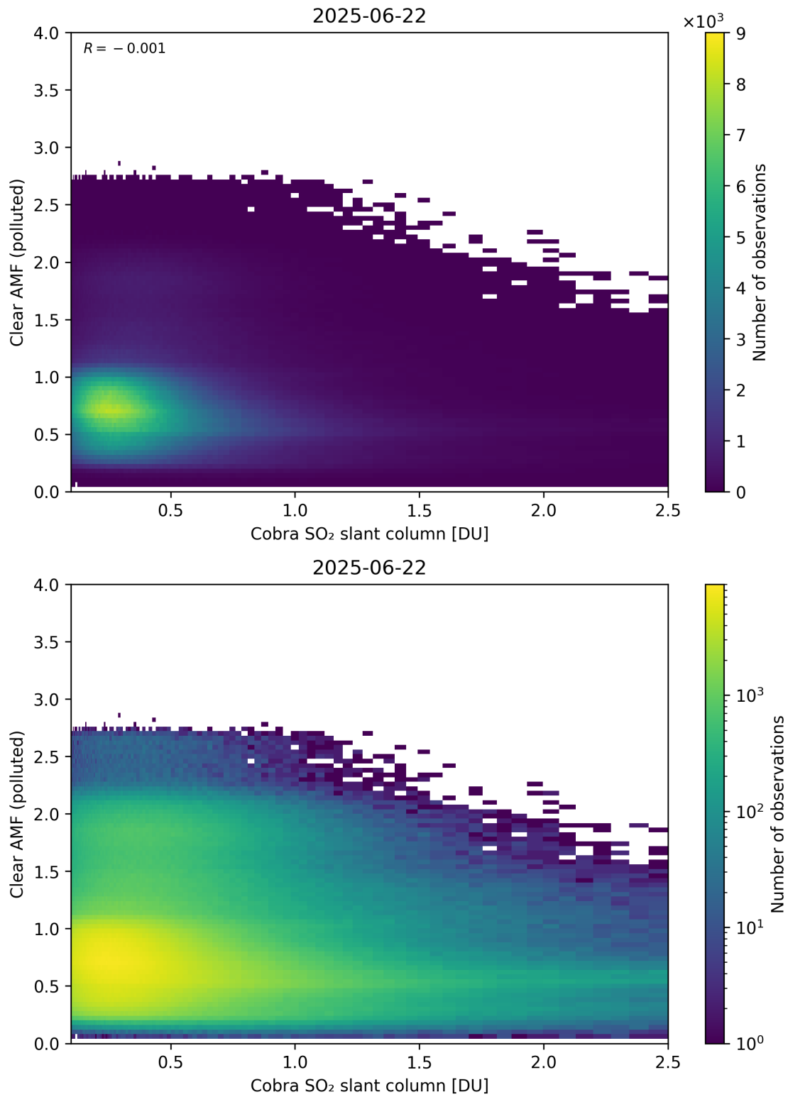
Figure 215: Scatter density plot of “Cobra SO 2 slant column” against “Clear AMF (polluted)” for 2025-06-22 to 2025-06-23.
