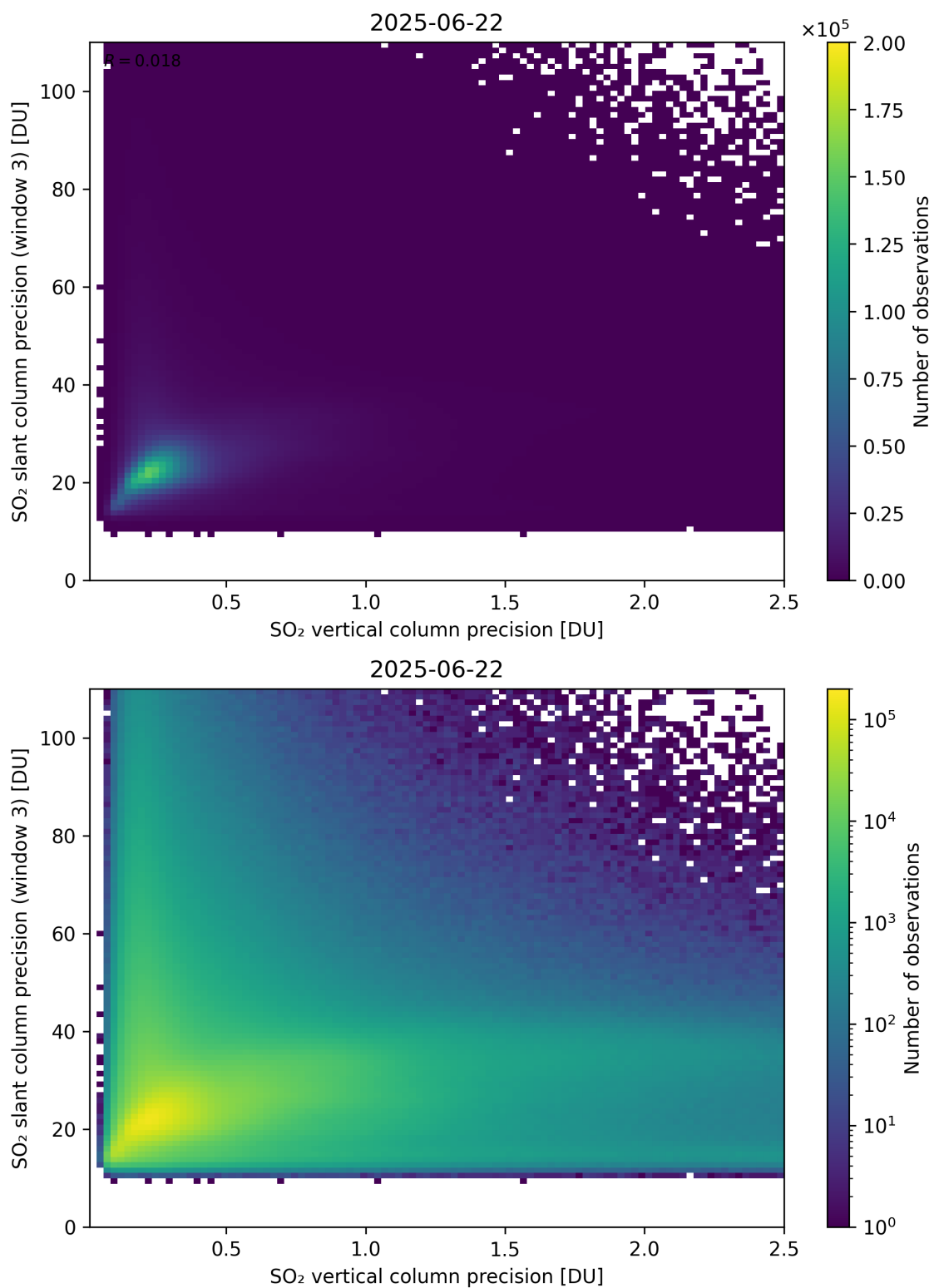
Figure 345: Scatter density plot of “SO 2 vertical column precision” against “SO 2 slant column precision (window 3)” for 2025-06-22 to 2025-06-23.
