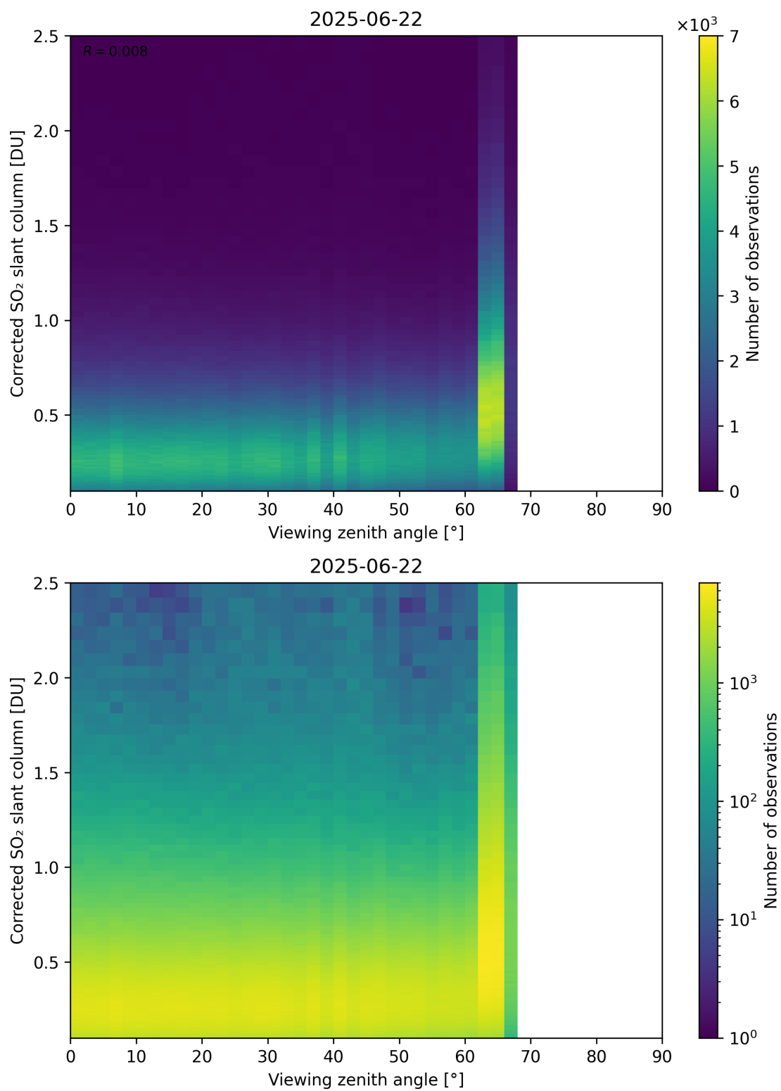
Figure 373: Scatter density plot of “Viewing zenith angle” against “Corrected SO 2 slant column” for 2025-06-22 to 2025-06-23.
