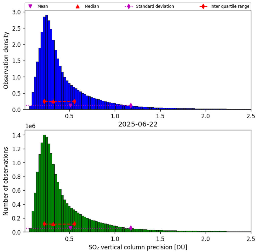
Figure 59: Histogram of “SO 2 vertical column precision” for 2025-06-22 to 2025-06-23
