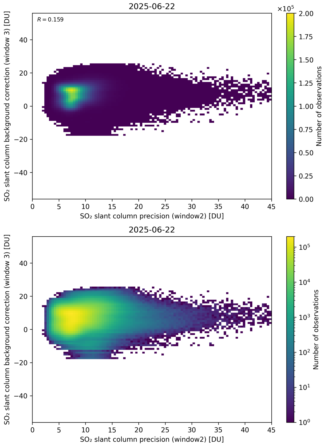
Figure 292: Scatter density plot of “SO 2 slant column precision (window2)” against “SO 2 slant column background correction (window 3)” for 2025-06-22 to 2025-06-23.
