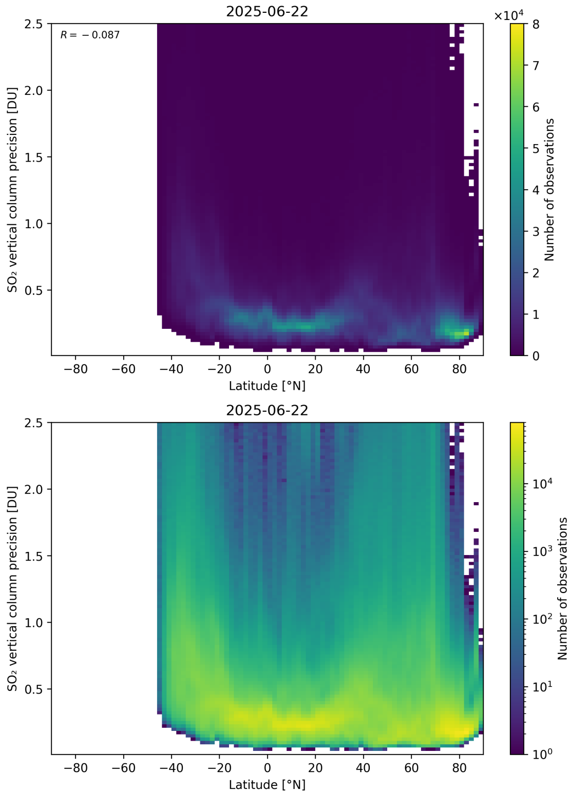
Figure 170: Scatter density plot of “Latitude” against “SO 2 vertical column precision” for 2025-06-22 to 2025-06-23.
