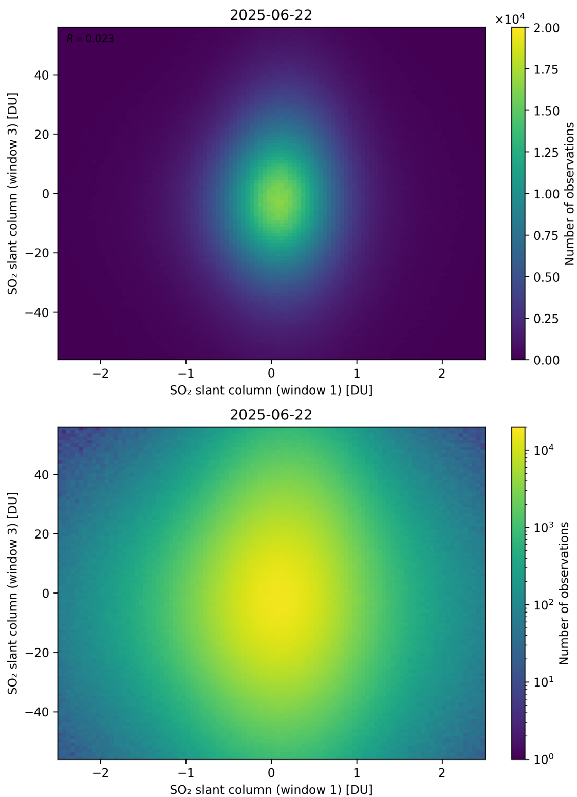
Figure 287: Scatter density plot of “SO 2 slant column (window 1)” against “SO 2 slant column (window 3)” for 2025-06-22 to 2025-06-23.
