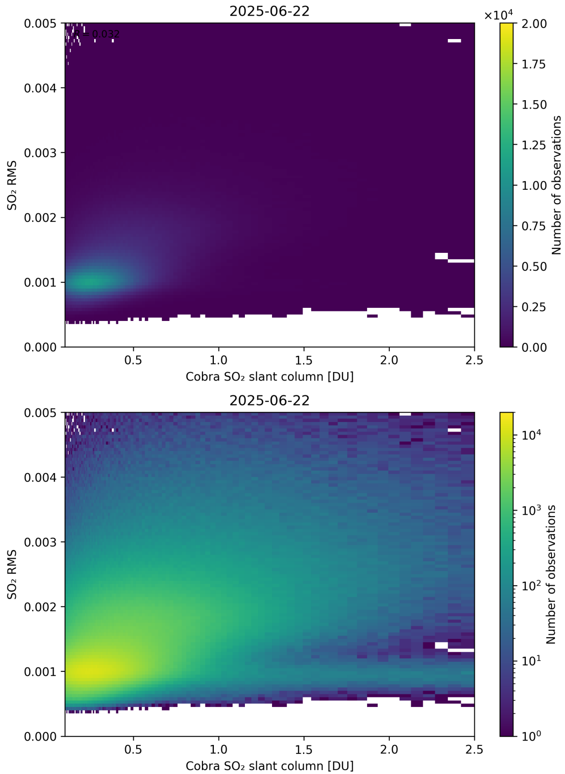
Figure 198: Scatter density plot of “Cobra SO 2 slant column” against “SO 2 RMS” for 2025-06-22 to 2025-06-23.
