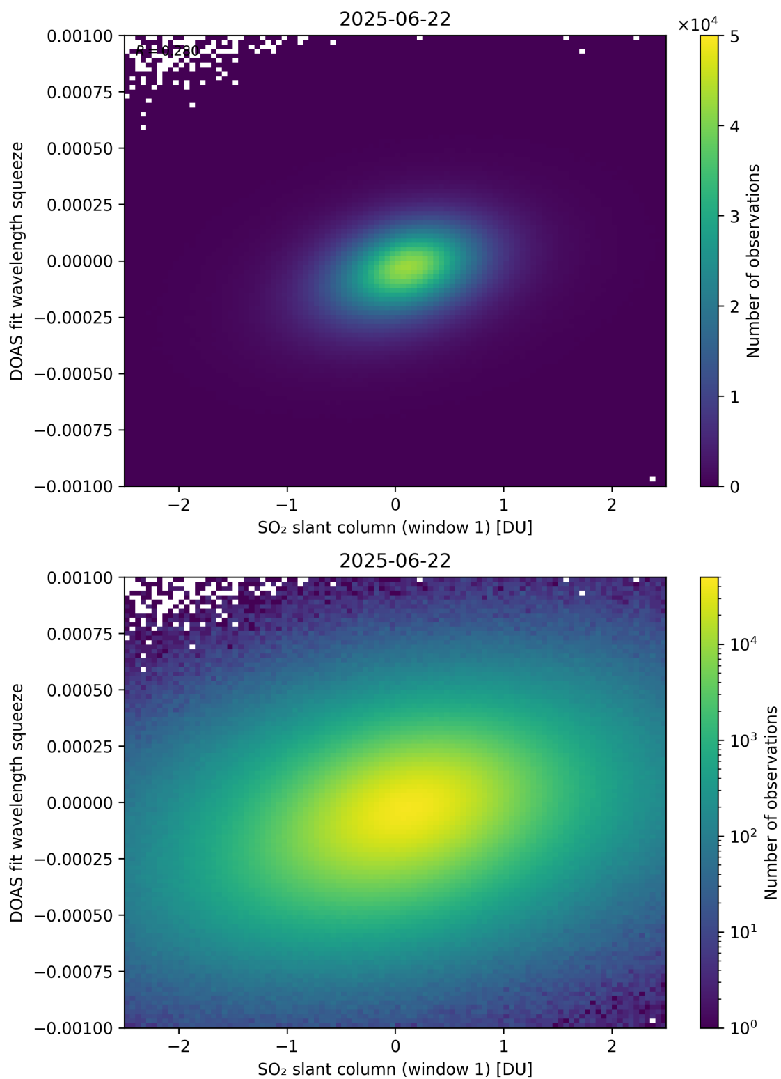
Figure 266: Scatter density plot of “SO 2 slant column (window 1)” against “DOAS fit wavelength squeeze” for 2025-06-22 to 2025-06-23.
