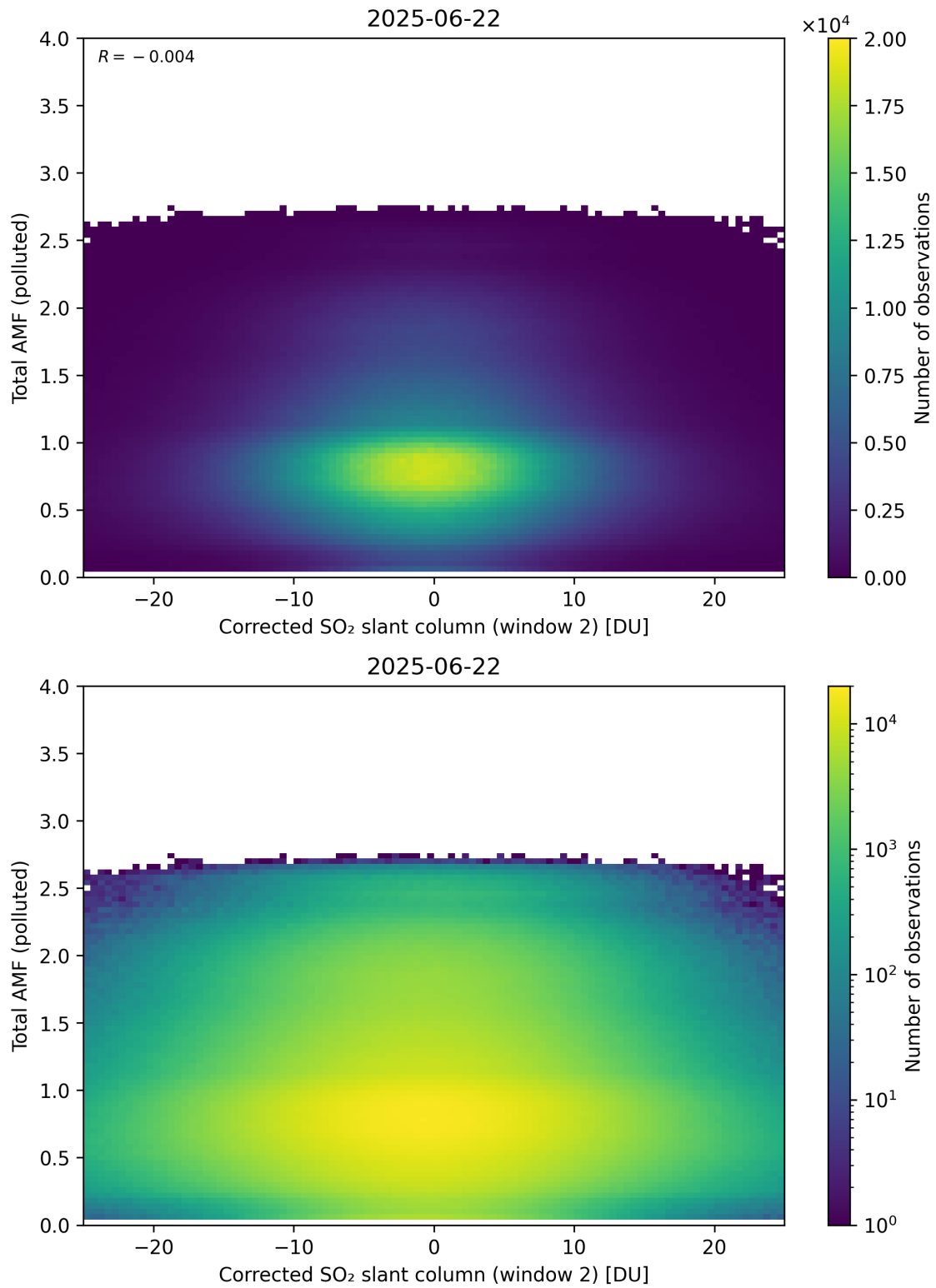
Figure 253: Scatter density plot of “Corrected SO 2 slant column (window 2)” against “Total AMF (polluted)” for 2025-06-22 to 2025-06-23.
