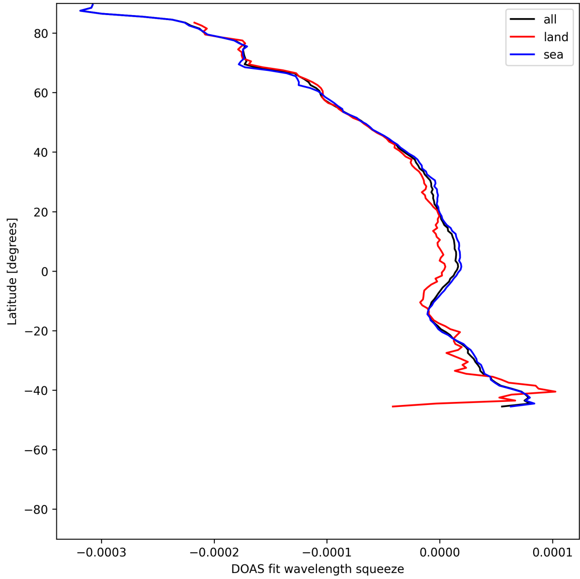
Figure 51: Zonal average of “DOAS fit wavelength squeeze” for 2025-06-22 to 2025-06-23.
