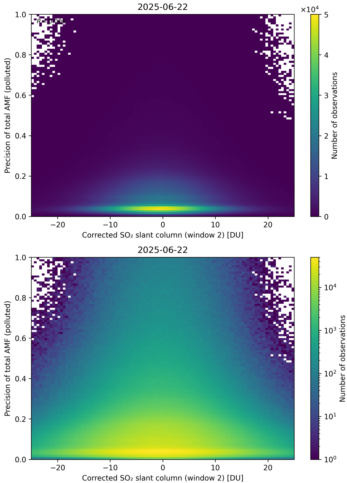
Figure 254: Scatter density plot of “Corrected SO 2 slant column (window 2)” against “Precision of total AMF (polluted)” for 2025-06-22 to 2025-06-23.
