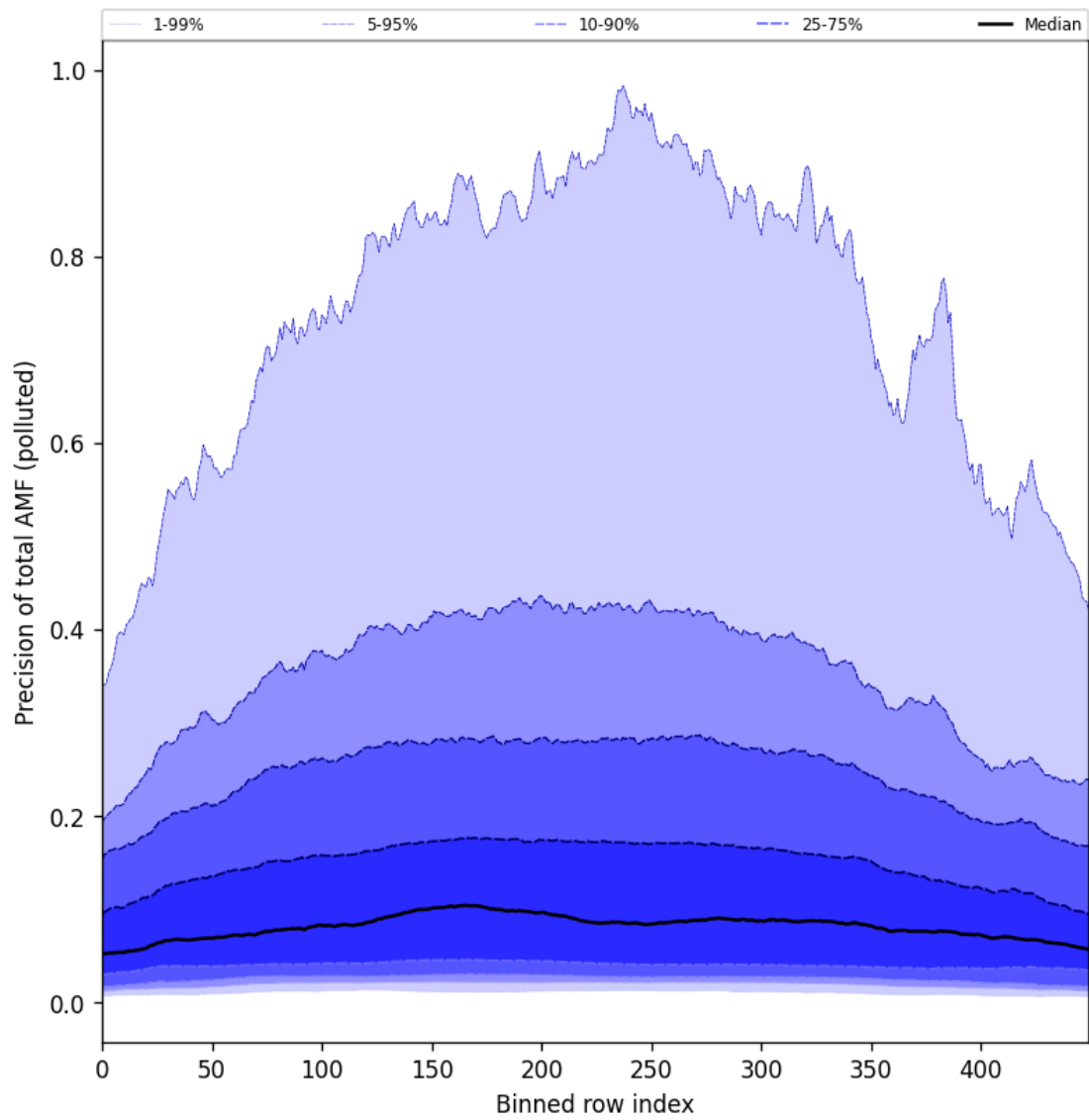
Figure 106: Along track statistics of “Precision of total AMF (polluted)” for 2025-06-22 to 2025-06-23
