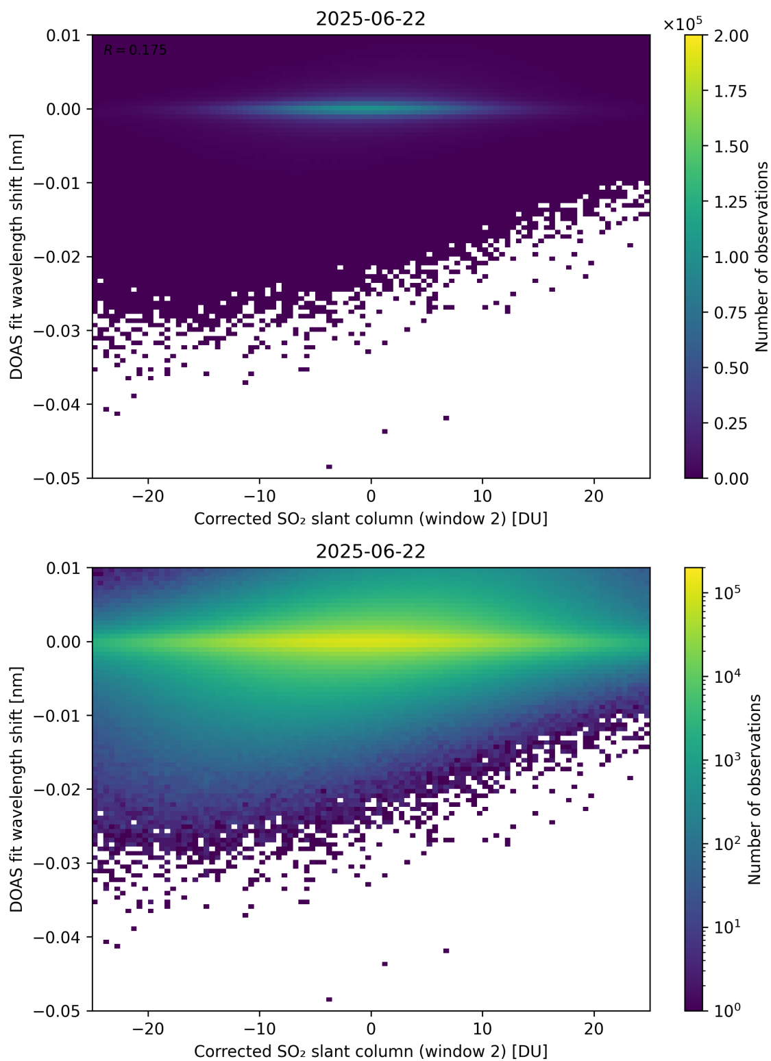
Figure 246: Scatter density plot of “Corrected SO 2 slant column (window 2)” against “DOAS fit wavelength shift” for 2025-06-22 to 2025-06-23.
