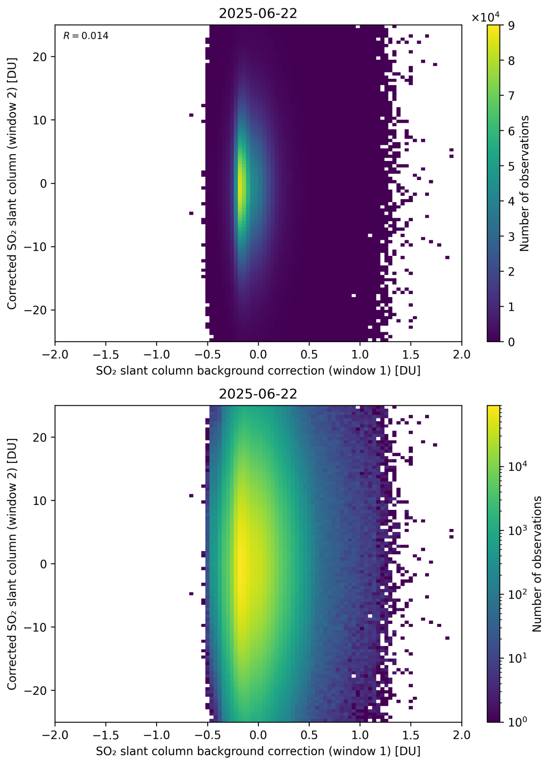
Figure 115: Scatter density plot of “SO 2 slant column background correction (window 1)” against “Corrected SO 2 slant column (window 2)” for 2025-06-22 to 2025-06-23.
