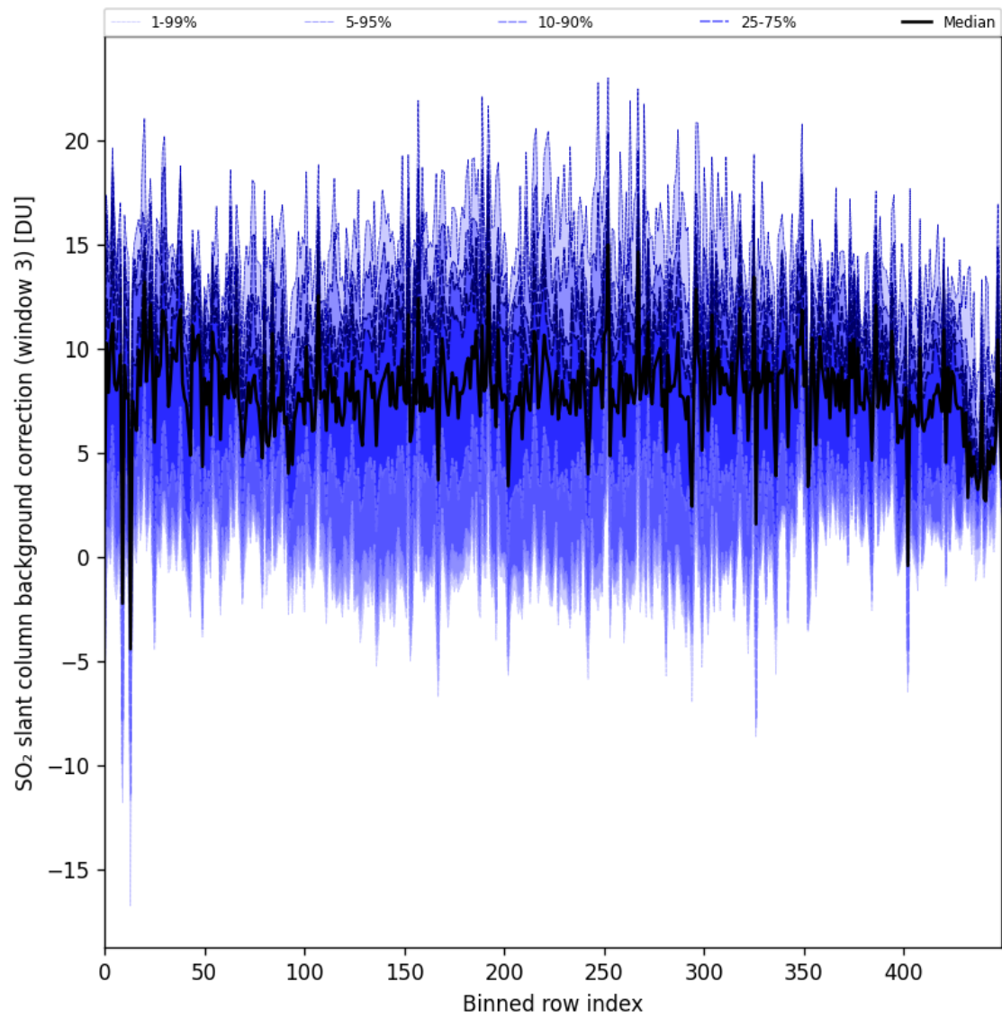
Figure 100: Along track statistics of “SO 2 slant column background correction (window 3)” for 2025-06-22 to 2025-06-23
