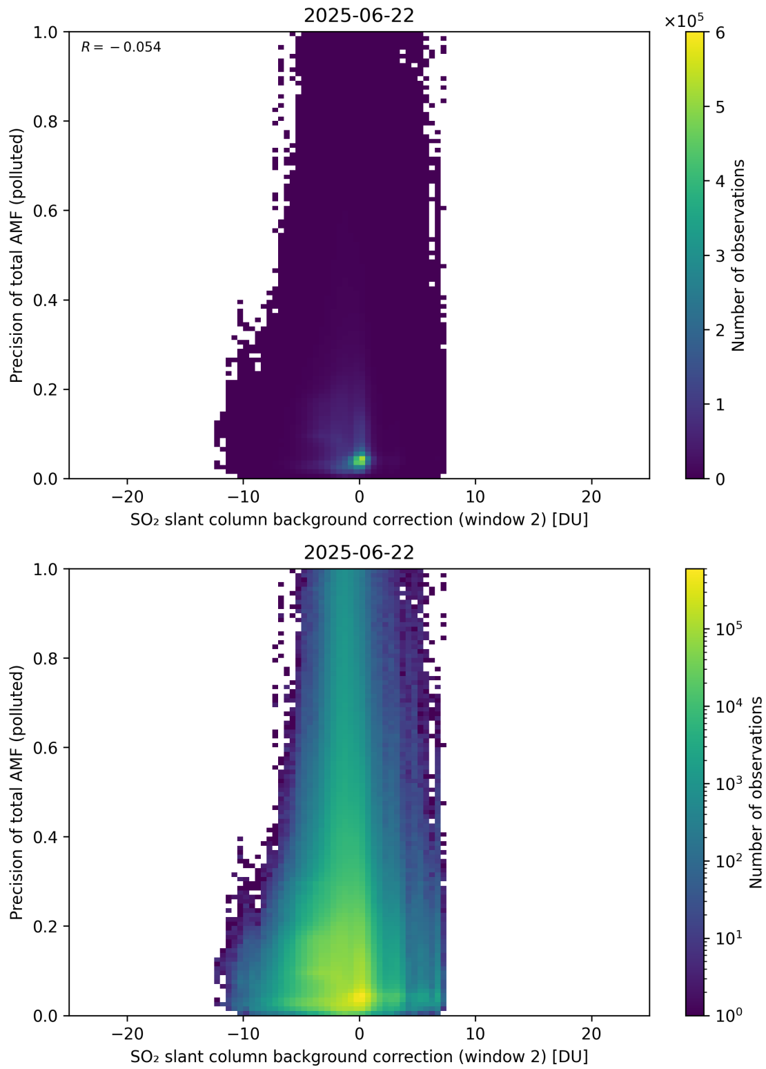
Figure 131: Scatter density plot of “SO 2 slant column background correction (window 2)” against “Precision of total AMF (polluted)” for 2025-06-22 to 2025-06-23.
