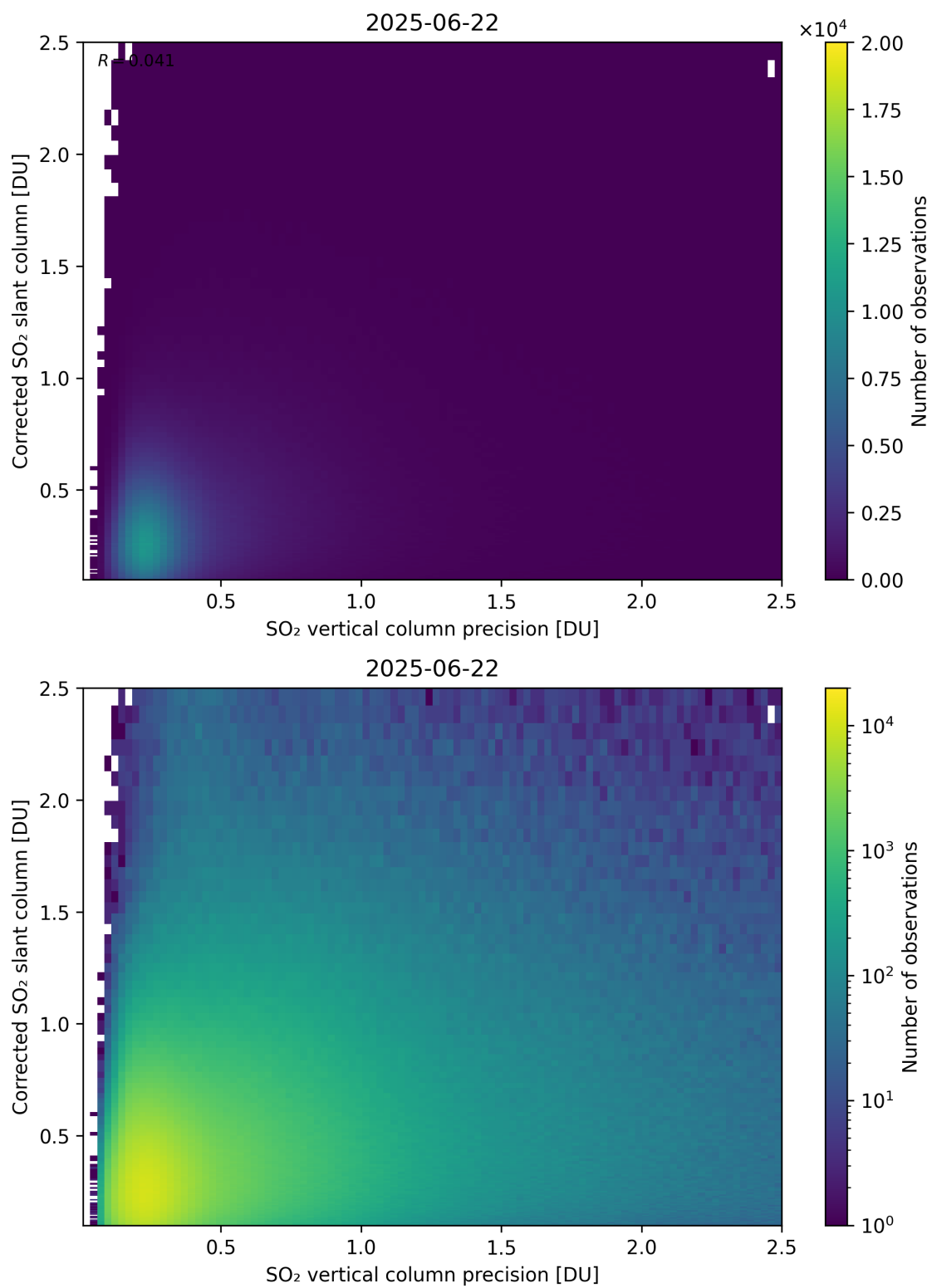
Figure 338: Scatter density plot of “SO 2 vertical column precision” against “Corrected SO 2 slant column” for 2025-06-22 to 2025-06-23.
