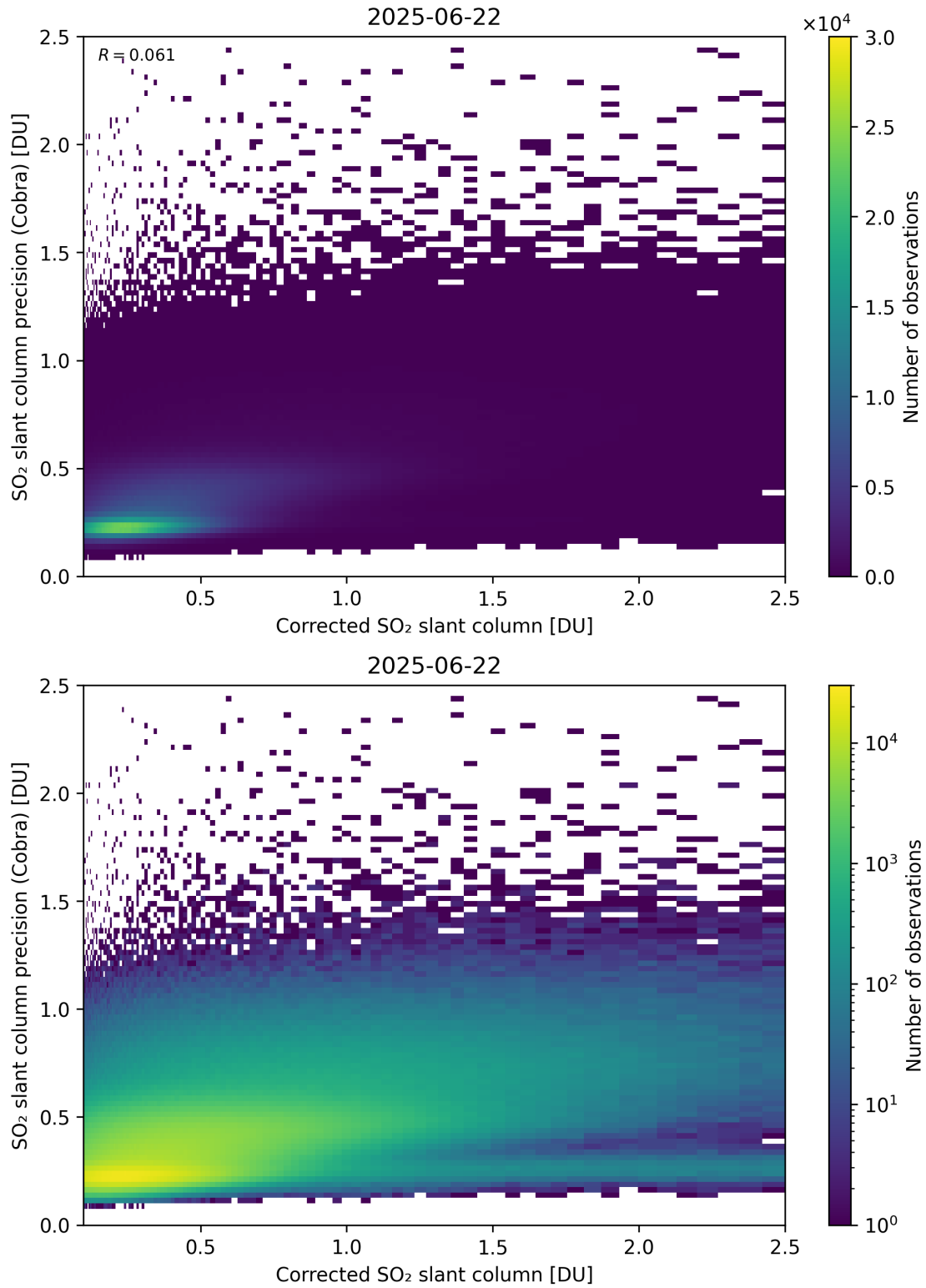
Figure 234: Scatter density plot of “Corrected SO 2 slant column” against “SO 2 slant column precision (Cobra)” for 2025-06-22 to 2025-06-23.
