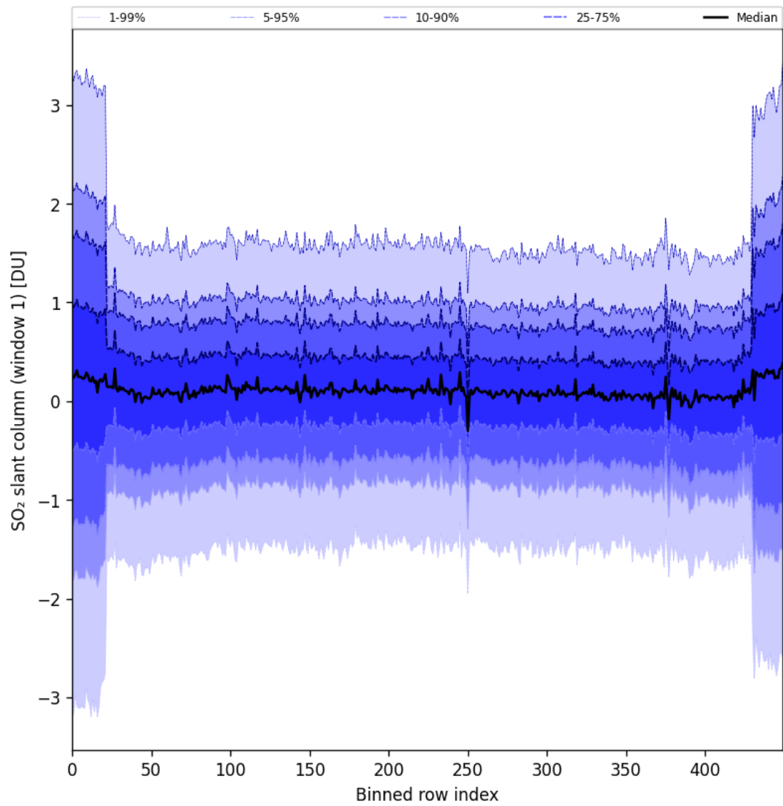
Figure 89: Along track statistics of “SO 2 slant column (window 1)” for 2025-06-22 to 2025-06-23
