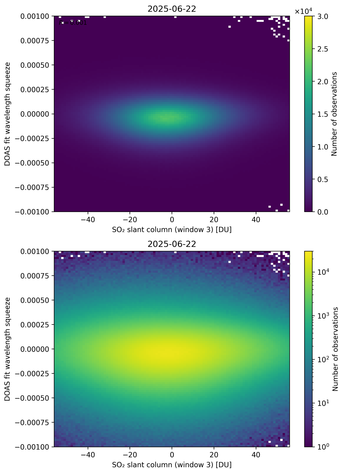
Figure 305: Scatter density plot of “SO 2 slant column (window 3)” against “DOAS fit wavelength squeeze” for 2025-06-22 to 2025-06-23.
