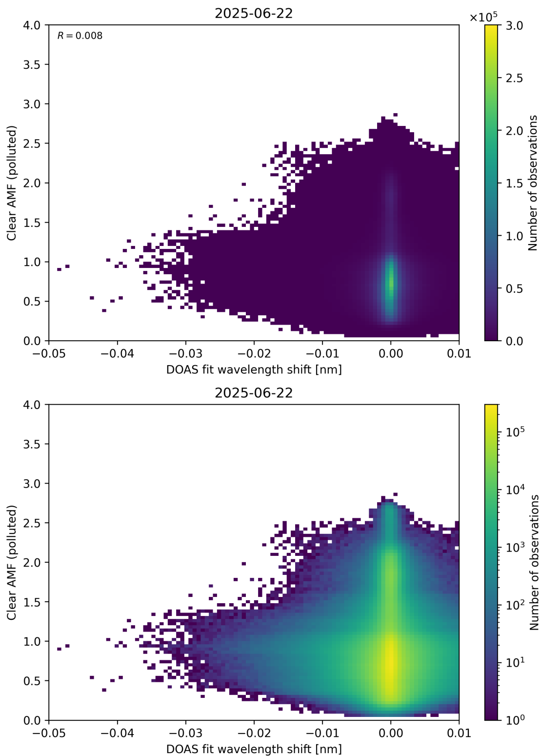
Figure 140: Scatter density plot of “DOAS fit wavelength shift” against “Clear AMF (polluted)” for 2025-06-22 to 2025-06-23.
