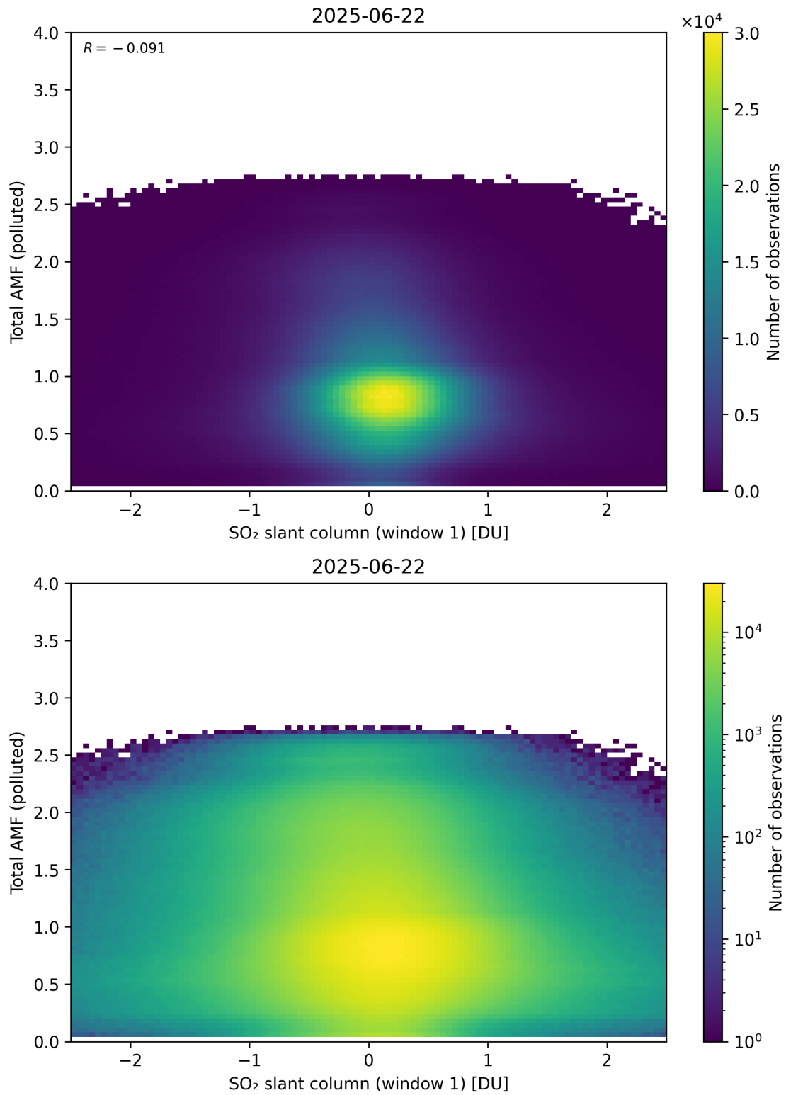
Figure 289: Scatter density plot of “SO 2 slant column (window 1)” against “Total AMF (polluted)” for 2025-06-22 to 2025-06-23.
