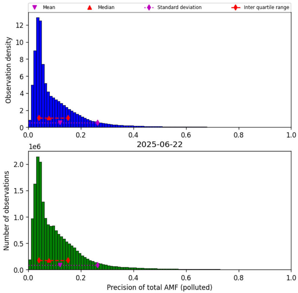
Figure 80: Histogram of “Precision of total AMF (polluted)” for 2025-06-22 to 2025-06-23
