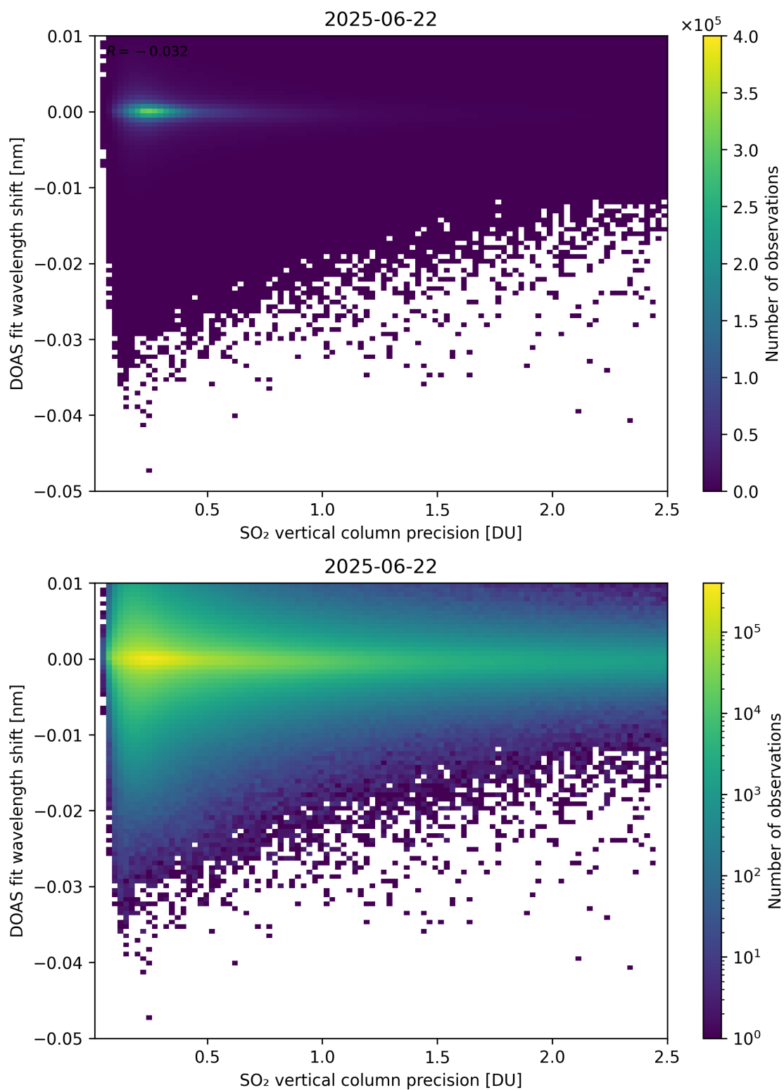
Figure 332: Scatter density plot of “SO 2 vertical column precision” against “DOAS fit wavelength shift” for 2025-06-22 to 2025-06-23.
