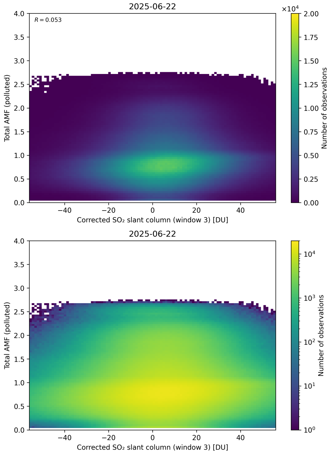
Figure 260: Scatter density plot of “Corrected SO 2 slant column (window 3)” against “Total AMF (polluted)” for 2025-06-22 to 2025-06-23.
