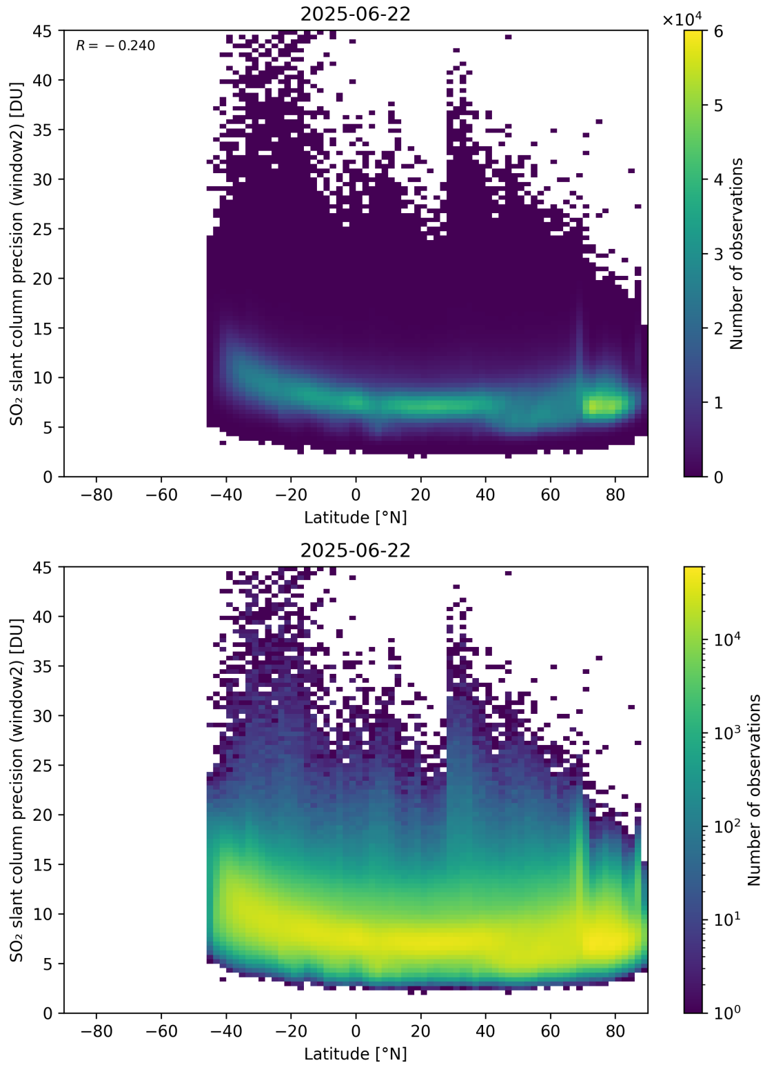
Figure 164: Scatter density plot of “Latitude” against “SO 2 slant column precision (window2)” for 2025-06-22 to 2025-06-23.
