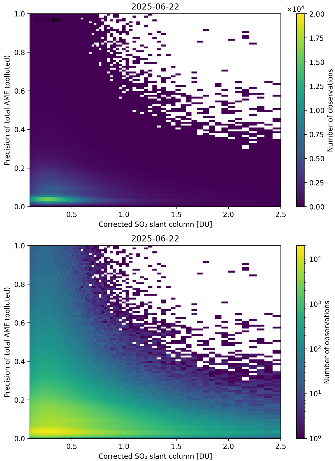
Figure 243: Scatter density plot of “Corrected SO 2 slant column” against “Precision of total AMF (polluted)” for 2025-06-22 to 2025-06-23.
