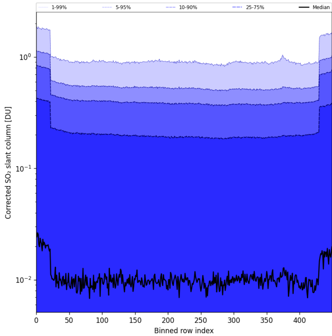
Figure 86: Along track statistics of "Corrected SO 2 slant column" for 2025-06-22 to 2025-06-23
