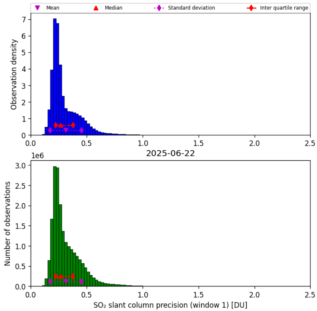
Figure 64: Histogram of “SO 2 slant column precision (window 1)” for 2025-06-22 to 2025-06-23
