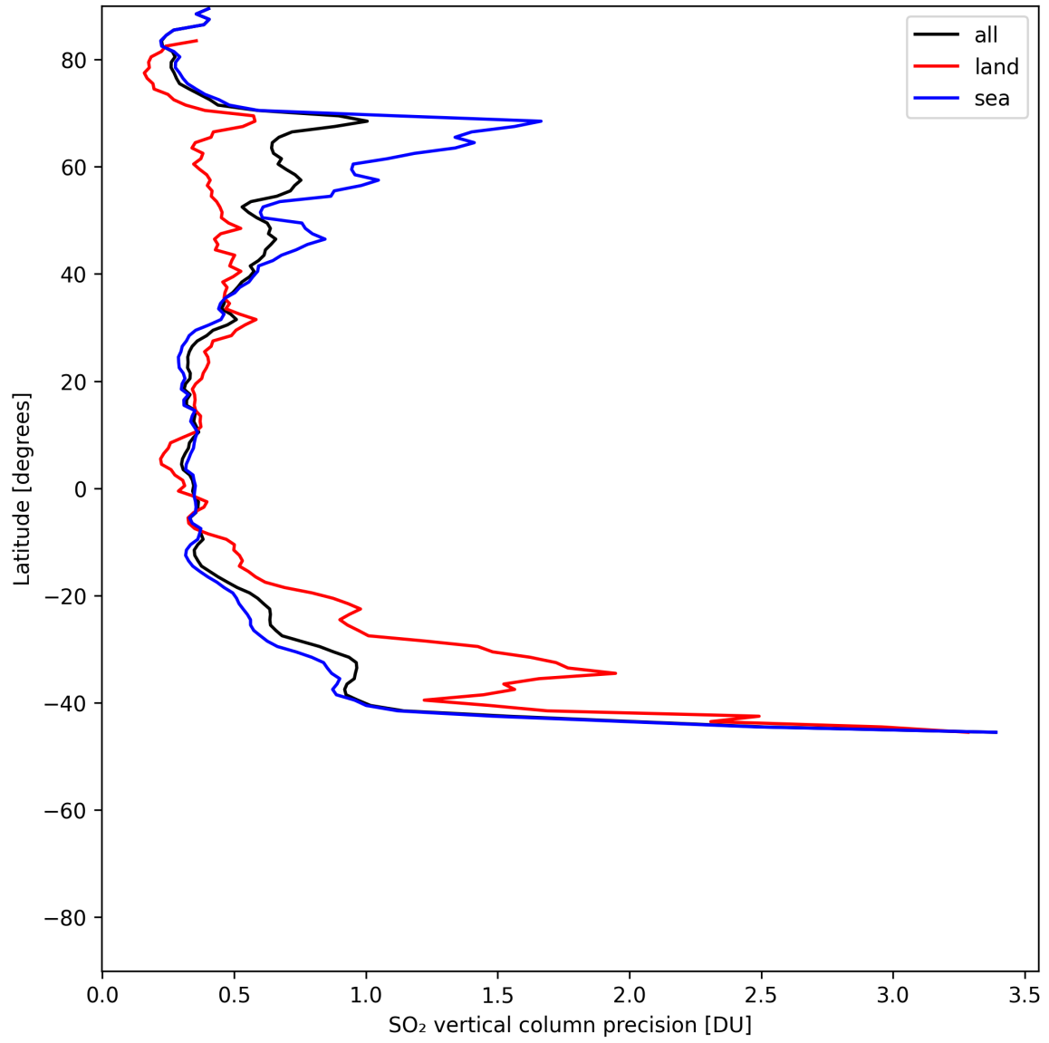
Figure 33: Zonal average of “SO 2 vertical column precision” for 2025-06-22 to 2025-06-23.
