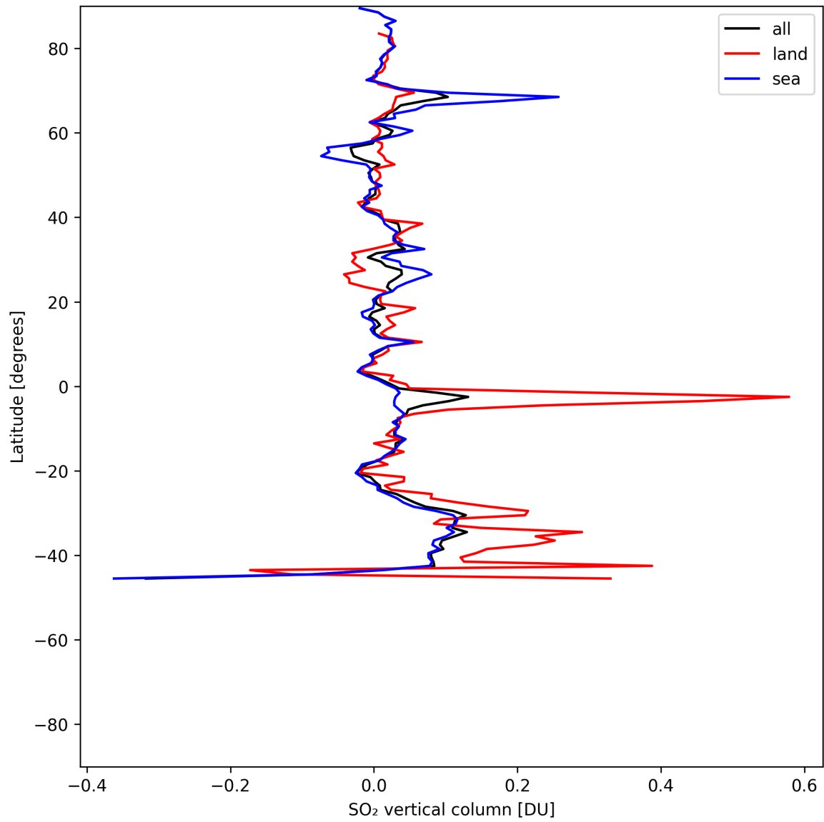
Figure 32: Zonal average of “SO 2 vertical column” for 2025-06-22 to 2025-06-23.
