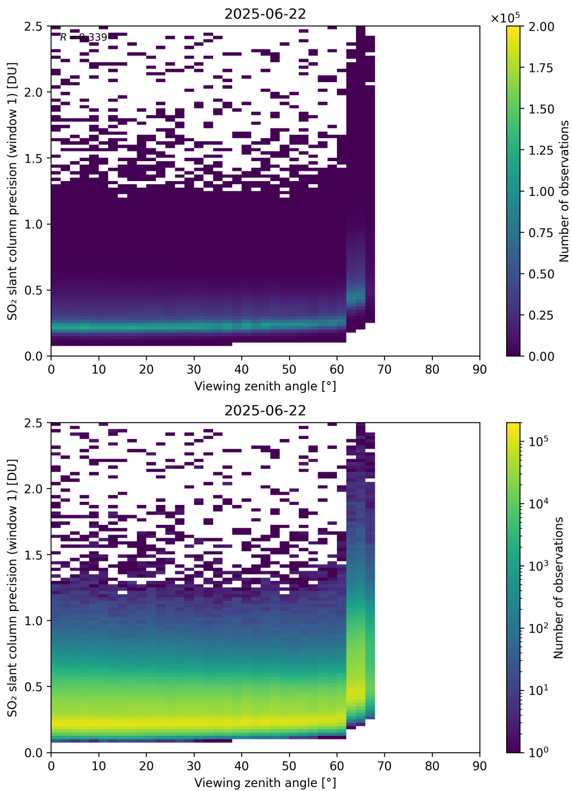
Figure 377: Scatter density plot of “Viewing zenith angle” against “SO 2 slant column precision (window 1)” for 2025-06-22 to 2025-06-23.
