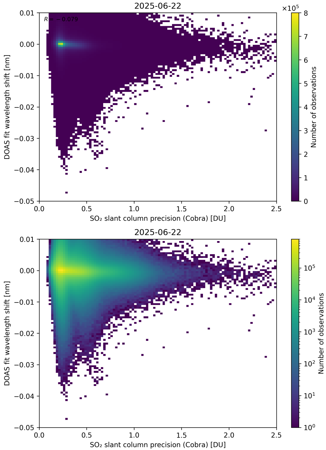
Figure 202: Scatter density plot of “SO 2 slant column precision (Cobra)” against “DOAS fit wavelength shift” for 2025-06-22 to 2025-06-23.
