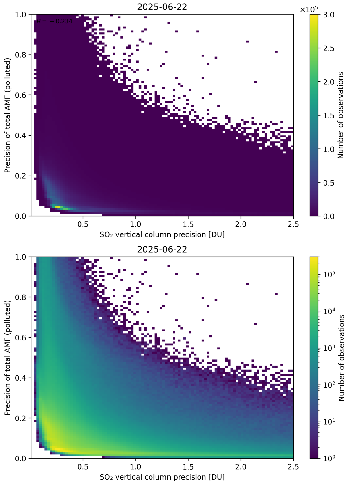
Figure 347: Scatter density plot of “SO 2 vertical column precision” against “Precision of total AMF (polluted)” for 2025-06-22 to 2025-06-23.
