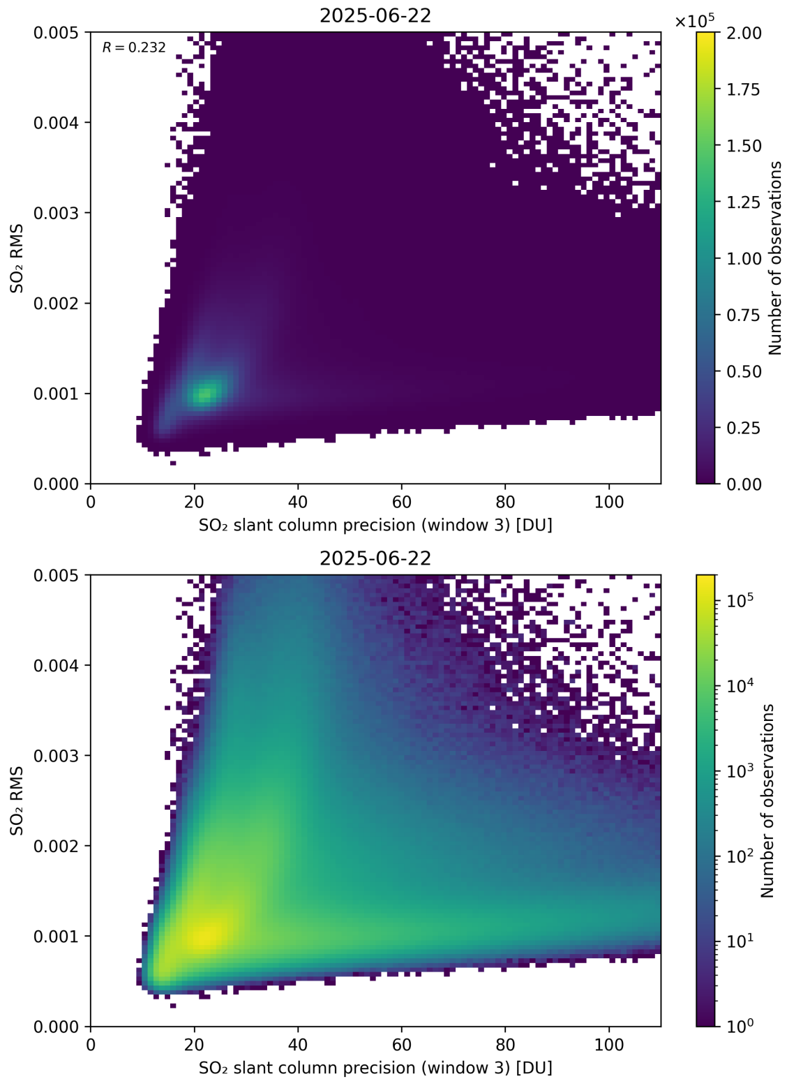
Figure 310: Scatter density plot of “SO 2 slant column precision (window 3)” against “SO 2 RMS” for 2025-06-22 to 2025-06-23.
