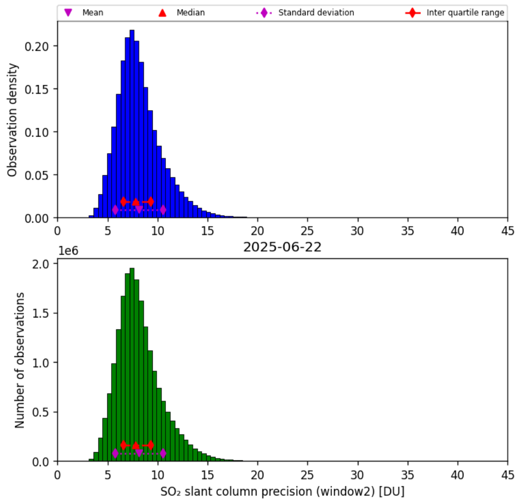
Figure 68: Histogram of “SO 2 slant column precision (window2)” for 2025-06-22 to 2025-06-23
