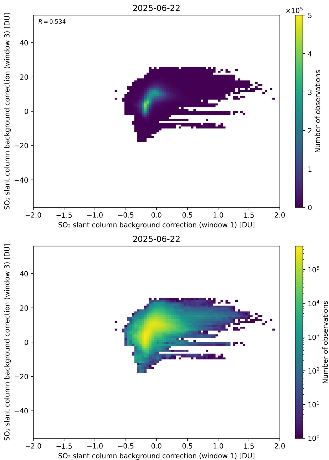
Figure 110: Scatter density plot of “SO 2 slant column background correction (window 1)” against “SO 2 slant column background correction (window 3)” for 2025-06-22 to 2025-06-23.
