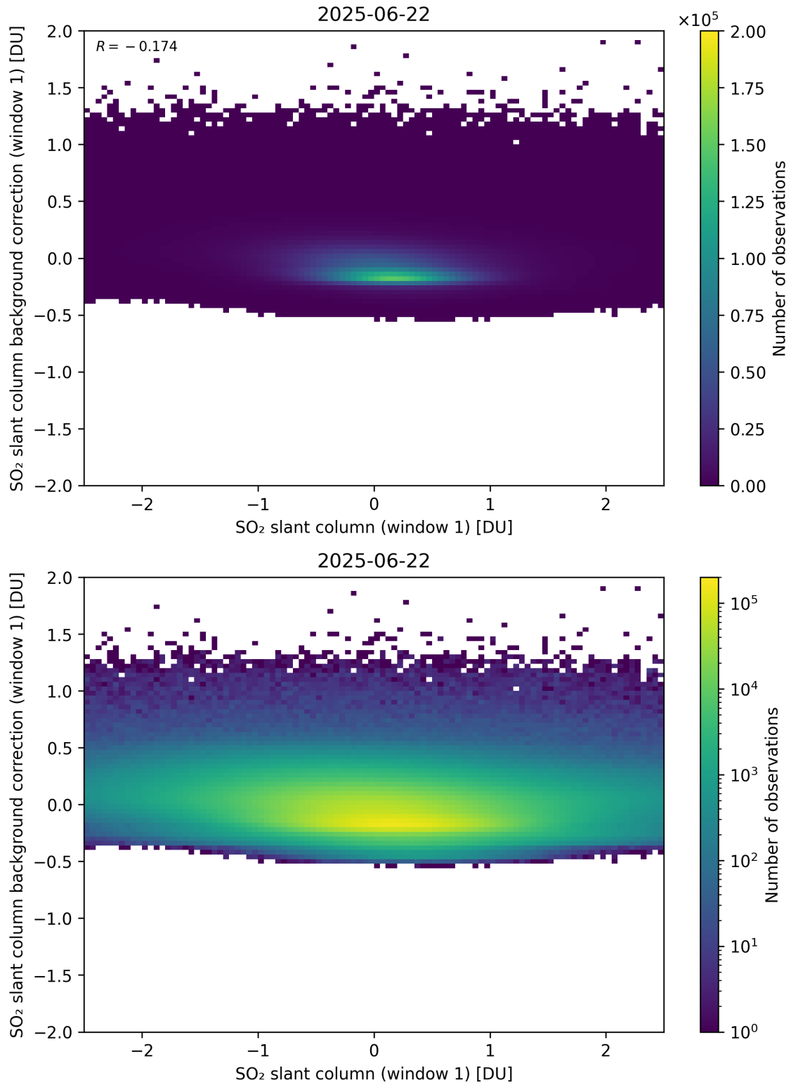
Figure 262: Scatter density plot of “SO 2 slant column (window 1)” against “SO 2 slant column background correction (window 1)” for 2025-06-22 to 2025-06-23.
