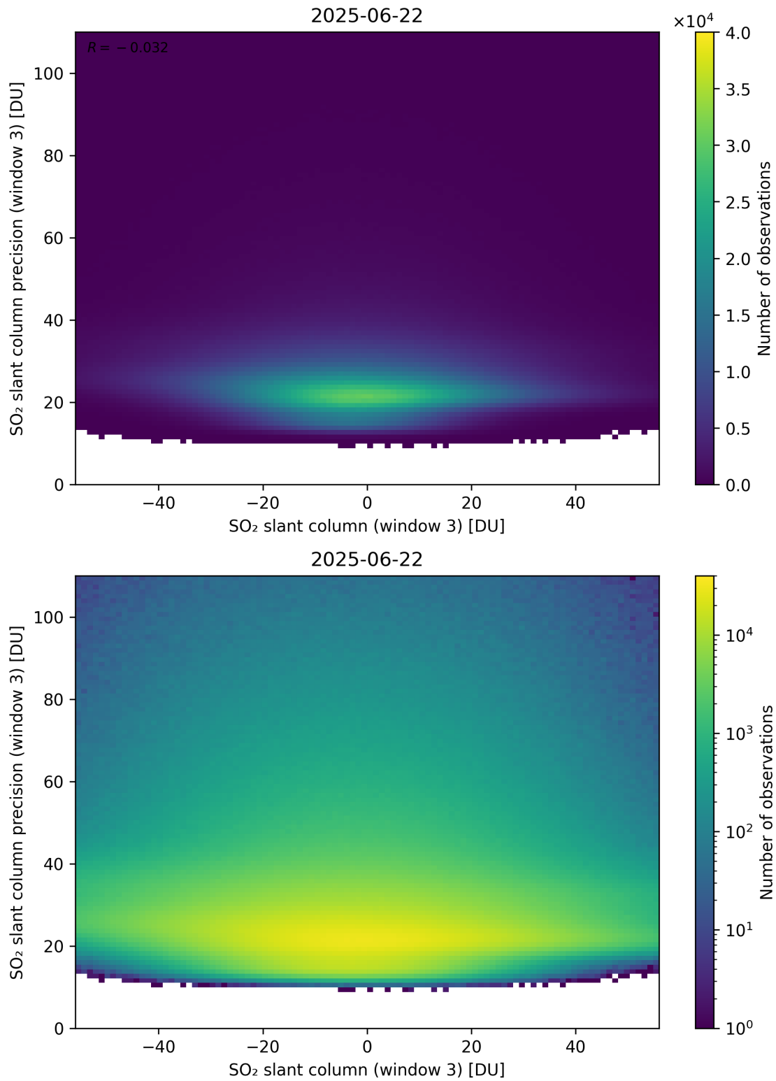
Figure 317: Scatter density plot of “SO 2 slant column (window 3)” against “SO 2 slant column precision (window 3)” for 2025-06-22 to 2025-06-23.
