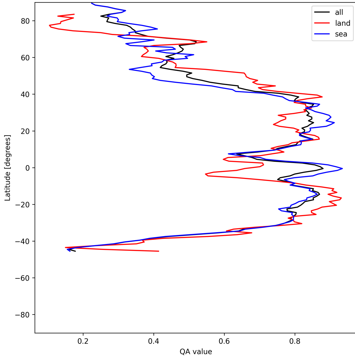
Figure 31: Zonal average of “QA value” for 2025-06-22 to 2025-06-23.
