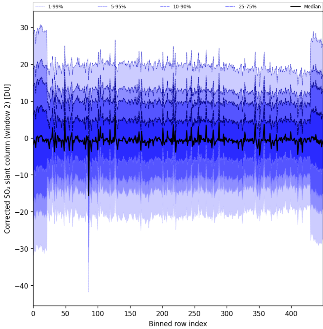
Figure 95: Along track statistics of “Corrected SO 2 slant column (window 2)” for 2025-06-22 to 2025-06-23
