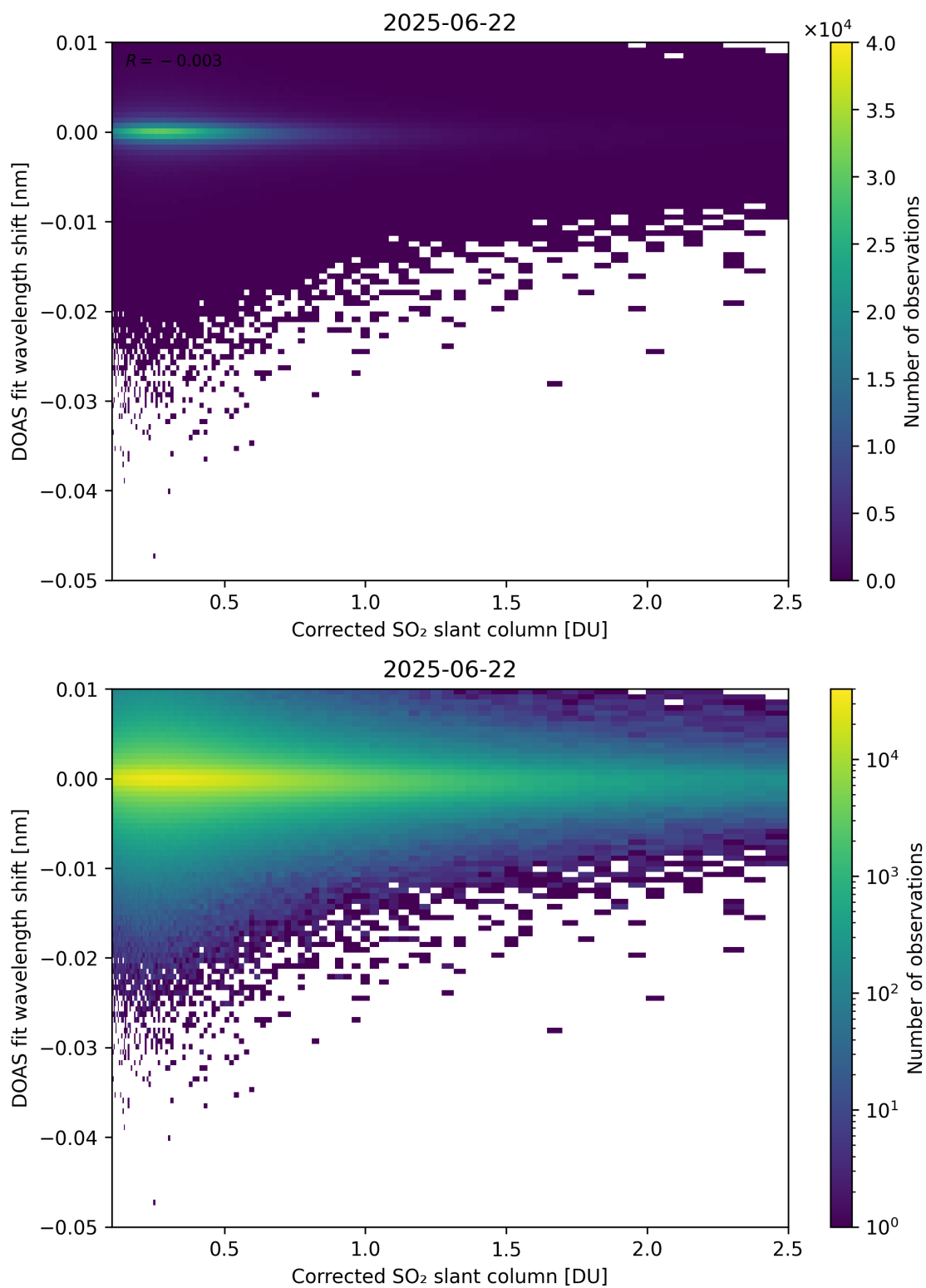
Figure 229: Scatter density plot of “Corrected SO 2 slant column” against “DOAS fit wavelength shift” for 2025-06-22 to 2025-06-23.
