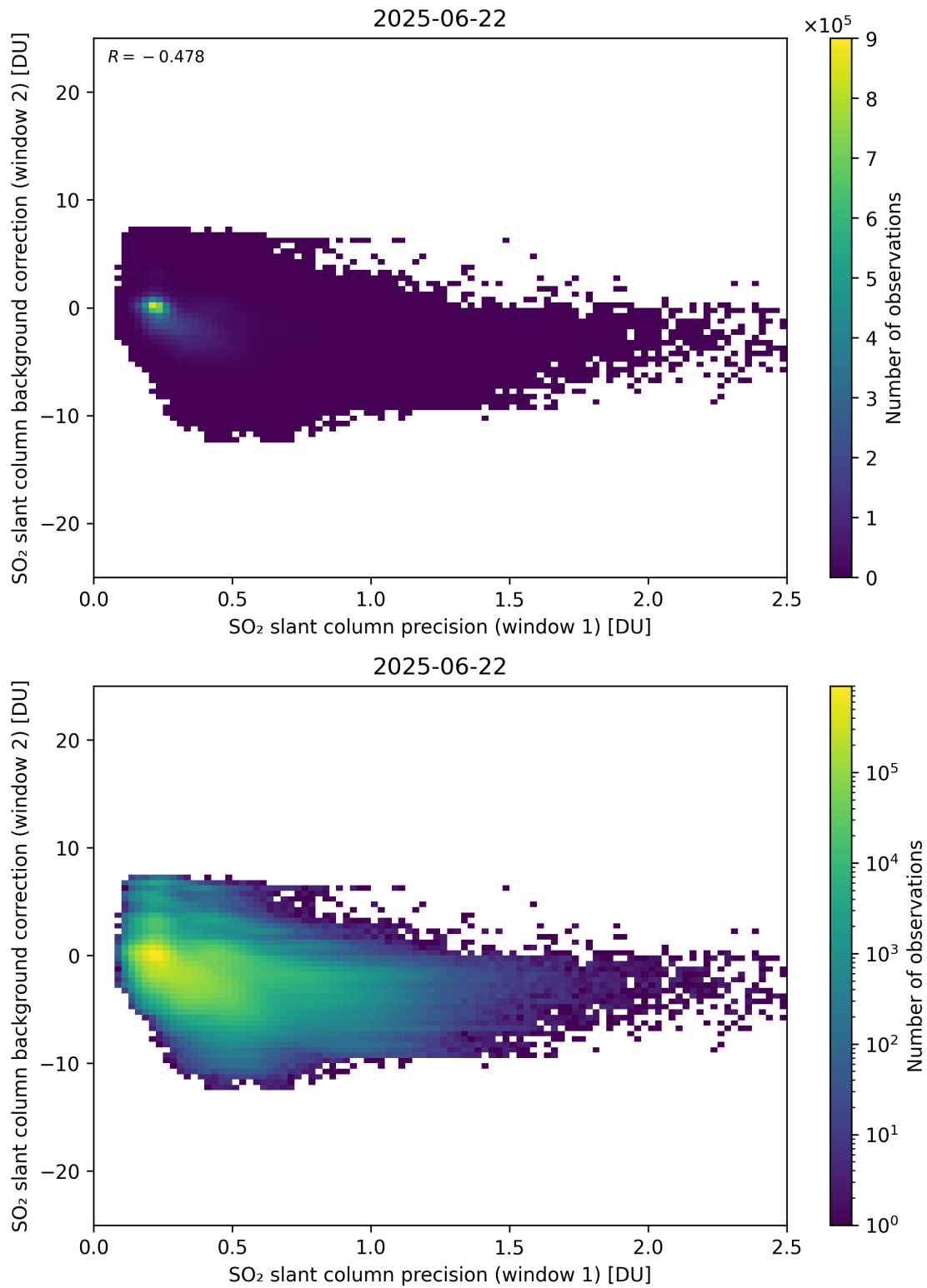
Figure 269: Scatter density plot of “SO 2 slant column precision (window 1)” against “SO 2 slant column background correction (window 2)” for 2025-06-22 to 2025-06-23.
