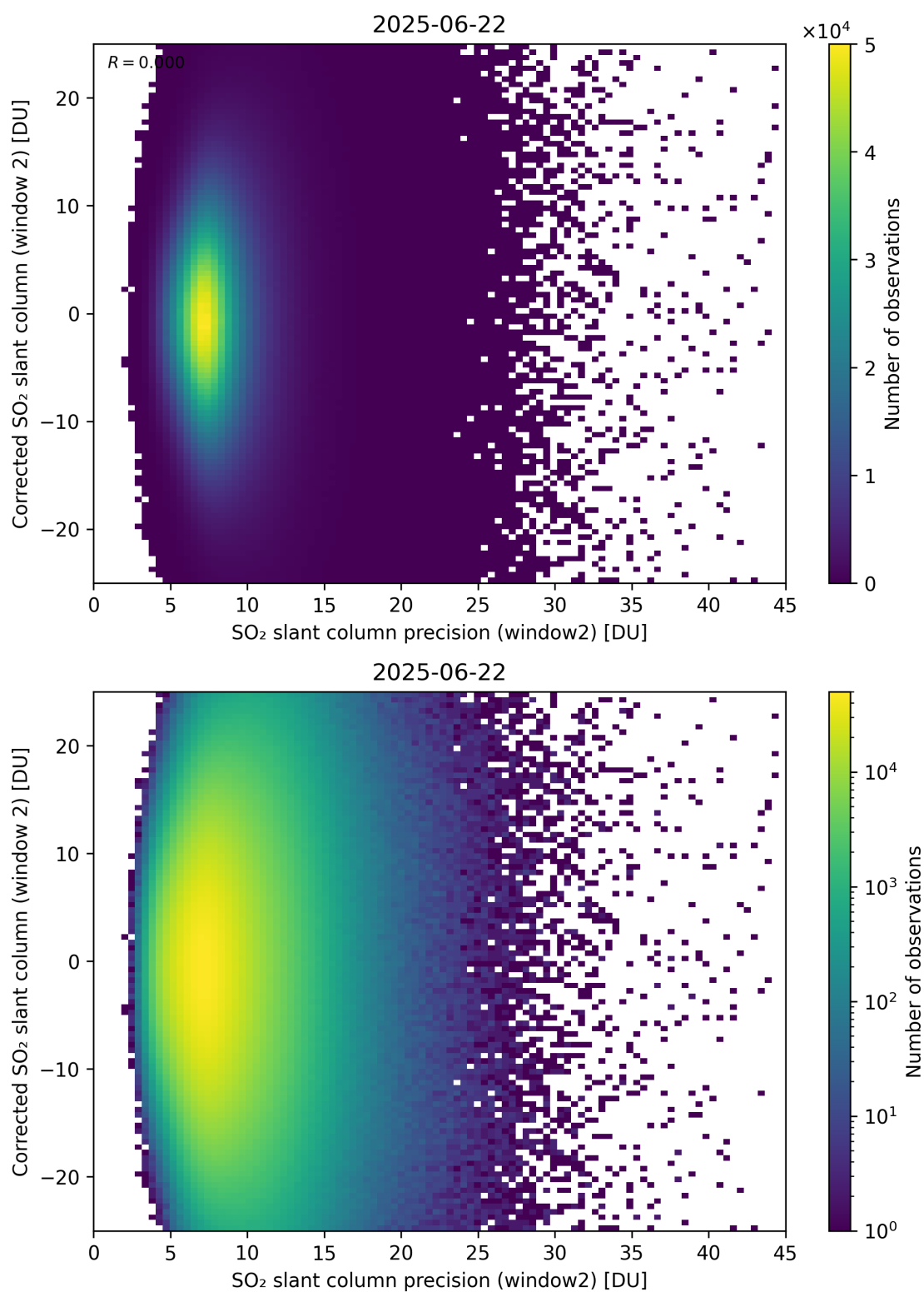
Figure 297: Scatter density plot of “SO 2 slant column precision (window2)” against “Corrected SO 2 slant column (window 2)” for 2025-06-22 to 2025-06-23.
