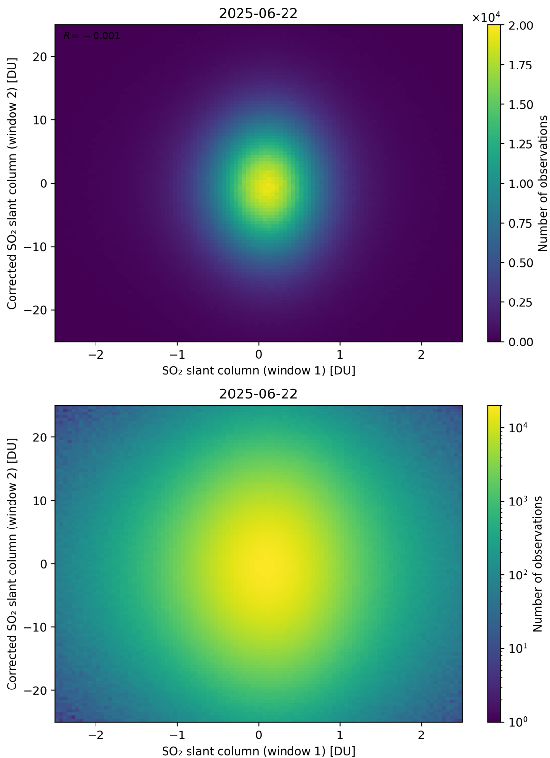
Figure 283: Scatter density plot of “SO 2 slant column (window 1)” against “Corrected SO 2 slant column (window 2)” for 2025-06-22 to 2025-06-23.
