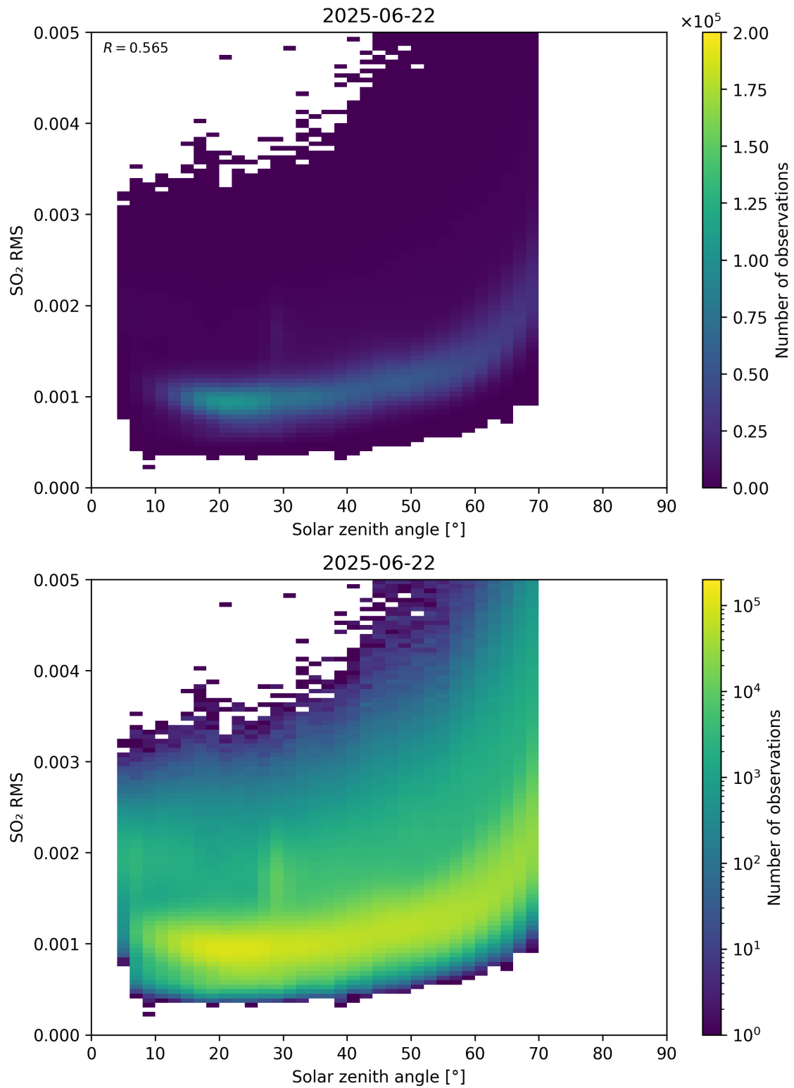
Figure 176: Scatter density plot of “Solar zenith angle” against “SO 2 RMS” for 2025-06-22 to 2025-06-23.
