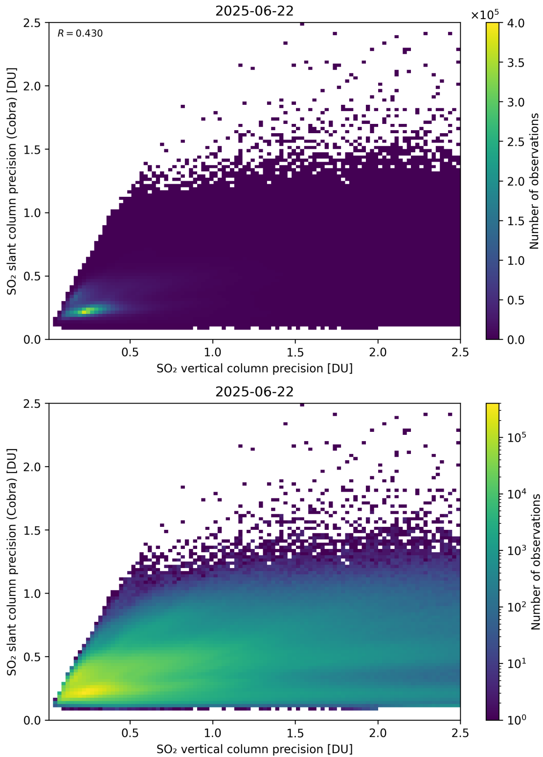
Figure 337: Scatter density plot of “SO 2 vertical column precision” against “SO 2 slant column precision (Cobra)” for 2025-06-22 to 2025-06-23.
