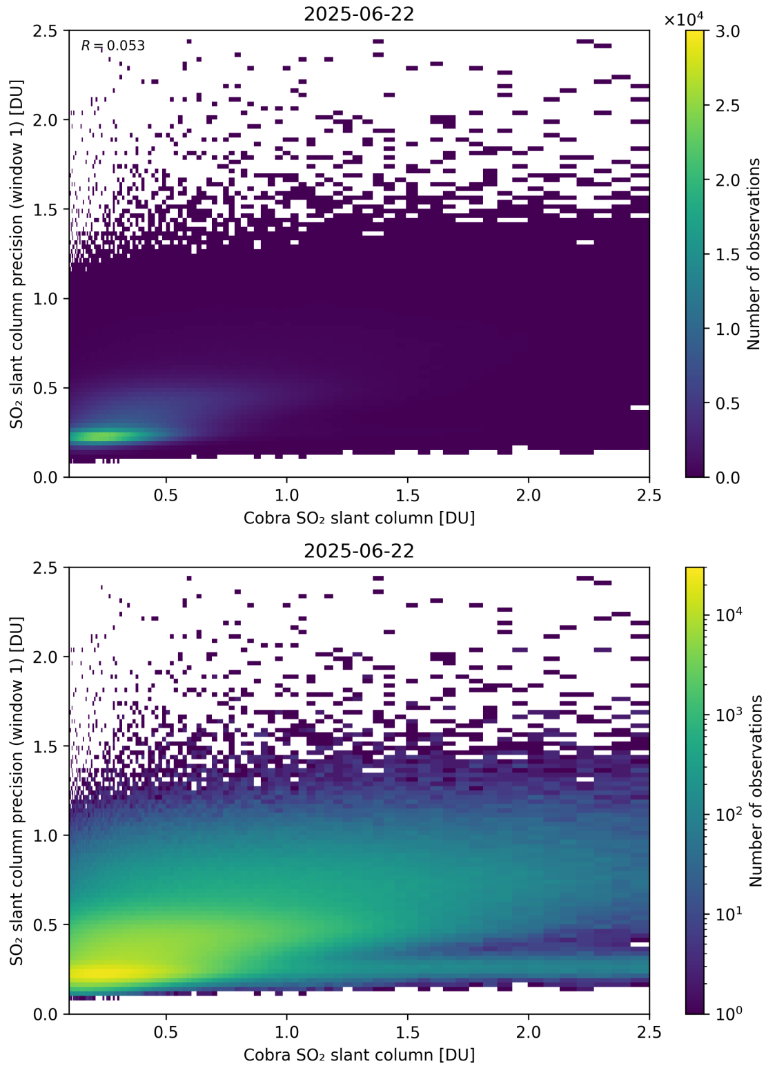
Figure 220: Scatter density plot of “Cobra SO 2 slant column” against “SO 2 slant column precision (window 1)” for 2025-06-22 to 2025-06-23.
