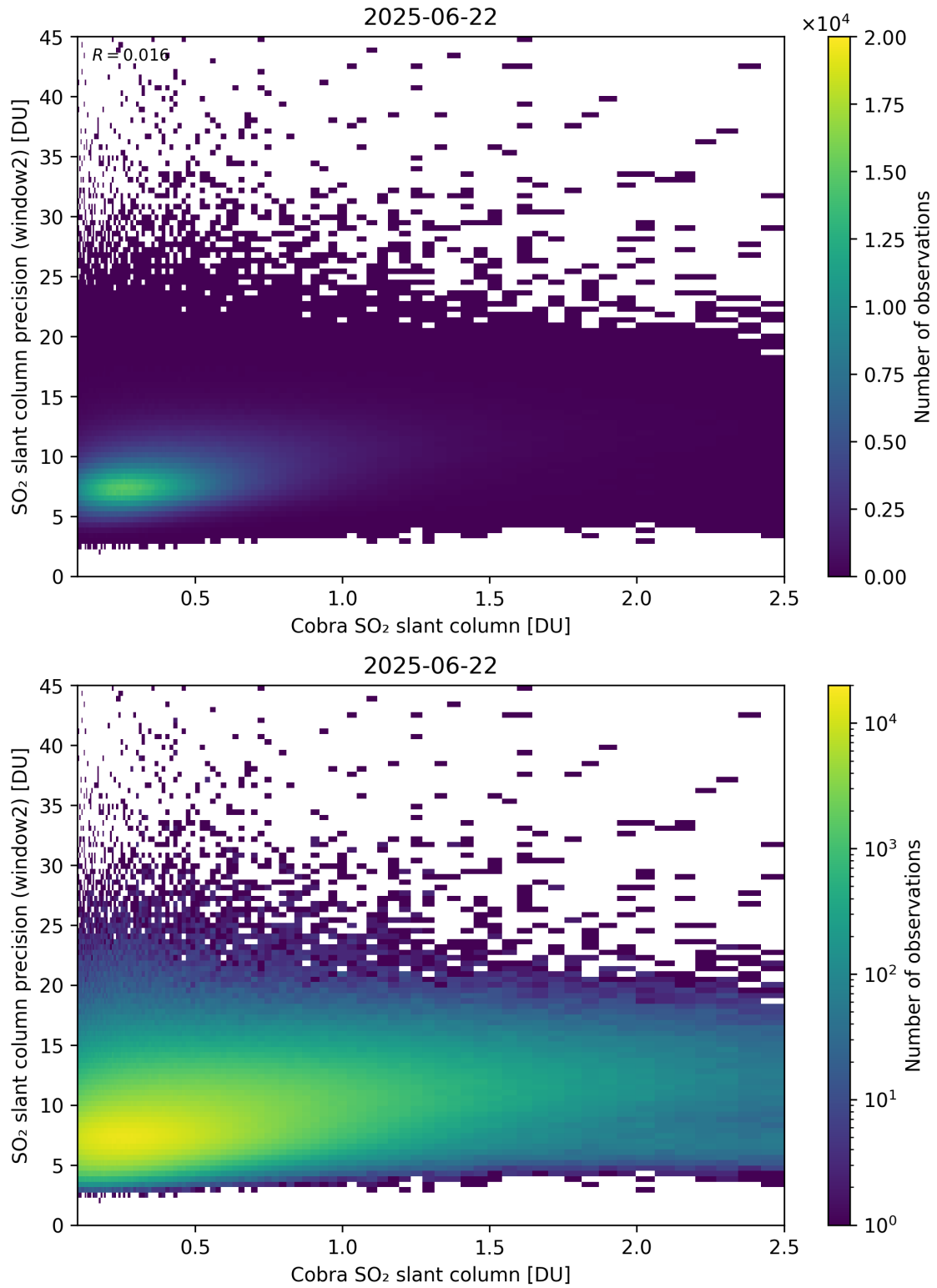
Figure 221: Scatter density plot of “Cobra SO 2 slant column” against “SO 2 slant column precision (window2)” for 2025-06-22 to 2025-06-23.
