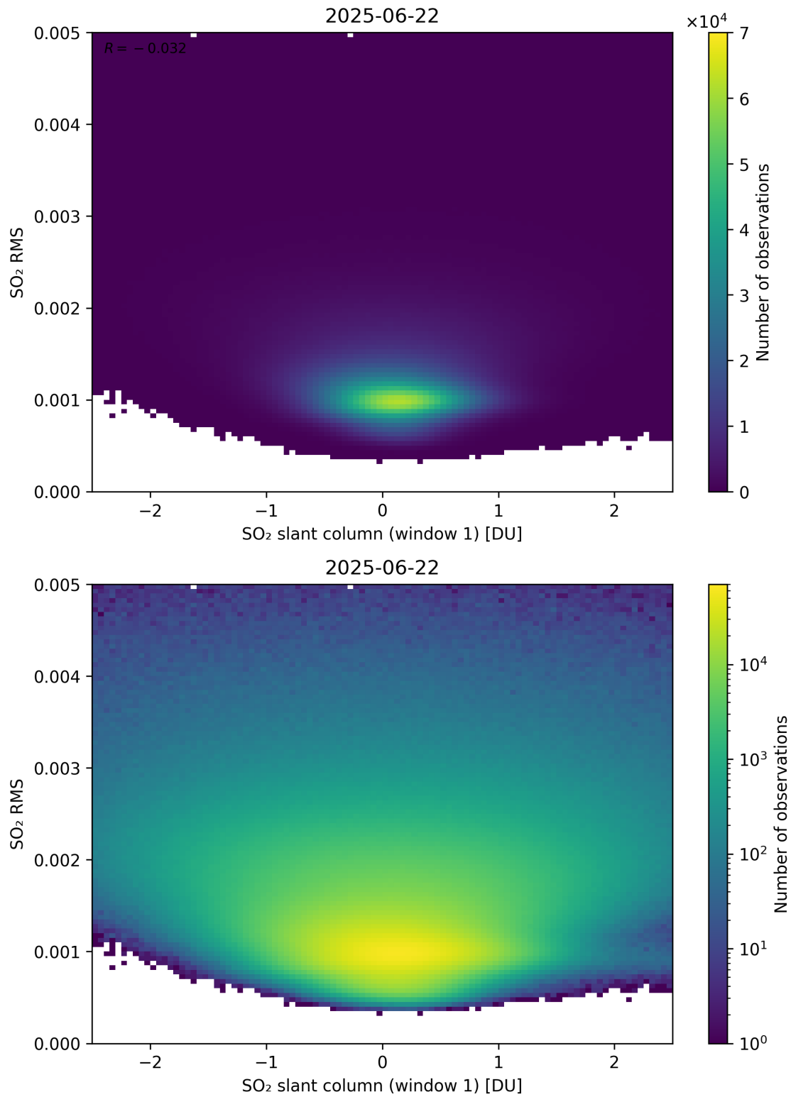
Figure 267: Scatter density plot of “SO 2 slant column (window 1)” against “SO 2 RMS” for 2025-06-22 to 2025-06-23.
