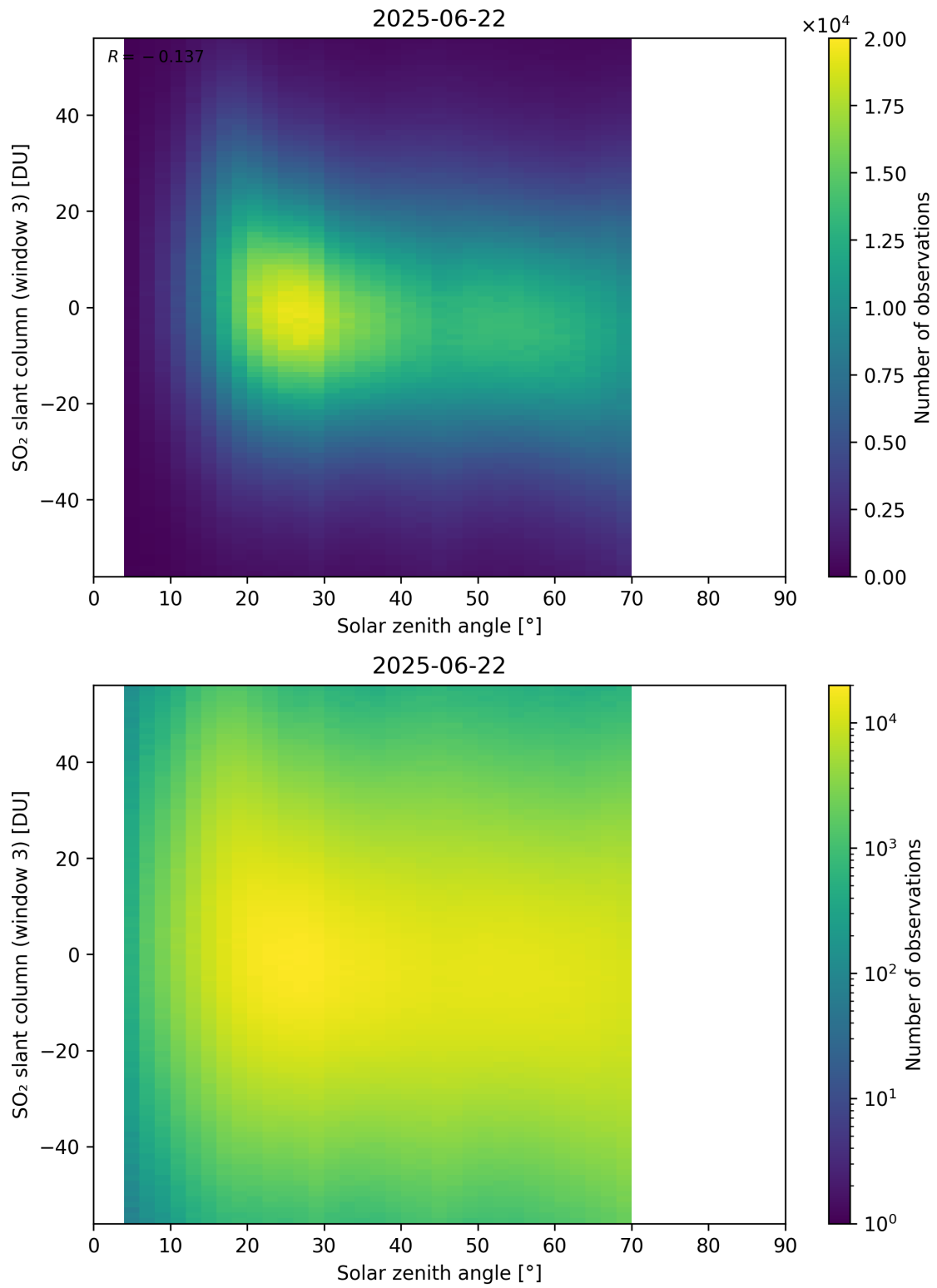
Figure 187: Scatter density plot of “Solar zenith angle” against “SO 2 slant column (window 3)” for 2025-06-22 to 2025-06-23.
