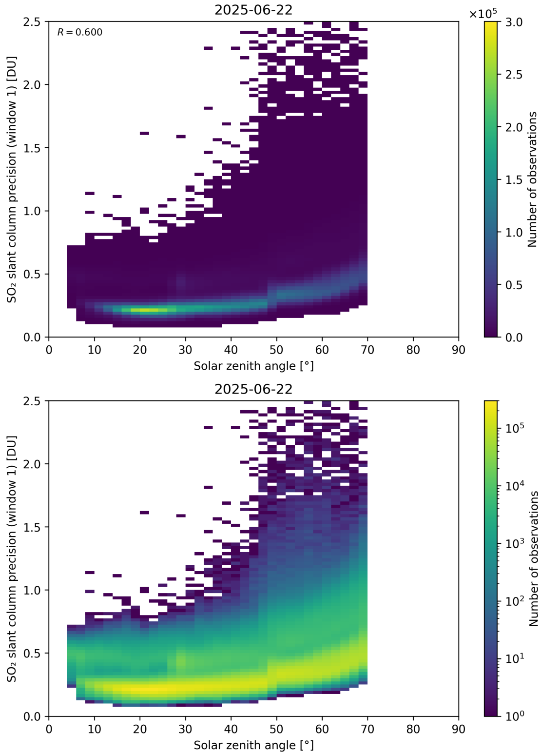
Figure 185: Scatter density plot of “Solar zenith angle” against “SO 2 slant column precision (window 1)” for 2025-06-22 to 2025-06-23.
