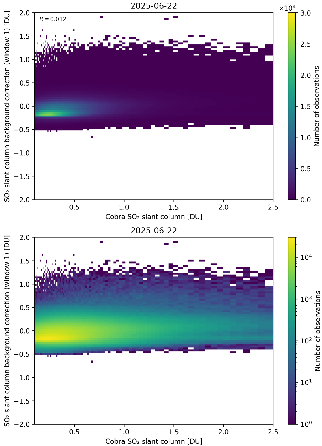
Figure 193: Scatter density plot of “Cobra SO 2 slant column” against “SO 2 slant column background correction (window 1)” for 2025-06-22 to 2025-06-23.
