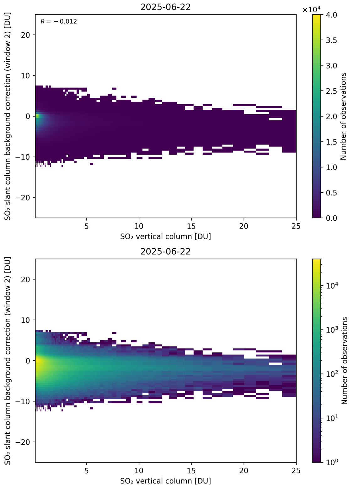
Figure 324: Scatter density plot of “SO 2 vertical column” against “SO 2 slant column background correction (window 2)” for 2025-06-22 to 2025-06-23.
