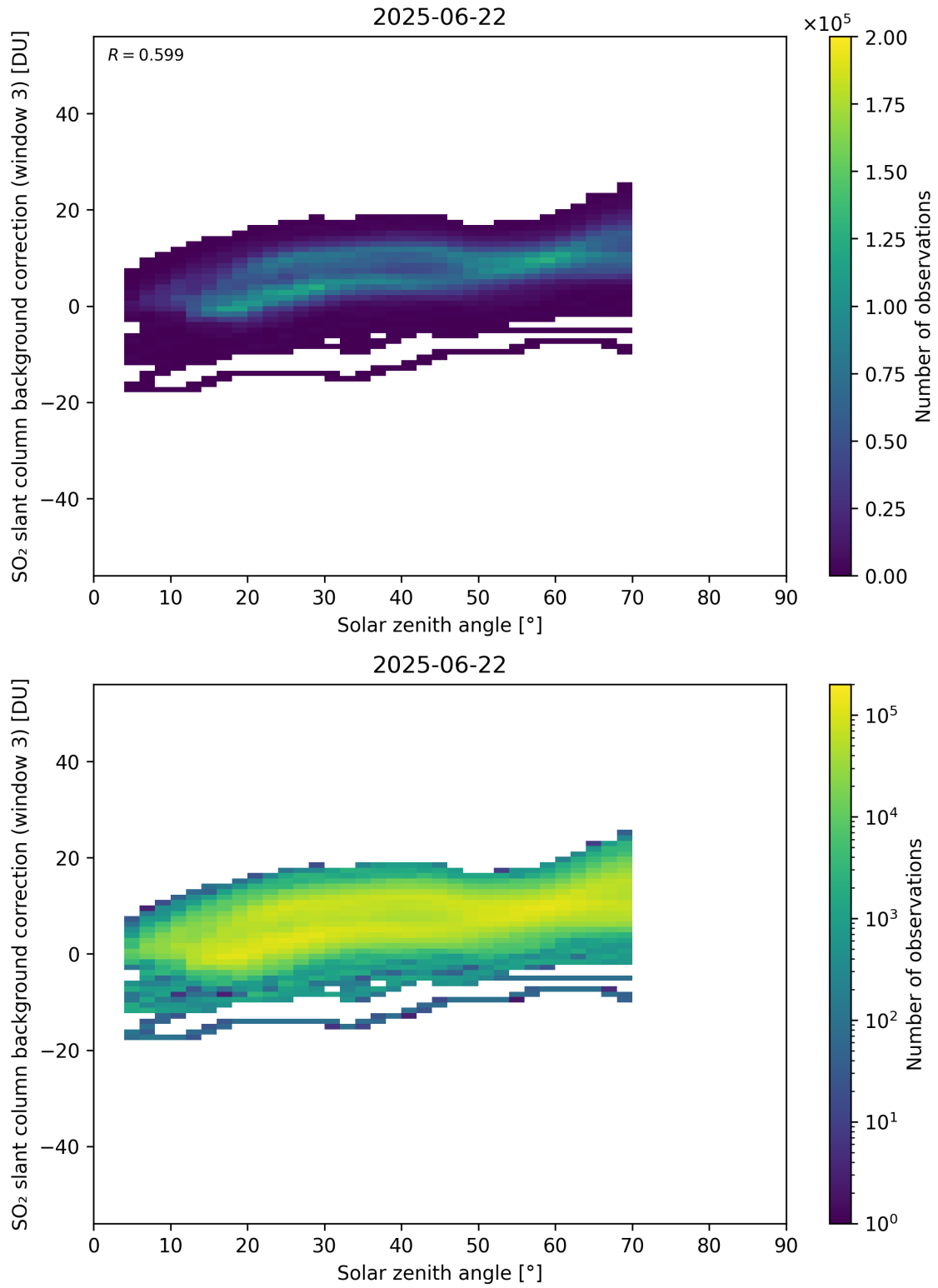
Figure 173: Scatter density plot of “Solar zenith angle” against “SO 2 slant column background correction (window 3)” for 2025-06-22 to 2025-06-23.
