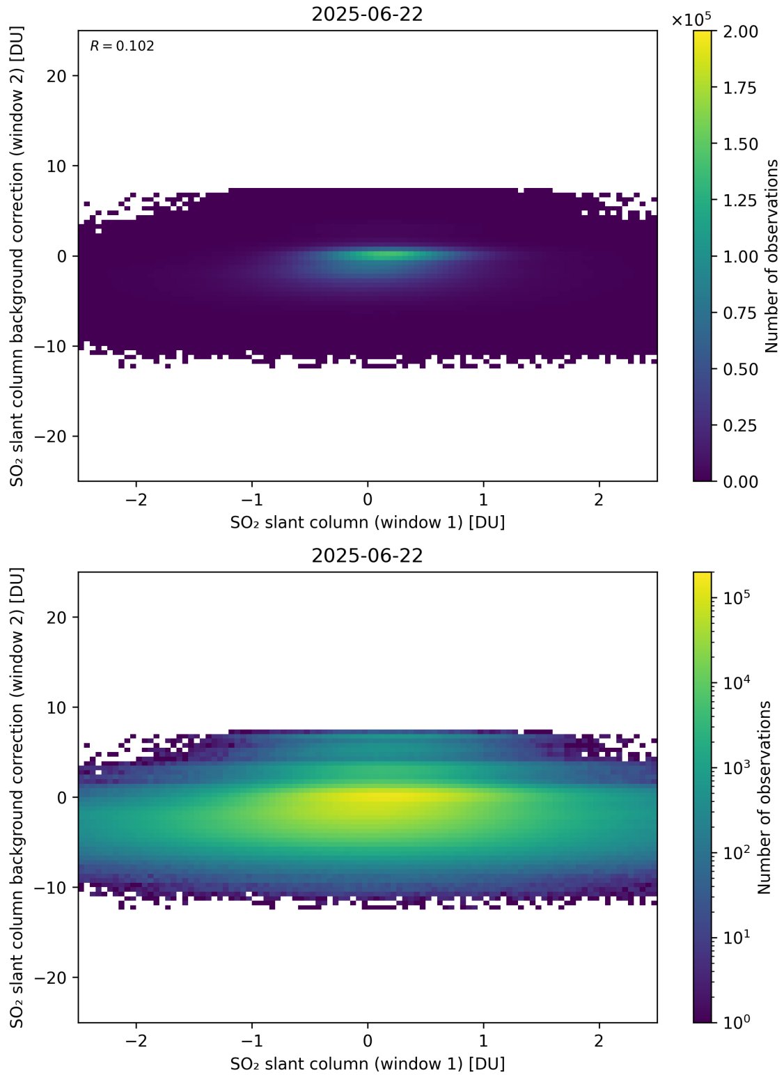
Figure 263: Scatter density plot of “SO 2 slant column (window 1)” against “SO 2 slant column background correction (window 2)” for 2025-06-22 to 2025-06-23.
