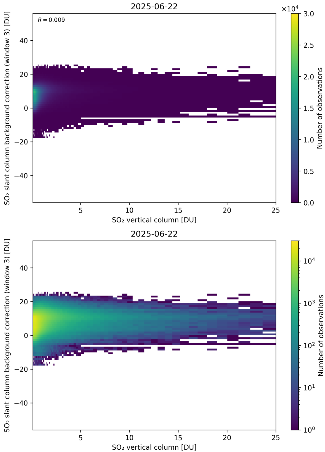
Figure 325: Scatter density plot of “SO 2 vertical column” against “SO 2 slant column background correction (window 3)” for 2025-06-22 to 2025-06-23.
