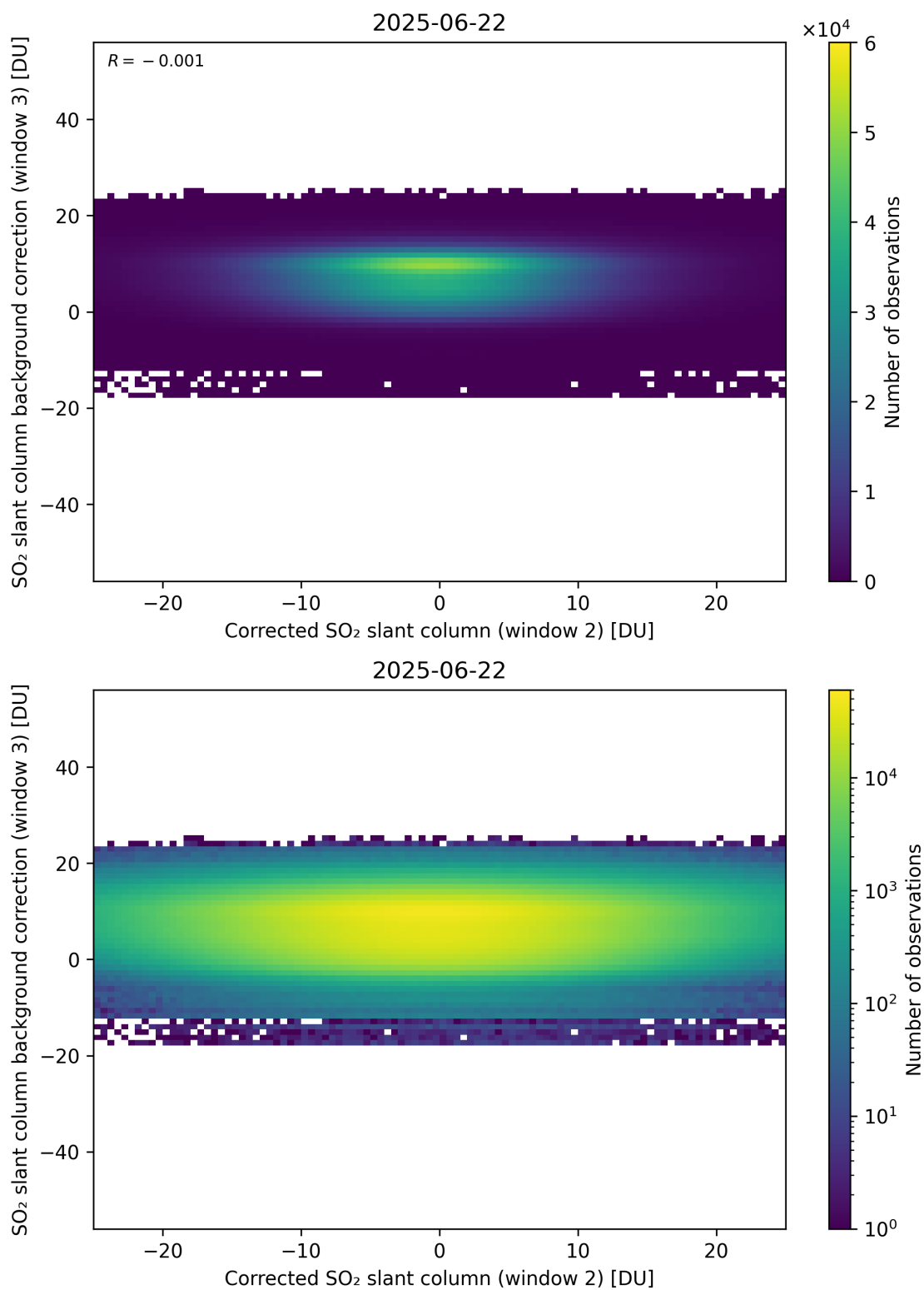
Figure 245: Scatter density plot of “Corrected SO 2 slant column (window 2)” against “SO 2 slant column background correction (window 3)” for 2025-06-22 to 2025-06-23.
