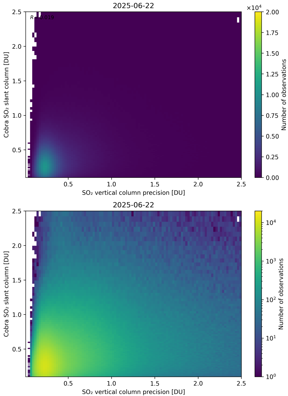
Figure 336: Scatter density plot of “SO 2 vertical column precision” against “Cobra SO 2 slant column” for 2025-06-22 to 2025-06-23.
