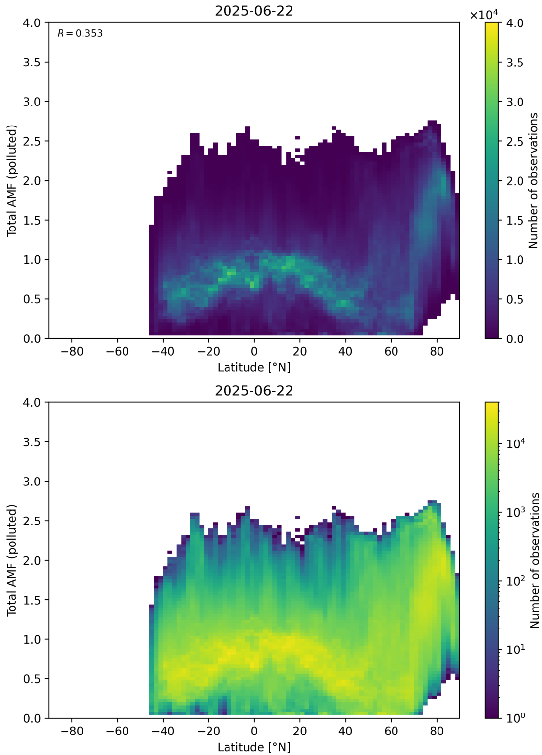
Figure 167: Scatter density plot of “Latitude” against “Total AMF (polluted)” for 2025-06-22 to 2025-06-23.
