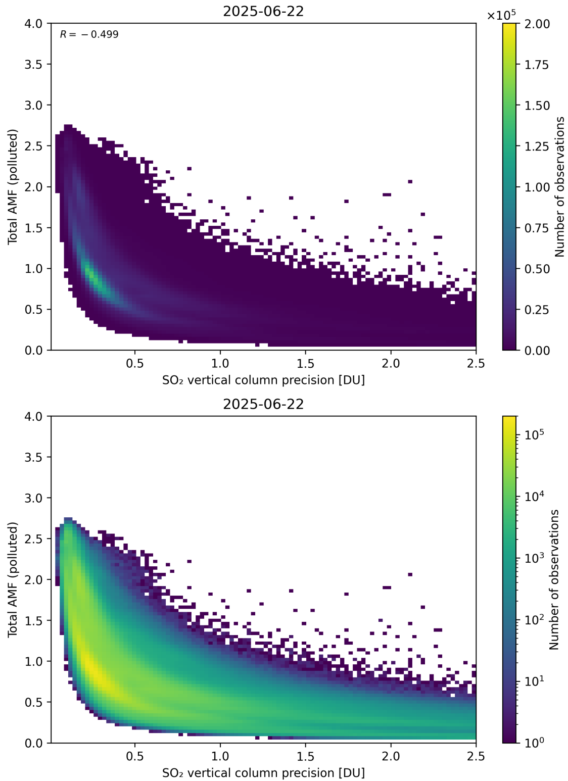
Figure 346: Scatter density plot of “SO 2 vertical column precision” against “Total AMF (polluted)” for 2025-06-22 to 2025-06-23.
