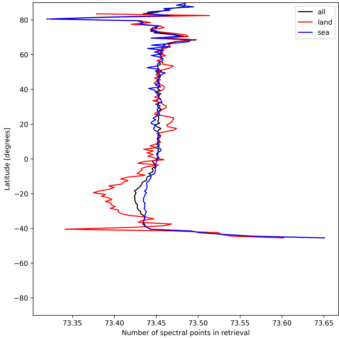
Figure 56: Zonal average of “Number of spectral points in retrieval” for 2025-06-22 to 2025-06-23.
