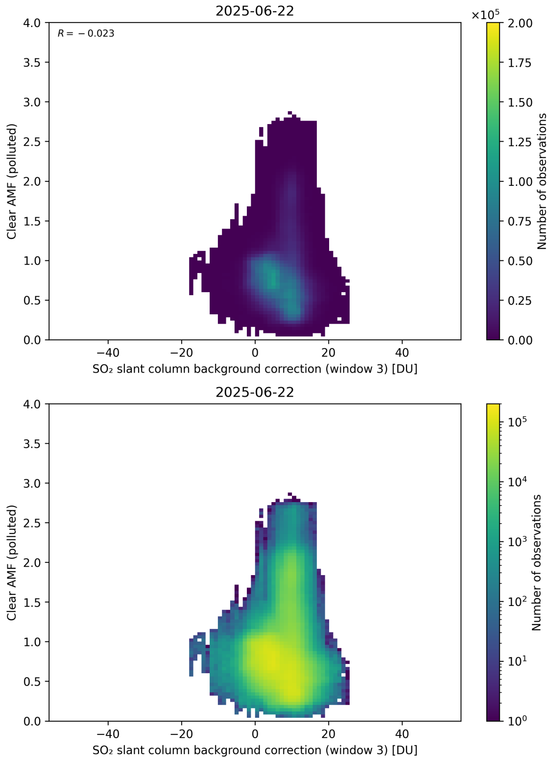
Figure 135: Scatter density plot of “SO 2 slant column background correction (window 3)” against “Clear AMF (polluted)” for 2025-06-22 to 2025-06-23.
