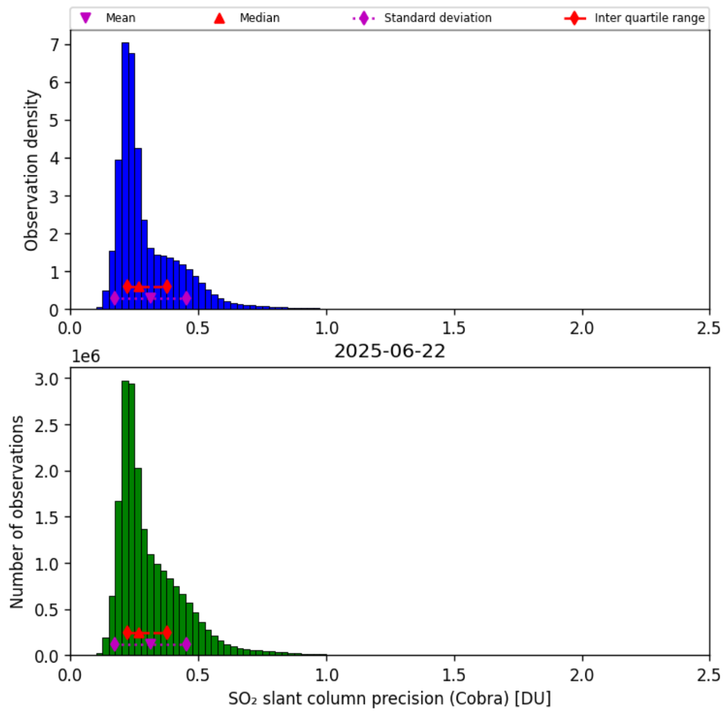
Figure 62: Histogram of “SO 2 slant column precision (Cobra)” for 2025-06-22 to 2025-06-23
