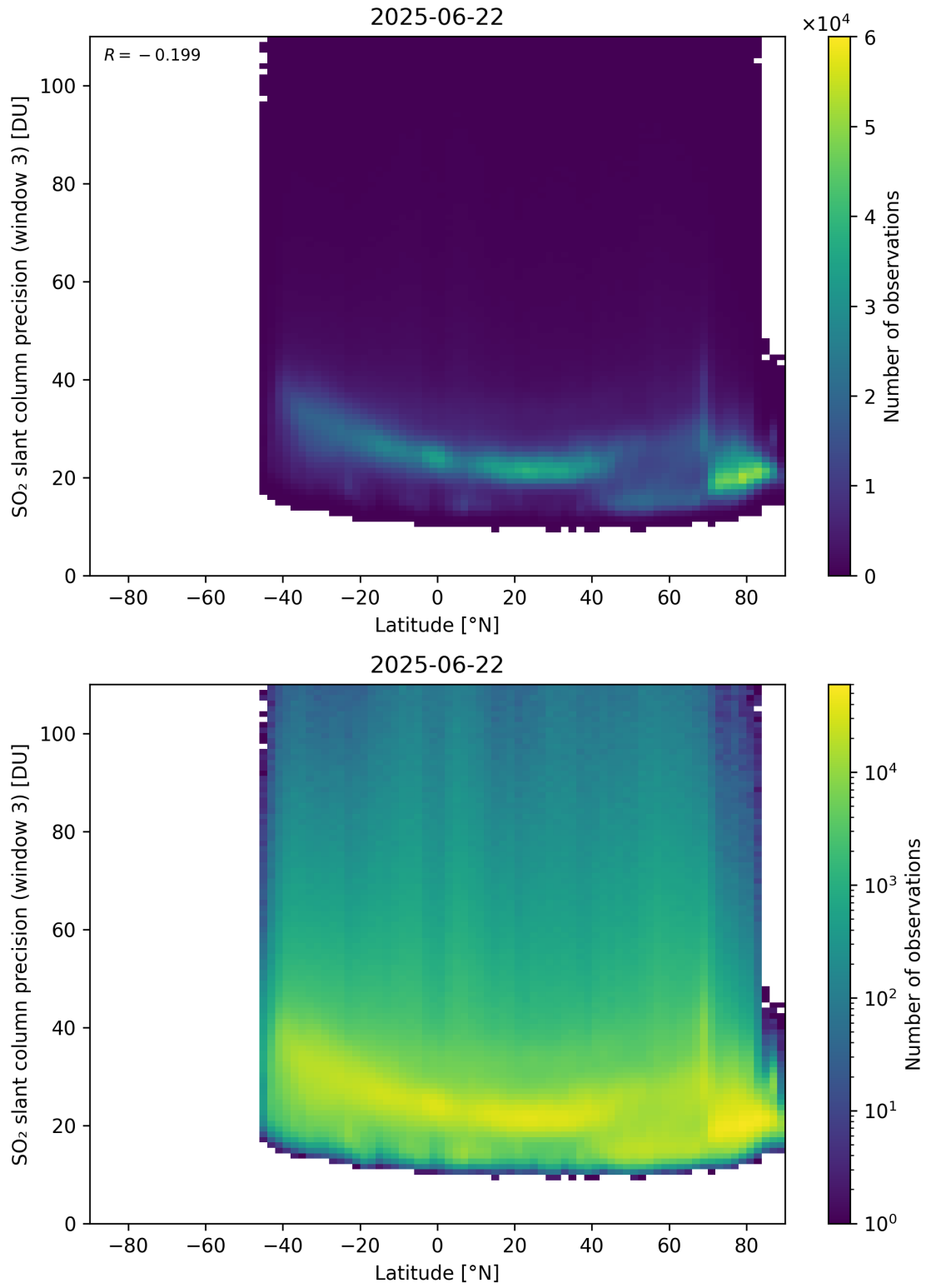
Figure 166: Scatter density plot of “Latitude” against “SO 2 slant column precision (window 3)” for 2025-06-22 to 2025-06-23.
