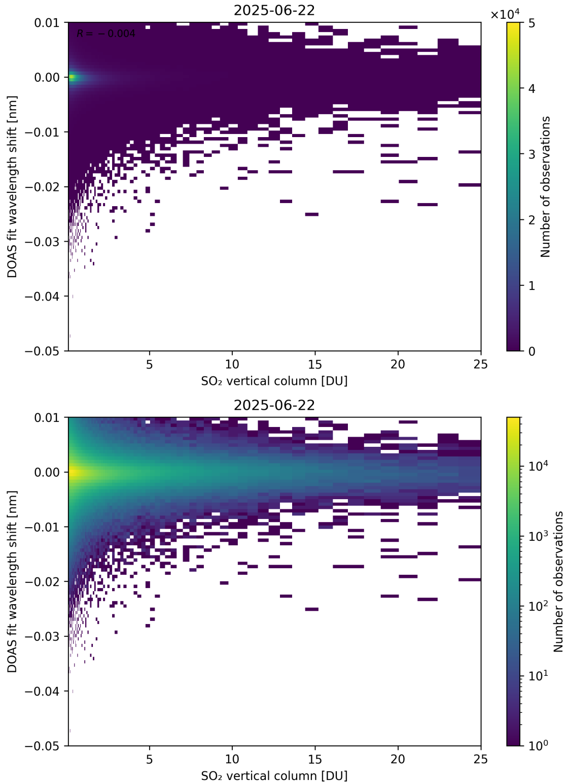
Figure 326: Scatter density plot of “SO 2 vertical column” against “DOAS fit wavelength shift” for 2025-06-22 to 2025-06-23.
