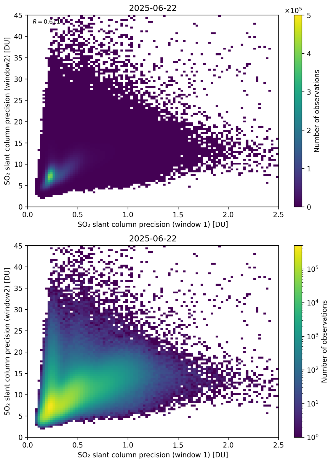
Figure 277: Scatter density plot of “SO 2 slant column precision (window 1)” against “SO 2 slant column precision (window2)” for 2025-06-22 to 2025-06-23.
