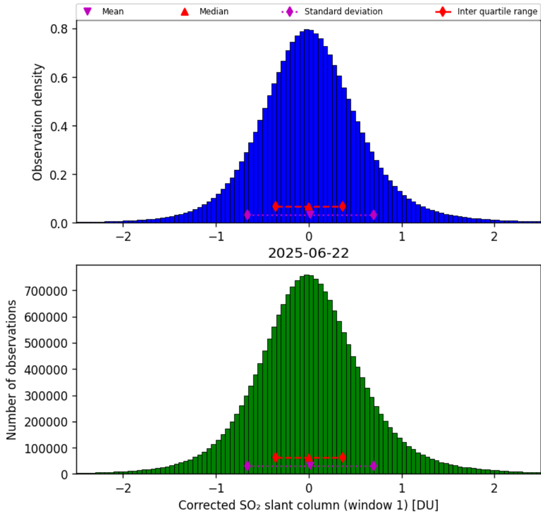
Figure 65: Histogram of “Corrected SO 2 slant column (window 1)” for 2025-06-22 to 2025-06-23
