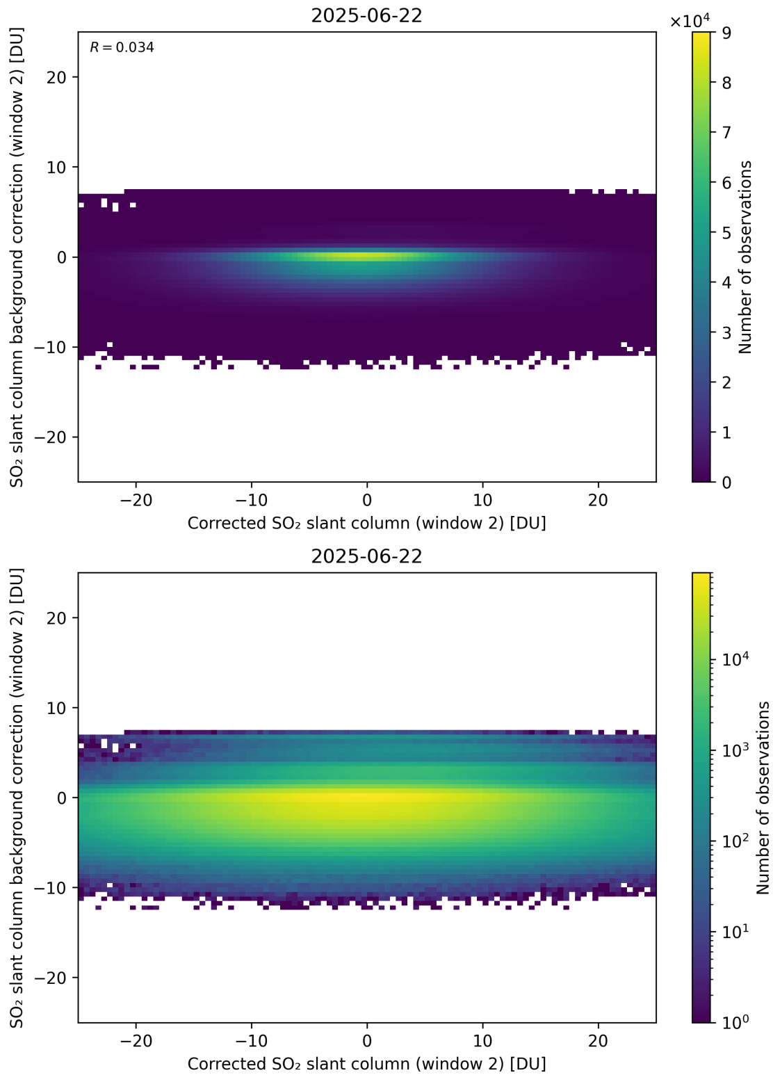
Figure 244: Scatter density plot of “Corrected SO 2 slant column (window 2)” against “SO 2 slant column background correction (window 2)” for 2025-06-22 to 2025-06-23.
