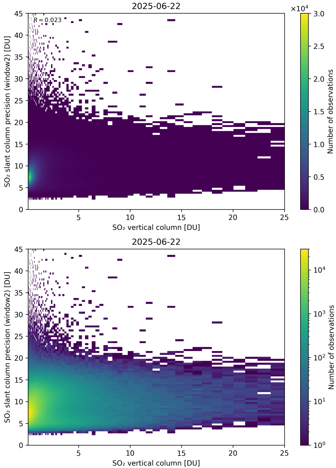
Figure 356: Scatter density plot of “SO 2 vertical column” against “SO 2 slant column precision (window2)” for 2025-06-22 to 2025-06-23.
