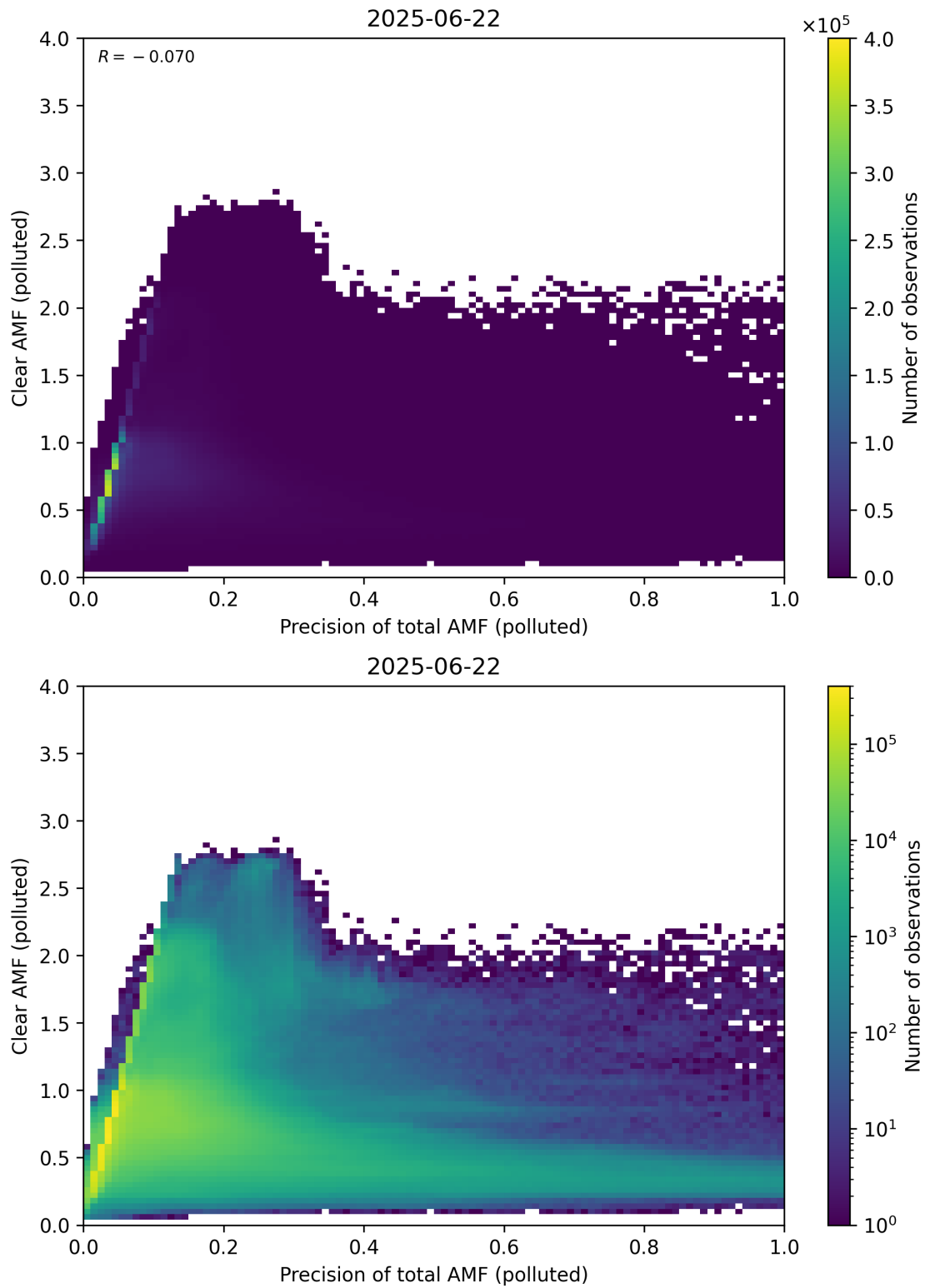
Figure 320: Scatter density plot of “Precision of total AMF (polluted)” against “Clear AMF (polluted)” for 2025-06-22 to 2025-06-23.
