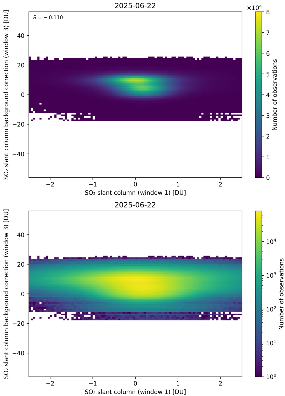
Figure 264: Scatter density plot of “SO 2 slant column (window 1)” against “SO 2 slant column background correction (window 3)” for 2025-06-22 to 2025-06-23.
