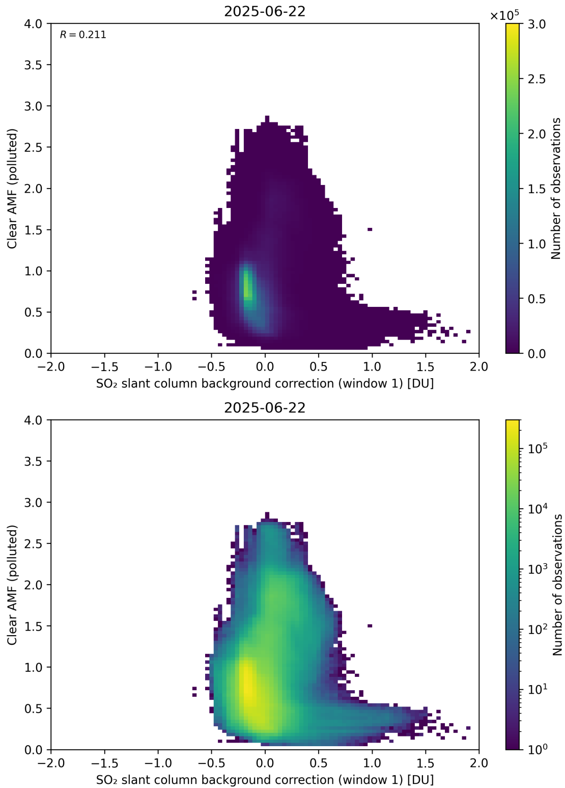
Figure 114: Scatter density plot of “SO 2 slant column background correction (window 1)” against “Clear AMF (polluted)” for 2025-06-22 to 2025-06-23.
