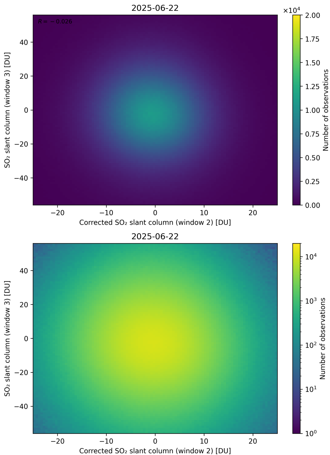
Figure 251: Scatter density plot of “Corrected SO 2 slant column (window 2)” against “SO 2 slant column (window 3)” for 2025-06-22 to 2025-06-23.
