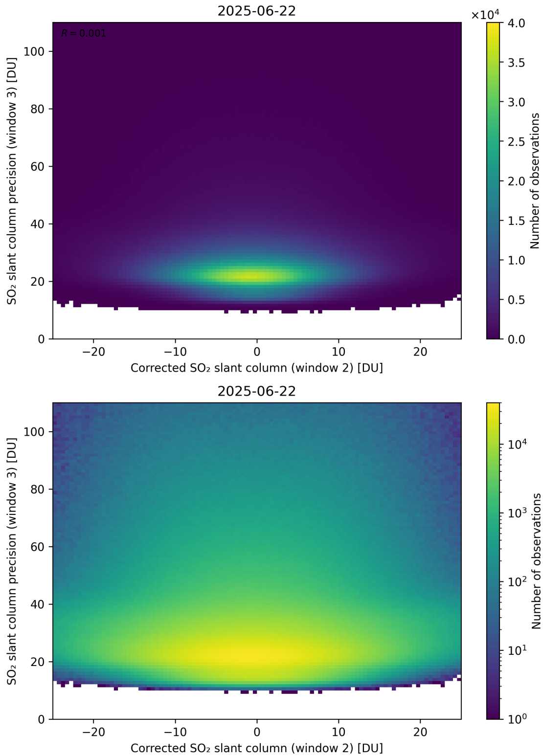
Figure 252: Scatter density plot of “Corrected SO 2 slant column (window 2)” against “SO 2 slant column precision (window 3)” for 2025-06-22 to 2025-06-23.
