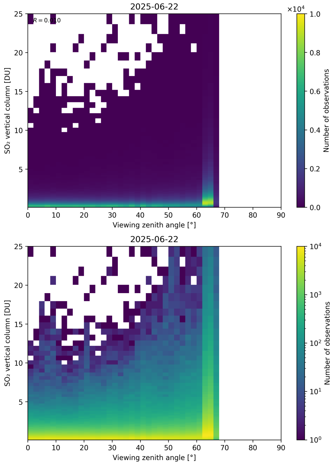
Figure 383: Scatter density plot of “Viewing zenith angle” against “SO 2 vertical column” for 2025-06-22 to 2025-06-23.
