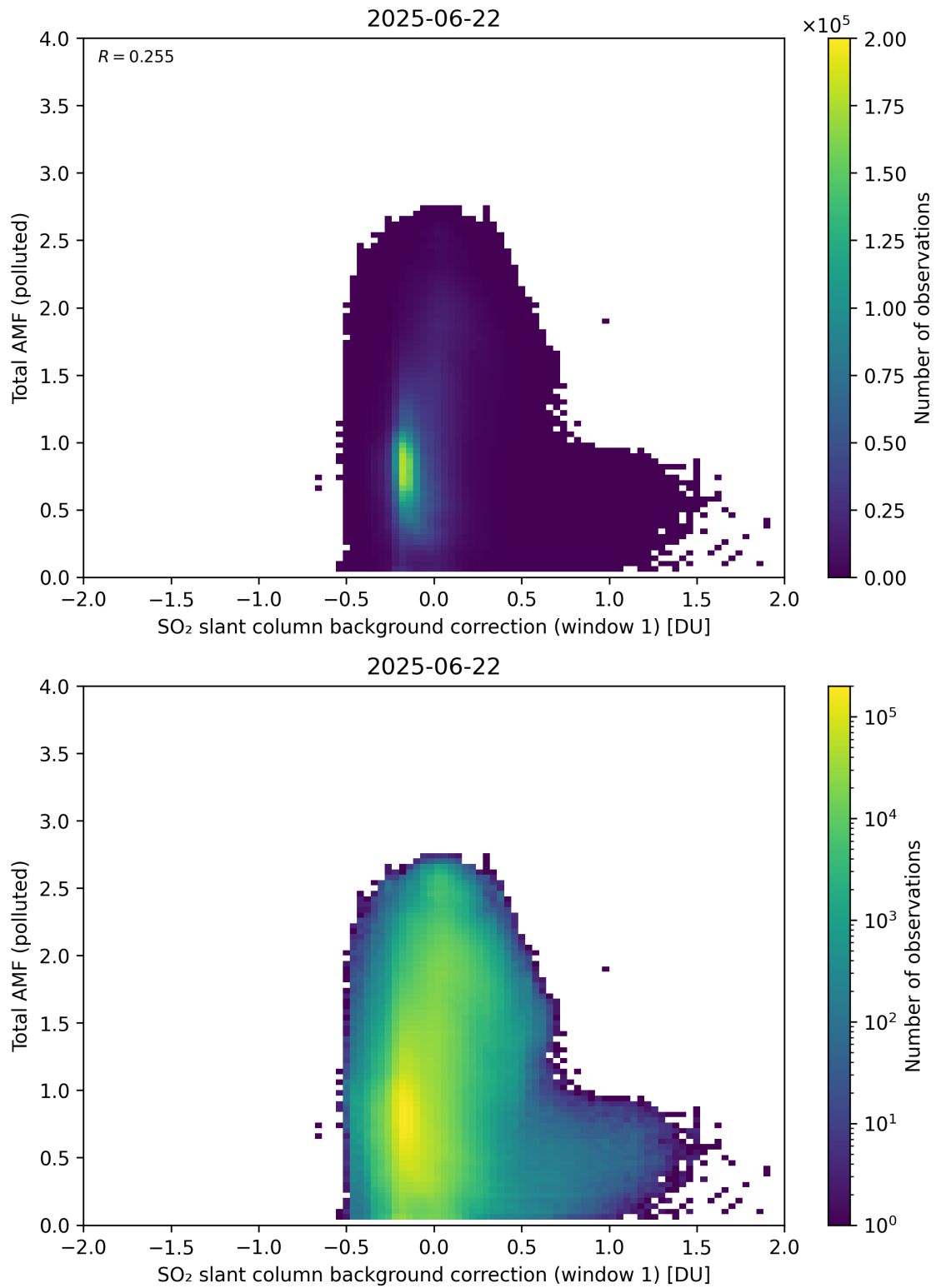
Figure 120: Scatter density plot of “SO 2 slant column background correction (window 1)” against “Total AMF (polluted)” for 2025-06-22 to 2025-06-23.
