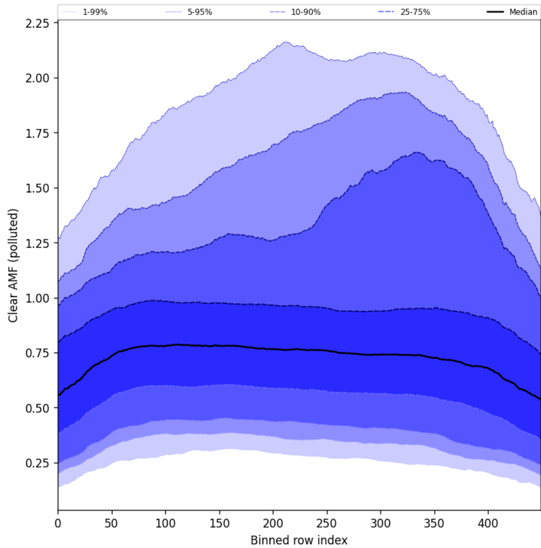
Figure 107: Along track statistics of “Clear AMF (polluted)” for 2025-06-22 to 2025-06-23
