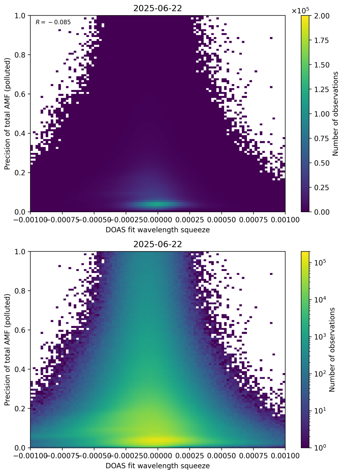
Figure 146: Scatter density plot of “DOAS fit wavelength squeeze” against “Precision of total AMF (polluted)” for 2025-06-22 to 2025-06-23.
