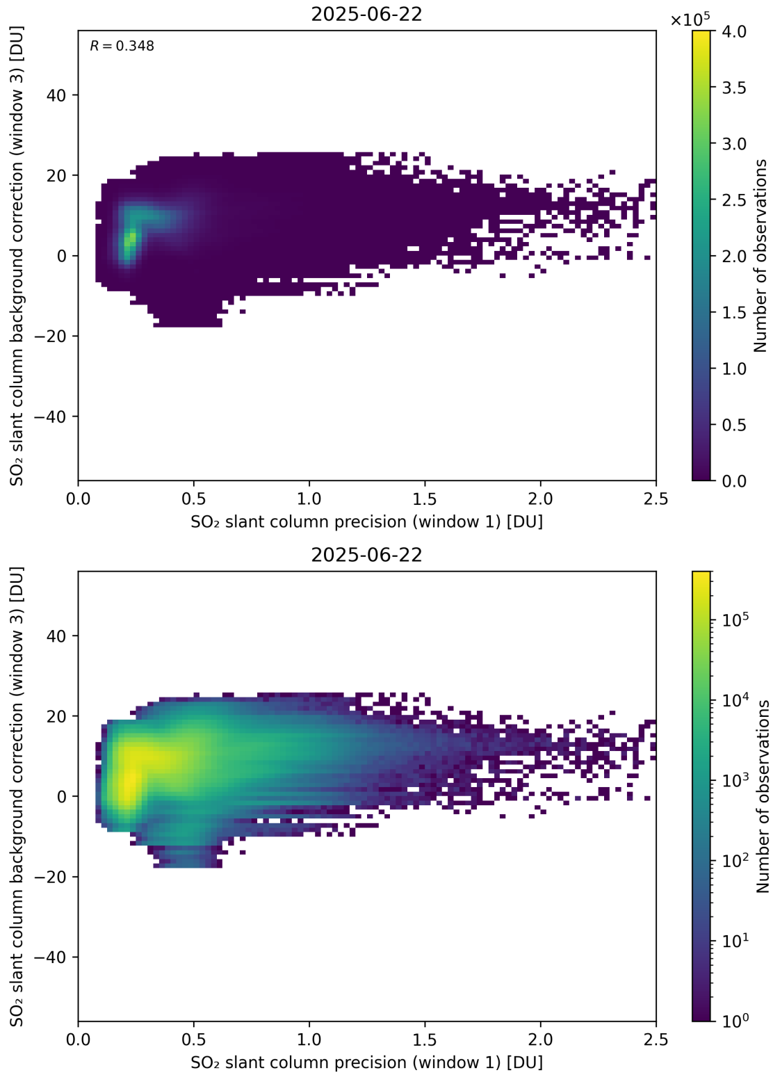
Figure 270: Scatter density plot of “SO 2 slant column precision (window 1)” against “SO 2 slant column background correction (window 3)” for 2025-06-22 to 2025-06-23.
