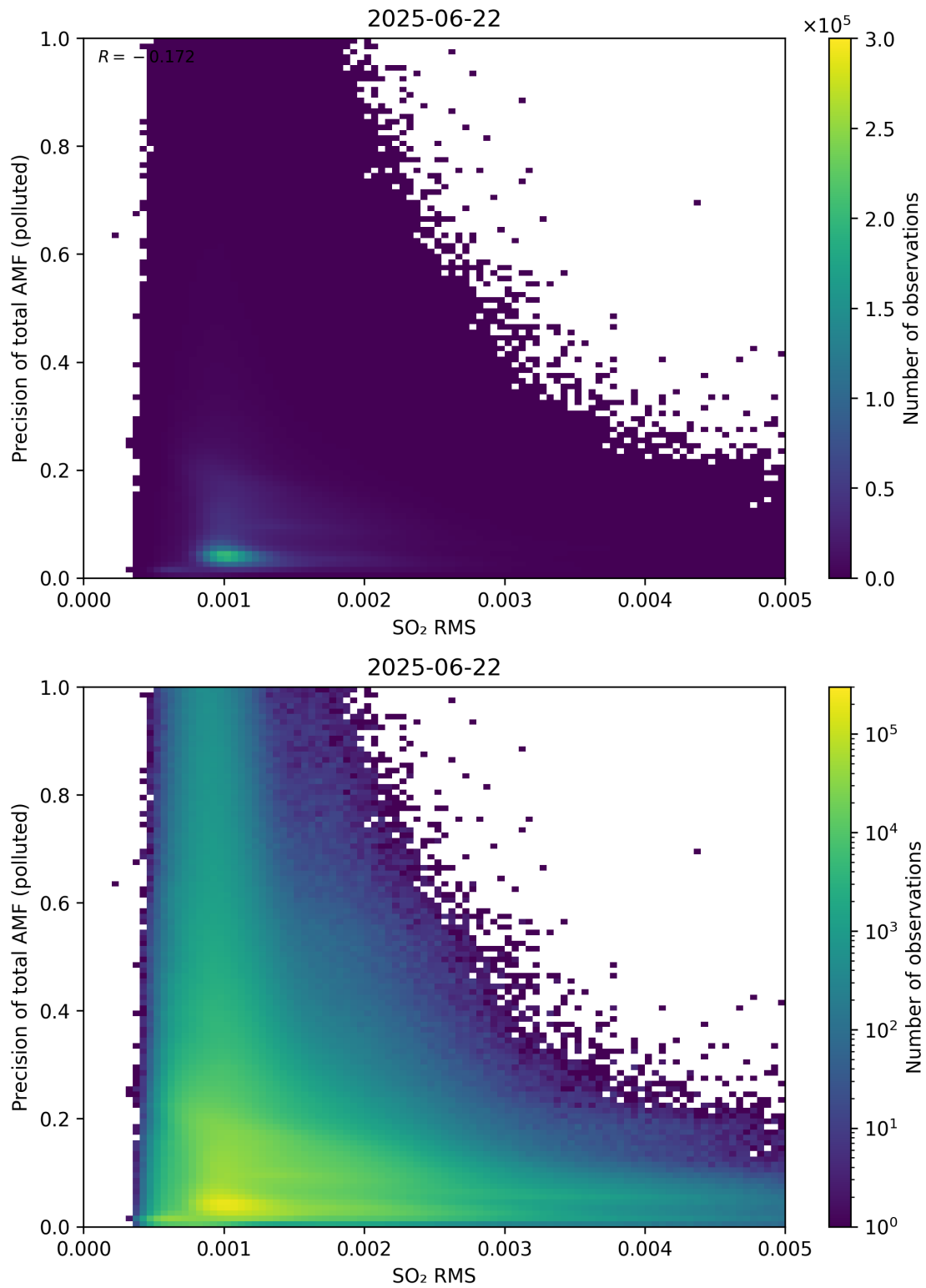
Figure 149: Scatter density plot of “SO 2 RMS” against “Precision of total AMF (polluted)” for 2025-06-22 to 2025-06-23.
