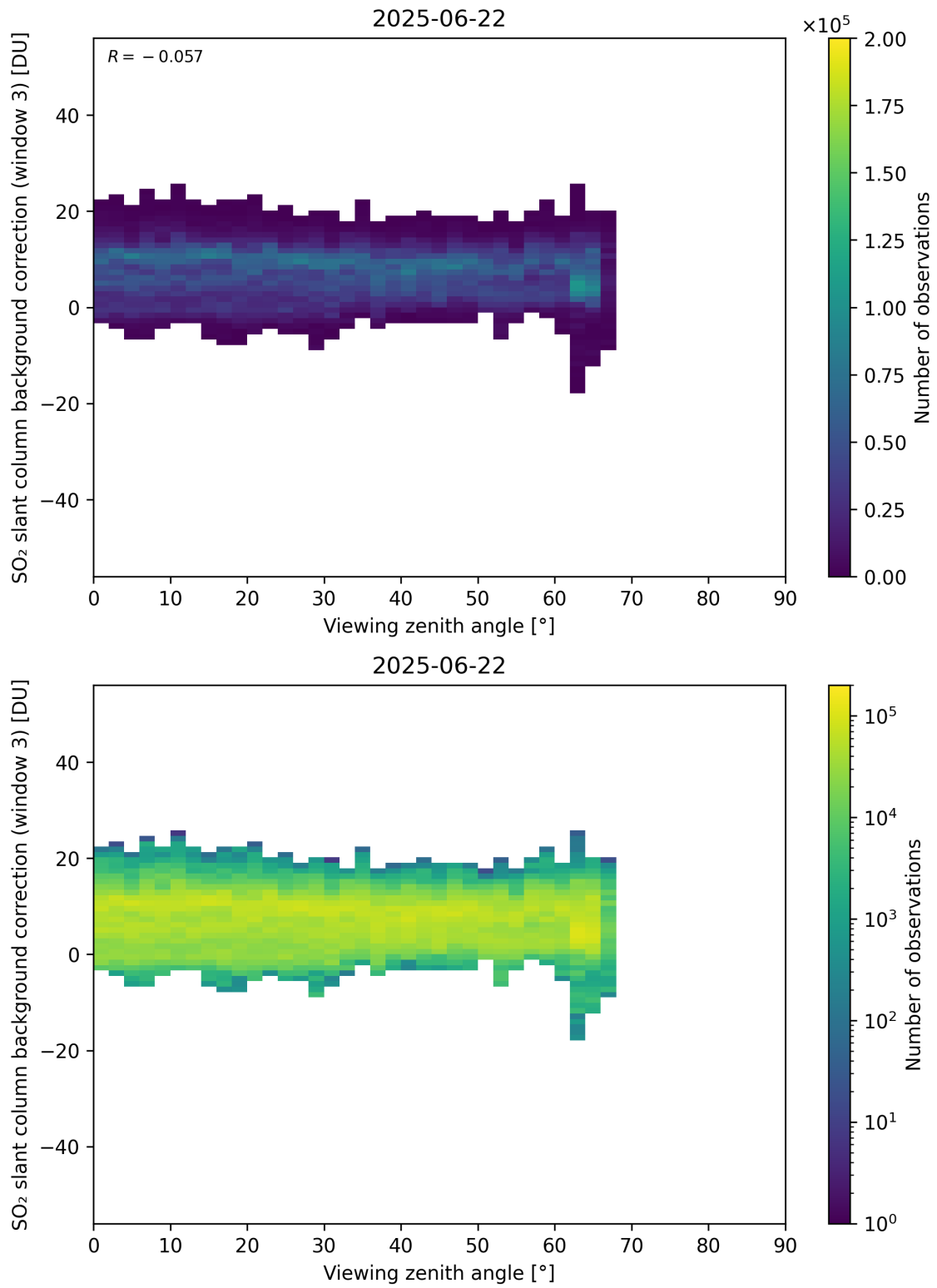
Figure 364: Scatter density plot of “Viewing zenith angle” against “SO 2 slant column background correction (window 3)” for 2025-06-22 to 2025-06-23.
