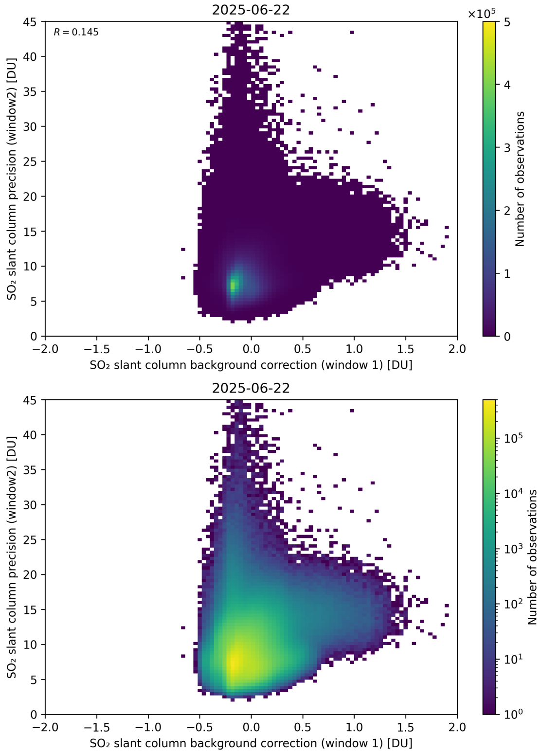
Figure 117: Scatter density plot of “SO 2 slant column background correction (window 1)” against “SO 2 slant column precision (window2)” for 2025-06-22 to 2025-06-23.
