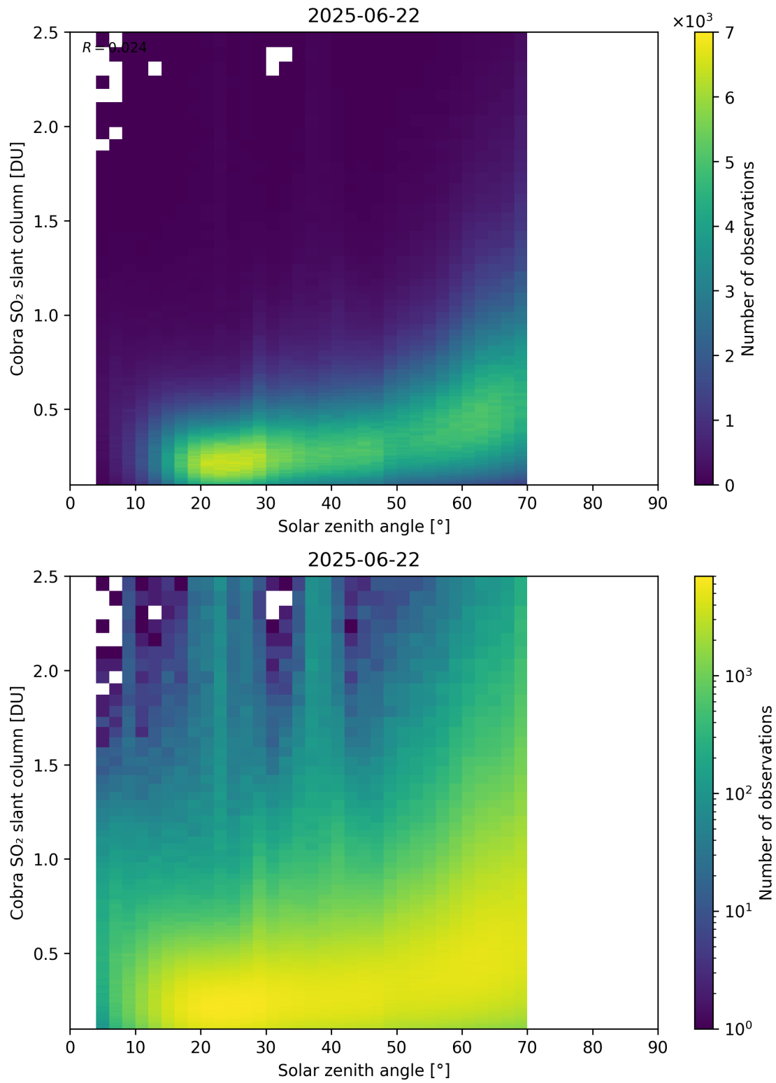
Figure 179: Scatter density plot of “Solar zenith angle” against “Cobra SO 2 slant column” for 2025-06-22 to 2025-06-23.
