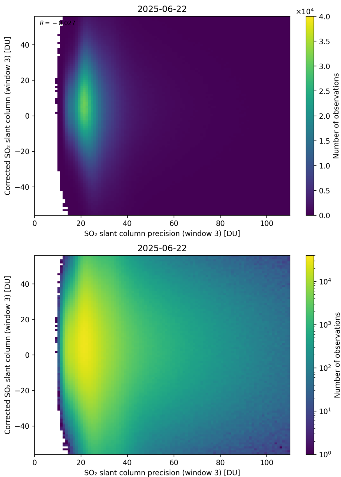
Figure 312: Scatter density plot of “SO 2 slant column precision (window 3)” against “Corrected SO 2 slant column (window 3)” for 2025-06-22 to 2025-06-23.
