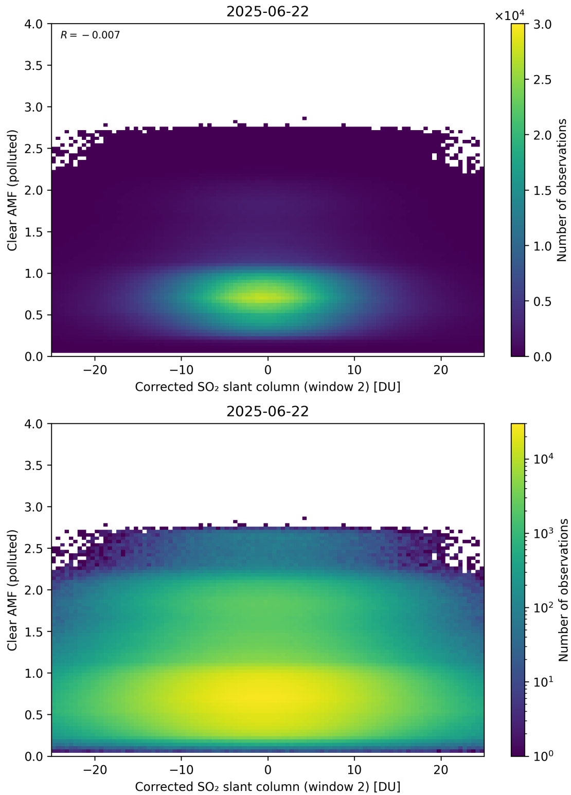
Figure 249: Scatter density plot of “Corrected SO 2 slant column (window 2)” against “Clear AMF (polluted)” for 2025-06-22 to 2025-06-23.
