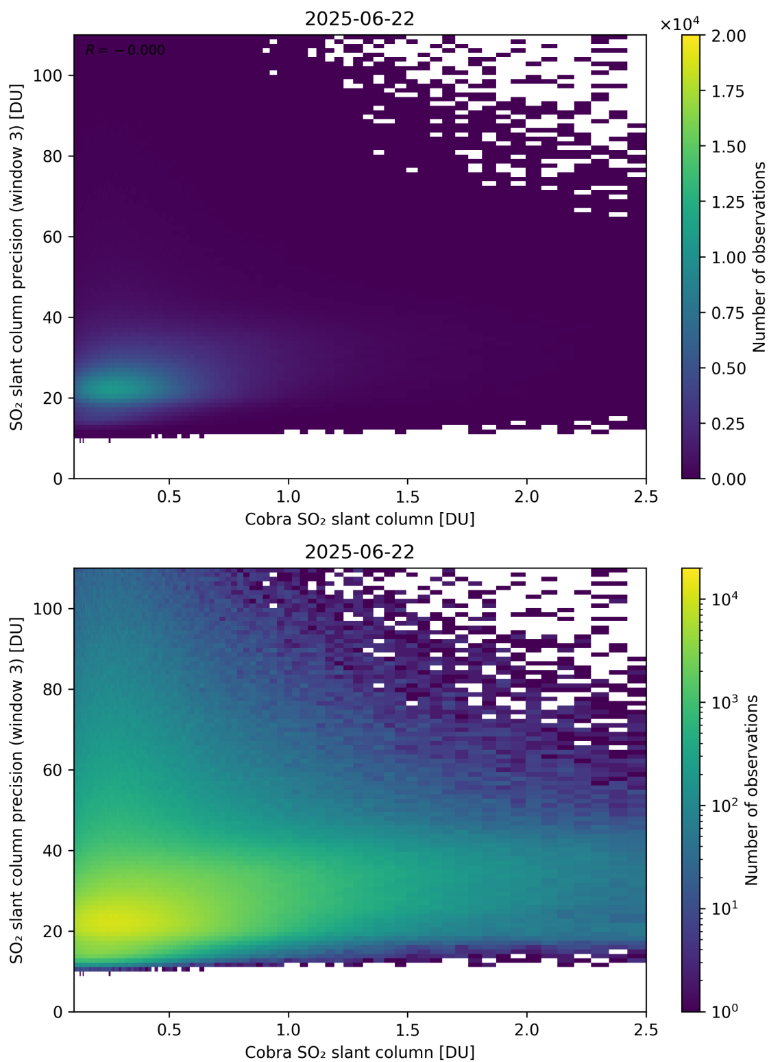
Figure 223: Scatter density plot of “Cobra SO 2 slant column” against “SO 2 slant column precision (window 3)” for 2025-06-22 to 2025-06-23.
