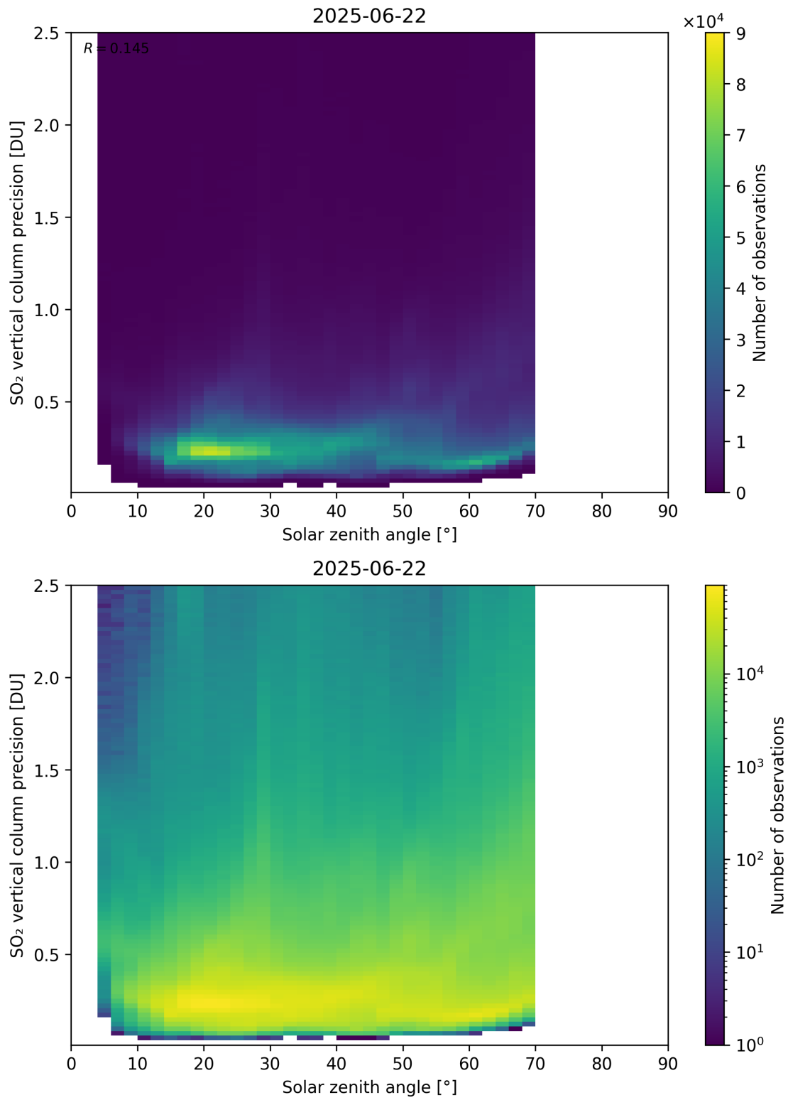
Figure 192: Scatter density plot of “Solar zenith angle” against “SO 2 vertical column precision” for 2025-06-22 to 2025-06-23.
