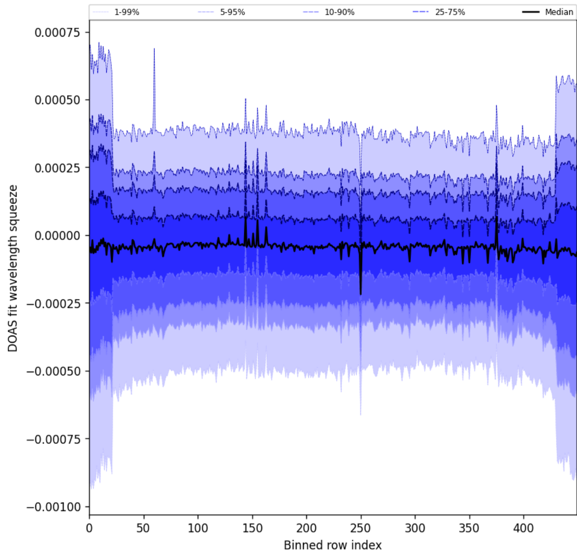
Figure 103: Along track statistics of “DOAS fit wavelength squeeze” for 2025-06-22 to 2025-06-23
