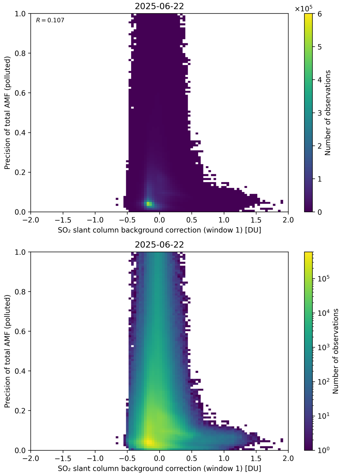
Figure 121: Scatter density plot of “SO 2 slant column background correction (window 1)” against “Precision of total AMF (polluted)” for 2025-06-22 to 2025-06-23.
