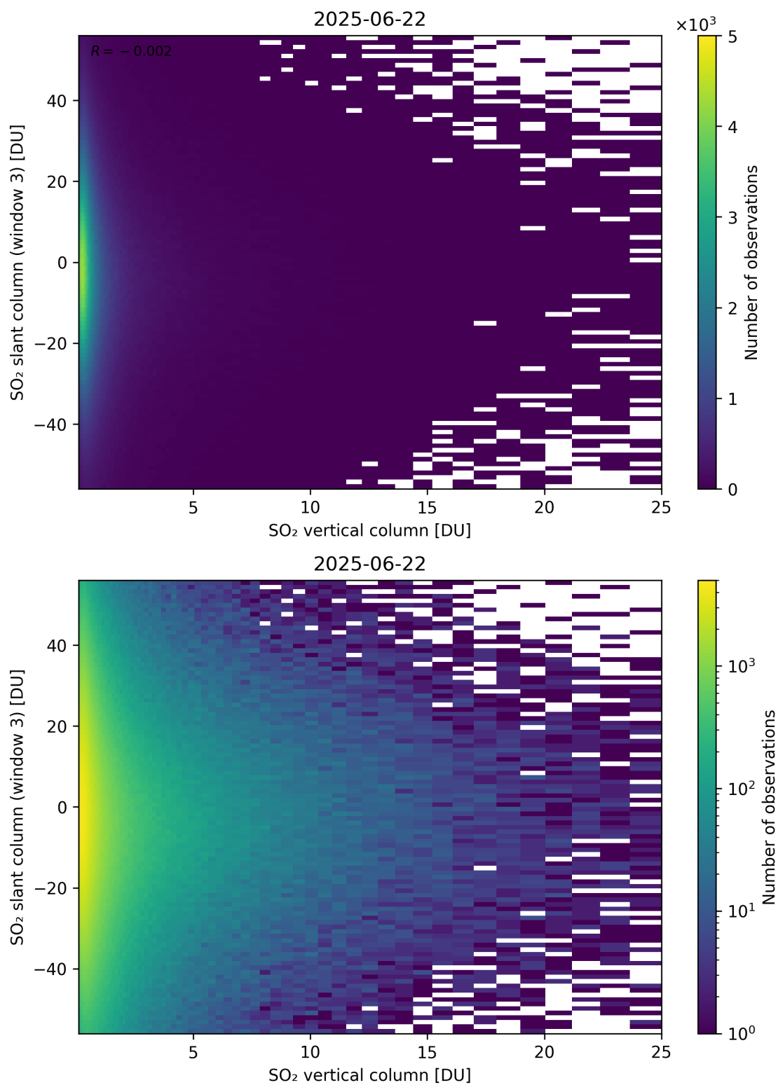
Figure 357: Scatter density plot of “SO 2 vertical column” against “SO 2 slant column (window 3)” for 2025-06-22 to 2025-06-23.
