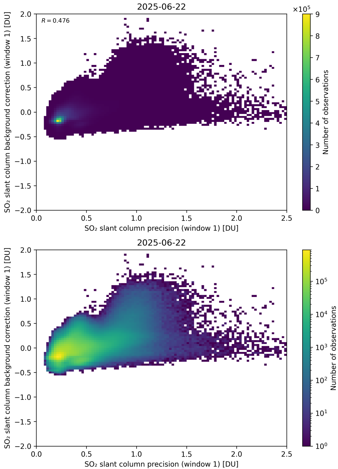
Figure 268: Scatter density plot of “SO 2 slant column precision (window 1)” against “SO 2 slant column background correction (window 1)” for 2025-06-22 to 2025-06-23.
