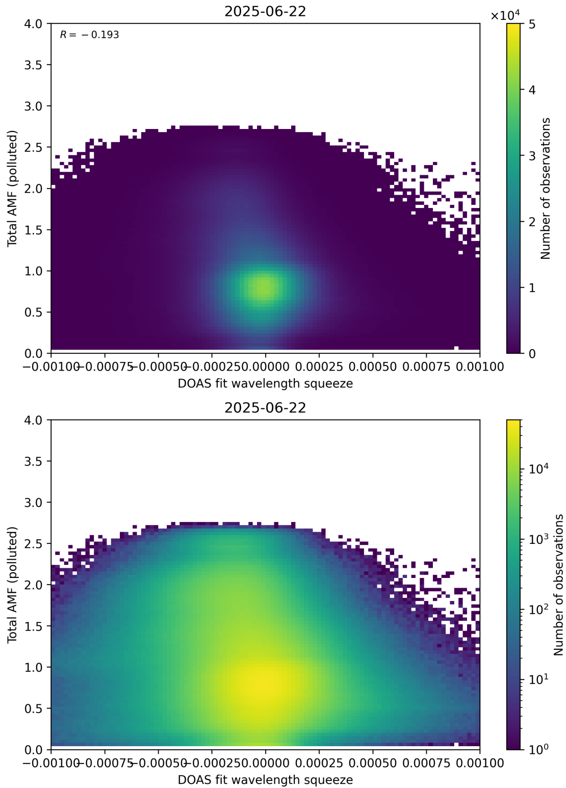
Figure 145: Scatter density plot of “DOAS fit wavelength squeeze” against “Total AMF (polluted)” for 2025-06-22 to 2025-06-23.
