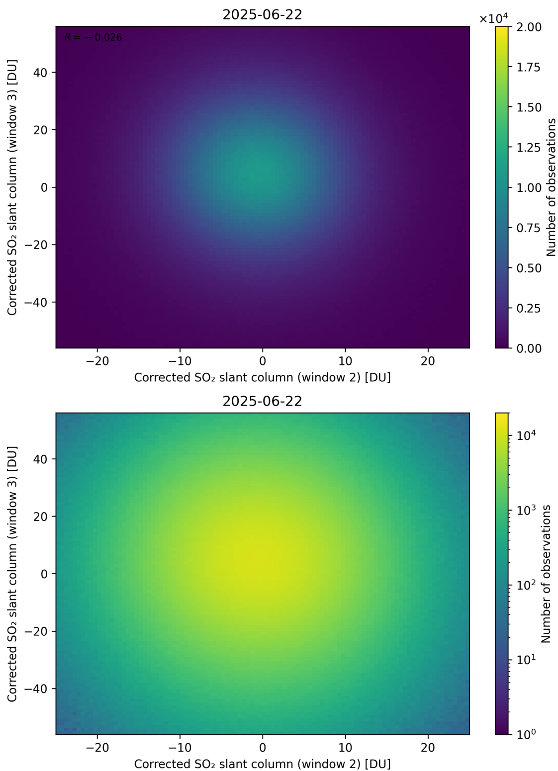
Figure 250: Scatter density plot of “Corrected SO 2 slant column (window 2)” against “Corrected SO 2 slant column (window 3)” for 2025-06-22 to 2025-06-23.
