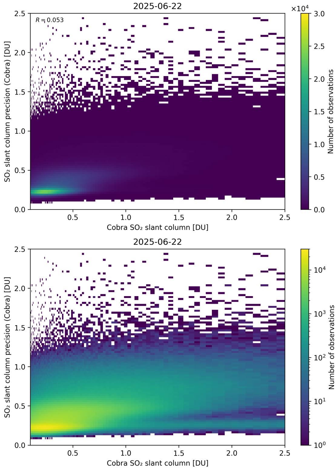
Figure 216: Scatter density plot of “Cobra SO 2 slant column” against “SO 2 slant column precision (Cobra)” for 2025-06-22 to 2025-06-23.
