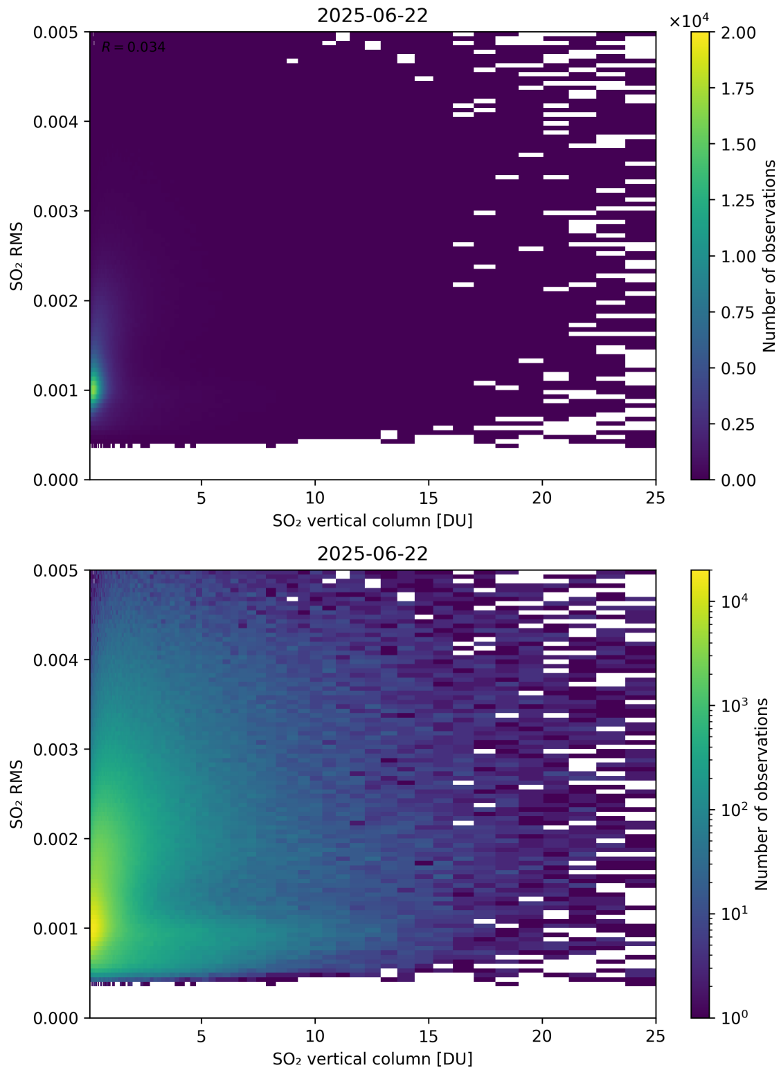
Figure 328: Scatter density plot of “SO 2 vertical column” against “SO 2 RMS” for 2025-06-22 to 2025-06-23.
