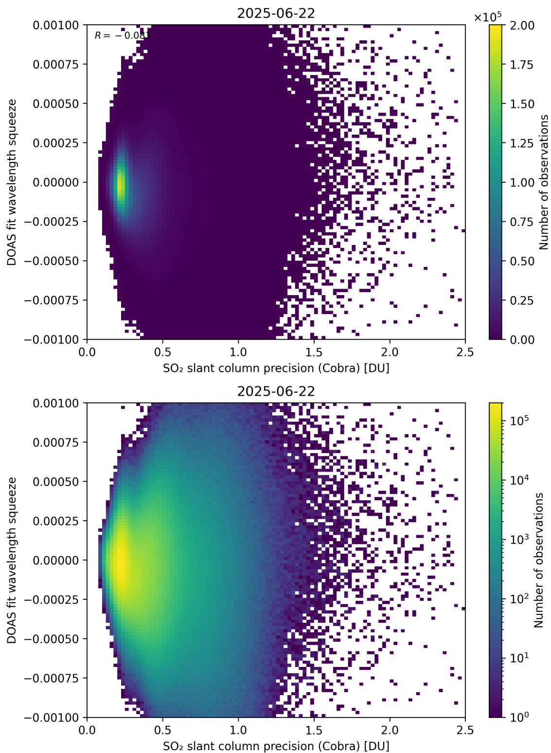
Figure 203: Scatter density plot of “SO 2 slant column precision (Cobra)” against “DOAS fit wavelength squeeze” for 2025-06-22 to 2025-06-23.
