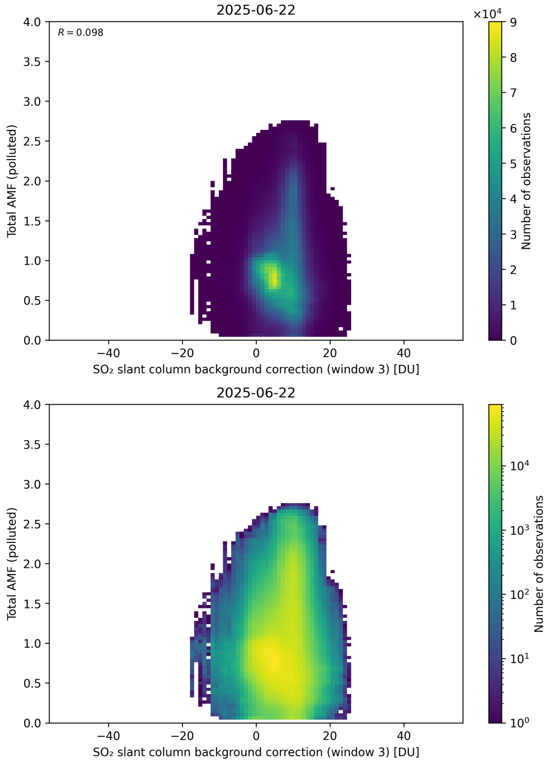
Figure 136: Scatter density plot of “SO 2 slant column background correction (window 3)” against “Total AMF (polluted)” for 2025-06-22 to 2025-06-23.
