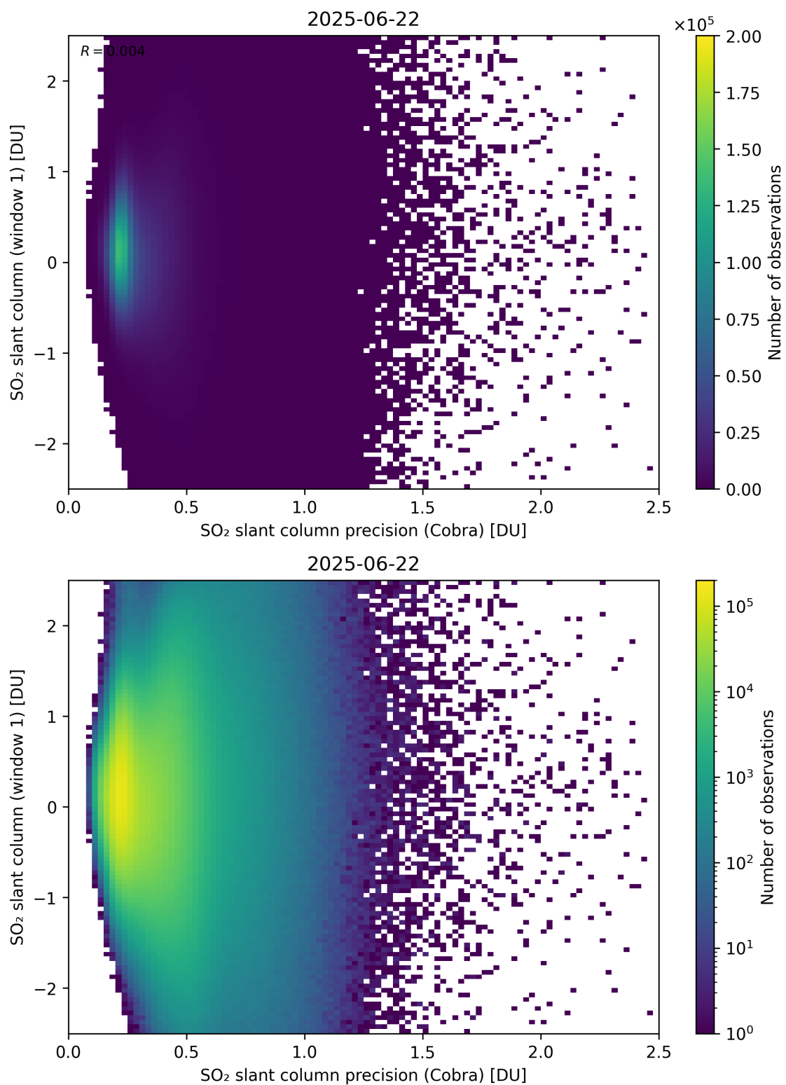
Figure 208: Scatter density plot of “SO 2 slant column precision (Cobra)” against “SO 2 slant column (window 1)” for 2025-06-22 to 2025-06-23.
