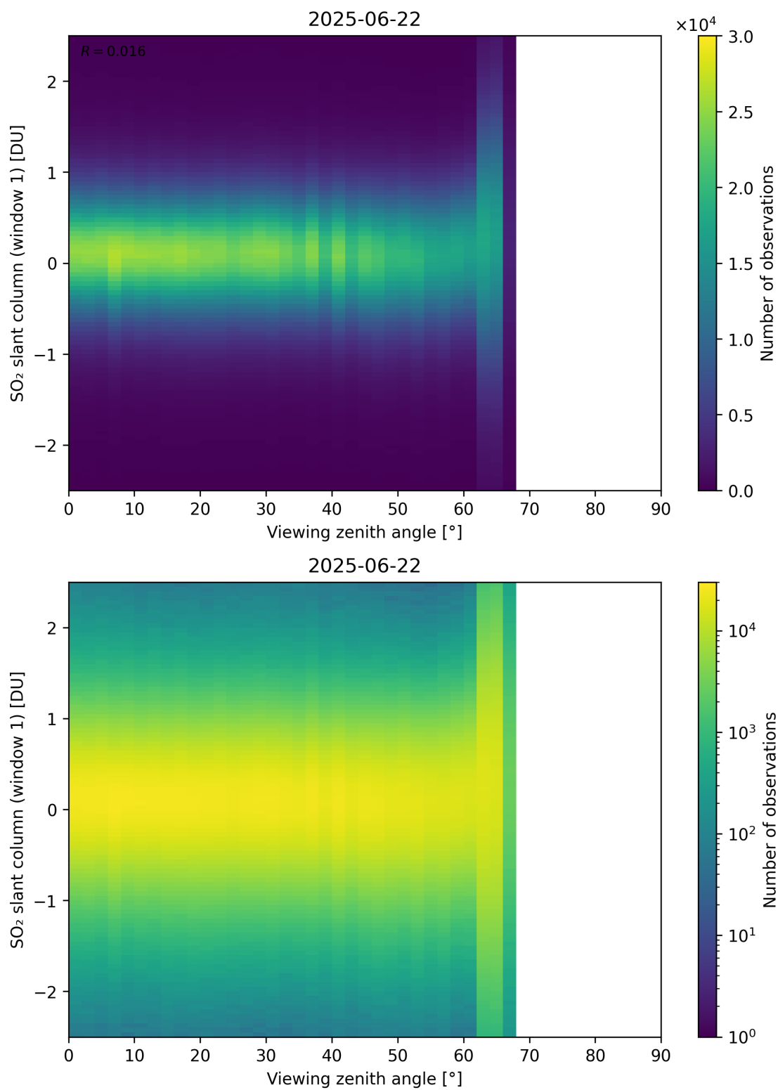
Figure 376: Scatter density plot of “Viewing zenith angle” against “SO 2 slant column (window 1)” for 2025-06-22 to 2025-06-23.
