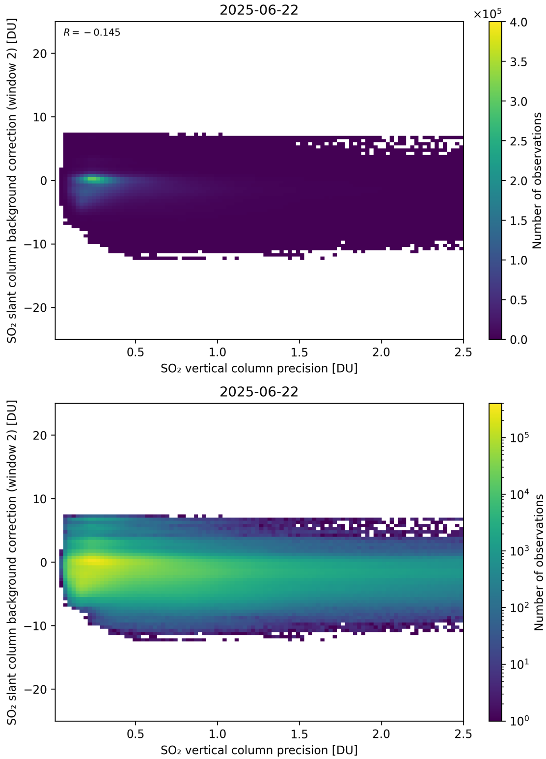
Figure 330: Scatter density plot of “SO 2 vertical column precision” against “SO 2 slant column background correction (window 2)” for 2025-06-22 to 2025-06-23.
