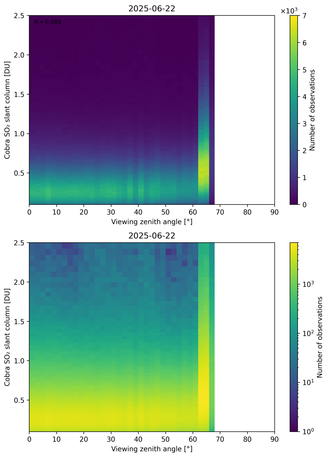
Figure 371: Scatter density plot of “Viewing zenith angle” against “Cobra SO 2 slant column” for 2025-06-22 to 2025-06-23.
