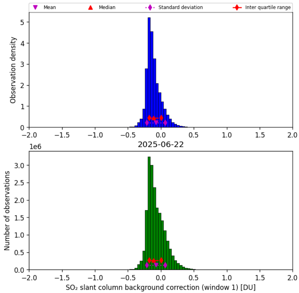
Figure 66: Histogram of “SO 2 slant column background correction (window 1)” for 2025-06-22 to 2025-06-23
