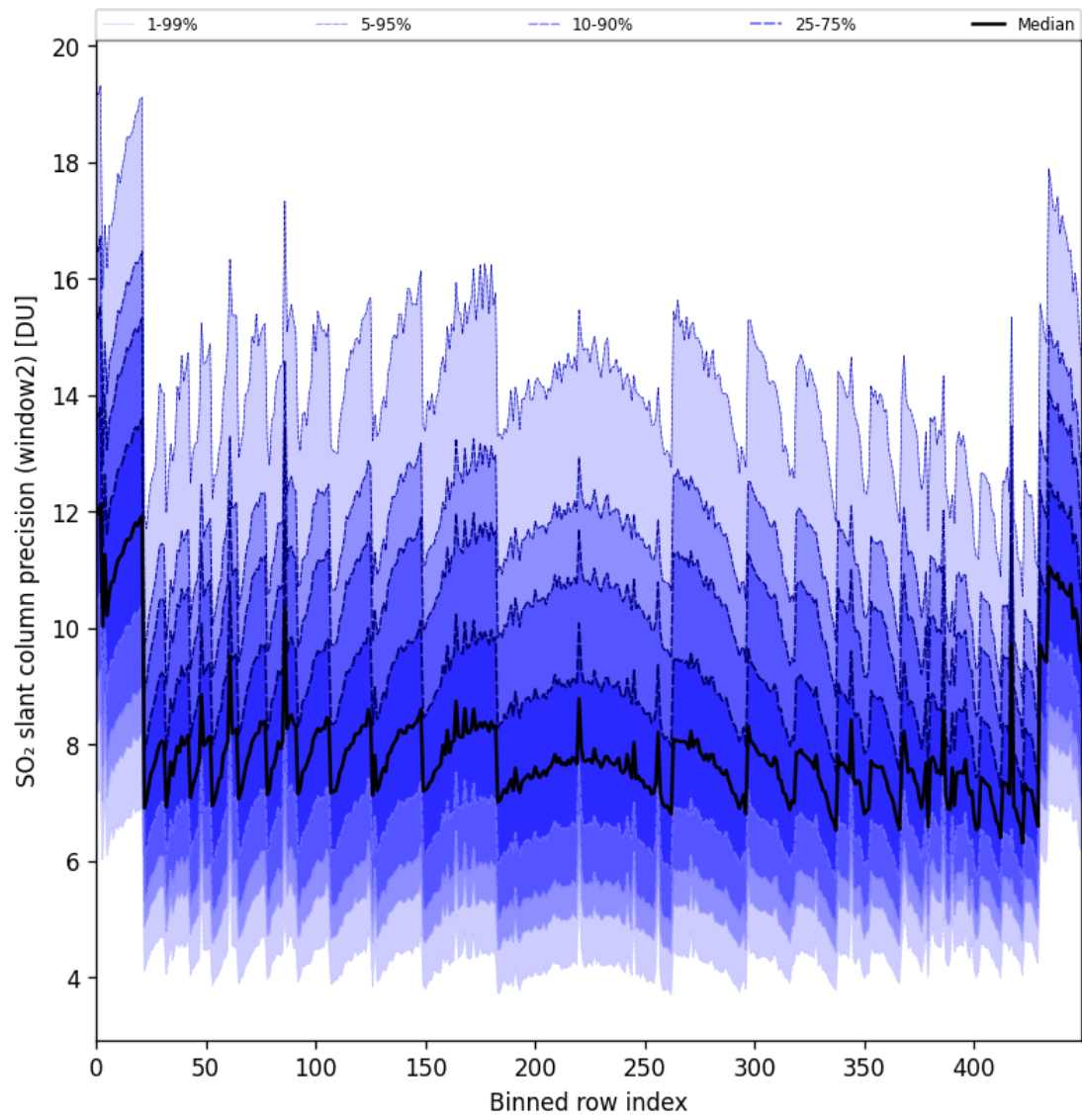
Figure 94: Along track statistics of “SO 2 slant column precision (window2)” for 2025-06-22 to 2025-06-23
