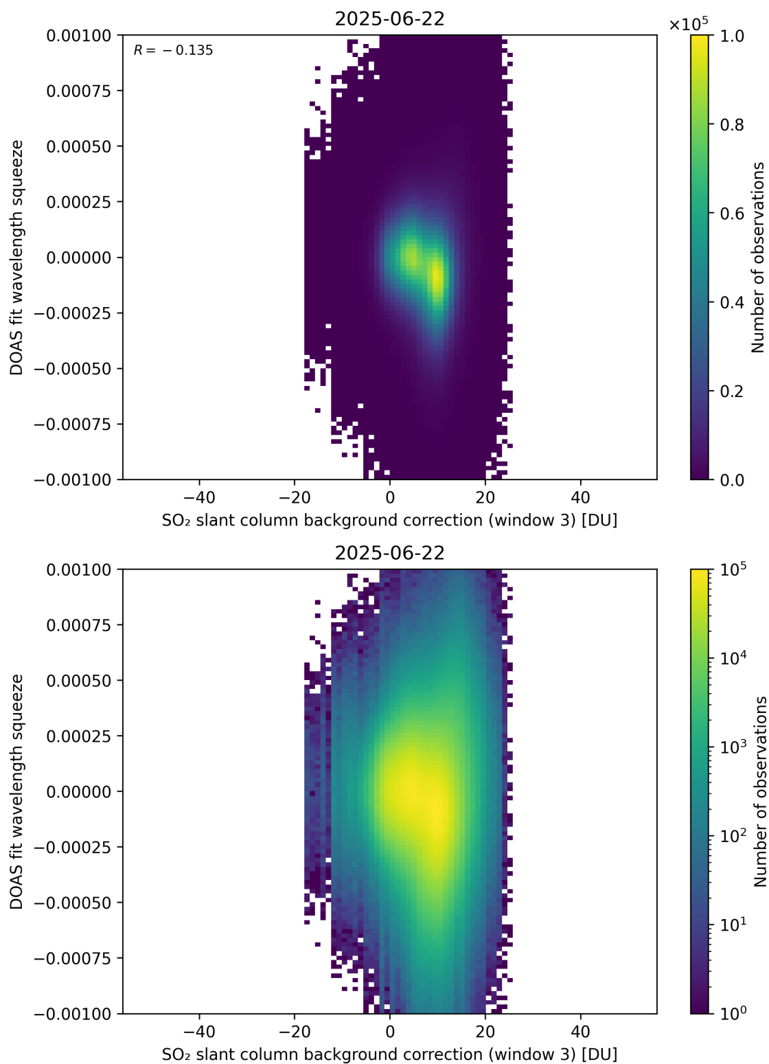
Figure 133: Scatter density plot of “SO 2 slant column background correction (window 3)” against “DOAS fit wavelength squeeze” for 2025-06-22 to 2025-06-23.
