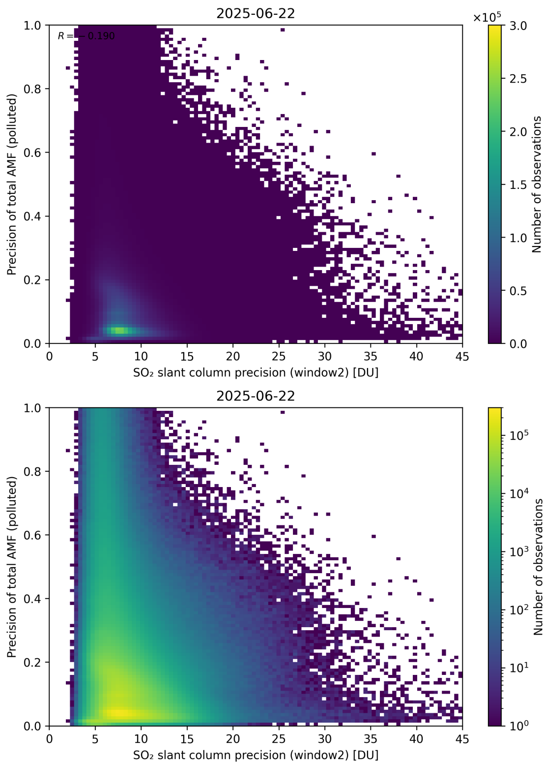
Figure 302: Scatter density plot of “SO 2 slant column precision (window2)” against “Precision of total AMF (polluted)” for 2025-06-22 to 2025-06-23.
