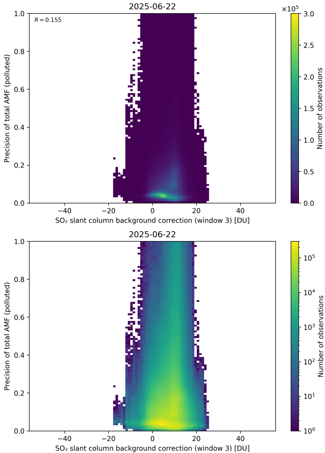
Figure 137: Scatter density plot of “SO 2 slant column background correction (window 3)” against “Precision of total AMF (polluted)” for 2025-06-22 to 2025-06-23.
