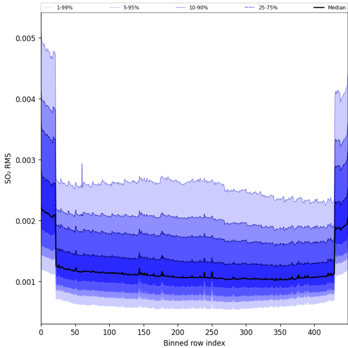
Figure 104: Along track statistics of “SO 2 RMS” for 2025-06-22 to 2025-06-23
