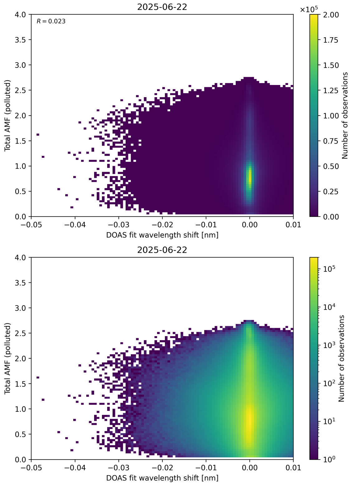
Figure 141: Scatter density plot of “DOAS fit wavelength shift” against “Total AMF (polluted)” for 2025-06-22 to 2025-06-23.
