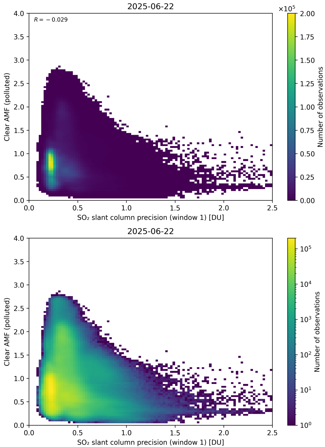
Figure 274: Scatter density plot of “SO 2 slant column precision (window 1)” against “Clear AMF (polluted)” for 2025-06-22 to 2025-06-23.
