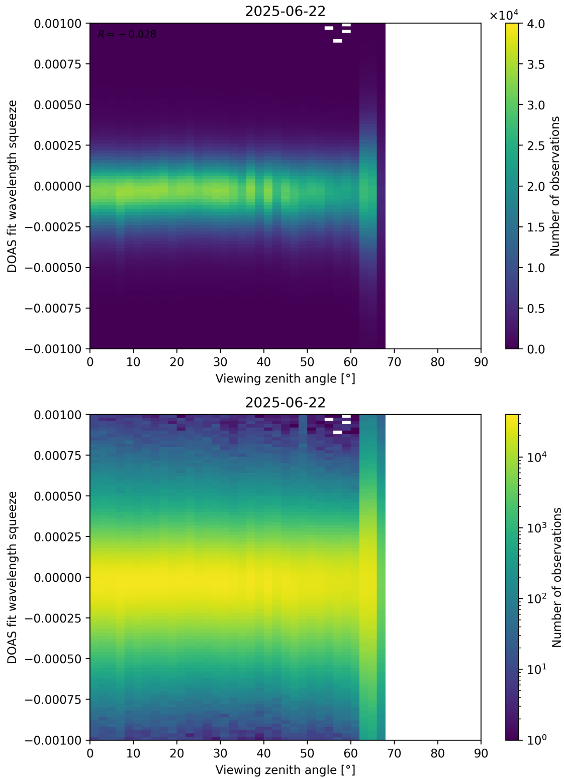
Figure 366: Scatter density plot of “Viewing zenith angle” against “DOAS fit wavelength squeeze” for 2025-06-22 to 2025-06-23.
