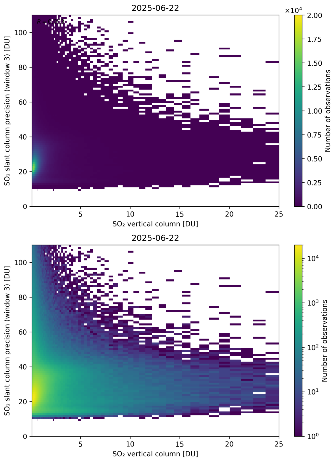
Figure 358: Scatter density plot of “SO 2 vertical column” against “SO 2 slant column precision (window 3)” for 2025-06-22 to 2025-06-23.
