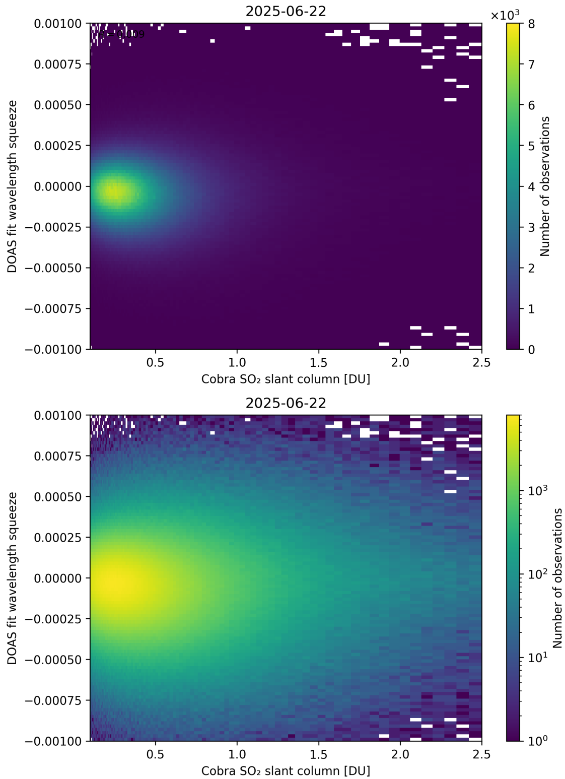
Figure 197: Scatter density plot of “Cobra SO 2 slant column” against “DOAS fit wavelength squeeze” for 2025-06-22 to 2025-06-23.
