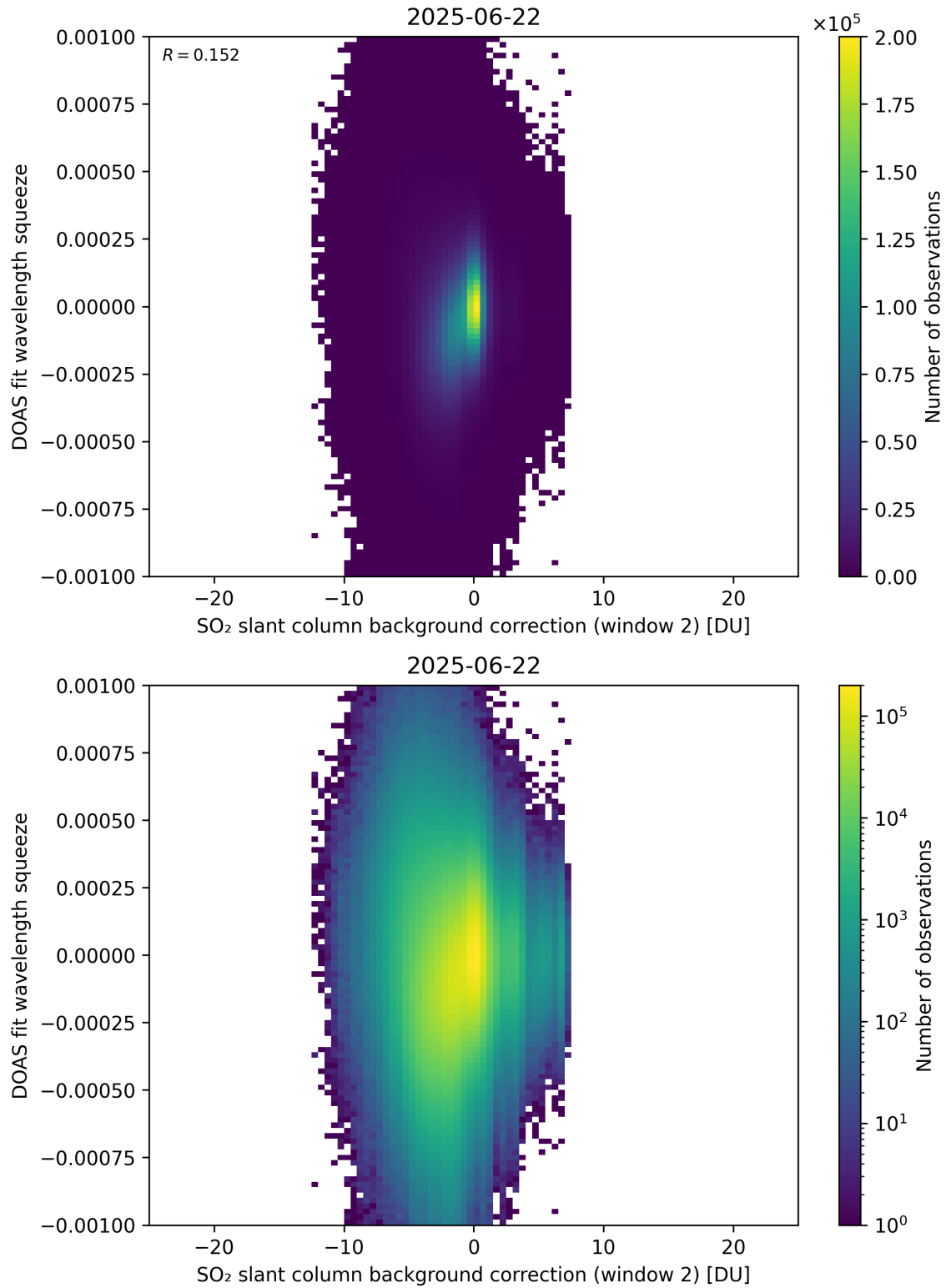
Figure 124: Scatter density plot of “SO 2 slant column background correction (window 2)” against “DOAS fit wavelength squeeze” for 2025-06-22 to 2025-06-23.
