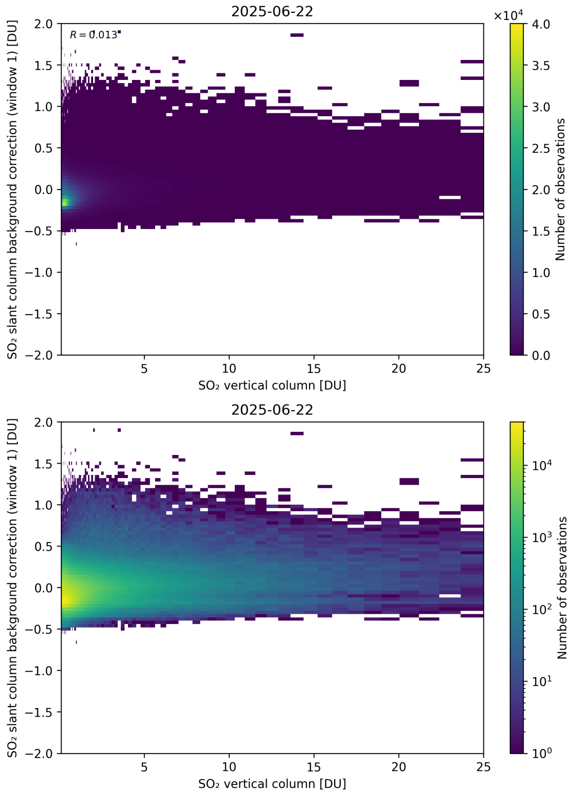
Figure 323: Scatter density plot of “SO 2 vertical column” against “SO 2 slant column background correction (window 1)” for 2025-06-22 to 2025-06-23.
