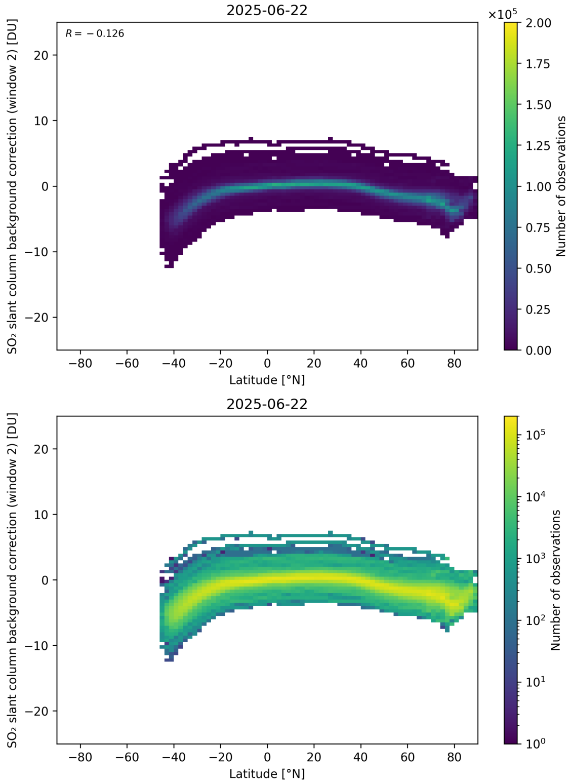
Figure 151: Scatter density plot of “Latitude” against “SO 2 slant column background correction (window 2)” for 2025-06-22 to 2025-06-23.
