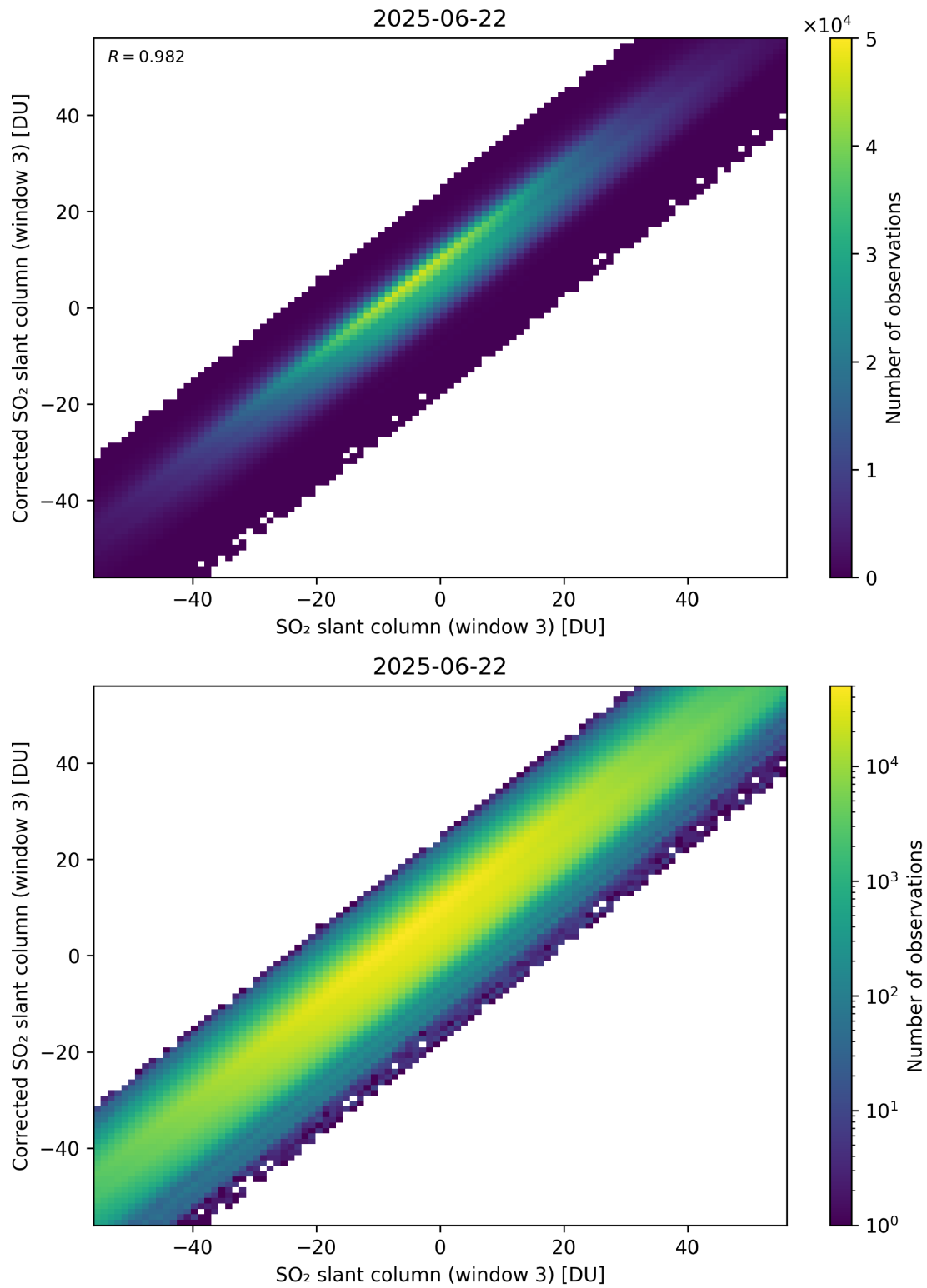
Figure 316: Scatter density plot of “SO 2 slant column (window 3)” against “Corrected SO 2 slant column (window 3)” for 2025-06-22 to 2025-06-23.
