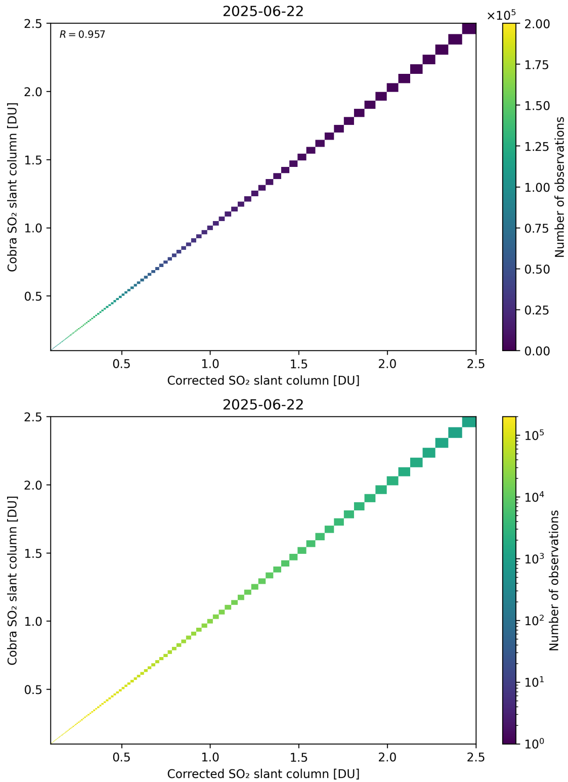
Figure 233: Scatter density plot of “Corrected SO 2 slant column” against “Cobra SO 2 slant column” for 2025-06-22 to 2025-06-23.
