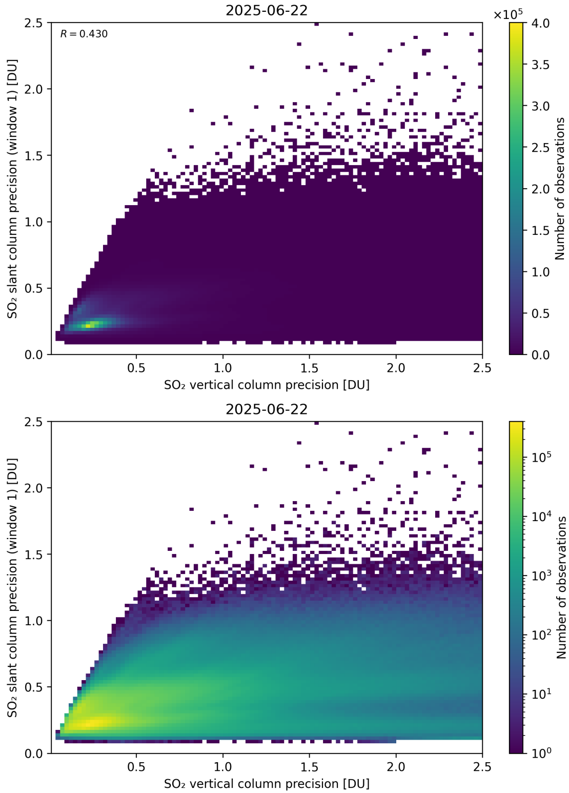
Figure 342: Scatter density plot of “SO 2 vertical column precision” against “SO 2 slant column precision (window 1)” for 2025-06-22 to 2025-06-23.
