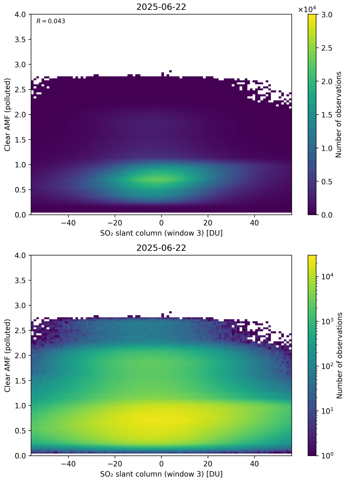
Figure 315: Scatter density plot of “SO 2 slant column (window 3)” against “Clear AMF (polluted)” for 2025-06-22 to 2025-06-23.
