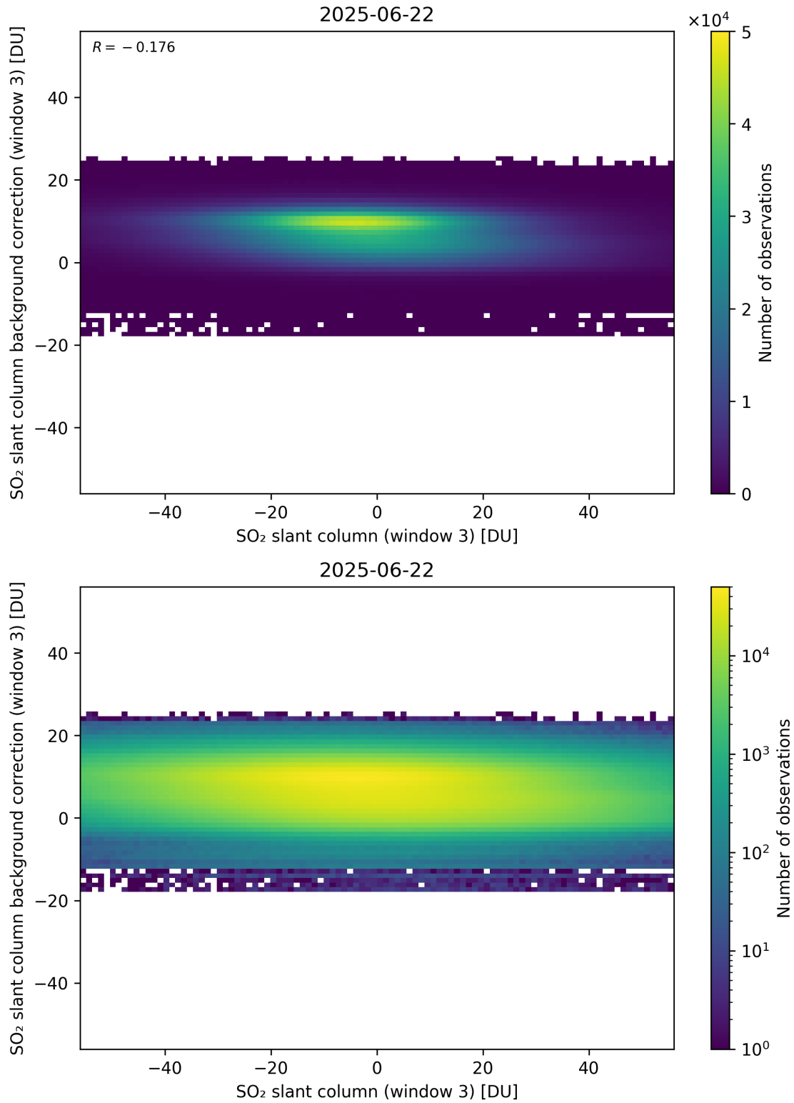
Figure 303: Scatter density plot of “SO 2 slant column (window 3)” against “SO 2 slant column background correction (window 3)” for 2025-06-22 to 2025-06-23.
