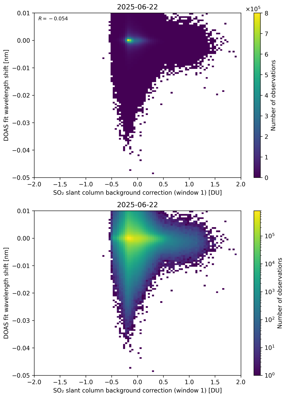
Figure 111: Scatter density plot of “SO 2 slant column background correction (window 1)” against “DOAS fit wavelength shift” for 2025-06-22 to 2025-06-23.
