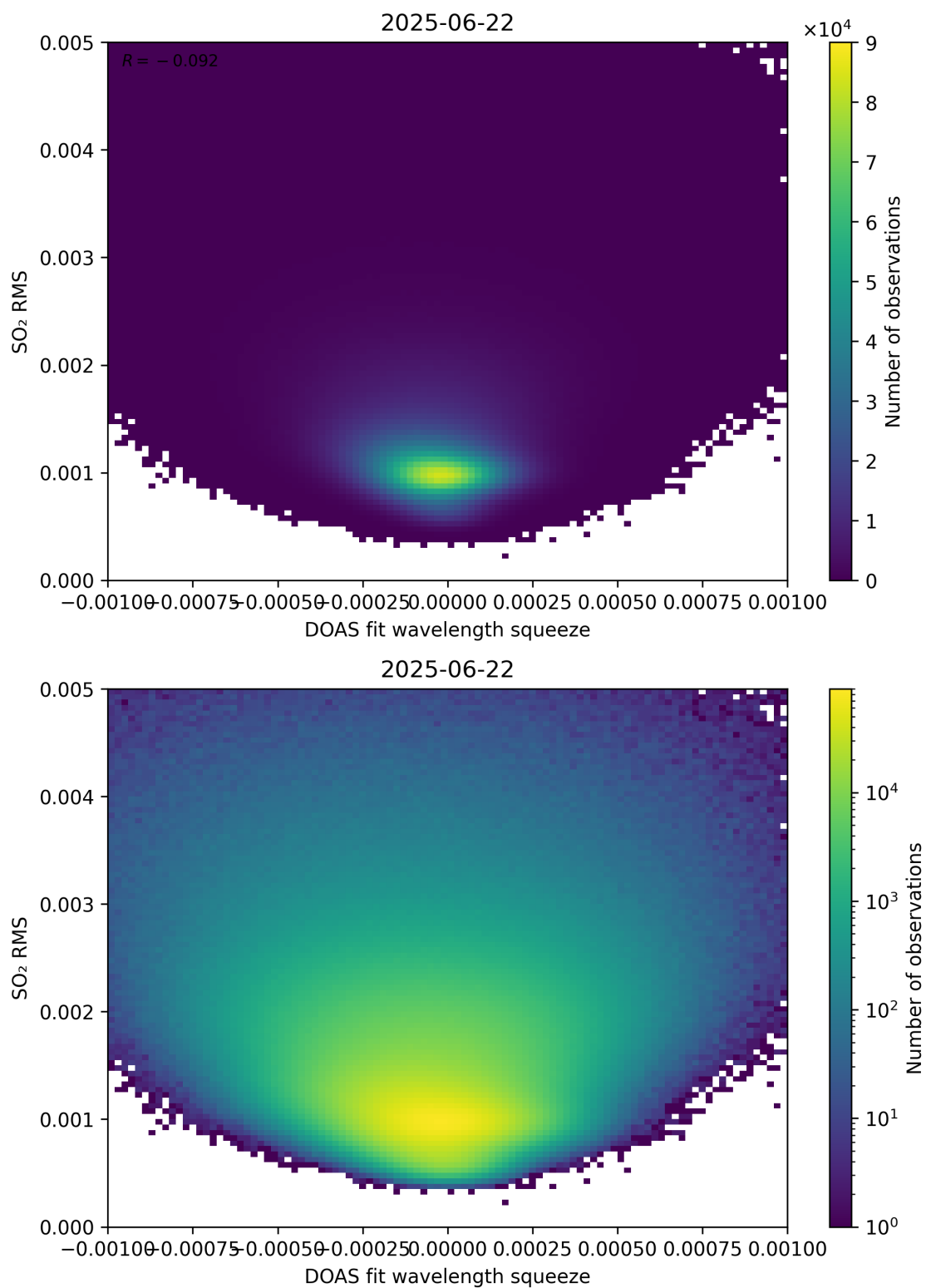
Figure 143: Scatter density plot of “DOAS fit wavelength squeeze” against “SO 2 RMS” for 2025-06-22 to 2025-06-23.
