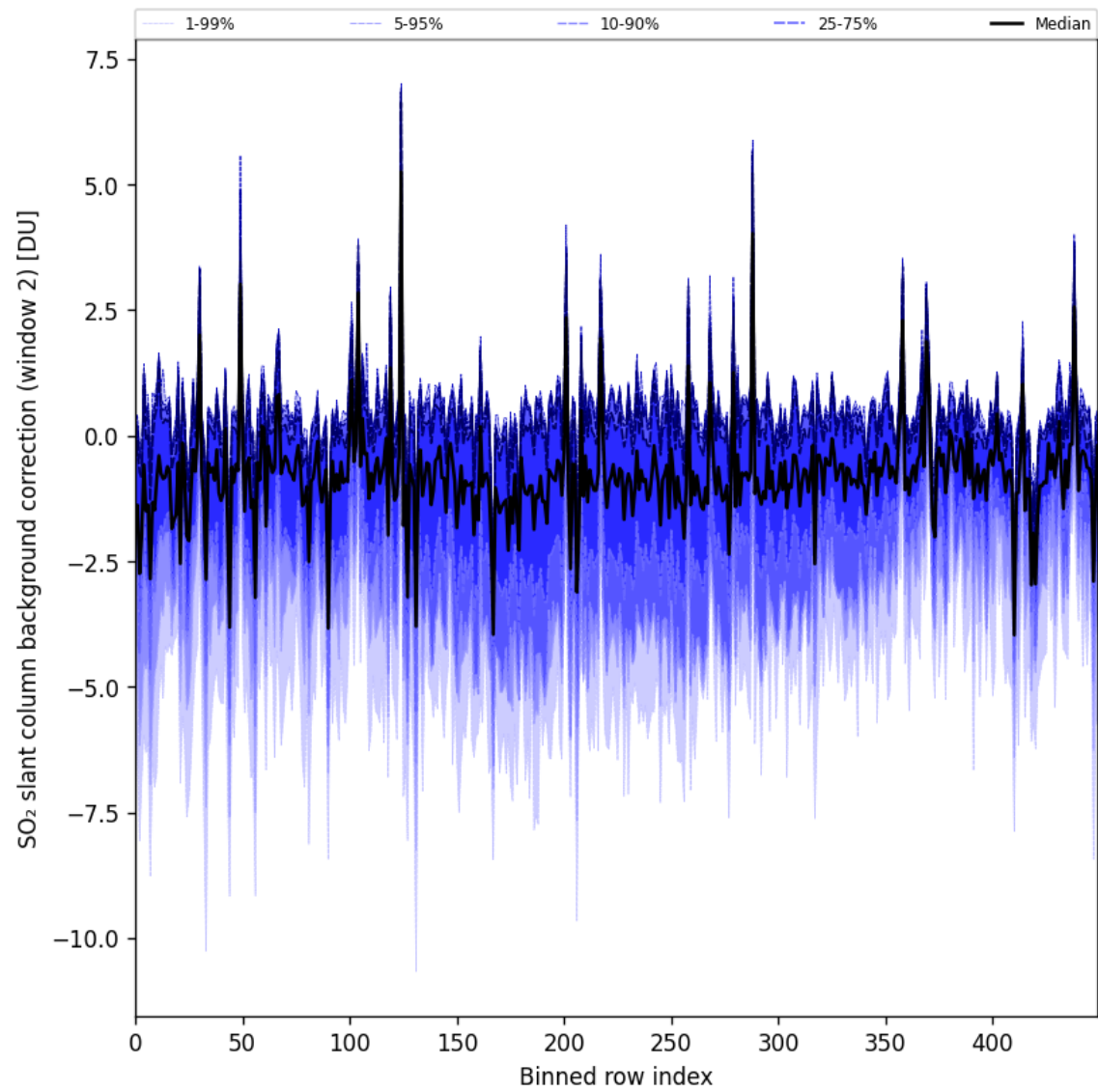
Figure 96: Along track statistics of “SO 2 slant column background correction (window 2)” for 2025-06-22 to 2025-06-23
