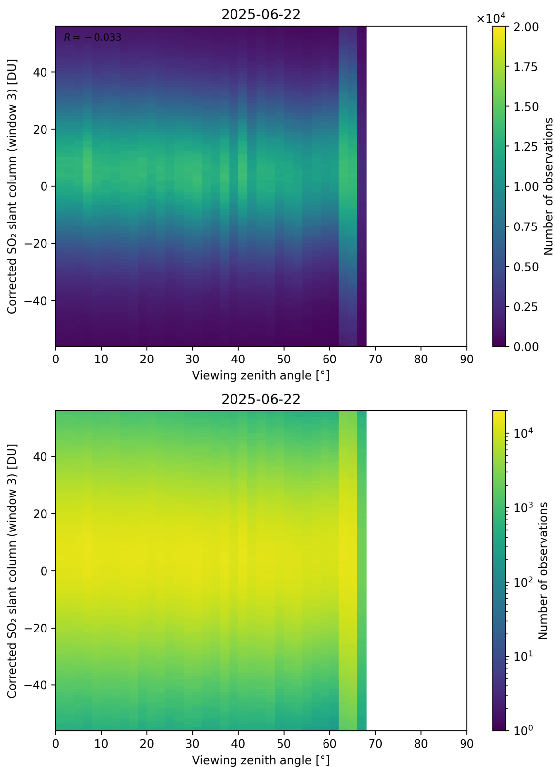
Figure 375: Scatter density plot of “Viewing zenith angle” against “Corrected SO 2 slant column (window 3)” for 2025-06-22 to 2025-06-23.
