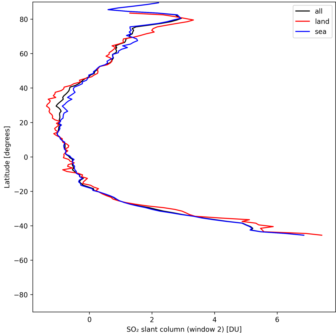
Figure 41: Zonal average of “SO 2 slant column (window 2)” for 2025-06-22 to 2025-06-23.
