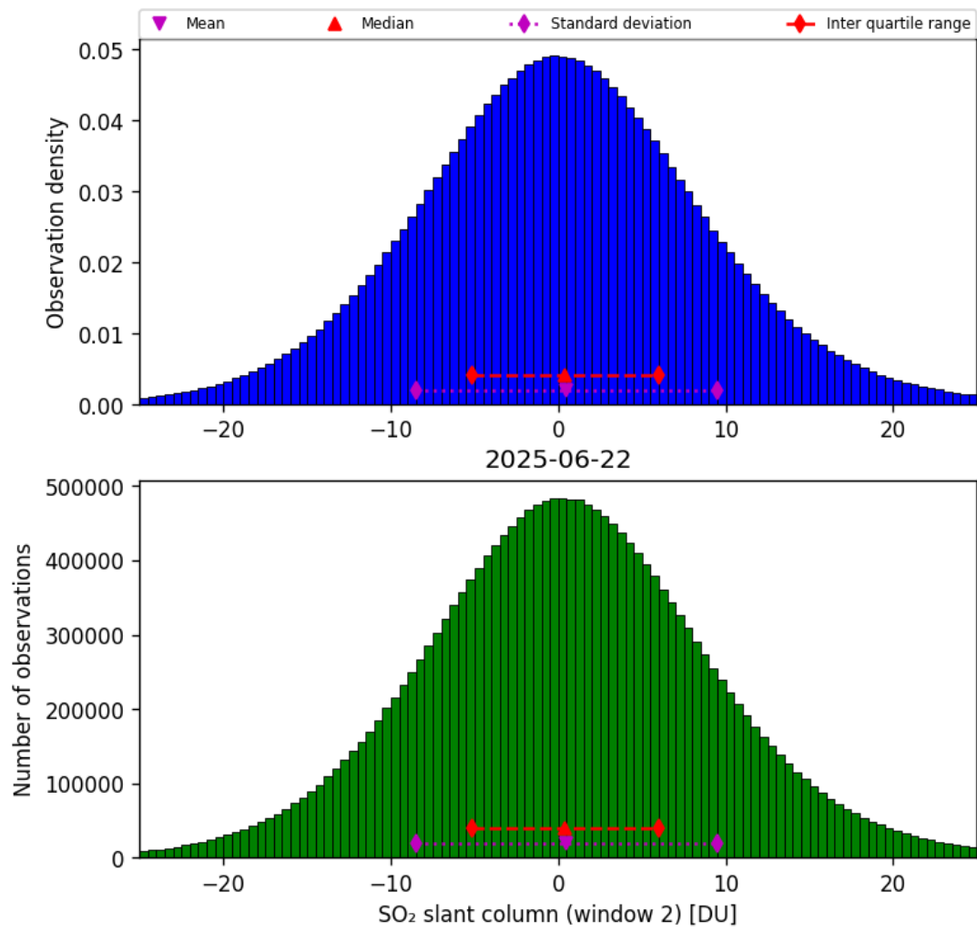
Figure 67: Histogram of “SO 2 slant column (window 2)” for 2025-06-22 to 2025-06-23
