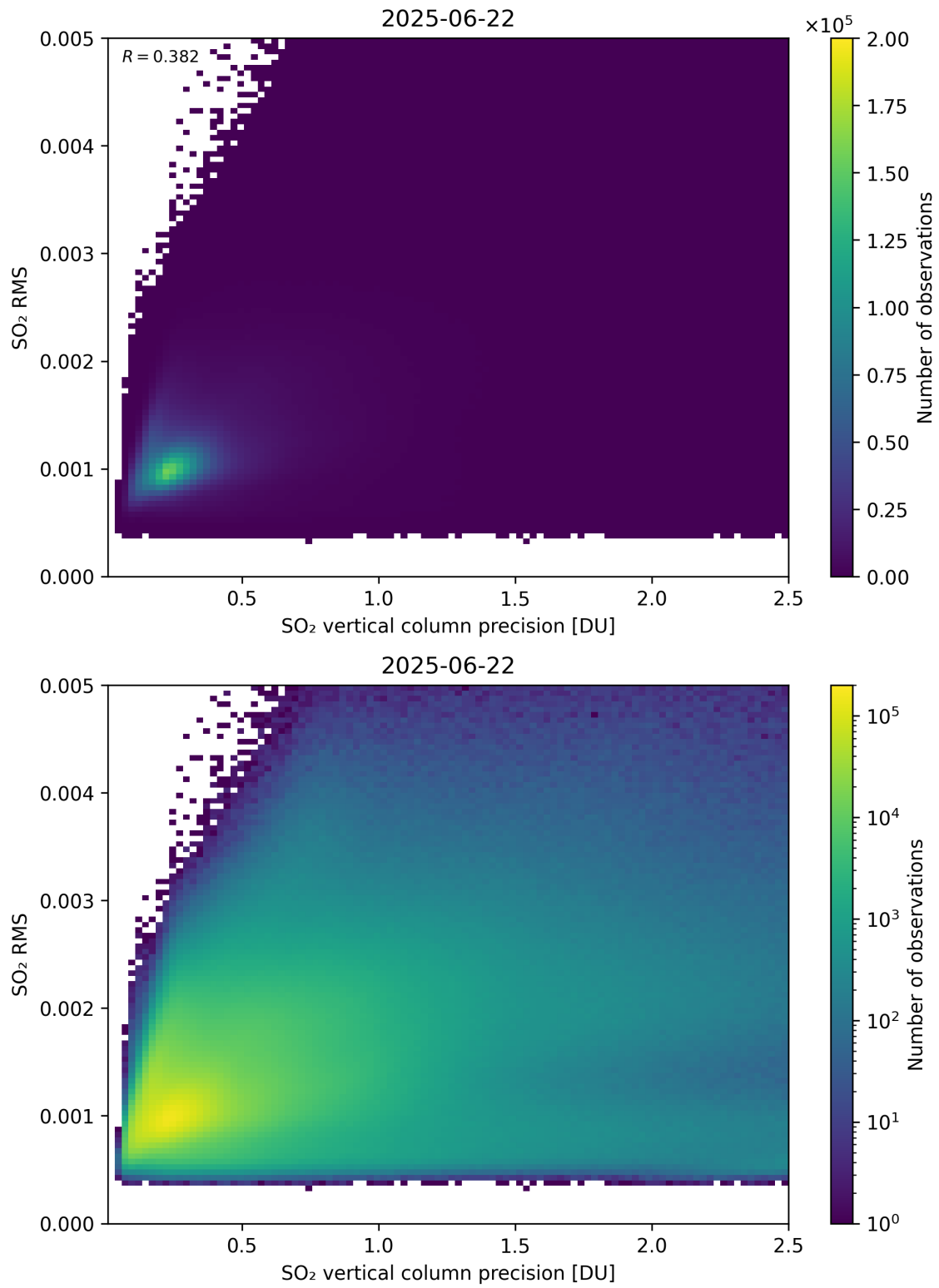
Figure 334: Scatter density plot of “SO 2 vertical column precision” against “SO 2 RMS” for 2025-06-22 to 2025-06-23.
