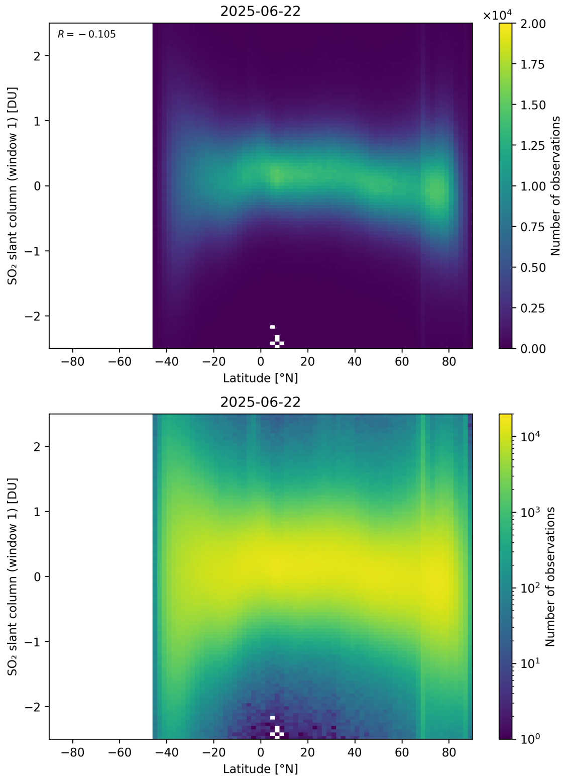
Figure 162: Scatter density plot of “Latitude” against “SO 2 slant column (window 1)” for 2025-06-22 to 2025-06-23.
