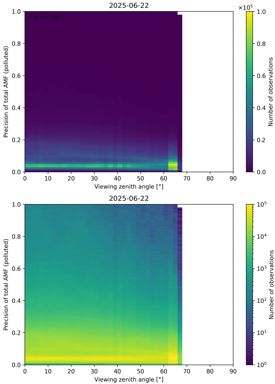
Figure 382: Scatter density plot of “Viewing zenith angle” against “Precision of total AMF (polluted)” for 2025-06-22 to 2025-06-23.
