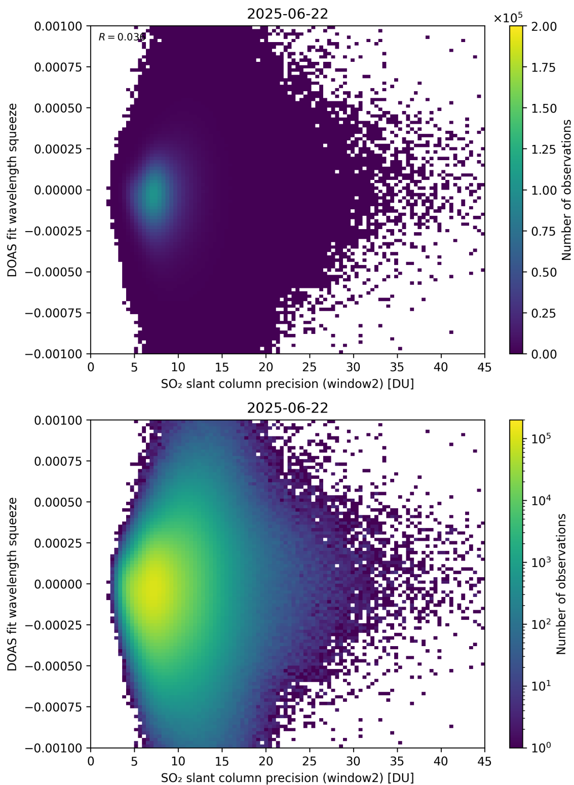
Figure 294: Scatter density plot of “SO 2 slant column precision (window2)” against “DOAS fit wavelength squeeze” for 2025-06-22 to 2025-06-23.
