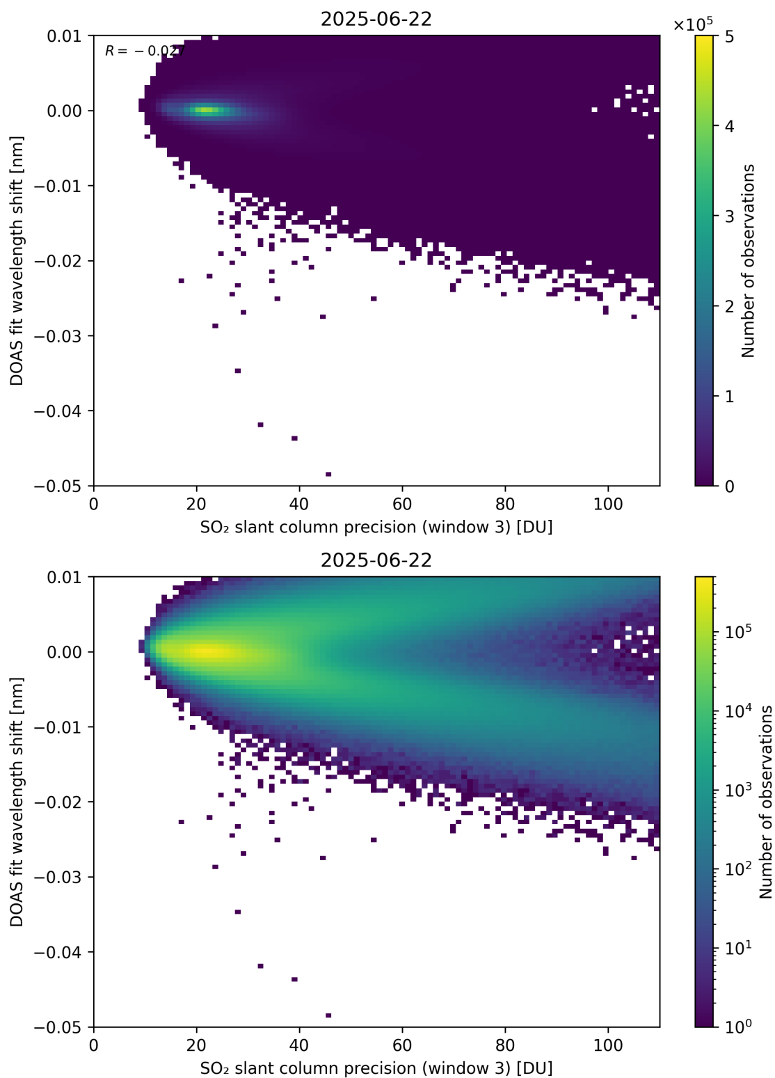
Figure 308: Scatter density plot of “SO 2 slant column precision (window 3)” against “DOAS fit wavelength shift” for 2025-06-22 to 2025-06-23.
