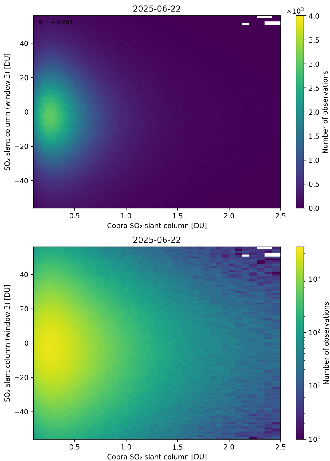
Figure 222: Scatter density plot of “Cobra SO 2 slant column” against “SO 2 slant column (window 3)” for 2025-06-22 to 2025-06-23.
