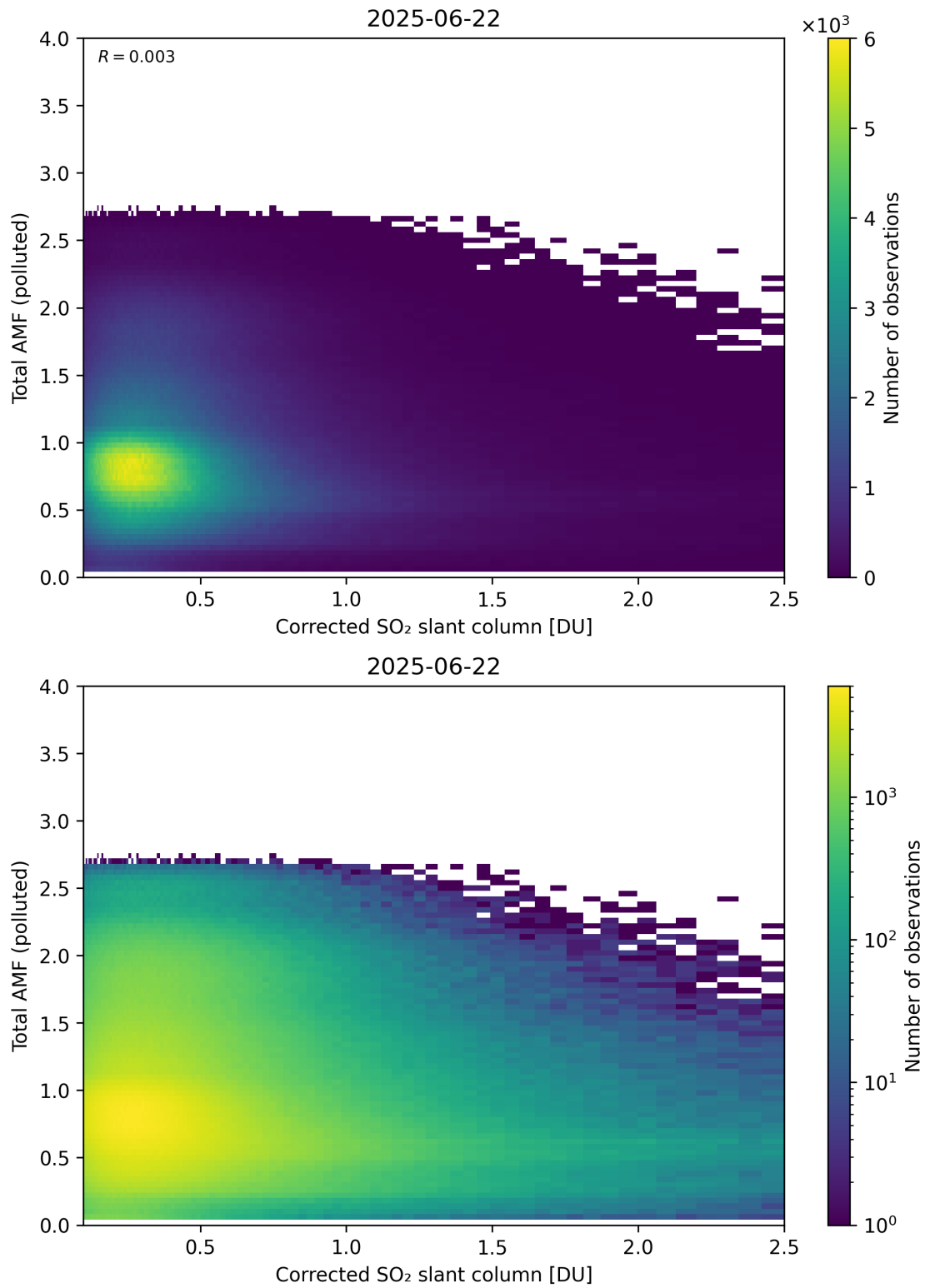
Figure 242: Scatter density plot of “Corrected SO 2 slant column” against “Total AMF (polluted)” for 2025-06-22 to 2025-06-23.
