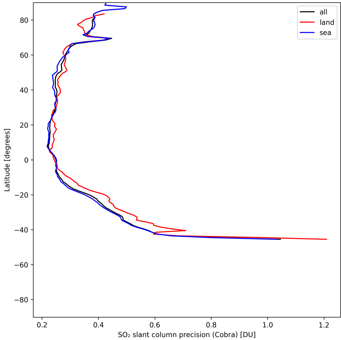
Figure 36: Zonal average of “SO 2 slant column precision (Cobra)” for 2025-06-22 to 2025-06-23.
