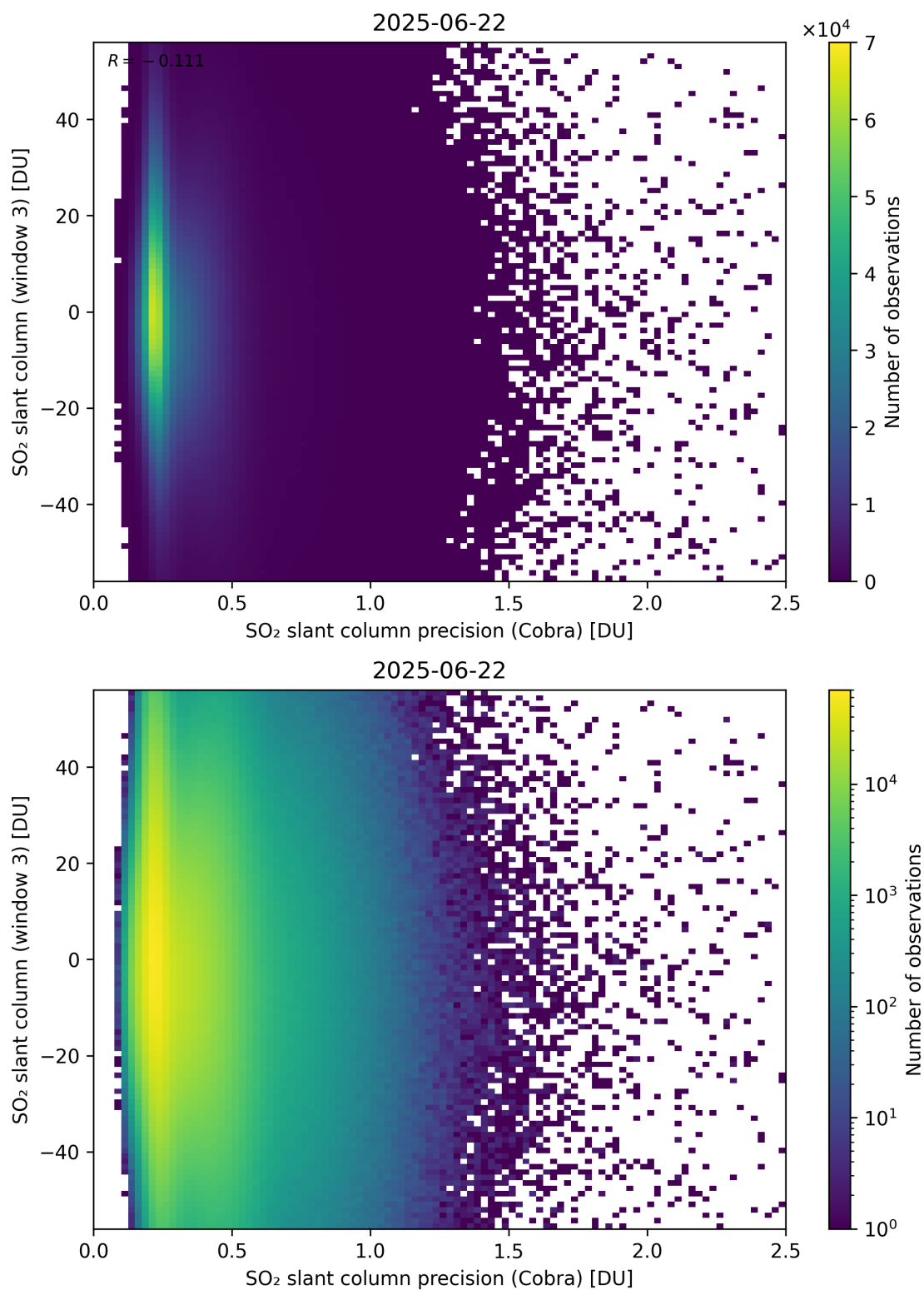
Figure 211: Scatter density plot of “SO 2 slant column precision (Cobra)” against “SO 2 slant column (window 3)” for 2025-06-22 to 2025-06-23.
