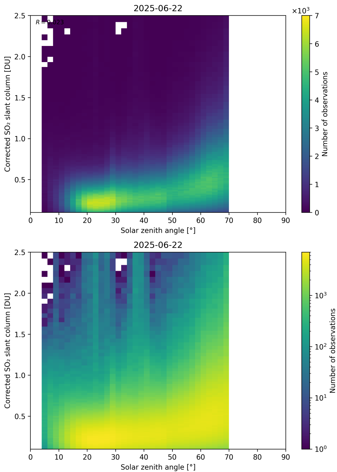
Figure 181: Scatter density plot of “Solar zenith angle” against “Corrected SO 2 slant column” for 2025-06-22 to 2025-06-23.
