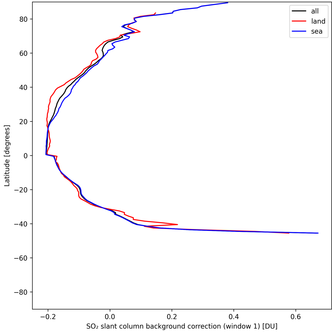
Figure 40: Zonal average of “SO 2 slant column background correction (window 1)” for 2025-06-22 to 2025-06-23.
