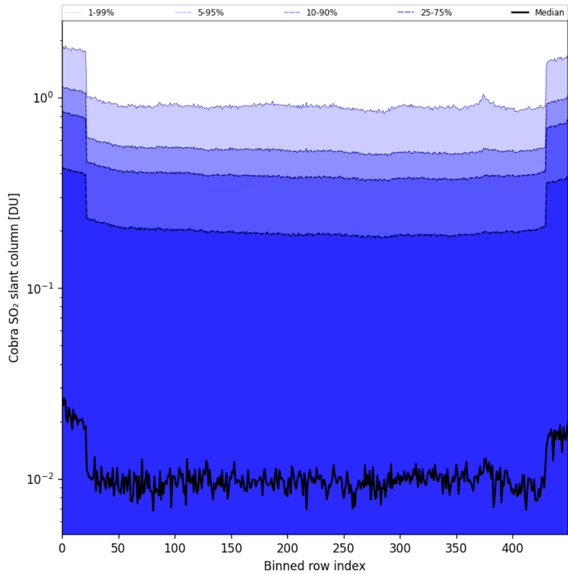
Figure 87: Along track statistics of “Cobra SO 2 slant column” for 2025-06-22 to 2025-06-23
