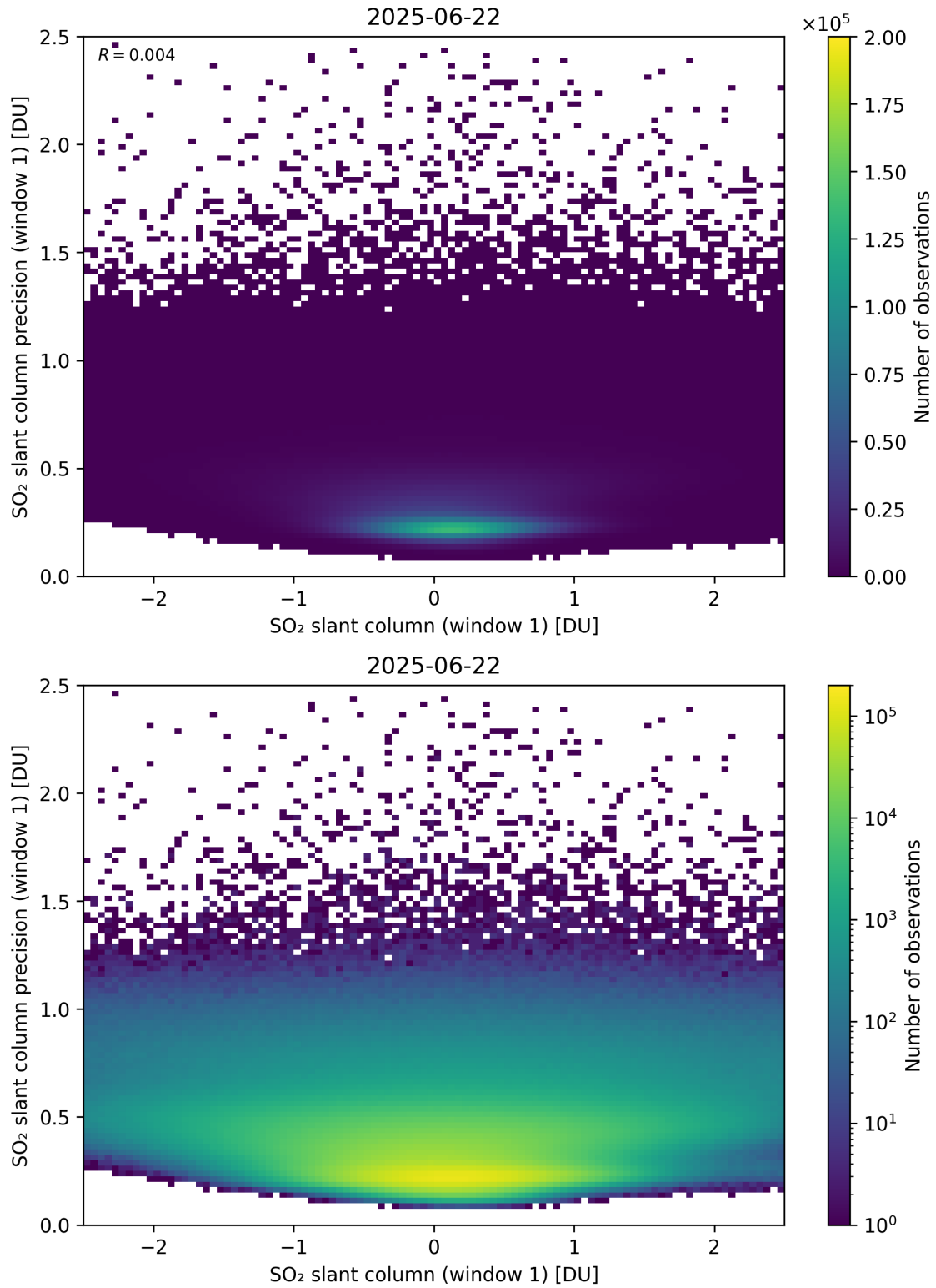
Figure 285: Scatter density plot of “SO 2 slant column (window 1)” against “SO 2 slant column precision (window 1)” for 2025-06-22 to 2025-06-23.
