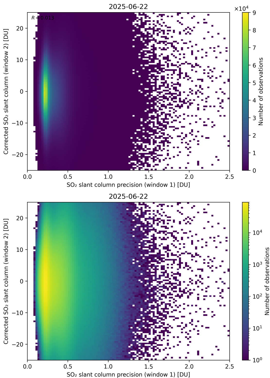
Figure 275: Scatter density plot of “SO 2 slant column precision (window 1)” against “Corrected SO 2 slant column (window 2)” for 2025-06-22 to 2025-06-23.
