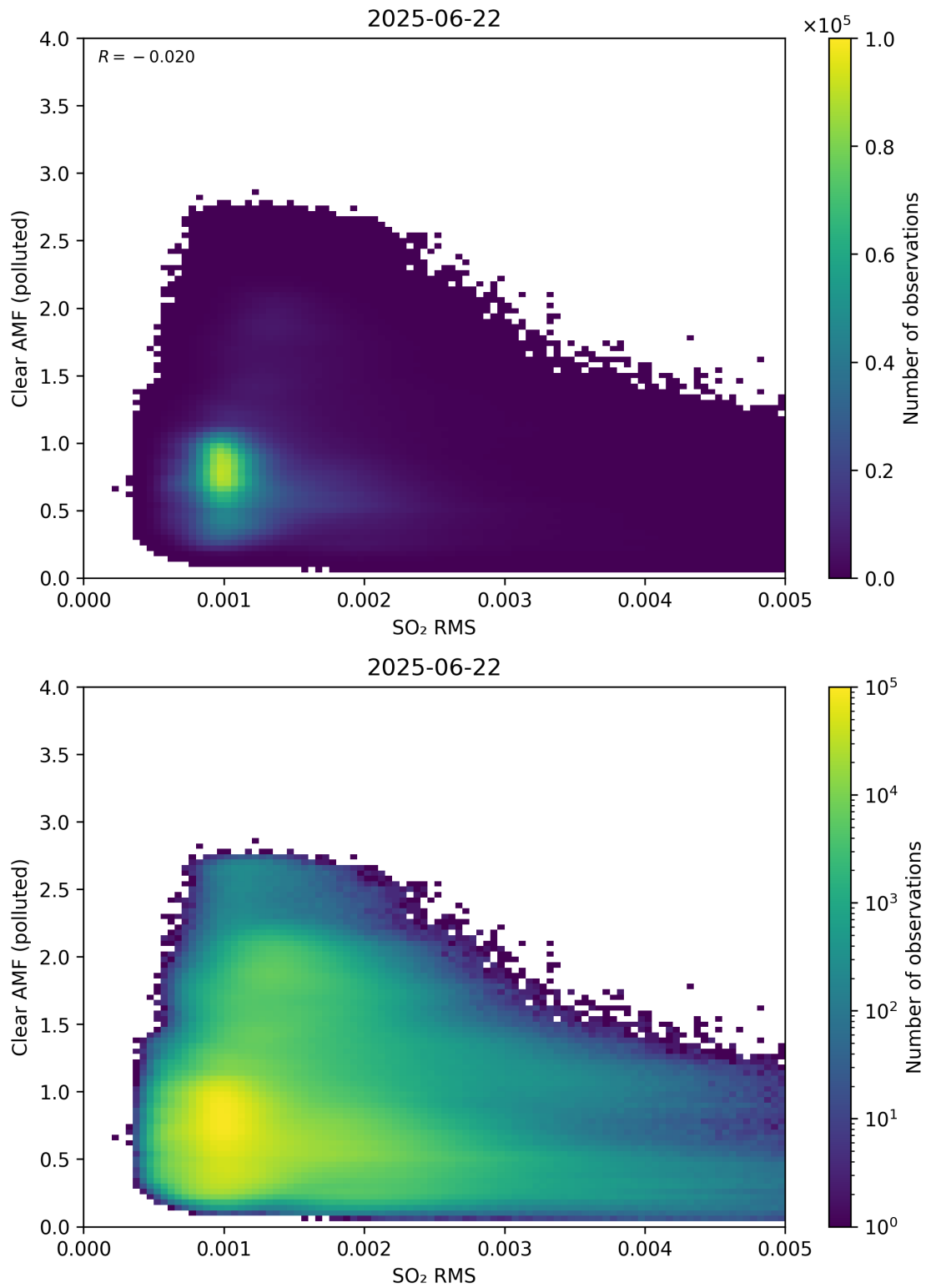
Figure 147: Scatter density plot of “SO 2 RMS” against “Clear AMF (polluted)” for 2025-06-22 to 2025-06-23.
