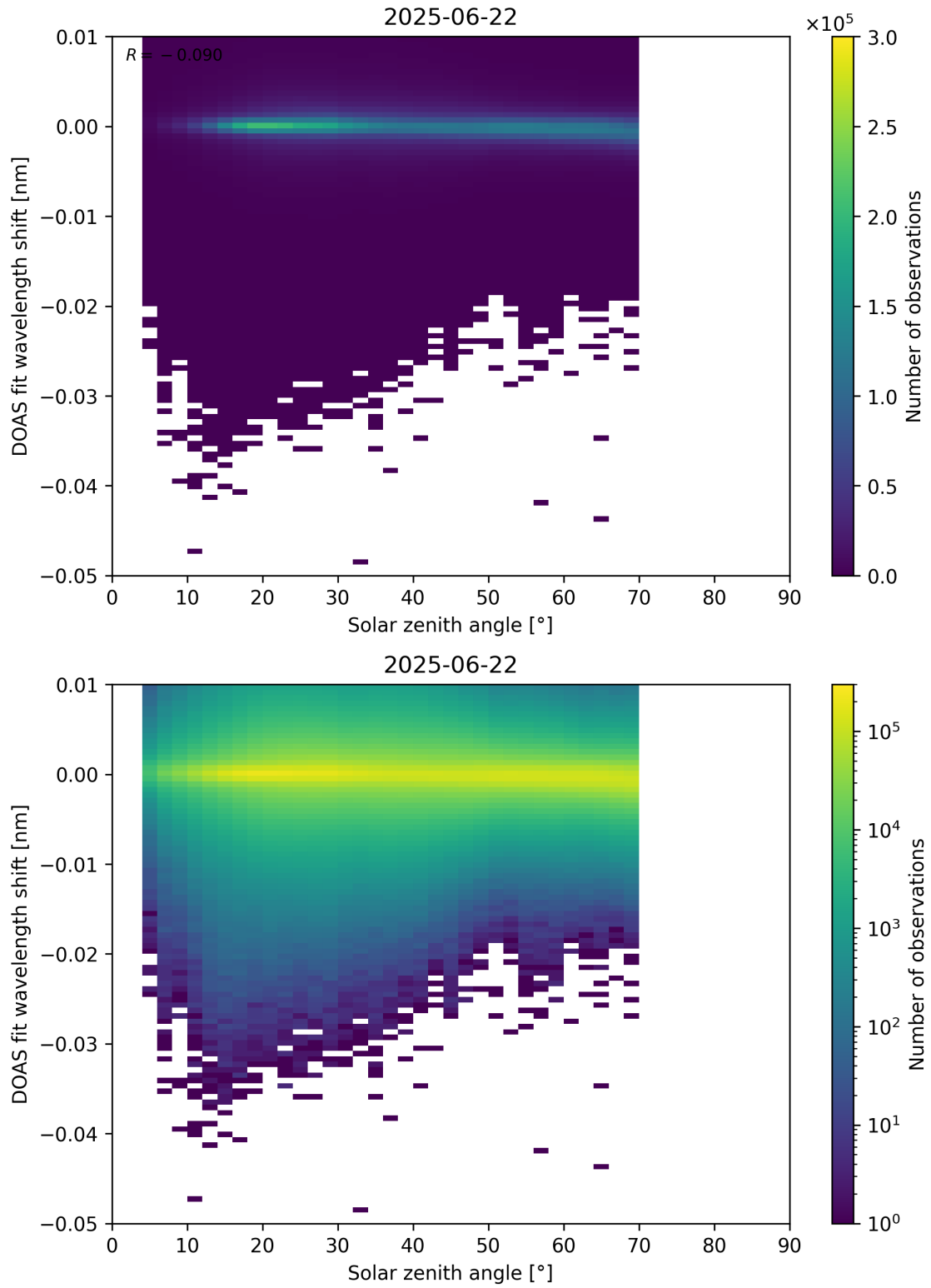
Figure 174: Scatter density plot of “Solar zenith angle” against “DOAS fit wavelength shift” for 2025-06-22 to 2025-06-23.
