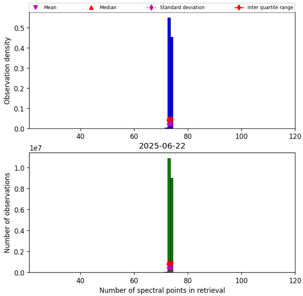
Figure 82: Histogram of “Number of spectral points in retrieval” for 2025-06-22 to 2025-06-23
