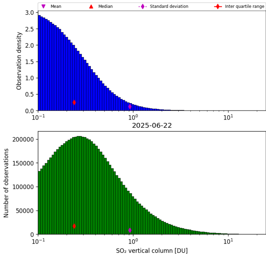
Figure 58: Histogram of “SO 2 vertical column” for 2025-06-22 to 2025-06-23
