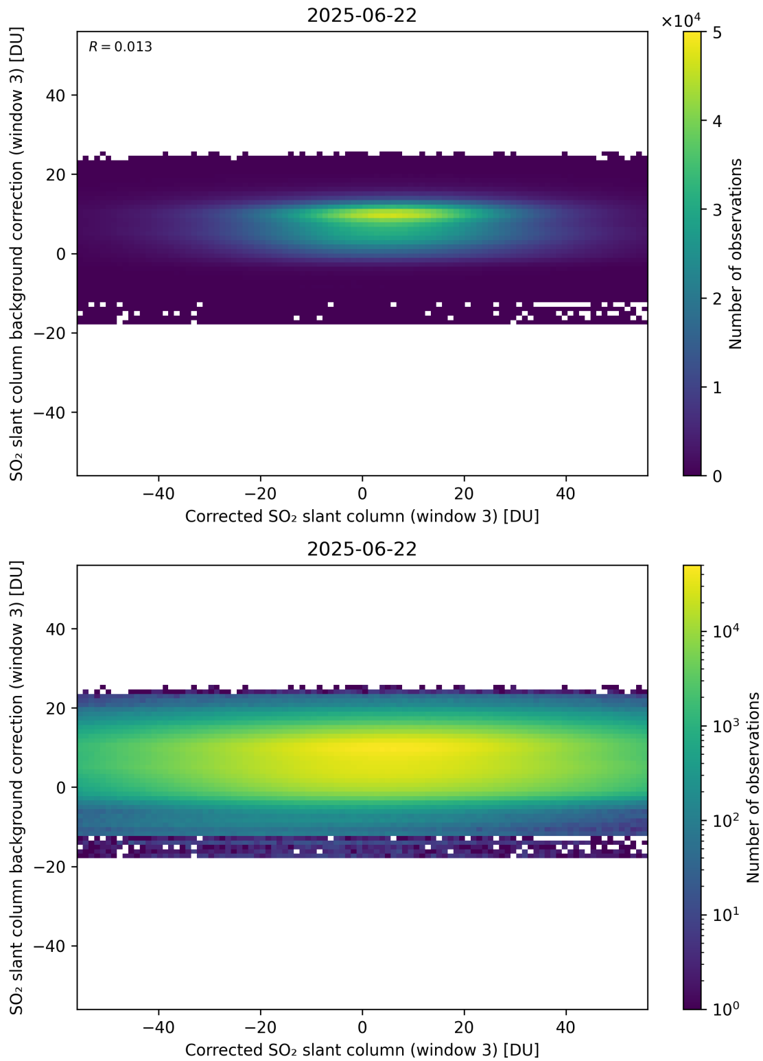
Figure 255: Scatter density plot of “Corrected SO 2 slant column (window 3)” against “SO 2 slant column background correction (window 3)” for 2025-06-22 to 2025-06-23.
