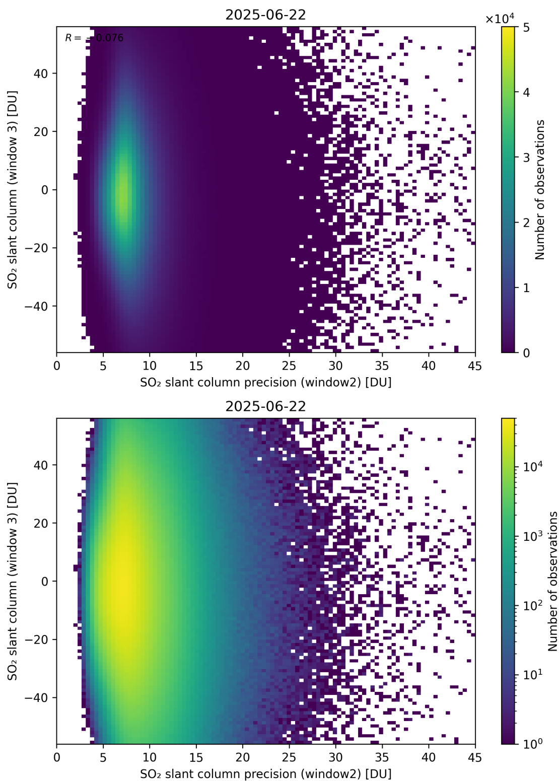
Figure 299: Scatter density plot of “SO 2 slant column precision (window2)” against “SO 2 slant column (window 3)” for 2025-06-22 to 2025-06-23.
