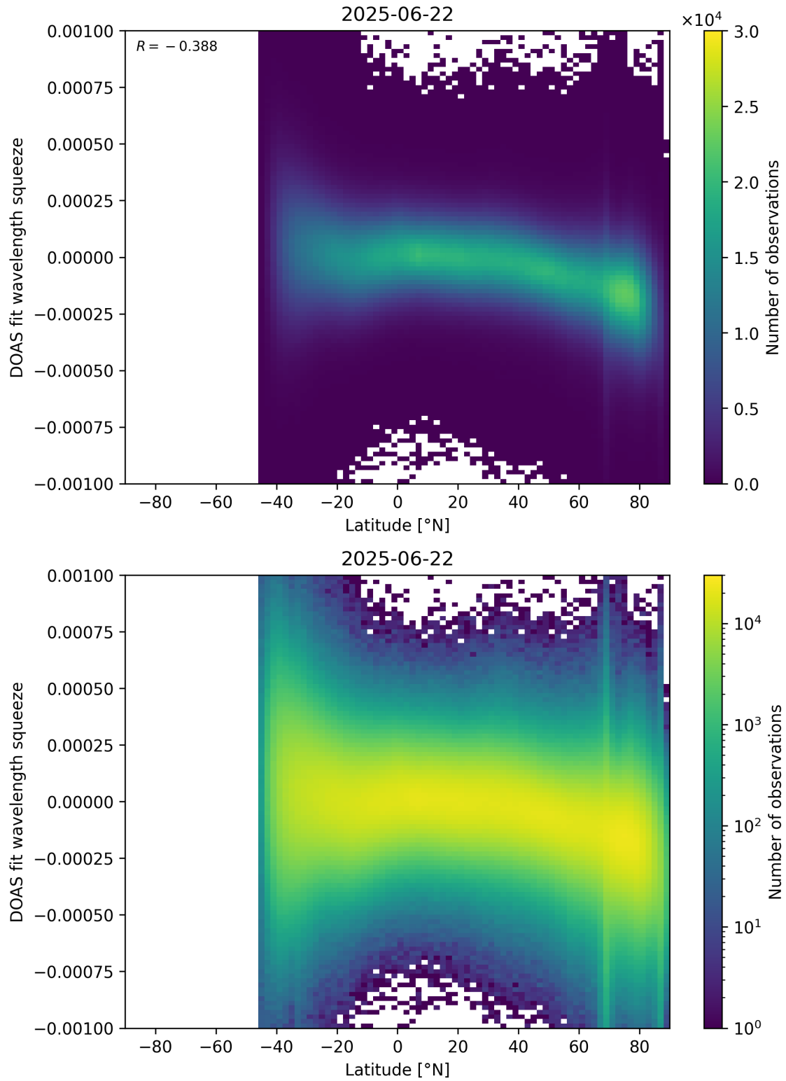
Figure 154: Scatter density plot of “Latitude” against “DOAS fit wavelength squeeze” for 2025-06-22 to 2025-06-23.
