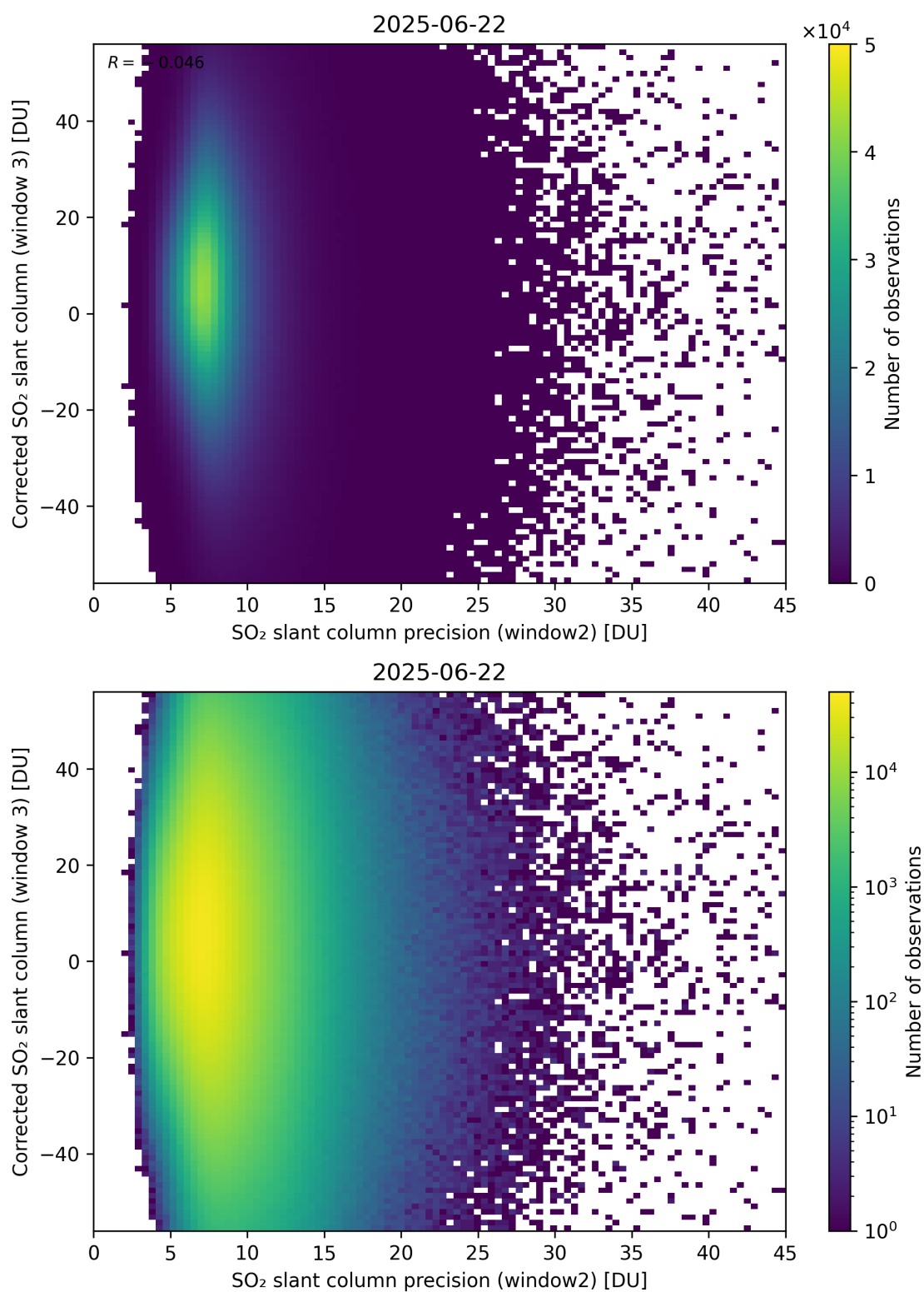
Figure 298: Scatter density plot of “SO 2 slant column precision (window2)” against “Corrected SO 2 slant column (window 3)” for 2025-06-22 to 2025-06-23.
