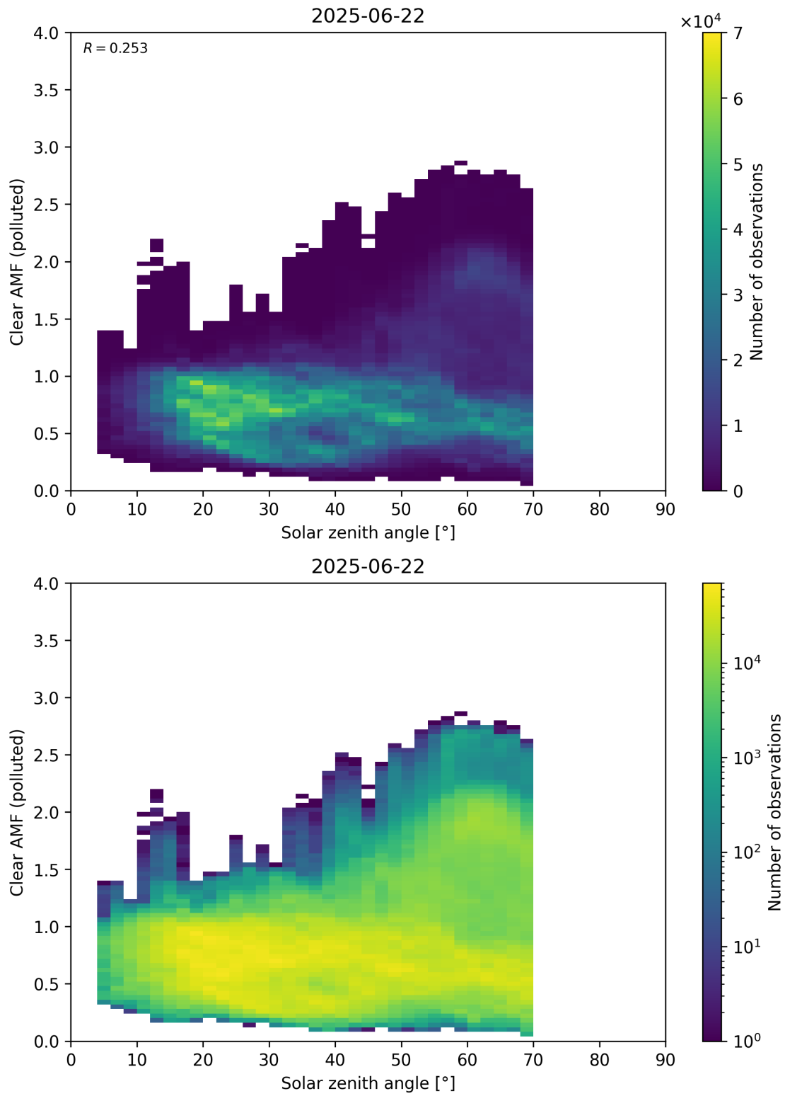
Figure 178: Scatter density plot of “Solar zenith angle” against “Clear AMF (polluted)” for 2025-06-22 to 2025-06-23.
