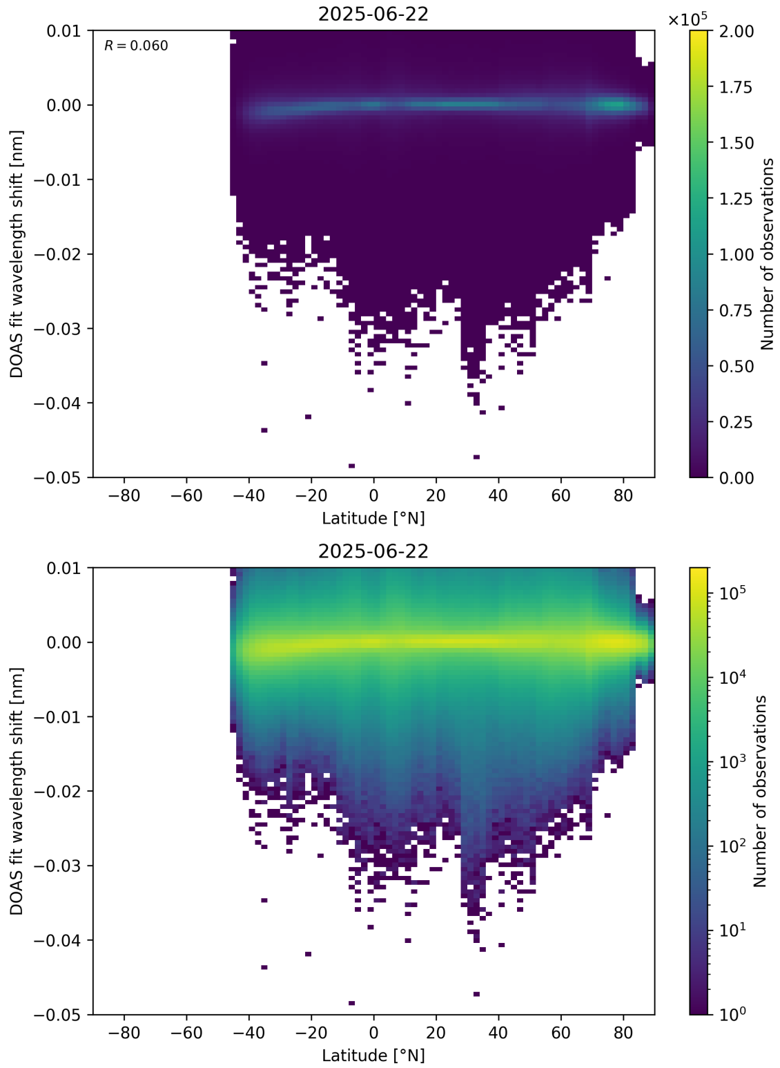
Figure 153: Scatter density plot of “Latitude” against “DOAS fit wavelength shift” for 2025-06-22 to 2025-06-23.
