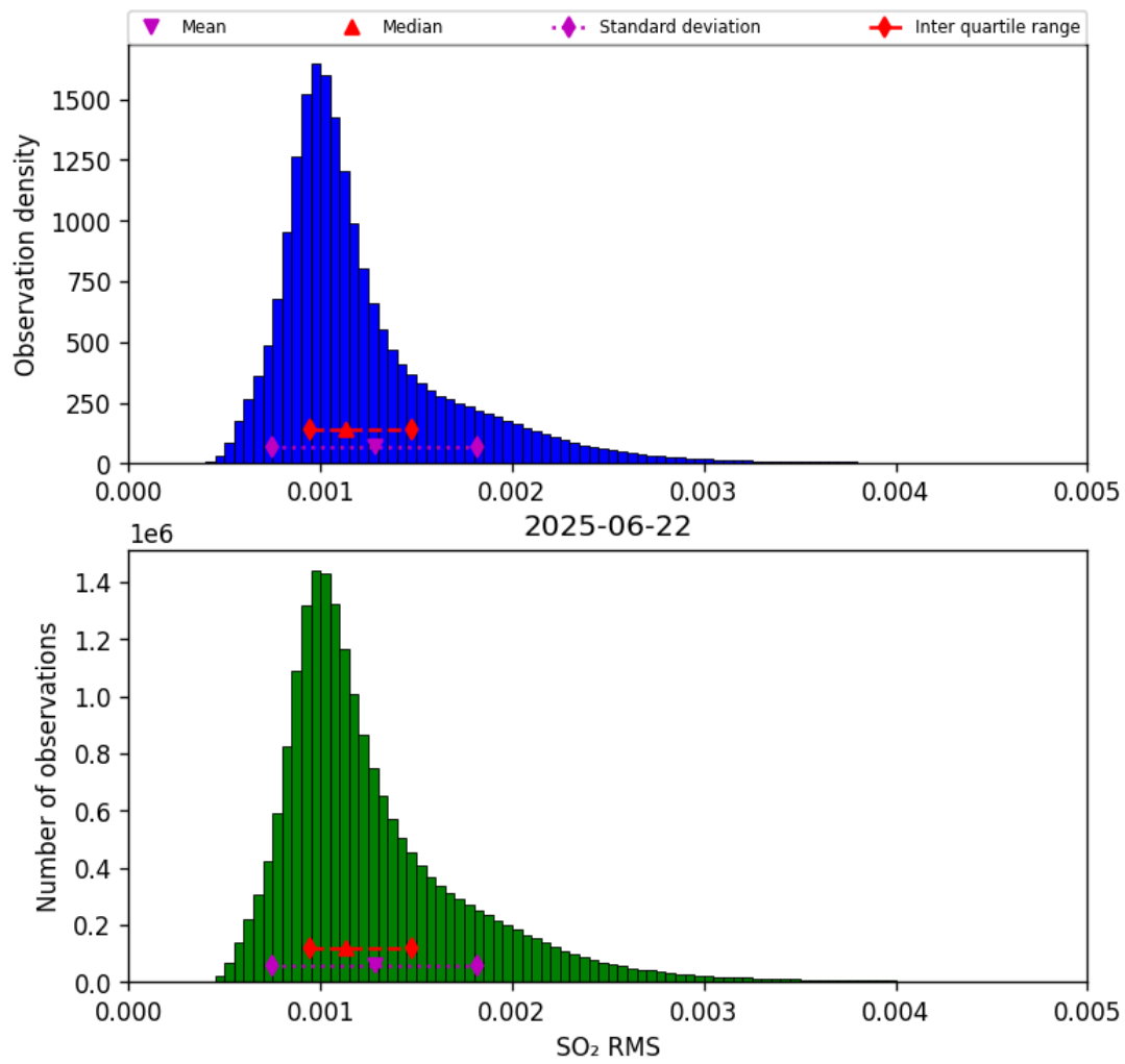
Figure 78: Histogram of “SO 2 RMS” for 2025-06-22 to 2025-06-23
