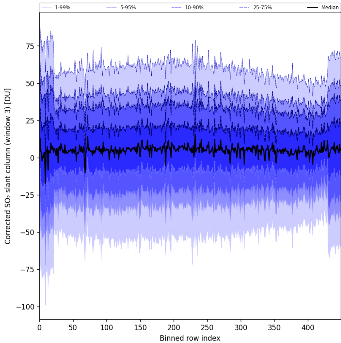
Figure 99: Along track statistics of “Corrected SO 2 slant column (window 3)” for 2025-06-22 to 2025-06-23
