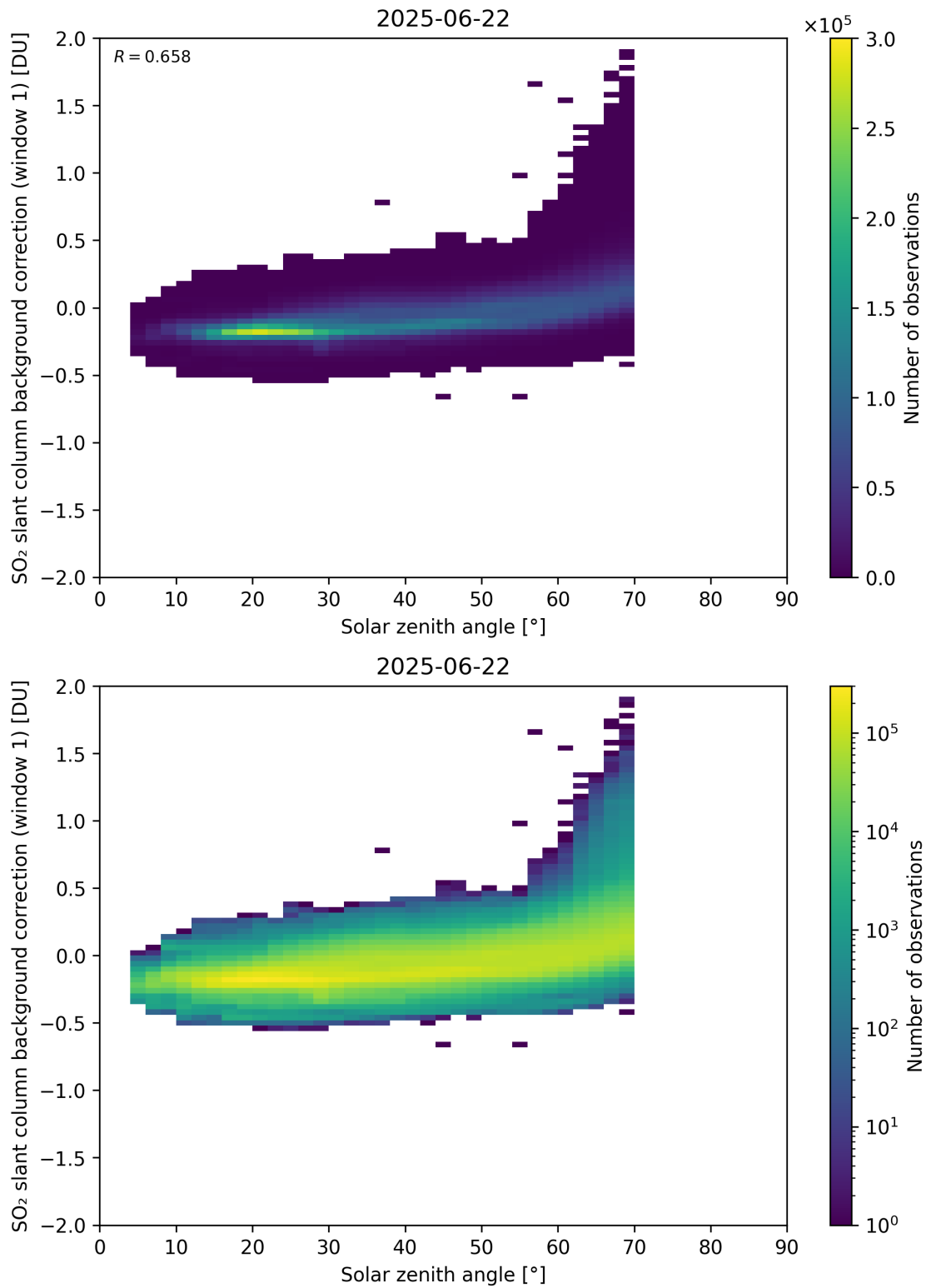
Figure 171: Scatter density plot of “Solar zenith angle” against “SO 2 slant column background correction (window 1)” for 2025-06-22 to 2025-06-23.
