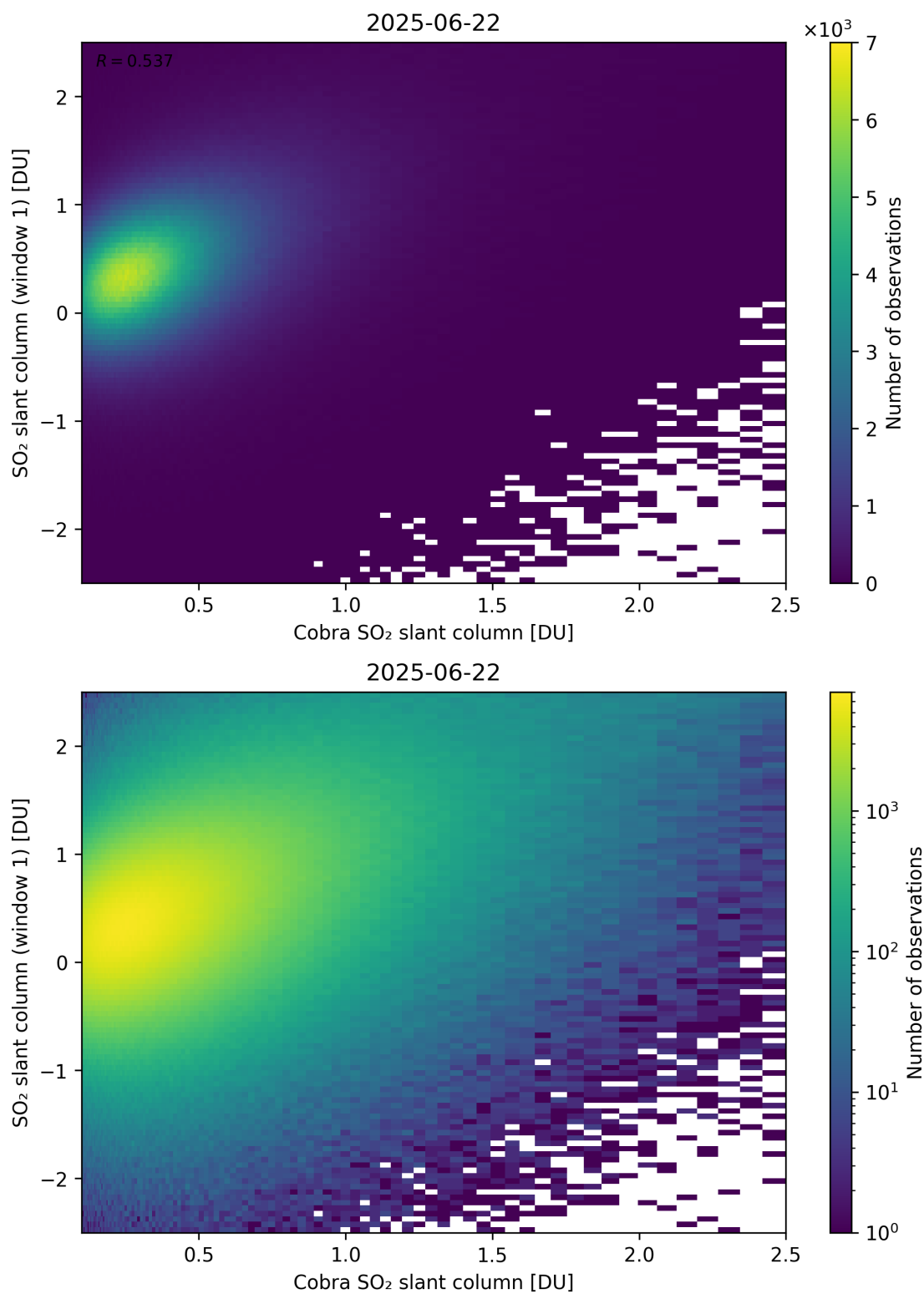
Figure 219: Scatter density plot of “Cobra SO 2 slant column” against “SO 2 slant column (window 1)” for 2025-06-22 to 2025-06-23.
