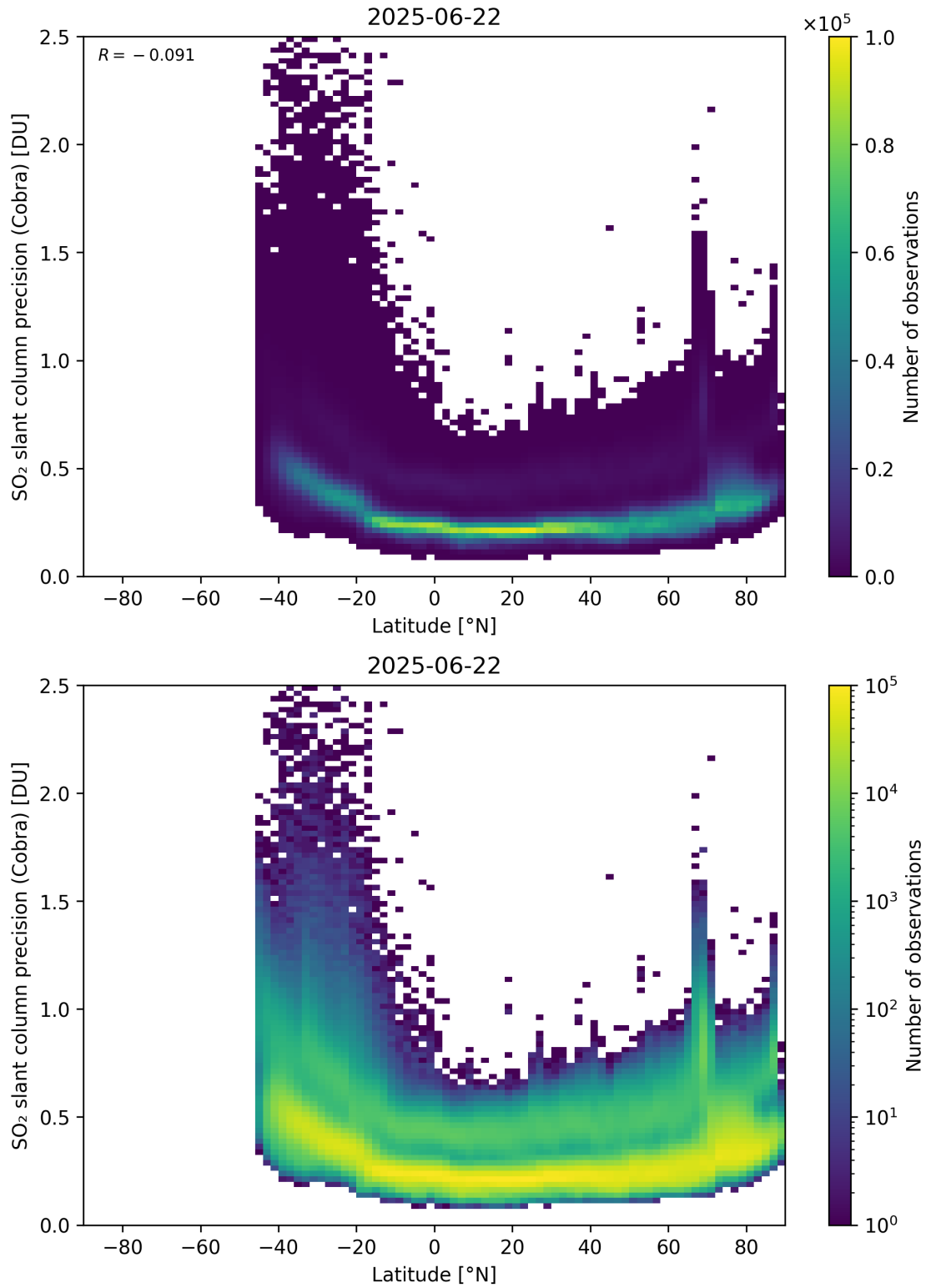
Figure 158: Scatter density plot of “Latitude” against “SO 2 slant column precision (Cobra)” for 2025-06-22 to 2025-06-23.
