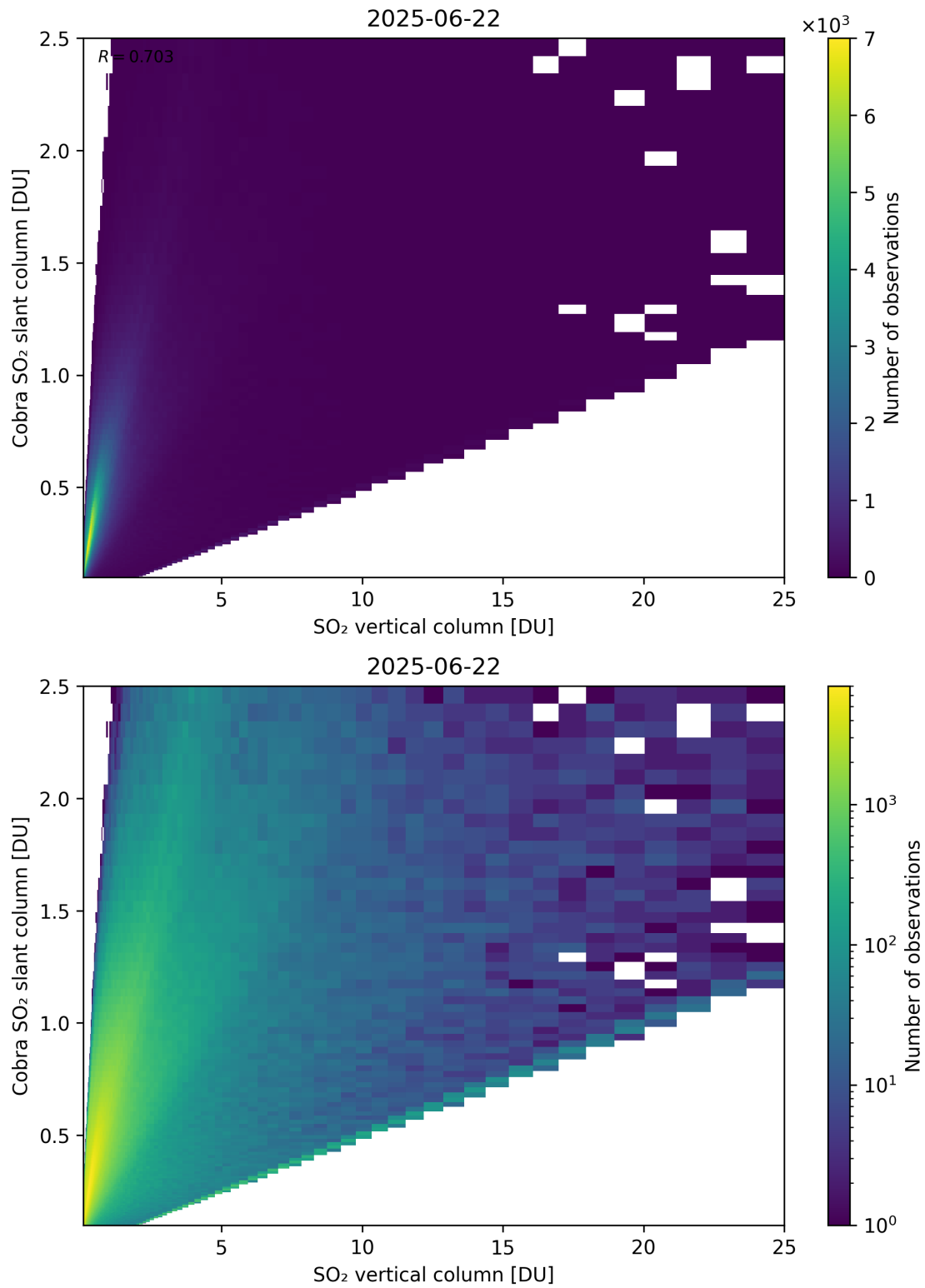
Figure 349: Scatter density plot of “SO 2 vertical column” against “Cobra SO 2 slant column” for 2025-06-22 to 2025-06-23.
