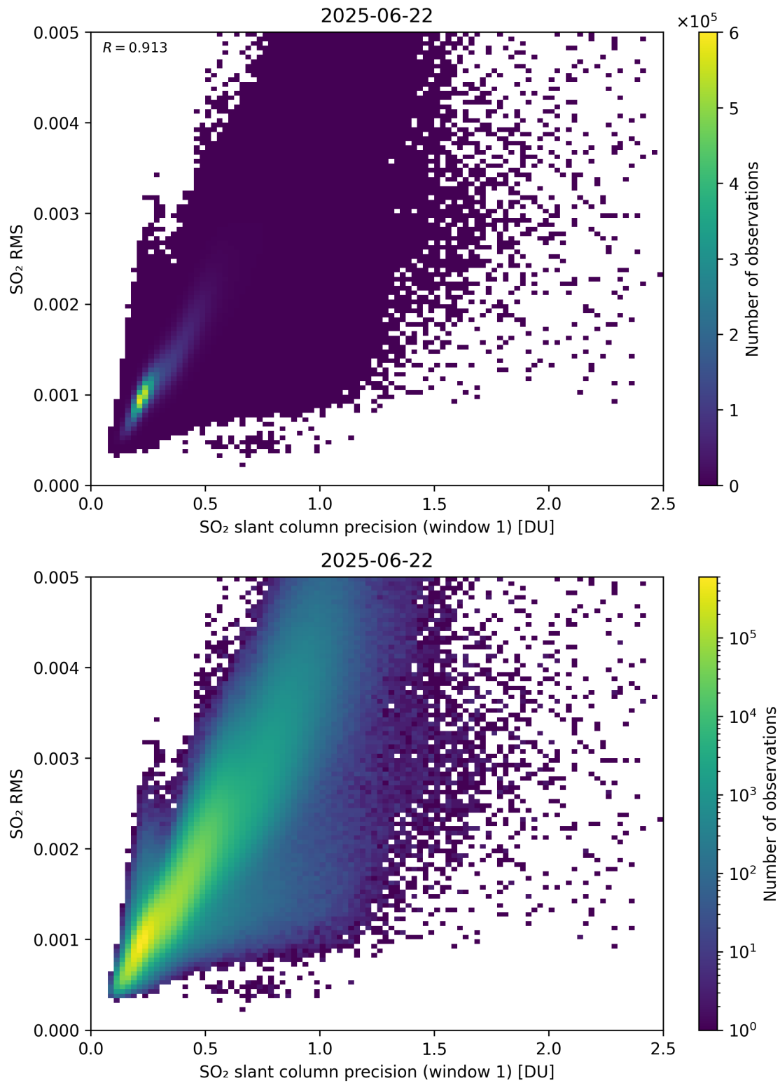
Figure 273: Scatter density plot of “SO 2 slant column precision (window 1)” against “SO 2 RMS” for 2025-06-22 to 2025-06-23.
