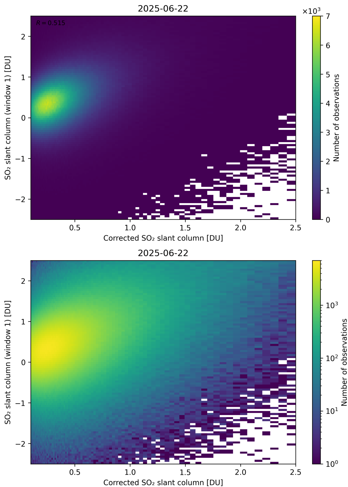
Figure 237: Scatter density plot of “Corrected SO 2 slant column” against “SO 2 slant column (window 1)” for 2025-06-22 to 2025-06-23.
