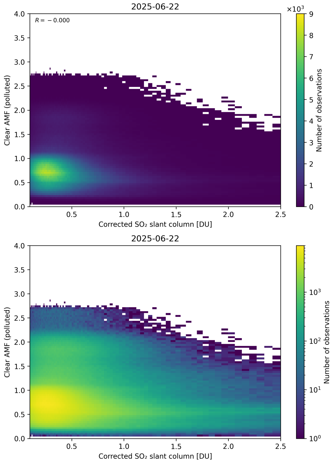
Figure 232: Scatter density plot of “Corrected SO 2 slant column” against “Clear AMF (polluted)” for 2025-06-22 to 2025-06-23.
