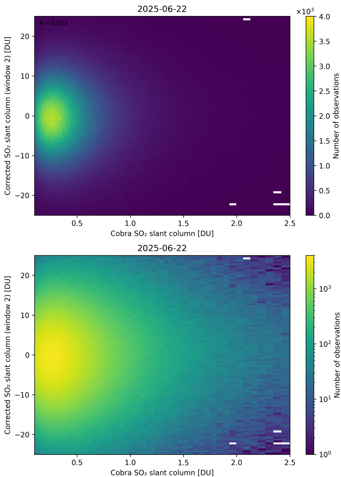
Figure 217: Scatter density plot of “Cobra SO 2 slant column” against “Corrected SO 2 slant column (window 2)” for 2025-06-22 to 2025-06-23.
