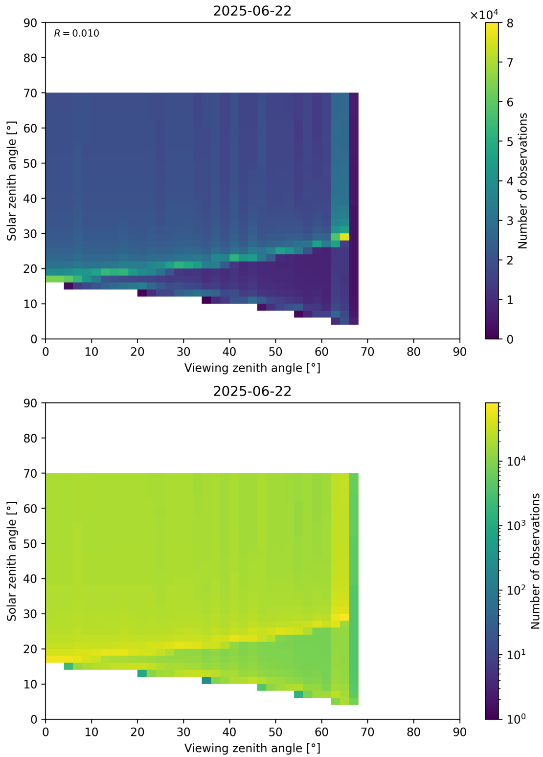
Figure 369: Scatter density plot of “Viewing zenith angle” against “Solar zenith angle” for 2025-06-22 to 2025-06-23.
