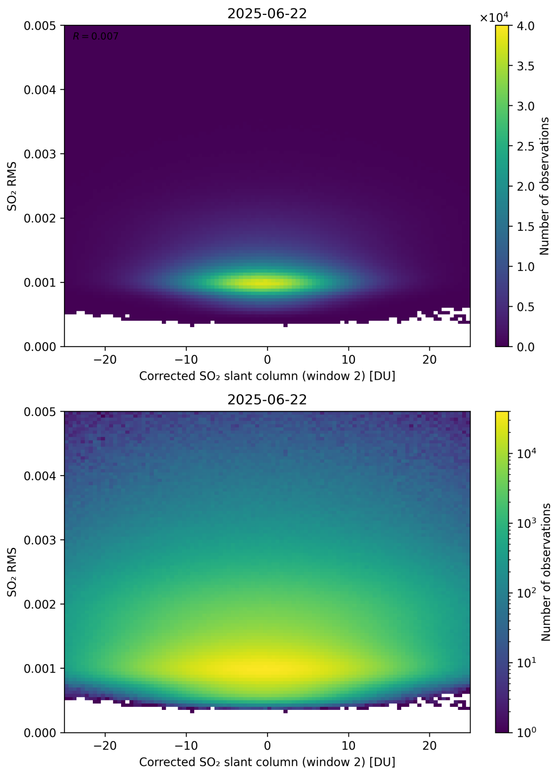
Figure 248: Scatter density plot of “Corrected SO 2 slant column (window 2)” against “SO 2 RMS” for 2025-06-22 to 2025-06-23.
