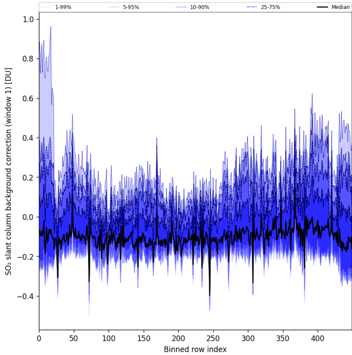
Figure 92: Along track statistics of “SO 2 slant column background correction (window 1)” for 2025-06-22 to 2025-06-23
