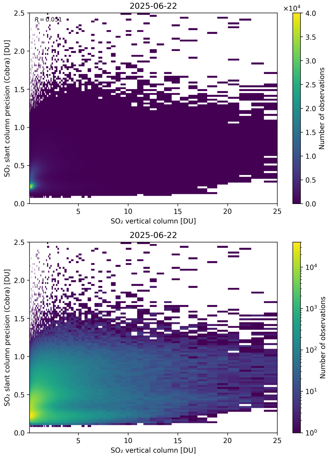
Figure 350: Scatter density plot of “SO 2 vertical column” against “SO 2 slant column precision (Cobra)” for 2025-06-22 to 2025-06-23.
