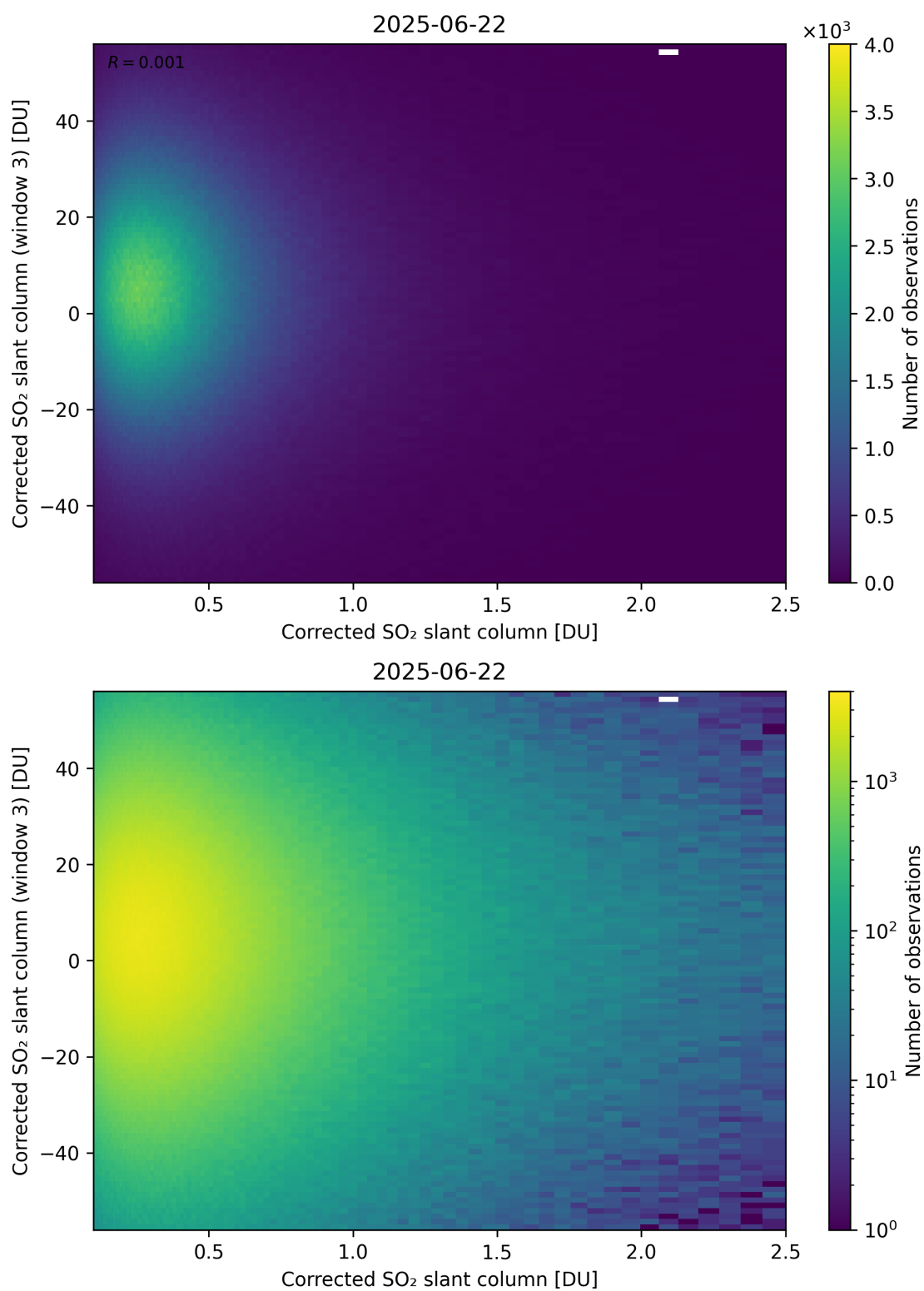
Figure 236: Scatter density plot of “Corrected SO 2 slant column” against “Corrected SO 2 slant column (window 3)” for 2025-06-22 to 2025-06-23.
