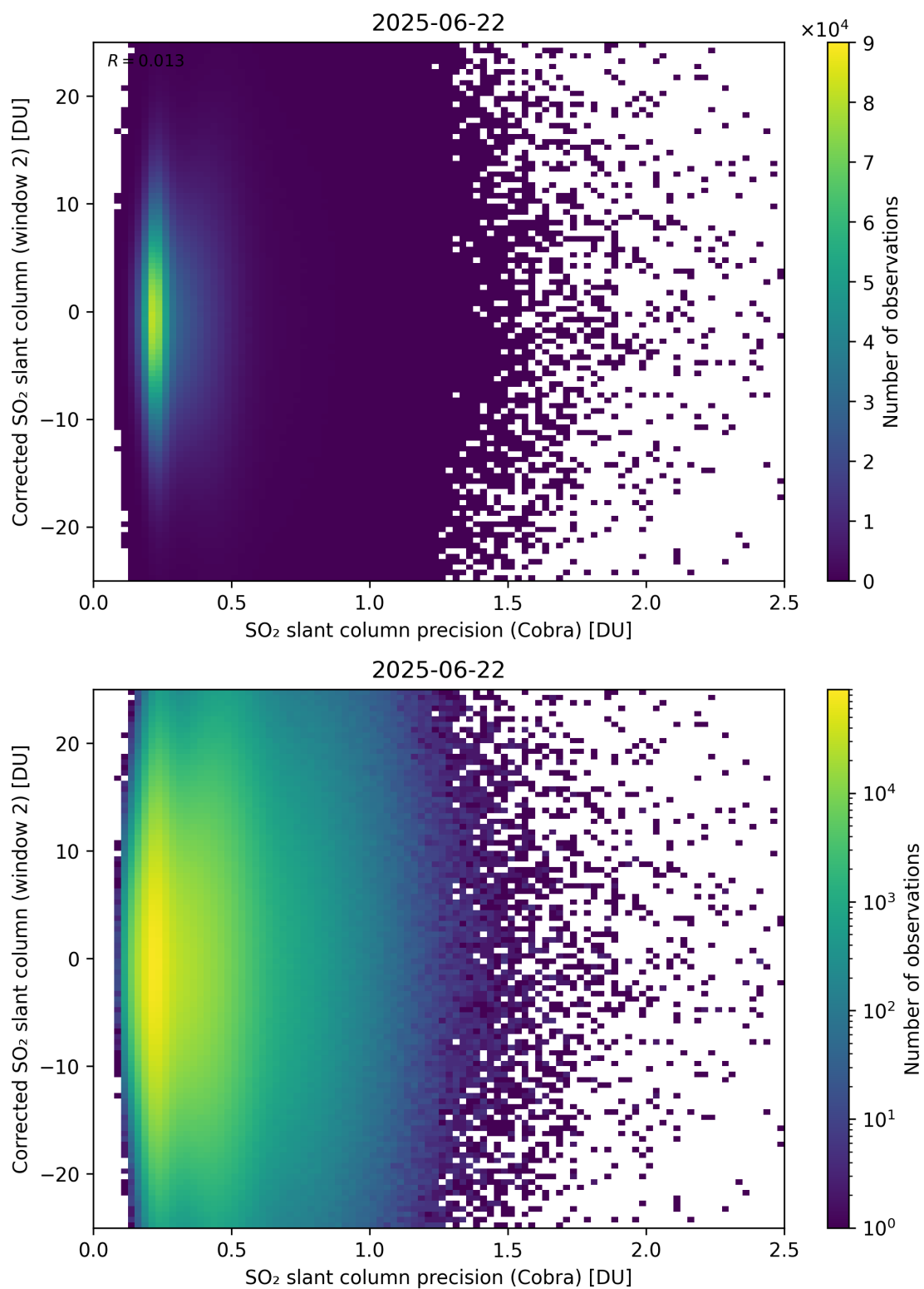
Figure 206: Scatter density plot of “SO 2 slant column precision (Cobra)” against “Corrected SO 2 slant column (window 2)” for 2025-06-22 to 2025-06-23.
