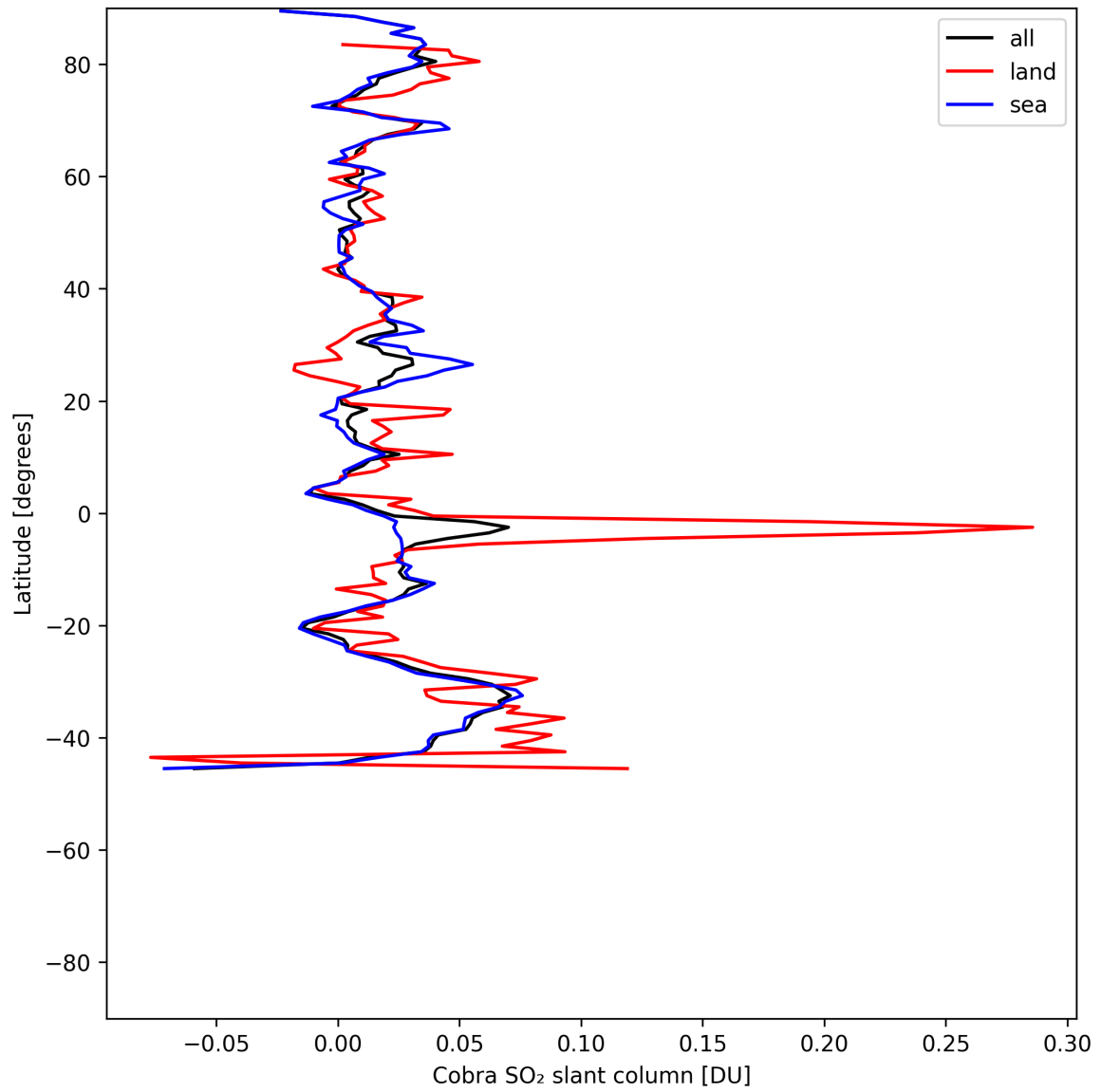
Figure 35: Zonal average of “Cobra SO 2 slant column” for 2025-06-22 to 2025-06-23.
