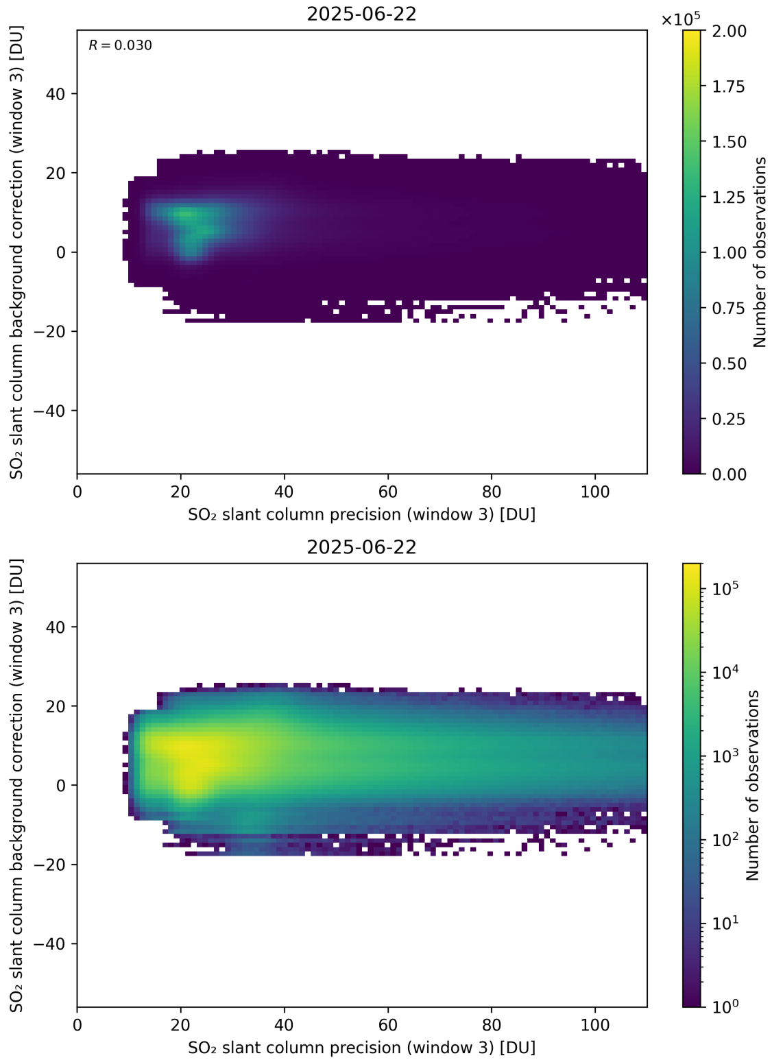
Figure 307: Scatter density plot of “SO 2 slant column precision (window 3)” against “SO 2 slant column background correction (window 3)” for 2025-06-22 to 2025-06-23.
