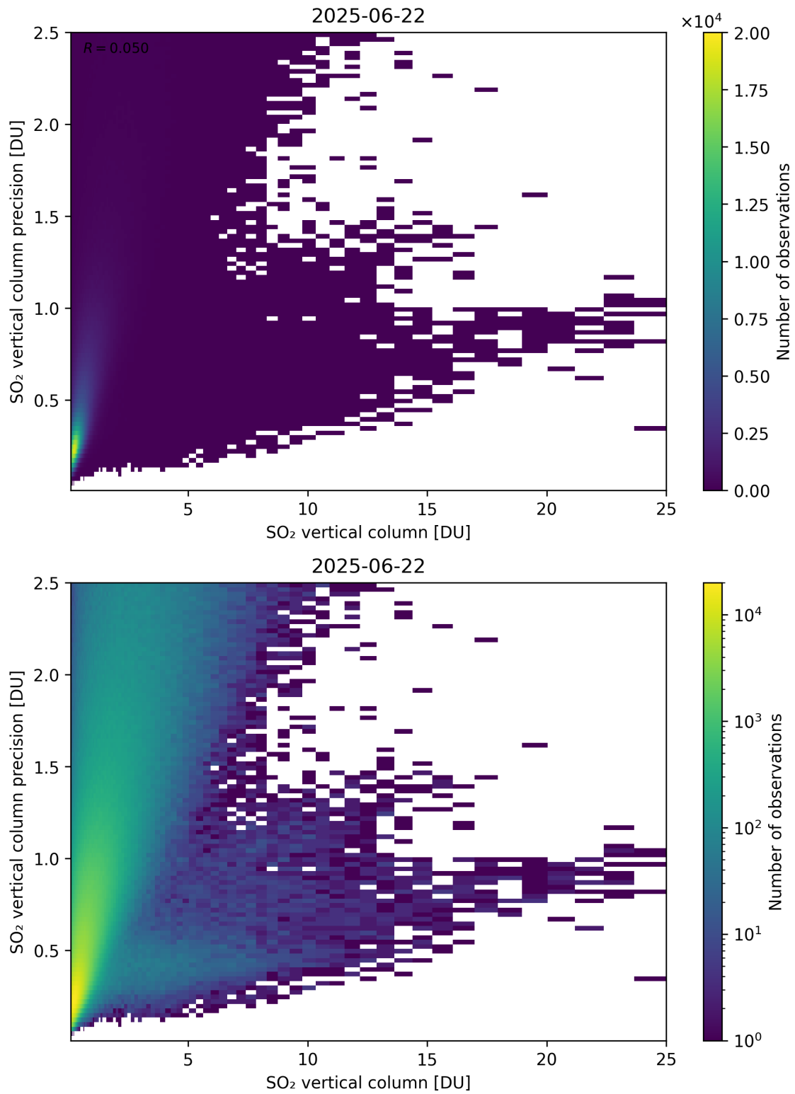
Figure 361: Scatter density plot of “SO 2 vertical column” against “SO 2 vertical column precision” for 2025-06-22 to 2025-06-23.
