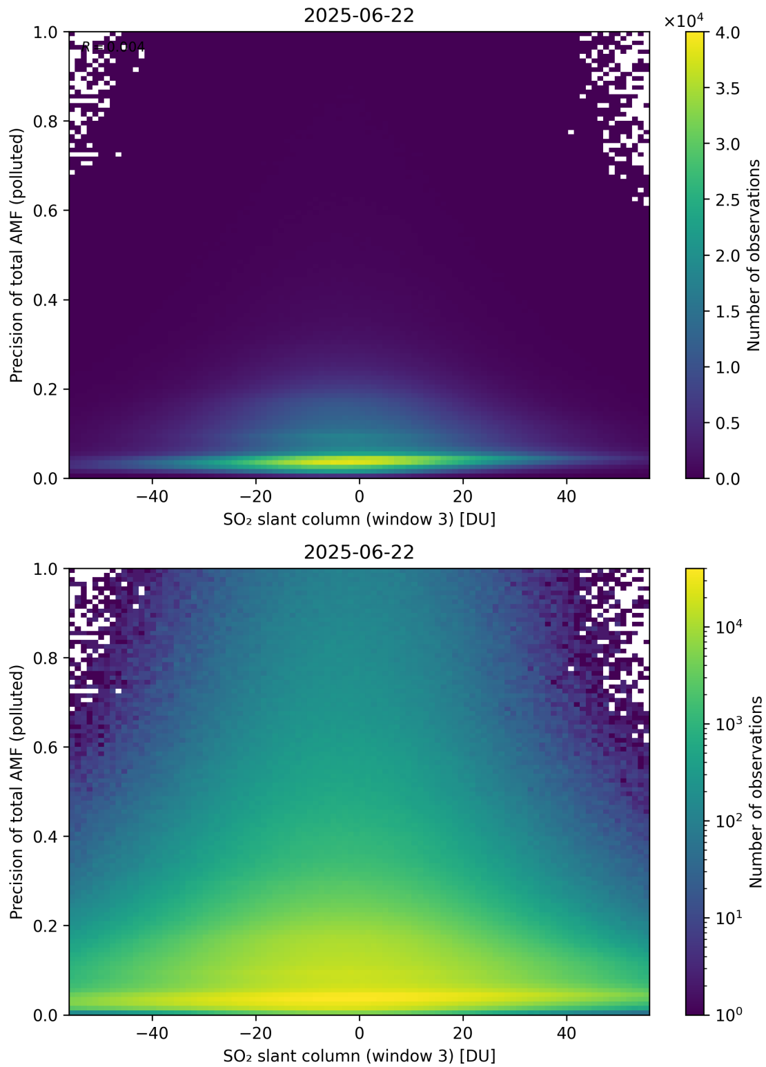
Figure 319: Scatter density plot of “SO 2 slant column (window 3)” against “Precision of total AMF (polluted)” for 2025-06-22 to 2025-06-23.
