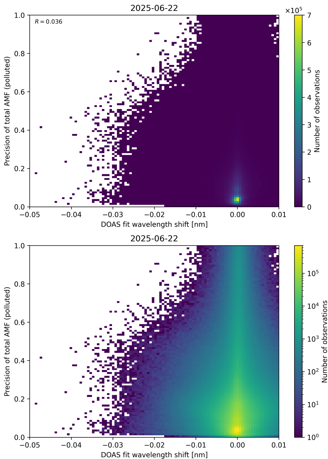
Figure 142: Scatter density plot of “DOAS fit wavelength shift” against “Precision of total AMF (polluted)” for 2025-06-22 to 2025-06-23.
