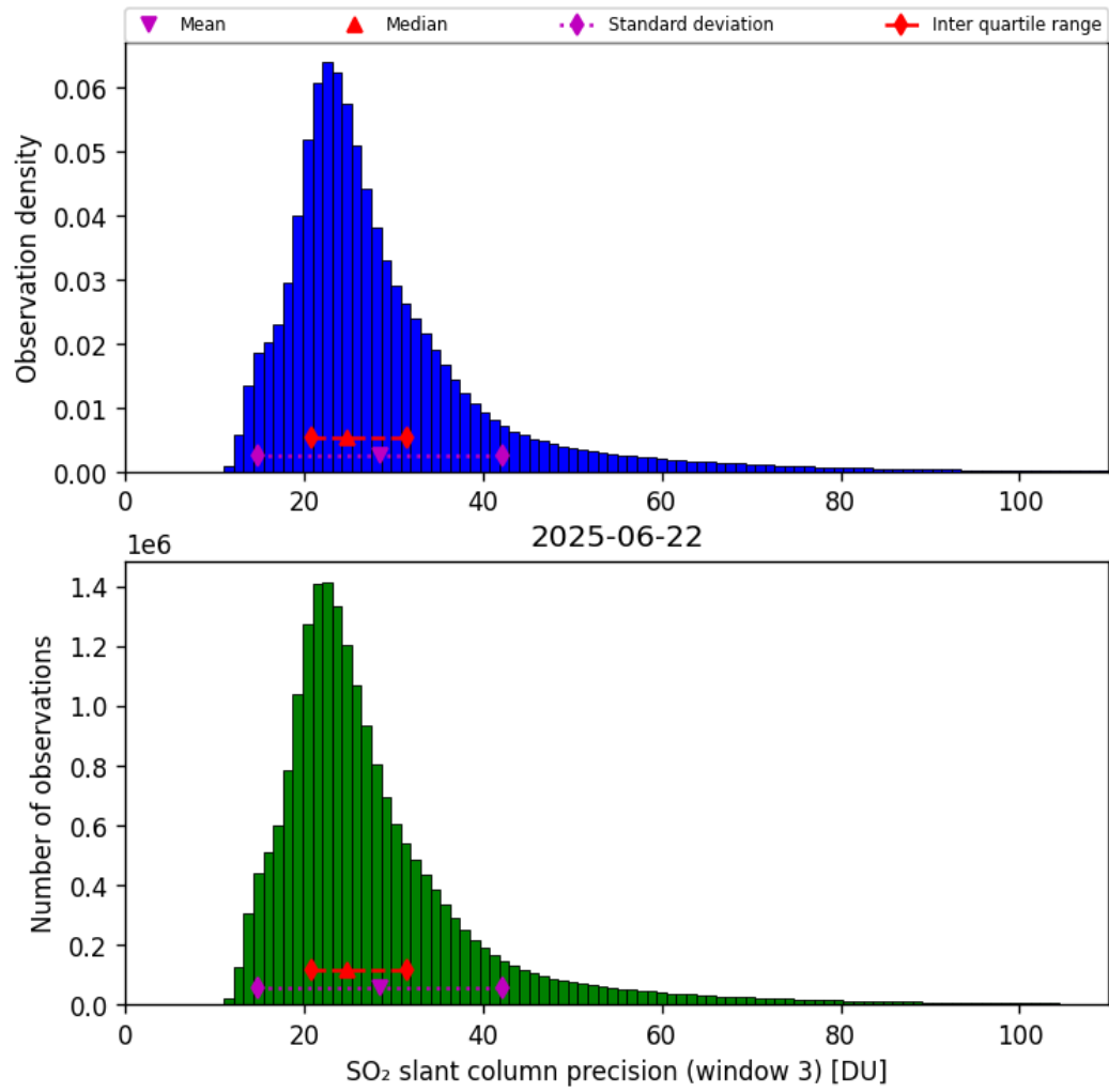
Figure 72: Histogram of “SO 2 slant column precision (window 3)” for 2025-06-22 to 2025-06-23
