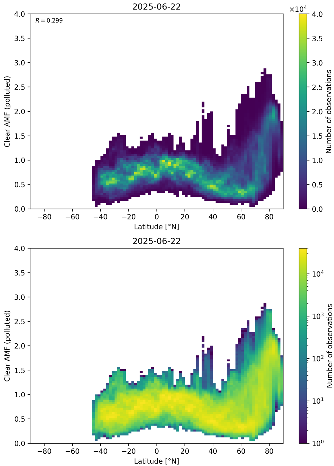
Figure 156: Scatter density plot of “Latitude” against “Clear AMF (polluted)” for 2025-06-22 to 2025-06-23.
