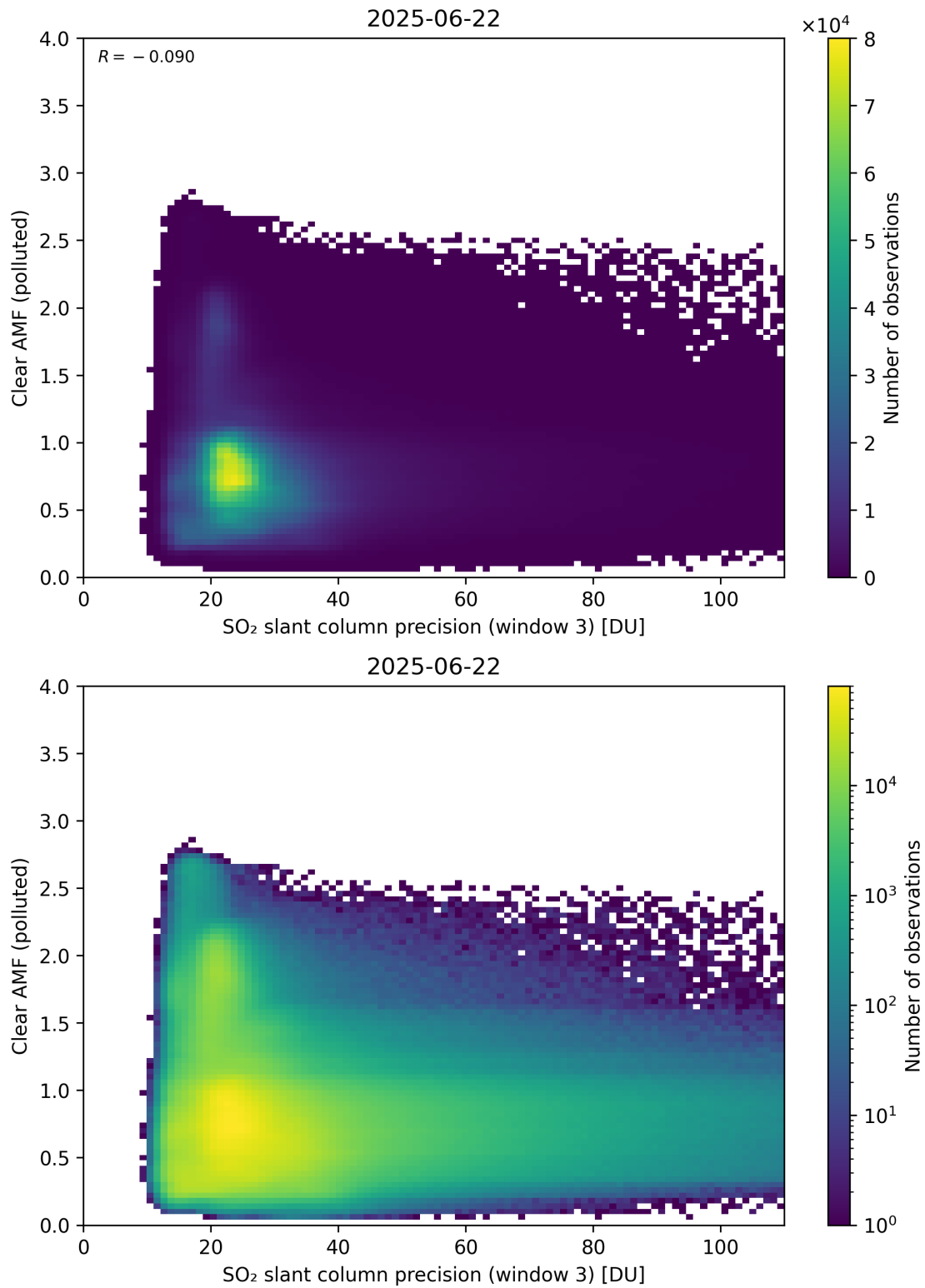
Figure 311: Scatter density plot of “SO 2 slant column precision (window 3)” against “Clear AMF (polluted)” for 2025-06-22 to 2025-06-23.
