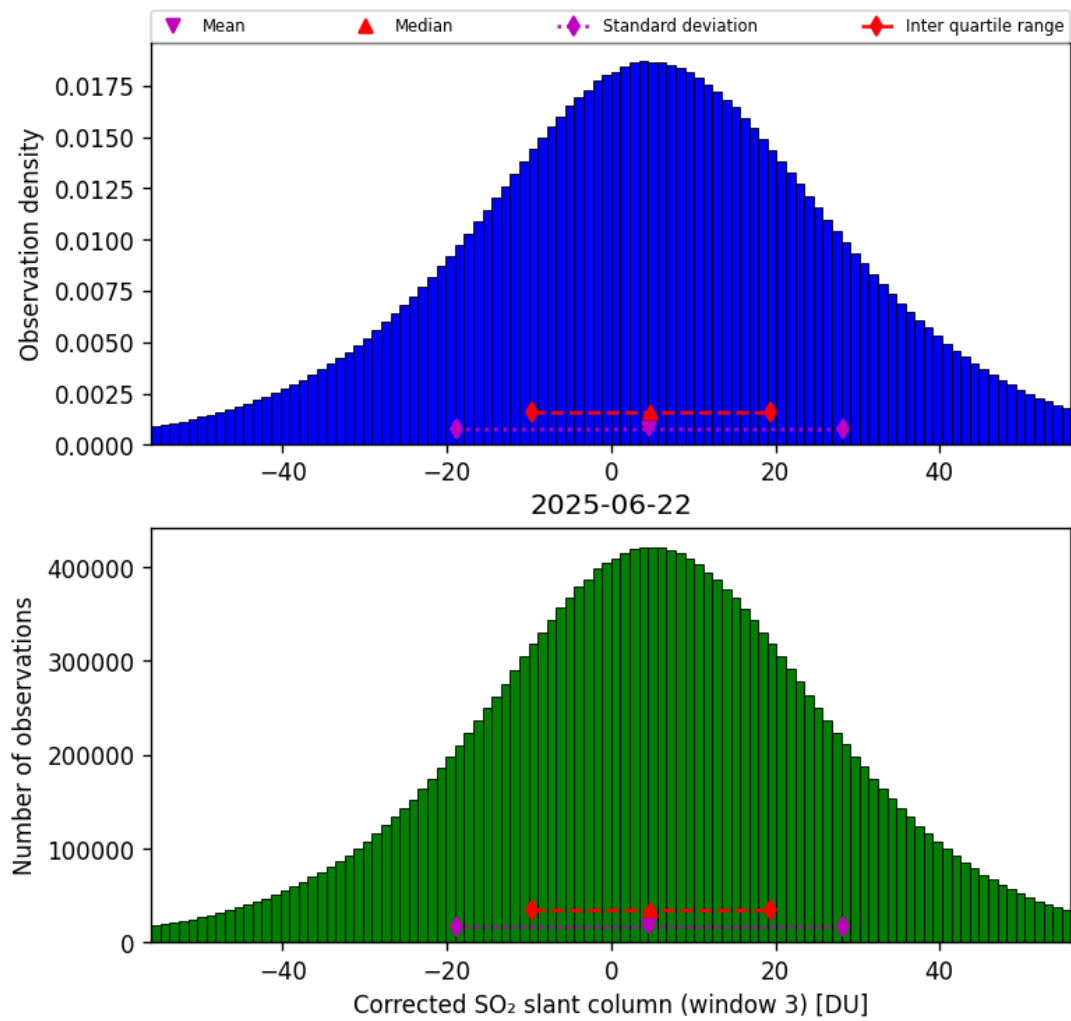
Figure 73: Histogram of “Corrected SO 2 slant column (window 3)” for 2025-06-22 to 2025-06-23
