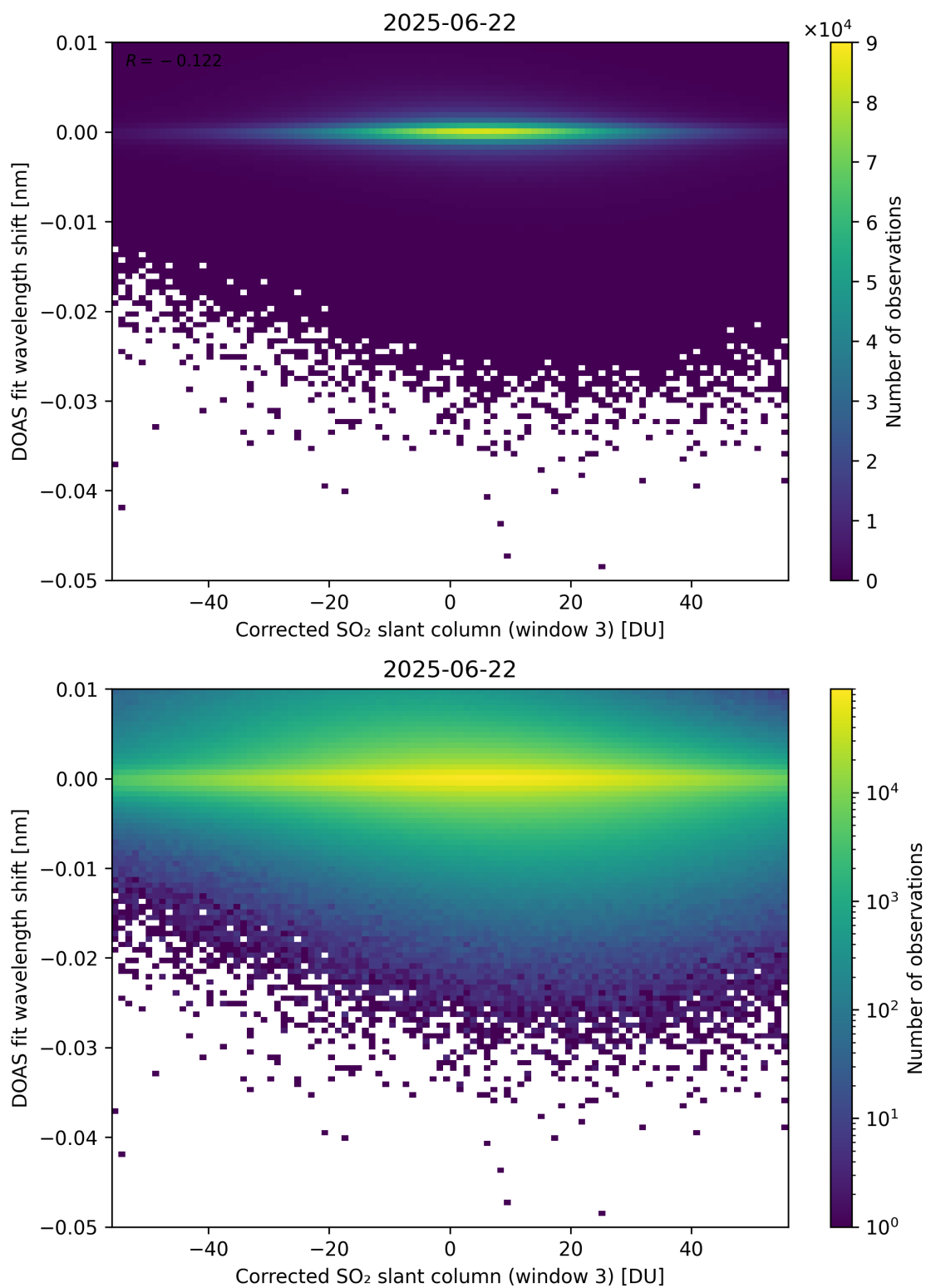
Figure 256: Scatter density plot of “Corrected SO 2 slant column (window 3)” against “DOAS fit wavelength shift” for 2025-06-22 to 2025-06-23.
