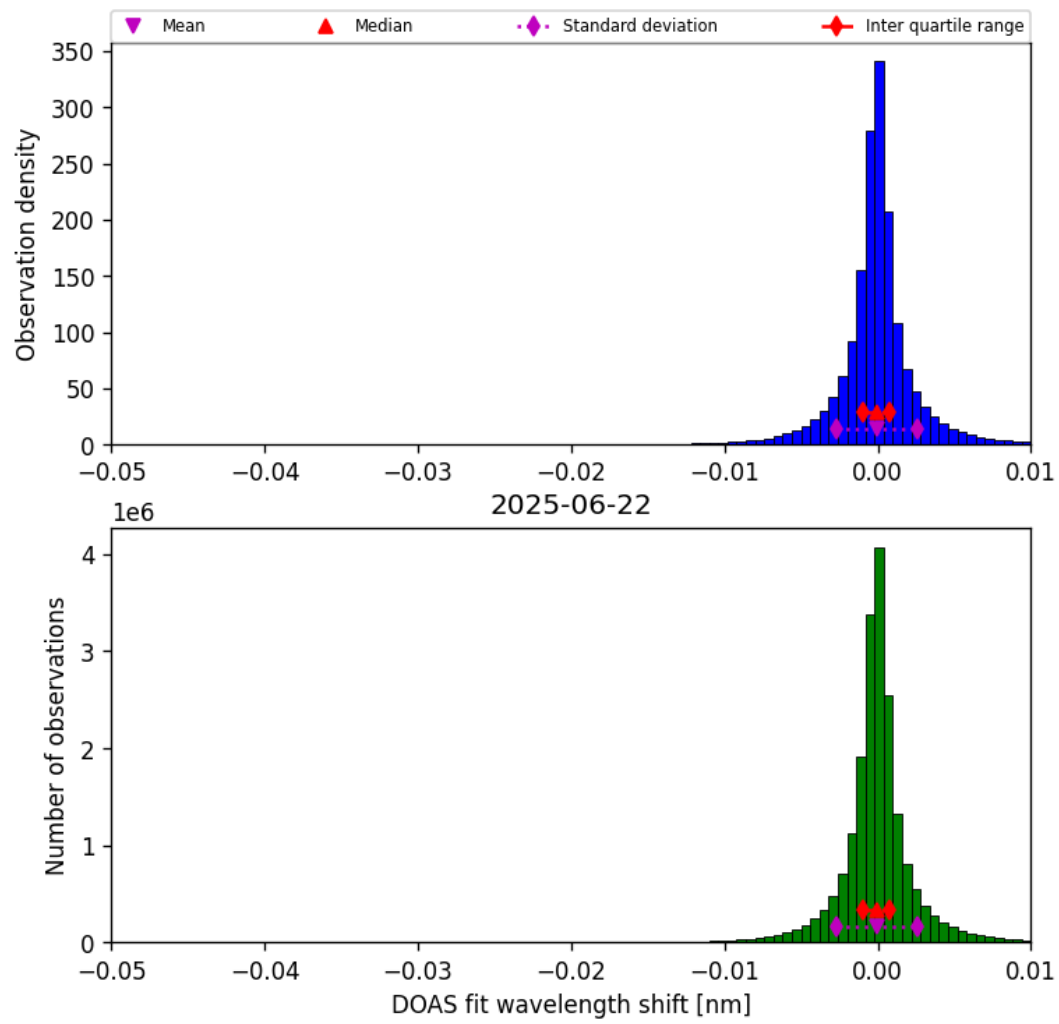
Figure 76: Histogram of “DOAS fit wavelength shift” for 2025-06-22 to 2025-06-23
