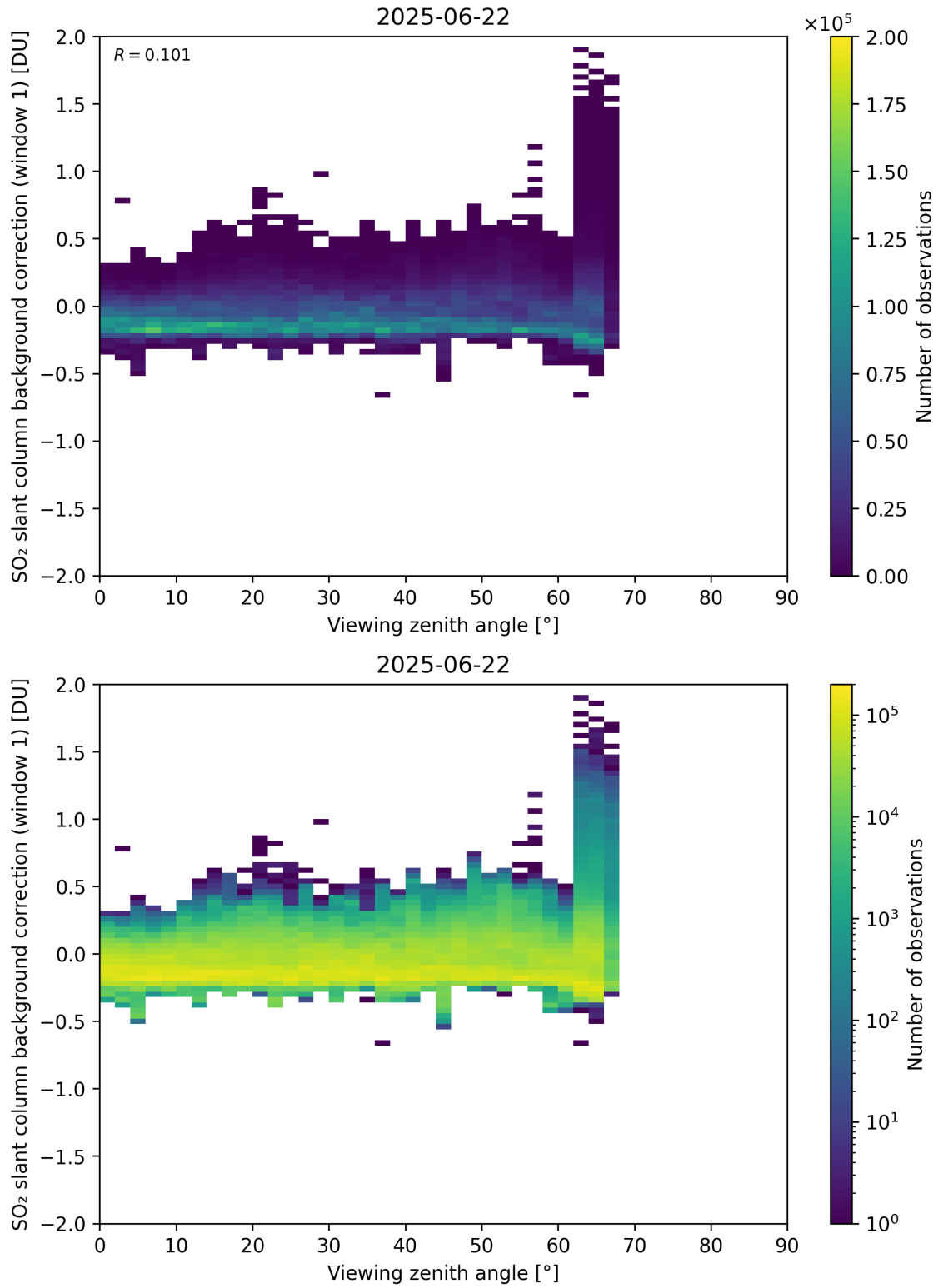
Figure 362: Scatter density plot of “Viewing zenith angle” against “SO 2 slant column background correction (window 1)” for 2025-06-22 to 2025-06-23.
