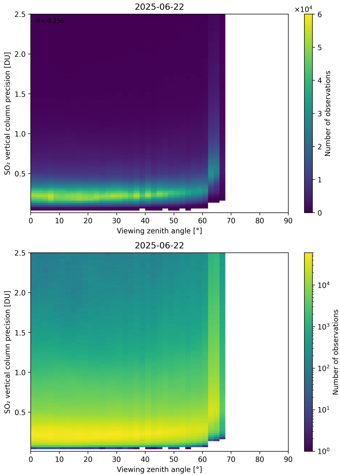
Figure 384: Scatter density plot of “Viewing zenith angle” against “SO 2 vertical column precision” for 2025-06-22 to 2025-06-23.
