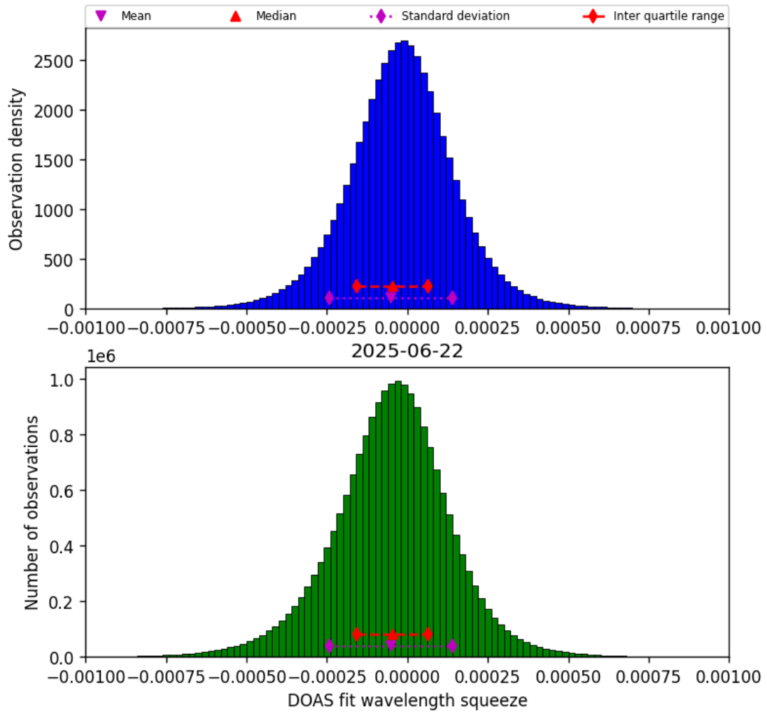
Figure 77: Histogram of “DOAS fit wavelength squeeze” for 2025-06-22 to 2025-06-23
