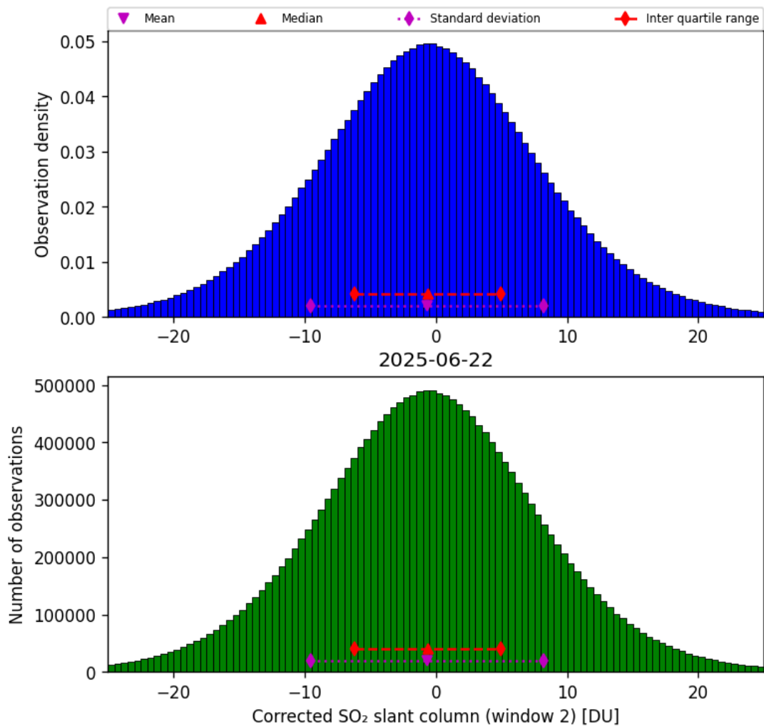
Figure 69: Histogram of “Corrected SO 2 slant column (window 2)” for 2025-06-22 to 2025-06-23
