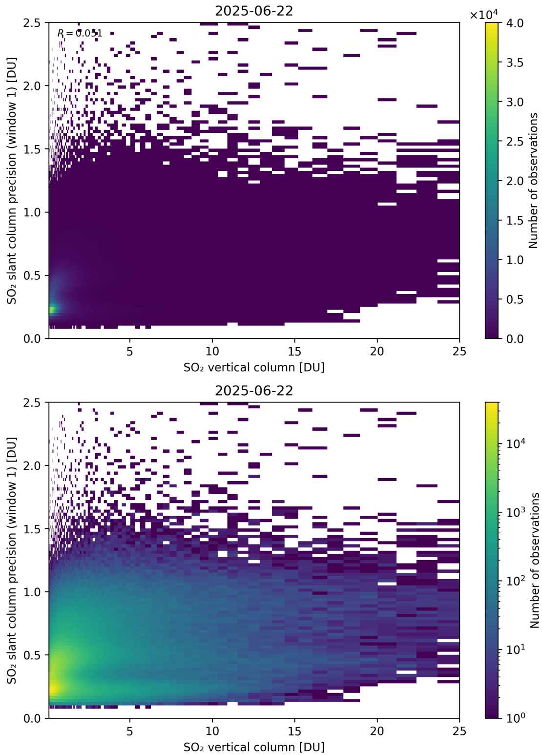
Figure 355: Scatter density plot of “SO 2 vertical column” against “SO 2 slant column precision (window 1)” for 2025-06-22 to 2025-06-23.
