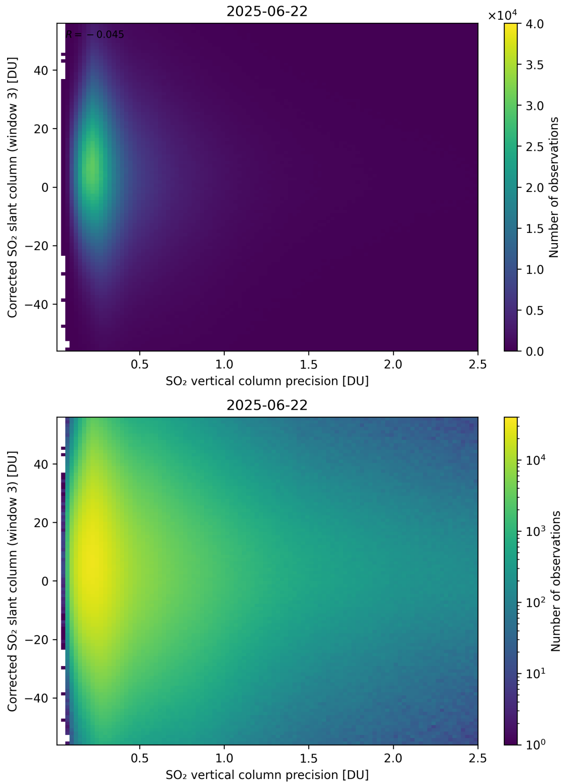
Figure 340: Scatter density plot of “SO 2 vertical column precision” against “Corrected SO 2 slant column (window 3)” for 2025-06-22 to 2025-06-23.
