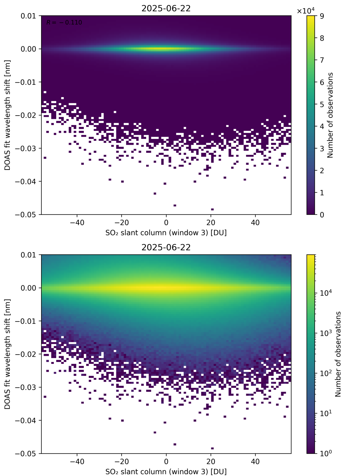
Figure 304: Scatter density plot of “SO 2 slant column (window 3)” against “DOAS fit wavelength shift” for 2025-06-22 to 2025-06-23.
