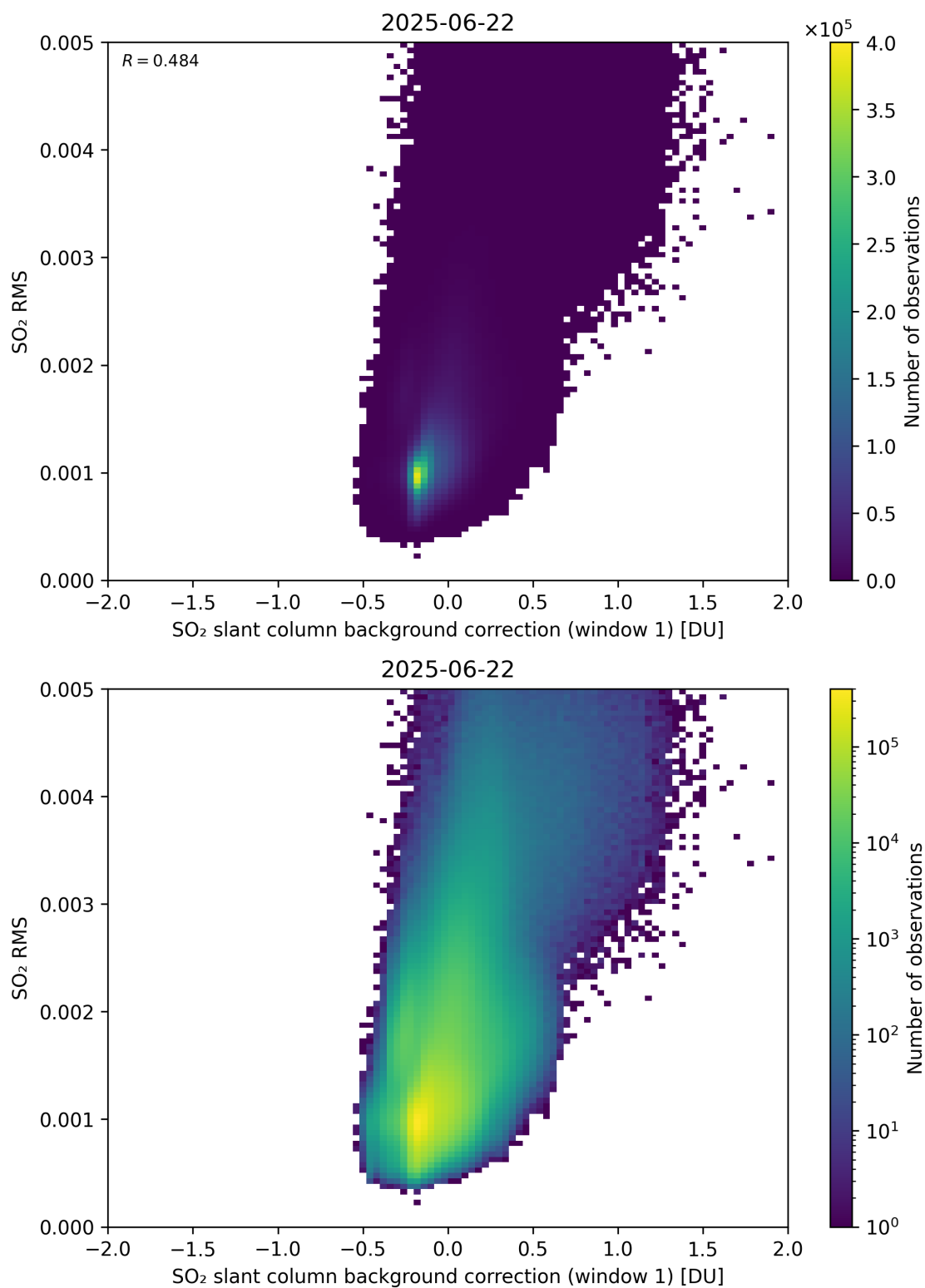
Figure 113: Scatter density plot of “SO 2 slant column background correction (window 1)” against “SO 2 RMS” for 2025-06-22 to 2025-06-23.
