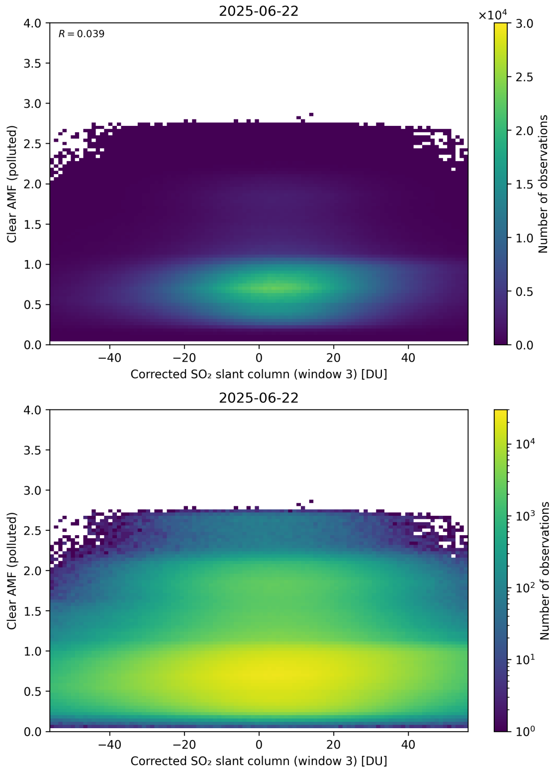
Figure 259: Scatter density plot of “Corrected SO 2 slant column (window 3)” against “Clear AMF (polluted)” for 2025-06-22 to 2025-06-23.
