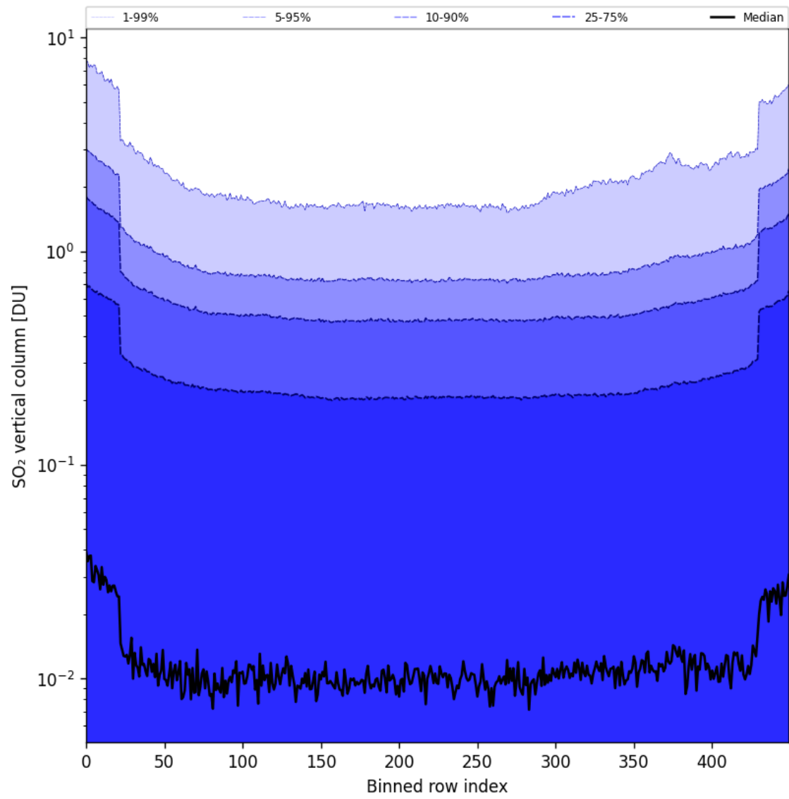
Figure 84: Along track statistics of “SO 2 vertical column” for 2025-06-22 to 2025-06-23
