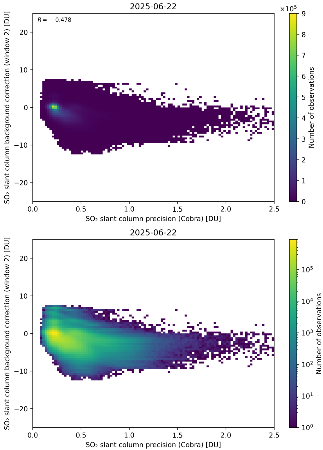
Figure 200: Scatter density plot of “SO 2 slant column precision (Cobra)” against “SO 2 slant column background correction (window 2)” for 2025-06-22 to 2025-06-23.
