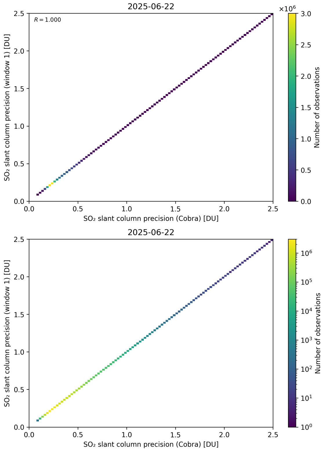
Figure 209: Scatter density plot of “SO 2 slant column precision (Cobra)” against “SO 2 slant column precision (window 1)” for 2025-06-22 to 2025-06-23.
