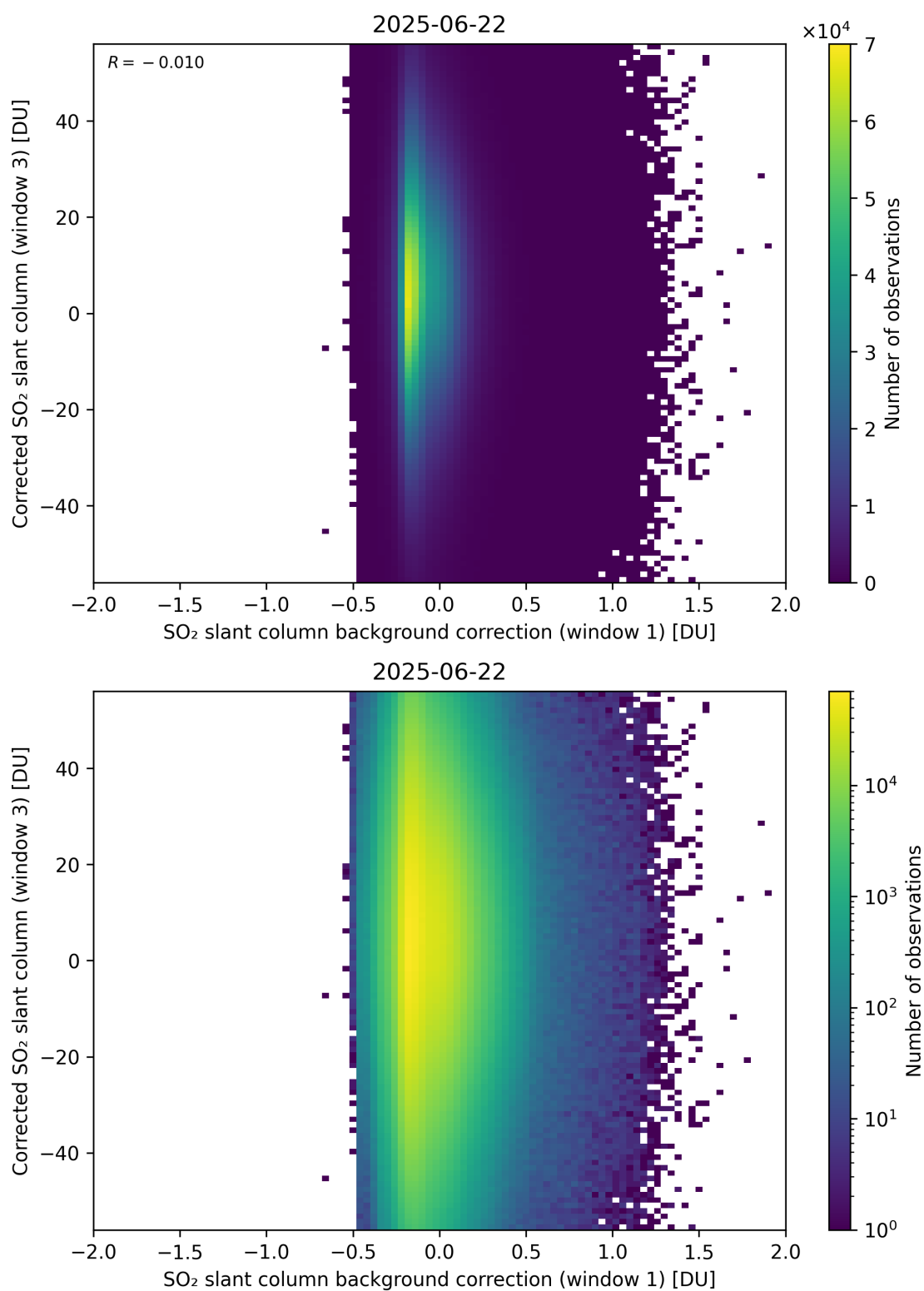
Figure 116: Scatter density plot of “SO 2 slant column background correction (window 1)” against “Corrected SO 2 slant column (window 3)” for 2025-06-22 to 2025-06-23.
