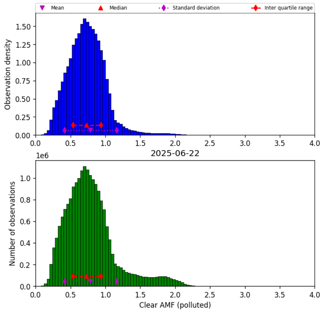
Figure 81: Histogram of “Clear AMF (polluted)” for 2025-06-22 to 2025-06-23
