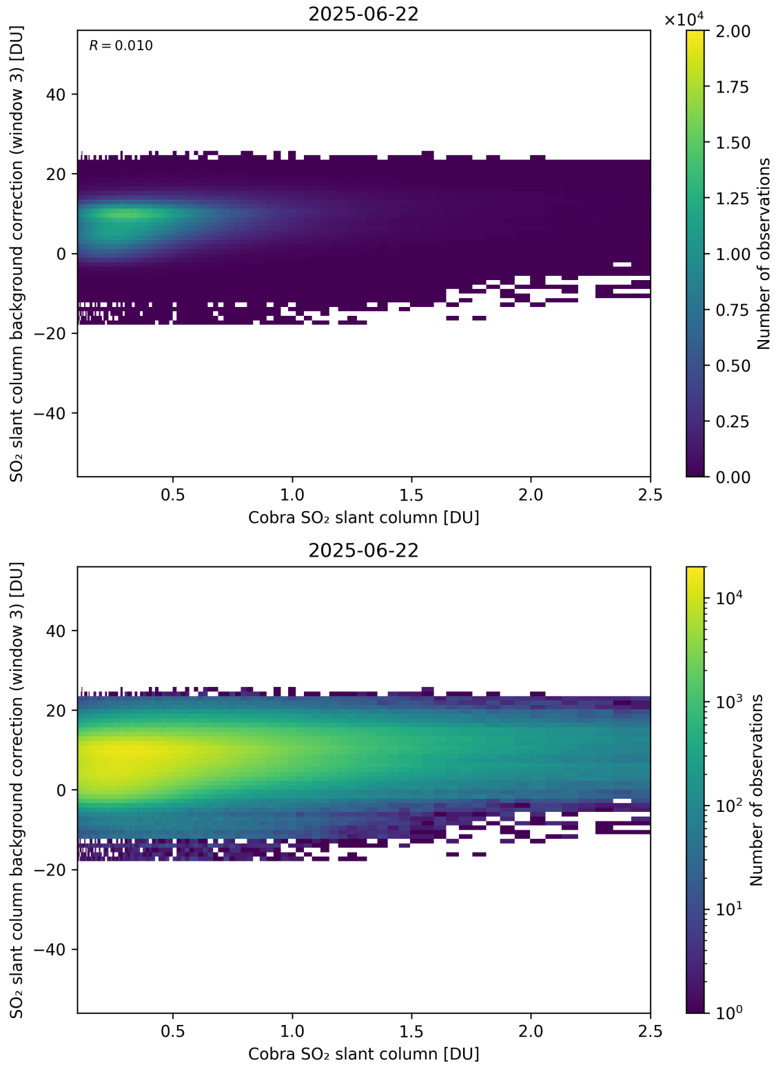
Figure 195: Scatter density plot of “Cobra SO 2 slant column” against “SO 2 slant column background correction (window 3)” for 2025-06-22 to 2025-06-23.
