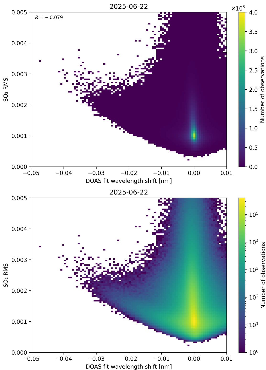
Figure 139: Scatter density plot of “DOAS fit wavelength shift” against “SO 2 RMS” for 2025-06-22 to 2025-06-23.
