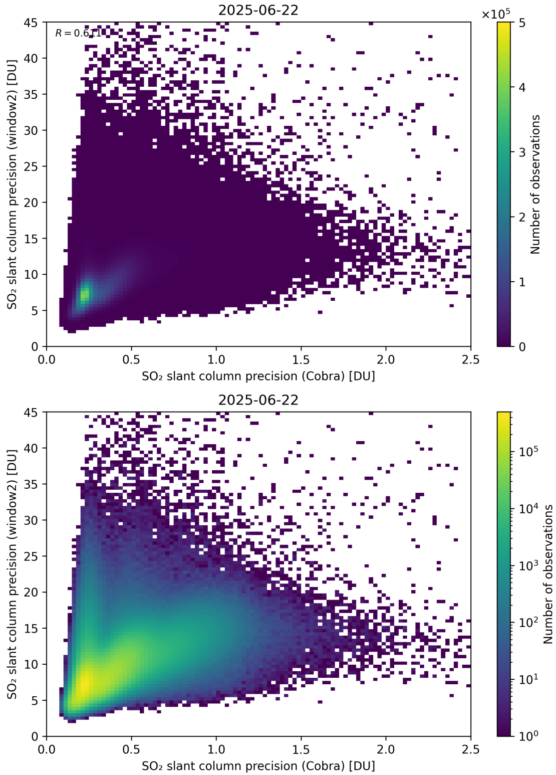
Figure 210: Scatter density plot of “SO 2 slant column precision (Cobra)” against “SO 2 slant column precision (window2)” for 2025-06-22 to 2025-06-23.
