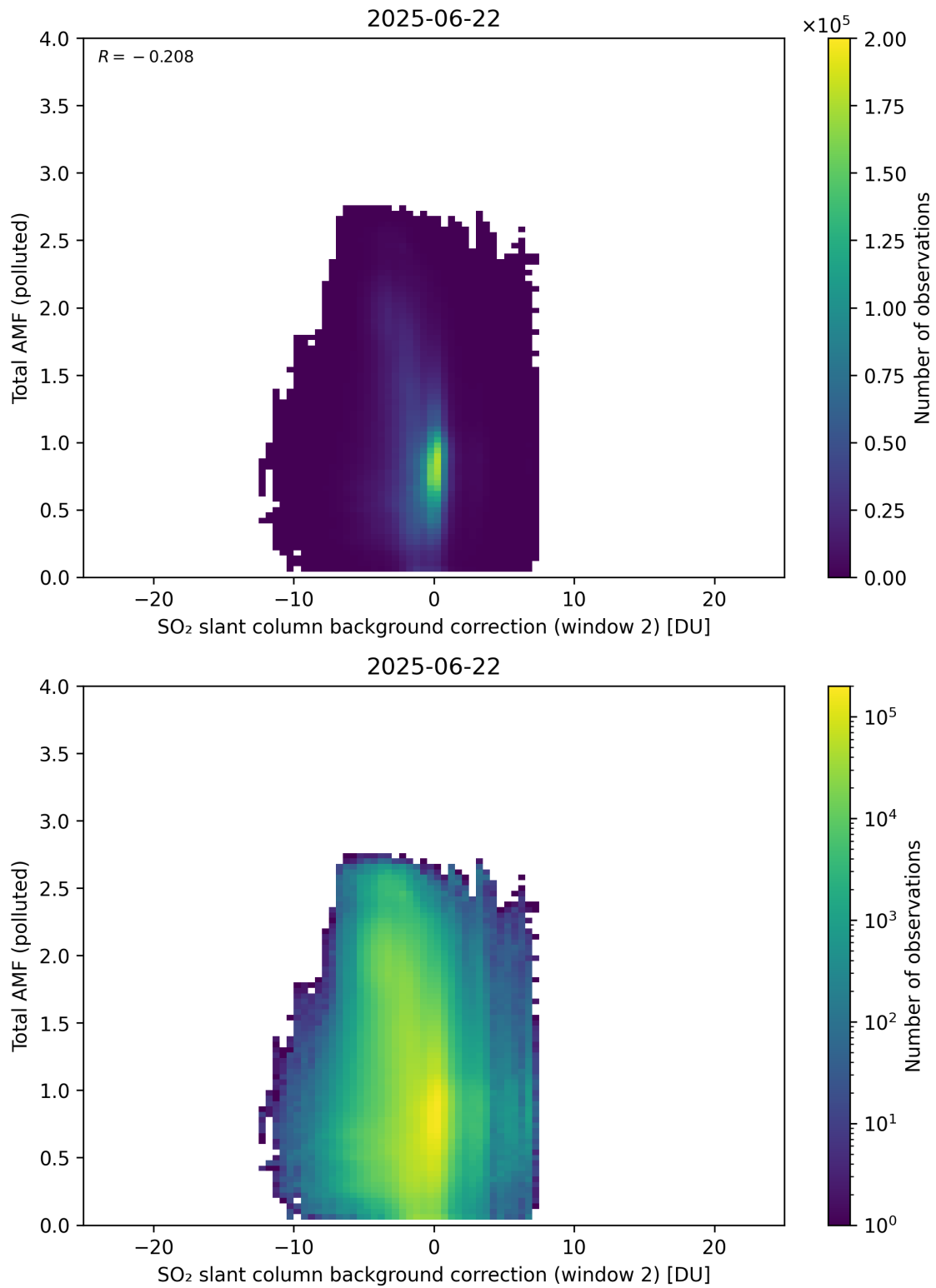
Figure 130: Scatter density plot of “SO 2 slant column background correction (window 2)” against “Total AMF (polluted)” for 2025-06-22 to 2025-06-23.
