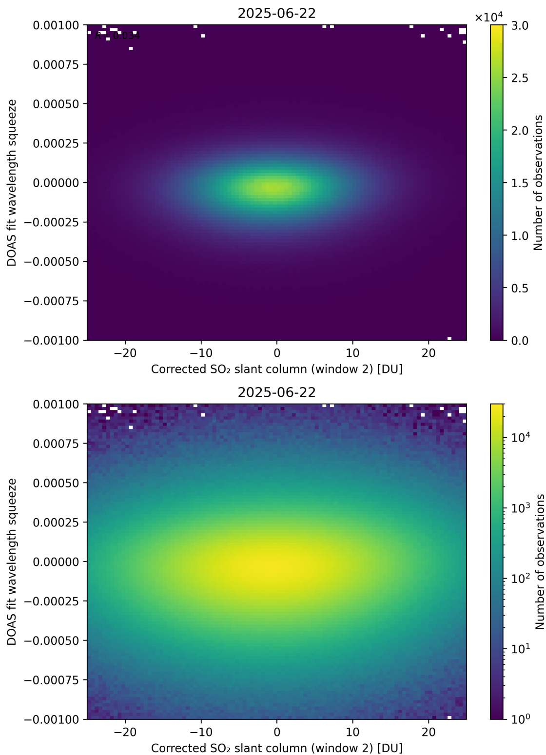
Figure 247: Scatter density plot of “Corrected SO 2 slant column (window 2)” against “DOAS fit wavelength squeeze” for 2025-06-22 to 2025-06-23.
