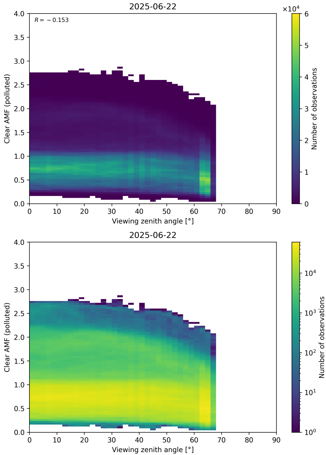
Figure 370: Scatter density plot of “Viewing zenith angle” against “Clear AMF (polluted)” for 2025-06-22 to 2025-06-23.
