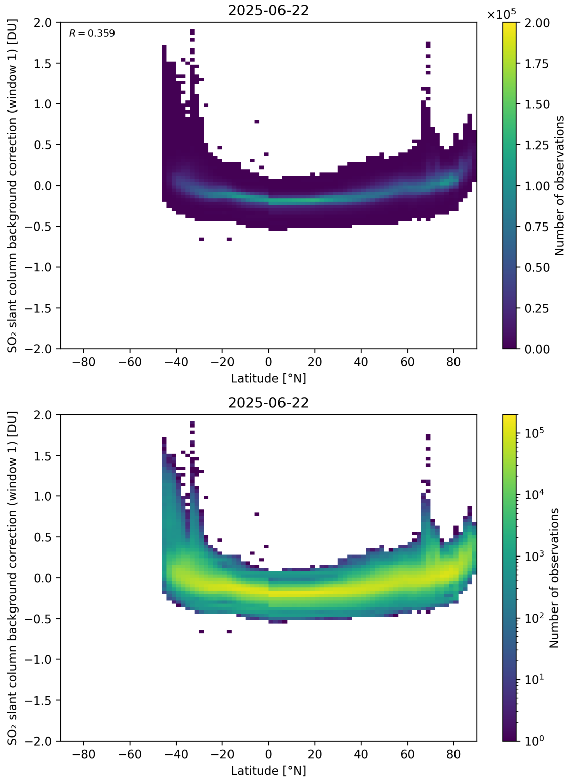
Figure 150: Scatter density plot of “Latitude” against “SO 2 slant column background correction (window 1)” for 2025-06-22 to 2025-06-23.
