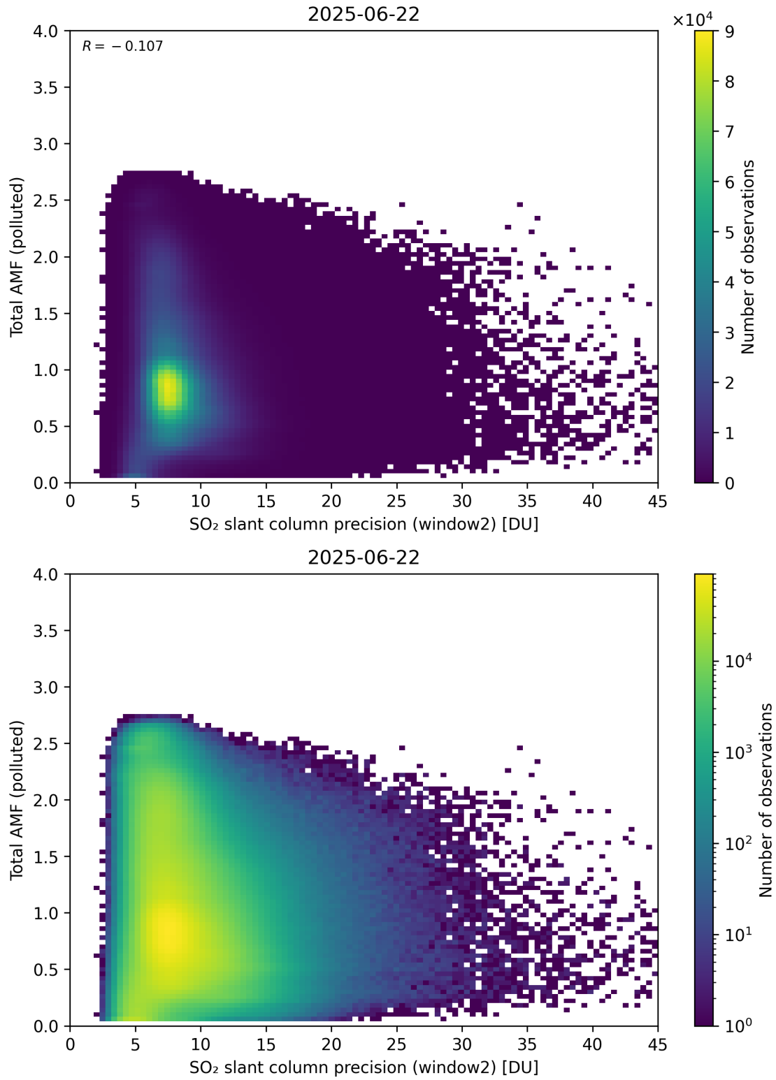
Figure 301: Scatter density plot of “SO 2 slant column precision (window2)” against “Total AMF (polluted)” for 2025-06-22 to 2025-06-23.
