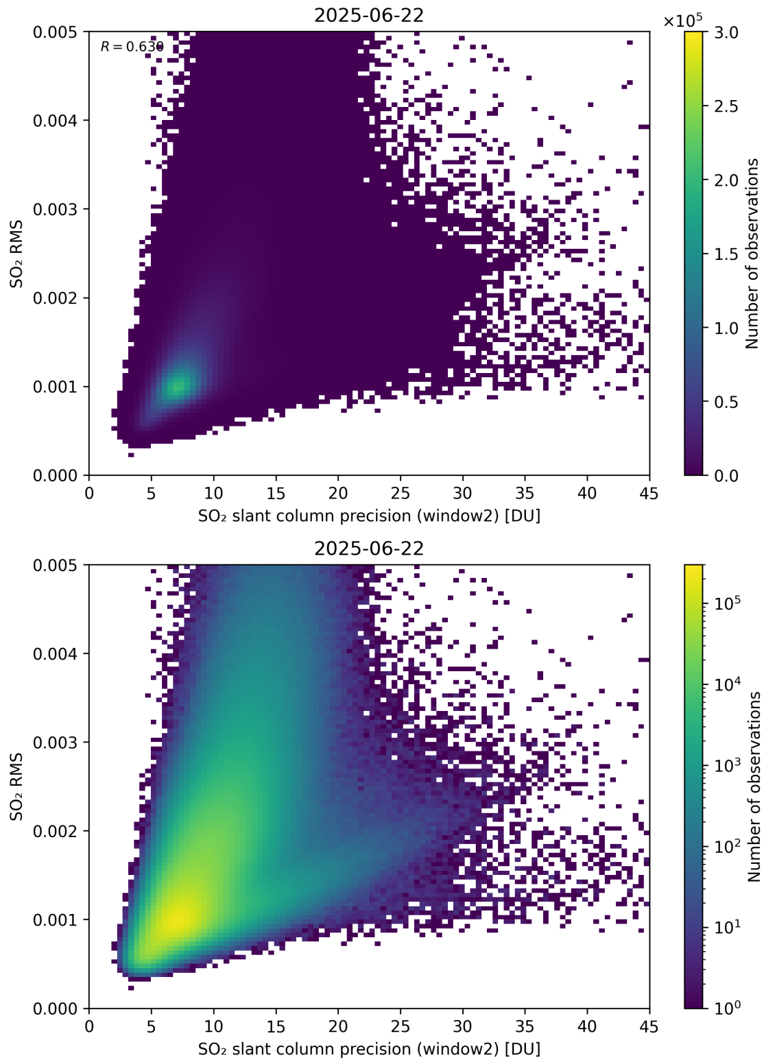
Figure 295: Scatter density plot of “SO 2 slant column precision (window2)” against “SO 2 RMS” for 2025-06-22 to 2025-06-23.
