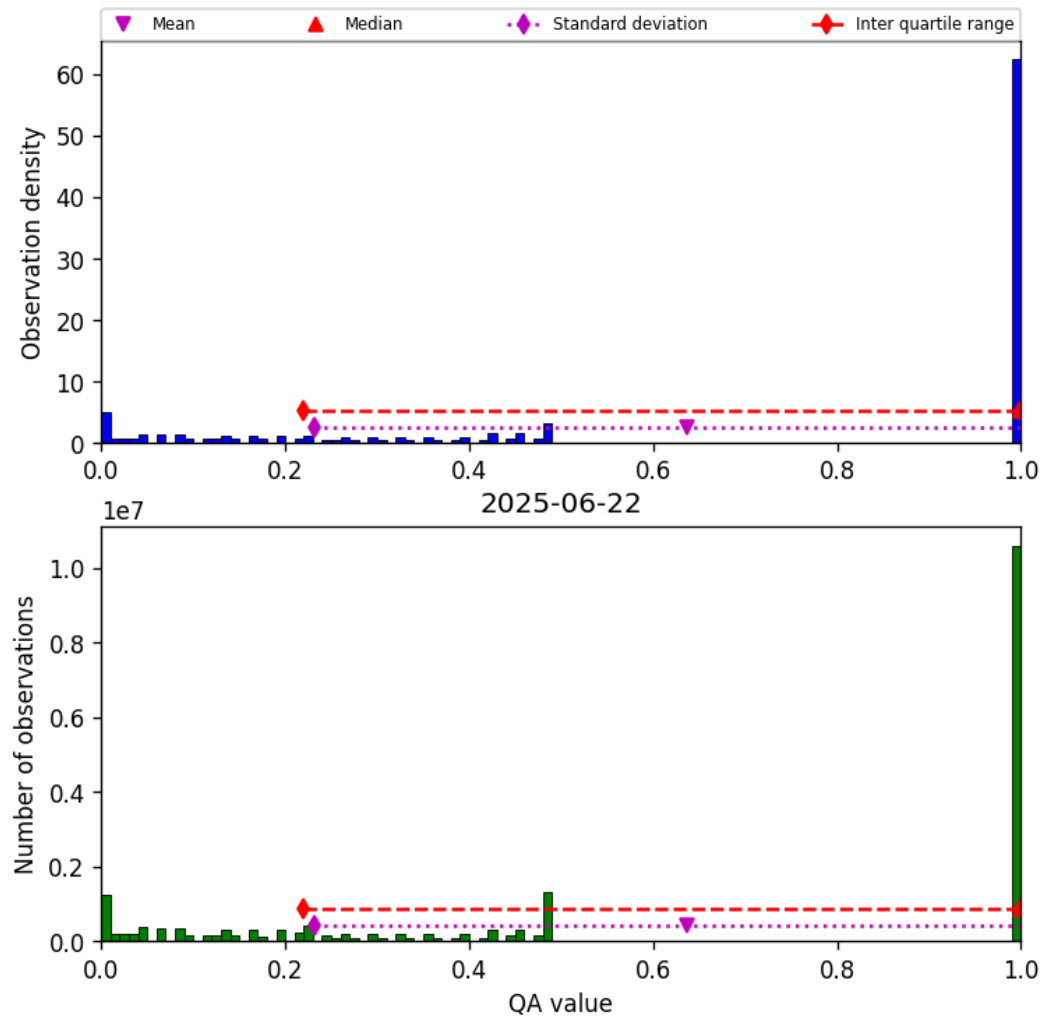
Figure 57: Histogram of “QA value” for 2025-06-22 to 2025-06-23
