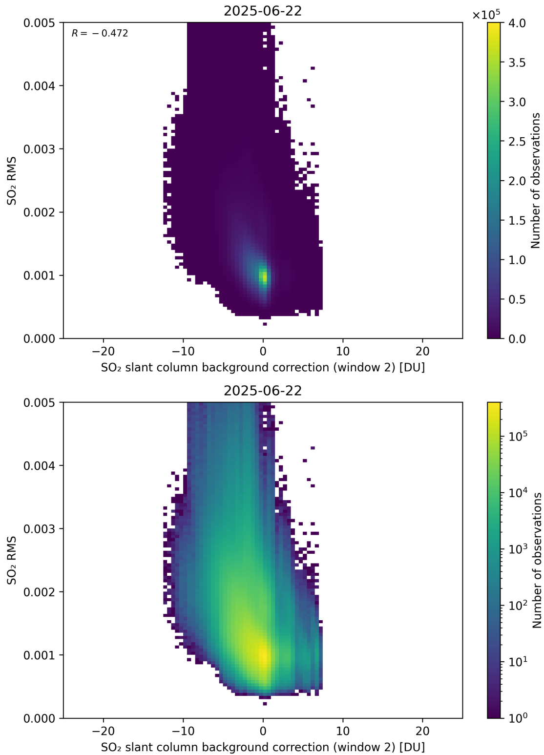
Figure 125: Scatter density plot of “SO 2 slant column background correction (window 2)” against “SO 2 RMS” for 2025-06-22 to 2025-06-23.
