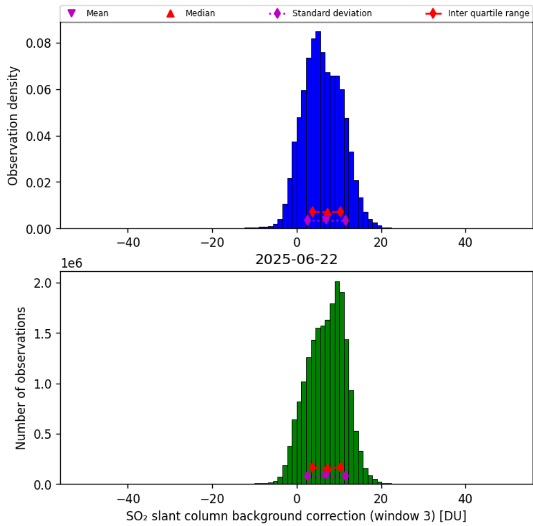
Figure 74: Histogram of “SO 2 slant column background correction (window 3)” for 2025-06-22 to 2025-06-23
