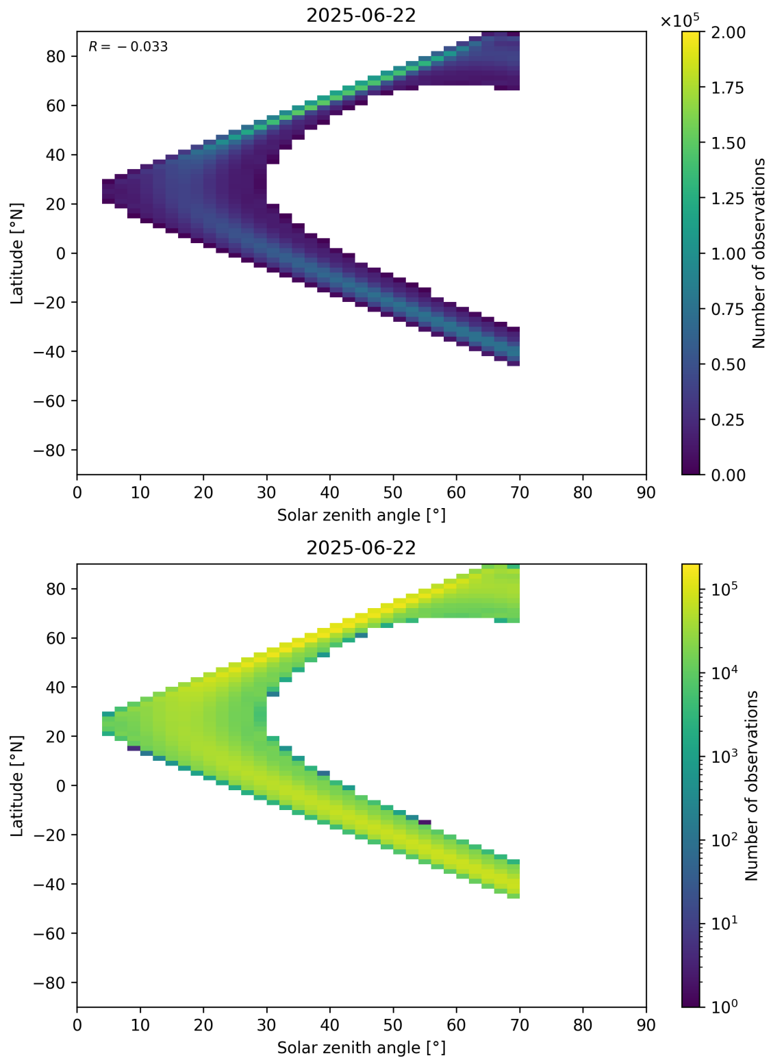
Figure 177: Scatter density plot of “Solar zenith angle” against “Latitude” for 2025-06-22 to 2025-06-23.
