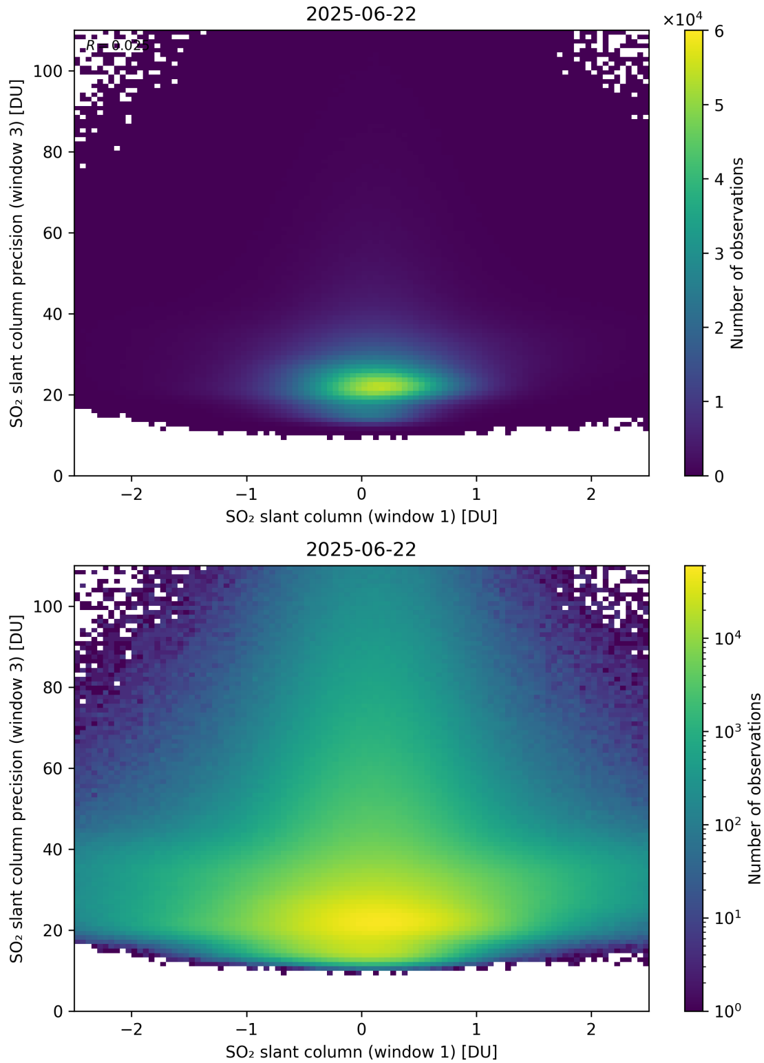
Figure 288: Scatter density plot of “SO 2 slant column (window 1)” against “SO 2 slant column precision (window 3)” for 2025-06-22 to 2025-06-23.
