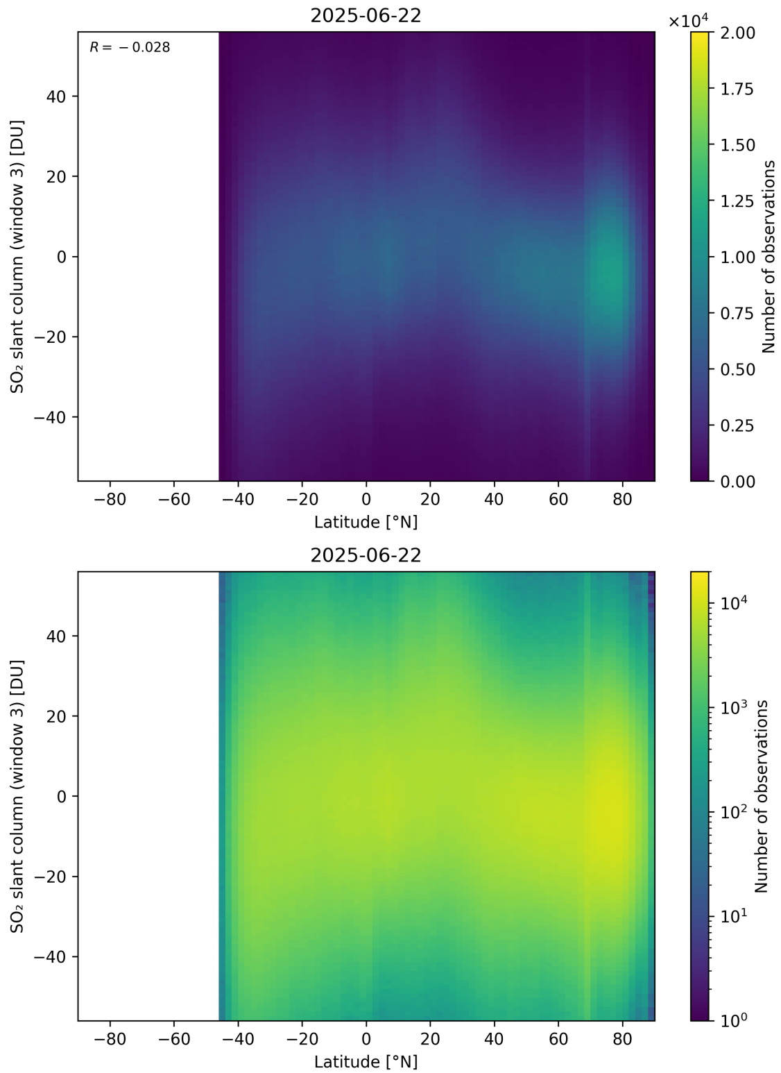
Figure 165: Scatter density plot of “Latitude” against “SO 2 slant column (window 3)” for 2025-06-22 to 2025-06-23.
