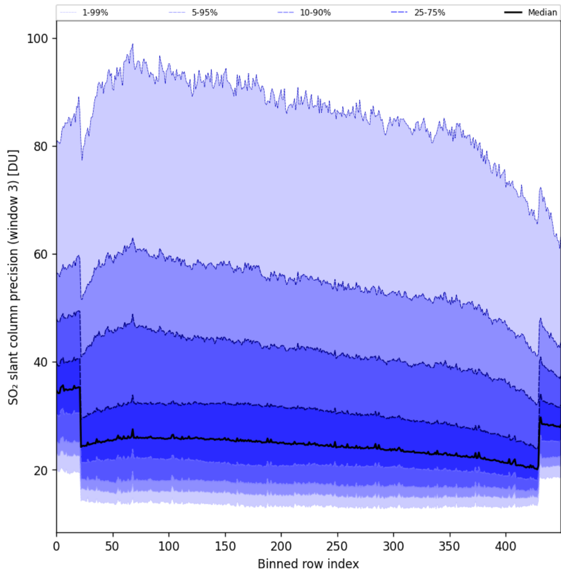
Figure 98: Along track statistics of “SO 2 slant column precision (window 3)” for 2025-06-22 to 2025-06-23
