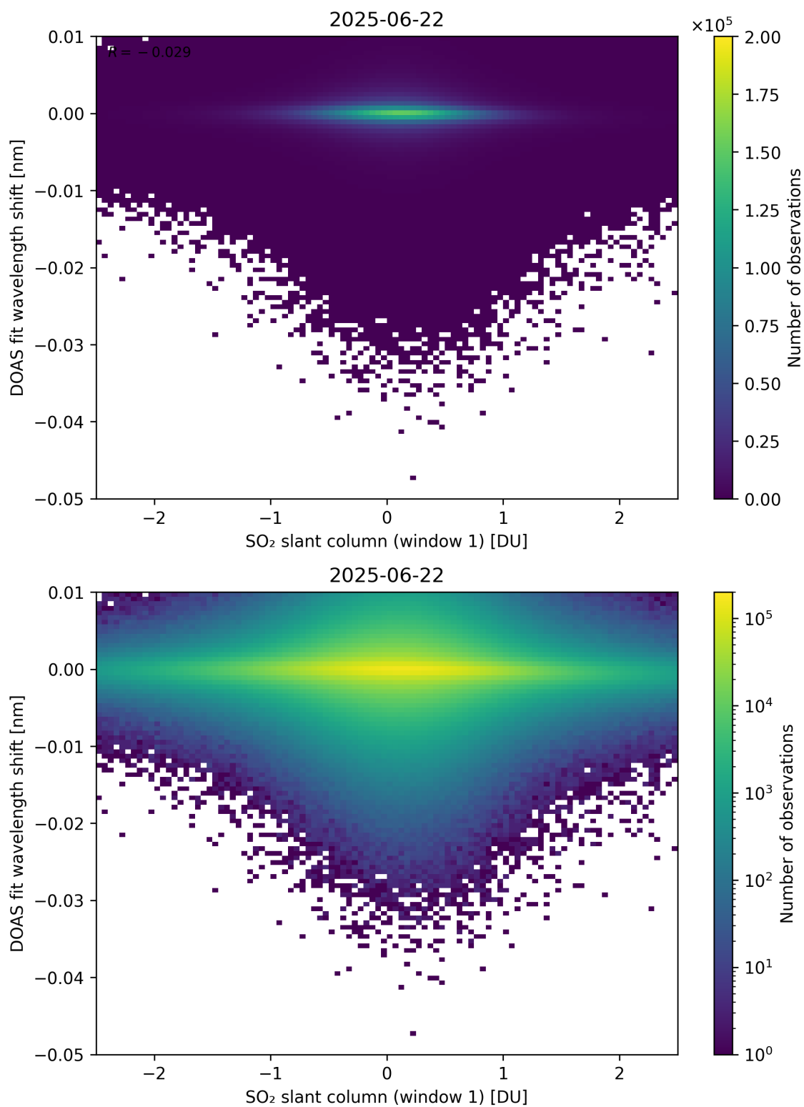
Figure 265: Scatter density plot of “SO 2 slant column (window 1)” against “DOAS fit wavelength shift” for 2025-06-22 to 2025-06-23.
