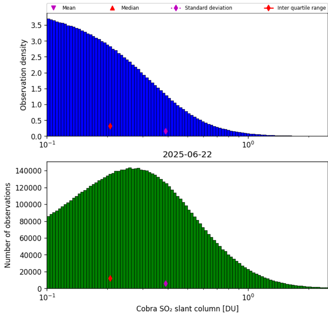
Figure 61: Histogram of “Cobra SO 2 slant column” for 2025-06-22 to 2025-06-23
