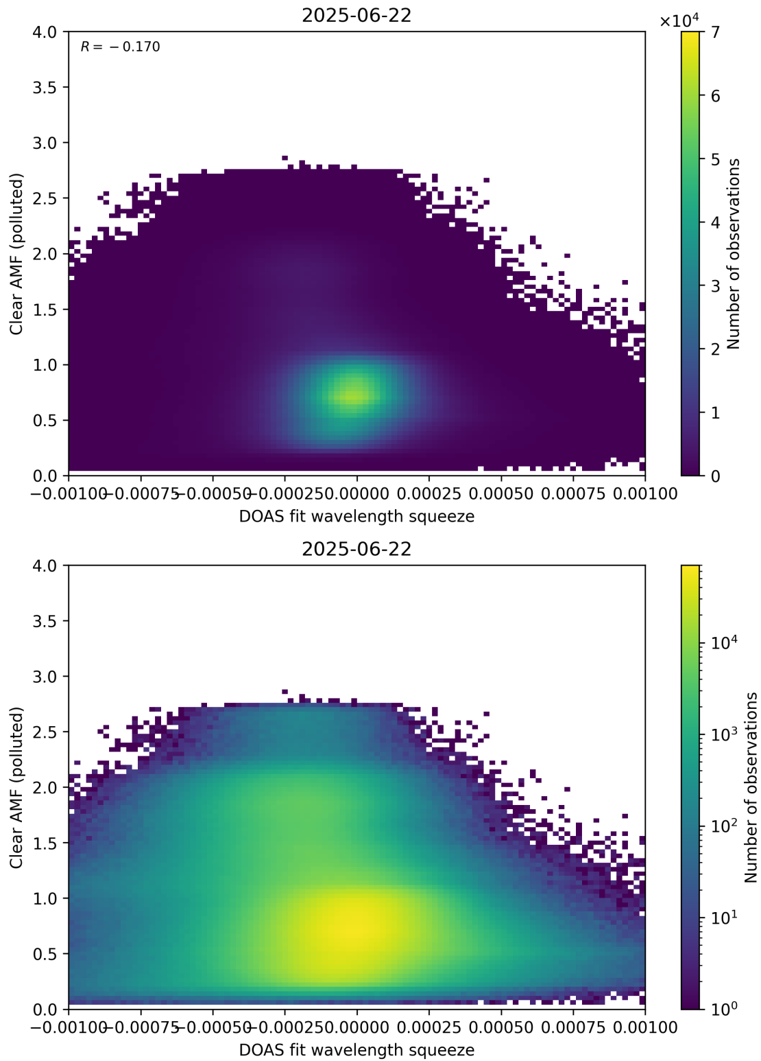
Figure 144: Scatter density plot of “DOAS fit wavelength squeeze” against “Clear AMF (polluted)” for 2025-06-22 to 2025-06-23.
