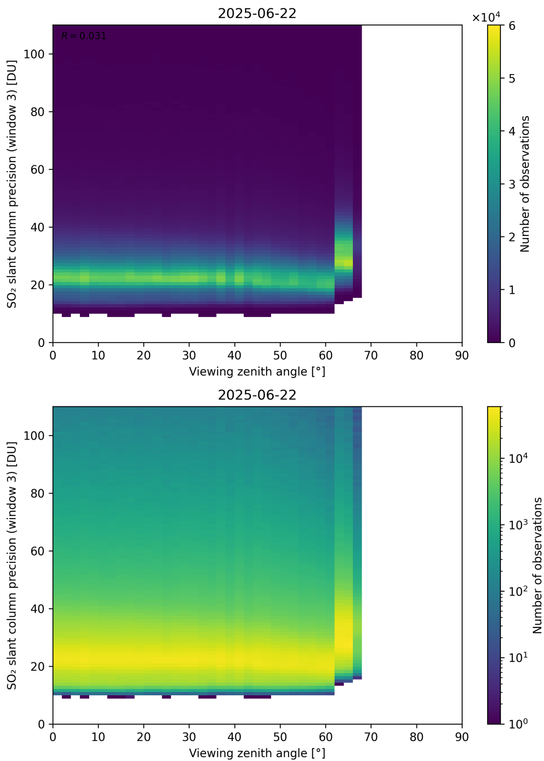
Figure 380: Scatter density plot of “Viewing zenith angle” against “SO 2 slant column precision (window 3)” for 2025-06-22 to 2025-06-23.
