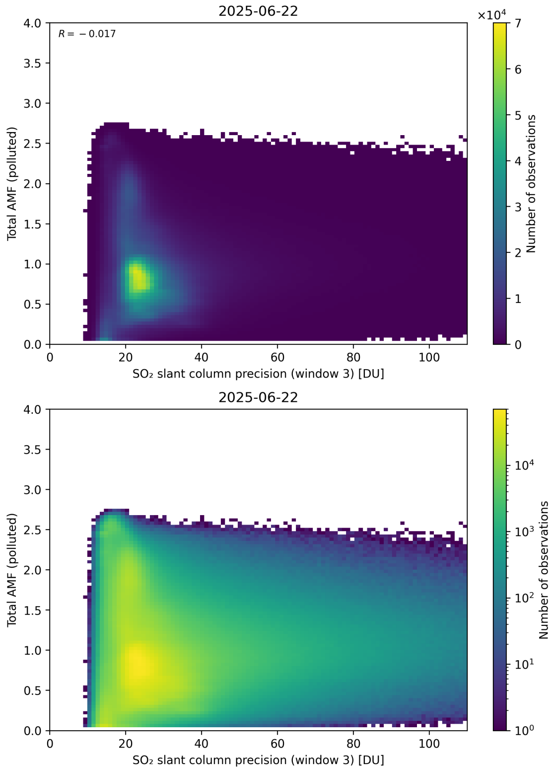
Figure 313: Scatter density plot of “SO 2 slant column precision (window 3)” against “Total AMF (polluted)” for 2025-06-22 to 2025-06-23.
