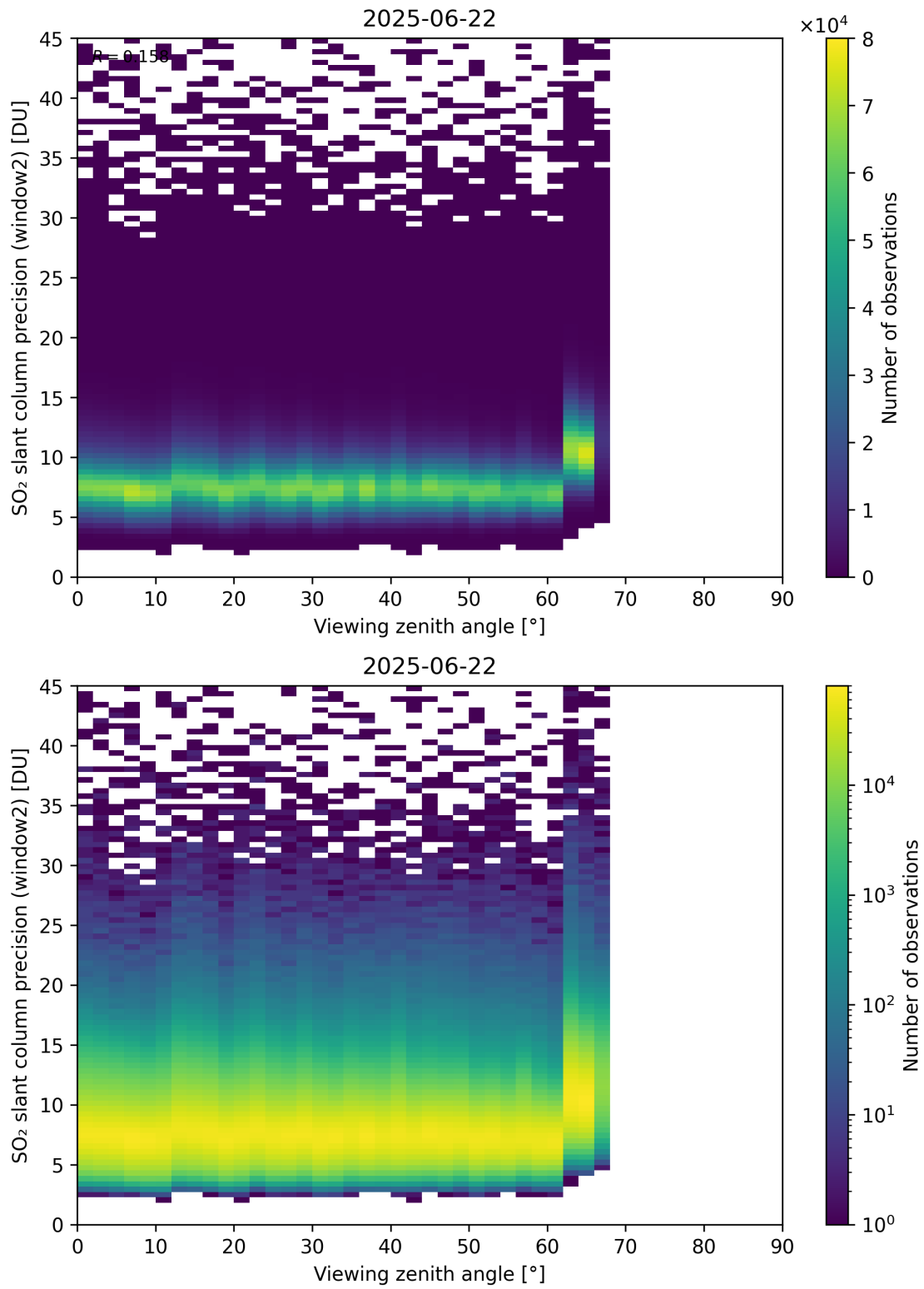
Figure 378: Scatter density plot of “Viewing zenith angle” against “SO 2 slant column precision (window2)” for 2025-06-22 to 2025-06-23.
