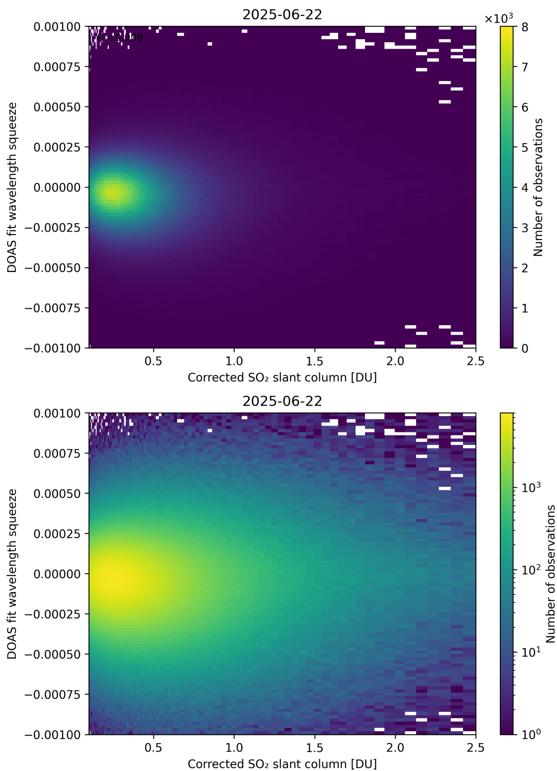
Figure 230: Scatter density plot of “Corrected SO 2 slant column” against “DOAS fit wavelength squeeze” for 2025-06-22 to 2025-06-23.
