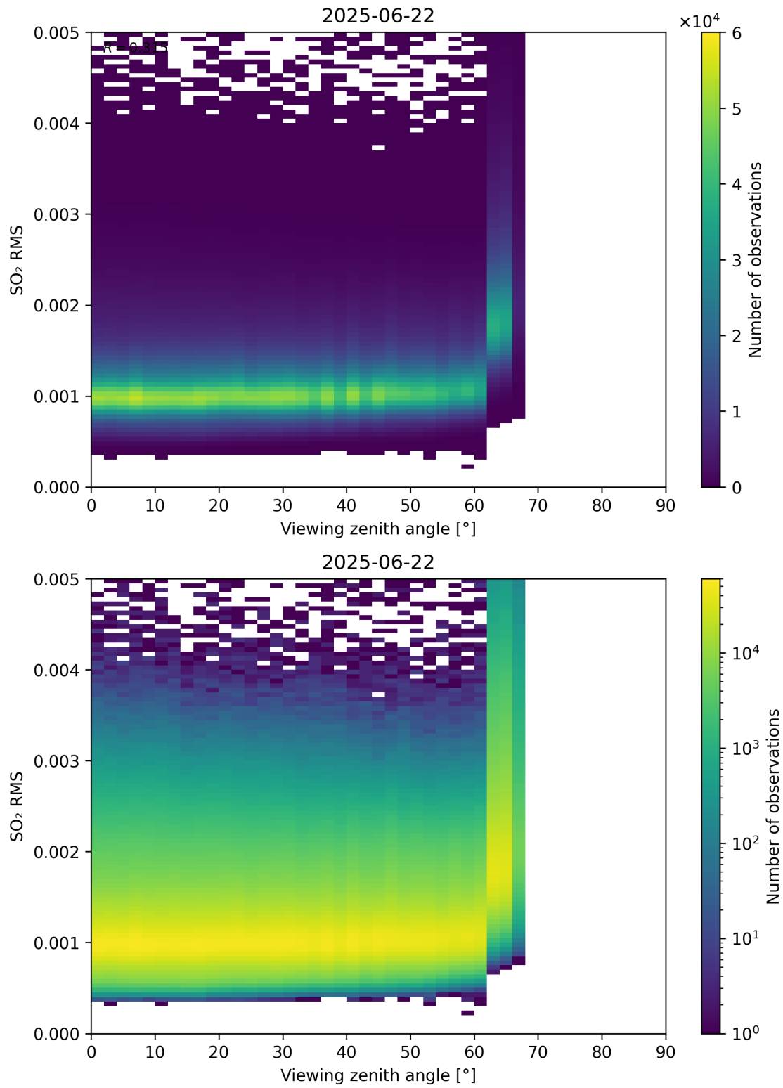
Figure 367: Scatter density plot of “Viewing zenith angle” against “SO 2 RMS” for 2025-06-22 to 2025-06-23.
