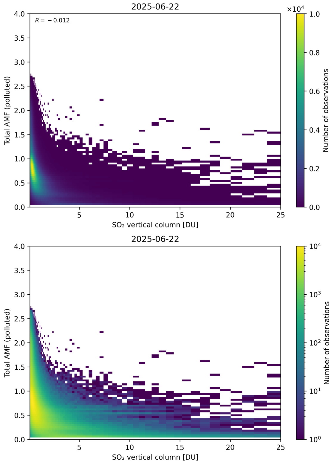
Figure 359: Scatter density plot of “SO 2 vertical column” against “Total AMF (polluted)” for 2025-06-22 to 2025-06-23.
