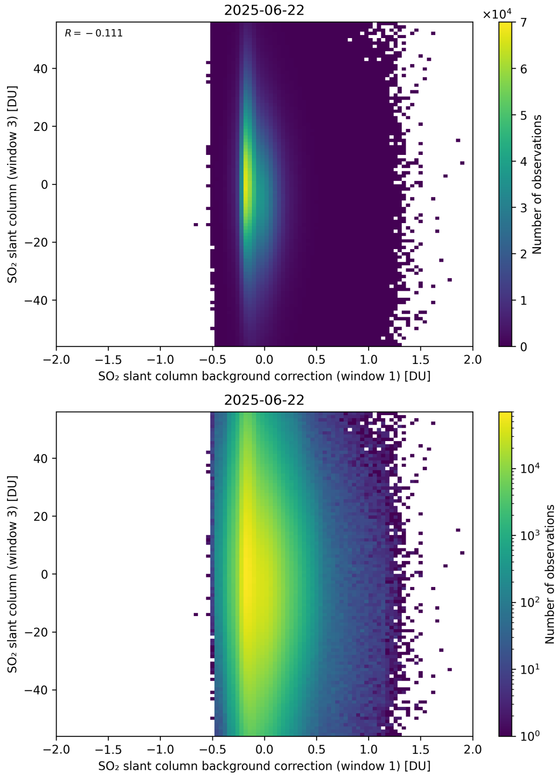
Figure 118: Scatter density plot of “SO 2 slant column background correction (window 1)” against “SO 2 slant column (window 3)” for 2025-06-22 to 2025-06-23.
