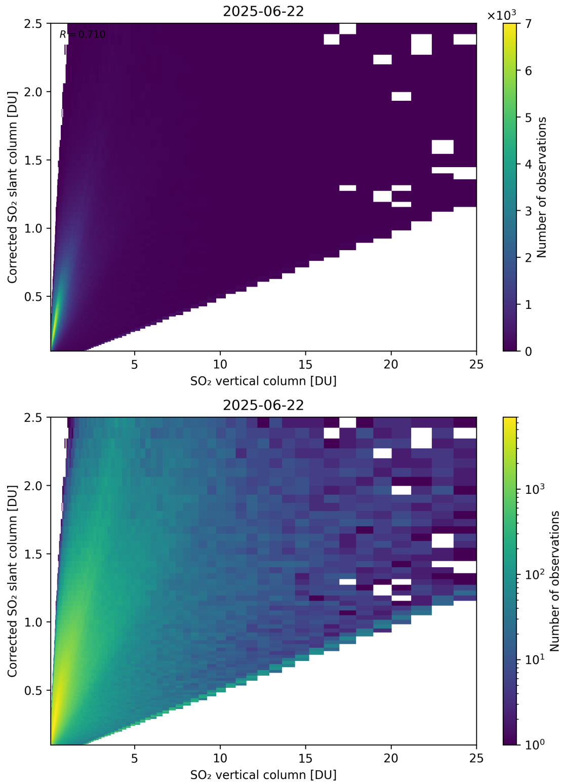
Figure 351: Scatter density plot of “SO 2 vertical column” against “Corrected SO 2 slant column” for 2025-06-22 to 2025-06-23.
