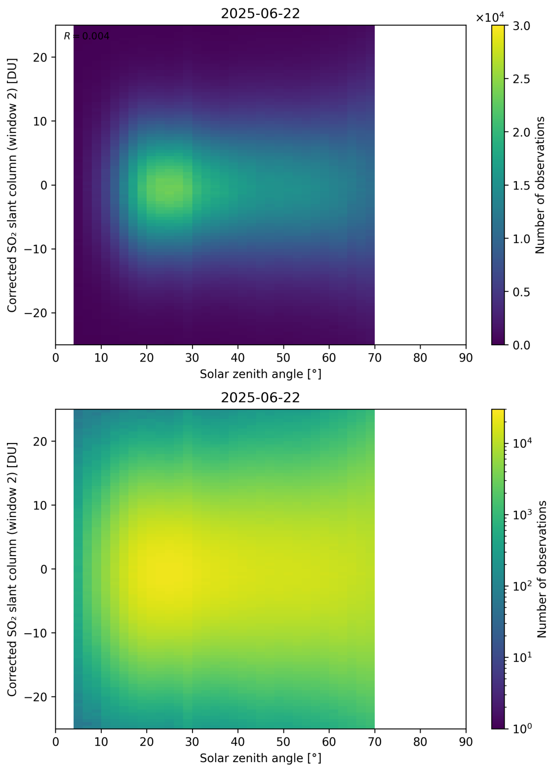
Figure 182: Scatter density plot of “Solar zenith angle” against “Corrected SO 2 slant column (window 2)” for 2025-06-22 to 2025-06-23.
