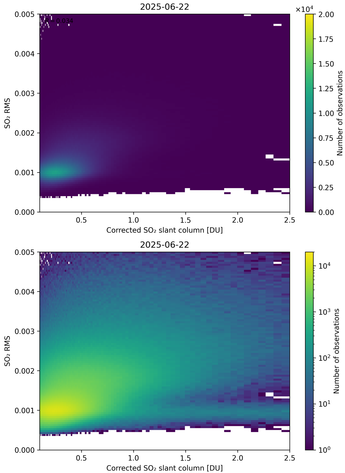
Figure 231: Scatter density plot of “Corrected SO 2 slant column” against “SO 2 RMS” for 2025-06-22 to 2025-06-23.
