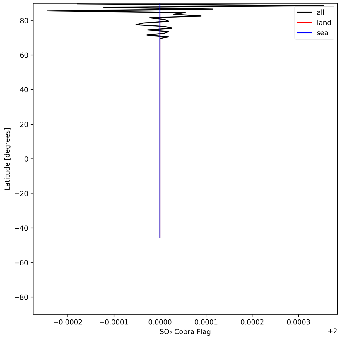
Figure 49: Zonal average of “SO 2 Cobra Flag” for 2025-06-22 to 2025-06-23.
