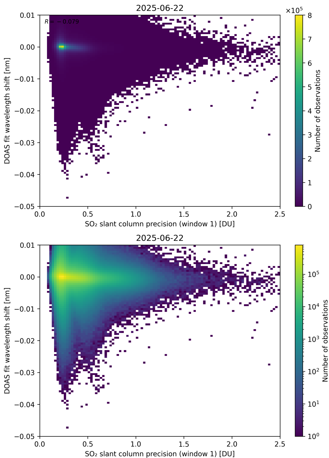
Figure 271: Scatter density plot of “SO 2 slant column precision (window 1)” against “DOAS fit wavelength shift” for 2025-06-22 to 2025-06-23.
