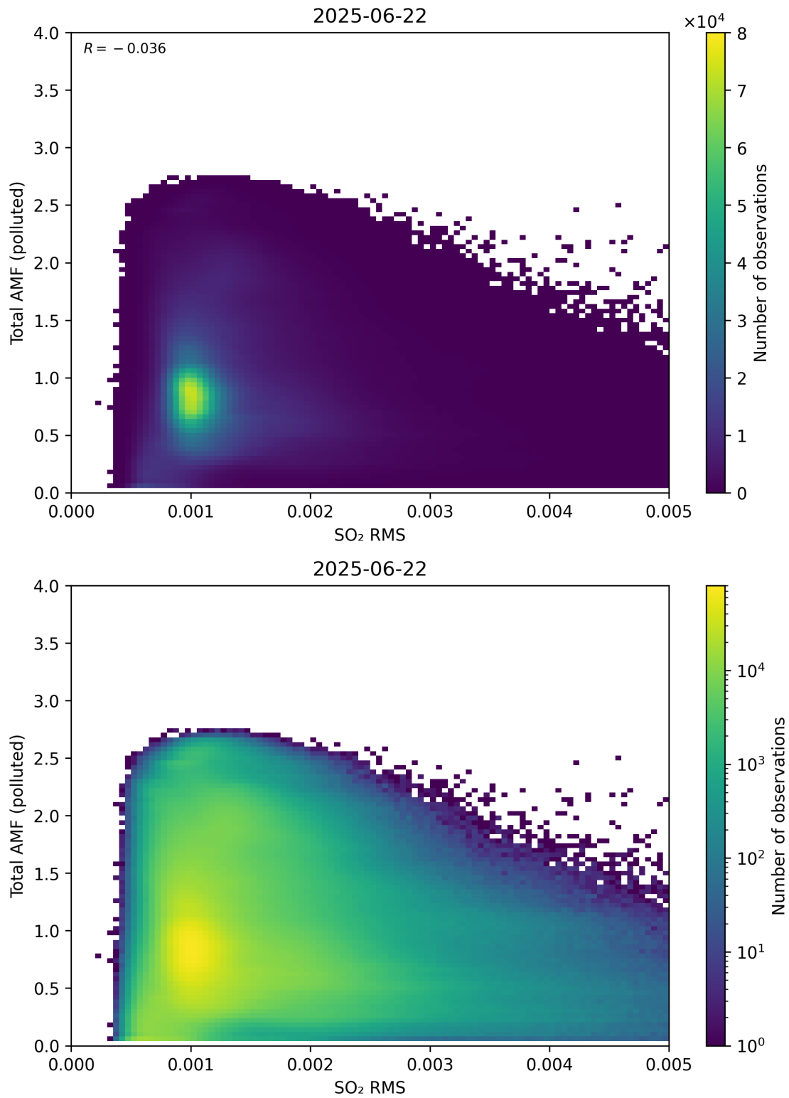
Figure 148: Scatter density plot of “SO 2 RMS” against “Total AMF (polluted)” for 2025-06-22 to 2025-06-23.
