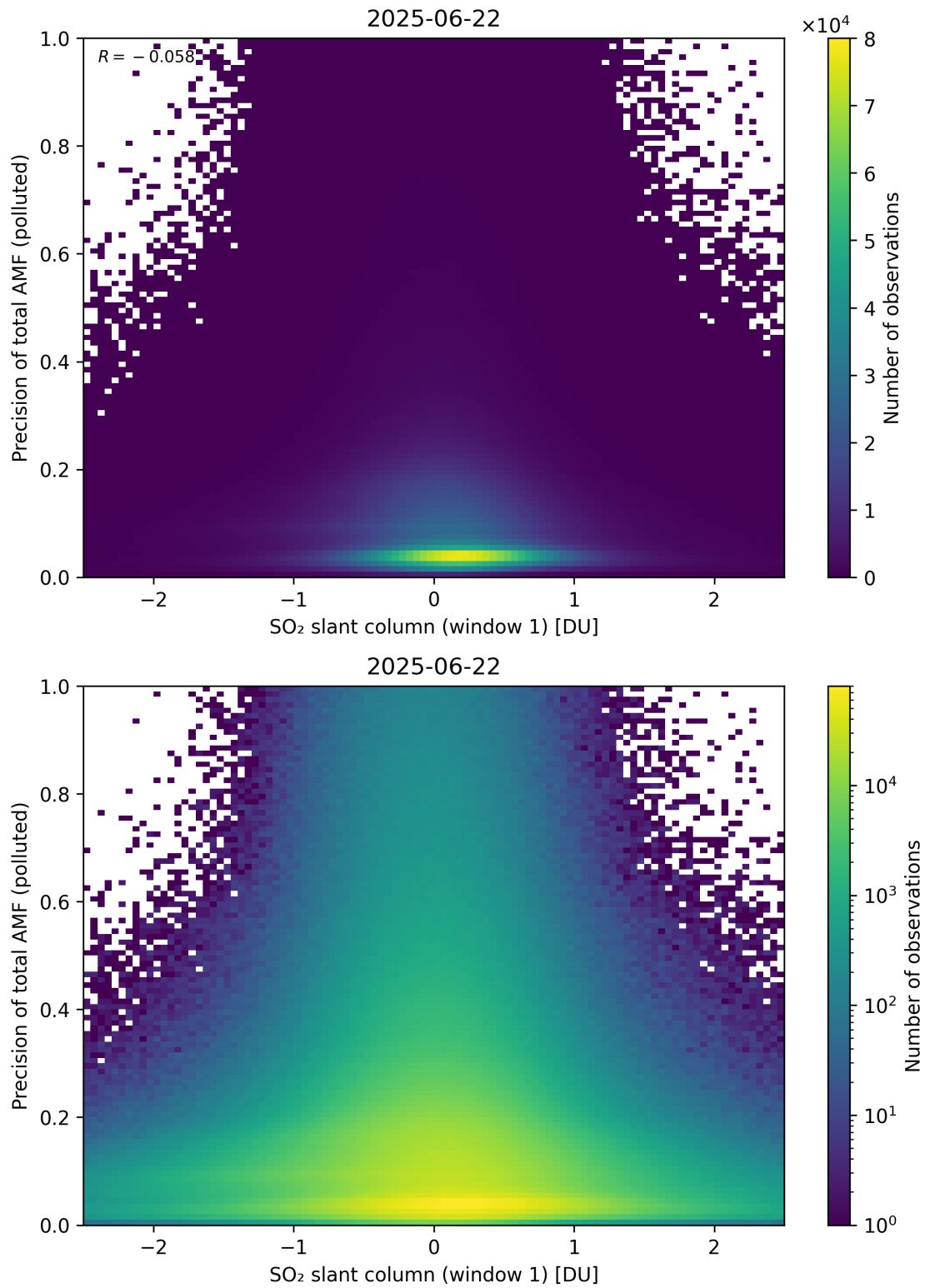
Figure 290: Scatter density plot of “SO 2 slant column (window 1)” against “Precision of total AMF (polluted)” for 2025-06-22 to 2025-06-23.
