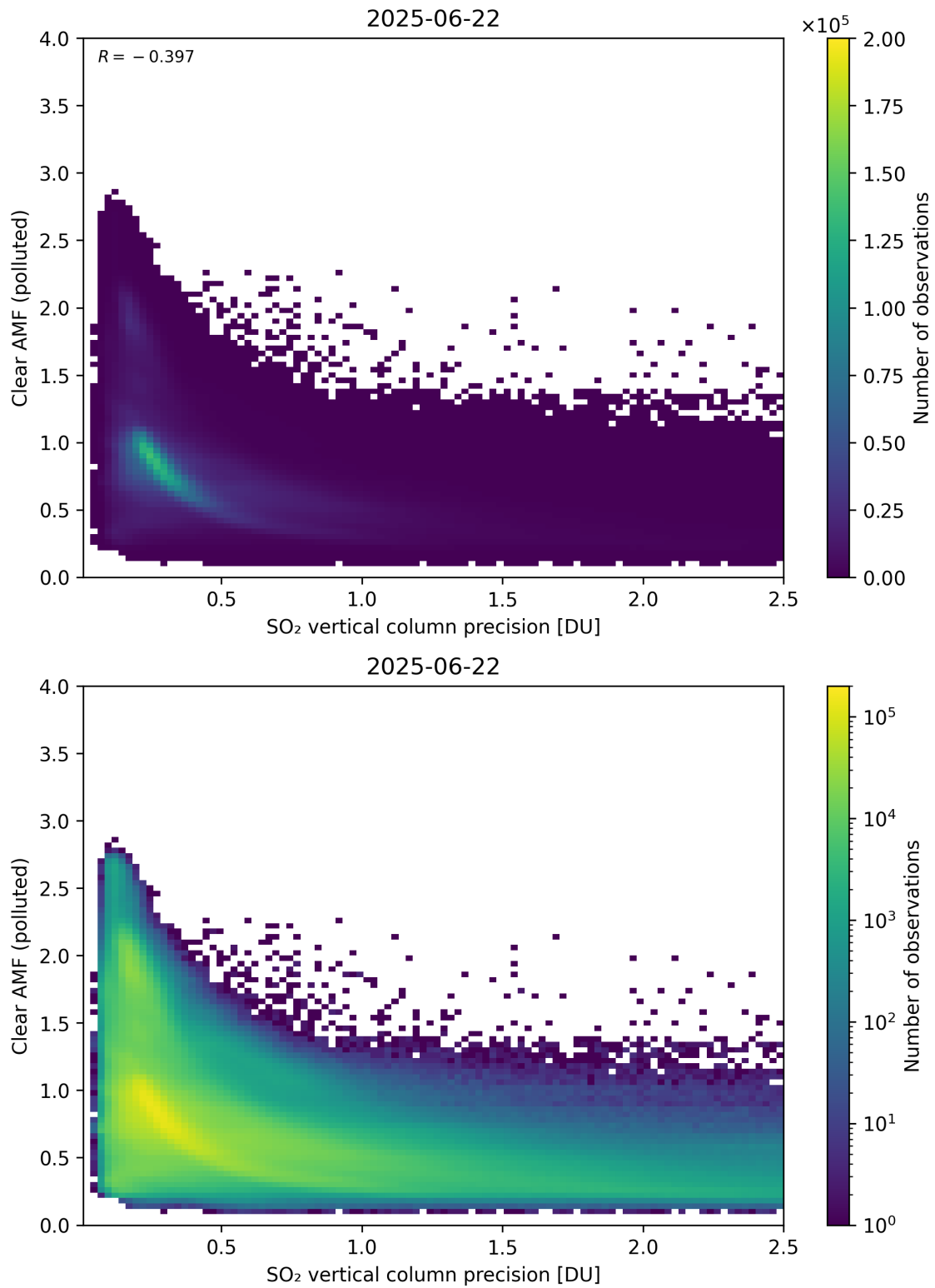
Figure 335: Scatter density plot of “SO 2 vertical column precision” against “Clear AMF (polluted)” for 2025-06-22 to 2025-06-23.
