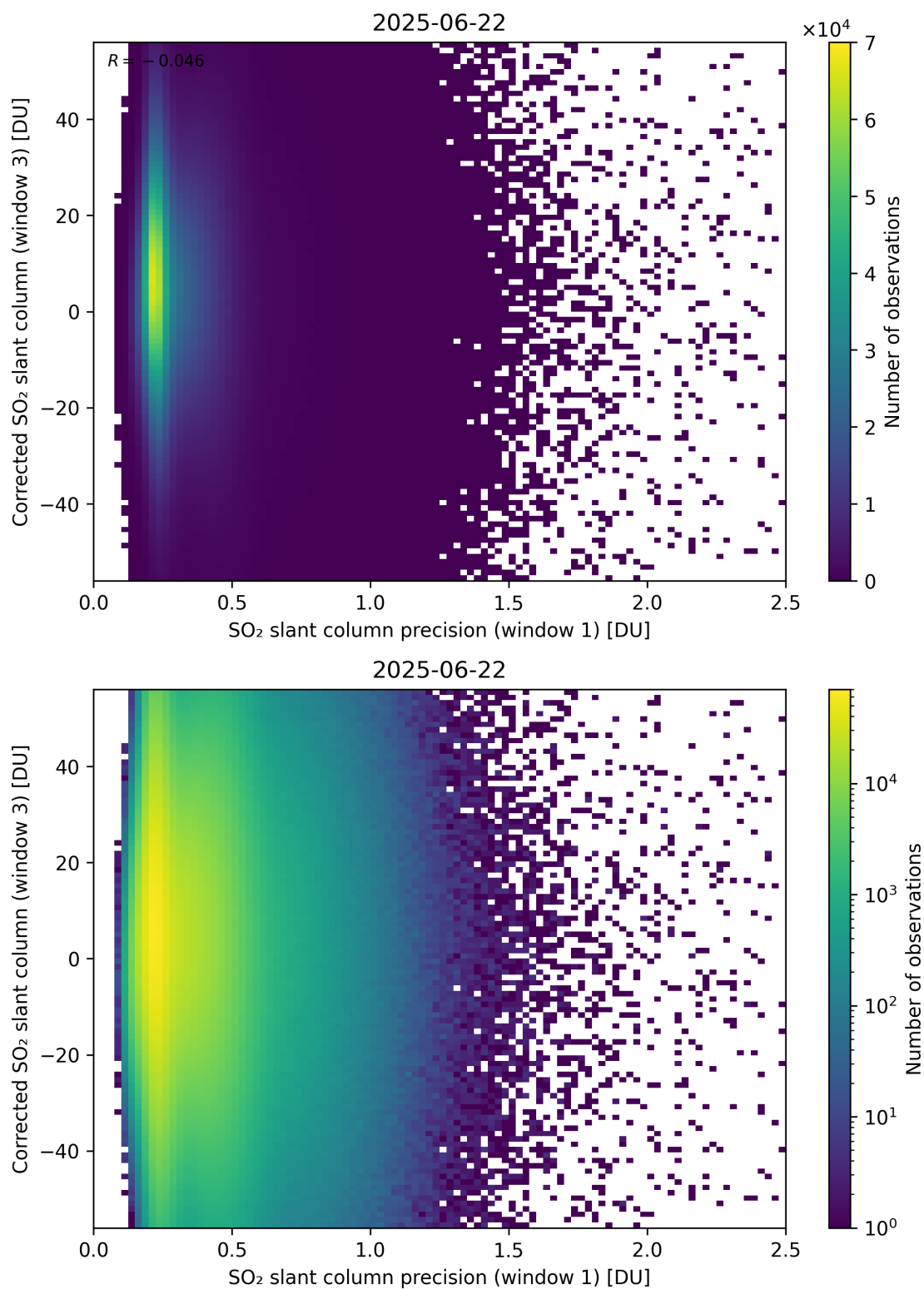
Figure 276: Scatter density plot of “SO 2 slant column precision (window 1)” against “Corrected SO 2 slant column (window 3)” for 2025-06-22 to 2025-06-23.
