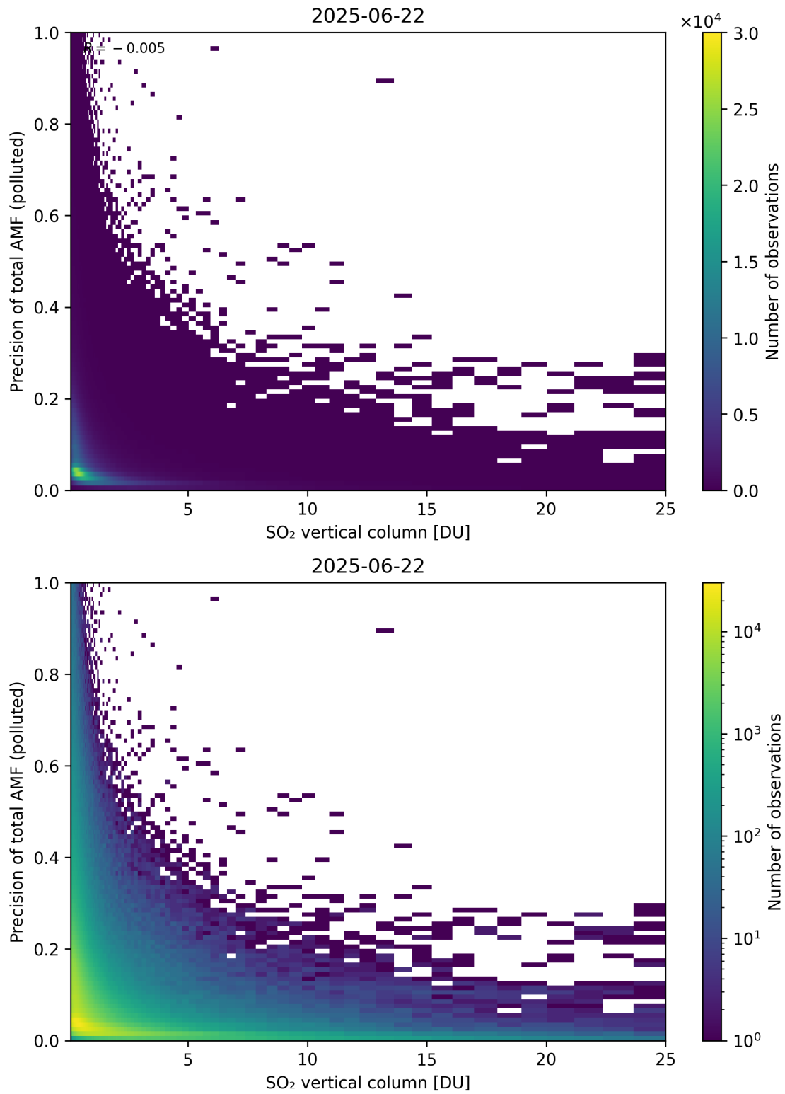
Figure 360: Scatter density plot of “SO 2 vertical column” against “Precision of total AMF (polluted)” for 2025-06-22 to 2025-06-23.
