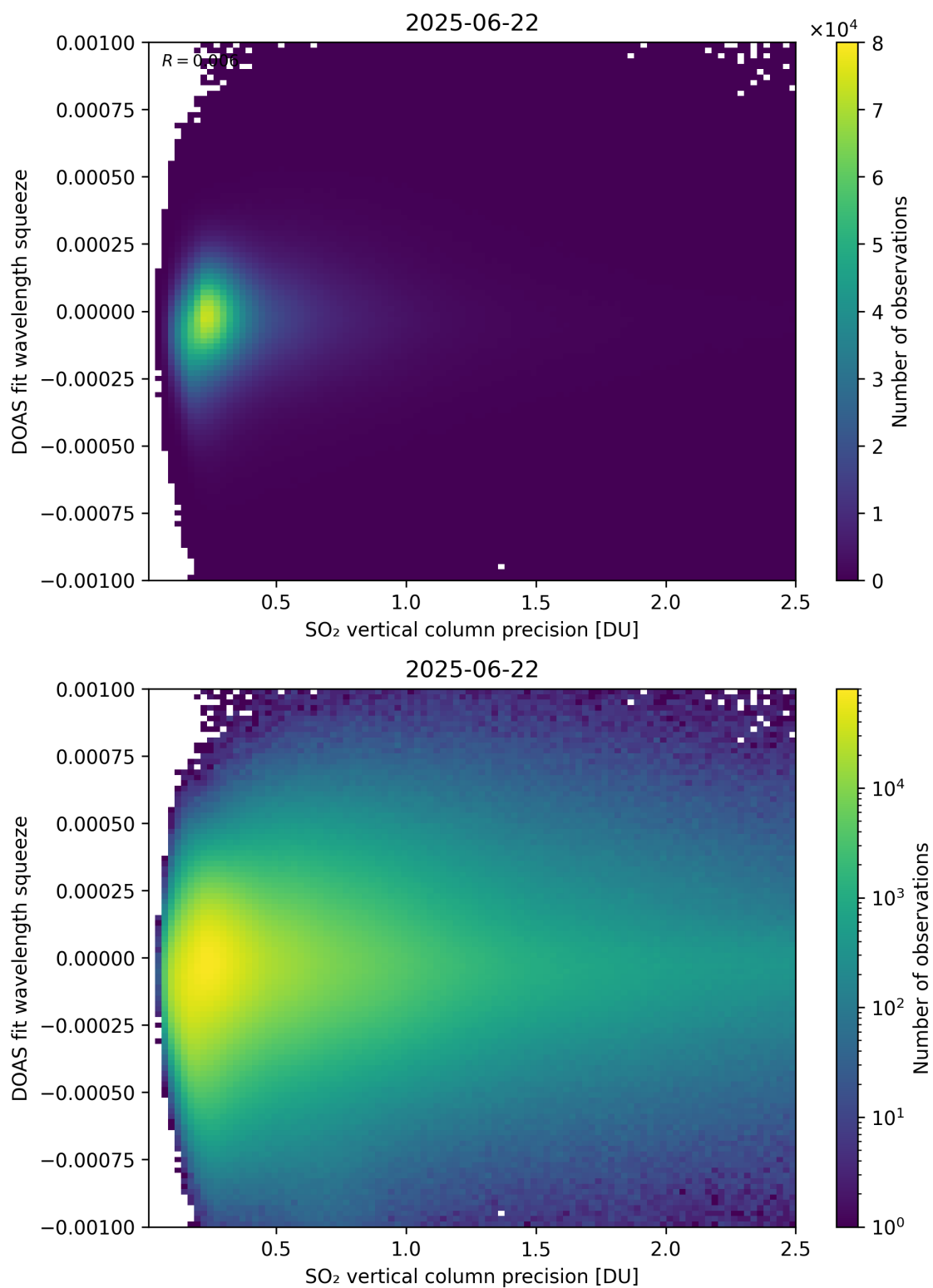
Figure 333: Scatter density plot of “SO 2 vertical column precision” against “DOAS fit wavelength squeeze” for 2025-06-22 to 2025-06-23.
