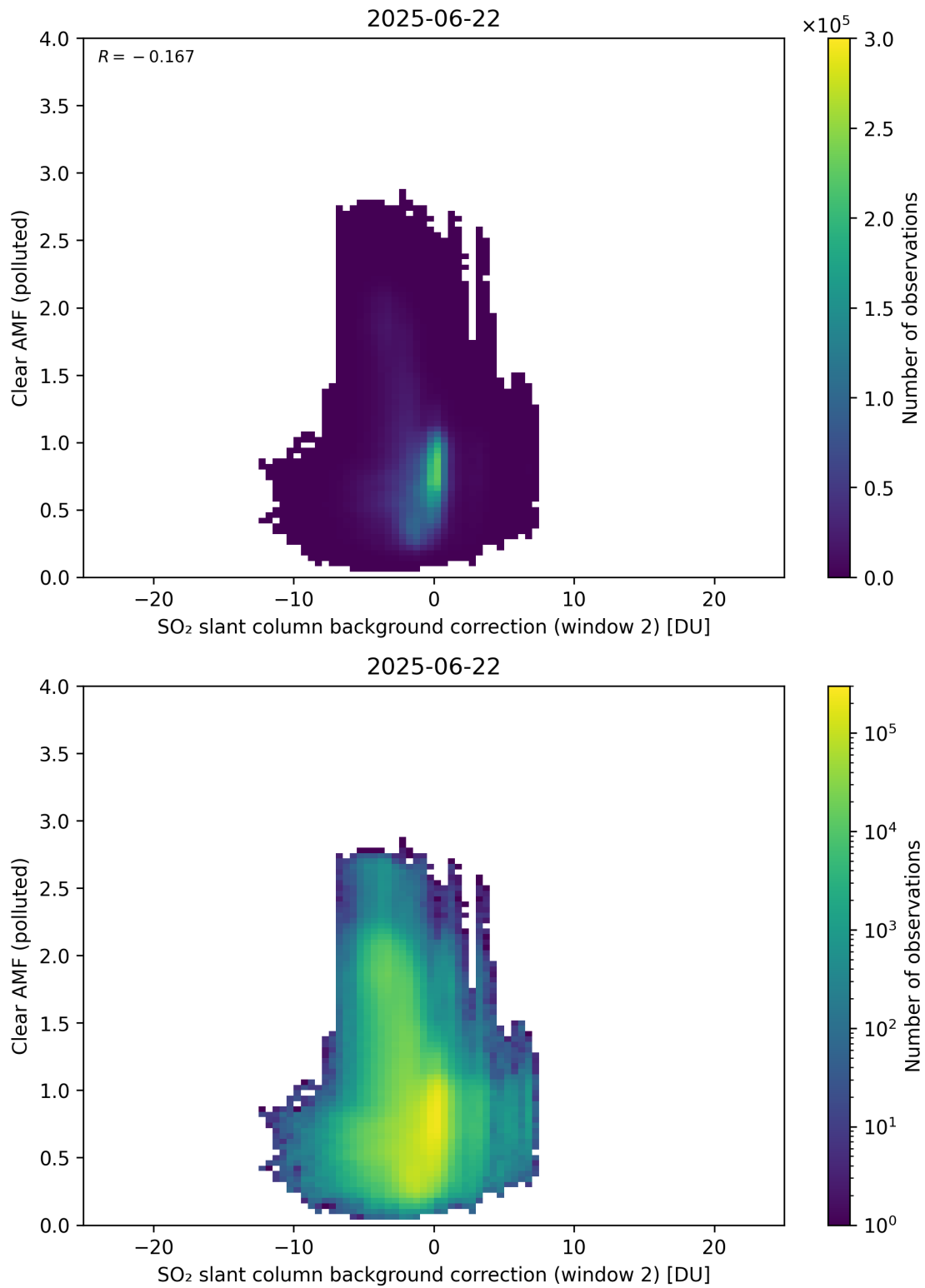
Figure 126: Scatter density plot of “SO 2 slant column background correction (window 2)” against “Clear AMF (polluted)” for 2025-06-22 to 2025-06-23.
