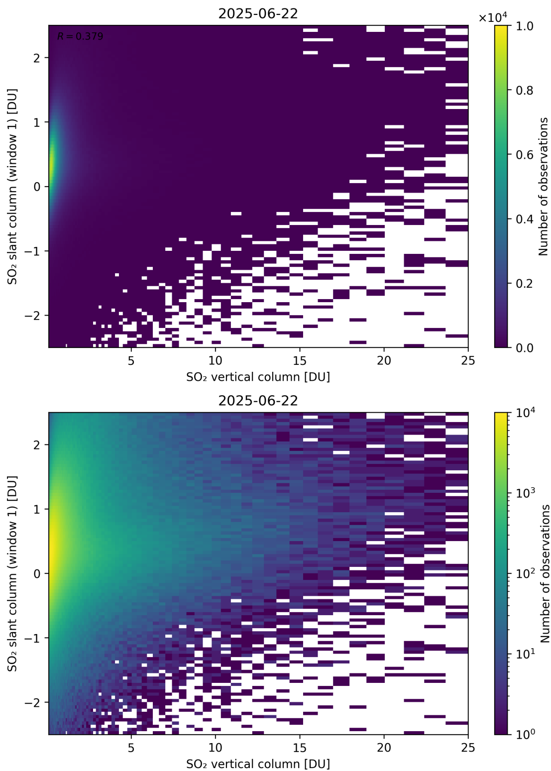
Figure 354: Scatter density plot of “SO 2 vertical column” against “SO 2 slant column (window 1)” for 2025-06-22 to 2025-06-23.
