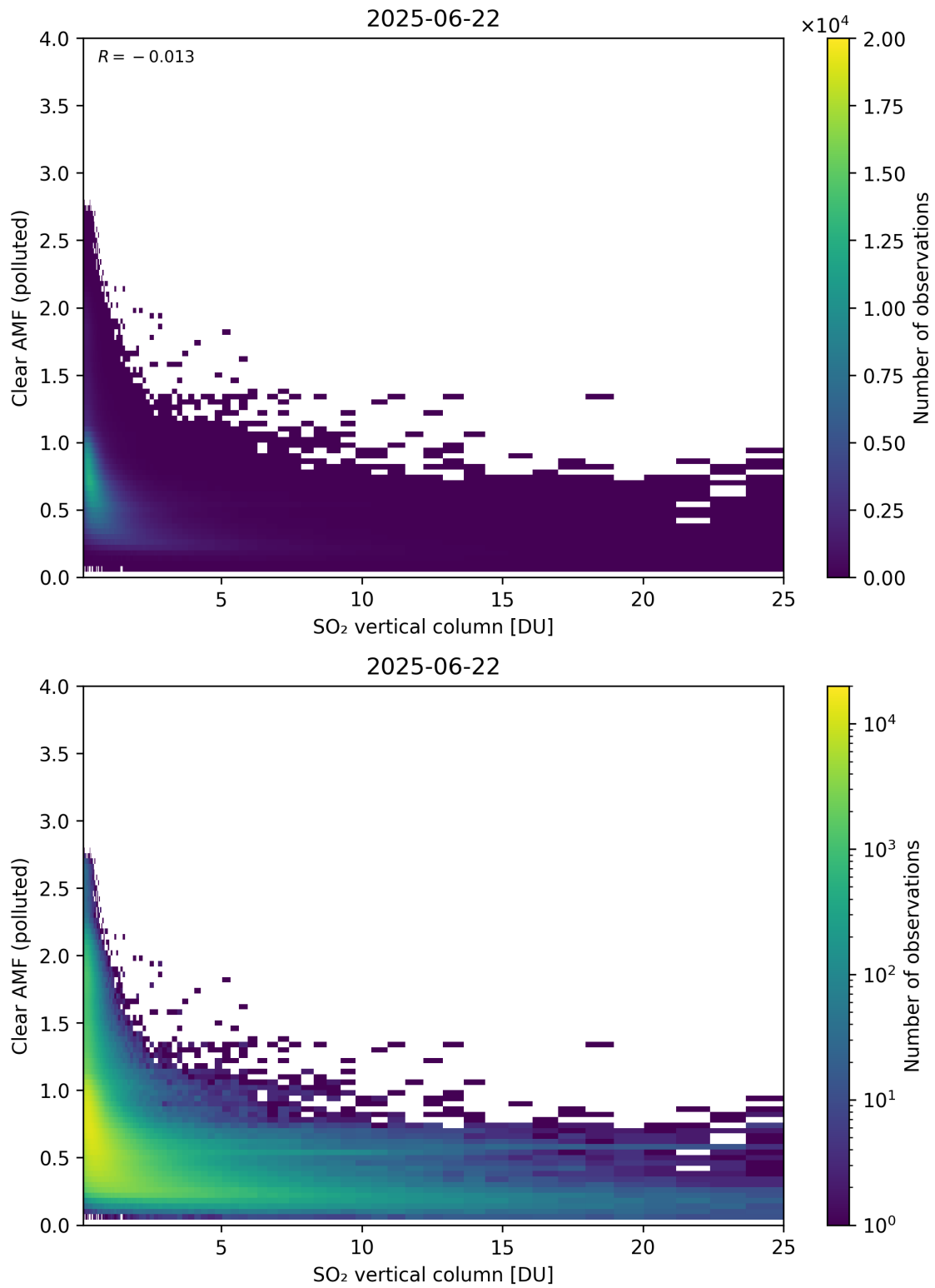
Figure 348: Scatter density plot of “SO 2 vertical column” against “Clear AMF (polluted)” for 2025-06-22 to 2025-06-23.
