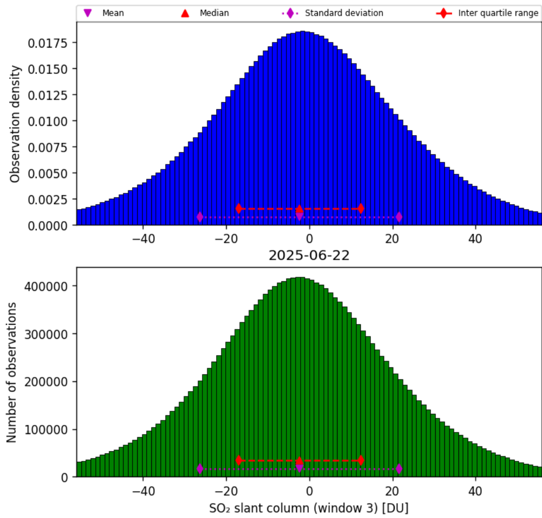
Figure 71: Histogram of “SO 2 slant column (window 3)” for 2025-06-22 to 2025-06-23
