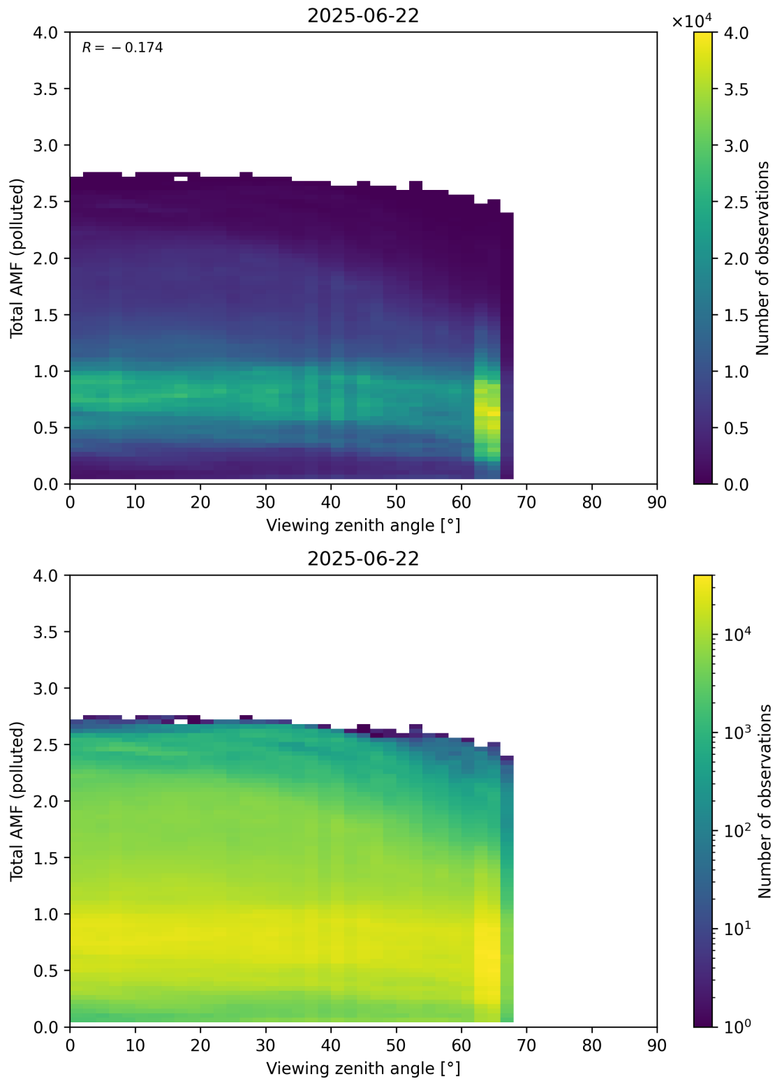
Figure 381: Scatter density plot of “Viewing zenith angle” against “Total AMF (polluted)” for 2025-06-22 to 2025-06-23.
