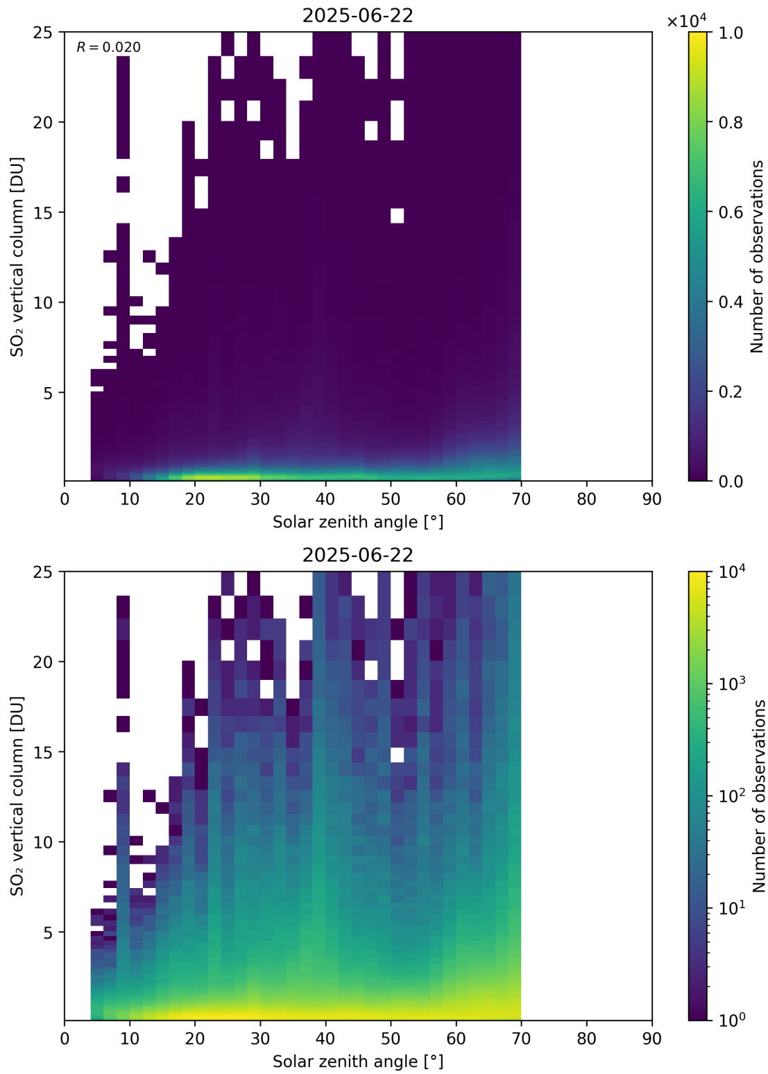
Figure 191: Scatter density plot of “Solar zenith angle” against “SO 2 vertical column” for 2025-06-22 to 2025-06-23.
