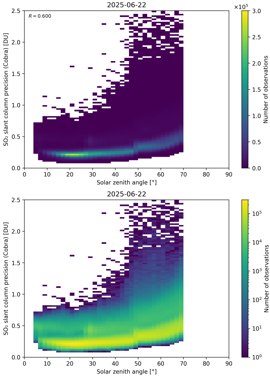
Figure 180: Scatter density plot of “Solar zenith angle” against “SO 2 slant column precision (Cobra)” for 2025-06-22 to 2025-06-23.
