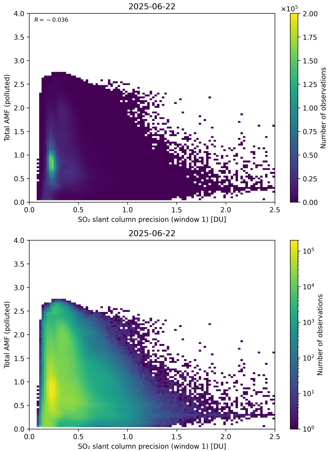
Figure 280: Scatter density plot of “SO 2 slant column precision (window 1)” against “Total AMF (polluted)” for 2025-06-22 to 2025-06-23.
