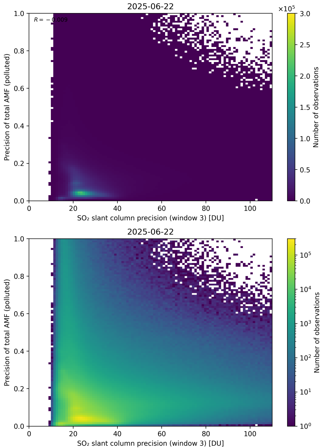
Figure 314: Scatter density plot of “SO 2 slant column precision (window 3)” against “Precision of total AMF (polluted)” for 2025-06-22 to 2025-06-23.
