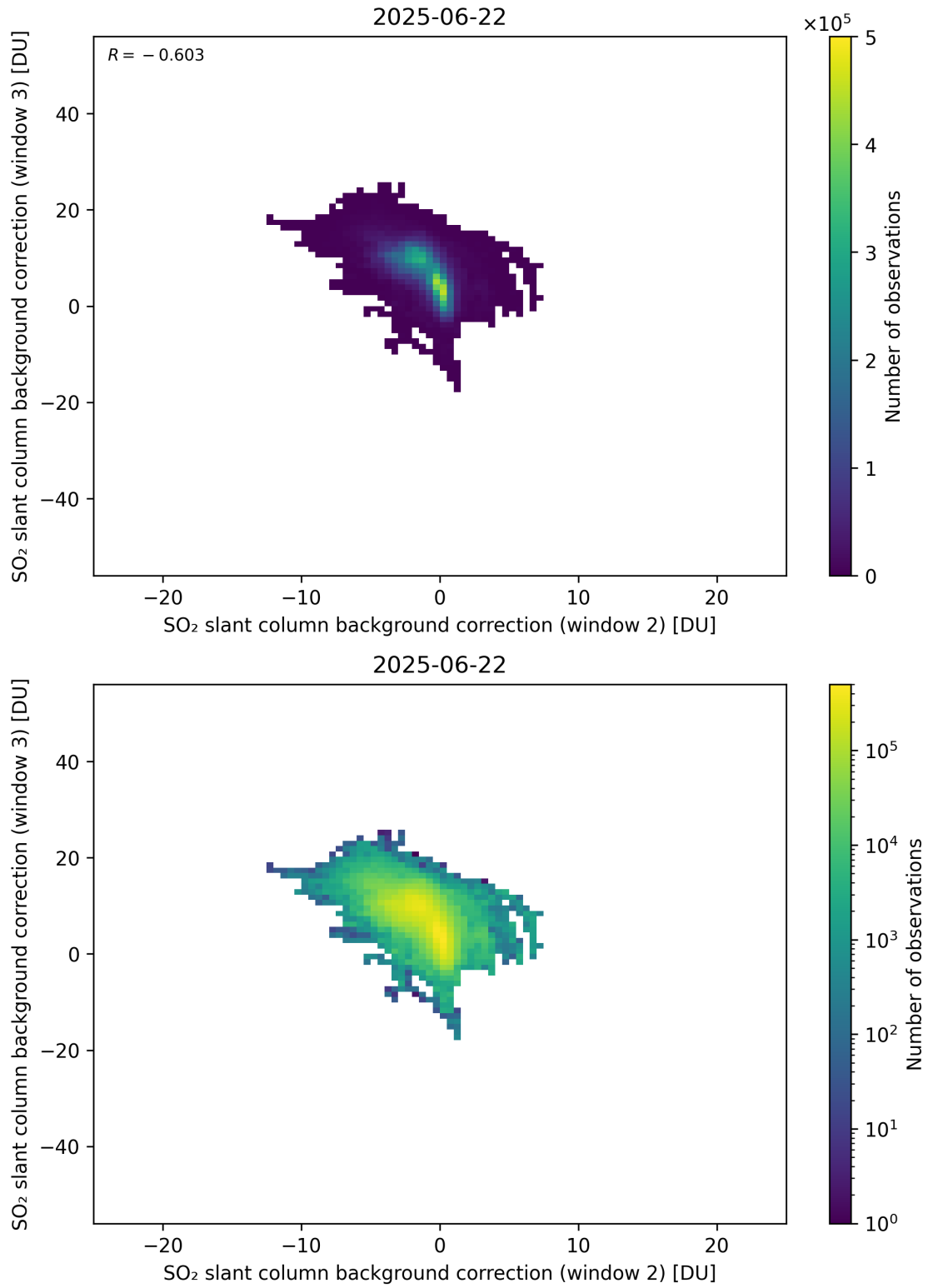
Figure 122: Scatter density plot of “SO 2 slant column background correction (window 2)” against “SO 2 slant column background correction (window 3)” for 2025-06-22 to 2025-06-23.
