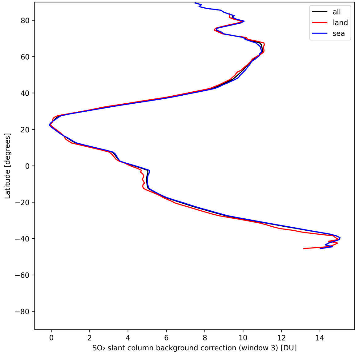
Figure 48: Zonal average of “SO 2 slant column background correction (window 3)” for 2025-06-22 to 2025-06-23.
