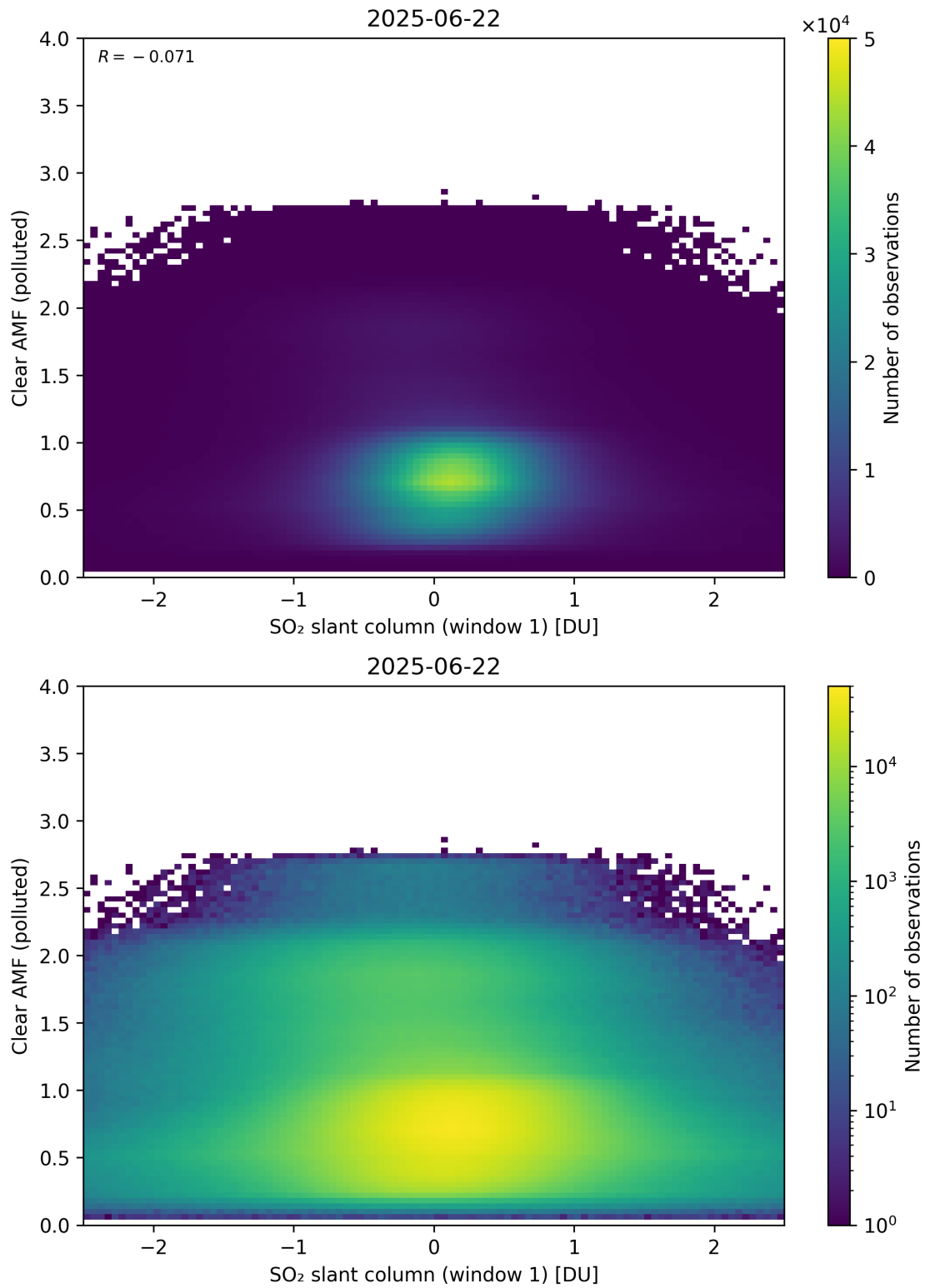
Figure 282: Scatter density plot of “SO 2 slant column (window 1)” against “Clear AMF (polluted)” for 2025-06-22 to 2025-06-23.
