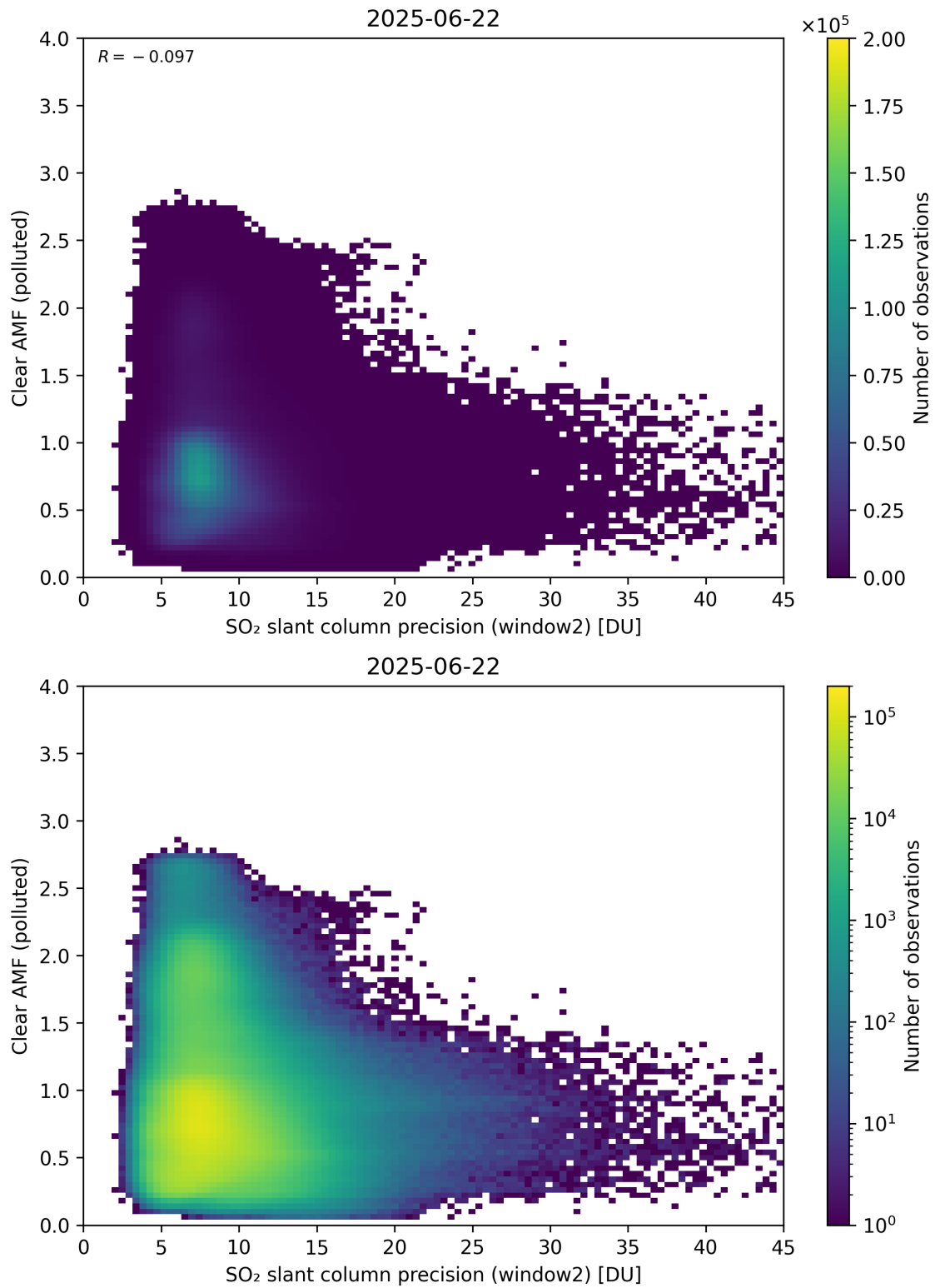
Figure 296: Scatter density plot of “SO 2 slant column precision (window2)” against “Clear AMF (polluted)” for 2025-06-22 to 2025-06-23.
