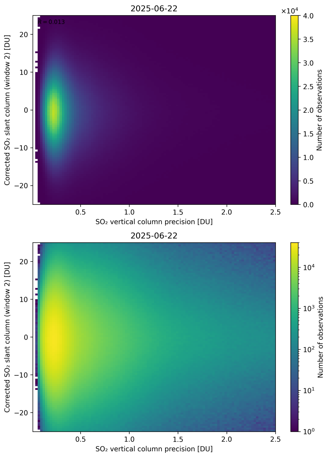
Figure 339: Scatter density plot of “SO 2 vertical column precision” against “Corrected SO 2 slant column (window 2)” for 2025-06-22 to 2025-06-23.
