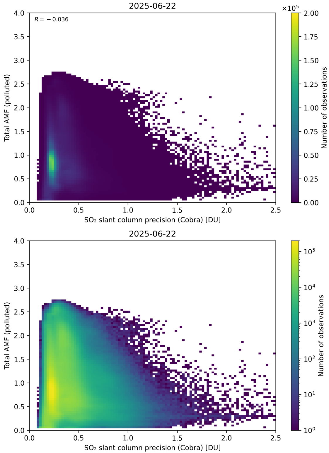
Figure 213: Scatter density plot of “SO 2 slant column precision (Cobra)” against “Total AMF (polluted)” for 2025-06-22 to 2025-06-23.
