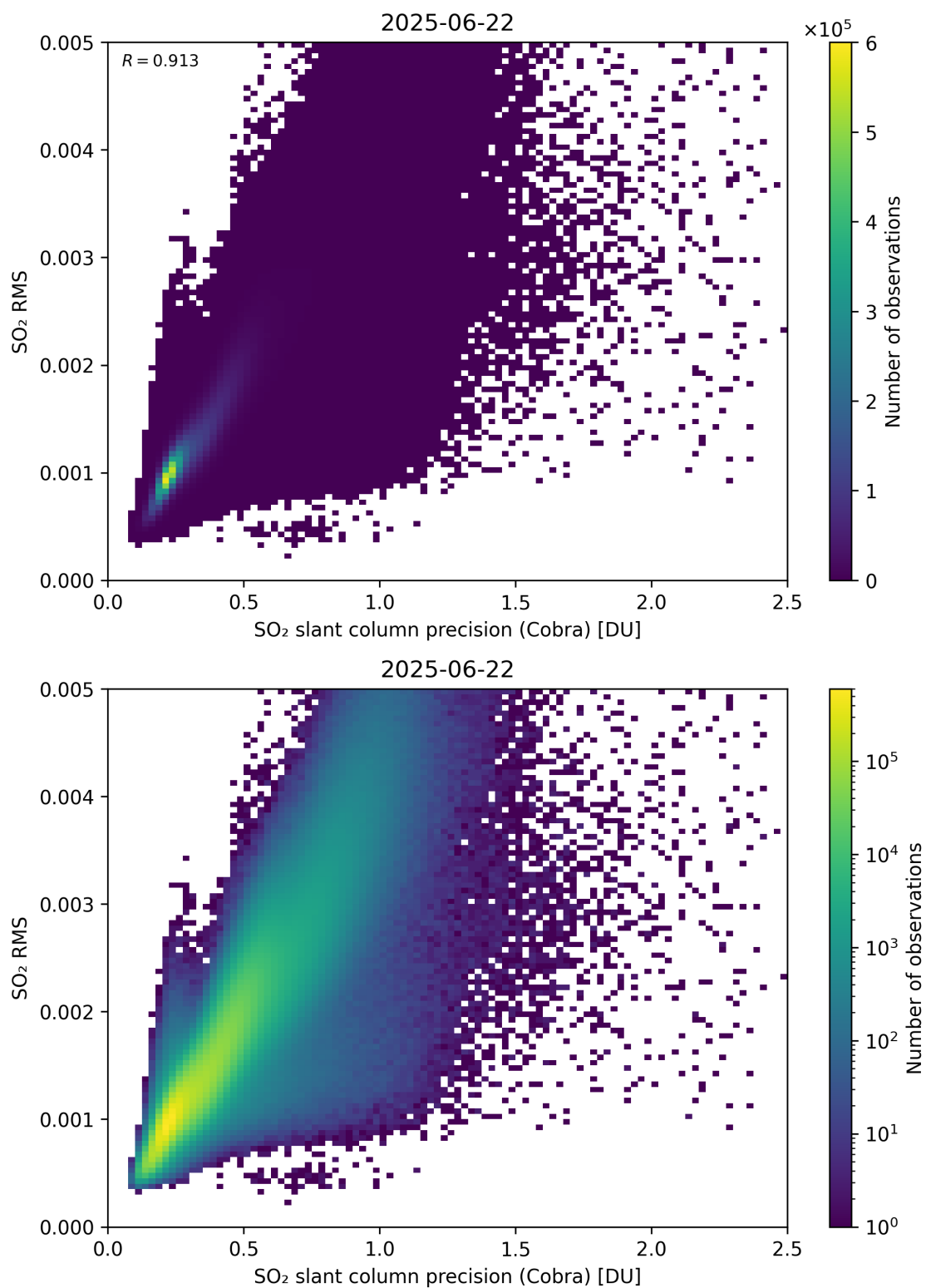
Figure 204: Scatter density plot of “SO 2 slant column precision (Cobra)” against “SO 2 RMS” for 2025-06-22 to 2025-06-23.
