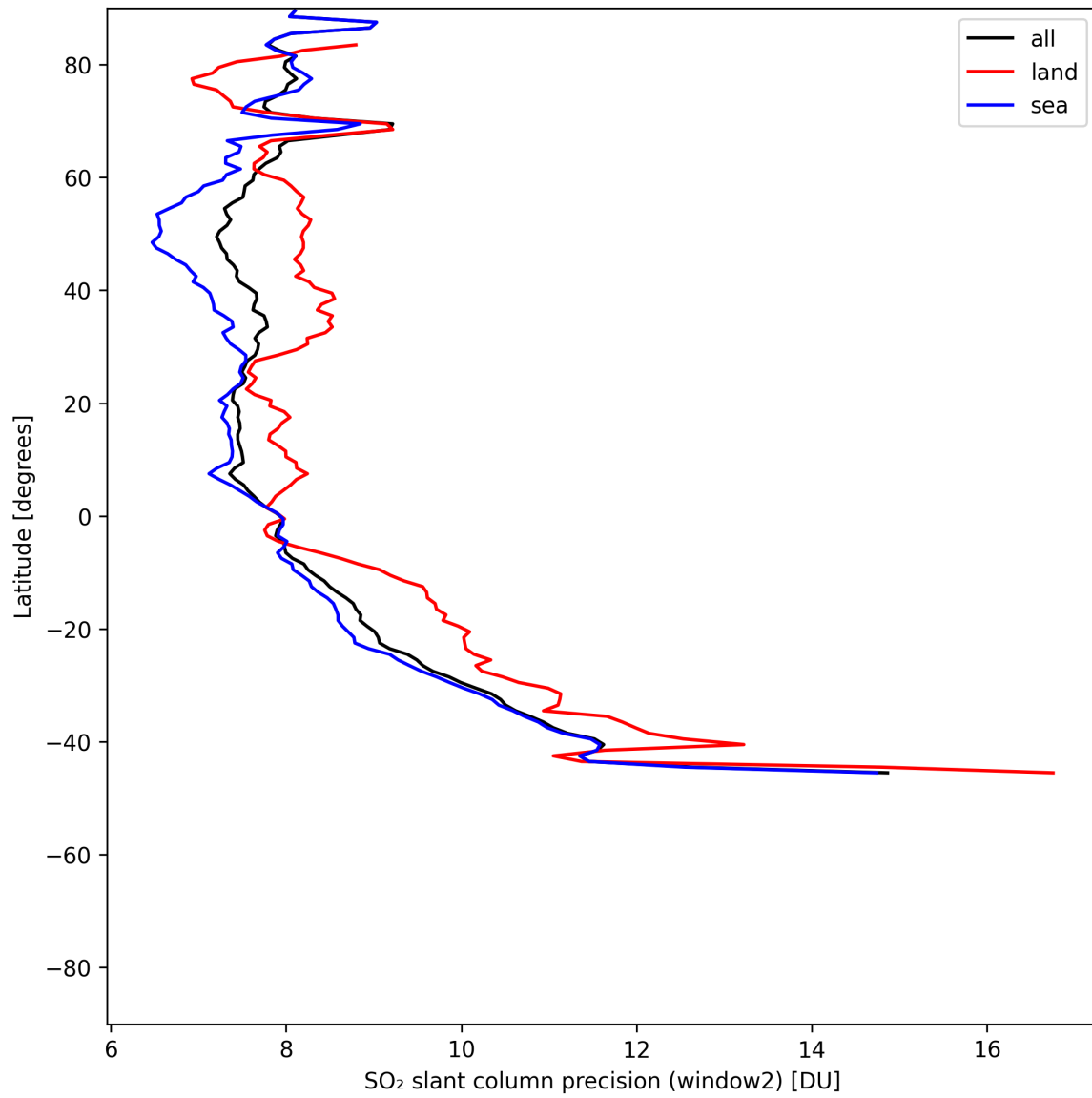
Figure 42: Zonal average of “SO 2 slant column precision (window2)” for 2025-06-22 to 2025-06-23.
