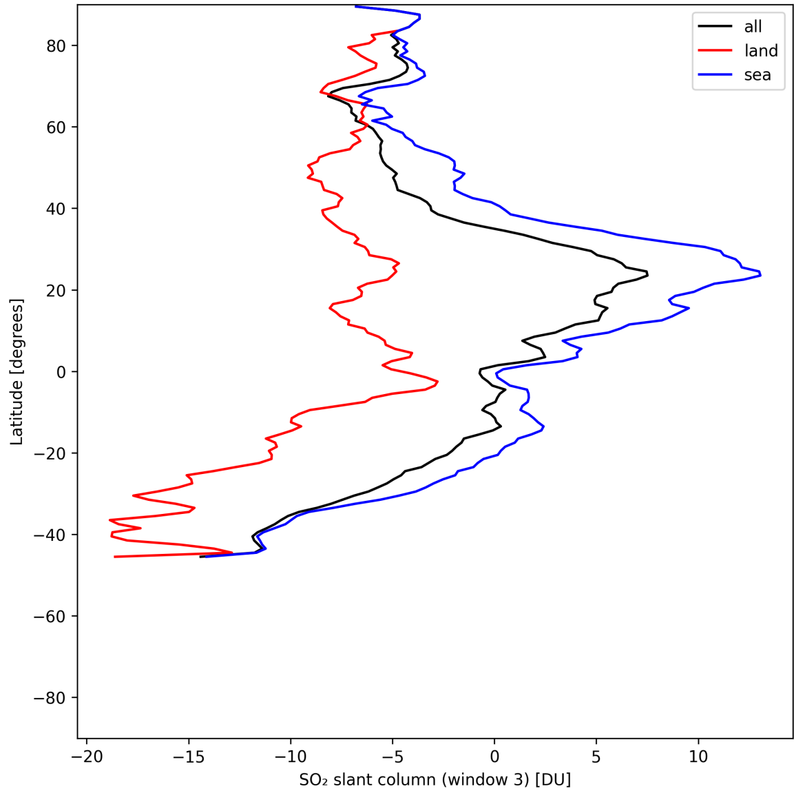
Figure 45: Zonal average of “SO 2 slant column (window 3)” for 2025-06-22 to 2025-06-23.
