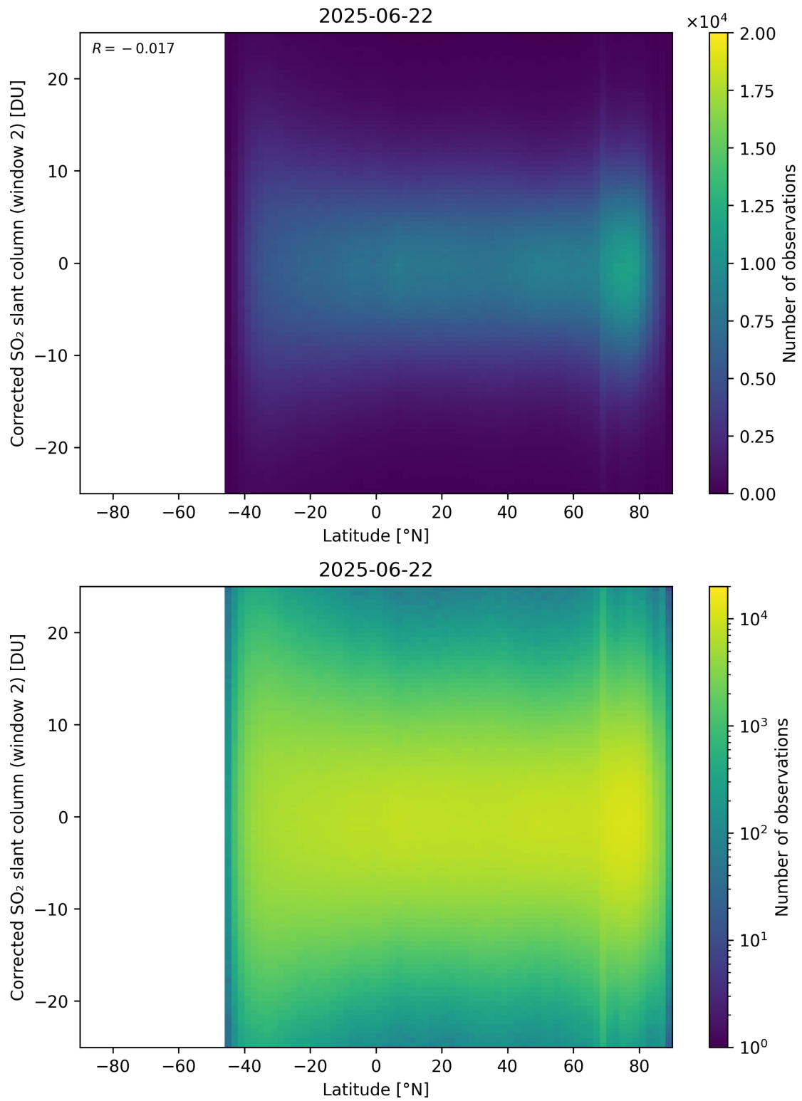
Figure 160: Scatter density plot of “Latitude” against “Corrected SO 2 slant column (window 2)” for 2025-06-22 to 2025-06-23.
