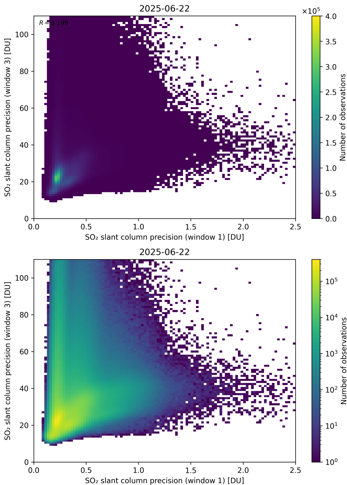
Figure 279: Scatter density plot of “SO 2 slant column precision (window 1)” against “SO 2 slant column precision (window 3)” for 2025-06-22 to 2025-06-23.
