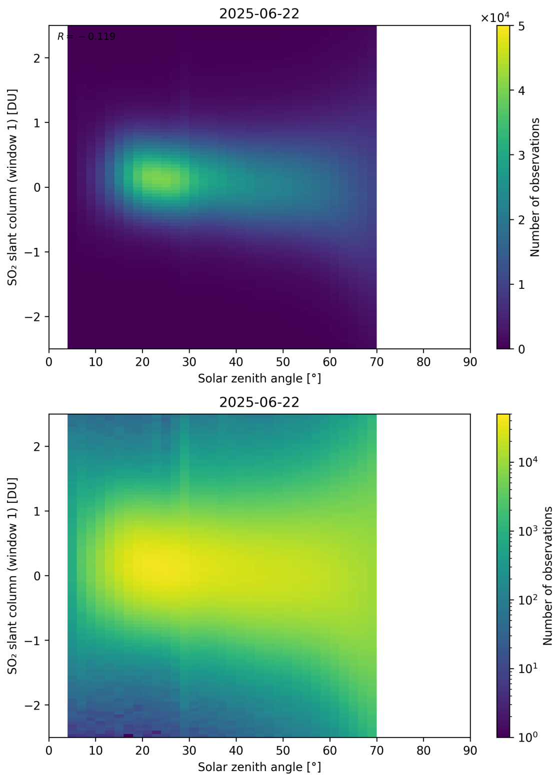
Figure 184: Scatter density plot of “Solar zenith angle” against “SO 2 slant column (window 1)” for 2025-06-22 to 2025-06-23.
