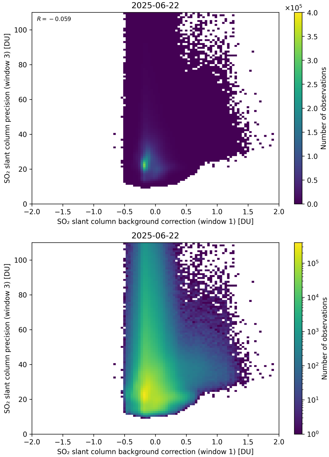
Figure 119: Scatter density plot of “SO 2 slant column background correction (window 1)” against “SO 2 slant column precision (window 3)” for 2025-06-22 to 2025-06-23.
