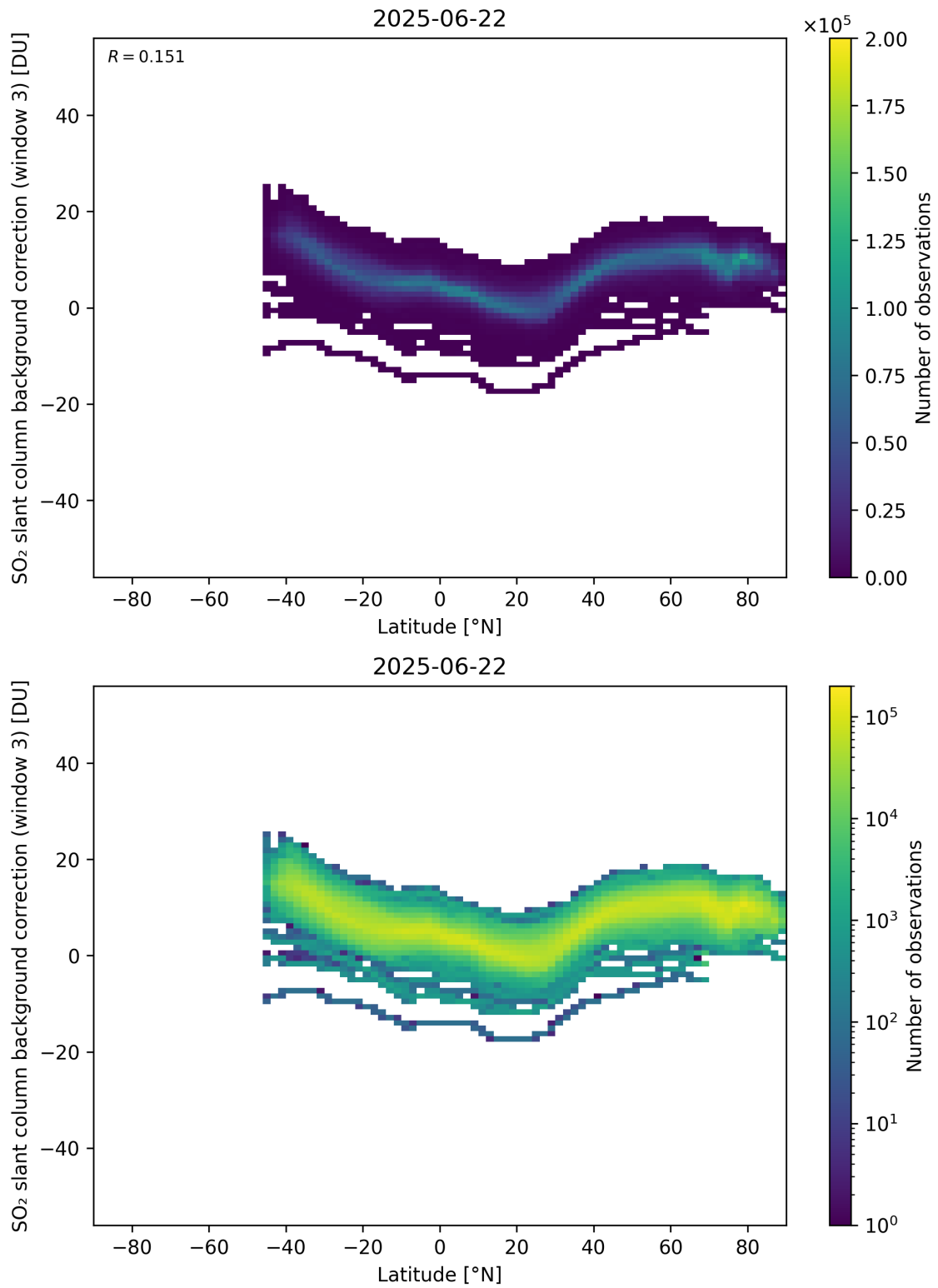
Figure 152: Scatter density plot of “Latitude” against “SO 2 slant column background correction (window 3)” for 2025-06-22 to 2025-06-23.
