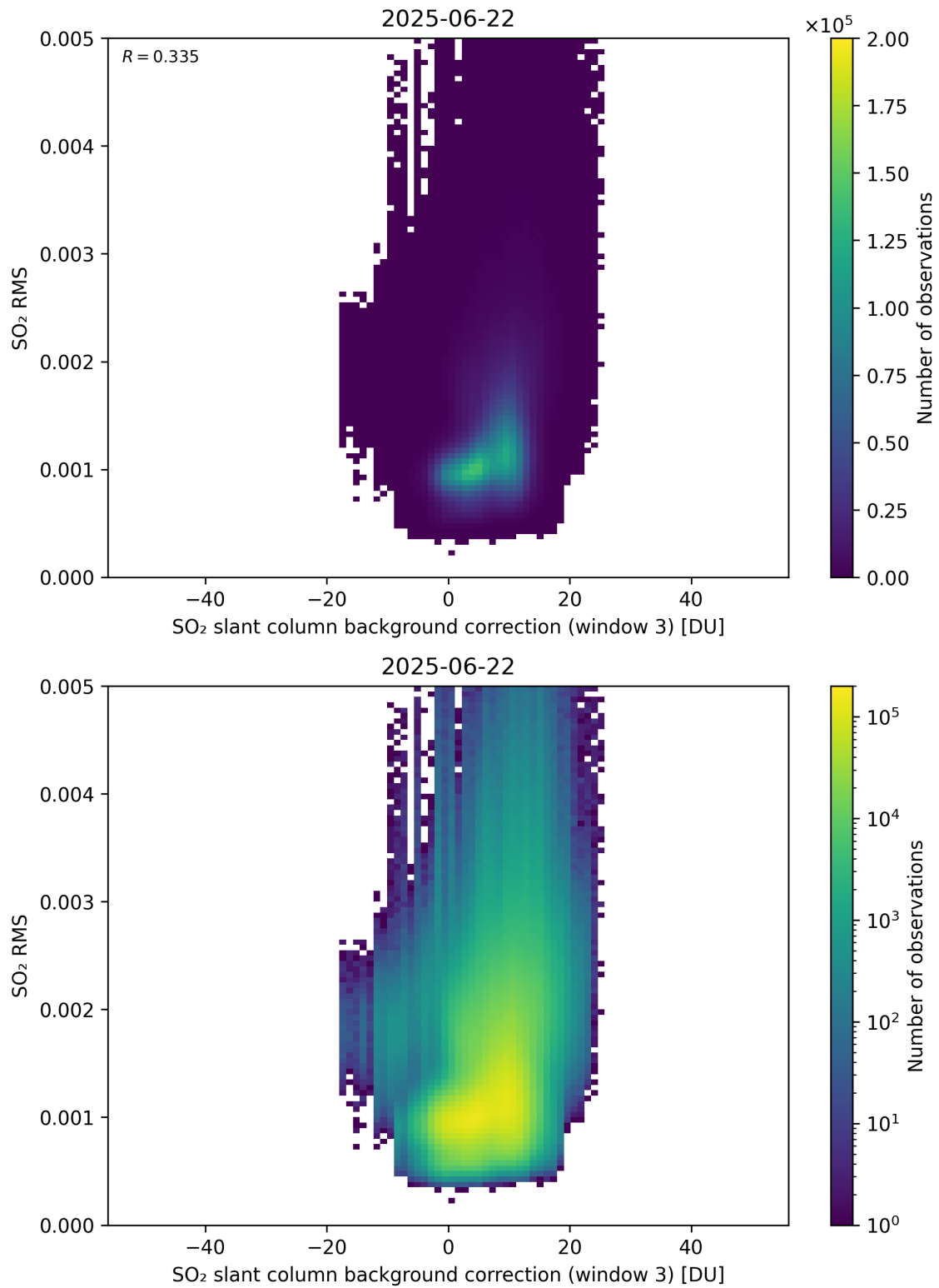
Figure 134: Scatter density plot of “SO 2 slant column background correction (window 3)” against “SO 2 RMS” for 2025-06-22 to 2025-06-23.
