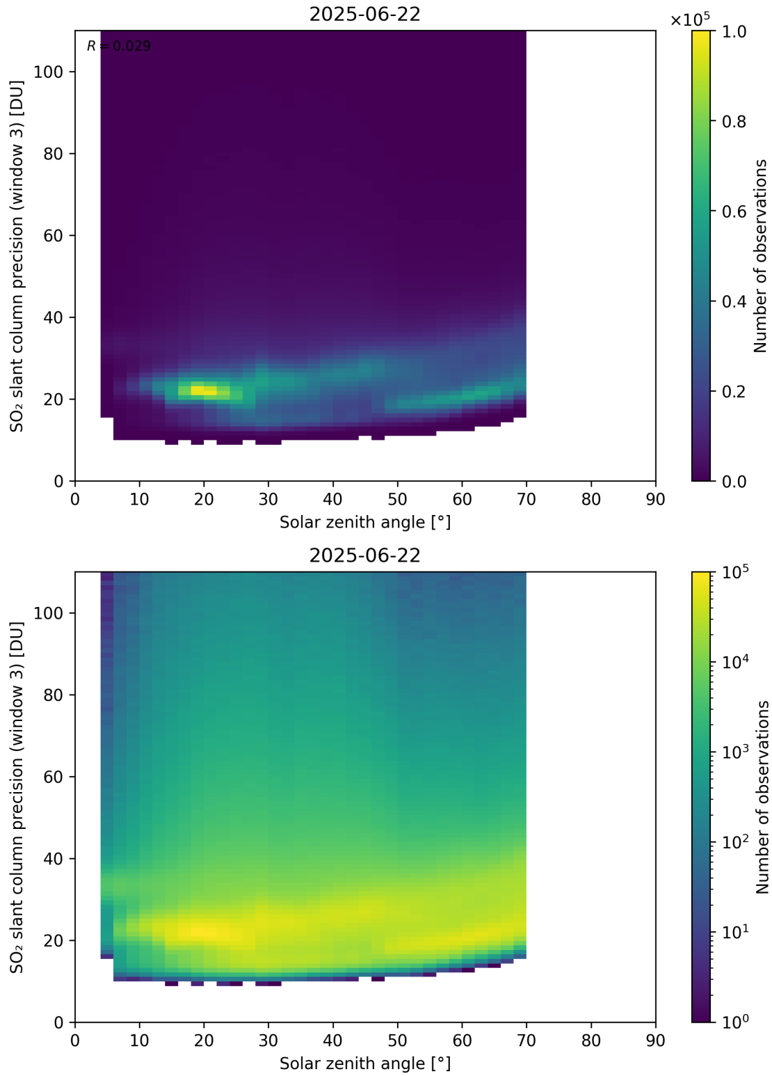
Figure 188: Scatter density plot of “Solar zenith angle” against “SO 2 slant column precision (window 3)” for 2025-06-22 to 2025-06-23.
