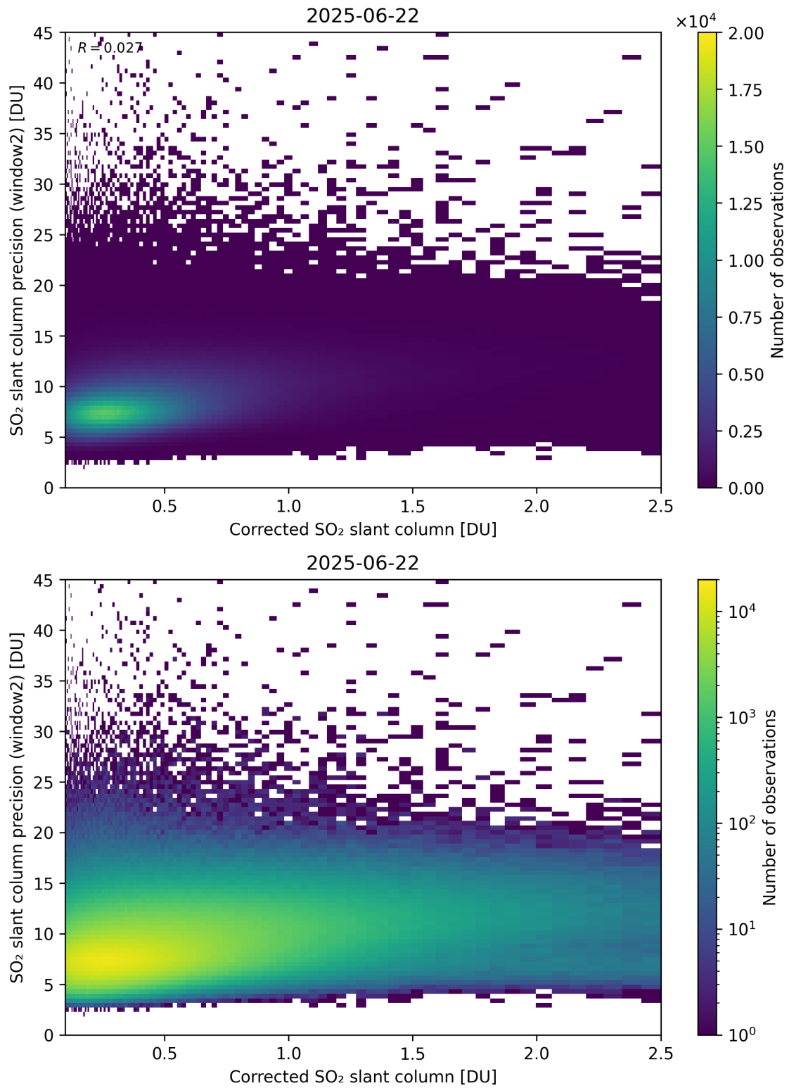
Figure 239: Scatter density plot of “Corrected SO 2 slant column” against “SO 2 slant column precision (window2)” for 2025-06-22 to 2025-06-23.
