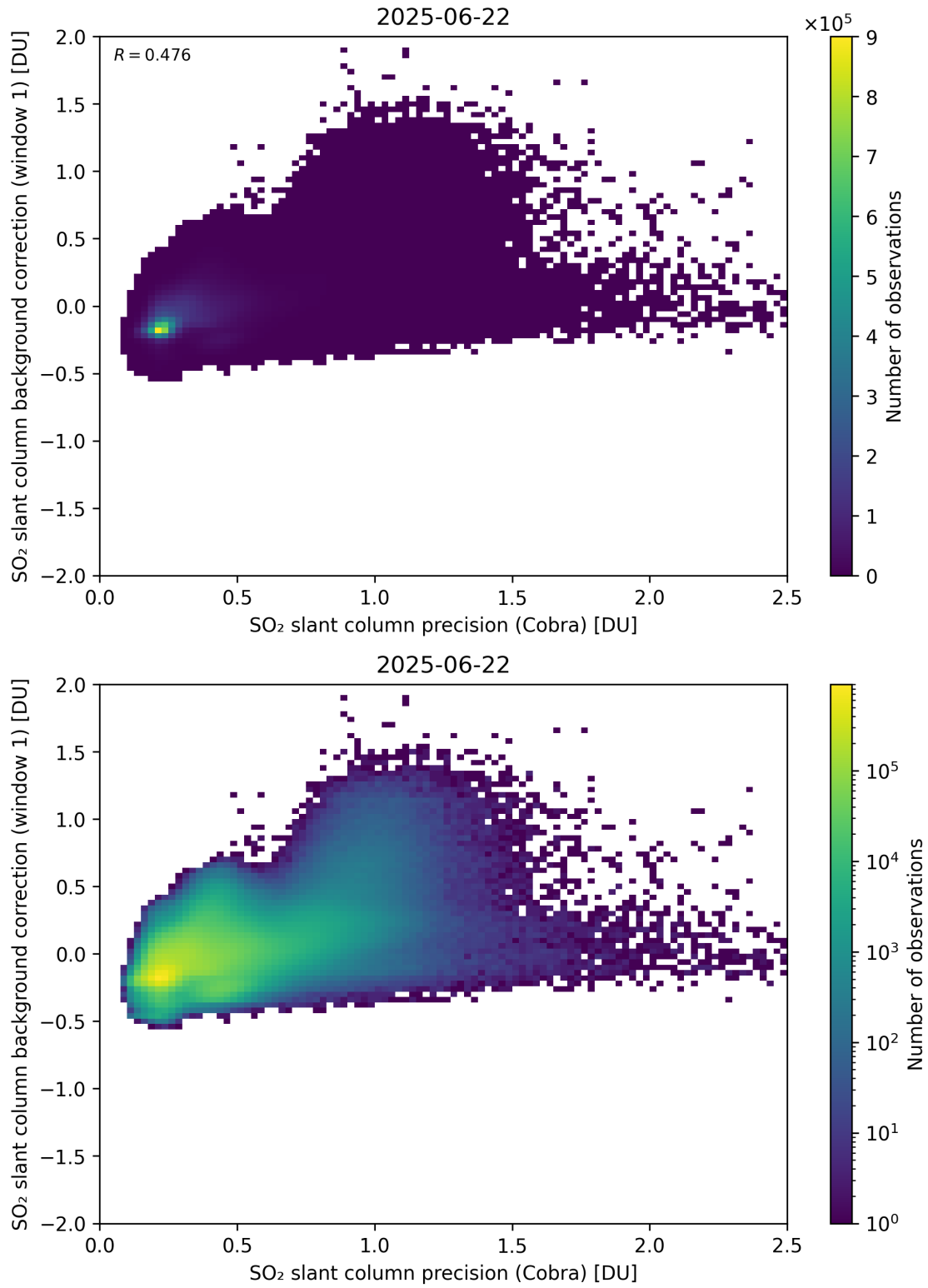
Figure 199: Scatter density plot of “SO 2 slant column precision (Cobra)” against “SO 2 slant column background correction (window 1)” for 2025-06-22 to 2025-06-23.
