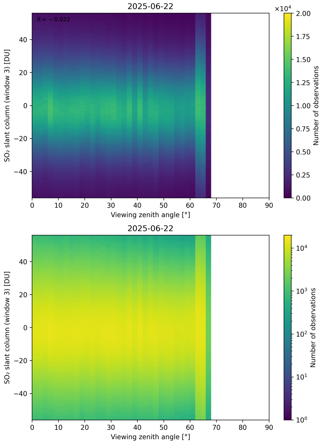
Figure 379: Scatter density plot of “Viewing zenith angle” against “SO 2 slant column (window 3)” for 2025-06-22 to 2025-06-23.
