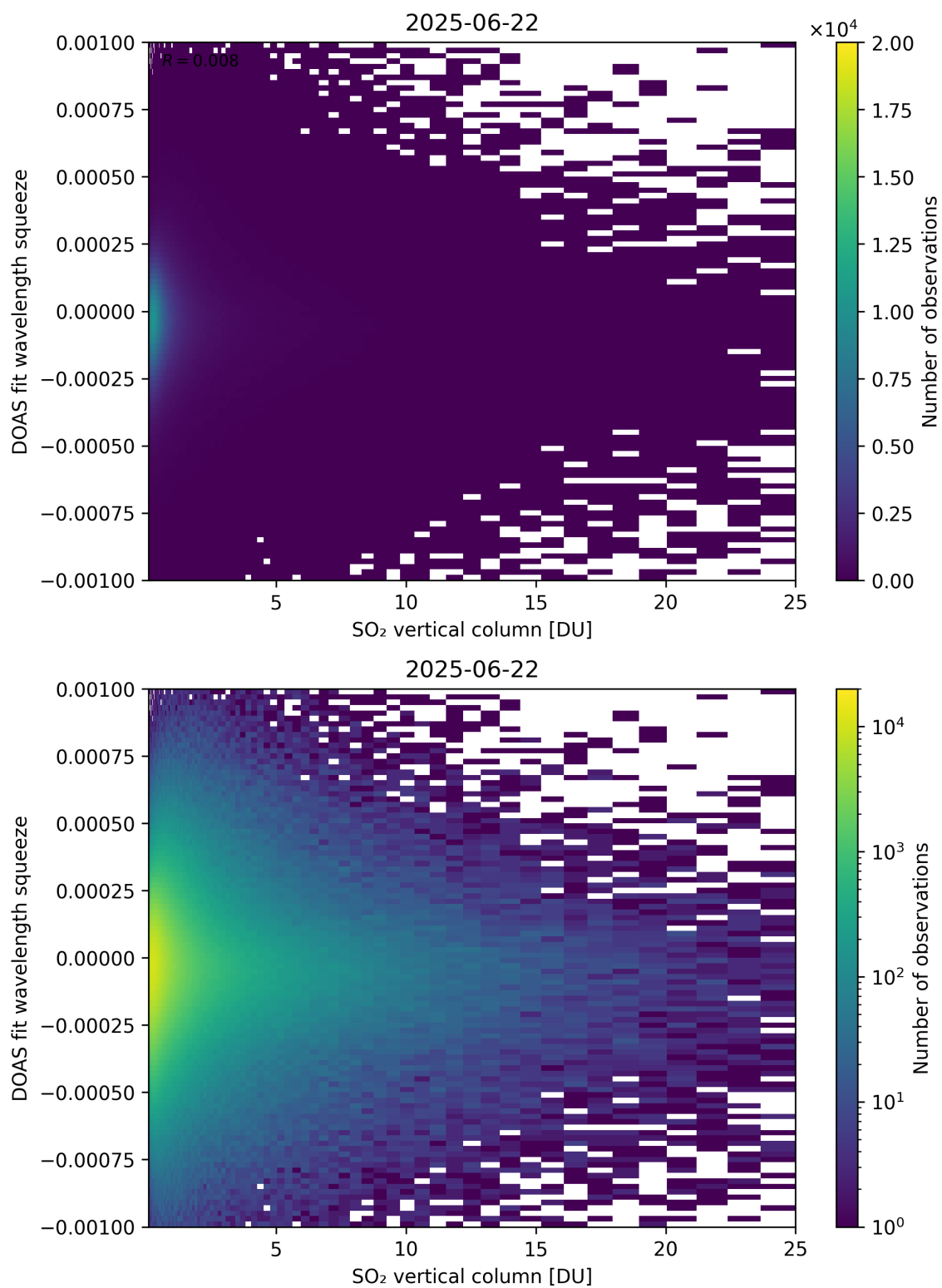
Figure 327: Scatter density plot of “SO 2 vertical column” against “DOAS fit wavelength squeeze” for 2025-06-22 to 2025-06-23.
