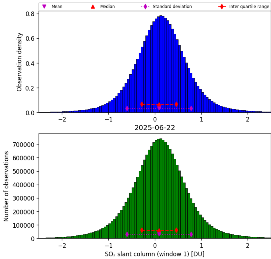
Figure 63: Histogram of “SO 2 slant column (window 1)” for 2025-06-22 to 2025-06-23
