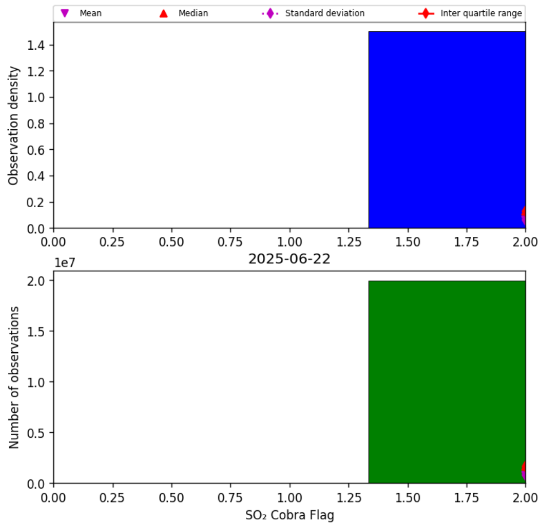
Figure 75: Histogram of “SO 2 Cobra Flag” for 2025-06-22 to 2025-06-23
