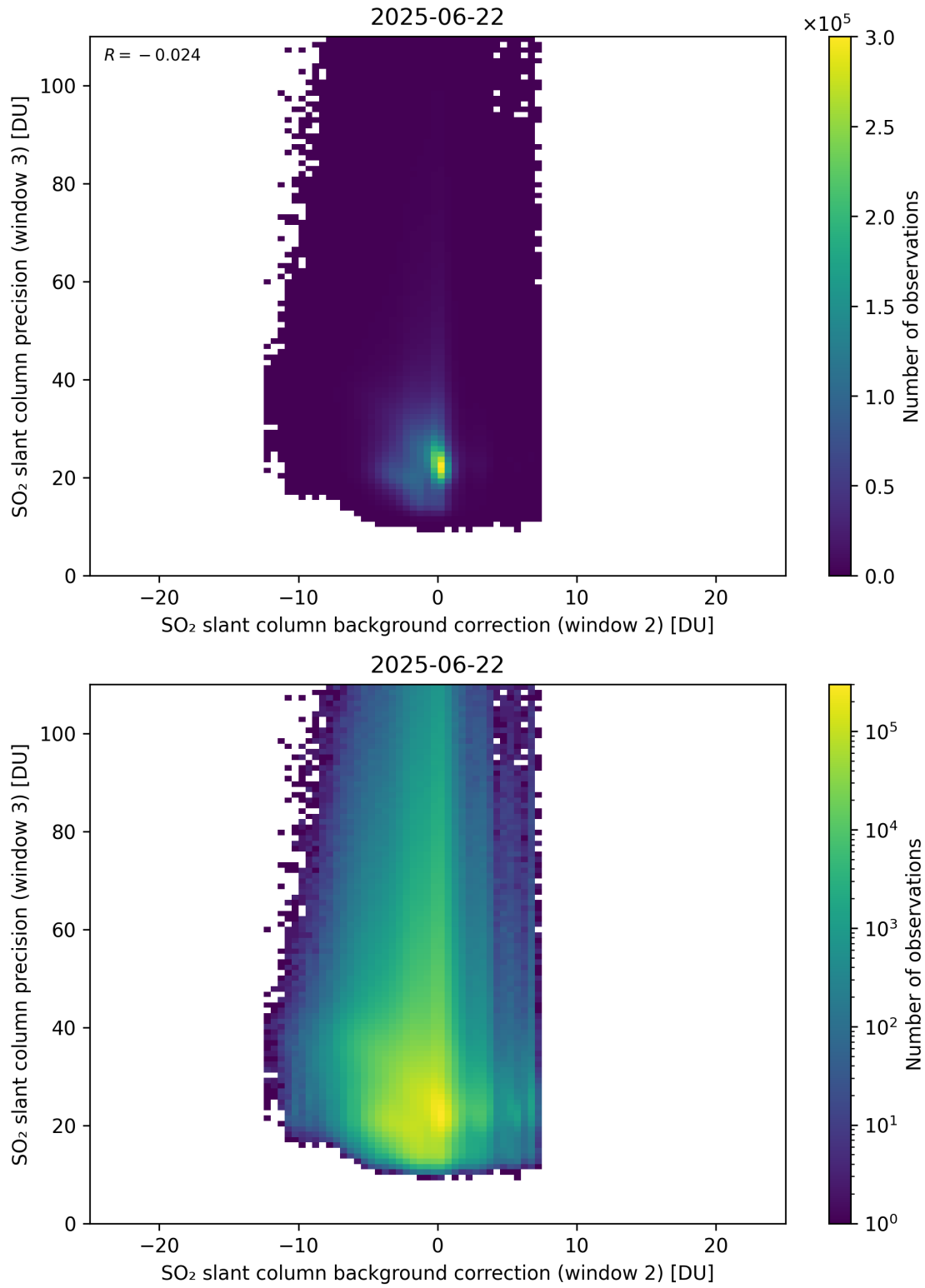
Figure 129: Scatter density plot of “SO 2 slant column background correction (window 2)” against “SO 2 slant column precision (window 3)” for 2025-06-22 to 2025-06-23.
