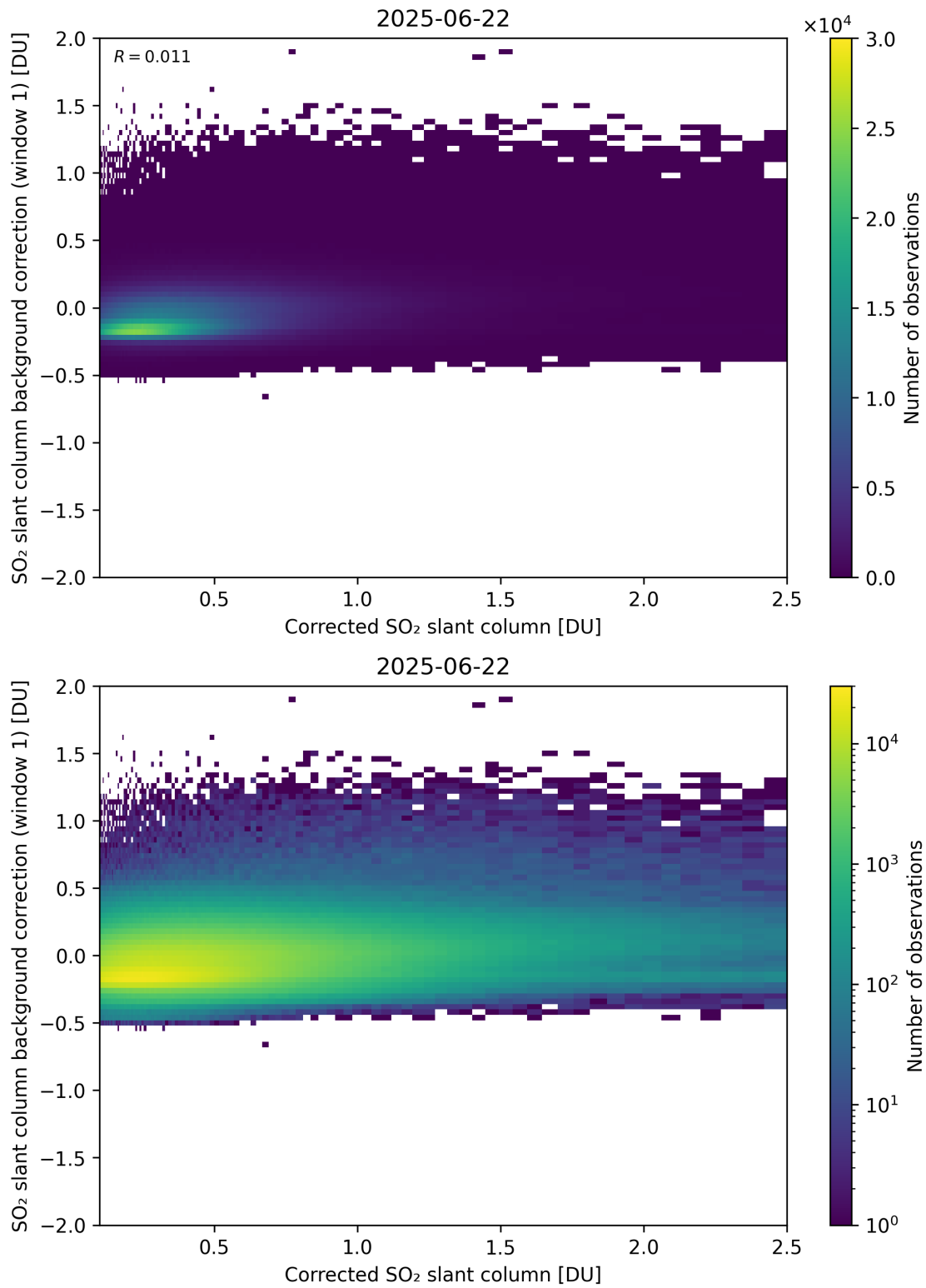
Figure 226: Scatter density plot of “Corrected SO 2 slant column” against “SO 2 slant column background correction (window 1)” for 2025-06-22 to 2025-06-23.
