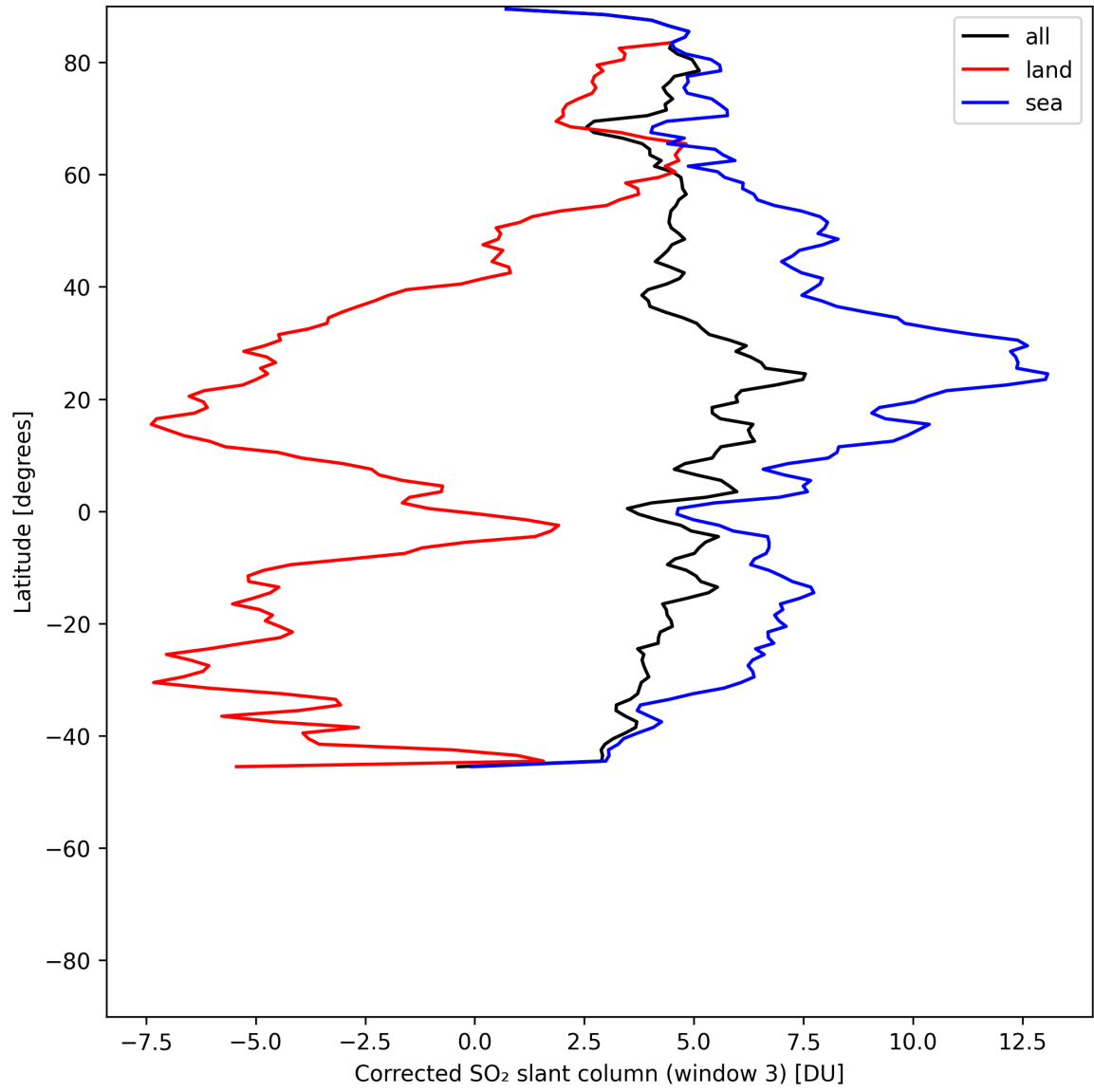
Figure 47: Zonal average of “Corrected SO 2 slant column (window 3)” for 2025-06-22 to 2025-06-23.
