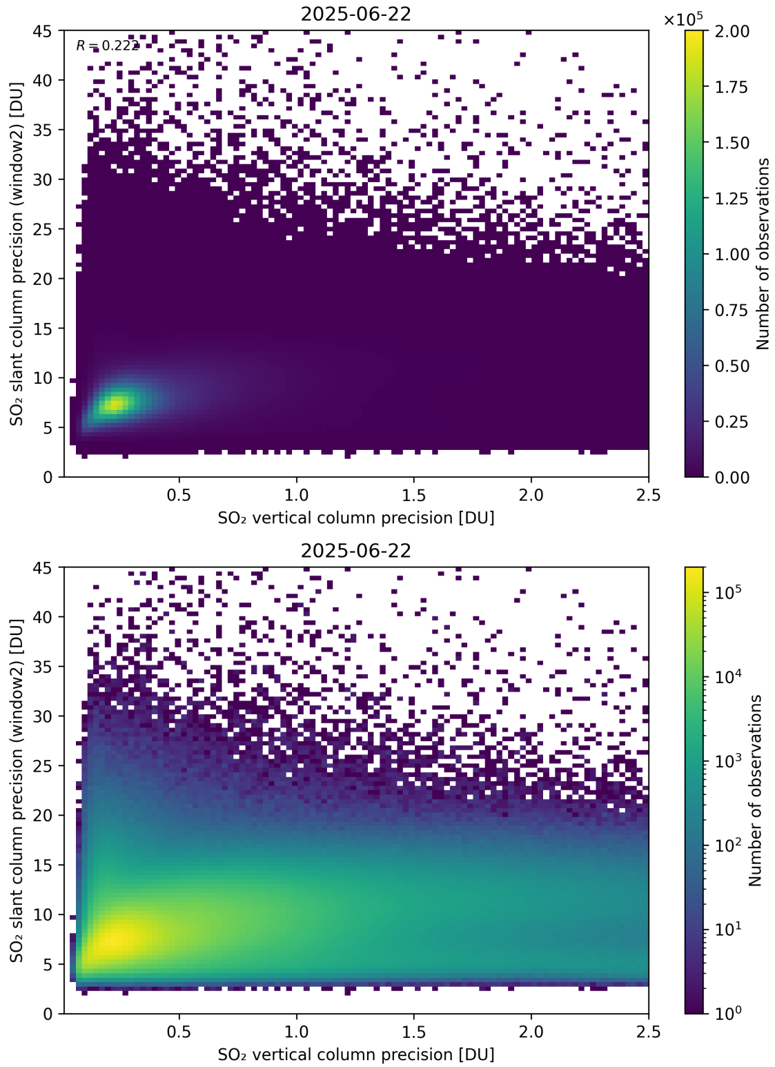
Figure 343: Scatter density plot of “SO 2 vertical column precision” against “SO 2 slant column precision (window2)” for 2025-06-22 to 2025-06-23.
