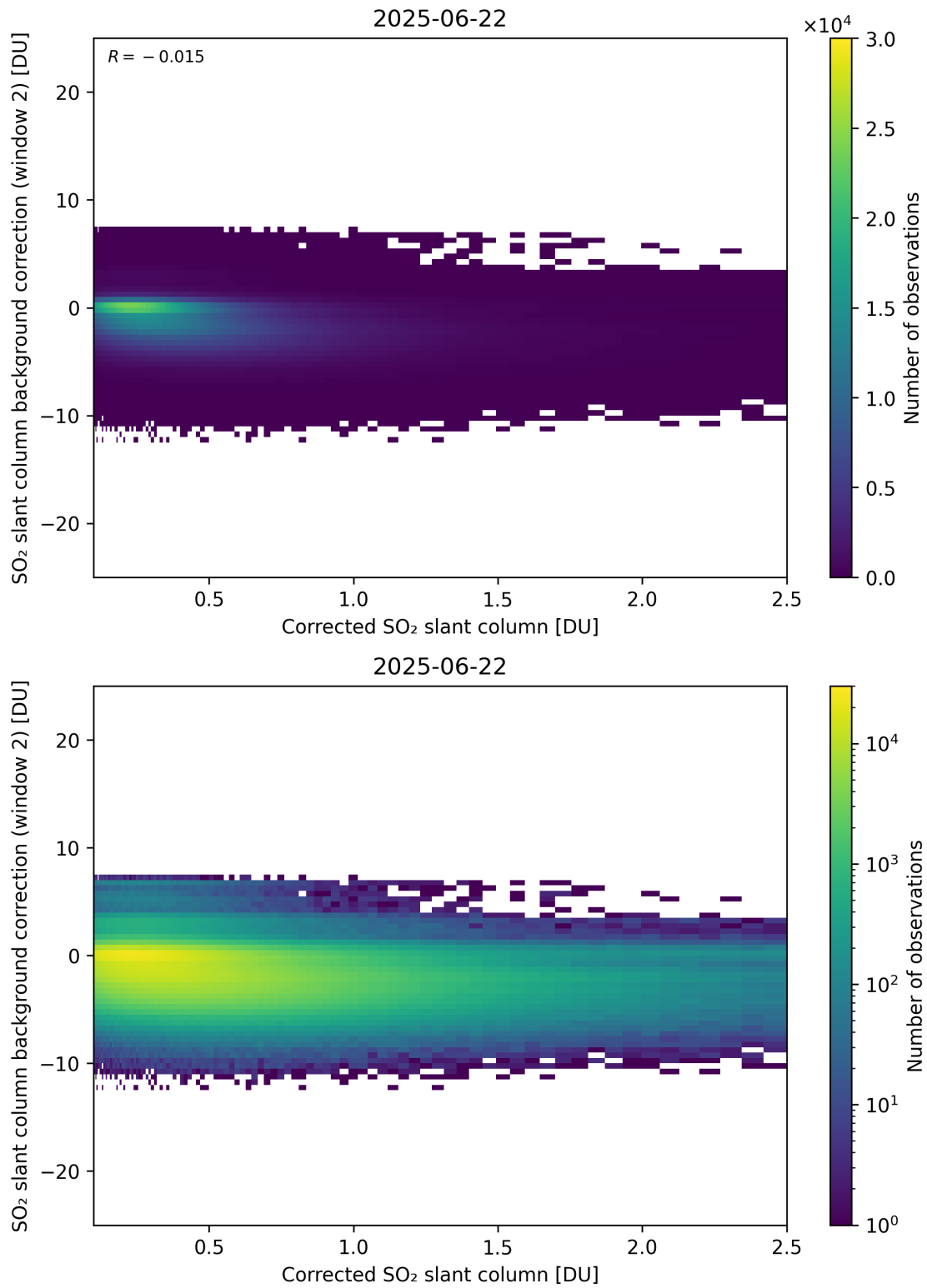
Figure 227: Scatter density plot of “Corrected SO 2 slant column” against “SO 2 slant column background correction (window 2)” for 2025-06-22 to 2025-06-23.
