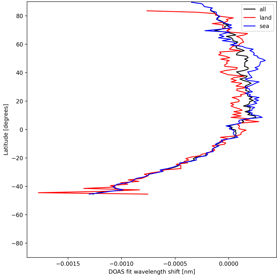
Figure 50: Zonal average of “DOAS fit wavelength shift” for 2025-06-22 to 2025-06-23.
