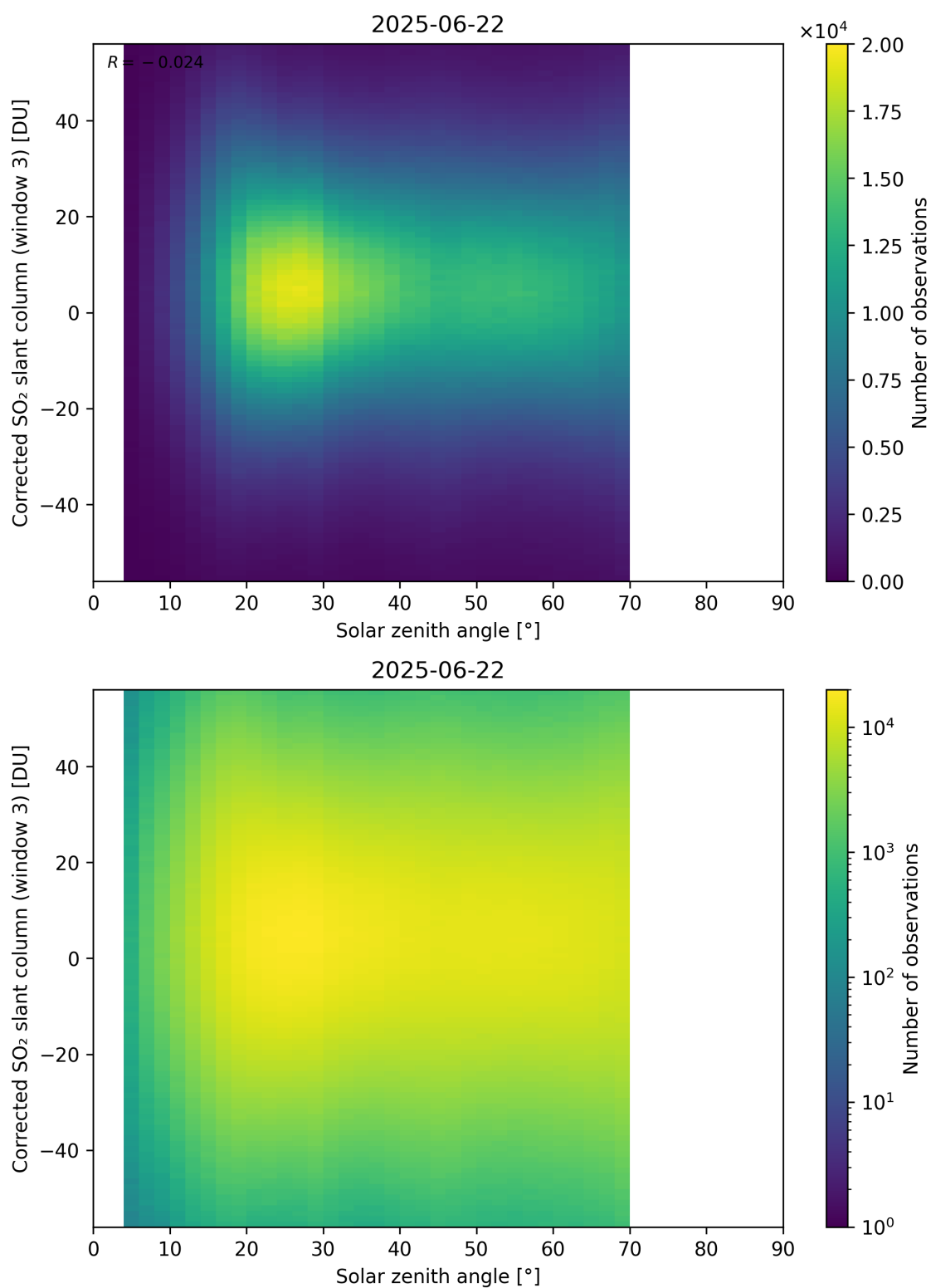
Figure 183: Scatter density plot of “Solar zenith angle” against “Corrected SO 2 slant column (window 3)” for 2025-06-22 to 2025-06-23.
