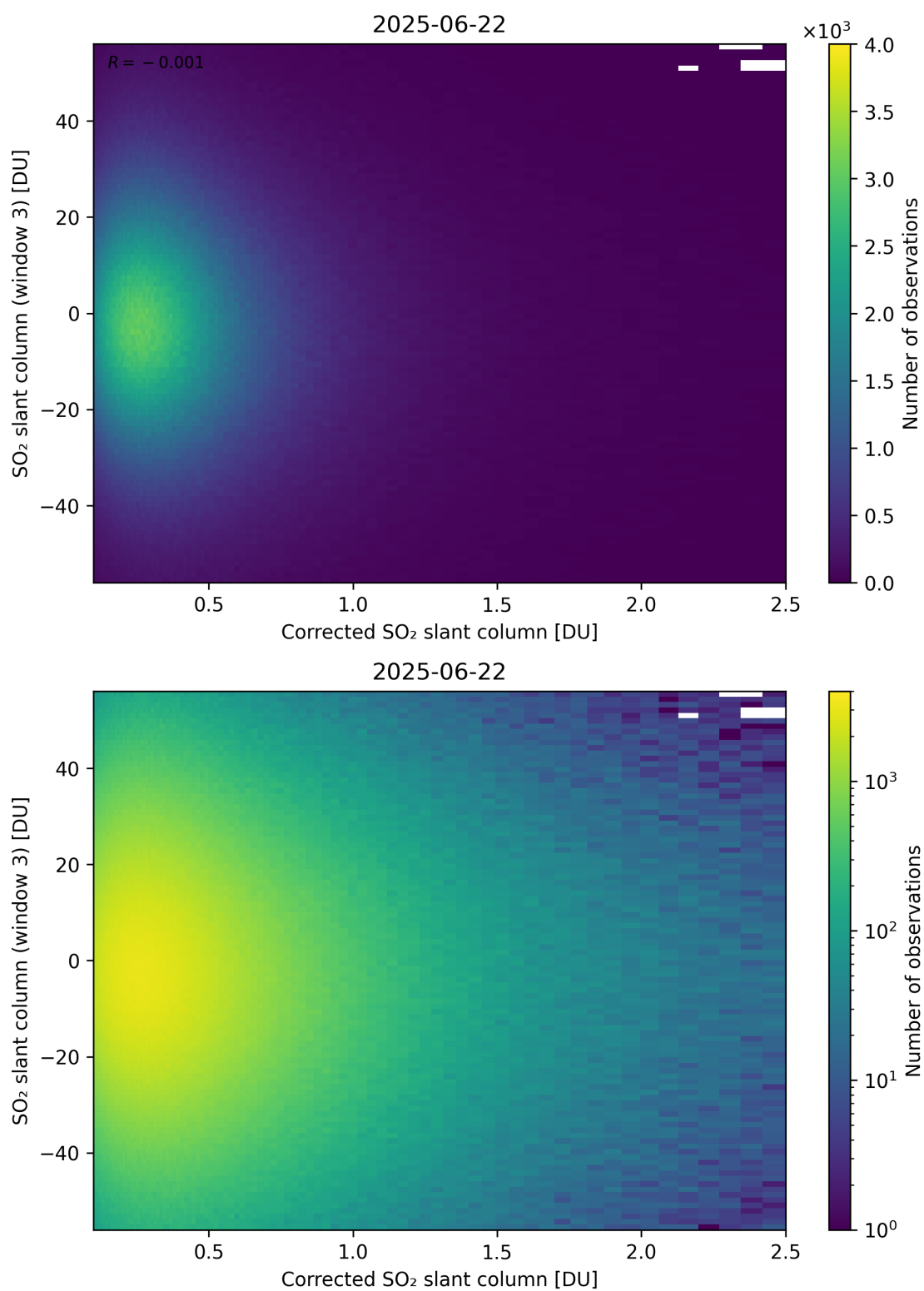
Figure 240: Scatter density plot of “Corrected SO 2 slant column” against “SO 2 slant column (window 3)” for 2025-06-22 to 2025-06-23.
