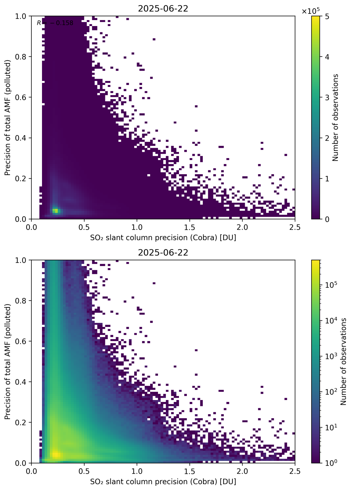
Figure 214: Scatter density plot of “SO 2 slant column precision (Cobra)” against “Precision of total AMF (polluted)” for 2025-06-22 to 2025-06-23.
