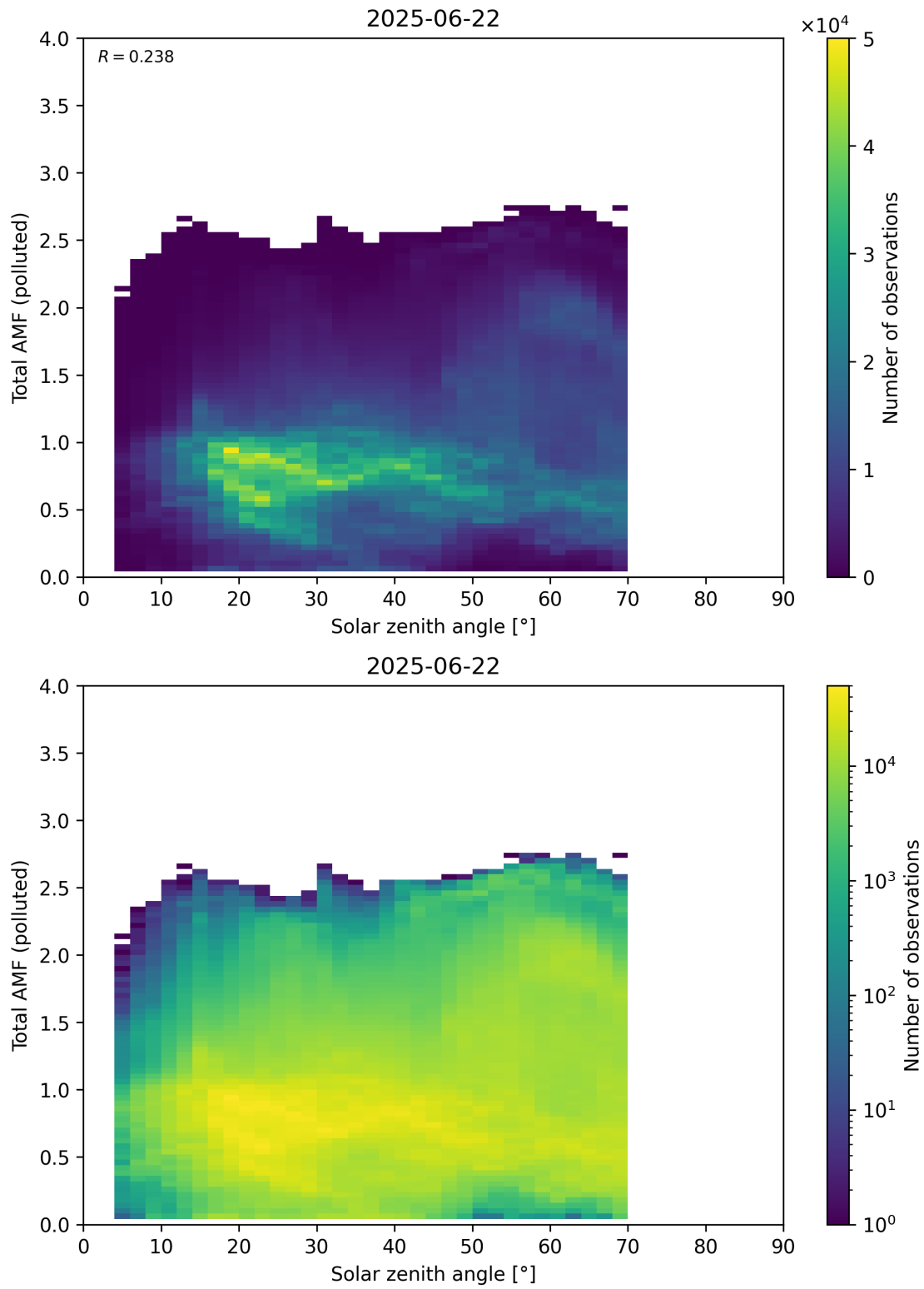
Figure 189: Scatter density plot of “Solar zenith angle” against “Total AMF (polluted)” for 2025-06-22 to 2025-06-23.
