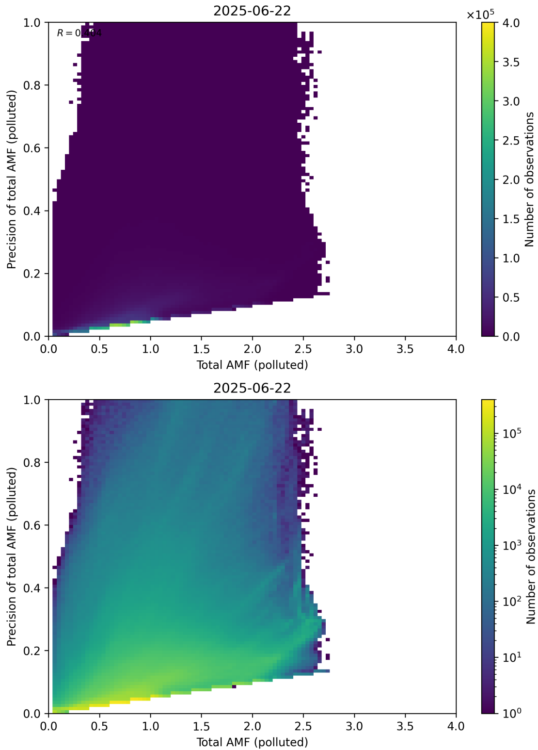
Figure 322: Scatter density plot of “Total AMF (polluted)” against “Precision of total AMF (polluted)” for 2025-06-22 to 2025-06-23.
