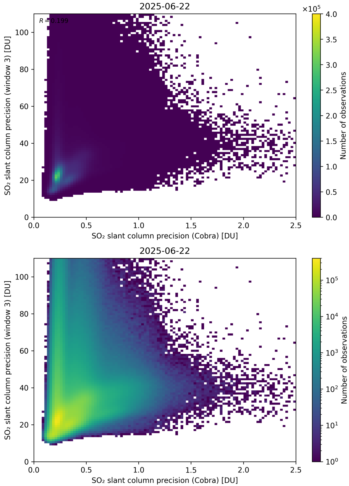
Figure 212: Scatter density plot of “SO 2 slant column precision (Cobra)” against “SO 2 slant column precision (window 3)” for 2025-06-22 to 2025-06-23.
