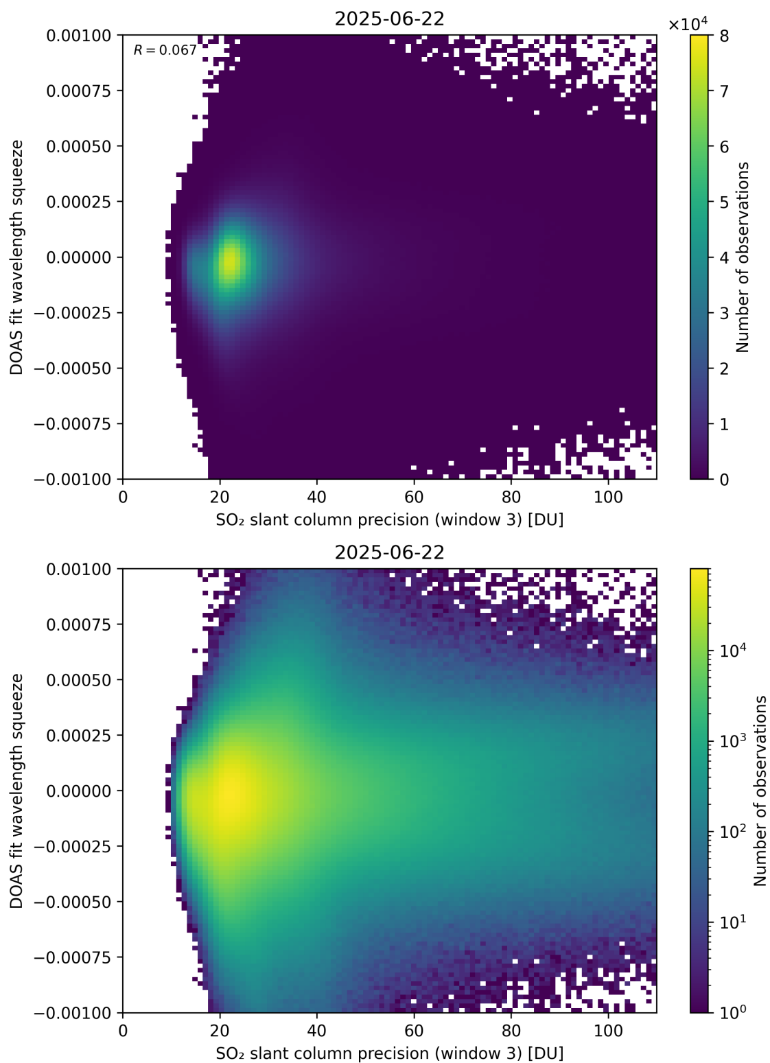
Figure 309: Scatter density plot of “SO 2 slant column precision (window 3)” against “DOAS fit wavelength squeeze” for 2025-06-22 to 2025-06-23.
