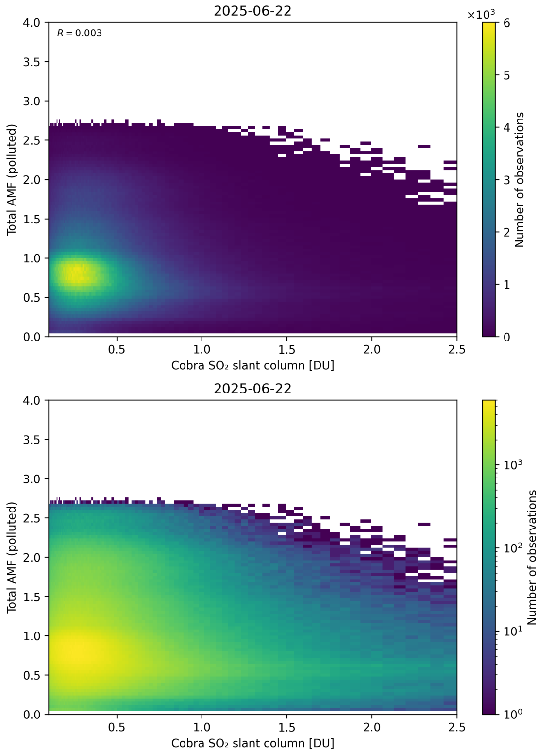
Figure 224: Scatter density plot of “Cobra SO 2 slant column” against “Total AMF (polluted)” for 2025-06-22 to 2025-06-23.
