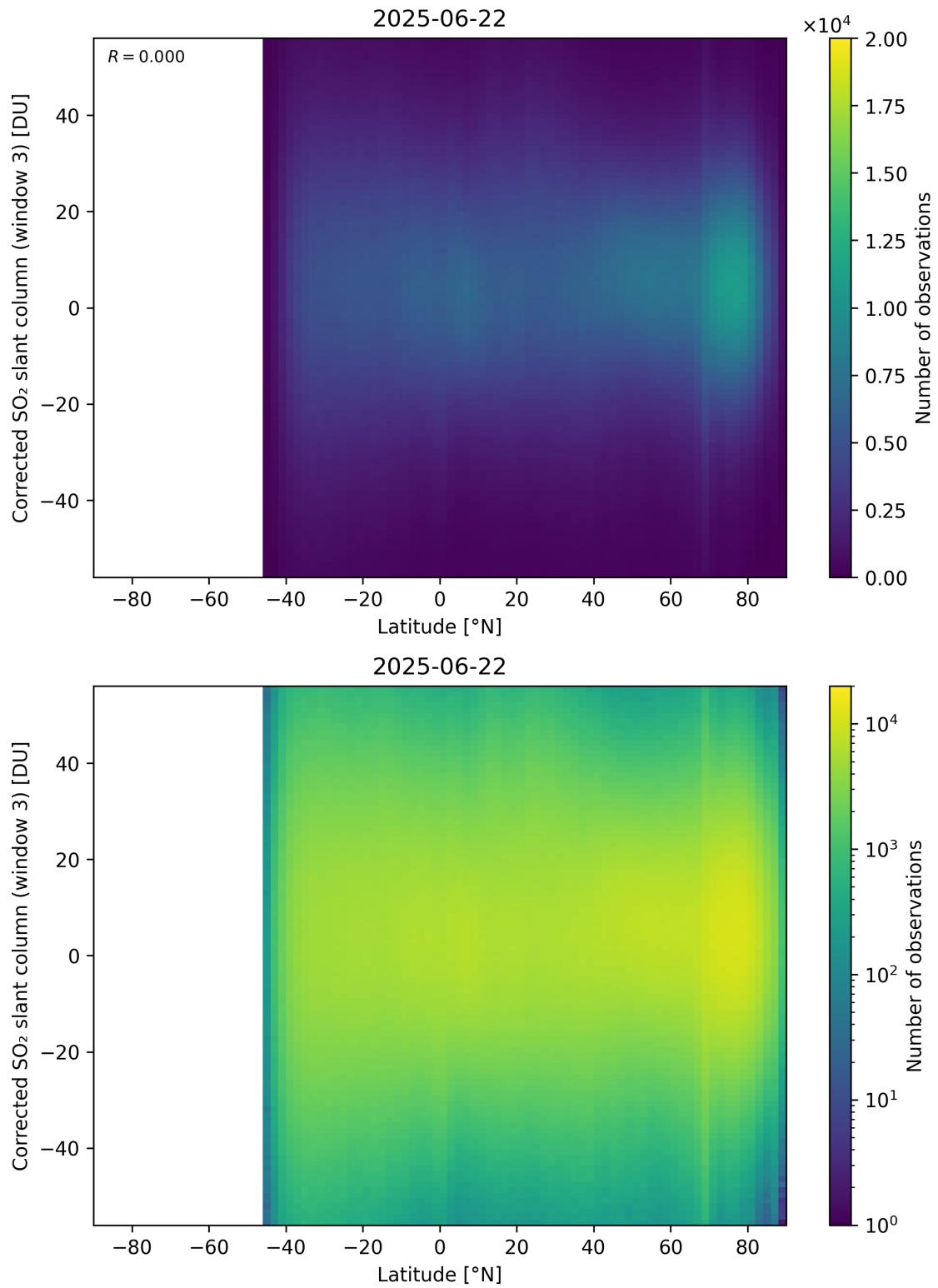
Figure 161: Scatter density plot of “Latitude” against “Corrected SO 2 slant column (window 3)” for 2025-06-22 to 2025-06-23.
