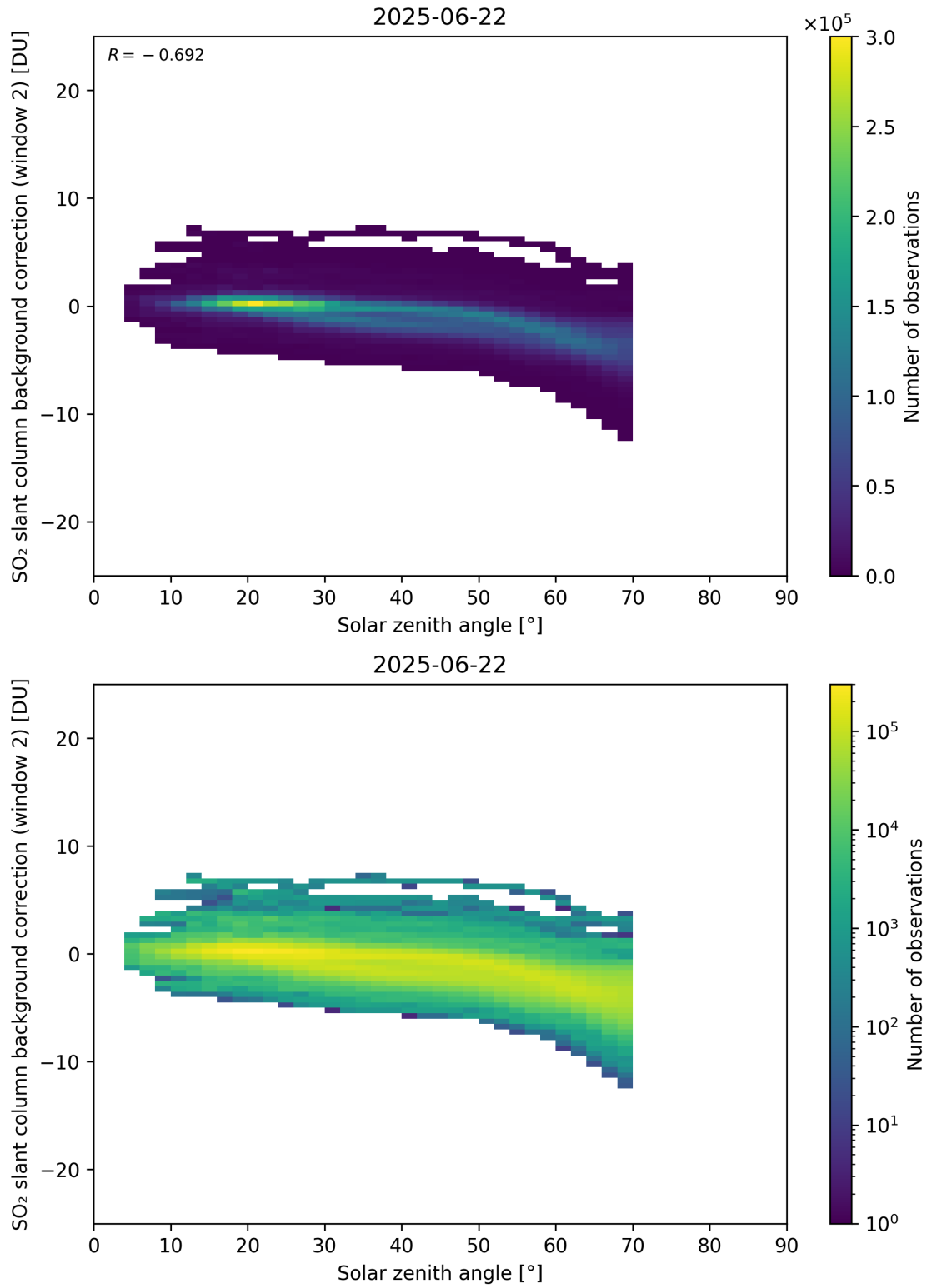
Figure 172: Scatter density plot of “Solar zenith angle” against “SO 2 slant column background correction (window 2)” for 2025-06-22 to 2025-06-23.
