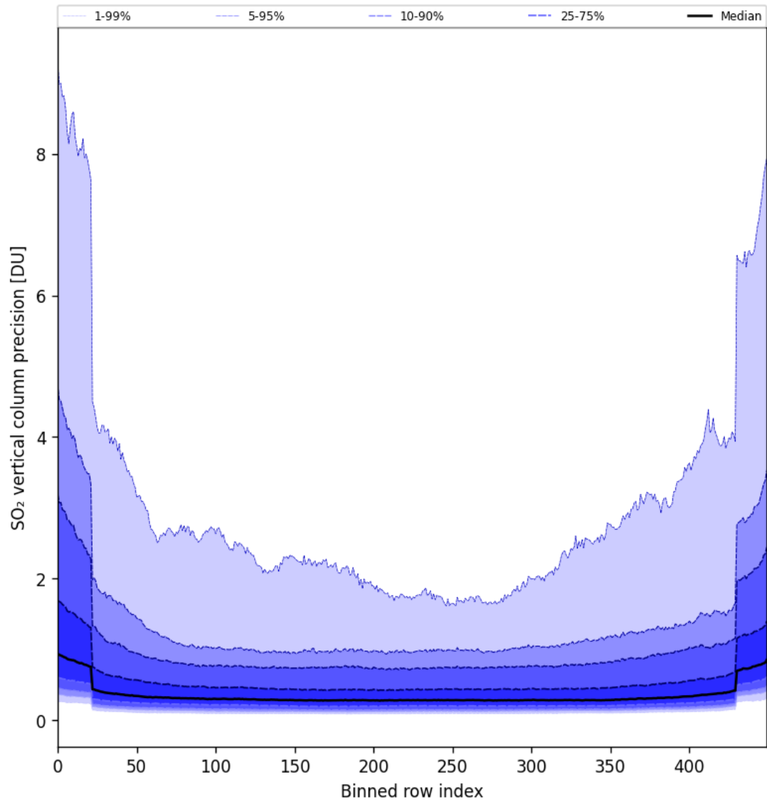
Figure 85: Along track statistics of “SO 2 vertical column precision” for 2025-06-22 to 2025-06-23
