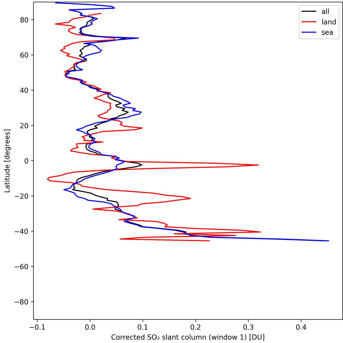
Figure 39: Zonal average of “Corrected SO 2 slant column (window 1)” for 2025-06-22 to 2025-06-23.
