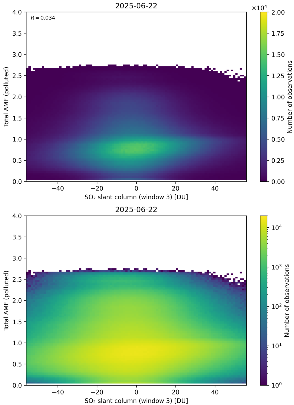
Figure 318: Scatter density plot of “SO 2 slant column (window 3)” against “Total AMF (polluted)” for 2025-06-22 to 2025-06-23.
