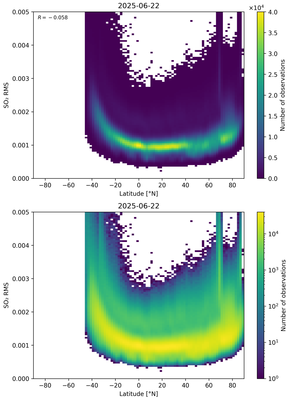
Figure 155: Scatter density plot of “Latitude” against “SO 2 RMS” for 2025-06-22 to 2025-06-23.
