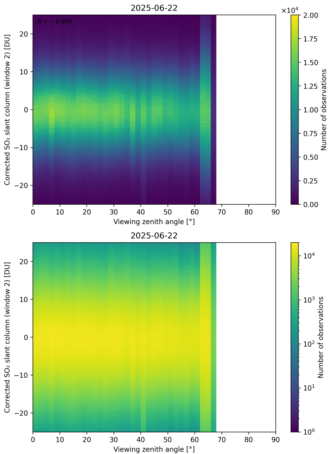
Figure 374: Scatter density plot of “Viewing zenith angle” against “Corrected SO 2 slant column (window 2)” for 2025-06-22 to 2025-06-23.
