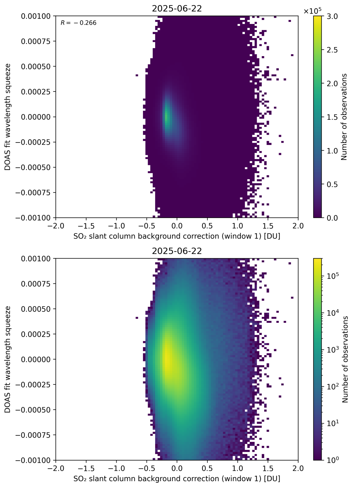
Figure 112: Scatter density plot of “SO 2 slant column background correction (window 1)” against “DOAS fit wavelength squeeze” for 2025-06-22 to 2025-06-23.
