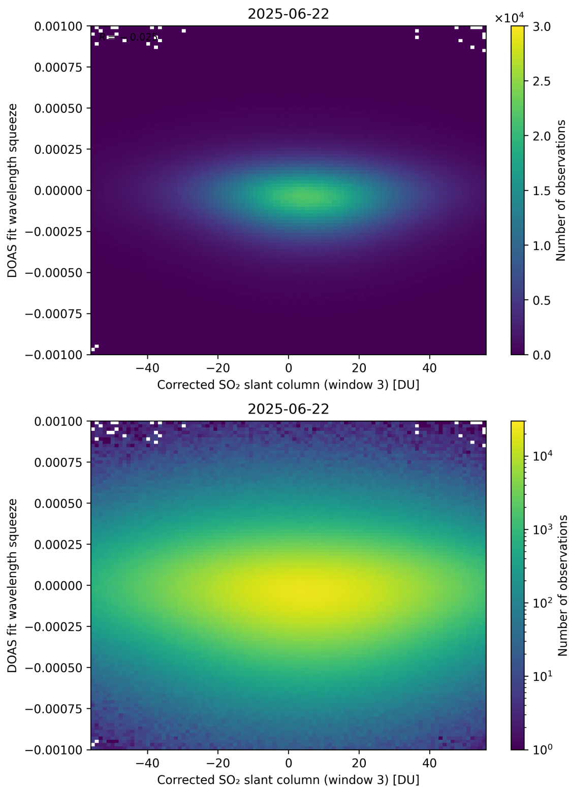
Figure 257: Scatter density plot of “Corrected SO 2 slant column (window 3)” against “DOAS fit wavelength squeeze” for 2025-06-22 to 2025-06-23.
