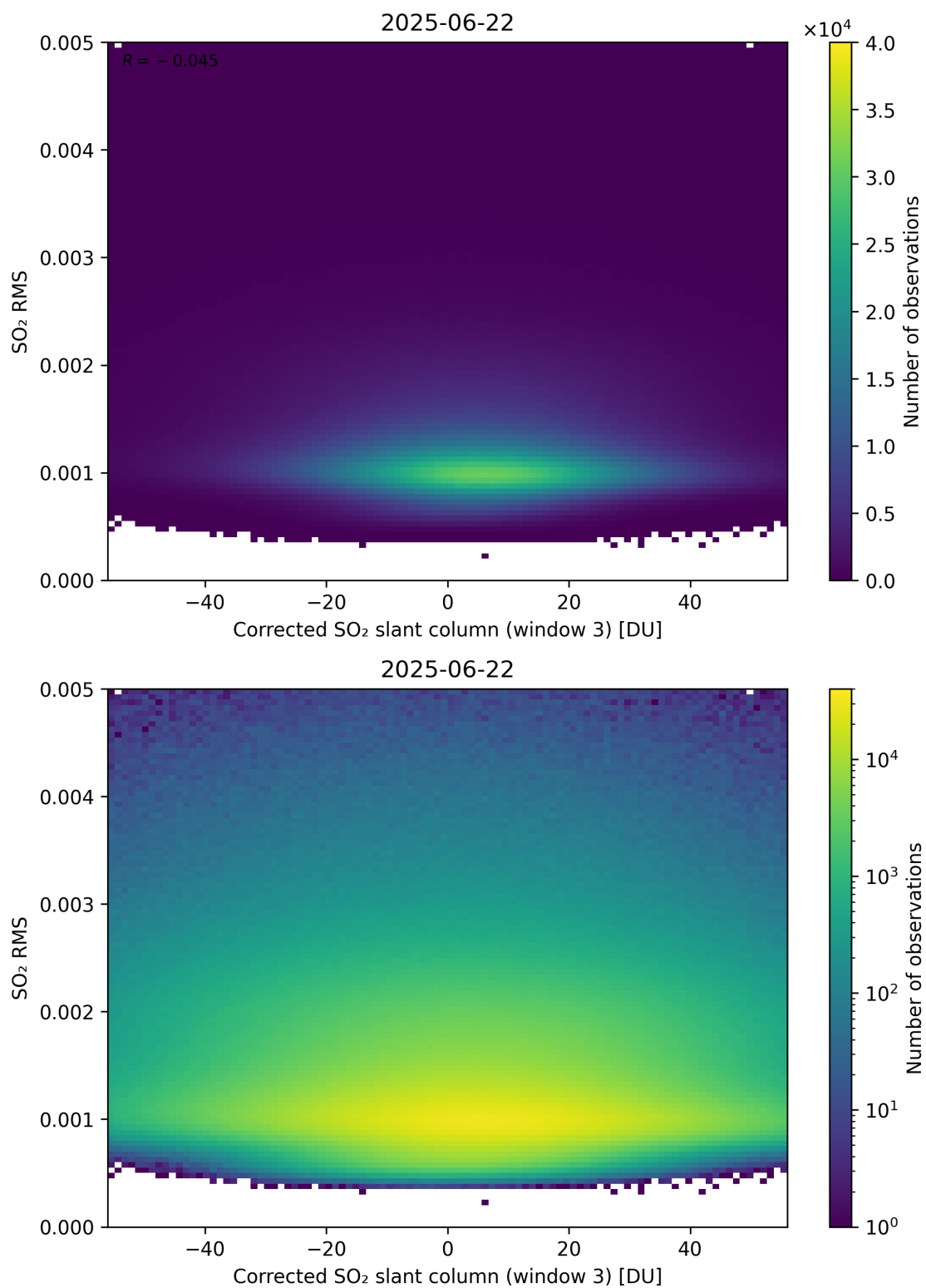
Figure 258: Scatter density plot of “Corrected SO 2 slant column (window 3)” against “SO 2 RMS” for 2025-06-22 to 2025-06-23.
