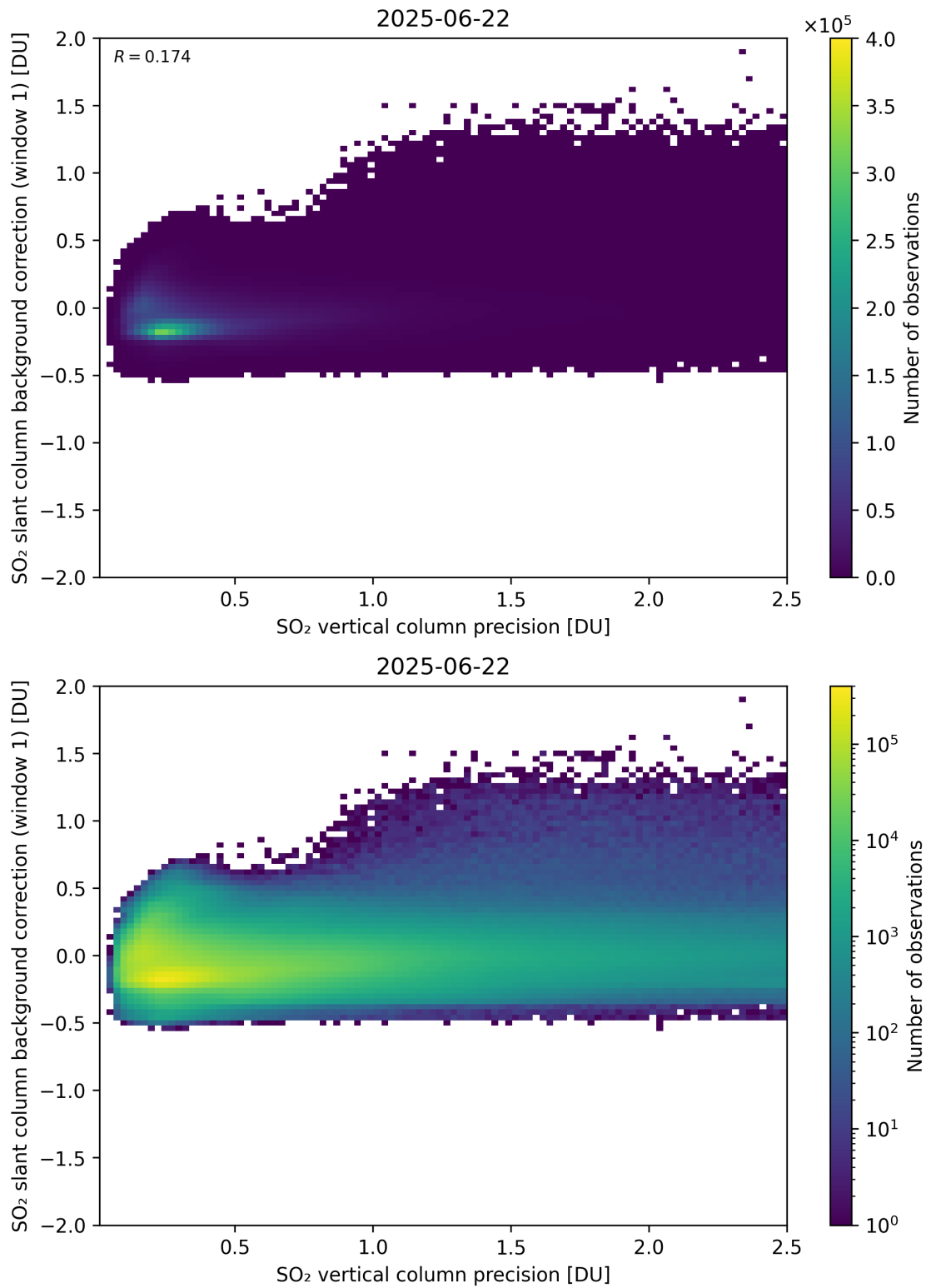
Figure 329: Scatter density plot of “SO 2 vertical column precision” against “SO 2 slant column background correction (window 1)” for 2025-06-22 to 2025-06-23.
