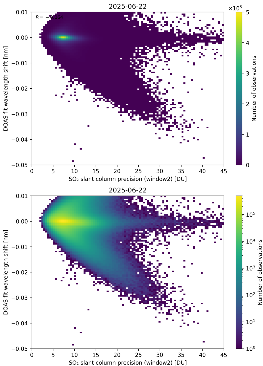
Figure 293: Scatter density plot of “SO 2 slant column precision (window2)” against “DOAS fit wavelength shift” for 2025-06-22 to 2025-06-23.
