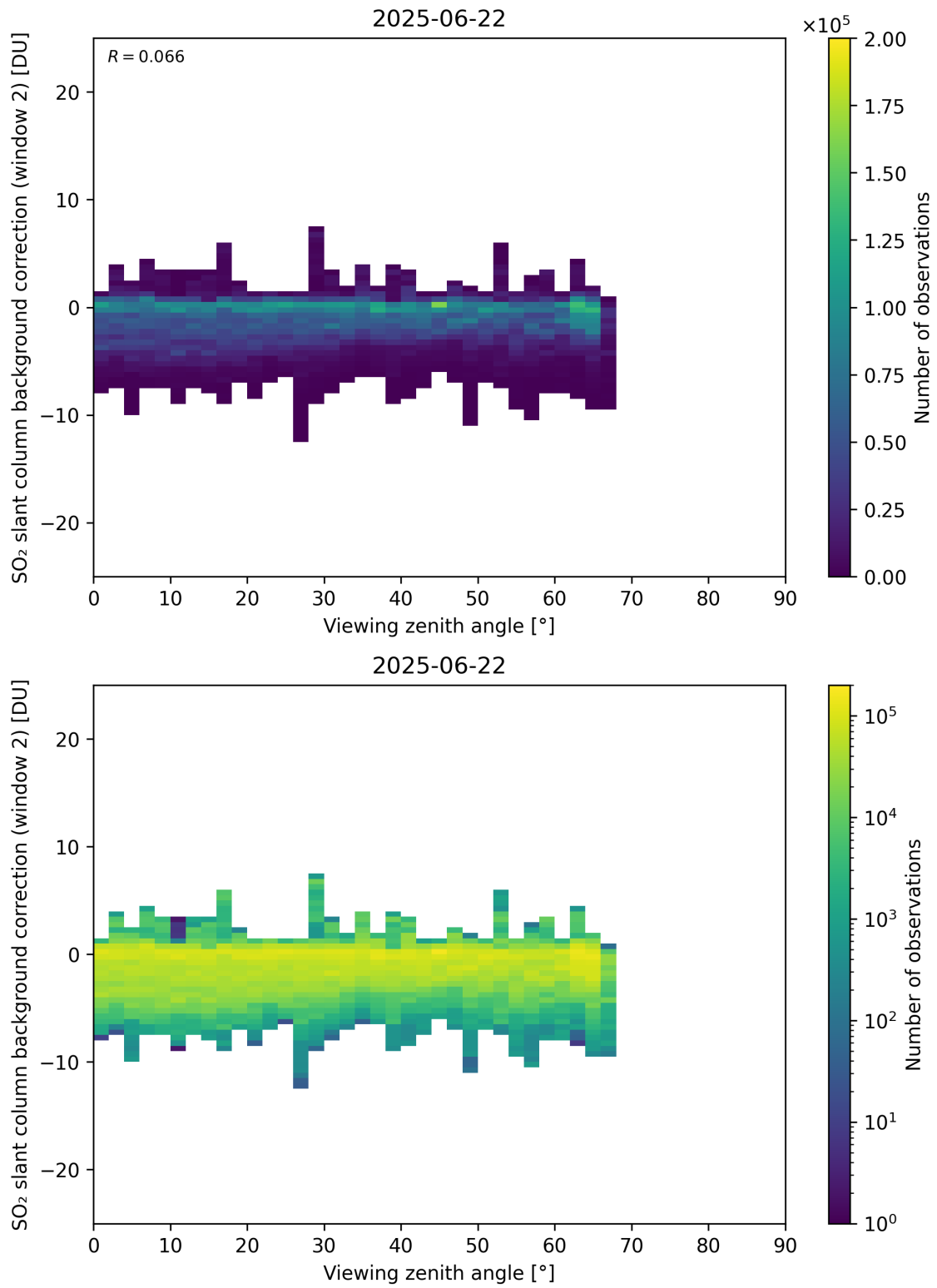
Figure 363: Scatter density plot of “Viewing zenith angle” against “SO 2 slant column background correction (window 2)” for 2025-06-22 to 2025-06-23.
