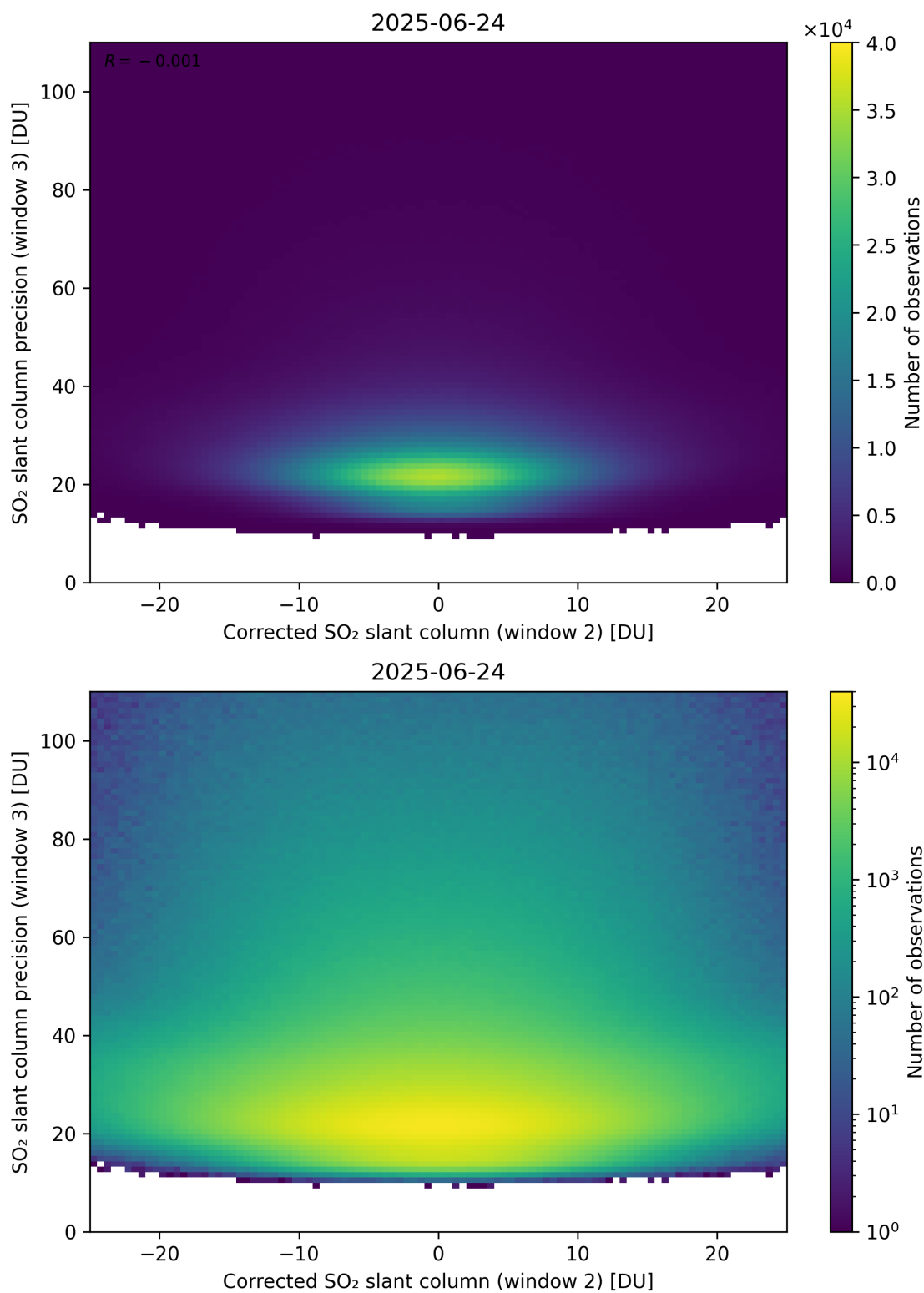
Figure 252: Scatter density plot of “Corrected SO 2 slant column (window 2)” against “SO 2 slant column precision (window 3)” for 2025-06-23 to 2025-06-25.
