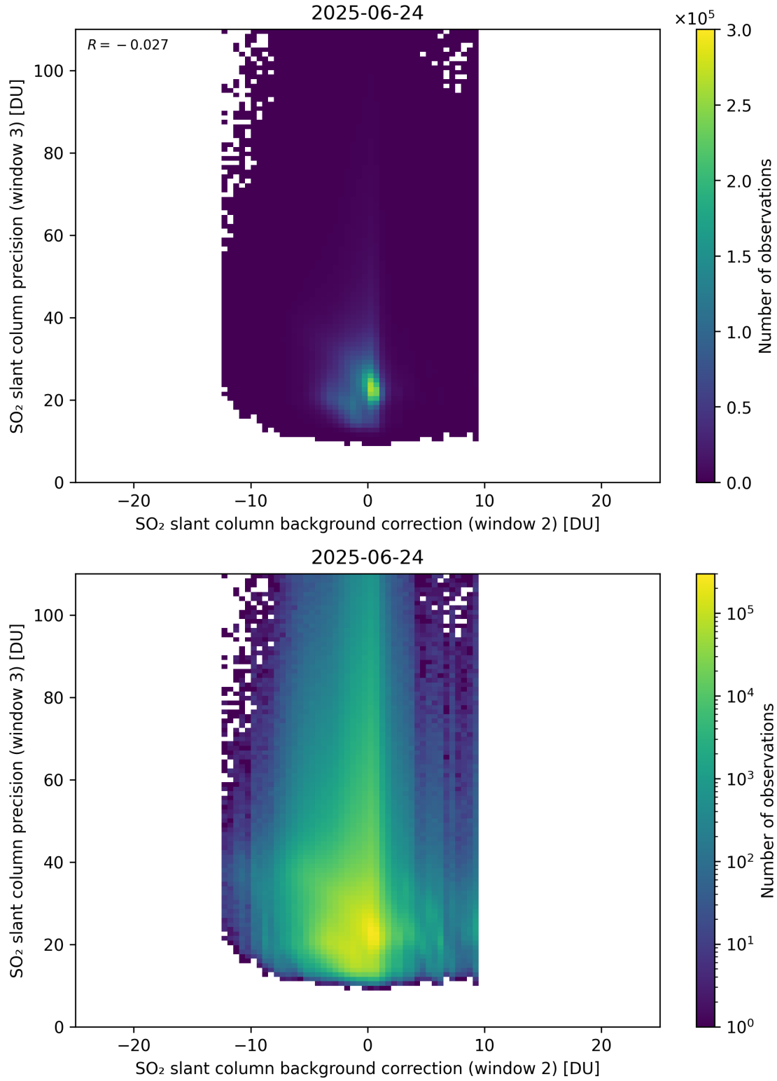
Figure 129: Scatter density plot of “SO 2 slant column background correction (window 2)” against “SO 2 slant column precision (window 3)” for 2025-06-23 to 2025-06-25.
