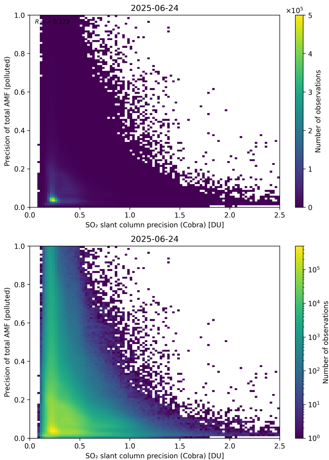
Figure 214: Scatter density plot of “SO 2 slant column precision (Cobra)” against “Precision of total AMF (polluted)” for 2025-06-23 to 2025-06-25.
