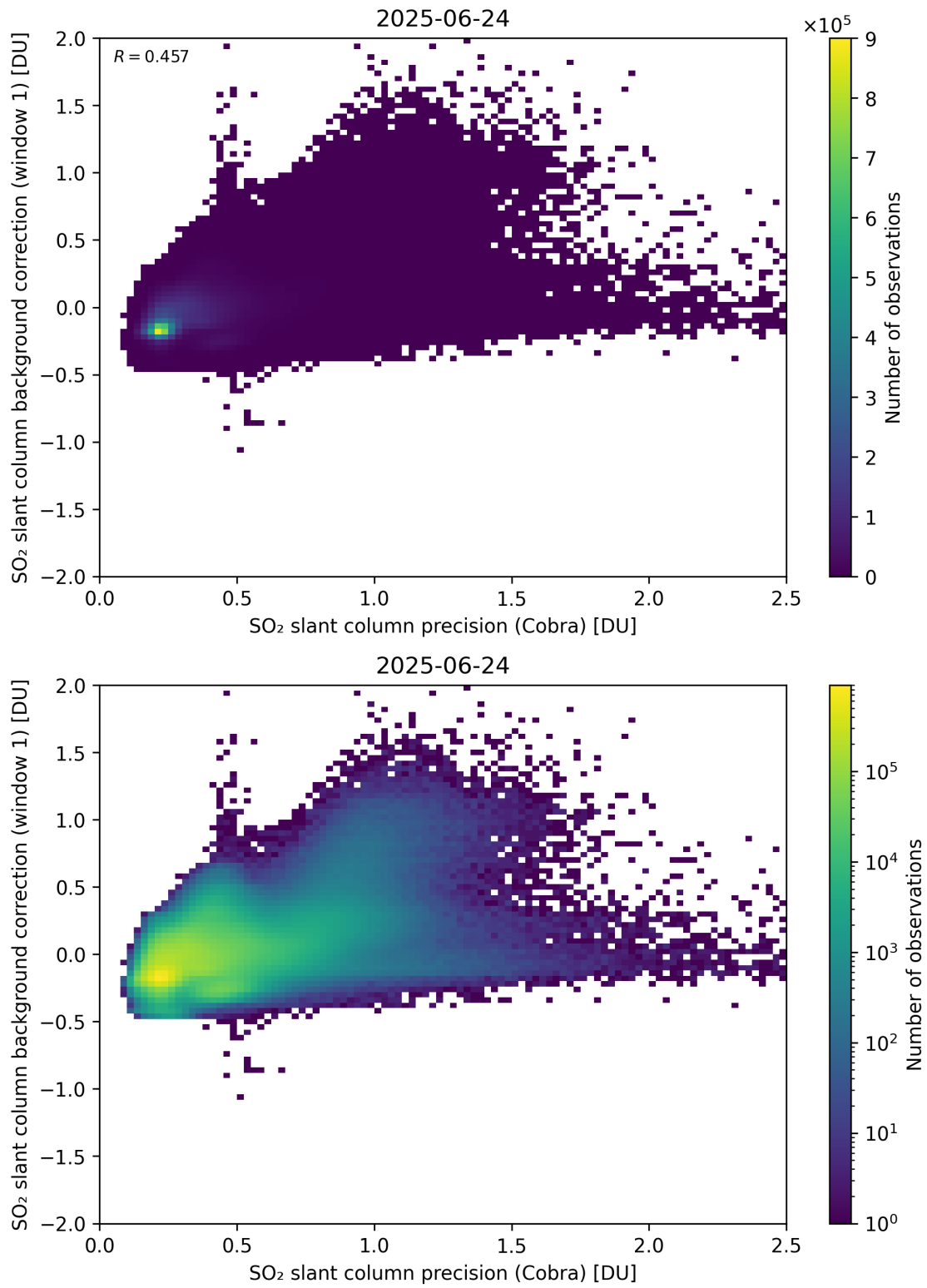
Figure 199: Scatter density plot of “SO 2 slant column precision (Cobra)” against “SO 2 slant column background correction (window 1)” for 2025-06-23 to 2025-06-25.
