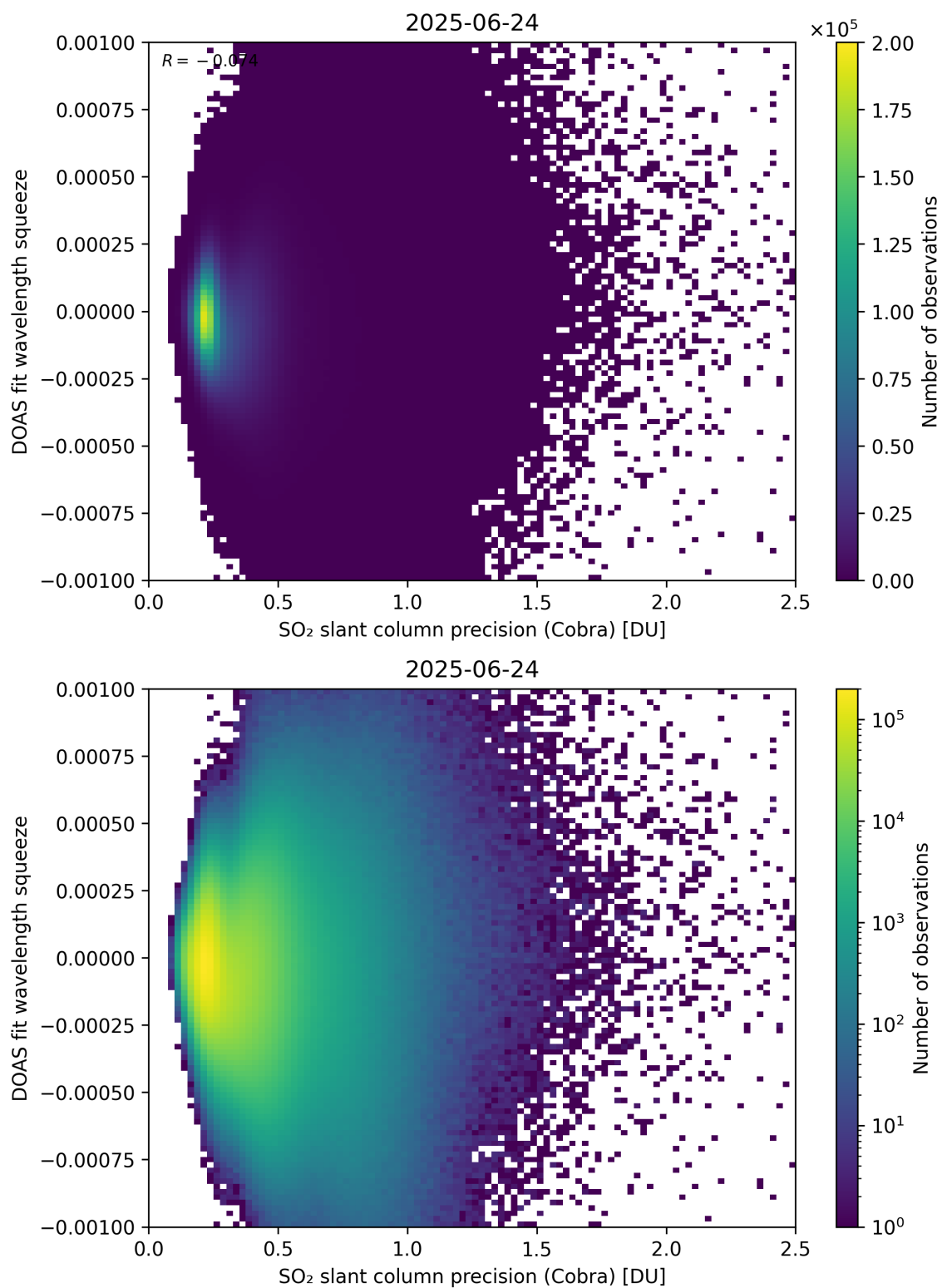
Figure 203: Scatter density plot of “SO 2 slant column precision (Cobra)” against “DOAS fit wavelength squeeze” for 2025-06-23 to 2025-06-25.
