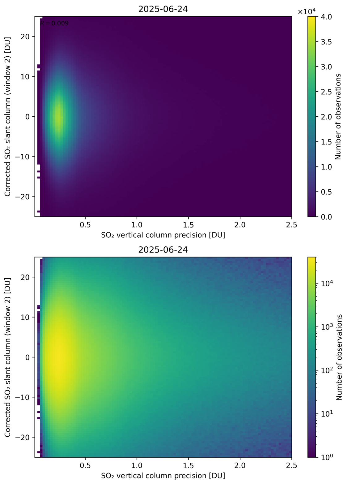
Figure 339: Scatter density plot of “SO 2 vertical column precision” against “Corrected SO 2 slant column (window 2)” for 2025-06-23 to 2025-06-25.
