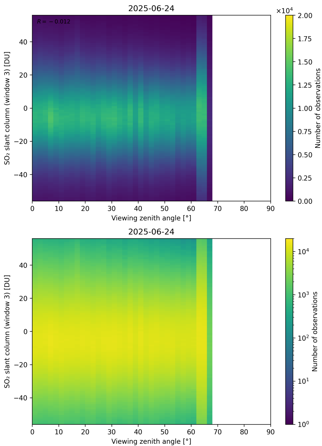
Figure 379: Scatter density plot of “Viewing zenith angle” against “SO 2 slant column (window 3)” for 2025-06-23 to 2025-06-25.
