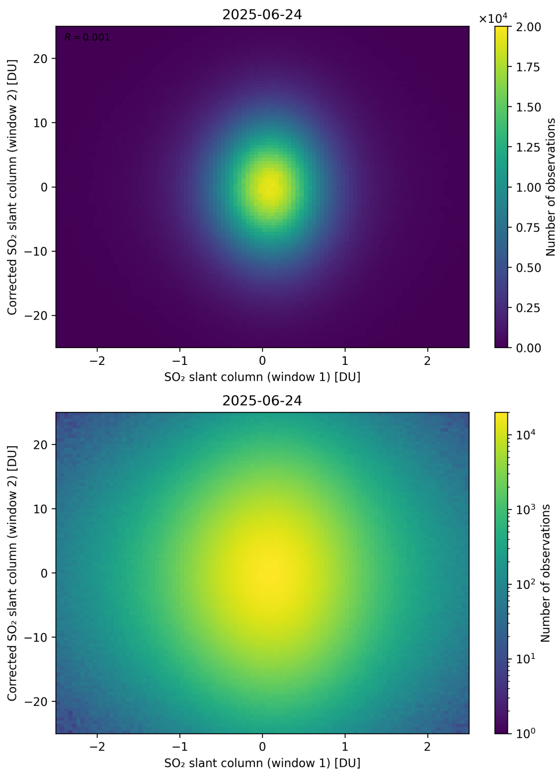
Figure 283: Scatter density plot of “SO 2 slant column (window 1)” against “Corrected SO 2 slant column (window 2)” for 2025-06-23 to 2025-06-25.
