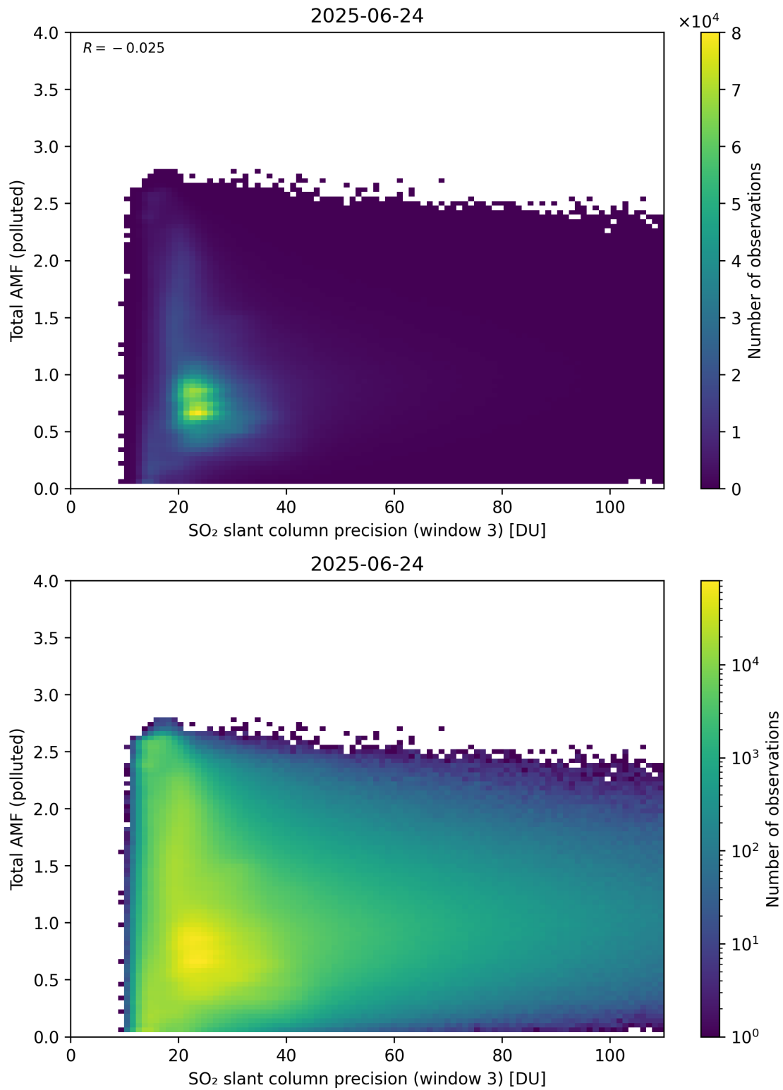
Figure 313: Scatter density plot of “SO 2 slant column precision (window 3)” against “Total AMF (polluted)” for 2025-06-23 to 2025-06-25.
