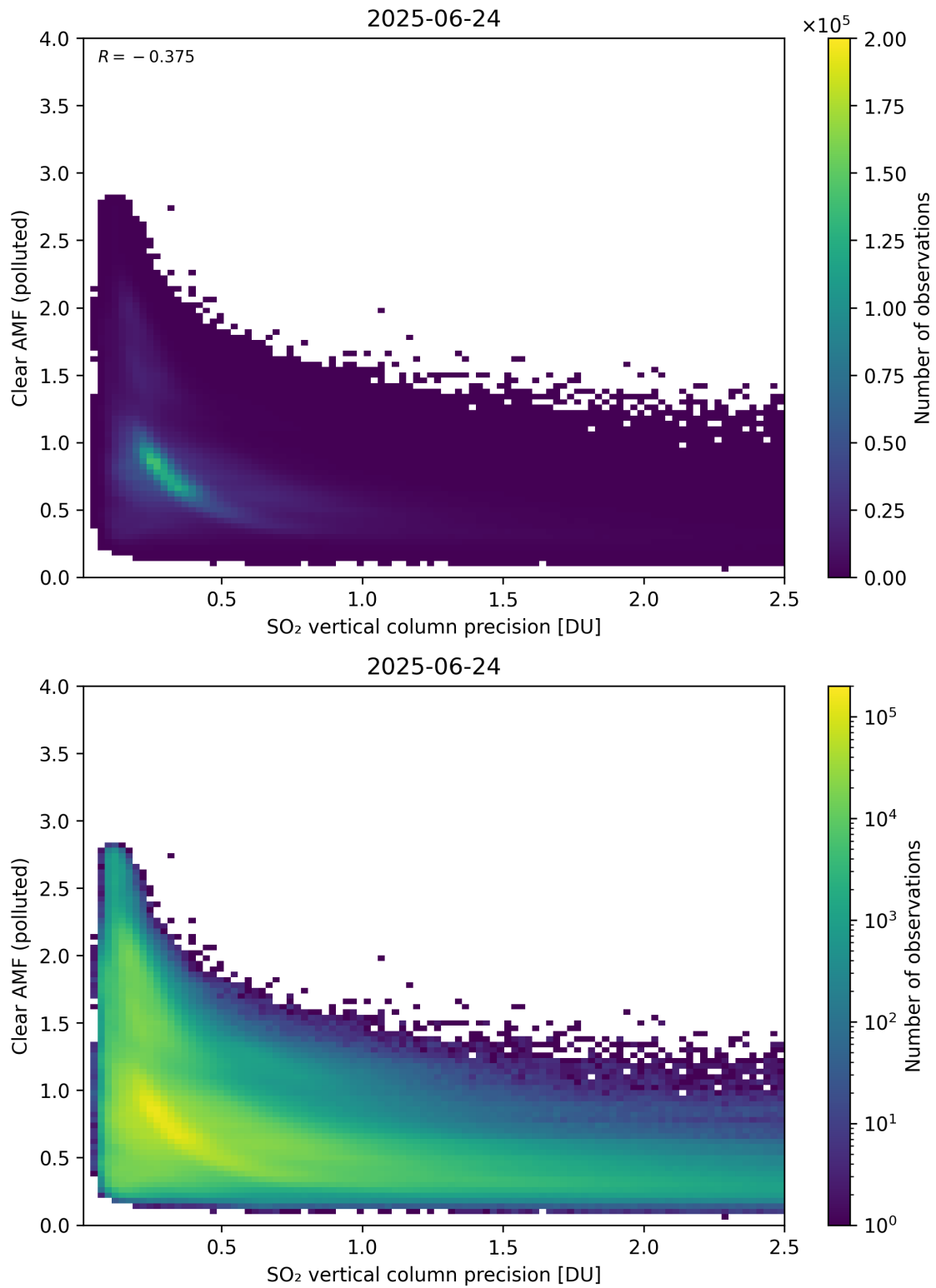
Figure 335: Scatter density plot of “SO 2 vertical column precision” against “Clear AMF (polluted)” for 2025-06-23 to 2025-06-25.
