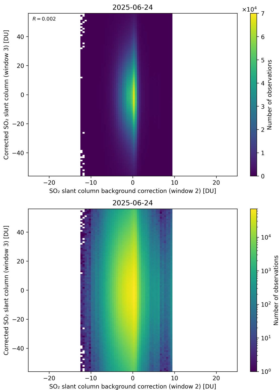
Figure 127: Scatter density plot of “SO 2 slant column background correction (window 2)” against “Corrected SO 2 slant column (window 3)” for 2025-06-23 to 2025-06-25.
