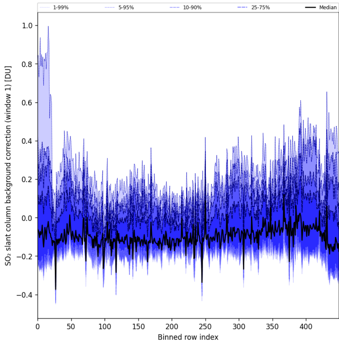
Figure 92: Along track statistics of “SO 2 slant column background correction (window 1)” for 2025-06-23 to 2025-06-25
