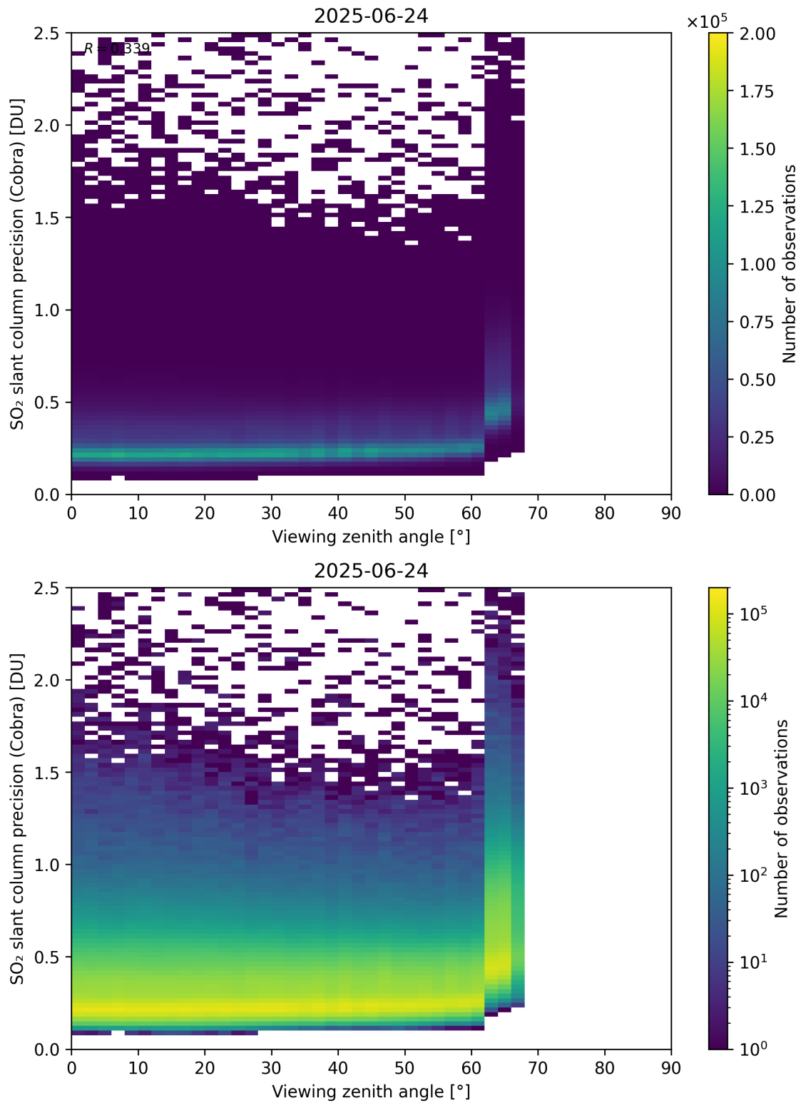
Figure 372: Scatter density plot of “Viewing zenith angle” against “SO 2 slant column precision (Cobra)” for 2025-06-23 to 2025-06-25.
