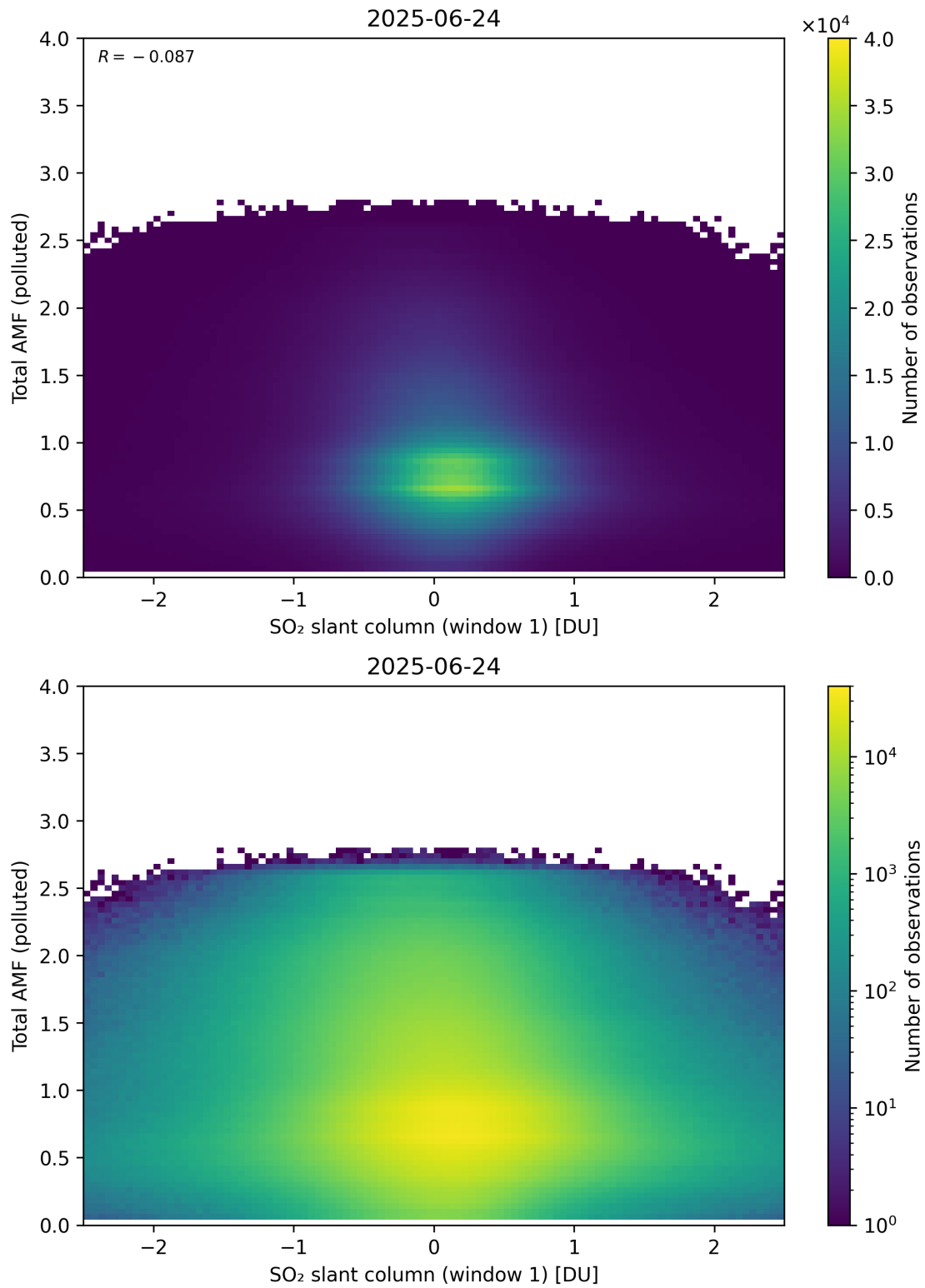
Figure 289: Scatter density plot of “SO 2 slant column (window 1)” against “Total AMF (polluted)” for 2025-06-23 to 2025-06-25.
