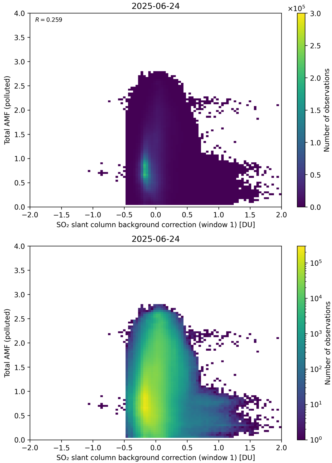
Figure 120: Scatter density plot of “SO 2 slant column background correction (window 1)” against “Total AMF (polluted)” for 2025-06-23 to 2025-06-25.
