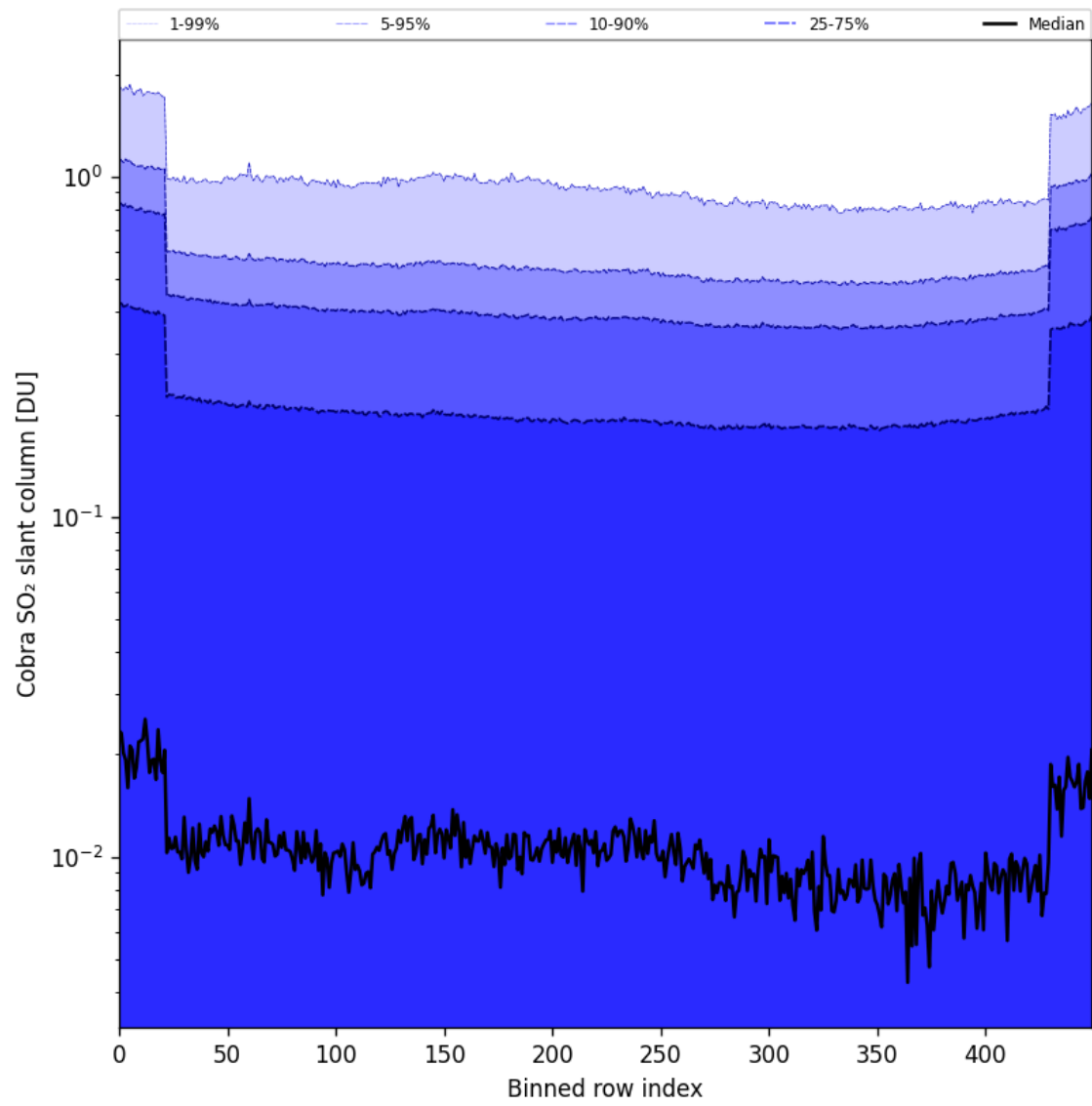
Figure 87: Along track statistics of “Cobra SO 2 slant column” for 2025-06-23 to 2025-06-25
