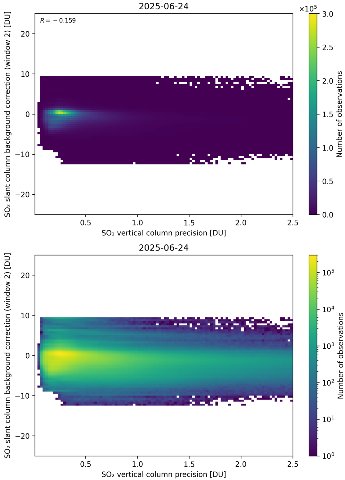
Figure 330: Scatter density plot of “SO 2 vertical column precision” against “SO 2 slant column background correction (window 2)” for 2025-06-23 to 2025-06-25.
