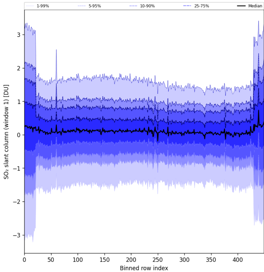
Figure 89: Along track statistics of “SO 2 slant column (window 1)” for 2025-06-23 to 2025-06-25
