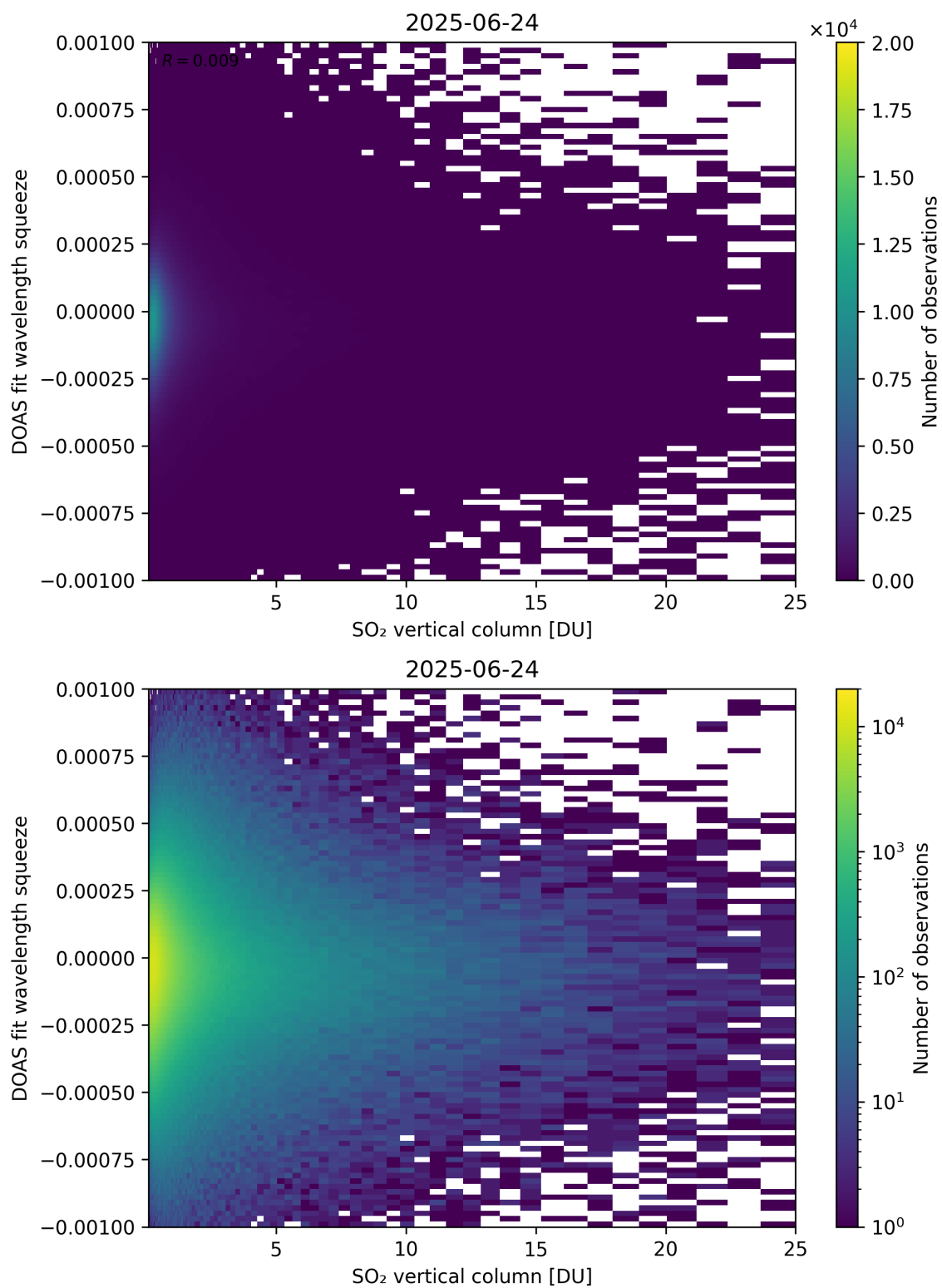
Figure 327: Scatter density plot of “SO 2 vertical column” against “DOAS fit wavelength squeeze” for 2025-06-23 to 2025-06-25.
