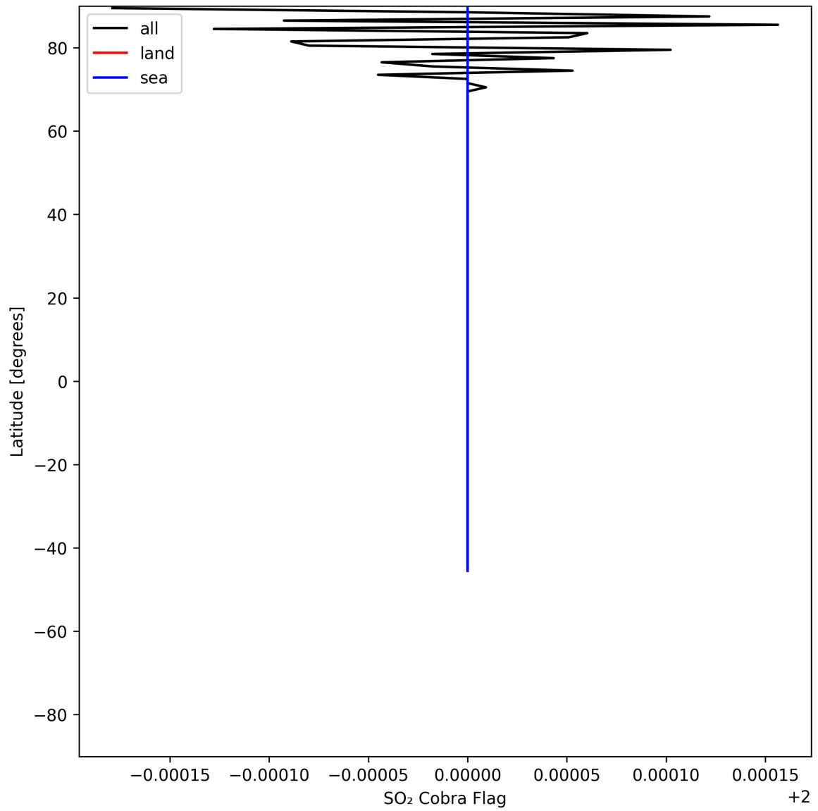
Figure 49: Zonal average of "SO 2 Cobra Flag" for 2025-06-23 to 2025-06-25.
