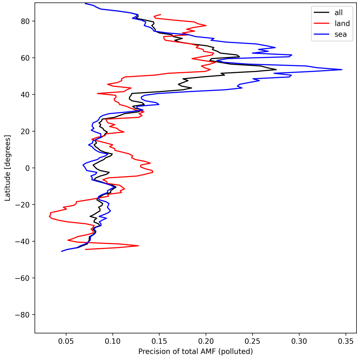
Figure 54: Zonal average of “Precision of total AMF (polluted)” for 2025-06-23 to 2025-06-25.
