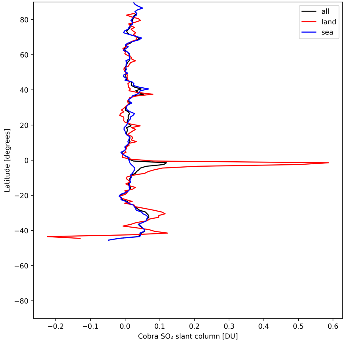
Figure 35: Zonal average of “Cobra SO 2 slant column” for 2025-06-23 to 2025-06-25.
