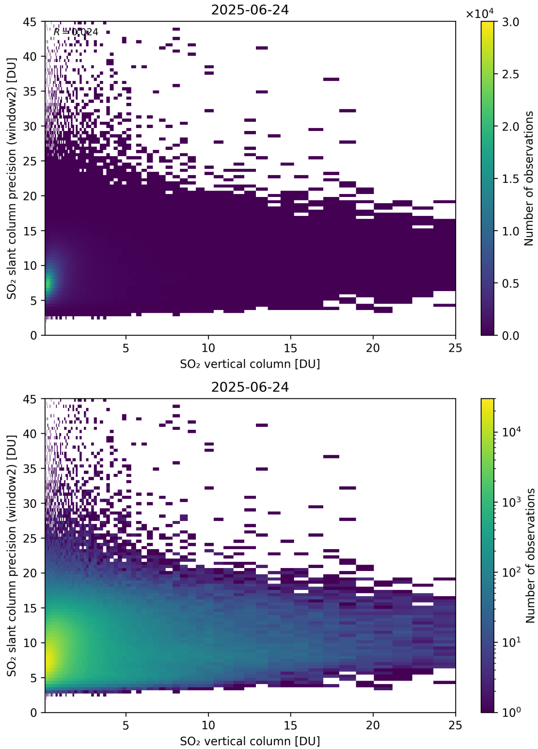
Figure 356: Scatter density plot of “SO 2 vertical column” against “SO 2 slant column precision (window2)” for 2025-06-23 to 2025-06-25.
