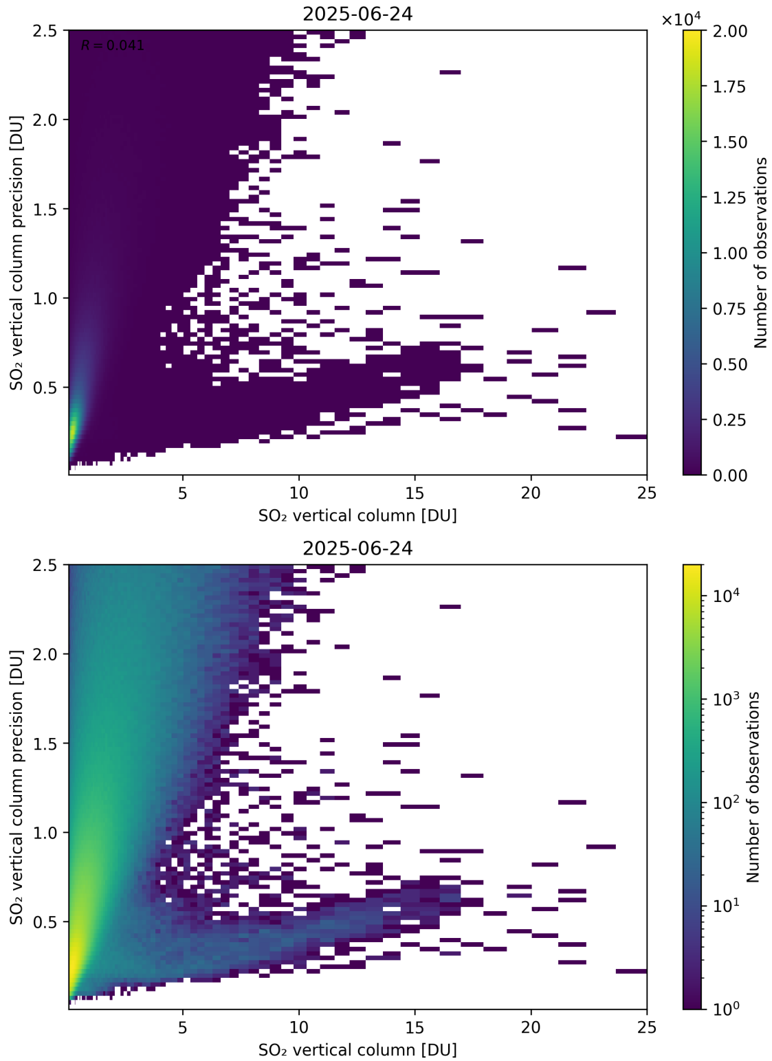
Figure 361: Scatter density plot of “SO 2 vertical column” against “SO 2 vertical column precision” for 2025-06-23 to 2025-06-25.
