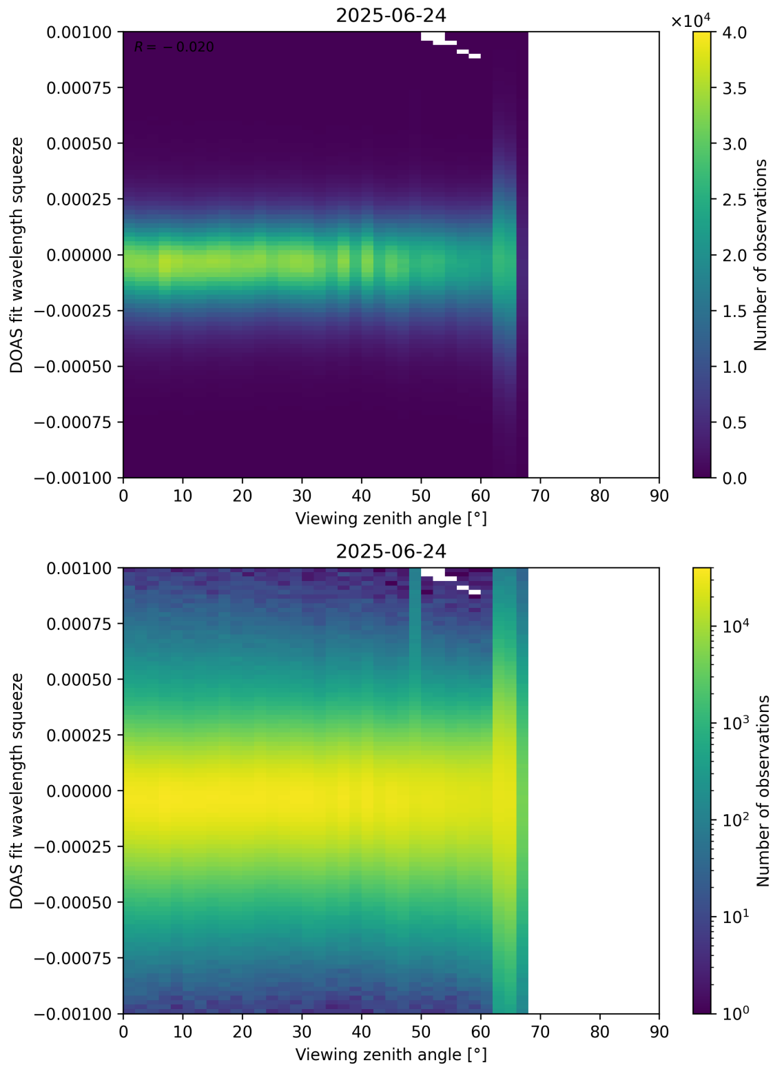
Figure 366: Scatter density plot of “Viewing zenith angle” against “DOAS fit wavelength squeeze” for 2025-06-23 to 2025-06-25.
