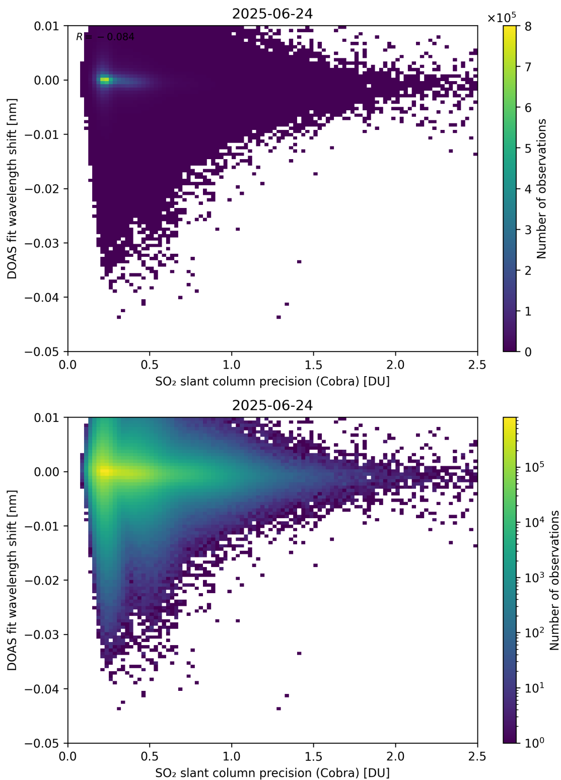
Figure 202: Scatter density plot of “SO 2 slant column precision (Cobra)” against “DOAS fit wavelength shift” for 2025-06-23 to 2025-06-25.
