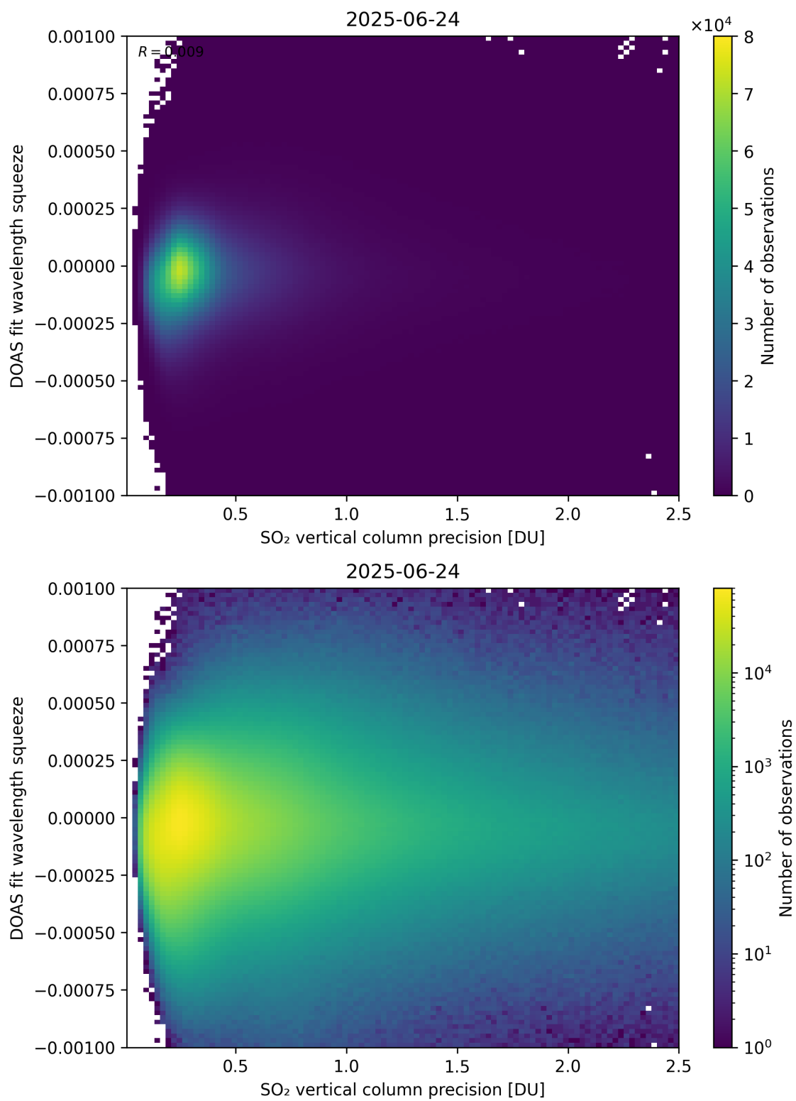
Figure 333: Scatter density plot of “SO 2 vertical column precision” against “DOAS fit wavelength squeeze” for 2025-06-23 to 2025-06-25.
