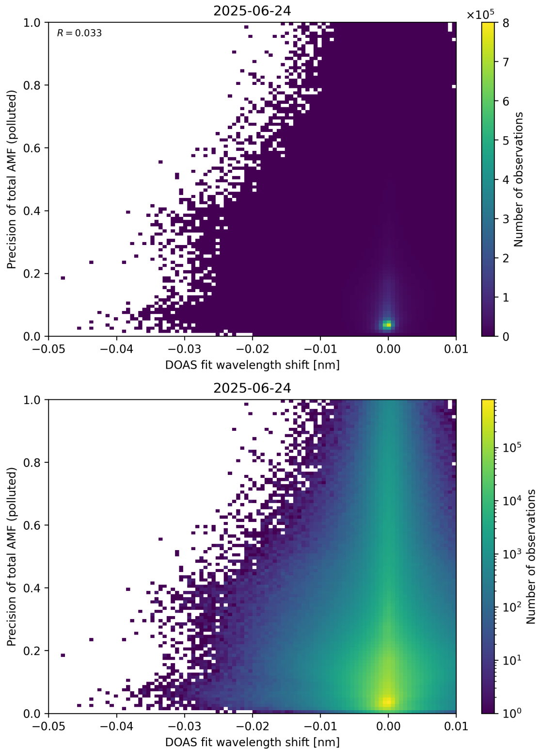
Figure 142: Scatter density plot of “DOAS fit wavelength shift” against “Precision of total AMF (polluted)” for 2025-06-23 to 2025-06-25.
