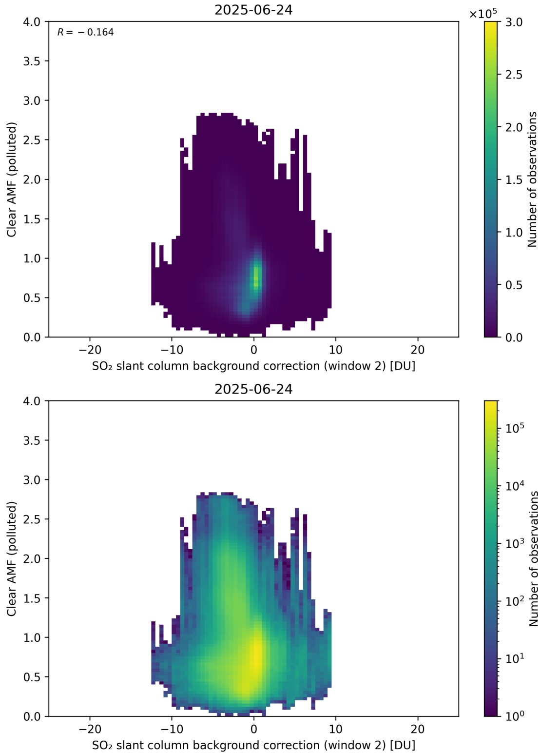
Figure 126: Scatter density plot of “SO 2 slant column background correction (window 2)” against “Clear AMF (polluted)” for 2025-06-23 to 2025-06-25.
