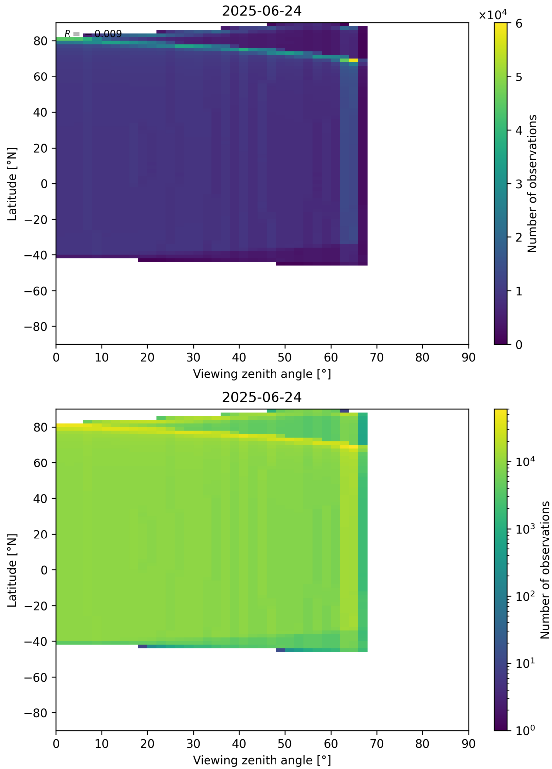
Figure 368: Scatter density plot of “Viewing zenith angle” against “Latitude” for 2025-06-23 to 2025-06-25.
