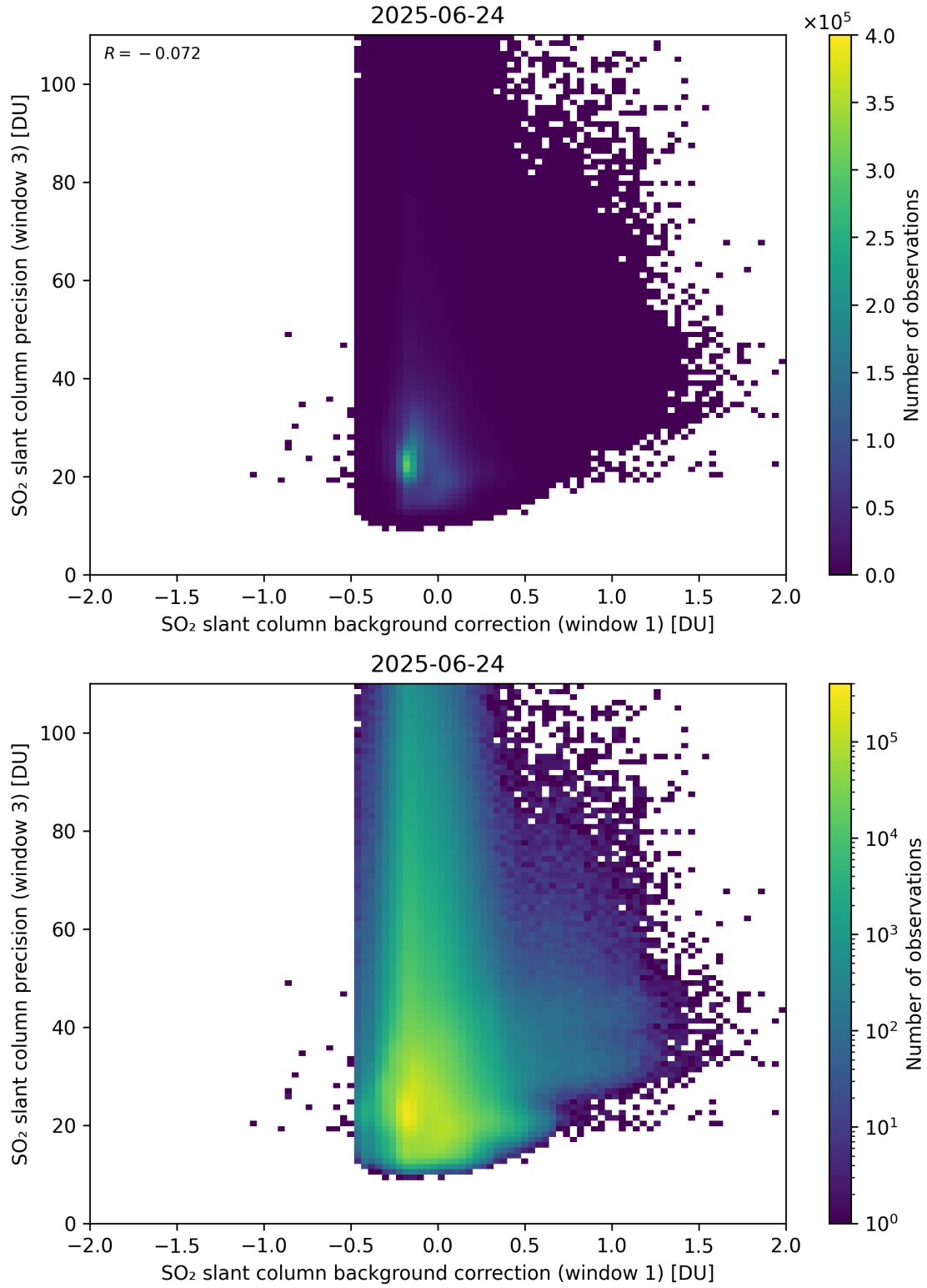
Figure 119: Scatter density plot of “SO 2 slant column background correction (window 1)” against “SO 2 slant column precision (window 3)” for 2025-06-23 to 2025-06-25.
