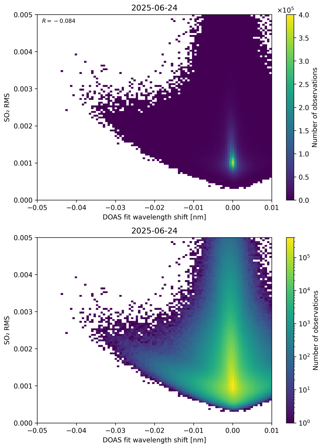
Figure 139: Scatter density plot of “DOAS fit wavelength shift” against “SO 2 RMS” for 2025-06-23 to 2025-06-25.
