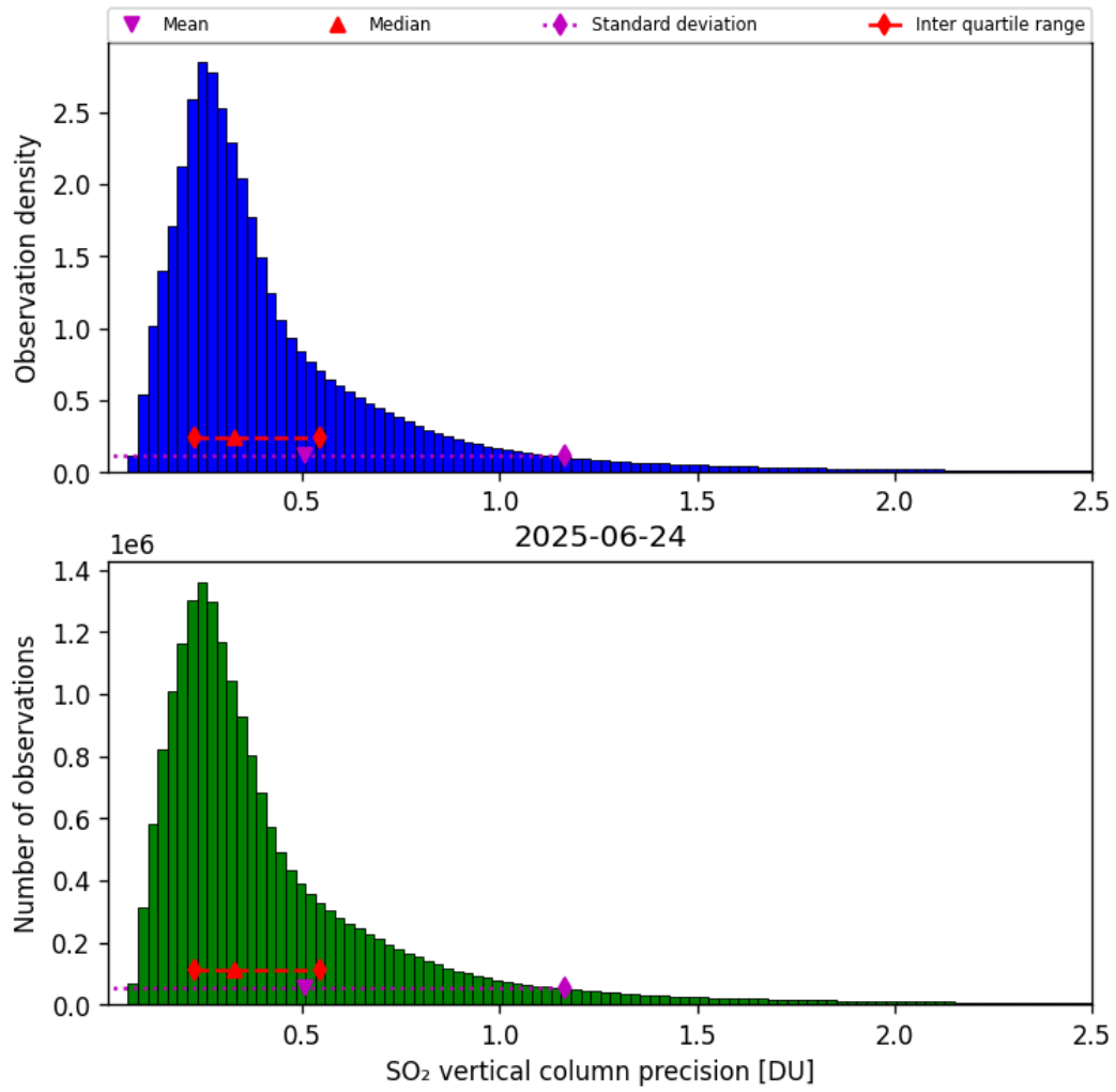
Figure 59: Histogram of “SO 2 vertical column precision” for 2025-06-23 to 2025-06-25
