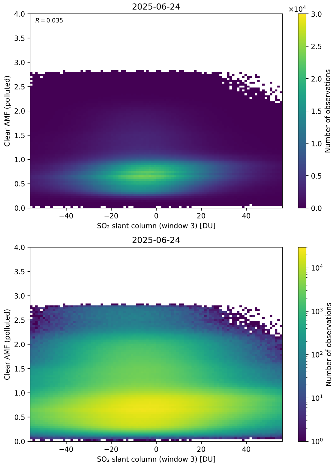
Figure 315: Scatter density plot of “SO 2 slant column (window 3)” against “Clear AMF (polluted)” for 2025-06-23 to 2025-06-25.
