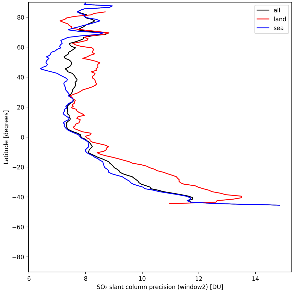
Figure 42: Zonal average of “SO 2 slant column precision (window2)” for 2025-06-23 to 2025-06-25.
