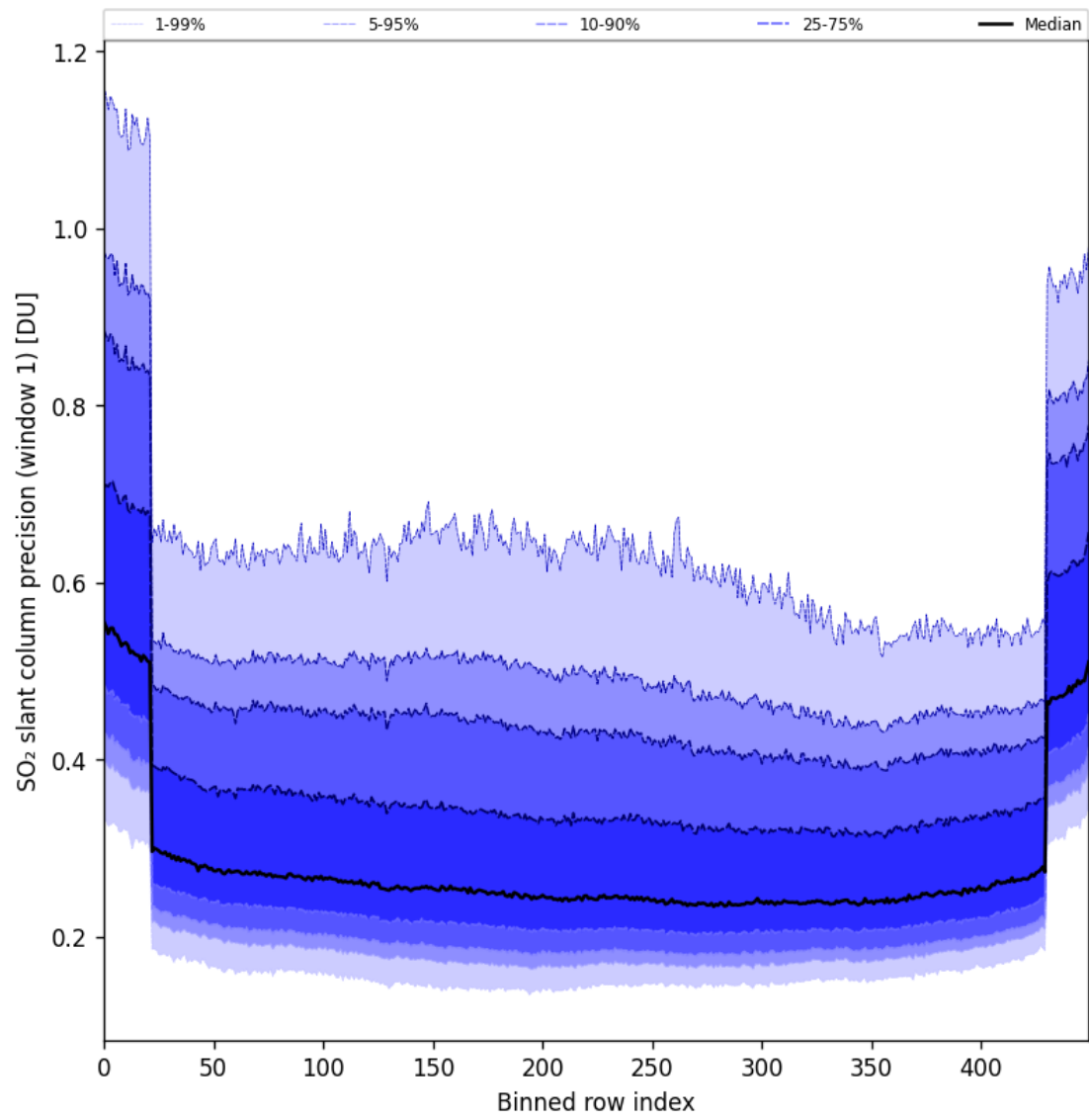
Figure 90: Along track statistics of “SO 2 slant column precision (window 1)” for 2025-06-23 to 2025-06-25
