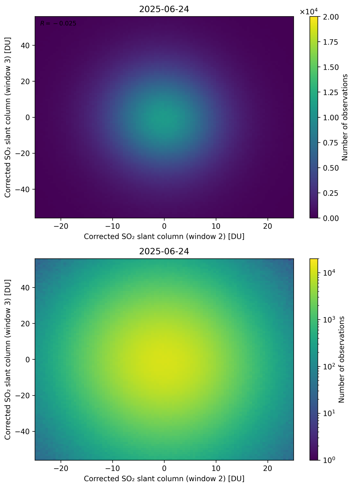
Figure 250: Scatter density plot of “Corrected SO 2 slant column (window 2)” against “Corrected SO 2 slant column (window 3)” for 2025-06-23 to 2025-06-25.
