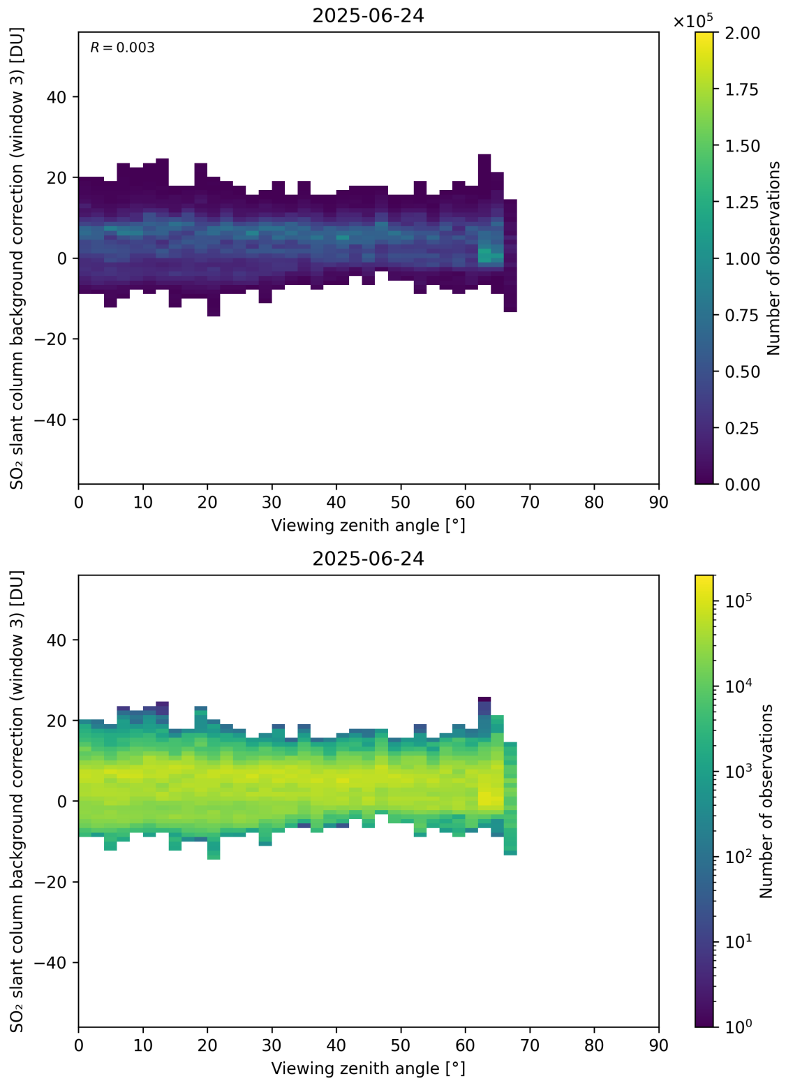
Figure 364: Scatter density plot of “Viewing zenith angle” against “SO 2 slant column background correction (window 3)” for 2025-06-23 to 2025-06-25.
