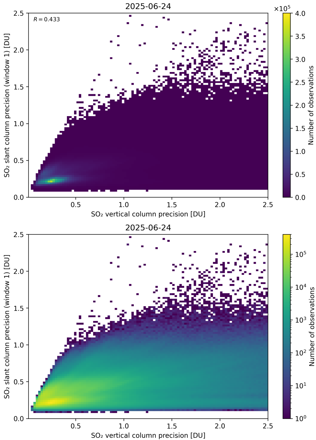
Figure 342: Scatter density plot of “SO 2 vertical column precision” against “SO 2 slant column precision (window 1)” for 2025-06-23 to 2025-06-25.
