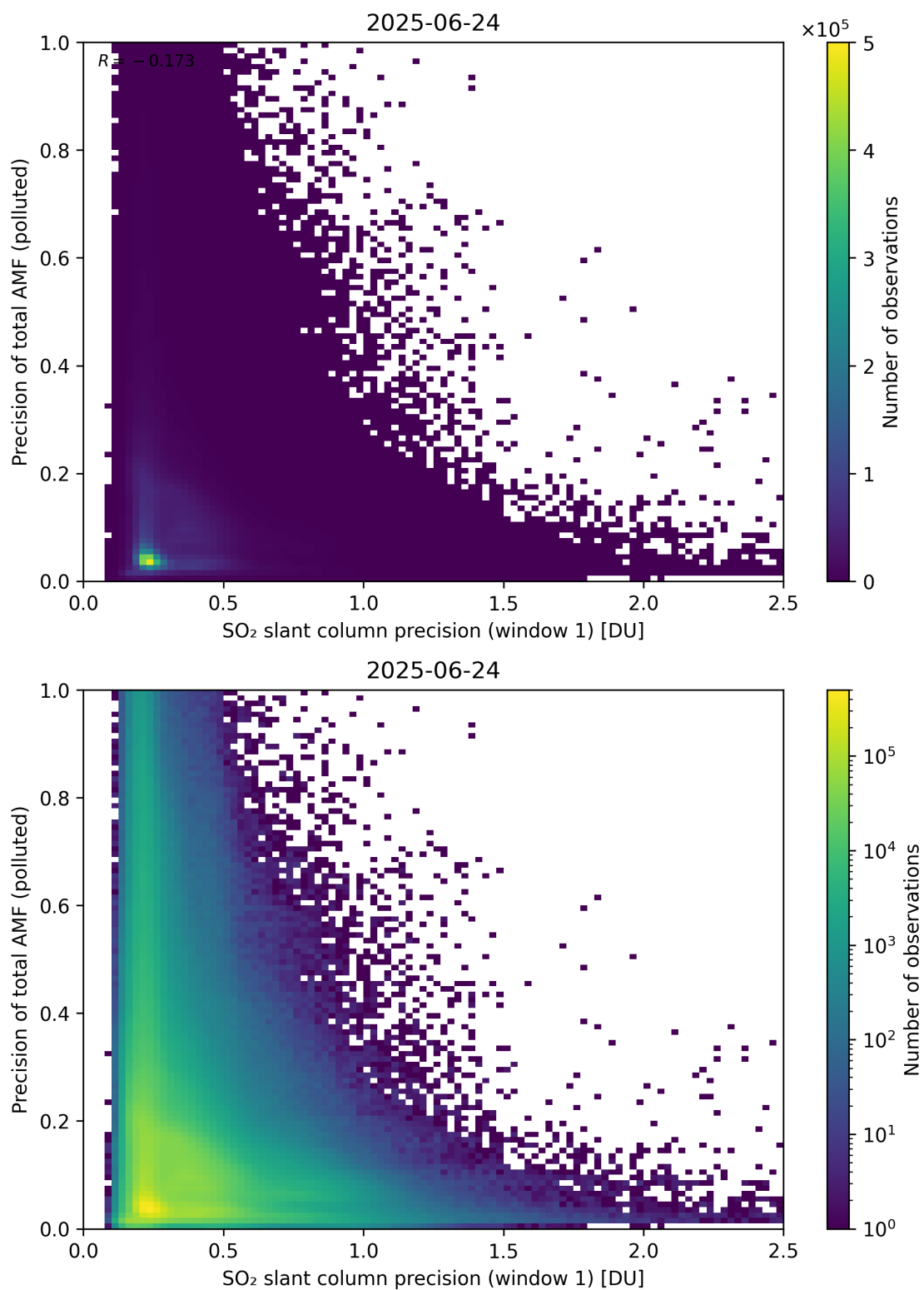
Figure 281: Scatter density plot of “SO 2 slant column precision (window 1)” against “Precision of total AMF (polluted)” for 2025-06-23 to 2025-06-25.
