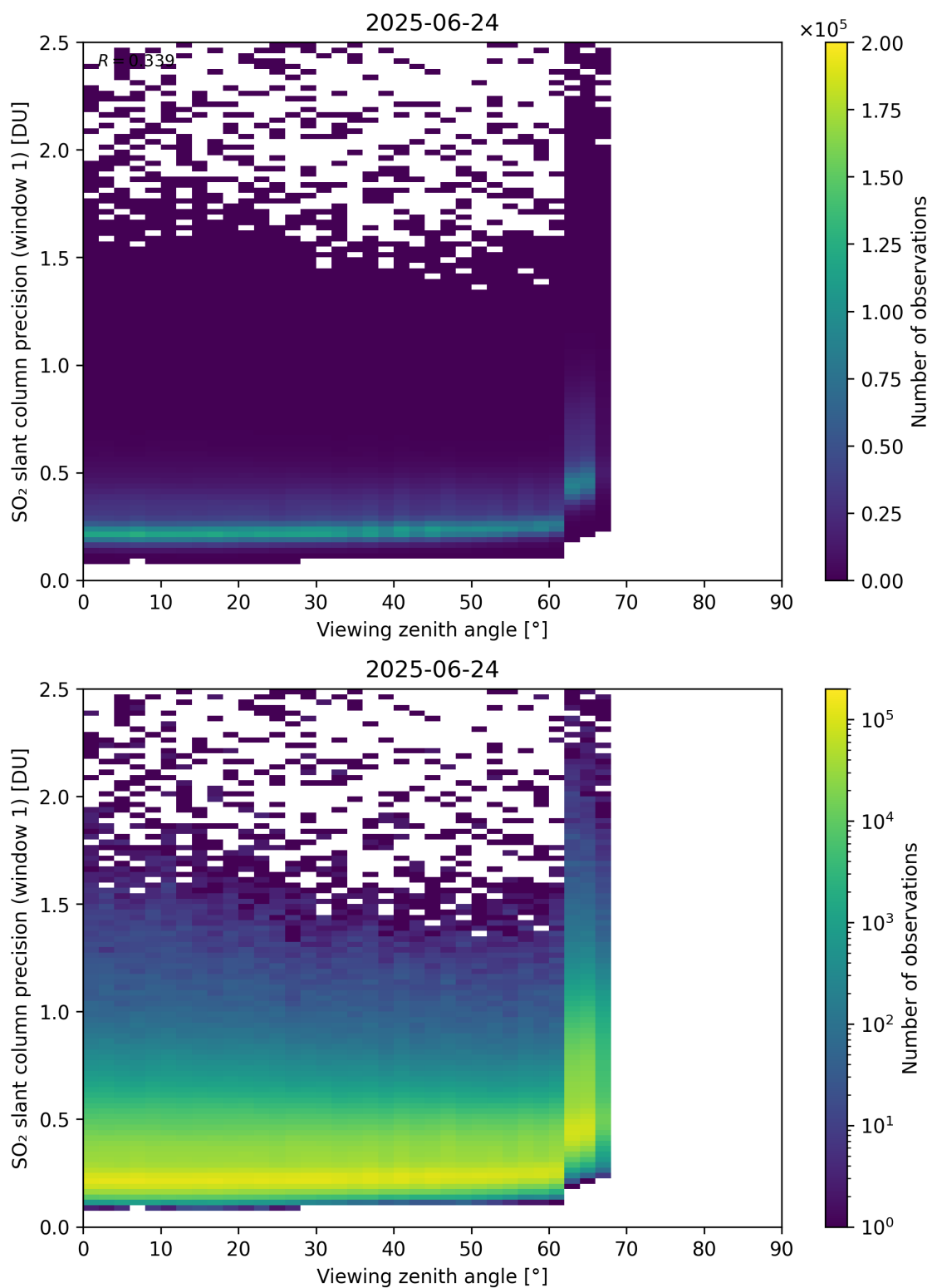
Figure 377: Scatter density plot of “Viewing zenith angle” against “SO 2 slant column precision (window 1)” for 2025-06-23 to 2025-06-25.
