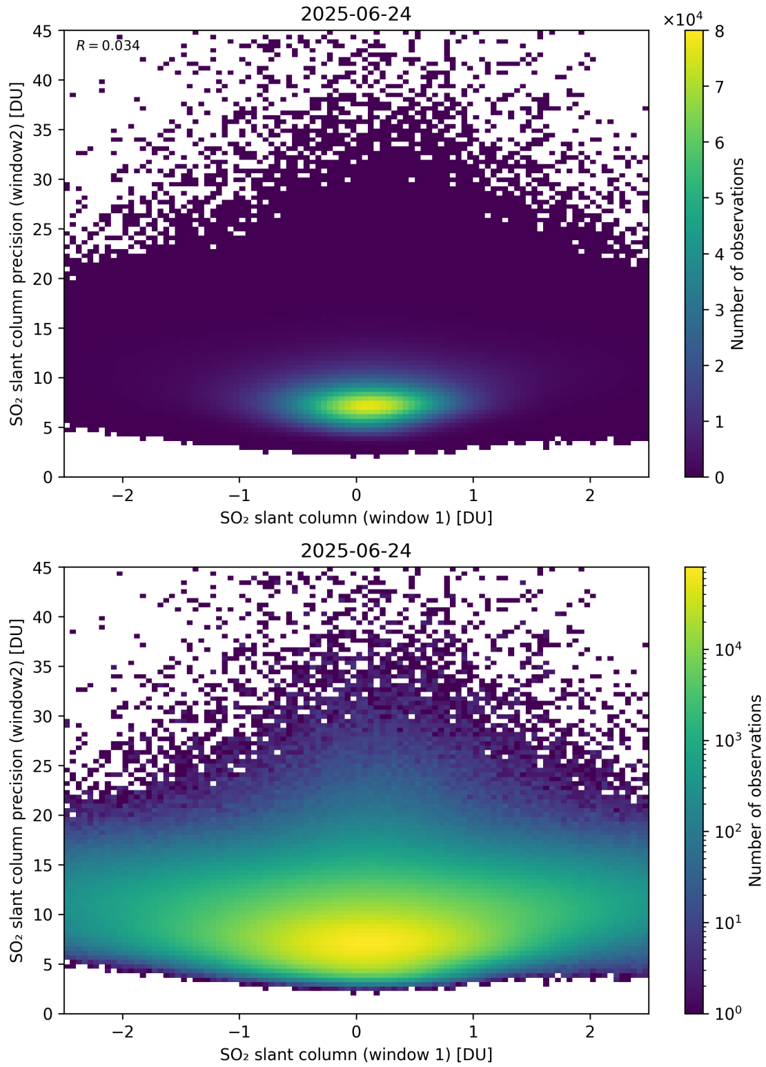
Figure 286: Scatter density plot of “SO 2 slant column (window 1)” against “SO 2 slant column precision (window2)” for 2025-06-23 to 2025-06-25.
