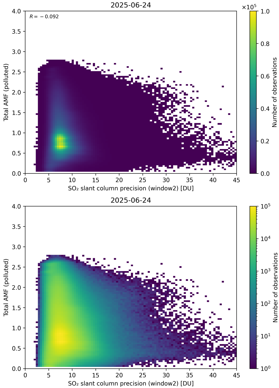
Figure 301: Scatter density plot of “SO 2 slant column precision (window2)” against “Total AMF (polluted)” for 2025-06-23 to 2025-06-25.
