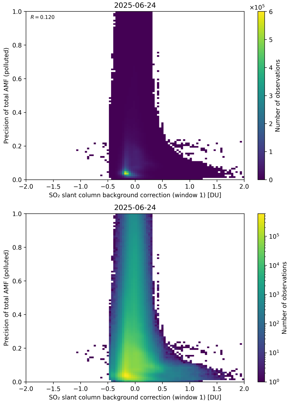
Figure 121: Scatter density plot of “SO 2 slant column background correction (window 1)” against “Precision of total AMF (polluted)” for 2025-06-23 to 2025-06-25.
