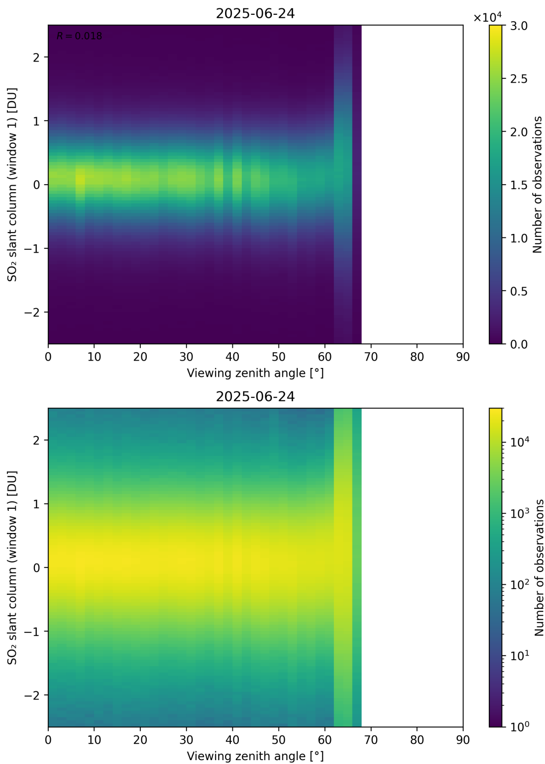
Figure 376: Scatter density plot of “Viewing zenith angle” against “SO 2 slant column (window 1)” for 2025-06-23 to 2025-06-25.
