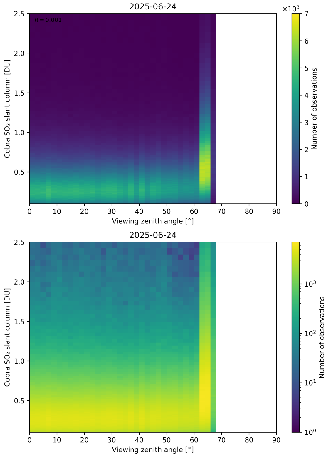
Figure 371: Scatter density plot of “Viewing zenith angle” against “Cobra SO 2 slant column” for 2025-06-23 to 2025-06-25.
