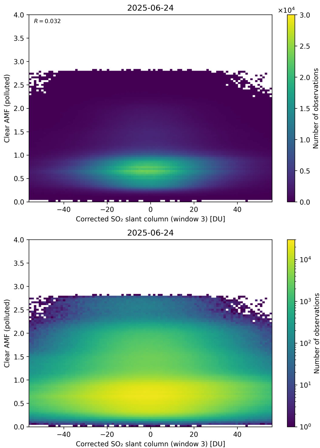
Figure 259: Scatter density plot of “Corrected SO 2 slant column (window 3)” against “Clear AMF (polluted)” for 2025-06-23 to 2025-06-25.
