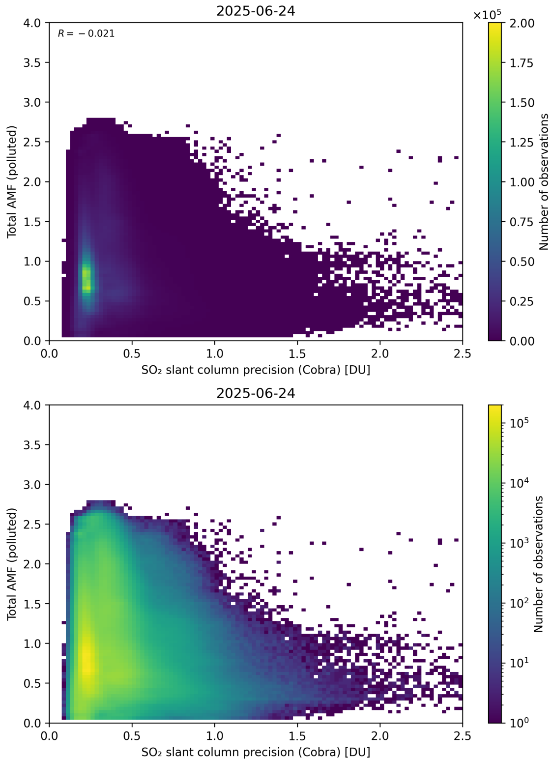
Figure 213: Scatter density plot of “SO 2 slant column precision (Cobra)” against “Total AMF (polluted)” for 2025-06-23 to 2025-06-25.
