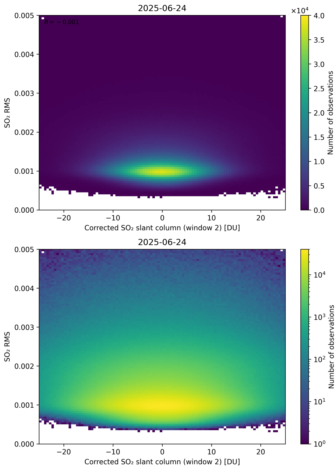
Figure 248: Scatter density plot of “Corrected SO 2 slant column (window 2)” against “SO 2 RMS” for 2025-06-23 to 2025-06-25.
