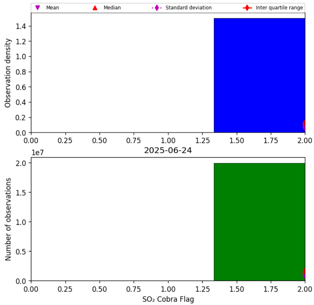
Figure 75: Histogram of “SO 2 Cobra Flag” for 2025-06-23 to 2025-06-25
