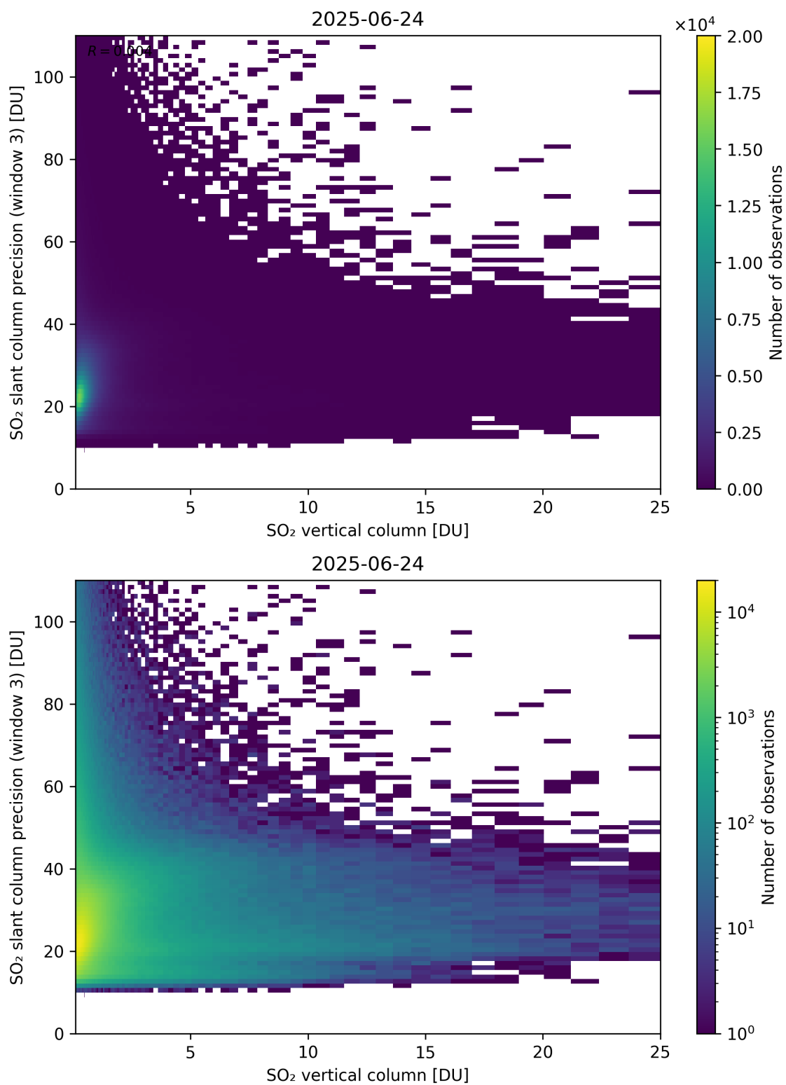
Figure 358: Scatter density plot of “SO 2 vertical column” against “SO 2 slant column precision (window 3)” for 2025-06-23 to 2025-06-25.
