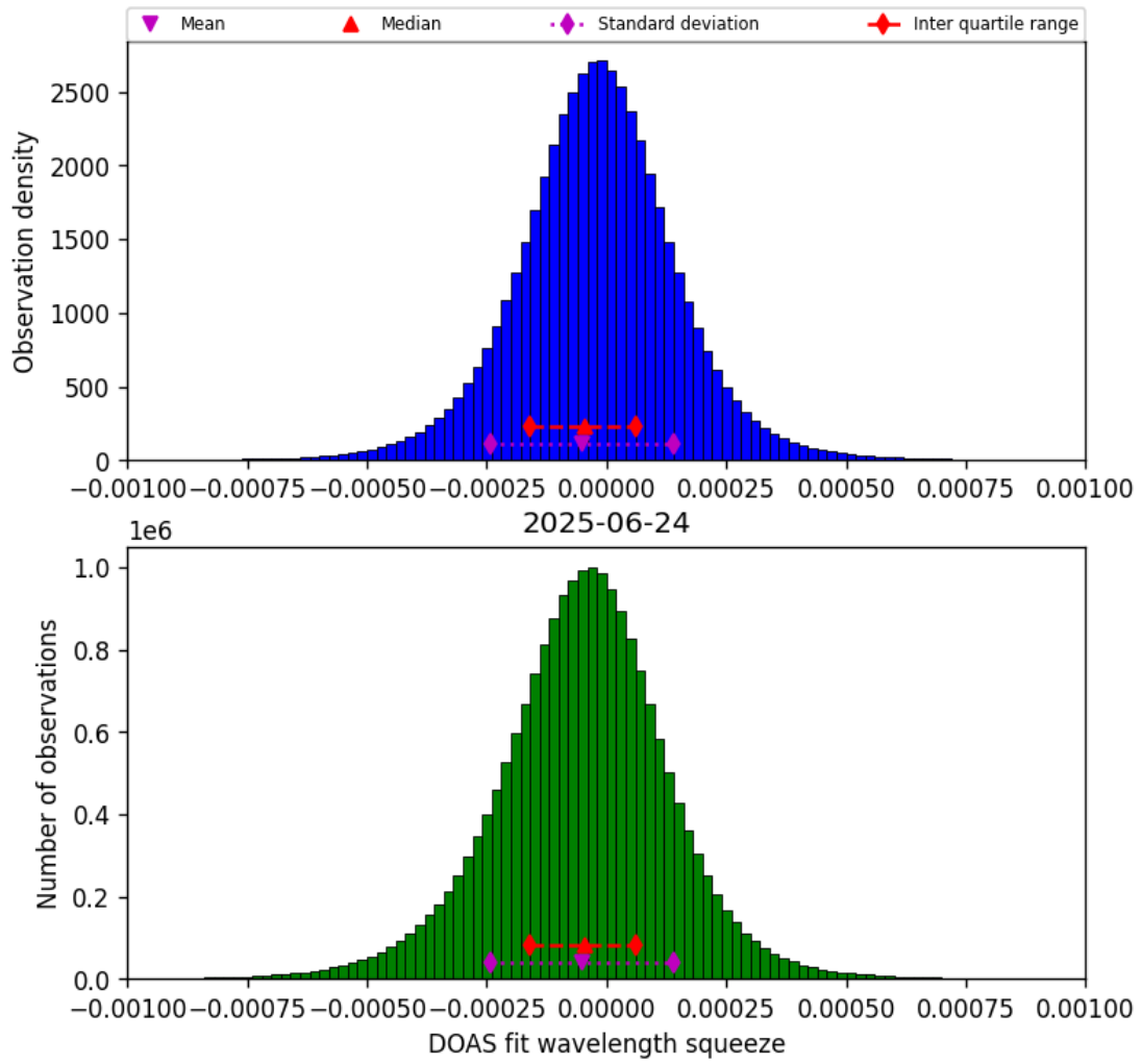
Figure 77: Histogram of “DOAS fit wavelength squeeze” for 2025-06-23 to 2025-06-25
