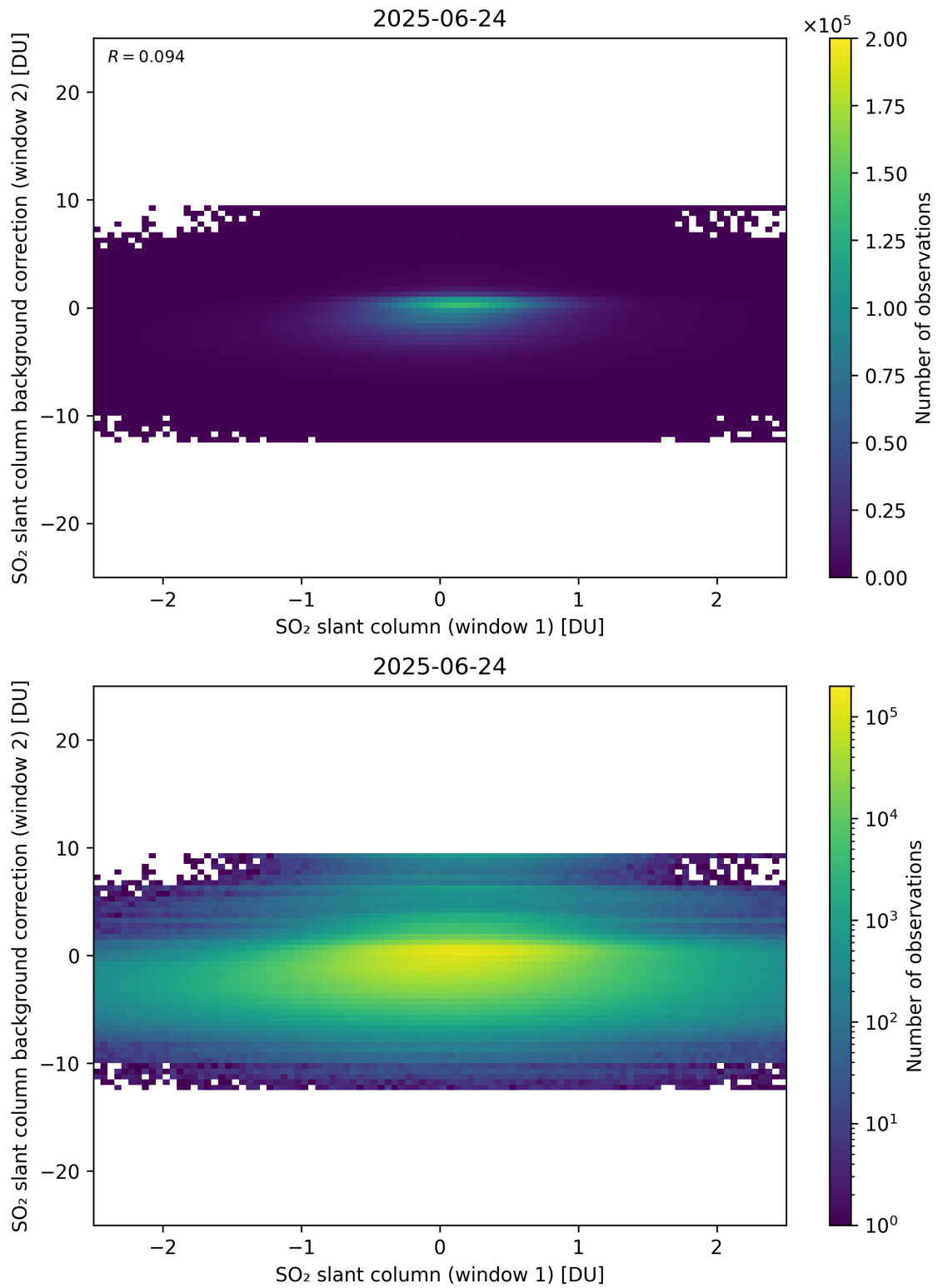
Figure 263: Scatter density plot of “SO 2 slant column (window 1)” against “SO 2 slant column background correction (window 2)” for 2025-06-23 to 2025-06-25.
