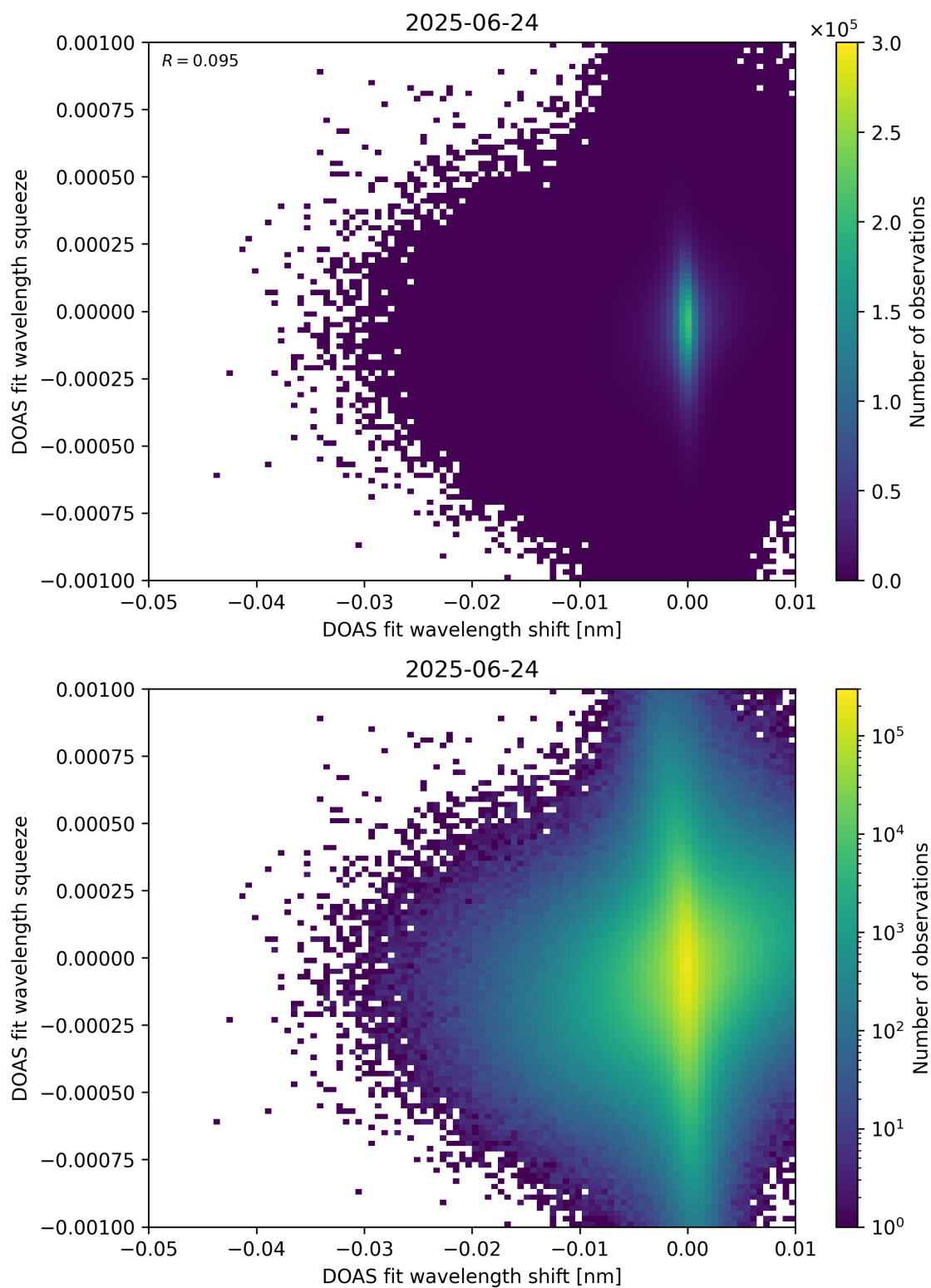
Figure 138: Scatter density plot of “DOAS fit wavelength shift” against “DOAS fit wavelength squeeze” for 2025-06-23 to 2025-06-25.
