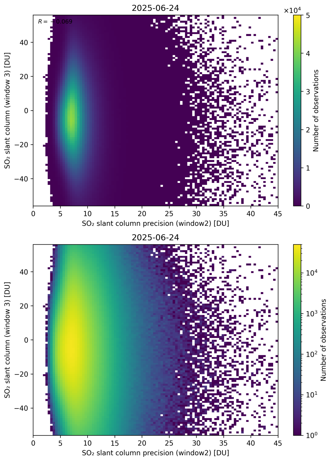
Figure 299: Scatter density plot of “SO 2 slant column precision (window2)” against “SO 2 slant column (window 3)” for 2025-06-23 to 2025-06-25.
