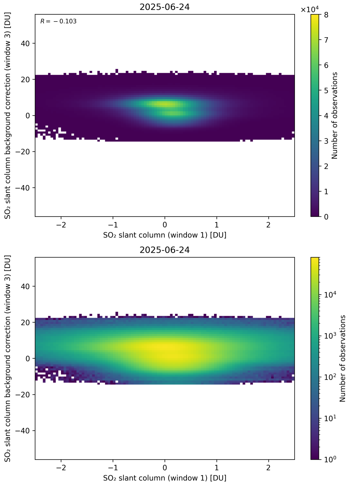
Figure 264: Scatter density plot of “SO 2 slant column (window 1)” against “SO 2 slant column background correction (window 3)” for 2025-06-23 to 2025-06-25.
