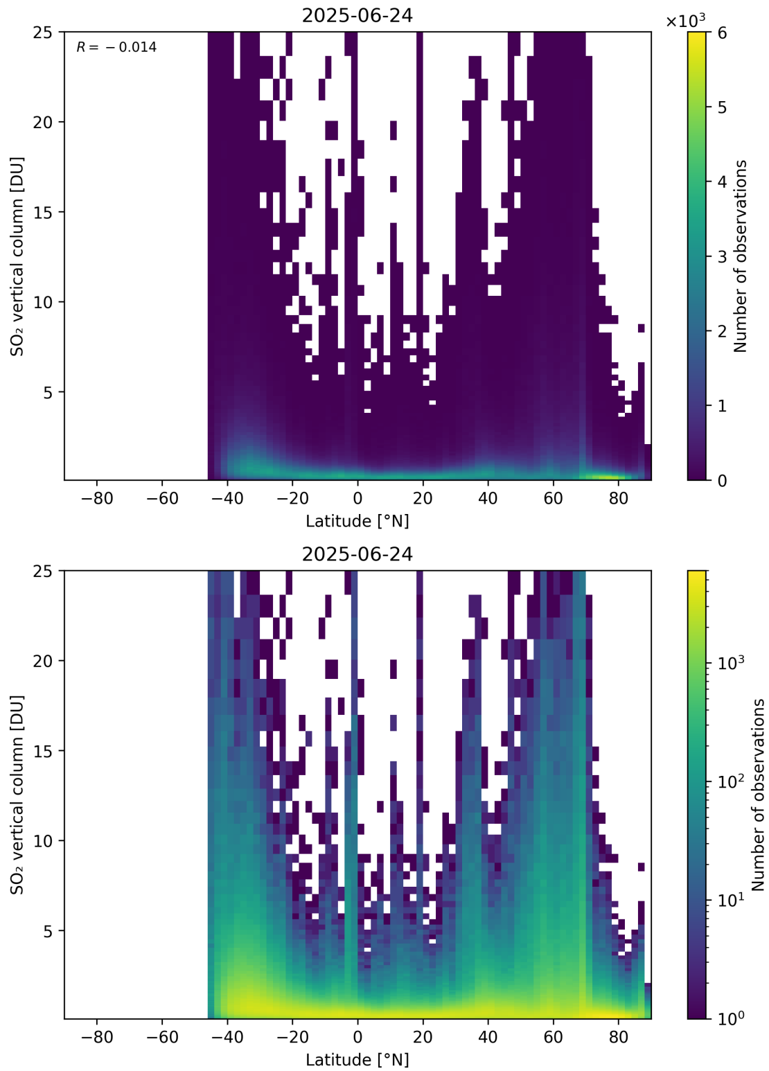
Figure 169: Scatter density plot of “Latitude” against “SO 2 vertical column” for 2025-06-23 to 2025-06-25.
