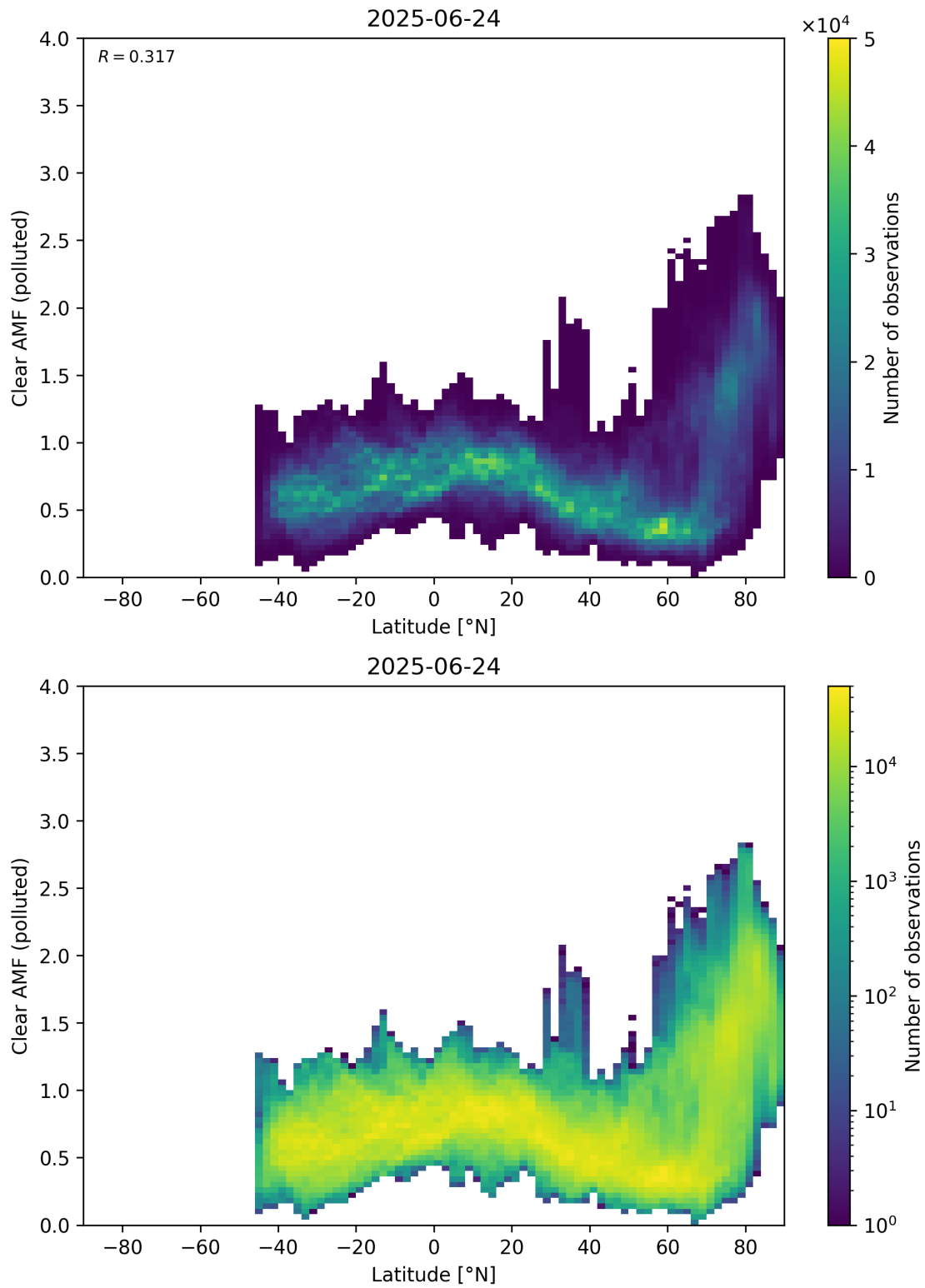
Figure 156: Scatter density plot of “Latitude” against “Clear AMF (polluted)” for 2025-06-23 to 2025-06-25.
