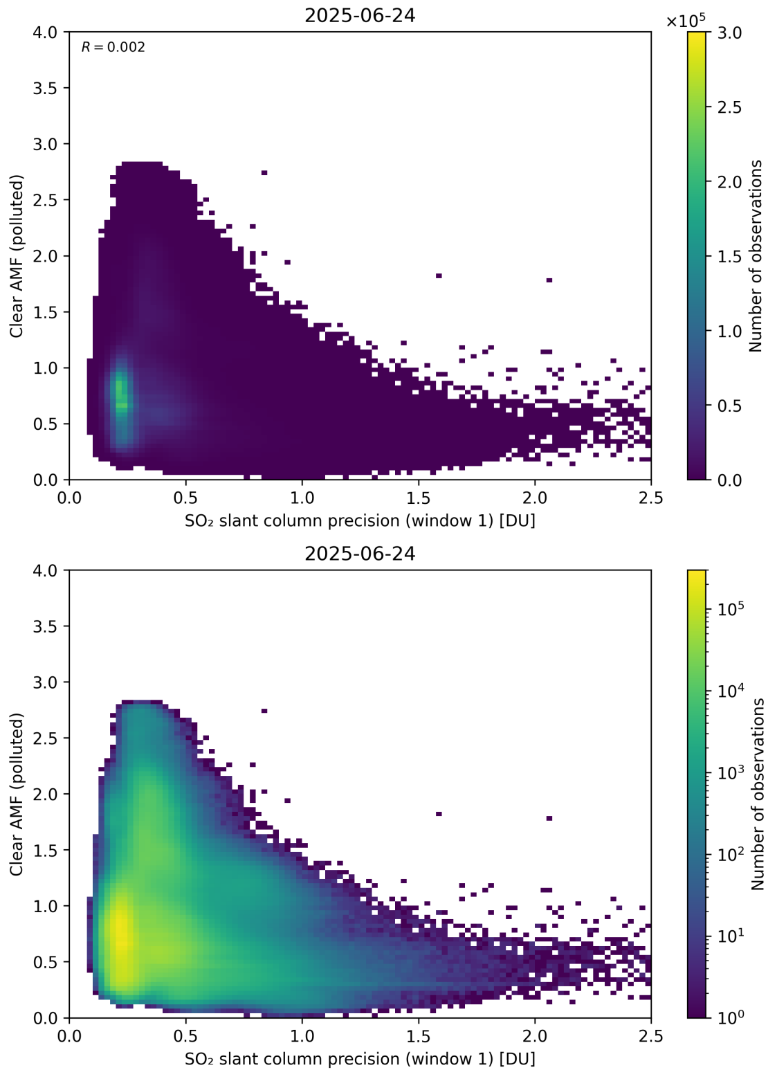
Figure 274: Scatter density plot of “SO 2 slant column precision (window 1)” against “Clear AMF (polluted)” for 2025-06-23 to 2025-06-25.
