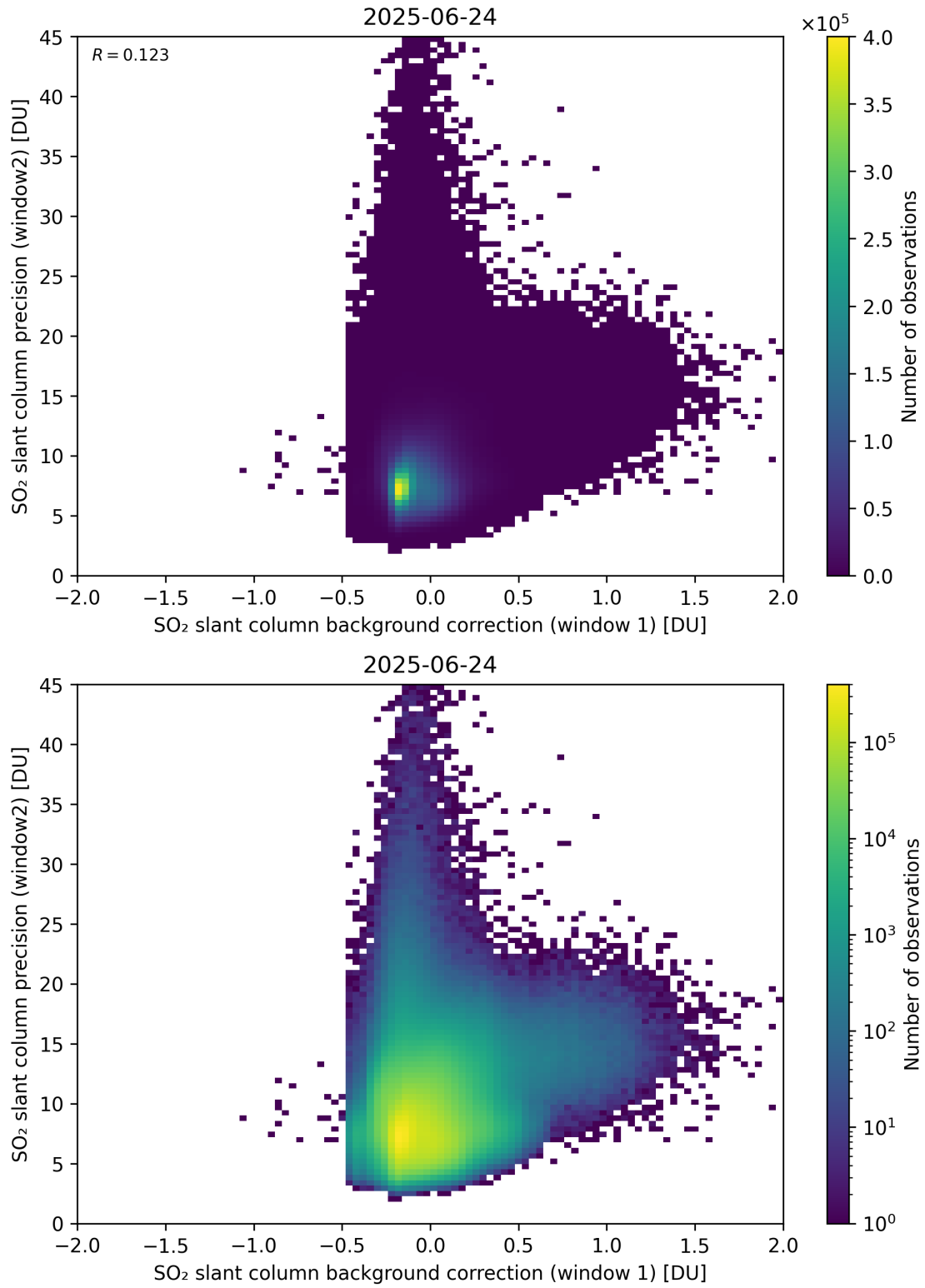
Figure 117: Scatter density plot of “SO 2 slant column background correction (window 1)” against “SO 2 slant column precision (window2)” for 2025-06-23 to 2025-06-25.
