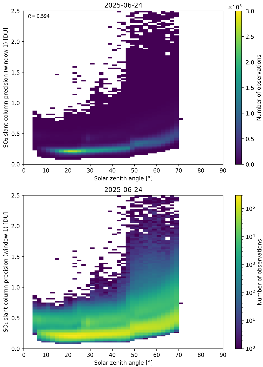
Figure 185: Scatter density plot of “Solar zenith angle” against “SO 2 slant column precision (window 1)” for 2025-06-23 to 2025-06-25.
