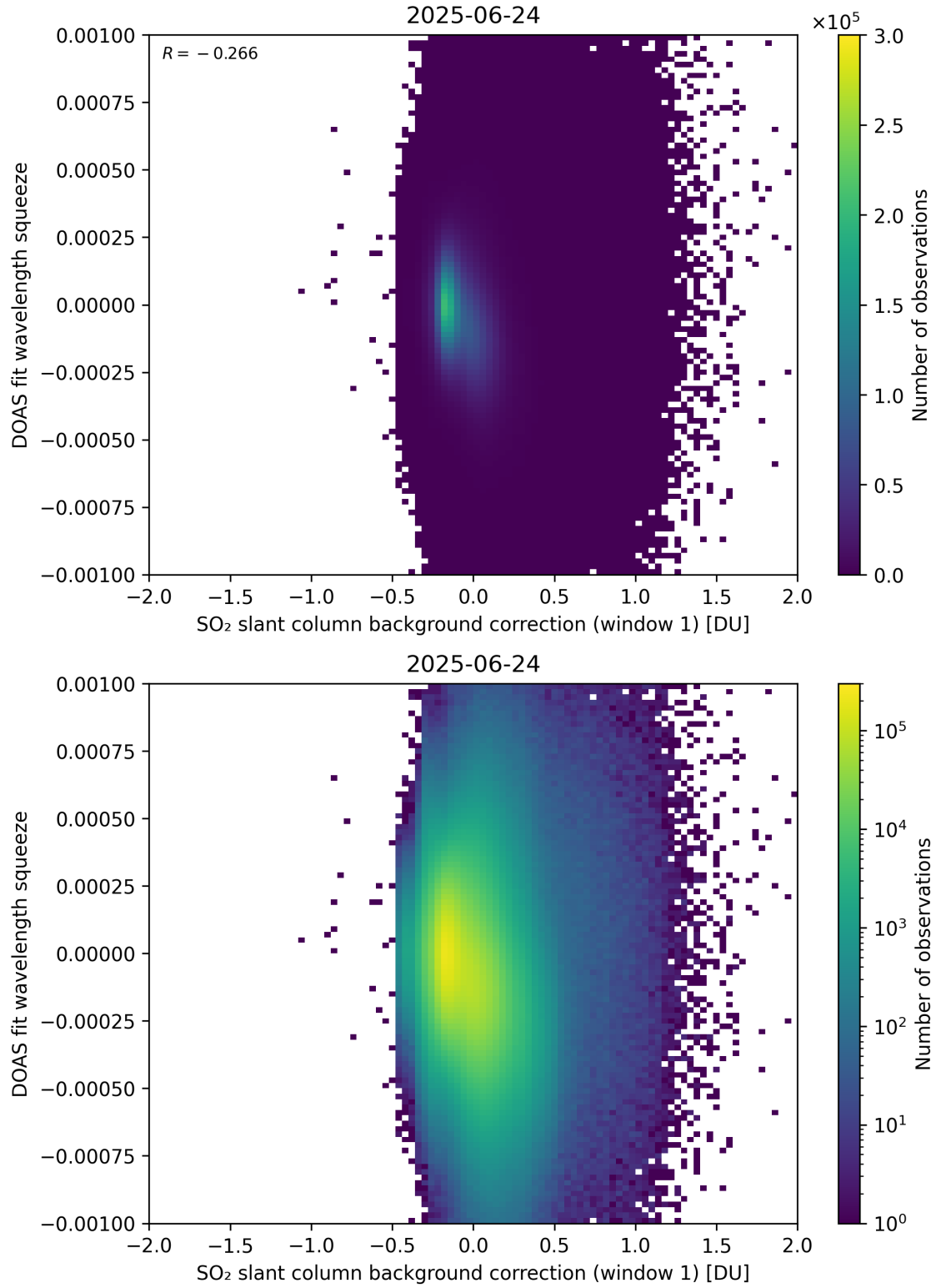
Figure 112: Scatter density plot of “SO 2 slant column background correction (window 1)” against “DOAS fit wavelength squeeze” for 2025-06-23 to 2025-06-25.
