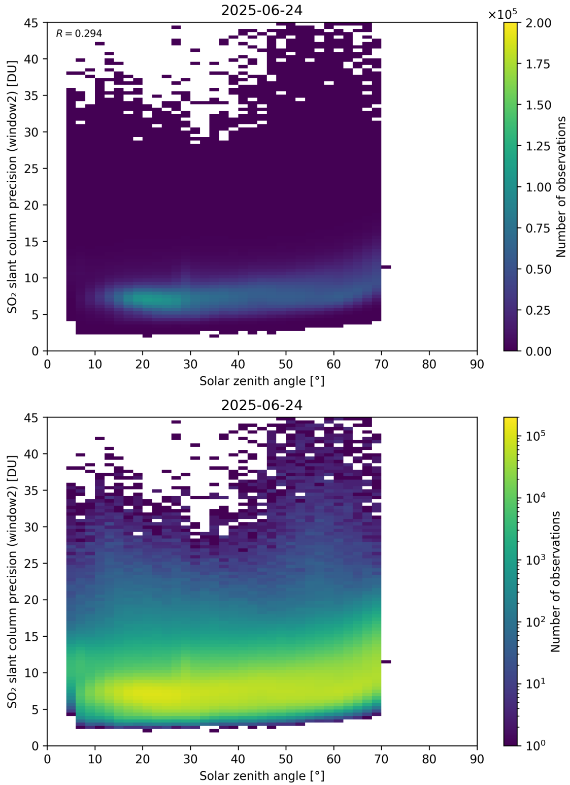
Figure 186: Scatter density plot of “Solar zenith angle” against “SO 2 slant column precision (window2)” for 2025-06-23 to 2025-06-25.
