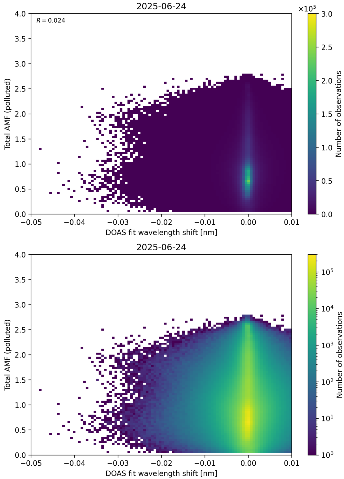
Figure 141: Scatter density plot of “DOAS fit wavelength shift” against “Total AMF (polluted)” for 2025-06-23 to 2025-06-25.
