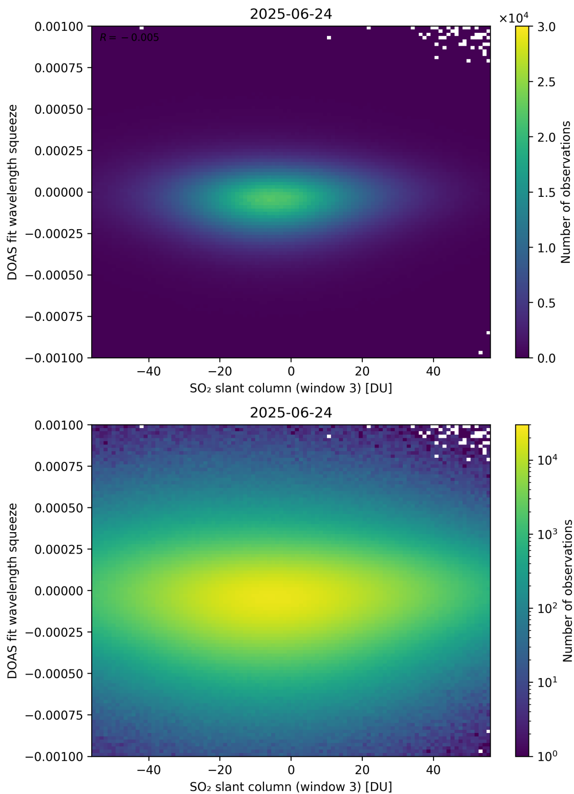
Figure 305: Scatter density plot of “SO 2 slant column (window 3)” against “DOAS fit wavelength squeeze” for 2025-06-23 to 2025-06-25.
