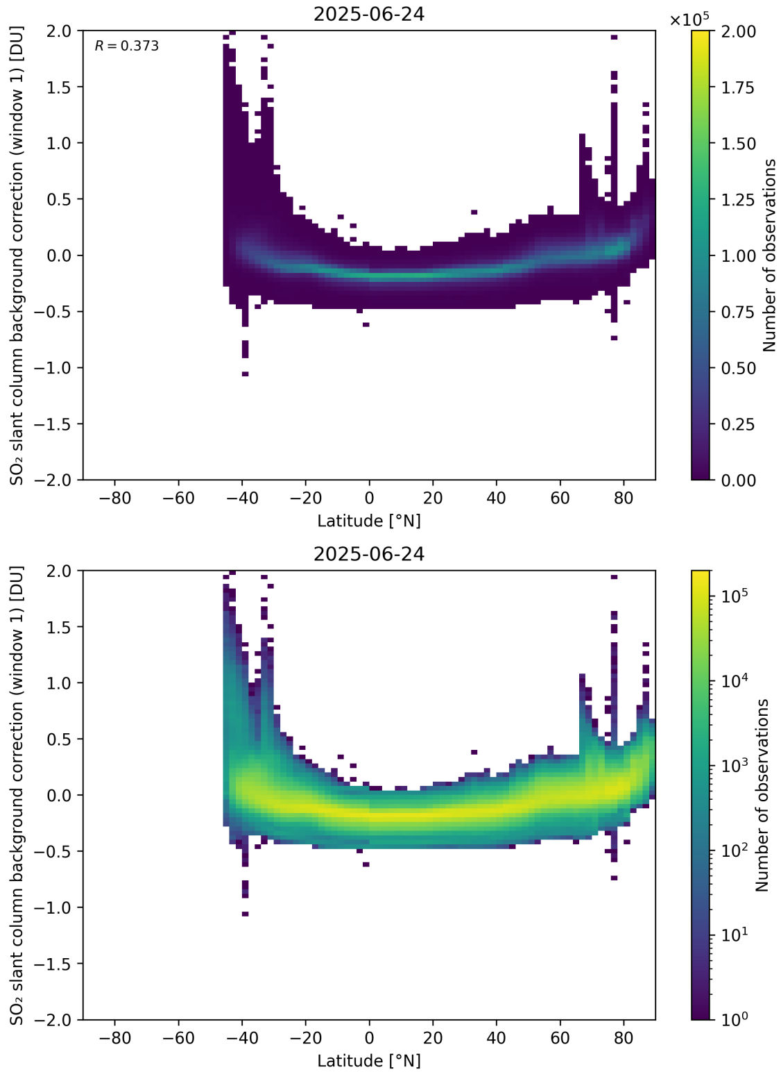
Figure 150: Scatter density plot of “Latitude” against “SO 2 slant column background correction (window 1)” for 2025-06-23 to 2025-06-25.
