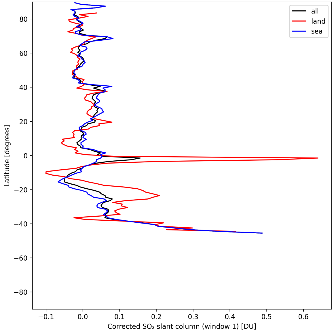
Figure 39: Zonal average of “Corrected SO 2 slant column (window 1)” for 2025-06-23 to 2025-06-25.
