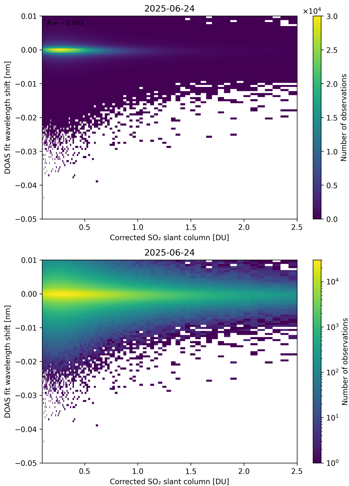
Figure 229: Scatter density plot of “Corrected SO 2 slant column” against “DOAS fit wavelength shift” for 2025-06-23 to 2025-06-25.
