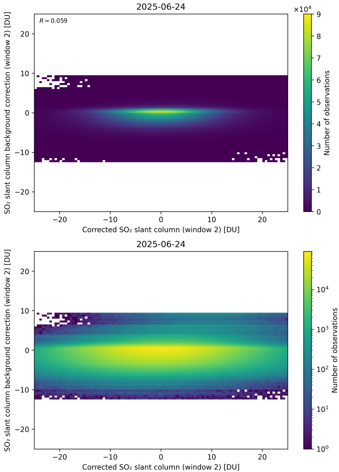
Figure 244: Scatter density plot of “Corrected SO 2 slant column (window 2)” against “SO 2 slant column background correction (window 2)” for 2025-06-23 to 2025-06-25.
