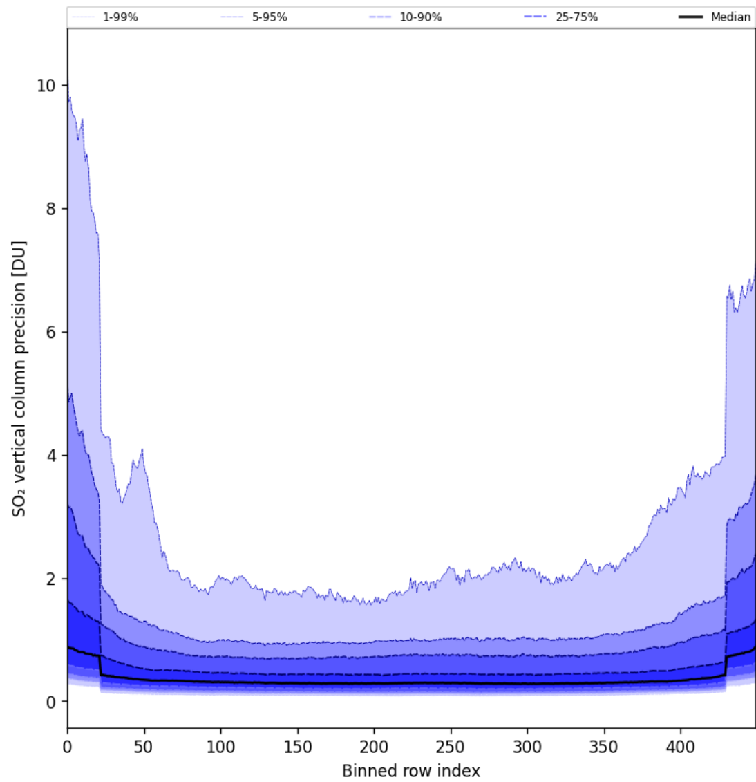
Figure 85: Along track statistics of “SO 2 vertical column precision” for 2025-06-23 to 2025-06-25
