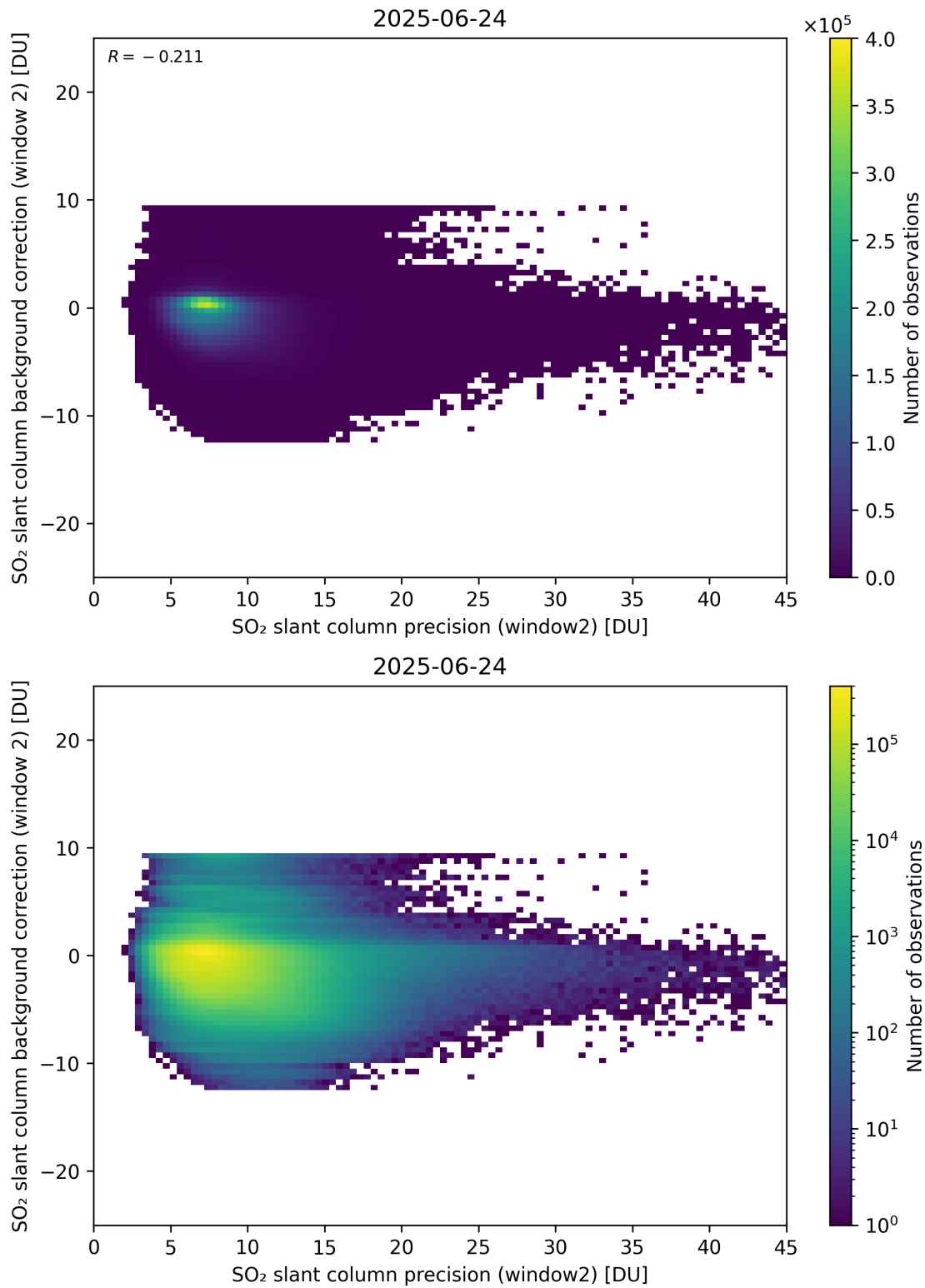
Figure 291: Scatter density plot of “SO 2 slant column precision (window2)” against “SO 2 slant column background correction (window 2)” for 2025-06-23 to 2025-06-25.
