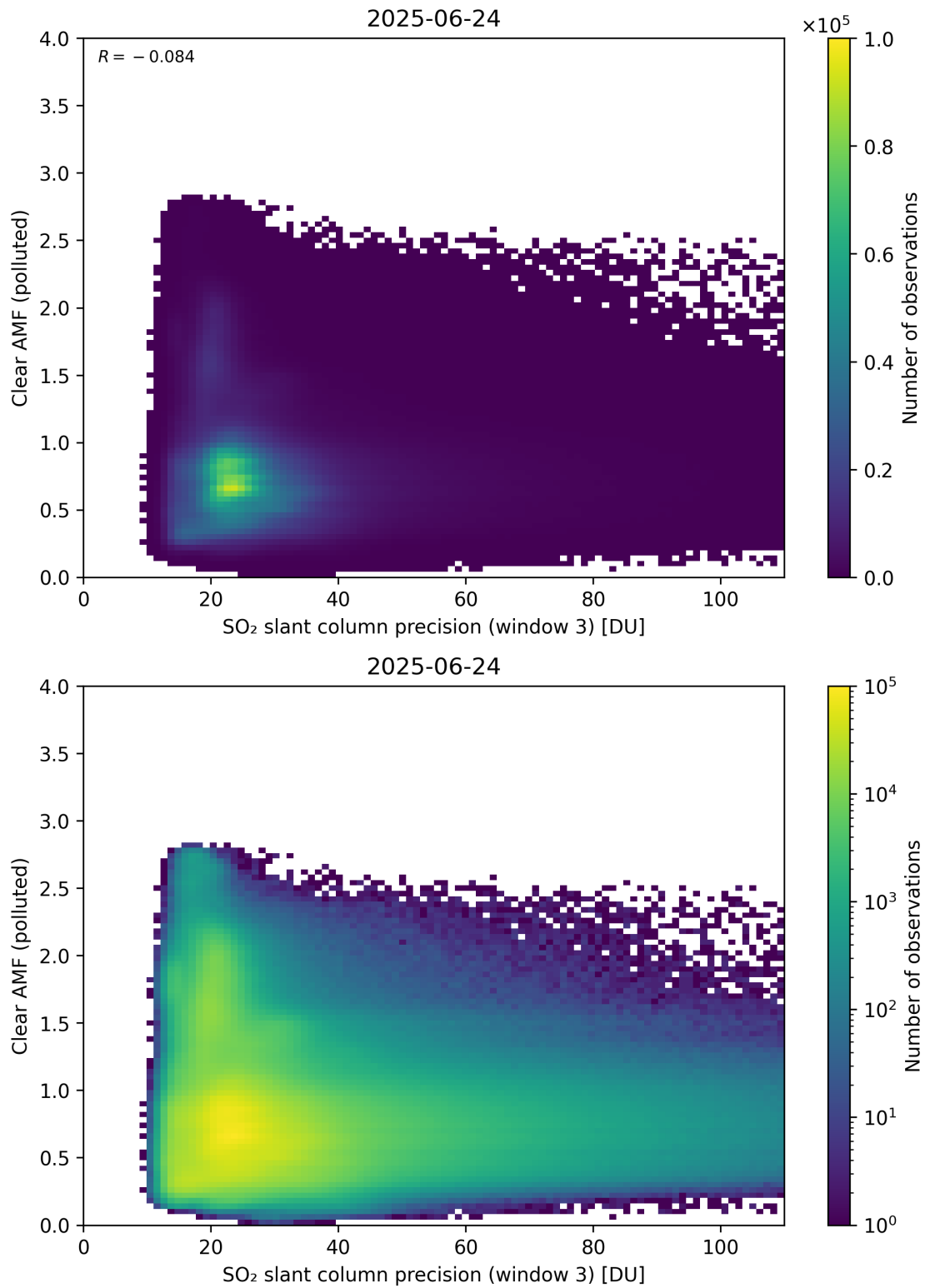
Figure 311: Scatter density plot of “SO 2 slant column precision (window 3)” against “Clear AMF (polluted)” for 2025-06-23 to 2025-06-25.
