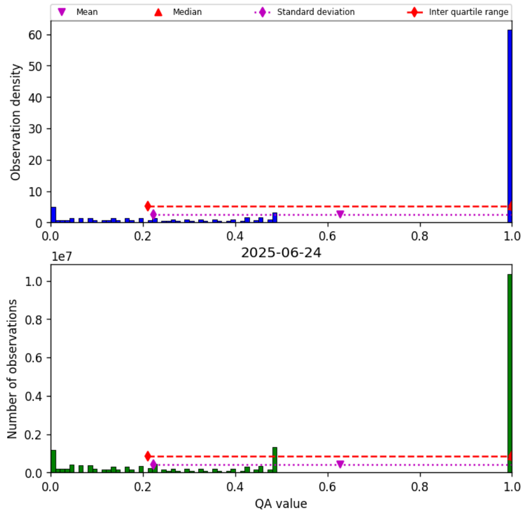
Figure 57: Histogram of “QA value” for 2025-06-23 to 2025-06-25
