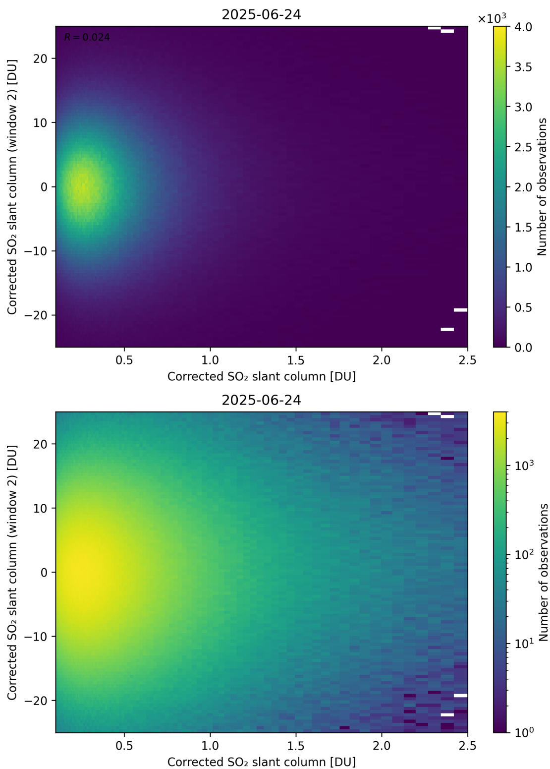
Figure 235: Scatter density plot of “Corrected SO 2 slant column” against “Corrected SO 2 slant column (window 2)” for 2025-06-23 to 2025-06-25.
