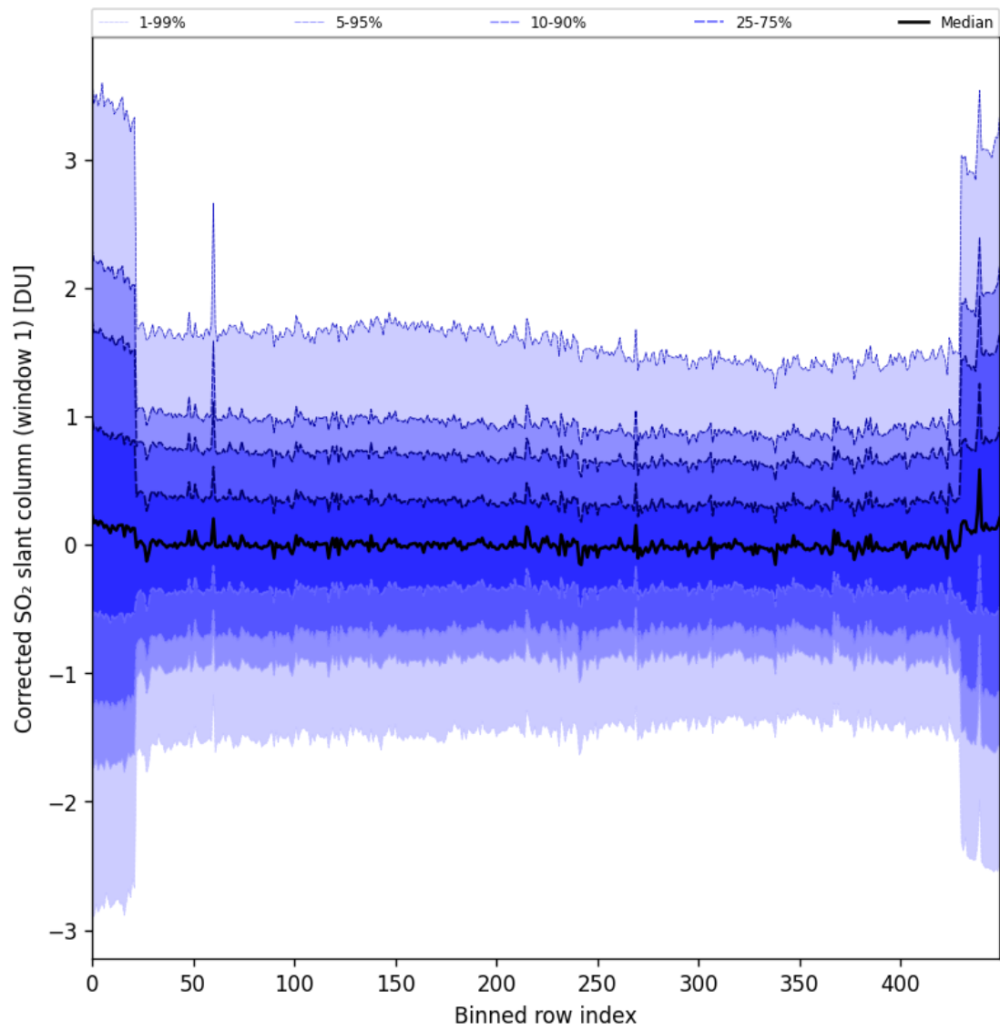
Figure 91: Along track statistics of “Corrected SO 2 slant column (window 1)” for 2025-06-23 to 2025-06-25
