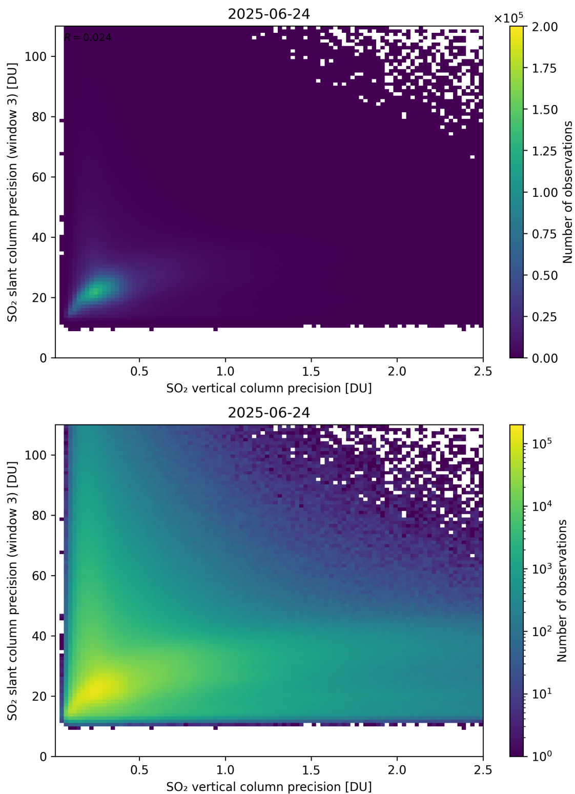
Figure 345: Scatter density plot of “SO 2 vertical column precision” against “SO 2 slant column precision (window 3)” for 2025-06-23 to 2025-06-25.
