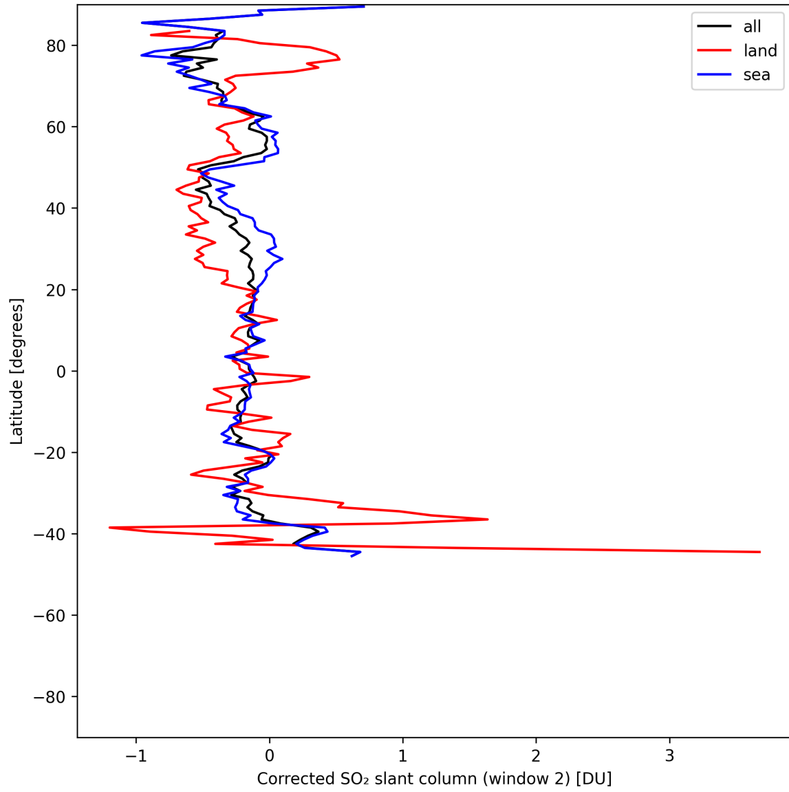
Figure 43: Zonal average of “Corrected SO 2 slant column (window 2)” for 2025-06-23 to 2025-06-25.
