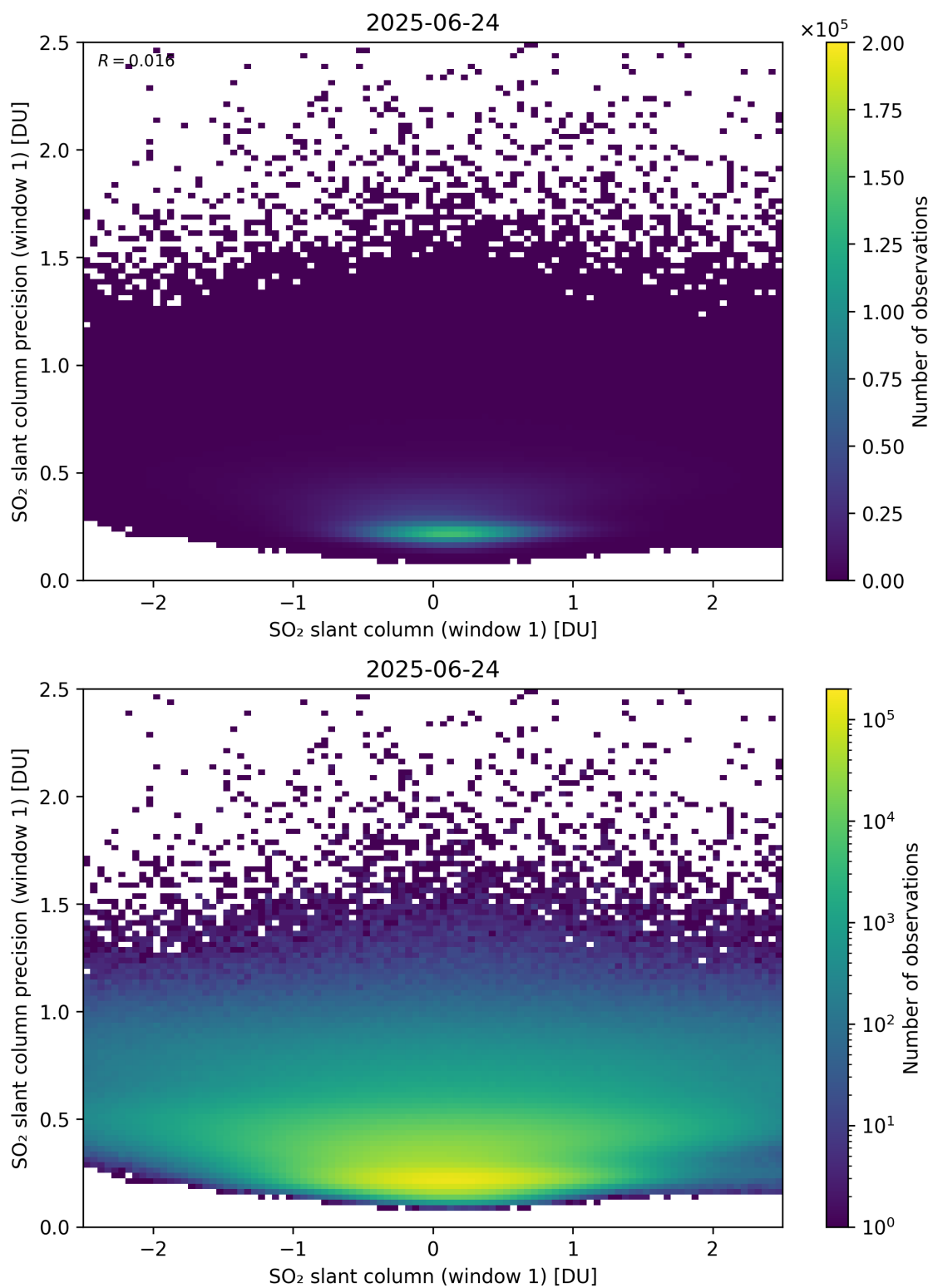
Figure 285: Scatter density plot of “SO 2 slant column (window 1)” against “SO 2 slant column precision (window 1)” for 2025-06-23 to 2025-06-25.
