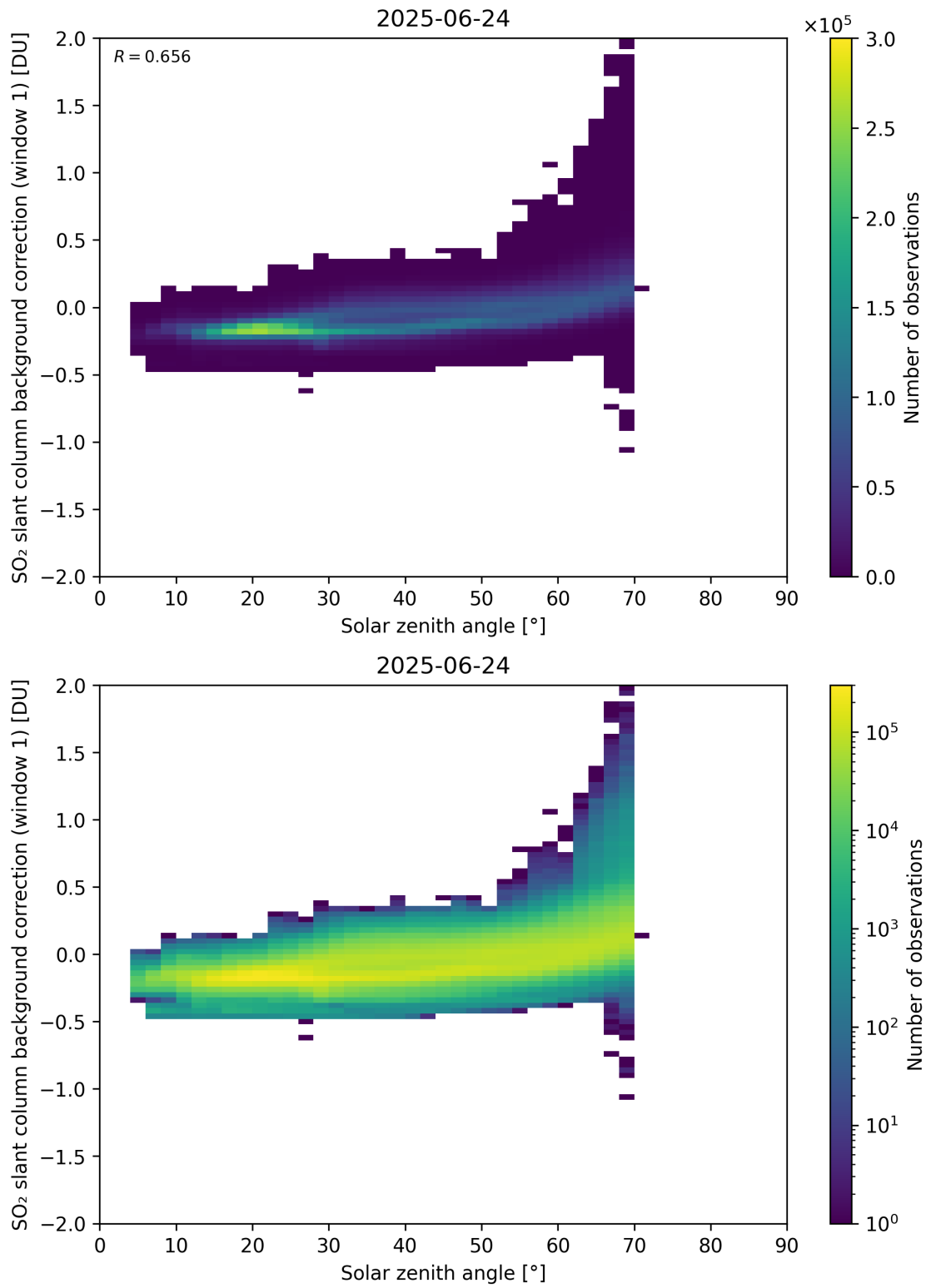
Figure 171: Scatter density plot of “Solar zenith angle” against “SO 2 slant column background correction (window 1)” for 2025-06-23 to 2025-06-25.
