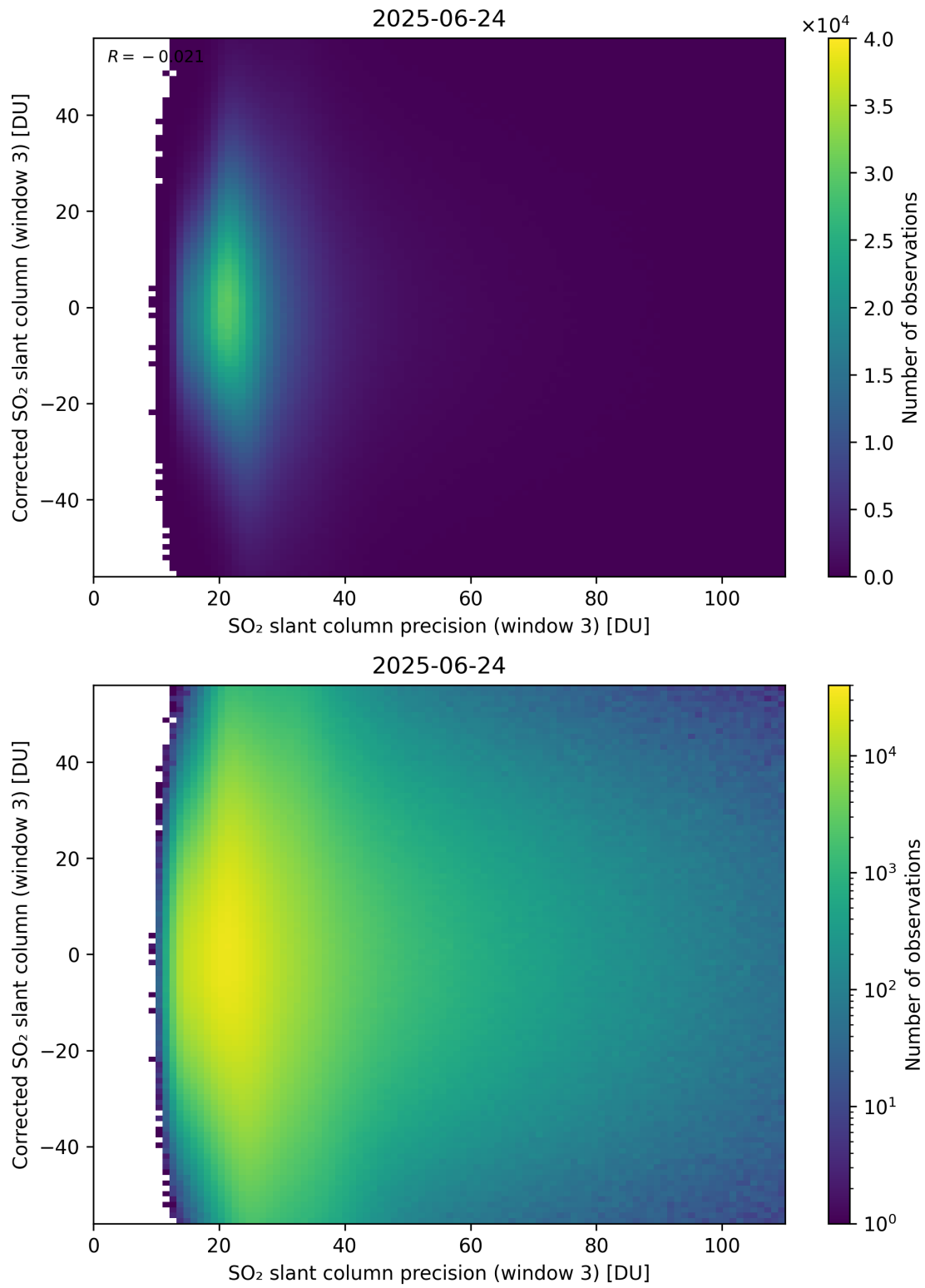
Figure 312: Scatter density plot of “SO 2 slant column precision (window 3)” against “Corrected SO 2 slant column (window 3)” for 2025-06-23 to 2025-06-25.
