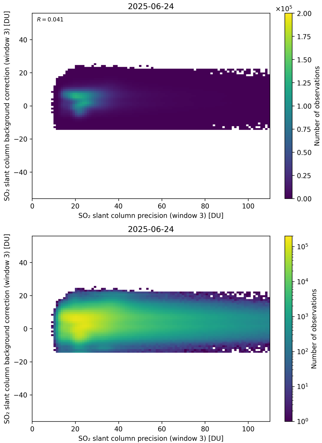
Figure 307: Scatter density plot of “SO 2 slant column precision (window 3)” against “SO 2 slant column background correction (window 3)” for 2025-06-23 to 2025-06-25.
