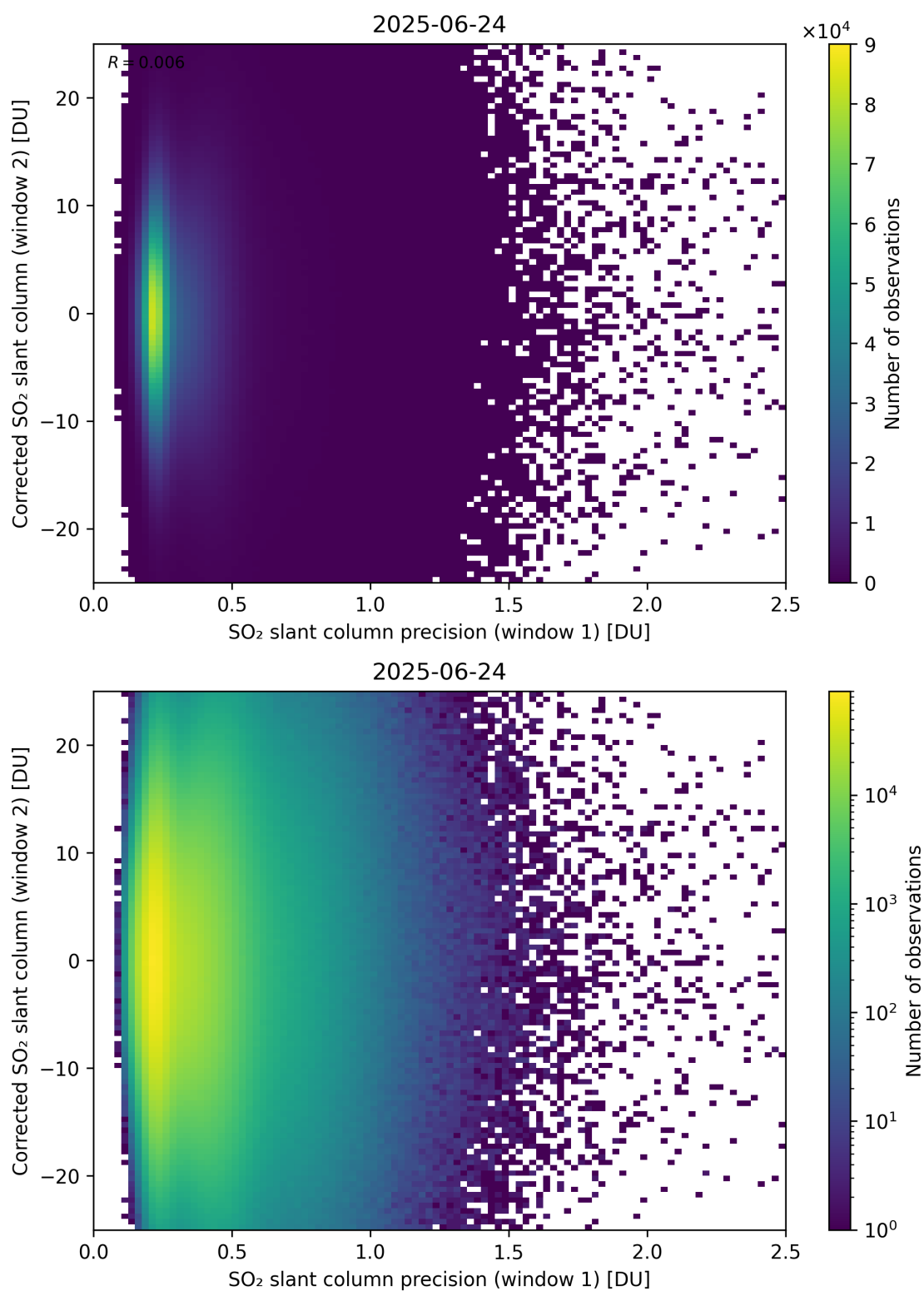
Figure 275: Scatter density plot of “SO 2 slant column precision (window 1)” against “Corrected SO 2 slant column (window 2)” for 2025-06-23 to 2025-06-25.
