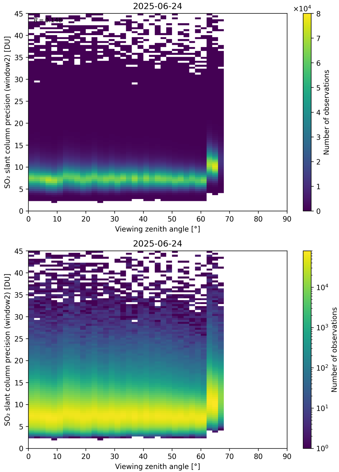
Figure 378: Scatter density plot of “Viewing zenith angle” against “SO 2 slant column precision (window2)” for 2025-06-23 to 2025-06-25.
