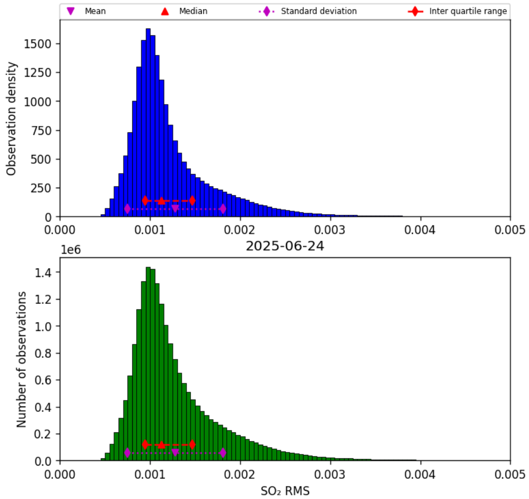
Figure 78: Histogram of “SO 2 RMS” for 2025-06-23 to 2025-06-25
