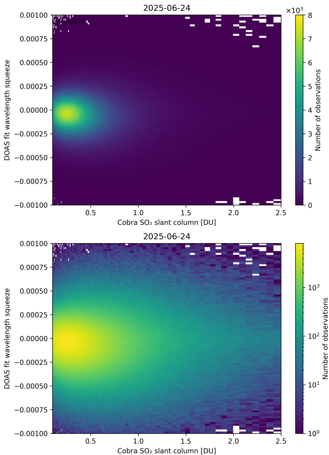
Figure 197: Scatter density plot of “Cobra SO 2 slant column” against “DOAS fit wavelength squeeze” for 2025-06-23 to 2025-06-25.
