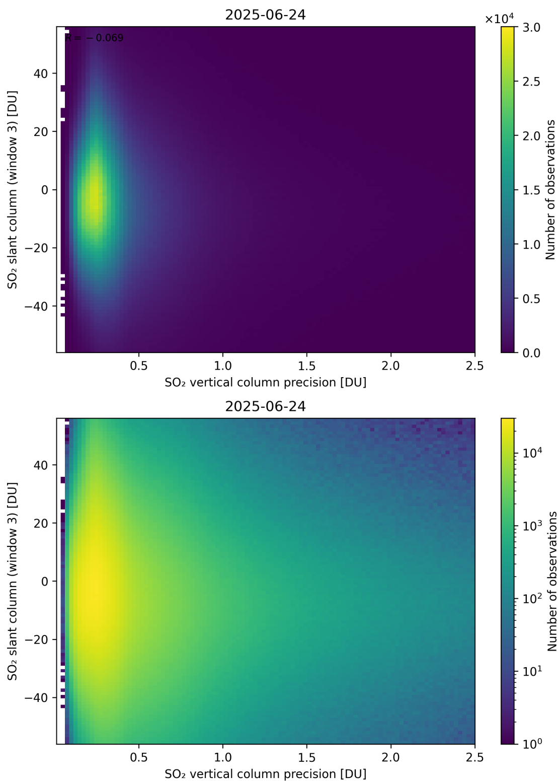
Figure 344: Scatter density plot of “SO 2 vertical column precision” against “SO 2 slant column (window 3)” for 2025-06-23 to 2025-06-25.
