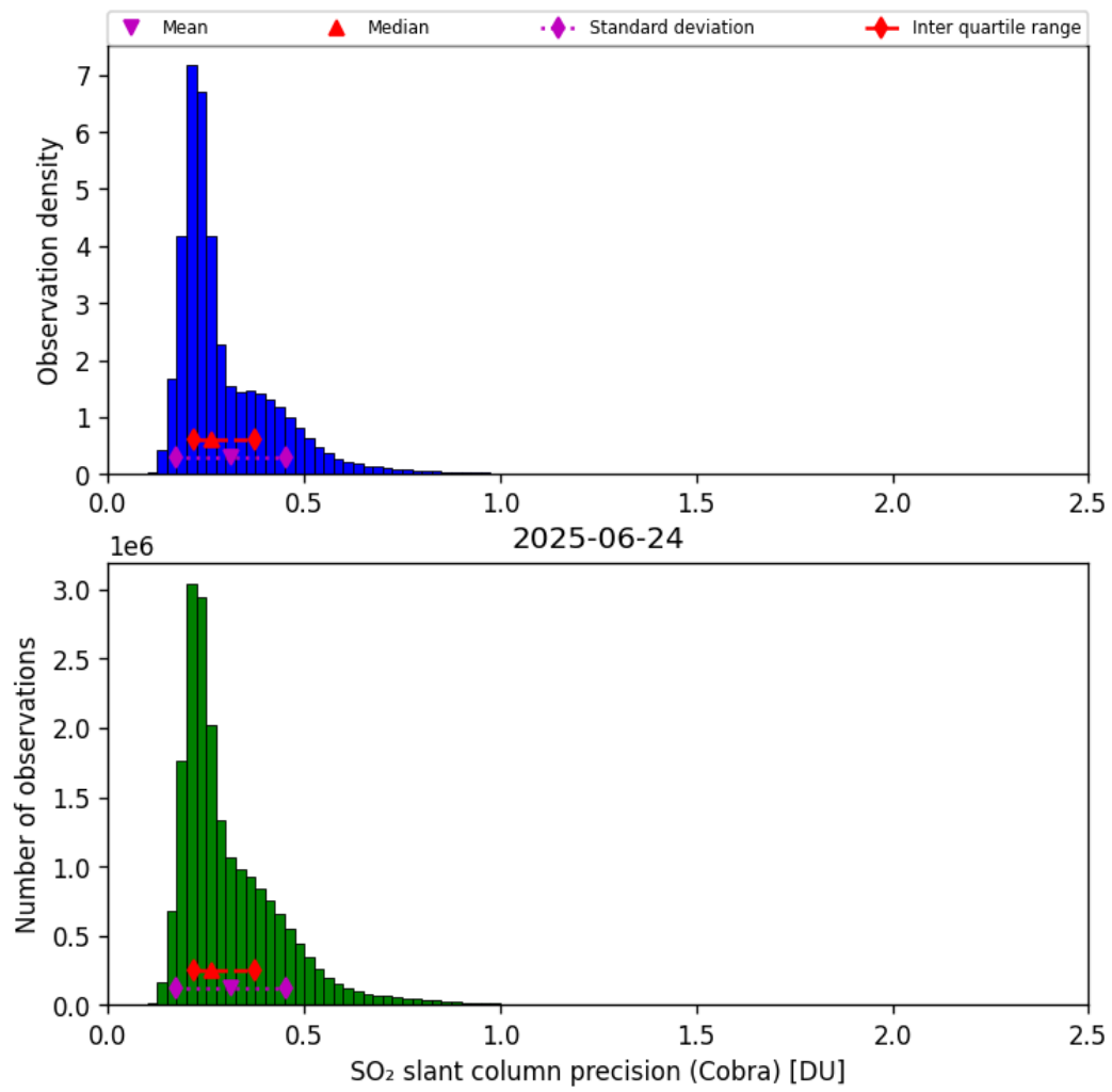
Figure 62: Histogram of “SO 2 slant column precision (Cobra)” for 2025-06-23 to 2025-06-25
