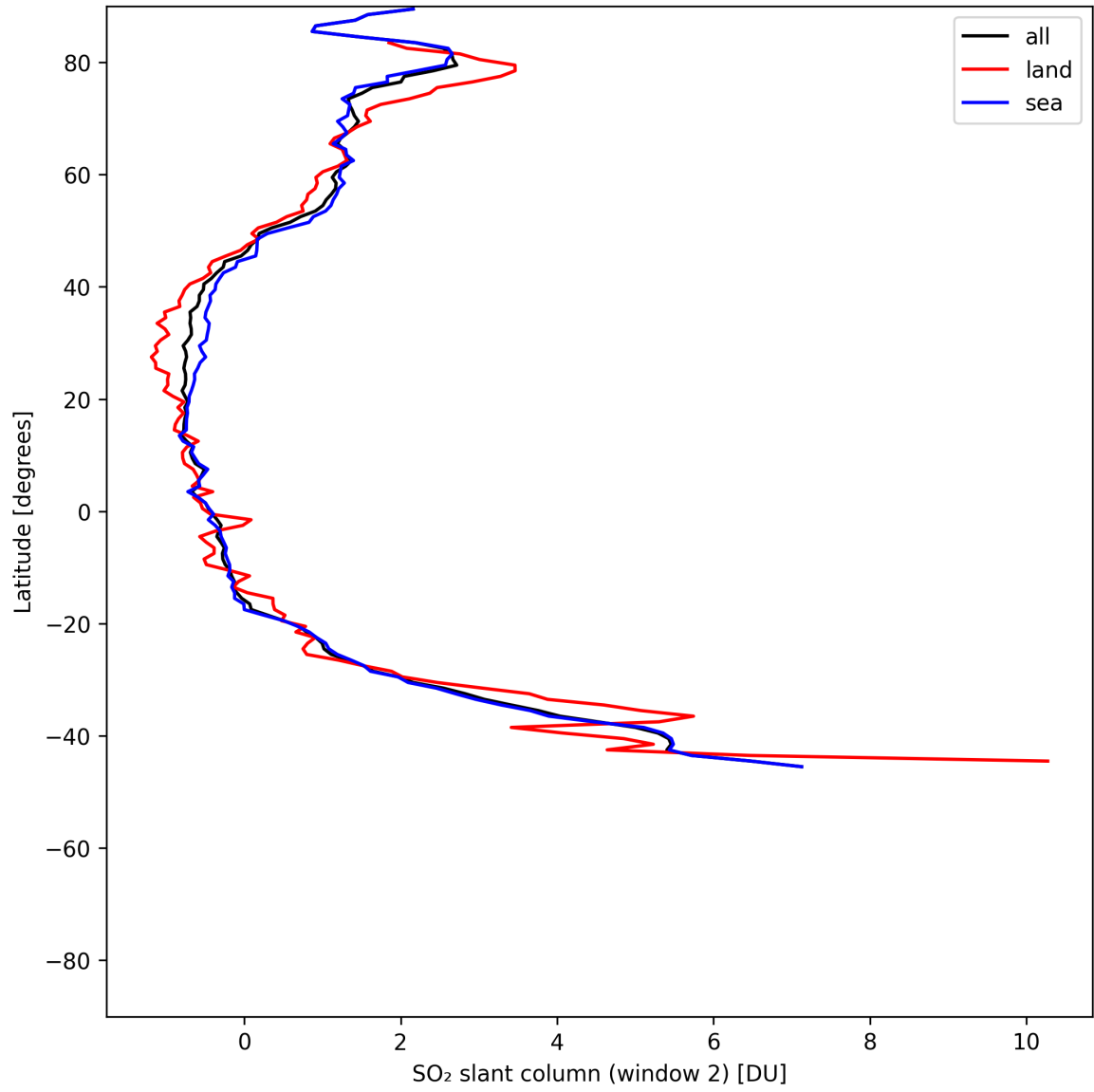
Figure 41: Zonal average of “SO 2 slant column (window 2)” for 2025-06-23 to 2025-06-25.
