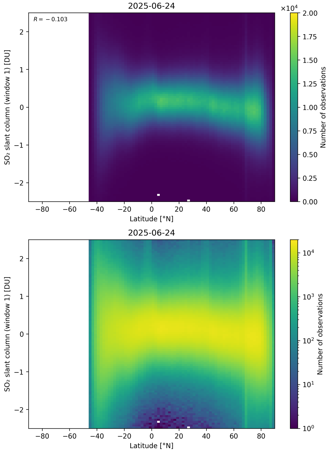
Figure 162: Scatter density plot of “Latitude” against “SO 2 slant column (window 1)” for 2025-06-23 to 2025-06-25.
