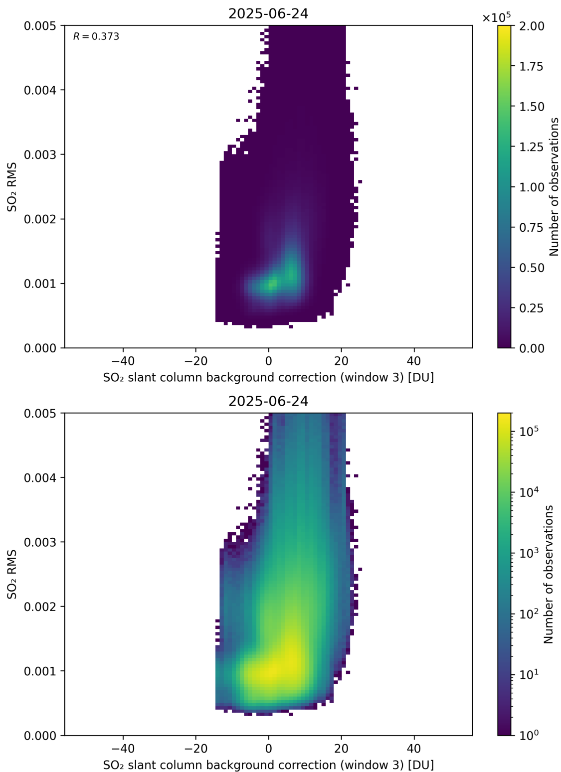
Figure 134: Scatter density plot of “SO 2 slant column background correction (window 3)” against “SO 2 RMS” for 2025-06-23 to 2025-06-25.
