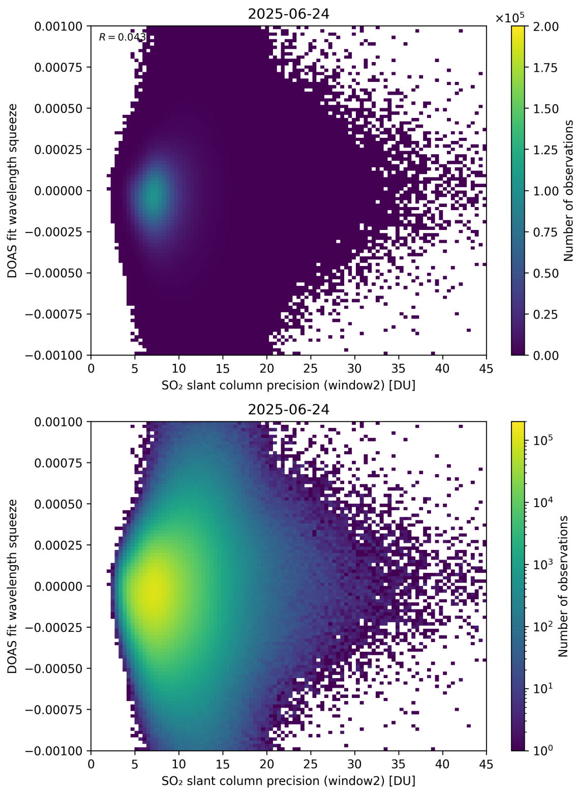
Figure 294: Scatter density plot of “SO 2 slant column precision (window2)” against “DOAS fit wavelength squeeze” for 2025-06-23 to 2025-06-25.
