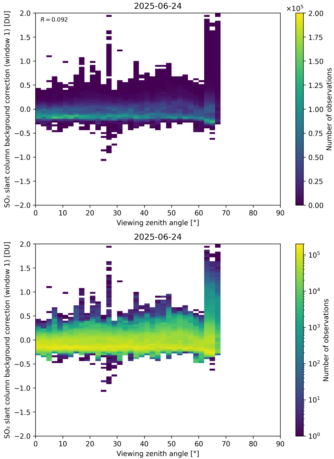
Figure 362: Scatter density plot of “Viewing zenith angle” against “SO 2 slant column background correction (window 1)” for 2025-06-23 to 2025-06-25.
