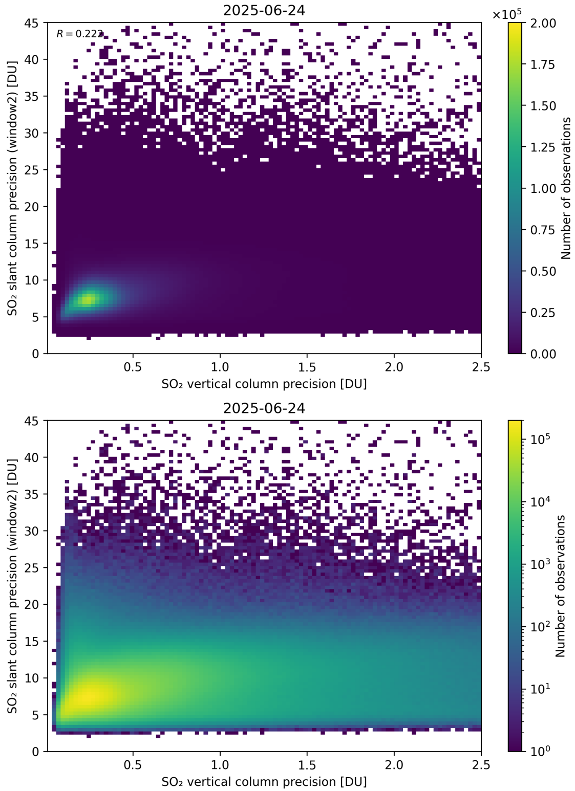
Figure 343: Scatter density plot of “SO 2 vertical column precision” against “SO 2 slant column precision (window2)” for 2025-06-23 to 2025-06-25.
