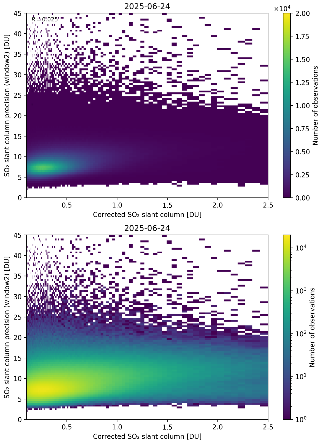
Figure 239: Scatter density plot of “Corrected SO 2 slant column” against “SO 2 slant column precision (window2)” for 2025-06-23 to 2025-06-25.
