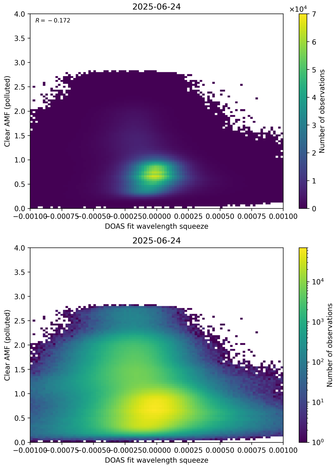
Figure 144: Scatter density plot of “DOAS fit wavelength squeeze” against “Clear AMF (polluted)” for 2025-06-23 to 2025-06-25.
