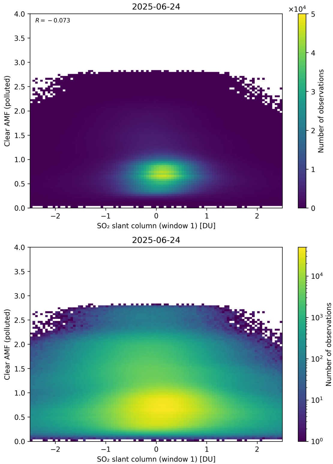
Figure 282: Scatter density plot of “SO 2 slant column (window 1)” against “Clear AMF (polluted)” for 2025-06-23 to 2025-06-25.
