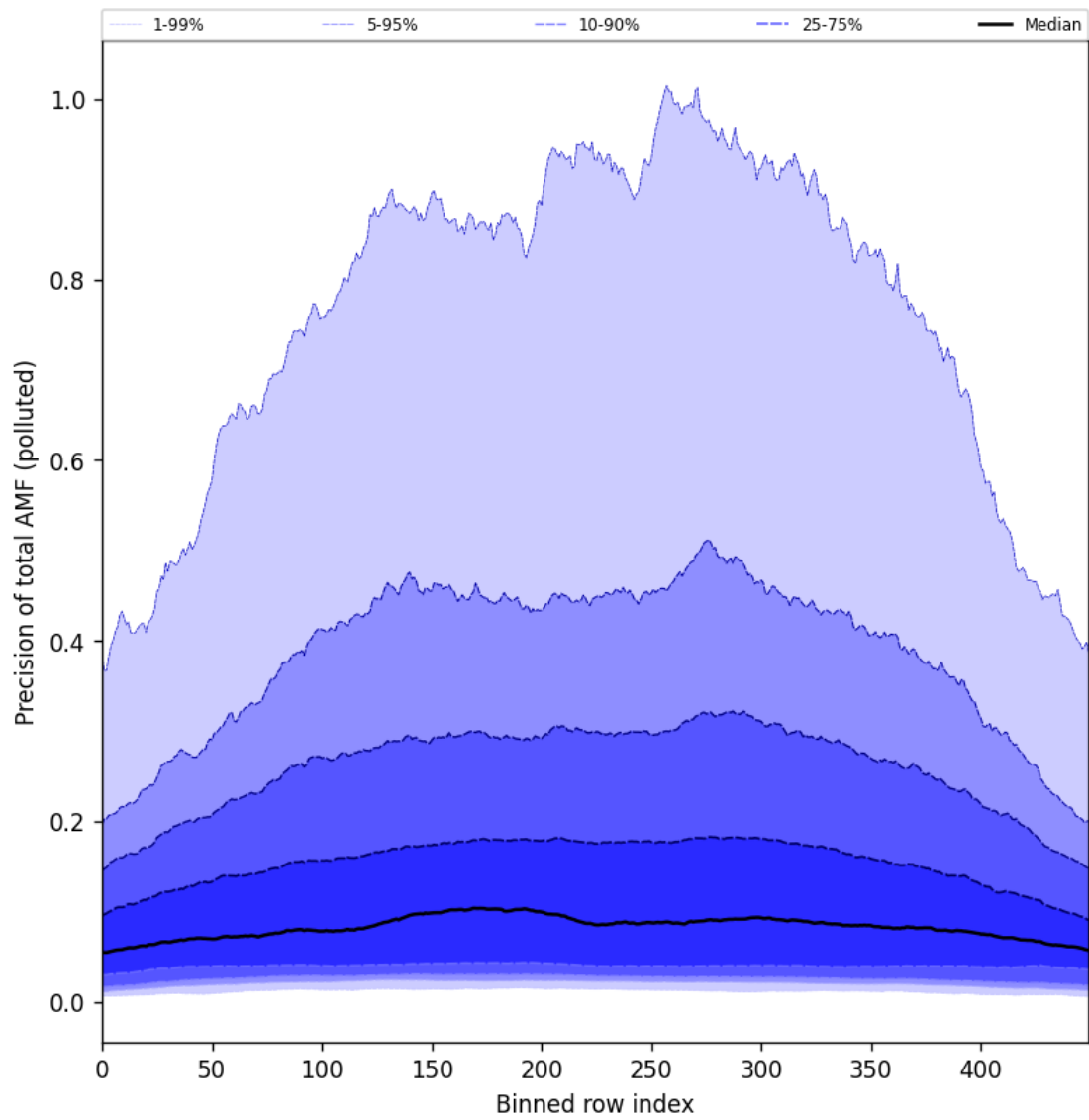
Figure 106: Along track statistics of “Precision of total AMF (polluted)” for 2025-06-23 to 2025-06-25
