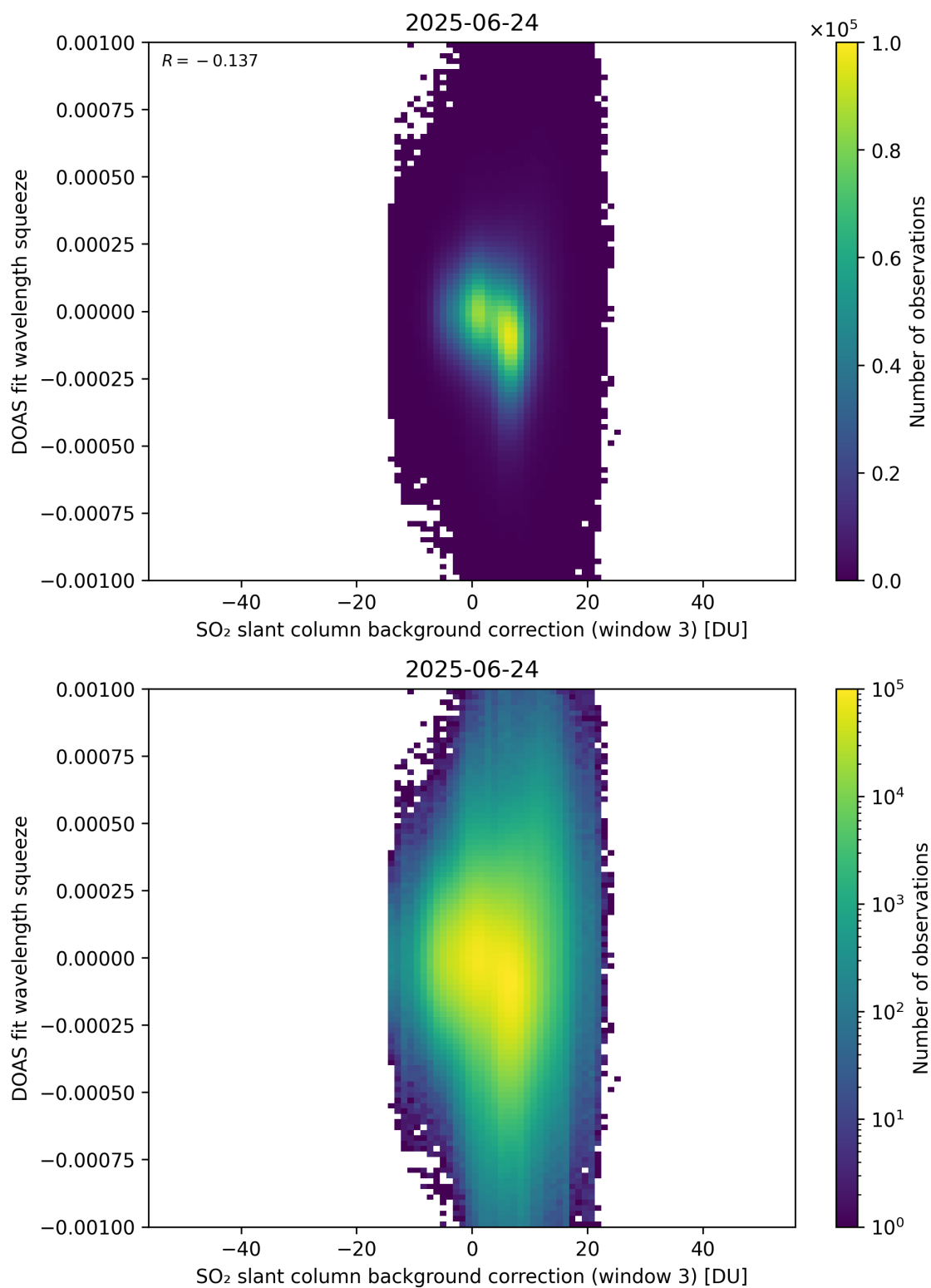
Figure 133: Scatter density plot of “SO 2 slant column background correction (window 3)” against “DOAS fit wavelength squeeze” for 2025-06-23 to 2025-06-25.
