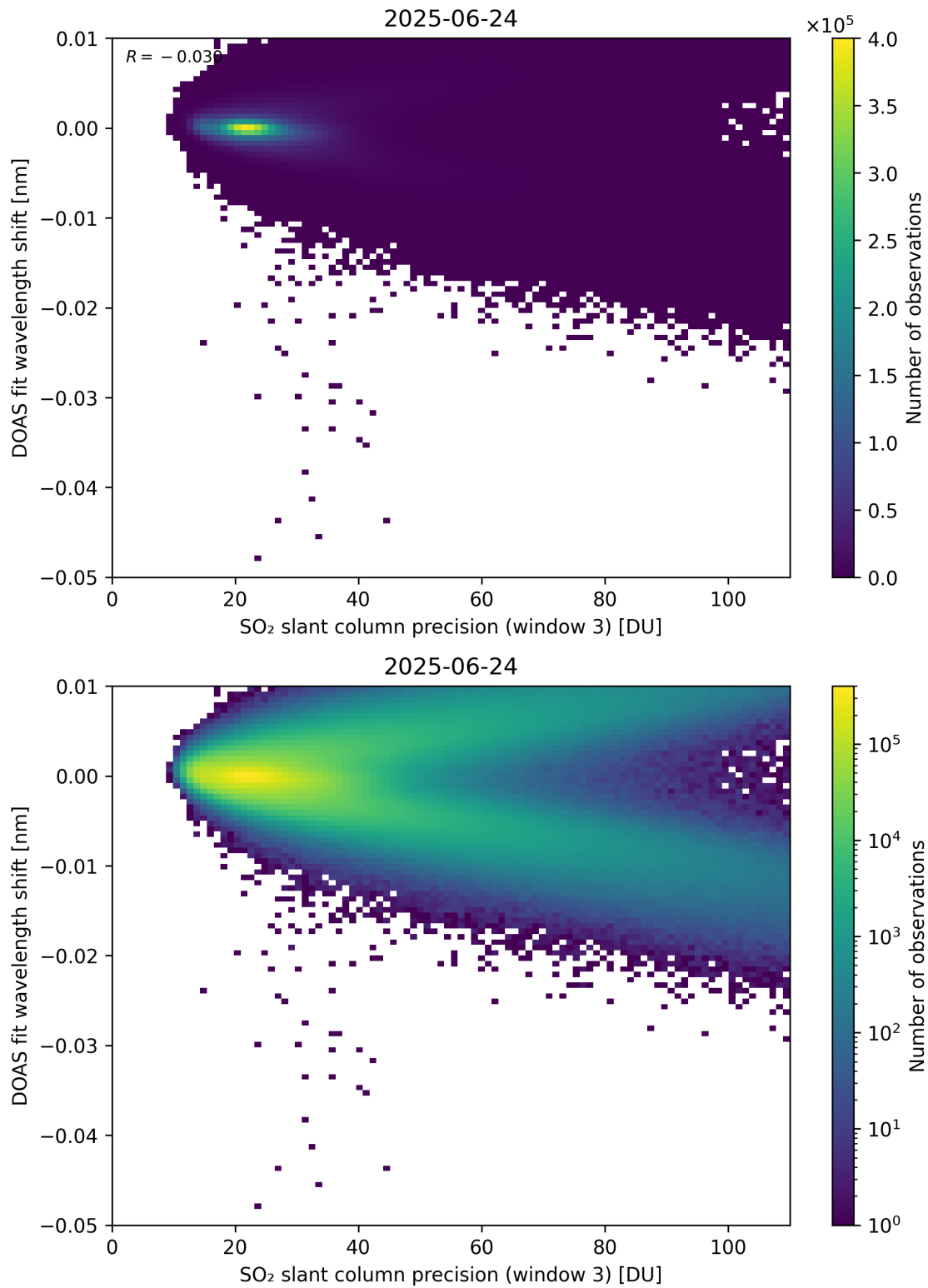
Figure 308: Scatter density plot of “SO 2 slant column precision (window 3)” against “DOAS fit wavelength shift” for 2025-06-23 to 2025-06-25.
