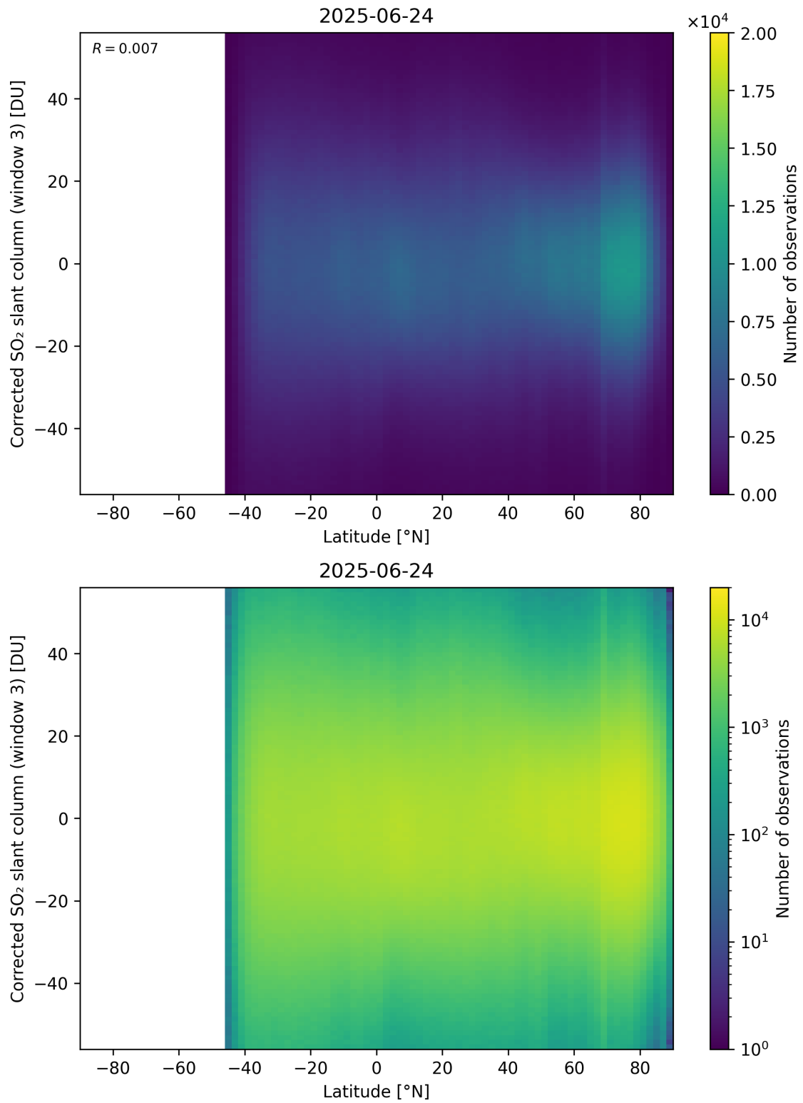
Figure 161: Scatter density plot of “Latitude” against “Corrected SO 2 slant column (window 3)” for 2025-06-23 to 2025-06-25.
