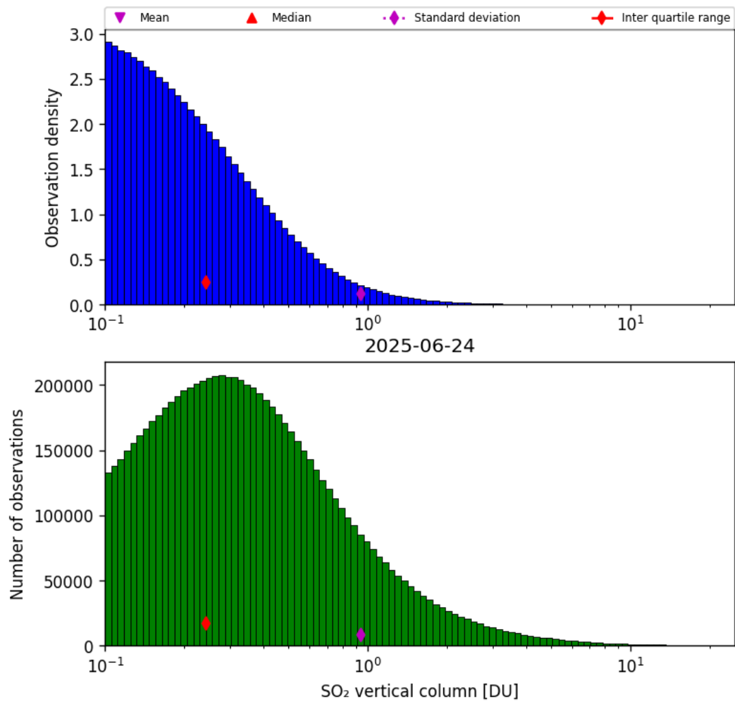
Figure 58: Histogram of “SO 2 vertical column” for 2025-06-23 to 2025-06-25
