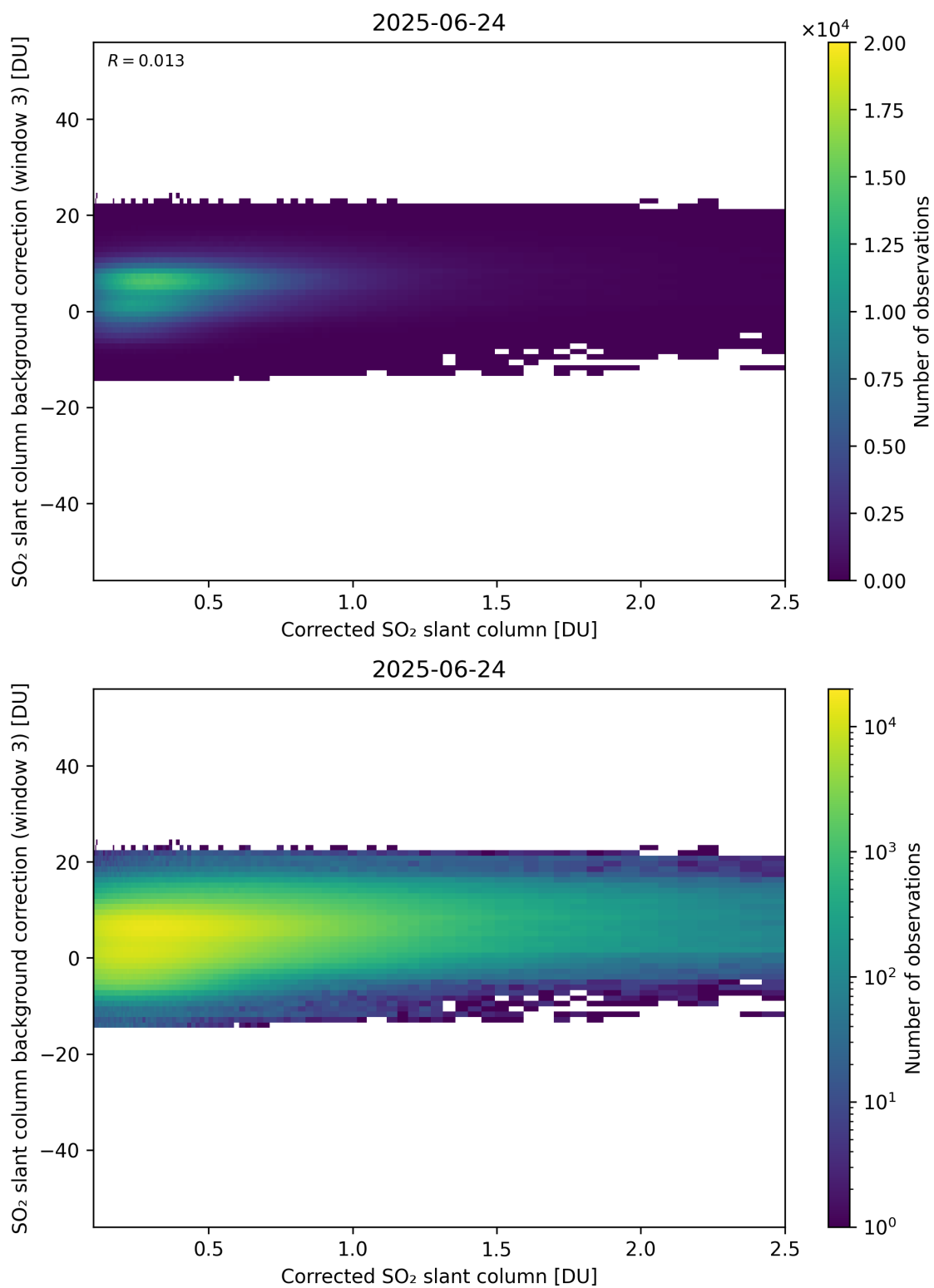
Figure 228: Scatter density plot of “Corrected SO 2 slant column” against “SO 2 slant column background correction (window 3)” for 2025-06-23 to 2025-06-25.
