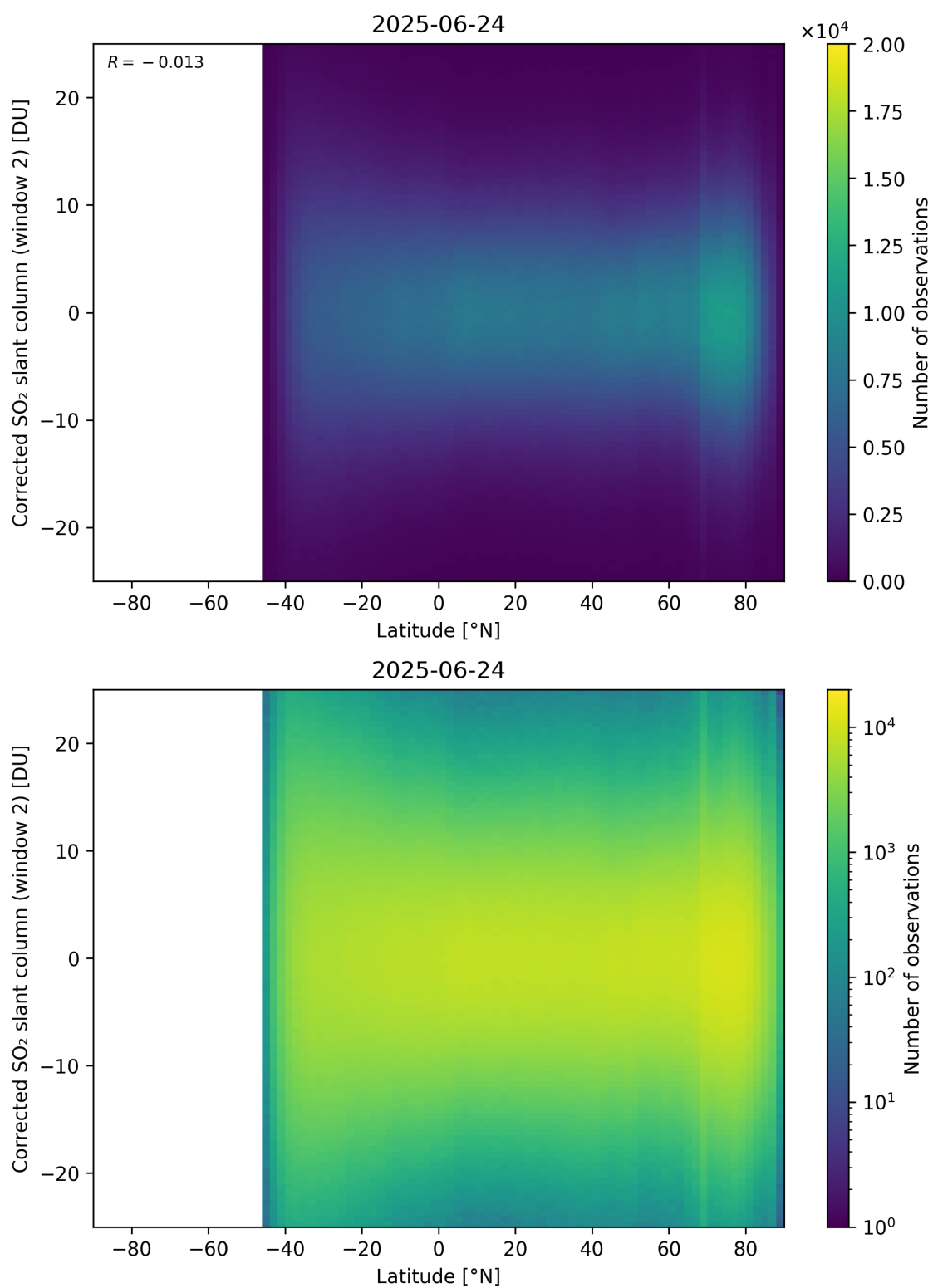
Figure 160: Scatter density plot of “Latitude” against “Corrected SO 2 slant column (window 2)” for 2025-06-23 to 2025-06-25.
