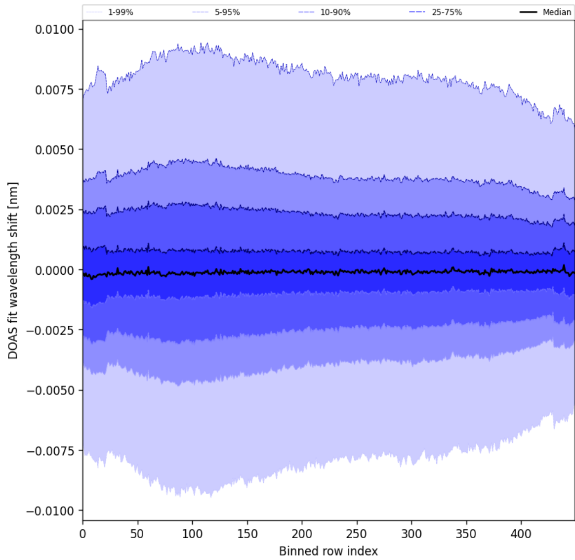
Figure 102: Along track statistics of “DOAS fit wavelength shift” for 2025-06-23 to 2025-06-25
