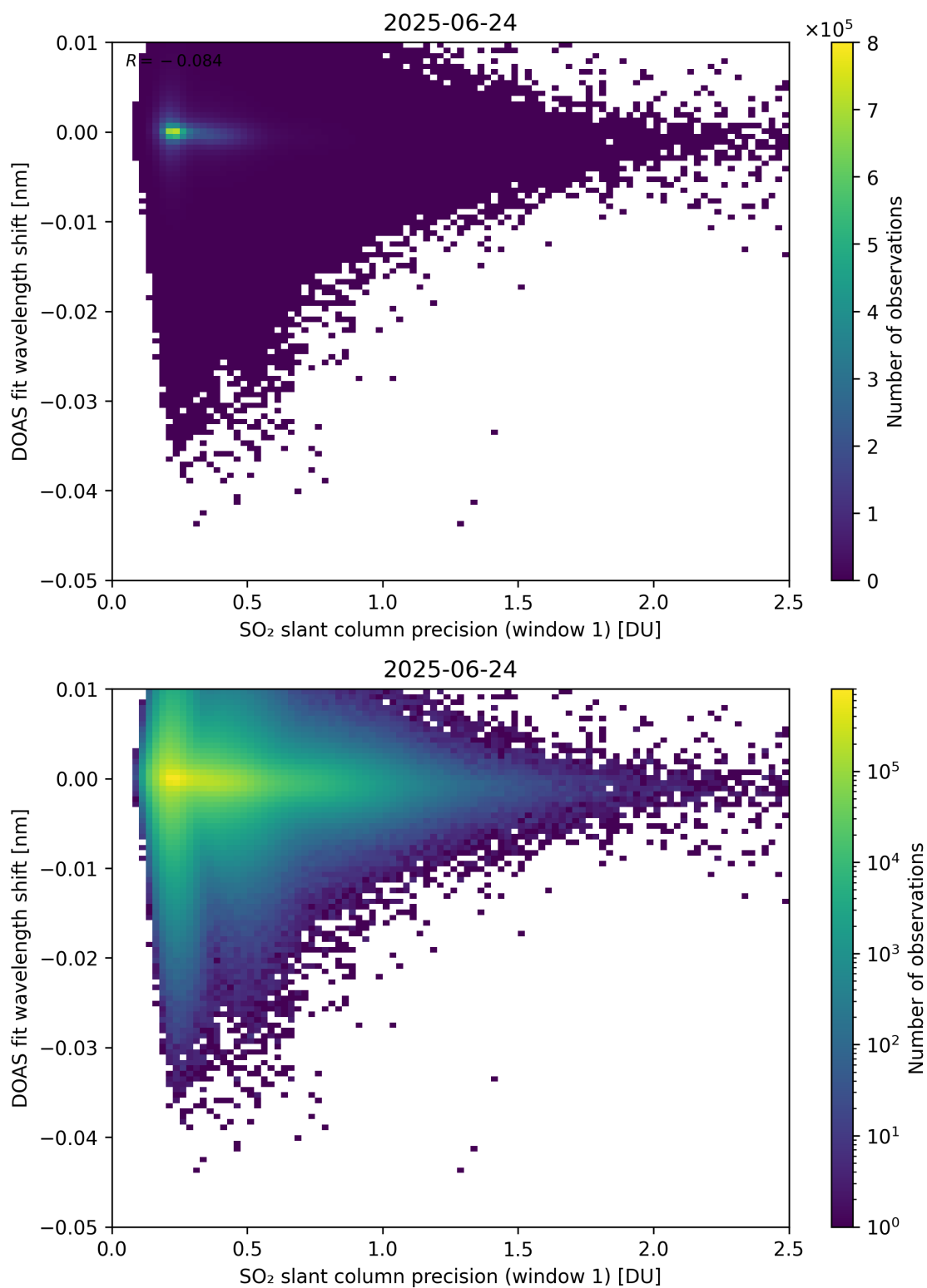
Figure 271: Scatter density plot of “SO 2 slant column precision (window 1)” against “DOAS fit wavelength shift” for 2025-06-23 to 2025-06-25.
