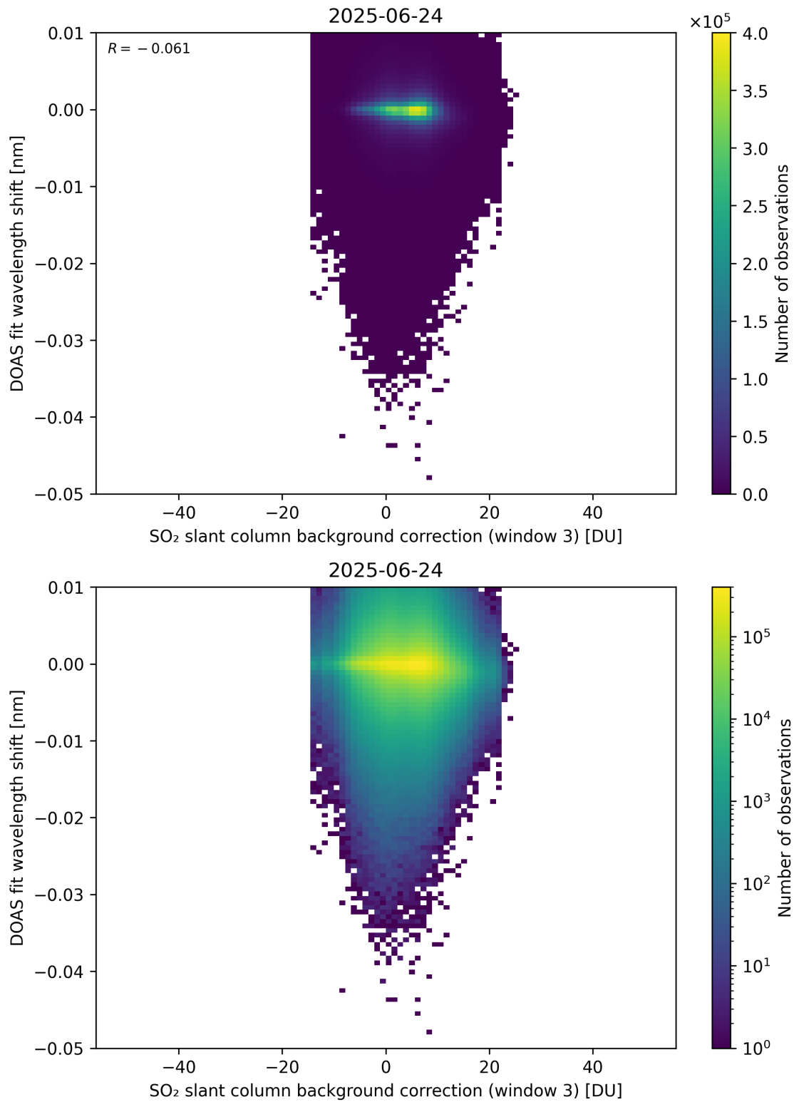
Figure 132: Scatter density plot of “SO 2 slant column background correction (window 3)” against “DOAS fit wavelength shift” for 2025-06-23 to 2025-06-25.
