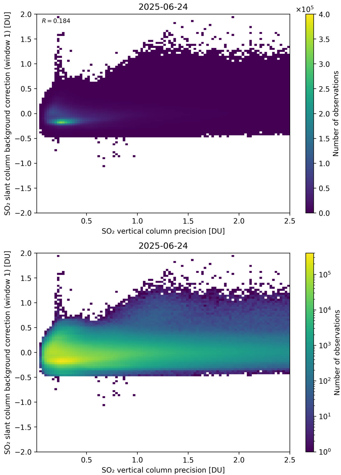
Figure 329: Scatter density plot of “SO 2 vertical column precision” against “SO 2 slant column background correction (window 1)” for 2025-06-23 to 2025-06-25.
