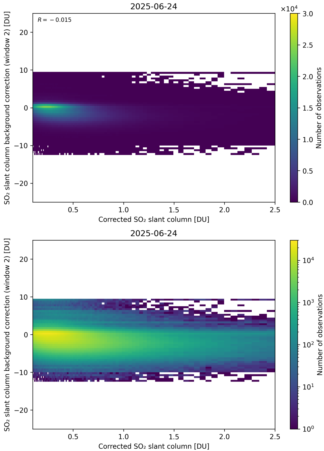
Figure 227: Scatter density plot of “Corrected SO 2 slant column” against “SO 2 slant column background correction (window 2)” for 2025-06-23 to 2025-06-25.
