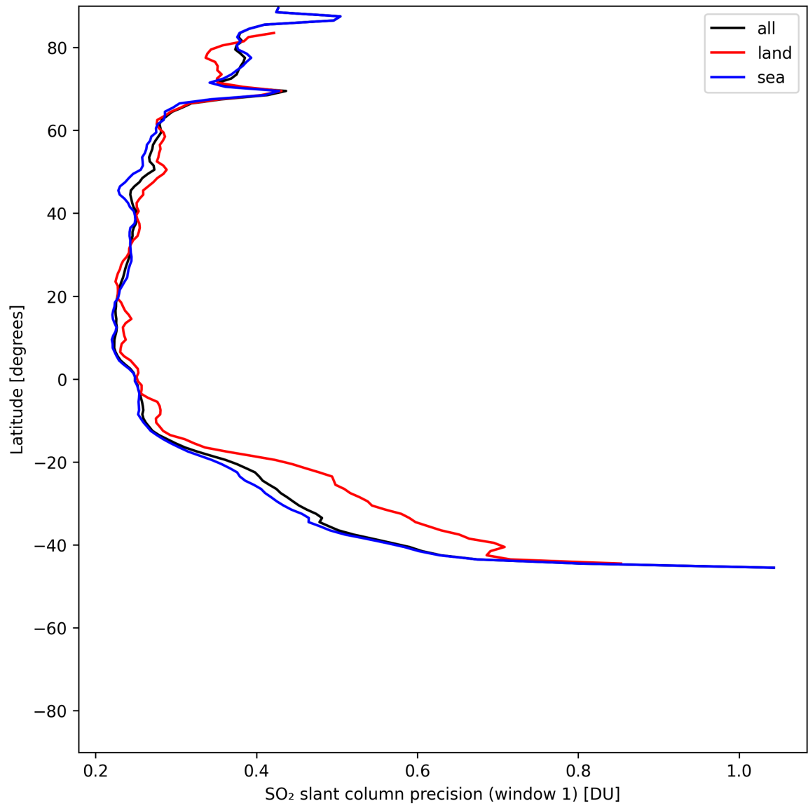
Figure 38: Zonal average of “SO 2 slant column precision (window 1)” for 2025-06-23 to 2025-06-25.
