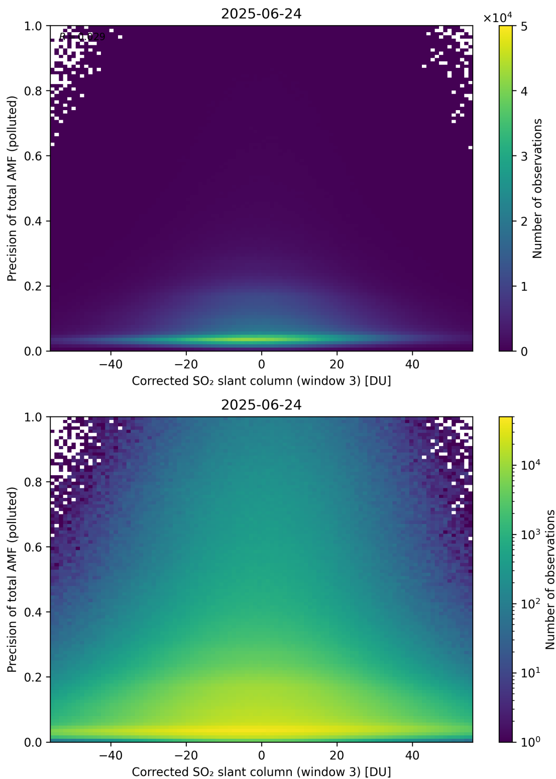
Figure 261: Scatter density plot of “Corrected SO 2 slant column (window 3)” against “Precision of total AMF (polluted)” for 2025-06-23 to 2025-06-25.
