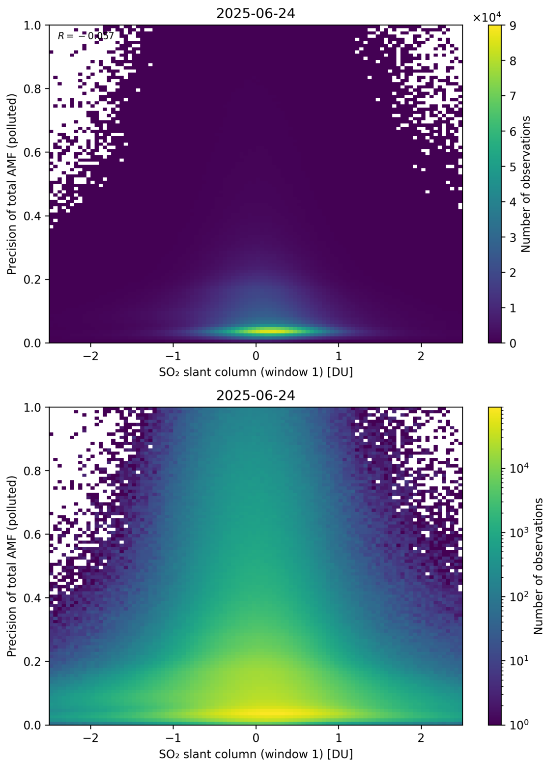
Figure 290: Scatter density plot of “SO 2 slant column (window 1)” against “Precision of total AMF (polluted)” for 2025-06-23 to 2025-06-25.
