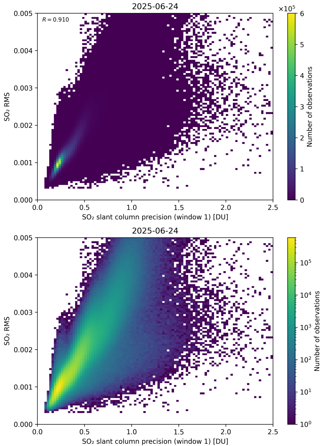
Figure 273: Scatter density plot of “SO 2 slant column precision (window 1)” against “SO 2 RMS” for 2025-06-23 to 2025-06-25.
