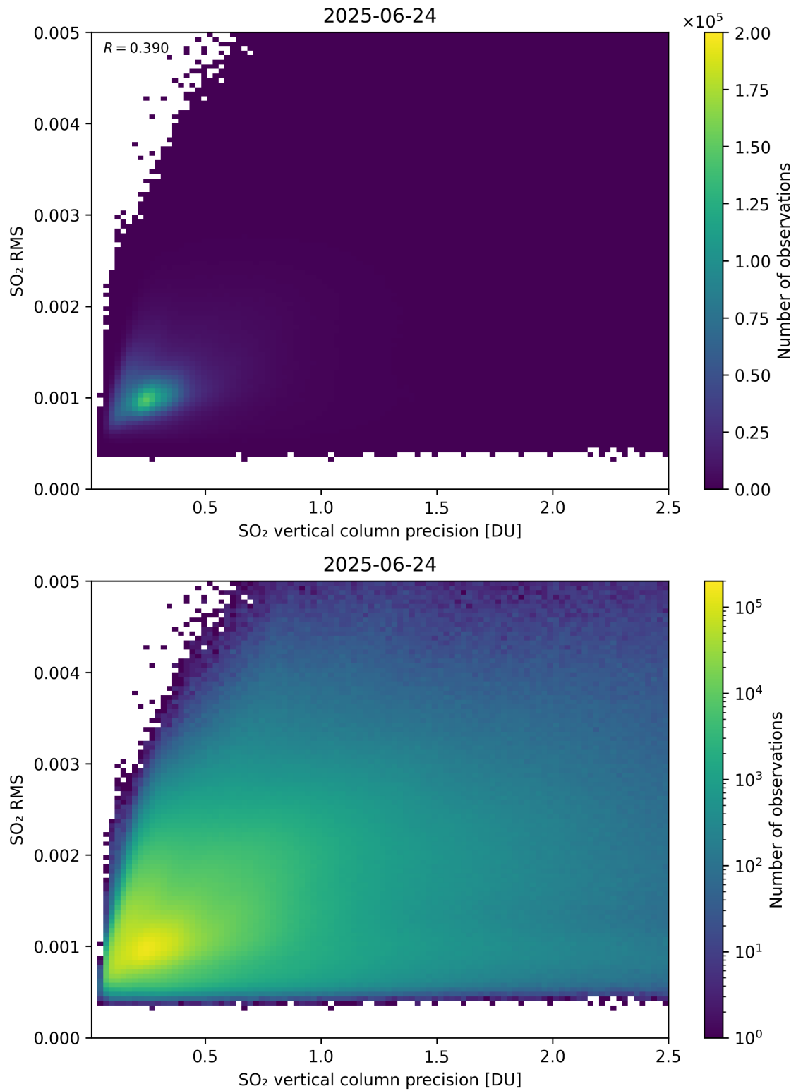
Figure 334: Scatter density plot of “SO 2 vertical column precision” against “SO 2 RMS” for 2025-06-23 to 2025-06-25.
