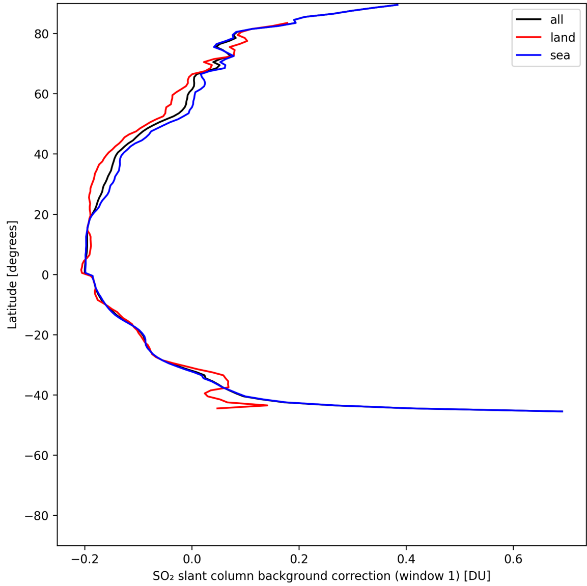
Figure 40: Zonal average of “SO 2 slant column background correction (window 1)” for 2025-06-23 to 2025-06-25.
