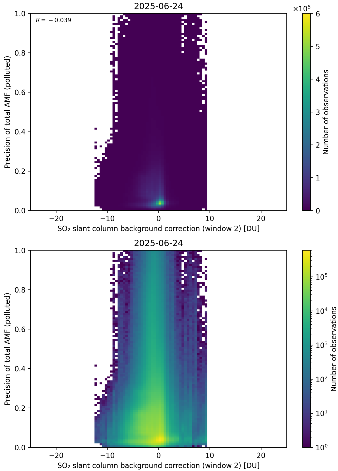
Figure 131: Scatter density plot of “SO 2 slant column background correction (window 2)” against “Precision of total AMF (polluted)” for 2025-06-23 to 2025-06-25.
