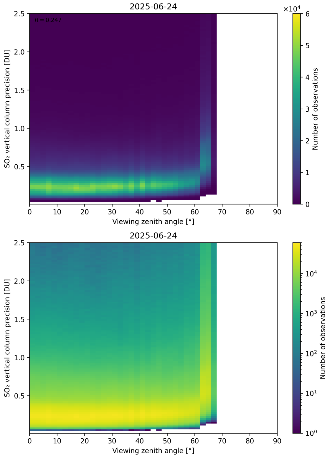
Figure 384: Scatter density plot of “Viewing zenith angle” against “SO 2 vertical column precision” for 2025-06-23 to 2025-06-25.
