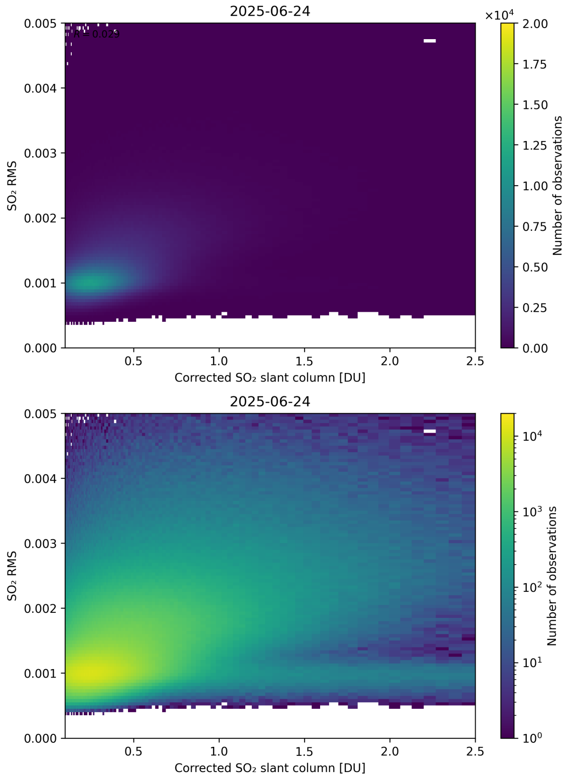
Figure 231: Scatter density plot of “Corrected SO 2 slant column” against “SO 2 RMS” for 2025-06-23 to 2025-06-25.
