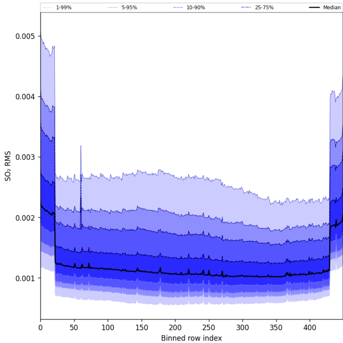
Figure 104: Along track statistics of “SO 2 RMS” for 2025-06-23 to 2025-06-25
