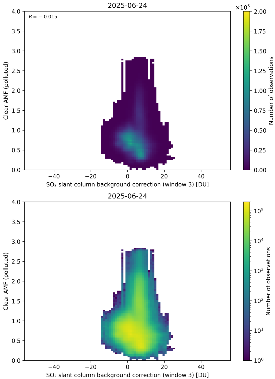
Figure 135: Scatter density plot of “SO 2 slant column background correction (window 3)” against “Clear AMF (polluted)” for 2025-06-23 to 2025-06-25.
