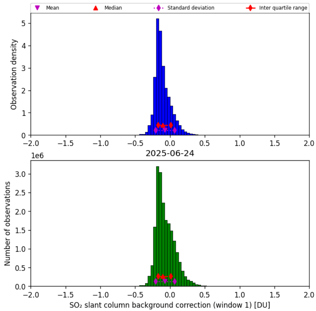
Figure 66: Histogram of “SO 2 slant column background correction (window 1)” for 2025-06-23 to 2025-06-25
