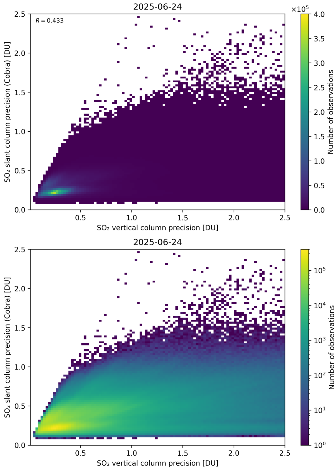
Figure 337: Scatter density plot of “SO 2 vertical column precision” against “SO 2 slant column precision (Cobra)” for 2025-06-23 to 2025-06-25.
