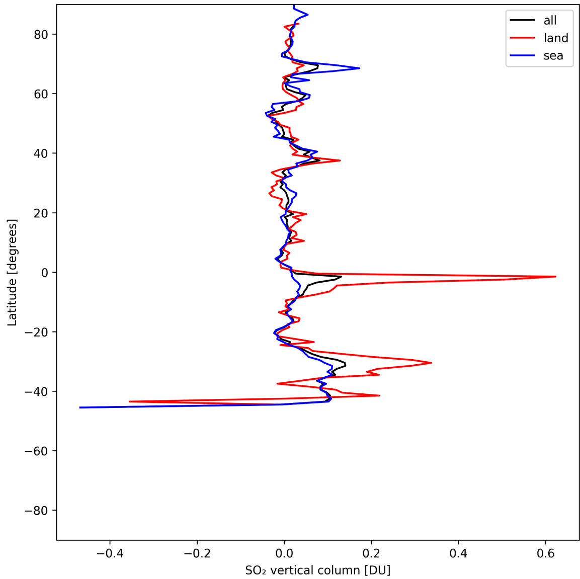
Figure 32: Zonal average of “SO 2 vertical column” for 2025-06-23 to 2025-06-25.
