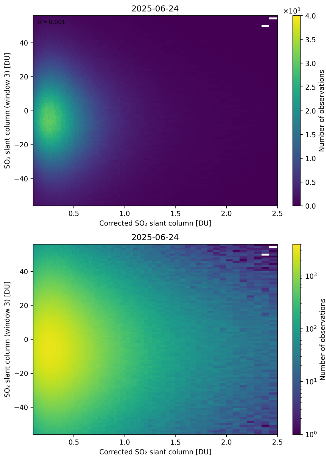
Figure 240: Scatter density plot of “Corrected SO 2 slant column” against “SO 2 slant column (window 3)” for 2025-06-23 to 2025-06-25.
