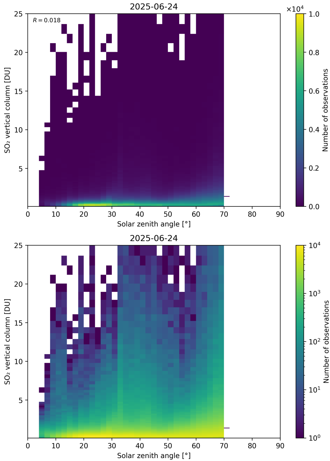
Figure 191: Scatter density plot of “Solar zenith angle” against “SO 2 vertical column” for 2025-06-23 to 2025-06-25.
