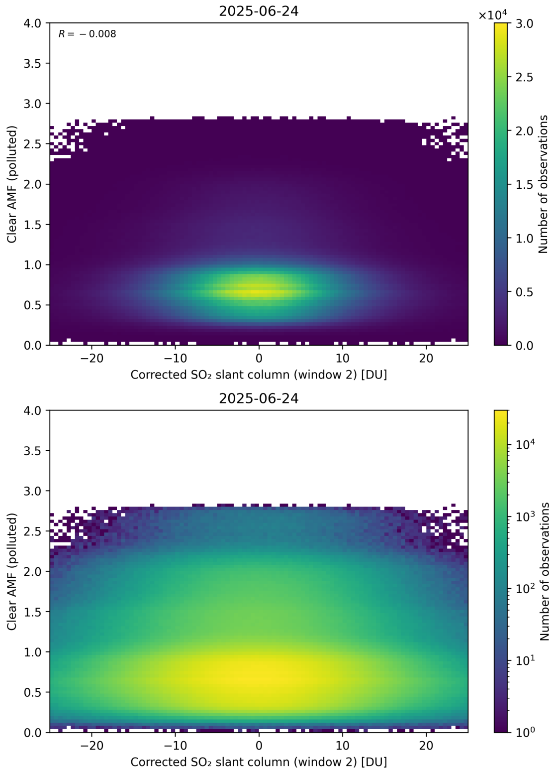
Figure 249: Scatter density plot of “Corrected SO 2 slant column (window 2)” against “Clear AMF (polluted)” for 2025-06-23 to 2025-06-25.
