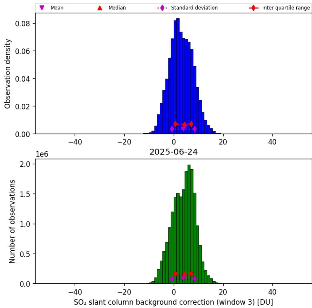
Figure 74: Histogram of “SO 2 slant column background correction (window 3)” for 2025-06-23 to 2025-06-25
