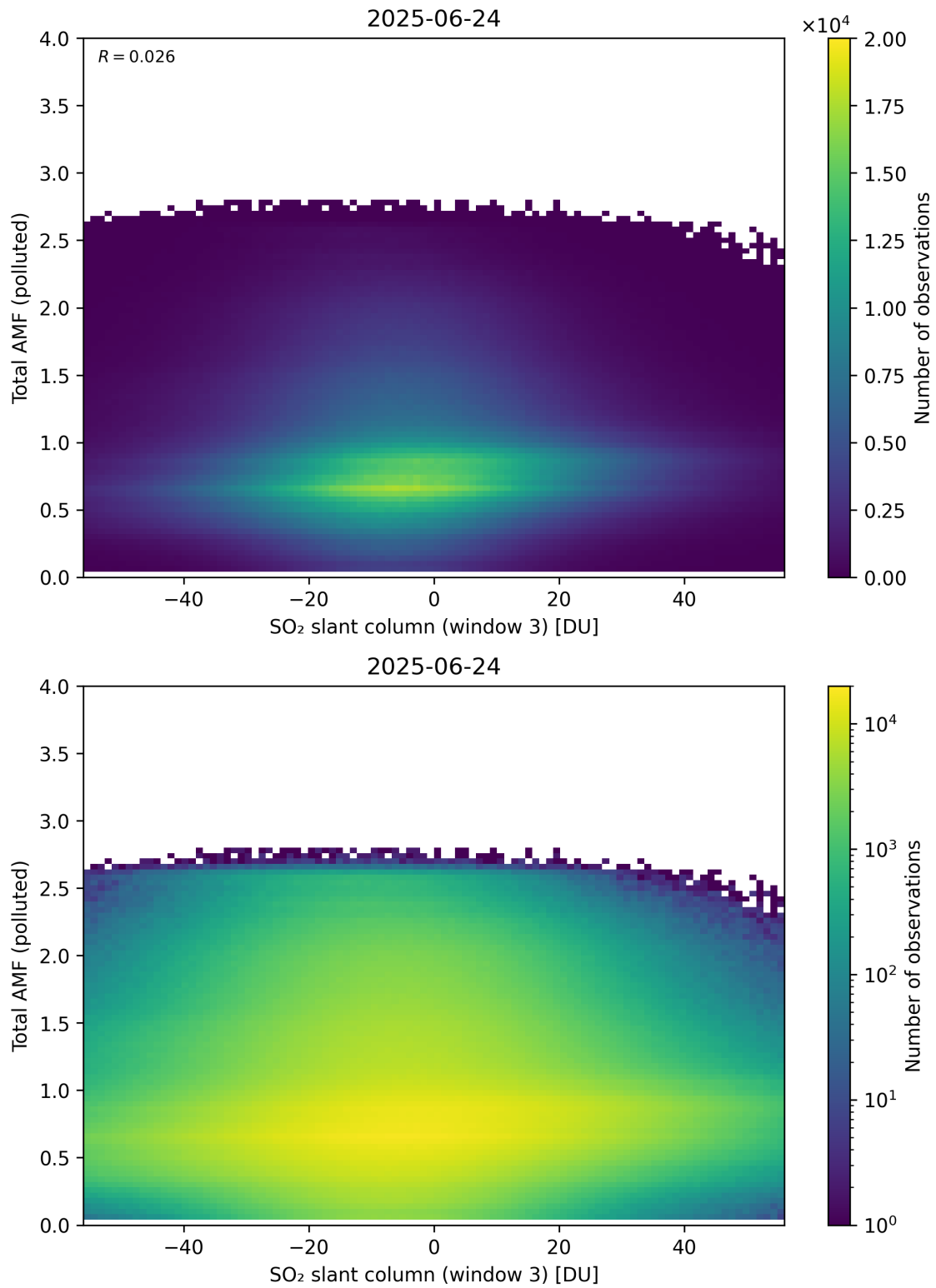
Figure 318: Scatter density plot of “SO 2 slant column (window 3)” against “Total AMF (polluted)” for 2025-06-23 to 2025-06-25.
