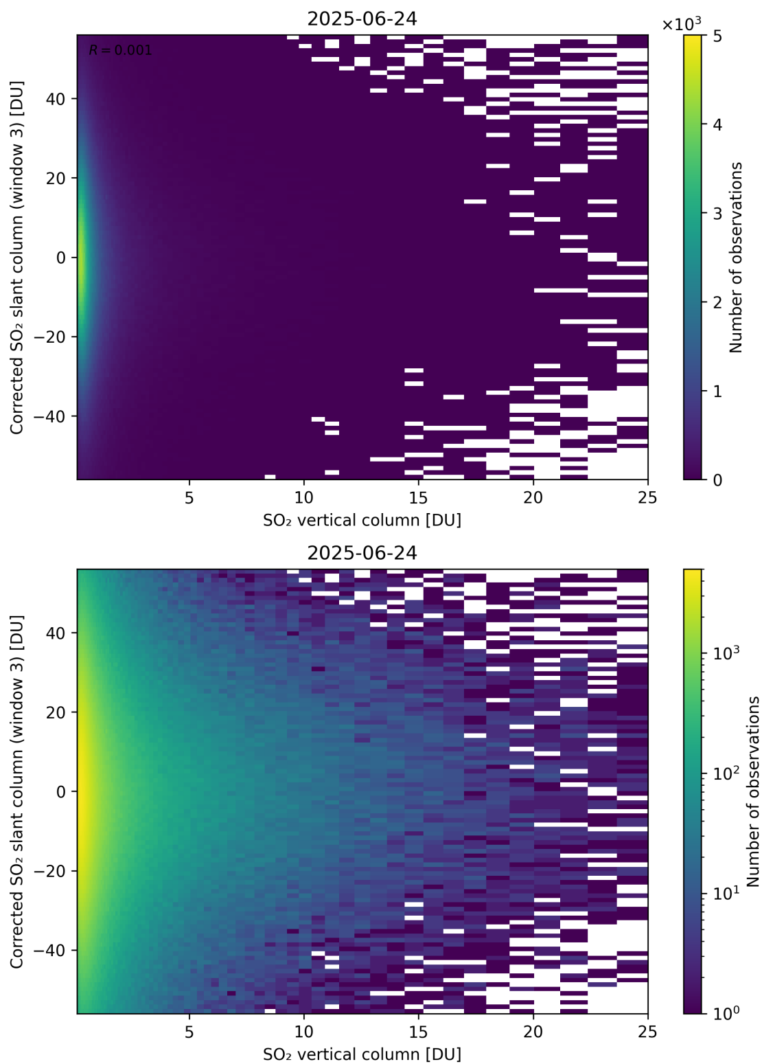
Figure 353: Scatter density plot of “SO 2 vertical column” against “Corrected SO 2 slant column (window 3)” for 2025-06-23 to 2025-06-25.
