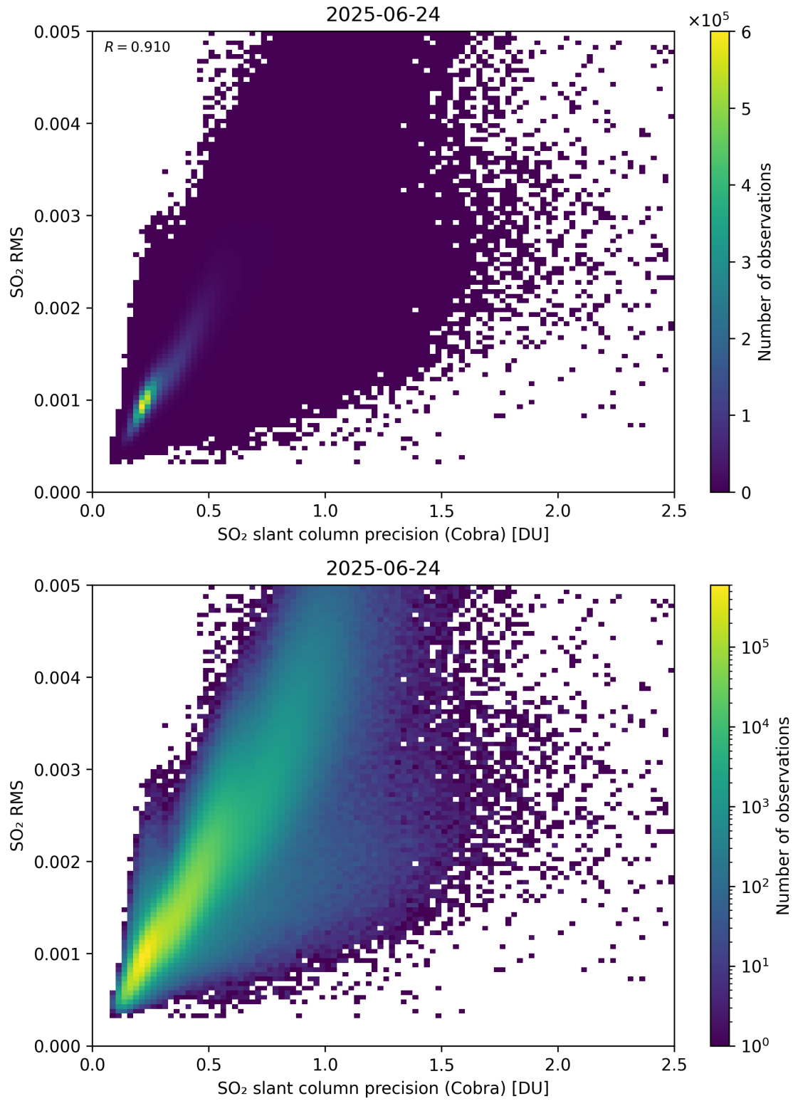
Figure 204: Scatter density plot of “SO 2 slant column precision (Cobra)” against “SO 2 RMS” for 2025-06-23 to 2025-06-25.
