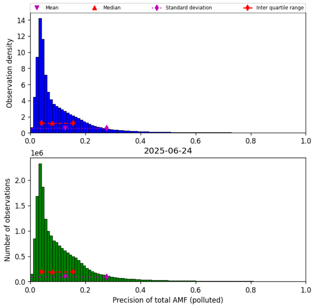
Figure 80: Histogram of “Precision of total AMF (polluted)” for 2025-06-23 to 2025-06-25
