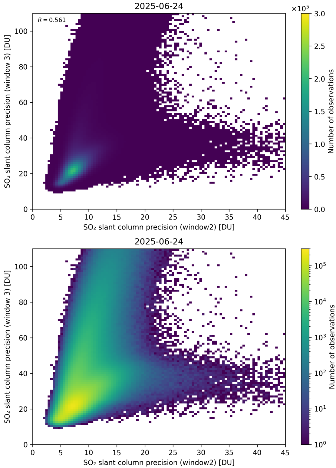
Figure 300: Scatter density plot of “SO 2 slant column precision (window2)” against “SO 2 slant column precision (window 3)” for 2025-06-23 to 2025-06-25.
