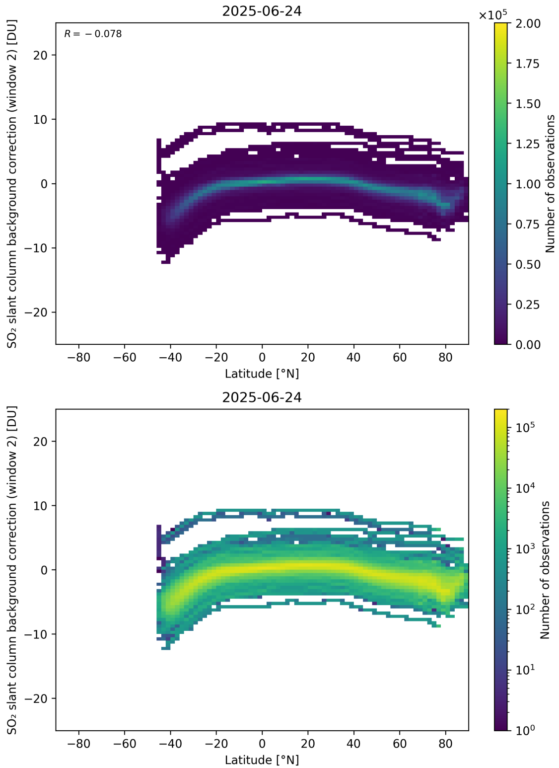
Figure 151: Scatter density plot of “Latitude” against “SO 2 slant column background correction (window 2)” for 2025-06-23 to 2025-06-25.
