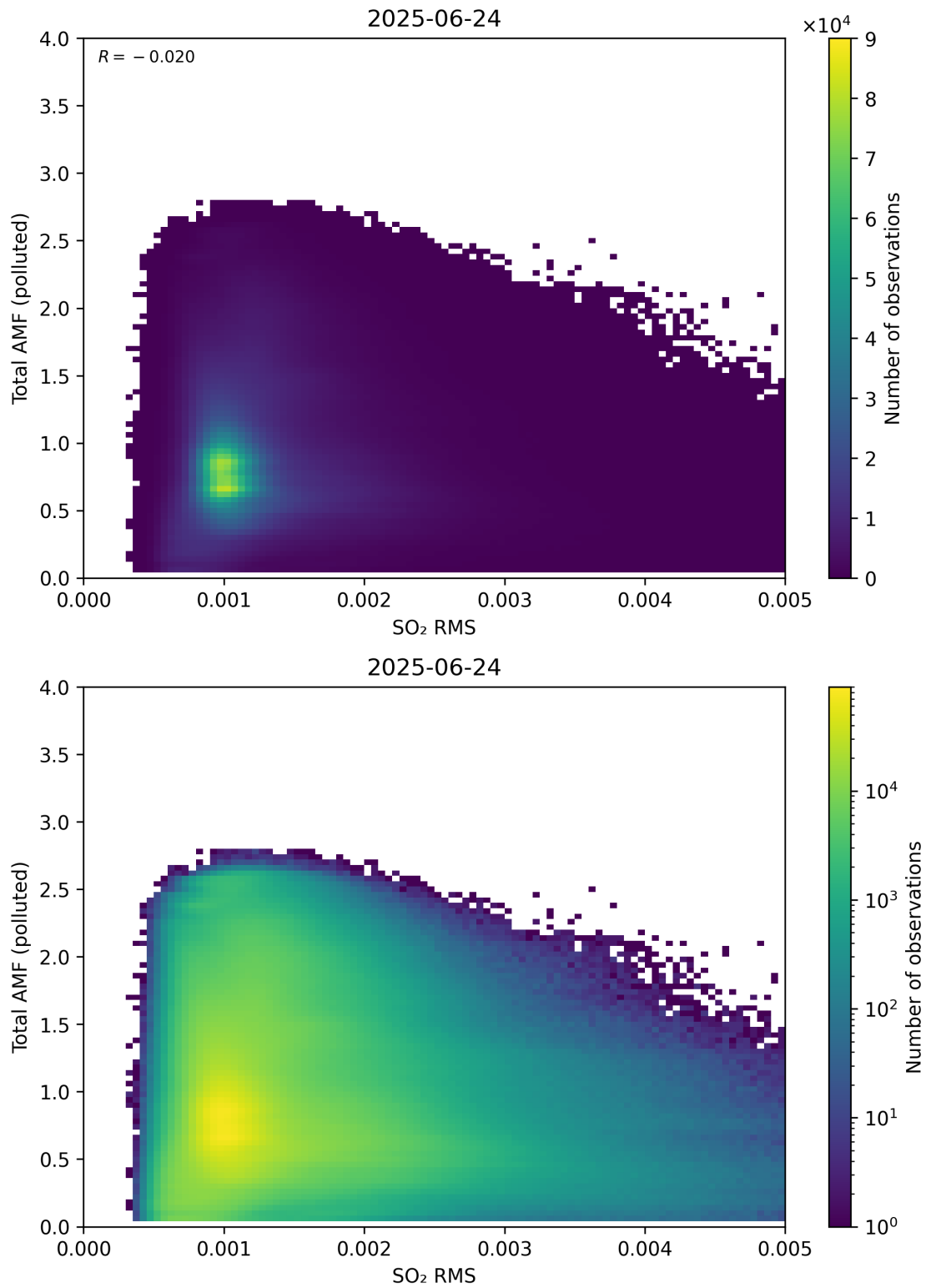
Figure 148: Scatter density plot of “SO 2 RMS” against “Total AMF (polluted)” for 2025-06-23 to 2025-06-25.
