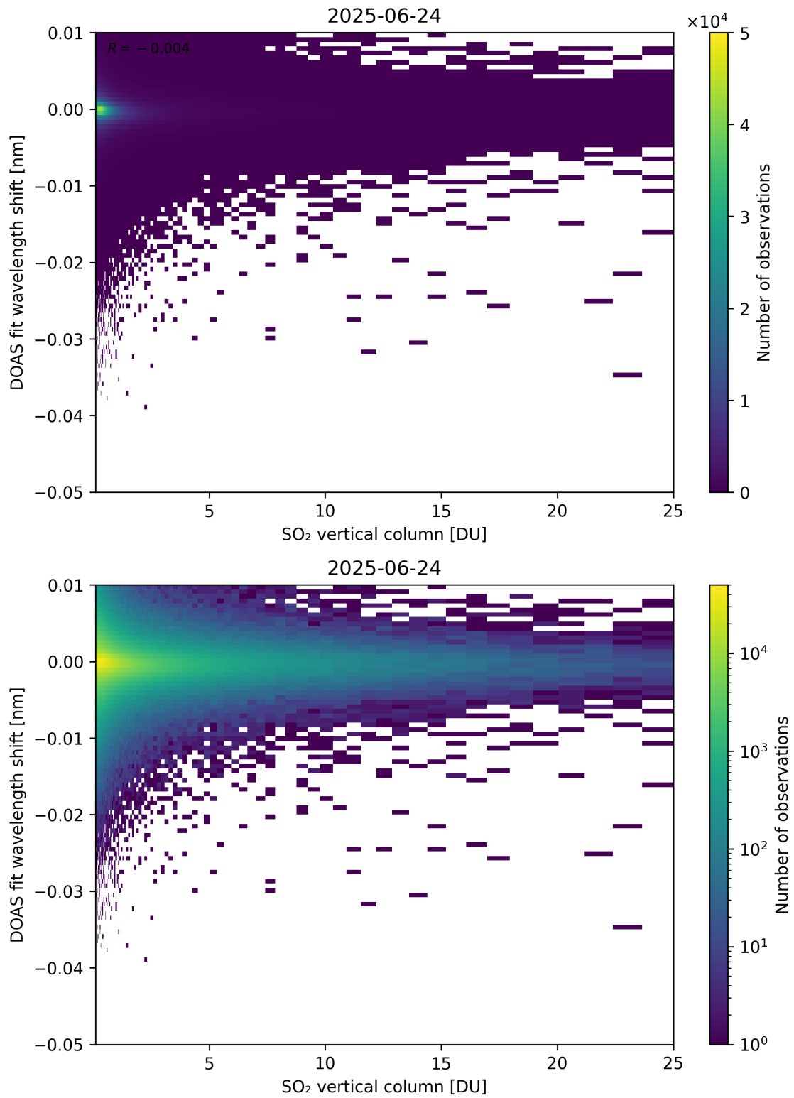
Figure 326: Scatter density plot of “SO 2 vertical column” against “DOAS fit wavelength shift” for 2025-06-23 to 2025-06-25.
