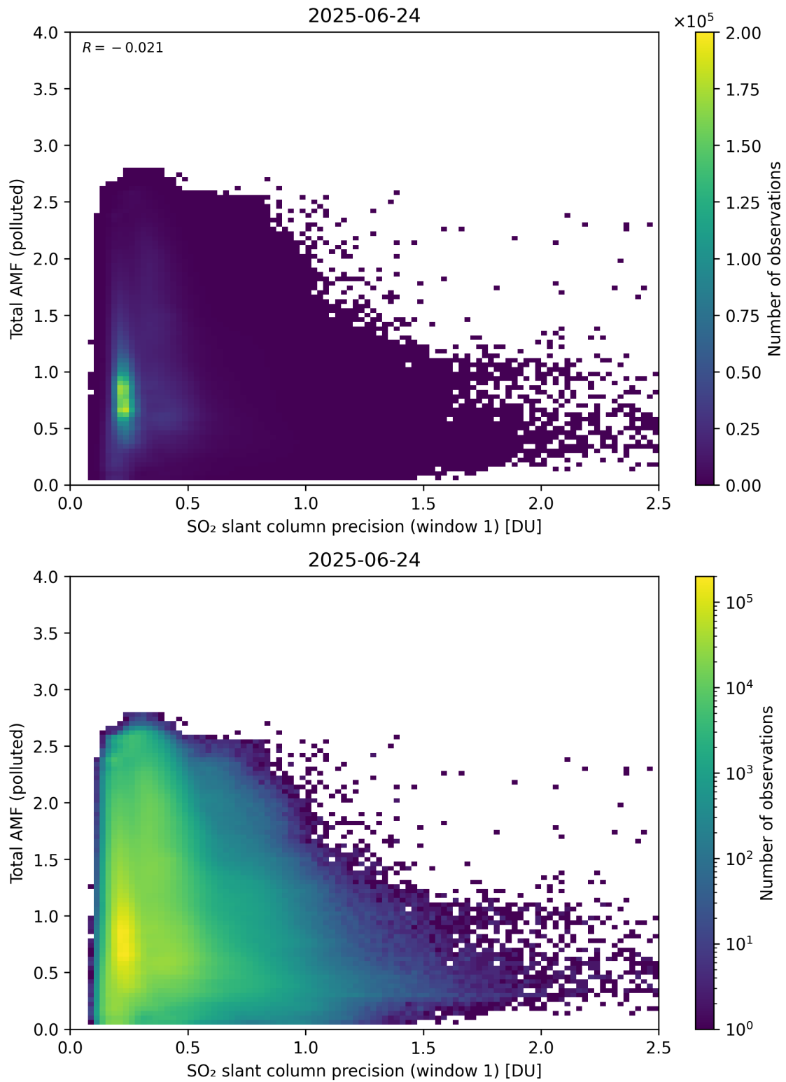
Figure 280: Scatter density plot of “SO 2 slant column precision (window 1)” against “Total AMF (polluted)” for 2025-06-23 to 2025-06-25.
