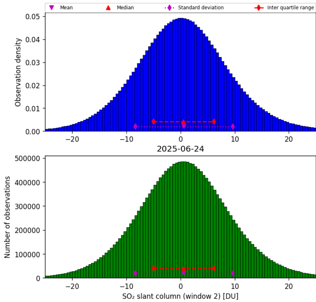
Figure 67: Histogram of “SO 2 slant column (window 2)” for 2025-06-23 to 2025-06-25
