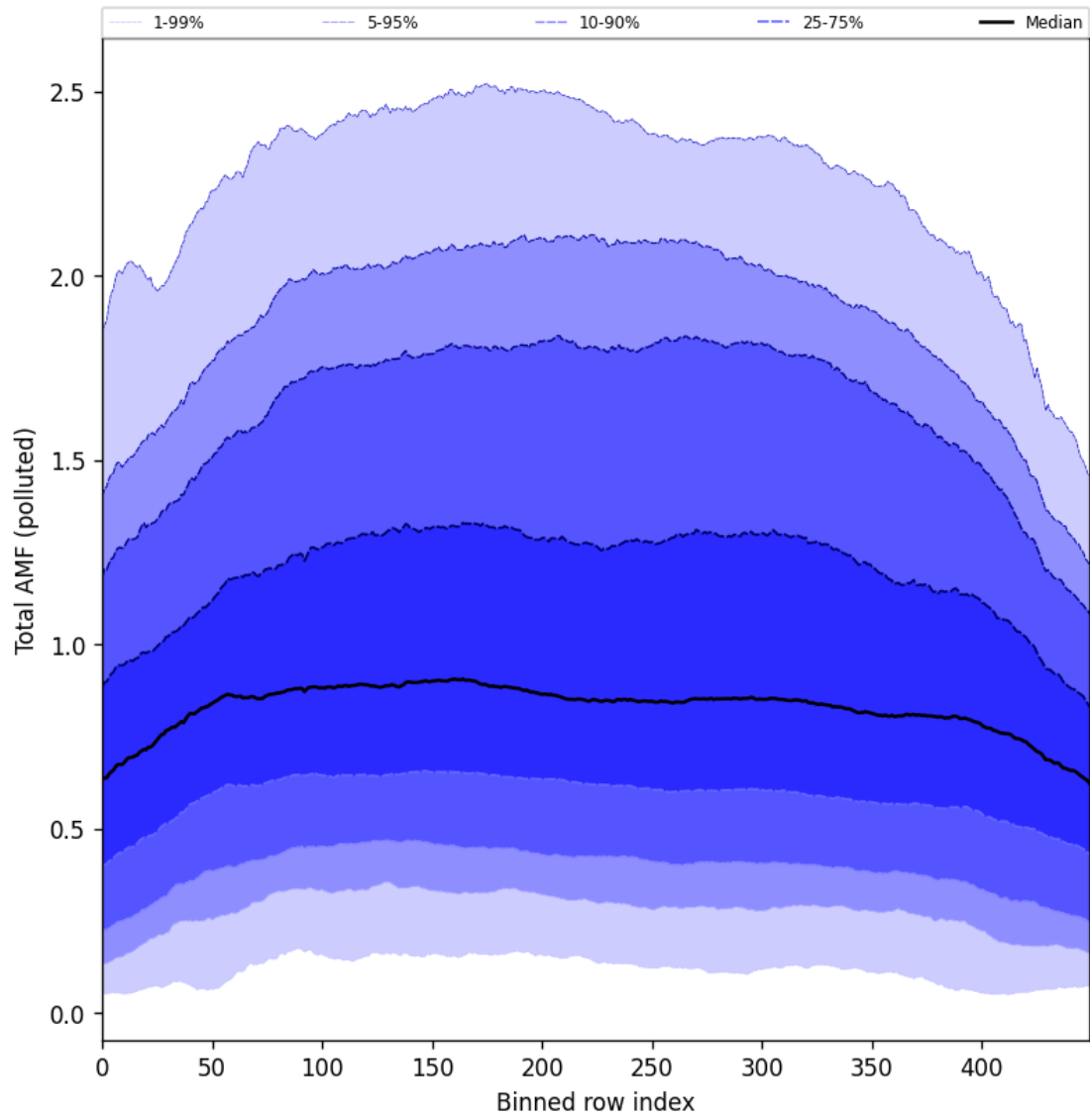
Figure 105: Along track statistics of “Total AMF (polluted)” for 2025-06-23 to 2025-06-25
