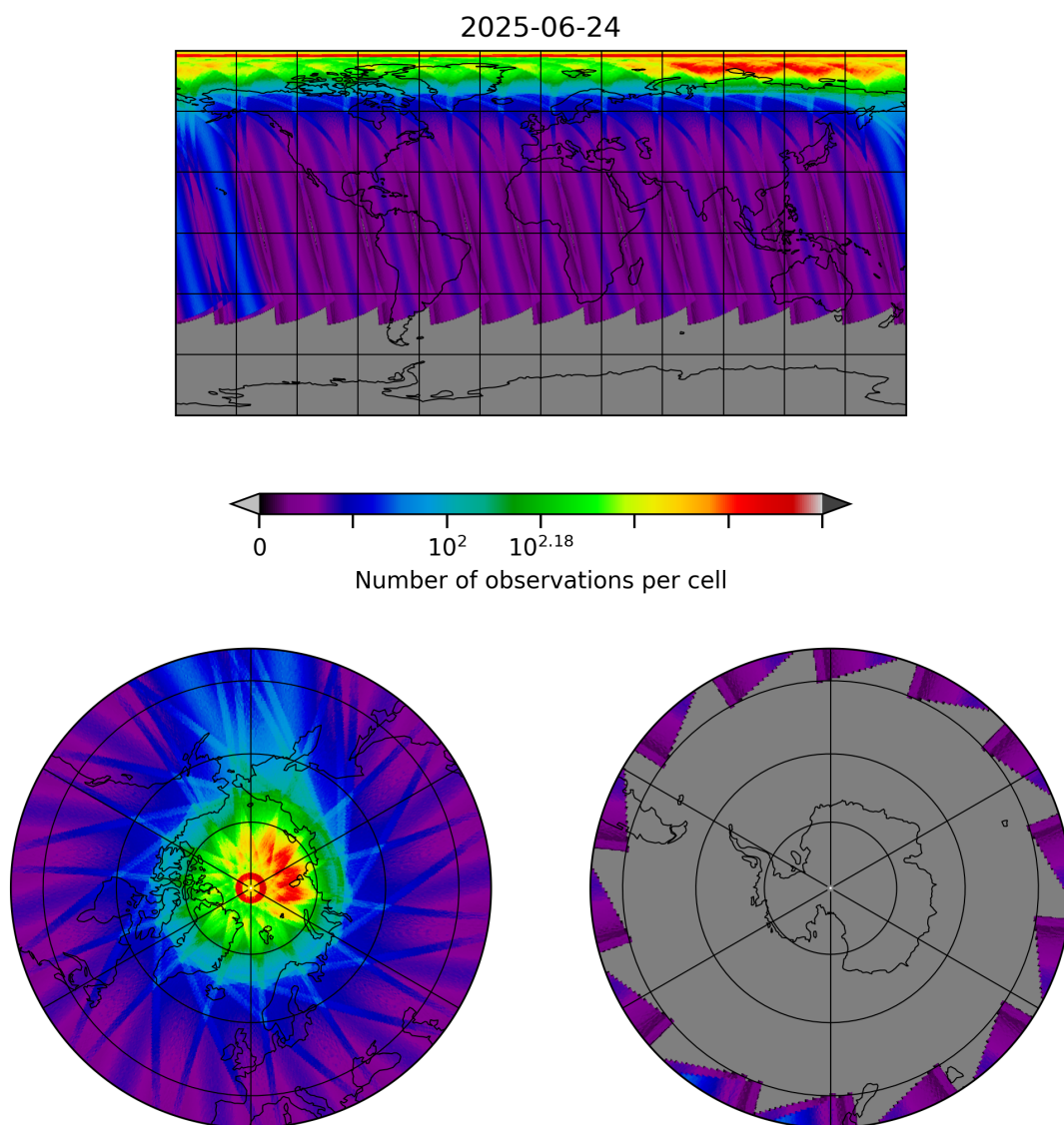
Figure 30: Map of the number of observations for 2025-06-23 to 2025-06-25
