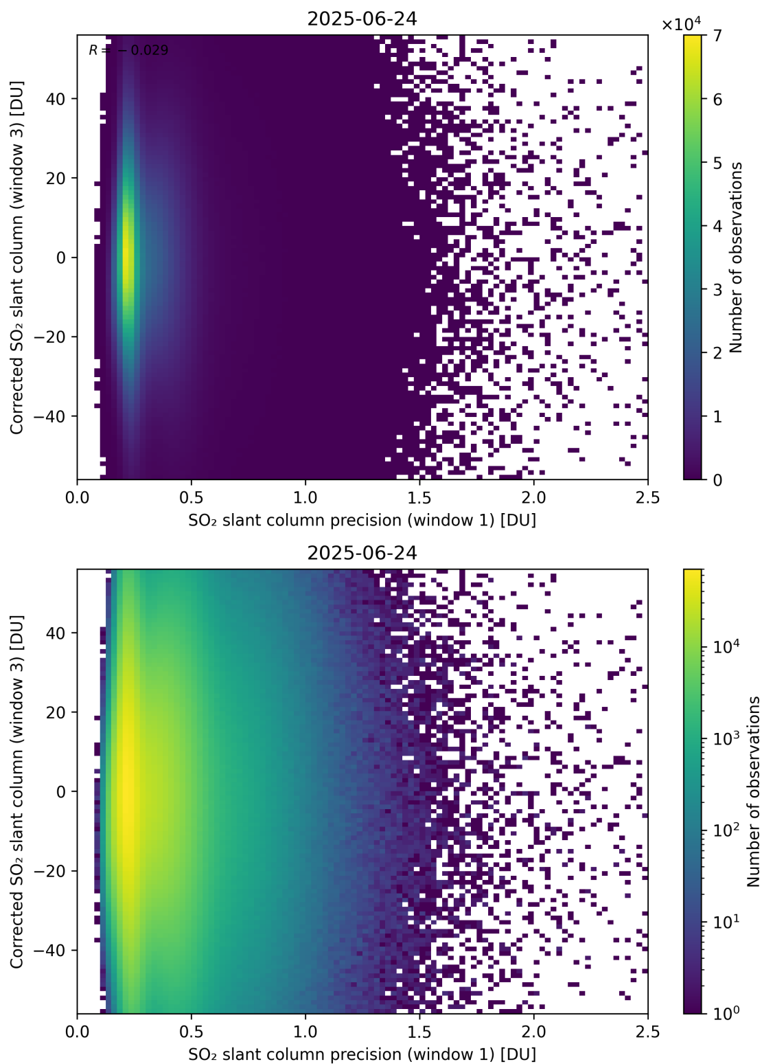
Figure 276: Scatter density plot of “SO 2 slant column precision (window 1)” against “Corrected SO 2 slant column (window 3)” for 2025-06-23 to 2025-06-25.
