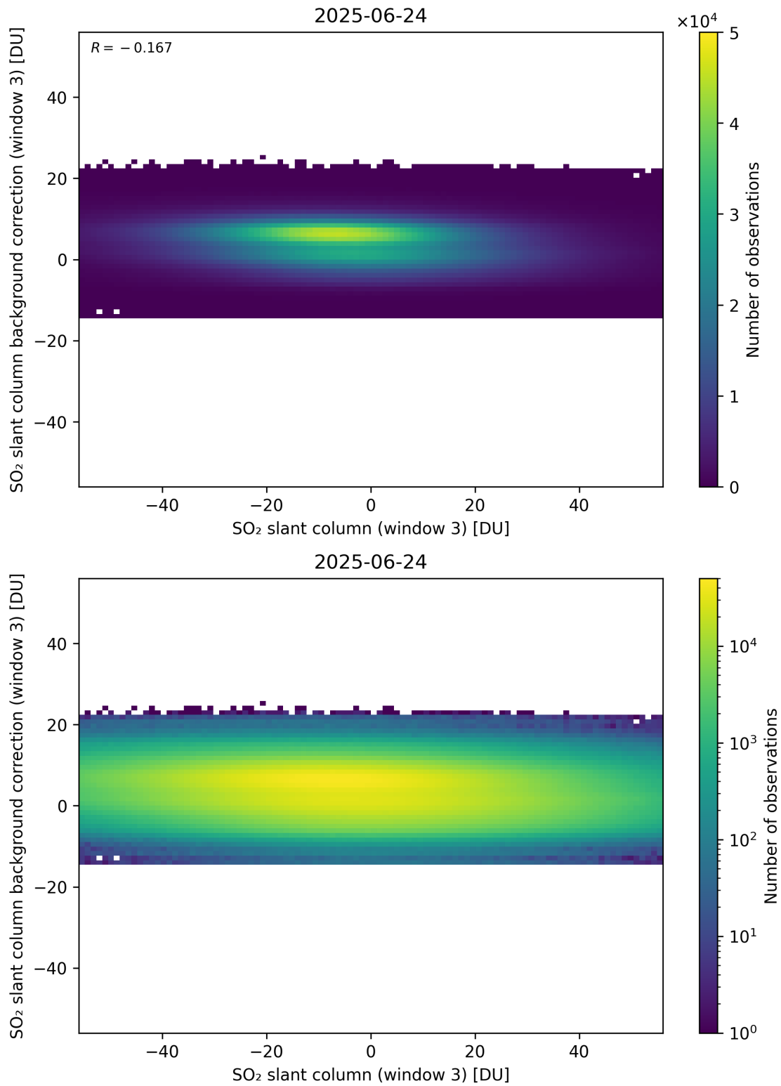
Figure 303: Scatter density plot of “SO 2 slant column (window 3)” against “SO 2 slant column background correction (window 3)” for 2025-06-23 to 2025-06-25.
