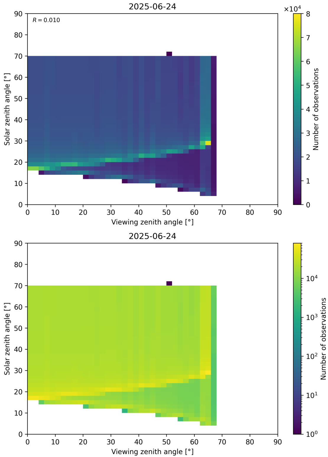
Figure 369: Scatter density plot of “Viewing zenith angle” against “Solar zenith angle” for 2025-06-23 to 2025-06-25.
