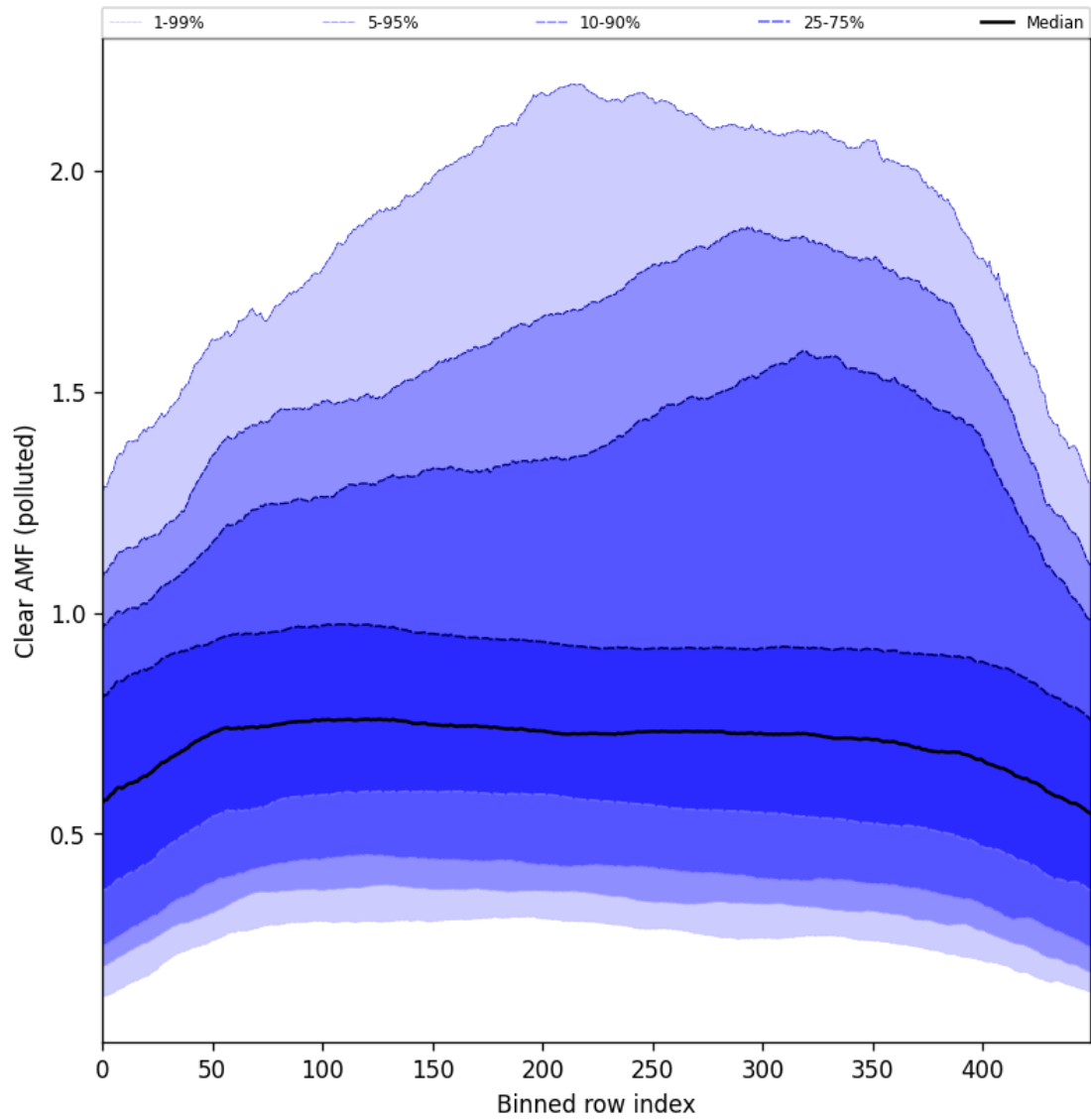
Figure 107: Along track statistics of “Clear AMF (polluted)” for 2025-06-23 to 2025-06-25
