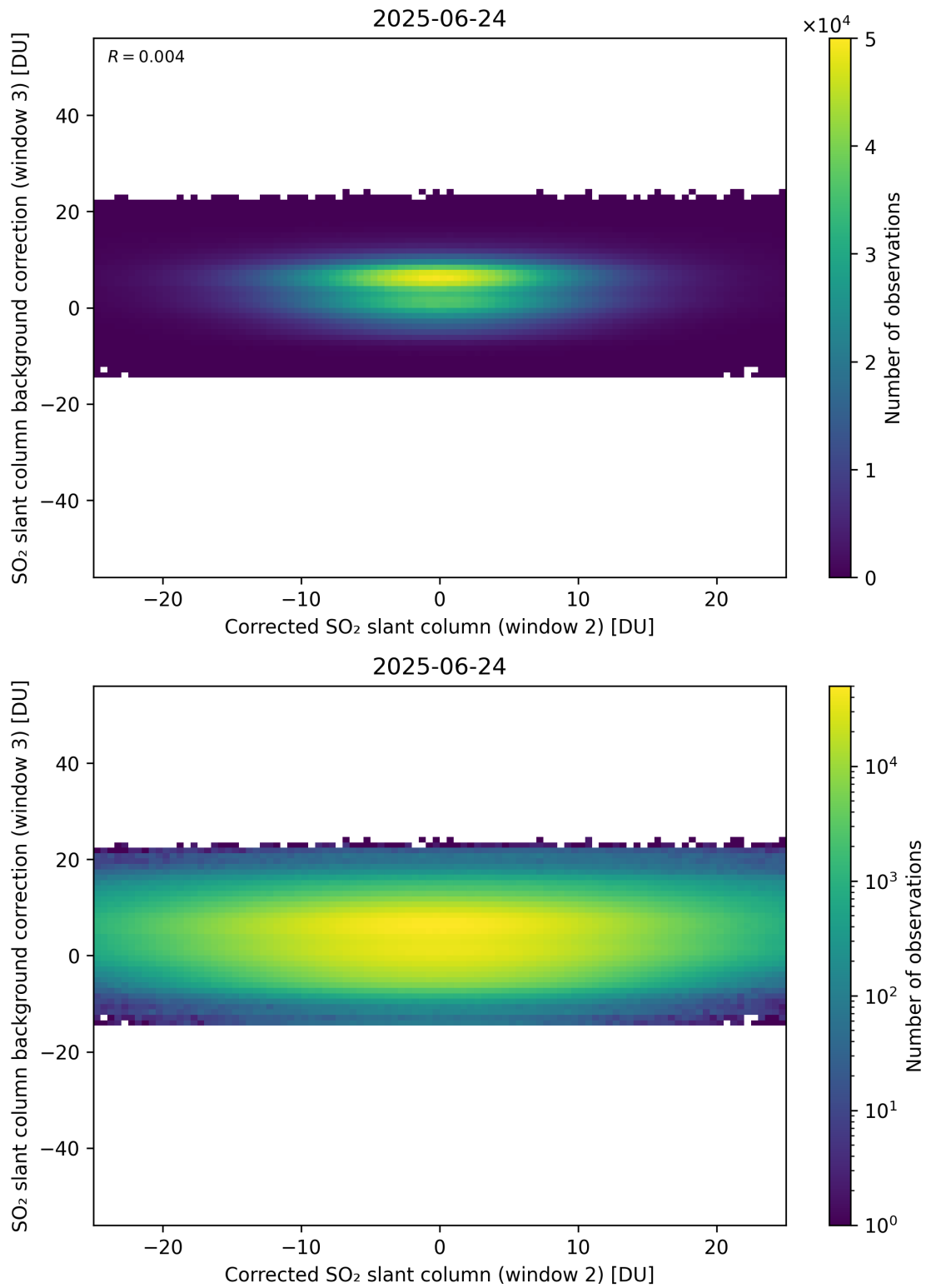
Figure 245: Scatter density plot of “Corrected SO 2 slant column (window 2)” against “SO 2 slant column background correction (window 3)” for 2025-06-23 to 2025-06-25.
