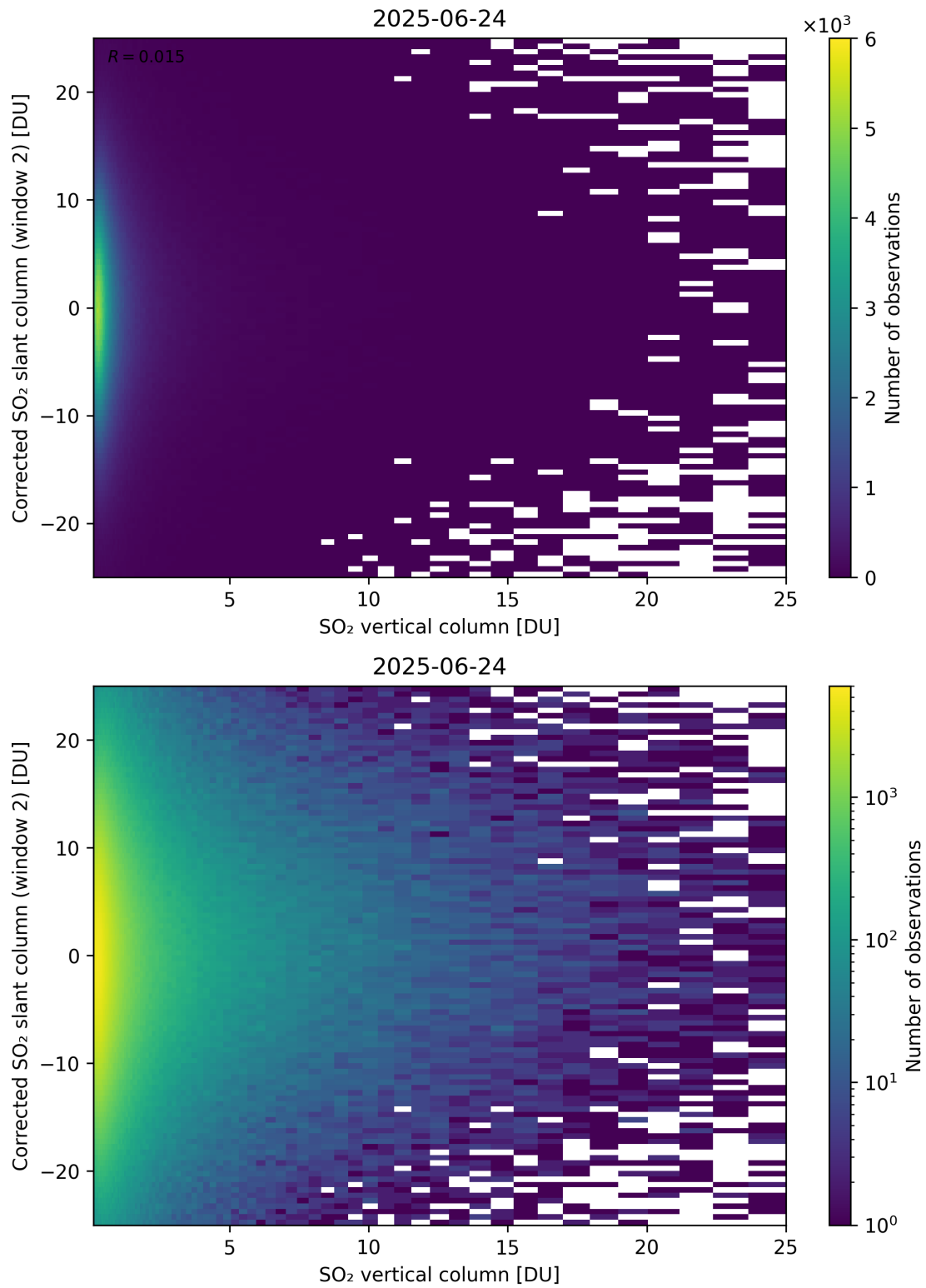
Figure 352: Scatter density plot of “SO 2 vertical column” against “Corrected SO 2 slant column (window 2)” for 2025-06-23 to 2025-06-25.
