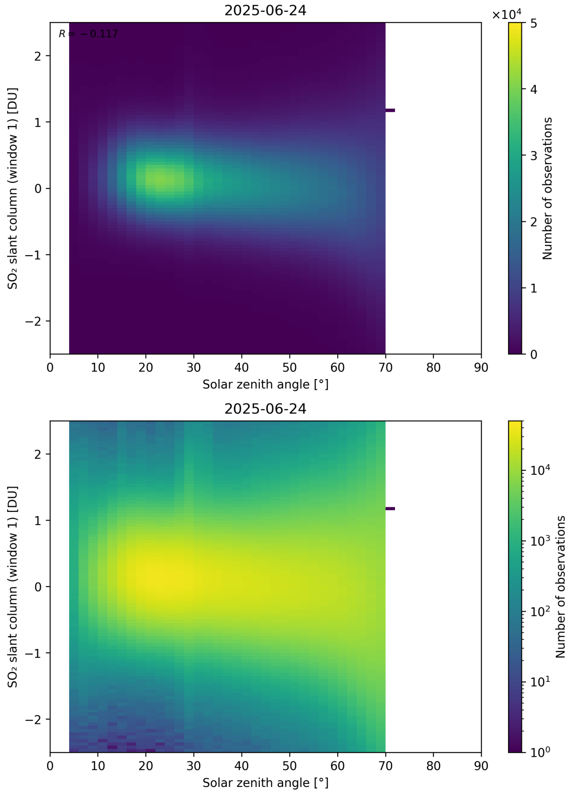
Figure 184: Scatter density plot of “Solar zenith angle” against “SO 2 slant column (window 1)” for 2025-06-23 to 2025-06-25.
