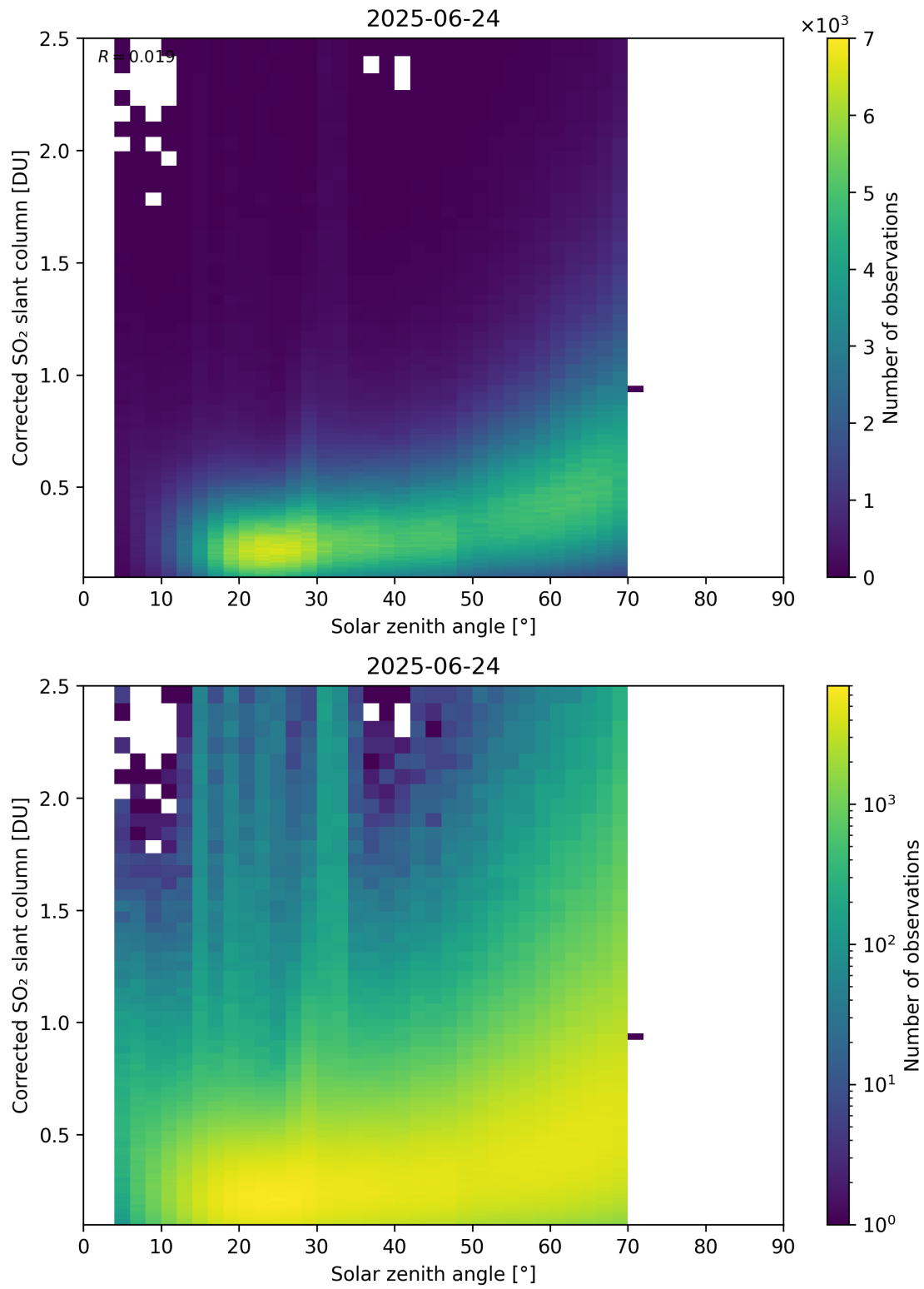
Figure 181: Scatter density plot of “Solar zenith angle” against “Corrected SO 2 slant column” for 2025-06-23 to 2025-06-25.
