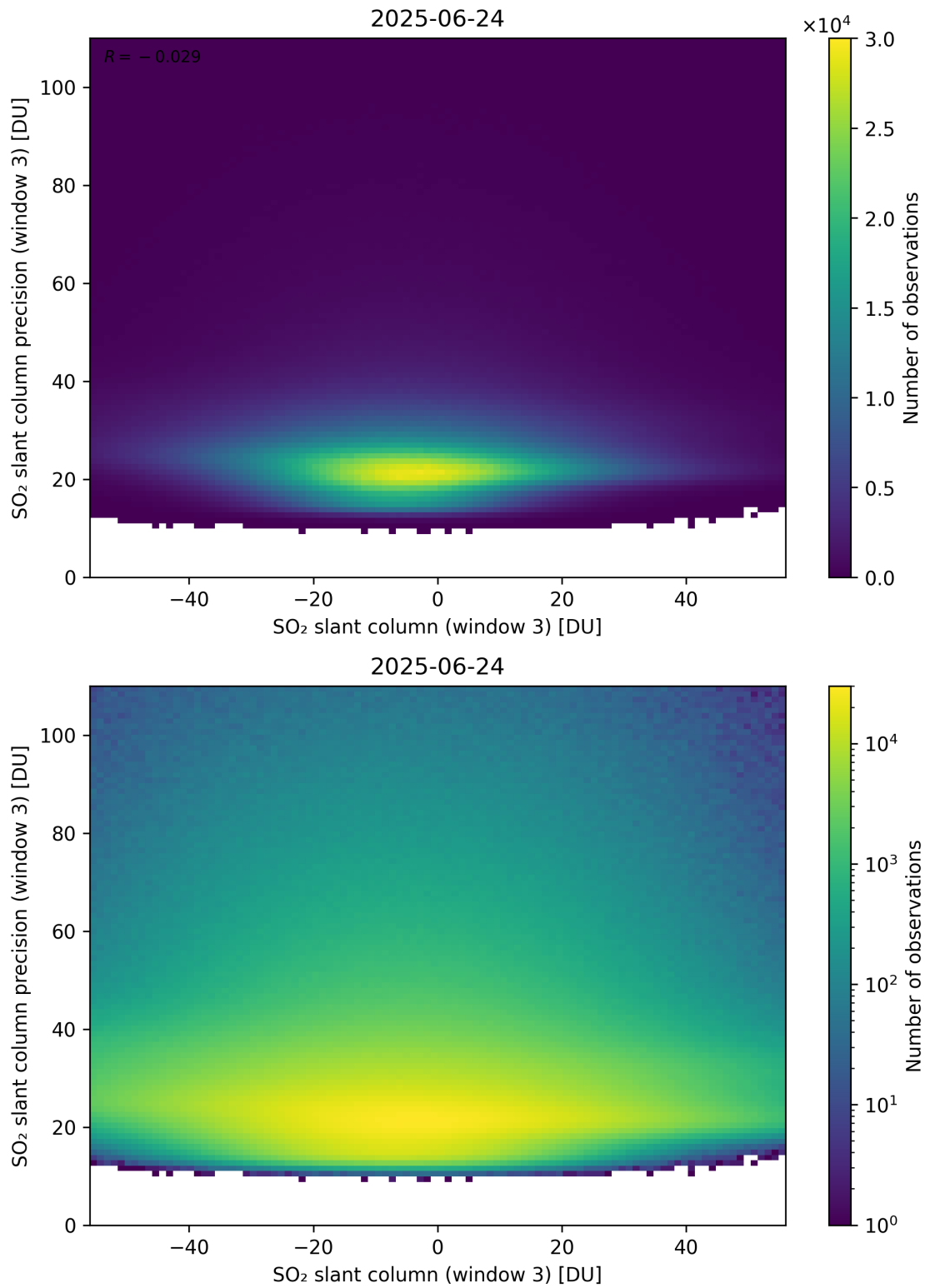
Figure 317: Scatter density plot of “SO 2 slant column (window 3)” against “SO 2 slant column precision (window 3)” for 2025-06-23 to 2025-06-25.
