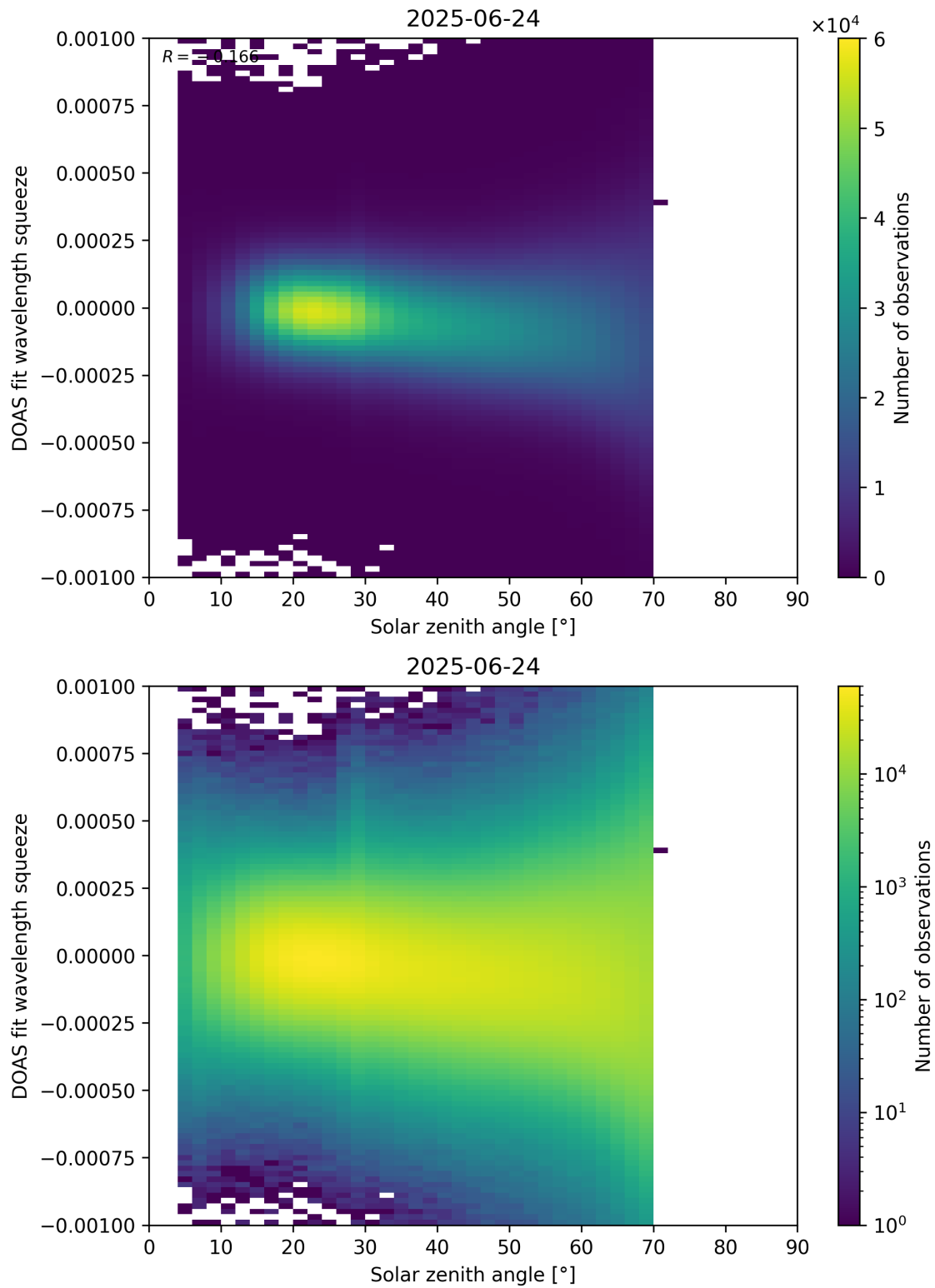
Figure 175: Scatter density plot of “Solar zenith angle” against “DOAS fit wavelength squeeze” for 2025-06-23 to 2025-06-25.
