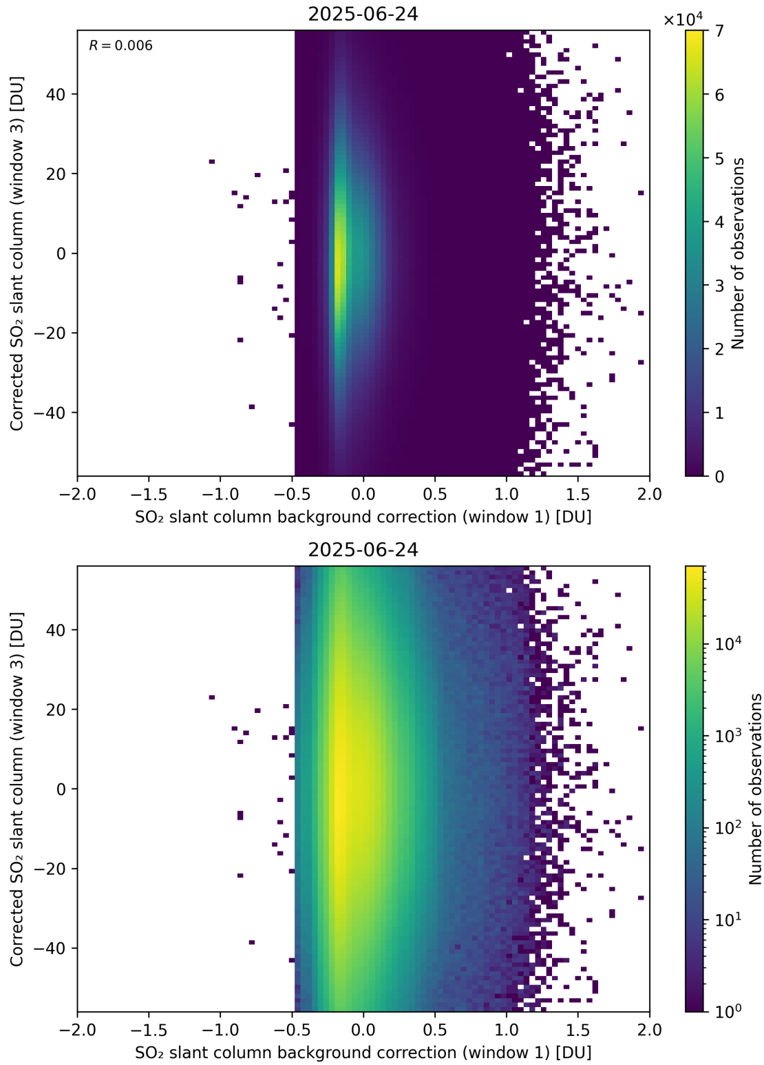
Figure 116: Scatter density plot of “SO 2 slant column background correction (window 1)” against “Corrected SO 2 slant column (window 3)” for 2025-06-23 to 2025-06-25.
