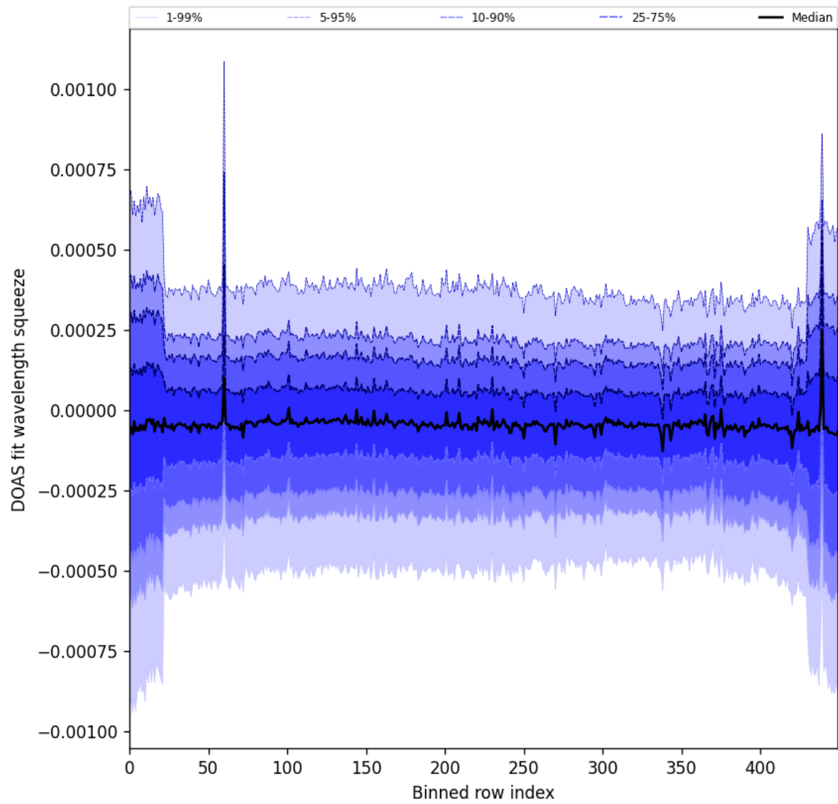
Figure 103: Along track statistics of “DOAS fit wavelength squeeze” for 2025-06-23 to 2025-06-25
