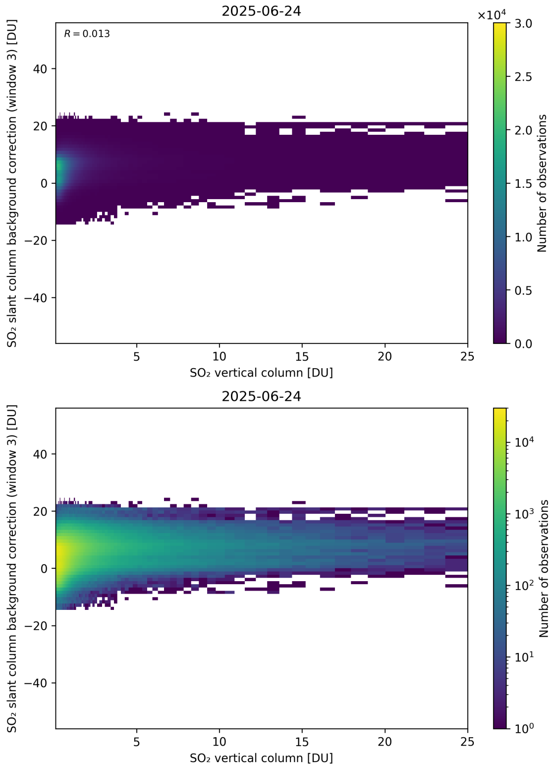
Figure 325: Scatter density plot of “SO 2 vertical column” against “SO 2 slant column background correction (window 3)” for 2025-06-23 to 2025-06-25.
