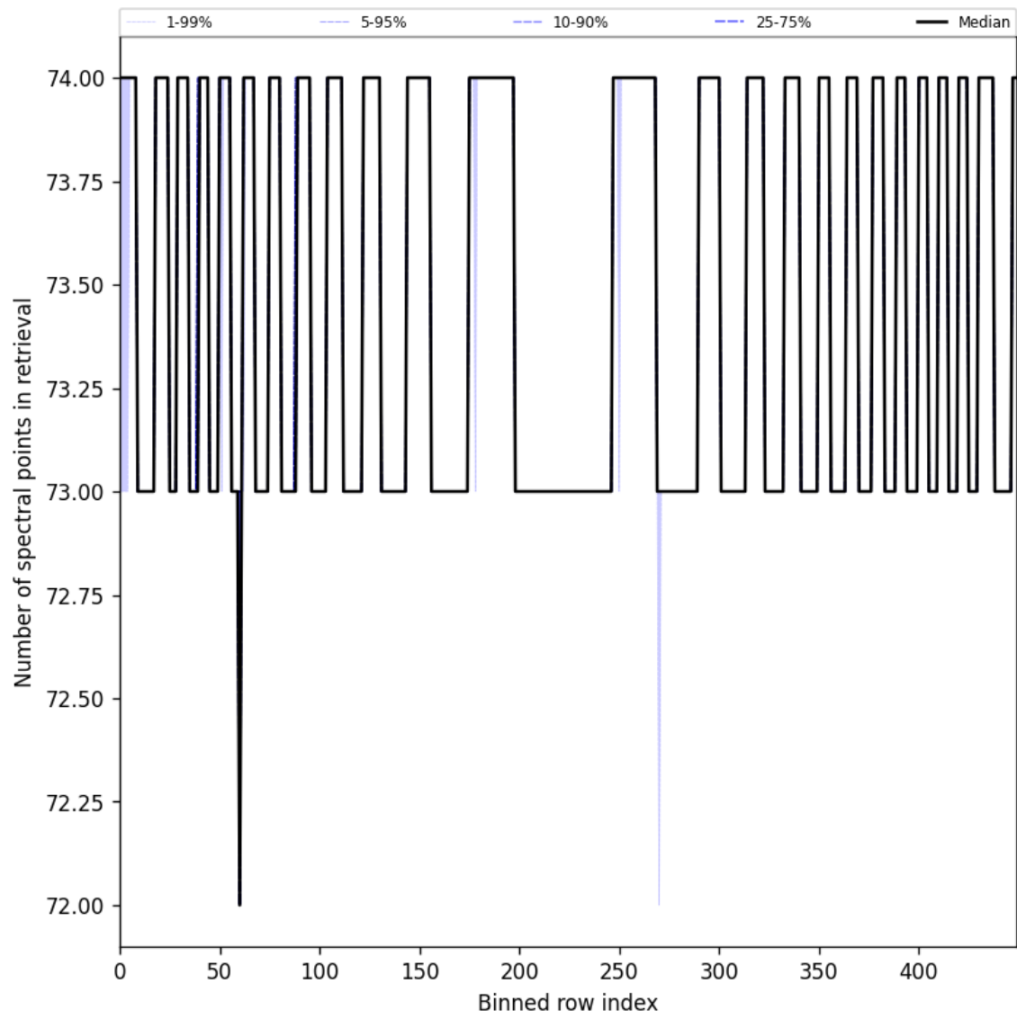
Figure 108: Along track statistics of “Number of spectral points in retrieval” for 2025-06-23 to 2025-06-25
