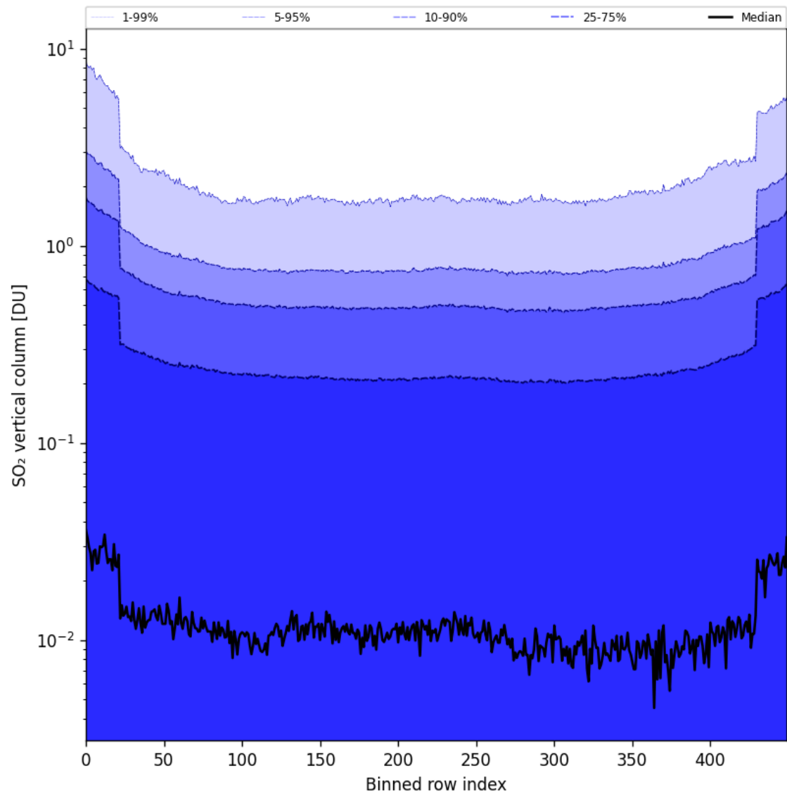
Figure 84: Along track statistics of “SO 2 vertical column” for 2025-06-23 to 2025-06-25
