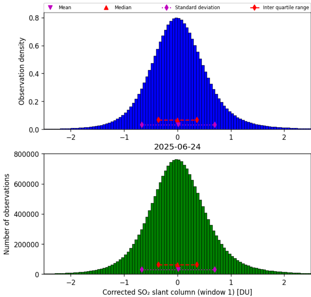
Figure 65: Histogram of “Corrected SO 2 slant column (window 1)” for 2025-06-23 to 2025-06-25
