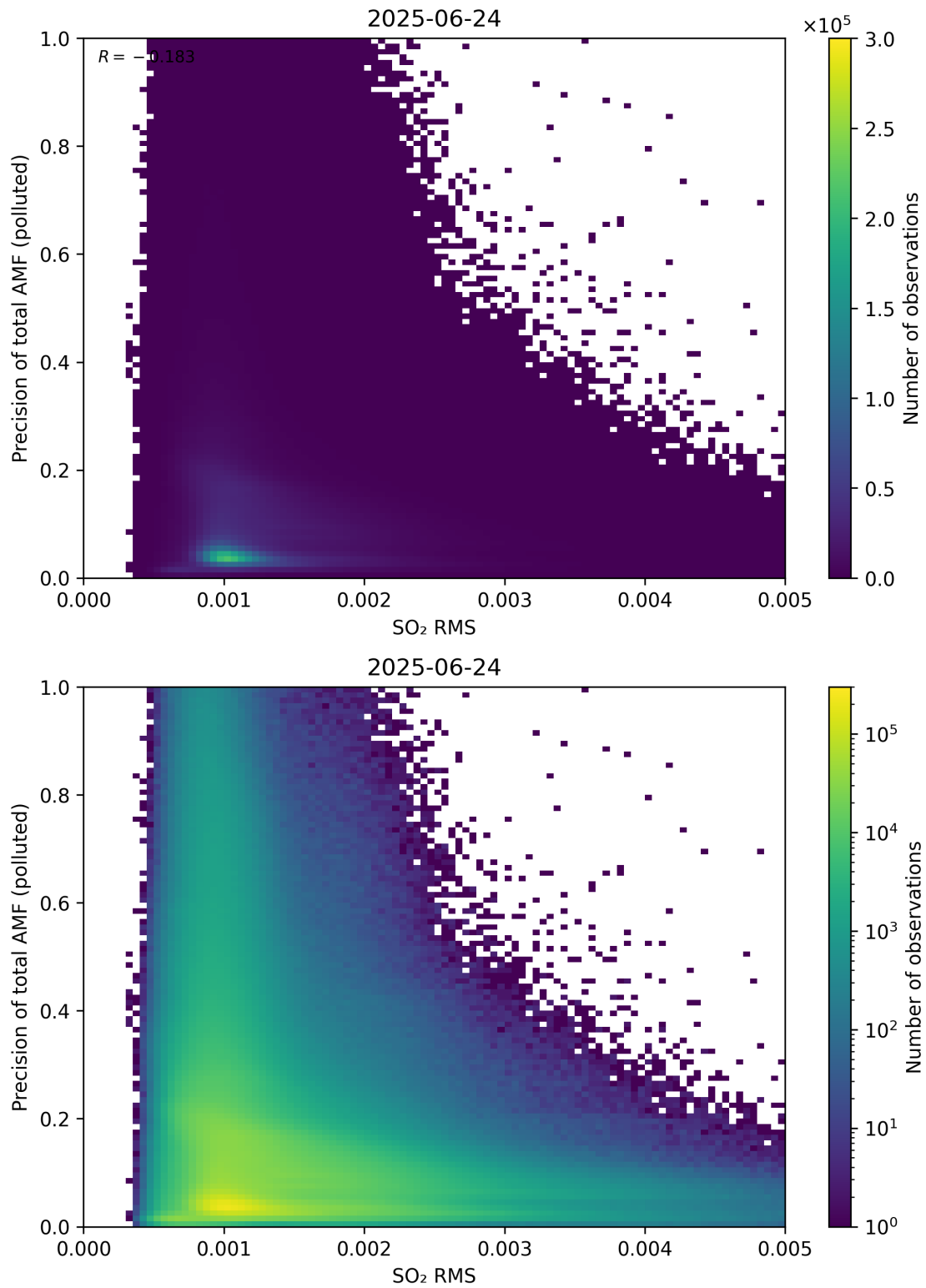
Figure 149: Scatter density plot of “SO 2 RMS” against “Precision of total AMF (polluted)” for 2025-06-23 to 2025-06-25.
