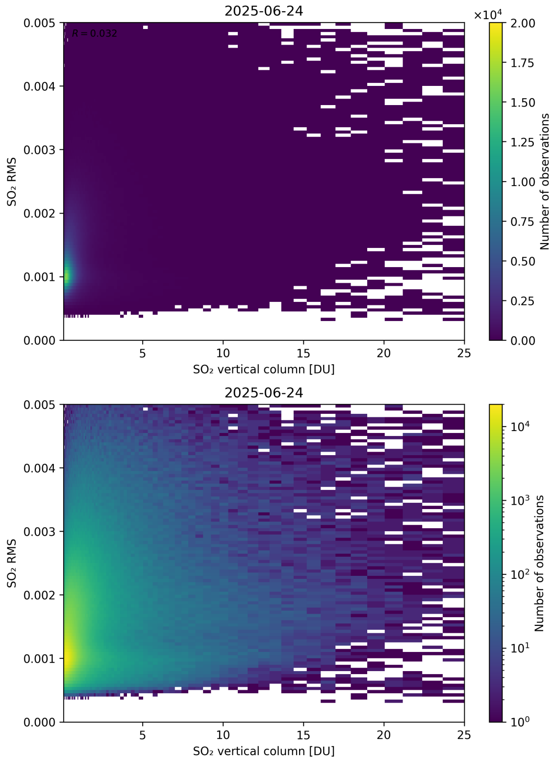
Figure 328: Scatter density plot of “SO 2 vertical column” against “SO 2 RMS” for 2025-06-23 to 2025-06-25.
