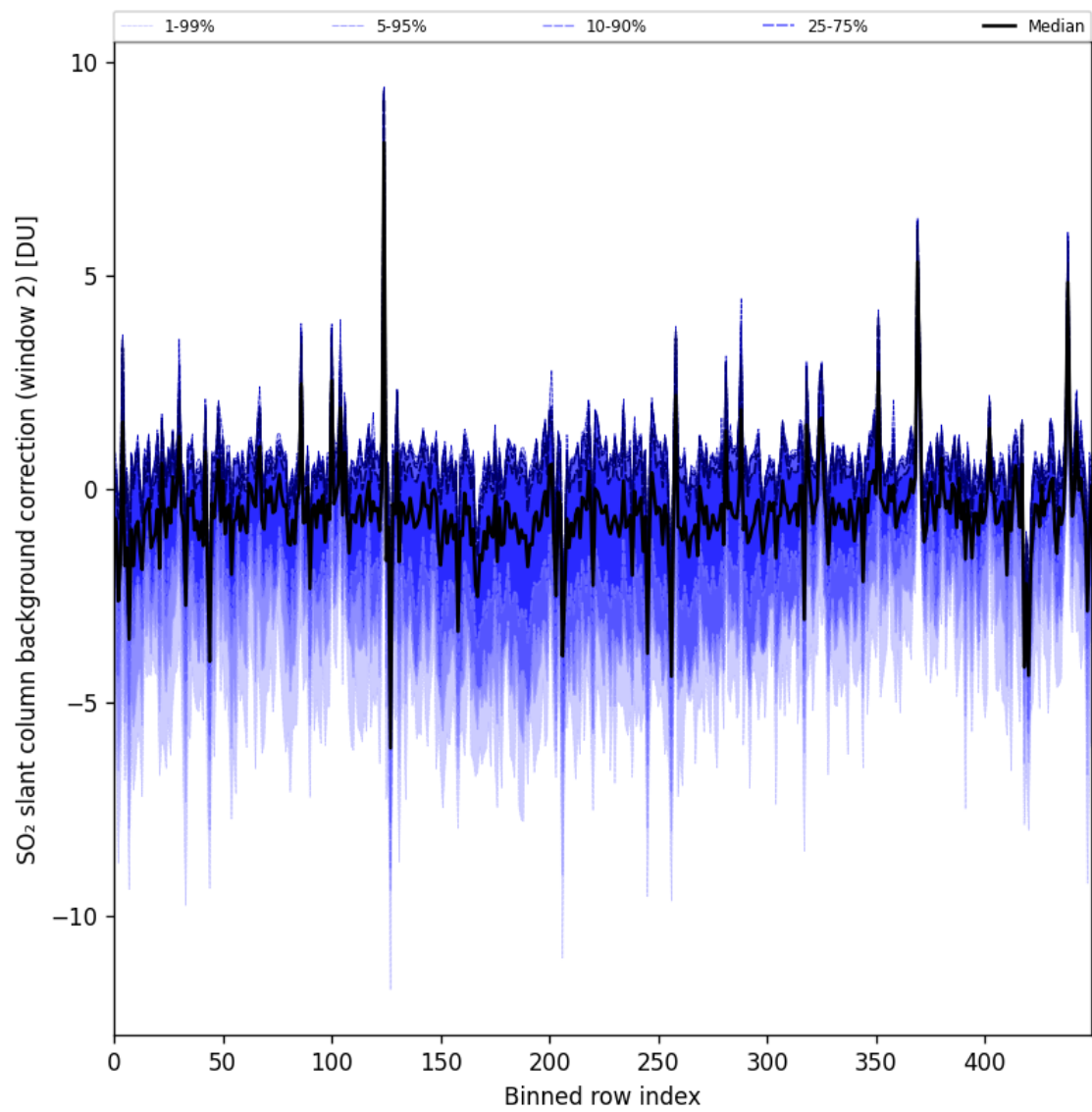
Figure 96: Along track statistics of “SO 2 slant column background correction (window 2)” for 2025-06-23 to 2025-06-25
