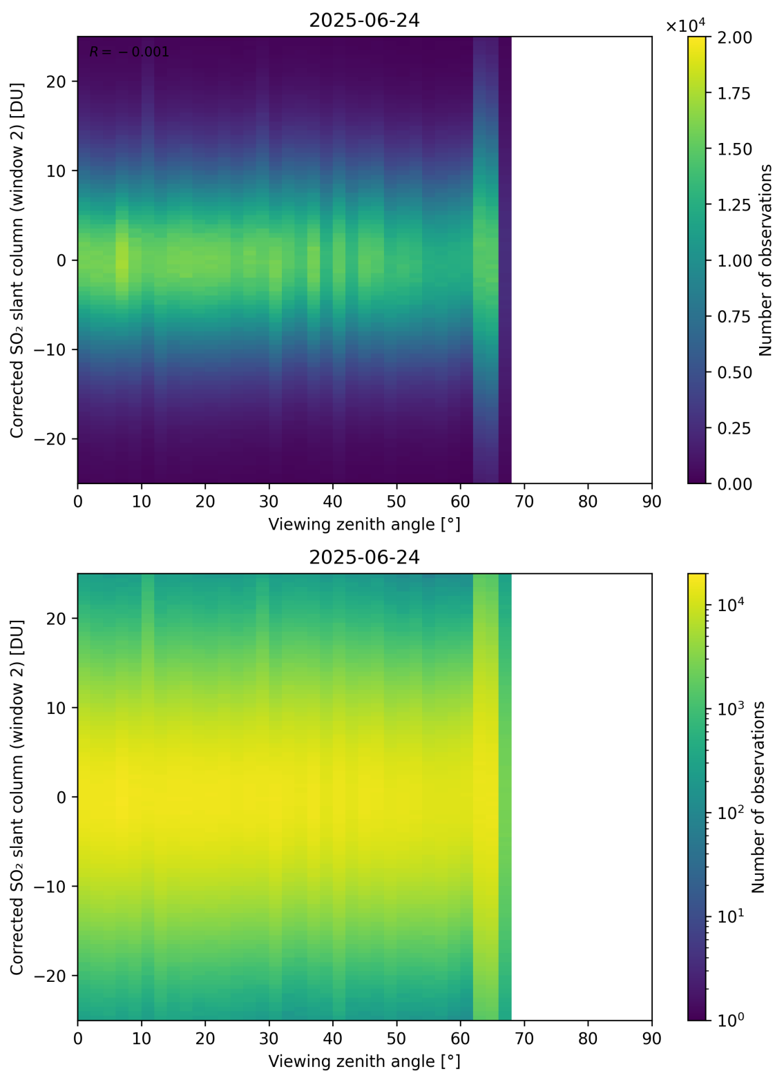
Figure 374: Scatter density plot of “Viewing zenith angle” against “Corrected SO 2 slant column (window 2)” for 2025-06-23 to 2025-06-25.
