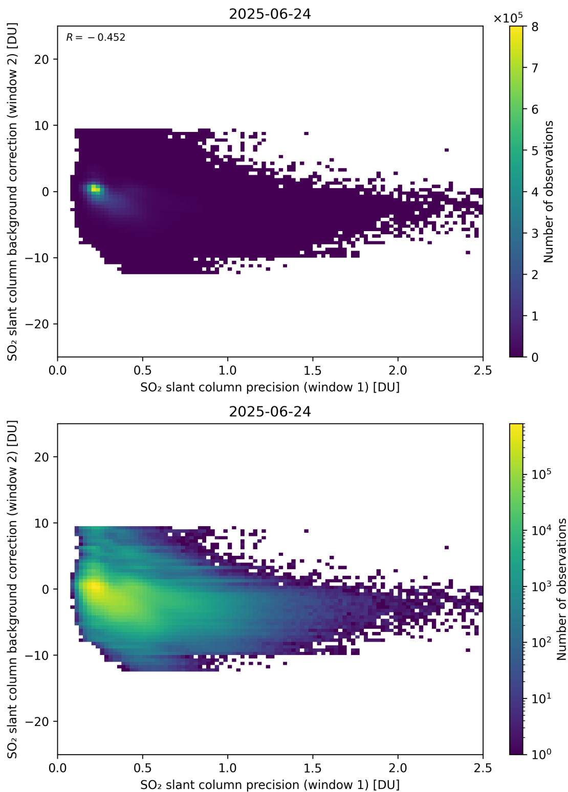
Figure 269: Scatter density plot of “SO 2 slant column precision (window 1)” against “SO 2 slant column background correction (window 2)” for 2025-06-23 to 2025-06-25.
