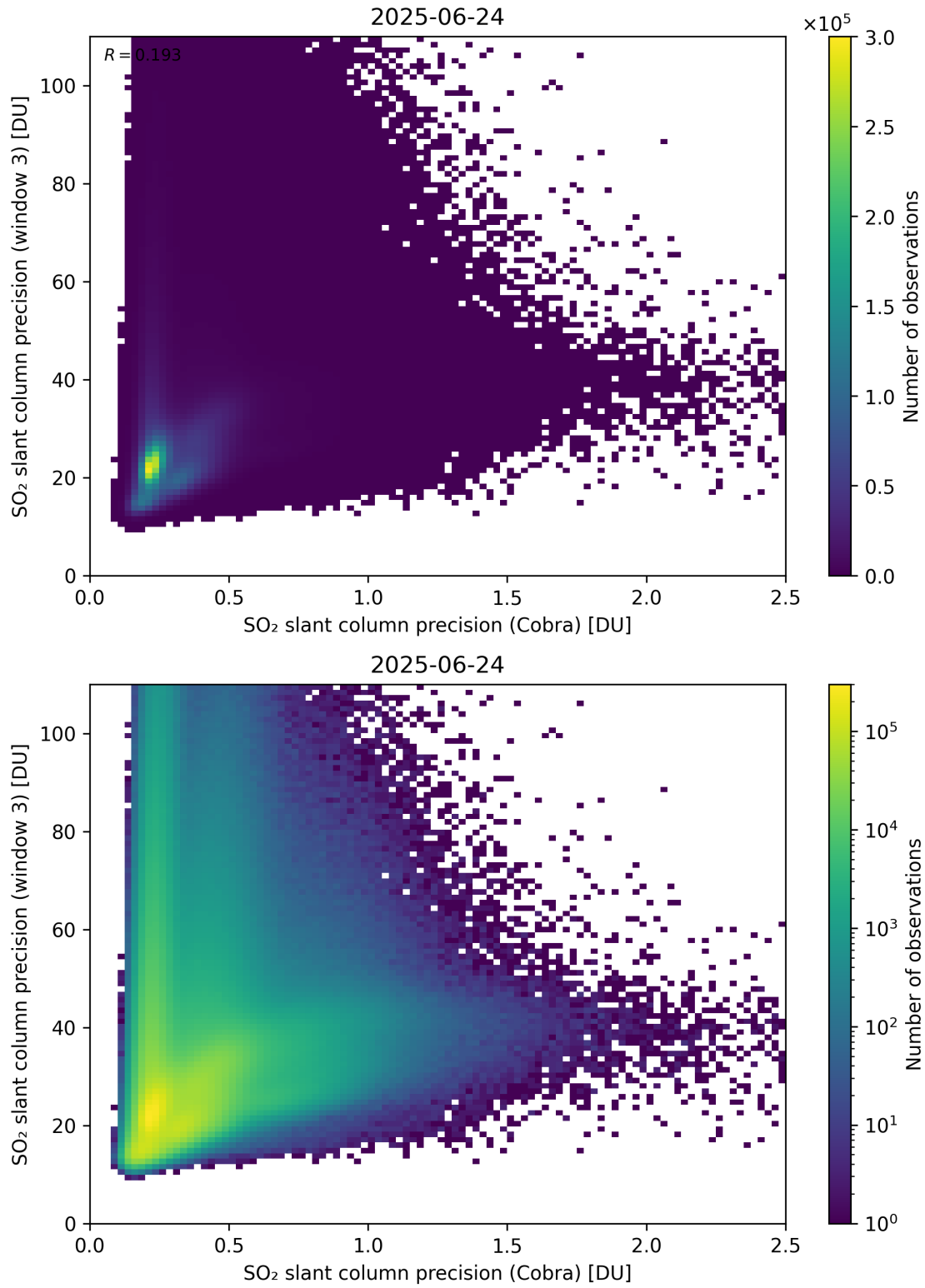
Figure 212: Scatter density plot of “SO 2 slant column precision (Cobra)” against “SO 2 slant column precision (window 3)” for 2025-06-23 to 2025-06-25.
