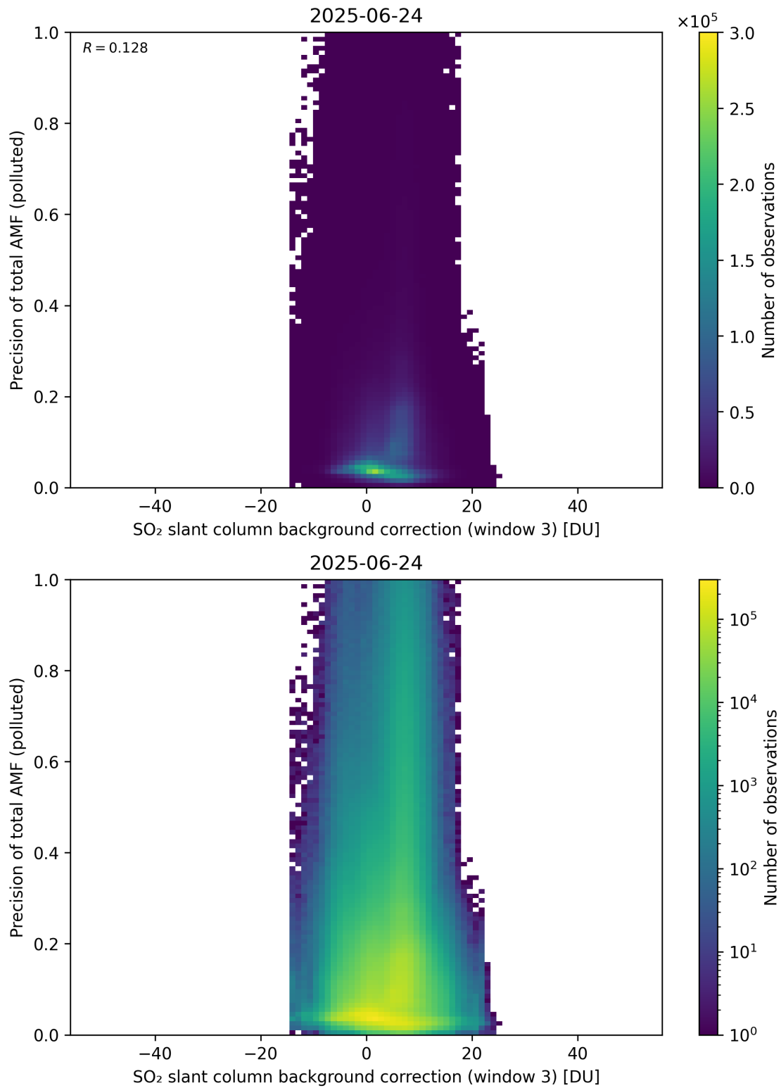
Figure 137: Scatter density plot of “SO 2 slant column background correction (window 3)” against “Precision of total AMF (polluted)” for 2025-06-23 to 2025-06-25.
