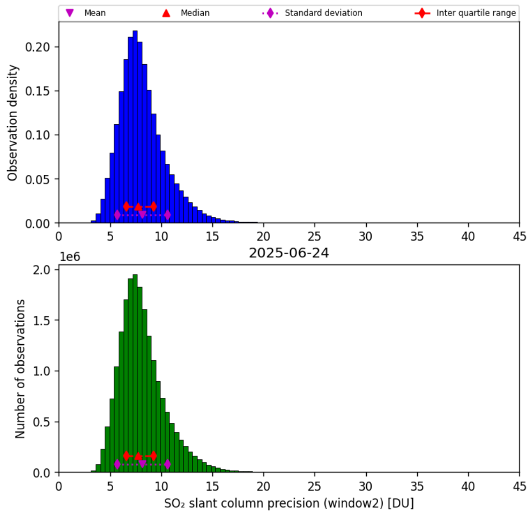
Figure 68: Histogram of “SO 2 slant column precision (window2)” for 2025-06-23 to 2025-06-25
