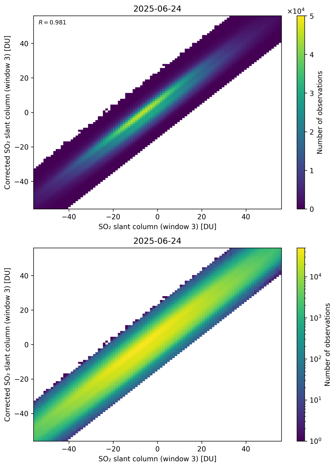
Figure 316: Scatter density plot of “SO 2 slant column (window 3)” against “Corrected SO 2 slant column (window 3)” for 2025-06-23 to 2025-06-25.
