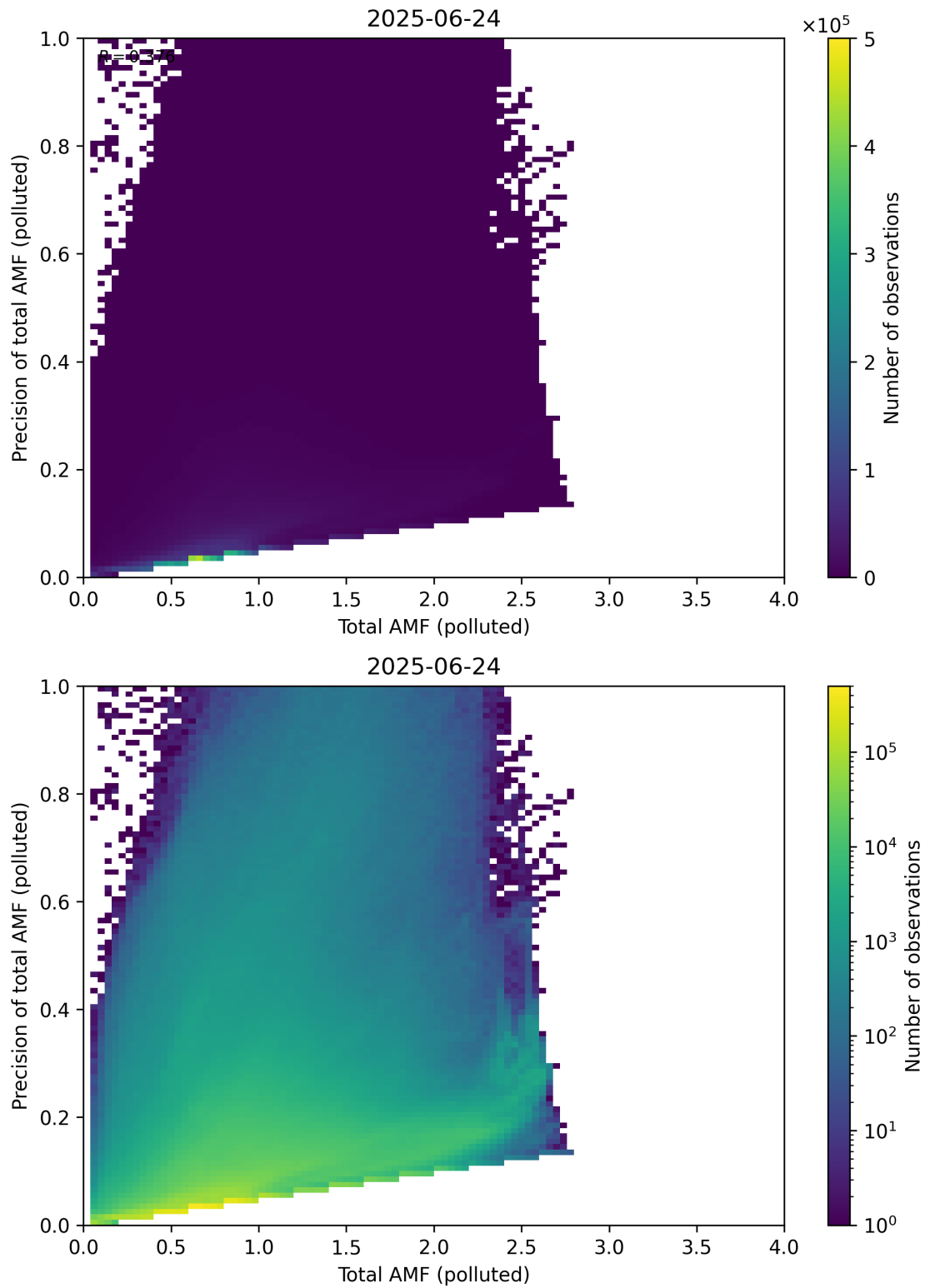
Figure 322: Scatter density plot of “Total AMF (polluted)” against “Precision of total AMF (polluted)” for 2025-06-23 to 2025-06-25.
