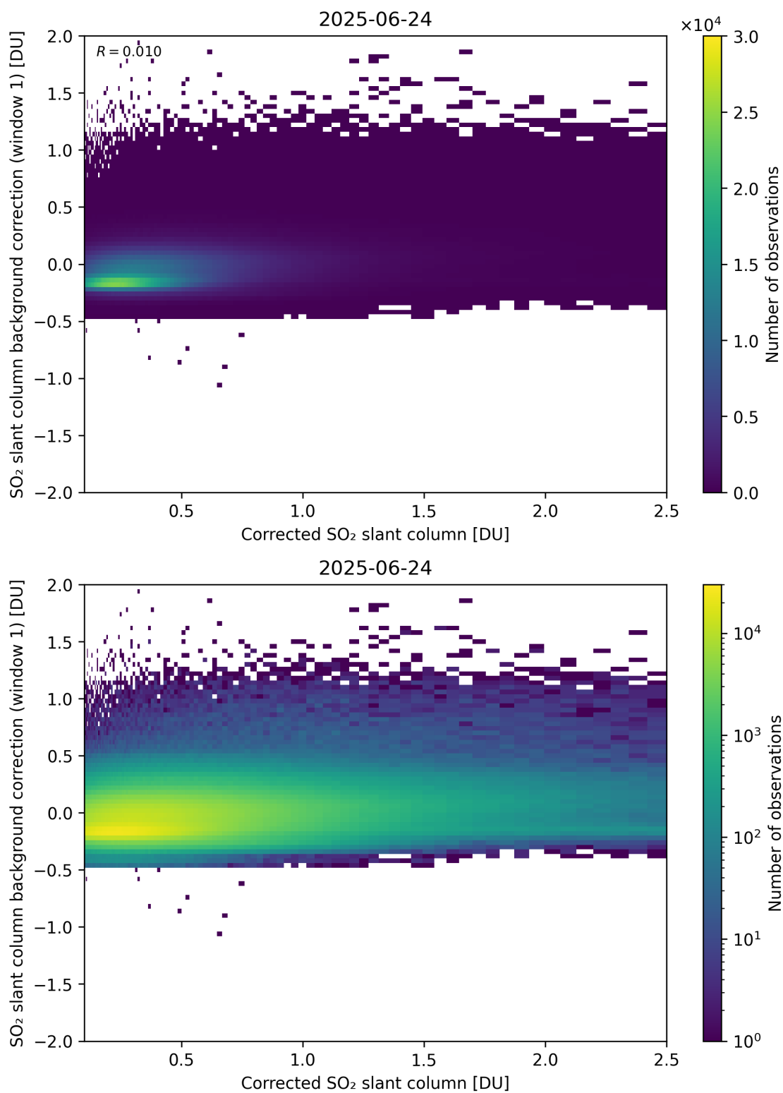
Figure 226: Scatter density plot of “Corrected SO 2 slant column” against “SO 2 slant column background correction (window 1)” for 2025-06-23 to 2025-06-25.
