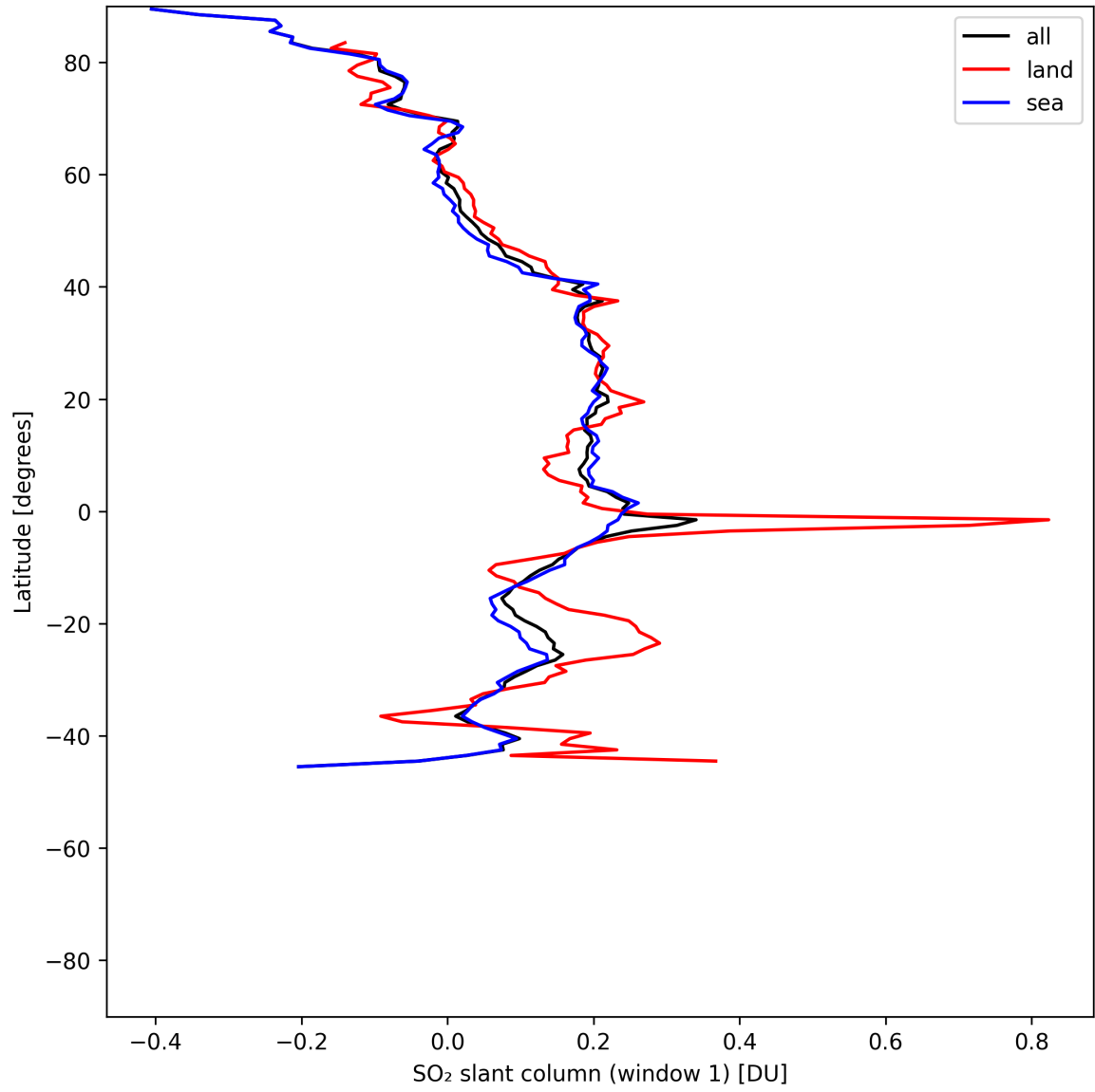
Figure 37: Zonal average of “SO 2 slant column (window 1)” for 2025-06-23 to 2025-06-25.
