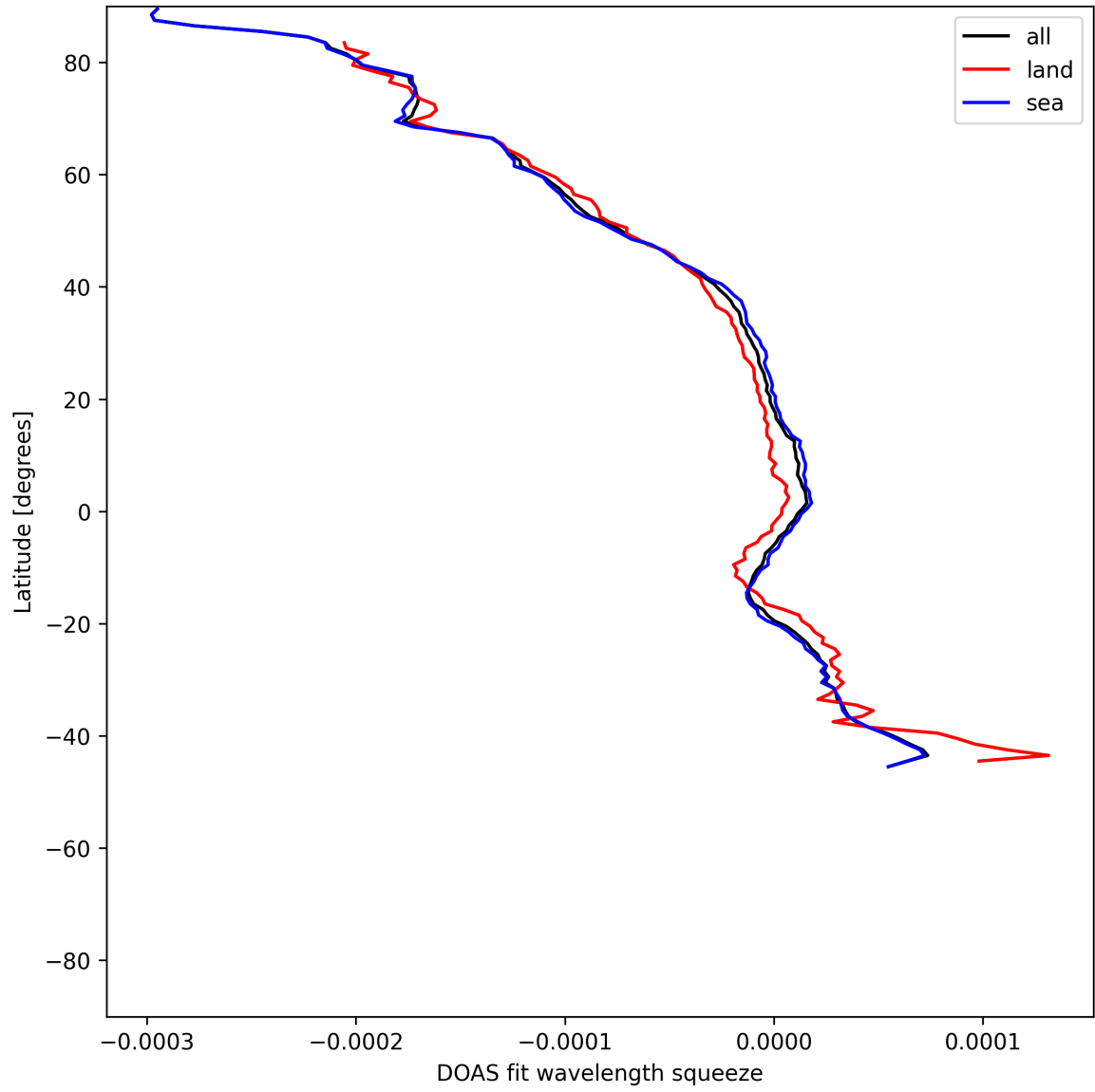
Figure 51: Zonal average of “DOAS fit wavelength squeeze” for 2025-06-23 to 2025-06-25.
