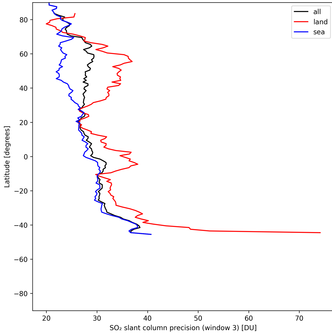
Figure 46: Zonal average of “SO 2 slant column precision (window 3)” for 2025-06-23 to 2025-06-25.
