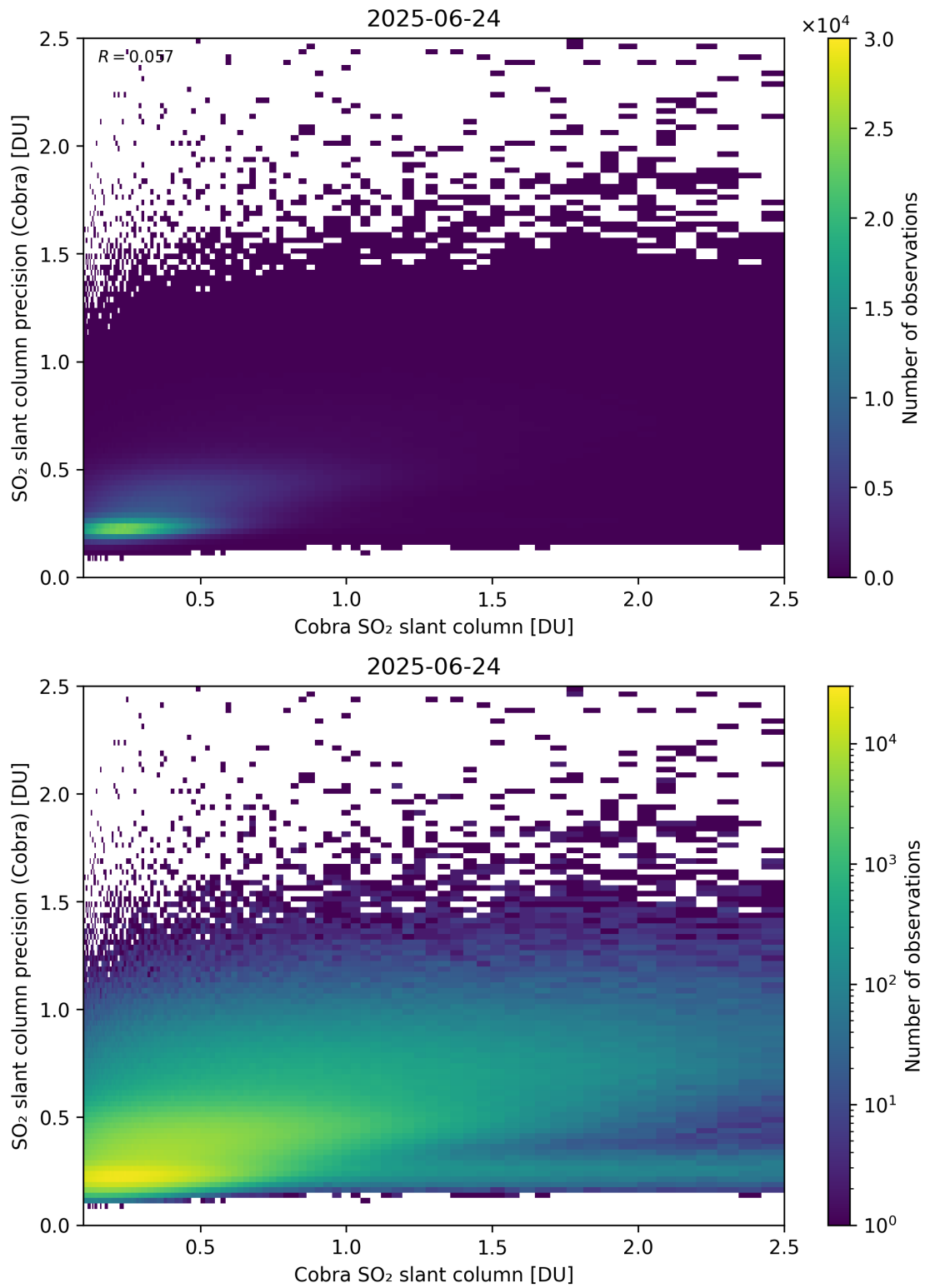
Figure 216: Scatter density plot of “Cobra SO 2 slant column” against “SO 2 slant column precision (Cobra)” for 2025-06-23 to 2025-06-25.
