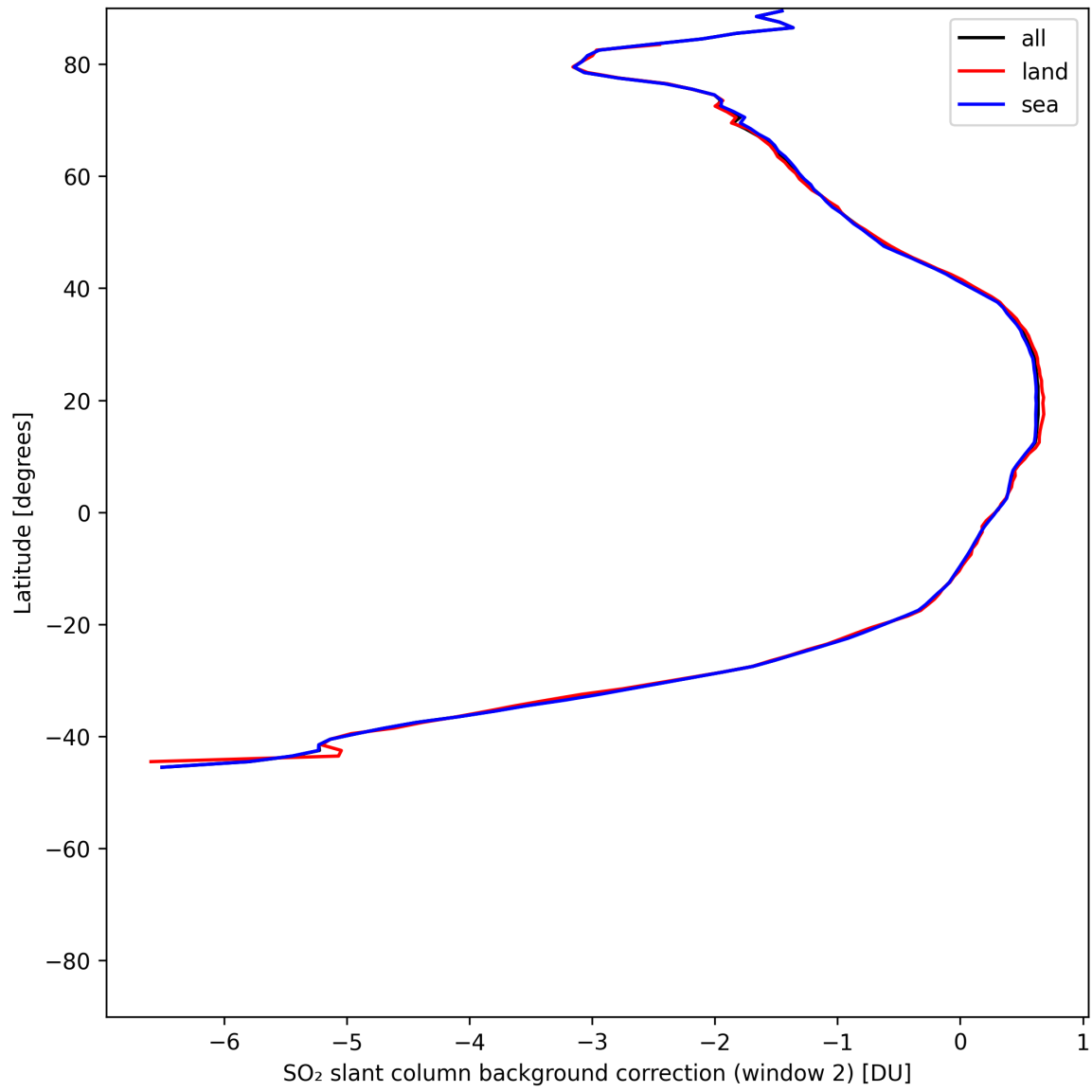
Figure 44: Zonal average of “SO 2 slant column background correction (window 2)” for 2025-06-23 to 2025-06-25.
