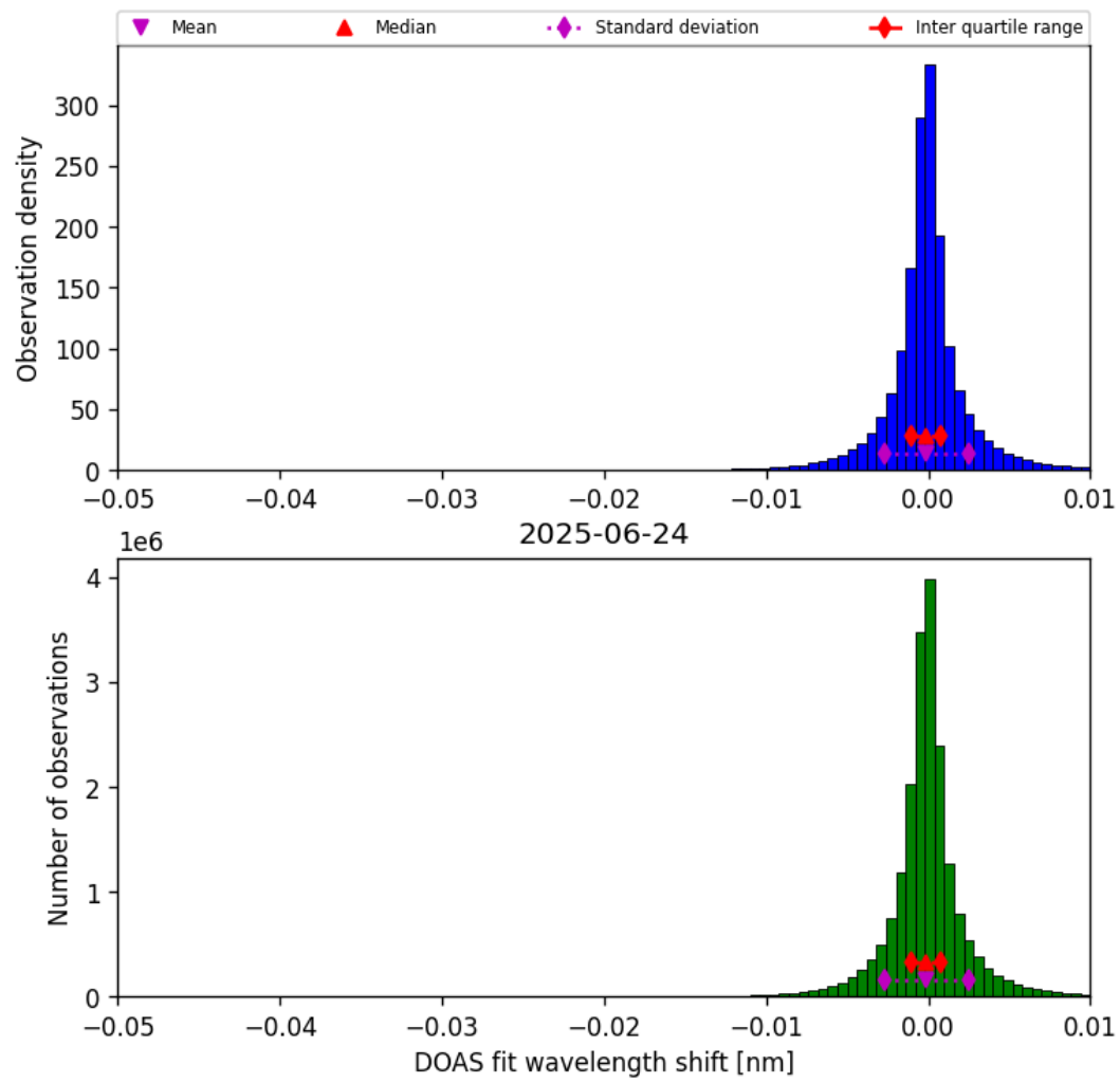
Figure 76: Histogram of “DOAS fit wavelength shift” for 2025-06-23 to 2025-06-25
