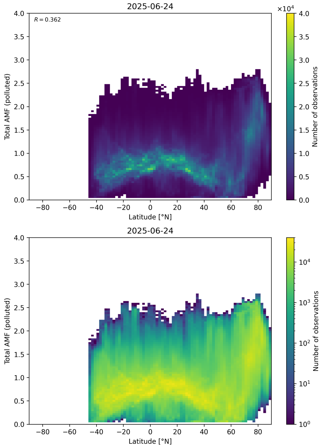
Figure 167: Scatter density plot of “Latitude” against “Total AMF (polluted)” for 2025-06-23 to 2025-06-25.
