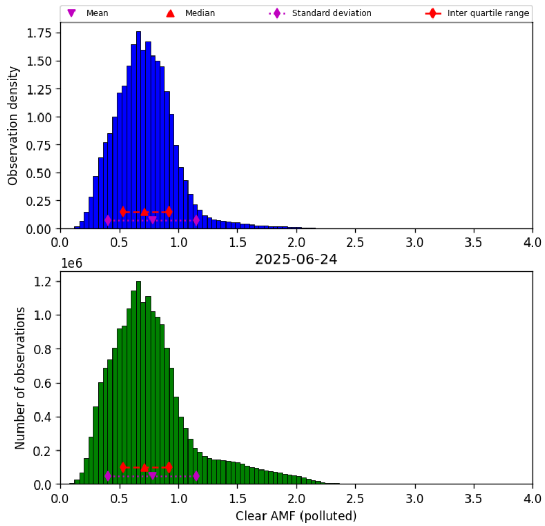
Figure 81: Histogram of “Clear AMF (polluted)” for 2025-06-23 to 2025-06-25
