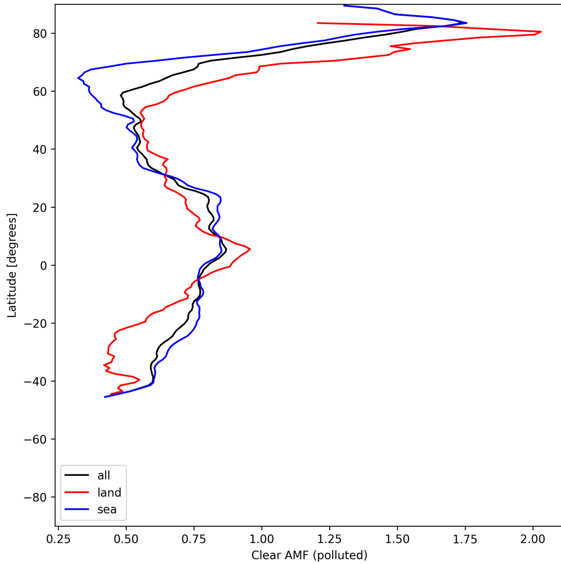
Figure 55: Zonal average of “Clear AMF (polluted)” for 2025-06-23 to 2025-06-25.
