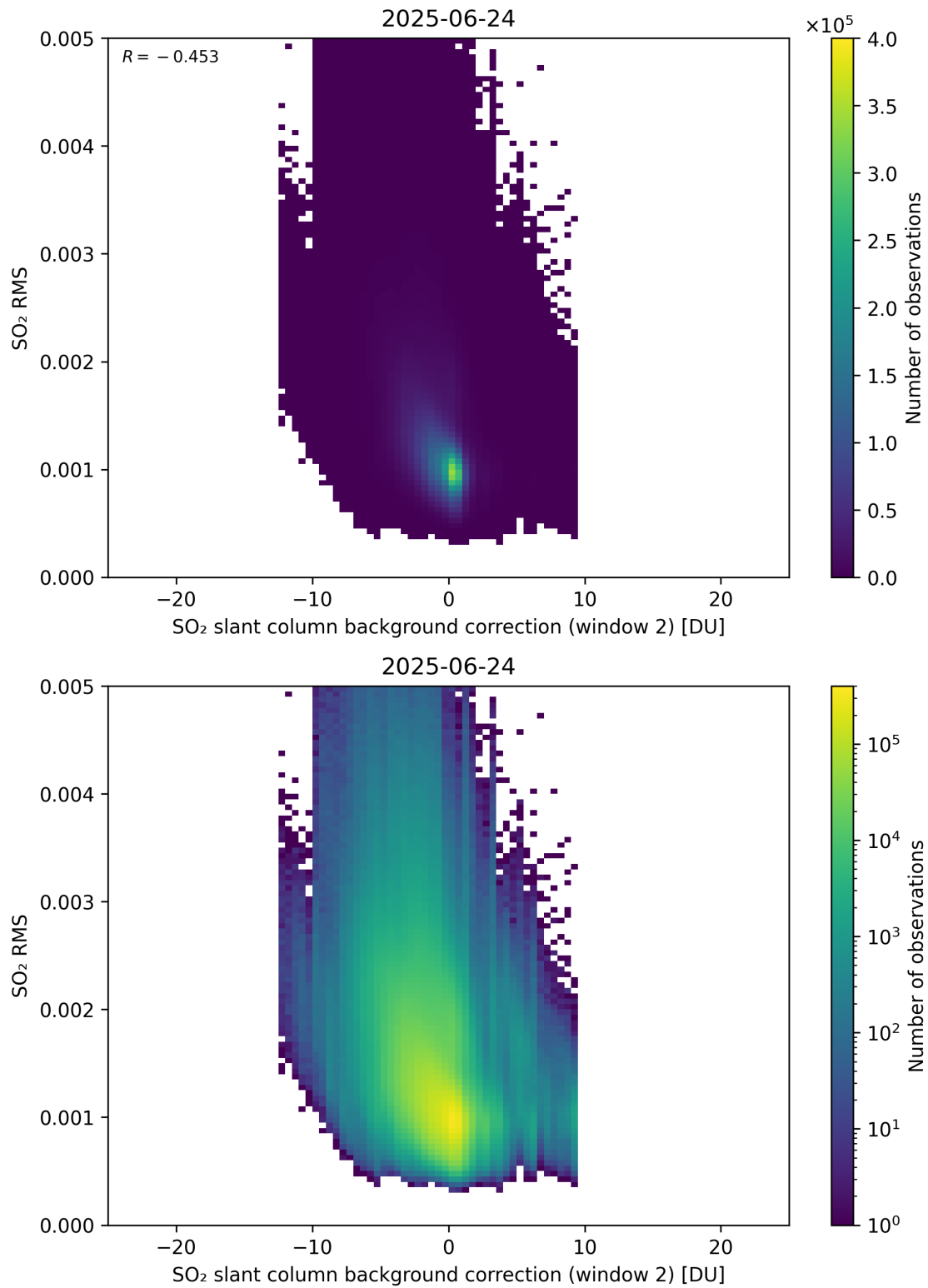
Figure 125: Scatter density plot of “SO 2 slant column background correction (window 2)” against “SO 2 RMS” for 2025-06-23 to 2025-06-25.
