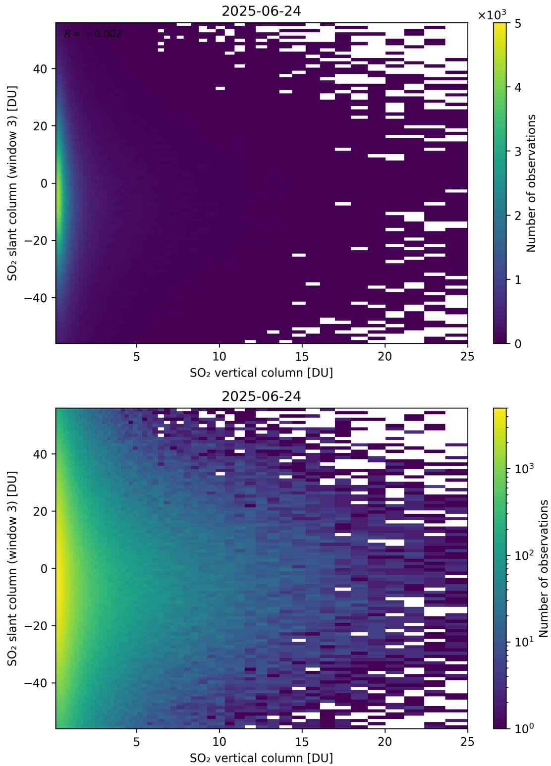
Figure 357: Scatter density plot of “SO 2 vertical column” against “SO 2 slant column (window 3)” for 2025-06-23 to 2025-06-25.
