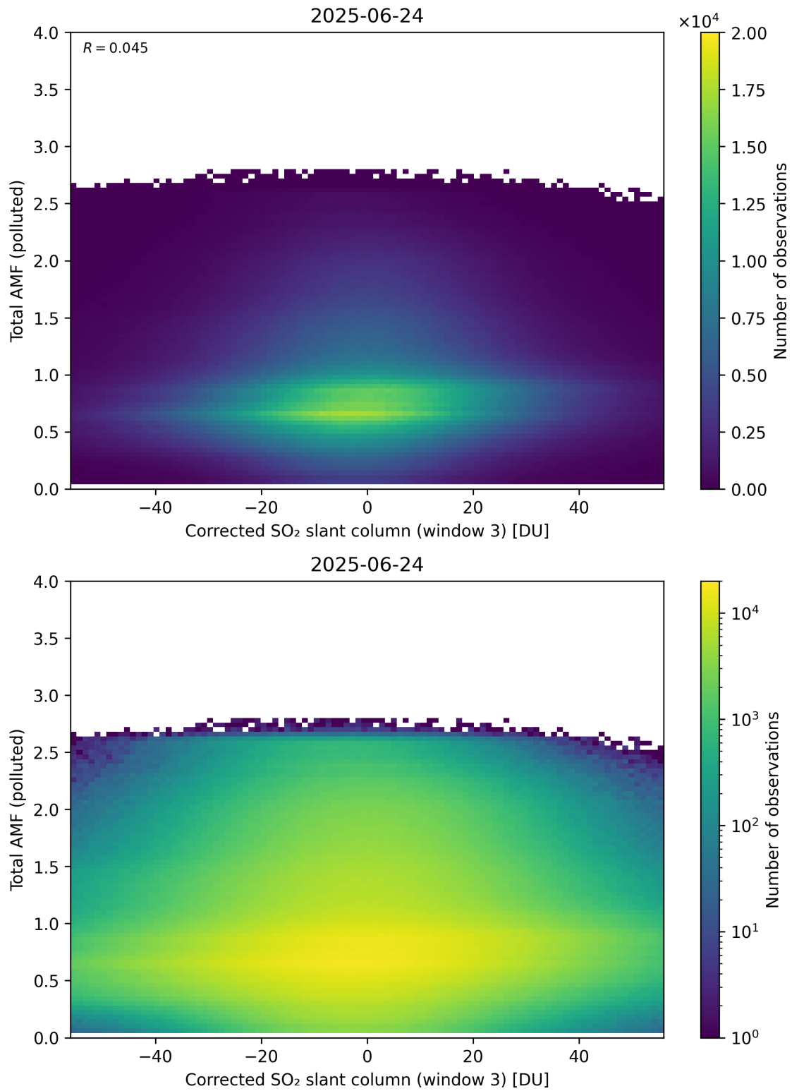
Figure 260: Scatter density plot of “Corrected SO 2 slant column (window 3)” against “Total AMF (polluted)” for 2025-06-23 to 2025-06-25.
