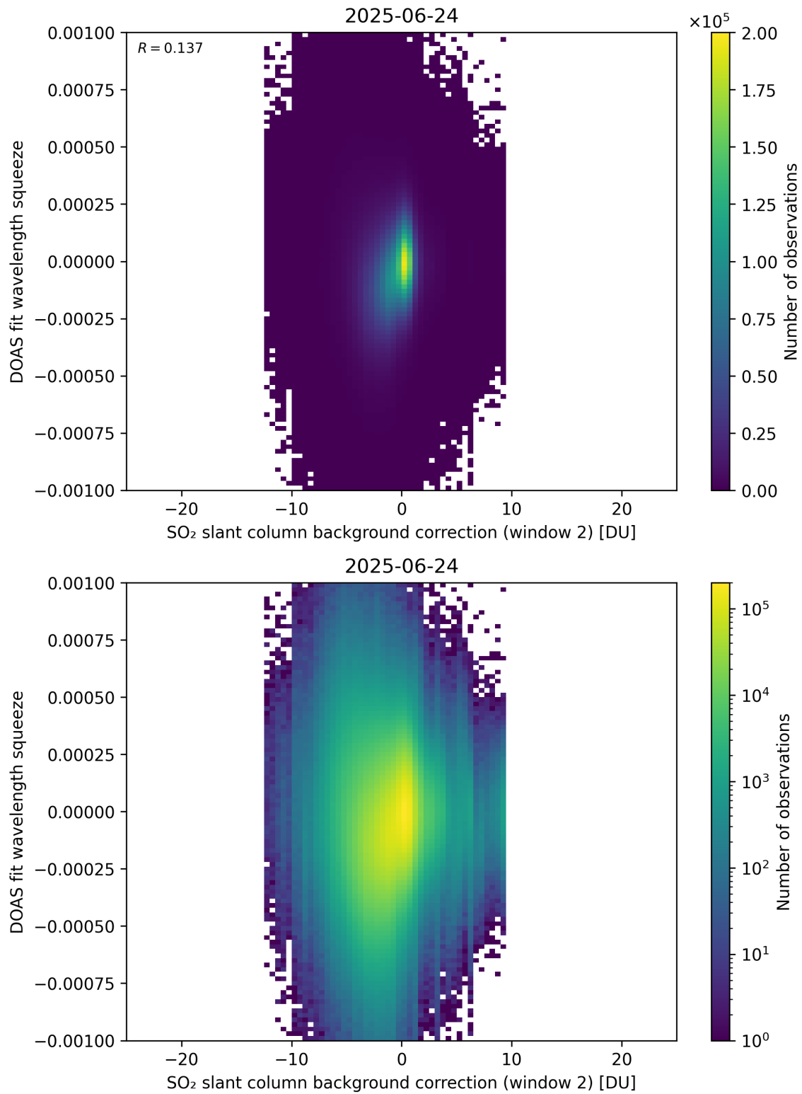
Figure 124: Scatter density plot of “SO 2 slant column background correction (window 2)” against “DOAS fit wavelength squeeze” for 2025-06-23 to 2025-06-25.
