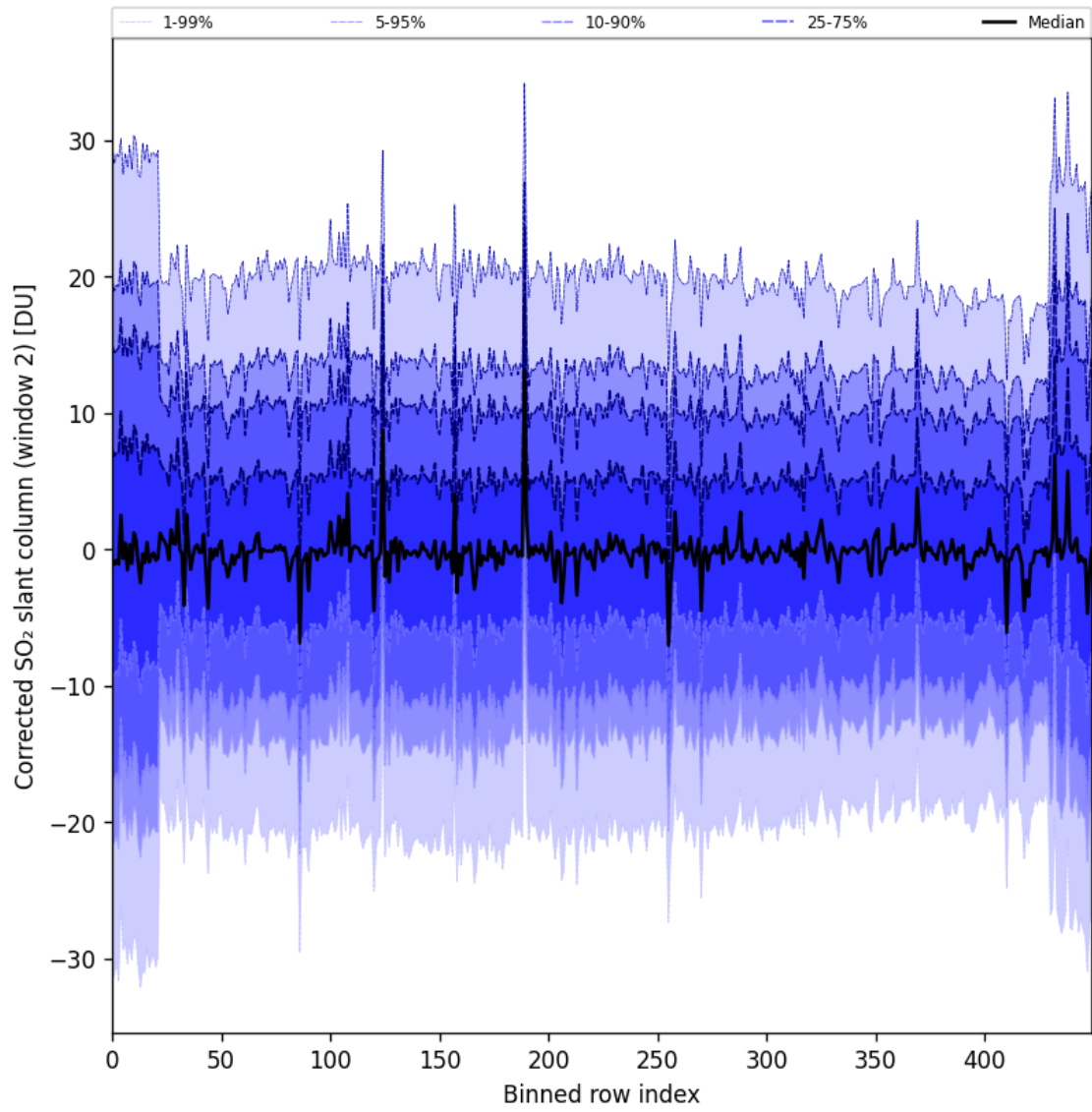
Figure 95: Along track statistics of “Corrected SO 2 slant column (window 2)” for 2025-06-23 to 2025-06-25
