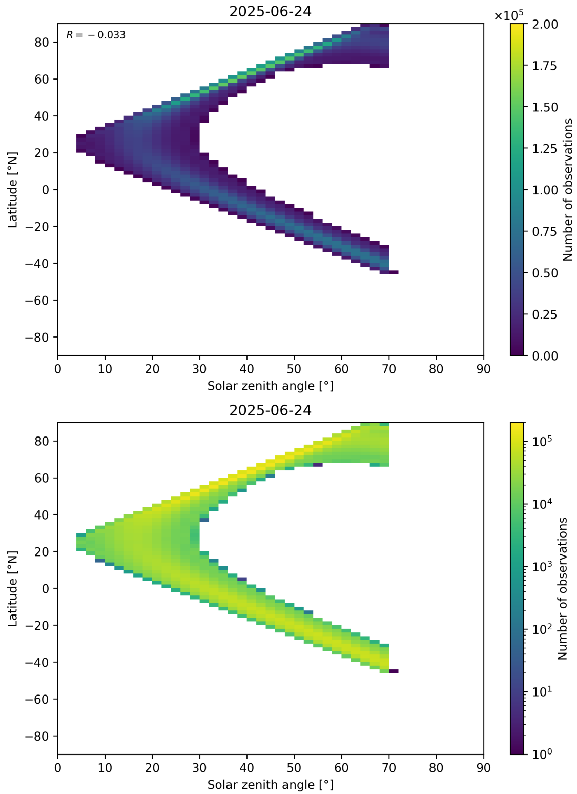
Figure 177: Scatter density plot of “Solar zenith angle” against “Latitude” for 2025-06-23 to 2025-06-25.
