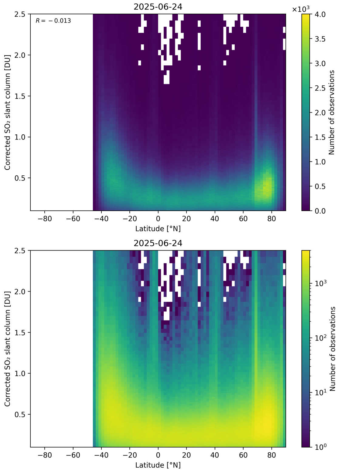
Figure 159: Scatter density plot of “Latitude” against “Corrected SO 2 slant column” for 2025-06-23 to 2025-06-25.
