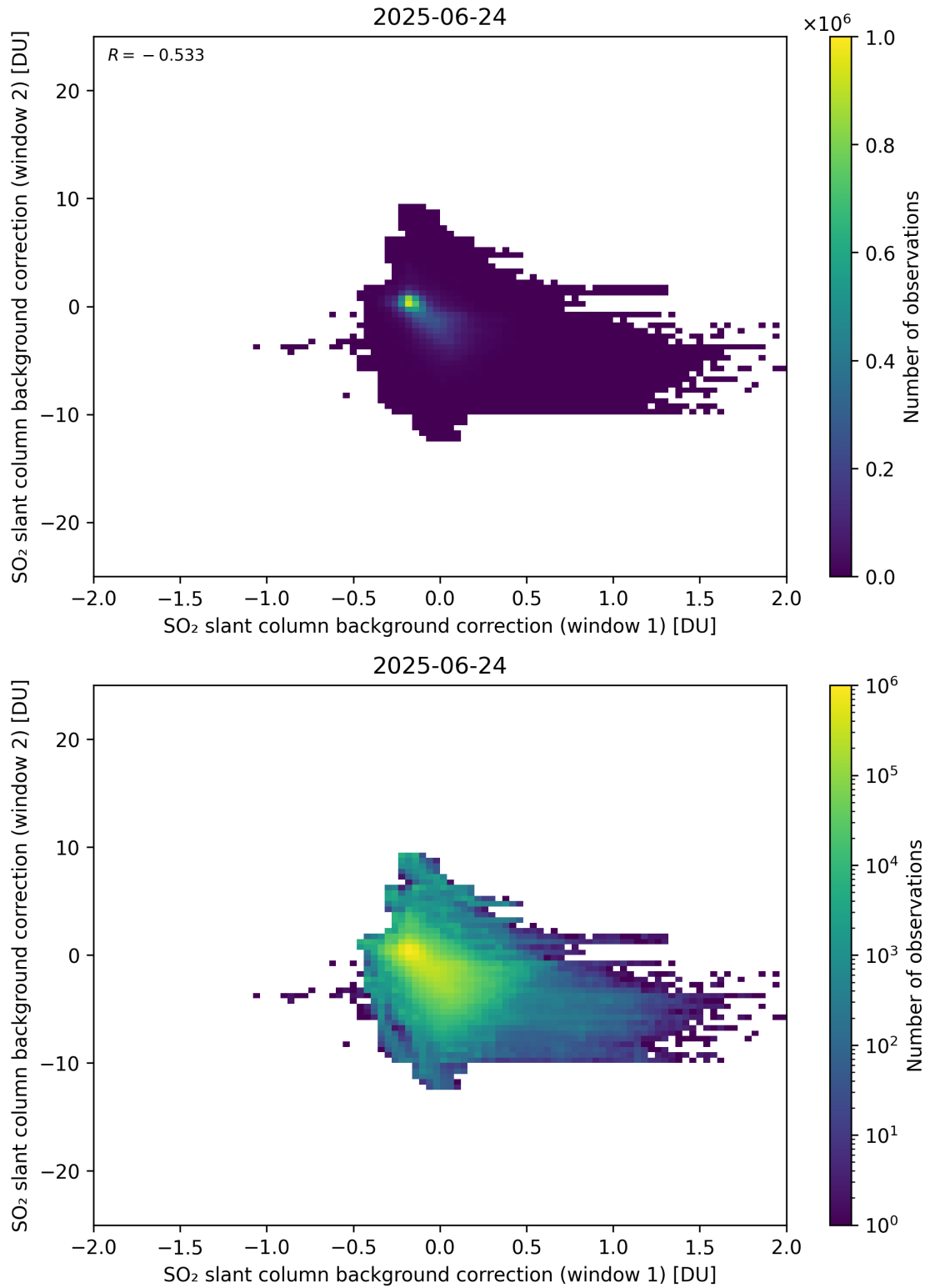
Figure 109: Scatter density plot of “SO 2 slant column background correction (window 1)” against “SO 2 slant column background correction (window 2)” for 2025-06-23 to 2025-06-25.
