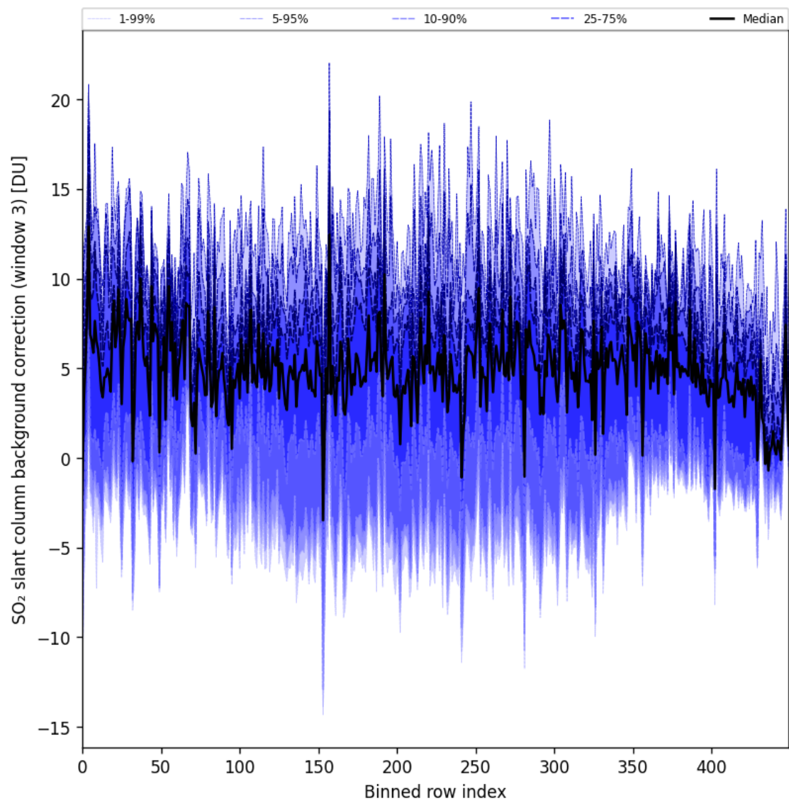
Figure 100: Along track statistics of “SO 2 slant column background correction (window 3)” for 2025-06-23 to 2025-06-25
