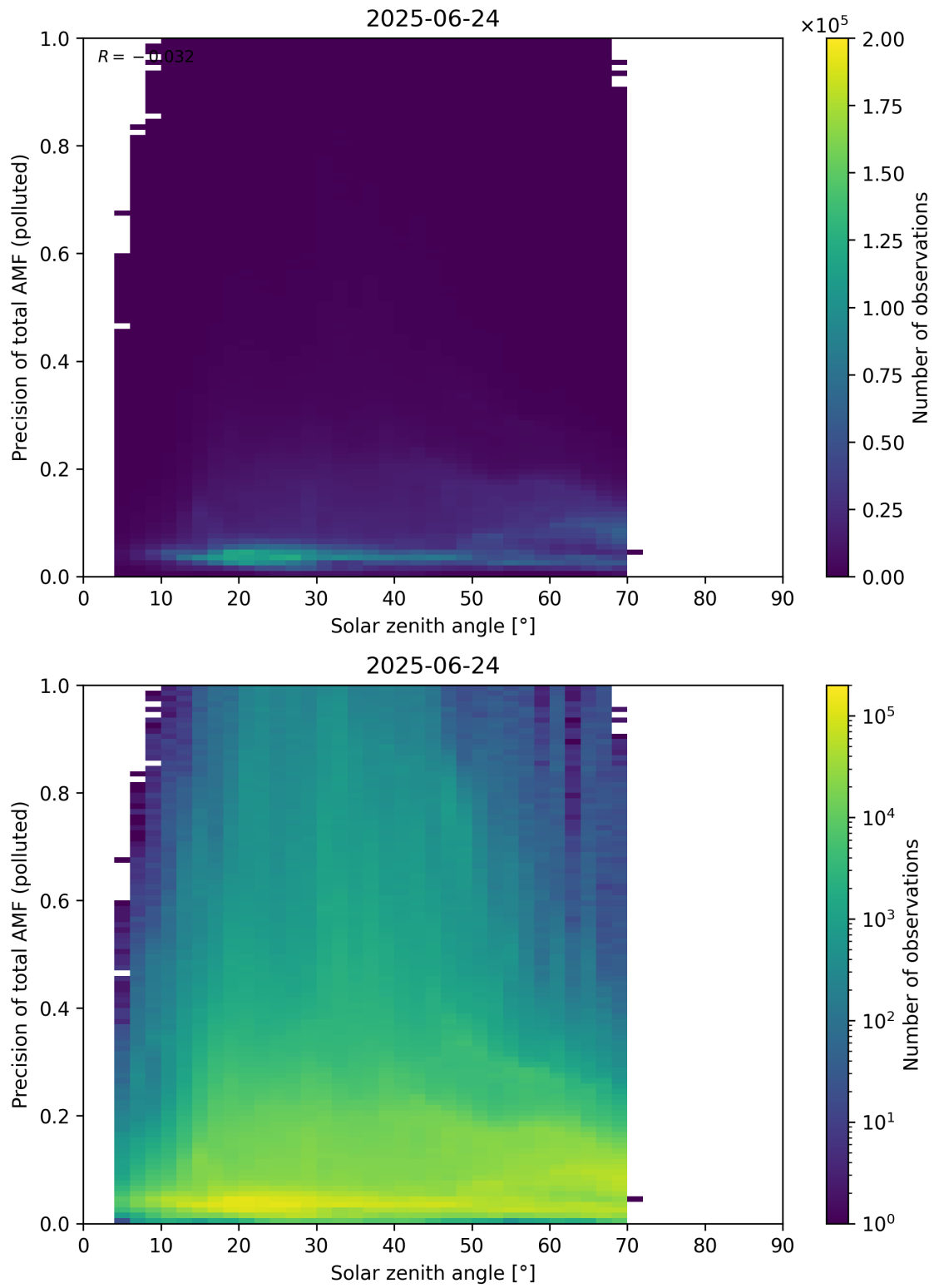
Figure 190: Scatter density plot of “Solar zenith angle” against “Precision of total AMF (polluted)” for 2025-06-23 to 2025-06-25.
