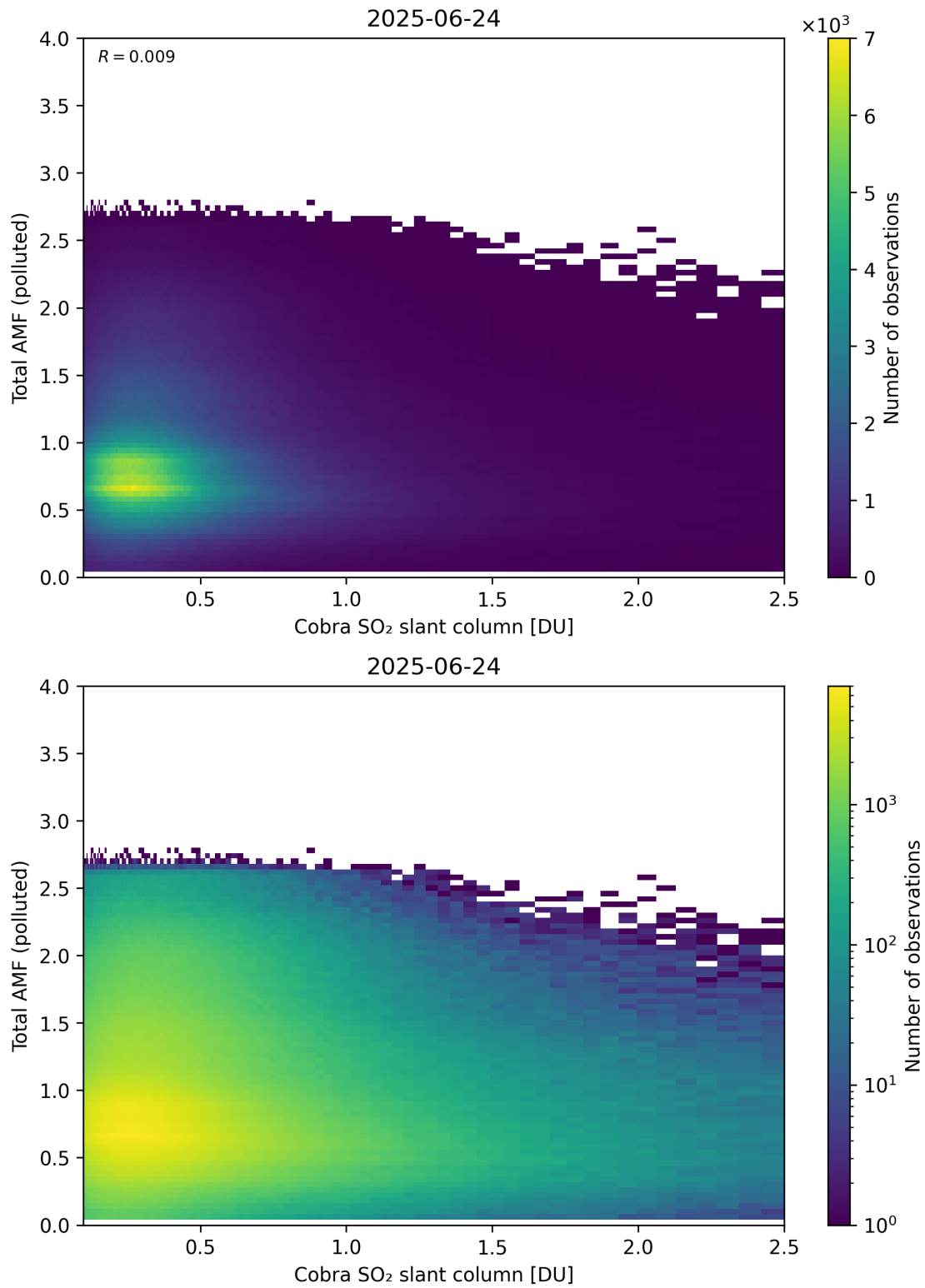
Figure 224: Scatter density plot of “Cobra SO 2 slant column” against “Total AMF (polluted)” for 2025-06-23 to 2025-06-25.
