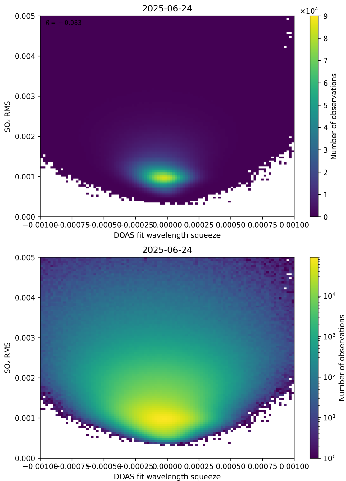
Figure 143: Scatter density plot of “DOAS fit wavelength squeeze” against “SO 2 RMS” for 2025-06-23 to 2025-06-25.
