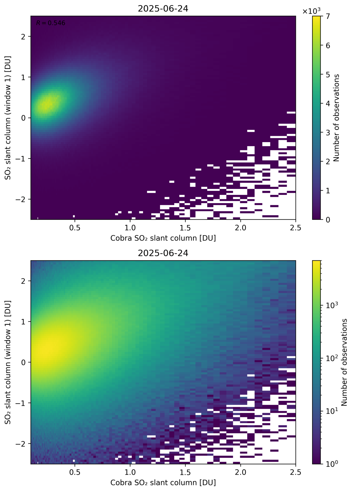
Figure 219: Scatter density plot of “Cobra SO 2 slant column” against “SO 2 slant column (window 1)” for 2025-06-23 to 2025-06-25.
