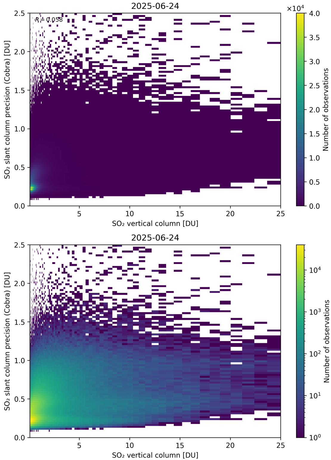
Figure 350: Scatter density plot of “SO 2 vertical column” against “SO 2 slant column precision (Cobra)” for 2025-06-23 to 2025-06-25.
