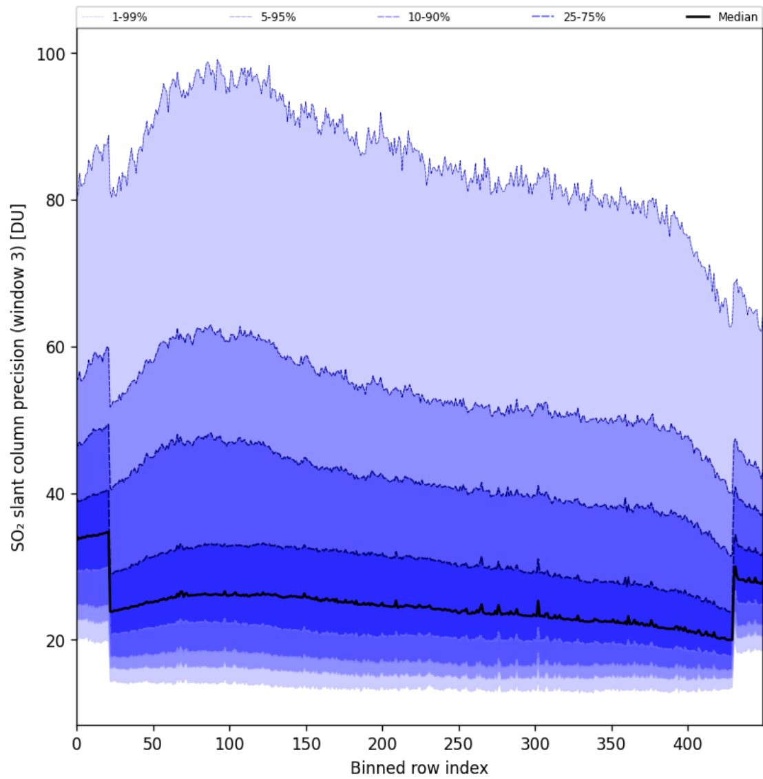
Figure 98: Along track statistics of “SO 2 slant column precision (window 3)” for 2025-06-23 to 2025-06-25
