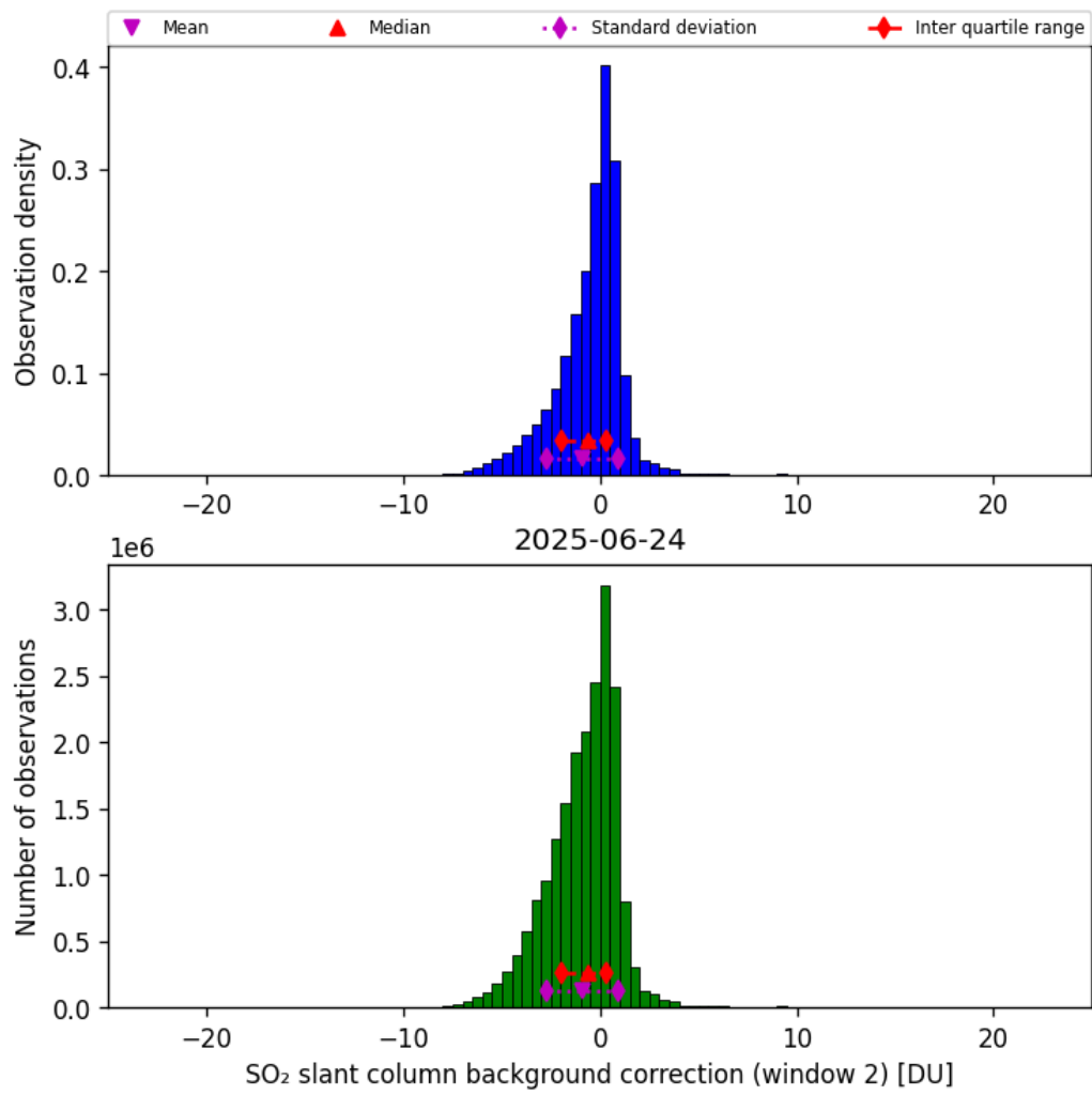
Figure 70: Histogram of “SO 2 slant column background correction (window 2)” for 2025-06-23 to 2025-06-25
