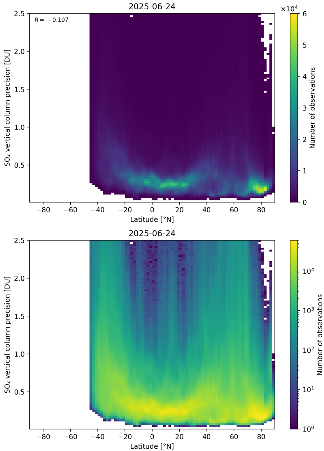
Figure 170: Scatter density plot of “Latitude” against “SO 2 vertical column precision” for 2025-06-23 to 2025-06-25.
