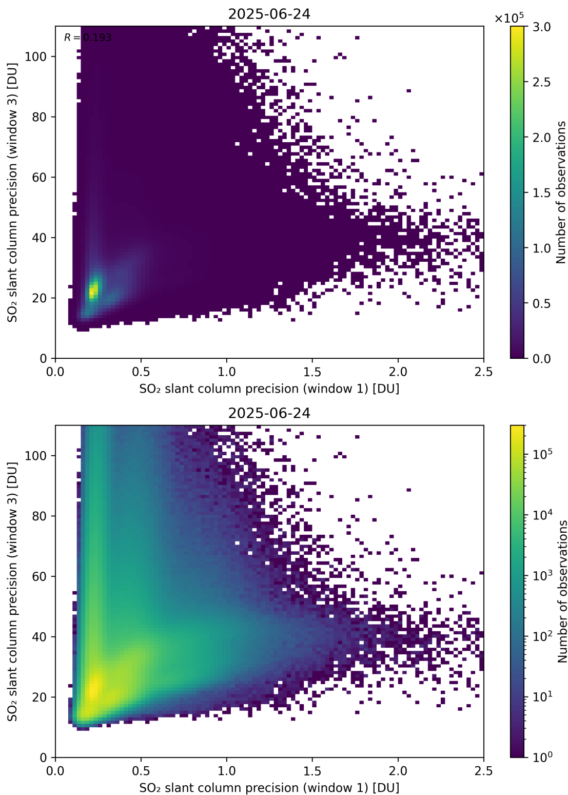
Figure 279: Scatter density plot of “SO 2 slant column precision (window 1)” against “SO 2 slant column precision (window 3)” for 2025-06-23 to 2025-06-25.
