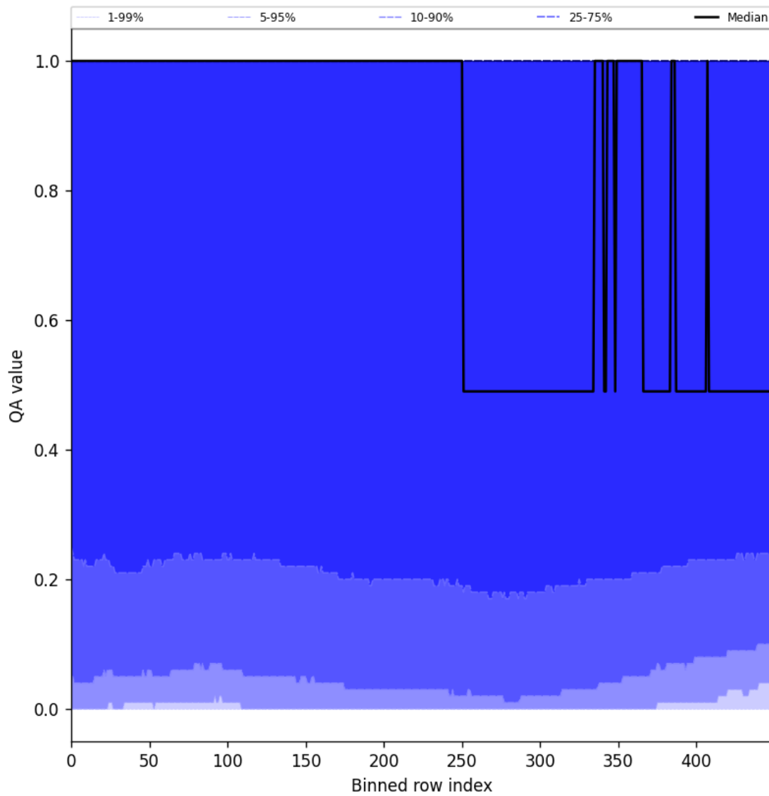
Figure 83: Along track statistics of “QA value” for 2025-06-23 to 2025-06-25
