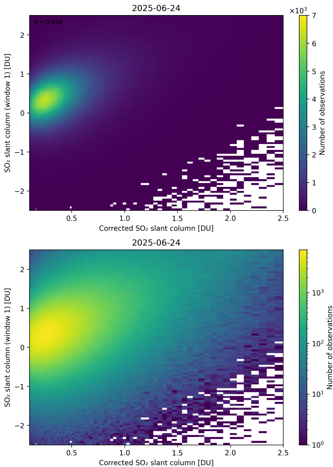
Figure 237: Scatter density plot of “Corrected SO 2 slant column” against “SO 2 slant column (window 1)” for 2025-06-23 to 2025-06-25.
