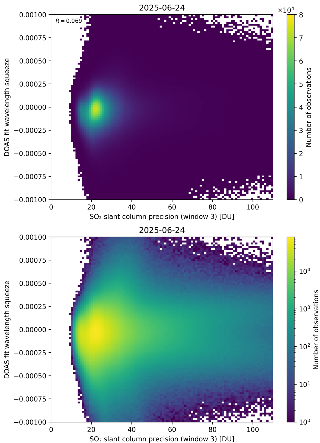
Figure 309: Scatter density plot of “SO 2 slant column precision (window 3)” against “DOAS fit wavelength squeeze” for 2025-06-23 to 2025-06-25.
