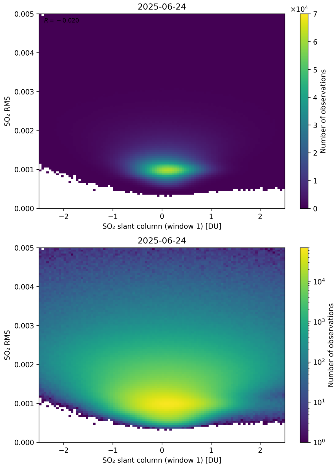
Figure 267: Scatter density plot of “SO 2 slant column (window 1)” against “SO 2 RMS” for 2025-06-23 to 2025-06-25.
