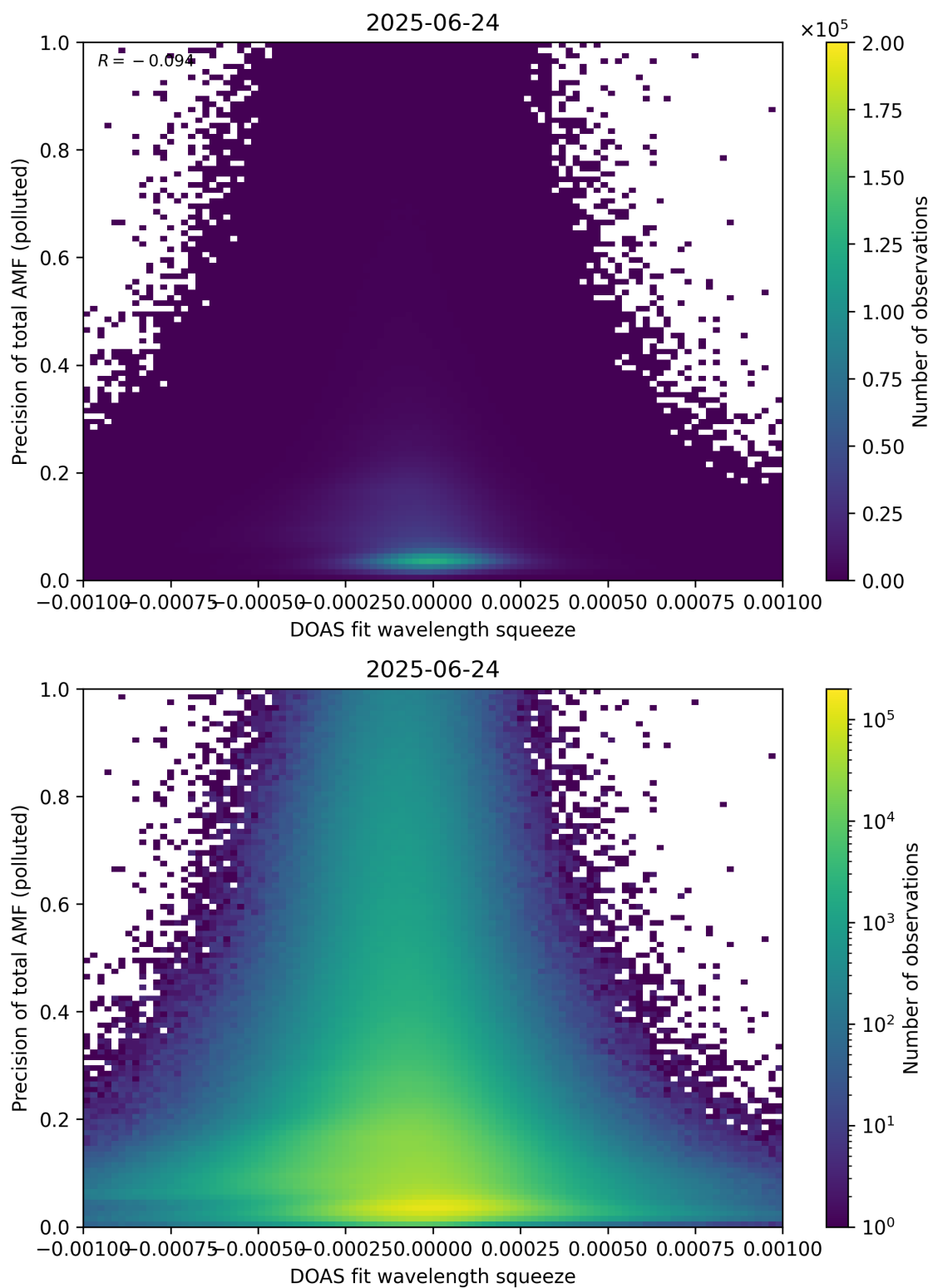
Figure 146: Scatter density plot of “DOAS fit wavelength squeeze” against “Precision of total AMF (polluted)” for 2025-06-23 to 2025-06-25.
