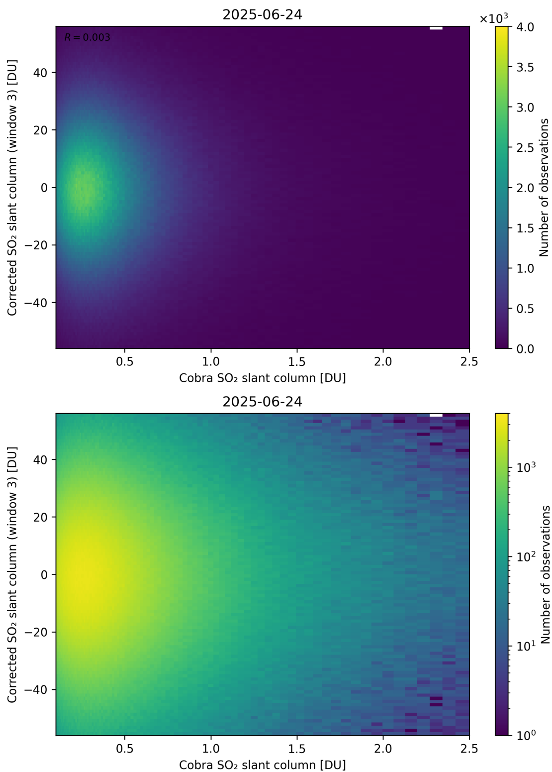
Figure 218: Scatter density plot of “Cobra SO 2 slant column” against “Corrected SO 2 slant column (window 3)” for 2025-06-23 to 2025-06-25.
