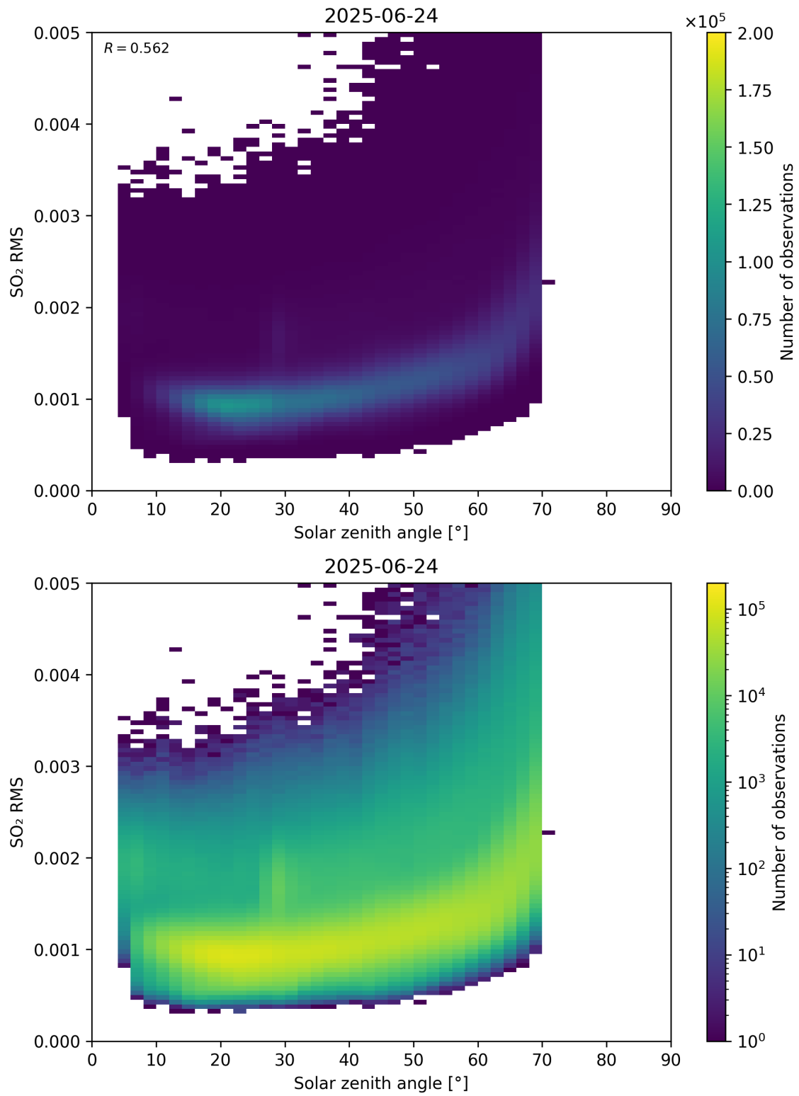
Figure 176: Scatter density plot of “Solar zenith angle” against “SO 2 RMS” for 2025-06-23 to 2025-06-25.
