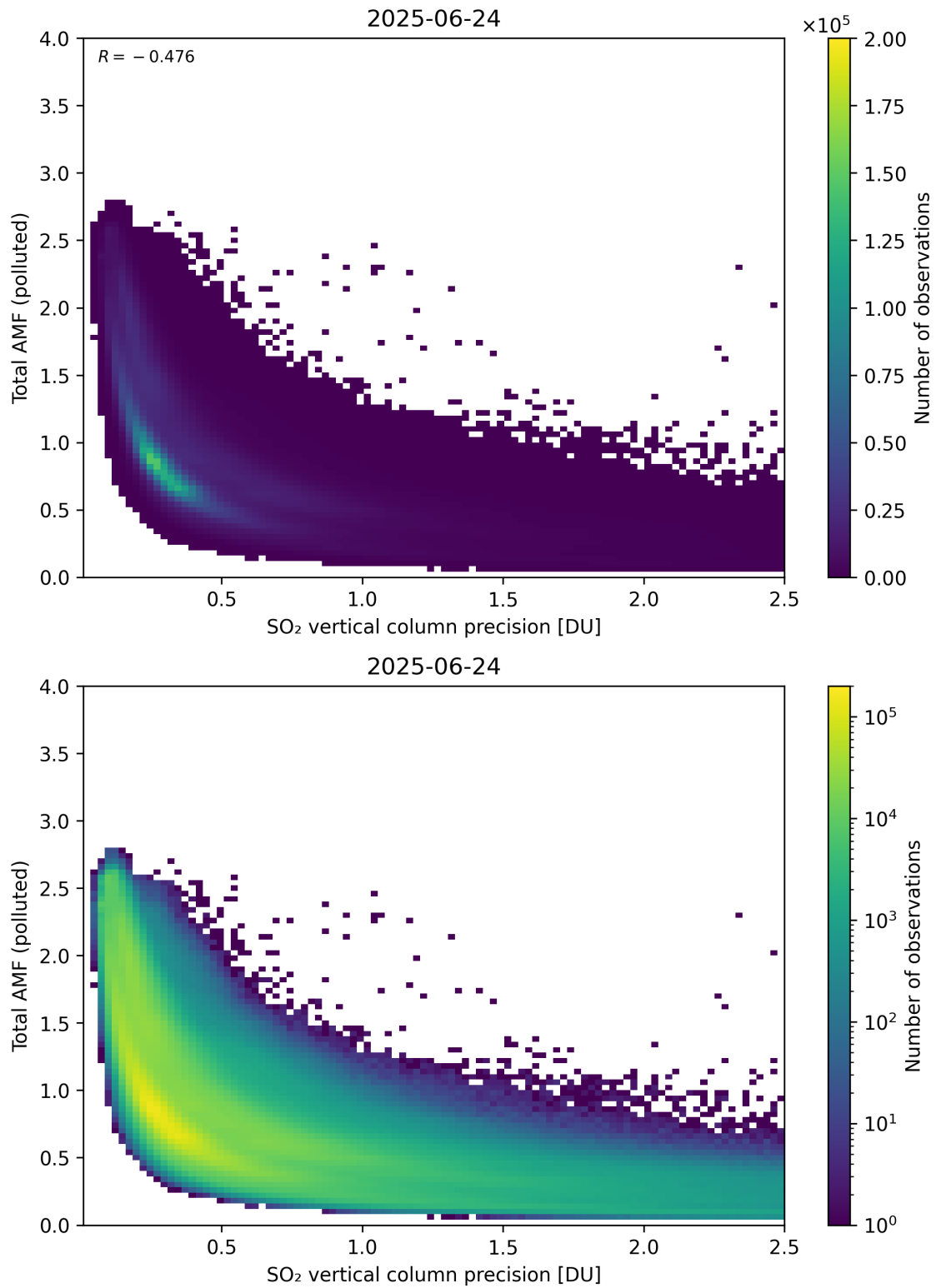
Figure 346: Scatter density plot of “SO 2 vertical column precision” against “Total AMF (polluted)” for 2025-06-23 to 2025-06-25.
