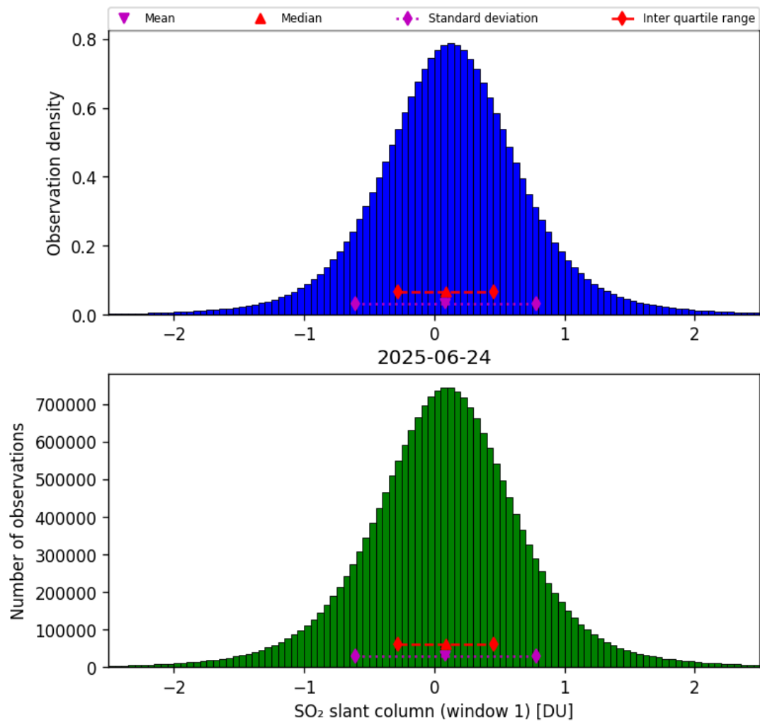
Figure 63: Histogram of “SO 2 slant column (window 1)” for 2025-06-23 to 2025-06-25
