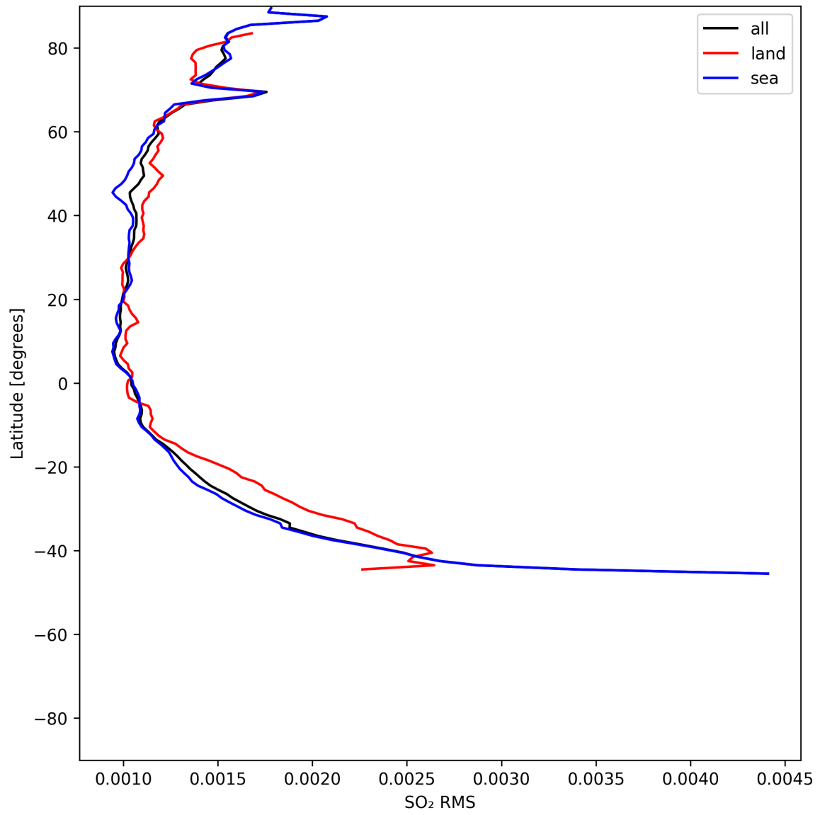
Figure 52: Zonal average of “SO 2 RMS” for 2025-06-23 to 2025-06-25.
