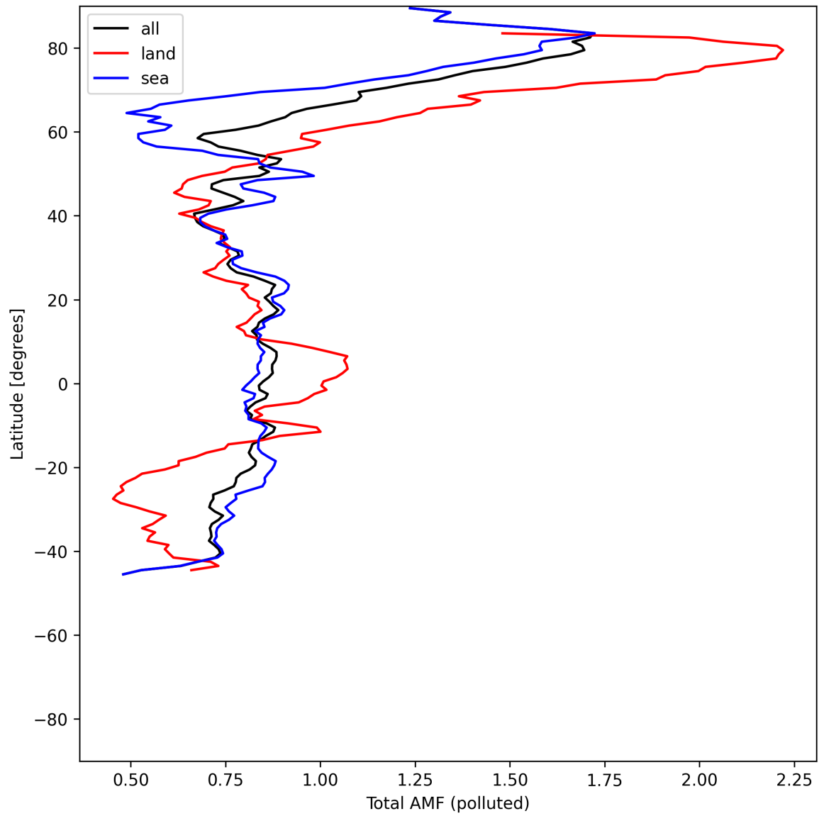
Figure 53: Zonal average of “Total AMF (polluted)” for 2025-06-23 to 2025-06-25.
