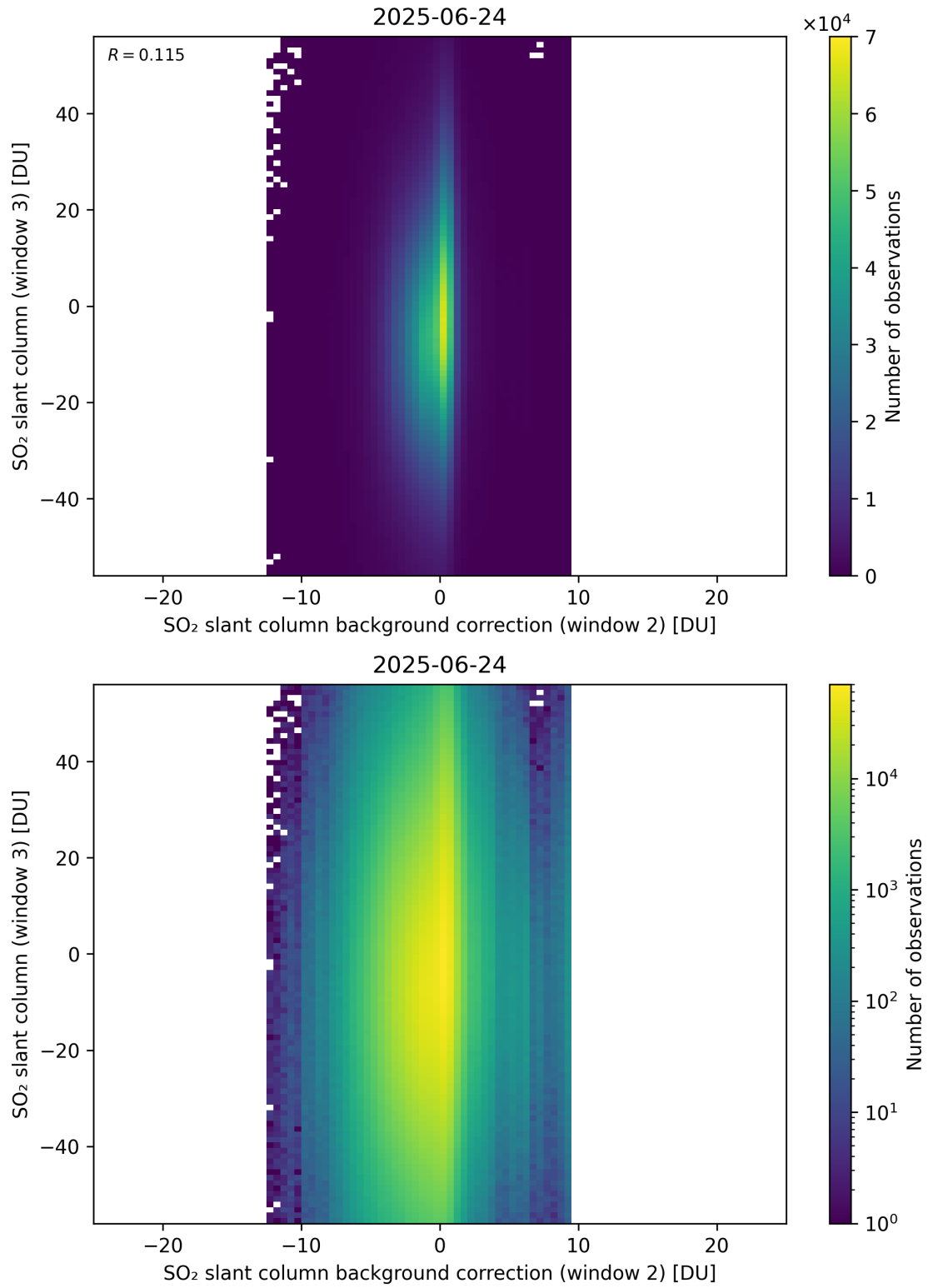
Figure 128: Scatter density plot of “SO 2 slant column background correction (window 2)” against “SO 2 slant column (window 3)” for 2025-06-23 to 2025-06-25.
