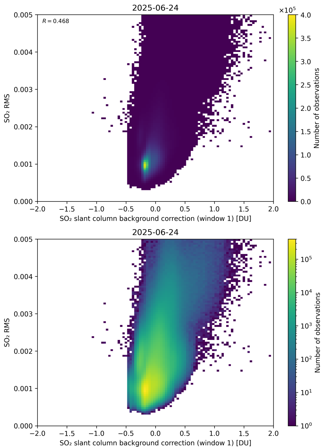
Figure 113: Scatter density plot of “SO 2 slant column background correction (window 1)” against “SO 2 RMS” for 2025-06-23 to 2025-06-25.
