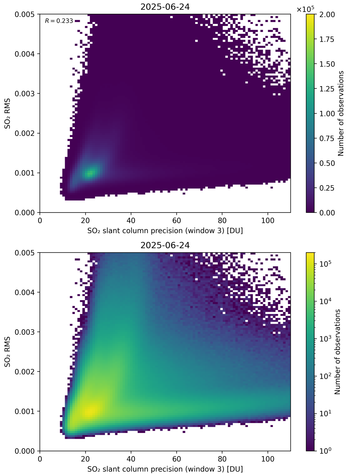
Figure 310: Scatter density plot of “SO 2 slant column precision (window 3)” against “SO 2 RMS” for 2025-06-23 to 2025-06-25.
