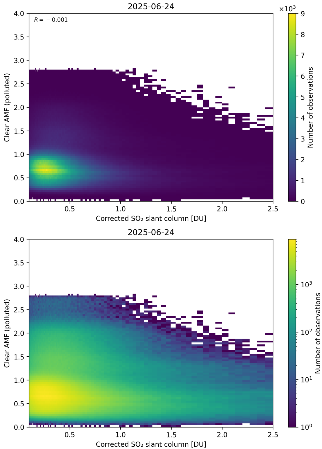
Figure 232: Scatter density plot of “Corrected SO 2 slant column” against “Clear AMF (polluted)” for 2025-06-23 to 2025-06-25.
