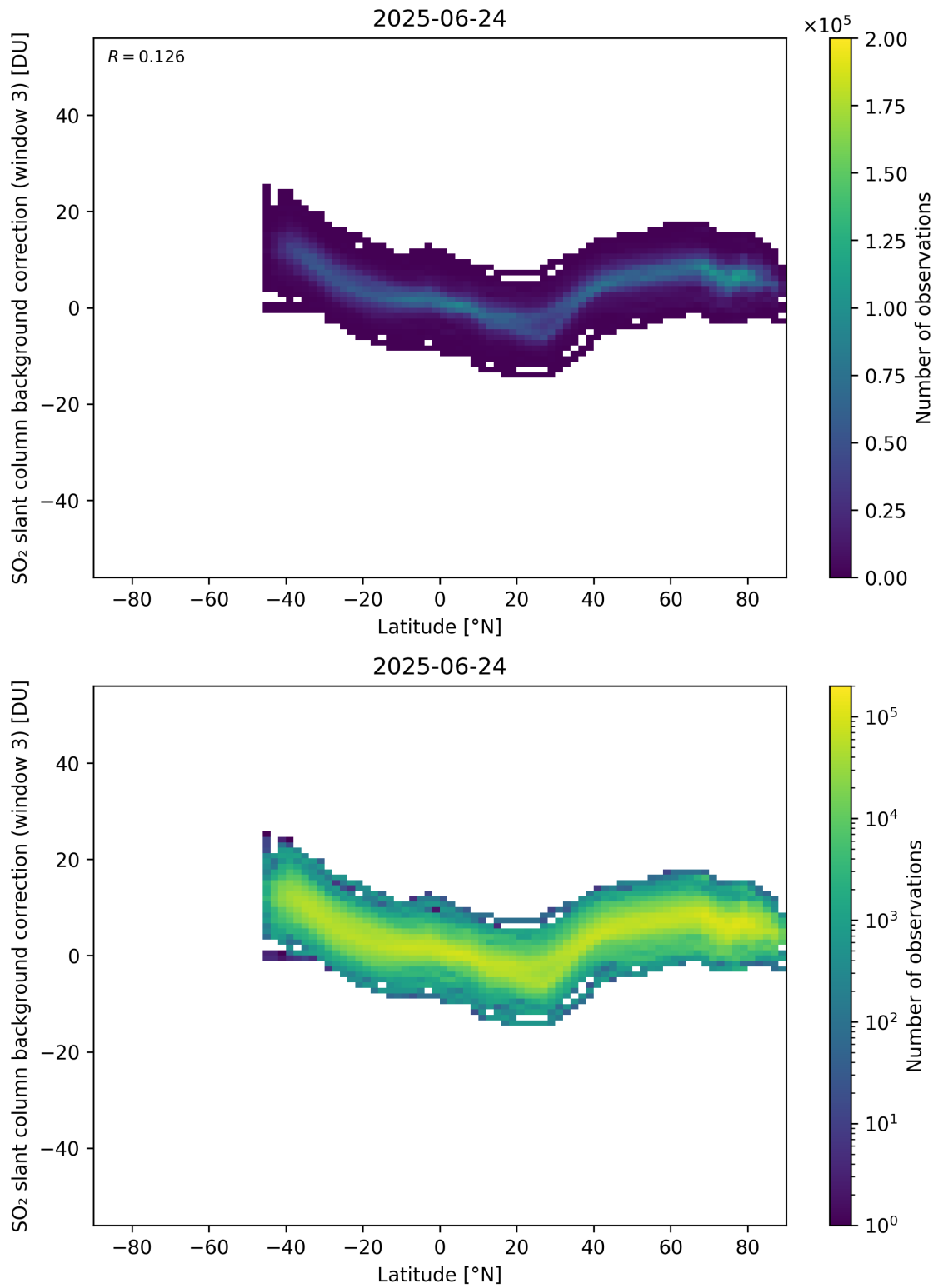
Figure 152: Scatter density plot of “Latitude” against “SO 2 slant column background correction (window 3)” for 2025-06-23 to 2025-06-25.
