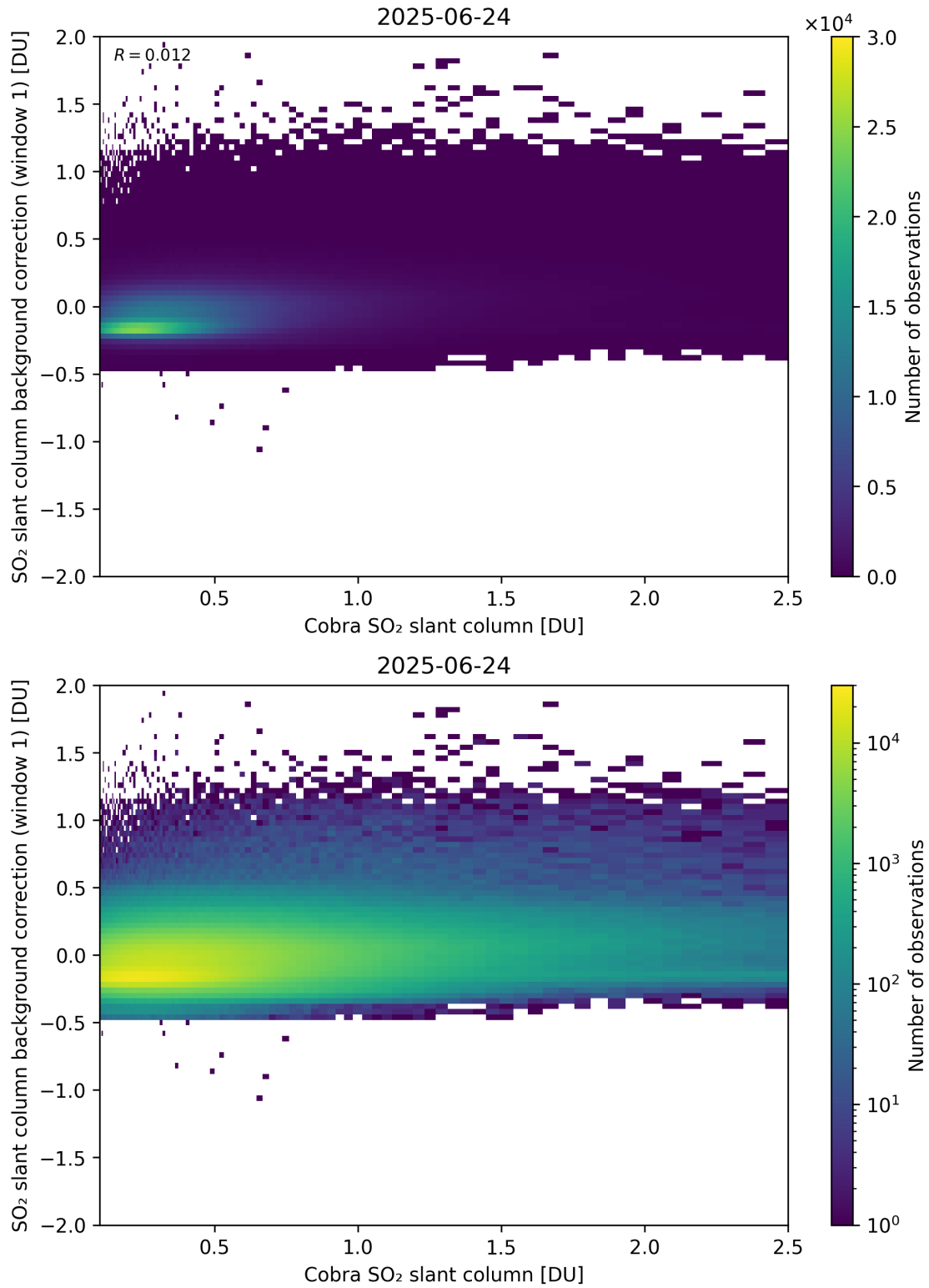
Figure 193: Scatter density plot of “Cobra SO 2 slant column” against “SO 2 slant column background correction (window 1)” for 2025-06-23 to 2025-06-25.
