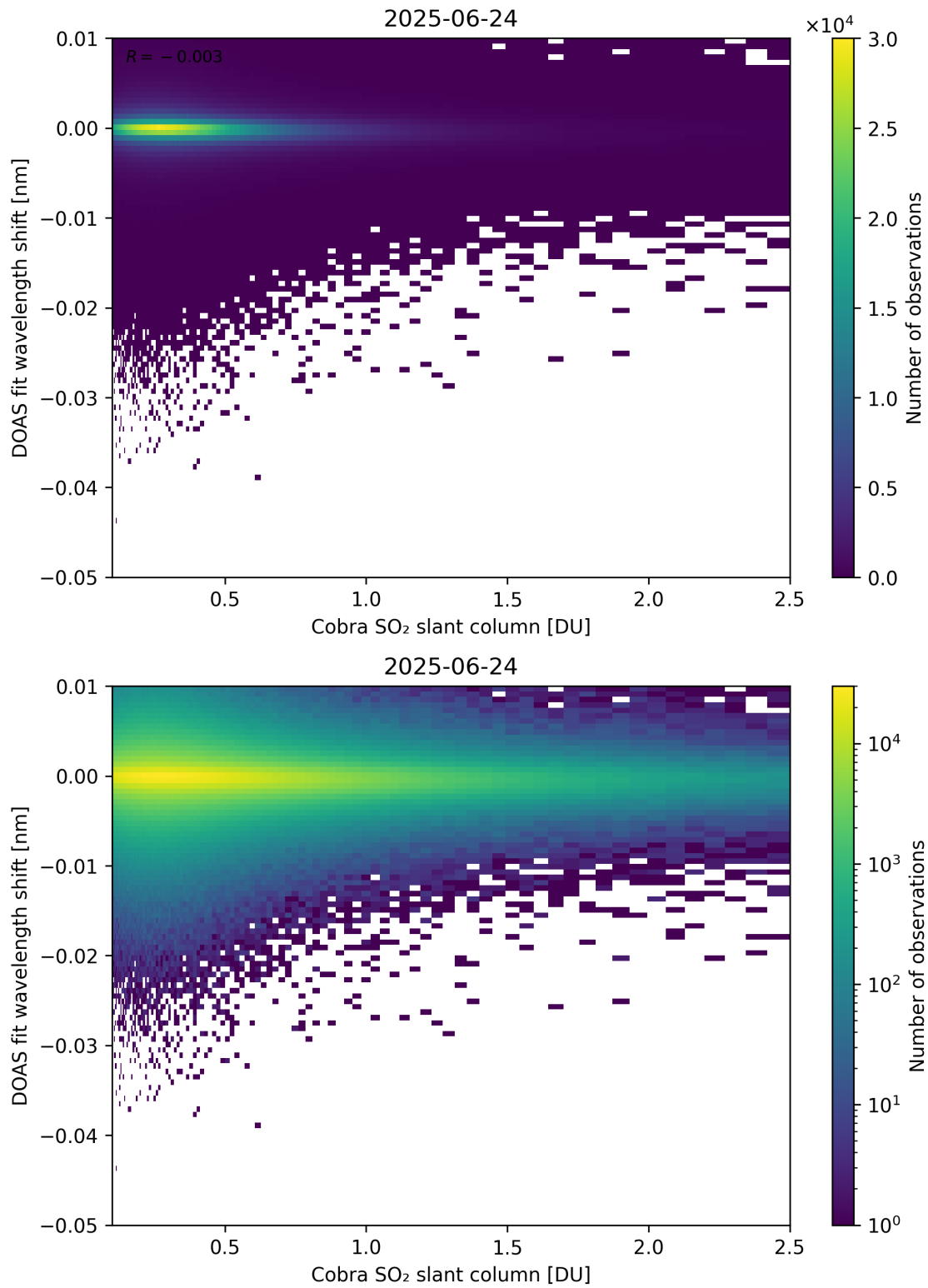
Figure 196: Scatter density plot of “Cobra SO 2 slant column” against “DOAS fit wavelength shift” for 2025-06-23 to 2025-06-25.
