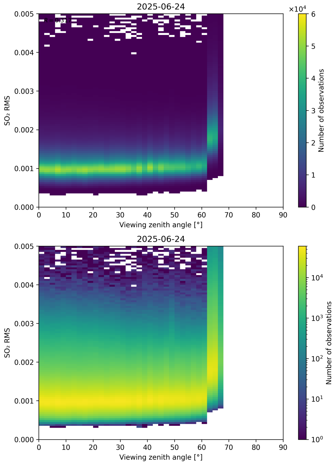
Figure 367: Scatter density plot of “Viewing zenith angle” against “SO 2 RMS” for 2025-06-23 to 2025-06-25.
