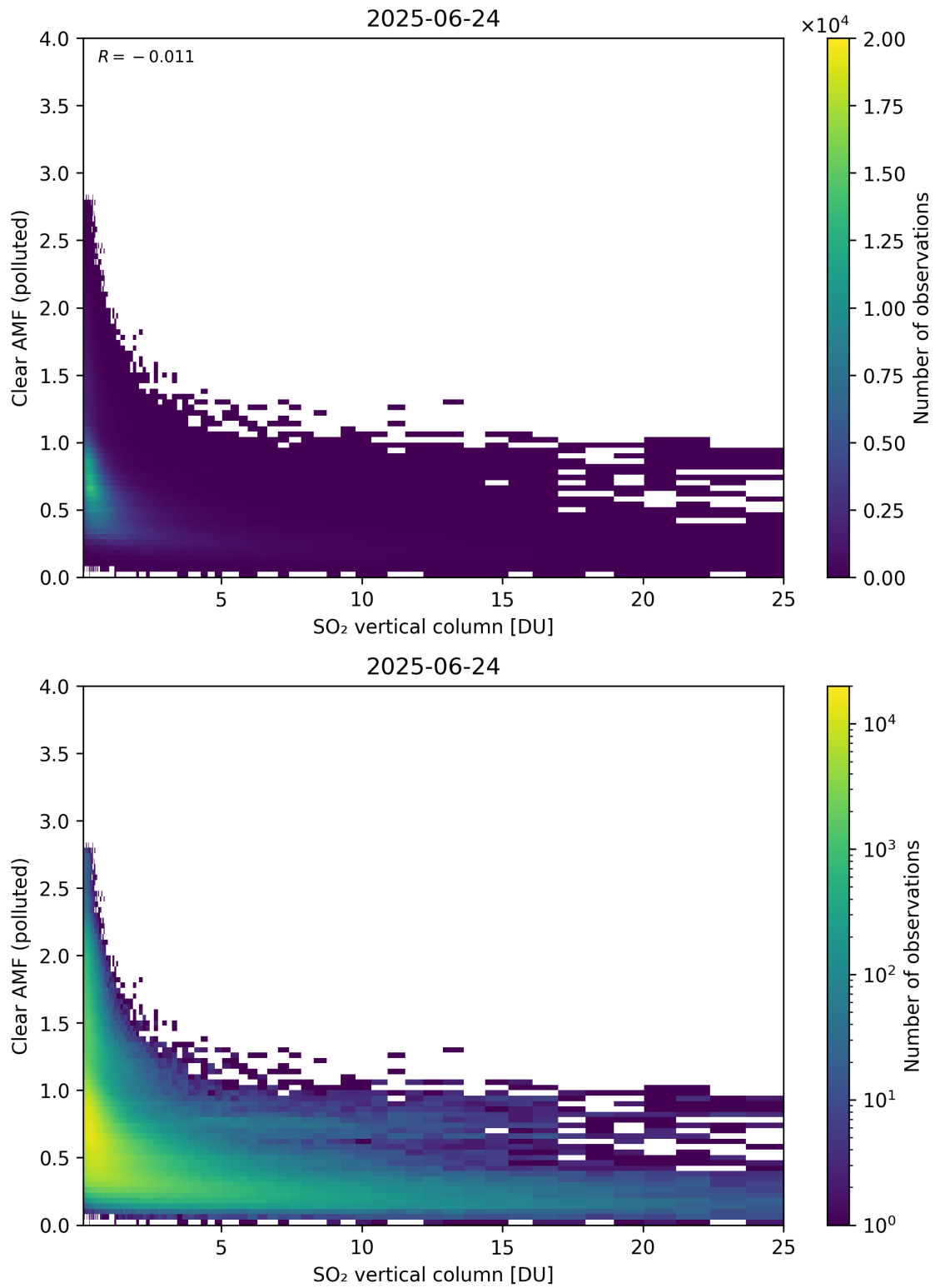
Figure 348: Scatter density plot of “SO 2 vertical column” against “Clear AMF (polluted)” for 2025-06-23 to 2025-06-25.
