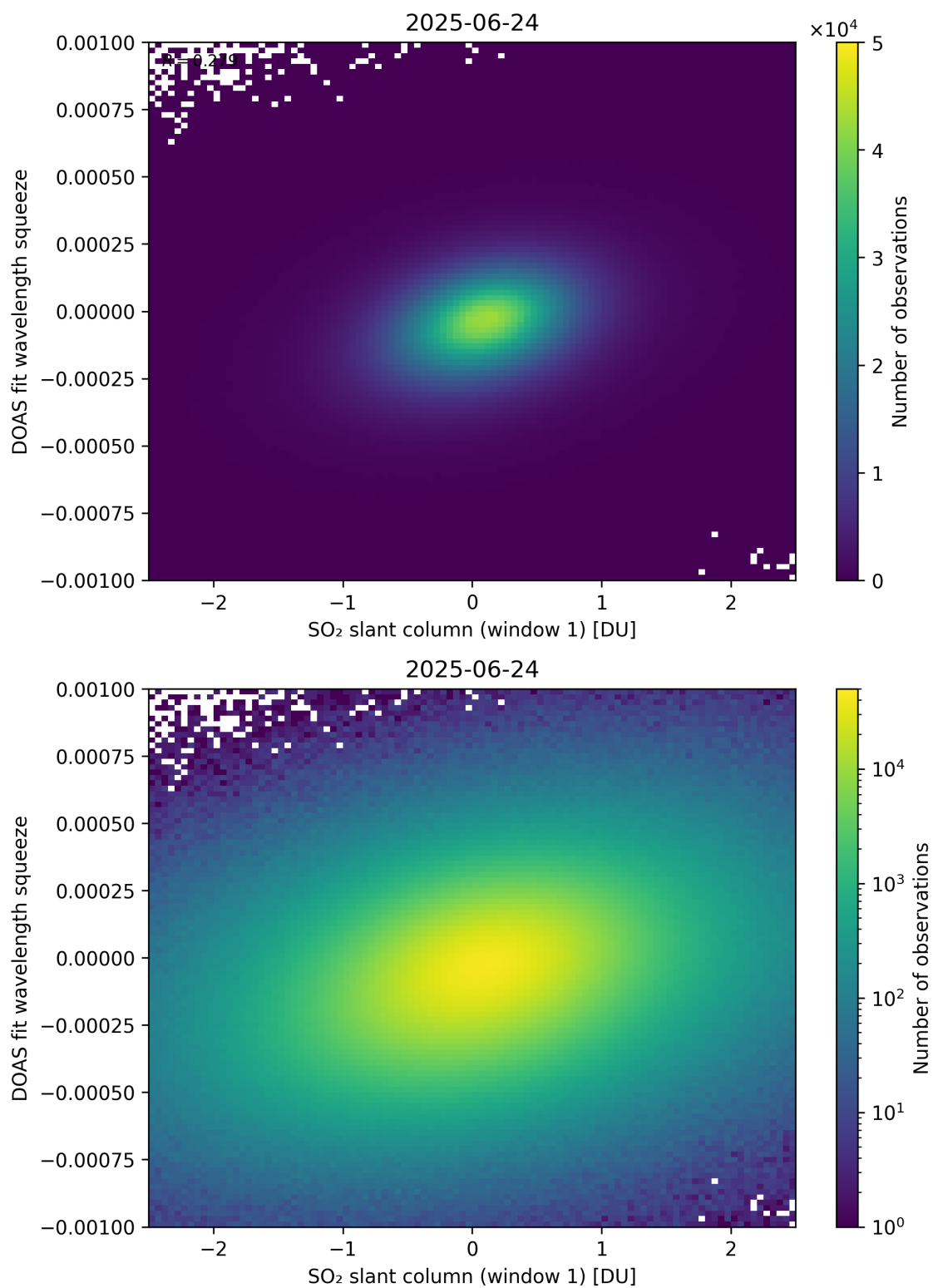
Figure 266: Scatter density plot of “SO 2 slant column (window 1)” against “DOAS fit wavelength squeeze” for 2025-06-23 to 2025-06-25.
