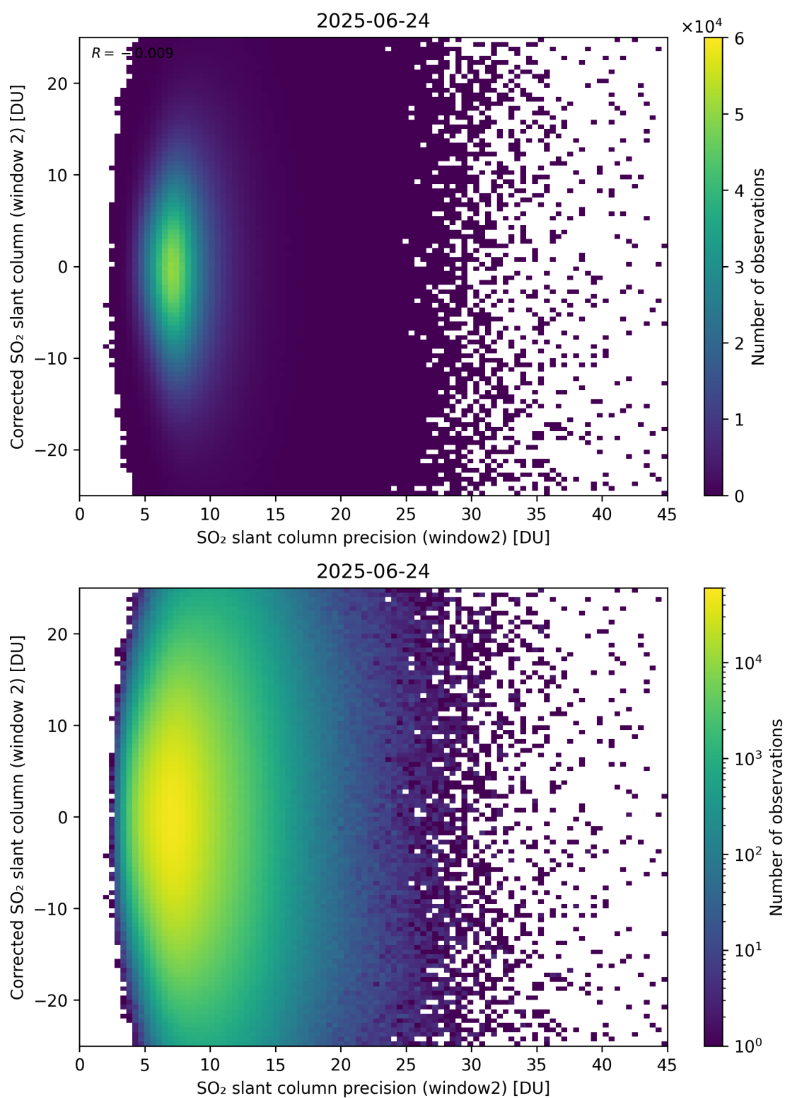
Figure 297: Scatter density plot of “SO 2 slant column precision (window2)” against “Corrected SO 2 slant column (window 2)” for 2025-06-23 to 2025-06-25.
