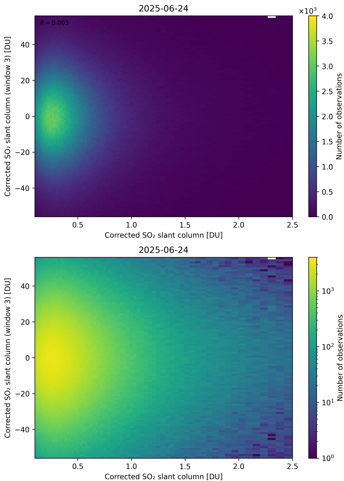
Figure 236: Scatter density plot of “Corrected SO 2 slant column” against “Corrected SO 2 slant column (window 3)” for 2025-06-23 to 2025-06-25.
