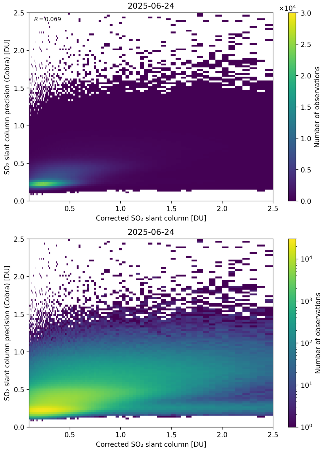
Figure 234: Scatter density plot of “Corrected SO 2 slant column” against “SO 2 slant column precision (Cobra)” for 2025-06-23 to 2025-06-25.
