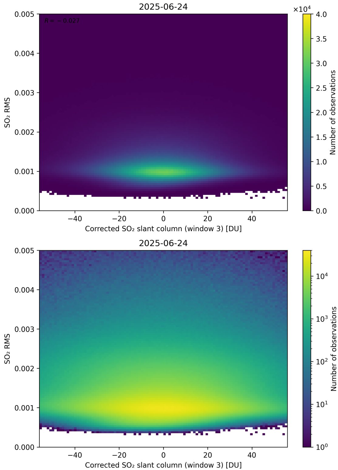
Figure 258: Scatter density plot of “Corrected SO 2 slant column (window 3)” against “SO 2 RMS” for 2025-06-23 to 2025-06-25.
