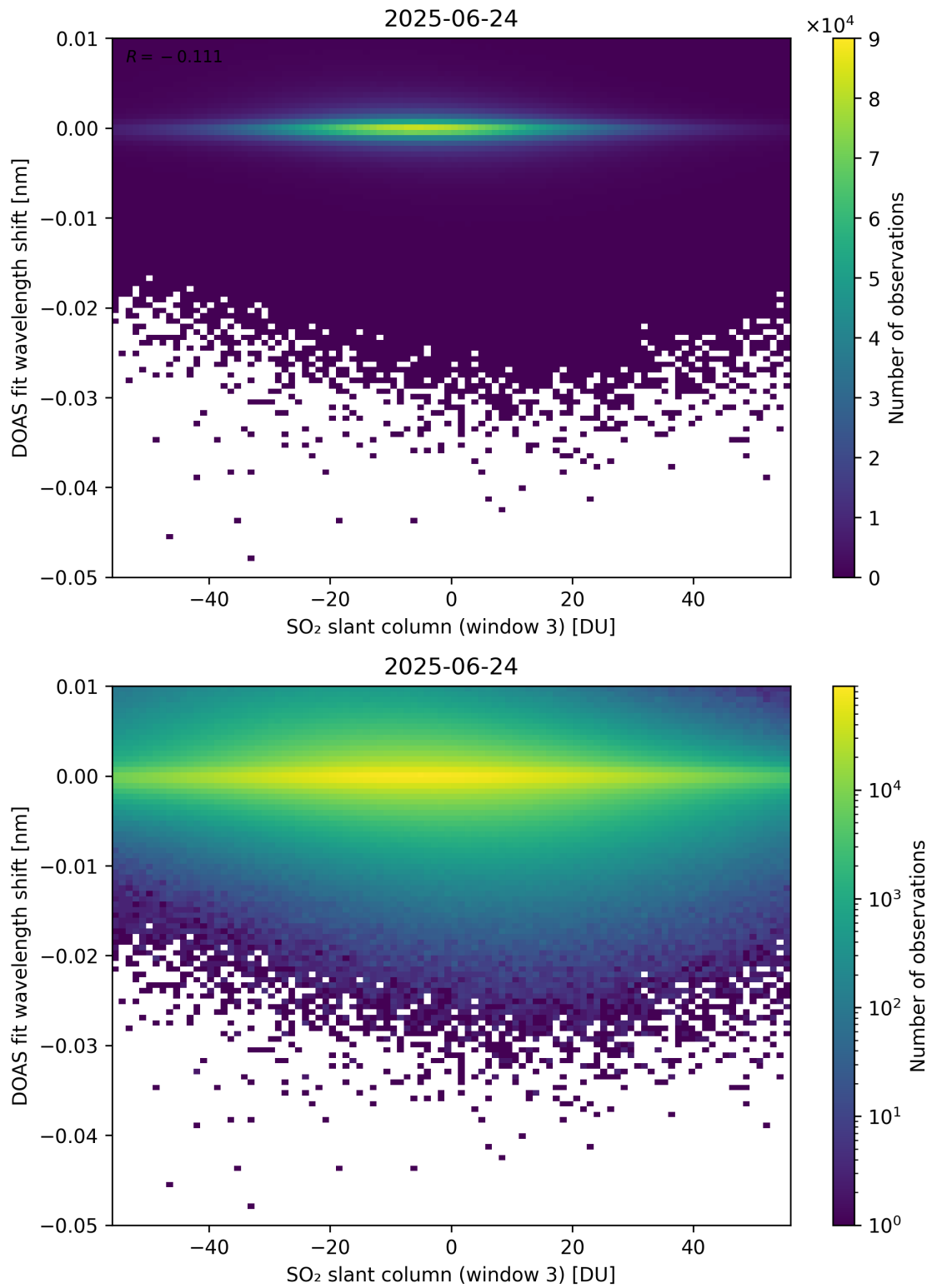
Figure 304: Scatter density plot of “SO 2 slant column (window 3)” against “DOAS fit wavelength shift” for 2025-06-23 to 2025-06-25.
