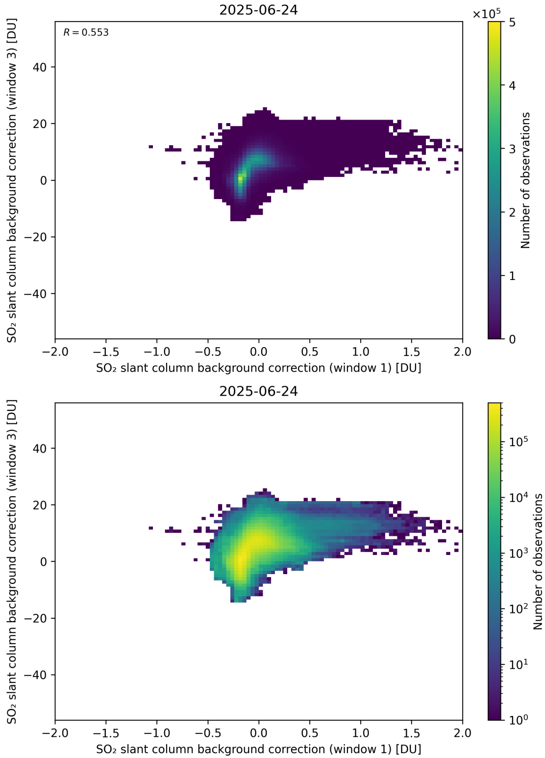
Figure 110: Scatter density plot of “SO 2 slant column background correction (window 1)” against “SO 2 slant column background correction (window 3)” for 2025-06-23 to 2025-06-25.
