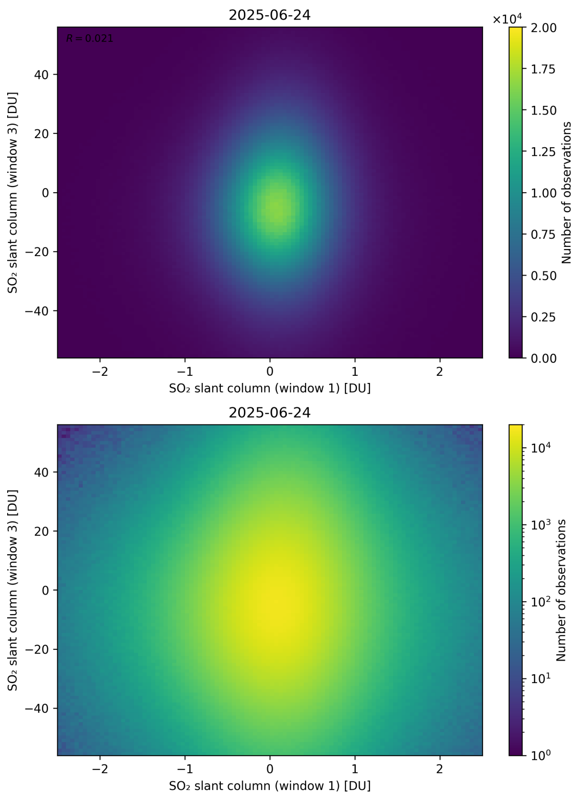
Figure 287: Scatter density plot of “SO 2 slant column (window 1)” against “SO 2 slant column (window 3)” for 2025-06-23 to 2025-06-25.
