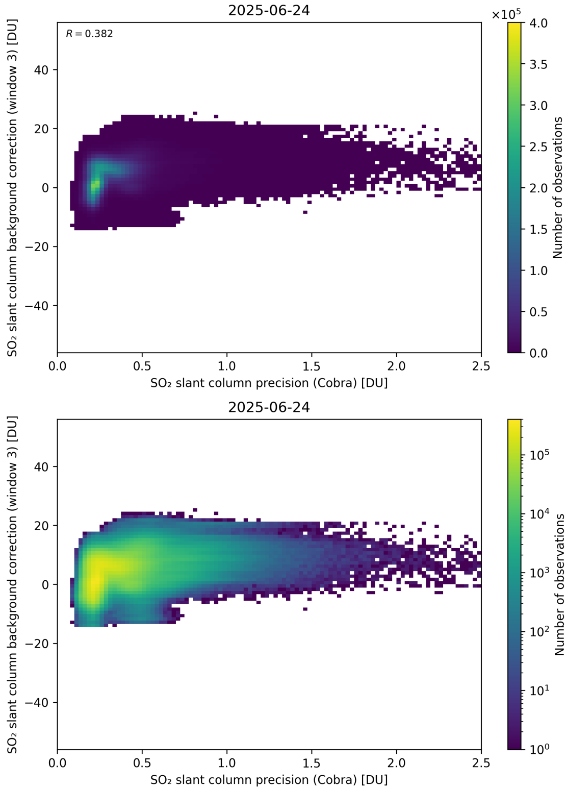
Figure 201: Scatter density plot of “SO 2 slant column precision (Cobra)” against “SO 2 slant column background correction (window 3)” for 2025-06-23 to 2025-06-25.
