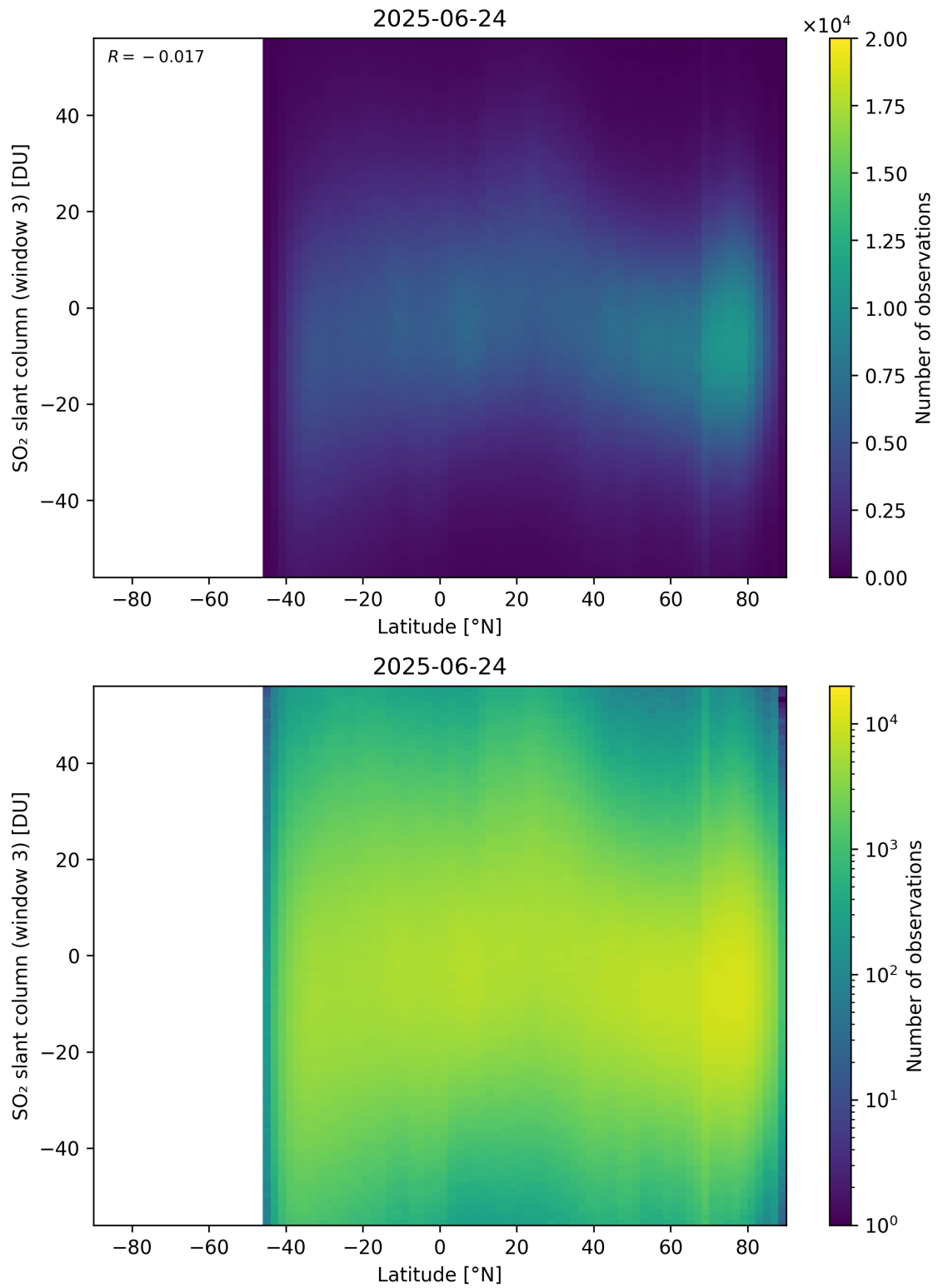
Figure 165: Scatter density plot of “Latitude” against “SO 2 slant column (window 3)” for 2025-06-23 to 2025-06-25.
