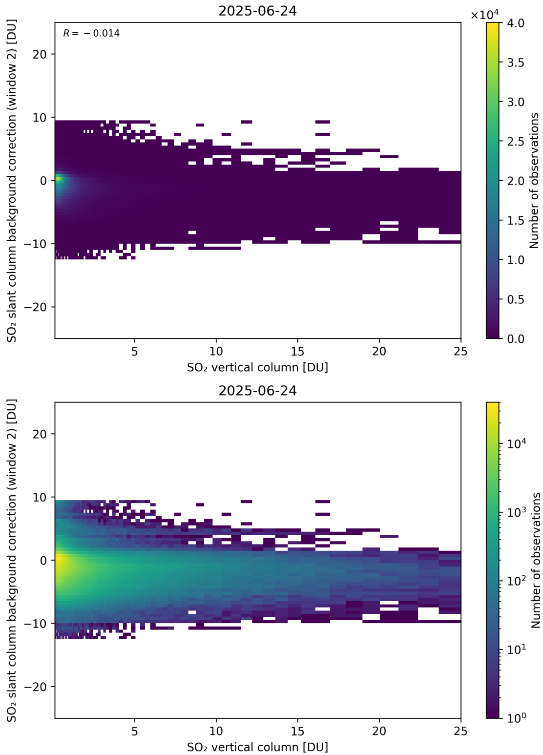
Figure 324: Scatter density plot of “SO 2 vertical column” against “SO 2 slant column background correction (window 2)” for 2025-06-23 to 2025-06-25.
