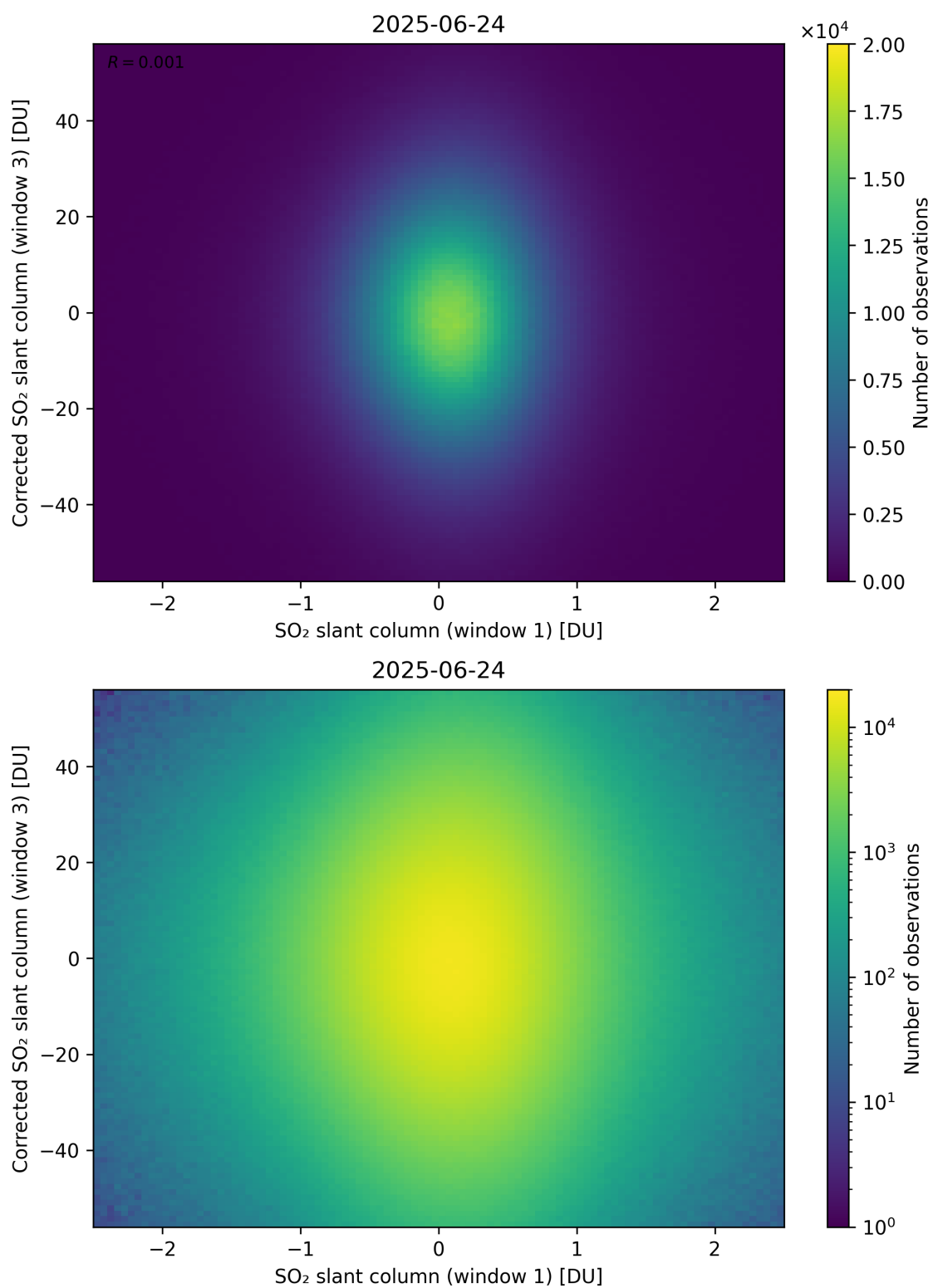
Figure 284: Scatter density plot of “SO 2 slant column (window 1)” against “Corrected SO 2 slant column (window 3)” for 2025-06-23 to 2025-06-25.
