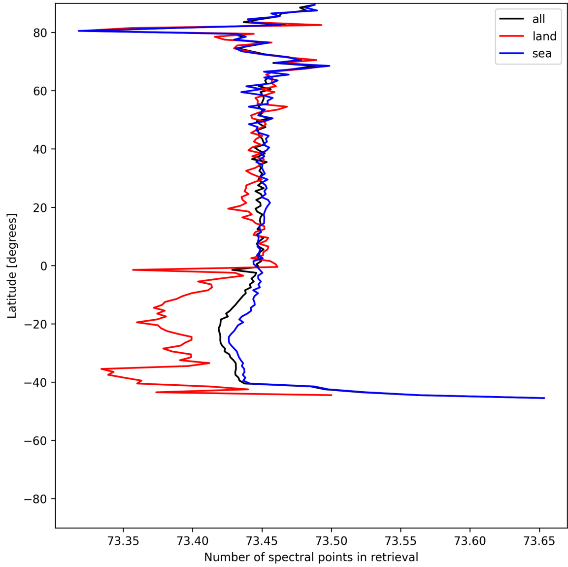
Figure 56: Zonal average of “Number of spectral points in retrieval” for 2025-06-23 to 2025-06-25.
