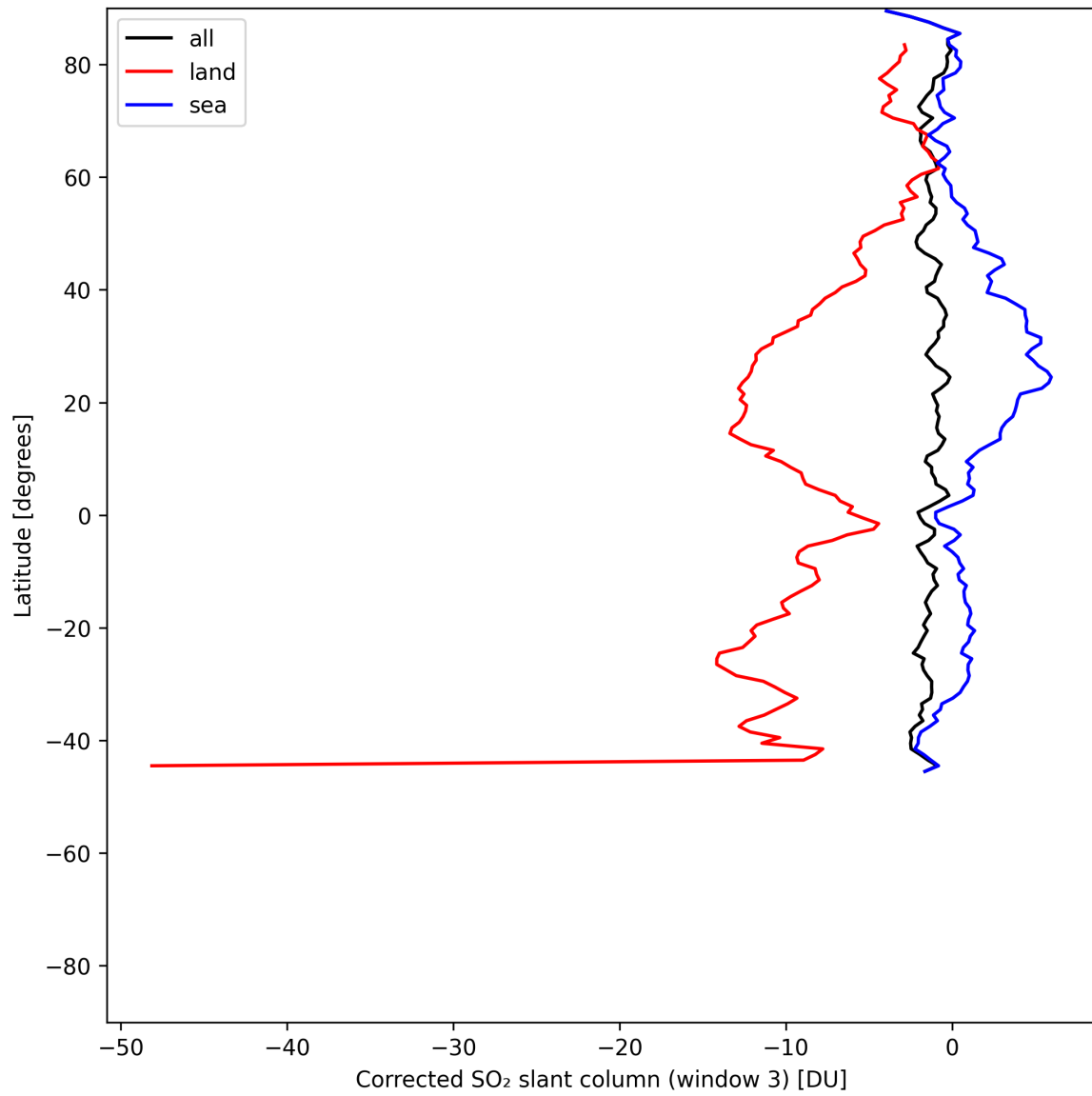
Figure 47: Zonal average of “Corrected SO 2 slant column (window 3)” for 2025-06-23 to 2025-06-25.
