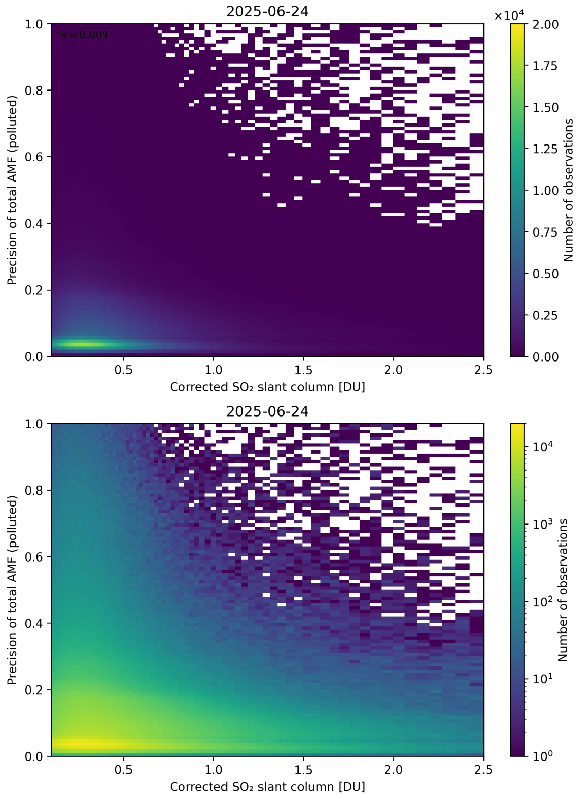
Figure 243: Scatter density plot of “Corrected SO 2 slant column” against “Precision of total AMF (polluted)” for 2025-06-23 to 2025-06-25.
