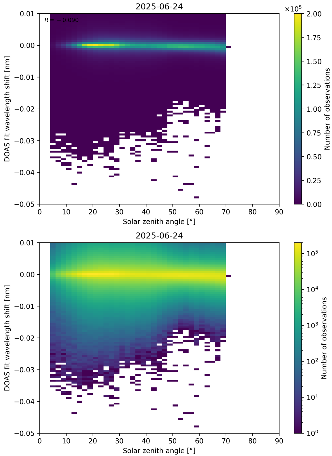
Figure 174: Scatter density plot of “Solar zenith angle” against “DOAS fit wavelength shift” for 2025-06-23 to 2025-06-25.
