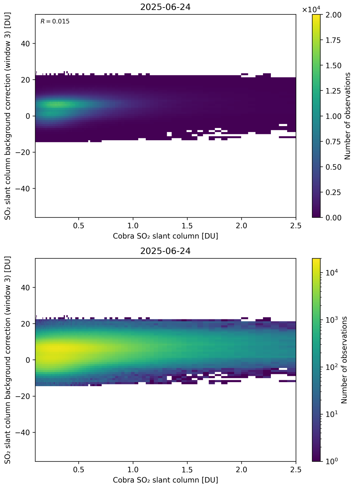
Figure 195: Scatter density plot of “Cobra SO 2 slant column” against “SO 2 slant column background correction (window 3)” for 2025-06-23 to 2025-06-25.
