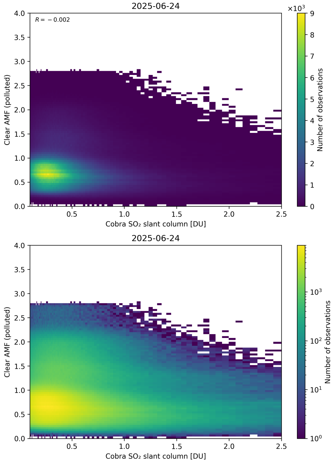
Figure 215: Scatter density plot of “Cobra SO 2 slant column” against “Clear AMF (polluted)” for 2025-06-23 to 2025-06-25.
