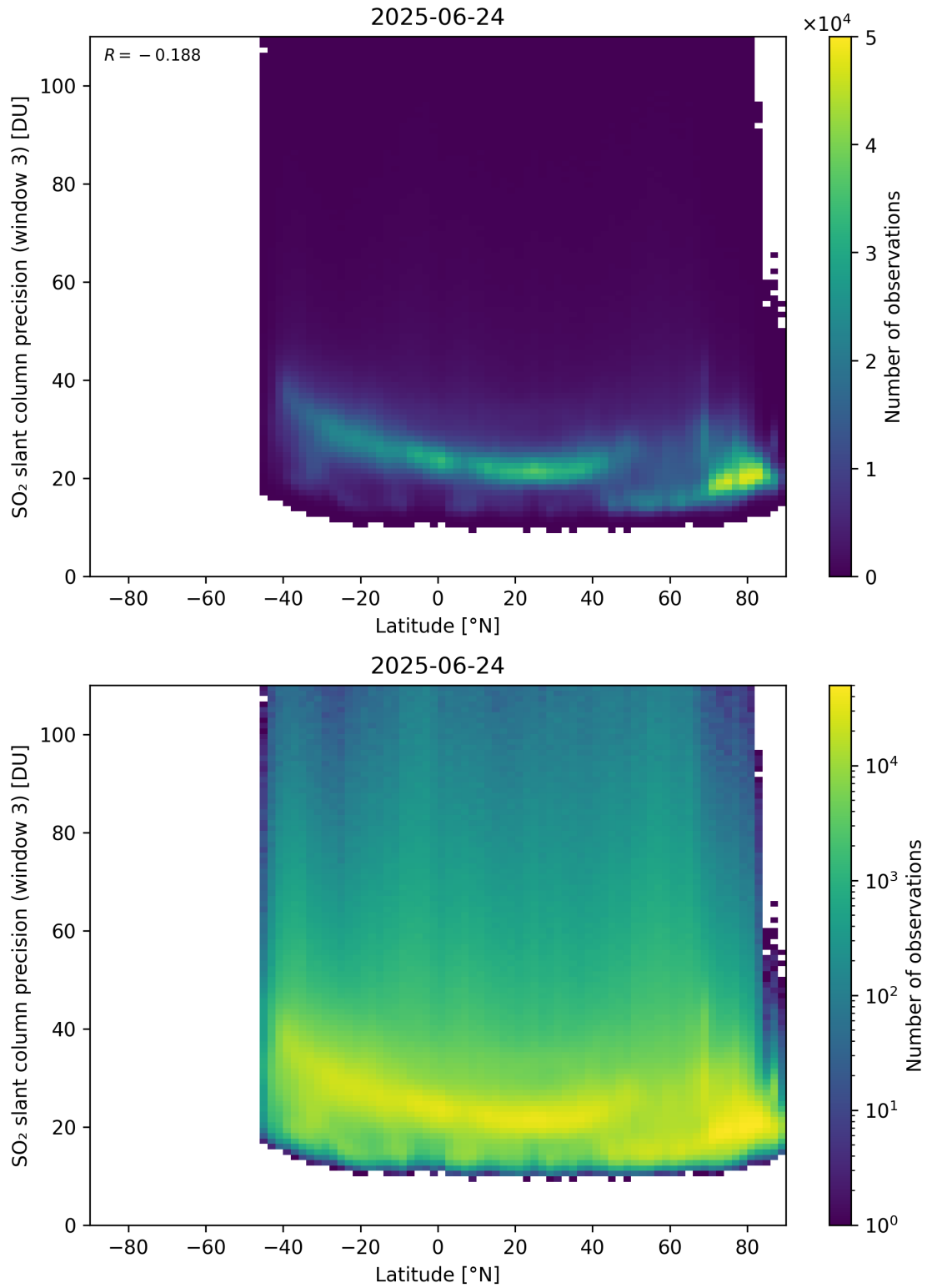
Figure 166: Scatter density plot of “Latitude” against “SO 2 slant column precision (window 3)” for 2025-06-23 to 2025-06-25.
