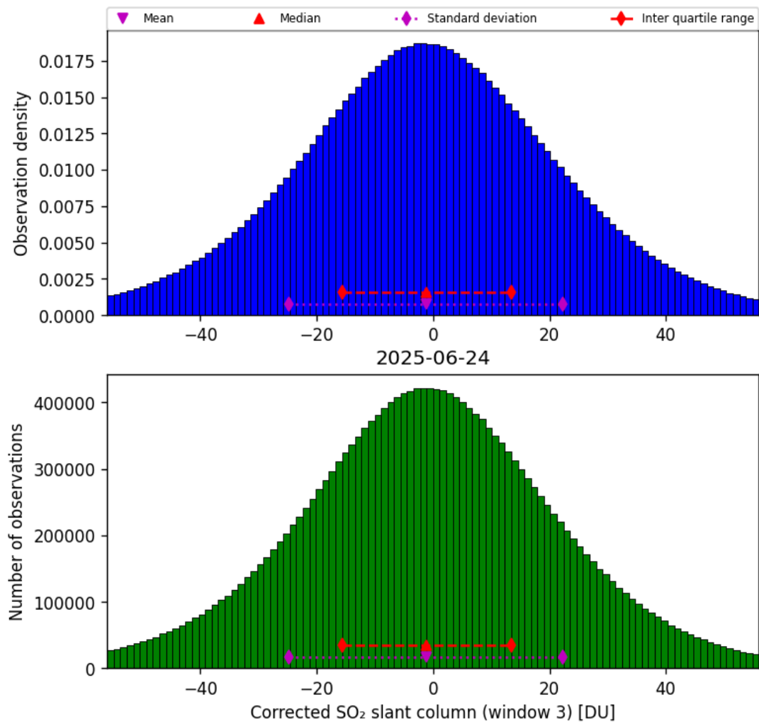
Figure 73: Histogram of “Corrected SO 2 slant column (window 3)” for 2025-06-23 to 2025-06-25
