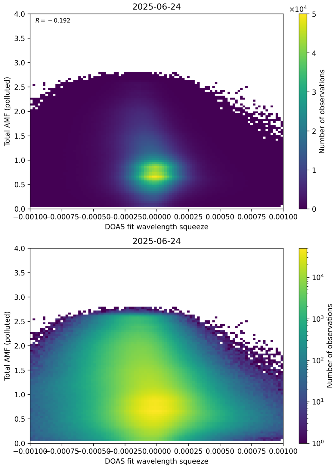
Figure 145: Scatter density plot of “DOAS fit wavelength squeeze” against “Total AMF (polluted)” for 2025-06-23 to 2025-06-25.
