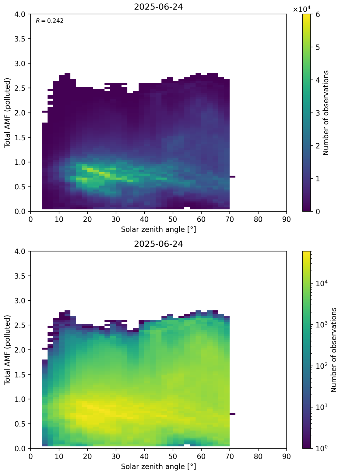
Figure 189: Scatter density plot of “Solar zenith angle” against “Total AMF (polluted)” for 2025-06-23 to 2025-06-25.
