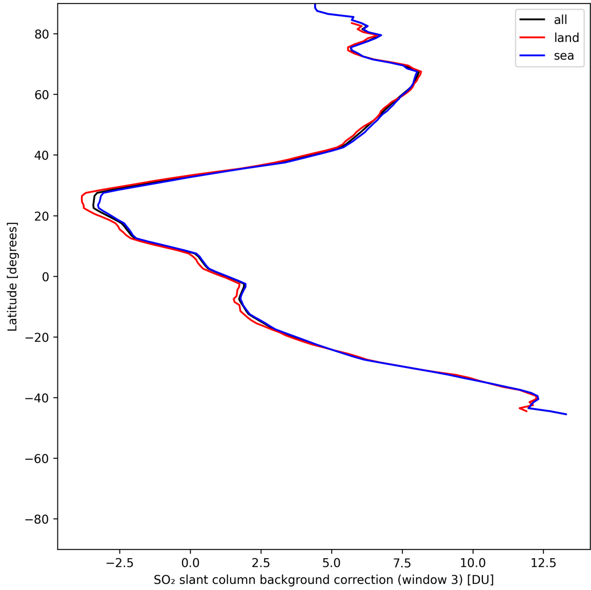
Figure 48: Zonal average of “SO 2 slant column background correction (window 3)” for 2025-06-23 to 2025-06-25.
