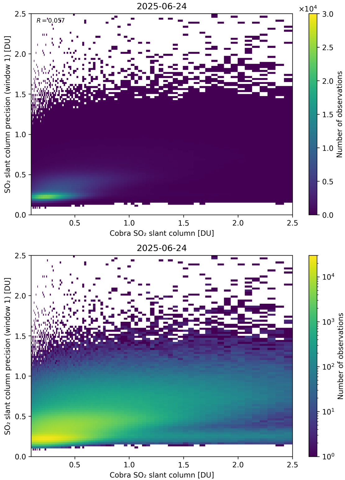
Figure 220: Scatter density plot of “Cobra SO 2 slant column” against “SO 2 slant column precision (window 1)” for 2025-06-23 to 2025-06-25.
