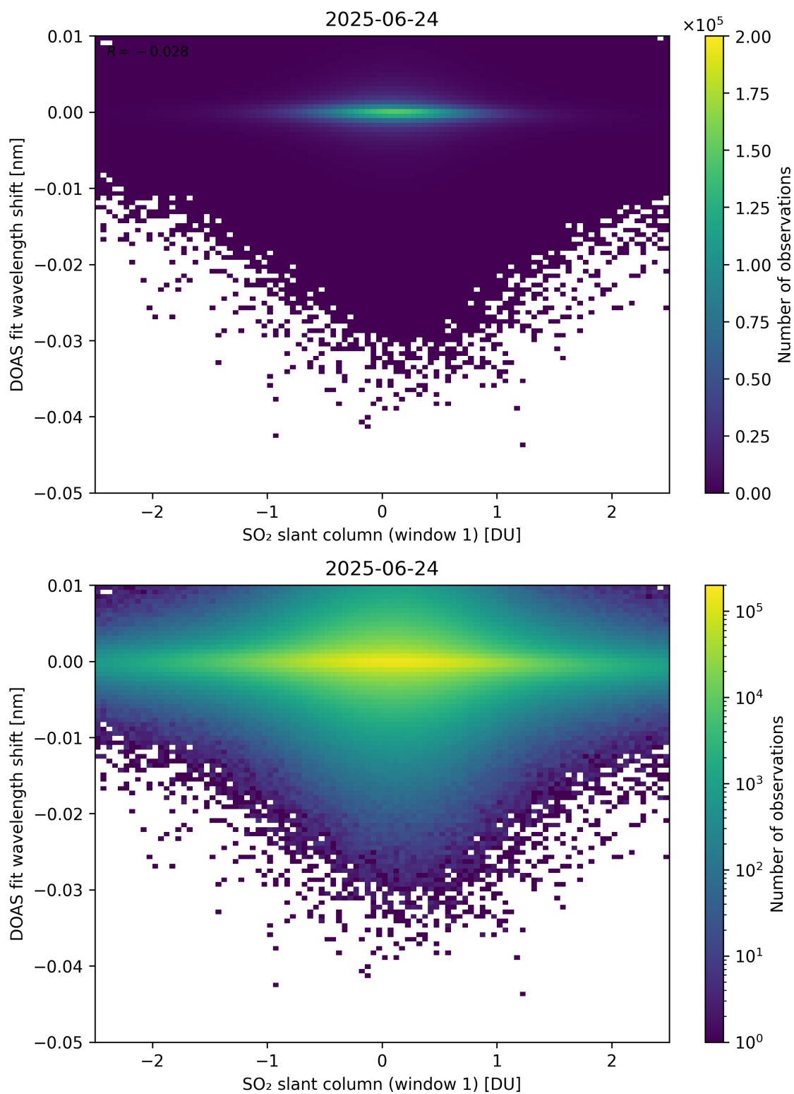
Figure 265: Scatter density plot of “SO 2 slant column (window 1)” against “DOAS fit wavelength shift” for 2025-06-23 to 2025-06-25.
