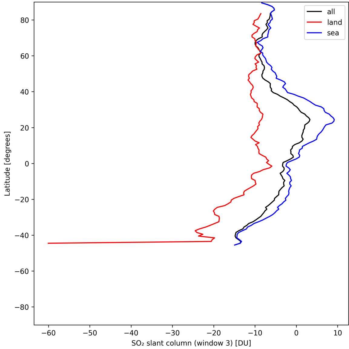
Figure 45: Zonal average of “SO 2 slant column (window 3)” for 2025-06-23 to 2025-06-25.
