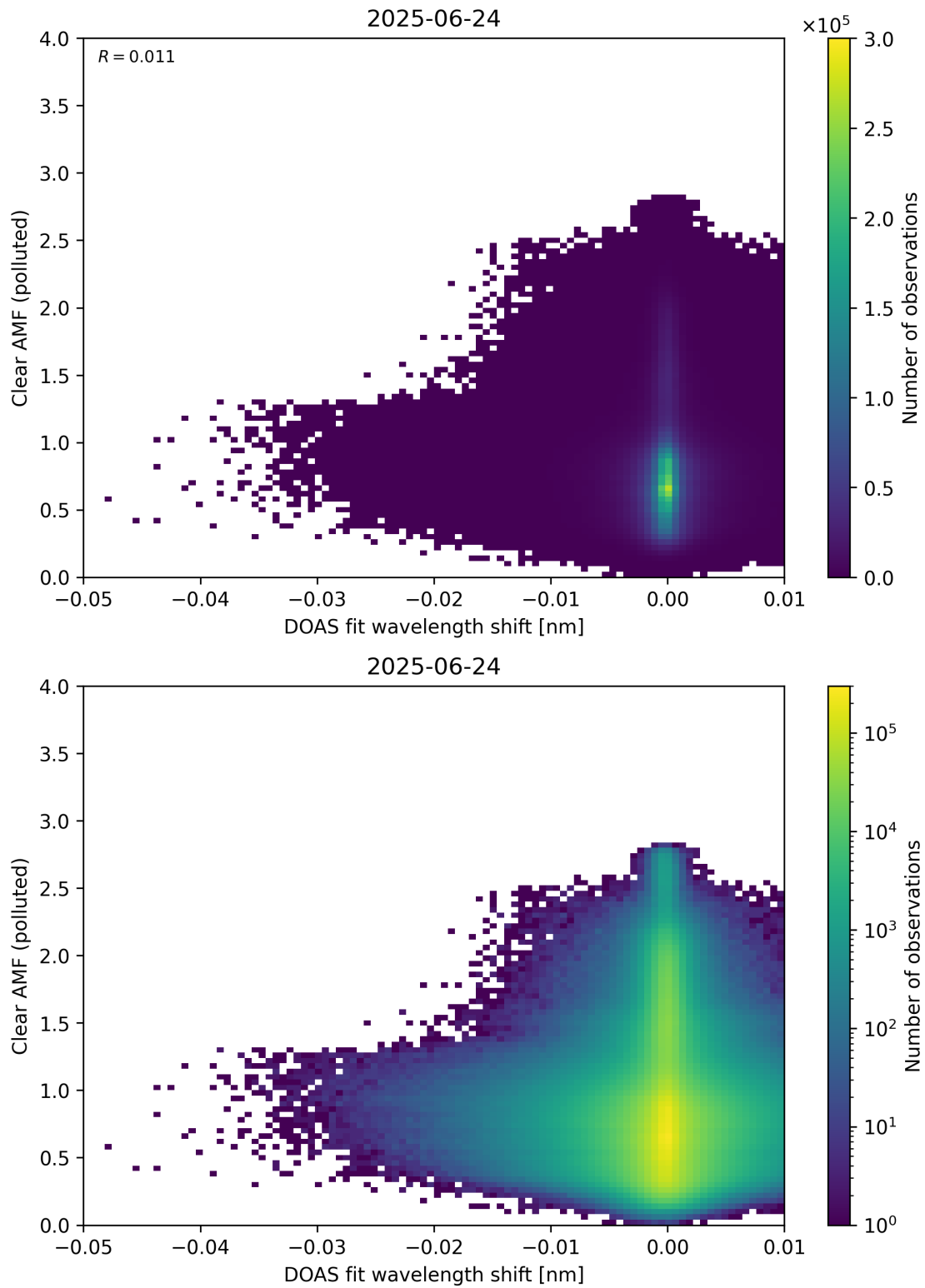
Figure 140: Scatter density plot of “DOAS fit wavelength shift” against “Clear AMF (polluted)” for 2025-06-23 to 2025-06-25.
