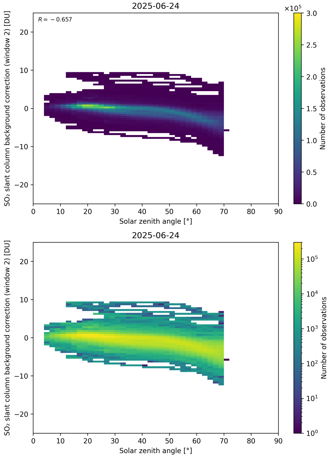
Figure 172: Scatter density plot of “Solar zenith angle” against “SO 2 slant column background correction (window 2)” for 2025-06-23 to 2025-06-25.
