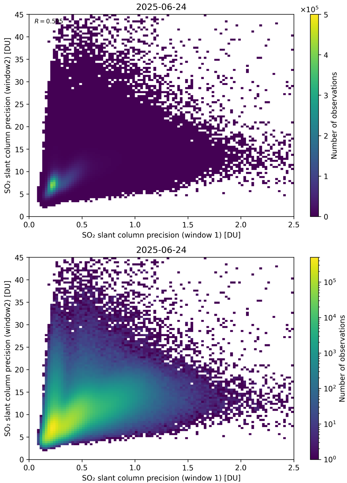
Figure 277: Scatter density plot of “SO 2 slant column precision (window 1)” against “SO 2 slant column precision (window2)” for 2025-06-23 to 2025-06-25.
