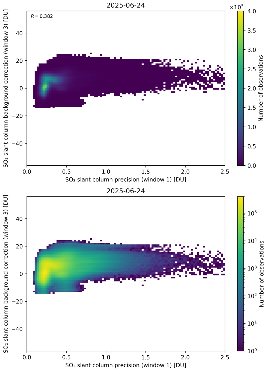
Figure 270: Scatter density plot of “SO 2 slant column precision (window 1)” against “SO 2 slant column background correction (window 3)” for 2025-06-23 to 2025-06-25.
