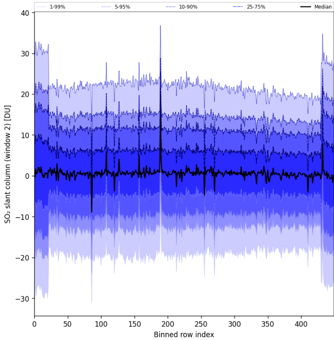
Figure 93: Along track statistics of “SO 2 slant column (window 2)” for 2025-06-23 to 2025-06-25
