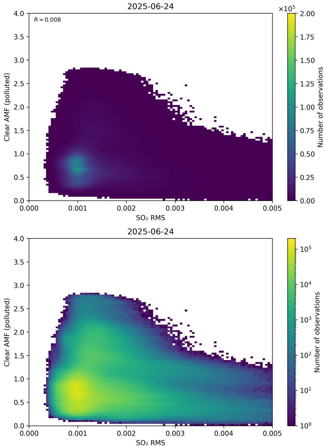
Figure 147: Scatter density plot of “SO 2 RMS” against “Clear AMF (polluted)” for 2025-06-23 to 2025-06-25.
