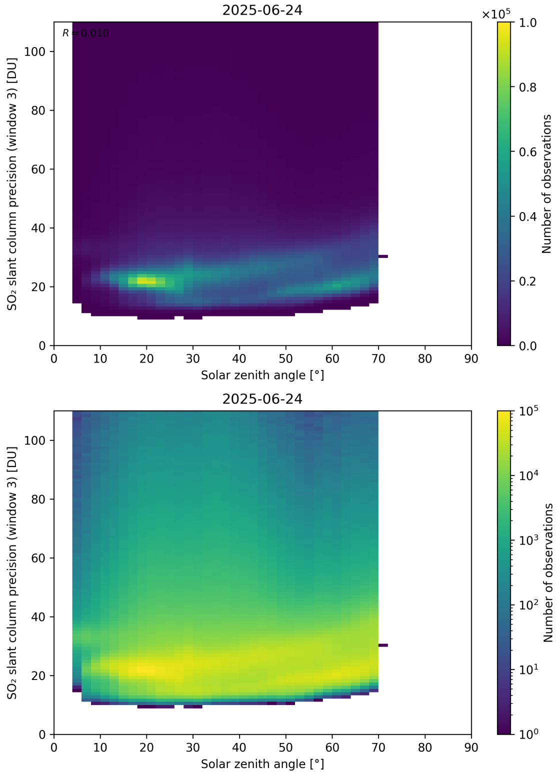
Figure 188: Scatter density plot of “Solar zenith angle” against “SO 2 slant column precision (window 3)” for 2025-06-23 to 2025-06-25.
