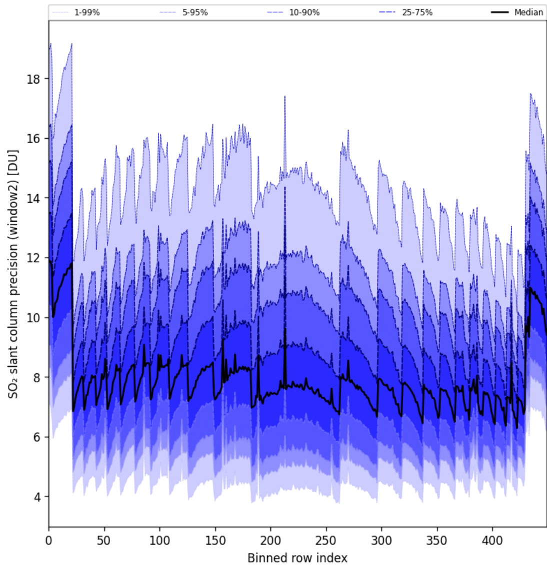
Figure 94: Along track statistics of “SO 2 slant column precision (window2)” for 2025-06-23 to 2025-06-25
