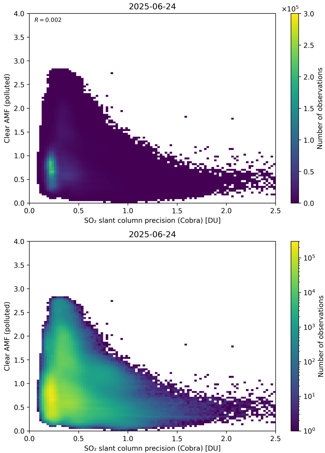
Figure 205: Scatter density plot of “SO 2 slant column precision (Cobra)” against “Clear AMF (polluted)” for 2025-06-23 to 2025-06-25.
