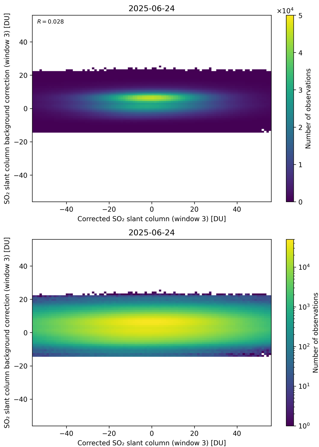
Figure 255: Scatter density plot of “Corrected SO 2 slant column (window 3)” against “SO 2 slant column background correction (window 3)” for 2025-06-23 to 2025-06-25.
