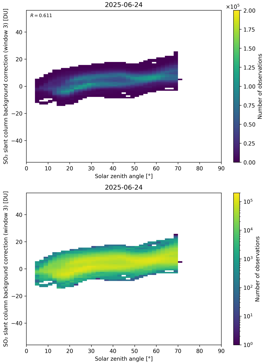
Figure 173: Scatter density plot of “Solar zenith angle” against “SO 2 slant column background correction (window 3)” for 2025-06-23 to 2025-06-25.
