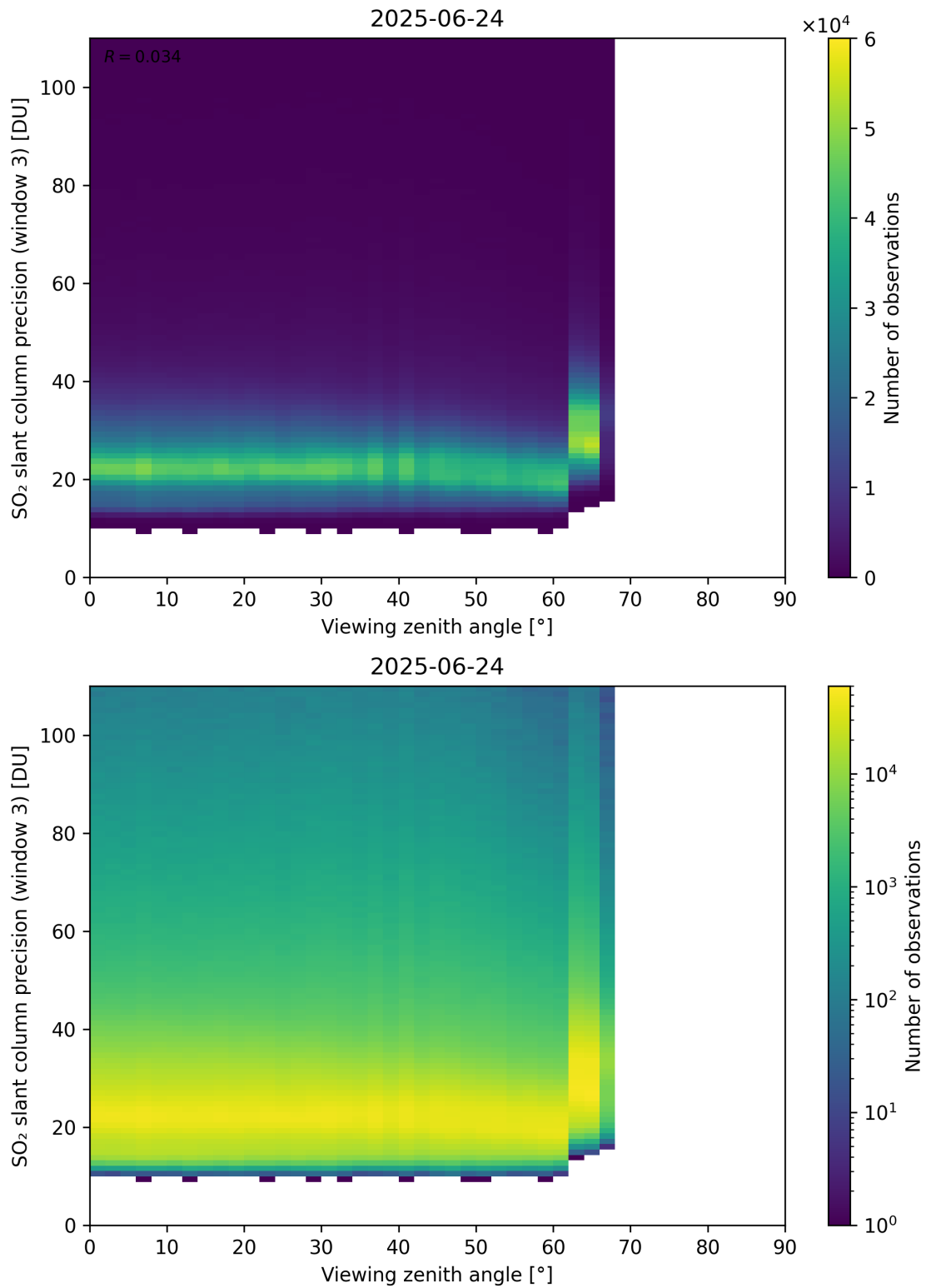
Figure 380: Scatter density plot of “Viewing zenith angle” against “SO 2 slant column precision (window 3)” for 2025-06-23 to 2025-06-25.
