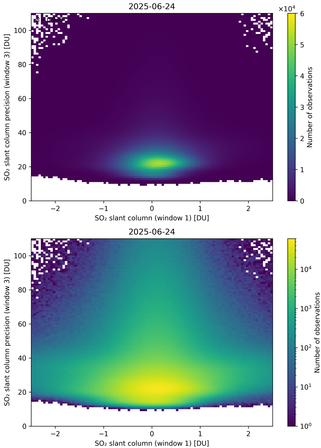
Figure 288: Scatter density plot of “SO 2 slant column (window 1)” against “SO 2 slant column precision (window 3)” for 2025-06-23 to 2025-06-25.
