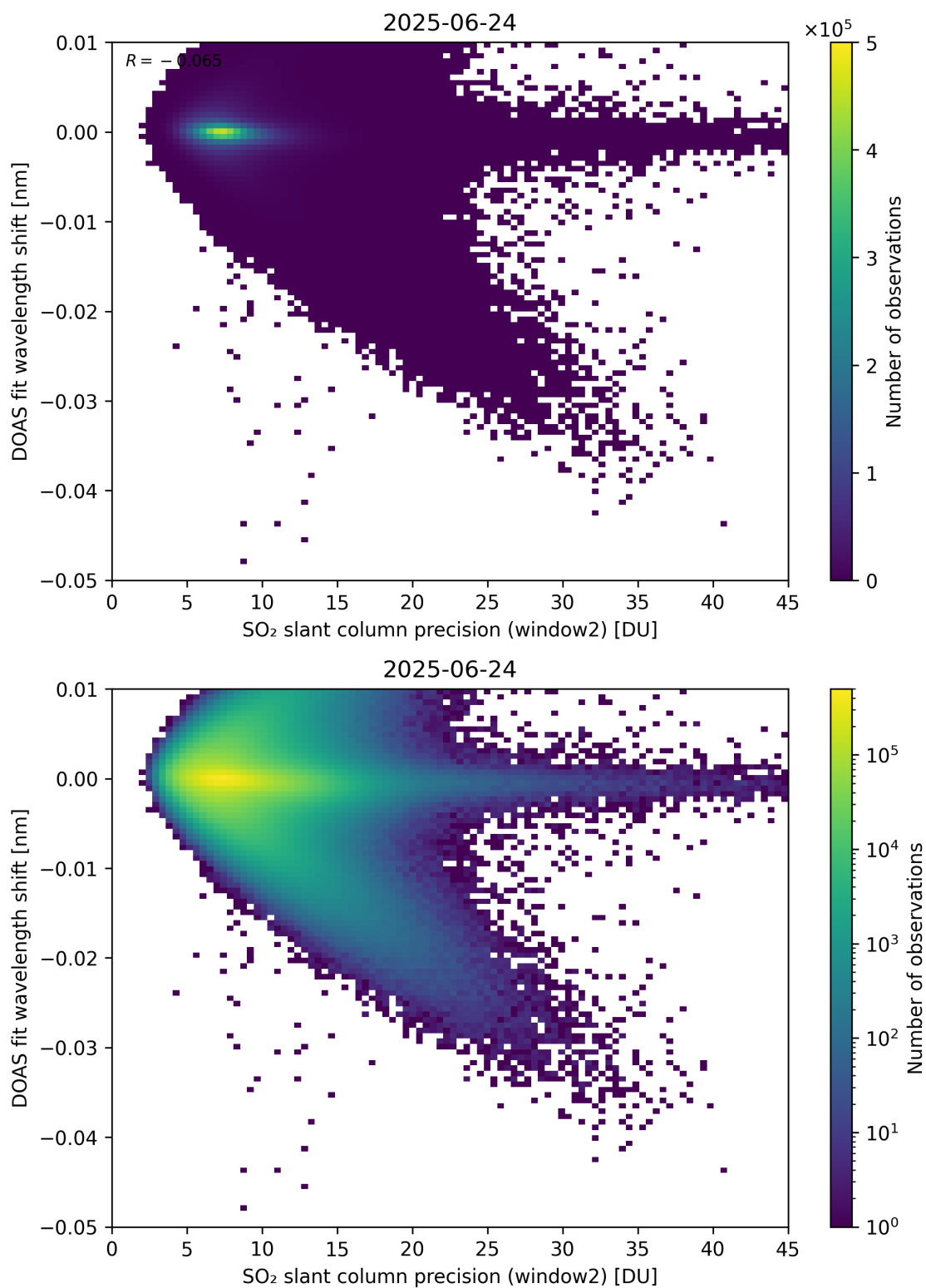
Figure 293: Scatter density plot of “SO 2 slant column precision (window2)” against “DOAS fit wavelength shift” for 2025-06-23 to 2025-06-25.
