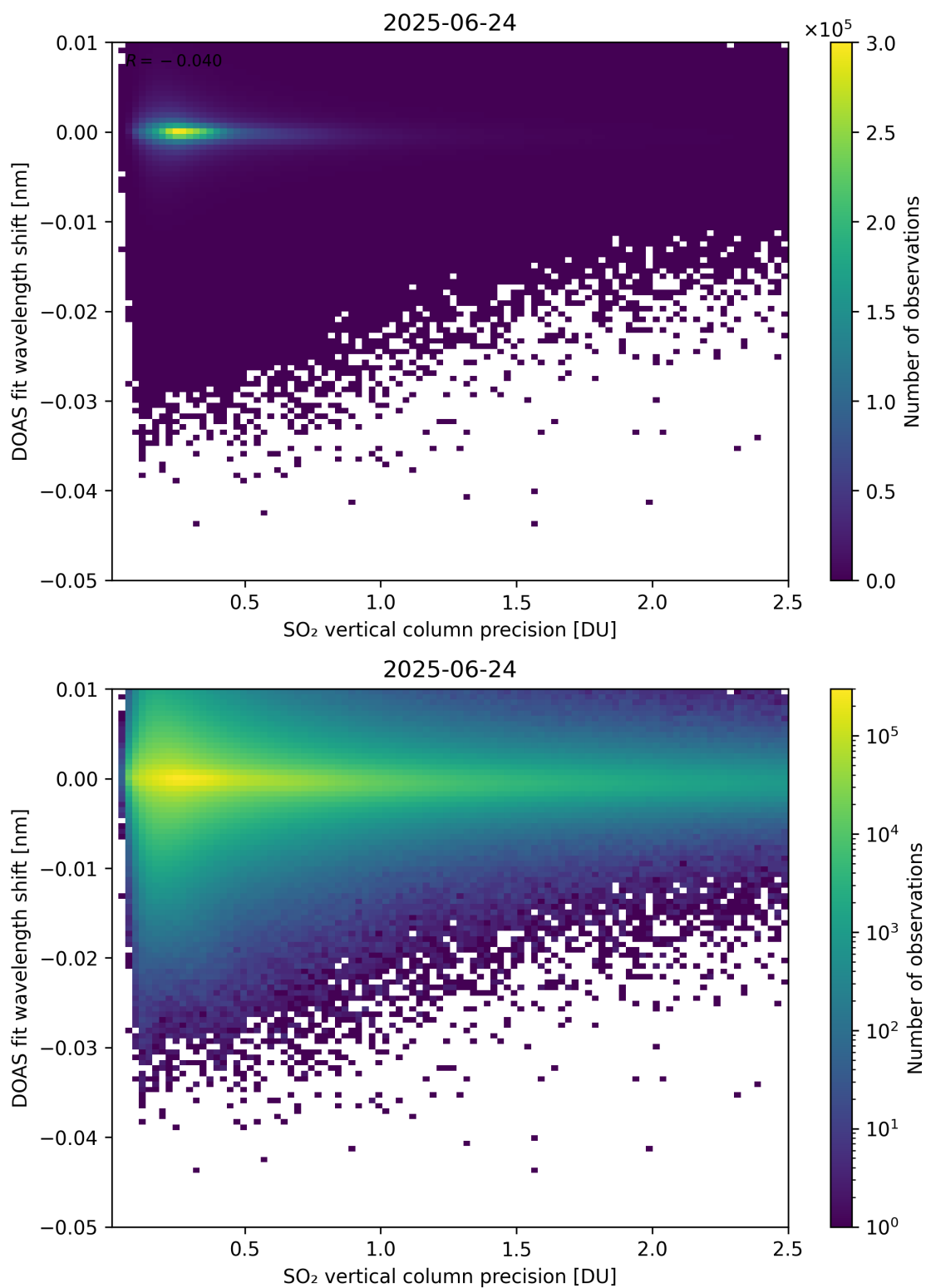
Figure 332: Scatter density plot of “SO 2 vertical column precision” against “DOAS fit wavelength shift” for 2025-06-23 to 2025-06-25.
