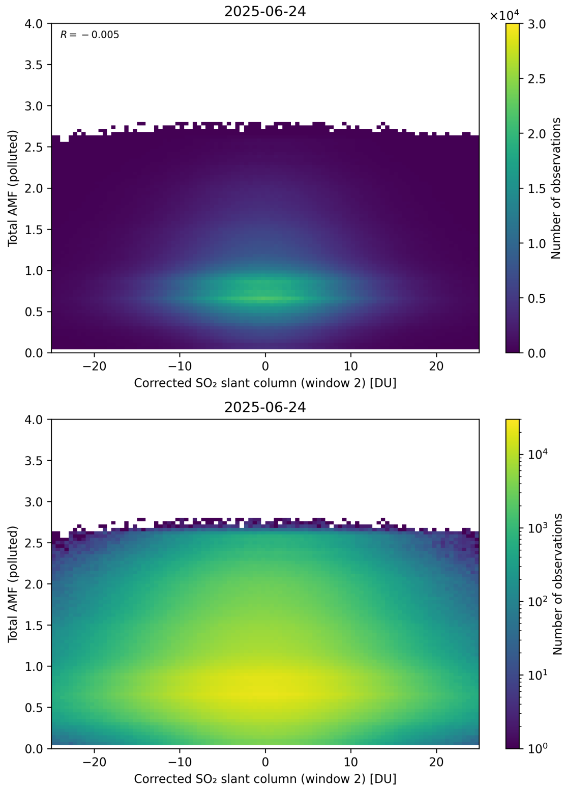
Figure 253: Scatter density plot of “Corrected SO 2 slant column (window 2)” against “Total AMF (polluted)” for 2025-06-23 to 2025-06-25.
