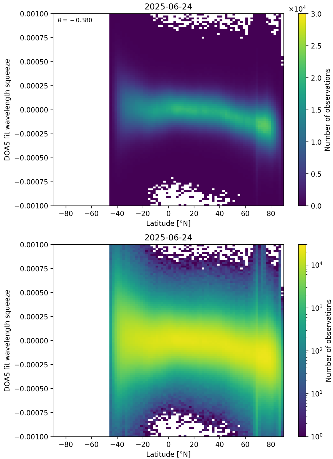
Figure 154: Scatter density plot of “Latitude” against “DOAS fit wavelength squeeze” for 2025-06-23 to 2025-06-25.
