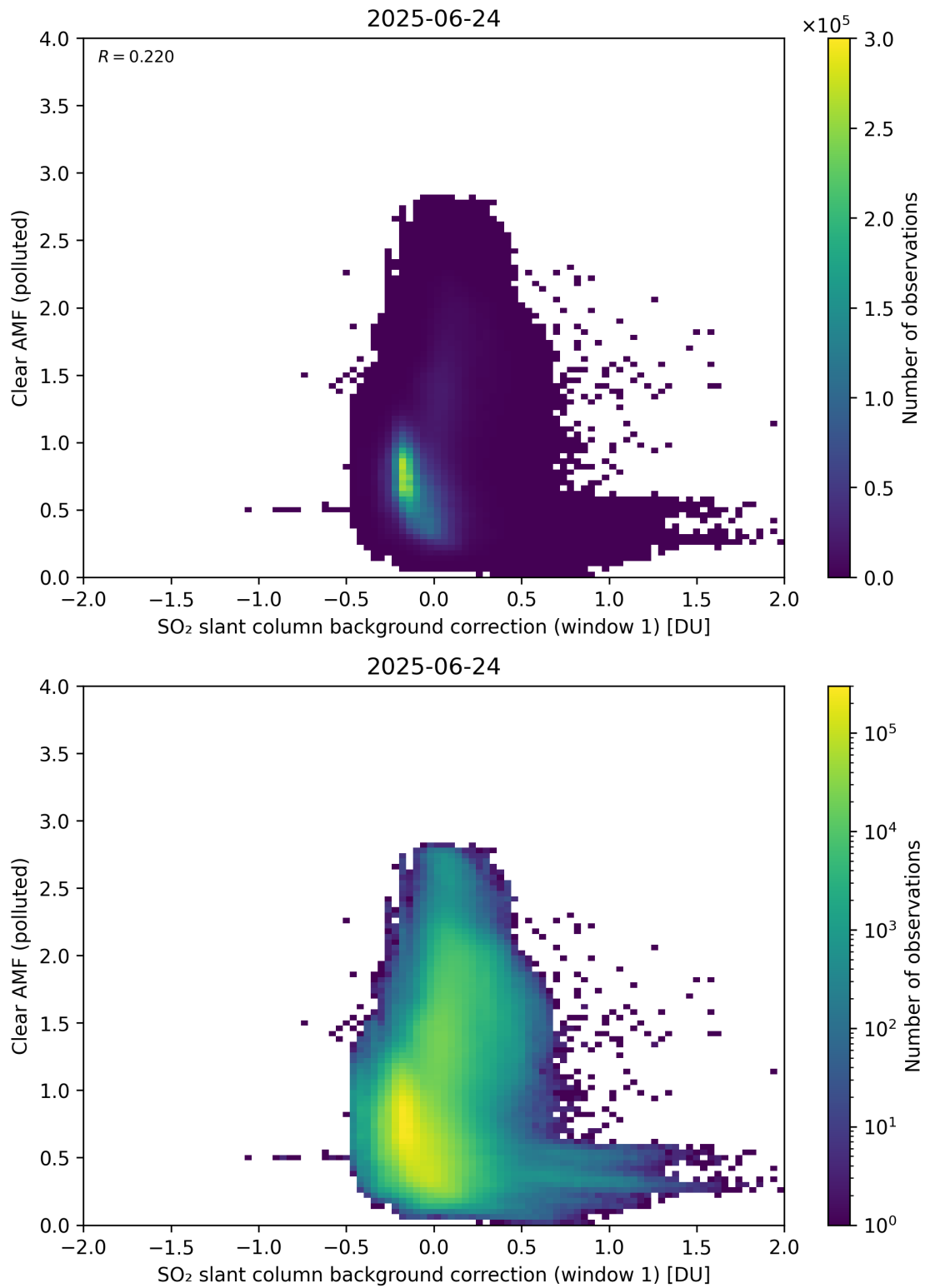
Figure 114: Scatter density plot of “SO 2 slant column background correction (window 1)” against “Clear AMF (polluted)” for 2025-06-23 to 2025-06-25.
