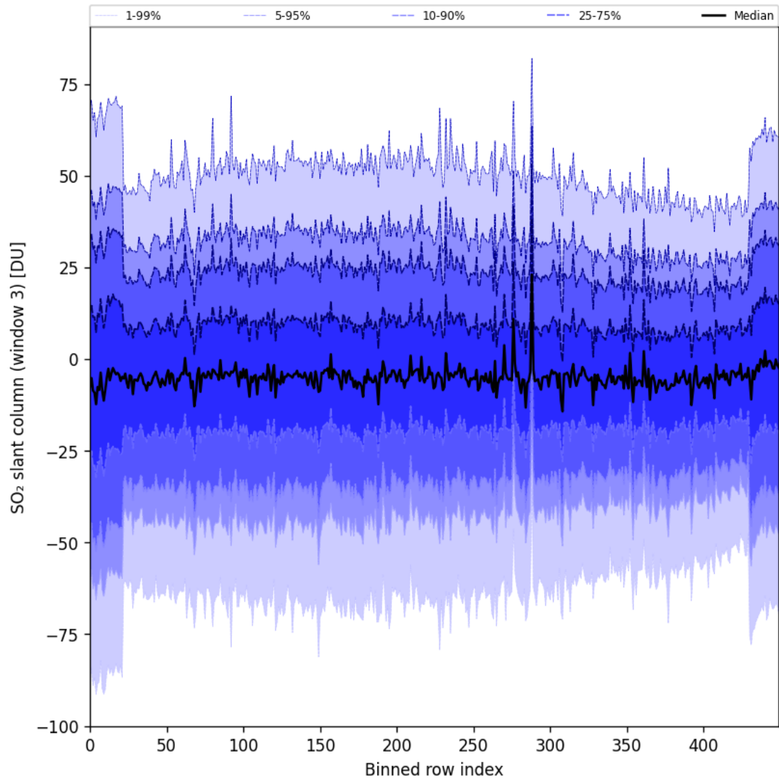
Figure 97: Along track statistics of “SO 2 slant column (window 3)” for 2025-06-23 to 2025-06-25
