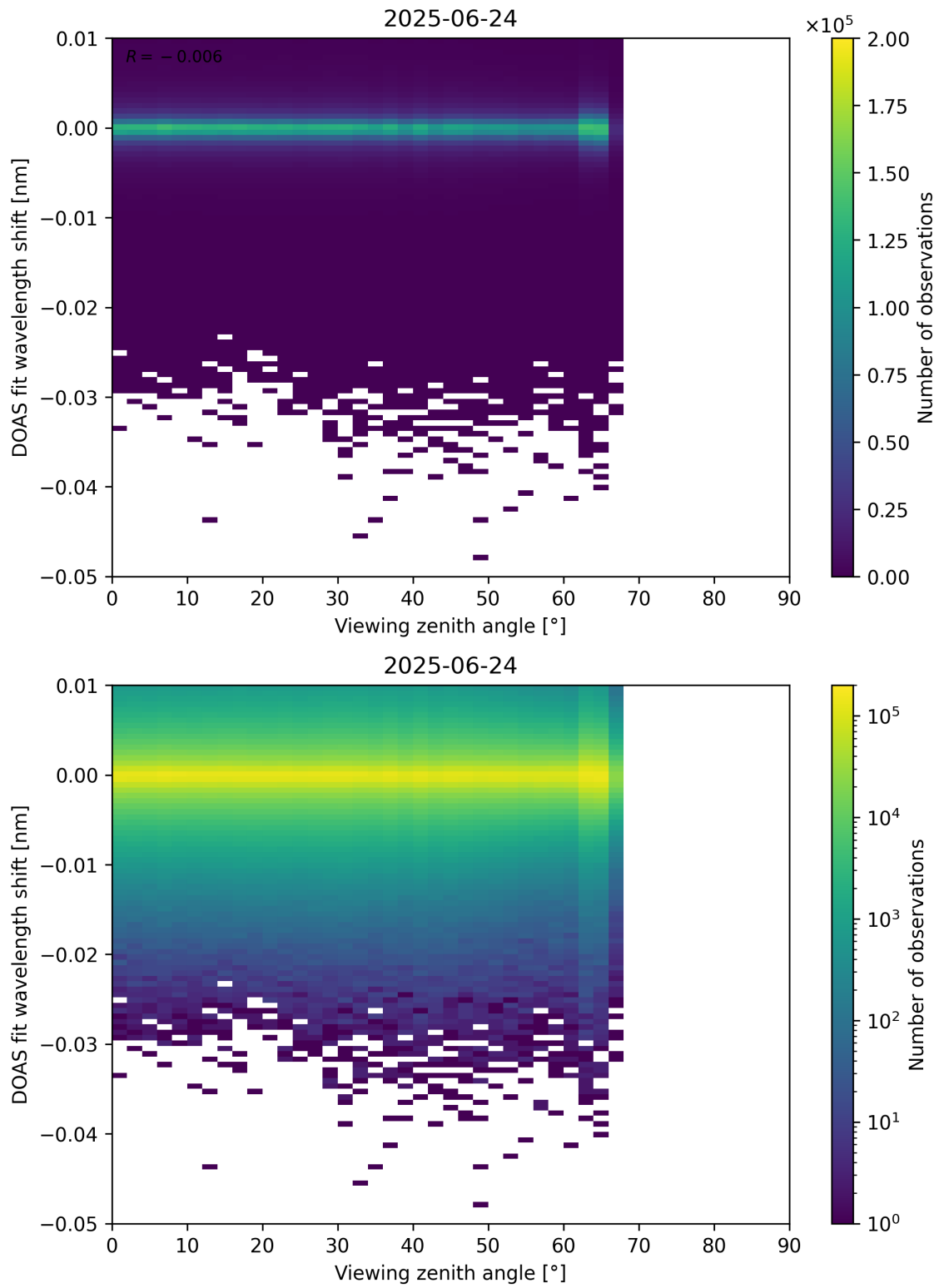
Figure 365: Scatter density plot of “Viewing zenith angle” against “DOAS fit wavelength shift” for 2025-06-23 to 2025-06-25.
