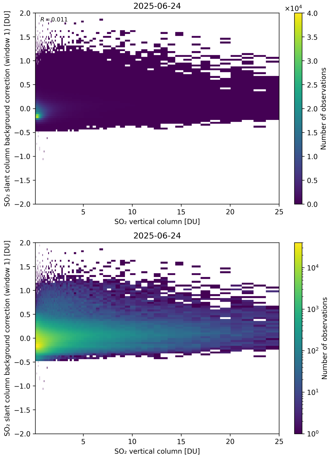
Figure 323: Scatter density plot of “SO 2 vertical column” against “SO 2 slant column background correction (window 1)” for 2025-06-23 to 2025-06-25.
