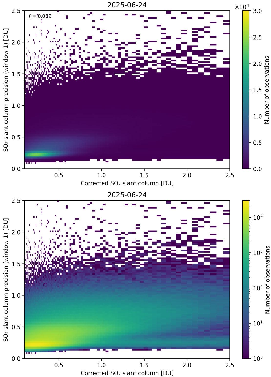
Figure 238: Scatter density plot of “Corrected SO 2 slant column” against “SO 2 slant column precision (window 1)” for 2025-06-23 to 2025-06-25.
