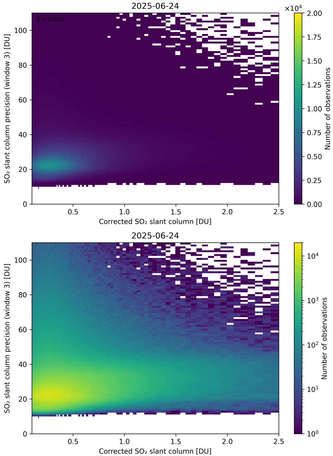
Figure 241: Scatter density plot of “Corrected SO 2 slant column” against “SO 2 slant column precision (window 3)” for 2025-06-23 to 2025-06-25.
