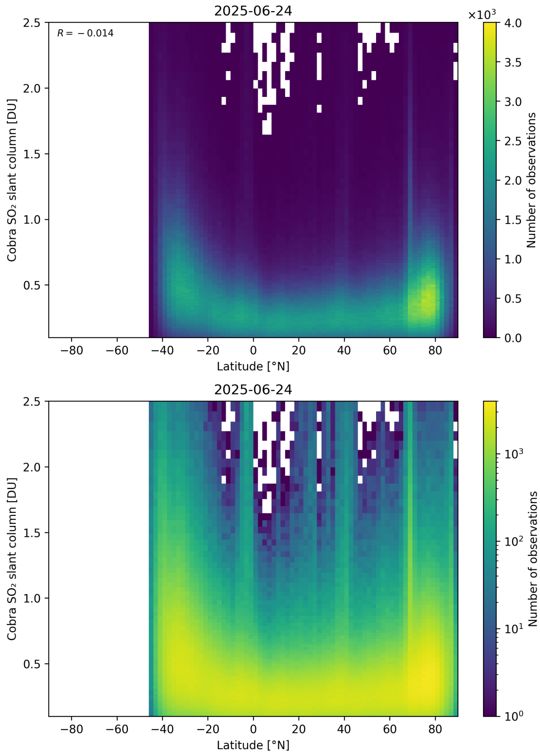
Figure 157: Scatter density plot of “Latitude” against “Cobra SO 2 slant column” for 2025-06-23 to 2025-06-25.
