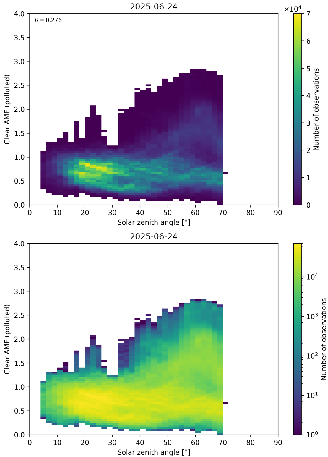
Figure 178: Scatter density plot of “Solar zenith angle” against “Clear AMF (polluted)” for 2025-06-23 to 2025-06-25.
