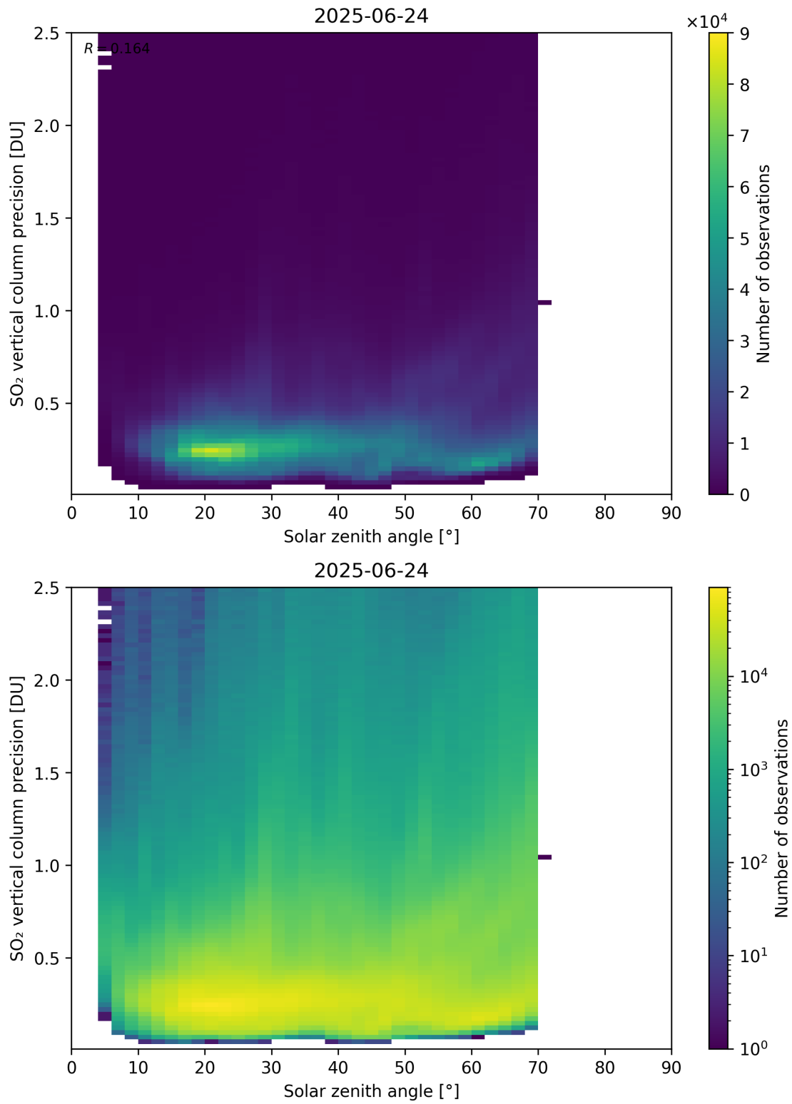
Figure 192: Scatter density plot of “Solar zenith angle” against “SO 2 vertical column precision” for 2025-06-23 to 2025-06-25.
