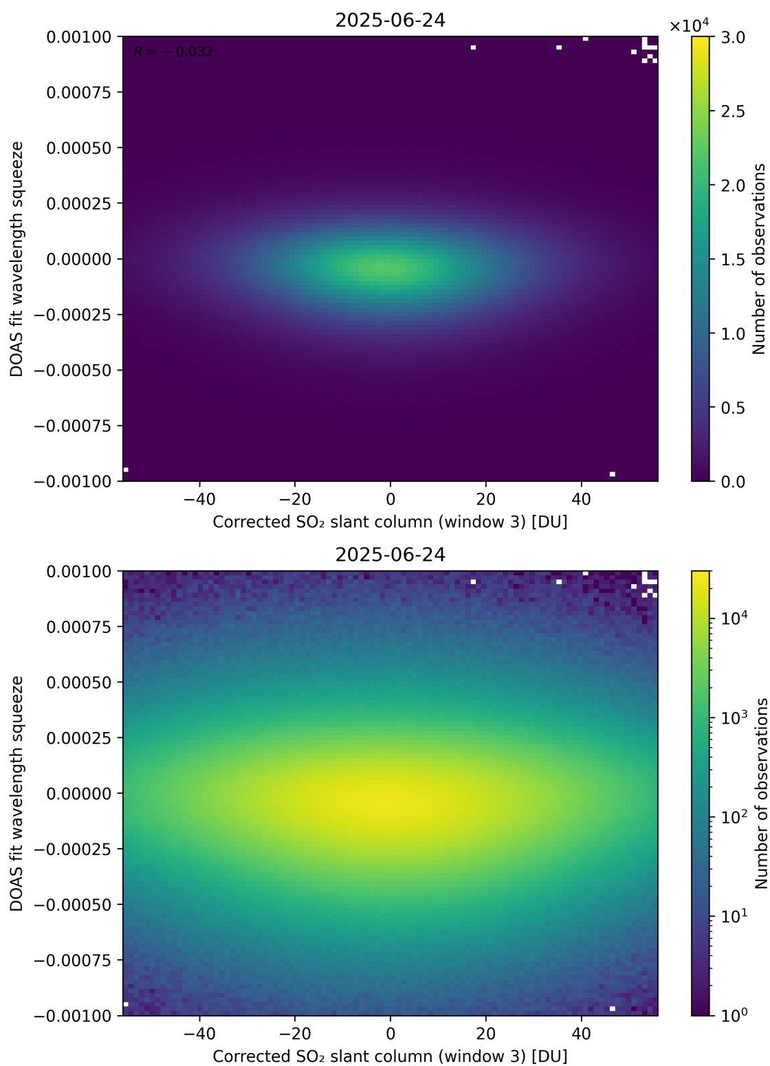
Figure 257: Scatter density plot of “Corrected SO 2 slant column (window 3)” against “DOAS fit wavelength squeeze” for 2025-06-23 to 2025-06-25.
