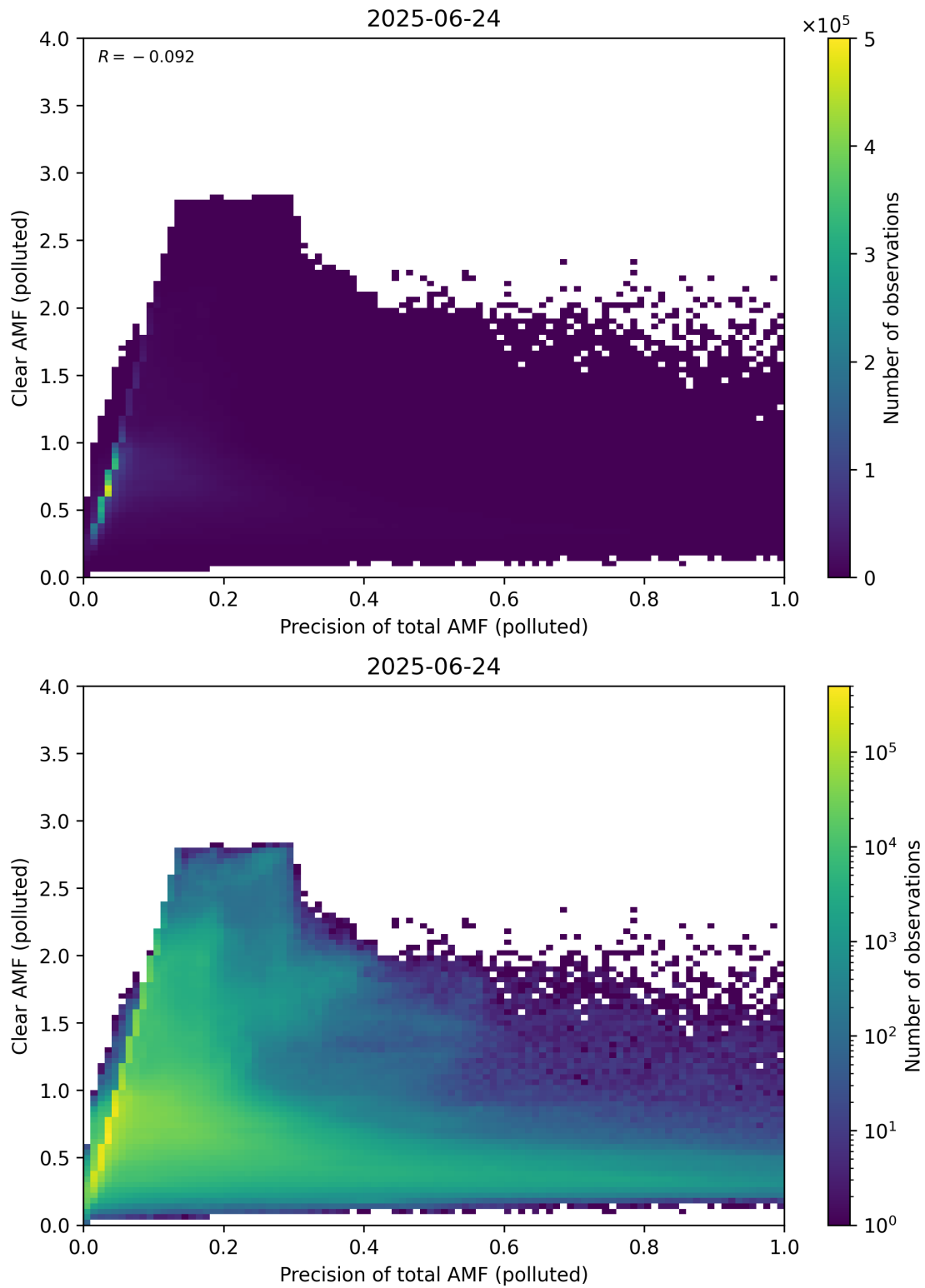
Figure 320: Scatter density plot of “Precision of total AMF (polluted)” against “Clear AMF (polluted)” for 2025-06-23 to 2025-06-25.
