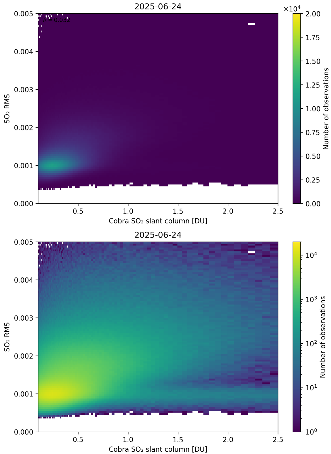
Figure 198: Scatter density plot of “Cobra SO 2 slant column” against “SO 2 RMS” for 2025-06-23 to 2025-06-25.
