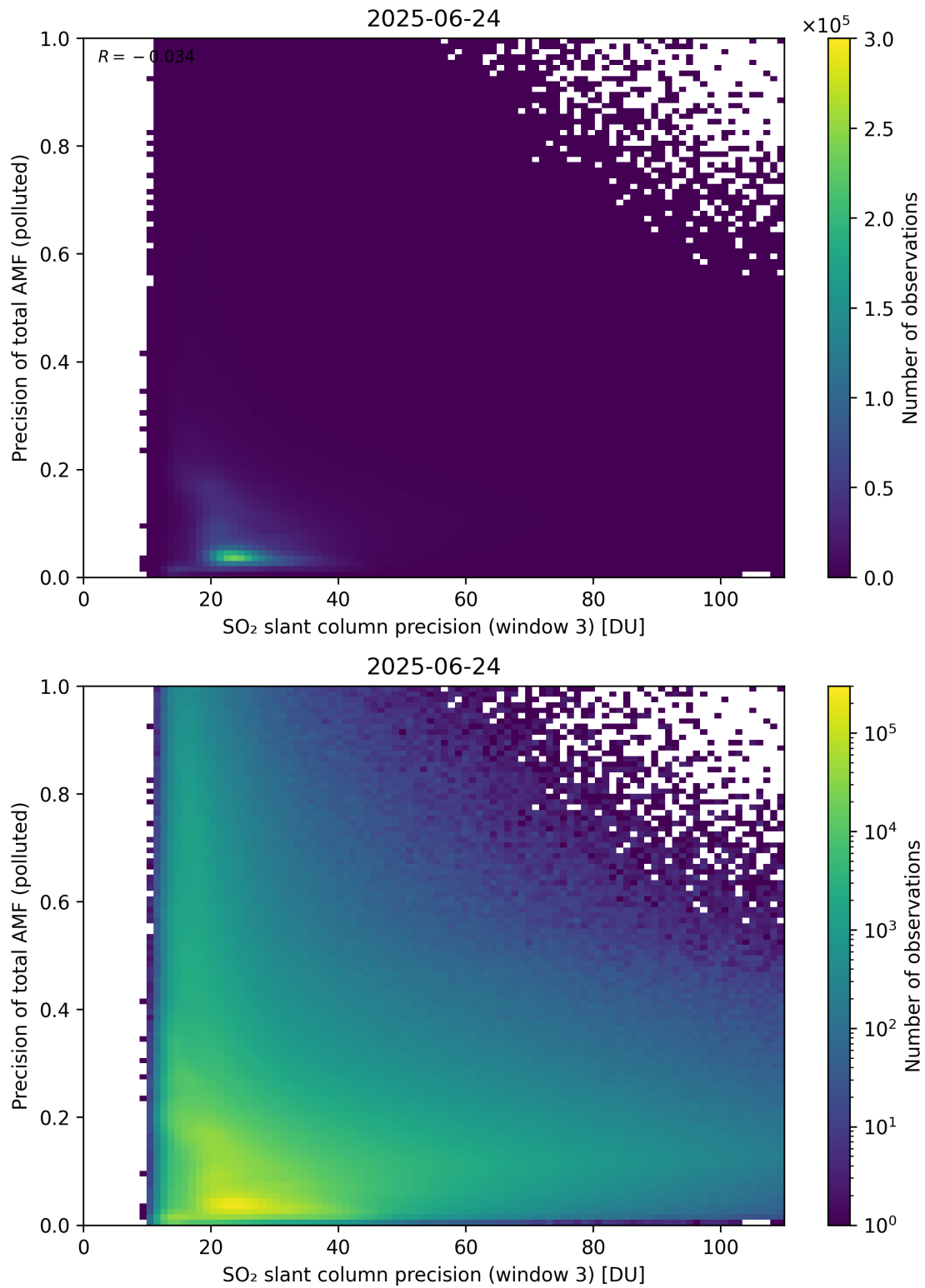
Figure 314: Scatter density plot of “SO 2 slant column precision (window 3)” against “Precision of total AMF (polluted)” for 2025-06-23 to 2025-06-25.
