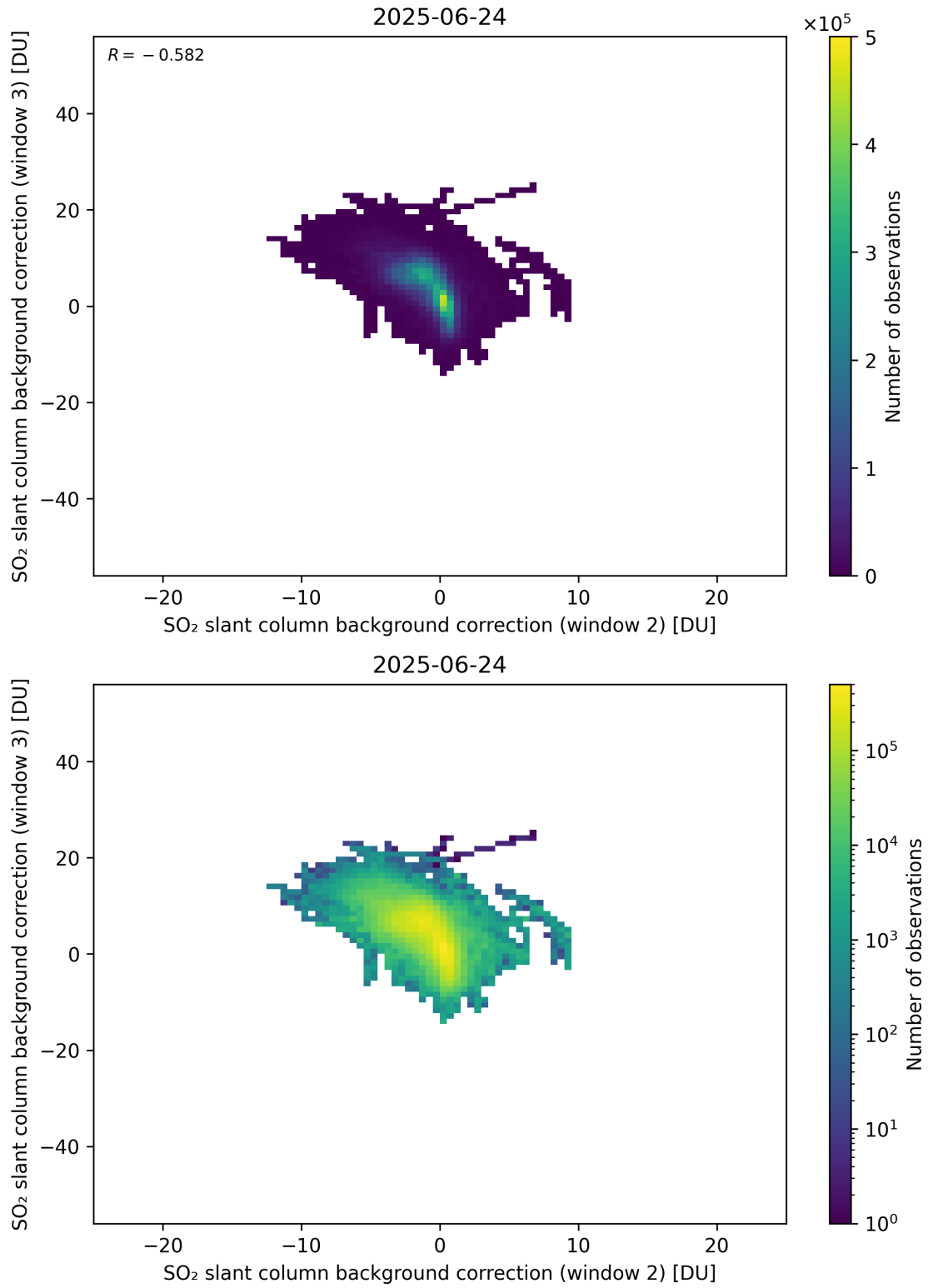
Figure 122: Scatter density plot of “SO 2 slant column background correction (window 2)” against “SO 2 slant column background correction (window 3)” for 2025-06-23 to 2025-06-25.
