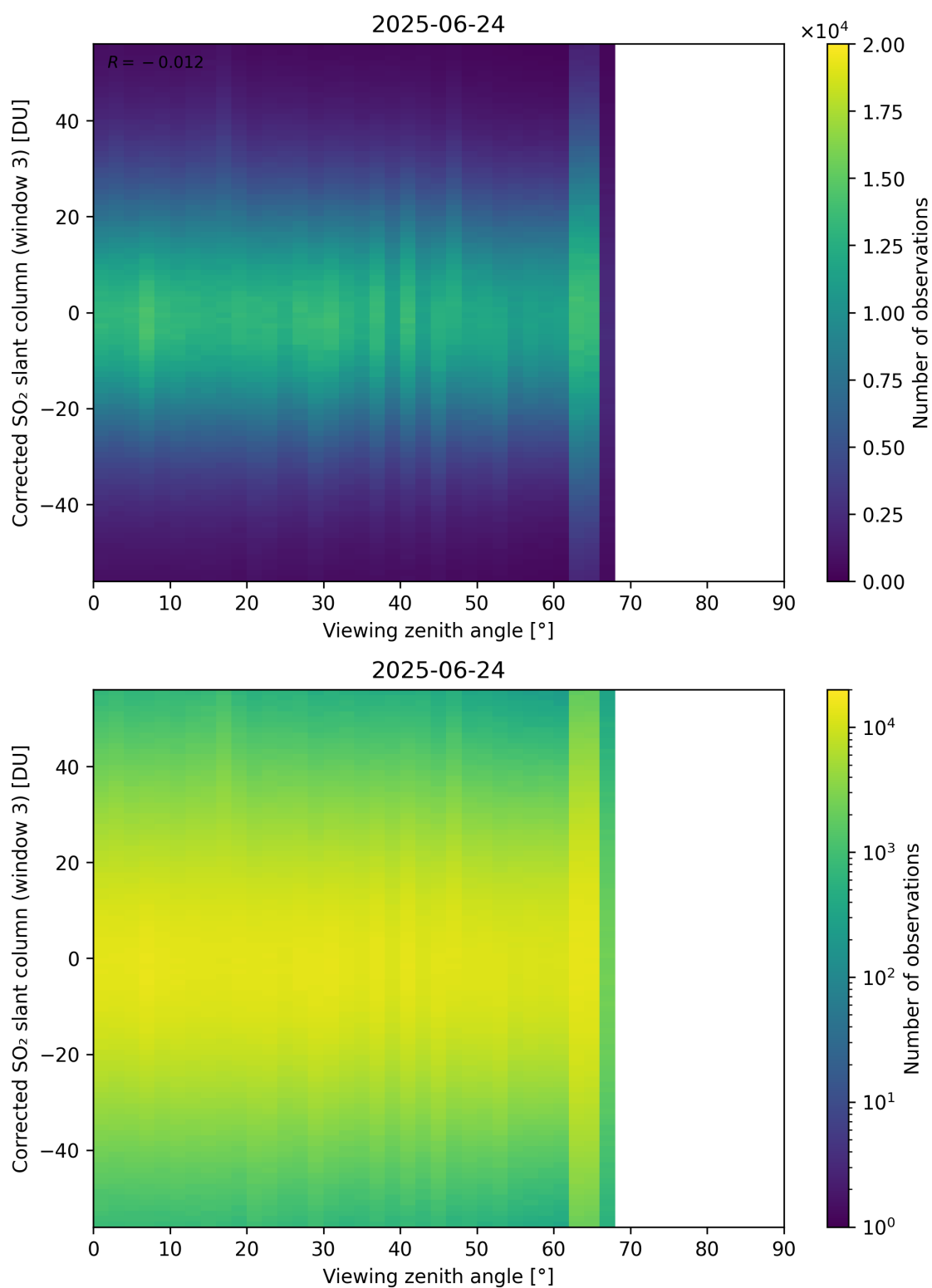
Figure 375: Scatter density plot of “Viewing zenith angle” against “Corrected SO 2 slant column (window 3)” for 2025-06-23 to 2025-06-25.
