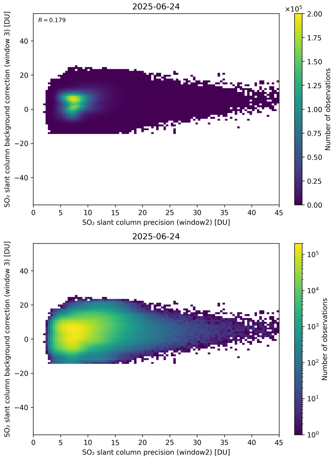
Figure 292: Scatter density plot of “SO 2 slant column precision (window2)” against “SO 2 slant column background correction (window 3)” for 2025-06-23 to 2025-06-25.
