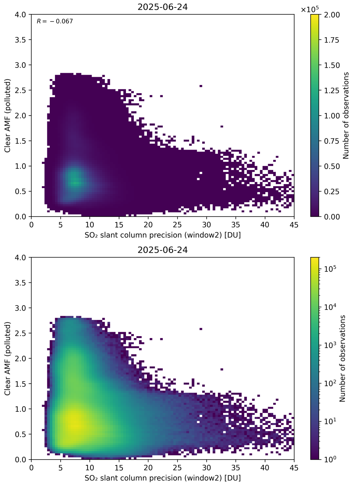
Figure 296: Scatter density plot of “SO 2 slant column precision (window2)” against “Clear AMF (polluted)” for 2025-06-23 to 2025-06-25.
