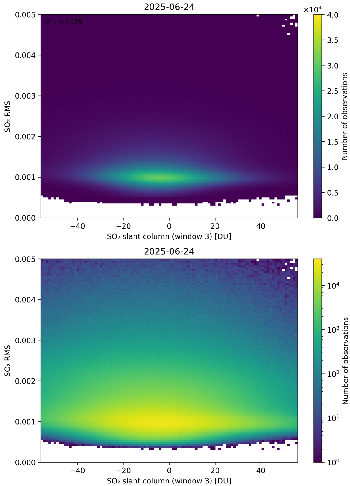
Figure 306: Scatter density plot of “SO 2 slant column (window 3)” against “SO 2 RMS” for 2025-06-23 to 2025-06-25.
