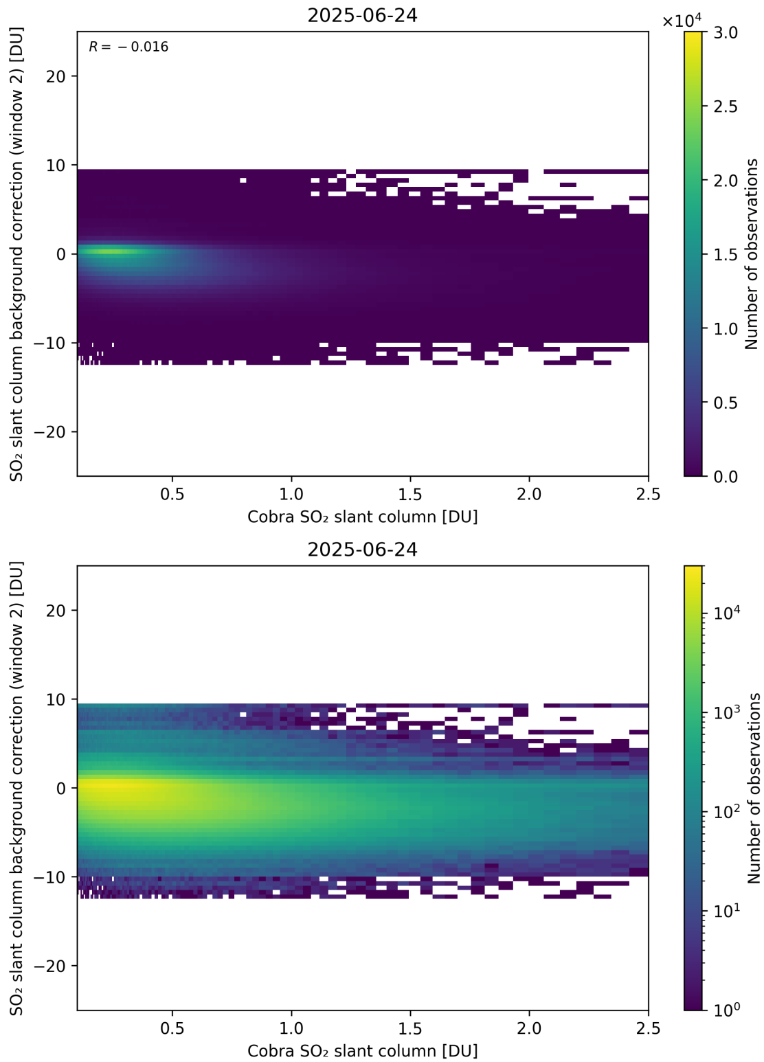
Figure 194: Scatter density plot of “Cobra SO 2 slant column” against “SO 2 slant column background correction (window 2)” for 2025-06-23 to 2025-06-25.
