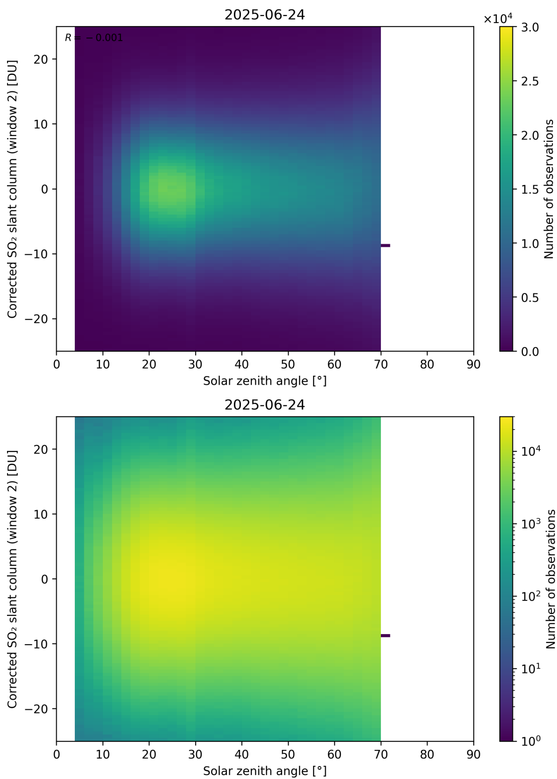
Figure 182: Scatter density plot of “Solar zenith angle” against “Corrected SO 2 slant column (window 2)” for 2025-06-23 to 2025-06-25.
