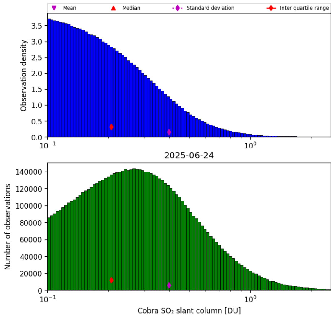
Figure 61: Histogram of “Cobra SO 2 slant column” for 2025-06-23 to 2025-06-25
