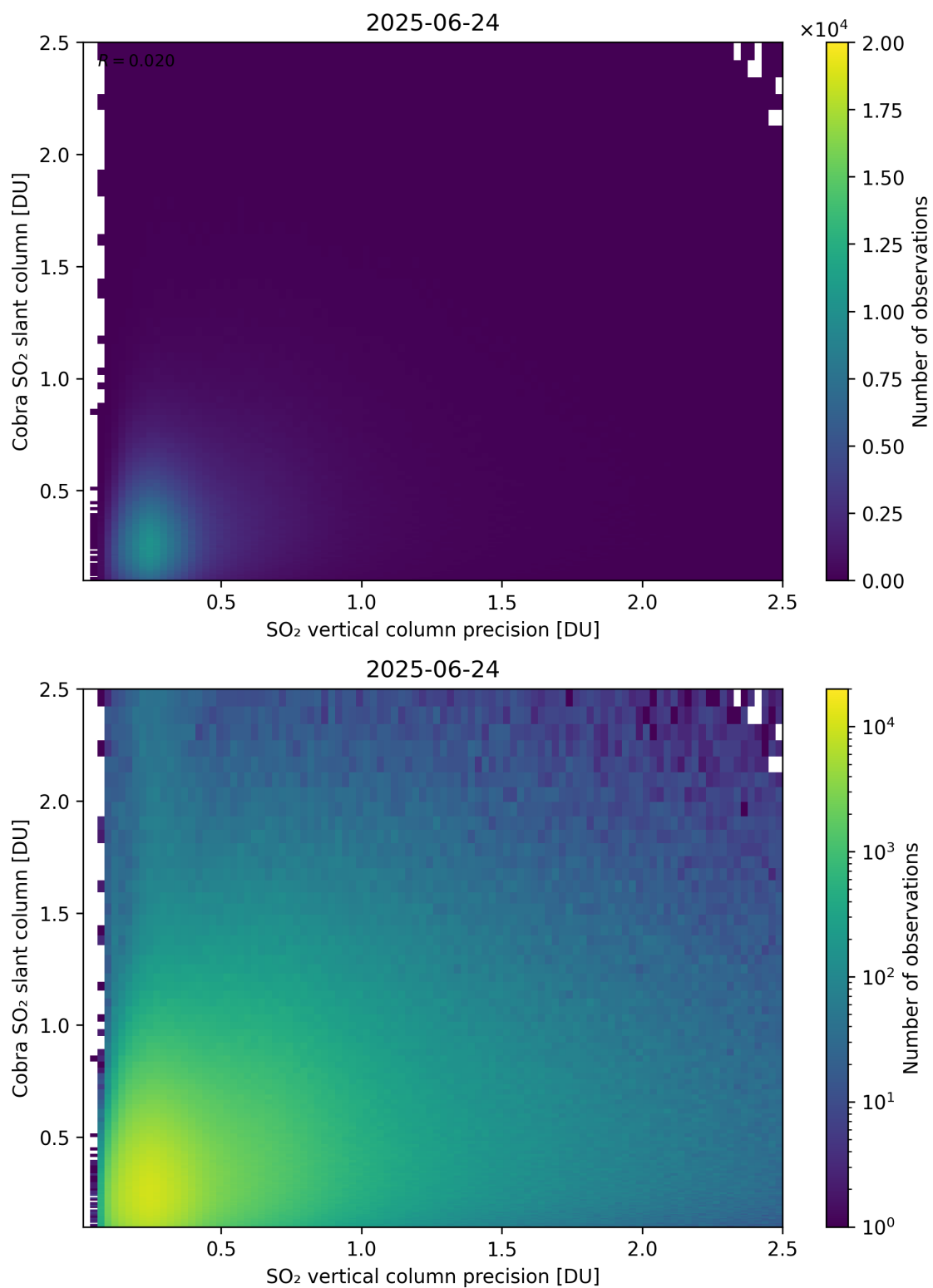
Figure 336: Scatter density plot of “SO 2 vertical column precision” against “Cobra SO 2 slant column” for 2025-06-23 to 2025-06-25.
