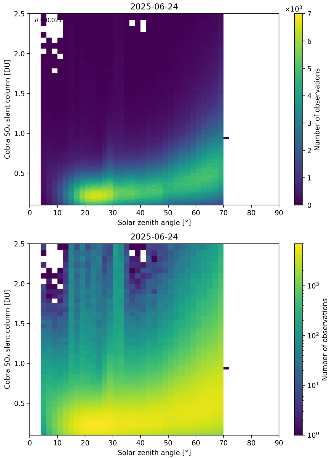
Figure 179: Scatter density plot of “Solar zenith angle” against “Cobra SO 2 slant column” for 2025-06-23 to 2025-06-25.
