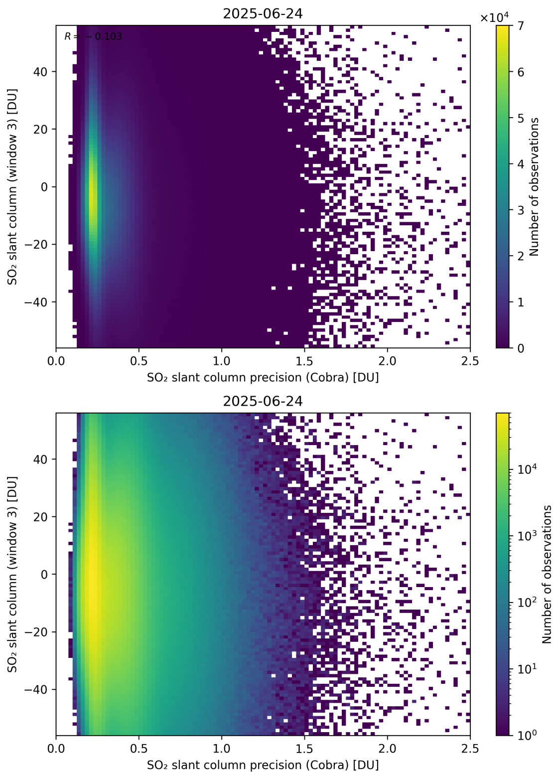
Figure 211: Scatter density plot of “SO 2 slant column precision (Cobra)” against “SO 2 slant column (window 3)” for 2025-06-23 to 2025-06-25.
