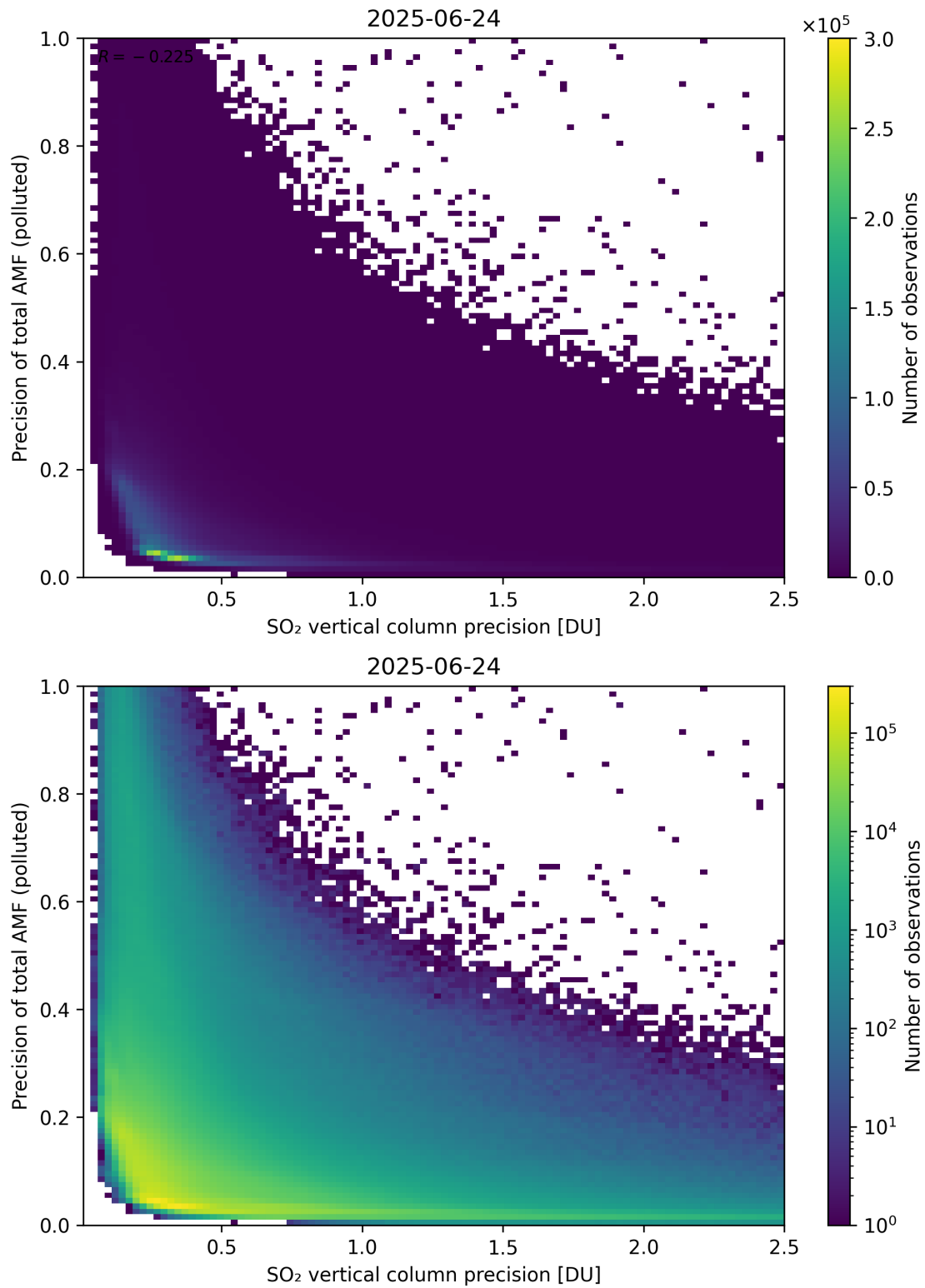
Figure 347: Scatter density plot of “SO 2 vertical column precision” against “Precision of total AMF (polluted)” for 2025-06-23 to 2025-06-25.
