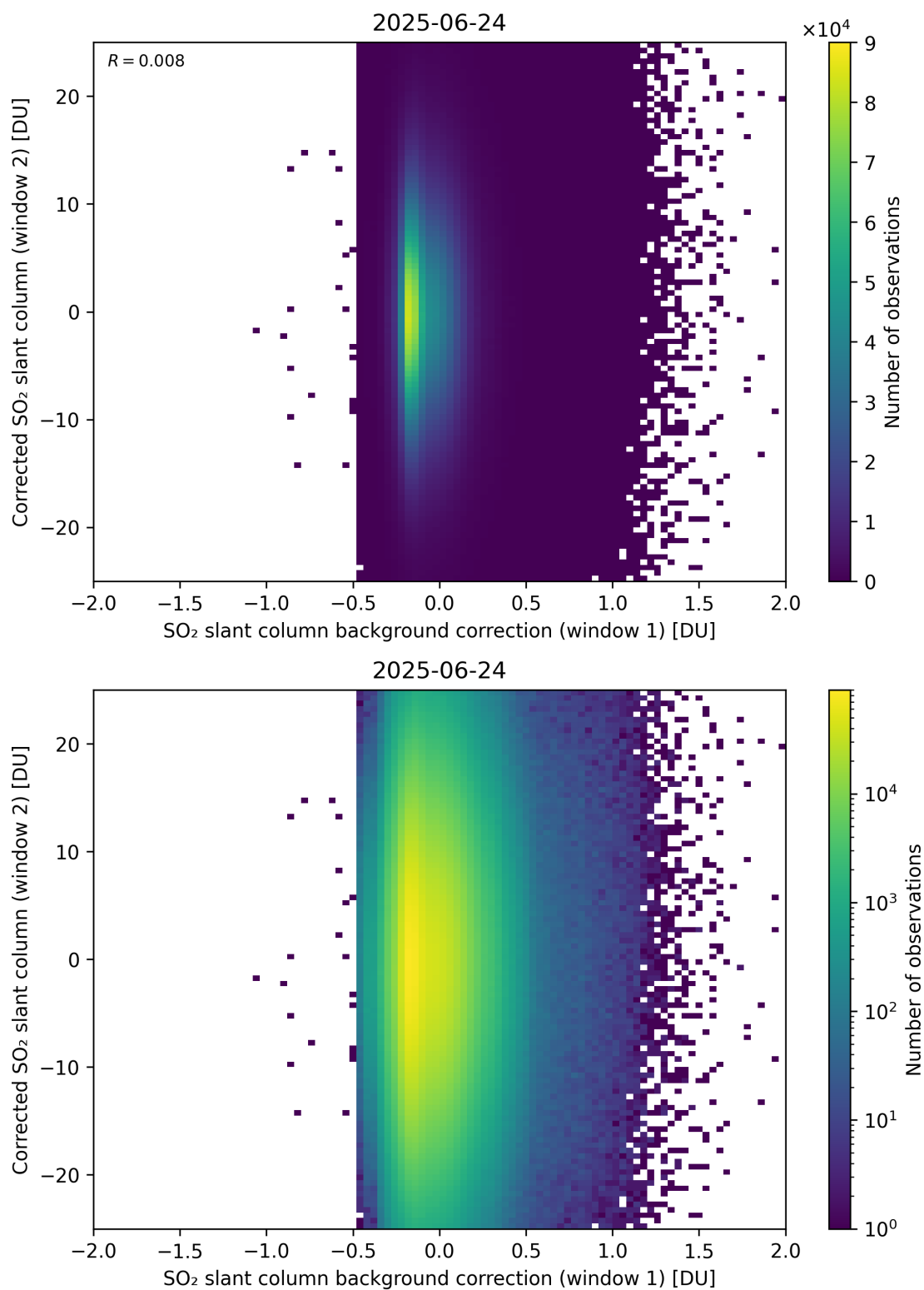
Figure 115: Scatter density plot of “SO 2 slant column background correction (window 1)” against “Corrected SO 2 slant column (window 2)” for 2025-06-23 to 2025-06-25.
