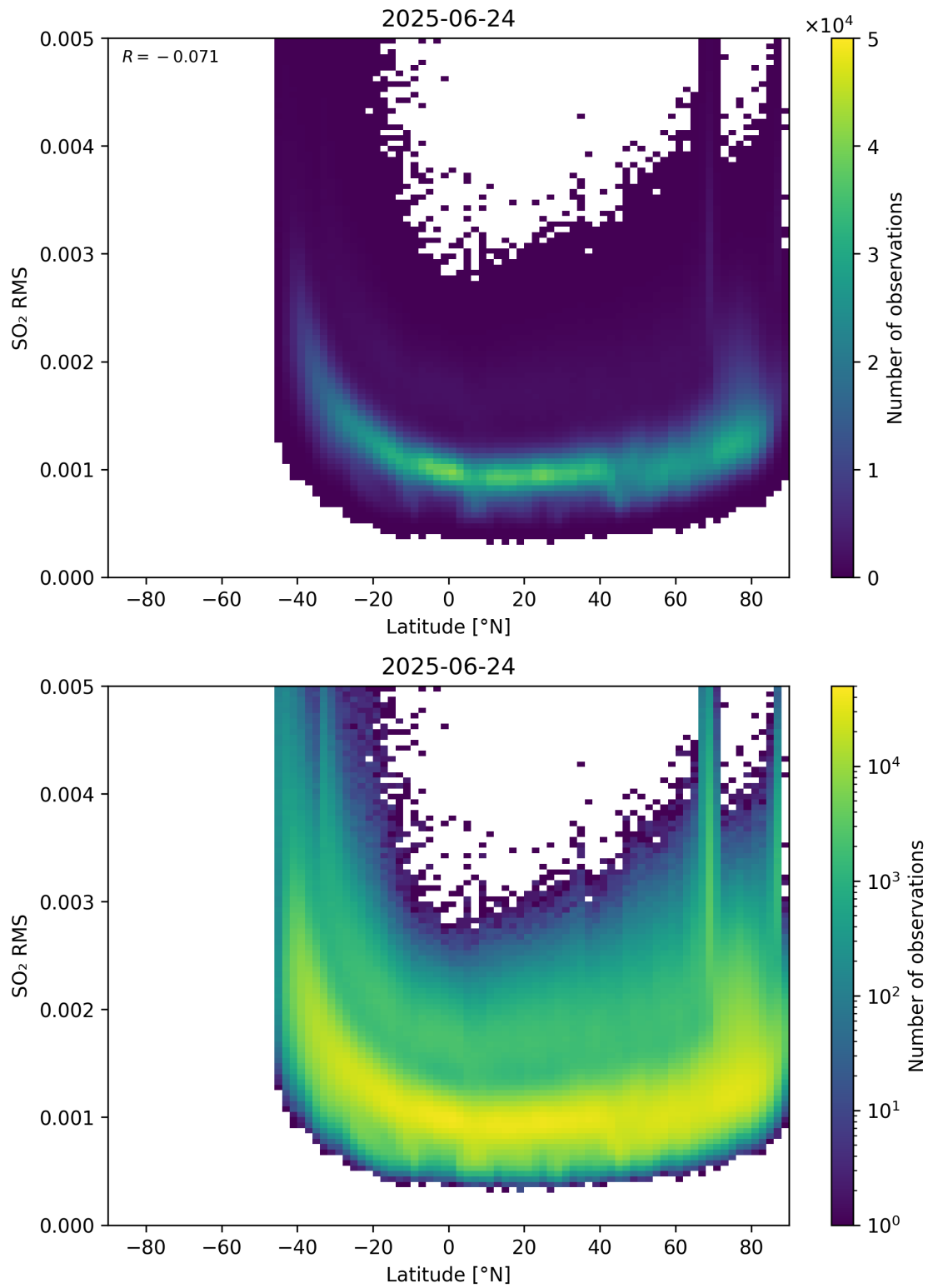
Figure 155: Scatter density plot of “Latitude” against “SO 2 RMS” for 2025-06-23 to 2025-06-25.
