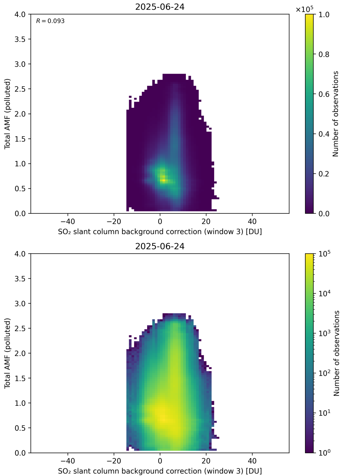
Figure 136: Scatter density plot of “SO 2 slant column background correction (window 3)” against “Total AMF (polluted)” for 2025-06-23 to 2025-06-25.
