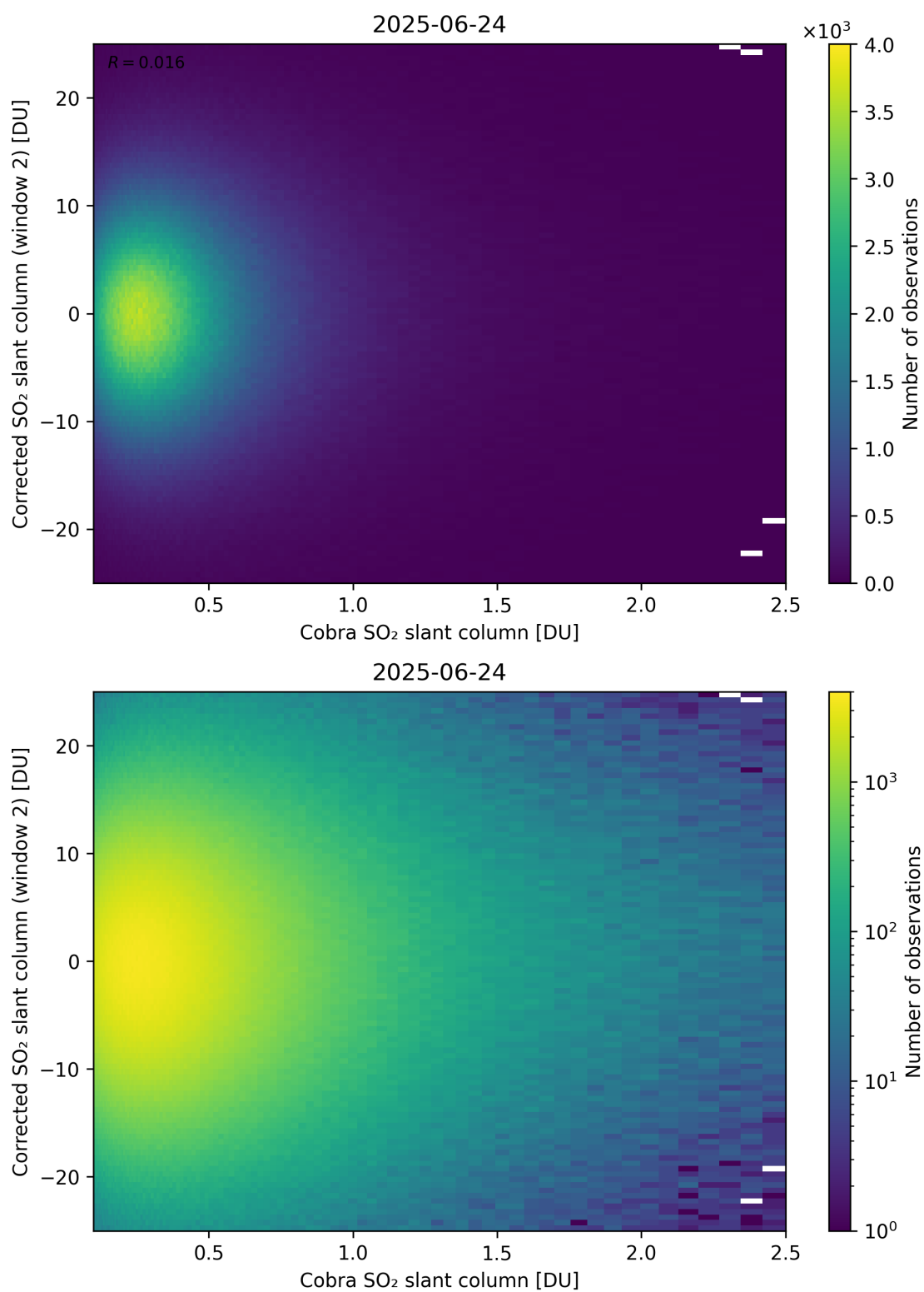
Figure 217: Scatter density plot of “Cobra SO 2 slant column” against “Corrected SO 2 slant column (window 2)” for 2025-06-23 to 2025-06-25.
