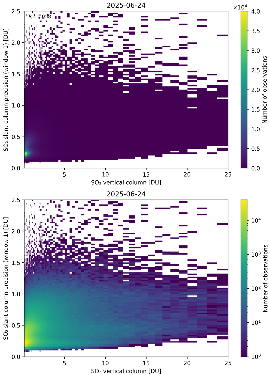
Figure 355: Scatter density plot of “SO 2 vertical column” against “SO 2 slant column precision (window 1)” for 2025-06-23 to 2025-06-25.
