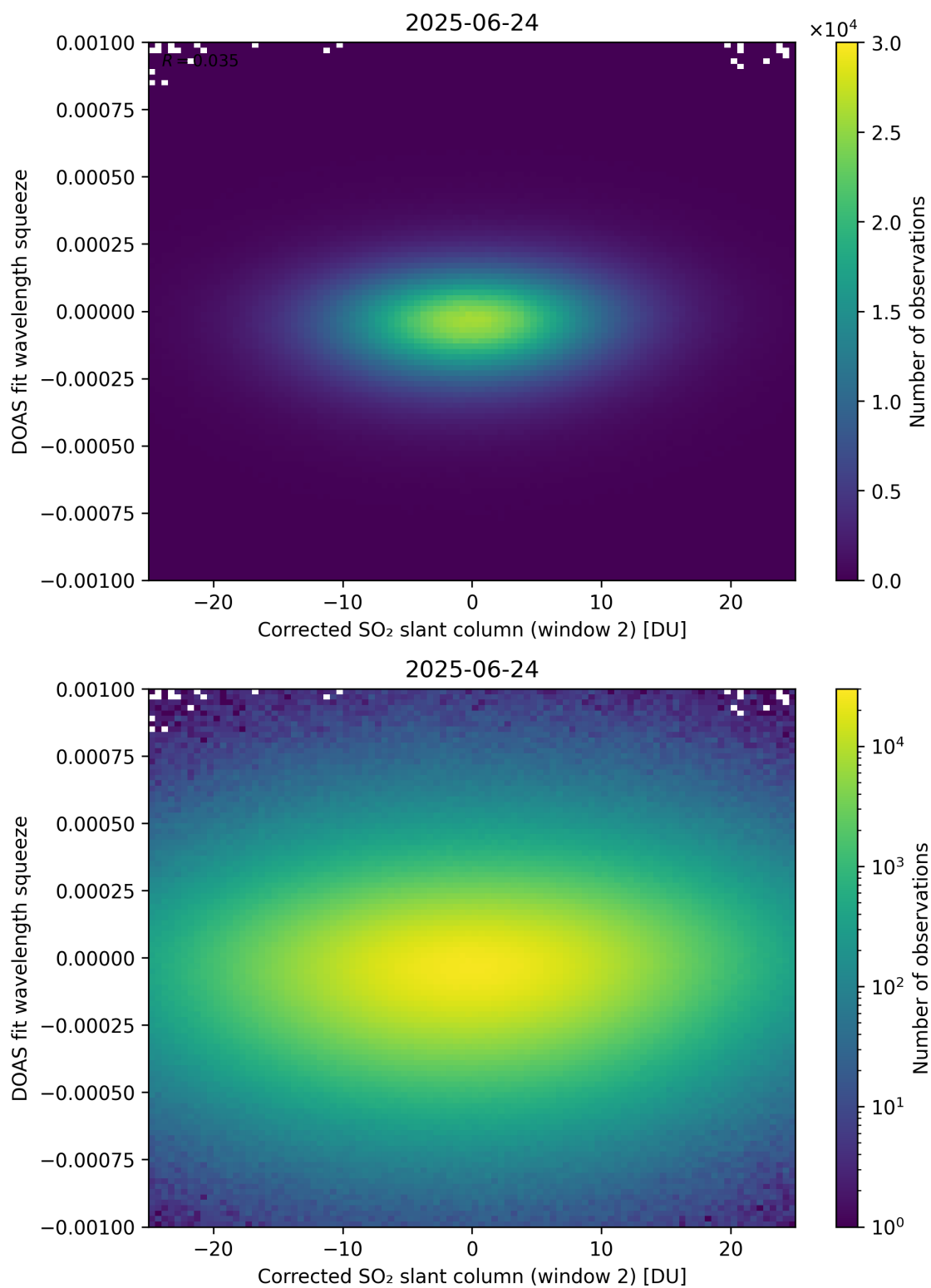
Figure 247: Scatter density plot of “Corrected SO 2 slant column (window 2)” against “DOAS fit wavelength squeeze” for 2025-06-23 to 2025-06-25.
