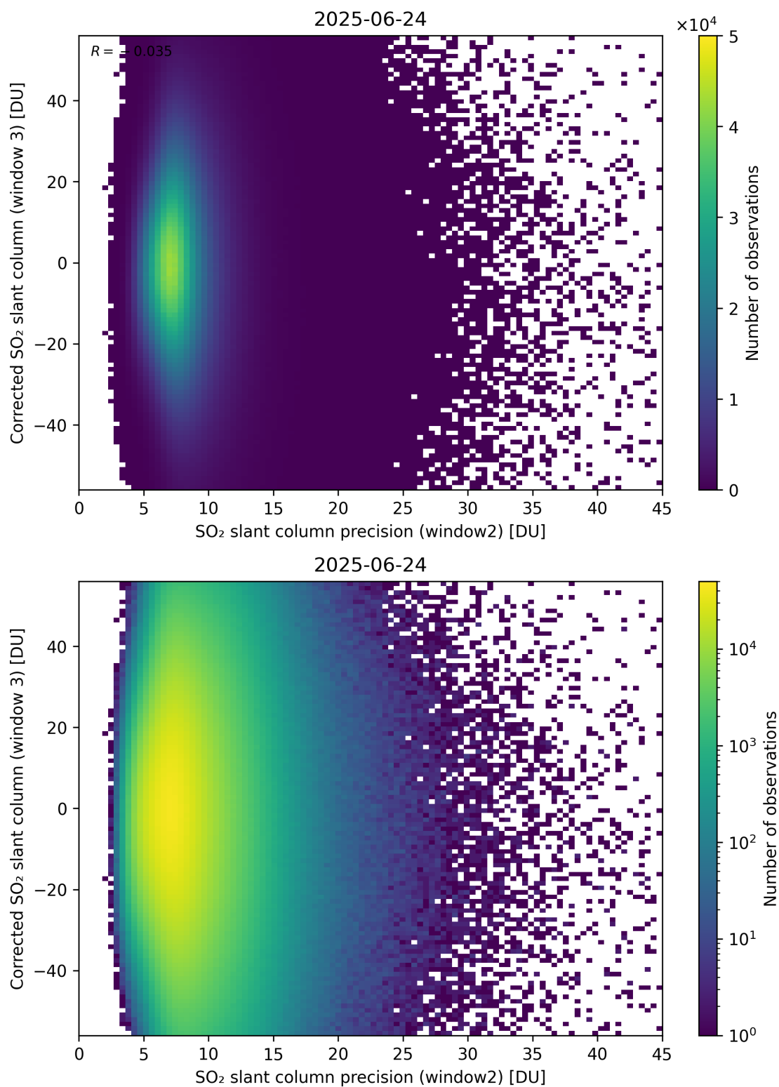
Figure 298: Scatter density plot of “SO 2 slant column precision (window2)” against “Corrected SO 2 slant column (window 3)” for 2025-06-23 to 2025-06-25.
