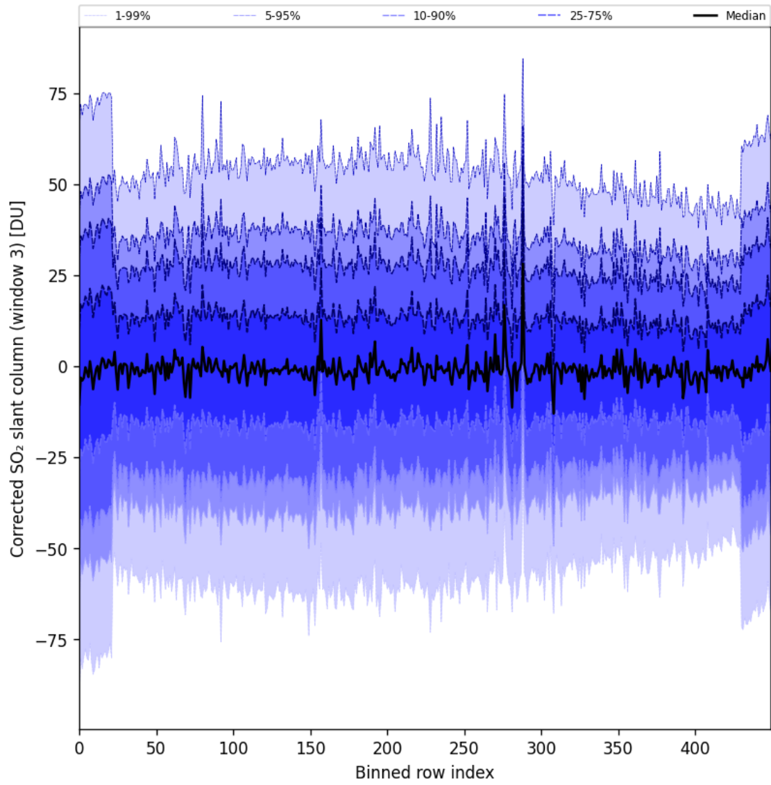
Figure 99: Along track statistics of “Corrected SO 2 slant column (window 3)” for 2025-06-23 to 2025-06-25
