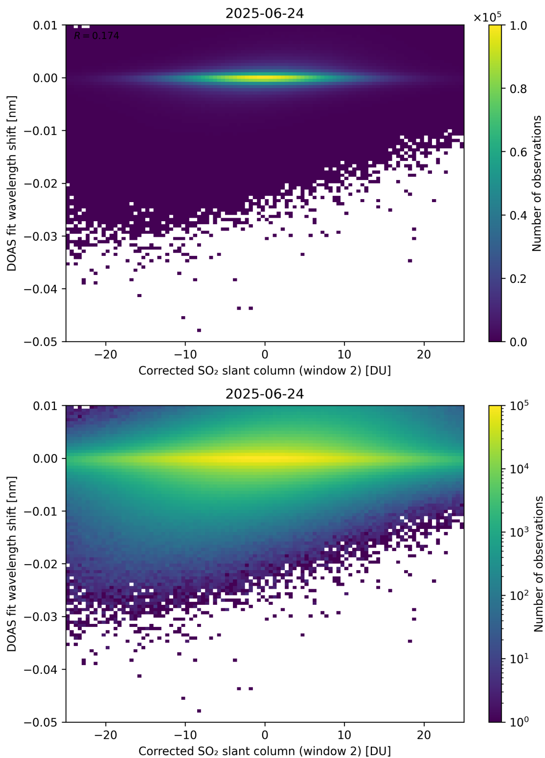
Figure 246: Scatter density plot of “Corrected SO 2 slant column (window 2)” against “DOAS fit wavelength shift” for 2025-06-23 to 2025-06-25.
