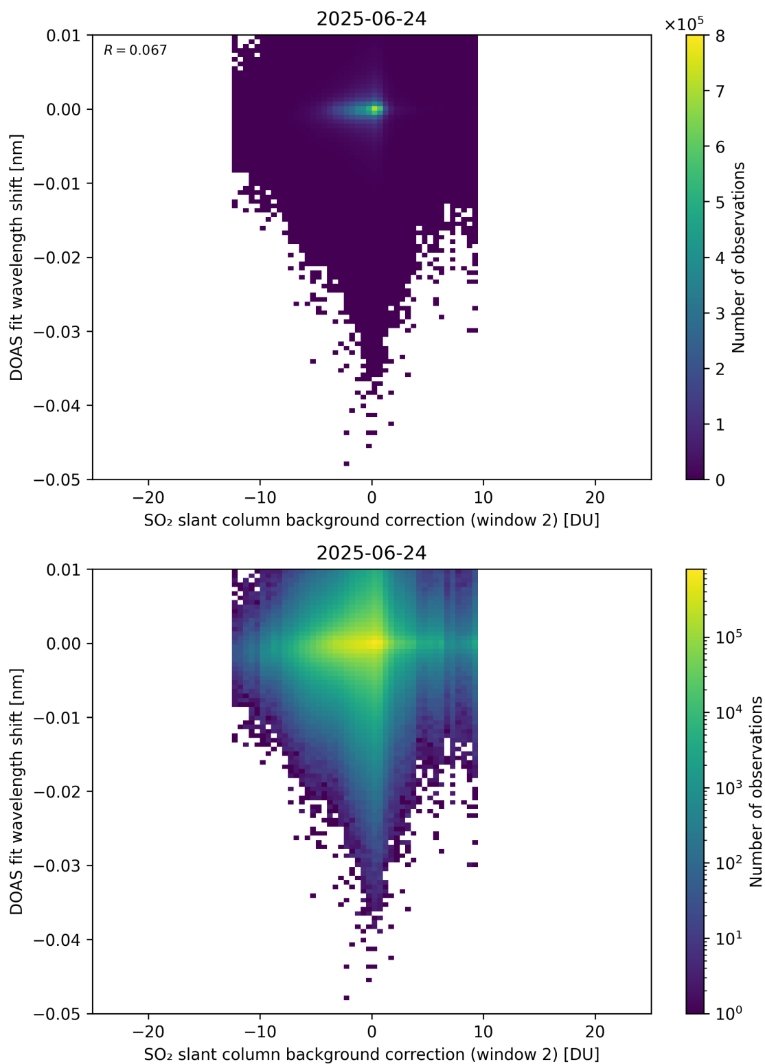
Figure 123: Scatter density plot of “SO 2 slant column background correction (window 2)” against “DOAS fit wavelength shift” for 2025-06-23 to 2025-06-25.
