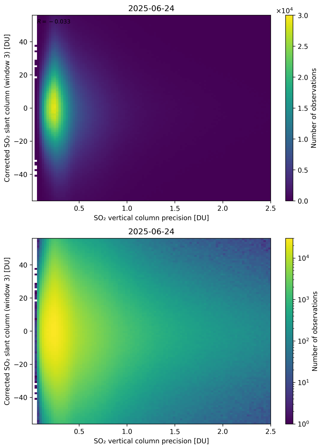
Figure 340: Scatter density plot of “SO 2 vertical column precision” against “Corrected SO 2 slant column (window 3)” for 2025-06-23 to 2025-06-25.
