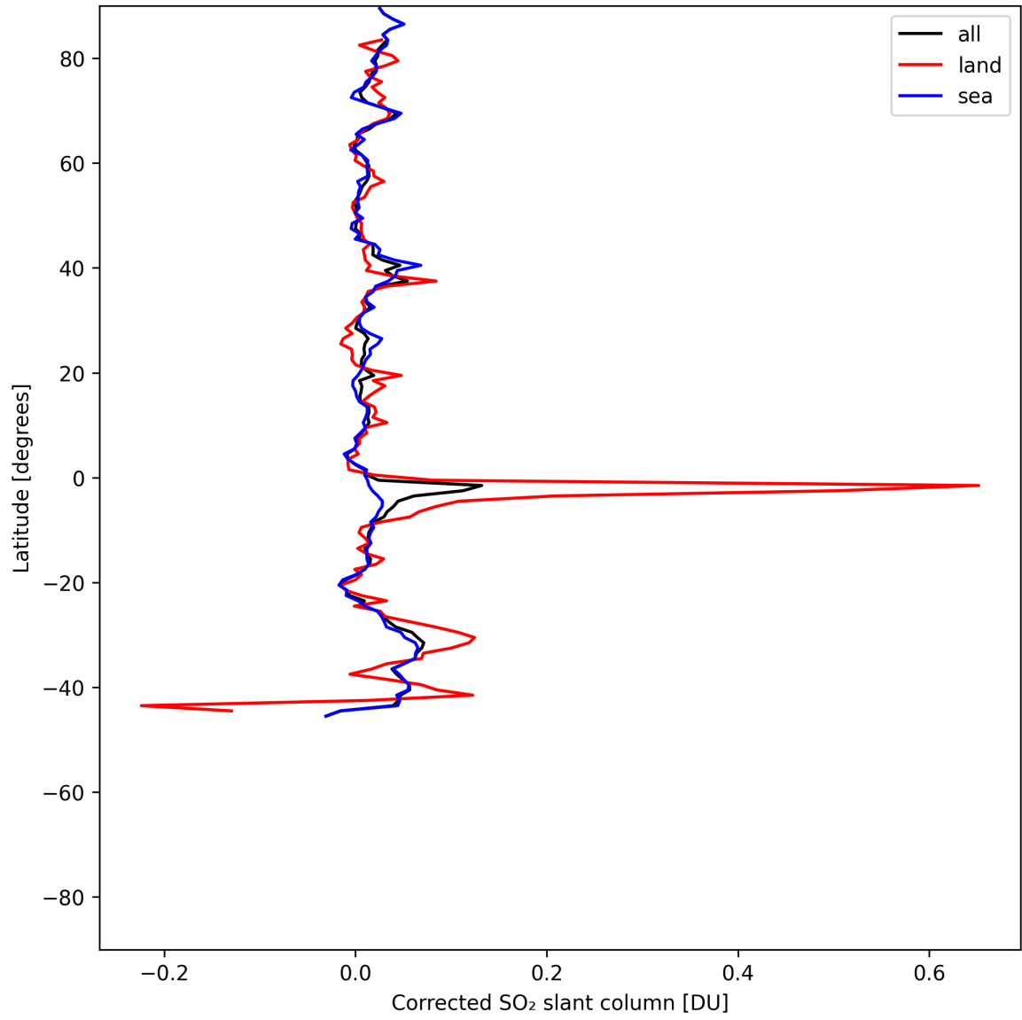
Figure 34: Zonal average of “Corrected SO 2 slant column” for 2025-06-23 to 2025-06-25.
