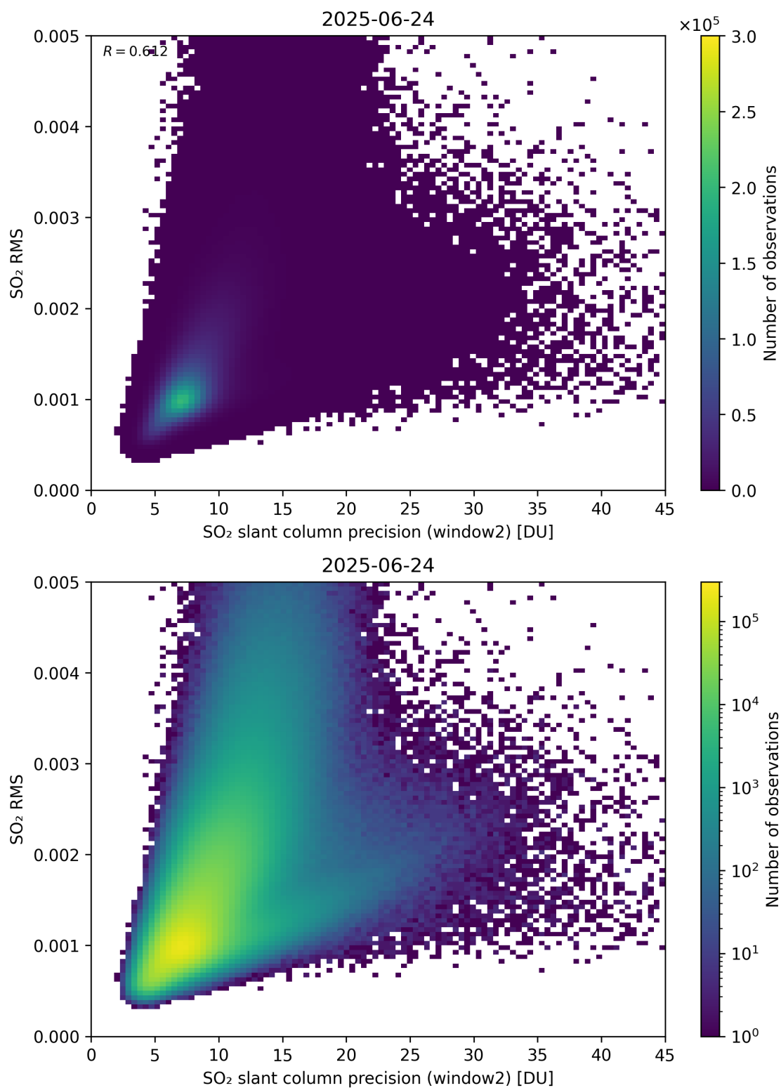
Figure 295: Scatter density plot of “SO 2 slant column precision (window2)” against “SO 2 RMS” for 2025-06-23 to 2025-06-25.
