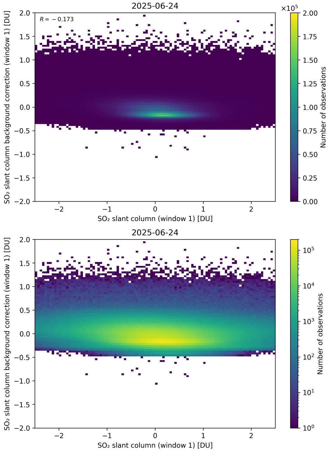
Figure 262: Scatter density plot of “SO 2 slant column (window 1)” against “SO 2 slant column background correction (window 1)” for 2025-06-23 to 2025-06-25.
