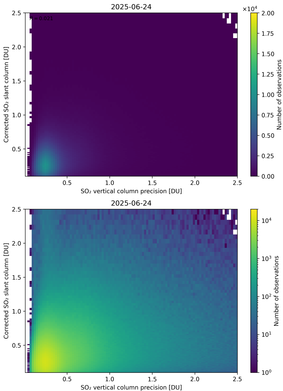
Figure 338: Scatter density plot of “SO 2 vertical column precision” against “Corrected SO 2 slant column” for 2025-06-23 to 2025-06-25.
