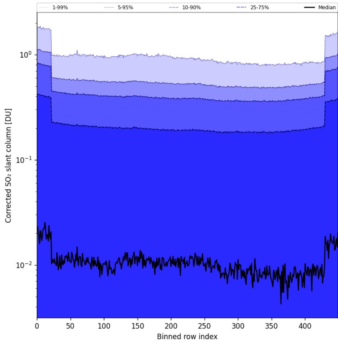
Figure 86: Along track statistics of “Corrected SO 2 slant column” for 2025-06-23 to 2025-06-25
