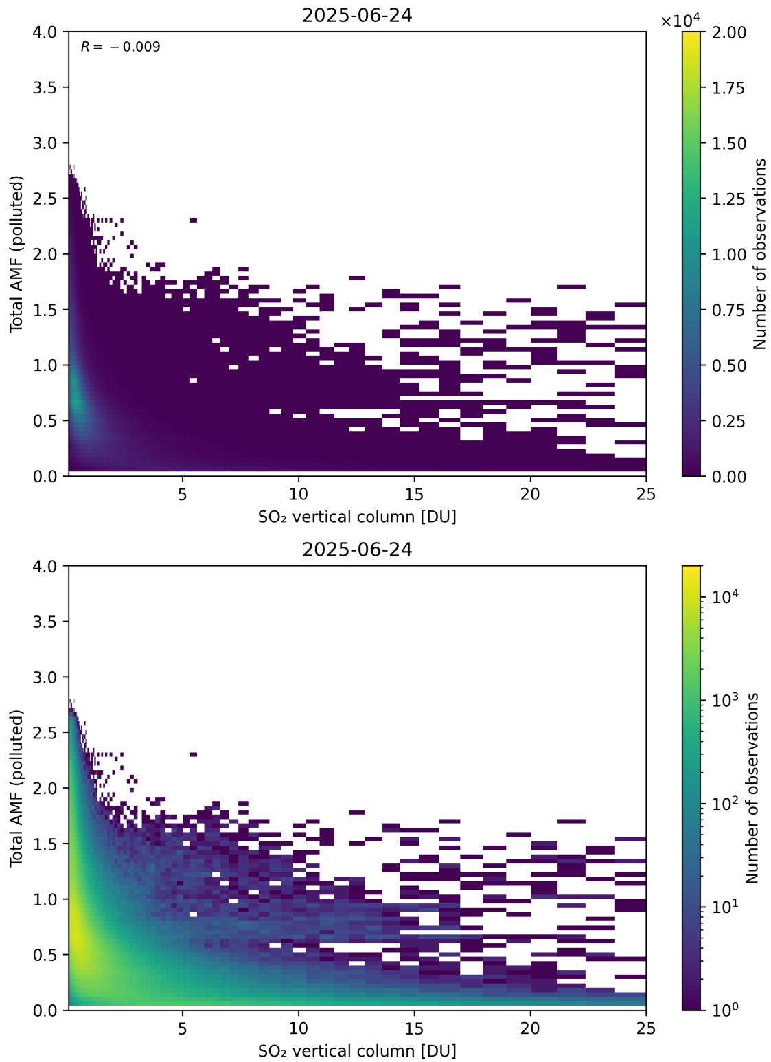
Figure 359: Scatter density plot of “SO 2 vertical column” against “Total AMF (polluted)” for 2025-06-23 to 2025-06-25.
