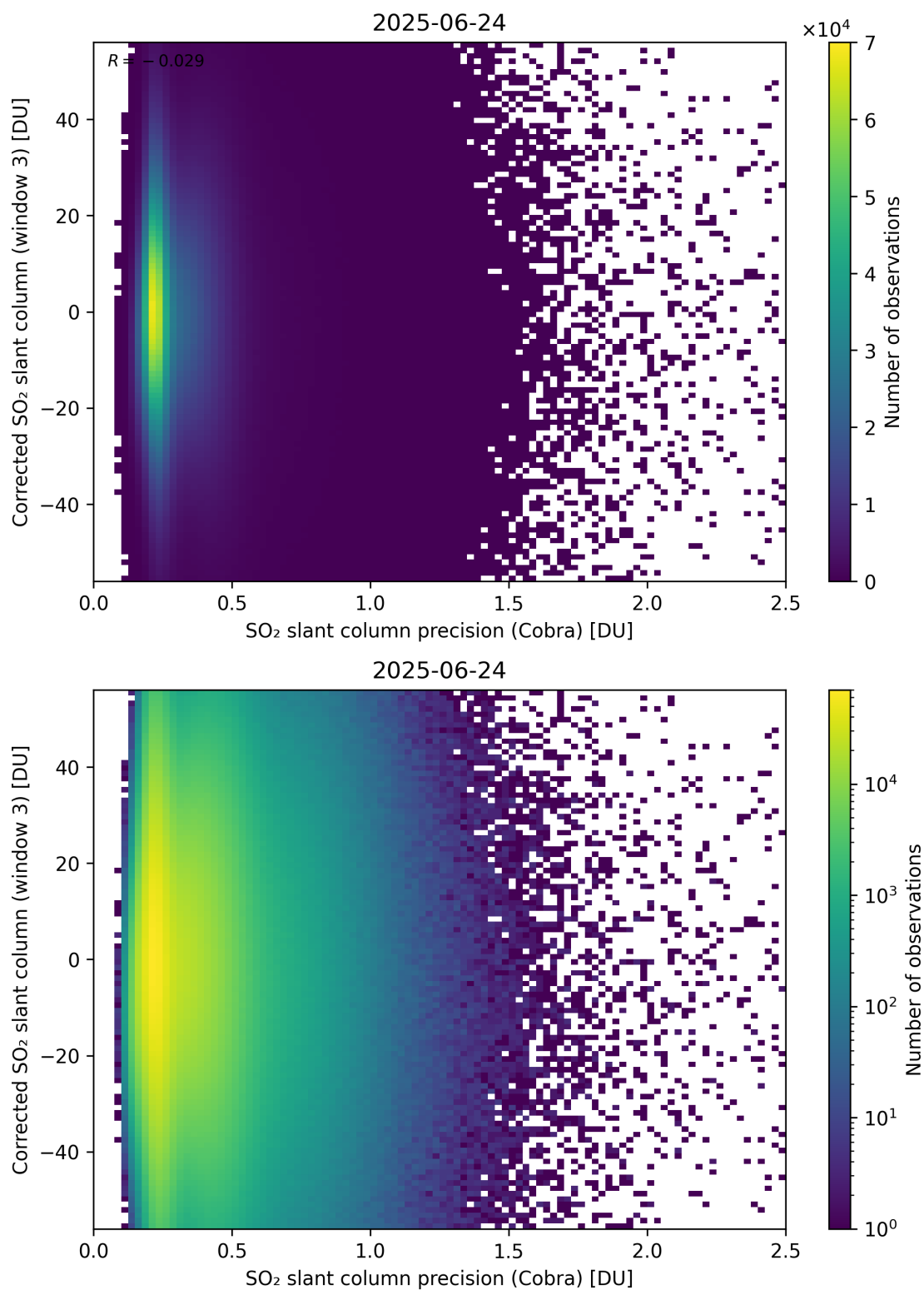
Figure 207: Scatter density plot of “SO 2 slant column precision (Cobra)” against “Corrected SO 2 slant column (window 3)” for 2025-06-23 to 2025-06-25.
