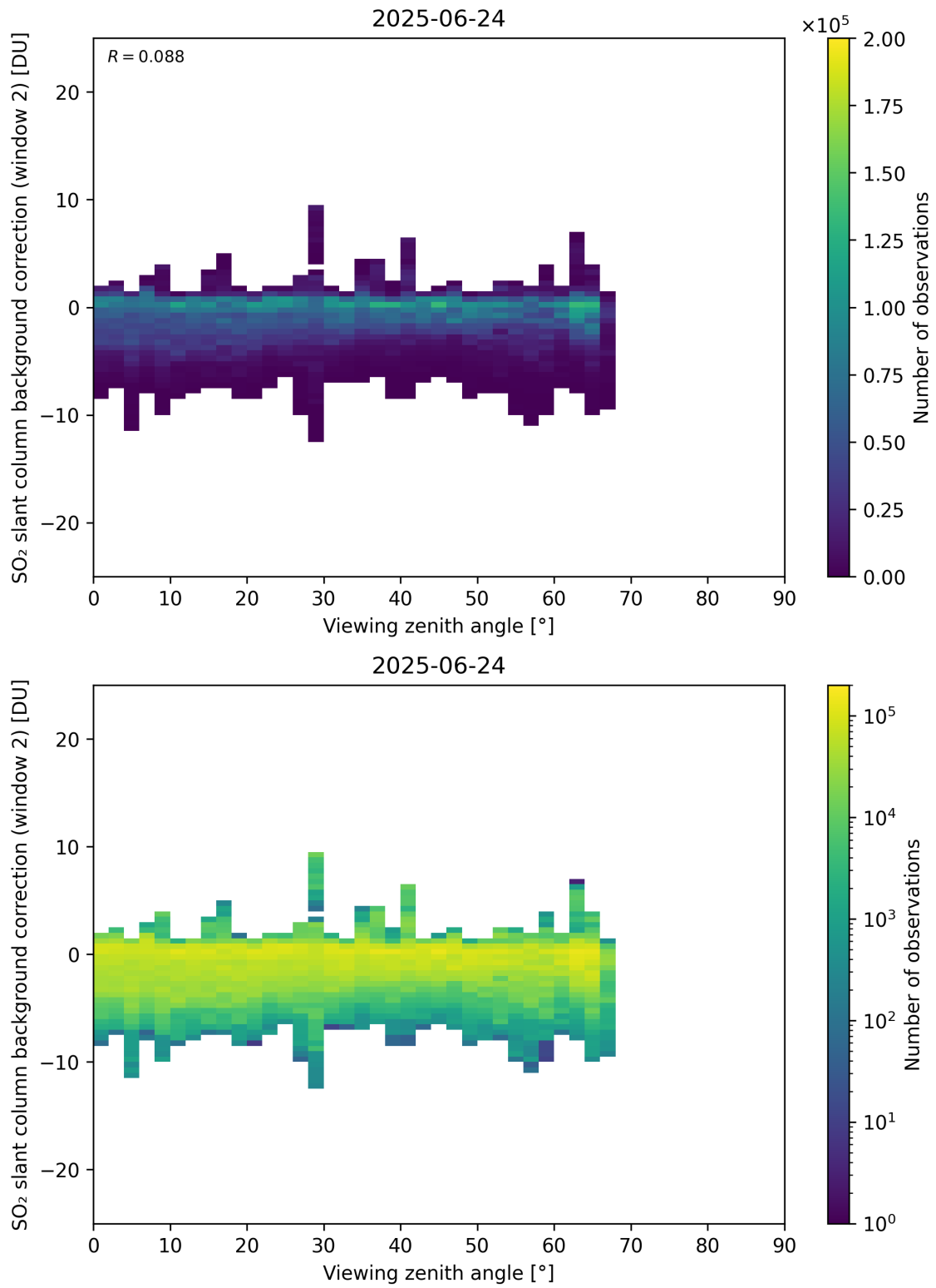
Figure 363: Scatter density plot of “Viewing zenith angle” against “SO 2 slant column background correction (window 2)” for 2025-06-23 to 2025-06-25.
