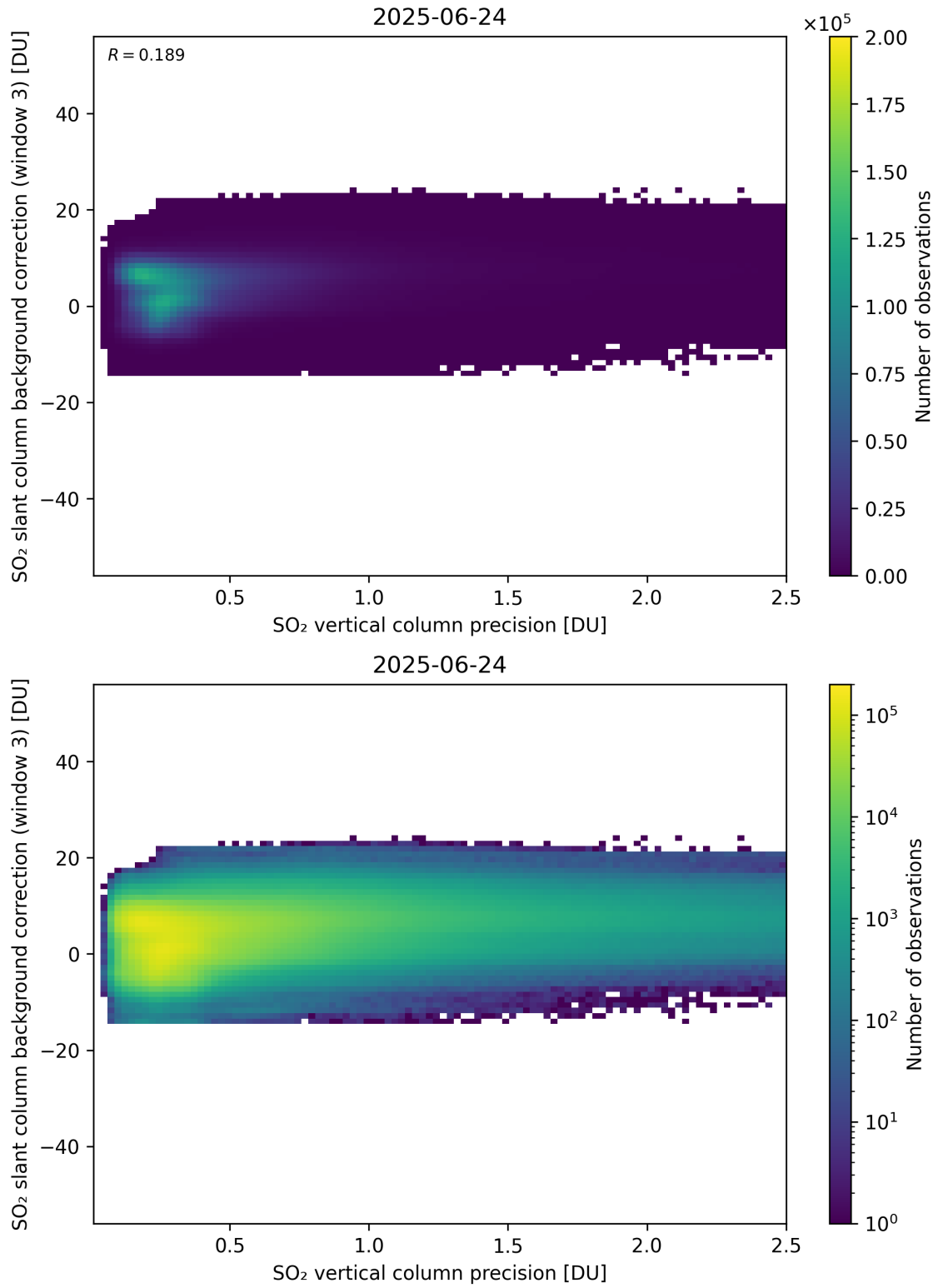
Figure 331: Scatter density plot of “SO 2 vertical column precision” against “SO 2 slant column background correction (window 3)” for 2025-06-23 to 2025-06-25.
