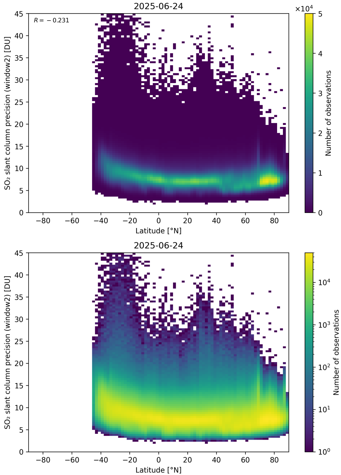
Figure 164: Scatter density plot of “Latitude” against “SO 2 slant column precision (window2)” for 2025-06-23 to 2025-06-25.
