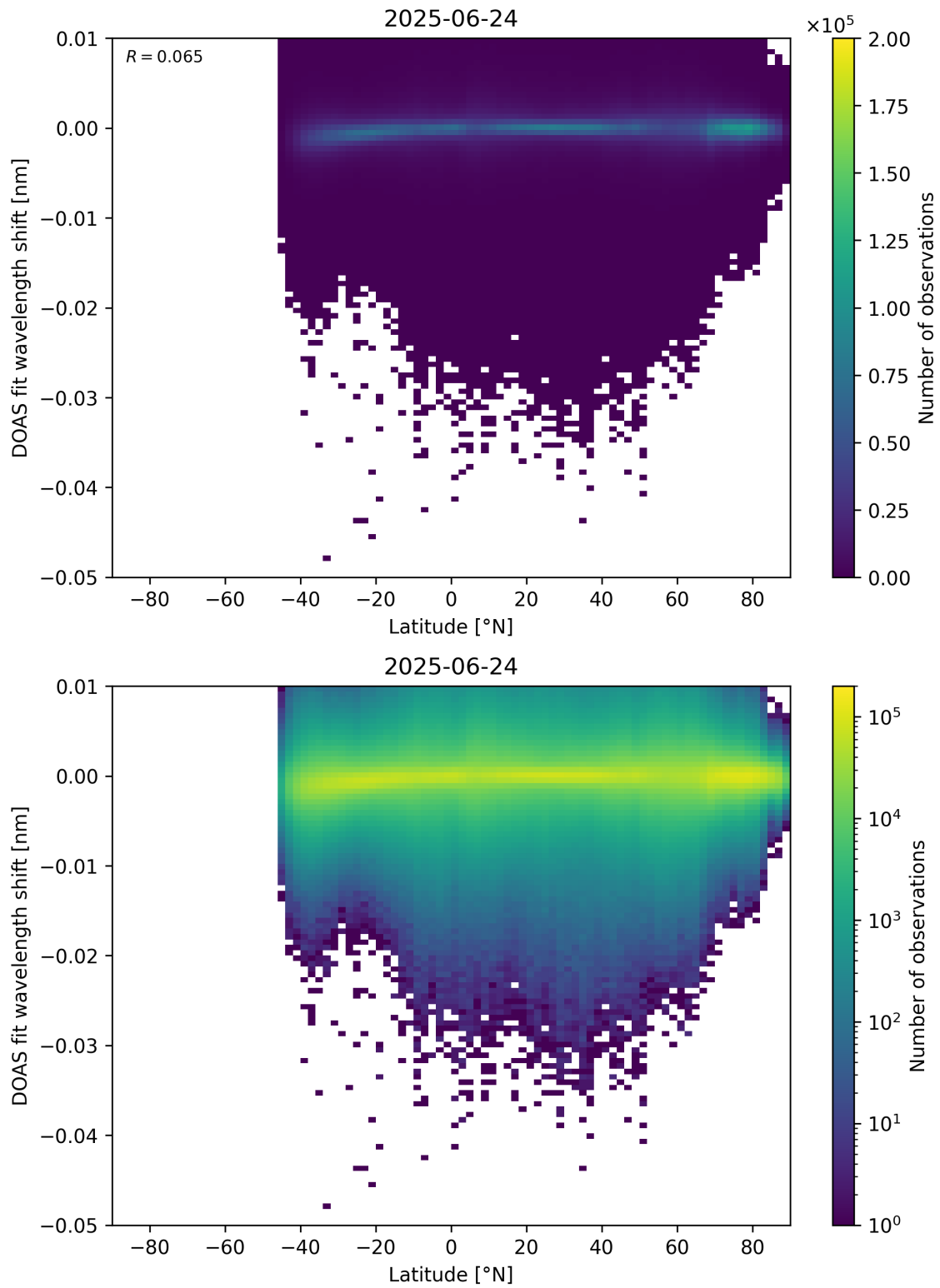
Figure 153: Scatter density plot of “Latitude” against “DOAS fit wavelength shift” for 2025-06-23 to 2025-06-25.
