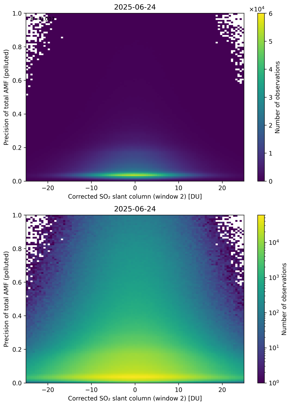
Figure 254: Scatter density plot of “Corrected SO 2 slant column (window 2)” against “Precision of total AMF (polluted)” for 2025-06-23 to 2025-06-25.
