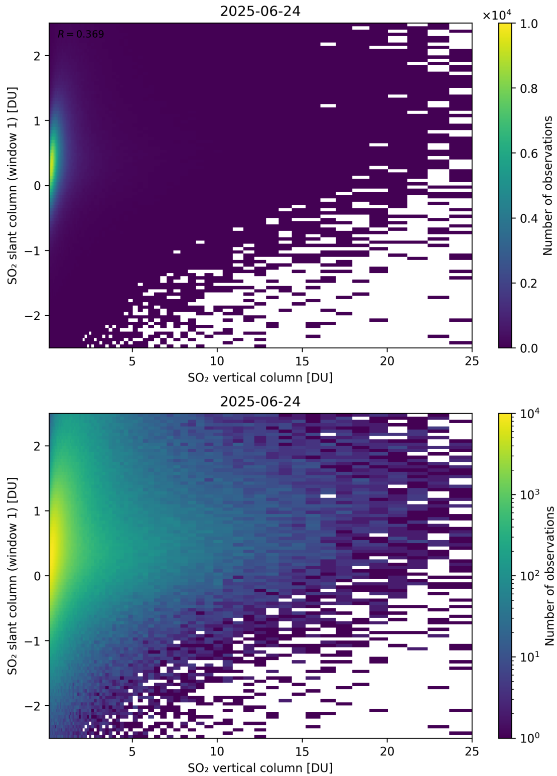
Figure 354: Scatter density plot of “SO 2 vertical column” against “SO 2 slant column (window 1)” for 2025-06-23 to 2025-06-25.
