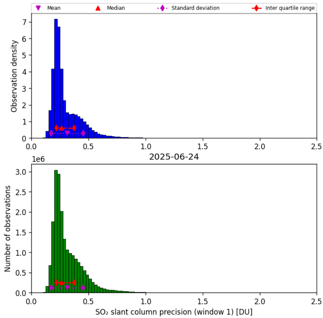
Figure 64: Histogram of “SO 2 slant column precision (window 1)” for 2025-06-23 to 2025-06-25
