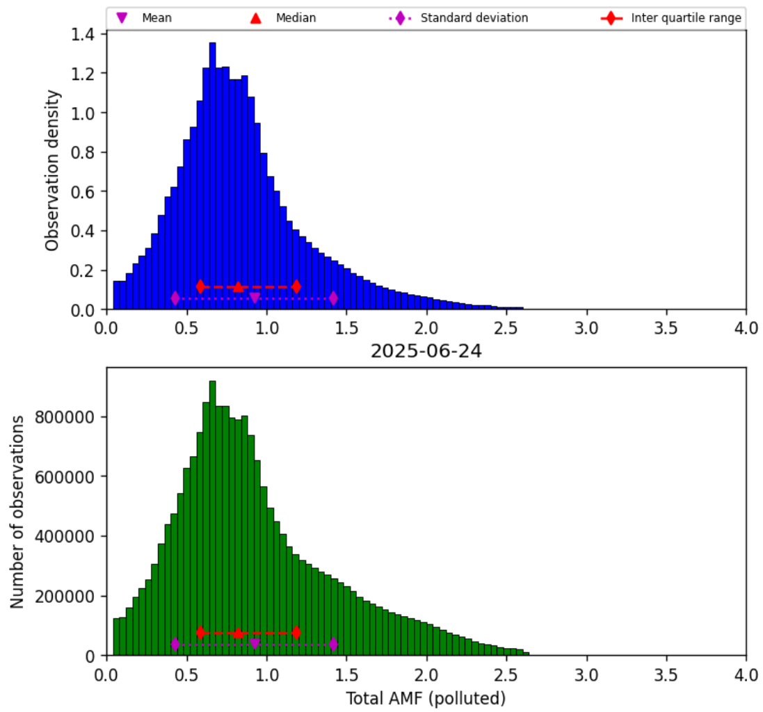
Figure 79: Histogram of “Total AMF (polluted)” for 2025-06-23 to 2025-06-25
