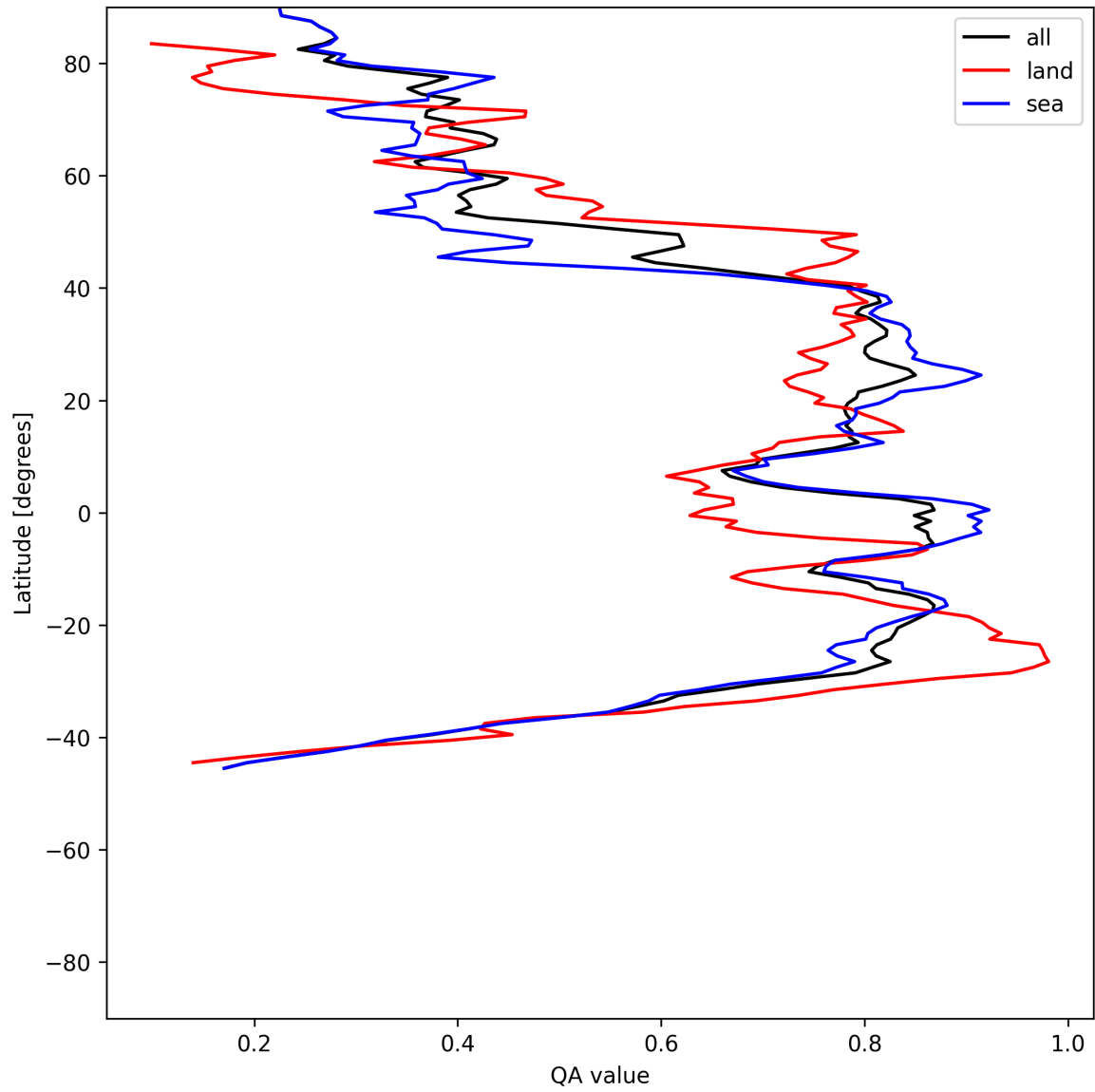
Figure 31: Zonal average of “QA value” for 2025-06-23 to 2025-06-25.
