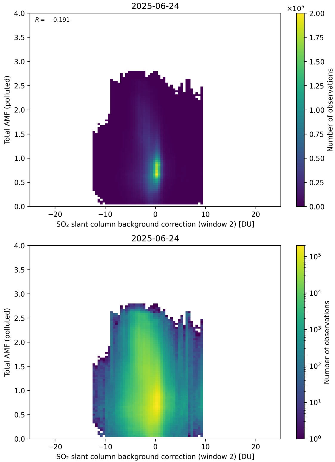
Figure 130: Scatter density plot of “SO 2 slant column background correction (window 2)” against “Total AMF (polluted)” for 2025-06-23 to 2025-06-25.
