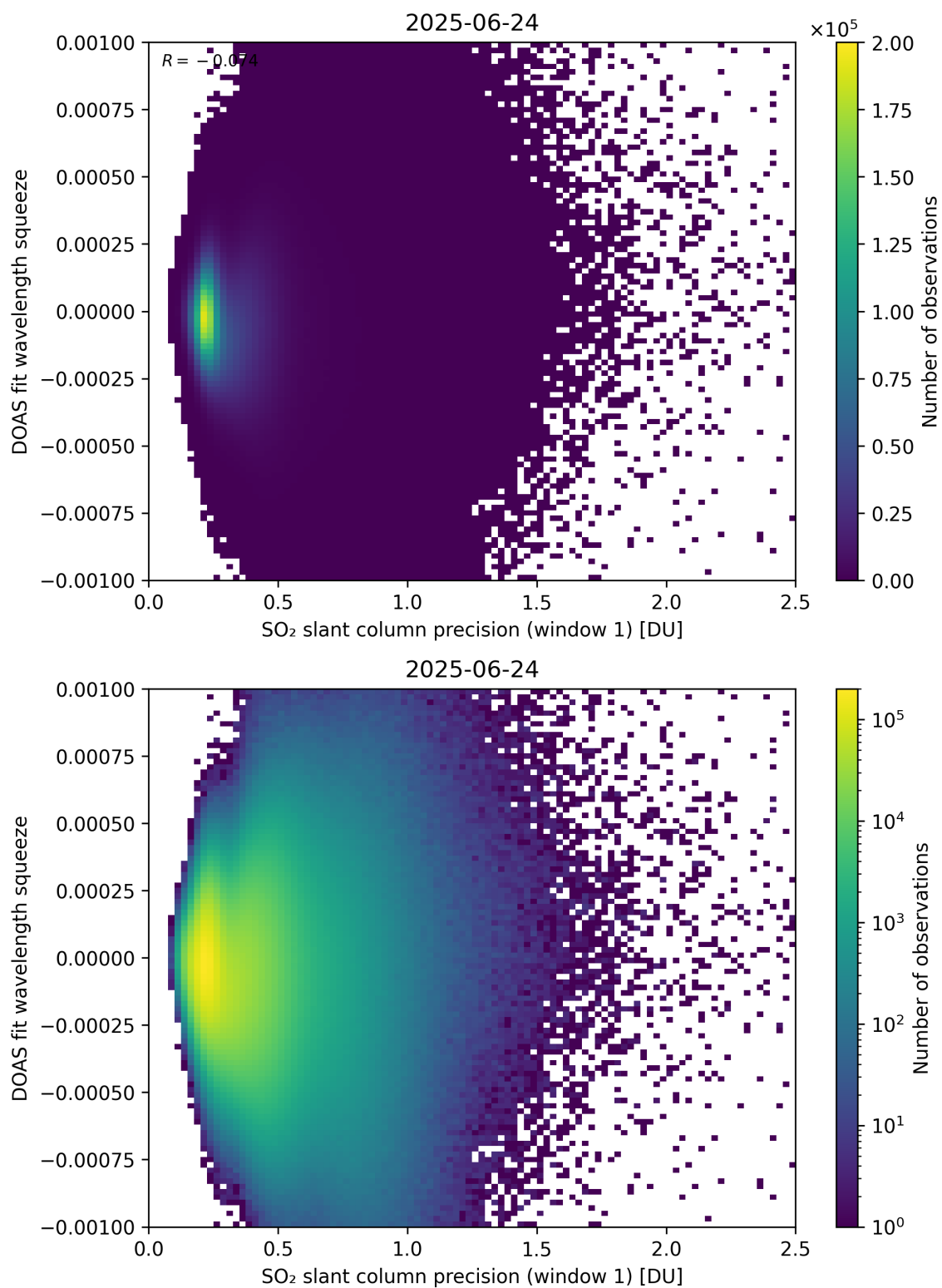
Figure 272: Scatter density plot of “SO 2 slant column precision (window 1)” against “DOAS fit wavelength squeeze” for 2025-06-23 to 2025-06-25.
