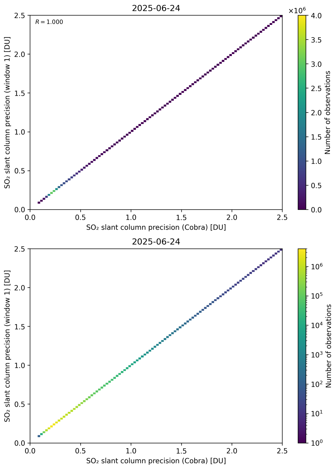
Figure 209: Scatter density plot of “SO 2 slant column precision (Cobra)” against “SO 2 slant column precision (window 1)” for 2025-06-23 to 2025-06-25.
