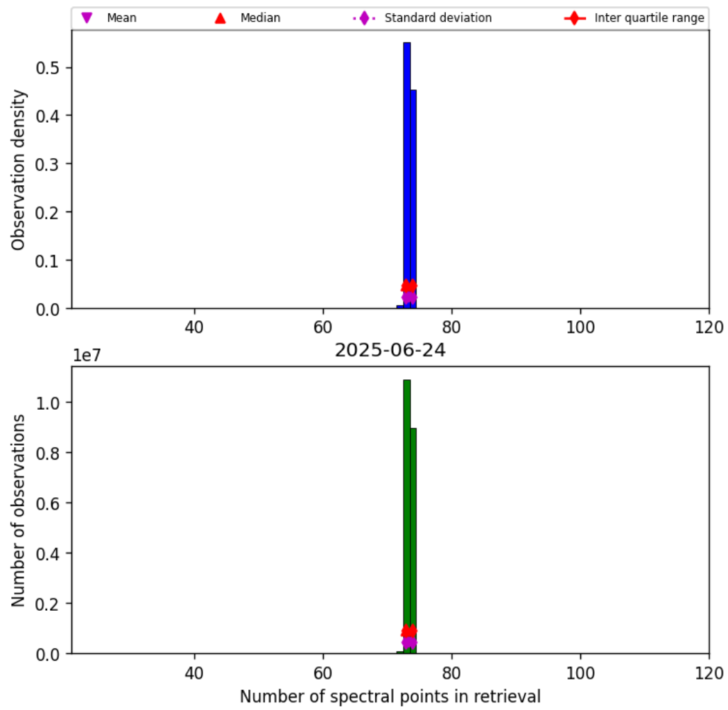
Figure 82: Histogram of “Number of spectral points in retrieval” for 2025-06-23 to 2025-06-25
