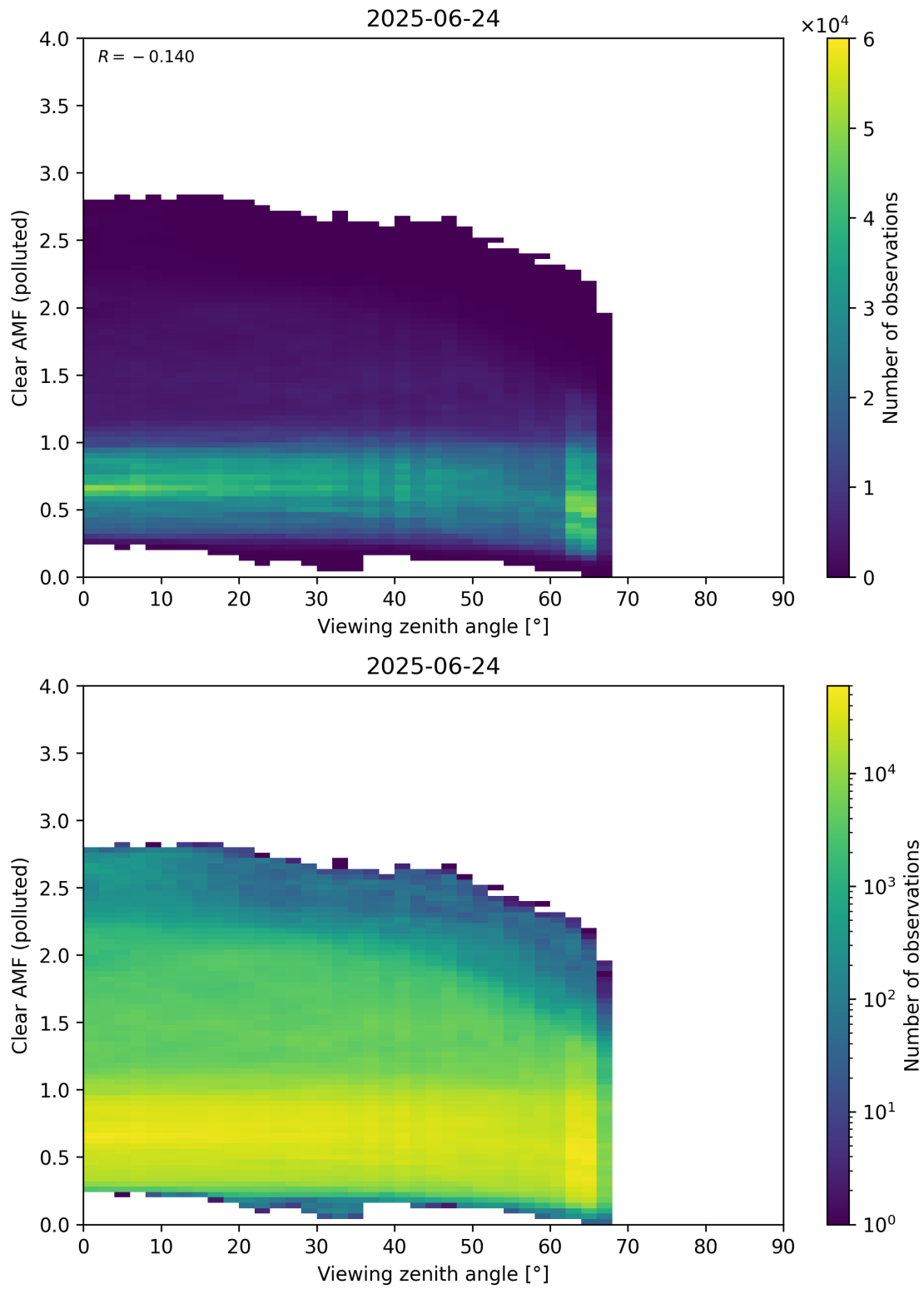
Figure 370: Scatter density plot of “Viewing zenith angle” against “Clear AMF (polluted)” for 2025-06-23 to 2025-06-25.
