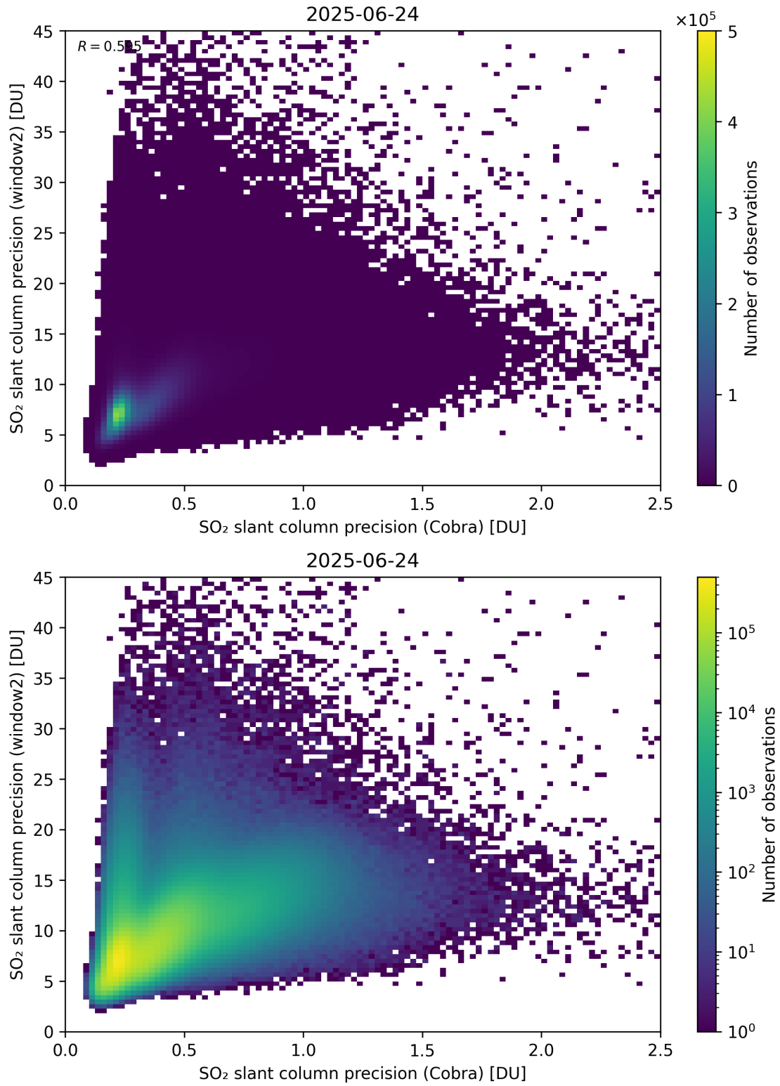
Figure 210: Scatter density plot of “SO 2 slant column precision (Cobra)” against “SO 2 slant column precision (window2)” for 2025-06-23 to 2025-06-25.
