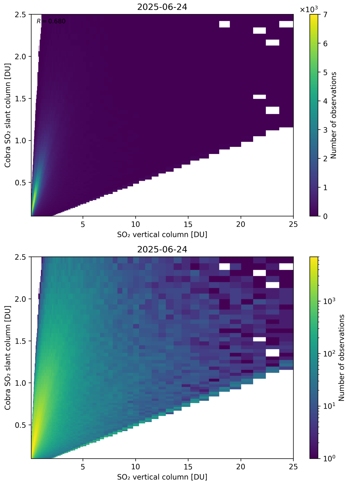
Figure 349: Scatter density plot of “SO 2 vertical column” against “Cobra SO 2 slant column” for 2025-06-23 to 2025-06-25.
