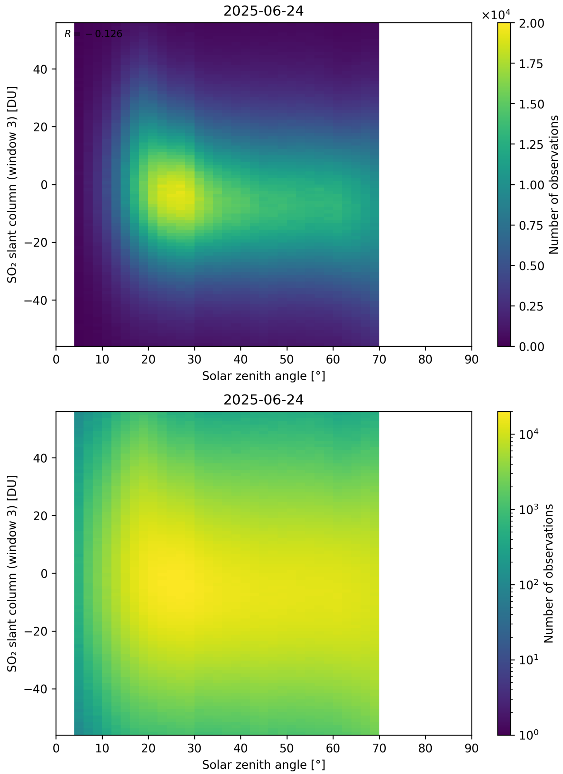
Figure 187: Scatter density plot of “Solar zenith angle” against “SO 2 slant column (window 3)” for 2025-06-23 to 2025-06-25.
