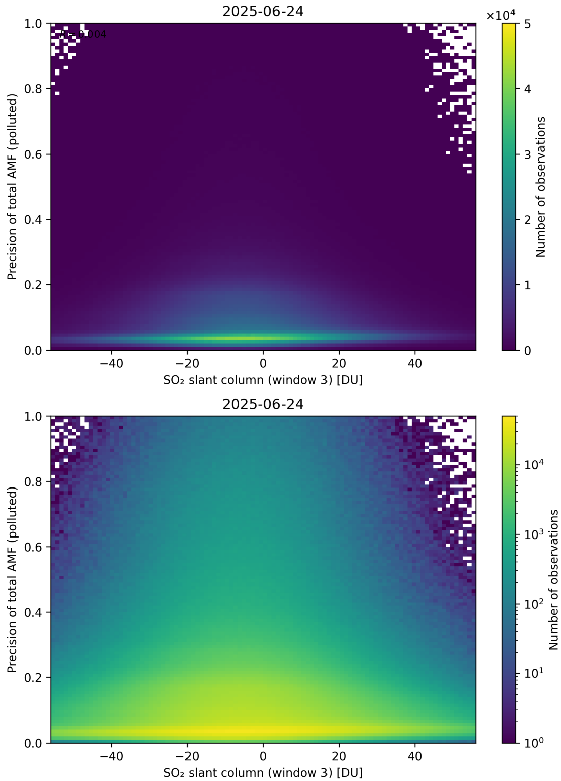
Figure 319: Scatter density plot of “SO 2 slant column (window 3)” against “Precision of total AMF (polluted)” for 2025-06-23 to 2025-06-25.
