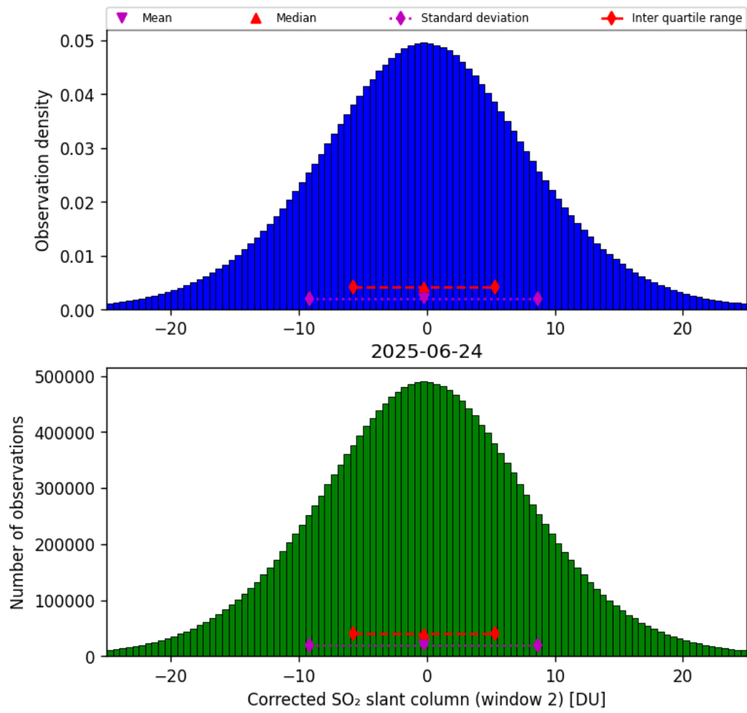
Figure 69: Histogram of “Corrected SO 2 slant column (window 2)” for 2025-06-23 to 2025-06-25
