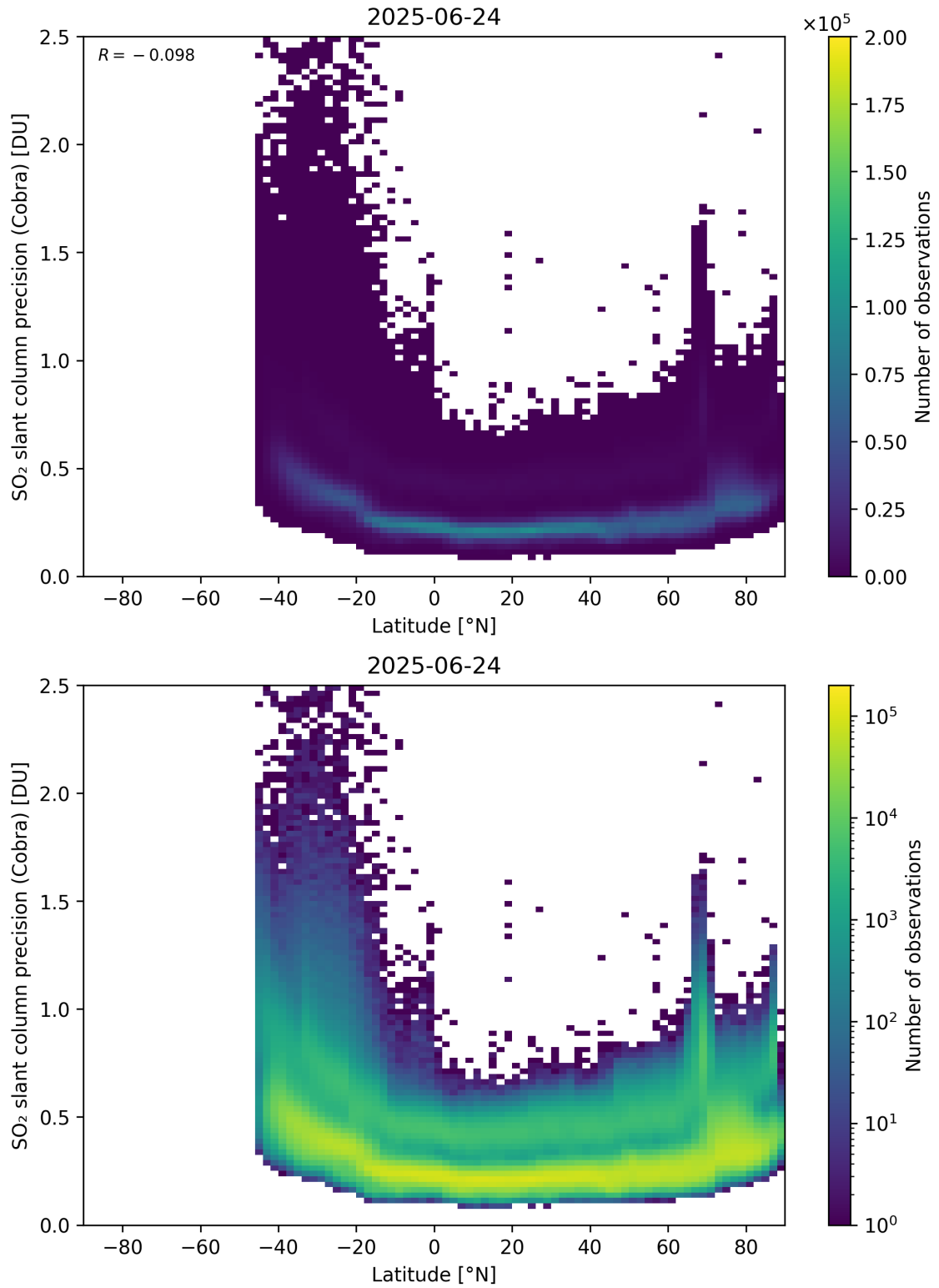
Figure 158: Scatter density plot of “Latitude” against “SO 2 slant column precision (Cobra)” for 2025-06-23 to 2025-06-25.
