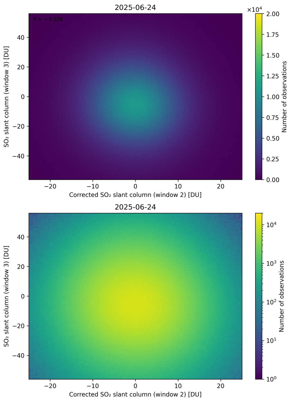
Figure 251: Scatter density plot of “Corrected SO 2 slant column (window 2)” against “SO 2 slant column (window 3)” for 2025-06-23 to 2025-06-25.
