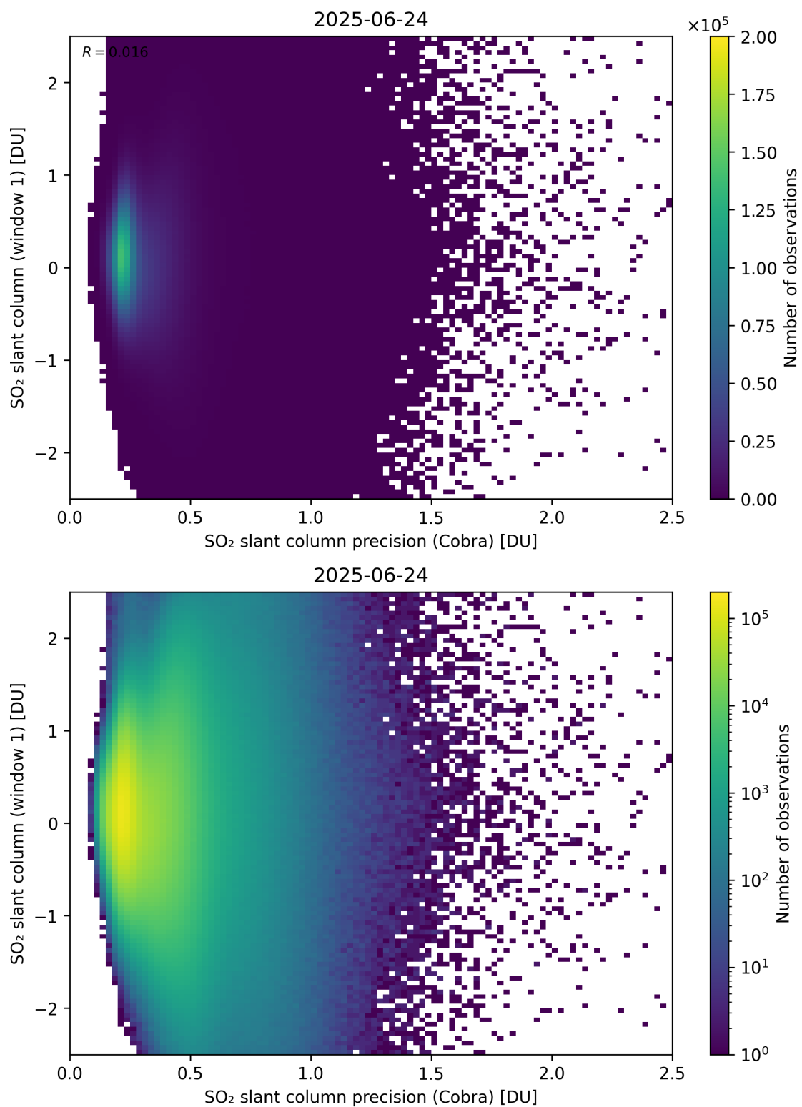
Figure 208: Scatter density plot of “SO 2 slant column precision (Cobra)” against “SO 2 slant column (window 1)” for 2025-06-23 to 2025-06-25.
