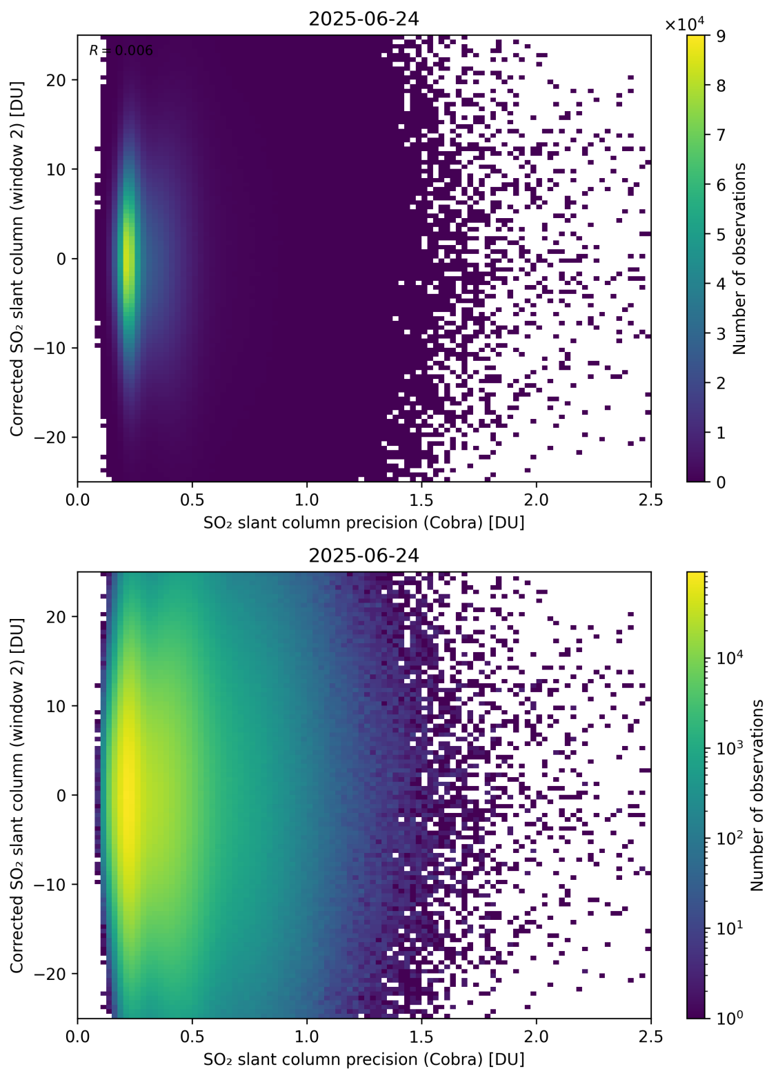
Figure 206: Scatter density plot of “SO 2 slant column precision (Cobra)” against “Corrected SO 2 slant column (window 2)” for 2025-06-23 to 2025-06-25.
