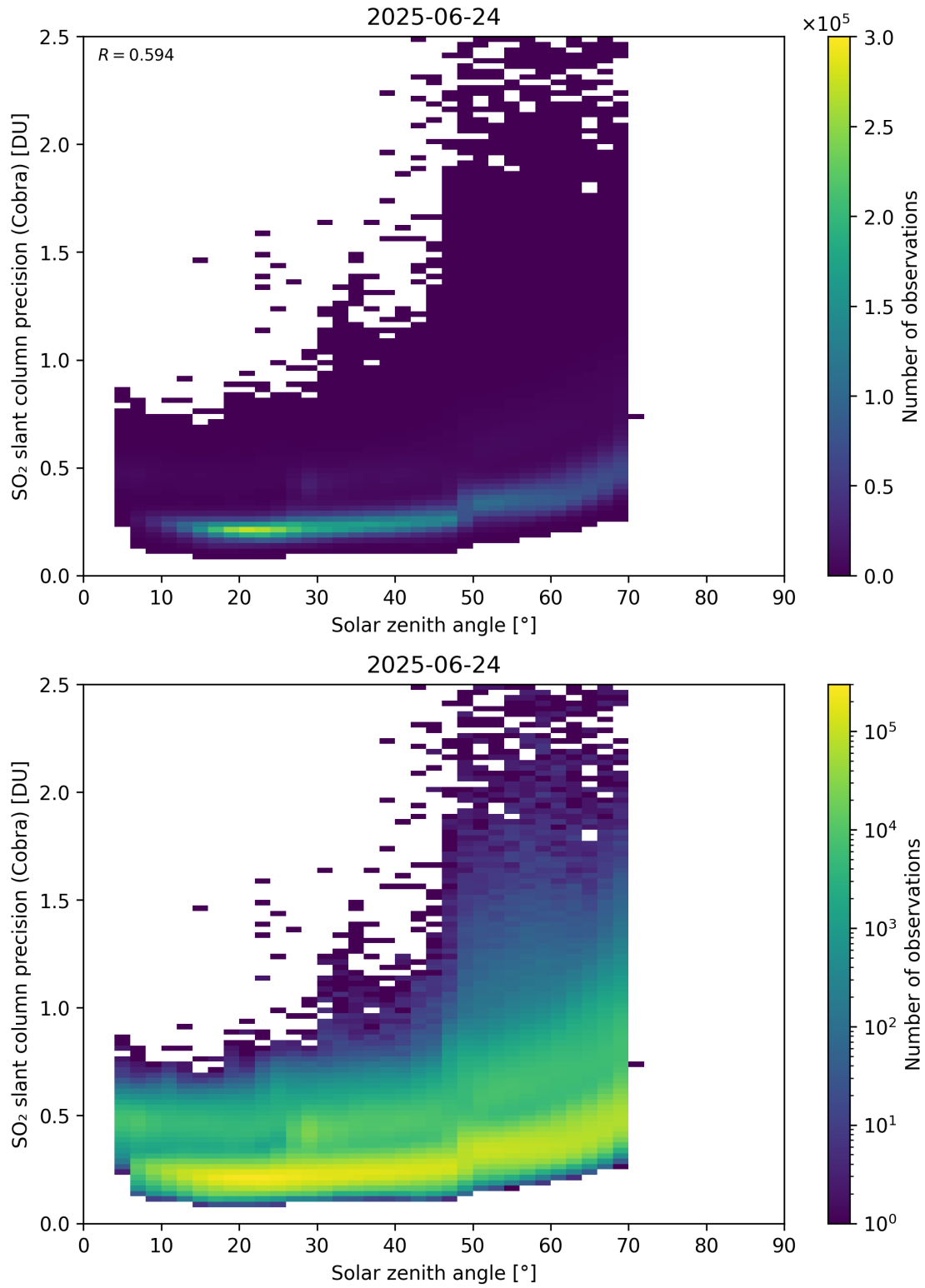
Figure 180: Scatter density plot of “Solar zenith angle” against “SO 2 slant column precision (Cobra)” for 2025-06-23 to 2025-06-25.
