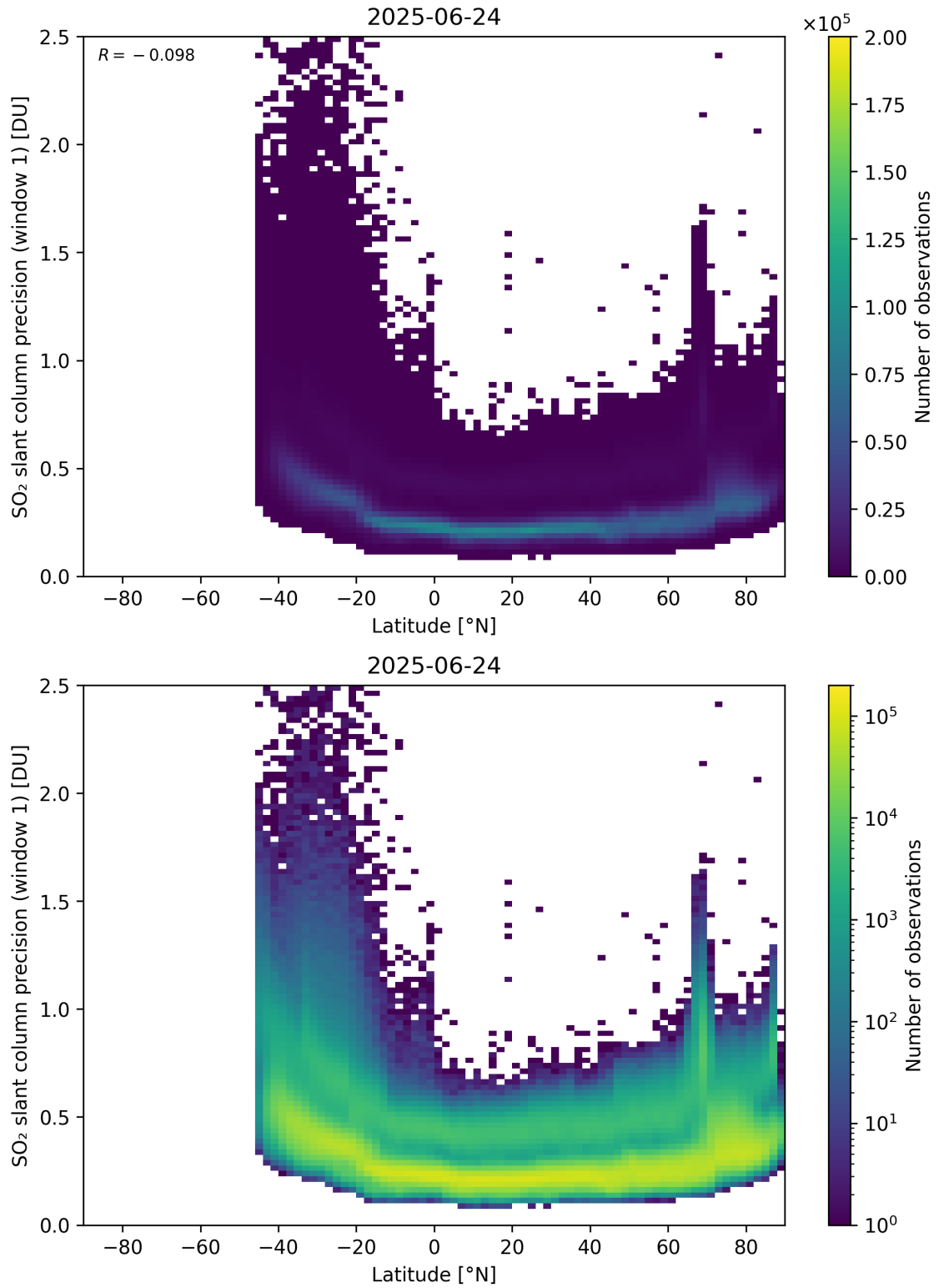
Figure 163: Scatter density plot of “Latitude” against “SO 2 slant column precision (window 1)” for 2025-06-23 to 2025-06-25.
