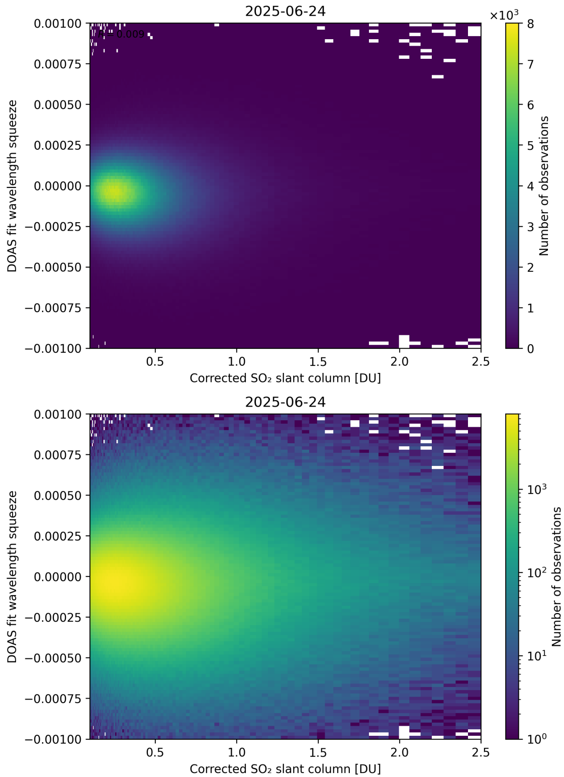
Figure 230: Scatter density plot of “Corrected SO 2 slant column” against “DOAS fit wavelength squeeze” for 2025-06-23 to 2025-06-25.
