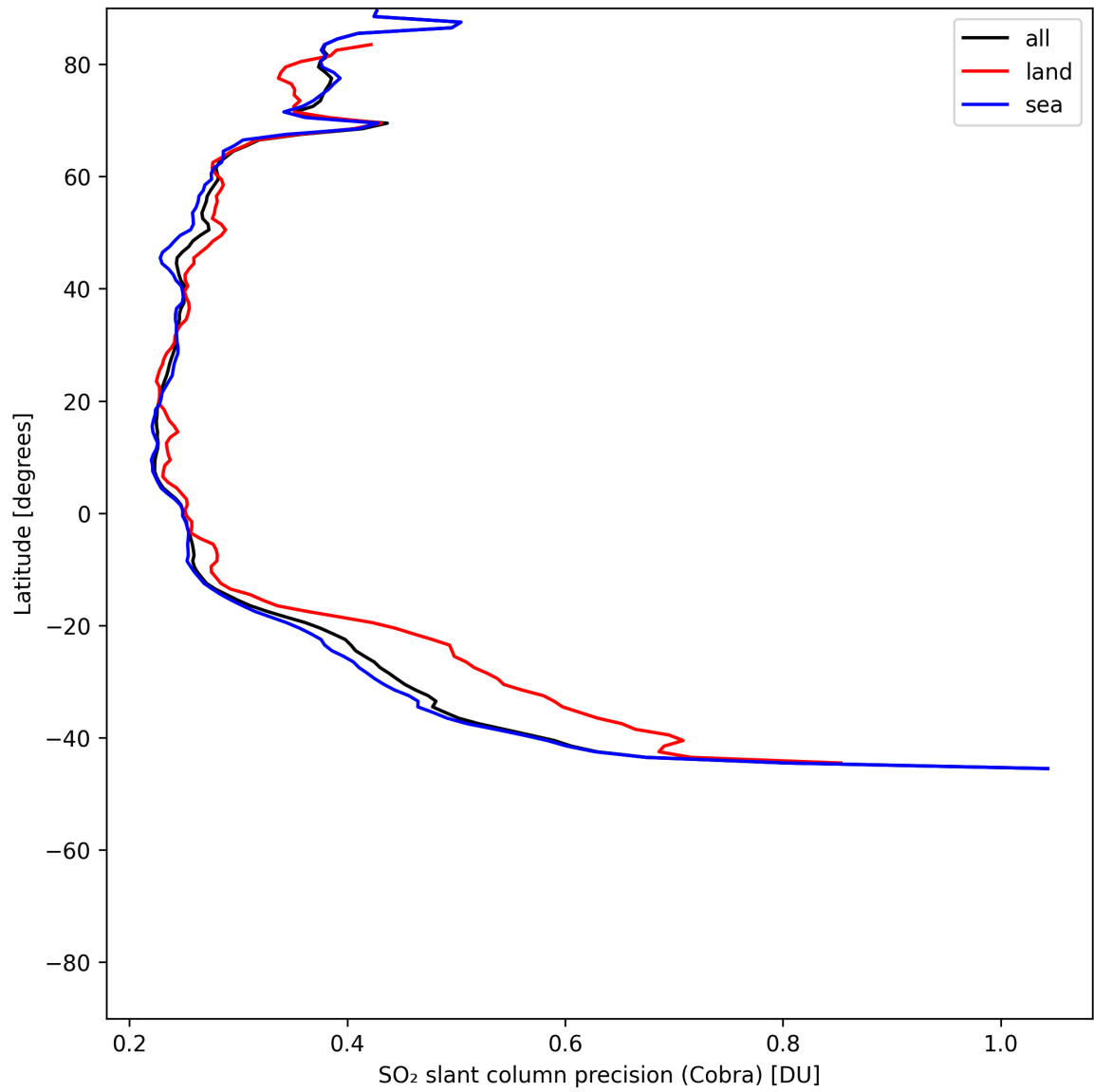
Figure 36: Zonal average of “SO 2 slant column precision (Cobra)” for 2025-06-23 to 2025-06-25.
