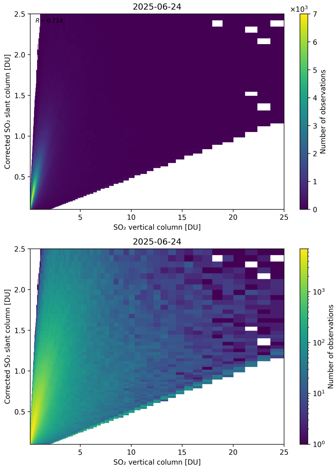
Figure 351: Scatter density plot of “SO 2 vertical column” against “Corrected SO 2 slant column” for 2025-06-23 to 2025-06-25.
