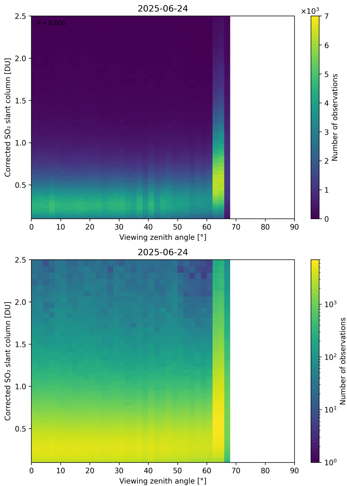
Figure 373: Scatter density plot of “Viewing zenith angle” against “Corrected SO 2 slant column” for 2025-06-23 to 2025-06-25.
