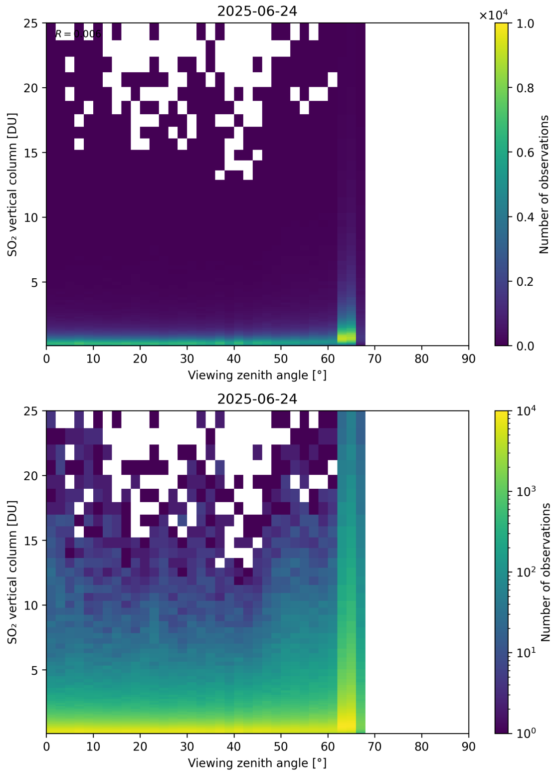
Figure 383: Scatter density plot of “Viewing zenith angle” against “SO 2 vertical column” for 2025-06-23 to 2025-06-25.
