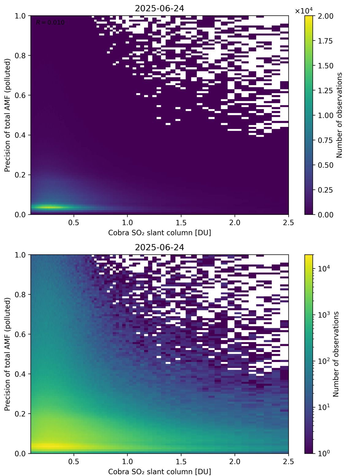
Figure 225: Scatter density plot of “Cobra SO 2 slant column” against “Precision of total AMF (polluted)” for 2025-06-23 to 2025-06-25.
