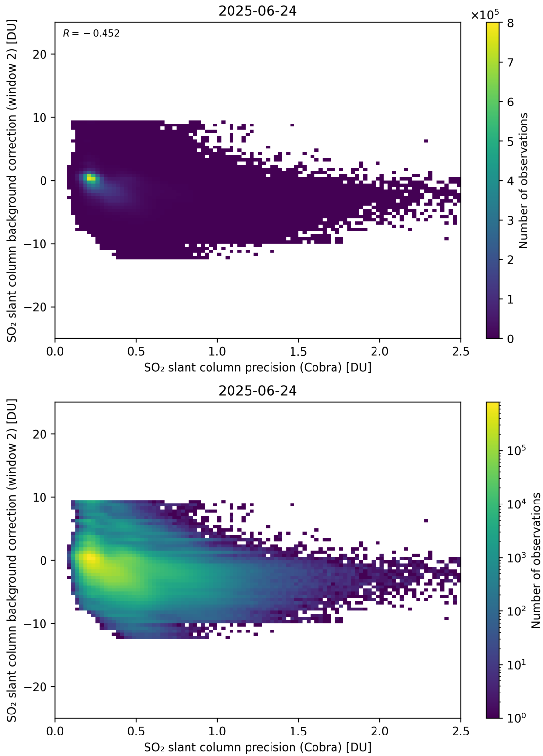
Figure 200: Scatter density plot of “SO 2 slant column precision (Cobra)” against “SO 2 slant column background correction (window 2)” for 2025-06-23 to 2025-06-25.
