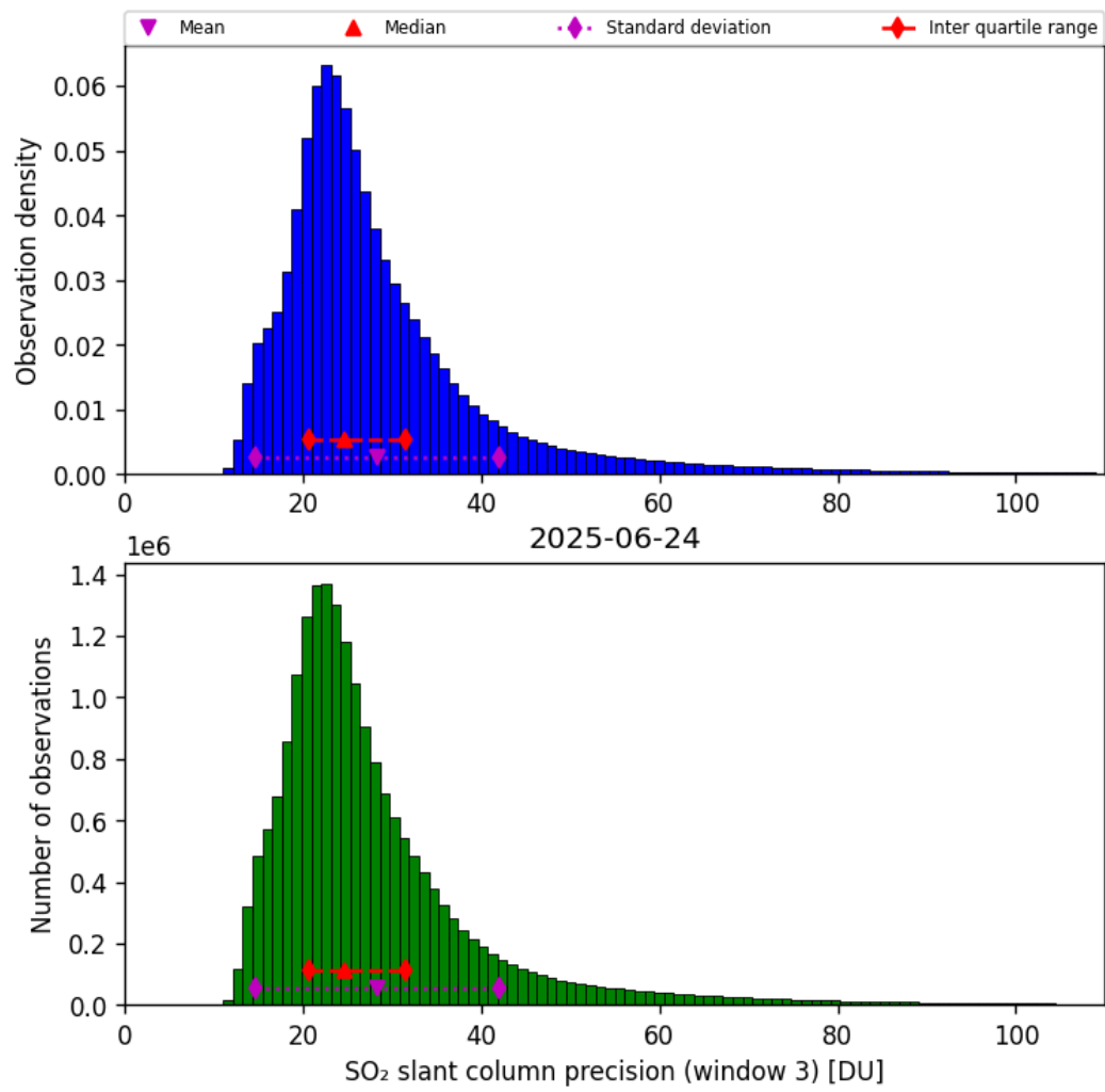
Figure 72: Histogram of “SO 2 slant column precision (window 3)” for 2025-06-23 to 2025-06-25
