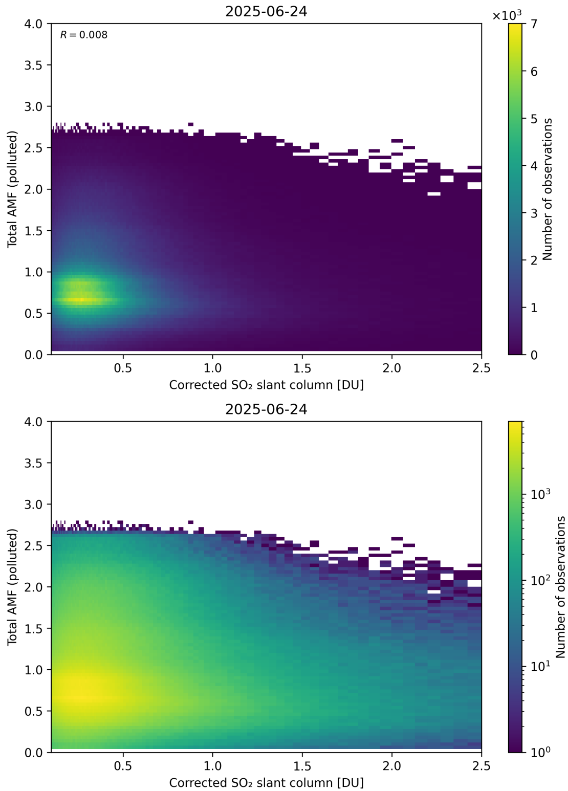
Figure 242: Scatter density plot of “Corrected SO 2 slant column” against “Total AMF (polluted)” for 2025-06-23 to 2025-06-25.
