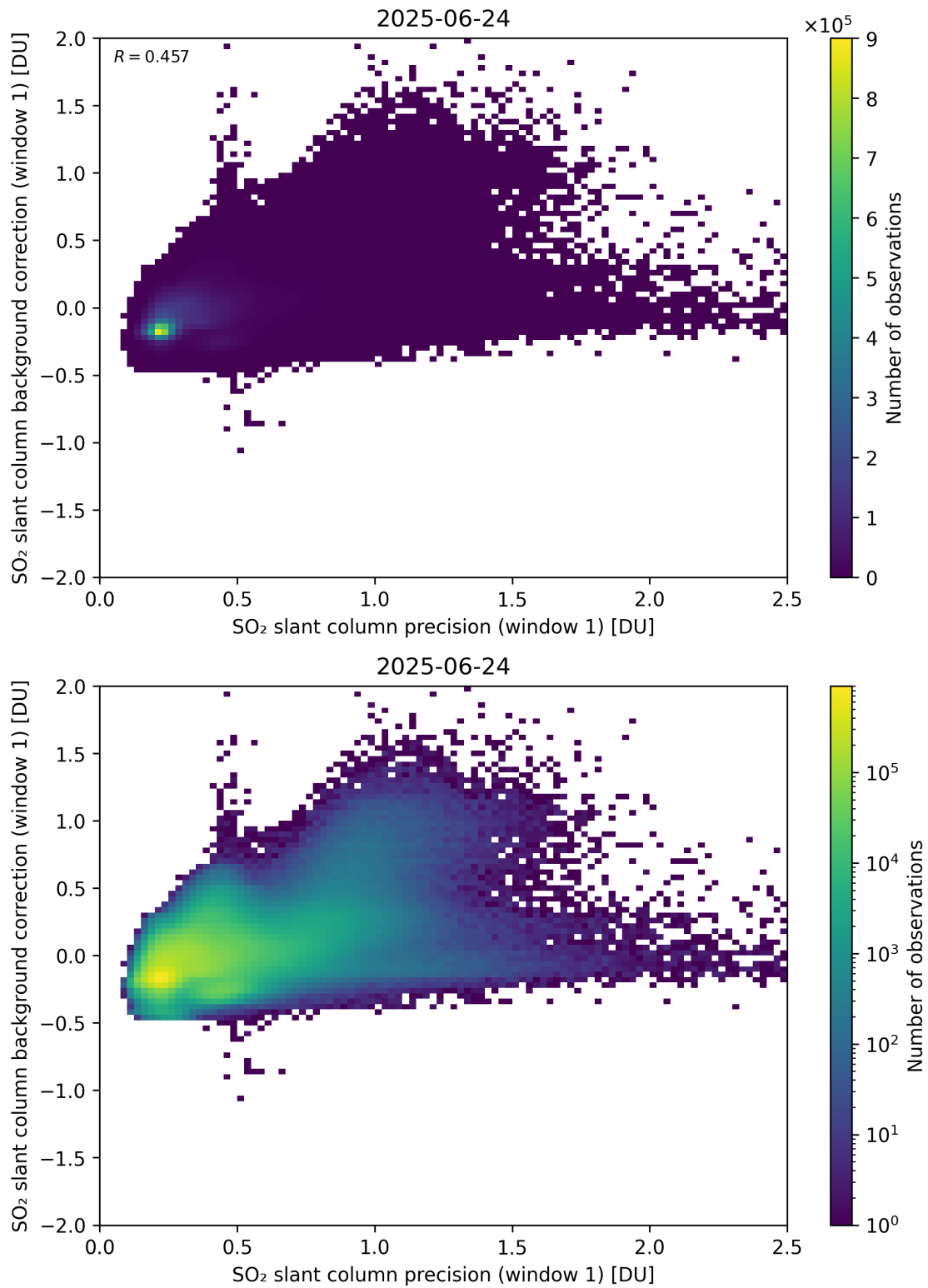
Figure 268: Scatter density plot of “SO 2 slant column precision (window 1)” against “SO 2 slant column background correction (window 1)” for 2025-06-23 to 2025-06-25.
