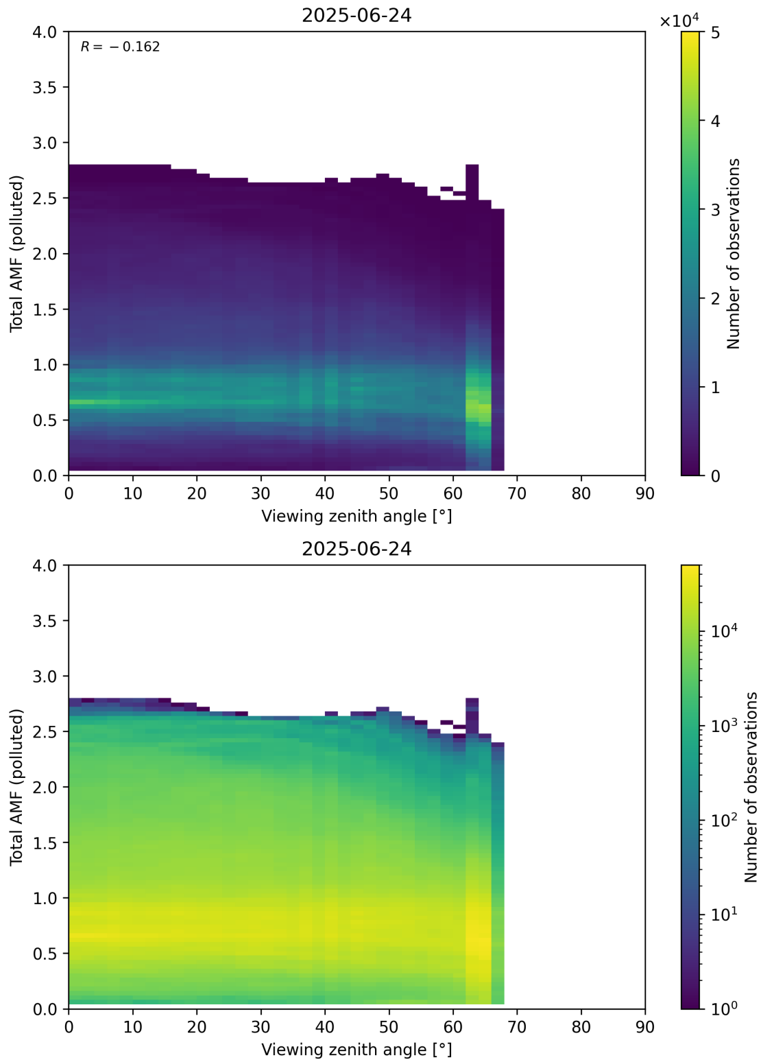
Figure 381: Scatter density plot of “Viewing zenith angle” against “Total AMF (polluted)” for 2025-06-23 to 2025-06-25.
