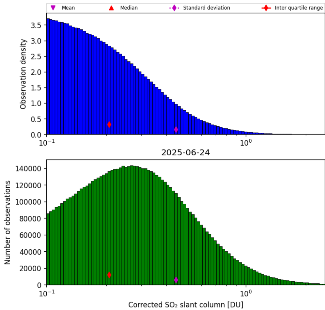
Figure 60: Histogram of "Corrected SO 2 slant column" for 2025-06-23 to 2025-06-25
