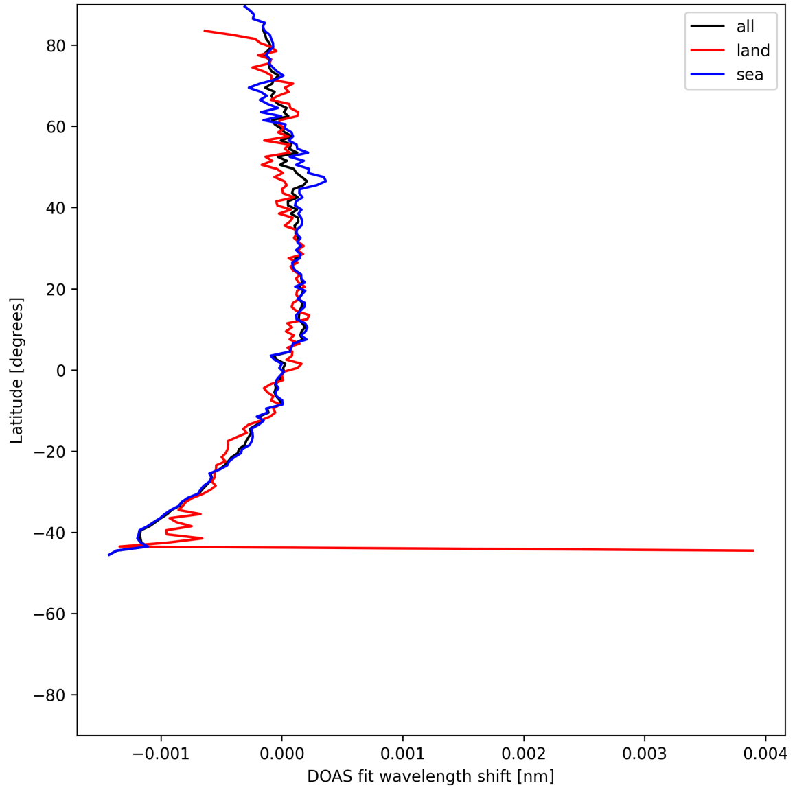
Figure 50: Zonal average of "DOAS fit wavelength shift" for 2025-06-23 to 2025-06-25.
