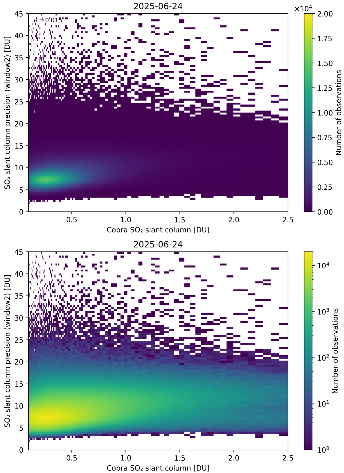
Figure 221: Scatter density plot of “Cobra SO 2 slant column” against “SO 2 slant column precision (window2)” for 2025-06-23 to 2025-06-25.
