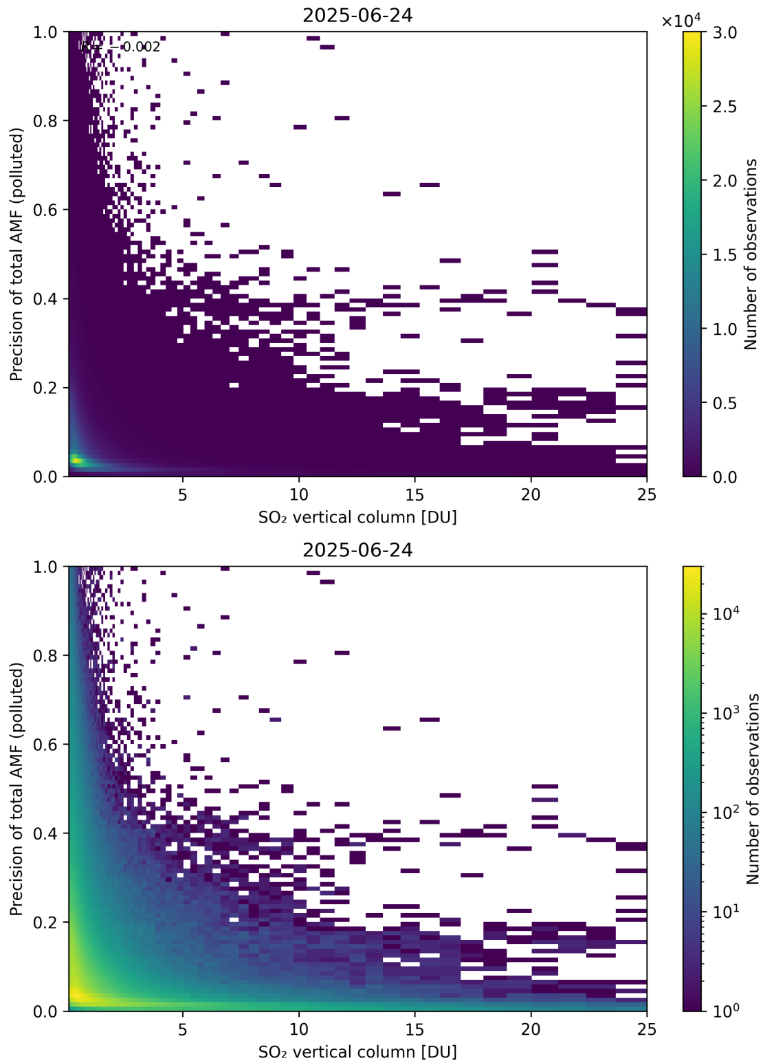
Figure 360: Scatter density plot of “SO 2 vertical column” against “Precision of total AMF (polluted)” for 2025-06-23 to 2025-06-25.
