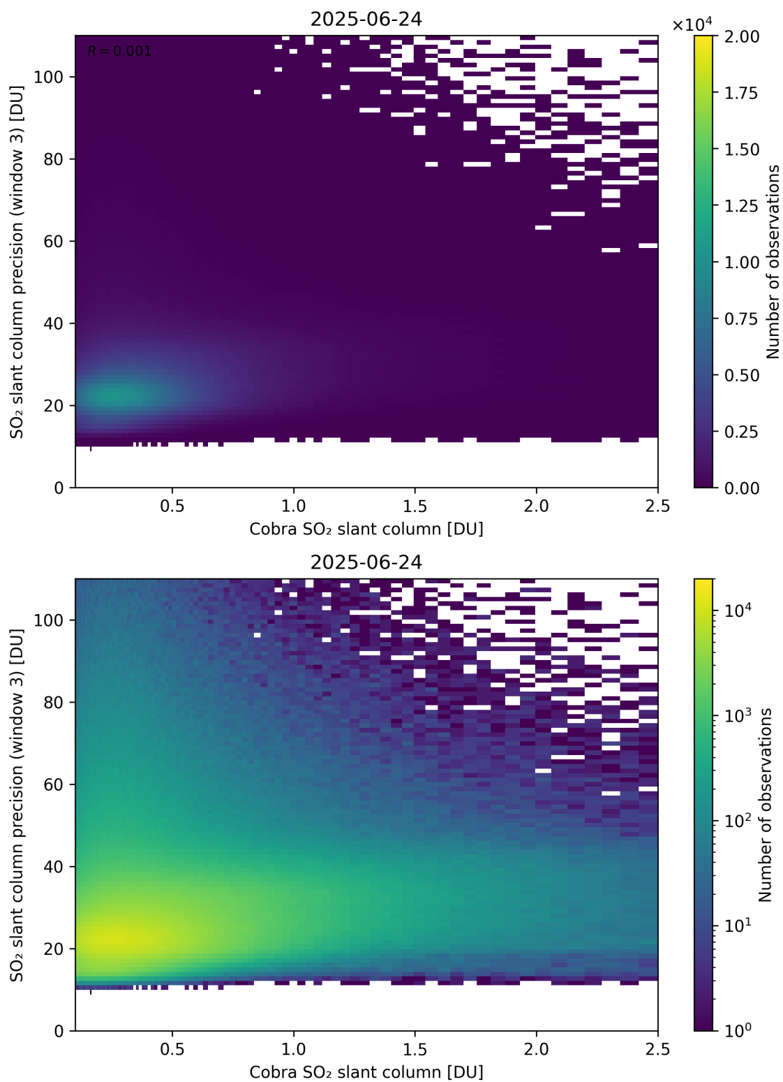
Figure 223: Scatter density plot of “Cobra SO 2 slant column” against “SO 2 slant column precision (window 3)” for 2025-06-23 to 2025-06-25.
