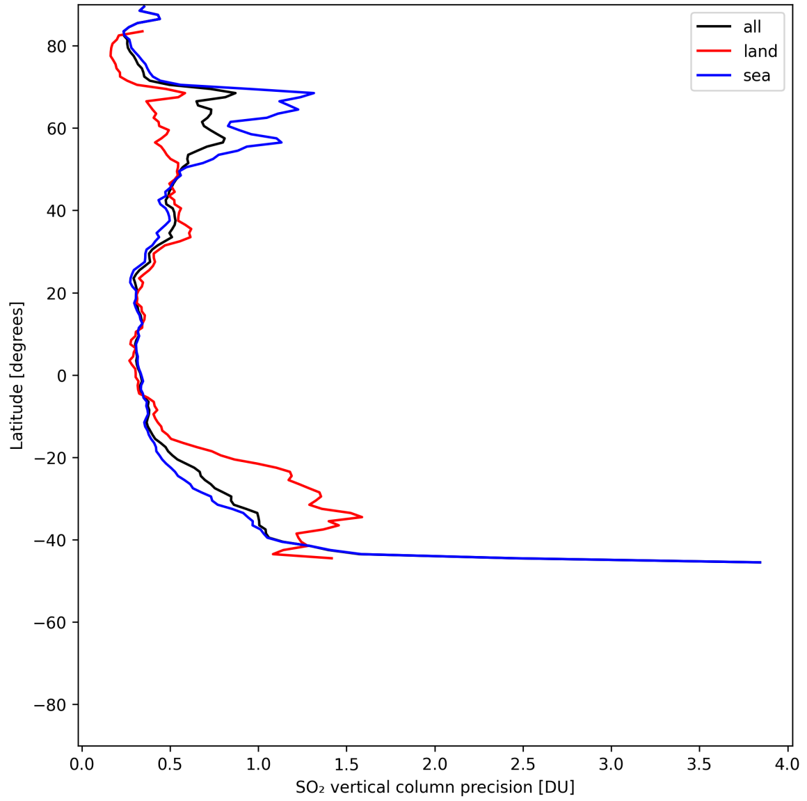
Figure 33: Zonal average of “SO 2 vertical column precision” for 2025-06-23 to 2025-06-25.
