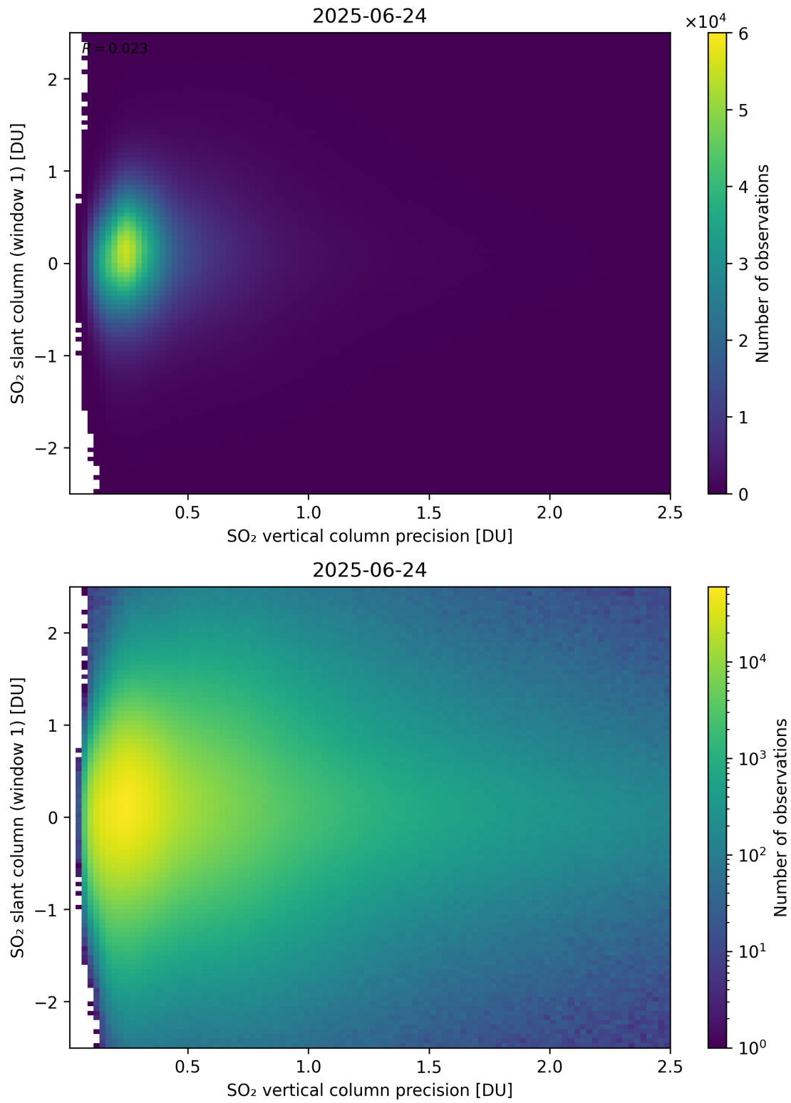
Figure 341: Scatter density plot of “SO 2 vertical column precision” against “SO 2 slant column (window 1)” for 2025-06-23 to 2025-06-25.
