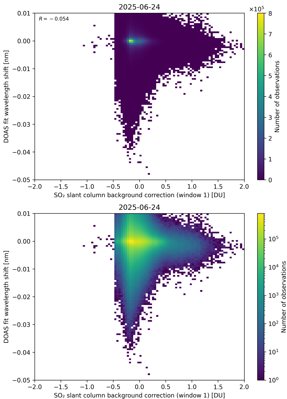
Figure 111: Scatter density plot of “SO 2 slant column background correction (window 1)” against “DOAS fit wavelength shift” for 2025-06-23 to 2025-06-25.
