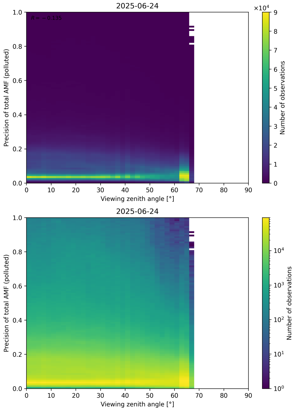
Figure 382: Scatter density plot of “Viewing zenith angle” against “Precision of total AMF (polluted)” for 2025-06-23 to 2025-06-25.
