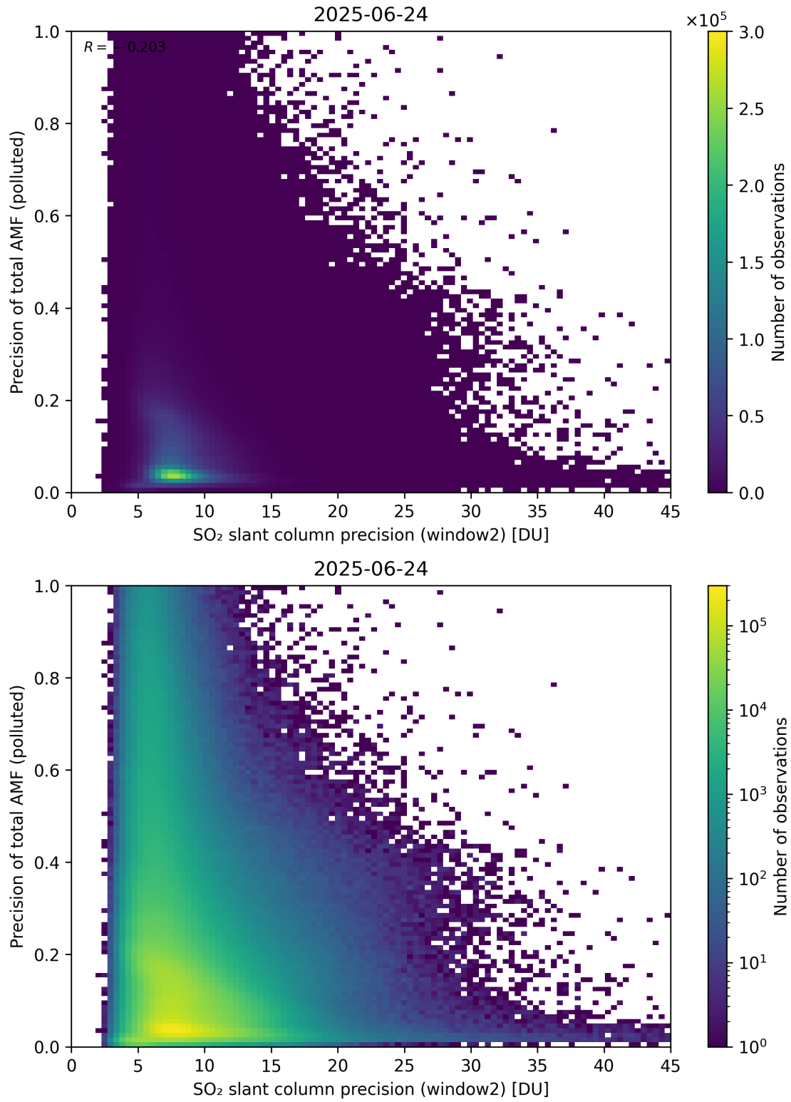
Figure 302: Scatter density plot of “SO 2 slant column precision (window2)” against “Precision of total AMF (polluted)” for 2025-06-23 to 2025-06-25.
