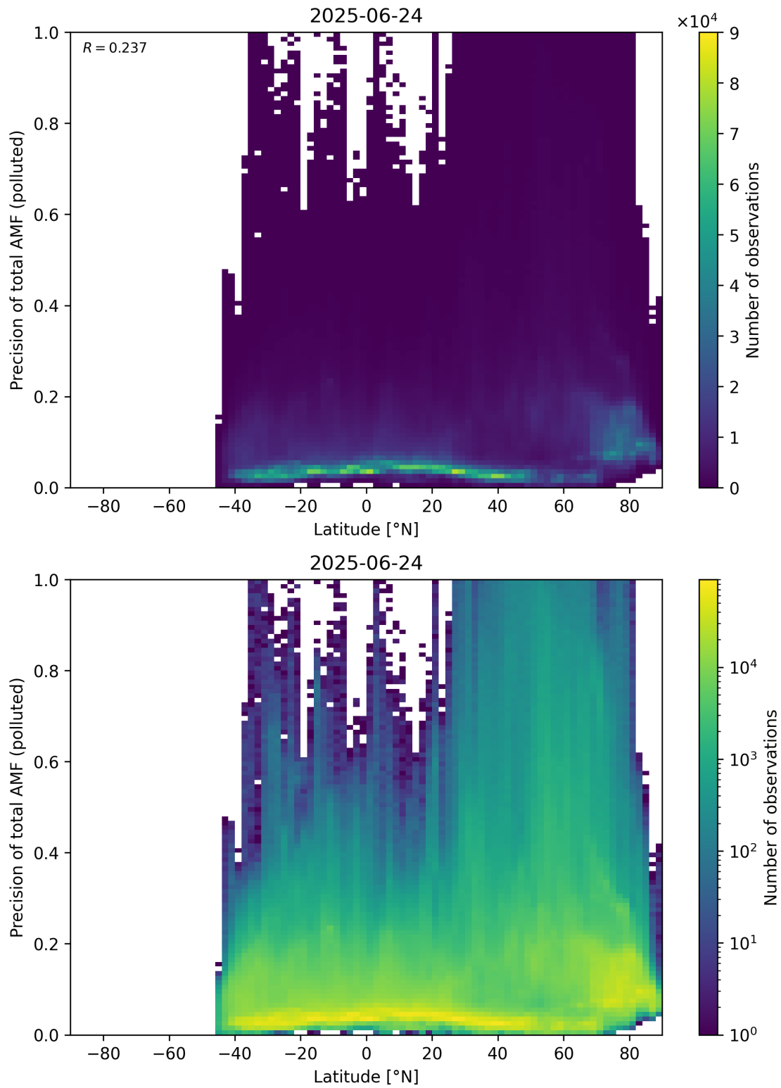
Figure 168: Scatter density plot of “Latitude” against “Precision of total AMF (polluted)” for 2025-06-23 to 2025-06-25.
