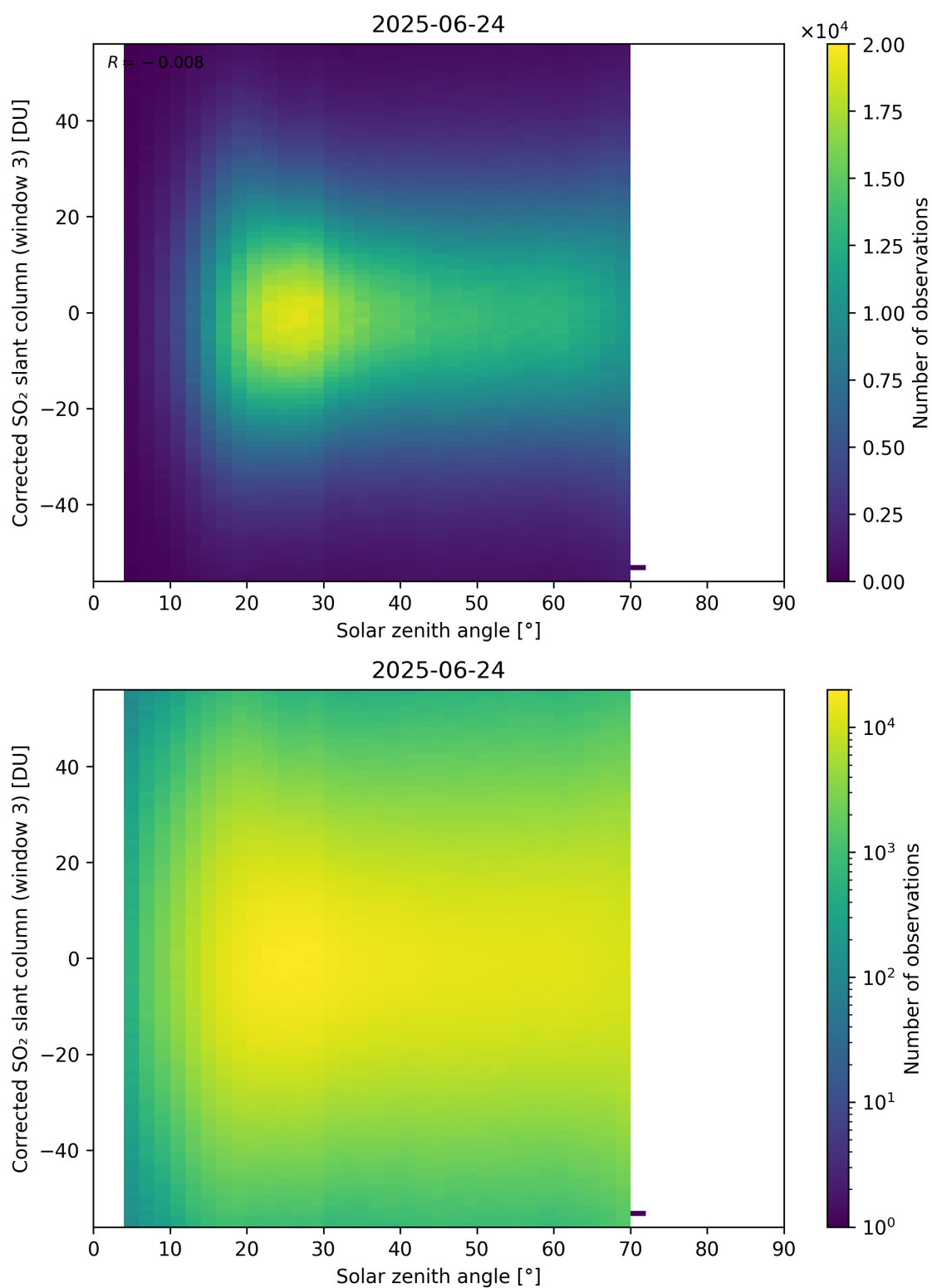
Figure 183: Scatter density plot of “Solar zenith angle” against “Corrected SO 2 slant column (window 3)” for 2025-06-23 to 2025-06-25.
