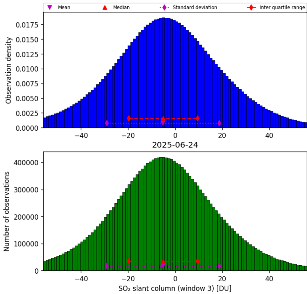
Figure 71: Histogram of “SO 2 slant column (window 3)” for 2025-06-23 to 2025-06-25
