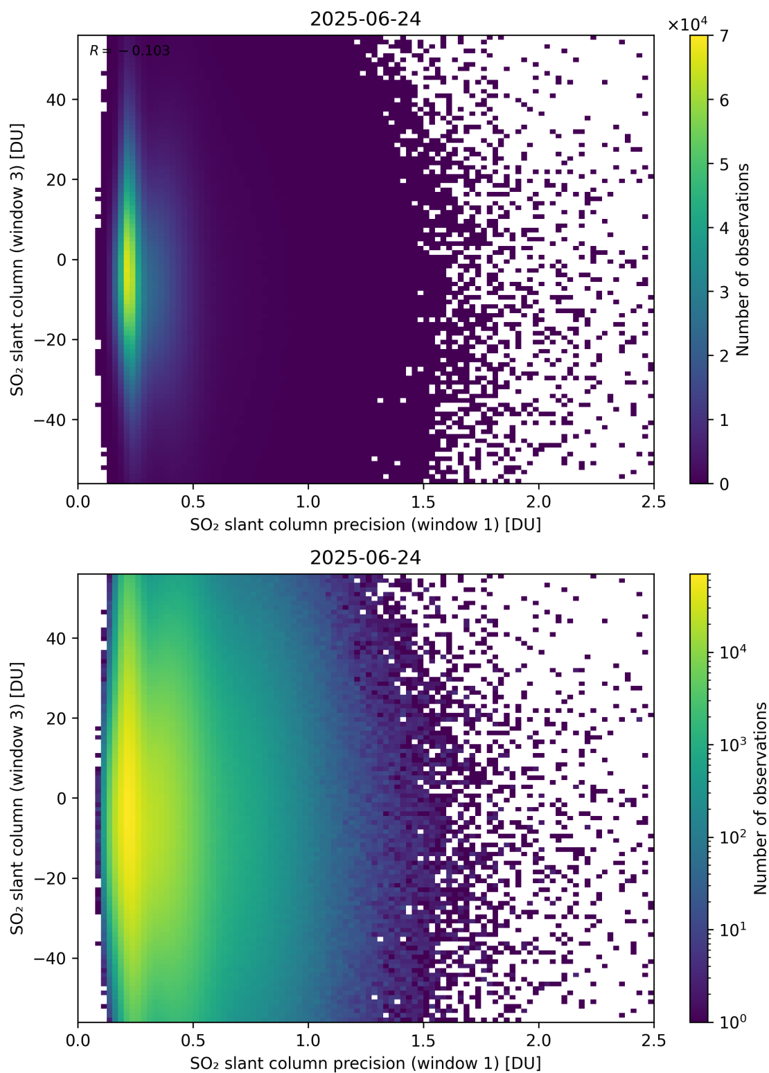
Figure 278: Scatter density plot of “SO 2 slant column precision (window 1)” against “SO 2 slant column (window 3)” for 2025-06-23 to 2025-06-25.
