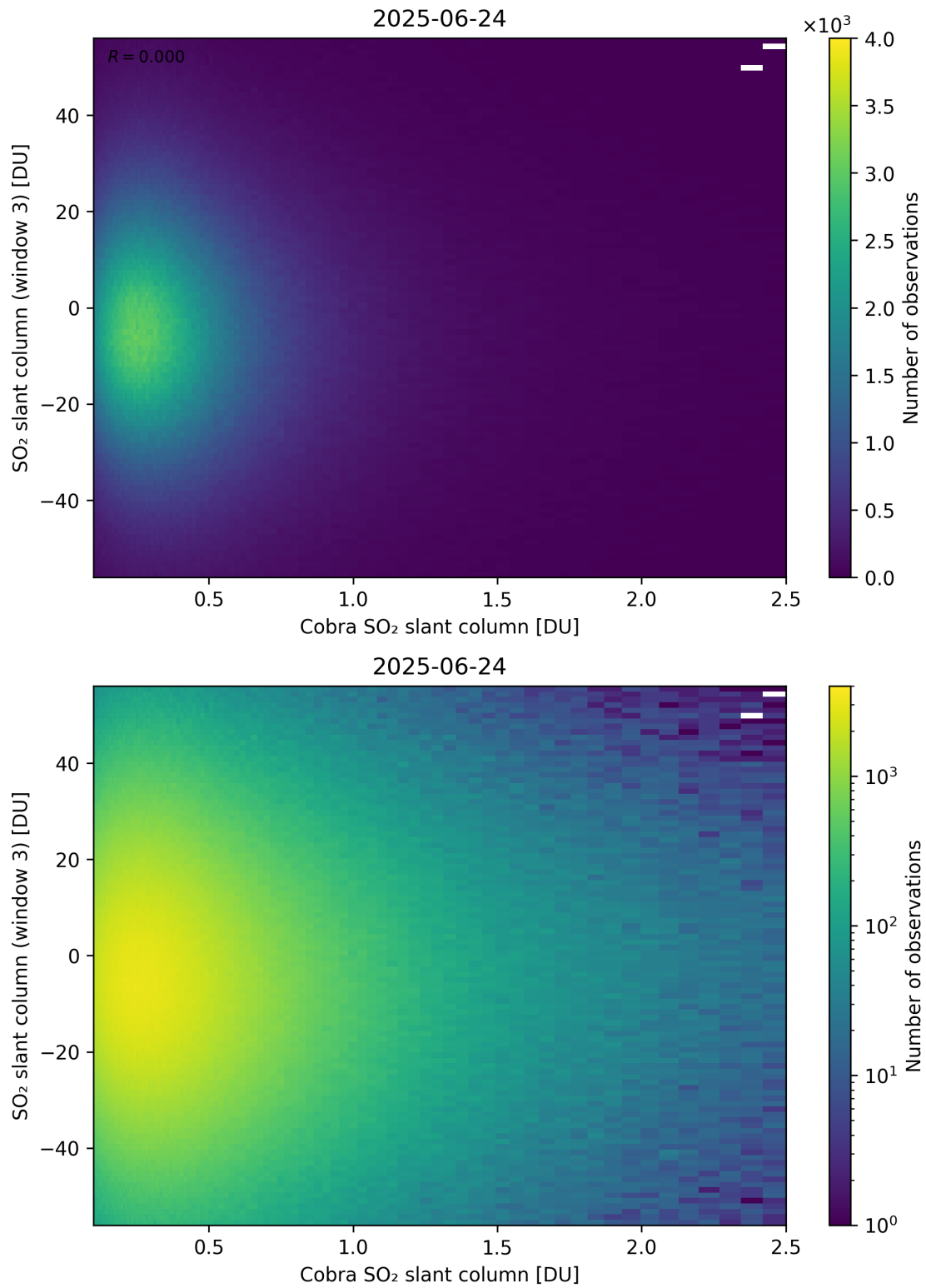
Figure 222: Scatter density plot of “Cobra SO 2 slant column” against “SO 2 slant column (window 3)” for 2025-06-23 to 2025-06-25.
