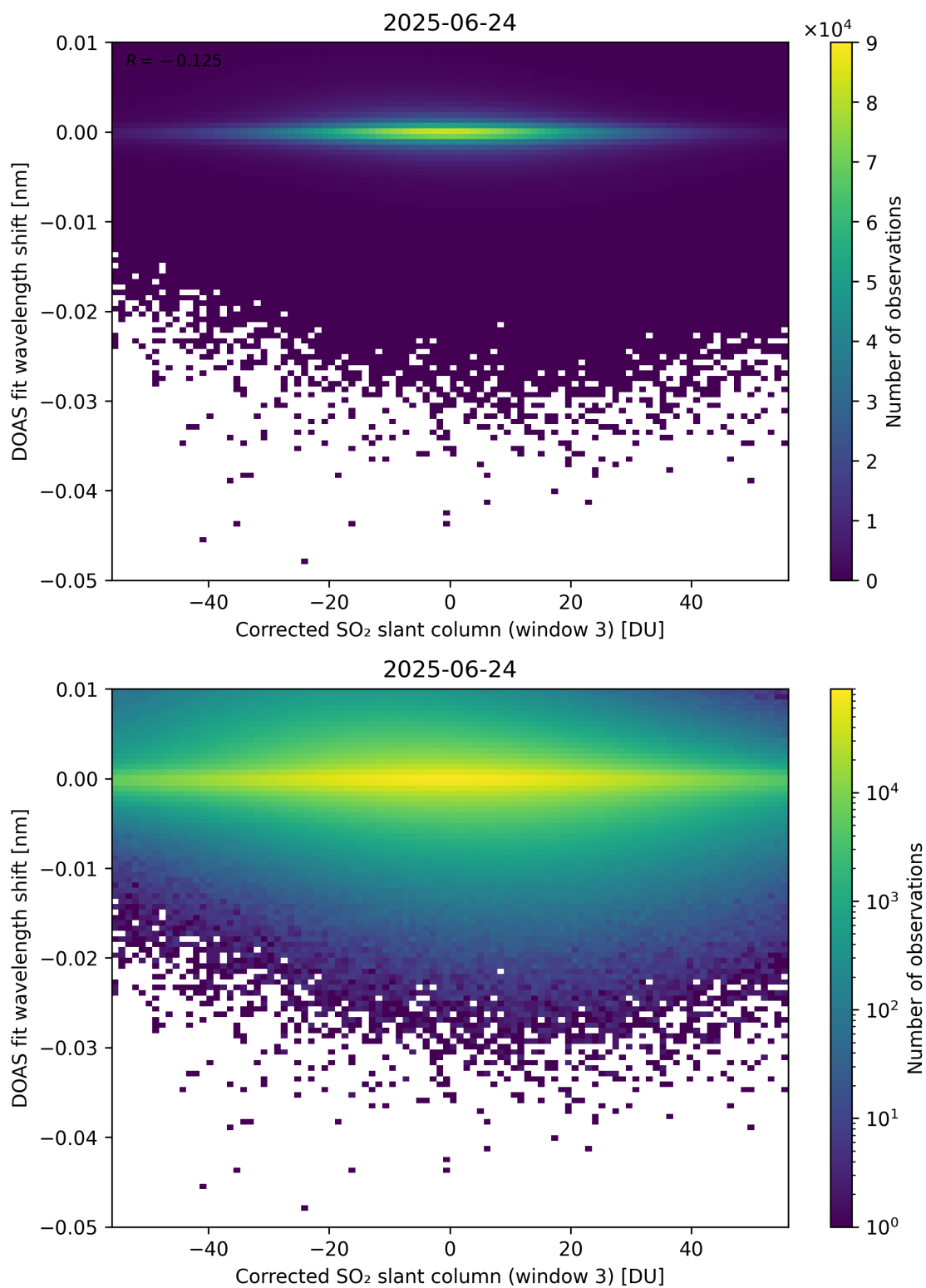
Figure 256: Scatter density plot of “Corrected SO 2 slant column (window 3)” against “DOAS fit wavelength shift” for 2025-06-23 to 2025-06-25.
