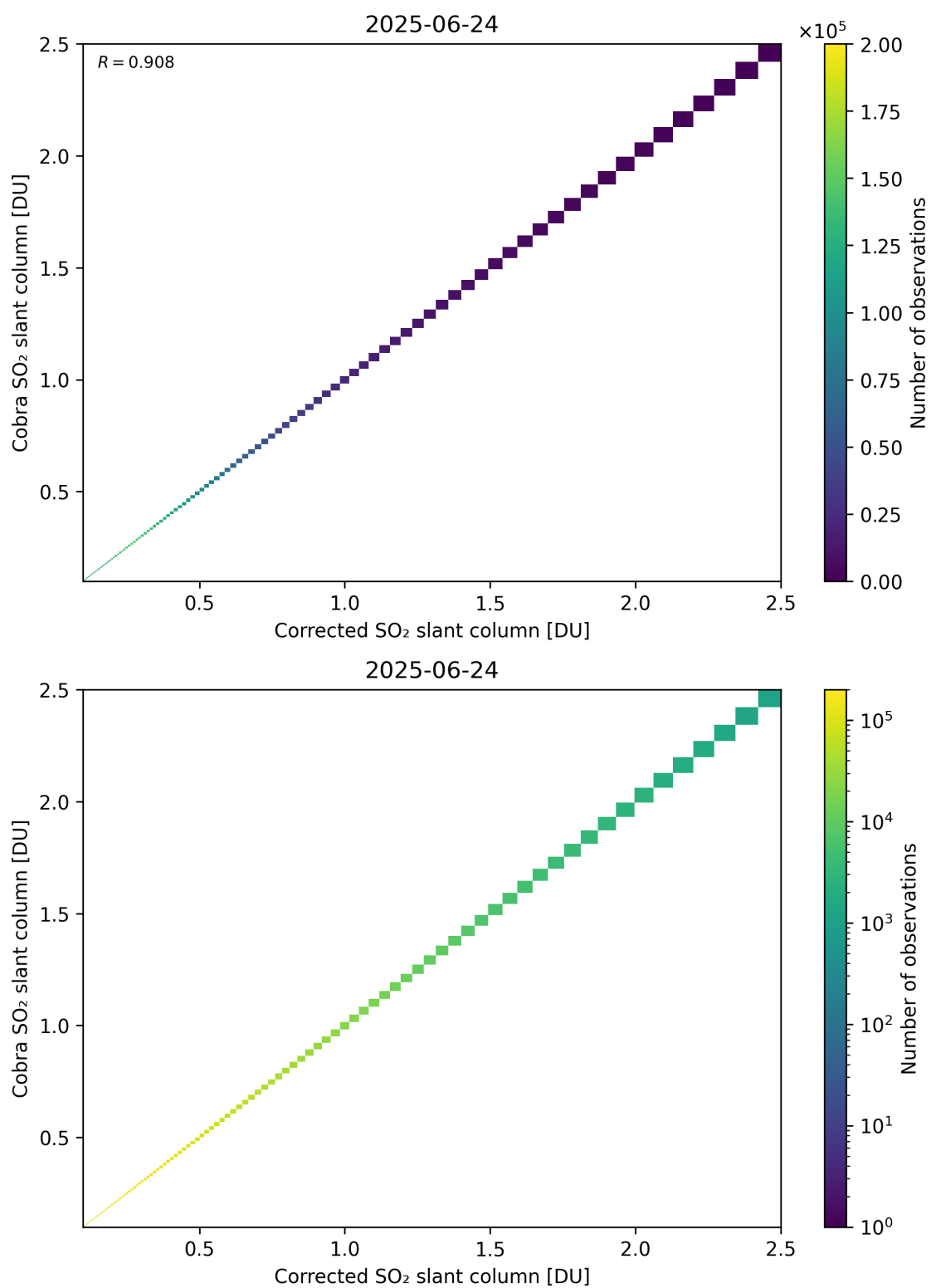
Figure 233: Scatter density plot of “Corrected SO 2 slant column” against “Cobra SO 2 slant column” for 2025-06-23 to 2025-06-25.
