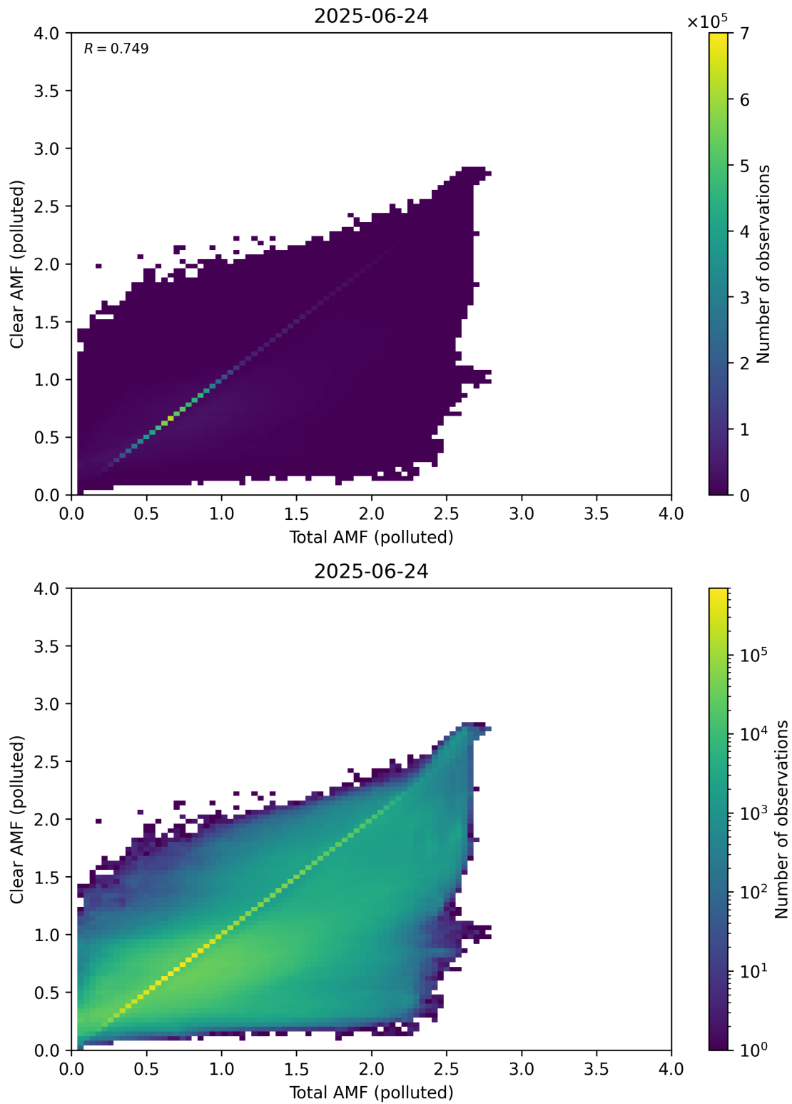
Figure 321: Scatter density plot of “Total AMF (polluted)” against “Clear AMF (polluted)” for 2025-06-23 to 2025-06-25.
