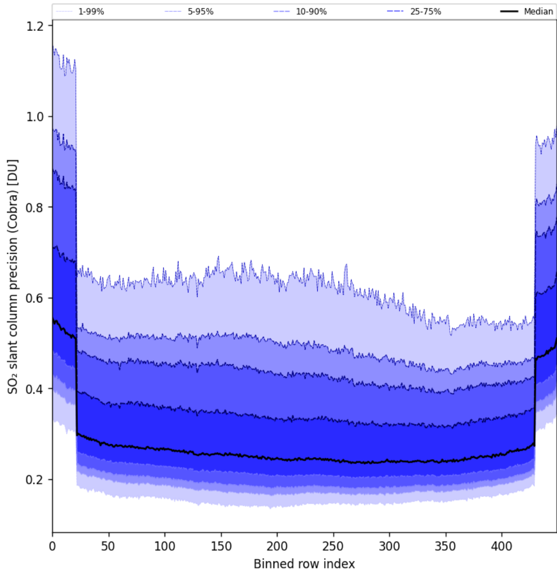
Figure 88: Along track statistics of “SO 2 slant column precision (Cobra)” for 2025-06-23 to 2025-06-25
