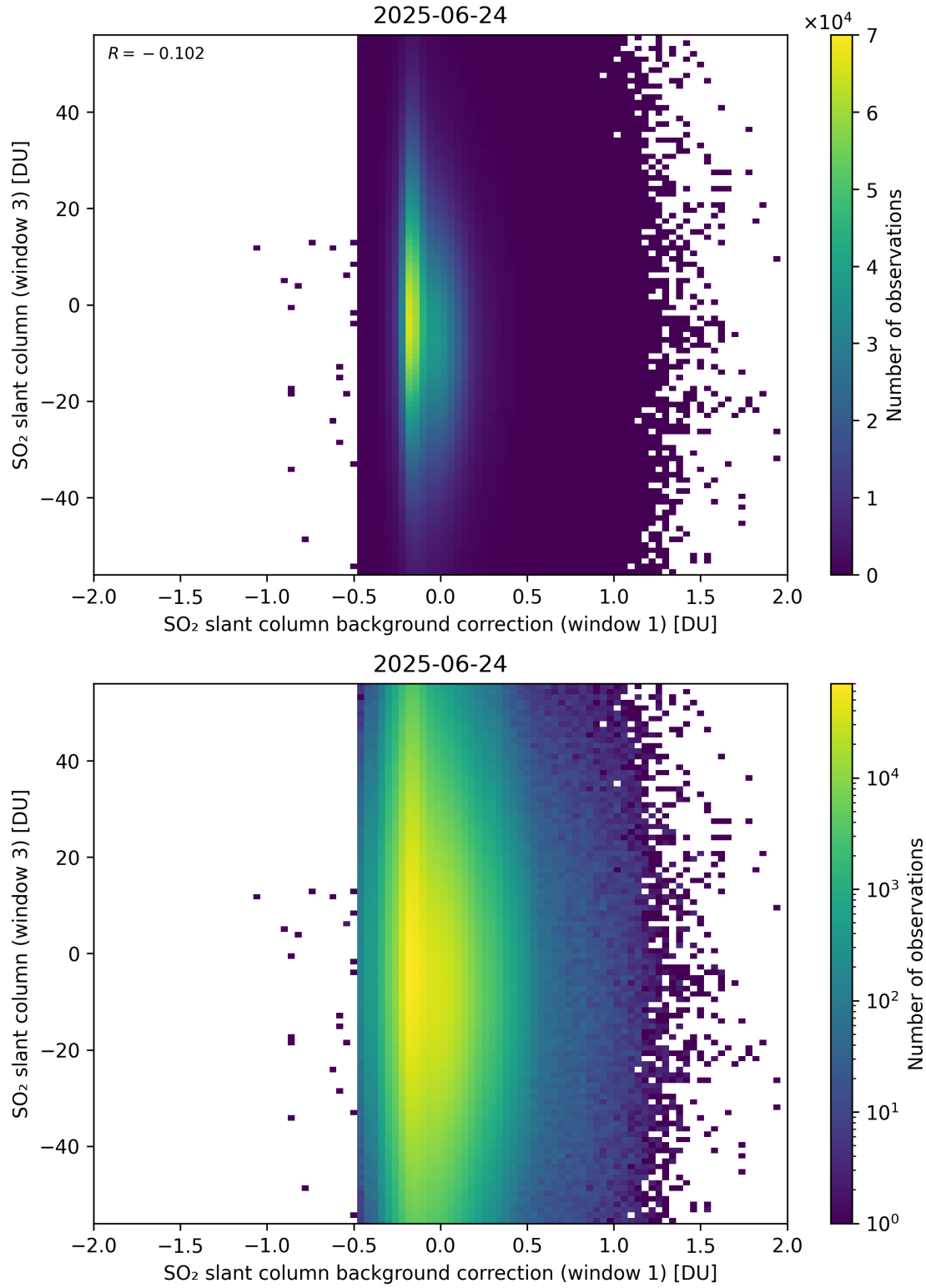
Figure 118: Scatter density plot of “SO 2 slant column background correction (window 1)” against “SO 2 slant column (window 3)” for 2025-06-23 to 2025-06-25.
