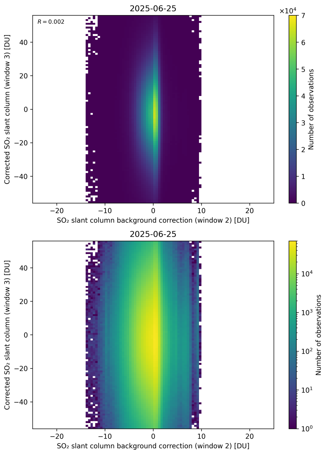
Figure 127: Scatter density plot of “SO 2 slant column background correction (window 2)” against “Corrected SO 2 slant column (window 3)” for 2025-06-24 to 2025-06-26.
