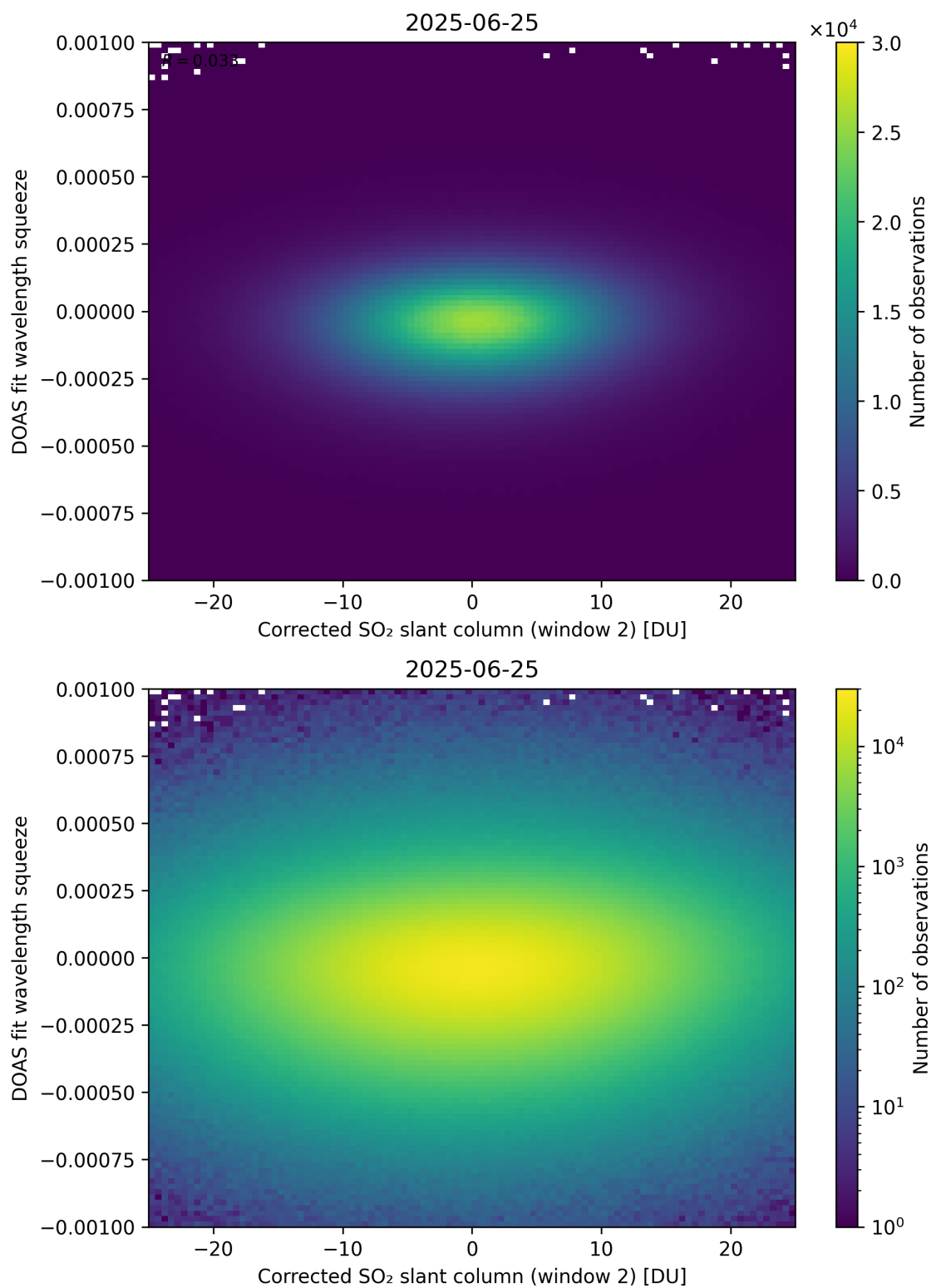
Figure 247: Scatter density plot of “Corrected SO 2 slant column (window 2)” against “DOAS fit wavelength squeeze” for 2025-06-24 to 2025-06-26.
