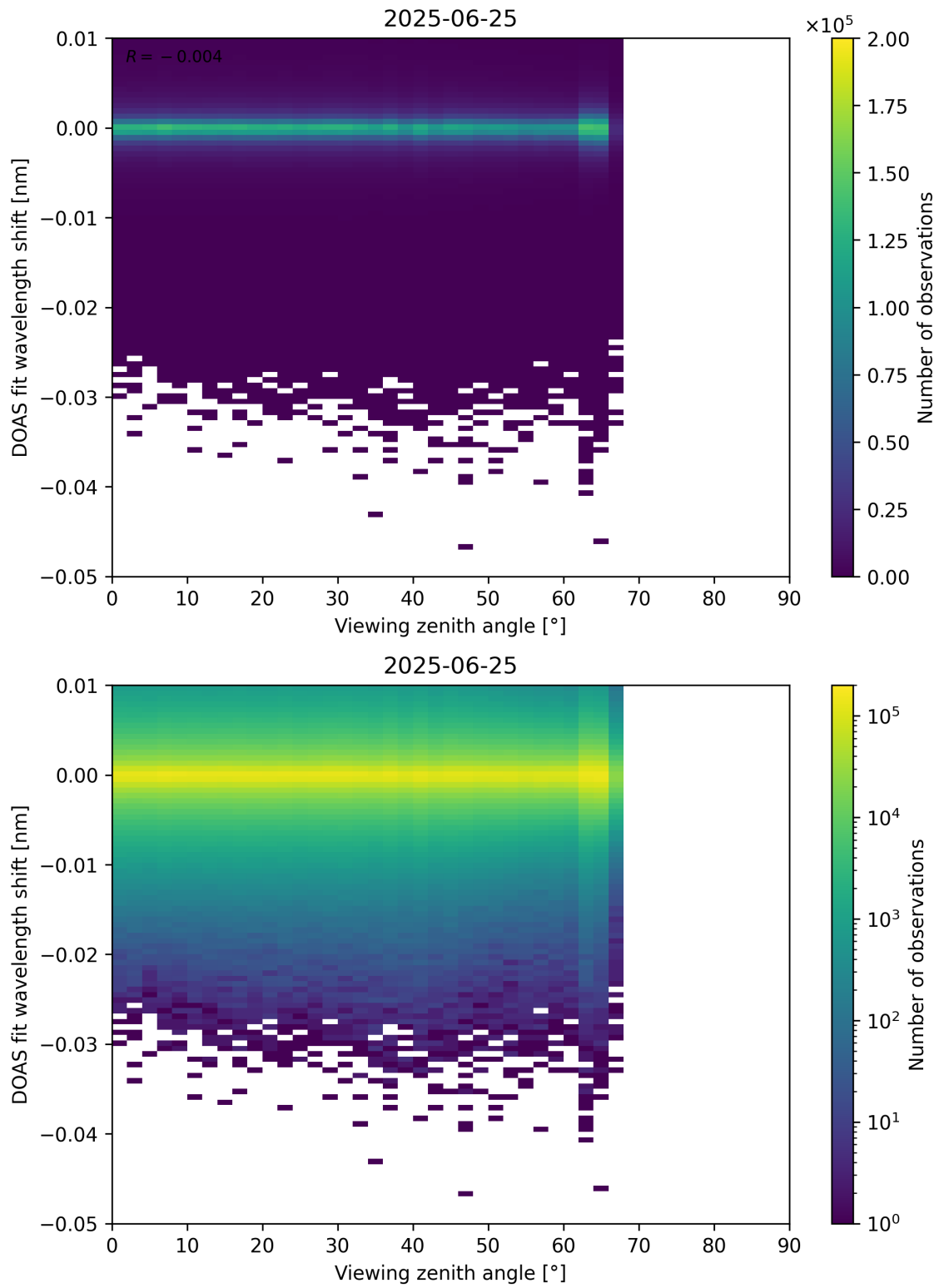
Figure 365: Scatter density plot of “Viewing zenith angle” against “DOAS fit wavelength shift” for 2025-06-24 to 2025-06-26.
