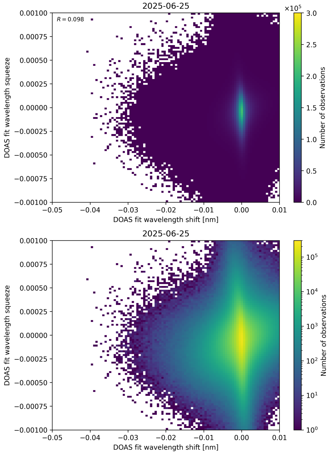
Figure 138: Scatter density plot of “DOAS fit wavelength shift” against “DOAS fit wavelength squeeze” for 2025-06-24 to 2025-06-26.
