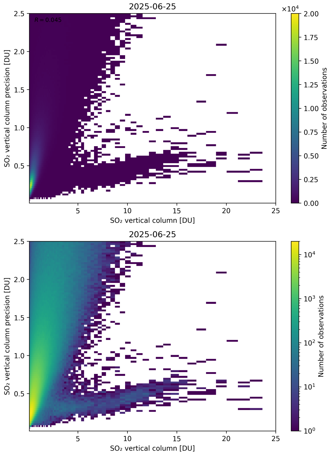
Figure 361: Scatter density plot of “SO 2 vertical column” against “SO 2 vertical column precision” for 2025-06-24 to 2025-06-26.
