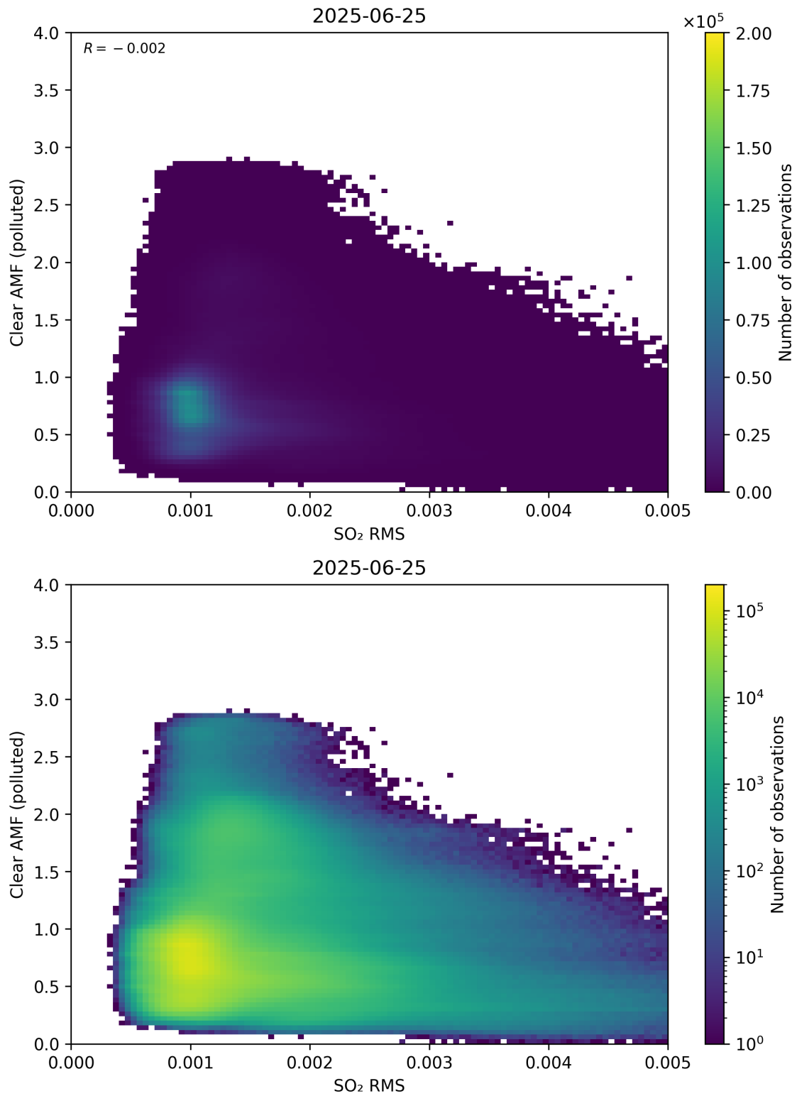
Figure 147: Scatter density plot of “SO 2 RMS” against “Clear AMF (polluted)” for 2025-06-24 to 2025-06-26.
