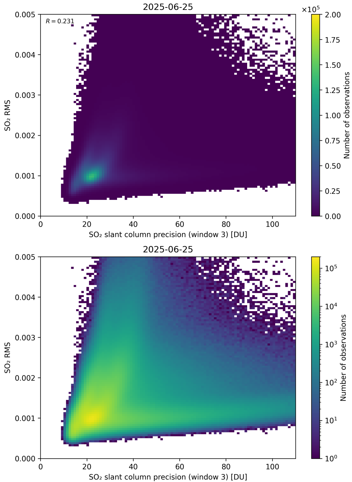
Figure 310: Scatter density plot of “SO 2 slant column precision (window 3)” against “SO 2 RMS” for 2025-06-24 to 2025-06-26.
