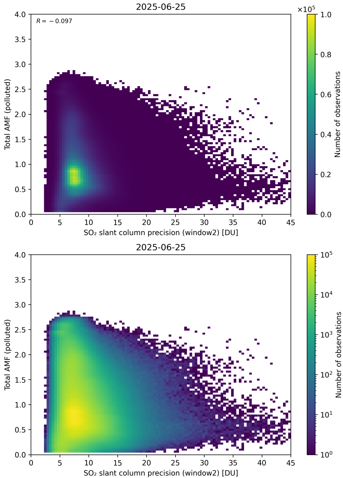
Figure 301: Scatter density plot of “SO 2 slant column precision (window2)” against “Total AMF (polluted)” for 2025-06-24 to 2025-06-26.
