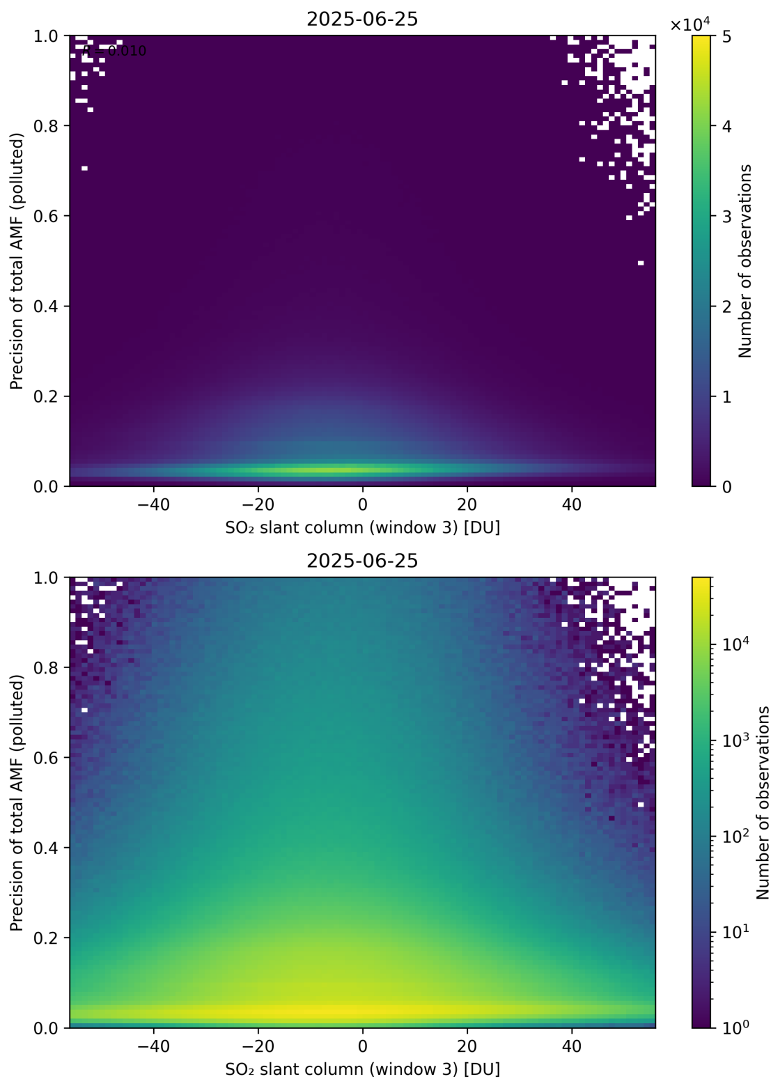
Figure 319: Scatter density plot of “SO 2 slant column (window 3)” against “Precision of total AMF (polluted)” for 2025-06-24 to 2025-06-26.
