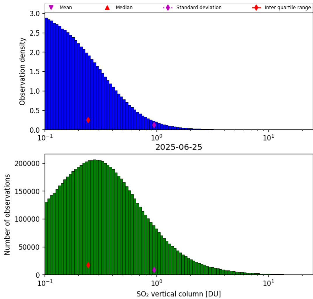
Figure 58: Histogram of “SO 2 vertical column” for 2025-06-24 to 2025-06-26
