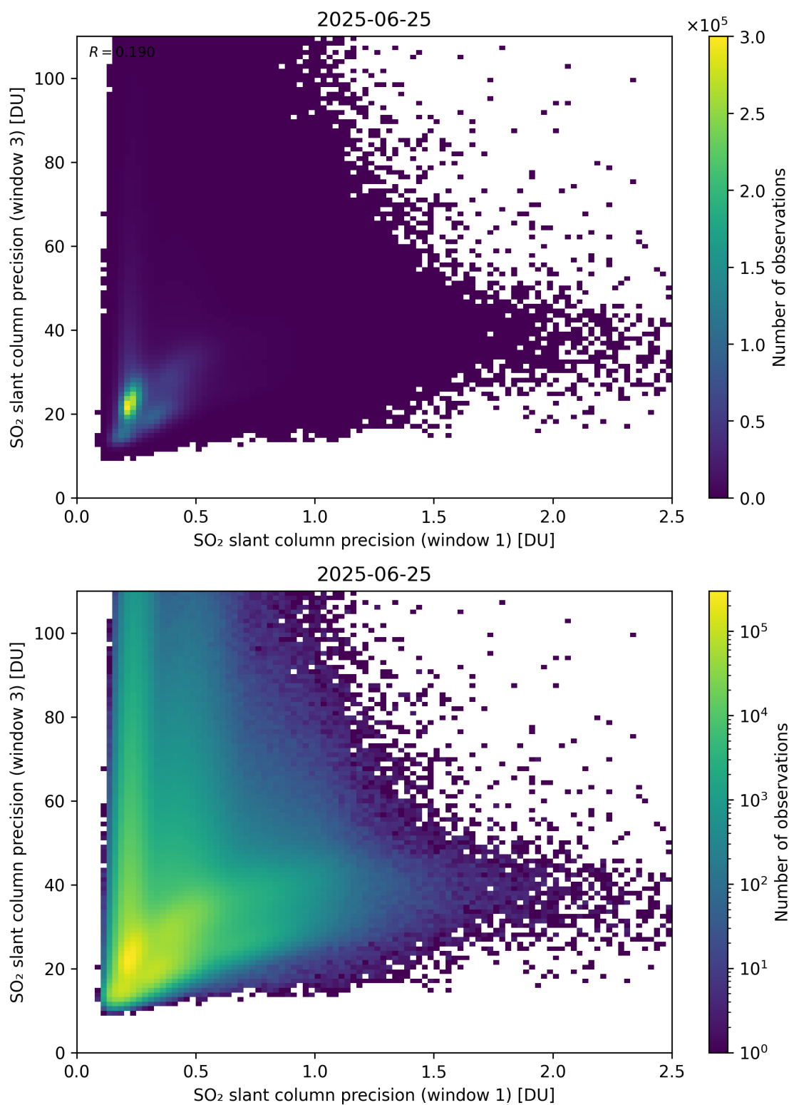
Figure 279: Scatter density plot of “SO 2 slant column precision (window 1)” against “SO 2 slant column precision (window 3)” for 2025-06-24 to 2025-06-26.
