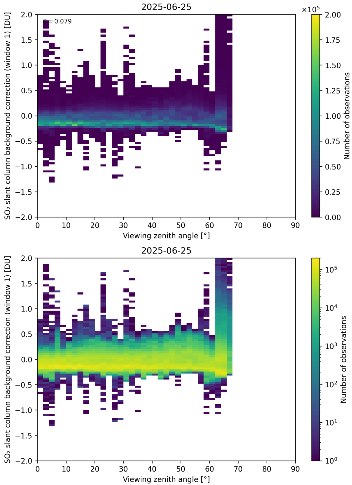
Figure 362: Scatter density plot of “Viewing zenith angle” against “SO 2 slant column background correction (window 1)” for 2025-06-24 to 2025-06-26.
