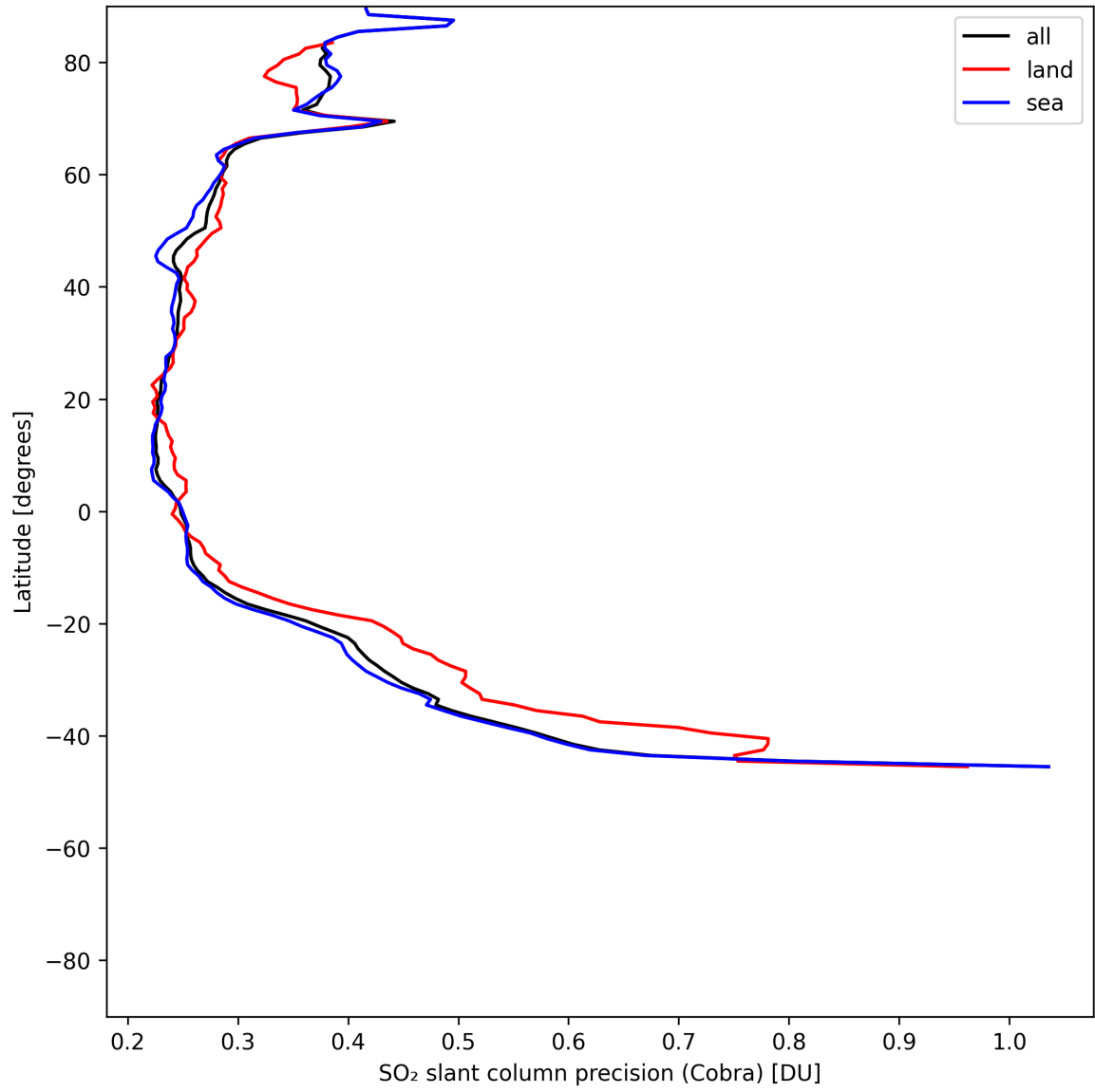
Figure 36: Zonal average of "SO 2 slant column precision (Cobra)" for 2025-06-24 to 2025-06-26.
