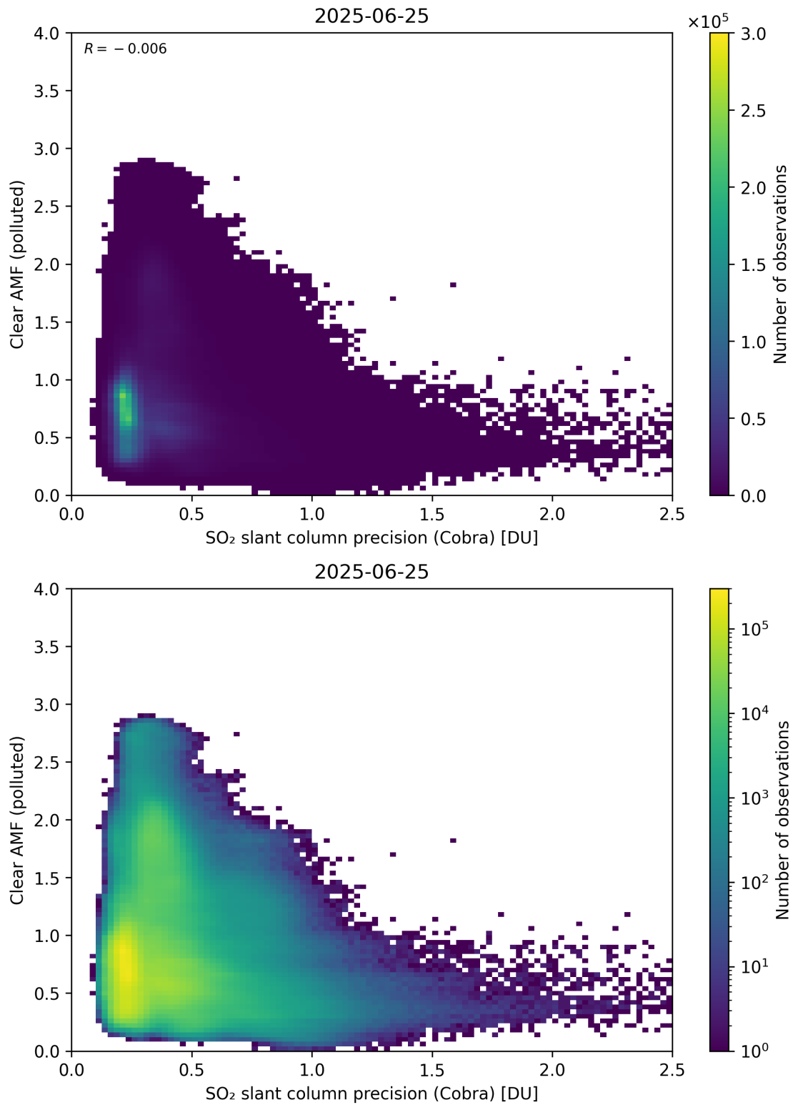
Figure 205: Scatter density plot of “SO 2 slant column precision (Cobra)” against “Clear AMF (polluted)” for 2025-06-24 to 2025-06-26.
