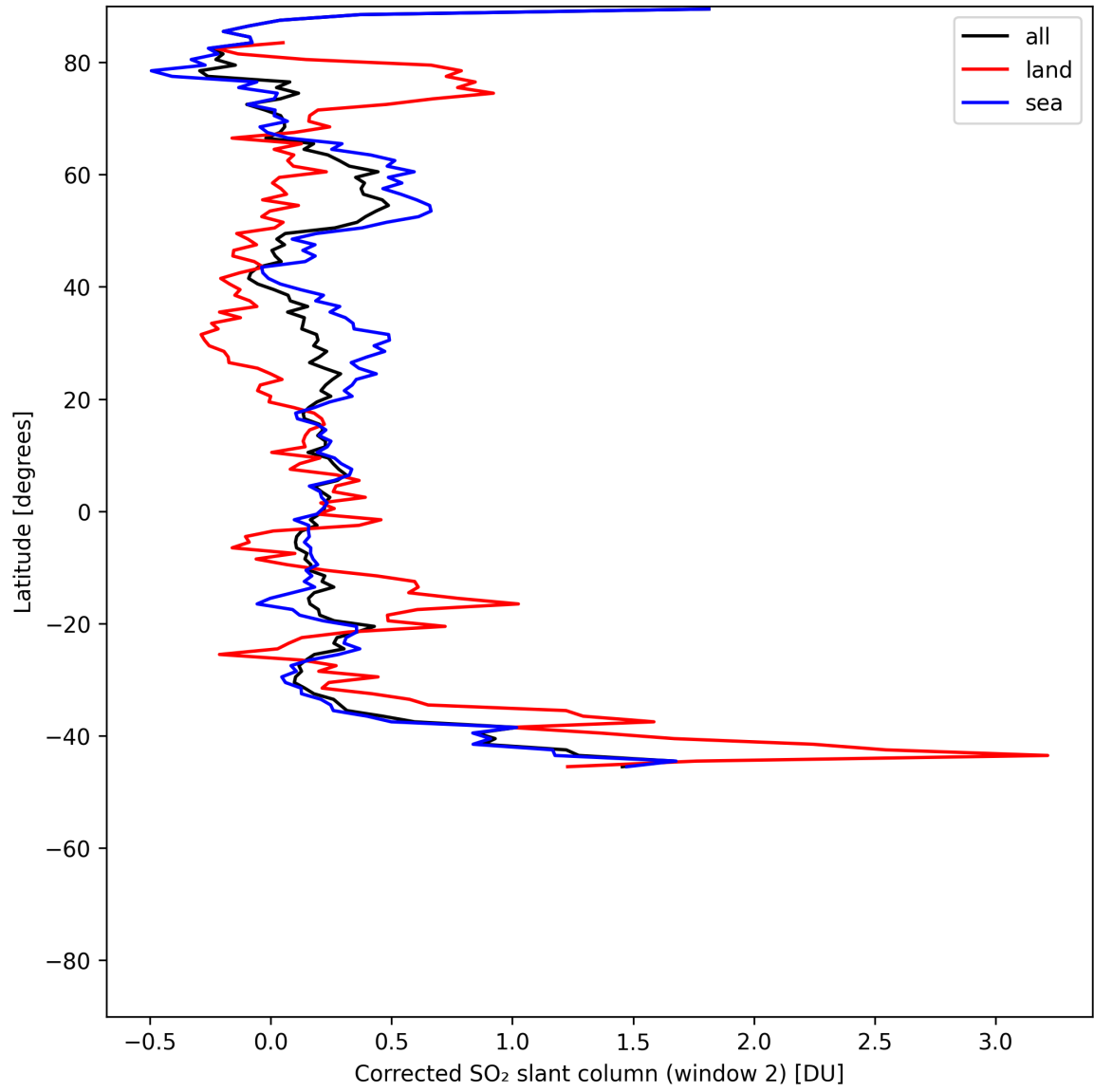
Figure 43: Zonal average of “Corrected SO 2 slant column (window 2)” for 2025-06-24 to 2025-06-26.
