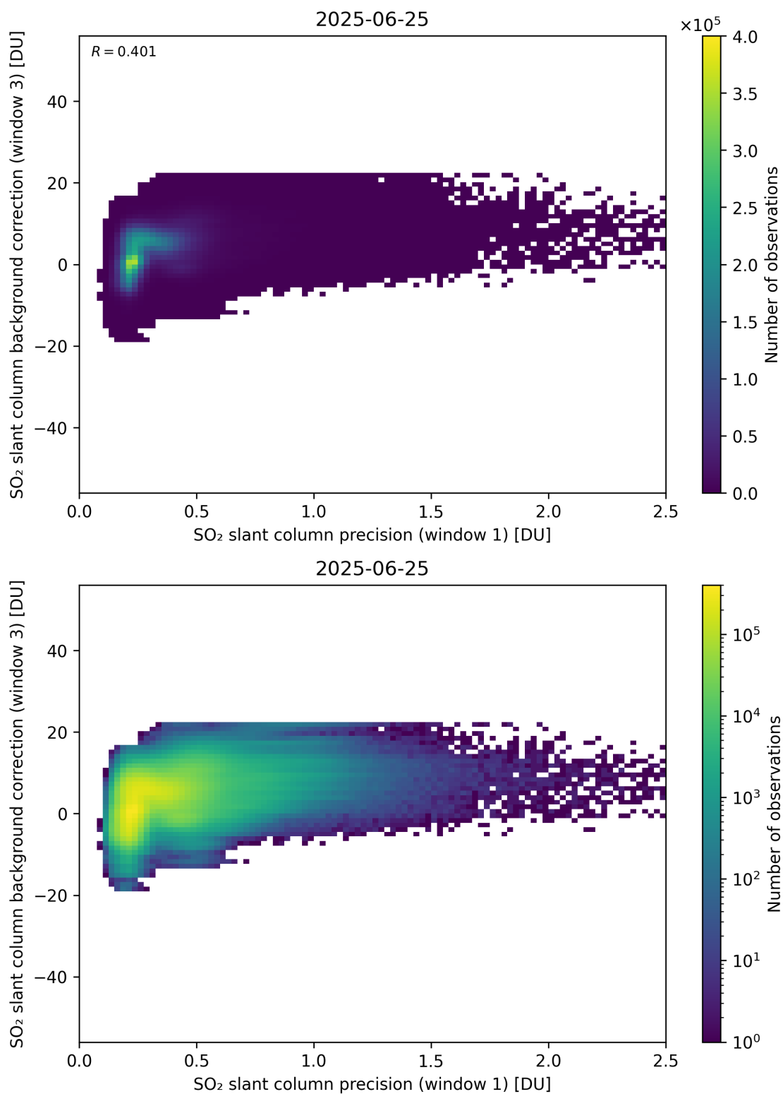
Figure 270: Scatter density plot of “SO 2 slant column precision (window 1)” against “SO 2 slant column background correction (window 3)” for 2025-06-24 to 2025-06-26.
