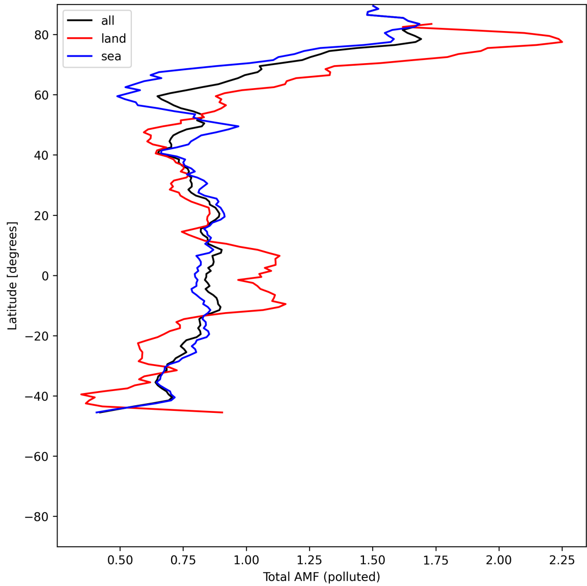
Figure 53: Zonal average of “Total AMF (polluted)” for 2025-06-24 to 2025-06-26.
