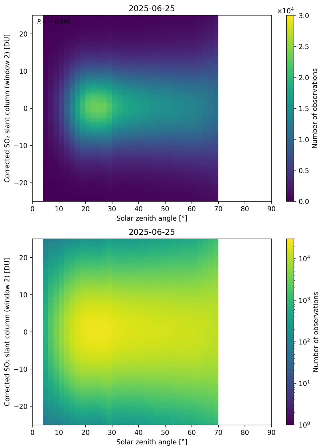
Figure 182: Scatter density plot of “Solar zenith angle” against “Corrected SO 2 slant column (window 2)” for 2025-06-24 to 2025-06-26.
