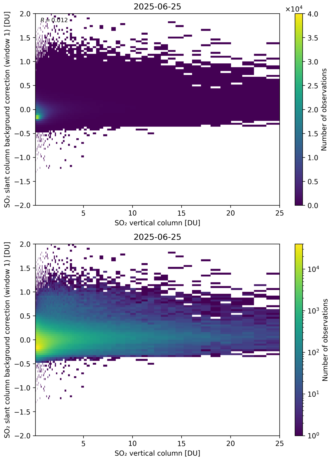
Figure 323: Scatter density plot of “SO 2 vertical column” against “SO 2 slant column background correction (window 1)” for 2025-06-24 to 2025-06-26.
