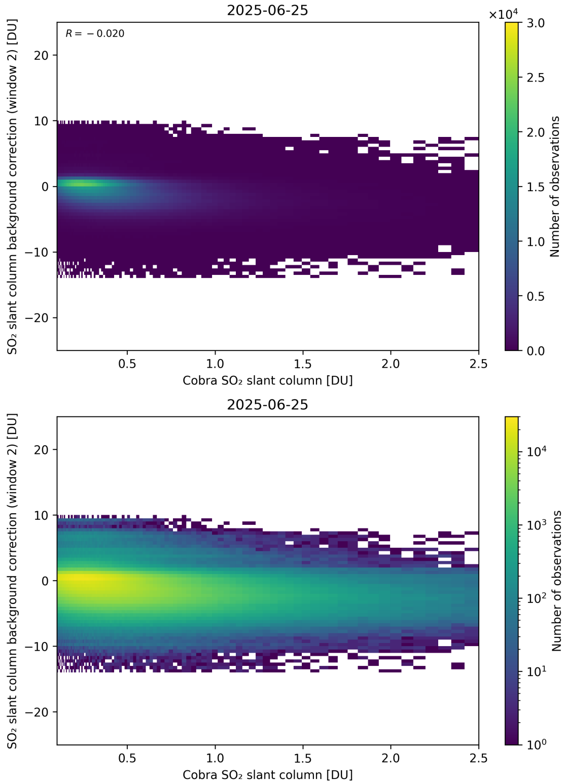
Figure 194: Scatter density plot of “Cobra SO 2 slant column” against “SO 2 slant column background correction (window 2)” for 2025-06-24 to 2025-06-26.
