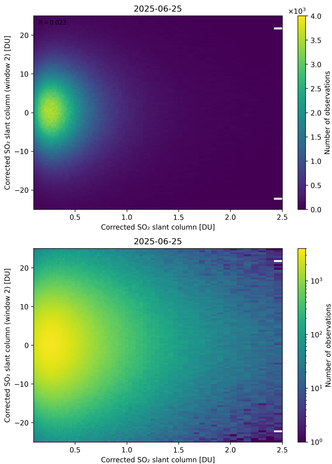
Figure 235: Scatter density plot of “Corrected SO 2 slant column” against “Corrected SO 2 slant column (window 2)” for 2025-06-24 to 2025-06-26.
