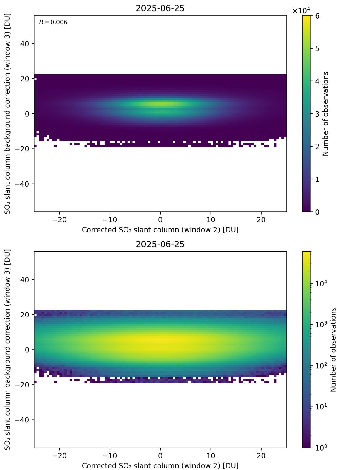
Figure 245: Scatter density plot of “Corrected SO 2 slant column (window 2)” against “SO 2 slant column background correction (window 3)” for 2025-06-24 to 2025-06-26.
