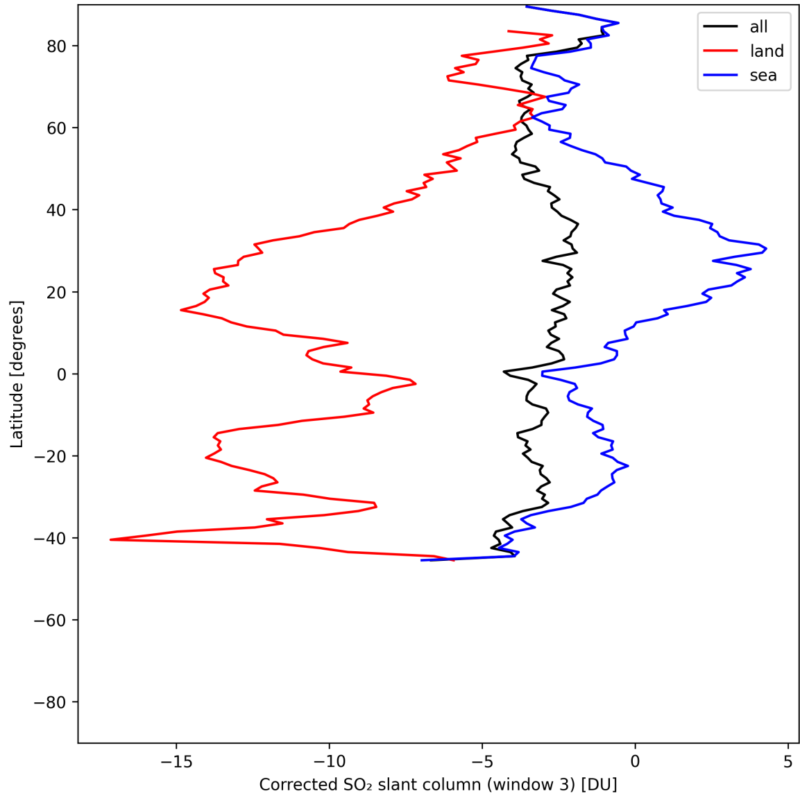
Figure 47: Zonal average of “Corrected SO 2 slant column (window 3)” for 2025-06-24 to 2025-06-26.
