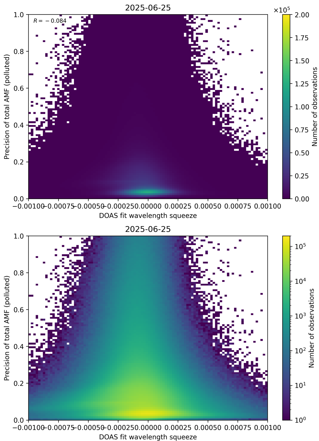
Figure 146: Scatter density plot of “DOAS fit wavelength squeeze” against “Precision of total AMF (polluted)” for 2025-06-24 to 2025-06-26.
