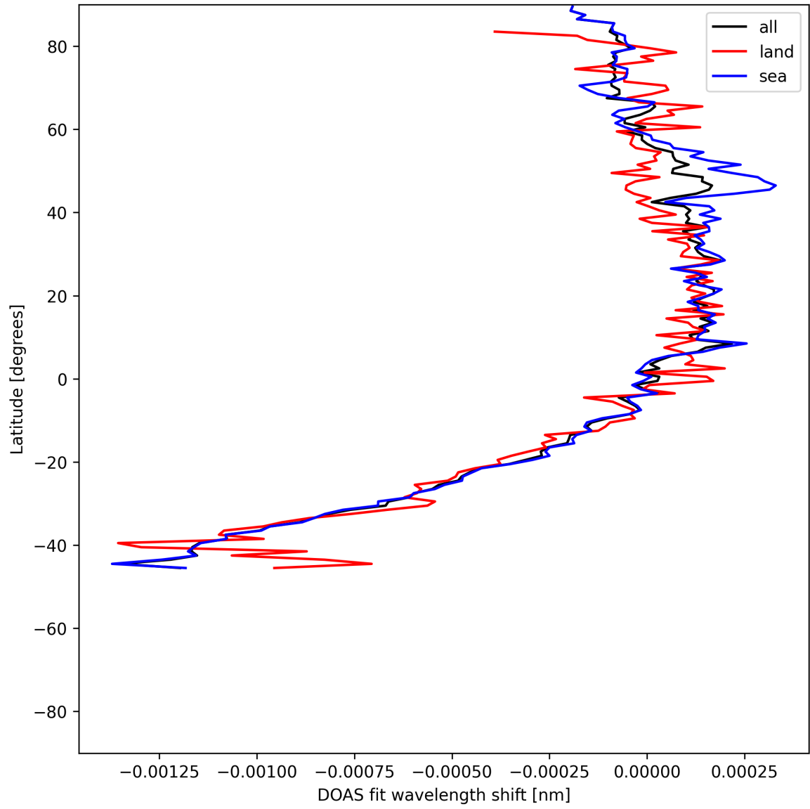
Figure 50: Zonal average of “DOAS fit wavelength shift” for 2025-06-24 to 2025-06-26.
