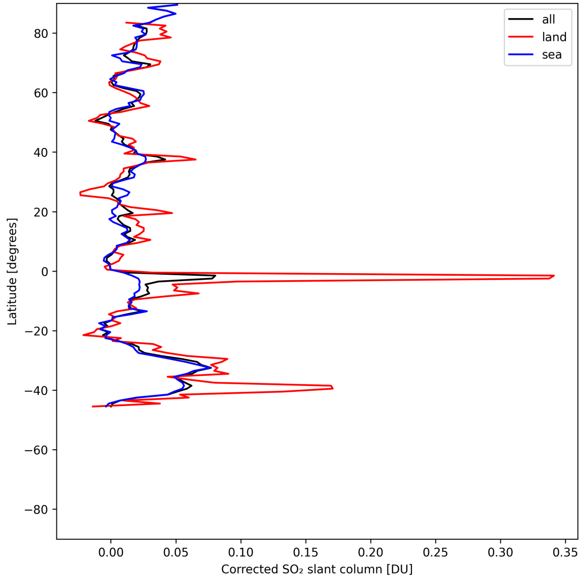
Figure 34: Zonal average of “Corrected SO 2 slant column” for 2025-06-24 to 2025-06-26.
