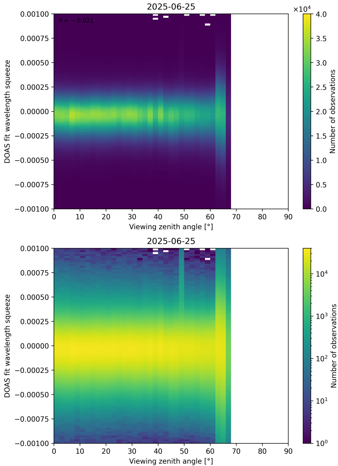
Figure 366: Scatter density plot of “Viewing zenith angle” against “DOAS fit wavelength squeeze” for 2025-06-24 to 2025-06-26.
