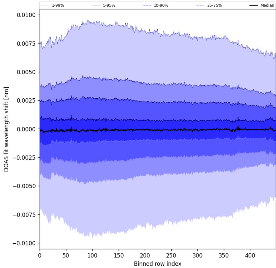
Figure 102: Along track statistics of “DOAS fit wavelength shift” for 2025-06-24 to 2025-06-26
