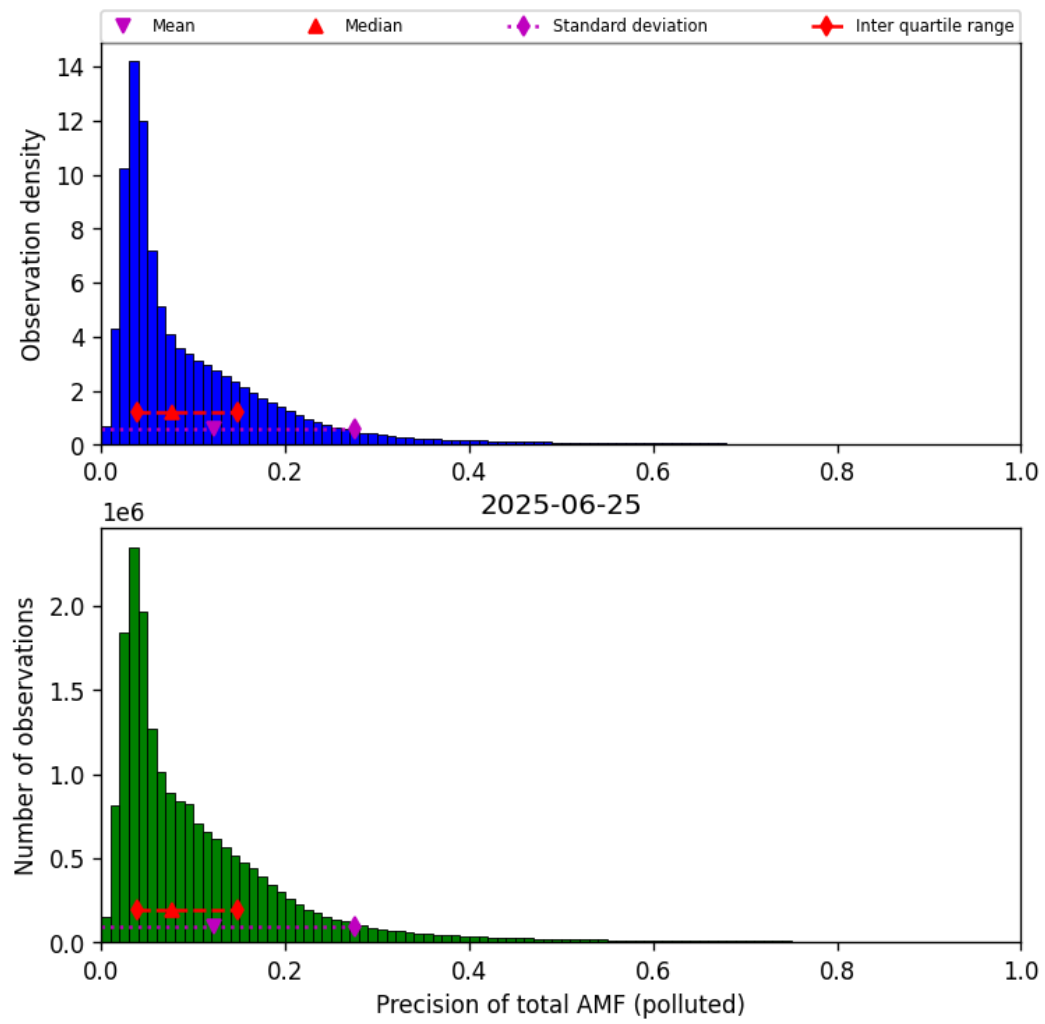
Figure 80: Histogram of “Precision of total AMF (polluted)” for 2025-06-24 to 2025-06-26
