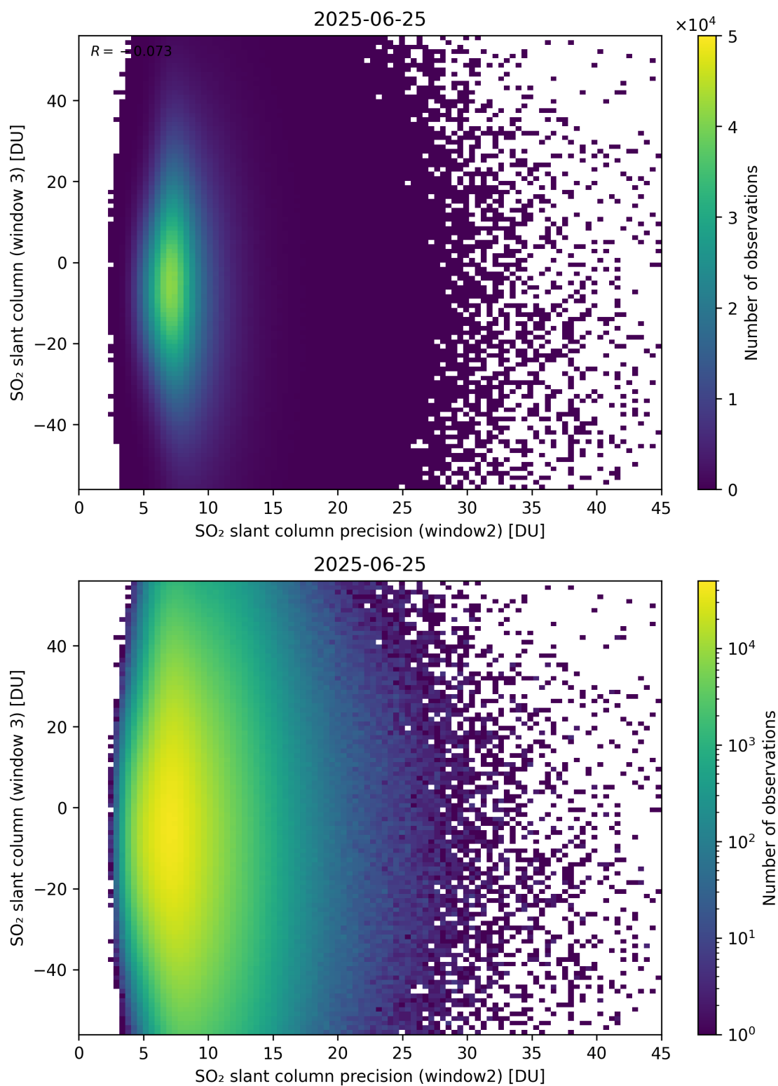
Figure 299: Scatter density plot of “SO 2 slant column precision (window2)” against “SO 2 slant column (window 3)” for 2025-06-24 to 2025-06-26.
