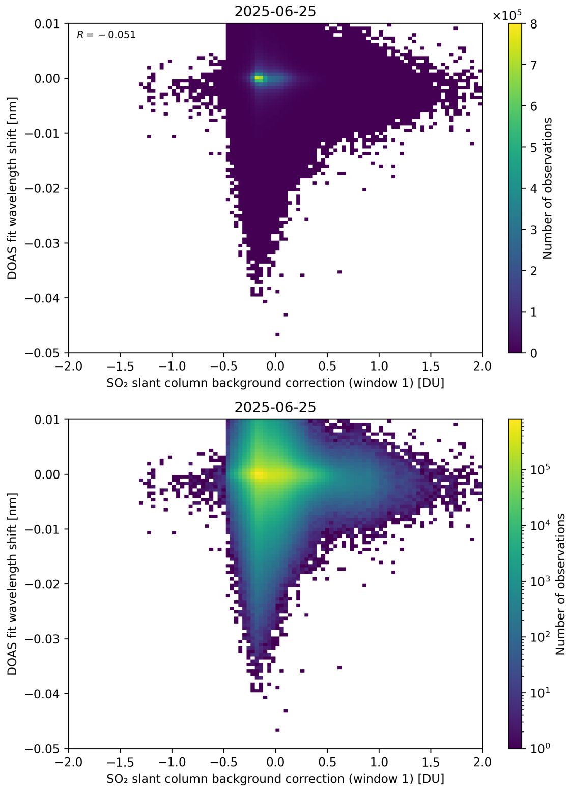
Figure 111: Scatter density plot of “SO 2 slant column background correction (window 1)” against “DOAS fit wavelength shift” for 2025-06-24 to 2025-06-26.
