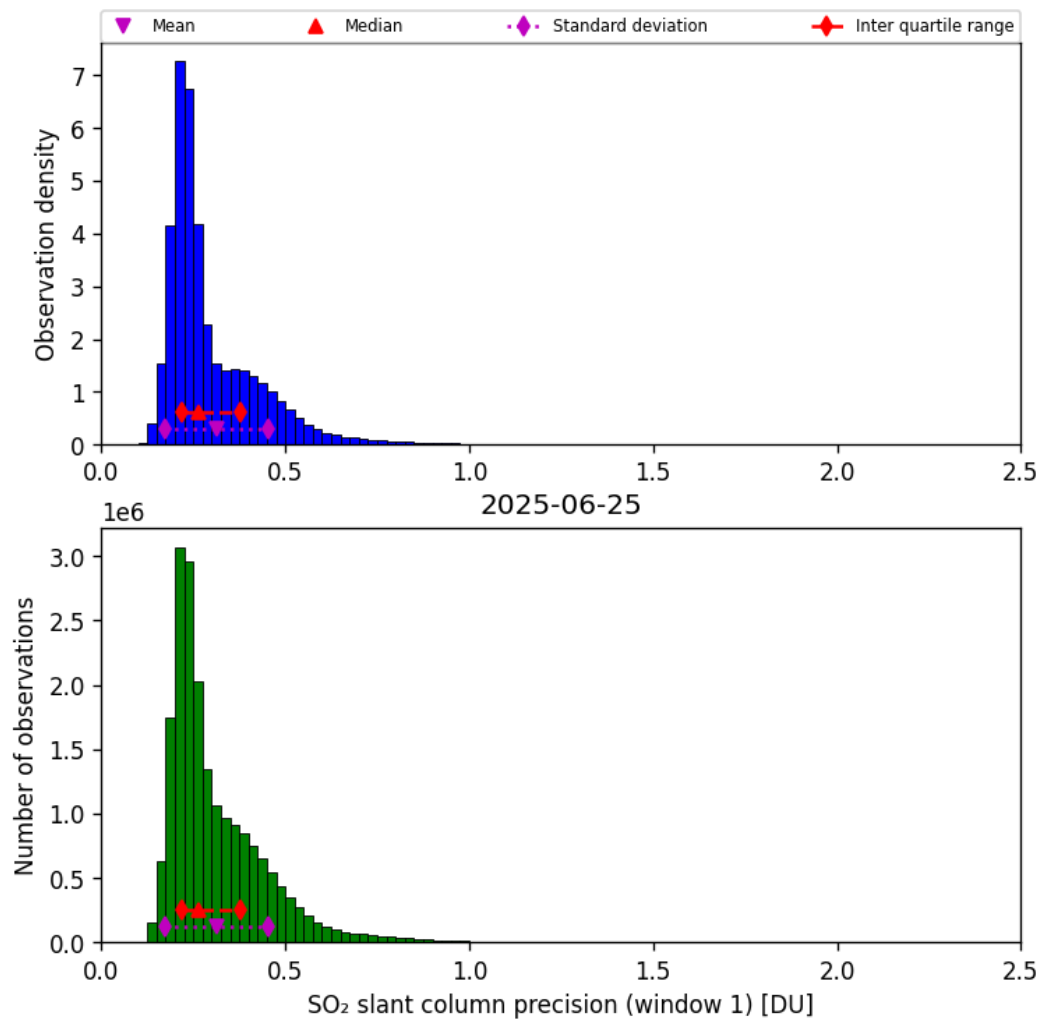
Figure 64: Histogram of “SO 2 slant column precision (window 1)” for 2025-06-24 to 2025-06-26
