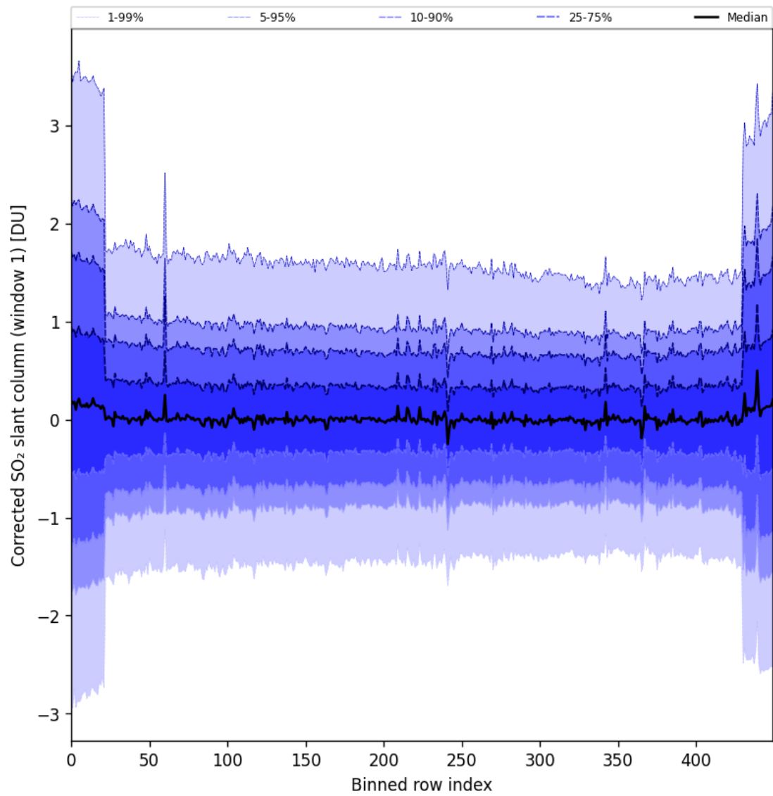
Figure 91: Along track statistics of “Corrected SO 2 slant column (window 1)” for 2025-06-24 to 2025-06-26
