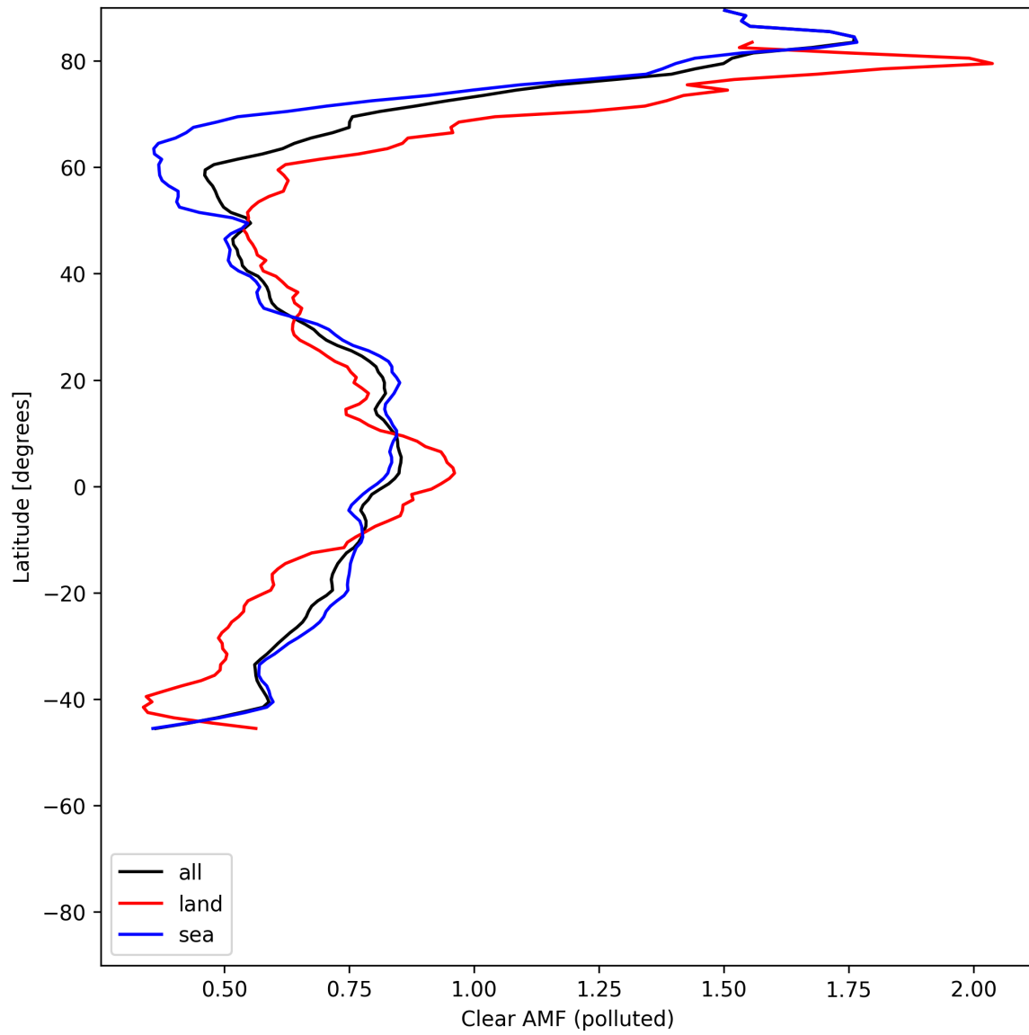
Figure 55: Zonal average of “Clear AMF (polluted)” for 2025-06-24 to 2025-06-26.
