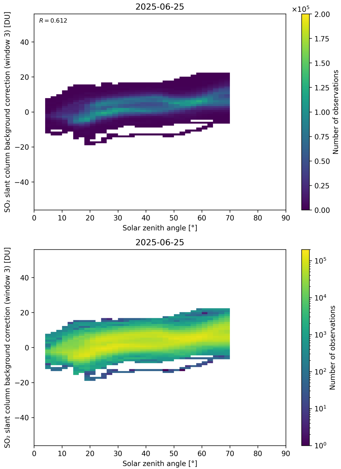
Figure 173: Scatter density plot of “Solar zenith angle” against “SO 2 slant column background correction (window 3)” for 2025-06-24 to 2025-06-26.
