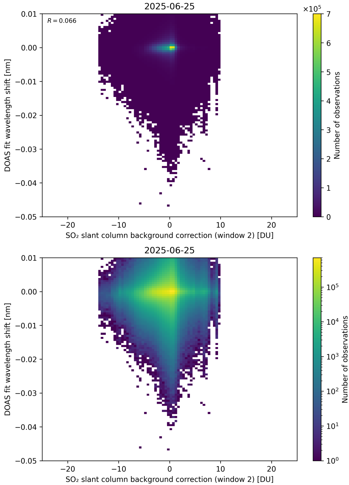
Figure 123: Scatter density plot of “SO 2 slant column background correction (window 2)” against “DOAS fit wavelength shift” for 2025-06-24 to 2025-06-26.
