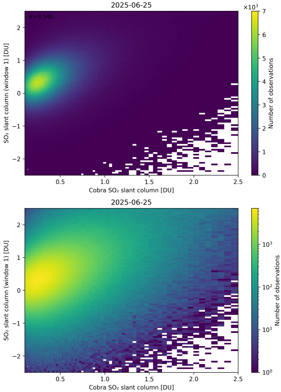
Figure 219: Scatter density plot of “Cobra SO 2 slant column” against “SO 2 slant column (window 1)” for 2025-06-24 to 2025-06-26.
