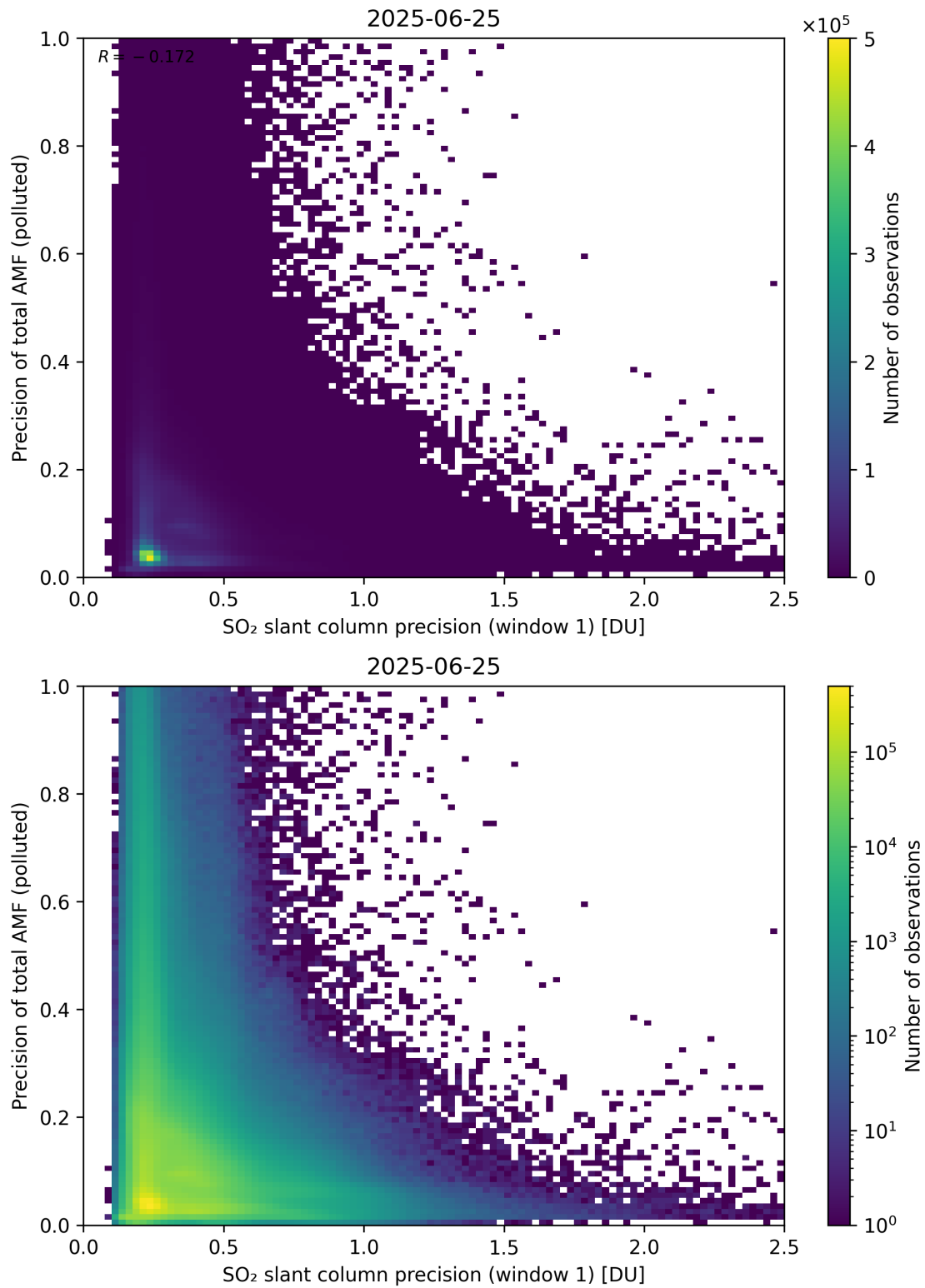
Figure 281: Scatter density plot of “SO 2 slant column precision (window 1)” against “Precision of total AMF (polluted)” for 2025-06-24 to 2025-06-26.
