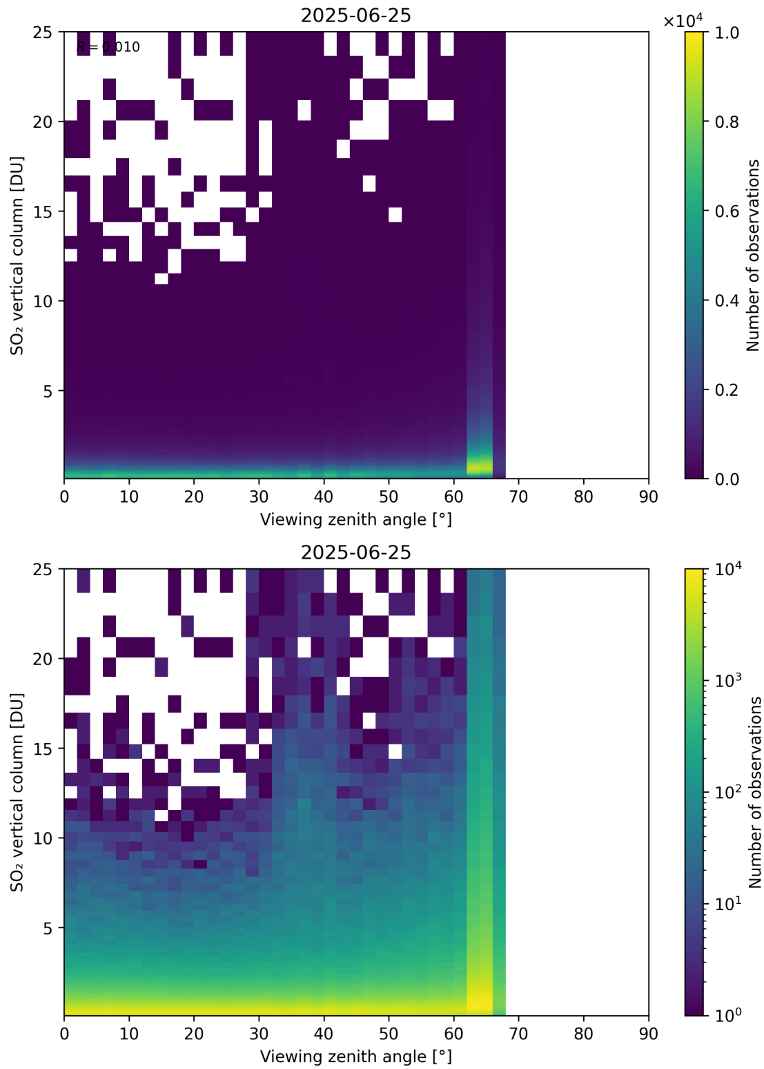
Figure 383: Scatter density plot of “Viewing zenith angle” against “SO 2 vertical column” for 2025-06-24 to 2025-06-26.
