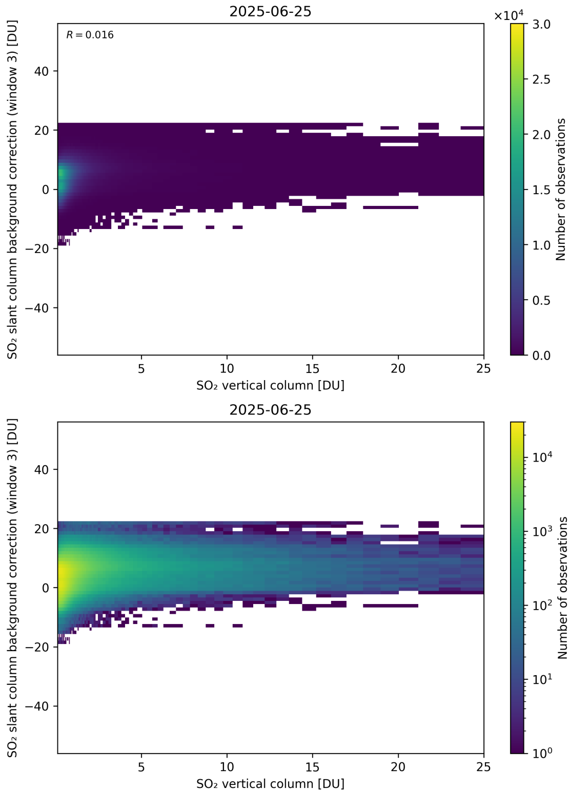
Figure 325: Scatter density plot of “SO 2 vertical column” against “SO 2 slant column background correction (window 3)” for 2025-06-24 to 2025-06-26.
