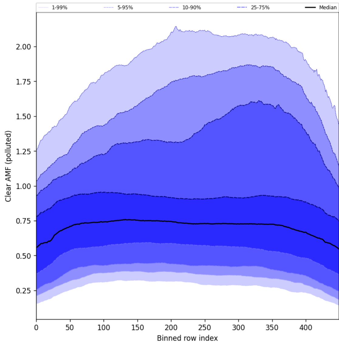
Figure 107: Along track statistics of “Clear AMF (polluted)” for 2025-06-24 to 2025-06-26
