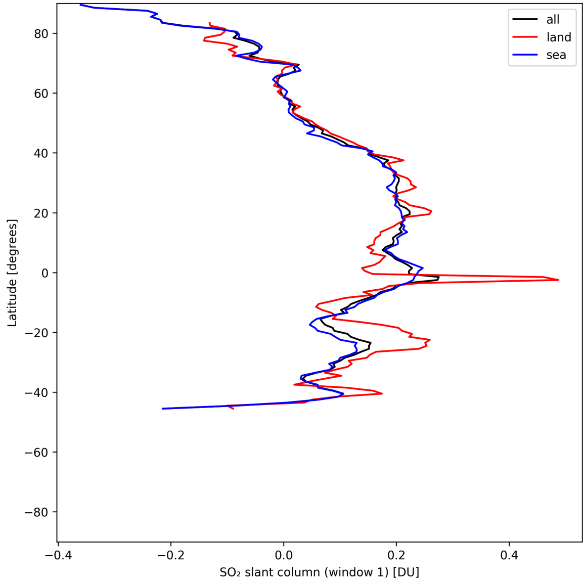
Figure 37: Zonal average of “SO 2 slant column (window 1)” for 2025-06-24 to 2025-06-26.
