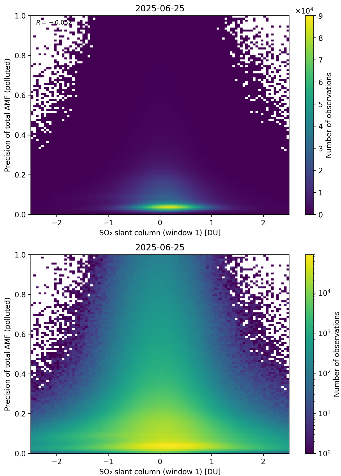
Figure 290: Scatter density plot of “SO 2 slant column (window 1)” against “Precision of total AMF (polluted)” for 2025-06-24 to 2025-06-26.
