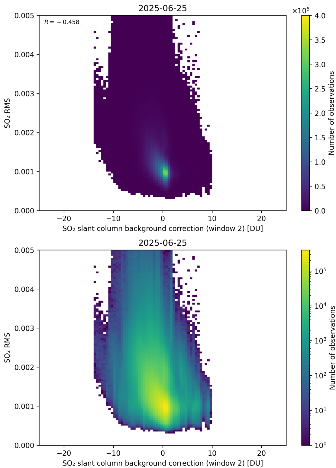
Figure 125: Scatter density plot of “SO 2 slant column background correction (window 2)” against “SO 2 RMS” for 2025-06-24 to 2025-06-26.
