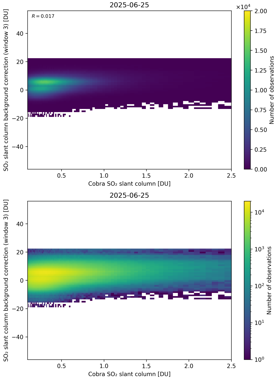
Figure 195: Scatter density plot of “Cobra SO 2 slant column” against “SO 2 slant column background correction (window 3)” for 2025-06-24 to 2025-06-26.
