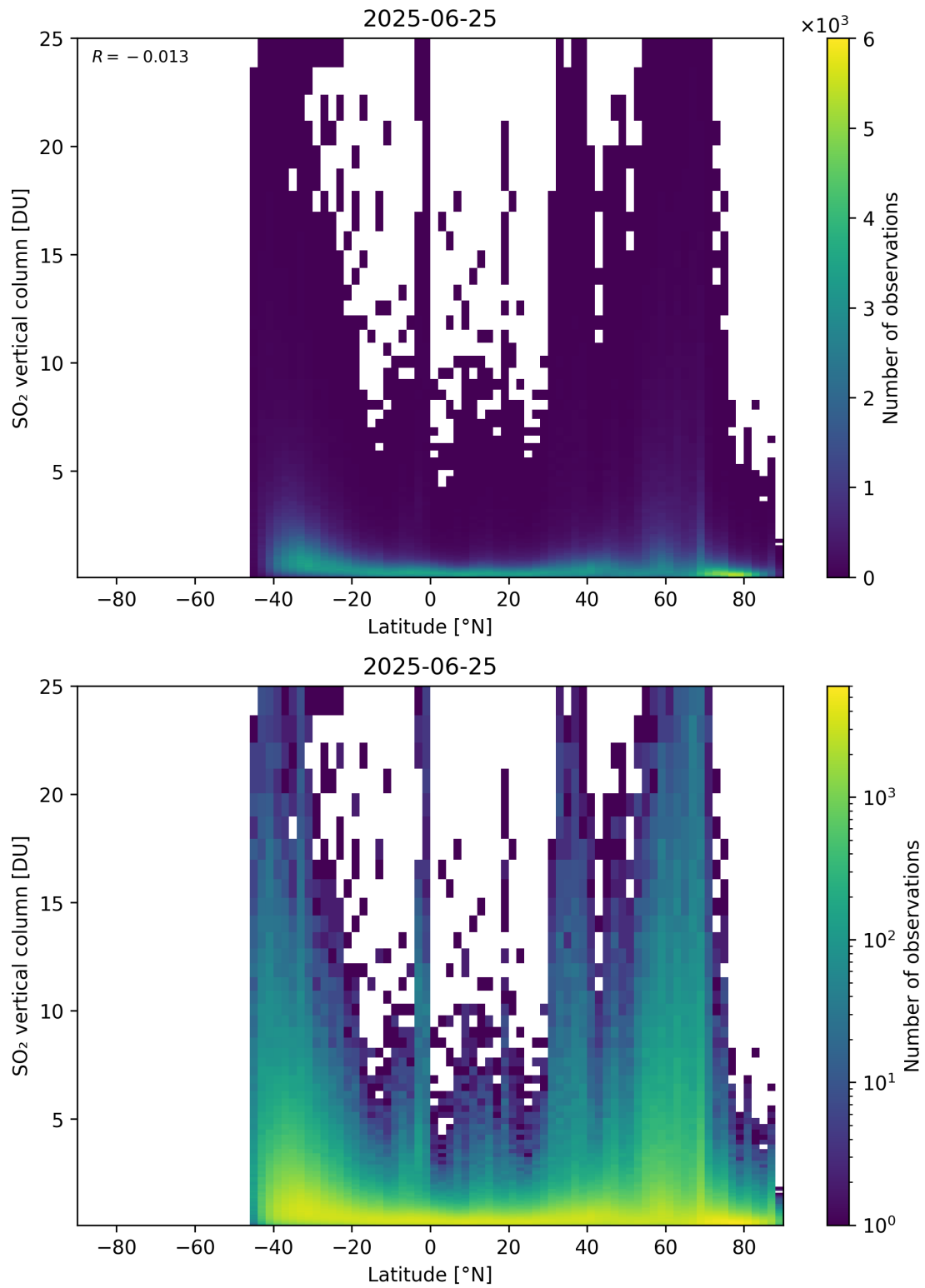
Figure 169: Scatter density plot of “Latitude” against “SO 2 vertical column” for 2025-06-24 to 2025-06-26.
