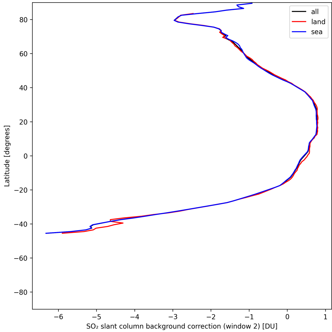
Figure 44: Zonal average of “SO 2 slant column background correction (window 2)” for 2025-06-24 to 2025-06-26.
