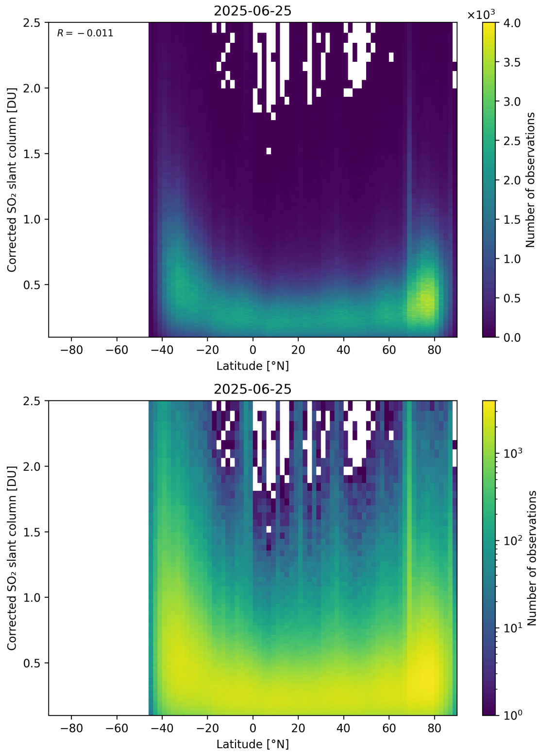
Figure 159: Scatter density plot of “Latitude” against “Corrected SO 2 slant column” for 2025-06-24 to 2025-06-26.
