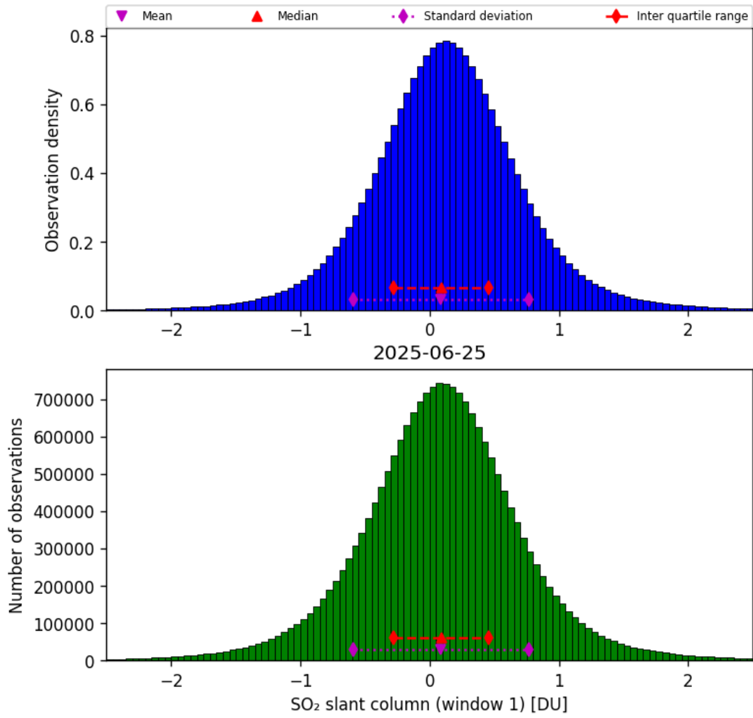
Figure 63: Histogram of “SO 2 slant column (window 1)” for 2025-06-24 to 2025-06-26
