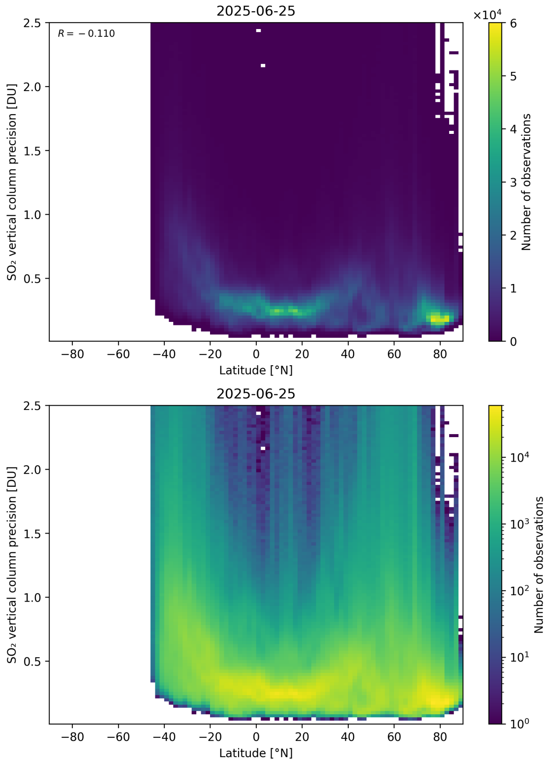
Figure 170: Scatter density plot of “Latitude” against “SO 2 vertical column precision” for 2025-06-24 to 2025-06-26.
