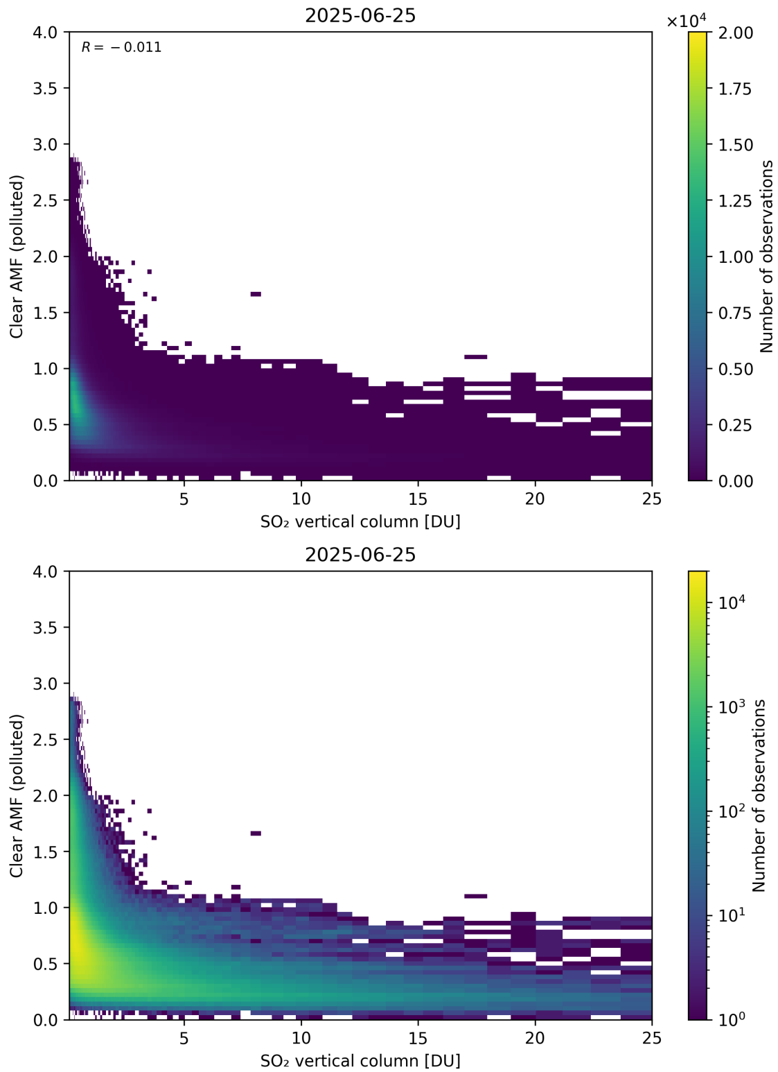
Figure 348: Scatter density plot of “SO 2 vertical column” against “Clear AMF (polluted)” for 2025-06-24 to 2025-06-26.
