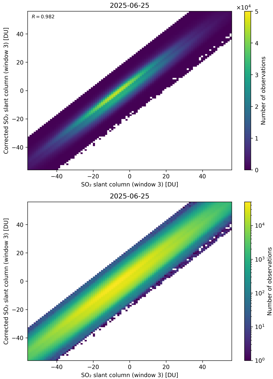
Figure 316: Scatter density plot of “SO 2 slant column (window 3)” against “Corrected SO 2 slant column (window 3)” for 2025-06-24 to 2025-06-26.
