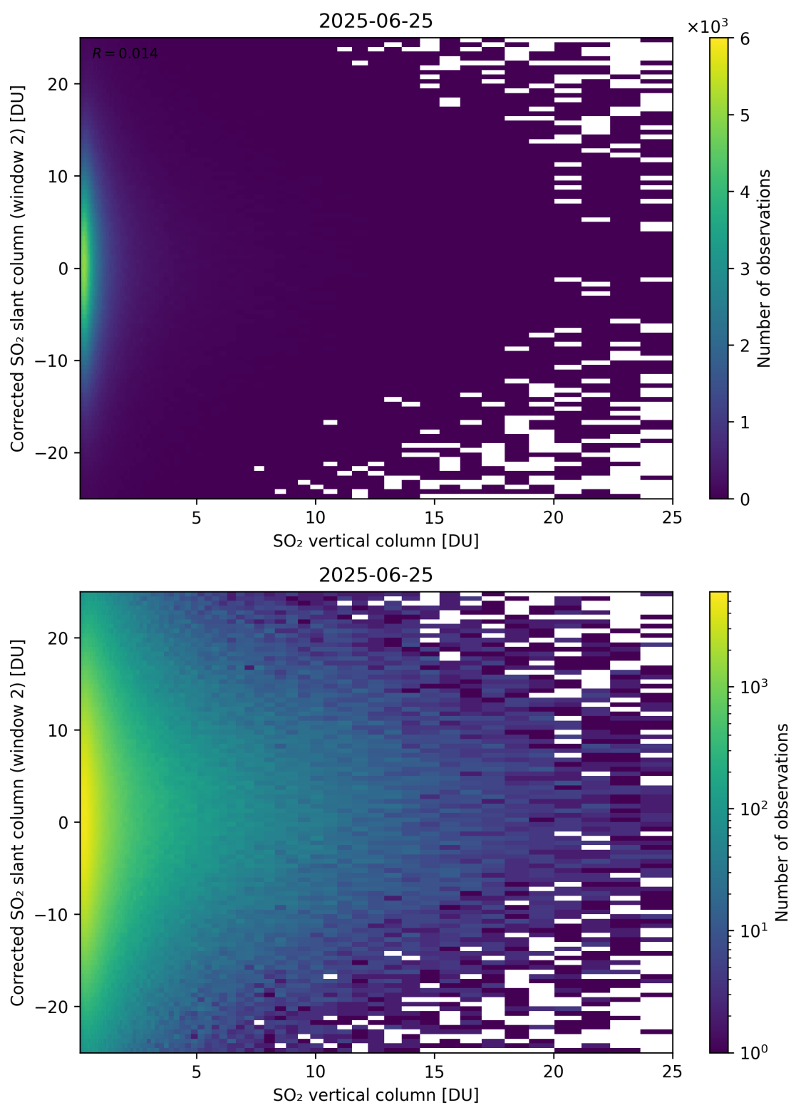
Figure 352: Scatter density plot of “SO 2 vertical column” against “Corrected SO 2 slant column (window 2)” for 2025-06-24 to 2025-06-26.
