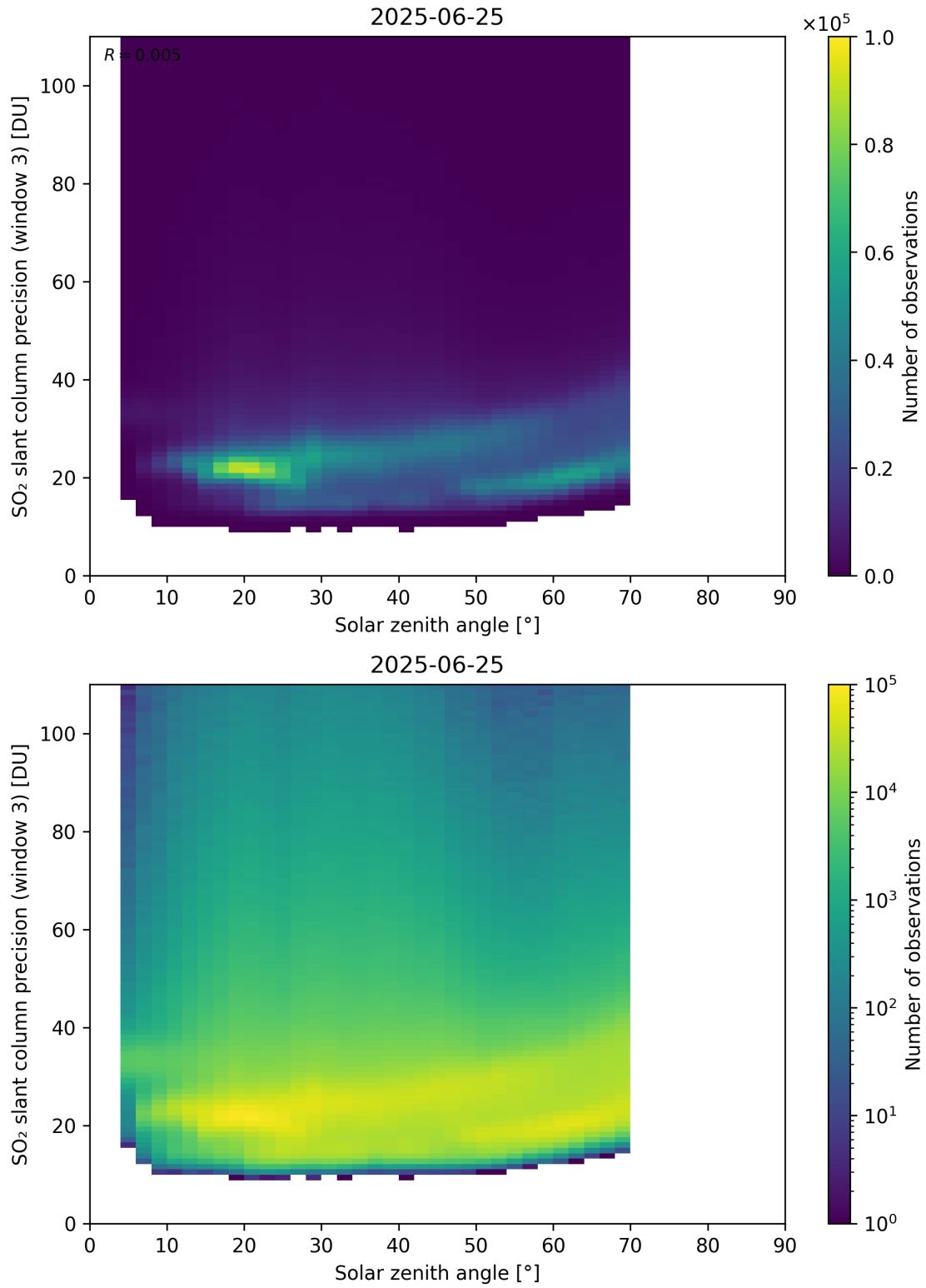
Figure 188: Scatter density plot of “Solar zenith angle” against “SO 2 slant column precision (window 3)” for 2025-06-24 to 2025-06-26.
