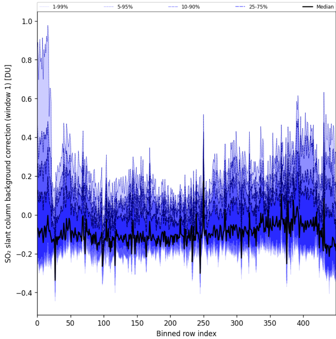
Figure 92: Along track statistics of “SO 2 slant column background correction (window 1)” for 2025-06-24 to 2025-06-26
