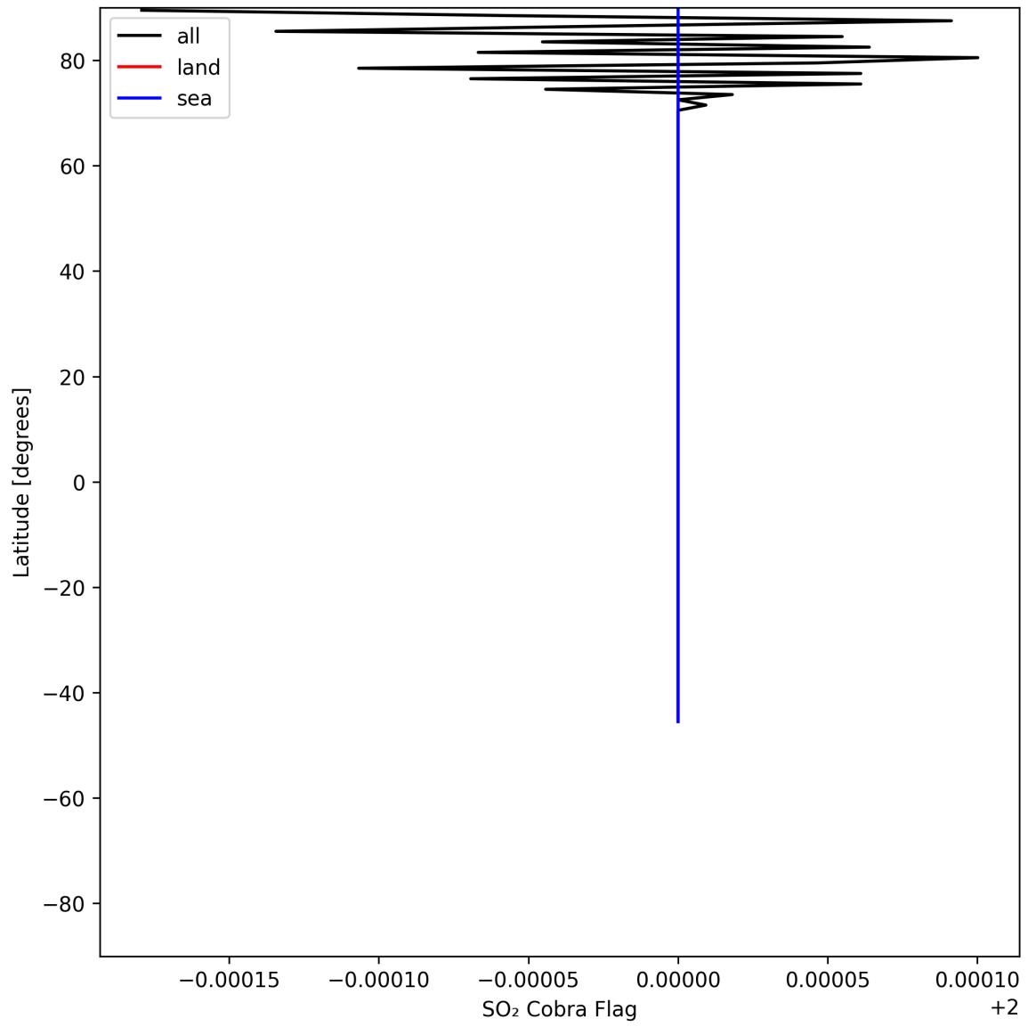
Figure 49: Zonal average of “SO 2 Cobra Flag” for 2025-06-24 to 2025-06-26.
