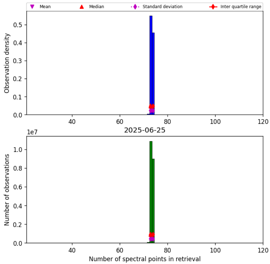
Figure 82: Histogram of “Number of spectral points in retrieval” for 2025-06-24 to 2025-06-26
