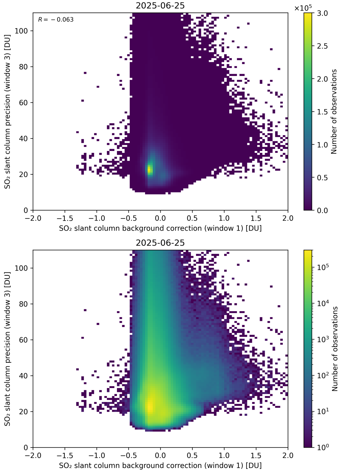
Figure 119: Scatter density plot of “SO 2 slant column background correction (window 1)” against “SO 2 slant column precision (window 3)” for 2025-06-24 to 2025-06-26.
