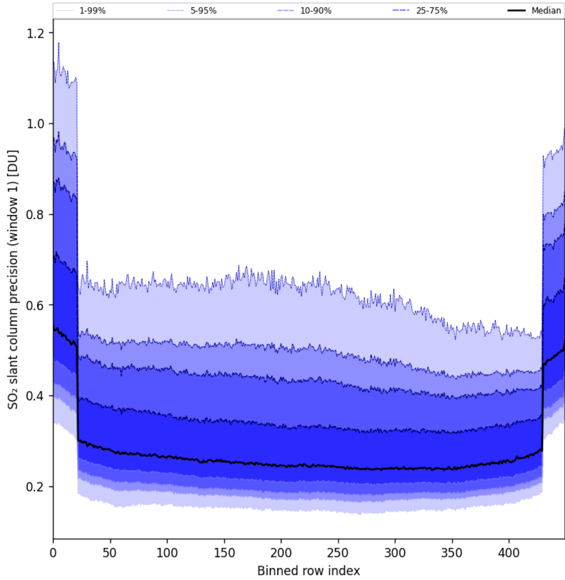
Figure 90: Along track statistics of “SO 2 slant column precision (window 1)” for 2025-06-24 to 2025-06-26
