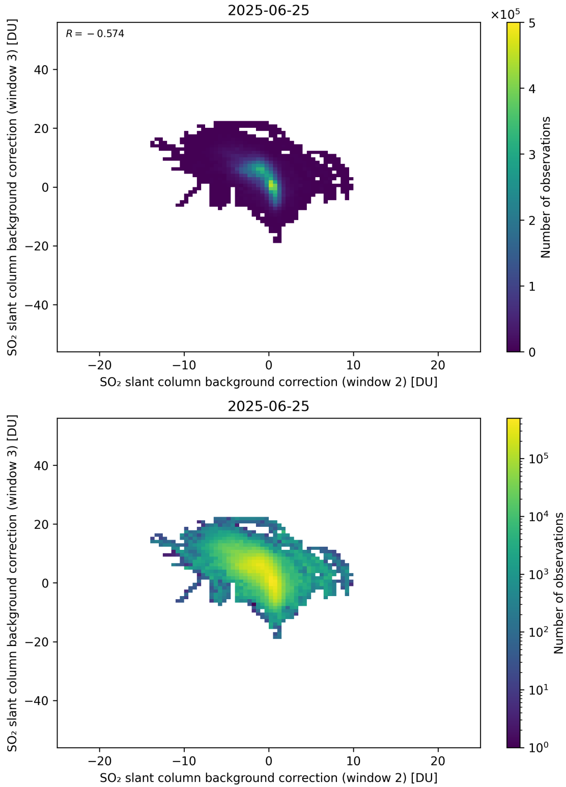
Figure 122: Scatter density plot of “SO 2 slant column background correction (window 2)” against “SO 2 slant column background correction (window 3)” for 2025-06-24 to 2025-06-26.
