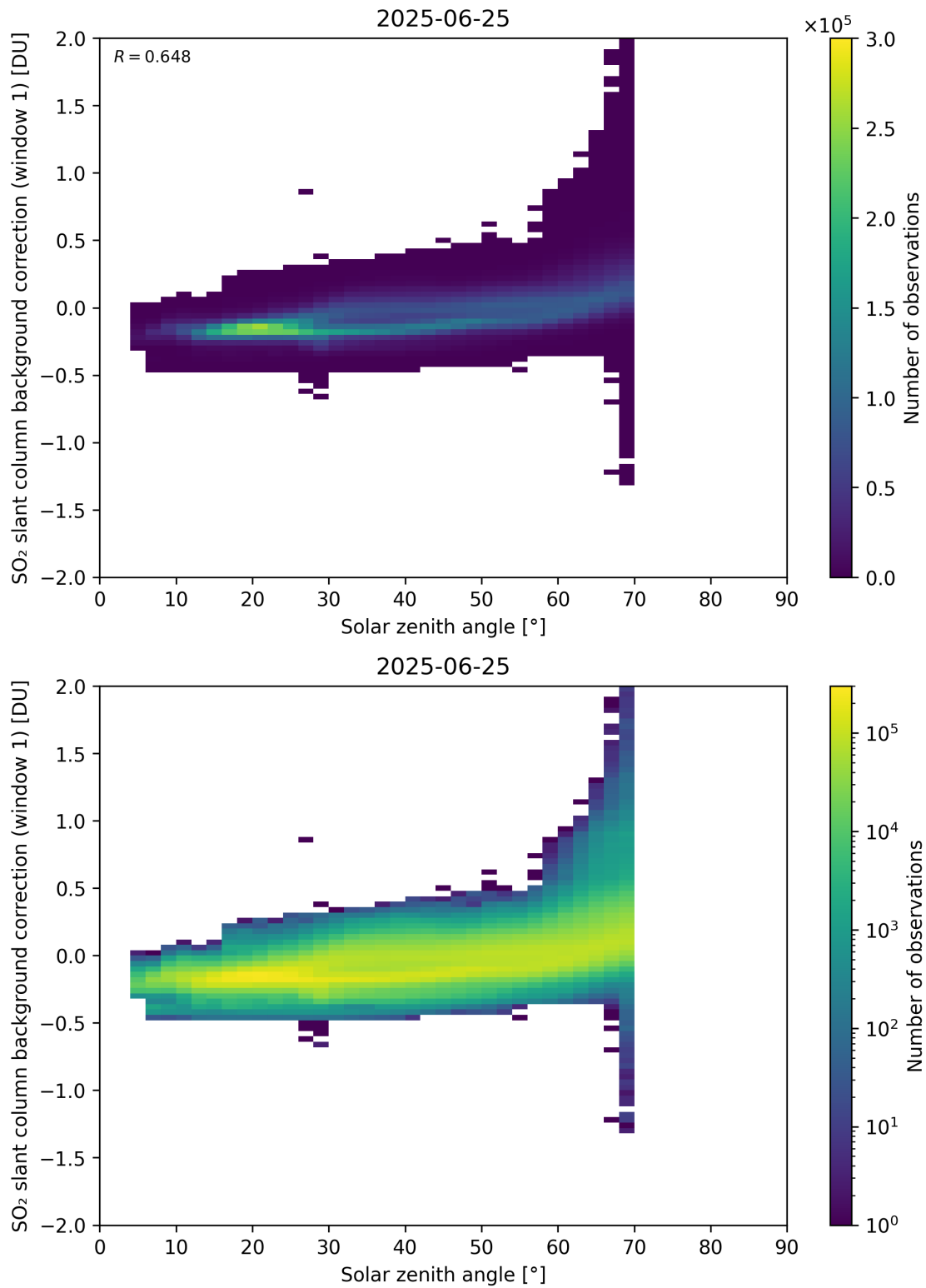
Figure 171: Scatter density plot of “Solar zenith angle” against “SO 2 slant column background correction (window 1)” for 2025-06-24 to 2025-06-26.
