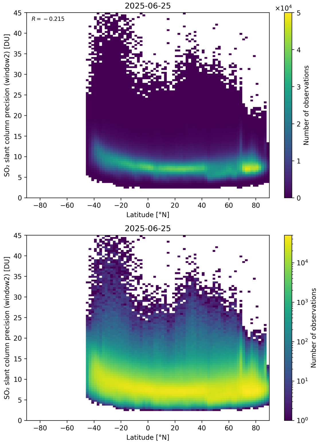
Figure 164: Scatter density plot of “Latitude” against “SO 2 slant column precision (window2)” for 2025-06-24 to 2025-06-26.
