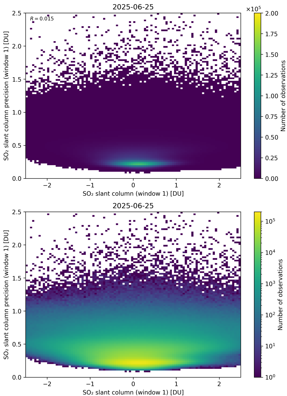
Figure 285: Scatter density plot of “SO 2 slant column (window 1)” against “SO 2 slant column precision (window 1)” for 2025-06-24 to 2025-06-26.
