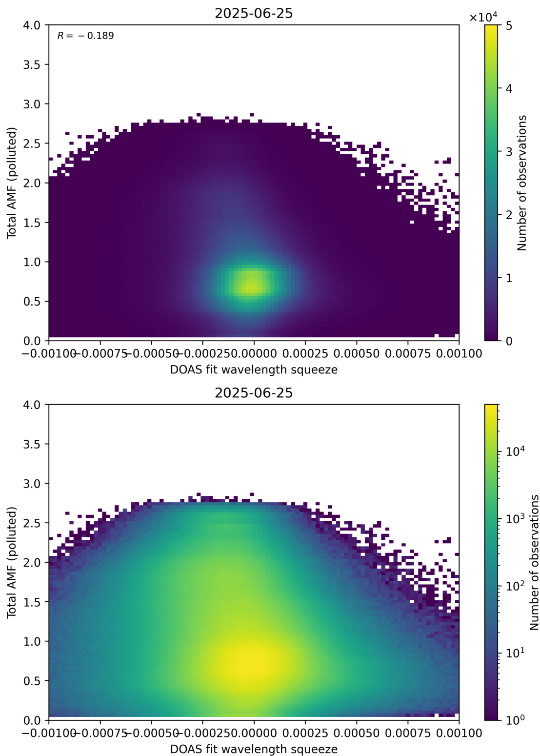
Figure 145: Scatter density plot of “DOAS fit wavelength squeeze” against “Total AMF (polluted)” for 2025-06-24 to 2025-06-26.
