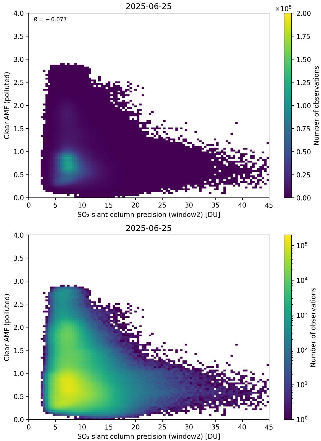
Figure 296: Scatter density plot of “SO 2 slant column precision (window2)” against “Clear AMF (polluted)” for 2025-06-24 to 2025-06-26.
