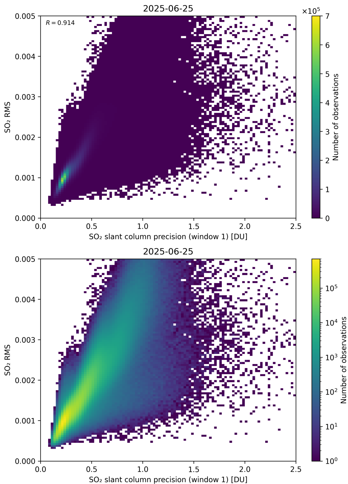
Figure 273: Scatter density plot of “SO 2 slant column precision (window 1)” against “SO 2 RMS” for 2025-06-24 to 2025-06-26.
