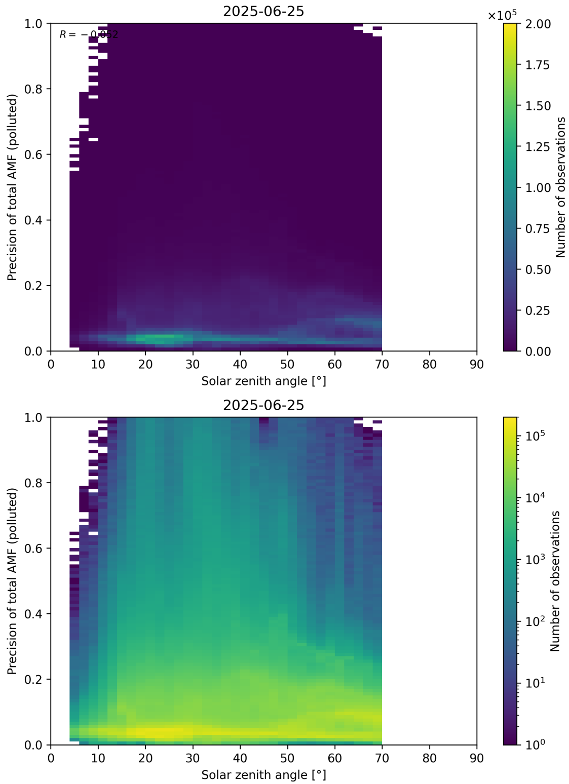
Figure 190: Scatter density plot of “Solar zenith angle” against “Precision of total AMF (polluted)” for 2025-06-24 to 2025-06-26.
