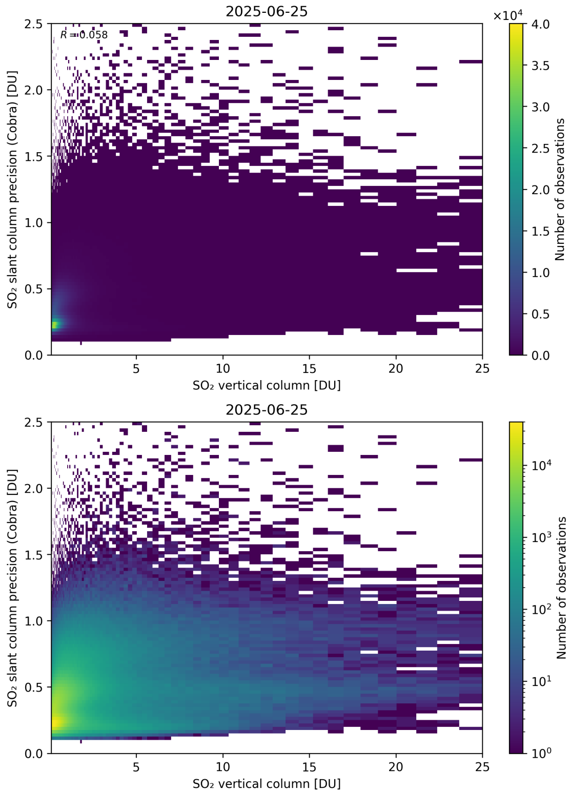
Figure 350: Scatter density plot of “SO 2 vertical column” against “SO 2 slant column precision (Cobra)” for 2025-06-24 to 2025-06-26.
