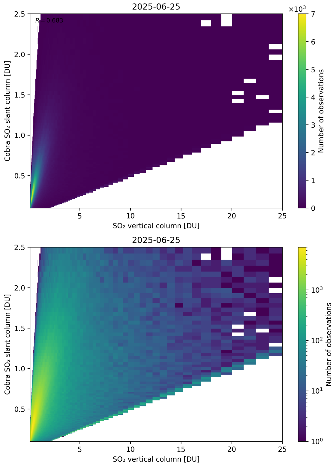
Figure 349: Scatter density plot of “SO 2 vertical column” against “Cobra SO 2 slant column” for 2025-06-24 to 2025-06-26.
