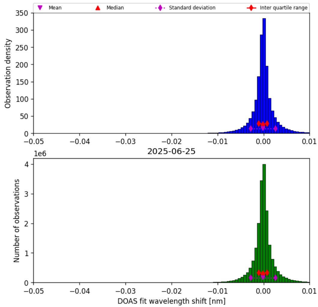
Figure 76: Histogram of “DOAS fit wavelength shift” for 2025-06-24 to 2025-06-26
