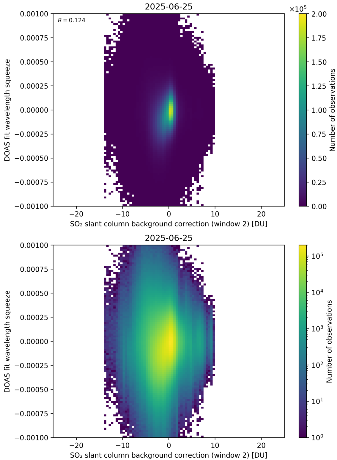
Figure 124: Scatter density plot of “SO 2 slant column background correction (window 2)” against “DOAS fit wavelength squeeze” for 2025-06-24 to 2025-06-26.
