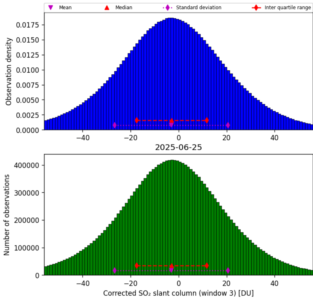
Figure 73: Histogram of “Corrected SO 2 slant column (window 3)” for 2025-06-24 to 2025-06-26
