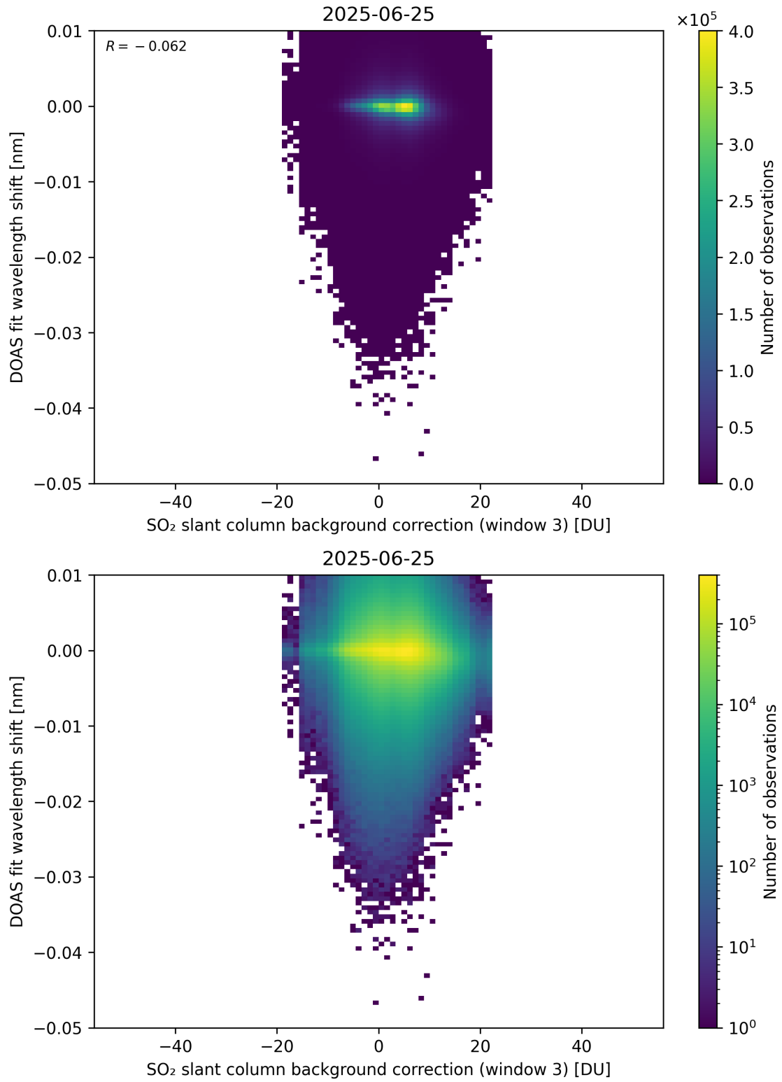
Figure 132: Scatter density plot of “SO 2 slant column background correction (window 3)” against “DOAS fit wavelength shift” for 2025-06-24 to 2025-06-26.
