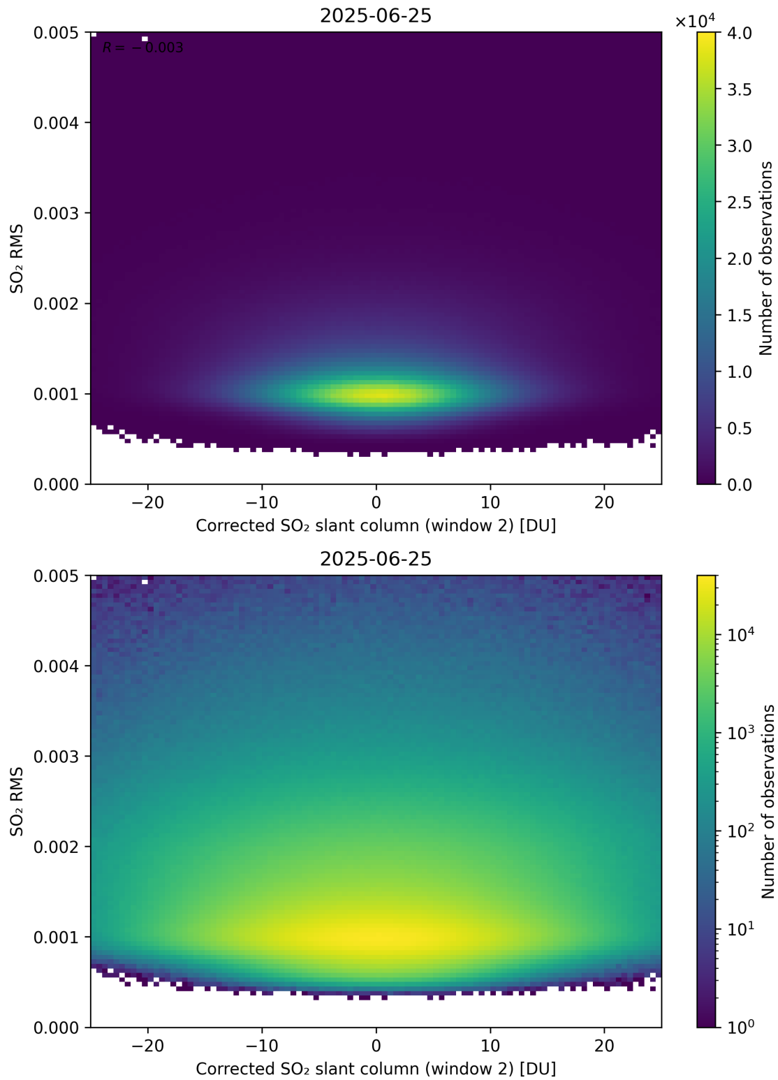
Figure 248: Scatter density plot of “Corrected SO 2 slant column (window 2)” against “SO 2 RMS” for 2025-06-24 to 2025-06-26.
