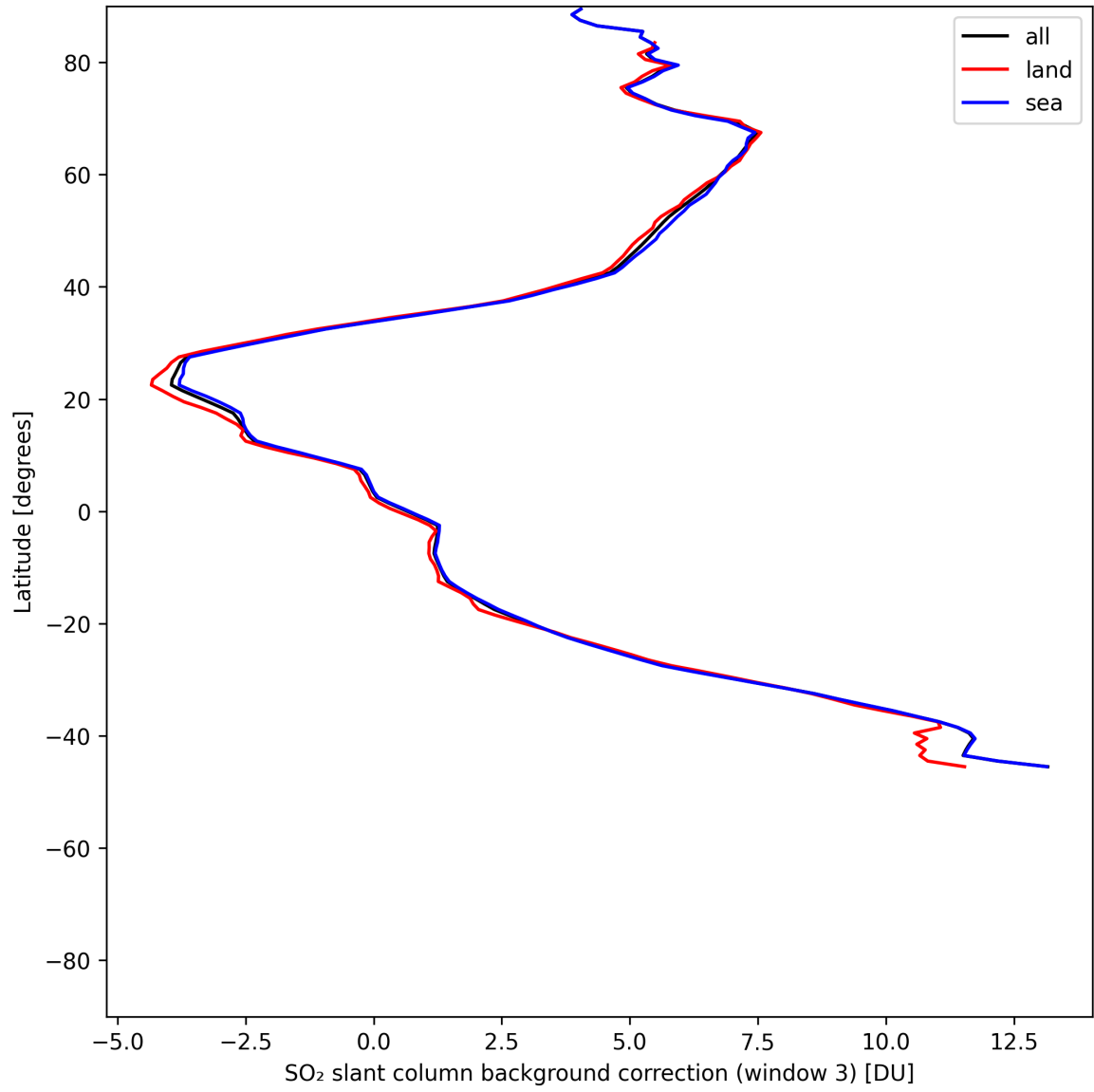
Figure 48: Zonal average of “SO 2 slant column background correction (window 3)” for 2025-06-24 to 2025-06-26.
