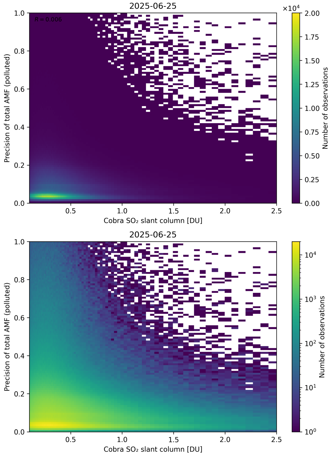
Figure 225: Scatter density plot of “Cobra SO 2 slant column” against “Precision of total AMF (polluted)” for 2025-06-24 to 2025-06-26.
