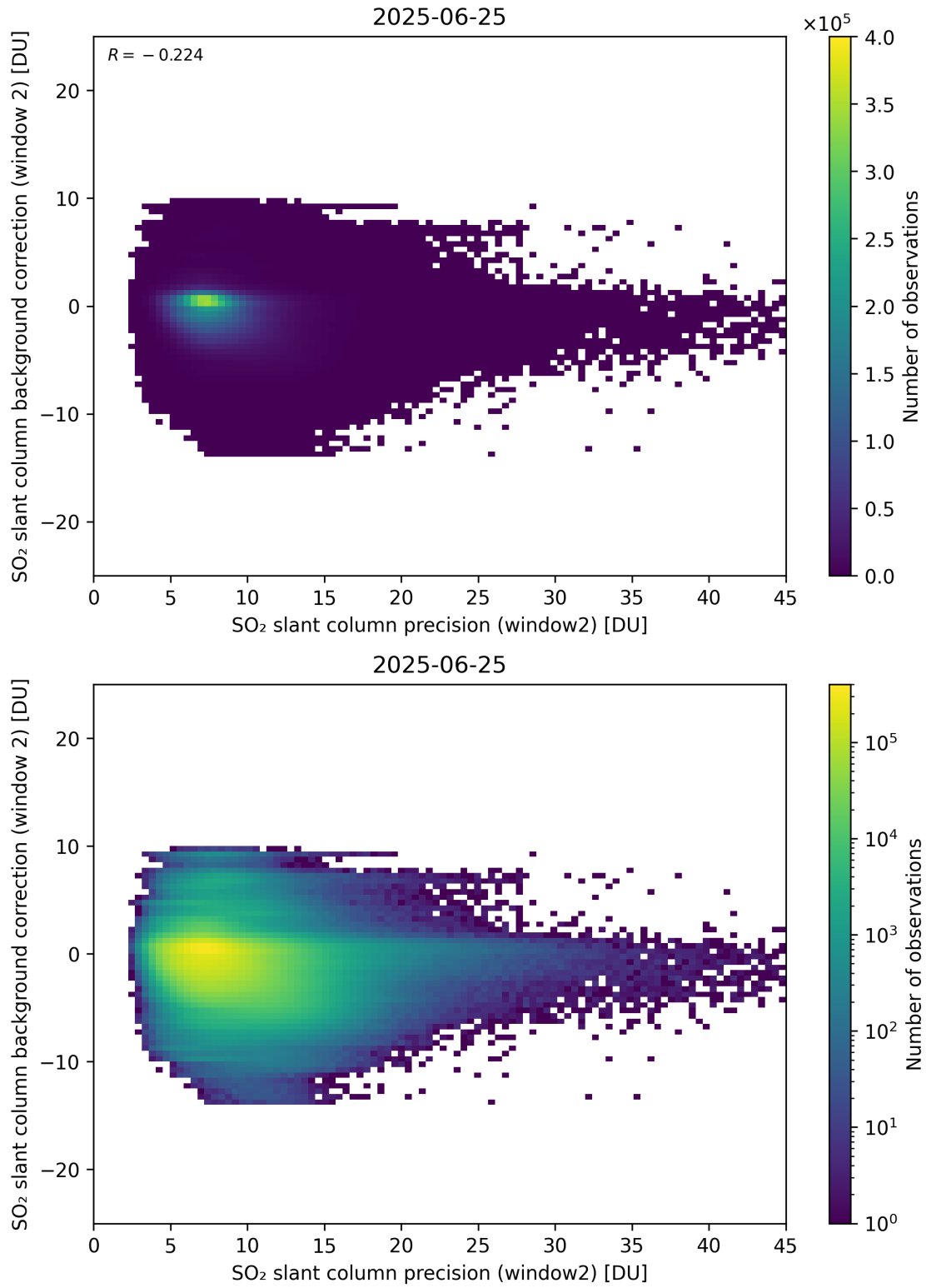
Figure 291: Scatter density plot of “SO 2 slant column precision (window2)” against “SO 2 slant column background correction (window 2)” for 2025-06-24 to 2025-06-26.
