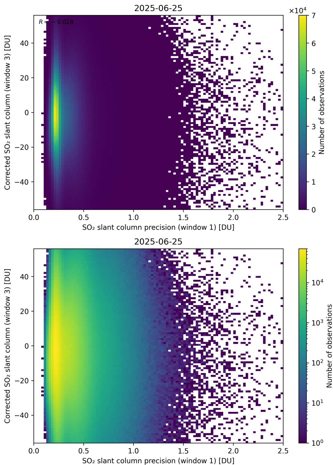
Figure 276: Scatter density plot of “SO 2 slant column precision (window 1)” against “Corrected SO 2 slant column (window 3)” for 2025-06-24 to 2025-06-26.
