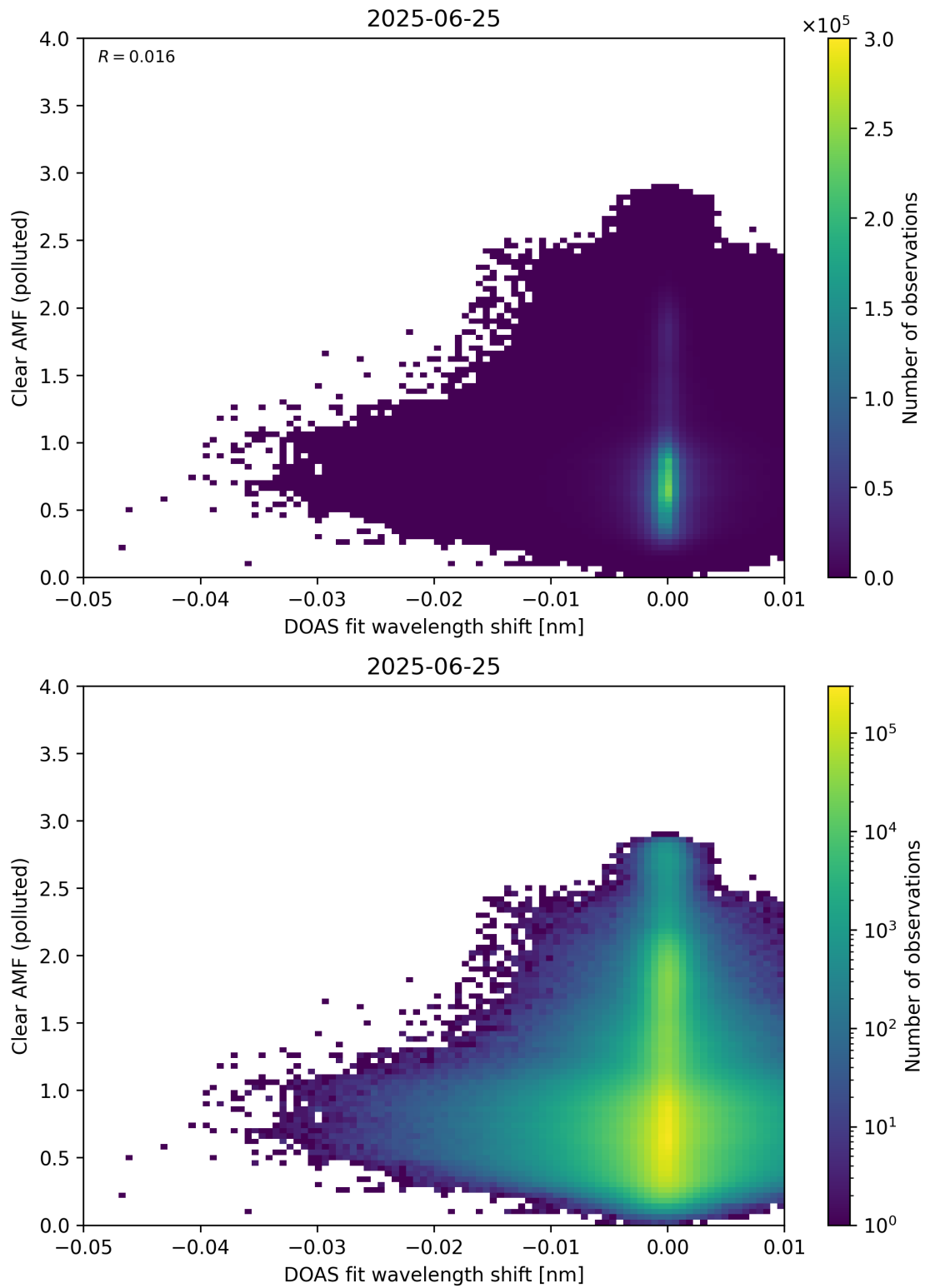
Figure 140: Scatter density plot of “DOAS fit wavelength shift” against “Clear AMF (polluted)” for 2025-06-24 to 2025-06-26.
