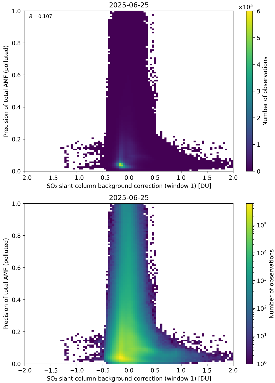
Figure 121: Scatter density plot of “SO 2 slant column background correction (window 1)” against “Precision of total AMF (polluted)” for 2025-06-24 to 2025-06-26.
