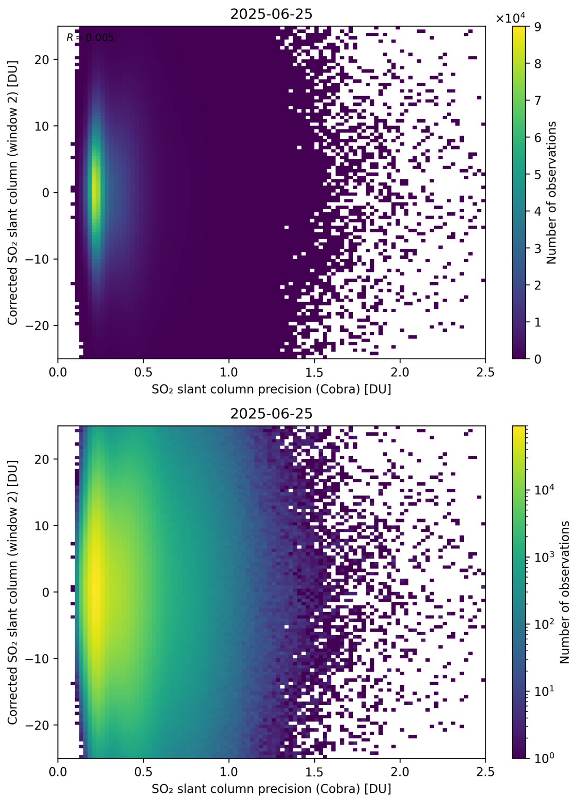
Figure 206: Scatter density plot of “SO 2 slant column precision (Cobra)” against “Corrected SO 2 slant column (window 2)” for 2025-06-24 to 2025-06-26.
