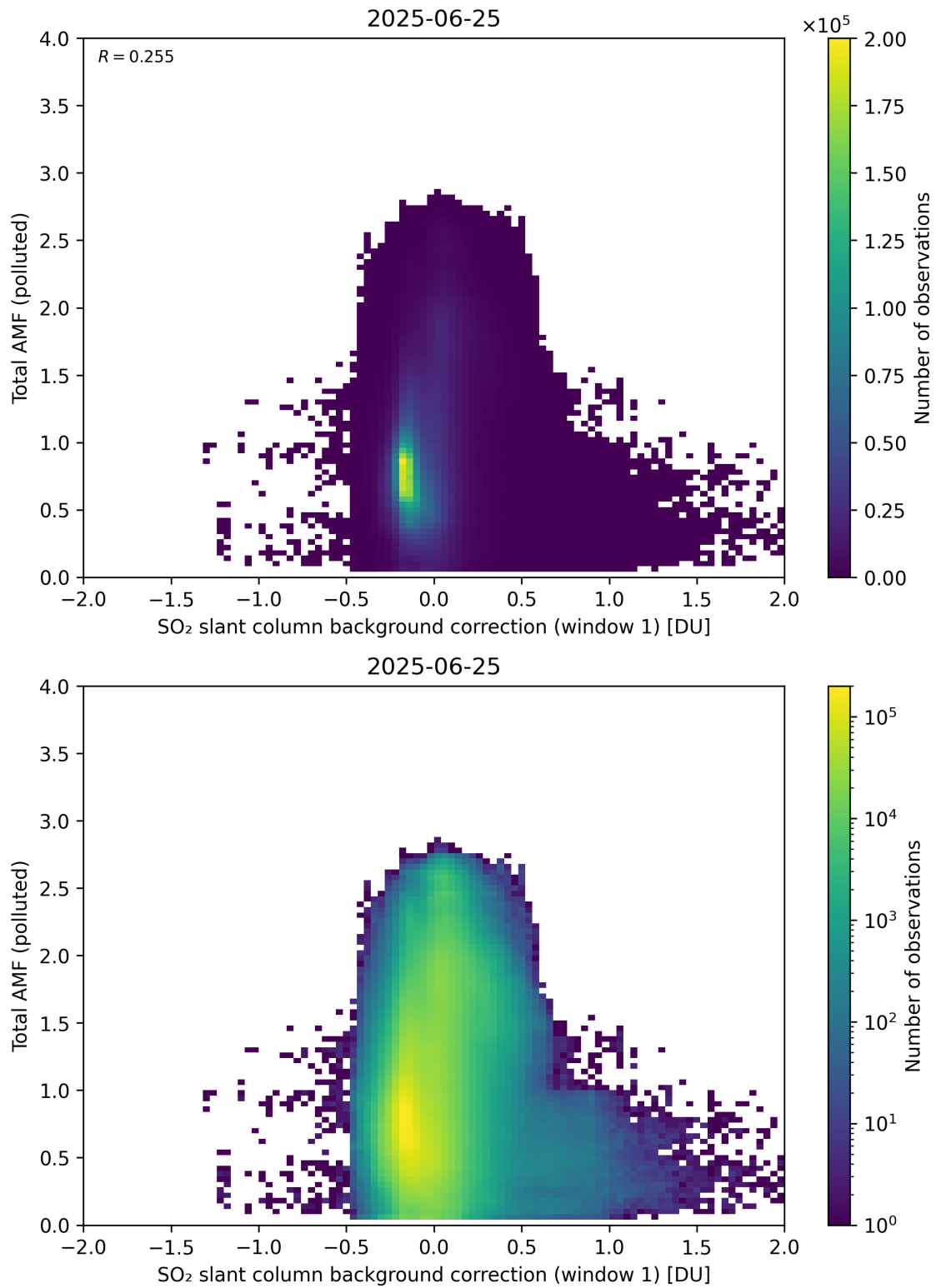
Figure 120: Scatter density plot of “SO 2 slant column background correction (window 1)” against “Total AMF (polluted)” for 2025-06-24 to 2025-06-26.
