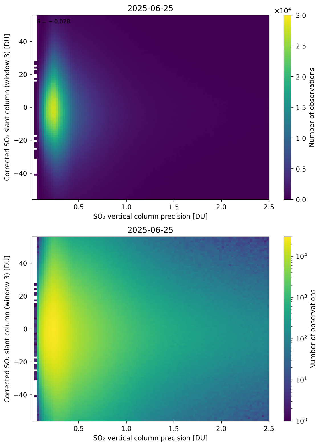
Figure 340: Scatter density plot of “SO 2 vertical column precision” against “Corrected SO 2 slant column (window 3)” for 2025-06-24 to 2025-06-26.
