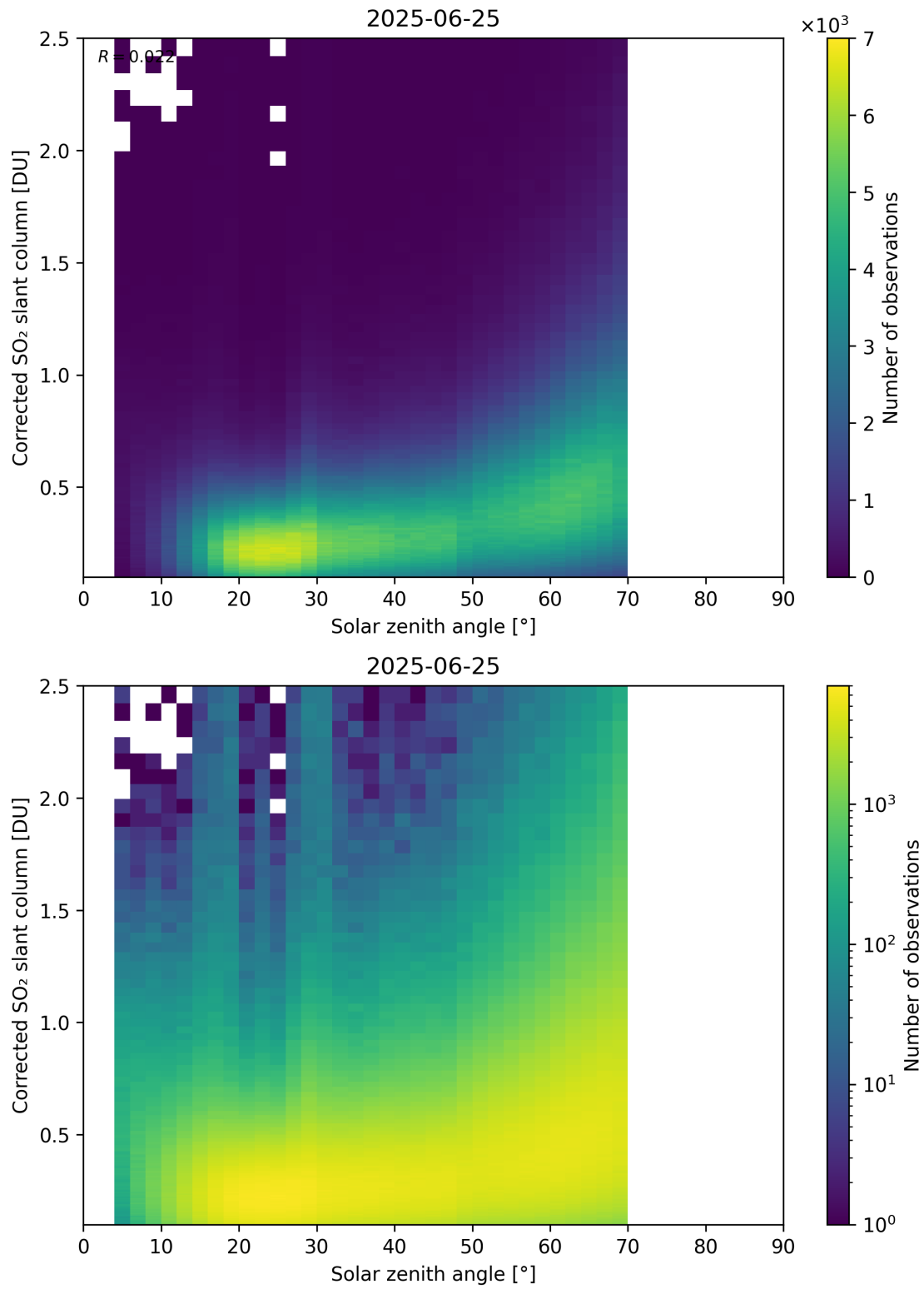
Figure 181: Scatter density plot of “Solar zenith angle” against “Corrected SO 2 slant column” for 2025-06-24 to 2025-06-26.
