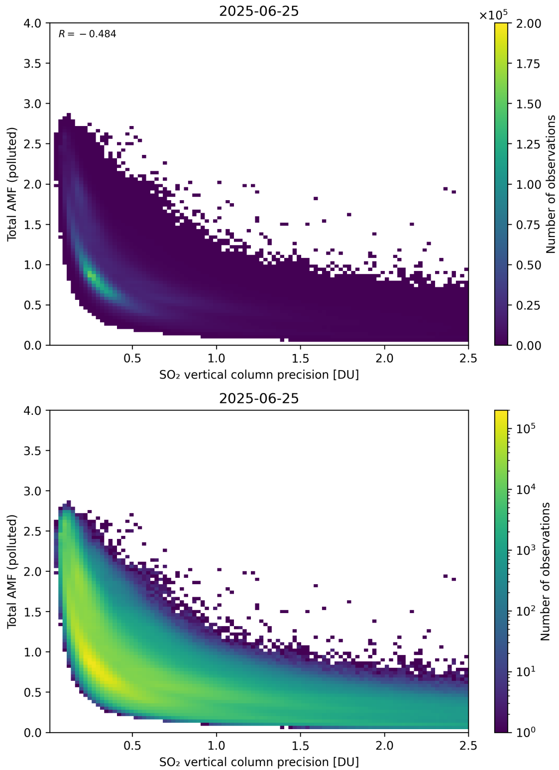
Figure 346: Scatter density plot of “SO 2 vertical column precision” against “Total AMF (polluted)” for 2025-06-24 to 2025-06-26.
