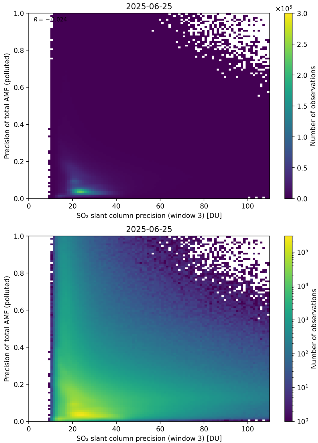
Figure 314: Scatter density plot of “SO 2 slant column precision (window 3)” against “Precision of total AMF (polluted)” for 2025-06-24 to 2025-06-26.
