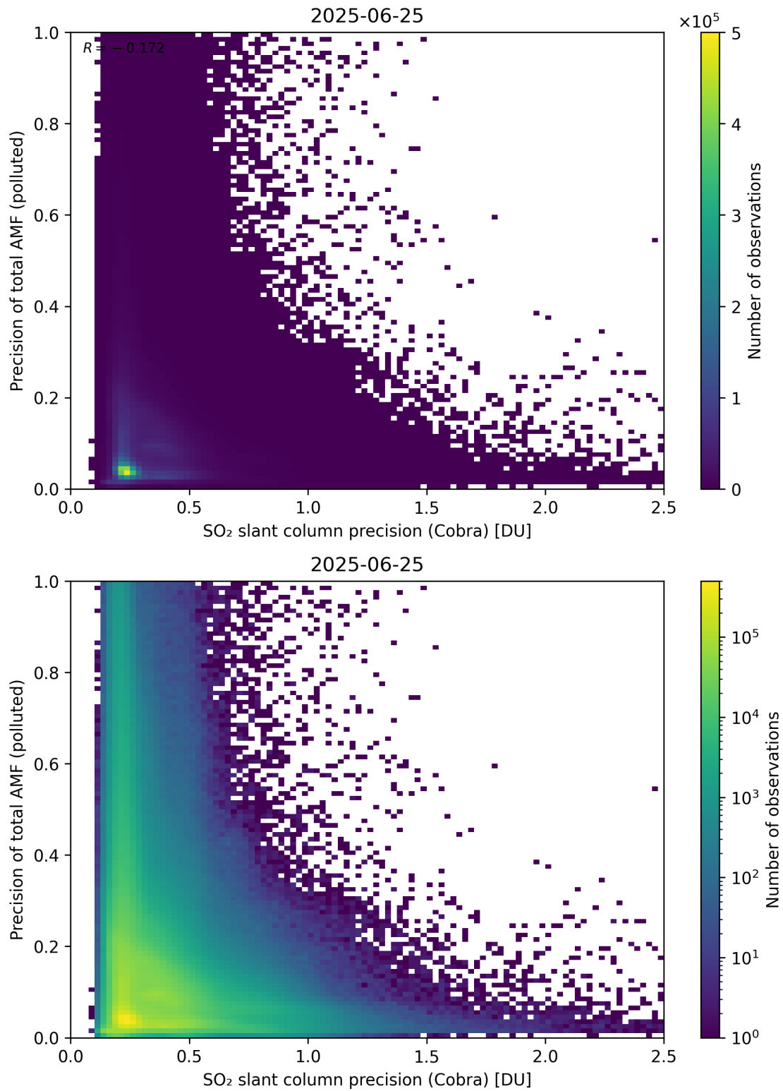
Figure 214: Scatter density plot of “SO 2 slant column precision (Cobra)” against “Precision of total AMF (polluted)” for 2025-06-24 to 2025-06-26.
