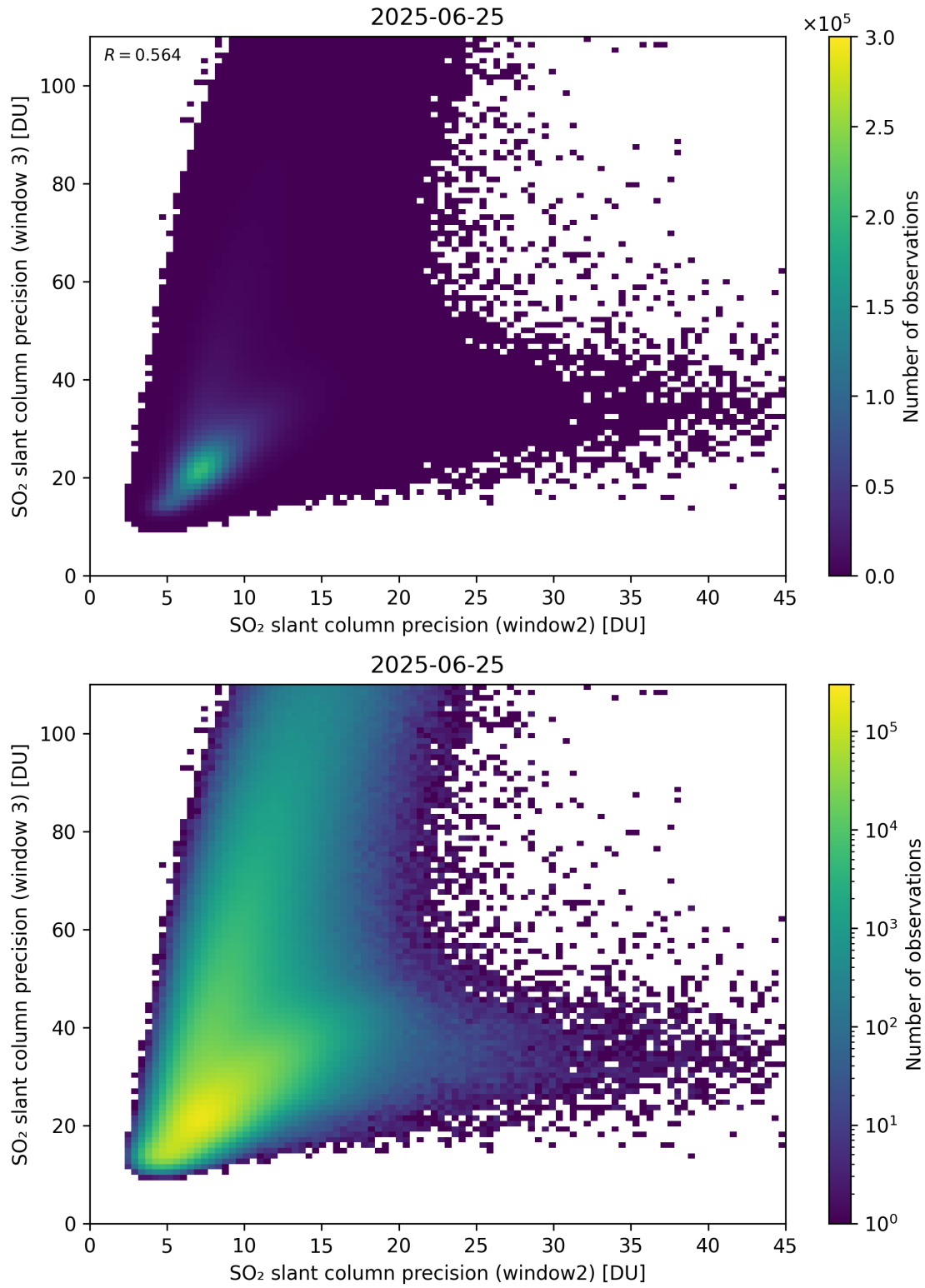
Figure 300: Scatter density plot of “SO 2 slant column precision (window2)” against “SO 2 slant column precision (window 3)” for 2025-06-24 to 2025-06-26.
