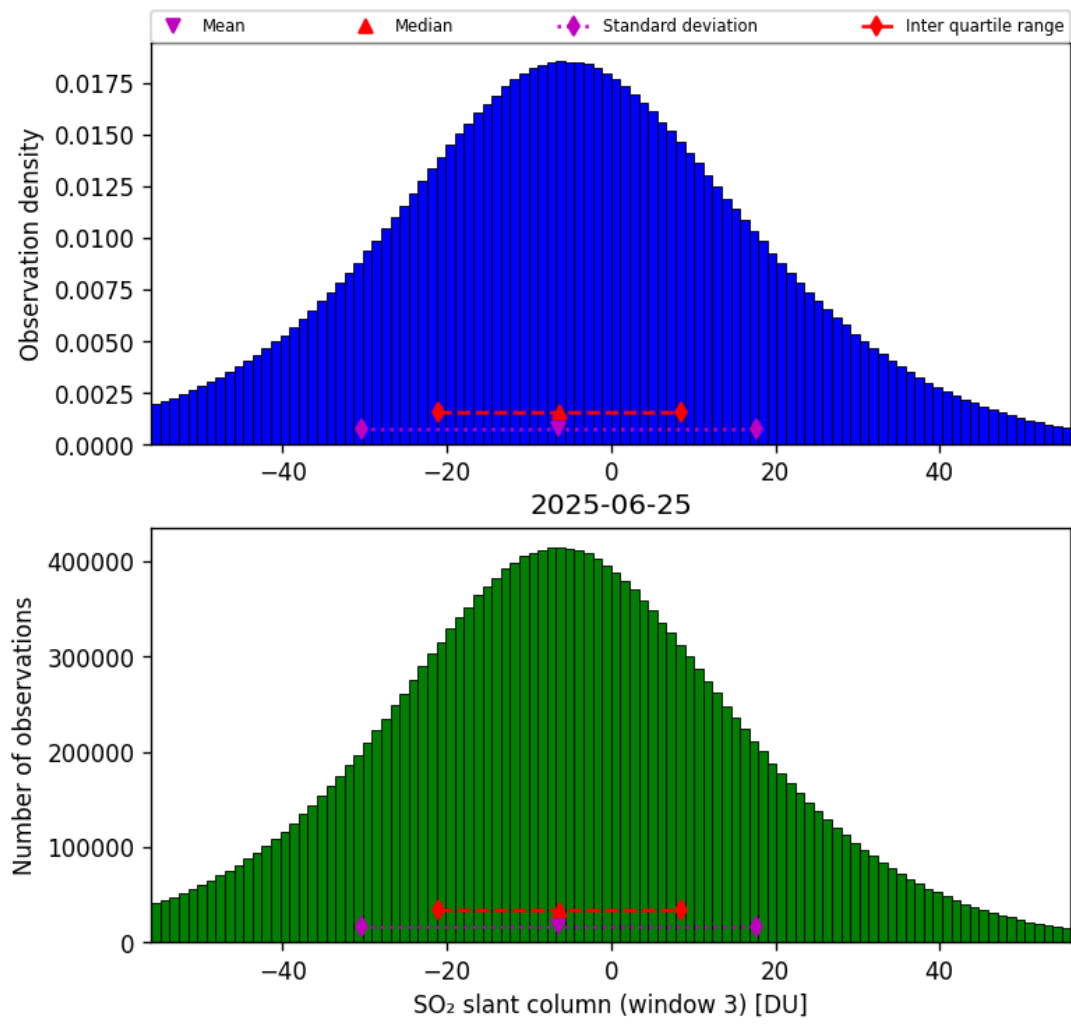
Figure 71: Histogram of “SO 2 slant column (window 3)” for 2025-06-24 to 2025-06-26
