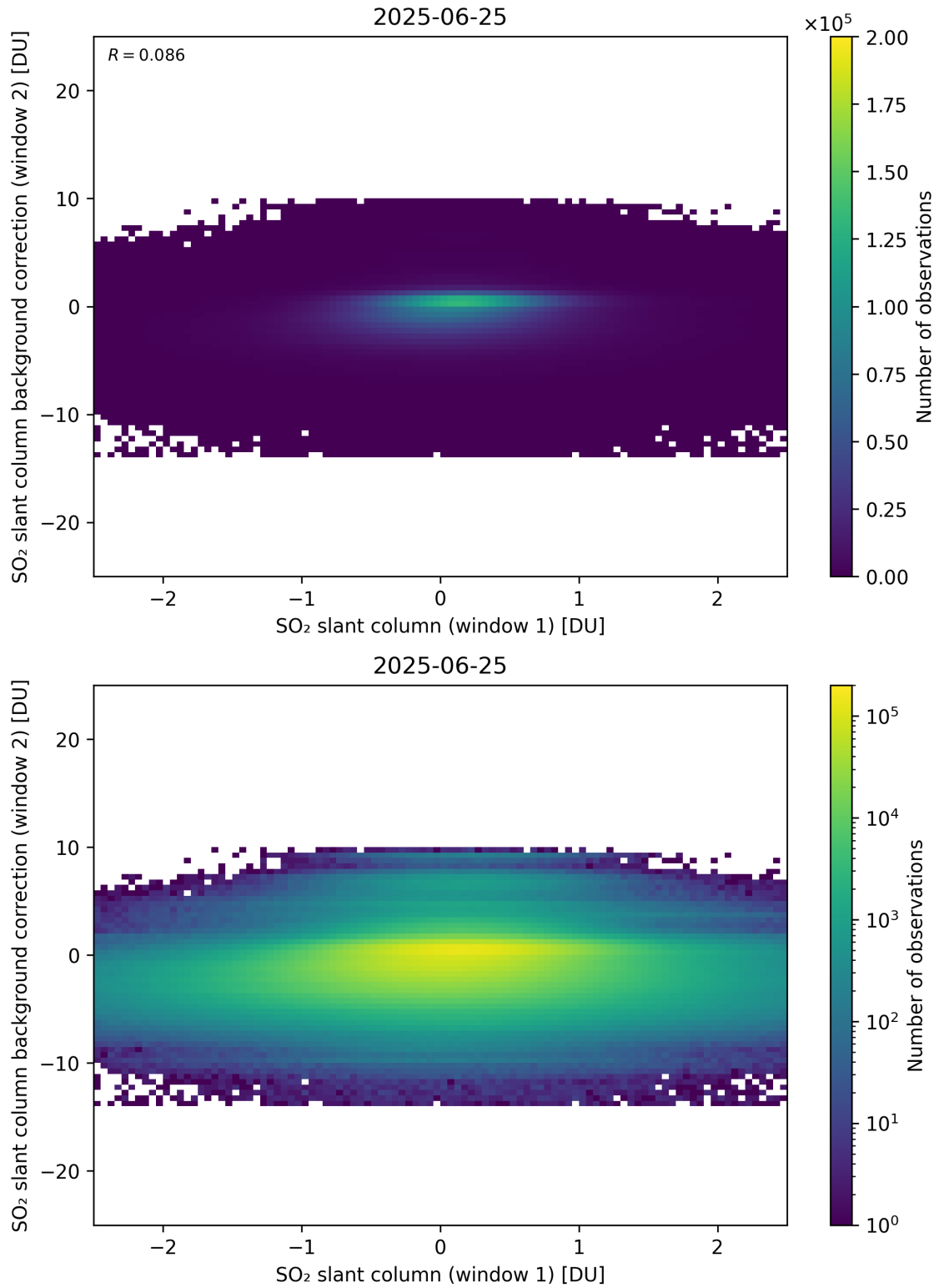
Figure 263: Scatter density plot of “SO 2 slant column (window 1)” against “SO 2 slant column background correction (window 2)” for 2025-06-24 to 2025-06-26.
