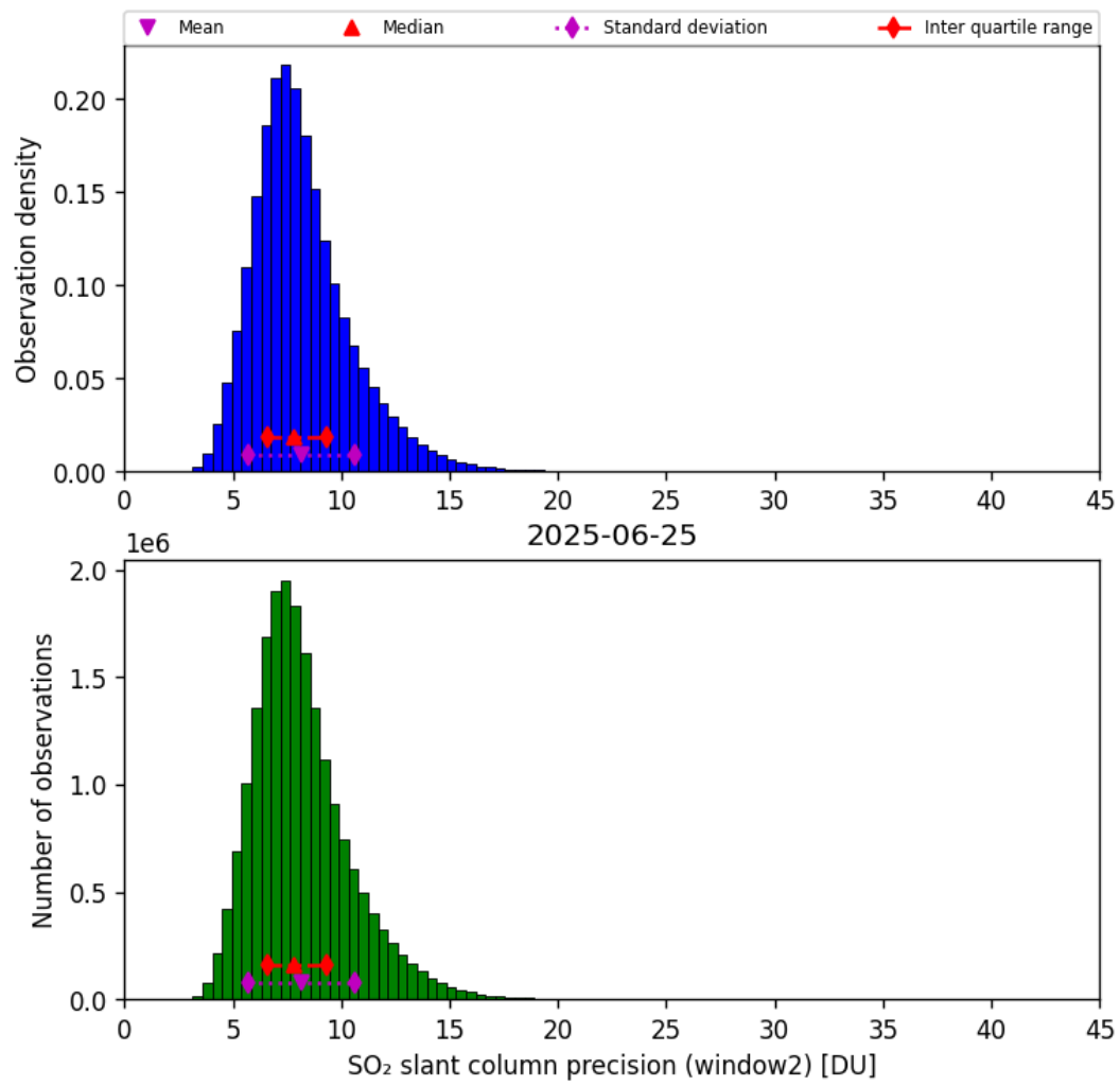
Figure 68: Histogram of “SO 2 slant column precision (window2)” for 2025-06-24 to 2025-06-26
