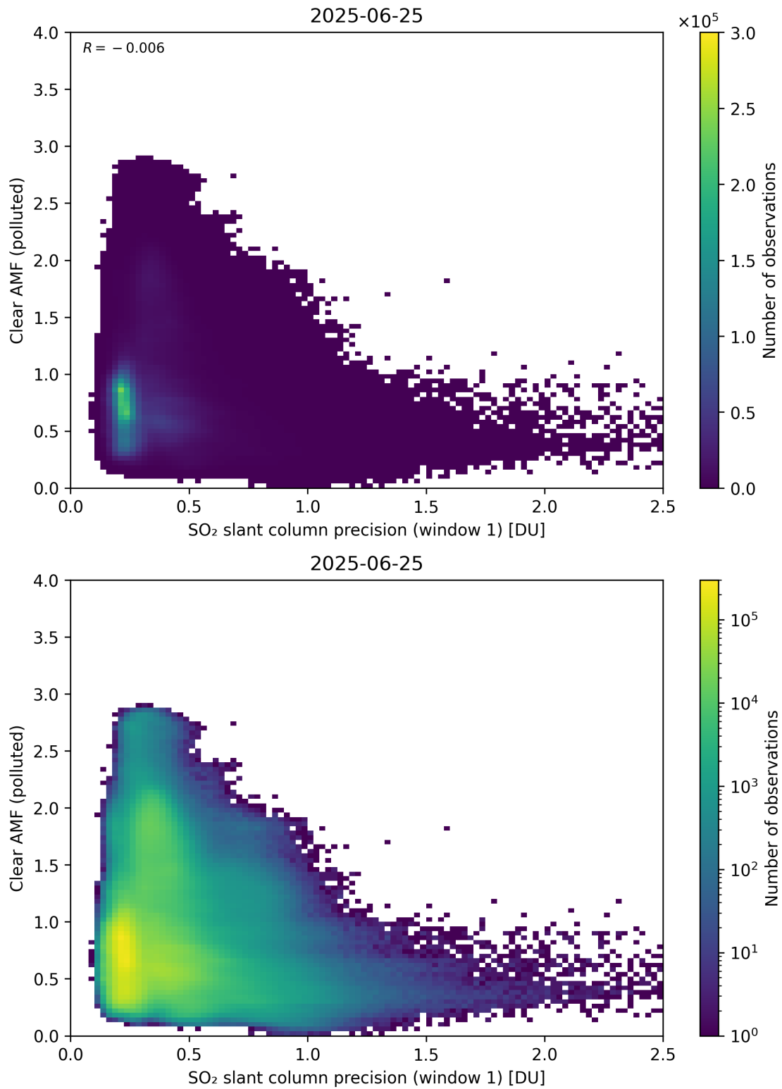
Figure 274: Scatter density plot of “SO 2 slant column precision (window 1)” against “Clear AMF (polluted)” for 2025-06-24 to 2025-06-26.
