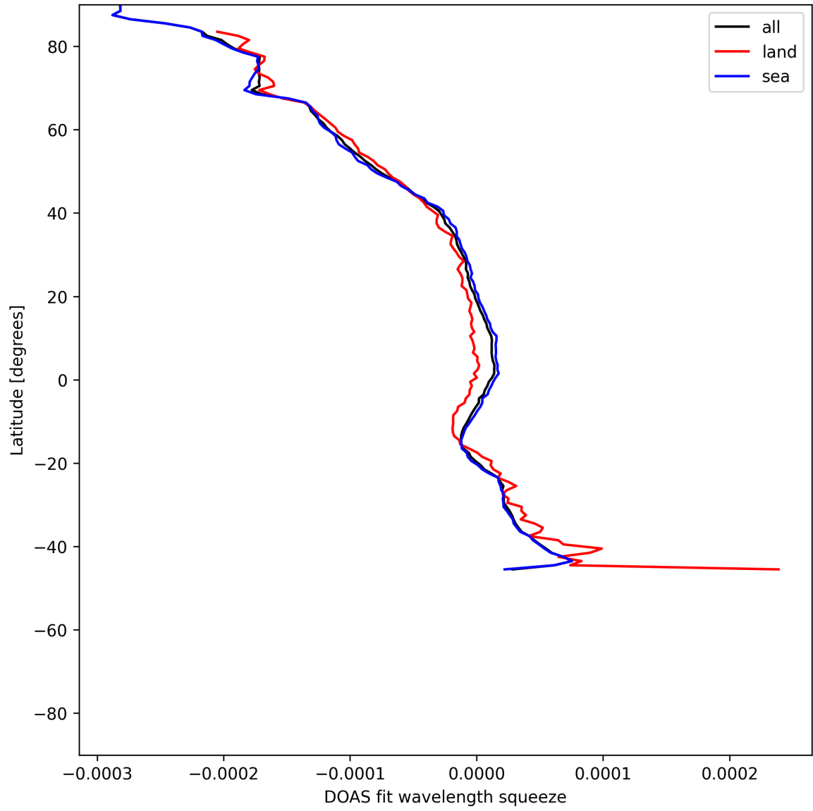
Figure 51: Zonal average of “DOAS fit wavelength squeeze” for 2025-06-24 to 2025-06-26.
