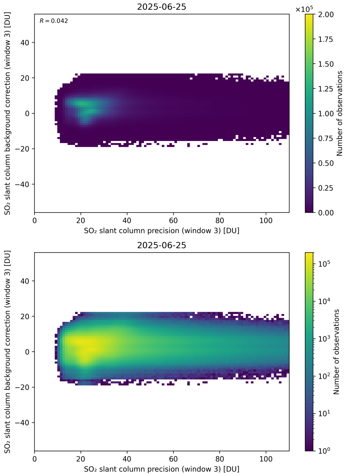
Figure 307: Scatter density plot of “SO 2 slant column precision (window 3)” against “SO 2 slant column background correction (window 3)” for 2025-06-24 to 2025-06-26.
