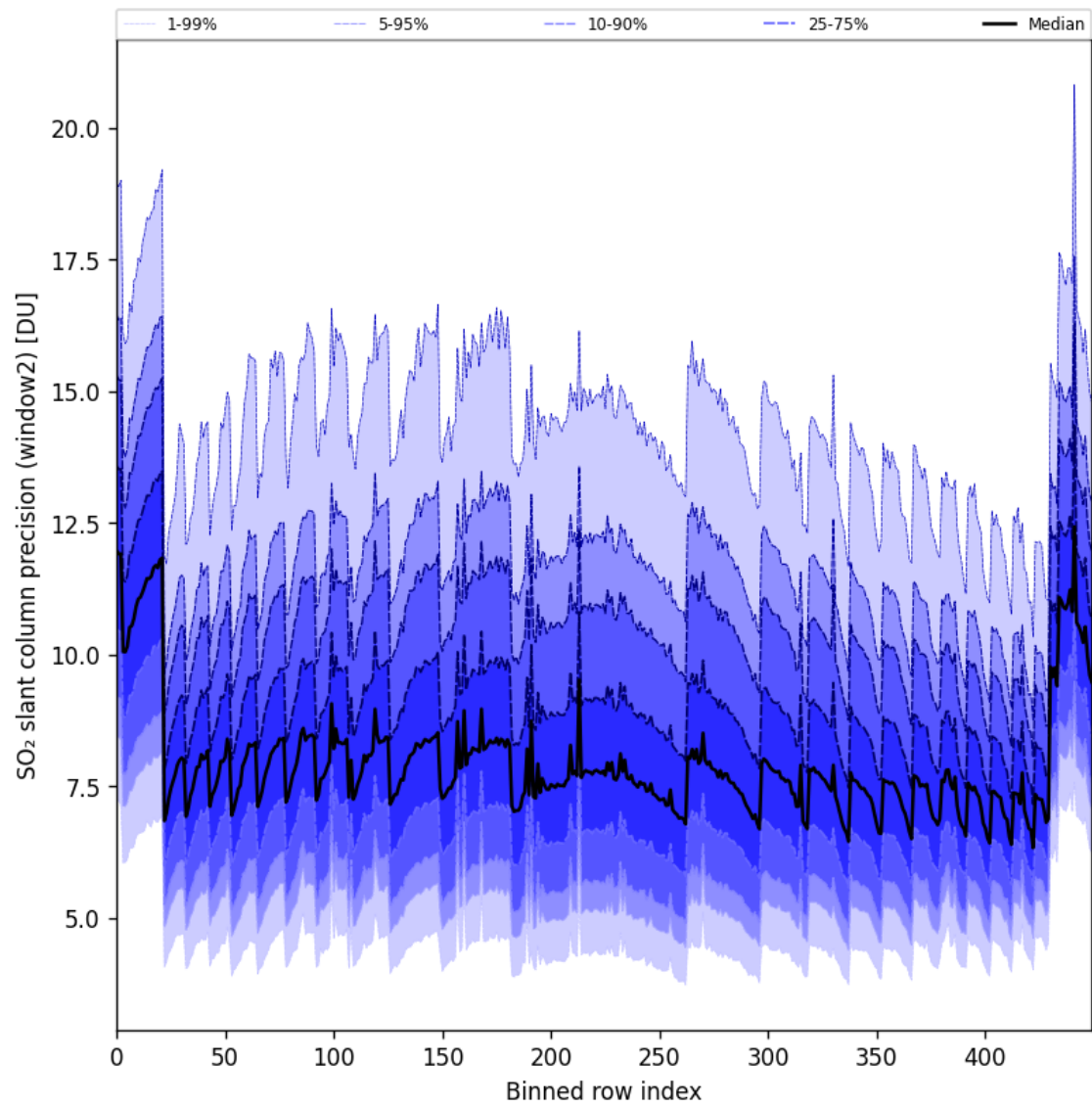
Figure 94: Along track statistics of “SO 2 slant column precision (window2)” for 2025-06-24 to 2025-06-26
