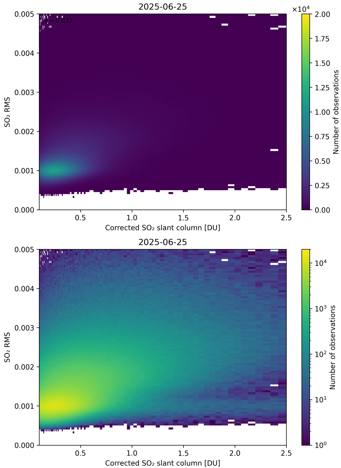
Figure 231: Scatter density plot of “Corrected SO 2 slant column” against “SO 2 RMS” for 2025-06-24 to 2025-06-26.
