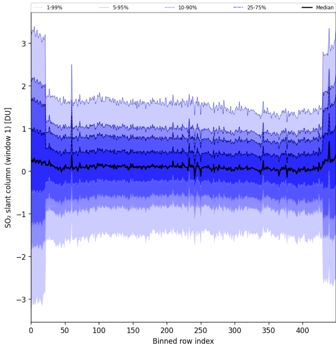
Figure 89: Along track statistics of “SO 2 slant column (window 1)” for 2025-06-24 to 2025-06-26
