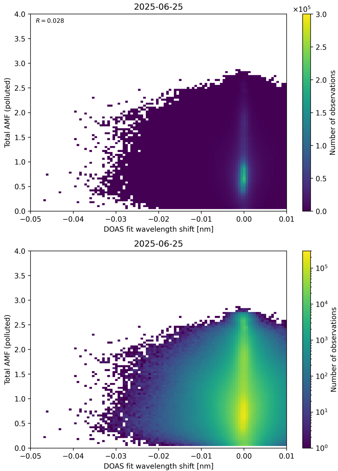
Figure 141: Scatter density plot of “DOAS fit wavelength shift” against “Total AMF (polluted)” for 2025-06-24 to 2025-06-26.
