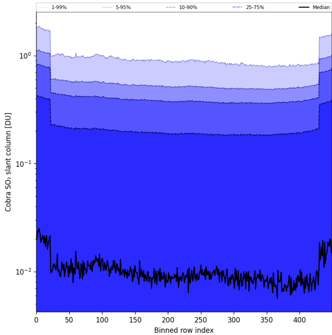
Figure 87: Along track statistics of “Cobra SO 2 slant column” for 2025-06-24 to 2025-06-26
