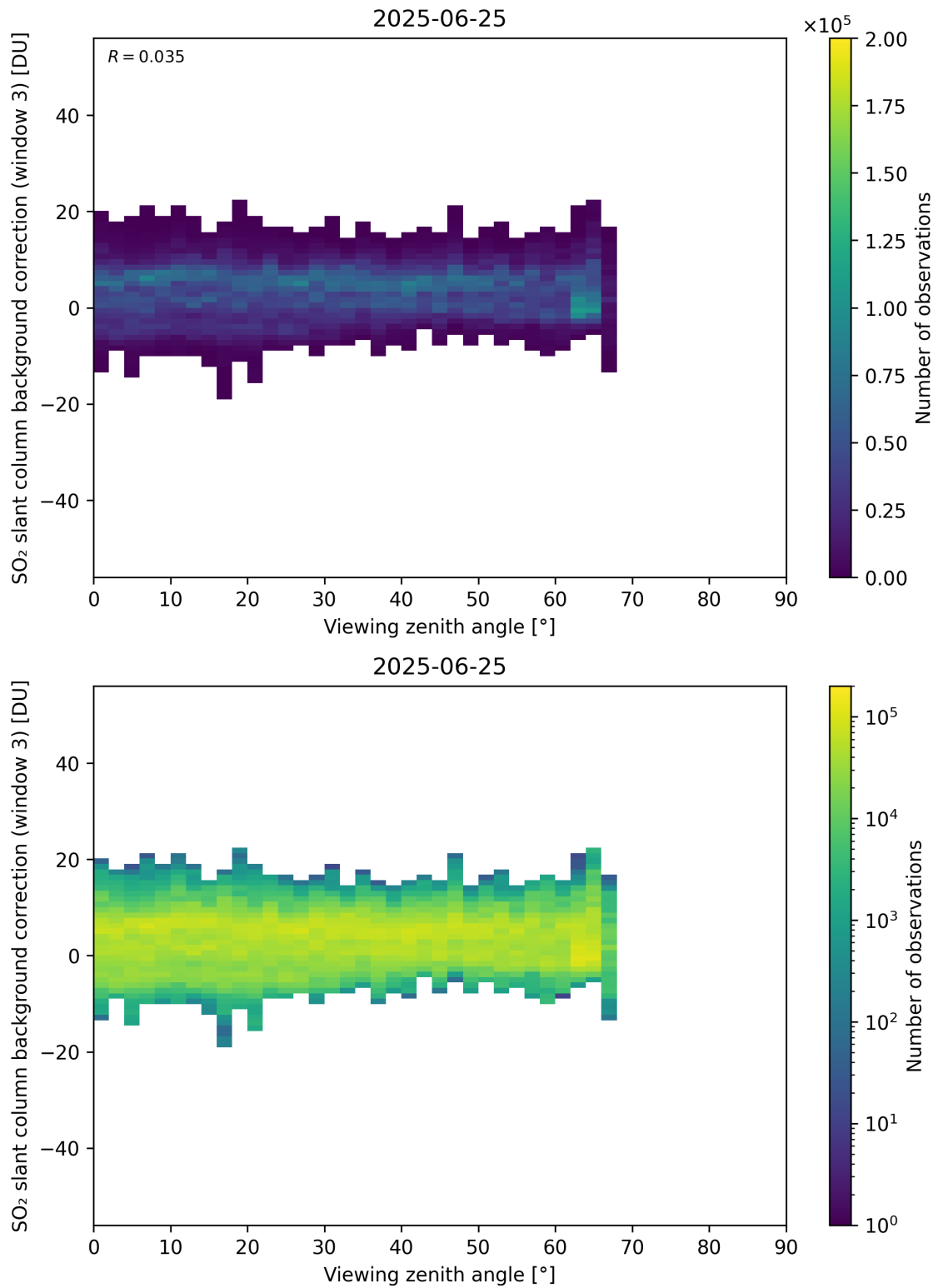
Figure 364: Scatter density plot of “Viewing zenith angle” against “SO 2 slant column background correction (window 3)” for 2025-06-24 to 2025-06-26.
