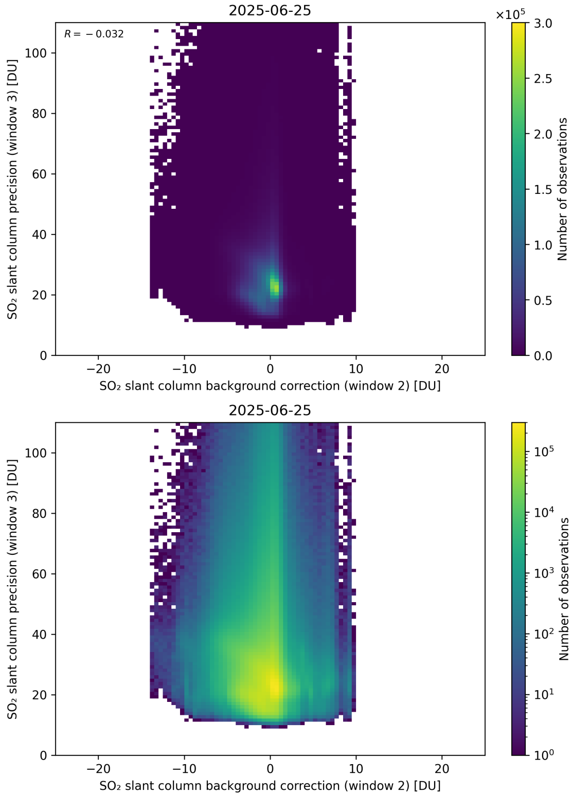
Figure 129: Scatter density plot of “SO 2 slant column background correction (window 2)” against “SO 2 slant column precision (window 3)” for 2025-06-24 to 2025-06-26.
