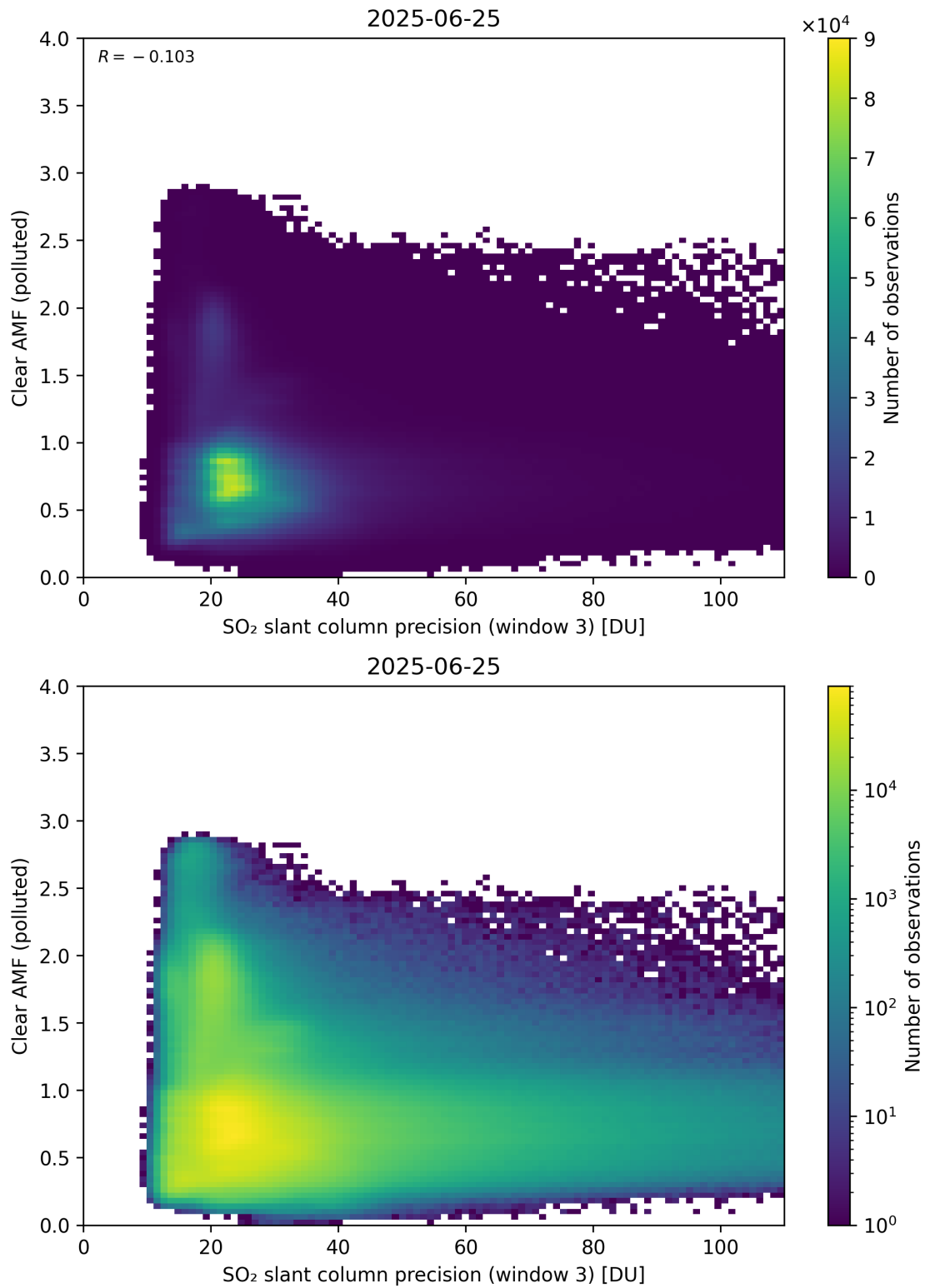
Figure 311: Scatter density plot of “SO 2 slant column precision (window 3)” against “Clear AMF (polluted)” for 2025-06-24 to 2025-06-26.
