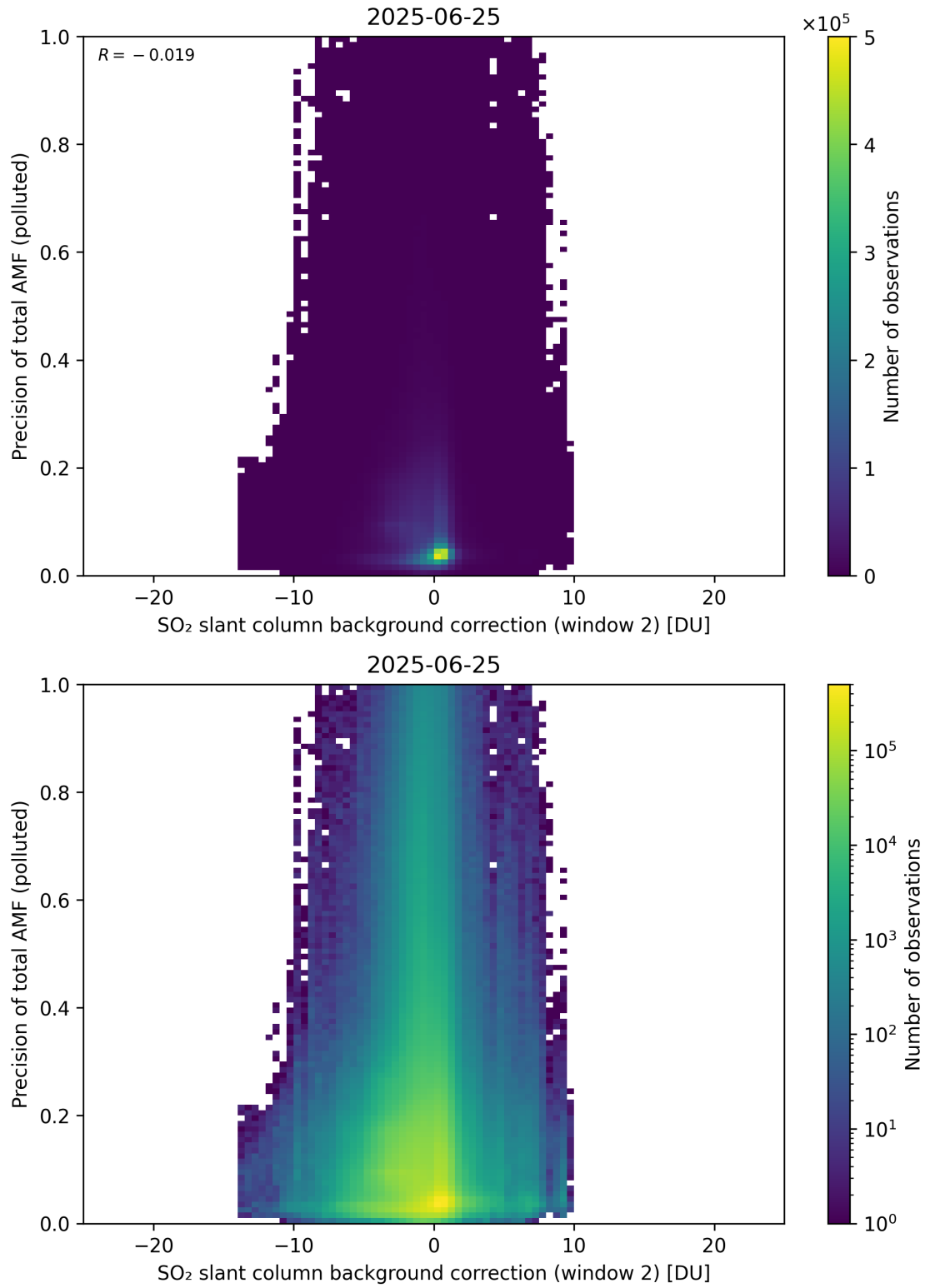
Figure 131: Scatter density plot of “SO 2 slant column background correction (window 2)” against “Precision of total AMF (polluted)” for 2025-06-24 to 2025-06-26.
