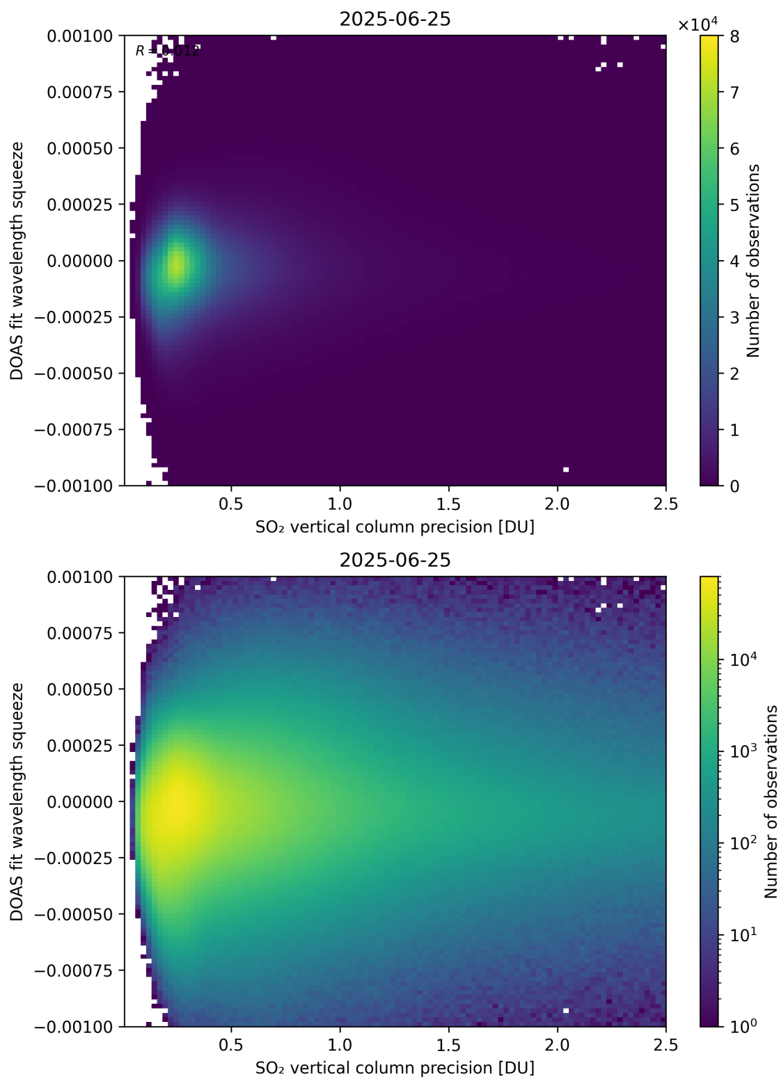
Figure 333: Scatter density plot of “SO 2 vertical column precision” against “DOAS fit wavelength squeeze” for 2025-06-24 to 2025-06-26.
