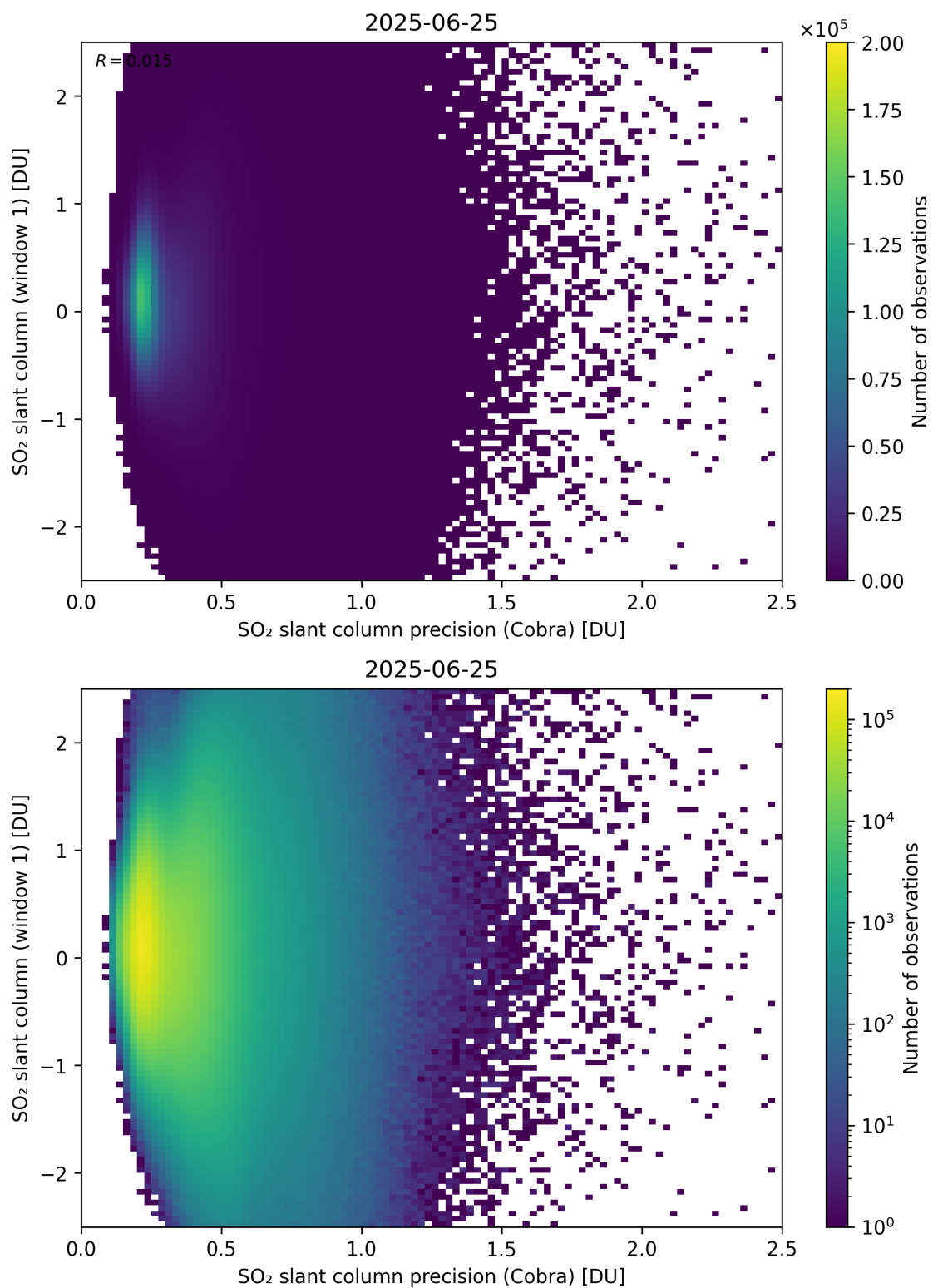
Figure 208: Scatter density plot of “SO 2 slant column precision (Cobra)” against “SO 2 slant column (window 1)” for 2025-06-24 to 2025-06-26.
