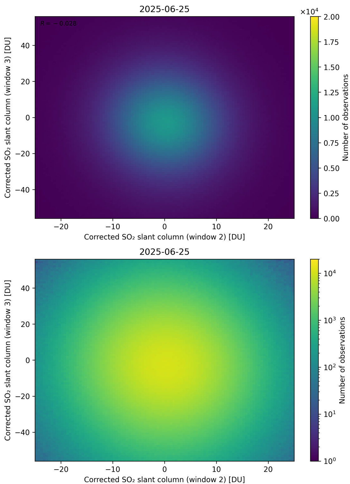
Figure 250: Scatter density plot of “Corrected SO 2 slant column (window 2)” against “Corrected SO 2 slant column (window 3)” for 2025-06-24 to 2025-06-26.
