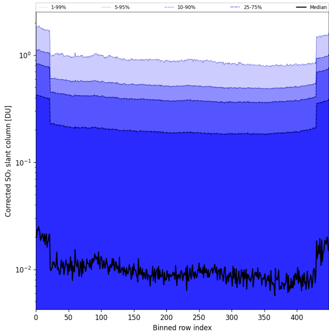
Figure 86: Along track statistics of “Corrected SO 2 slant column” for 2025-06-24 to 2025-06-26
