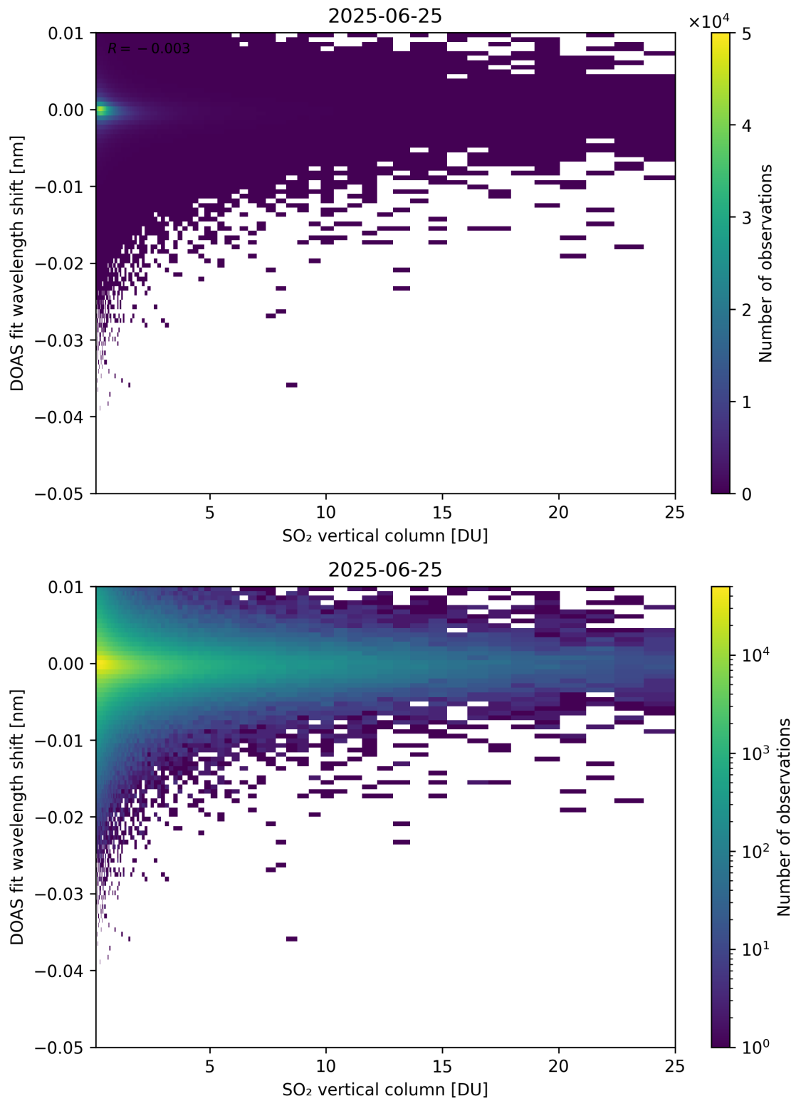
Figure 326: Scatter density plot of “SO 2 vertical column” against “DOAS fit wavelength shift” for 2025-06-24 to 2025-06-26.
