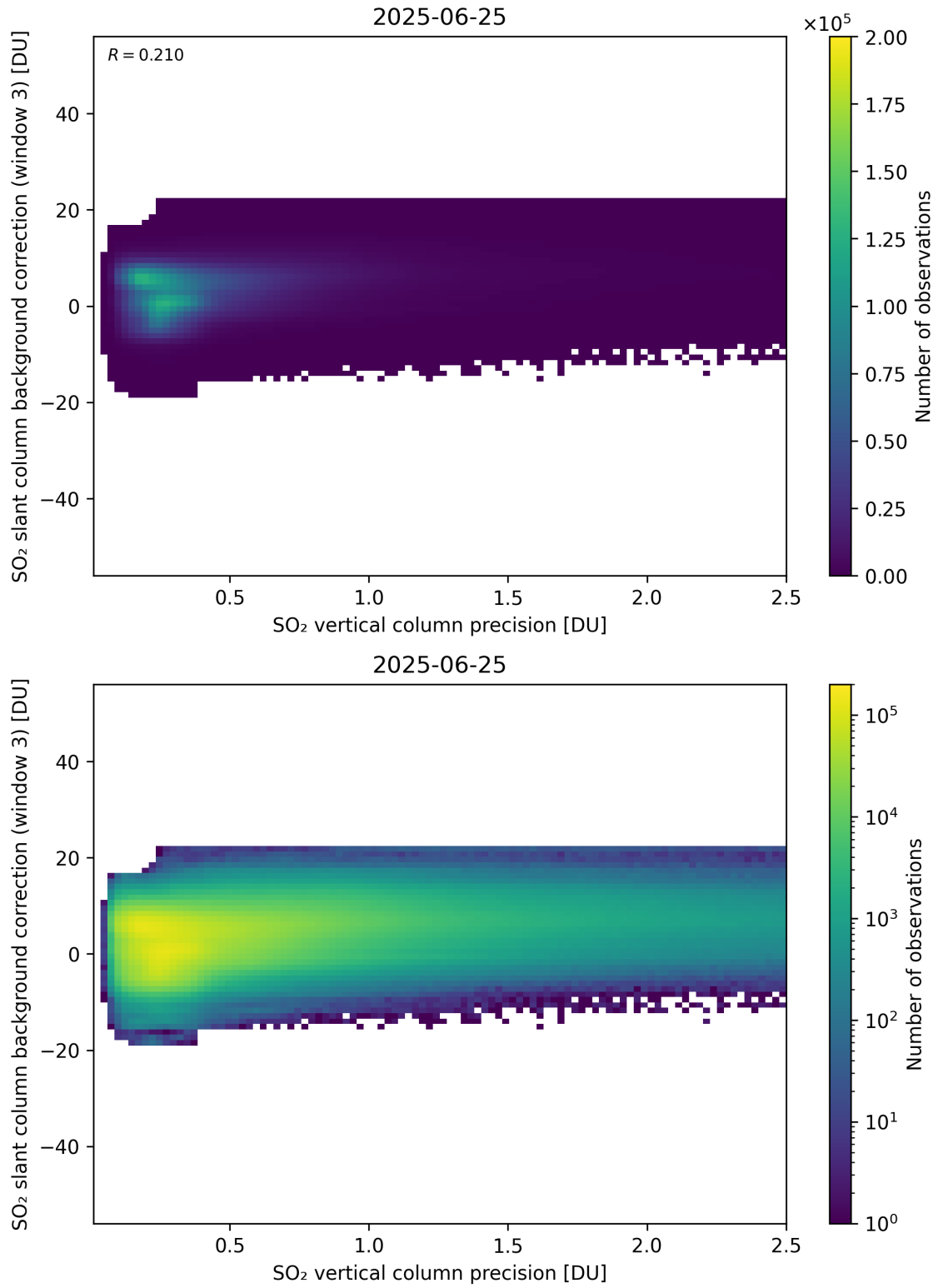
Figure 331: Scatter density plot of “SO 2 vertical column precision” against “SO 2 slant column background correction (window 3)” for 2025-06-24 to 2025-06-26.
