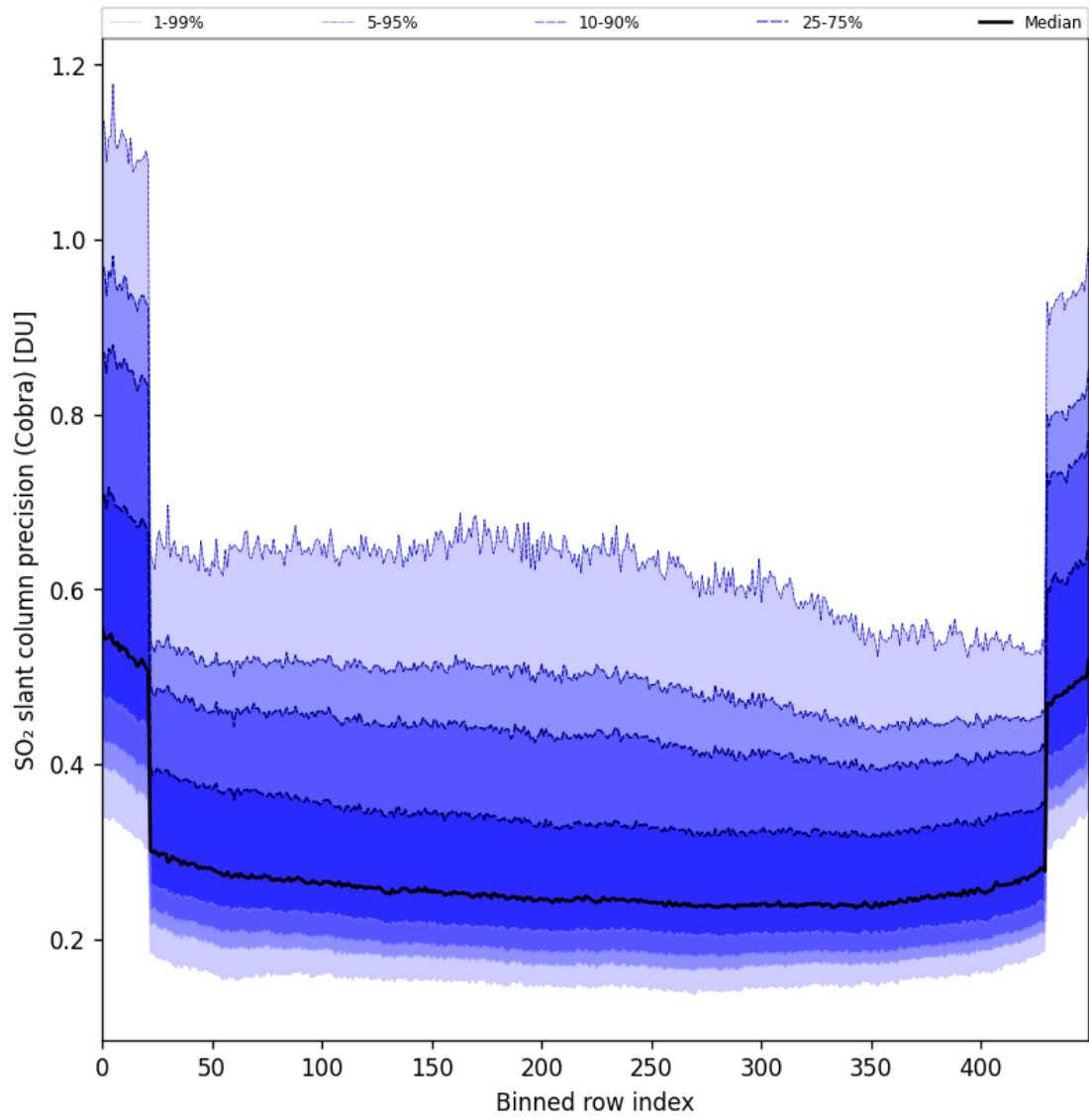
Figure 88: Along track statistics of “SO 2 slant column precision (Cobra)” for 2025-06-24 to 2025-06-26
