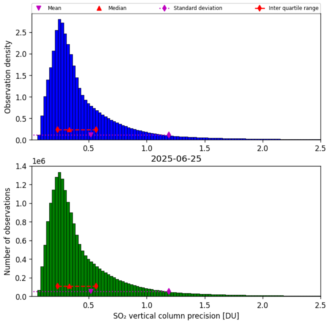
Figure 59: Histogram of “SO 2 vertical column precision” for 2025-06-24 to 2025-06-26
