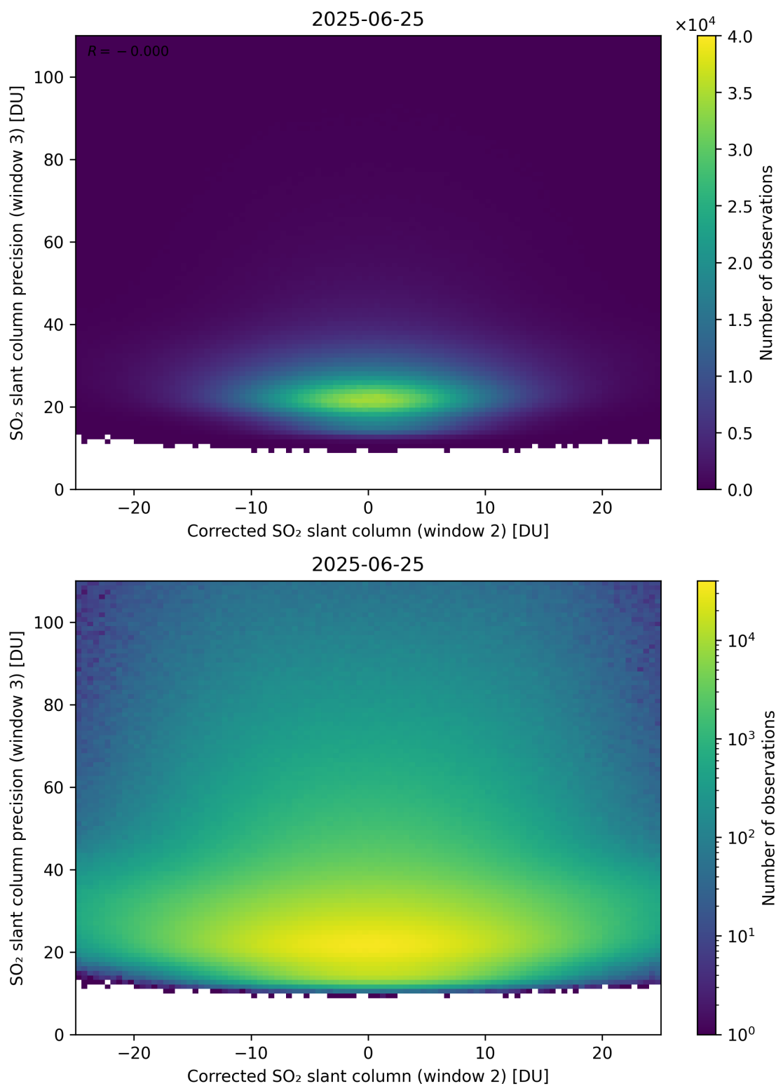
Figure 252: Scatter density plot of “Corrected SO 2 slant column (window 2)” against “SO 2 slant column precision (window 3)” for 2025-06-24 to 2025-06-26.
