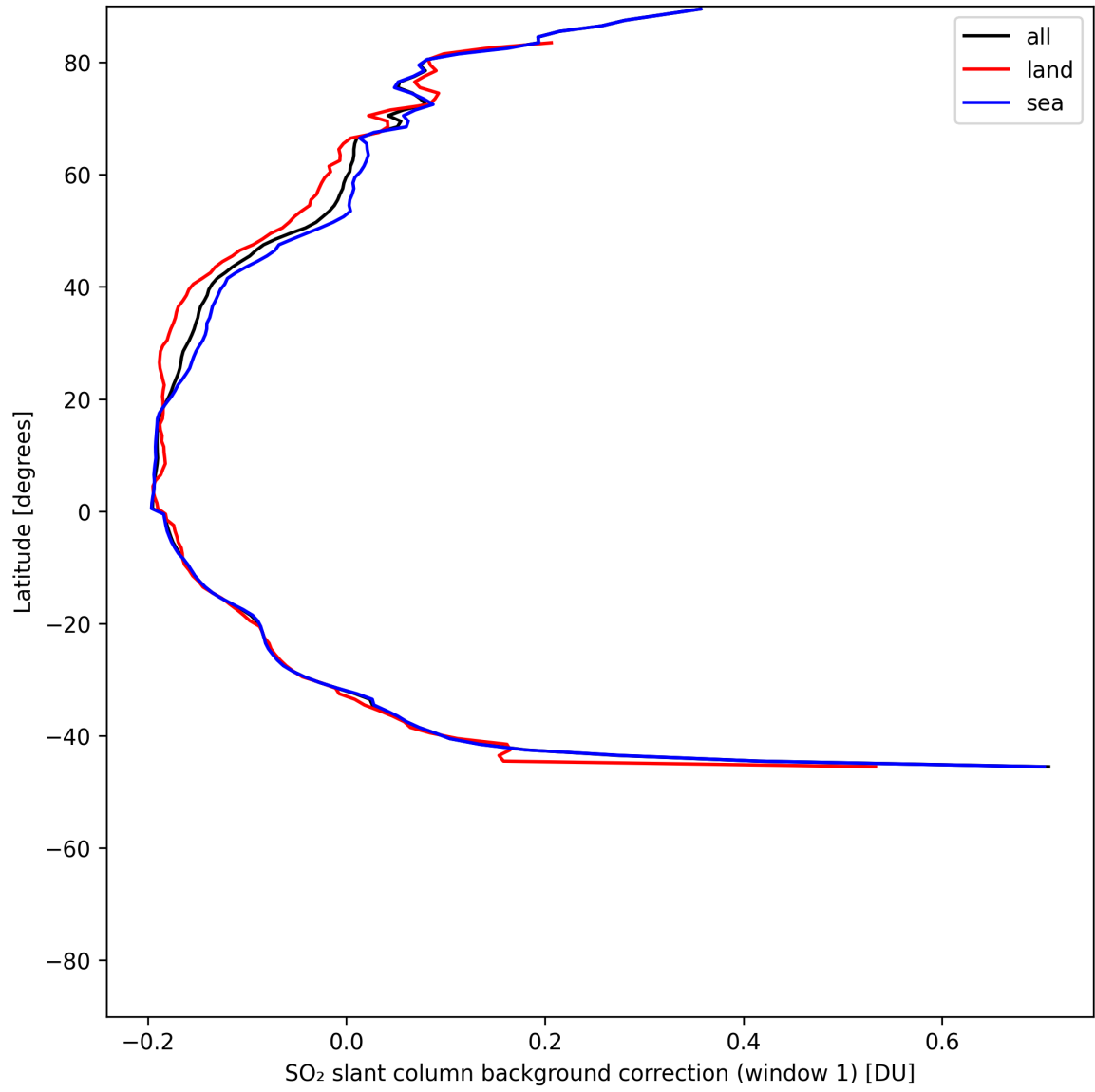
Figure 40: Zonal average of “SO 2 slant column background correction (window 1)” for 2025-06-24 to 2025-06-26.
