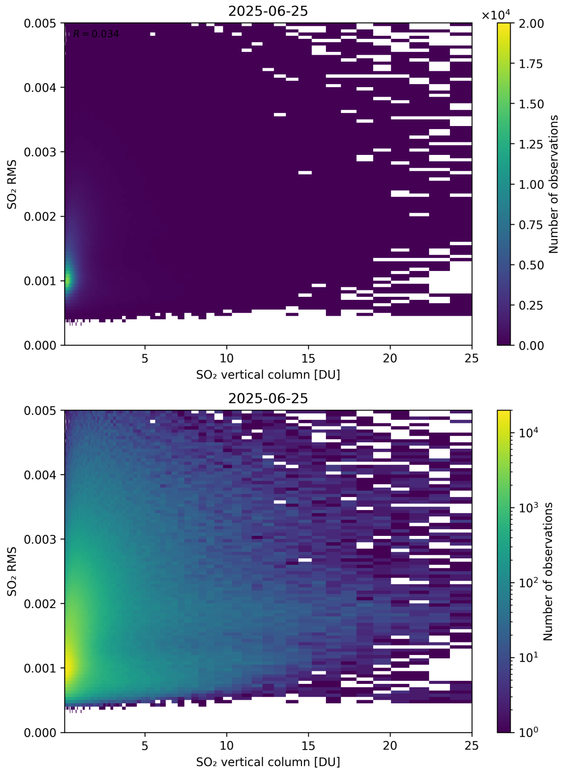
Figure 328: Scatter density plot of “SO 2 vertical column” against “SO 2 RMS” for 2025-06-24 to 2025-06-26.
