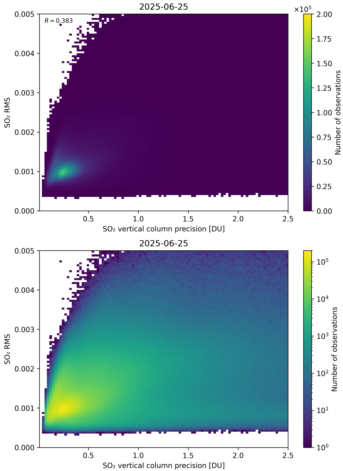
Figure 334: Scatter density plot of “SO 2 vertical column precision” against “SO 2 RMS” for 2025-06-24 to 2025-06-26.
