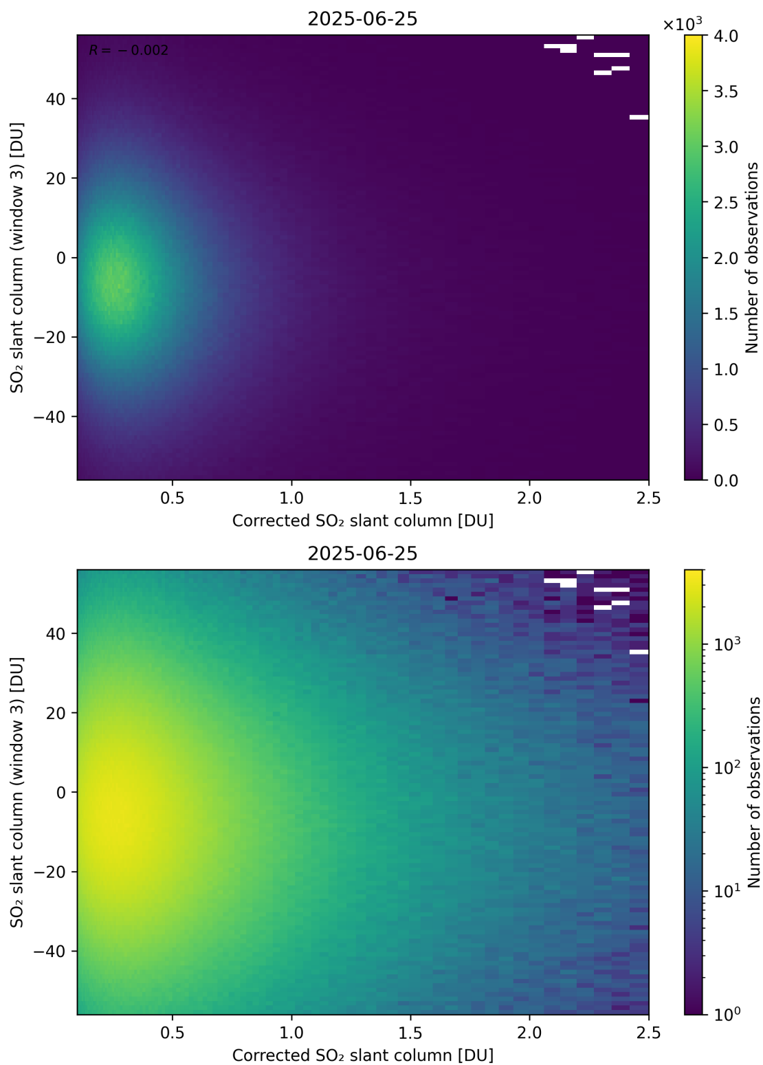
Figure 240: Scatter density plot of “Corrected SO 2 slant column” against “SO 2 slant column (window 3)” for 2025-06-24 to 2025-06-26.
