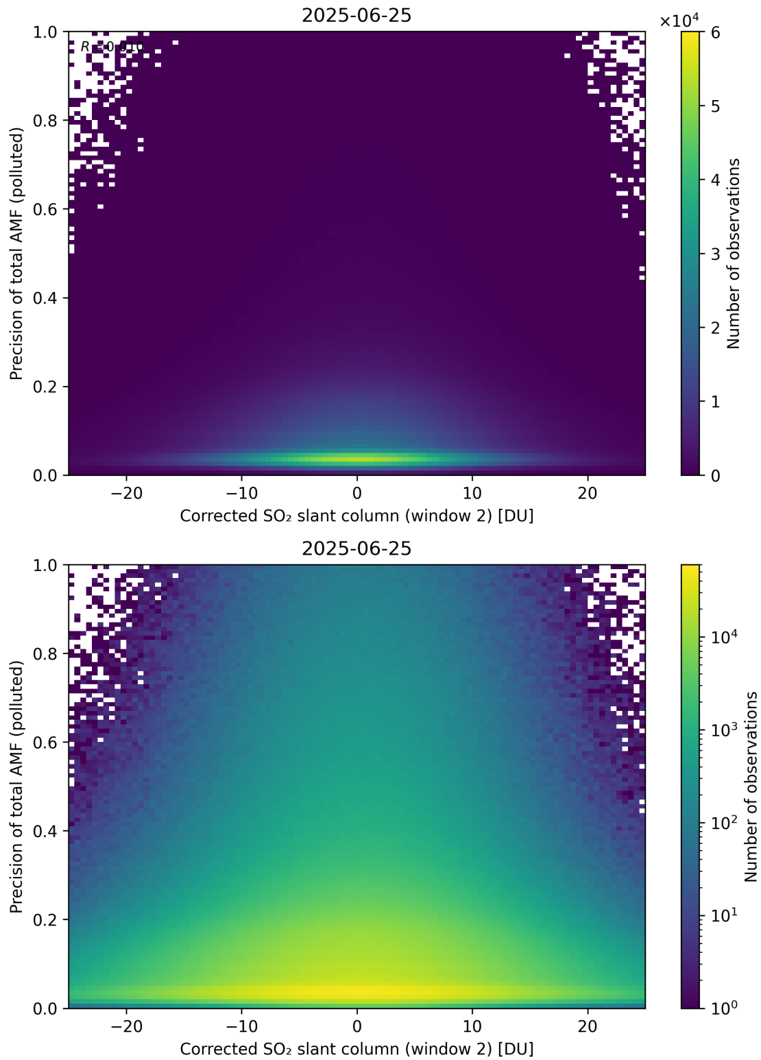
Figure 254: Scatter density plot of “Corrected SO 2 slant column (window 2)” against “Precision of total AMF (polluted)” for 2025-06-24 to 2025-06-26.
