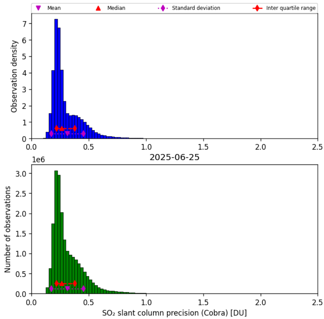
Figure 62: Histogram of “SO 2 slant column precision (Cobra)” for 2025-06-24 to 2025-06-26
