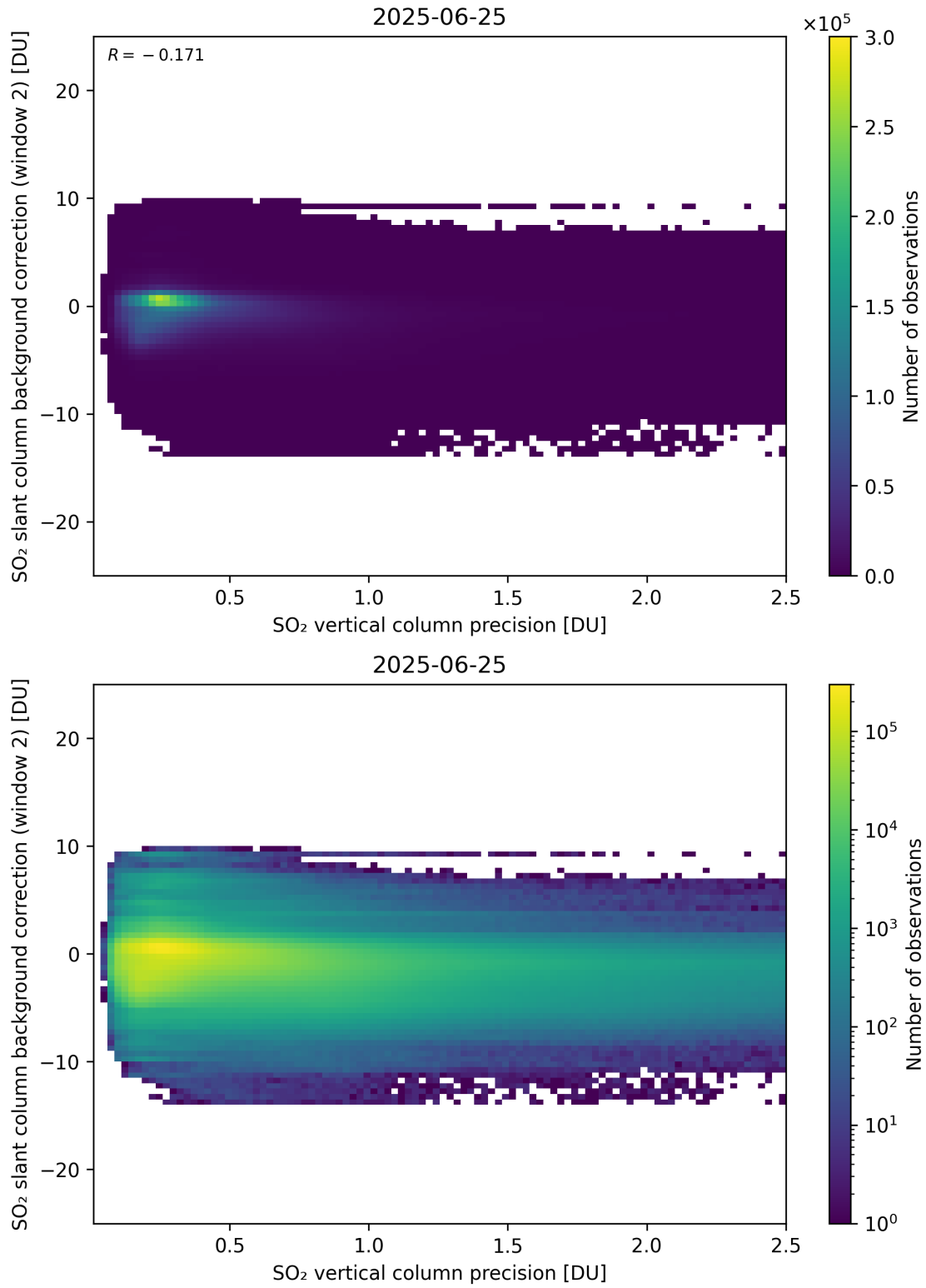
Figure 330: Scatter density plot of “SO 2 vertical column precision” against “SO 2 slant column background correction (window 2)” for 2025-06-24 to 2025-06-26.
