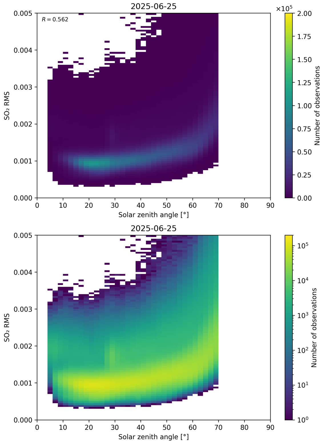
Figure 176: Scatter density plot of “Solar zenith angle” against “SO 2 RMS” for 2025-06-24 to 2025-06-26.
