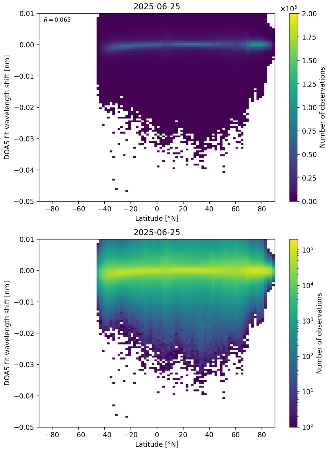
Figure 153: Scatter density plot of “Latitude” against “DOAS fit wavelength shift” for 2025-06-24 to 2025-06-26.
