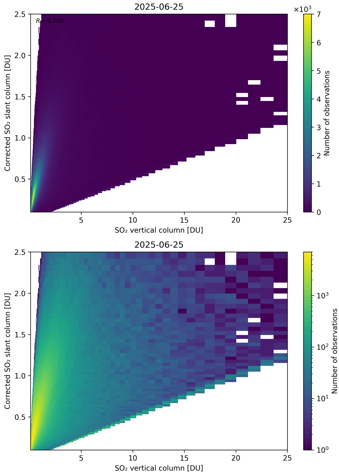
Figure 351: Scatter density plot of “SO 2 vertical column” against “Corrected SO 2 slant column” for 2025-06-24 to 2025-06-26.
