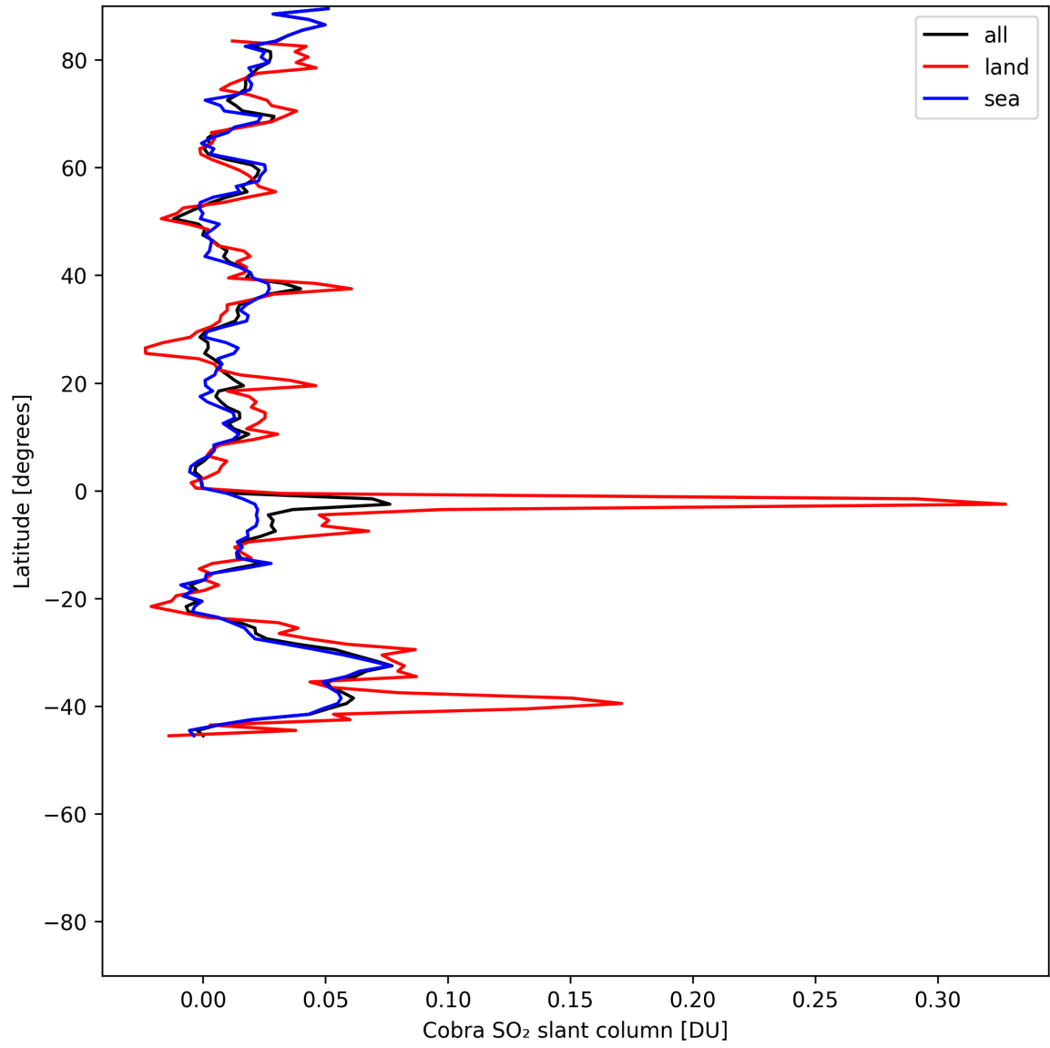
Figure 35: Zonal average of “Cobra SO 2 slant column” for 2025-06-24 to 2025-06-26.
