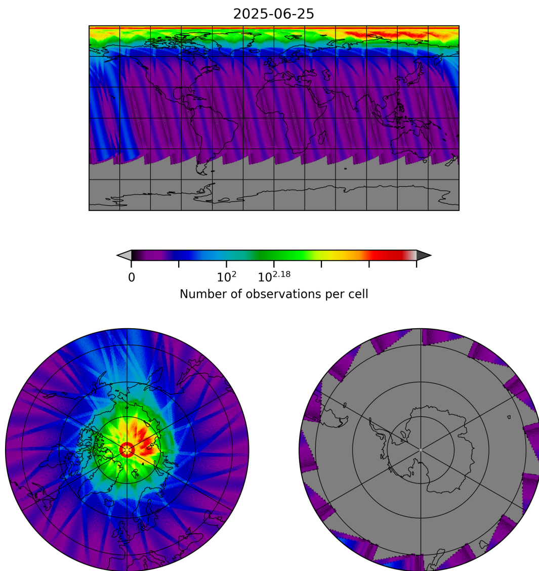
Figure 30: Map of the number of observations for 2025-06-24 to 2025-06-26
