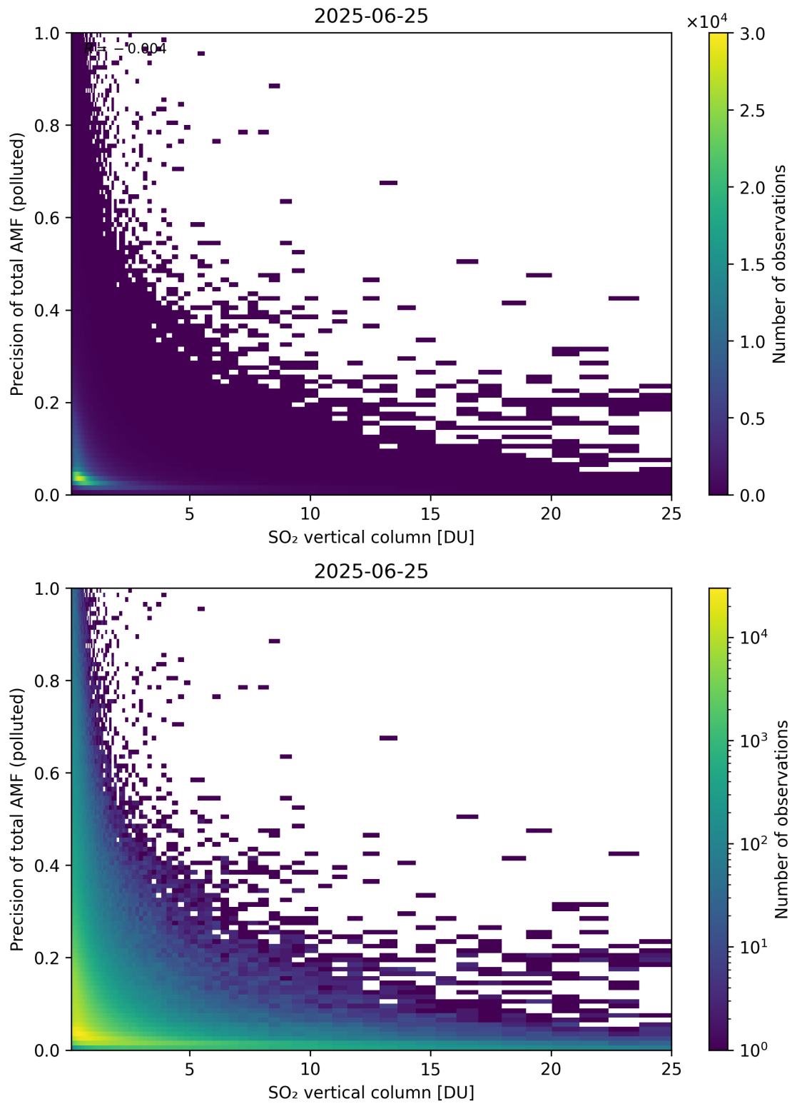
Figure 360: Scatter density plot of “SO 2 vertical column” against “Precision of total AMF (polluted)” for 2025-06-24 to 2025-06-26.
