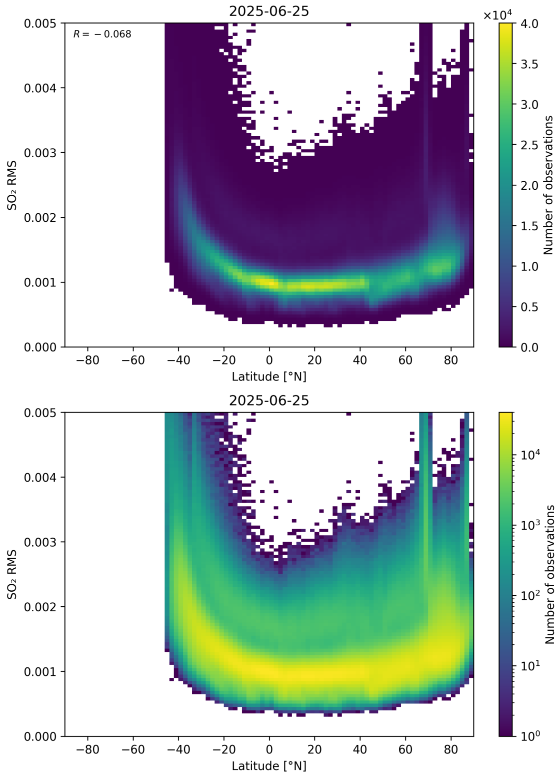
Figure 155: Scatter density plot of “Latitude” against “SO 2 RMS” for 2025-06-24 to 2025-06-26.
