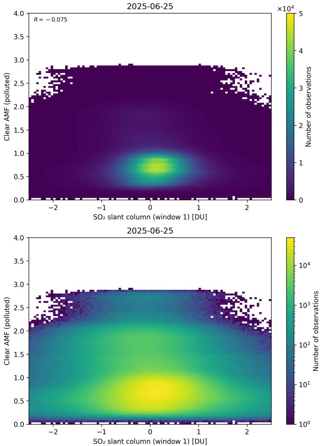
Figure 282: Scatter density plot of “SO 2 slant column (window 1)” against “Clear AMF (polluted)” for 2025-06-24 to 2025-06-26.
