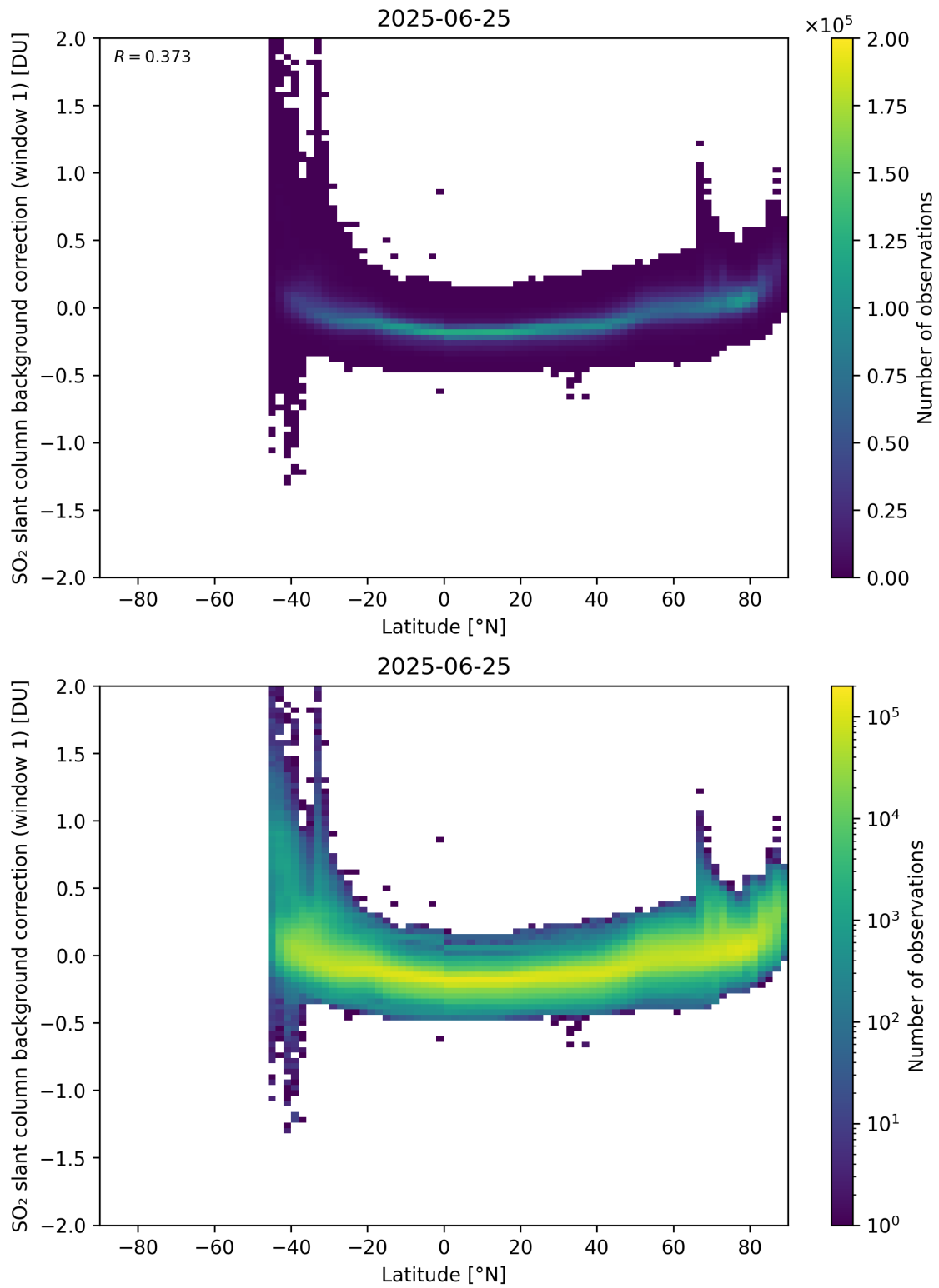
Figure 150: Scatter density plot of “Latitude” against “SO 2 slant column background correction (window 1)” for 2025-06-24 to 2025-06-26.
