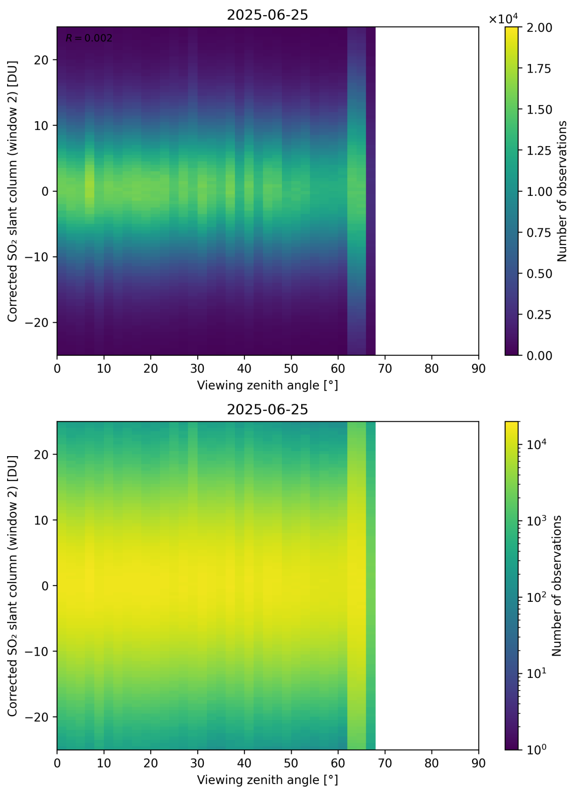
Figure 374: Scatter density plot of “Viewing zenith angle” against “Corrected SO 2 slant column (window 2)” for 2025-06-24 to 2025-06-26.
