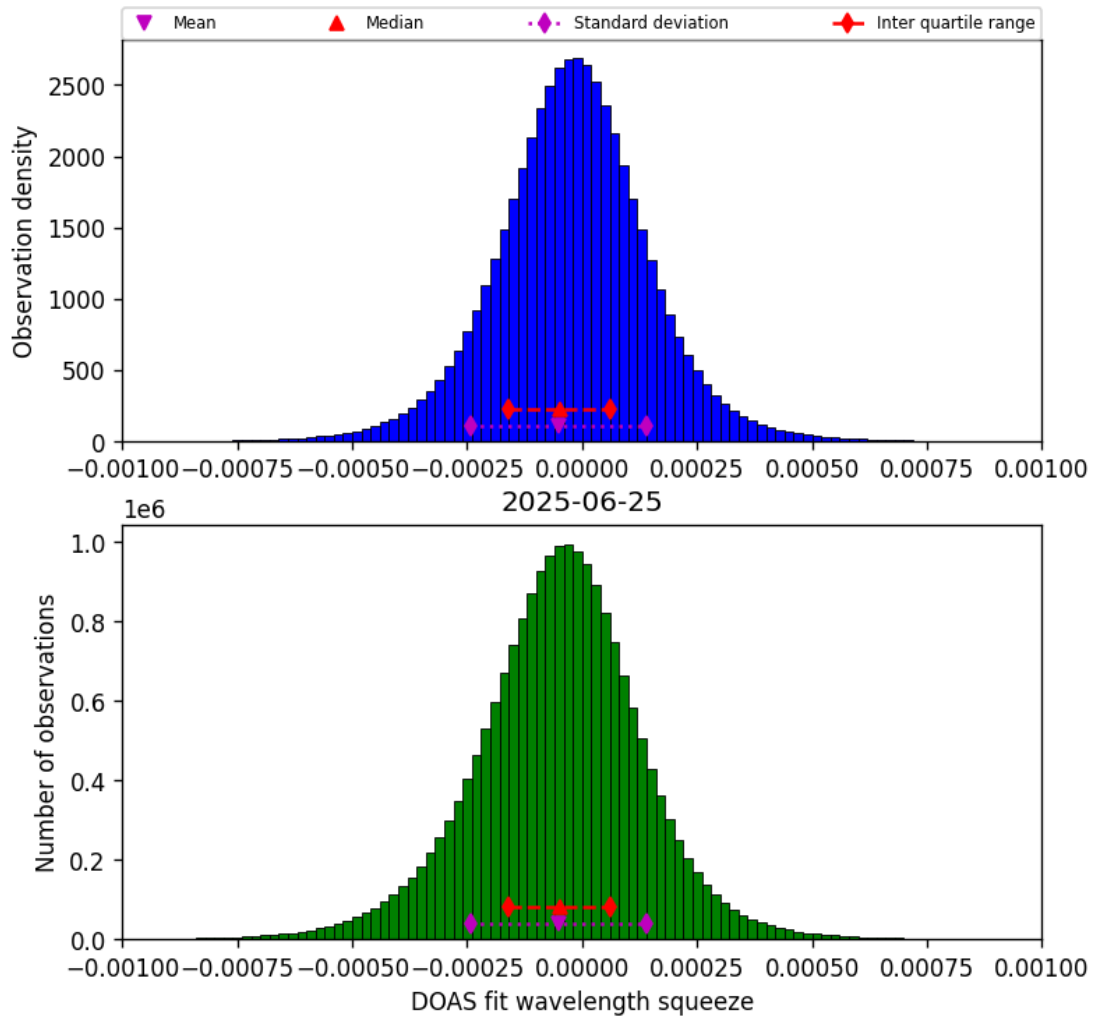
Figure 77: Histogram of “DOAS fit wavelength squeeze” for 2025-06-24 to 2025-06-26
