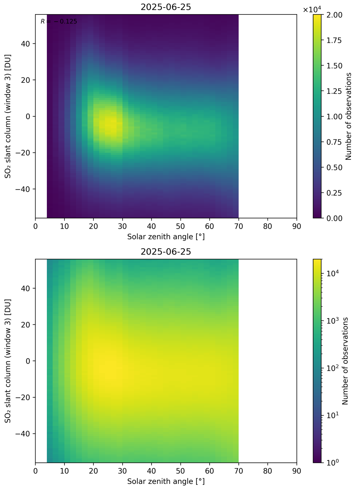
Figure 187: Scatter density plot of “Solar zenith angle” against “SO 2 slant column (window 3)” for 2025-06-24 to 2025-06-26.
