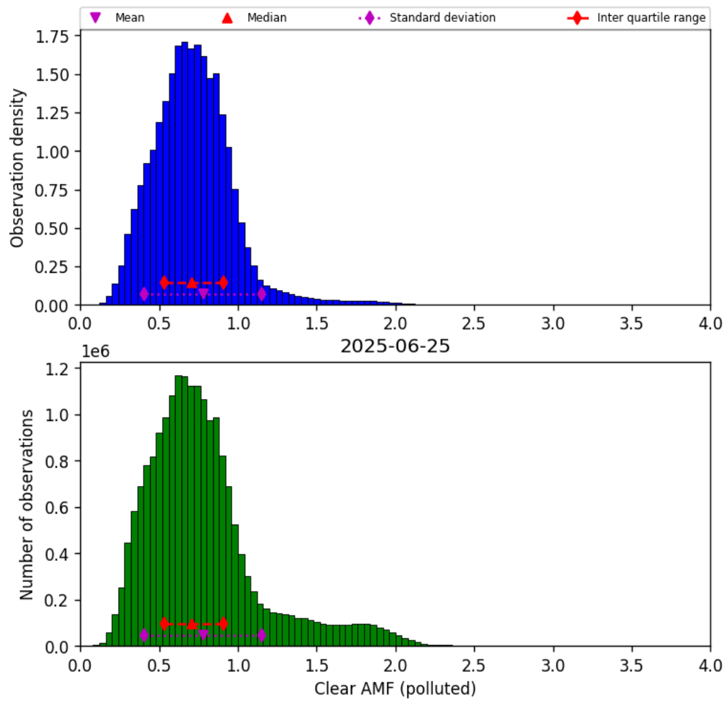
Figure 81: Histogram of “Clear AMF (polluted)” for 2025-06-24 to 2025-06-26
