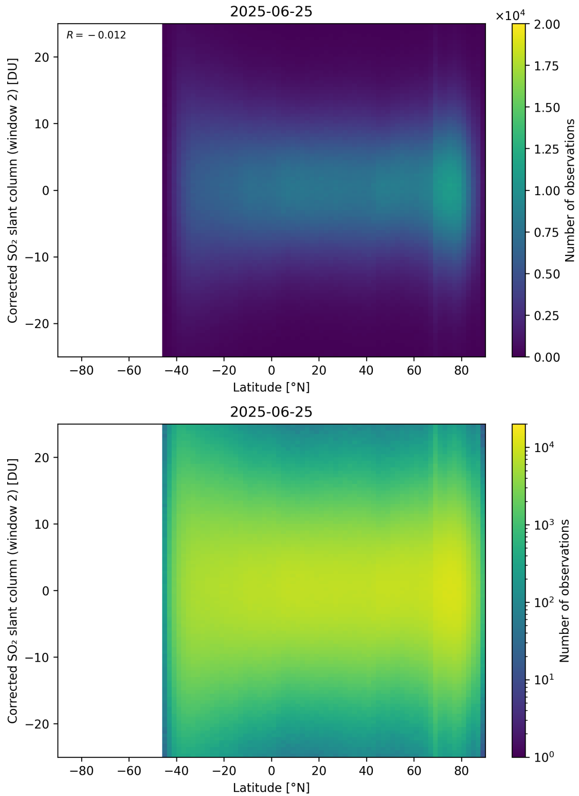
Figure 160: Scatter density plot of “Latitude” against “Corrected SO 2 slant column (window 2)” for 2025-06-24 to 2025-06-26.
