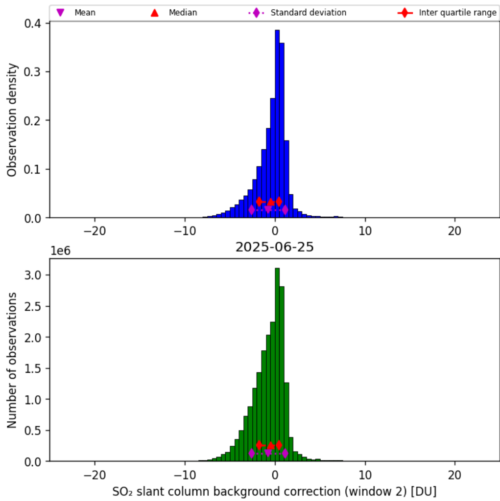
Figure 70: Histogram of “SO 2 slant column background correction (window 2)” for 2025-06-24 to 2025-06-26
