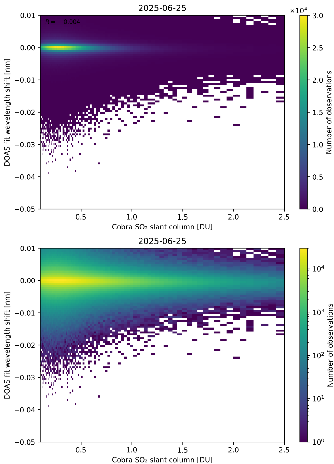
Figure 196: Scatter density plot of “Cobra SO 2 slant column” against “DOAS fit wavelength shift” for 2025-06-24 to 2025-06-26.
