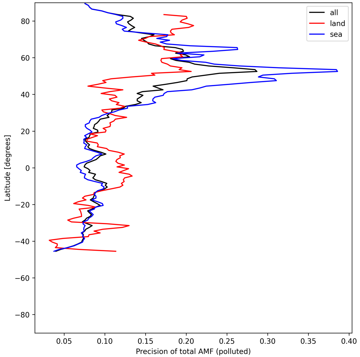
Figure 54: Zonal average of “Precision of total AMF (polluted)” for 2025-06-24 to 2025-06-26.
