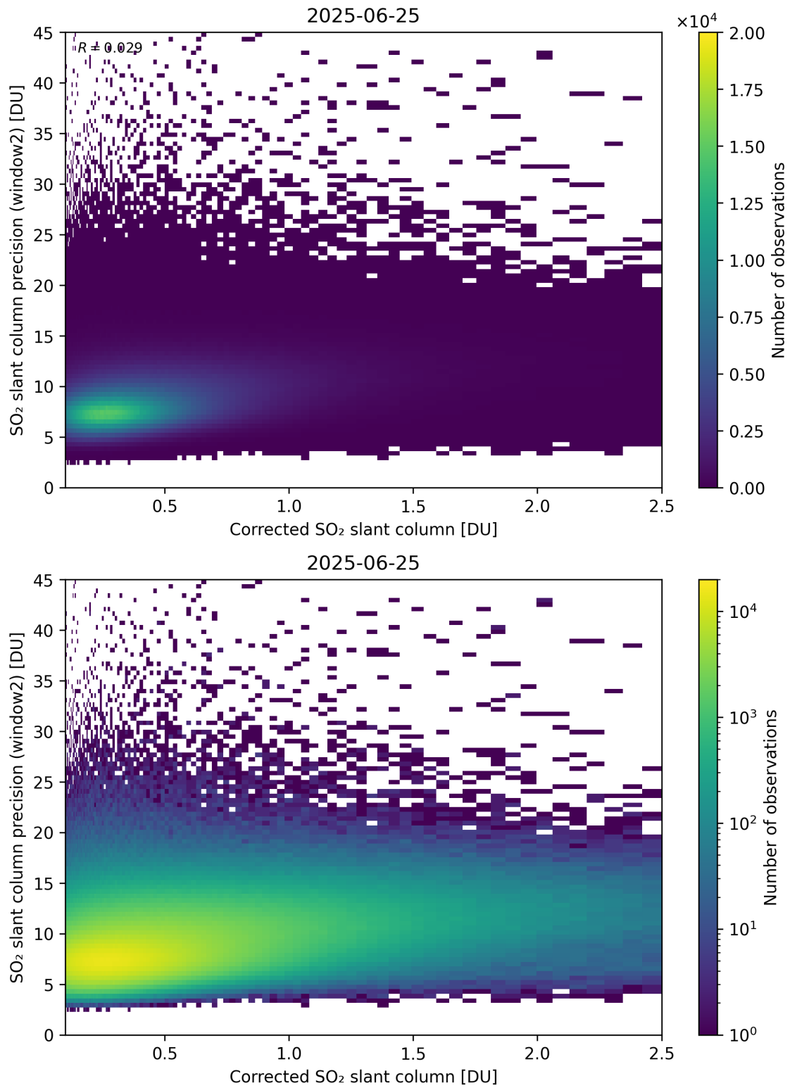
Figure 239: Scatter density plot of “Corrected SO 2 slant column” against “SO 2 slant column precision (window2)” for 2025-06-24 to 2025-06-26.
