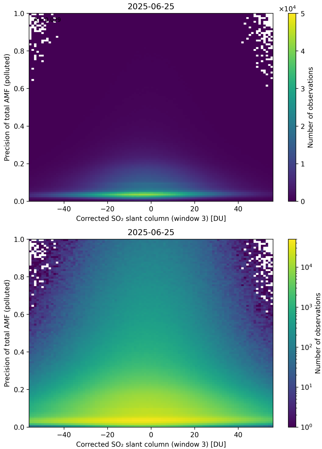
Figure 261: Scatter density plot of “Corrected SO 2 slant column (window 3)” against “Precision of total AMF (polluted)” for 2025-06-24 to 2025-06-26.
