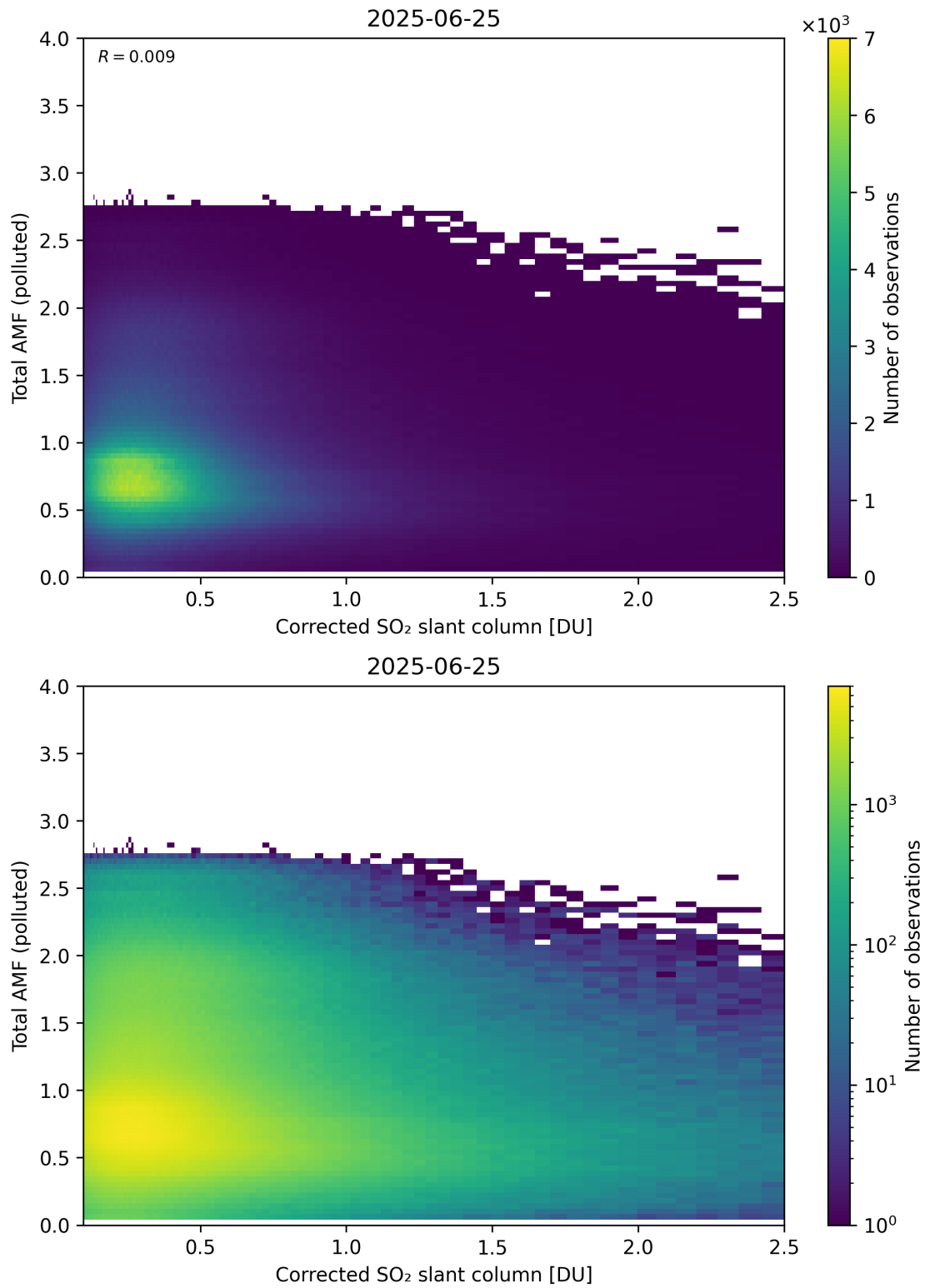
Figure 242: Scatter density plot of “Corrected SO 2 slant column” against “Total AMF (polluted)” for 2025-06-24 to 2025-06-26.
