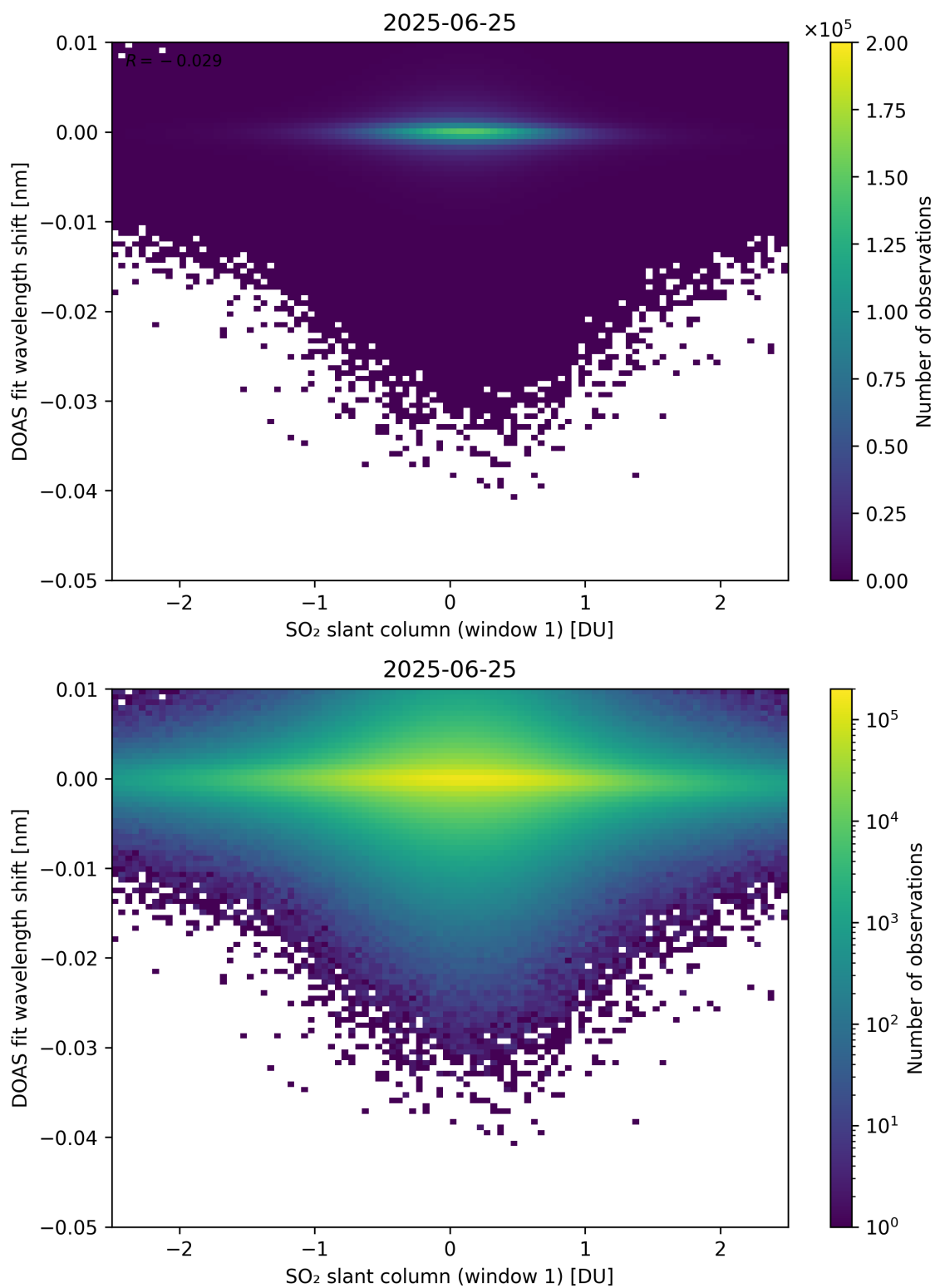
Figure 265: Scatter density plot of “SO 2 slant column (window 1)” against “DOAS fit wavelength shift” for 2025-06-24 to 2025-06-26.
