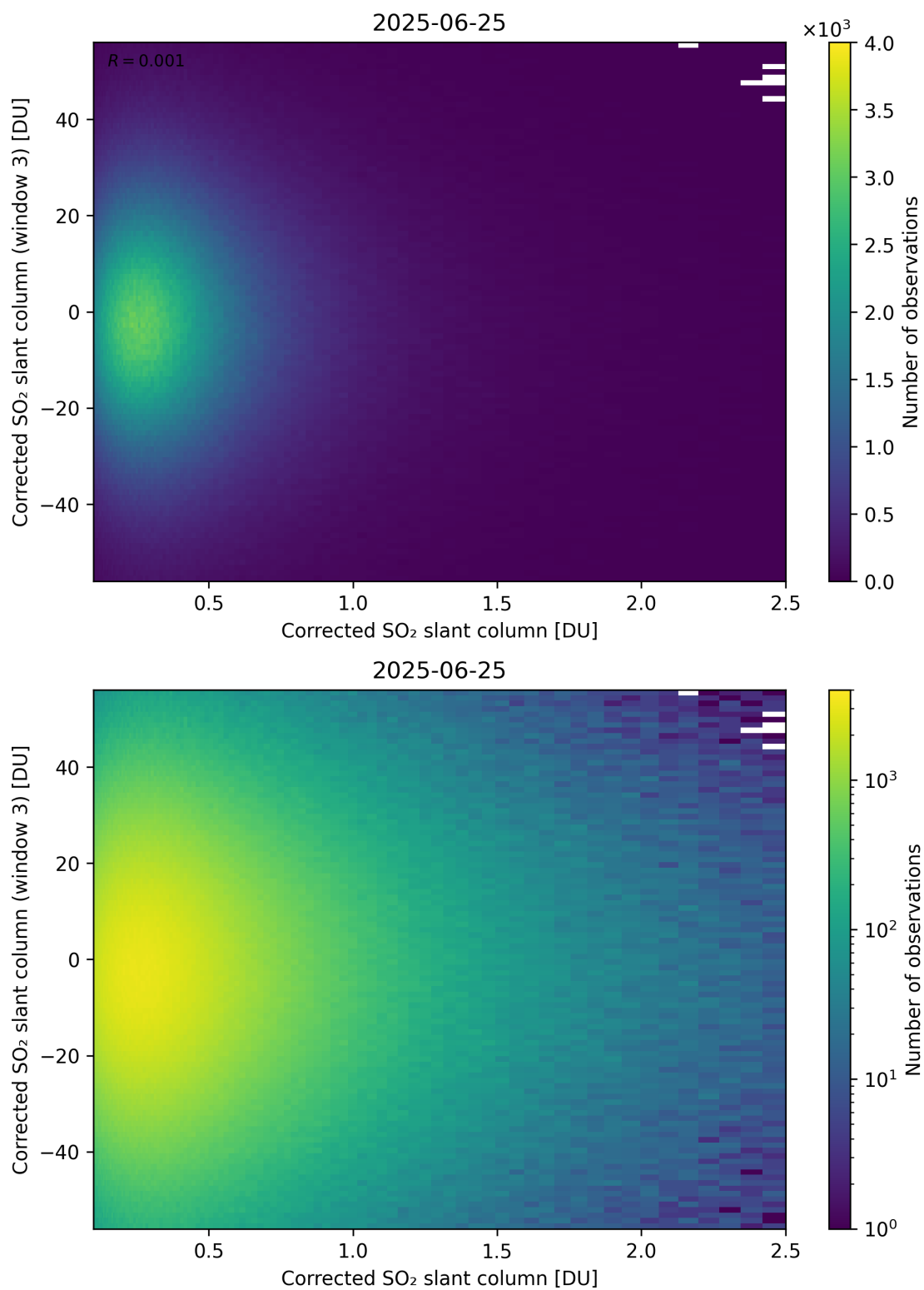
Figure 236: Scatter density plot of “Corrected SO 2 slant column” against “Corrected SO 2 slant column (window 3)” for 2025-06-24 to 2025-06-26.
