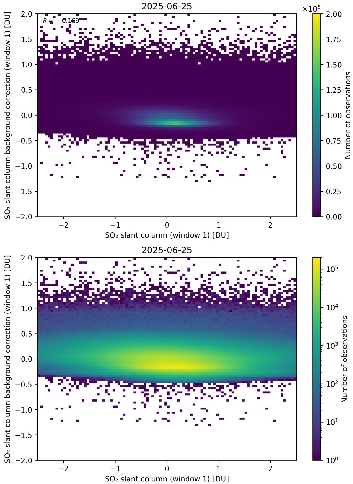
Figure 262: Scatter density plot of “SO 2 slant column (window 1)” against “SO 2 slant column background correction (window 1)” for 2025-06-24 to 2025-06-26.
