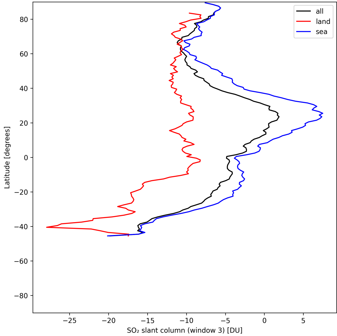
Figure 45: Zonal average of “SO 2 slant column (window 3)” for 2025-06-24 to 2025-06-26.
