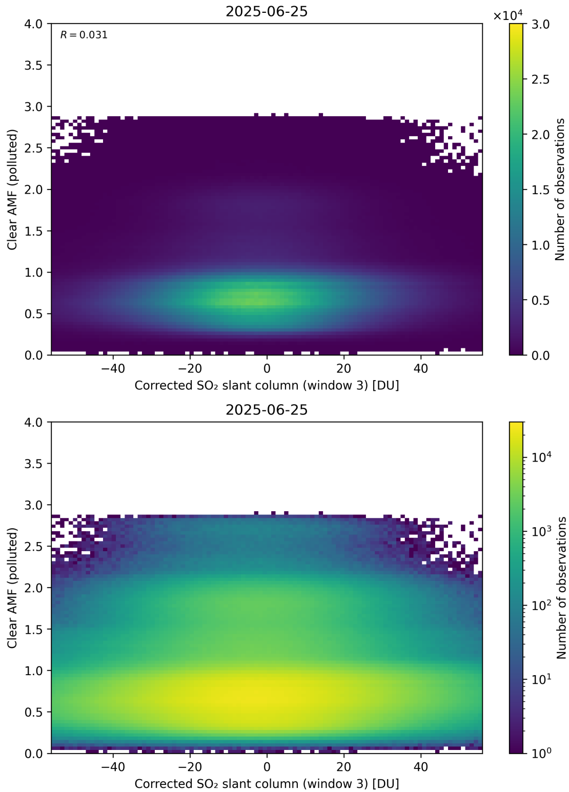
Figure 259: Scatter density plot of “Corrected SO 2 slant column (window 3)” against “Clear AMF (polluted)” for 2025-06-24 to 2025-06-26.
