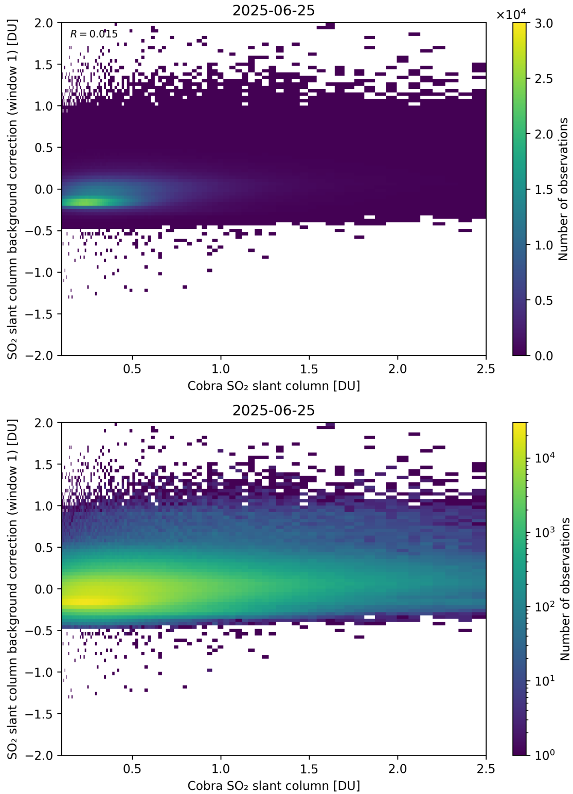
Figure 193: Scatter density plot of “Cobra SO 2 slant column” against “SO 2 slant column background correction (window 1)” for 2025-06-24 to 2025-06-26.
