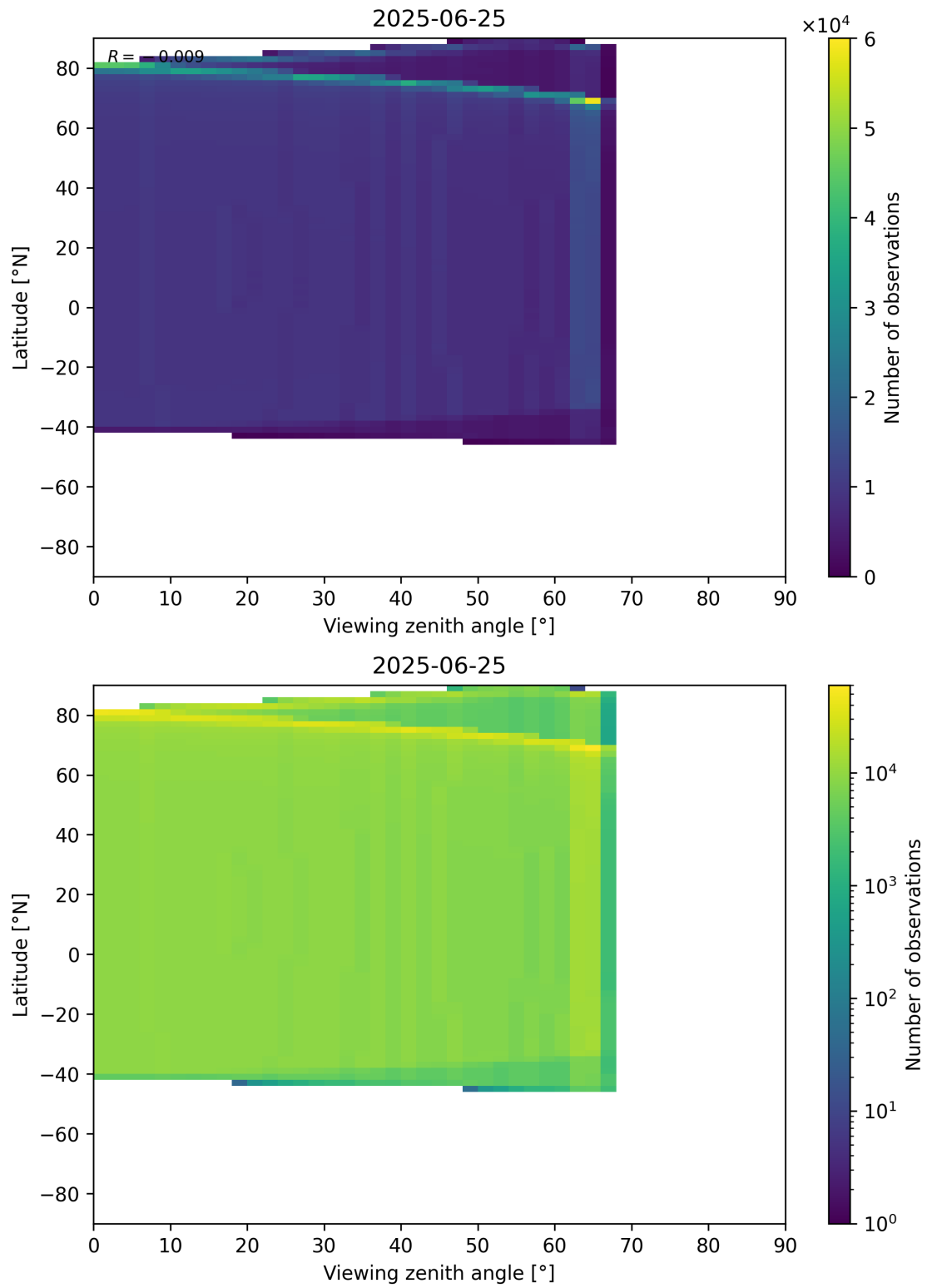
Figure 368: Scatter density plot of “Viewing zenith angle” against “Latitude” for 2025-06-24 to 2025-06-26.
