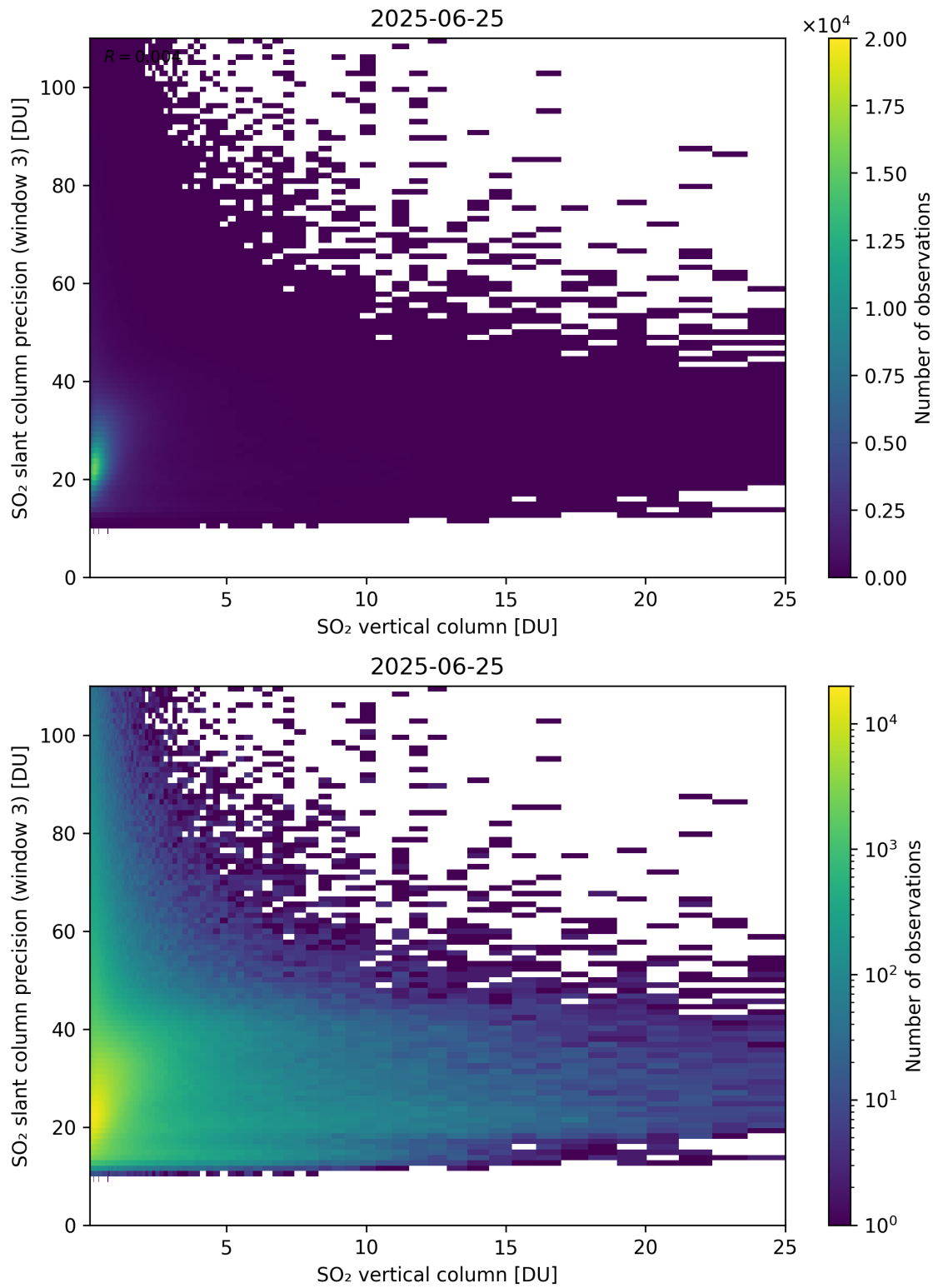
Figure 358: Scatter density plot of “SO 2 vertical column” against “SO 2 slant column precision (window 3)” for 2025-06-24 to 2025-06-26.
