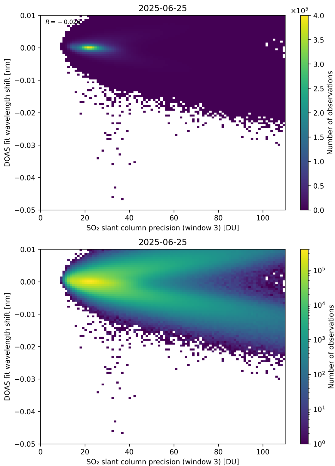
Figure 308: Scatter density plot of “SO 2 slant column precision (window 3)” against “DOAS fit wavelength shift” for 2025-06-24 to 2025-06-26.
