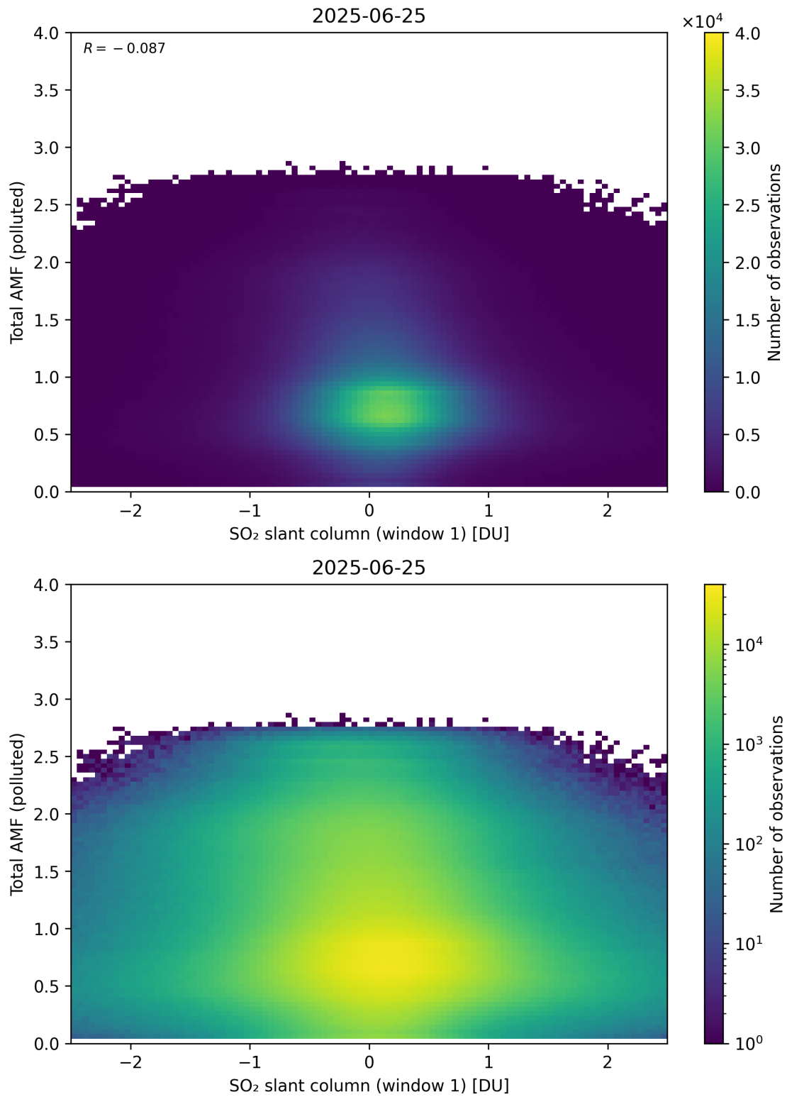
Figure 289: Scatter density plot of “SO 2 slant column (window 1)” against “Total AMF (polluted)” for 2025-06-24 to 2025-06-26.
