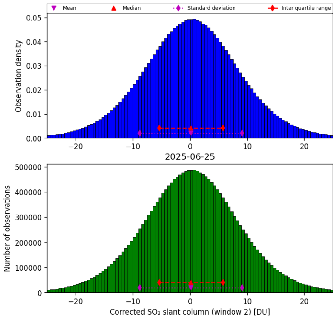
Figure 69: Histogram of “Corrected SO 2 slant column (window 2)” for 2025-06-24 to 2025-06-26
