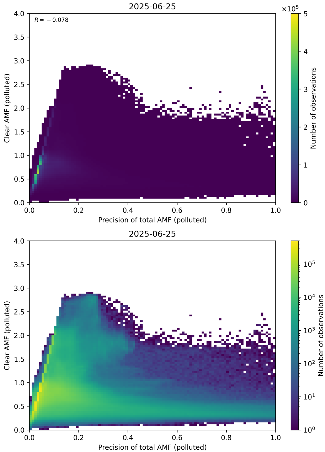
Figure 320: Scatter density plot of “Precision of total AMF (polluted)” against “Clear AMF (polluted)” for 2025-06-24 to 2025-06-26.
