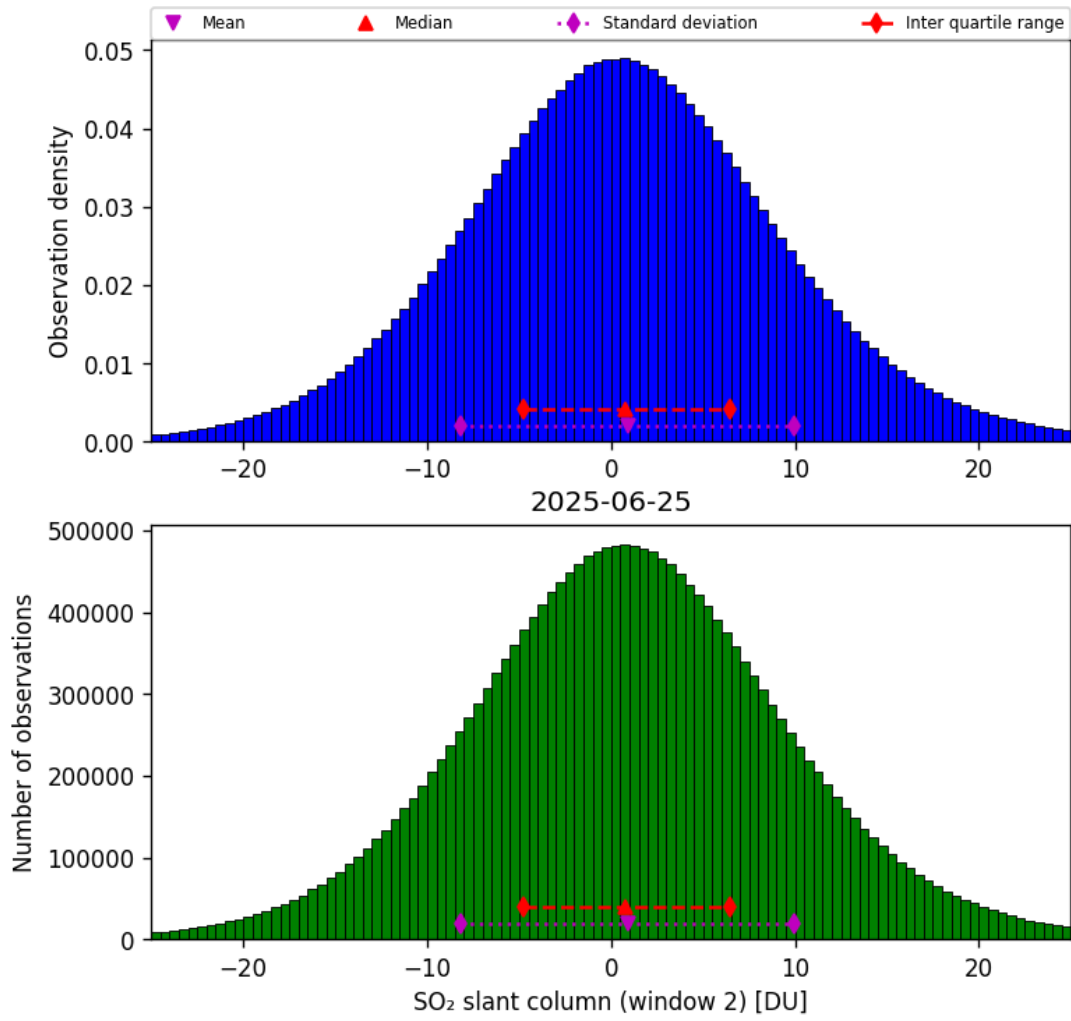
Figure 67: Histogram of “SO 2 slant column (window 2)” for 2025-06-24 to 2025-06-26
