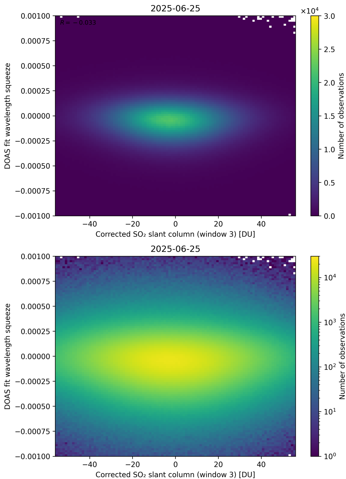
Figure 257: Scatter density plot of “Corrected SO 2 slant column (window 3)” against “DOAS fit wavelength squeeze” for 2025-06-24 to 2025-06-26.
