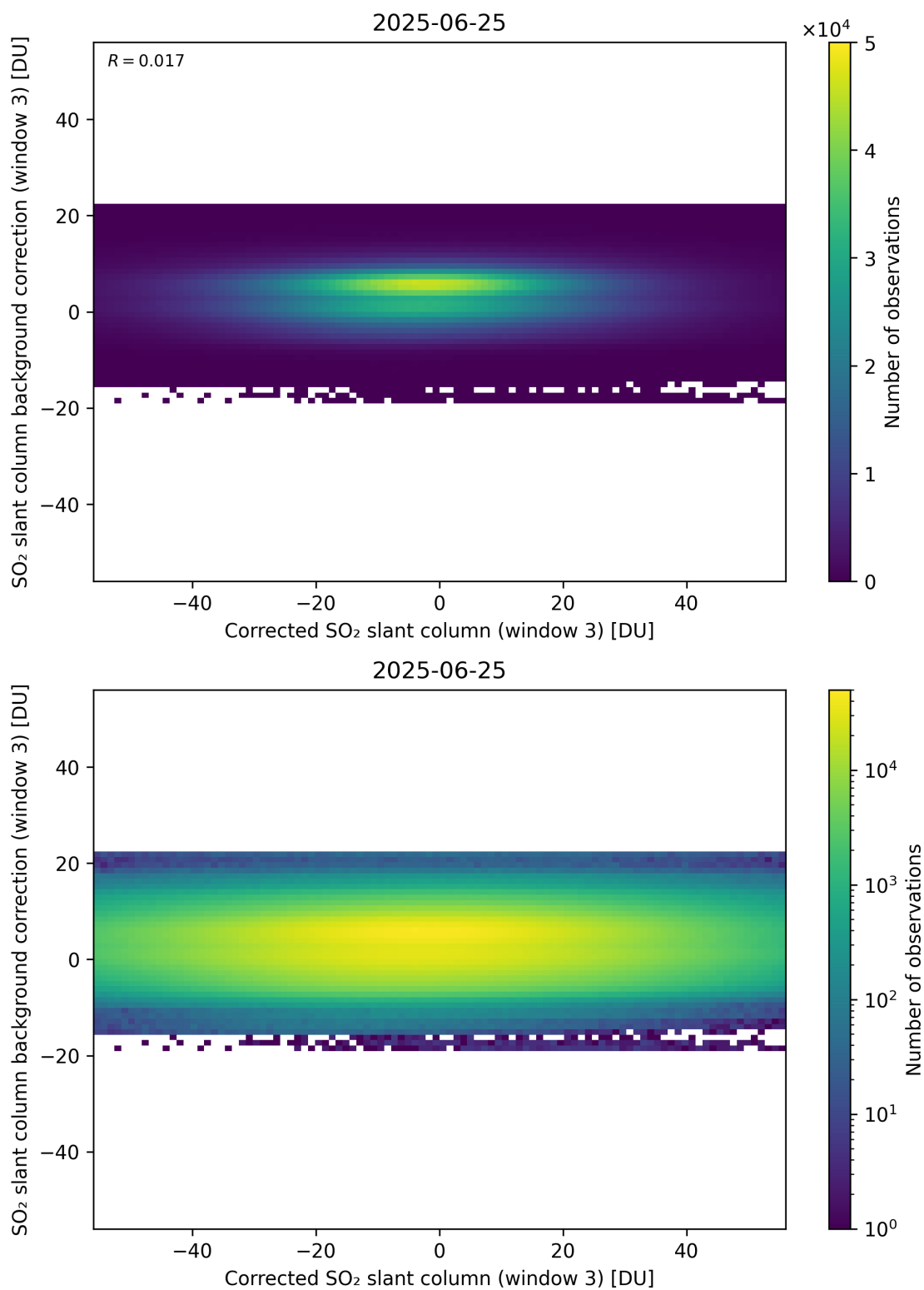
Figure 255: Scatter density plot of “Corrected SO 2 slant column (window 3)” against “SO 2 slant column background correction (window 3)” for 2025-06-24 to 2025-06-26.
