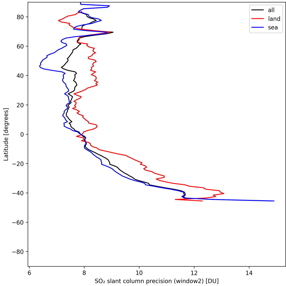
Figure 42: Zonal average of “SO 2 slant column precision (window2)” for 2025-06-24 to 2025-06-26.
