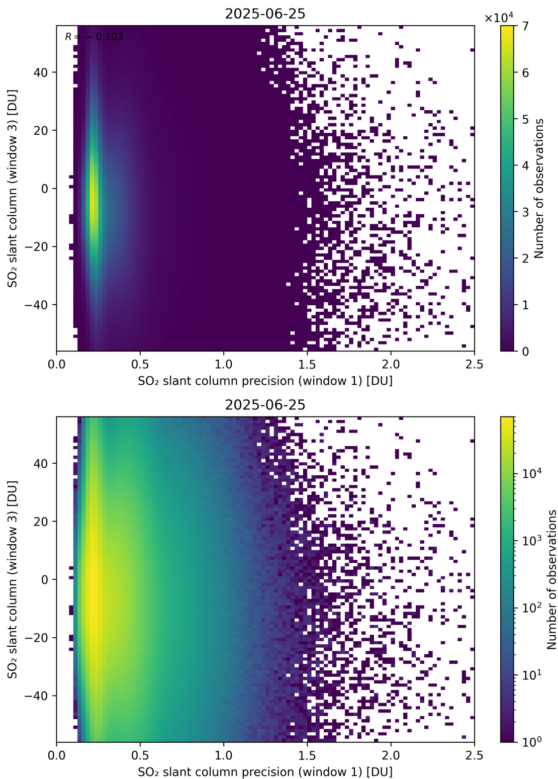
Figure 278: Scatter density plot of “SO 2 slant column precision (window 1)” against “SO 2 slant column (window 3)” for 2025-06-24 to 2025-06-26.
