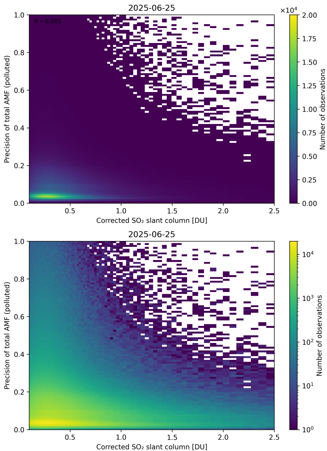
Figure 243: Scatter density plot of “Corrected SO 2 slant column” against “Precision of total AMF (polluted)” for 2025-06-24 to 2025-06-26.
