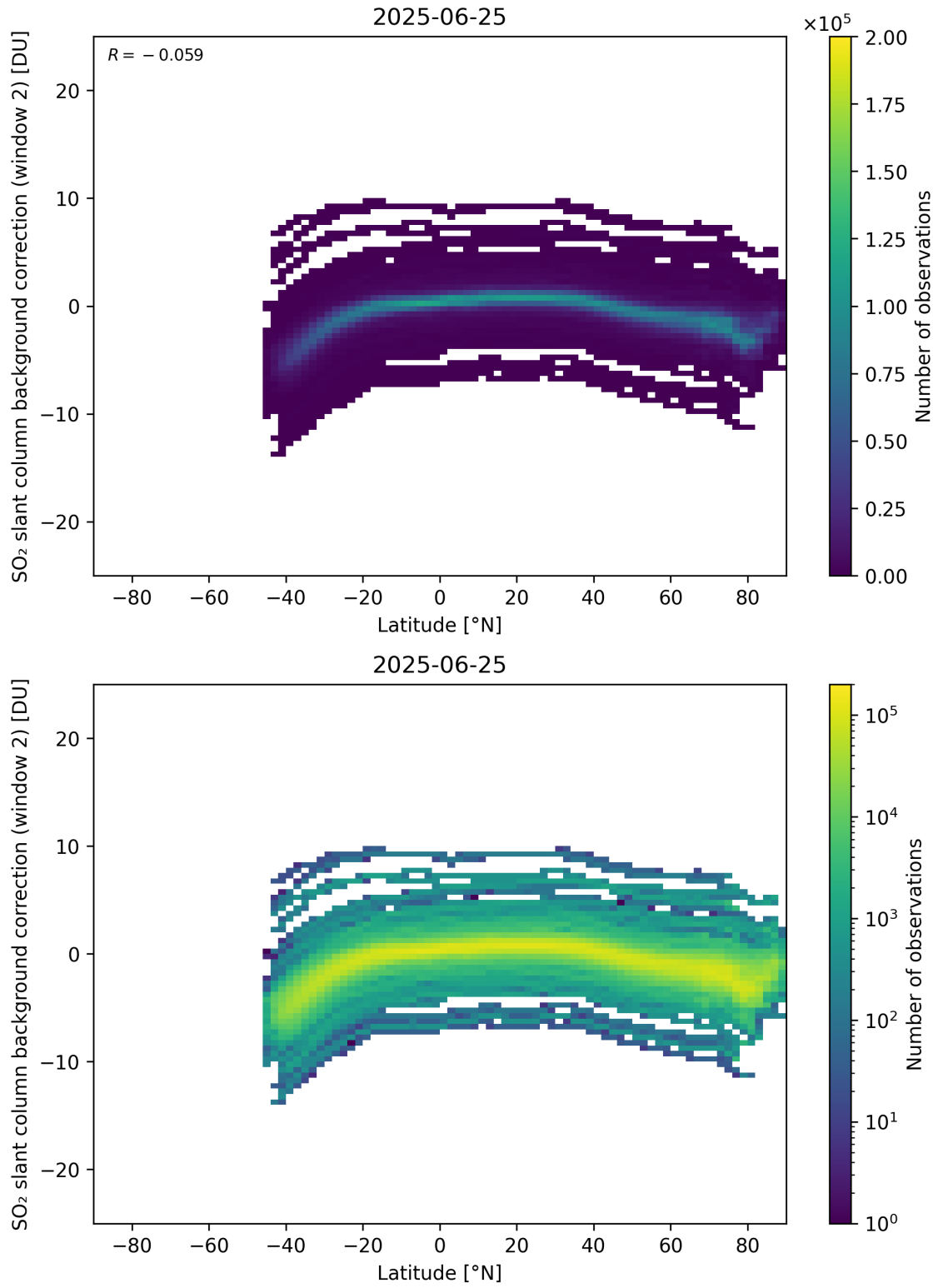
Figure 151: Scatter density plot of “Latitude” against “SO 2 slant column background correction (window 2)” for 2025-06-24 to 2025-06-26.
