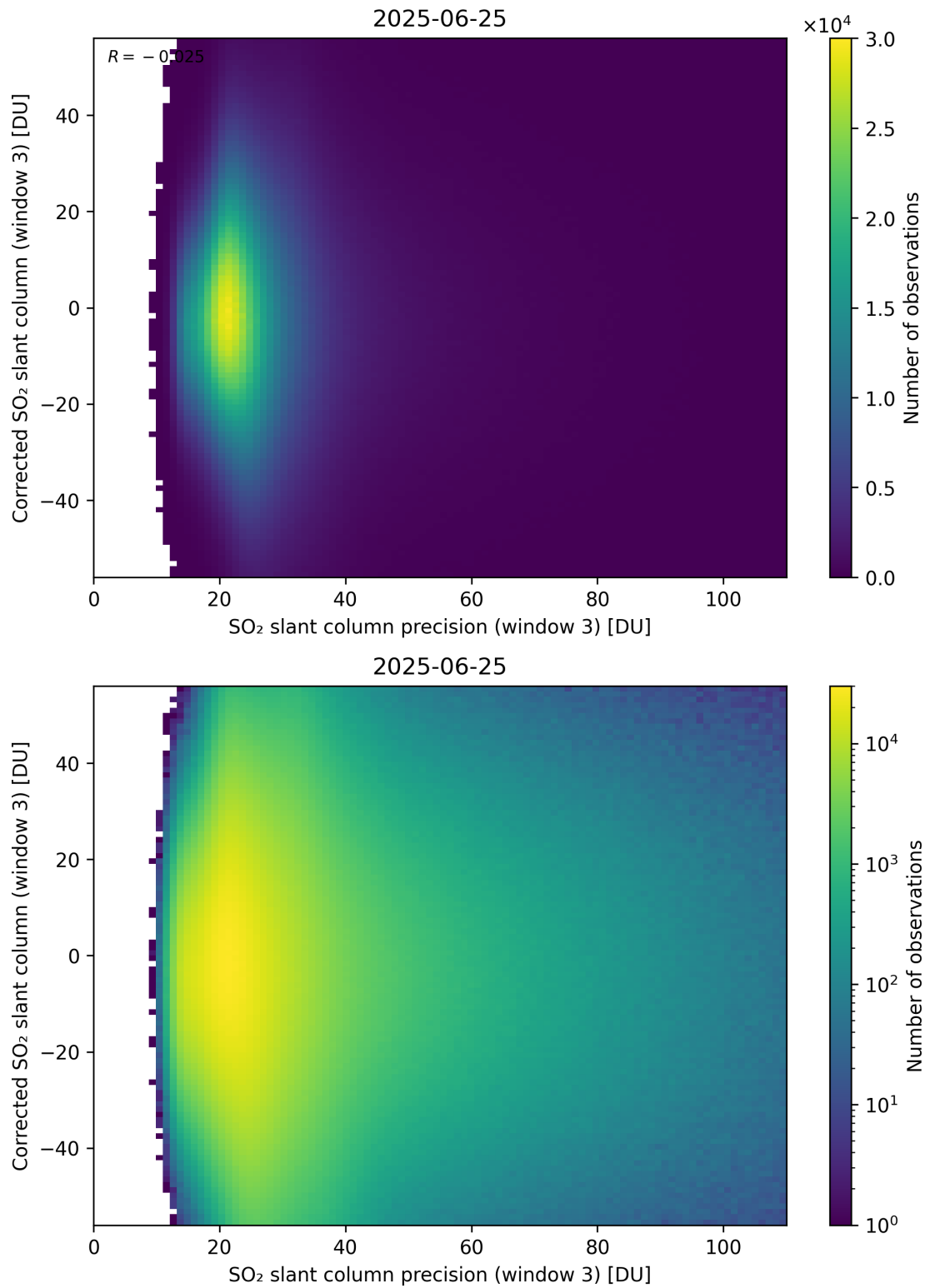
Figure 312: Scatter density plot of “SO 2 slant column precision (window 3)” against “Corrected SO 2 slant column (window 3)” for 2025-06-24 to 2025-06-26.
