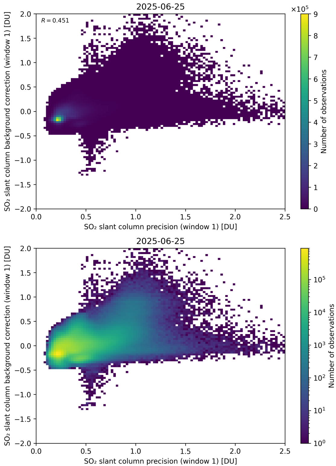
Figure 268: Scatter density plot of “SO 2 slant column precision (window 1)” against “SO 2 slant column background correction (window 1)” for 2025-06-24 to 2025-06-26.
