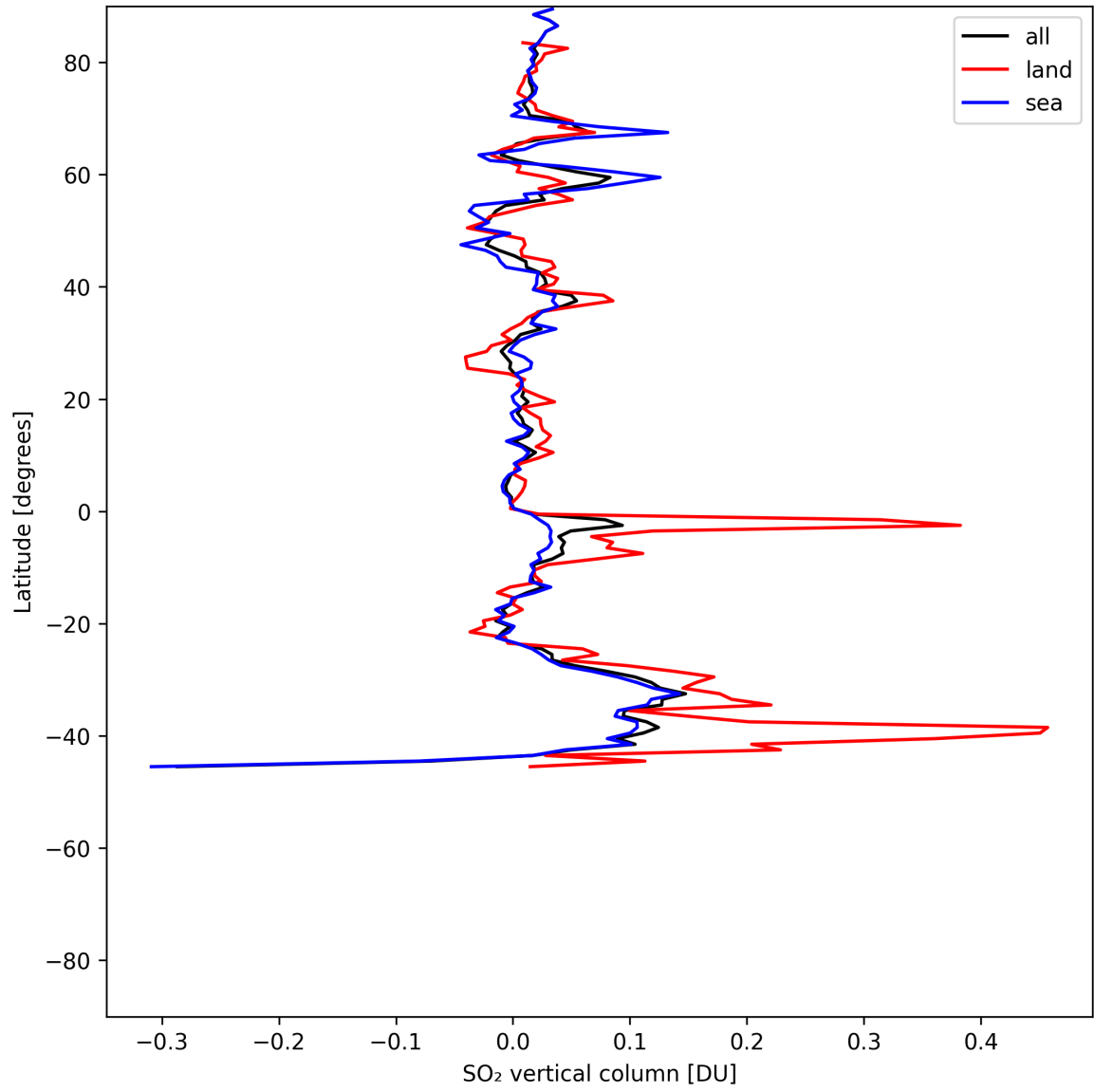
Figure 32: Zonal average of “SO 2 vertical column” for 2025-06-24 to 2025-06-26.
