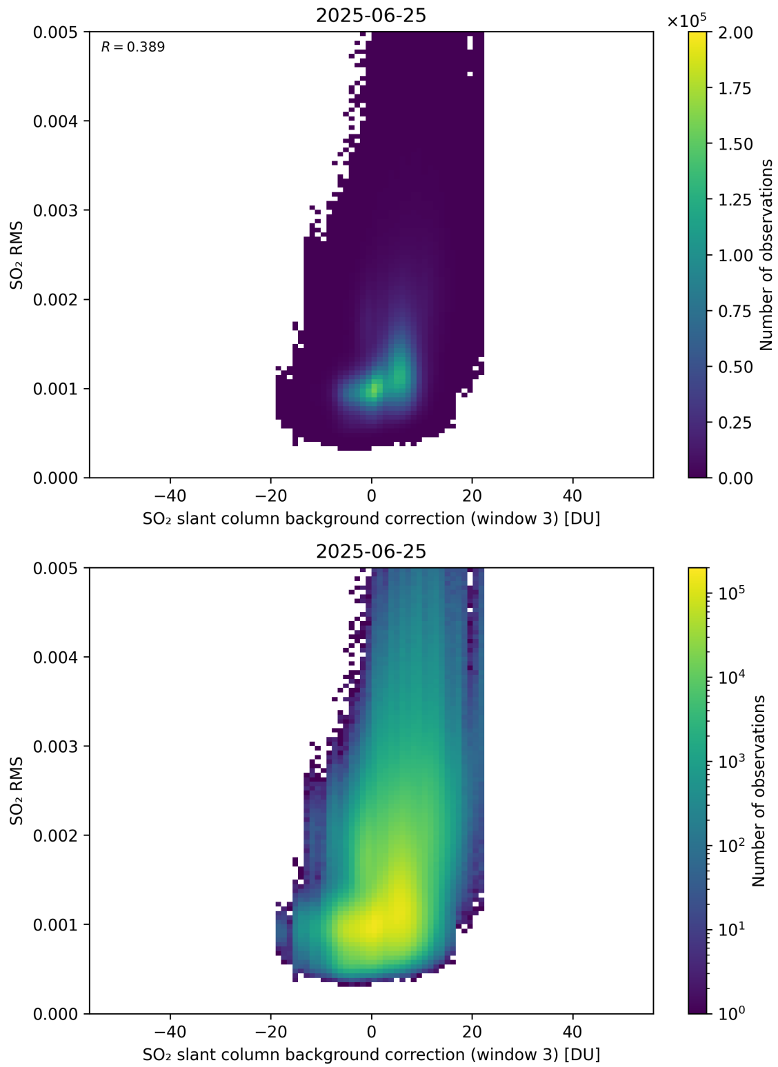
Figure 134: Scatter density plot of “SO 2 slant column background correction (window 3)” against “SO 2 RMS” for 2025-06-24 to 2025-06-26.
