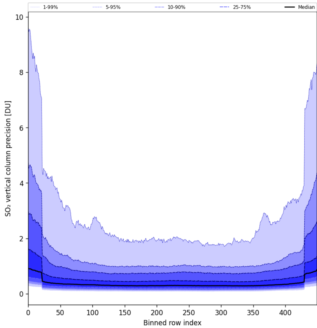
Figure 85: Along track statistics of “SO 2 vertical column precision” for 2025-06-24 to 2025-06-26
