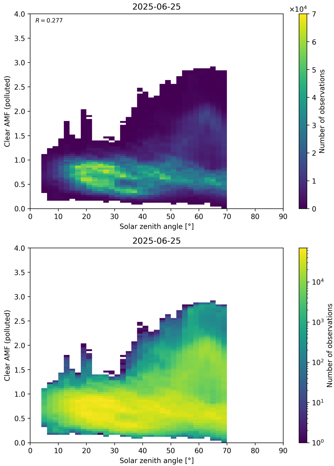
Figure 178: Scatter density plot of “Solar zenith angle” against “Clear AMF (polluted)” for 2025-06-24 to 2025-06-26.
