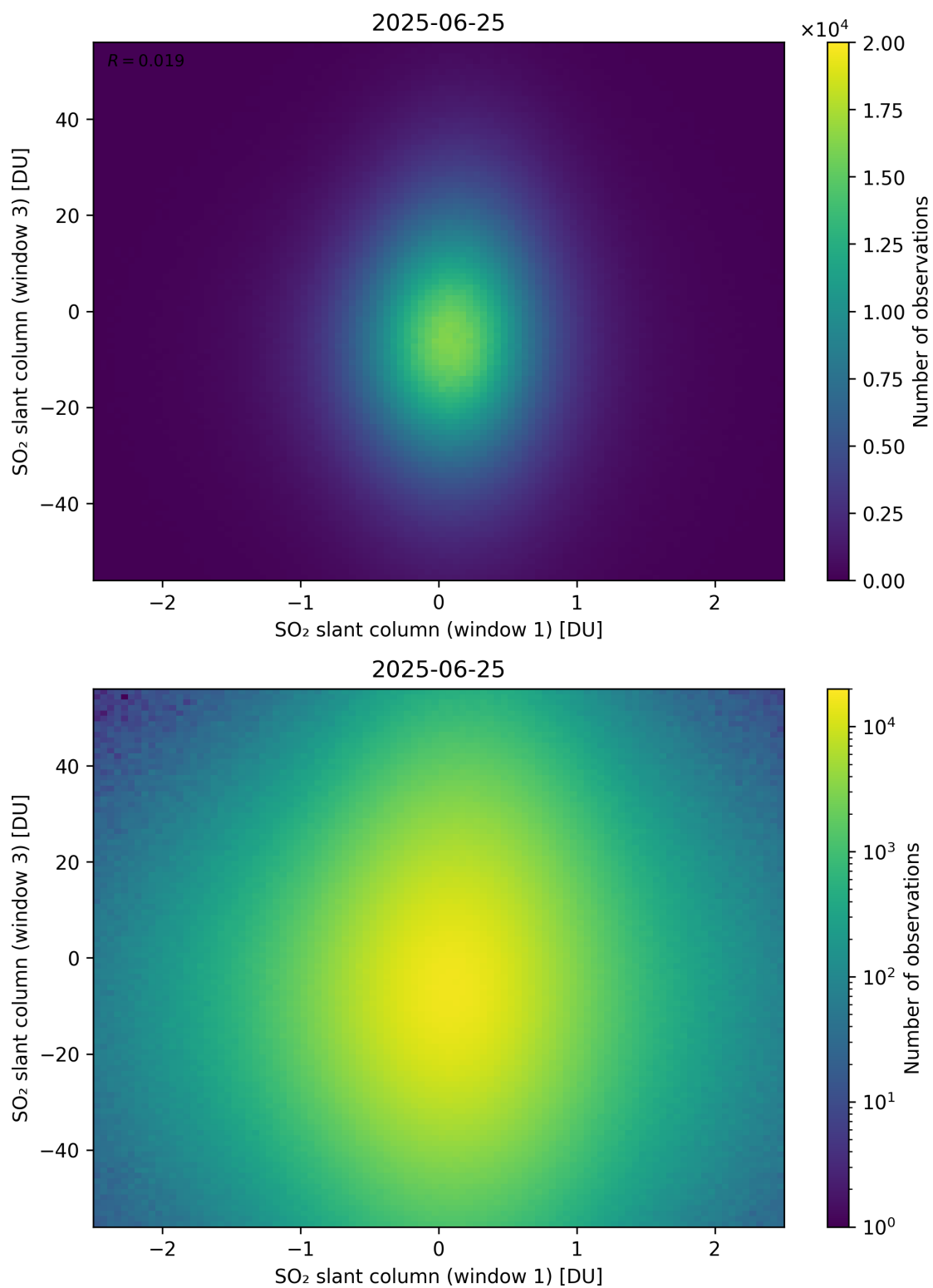
Figure 287: Scatter density plot of “SO 2 slant column (window 1)” against “SO 2 slant column (window 3)” for 2025-06-24 to 2025-06-26.
