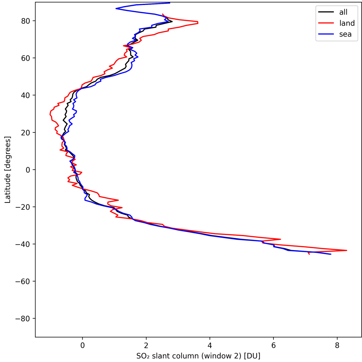
Figure 41: Zonal average of “SO 2 slant column (window 2)” for 2025-06-24 to 2025-06-26.
