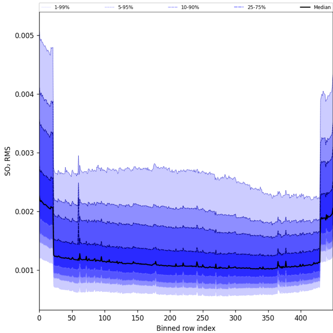
Figure 104: Along track statistics of “SO 2 RMS” for 2025-06-24 to 2025-06-26
