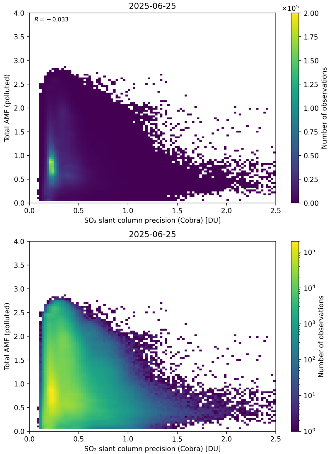
Figure 213: Scatter density plot of “SO 2 slant column precision (Cobra)” against “Total AMF (polluted)” for 2025-06-24 to 2025-06-26.
