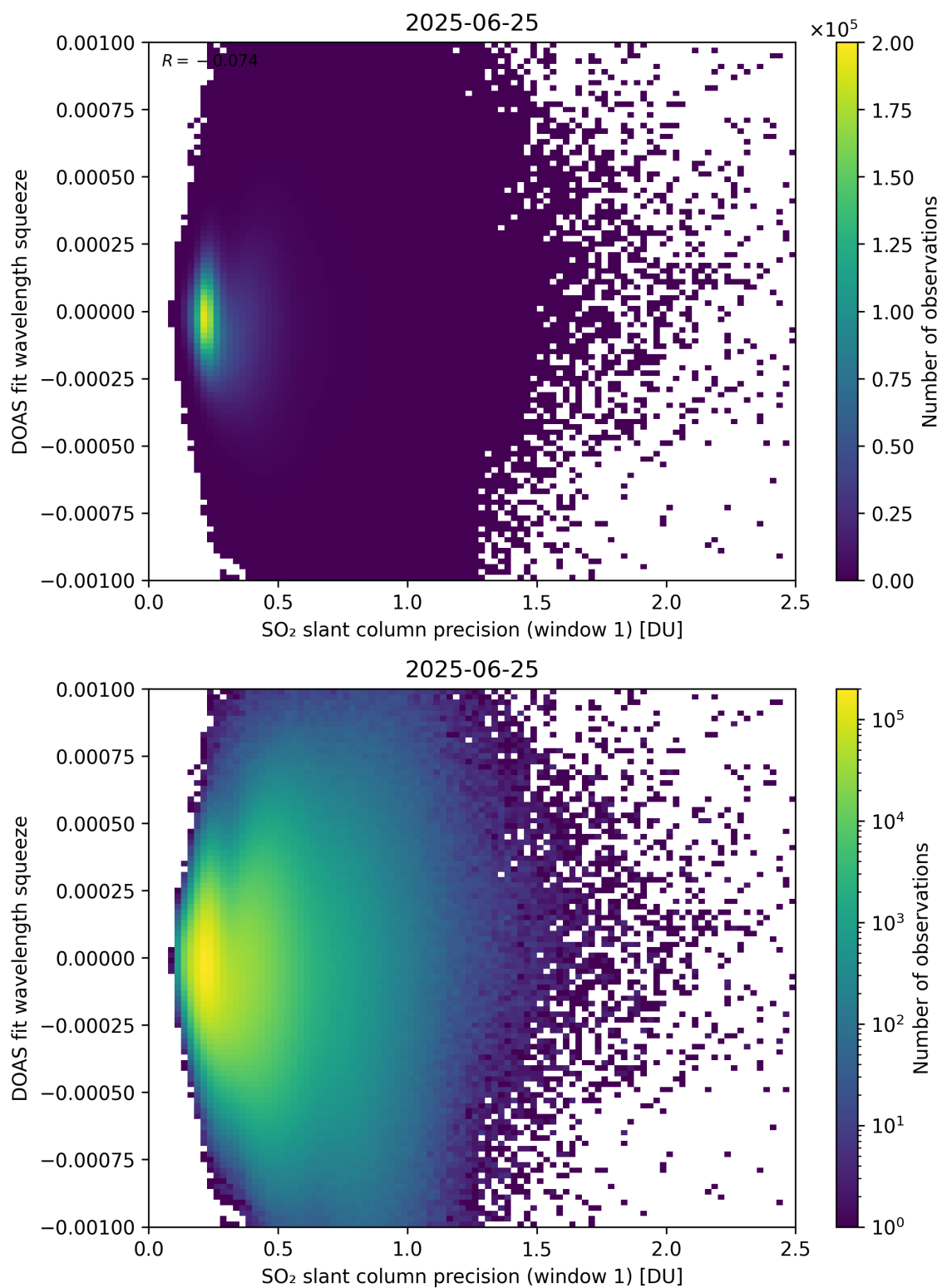
Figure 272: Scatter density plot of “SO 2 slant column precision (window 1)” against “DOAS fit wavelength squeeze” for 2025-06-24 to 2025-06-26.
