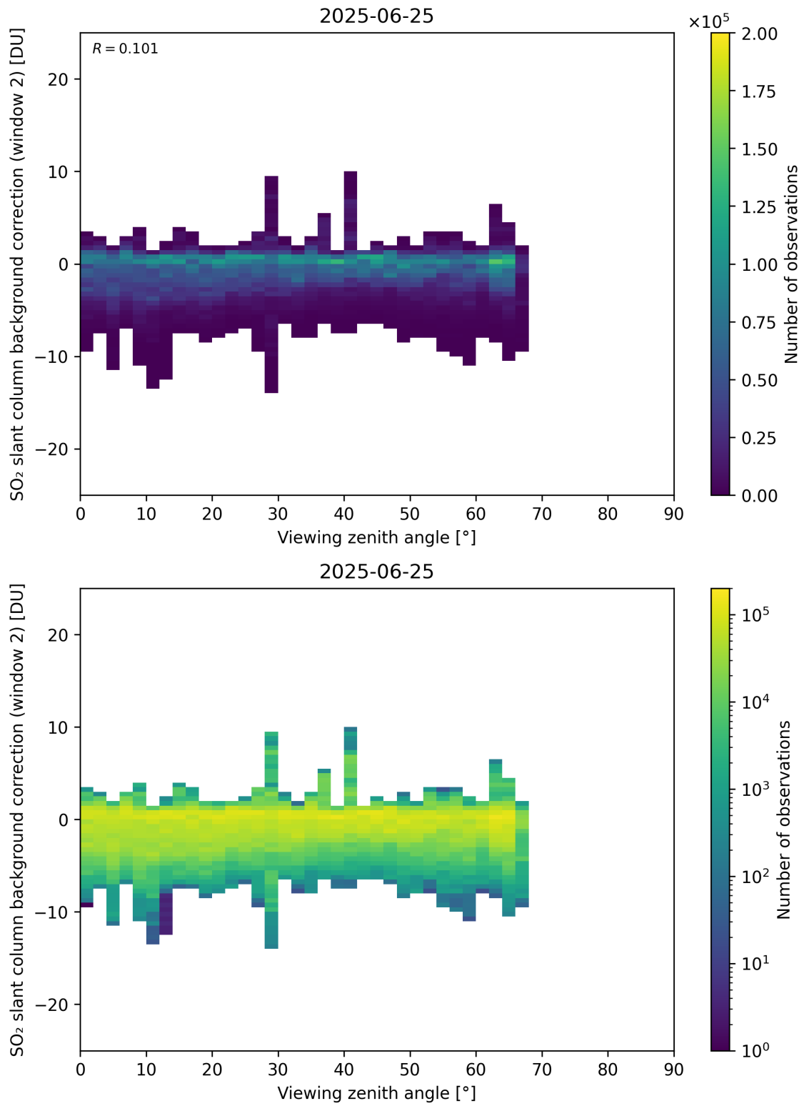
Figure 363: Scatter density plot of “Viewing zenith angle” against “SO 2 slant column background correction (window 2)” for 2025-06-24 to 2025-06-26.
