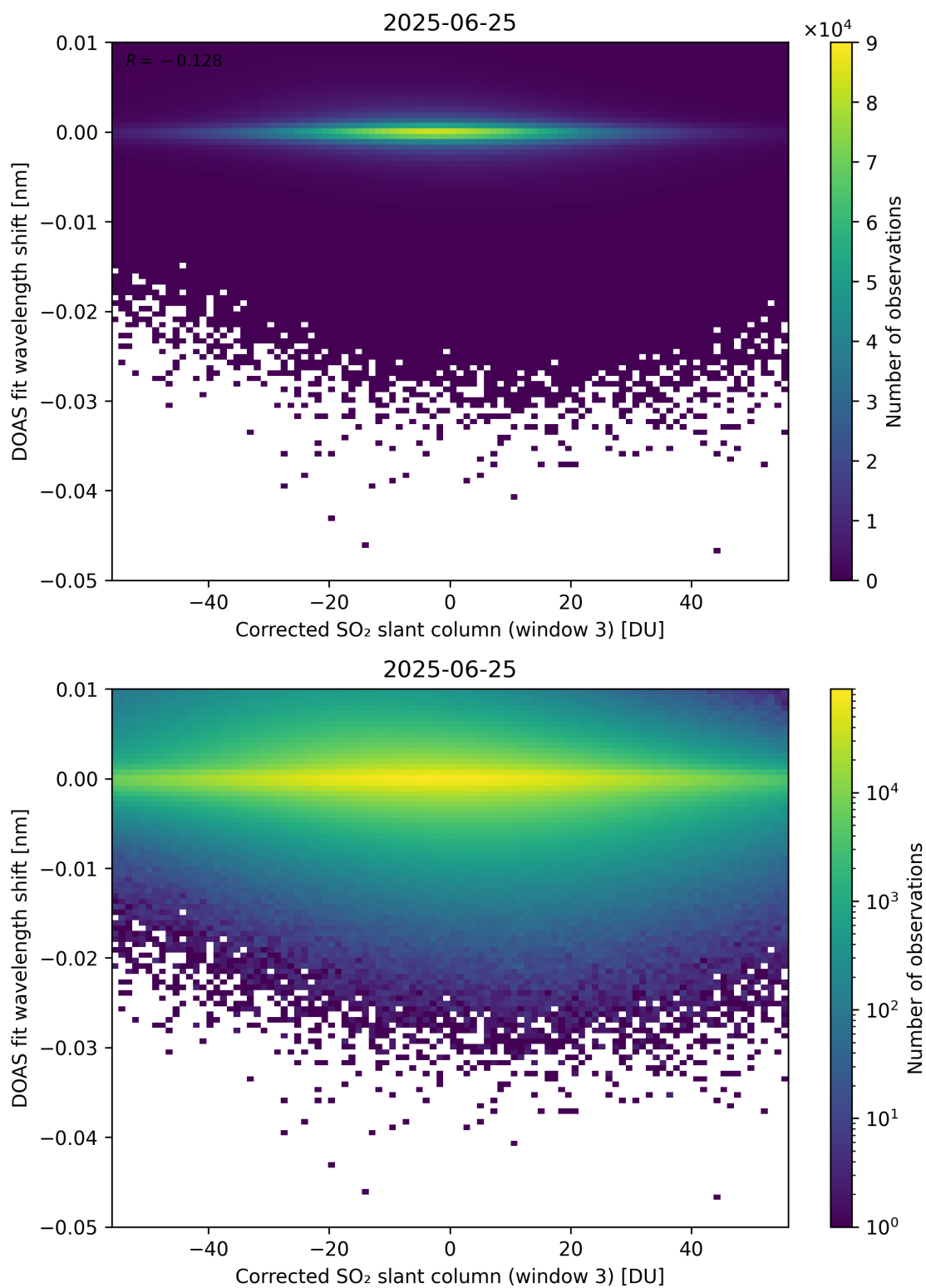
Figure 256: Scatter density plot of “Corrected SO 2 slant column (window 3)” against “DOAS fit wavelength shift” for 2025-06-24 to 2025-06-26.
