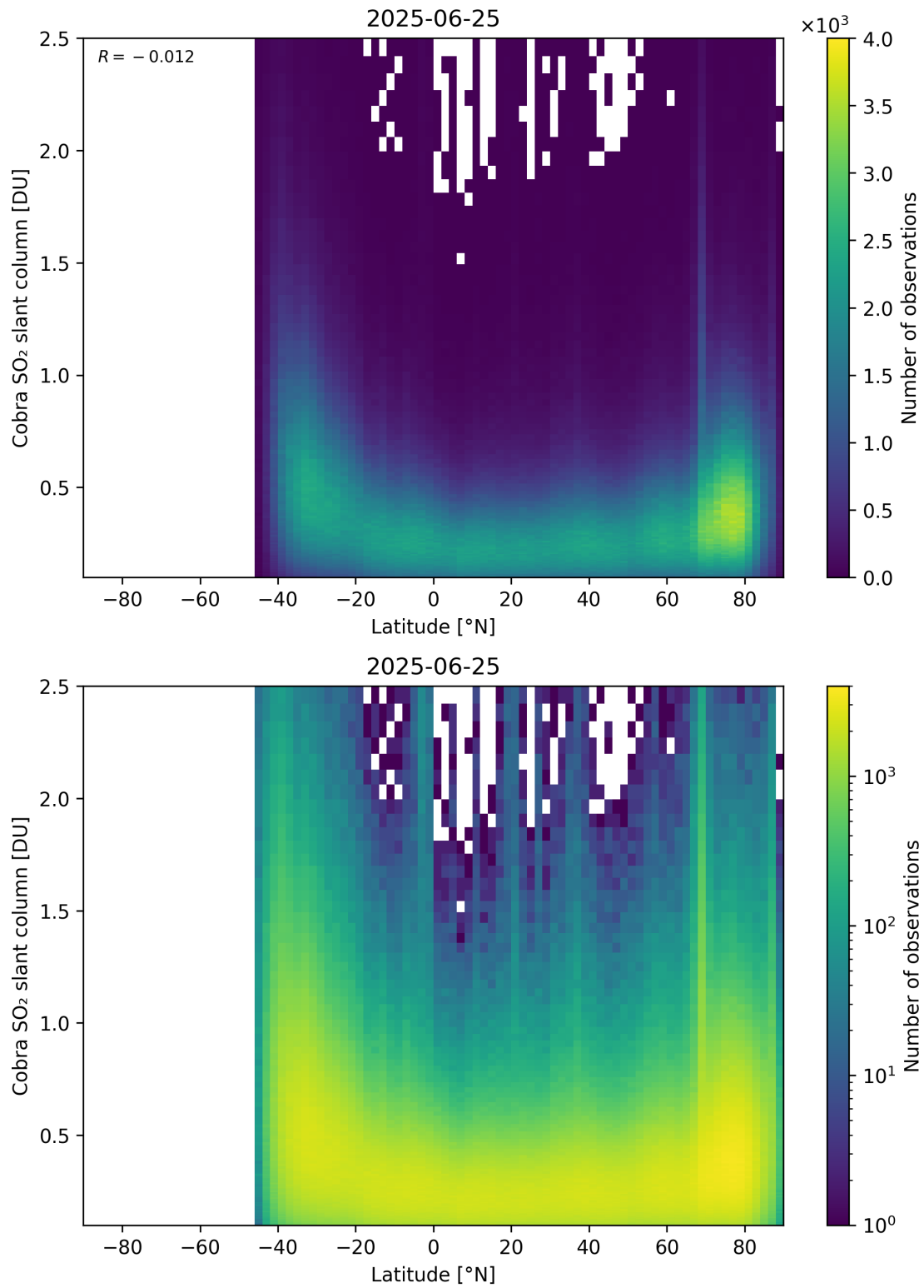
Figure 157: Scatter density plot of “Latitude” against “Cobra SO 2 slant column” for 2025-06-24 to 2025-06-26.
