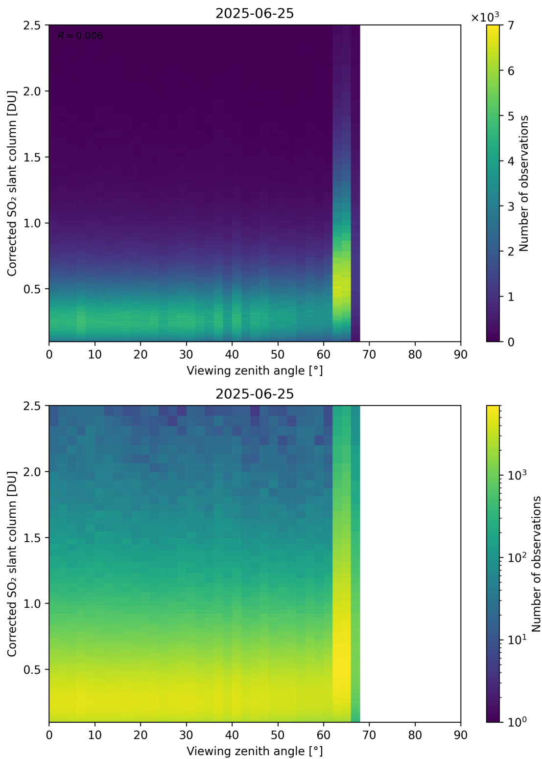
Figure 373: Scatter density plot of “Viewing zenith angle” against “Corrected SO 2 slant column” for 2025-06-24 to 2025-06-26.
