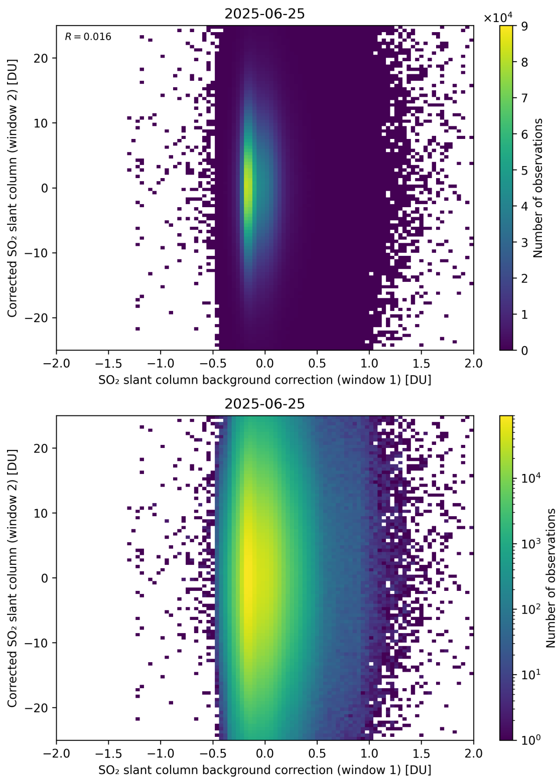
Figure 115: Scatter density plot of “SO 2 slant column background correction (window 1)” against “Corrected SO 2 slant column (window 2)” for 2025-06-24 to 2025-06-26.
