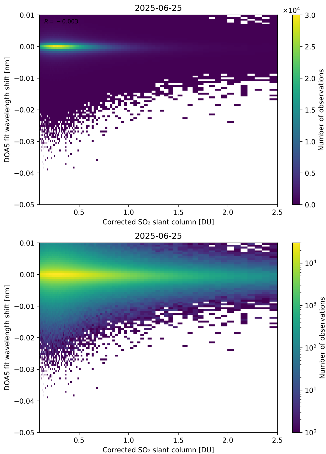
Figure 229: Scatter density plot of “Corrected SO 2 slant column” against “DOAS fit wavelength shift” for 2025-06-24 to 2025-06-26.
