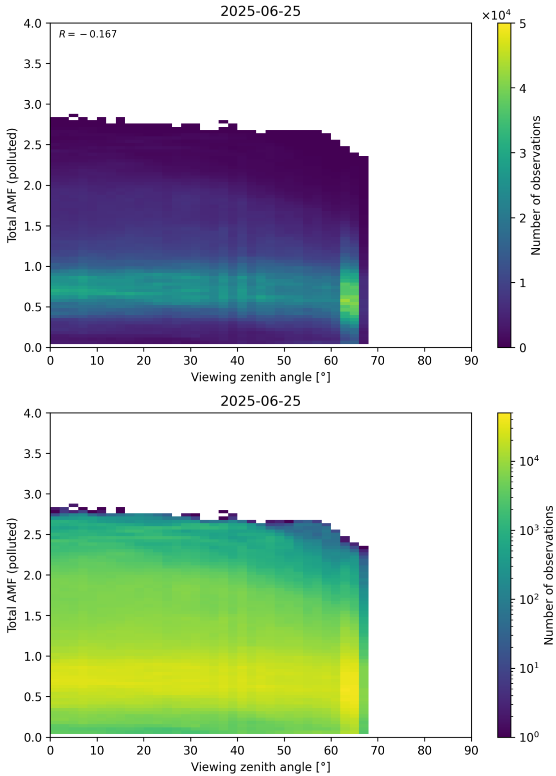
Figure 381: Scatter density plot of “Viewing zenith angle” against “Total AMF (polluted)” for 2025-06-24 to 2025-06-26.
