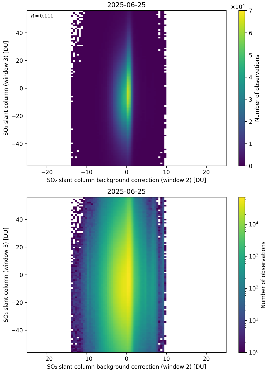
Figure 128: Scatter density plot of “SO 2 slant column background correction (window 2)” against “SO 2 slant column (window 3)” for 2025-06-24 to 2025-06-26.
