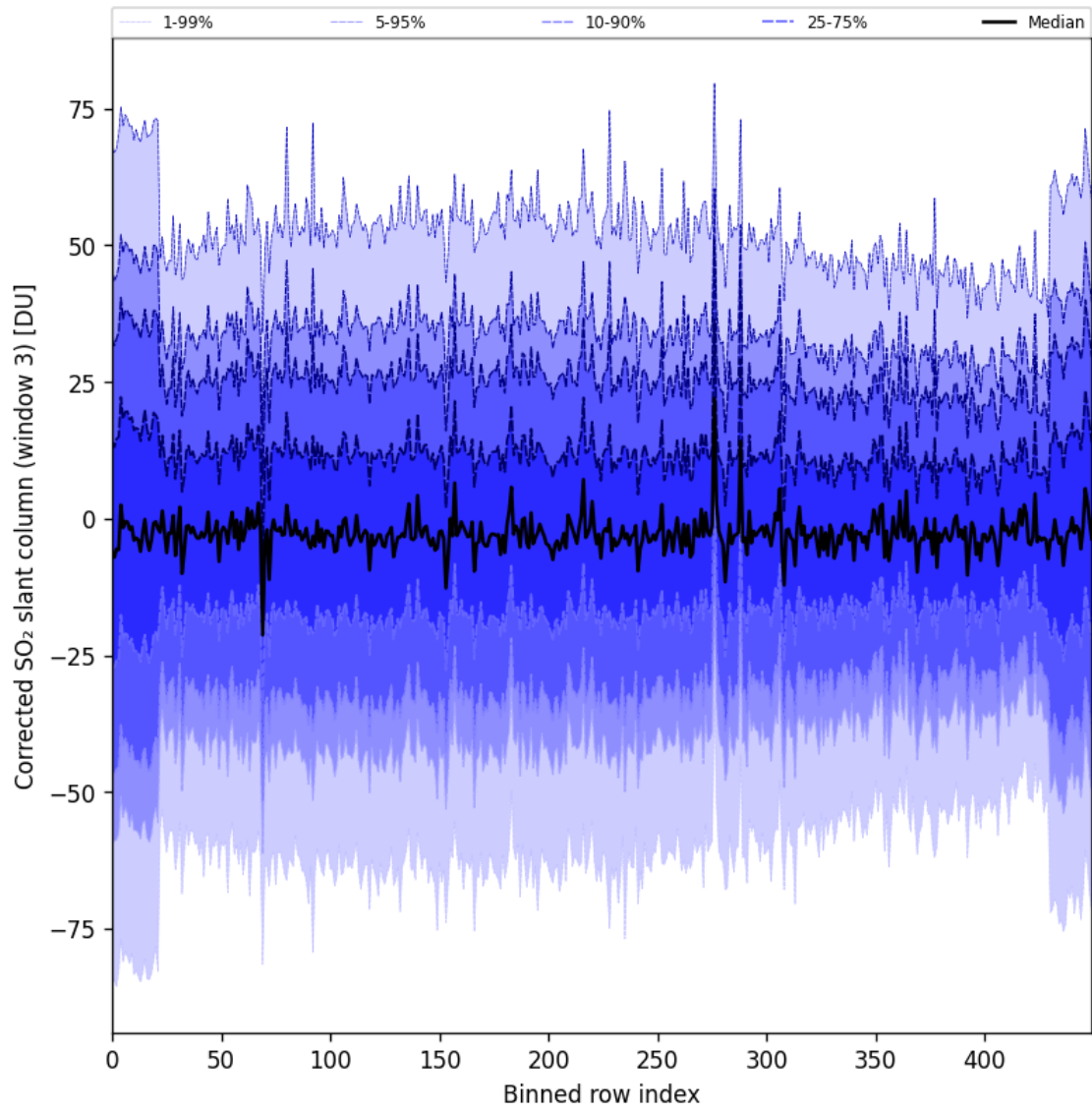
Figure 99: Along track statistics of “Corrected SO 2 slant column (window 3)” for 2025-06-24 to 2025-06-26
