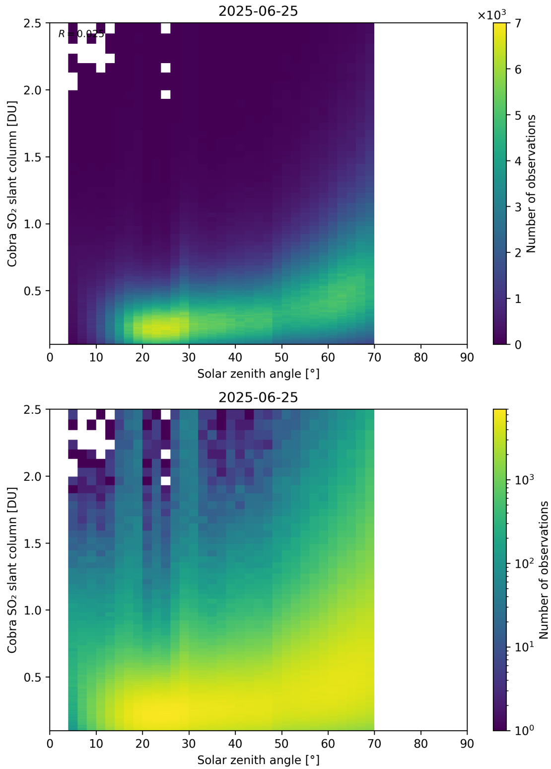
Figure 179: Scatter density plot of “Solar zenith angle” against “Cobra SO 2 slant column” for 2025-06-24 to 2025-06-26.
