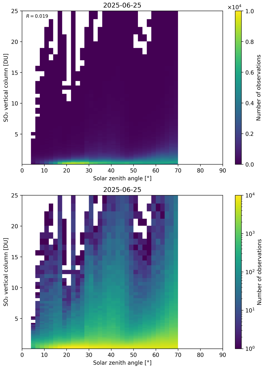
Figure 191: Scatter density plot of “Solar zenith angle” against “SO 2 vertical column” for 2025-06-24 to 2025-06-26.
