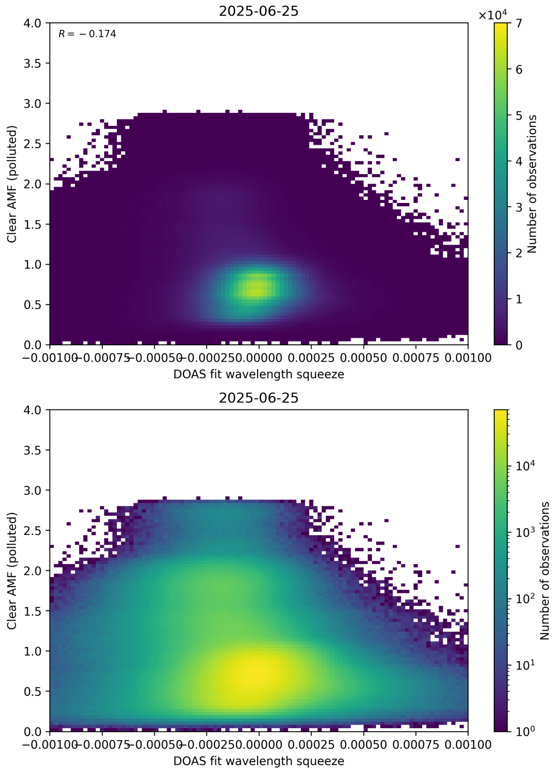
Figure 144: Scatter density plot of “DOAS fit wavelength squeeze” against “Clear AMF (polluted)” for 2025-06-24 to 2025-06-26.
