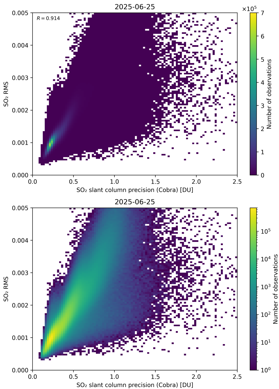
Figure 204: Scatter density plot of “SO 2 slant column precision (Cobra)” against “SO 2 RMS” for 2025-06-24 to 2025-06-26.
