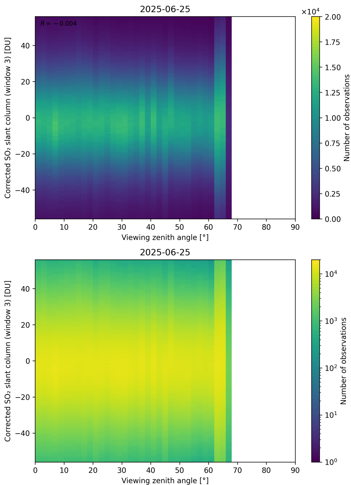
Figure 375: Scatter density plot of “Viewing zenith angle” against “Corrected SO 2 slant column (window 3)” for 2025-06-24 to 2025-06-26.
