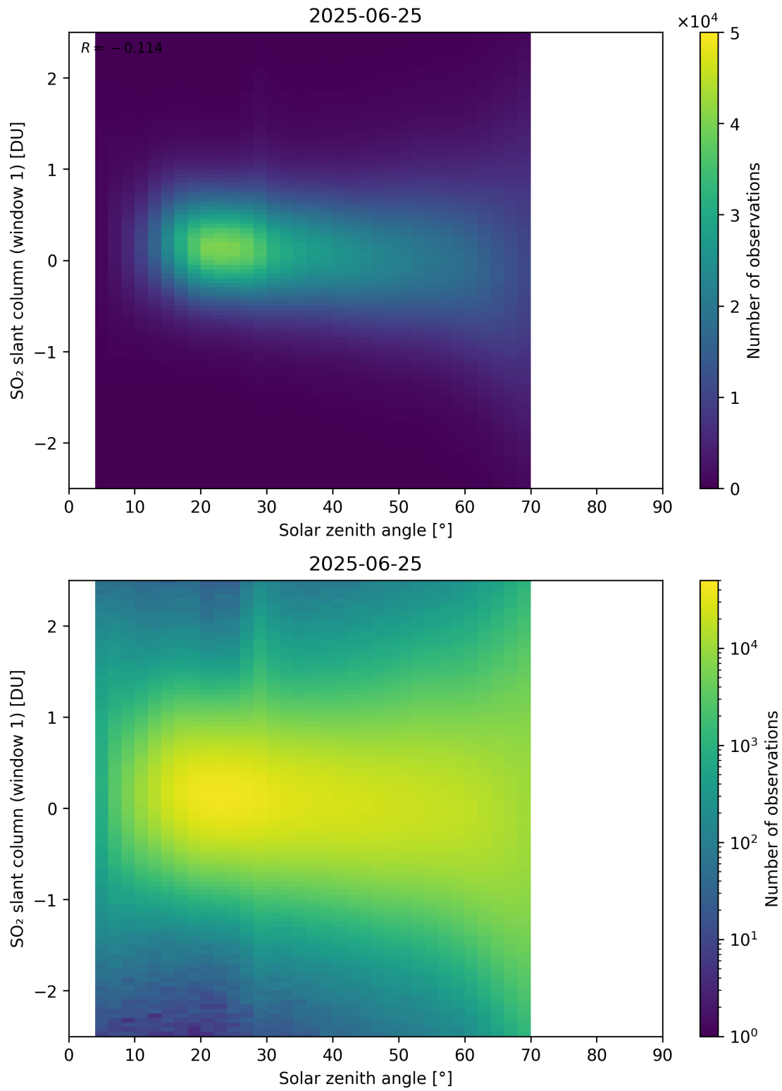
Figure 184: Scatter density plot of “Solar zenith angle” against “SO 2 slant column (window 1)” for 2025-06-24 to 2025-06-26.
