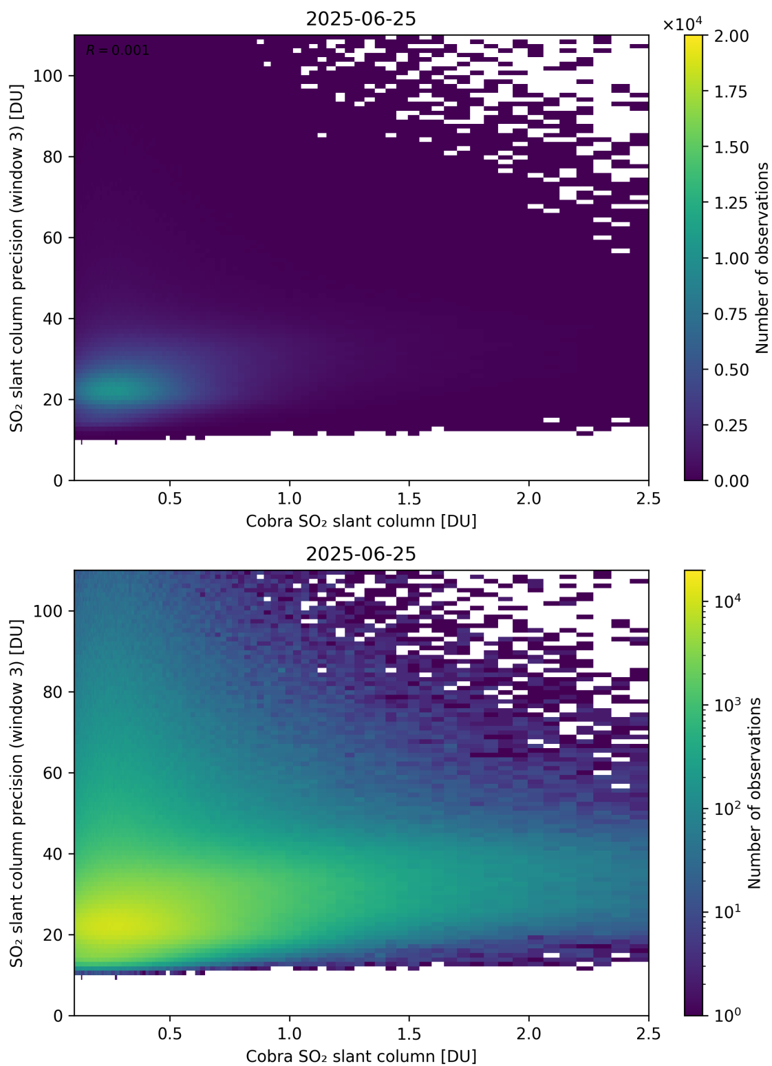
Figure 223: Scatter density plot of “Cobra SO 2 slant column” against “SO 2 slant column precision (window 3)” for 2025-06-24 to 2025-06-26.
