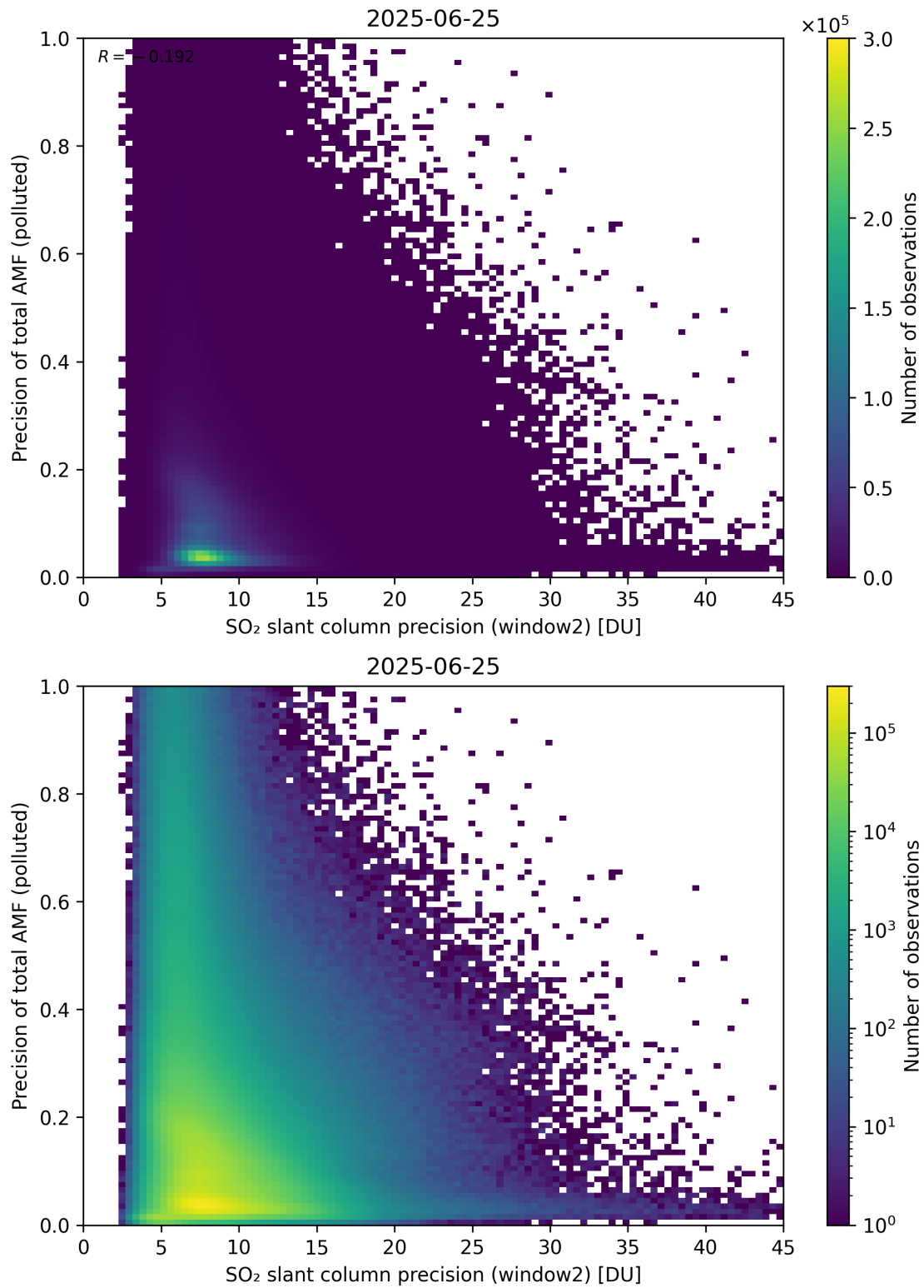
Figure 302: Scatter density plot of “SO 2 slant column precision (window2)” against “Precision of total AMF (polluted)” for 2025-06-24 to 2025-06-26.
