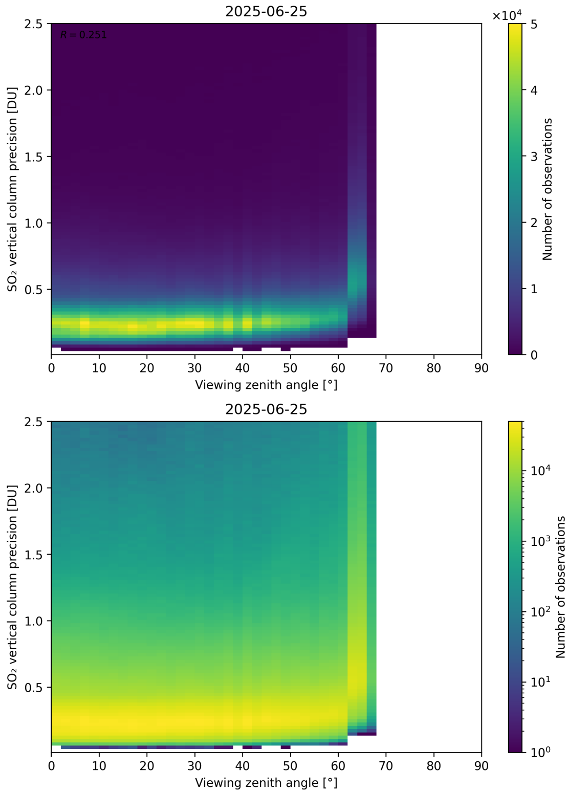
Figure 384: Scatter density plot of “Viewing zenith angle” against “SO 2 vertical column precision” for 2025-06-24 to 2025-06-26.
