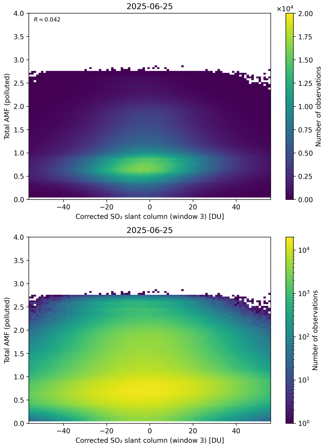
Figure 260: Scatter density plot of “Corrected SO 2 slant column (window 3)” against “Total AMF (polluted)” for 2025-06-24 to 2025-06-26.
