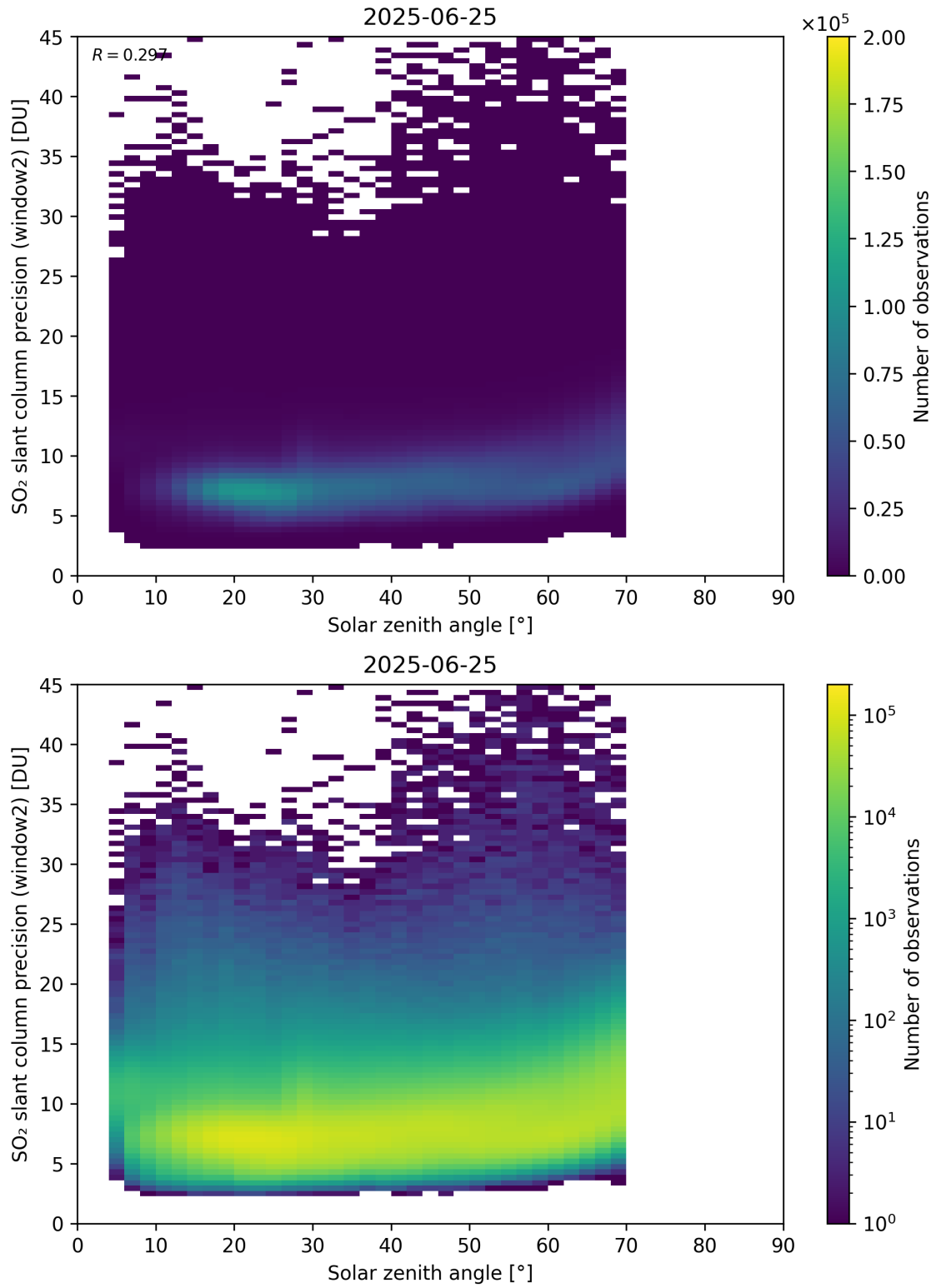
Figure 186: Scatter density plot of “Solar zenith angle” against “SO 2 slant column precision (window2)” for 2025-06-24 to 2025-06-26.
