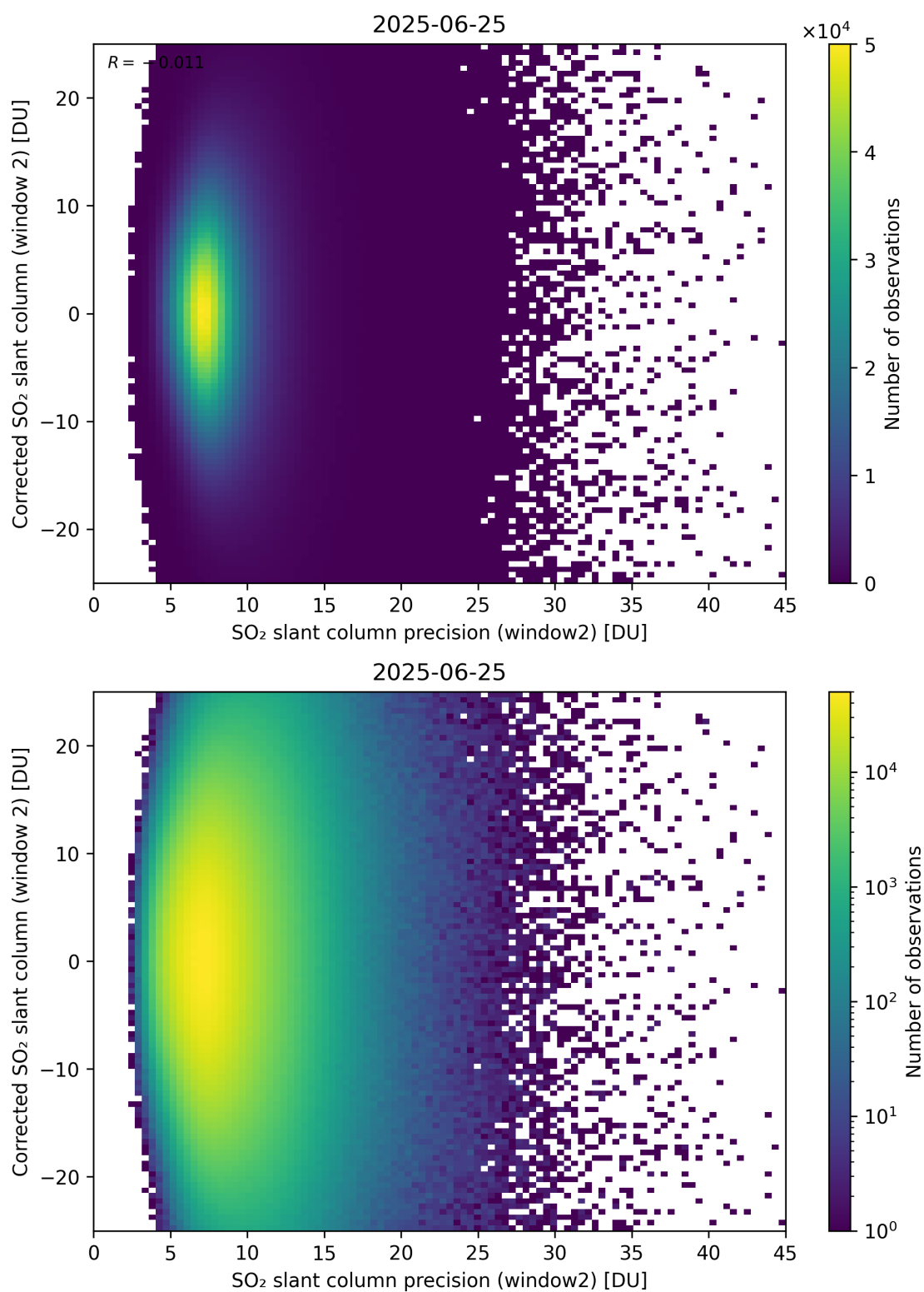
Figure 297: Scatter density plot of “SO 2 slant column precision (window2)” against “Corrected SO 2 slant column (window 2)” for 2025-06-24 to 2025-06-26.
