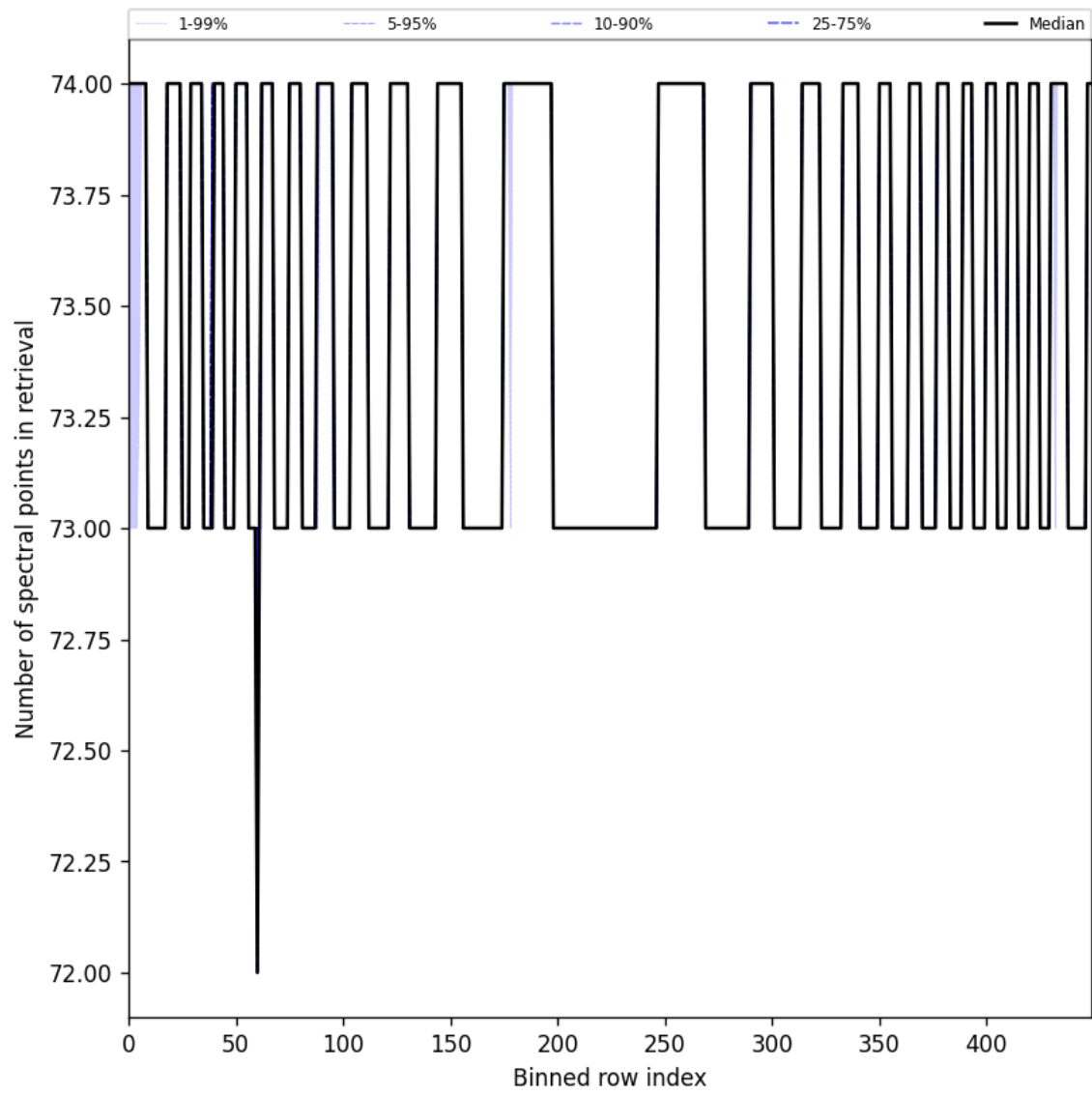
Figure 108: Along track statistics of “Number of spectral points in retrieval” for 2025-06-24 to 2025-06-26
