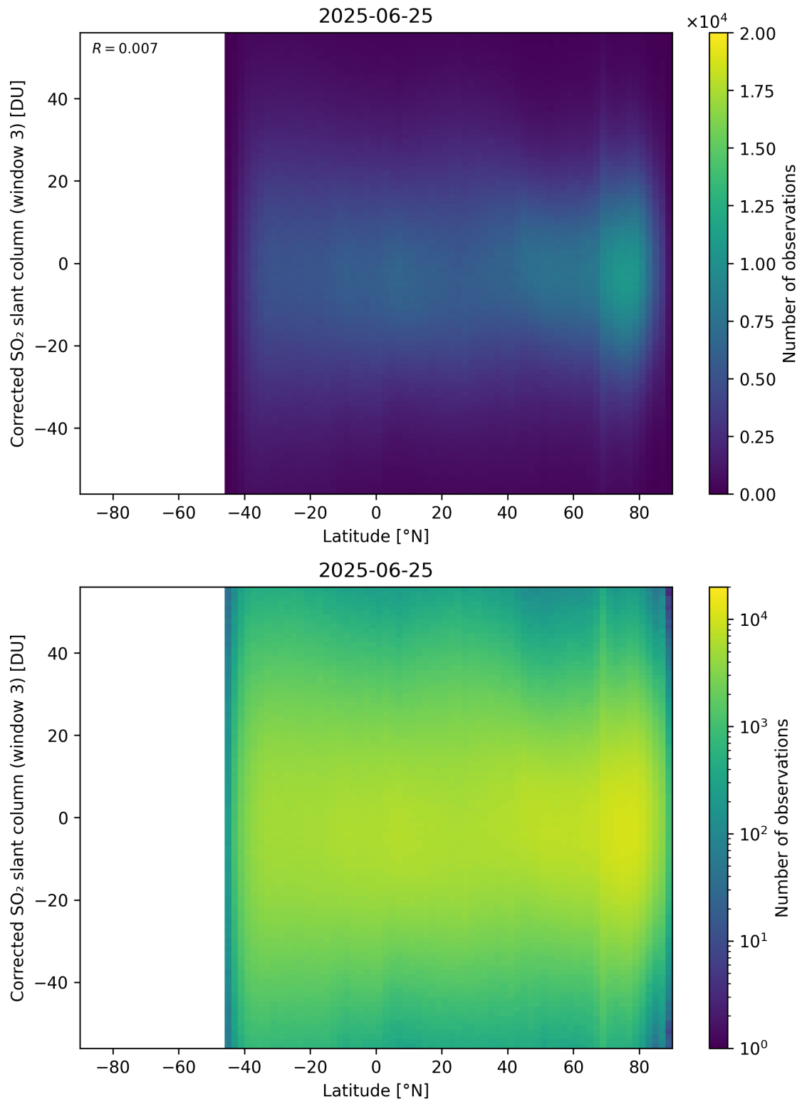
Figure 161: Scatter density plot of “Latitude” against “Corrected SO 2 slant column (window 3)” for 2025-06-24 to 2025-06-26.
