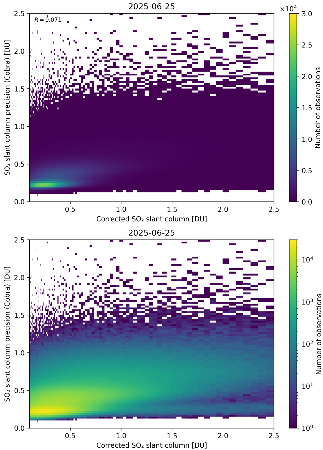
Figure 234: Scatter density plot of “Corrected SO 2 slant column” against “SO 2 slant column precision (Cobra)” for 2025-06-24 to 2025-06-26.
