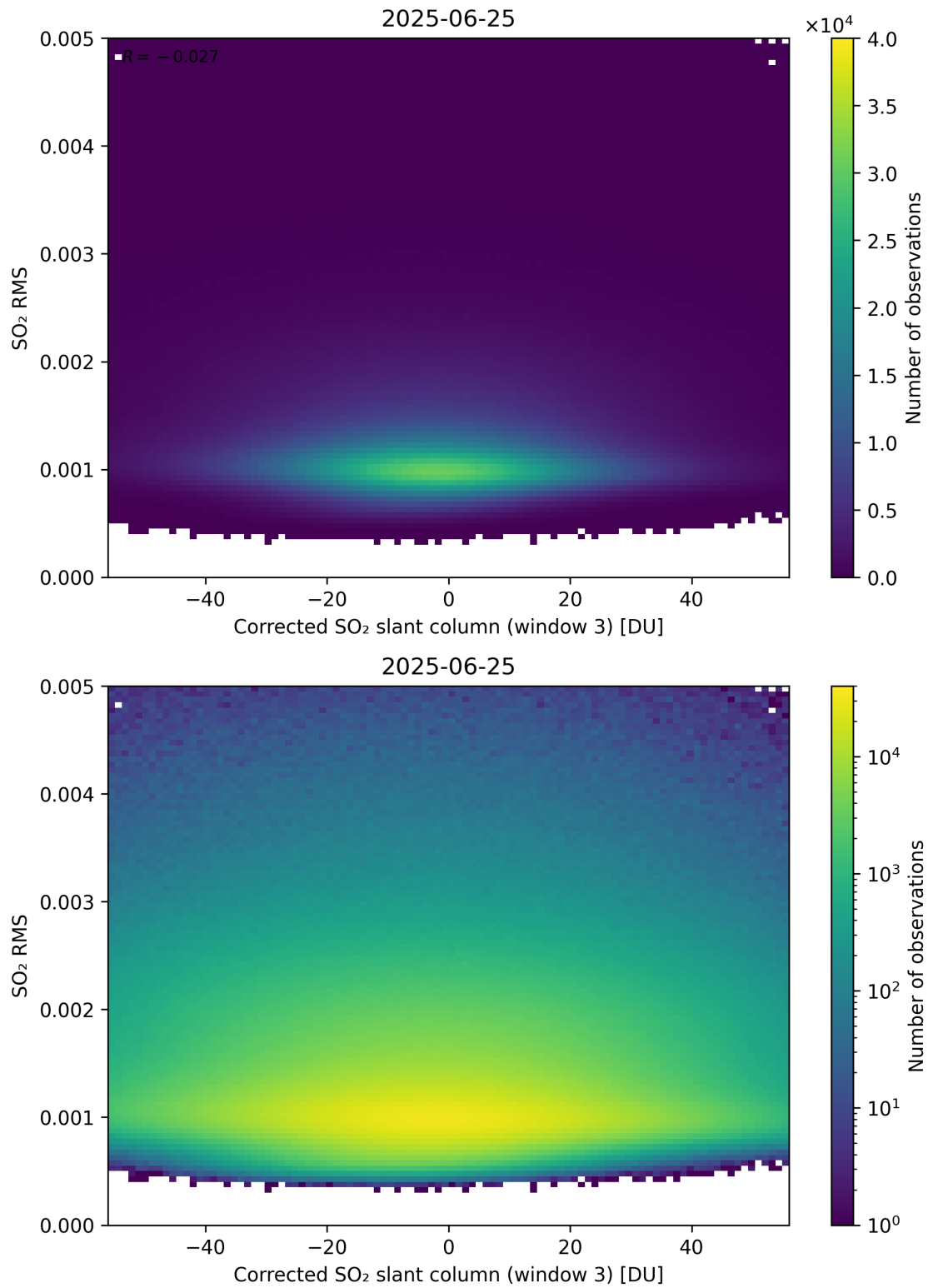
Figure 258: Scatter density plot of “Corrected SO 2 slant column (window 3)” against “SO 2 RMS” for 2025-06-24 to 2025-06-26.
