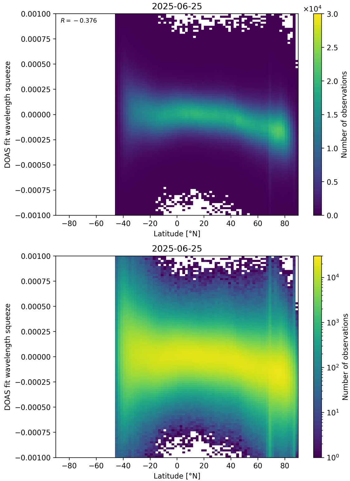
Figure 154: Scatter density plot of “Latitude” against “DOAS fit wavelength squeeze” for 2025-06-24 to 2025-06-26.
