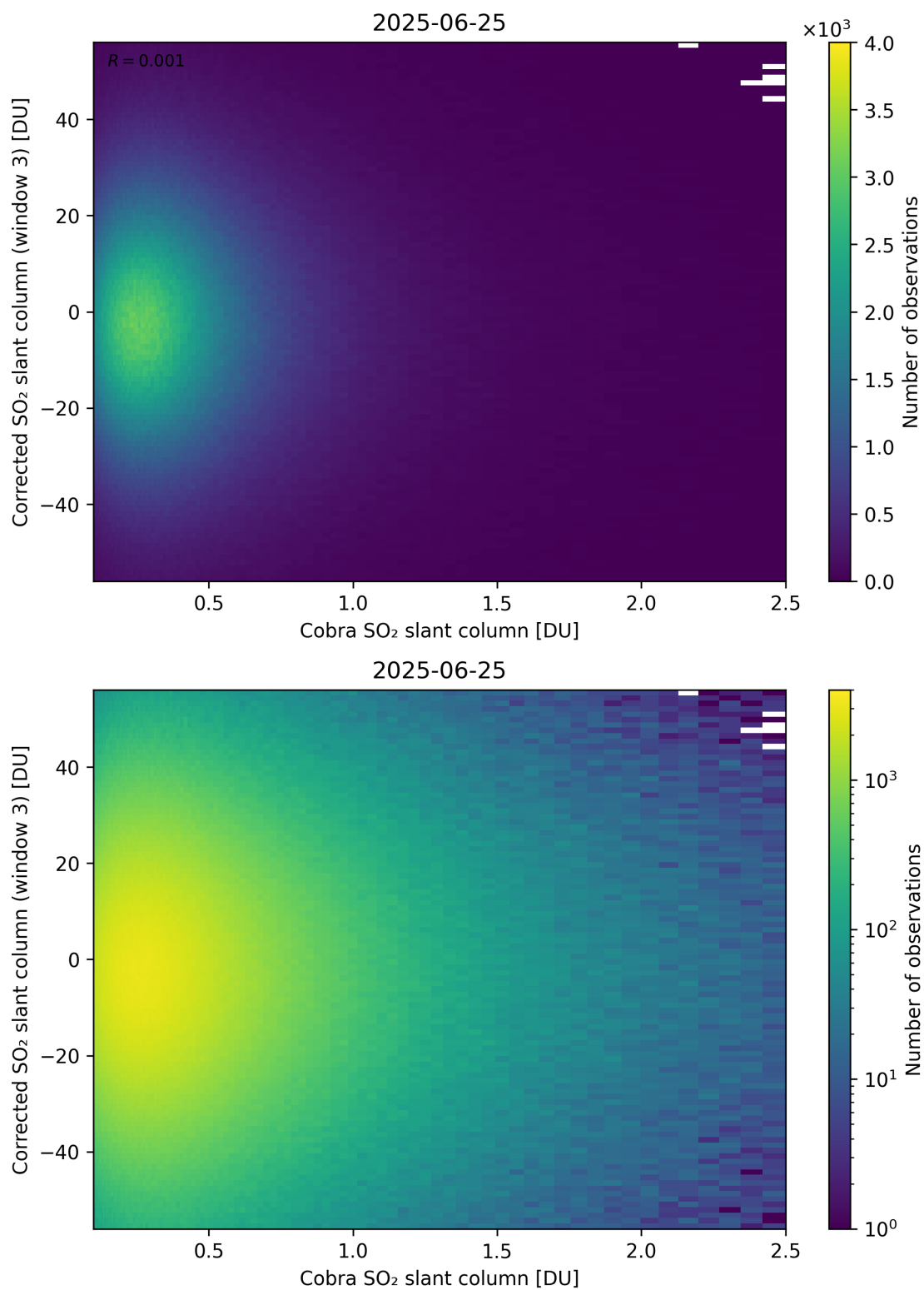
Figure 218: Scatter density plot of “Cobra SO 2 slant column” against “Corrected SO 2 slant column (window 3)” for 2025-06-24 to 2025-06-26.
