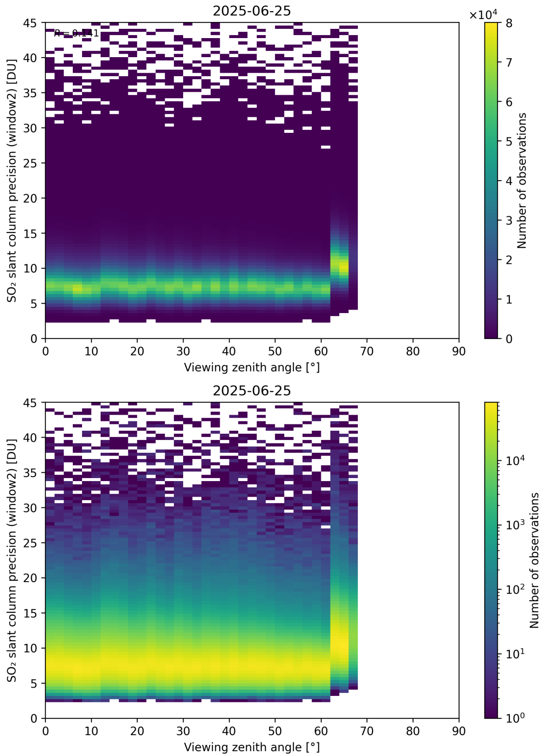
Figure 378: Scatter density plot of “Viewing zenith angle” against “SO 2 slant column precision (window2)” for 2025-06-24 to 2025-06-26.
