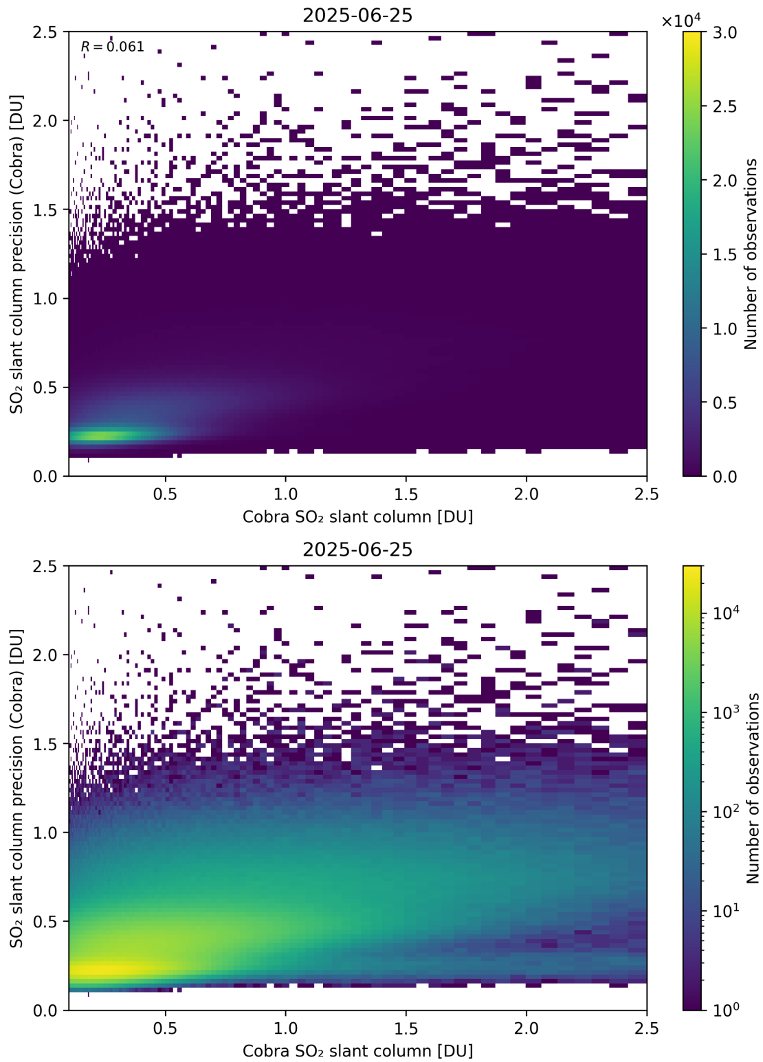
Figure 216: Scatter density plot of “Cobra SO 2 slant column” against “SO 2 slant column precision (Cobra)” for 2025-06-24 to 2025-06-26.
