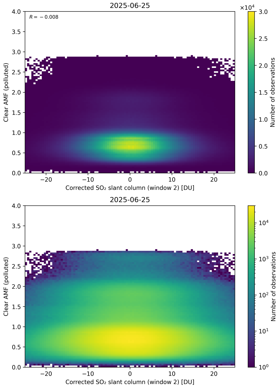
Figure 249: Scatter density plot of “Corrected SO 2 slant column (window 2)” against “Clear AMF (polluted)” for 2025-06-24 to 2025-06-26.
