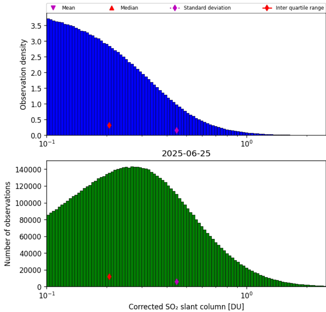
Figure 60: Histogram of “Corrected SO 2 slant column” for 2025-06-24 to 2025-06-26
