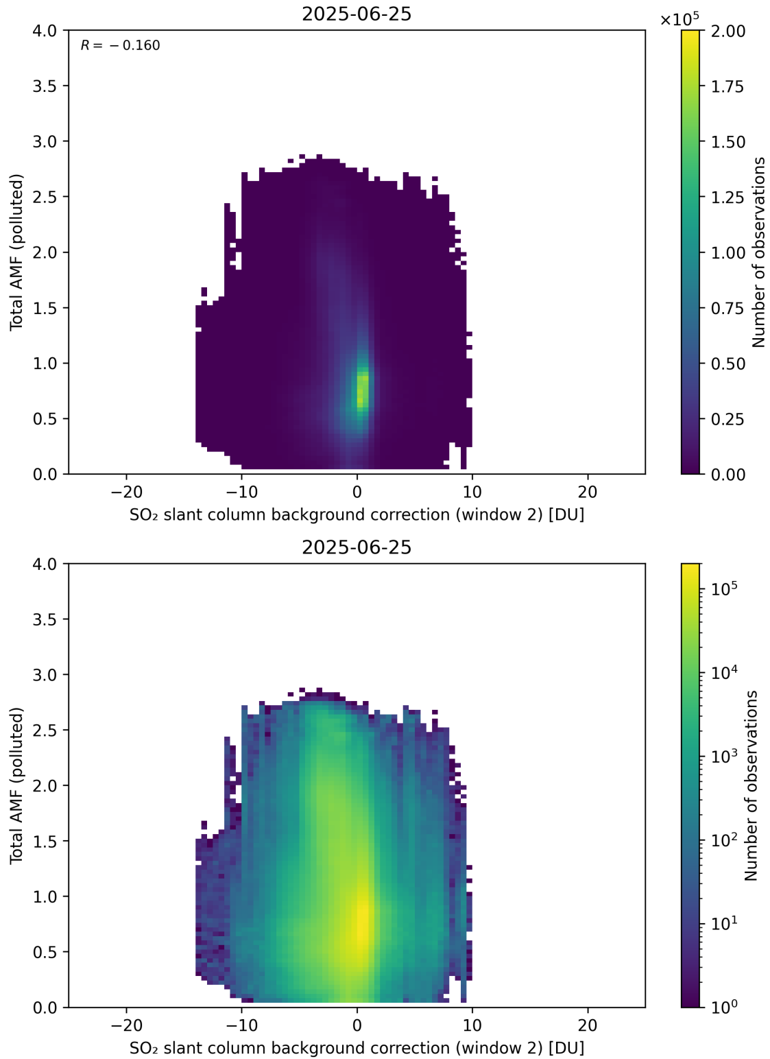
Figure 130: Scatter density plot of “SO 2 slant column background correction (window 2)” against “Total AMF (polluted)” for 2025-06-24 to 2025-06-26.
