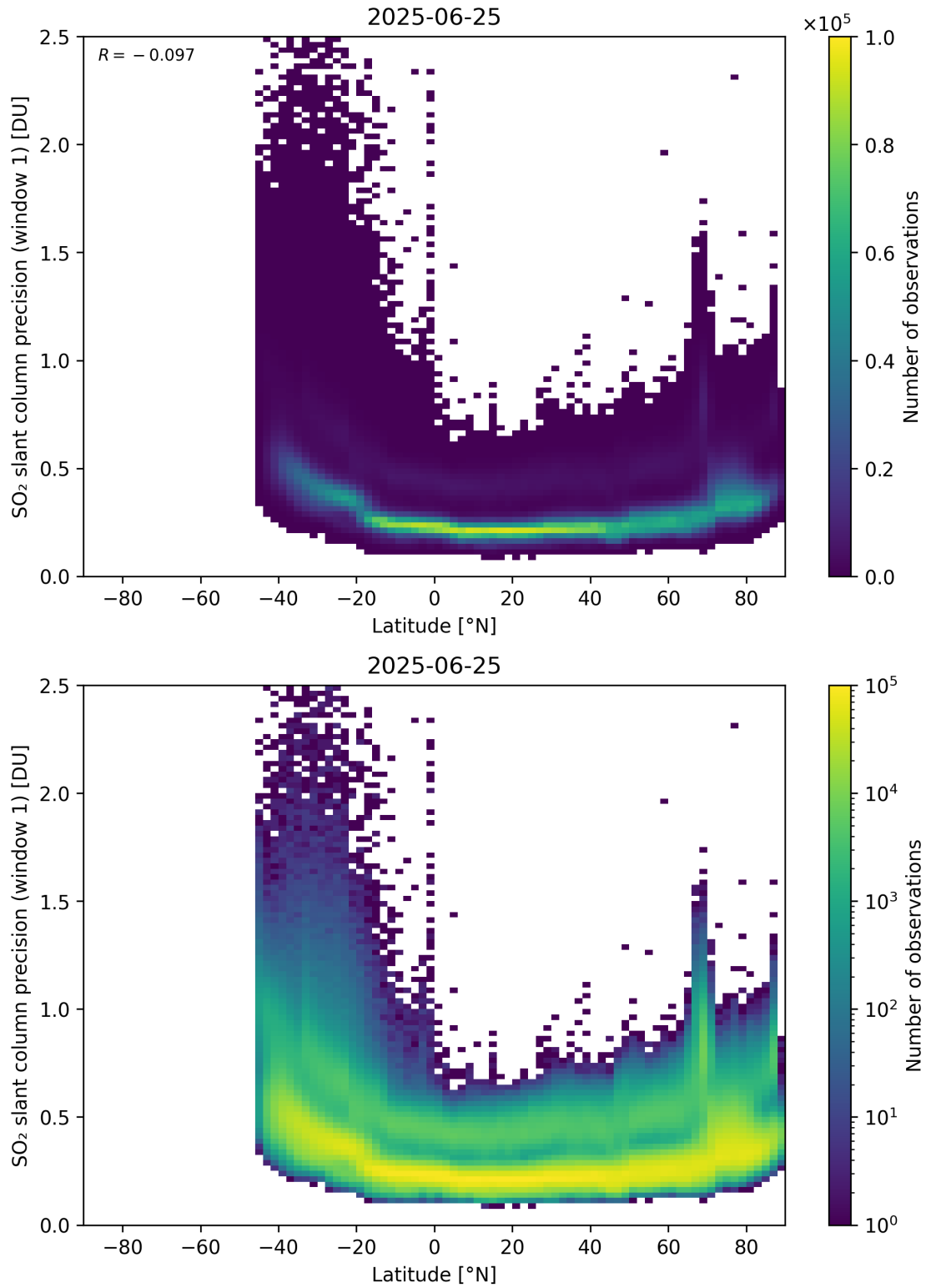
Figure 163: Scatter density plot of “Latitude” against “SO 2 slant column precision (window 1)” for 2025-06-24 to 2025-06-26.
