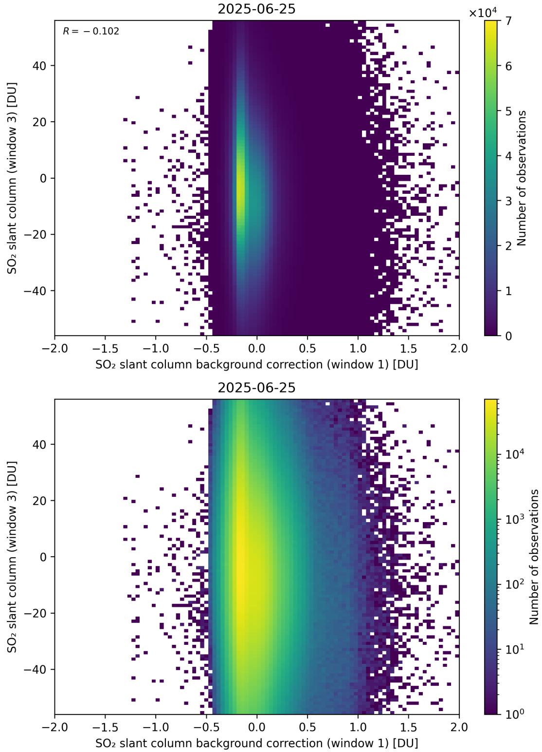
Figure 118: Scatter density plot of “SO 2 slant column background correction (window 1)” against “SO 2 slant column (window 3)” for 2025-06-24 to 2025-06-26.
