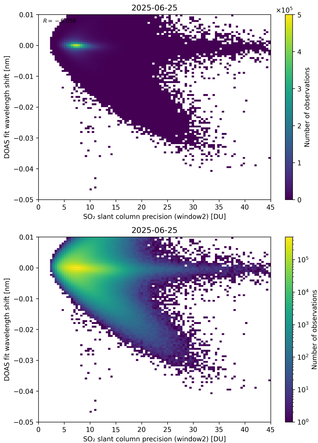
Figure 293: Scatter density plot of “SO 2 slant column precision (window2)” against “DOAS fit wavelength shift” for 2025-06-24 to 2025-06-26.
