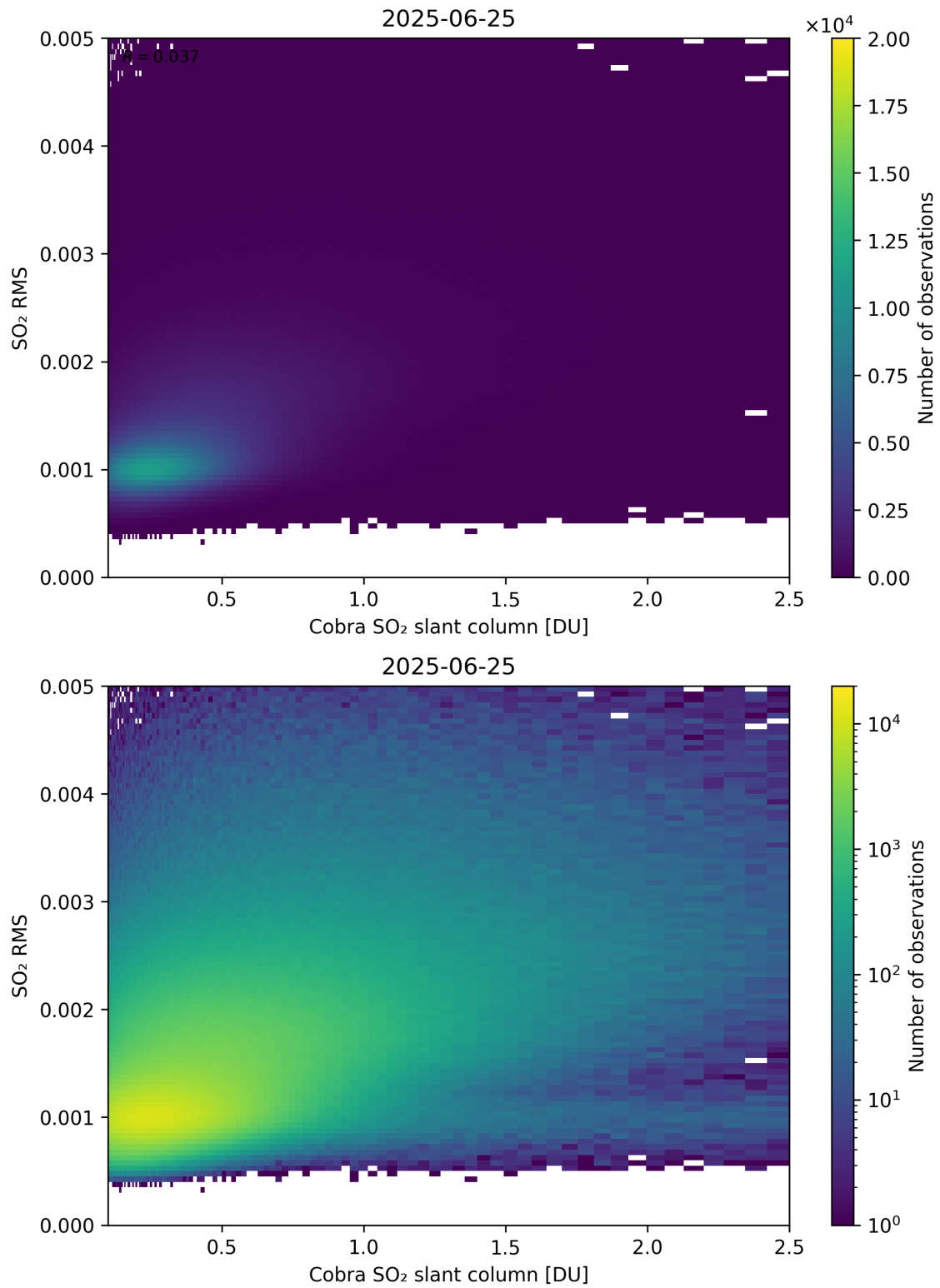
Figure 198: Scatter density plot of “Cobra SO 2 slant column” against “SO 2 RMS” for 2025-06-24 to 2025-06-26.
