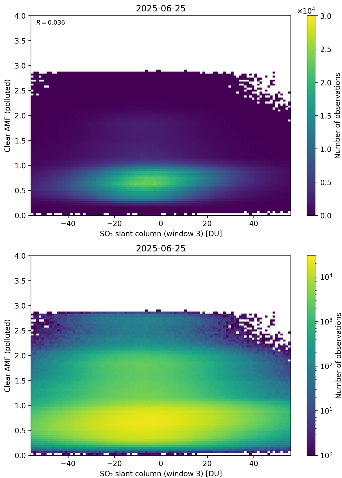
Figure 315: Scatter density plot of “SO 2 slant column (window 3)” against “Clear AMF (polluted)” for 2025-06-24 to 2025-06-26.
