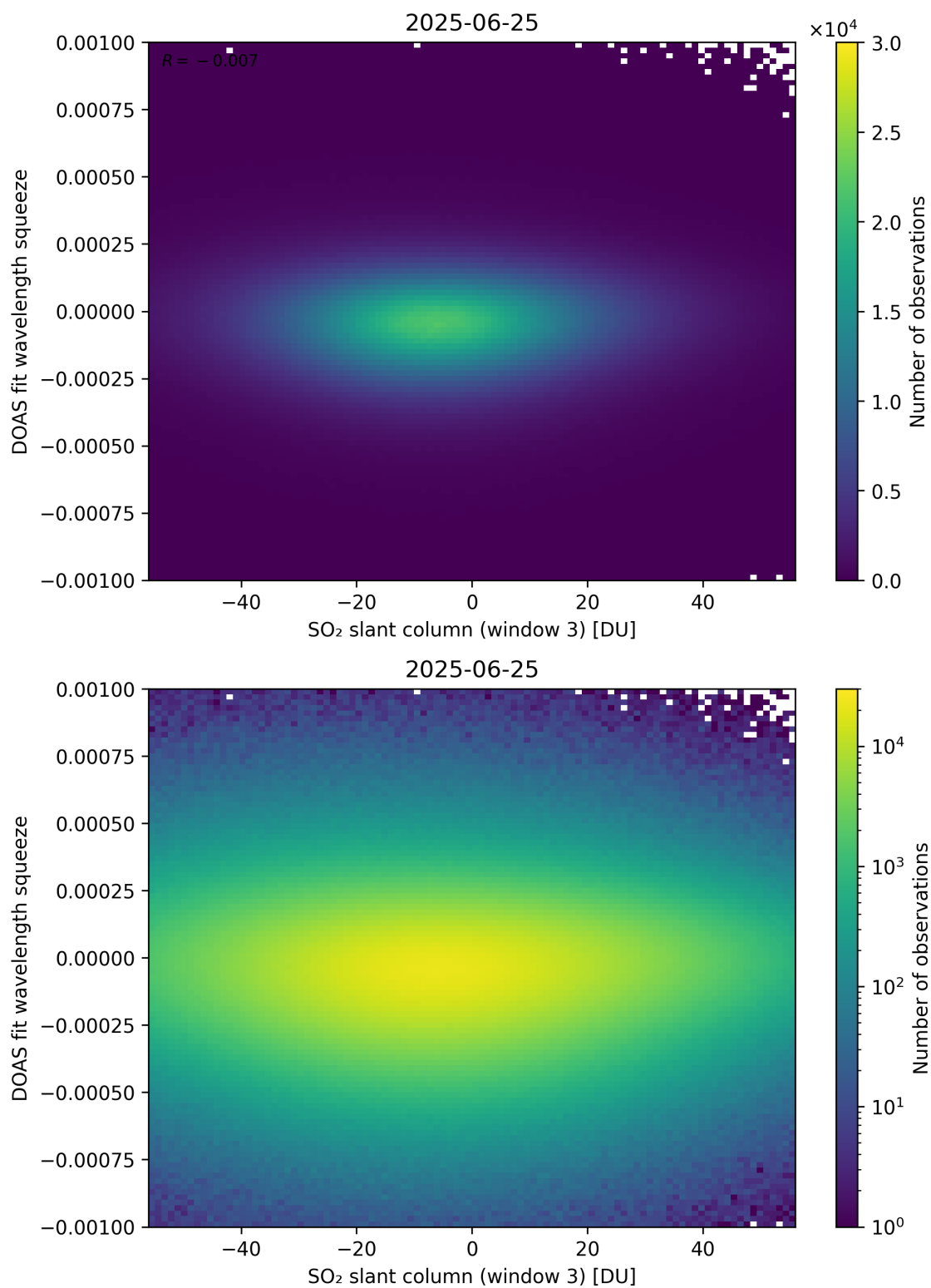
Figure 305: Scatter density plot of “SO 2 slant column (window 3)” against “DOAS fit wavelength squeeze” for 2025-06-24 to 2025-06-26.
