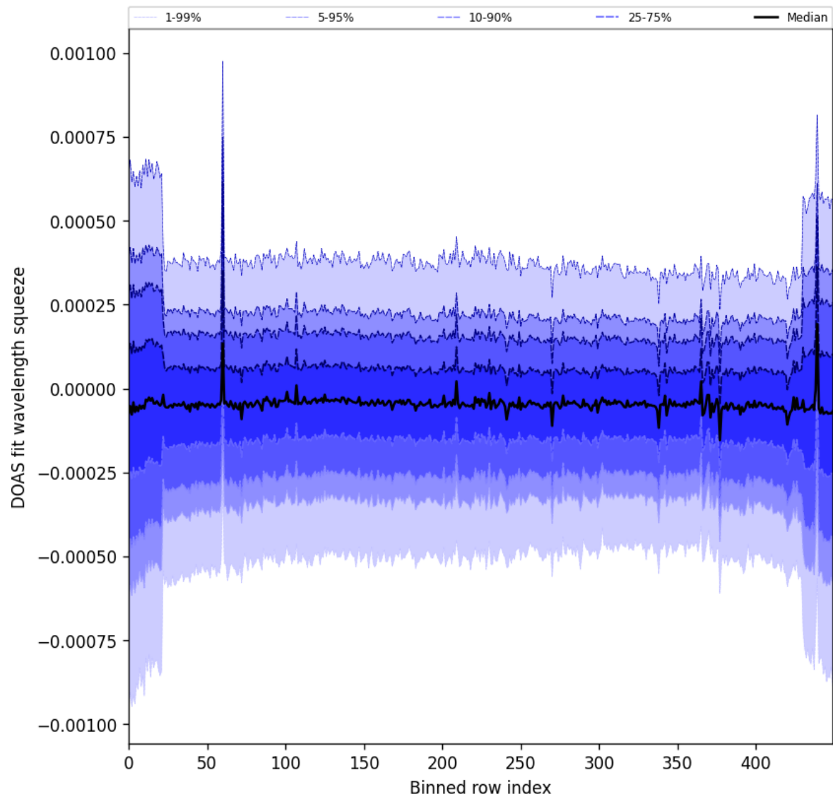
Figure 103: Along track statistics of “DOAS fit wavelength squeeze” for 2025-06-24 to 2025-06-26
