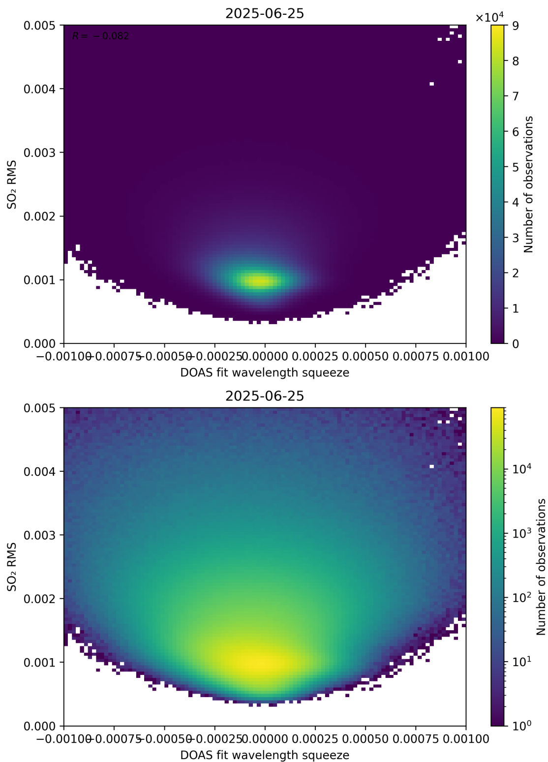
Figure 143: Scatter density plot of “DOAS fit wavelength squeeze” against “SO 2 RMS” for 2025-06-24 to 2025-06-26.
