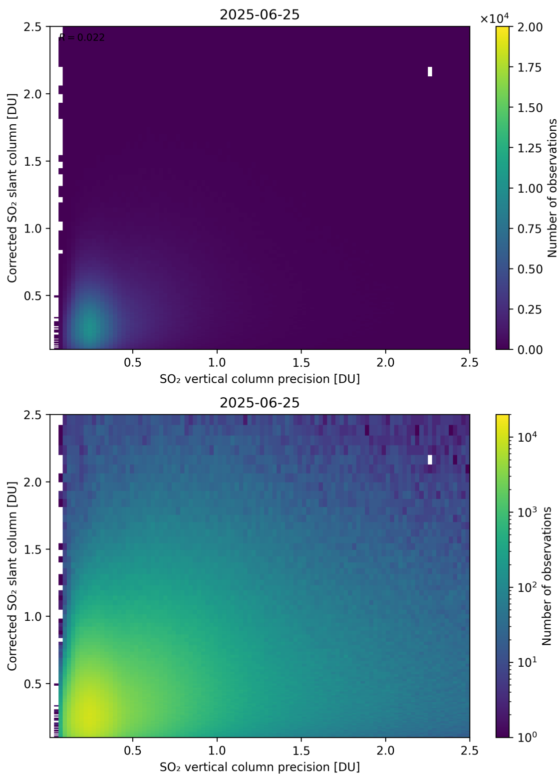
Figure 338: Scatter density plot of “SO 2 vertical column precision” against “Corrected SO 2 slant column” for 2025-06-24 to 2025-06-26.
