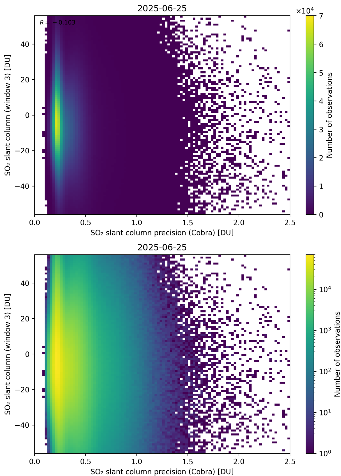
Figure 211: Scatter density plot of “SO 2 slant column precision (Cobra)” against “SO 2 slant column (window 3)” for 2025-06-24 to 2025-06-26.
