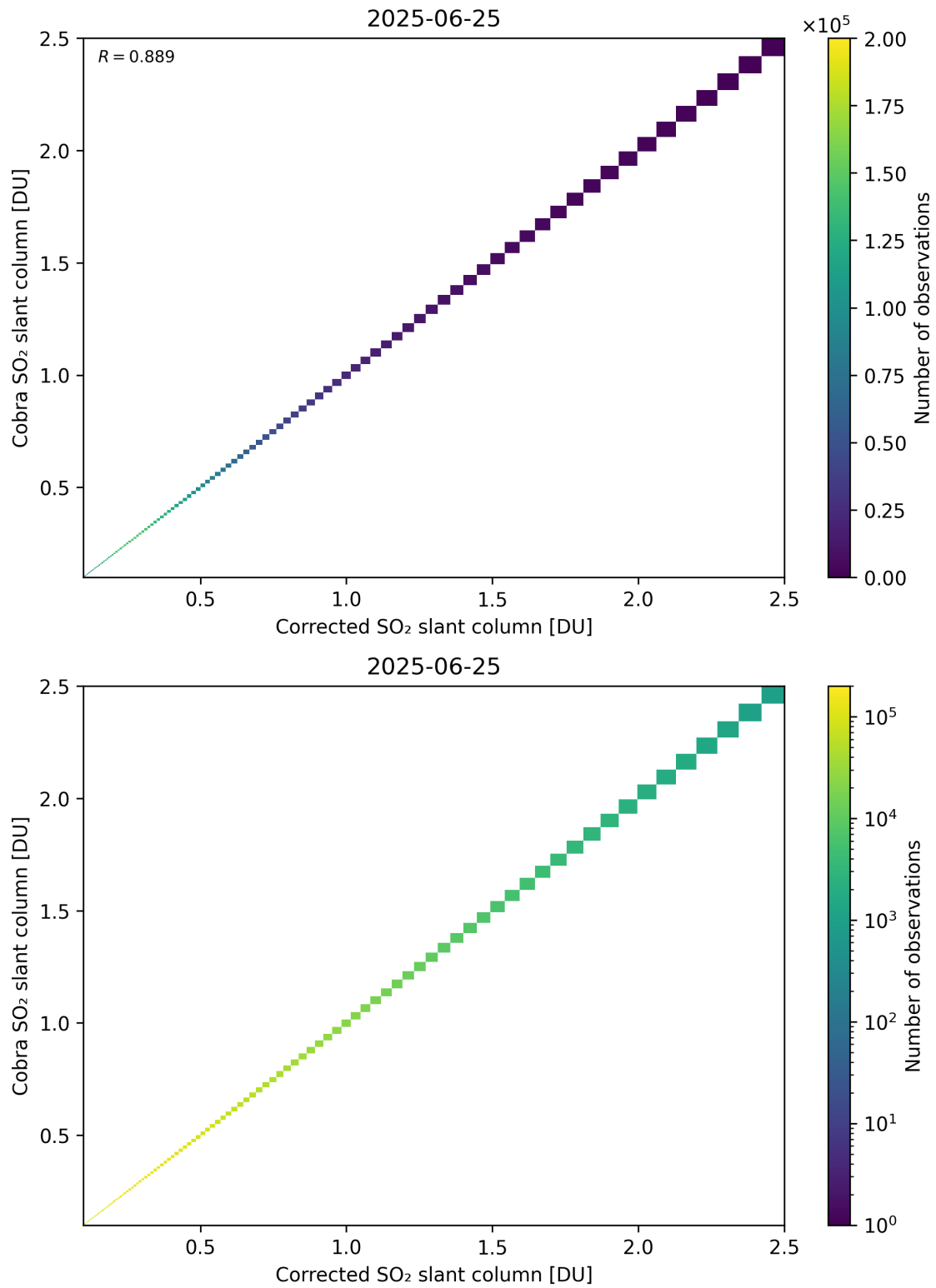
Figure 233: Scatter density plot of “Corrected SO 2 slant column” against “Cobra SO 2 slant column” for 2025-06-24 to 2025-06-26.
