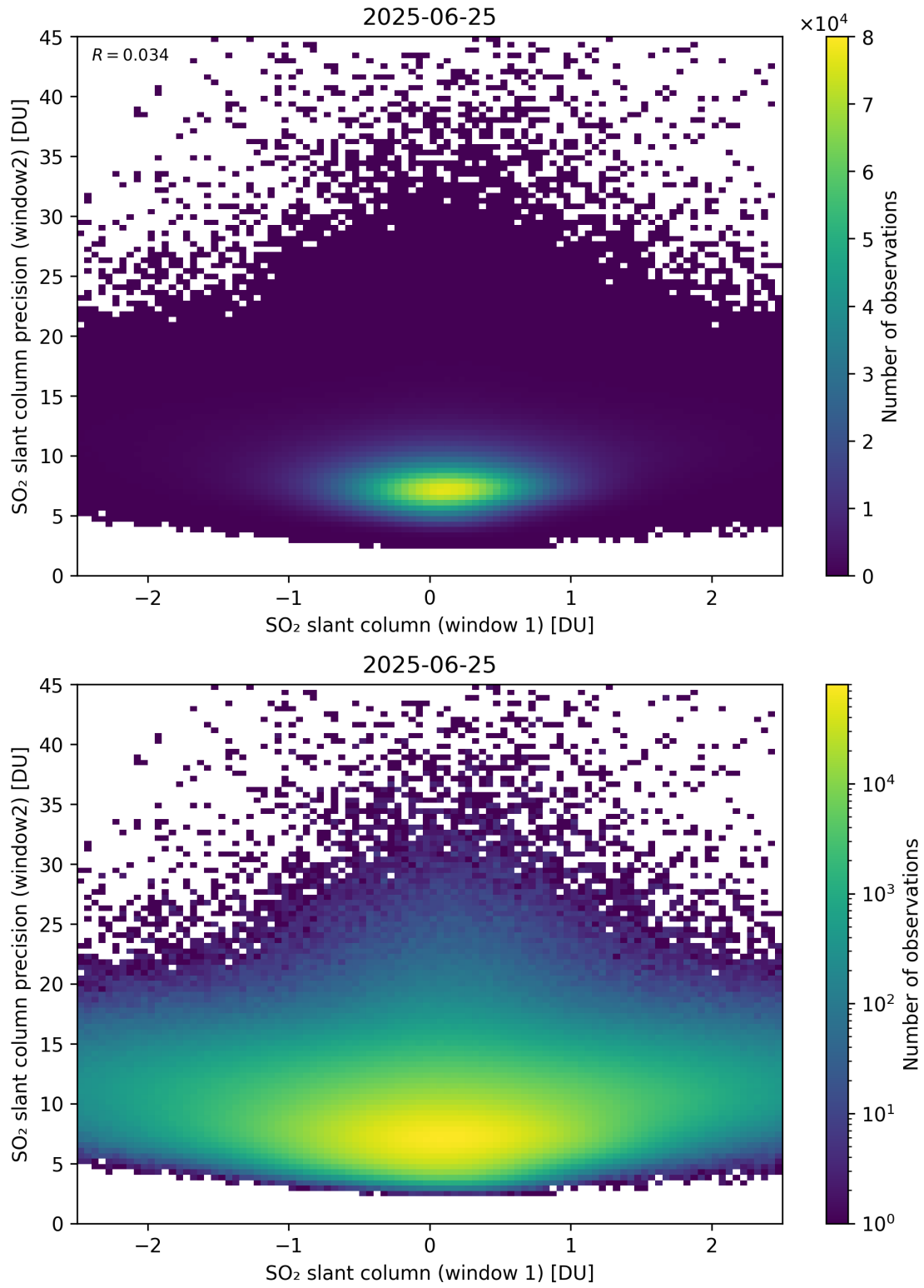
Figure 286: Scatter density plot of “SO 2 slant column (window 1)” against “SO 2 slant column precision (window2)” for 2025-06-24 to 2025-06-26.
