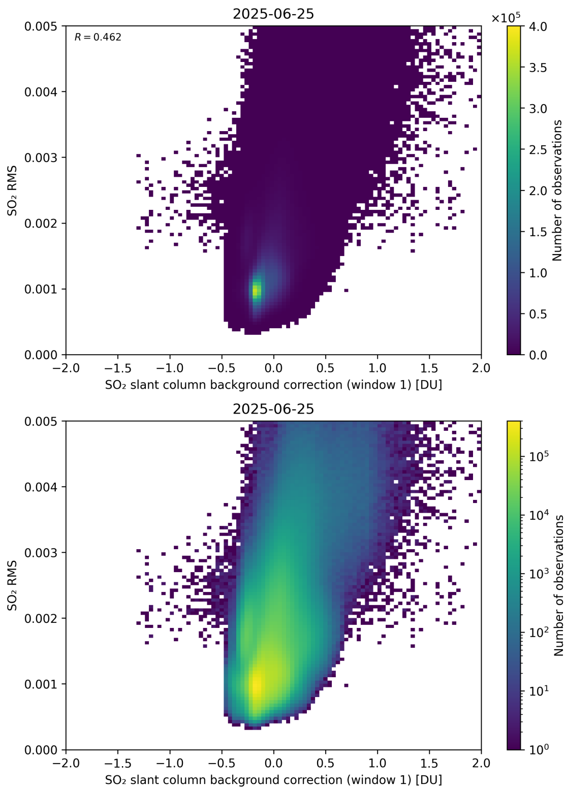
Figure 113: Scatter density plot of “SO 2 slant column background correction (window 1)” against “SO 2 RMS” for 2025-06-24 to 2025-06-26.
