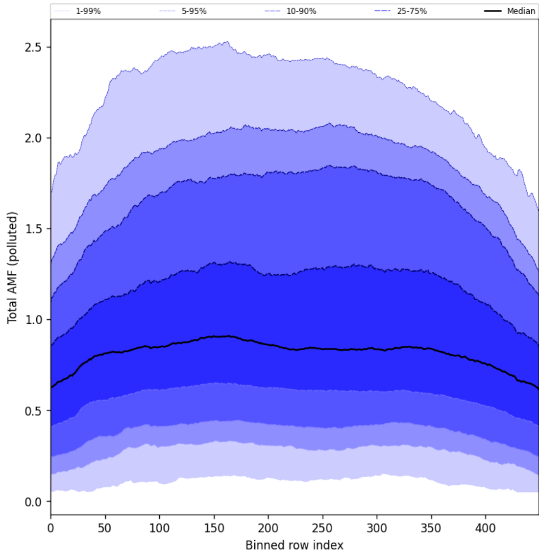
Figure 105: Along track statistics of “Total AMF (polluted)” for 2025-06-24 to 2025-06-26
