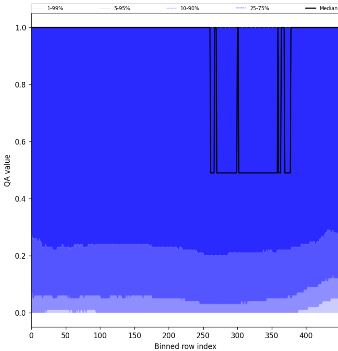
Figure 83: Along track statistics of “QA value” for 2025-06-24 to 2025-06-26
