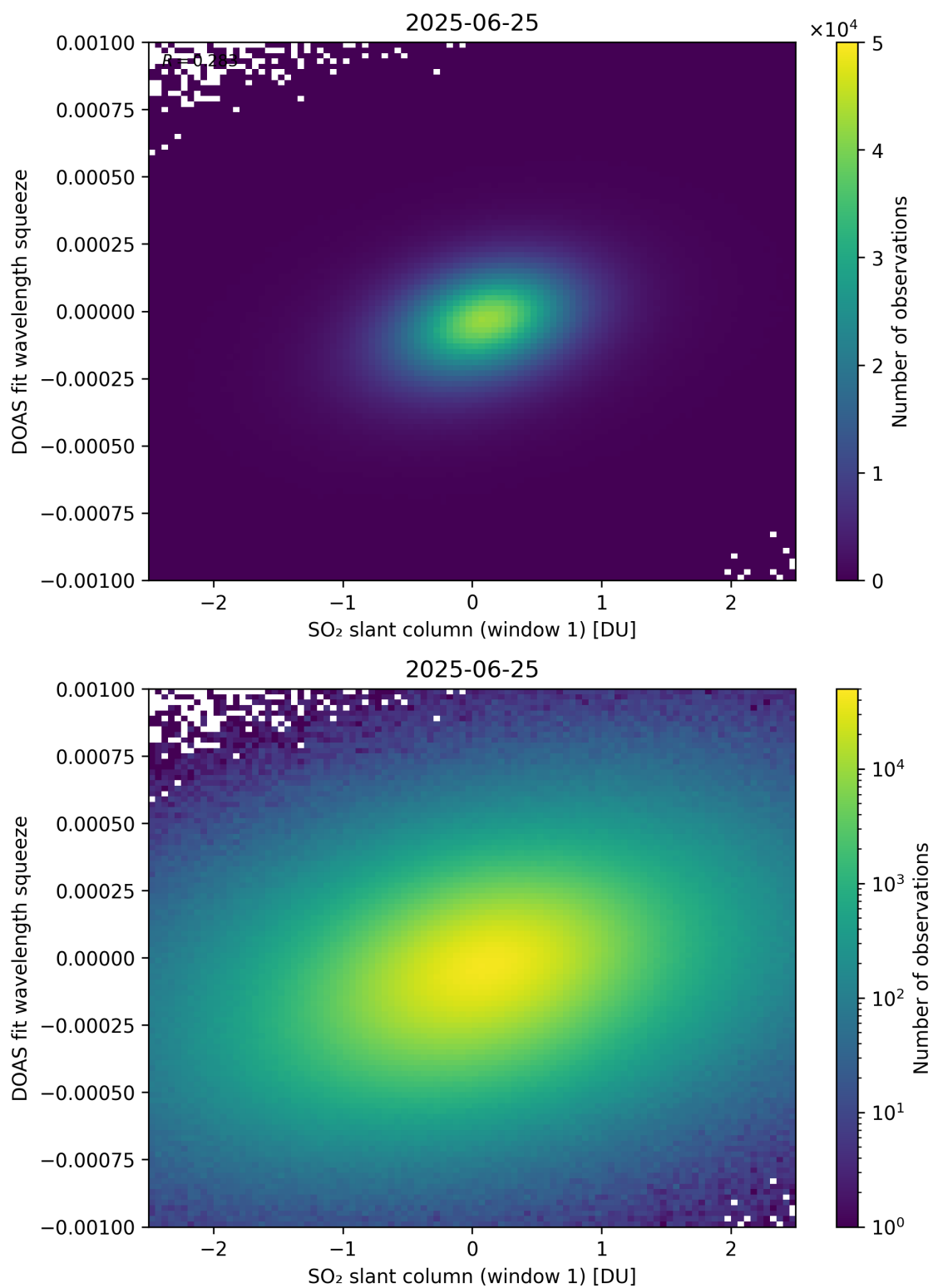
Figure 266: Scatter density plot of “SO 2 slant column (window 1)” against “DOAS fit wavelength squeeze” for 2025-06-24 to 2025-06-26.
