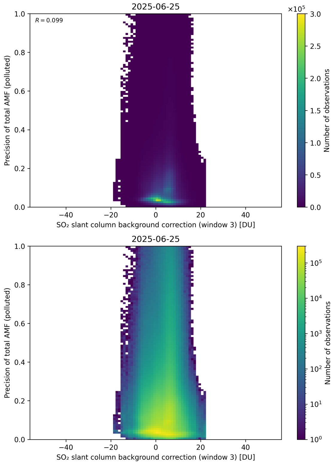
Figure 137: Scatter density plot of “SO 2 slant column background correction (window 3)” against “Precision of total AMF (polluted)” for 2025-06-24 to 2025-06-26.
