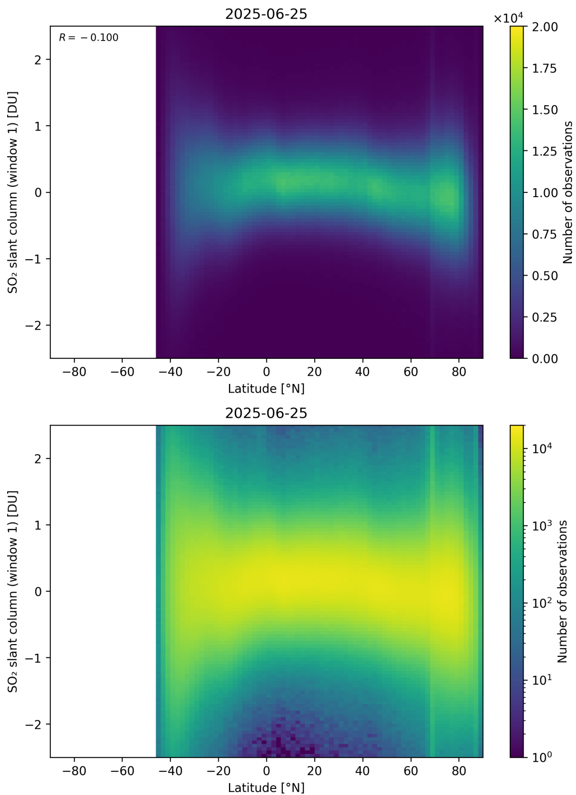
Figure 162: Scatter density plot of “Latitude” against “SO 2 slant column (window 1)” for 2025-06-24 to 2025-06-26.
