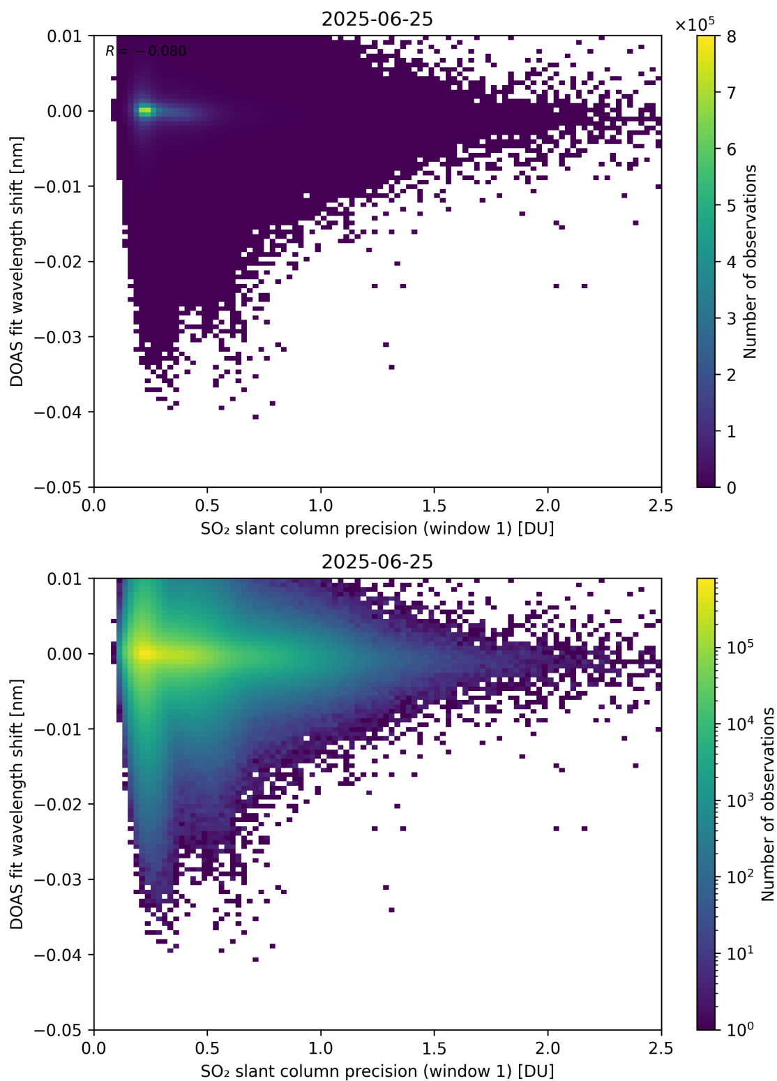
Figure 271: Scatter density plot of “SO 2 slant column precision (window 1)” against “DOAS fit wavelength shift” for 2025-06-24 to 2025-06-26.
