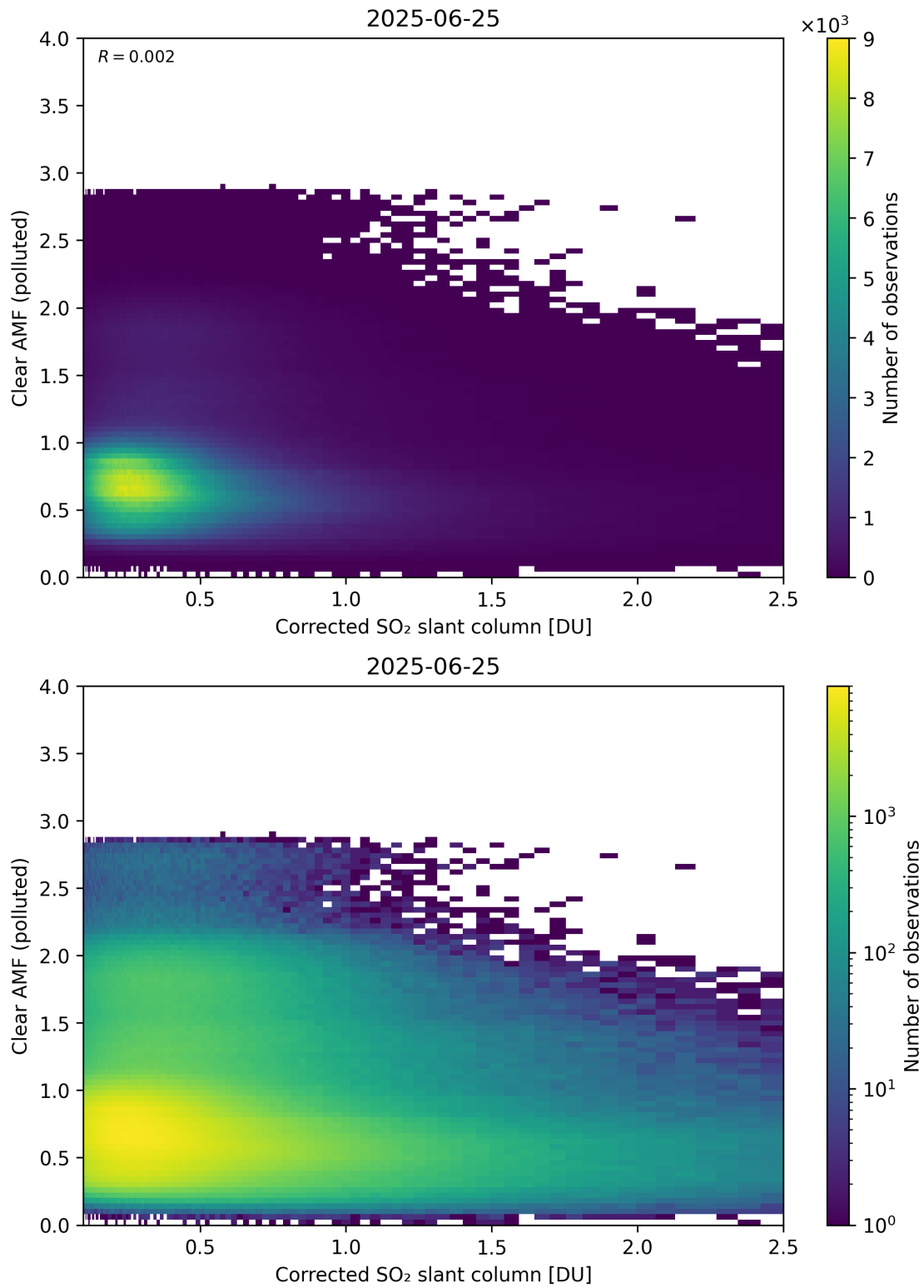
Figure 232: Scatter density plot of “Corrected SO 2 slant column” against “Clear AMF (polluted)” for 2025-06-24 to 2025-06-26.
