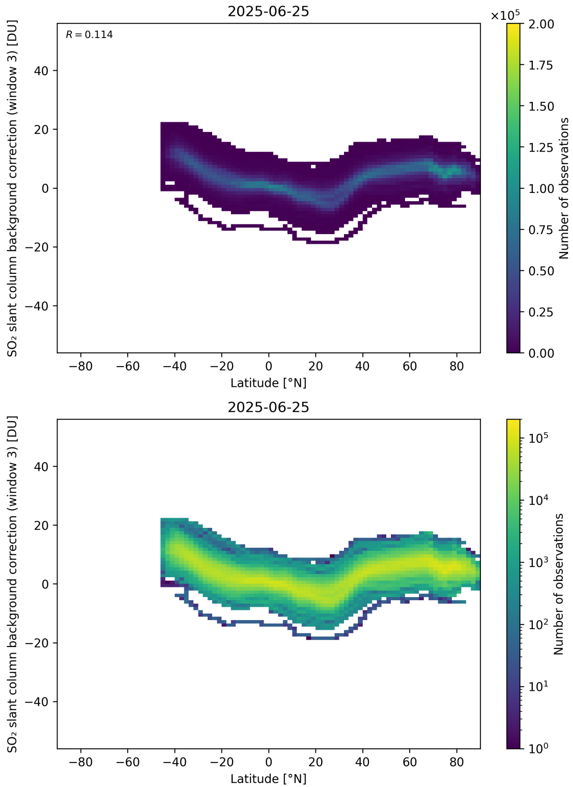
Figure 152: Scatter density plot of “Latitude” against “SO 2 slant column background correction (window 3)” for 2025-06-24 to 2025-06-26.
