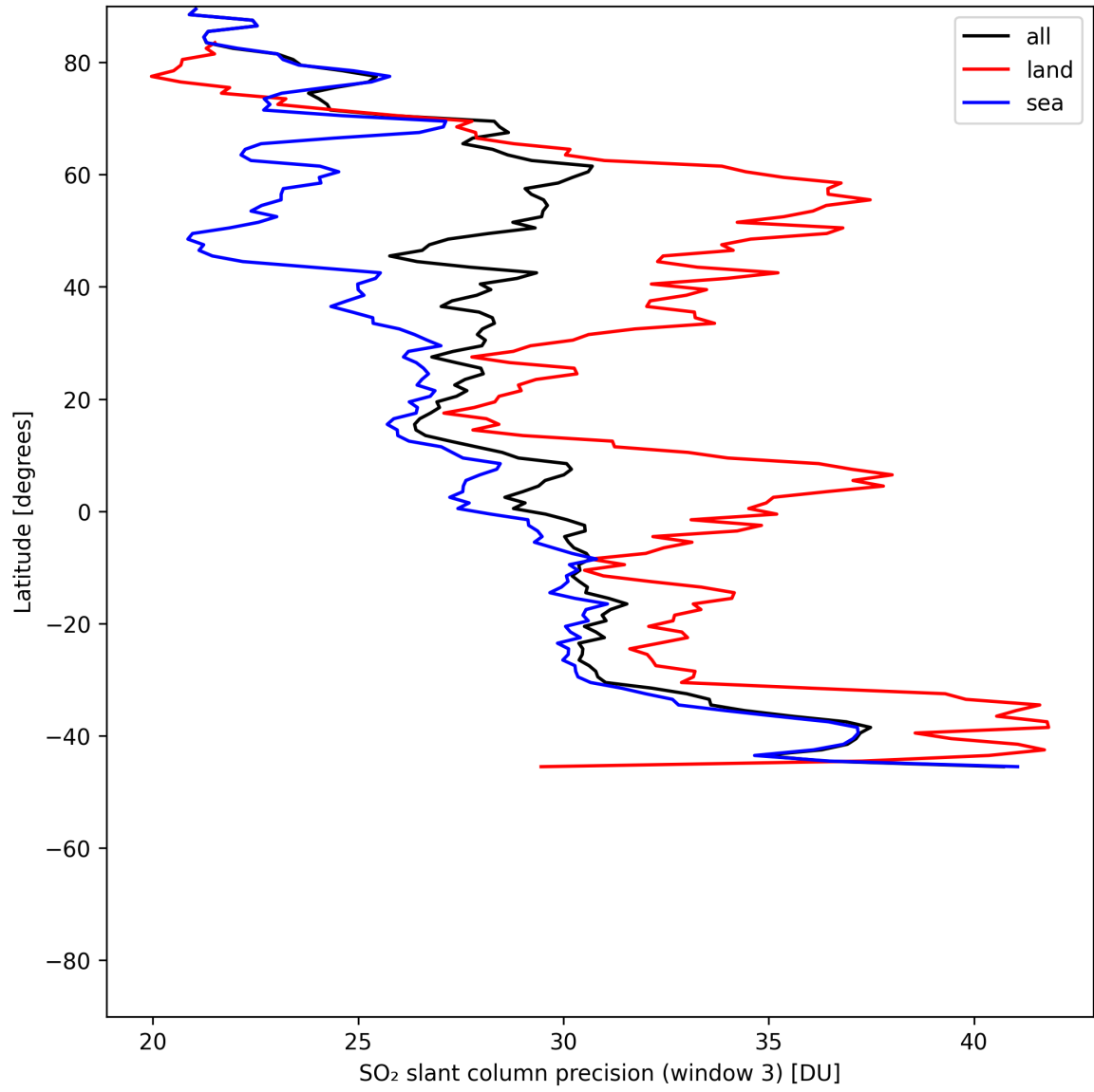
Figure 46: Zonal average of “SO 2 slant column precision (window 3)” for 2025-06-24 to 2025-06-26.
