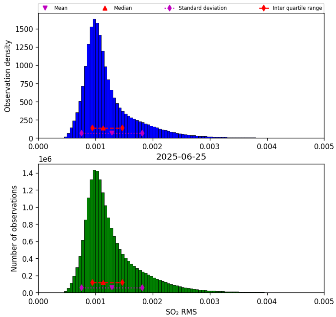
Figure 78: Histogram of “SO 2 RMS” for 2025-06-24 to 2025-06-26
