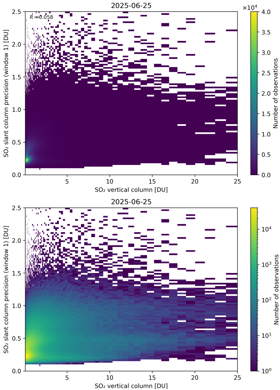
Figure 355: Scatter density plot of “SO 2 vertical column” against “SO 2 slant column precision (window 1)” for 2025-06-24 to 2025-06-26.
