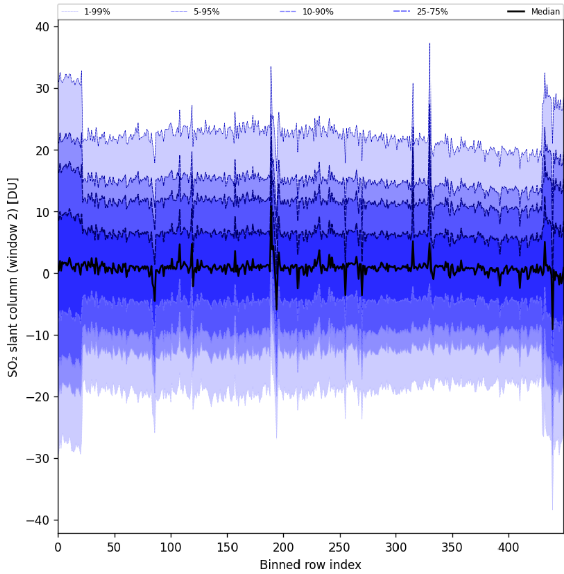
Figure 93: Along track statistics of “SO 2 slant column (window 2)” for 2025-06-24 to 2025-06-26
