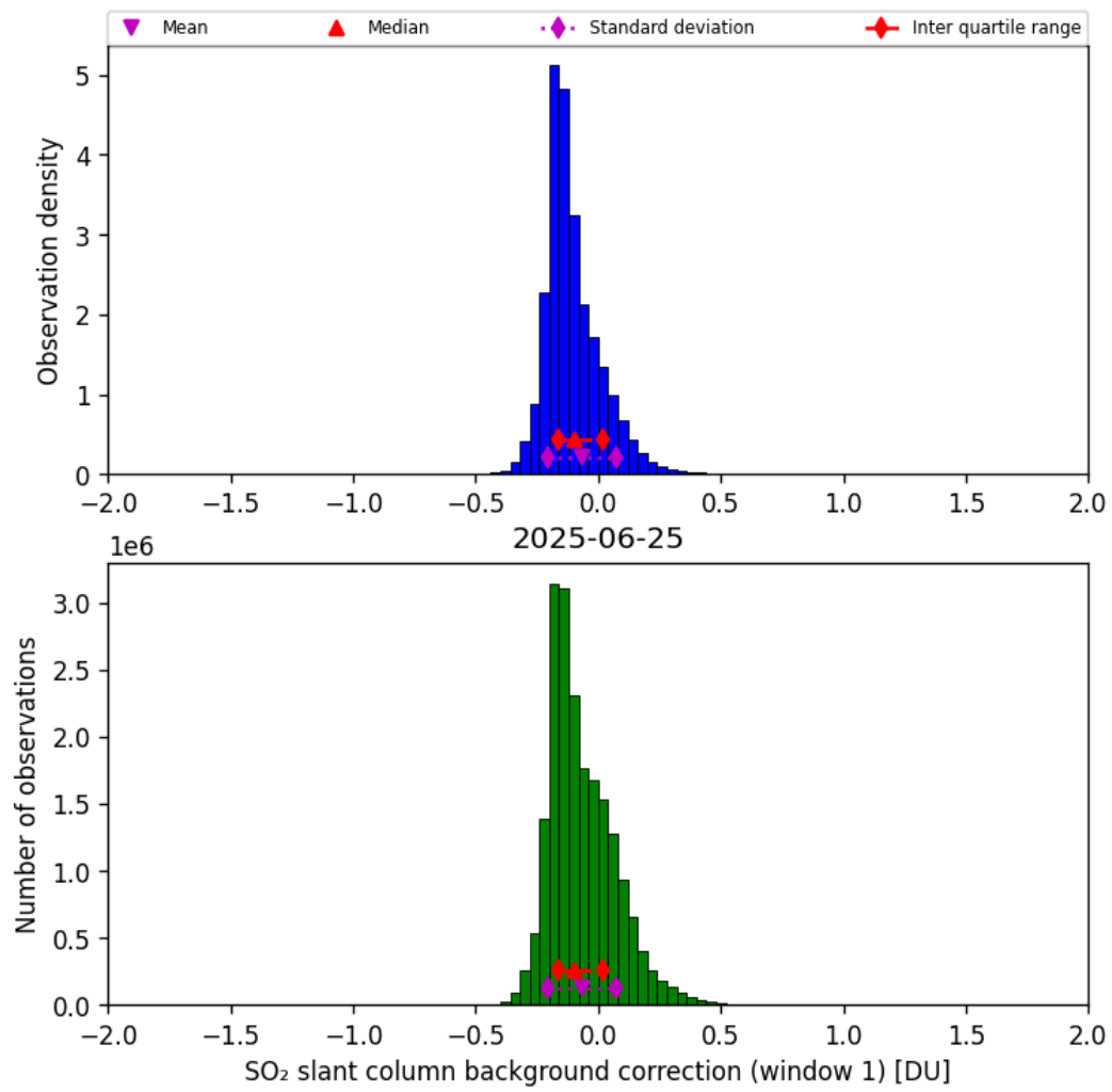
Figure 66: Histogram of “SO 2 slant column background correction (window 1)” for 2025-06-24 to 2025-06-26
