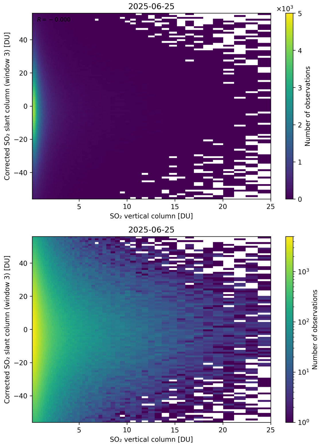
Figure 353: Scatter density plot of “SO 2 vertical column” against “Corrected SO 2 slant column (window 3)” for 2025-06-24 to 2025-06-26.
