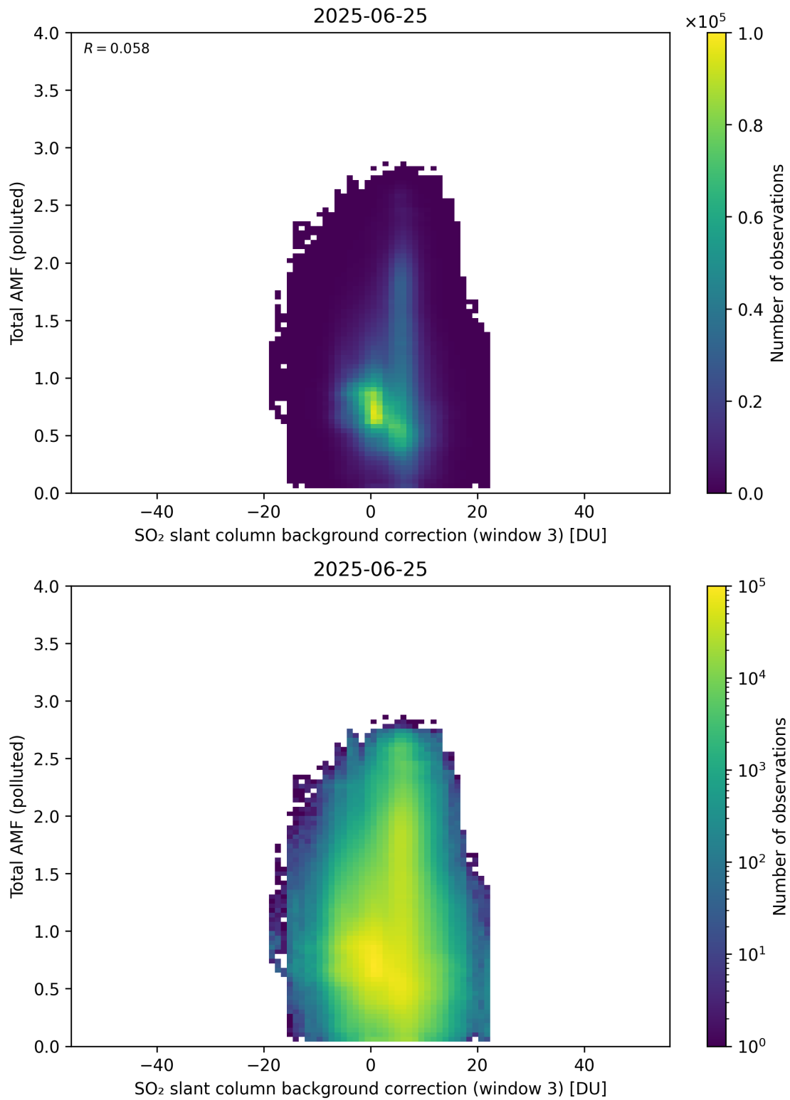
Figure 136: Scatter density plot of “SO 2 slant column background correction (window 3)” against “Total AMF (polluted)” for 2025-06-24 to 2025-06-26.
