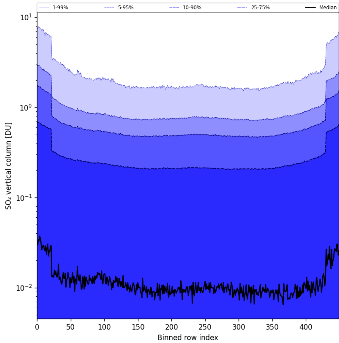
Figure 84: Along track statistics of "SO 2 vertical column" for 2025-06-24 to 2025-06-26
