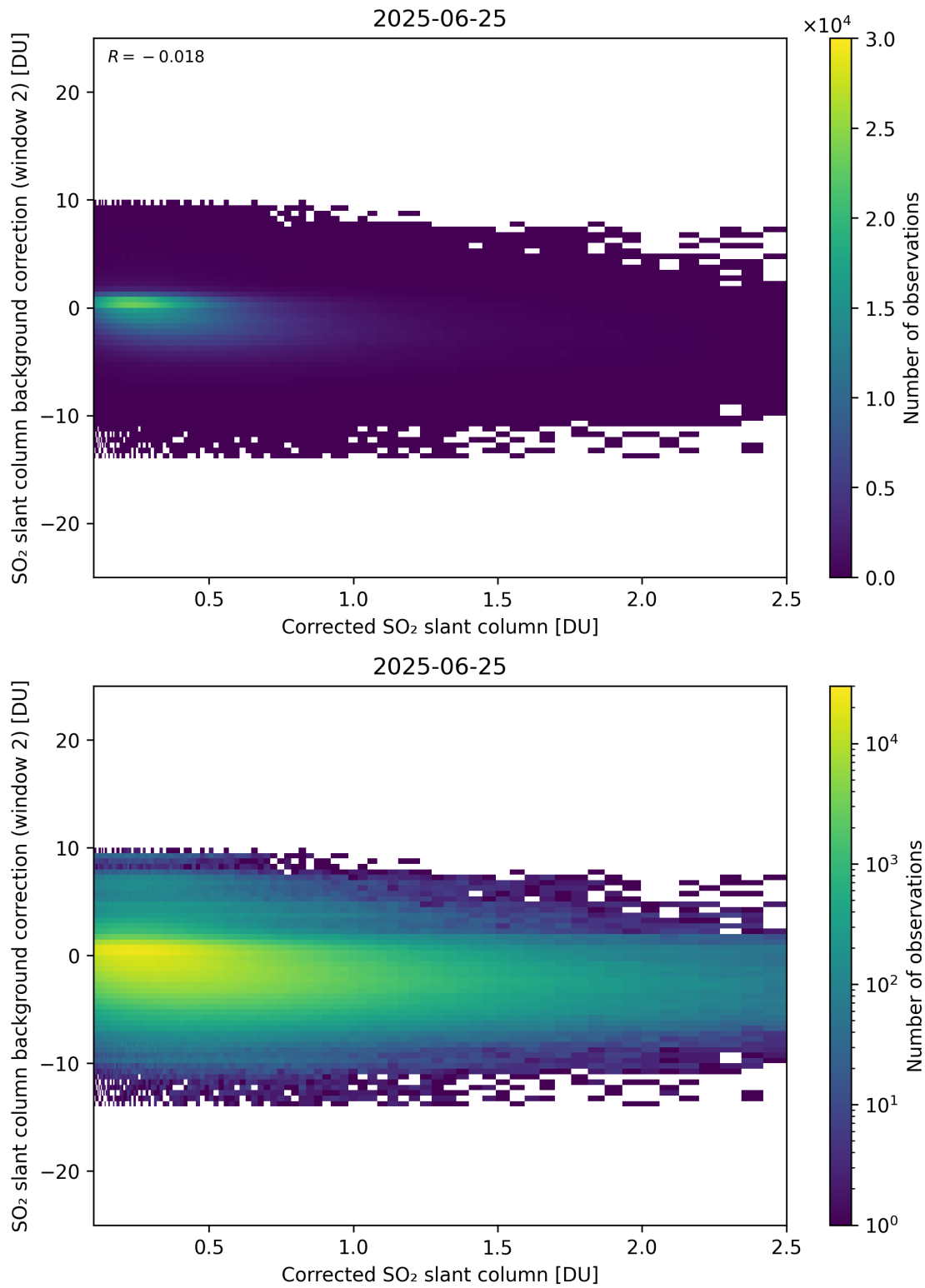
Figure 227: Scatter density plot of “Corrected SO 2 slant column” against “SO 2 slant column background correction (window 2)” for 2025-06-24 to 2025-06-26.
