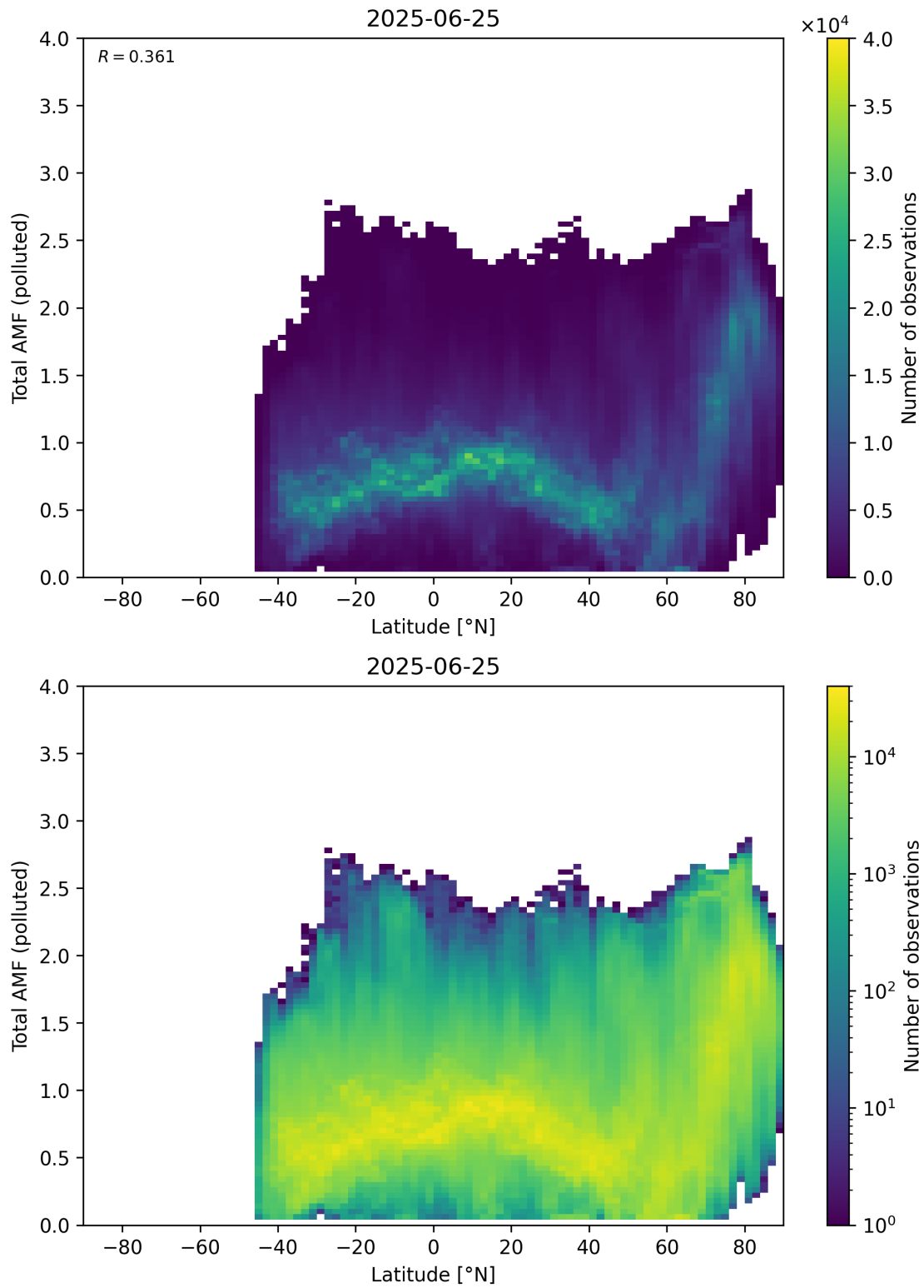
Figure 167: Scatter density plot of “Latitude” against “Total AMF (polluted)” for 2025-06-24 to 2025-06-26.
