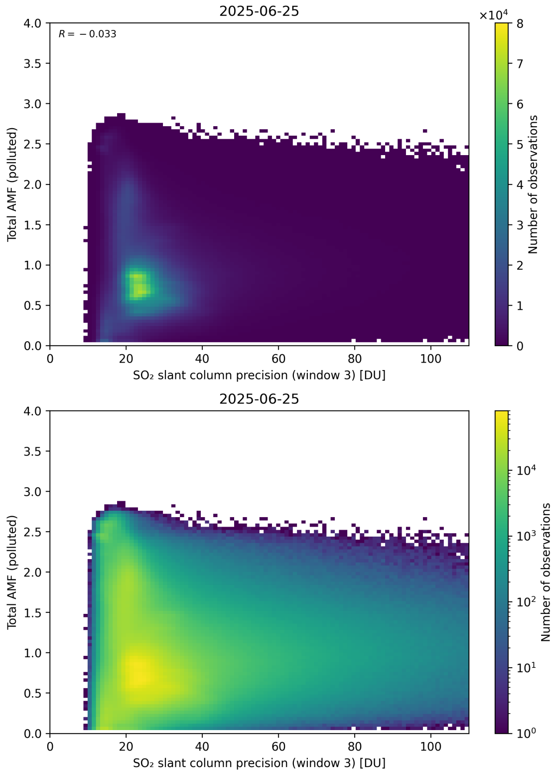
Figure 313: Scatter density plot of “SO 2 slant column precision (window 3)” against “Total AMF (polluted)” for 2025-06-24 to 2025-06-26.
