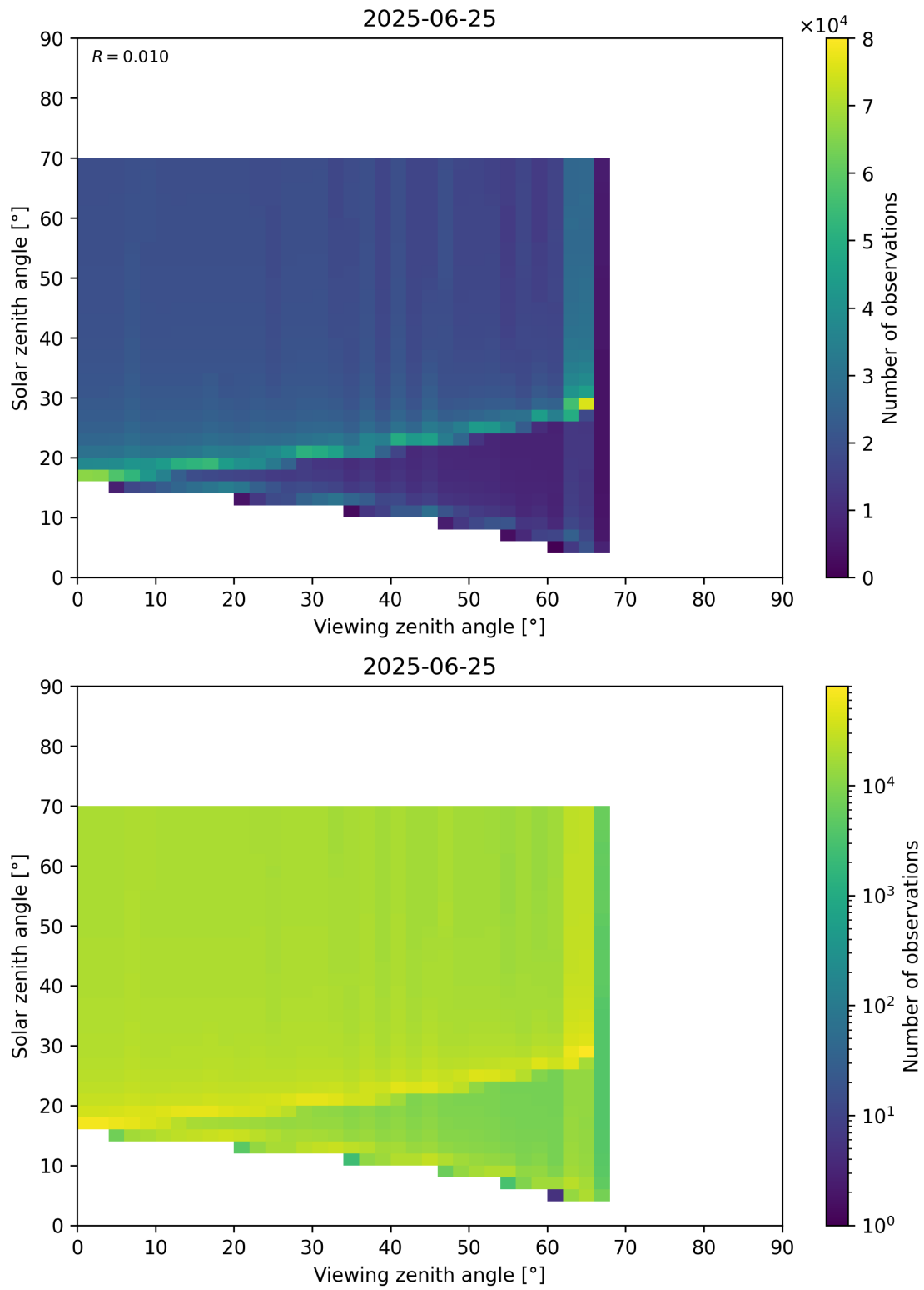
Figure 369: Scatter density plot of “Viewing zenith angle” against “Solar zenith angle” for 2025-06-24 to 2025-06-26.
