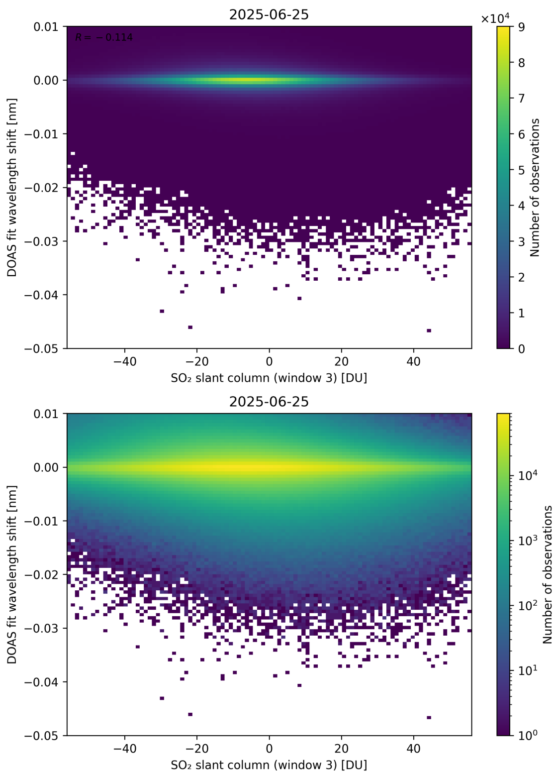
Figure 304: Scatter density plot of “SO 2 slant column (window 3)” against “DOAS fit wavelength shift” for 2025-06-24 to 2025-06-26.
