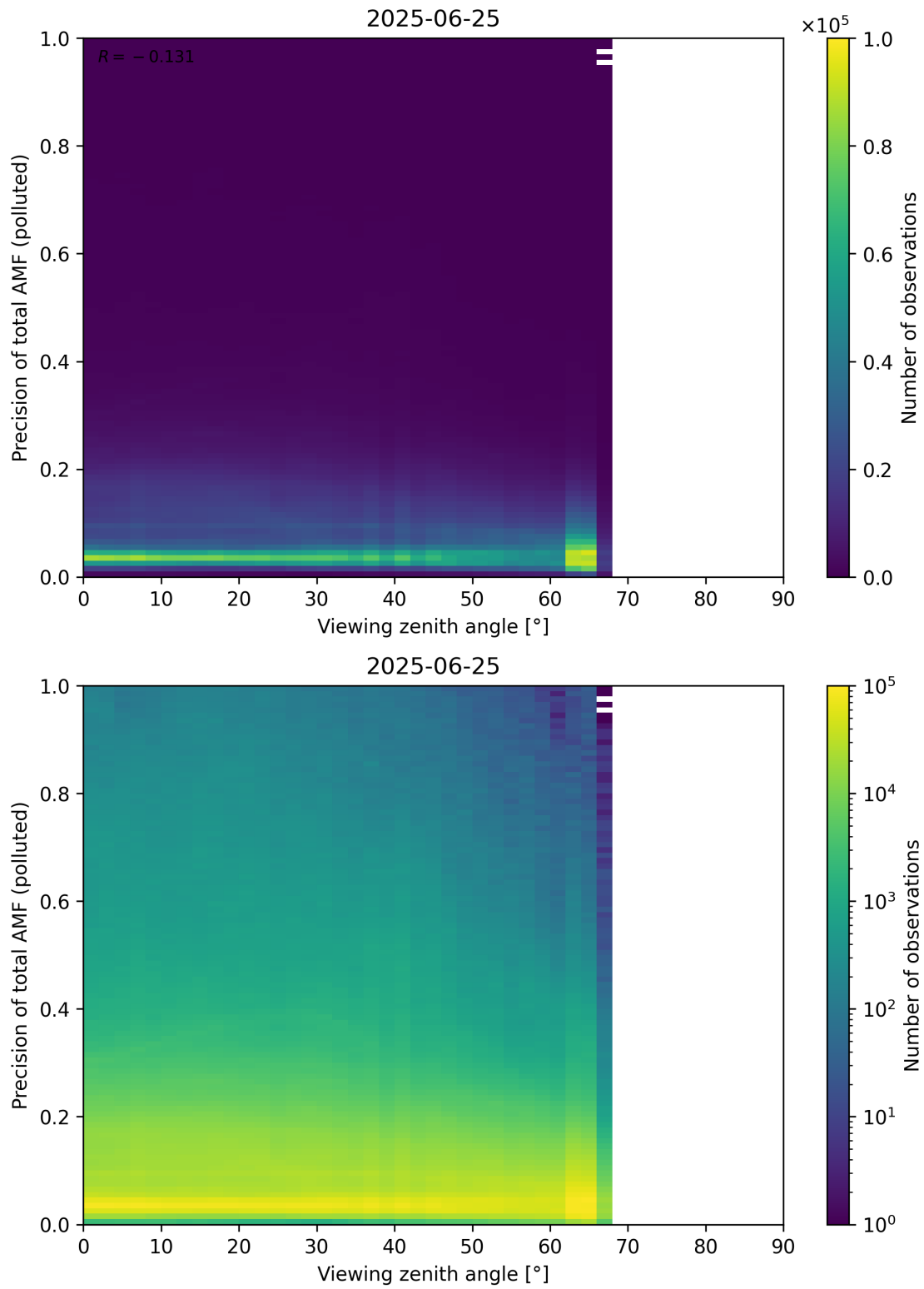
Figure 382: Scatter density plot of “Viewing zenith angle” against “Precision of total AMF (polluted)” for 2025-06-24 to 2025-06-26.
