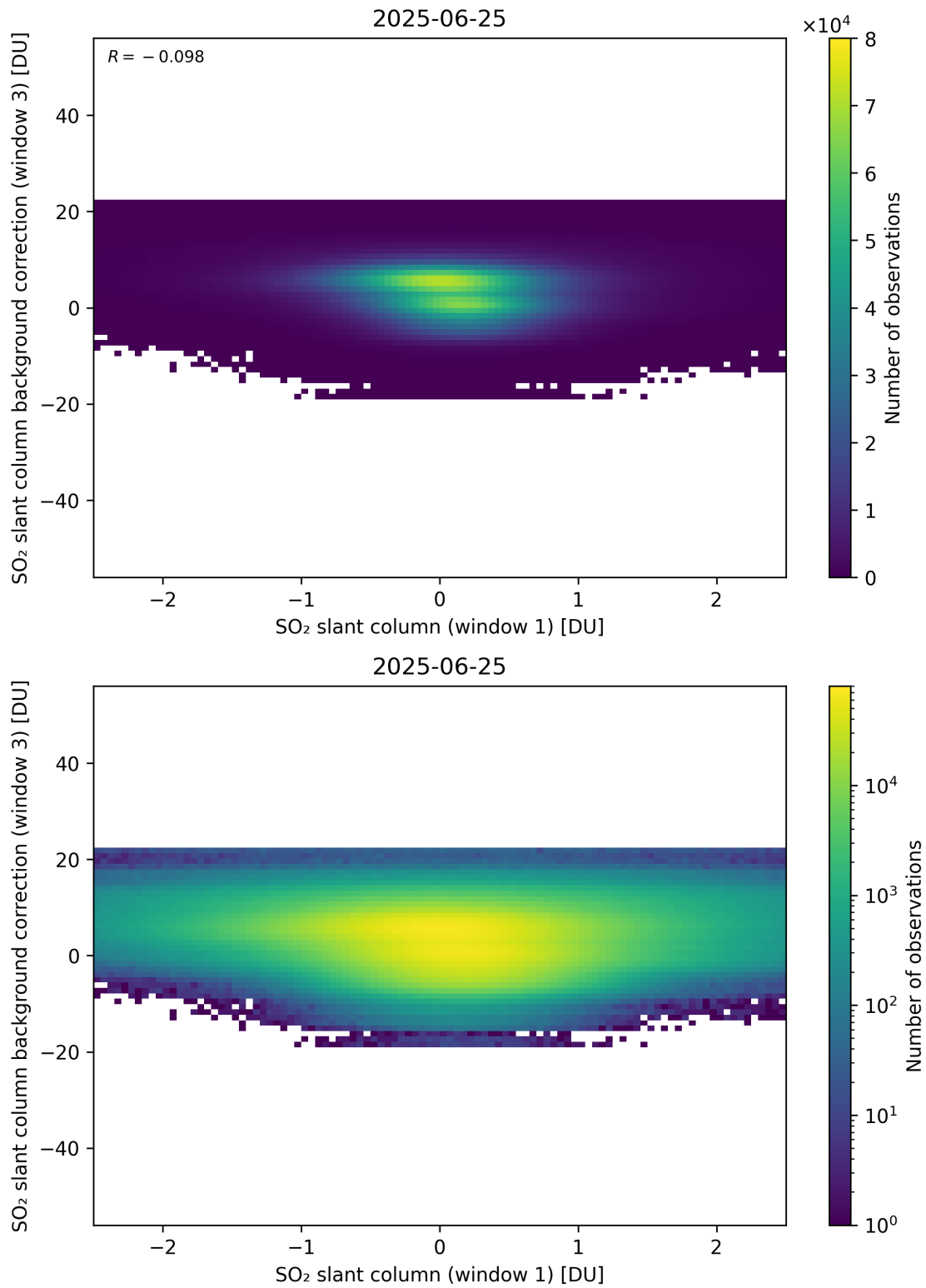
Figure 264: Scatter density plot of “SO 2 slant column (window 1)” against “SO 2 slant column background correction (window 3)” for 2025-06-24 to 2025-06-26.
