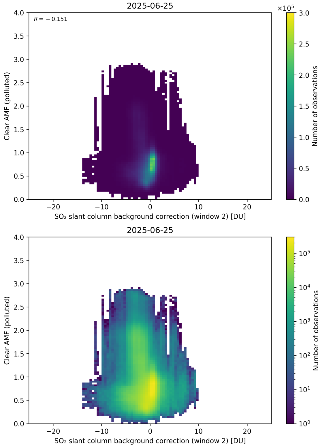
Figure 126: Scatter density plot of “SO 2 slant column background correction (window 2)” against “Clear AMF (polluted)” for 2025-06-24 to 2025-06-26.
