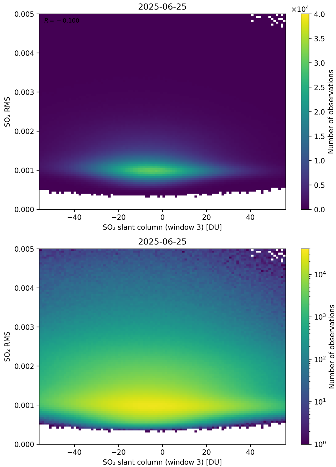
Figure 306: Scatter density plot of “SO 2 slant column (window 3)” against “SO 2 RMS” for 2025-06-24 to 2025-06-26.
