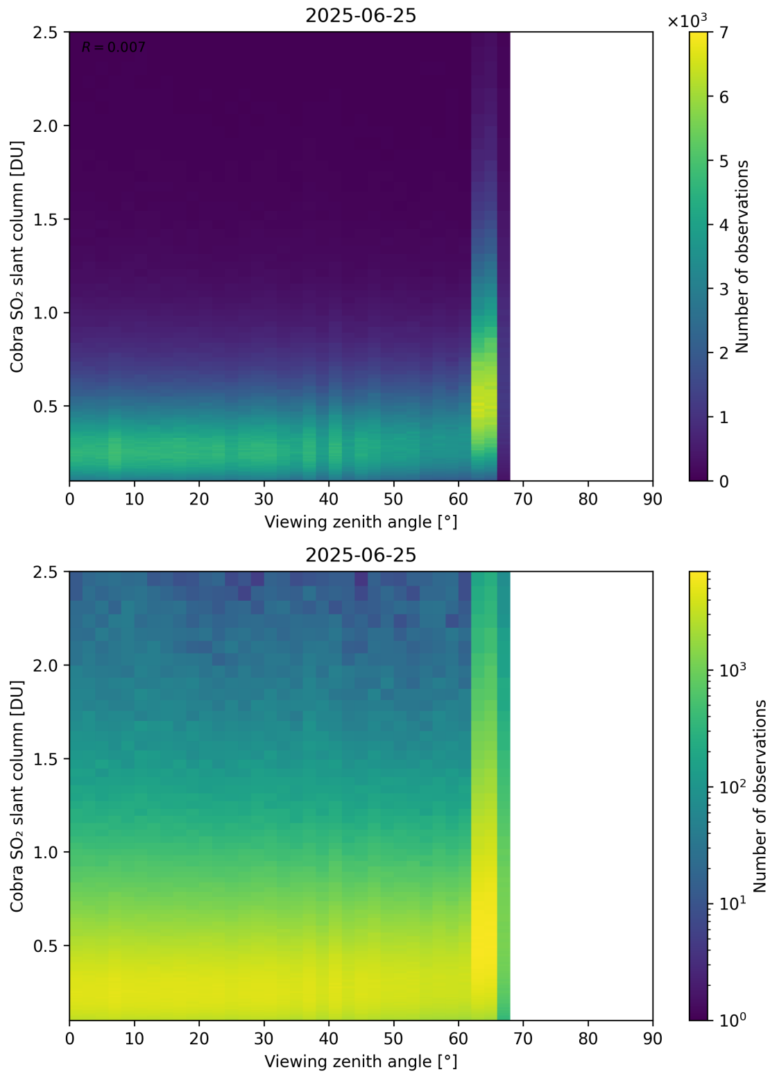
Figure 371: Scatter density plot of “Viewing zenith angle” against “Cobra SO 2 slant column” for 2025-06-24 to 2025-06-26.
