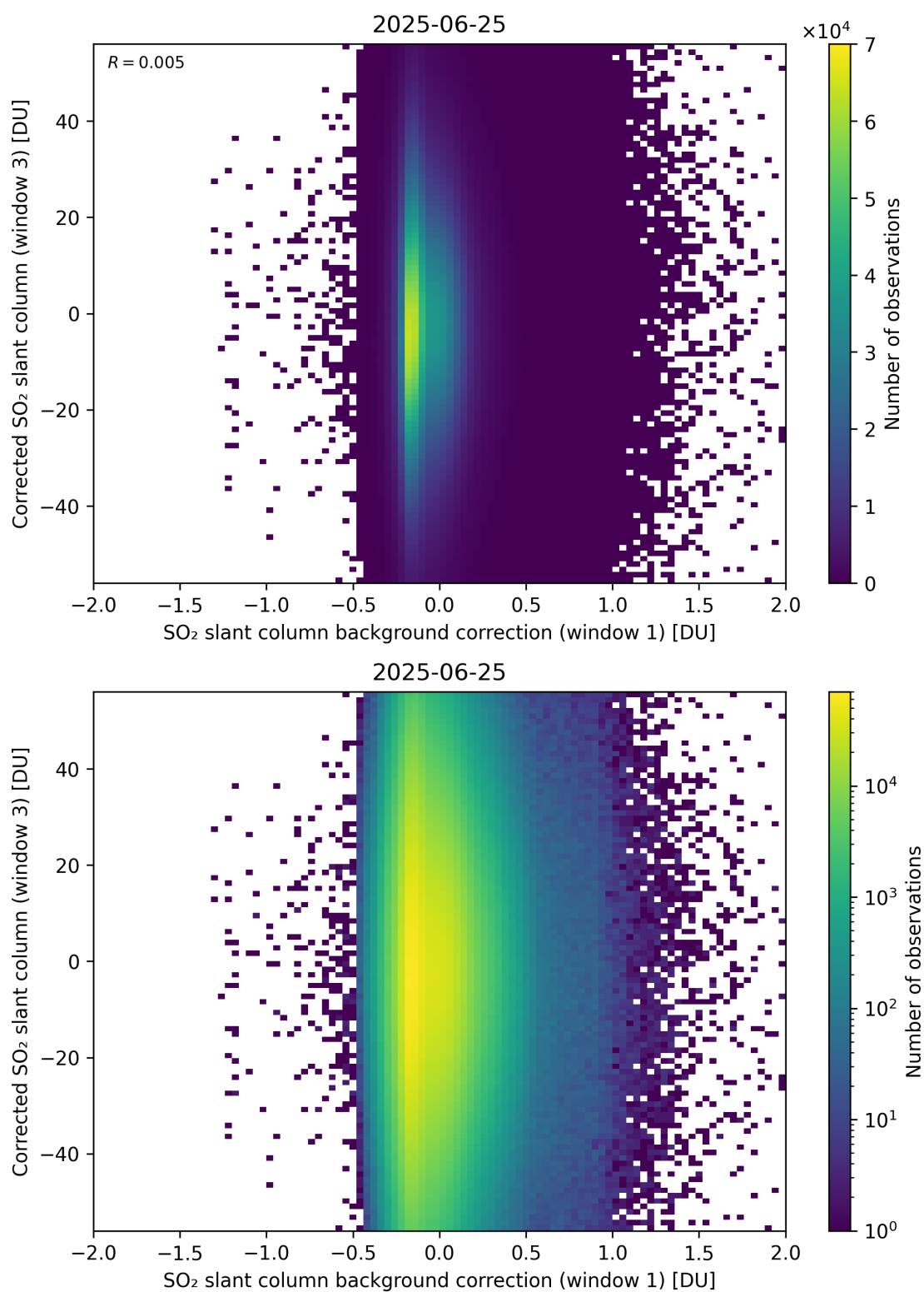
Figure 116: Scatter density plot of “SO 2 slant column background correction (window 1)” against “Corrected SO 2 slant column (window 3)” for 2025-06-24 to 2025-06-26.
