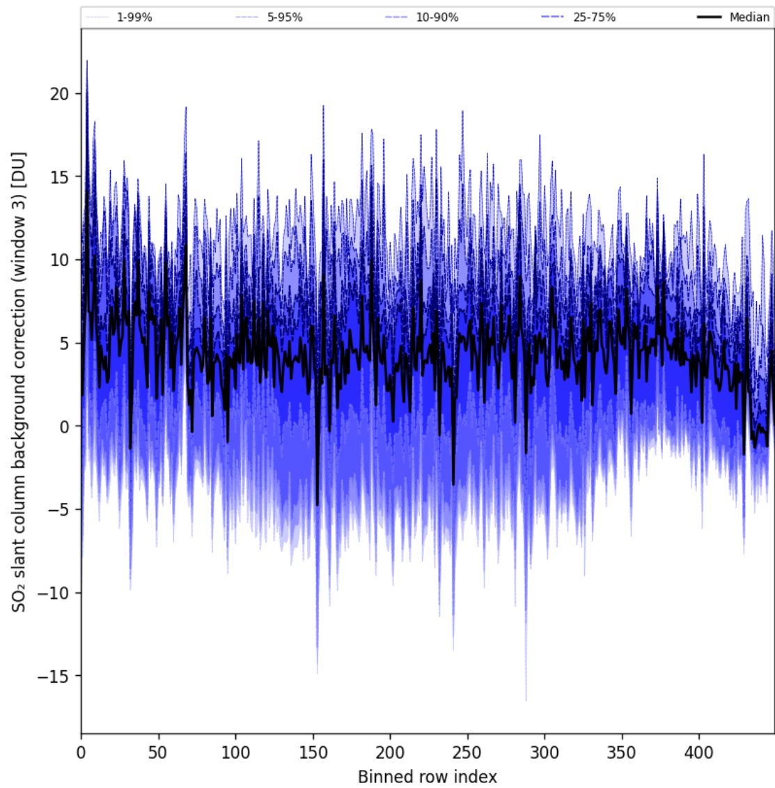
Figure 100: Along track statistics of “SO 2 slant column background correction (window 3)” for 2025-06-24 to 2025-06-26
