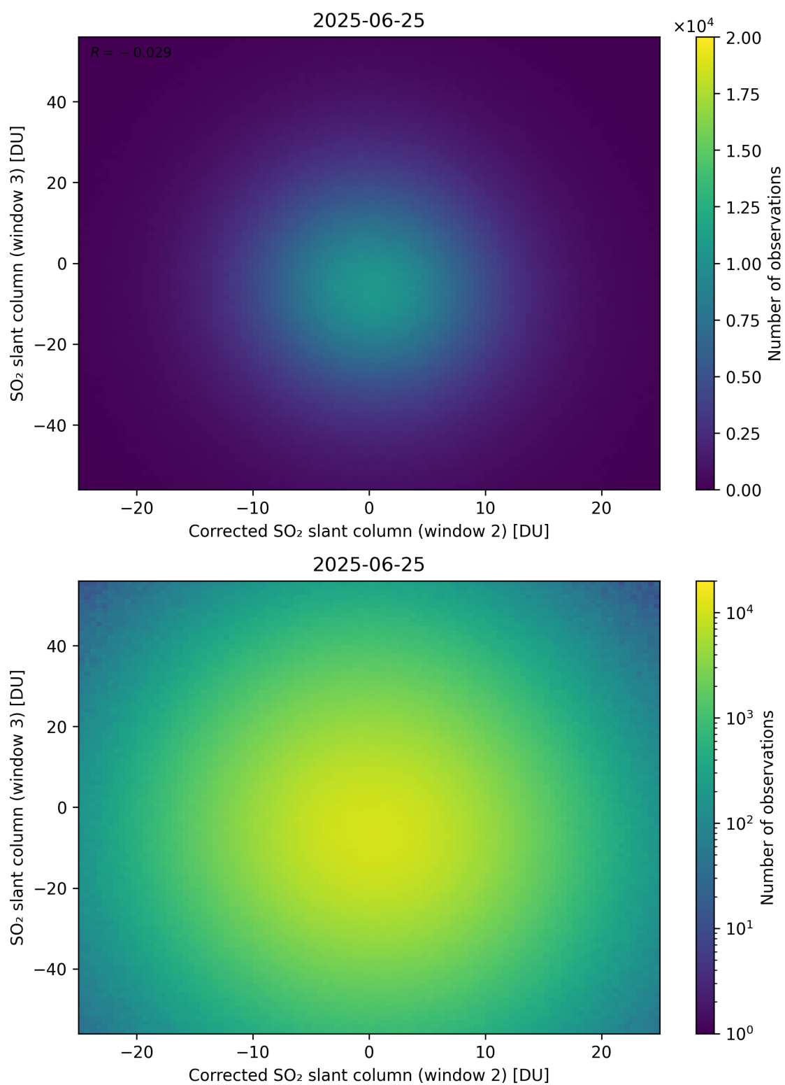
Figure 251: Scatter density plot of “Corrected SO 2 slant column (window 2)” against “SO 2 slant column (window 3)” for 2025-06-24 to 2025-06-26.
