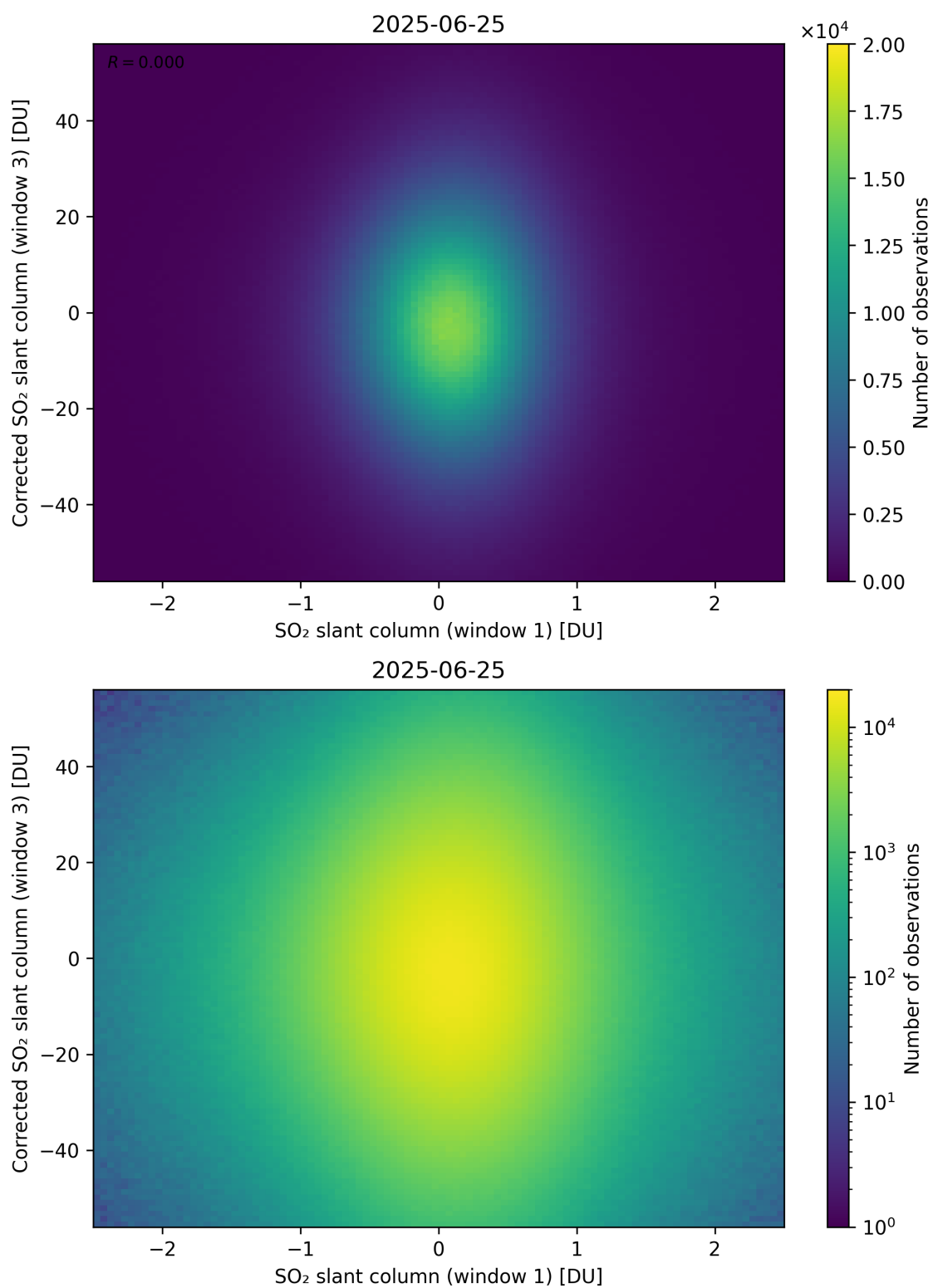
Figure 284: Scatter density plot of “SO 2 slant column (window 1)” against “Corrected SO 2 slant column (window 3)” for 2025-06-24 to 2025-06-26.
