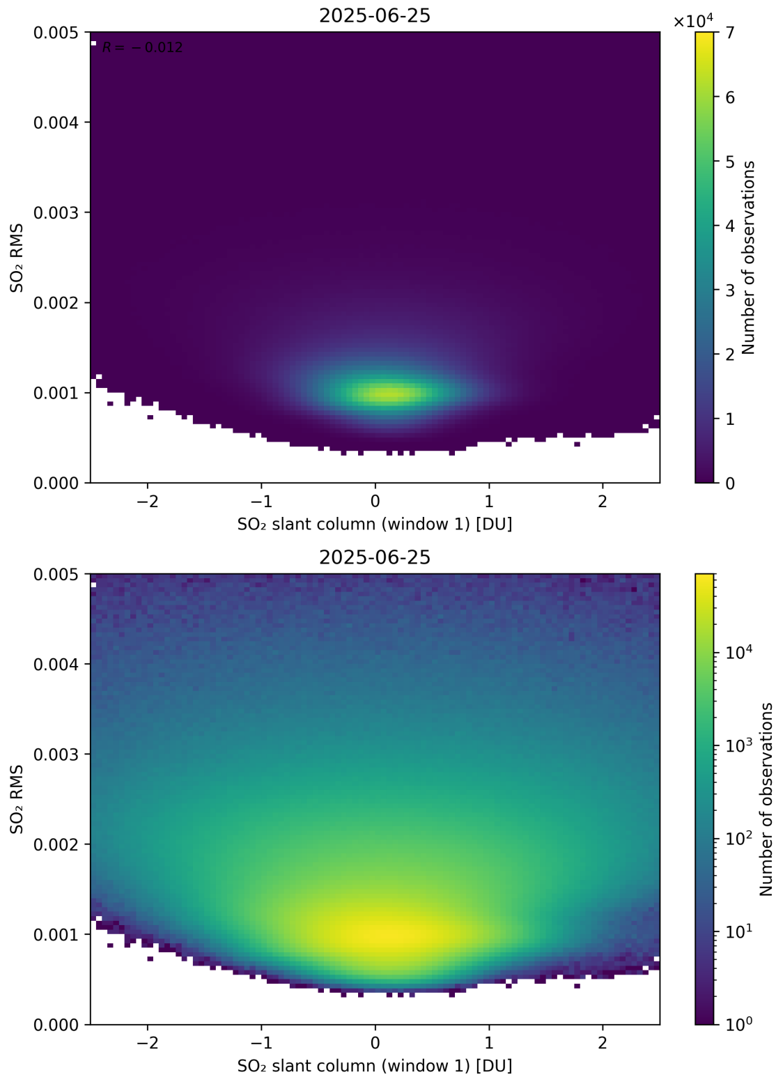
Figure 267: Scatter density plot of “SO 2 slant column (window 1)” against “SO 2 RMS” for 2025-06-24 to 2025-06-26.
