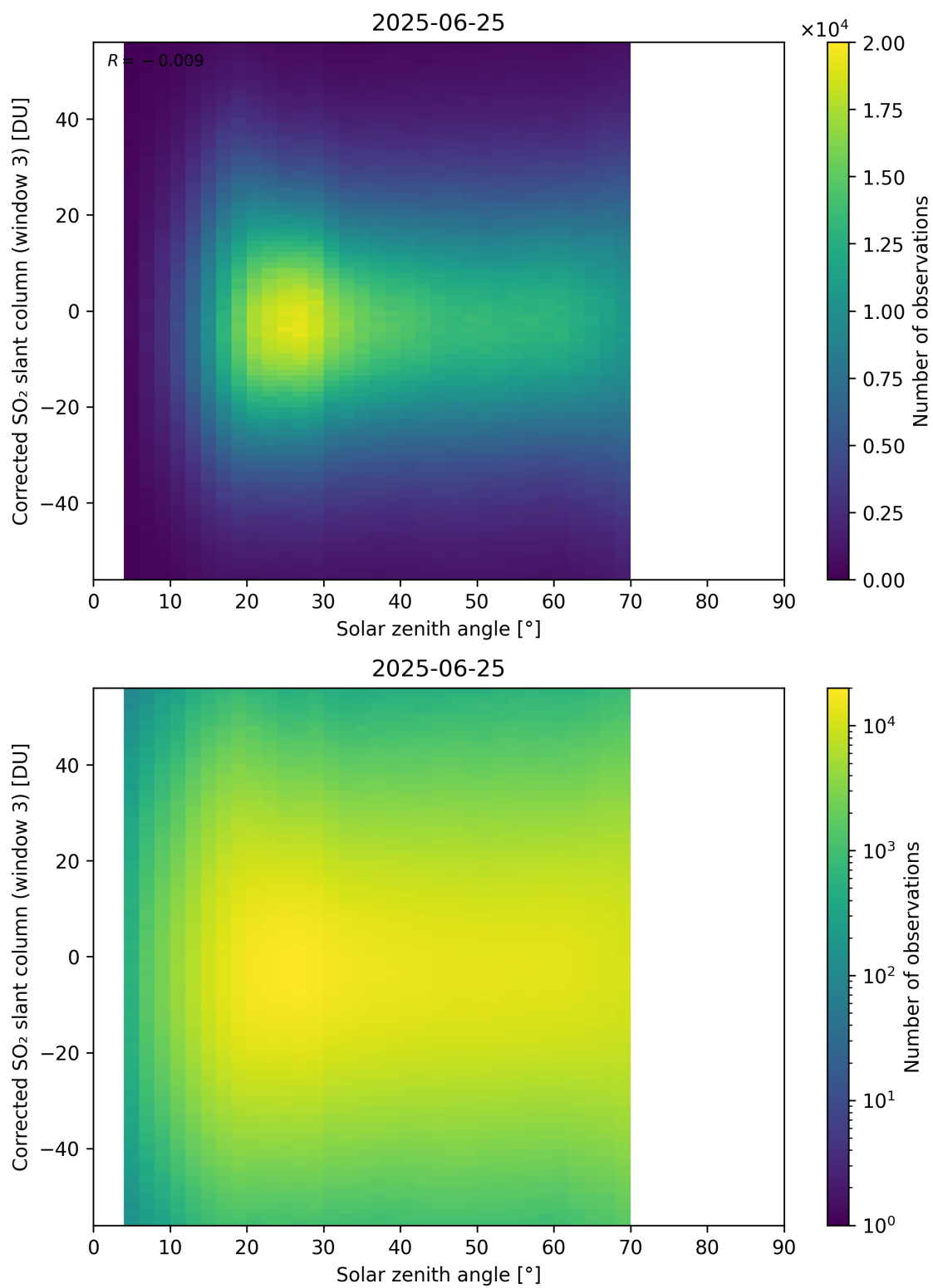
Figure 183: Scatter density plot of “Solar zenith angle” against “Corrected SO 2 slant column (window 3)” for 2025-06-24 to 2025-06-26.
