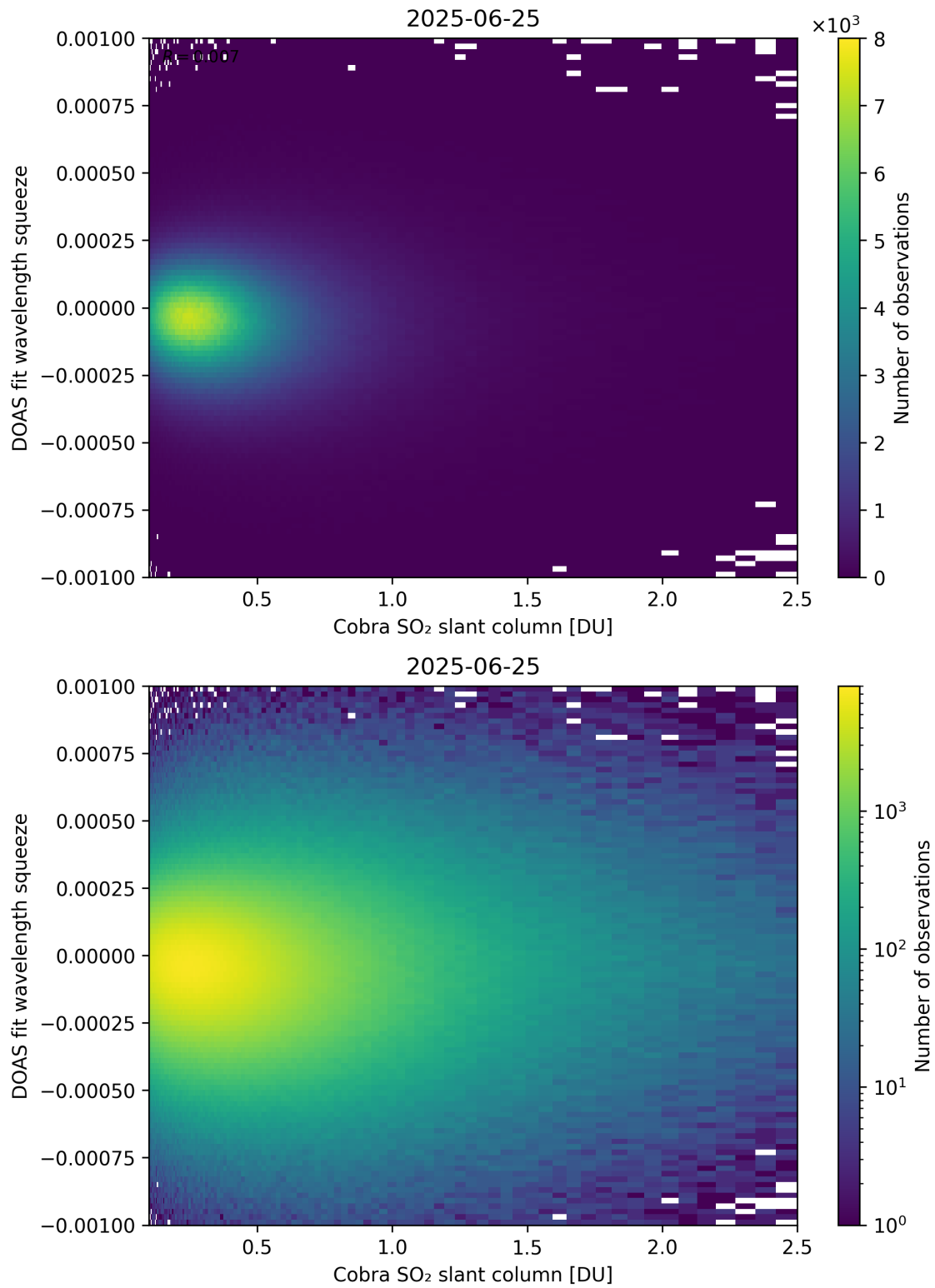
Figure 197: Scatter density plot of “Cobra SO 2 slant column” against “DOAS fit wavelength squeeze” for 2025-06-24 to 2025-06-26.
