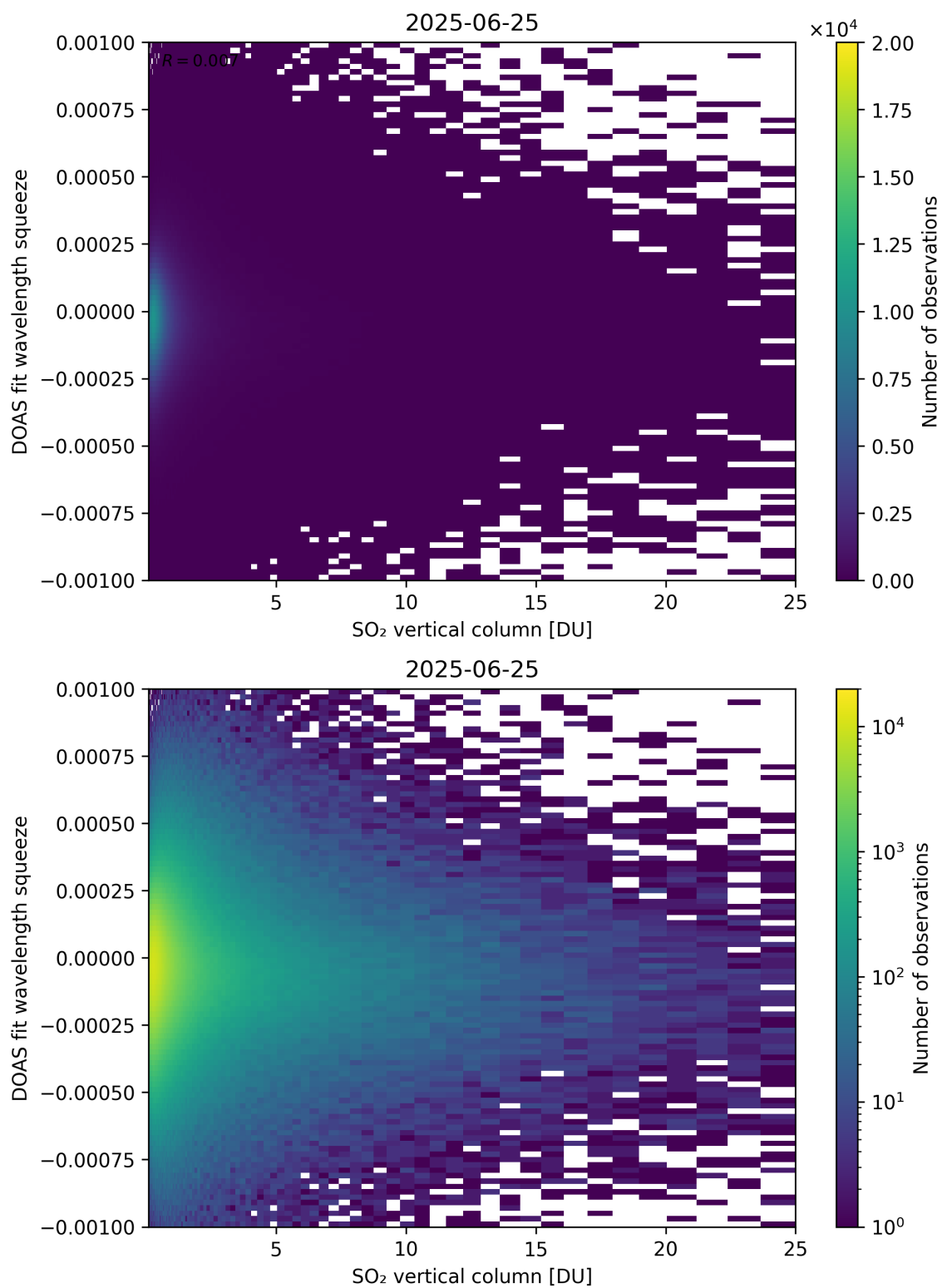
Figure 327: Scatter density plot of “SO 2 vertical column” against “DOAS fit wavelength squeeze” for 2025-06-24 to 2025-06-26.
