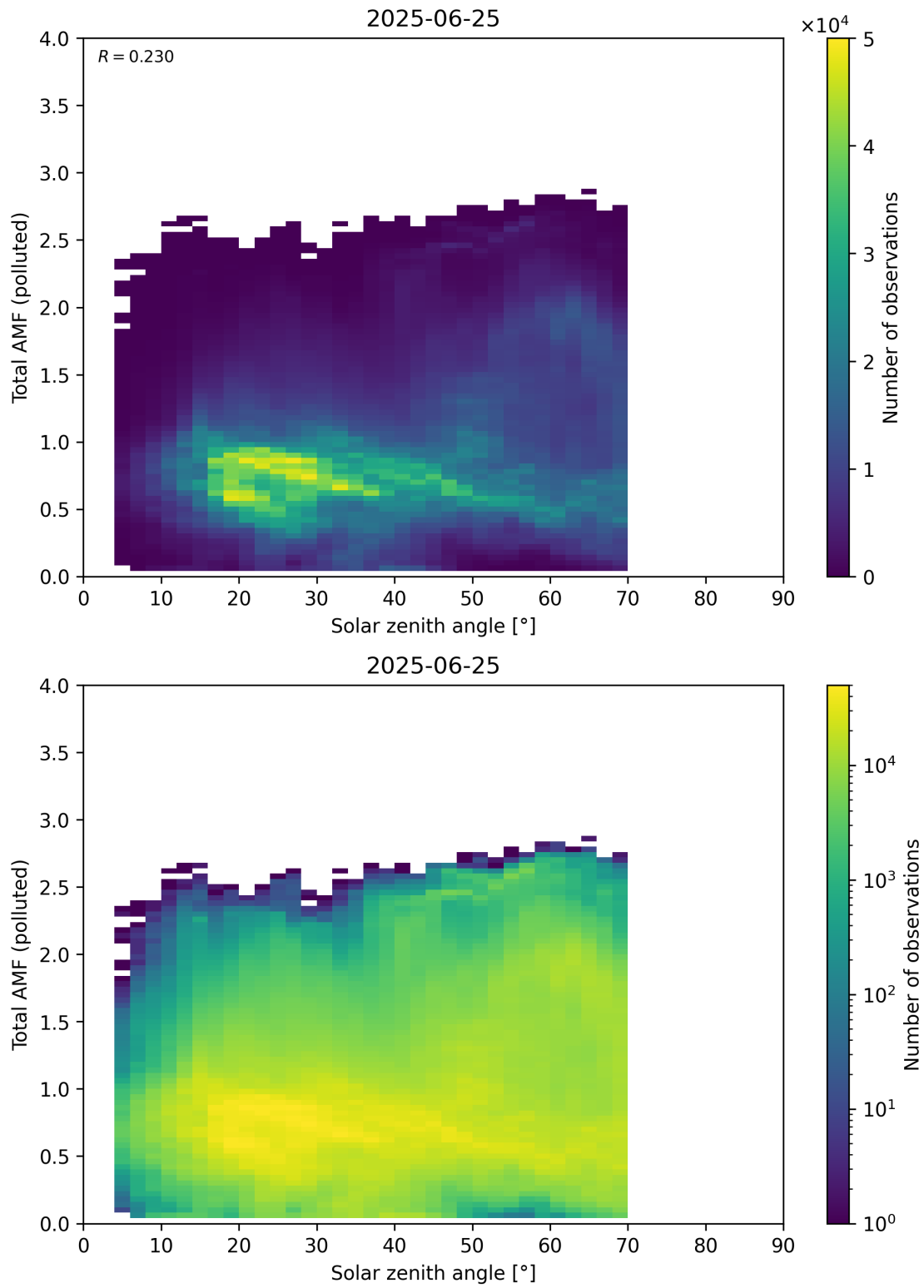
Figure 189: Scatter density plot of “Solar zenith angle” against “Total AMF (polluted)” for 2025-06-24 to 2025-06-26.
