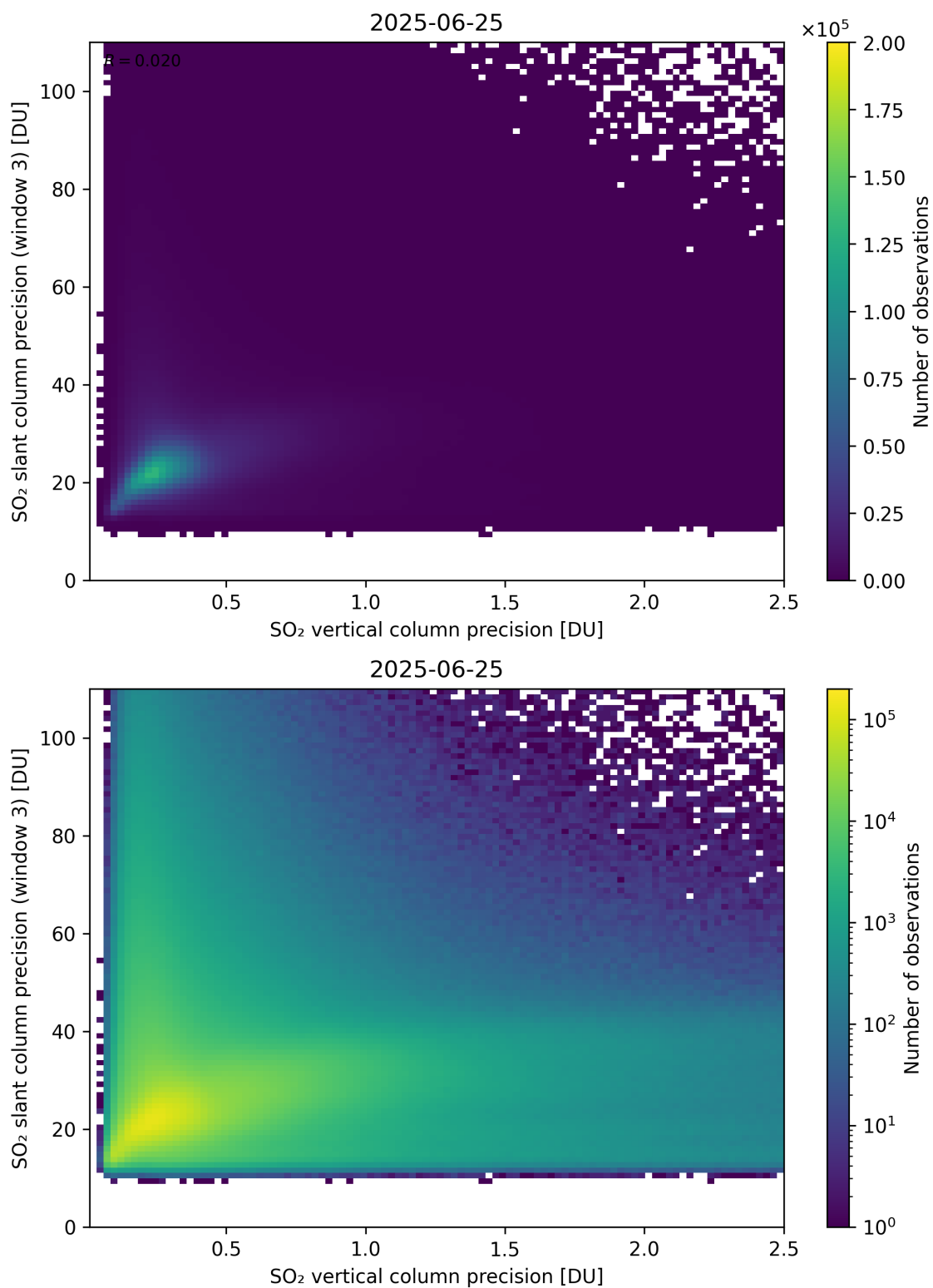
Figure 345: Scatter density plot of “SO 2 vertical column precision” against “SO 2 slant column precision (window 3)” for 2025-06-24 to 2025-06-26.
