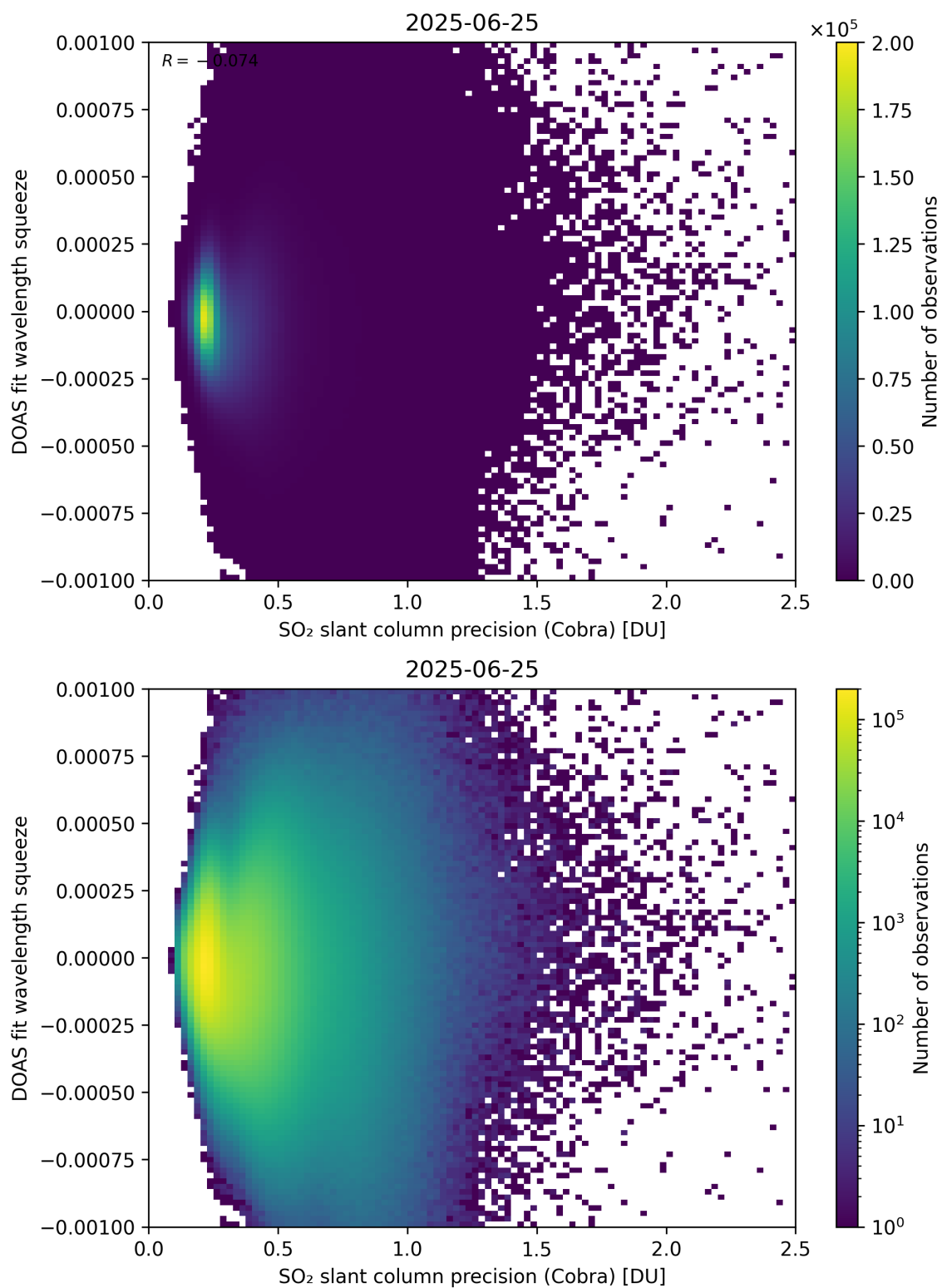
Figure 203: Scatter density plot of “SO 2 slant column precision (Cobra)” against “DOAS fit wavelength squeeze” for 2025-06-24 to 2025-06-26.
