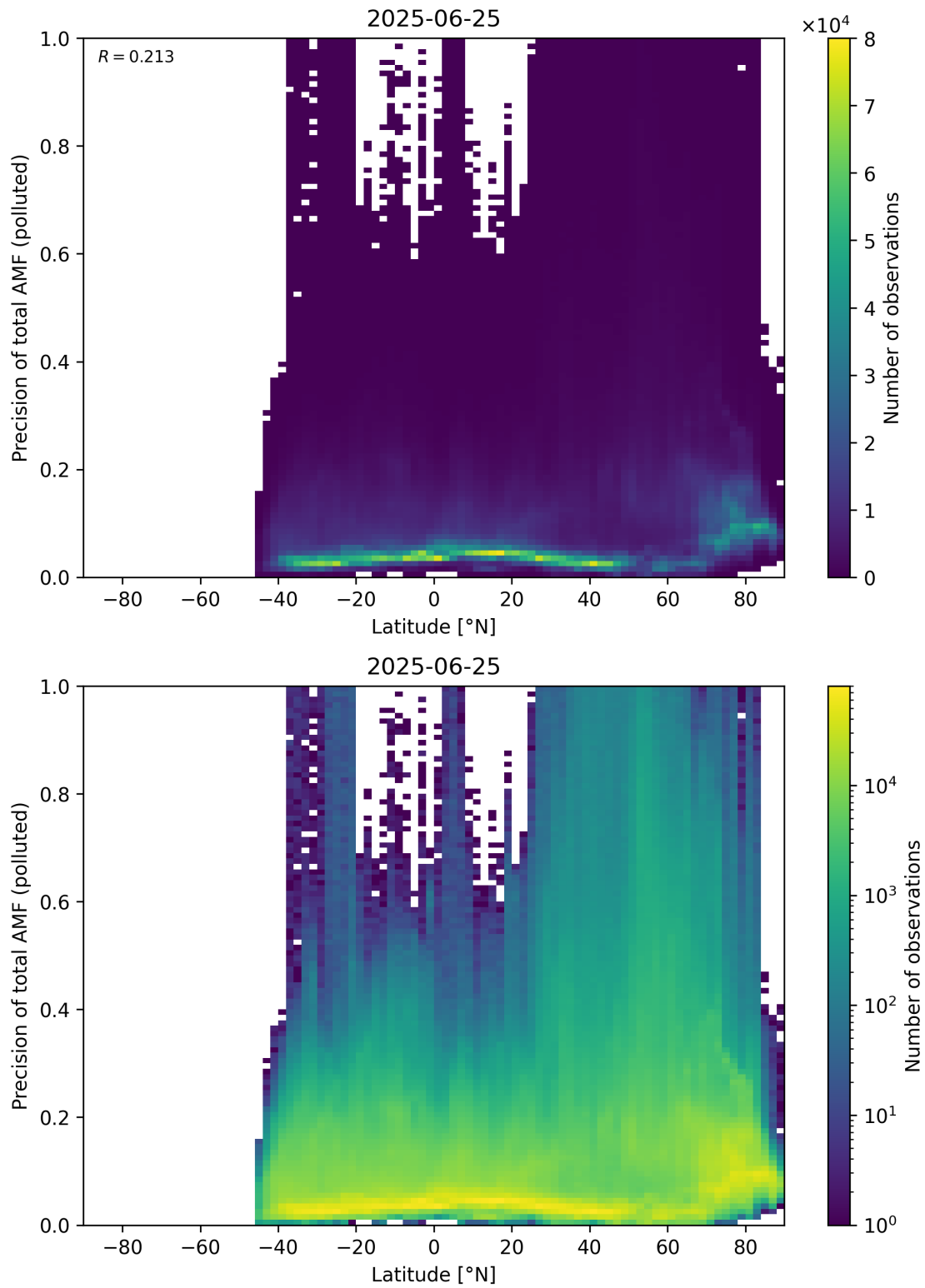
Figure 168: Scatter density plot of “Latitude” against “Precision of total AMF (polluted)” for 2025-06-24 to 2025-06-26.
