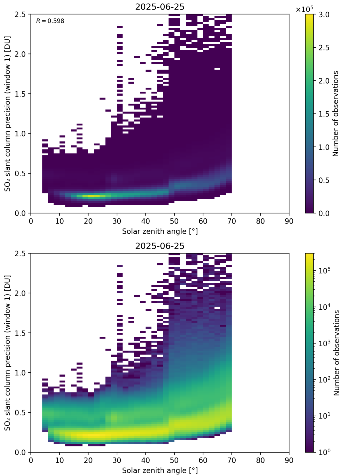
Figure 185: Scatter density plot of “Solar zenith angle” against “SO 2 slant column precision (window 1)” for 2025-06-24 to 2025-06-26.
