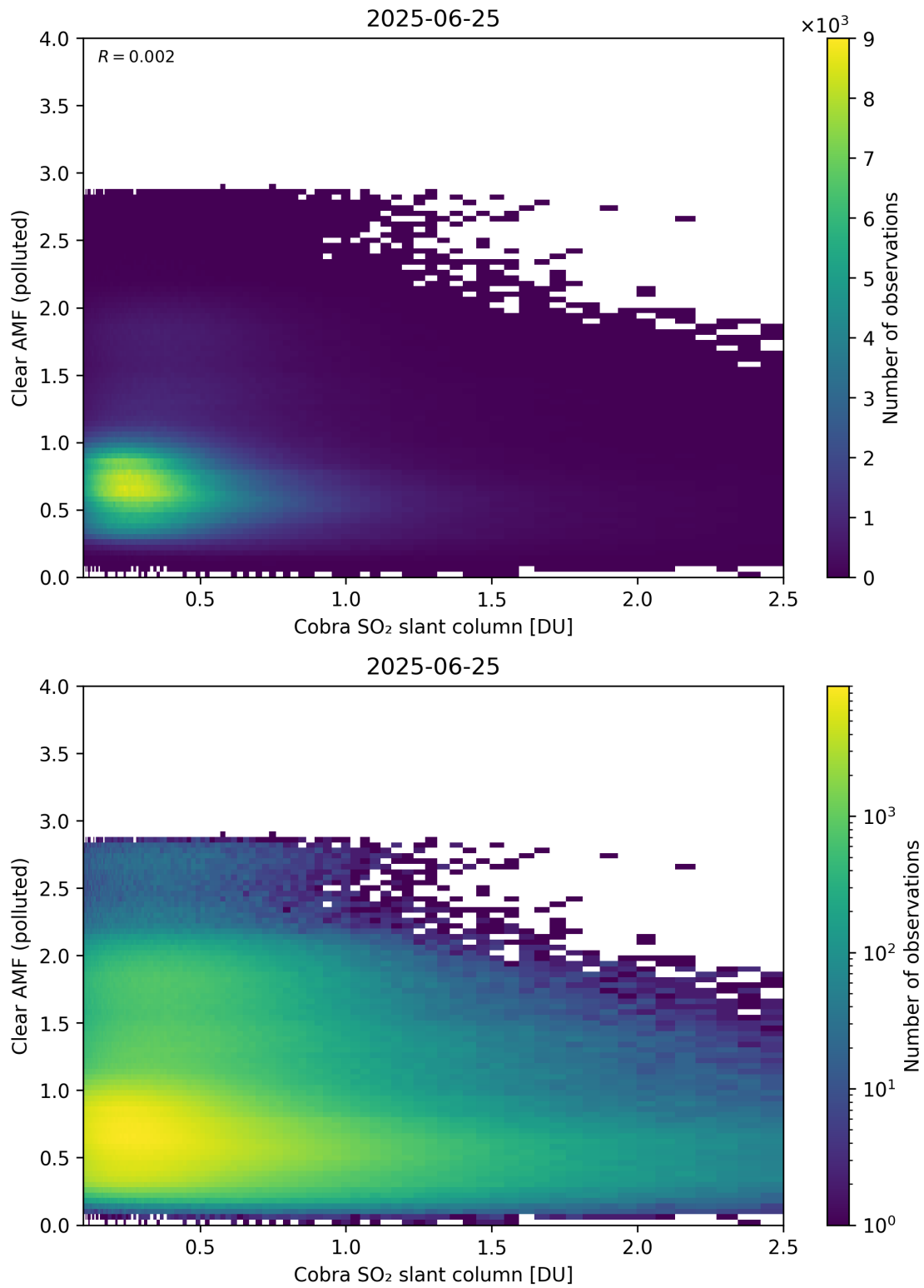
Figure 215: Scatter density plot of “Cobra SO 2 slant column” against “Clear AMF (polluted)” for 2025-06-24 to 2025-06-26.
