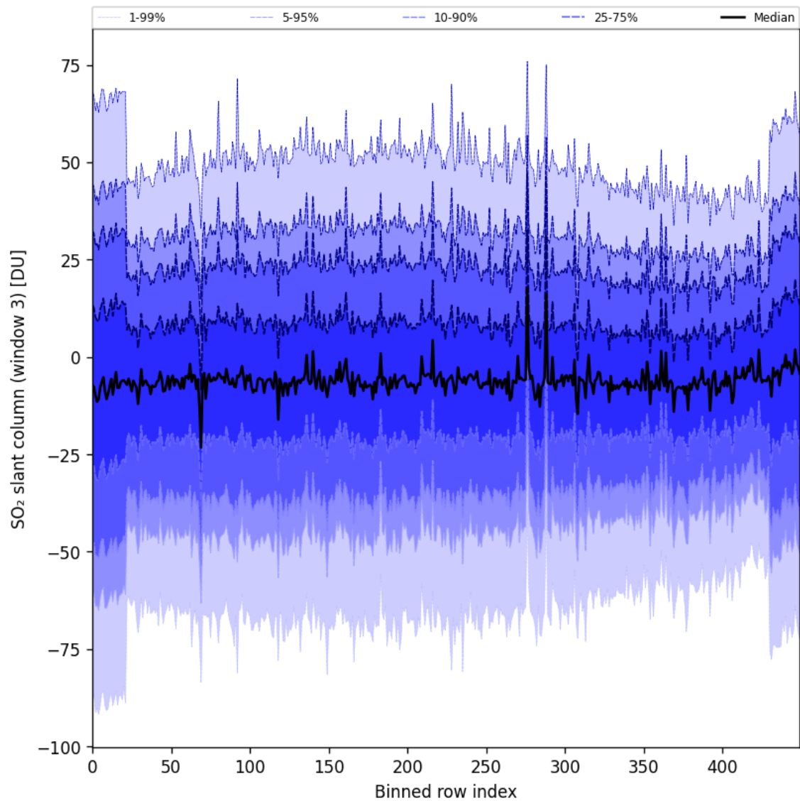
Figure 97: Along track statistics of “SO 2 slant column (window 3)” for 2025-06-24 to 2025-06-26
