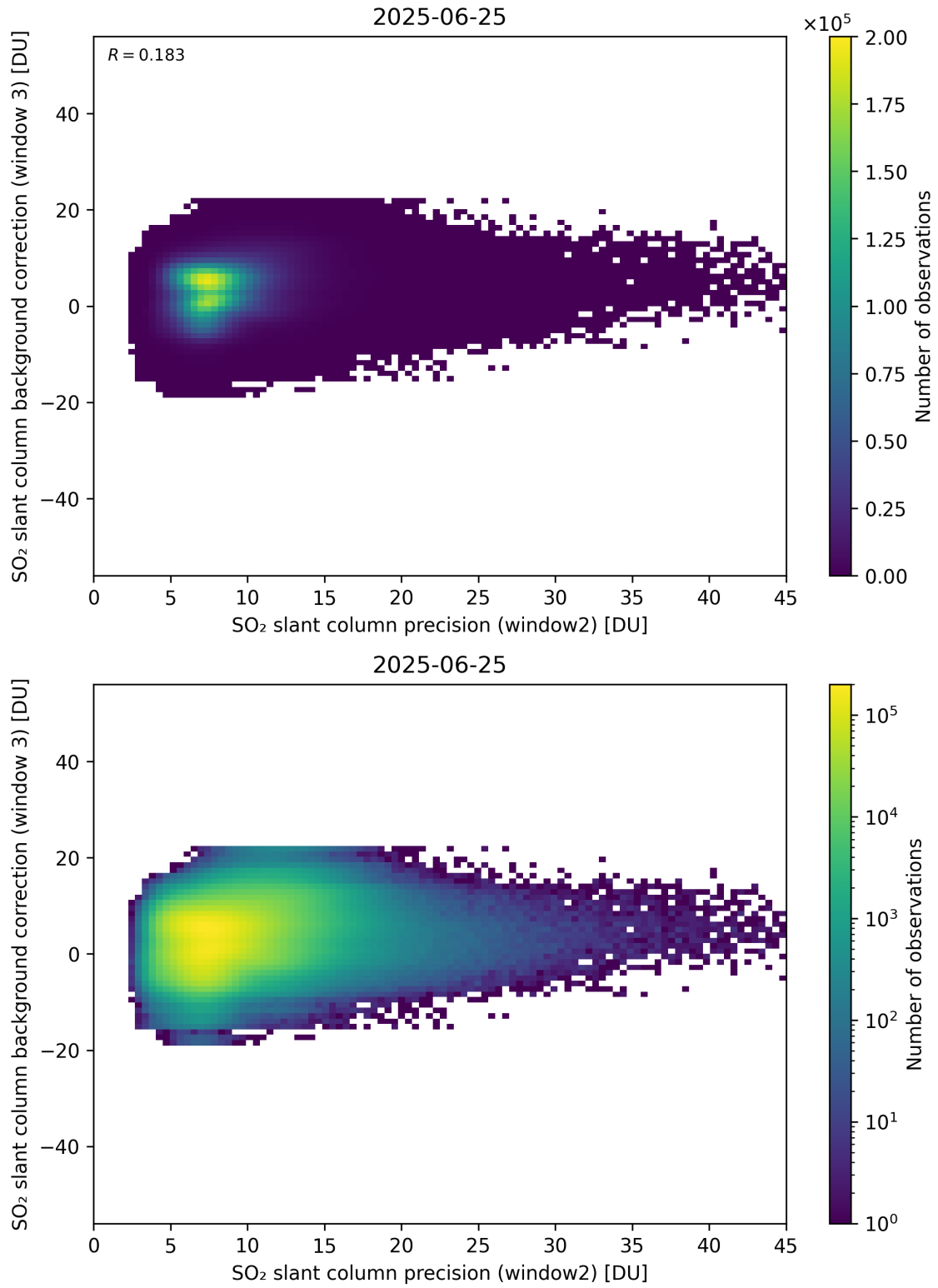
Figure 292: Scatter density plot of “SO 2 slant column precision (window2)” against “SO 2 slant column background correction (window 3)” for 2025-06-24 to 2025-06-26.
