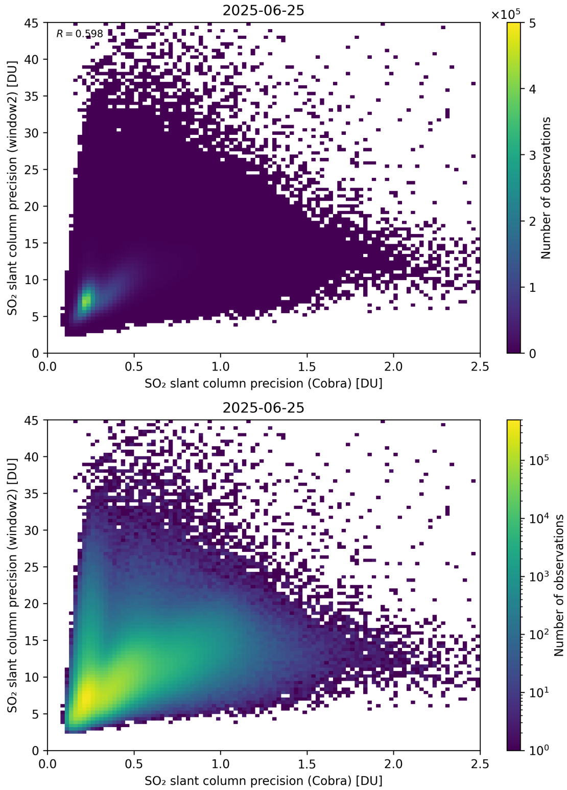
Figure 210: Scatter density plot of “SO 2 slant column precision (Cobra)” against “SO 2 slant column precision (window2)” for 2025-06-24 to 2025-06-26.
