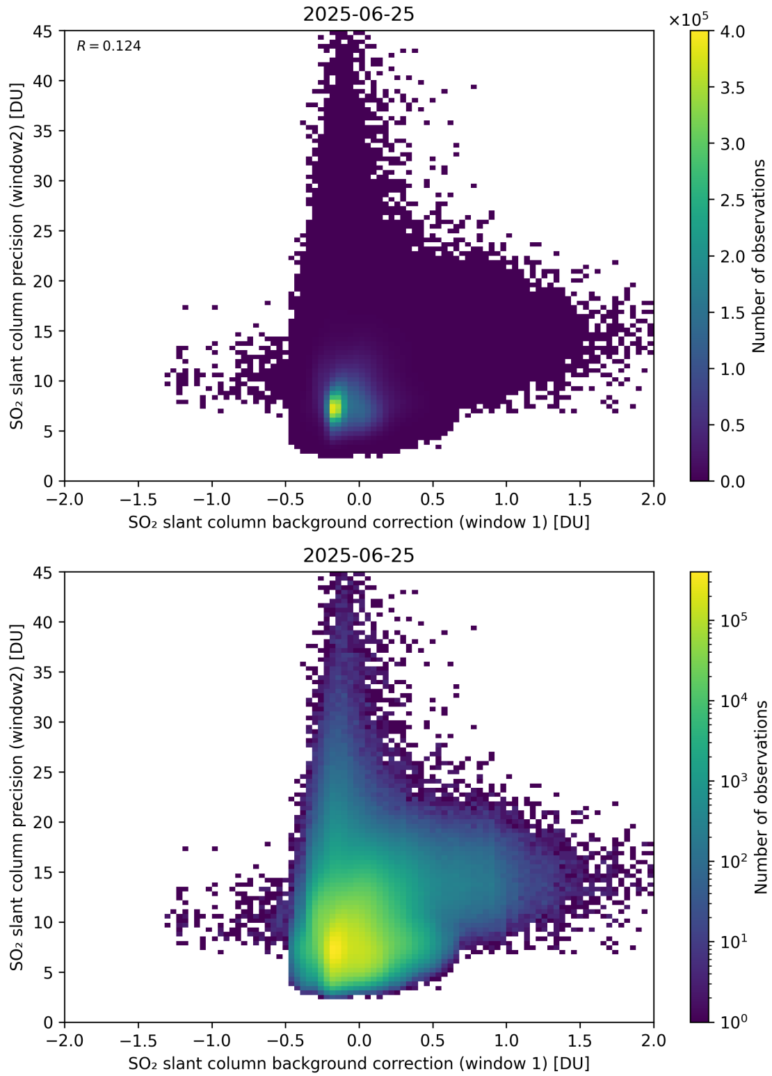
Figure 117: Scatter density plot of “SO 2 slant column background correction (window 1)” against “SO 2 slant column precision (window2)” for 2025-06-24 to 2025-06-26.
