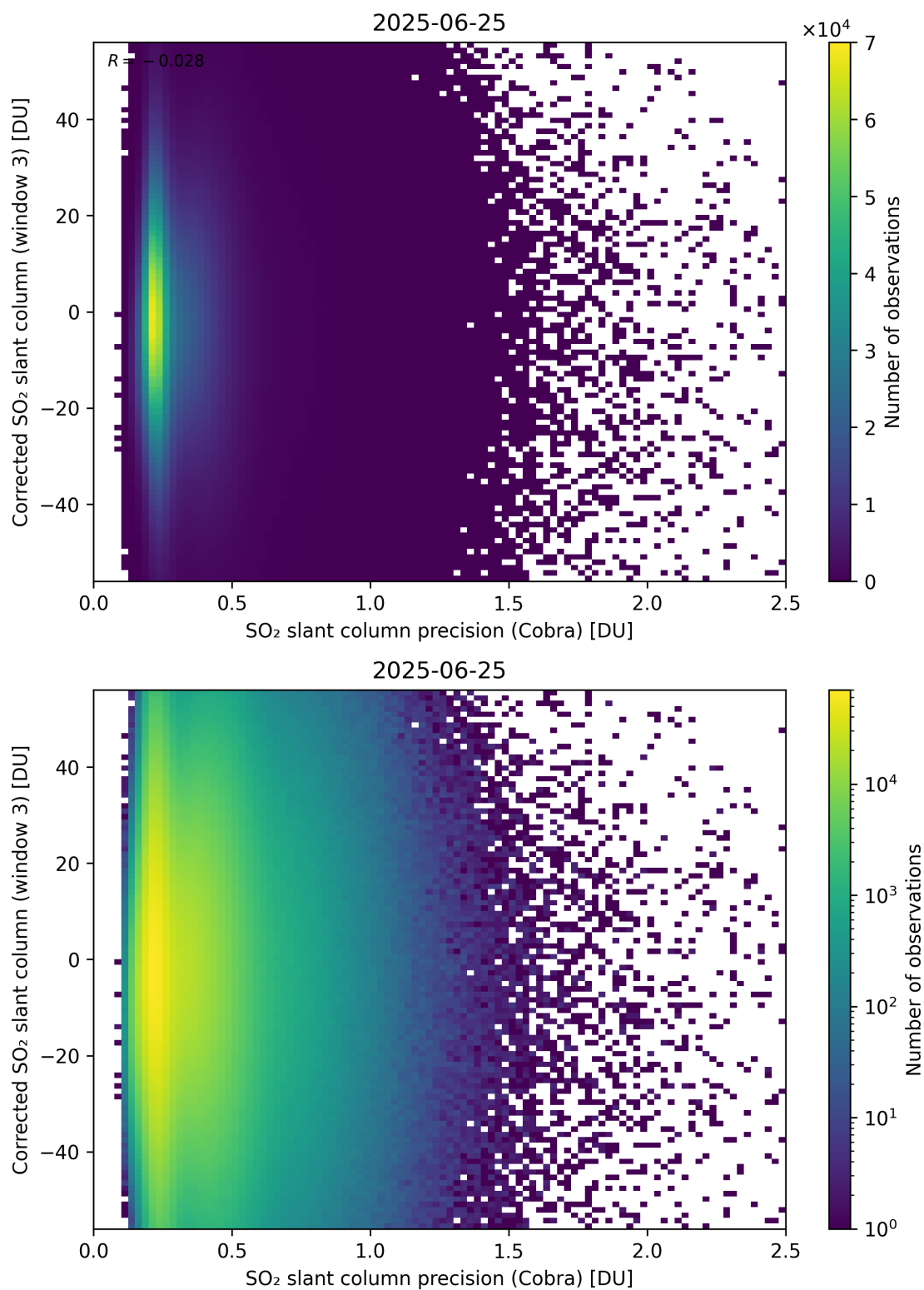
Figure 207: Scatter density plot of “SO 2 slant column precision (Cobra)” against “Corrected SO 2 slant column (window 3)” for 2025-06-24 to 2025-06-26.
