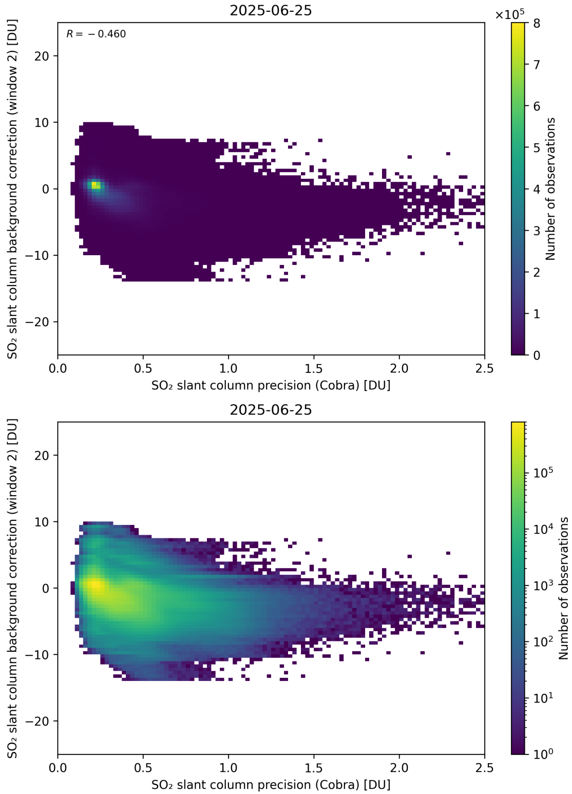
Figure 200: Scatter density plot of “SO 2 slant column precision (Cobra)” against “SO 2 slant column background correction (window 2)” for 2025-06-24 to 2025-06-26.
