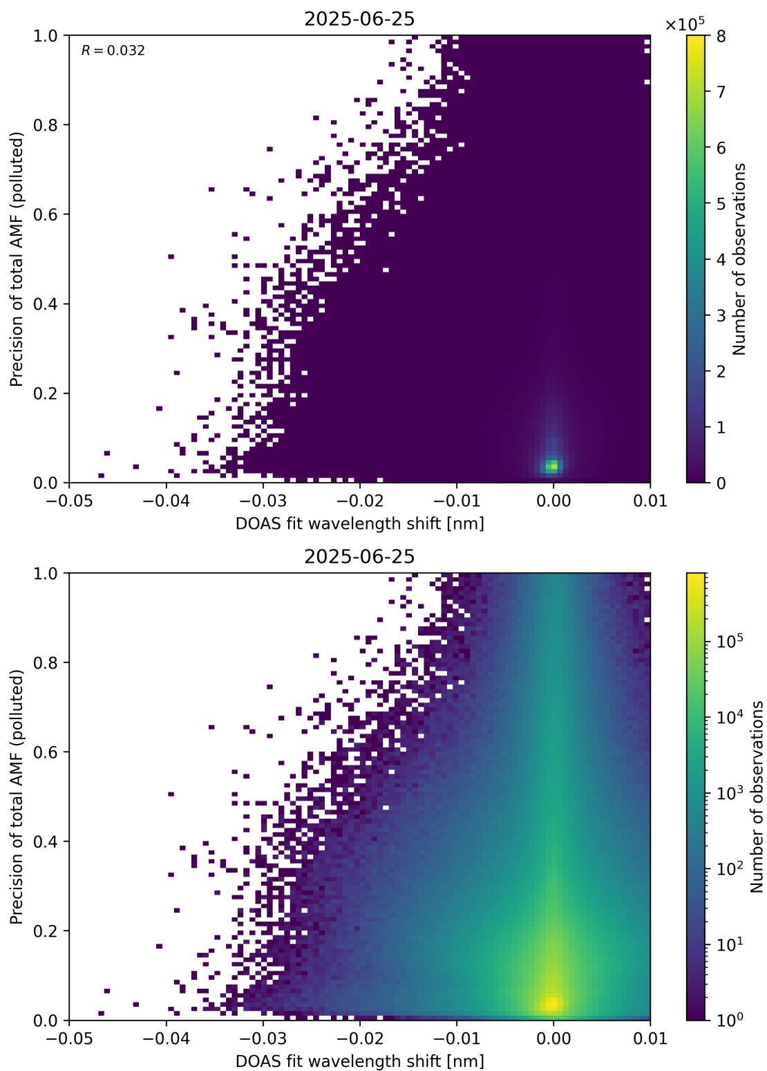
Figure 142: Scatter density plot of “DOAS fit wavelength shift” against “Precision of total AMF (polluted)” for 2025-06-24 to 2025-06-26.
