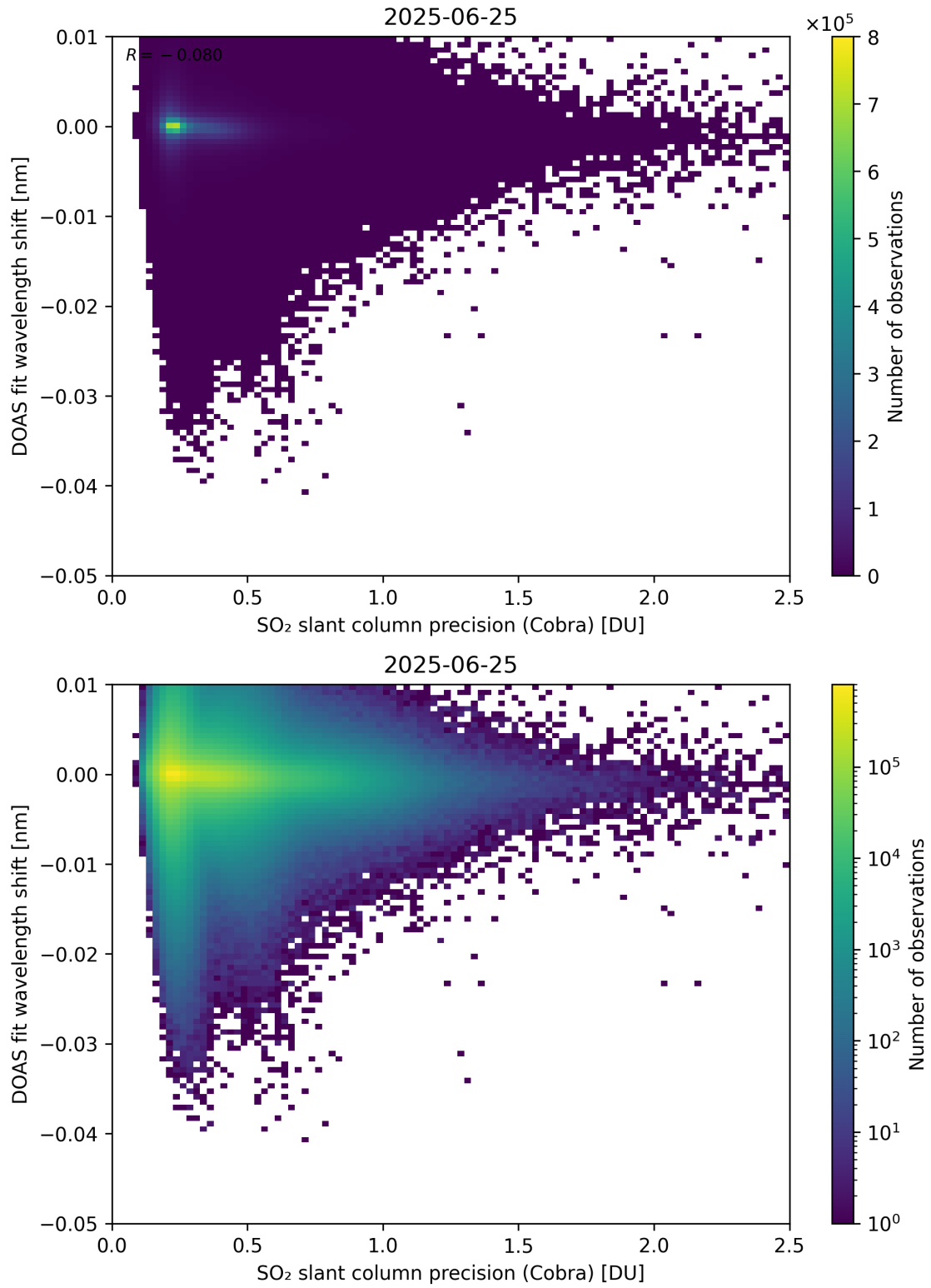
Figure 202: Scatter density plot of “SO 2 slant column precision (Cobra)” against “DOAS fit wavelength shift” for 2025-06-24 to 2025-06-26.
