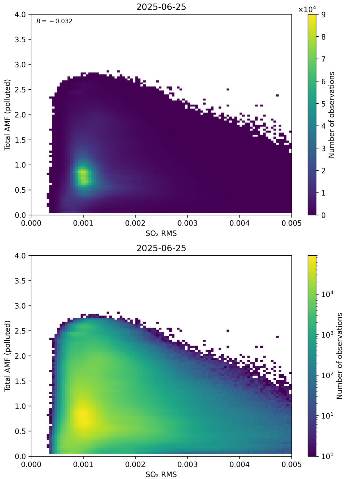
Figure 148: Scatter density plot of “SO 2 RMS” against “Total AMF (polluted)” for 2025-06-24 to 2025-06-26.
