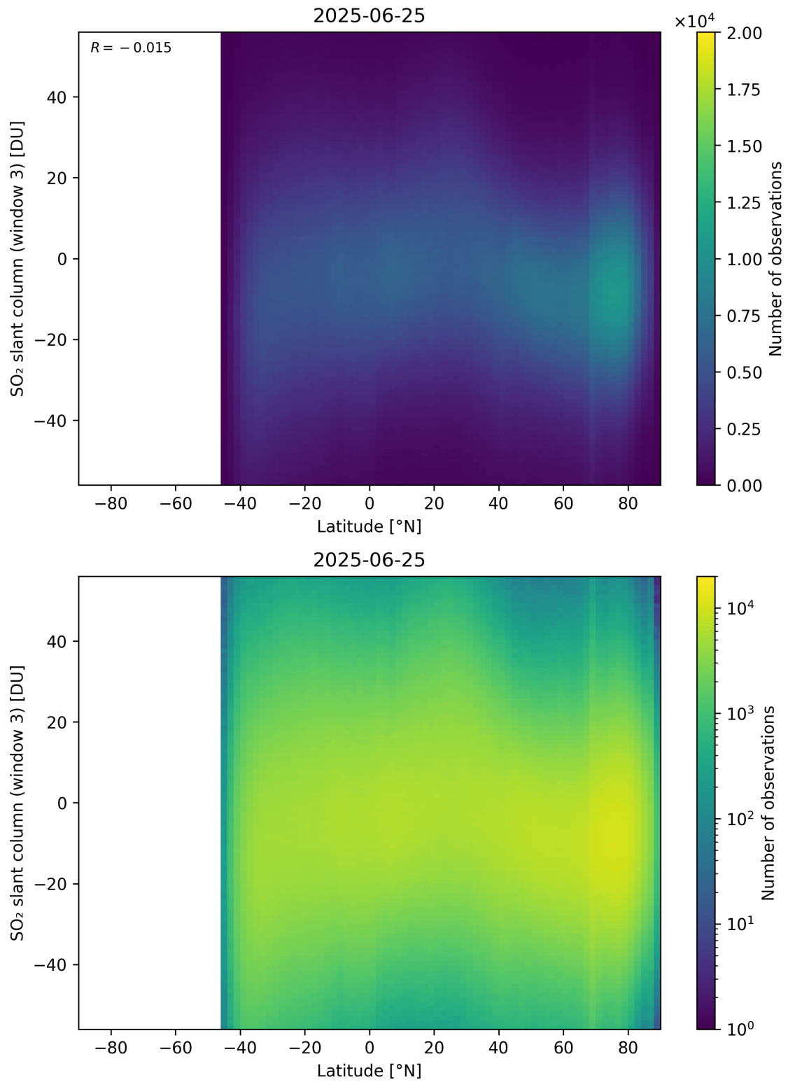
Figure 165: Scatter density plot of “Latitude” against “SO 2 slant column (window 3)” for 2025-06-24 to 2025-06-26.
