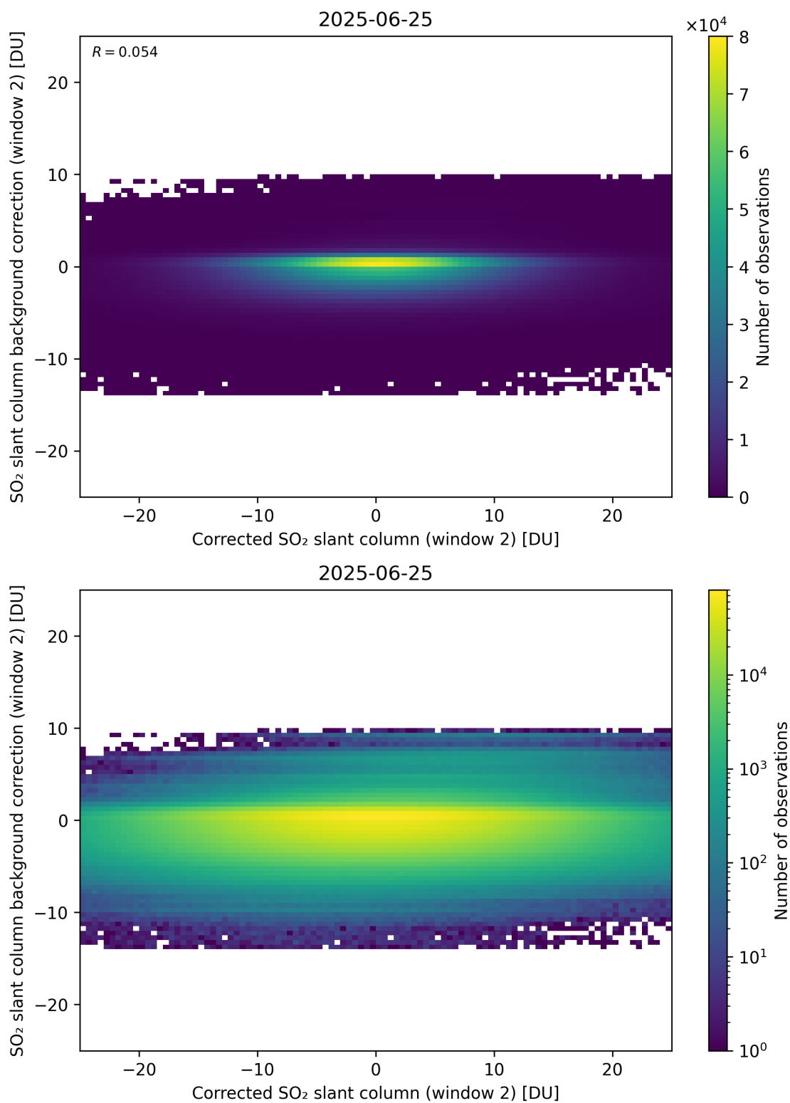
Figure 244: Scatter density plot of “Corrected SO 2 slant column (window 2)” against “SO 2 slant column background correction (window 2)” for 2025-06-24 to 2025-06-26.
