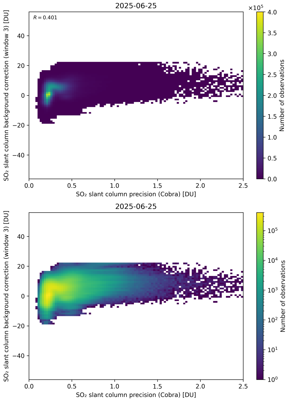
Figure 201: Scatter density plot of “SO 2 slant column precision (Cobra)” against “SO 2 slant column background correction (window 3)” for 2025-06-24 to 2025-06-26.
