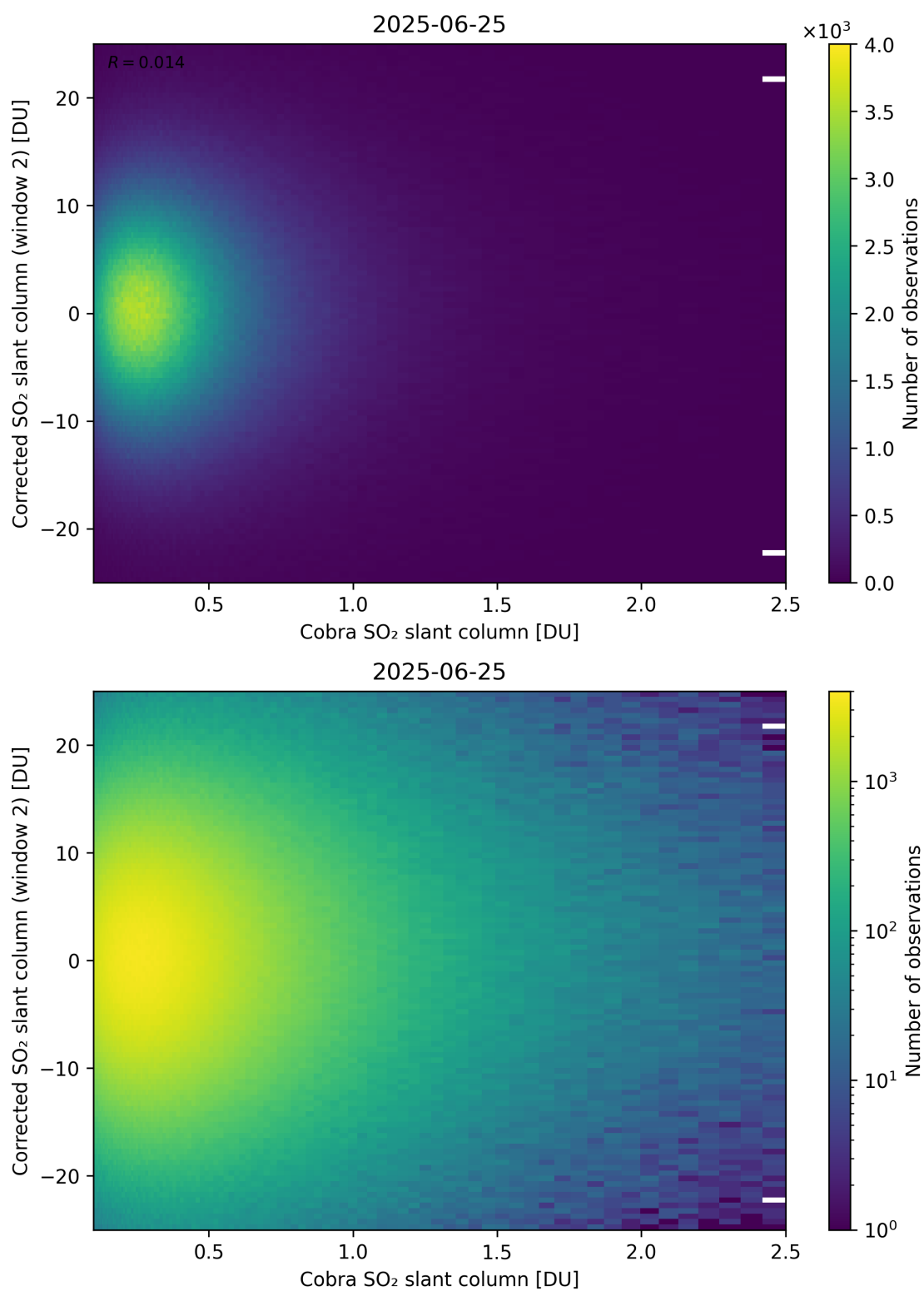
Figure 217: Scatter density plot of “Cobra SO 2 slant column” against “Corrected SO 2 slant column (window 2)” for 2025-06-24 to 2025-06-26.
