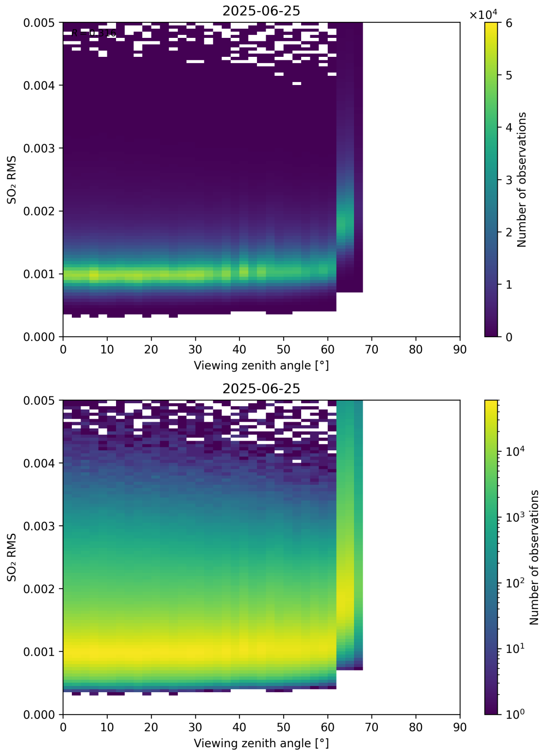
Figure 367: Scatter density plot of “Viewing zenith angle” against “SO 2 RMS” for 2025-06-24 to 2025-06-26.
