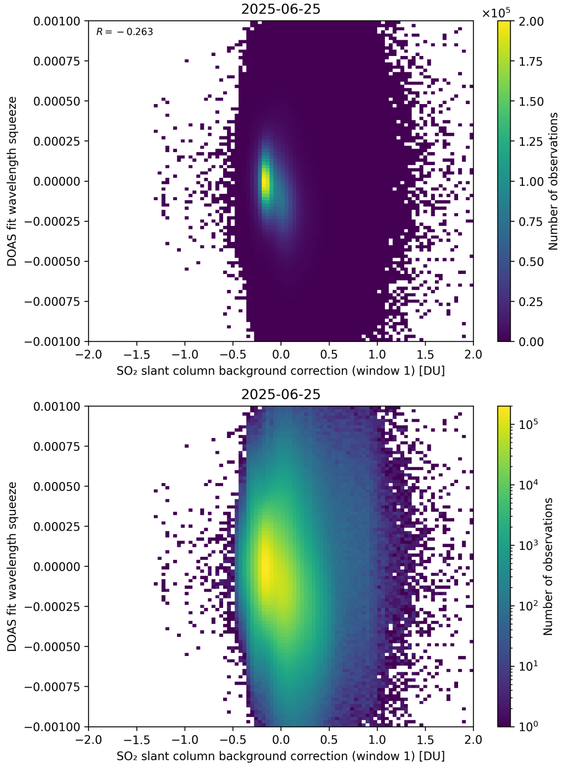
Figure 112: Scatter density plot of “SO 2 slant column background correction (window 1)” against “DOAS fit wavelength squeeze” for 2025-06-24 to 2025-06-26.
