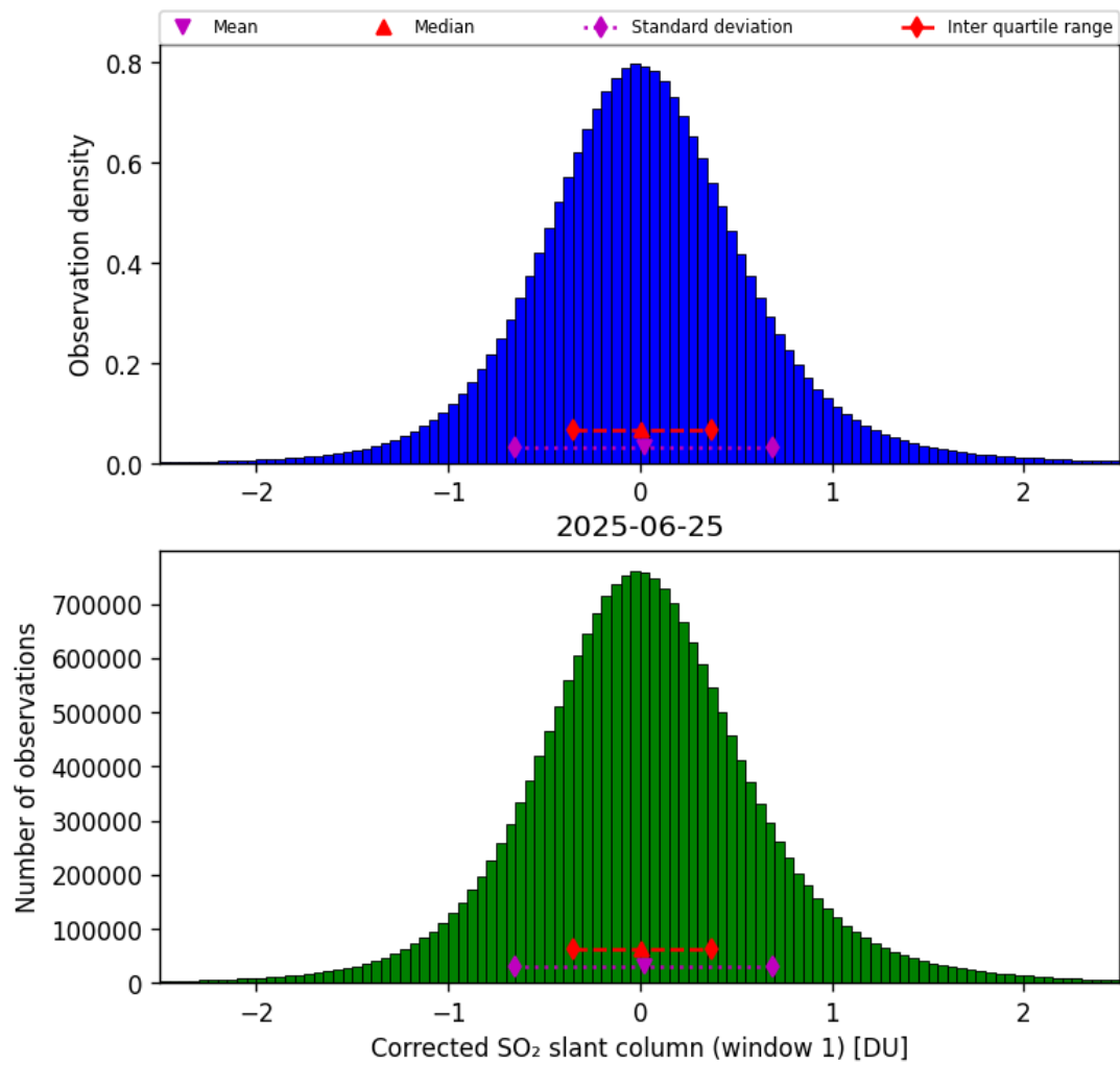
Figure 65: Histogram of “Corrected SO 2 slant column (window 1)” for 2025-06-24 to 2025-06-26
