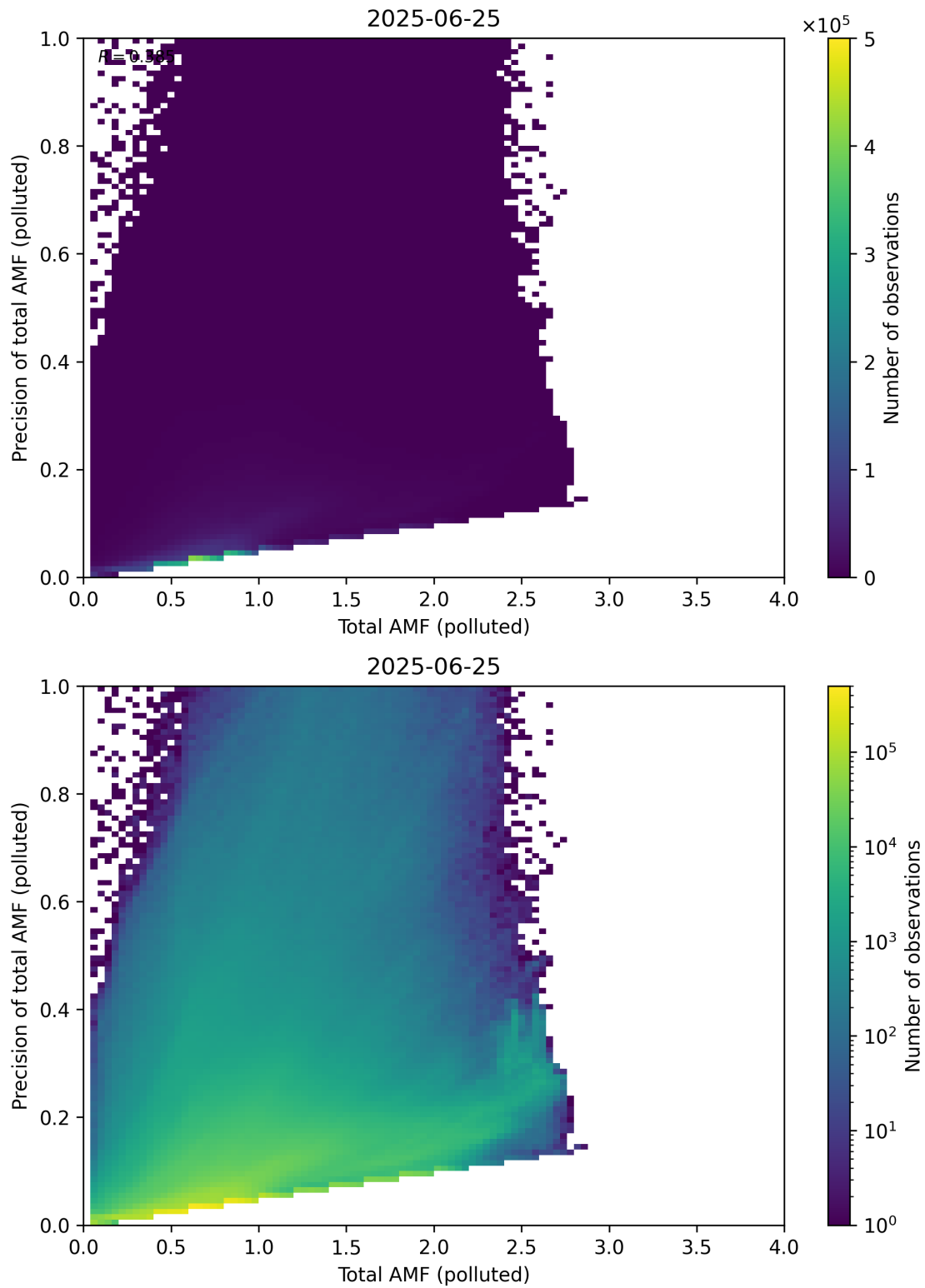
Figure 322: Scatter density plot of “Total AMF (polluted)” against “Precision of total AMF (polluted)” for 2025-06-24 to 2025-06-26.
