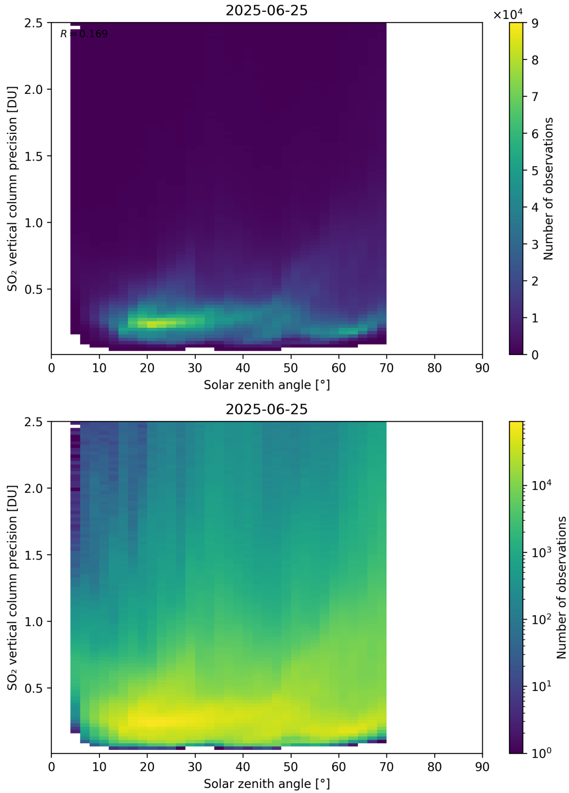
Figure 192: Scatter density plot of “Solar zenith angle” against “SO 2 vertical column precision” for 2025-06-24 to 2025-06-26.
