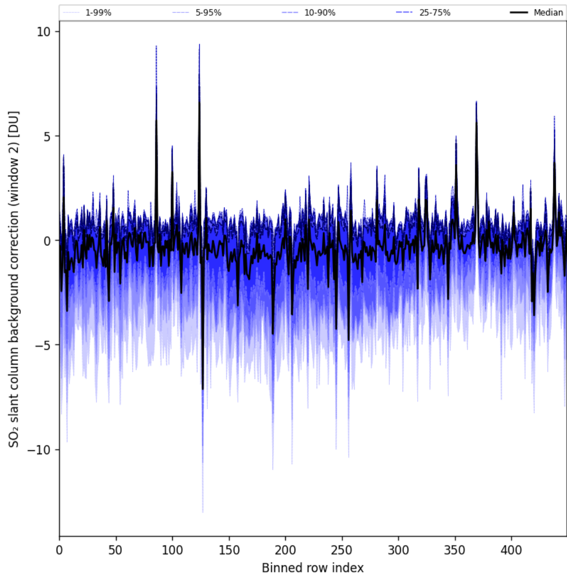
Figure 96: Along track statistics of “SO 2 slant column background correction (window 2)” for 2025-06-24 to 2025-06-26
