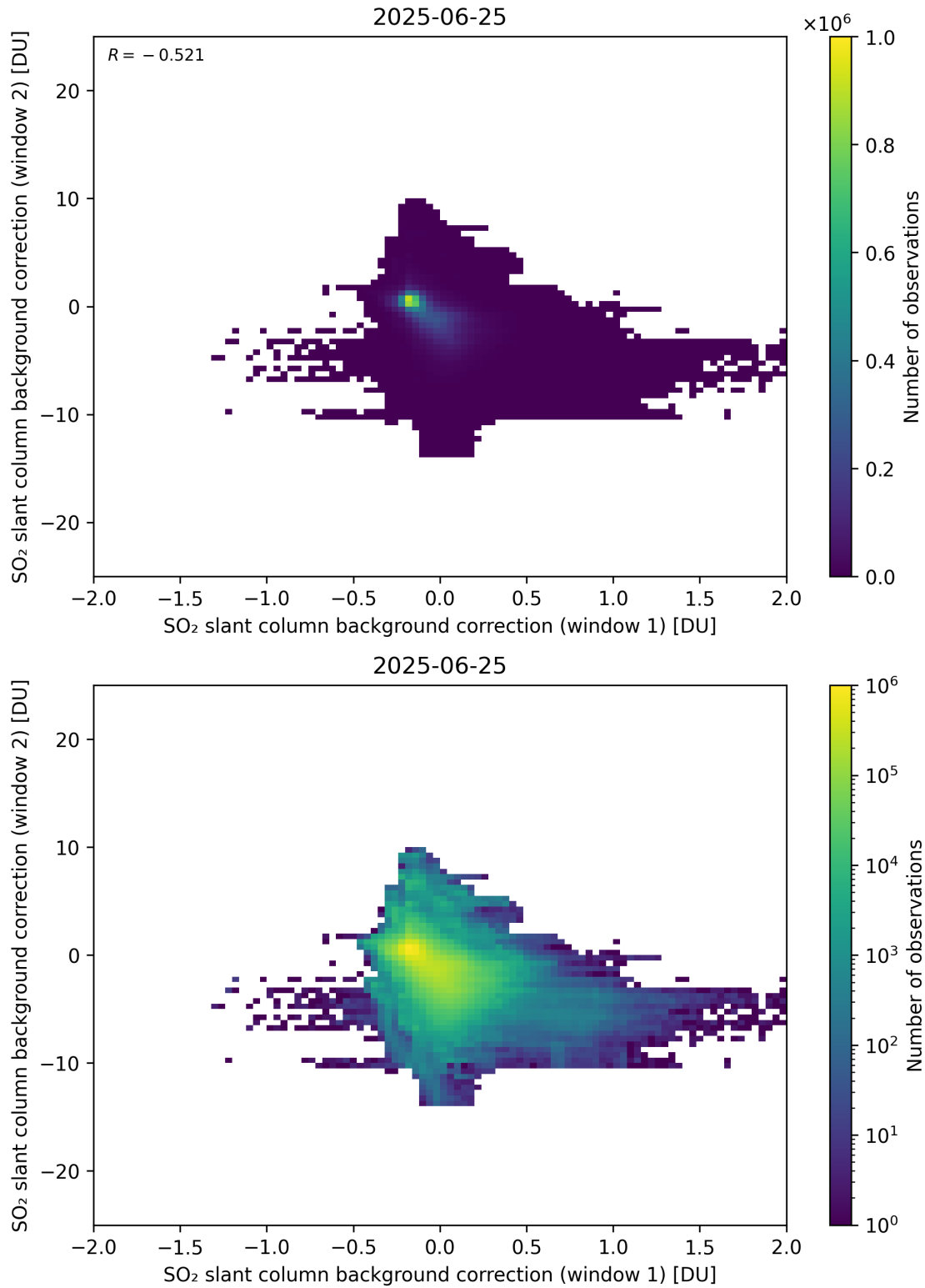
Figure 109: Scatter density plot of “SO 2 slant column background correction (window 1)” against “SO 2 slant column background correction (window 2)” for 2025-06-24 to 2025-06-26.
