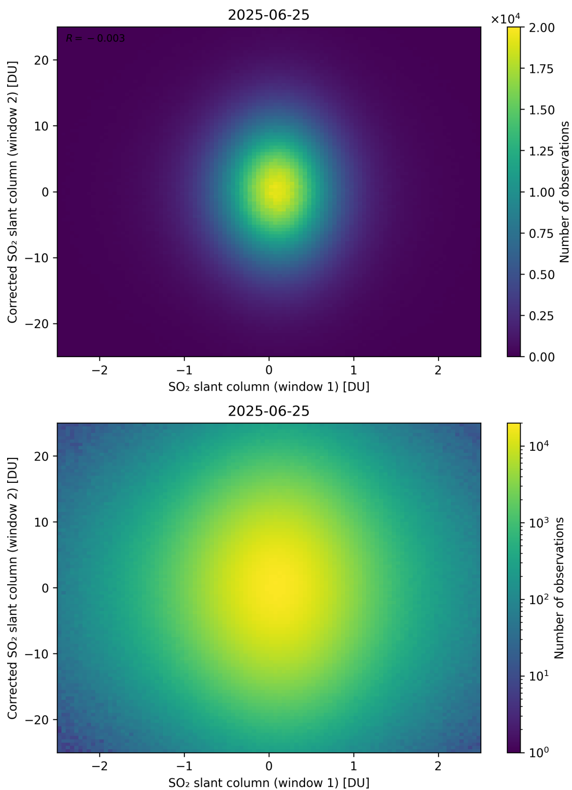
Figure 283: Scatter density plot of “SO 2 slant column (window 1)” against “Corrected SO 2 slant column (window 2)” for 2025-06-24 to 2025-06-26.
