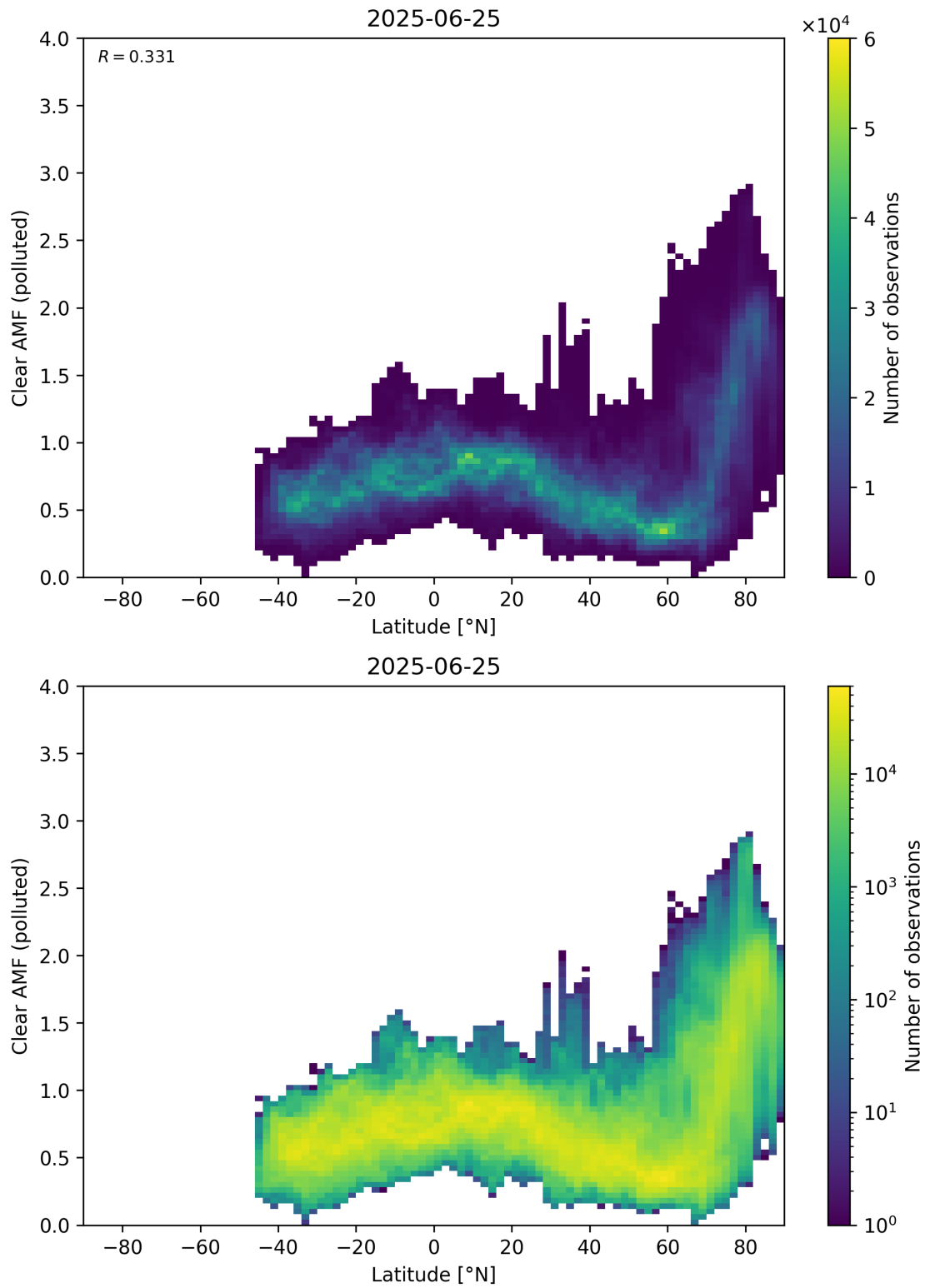
Figure 156: Scatter density plot of “Latitude” against “Clear AMF (polluted)” for 2025-06-24 to 2025-06-26.
