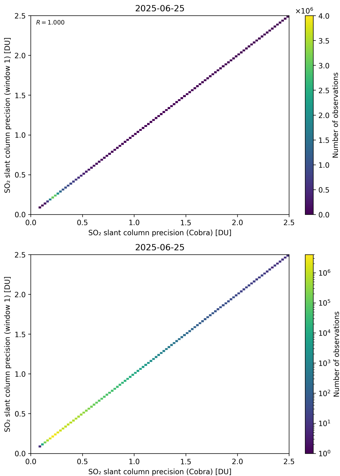
Figure 209: Scatter density plot of “SO 2 slant column precision (Cobra)” against “SO 2 slant column precision (window 1)” for 2025-06-24 to 2025-06-26.
