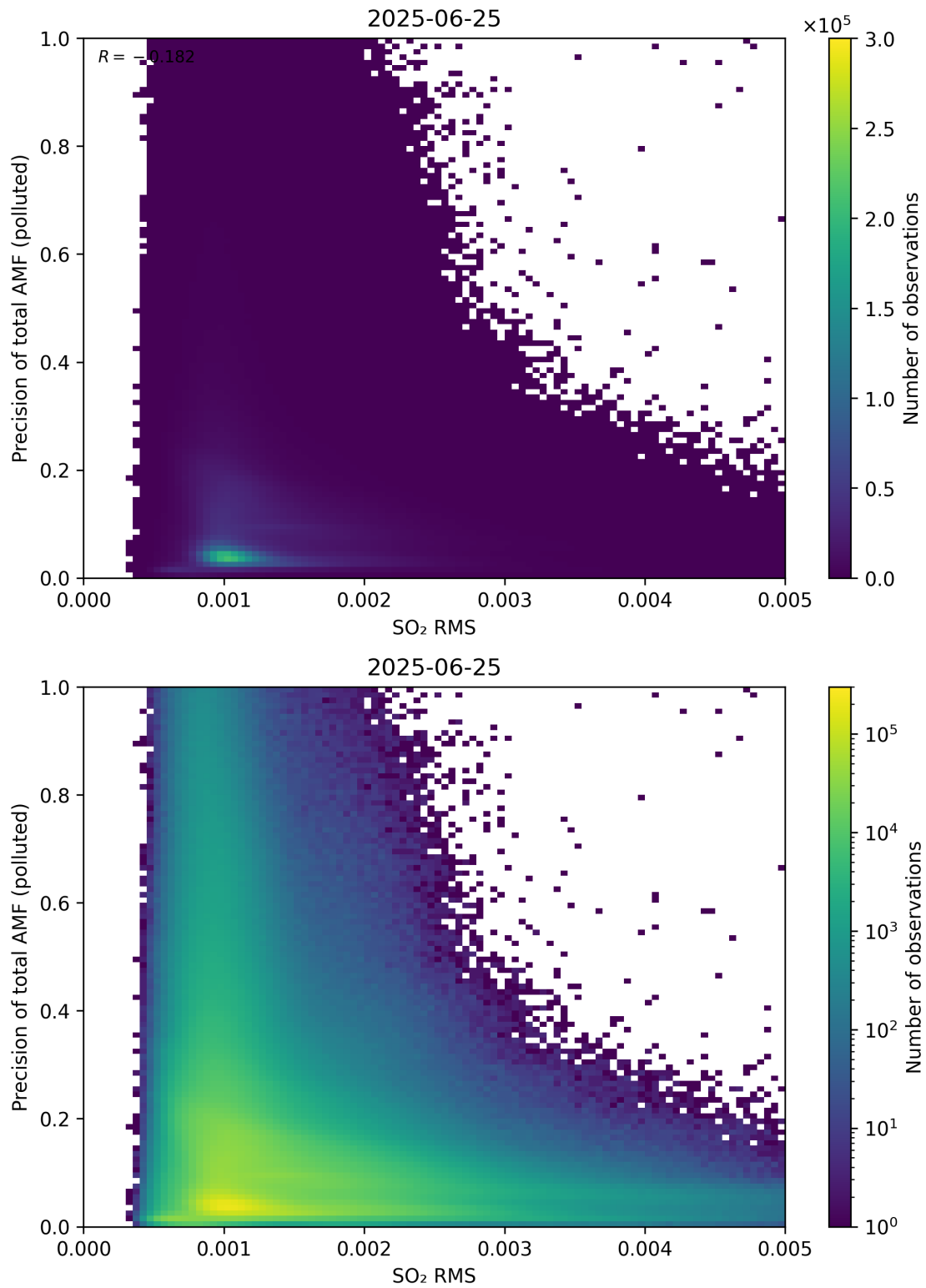
Figure 149: Scatter density plot of “SO 2 RMS” against “Precision of total AMF (polluted)” for 2025-06-24 to 2025-06-26.
