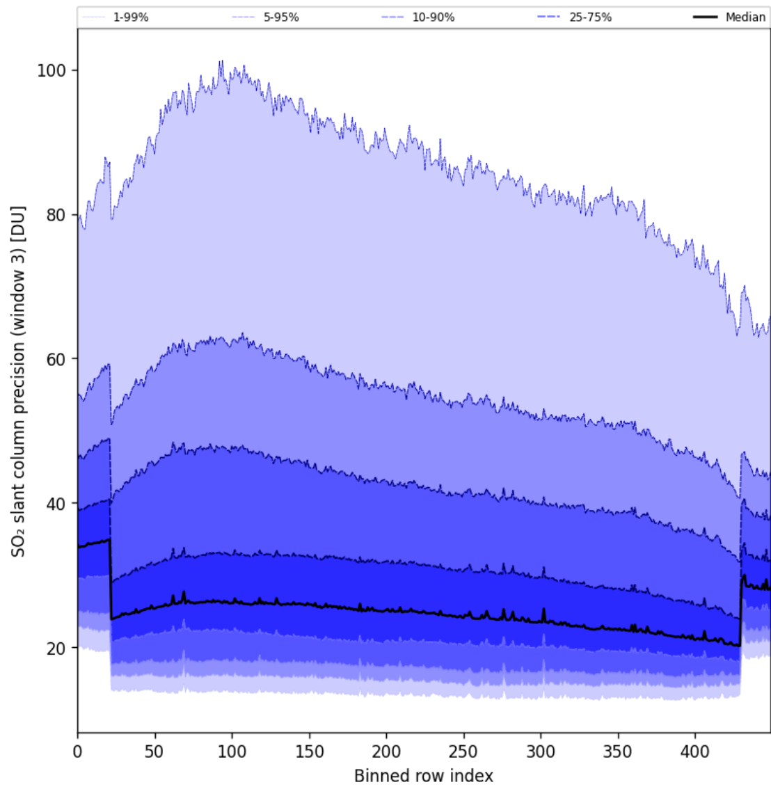
Figure 98: Along track statistics of “SO 2 slant column precision (window 3)” for 2025-06-24 to 2025-06-26
