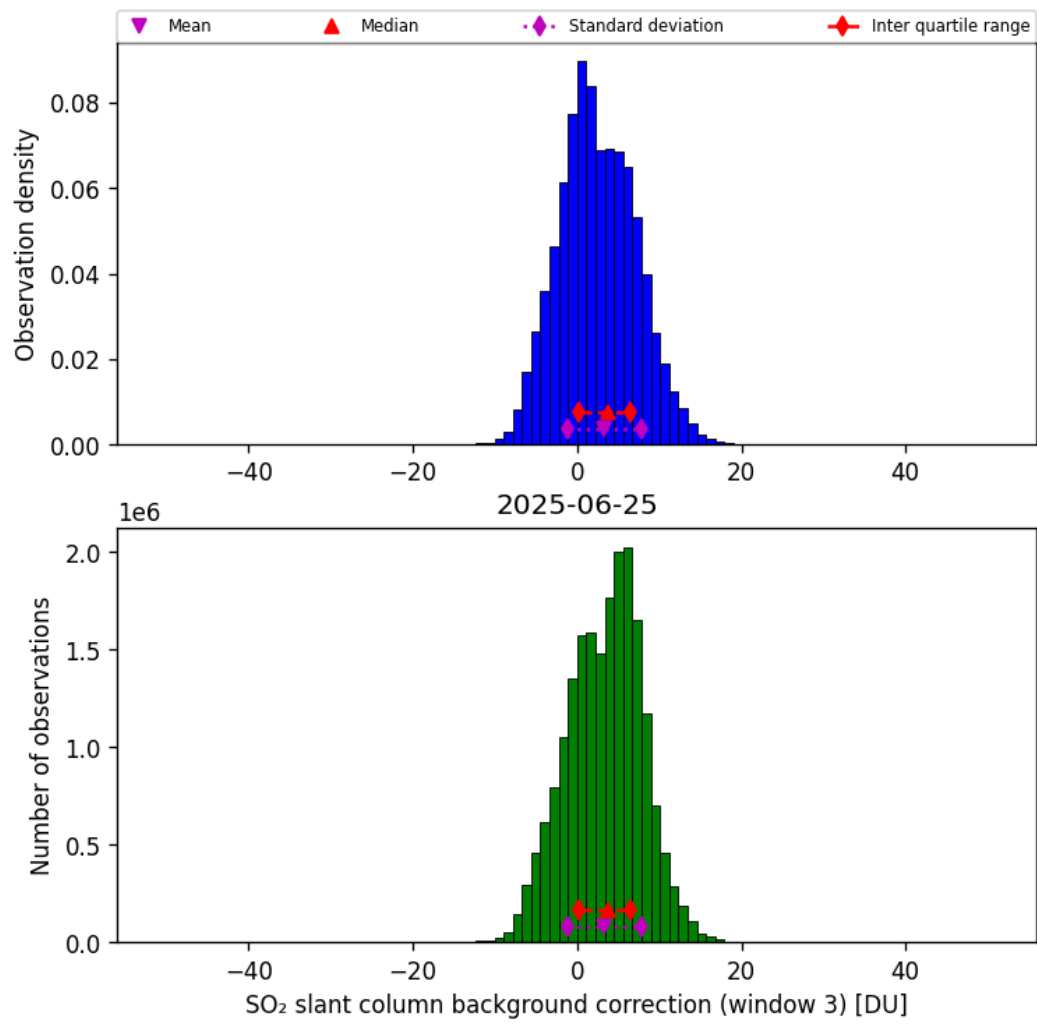
Figure 74: Histogram of “SO 2 slant column background correction (window 3)” for 2025-06-24 to 2025-06-26
