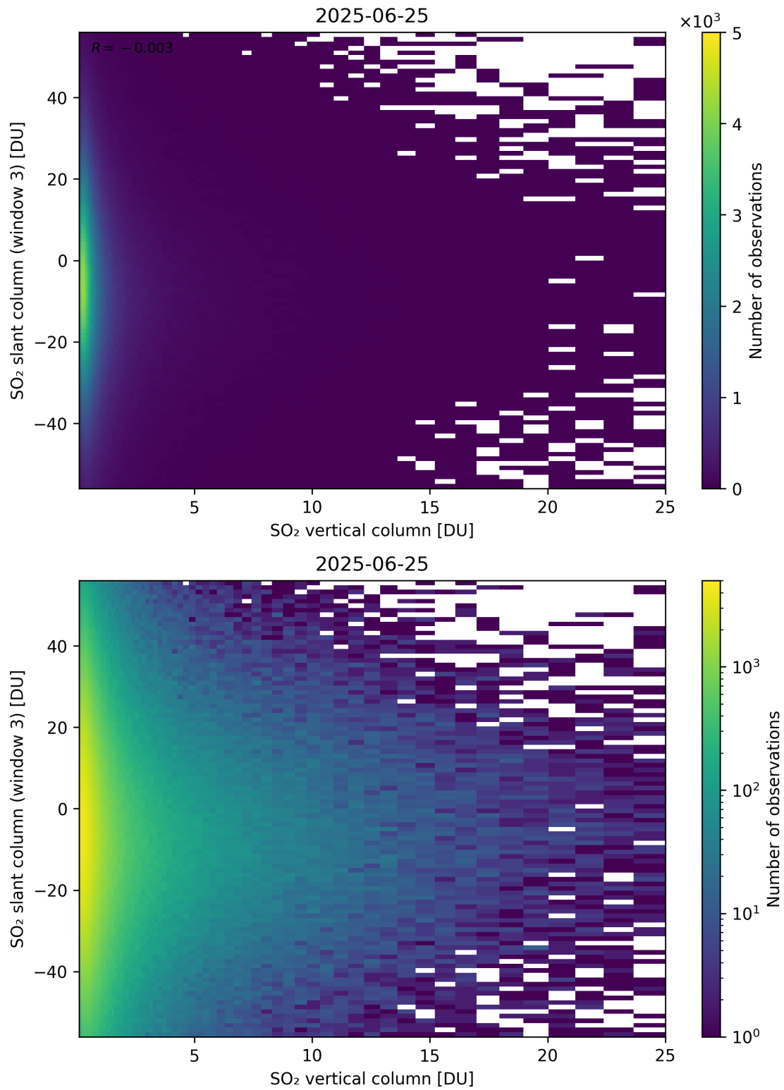
Figure 357: Scatter density plot of “SO 2 vertical column” against “SO 2 slant column (window 3)” for 2025-06-24 to 2025-06-26.
