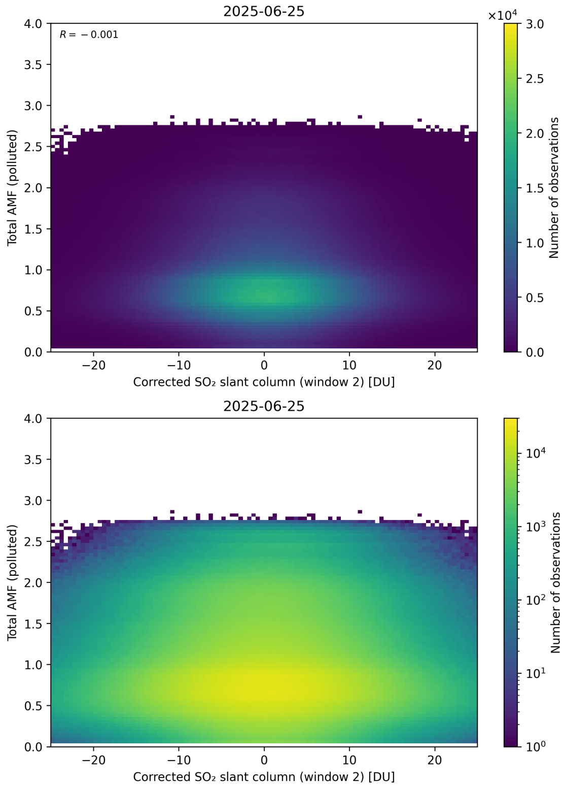
Figure 253: Scatter density plot of “Corrected SO 2 slant column (window 2)” against “Total AMF (polluted)” for 2025-06-24 to 2025-06-26.
