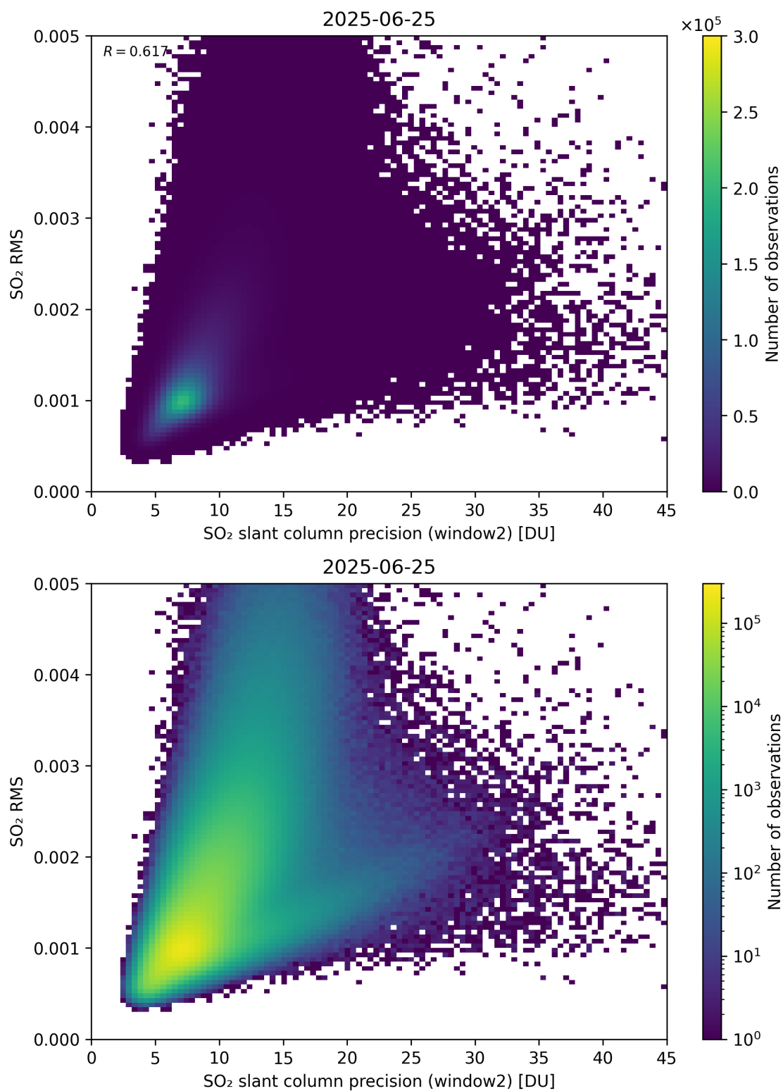
Figure 295: Scatter density plot of “SO 2 slant column precision (window2)” against “SO 2 RMS” for 2025-06-24 to 2025-06-26.
