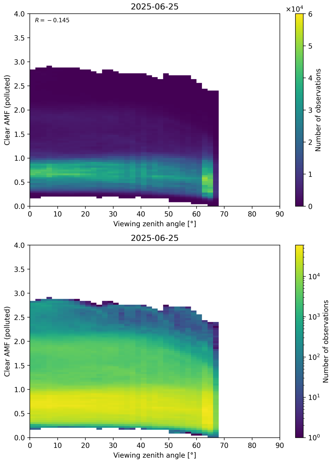
Figure 370: Scatter density plot of “Viewing zenith angle” against “Clear AMF (polluted)” for 2025-06-24 to 2025-06-26.
