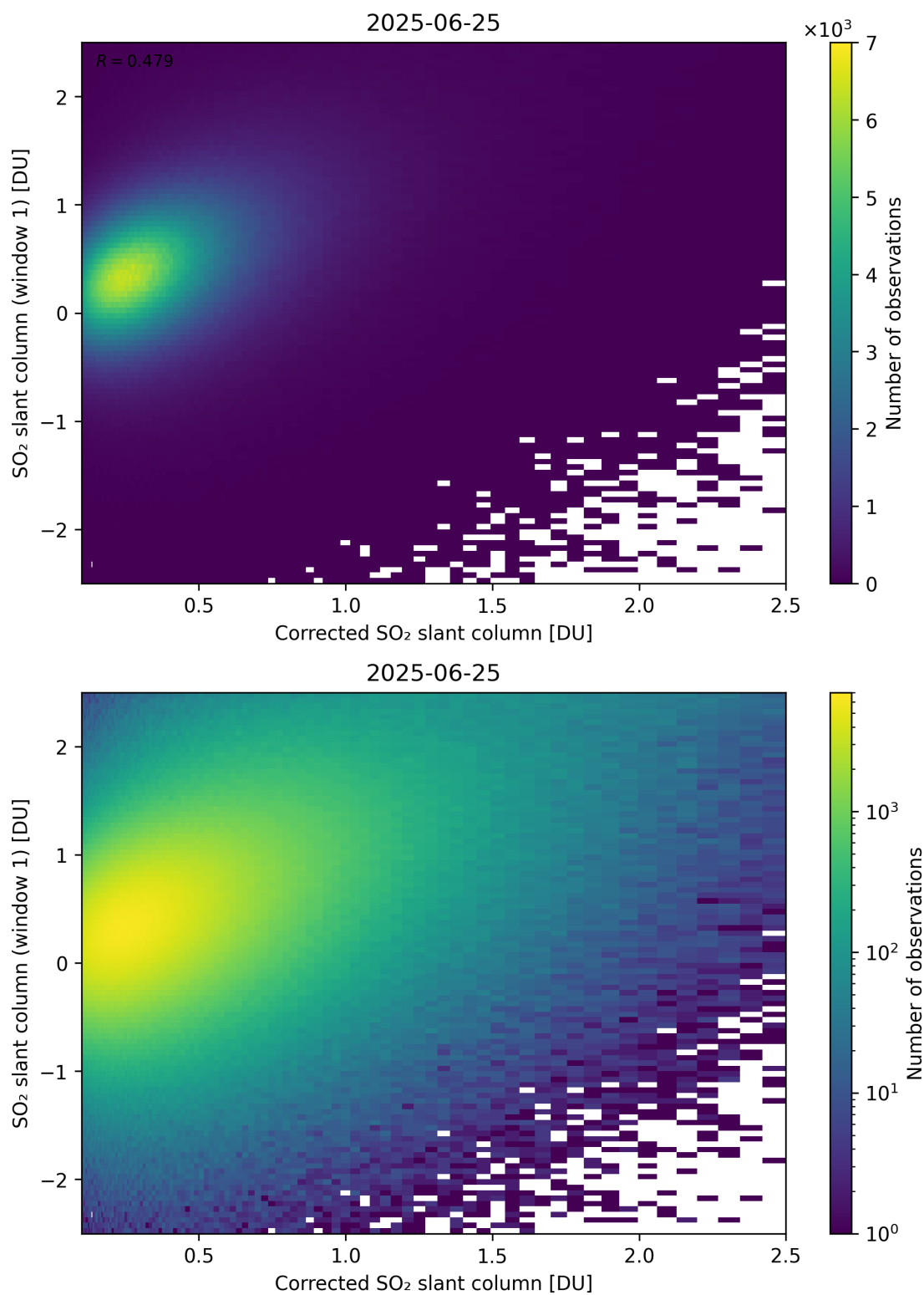
Figure 237: Scatter density plot of “Corrected SO 2 slant column” against “SO 2 slant column (window 1)” for 2025-06-24 to 2025-06-26.
