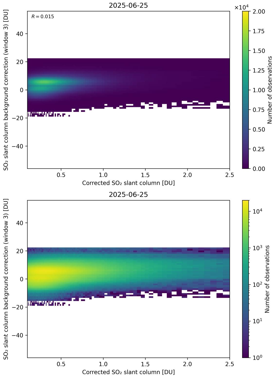
Figure 228: Scatter density plot of “Corrected SO 2 slant column” against “SO 2 slant column background correction (window 3)” for 2025-06-24 to 2025-06-26.
