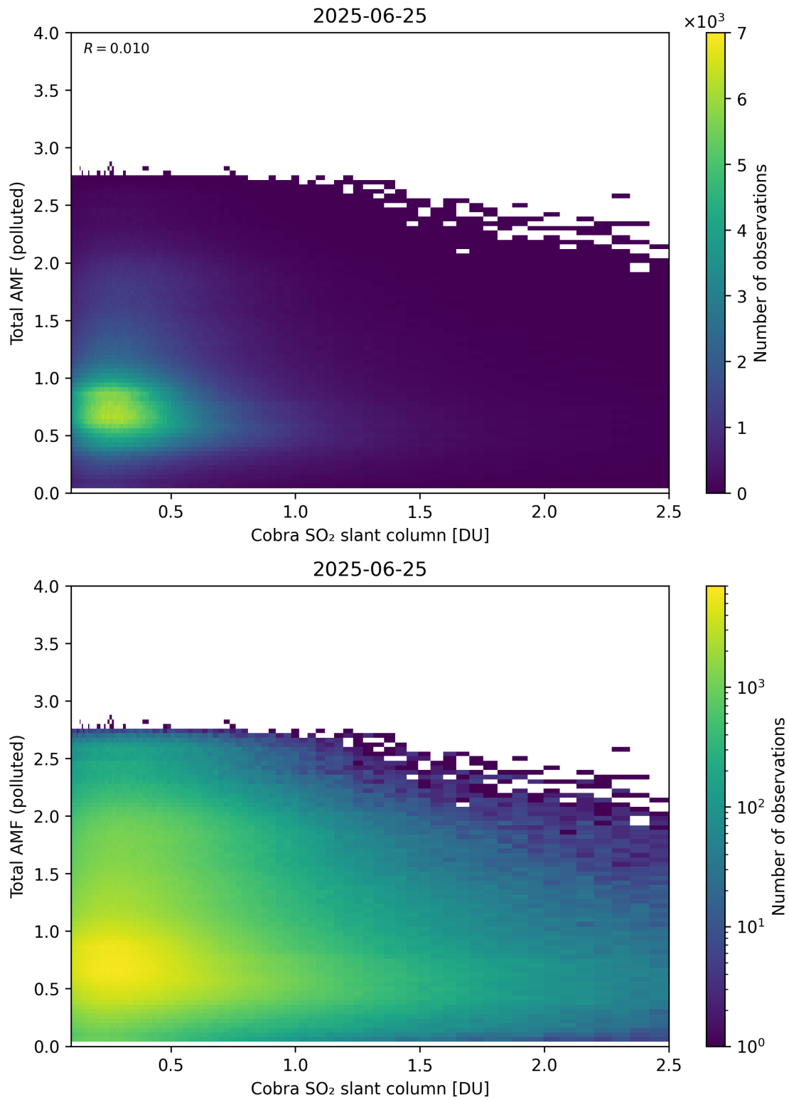
Figure 224: Scatter density plot of “Cobra SO 2 slant column” against “Total AMF (polluted)” for 2025-06-24 to 2025-06-26.
