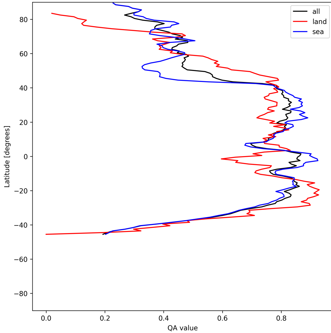
Figure 31: Zonal average of “QA value” for 2025-06-24 to 2025-06-26.
