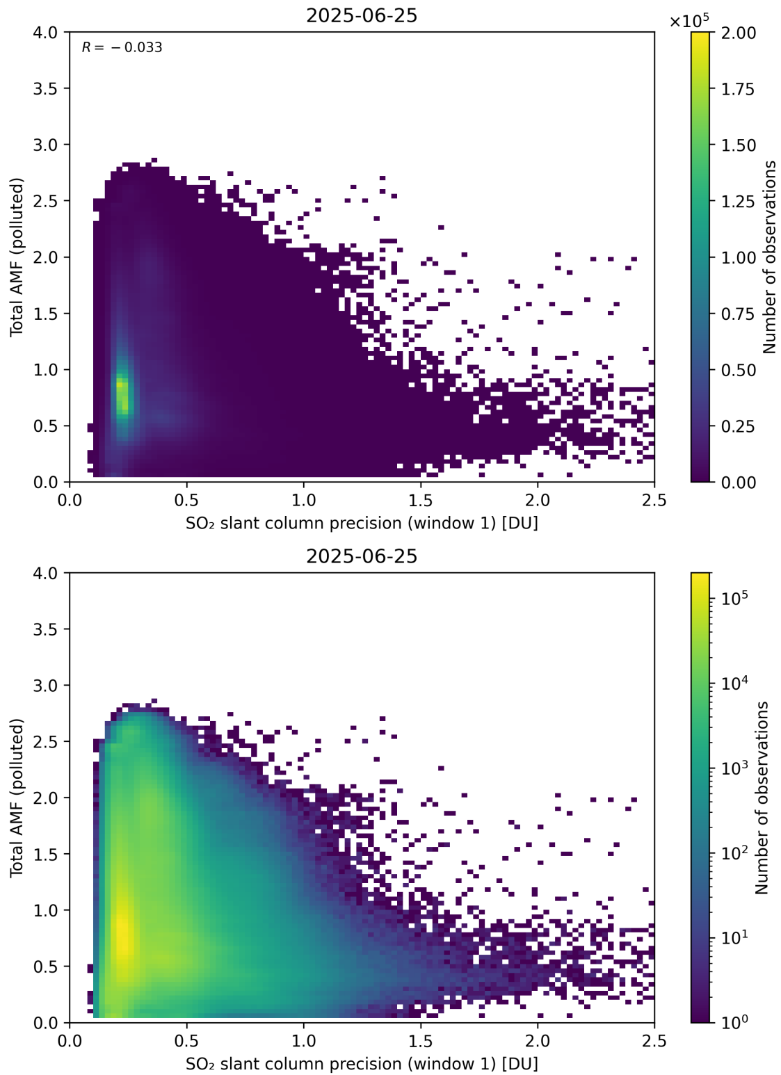
Figure 280: Scatter density plot of “SO 2 slant column precision (window 1)” against “Total AMF (polluted)” for 2025-06-24 to 2025-06-26.
