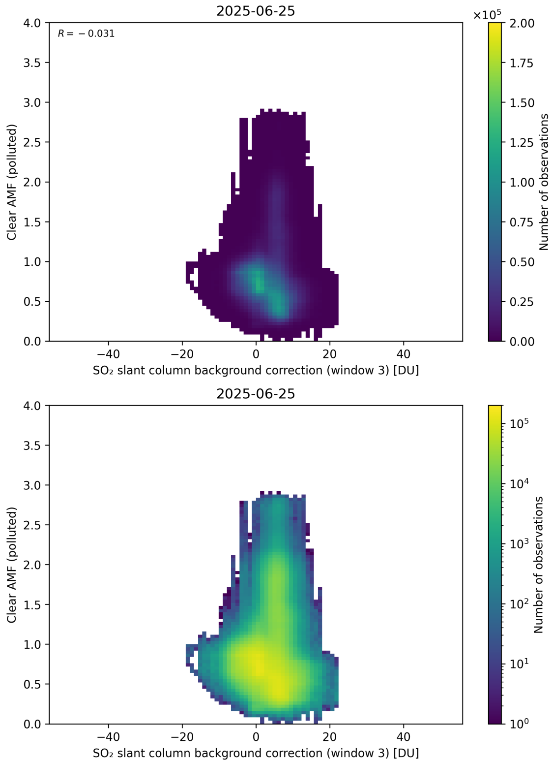
Figure 135: Scatter density plot of “SO 2 slant column background correction (window 3)” against “Clear AMF (polluted)” for 2025-06-24 to 2025-06-26.
