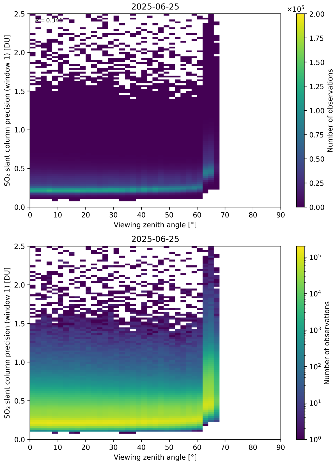
Figure 377: Scatter density plot of “Viewing zenith angle” against “SO 2 slant column precision (window 1)” for 2025-06-24 to 2025-06-26.
