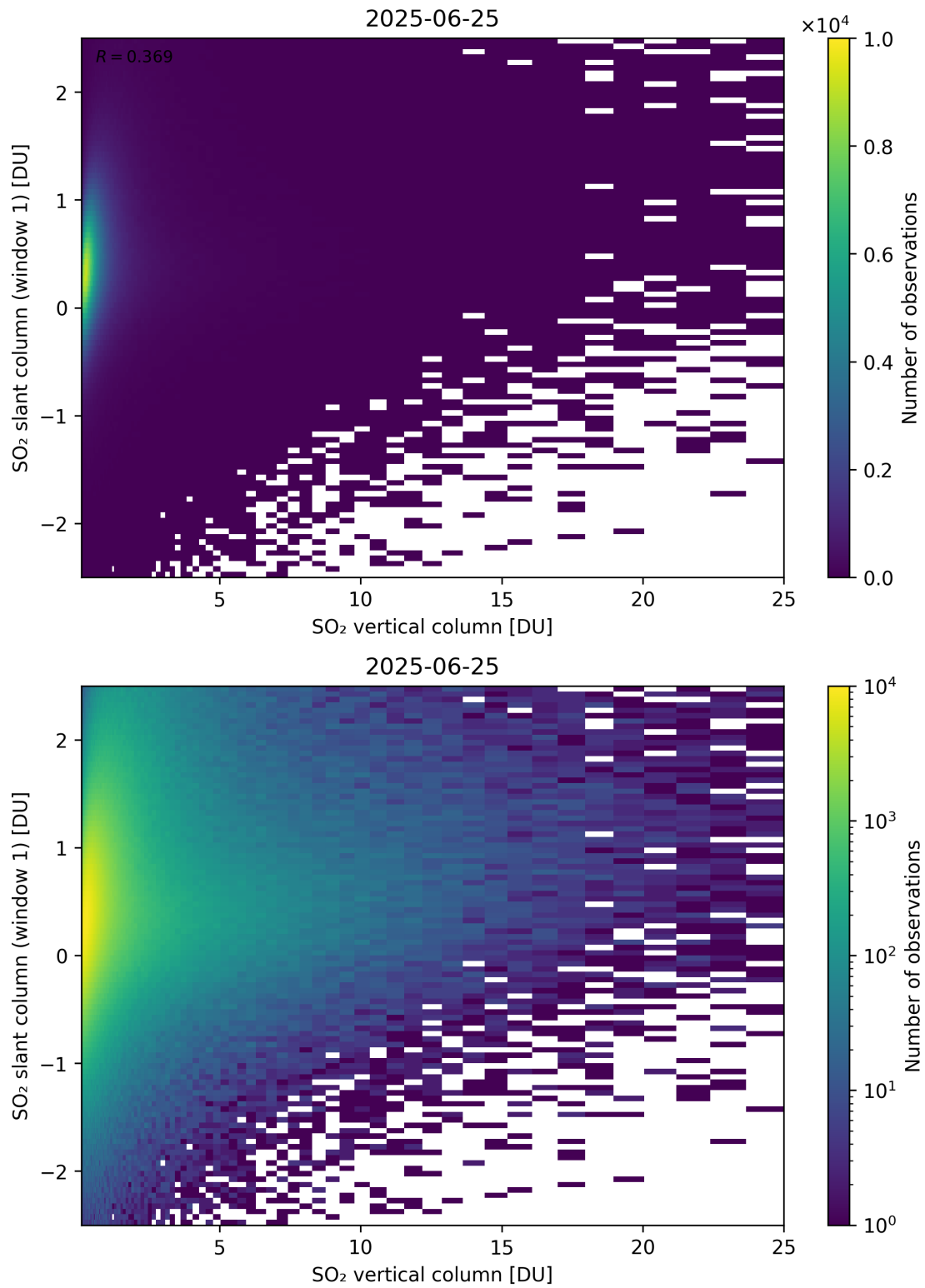
Figure 354: Scatter density plot of “SO 2 vertical column” against “SO 2 slant column (window 1)” for 2025-06-24 to 2025-06-26.
