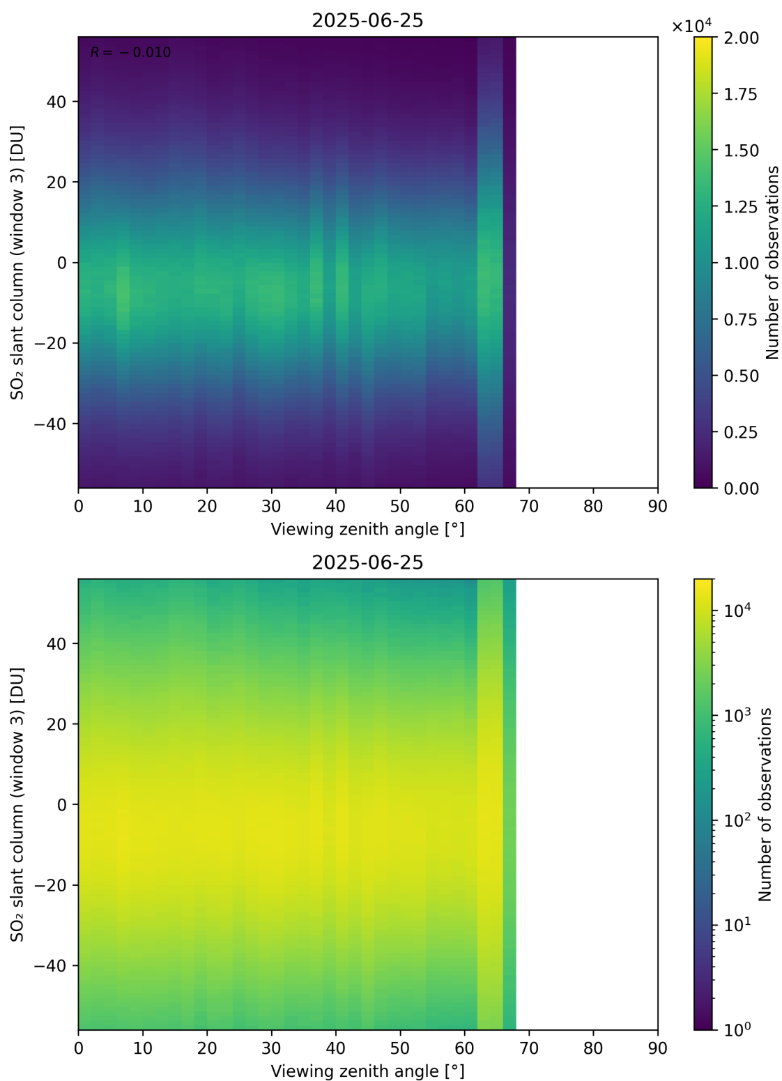
Figure 379: Scatter density plot of “Viewing zenith angle” against “SO 2 slant column (window 3)” for 2025-06-24 to 2025-06-26.
