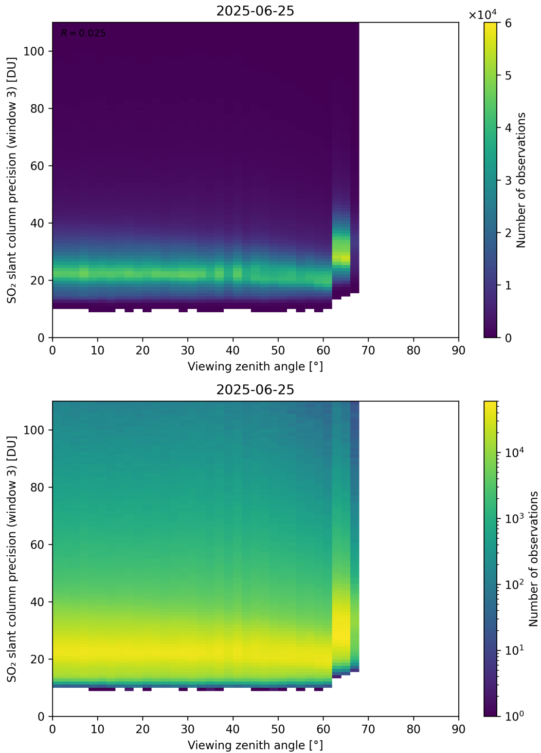
Figure 380: Scatter density plot of “Viewing zenith angle” against “SO 2 slant column precision (window 3)” for 2025-06-24 to 2025-06-26.
