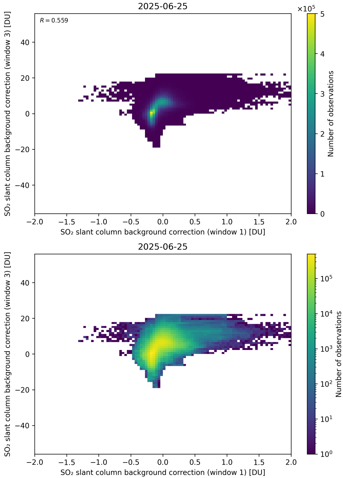
Figure 110: Scatter density plot of “SO 2 slant column background correction (window 1)” against “SO 2 slant column background correction (window 3)” for 2025-06-24 to 2025-06-26.
