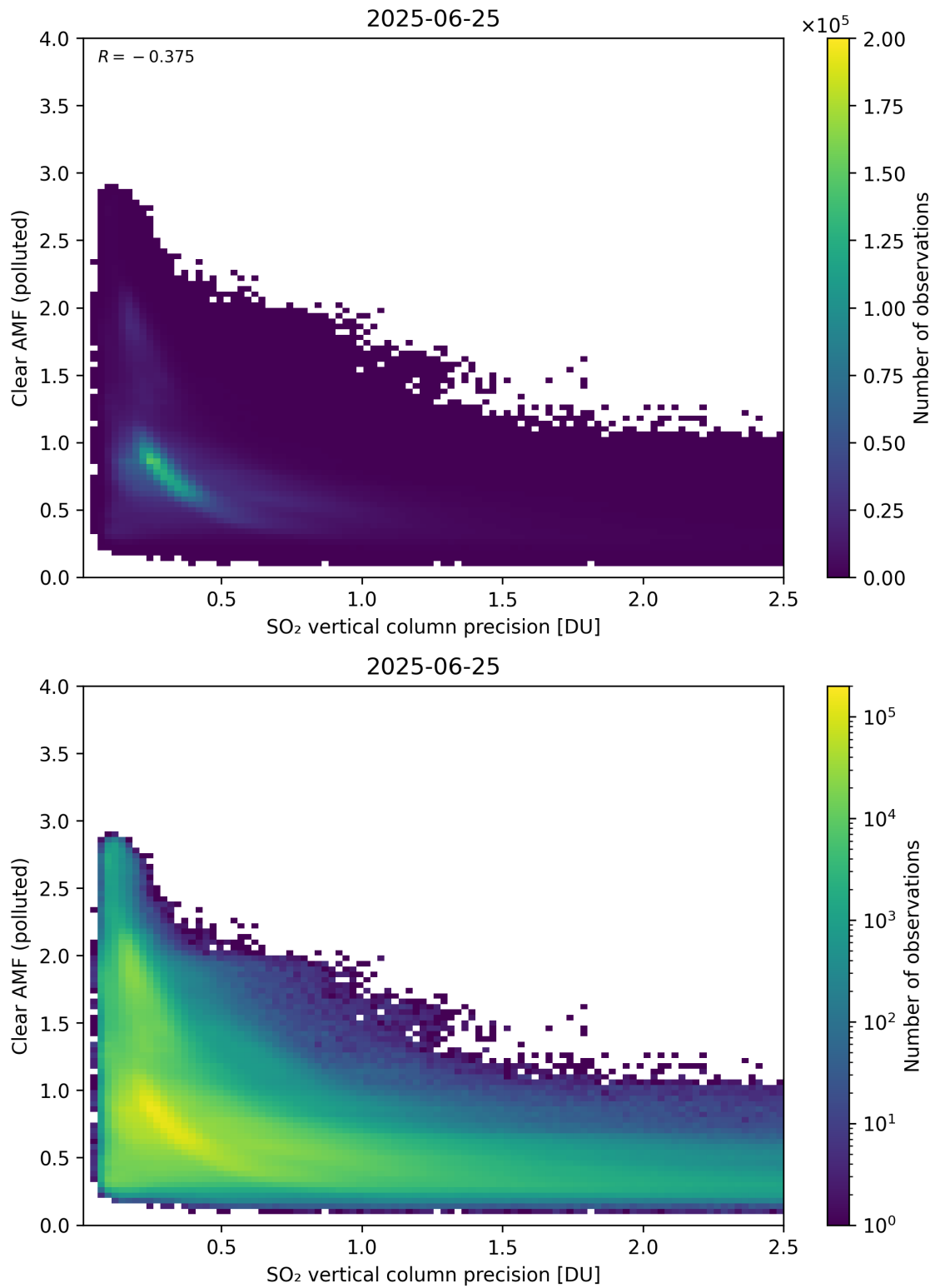
Figure 335: Scatter density plot of “SO 2 vertical column precision” against “Clear AMF (polluted)” for 2025-06-24 to 2025-06-26.
