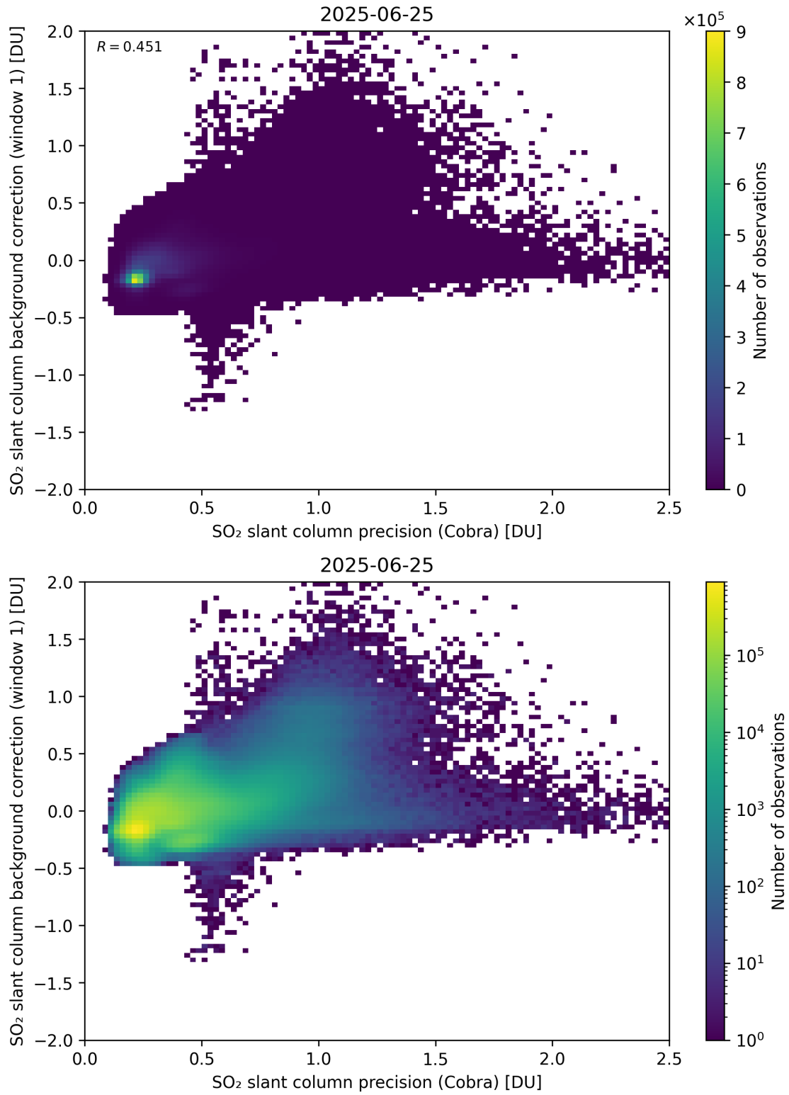
Figure 199: Scatter density plot of “SO 2 slant column precision (Cobra)” against “SO 2 slant column background correction (window 1)” for 2025-06-24 to 2025-06-26.
