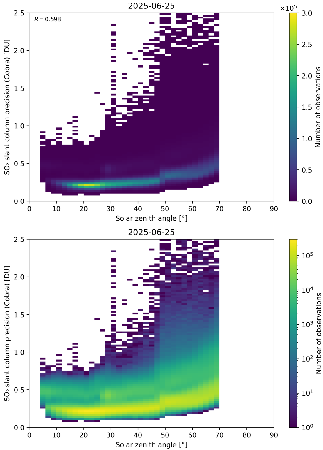
Figure 180: Scatter density plot of “Solar zenith angle” against “SO 2 slant column precision (Cobra)” for 2025-06-24 to 2025-06-26.
