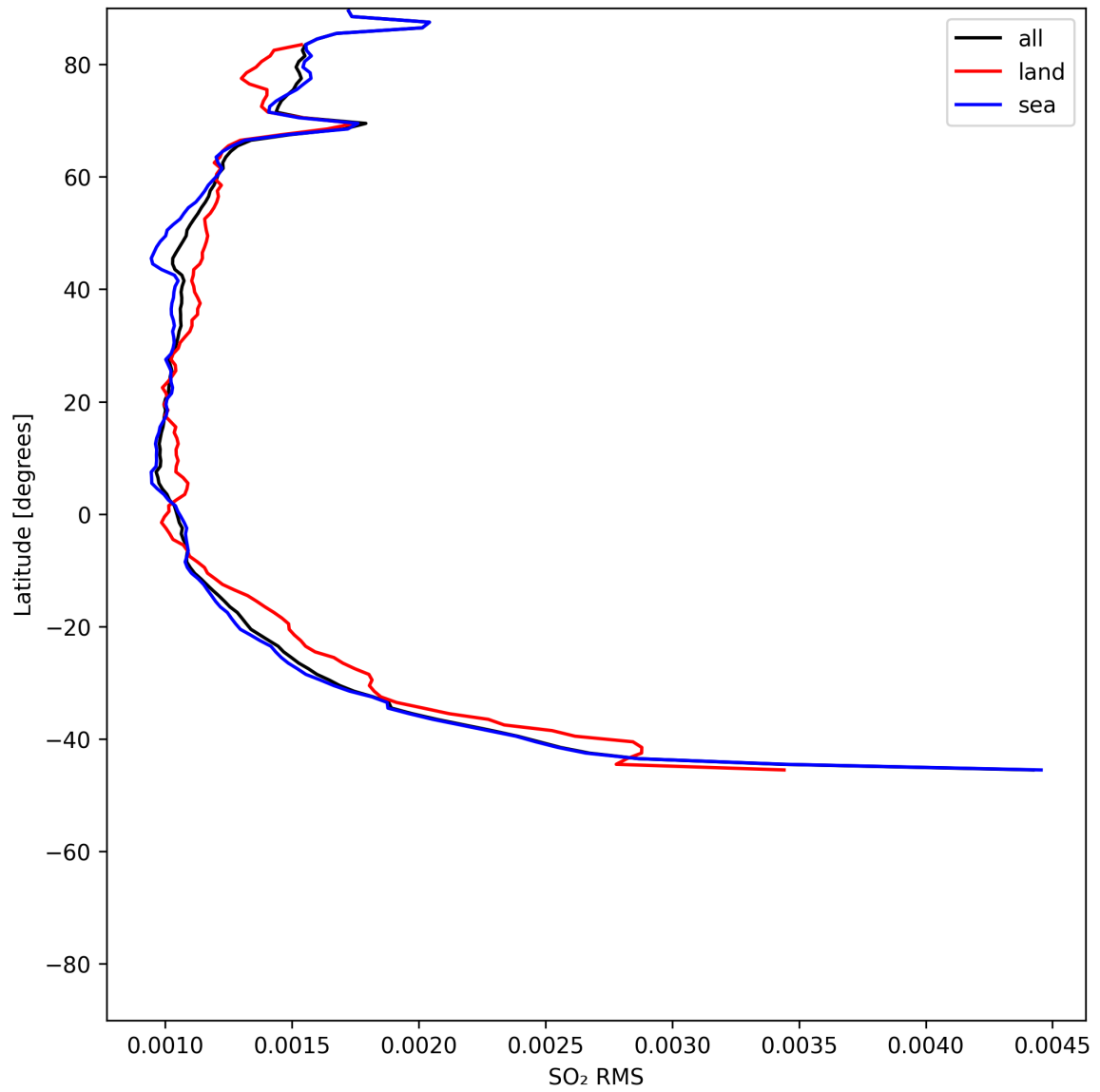
Figure 52: Zonal average of “SO 2 RMS” for 2025-06-24 to 2025-06-26.
