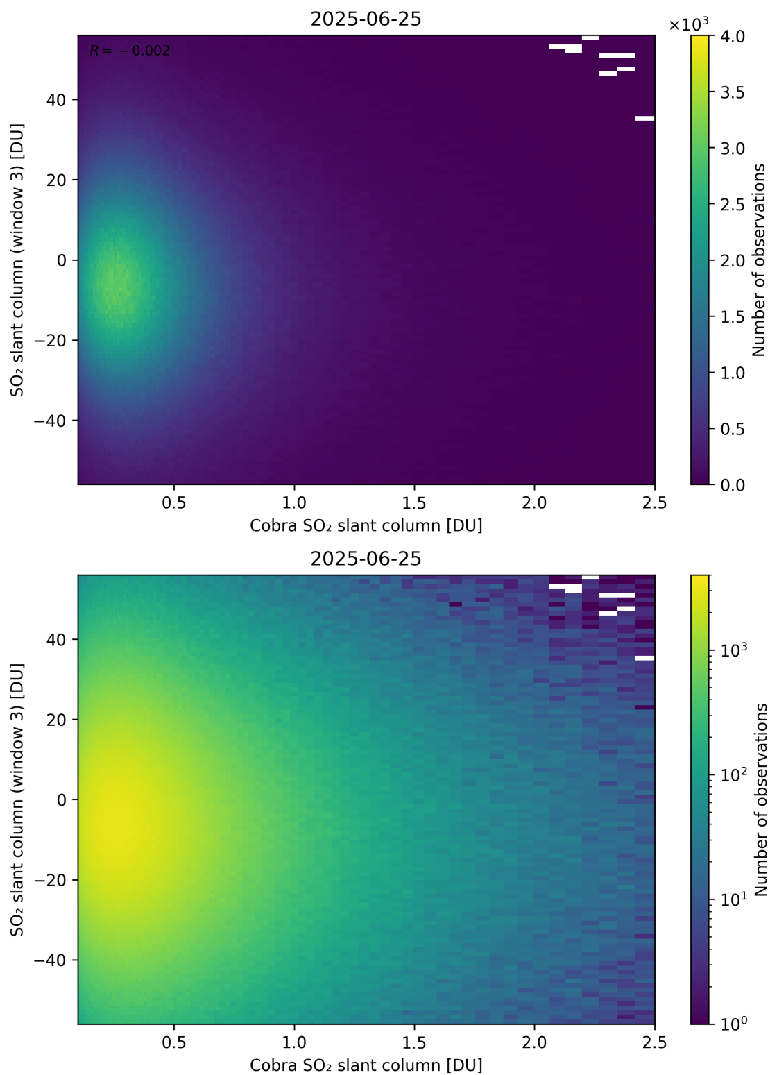
Figure 222: Scatter density plot of “Cobra SO 2 slant column” against “SO 2 slant column (window 3)” for 2025-06-24 to 2025-06-26.
