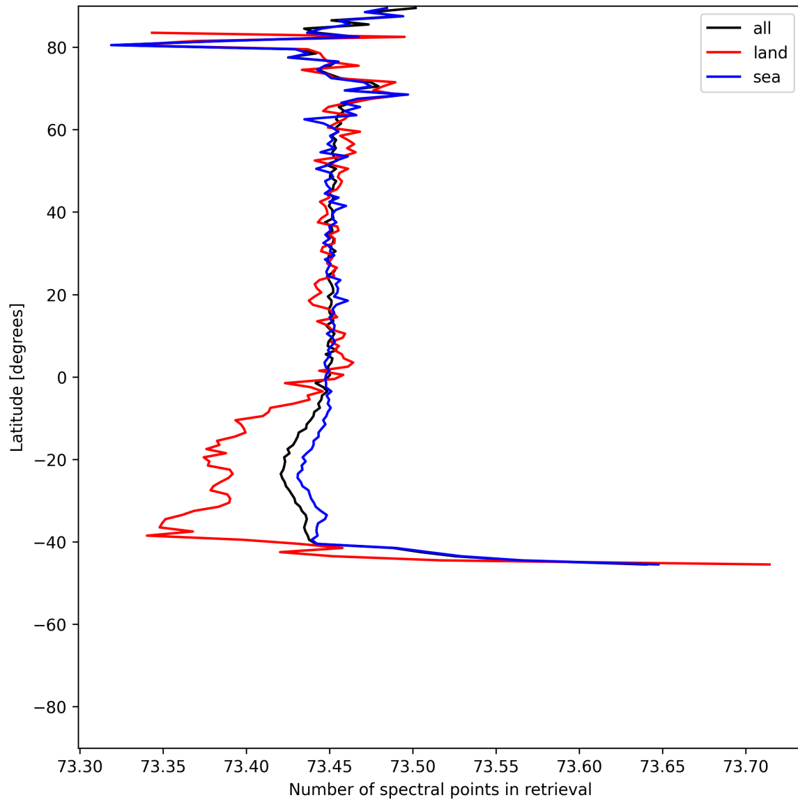
Figure 56: Zonal average of “Number of spectral points in retrieval” for 2025-06-24 to 2025-06-26.
