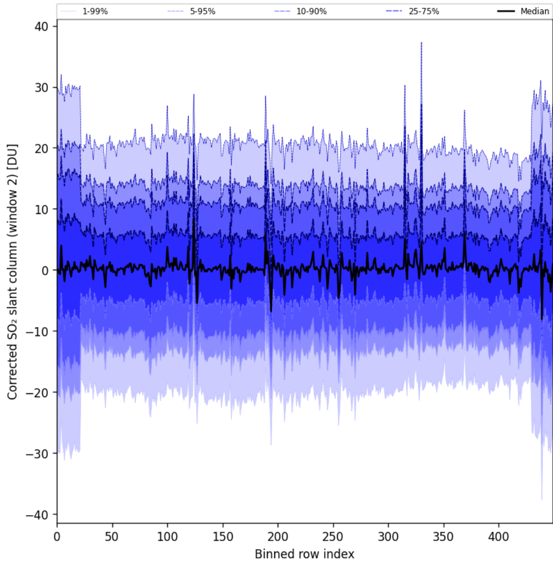
Figure 95: Along track statistics of “Corrected SO 2 slant column (window 2)” for 2025-06-24 to 2025-06-26
