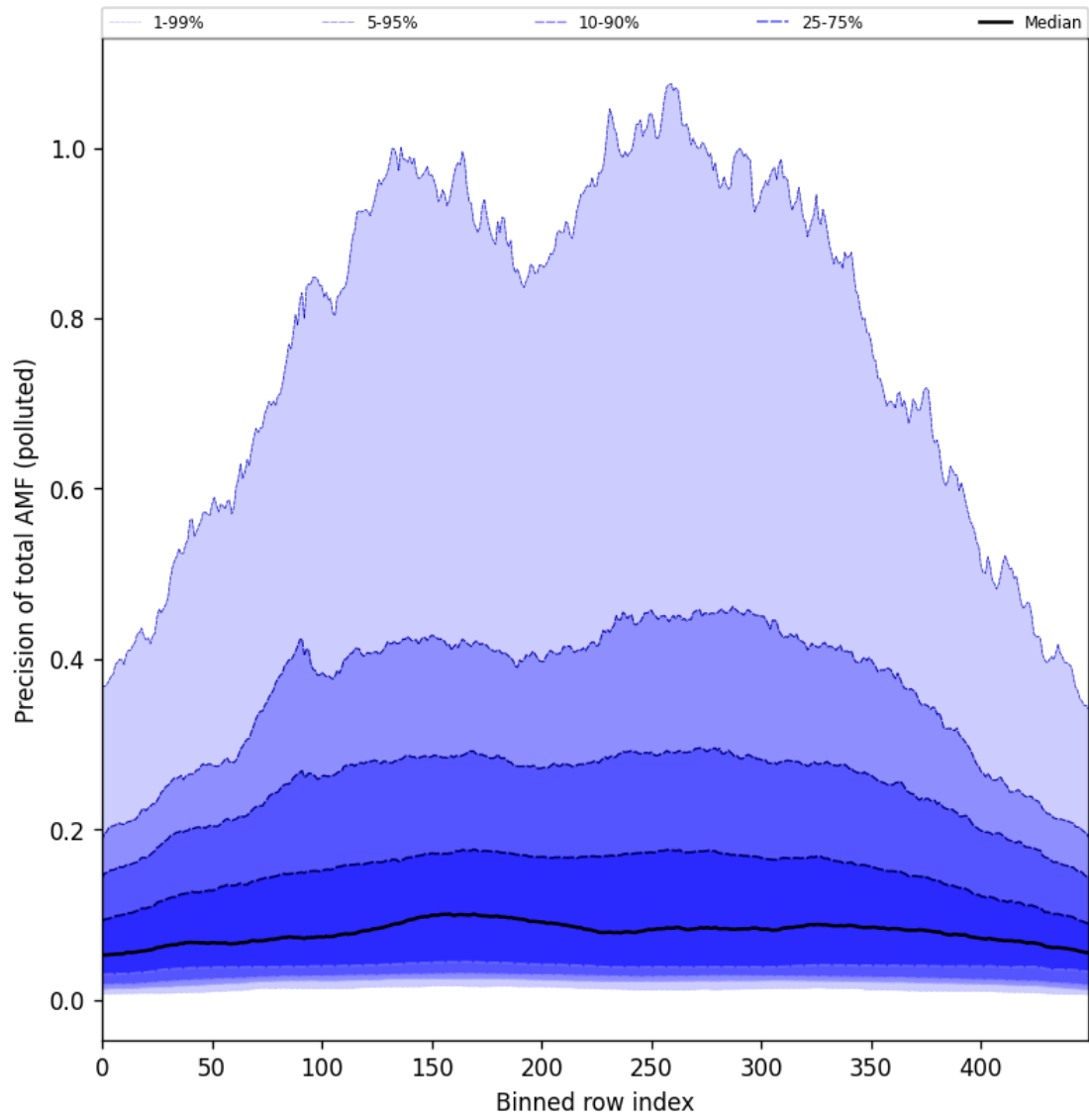
Figure 106: Along track statistics of “Precision of total AMF (polluted)” for 2025-06-24 to 2025-06-26
