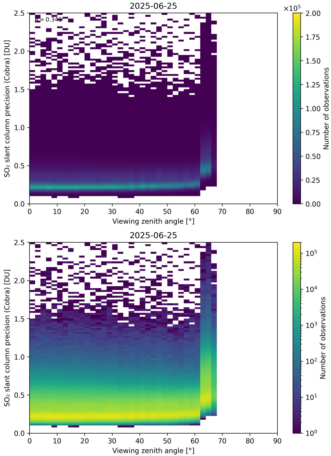
Figure 372: Scatter density plot of “Viewing zenith angle” against “SO 2 slant column precision (Cobra)” for 2025-06-24 to 2025-06-26.
