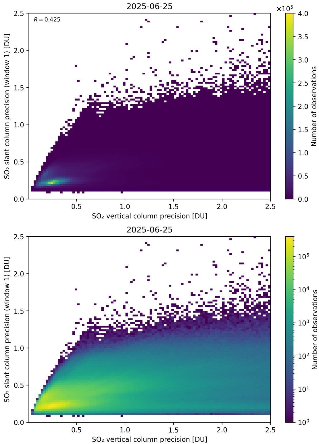
Figure 342: Scatter density plot of “SO 2 vertical column precision” against “SO 2 slant column precision (window 1)” for 2025-06-24 to 2025-06-26.
