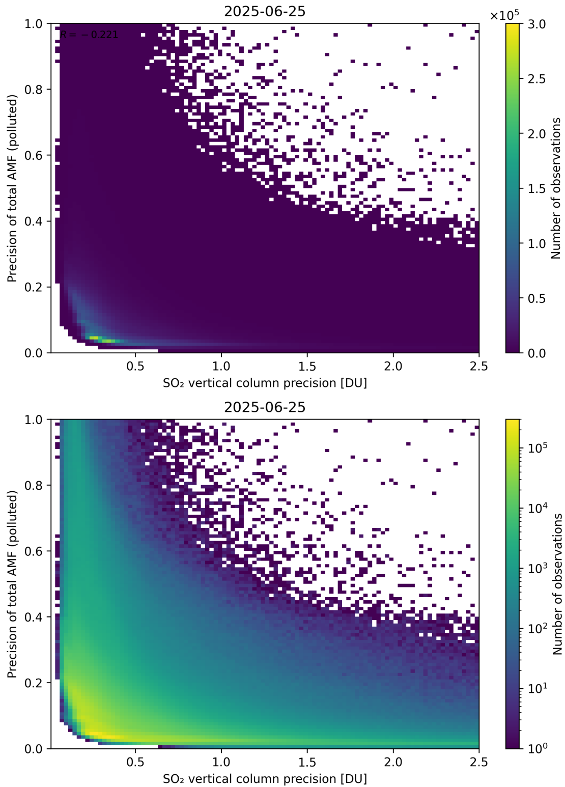
Figure 347: Scatter density plot of “SO 2 vertical column precision” against “Precision of total AMF (polluted)” for 2025-06-24 to 2025-06-26.
