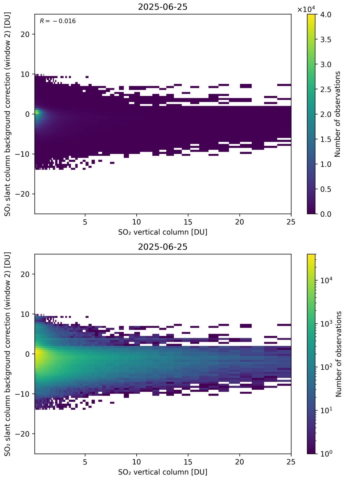
Figure 324: Scatter density plot of “SO 2 vertical column” against “SO 2 slant column background correction (window 2)” for 2025-06-24 to 2025-06-26.
