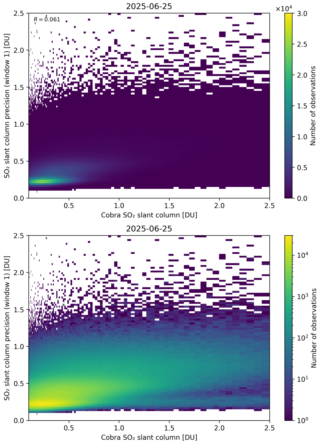
Figure 220: Scatter density plot of “Cobra SO 2 slant column” against “SO 2 slant column precision (window 1)” for 2025-06-24 to 2025-06-26.
