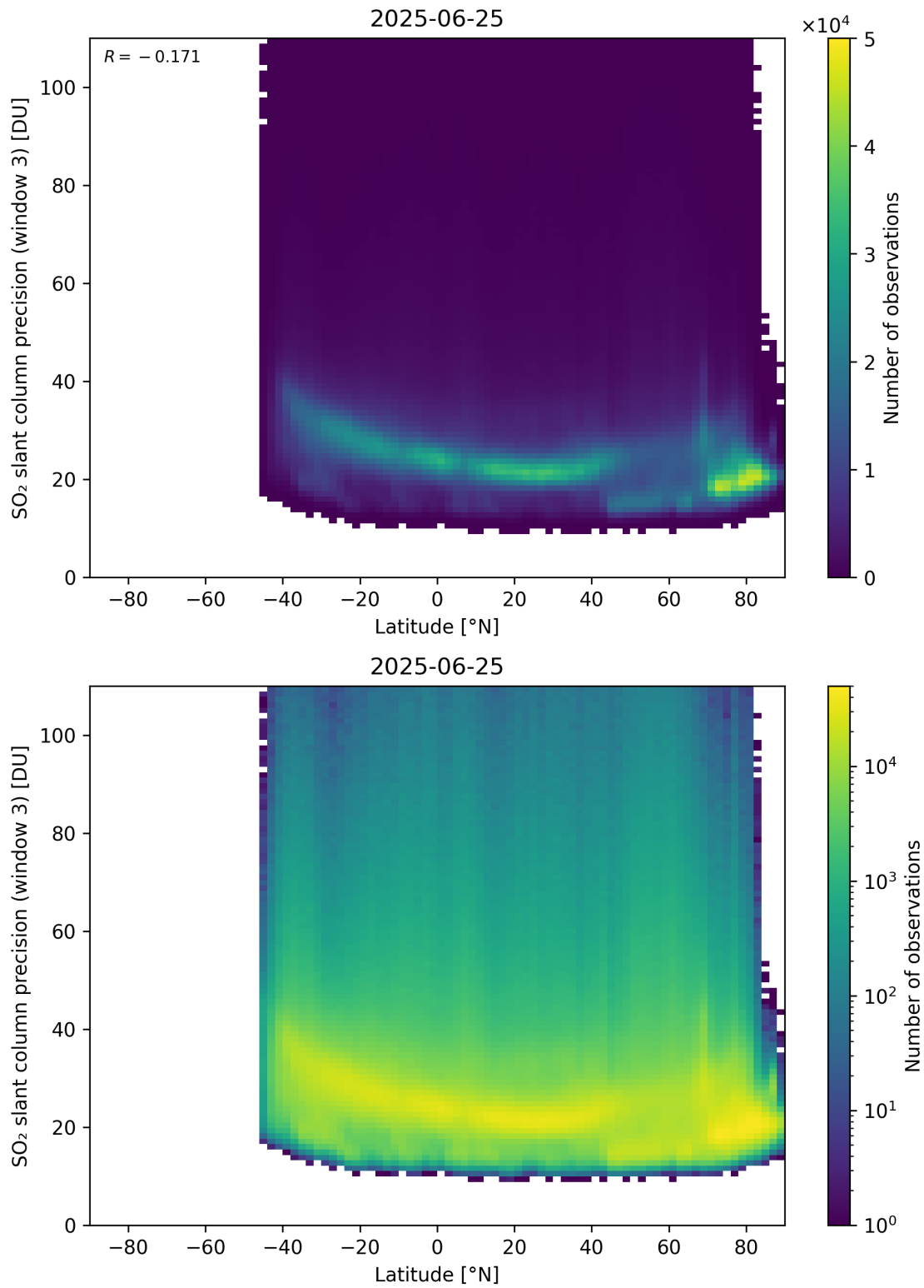
Figure 166: Scatter density plot of “Latitude” against “SO 2 slant column precision (window 3)” for 2025-06-24 to 2025-06-26.
