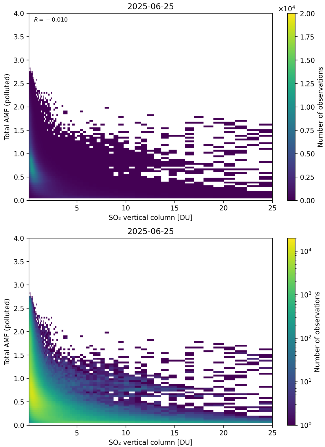
Figure 359: Scatter density plot of “SO 2 vertical column” against “Total AMF (polluted)” for 2025-06-24 to 2025-06-26.
