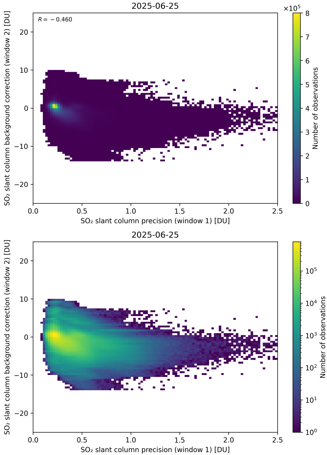
Figure 269: Scatter density plot of “SO 2 slant column precision (window 1)” against “SO 2 slant column background correction (window 2)” for 2025-06-24 to 2025-06-26.
