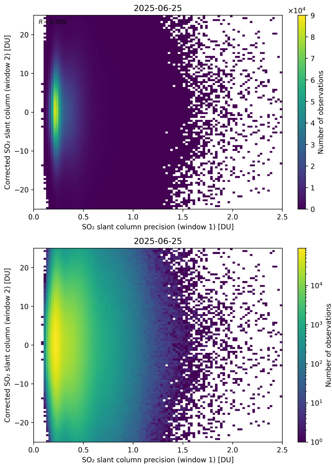
Figure 275: Scatter density plot of “SO 2 slant column precision (window 1)” against “Corrected SO 2 slant column (window 2)” for 2025-06-24 to 2025-06-26.
