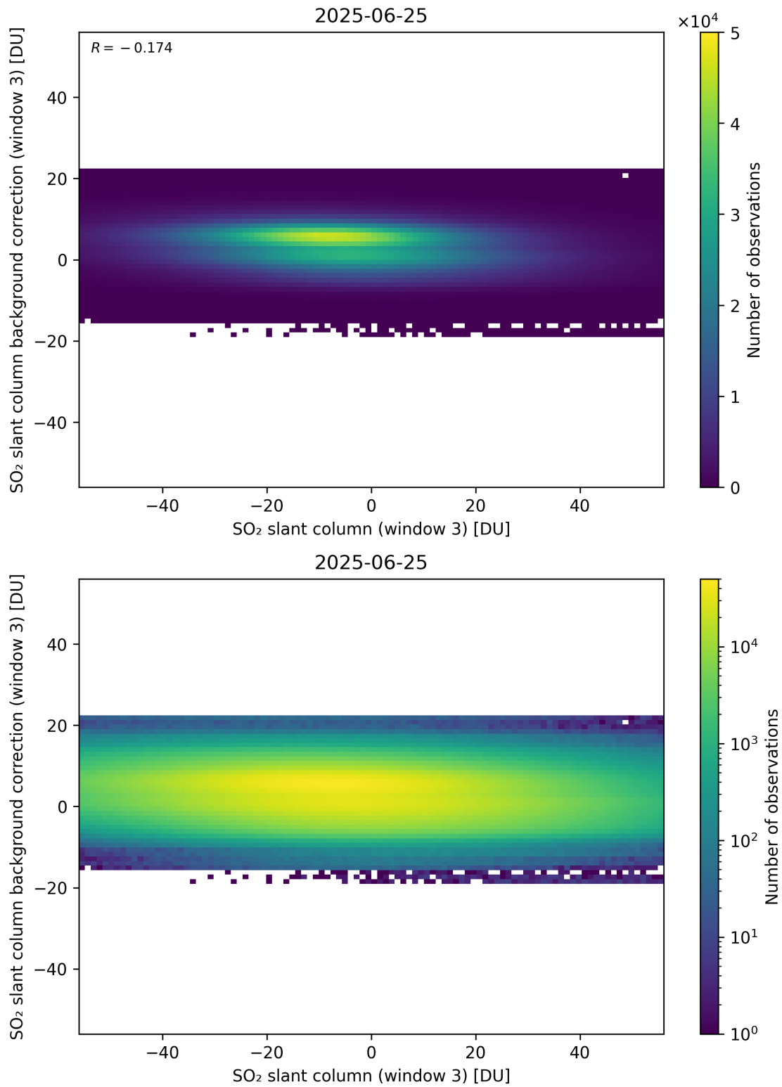
Figure 303: Scatter density plot of “SO 2 slant column (window 3)” against “SO 2 slant column background correction (window 3)” for 2025-06-24 to 2025-06-26.
