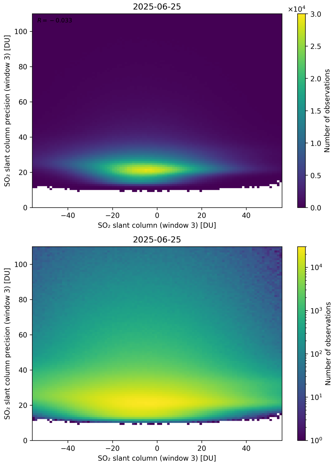
Figure 317: Scatter density plot of “SO 2 slant column (window 3)” against “SO 2 slant column precision (window 3)” for 2025-06-24 to 2025-06-26.
