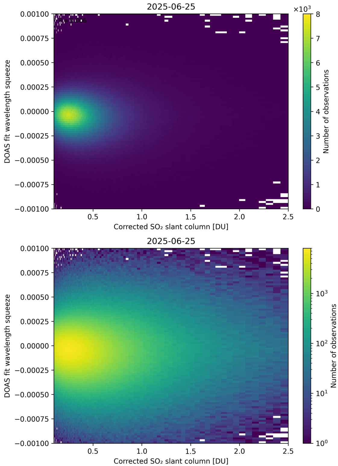
Figure 230: Scatter density plot of “Corrected SO 2 slant column” against “DOAS fit wavelength squeeze” for 2025-06-24 to 2025-06-26.
