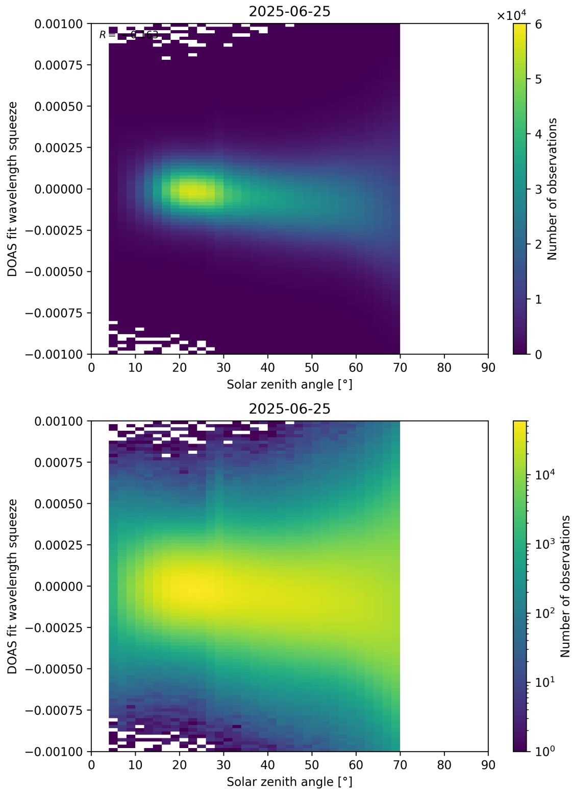
Figure 175: Scatter density plot of “Solar zenith angle” against “DOAS fit wavelength squeeze” for 2025-06-24 to 2025-06-26.
