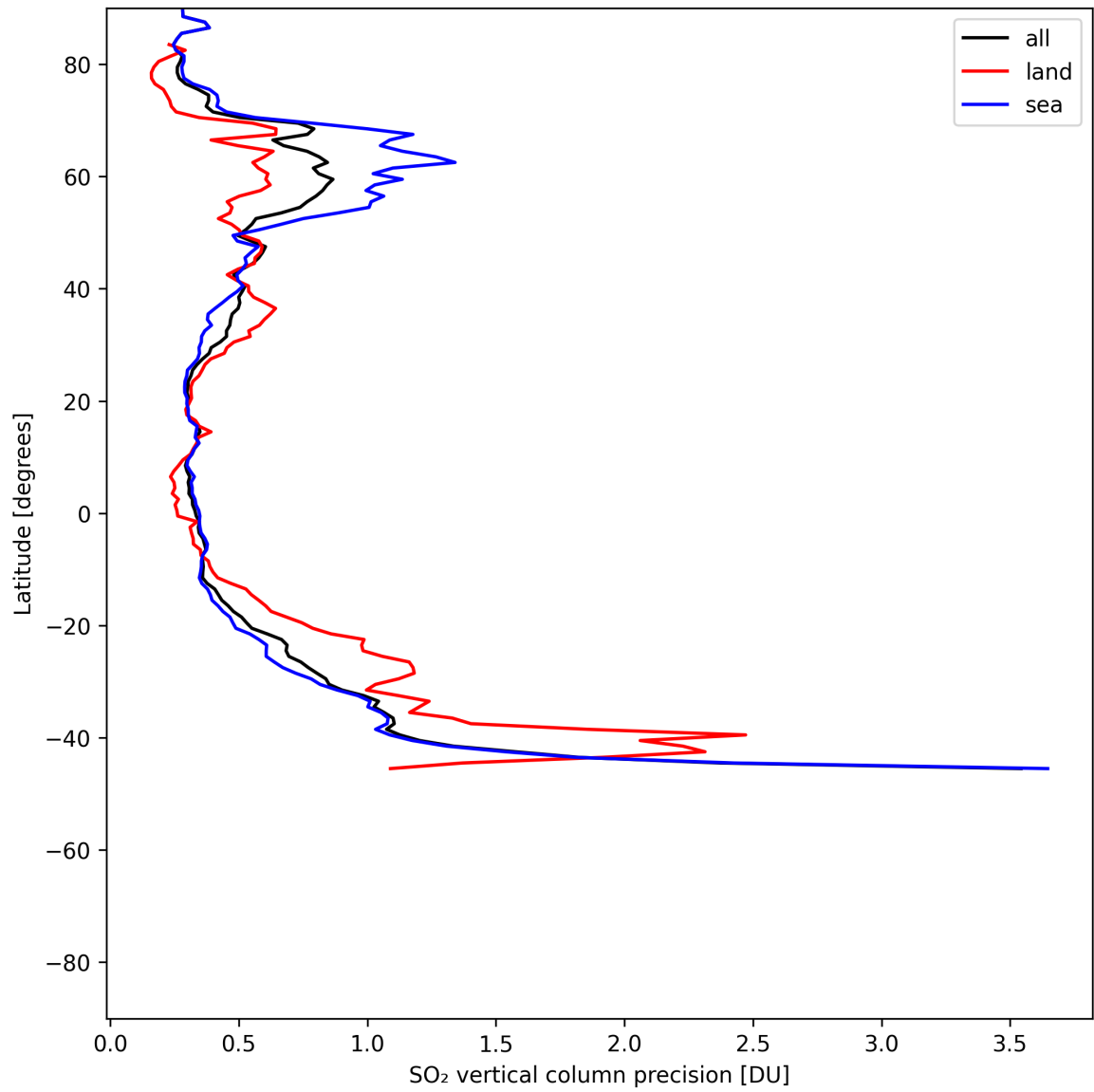
Figure 33: Zonal average of “SO 2 vertical column precision” for 2025-06-24 to 2025-06-26.
