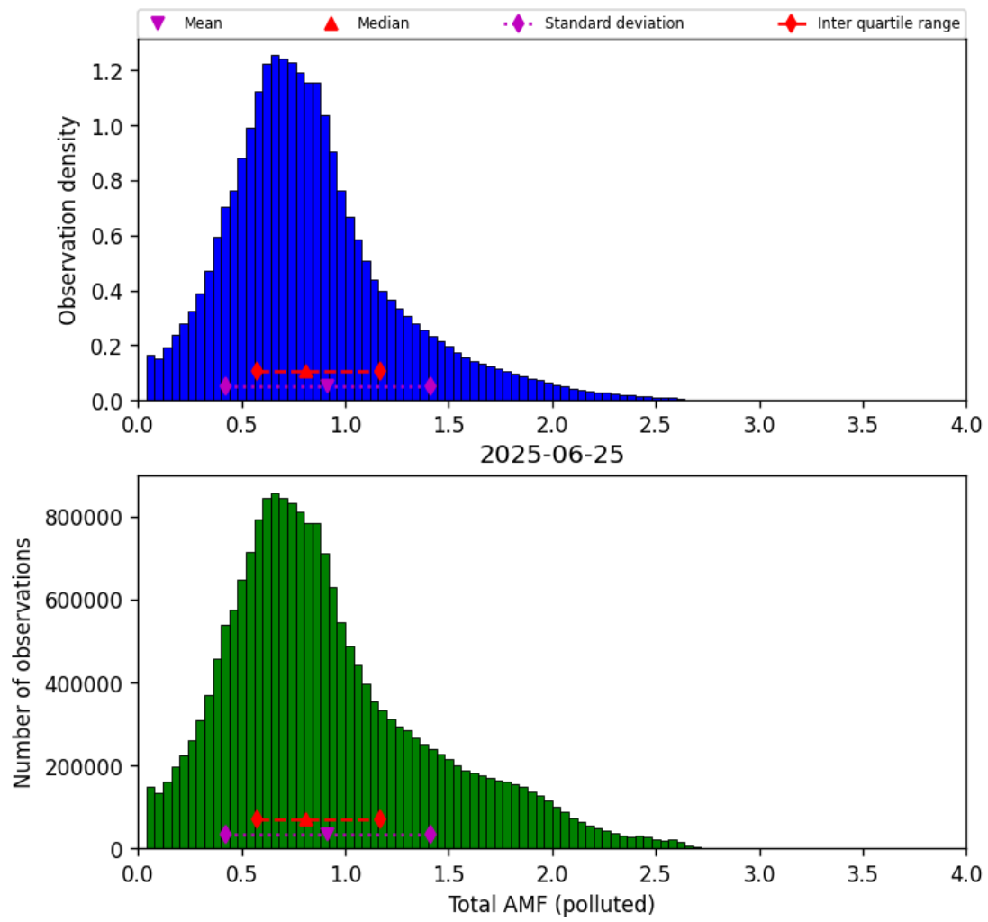
Figure 79: Histogram of “Total AMF (polluted)” for 2025-06-24 to 2025-06-26
