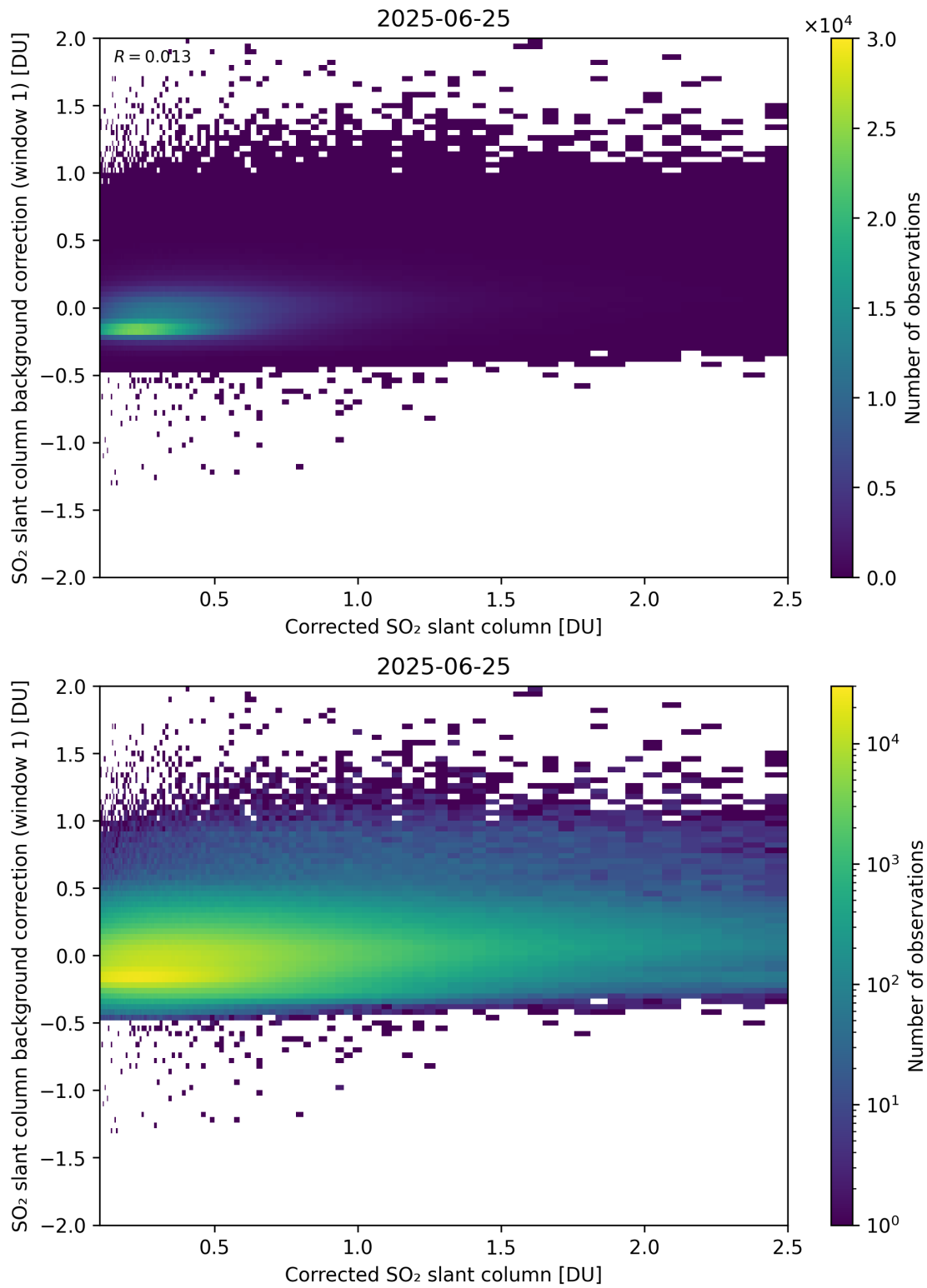
Figure 226: Scatter density plot of “Corrected SO 2 slant column” against “SO 2 slant column background correction (window 1)” for 2025-06-24 to 2025-06-26.
