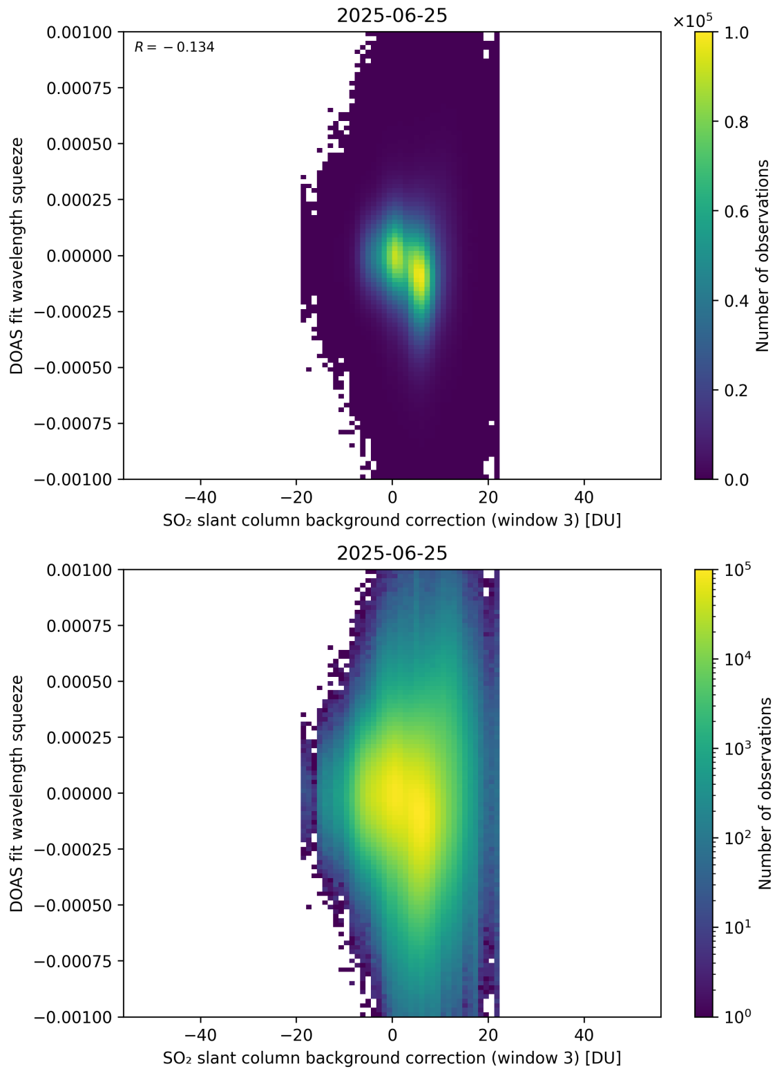
Figure 133: Scatter density plot of “SO 2 slant column background correction (window 3)” against “DOAS fit wavelength squeeze” for 2025-06-24 to 2025-06-26.
