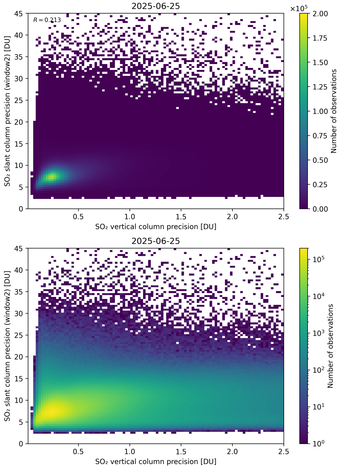
Figure 343: Scatter density plot of “SO 2 vertical column precision” against “SO 2 slant column precision (window2)” for 2025-06-24 to 2025-06-26.
