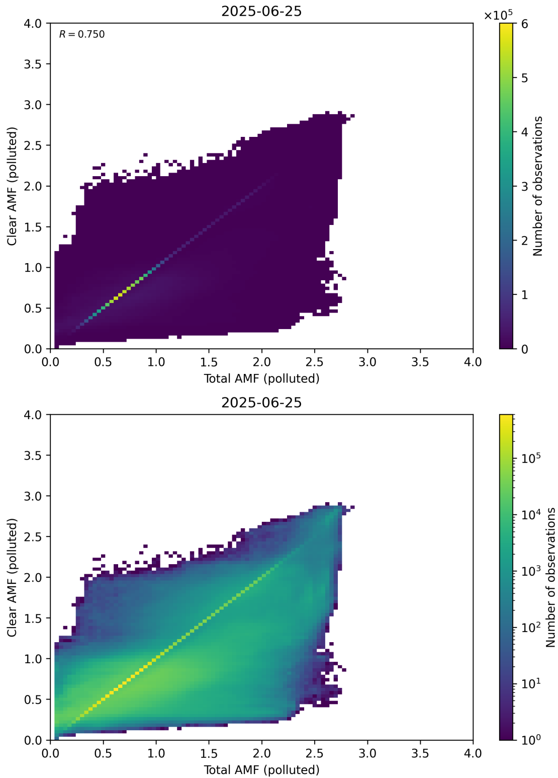
Figure 321: Scatter density plot of “Total AMF (polluted)” against “Clear AMF (polluted)” for 2025-06-24 to 2025-06-26.
