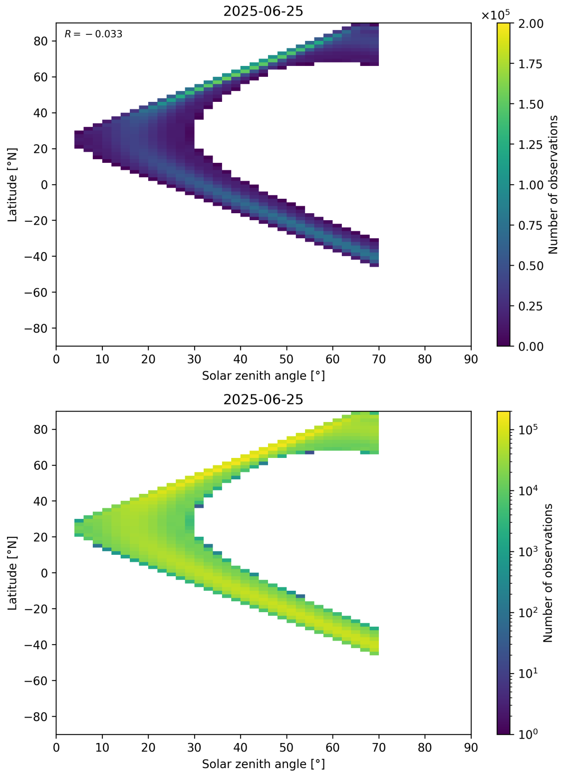
Figure 177: Scatter density plot of “Solar zenith angle” against “Latitude” for 2025-06-24 to 2025-06-26.
