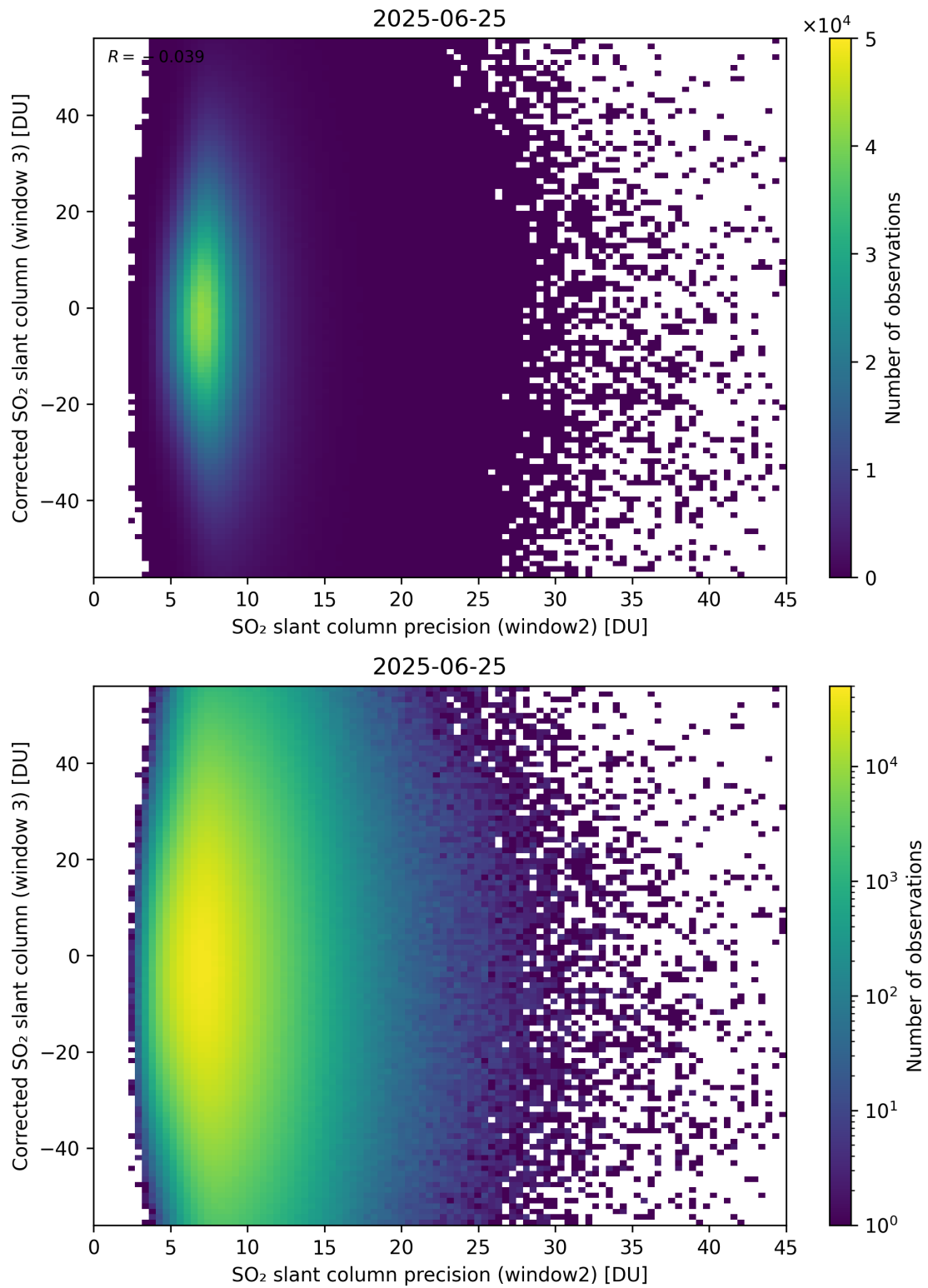
Figure 298: Scatter density plot of “SO 2 slant column precision (window2)” against “Corrected SO 2 slant column (window 3)” for 2025-06-24 to 2025-06-26.
