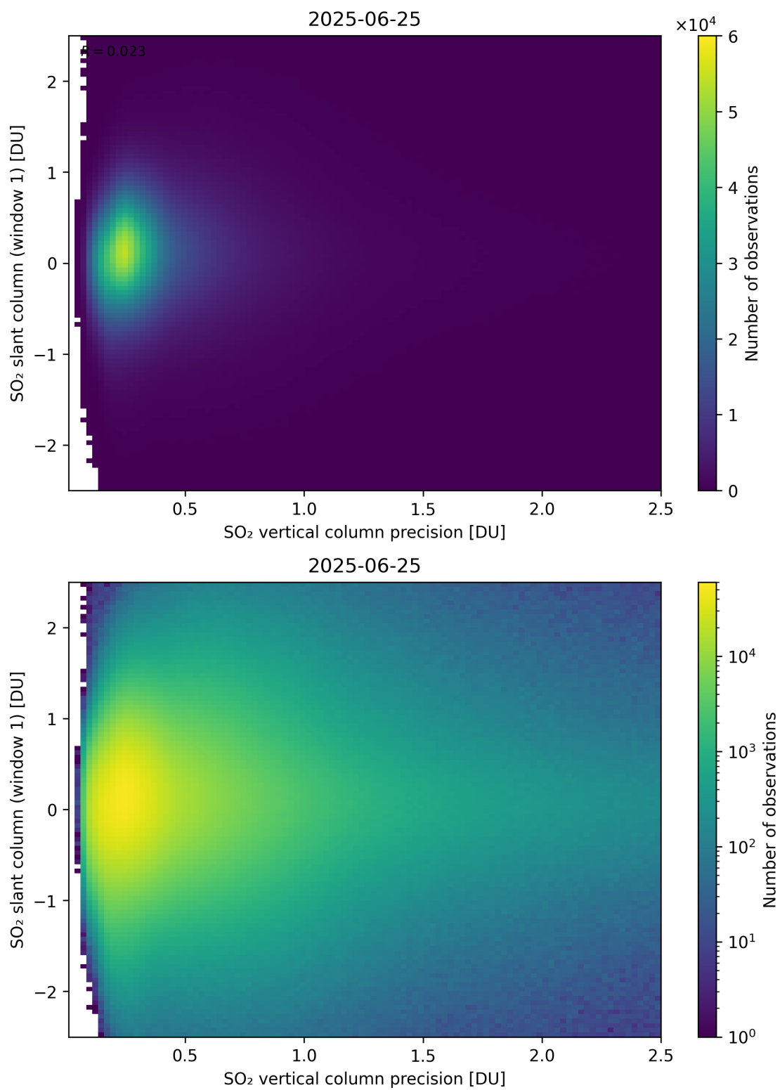
Figure 341: Scatter density plot of “SO 2 vertical column precision” against “SO 2 slant column (window 1)” for 2025-06-24 to 2025-06-26.
