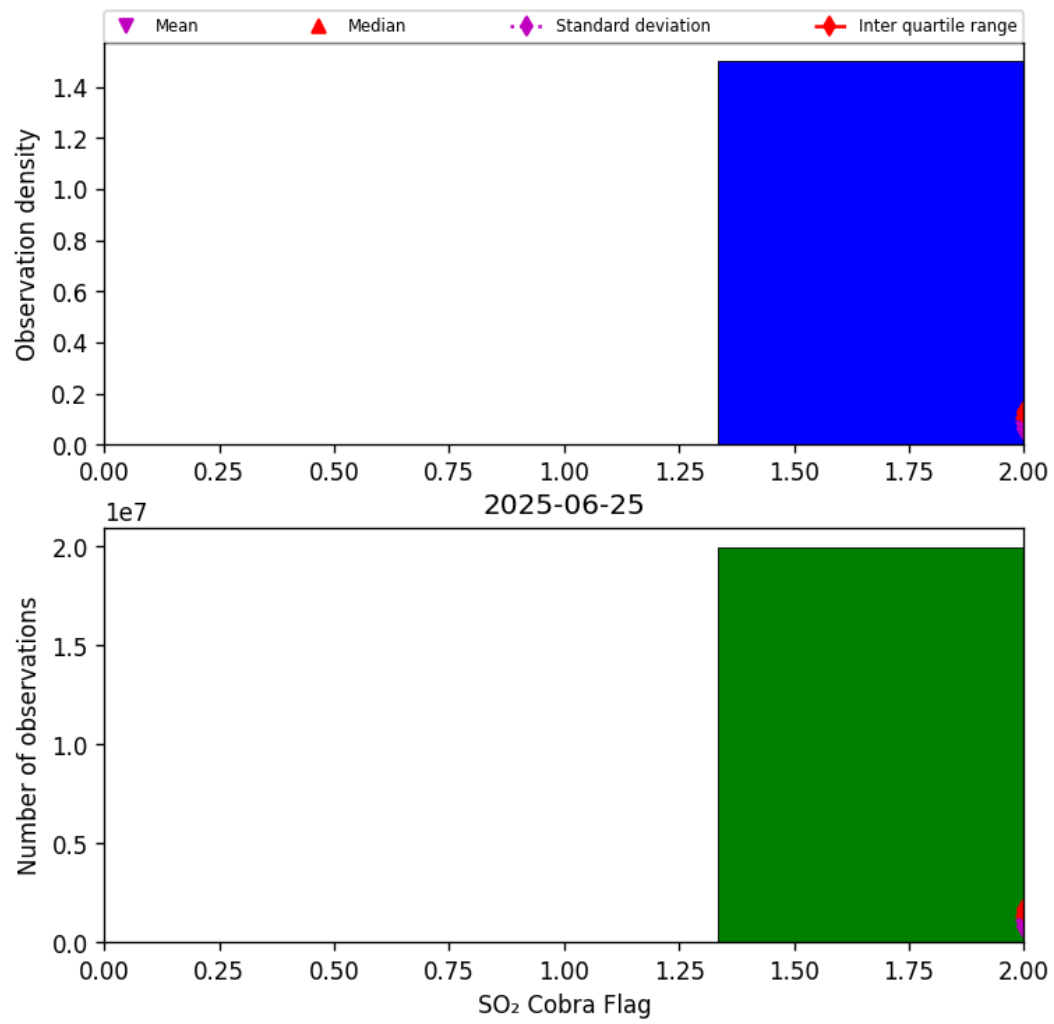
Figure 75: Histogram of “SO 2 Cobra Flag” for 2025-06-24 to 2025-06-26
