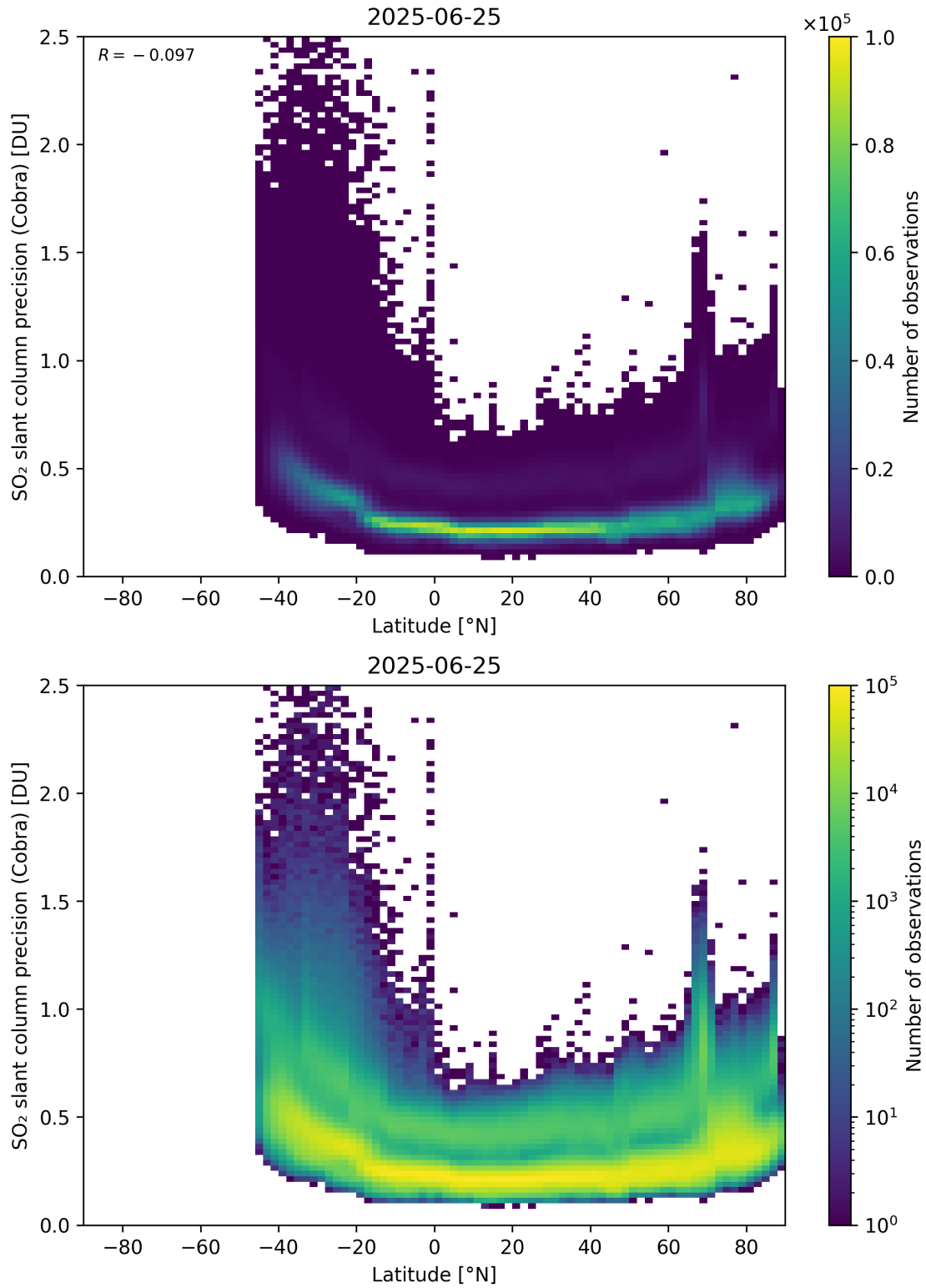
Figure 158: Scatter density plot of “Latitude” against “SO 2 slant column precision (Cobra)” for 2025-06-24 to 2025-06-26.
