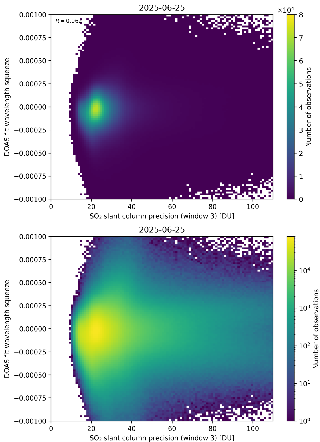
Figure 309: Scatter density plot of “SO 2 slant column precision (window 3)” against “DOAS fit wavelength squeeze” for 2025-06-24 to 2025-06-26.
