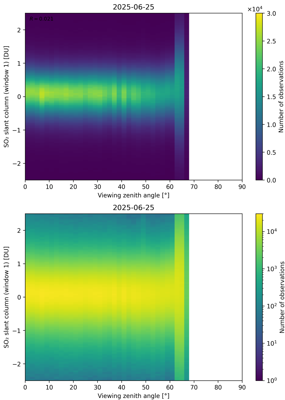
Figure 376: Scatter density plot of “Viewing zenith angle” against “SO 2 slant column (window 1)” for 2025-06-24 to 2025-06-26.
