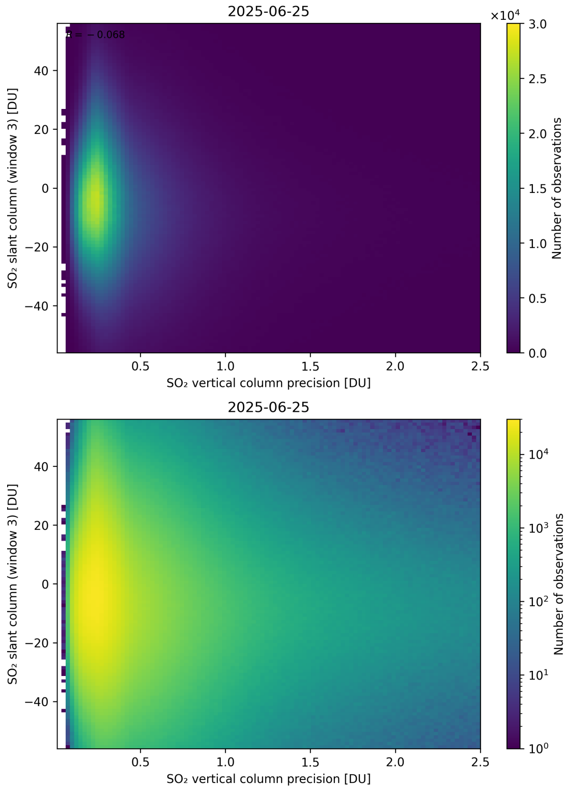
Figure 344: Scatter density plot of “SO 2 vertical column precision” against “SO 2 slant column (window 3)” for 2025-06-24 to 2025-06-26.
