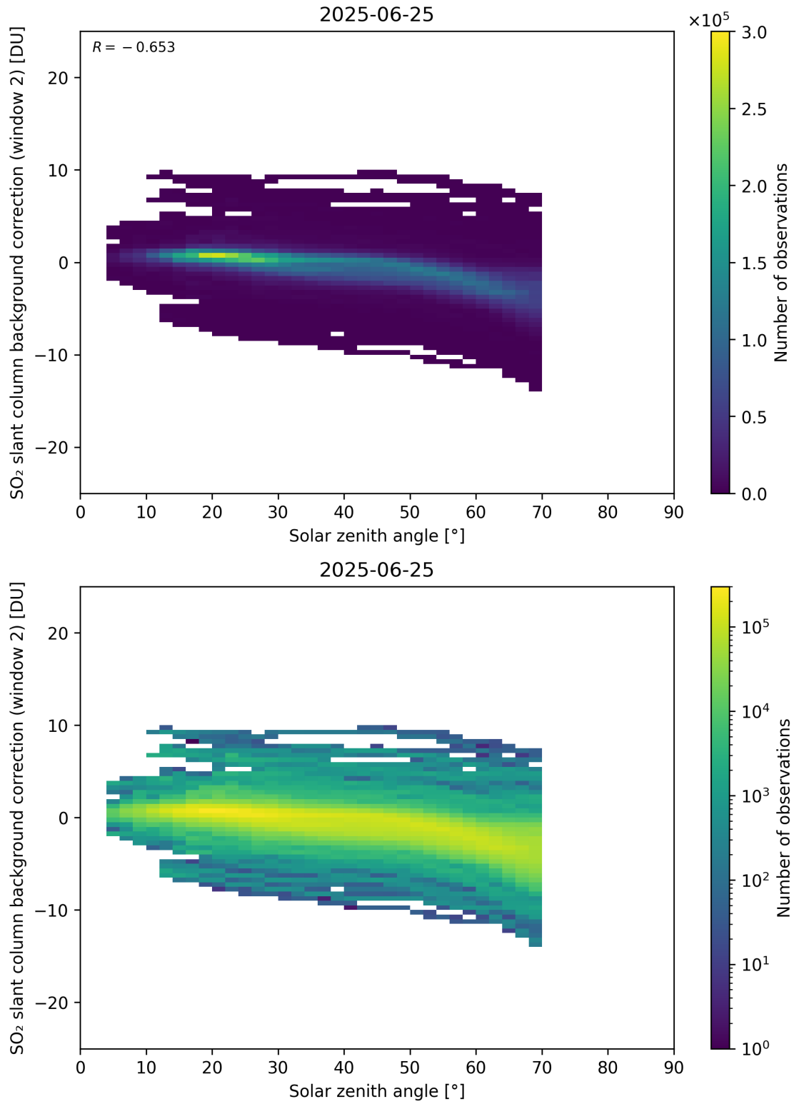
Figure 172: Scatter density plot of “Solar zenith angle” against “SO 2 slant column background correction (window 2)” for 2025-06-24 to 2025-06-26.
