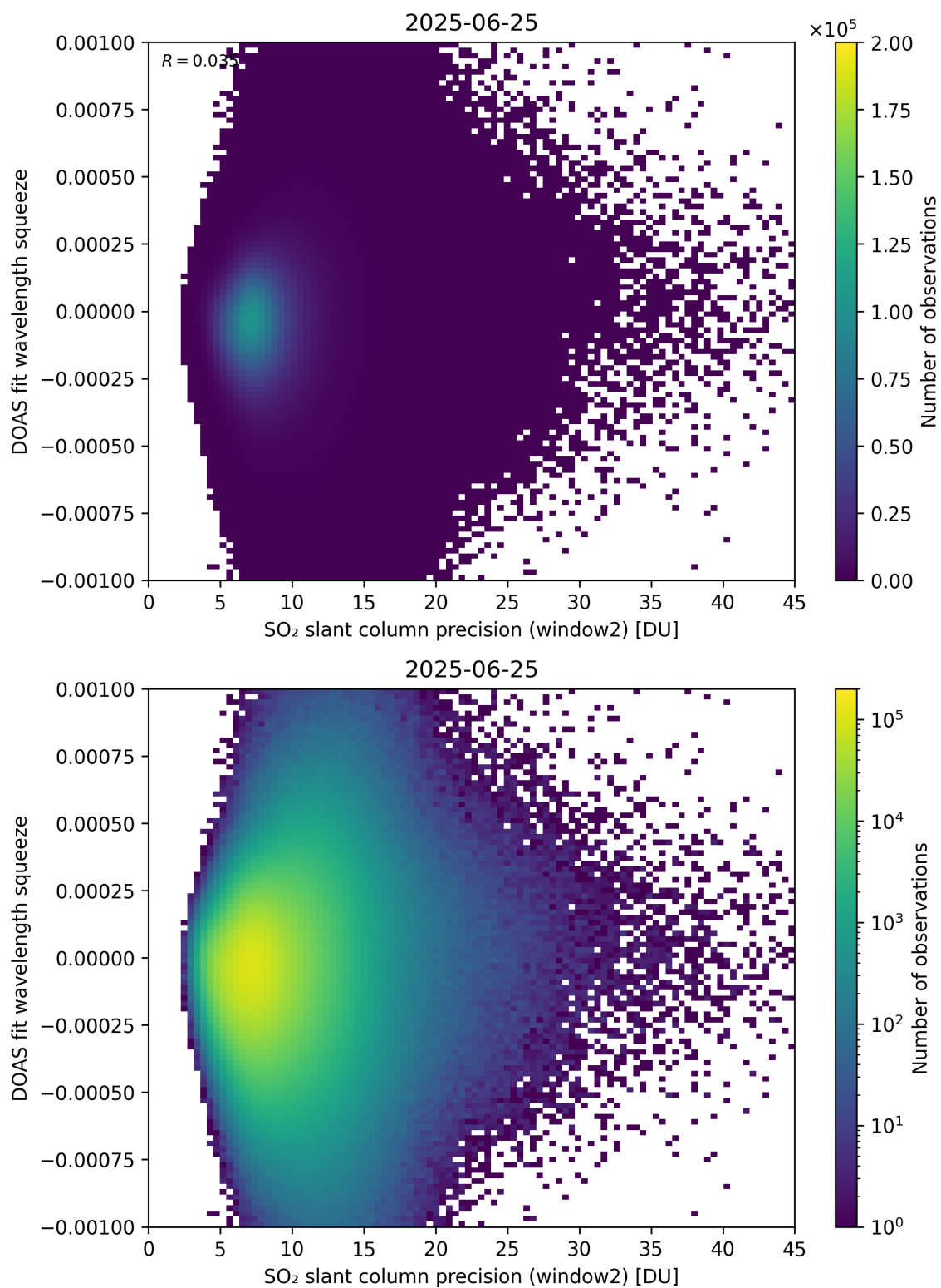
Figure 294: Scatter density plot of “SO 2 slant column precision (window2)” against “DOAS fit wavelength squeeze” for 2025-06-24 to 2025-06-26.
