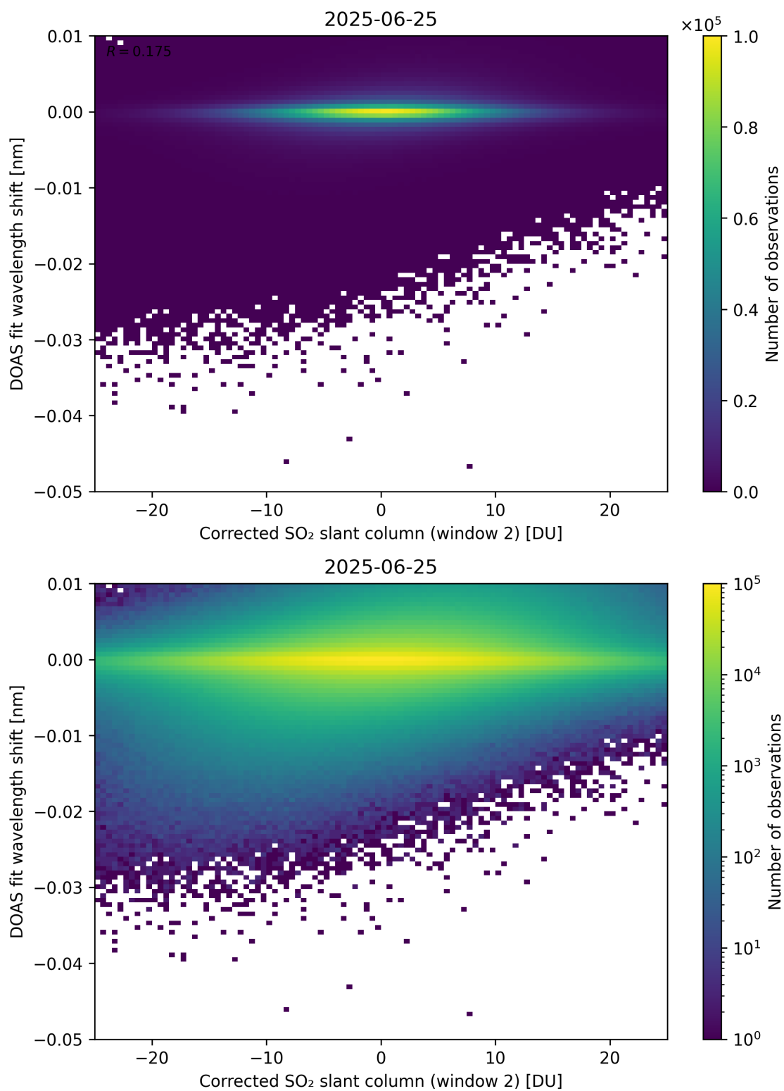
Figure 246: Scatter density plot of “Corrected SO 2 slant column (window 2)” against “DOAS fit wavelength shift” for 2025-06-24 to 2025-06-26.
