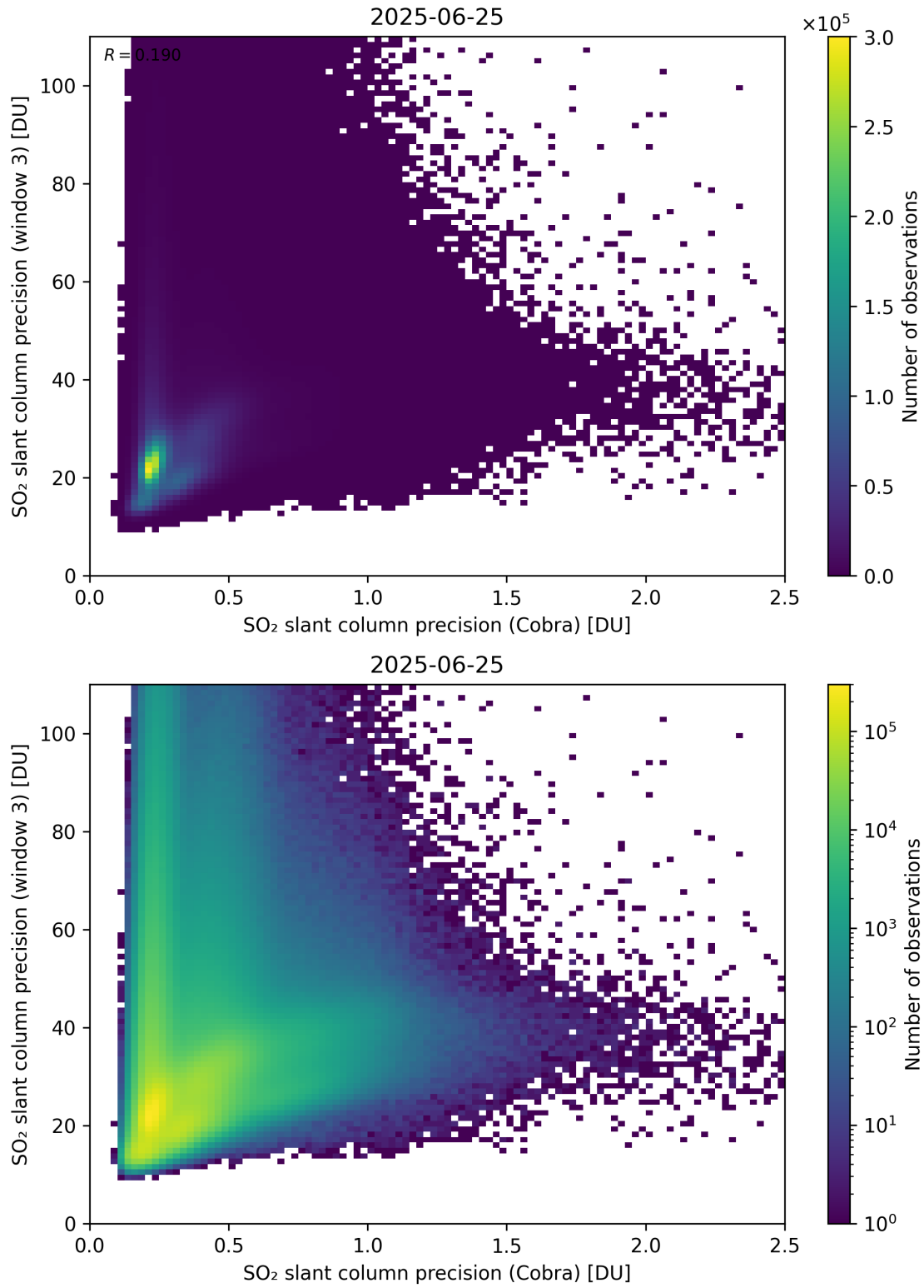
Figure 212: Scatter density plot of “SO 2 slant column precision (Cobra)” against “SO 2 slant column precision (window 3)” for 2025-06-24 to 2025-06-26.
