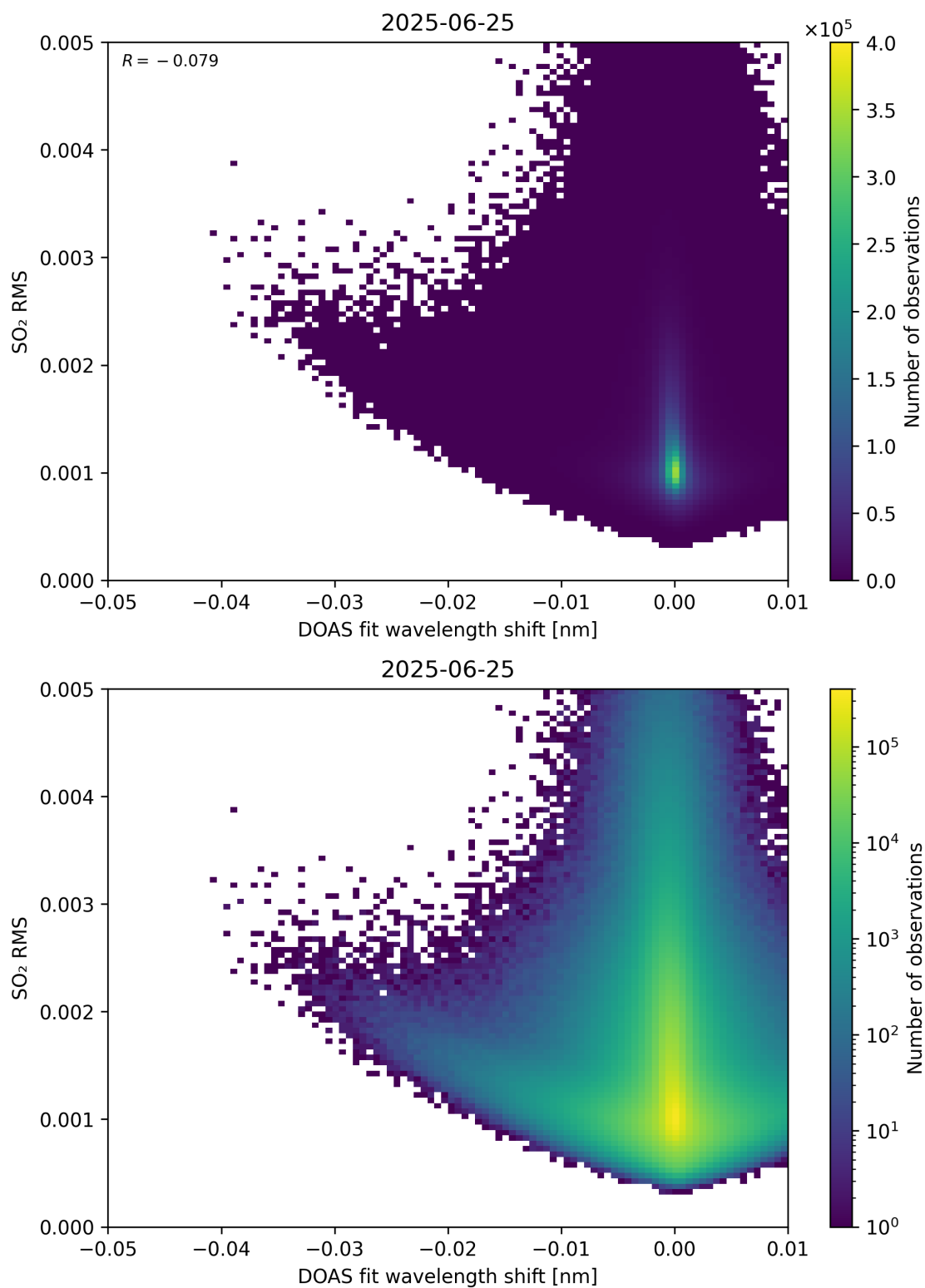
Figure 139: Scatter density plot of “DOAS fit wavelength shift” against “SO 2 RMS” for 2025-06-24 to 2025-06-26.
