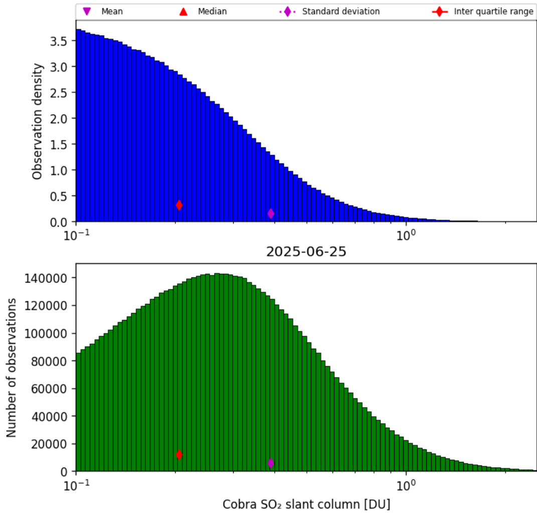
Figure 61: Histogram of “Cobra SO 2 slant column” for 2025-06-24 to 2025-06-26
