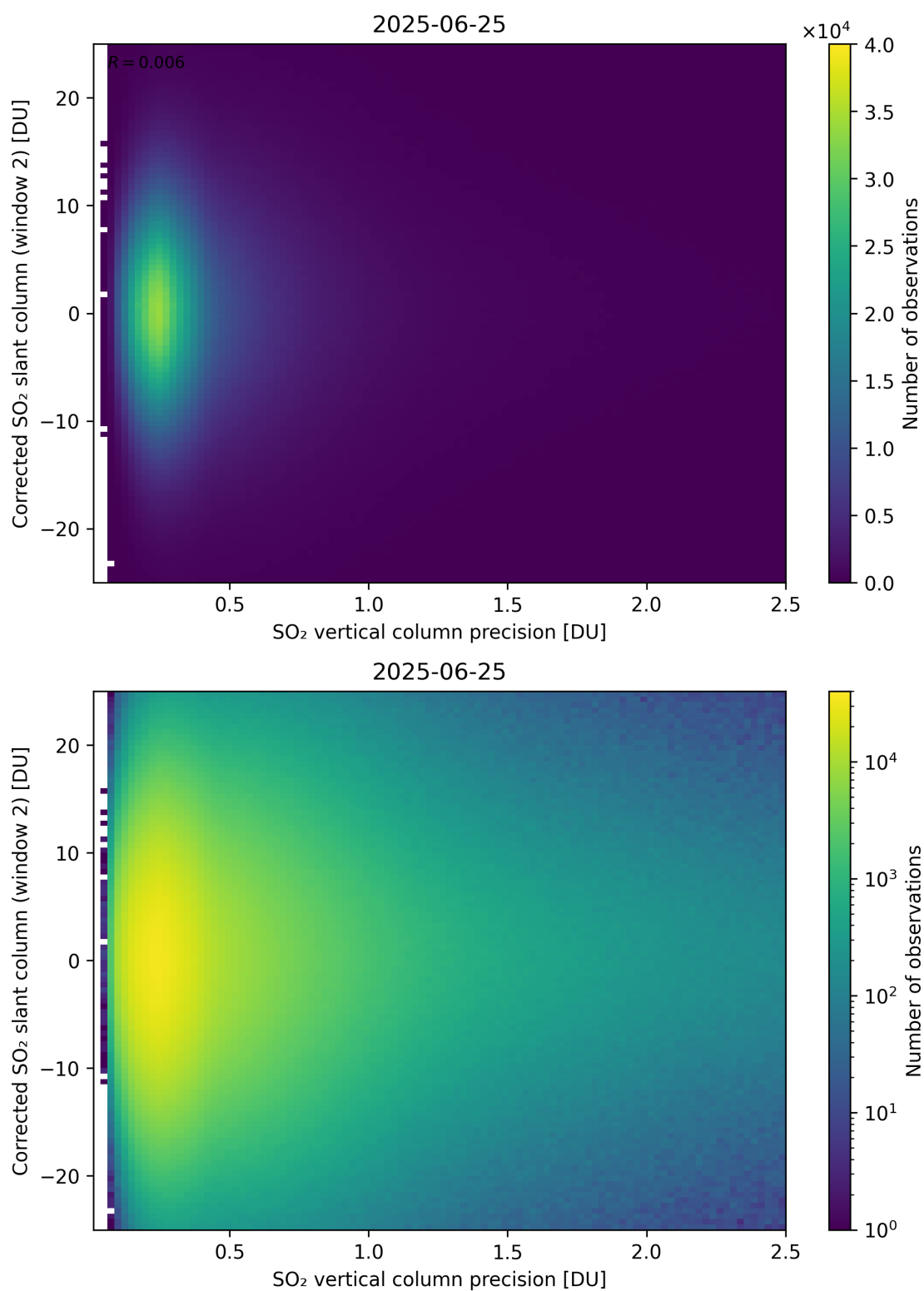
Figure 339: Scatter density plot of “SO 2 vertical column precision” against “Corrected SO 2 slant column (window 2)” for 2025-06-24 to 2025-06-26.
