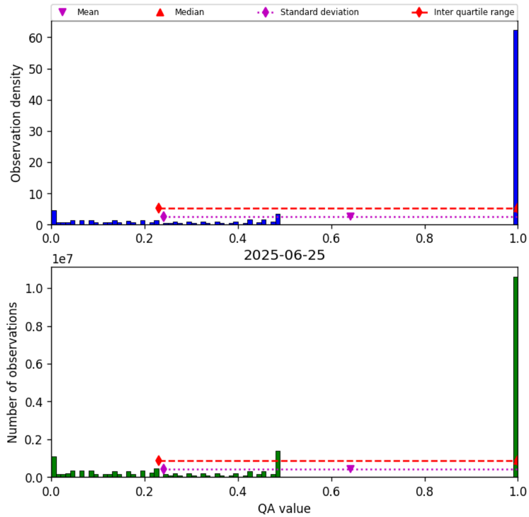
Figure 57: Histogram of “QA value” for 2025-06-24 to 2025-06-26
