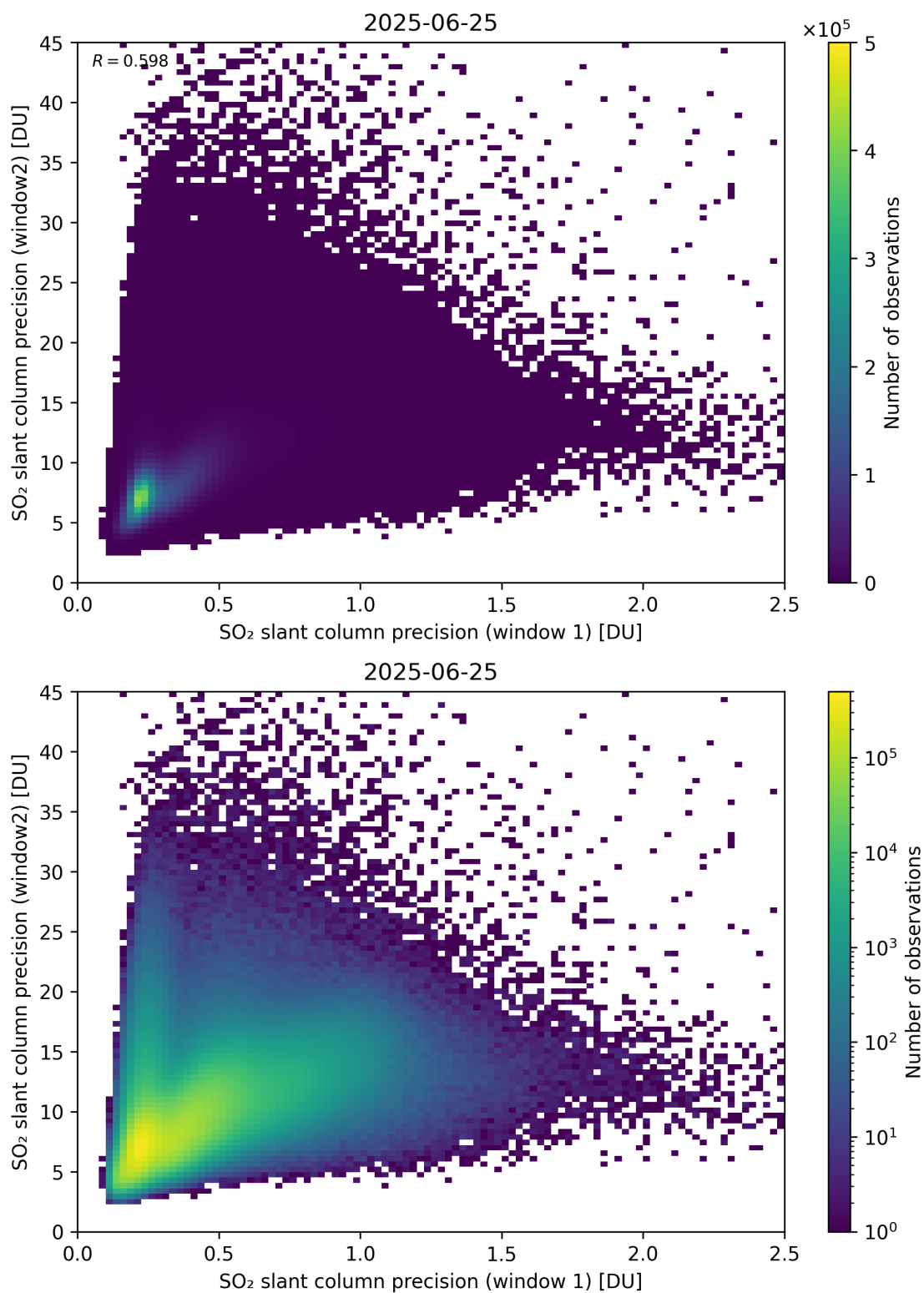
Figure 277: Scatter density plot of “SO 2 slant column precision (window 1)” against “SO 2 slant column precision (window2)” for 2025-06-24 to 2025-06-26.
