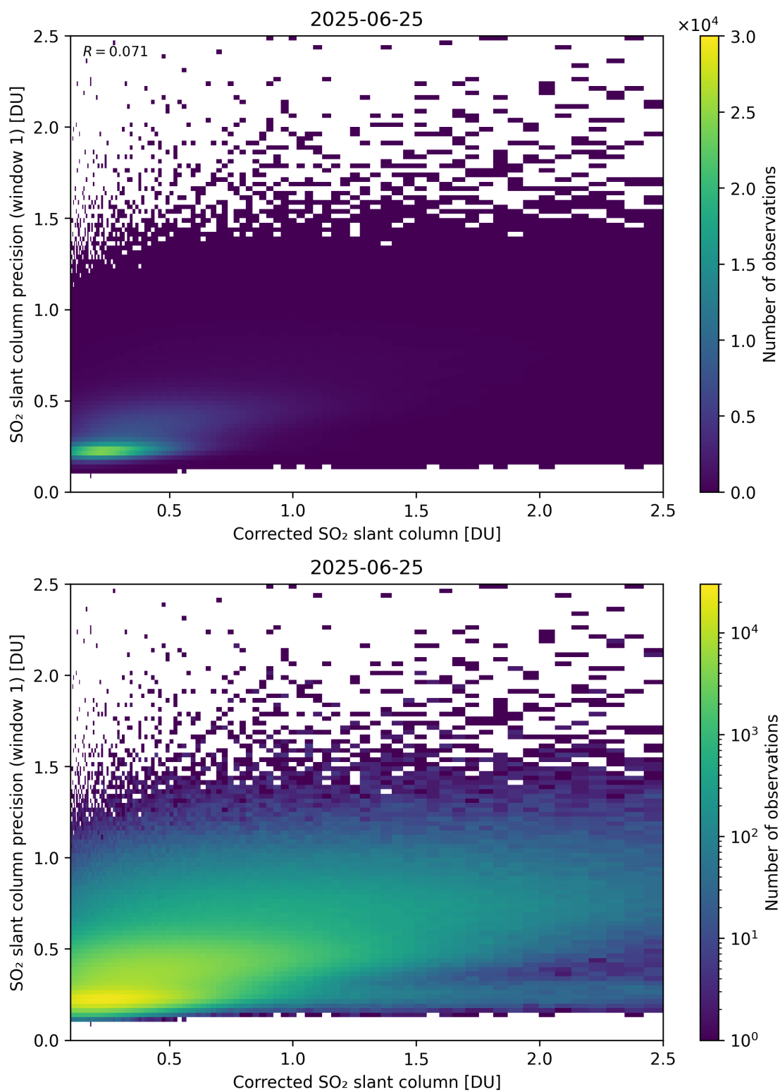
Figure 238: Scatter density plot of “Corrected SO 2 slant column” against “SO 2 slant column precision (window 1)” for 2025-06-24 to 2025-06-26.
