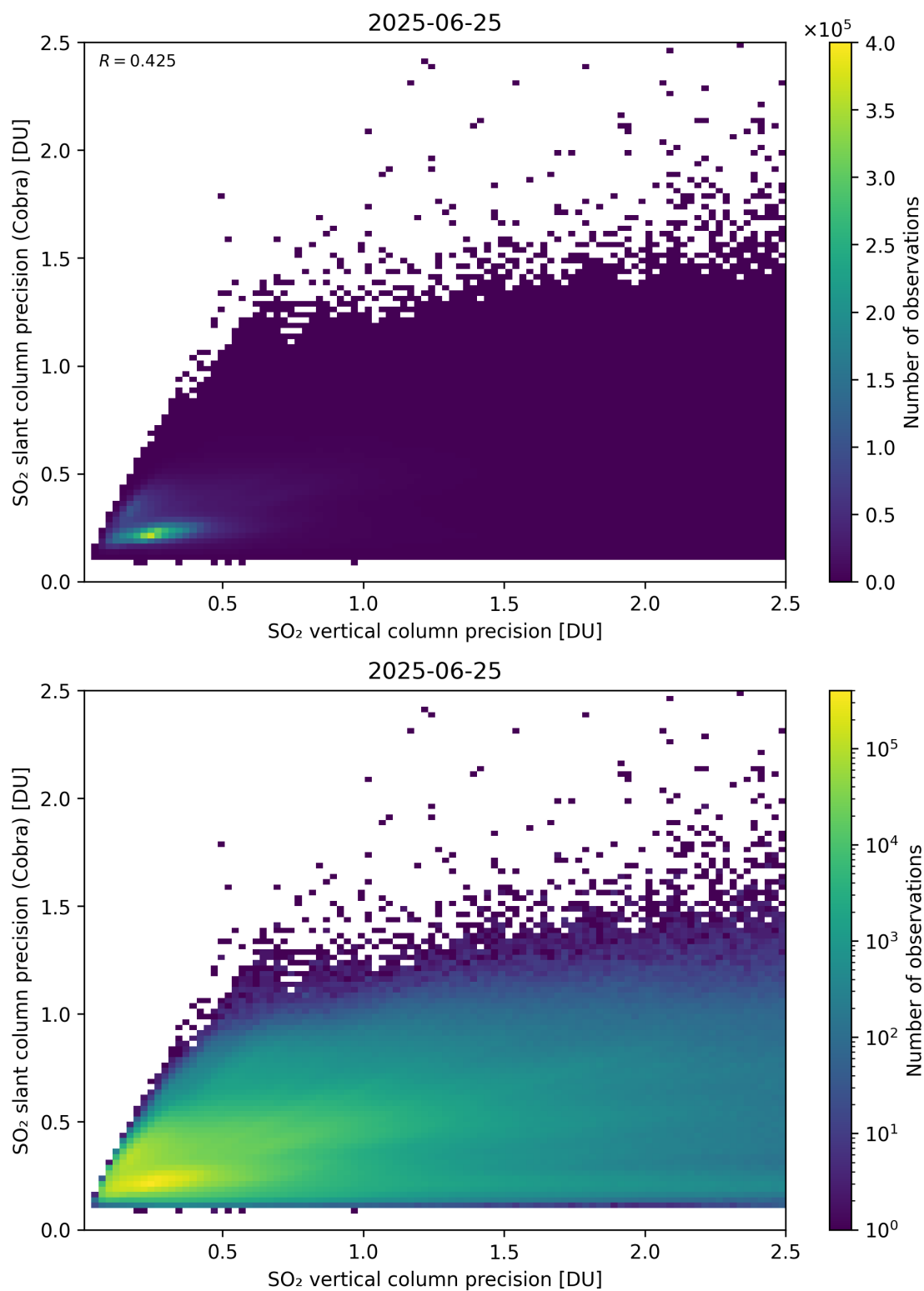
Figure 337: Scatter density plot of “SO 2 vertical column precision” against “SO 2 slant column precision (Cobra)” for 2025-06-24 to 2025-06-26.
