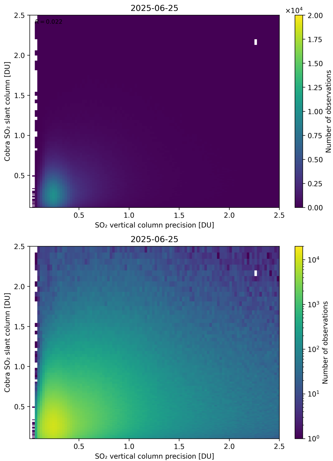
Figure 336: Scatter density plot of “SO 2 vertical column precision” against “Cobra SO 2 slant column” for 2025-06-24 to 2025-06-26.
