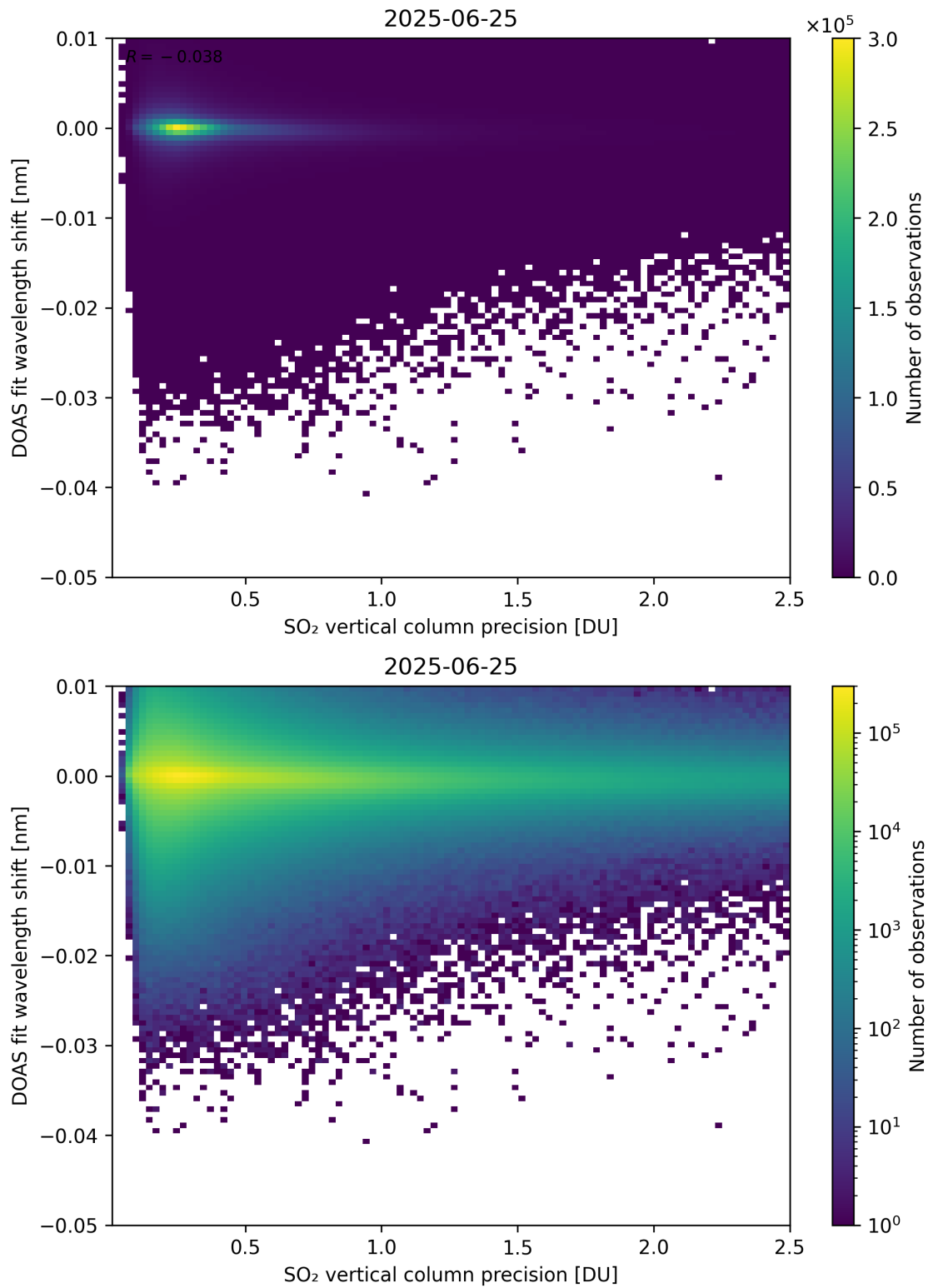
Figure 332: Scatter density plot of “SO 2 vertical column precision” against “DOAS fit wavelength shift” for 2025-06-24 to 2025-06-26.
