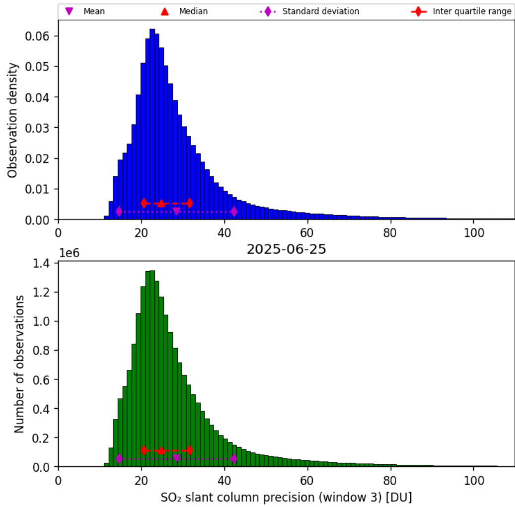
Figure 72: Histogram of “SO 2 slant column precision (window 3)” for 2025-06-24 to 2025-06-26
