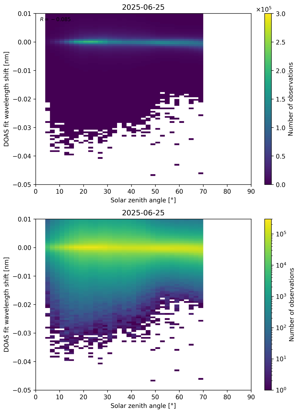
Figure 174: Scatter density plot of “Solar zenith angle” against “DOAS fit wavelength shift” for 2025-06-24 to 2025-06-26.
