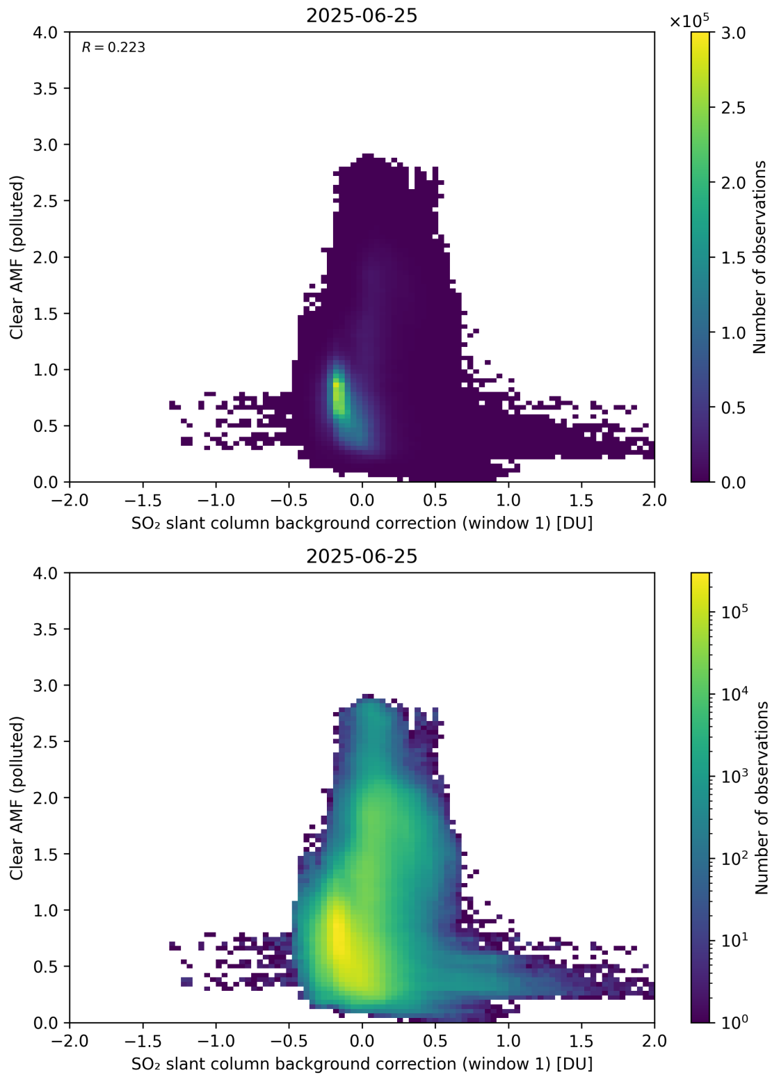
Figure 114: Scatter density plot of “SO 2 slant column background correction (window 1)” against “Clear AMF (polluted)” for 2025-06-24 to 2025-06-26.
