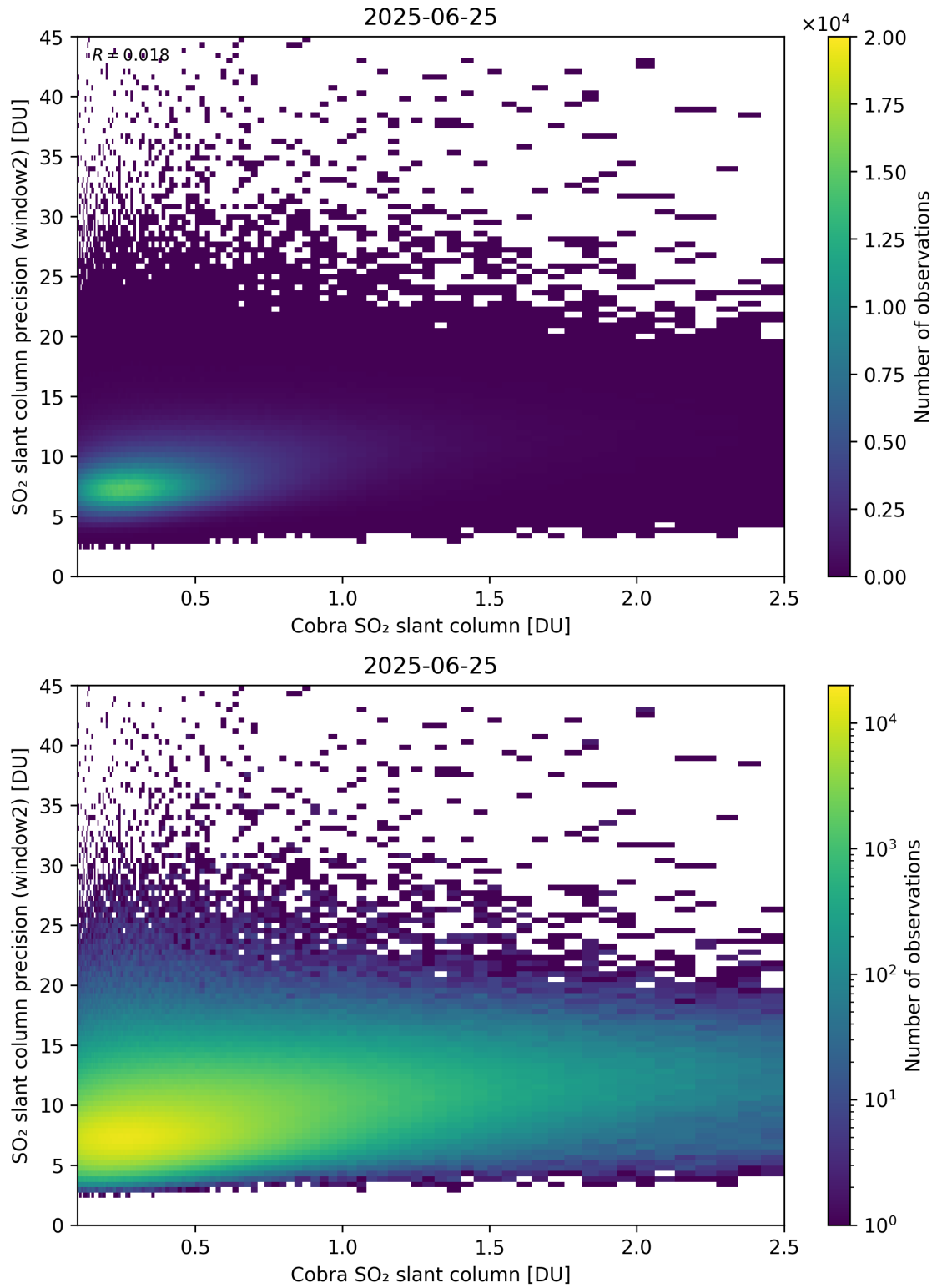
Figure 221: Scatter density plot of “Cobra SO 2 slant column” against “SO 2 slant column precision (window2)” for 2025-06-24 to 2025-06-26.
