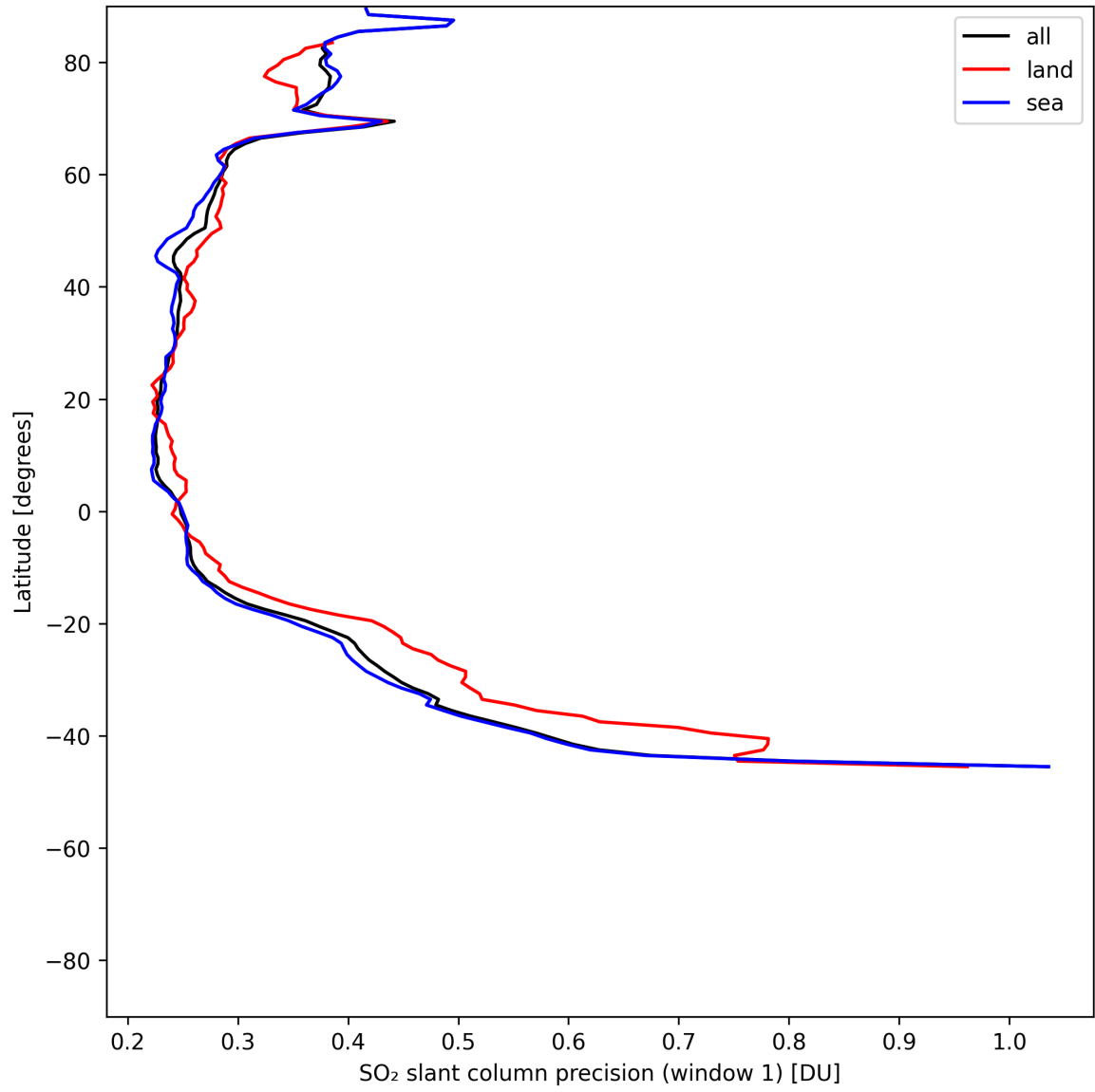
Figure 38: Zonal average of “SO 2 slant column precision (window 1)” for 2025-06-24 to 2025-06-26.
