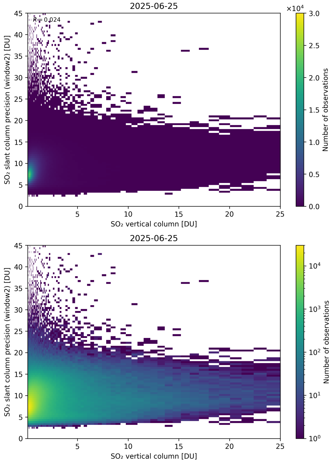
Figure 356: Scatter density plot of “SO 2 vertical column” against “SO 2 slant column precision (window2)” for 2025-06-24 to 2025-06-26.
