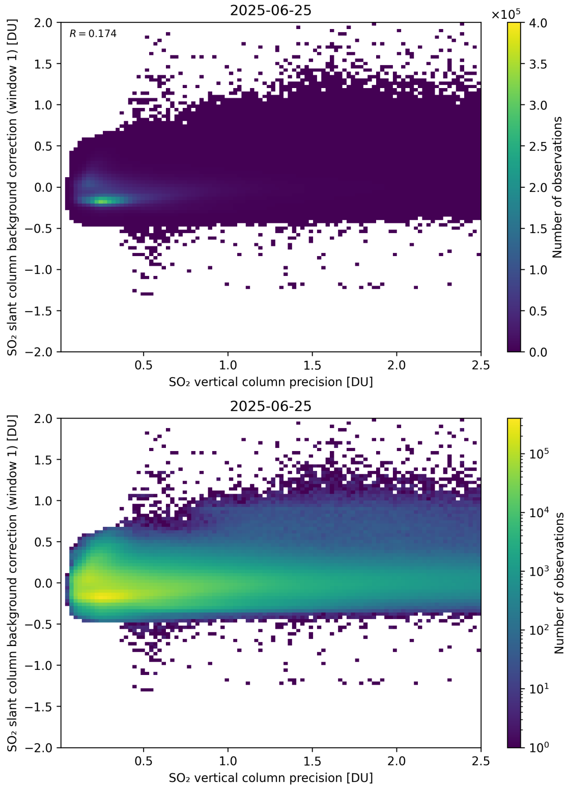
Figure 329: Scatter density plot of “SO 2 vertical column precision” against “SO 2 slant column background correction (window 1)” for 2025-06-24 to 2025-06-26.
