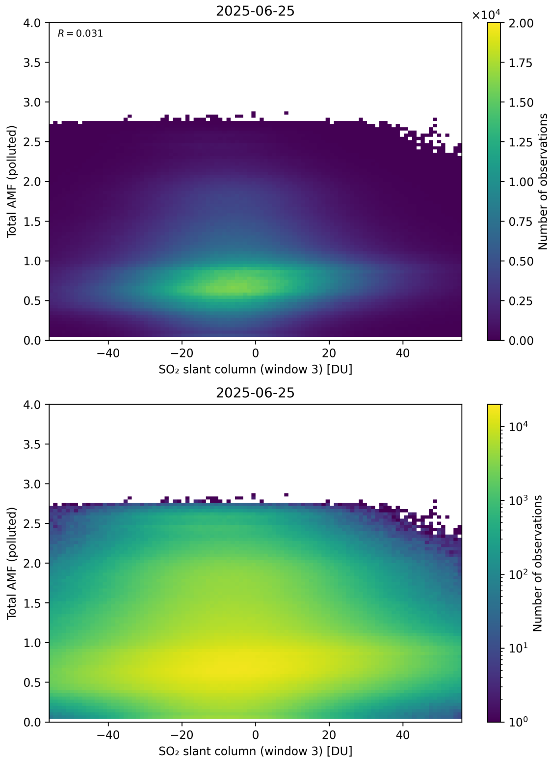
Figure 318: Scatter density plot of “SO 2 slant column (window 3)” against “Total AMF (polluted)” for 2025-06-24 to 2025-06-26.
