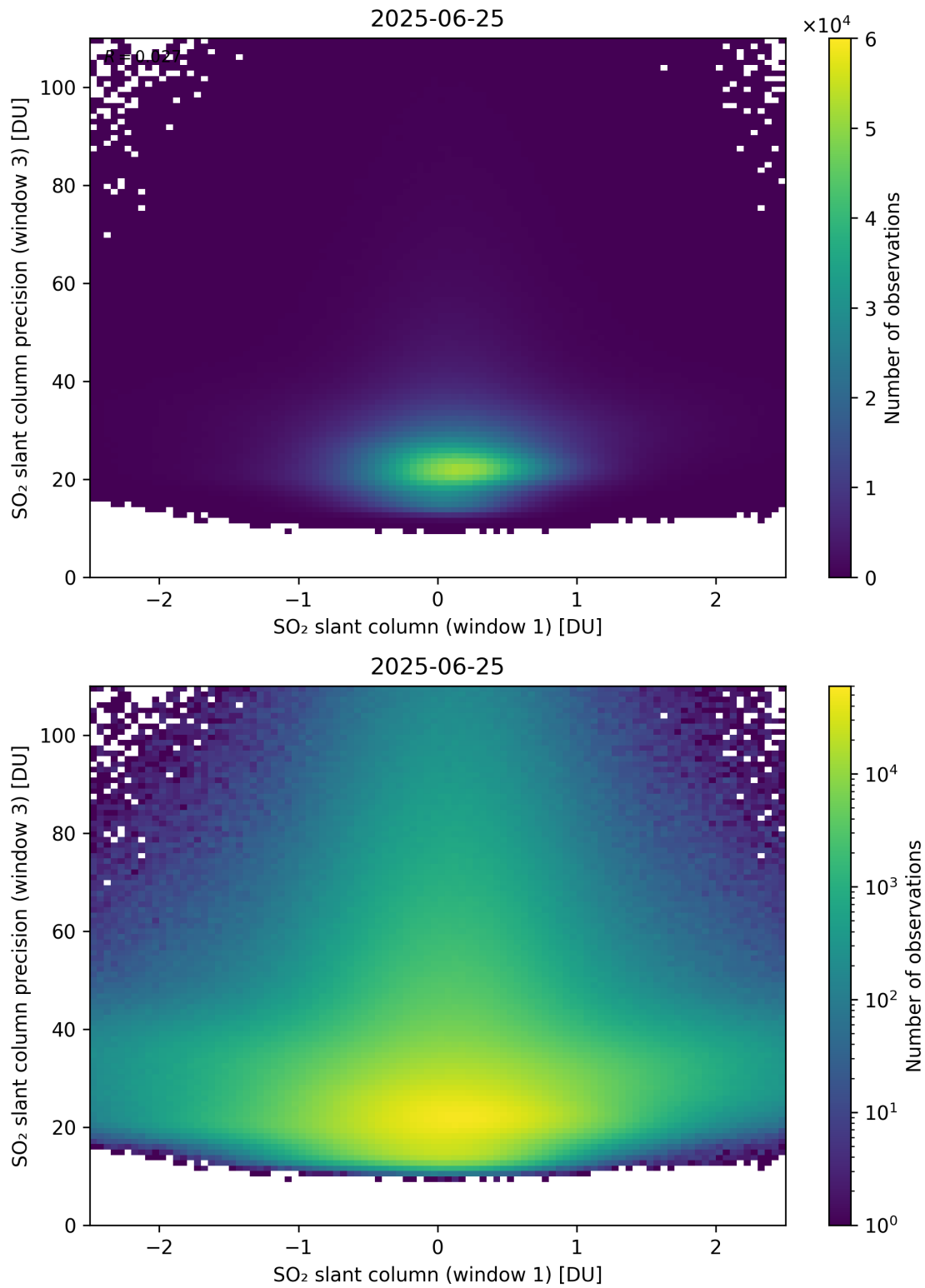
Figure 288: Scatter density plot of “SO 2 slant column (window 1)” against “SO 2 slant column precision (window 3)” for 2025-06-24 to 2025-06-26.
