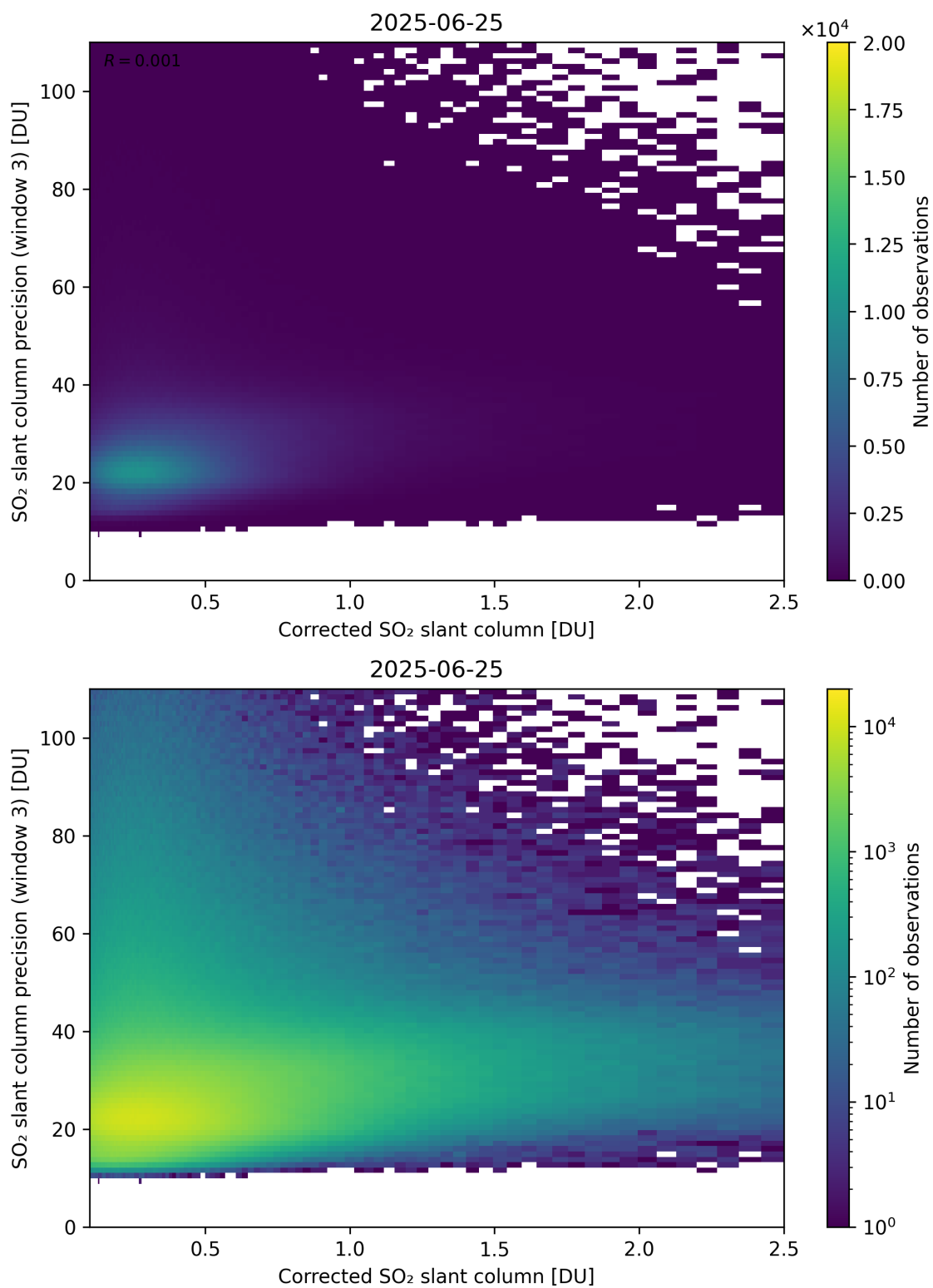
Figure 241: Scatter density plot of “Corrected SO 2 slant column” against “SO 2 slant column precision (window 3)” for 2025-06-24 to 2025-06-26.
