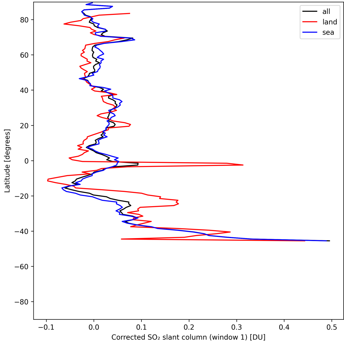
Figure 39: Zonal average of “Corrected SO 2 slant column (window 1)” for 2025-06-24 to 2025-06-26.
