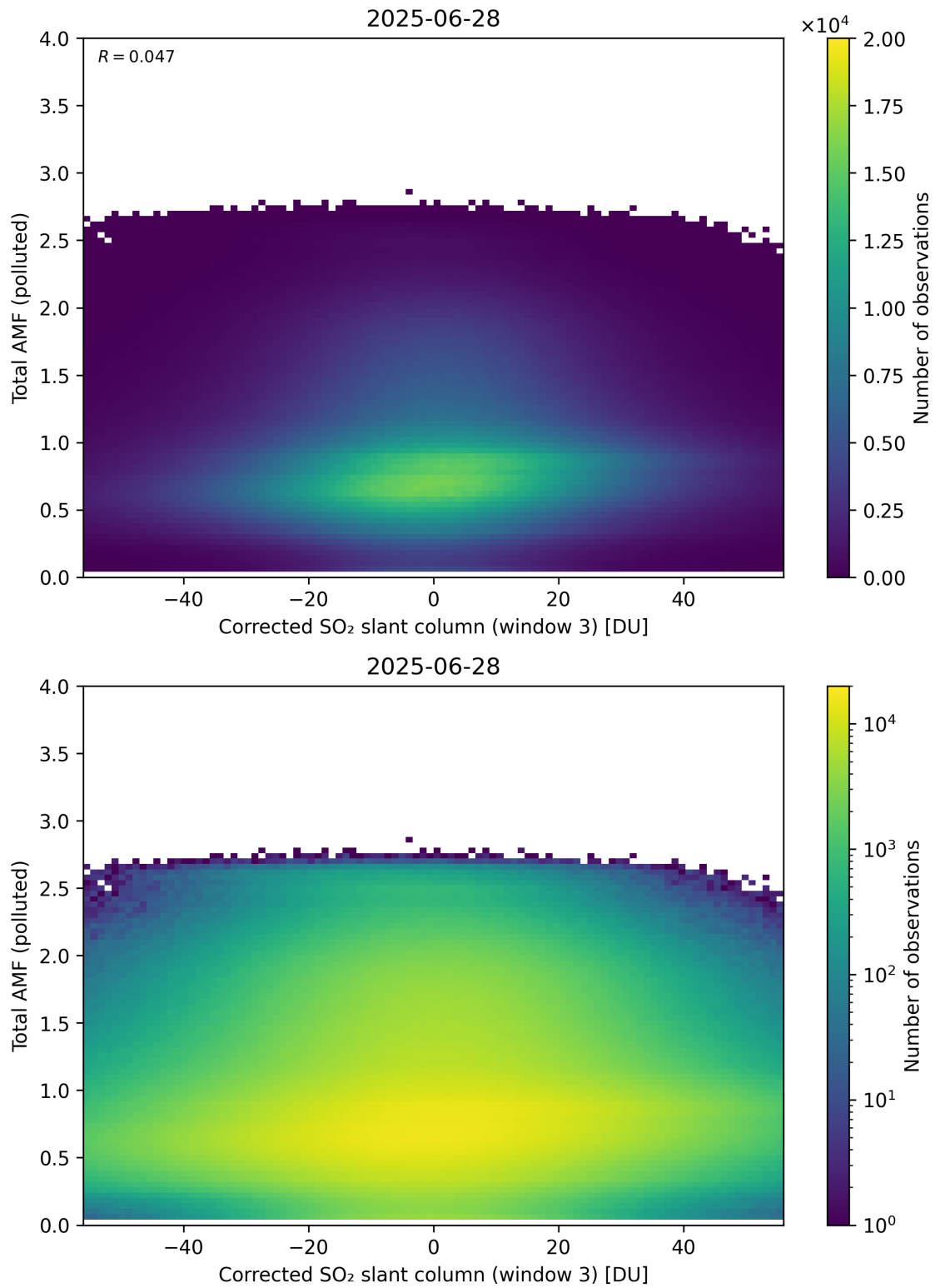
Figure 260: Scatter density plot of “Corrected SO 2 slant column (window 3)” against “Total AMF (polluted)” for 2025-06-27 to 2025-06-29.
