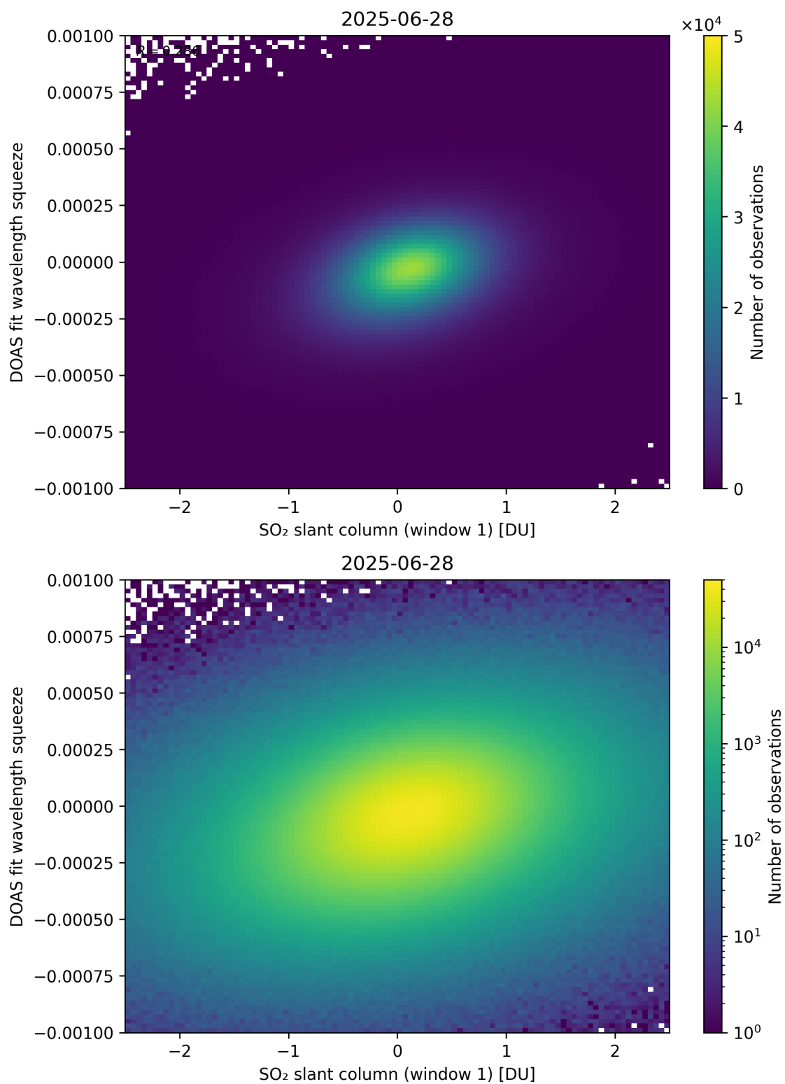
Figure 266: Scatter density plot of “SO 2 slant column (window 1)” against “DOAS fit wavelength squeeze” for 2025-06-27 to 2025-06-29.
