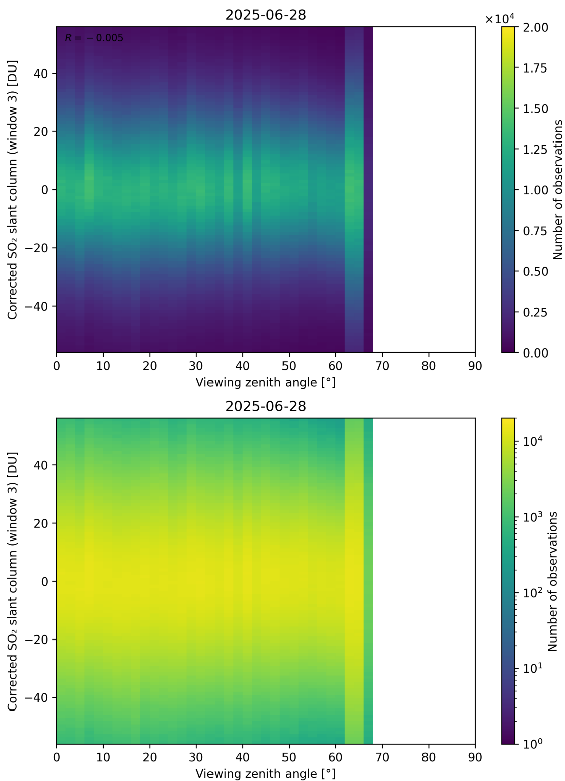
Figure 375: Scatter density plot of “Viewing zenith angle” against “Corrected SO 2 slant column (window 3)” for 2025-06-27 to 2025-06-29.
