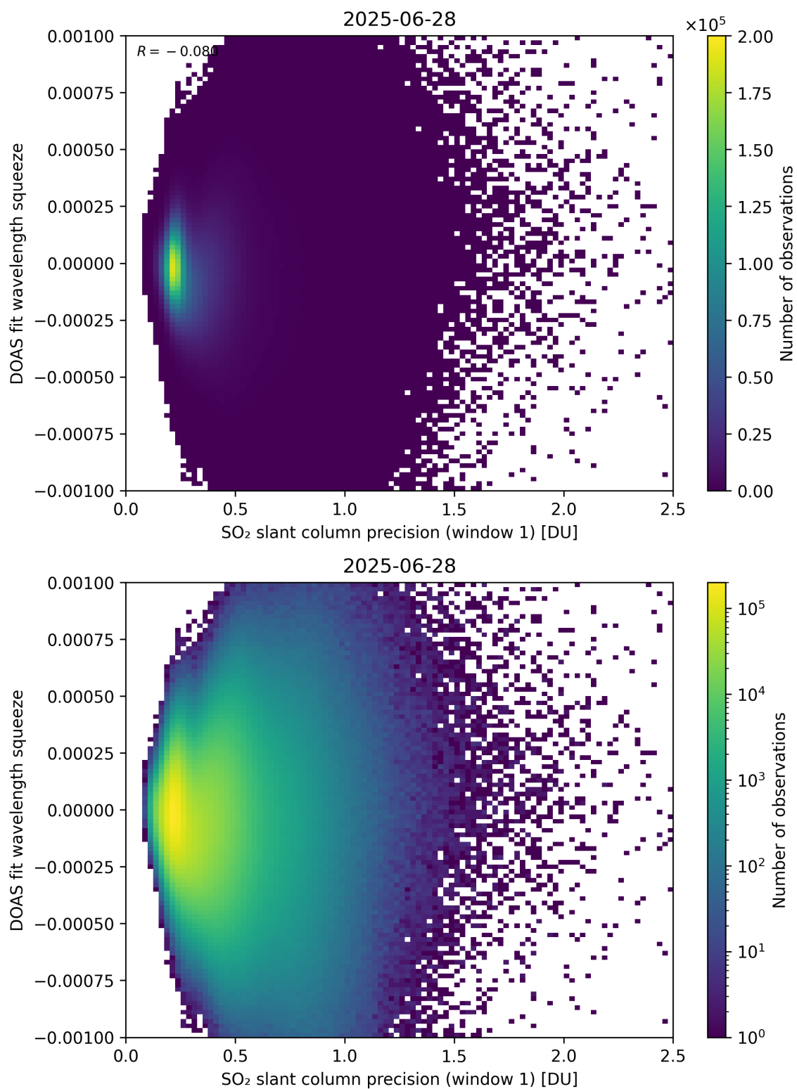
Figure 272: Scatter density plot of “SO 2 slant column precision (window 1)” against “DOAS fit wavelength squeeze” for 2025-06-27 to 2025-06-29.
