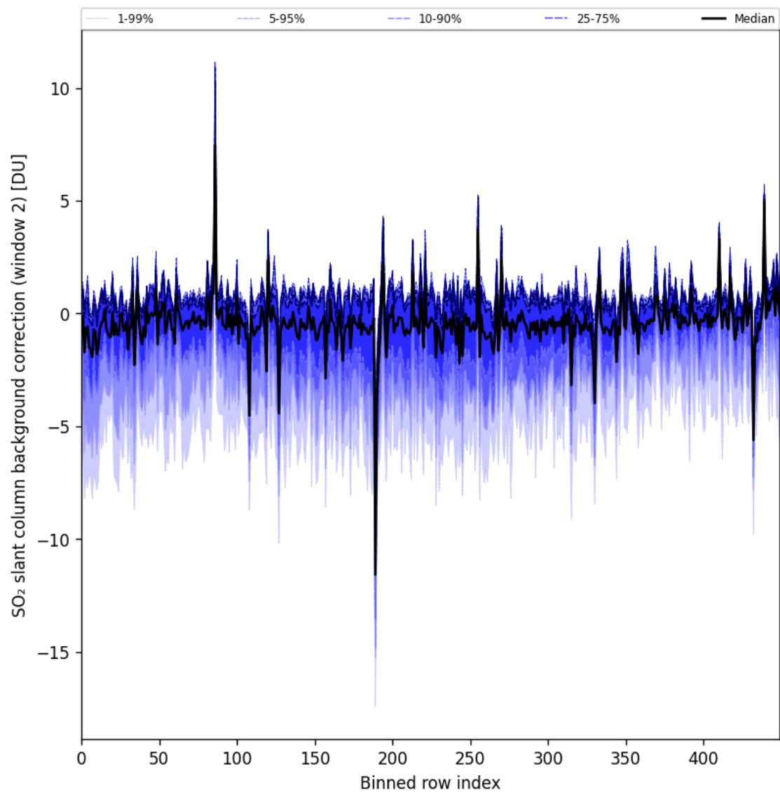
Figure 96: Along track statistics of “SO 2 slant column background correction (window 2)” for 2025-06-27 to 2025-06-29
