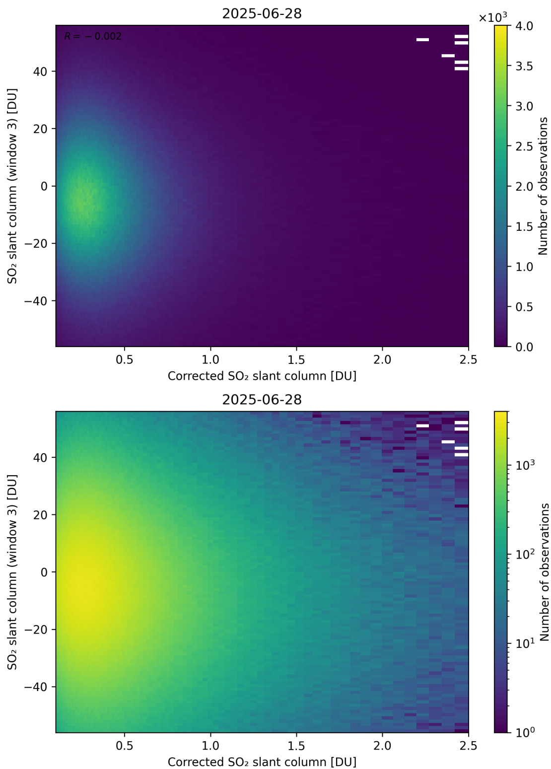
Figure 240: Scatter density plot of “Corrected SO 2 slant column” against “SO 2 slant column (window 3)” for 2025-06-27 to 2025-06-29.
