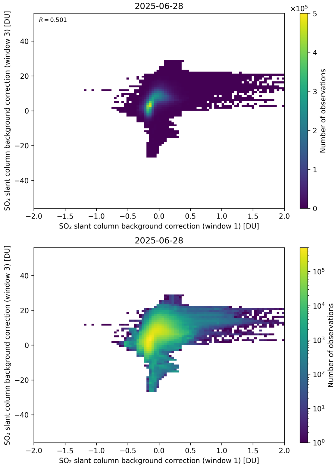
Figure 110: Scatter density plot of “SO 2 slant column background correction (window 1)” against “SO 2 slant column background correction (window 3)” for 2025-06-27 to 2025-06-29.
