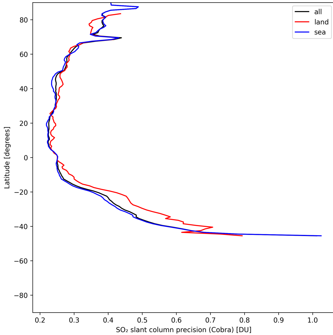
Figure 36: Zonal average of “SO 2 slant column precision (Cobra)” for 2025-06-27 to 2025-06-29.
