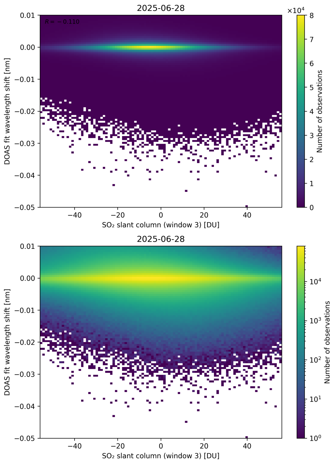
Figure 304: Scatter density plot of “SO 2 slant column (window 3)” against “DOAS fit wavelength shift” for 2025-06-27 to 2025-06-29.
