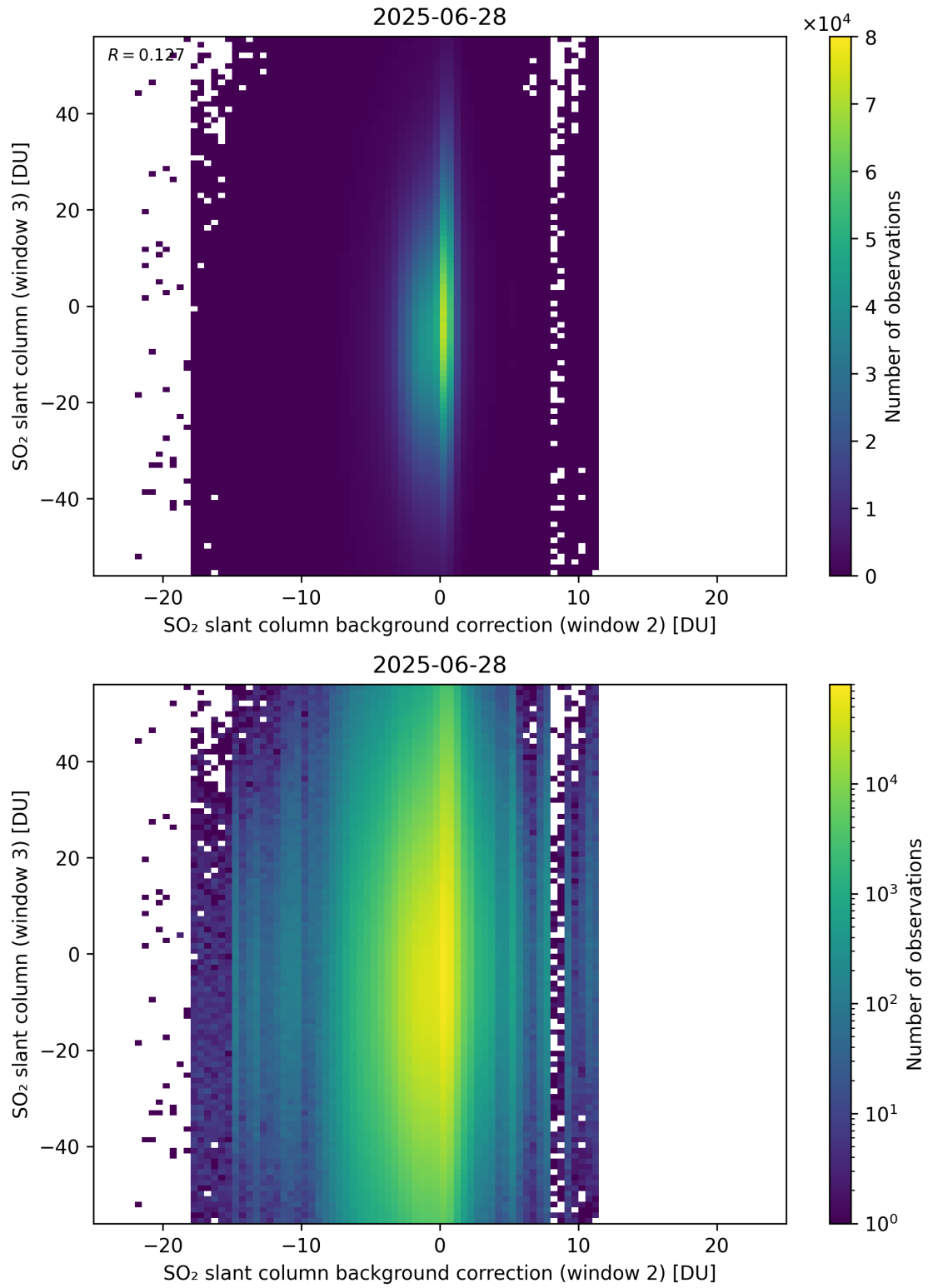
Figure 128: Scatter density plot of “SO 2 slant column background correction (window 2)” against “SO 2 slant column (window 3)” for 2025-06-27 to 2025-06-29.
