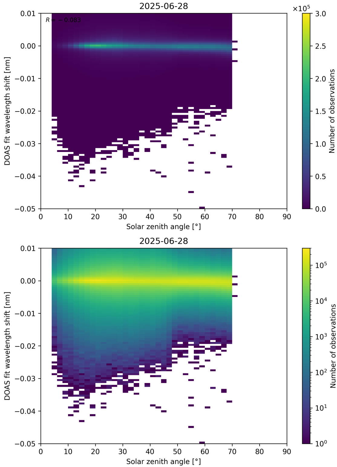
Figure 174: Scatter density plot of “Solar zenith angle” against “DOAS fit wavelength shift” for 2025-06-27 to 2025-06-29.
