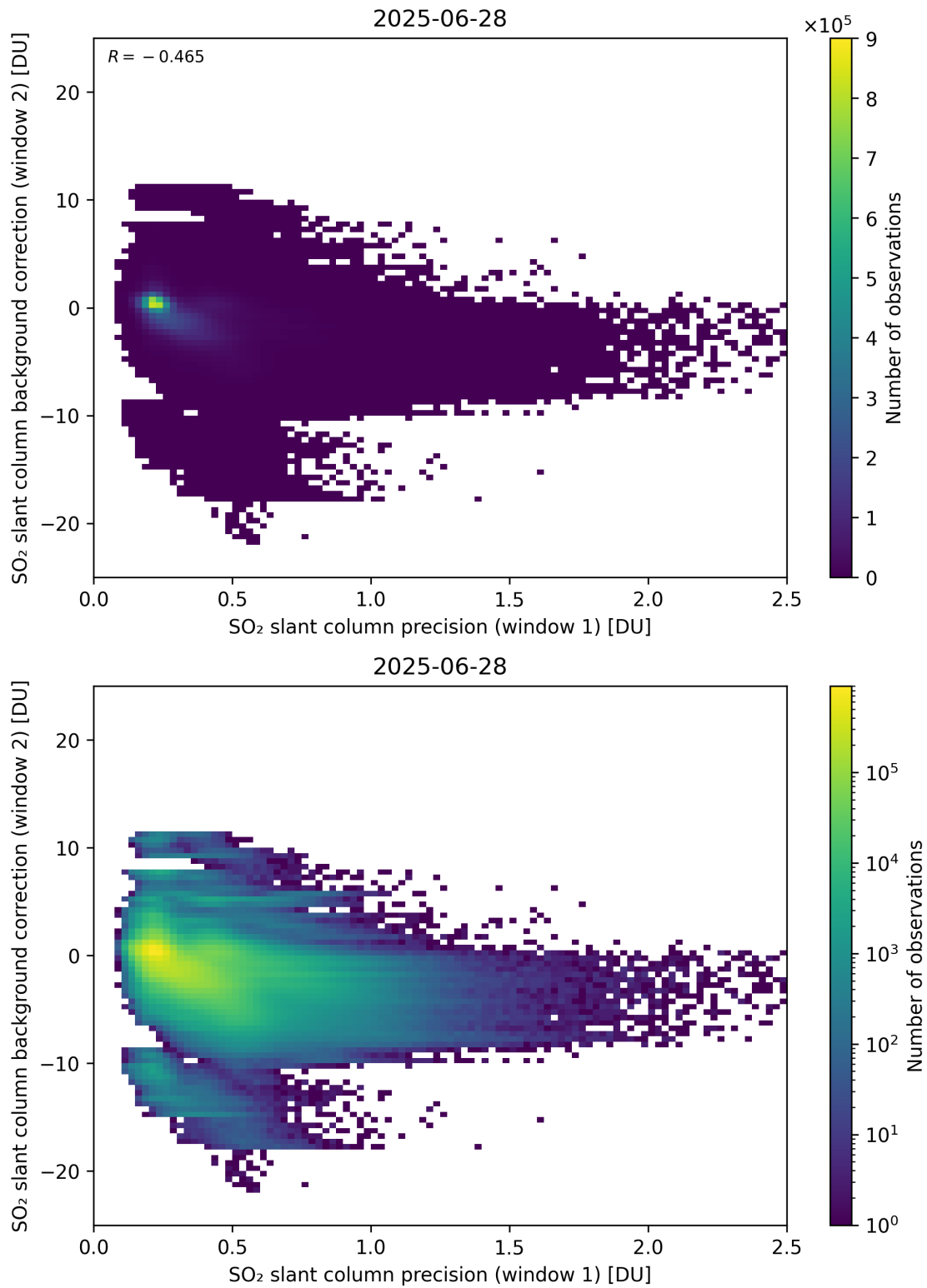
Figure 269: Scatter density plot of “SO 2 slant column precision (window 1)” against “SO 2 slant column background correction (window 2)” for 2025-06-27 to 2025-06-29.
