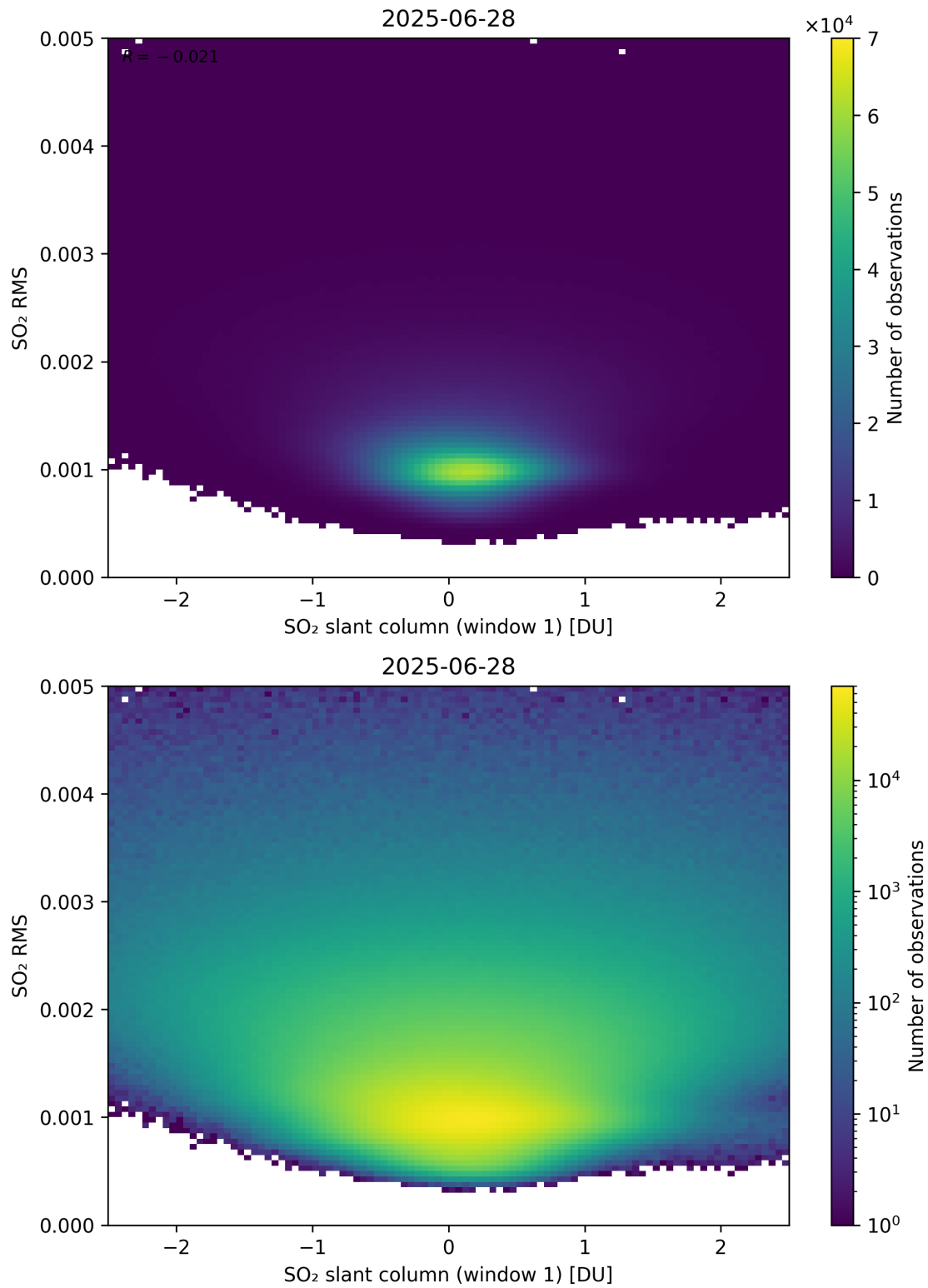
Figure 267: Scatter density plot of “SO 2 slant column (window 1)” against “SO 2 RMS” for 2025-06-27 to 2025-06-29.
