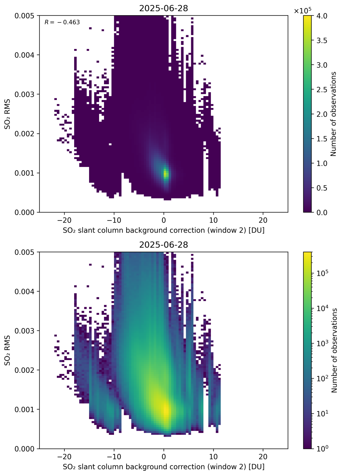
Figure 125: Scatter density plot of “SO 2 slant column background correction (window 2)” against “SO 2 RMS” for 2025-06-27 to 2025-06-29.
