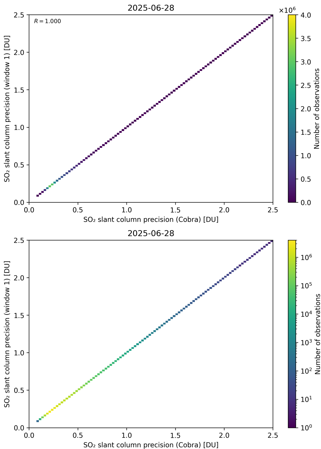
Figure 209: Scatter density plot of “SO 2 slant column precision (Cobra)” against “SO 2 slant column precision (window 1)” for 2025-06-27 to 2025-06-29.
