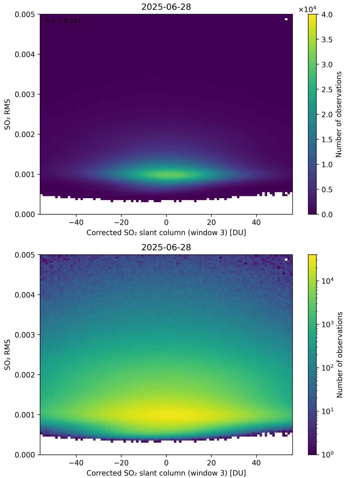
Figure 258: Scatter density plot of “Corrected SO 2 slant column (window 3)” against “SO 2 RMS” for 2025-06-27 to 2025-06-29.
