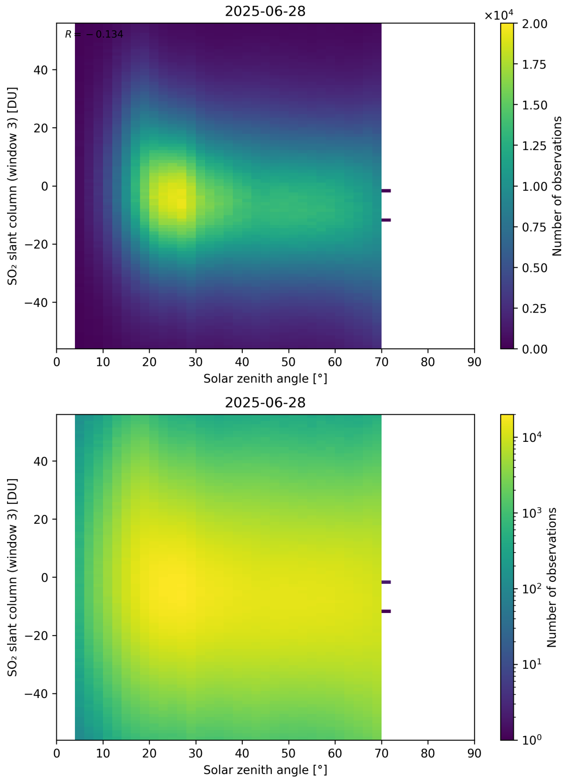
Figure 187: Scatter density plot of “Solar zenith angle” against “SO 2 slant column (window 3)” for 2025-06-27 to 2025-06-29.
