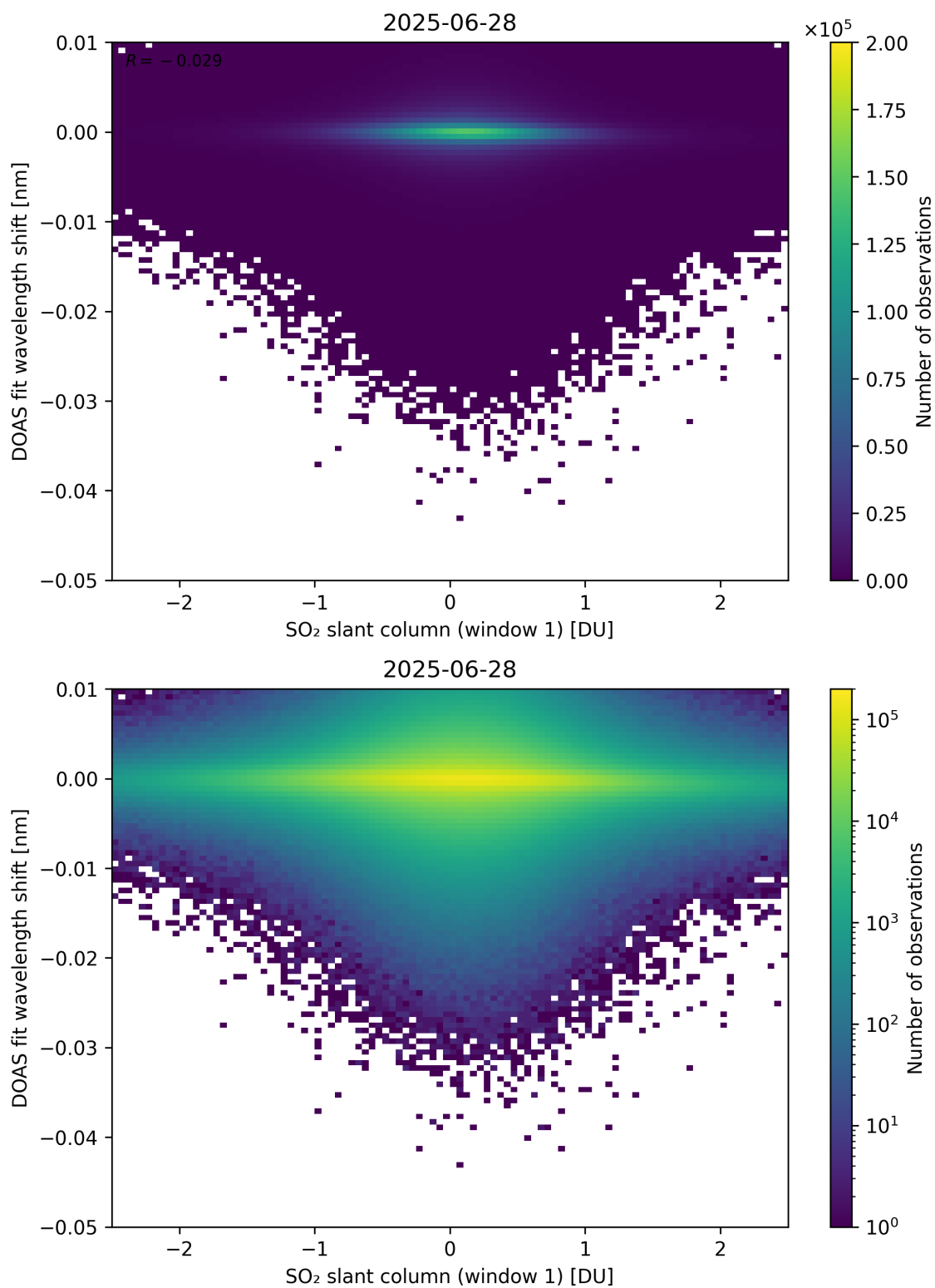
Figure 265: Scatter density plot of “SO 2 slant column (window 1)” against “DOAS fit wavelength shift” for 2025-06-27 to 2025-06-29.
