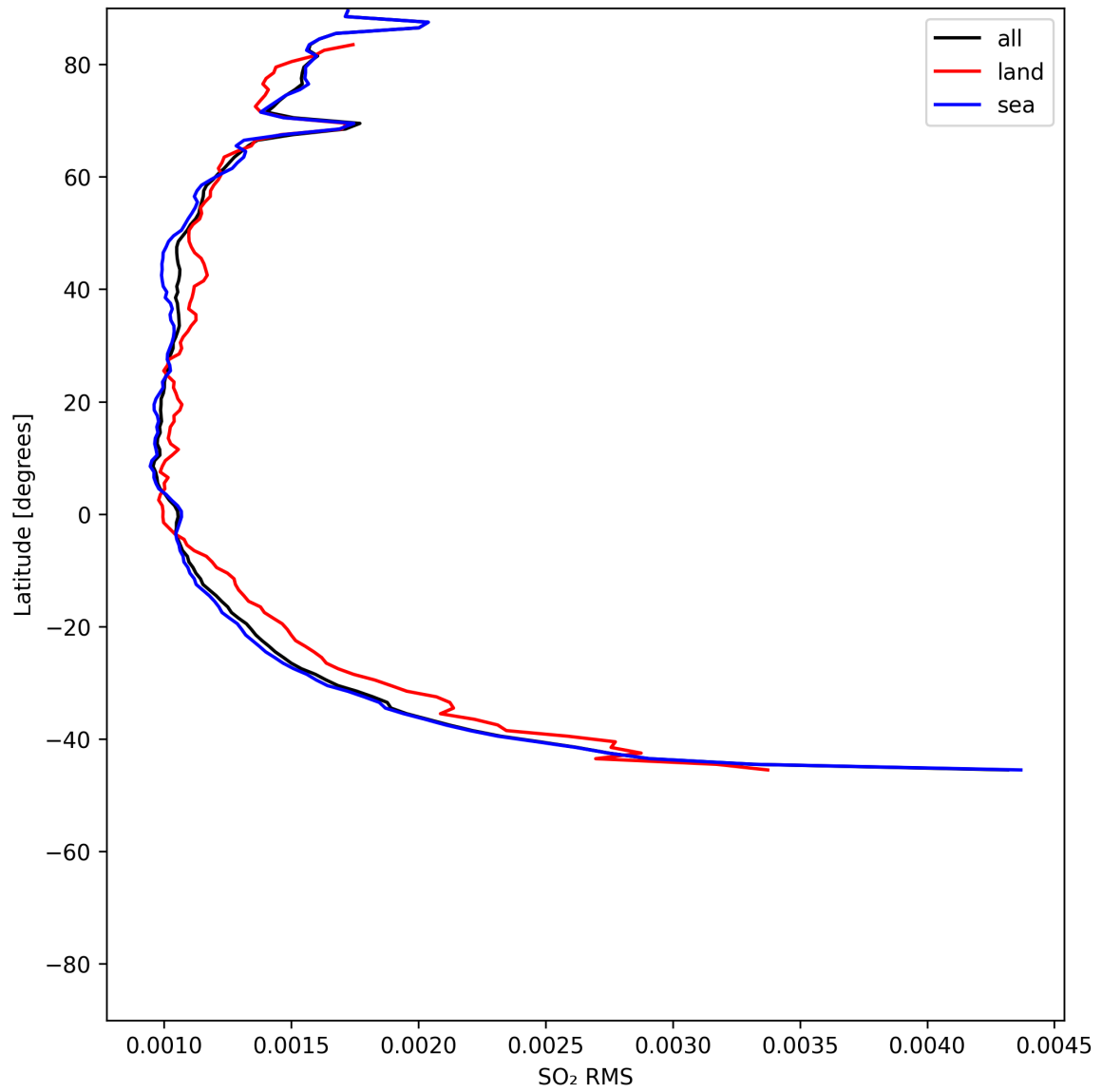
Figure 52: Zonal average of “SO 2 RMS” for 2025-06-27 to 2025-06-29.
