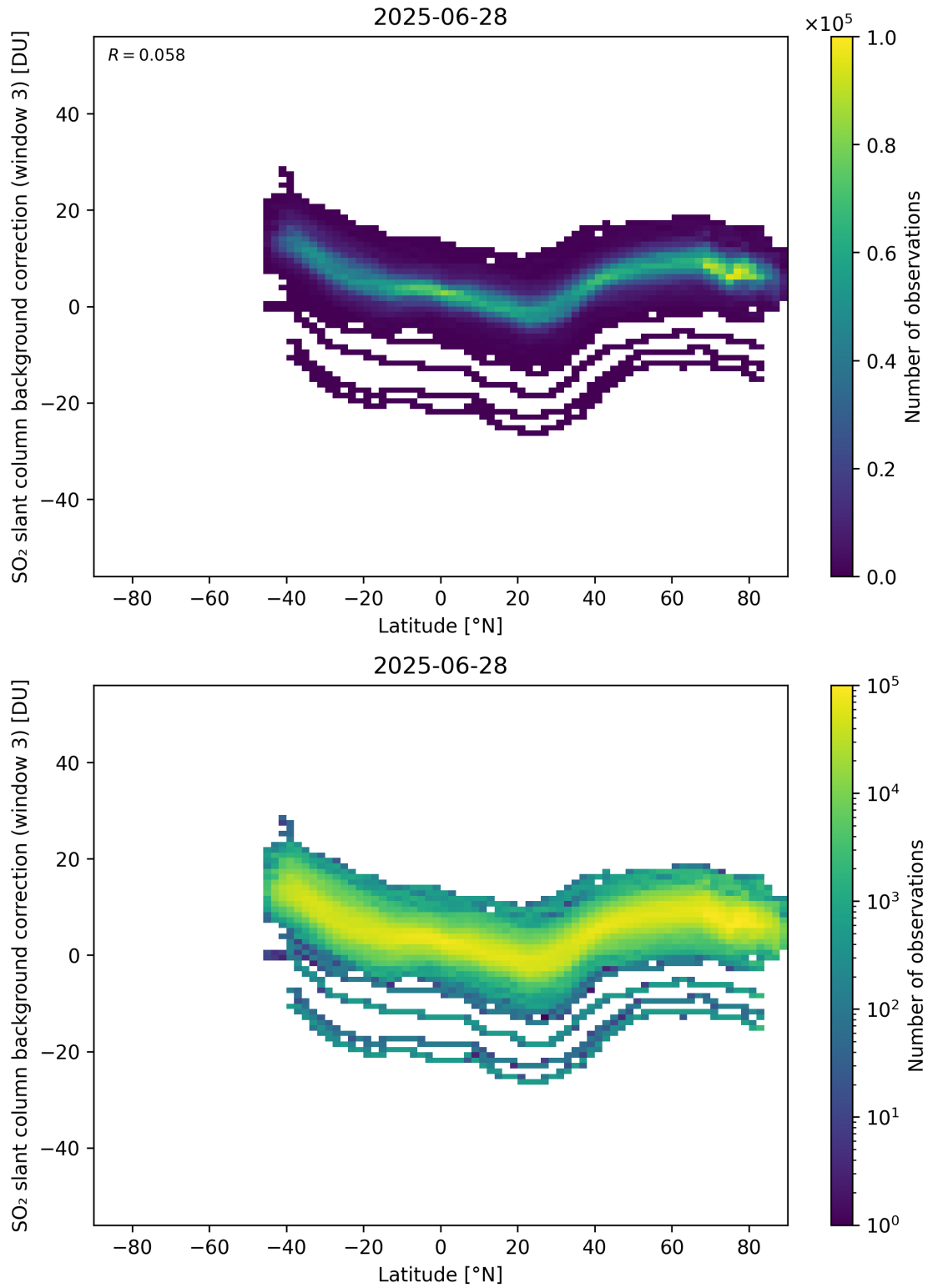
Figure 152: Scatter density plot of “Latitude” against “SO 2 slant column background correction (window 3)” for 2025-06-27 to 2025-06-29.
