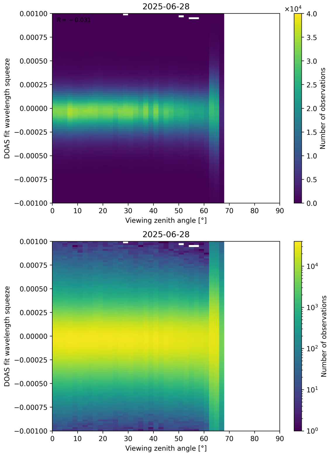
Figure 366: Scatter density plot of “Viewing zenith angle” against “DOAS fit wavelength squeeze” for 2025-06-27 to 2025-06-29.
