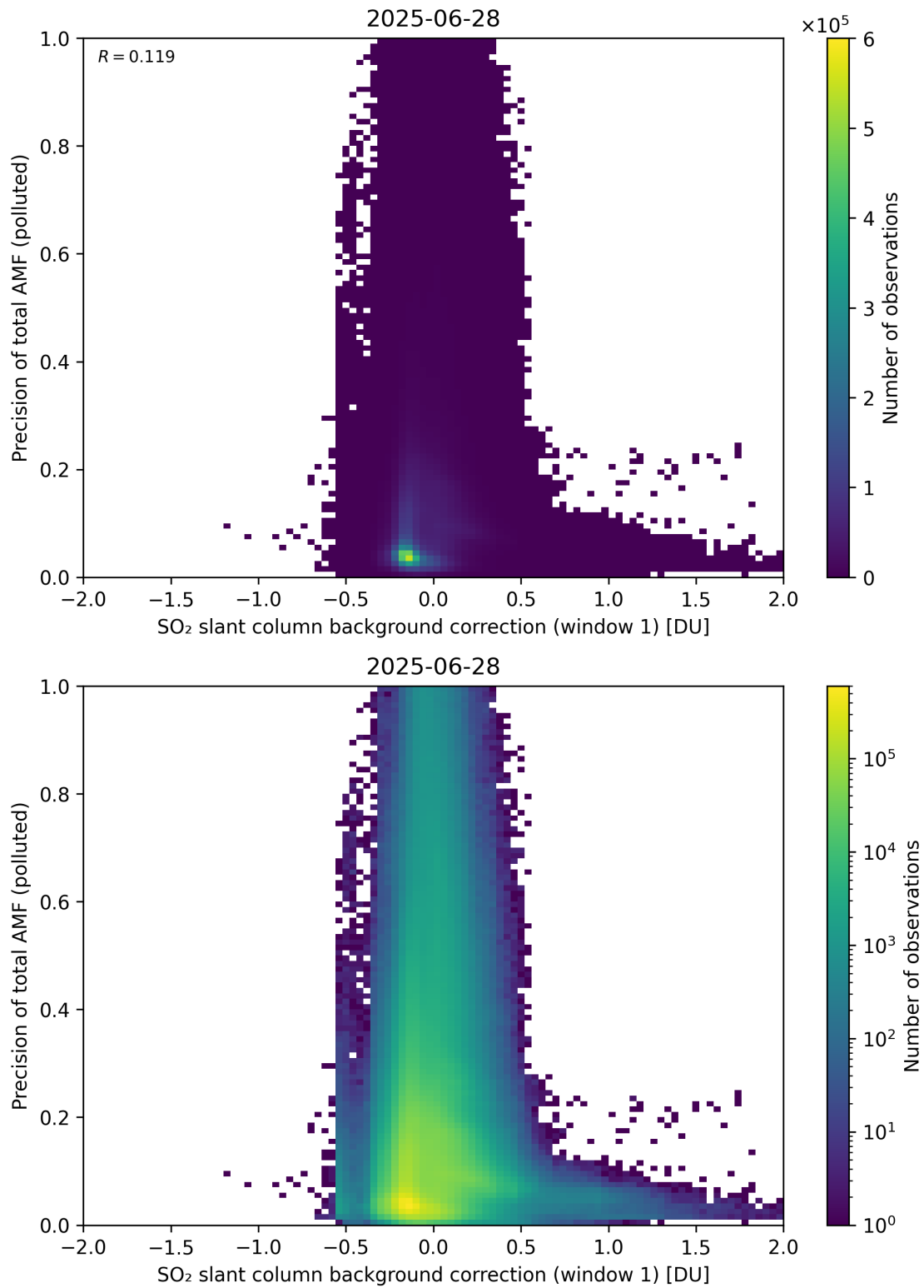
Figure 121: Scatter density plot of “SO 2 slant column background correction (window 1)” against “Precision of total AMF (polluted)” for 2025-06-27 to 2025-06-29.
