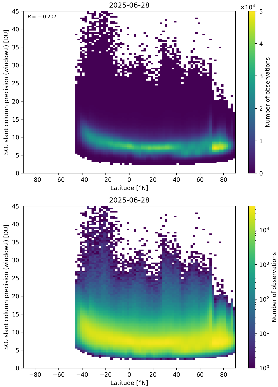
Figure 164: Scatter density plot of “Latitude” against “SO 2 slant column precision (window2)” for 2025-06-27 to 2025-06-29.
