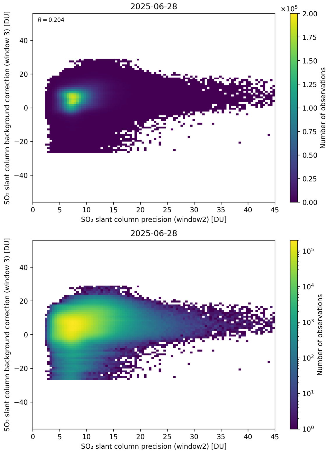
Figure 292: Scatter density plot of “SO 2 slant column precision (window2)” against “SO 2 slant column background correction (window 3)” for 2025-06-27 to 2025-06-29.
