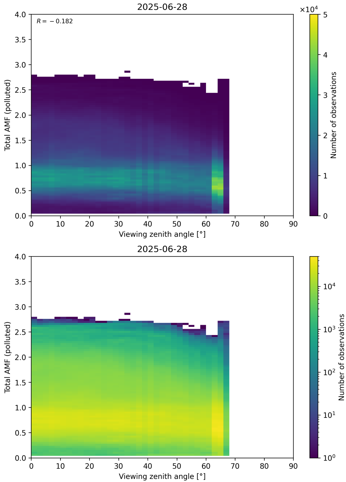
Figure 381: Scatter density plot of “Viewing zenith angle” against “Total AMF (polluted)” for 2025-06-27 to 2025-06-29.
