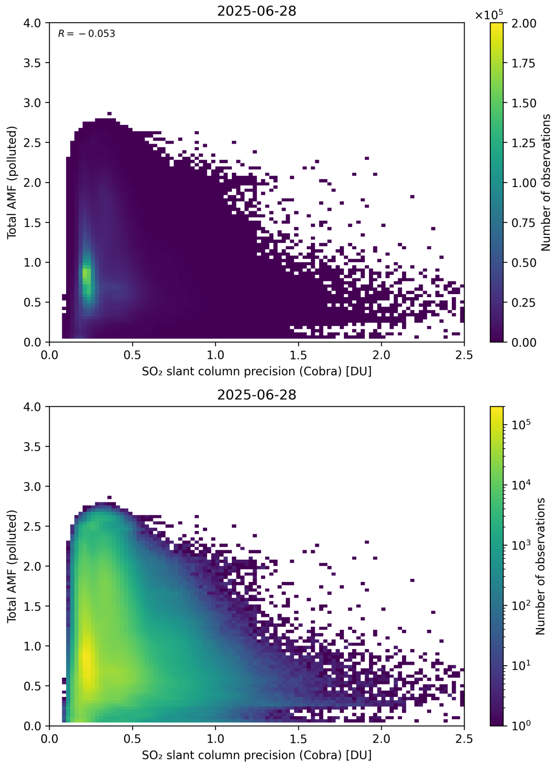
Figure 213: Scatter density plot of “SO 2 slant column precision (Cobra)” against “Total AMF (polluted)” for 2025-06-27 to 2025-06-29.
