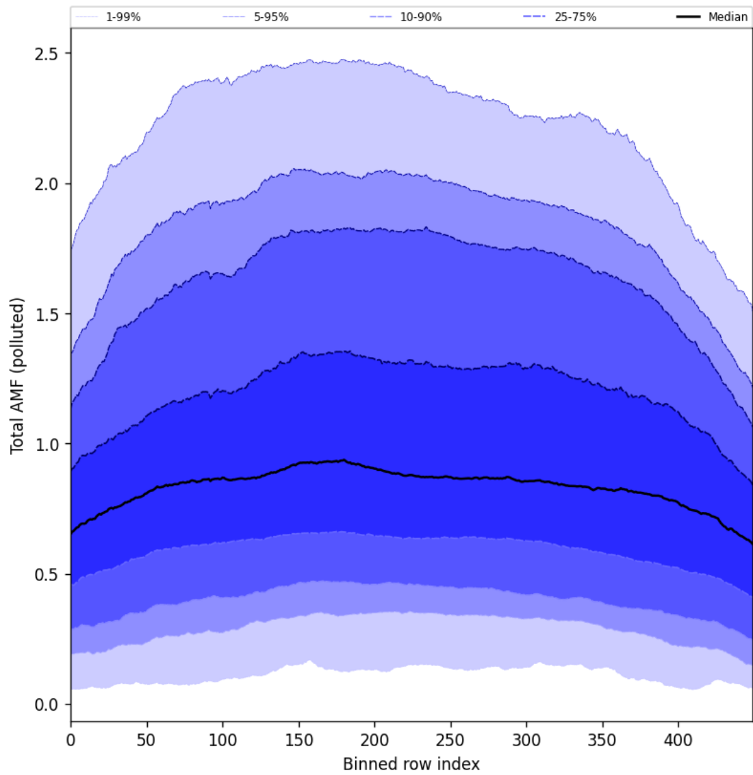
Figure 105: Along track statistics of “Total AMF (polluted)” for 2025-06-27 to 2025-06-29
