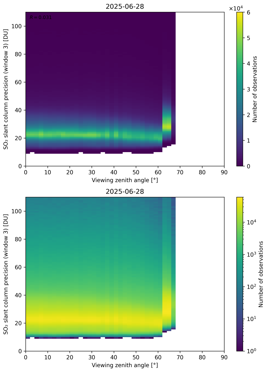
Figure 380: Scatter density plot of “Viewing zenith angle” against “SO 2 slant column precision (window 3)” for 2025-06-27 to 2025-06-29.
