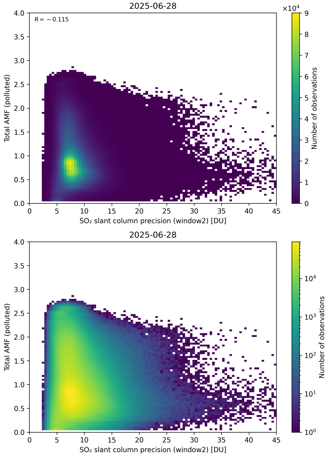
Figure 301: Scatter density plot of “SO 2 slant column precision (window2)” against “Total AMF (polluted)” for 2025-06-27 to 2025-06-29.
