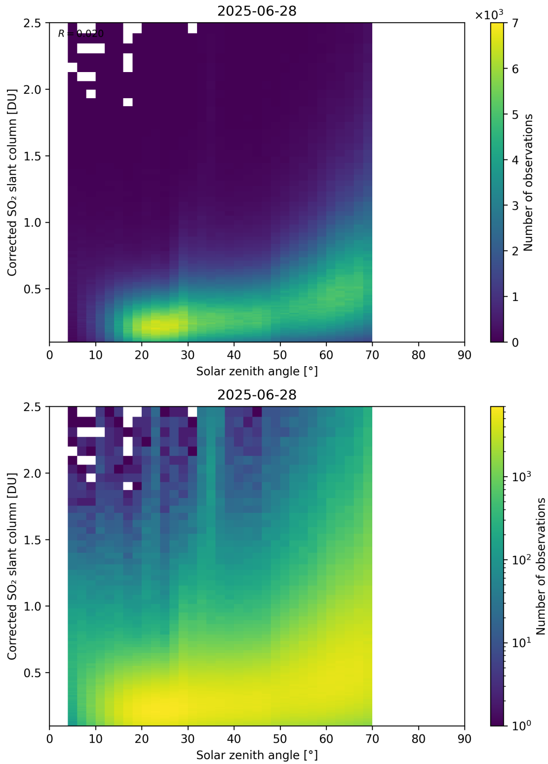
Figure 181: Scatter density plot of “Solar zenith angle” against “Corrected SO 2 slant column” for 2025-06-27 to 2025-06-29.
