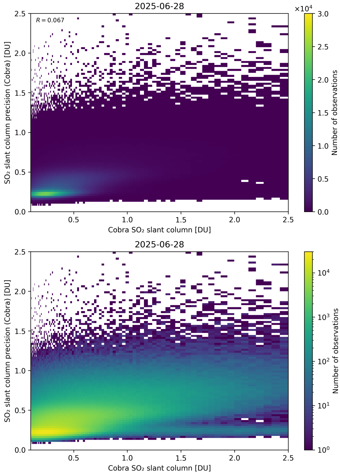
Figure 216: Scatter density plot of “Cobra SO 2 slant column” against “SO 2 slant column precision (Cobra)” for 2025-06-27 to 2025-06-29.
