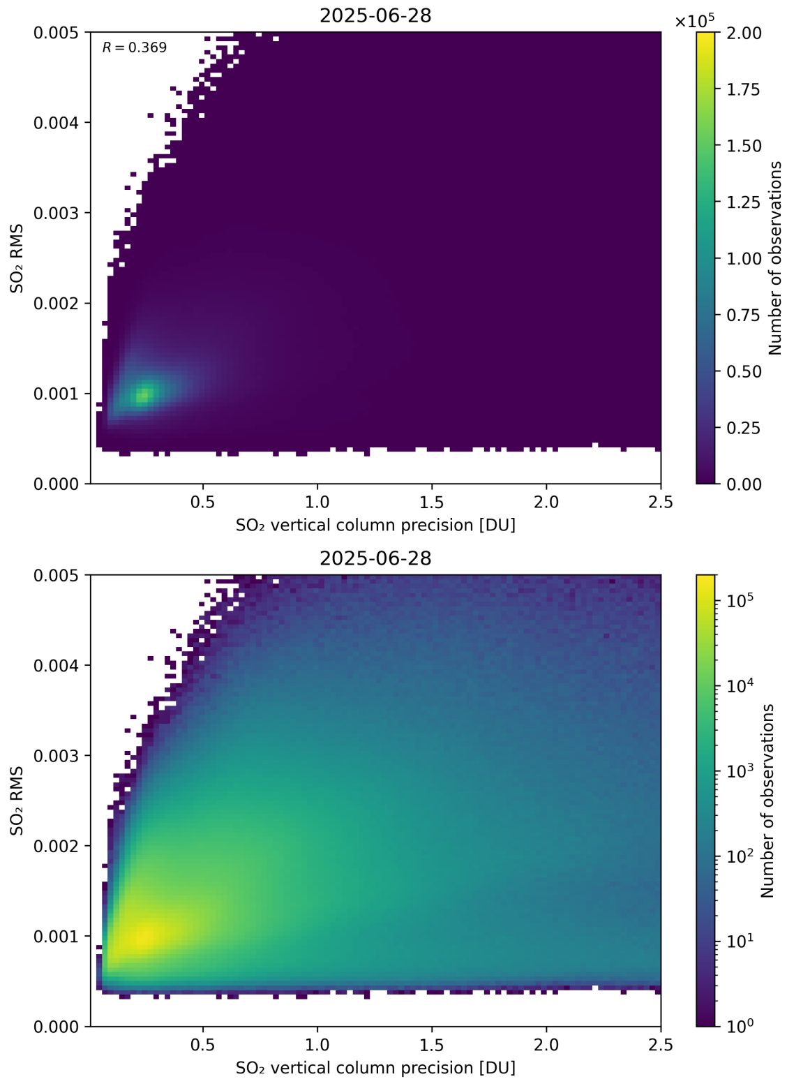
Figure 334: Scatter density plot of “SO 2 vertical column precision” against “SO 2 RMS” for 2025-06-27 to 2025-06-29.
