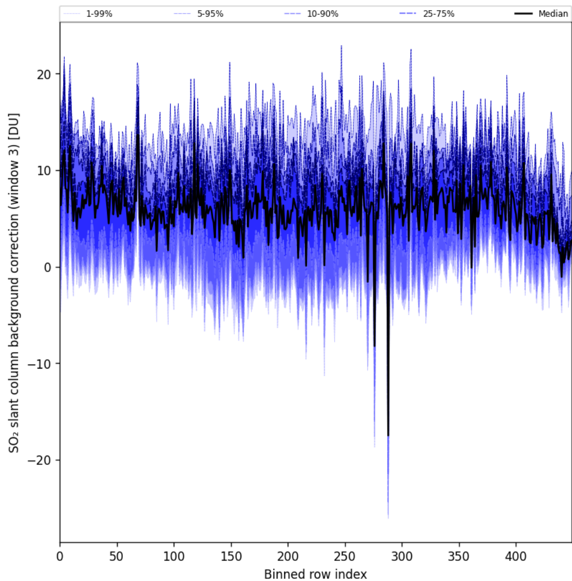
Figure 100: Along track statistics of “SO 2 slant column background correction (window 3)” for 2025-06-27 to 2025-06-29
