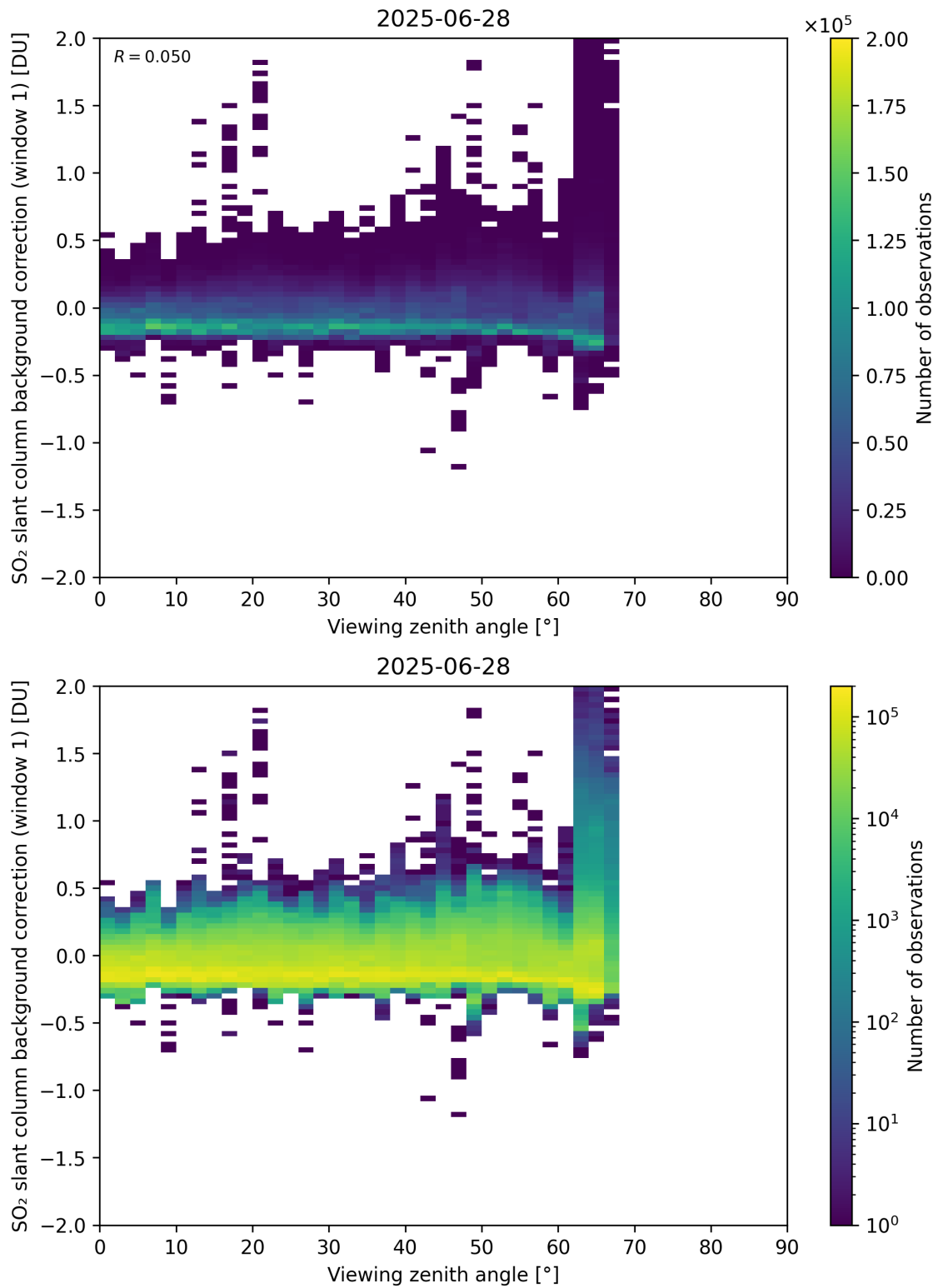
Figure 362: Scatter density plot of “Viewing zenith angle” against “SO 2 slant column background correction (window 1)” for 2025-06-27 to 2025-06-29.
