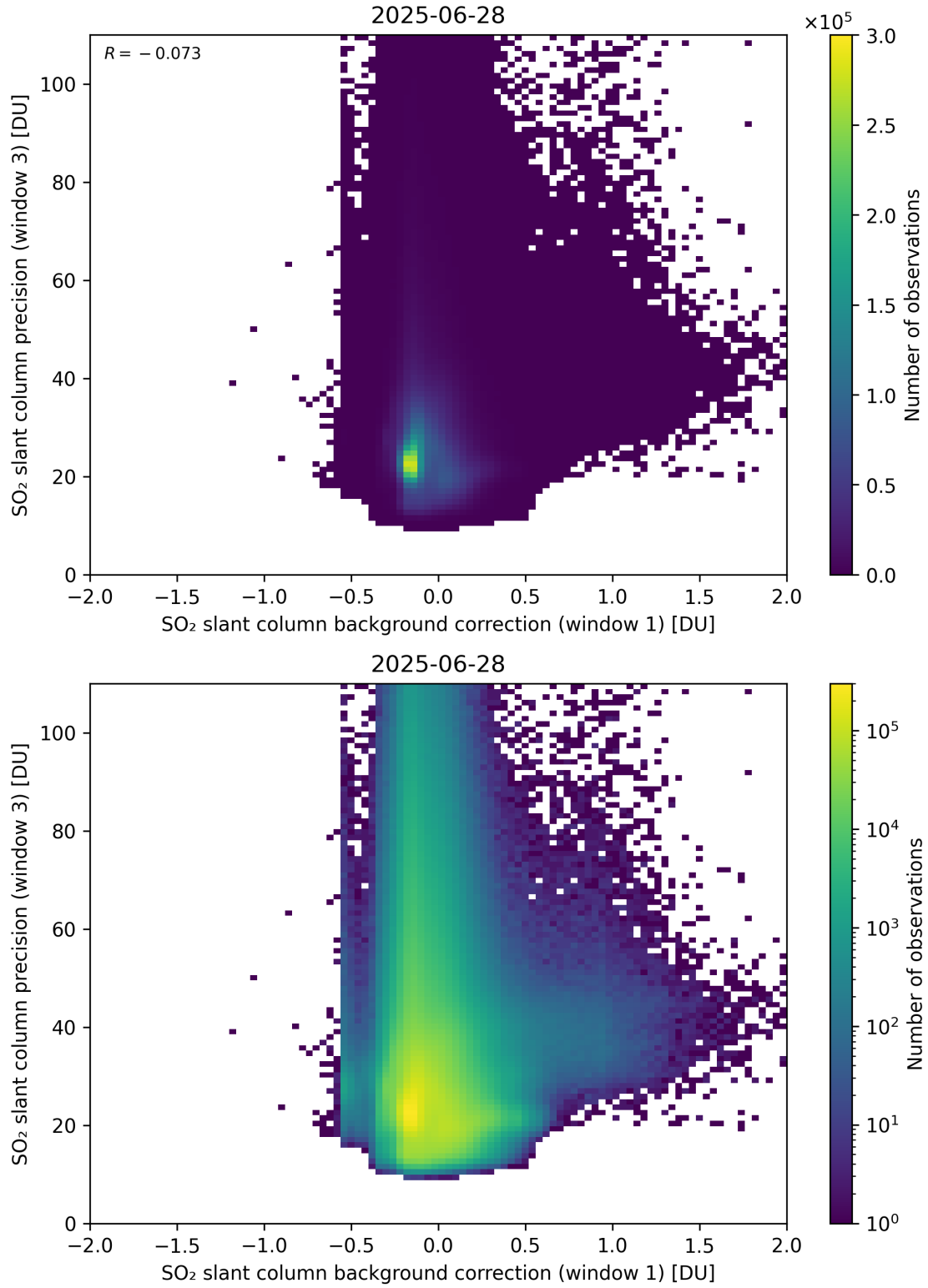
Figure 119: Scatter density plot of “SO 2 slant column background correction (window 1)” against “SO 2 slant column precision (window 3)” for 2025-06-27 to 2025-06-29.
