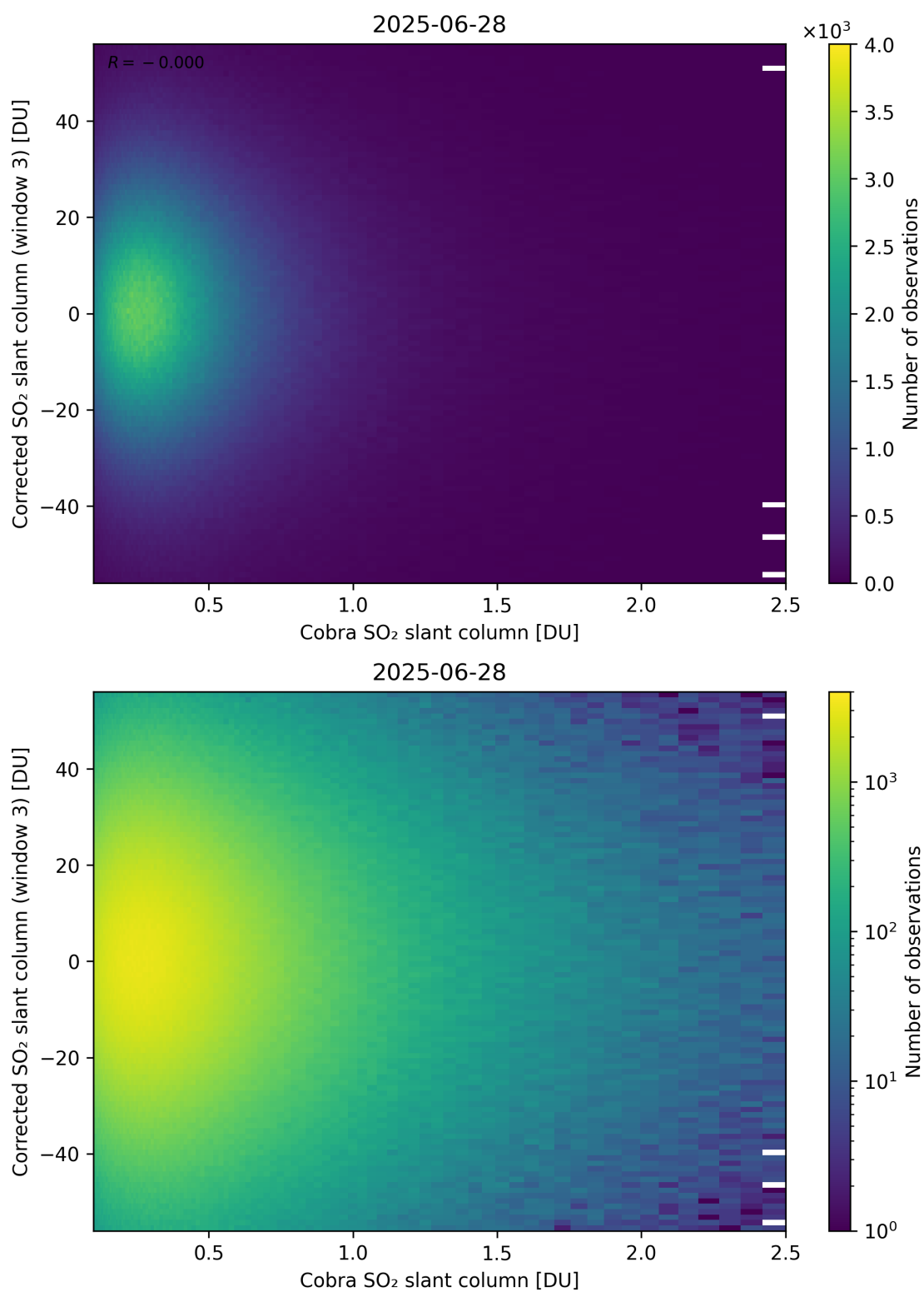
Figure 218: Scatter density plot of “Cobra SO 2 slant column” against “Corrected SO 2 slant column (window 3)” for 2025-06-27 to 2025-06-29.
