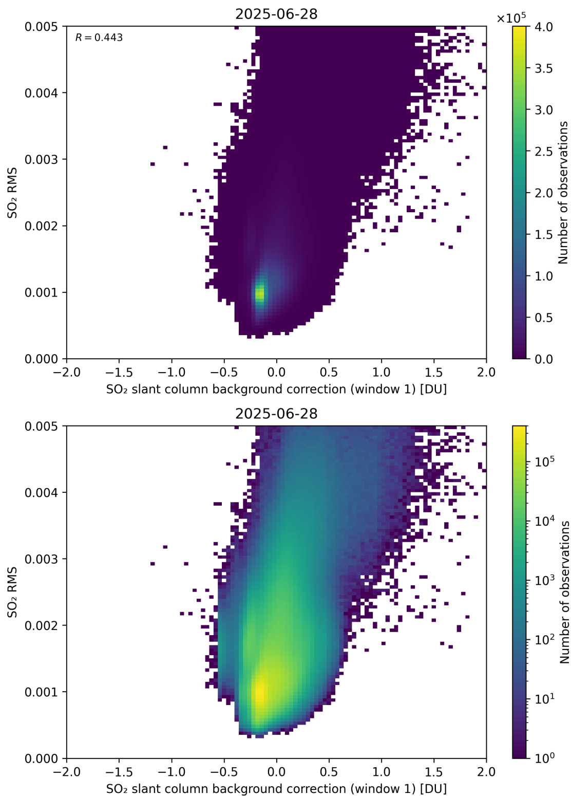
Figure 113: Scatter density plot of “SO 2 slant column background correction (window 1)” against “SO 2 RMS” for 2025-06-27 to 2025-06-29.
