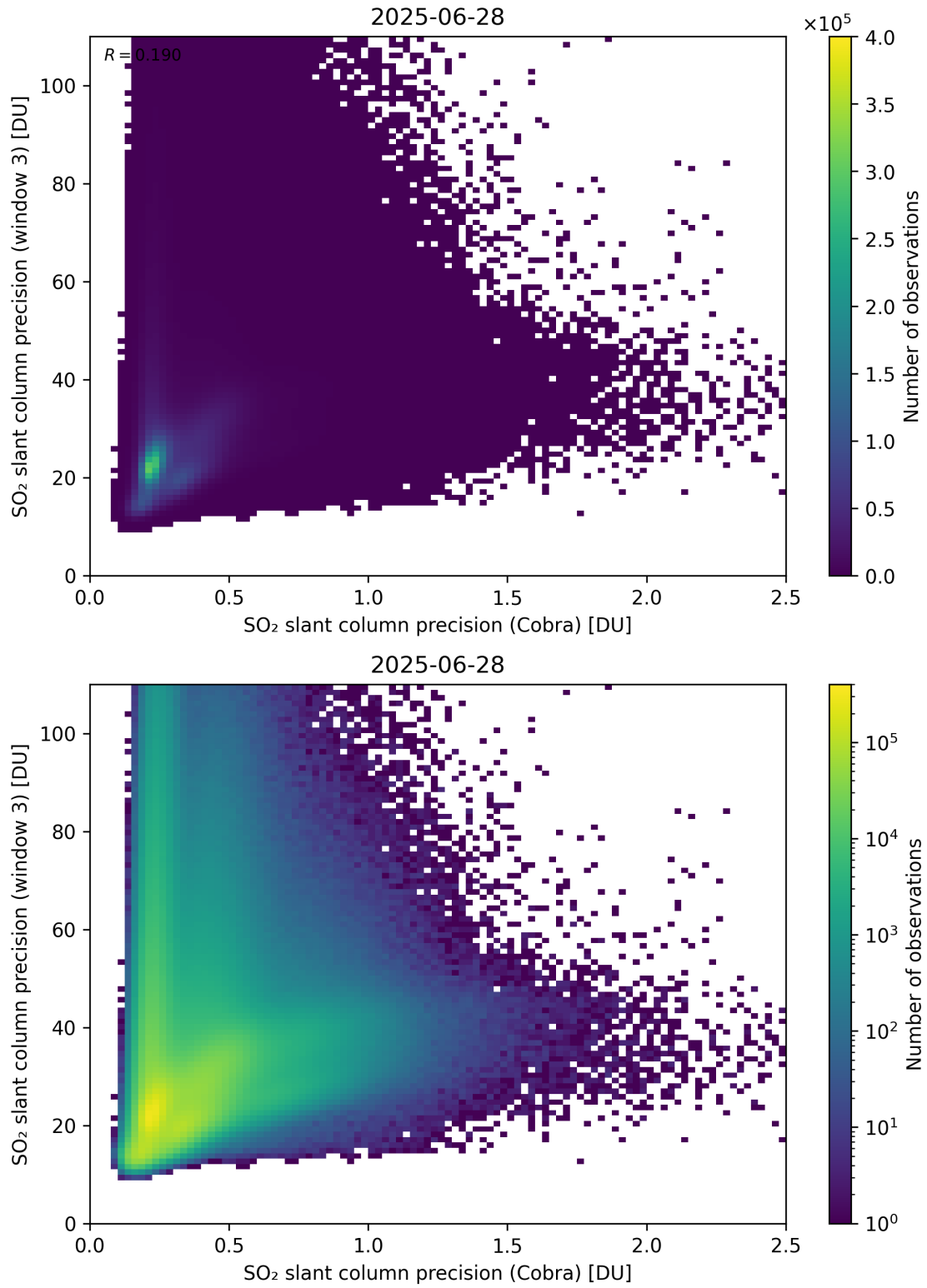
Figure 212: Scatter density plot of “SO 2 slant column precision (Cobra)” against “SO 2 slant column precision (window 3)” for 2025-06-27 to 2025-06-29.
