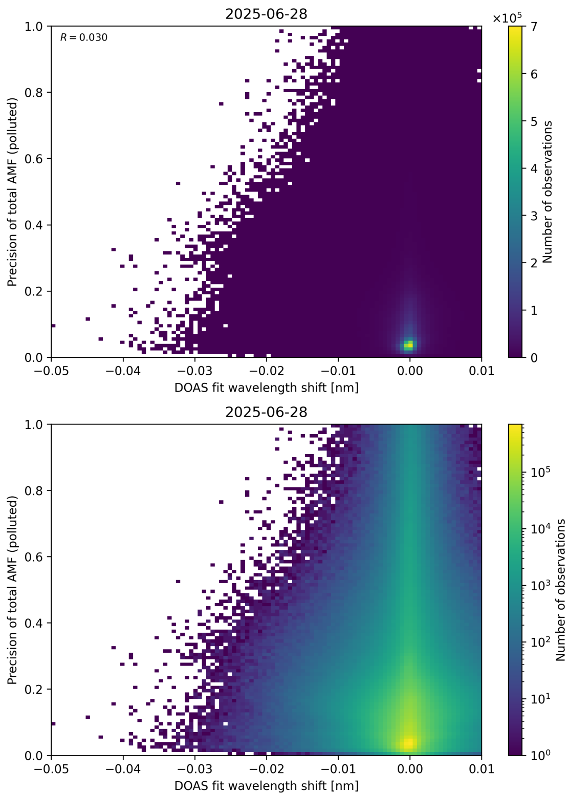
Figure 142: Scatter density plot of “DOAS fit wavelength shift” against “Precision of total AMF (polluted)” for 2025-06-27 to 2025-06-29.
