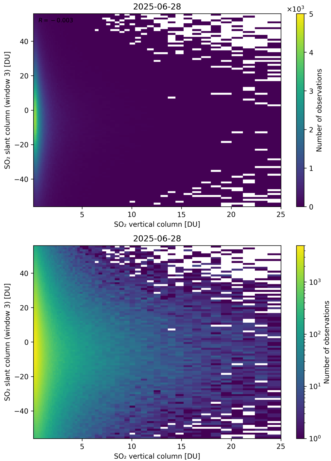
Figure 357: Scatter density plot of “SO 2 vertical column” against “SO 2 slant column (window 3)” for 2025-06-27 to 2025-06-29.
