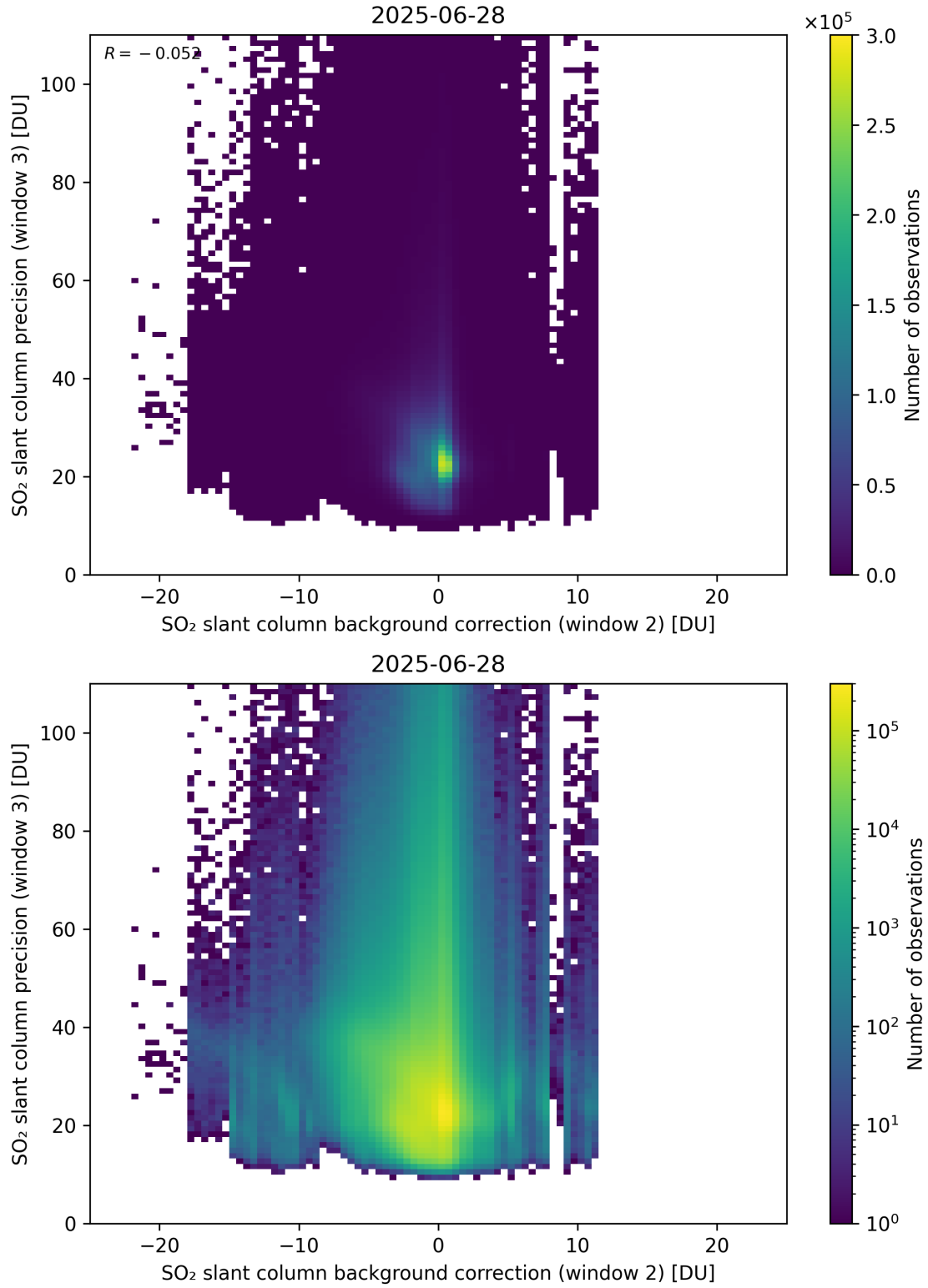
Figure 129: Scatter density plot of “SO 2 slant column background correction (window 2)” against “SO 2 slant column precision (window 3)” for 2025-06-27 to 2025-06-29.
