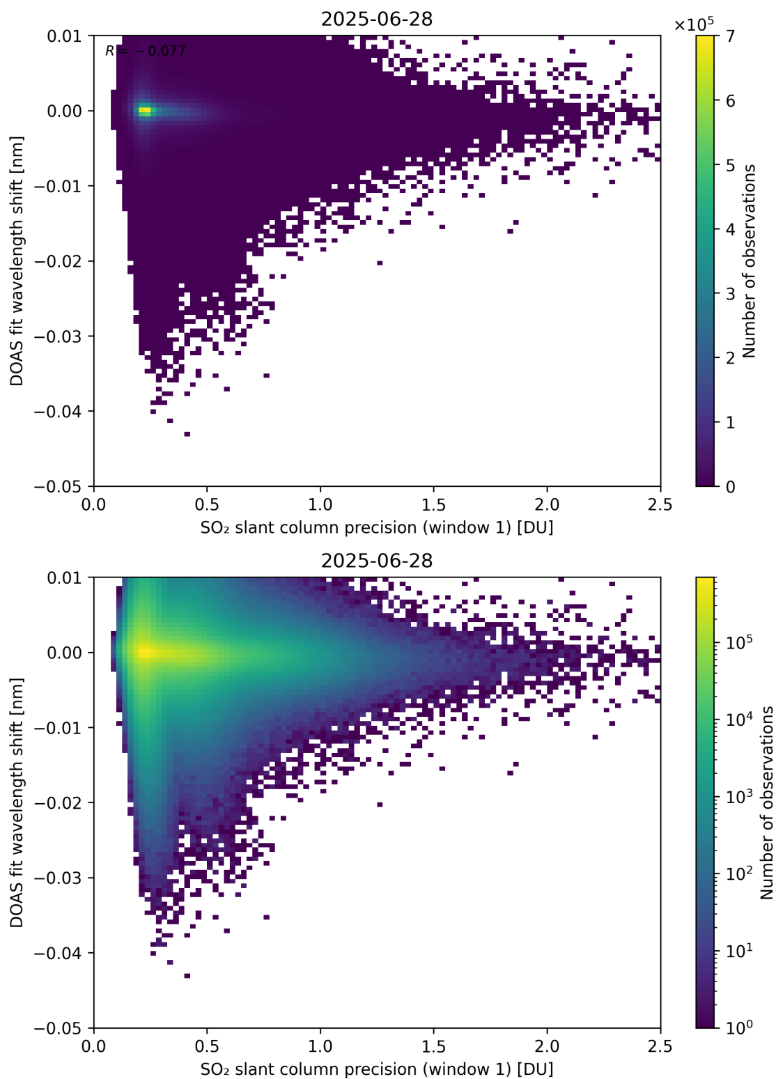
Figure 271: Scatter density plot of “SO 2 slant column precision (window 1)” against “DOAS fit wavelength shift” for 2025-06-27 to 2025-06-29.
