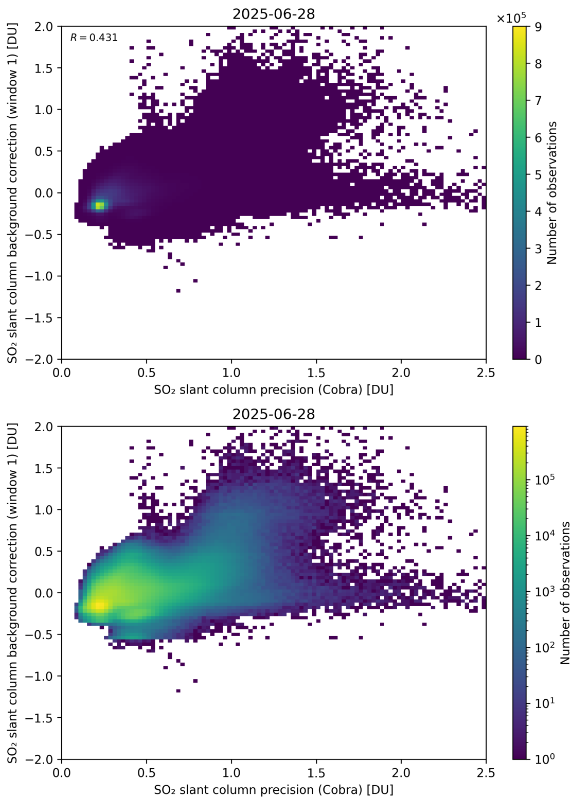
Figure 199: Scatter density plot of “SO 2 slant column precision (Cobra)” against “SO 2 slant column background correction (window 1)” for 2025-06-27 to 2025-06-29.
