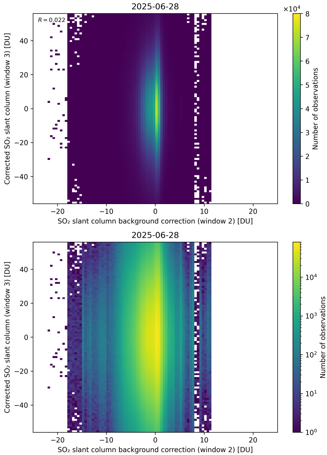
Figure 127: Scatter density plot of “SO 2 slant column background correction (window 2)” against “Corrected SO 2 slant column (window 3)” for 2025-06-27 to 2025-06-29.
