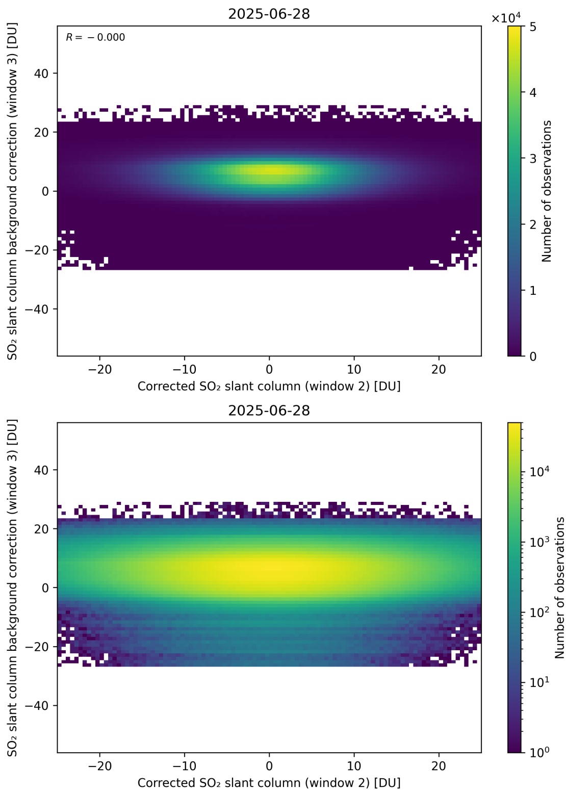
Figure 245: Scatter density plot of “Corrected SO 2 slant column (window 2)” against “SO 2 slant column background correction (window 3)” for 2025-06-27 to 2025-06-29.
