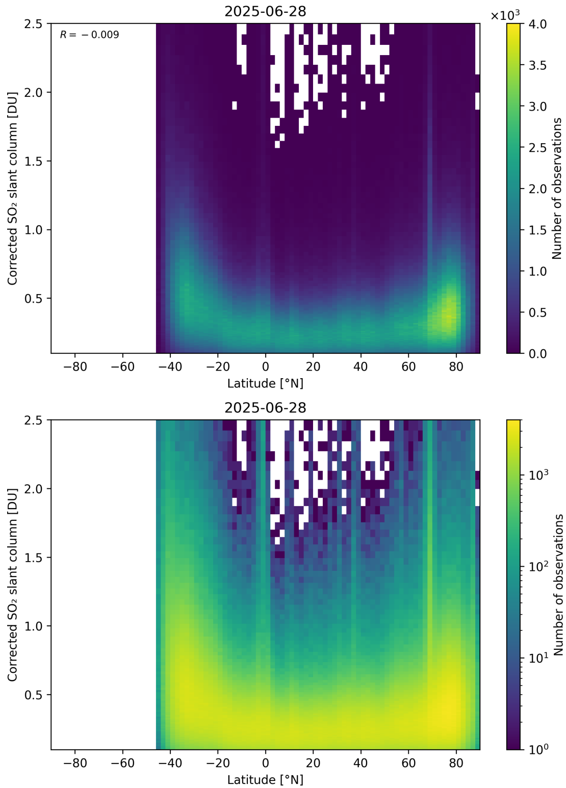
Figure 159: Scatter density plot of “Latitude” against “Corrected SO 2 slant column” for 2025-06-27 to 2025-06-29.
