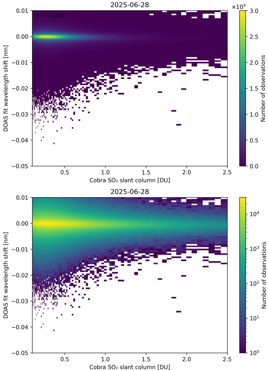
Figure 196: Scatter density plot of “Cobra SO 2 slant column” against “DOAS fit wavelength shift” for 2025-06-27 to 2025-06-29.
