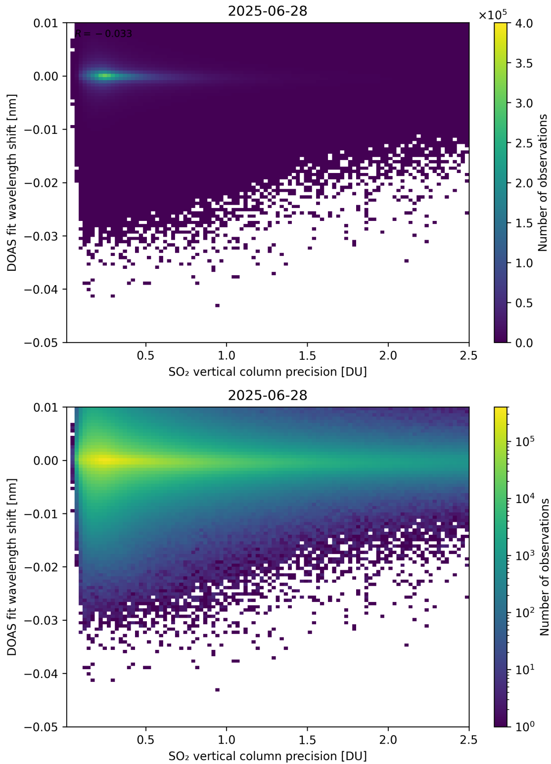
Figure 332: Scatter density plot of “SO 2 vertical column precision” against “DOAS fit wavelength shift” for 2025-06-27 to 2025-06-29.
