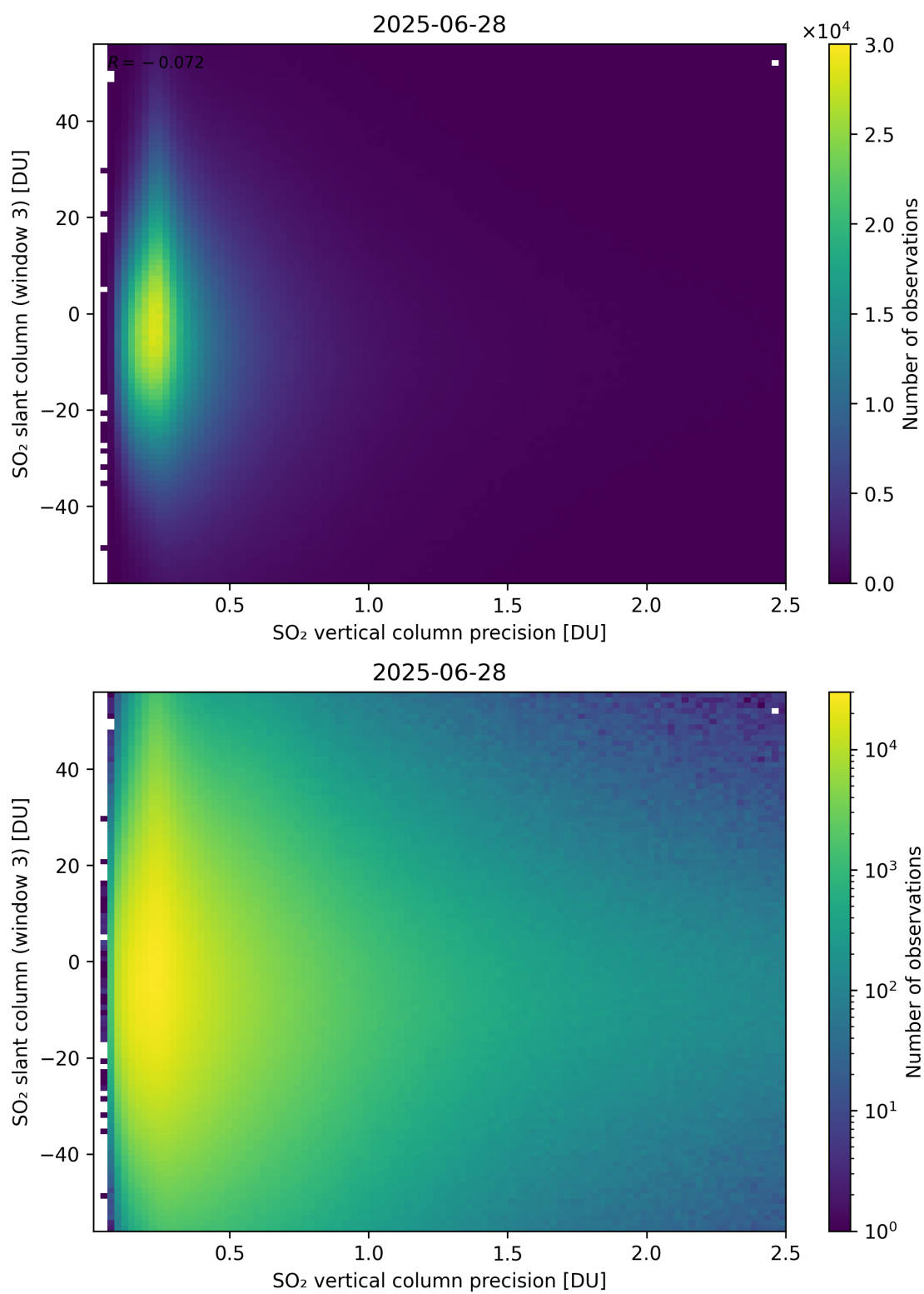
Figure 344: Scatter density plot of “SO 2 vertical column precision” against “SO 2 slant column (window 3)” for 2025-06-27 to 2025-06-29.
