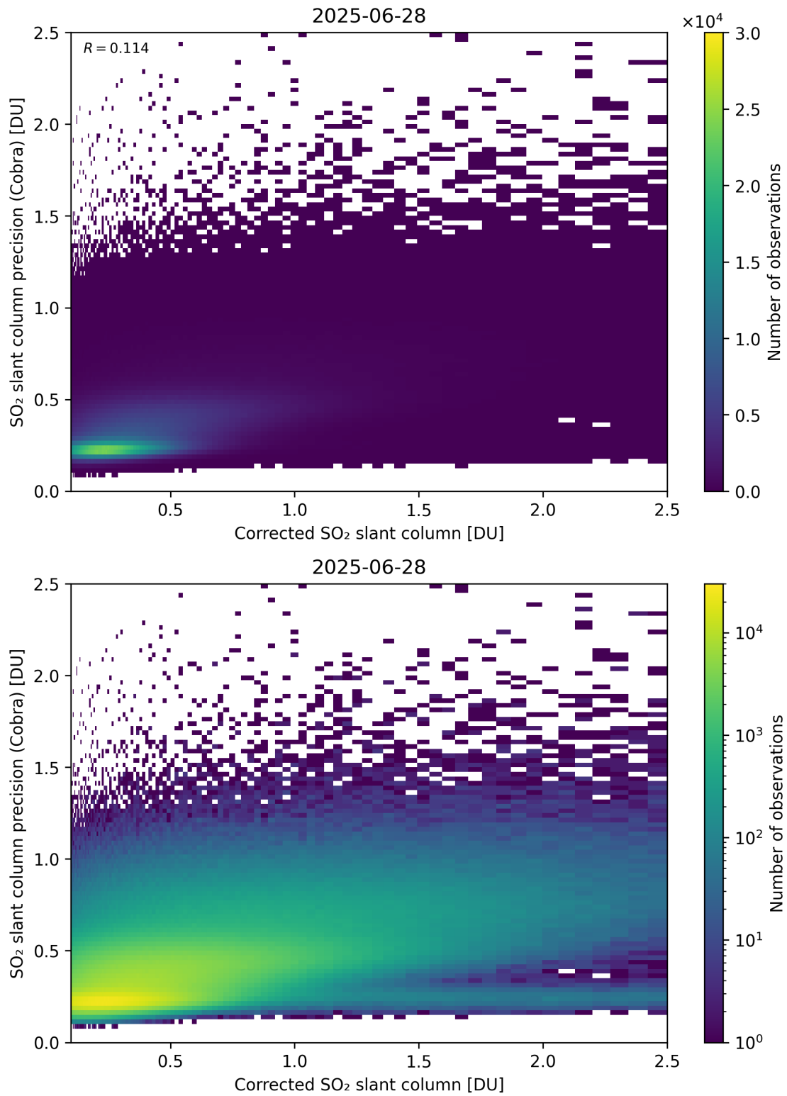
Figure 234: Scatter density plot of “Corrected SO 2 slant column” against “SO 2 slant column precision (Cobra)” for 2025-06-27 to 2025-06-29.
