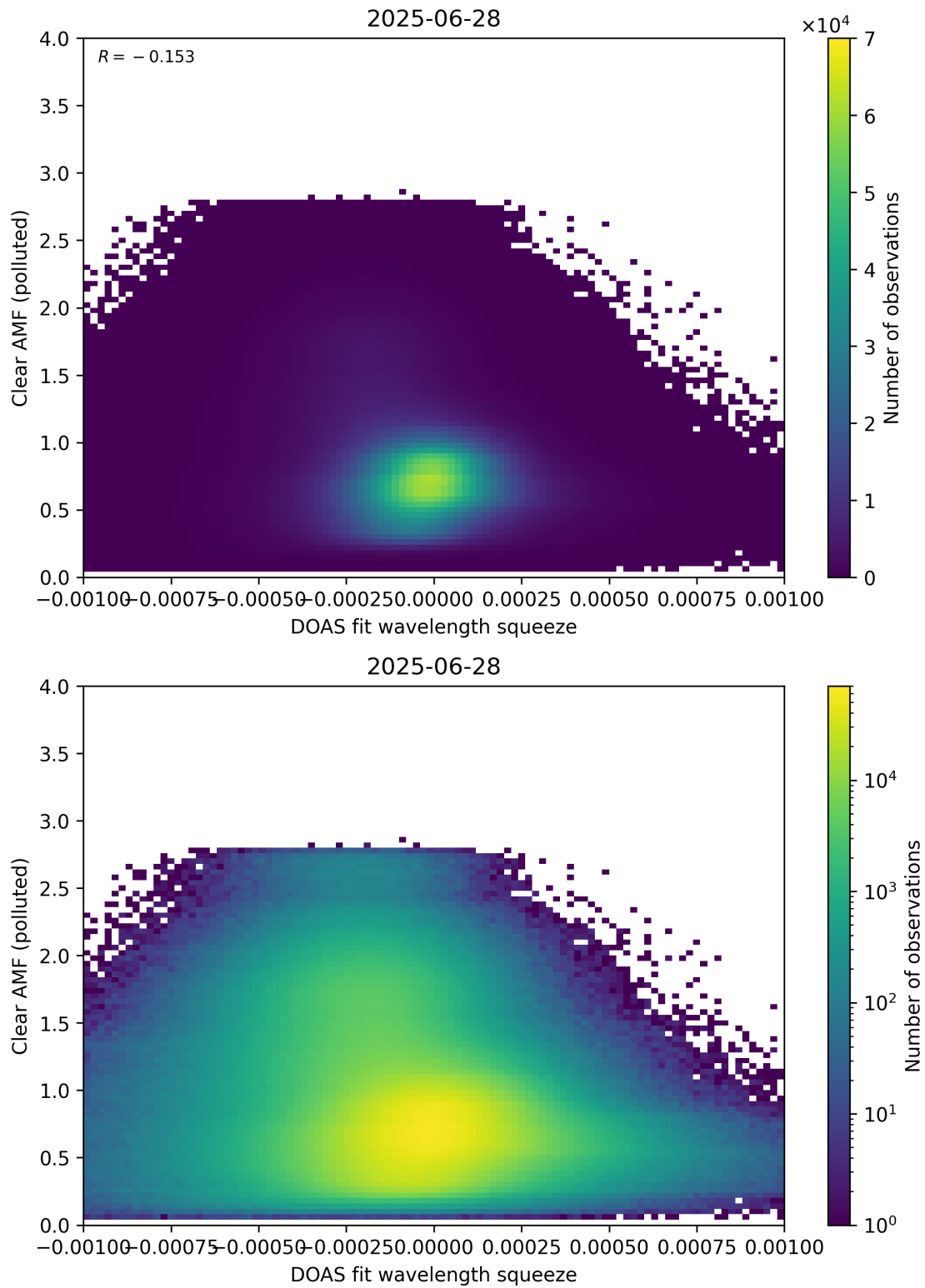
Figure 144: Scatter density plot of “DOAS fit wavelength squeeze” against “Clear AMF (polluted)” for 2025-06-27 to 2025-06-29.
