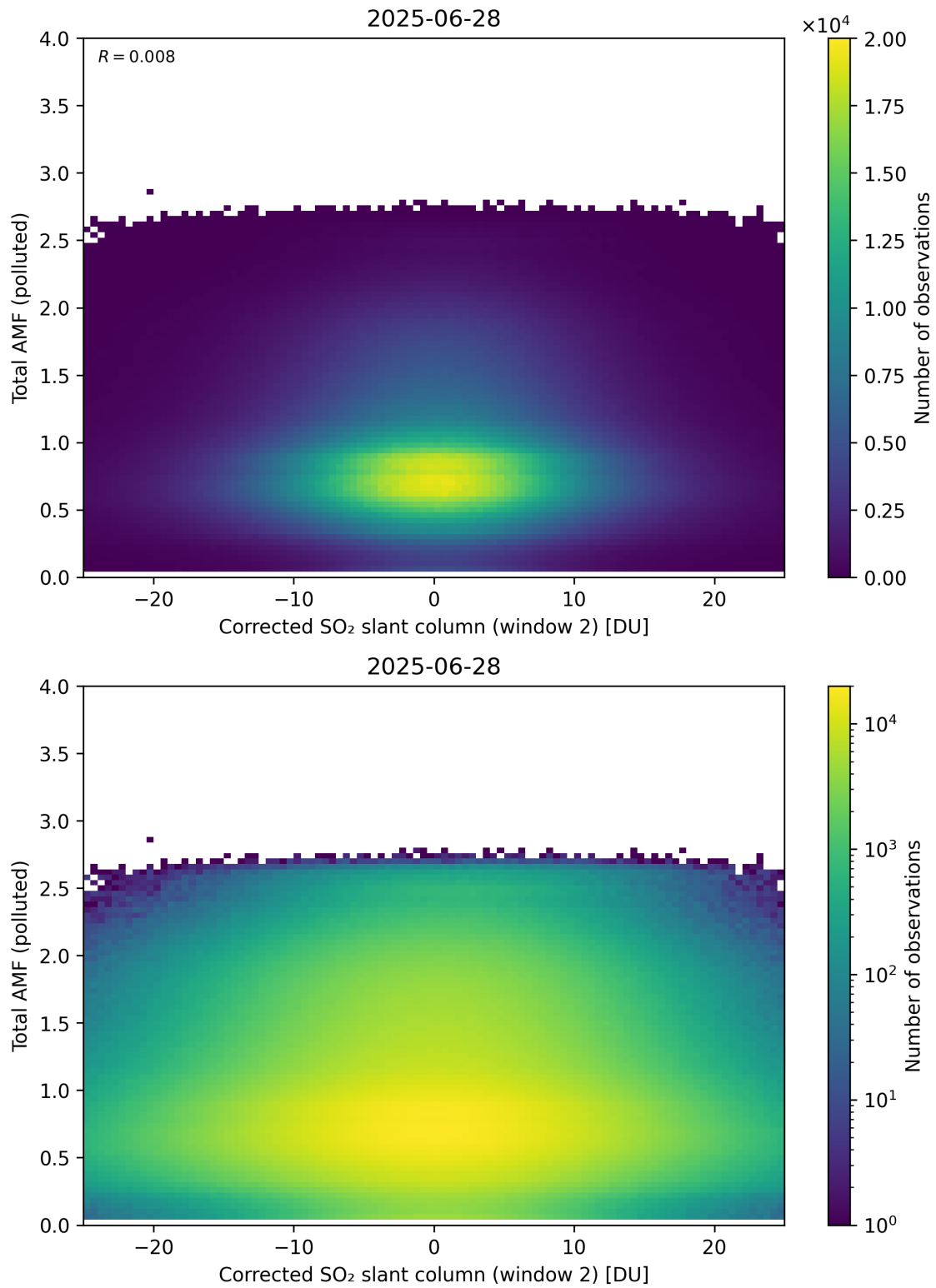
Figure 253: Scatter density plot of “Corrected SO 2 slant column (window 2)” against “Total AMF (polluted)” for 2025-06-27 to 2025-06-29.
