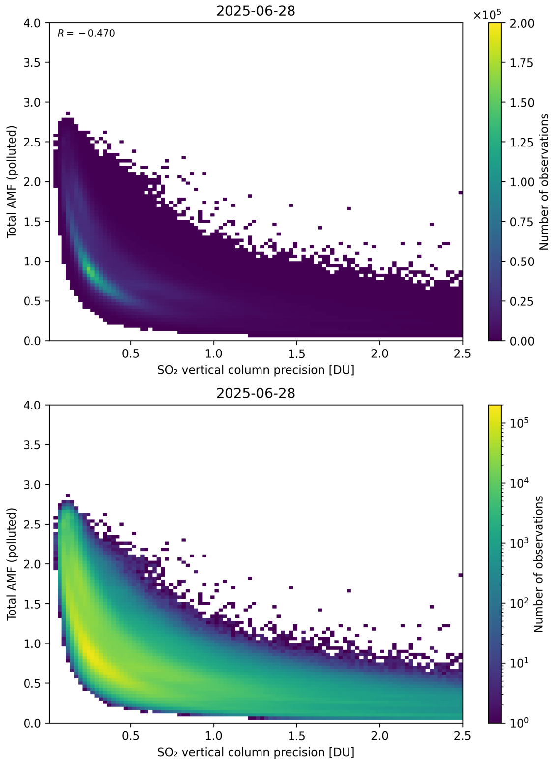
Figure 346: Scatter density plot of “SO 2 vertical column precision” against “Total AMF (polluted)” for 2025-06-27 to 2025-06-29.
