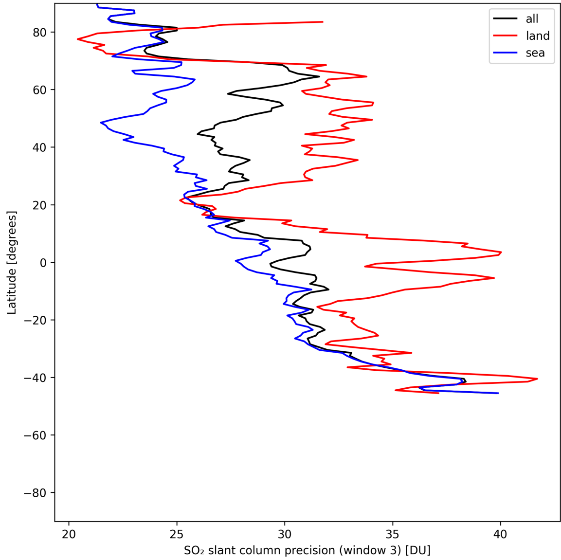
Figure 46: Zonal average of “SO 2 slant column precision (window 3)” for 2025-06-27 to 2025-06-29.
