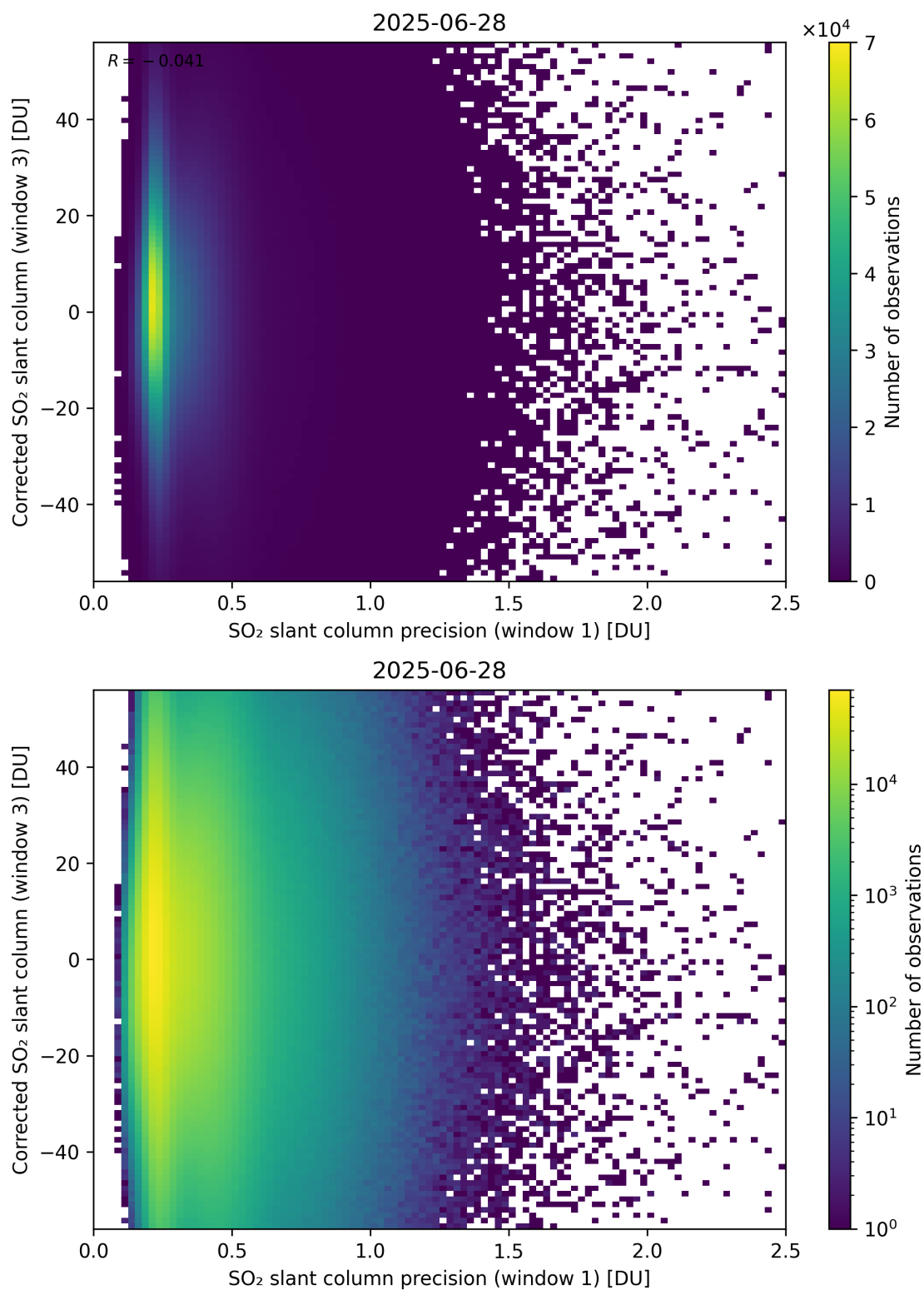
Figure 276: Scatter density plot of “SO 2 slant column precision (window 1)” against “Corrected SO 2 slant column (window 3)” for 2025-06-27 to 2025-06-29.
