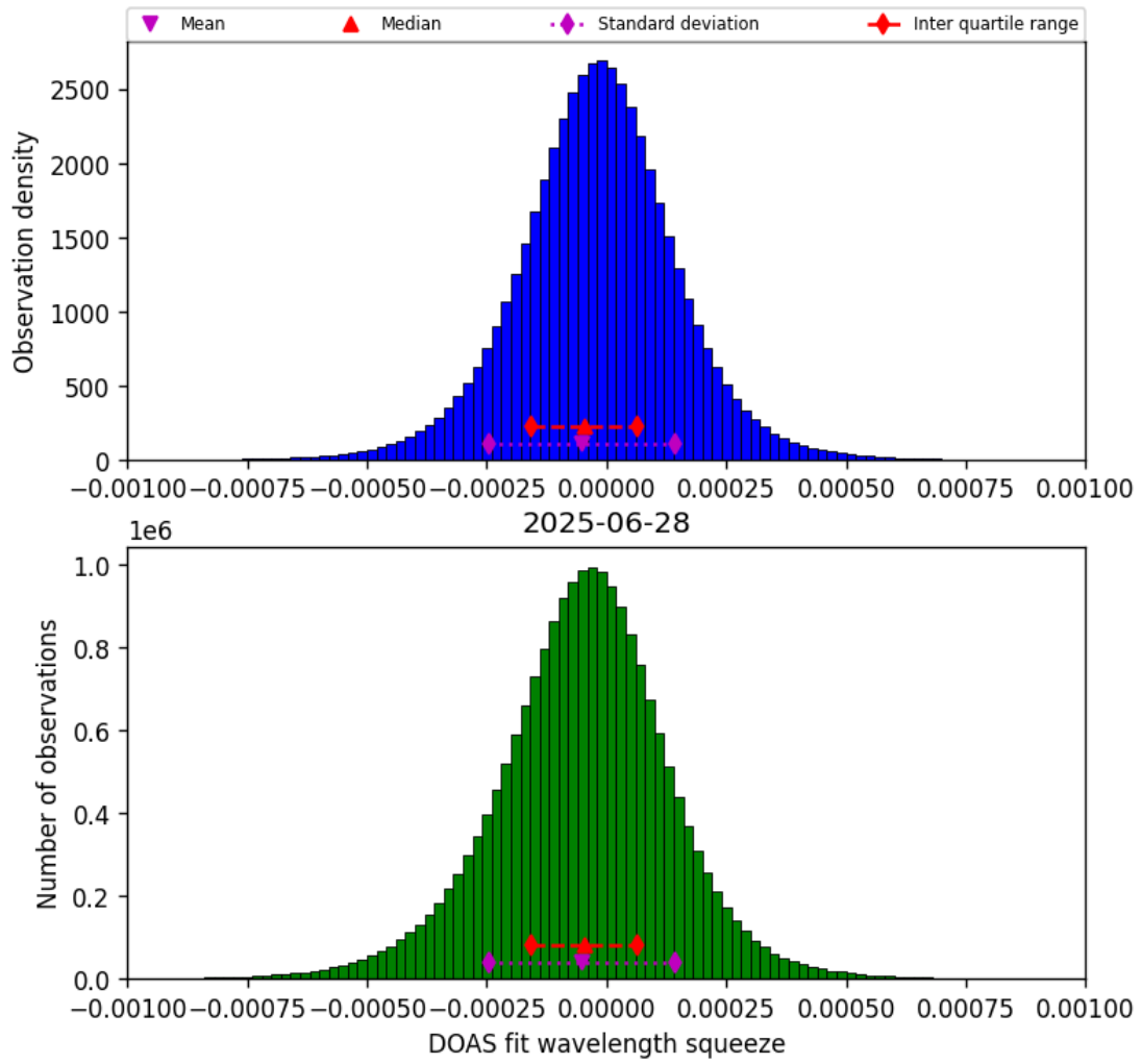
Figure 77: Histogram of “DOAS fit wavelength squeeze” for 2025-06-27 to 2025-06-29
