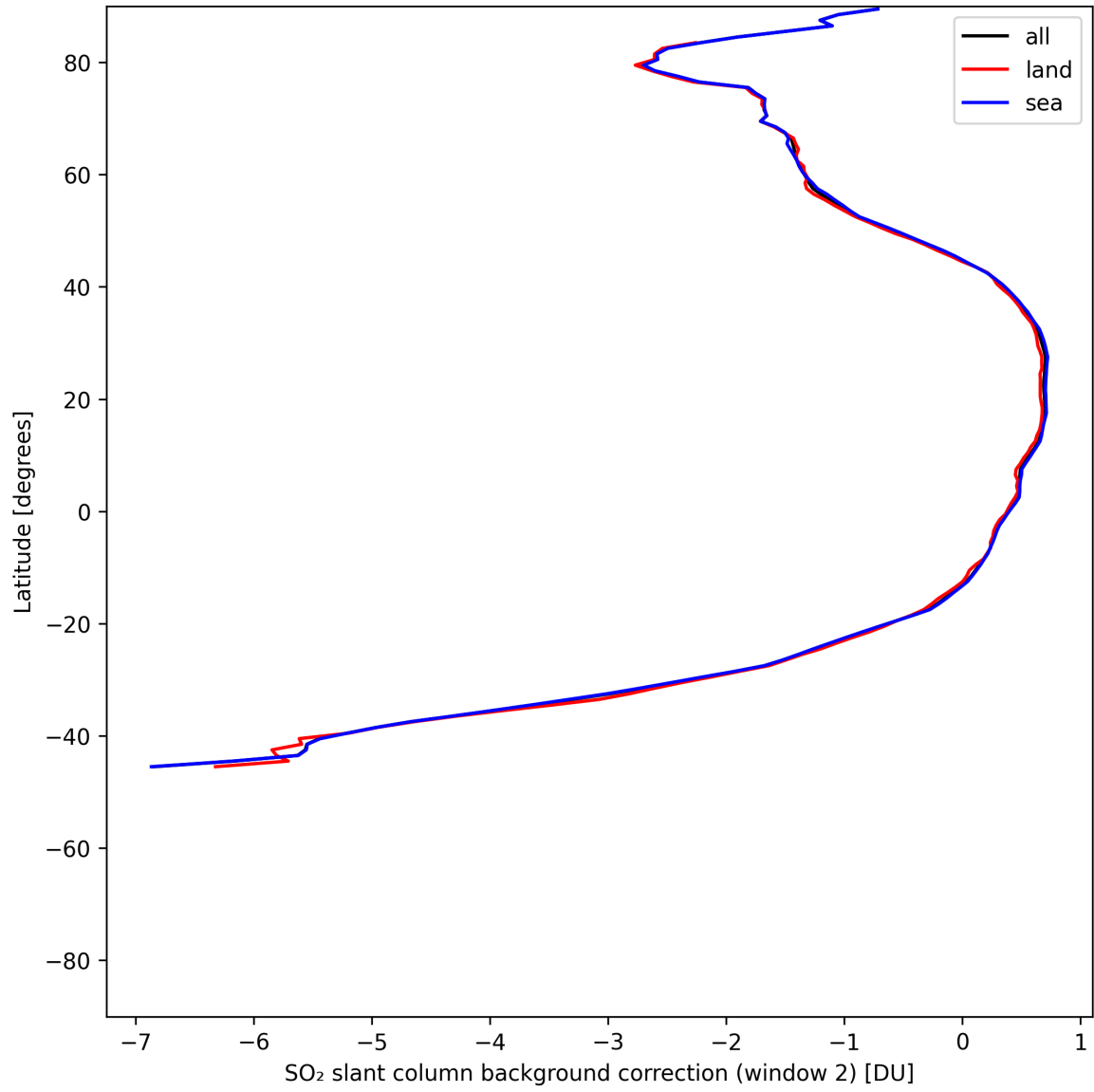
Figure 44: Zonal average of “SO 2 slant column background correction (window 2)” for 2025-06-27 to 2025-06-29.
