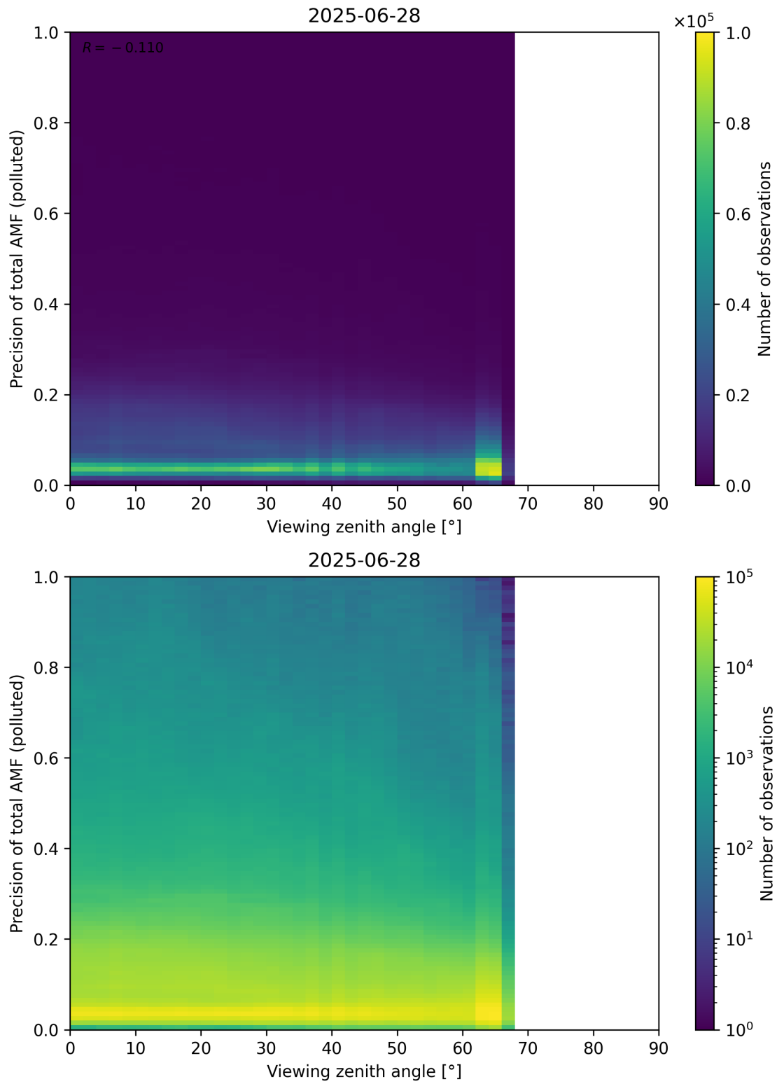
Figure 382: Scatter density plot of “Viewing zenith angle” against “Precision of total AMF (polluted)” for 2025-06-27 to 2025-06-29.
