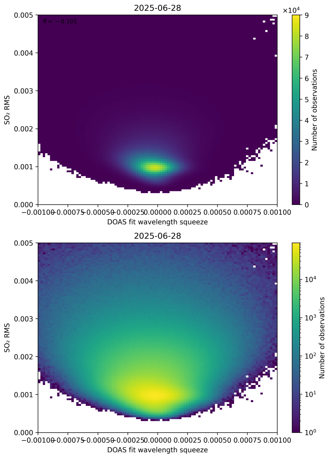
Figure 143: Scatter density plot of “DOAS fit wavelength squeeze” against “SO 2 RMS” for 2025-06-27 to 2025-06-29.
