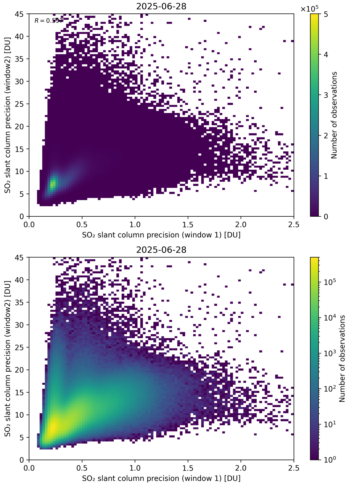
Figure 277: Scatter density plot of “SO 2 slant column precision (window 1)” against “SO 2 slant column precision (window 2)” for 2025-06-27 to 2025-06-29.
