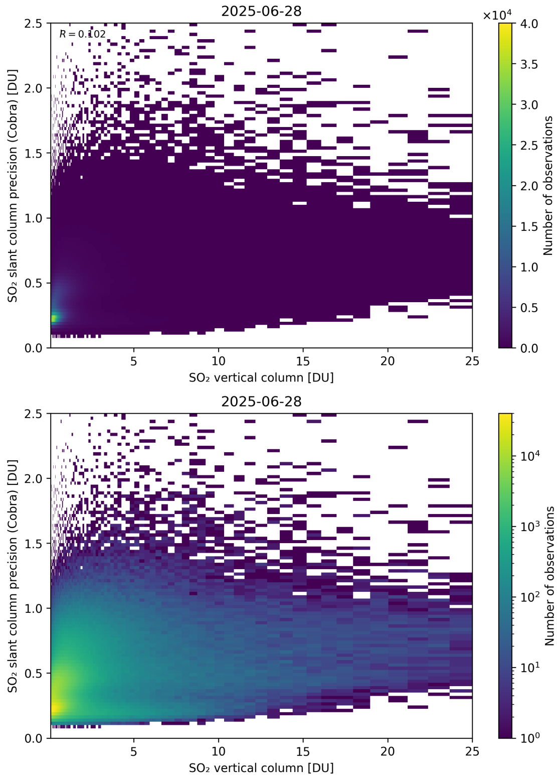
Figure 350: Scatter density plot of “SO 2 vertical column” against “SO 2 slant column precision (Cobra)” for 2025-06-27 to 2025-06-29.
