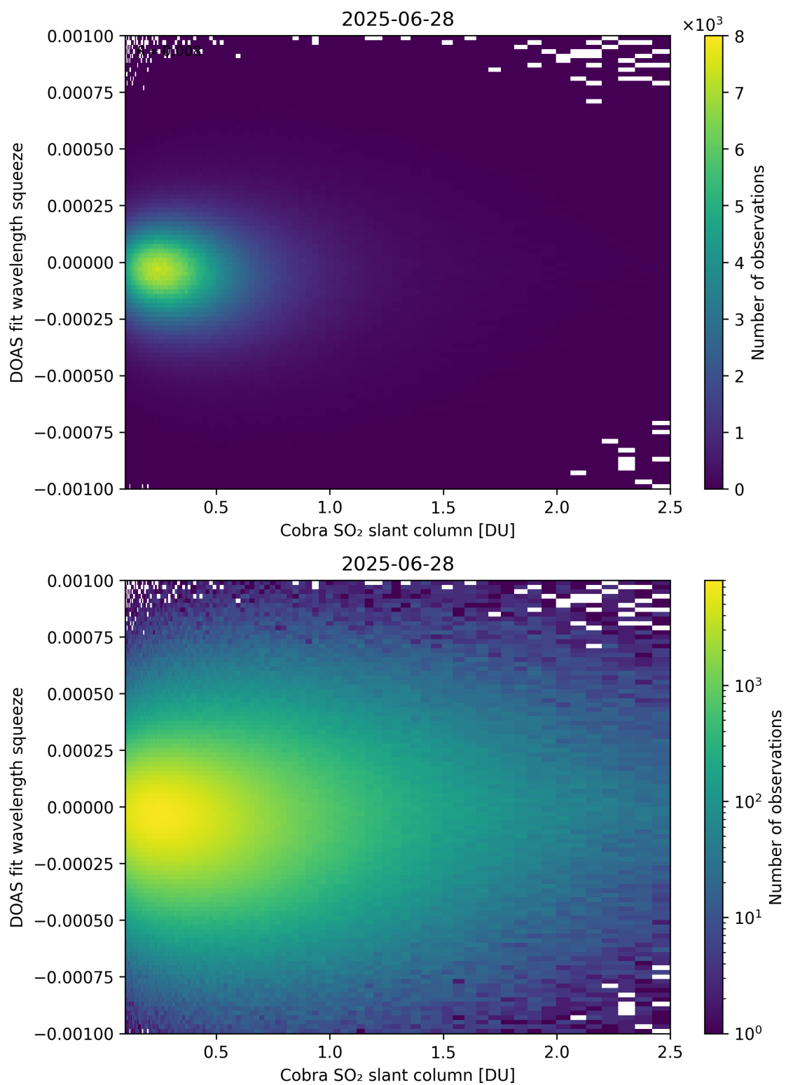
Figure 197: Scatter density plot of “Cobra SO 2 slant column” against “DOAS fit wavelength squeeze” for 2025-06-27 to 2025-06-29.
