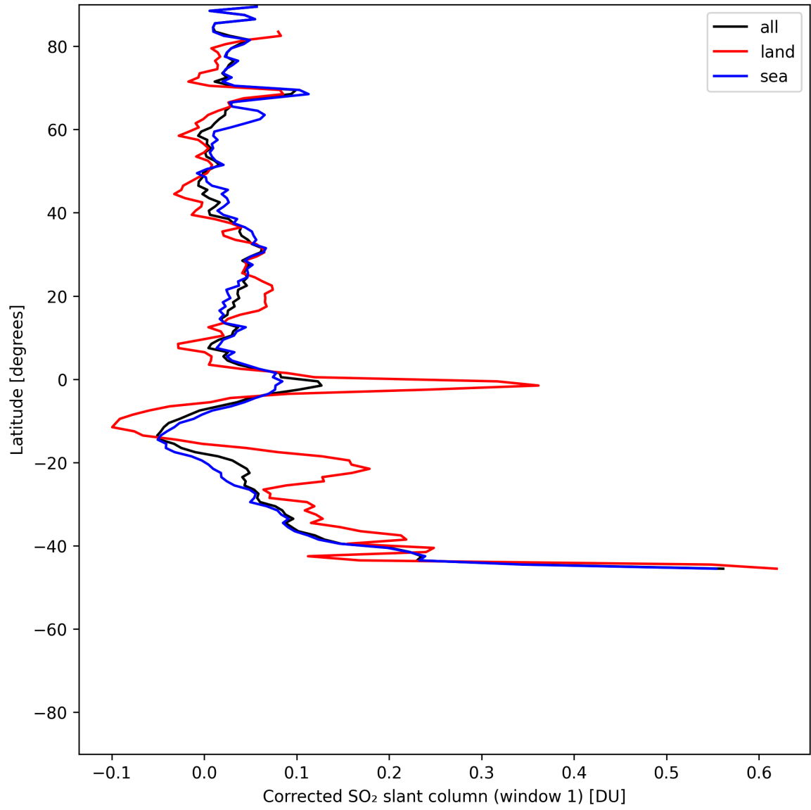
Figure 39: Zonal average of “Corrected SO 2 slant column (window 1)” for 2025-06-27 to 2025-06-29.
