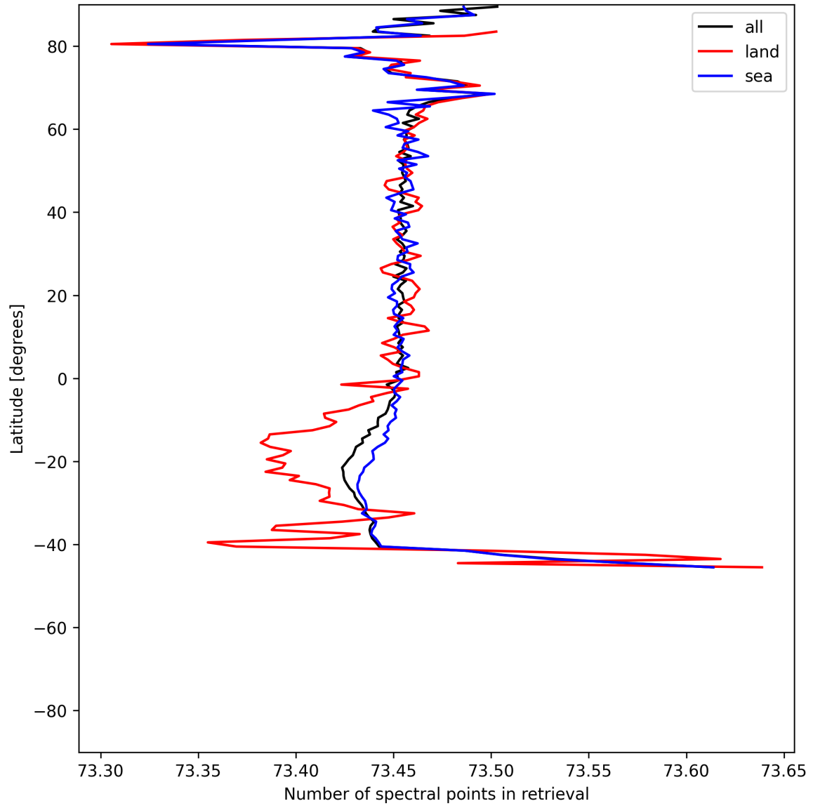
Figure 56: Zonal average of “Number of spectral points in retrieval” for 2025-06-27 to 2025-06-29.
