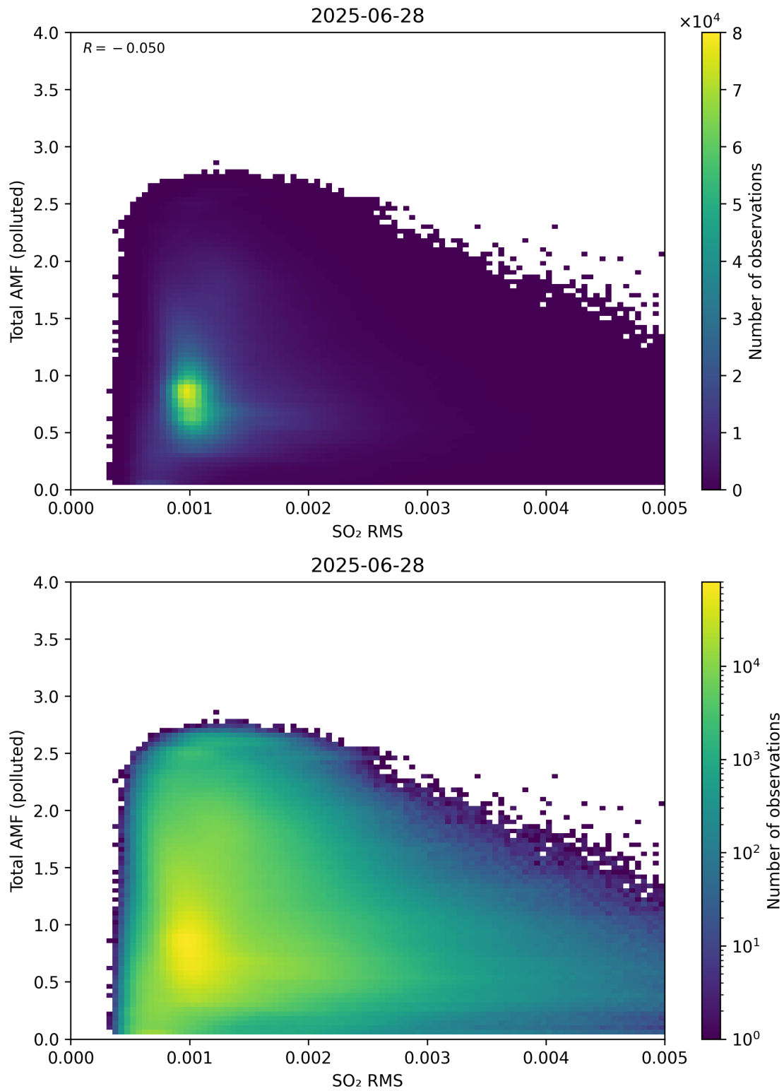
Figure 148: Scatter density plot of “SO 2 RMS” against “Total AMF (polluted)” for 2025-06-27 to 2025-06-29.
