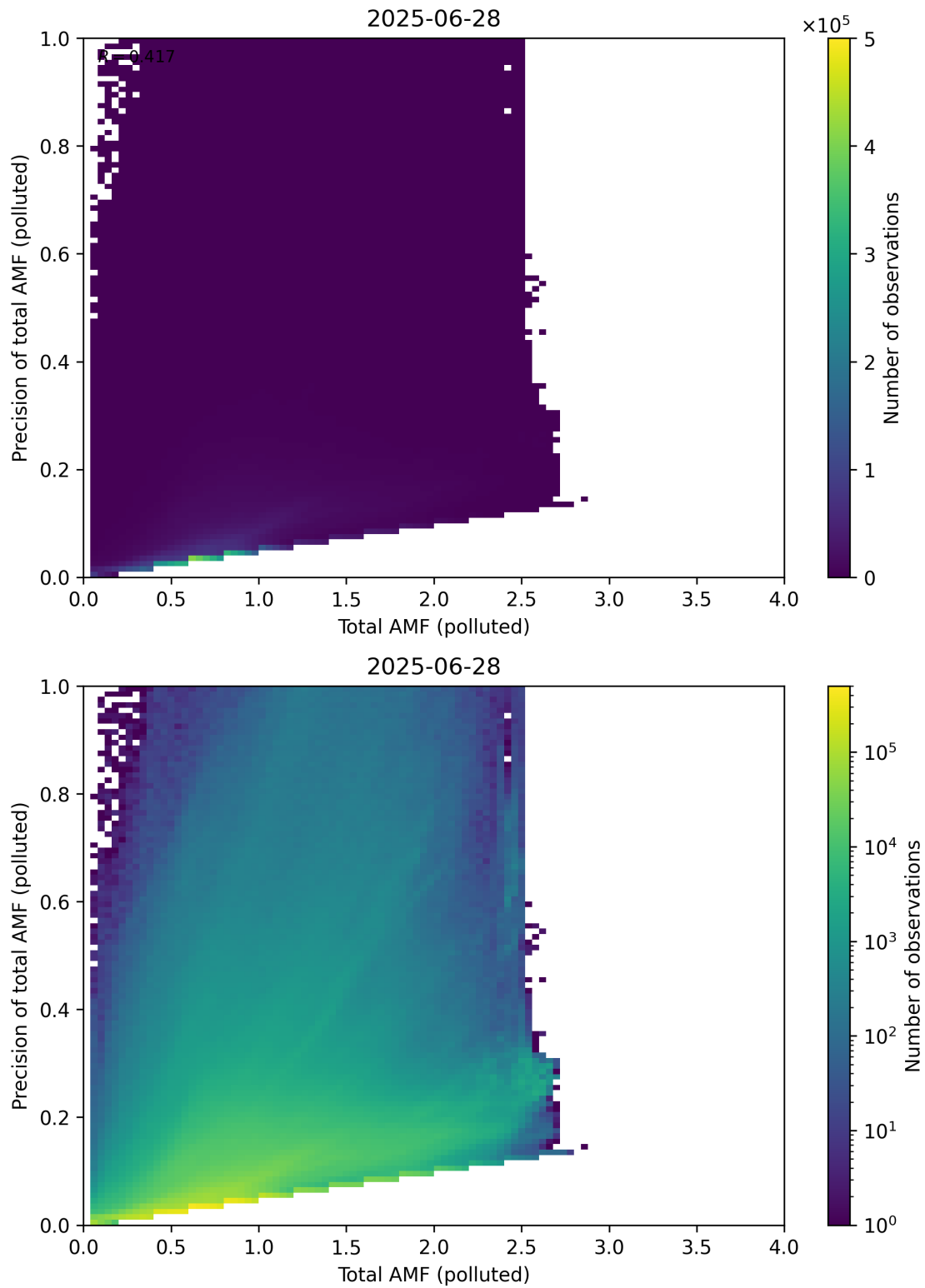
Figure 322: Scatter density plot of “Total AMF (polluted)” against “Precision of total AMF (polluted)” for 2025-06-27 to 2025-06-29.
