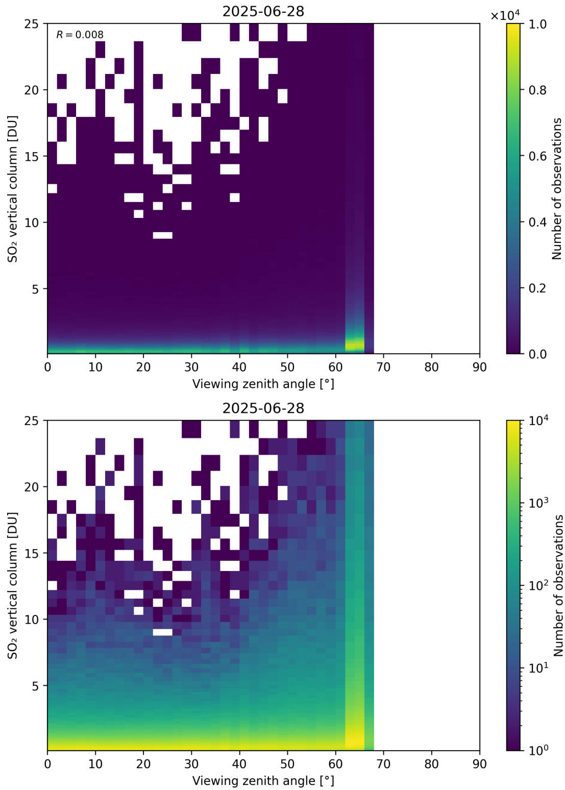
Figure 383: Scatter density plot of “Viewing zenith angle” against “SO 2 vertical column” for 2025-06-27 to 2025-06-29.
