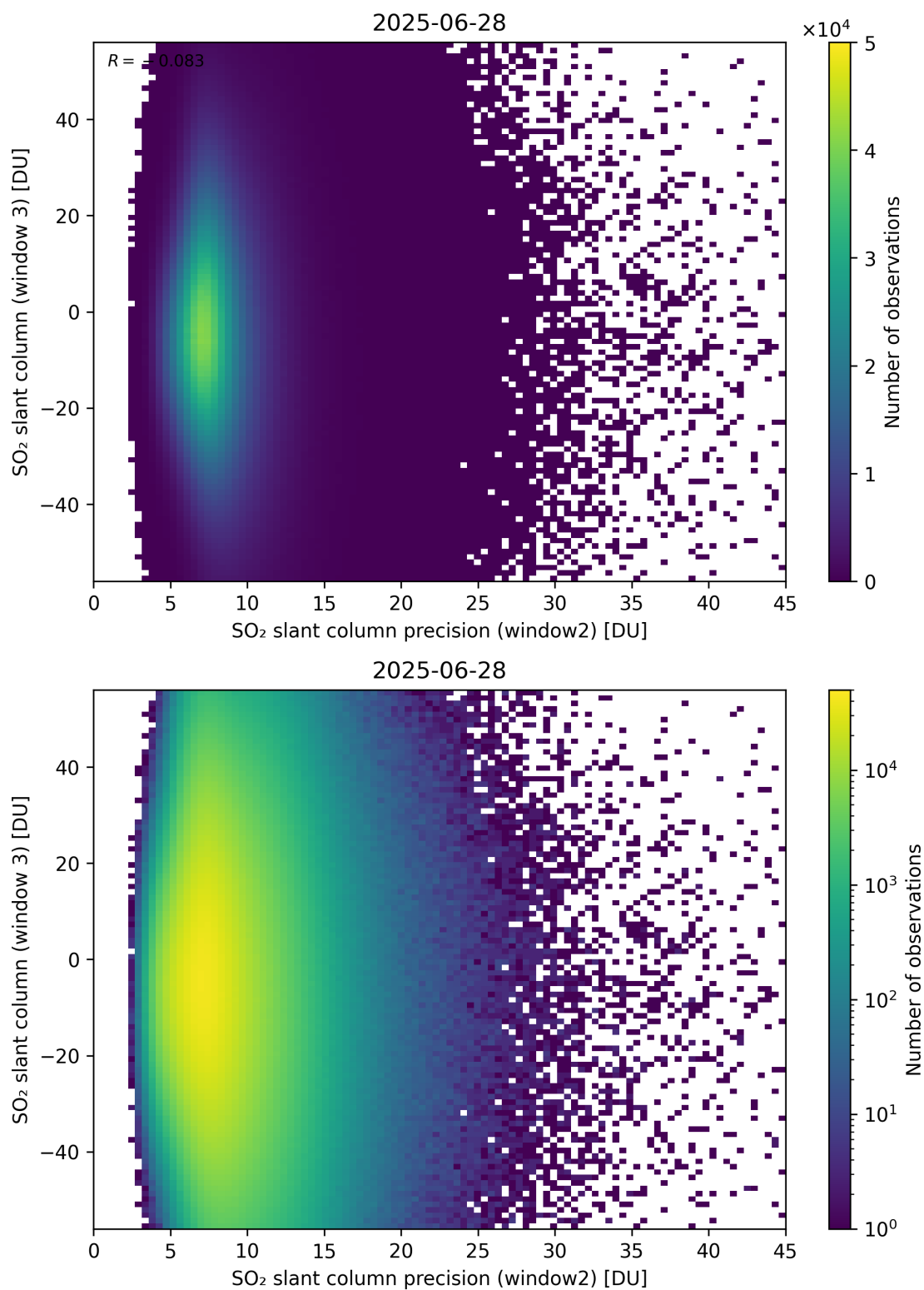
Figure 299: Scatter density plot of “SO 2 slant column precision (window2)” against “SO 2 slant column (window 3)” for 2025-06-27 to 2025-06-29.
