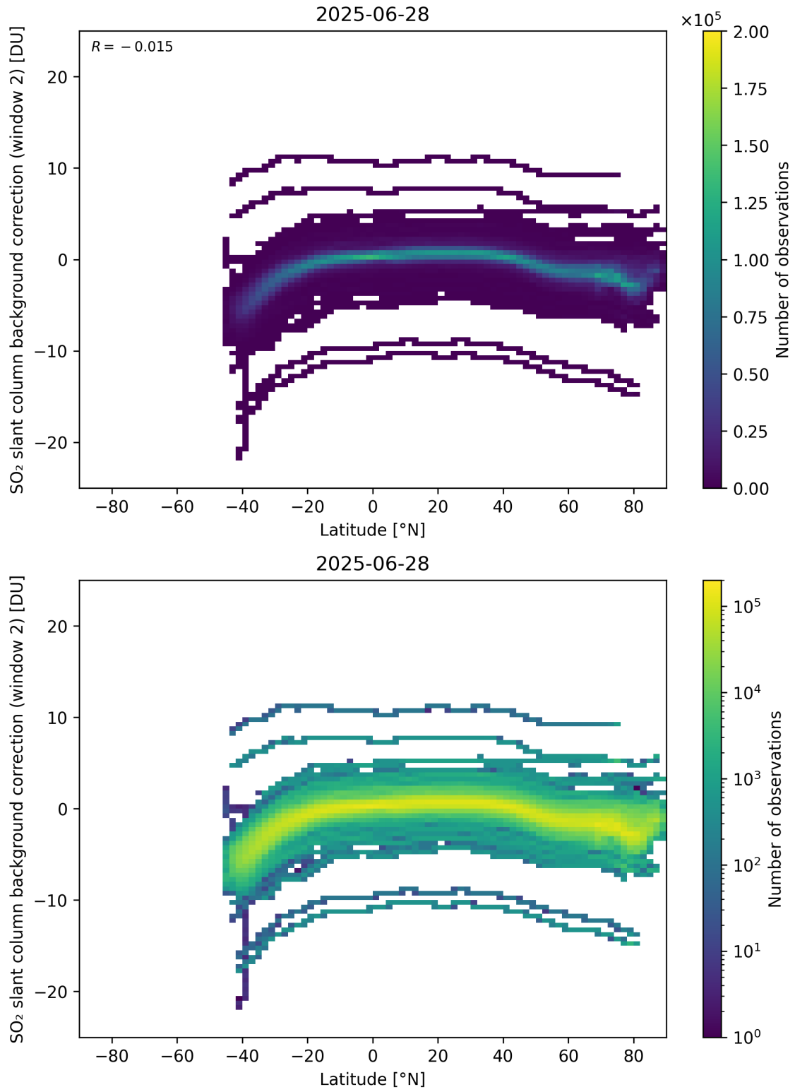
Figure 151: Scatter density plot of “Latitude” against “SO 2 slant column background correction (window 2)” for 2025-06-27 to 2025-06-29.
