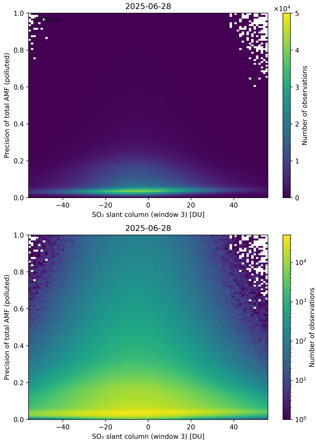
Figure 319: Scatter density plot of “SO 2 slant column (window 3)” against “Precision of total AMF (polluted)” for 2025-06-27 to 2025-06-29.
