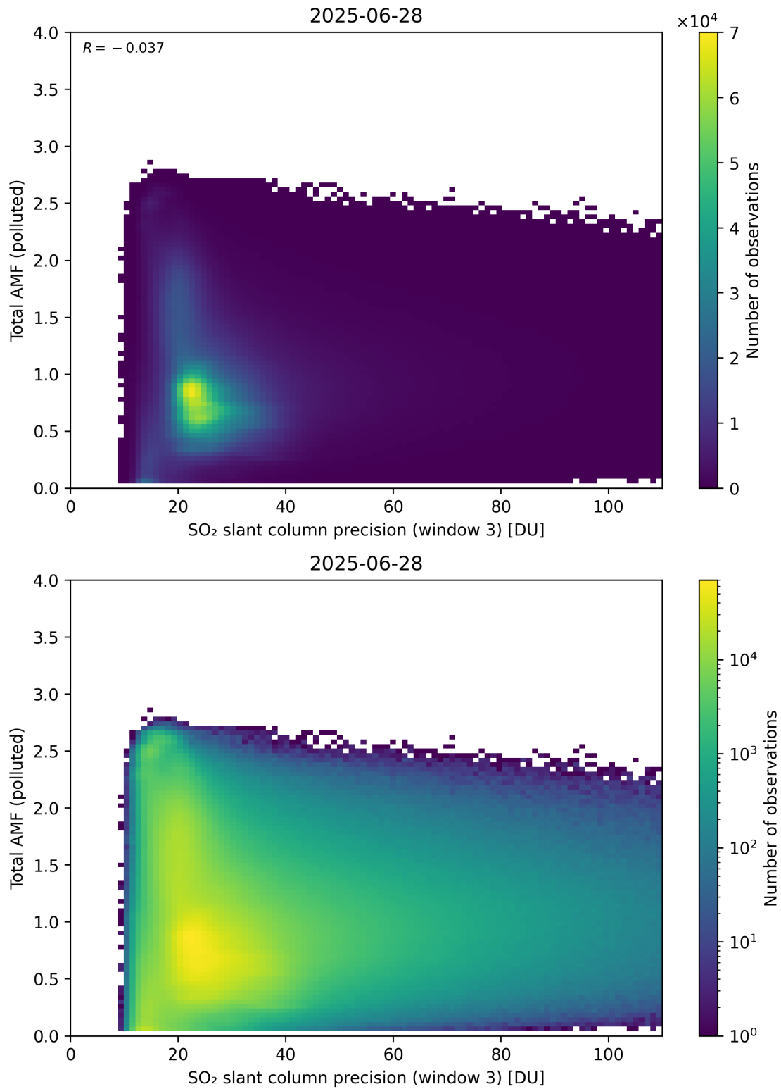
Figure 313: Scatter density plot of “SO 2 slant column precision (window 3)” against “Total AMF (polluted)” for 2025-06-27 to 2025-06-29.
