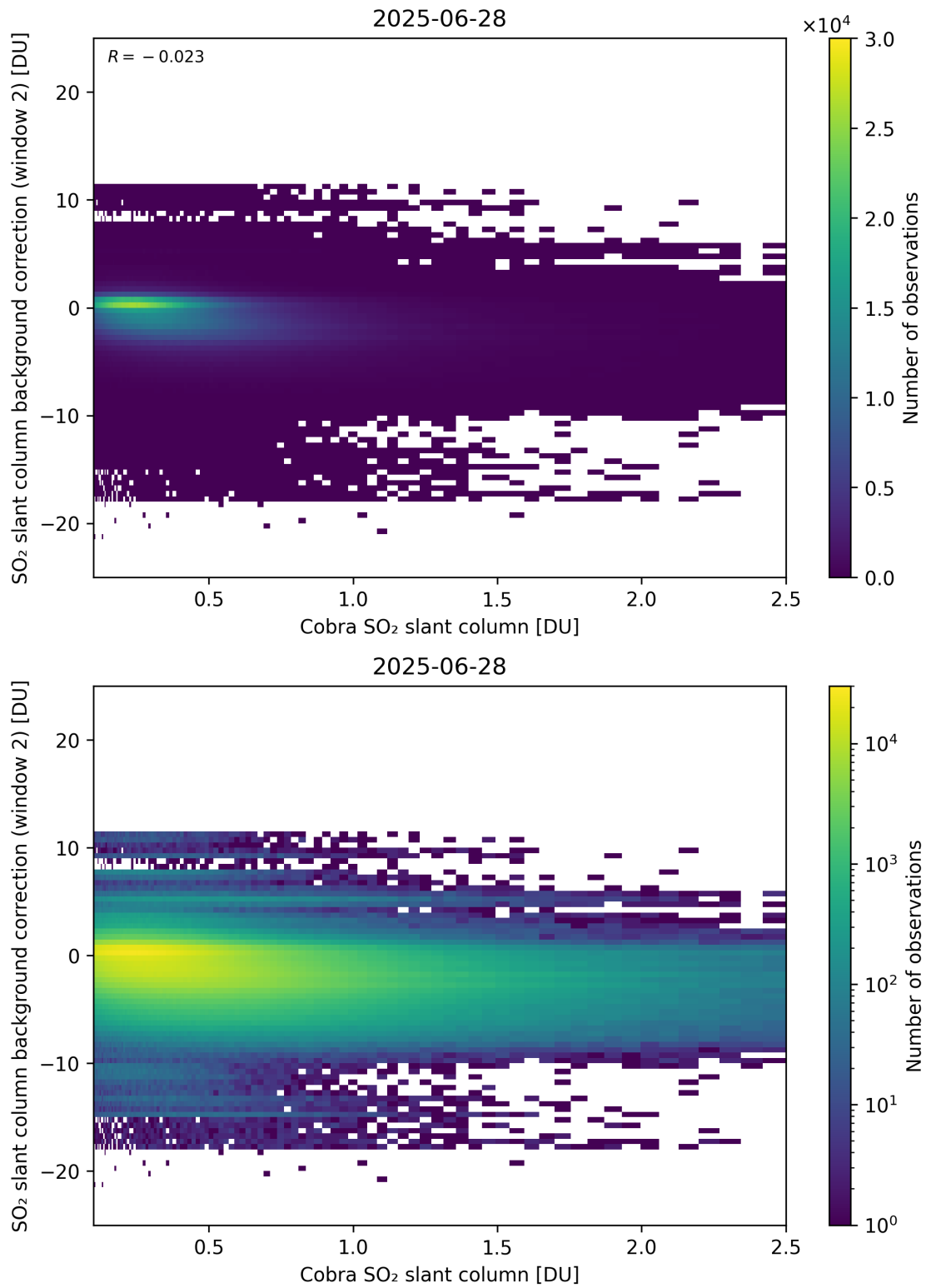
Figure 194: Scatter density plot of “Cobra SO 2 slant column” against “SO 2 slant column background correction (window 2)” for 2025-06-27 to 2025-06-29.
