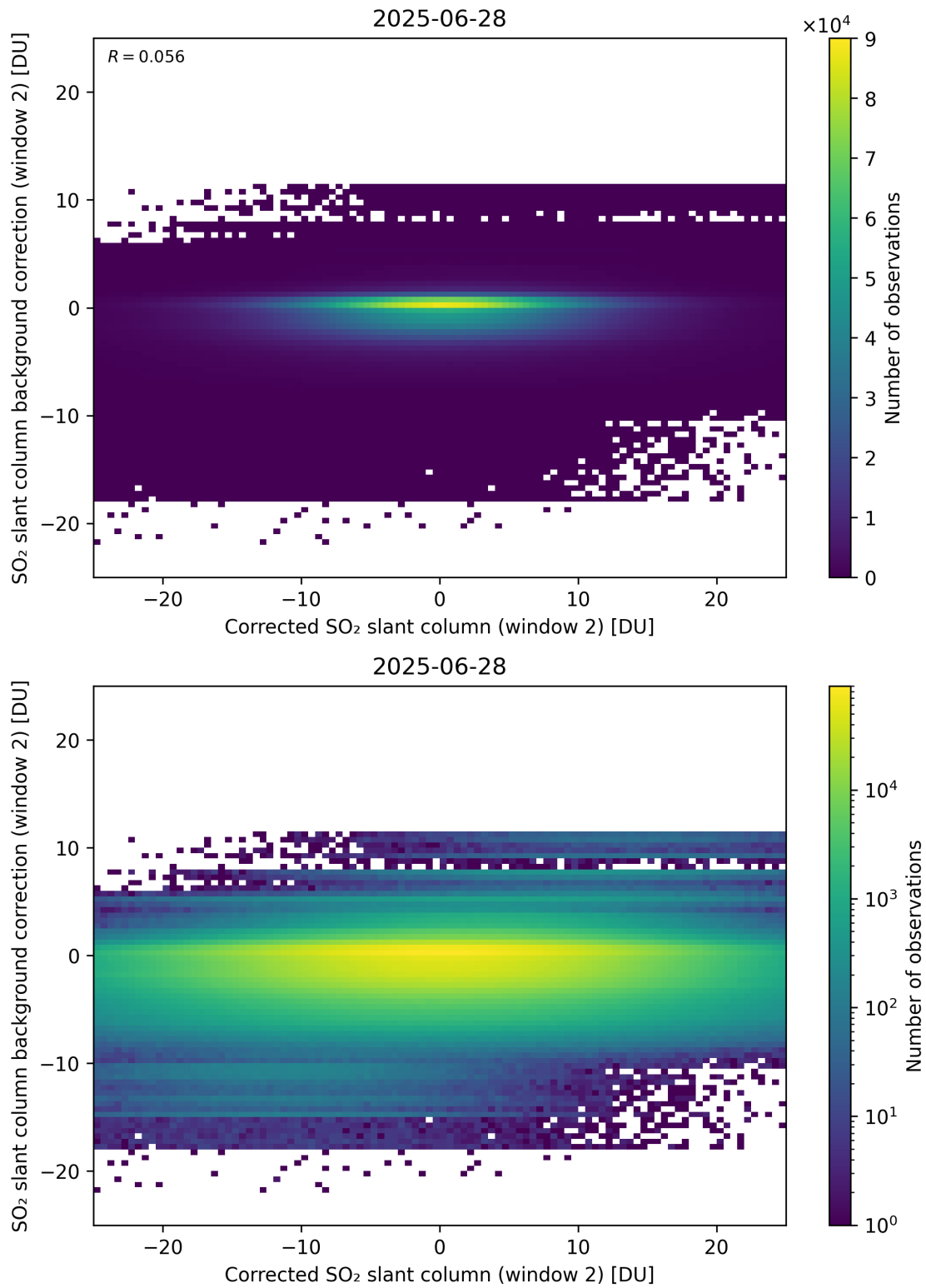
Figure 244: Scatter density plot of “Corrected SO 2 slant column (window 2)” against “SO 2 slant column background correction (window 2)” for 2025-06-27 to 2025-06-29.
