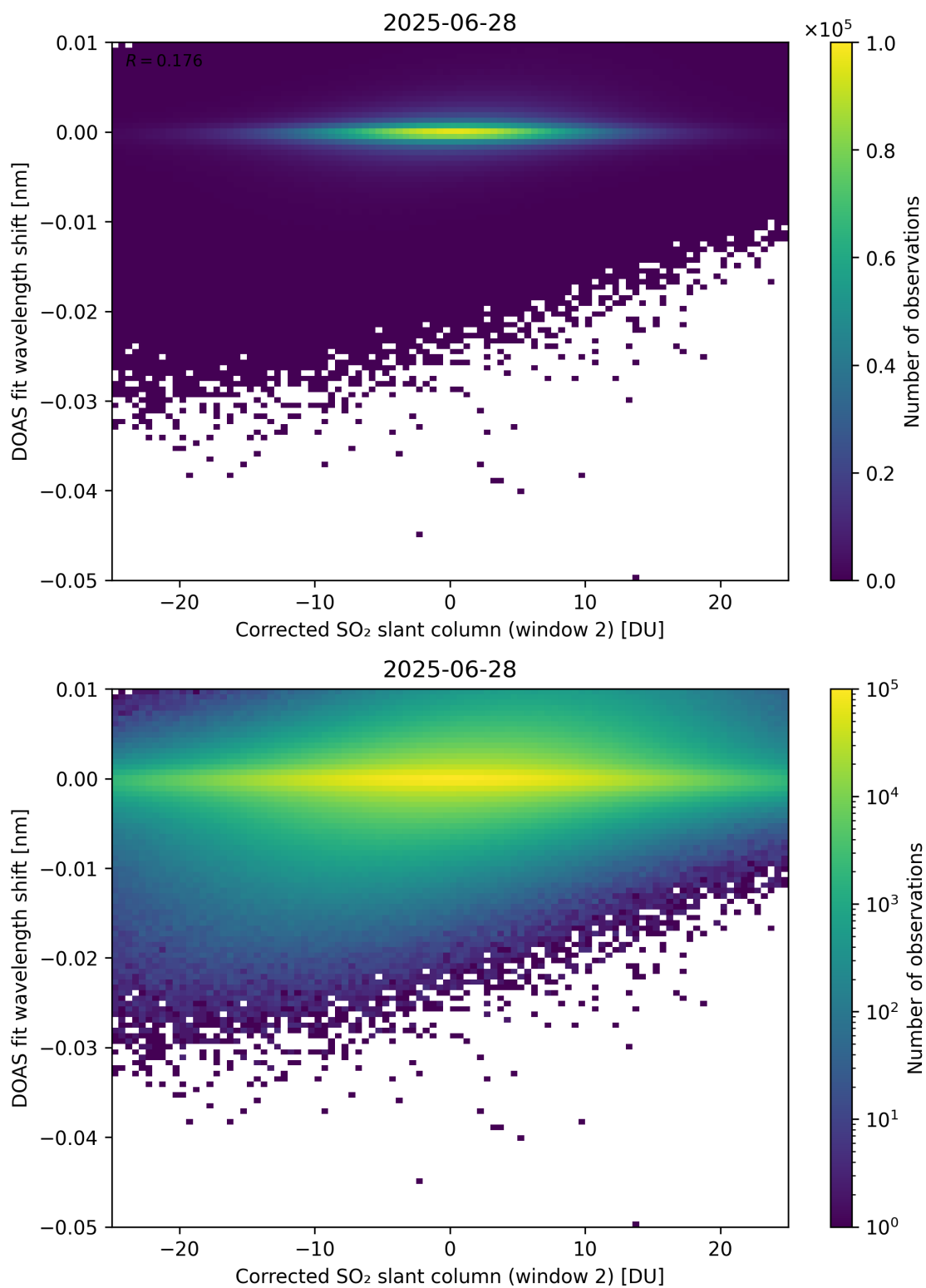
Figure 246: Scatter density plot of “Corrected SO 2 slant column (window 2)” against “DOAS fit wavelength shift” for 2025-06-27 to 2025-06-29.
