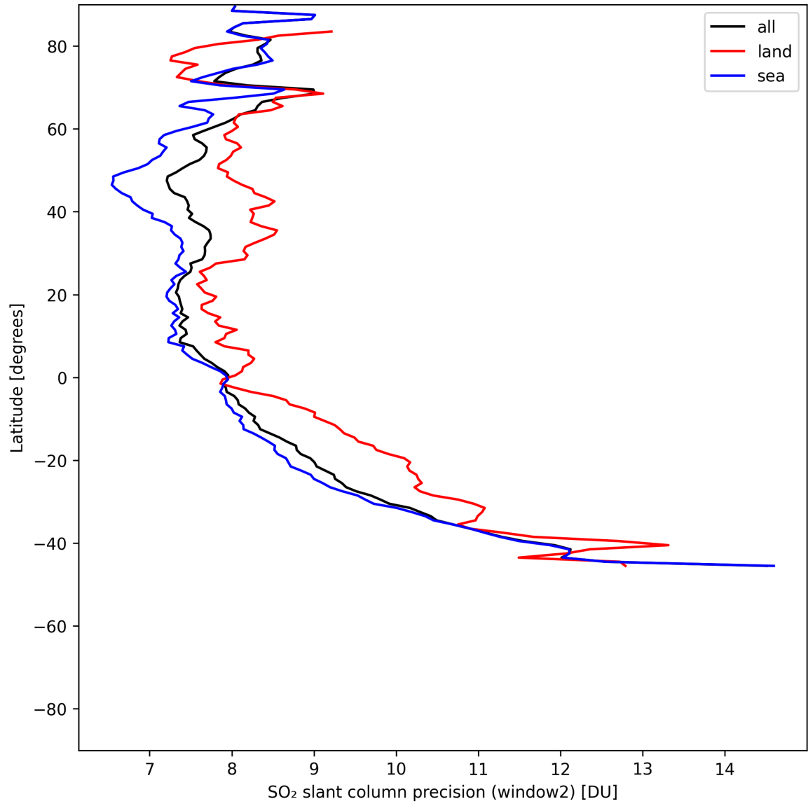
Figure 42: Zonal average of “SO 2 slant column precision (window2)” for 2025-06-27 to 2025-06-29.
