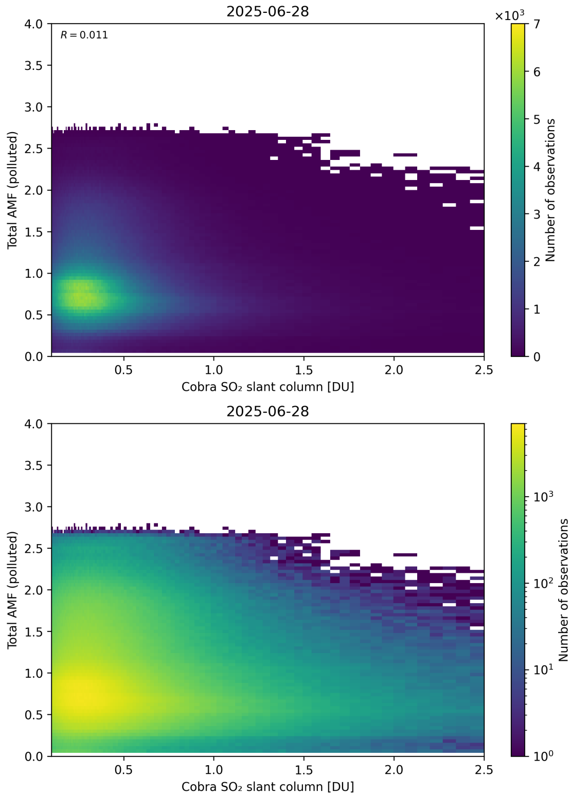
Figure 224: Scatter density plot of “Cobra SO 2 slant column” against “Total AMF (polluted)” for 2025-06-27 to 2025-06-29.
