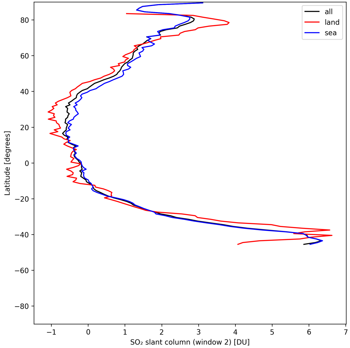
Figure 41: Zonal average of “SO 2 slant column (window 2)” for 2025-06-27 to 2025-06-29.
