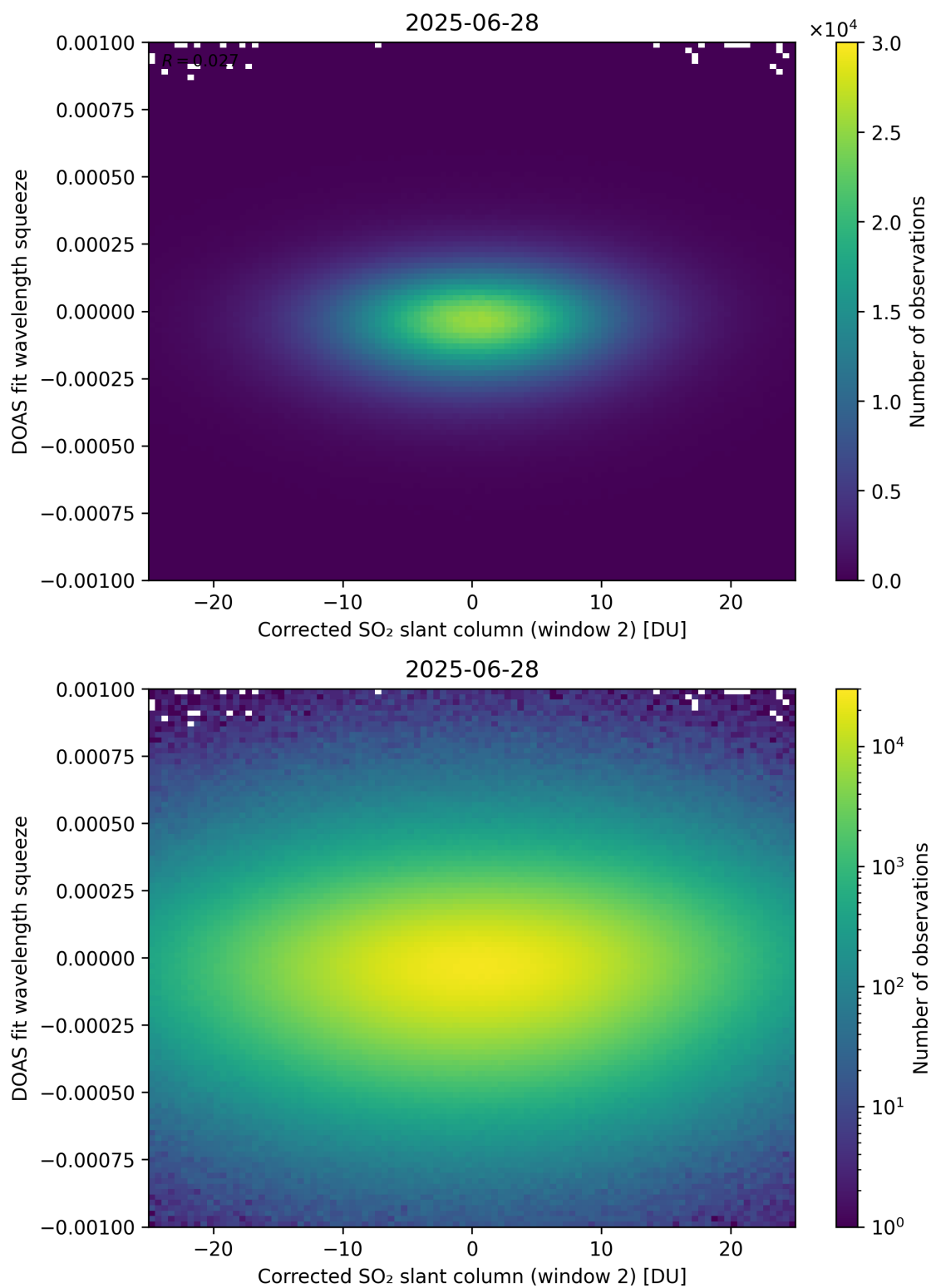
Figure 247: Scatter density plot of “Corrected SO 2 slant column (window 2)” against “DOAS fit wavelength squeeze” for 2025-06-27 to 2025-06-29.
