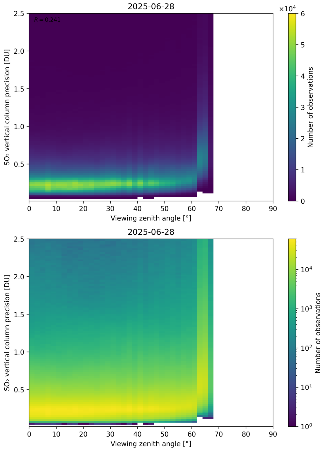
Figure 384: Scatter density plot of “Viewing zenith angle” against “SO 2 vertical column precision” for 2025-06-27 to 2025-06-29.
