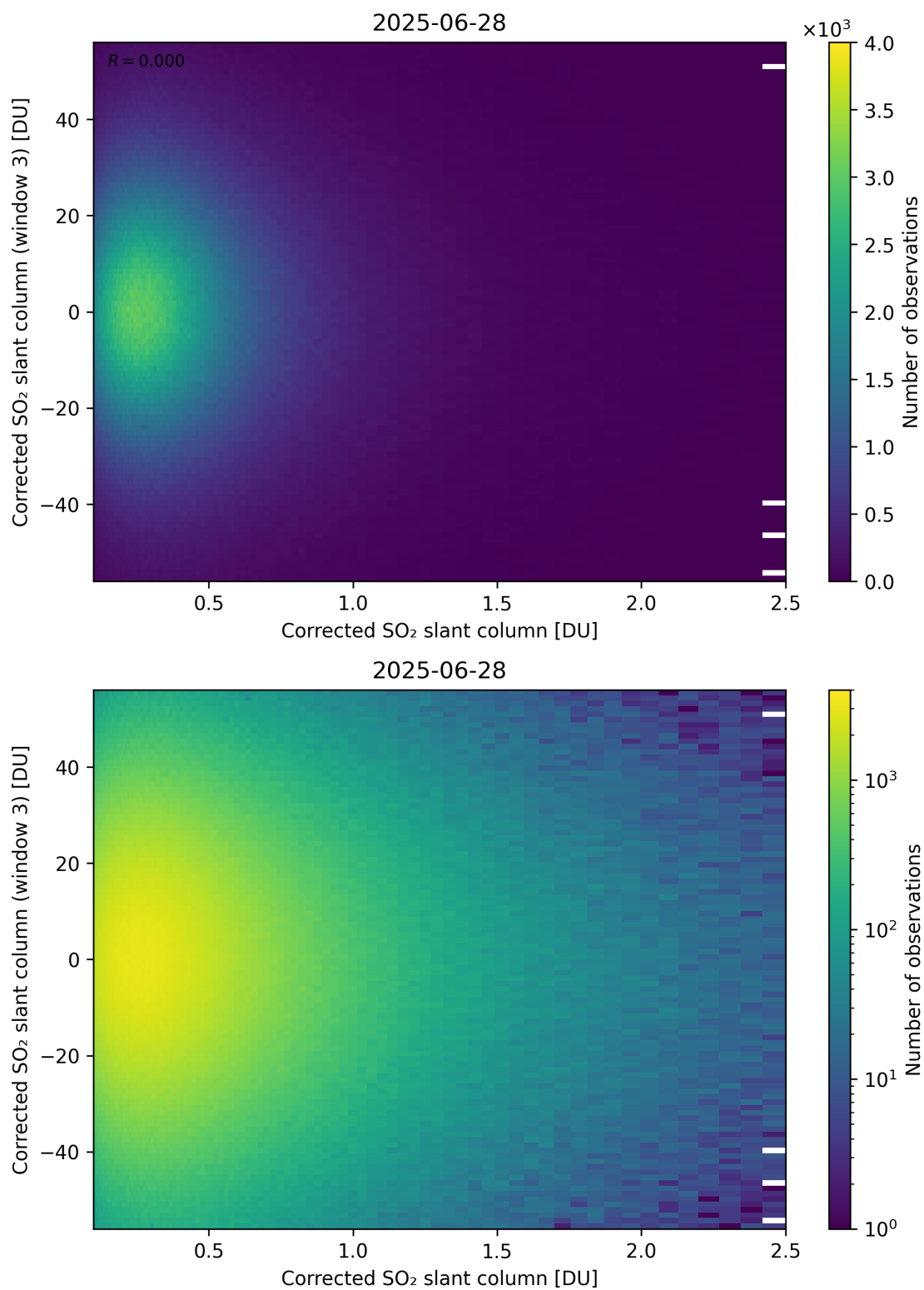
Figure 236: Scatter density plot of “Corrected SO 2 slant column” against “Corrected SO 2 slant column (window 3)” for 2025-06-27 to 2025-06-29.
