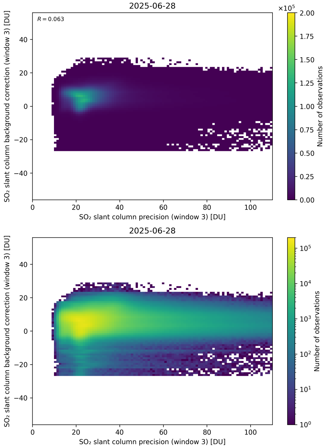
Figure 307: Scatter density plot of “SO 2 slant column precision (window 3)” against “SO 2 slant column background correction (window 3)” for 2025-06-27 to 2025-06-29.
