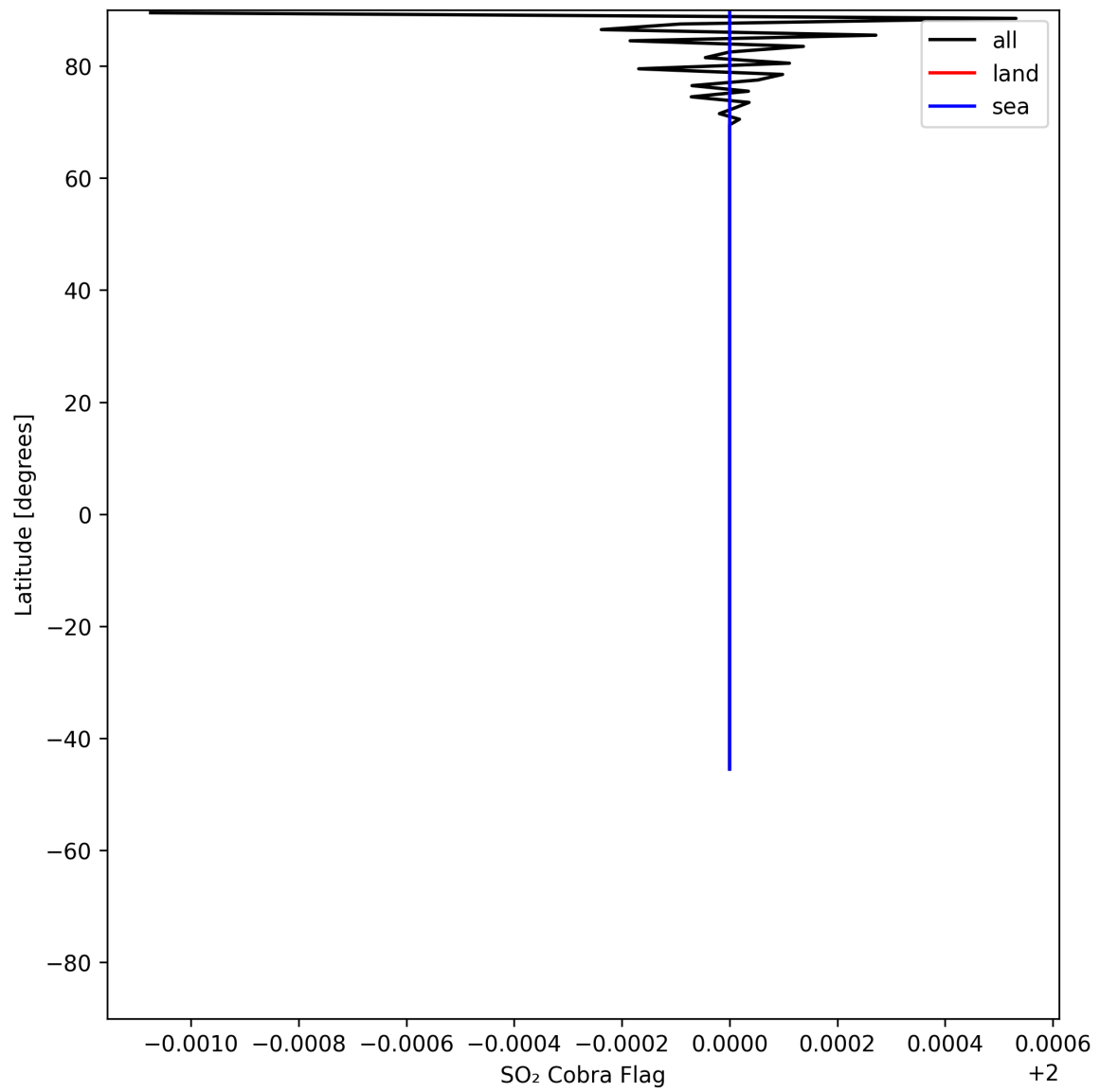
Figure 49: Zonal average of “SO 2 Cobra Flag” for 2025-06-27 to 2025-06-29.
