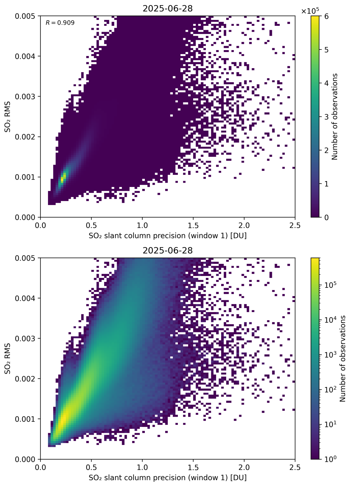
Figure 273: Scatter density plot of “SO 2 slant column precision (window 1)” against “SO 2 RMS” for 2025-06-27 to 2025-06-29.
