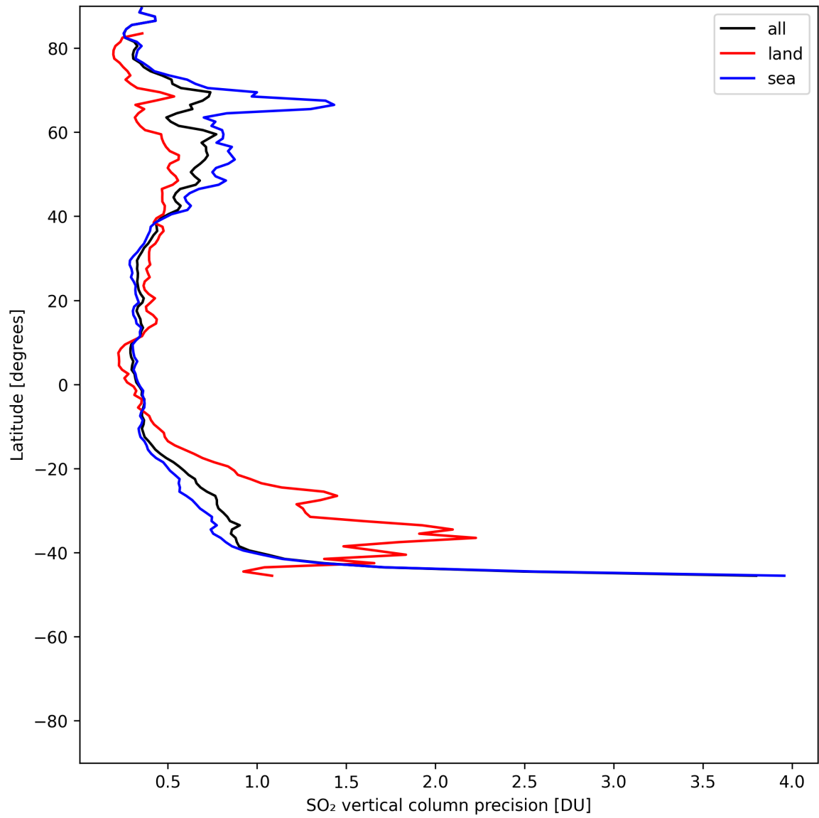
Figure 33: Zonal average of “SO 2 vertical column precision” for 2025-06-27 to 2025-06-29.
