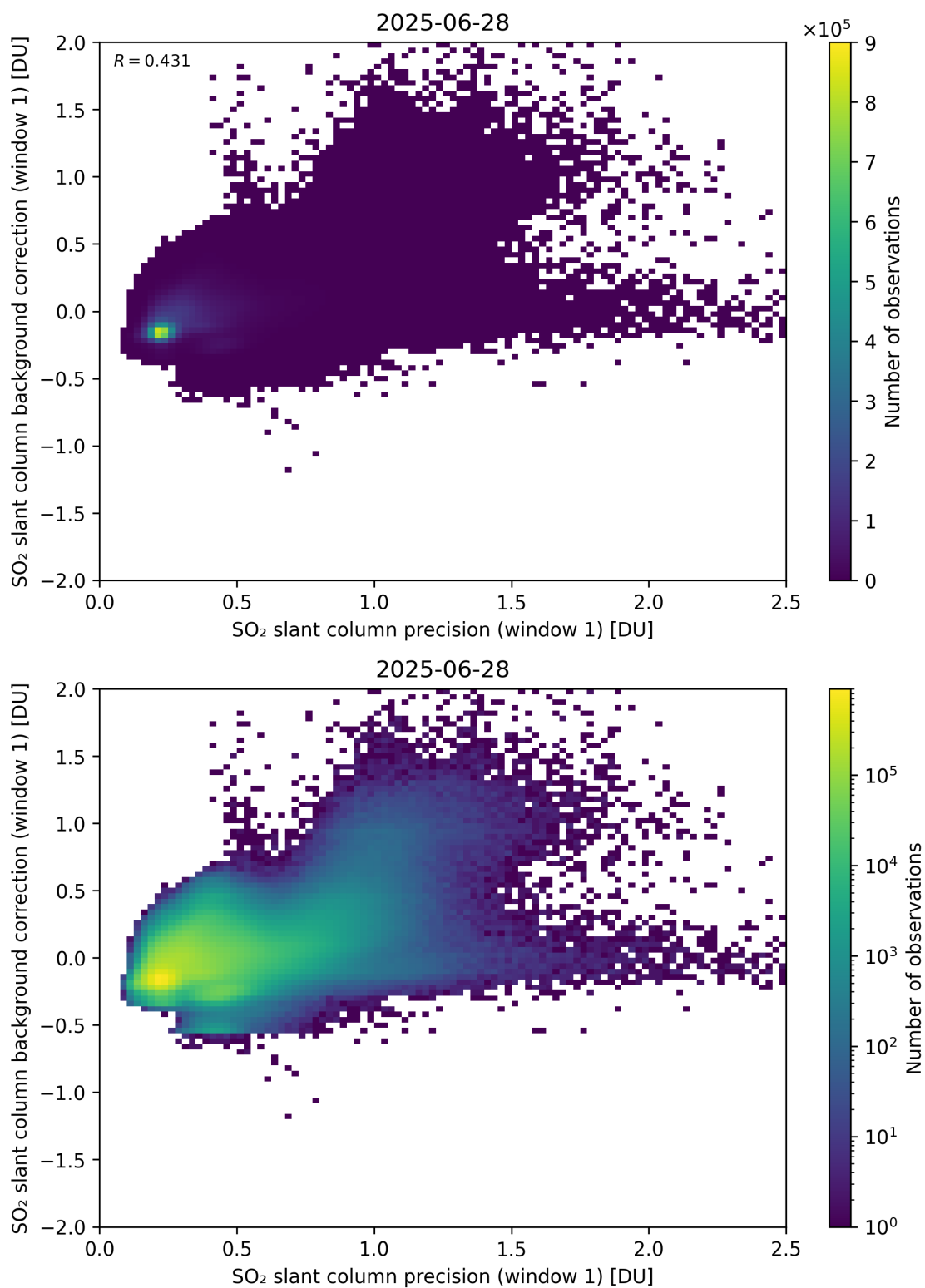
Figure 268: Scatter density plot of “SO 2 slant column precision (window 1)” against “SO 2 slant column background correction (window 1)” for 2025-06-27 to 2025-06-29.
