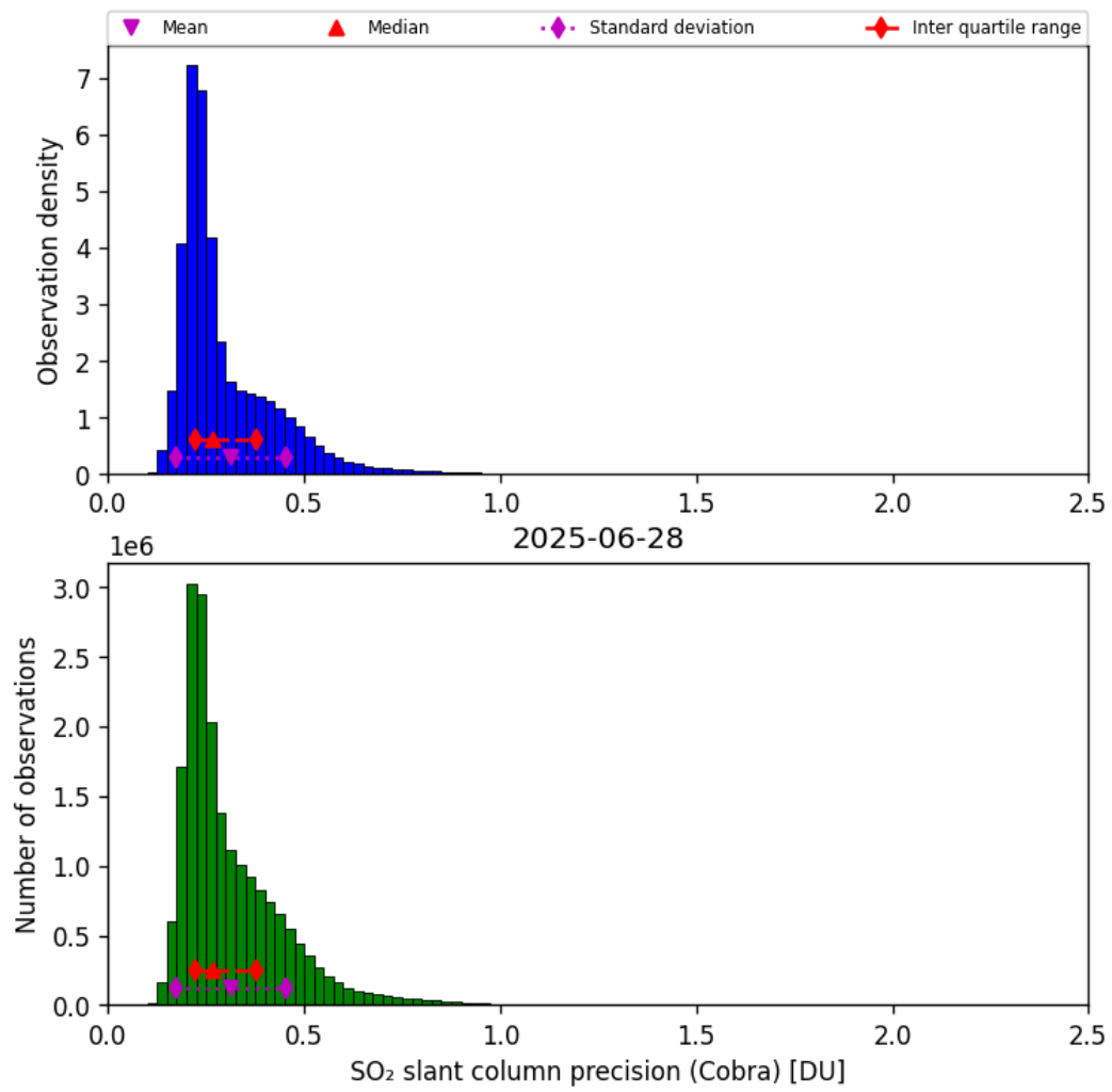
Figure 62: Histogram of “SO 2 slant column precision (Cobra)” for 2025-06-27 to 2025-06-29
