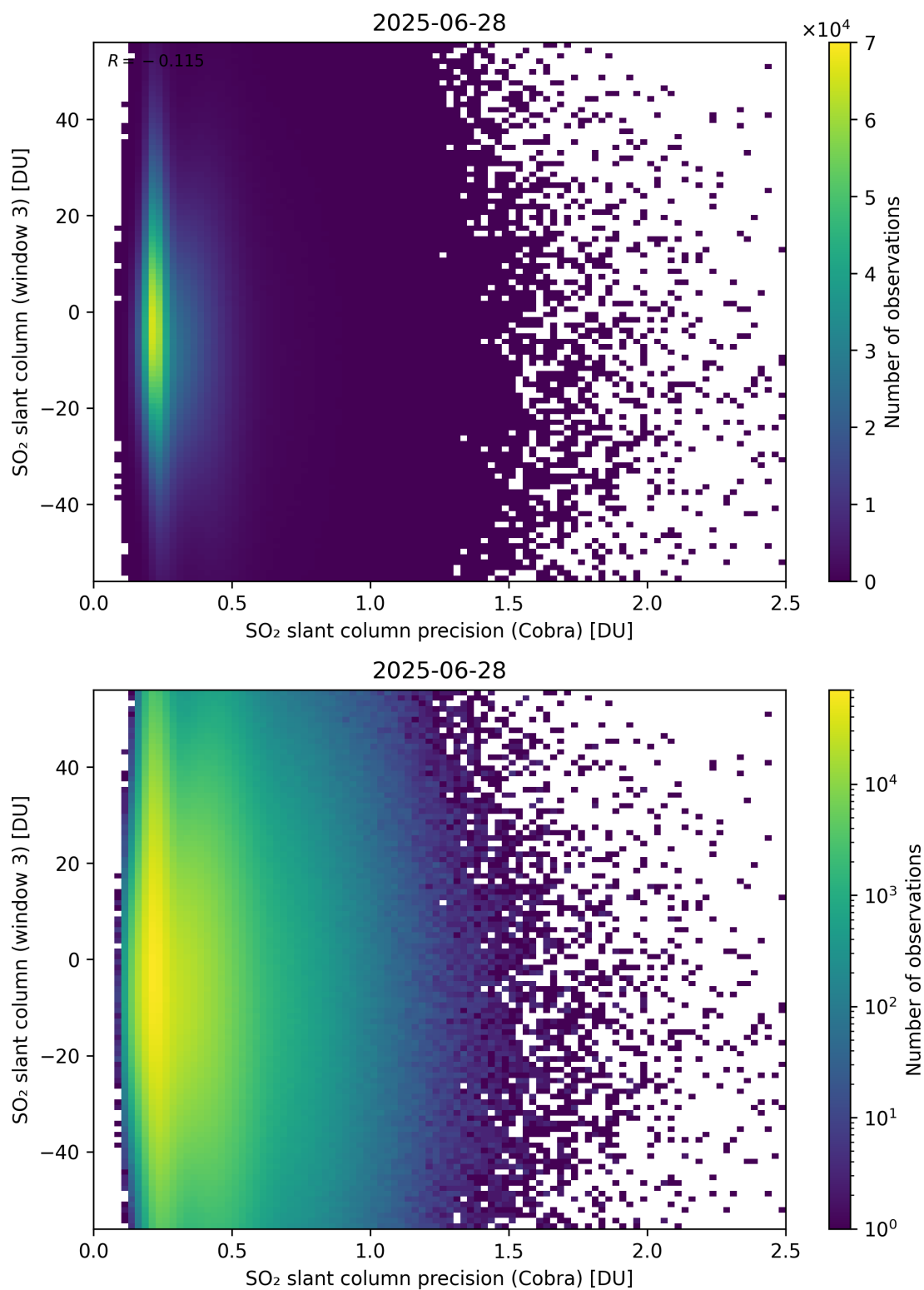
Figure 211: Scatter density plot of “SO 2 slant column precision (Cobra)” against “SO 2 slant column (window 3)” for 2025-06-27 to 2025-06-29.
