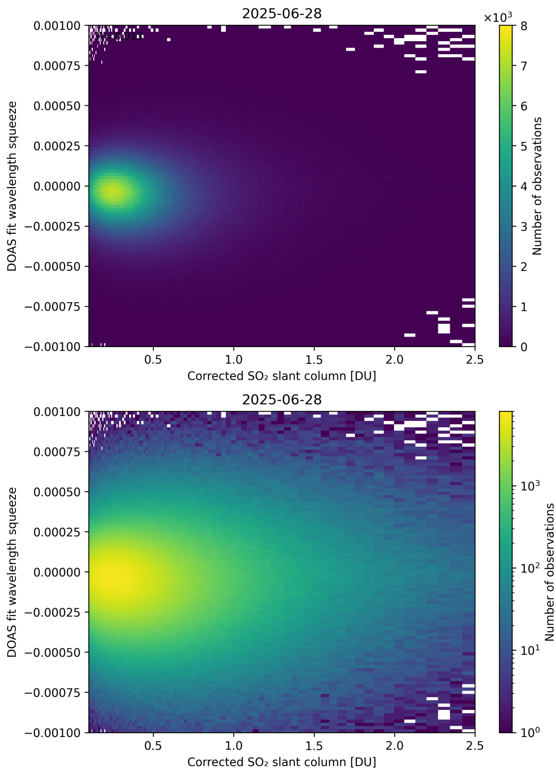
Figure 230: Scatter density plot of "Corrected SO 2 slant column" against "DOAS fit wavelength squeeze" for 2025-06-27 to 2025-06-29.
