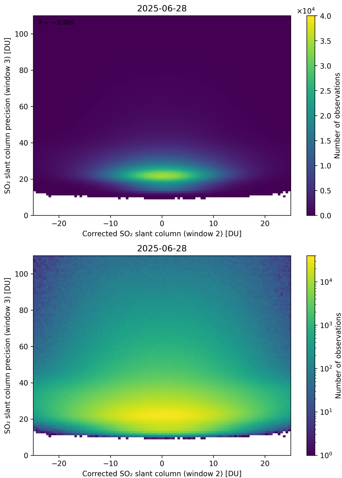
Figure 252: Scatter density plot of “Corrected SO 2 slant column (window 2)” against “SO 2 slant column precision (window 3)” for 2025-06-27 to 2025-06-29.
