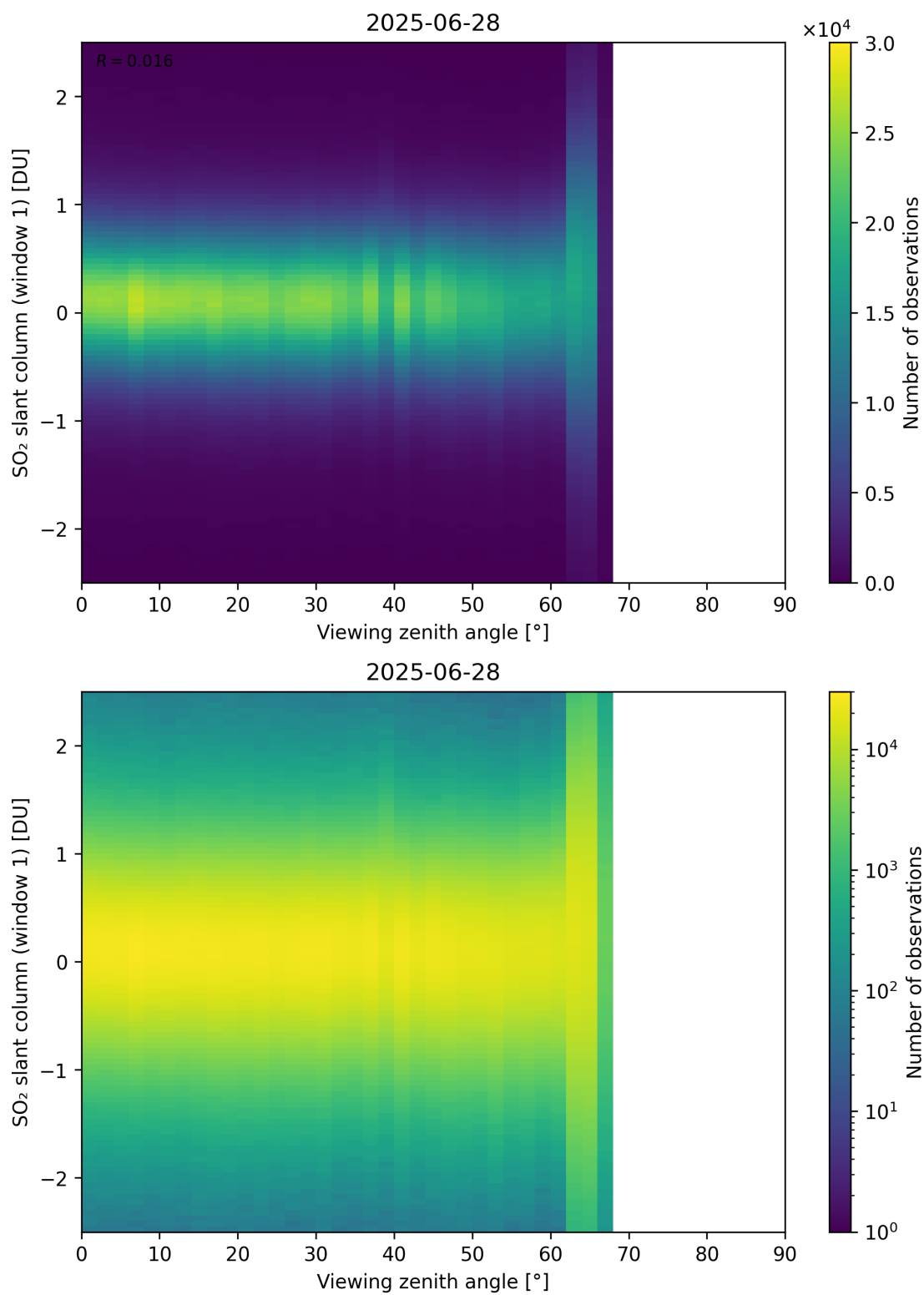
Figure 376: Scatter density plot of “Viewing zenith angle” against “SO 2 slant column (window 1)” for 2025-06-27 to 2025-06-29.
