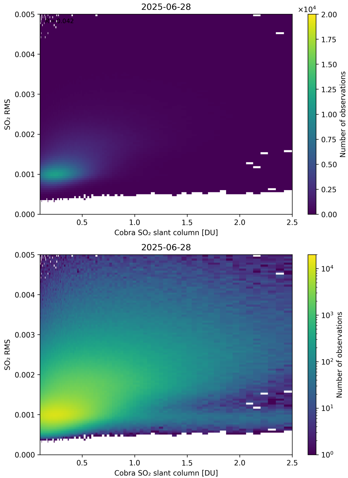
Figure 198: Scatter density plot of “Cobra SO 2 slant column” against “SO 2 RMS” for 2025-06-27 to 2025-06-29.
