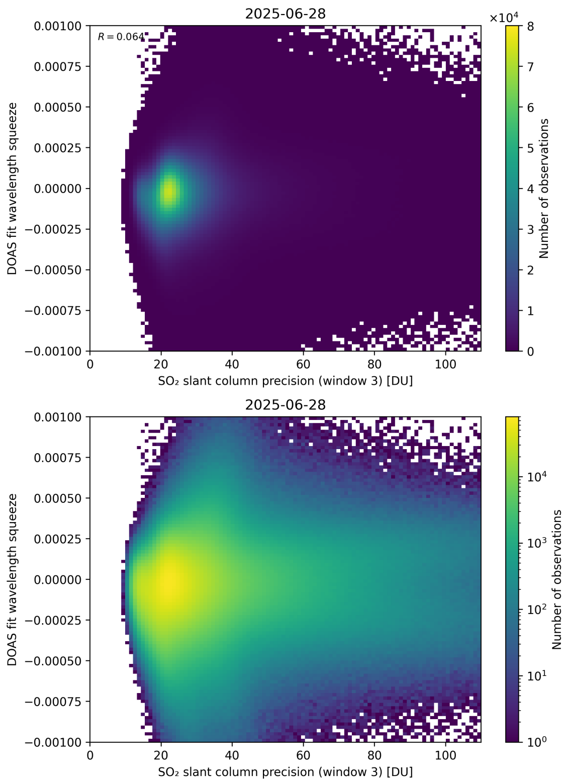
Figure 309: Scatter density plot of “SO 2 slant column precision (window 3)” against “DOAS fit wavelength squeeze” for 2025-06-27 to 2025-06-29.
