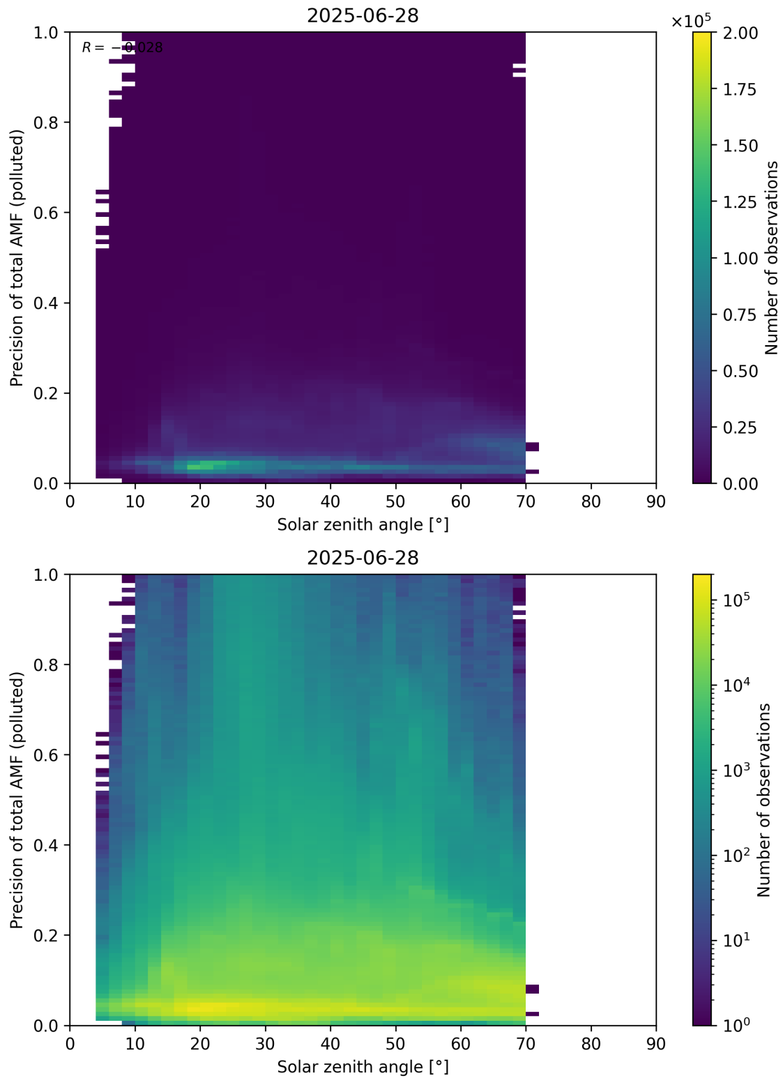
Figure 190: Scatter density plot of “Solar zenith angle” against “Precision of total AMF (polluted)” for 2025-06-27 to 2025-06-29.
