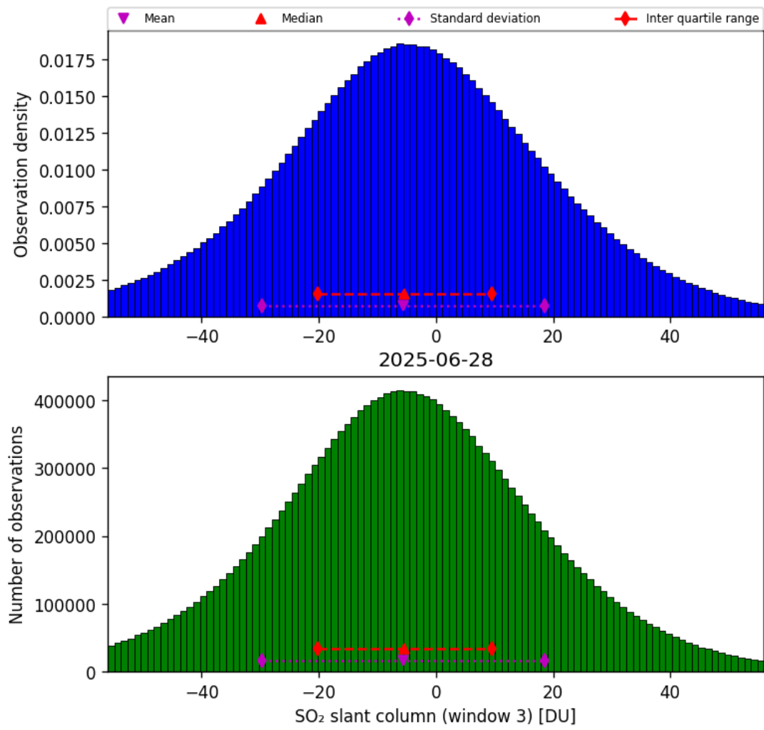
Figure 71: Histogram of “SO 2 slant column (window 3)” for 2025-06-27 to 2025-06-29
