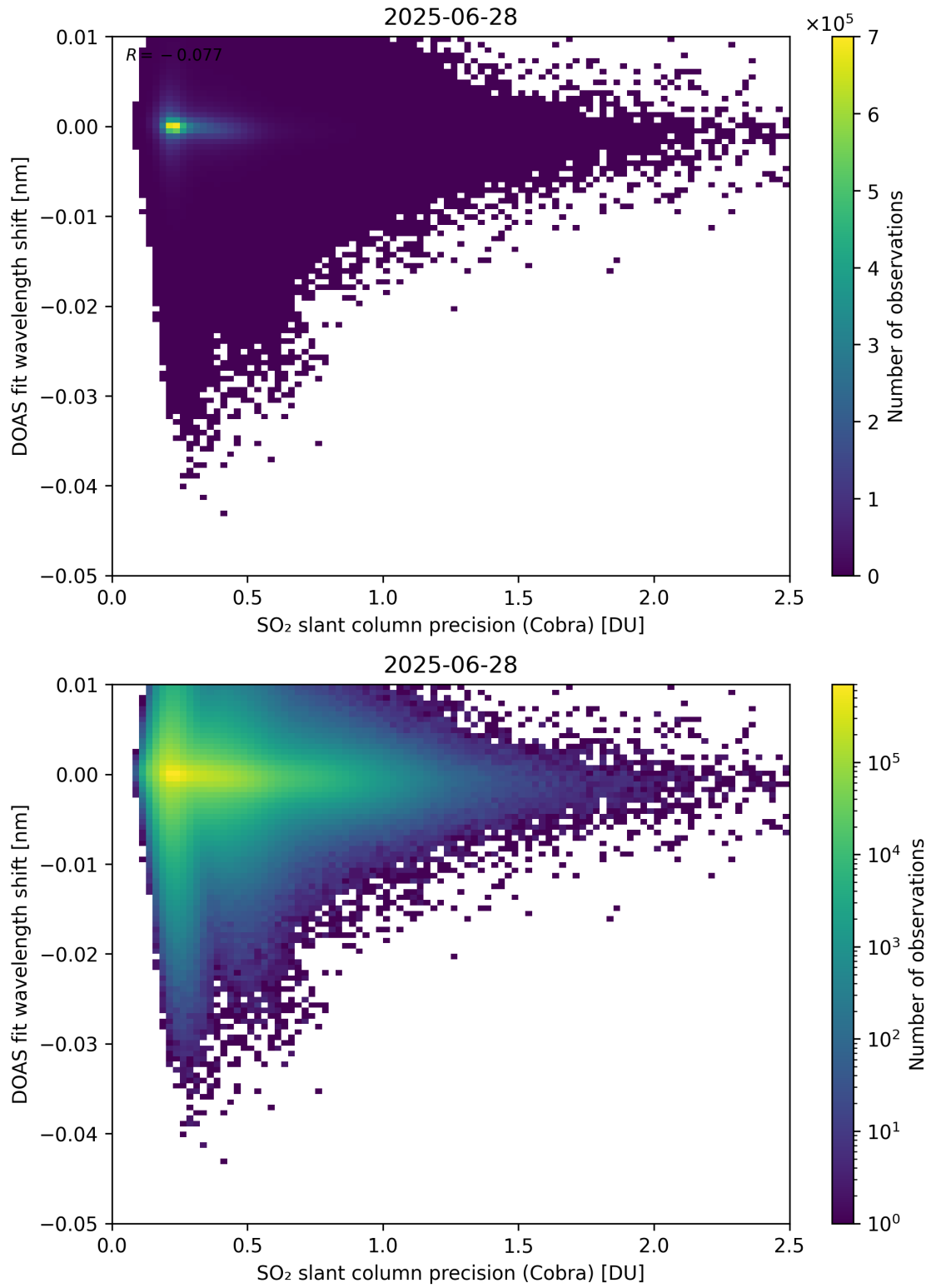
Figure 202: Scatter density plot of “SO 2 slant column precision (Cobra)” against “DOAS fit wavelength shift” for 2025-06-27 to 2025-06-29.
