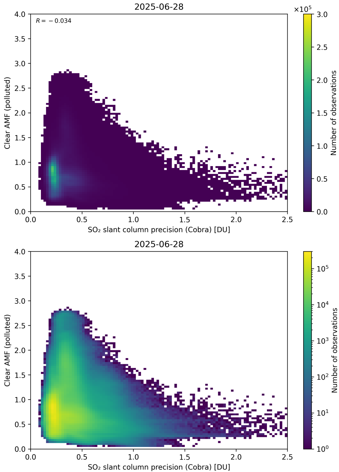
Figure 205: Scatter density plot of “SO 2 slant column precision (Cobra)” against “Clear AMF (polluted)” for 2025-06-27 to 2025-06-29.
