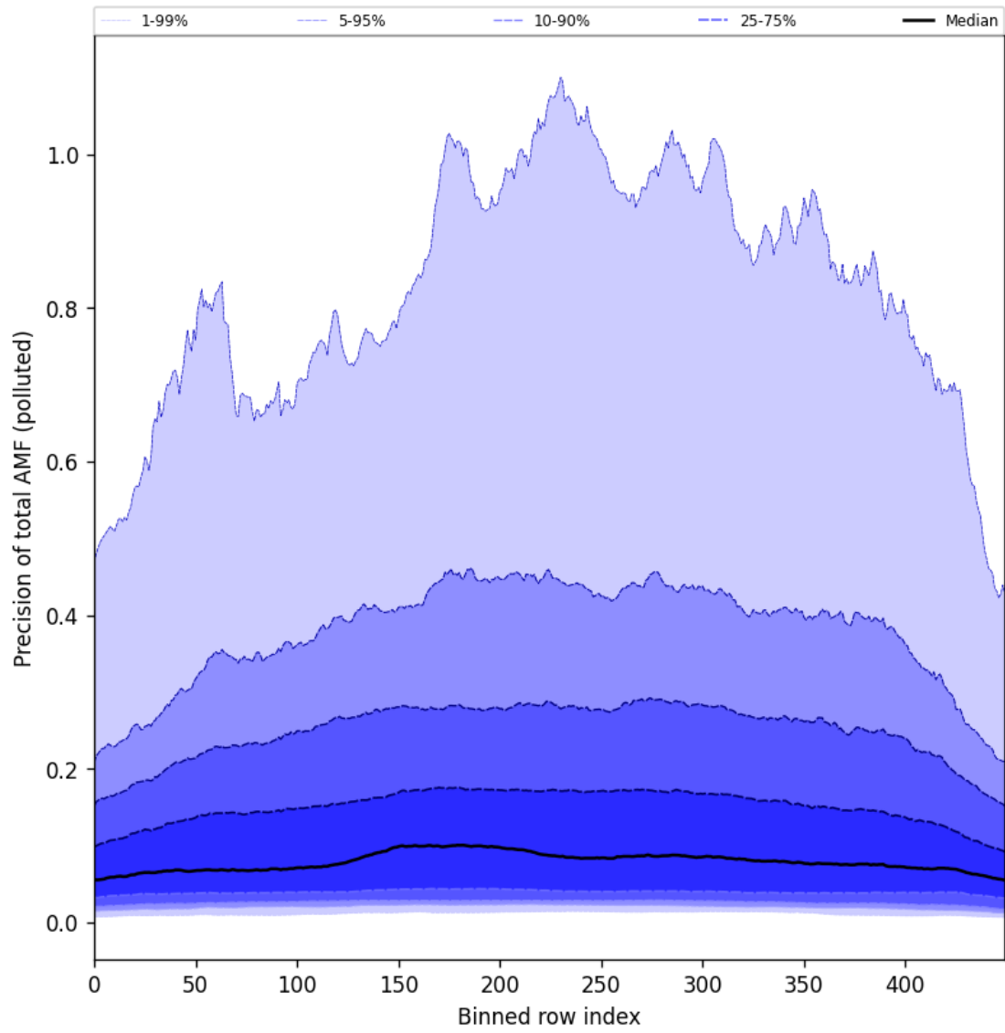
Figure 106: Along track statistics of “Precision of total AMF (polluted)” for 2025-06-27 to 2025-06-29
