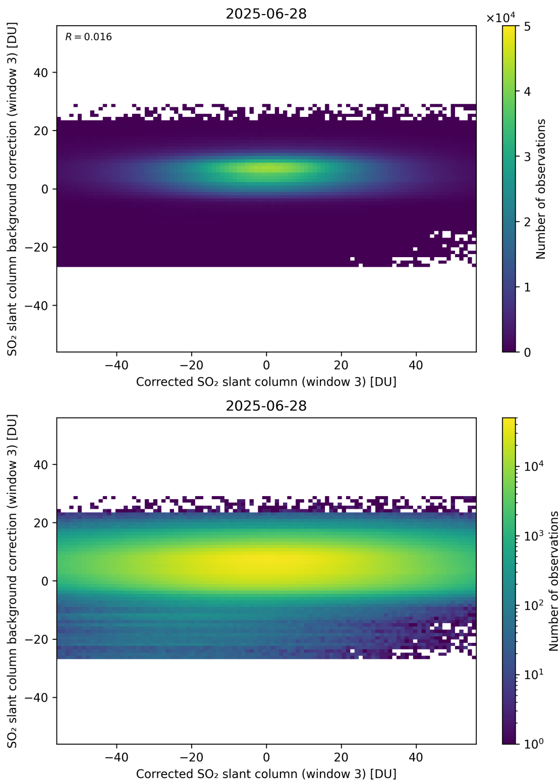
Figure 255: Scatter density plot of “Corrected SO 2 slant column (window 3)” against “SO 2 slant column background correction (window 3)” for 2025-06-27 to 2025-06-29.
