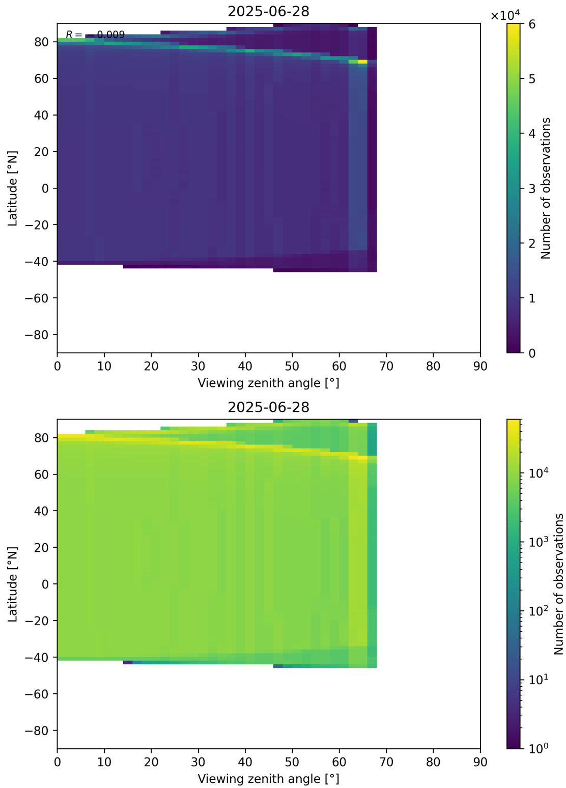
Figure 368: Scatter density plot of “Viewing zenith angle” against “Latitude” for 2025-06-27 to 2025-06-29.
