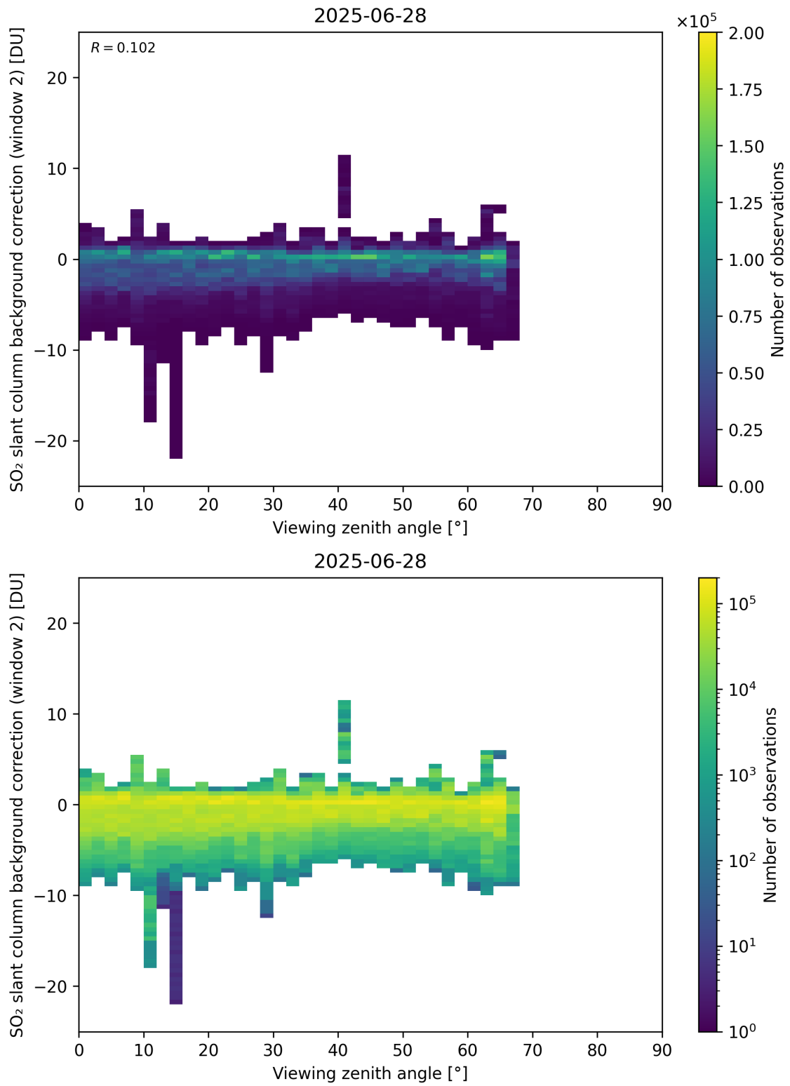
Figure 363: Scatter density plot of “Viewing zenith angle” against “SO 2 slant column background correction (window 2)” for 2025-06-27 to 2025-06-29.
