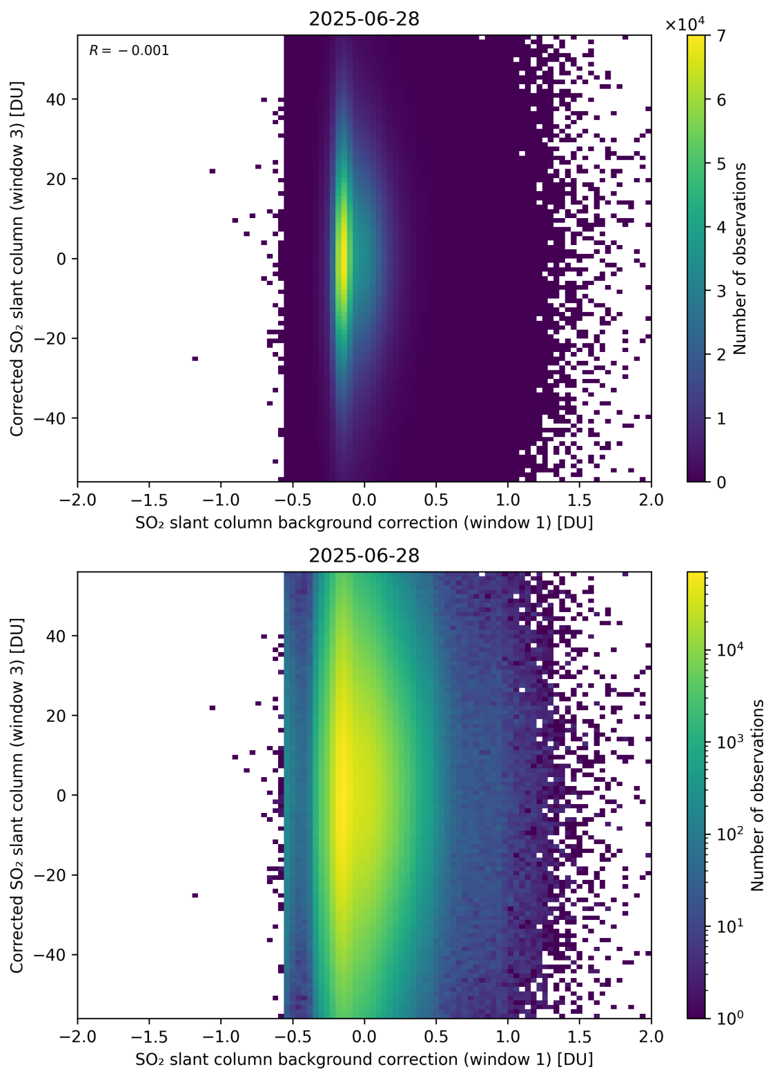
Figure 116: Scatter density plot of “SO 2 slant column background correction (window 1)” against “Corrected SO 2 slant column (window 3)” for 2025-06-27 to 2025-06-29.
