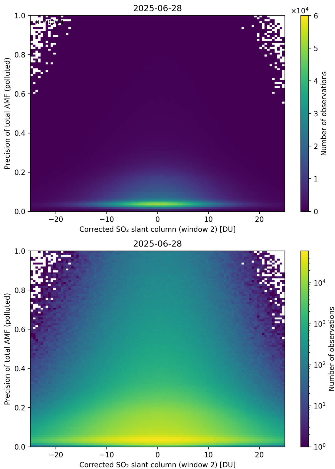
Figure 254: Scatter density plot of “Corrected SO 2 slant column (window 2)” against “Precision of total AMF (polluted)” for 2025-06-27 to 2025-06-29.
