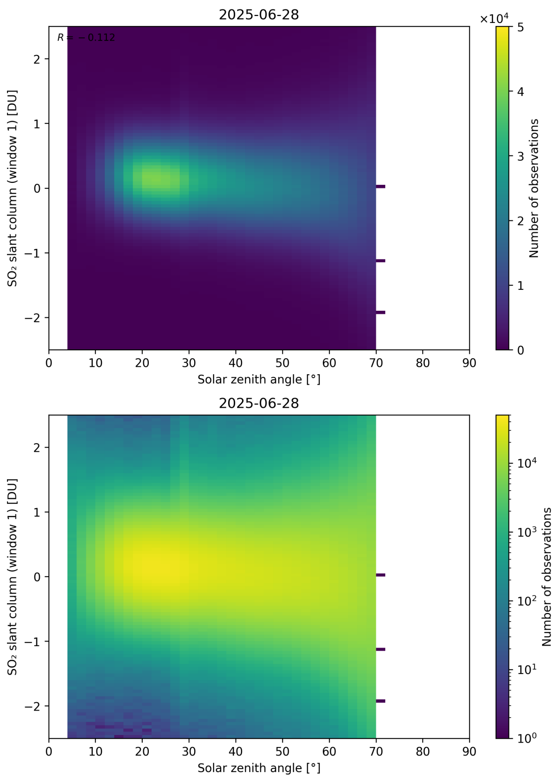
Figure 184: Scatter density plot of “Solar zenith angle” against “SO 2 slant column (window 1)” for 2025-06-27 to 2025-06-29.
