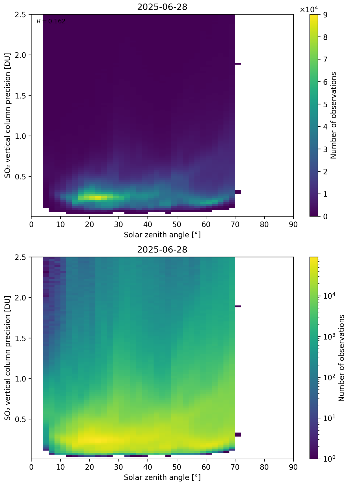
Figure 192: Scatter density plot of “Solar zenith angle” against “SO 2 vertical column precision” for 2025-06-27 to 2025-06-29.
