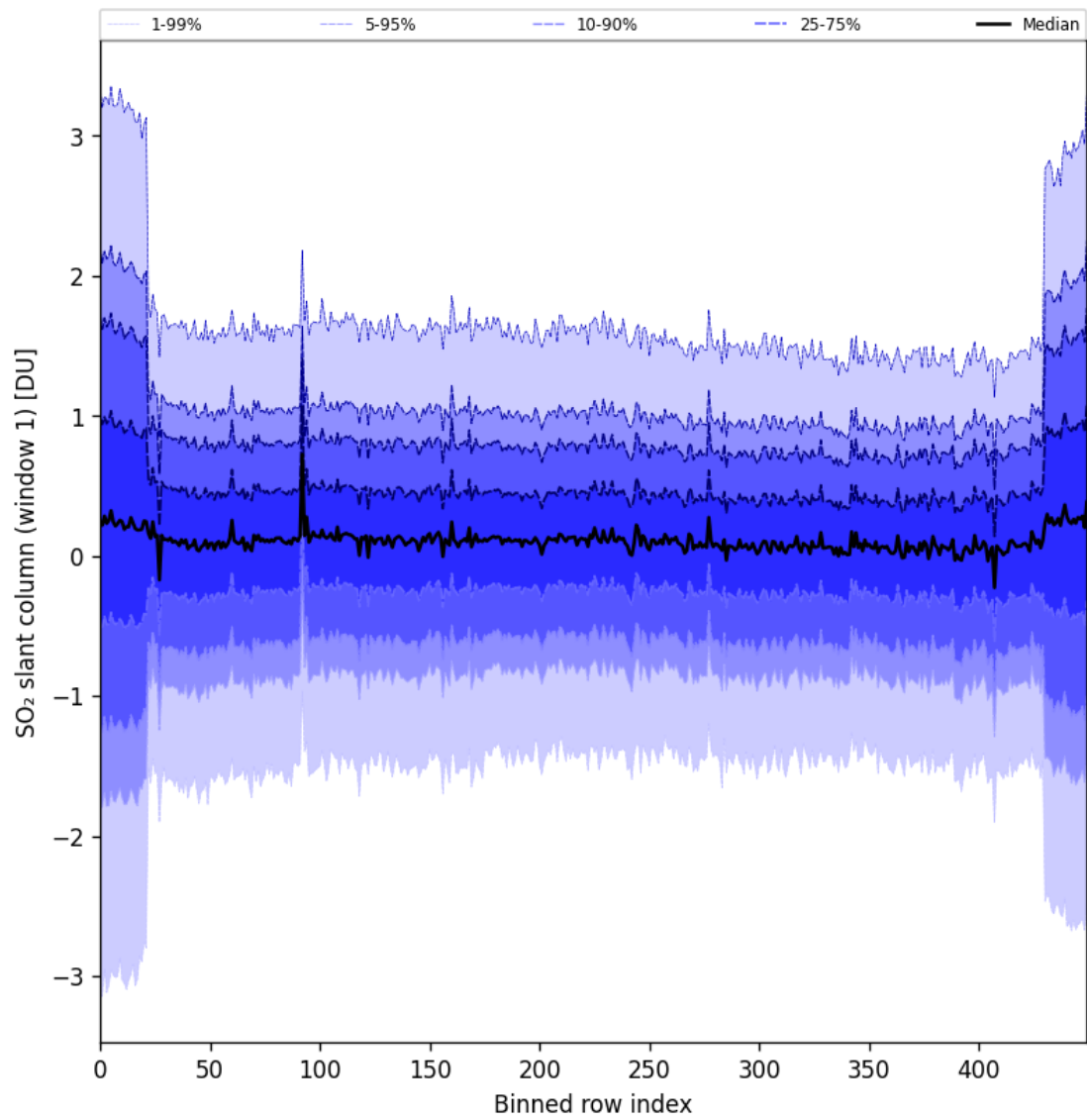
Figure 89: Along track statistics of “SO 2 slant column (window 1)” for 2025-06-27 to 2025-06-29
