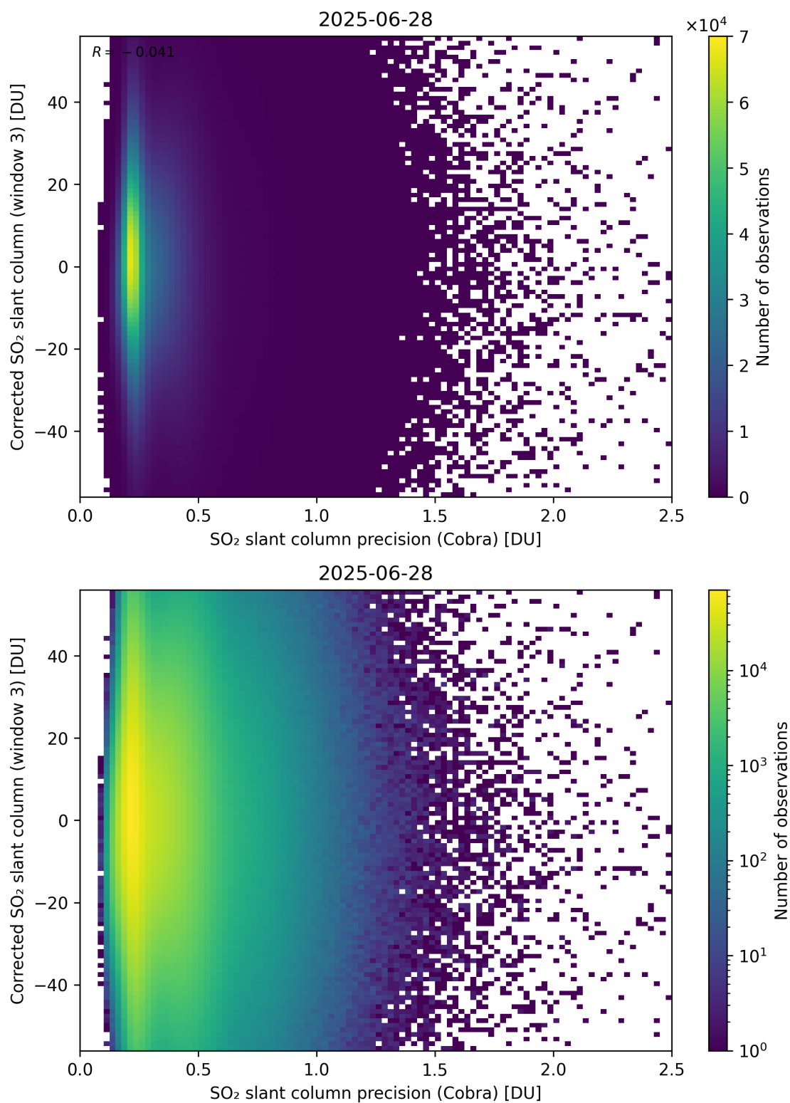
Figure 207: Scatter density plot of “SO 2 slant column precision (Cobra)” against “Corrected SO 2 slant column (window 3)” for 2025-06-27 to 2025-06-29.
