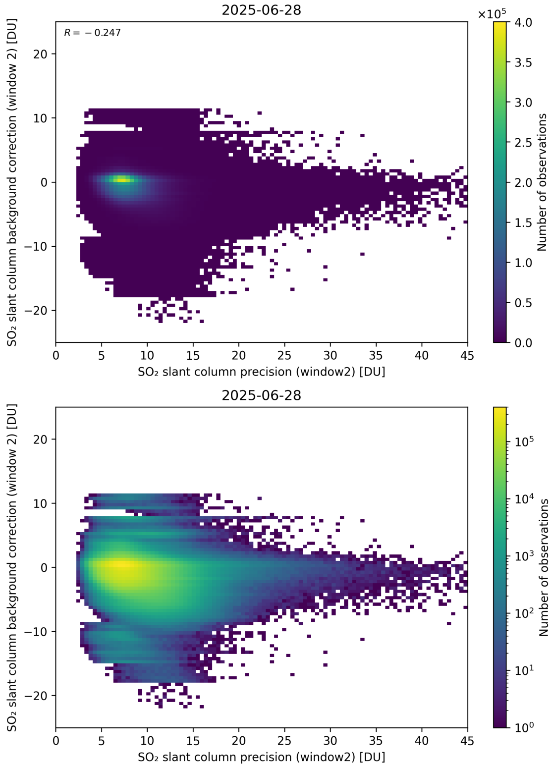
Figure 291: Scatter density plot of “SO 2 slant column precision (window2)” against “SO 2 slant column background correction (window 2)” for 2025-06-27 to 2025-06-29.
