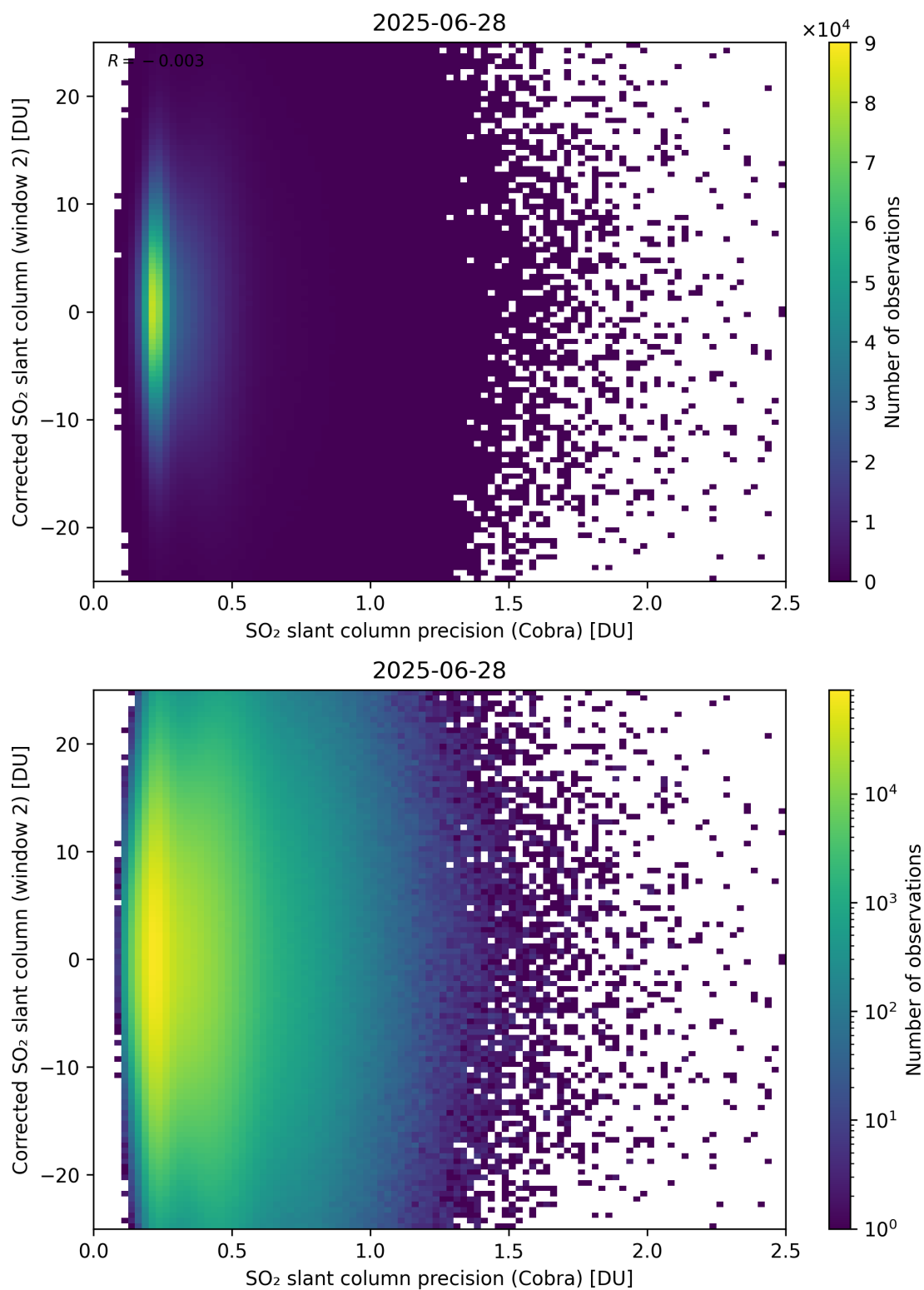
Figure 206: Scatter density plot of “SO 2 slant column precision (Cobra)” against “Corrected SO 2 slant column (window 2)” for 2025-06-27 to 2025-06-29.
