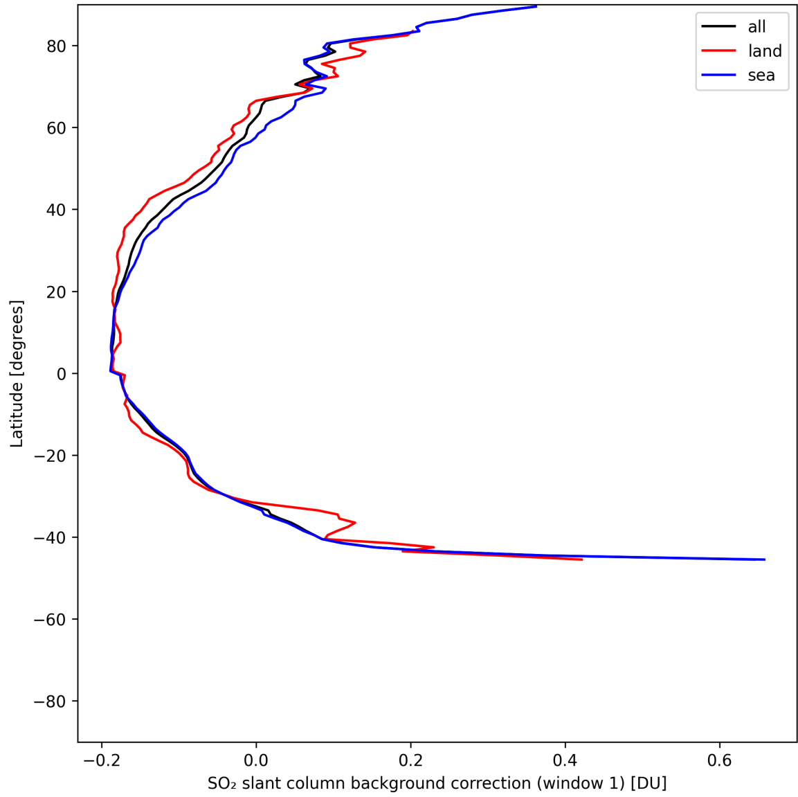
Figure 40: Zonal average of “SO 2 slant column background correction (window 1)” for 2025-06-27 to 2025-06-29.
