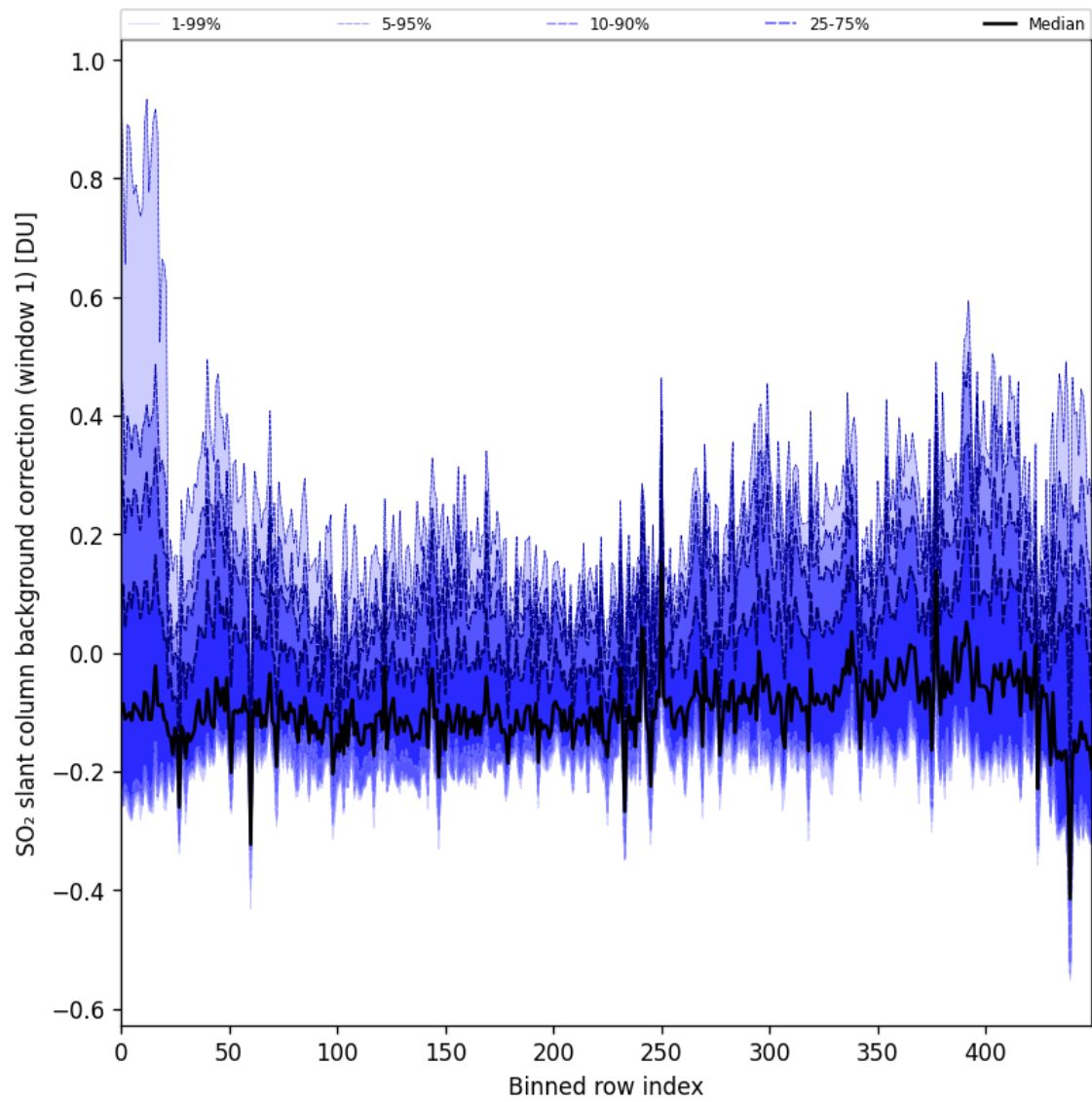
Figure 92: Along track statistics of “SO 2 slant column background correction (window 1)” for 2025-06-27 to 2025-06-29
