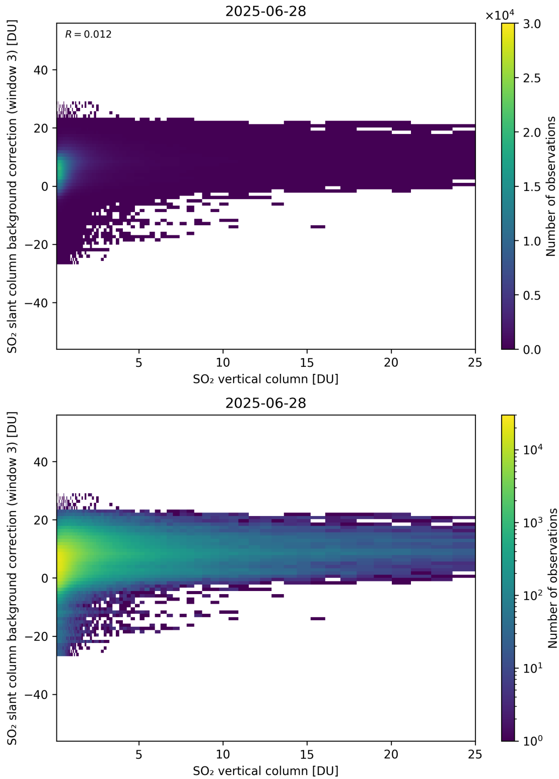
Figure 325: Scatter density plot of “SO 2 vertical column” against “SO 2 slant column background correction (window 3)” for 2025-06-27 to 2025-06-29.
