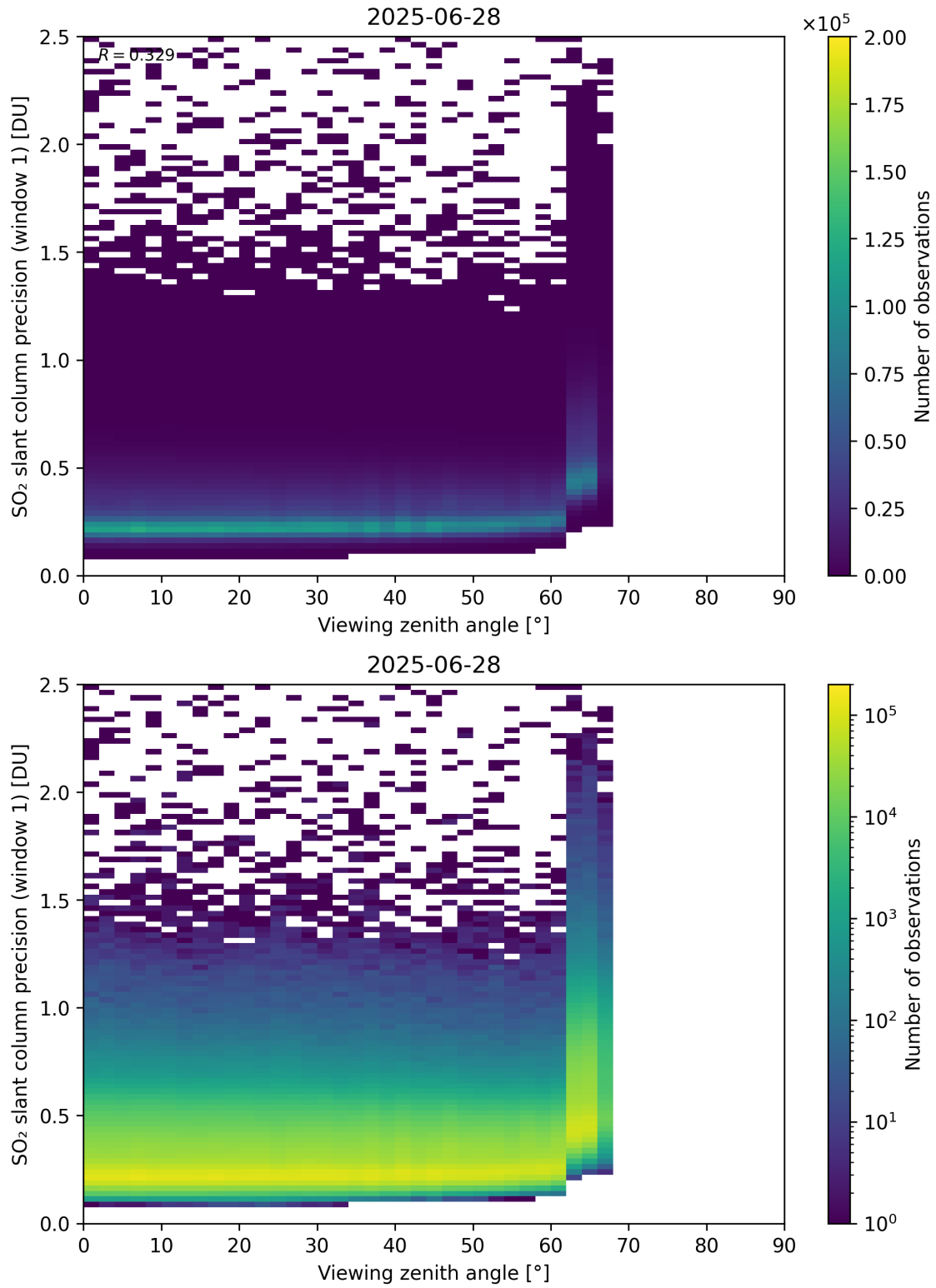
Figure 377: Scatter density plot of “Viewing zenith angle” against “SO 2 slant column precision (window 1)” for 2025-06-27 to 2025-06-29.
