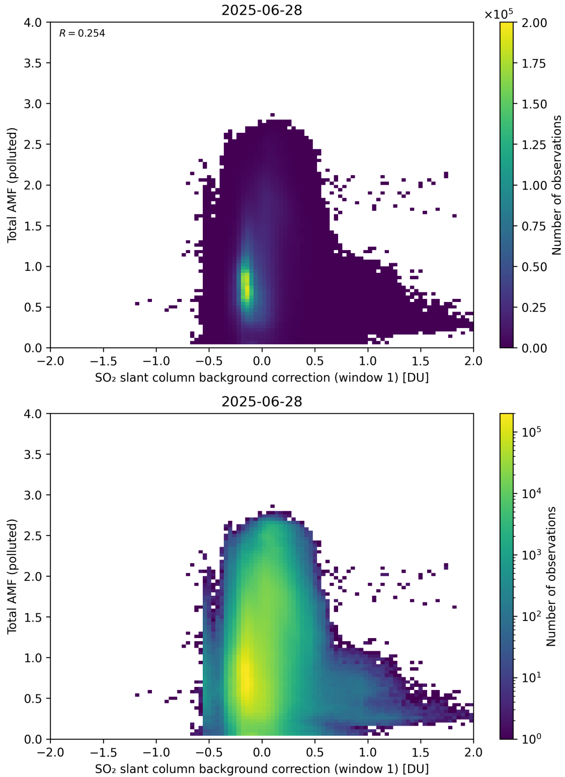
Figure 120: Scatter density plot of “SO 2 slant column background correction (window 1)” against “Total AMF (polluted)” for 2025-06-27 to 2025-06-29.
