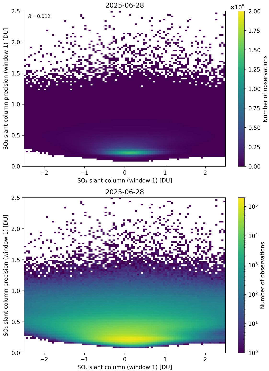
Figure 285: Scatter density plot of “SO 2 slant column (window 1)” against “SO 2 slant column precision (window 1)” for 2025-06-27 to 2025-06-29.
