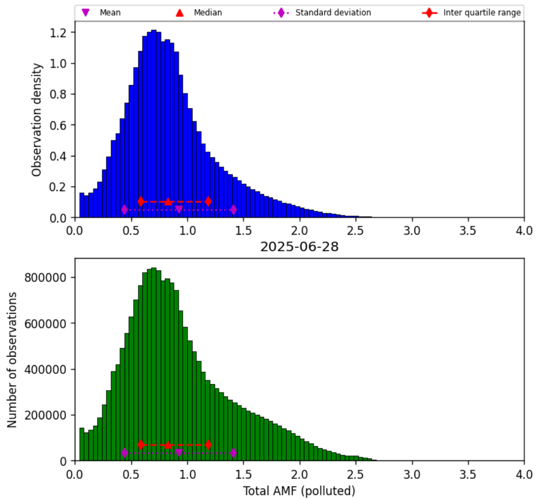
Figure 79: Histogram of “Total AMF (polluted)” for 2025-06-27 to 2025-06-29
