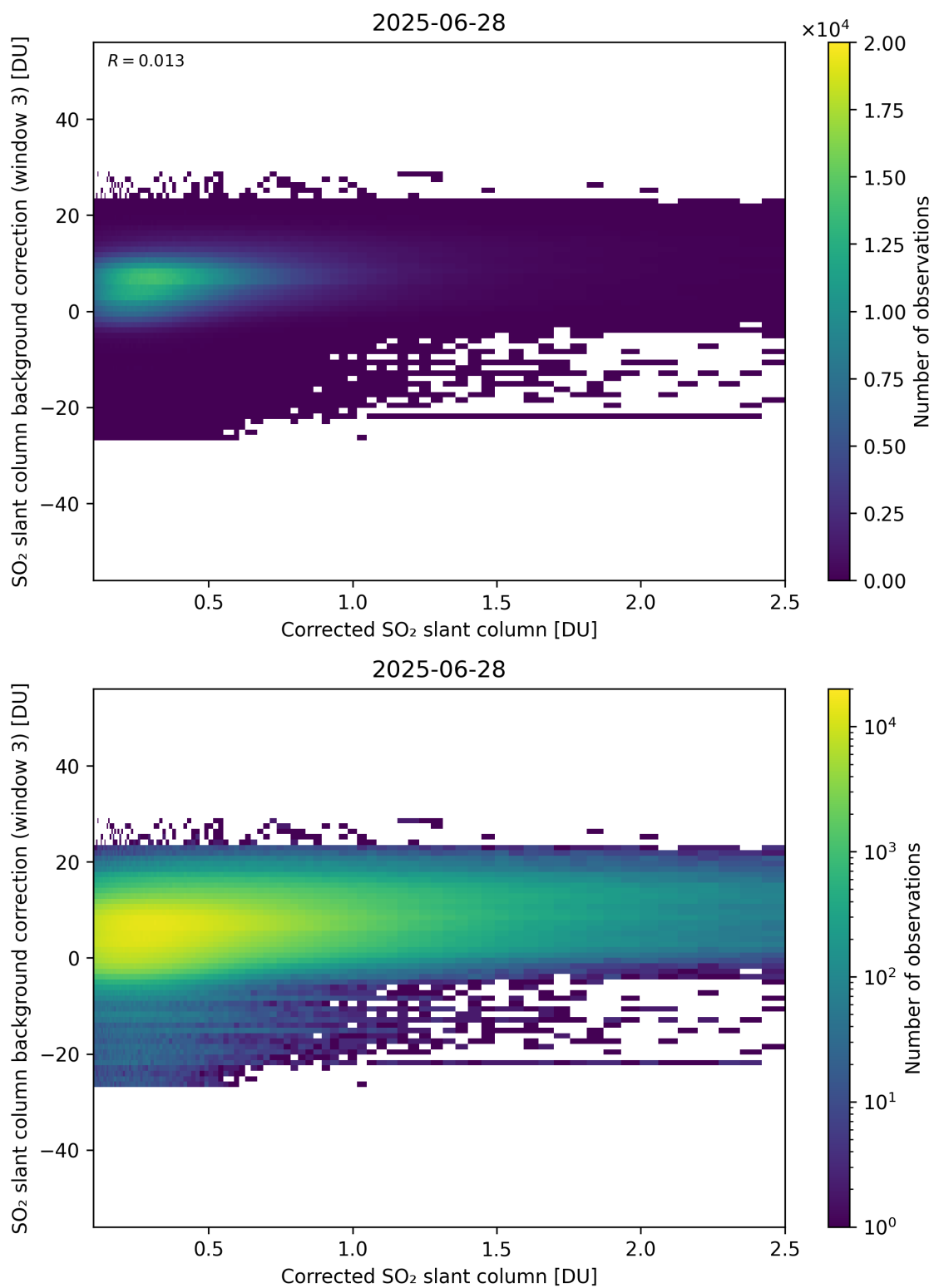
Figure 228: Scatter density plot of “Corrected SO 2 slant column” against “SO 2 slant column background correction (window 3)” for 2025-06-27 to 2025-06-29.
