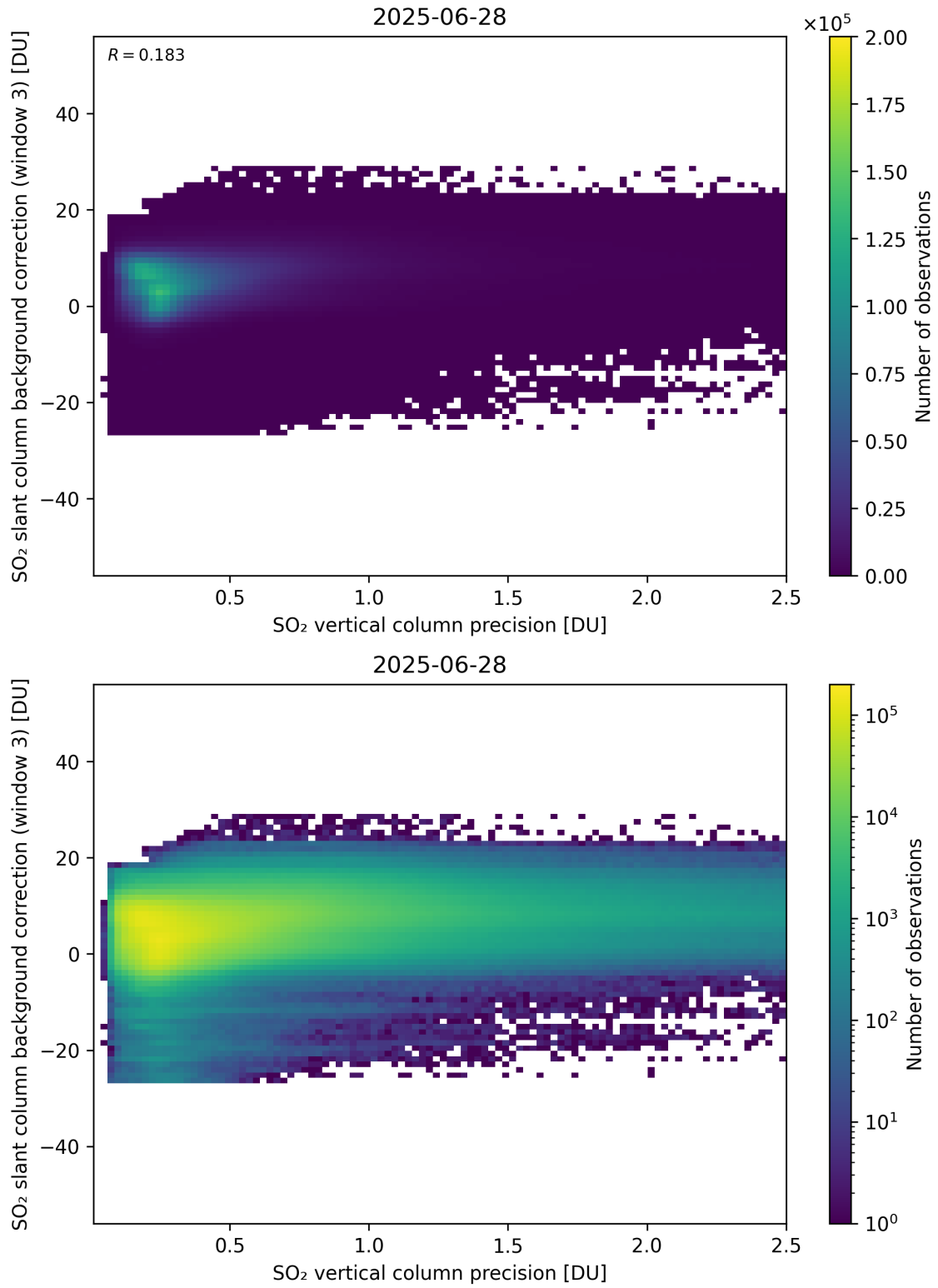
Figure 331: Scatter density plot of “SO 2 vertical column precision” against “SO 2 slant column background correction (window 3)” for 2025-06-27 to 2025-06-29.
