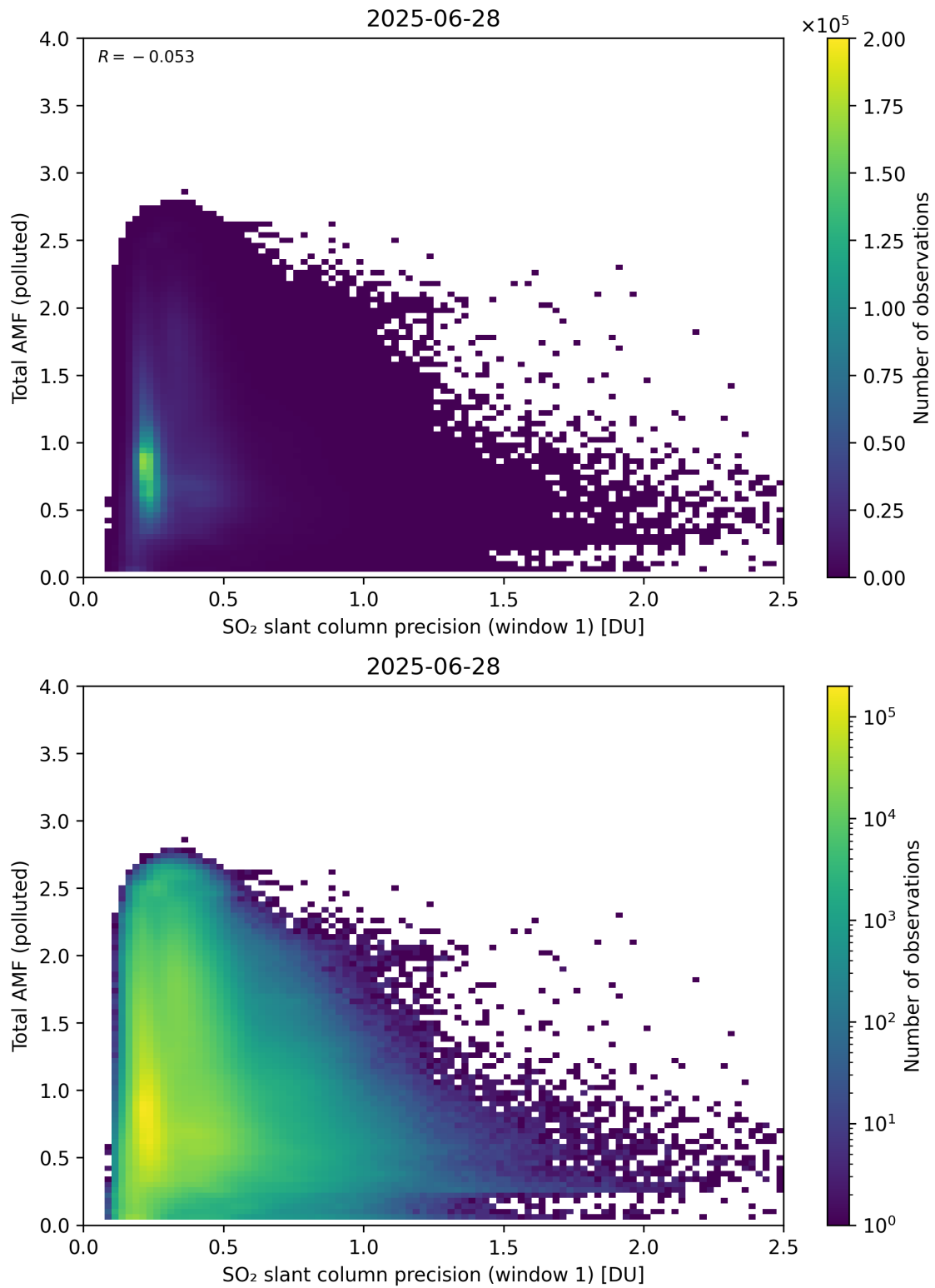
Figure 280: Scatter density plot of “SO 2 slant column precision (window 1)” against “Total AMF (polluted)” for 2025-06-27 to 2025-06-29.
