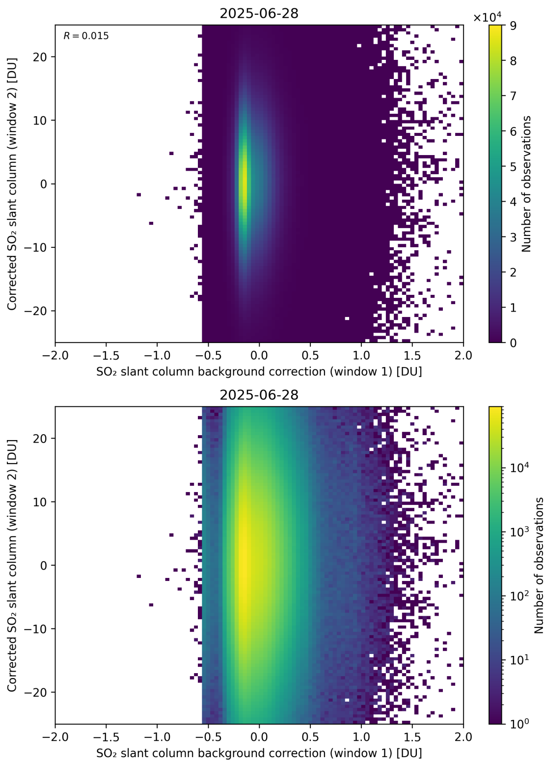
Figure 115: Scatter density plot of “SO 2 slant column background correction (window 1)” against “Corrected SO 2 slant column (window 2)” for 2025-06-27 to 2025-06-29.
