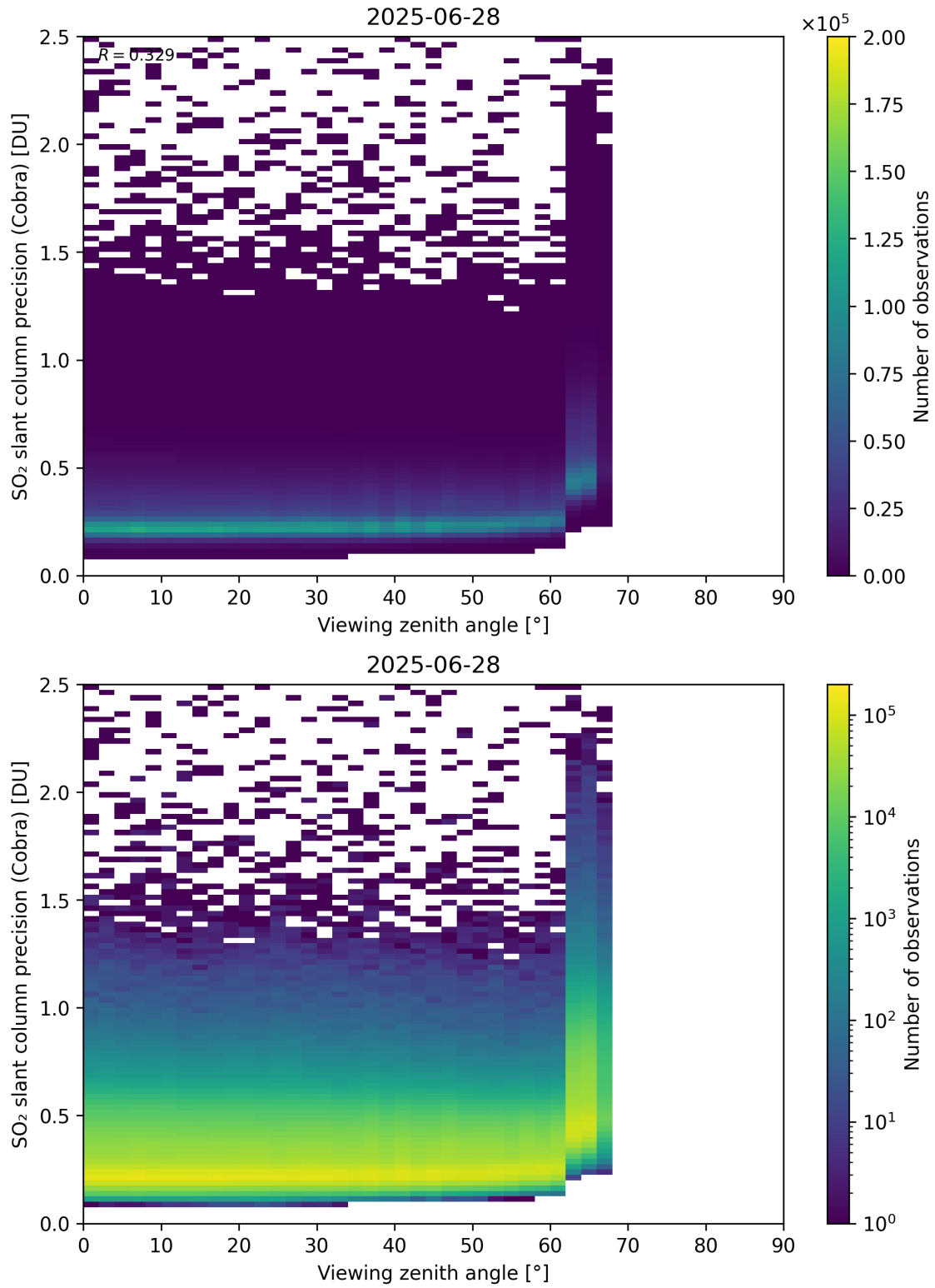
Figure 372: Scatter density plot of “Viewing zenith angle” against “SO 2 slant column precision (Cobra)” for 2025-06-27 to 2025-06-29.
