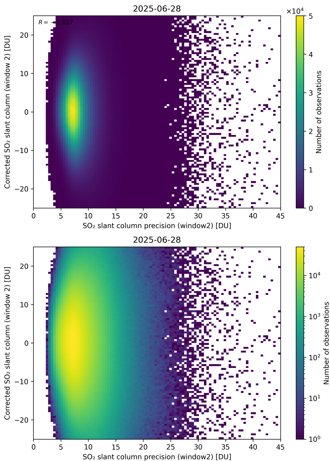
Figure 297: Scatter density plot of “SO 2 slant column precision (window2)” against “Corrected SO 2 slant column (window 2)” for 2025-06-27 to 2025-06-29.
