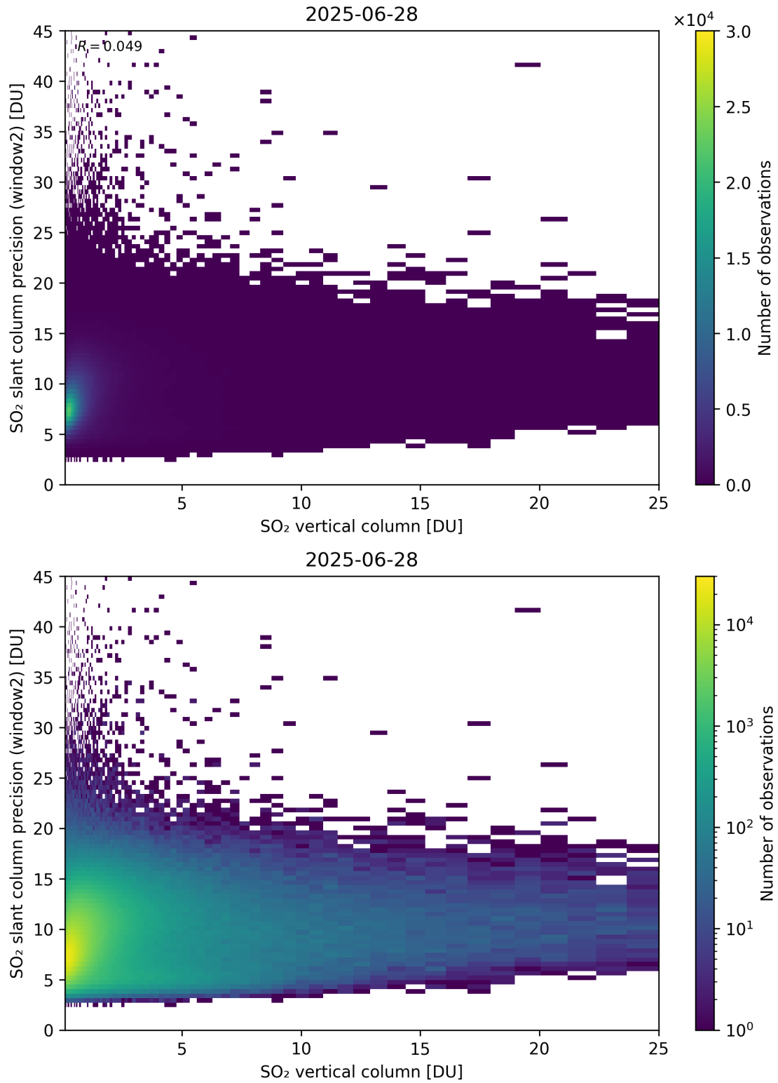
Figure 356: Scatter density plot of “SO 2 vertical column” against “SO 2 slant column precision (window2)” for 2025-06-27 to 2025-06-29.
