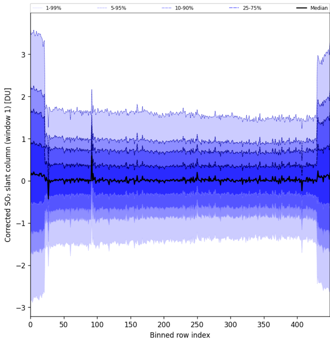
Figure 91: Along track statistics of “Corrected SO 2 slant column (window 1)” for 2025-06-27 to 2025-06-29
