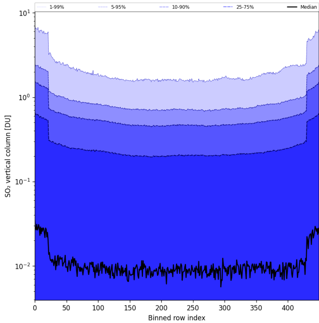
Figure 84: Along track statistics of “SO 2 vertical column” for 2025-06-27 to 2025-06-29
