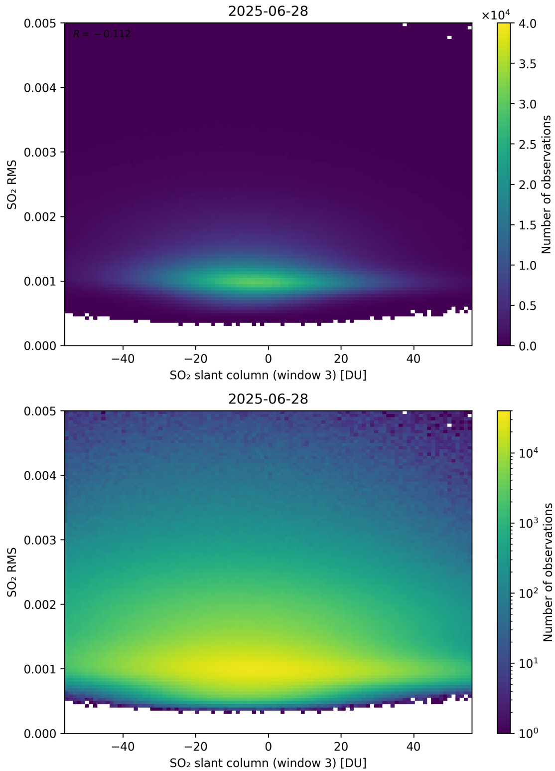
Figure 306: Scatter density plot of “SO 2 slant column (window 3)” against “SO 2 RMS” for 2025-06-27 to 2025-06-29.
