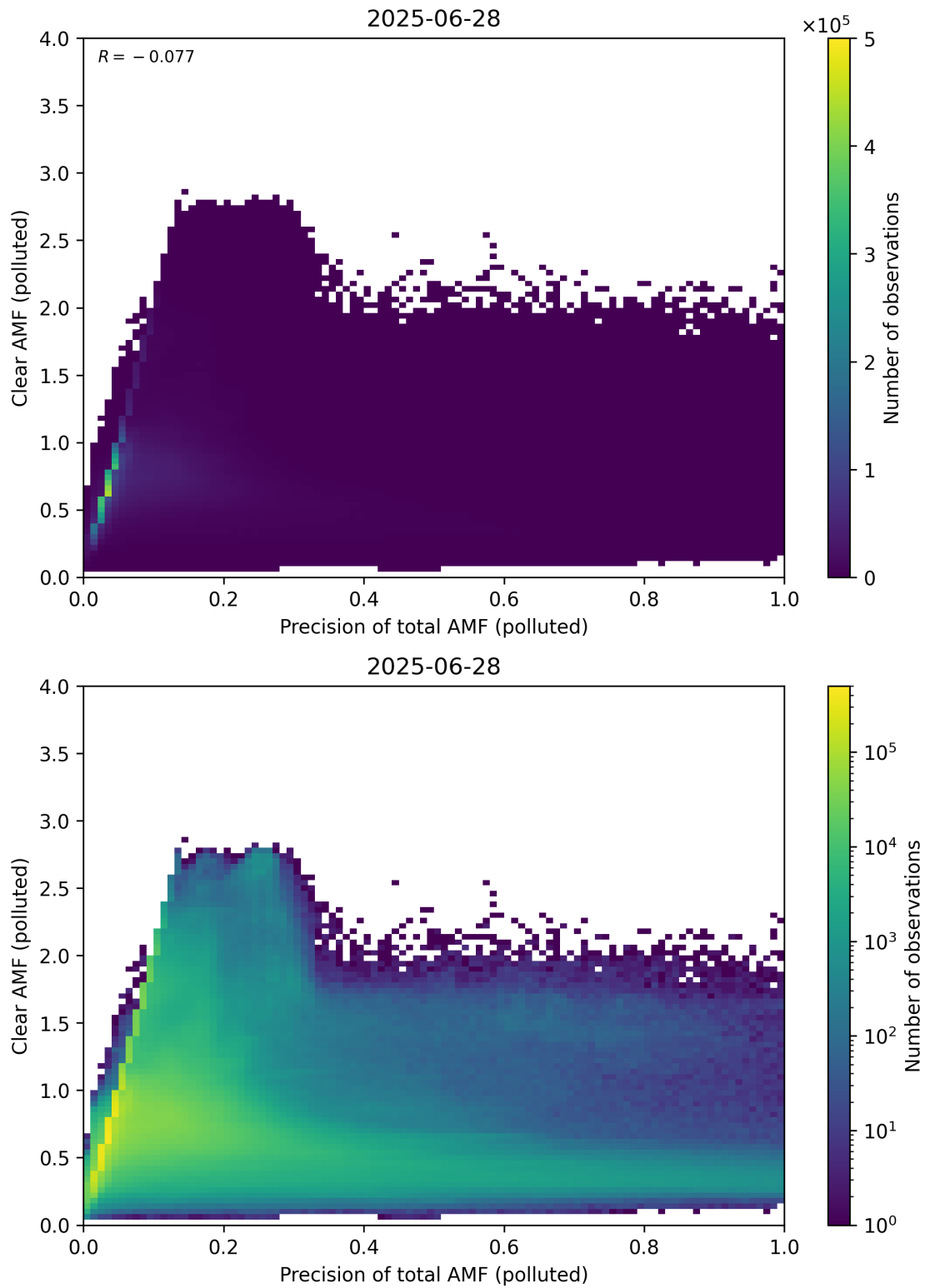
Figure 320: Scatter density plot of “Precision of total AMF (polluted)” against “Clear AMF (polluted)” for 2025-06-27 to 2025-06-29.
