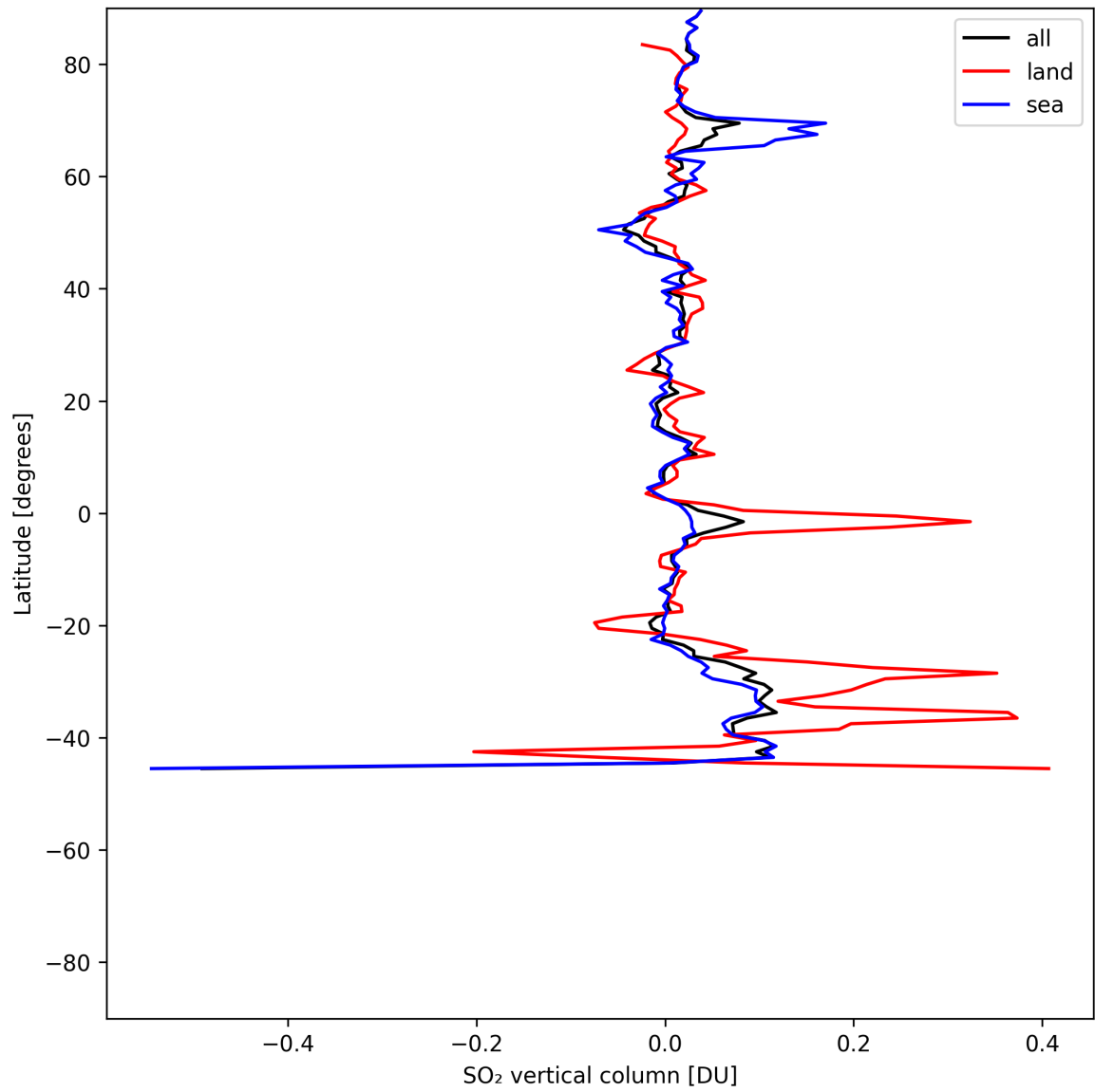
Figure 32: Zonal average of “SO 2 vertical column” for 2025-06-27 to 2025-06-29.
