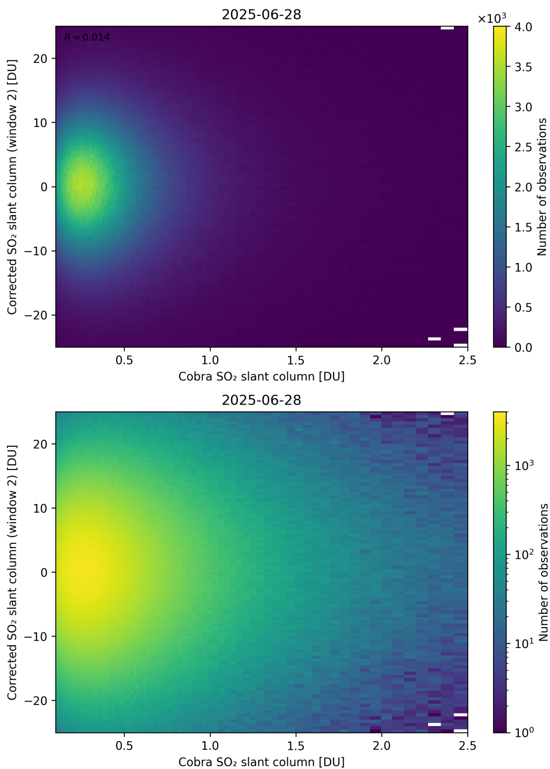
Figure 217: Scatter density plot of “Cobra SO 2 slant column” against “Corrected SO 2 slant column (window 2)” for 2025-06-27 to 2025-06-29.
