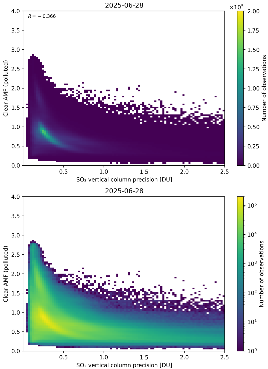
Figure 335: Scatter density plot of “SO 2 vertical column precision” against “Clear AMF (polluted)” for 2025-06-27 to 2025-06-29.
