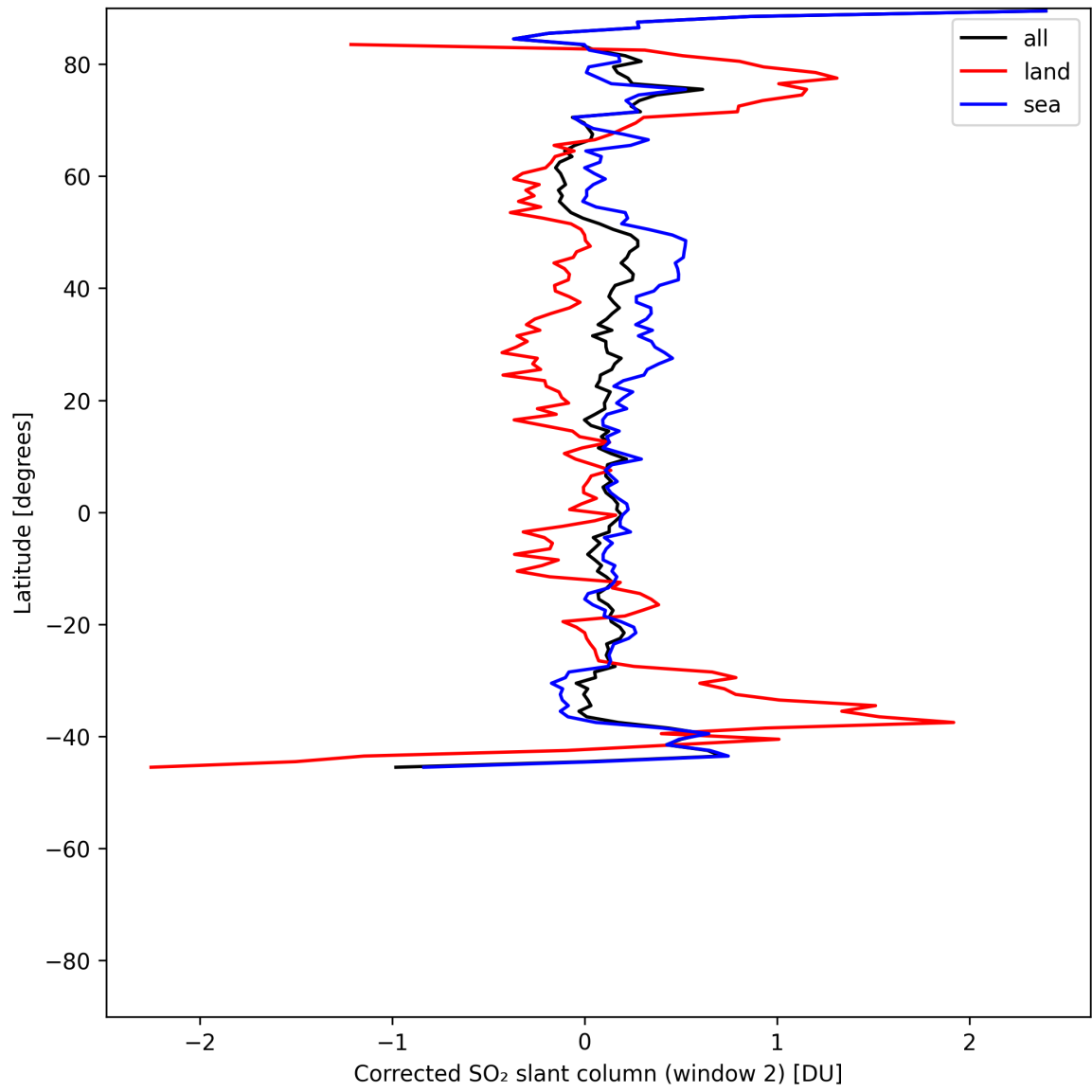
Figure 43: Zonal average of “Corrected SO 2 slant column (window 2)” for 2025-06-27 to 2025-06-29.
