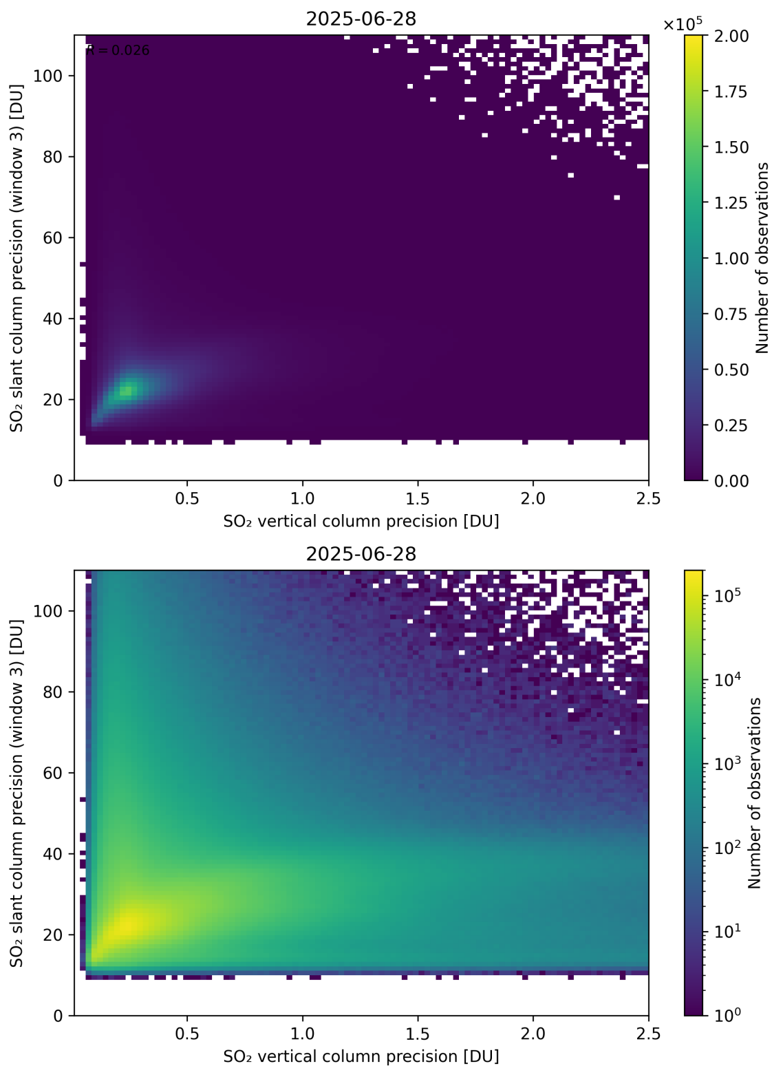
Figure 345: Scatter density plot of “SO 2 vertical column precision” against “SO 2 slant column precision (window 3)” for 2025-06-27 to 2025-06-29.
