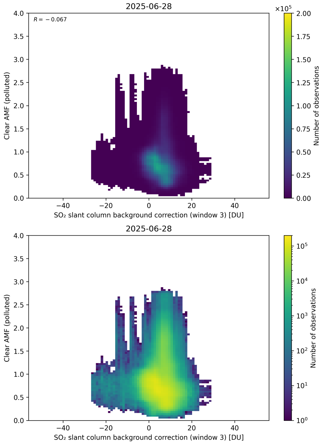
Figure 135: Scatter density plot of “SO 2 slant column background correction (window 3)” against “Clear AMF (polluted)” for 2025-06-27 to 2025-06-29.
