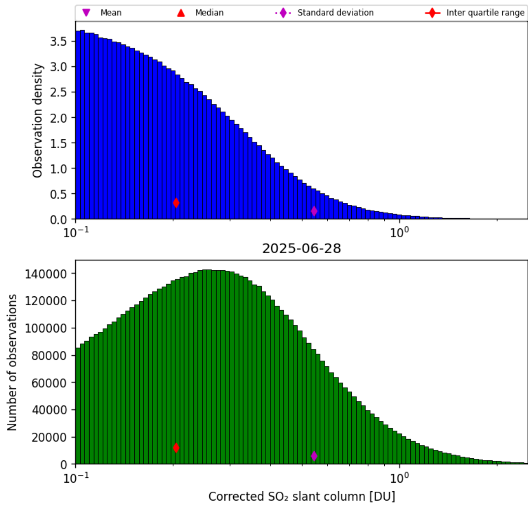
Figure 60: Histogram of “Corrected SO 2 slant column” for 2025-06-27 to 2025-06-29
