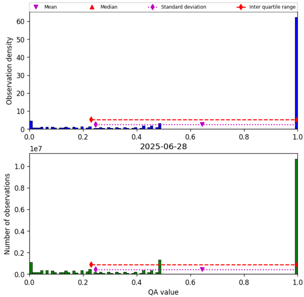
Figure 57: Histogram of “QA value” for 2025-06-27 to 2025-06-29
