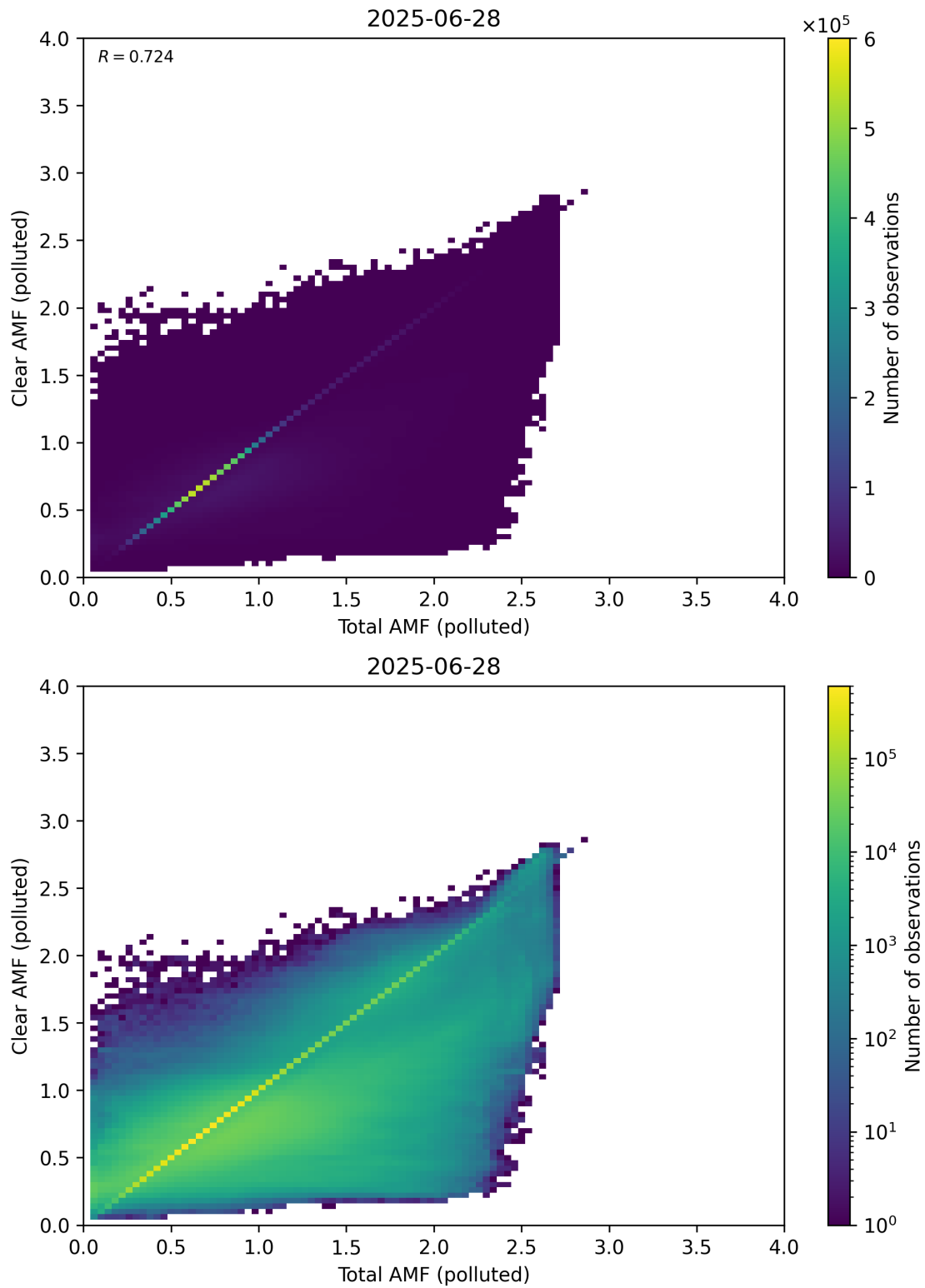
Figure 321: Scatter density plot of “Total AMF (polluted)” against “Clear AMF (polluted)” for 2025-06-27 to 2025-06-29.
