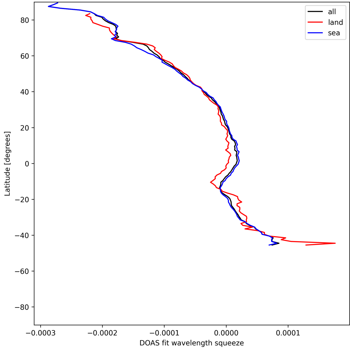
Figure 51: Zonal average of “DOAS fit wavelength squeeze” for 2025-06-27 to 2025-06-29.
