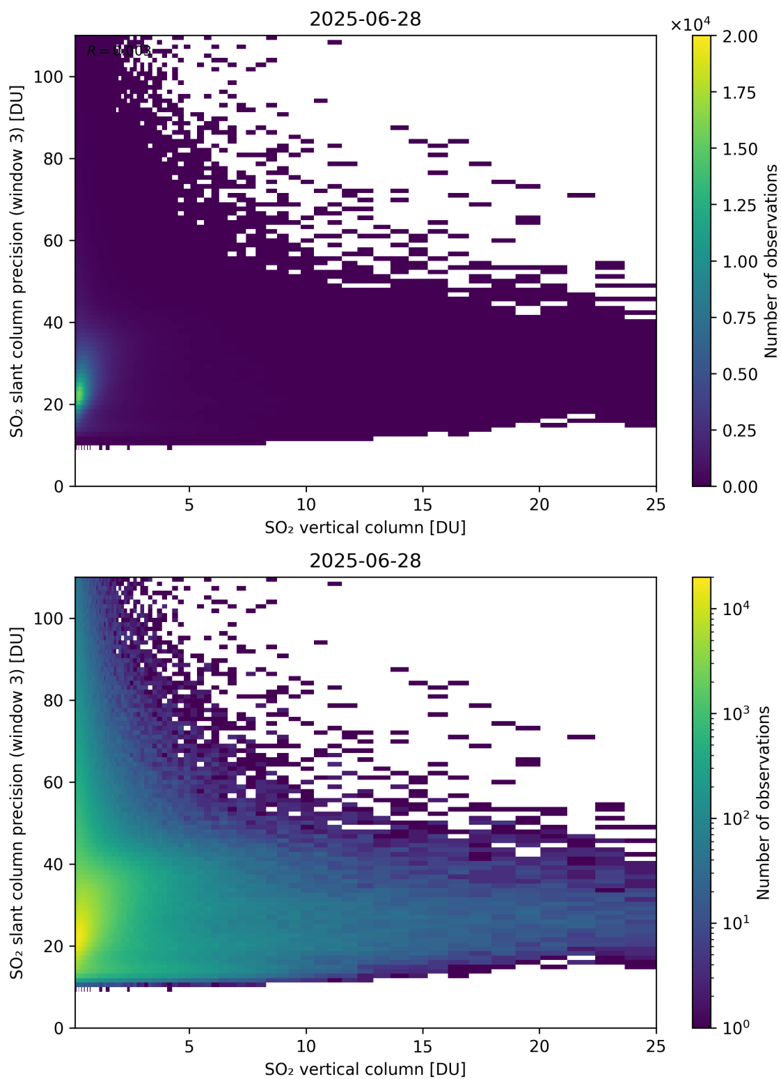
Figure 358: Scatter density plot of “SO 2 vertical column” against “SO 2 slant column precision (window 3)” for 2025-06-27 to 2025-06-29.
