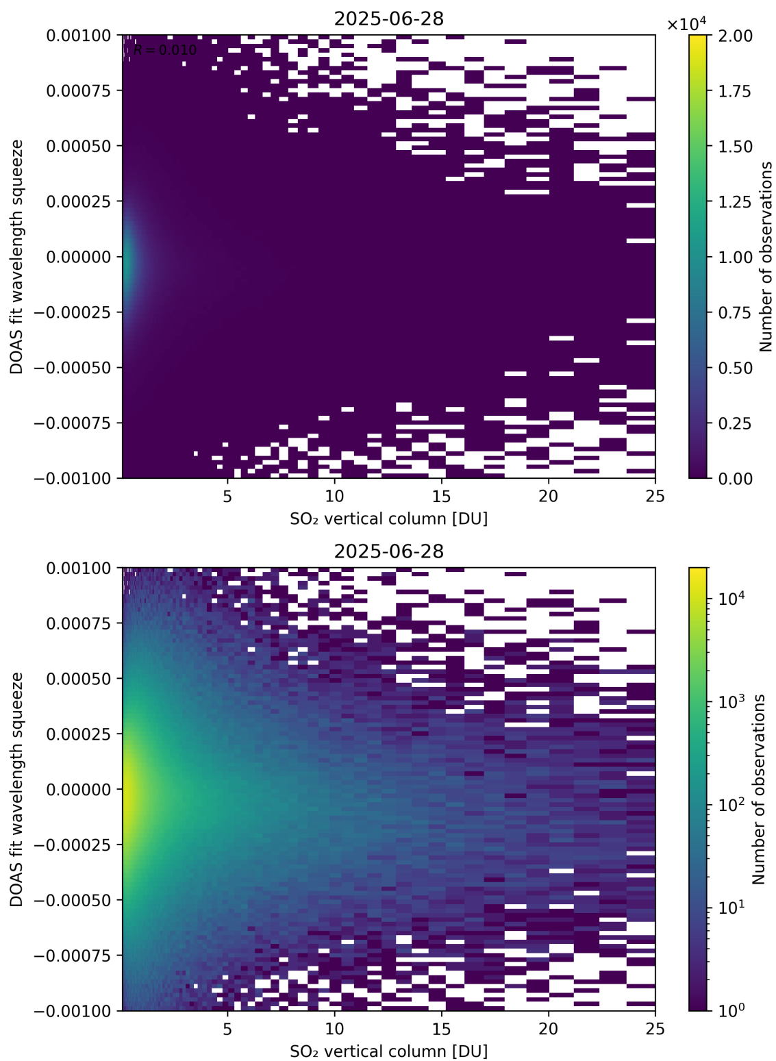
Figure 327: Scatter density plot of “SO 2 vertical column” against “DOAS fit wavelength squeeze” for 2025-06-27 to 2025-06-29.
