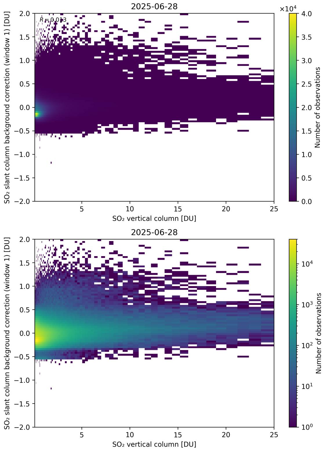
Figure 323: Scatter density plot of “SO 2 vertical column” against “SO 2 slant column background correction (window 1)” for 2025-06-27 to 2025-06-29.
