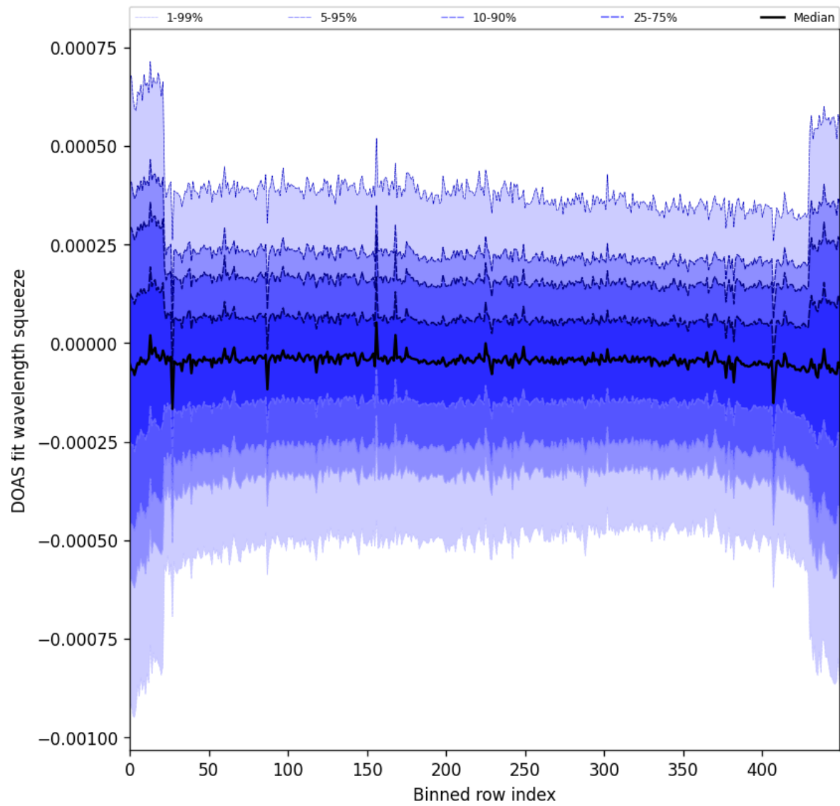
Figure 103: Along track statistics of “DOAS fit wavelength squeeze” for 2025-06-27 to 2025-06-29
