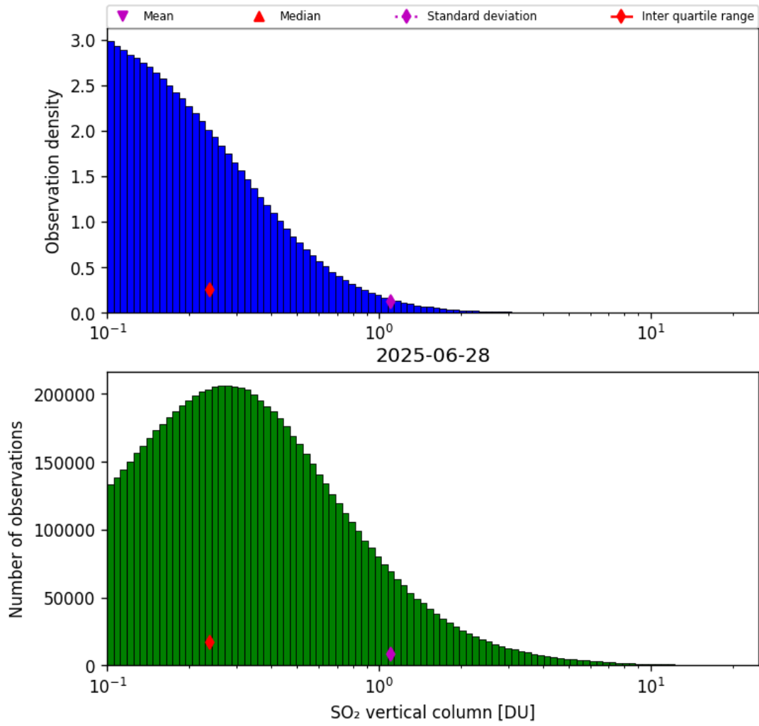
Figure 58: Histogram of “SO 2 vertical column” for 2025-06-27 to 2025-06-29
