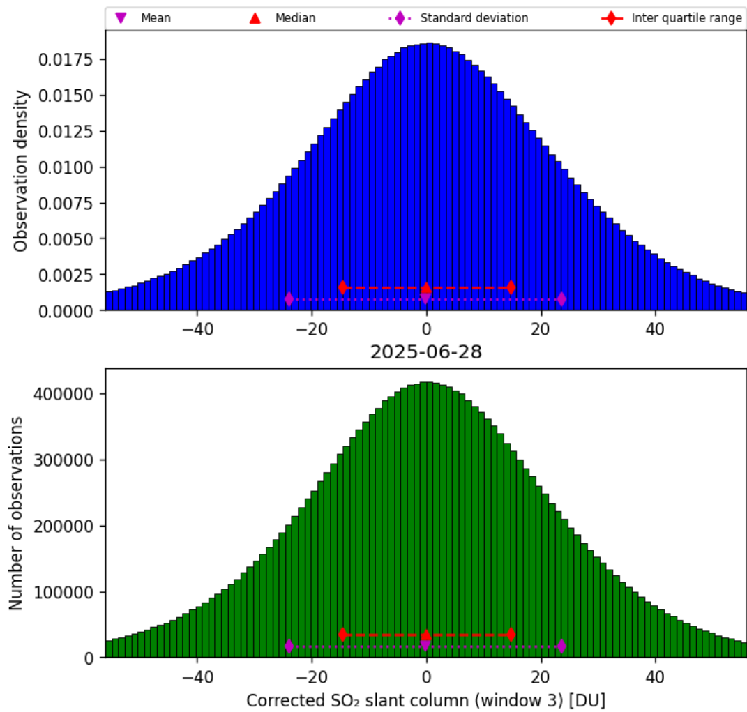
Figure 73: Histogram of “Corrected SO 2 slant column (window 3)” for 2025-06-27 to 2025-06-29
