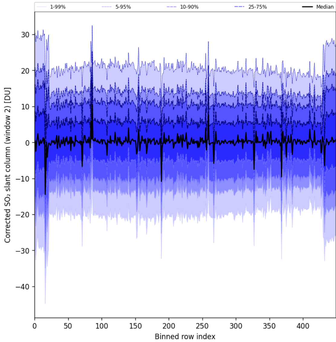
Figure 95: Along track statistics of “Corrected SO 2 slant column (window 2)” for 2025-06-27 to 2025-06-29
