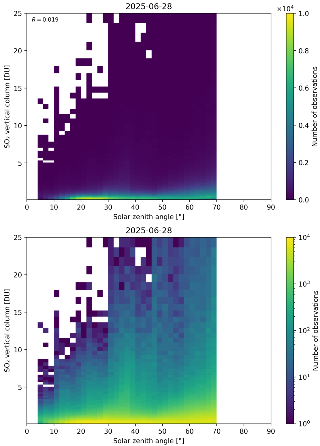
Figure 191: Scatter density plot of “Solar zenith angle” against “SO 2 vertical column” for 2025-06-27 to 2025-06-29.
