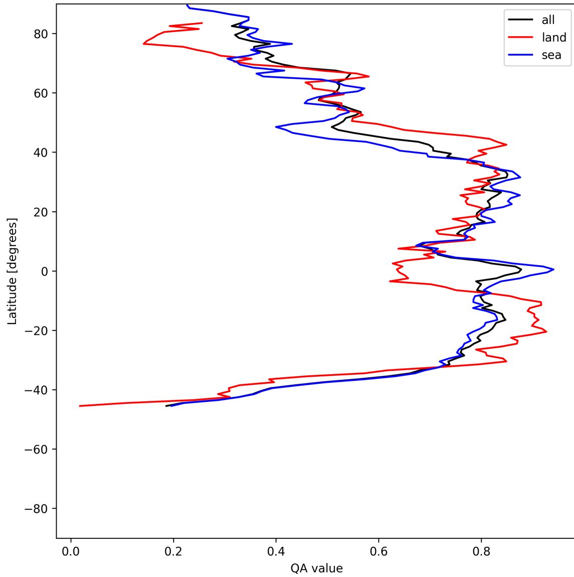
Figure 31: Zonal average of “QA value” for 2025-06-27 to 2025-06-29.
