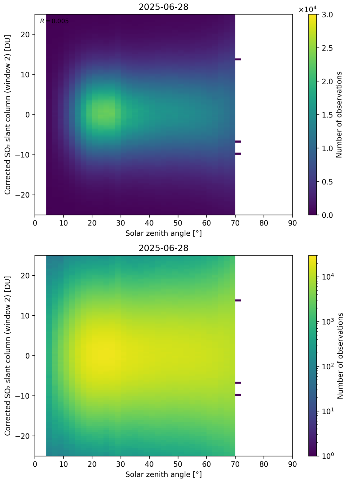
Figure 182: Scatter density plot of “Solar zenith angle” against “Corrected SO 2 slant column (window 2)” for 2025-06-27 to 2025-06-29.
