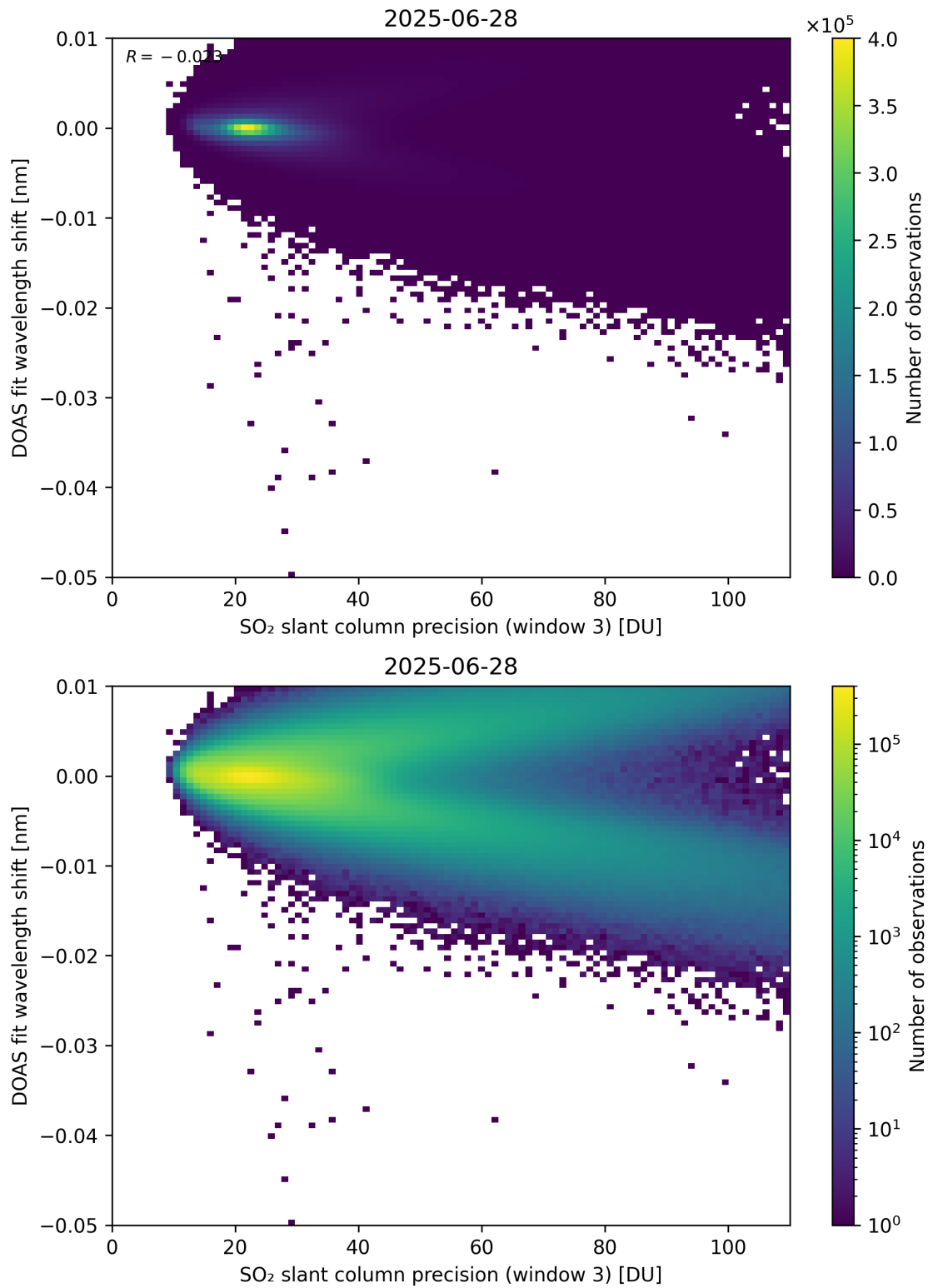
Figure 308: Scatter density plot of “SO 2 slant column precision (window 3)” against “DOAS fit wavelength shift” for 2025-06-27 to 2025-06-29.
