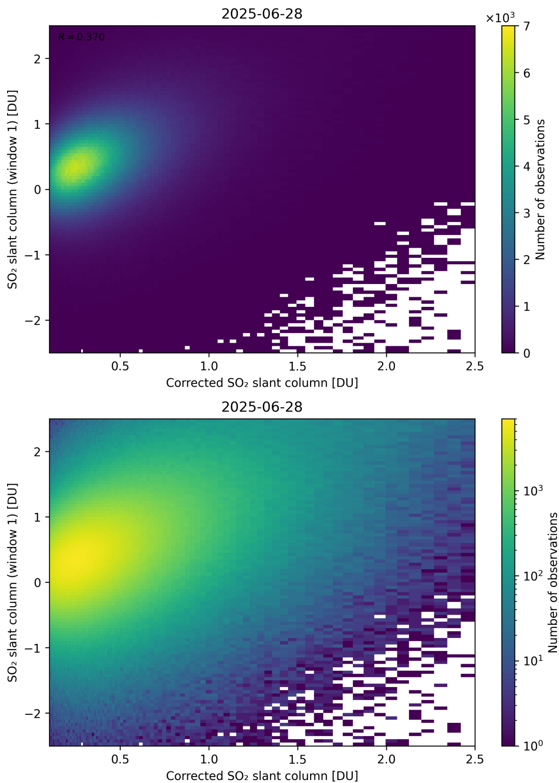
Figure 237: Scatter density plot of “Corrected SO 2 slant column” against “SO 2 slant column (window 1)” for 2025-06-27 to 2025-06-29.
