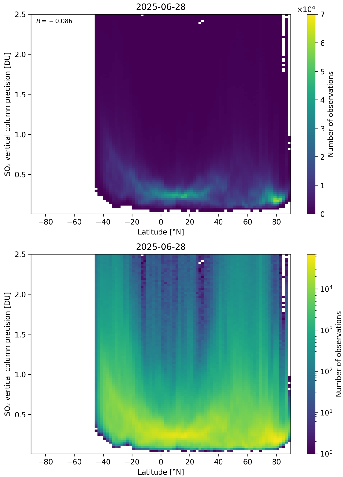
Figure 170: Scatter density plot of “Latitude” against “SO 2 vertical column precision” for 2025-06-27 to 2025-06-29.
