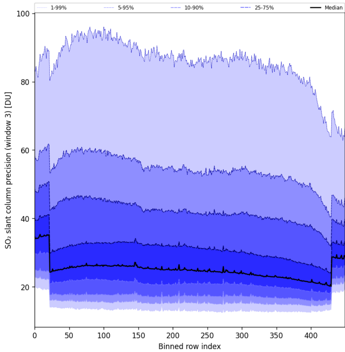
Figure 98: Along track statistics of “SO 2 slant column precision (window 3)” for 2025-06-27 to 2025-06-29
