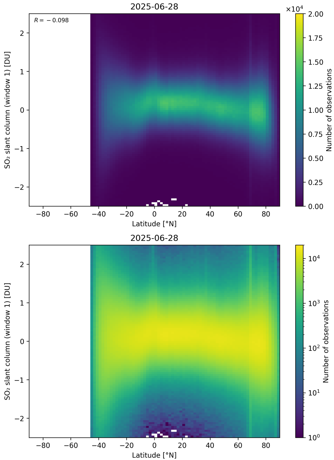
Figure 162: Scatter density plot of “Latitude” against “SO 2 slant column (window 1)” for 2025-06-27 to 2025-06-29.
