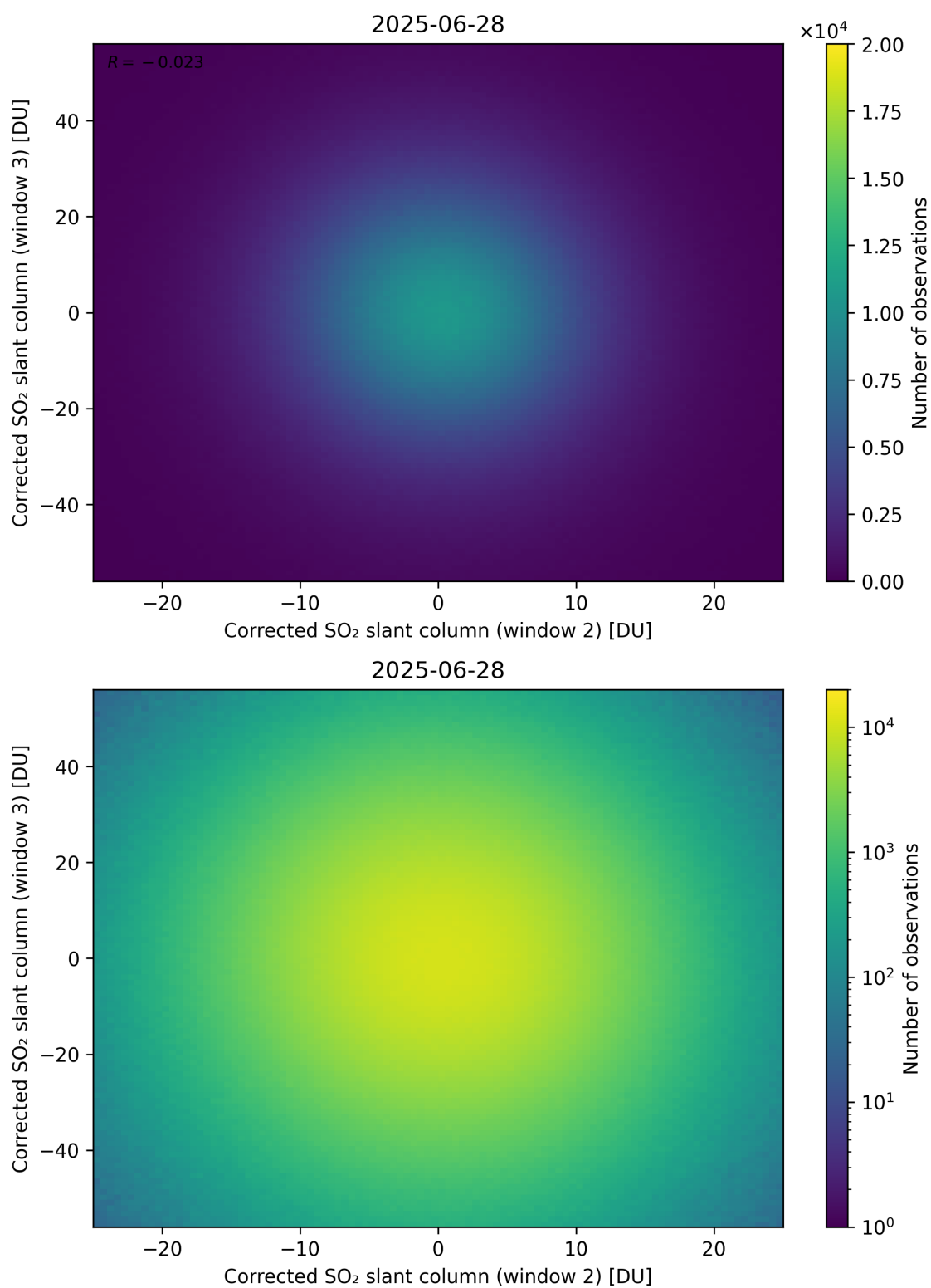
Figure 250: Scatter density plot of “Corrected SO 2 slant column (window 2)” against “Corrected SO 2 slant column (window 3)” for 2025-06-27 to 2025-06-29.
