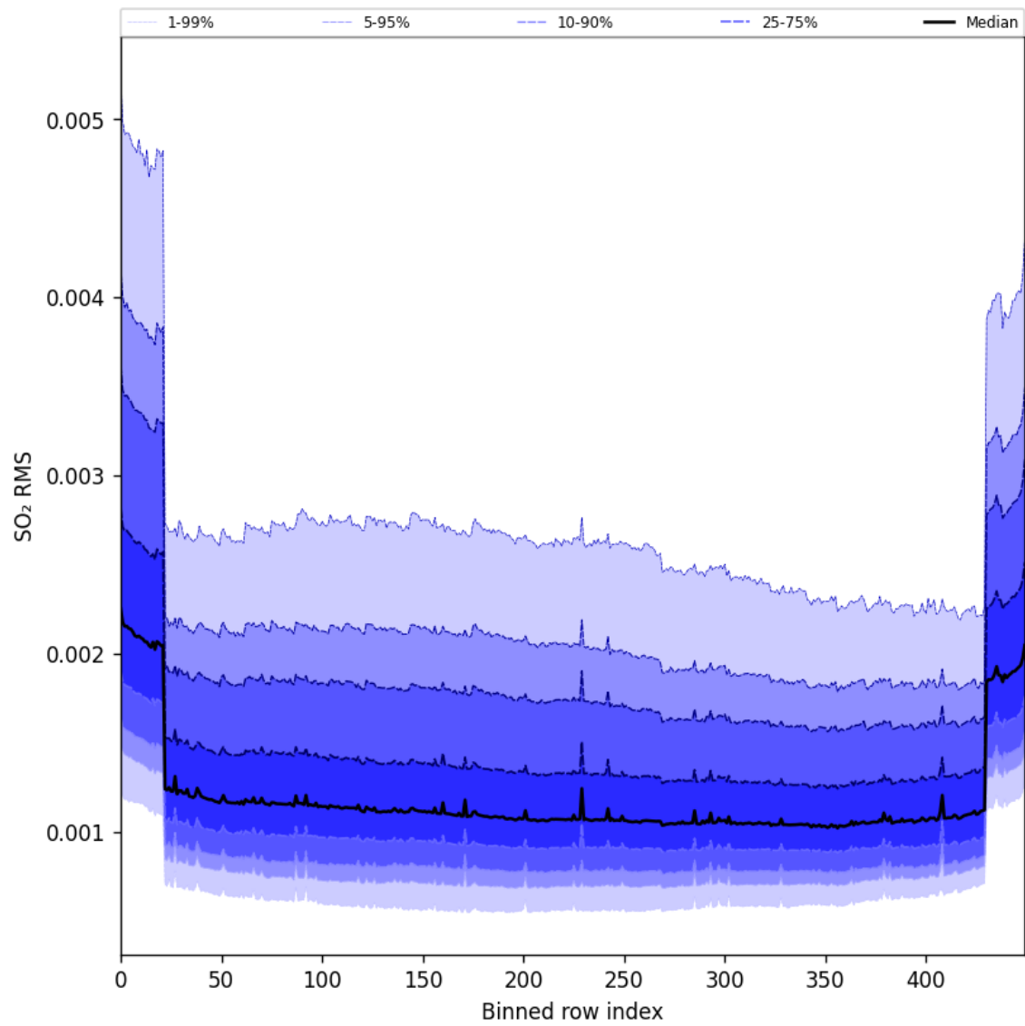
Figure 104: Along track statistics of “SO 2 RMS” for 2025-06-27 to 2025-06-29
