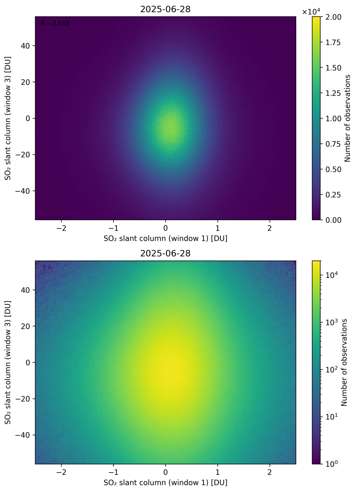
Figure 287: Scatter density plot of “SO 2 slant column (window 1)” against “SO 2 slant column (window 3)” for 2025-06-27 to 2025-06-29.
