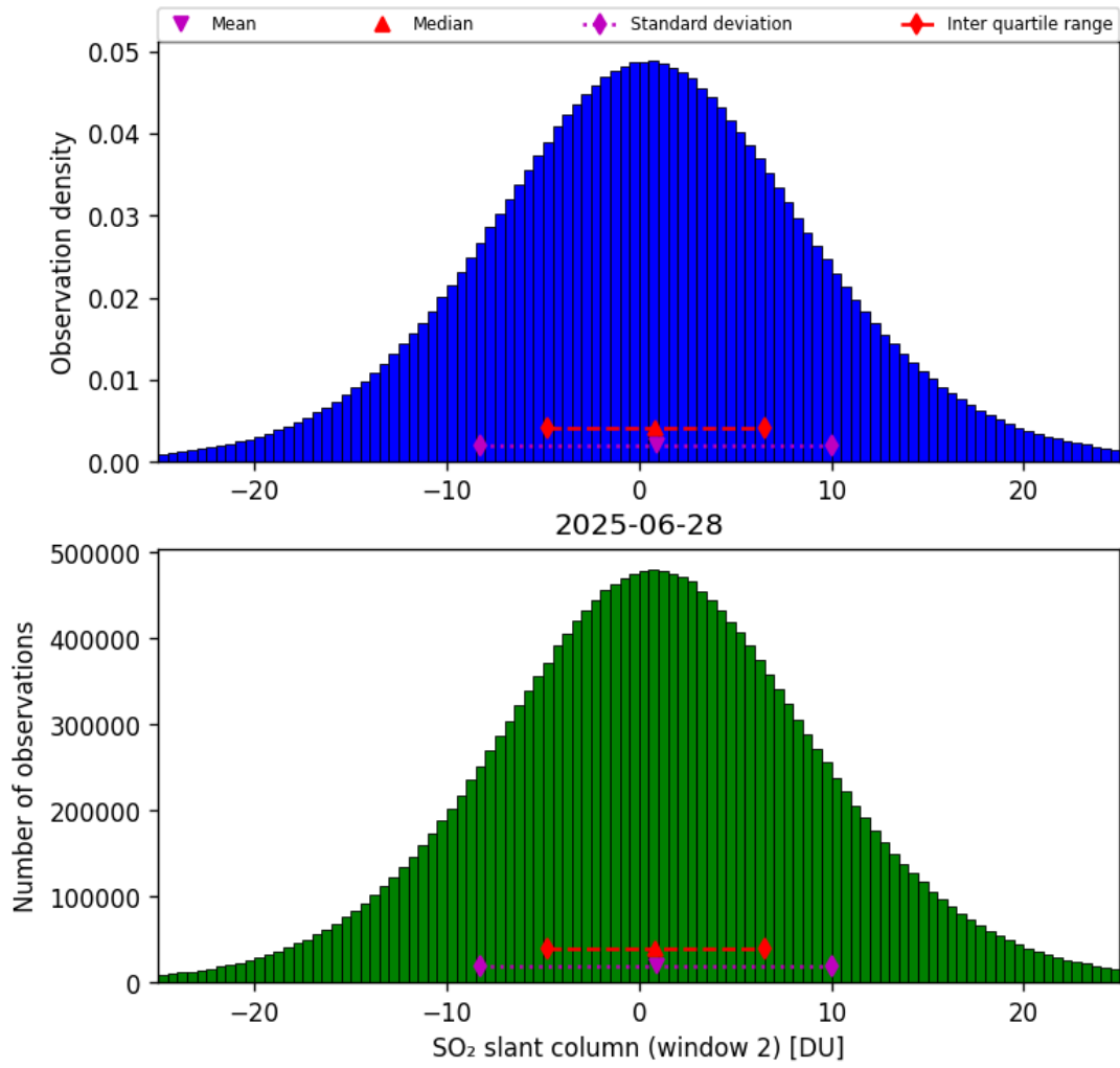
Figure 67: Histogram of “SO 2 slant column (window 2)” for 2025-06-27 to 2025-06-29
