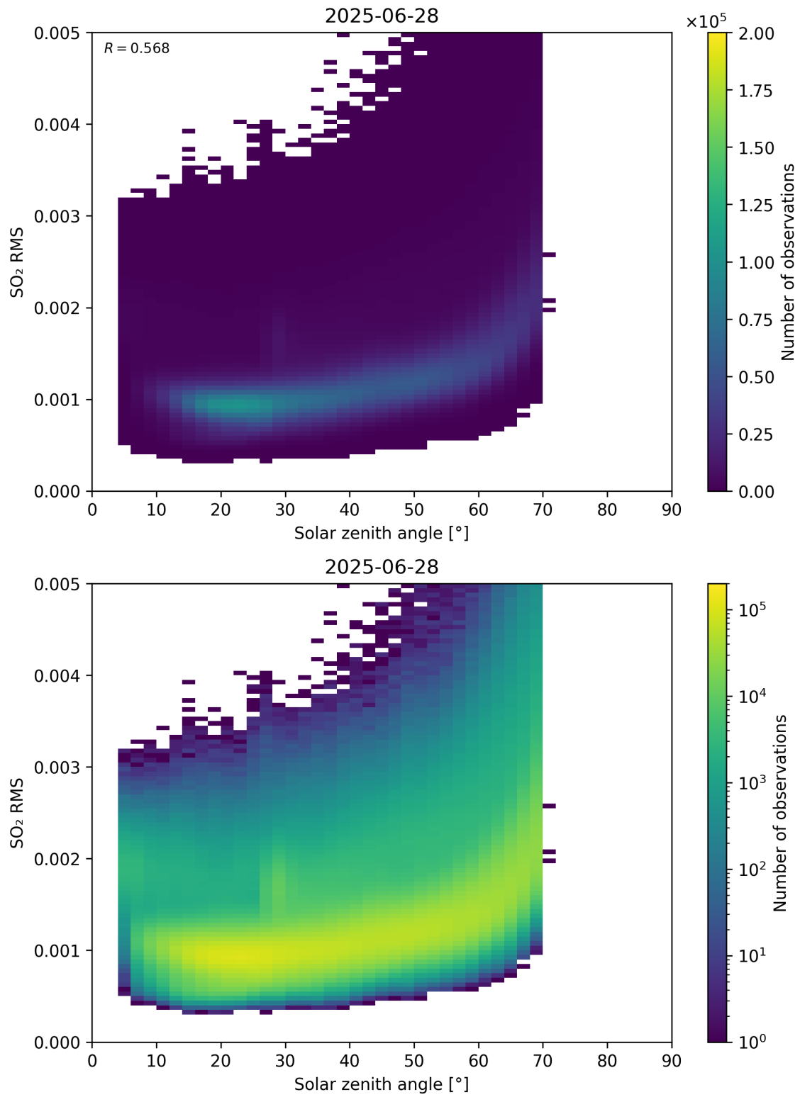
Figure 176: Scatter density plot of “Solar zenith angle” against “SO 2 RMS” for 2025-06-27 to 2025-06-29.
