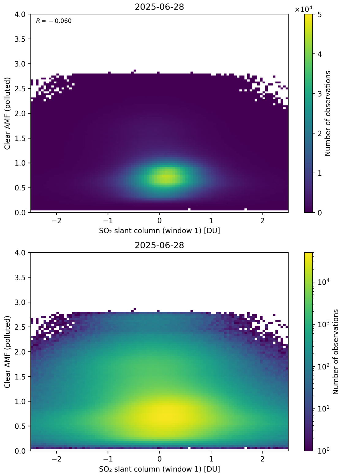
Figure 282: Scatter density plot of “SO 2 slant column (window 1)” against “Clear AMF (polluted)” for 2025-06-27 to 2025-06-29.
