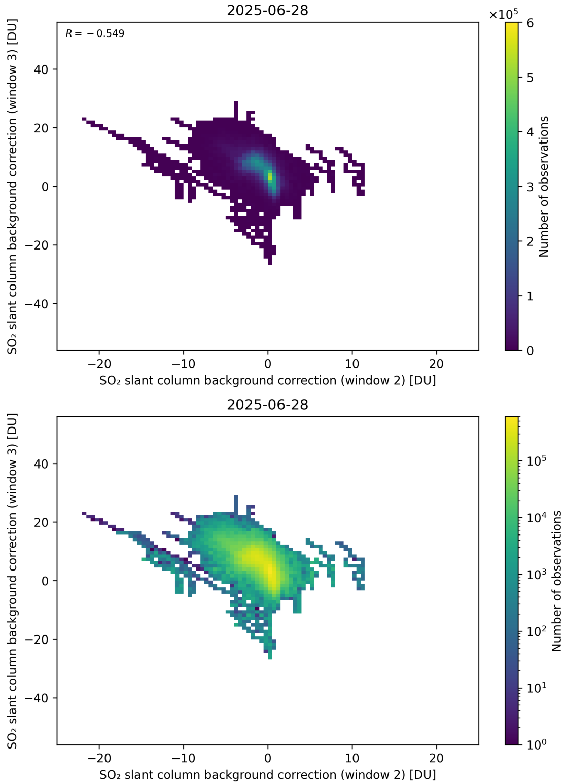
Figure 122: Scatter density plot of “SO 2 slant column background correction (window 2)” against “SO 2 slant column background correction (window 3)” for 2025-06-27 to 2025-06-29.
