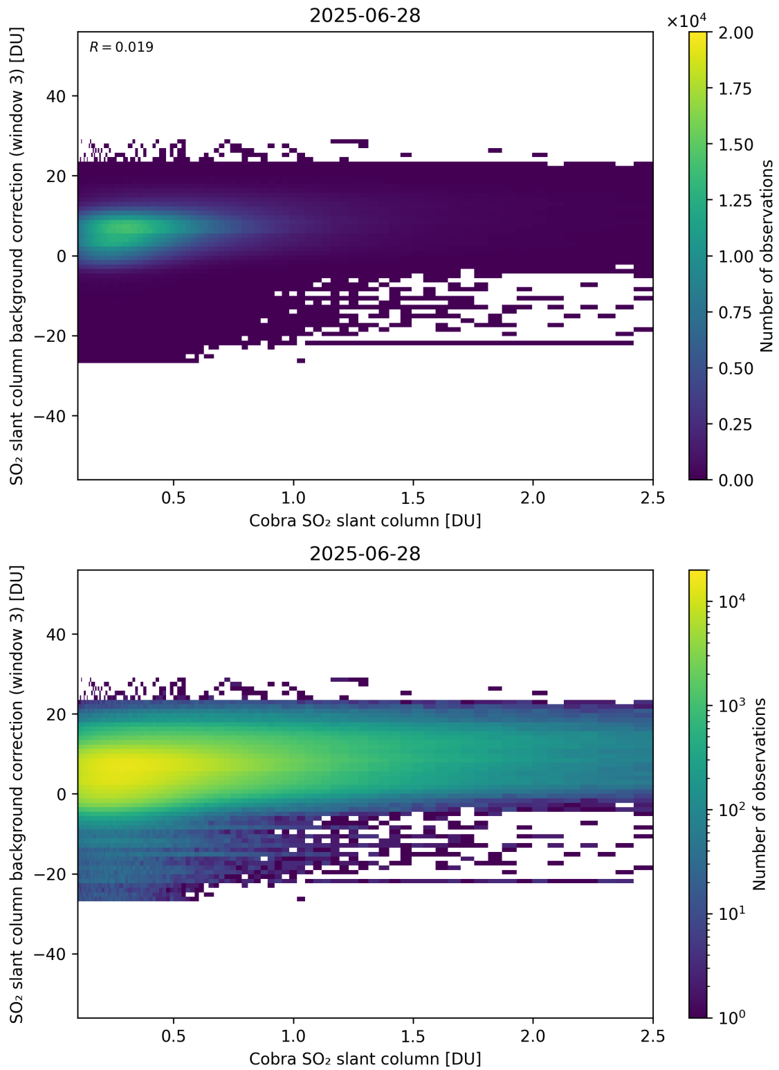
Figure 195: Scatter density plot of “Cobra SO 2 slant column” against “SO 2 slant column background correction (window 3)” for 2025-06-27 to 2025-06-29.
