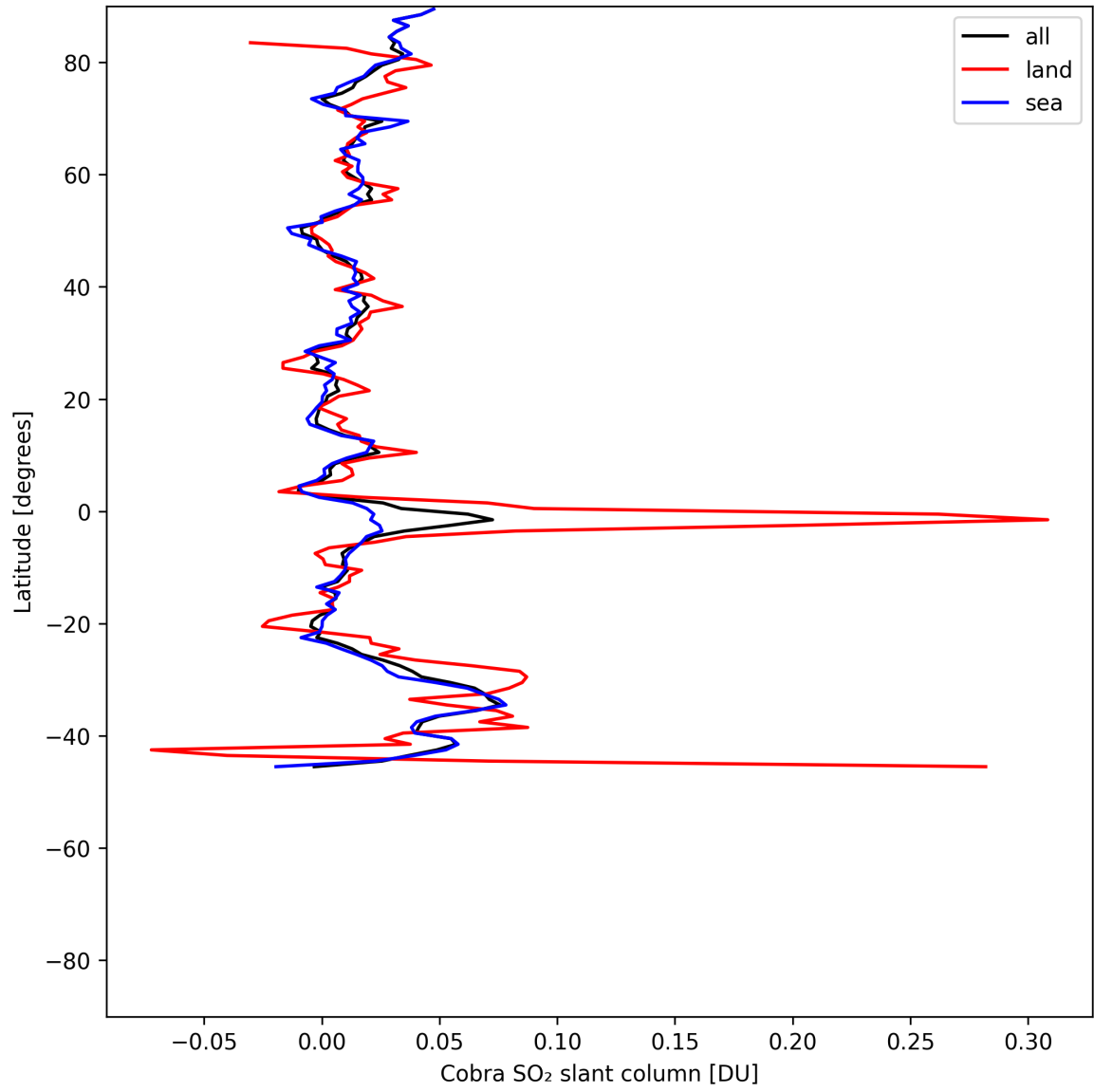
Figure 35: Zonal average of “Cobra SO 2 slant column” for 2025-06-27 to 2025-06-29.
