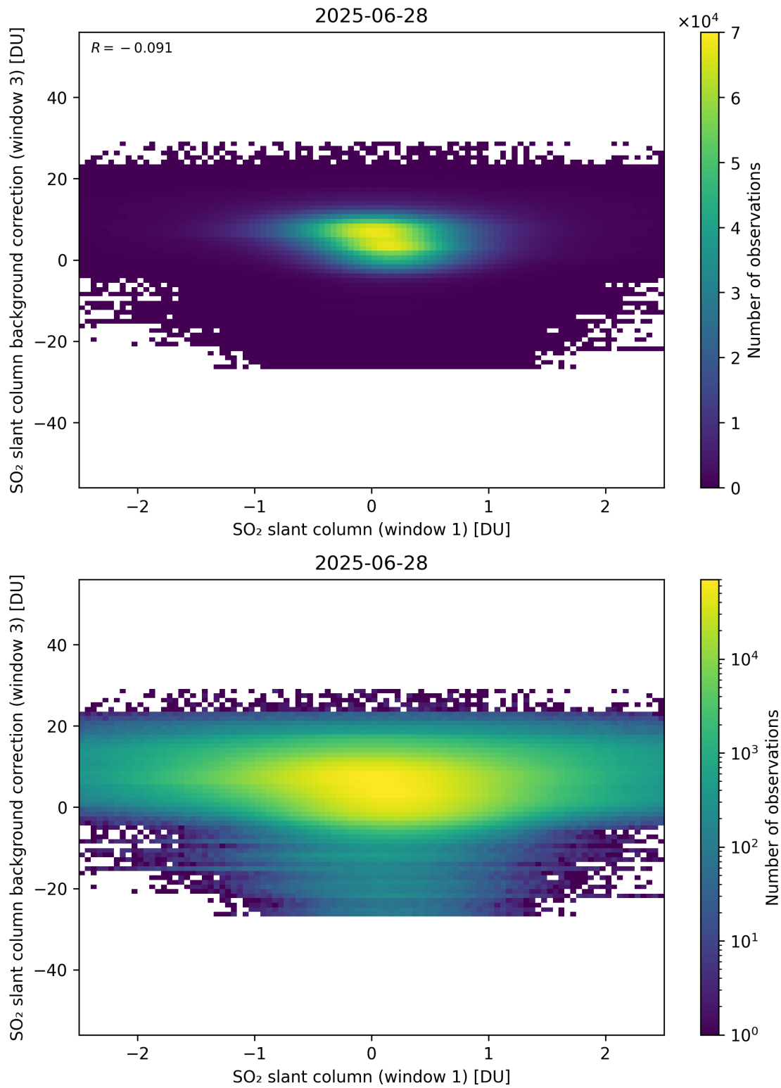
Figure 264: Scatter density plot of “SO 2 slant column (window 1)” against “SO 2 slant column background correction (window 3)” for 2025-06-27 to 2025-06-29.
