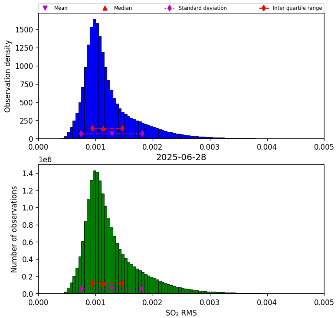
Figure 78: Histogram of “SO 2 RMS” for 2025-06-27 to 2025-06-29
