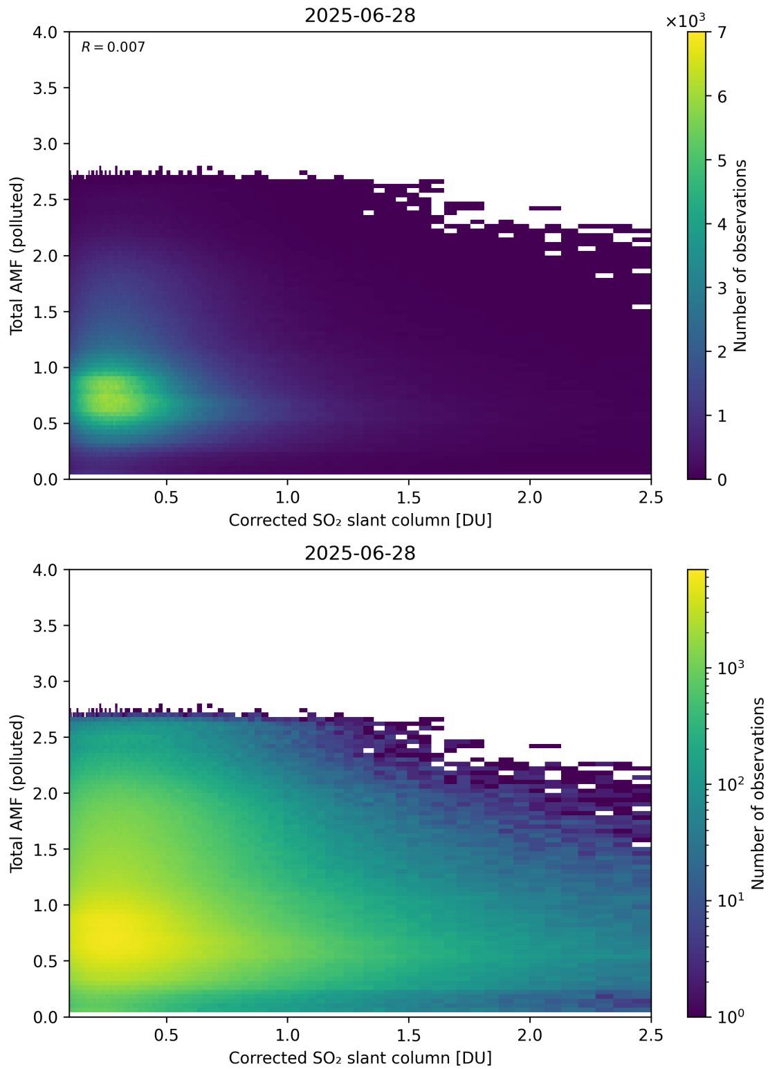
Figure 242: Scatter density plot of “Corrected SO 2 slant column” against “Total AMF (polluted)” for 2025-06-27 to 2025-06-29.
