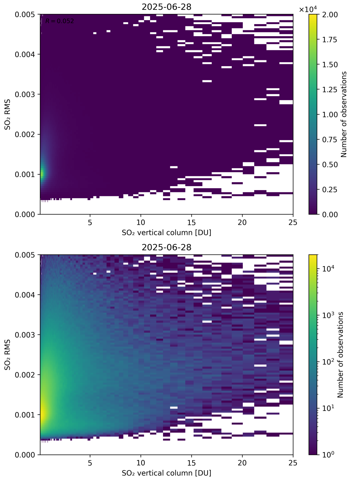
Figure 328: Scatter density plot of “SO 2 vertical column” against “SO 2 RMS” for 2025-06-27 to 2025-06-29.
