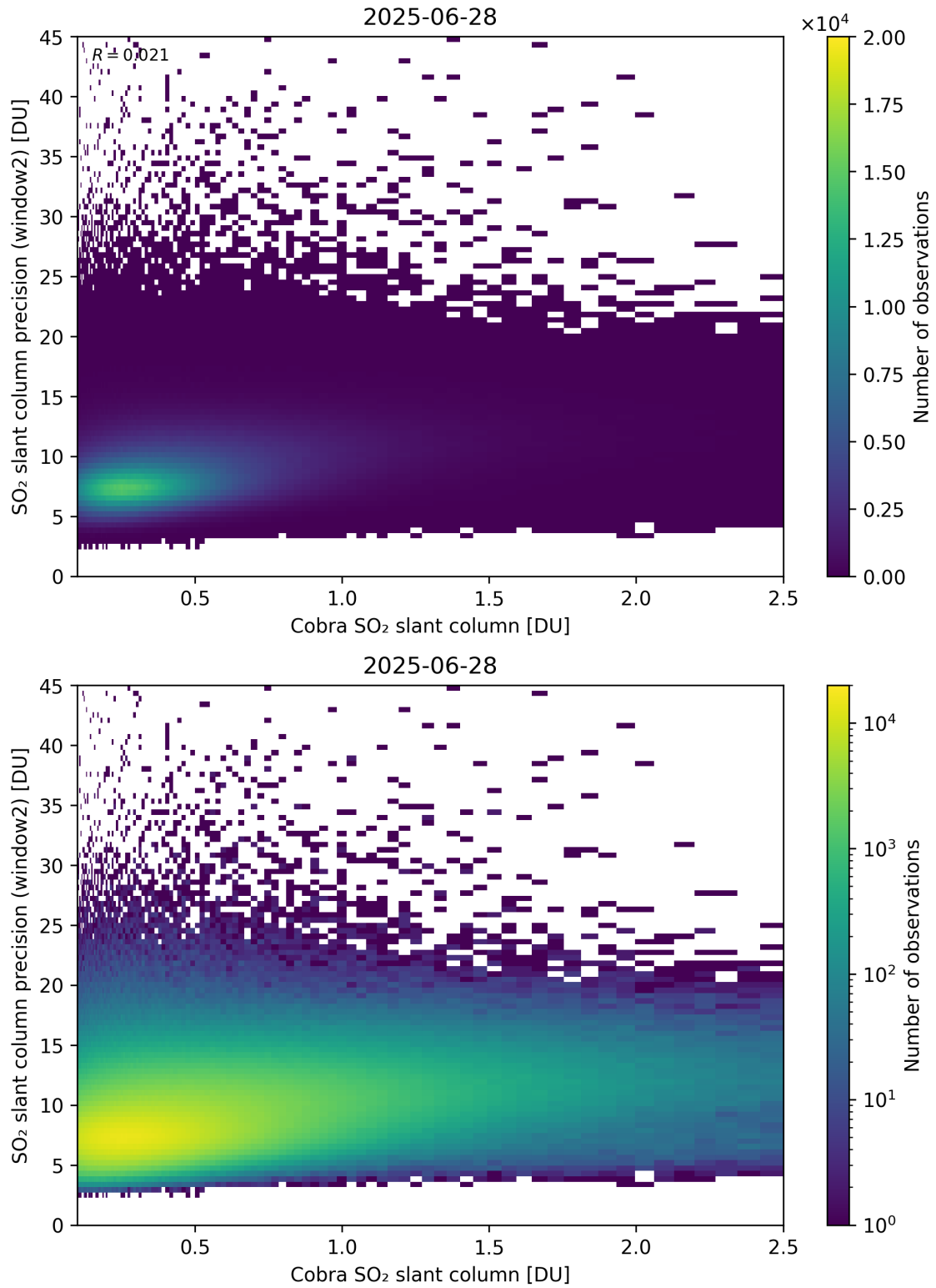
Figure 221: Scatter density plot of “Cobra SO 2 slant column” against “SO 2 slant column precision (window2)” for 2025-06-27 to 2025-06-29.
