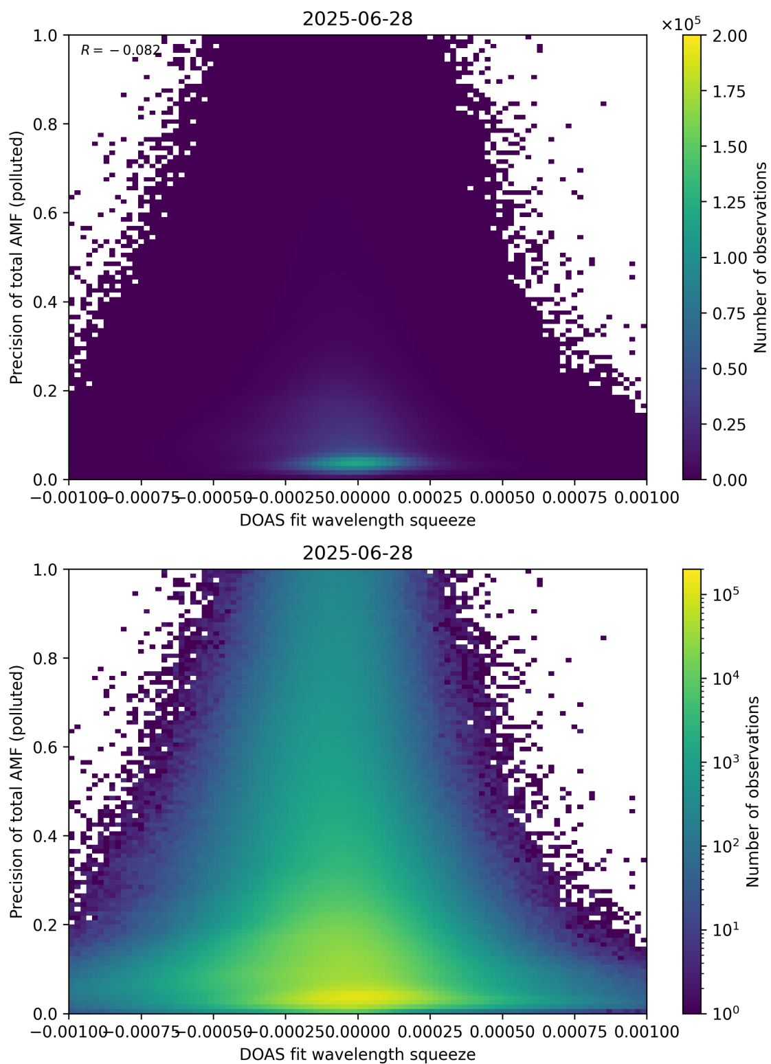
Figure 146: Scatter density plot of “DOAS fit wavelength squeeze” against “Precision of total AMF (polluted)” for 2025-06-27 to 2025-06-29.
