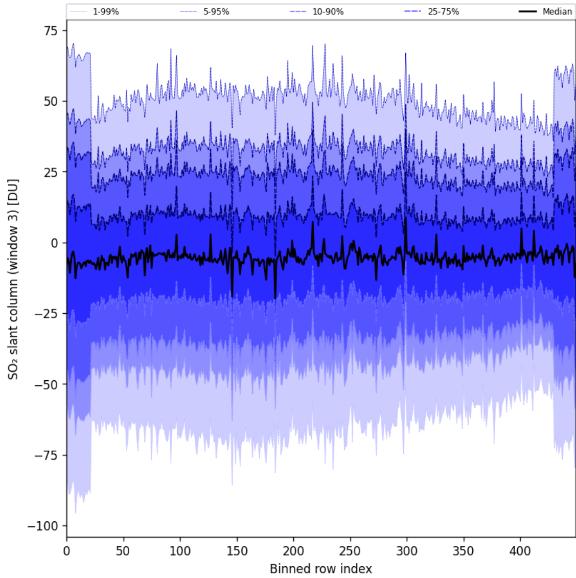
Figure 97: Along track statistics of “SO 2 slant column (window 3)” for 2025-06-27 to 2025-06-29
