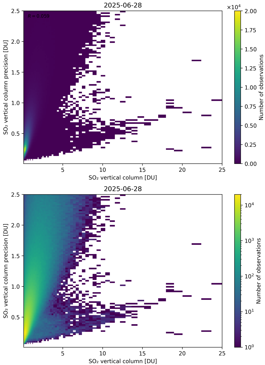
Figure 361: Scatter density plot of “SO 2 vertical column” against “SO 2 vertical column precision” for 2025-06-27 to 2025-06-29.
