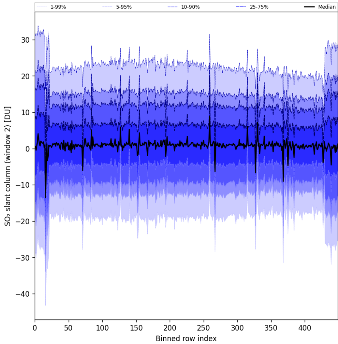
Figure 93: Along track statistics of “SO 2 slant column (window 2)” for 2025-06-27 to 2025-06-29
