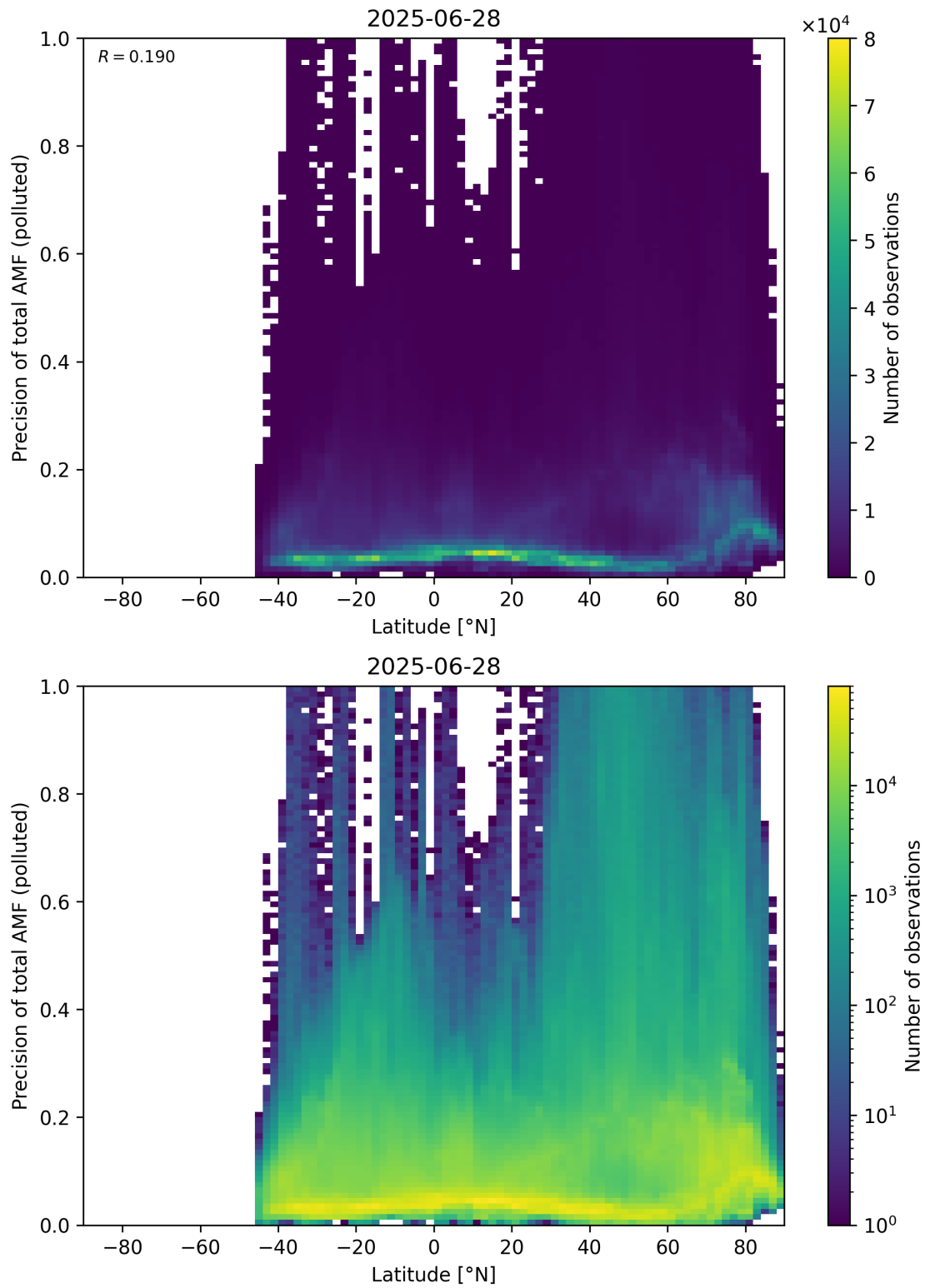
Figure 168: Scatter density plot of “Latitude” against “Precision of total AMF (polluted)” for 2025-06-27 to 2025-06-29.
