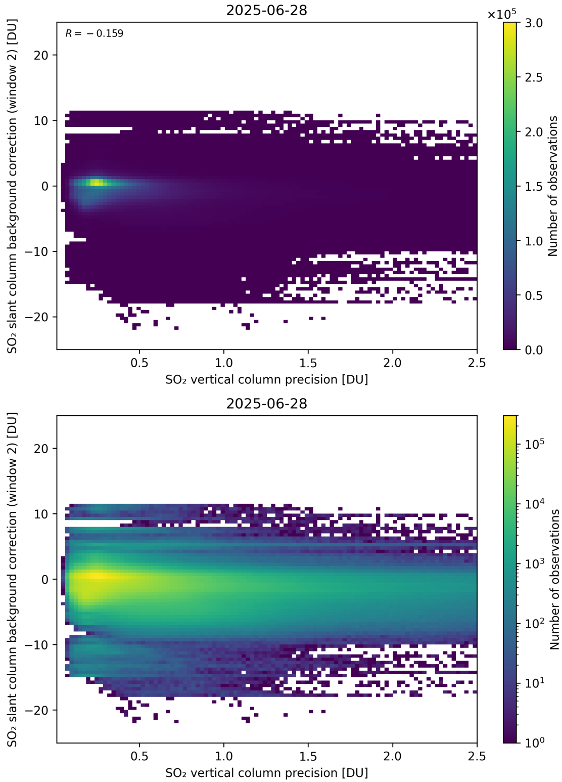
Figure 330: Scatter density plot of “SO 2 vertical column precision” against “SO 2 slant column background correction (window 2)” for 2025-06-27 to 2025-06-29.
