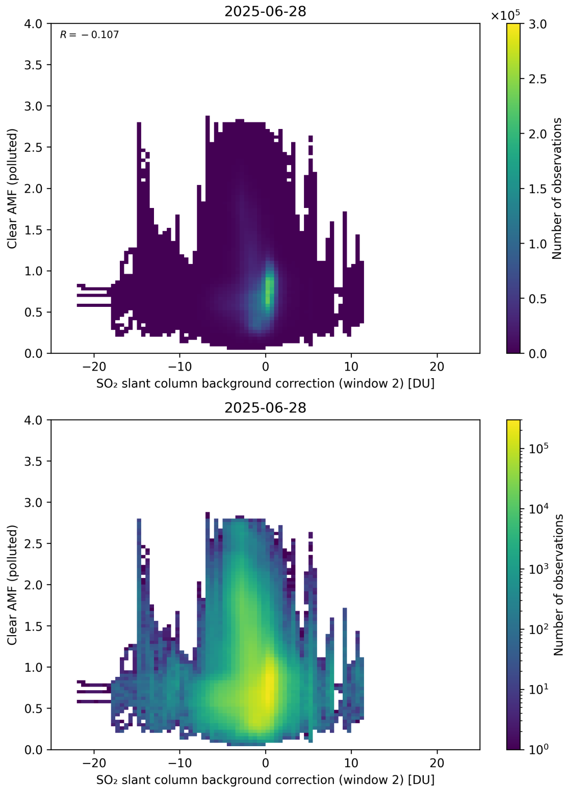
Figure 126: Scatter density plot of “SO 2 slant column background correction (window 2)” against “Clear AMF (polluted)” for 2025-06-27 to 2025-06-29.
