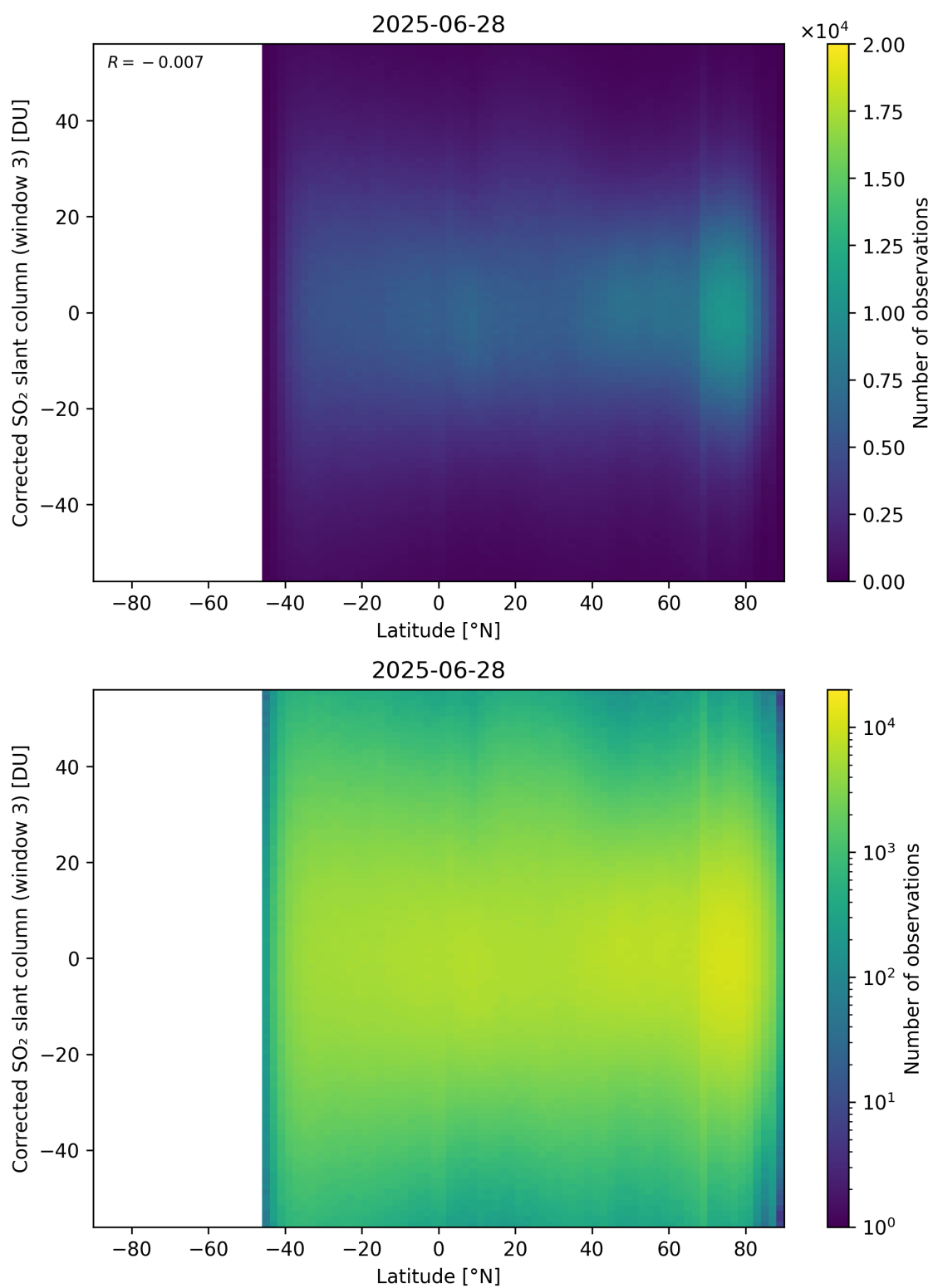
Figure 161: Scatter density plot of “Latitude” against “Corrected SO 2 slant column (window 3)” for 2025-06-27 to 2025-06-29.
