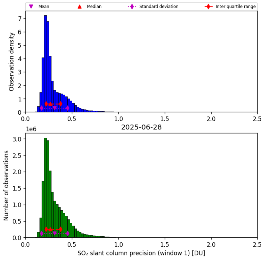
Figure 64: Histogram of “SO 2 slant column precision (window 1)” for 2025-06-27 to 2025-06-29
