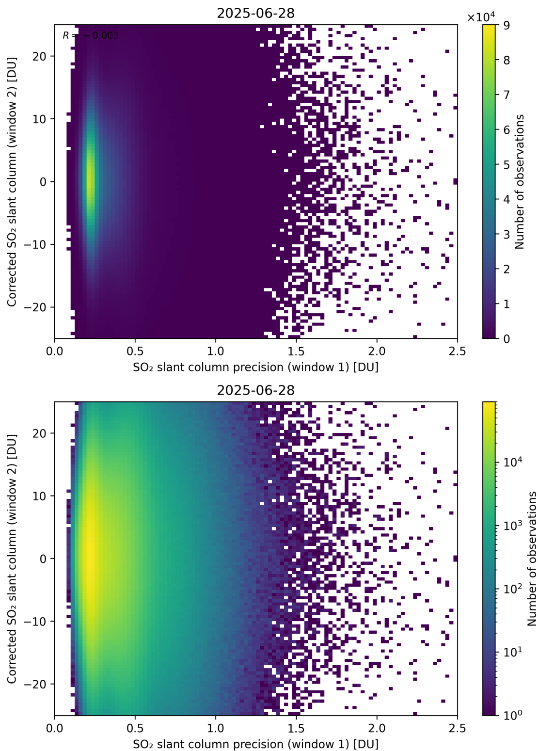
Figure 275: Scatter density plot of “SO 2 slant column precision (window 1)” against “Corrected SO 2 slant column (window 2)” for 2025-06-27 to 2025-06-29.
