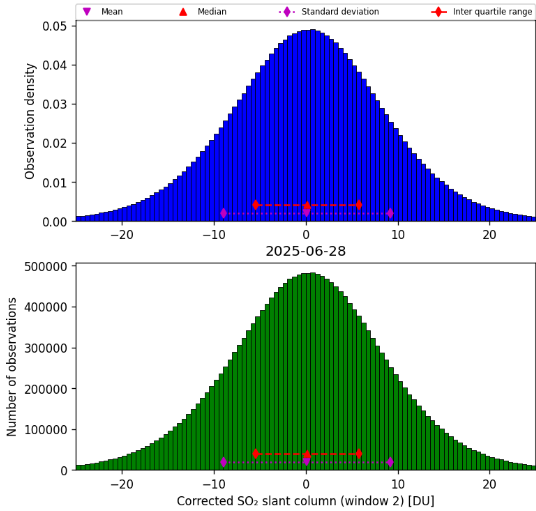
Figure 69: Histogram of “Corrected SO 2 slant column (window 2)” for 2025-06-27 to 2025-06-29
