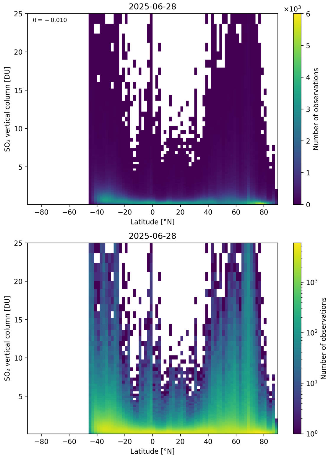
Figure 169: Scatter density plot of “Latitude” against “SO 2 vertical column” for 2025-06-27 to 2025-06-29.
