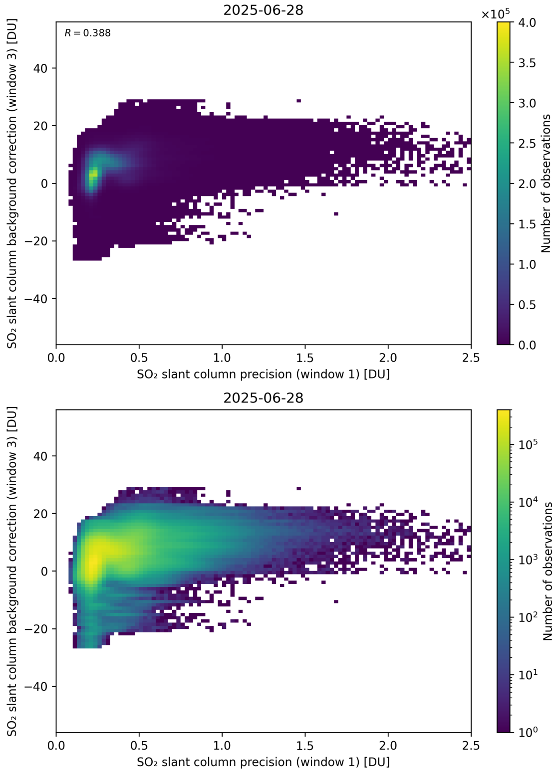
Figure 270: Scatter density plot of “SO 2 slant column precision (window 1)” against “SO 2 slant column background correction (window 3)” for 2025-06-27 to 2025-06-29.
