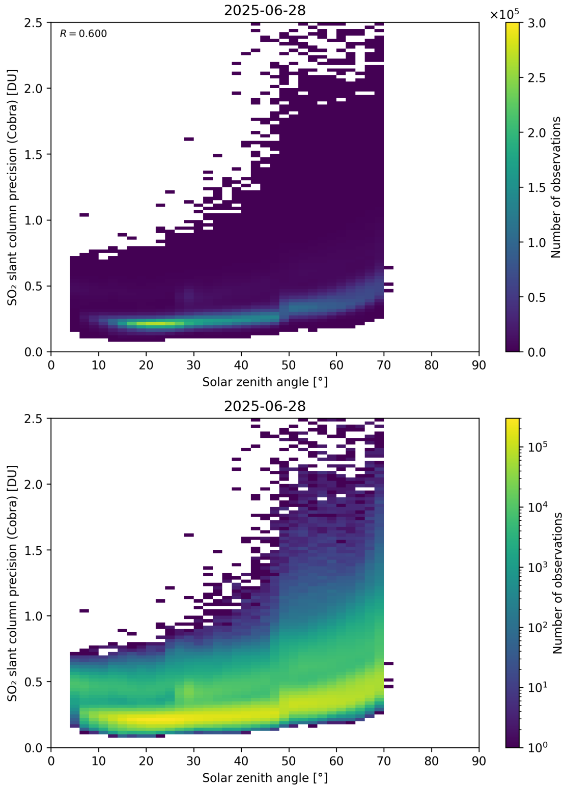
Figure 180: Scatter density plot of “Solar zenith angle” against “SO 2 slant column precision (Cobra)” for 2025-06-27 to 2025-06-29.
