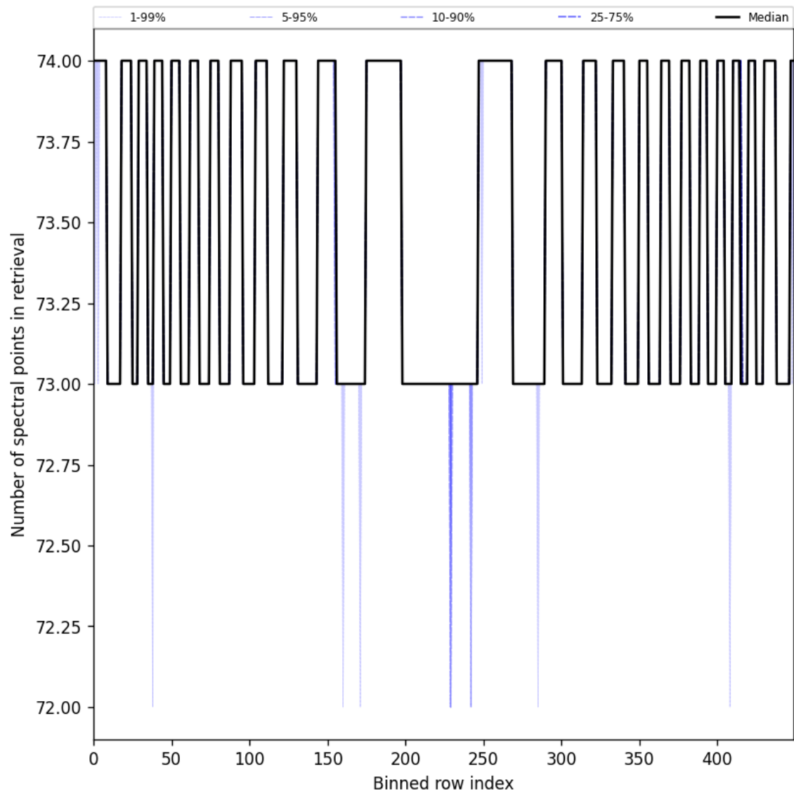
Figure 108: Along track statistics of “Number of spectral points in retrieval” for 2025-06-27 to 2025-06-29
