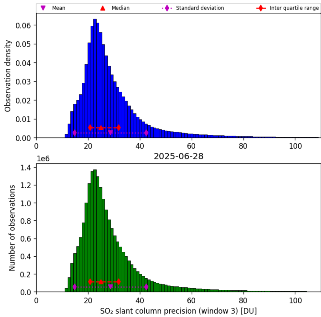
Figure 72: Histogram of “SO 2 slant column precision (window 3)” for 2025-06-27 to 2025-06-29
