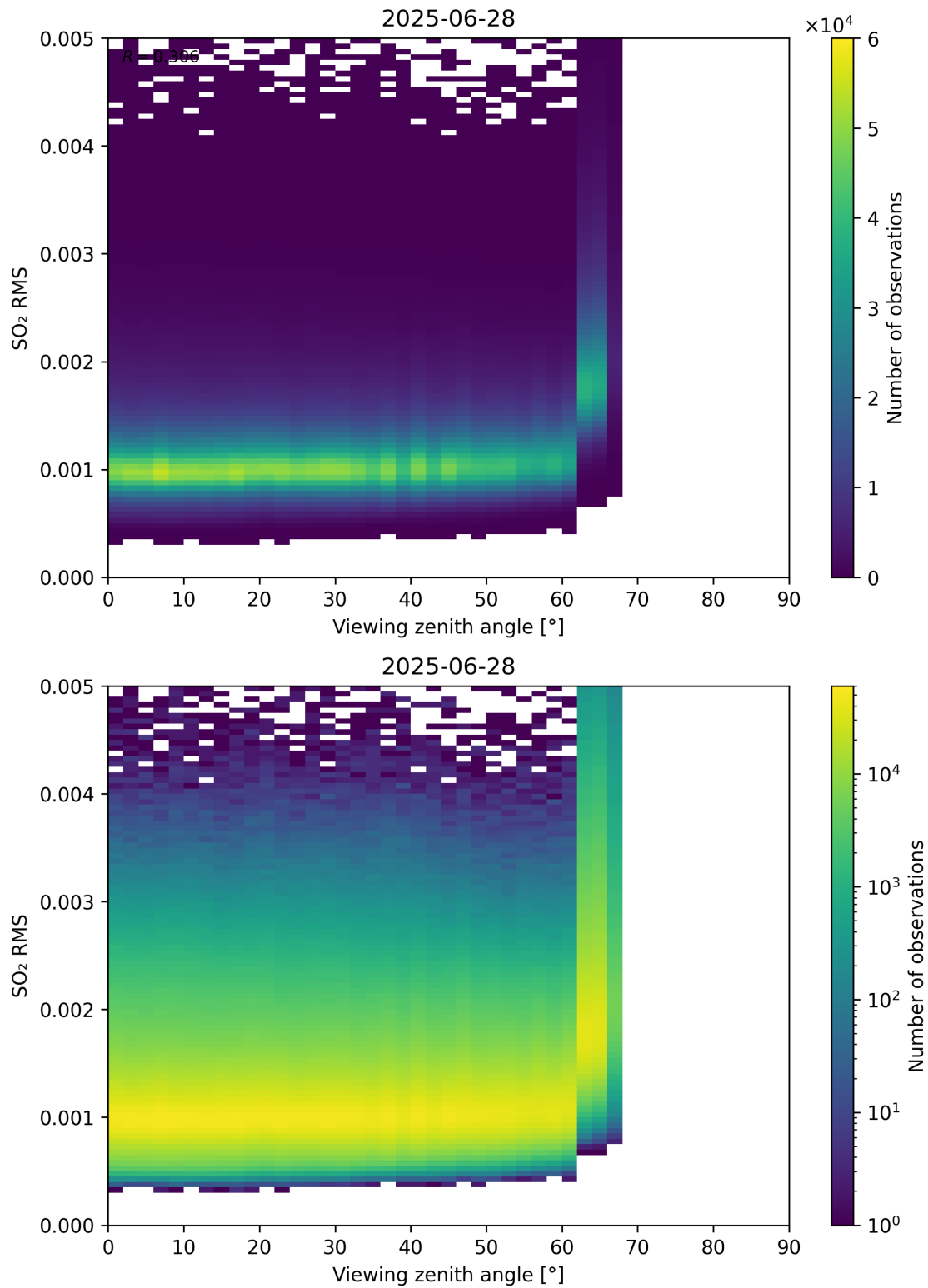
Figure 367: Scatter density plot of “Viewing zenith angle” against “SO 2 RMS” for 2025-06-27 to 2025-06-29.
