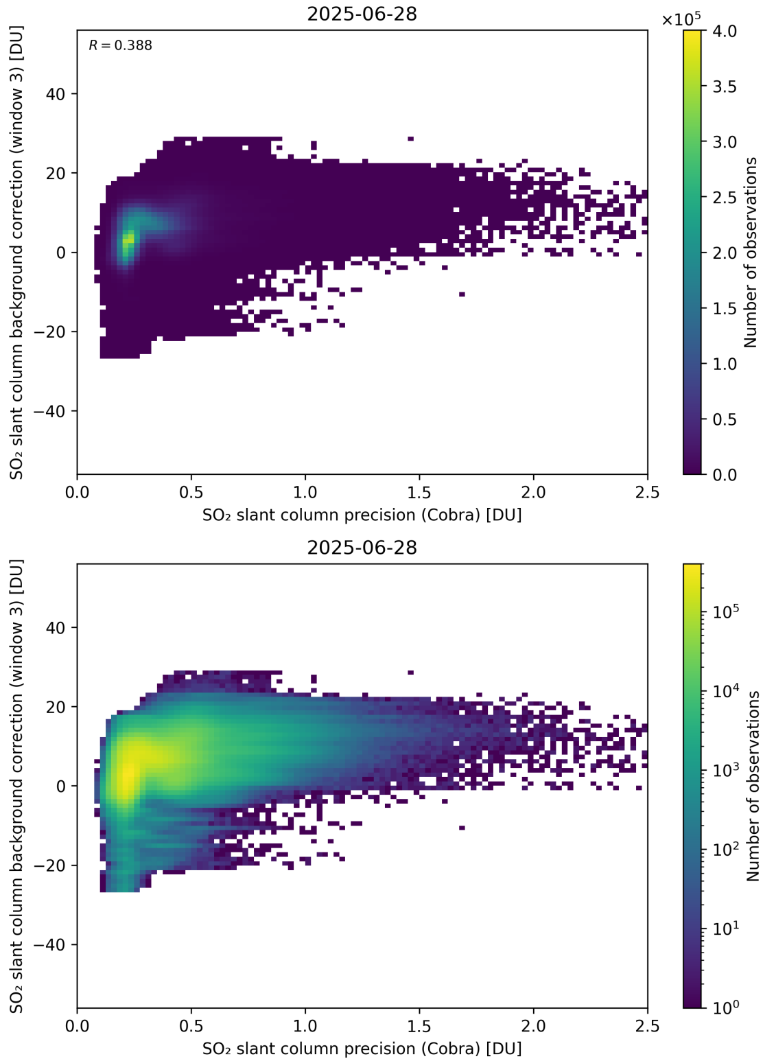
Figure 201: Scatter density plot of “SO 2 slant column precision (Cobra)” against “SO 2 slant column background correction (window 3)” for 2025-06-27 to 2025-06-29.
