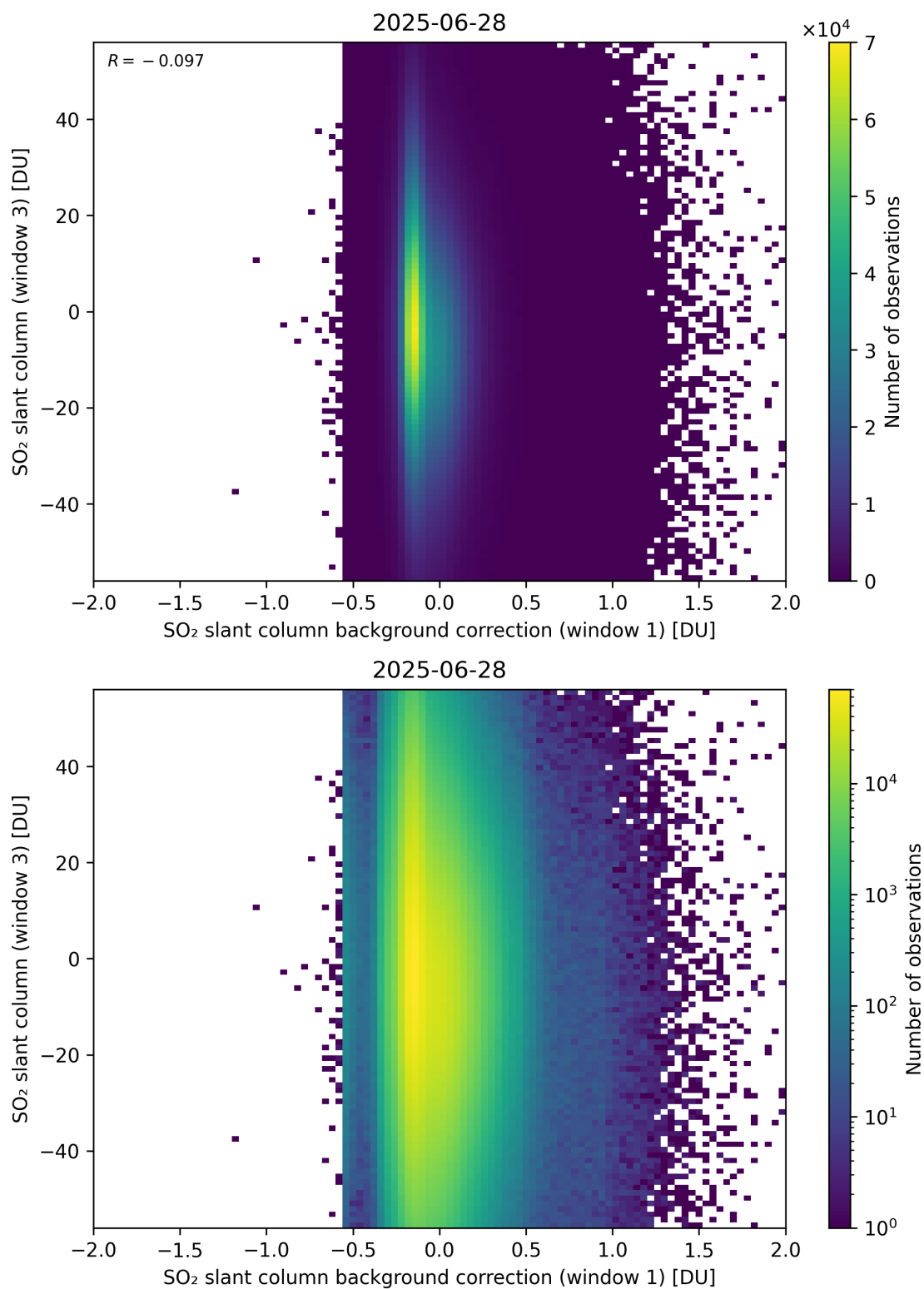
Figure 118: Scatter density plot of “SO 2 slant column background correction (window 1)” against “SO 2 slant column (window 3)” for 2025-06-27 to 2025-06-29.
