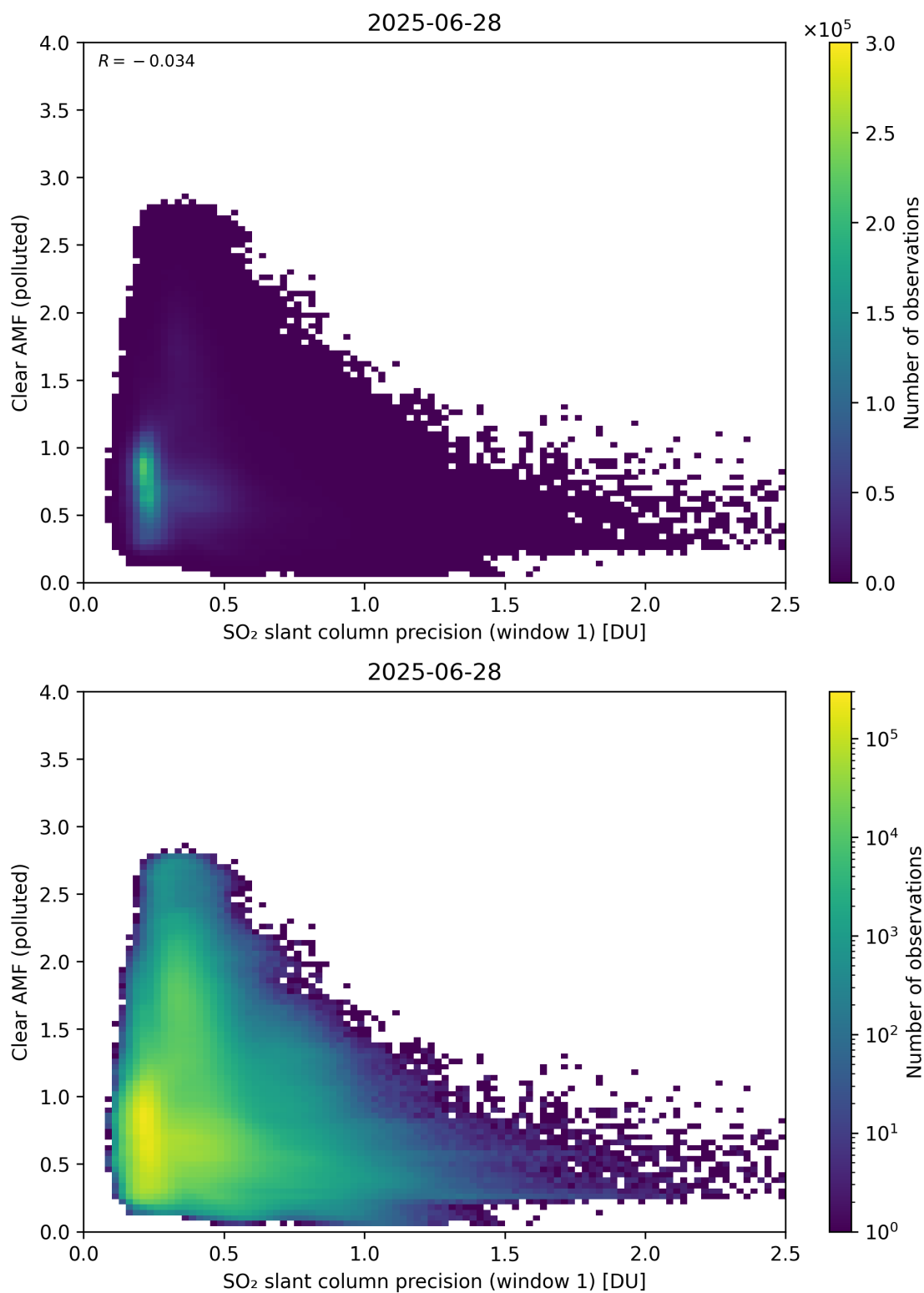
Figure 274: Scatter density plot of “SO 2 slant column precision (window 1)” against “Clear AMF (polluted)” for 2025-06-27 to 2025-06-29.
