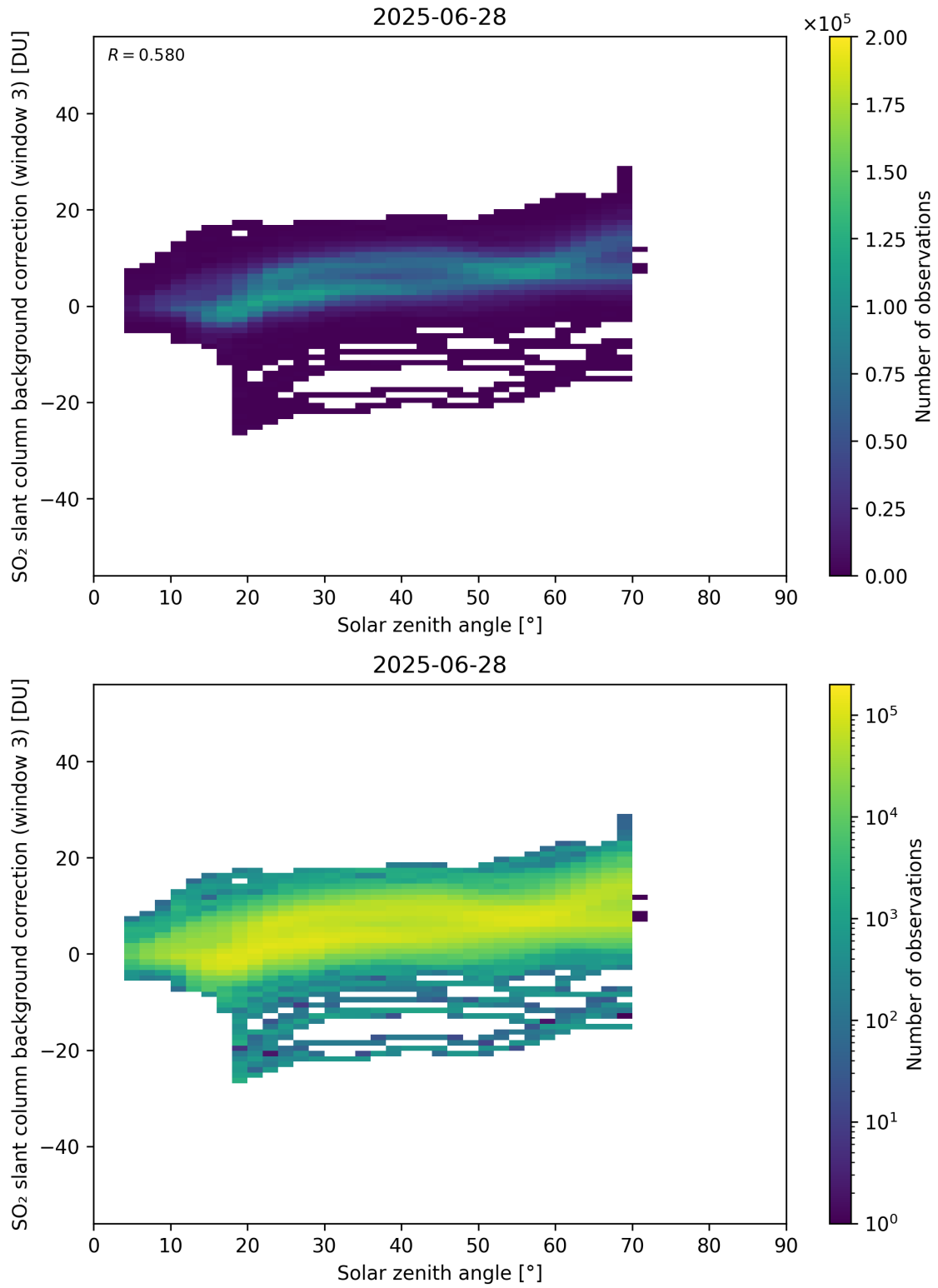
Figure 173: Scatter density plot of “Solar zenith angle” against “SO 2 slant column background correction (window 3)” for 2025-06-27 to 2025-06-29.
