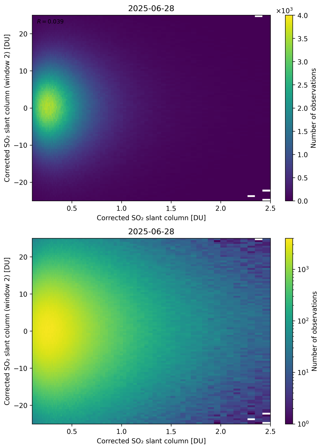
Figure 235: Scatter density plot of “Corrected SO 2 slant column” against “Corrected SO 2 slant column (window 2)” for 2025-06-27 to 2025-06-29.
