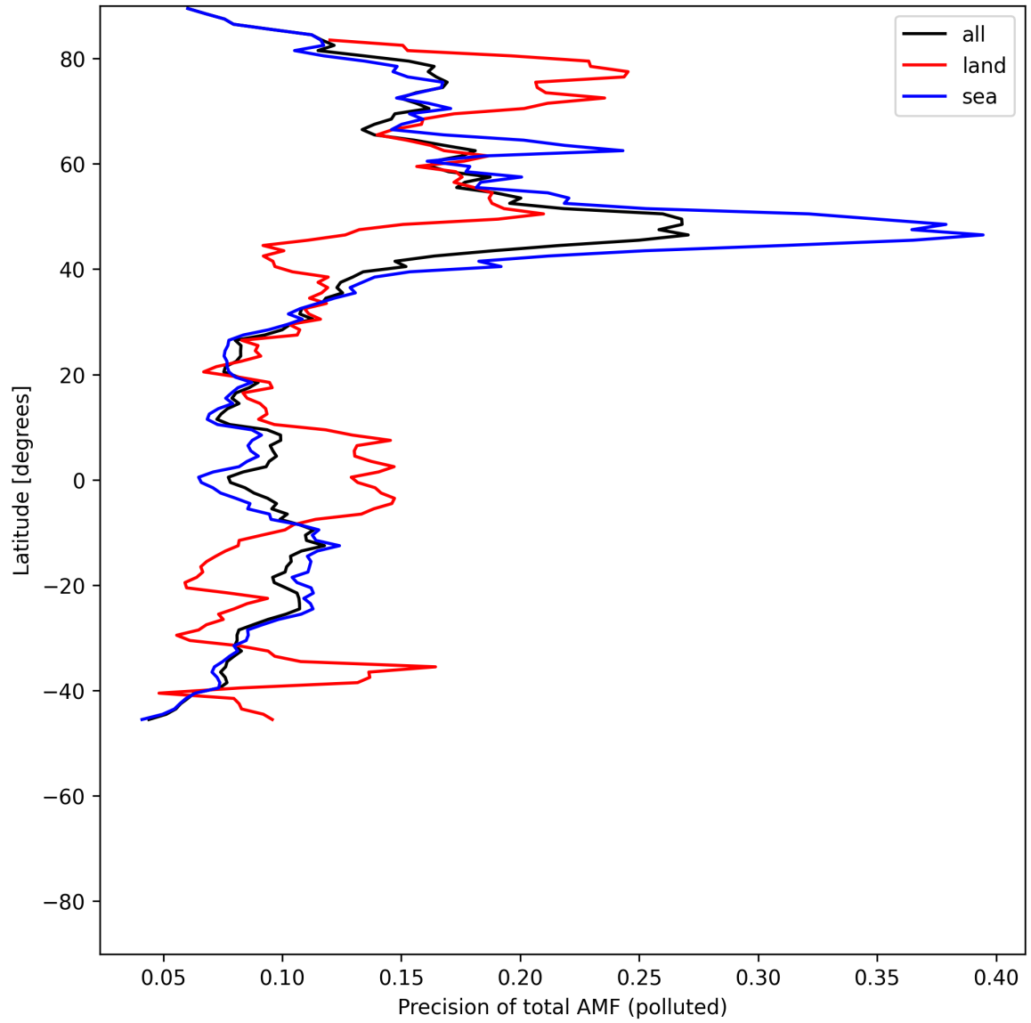
Figure 54: Zonal average of “Precision of total AMF (polluted)” for 2025-06-27 to 2025-06-29.
