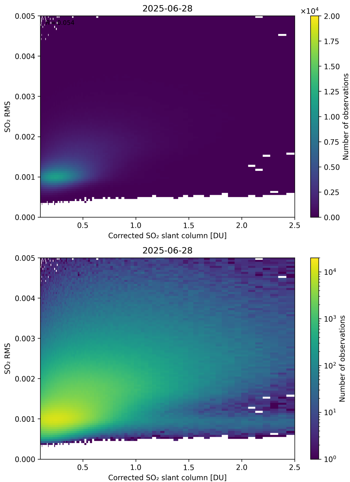
Figure 231: Scatter density plot of “Corrected SO 2 slant column” against “SO 2 RMS” for 2025-06-27 to 2025-06-29.
