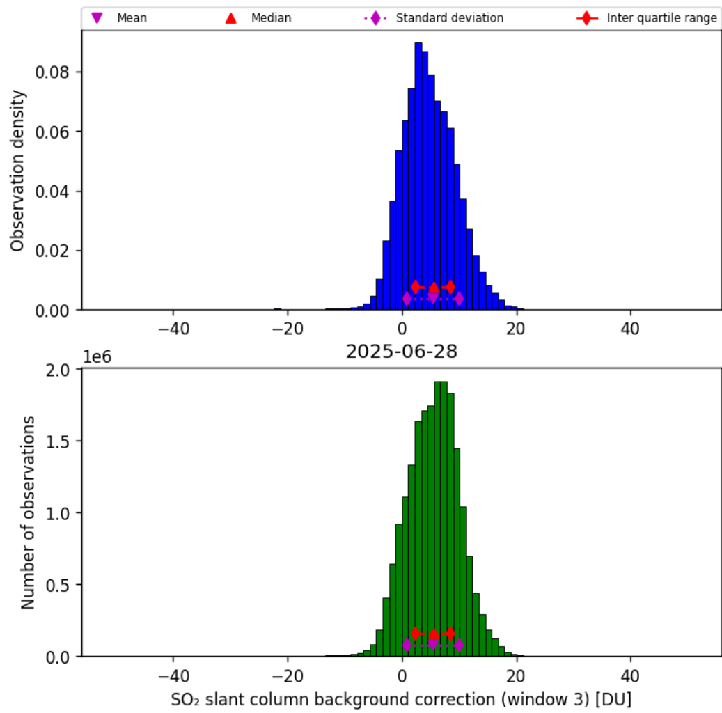
Figure 74: Histogram of “SO 2 slant column background correction (window 3)” for 2025-06-27 to 2025-06-29
