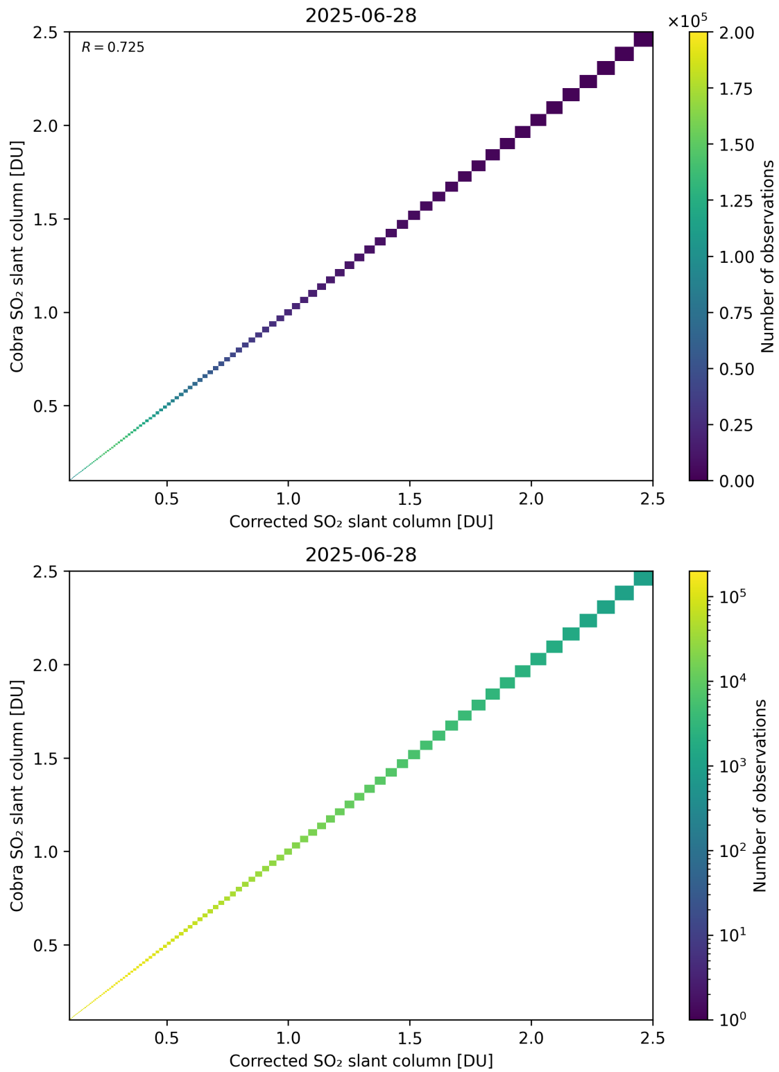
Figure 233: Scatter density plot of “Corrected SO 2 slant column” against “Cobra SO 2 slant column” for 2025-06-27 to 2025-06-29.
