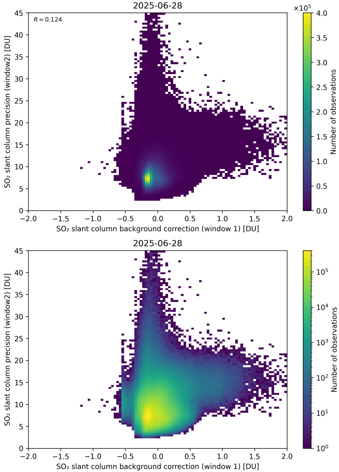
Figure 117: Scatter density plot of “SO 2 slant column background correction (window 1)” against “SO 2 slant column precision (window2)” for 2025-06-27 to 2025-06-29.
