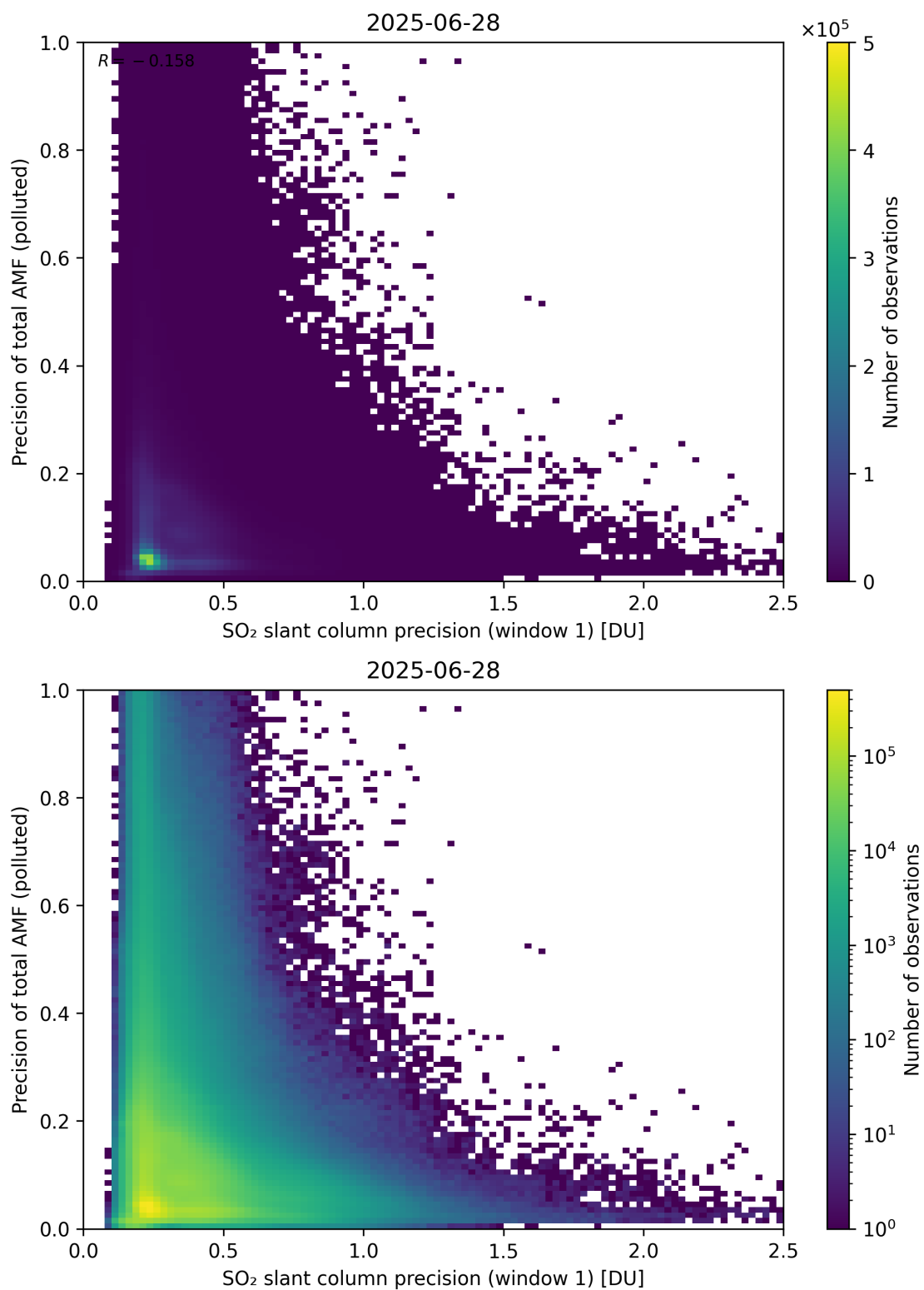
Figure 281: Scatter density plot of “SO 2 slant column precision (window 1)” against “Precision of total AMF (polluted)” for 2025-06-27 to 2025-06-29.
