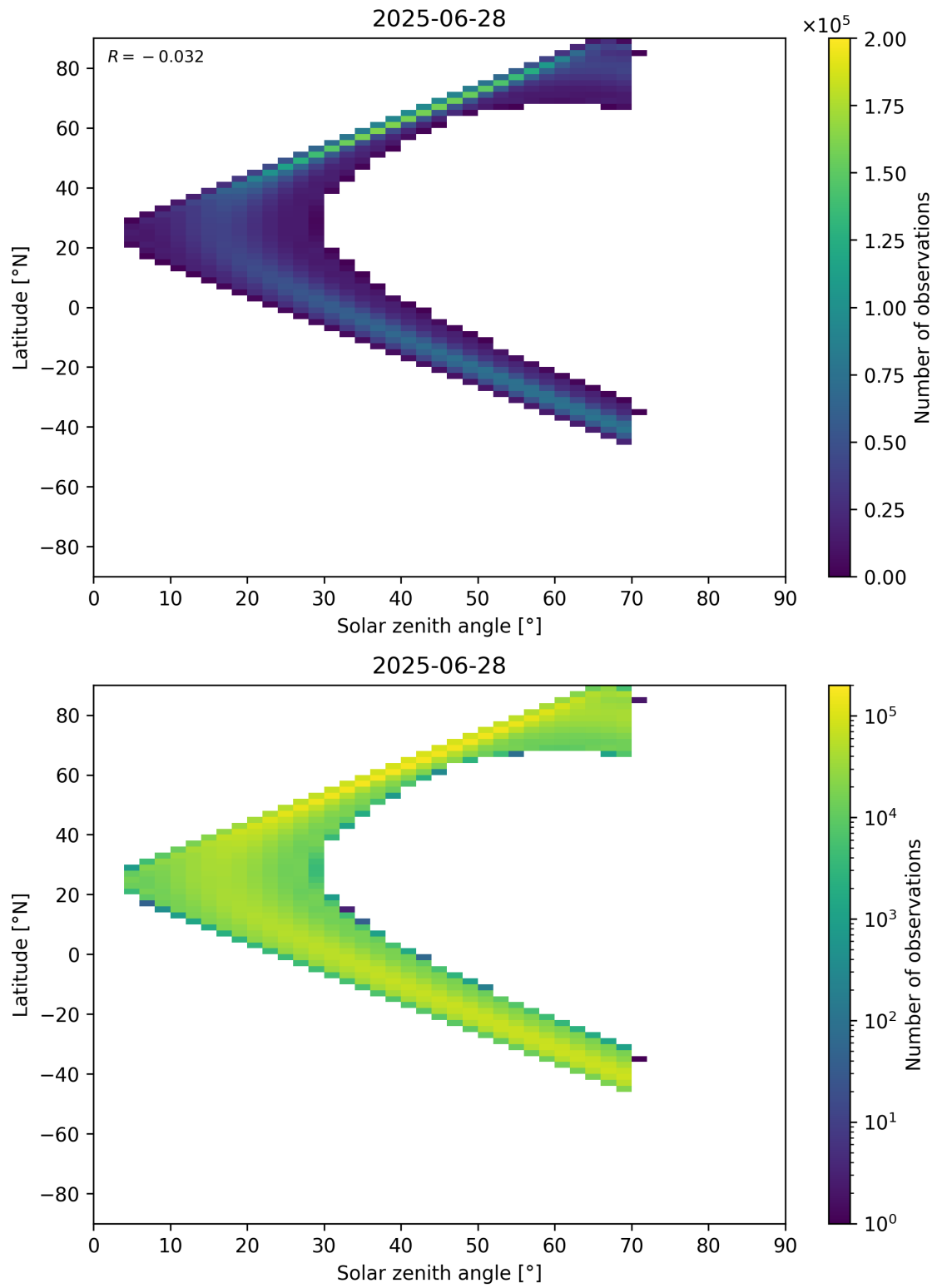
Figure 177: Scatter density plot of “Solar zenith angle” against “Latitude” for 2025-06-27 to 2025-06-29.
