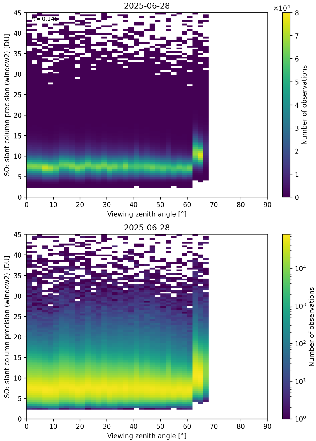
Figure 378: Scatter density plot of “Viewing zenith angle” against “SO 2 slant column precision (window2)” for 2025-06-27 to 2025-06-29.
