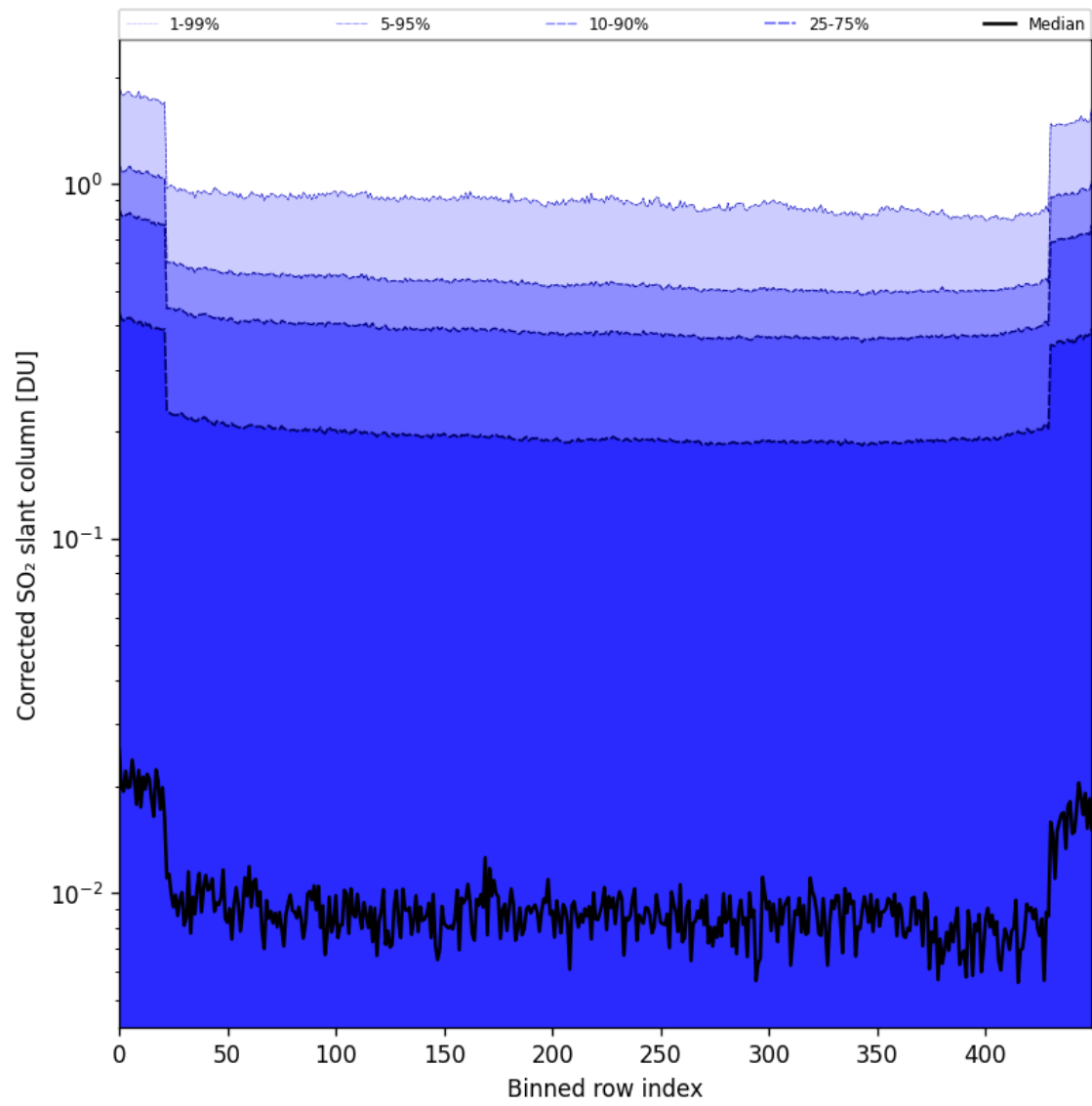
Figure 86: Along track statistics of “Corrected SO 2 slant column” for 2025-06-27 to 2025-06-29
