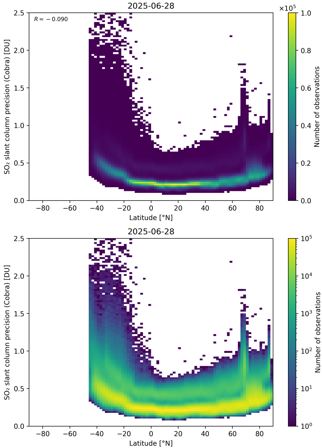
Figure 158: Scatter density plot of “Latitude” against “SO 2 slant column precision (Cobra)” for 2025-06-27 to 2025-06-29.
