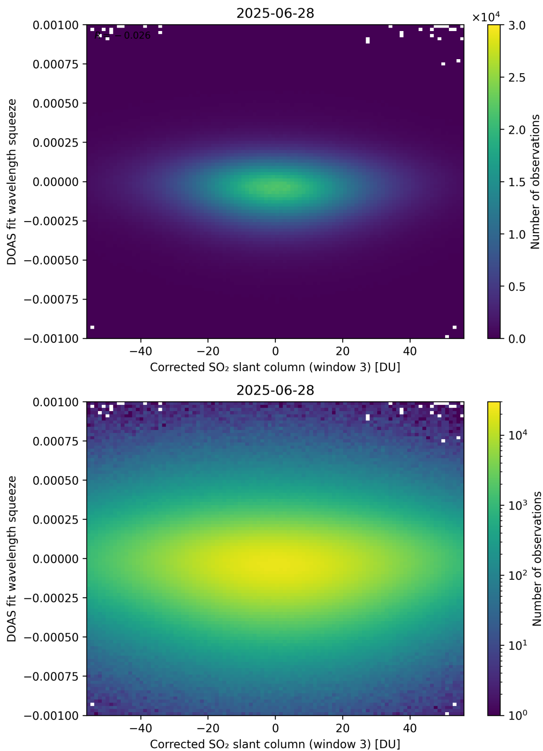
Figure 257: Scatter density plot of “Corrected SO 2 slant column (window 3)” against “DOAS fit wavelength squeeze” for 2025-06-27 to 2025-06-29.
