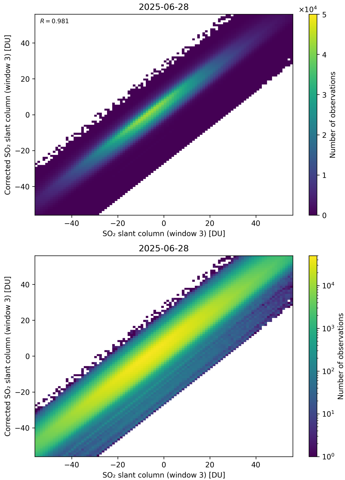
Figure 316: Scatter density plot of “SO 2 slant column (window 3)” against “Corrected SO 2 slant column (window 3)” for 2025-06-27 to 2025-06-29.
