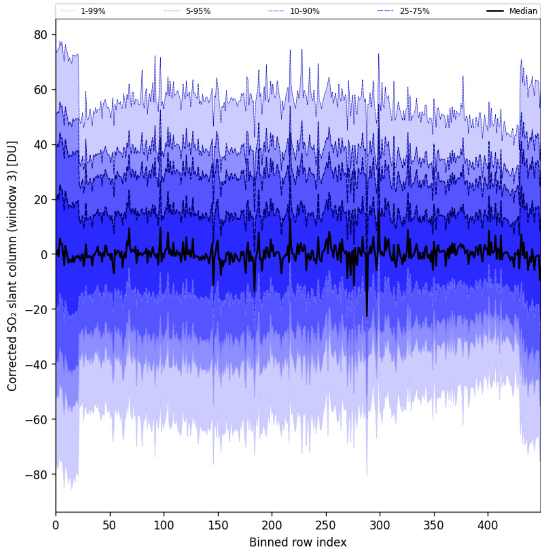
Figure 99: Along track statistics of “Corrected SO 2 slant column (window 3)” for 2025-06-27 to 2025-06-29
