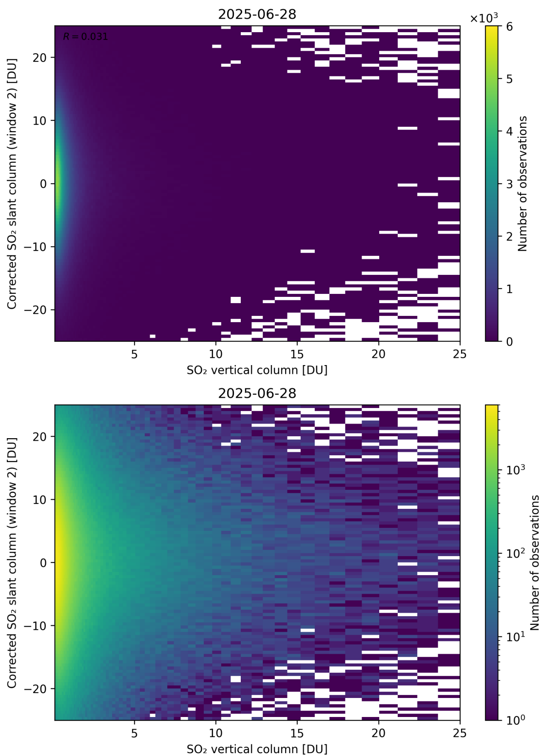
Figure 352: Scatter density plot of “SO 2 vertical column” against “Corrected SO 2 slant column (window 2)” for 2025-06-27 to 2025-06-29.
