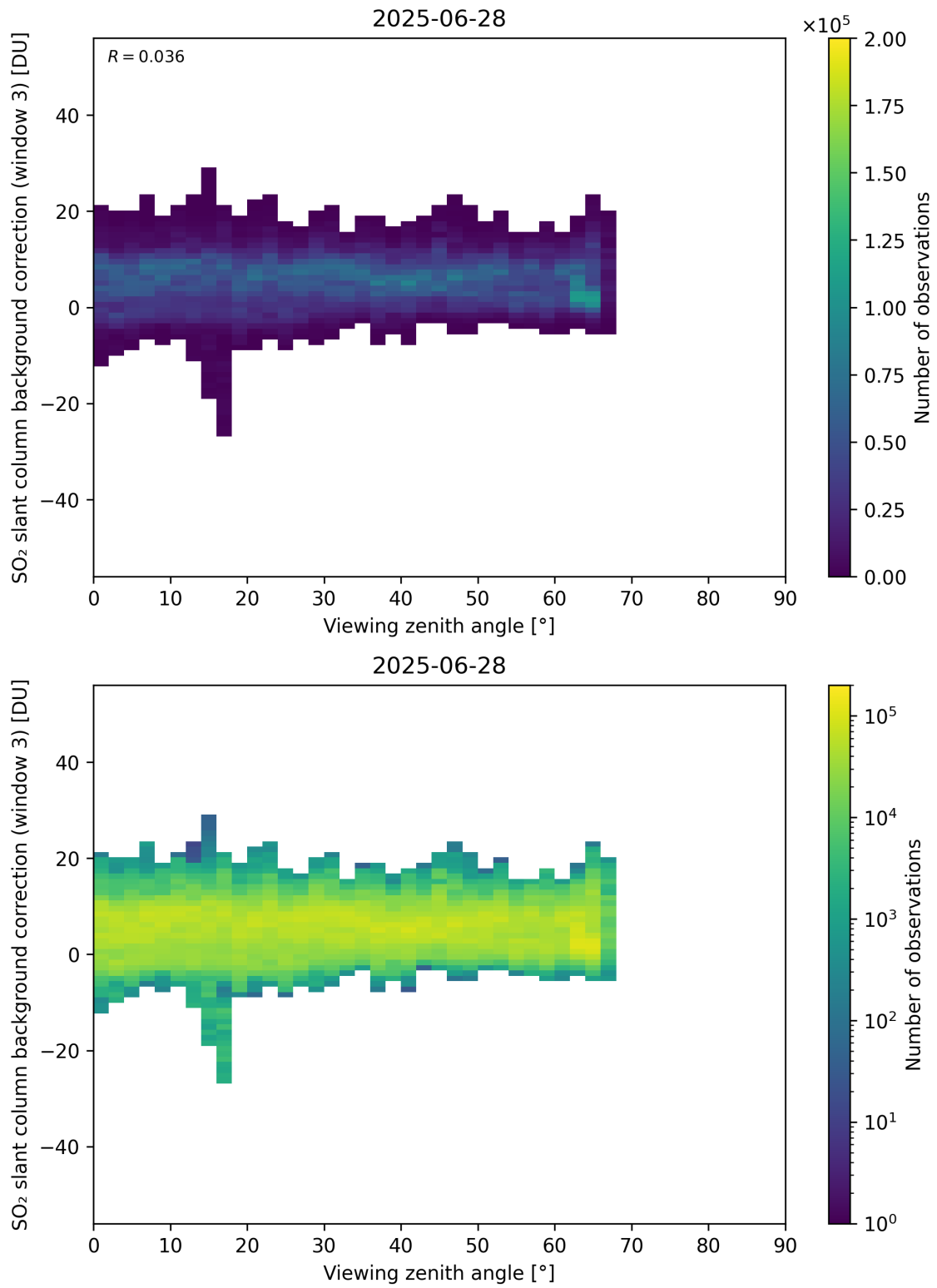
Figure 364: Scatter density plot of “Viewing zenith angle” against “SO 2 slant column background correction (window 3)” for 2025-06-27 to 2025-06-29.
