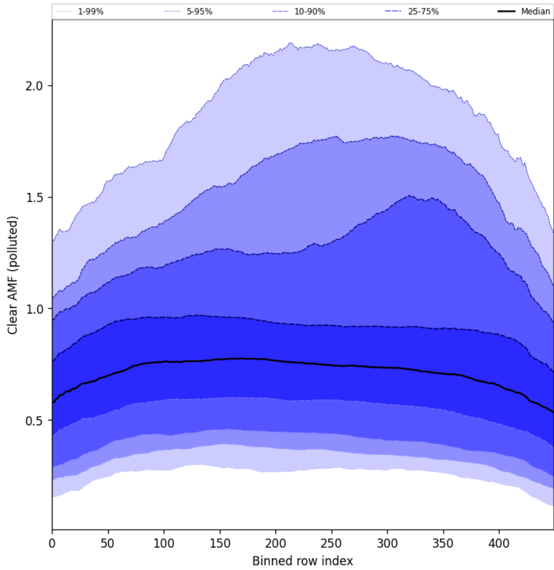
Figure 107: Along track statistics of “Clear AMF (polluted)” for 2025-06-27 to 2025-06-29
