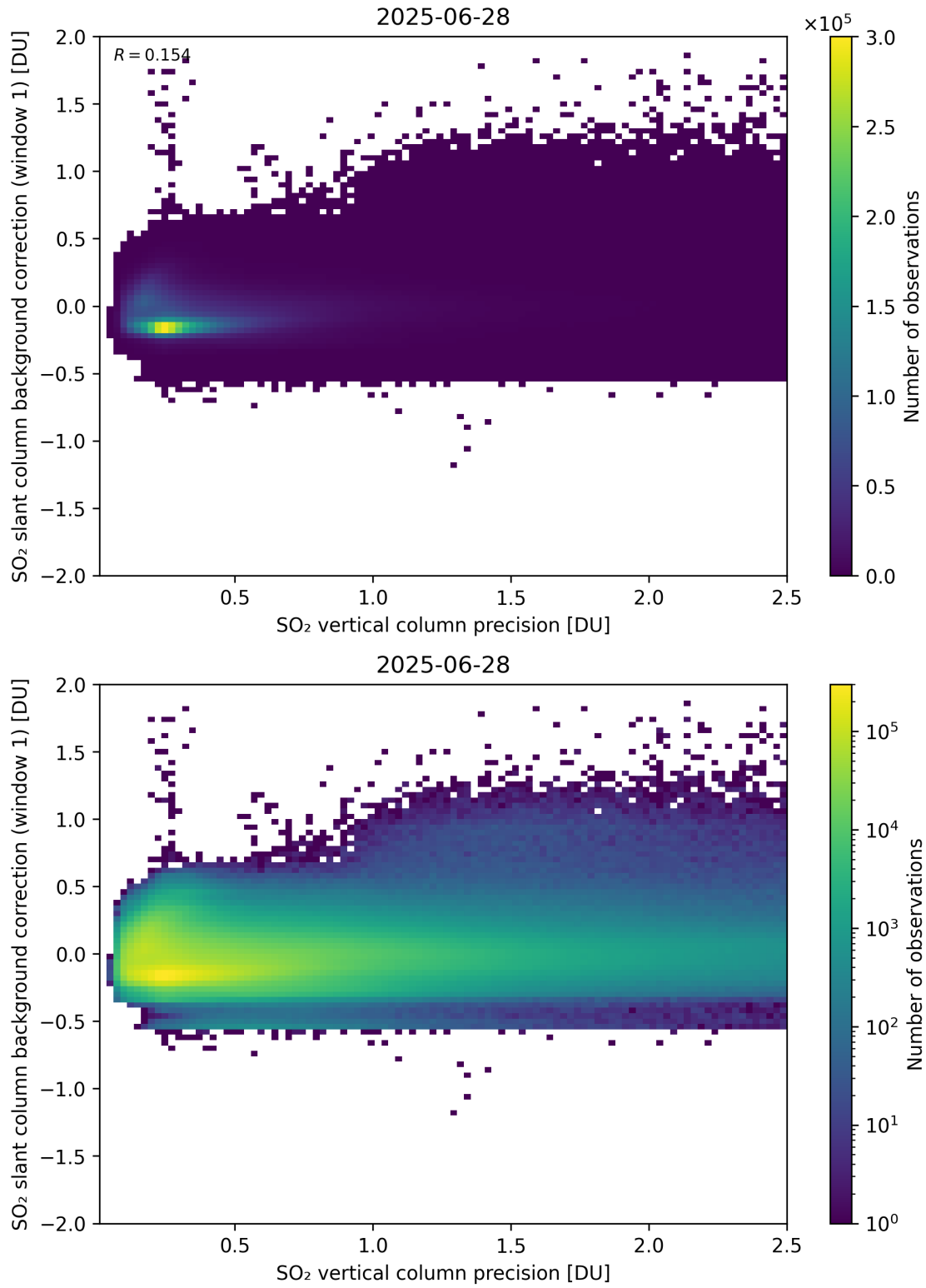
Figure 329: Scatter density plot of “SO 2 vertical column precision” against “SO 2 slant column background correction (window 1)” for 2025-06-27 to 2025-06-29.
