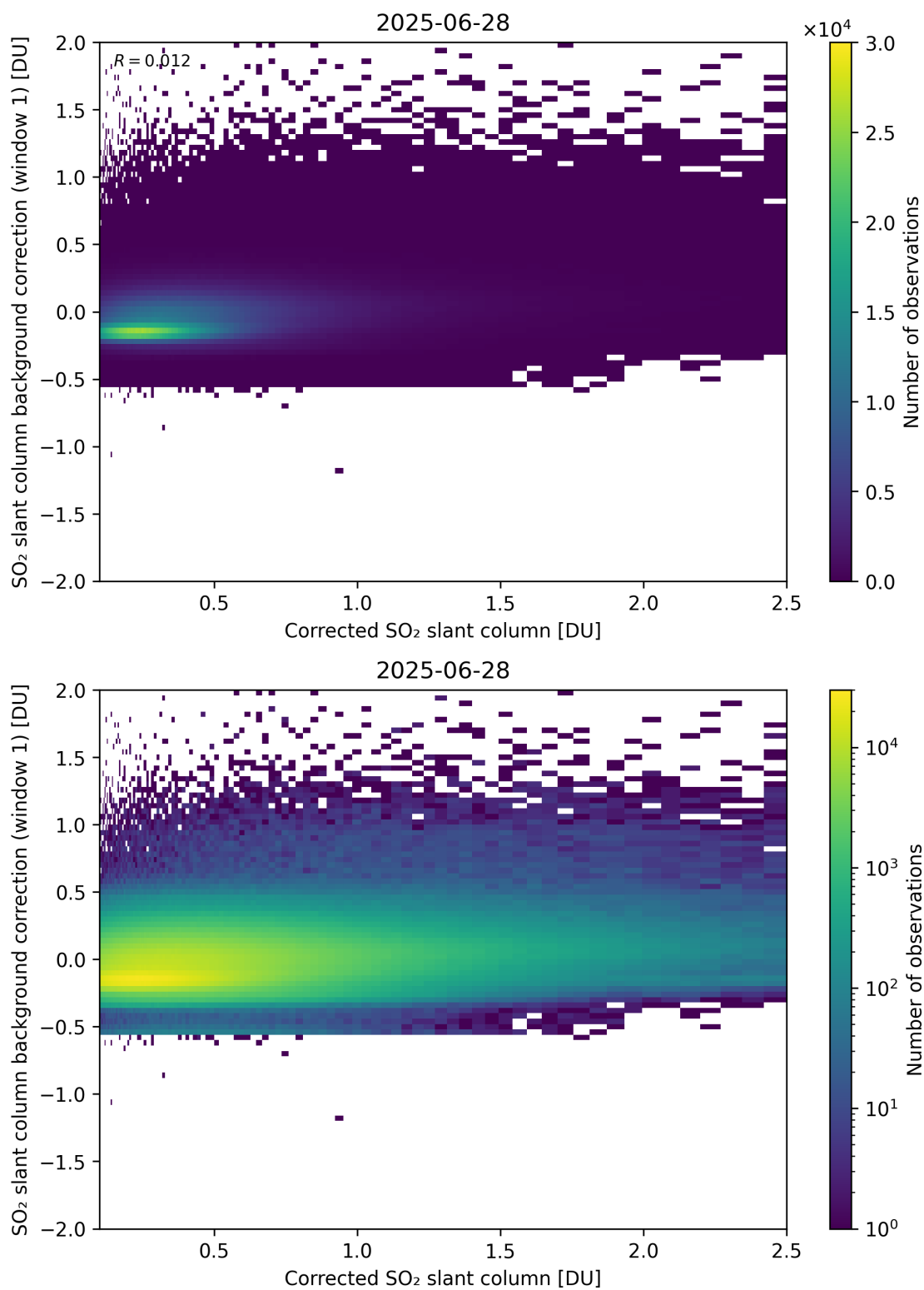
Figure 226: Scatter density plot of “Corrected SO 2 slant column” against “SO 2 slant column background correction (window 1)” for 2025-06-27 to 2025-06-29.
