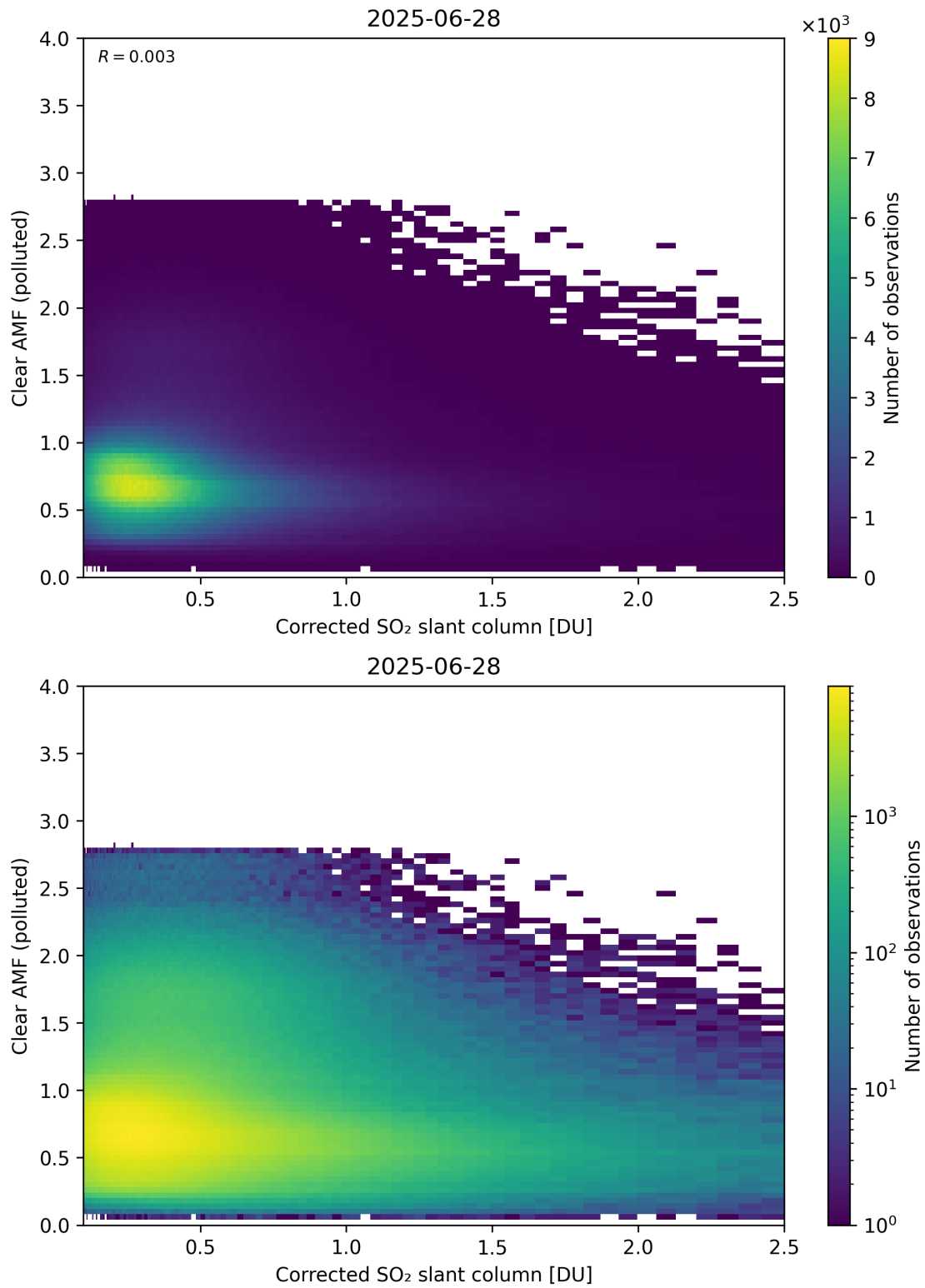
Figure 232: Scatter density plot of “Corrected SO 2 slant column” against “Clear AMF (polluted)” for 2025-06-27 to 2025-06-29.
