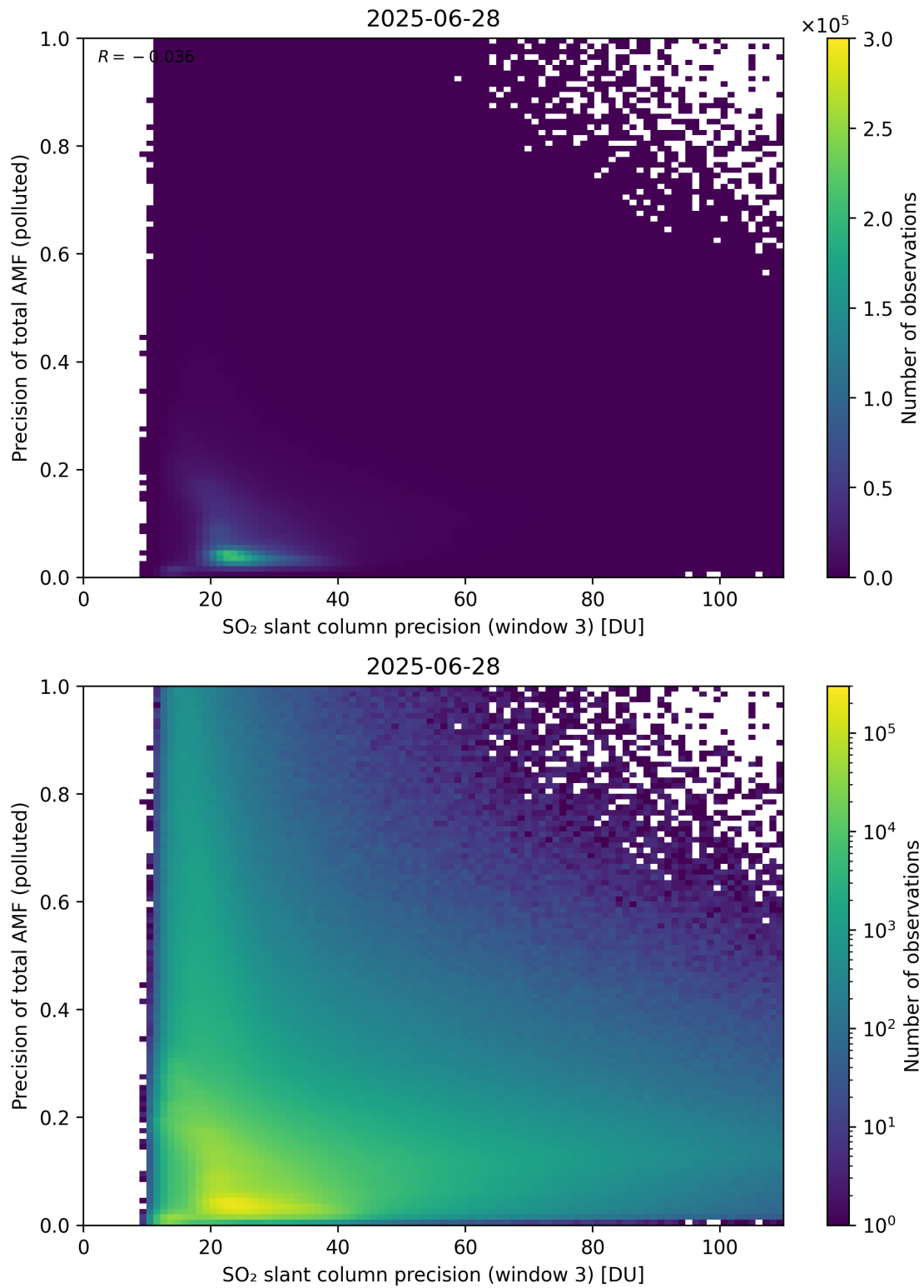
Figure 314: Scatter density plot of “SO 2 slant column precision (window 3)” against “Precision of total AMF (polluted)” for 2025-06-27 to 2025-06-29.
