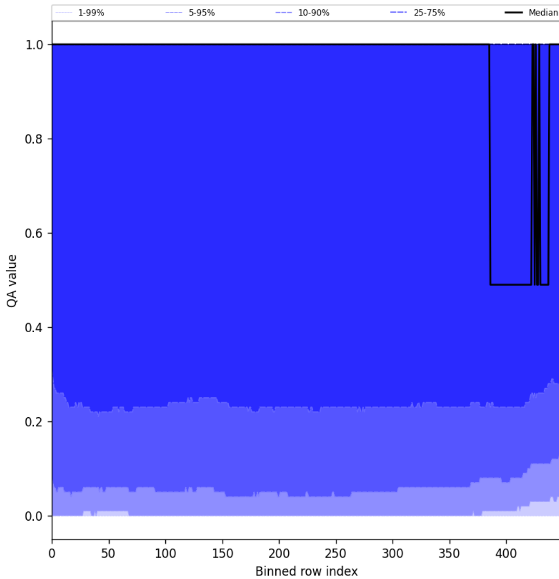
Figure 83: Along track statistics of “QA value” for 2025-06-27 to 2025-06-29
