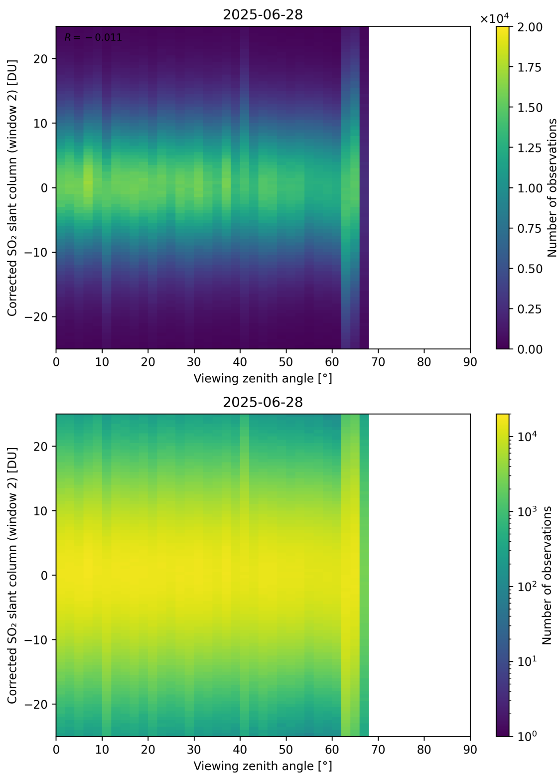
Figure 374: Scatter density plot of “Viewing zenith angle” against “Corrected SO 2 slant column (window 2)” for 2025-06-27 to 2025-06-29.
