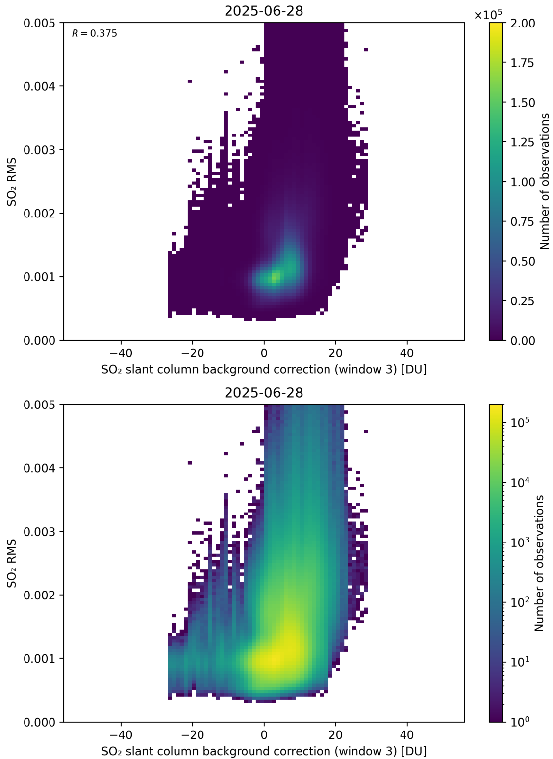
Figure 134: Scatter density plot of “SO 2 slant column background correction (window 3)” against “SO 2 RMS” for 2025-06-27 to 2025-06-29.
