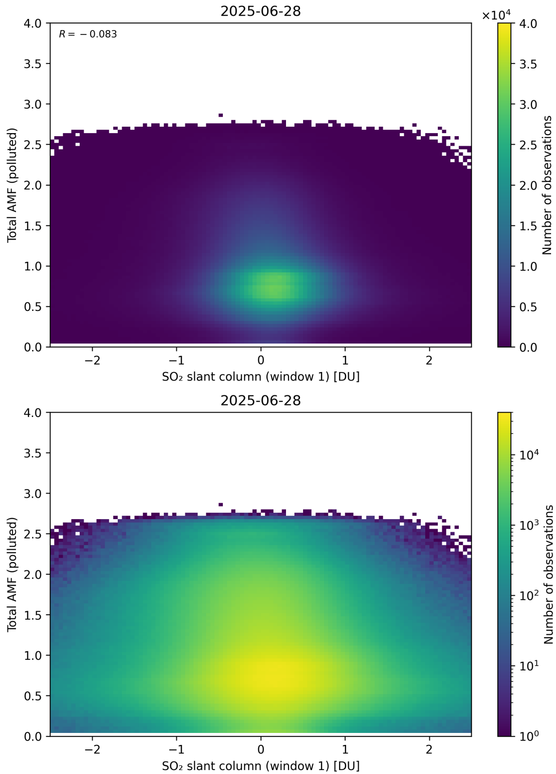
Figure 289: Scatter density plot of “SO 2 slant column (window 1)” against “Total AMF (polluted)” for 2025-06-27 to 2025-06-29.
