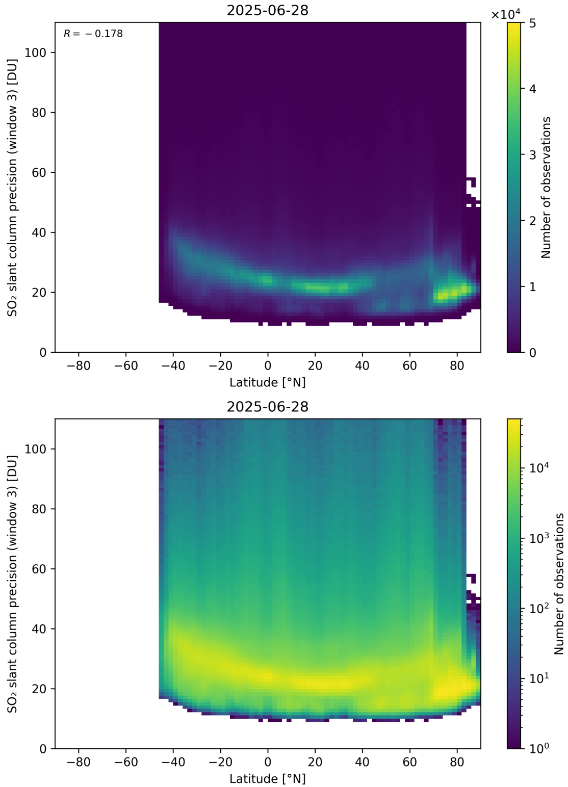
Figure 166: Scatter density plot of “Latitude” against “SO 2 slant column precision (window 3)” for 2025-06-27 to 2025-06-29.
