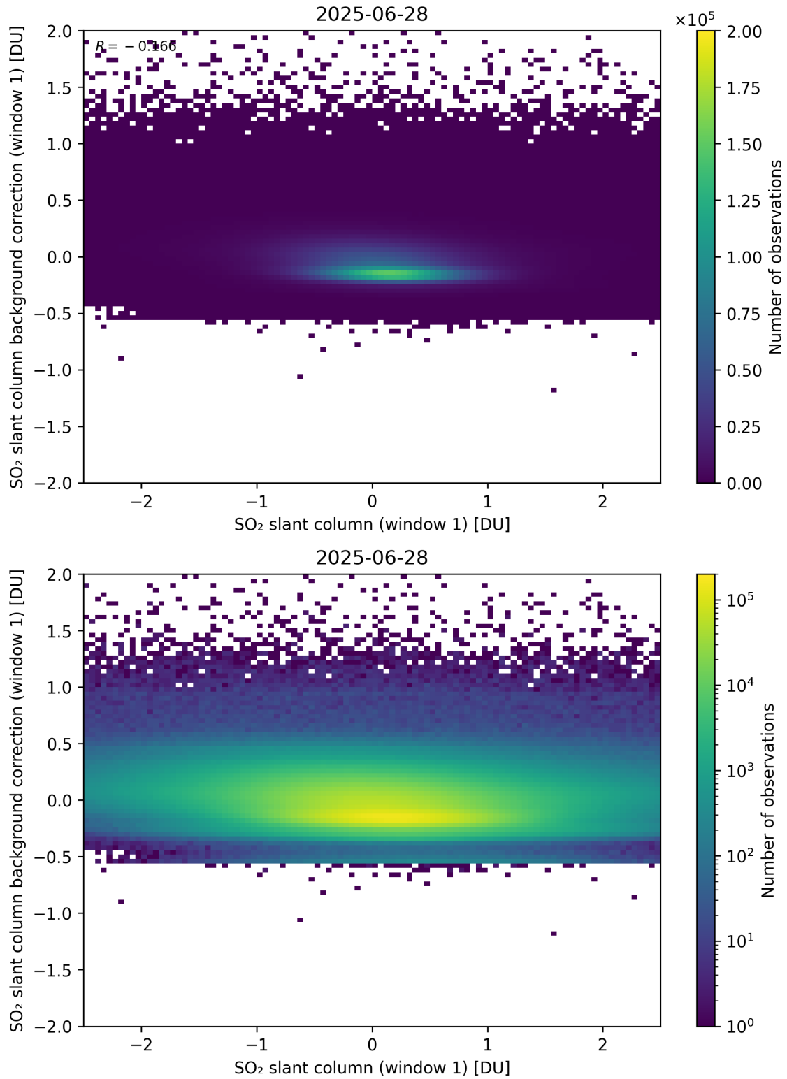
Figure 262: Scatter density plot of “SO 2 slant column (window 1)” against “SO 2 slant column background correction (window 1)” for 2025-06-27 to 2025-06-29.
