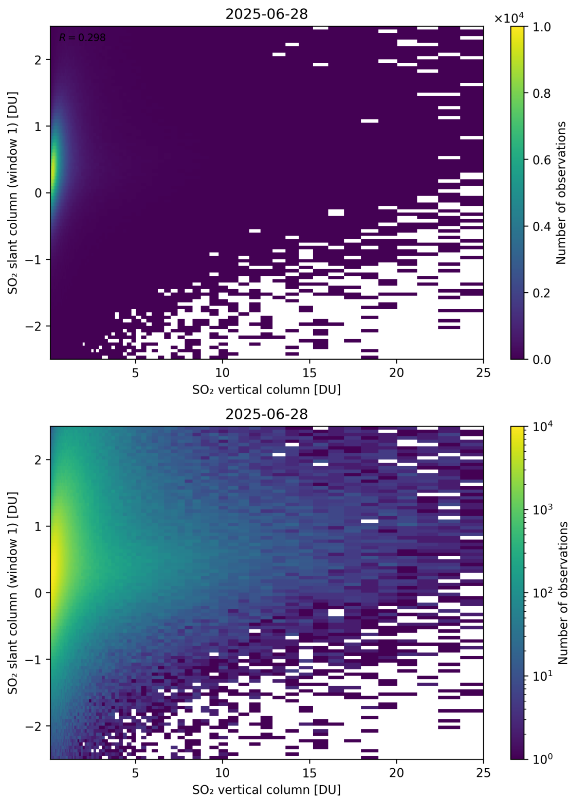
Figure 354: Scatter density plot of “SO 2 vertical column” against “SO 2 slant column (window 1)” for 2025-06-27 to 2025-06-29.
