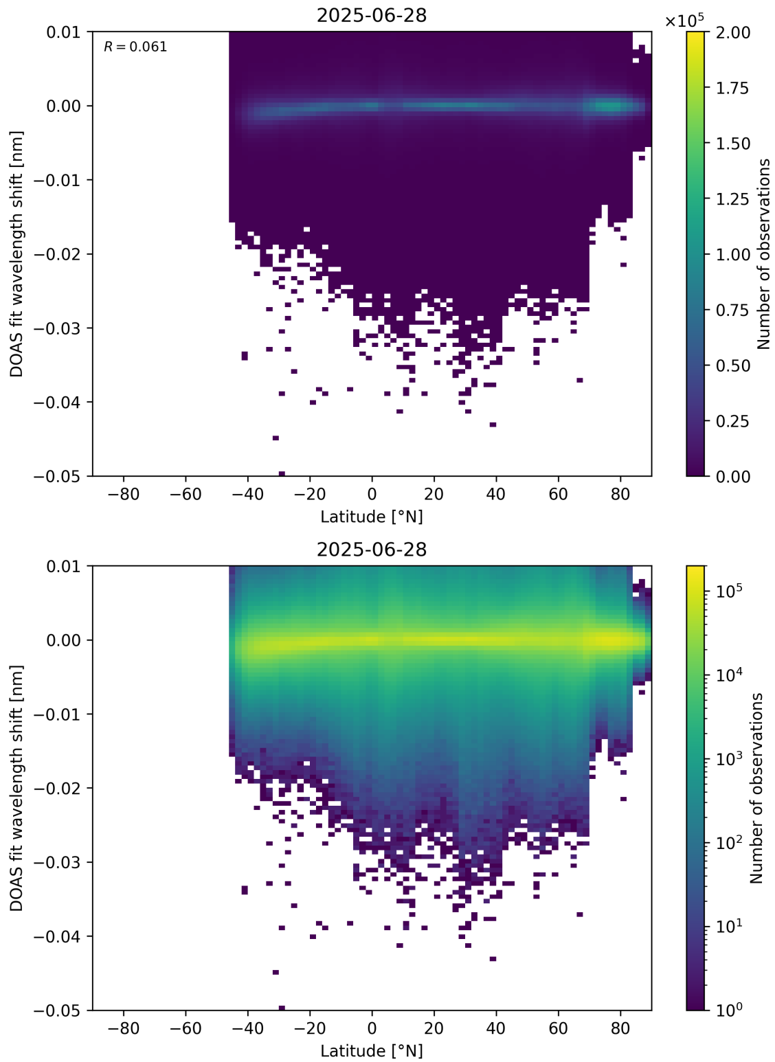
Figure 153: Scatter density plot of “Latitude” against “DOAS fit wavelength shift” for 2025-06-27 to 2025-06-29.
