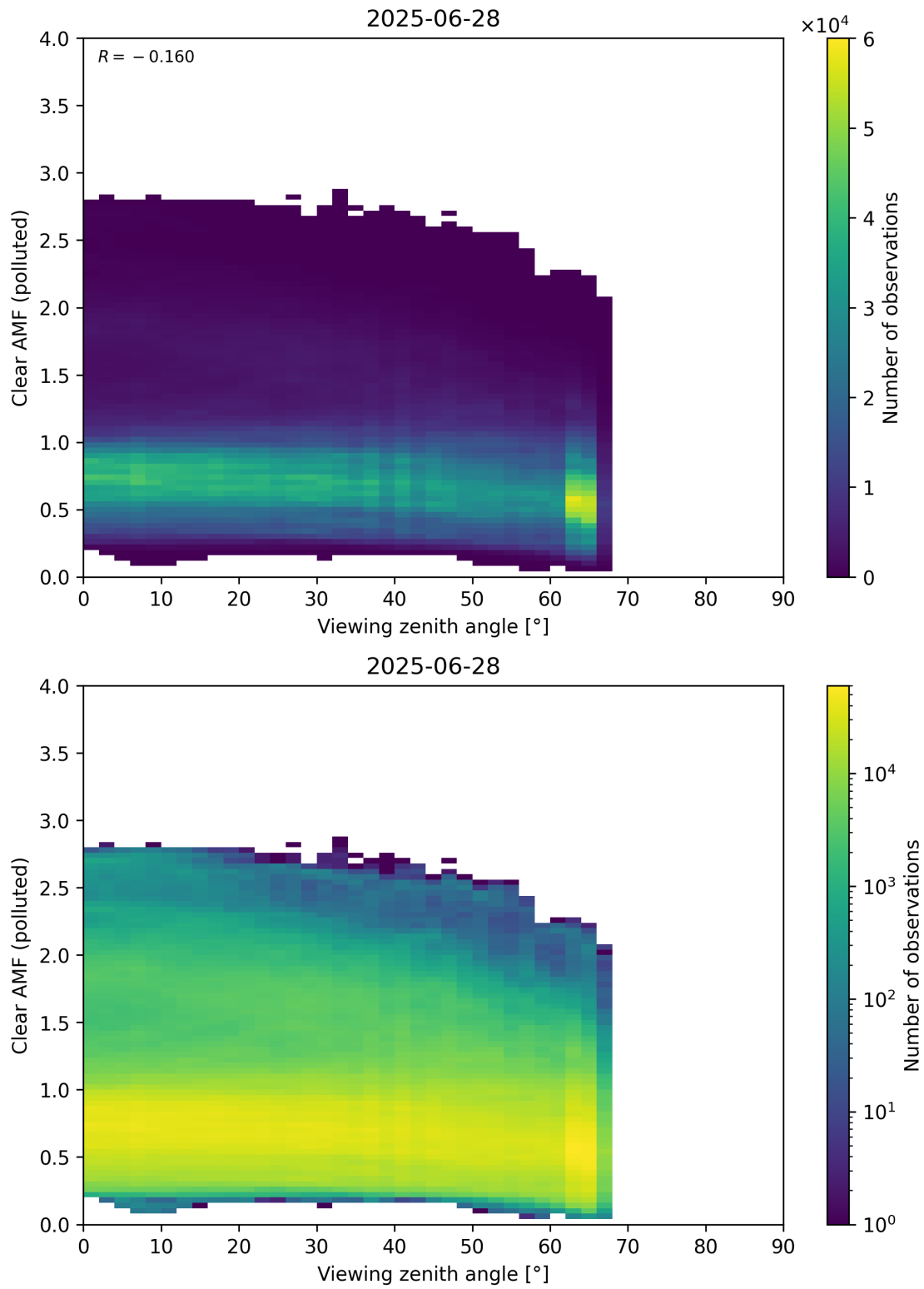
Figure 370: Scatter density plot of “Viewing zenith angle” against “Clear AMF (polluted)” for 2025-06-27 to 2025-06-29.
