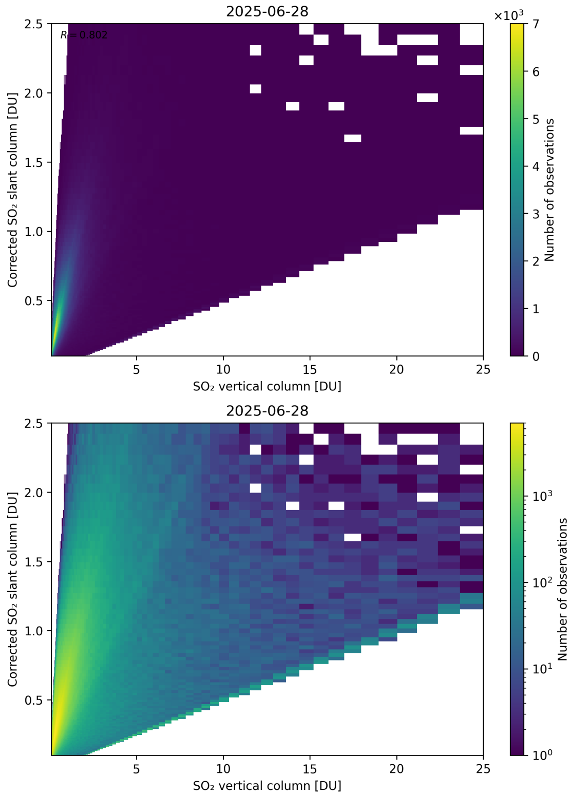
Figure 351: Scatter density plot of “SO 2 vertical column” against “Corrected SO 2 slant column” for 2025-06-27 to 2025-06-29.
