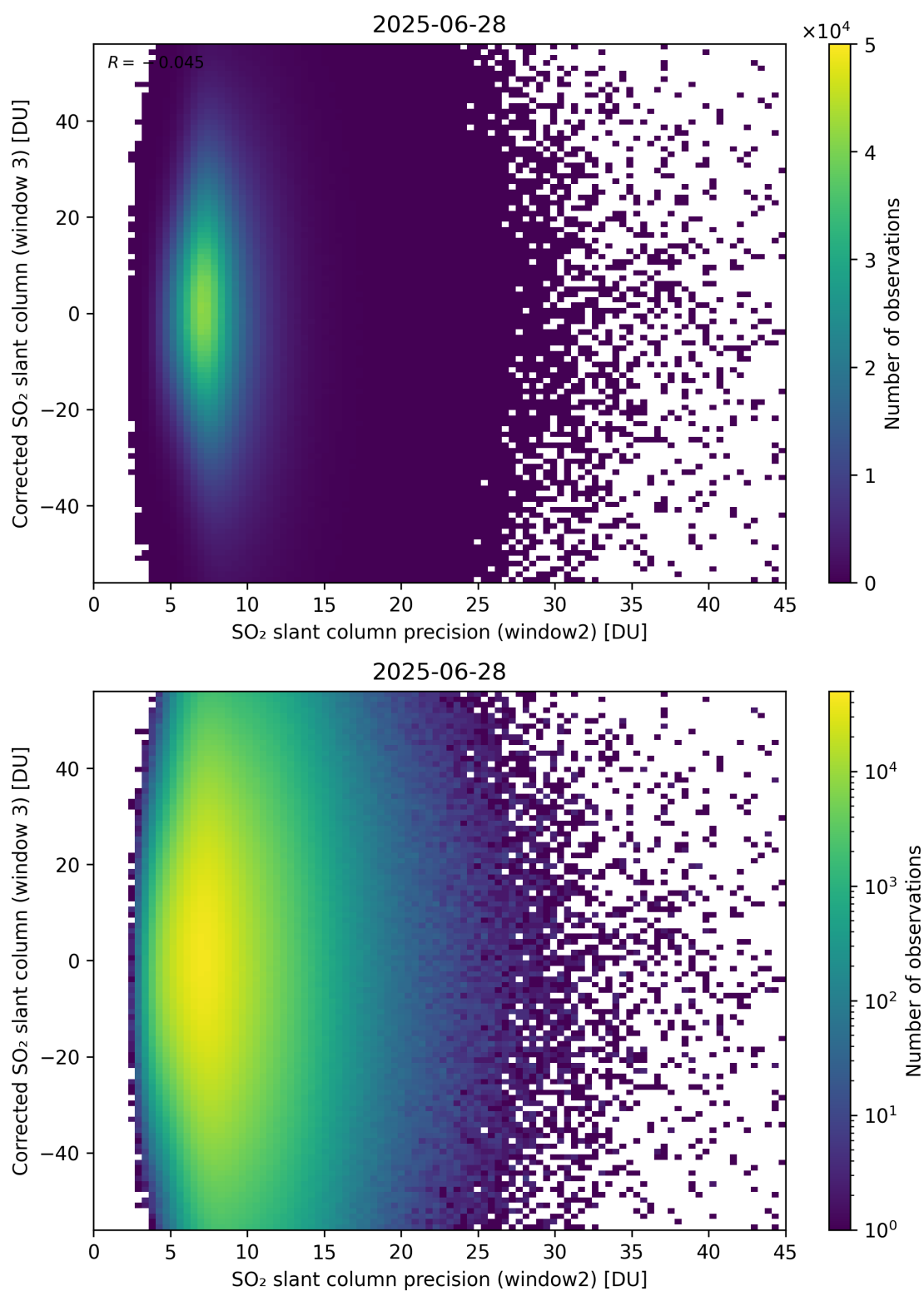
Figure 298: Scatter density plot of “SO 2 slant column precision (window2)” against “Corrected SO 2 slant column (window 3)” for 2025-06-27 to 2025-06-29.
