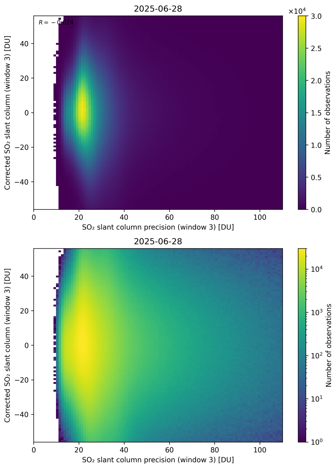
Figure 312: Scatter density plot of “SO 2 slant column precision (window 3)” against “Corrected SO 2 slant column (window 3)” for 2025-06-27 to 2025-06-29.
