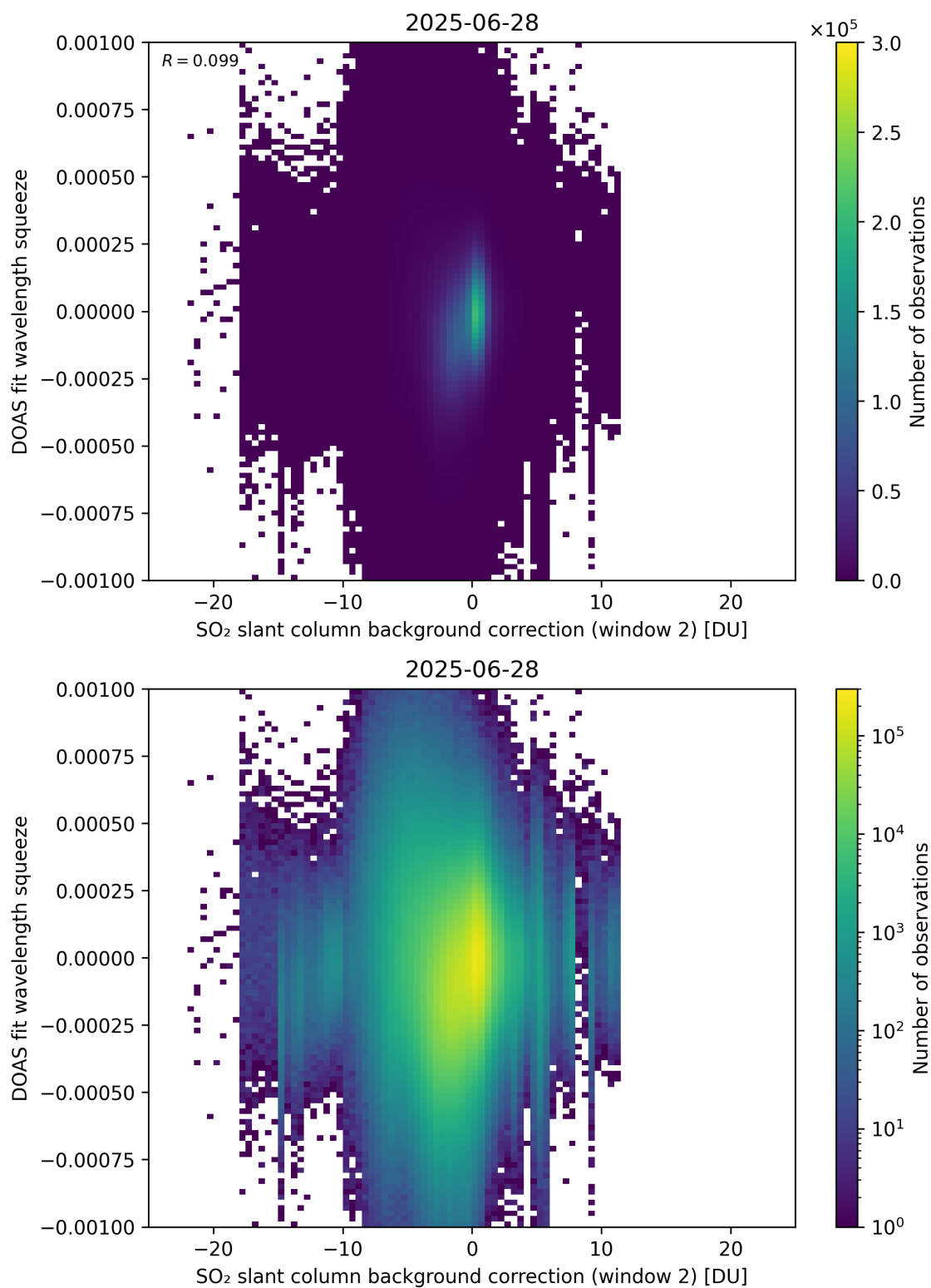
Figure 124: Scatter density plot of “SO 2 slant column background correction (window 2)” against “DOAS fit wavelength squeeze” for 2025-06-27 to 2025-06-29.
