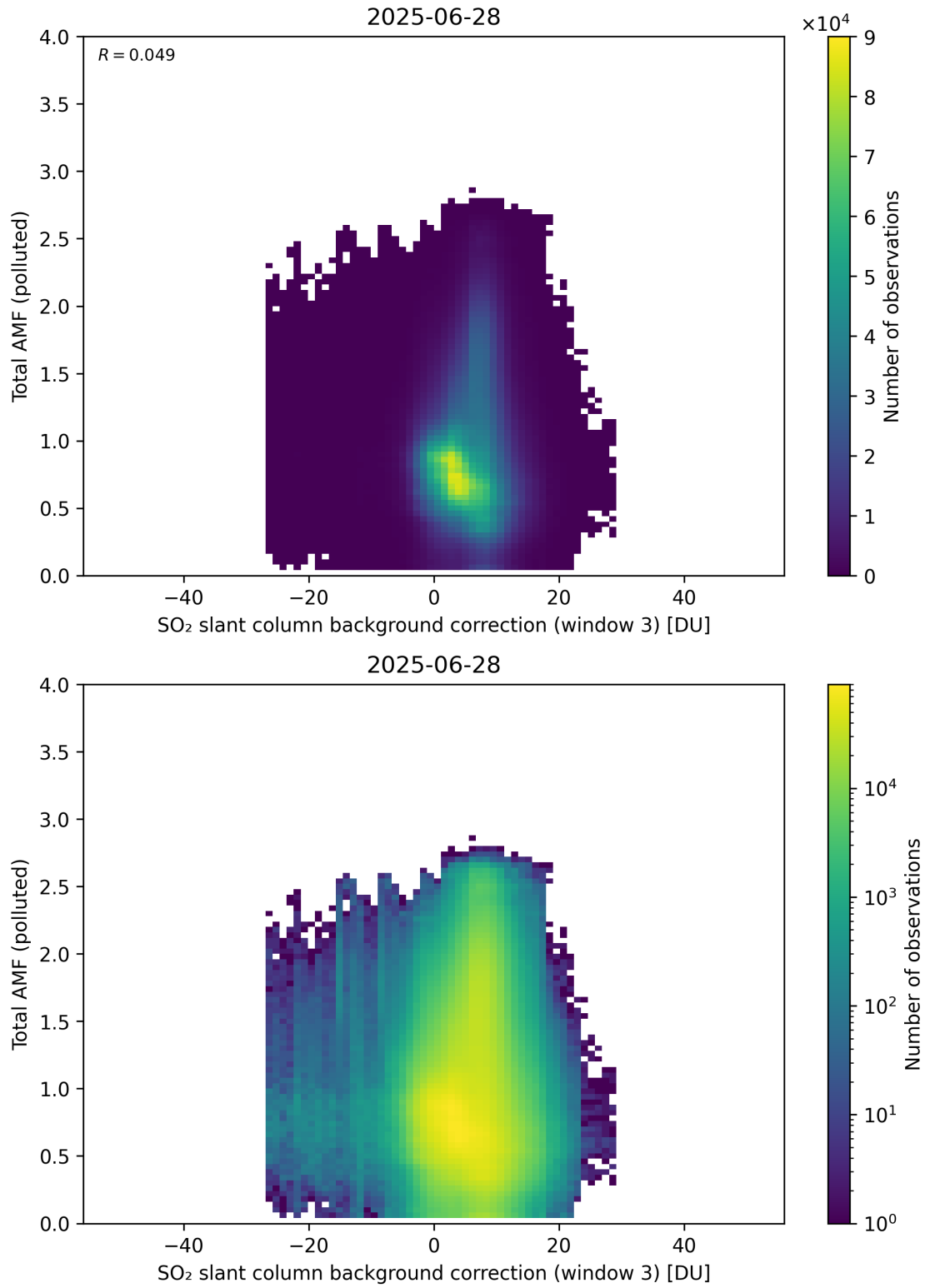
Figure 136: Scatter density plot of “SO 2 slant column background correction (window 3)” against “Total AMF (polluted)” for 2025-06-27 to 2025-06-29.
