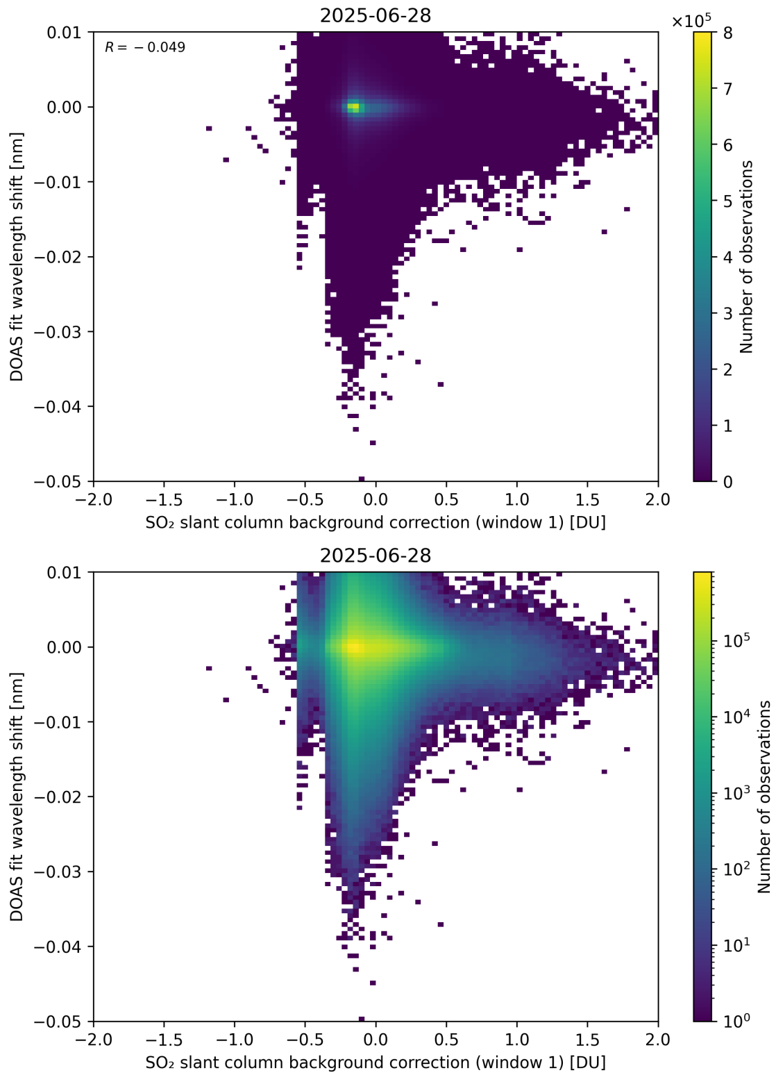
Figure 111: Scatter density plot of “SO 2 slant column background correction (window 1)” against “DOAS fit wavelength shift” for 2025-06-27 to 2025-06-29.
