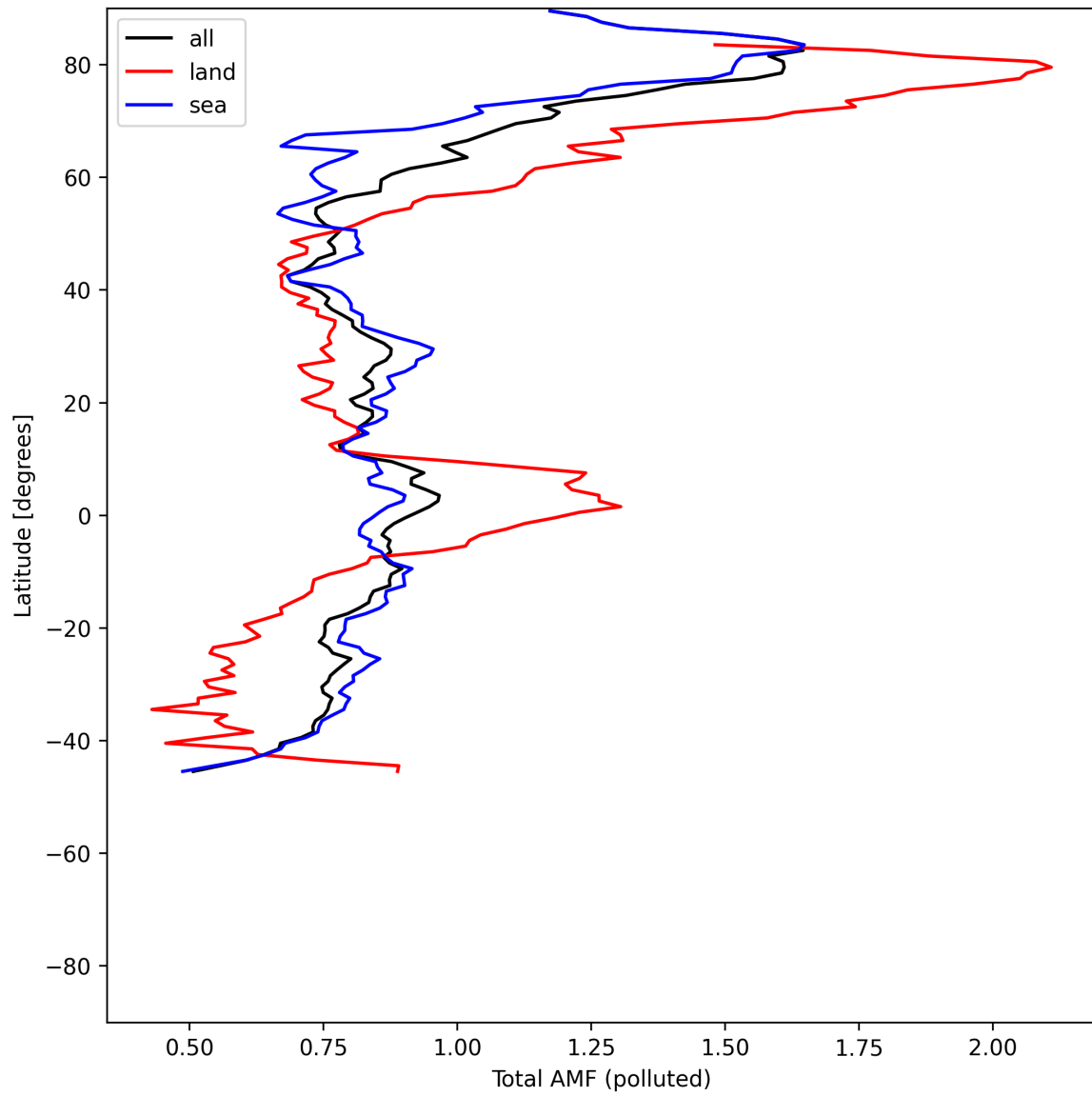
Figure 53: Zonal average of “Total AMF (polluted)” for 2025-06-27 to 2025-06-29.
