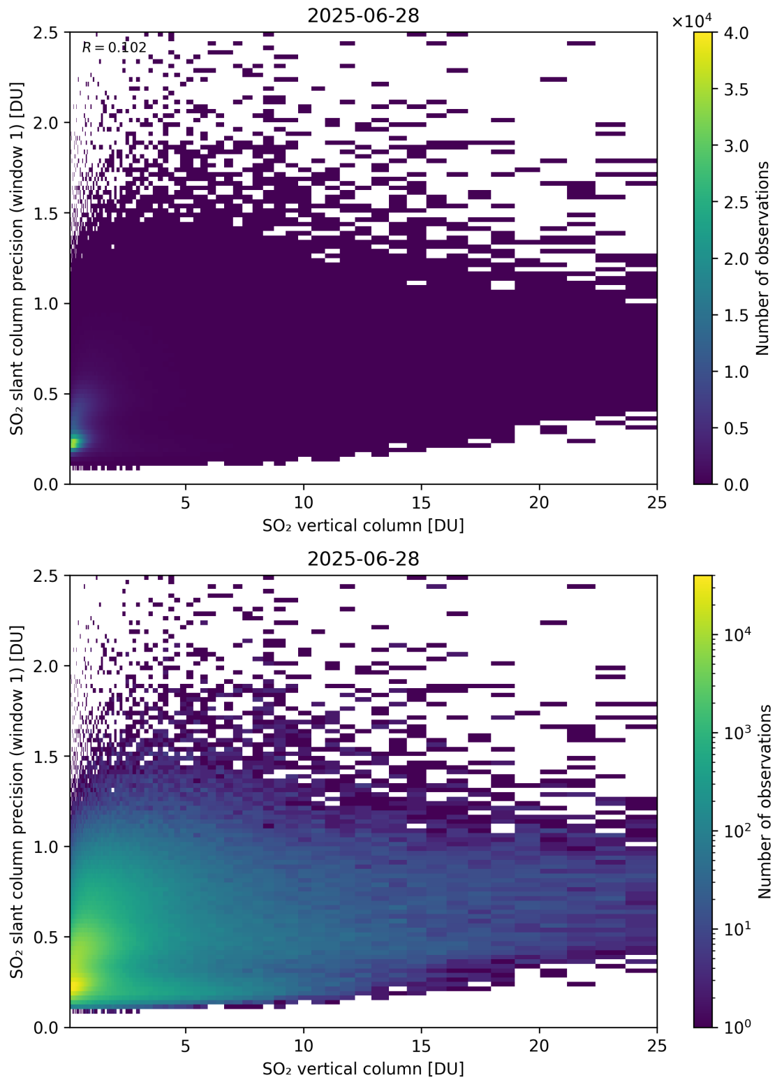
Figure 355: Scatter density plot of “SO 2 vertical column” against “SO 2 slant column precision (window 1)” for 2025-06-27 to 2025-06-29.
