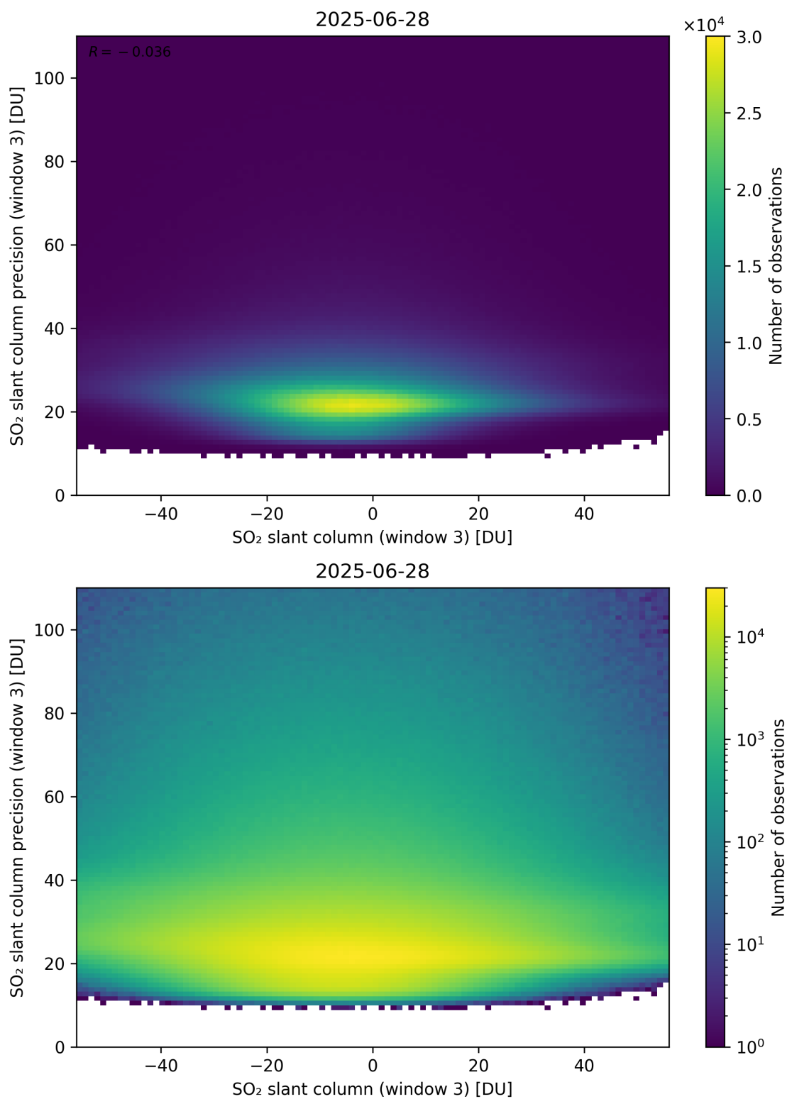
Figure 317: Scatter density plot of “SO 2 slant column (window 3)” against “SO 2 slant column precision (window 3)” for 2025-06-27 to 2025-06-29.
