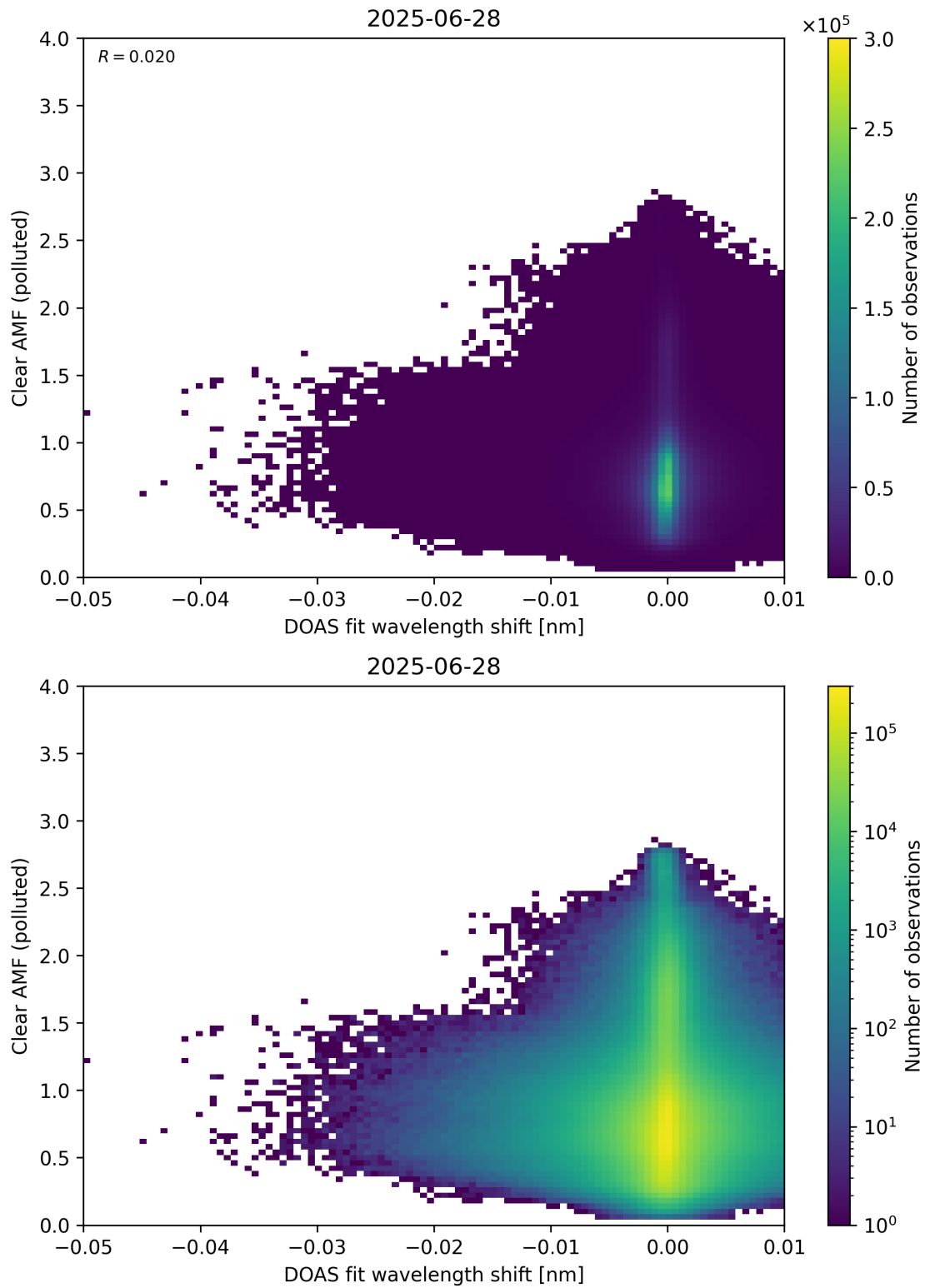
Figure 140: Scatter density plot of “DOAS fit wavelength shift” against “Clear AMF (polluted)” for 2025-06-27 to 2025-06-29.
