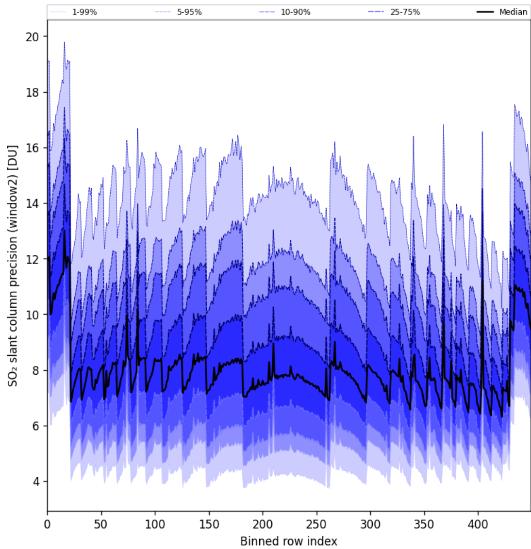
Figure 94: Along track statistics of “SO 2 slant column precision (window2)” for 2025-06-27 to 2025-06-29
