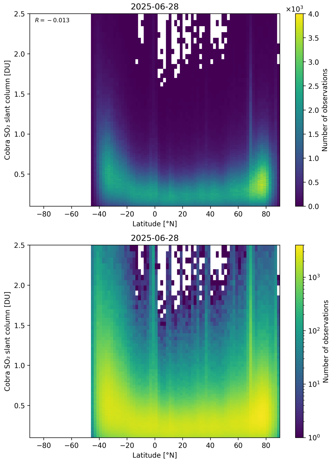
Figure 157: Scatter density plot of “Latitude” against “Cobra SO 2 slant column” for 2025-06-27 to 2025-06-29.
