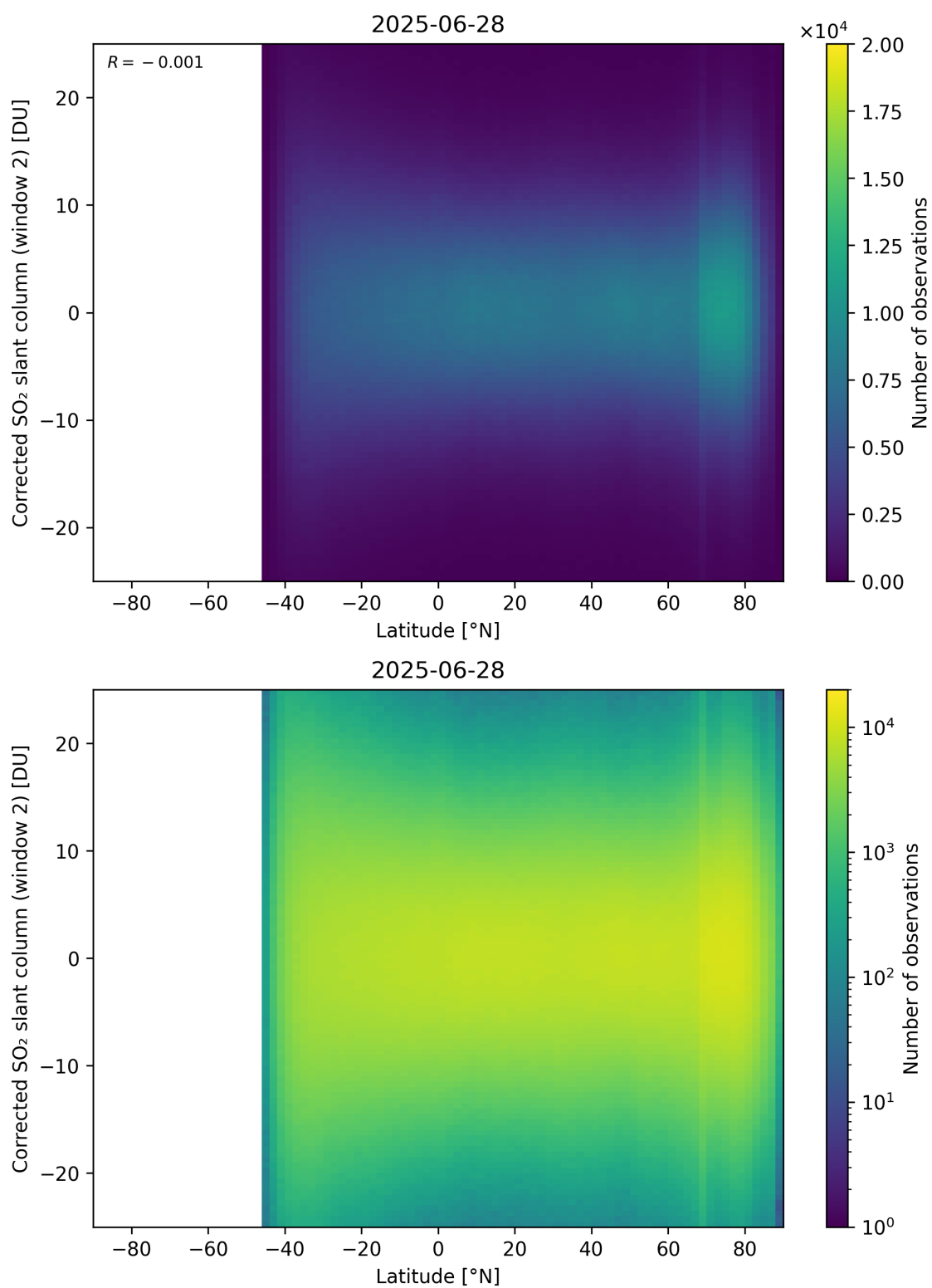
Figure 160: Scatter density plot of “Latitude” against “Corrected SO 2 slant column (window 2)” for 2025-06-27 to 2025-06-29.
