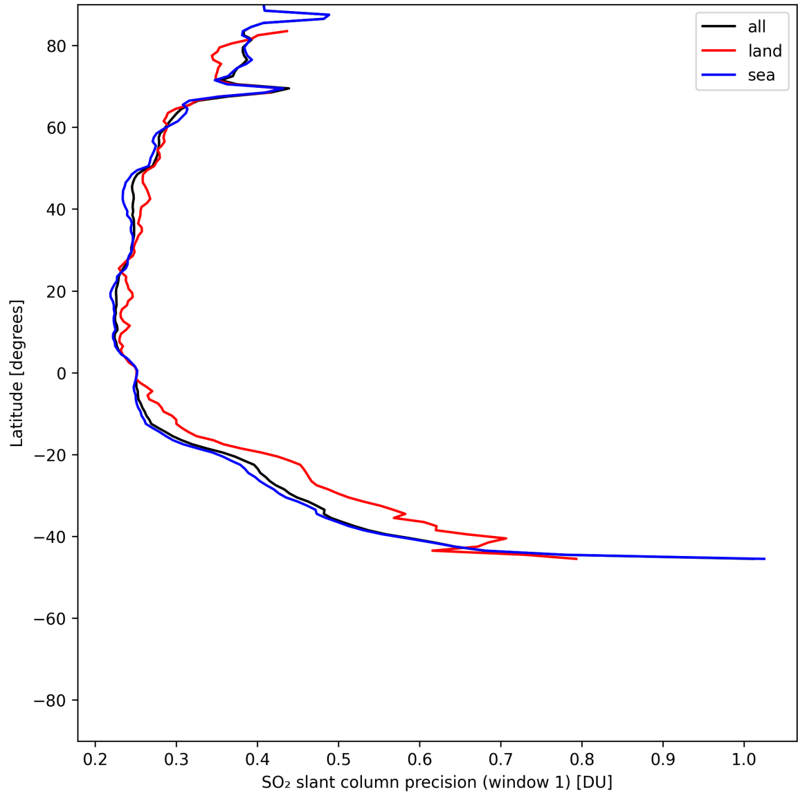
Figure 38: Zonal average of “SO 2 slant column precision (window 1)” for 2025-06-27 to 2025-06-29.
