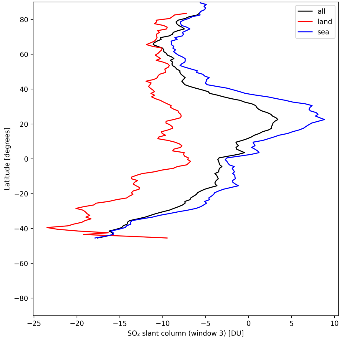
Figure 45: Zonal average of “SO 2 slant column (window 3)” for 2025-06-27 to 2025-06-29.
