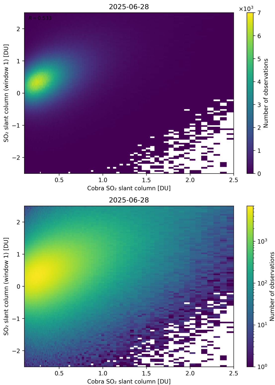
Figure 219: Scatter density plot of “Cobra SO 2 slant column” against “SO 2 slant column (window 1)” for 2025-06-27 to 2025-06-29.
