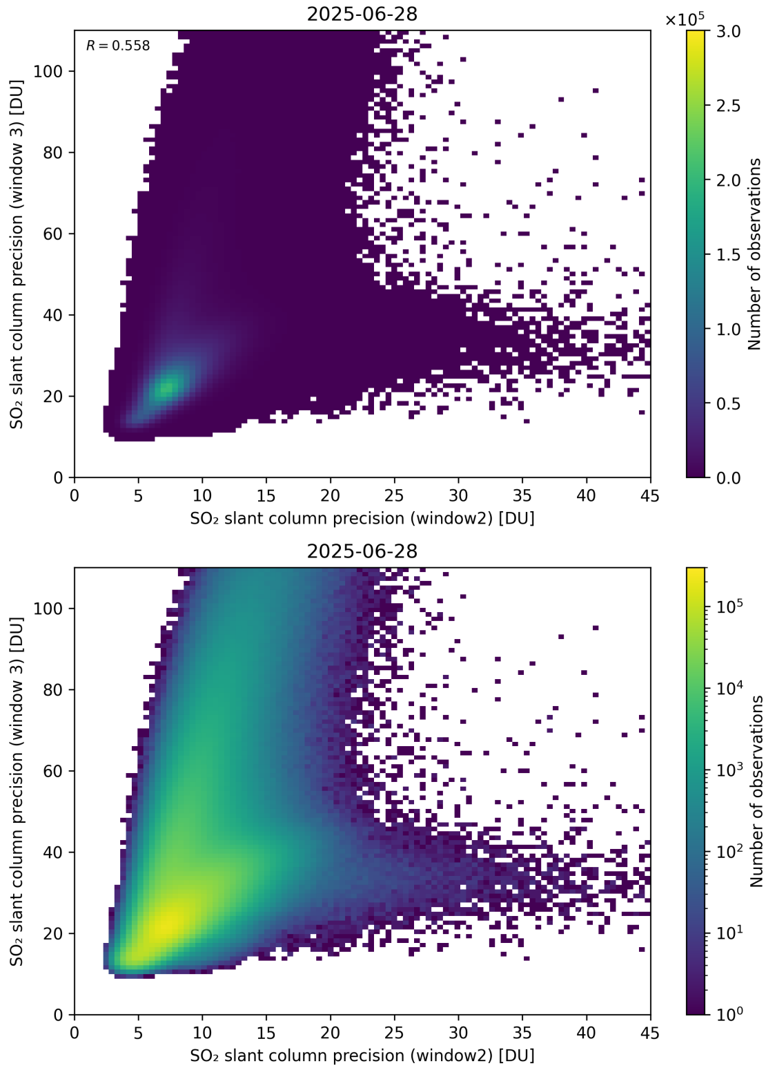
Figure 300: Scatter density plot of “SO 2 slant column precision (window2)” against “SO 2 slant column precision (window 3)” for 2025-06-27 to 2025-06-29.
