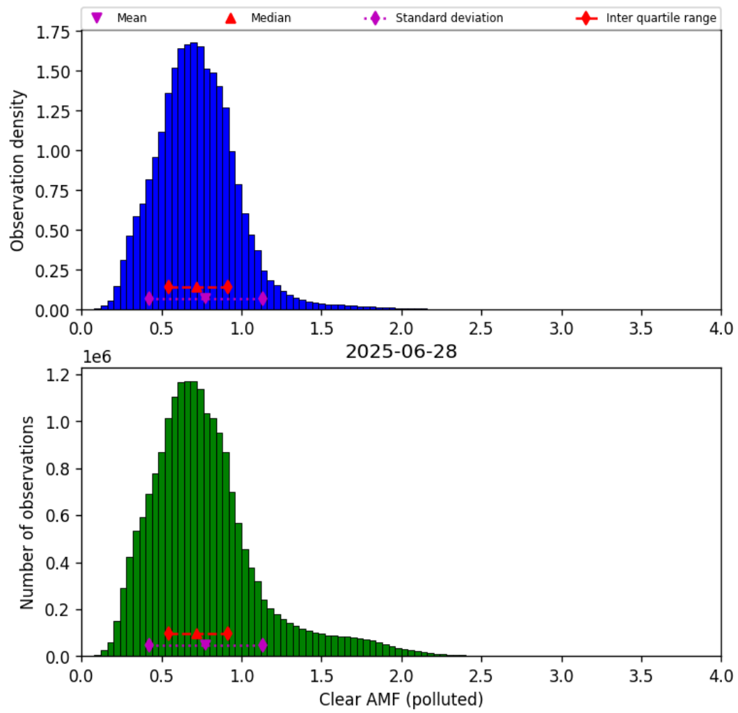
Figure 81: Histogram of “Clear AMF (polluted)” for 2025-06-27 to 2025-06-29
