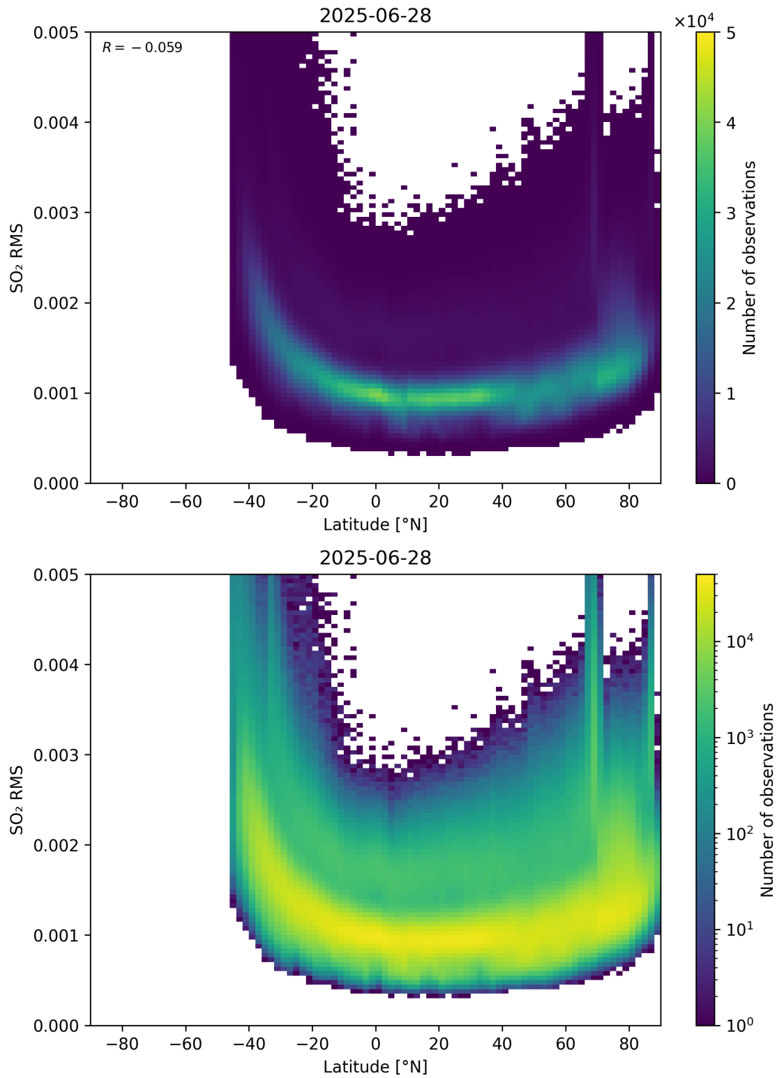
Figure 155: Scatter density plot of “Latitude” against “SO 2 RMS” for 2025-06-27 to 2025-06-29.
