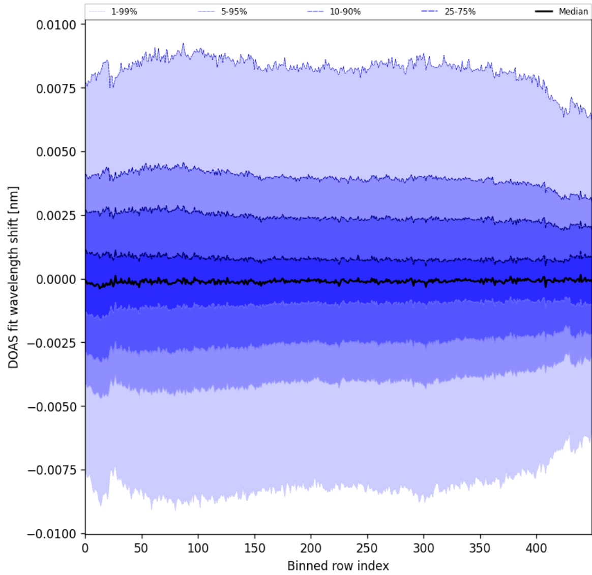
Figure 102: Along track statistics of “DOAS fit wavelength shift” for 2025-06-27 to 2025-06-29
