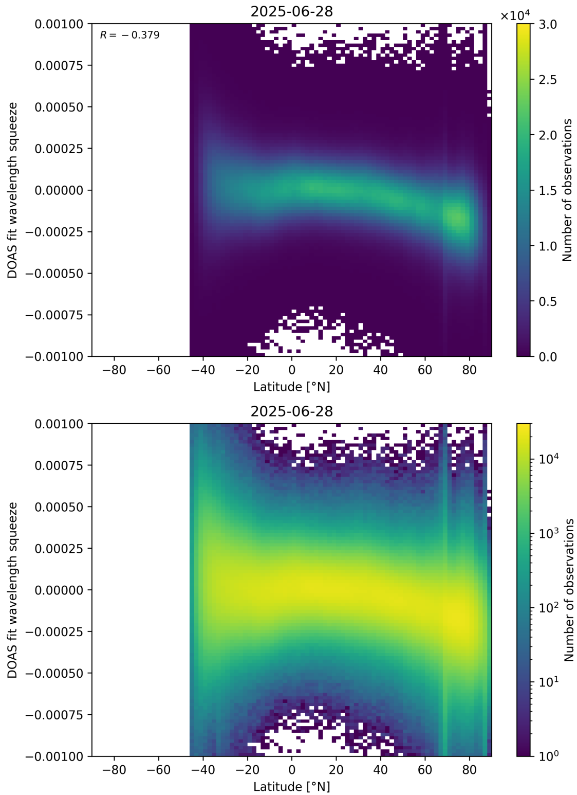
Figure 154: Scatter density plot of “Latitude” against “DOAS fit wavelength squeeze” for 2025-06-27 to 2025-06-29.
