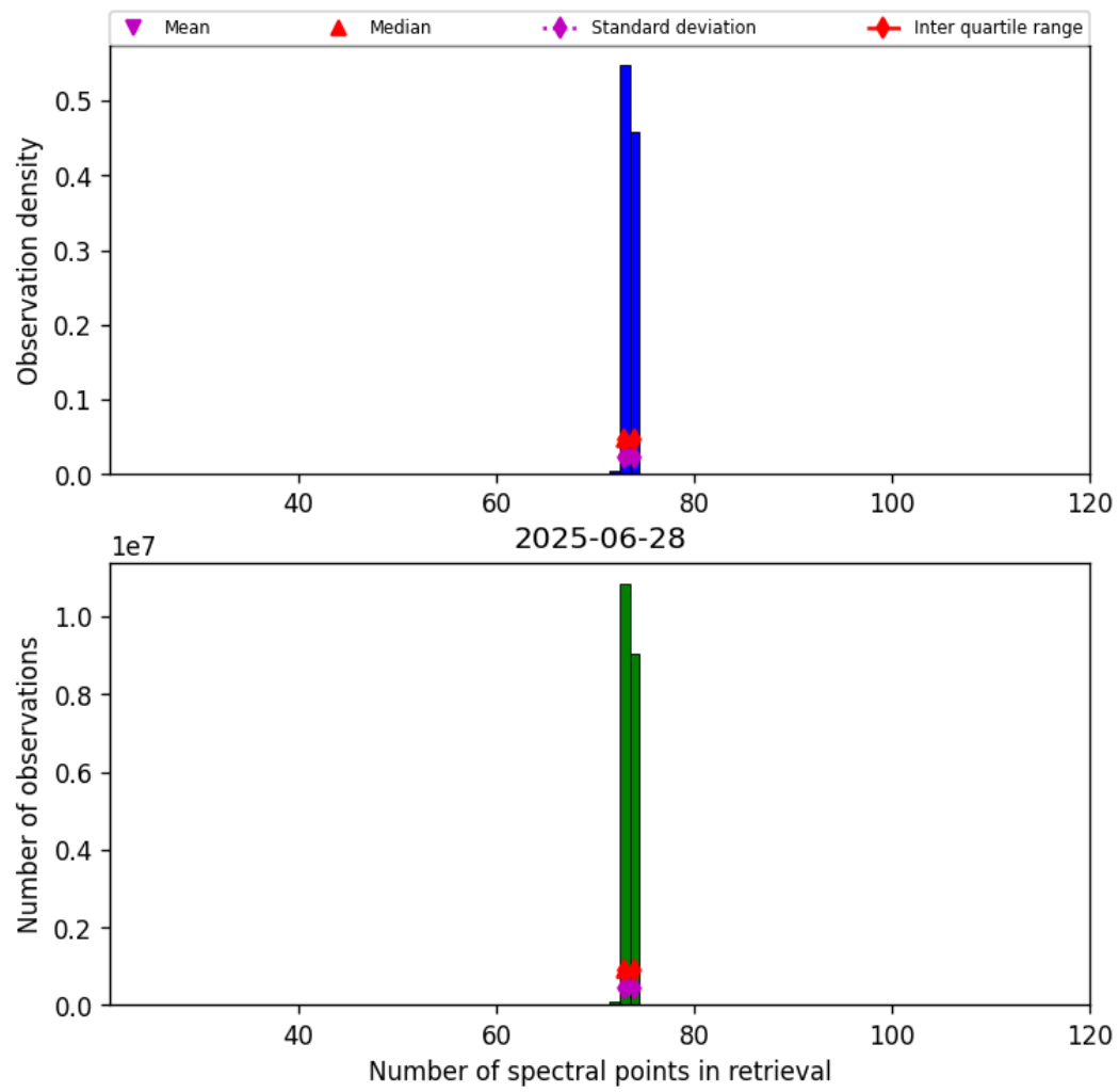
Figure 82: Histogram of “Number of spectral points in retrieval” for 2025-06-27 to 2025-06-29
