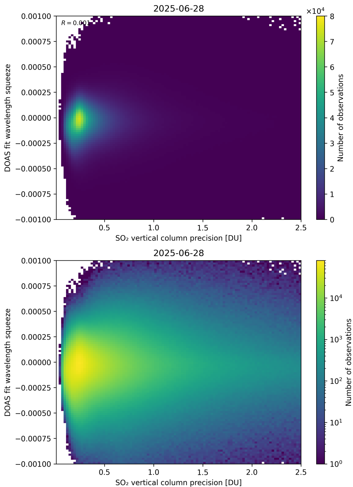
Figure 333: Scatter density plot of “SO 2 vertical column precision” against “DOAS fit wavelength squeeze” for 2025-06-27 to 2025-06-29.
