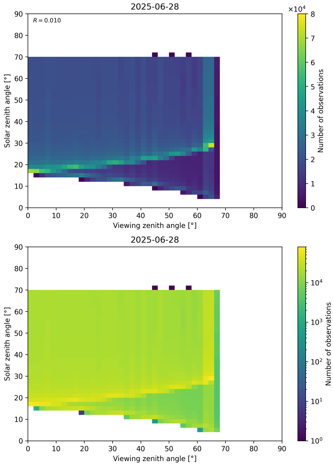
Figure 369: Scatter density plot of “Viewing zenith angle” against “Solar zenith angle” for 2025-06-27 to 2025-06-29.
