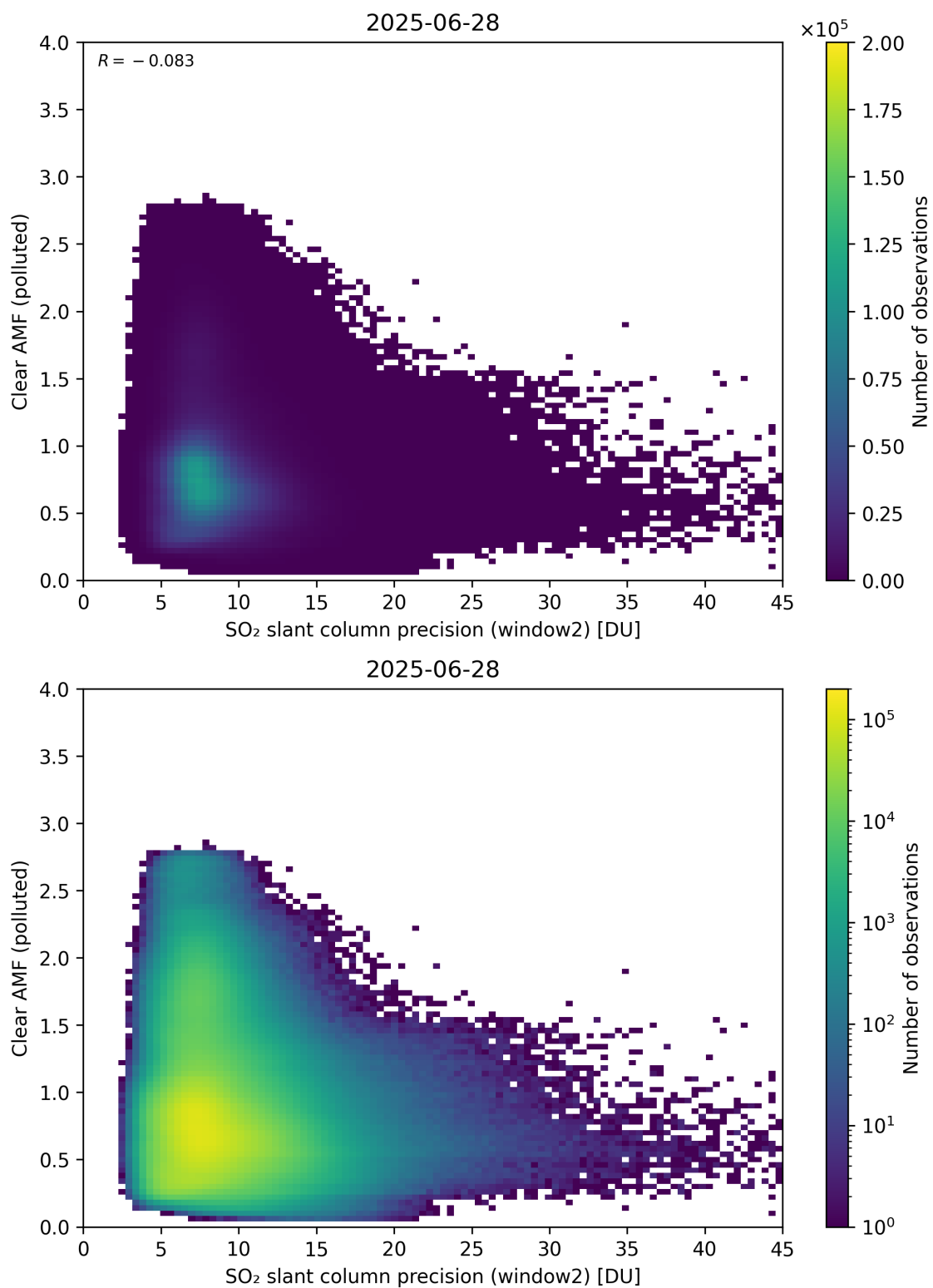
Figure 296: Scatter density plot of “SO 2 slant column precision (window2)” against “Clear AMF (polluted)” for 2025-06-27 to 2025-06-29.
