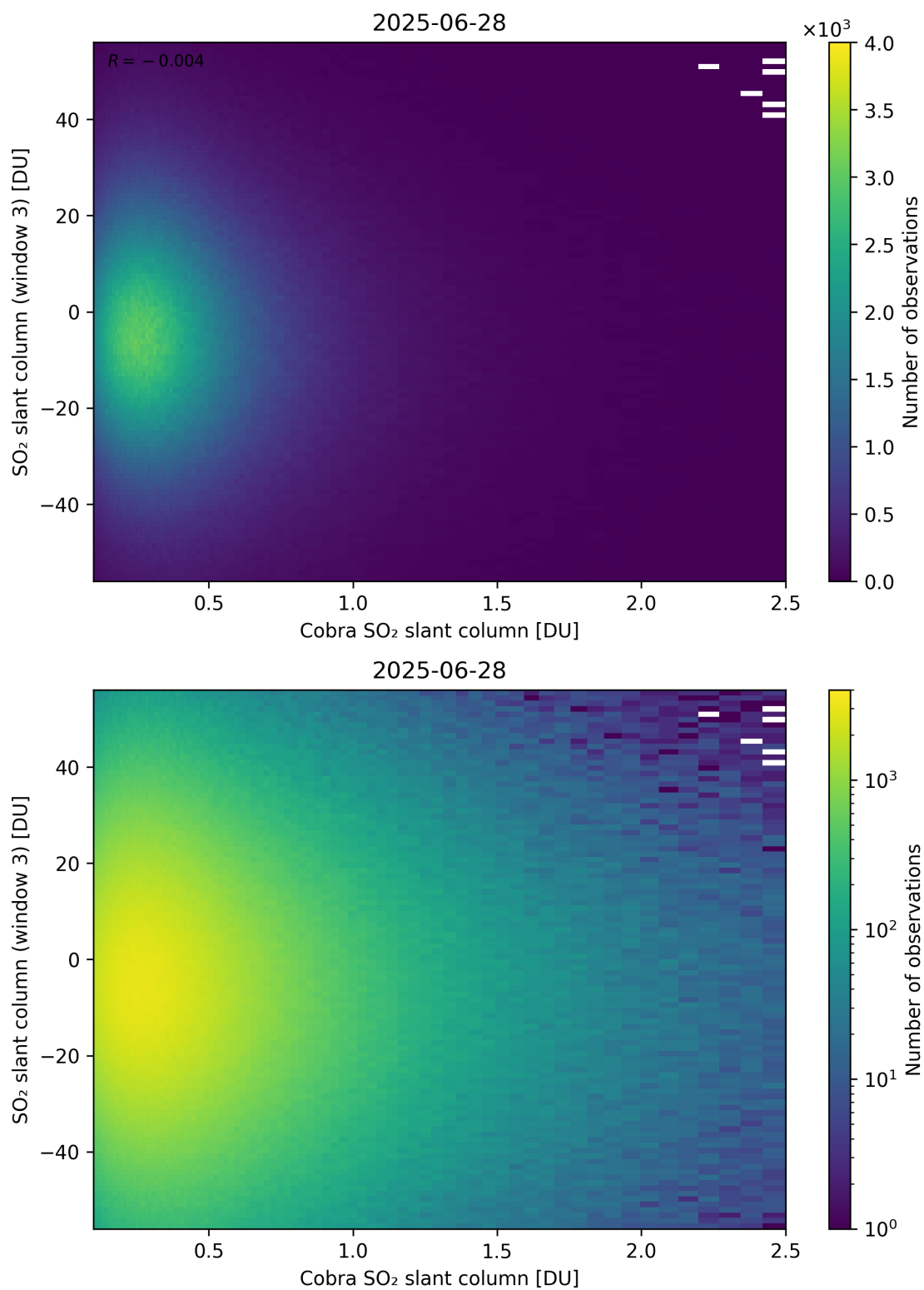
Figure 222: Scatter density plot of “Cobra SO 2 slant column” against “SO 2 slant column (window 3)” for 2025-06-27 to 2025-06-29.
