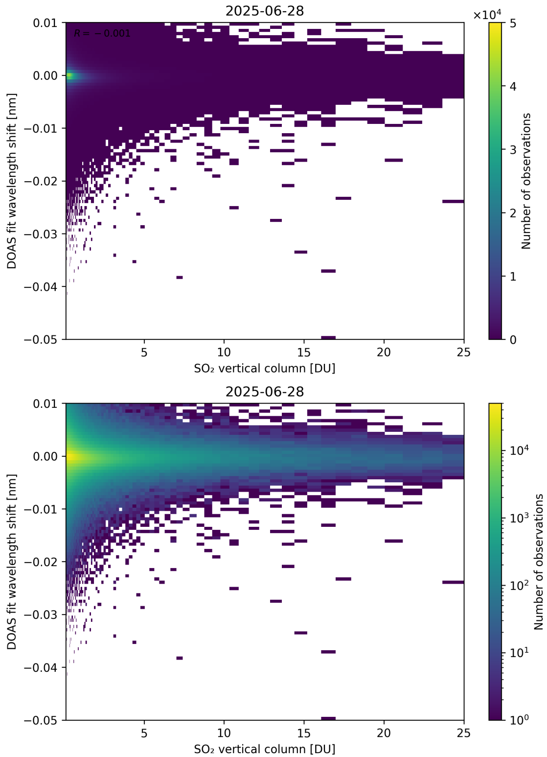
Figure 326: Scatter density plot of “SO 2 vertical column” against “DOAS fit wavelength shift” for 2025-06-27 to 2025-06-29.
