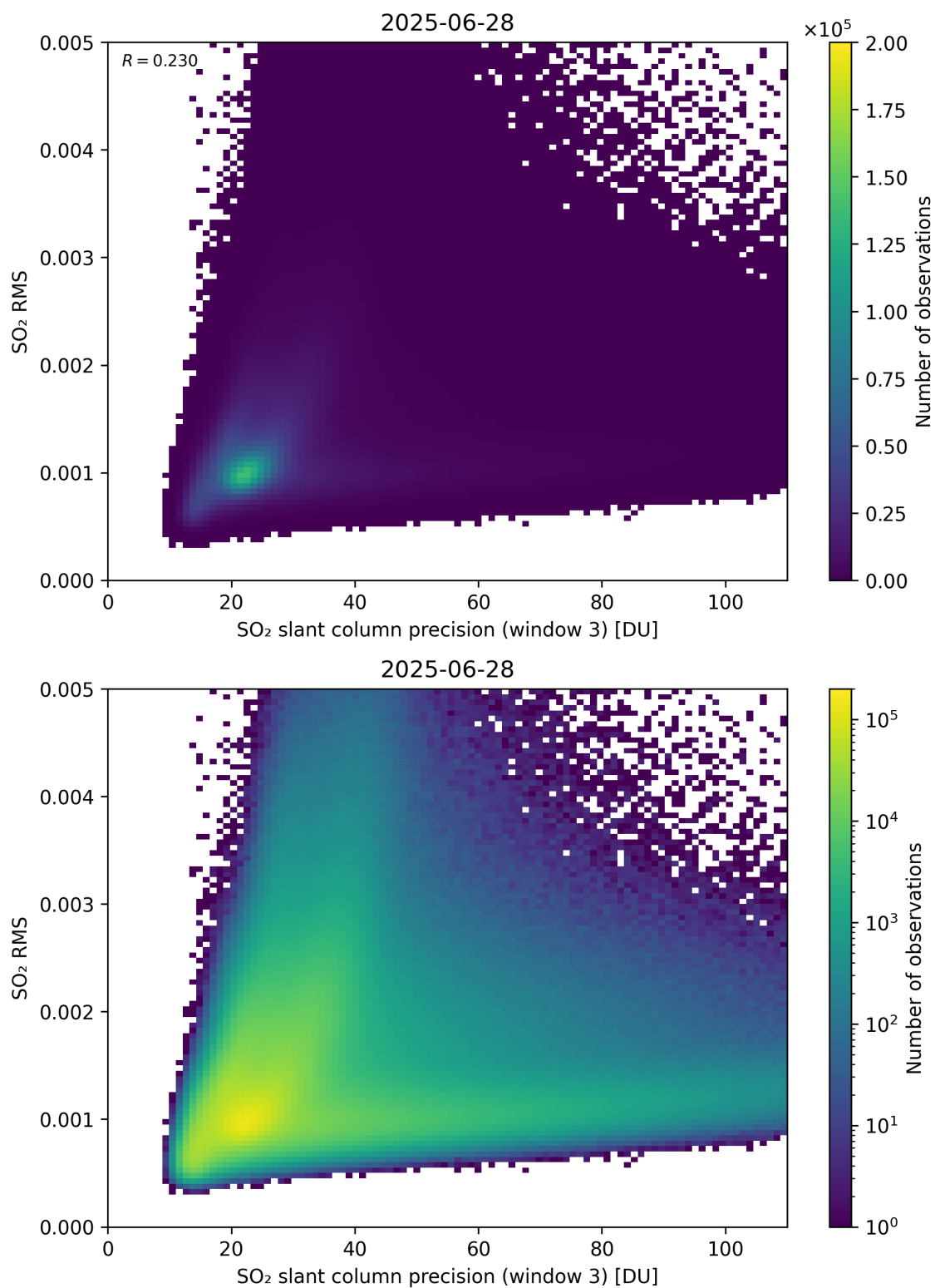
Figure 310: Scatter density plot of “SO 2 slant column precision (window 3)” against “SO 2 RMS” for 2025-06-27 to 2025-06-29.
