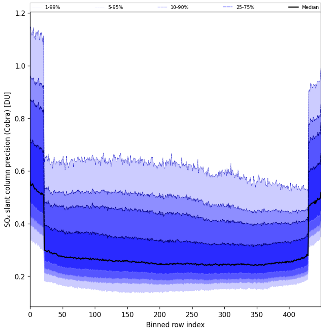
Figure 88: Along track statistics of “SO 2 slant column precision (Cobra)” for 2025-06-27 to 2025-06-29
