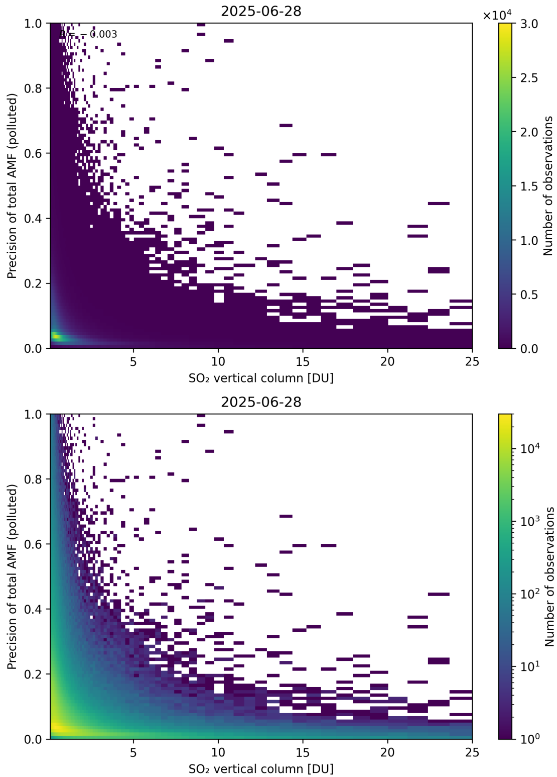
Figure 360: Scatter density plot of “SO 2 vertical column” against “Precision of total AMF (polluted)” for 2025-06-27 to 2025-06-29.
