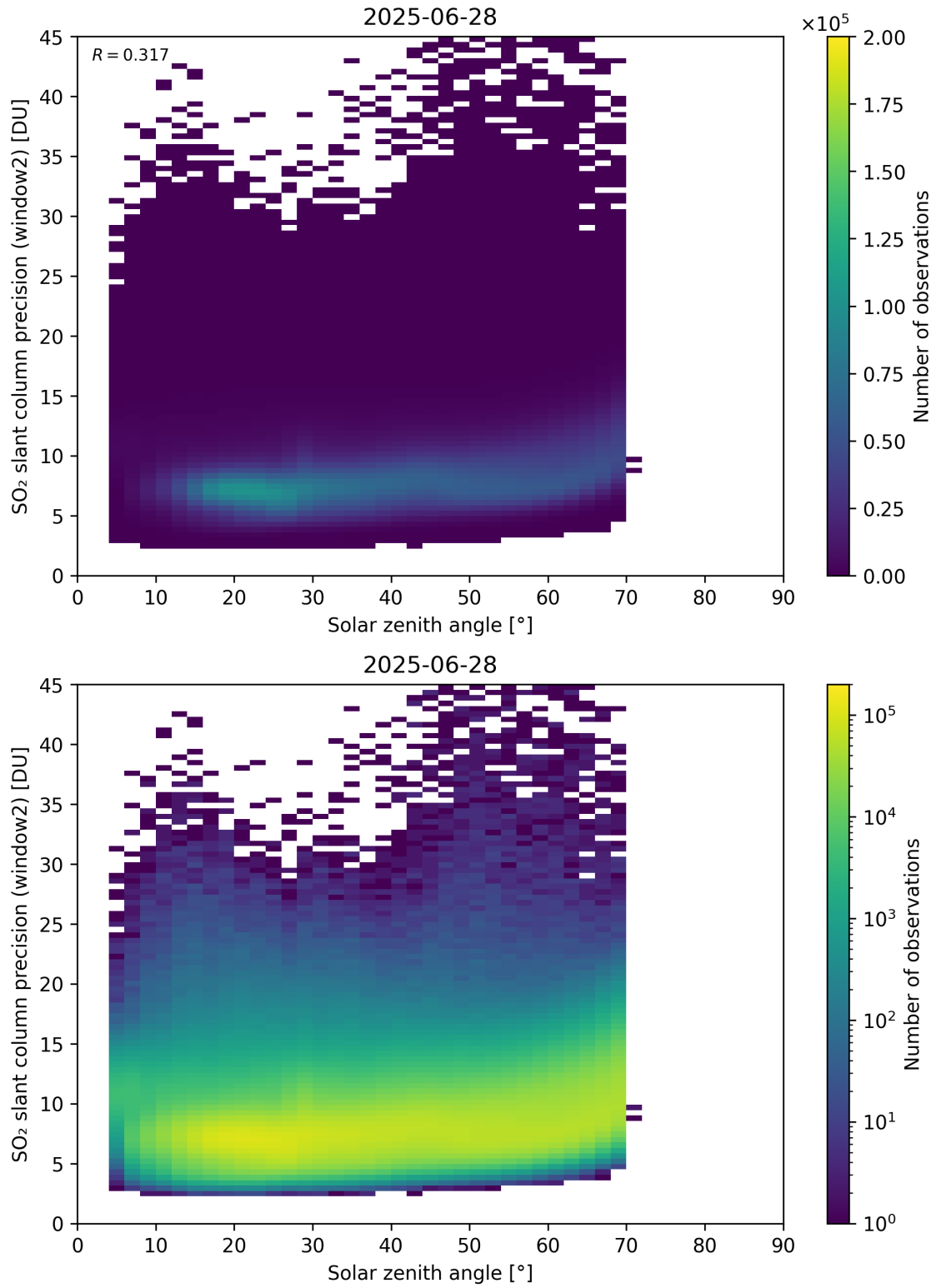
Figure 186: Scatter density plot of “Solar zenith angle” against “SO 2 slant column precision (window2)” for 2025-06-27 to 2025-06-29.
