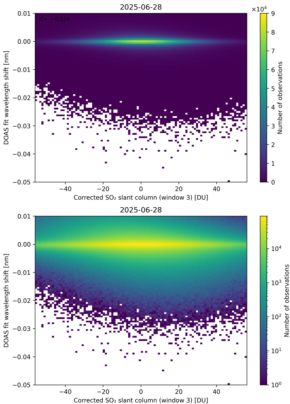
Figure 256: Scatter density plot of “Corrected SO 2 slant column (window 3)” against “DOAS fit wavelength shift” for 2025-06-27 to 2025-06-29.
