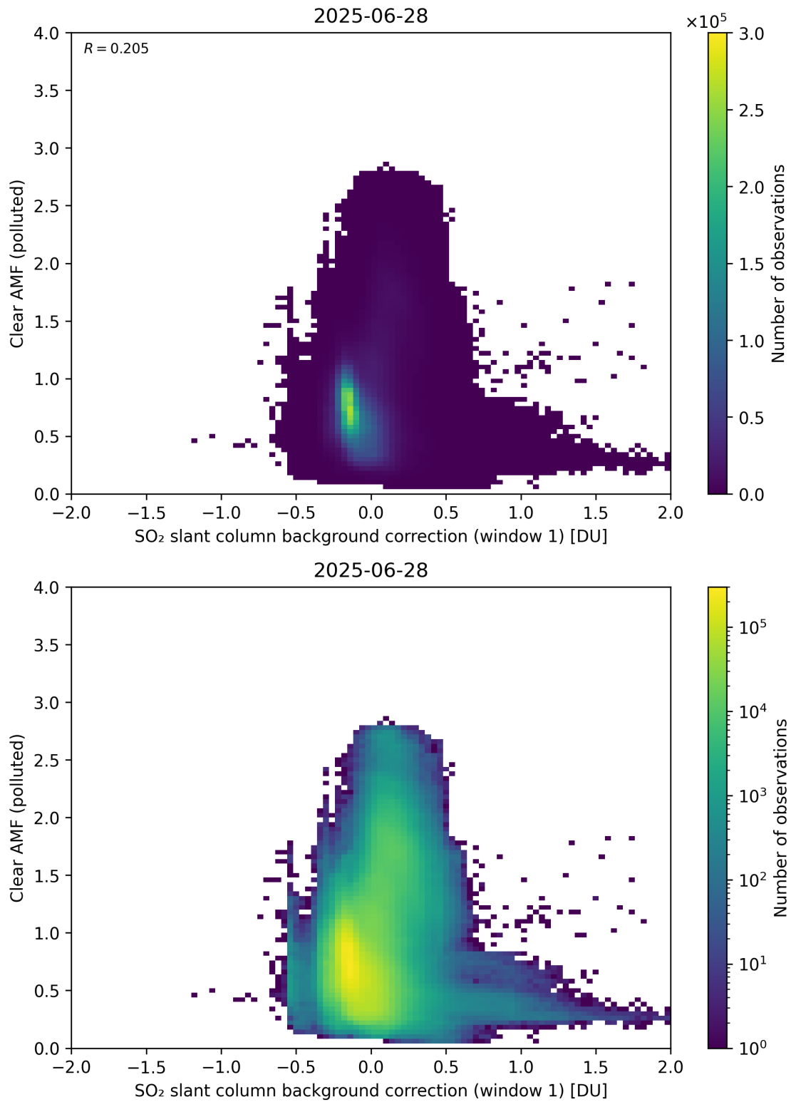
Figure 114: Scatter density plot of “SO 2 slant column background correction (window 1)” against “Clear AMF (polluted)” for 2025-06-27 to 2025-06-29.
