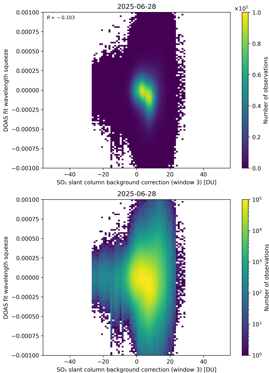
Figure 133: Scatter density plot of “SO 2 slant column background correction (window 3)” against “DOAS fit wavelength squeeze” for 2025-06-27 to 2025-06-29.
