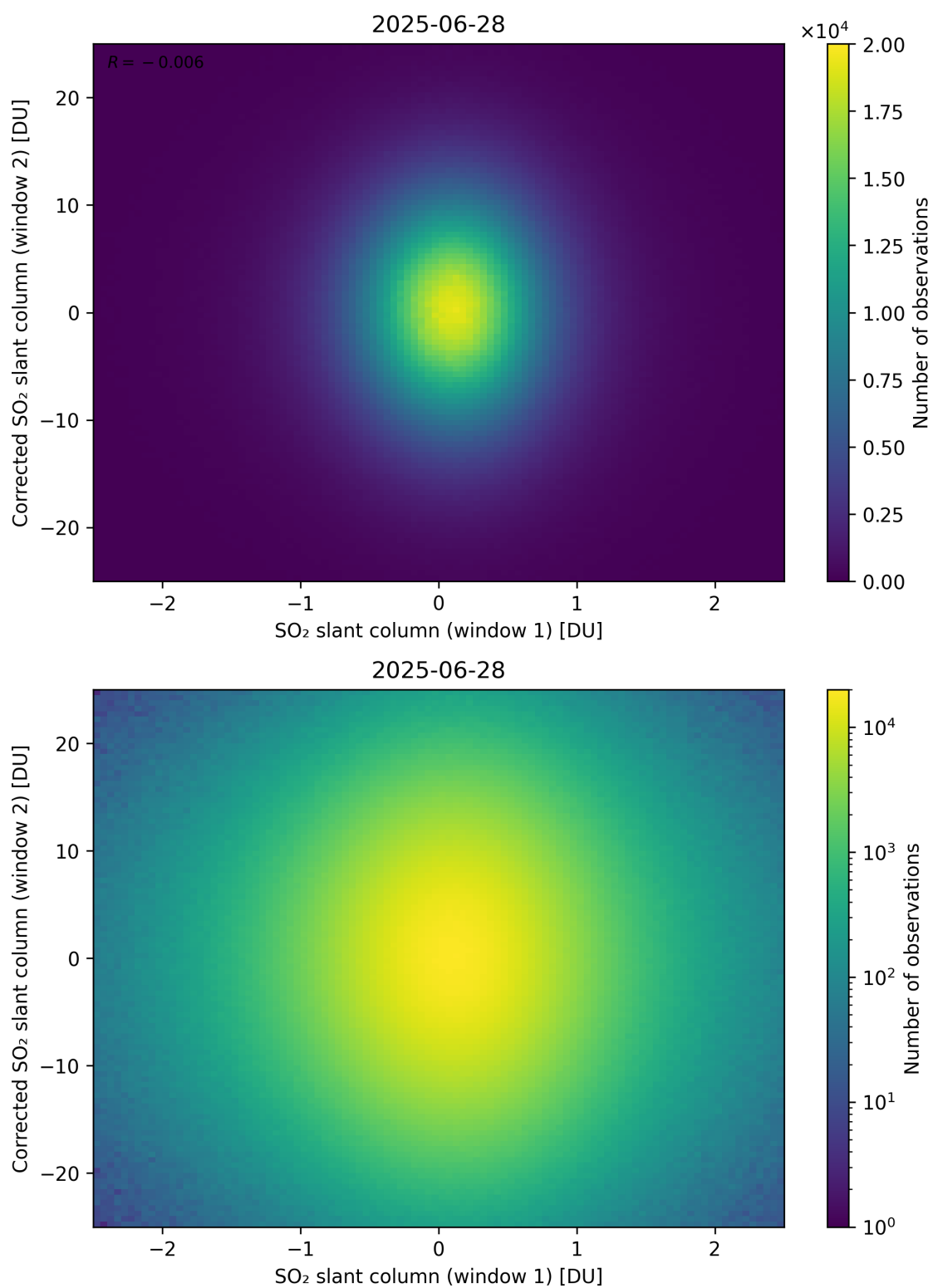
Figure 283: Scatter density plot of “SO 2 slant column (window 1)” against “Corrected SO 2 slant column (window 2)” for 2025-06-27 to 2025-06-29.
