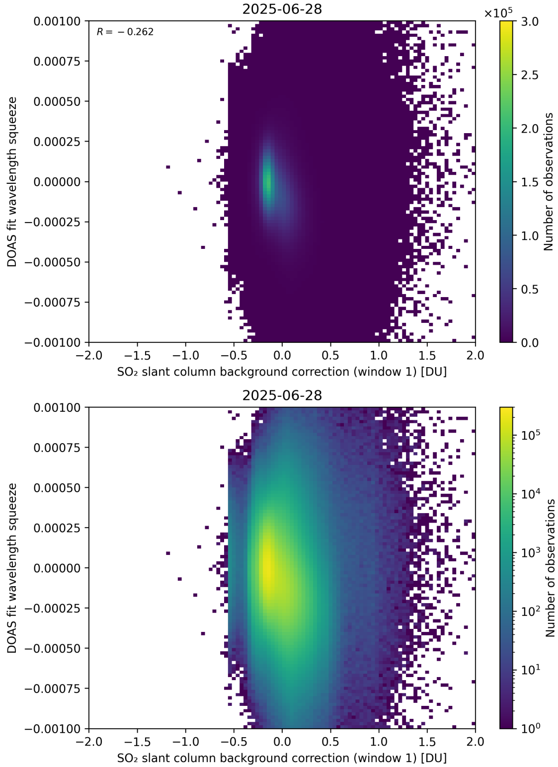
Figure 112: Scatter density plot of “SO 2 slant column background correction (window 1)” against “DOAS fit wavelength squeeze” for 2025-06-27 to 2025-06-29.
