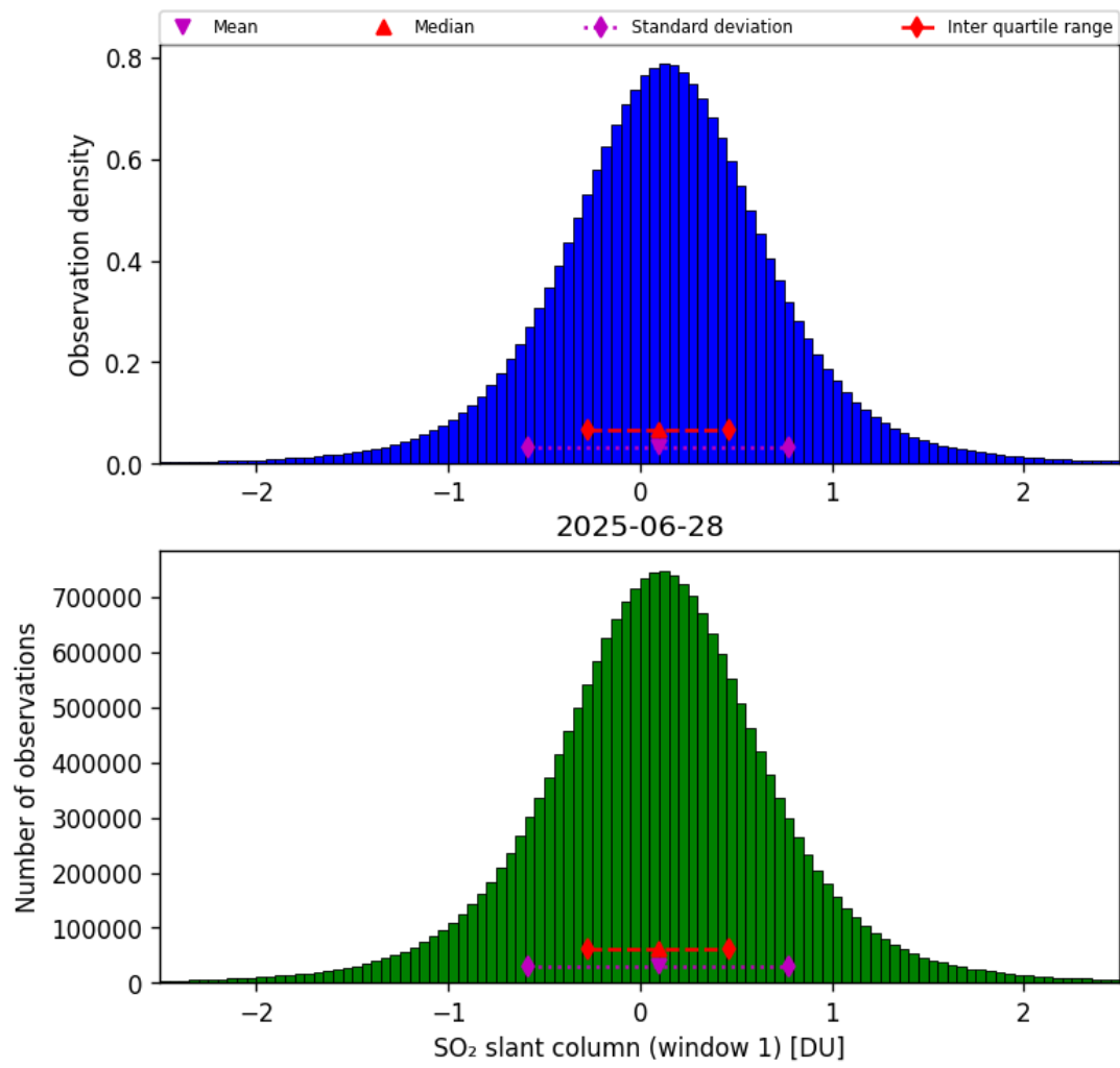
Figure 63: Histogram of “SO 2 slant column (window 1)” for 2025-06-27 to 2025-06-29
