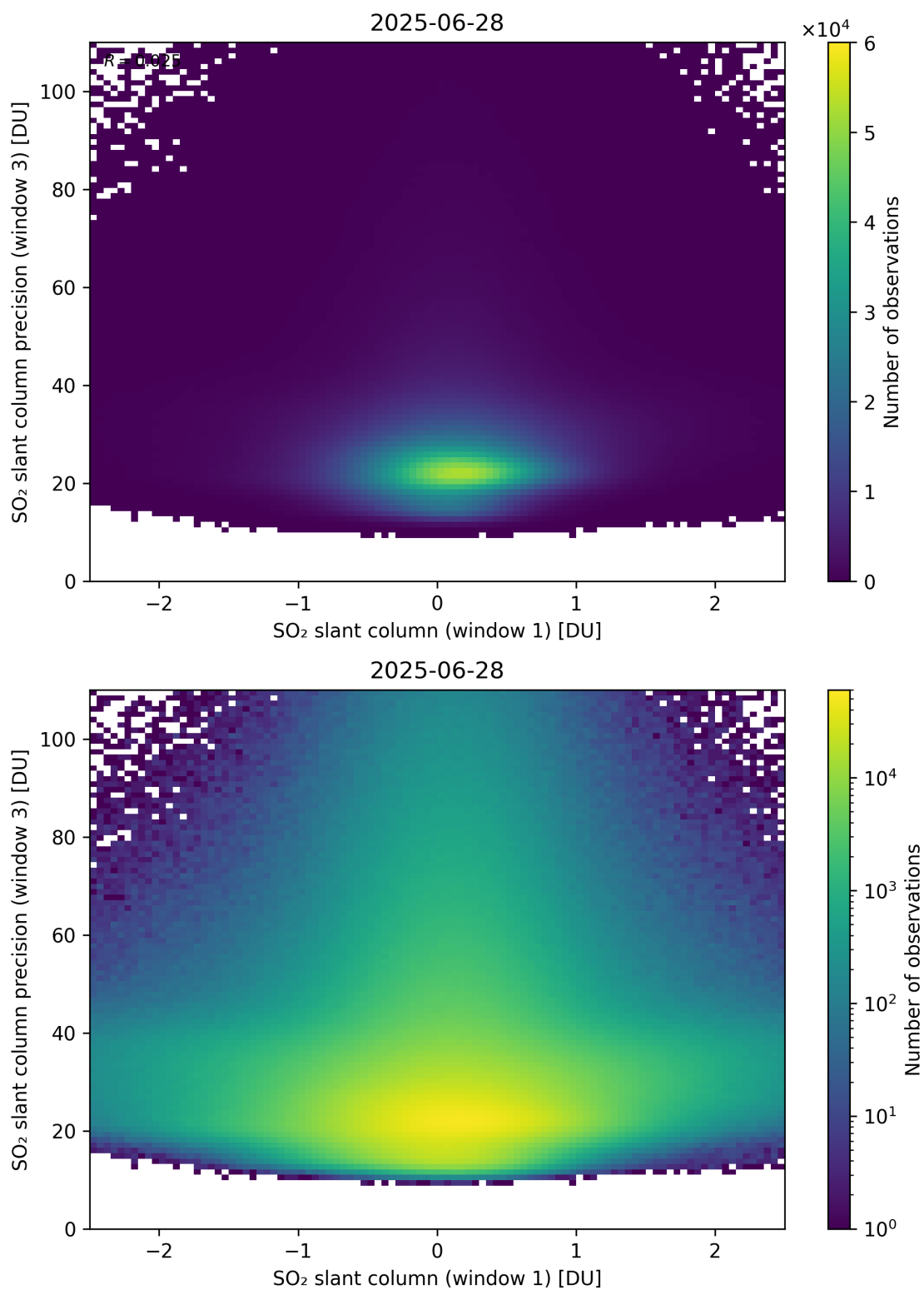
Figure 288: Scatter density plot of “SO 2 slant column (window 1)” against “SO 2 slant column precision (window 3)” for 2025-06-27 to 2025-06-29.
