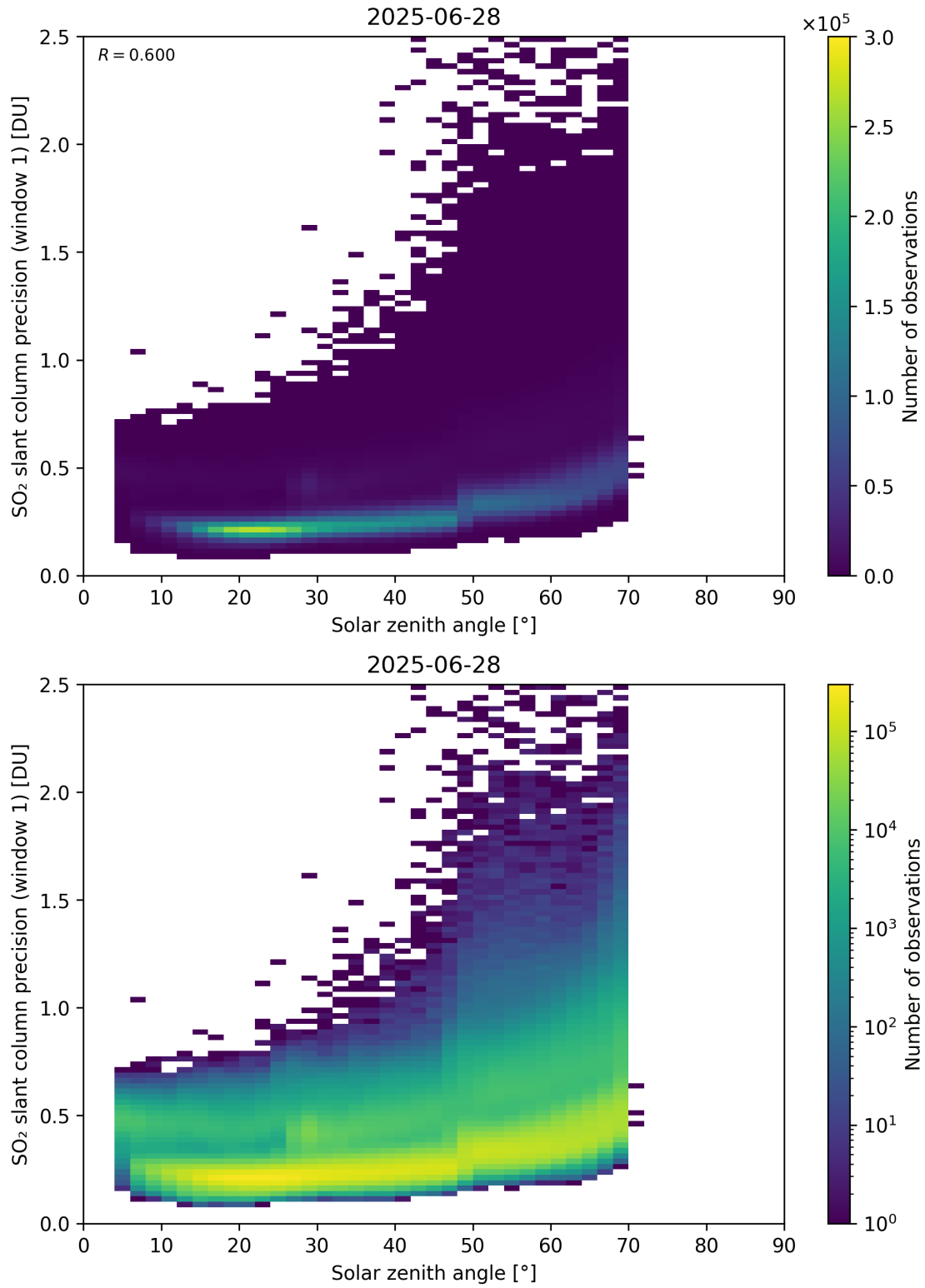
Figure 185: Scatter density plot of “Solar zenith angle” against “SO 2 slant column precision (window 1)” for 2025-06-27 to 2025-06-29.
