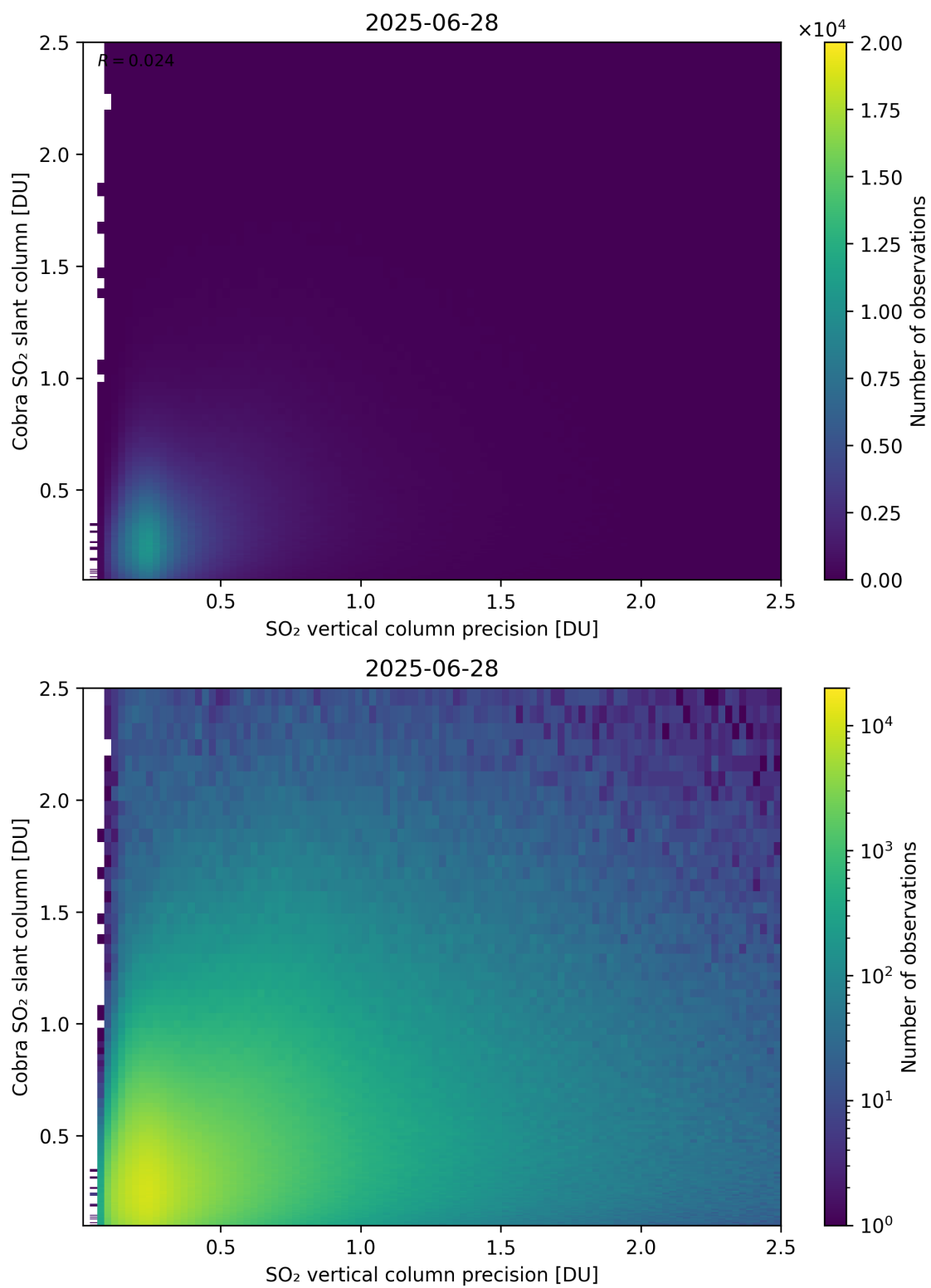
Figure 336: Scatter density plot of “SO 2 vertical column precision” against “Cobra SO 2 slant column” for 2025-06-27 to 2025-06-29.
