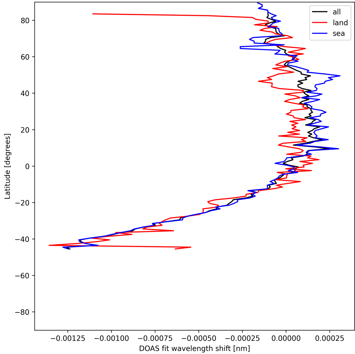
Figure 50: Zonal average of “DOAS fit wavelength shift” for 2025-06-27 to 2025-06-29.
