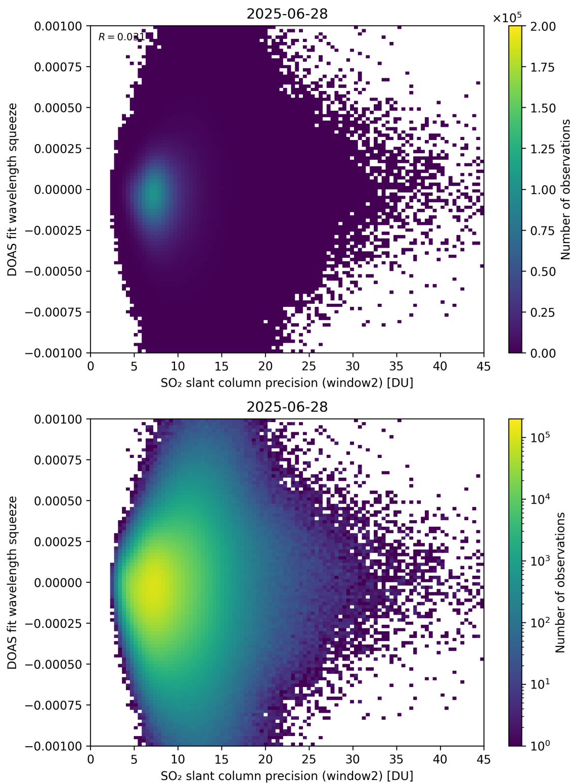
Figure 294: Scatter density plot of “SO 2 slant column precision (window2)” against “DOAS fit wavelength squeeze” for 2025-06-27 to 2025-06-29.
