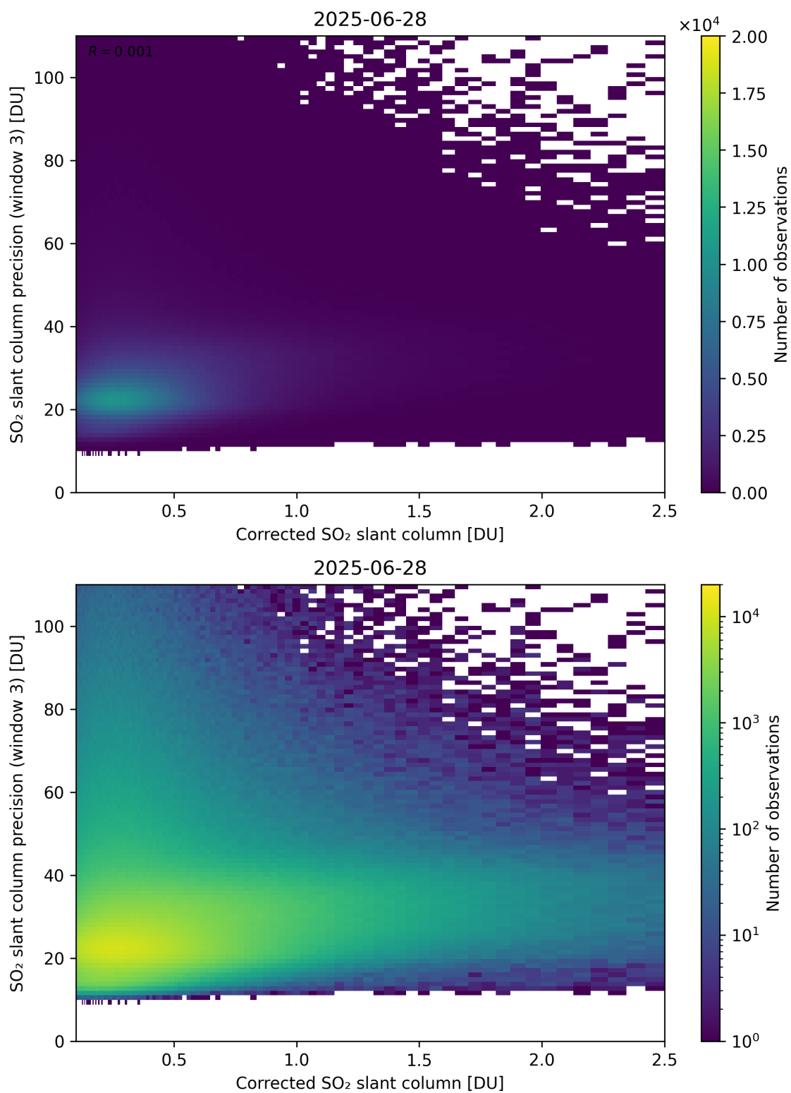
Figure 241: Scatter density plot of “Corrected SO 2 slant column” against “SO 2 slant column precision (window 3)” for 2025-06-27 to 2025-06-29.
