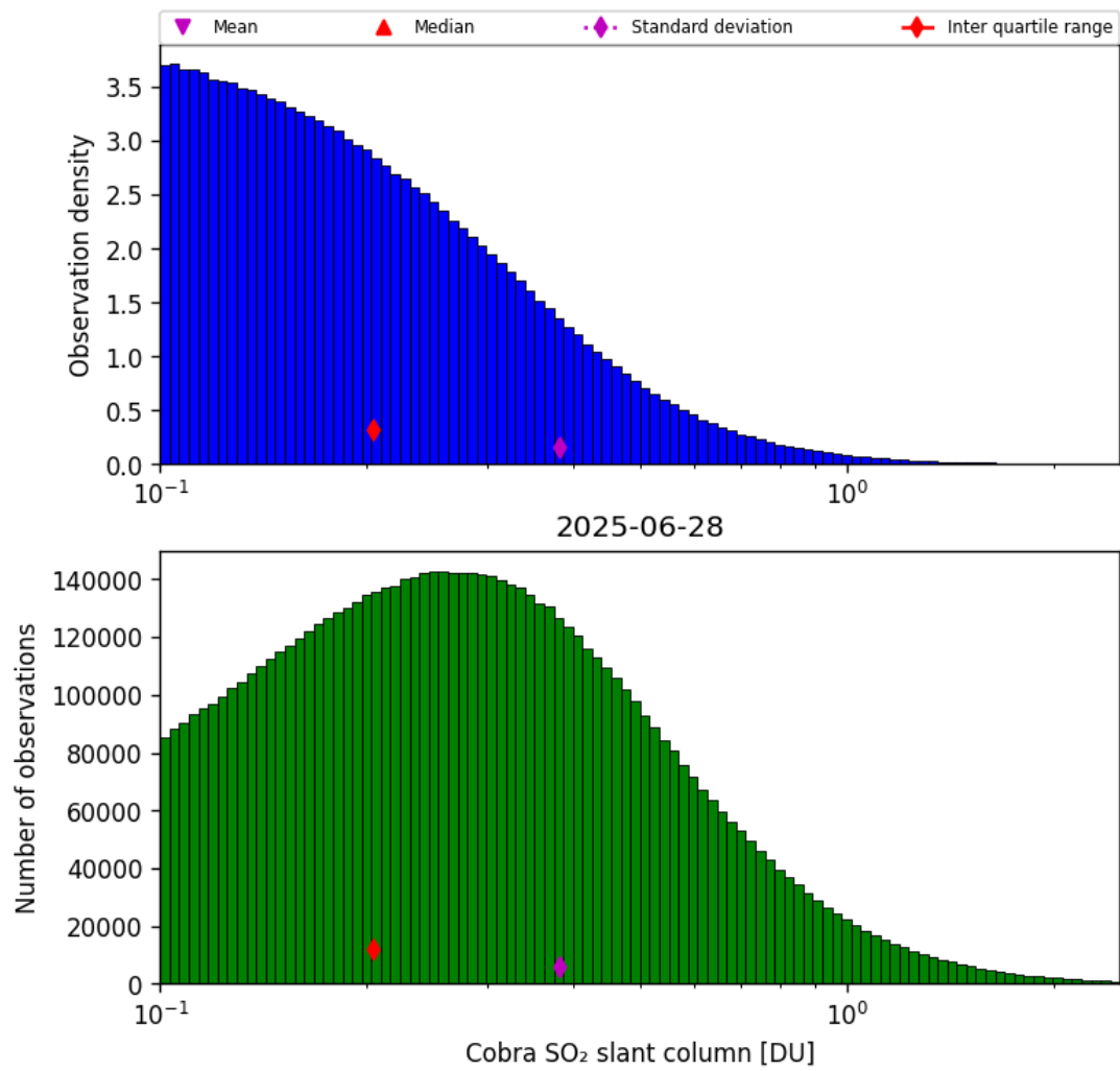
Figure 61: Histogram of “Cobra SO 2 slant column” for 2025-06-27 to 2025-06-29
