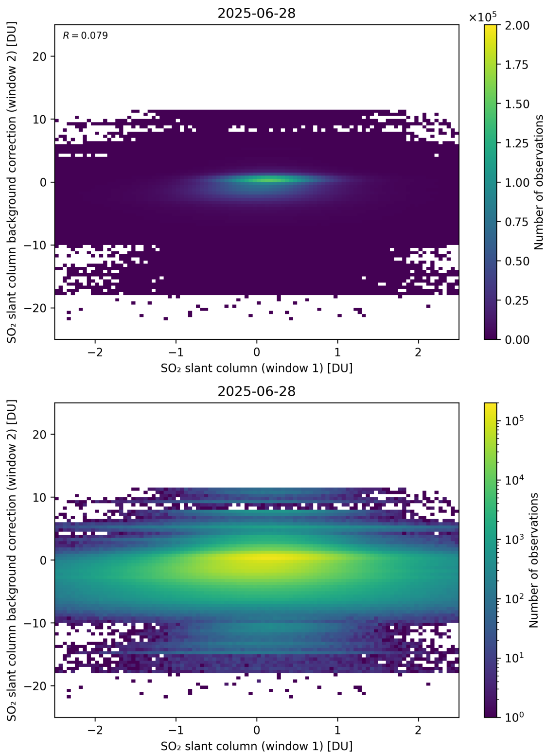
Figure 263: Scatter density plot of “SO 2 slant column (window 1)” against “SO 2 slant column background correction (window 2)” for 2025-06-27 to 2025-06-29.
