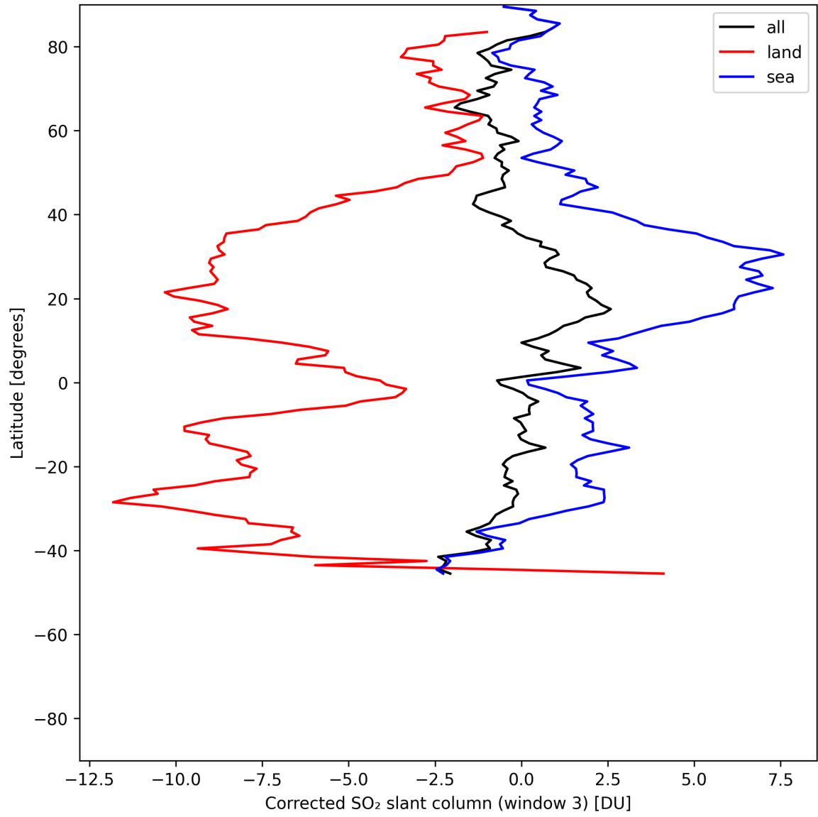
Figure 47: Zonal average of “Corrected SO 2 slant column (window 3)” for 2025-06-27 to 2025-06-29.
