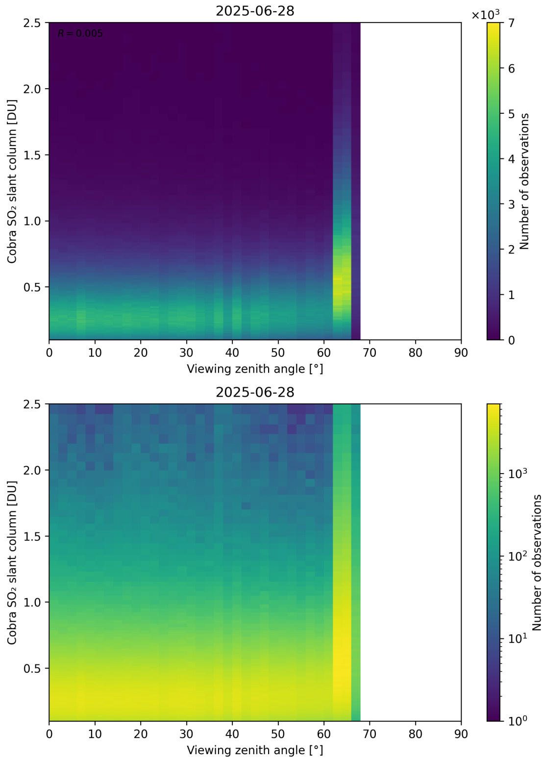
Figure 371: Scatter density plot of “Viewing zenith angle” against “Cobra SO 2 slant column” for 2025-06-27 to 2025-06-29.
