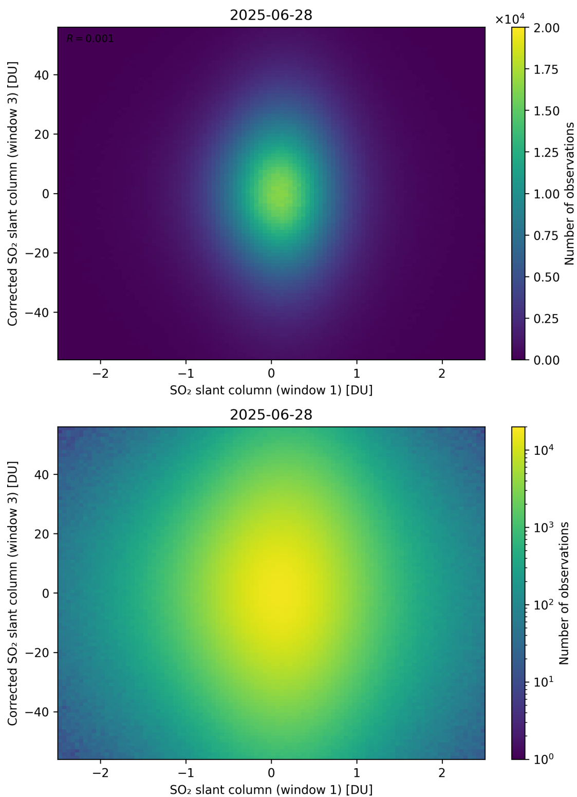
Figure 284: Scatter density plot of “SO 2 slant column (window 1)” against “Corrected SO 2 slant column (window 3)” for 2025-06-27 to 2025-06-29.
