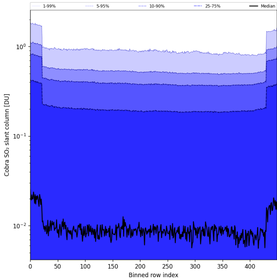
Figure 87: Along track statistics of “Cobra SO 2 slant column” for 2025-06-27 to 2025-06-29
