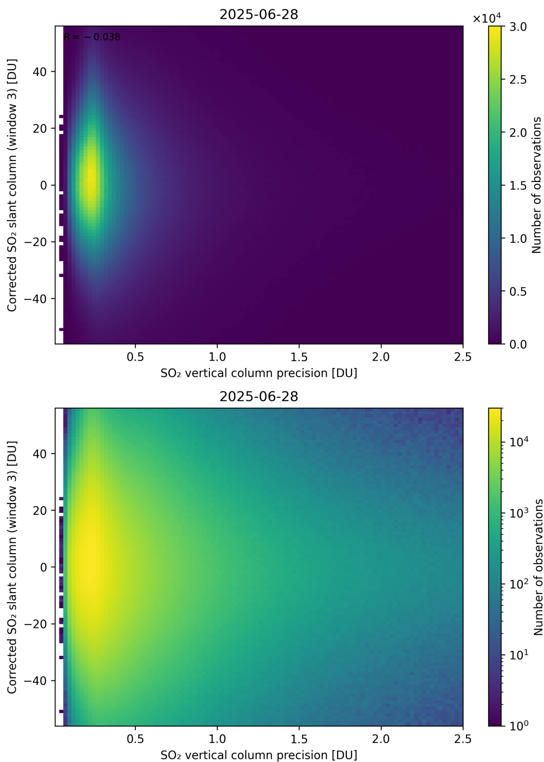
Figure 340: Scatter density plot of “SO 2 vertical column precision” against “Corrected SO 2 slant column (window 3)” for 2025-06-27 to 2025-06-29.
