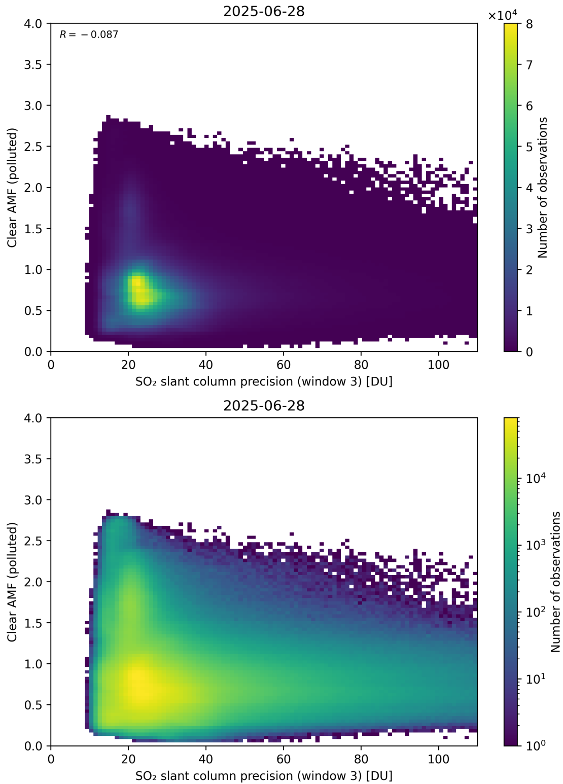
Figure 311: Scatter density plot of “SO 2 slant column precision (window 3)” against “Clear AMF (polluted)” for 2025-06-27 to 2025-06-29.
