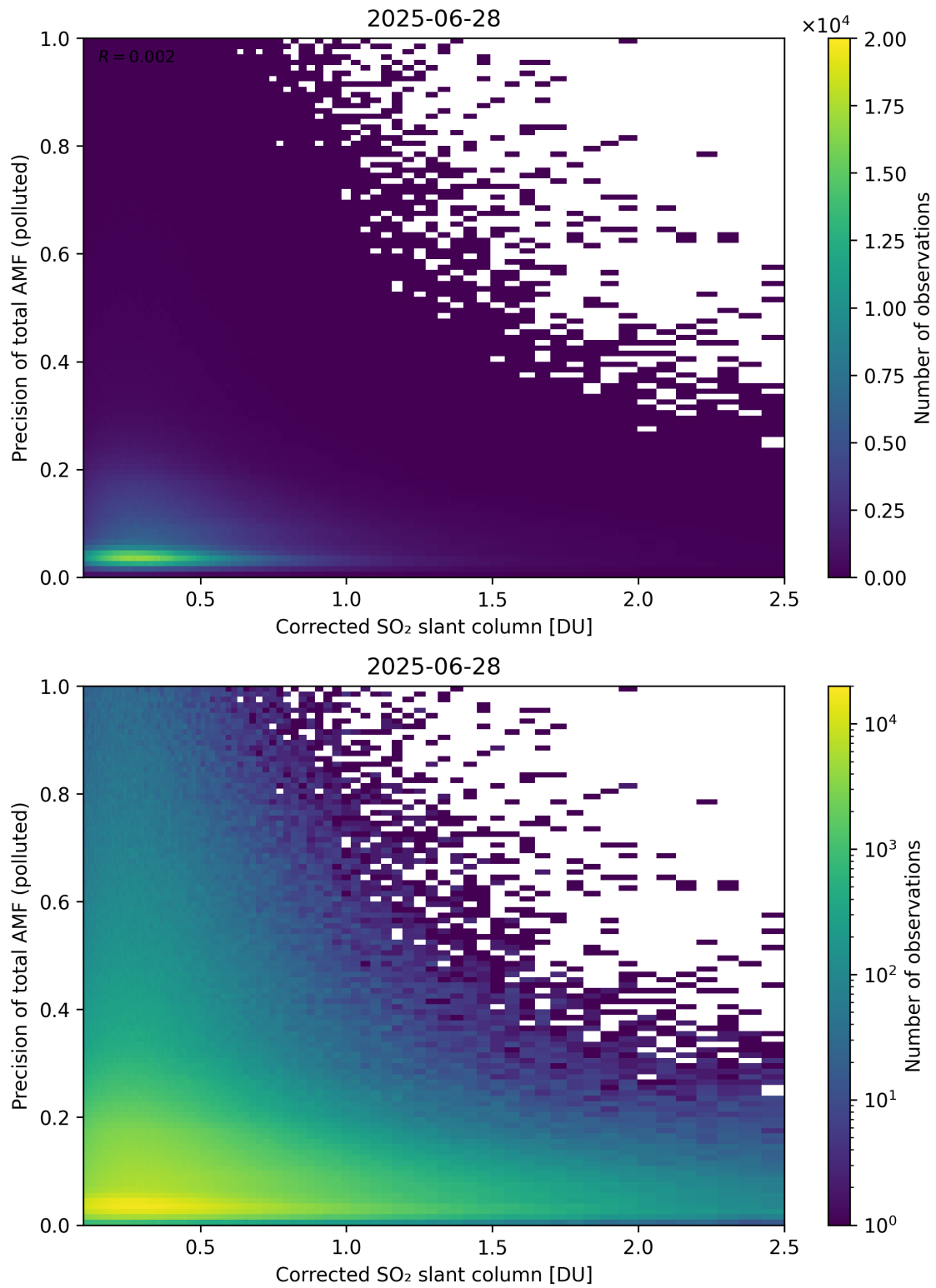
Figure 243: Scatter density plot of “Corrected SO 2 slant column” against “Precision of total AMF (polluted)” for 2025-06-27 to 2025-06-29.
