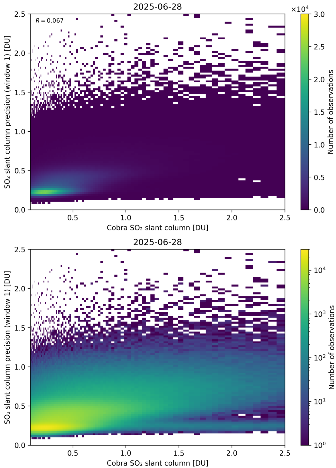
Figure 220: Scatter density plot of “Cobra SO 2 slant column” against “SO 2 slant column precision (window 1)” for 2025-06-27 to 2025-06-29.
