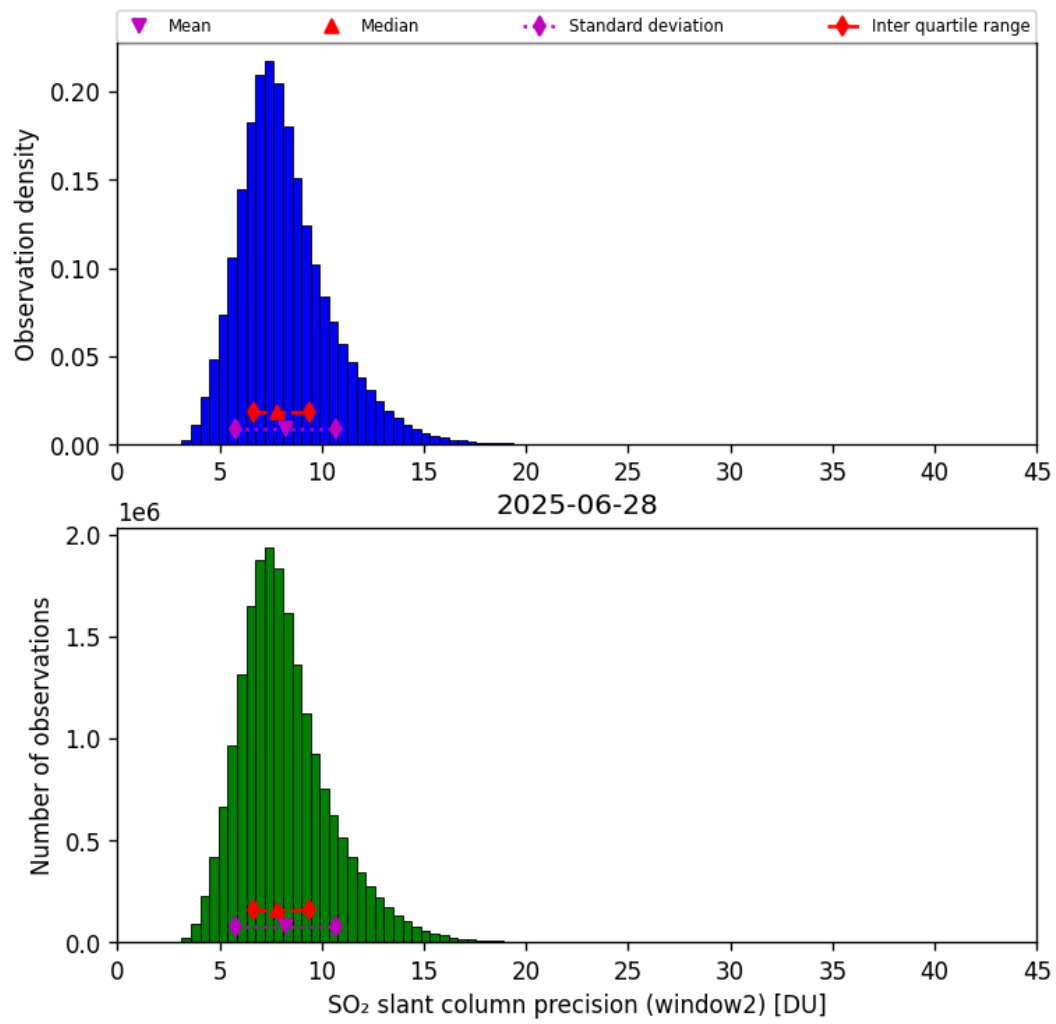
Figure 68: Histogram of “SO 2 slant column precision (window2)” for 2025-06-27 to 2025-06-29
