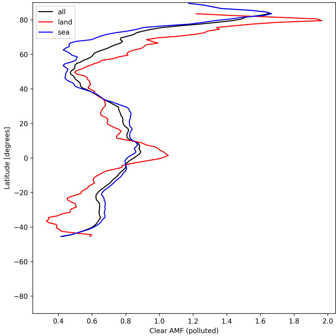
Figure 55: Zonal average of “Clear AMF (polluted)” for 2025-06-27 to 2025-06-29.
