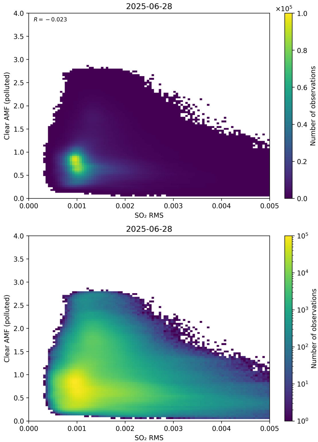
Figure 147: Scatter density plot of “SO 2 RMS” against “Clear AMF (polluted)” for 2025-06-27 to 2025-06-29.
