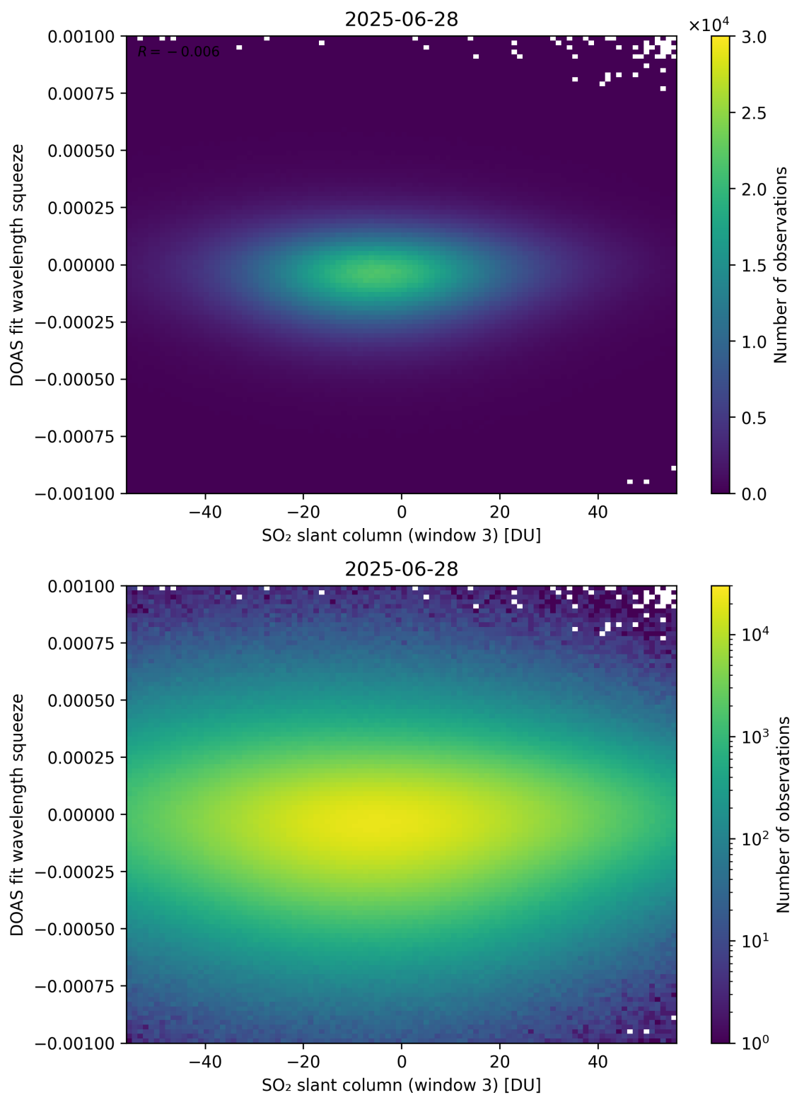
Figure 305: Scatter density plot of “SO 2 slant column (window 3)” against “DOAS fit wavelength squeeze” for 2025-06-27 to 2025-06-29.
