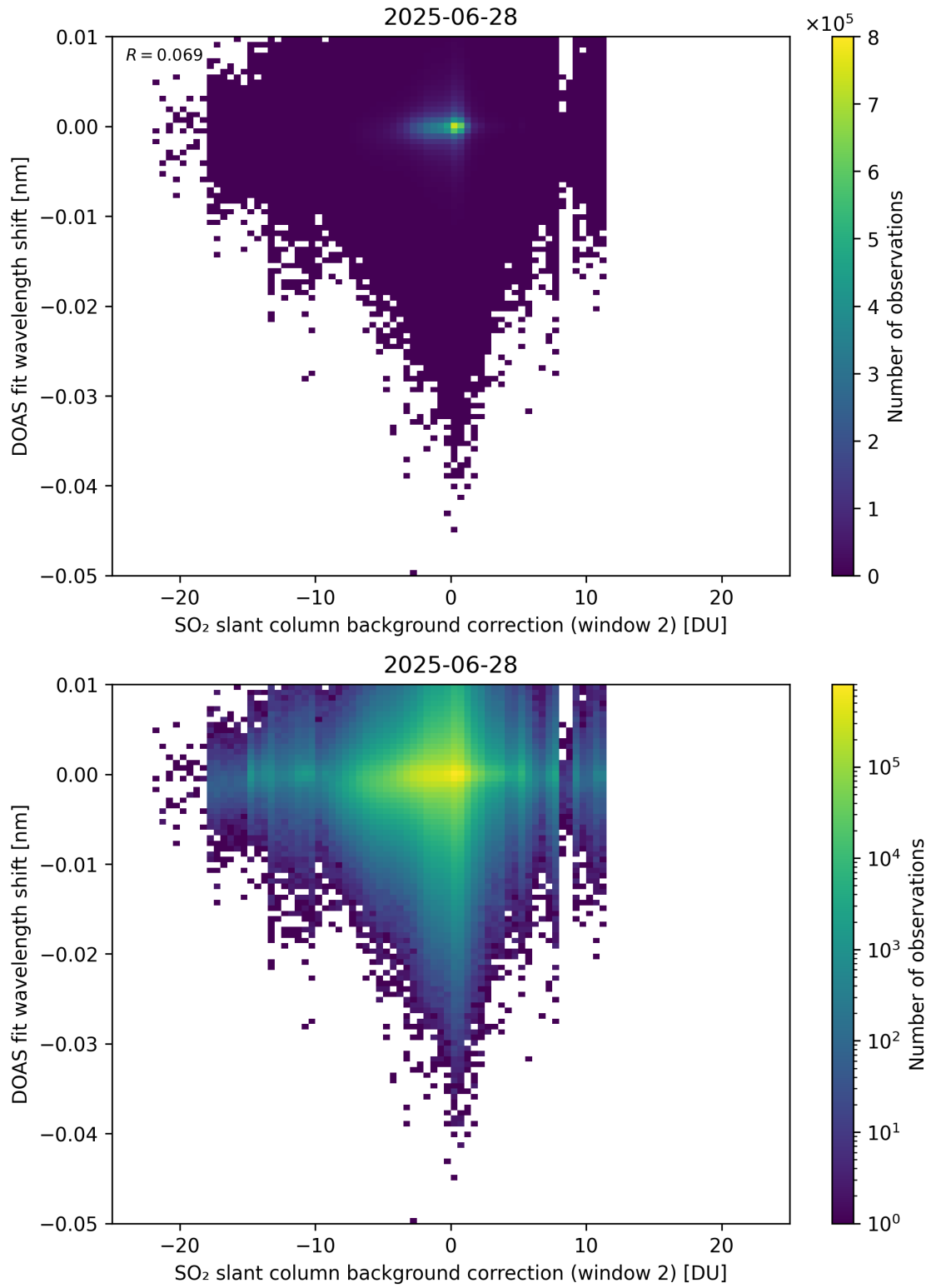
Figure 123: Scatter density plot of “SO 2 slant column background correction (window 2)” against “DOAS fit wavelength shift” for 2025-06-27 to 2025-06-29.
