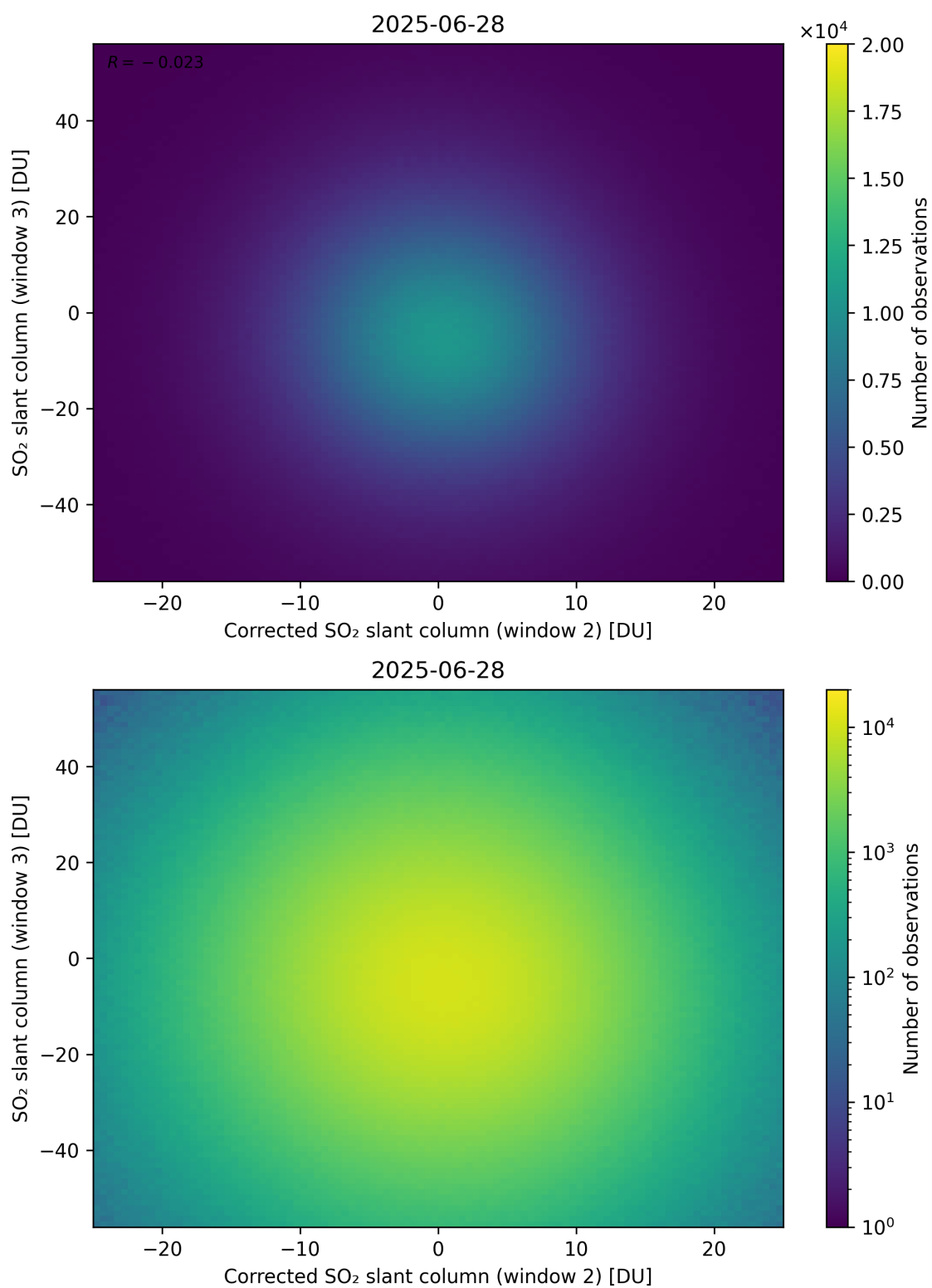
Figure 251: Scatter density plot of “Corrected SO 2 slant column (window 2)” against “SO 2 slant column (window 3)” for 2025-06-27 to 2025-06-29.
