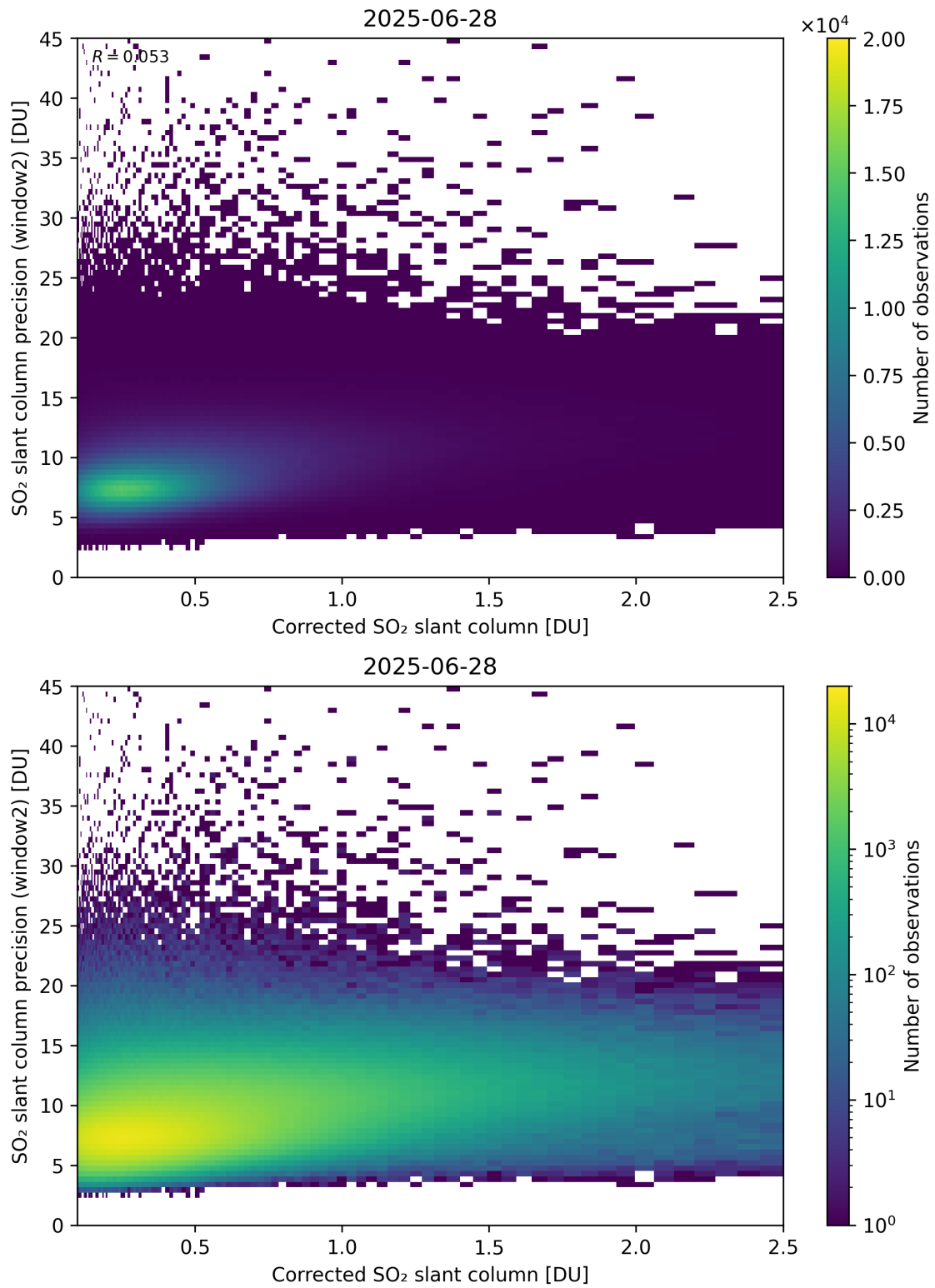
Figure 239: Scatter density plot of “Corrected SO 2 slant column” against “SO 2 slant column precision (window2)” for 2025-06-27 to 2025-06-29.
