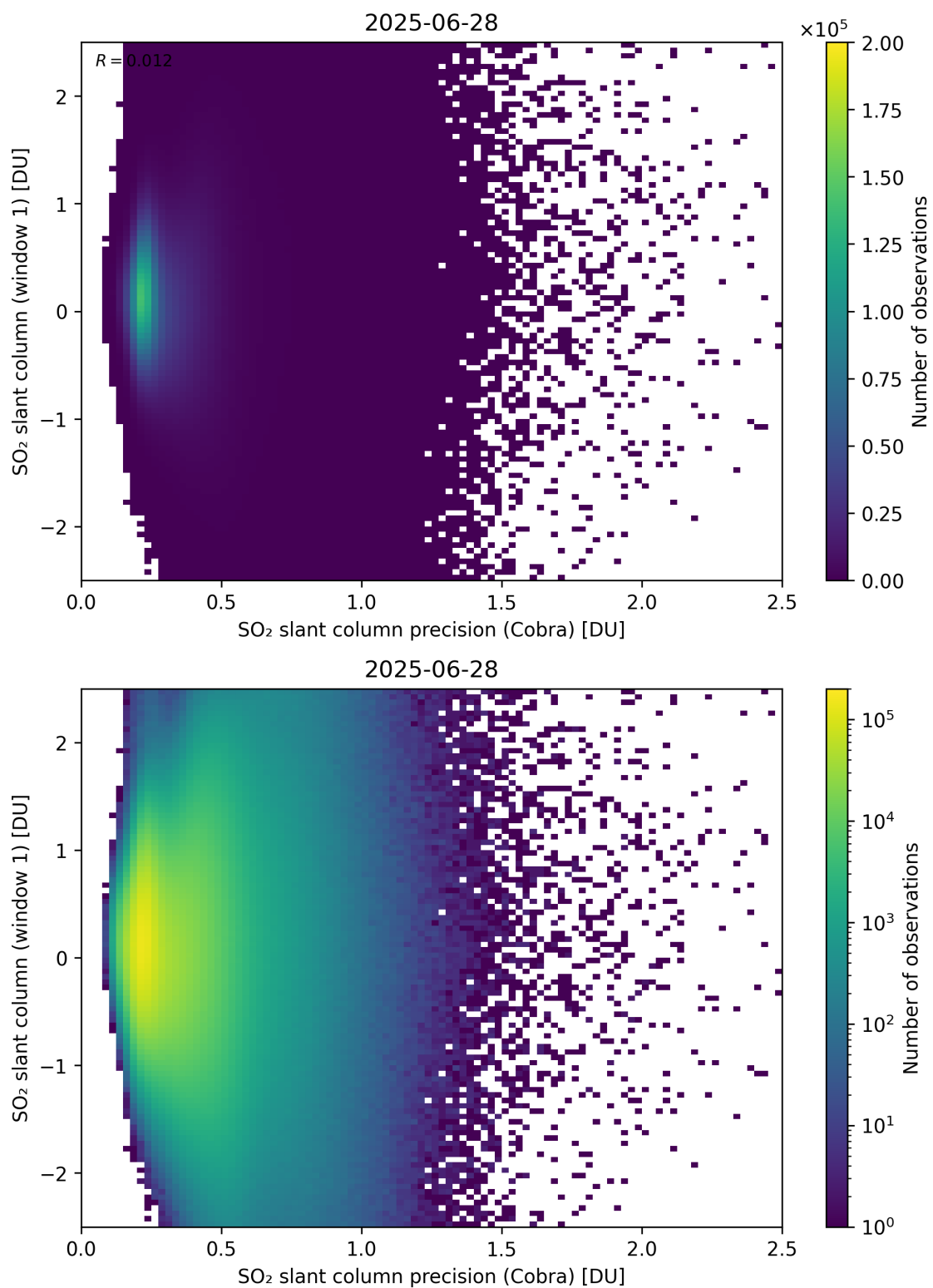
Figure 208: Scatter density plot of “SO 2 slant column precision (Cobra)” against “SO 2 slant column (window 1)” for 2025-06-27 to 2025-06-29.
