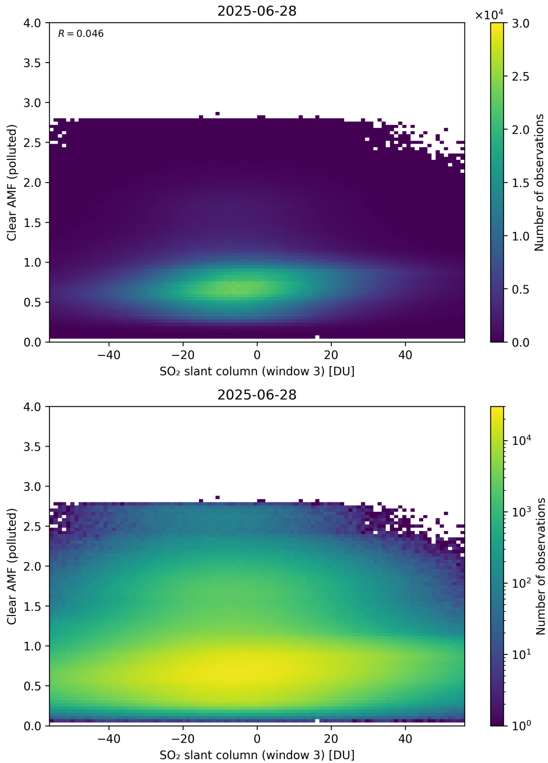
Figure 315: Scatter density plot of “SO 2 slant column (window 3)” against “Clear AMF (polluted)” for 2025-06-27 to 2025-06-29.
