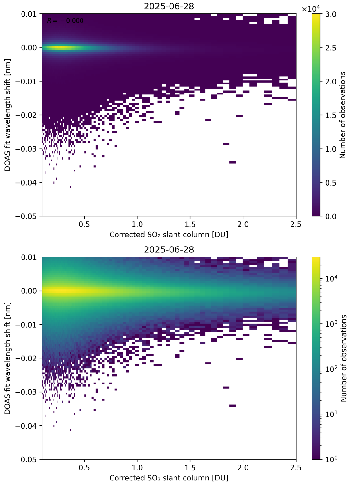
Figure 229: Scatter density plot of “Corrected SO 2 slant column” against “DOAS fit wavelength shift” for 2025-06-27 to 2025-06-29.
