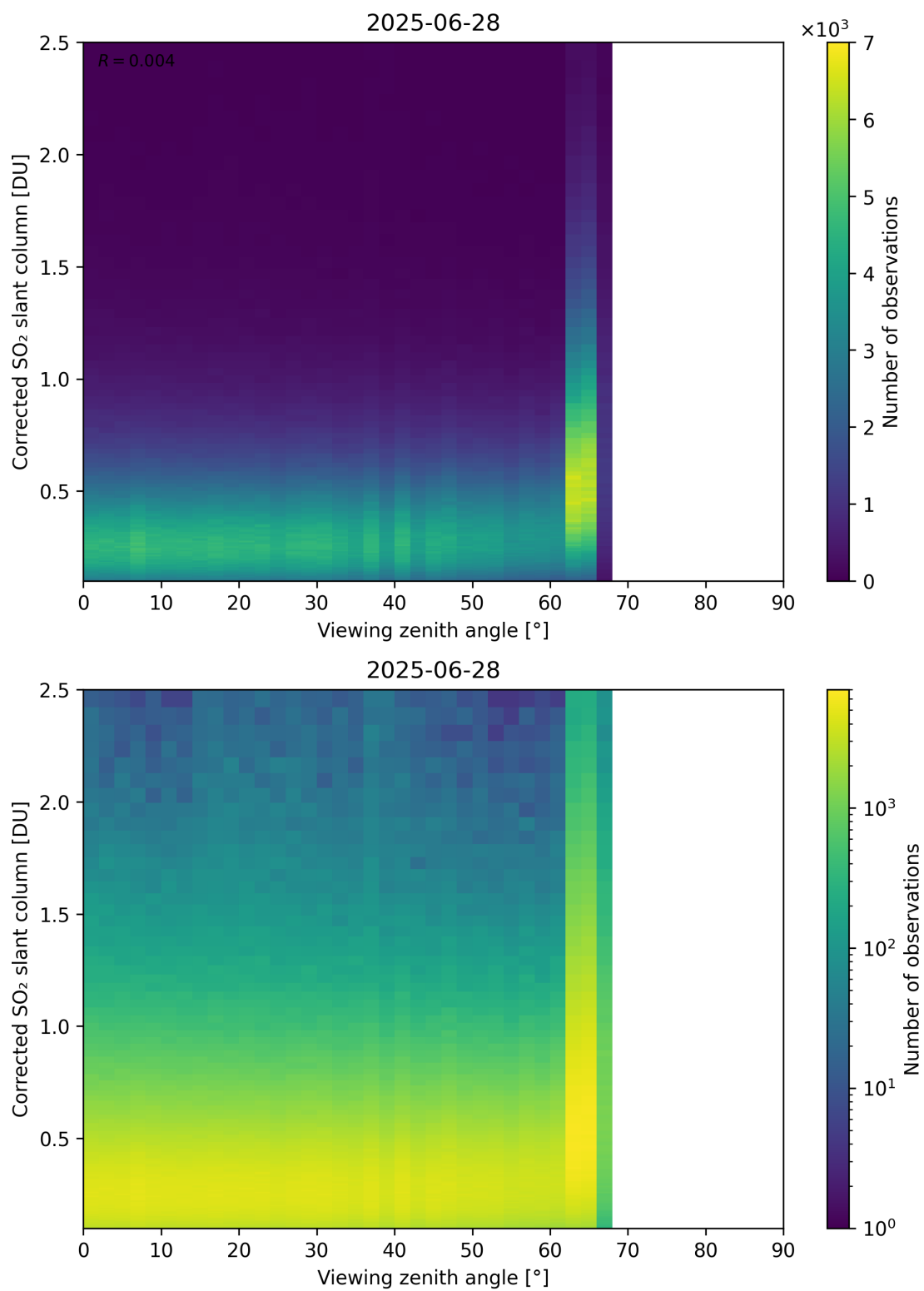
Figure 373: Scatter density plot of “Viewing zenith angle” against “Corrected SO 2 slant column” for 2025-06-27 to 2025-06-29.
