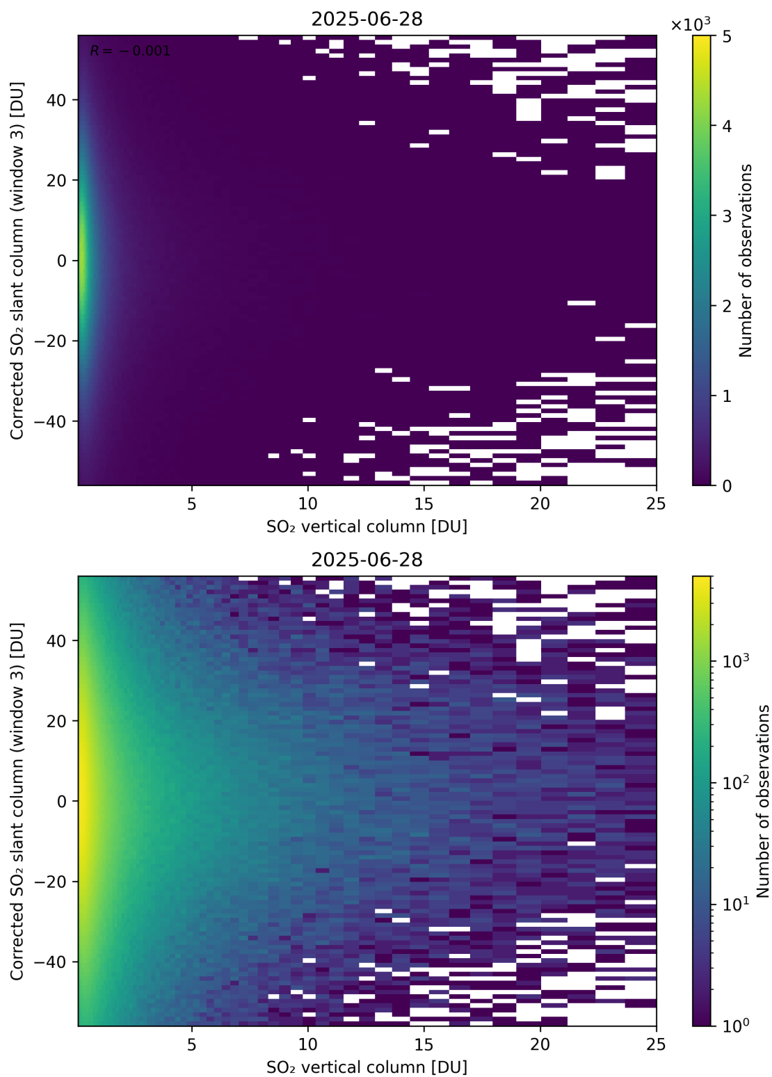
Figure 353: Scatter density plot of “SO 2 vertical column” against “Corrected SO 2 slant column (window 3)” for 2025-06-27 to 2025-06-29.
