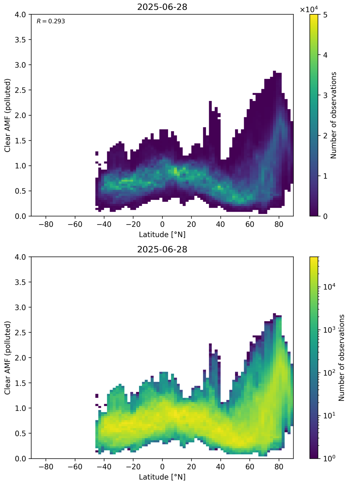
Figure 156: Scatter density plot of “Latitude” against “Clear AMF (polluted)” for 2025-06-27 to 2025-06-29.
