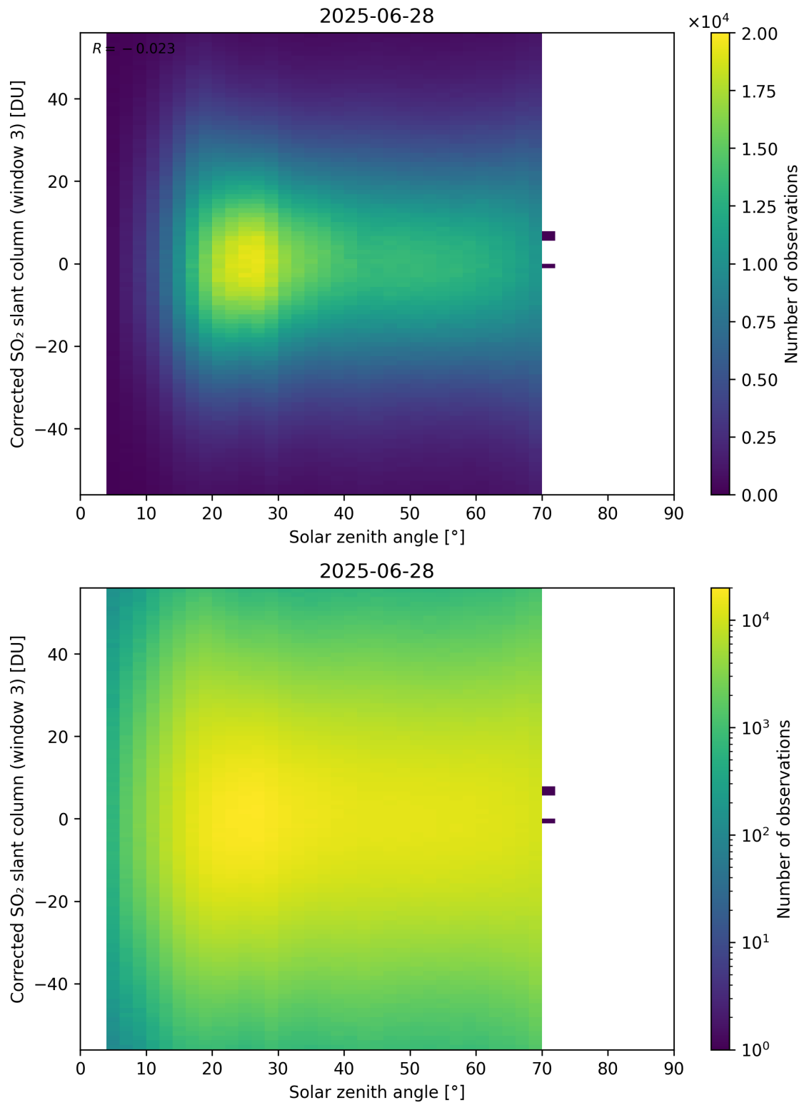
Figure 183: Scatter density plot of “Solar zenith angle” against “Corrected SO 2 slant column (window 3)” for 2025-06-27 to 2025-06-29.
