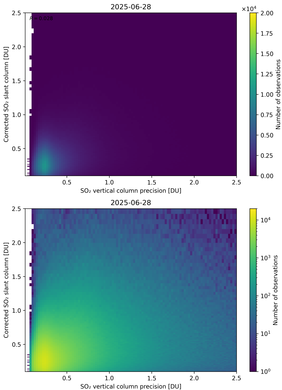
Figure 338: Scatter density plot of “SO 2 vertical column precision” against “Corrected SO 2 slant column” for 2025-06-27 to 2025-06-29.
