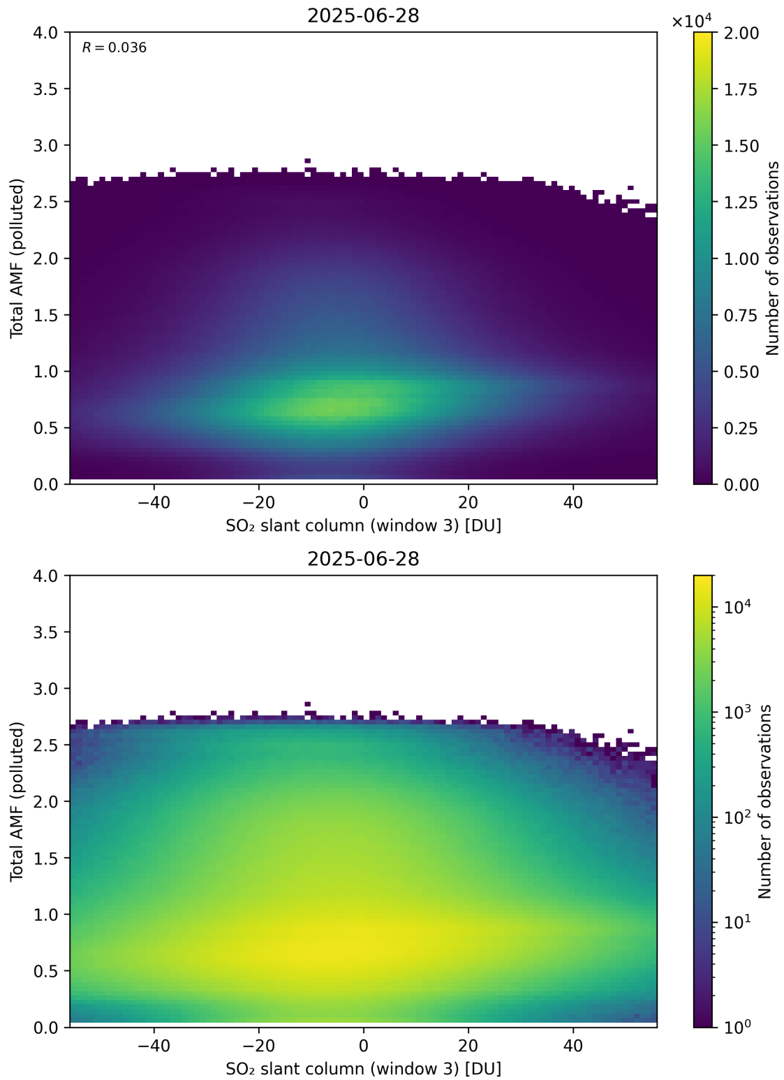
Figure 318: Scatter density plot of “SO 2 slant column (window 3)” against “Total AMF (polluted)” for 2025-06-27 to 2025-06-29.
