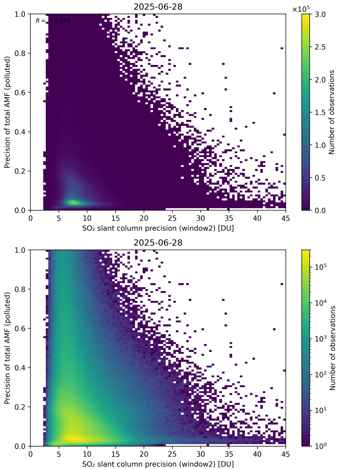
Figure 302: Scatter density plot of “SO 2 slant column precision (window2)” against “Precision of total AMF (polluted)” for 2025-06-27 to 2025-06-29.
