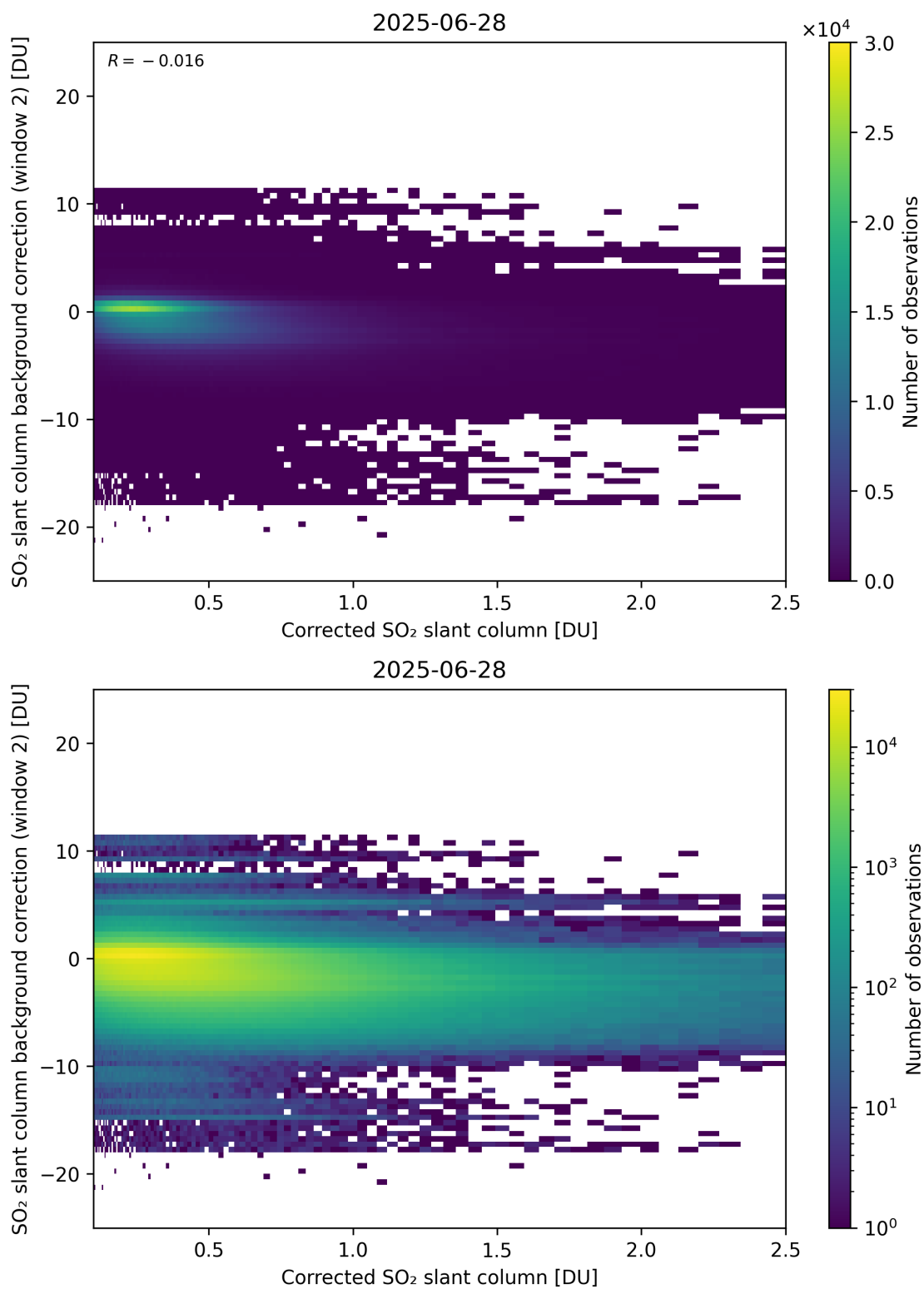
Figure 227: Scatter density plot of “Corrected SO 2 slant column” against “SO 2 slant column background correction (window 2)” for 2025-06-27 to 2025-06-29.
