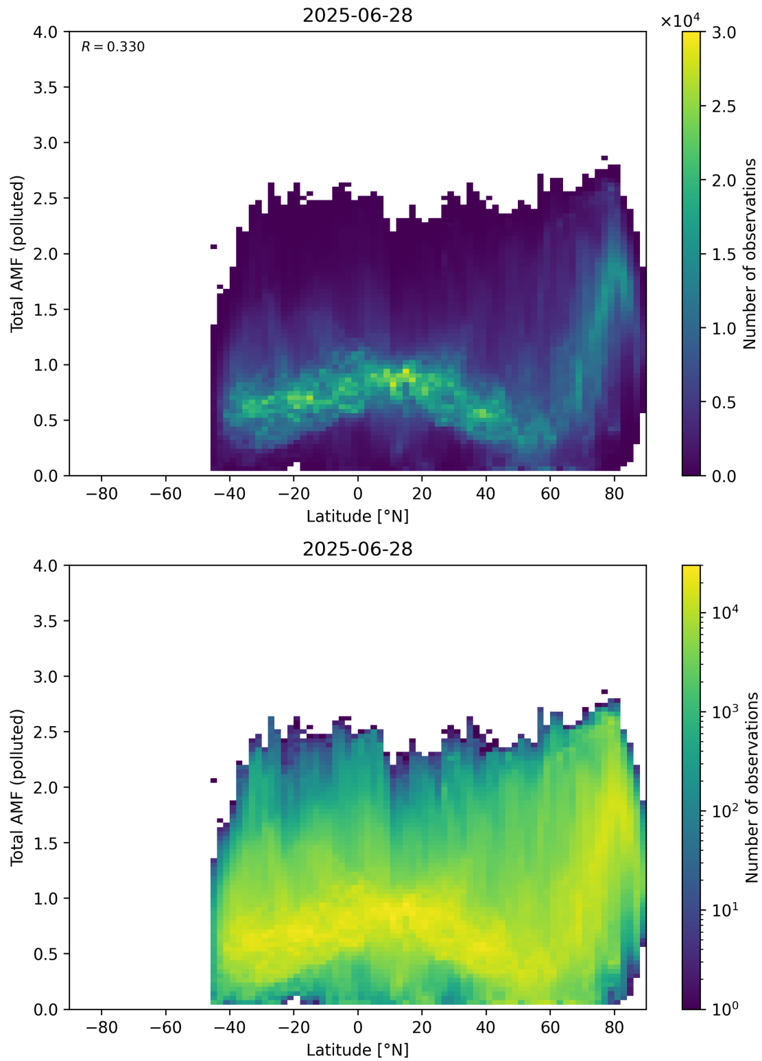
Figure 167: Scatter density plot of “Latitude” against “Total AMF (polluted)” for 2025-06-27 to 2025-06-29.
