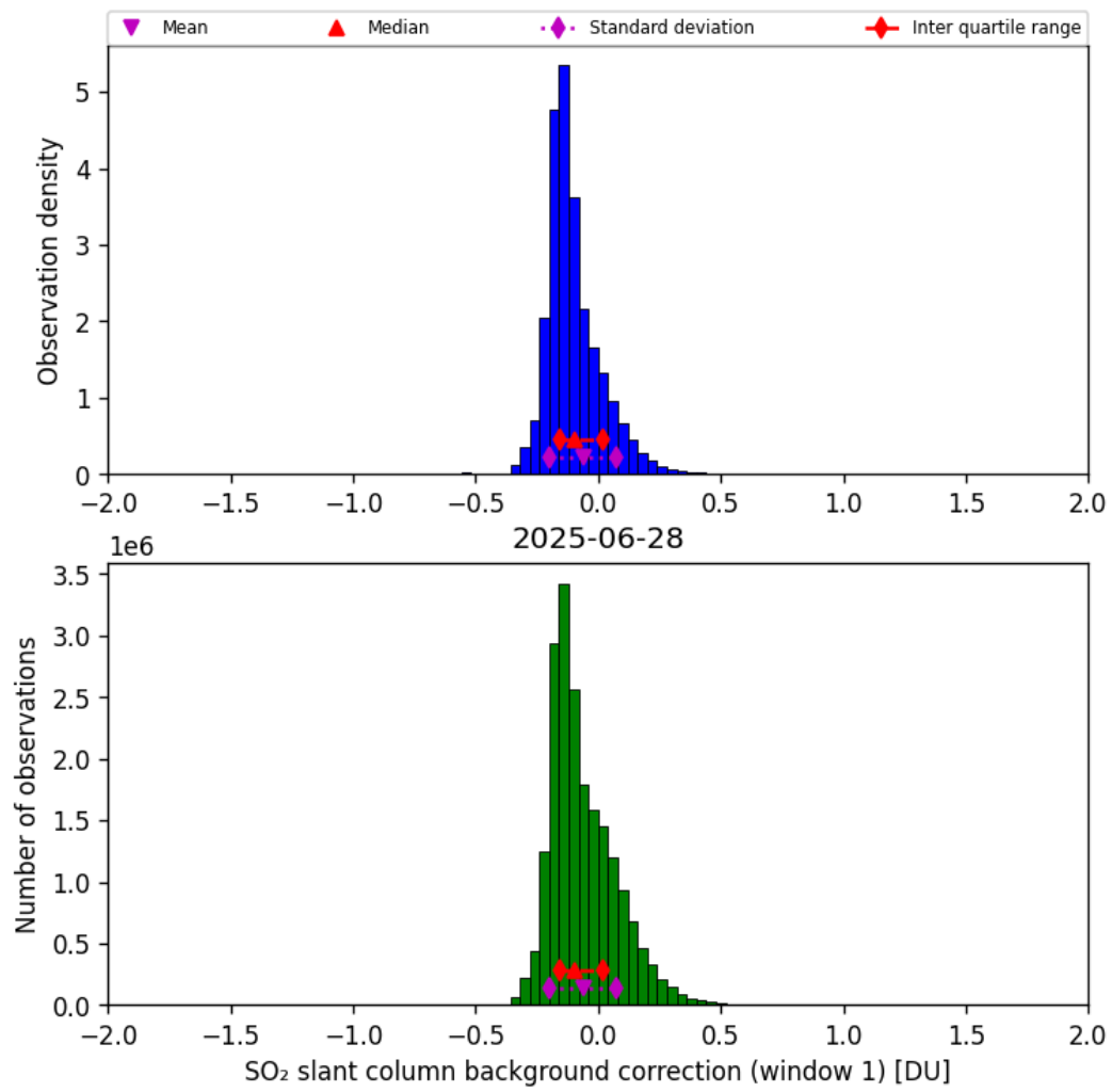
Figure 66: Histogram of “SO 2 slant column background correction (window 1)” for 2025-06-27 to 2025-06-29
