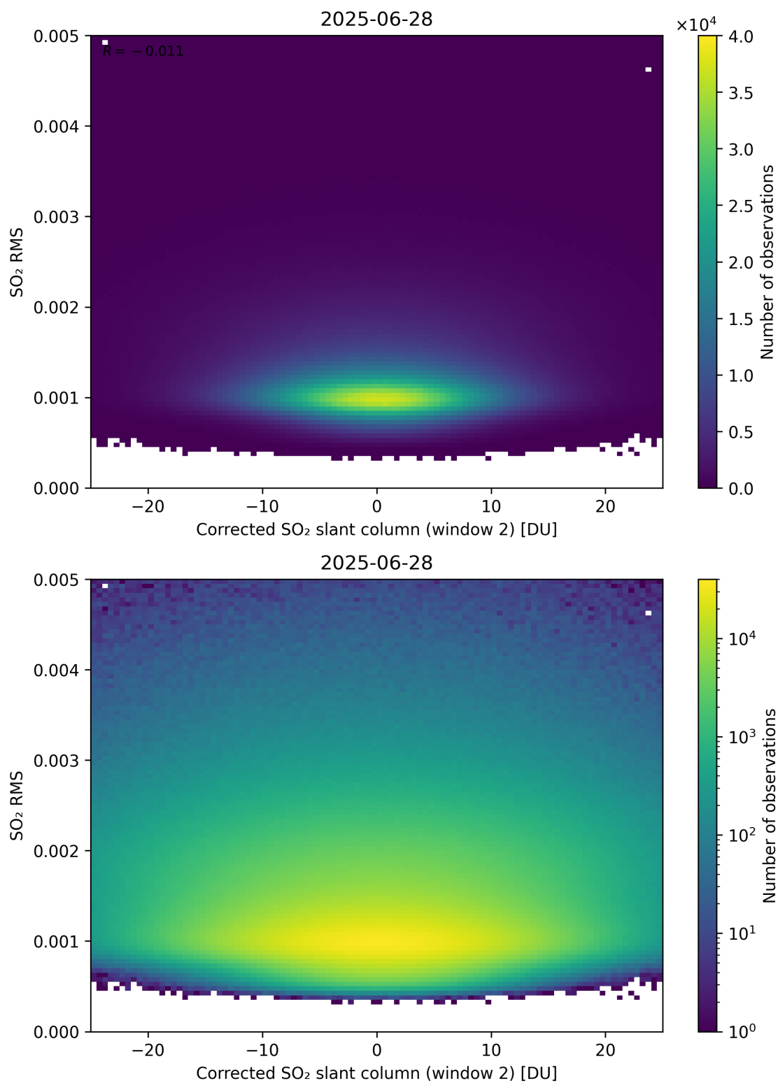
Figure 248: Scatter density plot of “Corrected SO 2 slant column (window 2)” against “SO 2 RMS” for 2025-06-27 to 2025-06-29.
