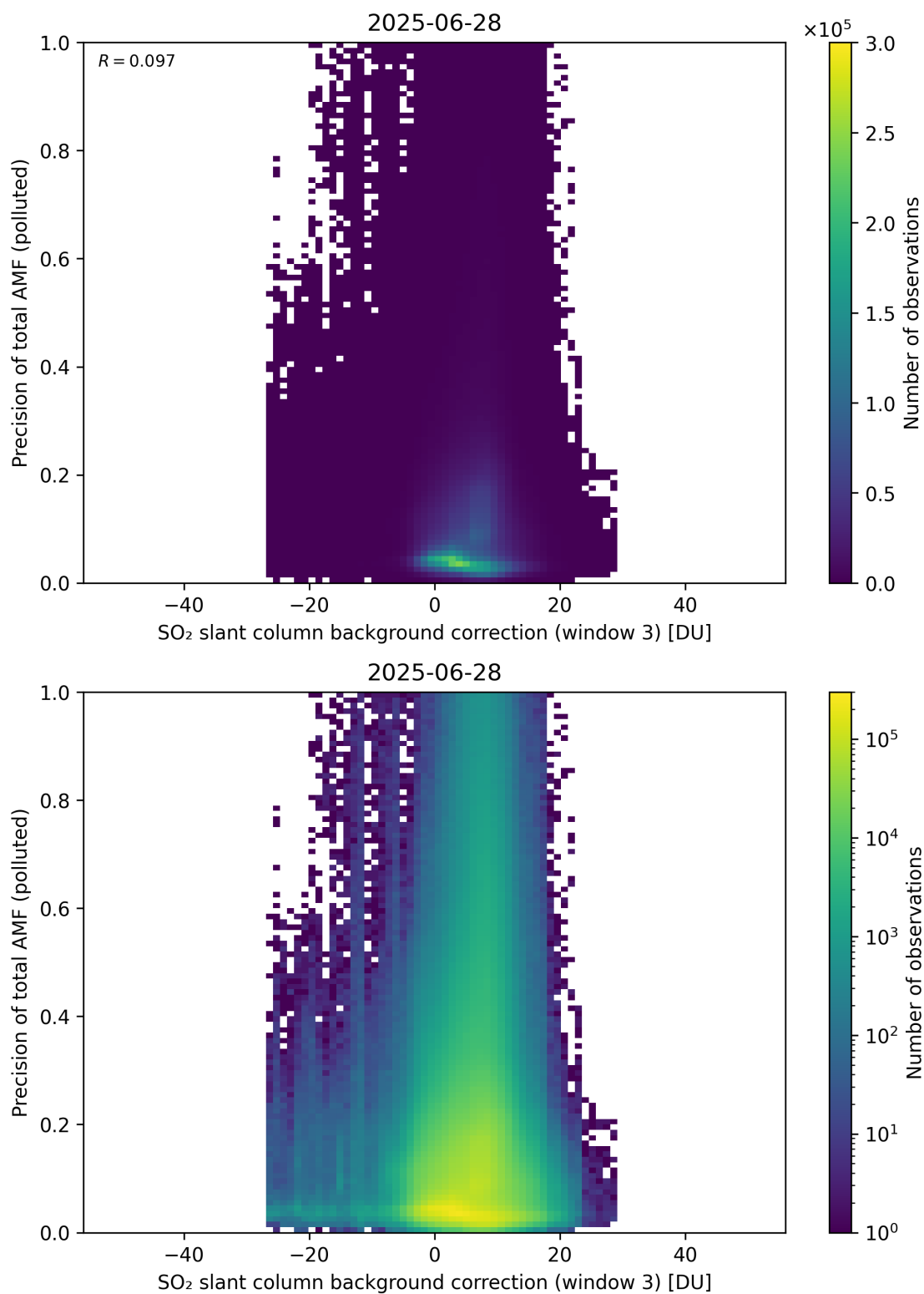
Figure 137: Scatter density plot of “SO 2 slant column background correction (window 3)” against “Precision of total AMF (polluted)” for 2025-06-27 to 2025-06-29.
