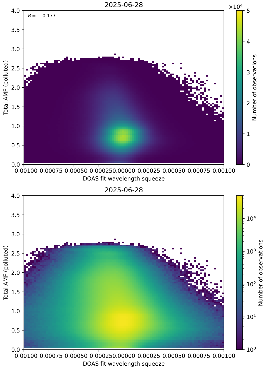
Figure 145: Scatter density plot of “DOAS fit wavelength squeeze” against “Total AMF (polluted)” for 2025-06-27 to 2025-06-29.
