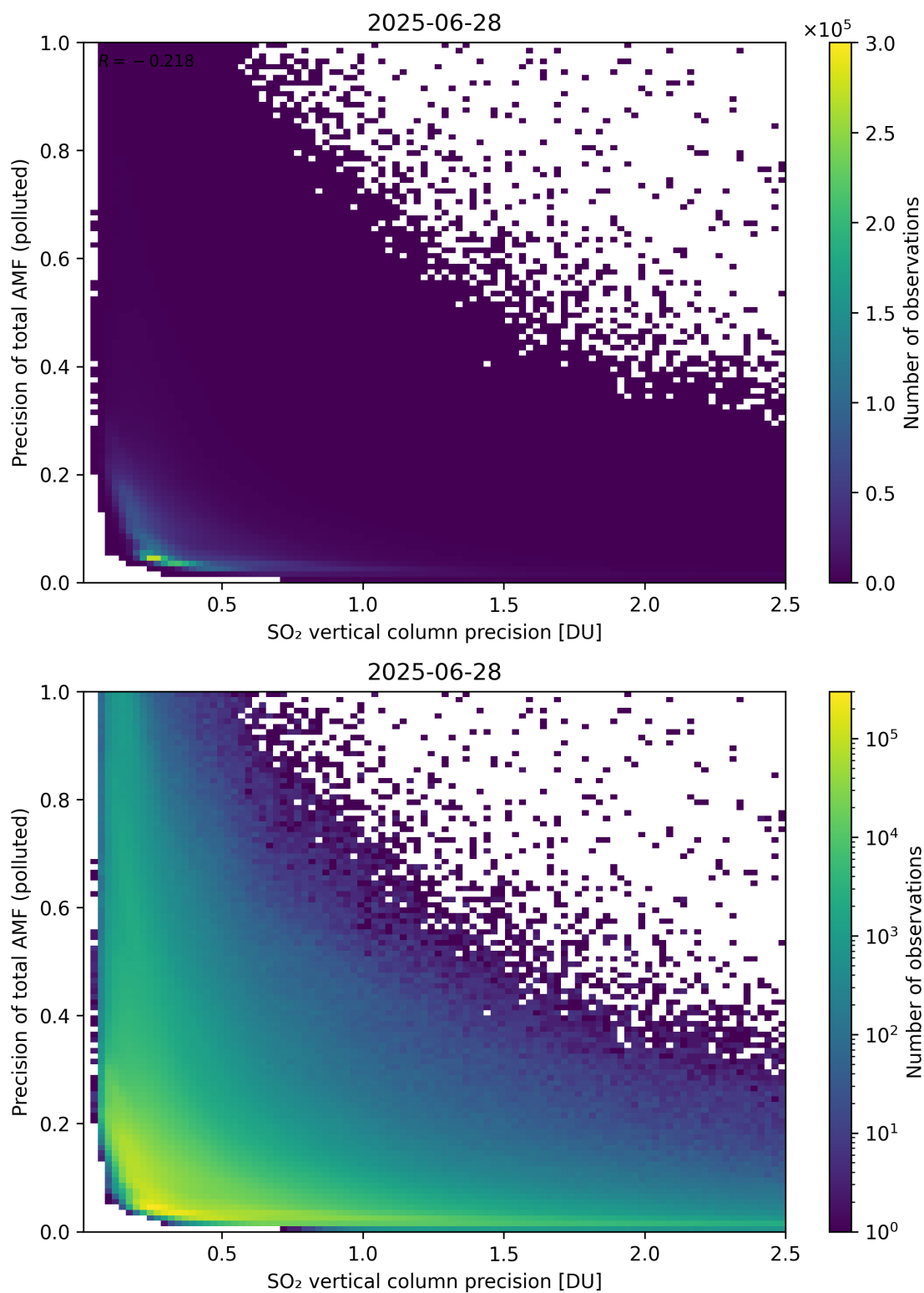
Figure 347: Scatter density plot of “SO 2 vertical column precision” against “Precision of total AMF (polluted)” for 2025-06-27 to 2025-06-29.
