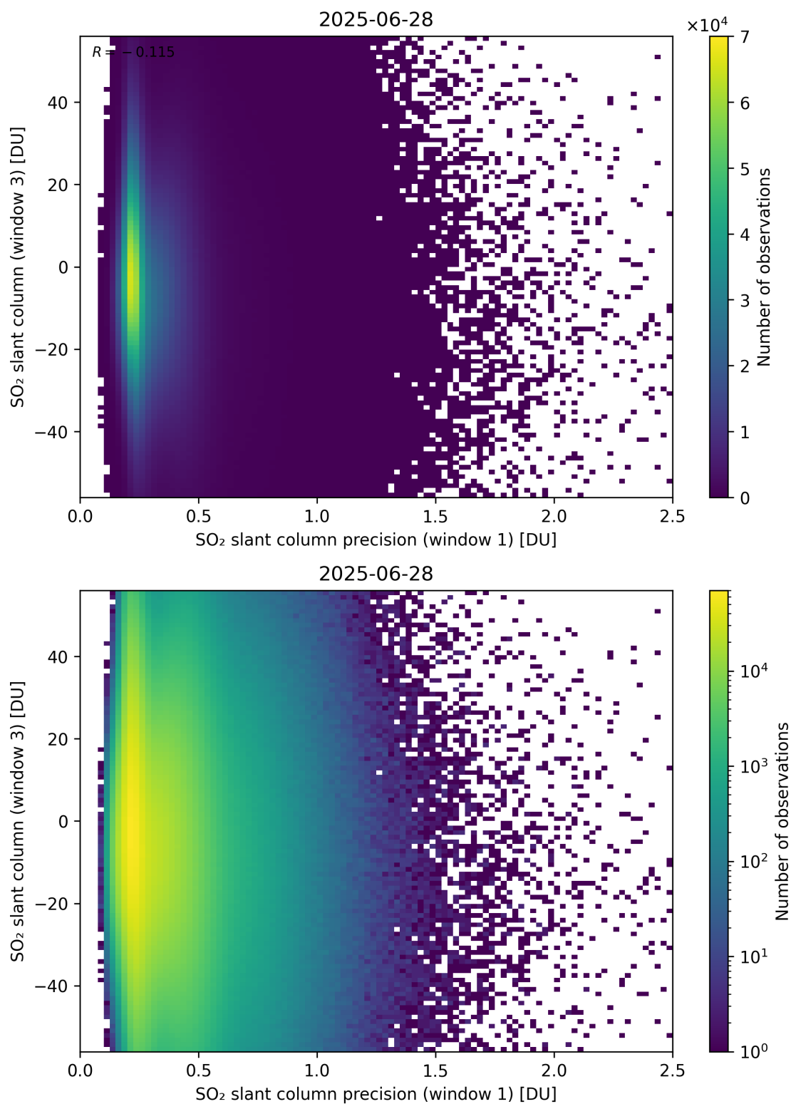
Figure 278: Scatter density plot of “SO 2 slant column precision (window 1)” against “SO 2 slant column (window 3)” for 2025-06-27 to 2025-06-29.
