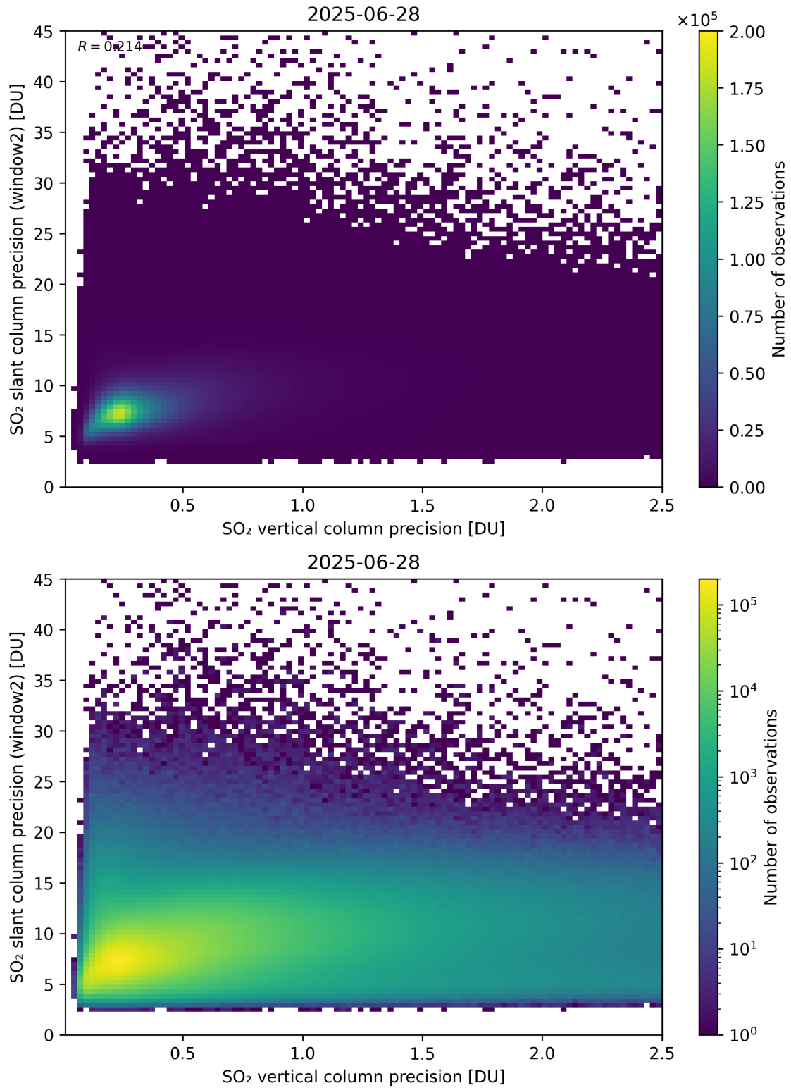
Figure 343: Scatter density plot of “SO 2 vertical column precision” against “SO 2 slant column precision (window2)” for 2025-06-27 to 2025-06-29.
