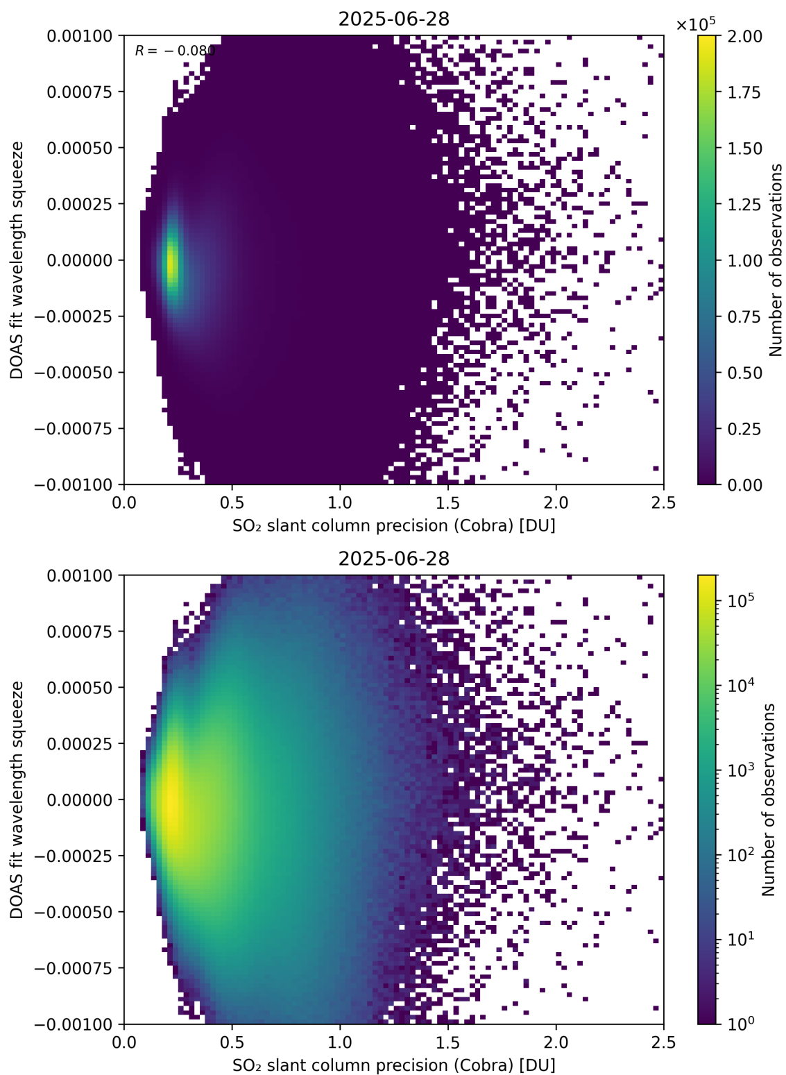
Figure 203: Scatter density plot of “SO 2 slant column precision (Cobra)” against “DOAS fit wavelength squeeze” for 2025-06-27 to 2025-06-29.
