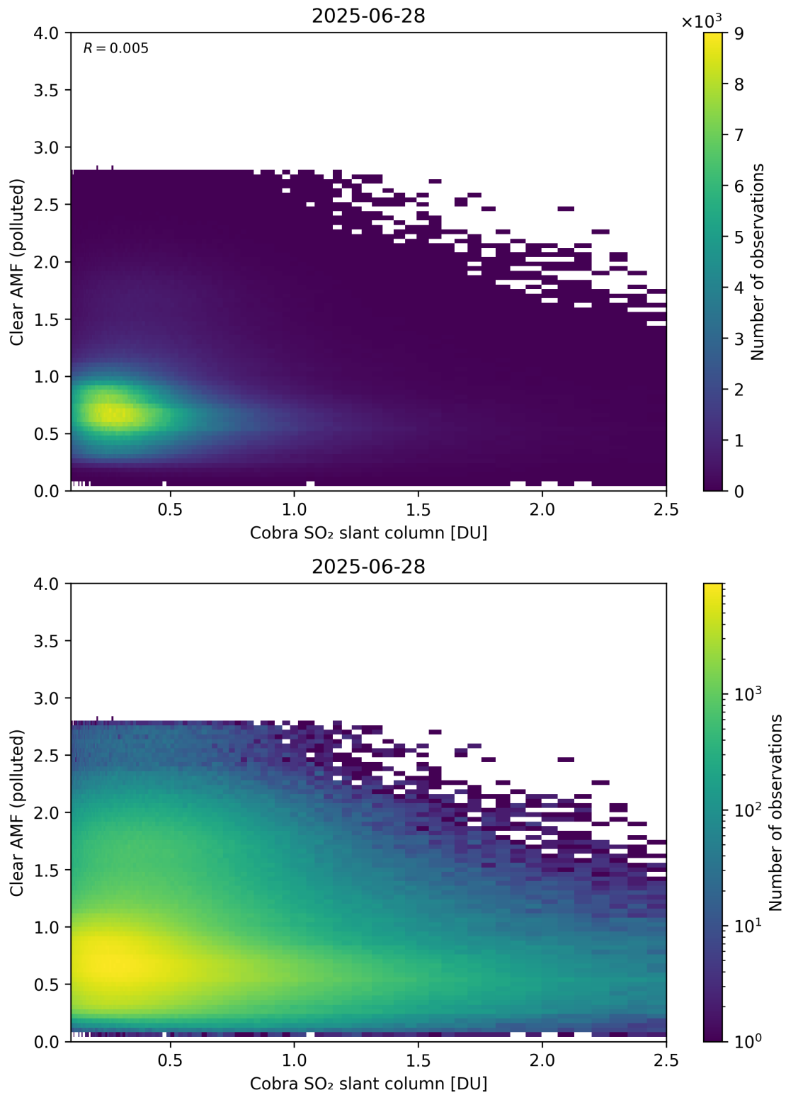
Figure 215: Scatter density plot of “Cobra SO 2 slant column” against “Clear AMF (polluted)” for 2025-06-27 to 2025-06-29.
