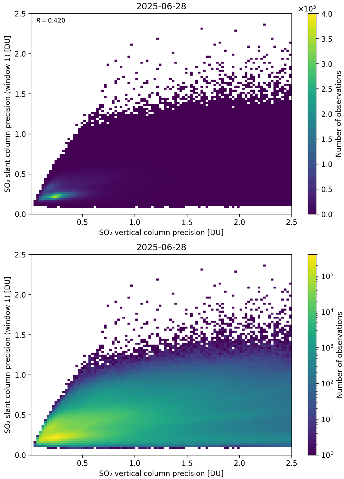
Figure 342: Scatter density plot of “SO 2 vertical column precision” against “SO 2 slant column precision (window 1)” for 2025-06-27 to 2025-06-29.
