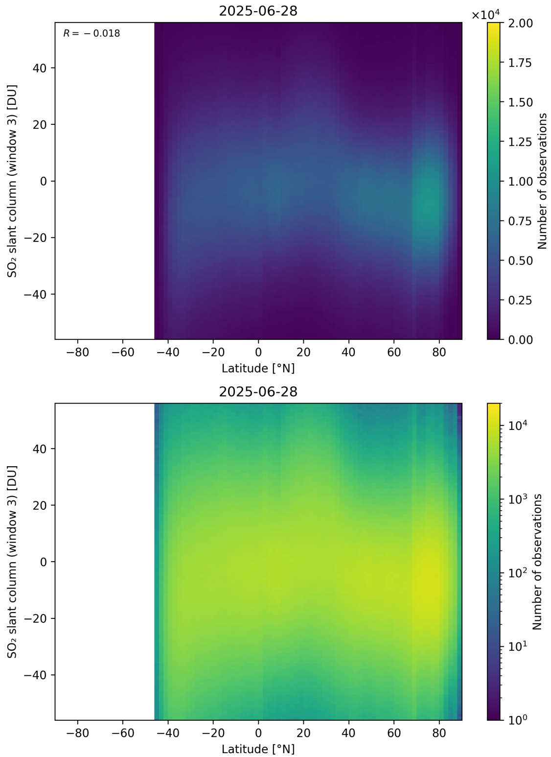
Figure 165: Scatter density plot of “Latitude” against “SO 2 slant column (window 3)” for 2025-06-27 to 2025-06-29.
