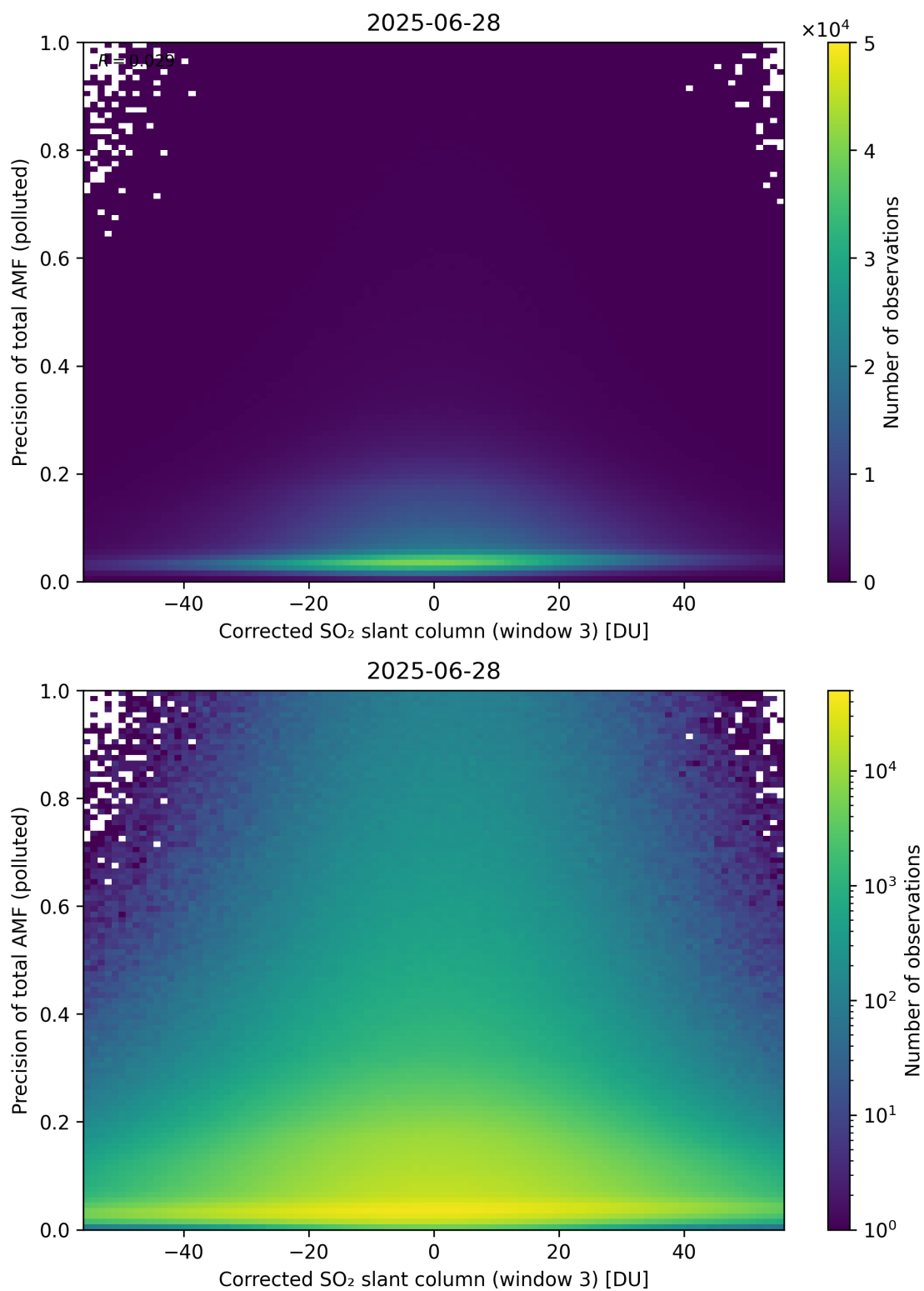
Figure 261: Scatter density plot of “Corrected SO 2 slant column (window 3)” against “Precision of total AMF (polluted)” for 2025-06-27 to 2025-06-29.
