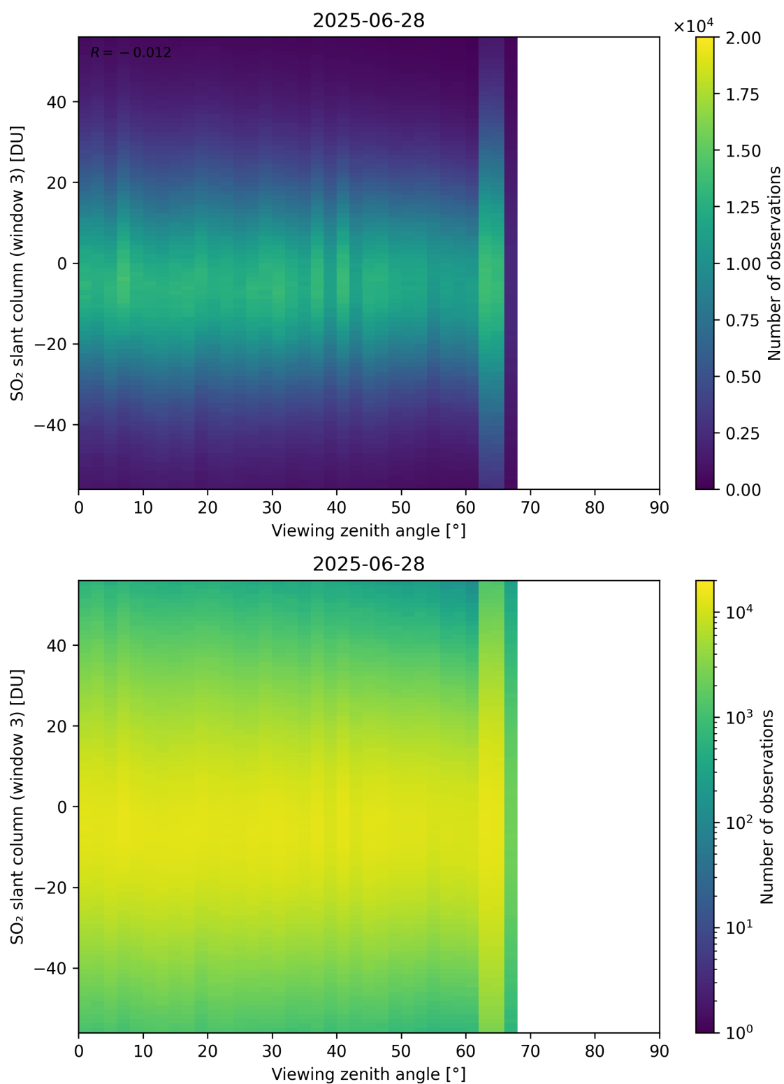
Figure 379: Scatter density plot of “Viewing zenith angle” against “SO 2 slant column (window 3)” for 2025-06-27 to 2025-06-29.
