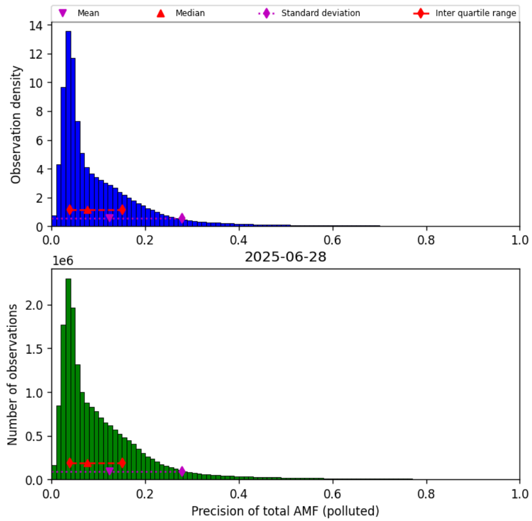
Figure 80: Histogram of “Precision of total AMF (polluted)” for 2025-06-27 to 2025-06-29
