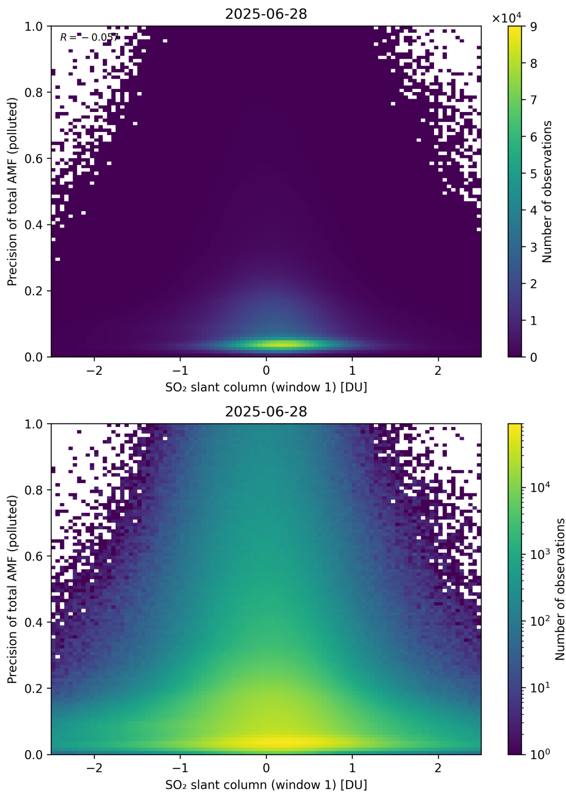
Figure 290: Scatter density plot of “SO 2 slant column (window 1)” against “Precision of total AMF (polluted)” for 2025-06-27 to 2025-06-29.
