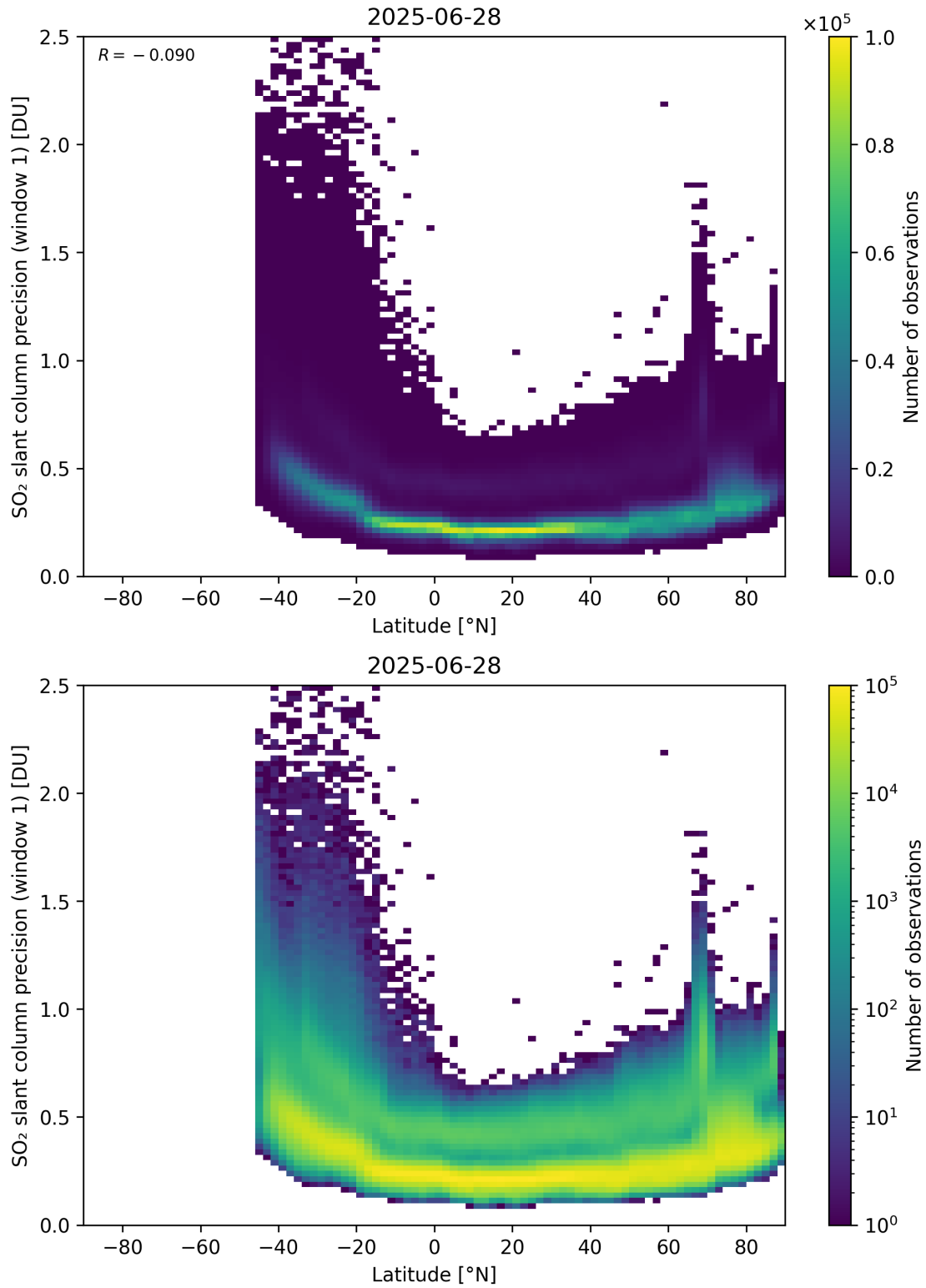
Figure 163: Scatter density plot of “Latitude” against “SO 2 slant column precision (window 1)” for 2025-06-27 to 2025-06-29.
