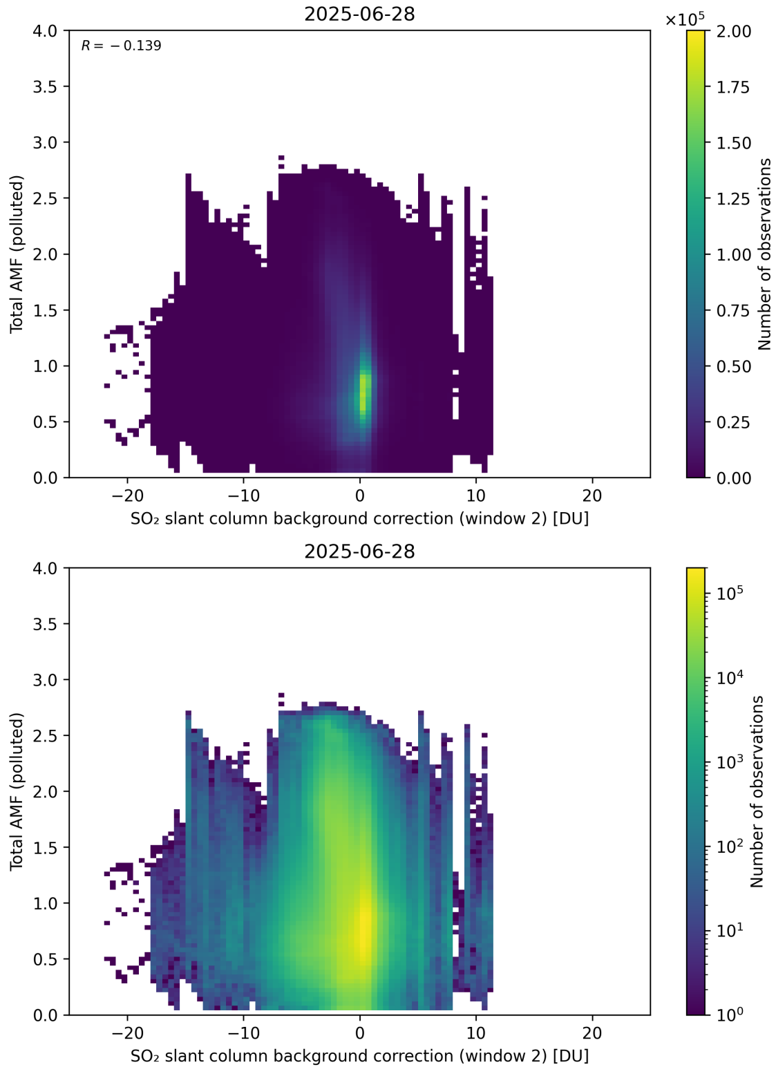
Figure 130: Scatter density plot of “SO 2 slant column background correction (window 2)” against “Total AMF (polluted)” for 2025-06-27 to 2025-06-29.
