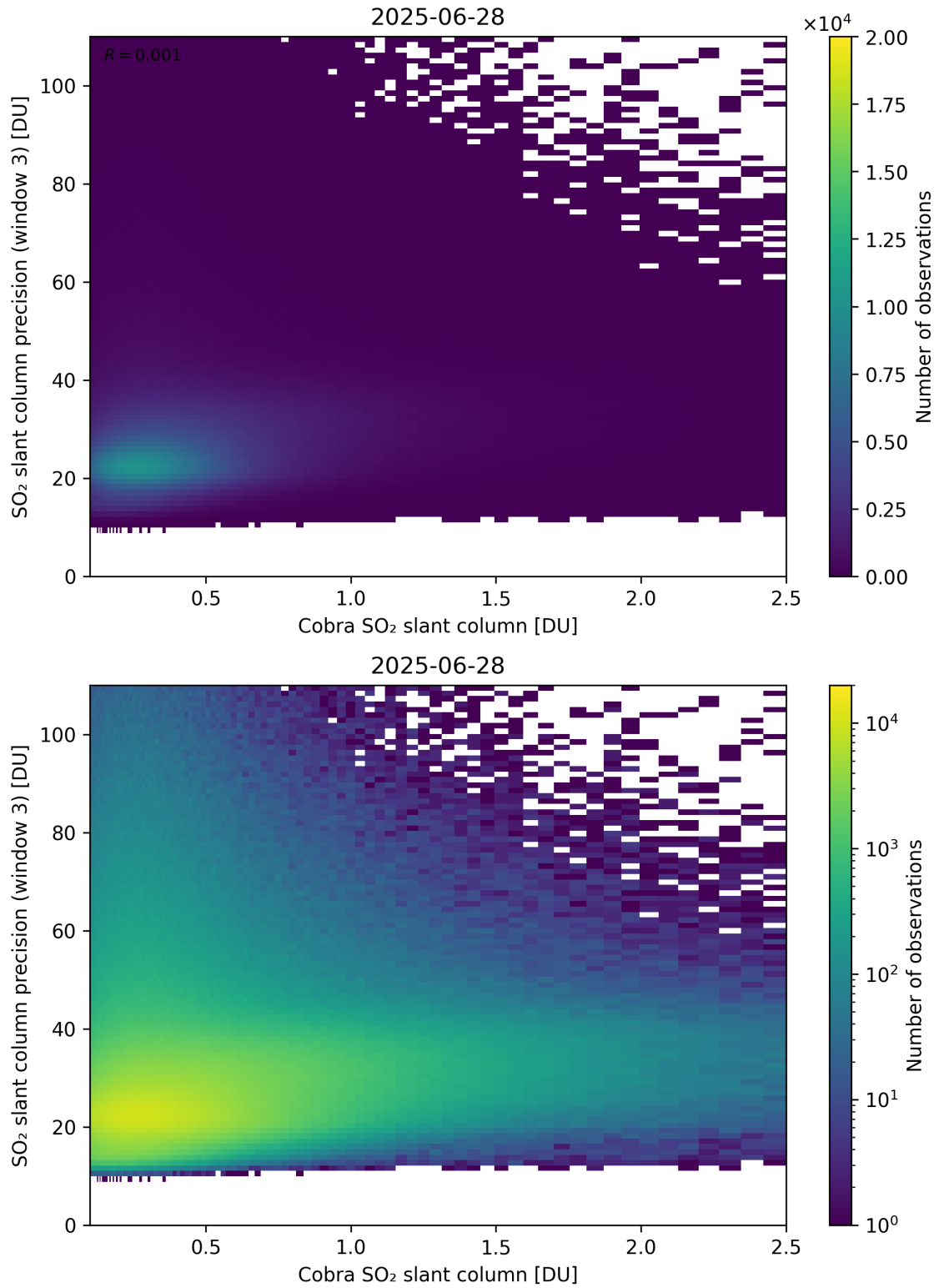
Figure 223: Scatter density plot of “Cobra SO 2 slant column” against “SO 2 slant column precision (window 3)” for 2025-06-27 to 2025-06-29.
