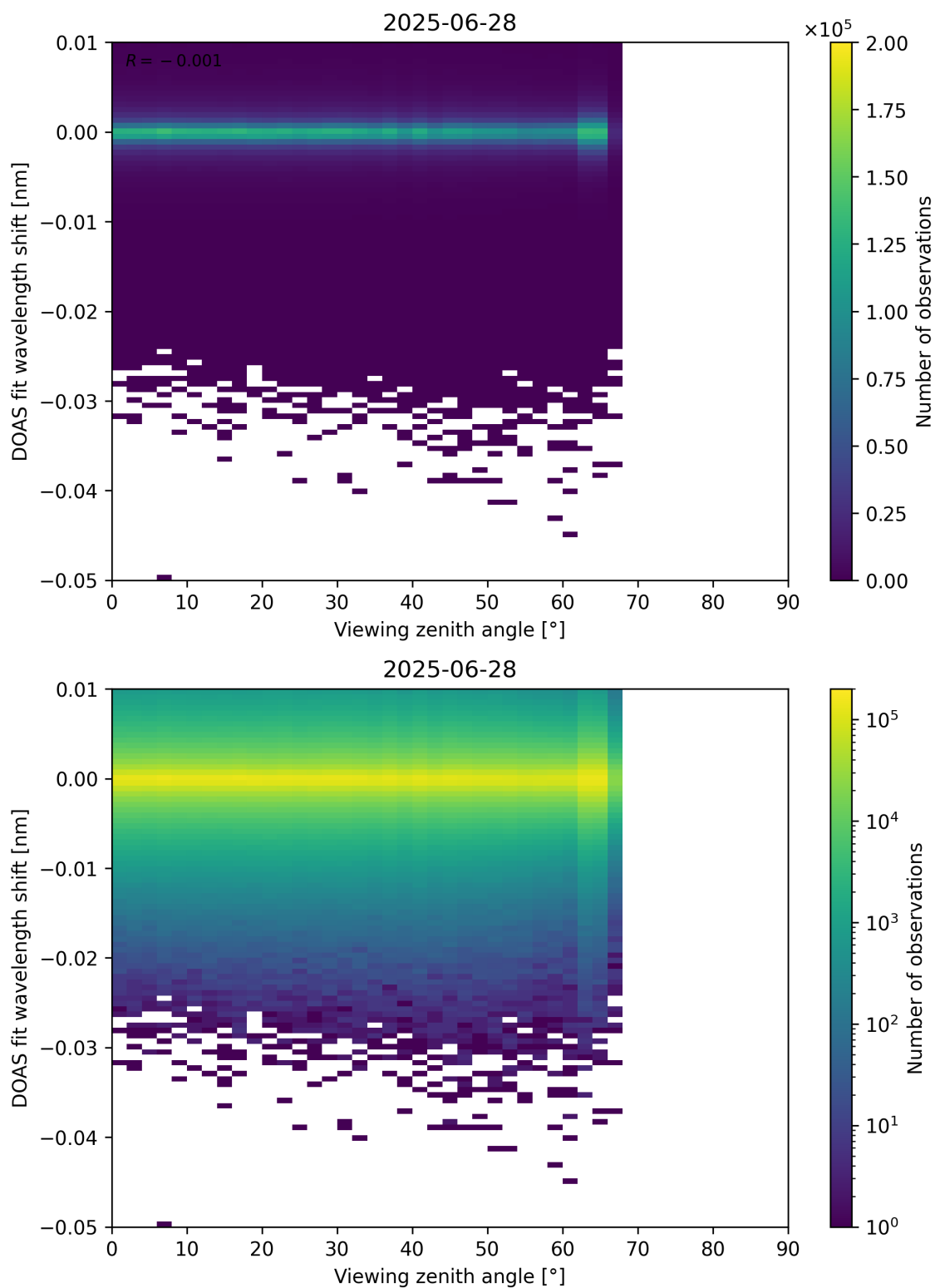
Figure 365: Scatter density plot of “Viewing zenith angle” against “DOAS fit wavelength shift” for 2025-06-27 to 2025-06-29.
