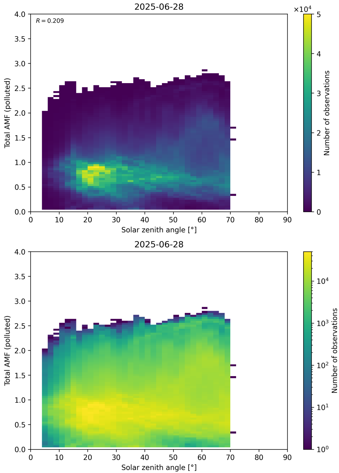
Figure 189: Scatter density plot of “Solar zenith angle” against “Total AMF (polluted)” for 2025-06-27 to 2025-06-29.
