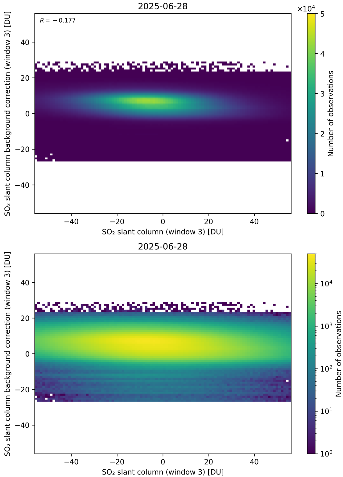
Figure 303: Scatter density plot of “SO 2 slant column (window 3)” against “SO 2 slant column background correction (window 3)” for 2025-06-27 to 2025-06-29.
