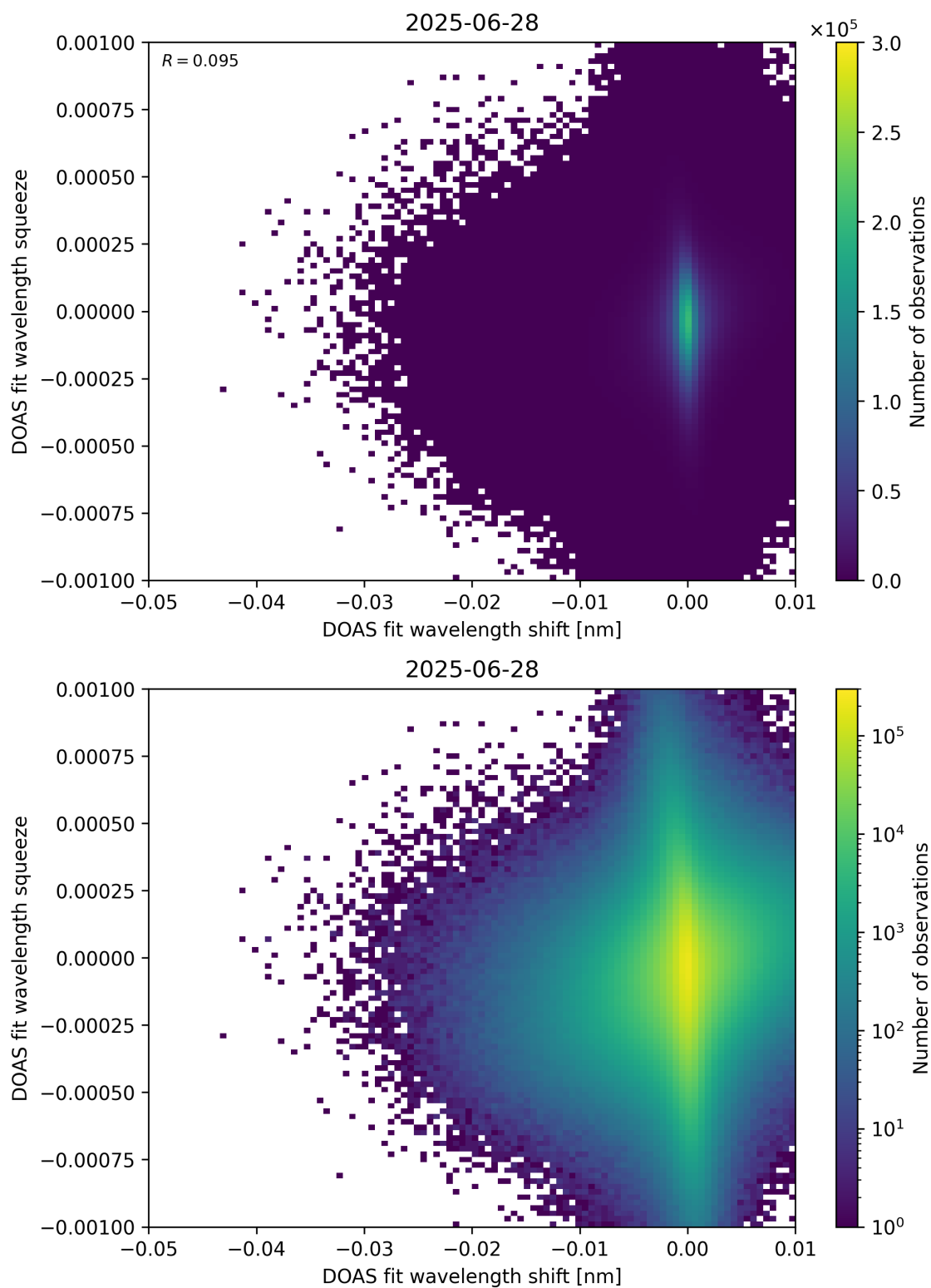
Figure 138: Scatter density plot of “DOAS fit wavelength shift” against “DOAS fit wavelength squeeze” for 2025-06-27 to 2025-06-29.
