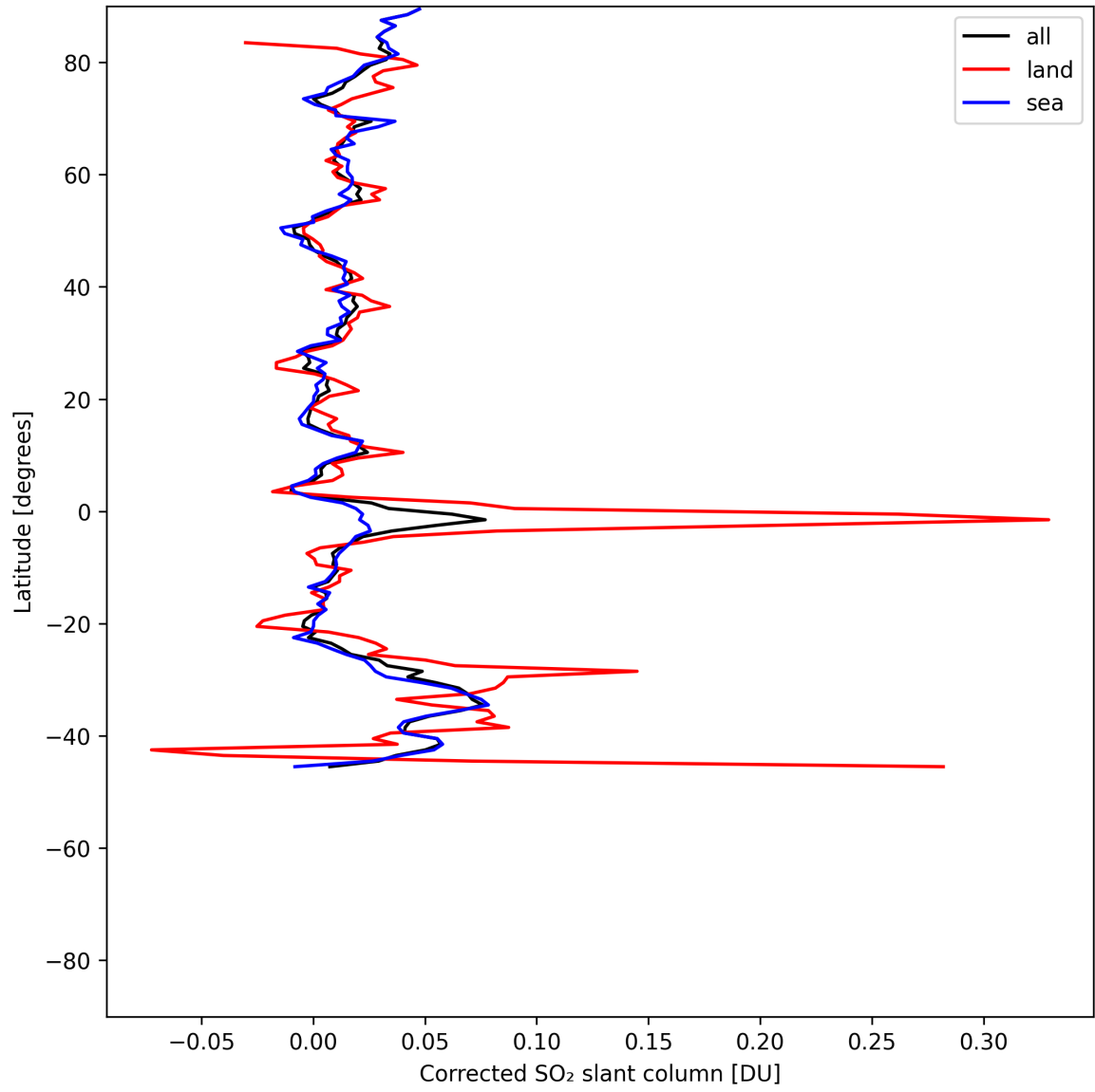
Figure 34: Zonal average of “Corrected SO 2 slant column” for 2025-06-27 to 2025-06-29.
