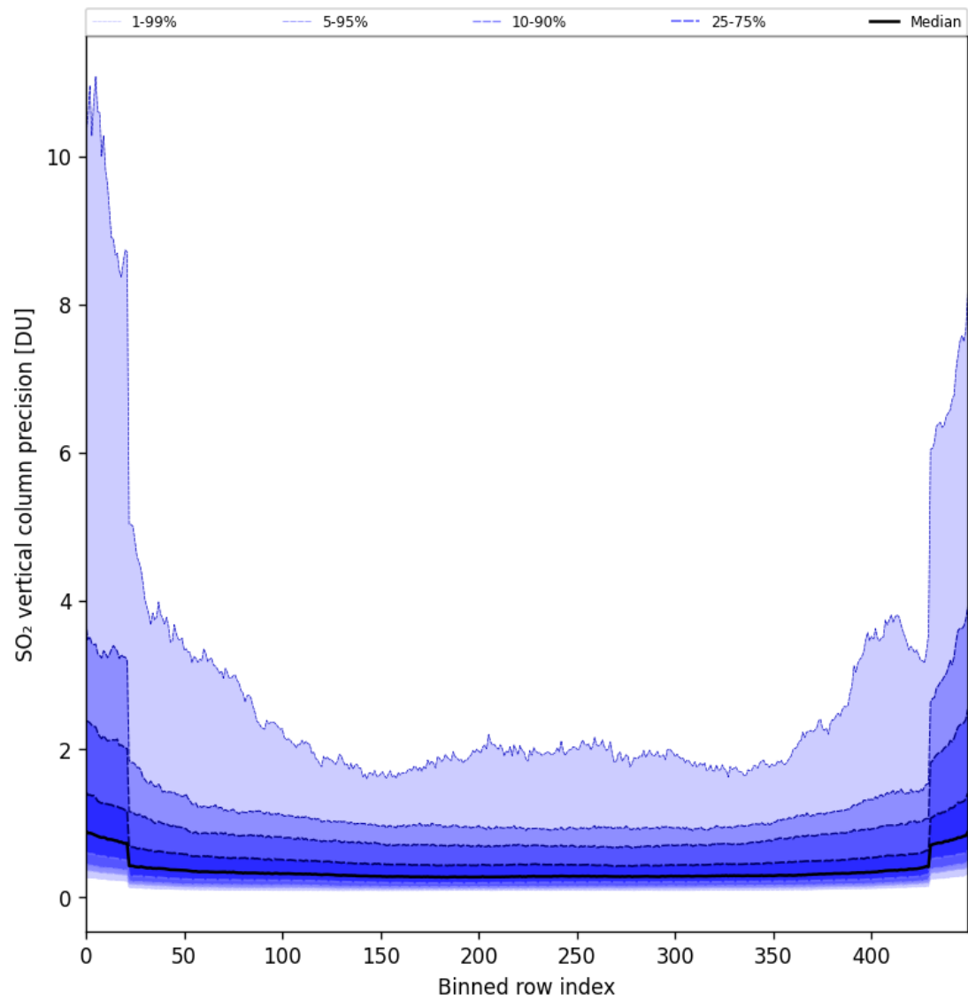
Figure 85: Along track statistics of “SO 2 vertical column precision” for 2025-06-27 to 2025-06-29
