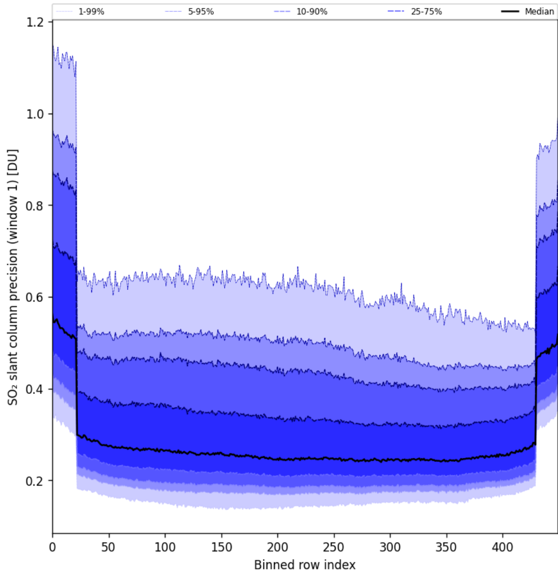
Figure 90: Along track statistics of “SO 2 slant column precision (window 1)” for 2025-06-27 to 2025-06-29
