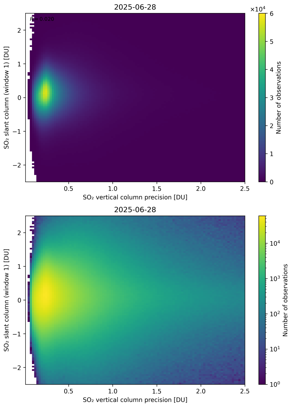
Figure 341: Scatter density plot of “SO 2 vertical column precision” against “SO 2 slant column (window 1)” for 2025-06-27 to 2025-06-29.
