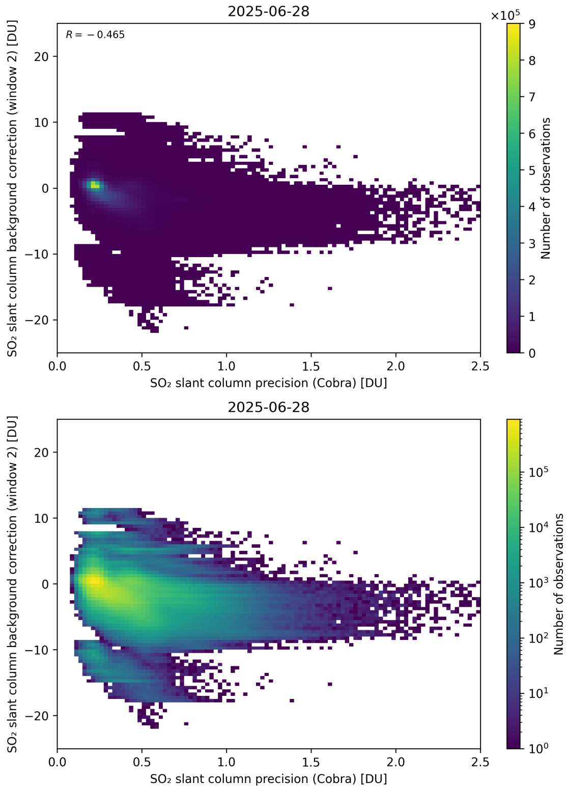
Figure 200: Scatter density plot of “SO 2 slant column precision (Cobra)” against “SO 2 slant column background correction (window 2)” for 2025-06-27 to 2025-06-29.
