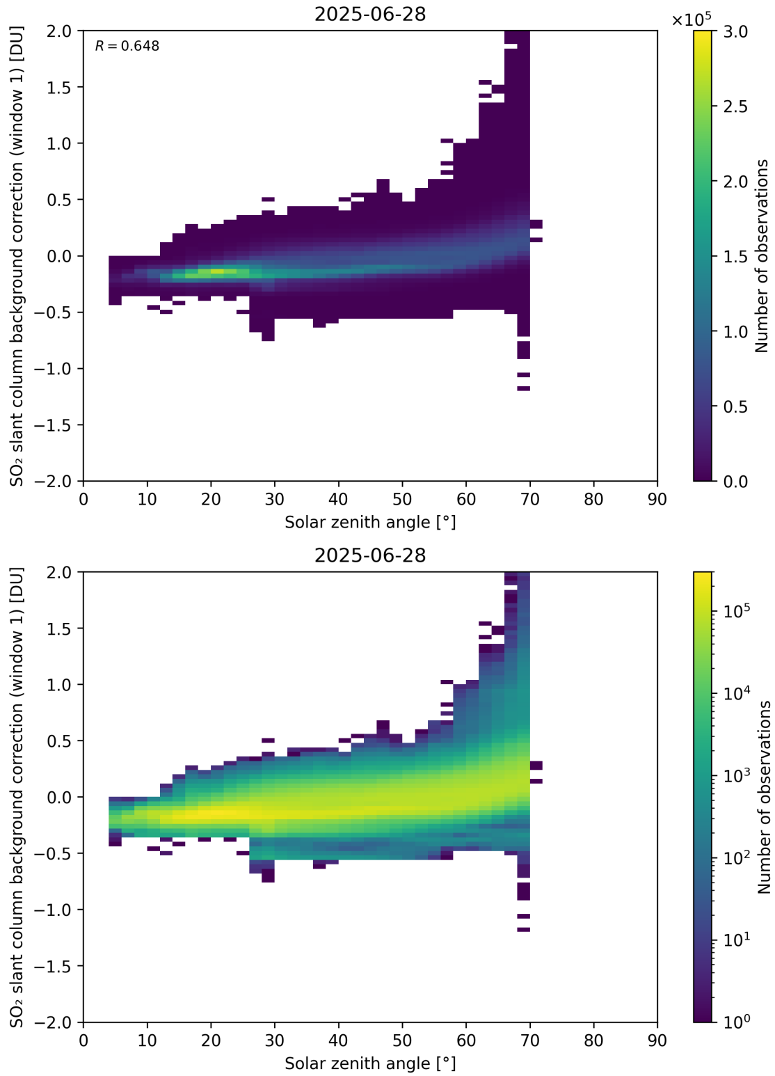
Figure 171: Scatter density plot of “Solar zenith angle” against “SO 2 slant column background correction (window 1)” for 2025-06-27 to 2025-06-29.
