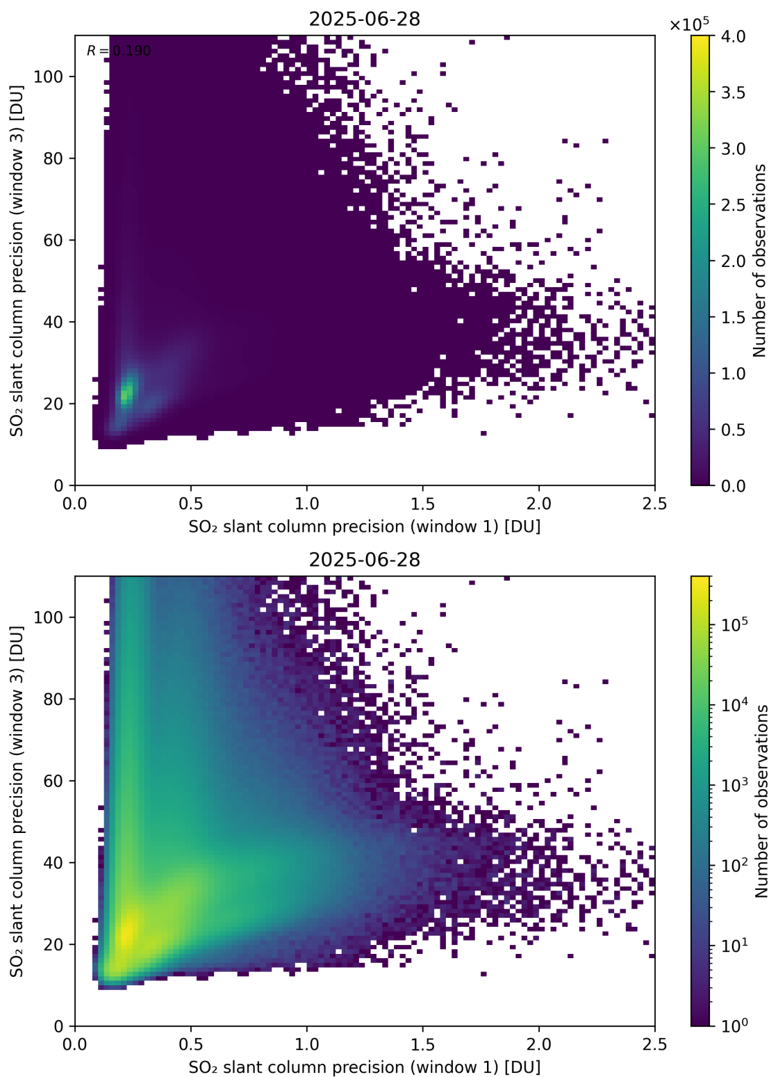
Figure 279: Scatter density plot of “SO 2 slant column precision (window 1)” against “SO 2 slant column precision (window 3)” for 2025-06-27 to 2025-06-29.
