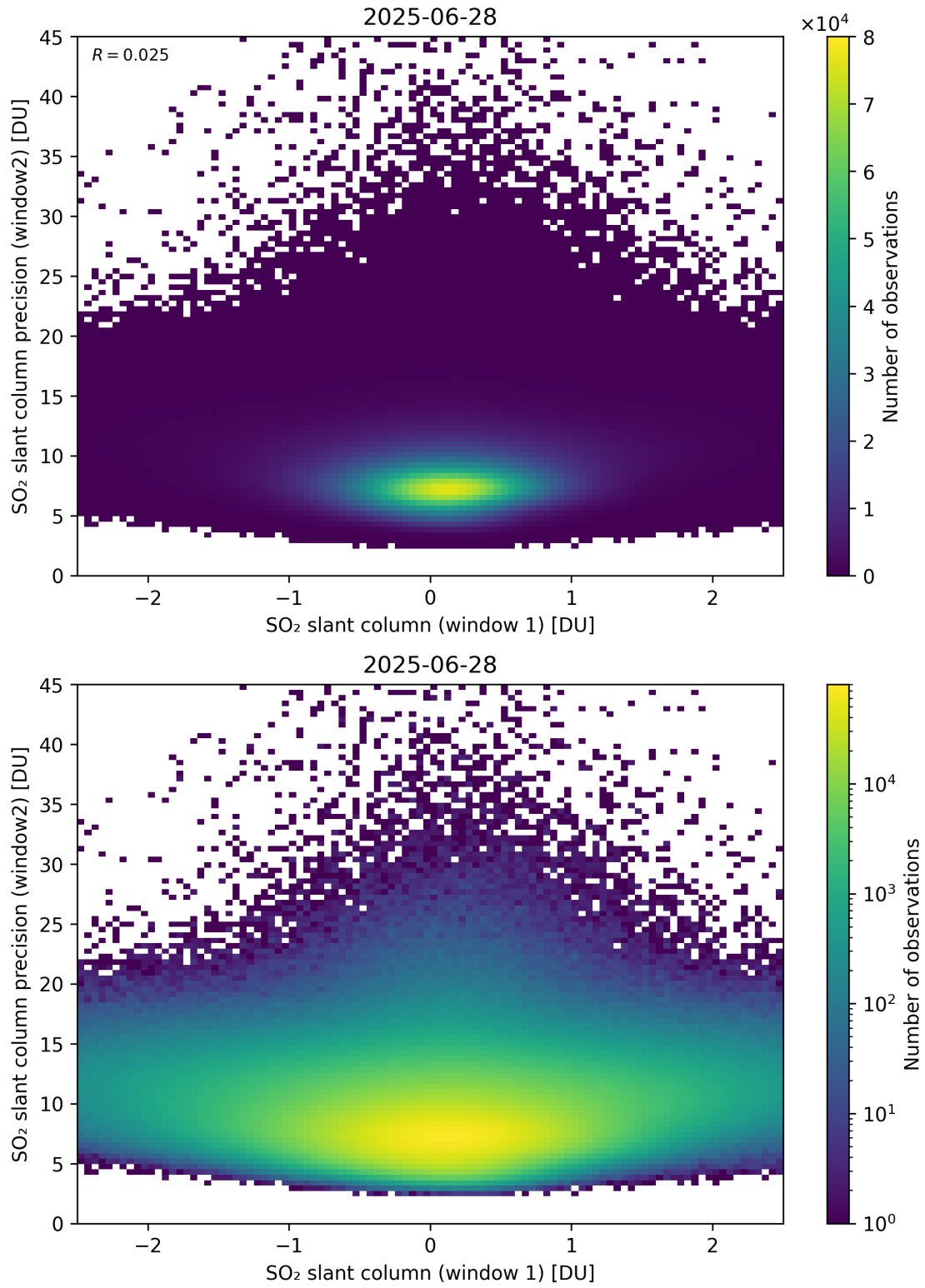
Figure 286: Scatter density plot of “SO 2 slant column (window 1)” against “SO 2 slant column precision (window2)” for 2025-06-27 to 2025-06-29.
