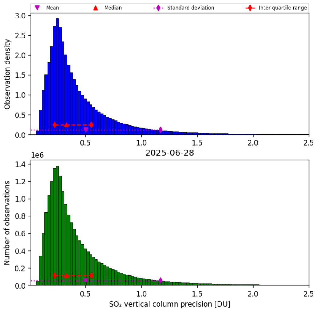
Figure 59: Histogram of “SO 2 vertical column precision” for 2025-06-27 to 2025-06-29
