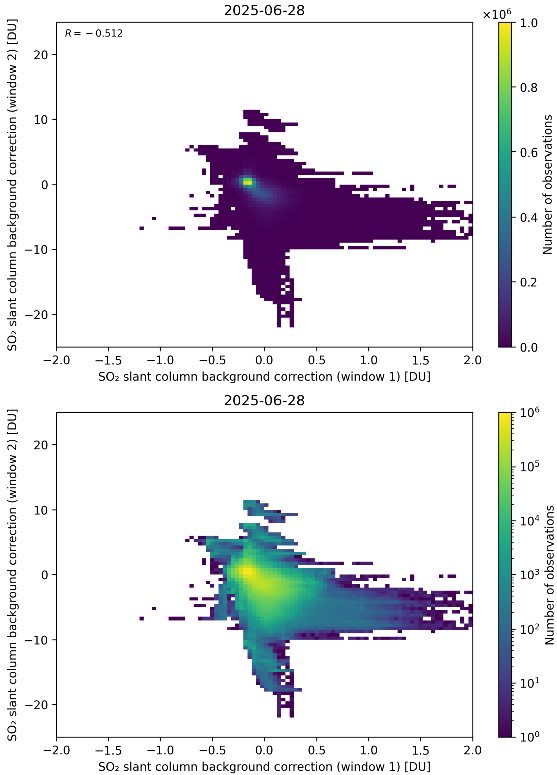
Figure 109: Scatter density plot of “SO 2 slant column background correction (window 1)” against “SO 2 slant column background correction (window 2)” for 2025-06-27 to 2025-06-29.
