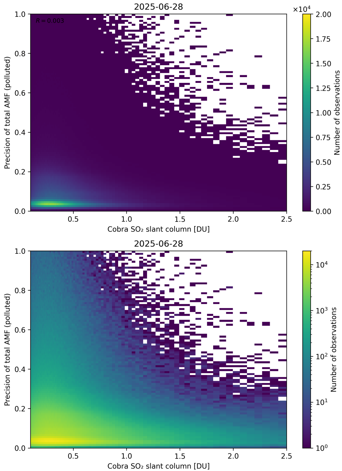
Figure 225: Scatter density plot of “Cobra SO 2 slant column” against “Precision of total AMF (polluted)” for 2025-06-27 to 2025-06-29.
