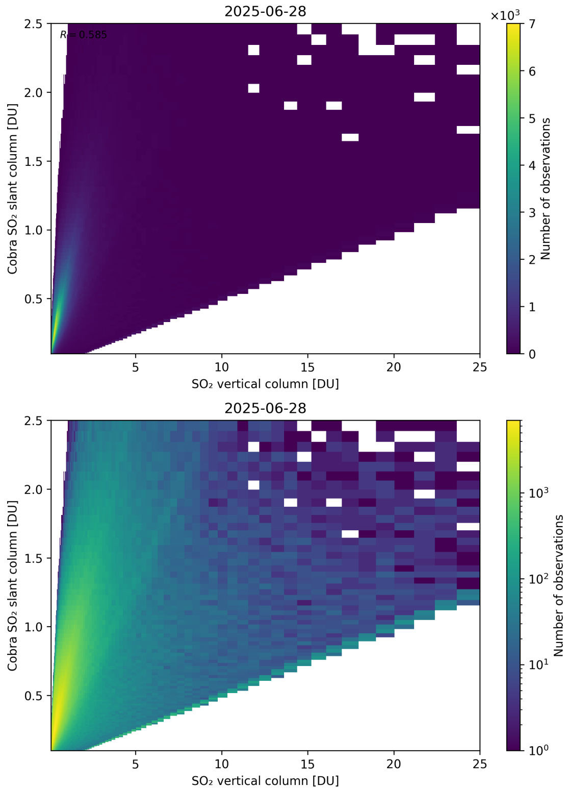
Figure 349: Scatter density plot of “SO 2 vertical column” against “Cobra SO 2 slant column” for 2025-06-27 to 2025-06-29.
