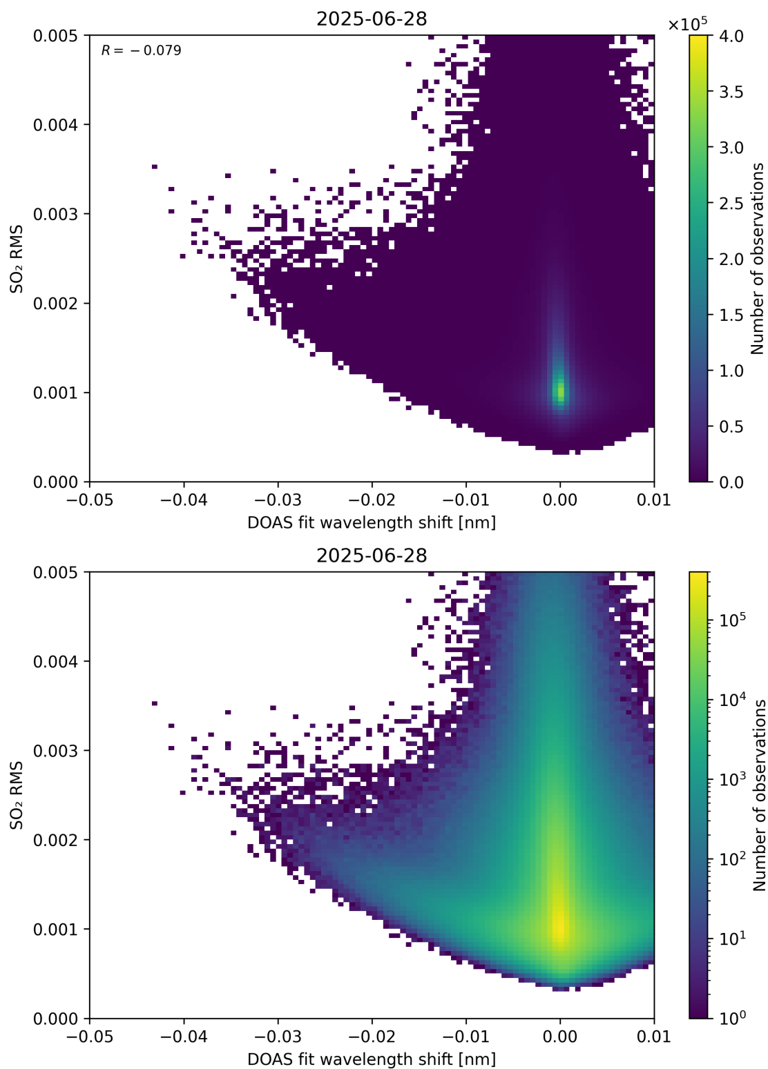
Figure 139: Scatter density plot of “DOAS fit wavelength shift” against “SO 2 RMS” for 2025-06-27 to 2025-06-29.
