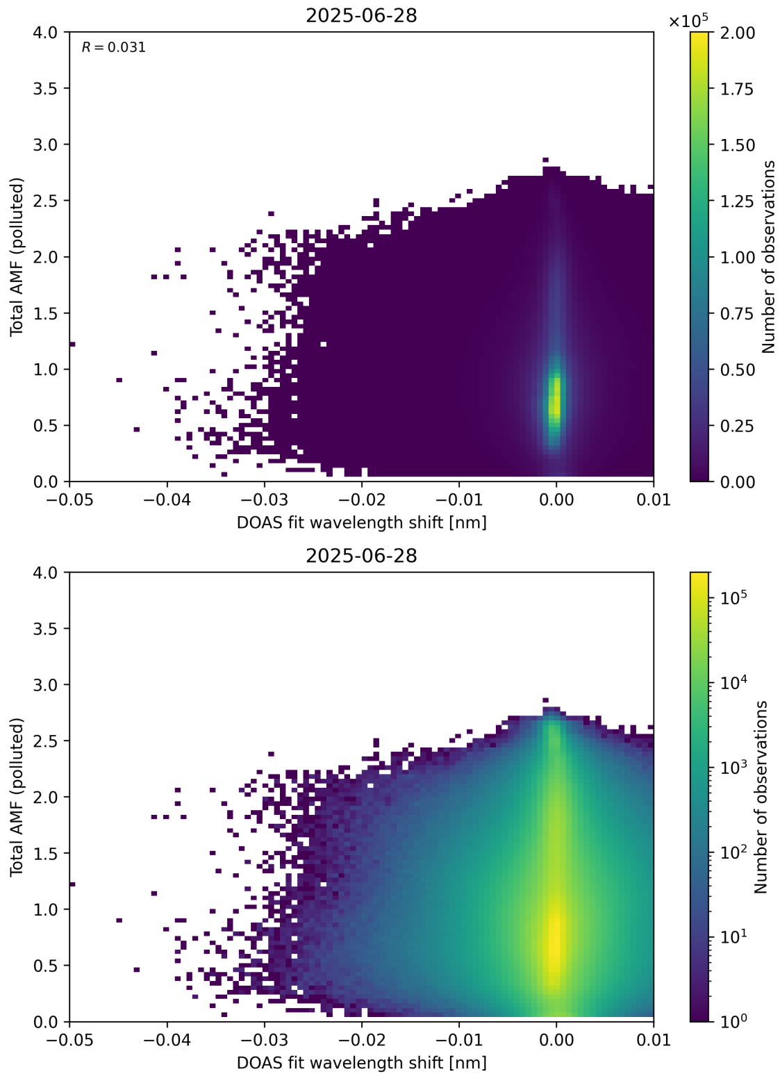
Figure 141: Scatter density plot of “DOAS fit wavelength shift” against “Total AMF (polluted)” for 2025-06-27 to 2025-06-29.
