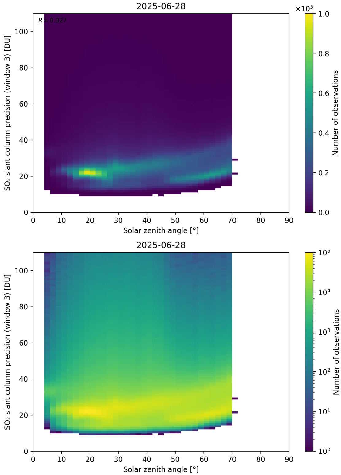
Figure 188: Scatter density plot of “Solar zenith angle” against “SO 2 slant column precision (window 3)” for 2025-06-27 to 2025-06-29.
