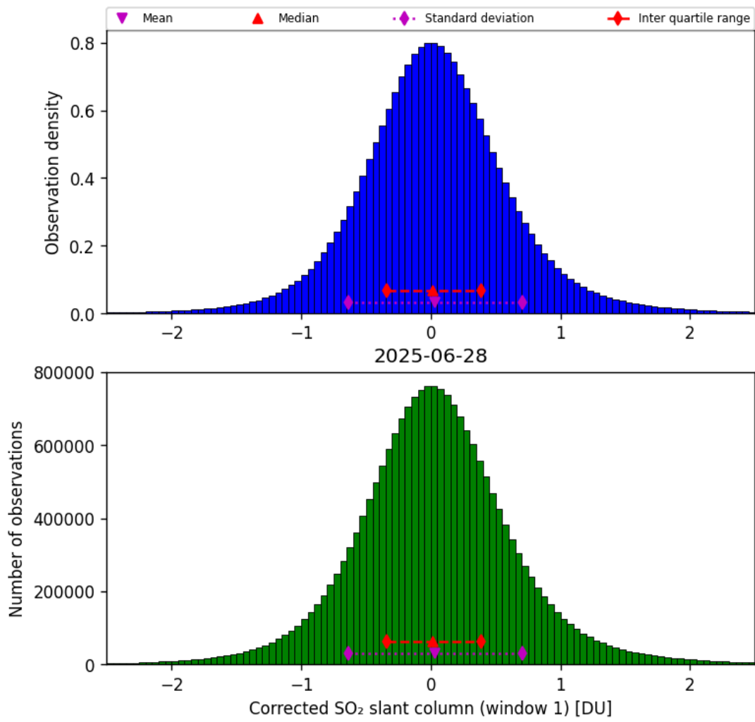
Figure 65: Histogram of “Corrected SO 2 slant column (window 1)” for 2025-06-27 to 2025-06-29
