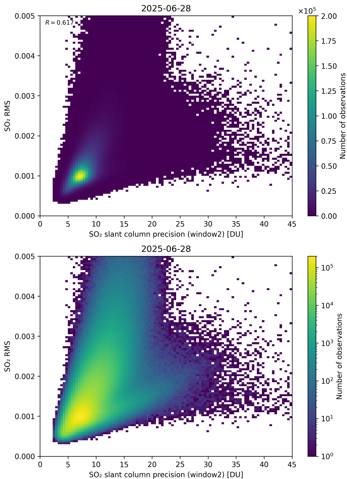
Figure 295: Scatter density plot of “SO 2 slant column precision (window2)” against “SO 2 RMS” for 2025-06-27 to 2025-06-29.
