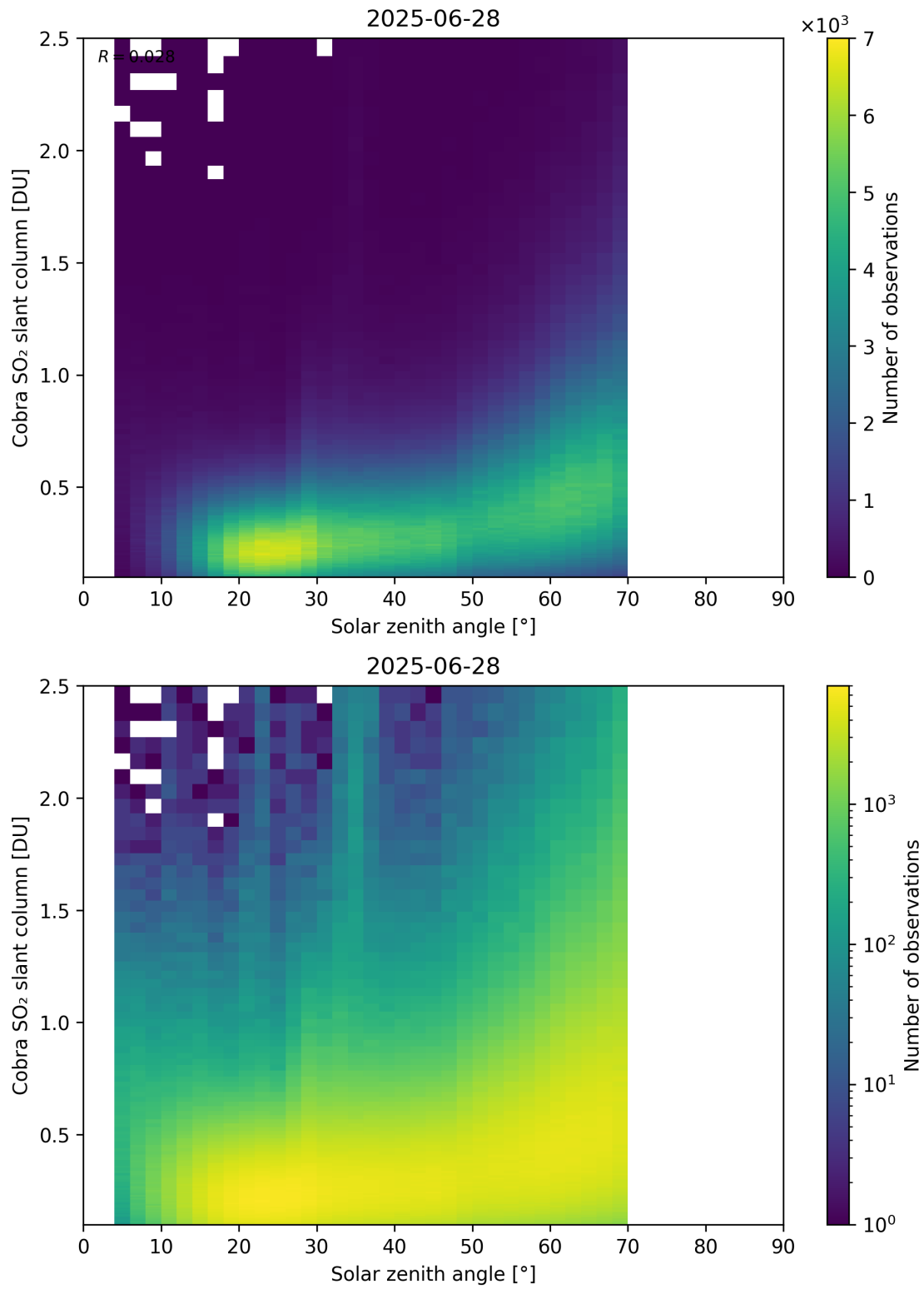
Figure 179: Scatter density plot of “Solar zenith angle” against “Cobra SO 2 slant column” for 2025-06-27 to 2025-06-29.
