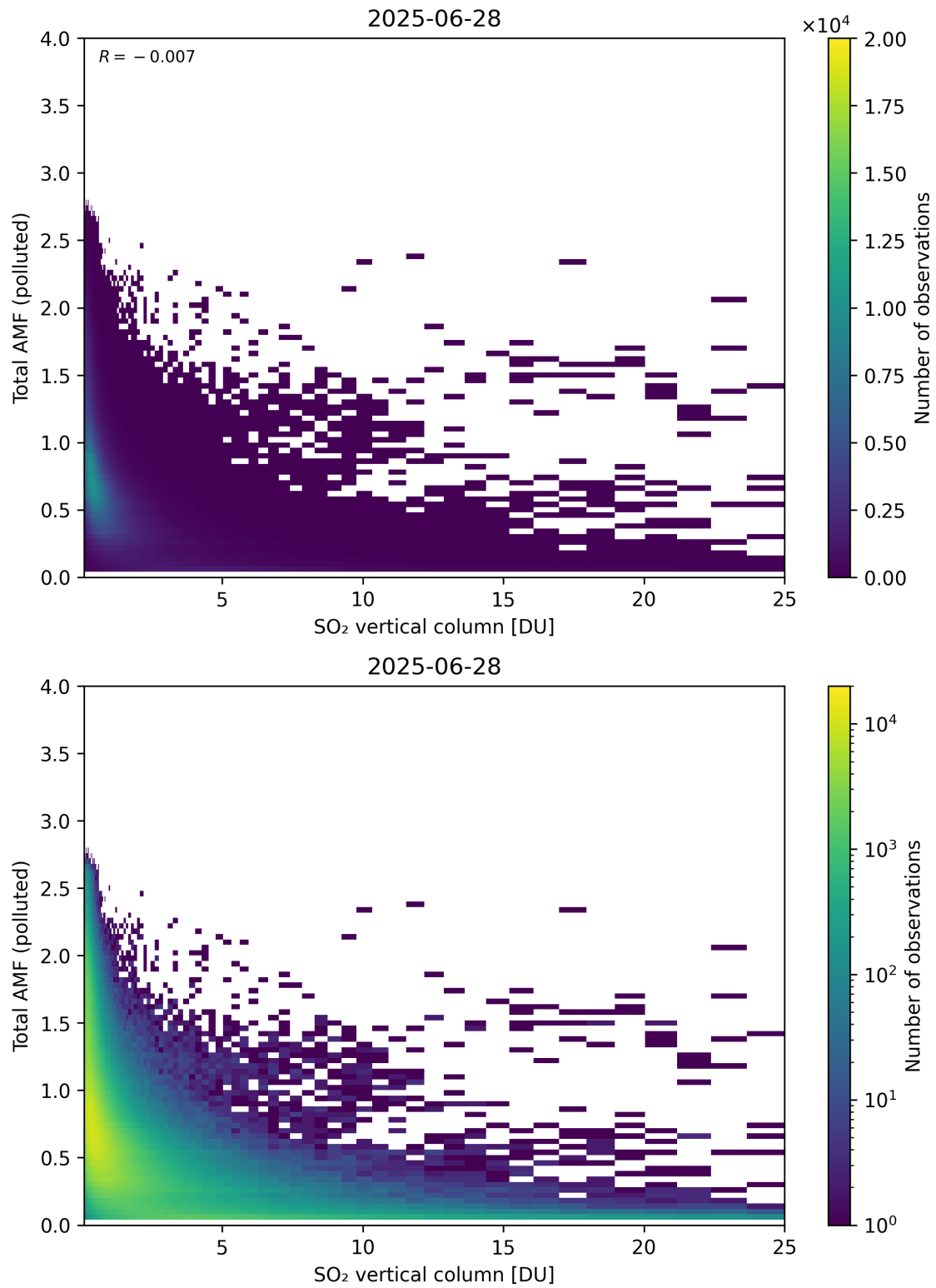
Figure 359: Scatter density plot of “SO 2 vertical column” against “Total AMF (polluted)” for 2025-06-27 to 2025-06-29.
