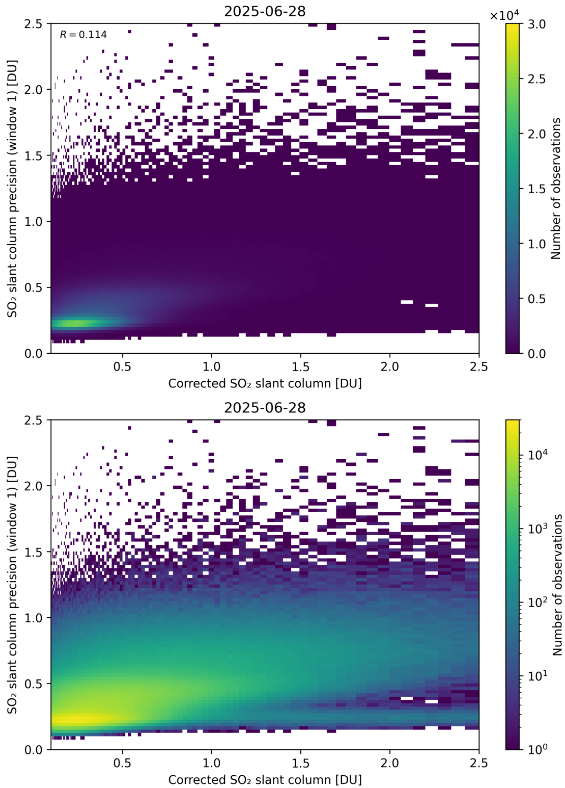
Figure 238: Scatter density plot of “Corrected SO 2 slant column” against “SO 2 slant column precision (window 1)” for 2025-06-27 to 2025-06-29.
