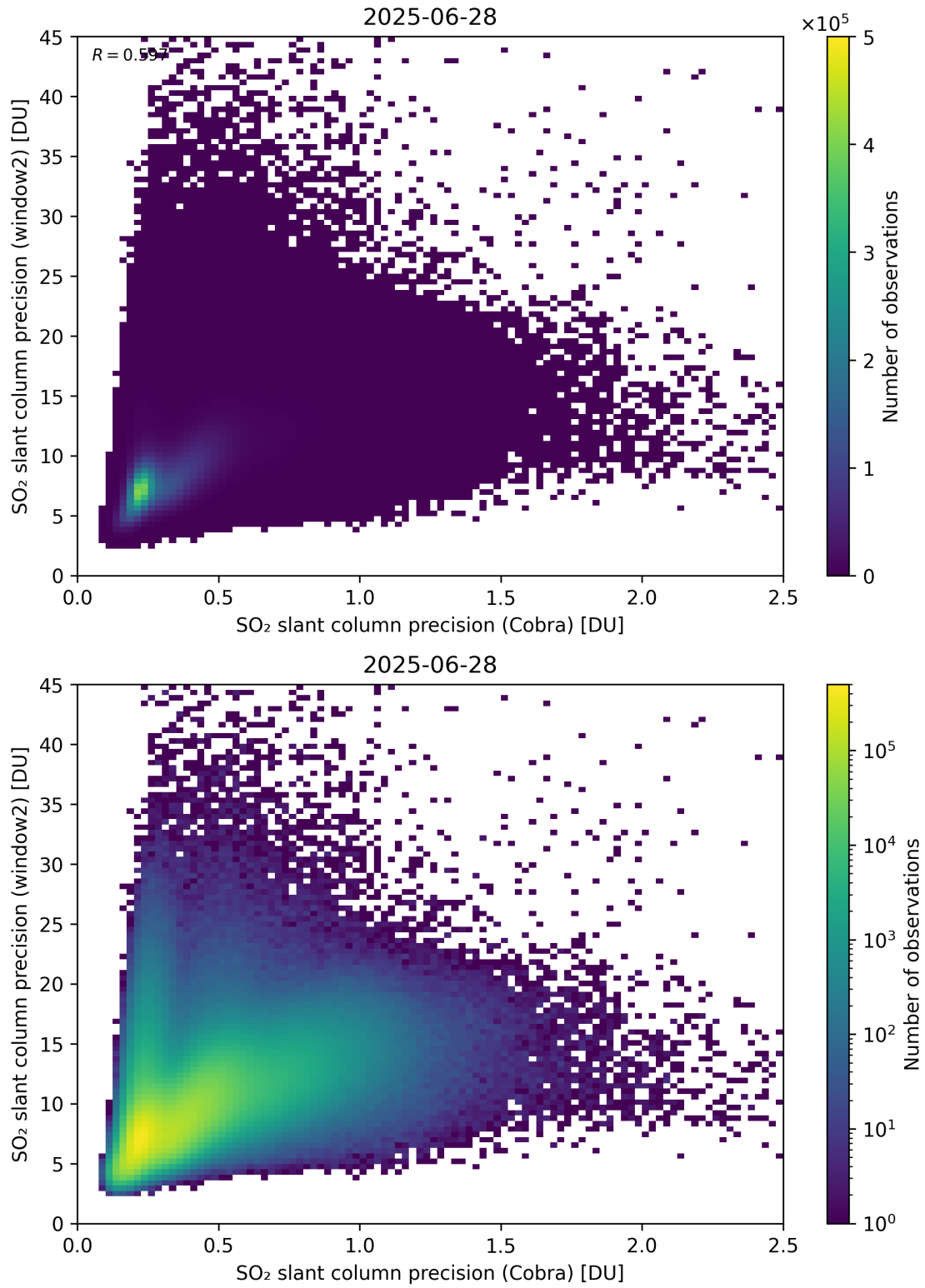
Figure 210: Scatter density plot of “SO 2 slant column precision (Cobra)” against “SO 2 slant column precision (window2)” for 2025-06-27 to 2025-06-29.
