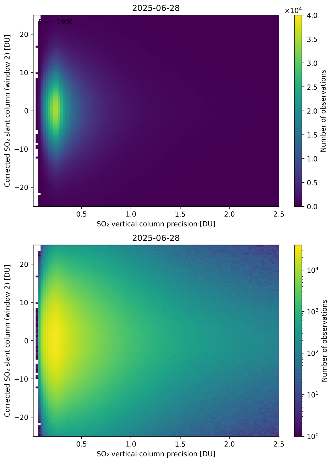
Figure 339: Scatter density plot of “SO 2 vertical column precision” against “Corrected SO 2 slant column (window 2)” for 2025-06-27 to 2025-06-29.
