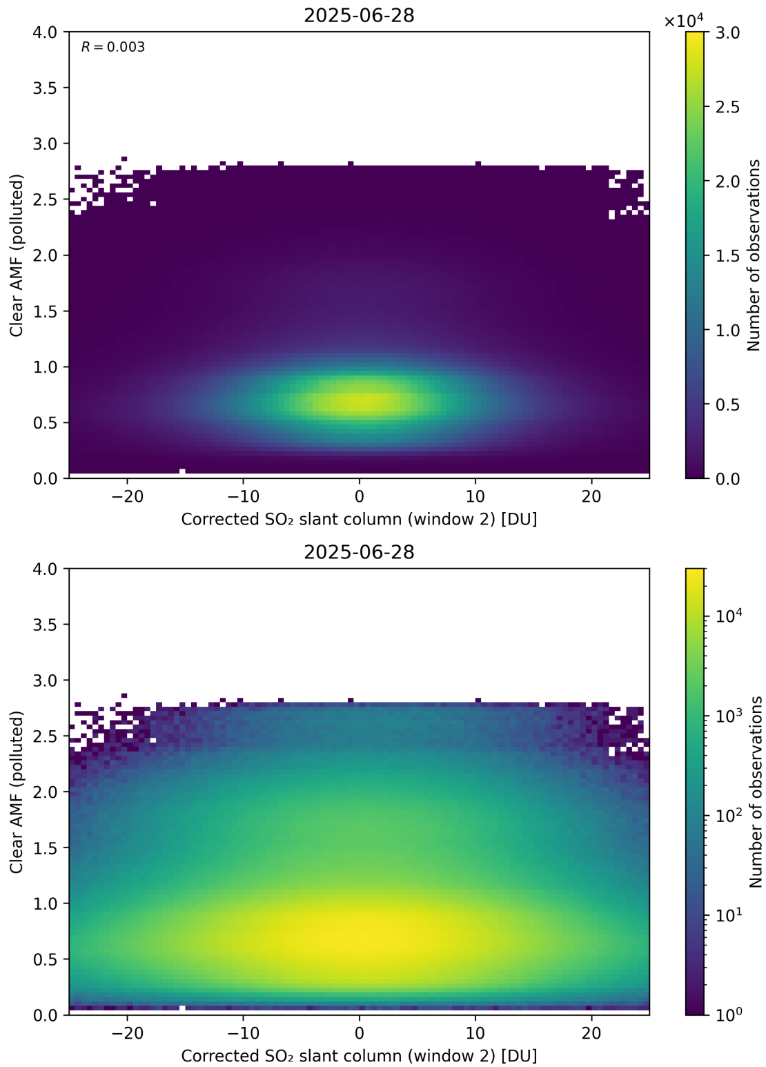
Figure 249: Scatter density plot of “Corrected SO 2 slant column (window 2)” against “Clear AMF (polluted)” for 2025-06-27 to 2025-06-29.
