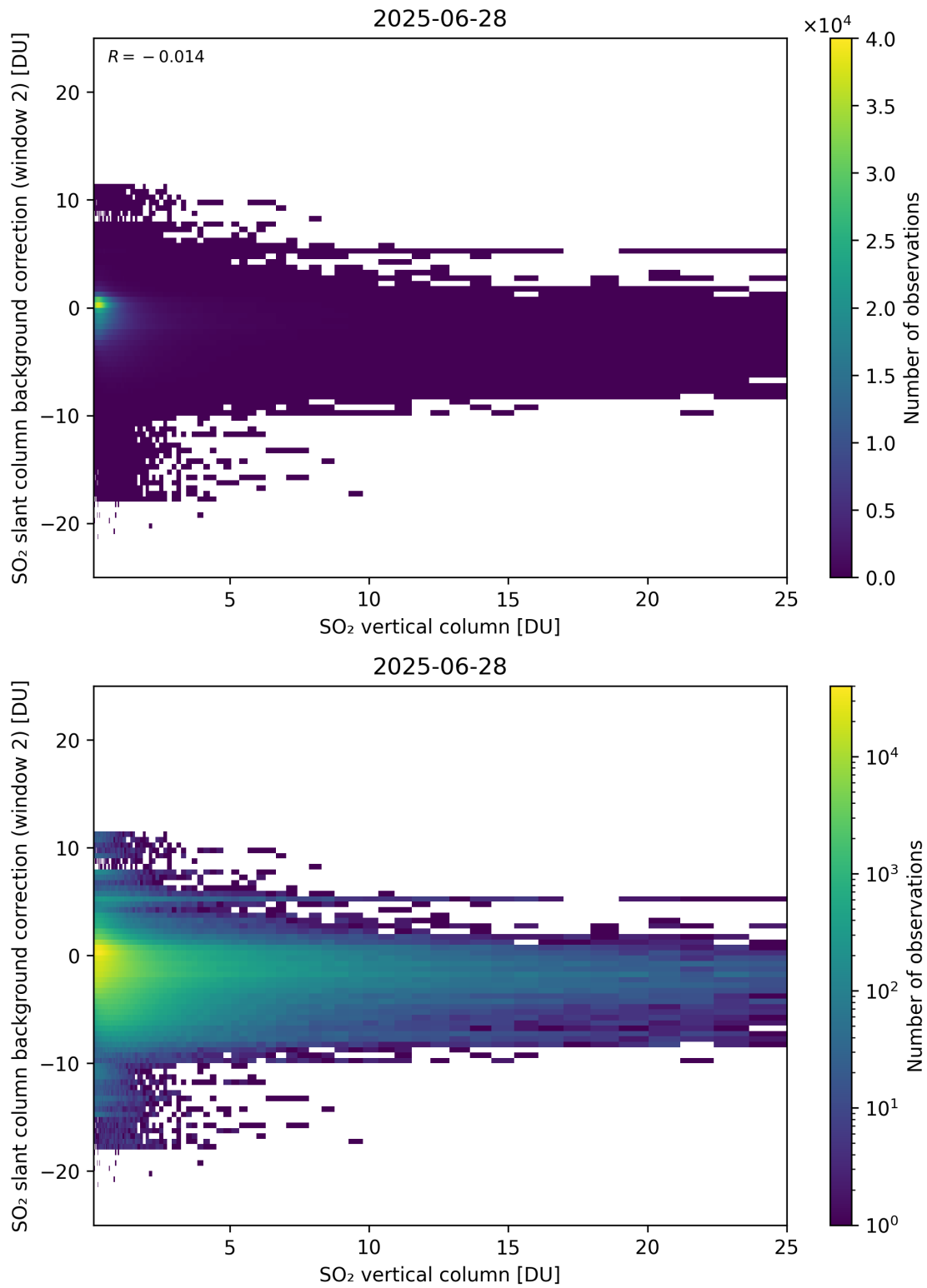
Figure 324: Scatter density plot of “SO 2 vertical column” against “SO 2 slant column background correction (window 2)” for 2025-06-27 to 2025-06-29.
