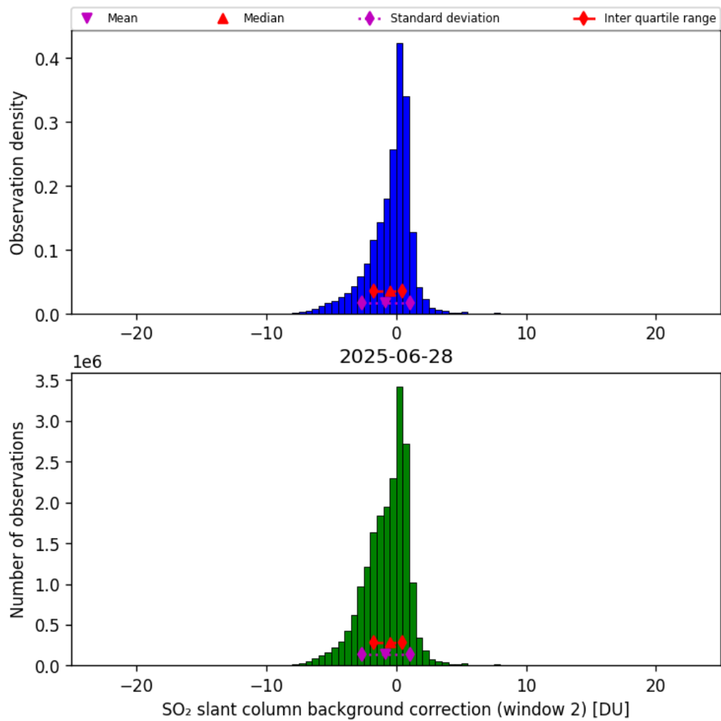
Figure 70: Histogram of “SO 2 slant column background correction (window 2)” for 2025-06-27 to 2025-06-29
