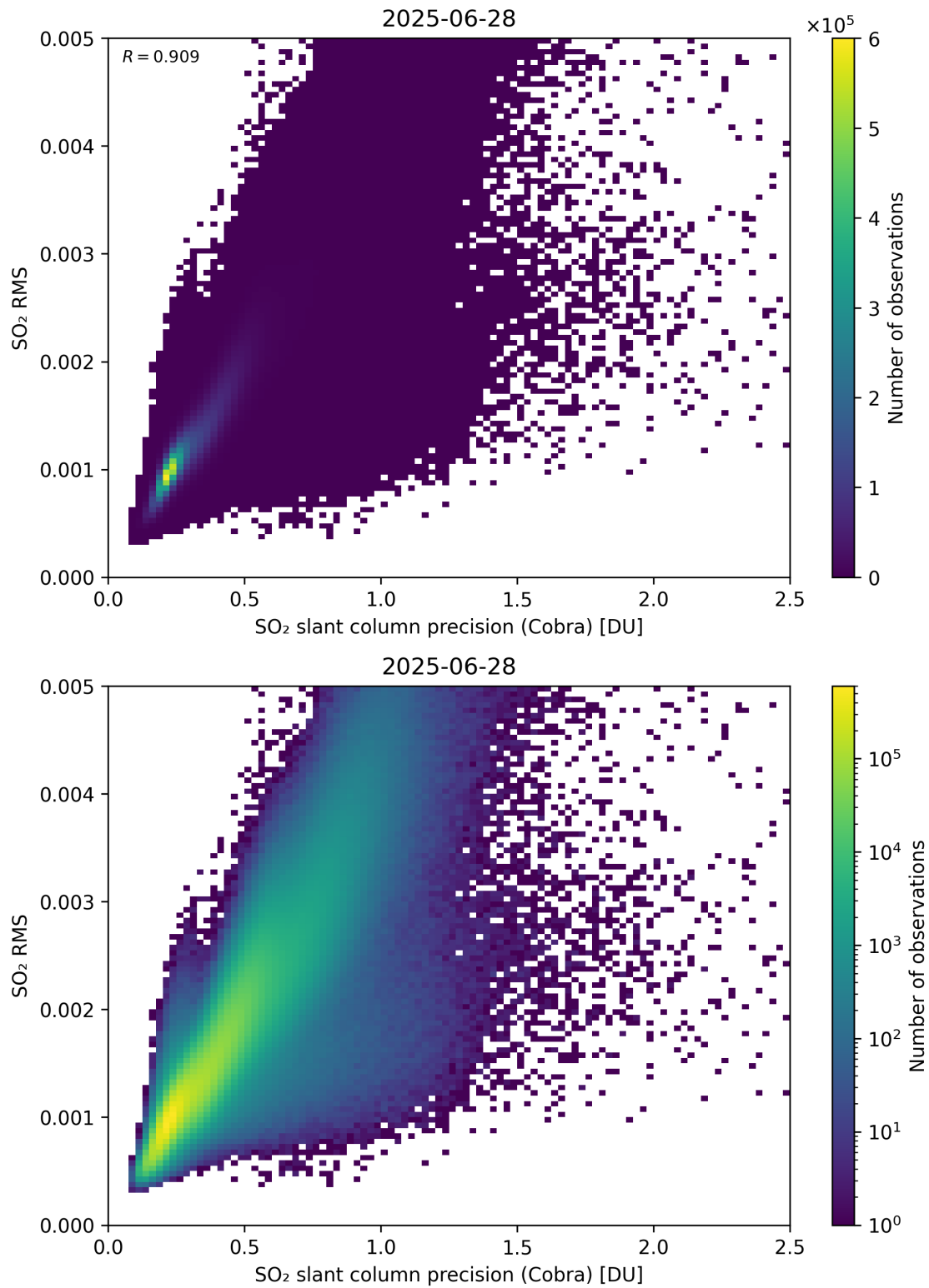
Figure 204: Scatter density plot of “SO 2 slant column precision (Cobra)” against “SO 2 RMS” for 2025-06-27 to 2025-06-29.
