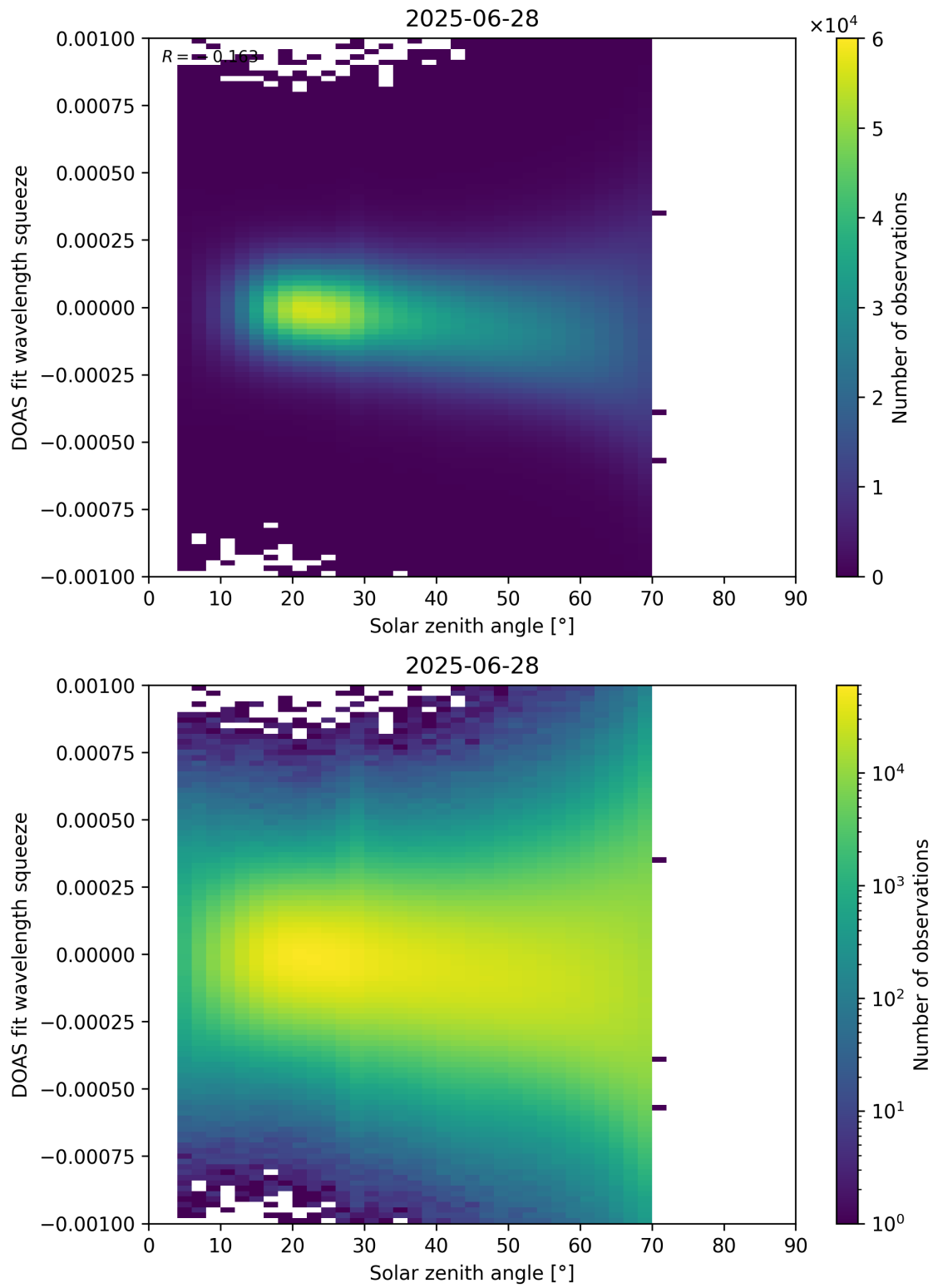
Figure 175: Scatter density plot of “Solar zenith angle” against “DOAS fit wavelength squeeze” for 2025-06-27 to 2025-06-29.
