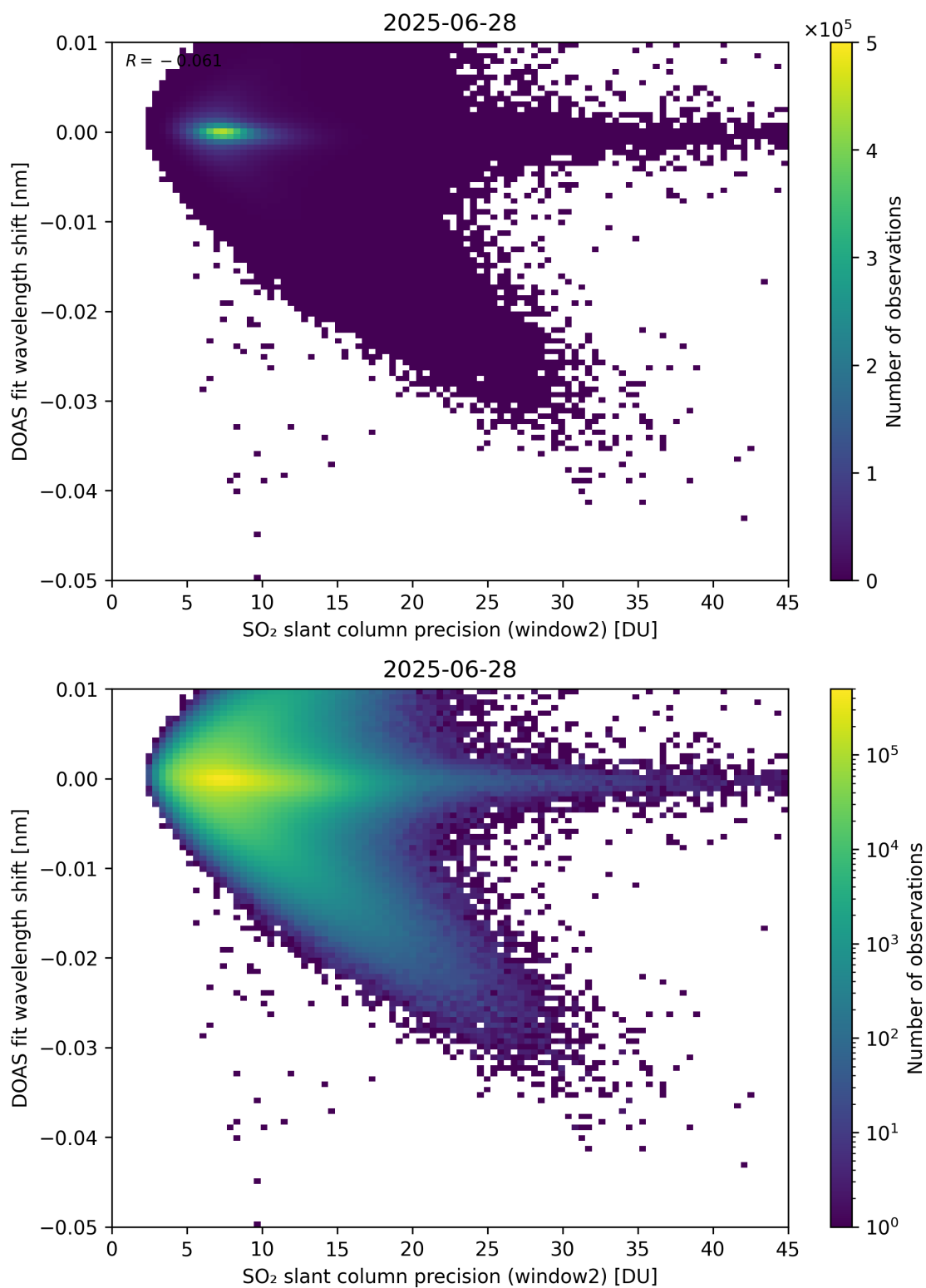
Figure 293: Scatter density plot of “SO 2 slant column precision (window2)” against “DOAS fit wavelength shift” for 2025-06-27 to 2025-06-29.
