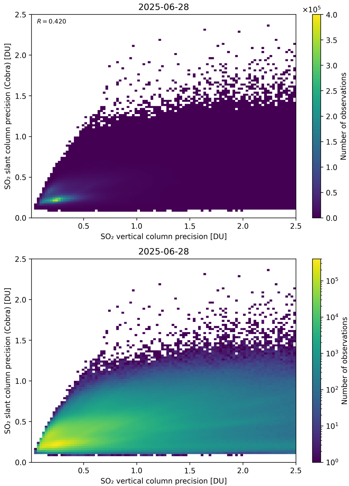
Figure 337: Scatter density plot of “SO 2 vertical column precision” against “SO 2 slant column precision (Cobra)” for 2025-06-27 to 2025-06-29.
