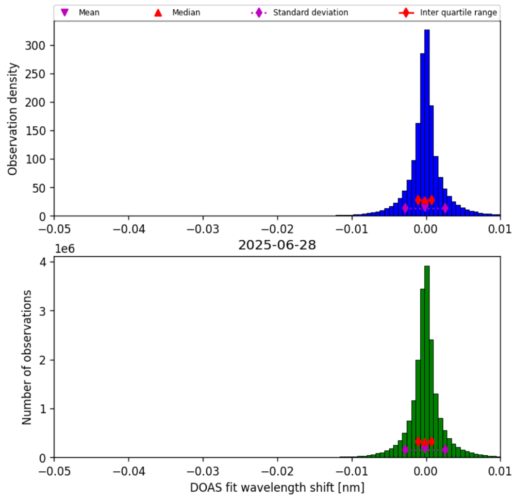
Figure 76: Histogram of “DOAS fit wavelength shift” for 2025-06-27 to 2025-06-29
