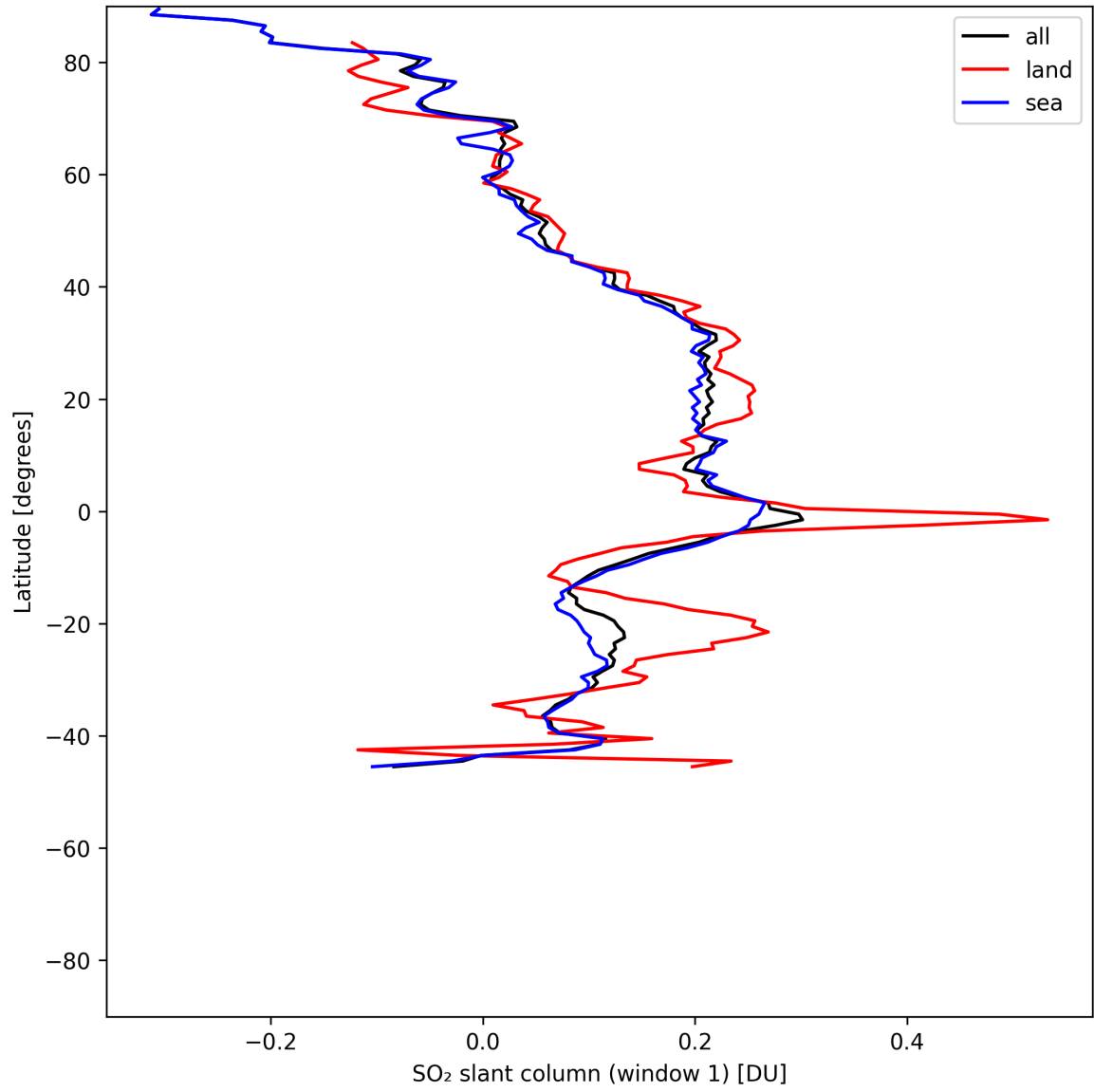
Figure 37: Zonal average of “SO 2 slant column (window 1)” for 2025-06-27 to 2025-06-29.
