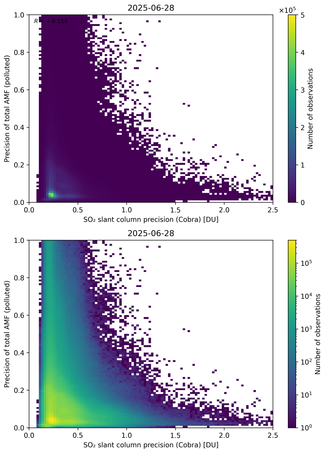
Figure 214: Scatter density plot of “SO 2 slant column precision (Cobra)” against “Precision of total AMF (polluted)” for 2025-06-27 to 2025-06-29.
