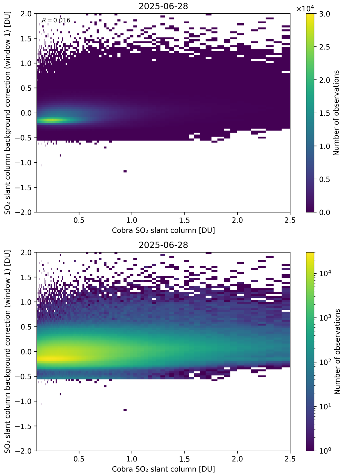
Figure 193: Scatter density plot of “Cobra SO 2 slant column” against “SO 2 slant column background correction (window 1)” for 2025-06-27 to 2025-06-29.
