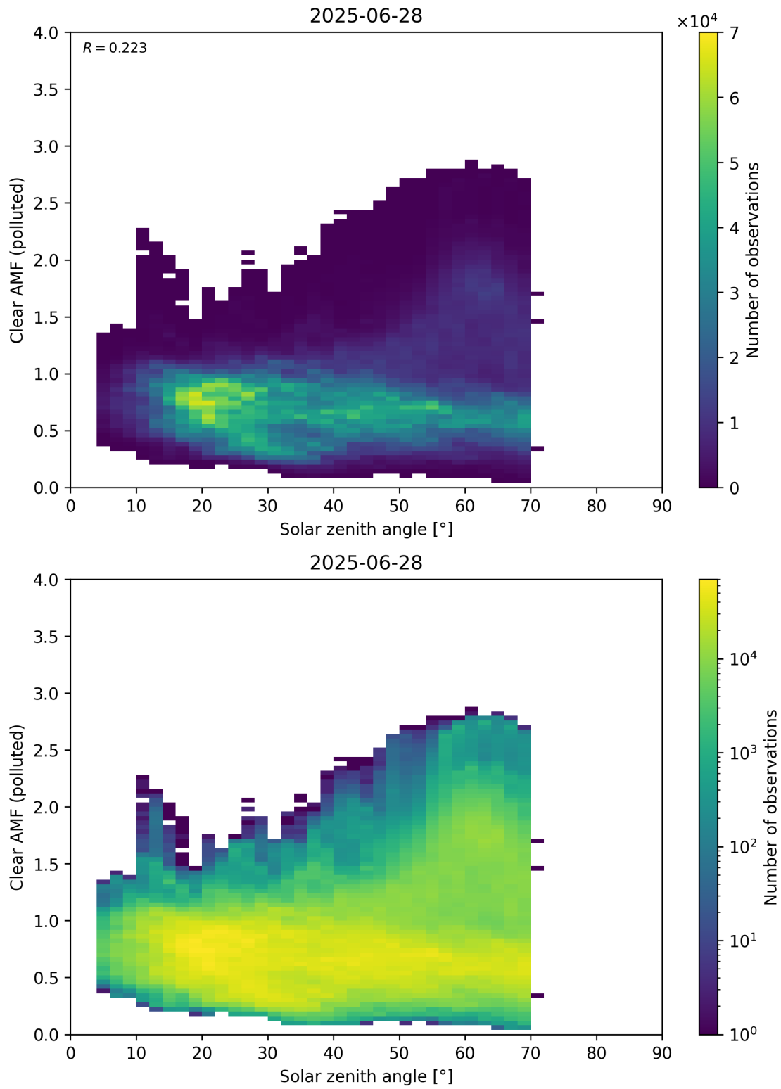
Figure 178: Scatter density plot of “Solar zenith angle” against “Clear AMF (polluted)” for 2025-06-27 to 2025-06-29.
