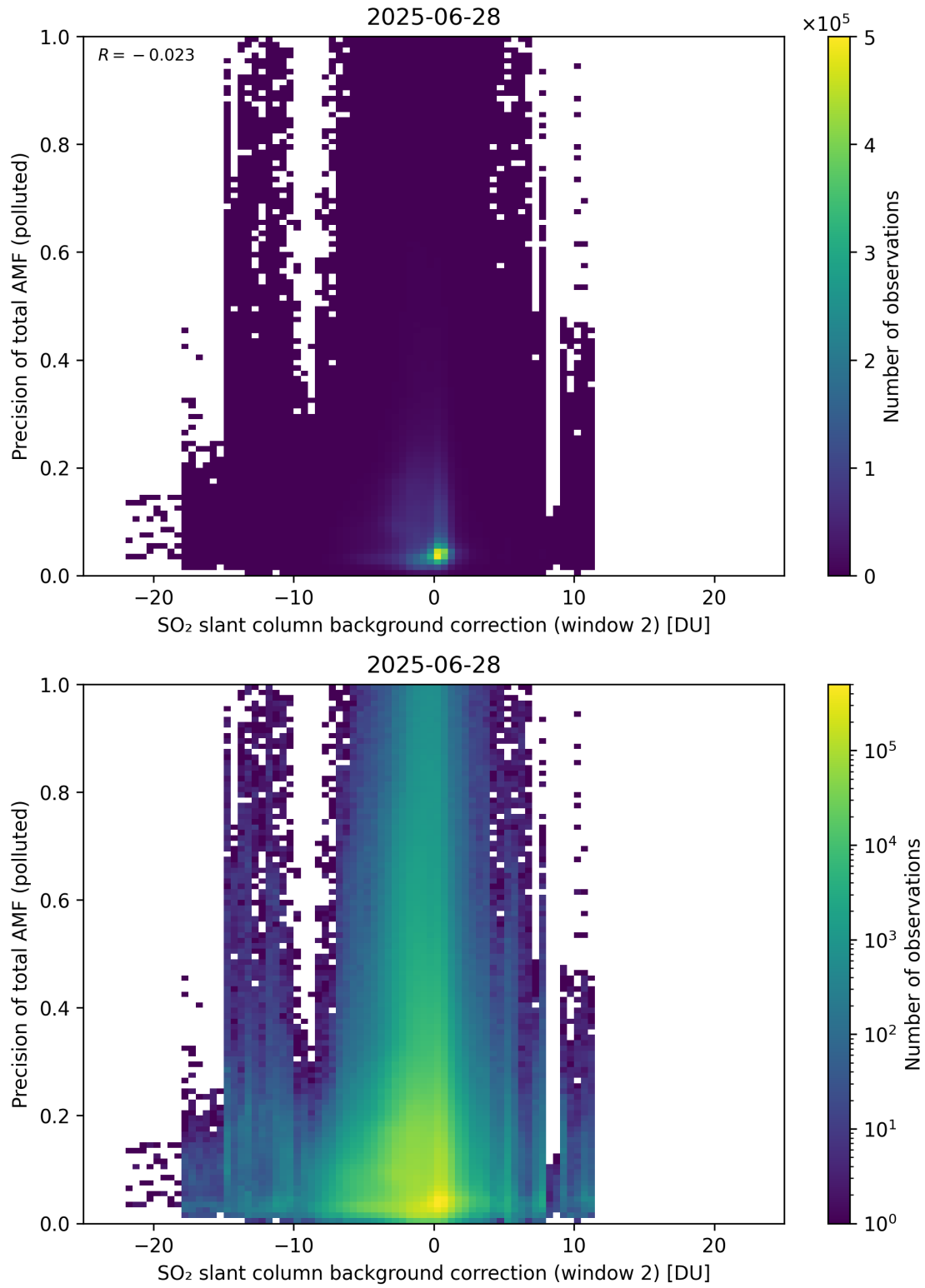
Figure 131: Scatter density plot of “SO 2 slant column background correction (window 2)” against “Precision of total AMF (polluted)” for 2025-06-27 to 2025-06-29.
