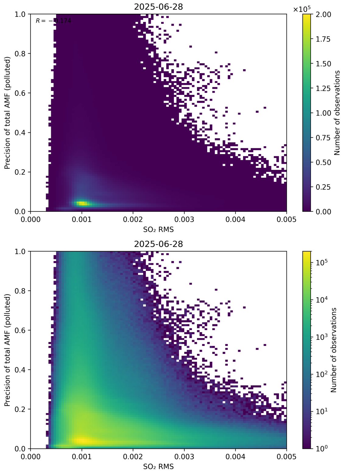
Figure 149: Scatter density plot of “SO 2 RMS” against “Precision of total AMF (polluted)” for 2025-06-27 to 2025-06-29.
