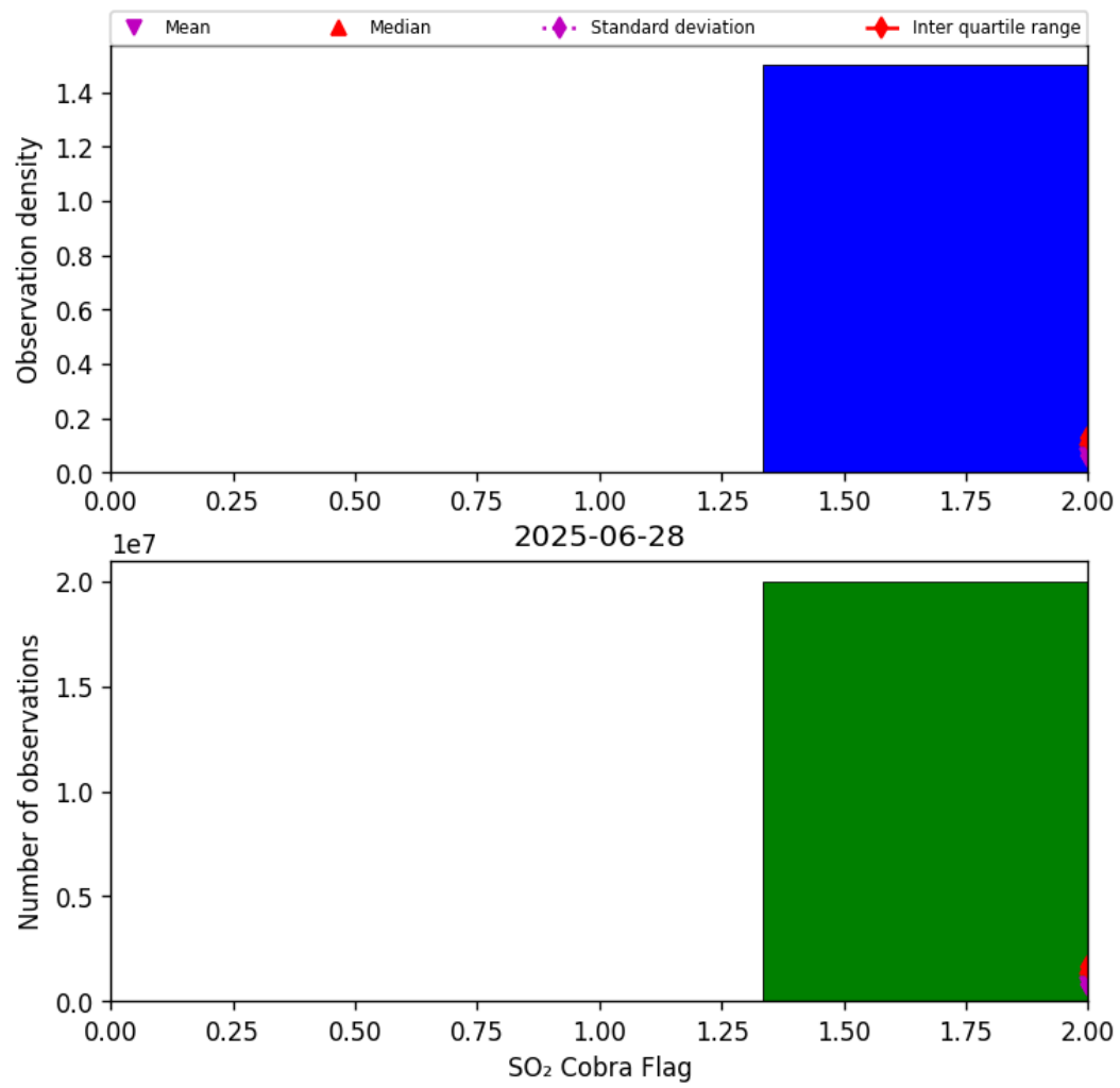
Figure 75: Histogram of “SO 2 Cobra Flag” for 2025-06-27 to 2025-06-29
