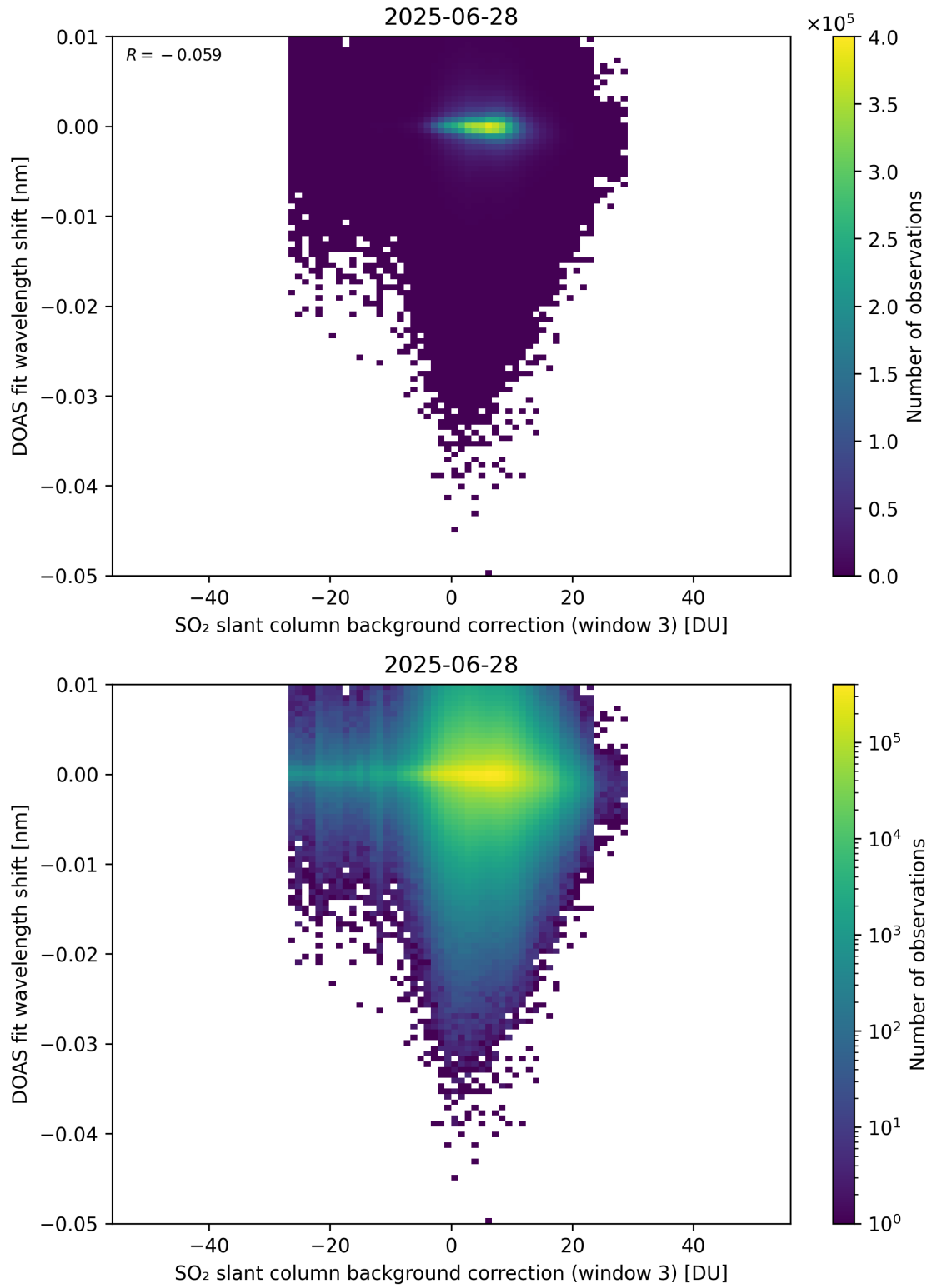
Figure 132: Scatter density plot of “SO 2 slant column background correction (window 3)” against “DOAS fit wavelength shift” for 2025-06-27 to 2025-06-29.
