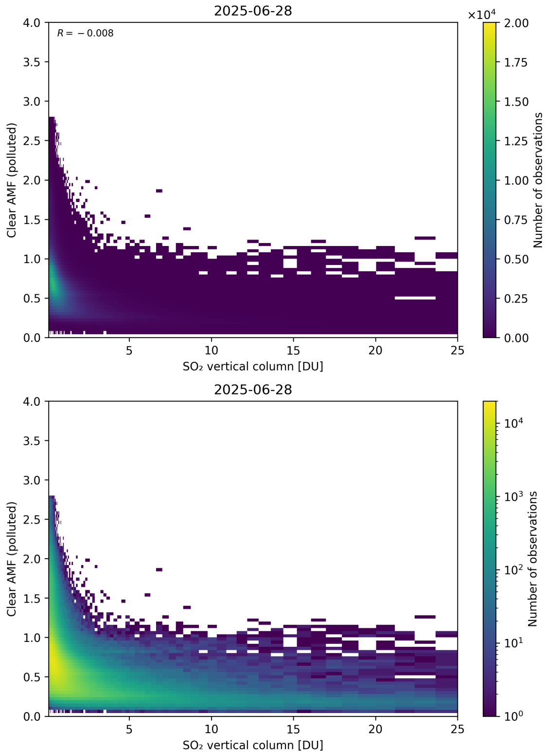
Figure 348: Scatter density plot of “SO 2 vertical column” against “Clear AMF (polluted)” for 2025-06-27 to 2025-06-29.
