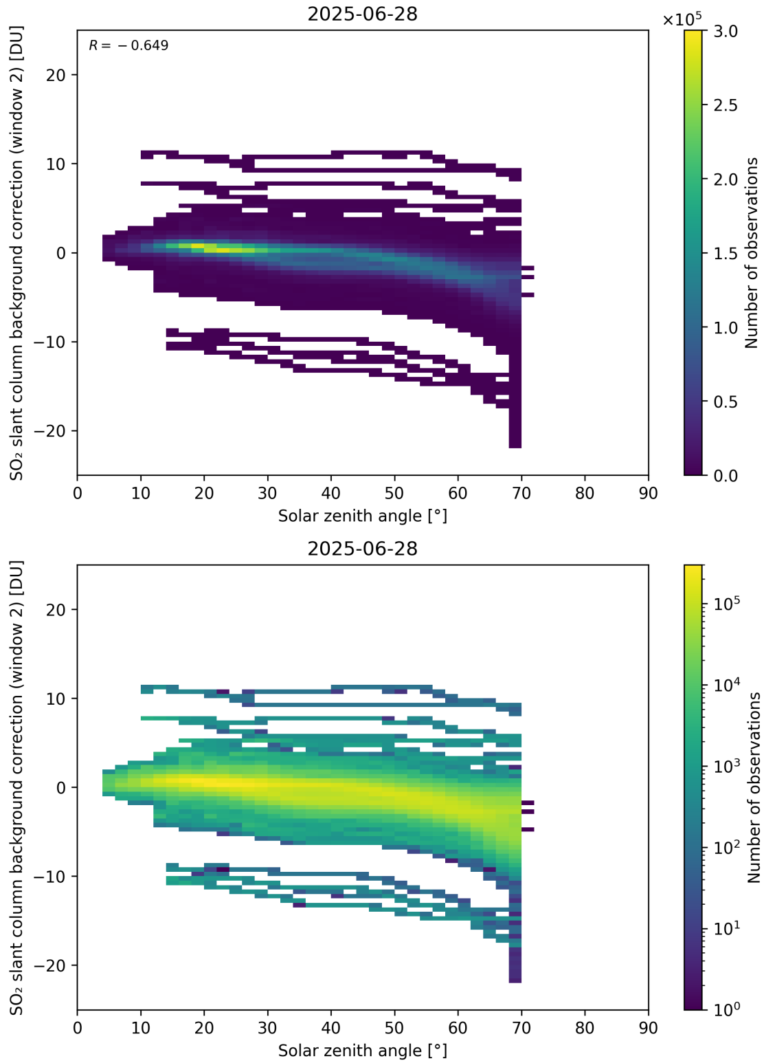
Figure 172: Scatter density plot of “Solar zenith angle” against “SO 2 slant column background correction (window 2)” for 2025-06-27 to 2025-06-29.
