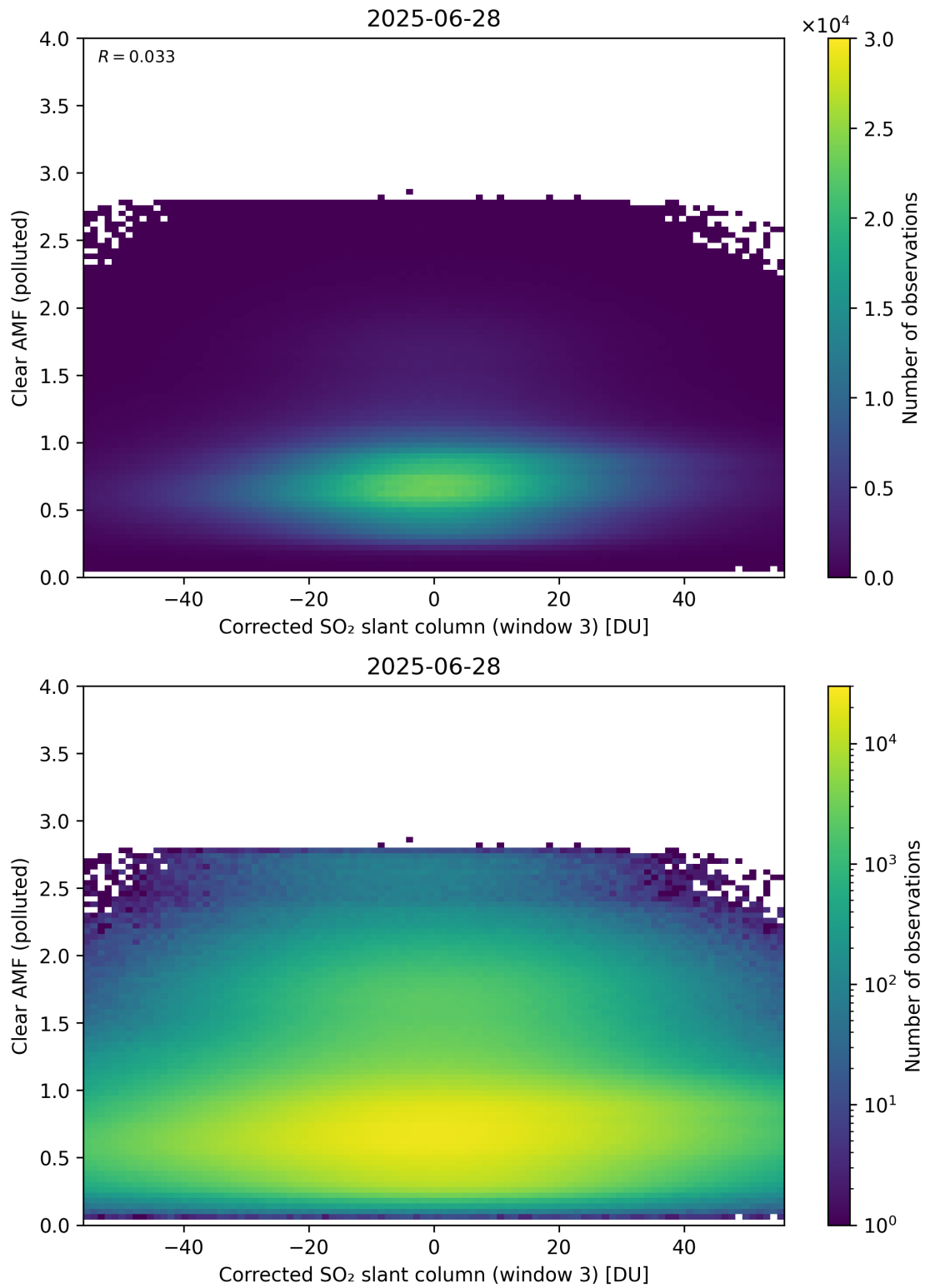
Figure 259: Scatter density plot of “Corrected SO 2 slant column (window 3)” against “Clear AMF (polluted)” for 2025-06-27 to 2025-06-29.
