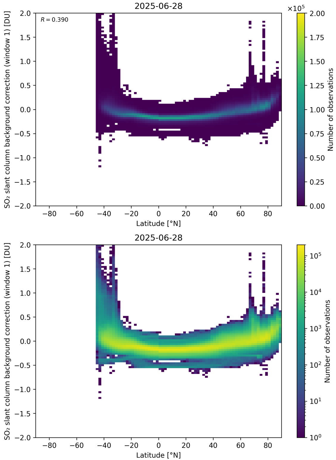
Figure 150: Scatter density plot of “Latitude” against “SO 2 slant column background correction (window 1)” for 2025-06-27 to 2025-06-29.
