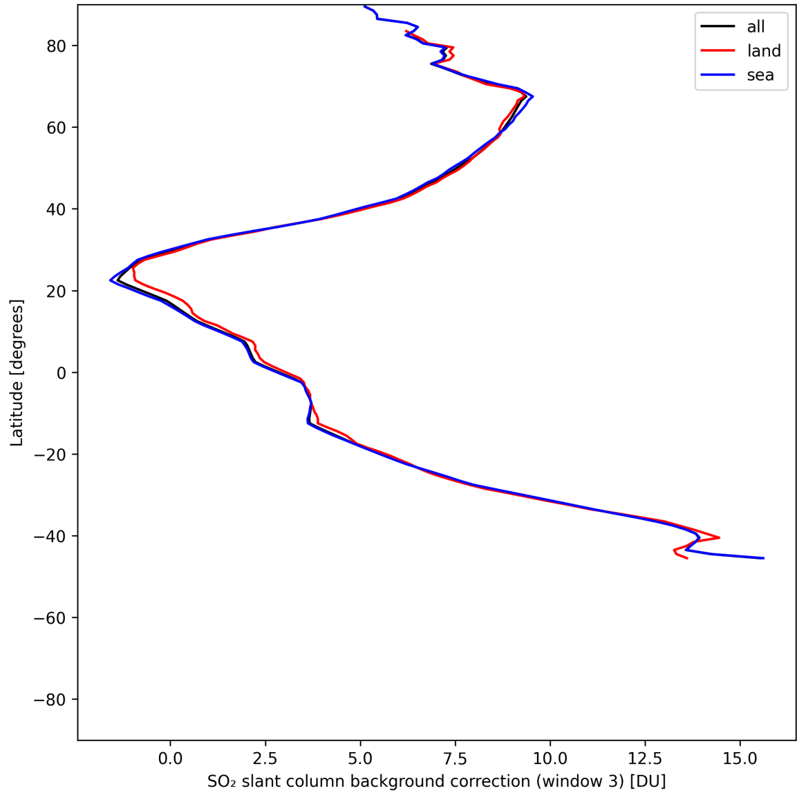
Figure 48: Zonal average of “SO 2 slant column background correction (window 3)” for 2025-06-27 to 2025-06-29.
