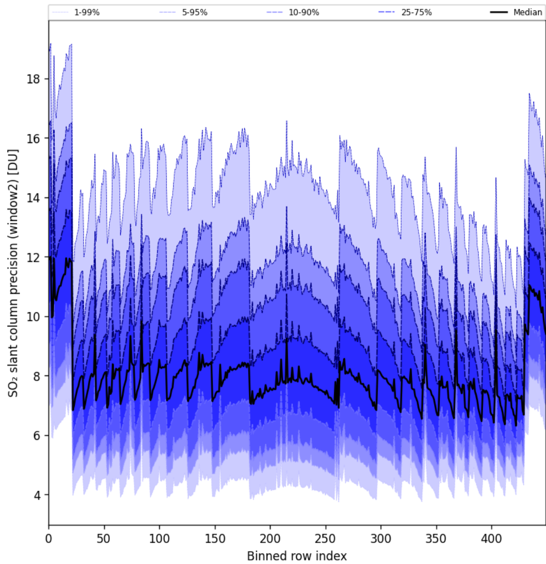
Figure 94: Along track statistics of “SO 2 slant column precision (window2)” for 2025-06-28 to 2025-06-30
