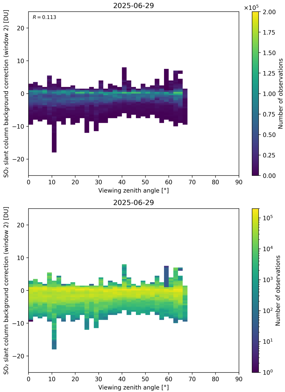
Figure 363: Scatter density plot of “Viewing zenith angle” against “SO 2 slant column background correction (window 2)” for 2025-06-28 to 2025-06-30.
