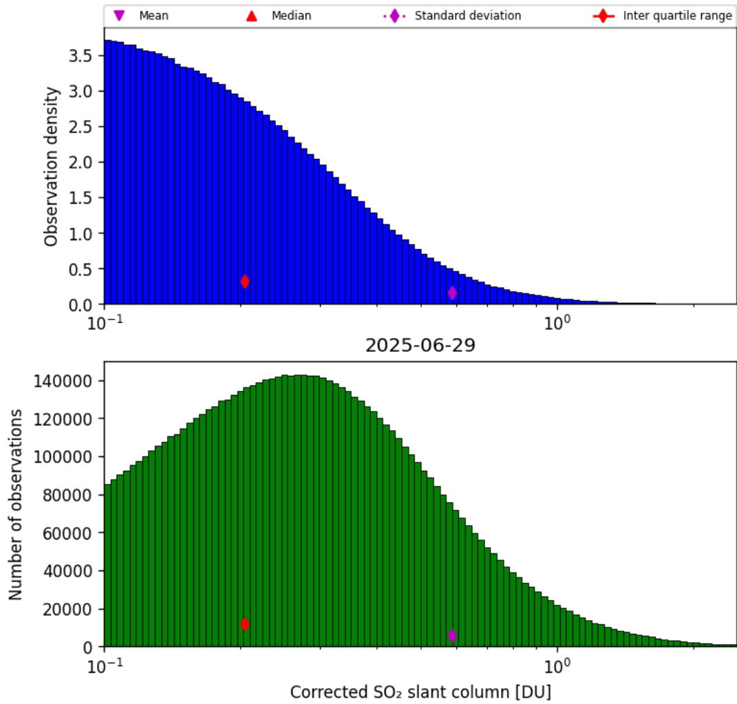
Figure 60: Histogram of “Corrected SO 2 slant column” for 2025-06-28 to 2025-06-30
