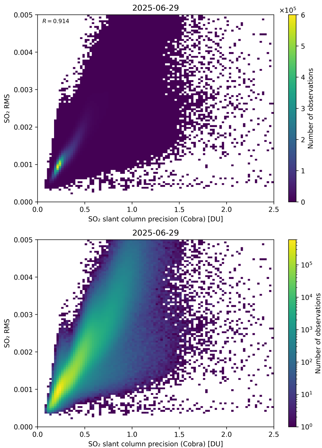
Figure 204: Scatter density plot of “SO 2 slant column precision (Cobra)” against “SO 2 RMS” for 2025-06-28 to 2025-06-30.
