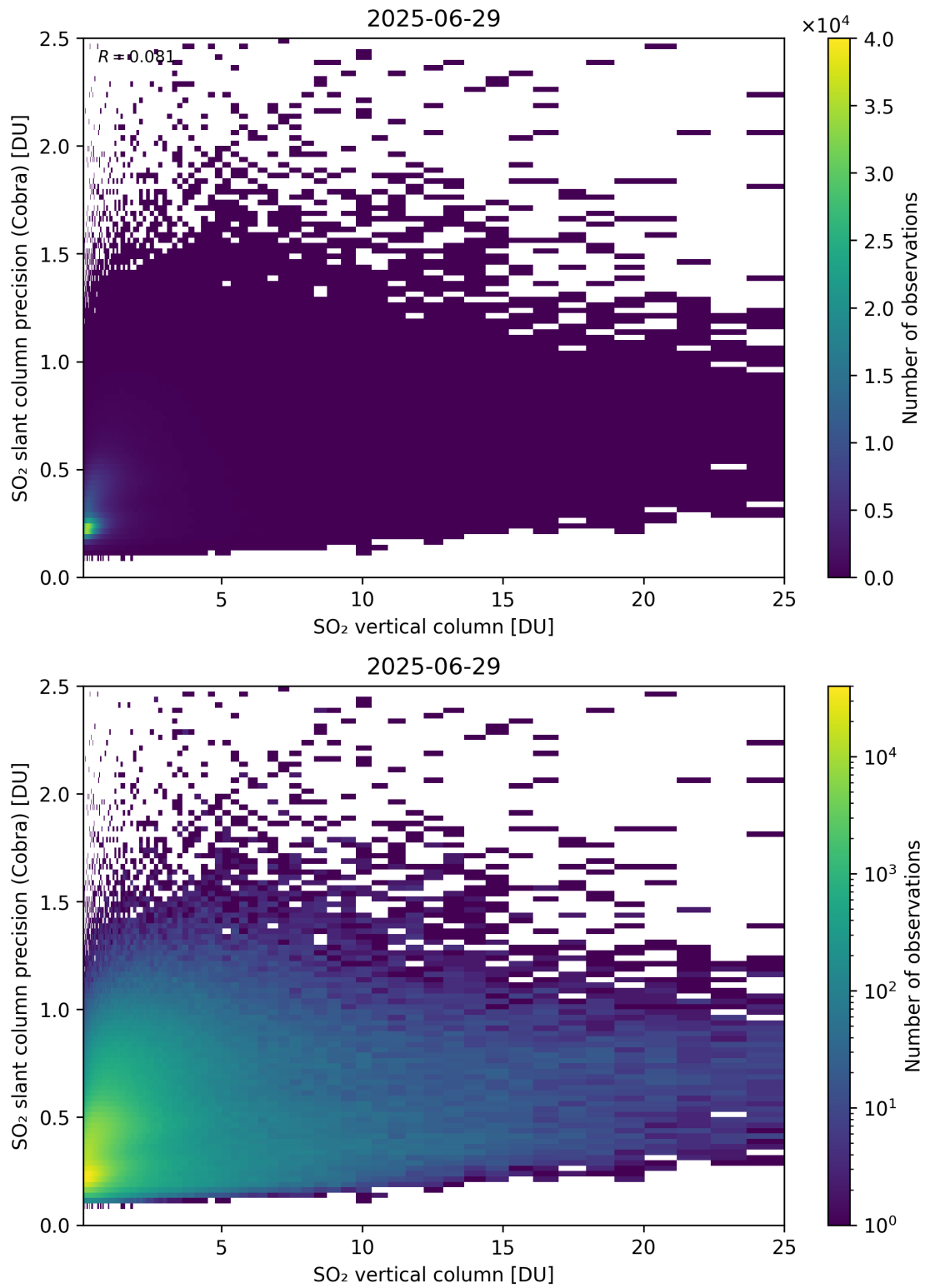
Figure 350: Scatter density plot of “SO 2 vertical column” against “SO 2 slant column precision (Cobra)” for 2025-06-28 to 2025-06-30.
