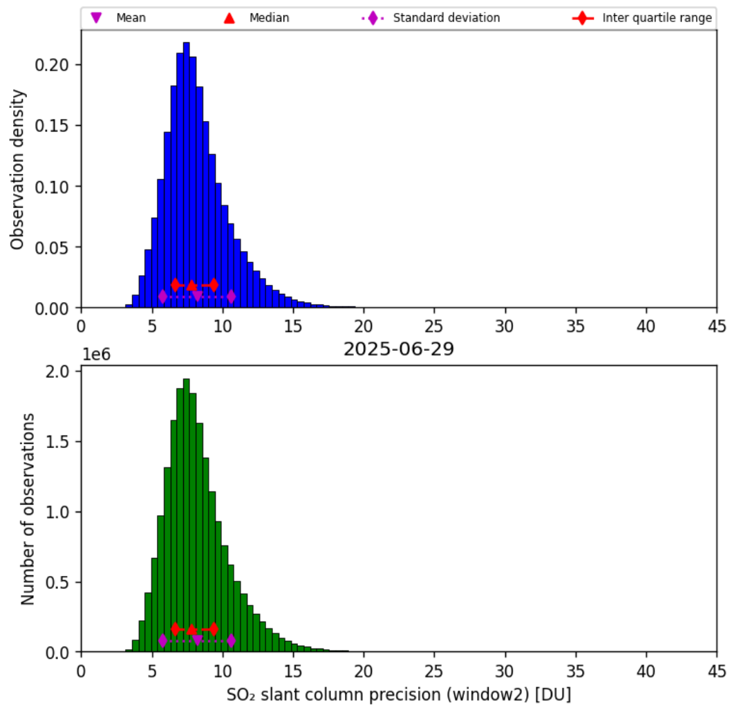
Figure 68: Histogram of “SO 2 slant column precision (window2)” for 2025-06-28 to 2025-06-30
