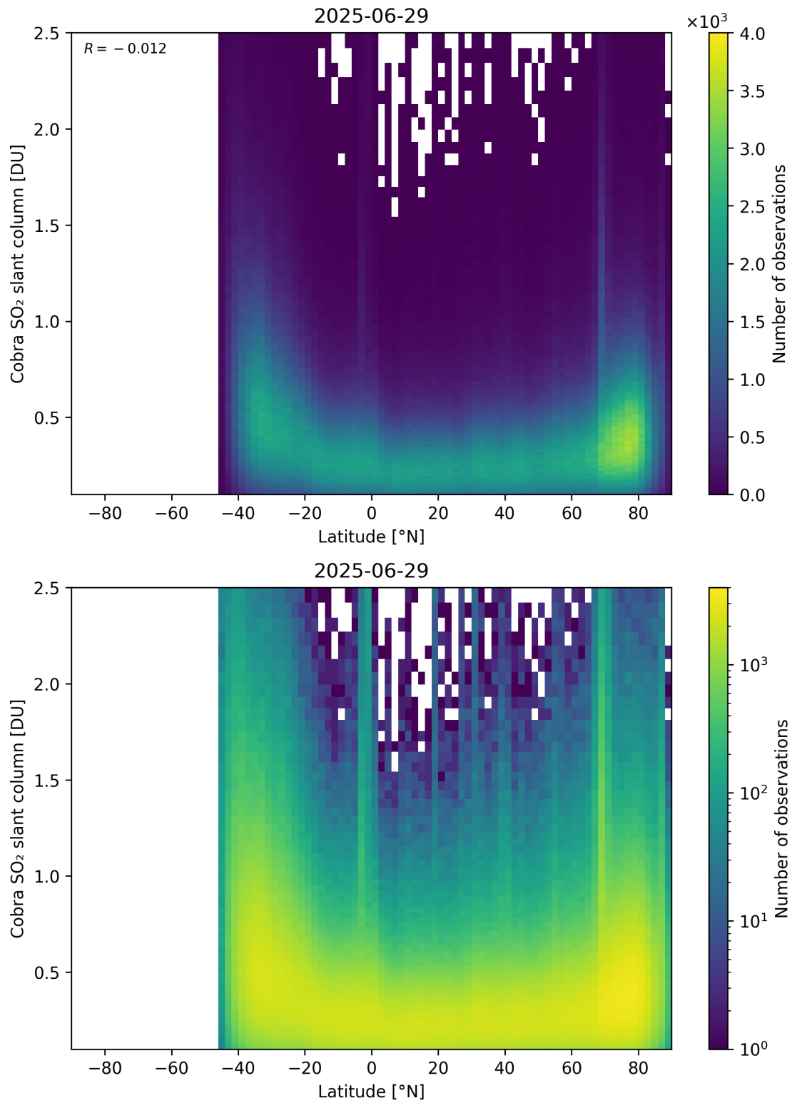
Figure 157: Scatter density plot of “Latitude” against “Cobra SO 2 slant column” for 2025-06-28 to 2025-06-30.
