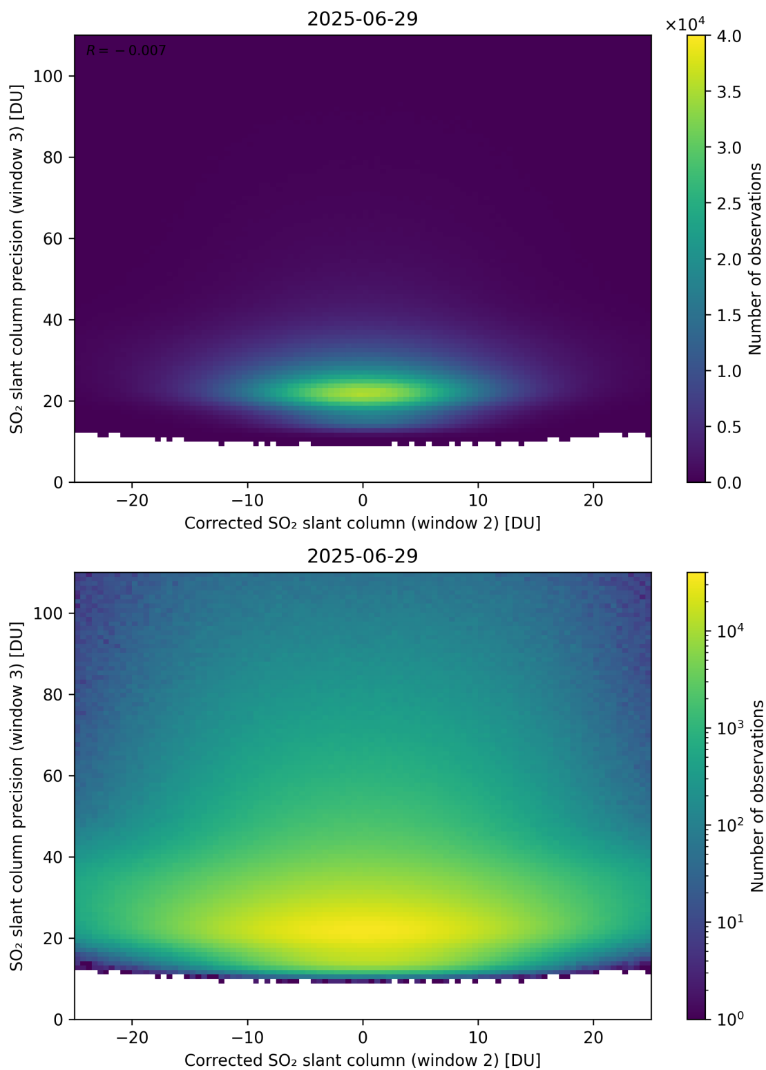
Figure 252: Scatter density plot of “Corrected SO 2 slant column (window 2)” against “SO 2 slant column precision (window 3)” for 2025-06-28 to 2025-06-30.
