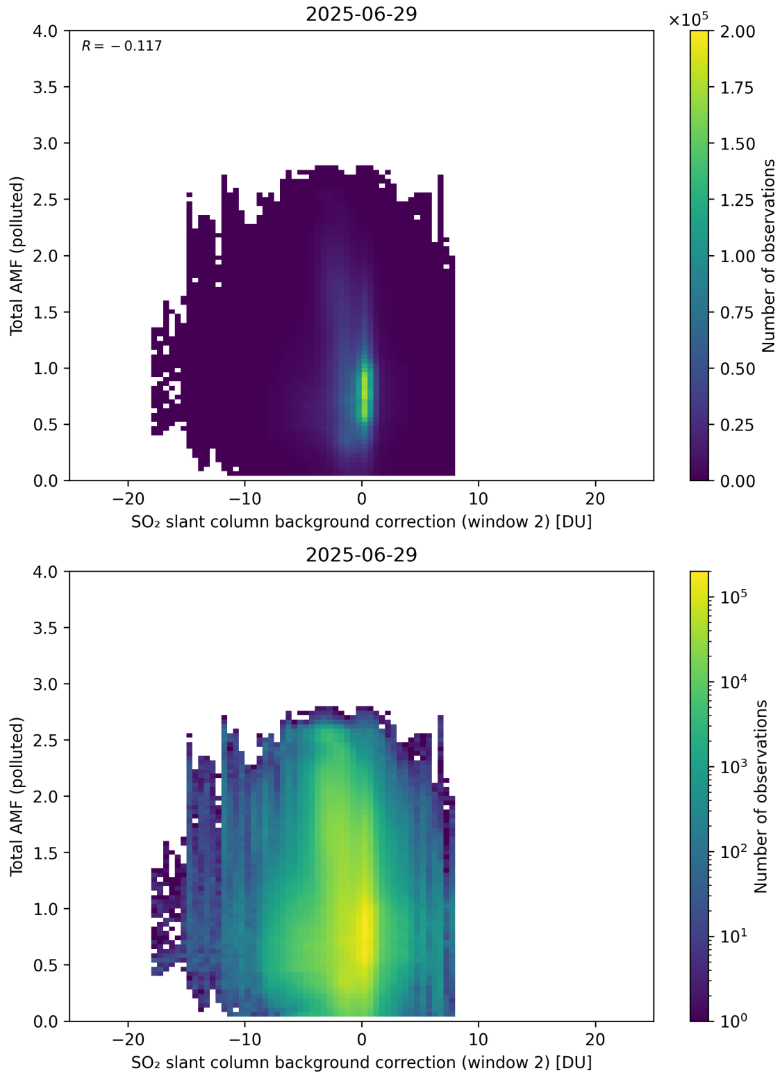
Figure 130: Scatter density plot of “SO 2 slant column background correction (window 2)” against “Total AMF (polluted)” for 2025-06-28 to 2025-06-30.
