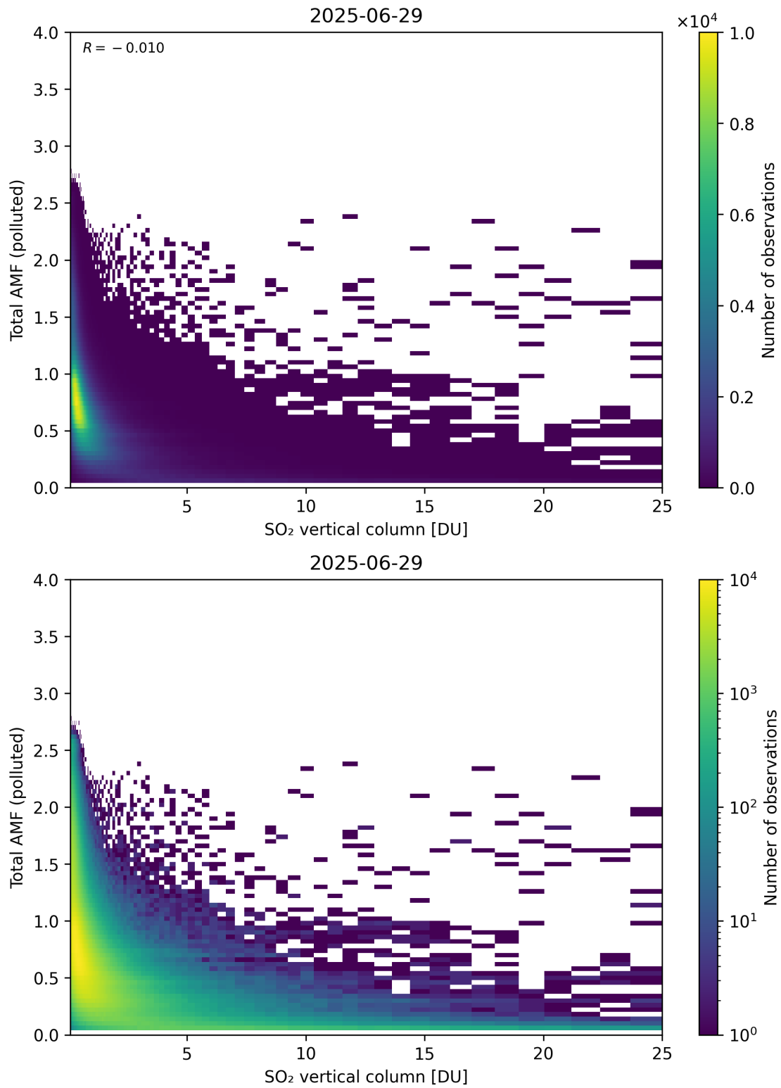
Figure 359: Scatter density plot of “SO 2 vertical column” against “Total AMF (polluted)” for 2025-06-28 to 2025-06-30.
