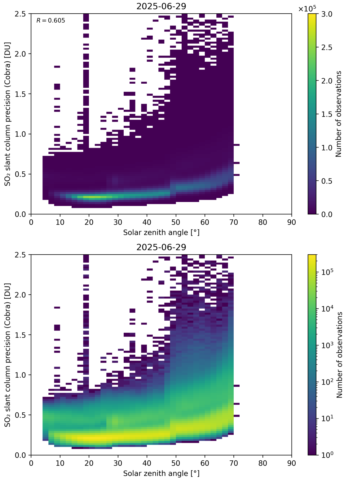
Figure 180: Scatter density plot of “Solar zenith angle” against “SO 2 slant column precision (Cobra)” for 2025-06-28 to 2025-06-30.
