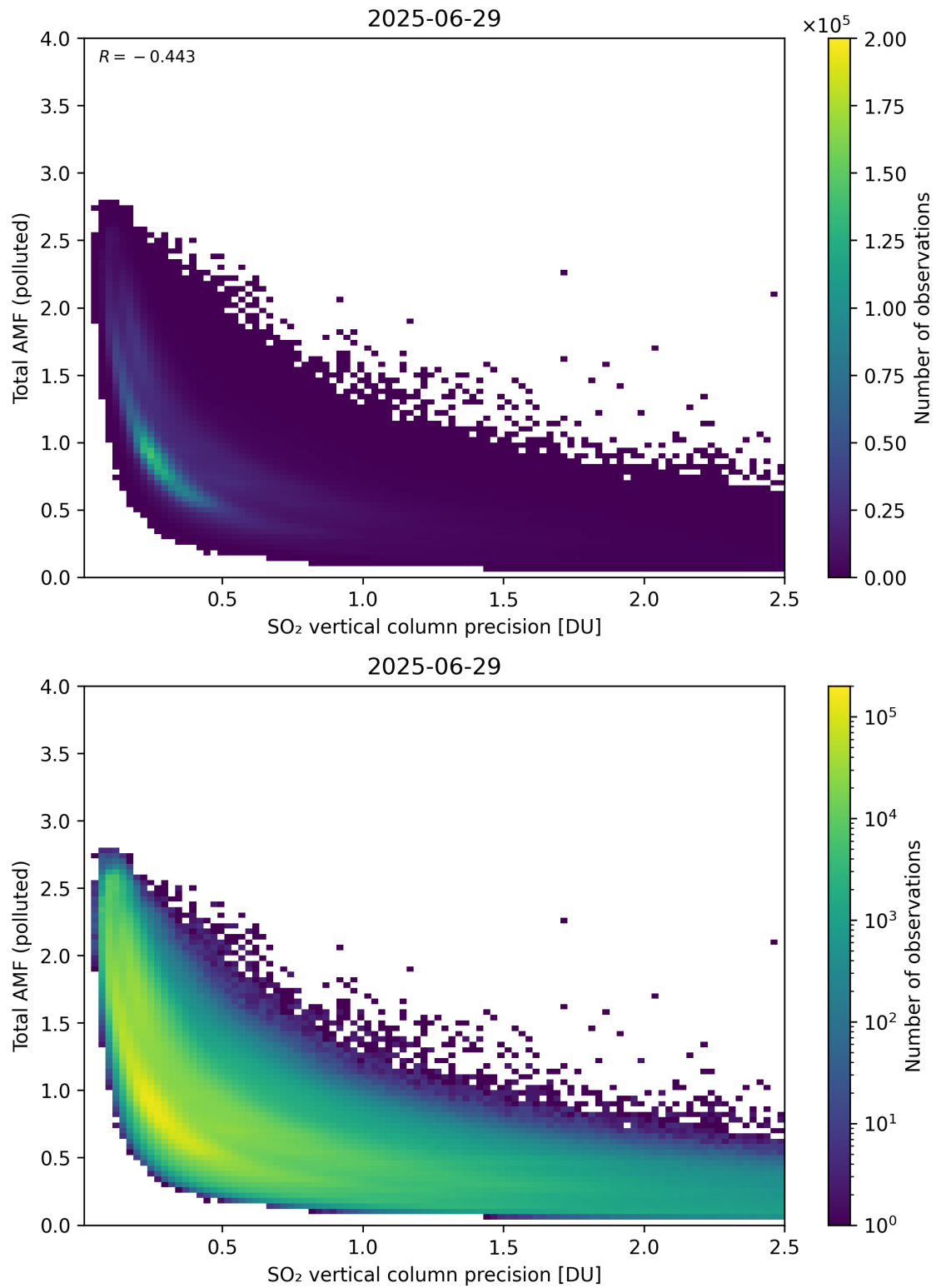
Figure 346: Scatter density plot of “SO 2 vertical column precision” against “Total AMF (polluted)” for 2025-06-28 to 2025-06-30.
