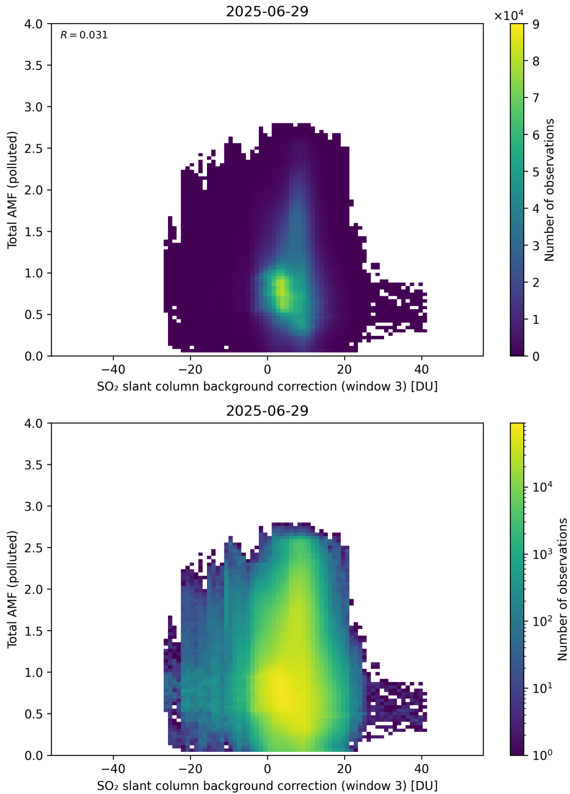
Figure 136: Scatter density plot of “SO 2 slant column background correction (window 3)” against “Total AMF (polluted)” for 2025-06-28 to 2025-06-30.
