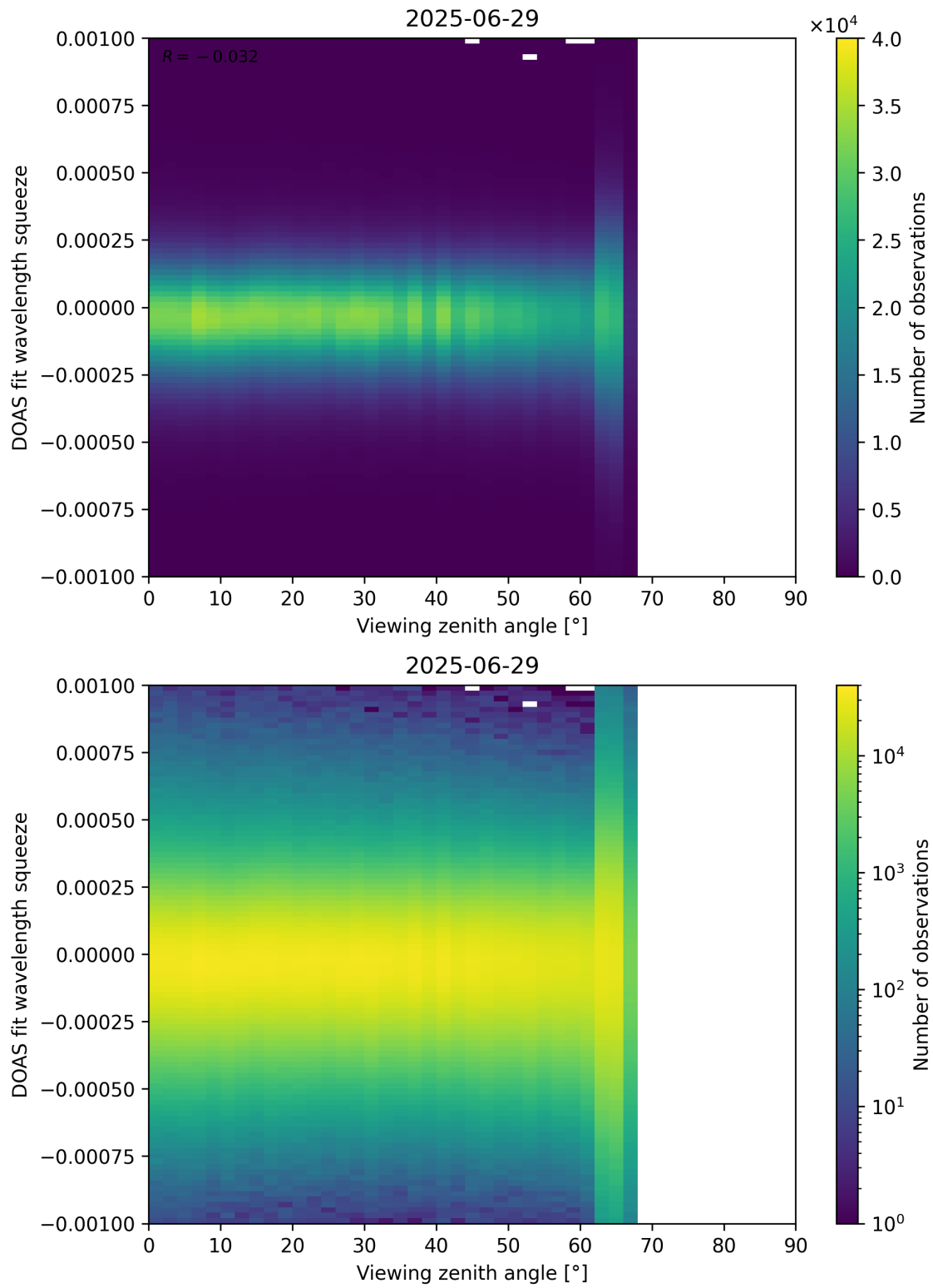
Figure 366: Scatter density plot of “Viewing zenith angle” against “DOAS fit wavelength squeeze” for 2025-06-28 to 2025-06-30.
