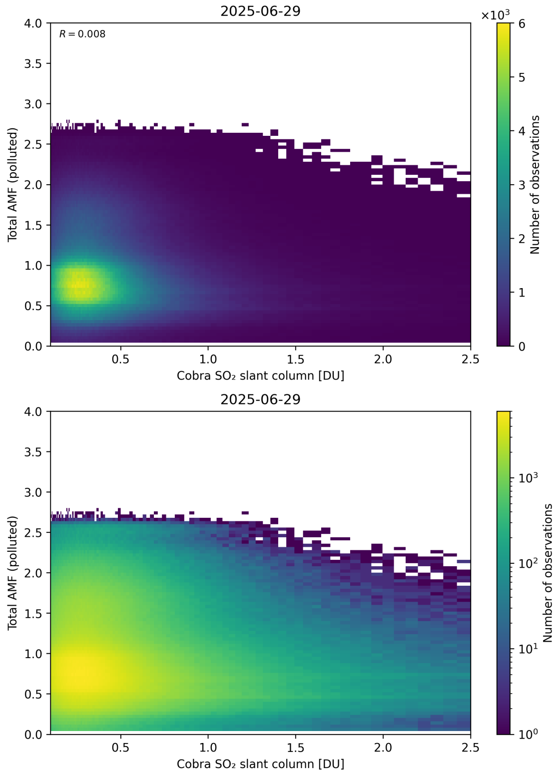
Figure 224: Scatter density plot of “Cobra SO 2 slant column” against “Total AMF (polluted)” for 2025-06-28 to 2025-06-30.
