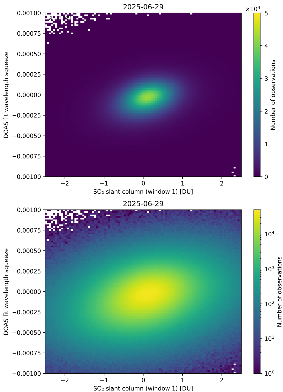
Figure 266: Scatter density plot of “SO 2 slant column (window 1)” against “DOAS fit wavelength squeeze” for 2025-06-28 to 2025-06-30.
