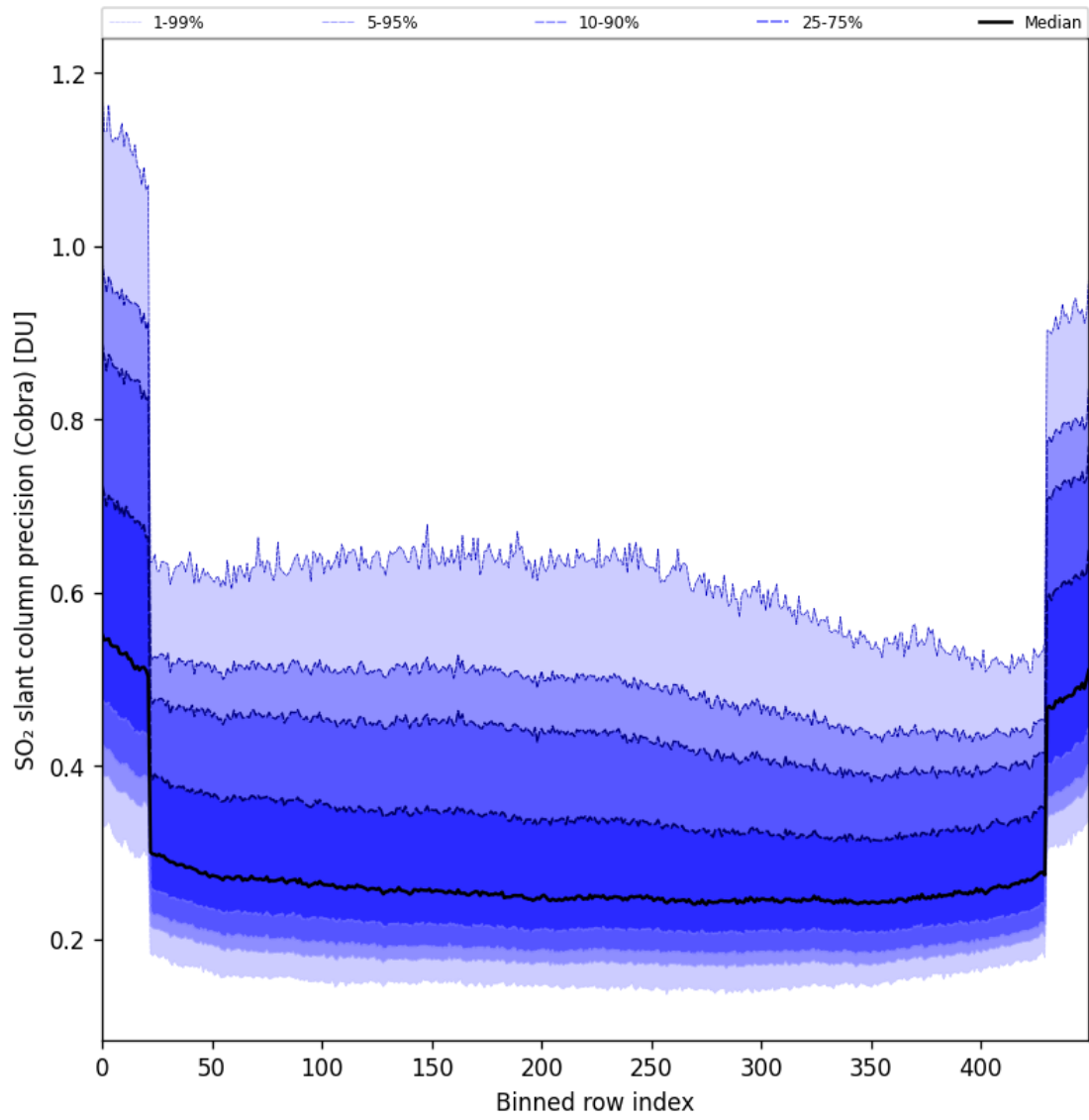
Figure 88: Along track statistics of “SO 2 slant column precision (Cobra)” for 2025-06-28 to 2025-06-30
