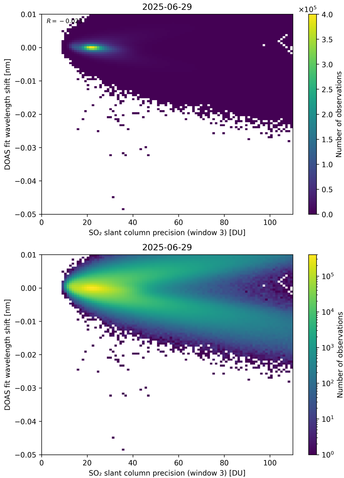
Figure 308: Scatter density plot of “SO 2 slant column precision (window 3)” against “DOAS fit wavelength shift” for 2025-06-28 to 2025-06-30.
