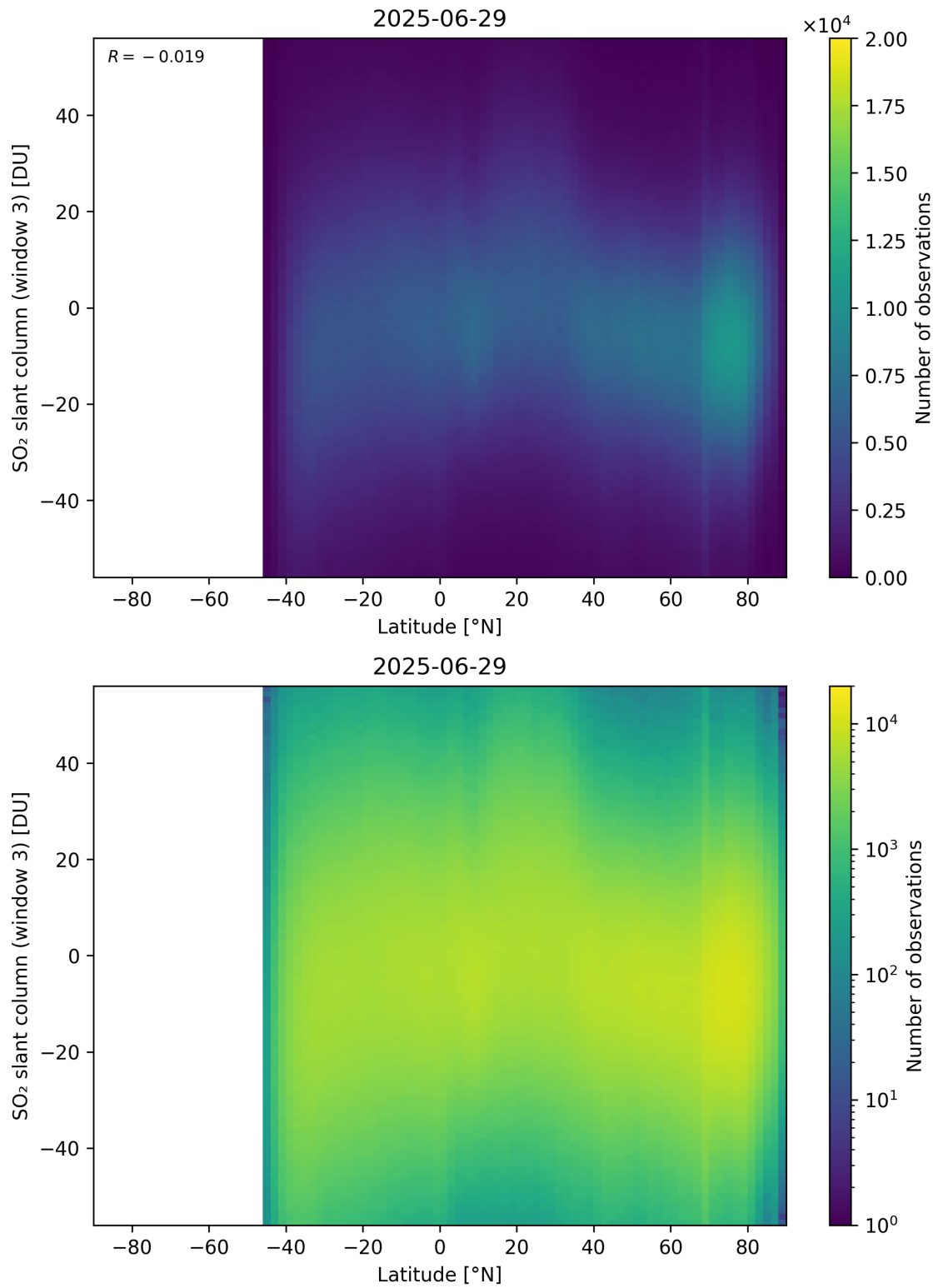
Figure 165: Scatter density plot of “Latitude” against “SO 2 slant column (window 3)” for 2025-06-28 to 2025-06-30.
