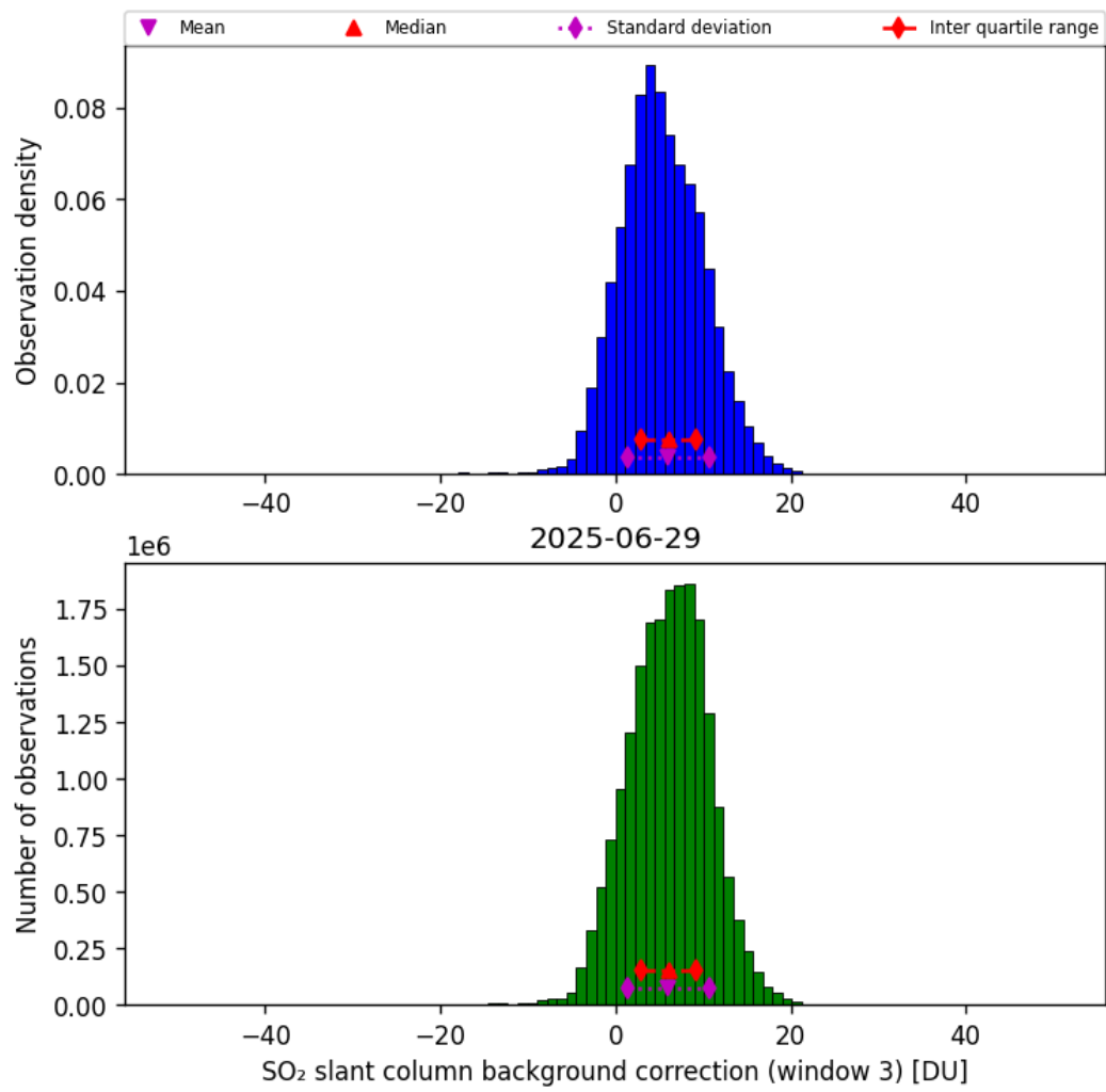
Figure 74: Histogram of “SO 2 slant column background correction (window 3)” for 2025-06-28 to 2025-06-30
