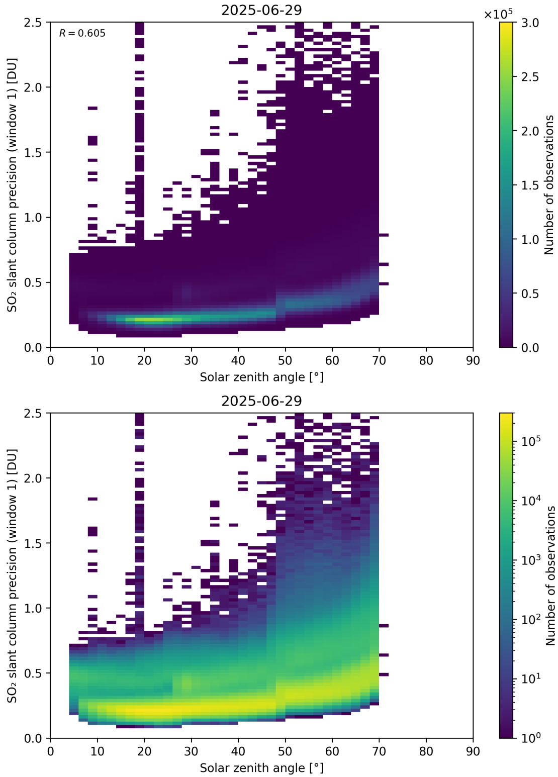
Figure 185: Scatter density plot of “Solar zenith angle” against “SO 2 slant column precision (window 1)” for 2025-06-28 to 2025-06-30.
