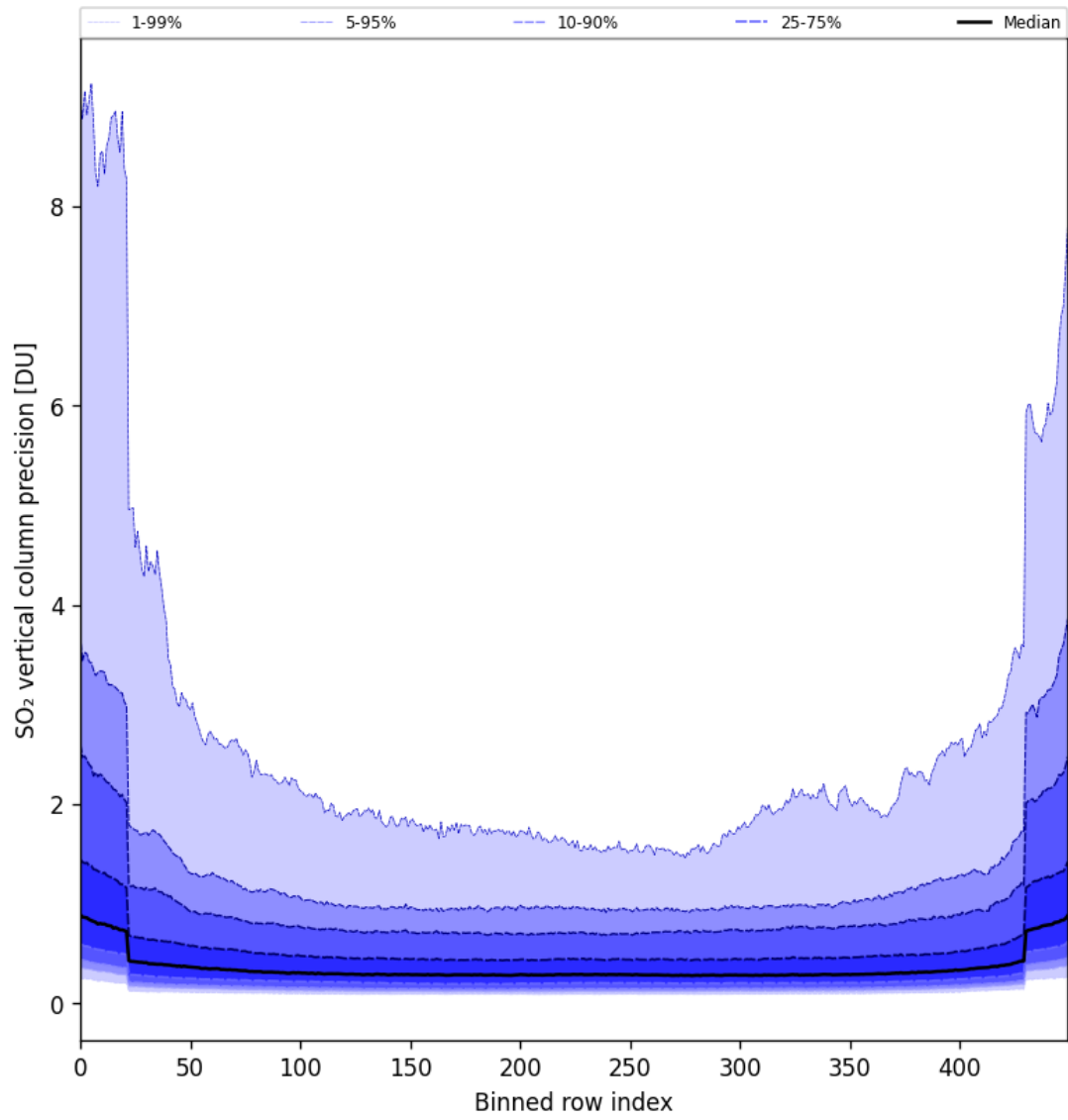
Figure 85: Along track statistics of “SO 2 vertical column precision” for 2025-06-28 to 2025-06-30
