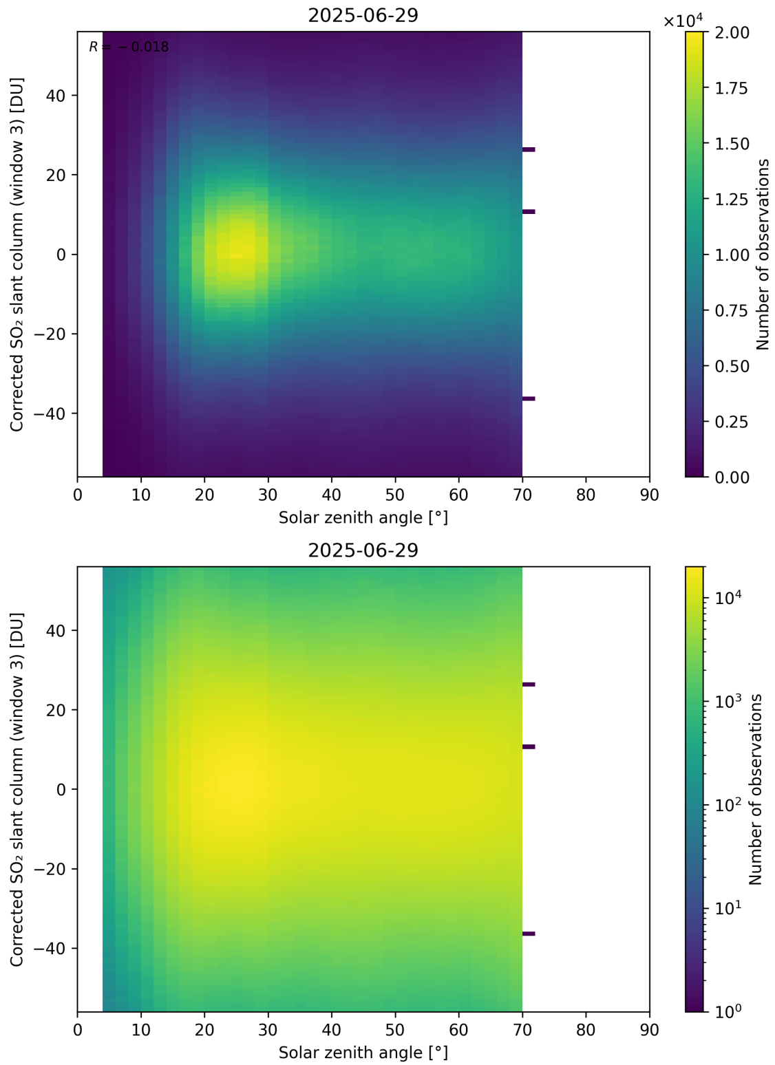
Figure 183: Scatter density plot of “Solar zenith angle” against “Corrected SO 2 slant column (window 3)” for 2025-06-28 to 2025-06-30.
