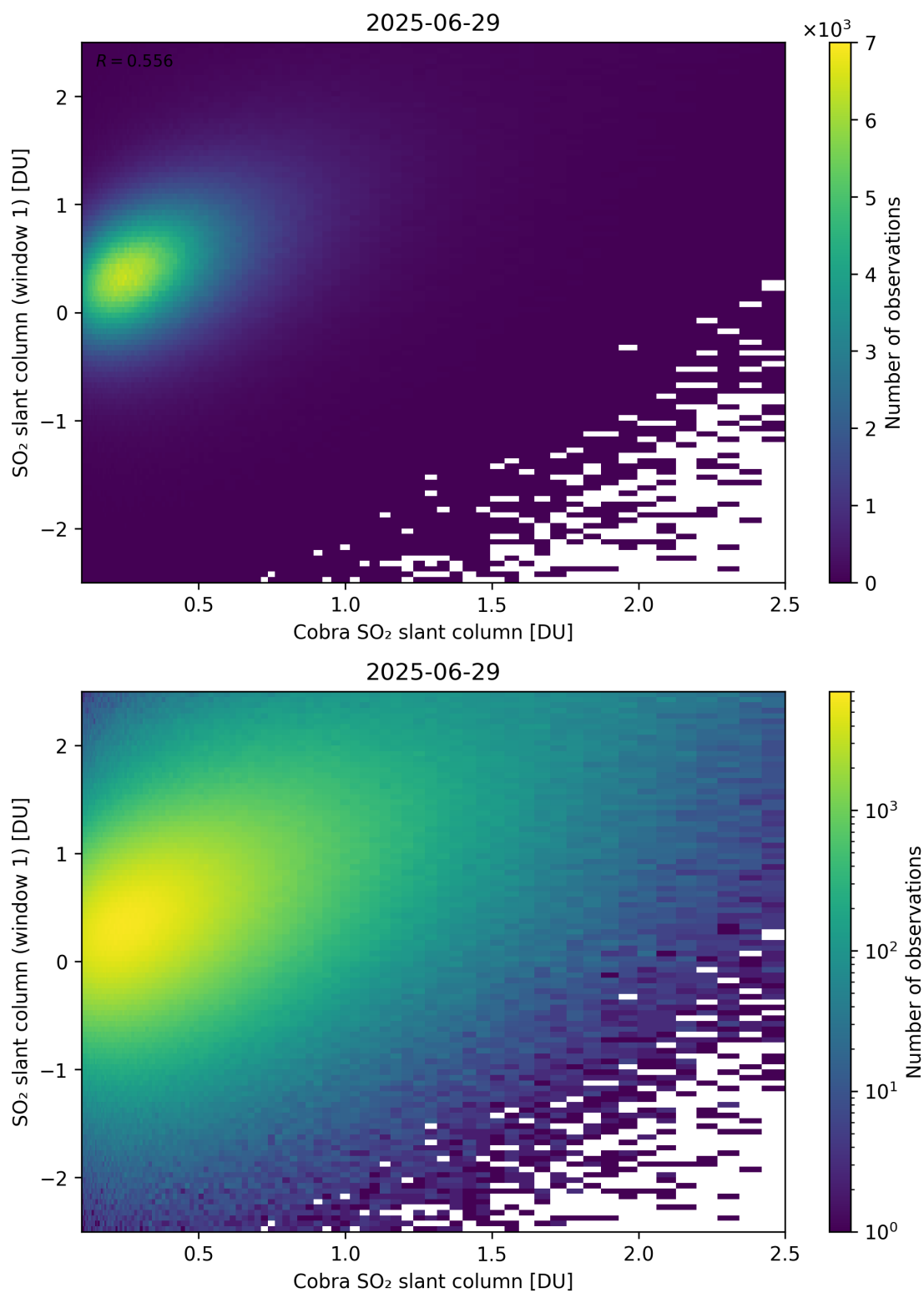
Figure 219: Scatter density plot of “Cobra SO 2 slant column” against “SO 2 slant column (window 1)” for 2025-06-28 to 2025-06-30.
