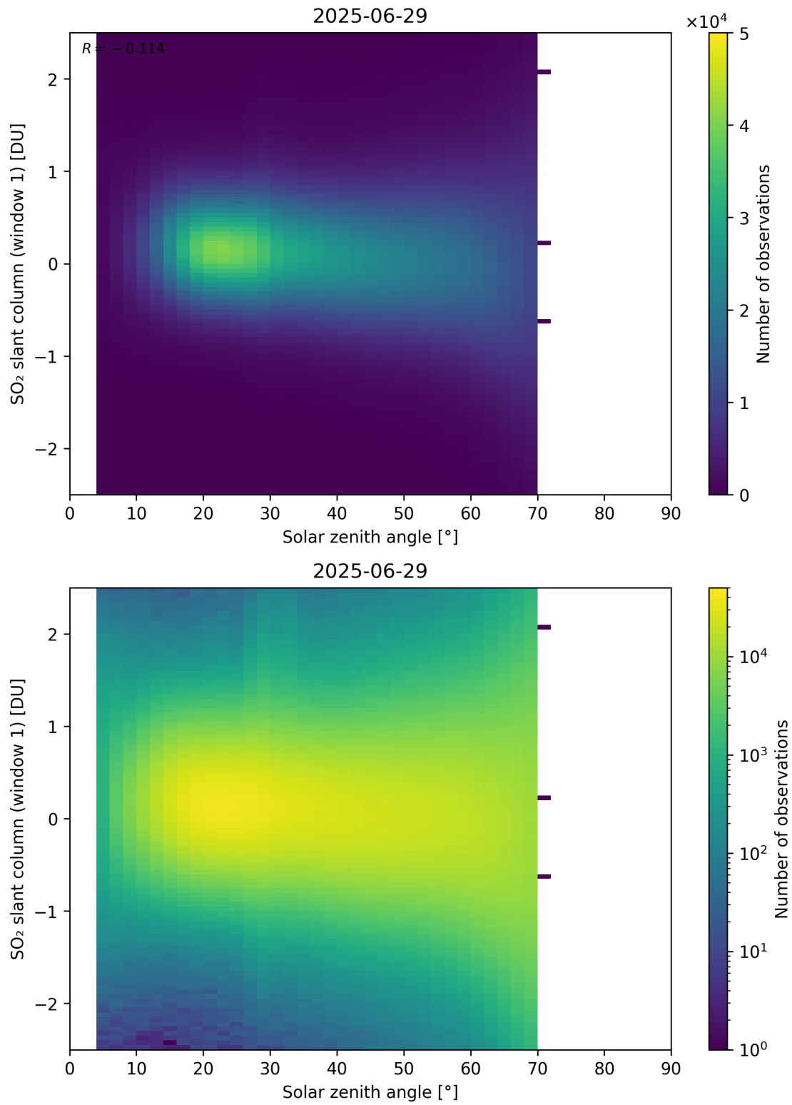
Figure 184: Scatter density plot of “Solar zenith angle” against “SO 2 slant column (window 1)” for 2025-06-28 to 2025-06-30.
