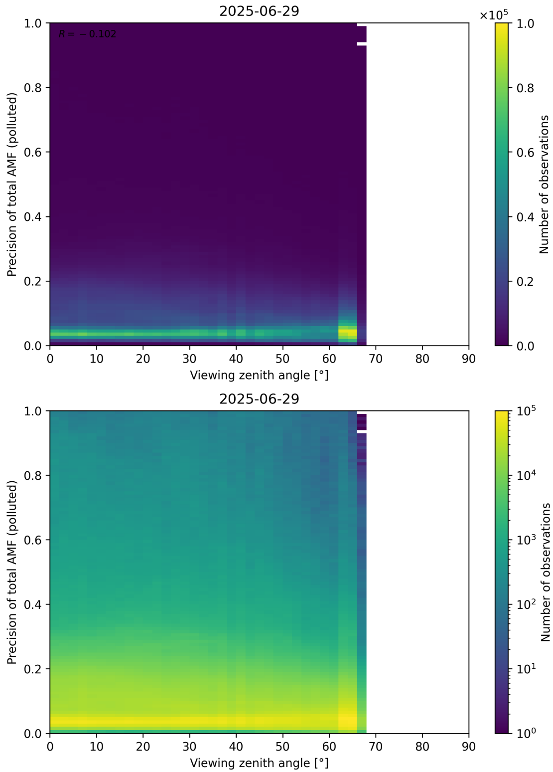
Figure 382: Scatter density plot of “Viewing zenith angle” against “Precision of total AMF (polluted)” for 2025-06-28 to 2025-06-30.
