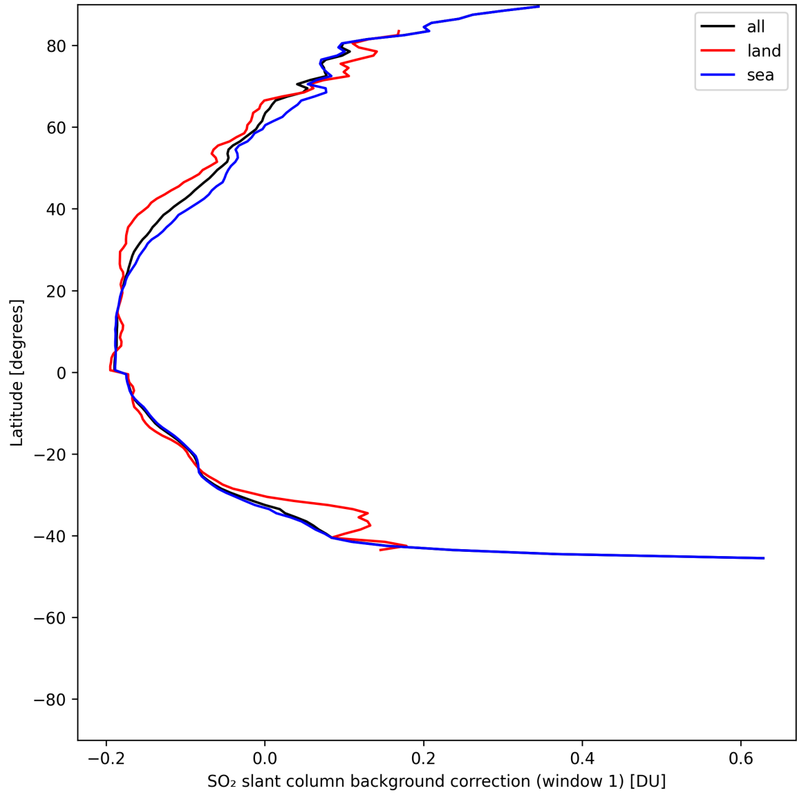
Figure 40: Zonal average of "SO 2 slant column background correction (window 1)" for 2025-06-28 to 2025-06-30.
