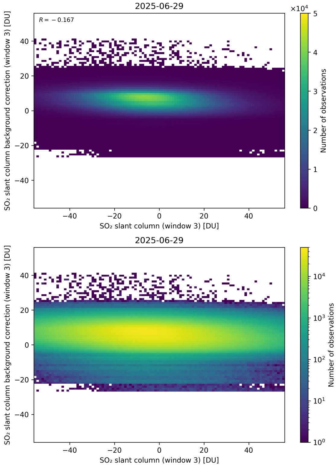
Figure 303: Scatter density plot of “SO 2 slant column (window 3)” against “SO 2 slant column background correction (window 3)” for 2025-06-28 to 2025-06-30.
