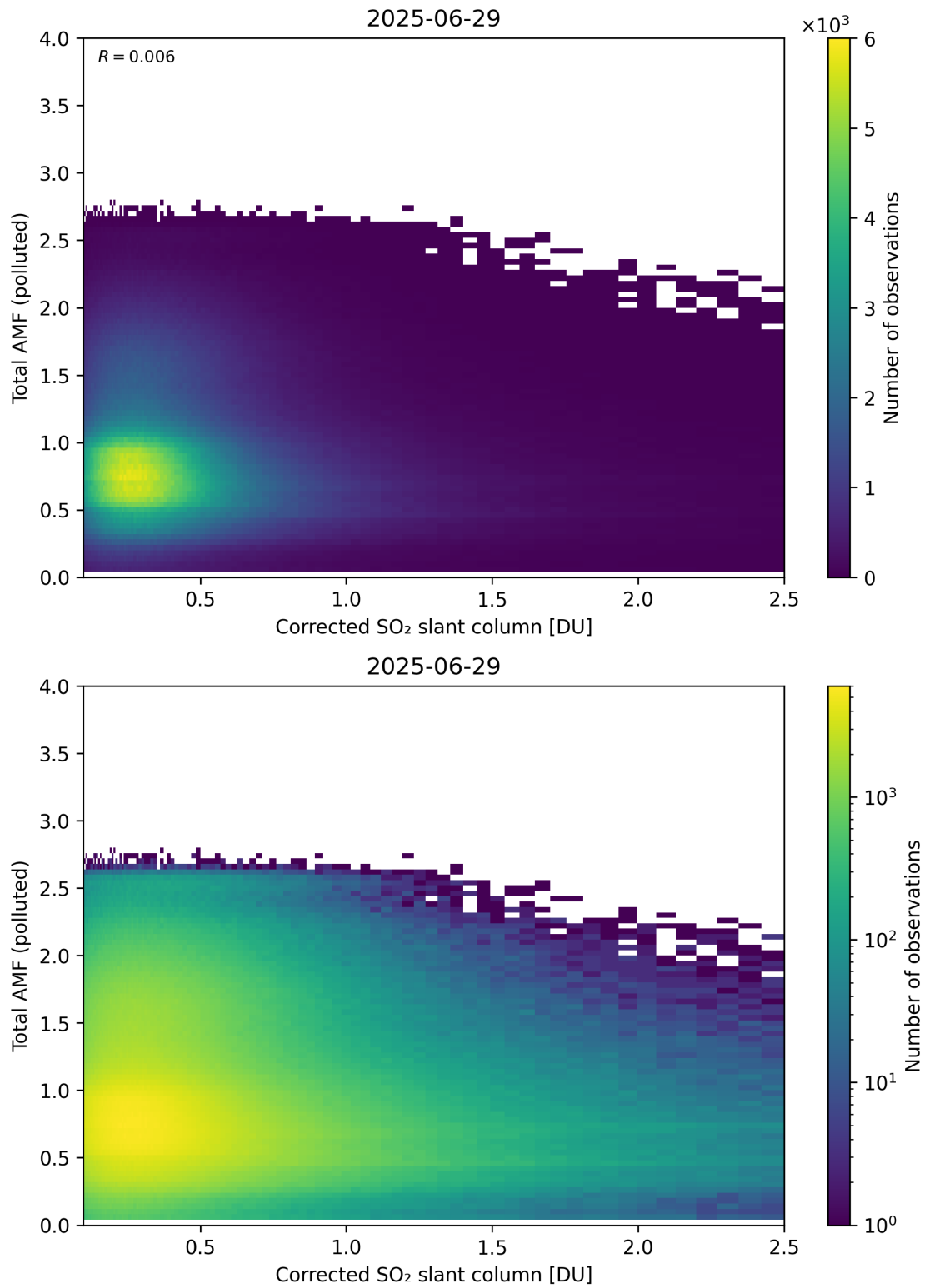
Figure 242: Scatter density plot of “Corrected SO 2 slant column” against “Total AMF (polluted)” for 2025-06-28 to 2025-06-30.
