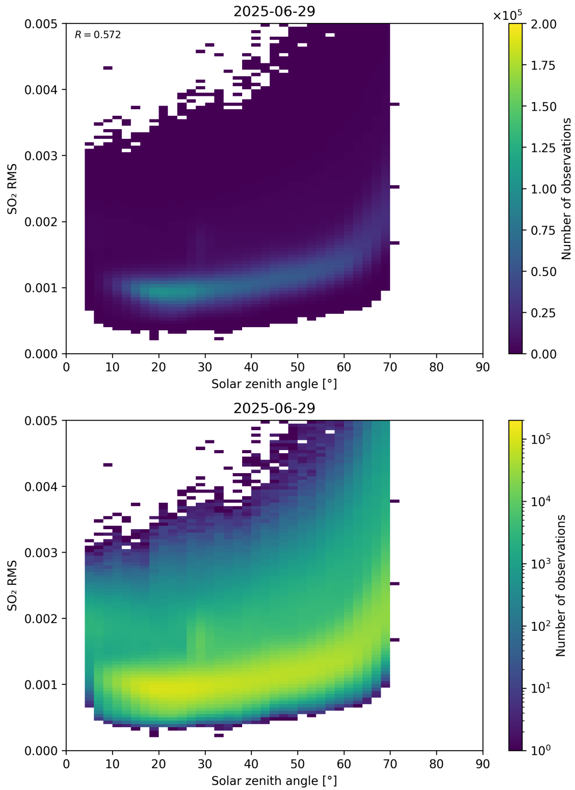
Figure 176: Scatter density plot of “Solar zenith angle” against “SO 2 RMS” for 2025-06-28 to 2025-06-30.
