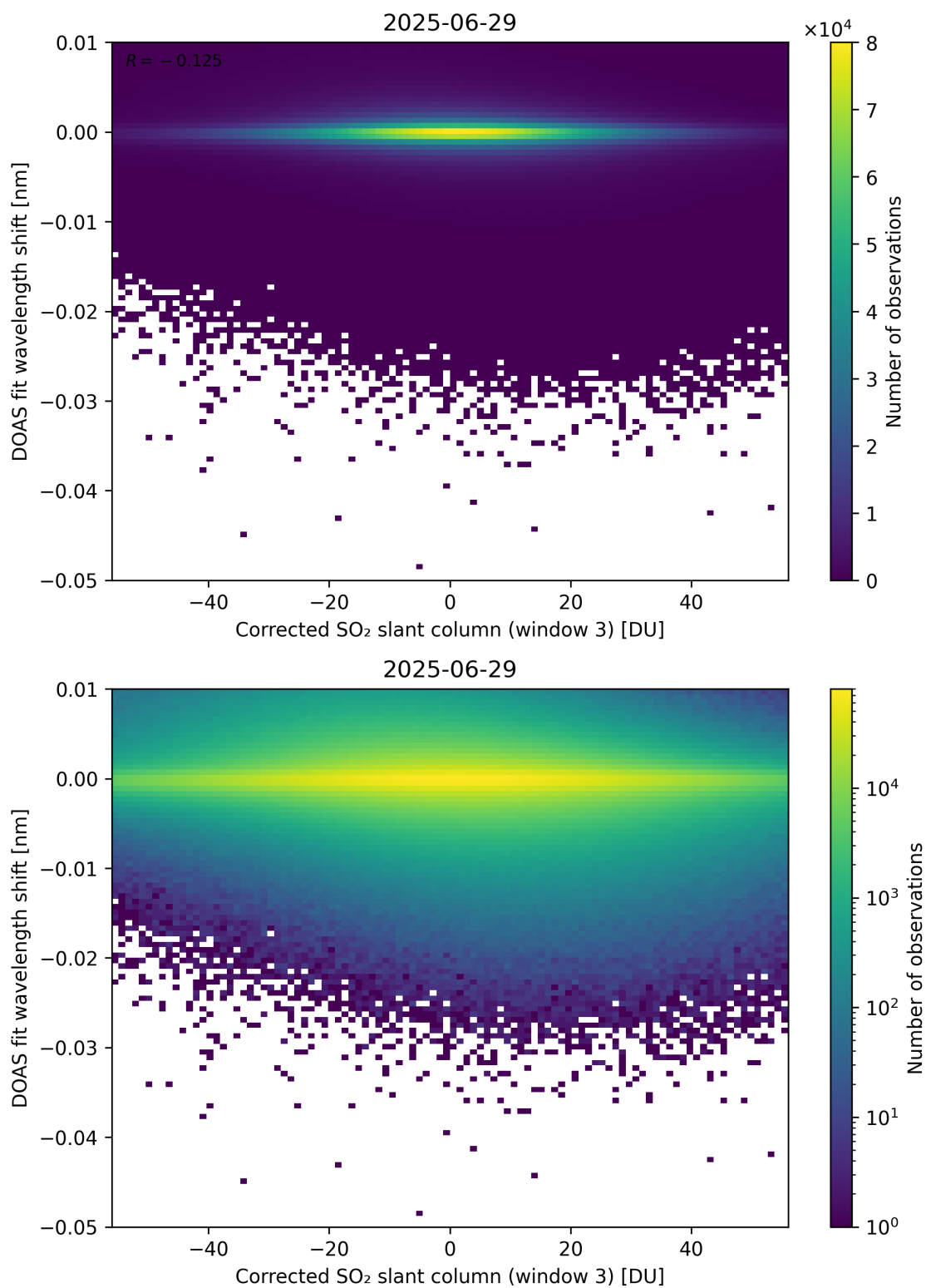
Figure 256: Scatter density plot of “Corrected SO 2 slant column (window 3)” against “DOAS fit wavelength shift” for 2025-06-28 to 2025-06-30.
