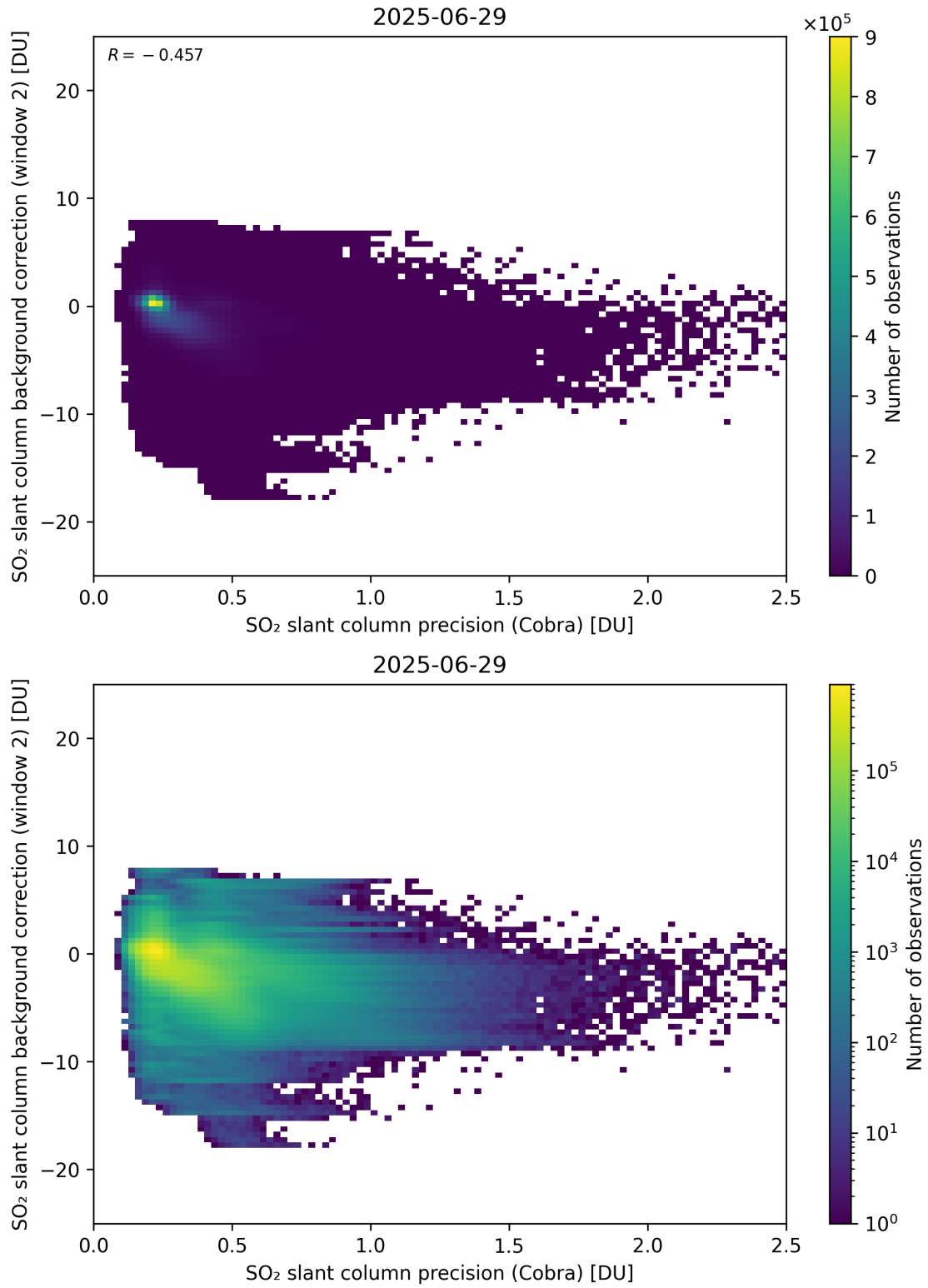
Figure 200: Scatter density plot of “SO 2 slant column precision (Cobra)” against “SO 2 slant column background correction (window 2)” for 2025-06-28 to 2025-06-30.
