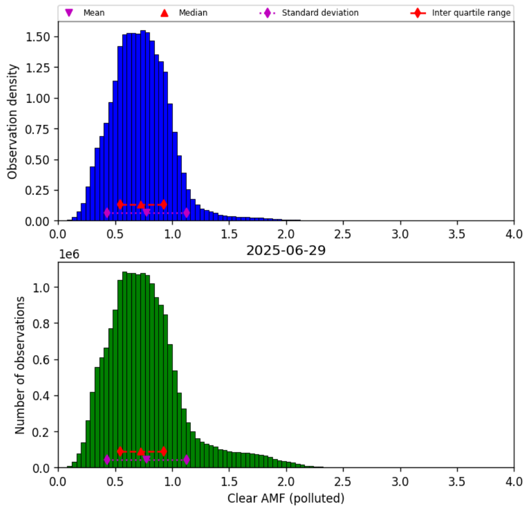
Figure 81: Histogram of “Clear AMF (polluted)” for 2025-06-28 to 2025-06-30
