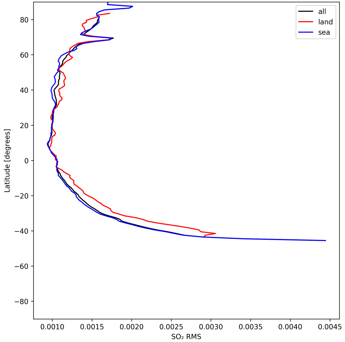
Figure 52: Zonal average of “SO 2 RMS” for 2025-06-28 to 2025-06-30.
