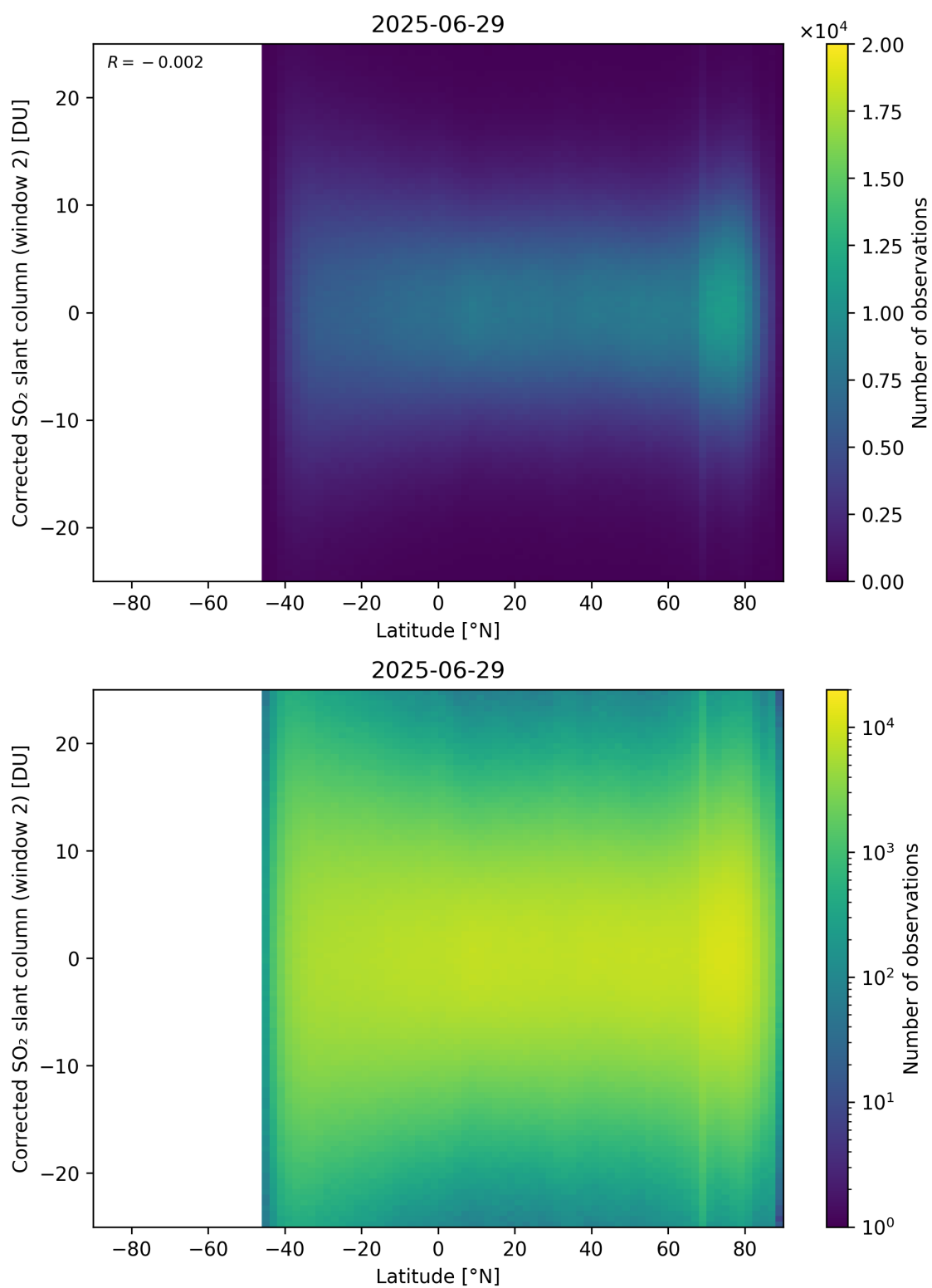
Figure 160: Scatter density plot of “Latitude” against “Corrected SO 2 slant column (window 2)” for 2025-06-28 to 2025-06-30.
