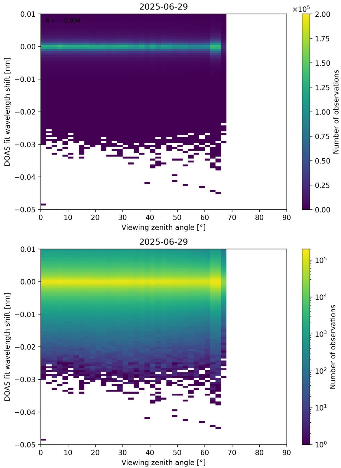
Figure 365: Scatter density plot of “Viewing zenith angle” against “DOAS fit wavelength shift” for 2025-06-28 to 2025-06-30.
