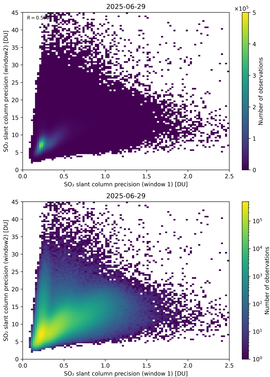
Figure 277: Scatter density plot of “SO 2 slant column precision (window 1)” against “SO 2 slant column precision (window2)” for 2025-06-28 to 2025-06-30.
