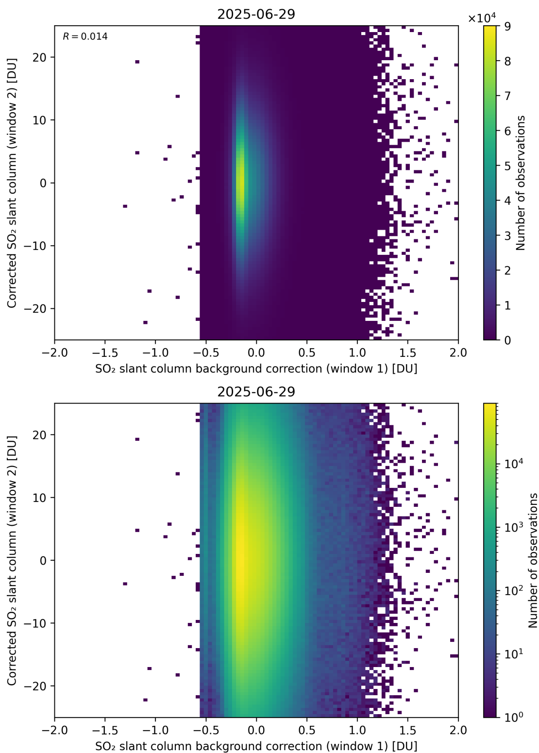
Figure 115: Scatter density plot of “SO 2 slant column background correction (window 1)” against “Corrected SO 2 slant column (window 2)” for 2025-06-28 to 2025-06-30.
