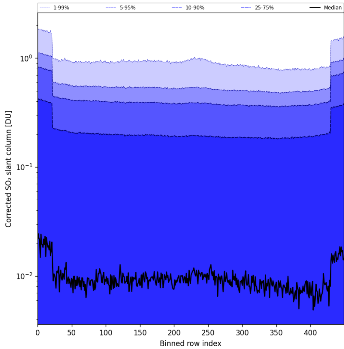
Figure 86: Along track statistics of “Corrected SO 2 slant column” for 2025-06-28 to 2025-06-30
