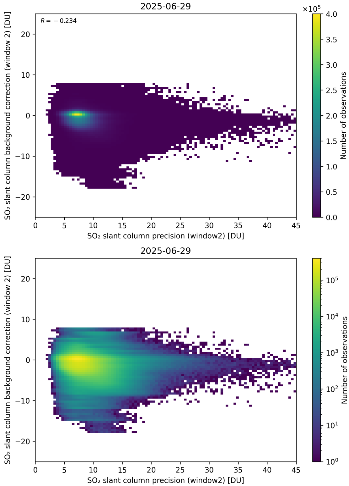
Figure 291: Scatter density plot of “SO 2 slant column precision (window2)” against “SO 2 slant column background correction (window 2)” for 2025-06-28 to 2025-06-30.
