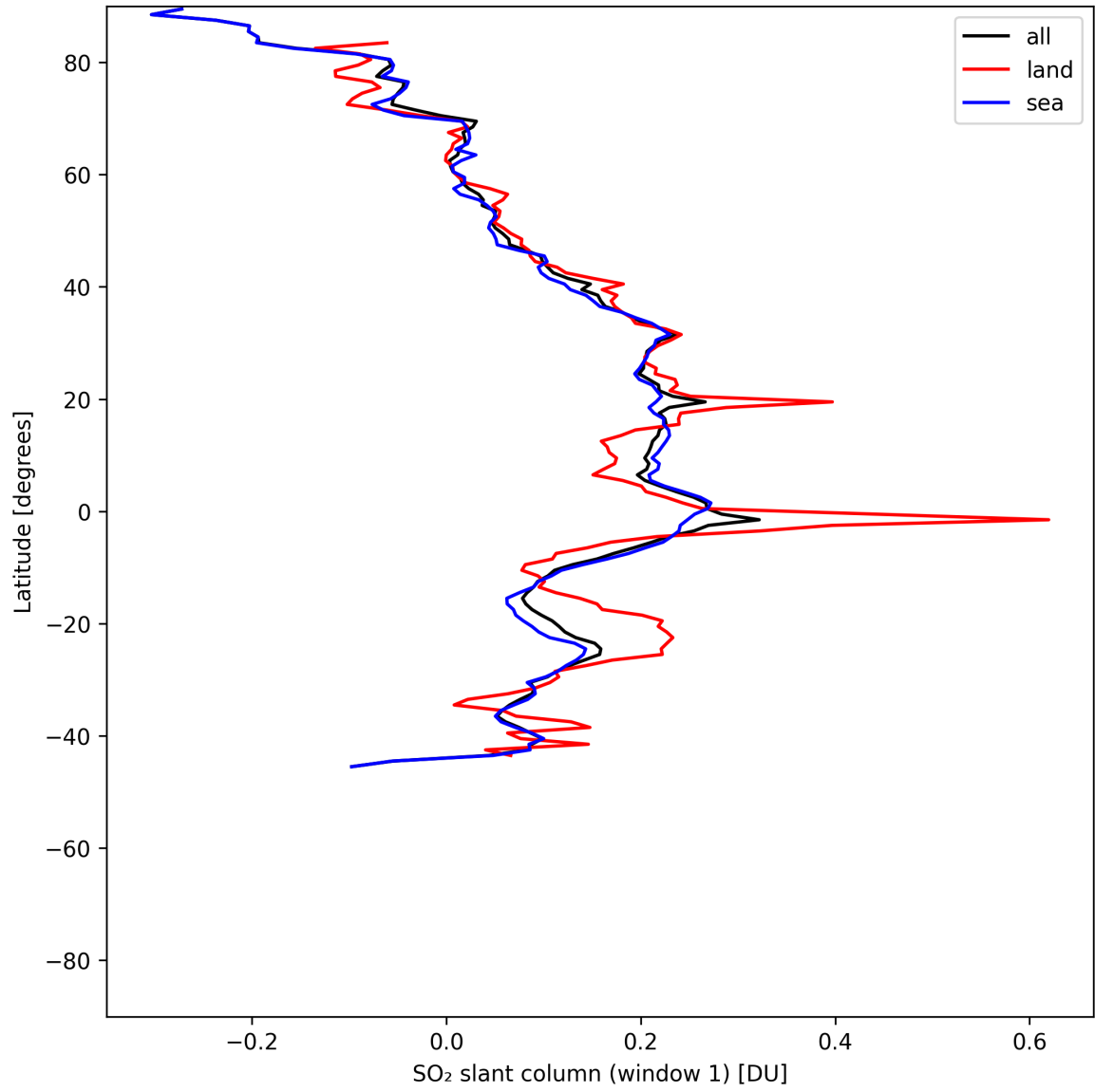
Figure 37: Zonal average of “SO 2 slant column (window 1)” for 2025-06-28 to 2025-06-30.
