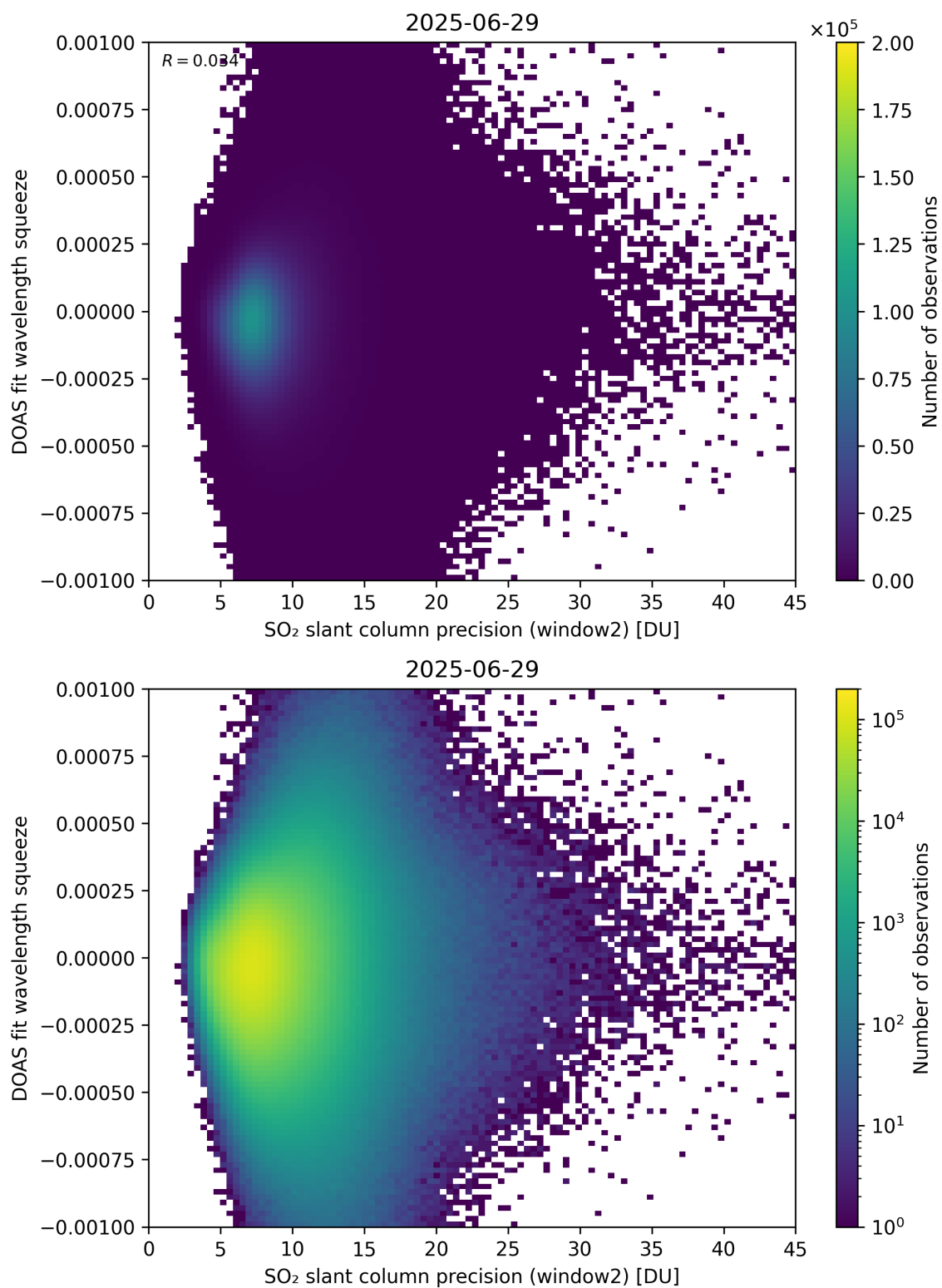
Figure 294: Scatter density plot of “SO 2 slant column precision (window2)” against “DOAS fit wavelength squeeze” for 2025-06-28 to 2025-06-30.
