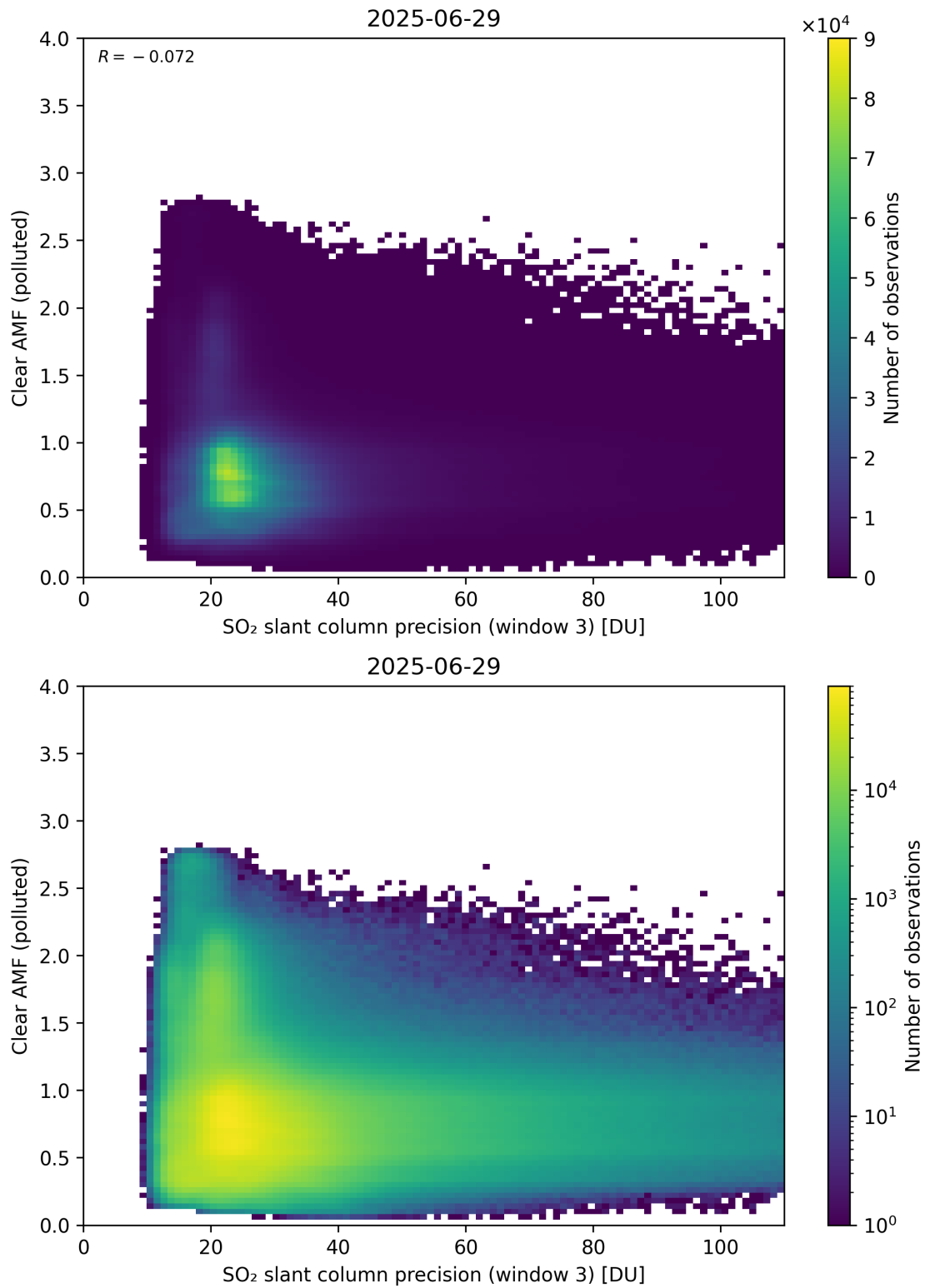
Figure 311: Scatter density plot of “SO 2 slant column precision (window 3)” against “Clear AMF (polluted)” for 2025-06-28 to 2025-06-30.
