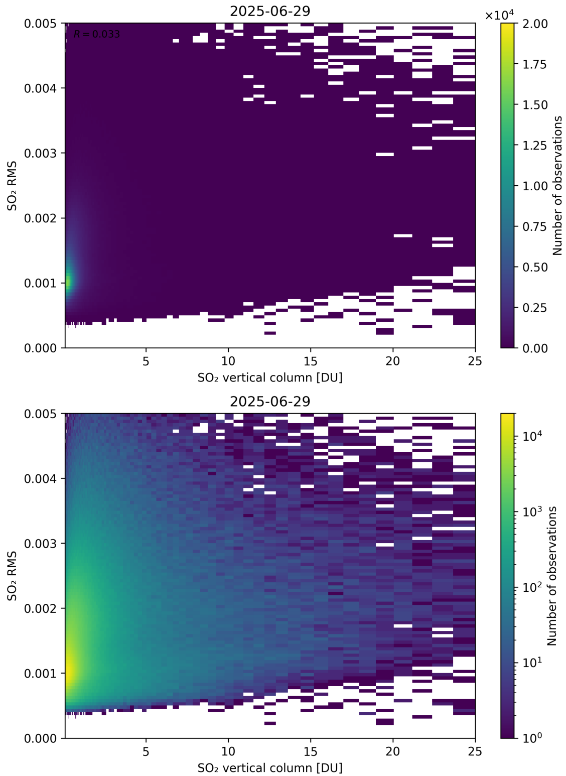
Figure 328: Scatter density plot of “SO 2 vertical column” against “SO 2 RMS” for 2025-06-28 to 2025-06-30.
