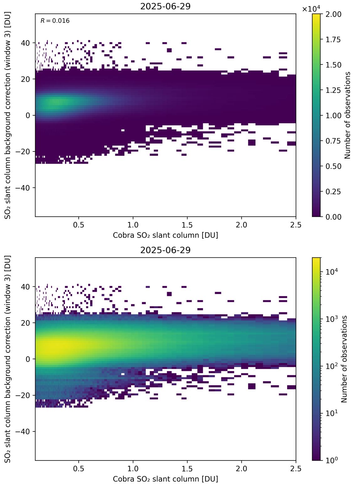
Figure 195: Scatter density plot of “Cobra SO 2 slant column” against “SO 2 slant column background correction (window 3)” for 2025-06-28 to 2025-06-30.
