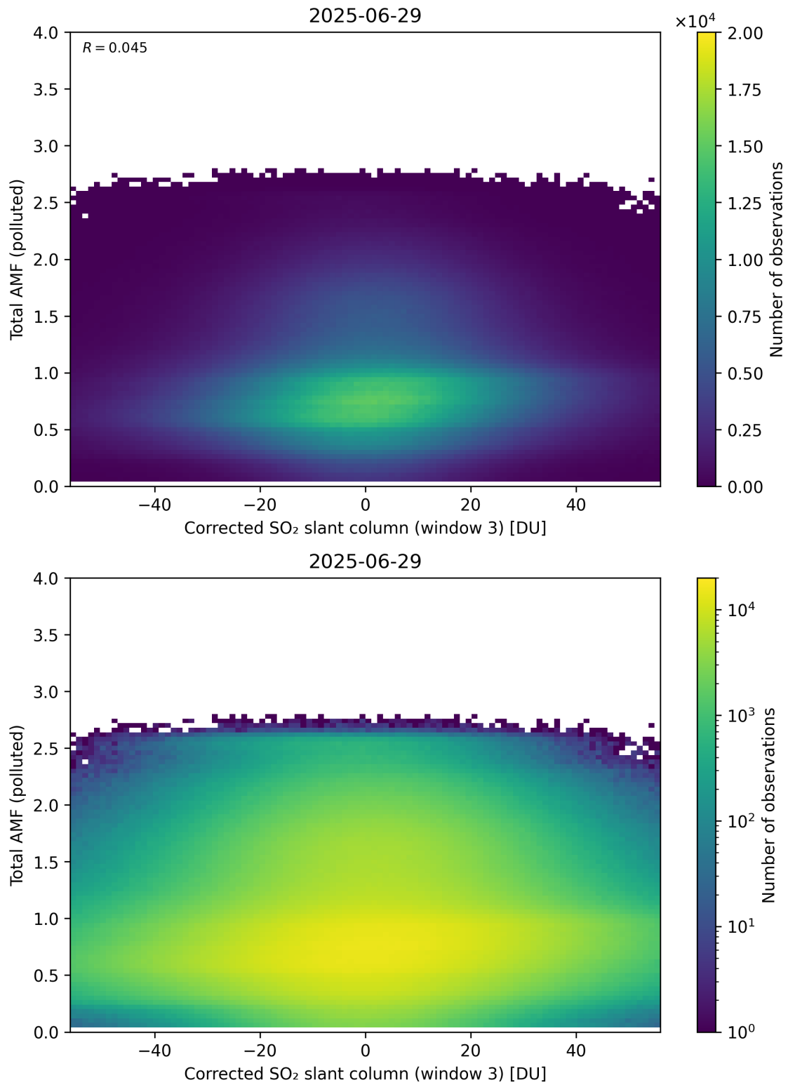
Figure 260: Scatter density plot of “Corrected SO 2 slant column (window 3)” against “Total AMF (polluted)” for 2025-06-28 to 2025-06-30.
