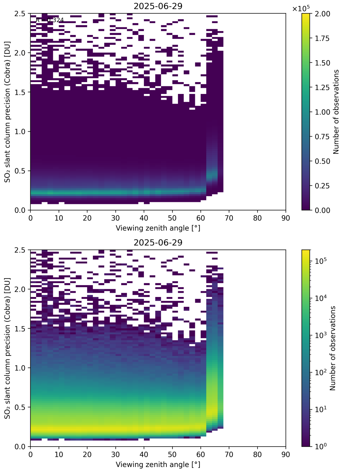
Figure 372: Scatter density plot of “Viewing zenith angle” against “SO 2 slant column precision (Cobra)” for 2025-06-28 to 2025-06-30.
