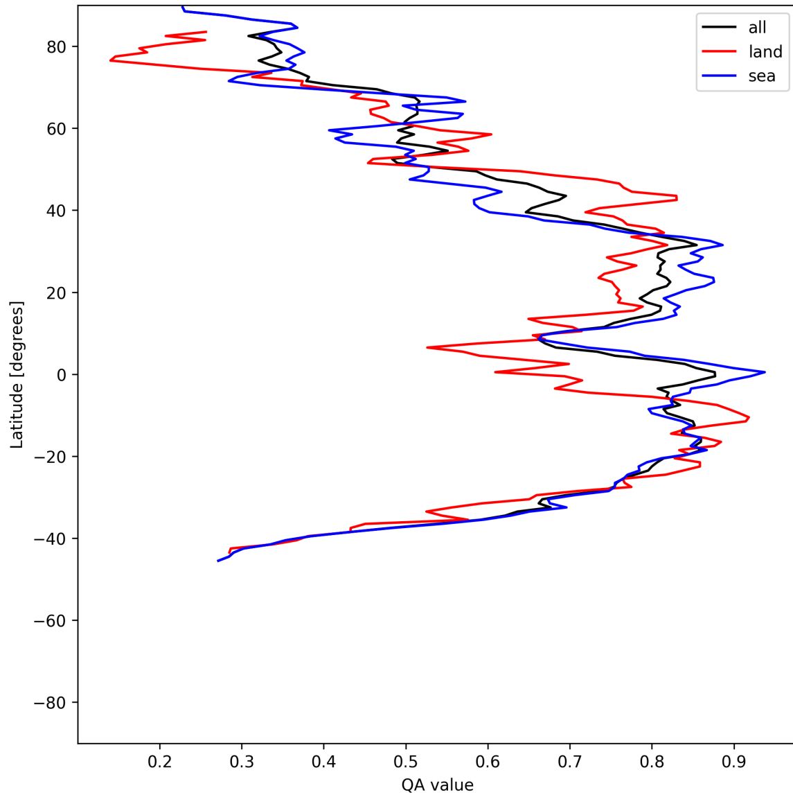
Figure 31: Zonal average of “QA value” for 2025-06-28 to 2025-06-30.
