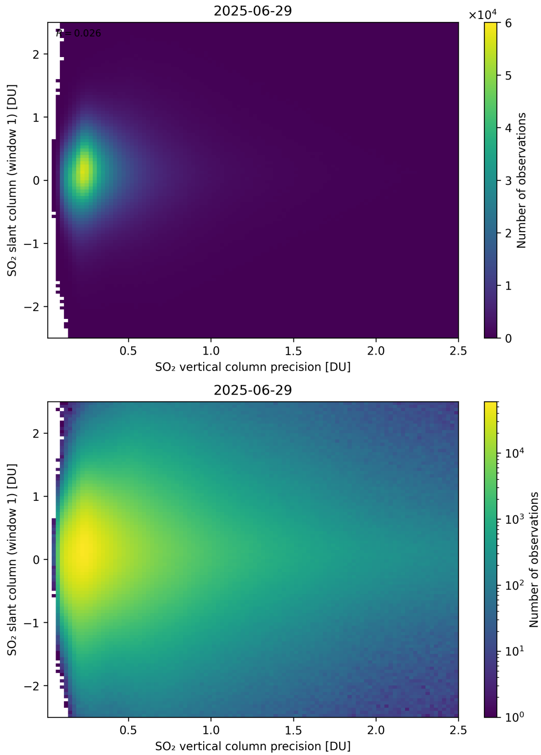
Figure 341: Scatter density plot of “SO 2 vertical column precision” against “SO 2 slant column (window 1)” for 2025-06-28 to 2025-06-30.
