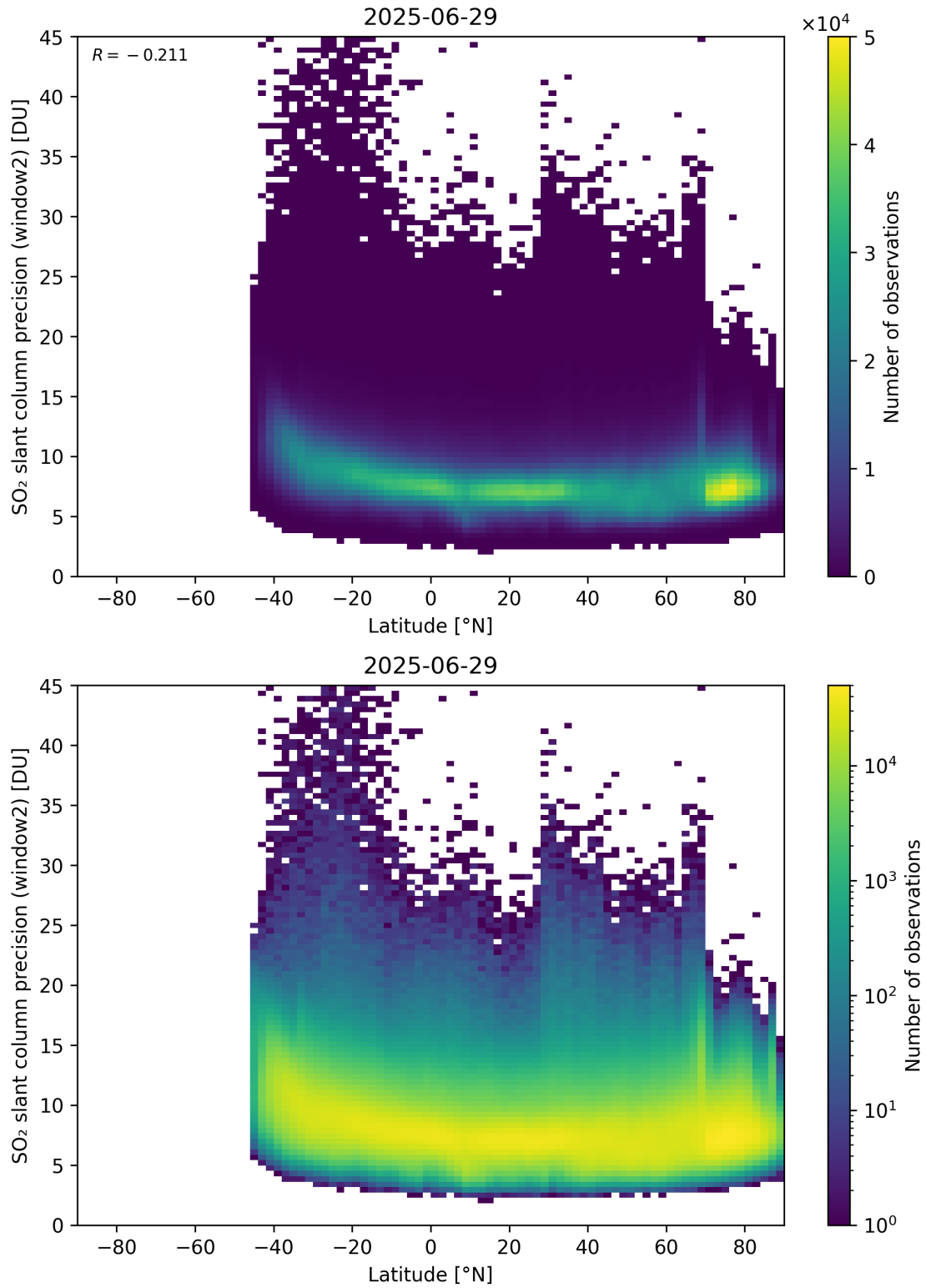
Figure 164: Scatter density plot of “Latitude” against “SO 2 slant column precision (window2)” for 2025-06-28 to 2025-06-30.
