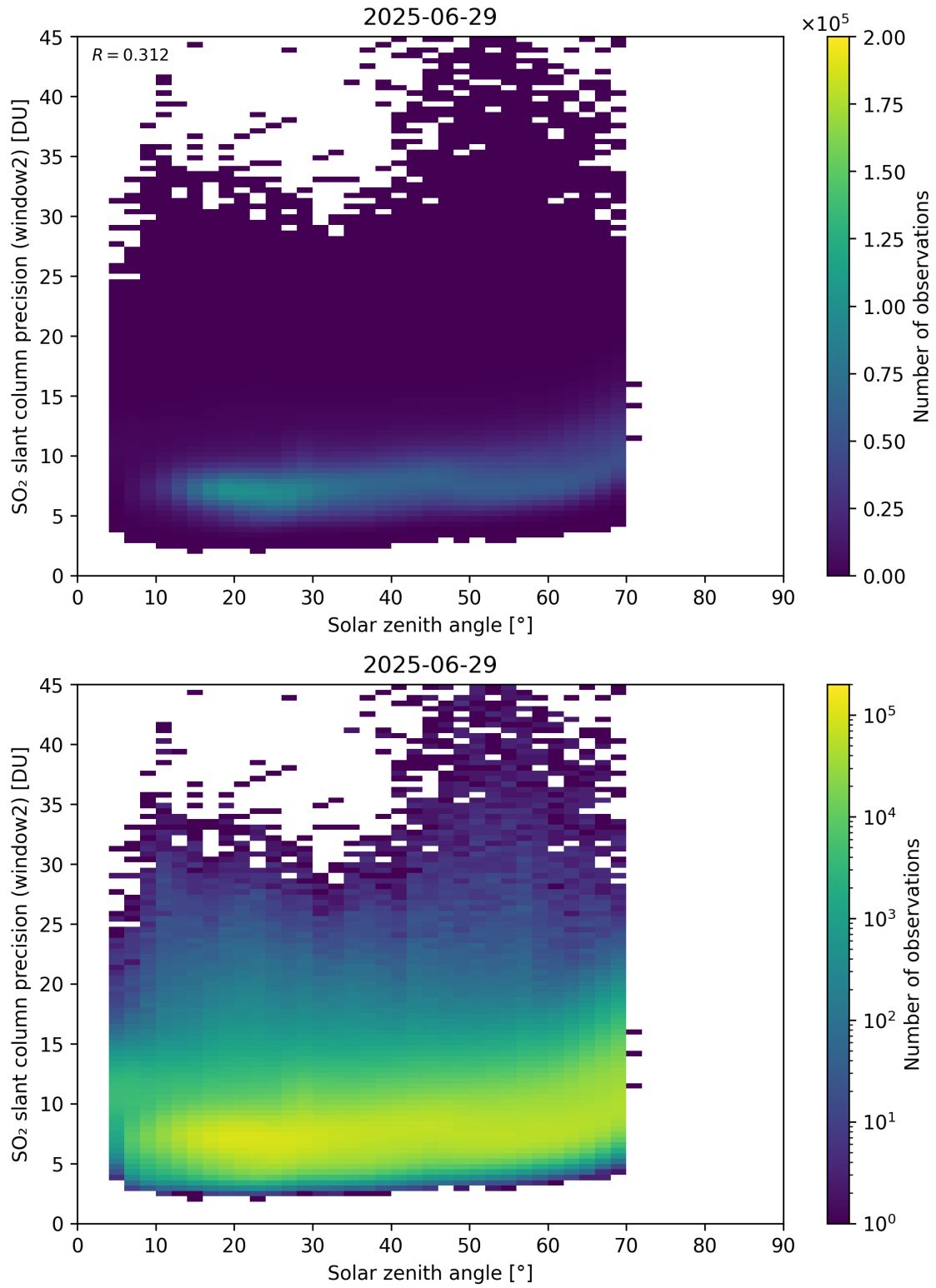
Figure 186: Scatter density plot of “Solar zenith angle” against “SO 2 slant column precision (window2)” for 2025-06-28 to 2025-06-30.
