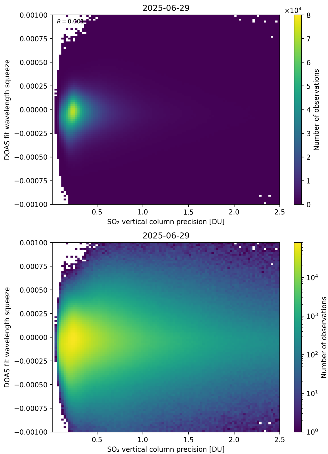
Figure 333: Scatter density plot of “SO 2 vertical column precision” against “DOAS fit wavelength squeeze” for 2025-06-28 to 2025-06-30.
