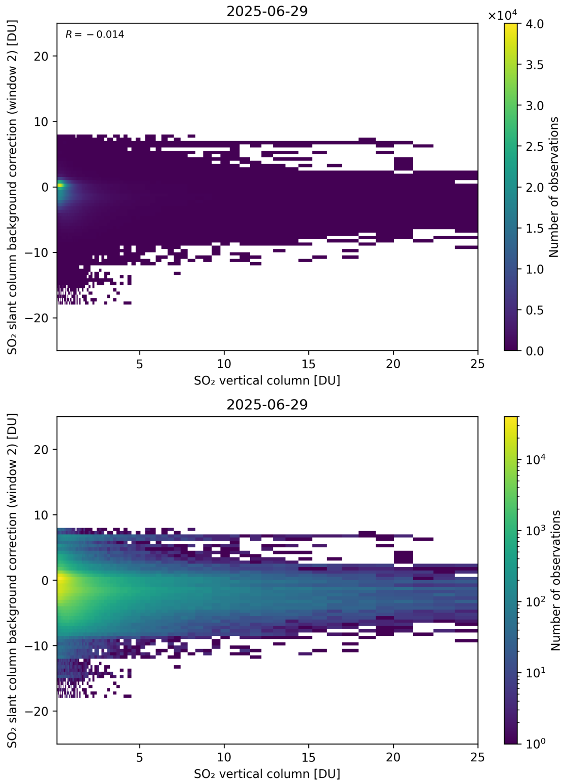
Figure 324: Scatter density plot of “SO 2 vertical column” against “SO 2 slant column background correction (window 2)” for 2025-06-28 to 2025-06-30.
