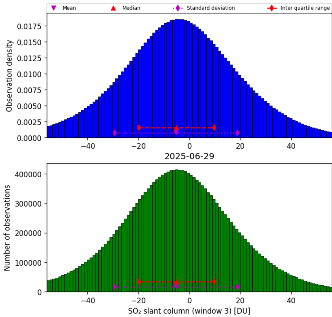
Figure 71: Histogram of “SO 2 slant column (window 3)” for 2025-06-28 to 2025-06-30
