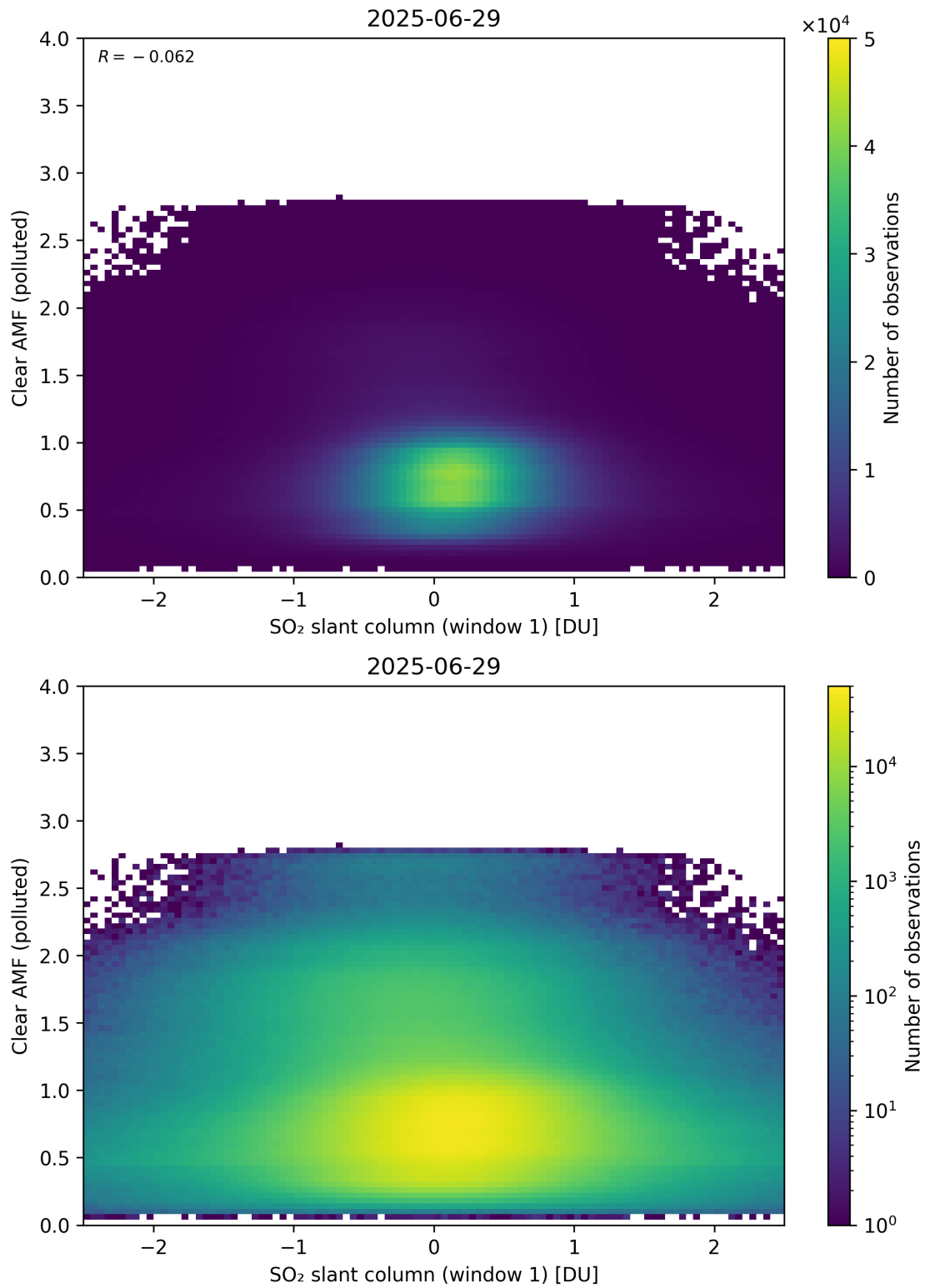
Figure 282: Scatter density plot of “SO 2 slant column (window 1)” against “Clear AMF (polluted)” for 2025-06-28 to 2025-06-30.
