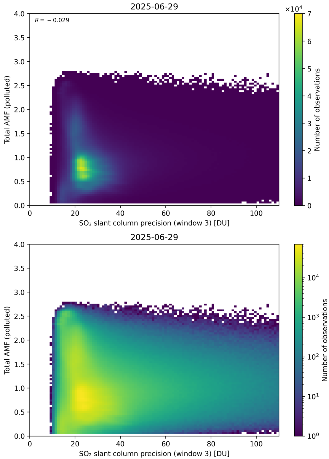
Figure 313: Scatter density plot of “SO 2 slant column precision (window 3)” against “Total AMF (polluted)” for 2025-06-28 to 2025-06-30.
