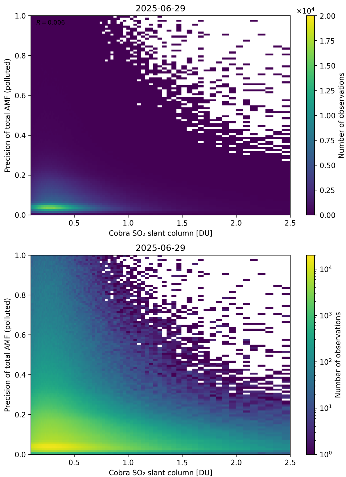
Figure 225: Scatter density plot of “Cobra SO 2 slant column” against “Precision of total AMF (polluted)” for 2025-06-28 to 2025-06-30.
