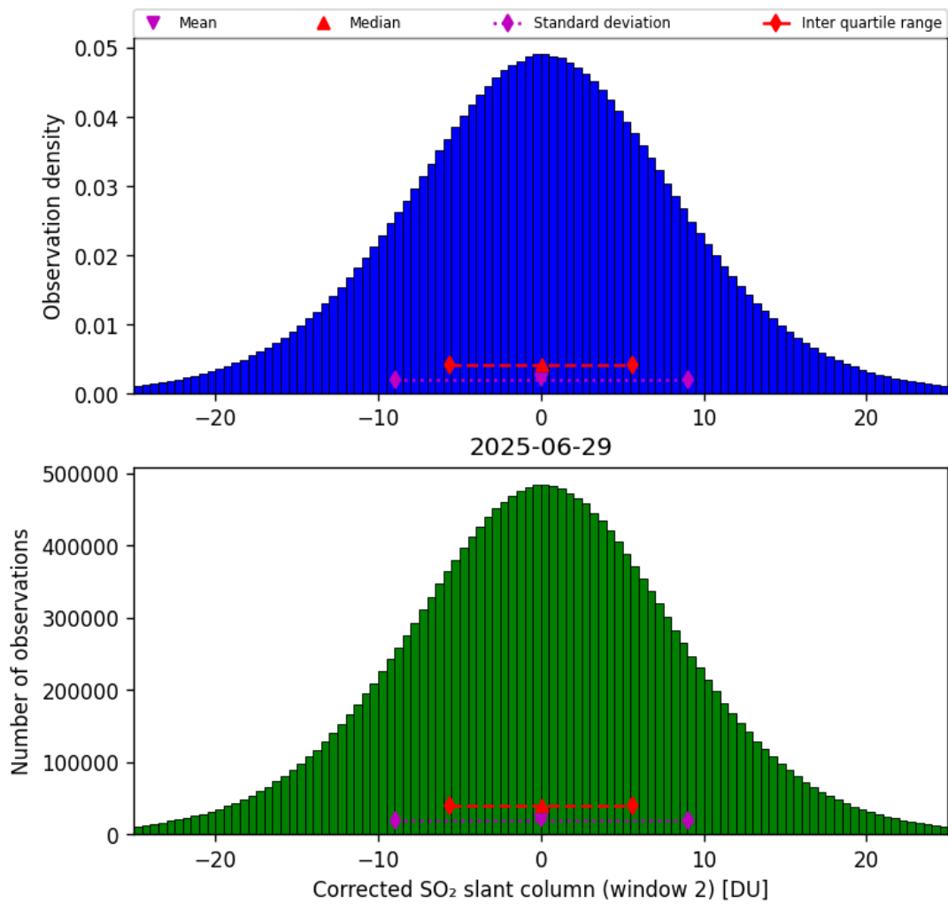
Figure 69: Histogram of “Corrected SO 2 slant column (window 2)” for 2025-06-28 to 2025-06-30
