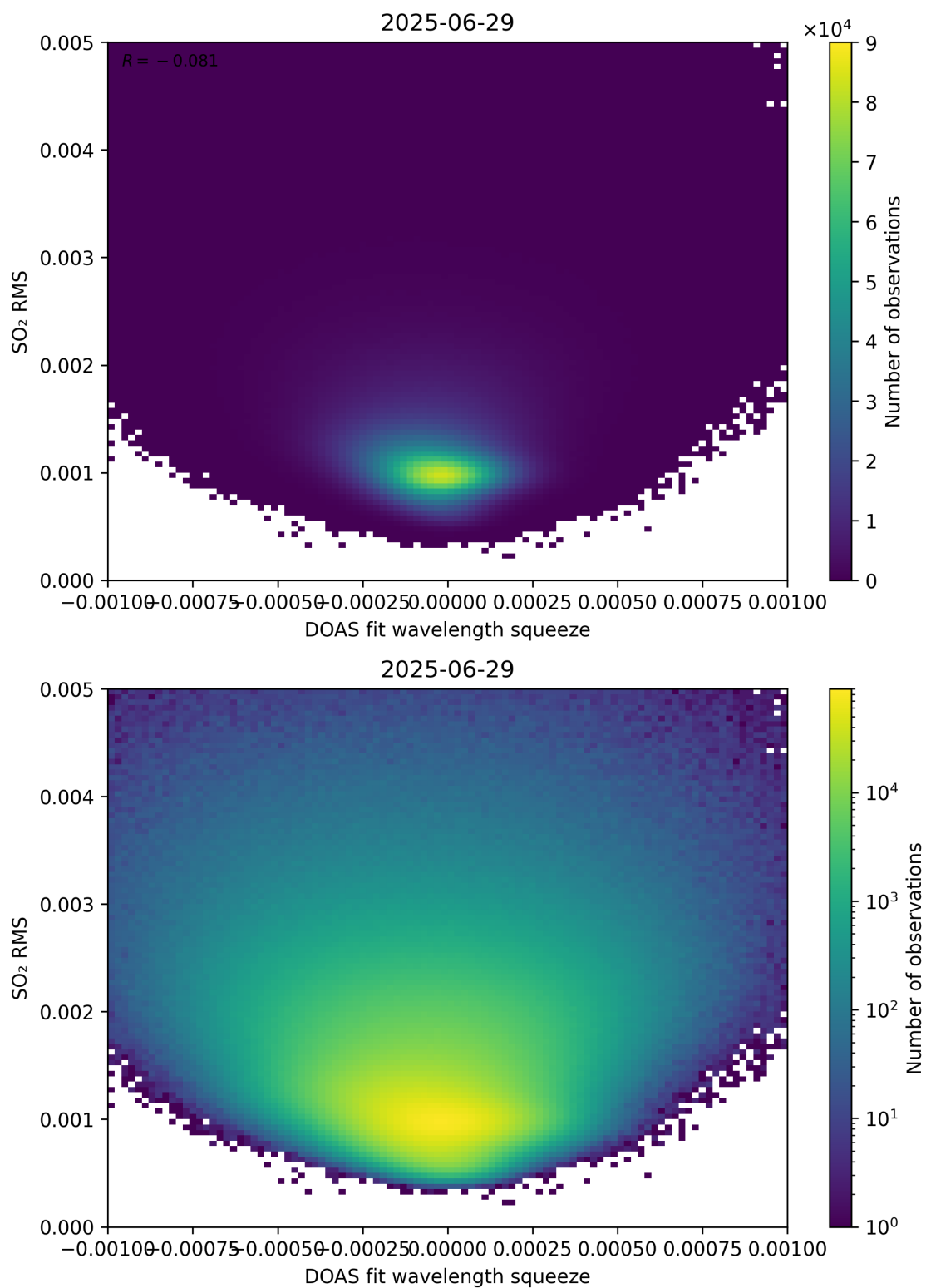
Figure 143: Scatter density plot of “DOAS fit wavelength squeeze” against “SO 2 RMS” for 2025-06-28 to 2025-06-30.
