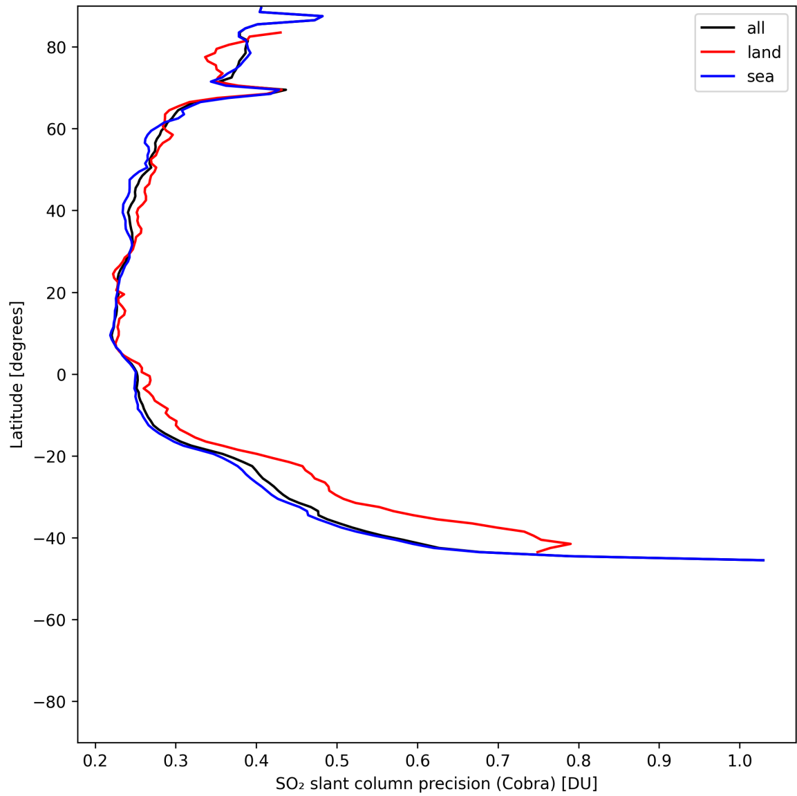
Figure 36: Zonal average of “SO 2 slant column precision (Cobra)” for 2025-06-28 to 2025-06-30.
