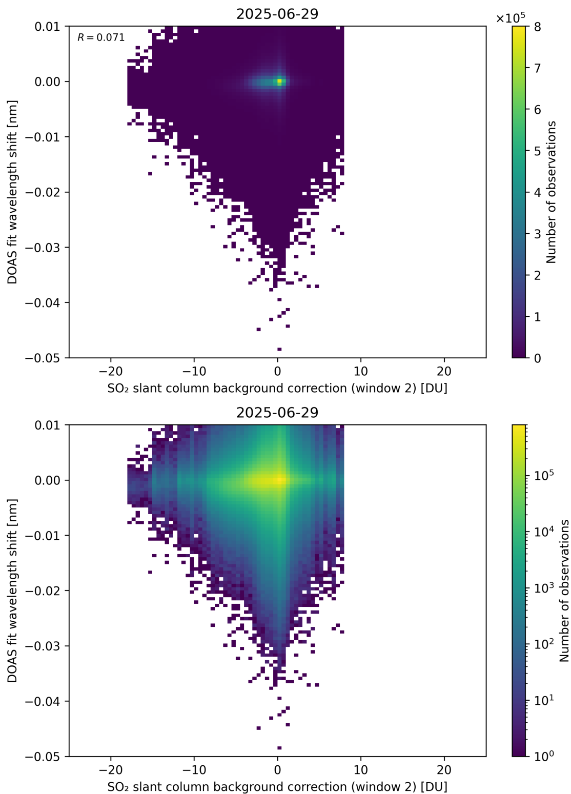
Figure 123: Scatter density plot of “SO 2 slant column background correction (window 2)” against “DOAS fit wavelength shift” for 2025-06-28 to 2025-06-30.
