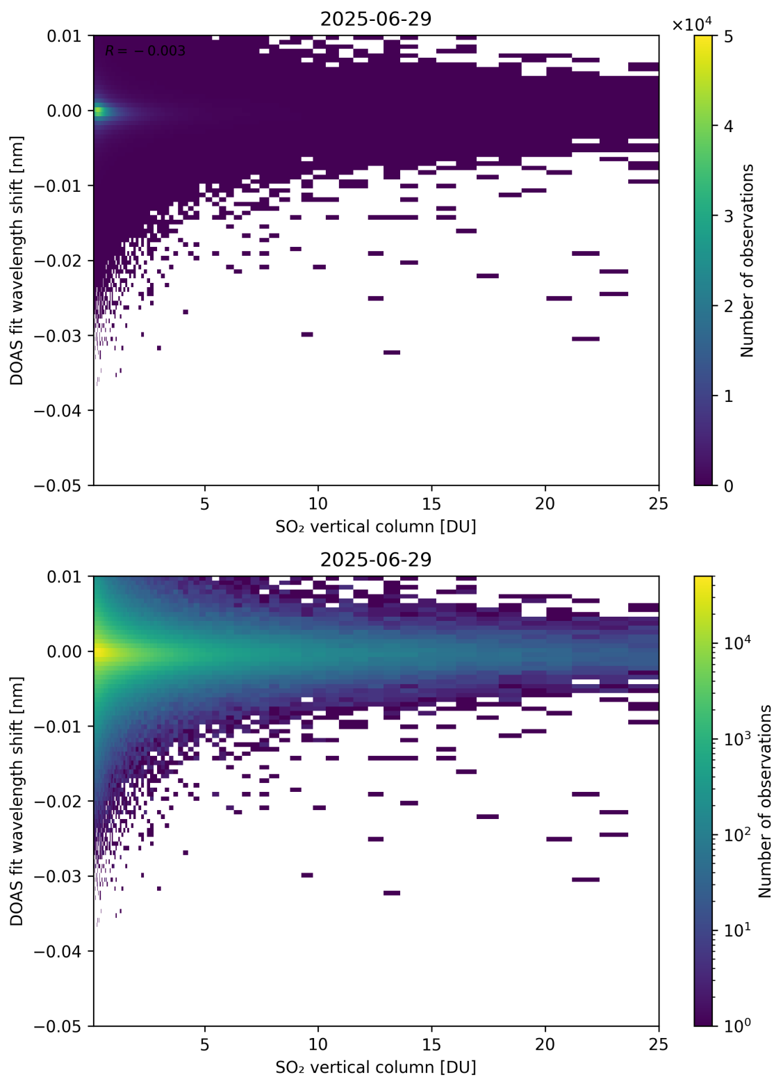
Figure 326: Scatter density plot of “SO 2 vertical column” against “DOAS fit wavelength shift” for 2025-06-28 to 2025-06-30.
