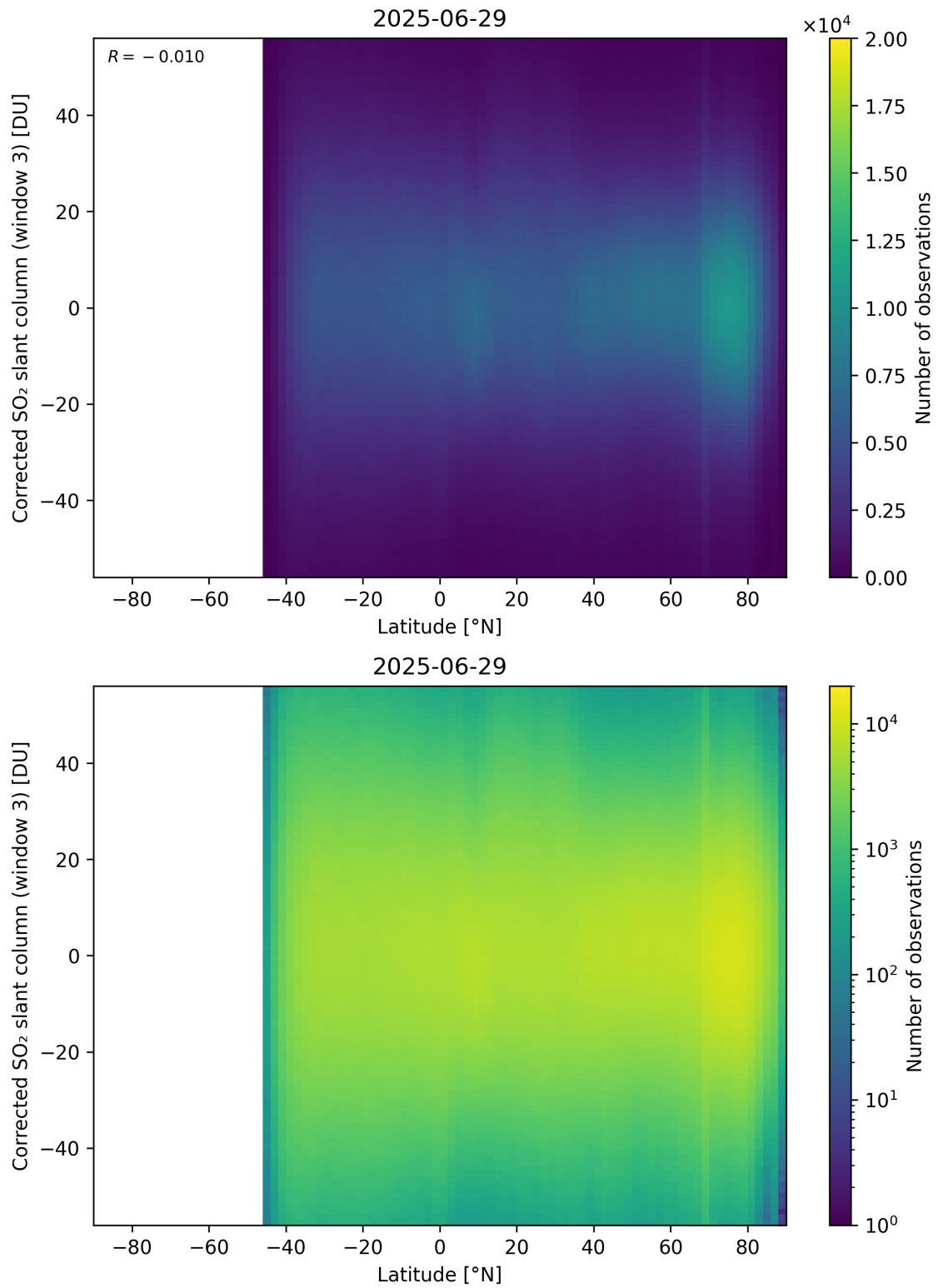
Figure 161: Scatter density plot of “Latitude” against “Corrected SO 2 slant column (window 3)” for 2025-06-28 to 2025-06-30.
