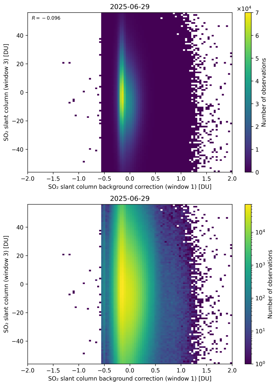
Figure 118: Scatter density plot of “SO 2 slant column background correction (window 1)” against “SO 2 slant column (window 3)” for 2025-06-28 to 2025-06-30.
