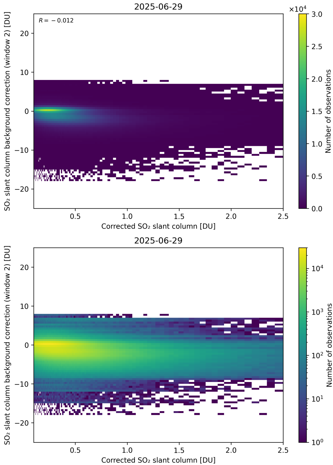
Figure 227: Scatter density plot of “Corrected SO 2 slant column” against “SO 2 slant column background correction (window 2)” for 2025-06-28 to 2025-06-30.
