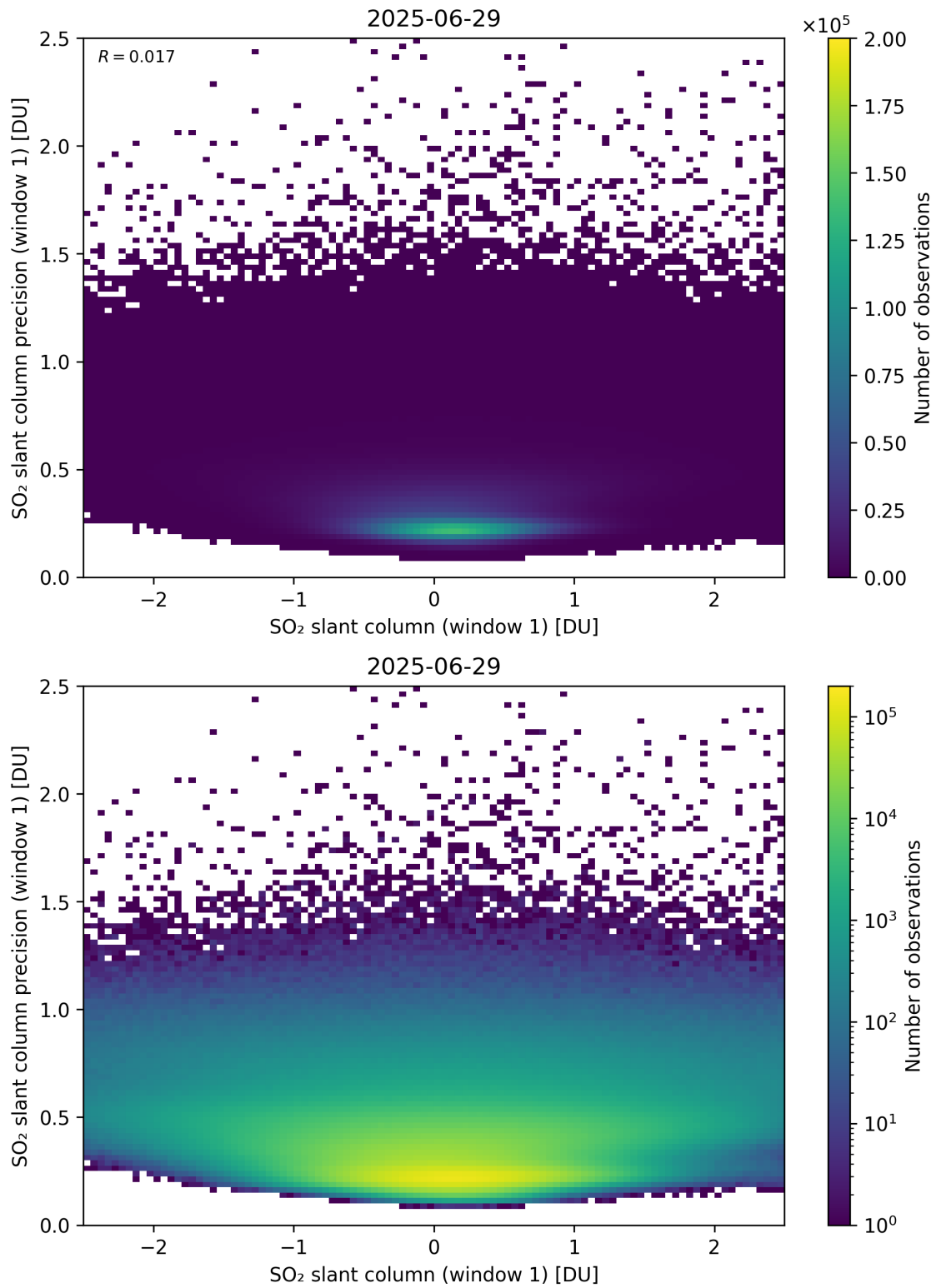
Figure 285: Scatter density plot of “SO 2 slant column (window 1)” against “SO 2 slant column precision (window 1)” for 2025-06-28 to 2025-06-30.
