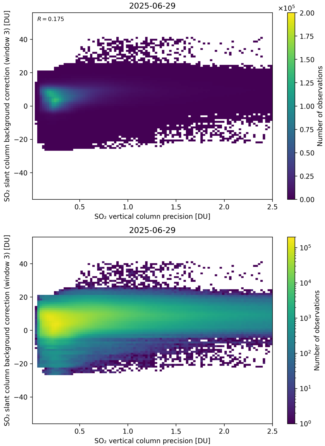
Figure 331: Scatter density plot of “SO 2 vertical column precision” against “SO 2 slant column background correction (window 3)” for 2025-06-28 to 2025-06-30.
