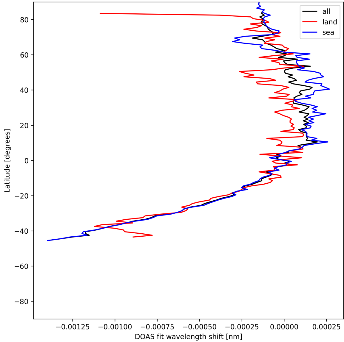
Figure 50: Zonal average of “DOAS fit wavelength shift” for 2025-06-28 to 2025-06-30.
