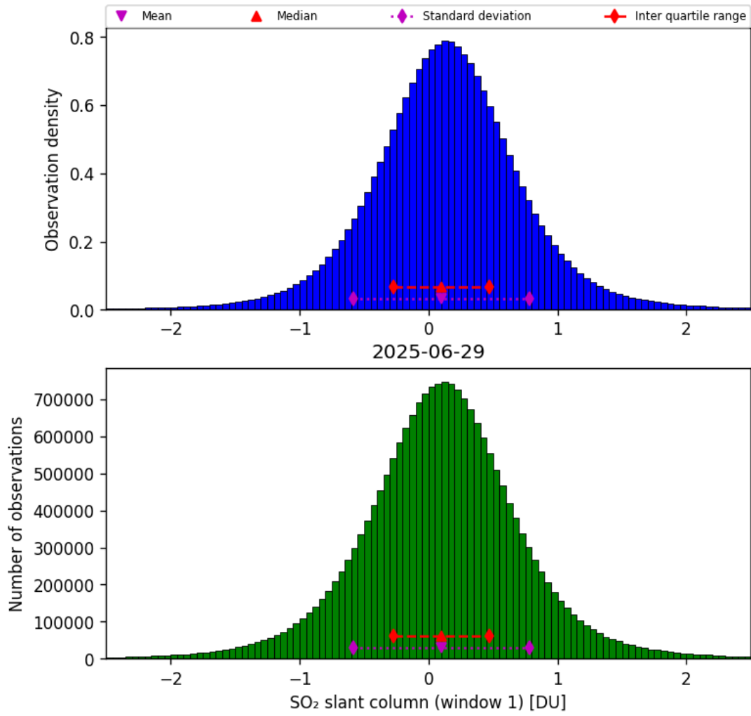
Figure 63: Histogram of “SO 2 slant column (window 1)” for 2025-06-28 to 2025-06-30
