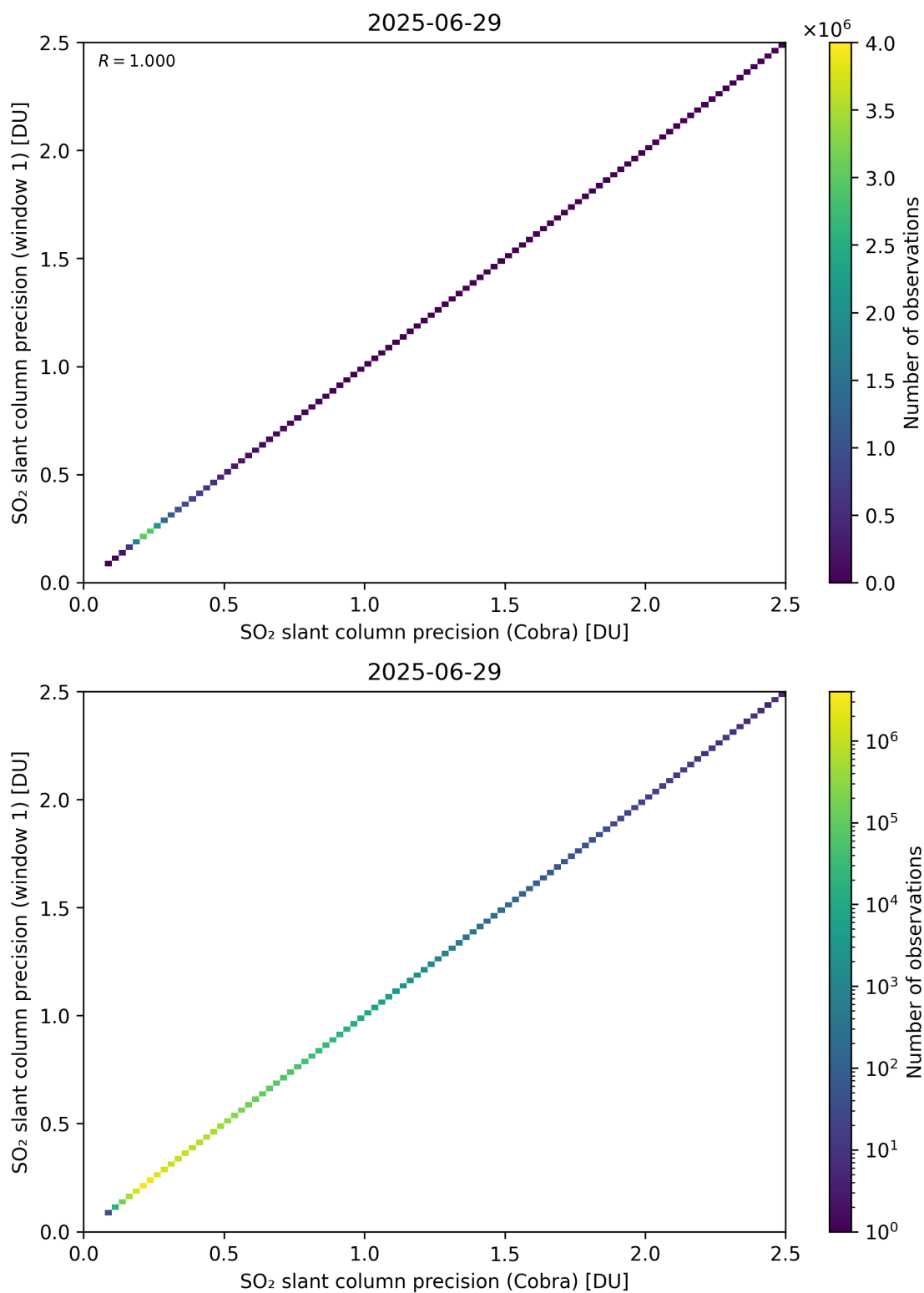
Figure 209: Scatter density plot of “SO 2 slant column precision (Cobra)” against “SO 2 slant column precision (window 1)” for 2025-06-28 to 2025-06-30.
