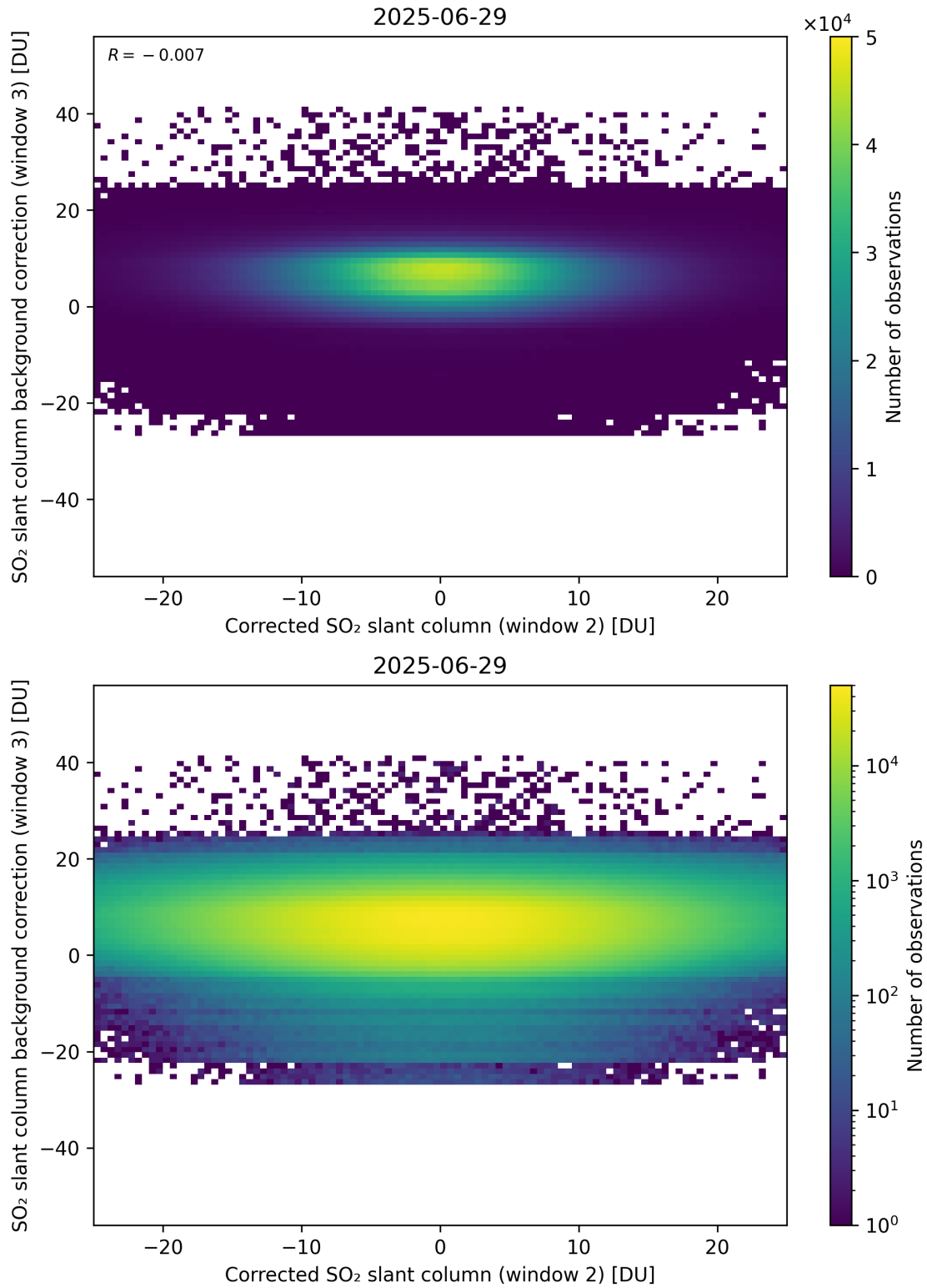
Figure 245: Scatter density plot of “Corrected SO 2 slant column (window 2)” against “SO 2 slant column background correction (window 3)” for 2025-06-28 to 2025-06-30.
