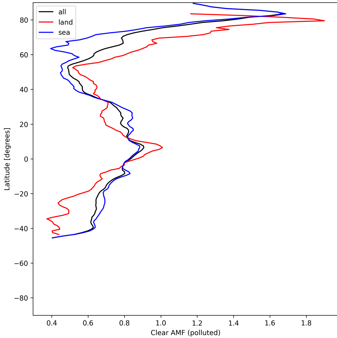
Figure 55: Zonal average of “Clear AMF (polluted)” for 2025-06-28 to 2025-06-30.
