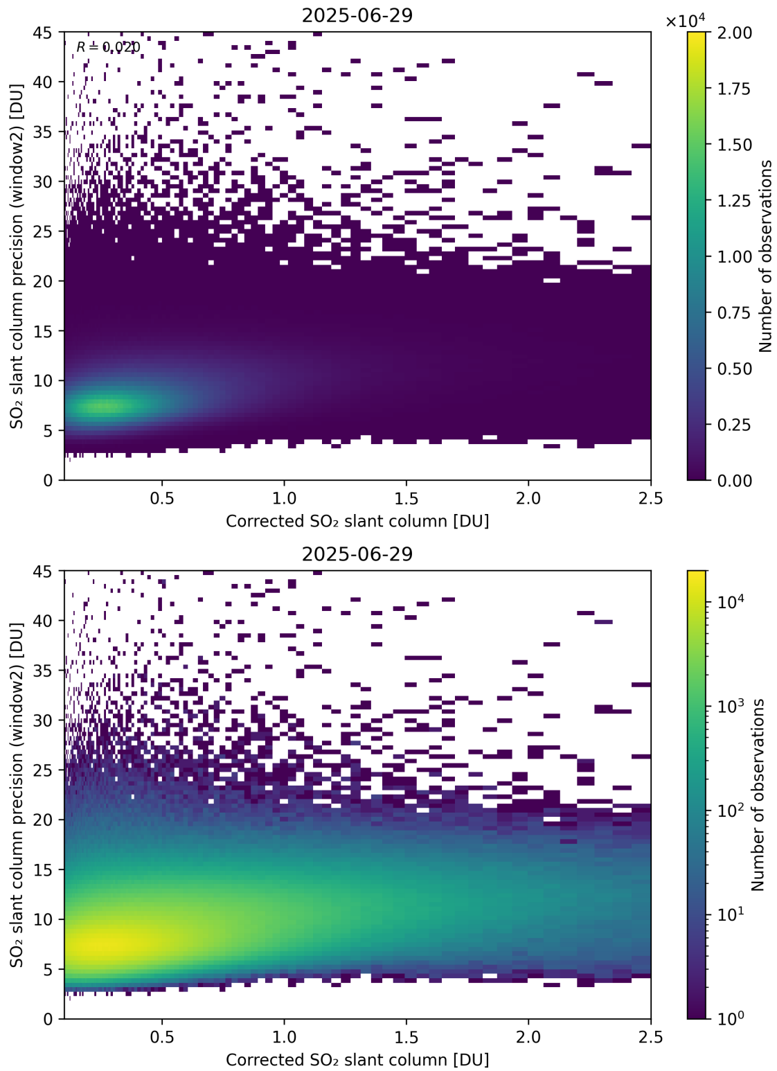
Figure 239: Scatter density plot of “Corrected SO 2 slant column” against “SO 2 slant column precision (window2)” for 2025-06-28 to 2025-06-30.
