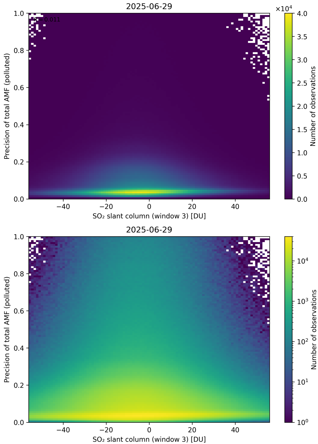
Figure 319: Scatter density plot of “SO 2 slant column (window 3)” against “Precision of total AMF (polluted)” for 2025-06-28 to 2025-06-30.
