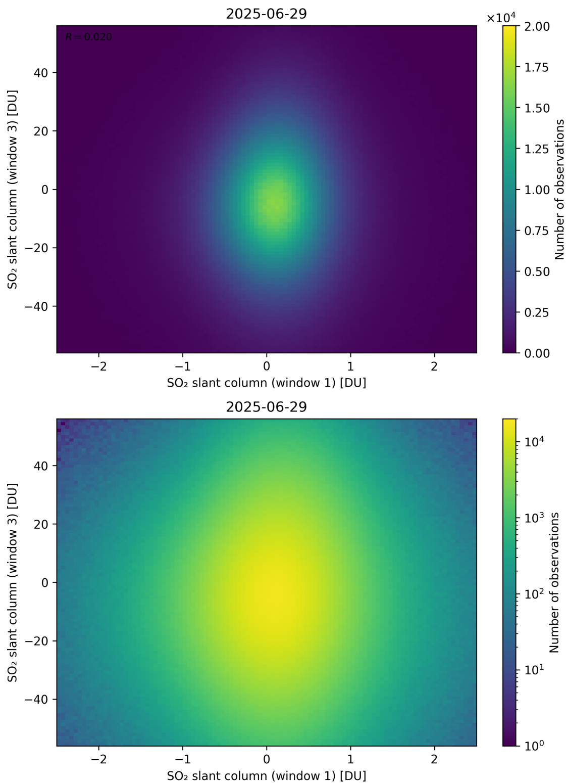
Figure 287: Scatter density plot of “SO 2 slant column (window 1)” against “SO 2 slant column (window 3)” for 2025-06-28 to 2025-06-30.
