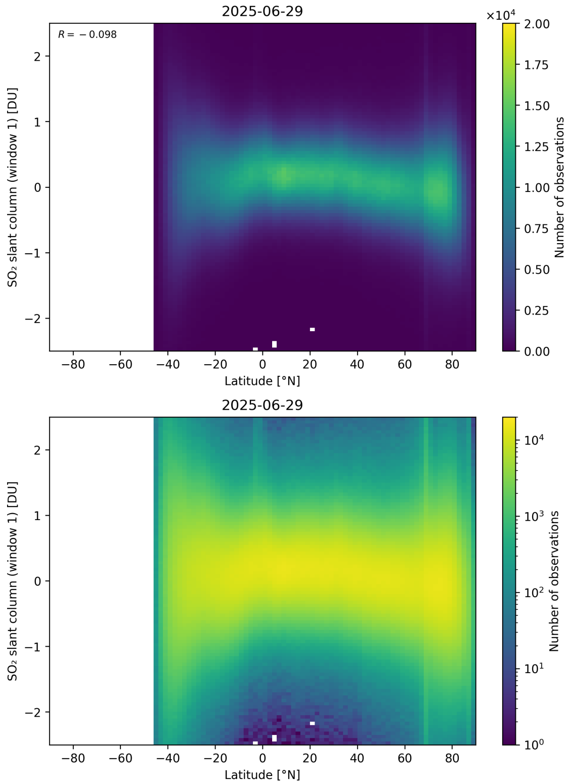
Figure 162: Scatter density plot of “Latitude” against “SO 2 slant column (window 1)” for 2025-06-28 to 2025-06-30.
