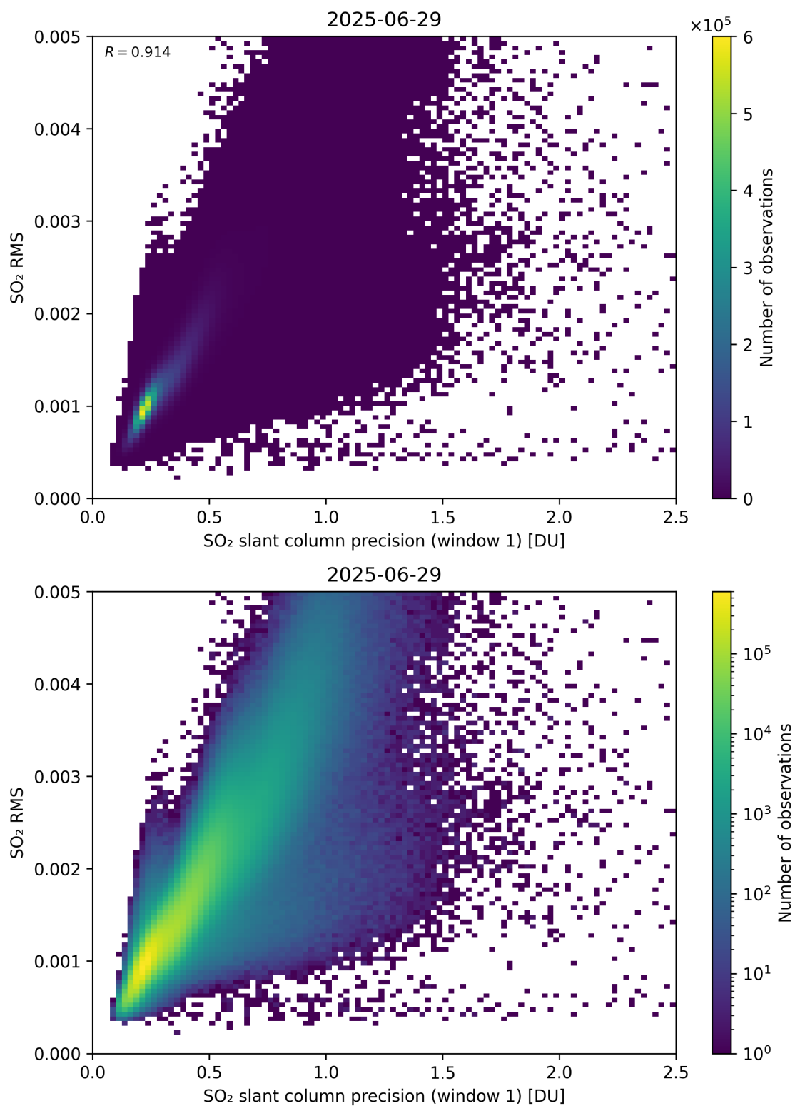
Figure 273: Scatter density plot of “SO 2 slant column precision (window 1)” against “SO 2 RMS” for 2025-06-28 to 2025-06-30.
