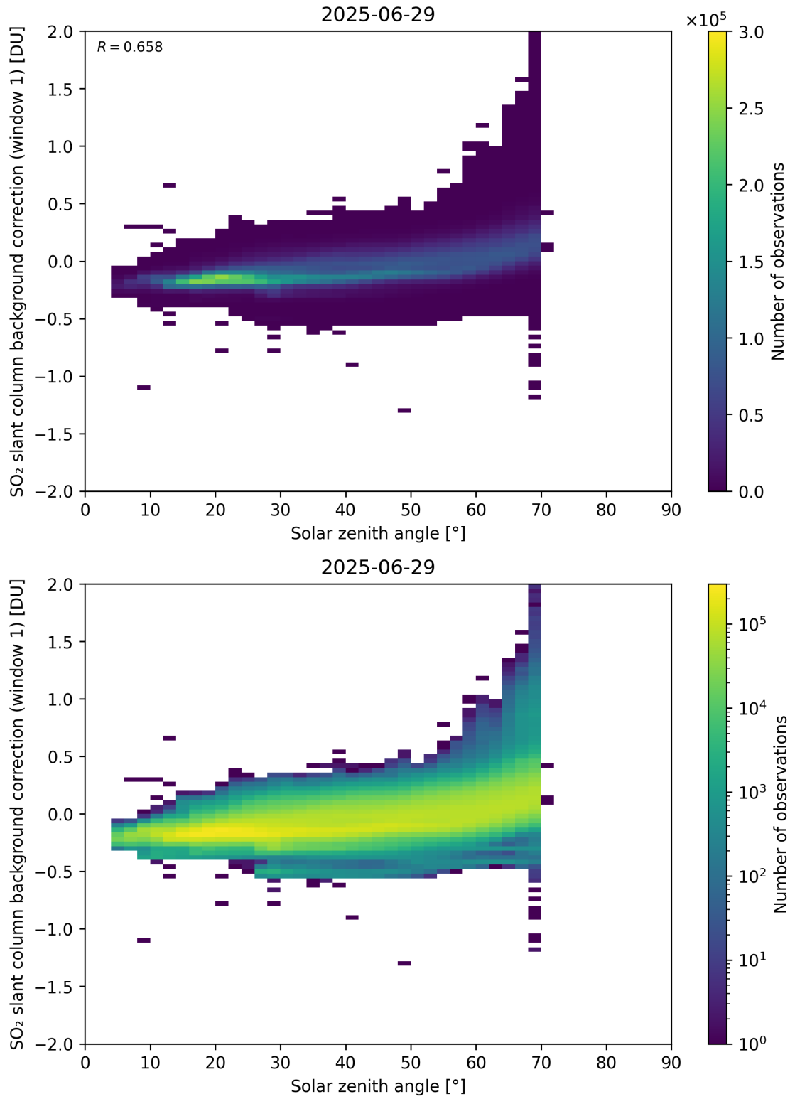
Figure 171: Scatter density plot of “Solar zenith angle” against “SO 2 slant column background correction (window 1)” for 2025-06-28 to 2025-06-30.
