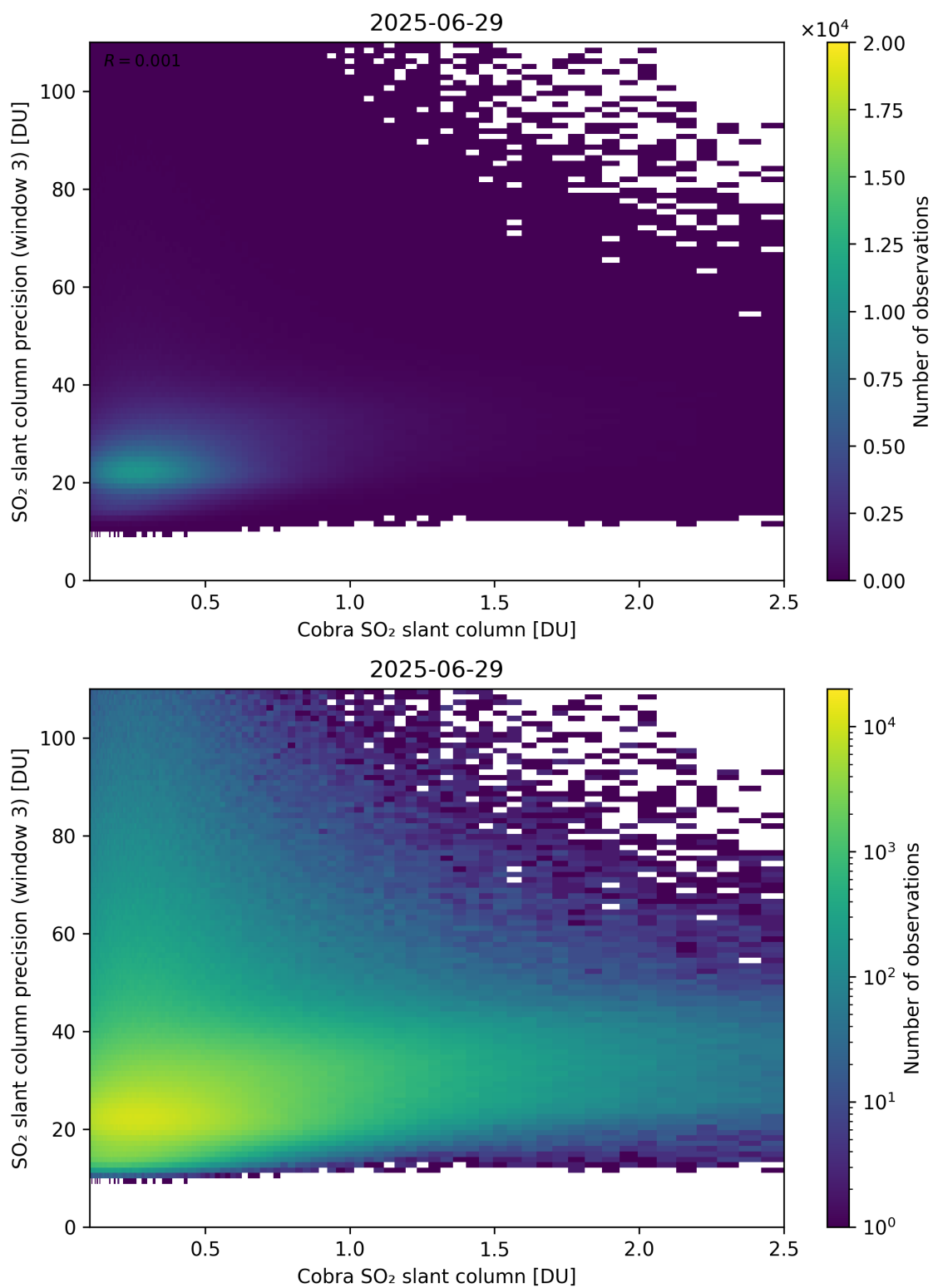
Figure 223: Scatter density plot of “Cobra SO 2 slant column” against “SO 2 slant column precision (window 3)” for 2025-06-28 to 2025-06-30.
