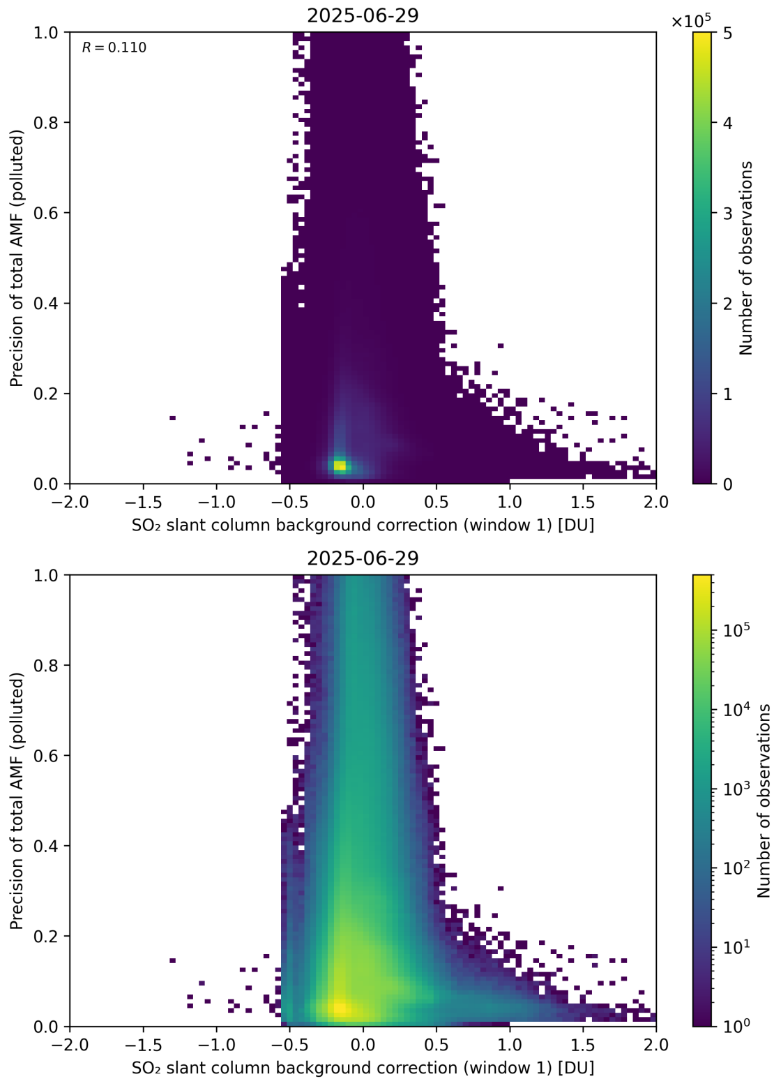
Figure 121: Scatter density plot of “SO 2 slant column background correction (window 1)” against “Precision of total AMF (polluted)” for 2025-06-28 to 2025-06-30.
