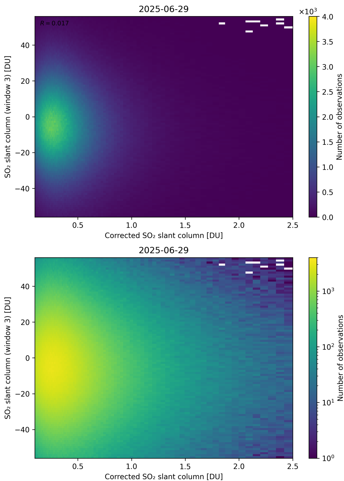
Figure 240: Scatter density plot of “Corrected SO 2 slant column” against “SO 2 slant column (window 3)” for 2025-06-28 to 2025-06-30.
