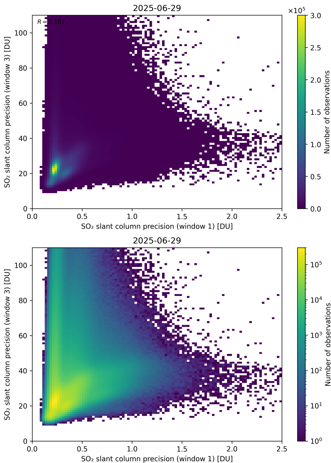
Figure 279: Scatter density plot of “SO 2 slant column precision (window 1)” against “SO 2 slant column precision (window 3)” for 2025-06-28 to 2025-06-30.
