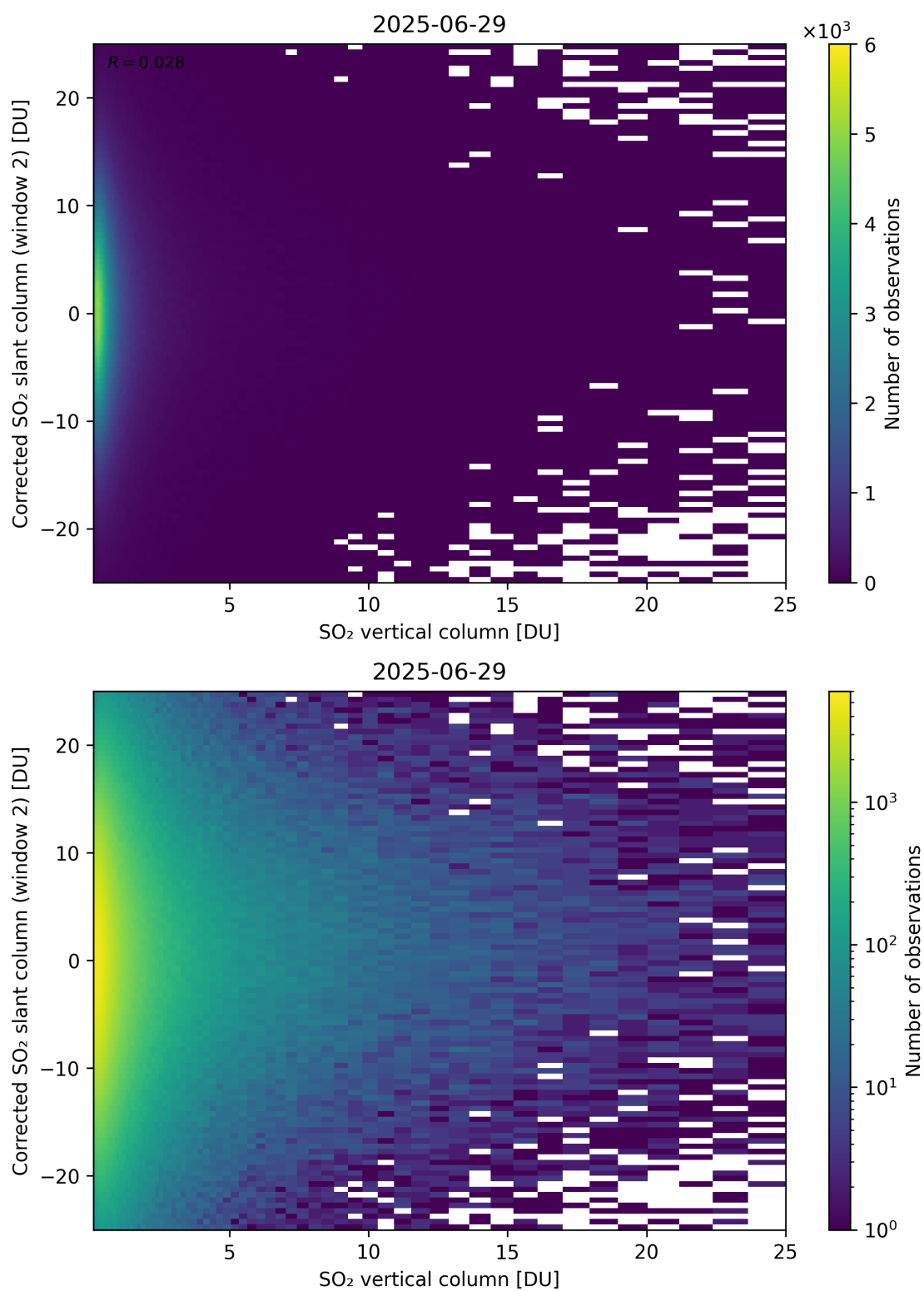
Figure 352: Scatter density plot of “SO 2 vertical column” against “Corrected SO 2 slant column (window 2)” for 2025-06-28 to 2025-06-30.
