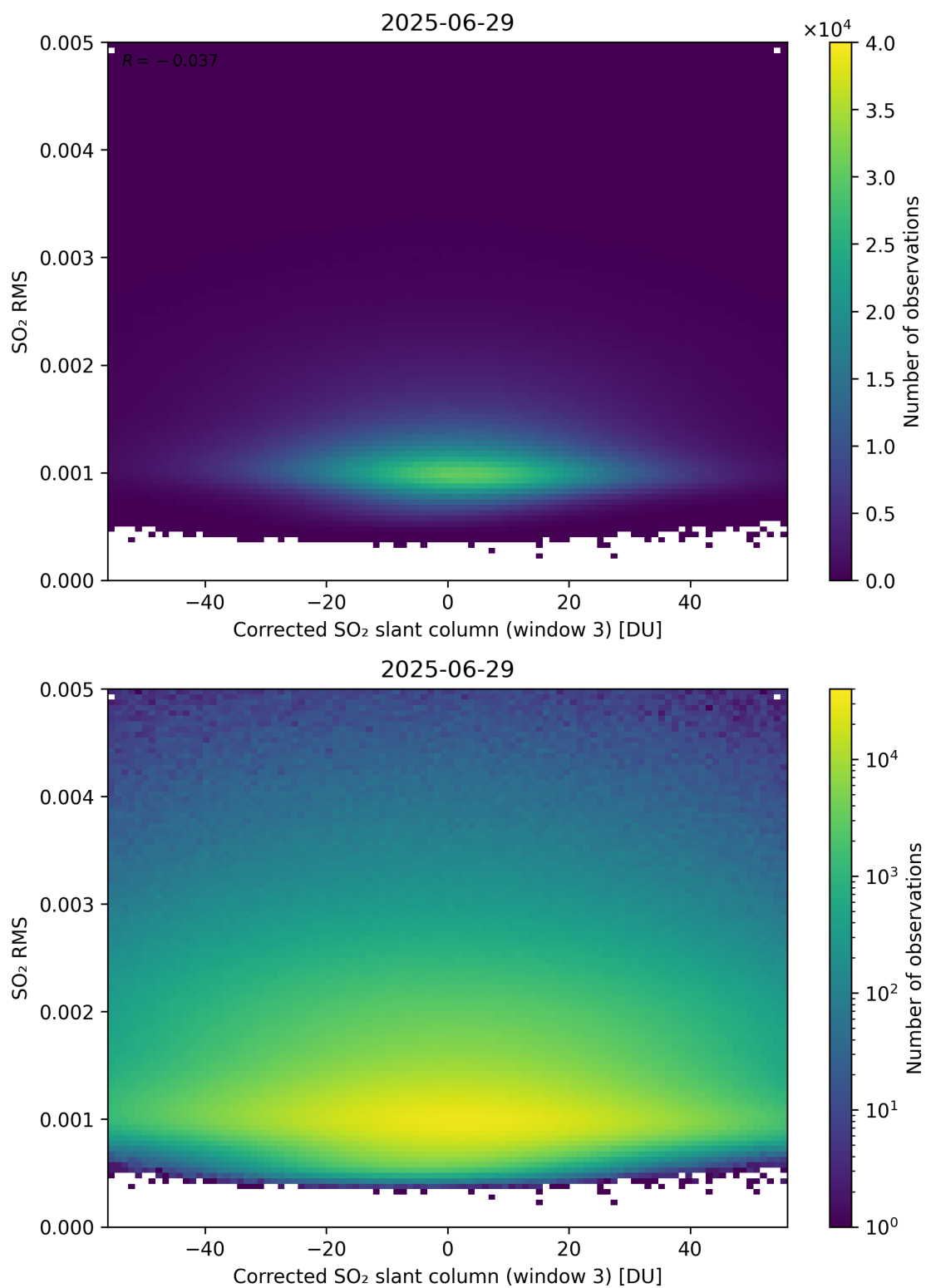
Figure 258: Scatter density plot of “Corrected SO 2 slant column (window 3)” against “SO 2 RMS” for 2025-06-28 to 2025-06-30.
