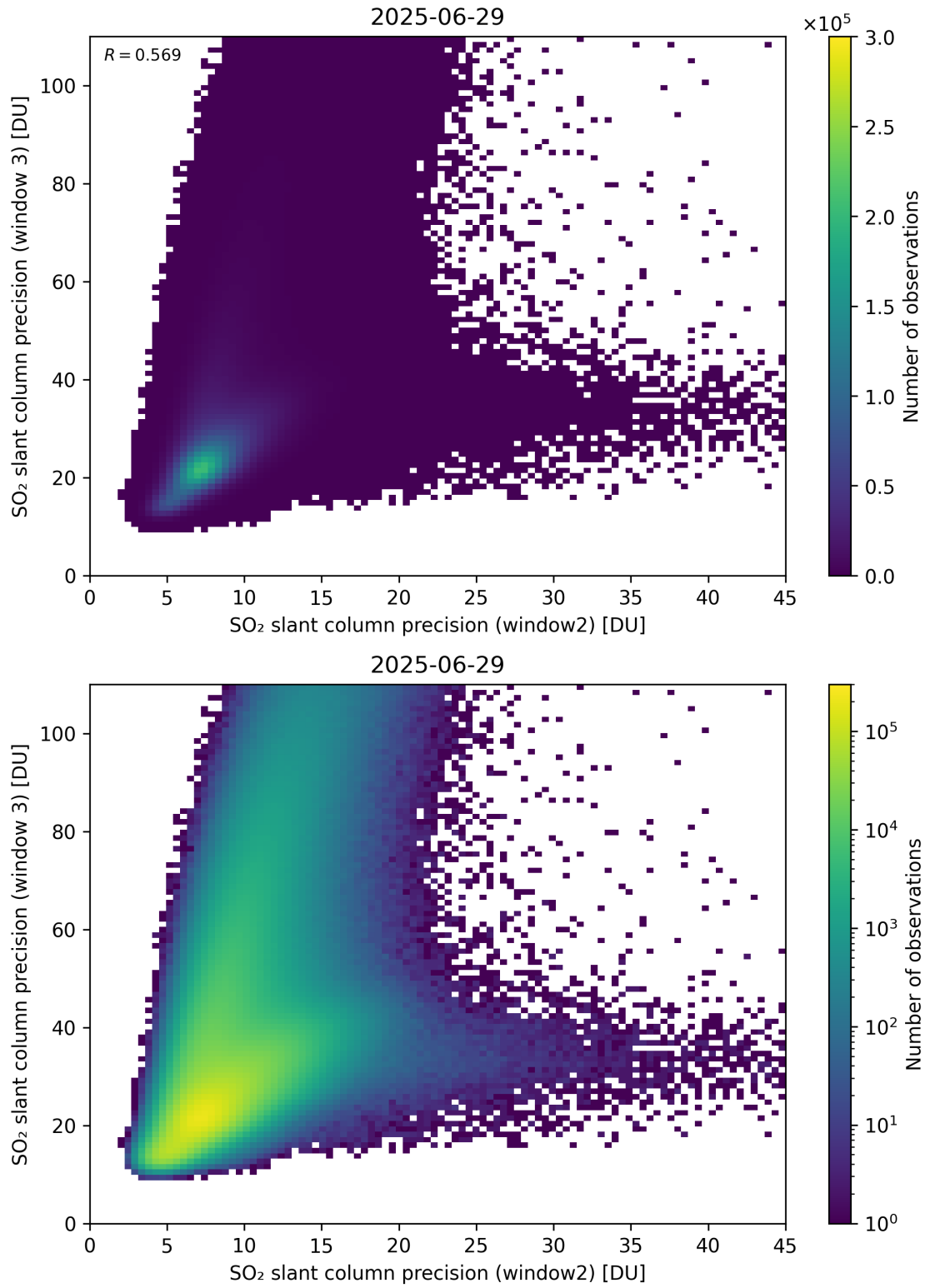
Figure 300: Scatter density plot of “SO 2 slant column precision (window2)” against “SO 2 slant column precision (window 3)” for 2025-06-28 to 2025-06-30.
