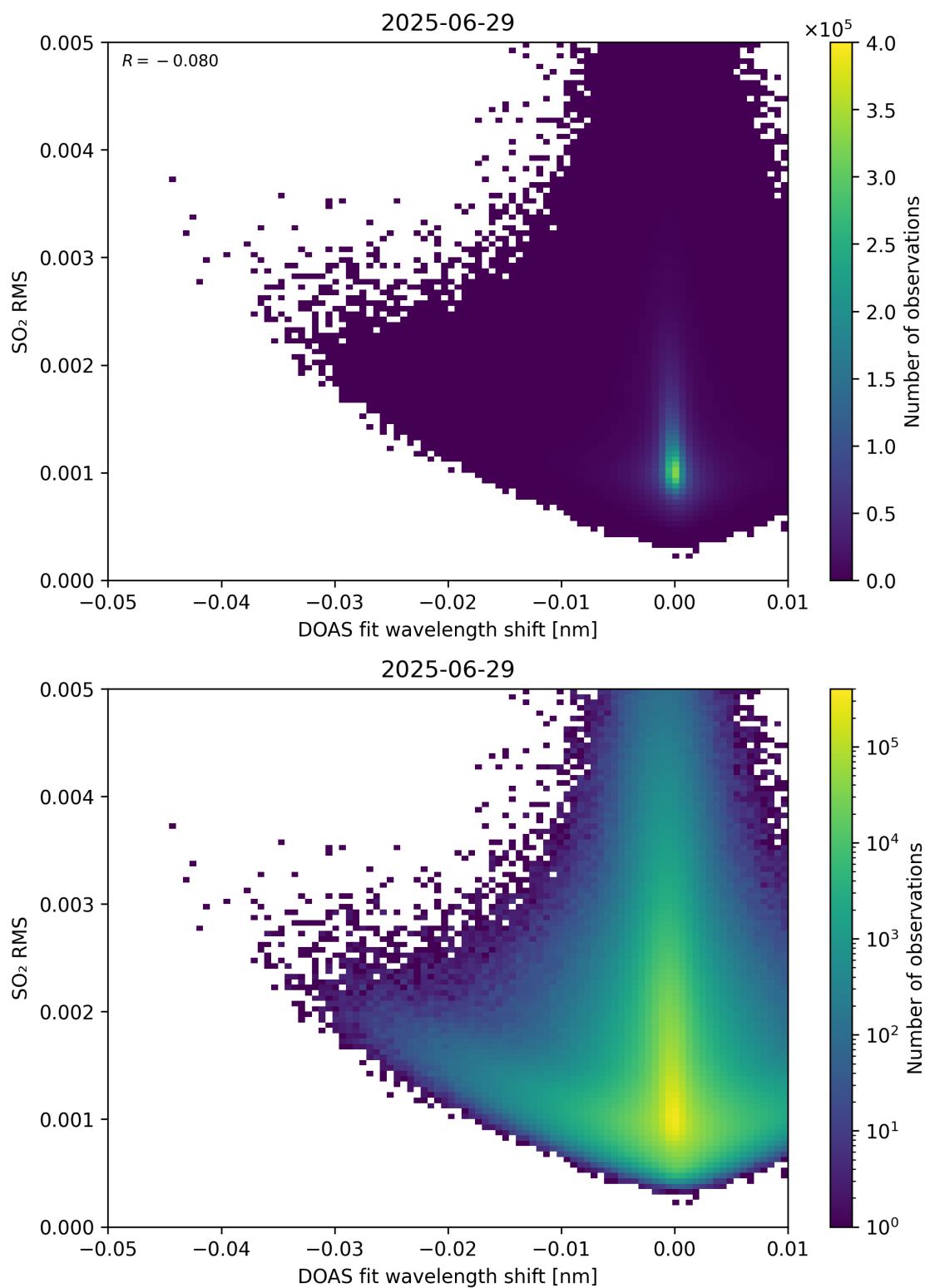
Figure 139: Scatter density plot of “DOAS fit wavelength shift” against “SO 2 RMS” for 2025-06-28 to 2025-06-30.
