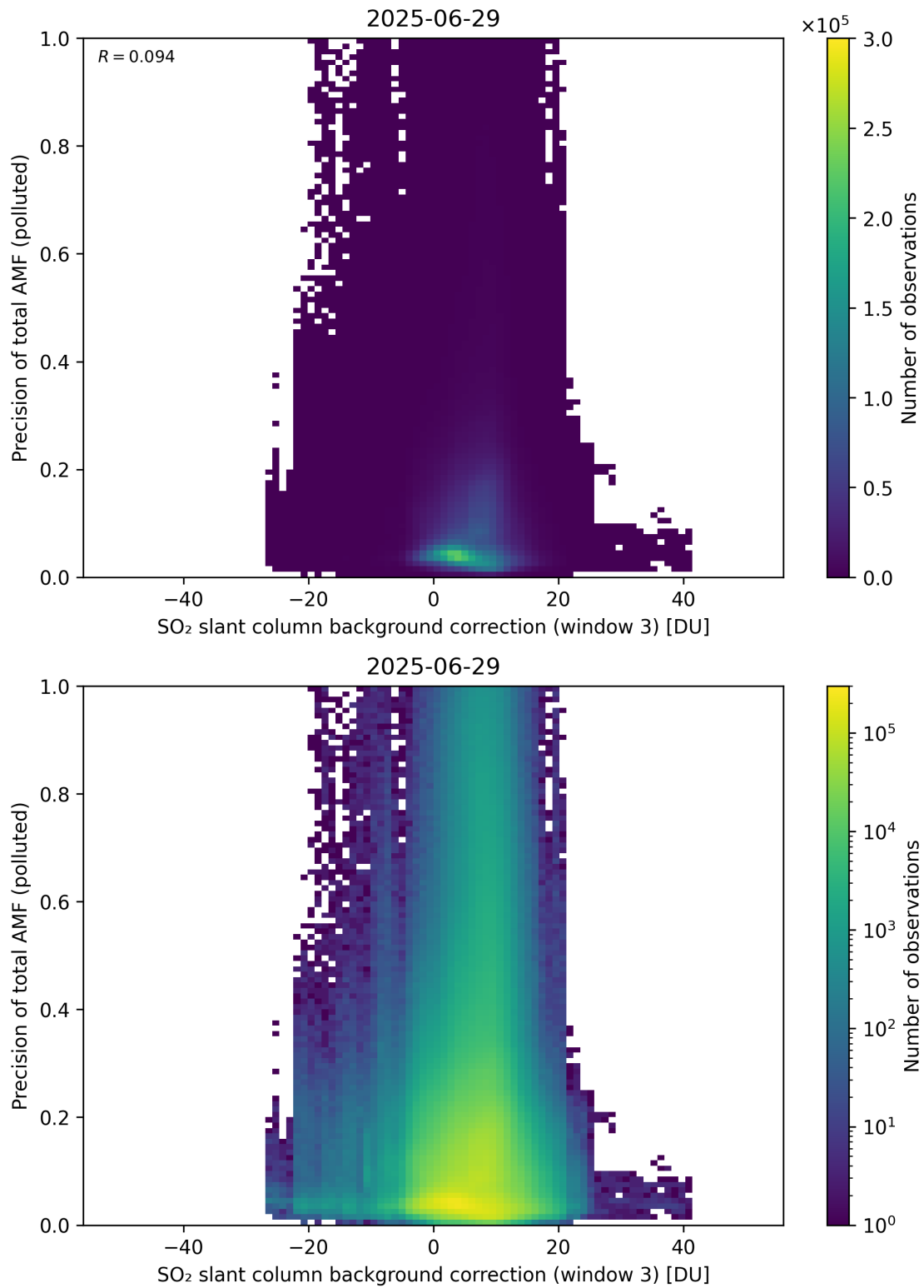
Figure 137: Scatter density plot of “SO 2 slant column background correction (window 3)” against “Precision of total AMF (polluted)” for 2025-06-28 to 2025-06-30.
