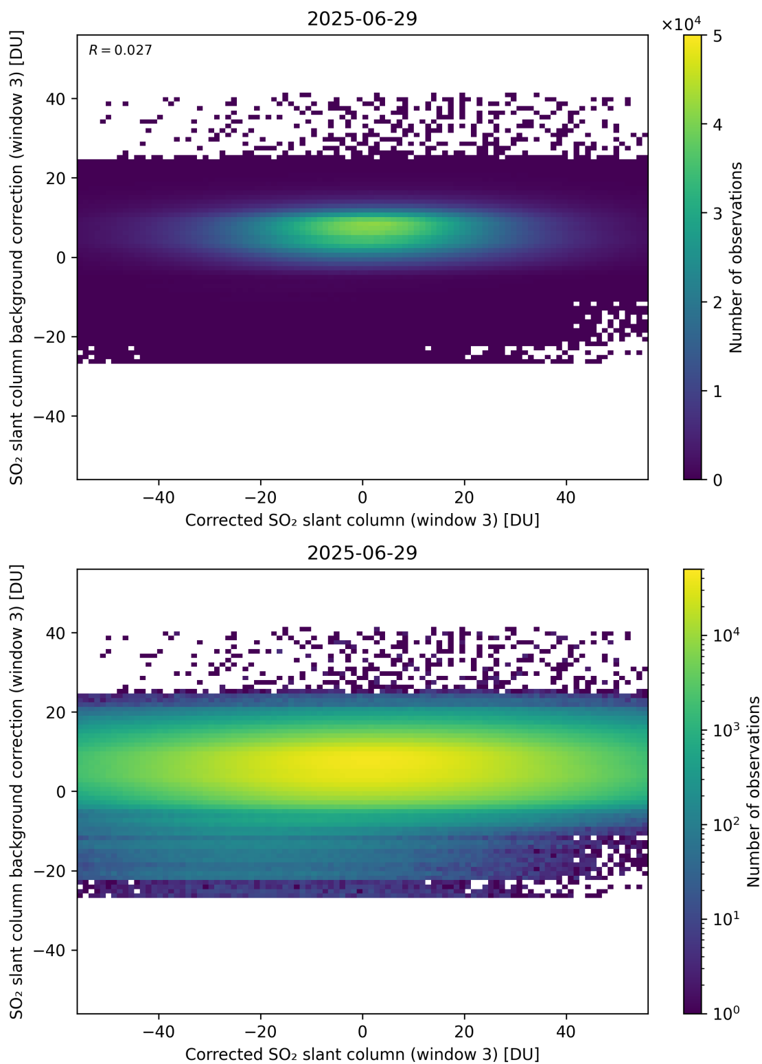
Figure 255: Scatter density plot of “Corrected SO 2 slant column (window 3)” against “SO 2 slant column background correction (window 3)” for 2025-06-28 to 2025-06-30.
