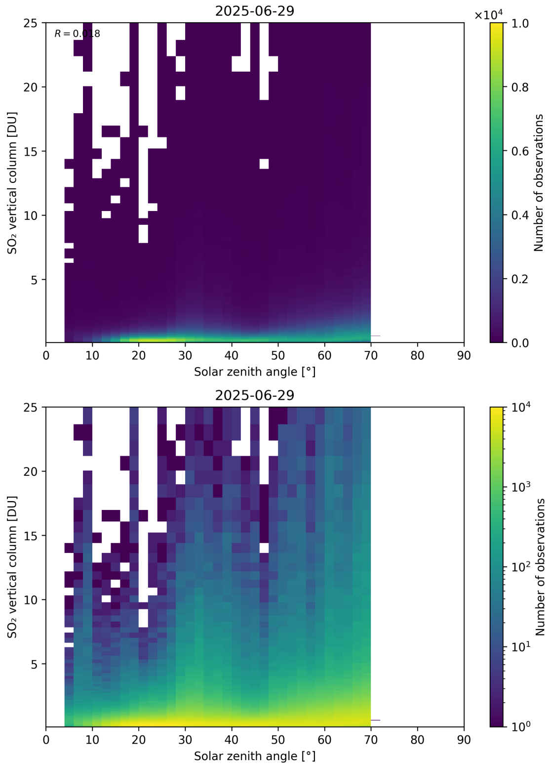
Figure 191: Scatter density plot of “Solar zenith angle” against “SO 2 vertical column” for 2025-06-28 to 2025-06-30.
