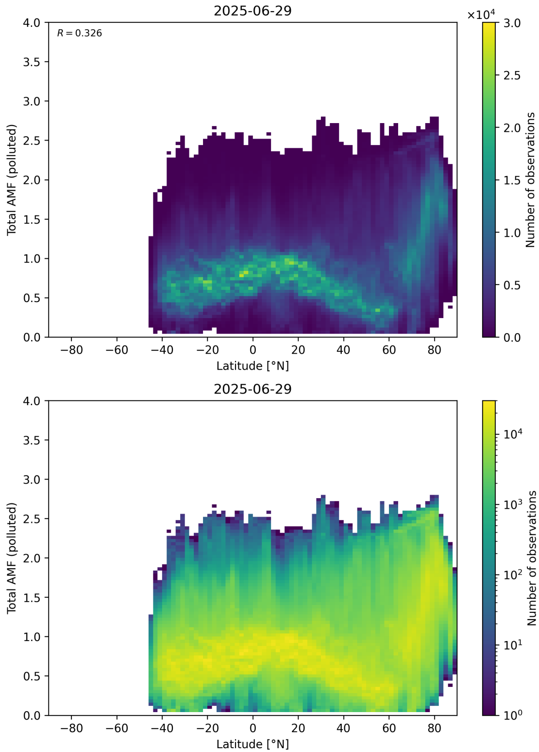
Figure 167: Scatter density plot of “Latitude” against “Total AMF (polluted)” for 2025-06-28 to 2025-06-30.
