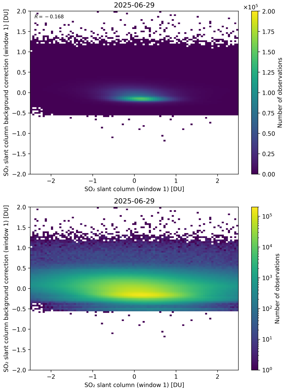
Figure 262: Scatter density plot of “SO 2 slant column (window 1)” against “SO 2 slant column background correction (window 1)” for 2025-06-28 to 2025-06-30.
