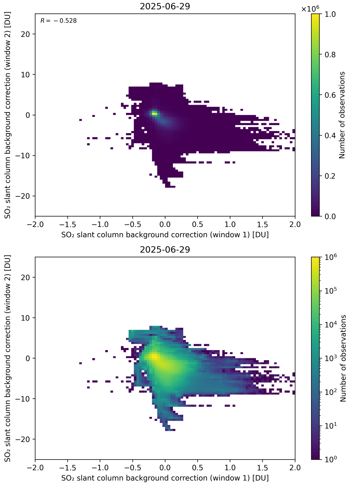
Figure 109: Scatter density plot of “SO 2 slant column background correction (window 1)” against “SO 2 slant column background correction (window 2)” for 2025-06-28 to 2025-06-30.
