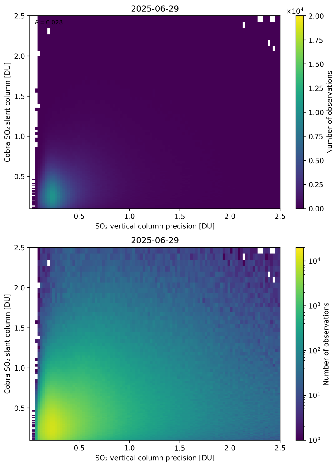
Figure 336: Scatter density plot of “SO 2 vertical column precision” against “Cobra SO 2 slant column” for 2025-06-28 to 2025-06-30.
