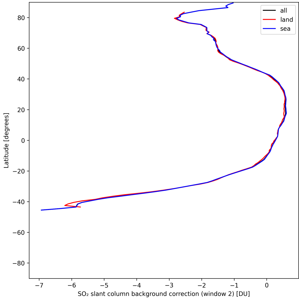
Figure 44: Zonal average of “SO 2 slant column background correction (window 2)” for 2025-06-28 to 2025-06-30.
