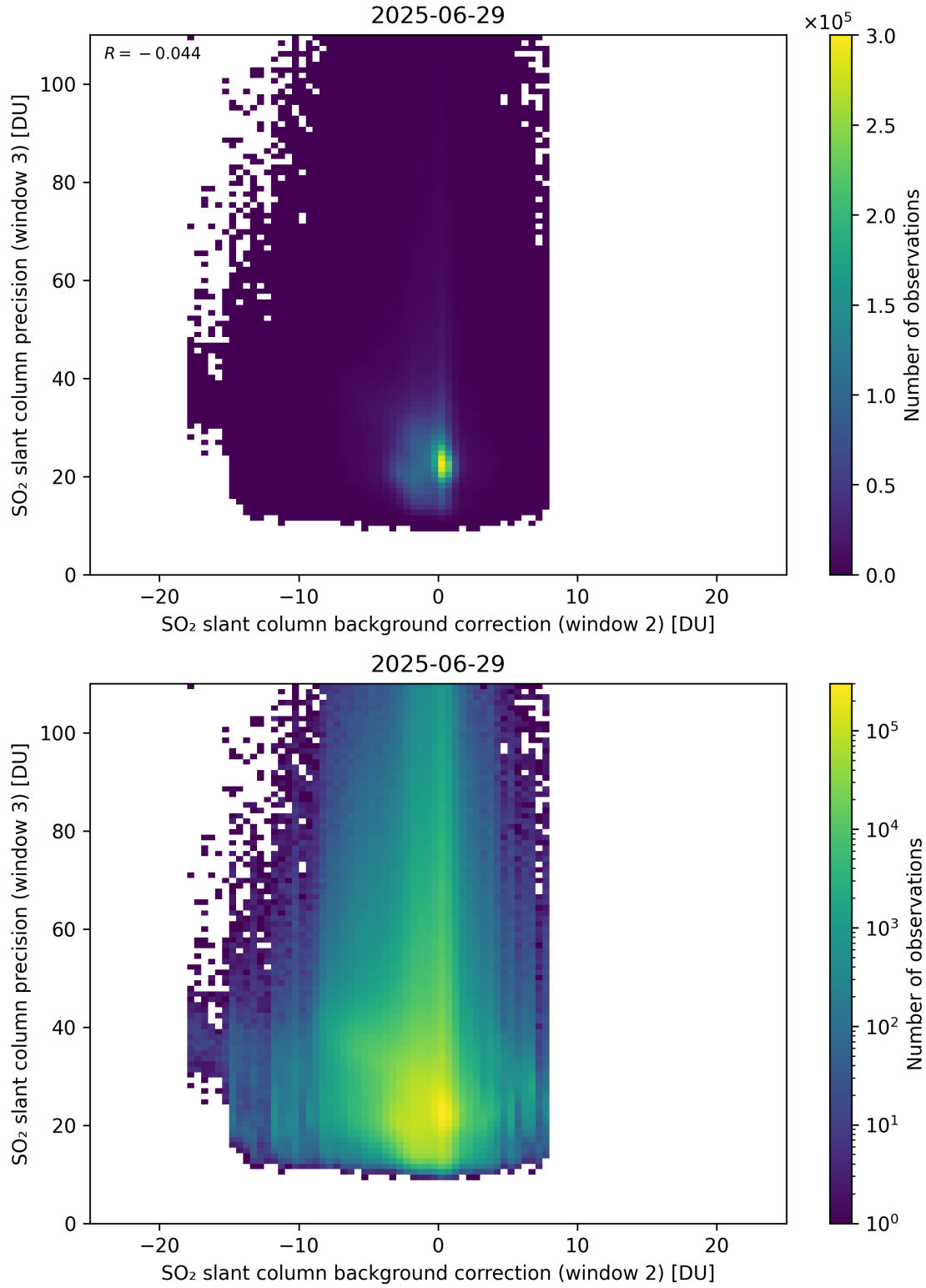
Figure 129: Scatter density plot of “SO 2 slant column background correction (window 2)” against “SO 2 slant column precision (window 3)” for 2025-06-28 to 2025-06-30.
