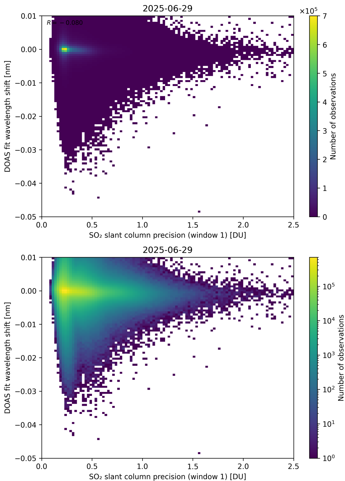
Figure 271: Scatter density plot of “SO 2 slant column precision (window 1)” against “DOAS fit wavelength shift” for 2025-06-28 to 2025-06-30.
