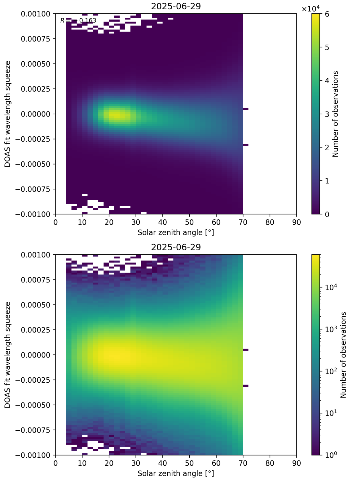
Figure 175: Scatter density plot of “Solar zenith angle” against “DOAS fit wavelength squeeze” for 2025-06-28 to 2025-06-30.
