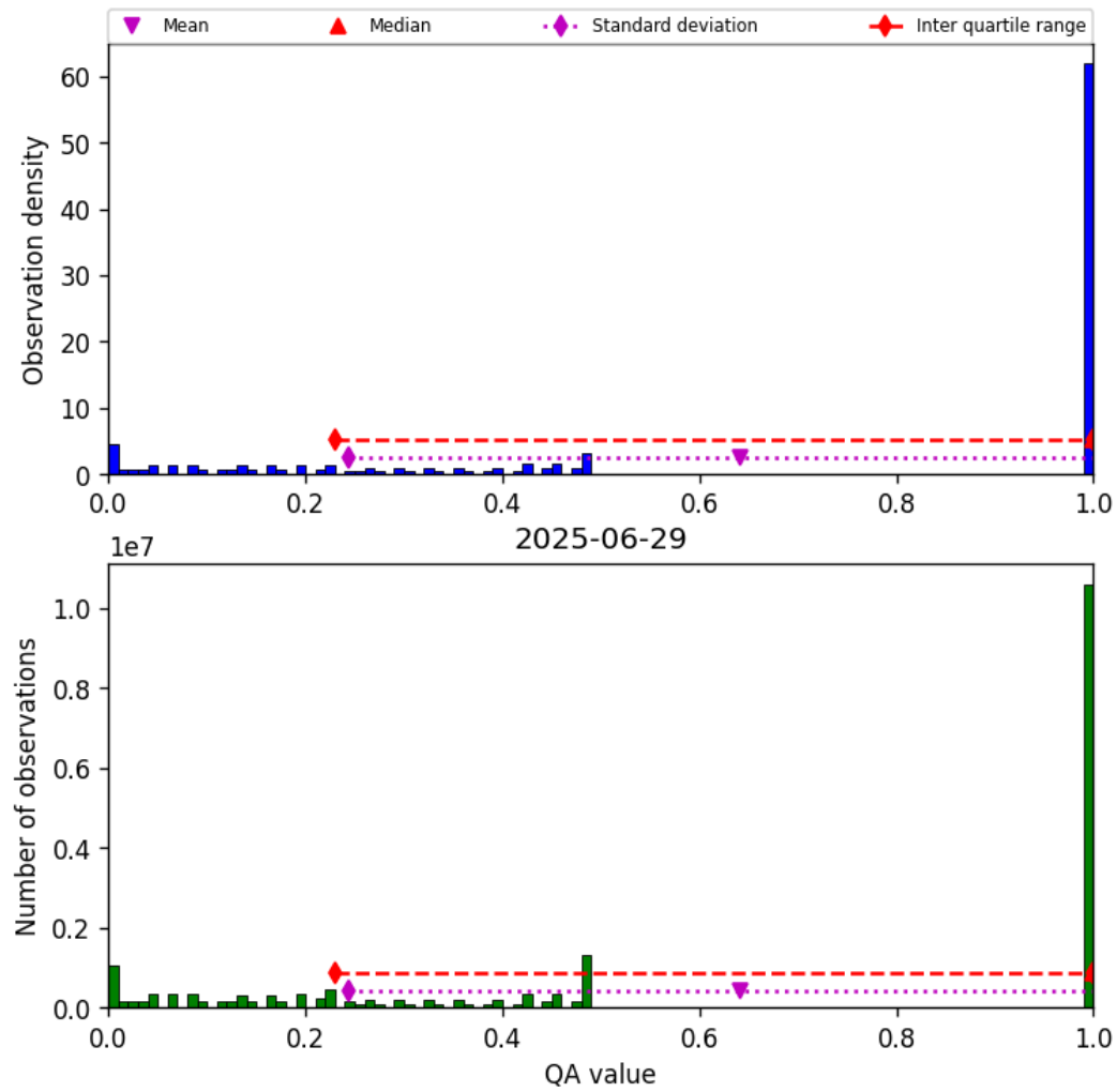
Figure 57: Histogram of “QA value” for 2025-06-28 to 2025-06-30
