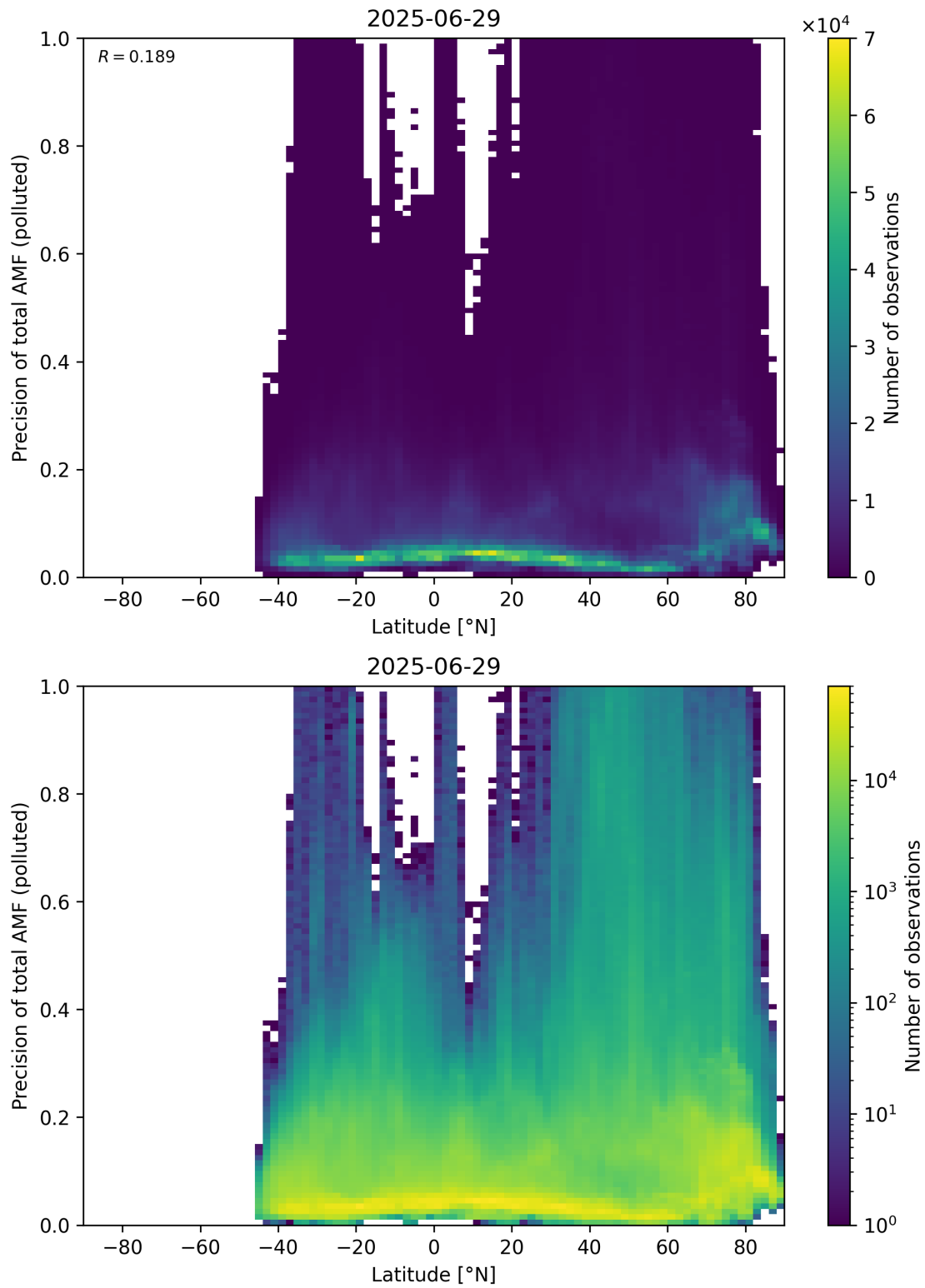
Figure 168: Scatter density plot of “Latitude” against “Precision of total AMF (polluted)” for 2025-06-28 to 2025-06-30.
