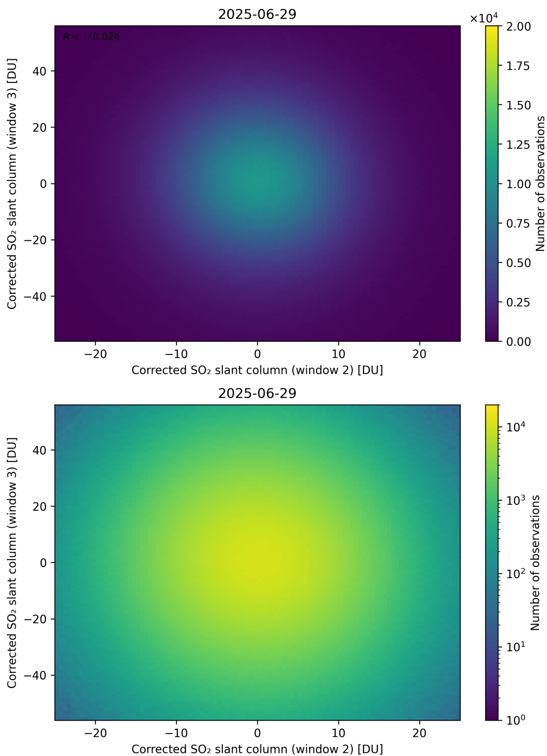
Figure 250: Scatter density plot of “Corrected SO 2 slant column (window 2)” against “Corrected SO 2 slant column (window 3)” for 2025-06-28 to 2025-06-30.
