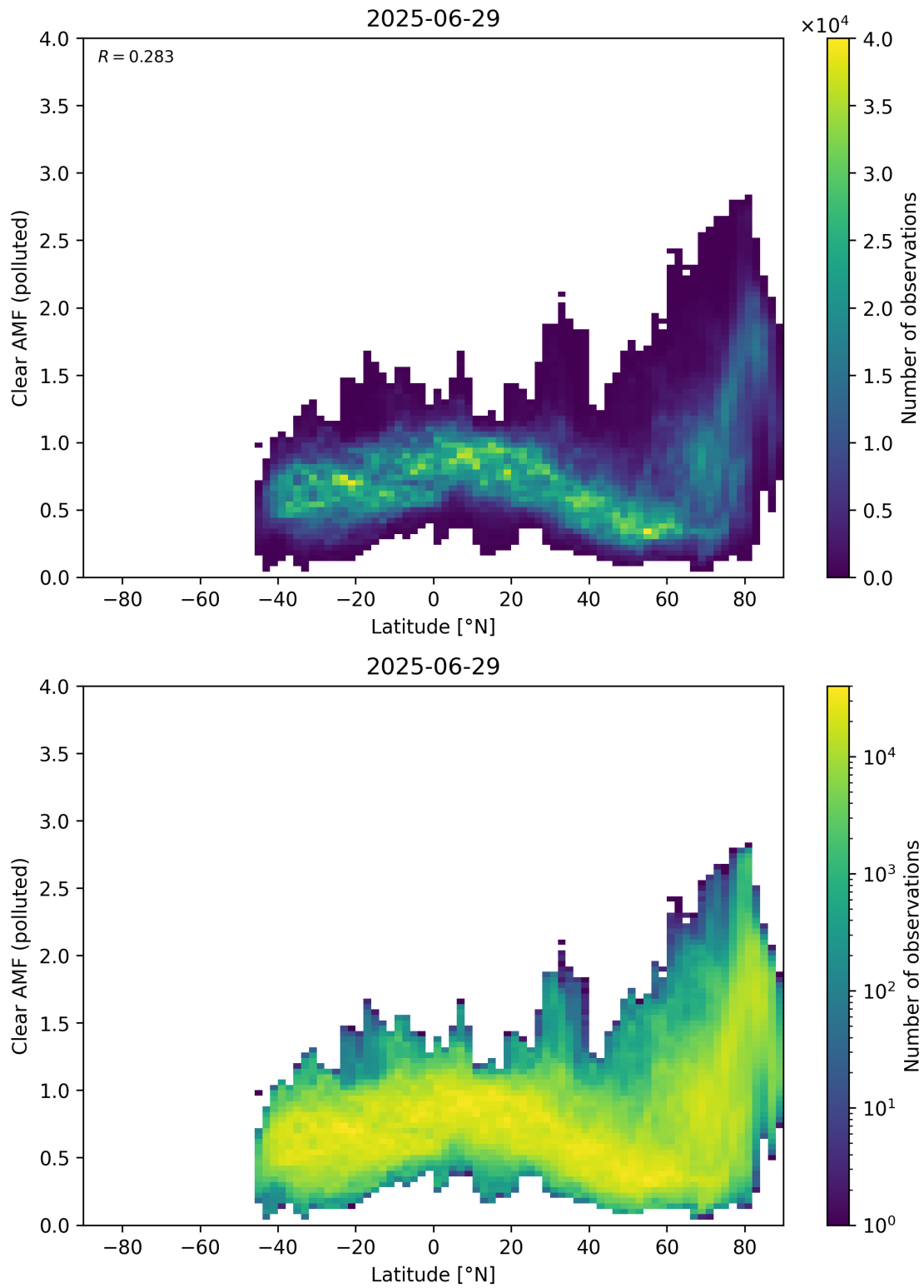
Figure 156: Scatter density plot of “Latitude” against “Clear AMF (polluted)” for 2025-06-28 to 2025-06-30.
