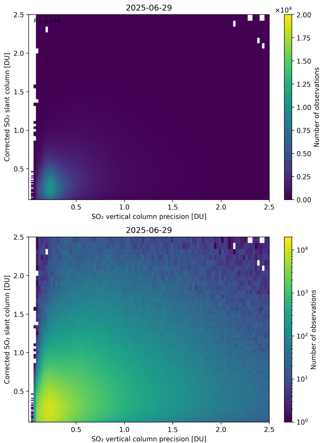
Figure 338: Scatter density plot of “SO 2 vertical column precision” against “Corrected SO 2 slant column” for 2025-06-28 to 2025-06-30.
