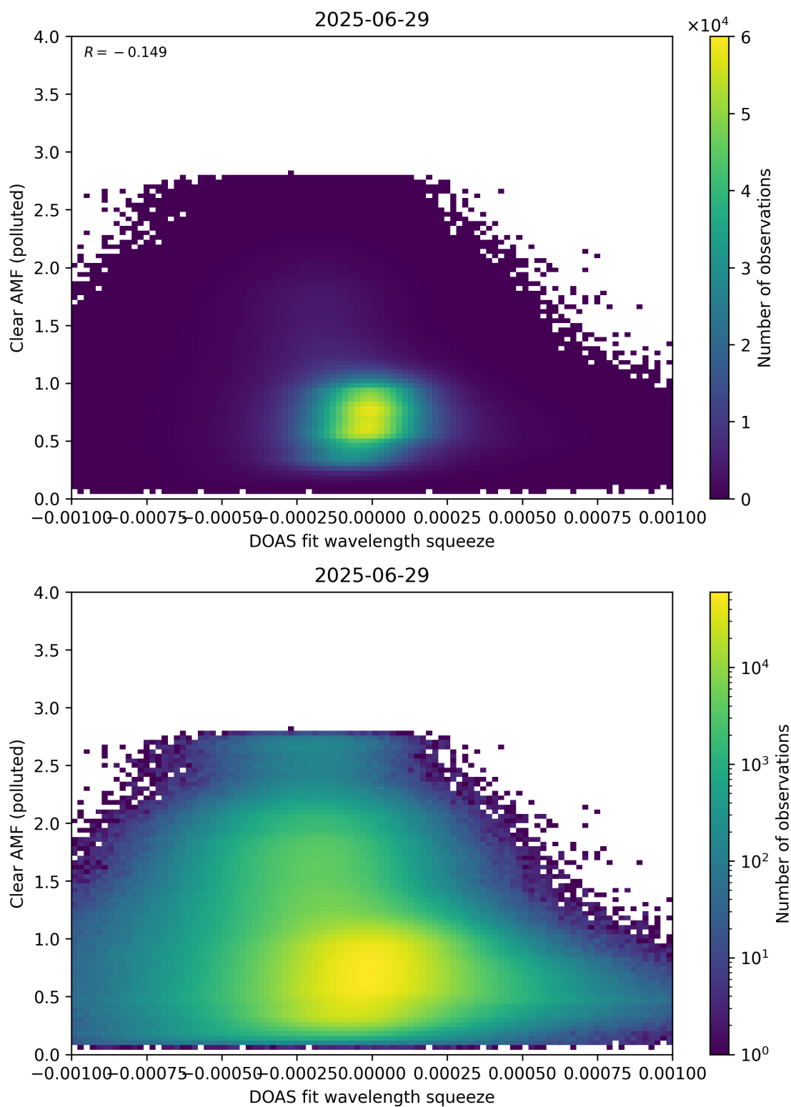
Figure 144: Scatter density plot of “DOAS fit wavelength squeeze” against “Clear AMF (polluted)” for 2025-06-28 to 2025-06-30.
