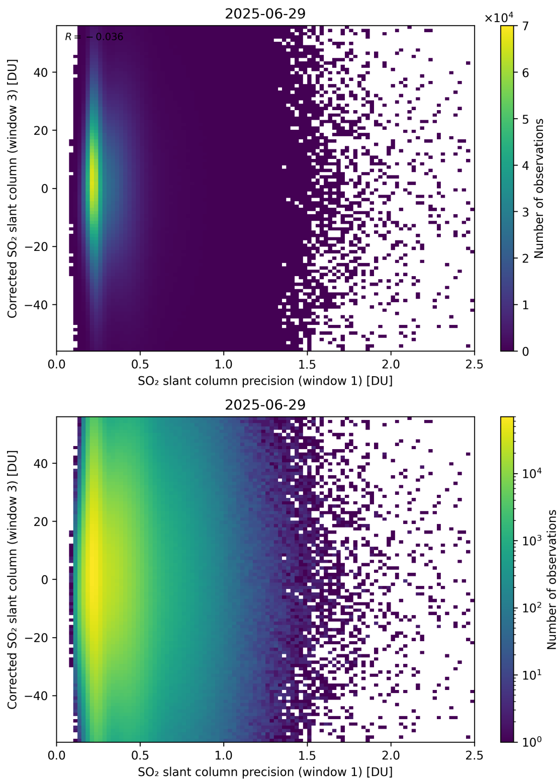
Figure 276: Scatter density plot of “SO 2 slant column precision (window 1)” against “Corrected SO 2 slant column (window 3)” for 2025-06-28 to 2025-06-30.
