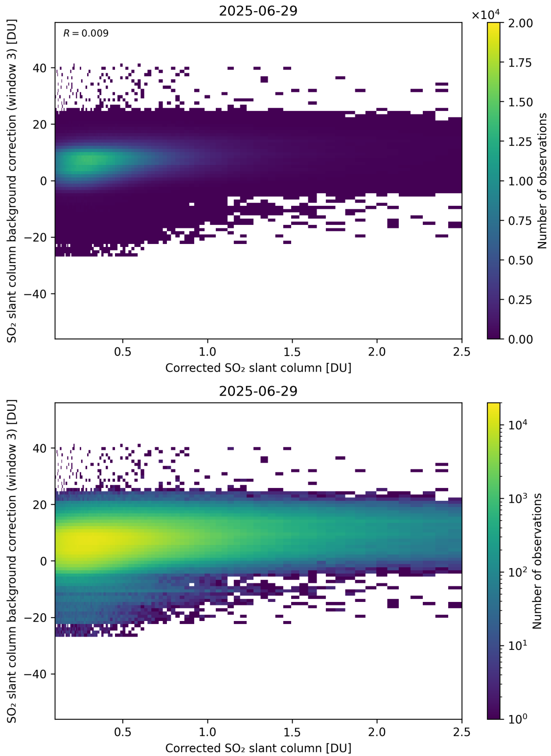
Figure 228: Scatter density plot of “Corrected SO 2 slant column” against “SO 2 slant column background correction (window 3)” for 2025-06-28 to 2025-06-30.
