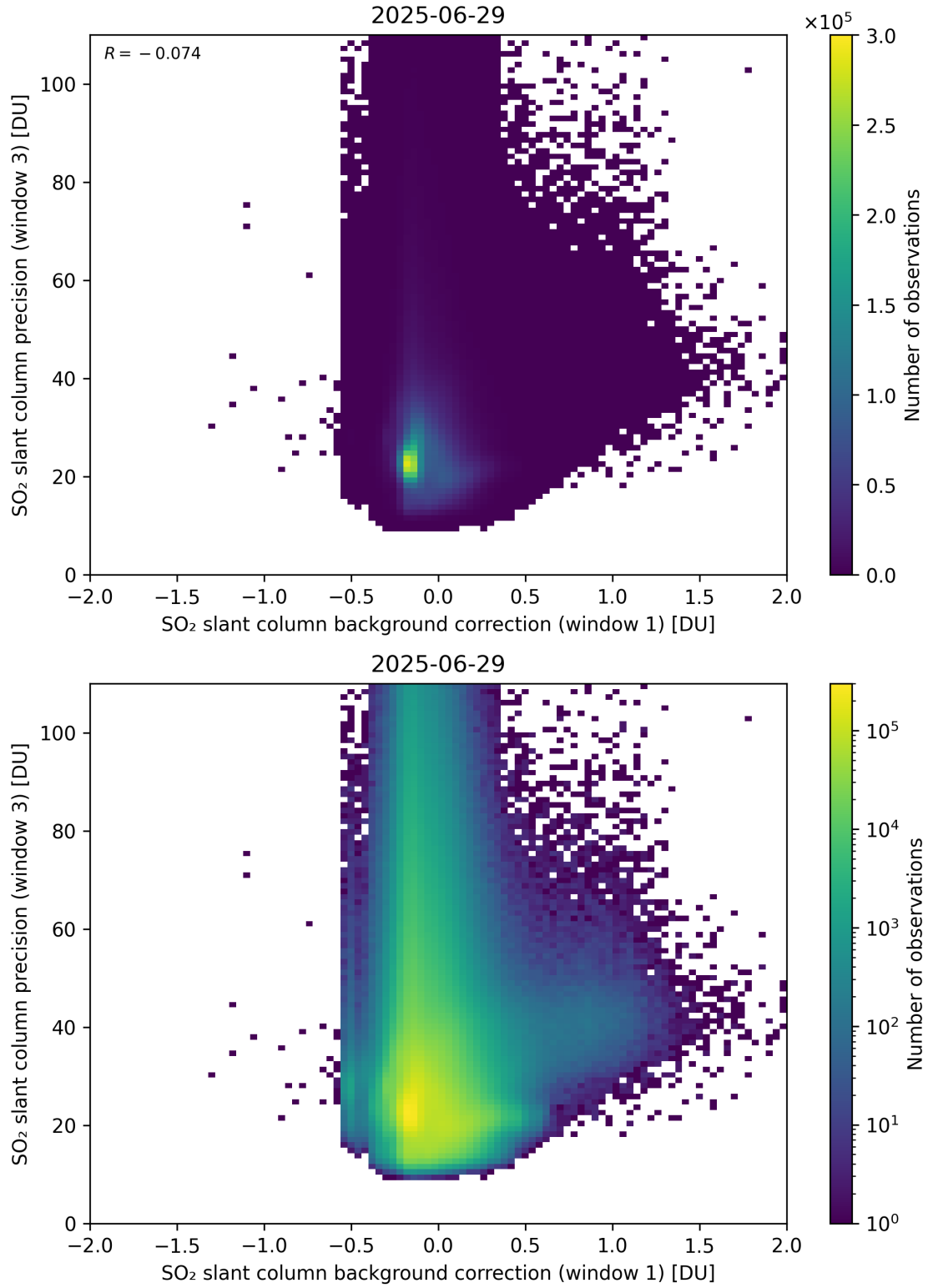
Figure 119: Scatter density plot of “SO 2 slant column background correction (window 1)” against “SO 2 slant column precision (window 3)” for 2025-06-28 to 2025-06-30.
