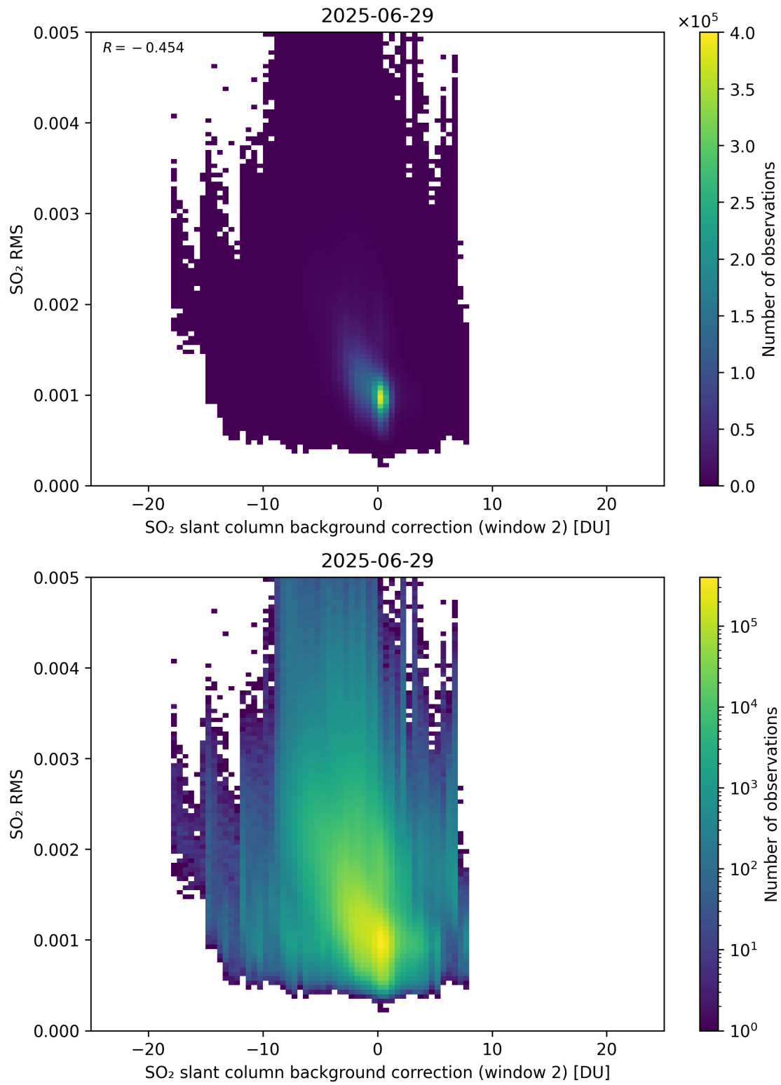
Figure 125: Scatter density plot of “SO 2 slant column background correction (window 2)” against “SO 2 RMS” for 2025-06-28 to 2025-06-30.
