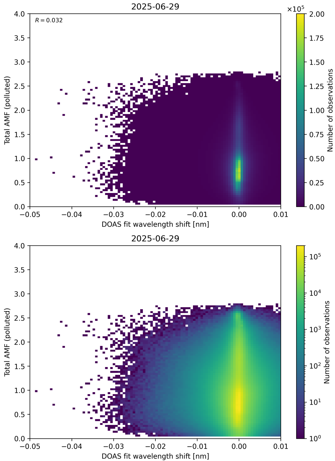
Figure 141: Scatter density plot of “DOAS fit wavelength shift” against “Total AMF (polluted)” for 2025-06-28 to 2025-06-30.
