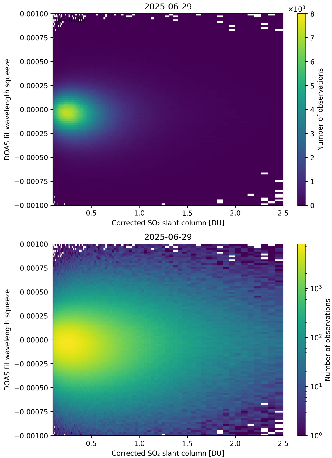
Figure 230: Scatter density plot of “Corrected SO 2 slant column” against “DOAS fit wavelength squeeze” for 2025-06-28 to 2025-06-30.
