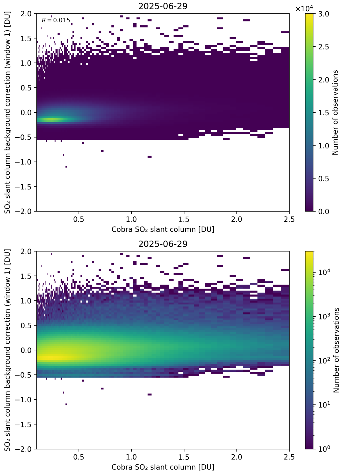
Figure 193: Scatter density plot of “Cobra SO 2 slant column” against “SO 2 slant column background correction (window 1)” for 2025-06-28 to 2025-06-30.
