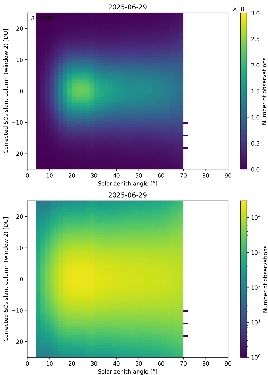
Figure 182: Scatter density plot of “Solar zenith angle” against “Corrected SO 2 slant column (window 2)” for 2025-06-28 to 2025-06-30.
