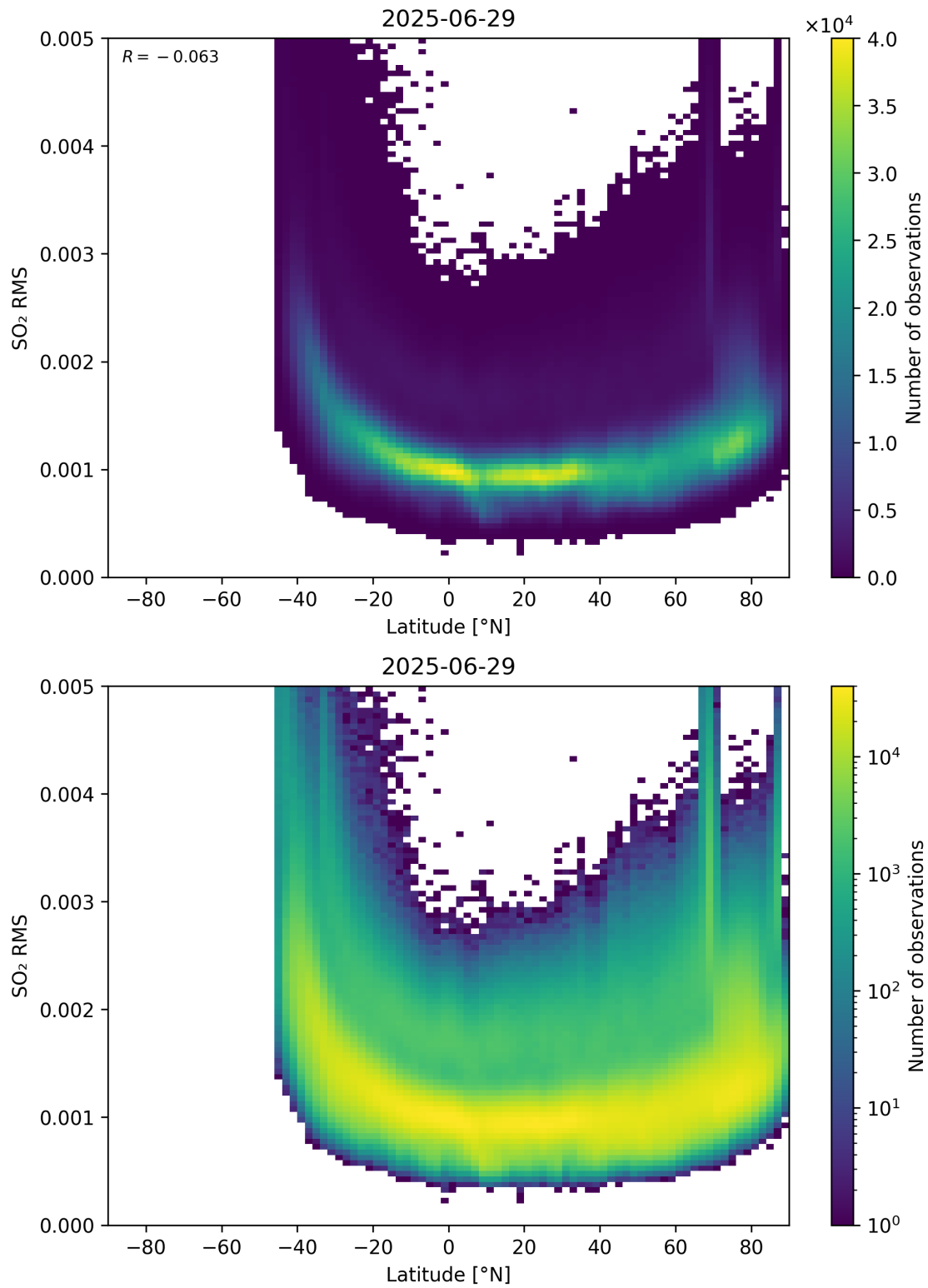
Figure 155: Scatter density plot of “Latitude” against “SO 2 RMS” for 2025-06-28 to 2025-06-30.
