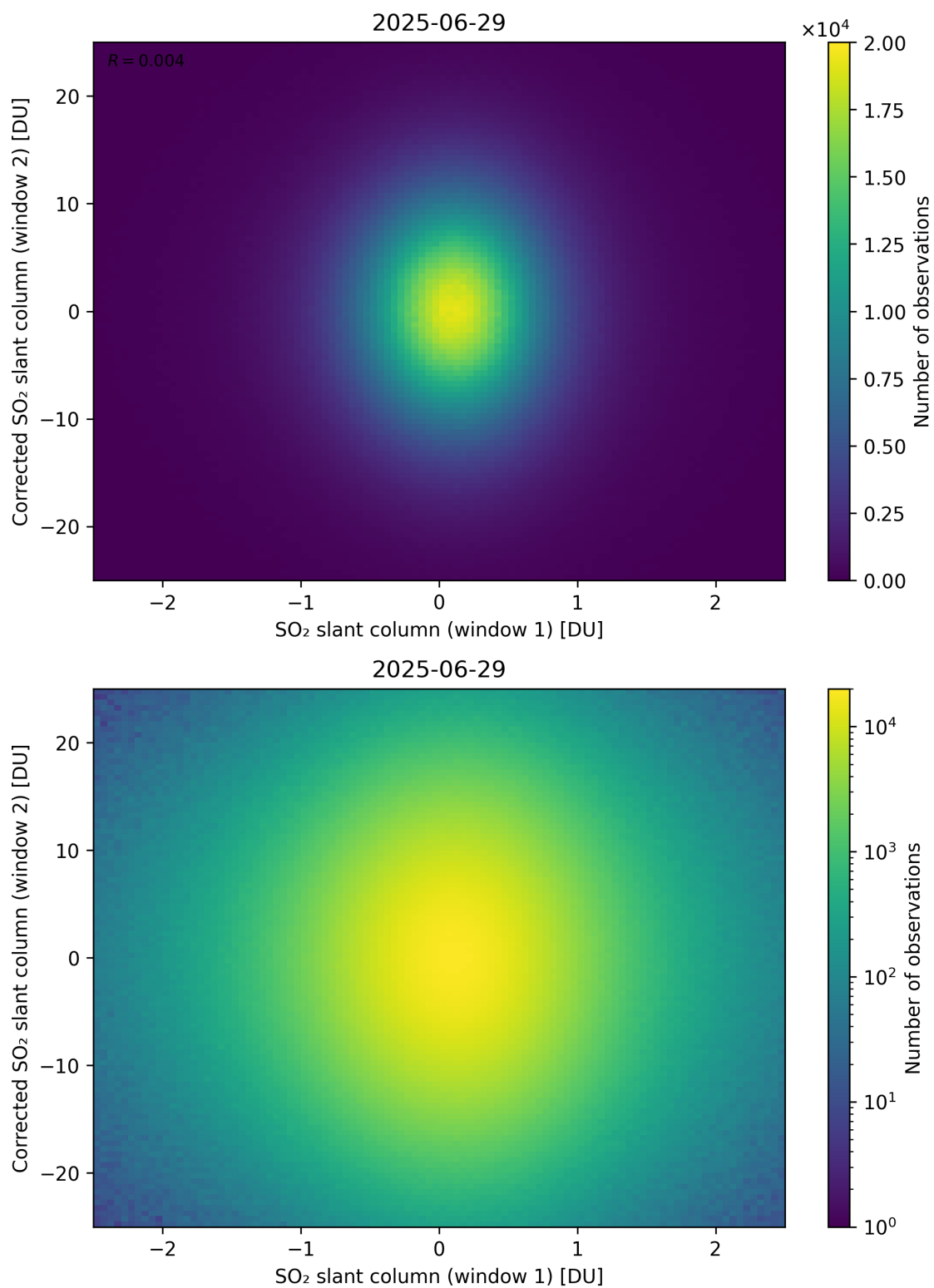
Figure 283: Scatter density plot of “SO 2 slant column (window 1)” against “Corrected SO 2 slant column (window 2)” for 2025-06-28 to 2025-06-30.
