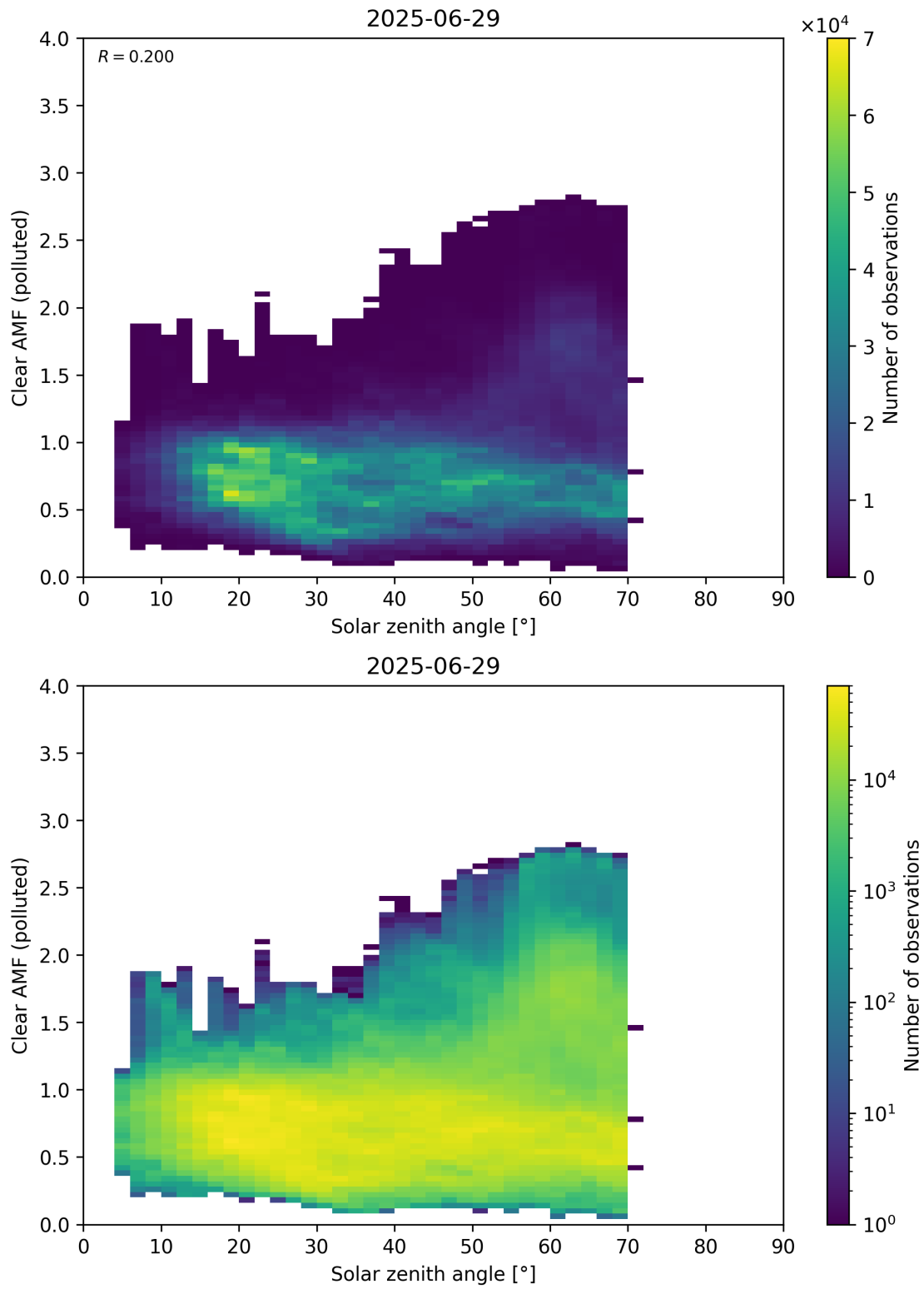
Figure 178: Scatter density plot of “Solar zenith angle” against “Clear AMF (polluted)” for 2025-06-28 to 2025-06-30.
