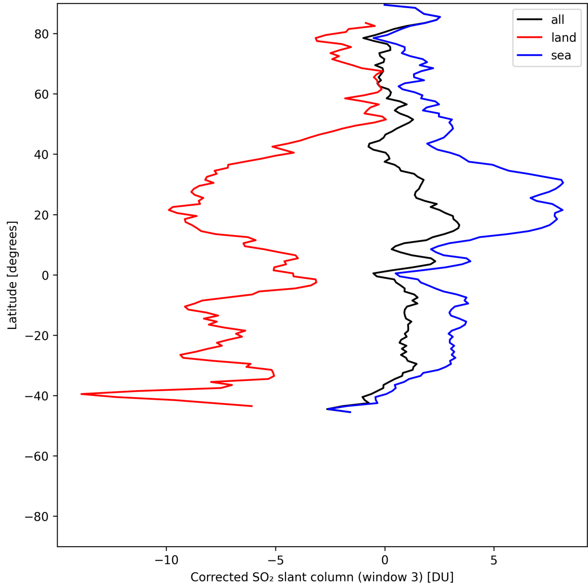
Figure 47: Zonal average of “Corrected SO 2 slant column (window 3)” for 2025-06-28 to 2025-06-30.
