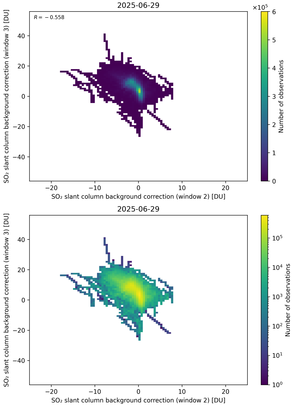
Figure 122: Scatter density plot of “SO 2 slant column background correction (window 2)” against “SO 2 slant column background correction (window 3)” for 2025-06-28 to 2025-06-30.
