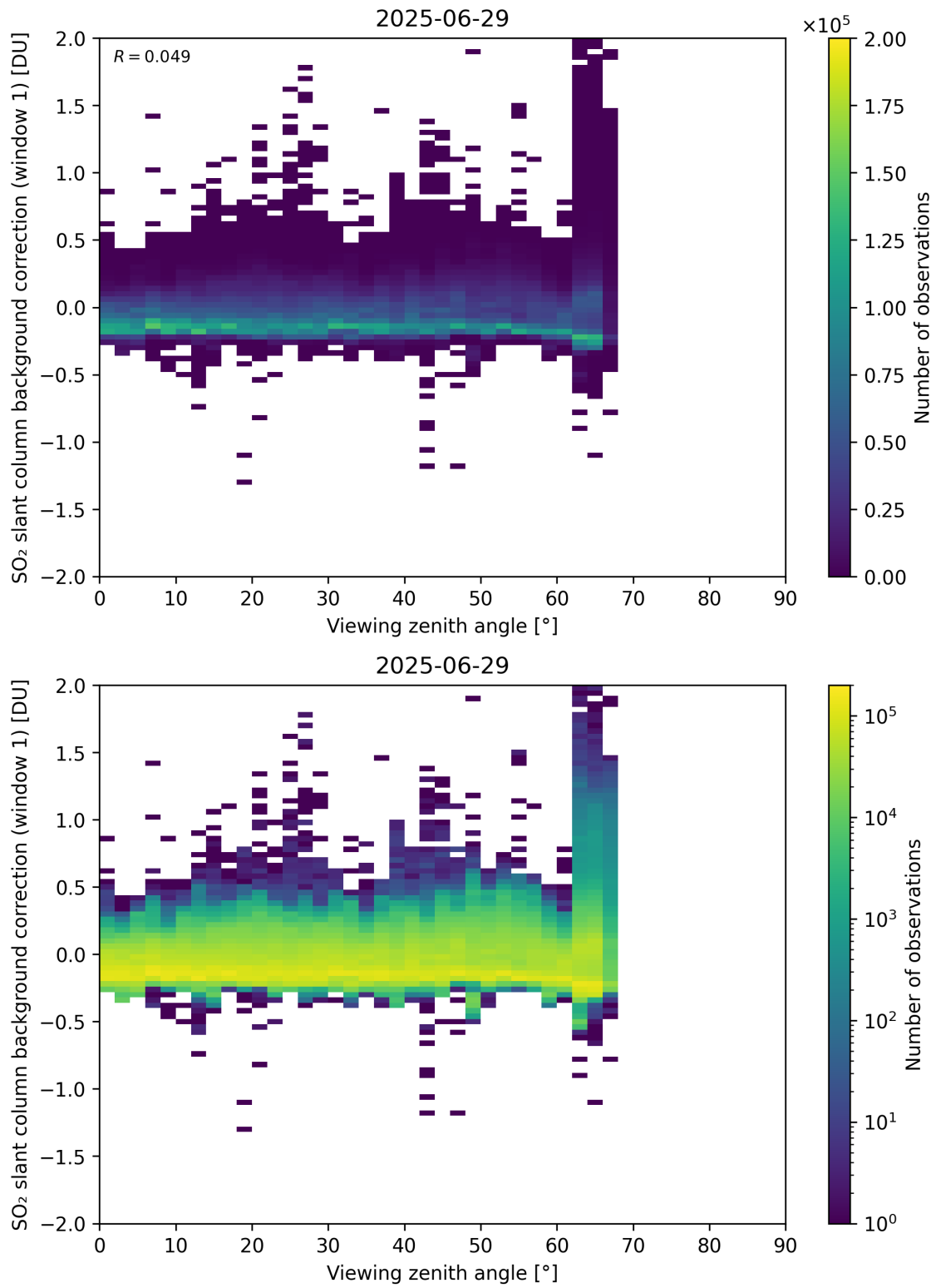
Figure 362: Scatter density plot of “Viewing zenith angle” against “SO 2 slant column background correction (window 1)” for 2025-06-28 to 2025-06-30.
