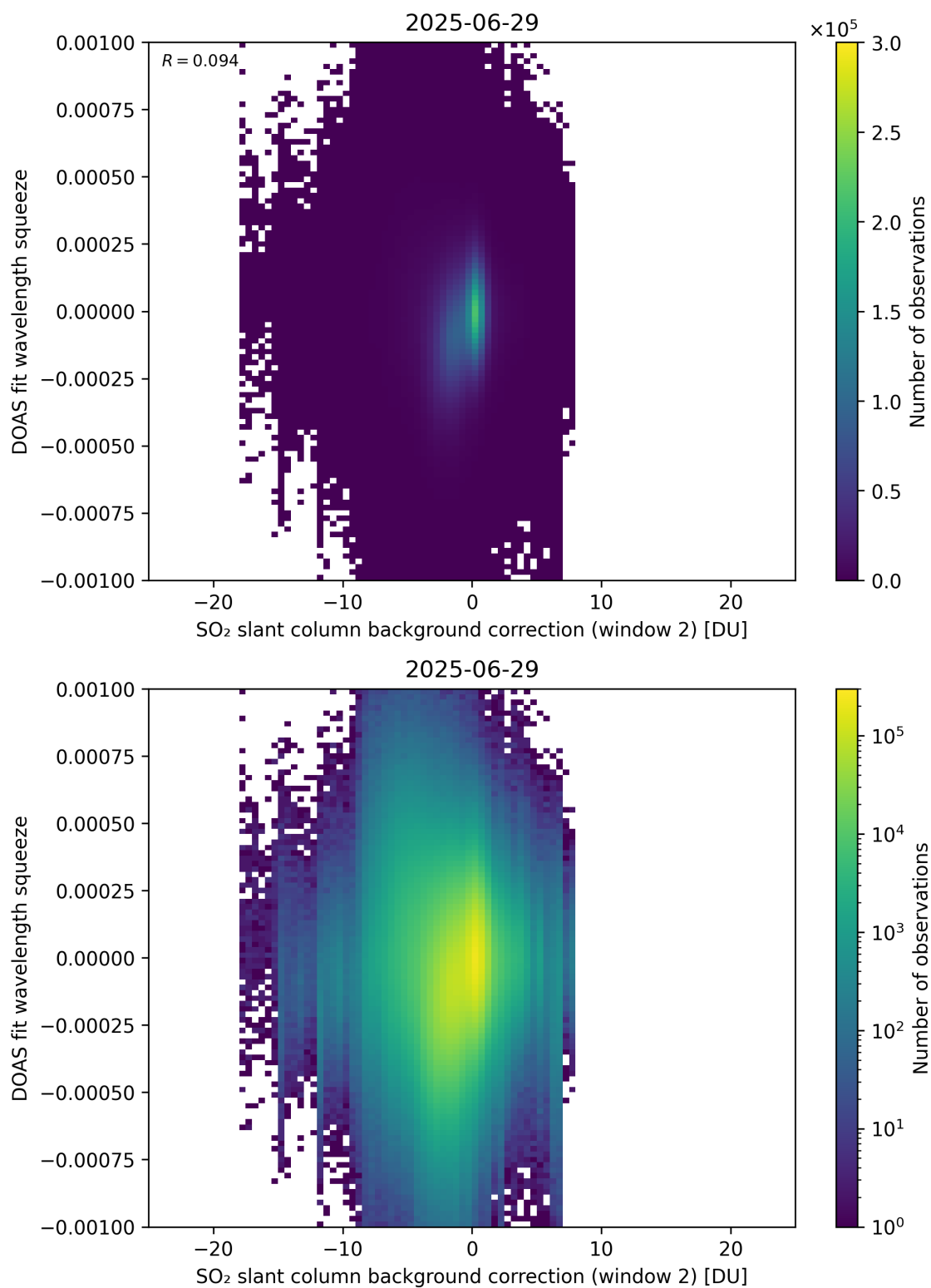
Figure 124: Scatter density plot of “SO 2 slant column background correction (window 2)” against “DOAS fit wavelength squeeze” for 2025-06-28 to 2025-06-30.
