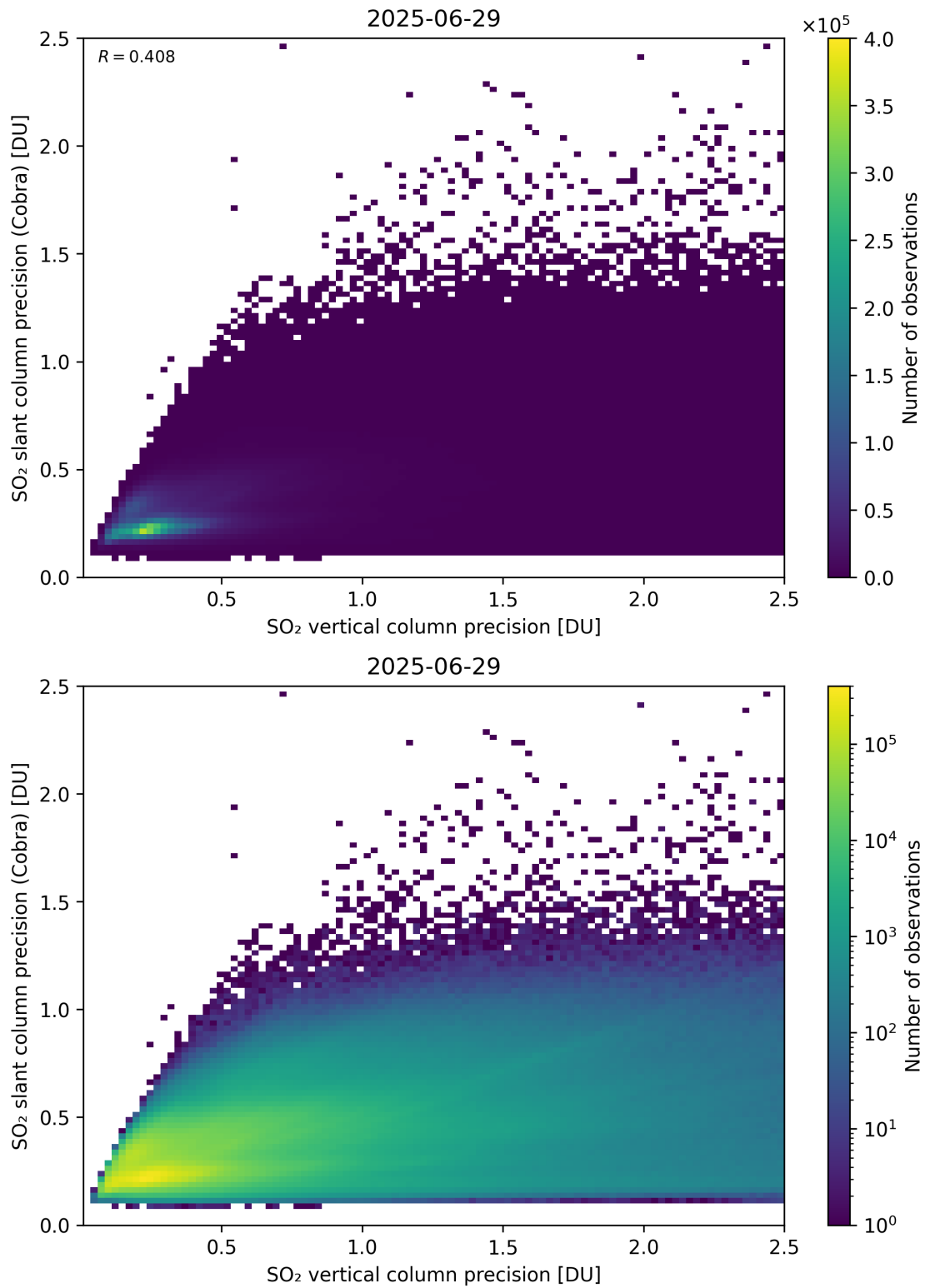
Figure 337: Scatter density plot of “SO 2 vertical column precision” against “SO 2 slant column precision (Cobra)” for 2025-06-28 to 2025-06-30.
