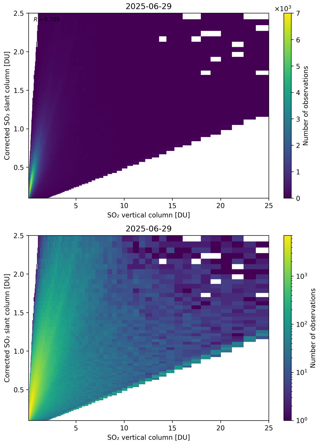
Figure 351: Scatter density plot of “SO 2 vertical column” against “Corrected SO 2 slant column” for 2025-06-28 to 2025-06-30.
