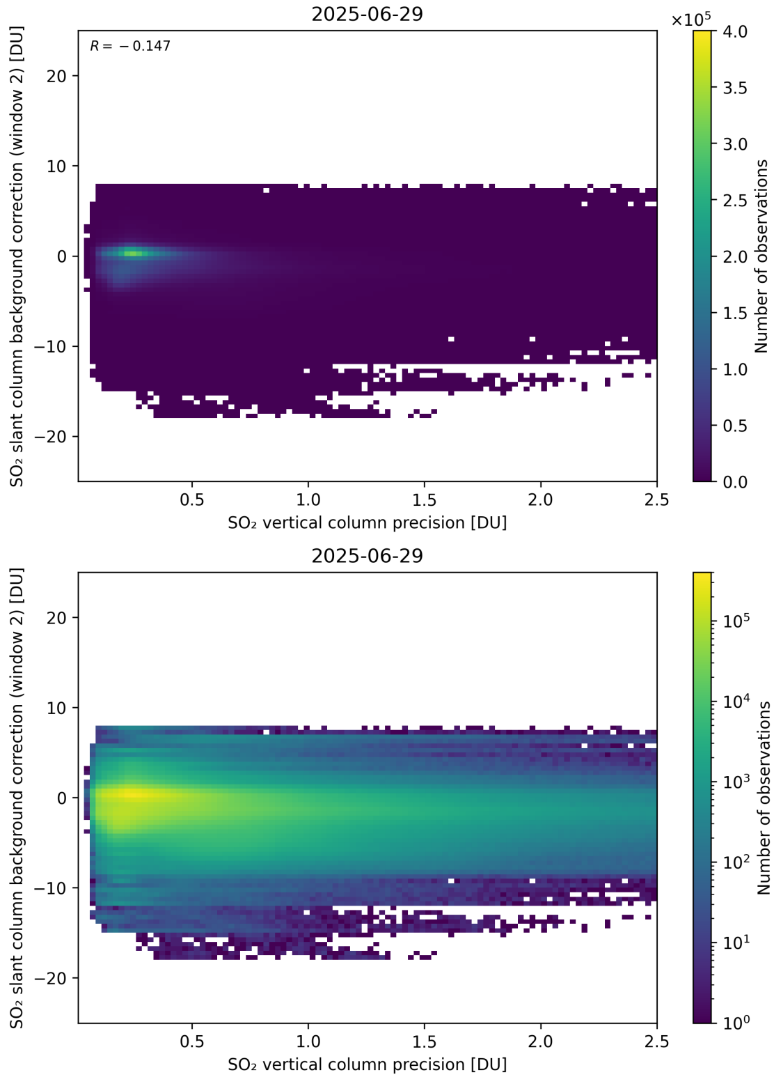
Figure 330: Scatter density plot of “SO 2 vertical column precision” against “SO 2 slant column background correction (window 2)” for 2025-06-28 to 2025-06-30.
