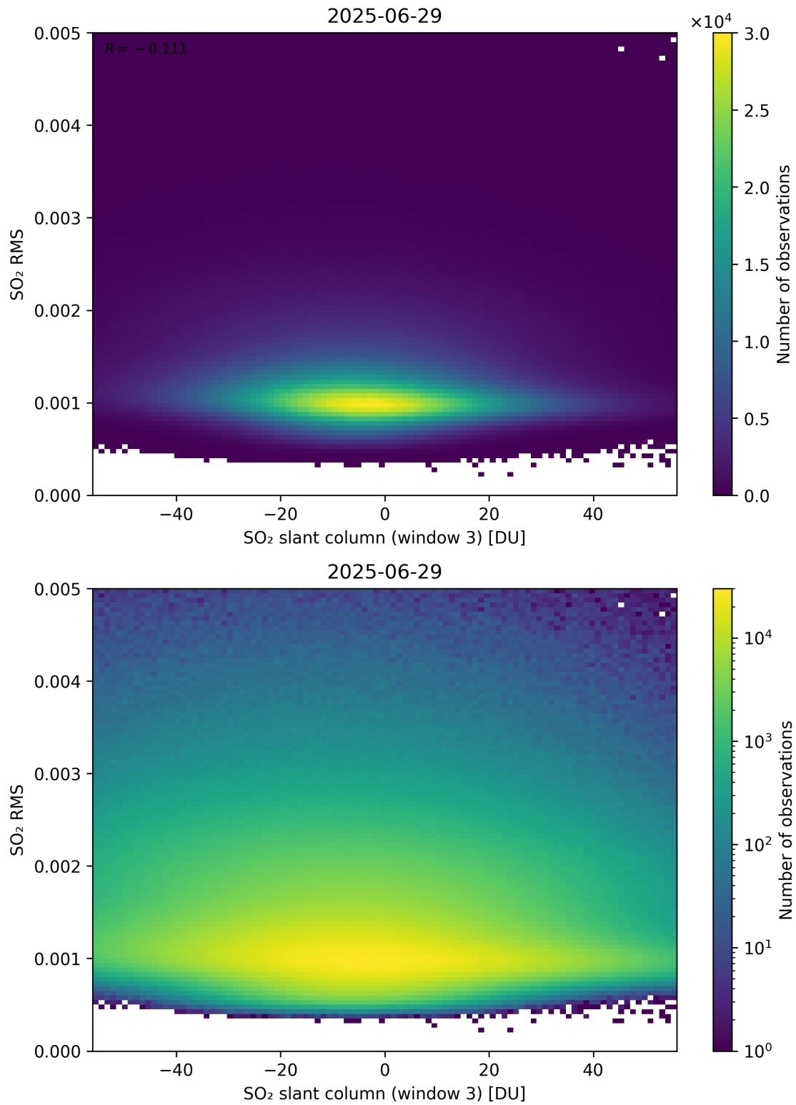
Figure 306: Scatter density plot of “SO 2 slant column (window 3)” against “SO 2 RMS” for 2025-06-28 to 2025-06-30.
