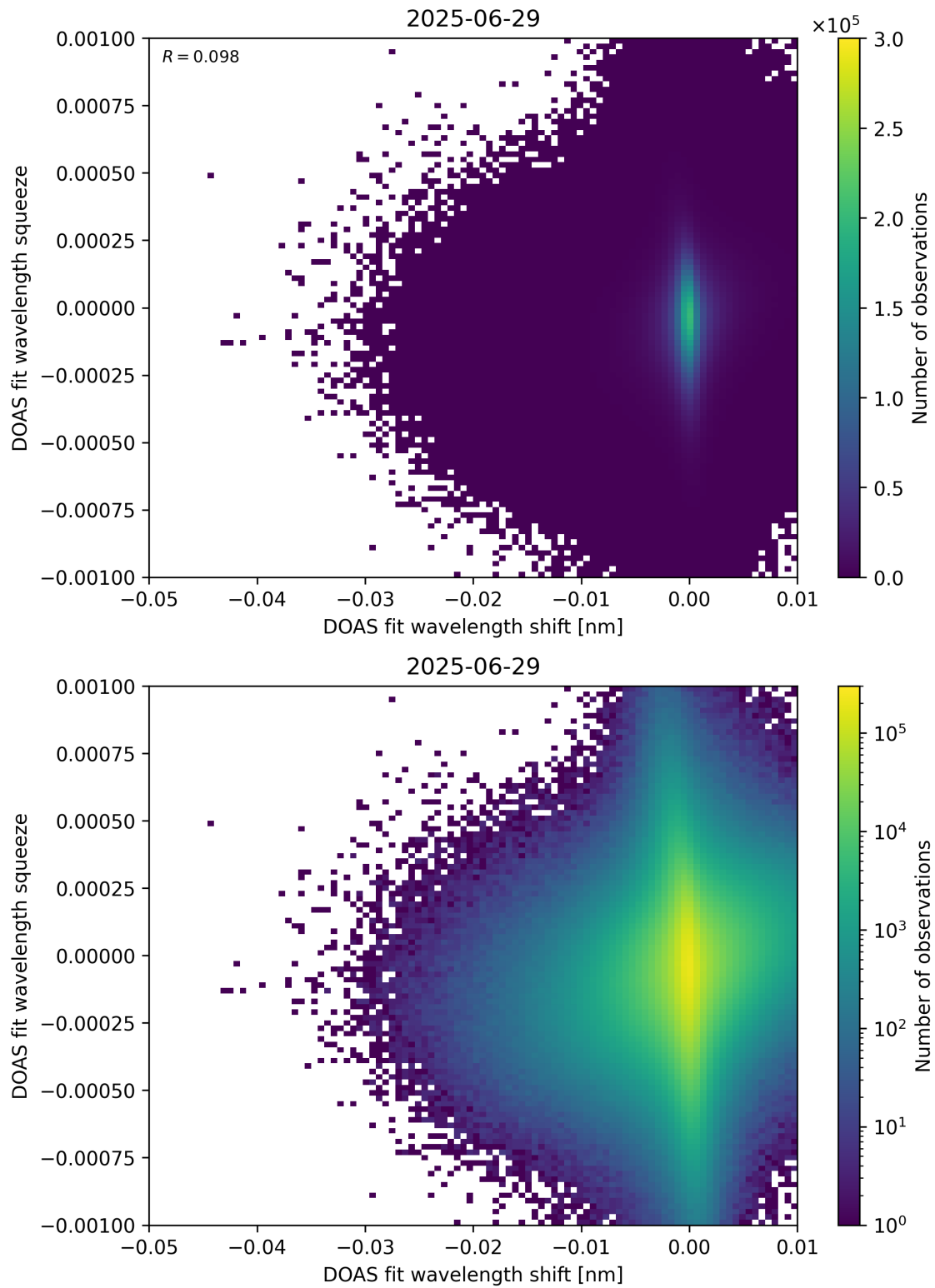
Figure 138: Scatter density plot of “DOAS fit wavelength shift” against “DOAS fit wavelength squeeze” for 2025-06-28 to 2025-06-30.
