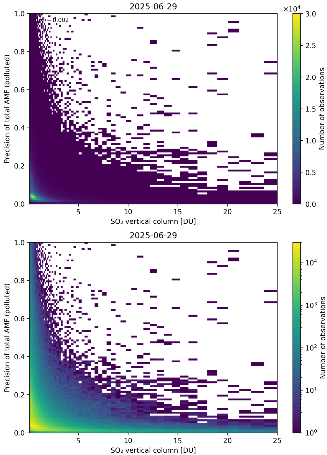
Figure 360: Scatter density plot of “SO 2 vertical column” against “Precision of total AMF (polluted)” for 2025-06-28 to 2025-06-30.
