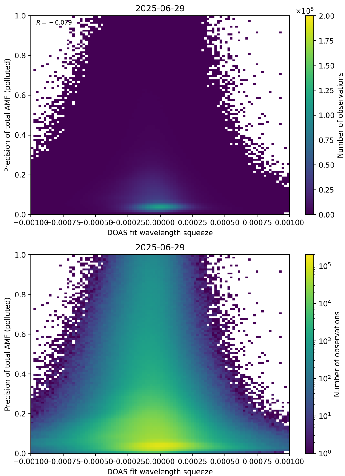
Figure 146: Scatter density plot of “DOAS fit wavelength squeeze” against “Precision of total AMF (polluted)” for 2025-06-28 to 2025-06-30.
