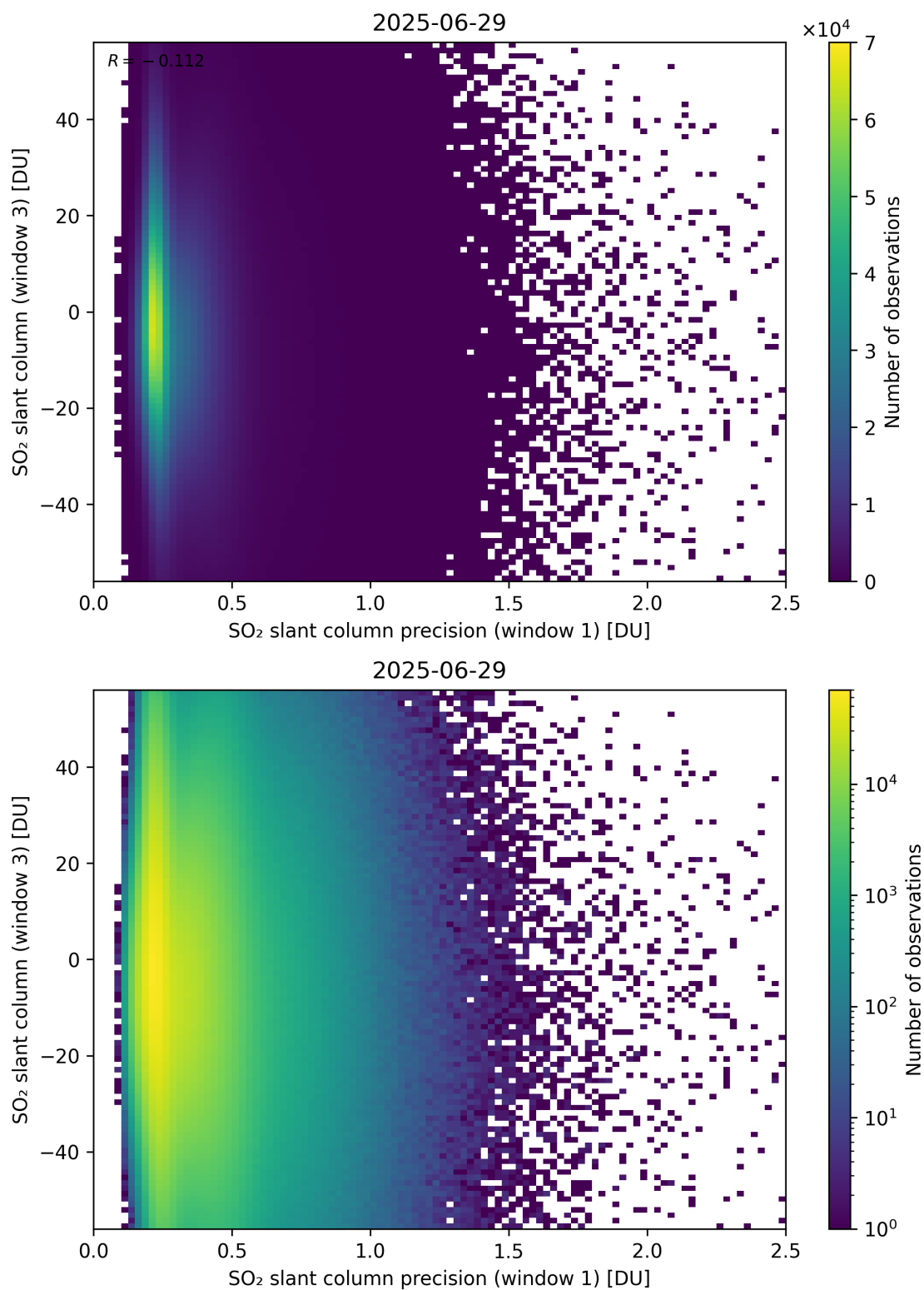
Figure 278: Scatter density plot of “SO 2 slant column precision (window 1)” against “SO 2 slant column (window 3)” for 2025-06-28 to 2025-06-30.
