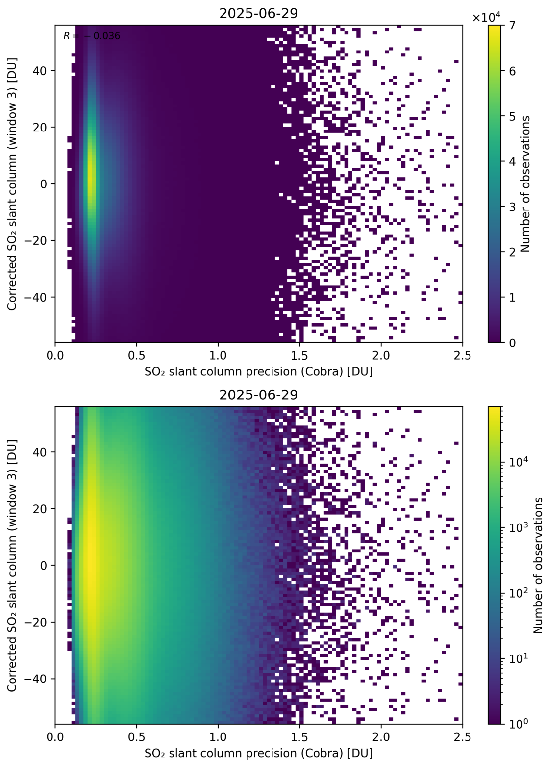
Figure 207: Scatter density plot of “SO 2 slant column precision (Cobra)” against “Corrected SO 2 slant column (window 3)” for 2025-06-28 to 2025-06-30.
