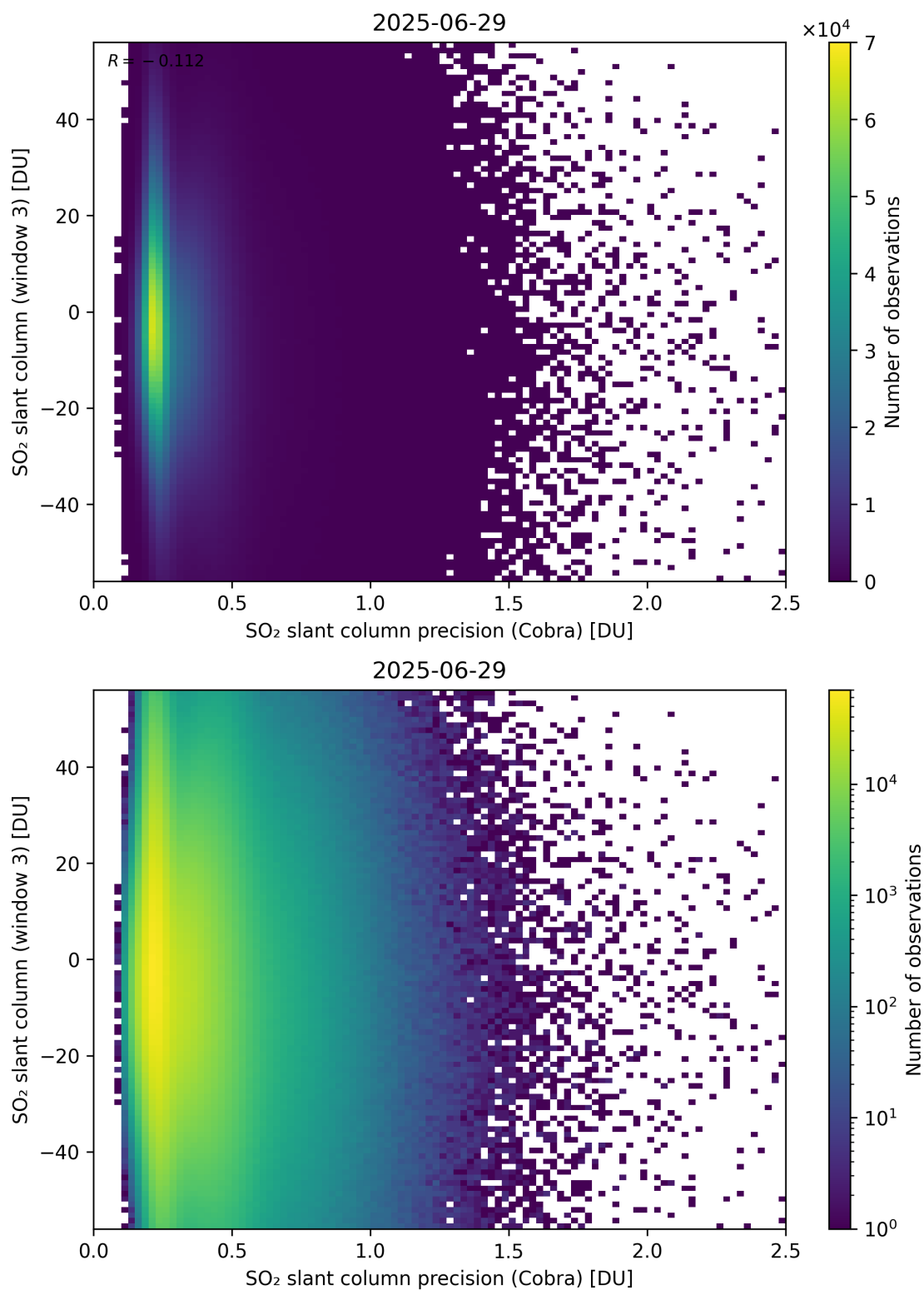
Figure 211: Scatter density plot of “SO 2 slant column precision (Cobra)” against “SO 2 slant column (window 3)” for 2025-06-28 to 2025-06-30.
