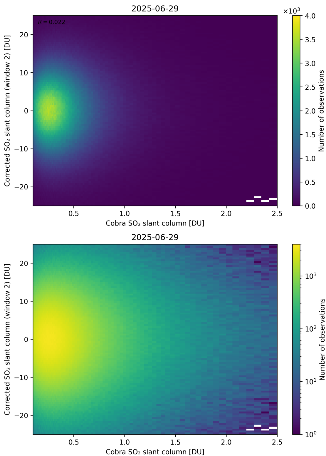
Figure 217: Scatter density plot of “Cobra SO 2 slant column” against “Corrected SO 2 slant column (window 2)” for 2025-06-28 to 2025-06-30.
