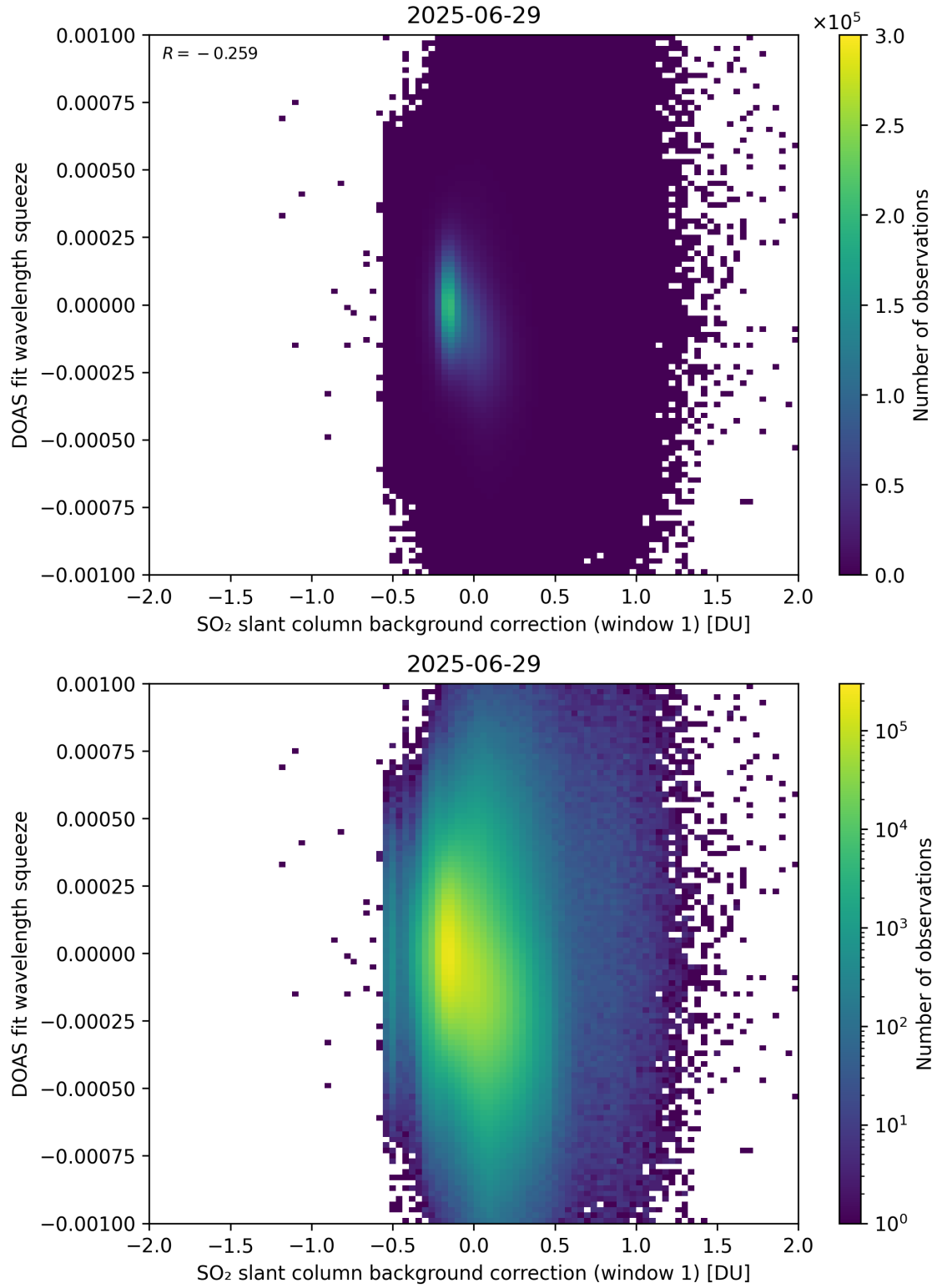
Figure 112: Scatter density plot of “SO 2 slant column background correction (window 1)” against “DOAS fit wavelength squeeze” for 2025-06-28 to 2025-06-30.
