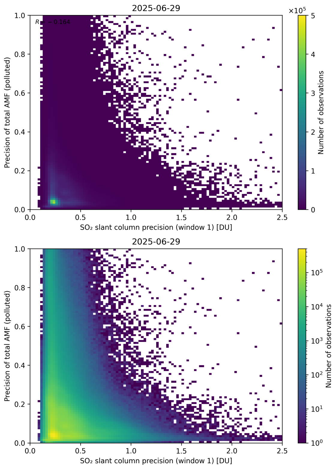
Figure 281: Scatter density plot of “SO 2 slant column precision (window 1)” against “Precision of total AMF (polluted)” for 2025-06-28 to 2025-06-30.
