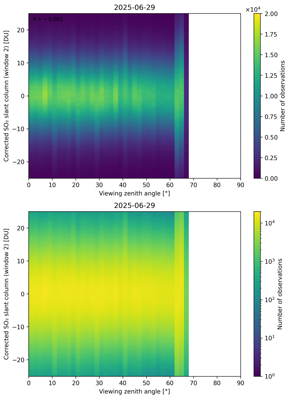
Figure 374: Scatter density plot of “Viewing zenith angle” against “Corrected SO 2 slant column (window 2)” for 2025-06-28 to 2025-06-30.
