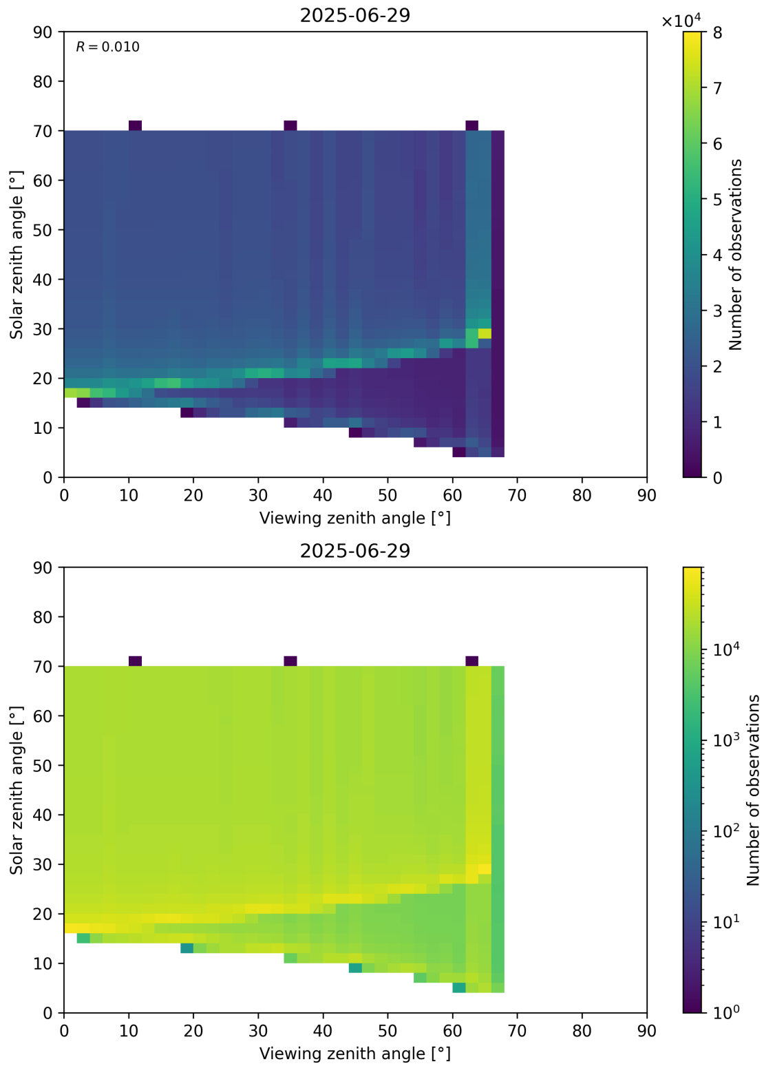
Figure 369: Scatter density plot of “Viewing zenith angle” against “Solar zenith angle” for 2025-06-28 to 2025-06-30.
