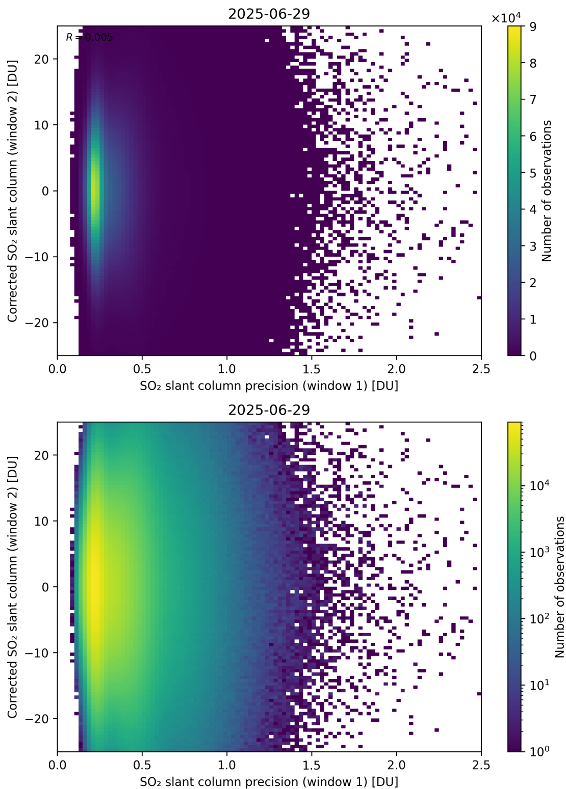
Figure 275: Scatter density plot of “SO 2 slant column precision (window 1)” against “Corrected SO 2 slant column (window 2)” for 2025-06-28 to 2025-06-30.
