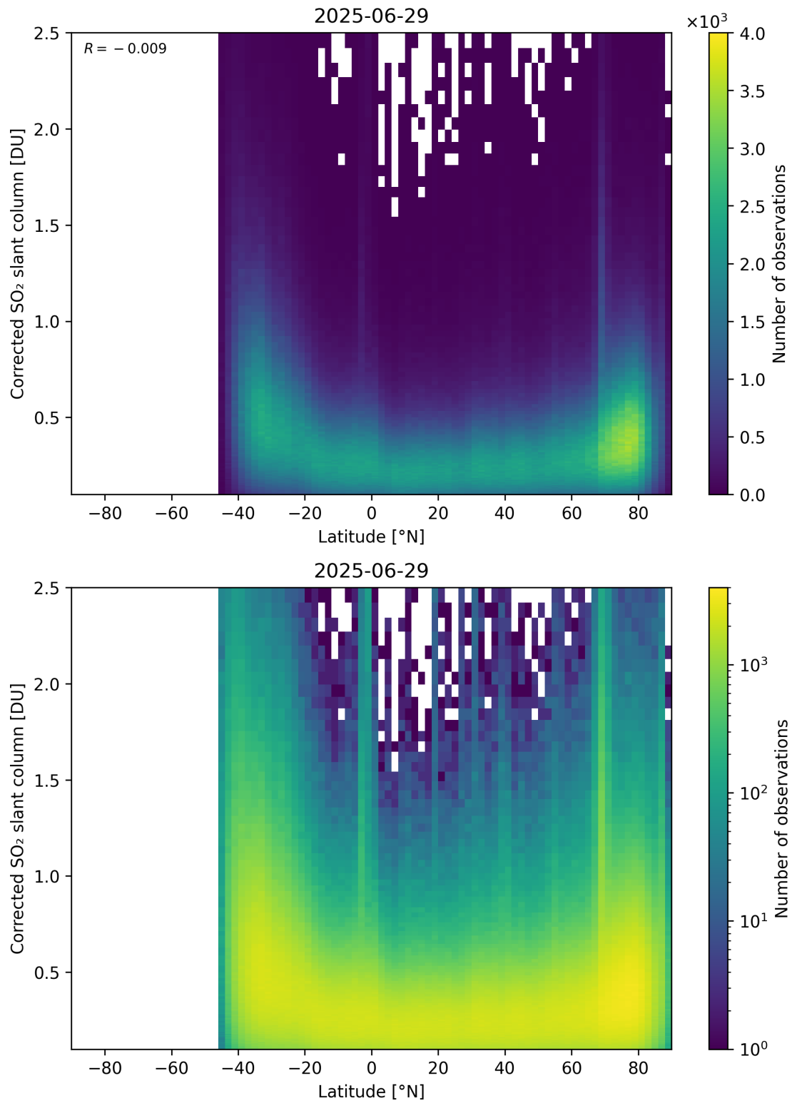
Figure 159: Scatter density plot of “Latitude” against “Corrected SO 2 slant column” for 2025-06-28 to 2025-06-30.
