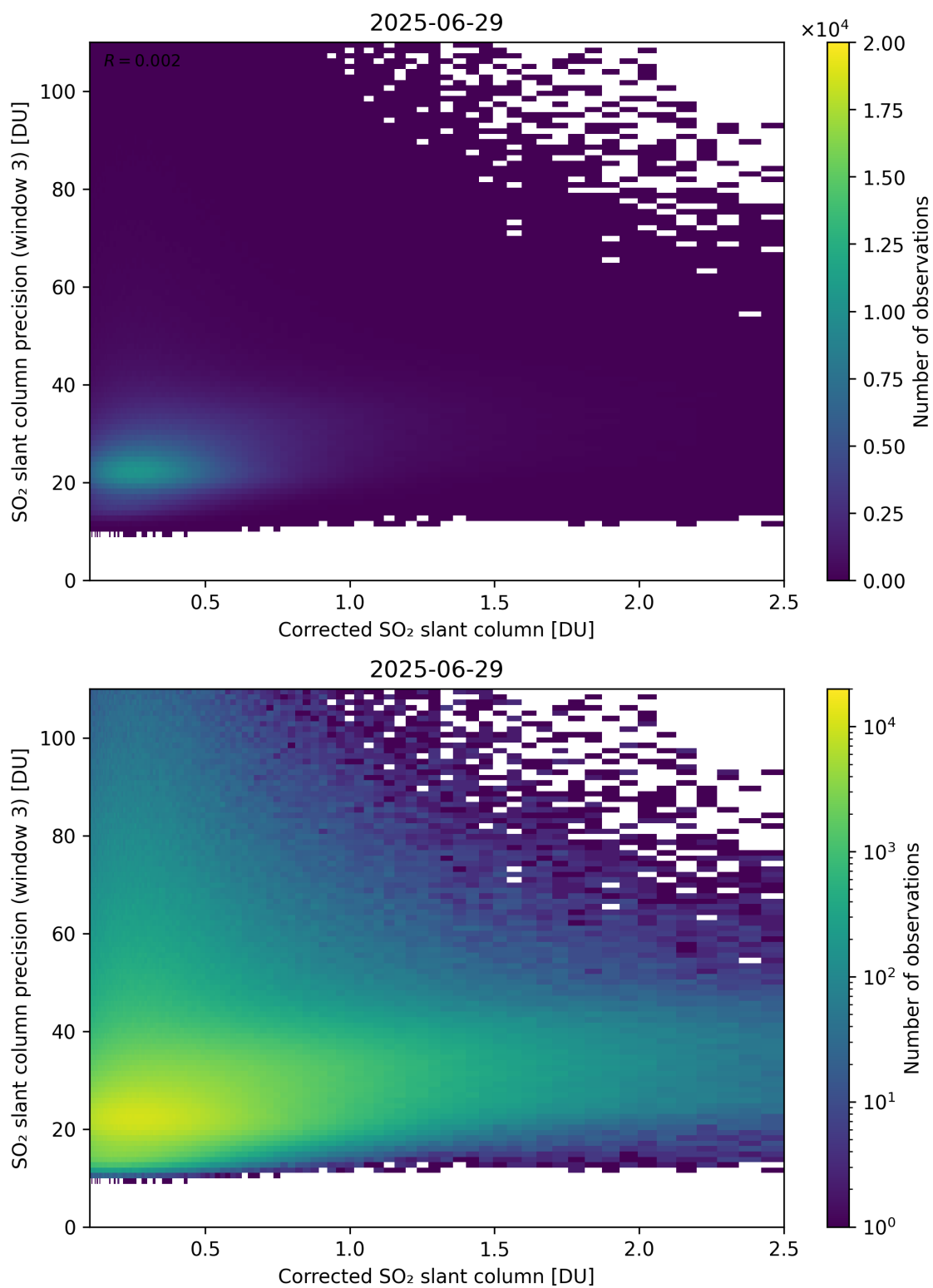
Figure 241: Scatter density plot of “Corrected SO 2 slant column” against “SO 2 slant column precision (window 3)” for 2025-06-28 to 2025-06-30.
