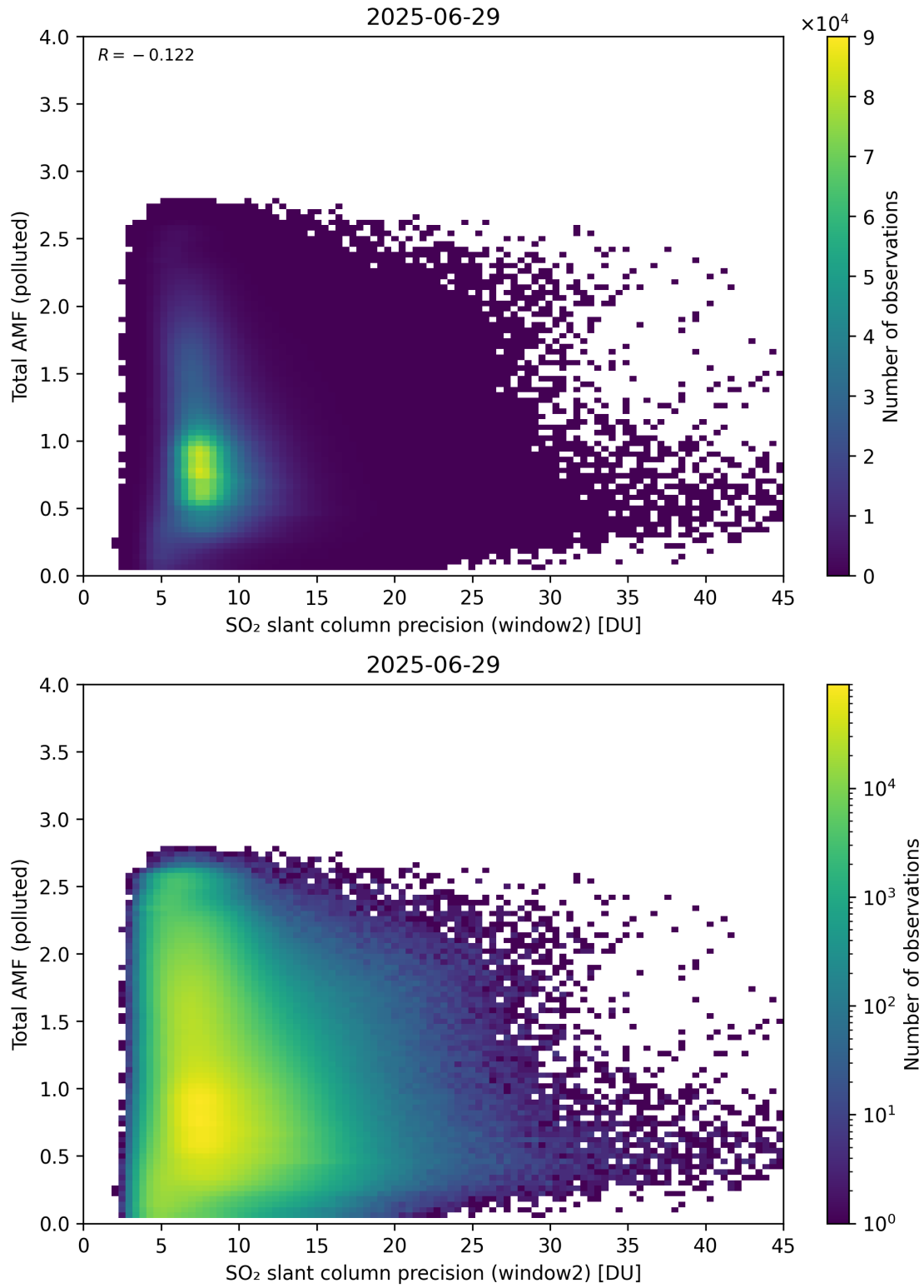
Figure 301: Scatter density plot of “SO 2 slant column precision (window2)” against “Total AMF (polluted)” for 2025-06-28 to 2025-06-30.
