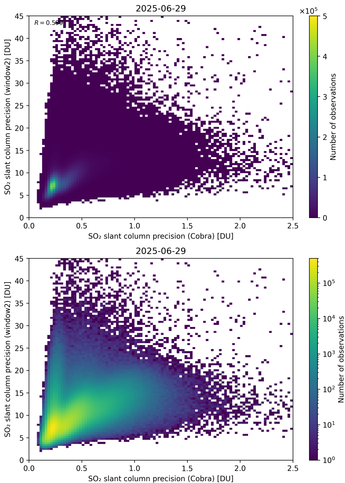
Figure 210: Scatter density plot of “SO 2 slant column precision (Cobra)” against “SO 2 slant column precision (window2)” for 2025-06-28 to 2025-06-30.
