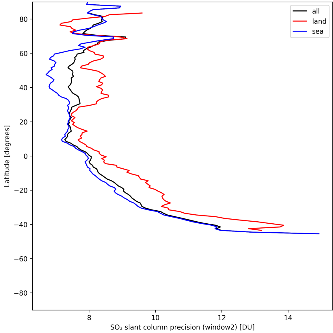
Figure 42: Zonal average of “SO 2 slant column precision (window2)” for 2025-06-28 to 2025-06-30.
