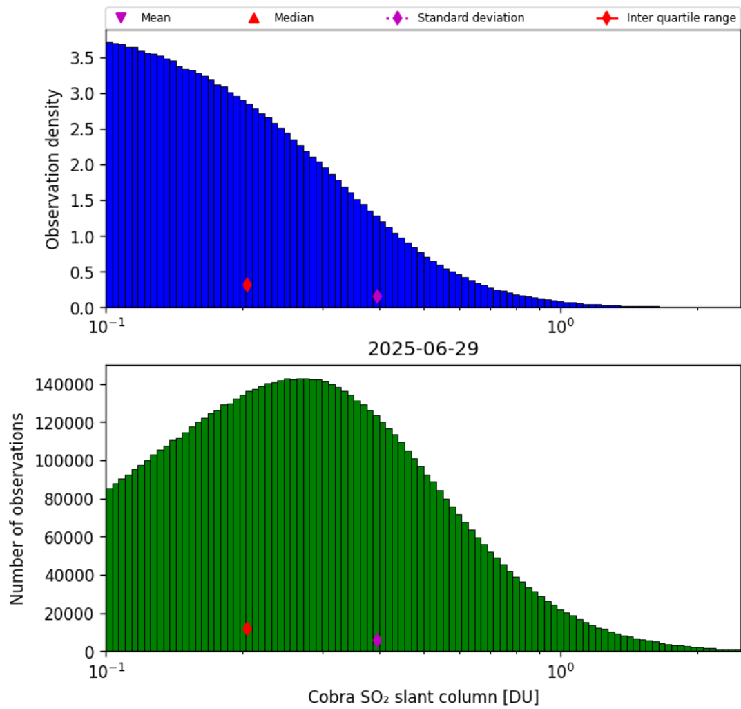
Figure 61: Histogram of “Cobra SO 2 slant column” for 2025-06-28 to 2025-06-30
