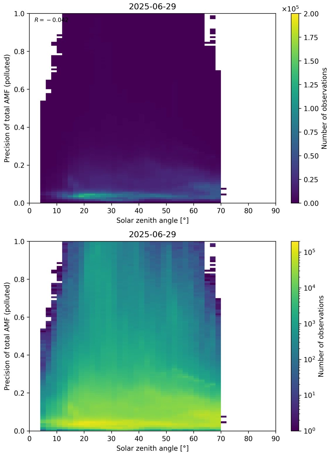
Figure 190: Scatter density plot of “Solar zenith angle” against “Precision of total AMF (polluted)” for 2025-06-28 to 2025-06-30.
