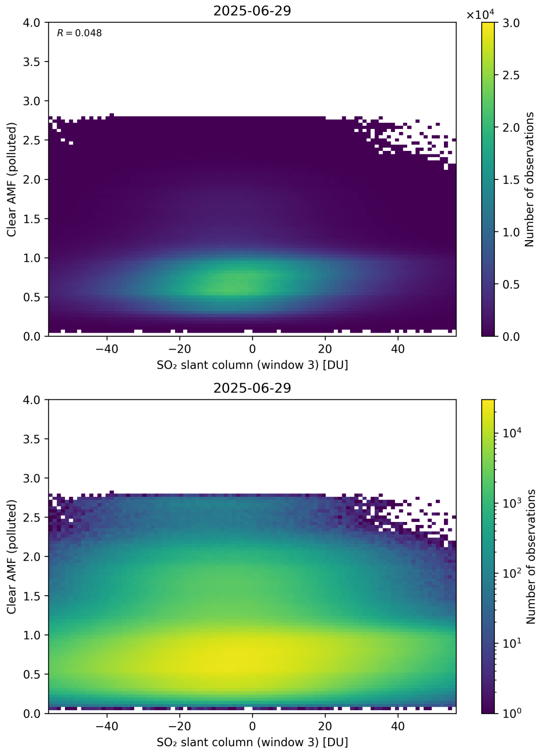
Figure 315: Scatter density plot of “SO 2 slant column (window 3)” against “Clear AMF (polluted)” for 2025-06-28 to 2025-06-30.
