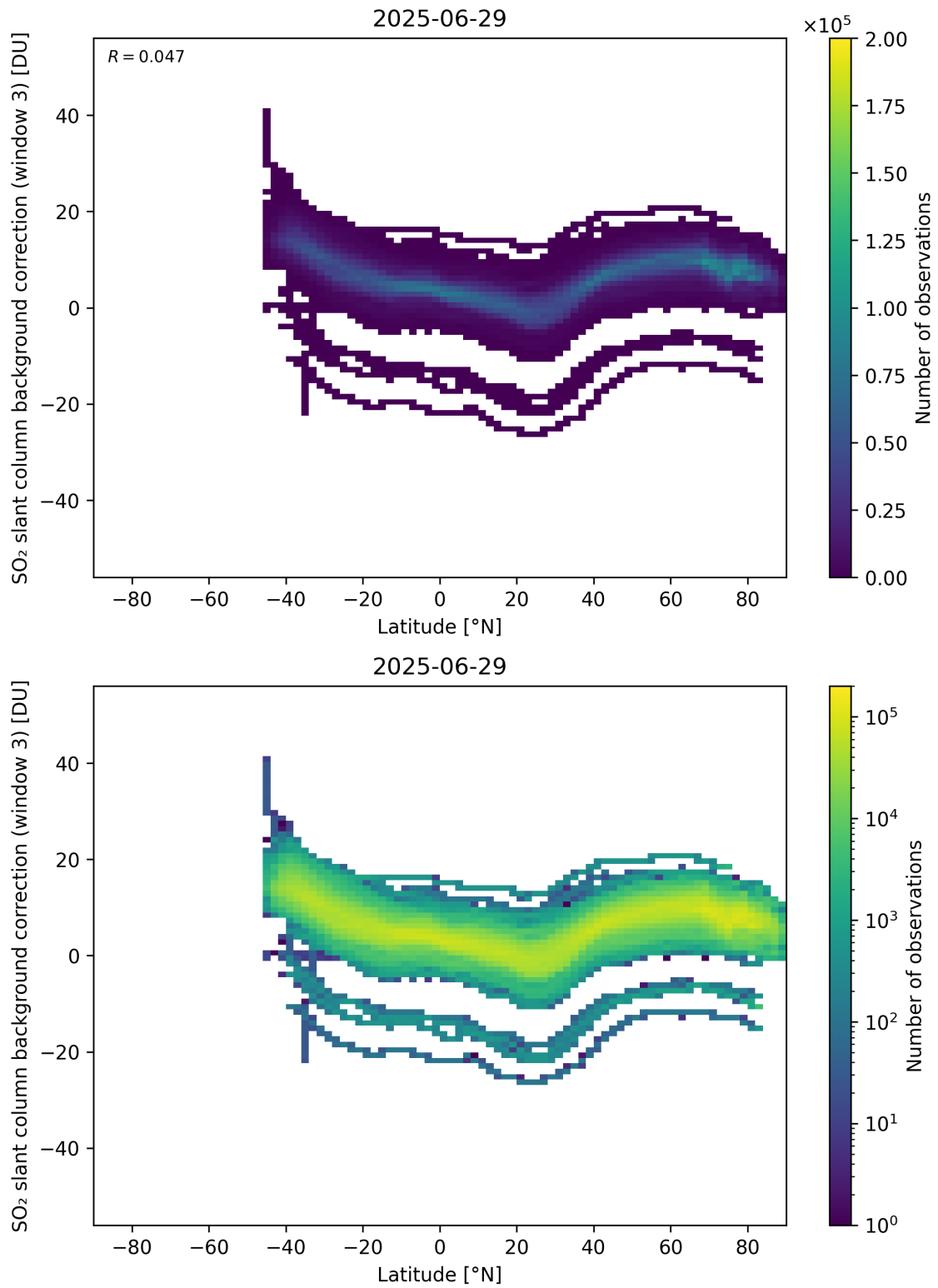
Figure 152: Scatter density plot of “Latitude” against “SO 2 slant column background correction (window 3)” for 2025-06-28 to 2025-06-30.
