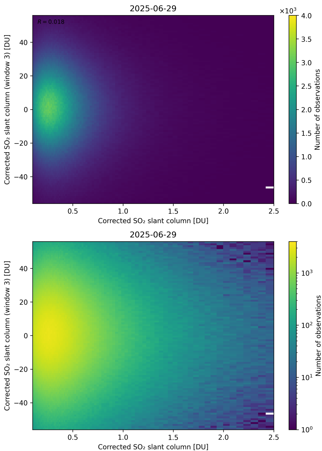
Figure 236: Scatter density plot of “Corrected SO 2 slant column” against “Corrected SO 2 slant column (window 3)” for 2025-06-28 to 2025-06-30.
