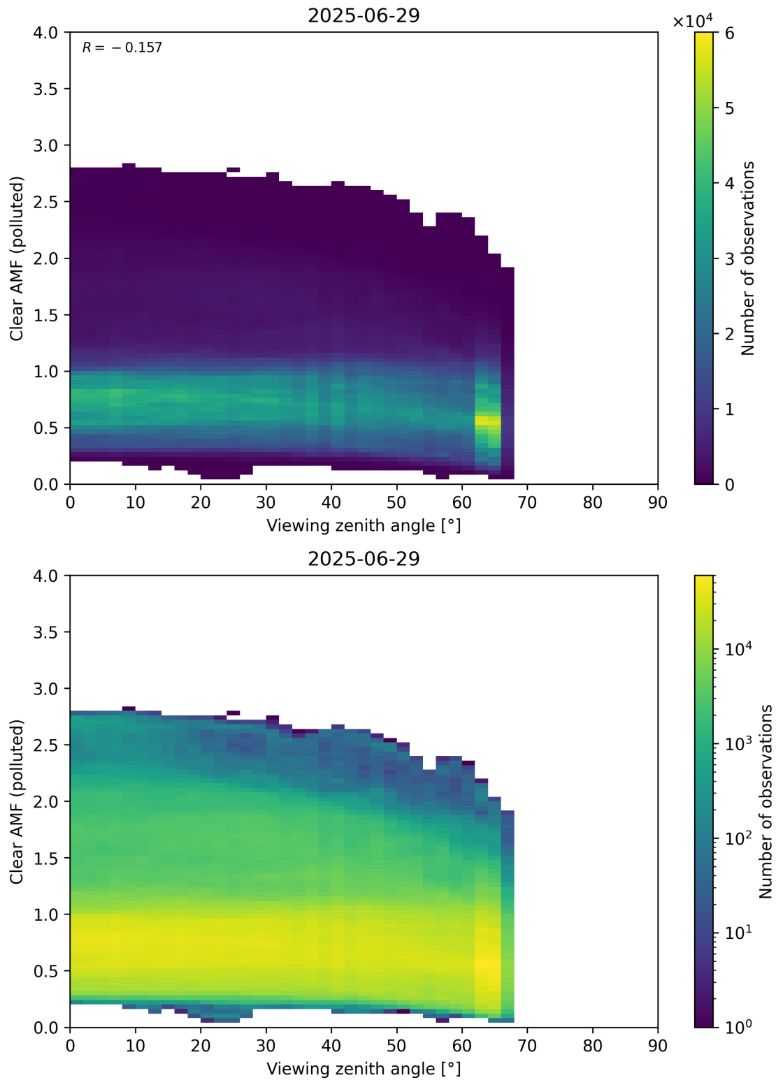
Figure 370: Scatter density plot of “Viewing zenith angle” against “Clear AMF (polluted)” for 2025-06-28 to 2025-06-30.
