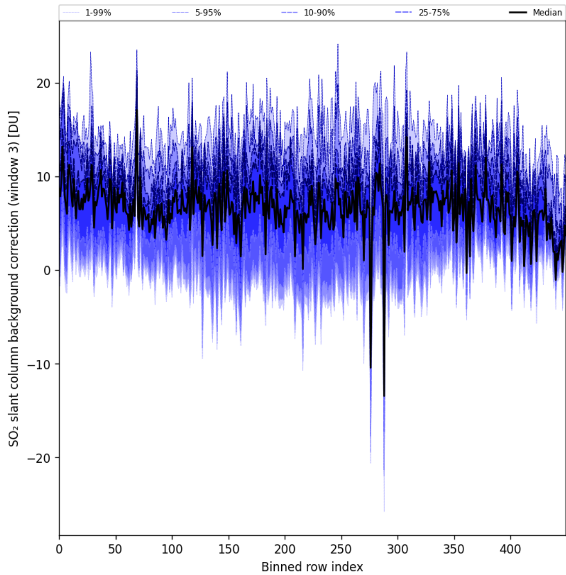
Figure 100: Along track statistics of “SO 2 slant column background correction (window 3)” for 2025-06-28 to 2025-06-30
