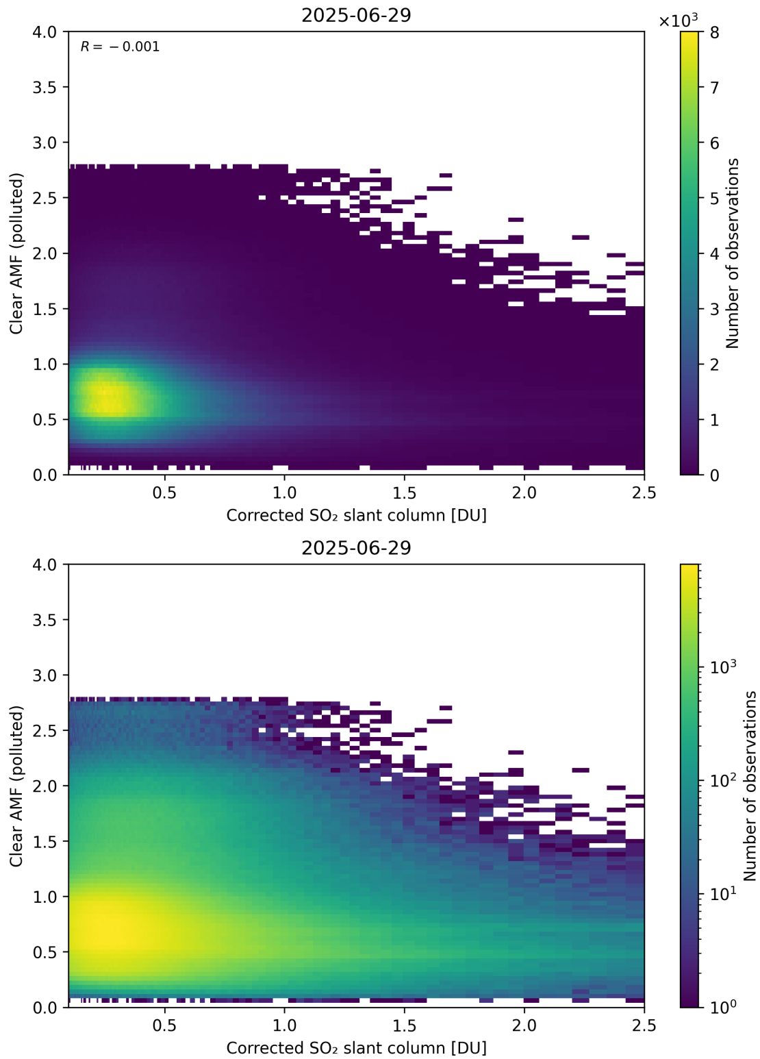
Figure 232: Scatter density plot of “Corrected SO 2 slant column” against “Clear AMF (polluted)” for 2025-06-28 to 2025-06-30.
