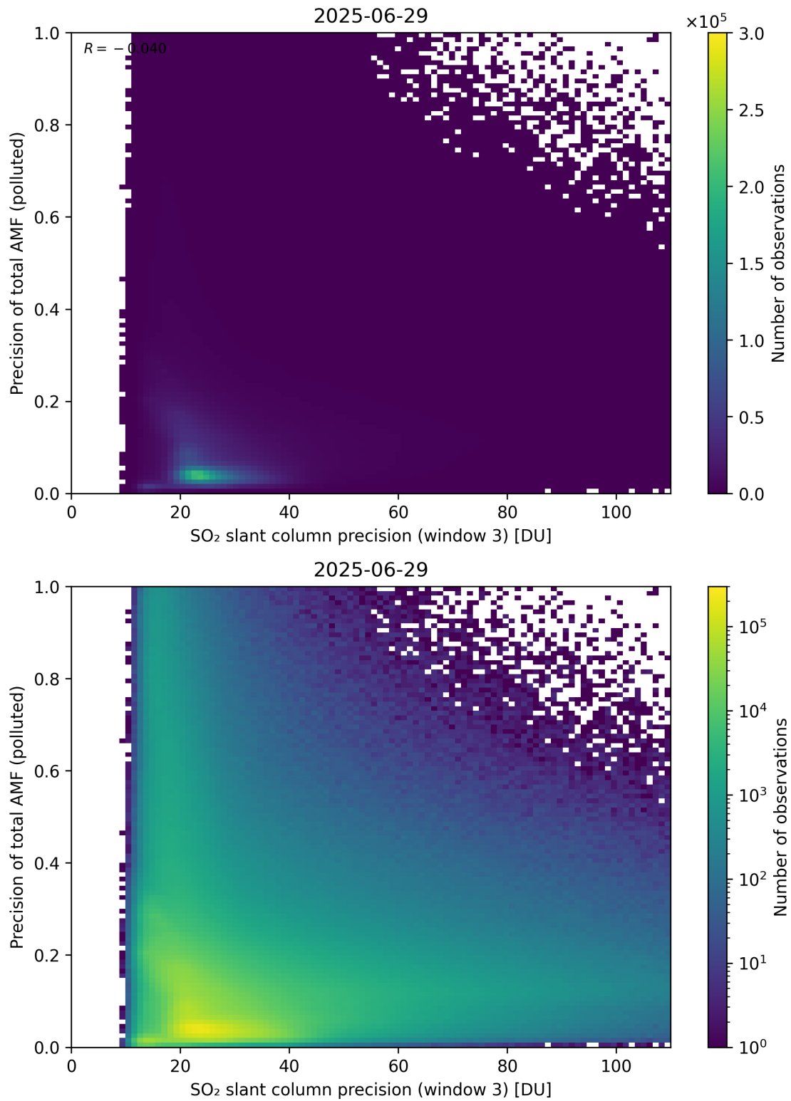
Figure 314: Scatter density plot of “SO 2 slant column precision (window 3)” against “Precision of total AMF (polluted)” for 2025-06-28 to 2025-06-30.
