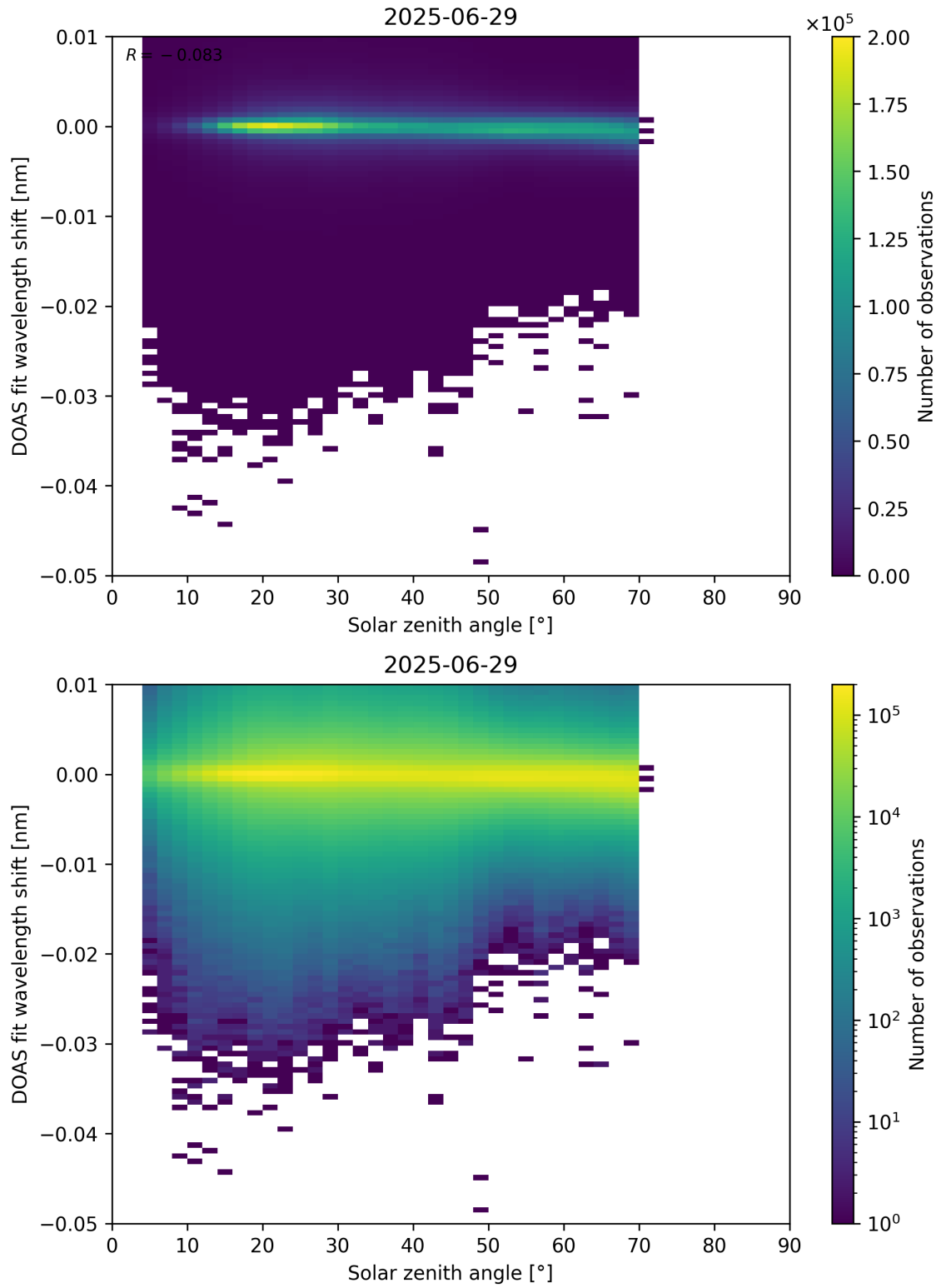
Figure 174: Scatter density plot of “Solar zenith angle” against “DOAS fit wavelength shift” for 2025-06-28 to 2025-06-30.
