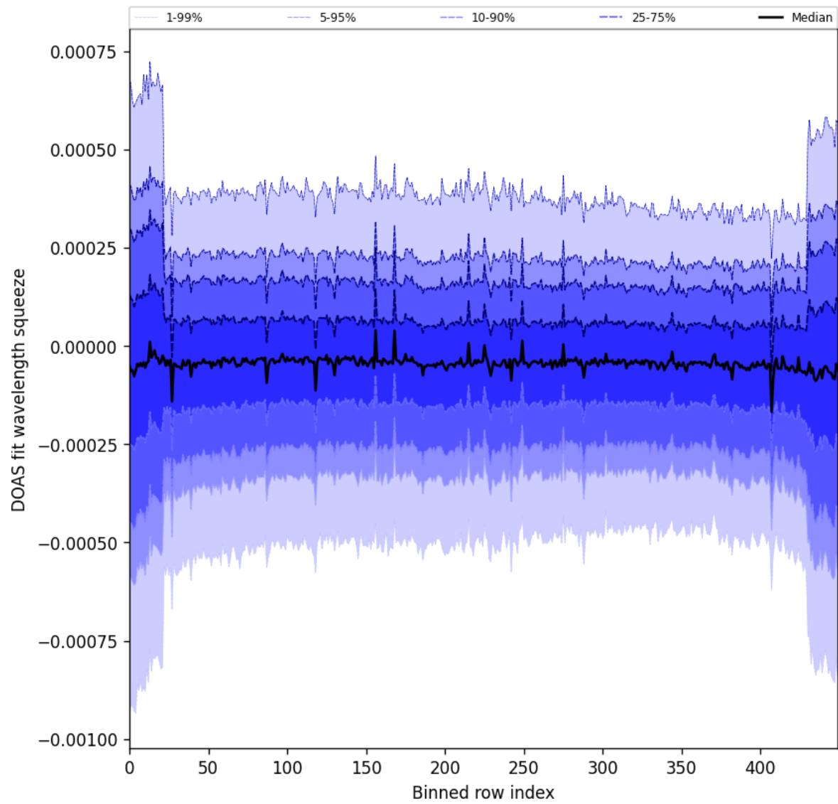
Figure 103: Along track statistics of “DOAS fit wavelength squeeze” for 2025-06-28 to 2025-06-30
