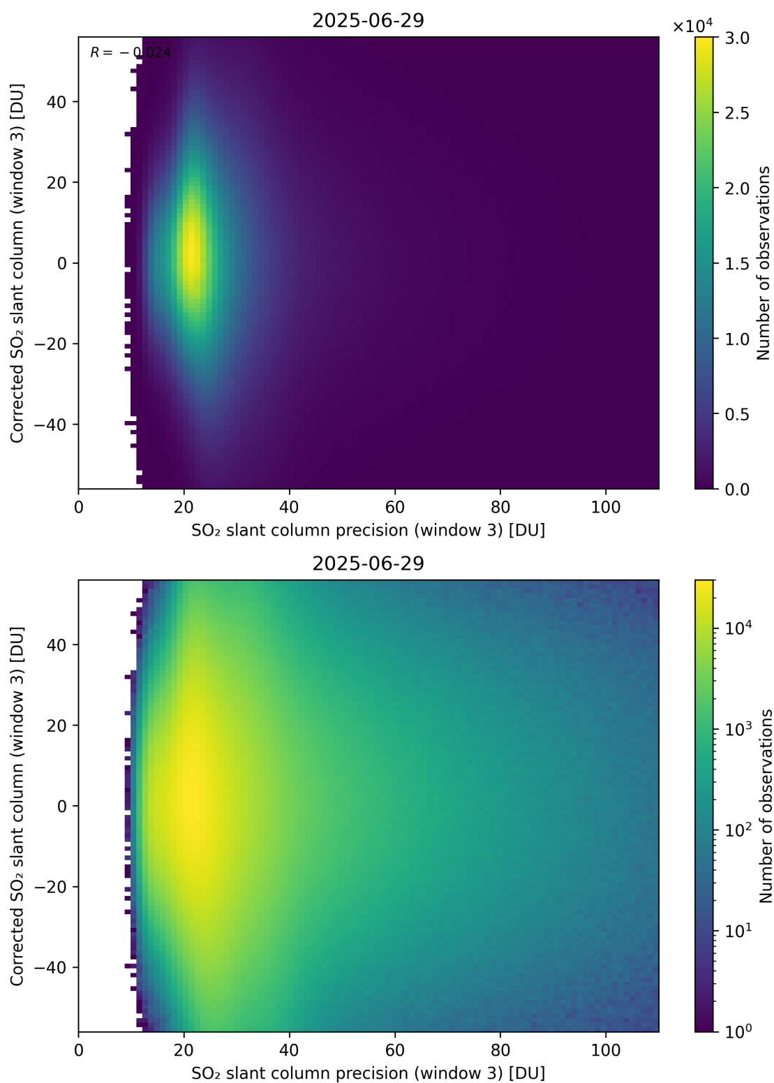
Figure 312: Scatter density plot of “SO 2 slant column precision (window 3)” against “Corrected SO 2 slant column (window 3)” for 2025-06-28 to 2025-06-30.
