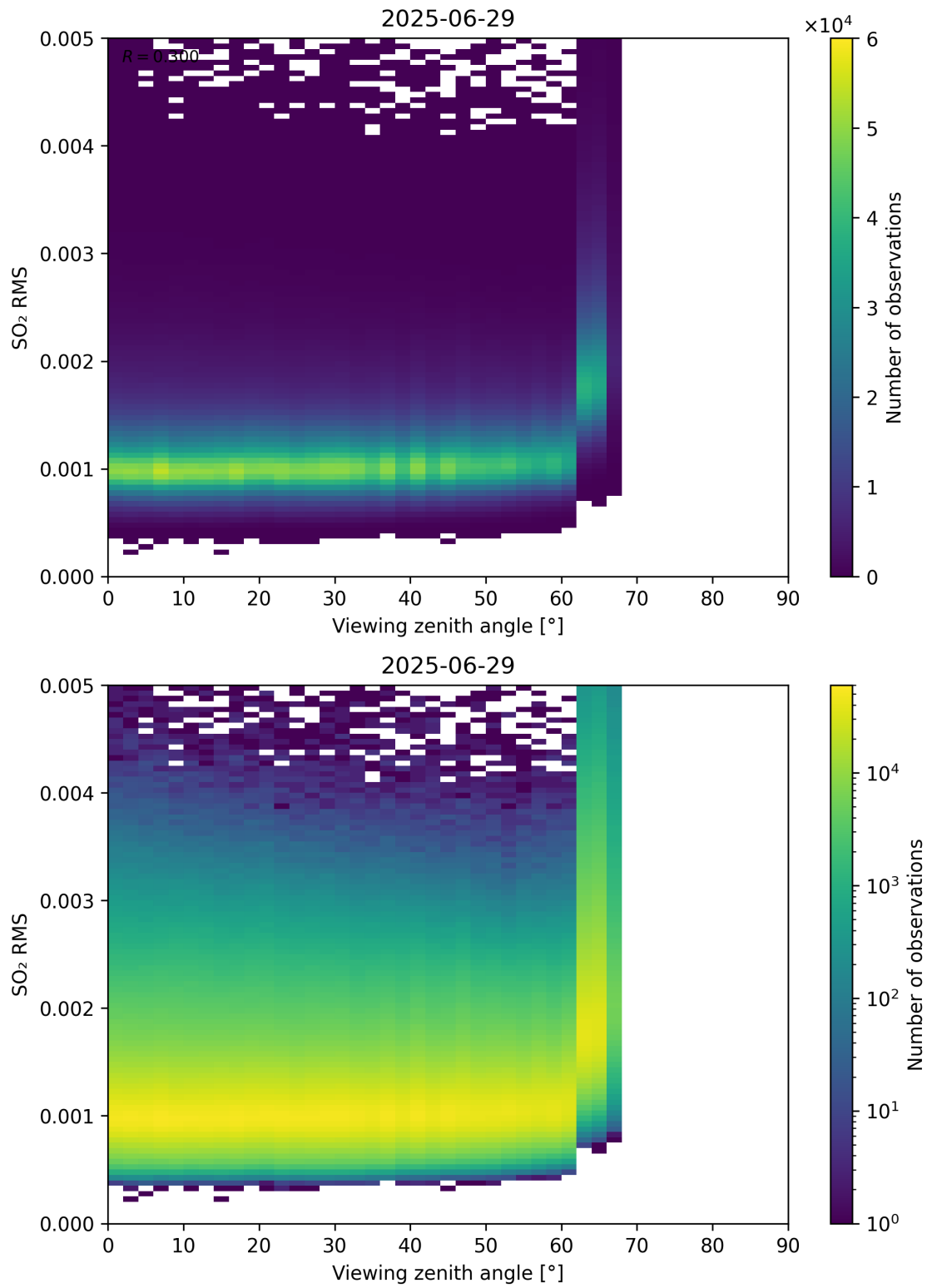
Figure 367: Scatter density plot of “Viewing zenith angle” against “SO 2 RMS” for 2025-06-28 to 2025-06-30.
