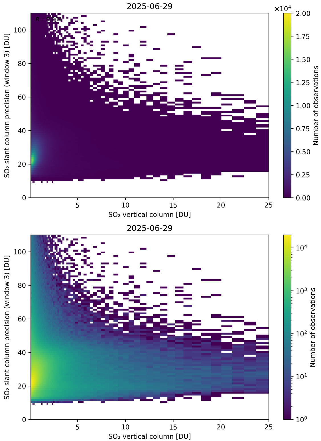
Figure 358: Scatter density plot of “SO 2 vertical column” against “SO 2 slant column precision (window 3)” for 2025-06-28 to 2025-06-30.
