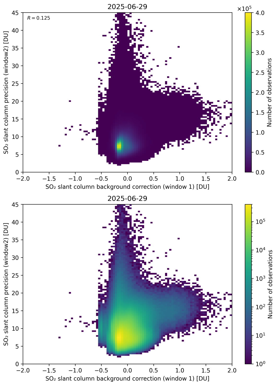
Figure 117: Scatter density plot of “SO 2 slant column background correction (window 1)” against “SO 2 slant column precision (window2)” for 2025-06-28 to 2025-06-30.
