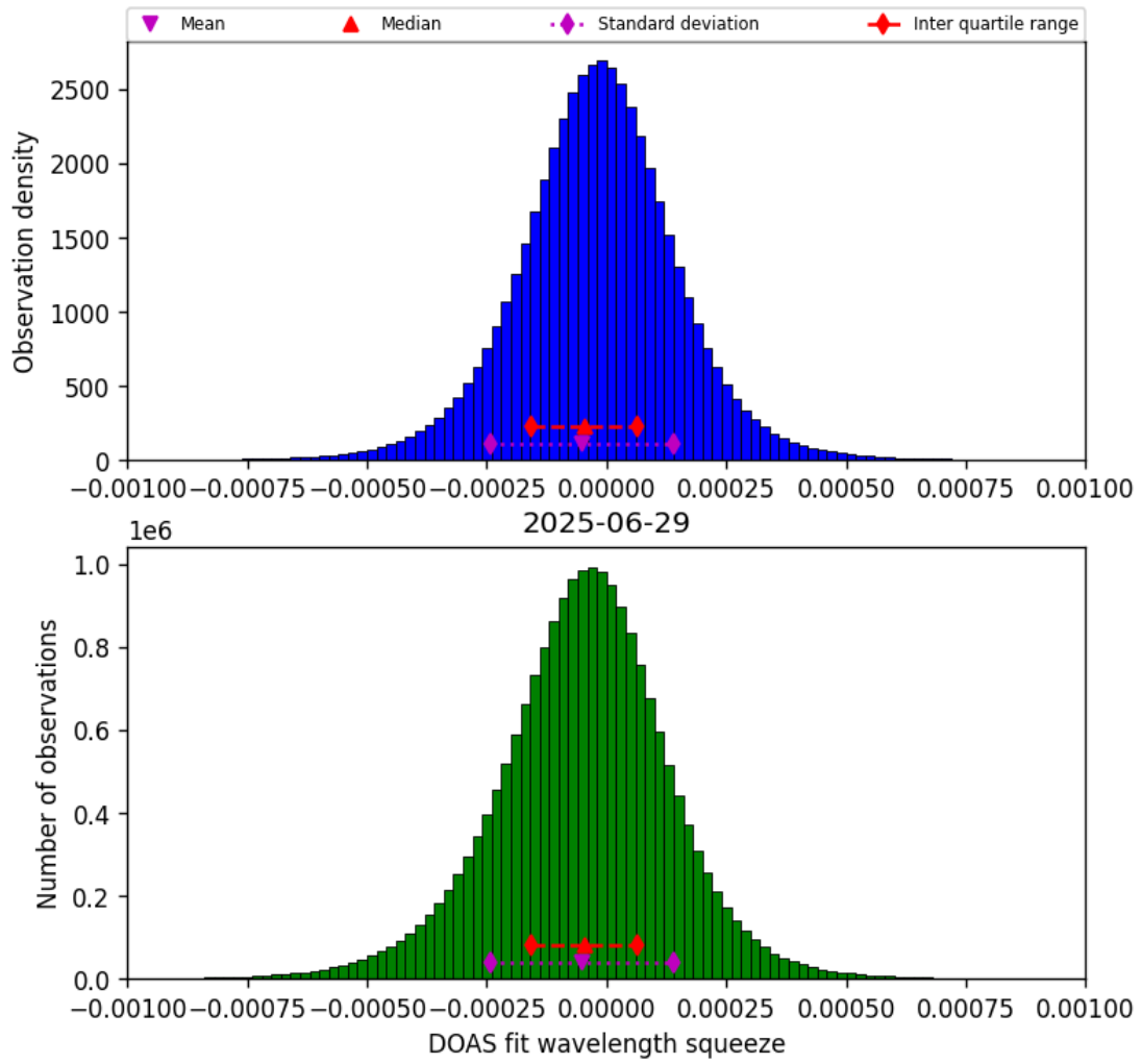
Figure 77: Histogram of “DOAS fit wavelength squeeze” for 2025-06-28 to 2025-06-30
