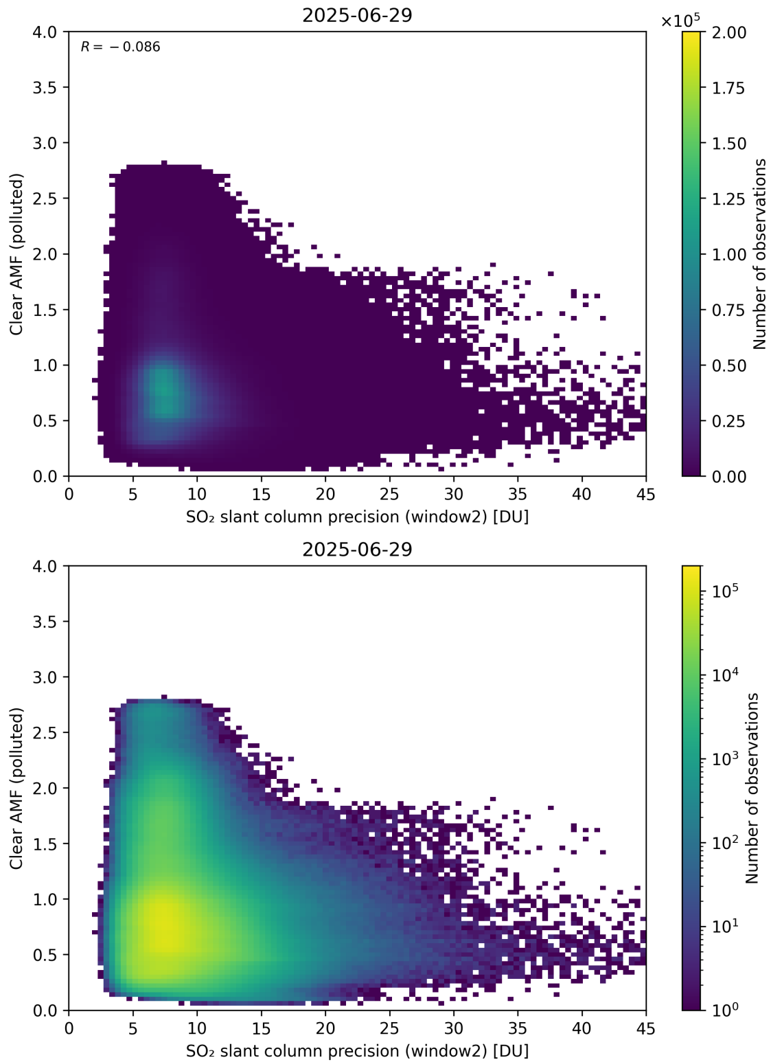
Figure 296: Scatter density plot of “SO 2 slant column precision (window2)” against “Clear AMF (polluted)” for 2025-06-28 to 2025-06-30.
