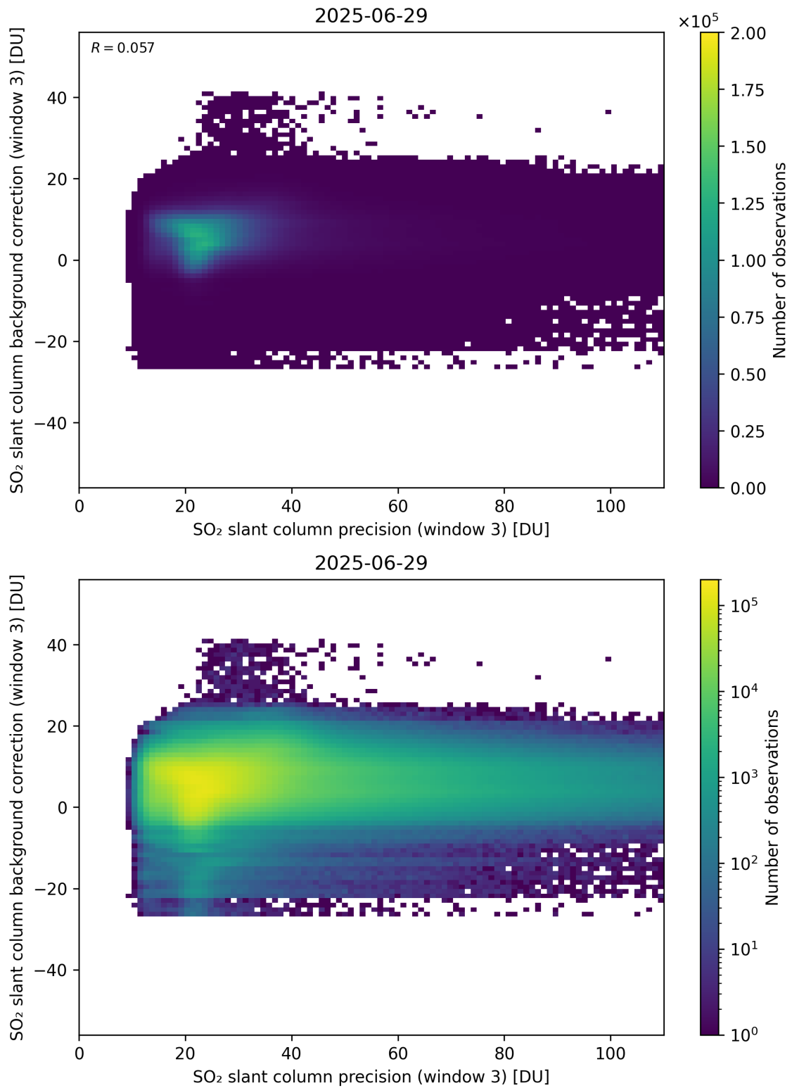
Figure 307: Scatter density plot of “SO 2 slant column precision (window 3)” against “SO 2 slant column background correction (window 3)” for 2025-06-28 to 2025-06-30.
