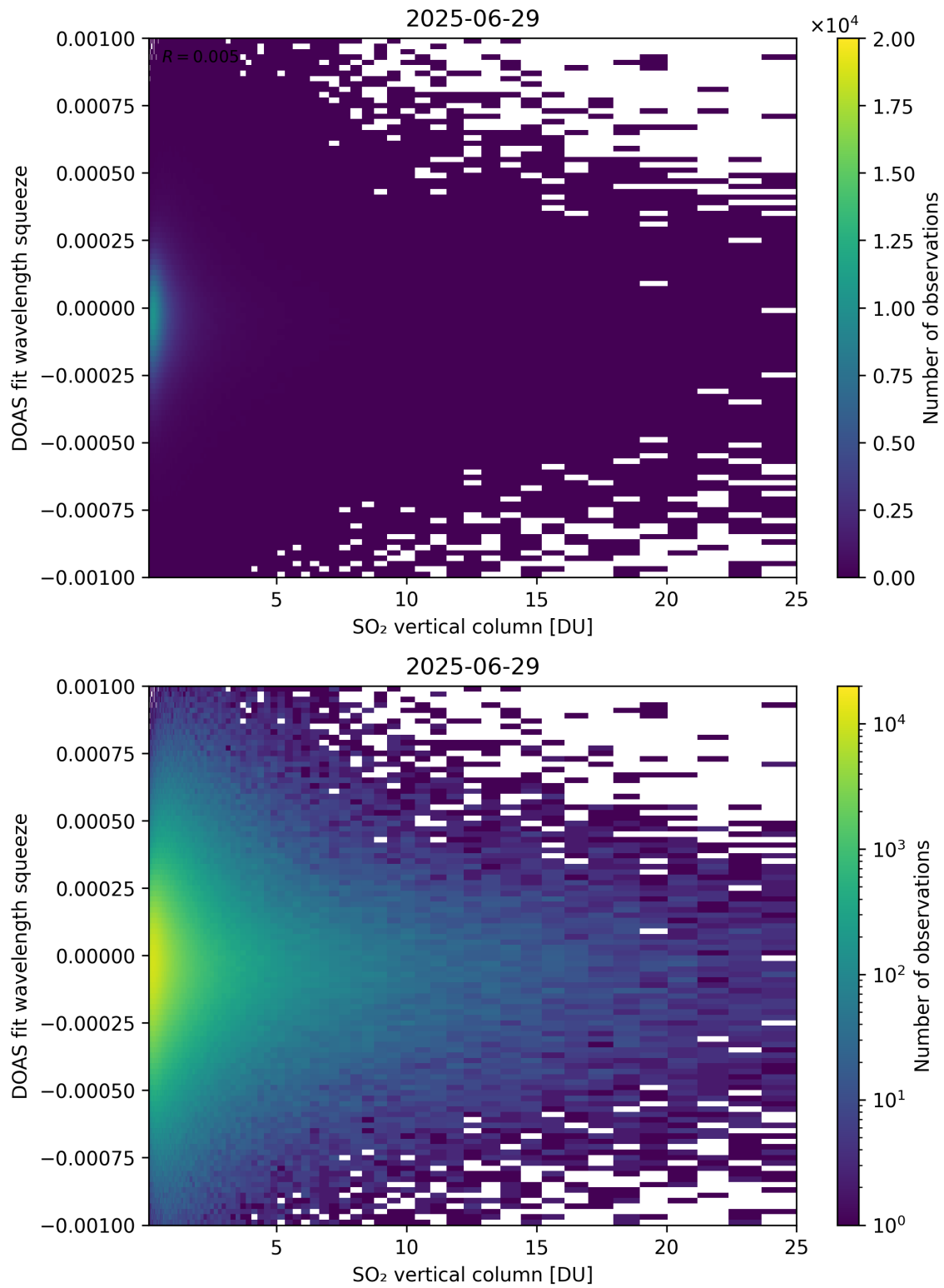
Figure 327: Scatter density plot of “SO 2 vertical column” against “DOAS fit wavelength squeeze” for 2025-06-28 to 2025-06-30.
