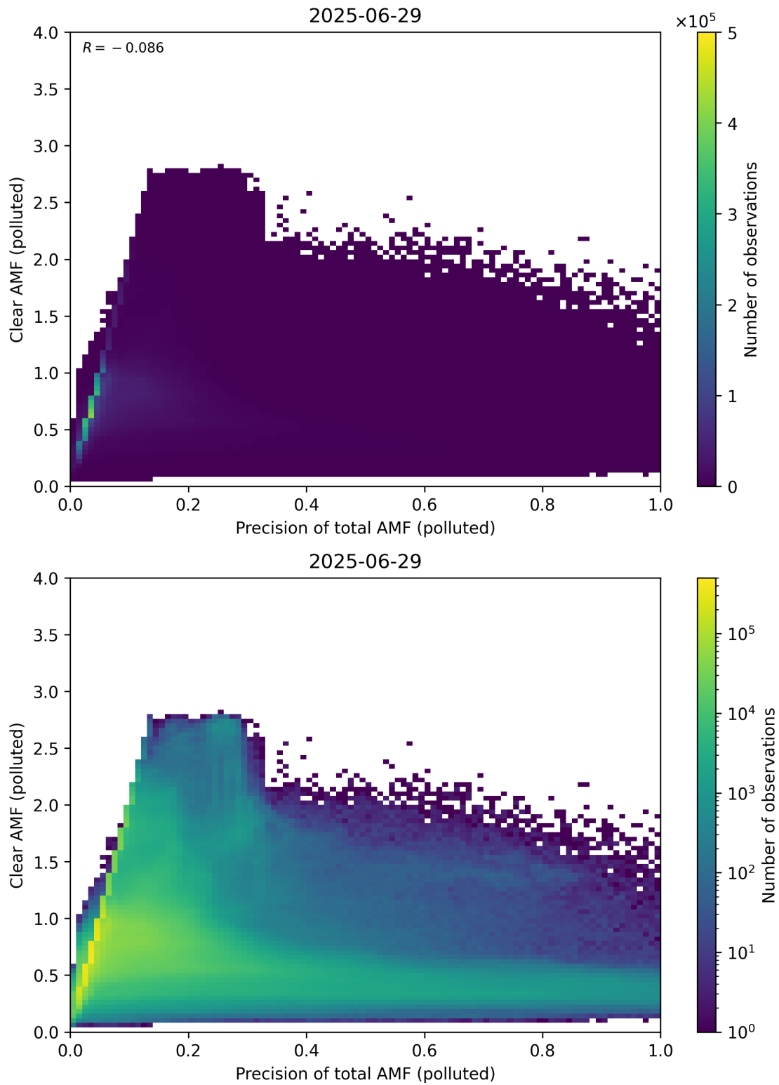
Figure 320: Scatter density plot of “Precision of total AMF (polluted)” against “Clear AMF (polluted)” for 2025-06-28 to 2025-06-30.
