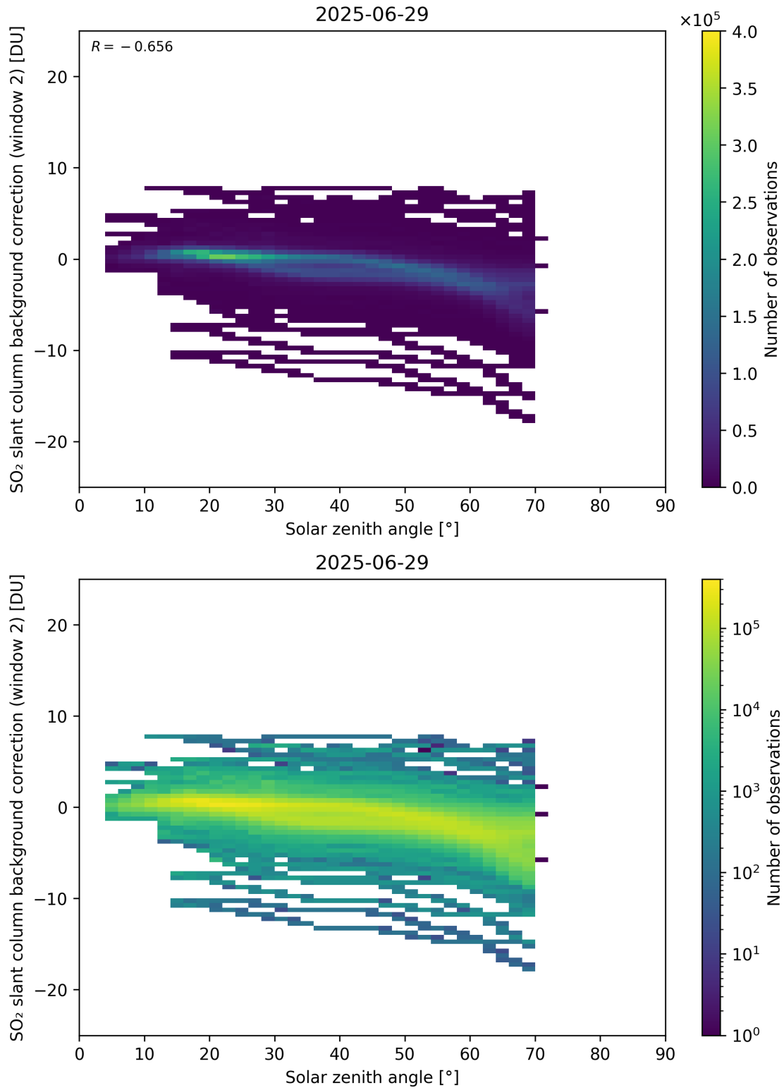
Figure 172: Scatter density plot of “Solar zenith angle” against “SO 2 slant column background correction (window 2)” for 2025-06-28 to 2025-06-30.
