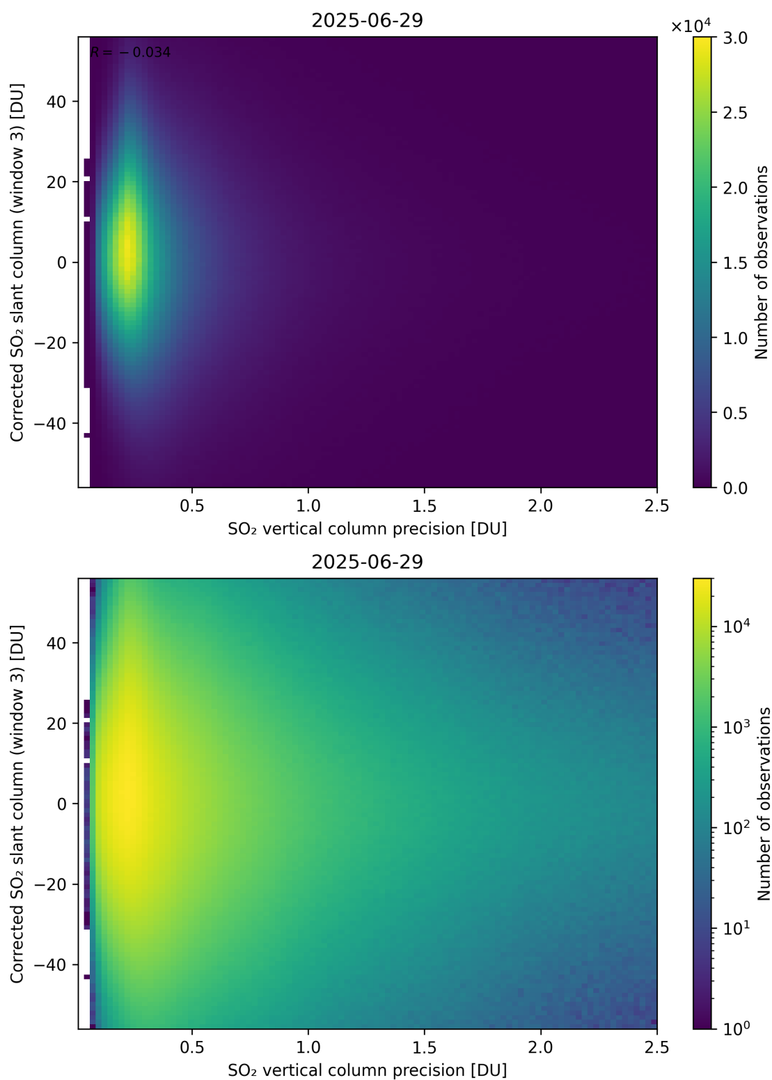
Figure 340: Scatter density plot of “SO 2 vertical column precision” against “Corrected SO 2 slant column (window 3)” for 2025-06-28 to 2025-06-30.
