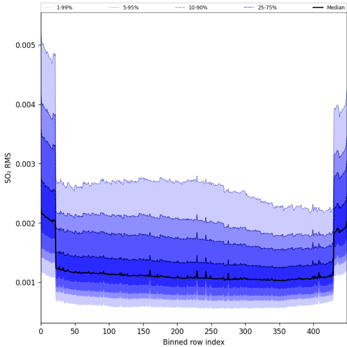
Figure 104: Along track statistics of “SO 2 RMS” for 2025-06-28 to 2025-06-30
