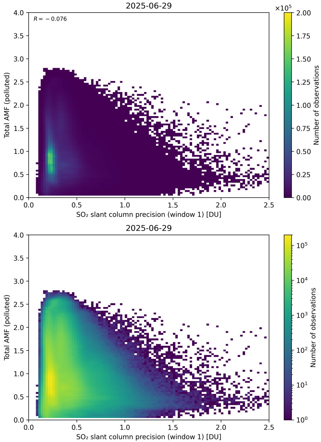
Figure 280: Scatter density plot of “SO 2 slant column precision (window 1)” against “Total AMF (polluted)” for 2025-06-28 to 2025-06-30.
