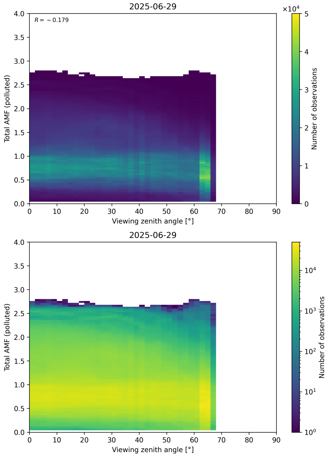
Figure 381: Scatter density plot of “Viewing zenith angle” against “Total AMF (polluted)” for 2025-06-28 to 2025-06-30.
