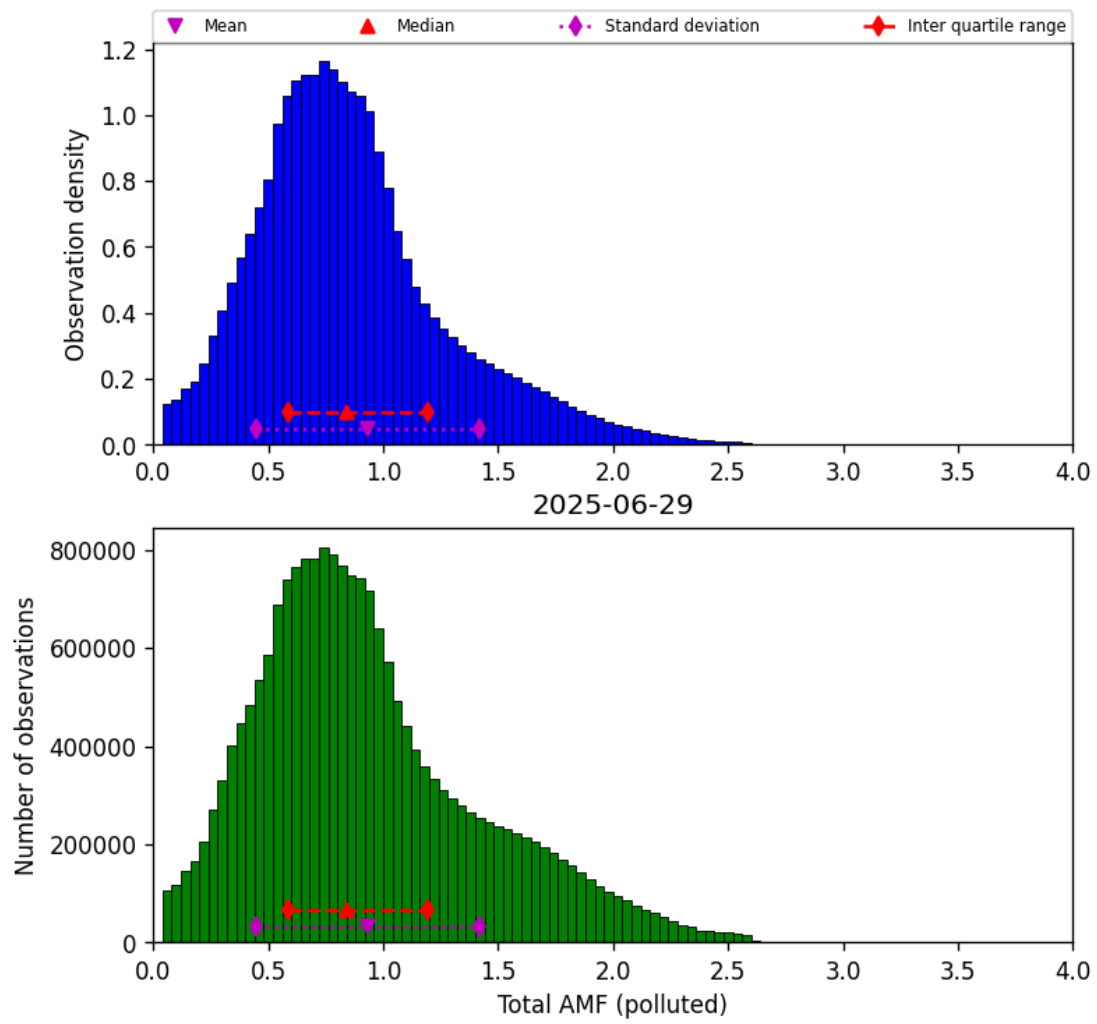
Figure 79: Histogram of “Total AMF (polluted)” for 2025-06-28 to 2025-06-30
