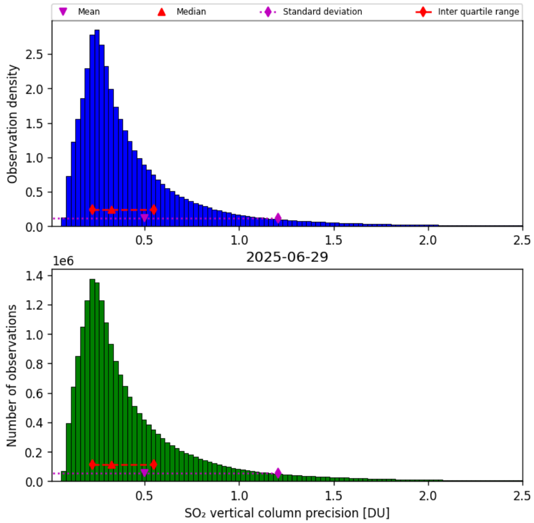
Figure 59: Histogram of “SO 2 vertical column precision” for 2025-06-28 to 2025-06-30
