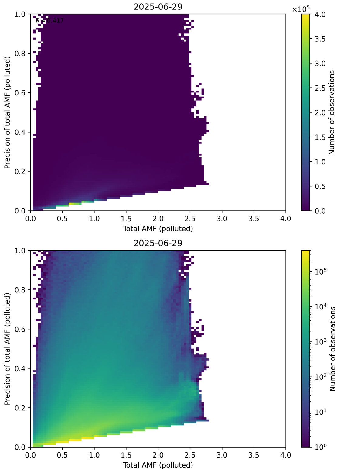
Figure 322: Scatter density plot of “Total AMF (polluted)” against “Precision of total AMF (polluted)” for 2025-06-28 to 2025-06-30.
