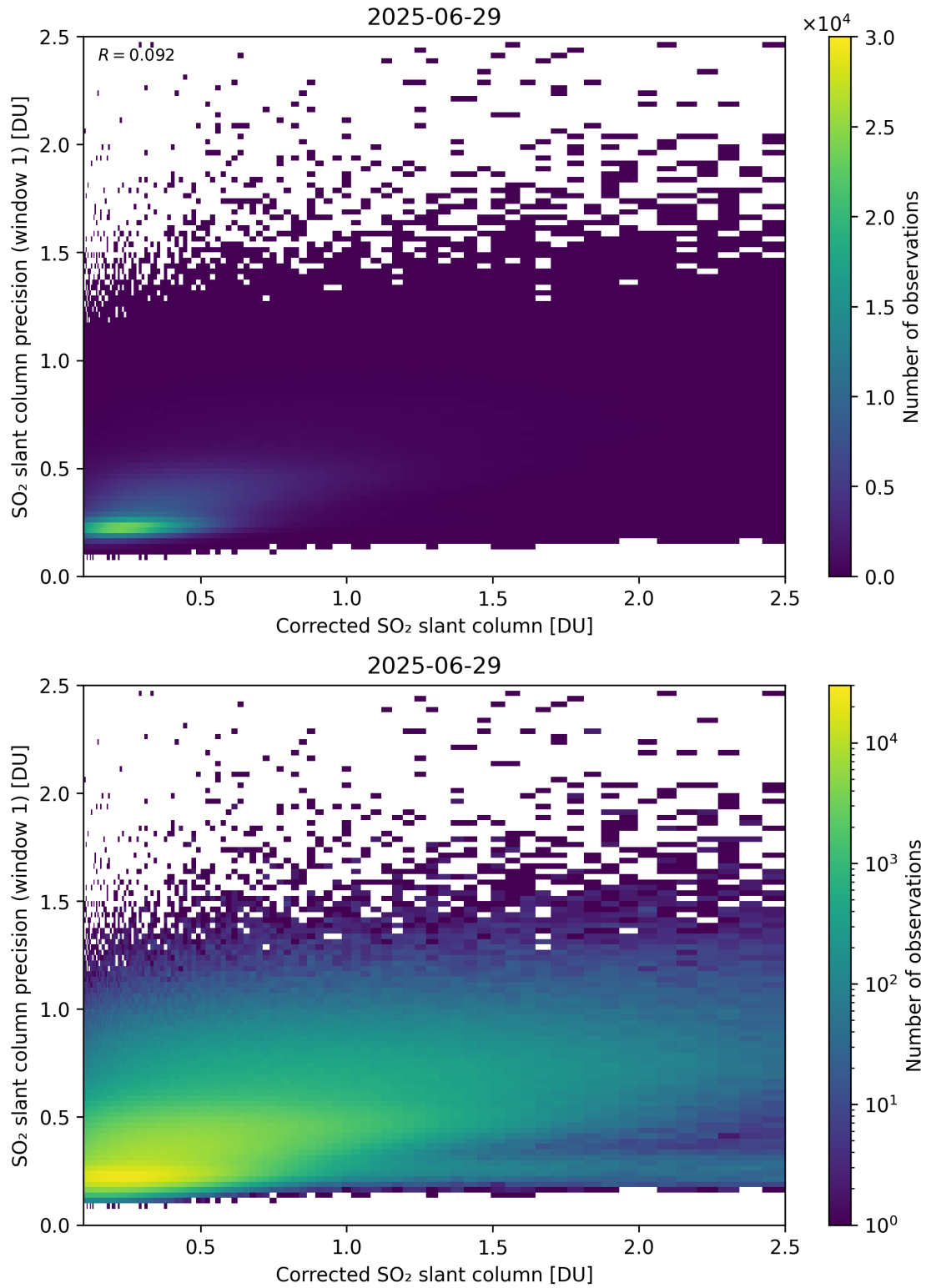
Figure 238: Scatter density plot of “Corrected SO 2 slant column” against “SO 2 slant column precision (window 1)” for 2025-06-28 to 2025-06-30.
