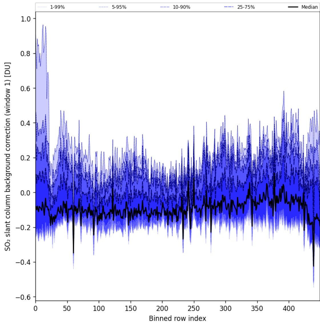
Figure 92: Along track statistics of “SO 2 slant column background correction (window 1)” for 2025-06-28 to 2025-06-30
