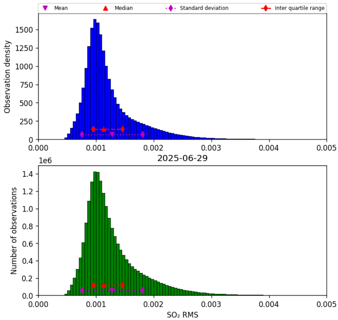
Figure 78: Histogram of “SO 2 RMS” for 2025-06-28 to 2025-06-30
