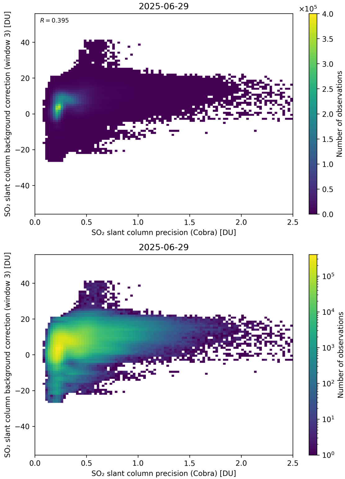
Figure 201: Scatter density plot of “SO 2 slant column precision (Cobra)” against “SO 2 slant column background correction (window 3)” for 2025-06-28 to 2025-06-30.
