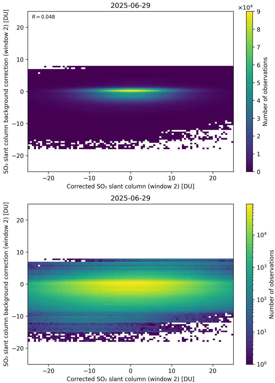
Figure 244: Scatter density plot of “Corrected SO 2 slant column (window 2)” against “SO 2 slant column background correction (window 2)” for 2025-06-28 to 2025-06-30.
