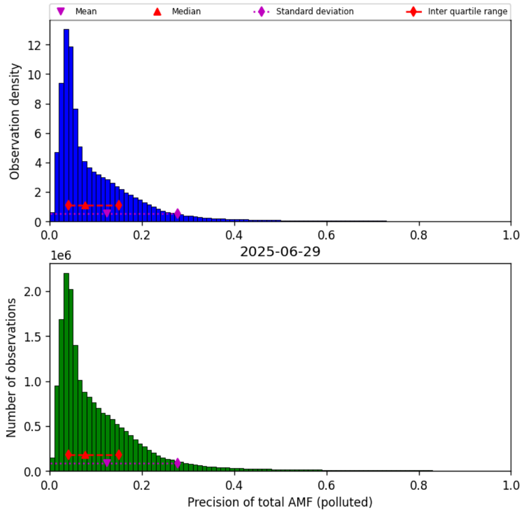
Figure 80: Histogram of “Precision of total AMF (polluted)” for 2025-06-28 to 2025-06-30
