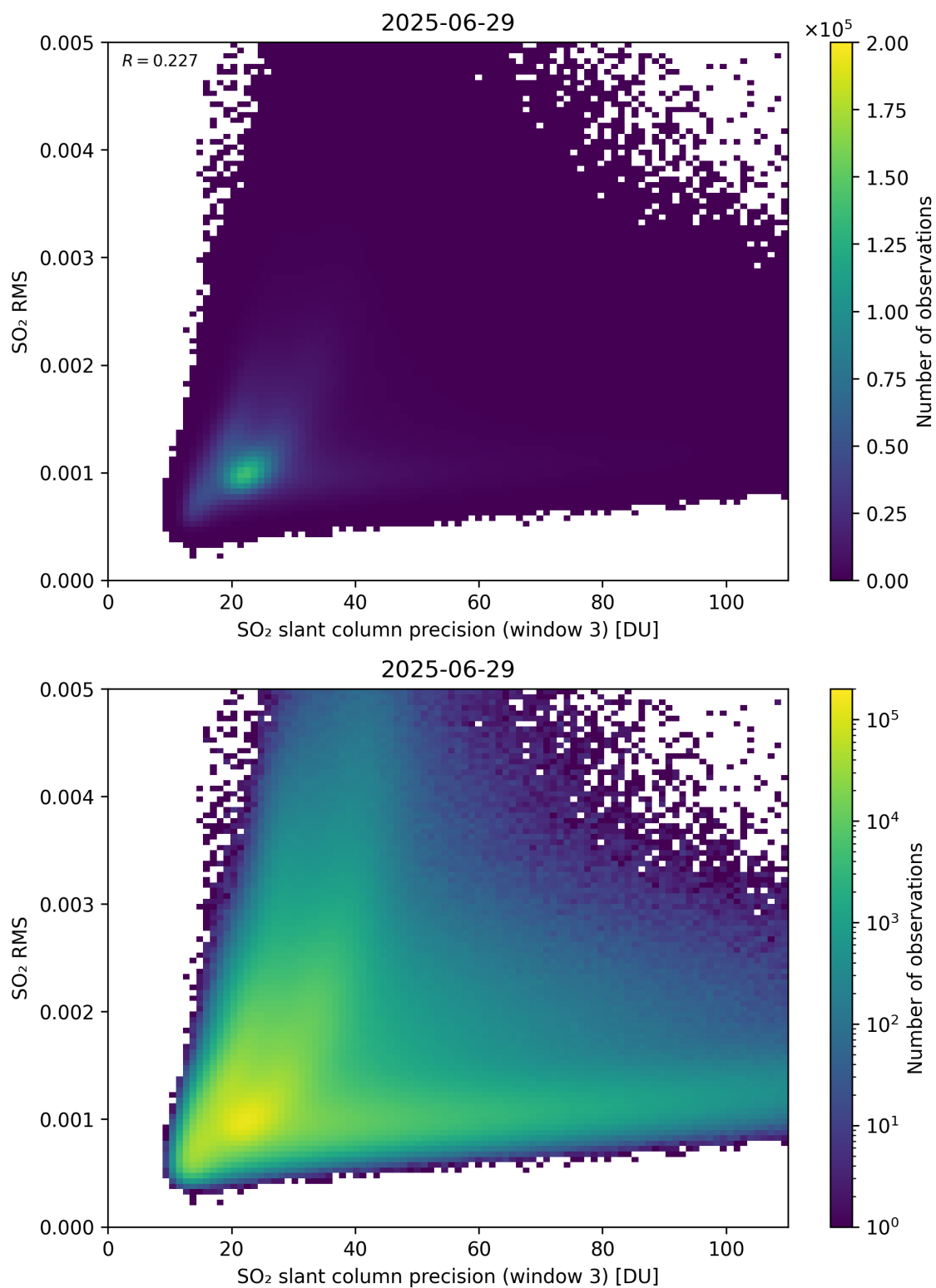
Figure 310: Scatter density plot of “SO 2 slant column precision (window 3)” against “SO 2 RMS” for 2025-06-28 to 2025-06-30.
