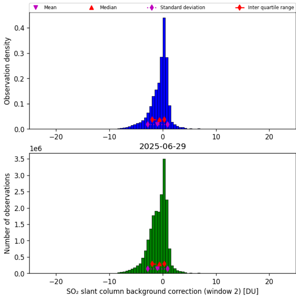
Figure 70: Histogram of “SO 2 slant column background correction (window 2)” for 2025-06-28 to 2025-06-30
