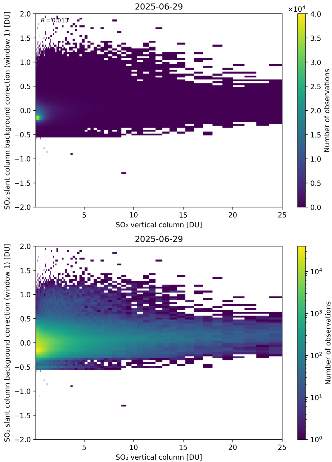
Figure 323: Scatter density plot of “SO 2 vertical column” against “SO 2 slant column background correction (window 1)” for 2025-06-28 to 2025-06-30.
