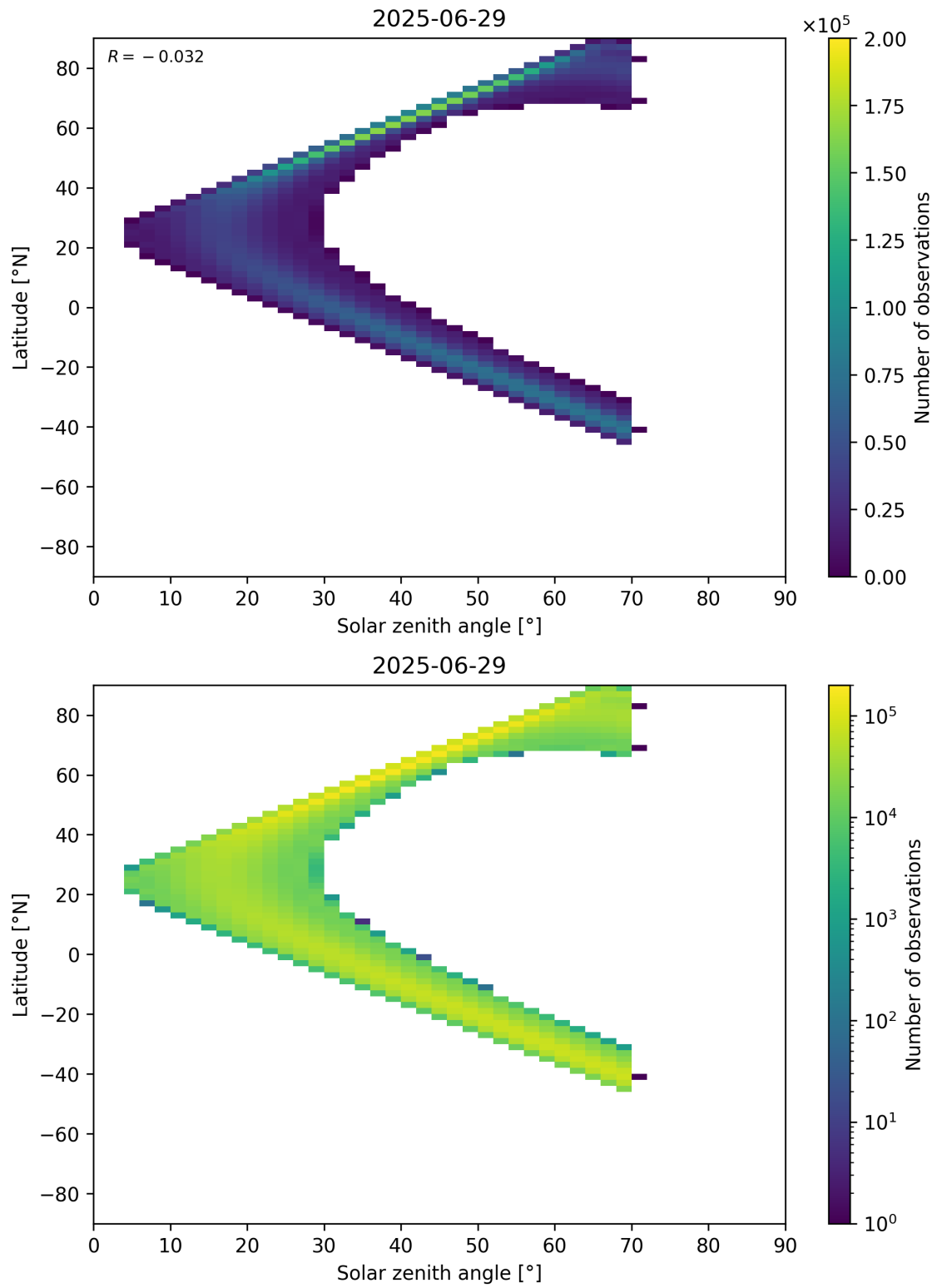
Figure 177: Scatter density plot of “Solar zenith angle” against “Latitude” for 2025-06-28 to 2025-06-30.
