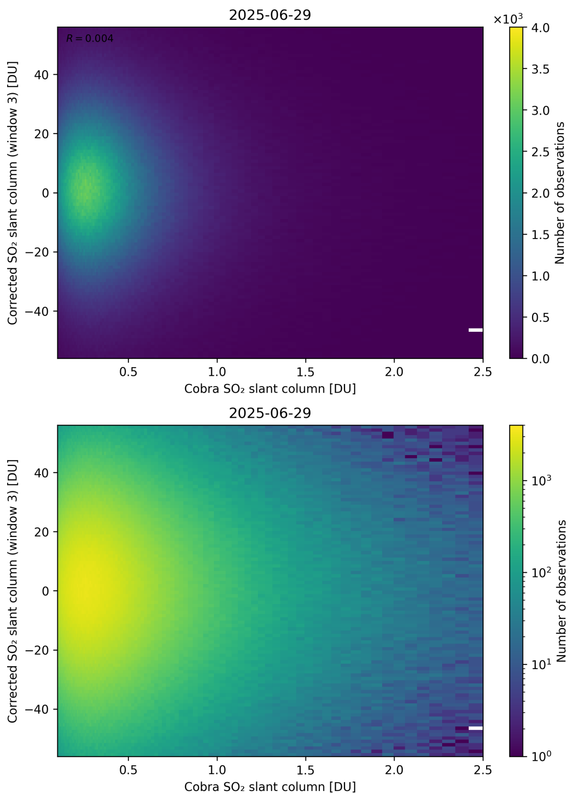
Figure 218: Scatter density plot of “Cobra SO 2 slant column” against “Corrected SO 2 slant column (window 3)” for 2025-06-28 to 2025-06-30.
