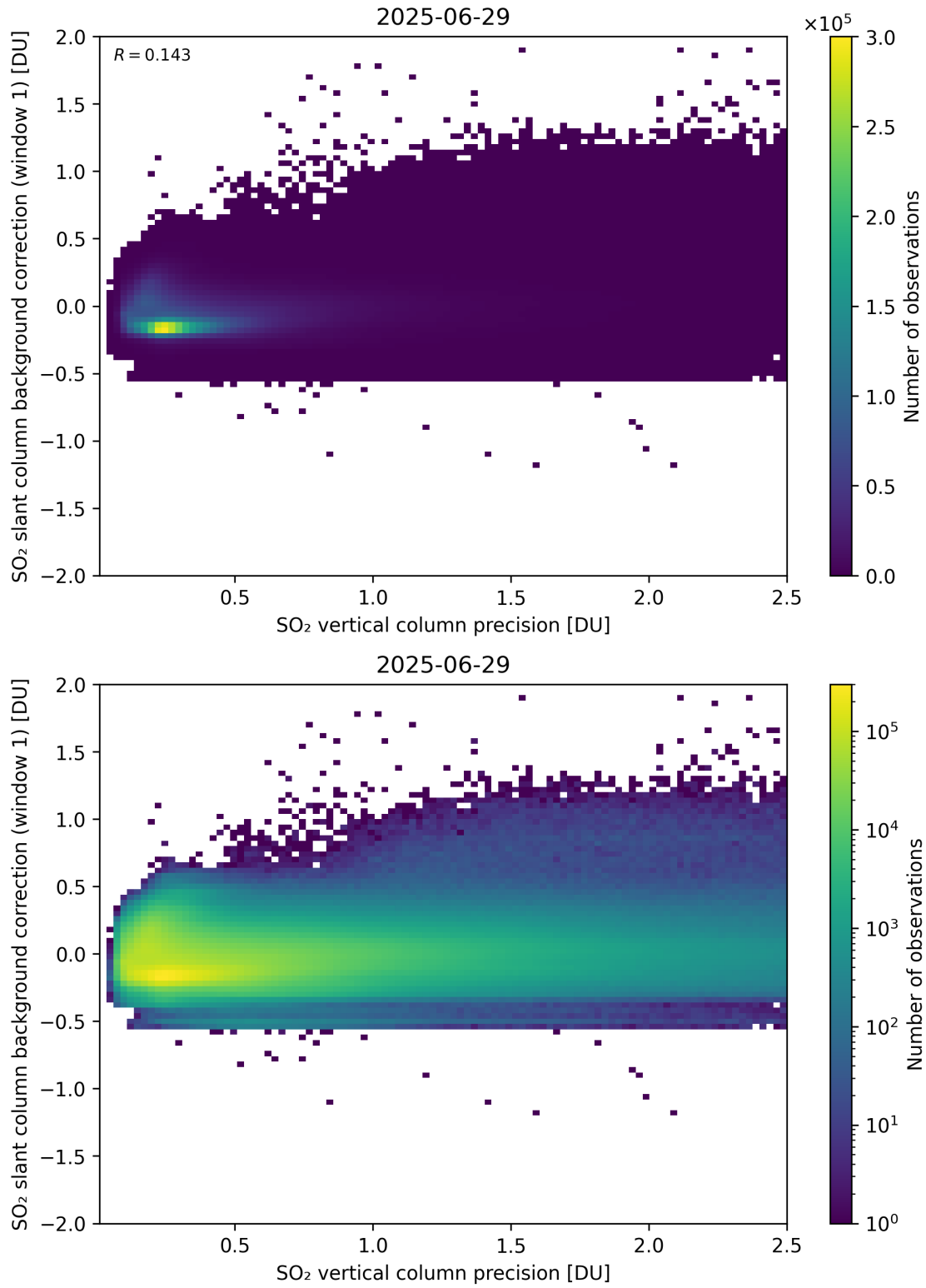
Figure 329: Scatter density plot of “SO 2 vertical column precision” against “SO 2 slant column background correction (window 1)” for 2025-06-28 to 2025-06-30.
