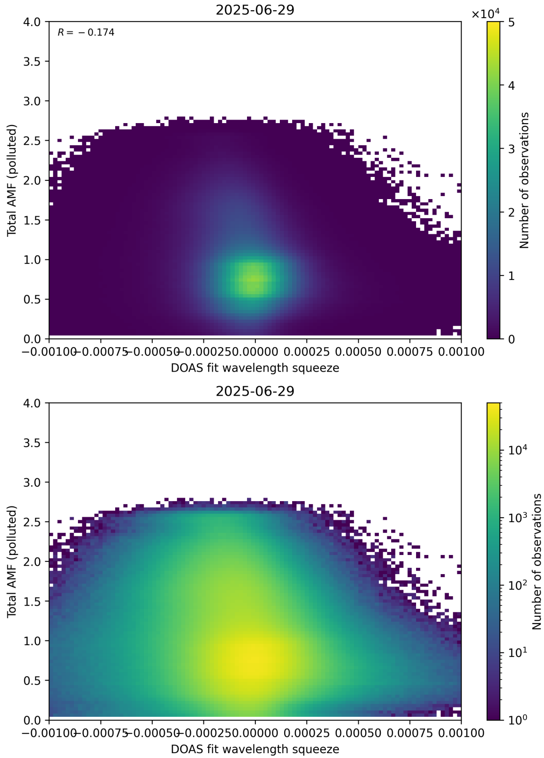
Figure 145: Scatter density plot of “DOAS fit wavelength squeeze” against “Total AMF (polluted)” for 2025-06-28 to 2025-06-30.
