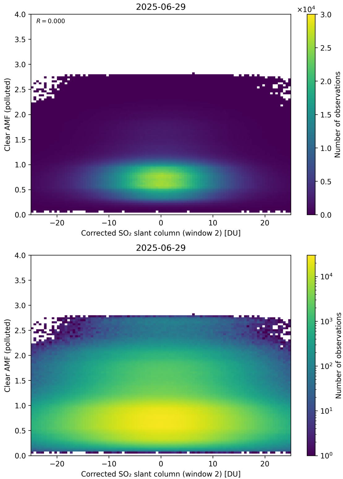
Figure 249: Scatter density plot of “Corrected SO 2 slant column (window 2)” against “Clear AMF (polluted)” for 2025-06-28 to 2025-06-30.
