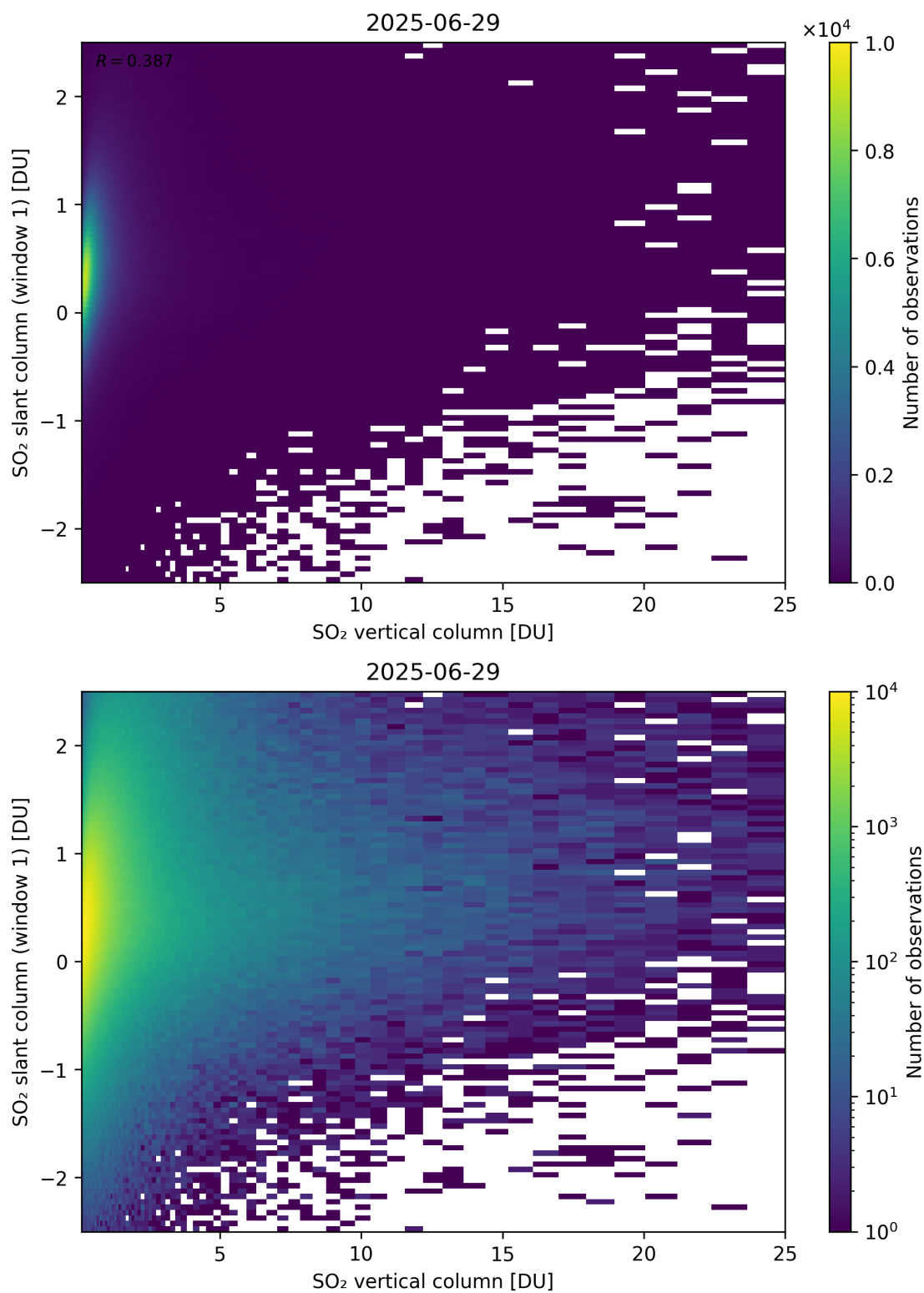
Figure 354: Scatter density plot of “SO 2 vertical column” against “SO 2 slant column (window 1)” for 2025-06-28 to 2025-06-30.
