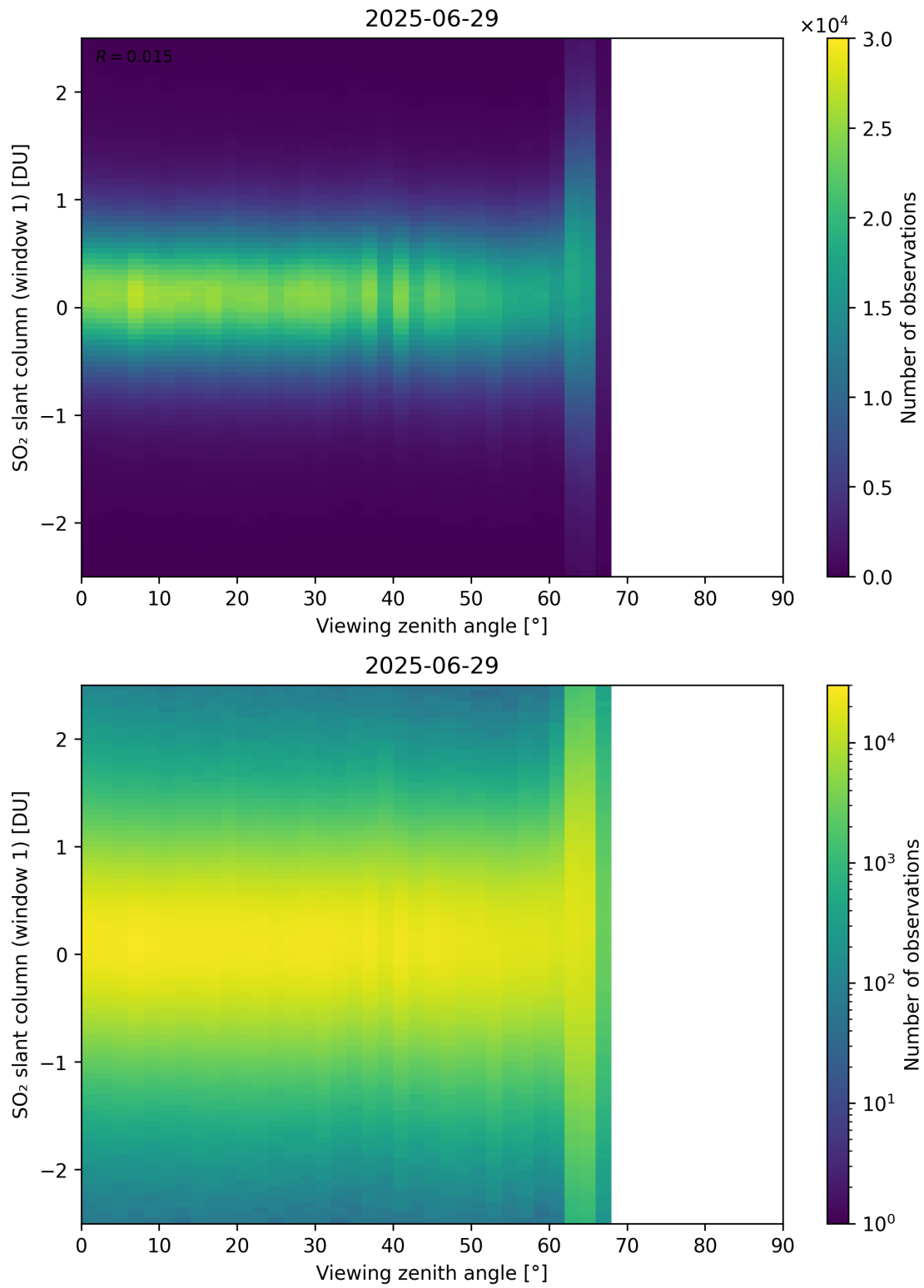
Figure 376: Scatter density plot of “Viewing zenith angle” against “SO 2 slant column (window 1)” for 2025-06-28 to 2025-06-30.
