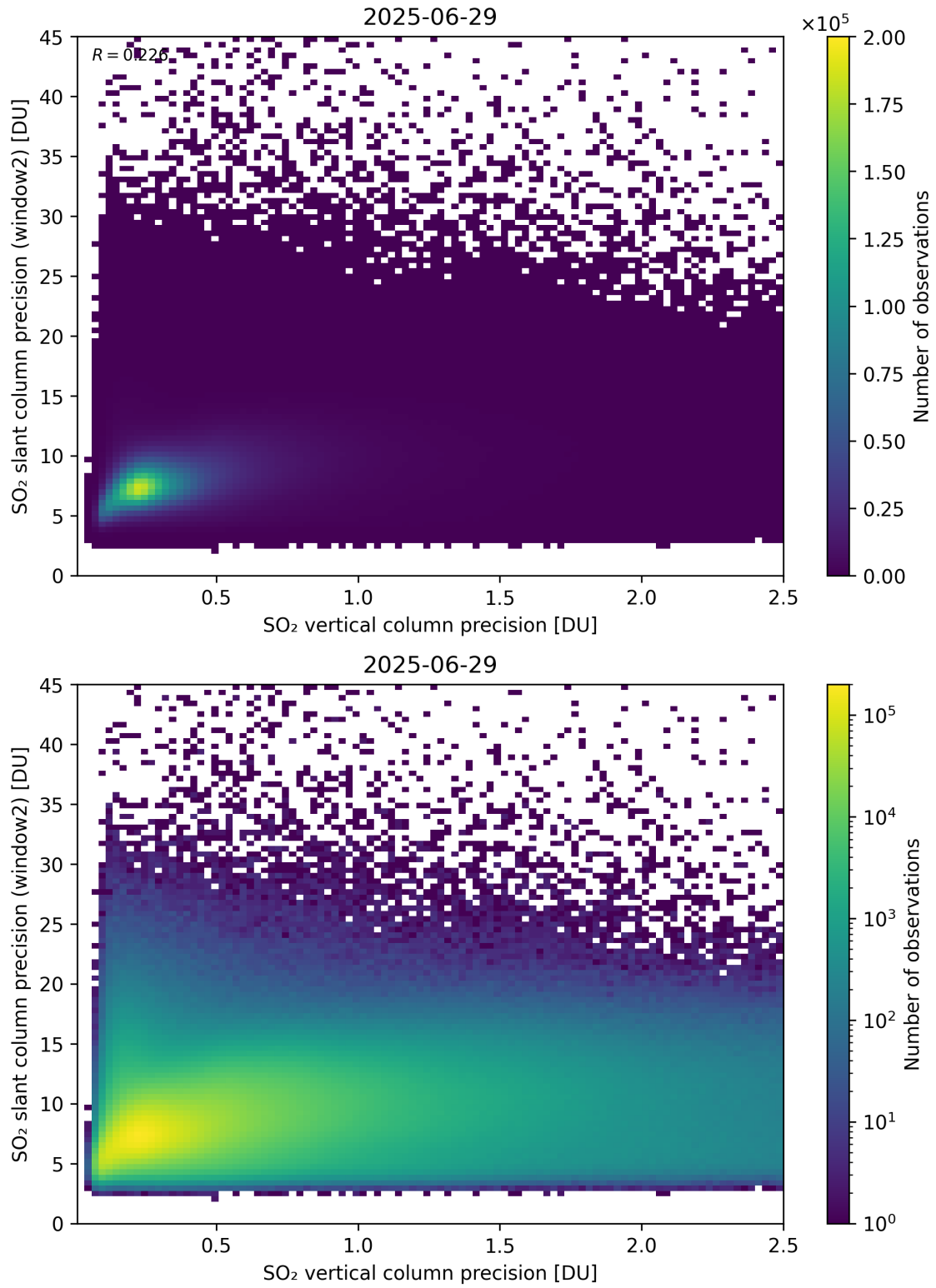
Figure 343: Scatter density plot of “SO 2 vertical column precision” against “SO 2 slant column precision (window2)” for 2025-06-28 to 2025-06-30.
