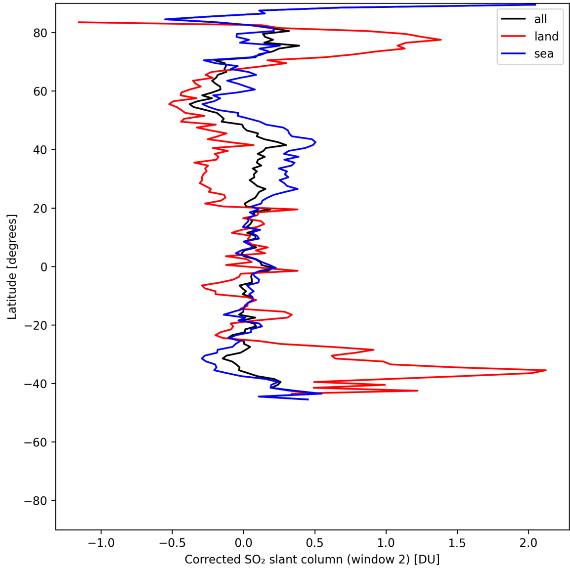
Figure 43: Zonal average of “Corrected SO 2 slant column (window 2)” for 2025-06-28 to 2025-06-30.
