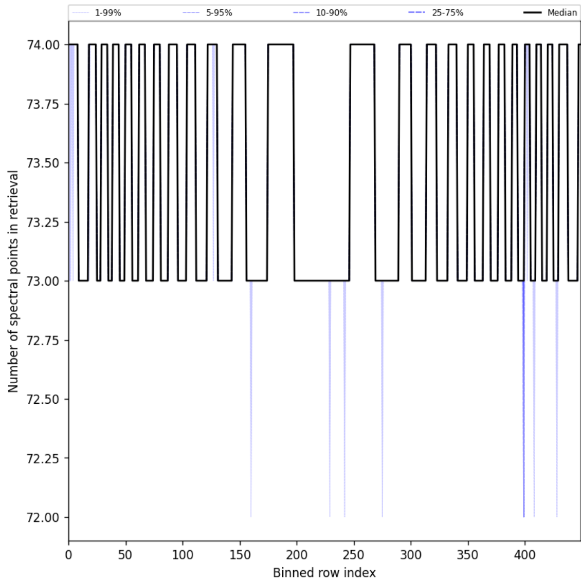
Figure 108: Along track statistics of “Number of spectral points in retrieval” for 2025-06-28 to 2025-06-30
