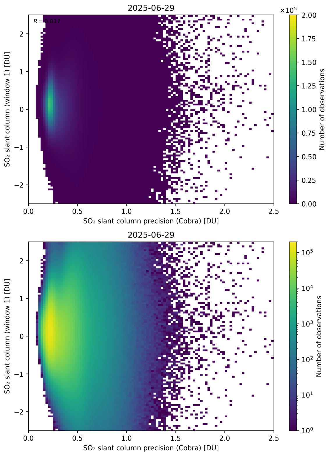
Figure 208: Scatter density plot of “SO 2 slant column precision (Cobra)” against “SO 2 slant column (window 1)” for 2025-06-28 to 2025-06-30.
