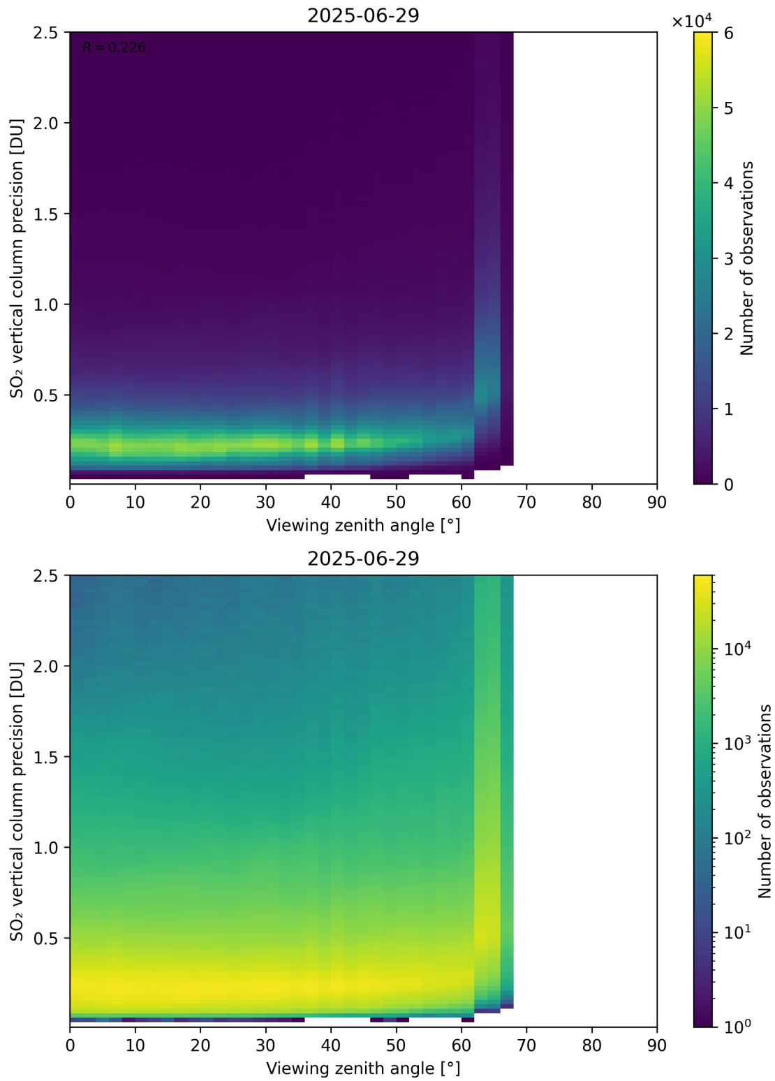
Figure 384: Scatter density plot of “Viewing zenith angle” against “SO 2 vertical column precision” for 2025-06-28 to 2025-06-30.
