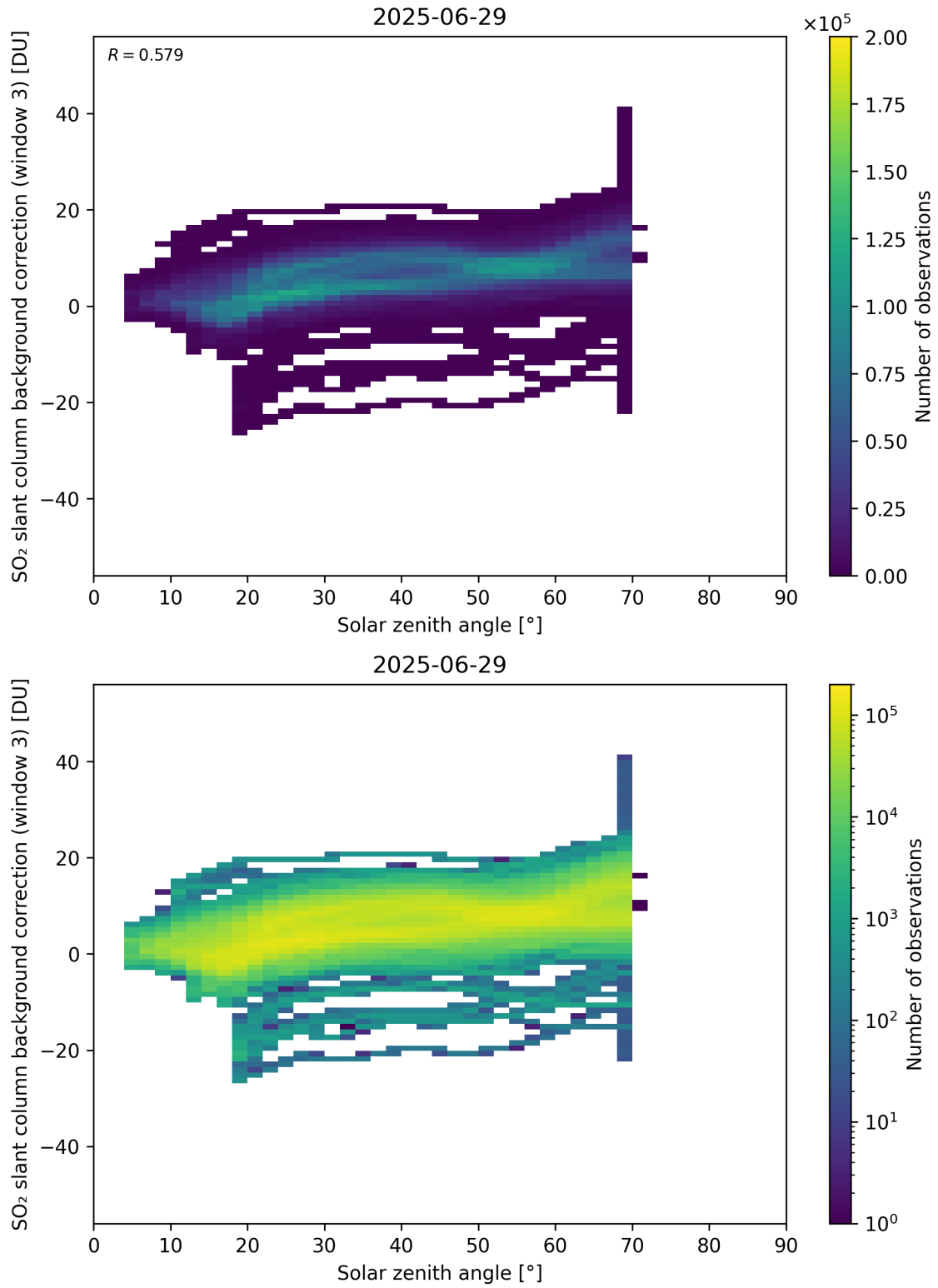
Figure 173: Scatter density plot of “Solar zenith angle” against “SO 2 slant column background correction (window 3)” for 2025-06-28 to 2025-06-30.
