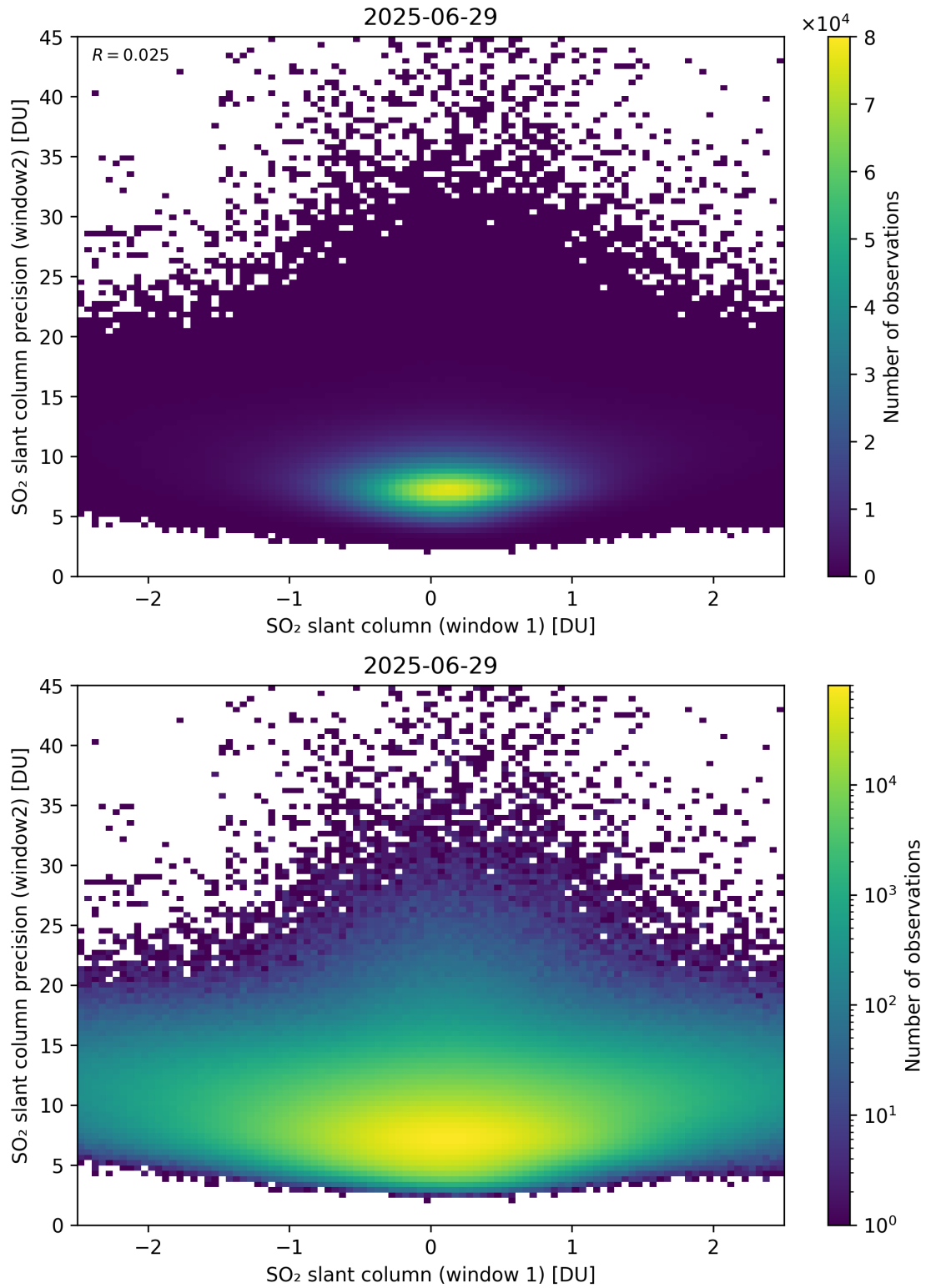
Figure 286: Scatter density plot of “SO 2 slant column (window 1)” against “SO 2 slant column precision (window2)” for 2025-06-28 to 2025-06-30.
