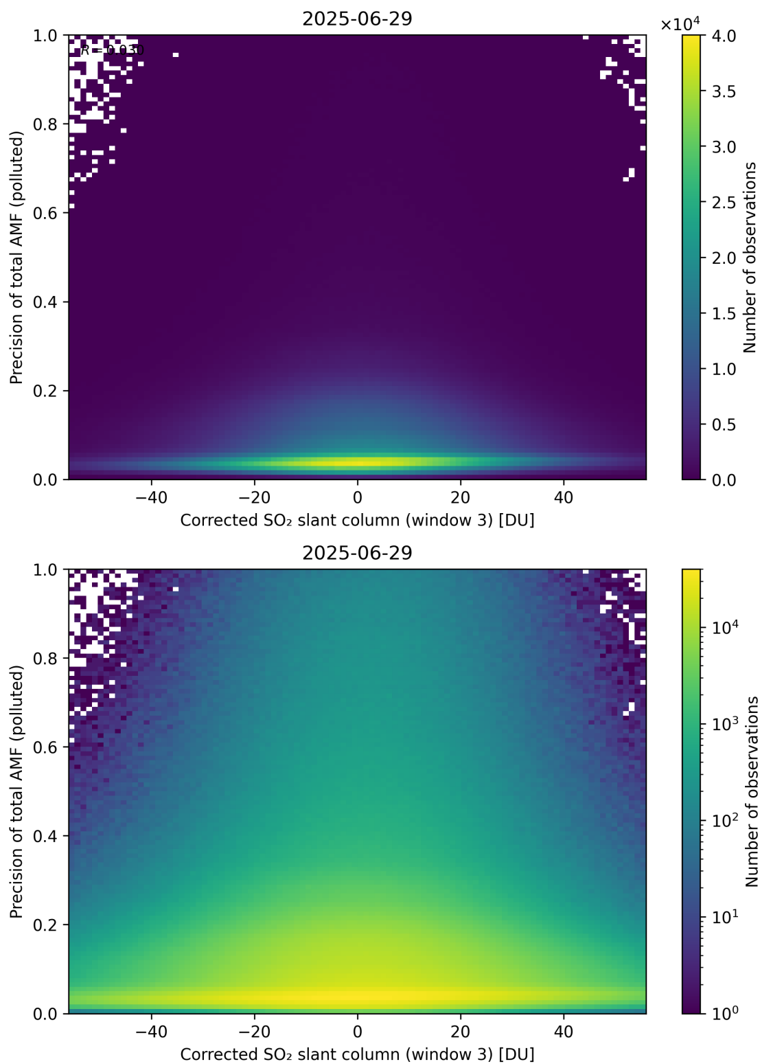
Figure 261: Scatter density plot of “Corrected SO 2 slant column (window 3)” against “Precision of total AMF (polluted)” for 2025-06-28 to 2025-06-30.
