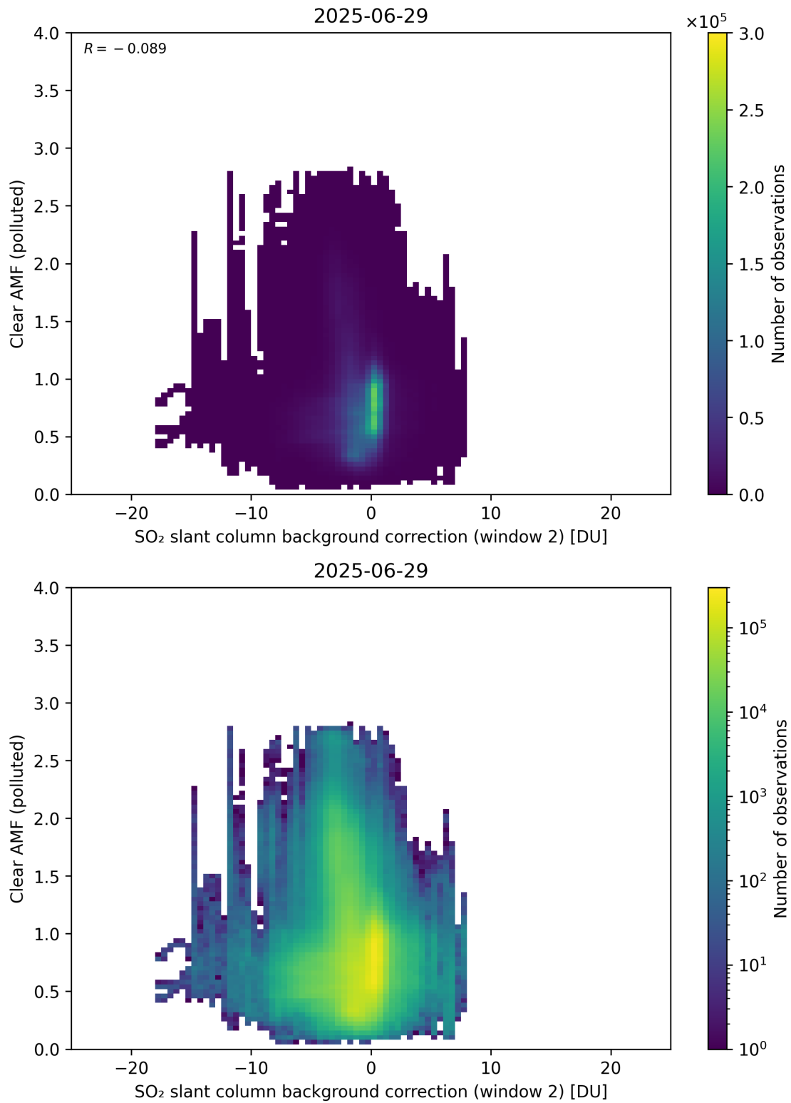
Figure 126: Scatter density plot of “SO 2 slant column background correction (window 2)” against “Clear AMF (polluted)” for 2025-06-28 to 2025-06-30.
