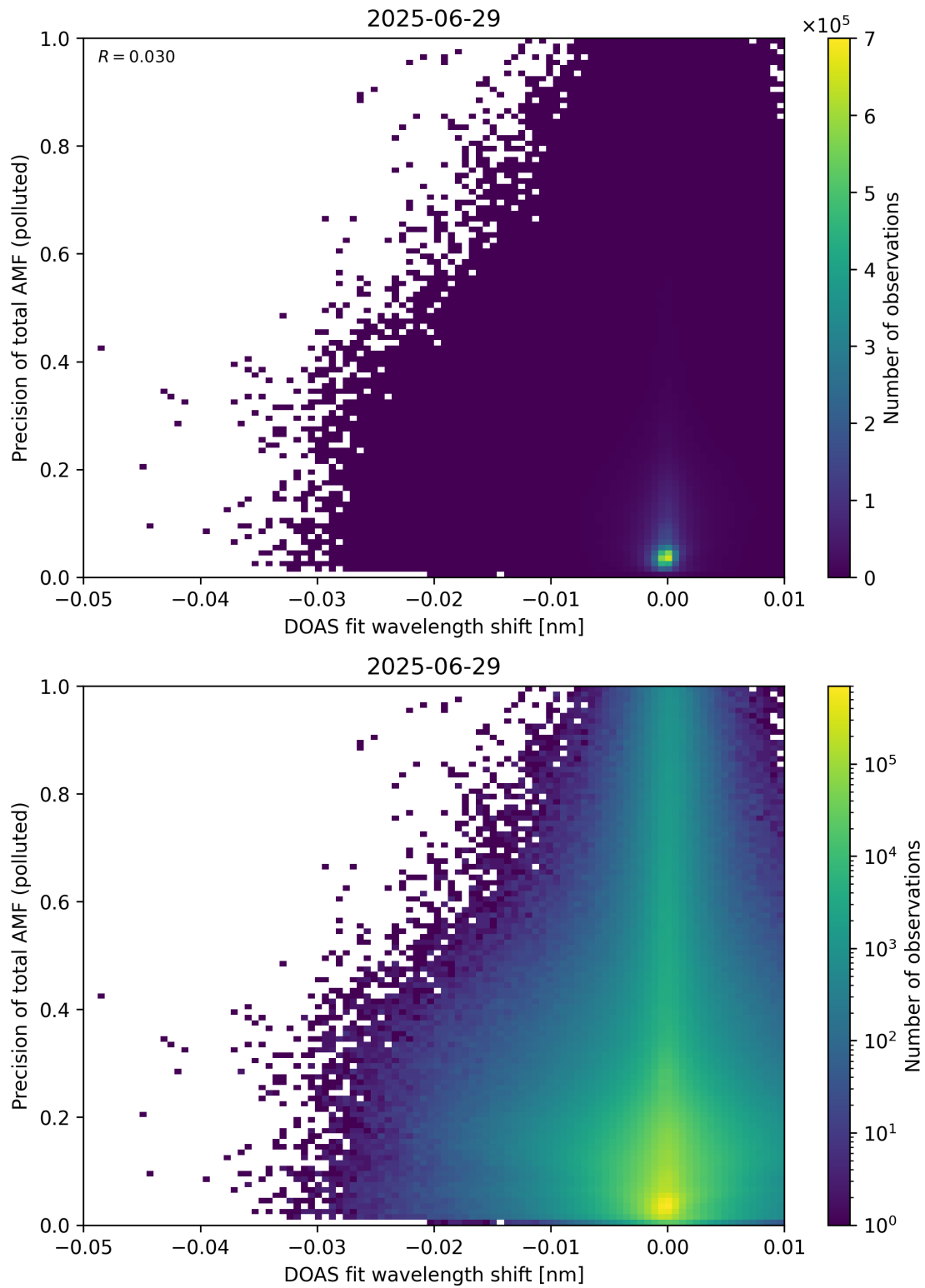
Figure 142: Scatter density plot of “DOAS fit wavelength shift” against “Precision of total AMF (polluted)” for 2025-06-28 to 2025-06-30.
