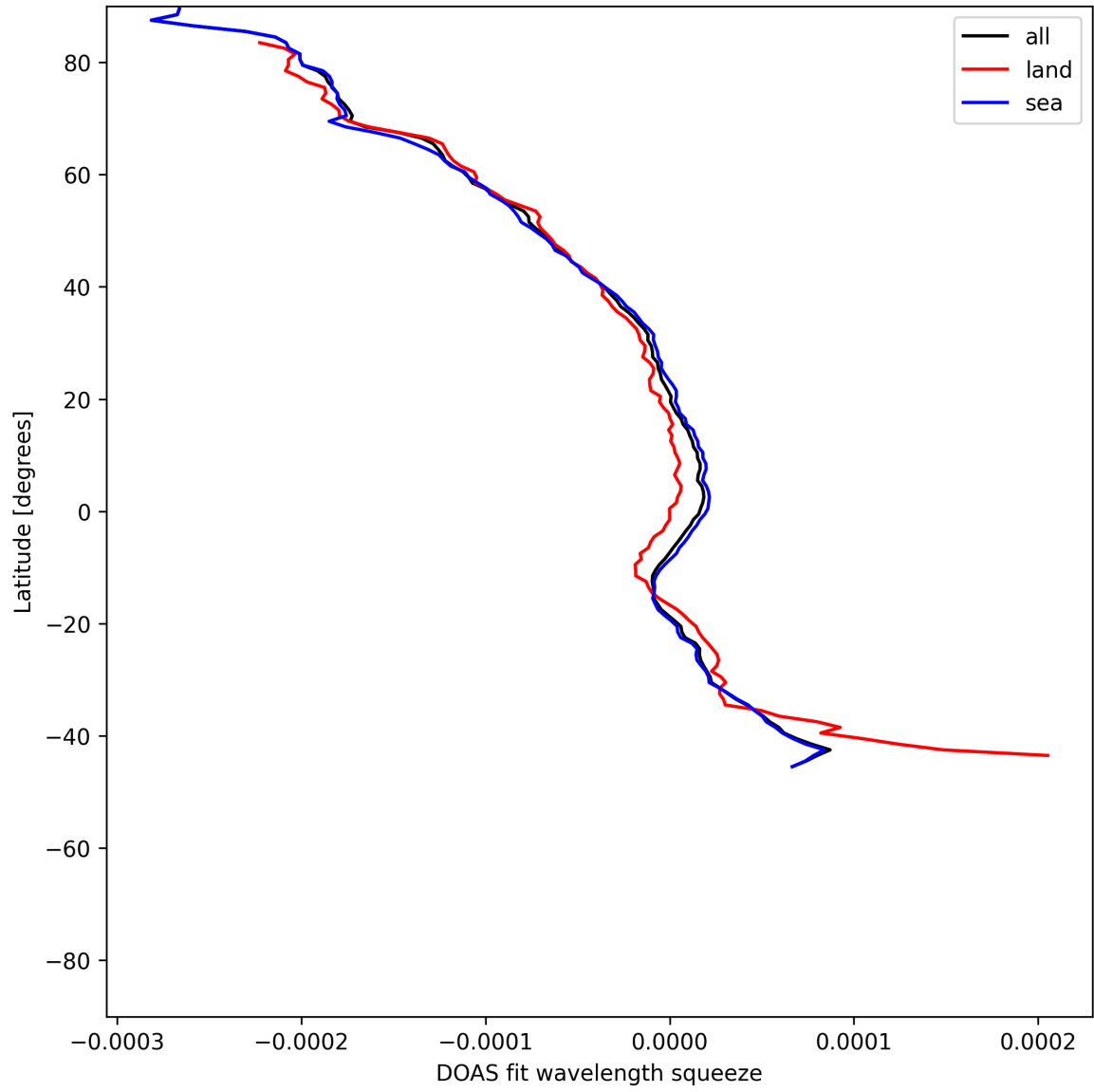
Figure 51: Zonal average of “DOAS fit wavelength squeeze” for 2025-06-28 to 2025-06-30.
