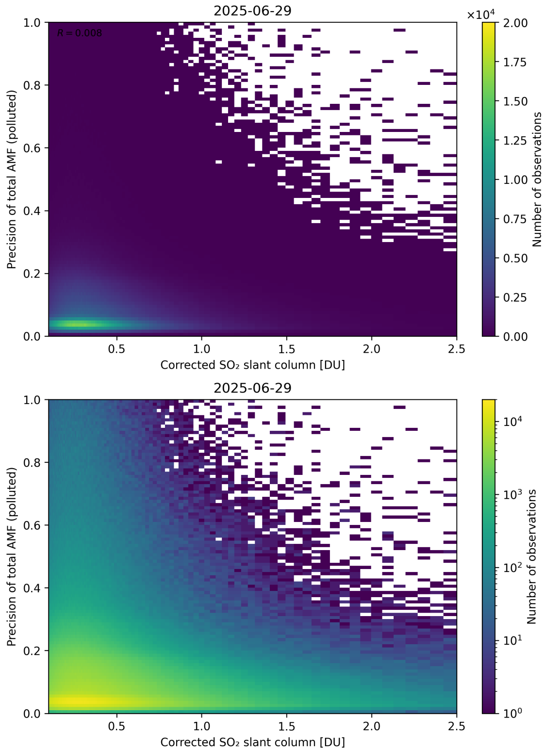
Figure 243: Scatter density plot of “Corrected SO 2 slant column” against “Precision of total AMF (polluted)” for 2025-06-28 to 2025-06-30.
