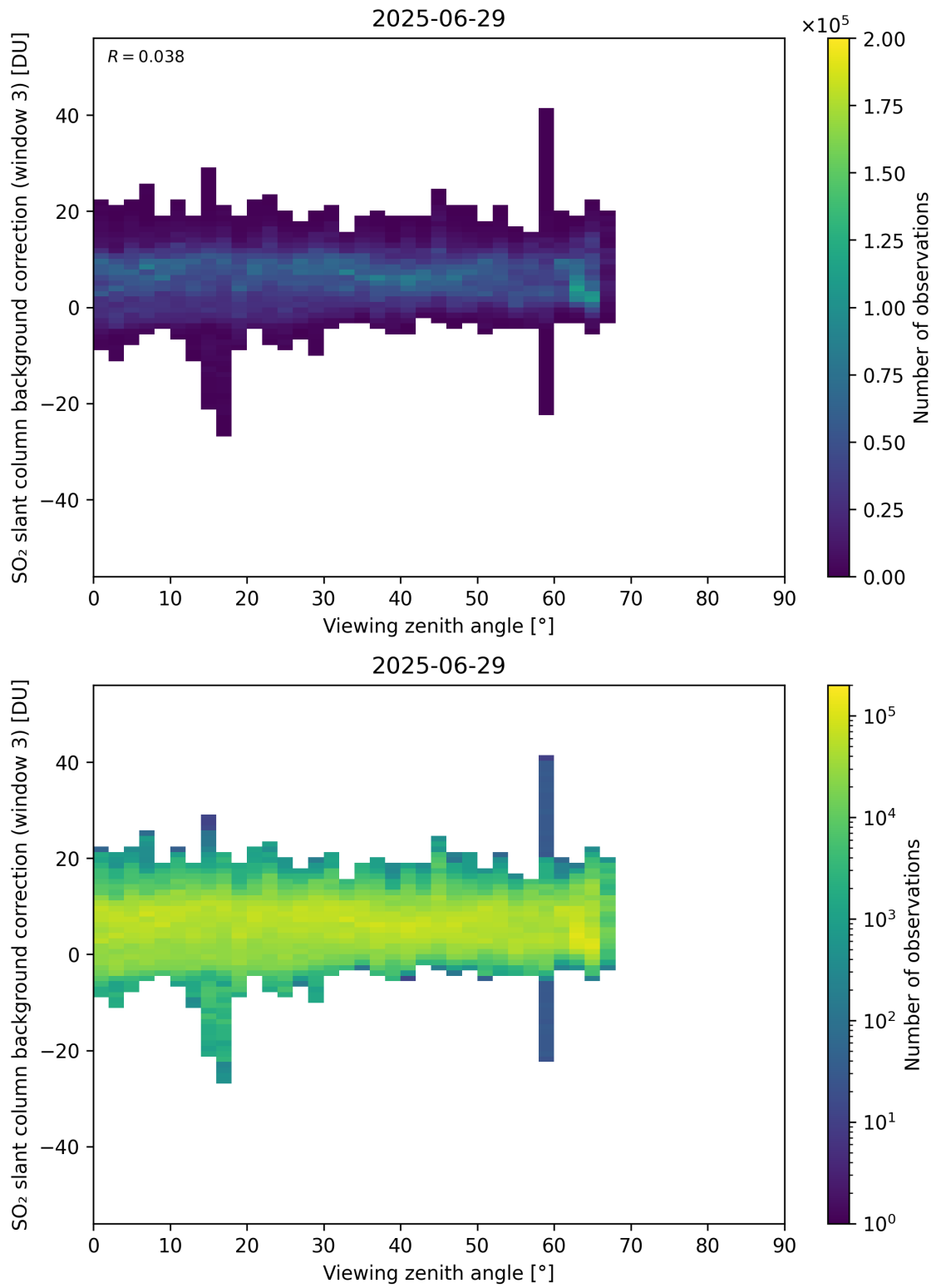
Figure 364: Scatter density plot of “Viewing zenith angle” against “SO 2 slant column background correction (window 3)” for 2025-06-28 to 2025-06-30.
