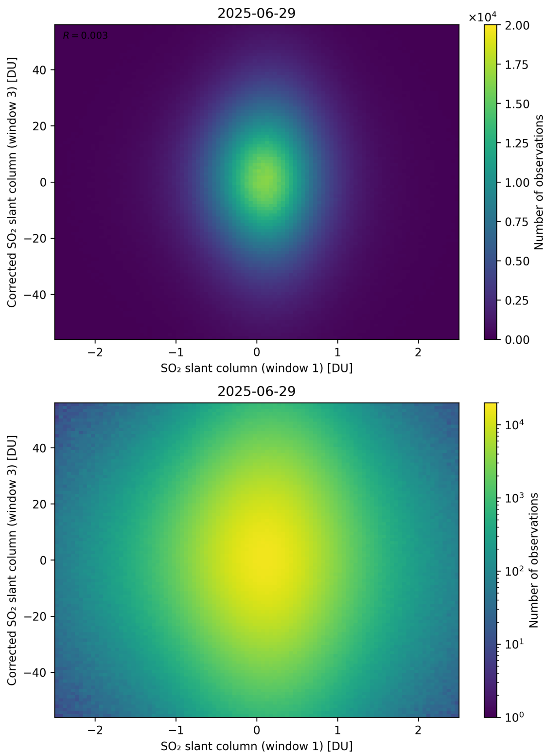
Figure 284: Scatter density plot of “SO 2 slant column (window 1)” against “Corrected SO 2 slant column (window 3)” for 2025-06-28 to 2025-06-30.
