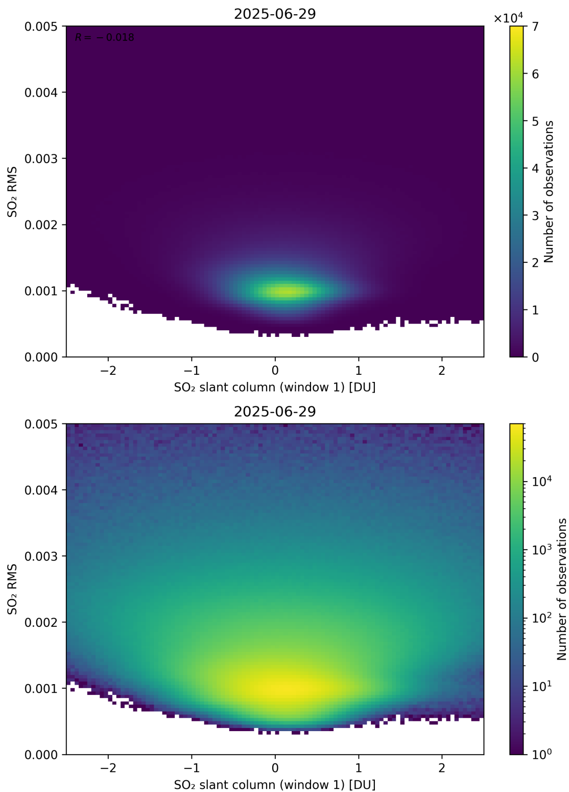
Figure 267: Scatter density plot of “SO 2 slant column (window 1)” against “SO 2 RMS” for 2025-06-28 to 2025-06-30.
