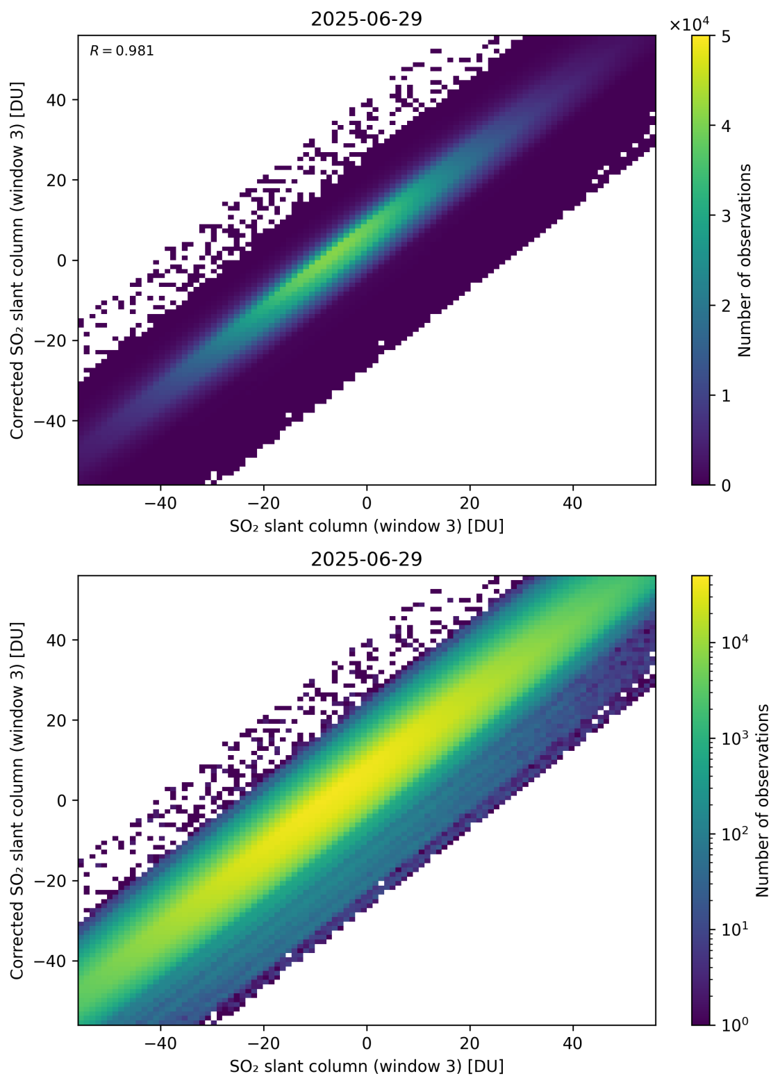
Figure 316: Scatter density plot of “SO 2 slant column (window 3)” against “Corrected SO 2 slant column (window 3)” for 2025-06-28 to 2025-06-30.
