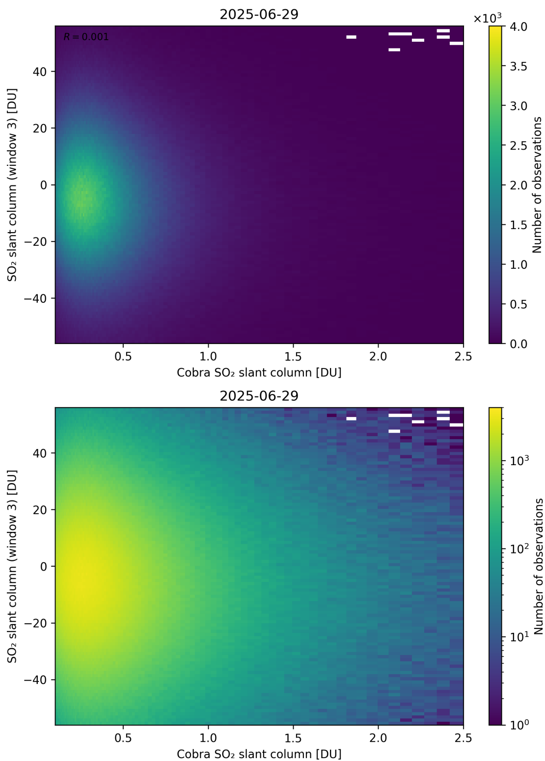
Figure 222: Scatter density plot of “Cobra SO 2 slant column” against “SO 2 slant column (window 3)” for 2025-06-28 to 2025-06-30.
