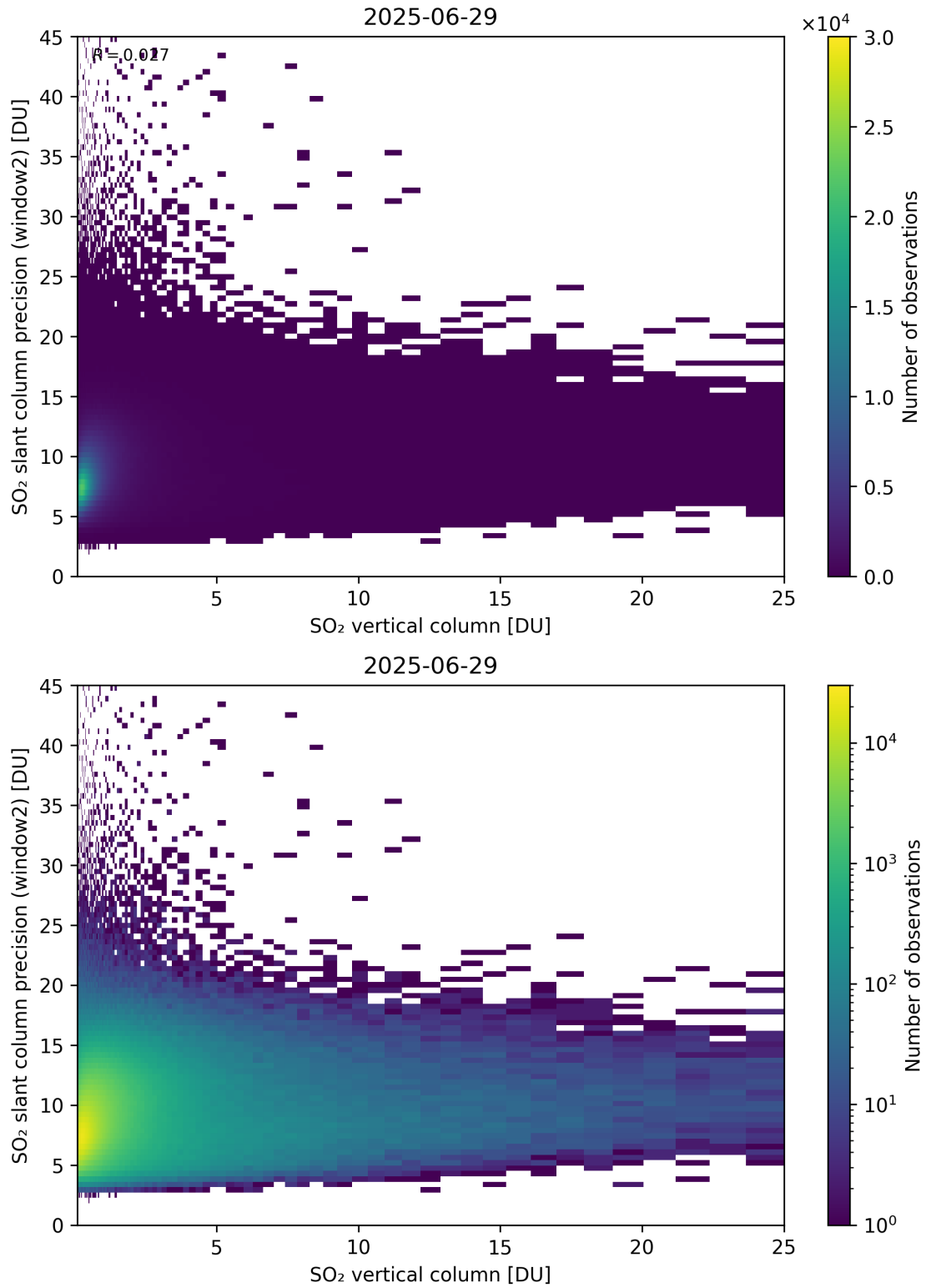
Figure 356: Scatter density plot of “SO 2 vertical column” against “SO 2 slant column precision (window2)” for 2025-06-28 to 2025-06-30.
