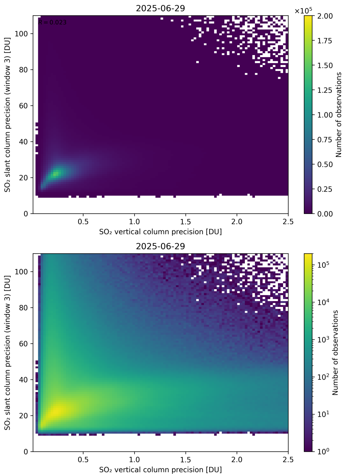
Figure 345: Scatter density plot of “SO 2 vertical column precision” against “SO 2 slant column precision (window 3)” for 2025-06-28 to 2025-06-30.
