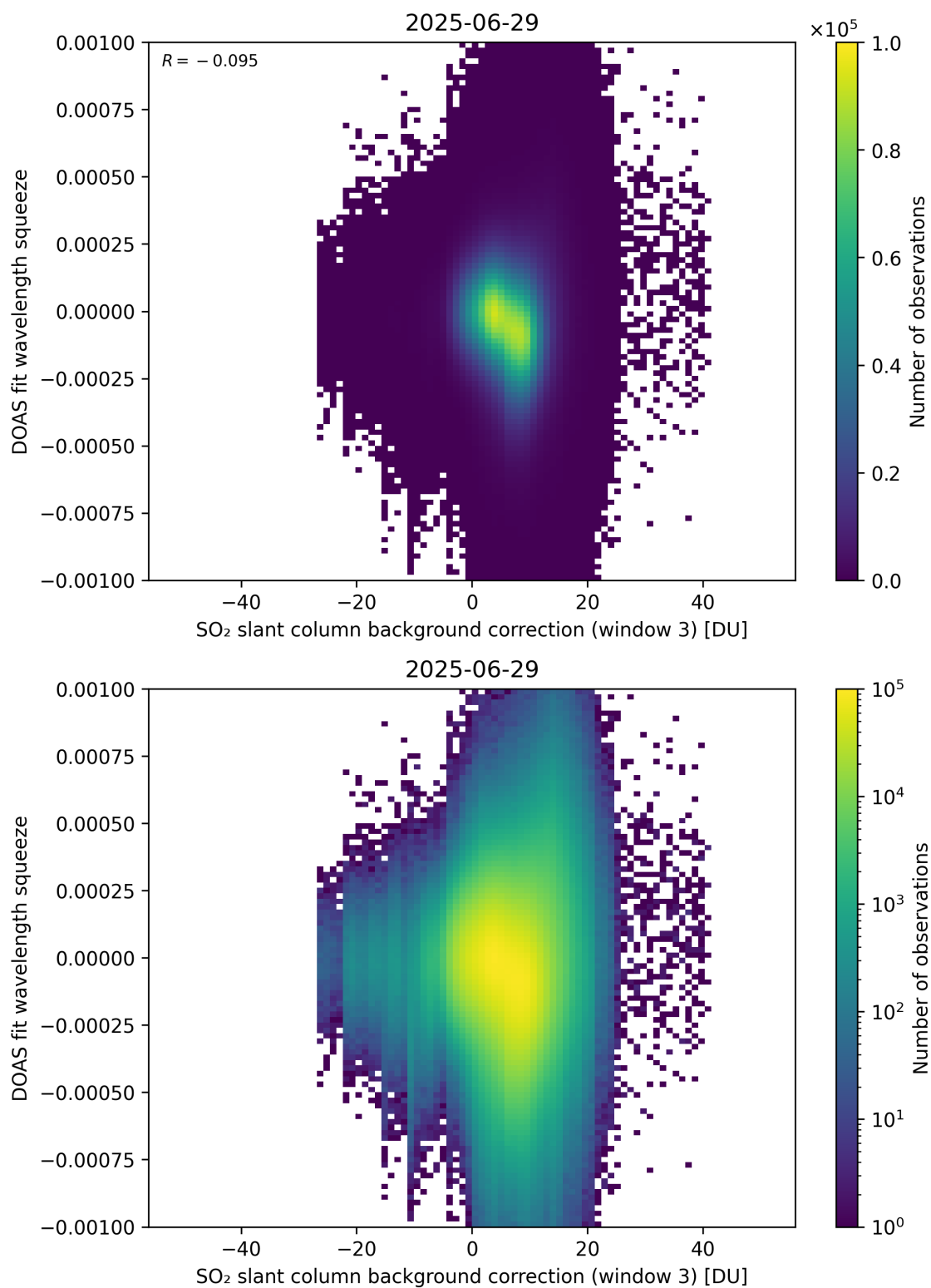
Figure 133: Scatter density plot of “SO 2 slant column background correction (window 3)” against “DOAS fit wavelength squeeze” for 2025-06-28 to 2025-06-30.
