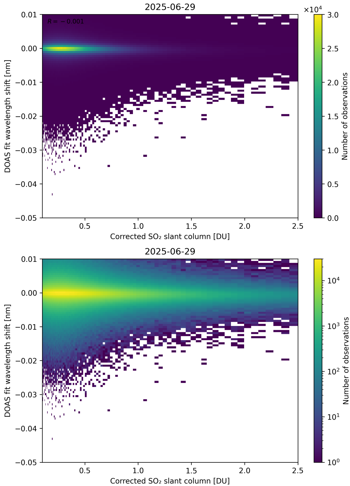
Figure 229: Scatter density plot of “Corrected SO 2 slant column” against “DOAS fit wavelength shift” for 2025-06-28 to 2025-06-30.
