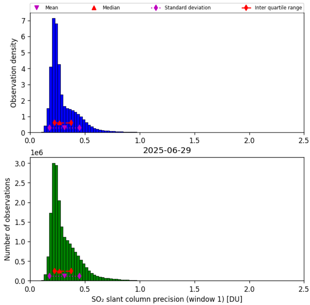
Figure 64: Histogram of “SO 2 slant column precision (window 1)” for 2025-06-28 to 2025-06-30
