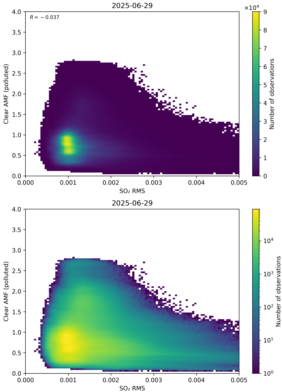
Figure 147: Scatter density plot of “SO 2 RMS” against “Clear AMF (polluted)” for 2025-06-28 to 2025-06-30.
