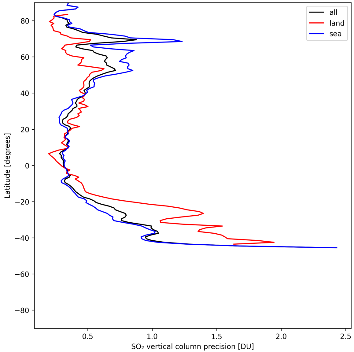
Figure 33: Zonal average of “SO 2 vertical column precision” for 2025-06-28 to 2025-06-30.
