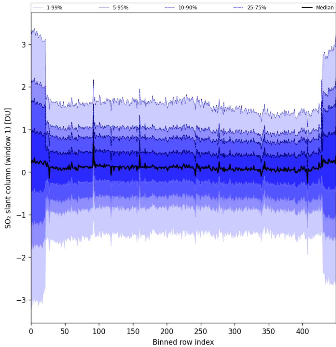
Figure 89: Along track statistics of “SO 2 slant column (window 1)” for 2025-06-28 to 2025-06-30
