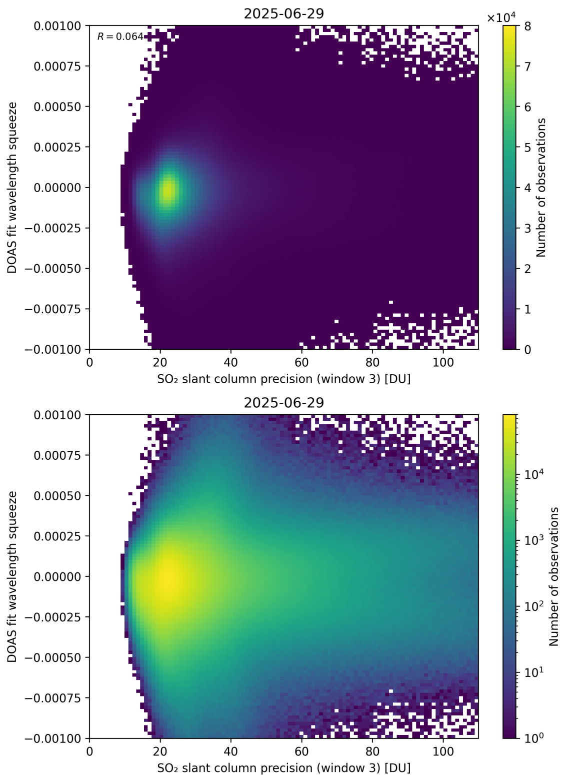
Figure 309: Scatter density plot of “SO 2 slant column precision (window 3)” against “DOAS fit wavelength squeeze” for 2025-06-28 to 2025-06-30.
