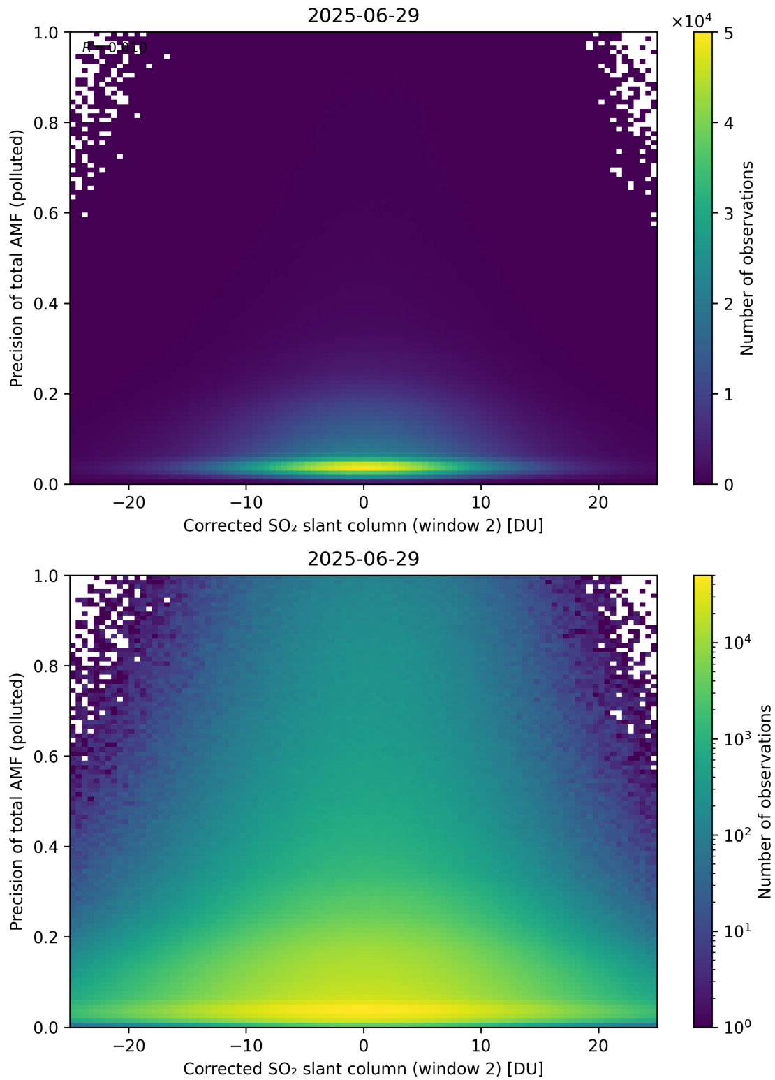
Figure 254: Scatter density plot of “Corrected SO 2 slant column (window 2)” against “Precision of total AMF (polluted)” for 2025-06-28 to 2025-06-30.
