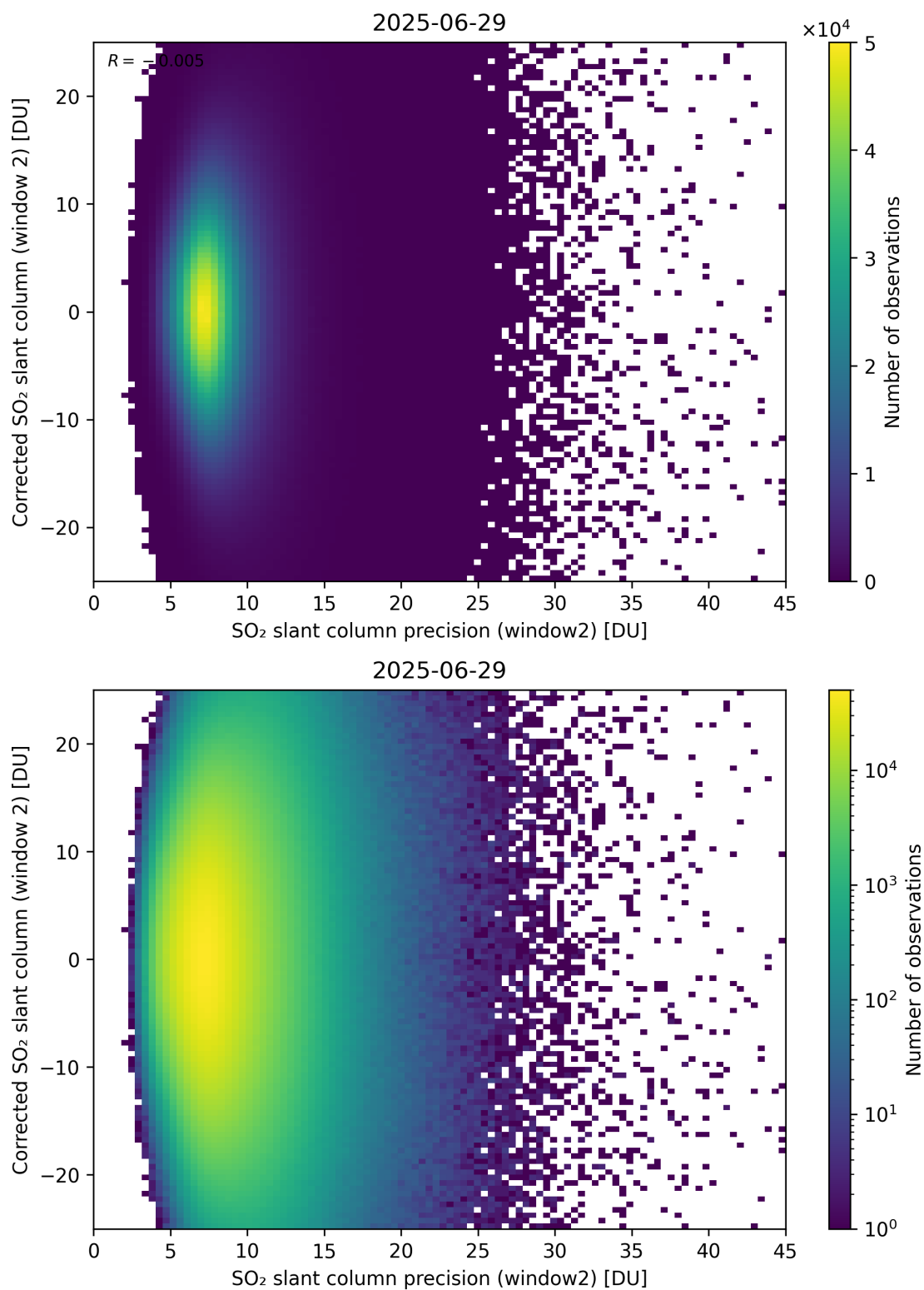
Figure 297: Scatter density plot of “SO 2 slant column precision (window2)” against “Corrected SO 2 slant column (window 2)” for 2025-06-28 to 2025-06-30.
