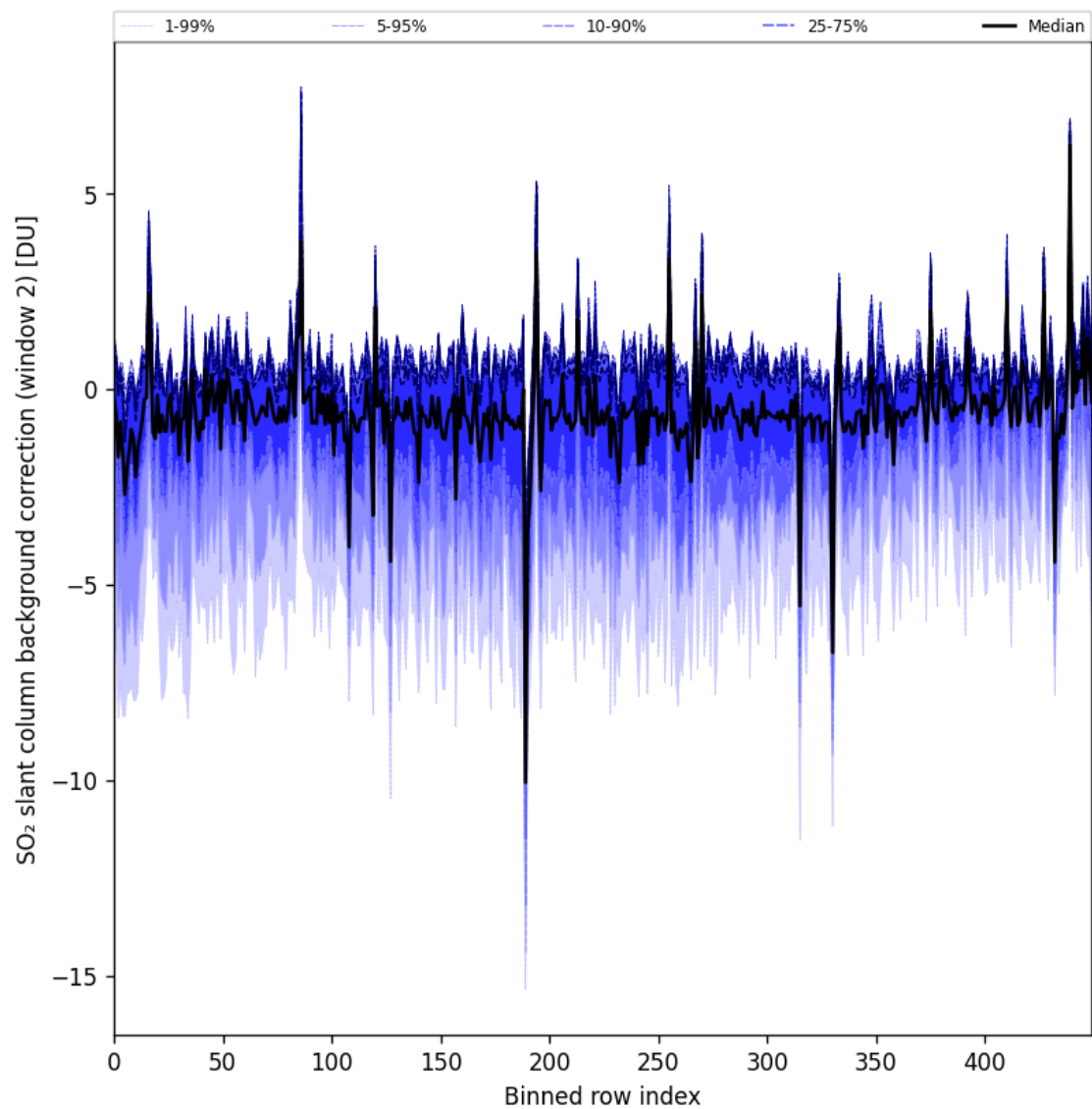
Figure 96: Along track statistics of “SO 2 slant column background correction (window 2)” for 2025-06-28 to 2025-06-30
