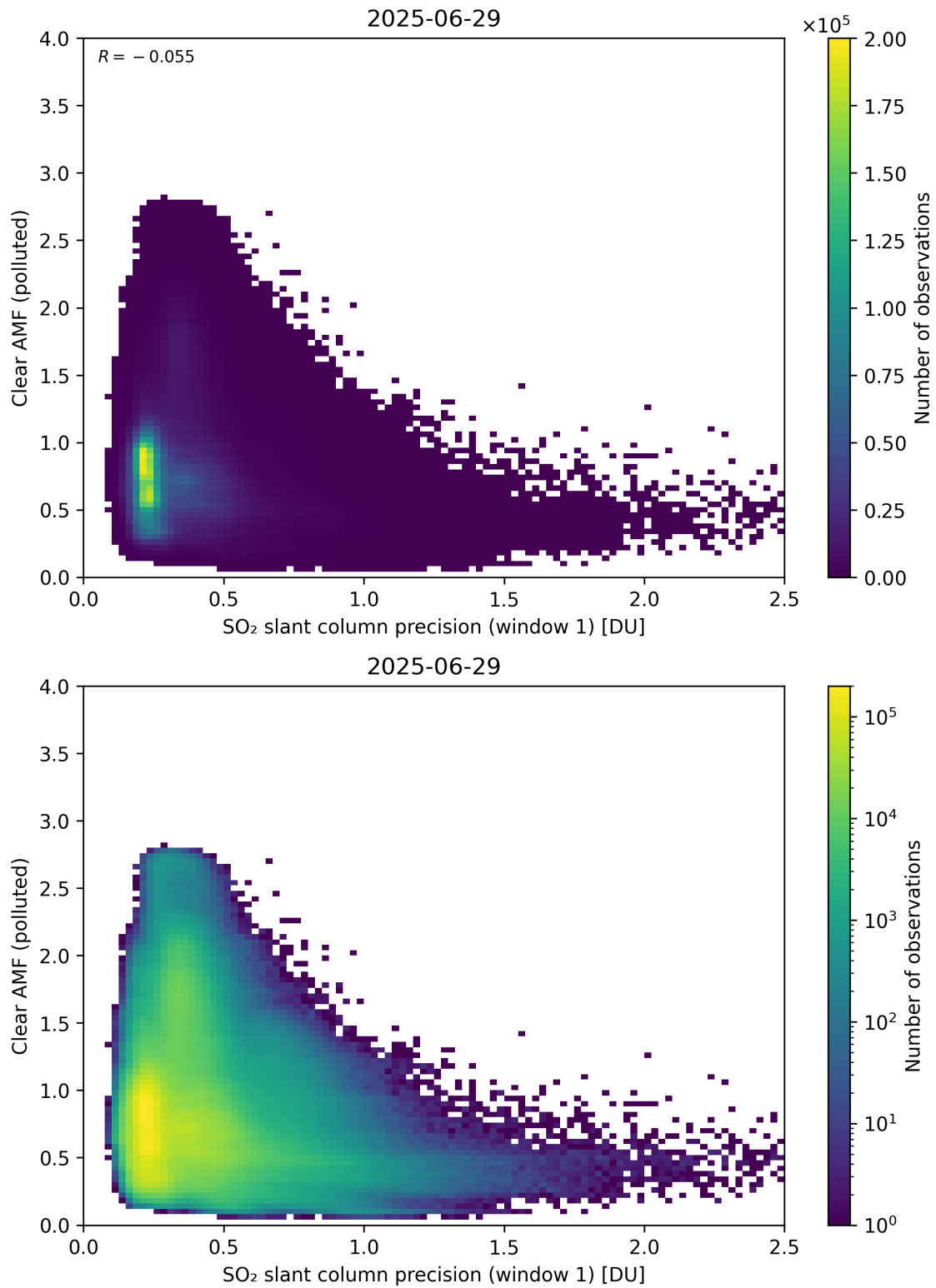
Figure 274: Scatter density plot of “SO 2 slant column precision (window 1)” against “Clear AMF (polluted)” for 2025-06-28 to 2025-06-30.
