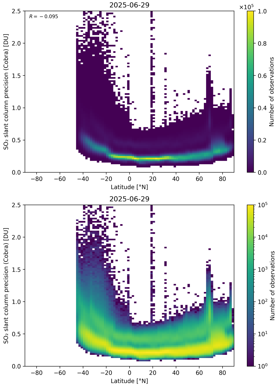
Figure 158: Scatter density plot of “Latitude” against “SO 2 slant column precision (Cobra)” for 2025-06-28 to 2025-06-30.
