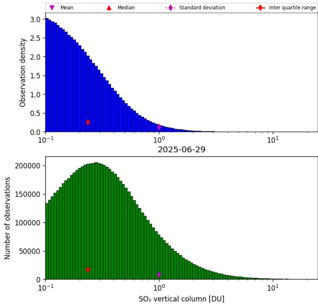
Figure 58: Histogram of “SO 2 vertical column” for 2025-06-28 to 2025-06-30
