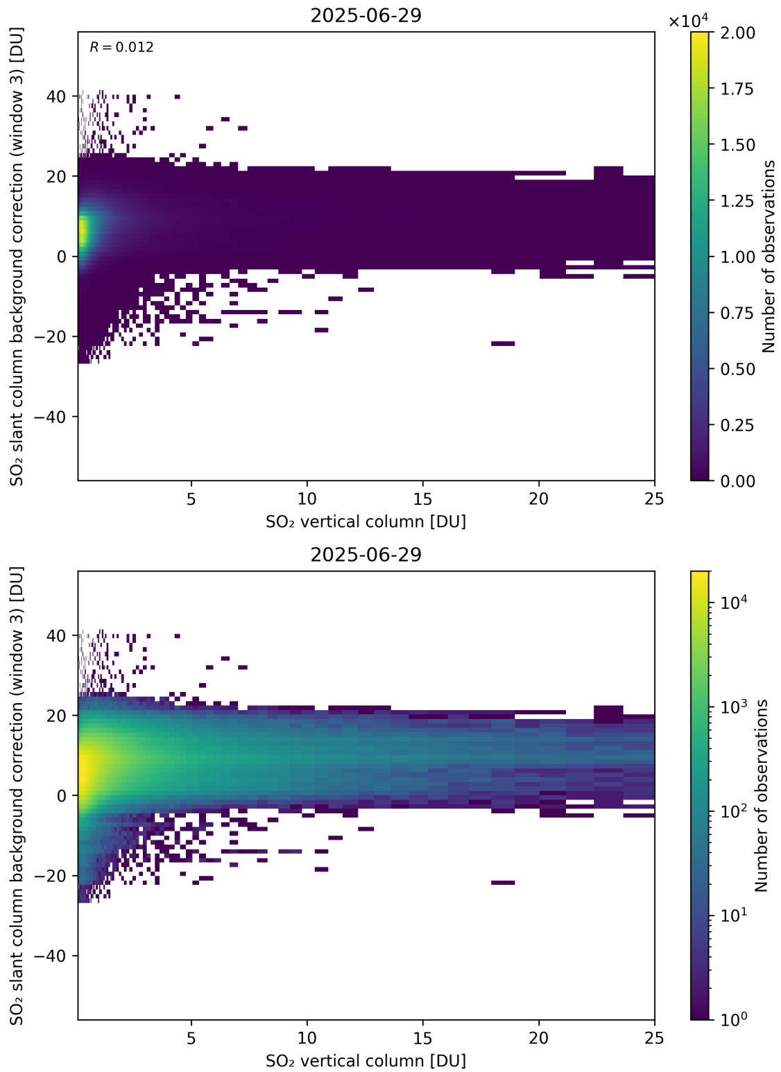
Figure 325: Scatter density plot of “SO 2 vertical column” against “SO 2 slant column background correction (window 3)” for 2025-06-28 to 2025-06-30.
