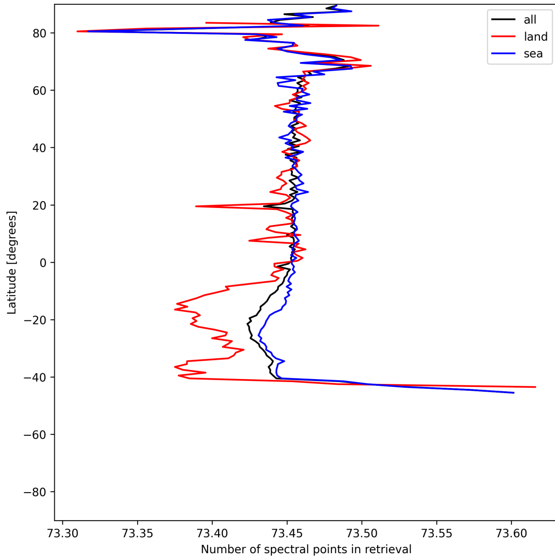
Figure 56: Zonal average of “Number of spectral points in retrieval” for 2025-06-28 to 2025-06-30.
