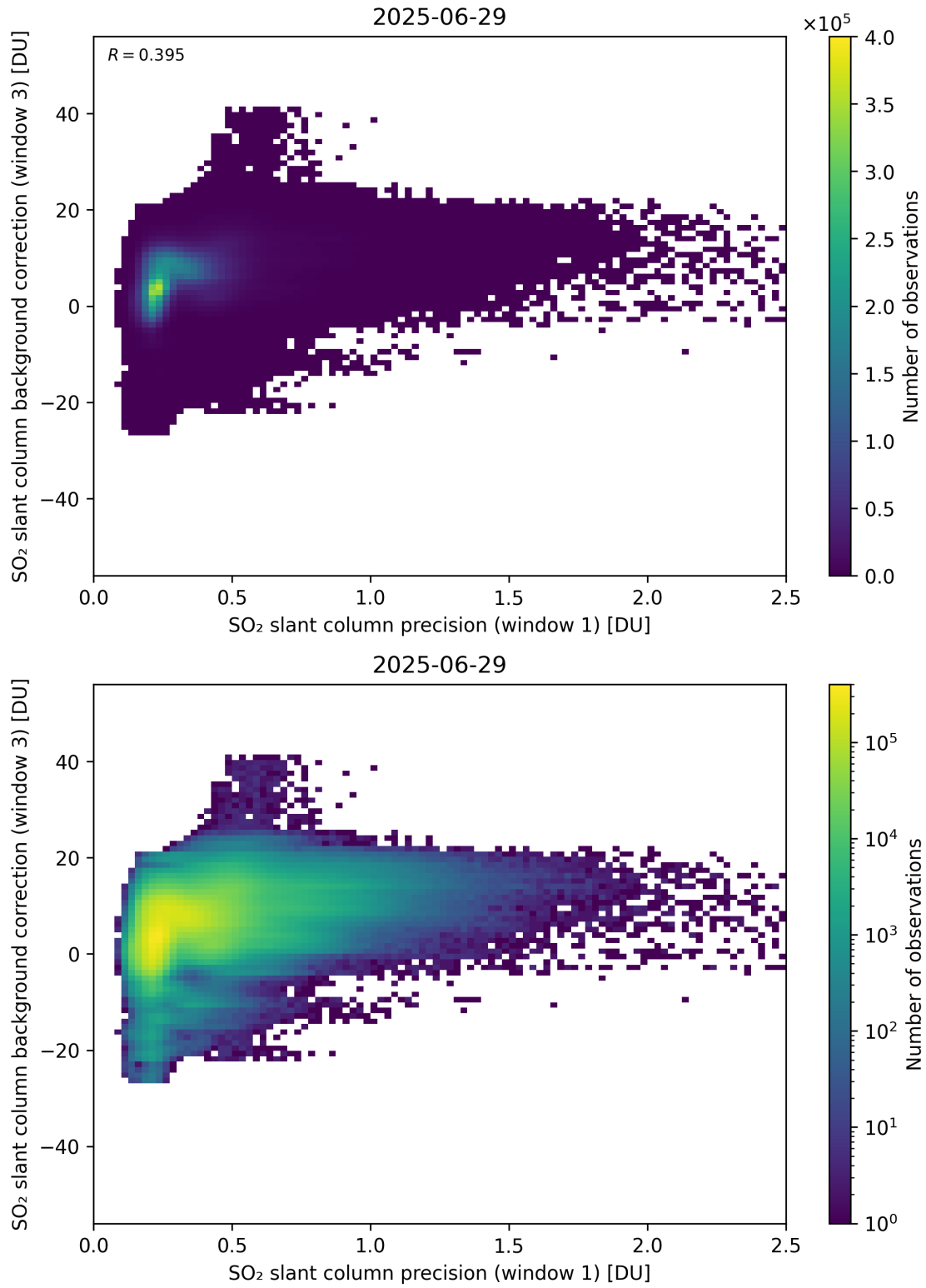
Figure 270: Scatter density plot of “SO 2 slant column precision (window 1)” against “SO 2 slant column background correction (window 3)” for 2025-06-28 to 2025-06-30.
