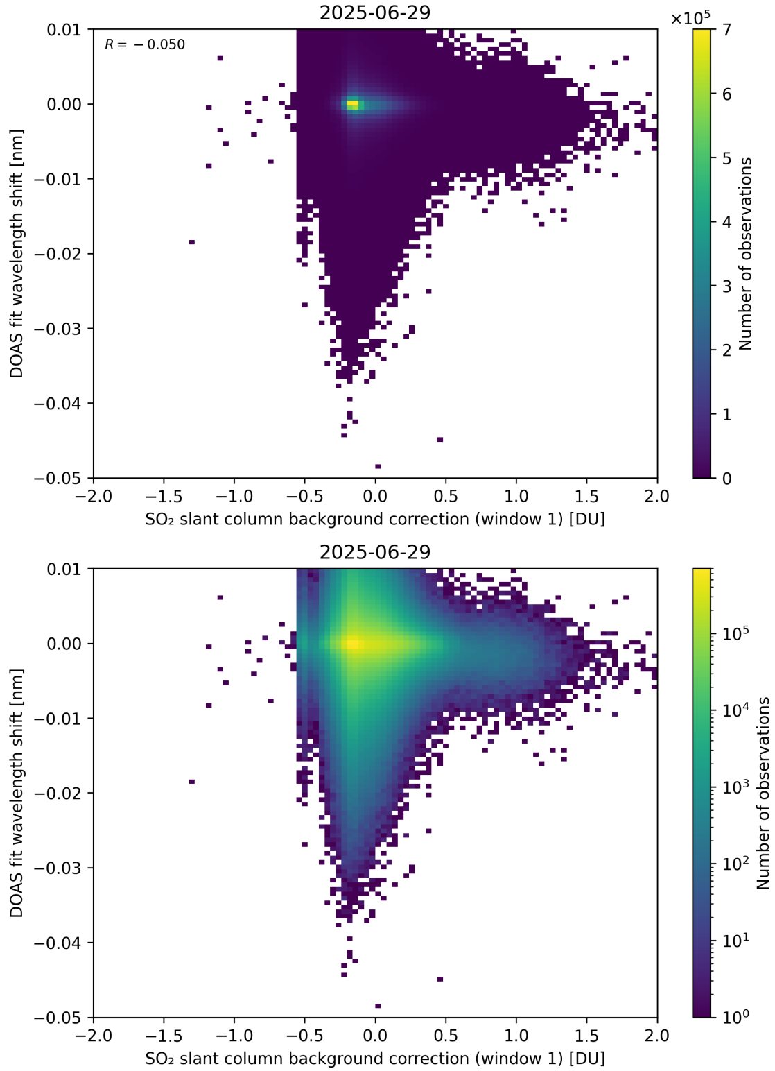
Figure 111: Scatter density plot of “SO 2 slant column background correction (window 1)” against “DOAS fit wavelength shift” for 2025-06-28 to 2025-06-30.
