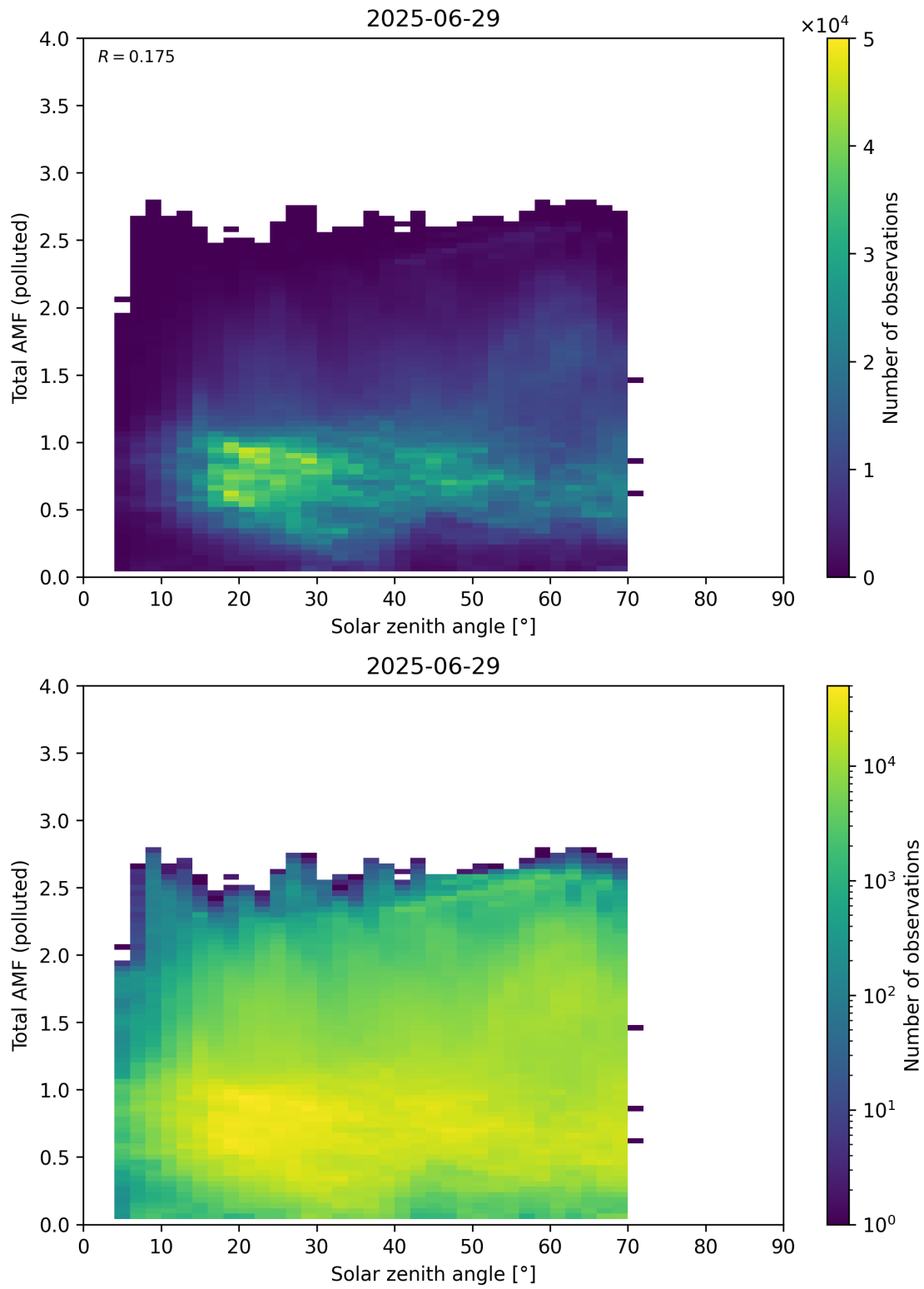
Figure 189: Scatter density plot of “Solar zenith angle” against “Total AMF (polluted)” for 2025-06-28 to 2025-06-30.
