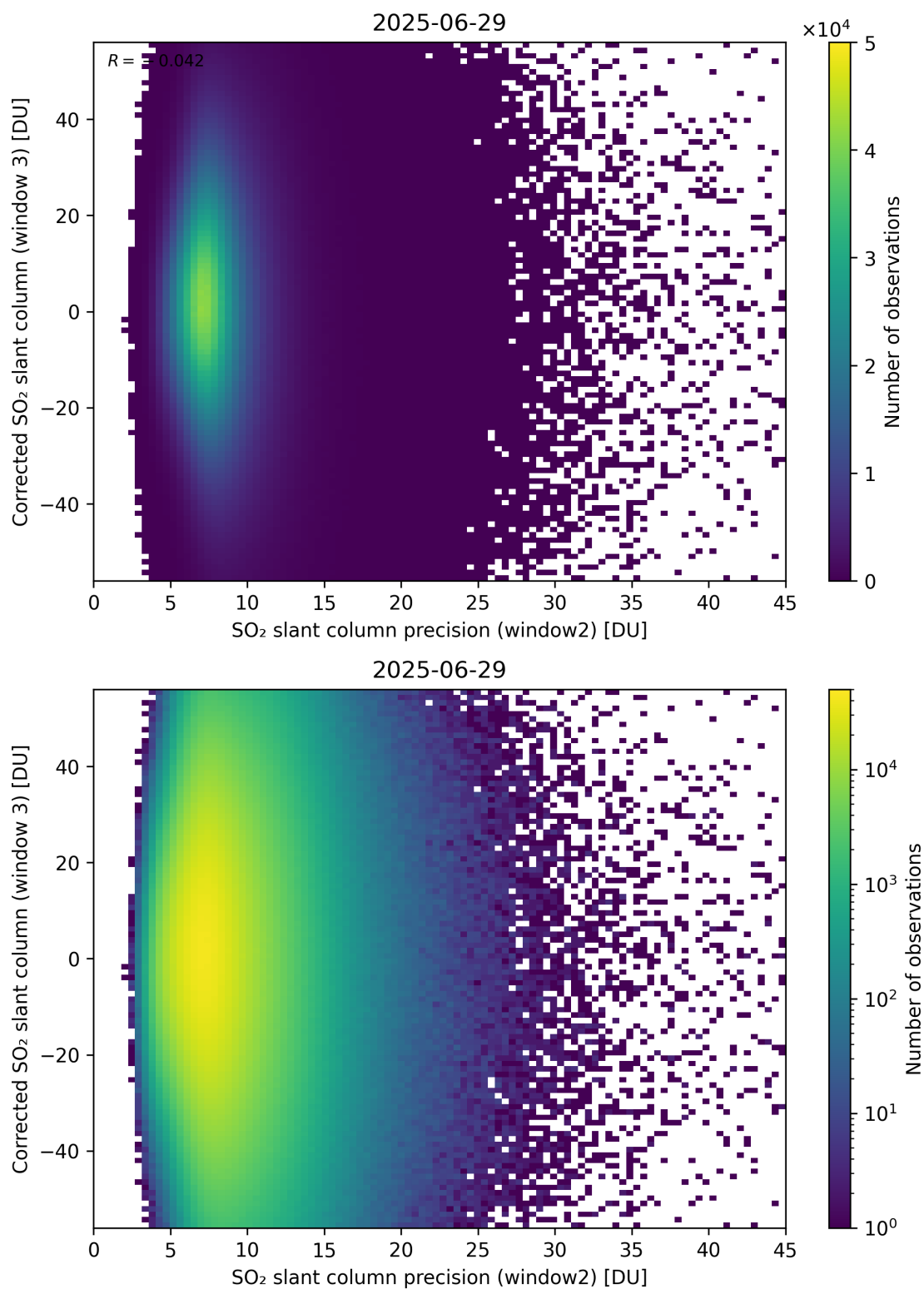
Figure 298: Scatter density plot of “SO 2 slant column precision (window2)” against “Corrected SO 2 slant column (window 3)” for 2025-06-28 to 2025-06-30.
