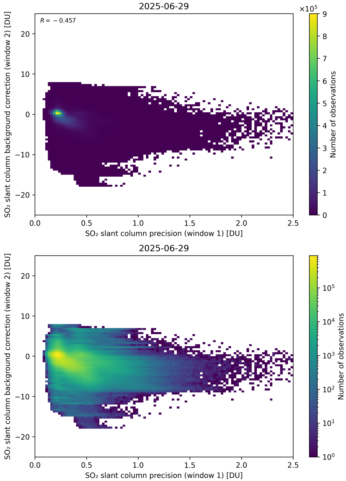
Figure 269: Scatter density plot of “SO 2 slant column precision (window 1)” against “SO 2 slant column background correction (window 2)” for 2025-06-28 to 2025-06-30.
