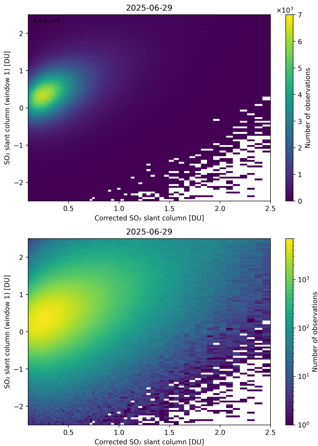
Figure 237: Scatter density plot of “Corrected SO 2 slant column” against “SO 2 slant column (window 1)” for 2025-06-28 to 2025-06-30.
