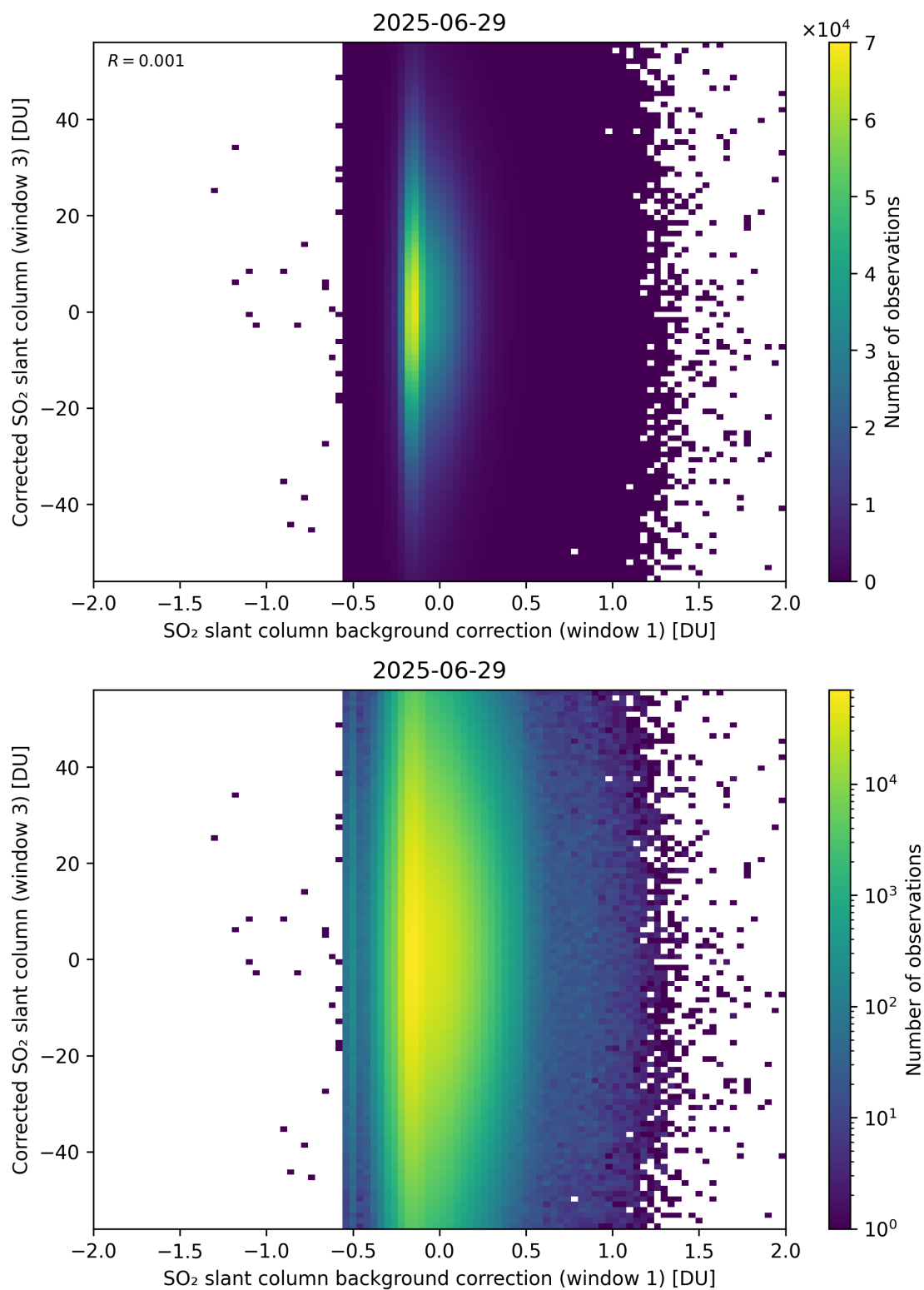
Figure 116: Scatter density plot of “SO 2 slant column background correction (window 1)” against “Corrected SO 2 slant column (window 3)” for 2025-06-28 to 2025-06-30.
