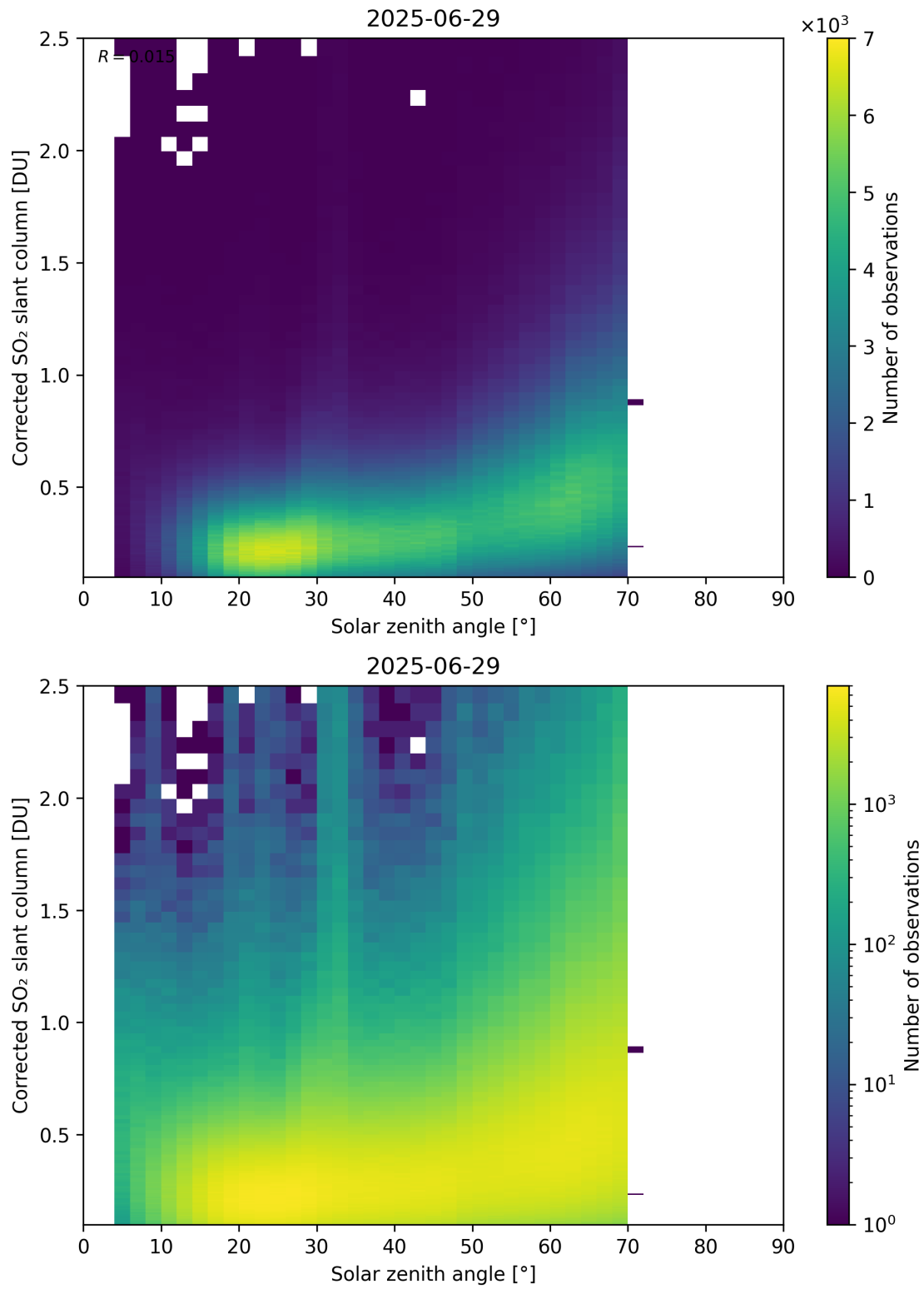
Figure 181: Scatter density plot of “Solar zenith angle” against “Corrected SO 2 slant column” for 2025-06-28 to 2025-06-30.
