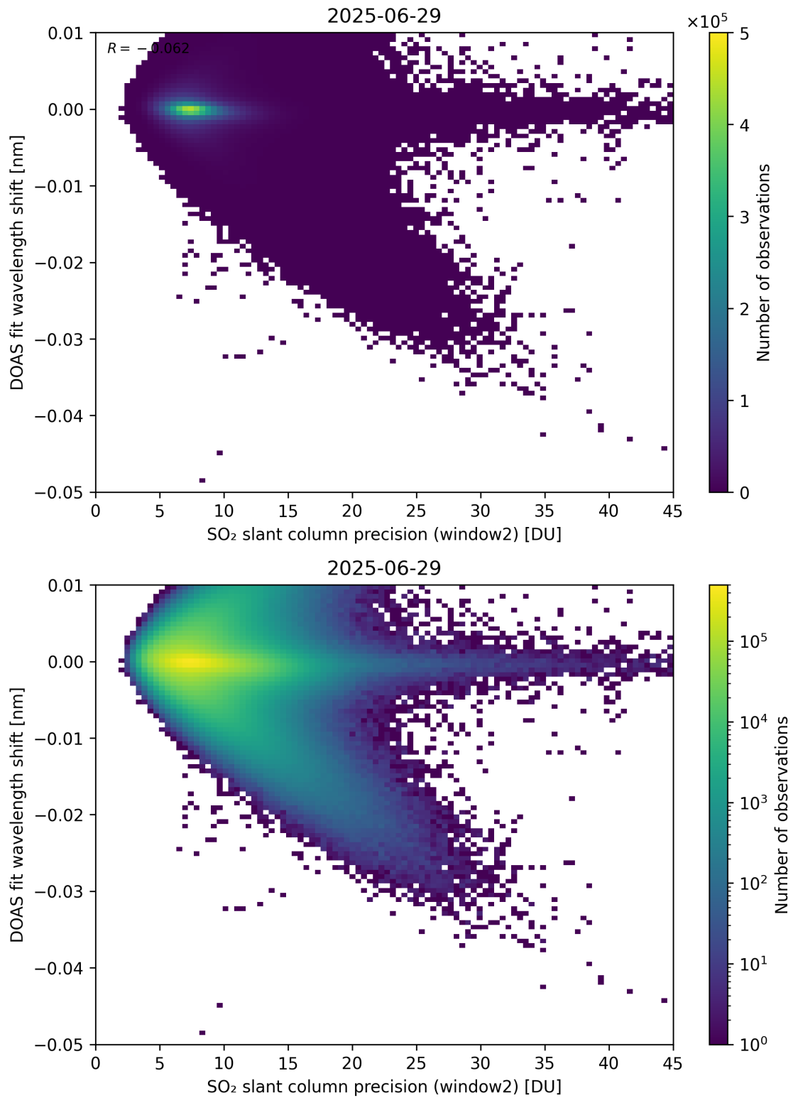
Figure 293: Scatter density plot of “SO 2 slant column precision (window2)” against “DOAS fit wavelength shift” for 2025-06-28 to 2025-06-30.
