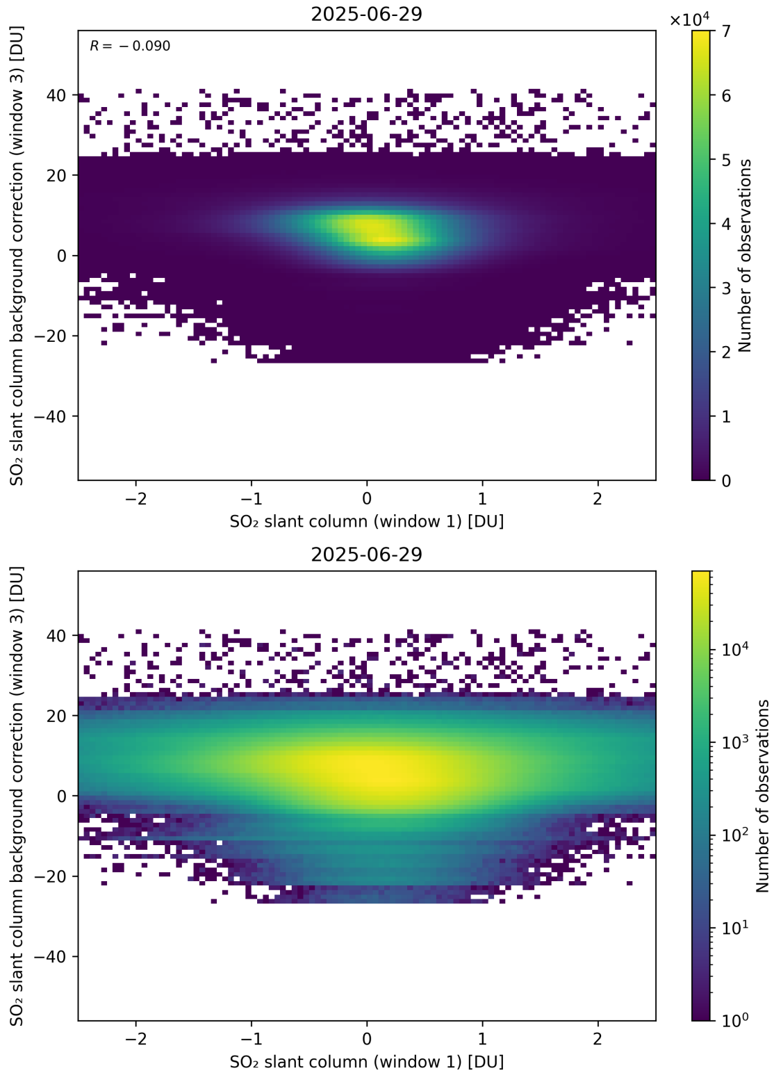
Figure 264: Scatter density plot of “SO 2 slant column (window 1)” against “SO 2 slant column background correction (window 3)” for 2025-06-28 to 2025-06-30.
