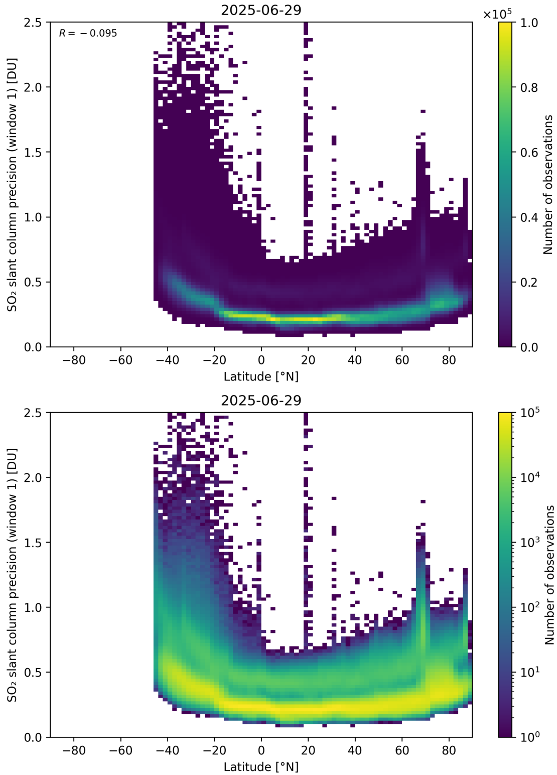
Figure 163: Scatter density plot of “Latitude” against “SO 2 slant column precision (window 1)” for 2025-06-28 to 2025-06-30.
