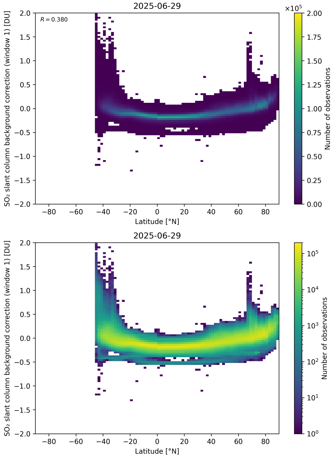
Figure 150: Scatter density plot of “Latitude” against “SO 2 slant column background correction (window 1)” for 2025-06-28 to 2025-06-30.
