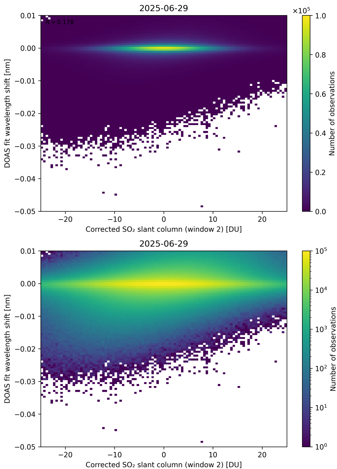
Figure 246: Scatter density plot of “Corrected SO 2 slant column (window 2)” against “DOAS fit wavelength shift” for 2025-06-28 to 2025-06-30.
