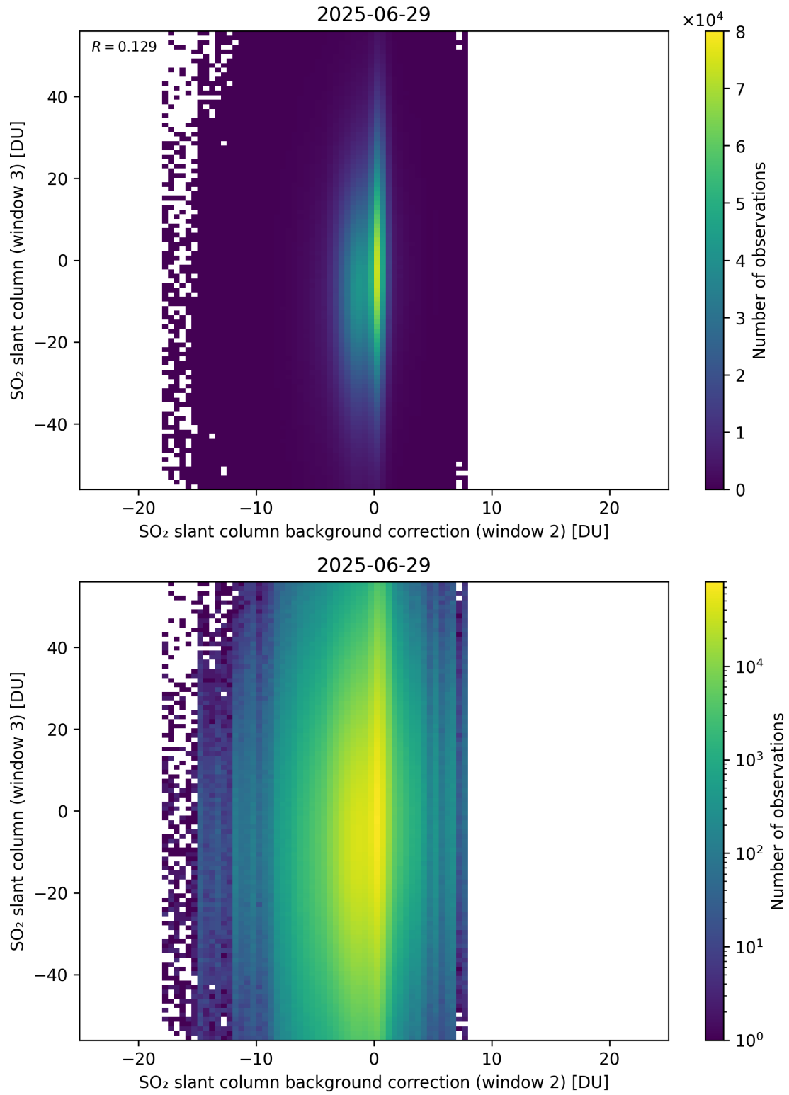
Figure 128: Scatter density plot of “SO 2 slant column background correction (window 2)” against “SO 2 slant column (window 3)” for 2025-06-28 to 2025-06-30.
