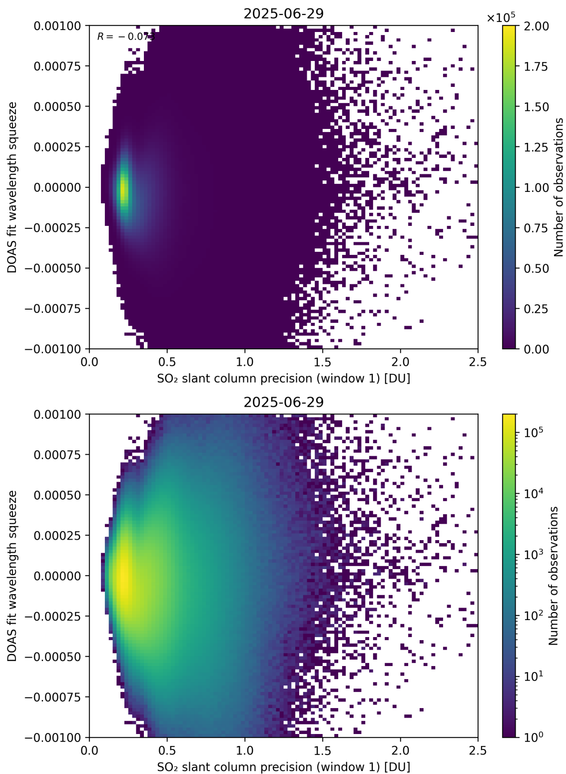
Figure 272: Scatter density plot of “SO 2 slant column precision (window 1)” against “DOAS fit wavelength squeeze” for 2025-06-28 to 2025-06-30.
