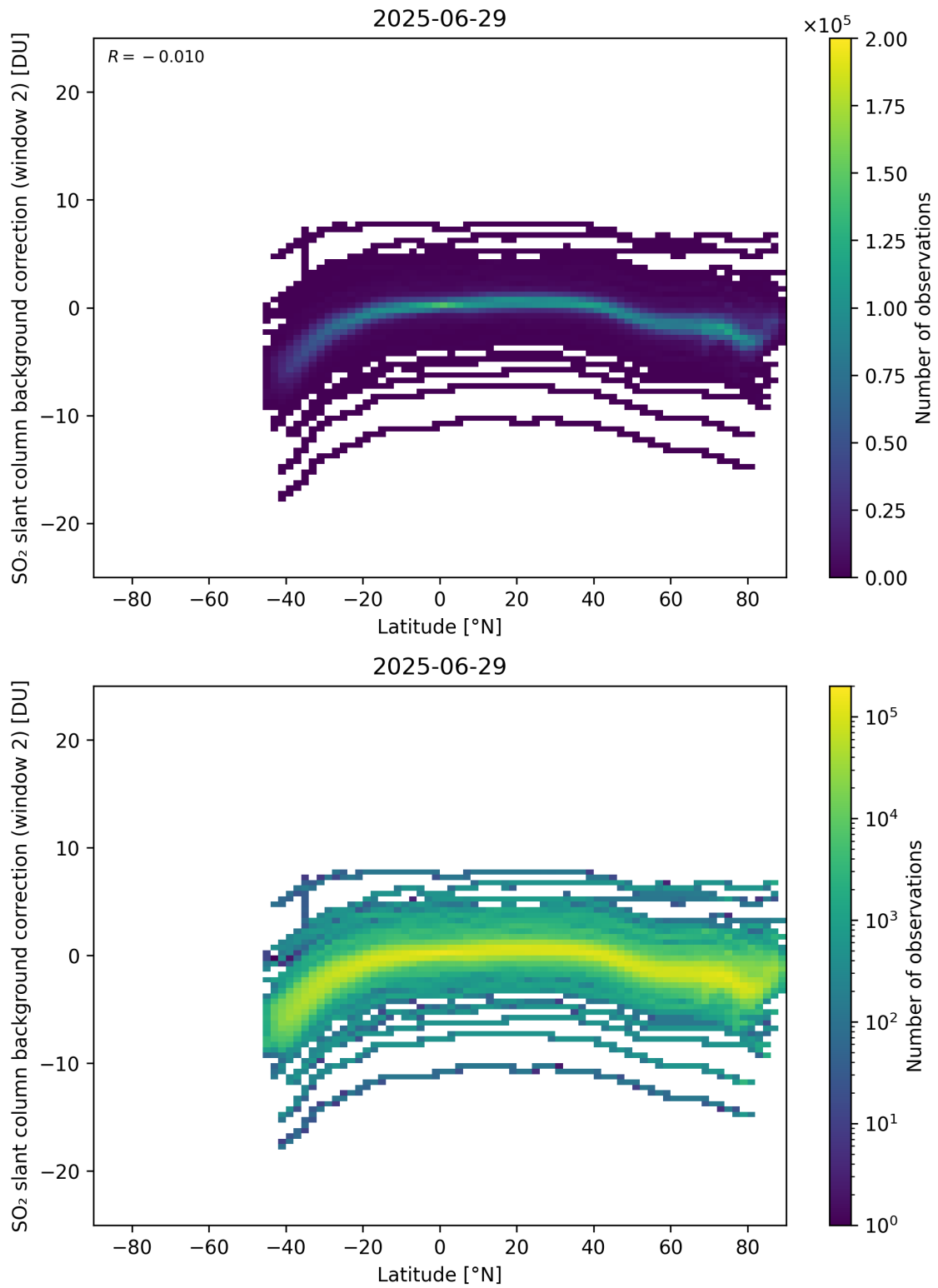
Figure 151: Scatter density plot of “Latitude” against “SO 2 slant column background correction (window 2)” for 2025-06-28 to 2025-06-30.
