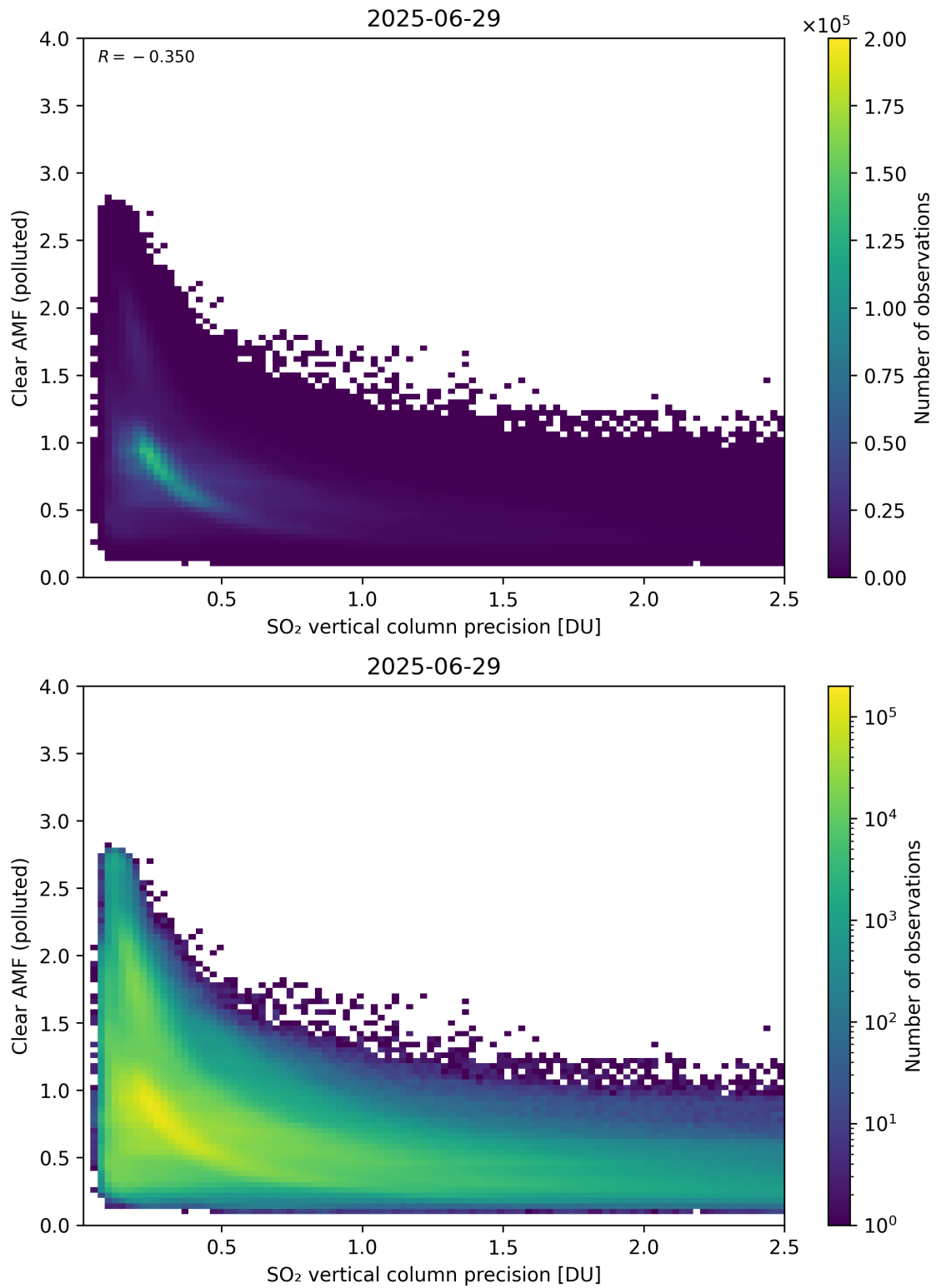
Figure 335: Scatter density plot of “SO 2 vertical column precision” against “Clear AMF (polluted)” for 2025-06-28 to 2025-06-30.
