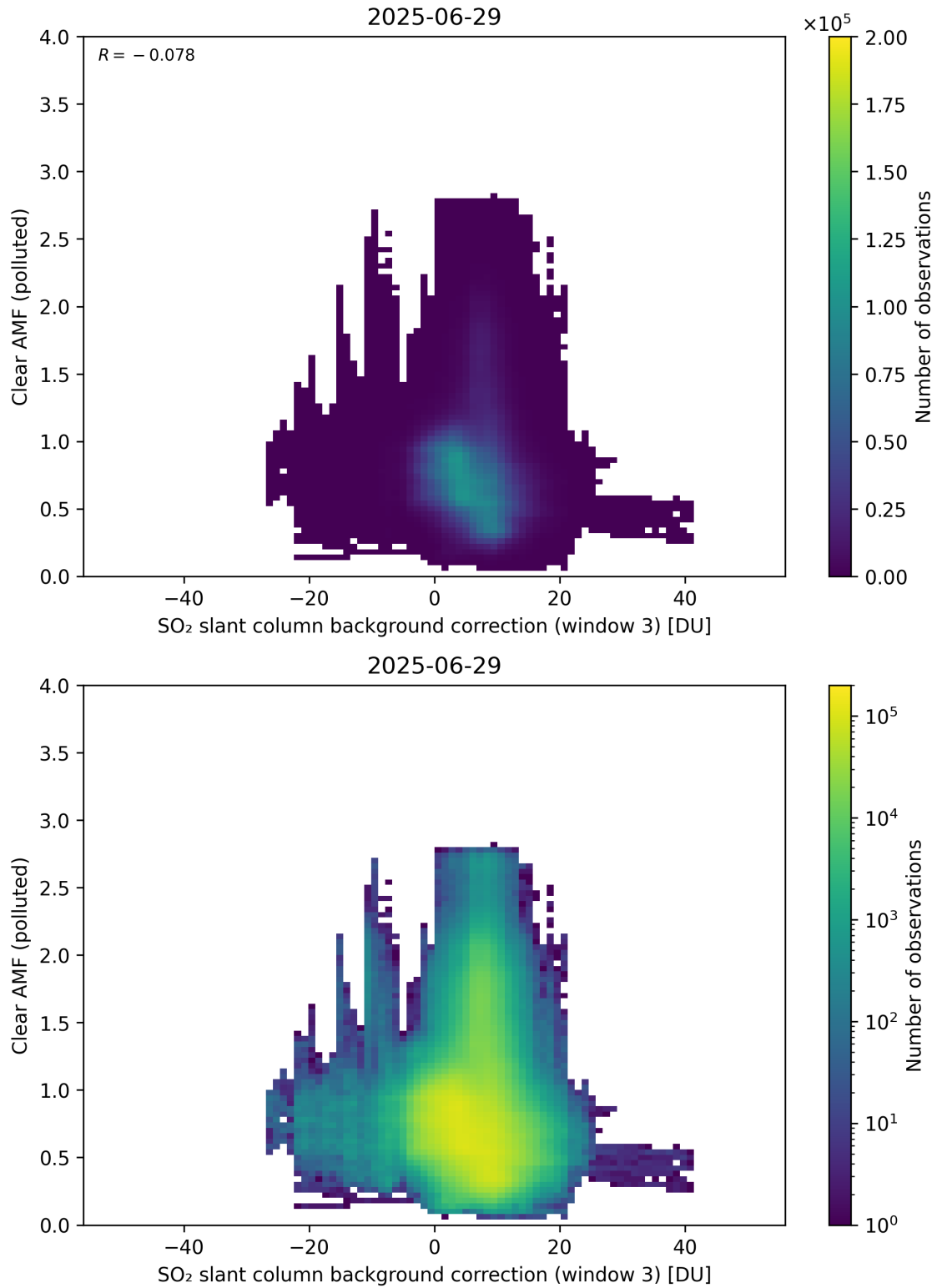
Figure 135: Scatter density plot of “SO 2 slant column background correction (window 3)” against “Clear AMF (polluted)” for 2025-06-28 to 2025-06-30.
