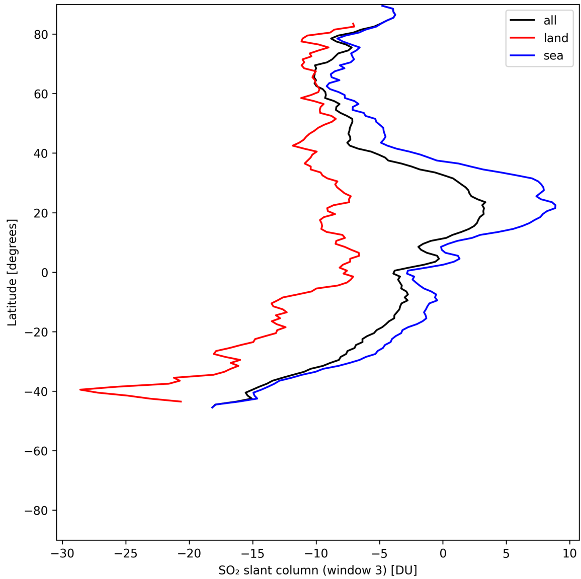
Figure 45: Zonal average of “SO 2 slant column (window 3)” for 2025-06-28 to 2025-06-30.
