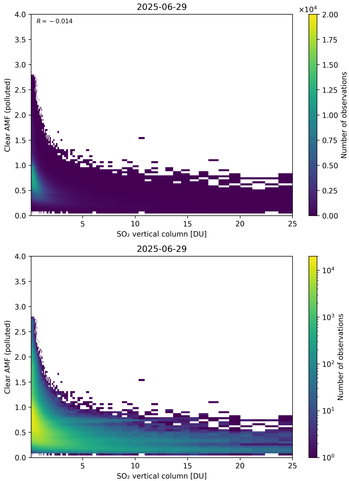
Figure 348: Scatter density plot of “SO 2 vertical column” against “Clear AMF (polluted)” for 2025-06-28 to 2025-06-30.
