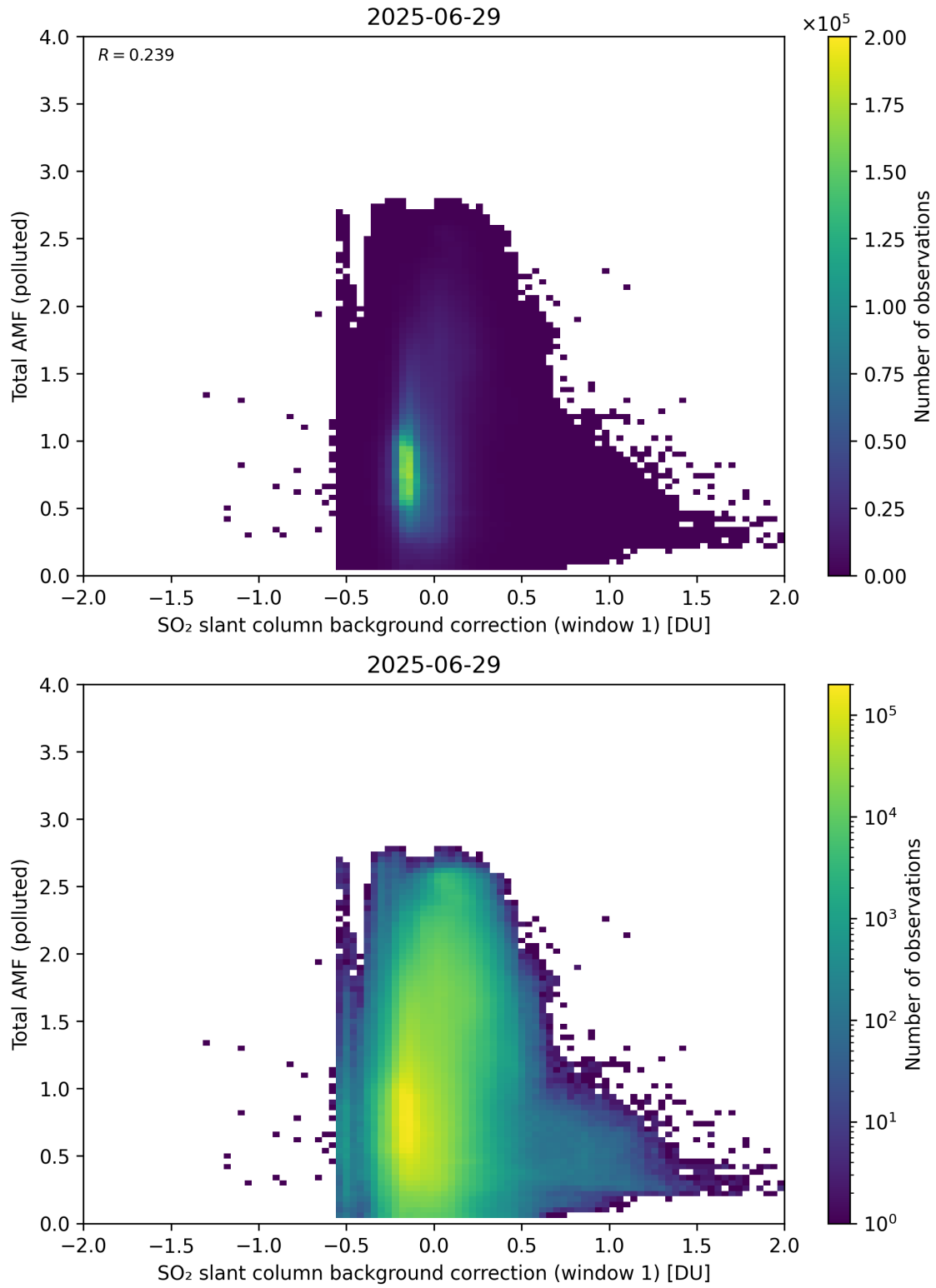
Figure 120: Scatter density plot of “SO 2 slant column background correction (window 1)” against “Total AMF (polluted)” for 2025-06-28 to 2025-06-30.
