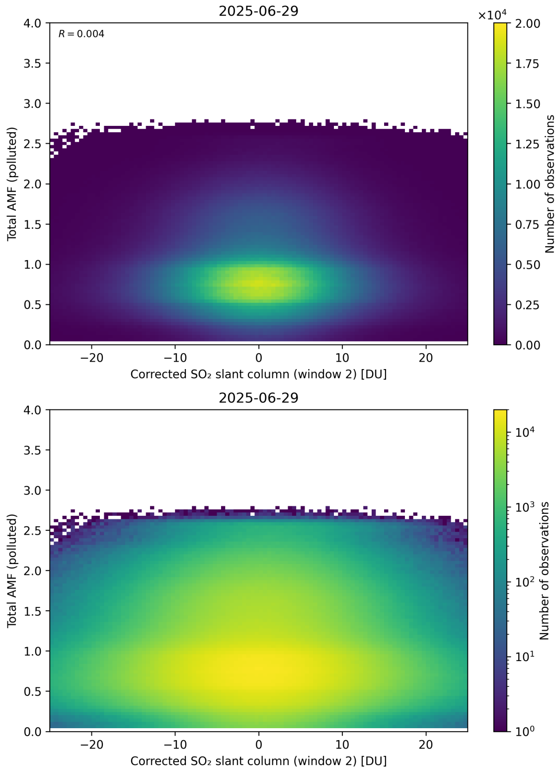
Figure 253: Scatter density plot of “Corrected SO 2 slant column (window 2)” against “Total AMF (polluted)” for 2025-06-28 to 2025-06-30.
