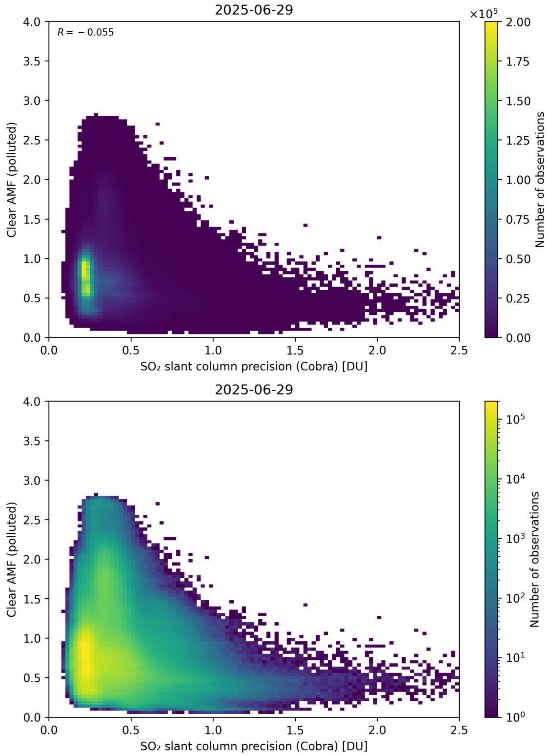
Figure 205: Scatter density plot of “SO 2 slant column precision (Cobra)” against “Clear AMF (polluted)” for 2025-06-28 to 2025-06-30.
