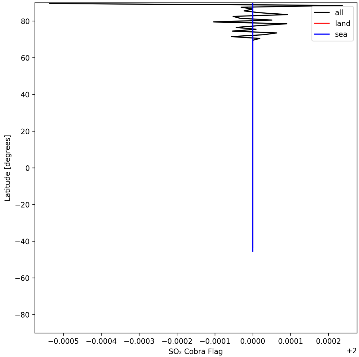
Figure 49: Zonal average of "SO 2 Cobra Flag" for 2025-06-28 to 2025-06-30.
