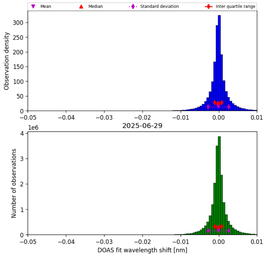
Figure 76: Histogram of “DOAS fit wavelength shift” for 2025-06-28 to 2025-06-30
