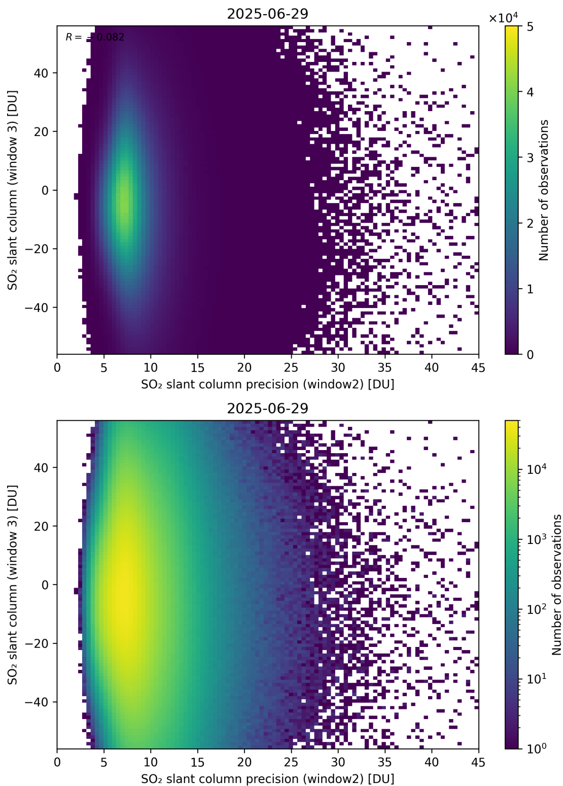
Figure 299: Scatter density plot of “SO 2 slant column precision (window2)” against “SO 2 slant column (window 3)” for 2025-06-28 to 2025-06-30.
