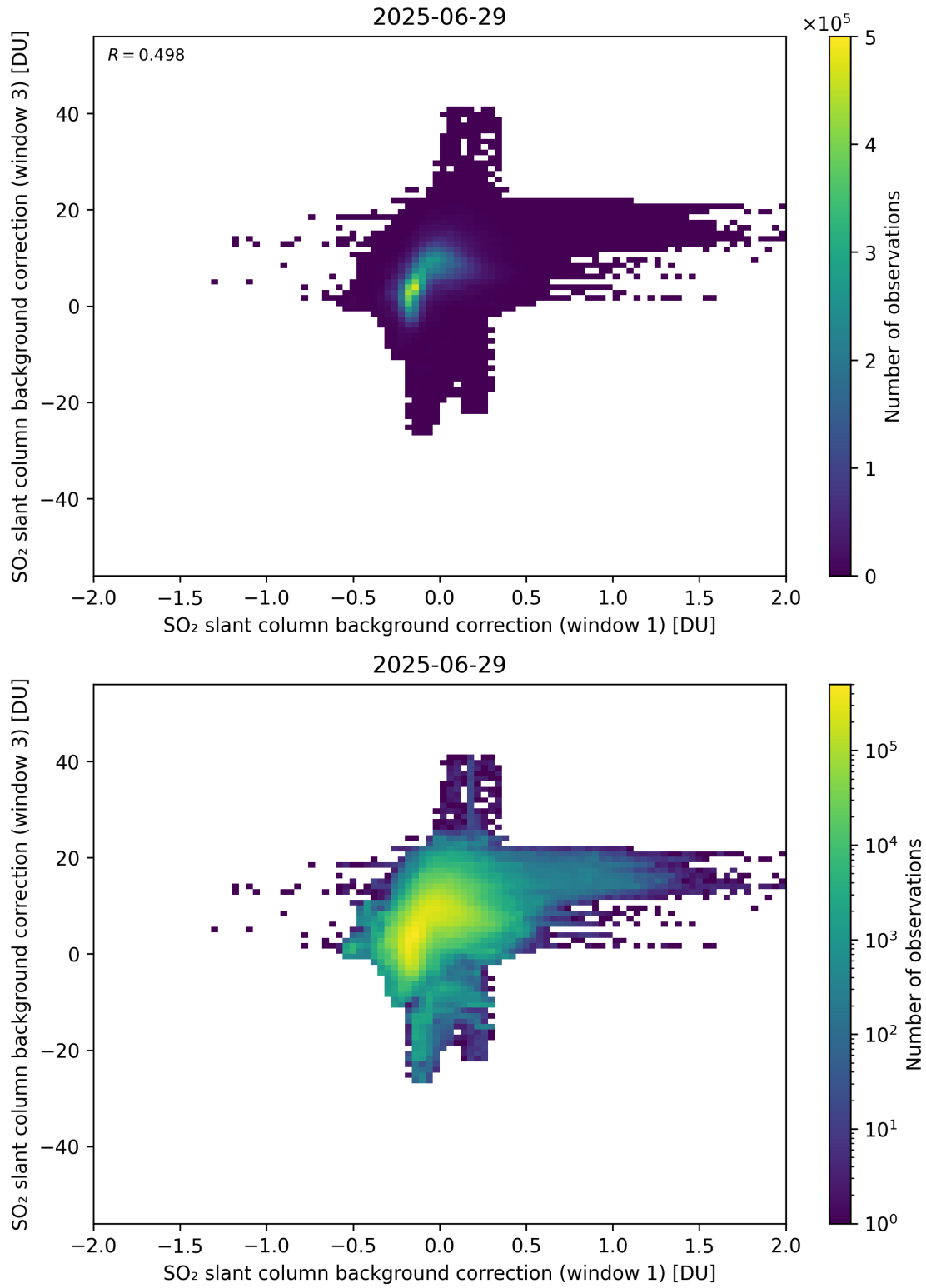
Figure 110: Scatter density plot of “SO 2 slant column background correction (window 1)” against “SO 2 slant column background correction (window 3)” for 2025-06-28 to 2025-06-30.
