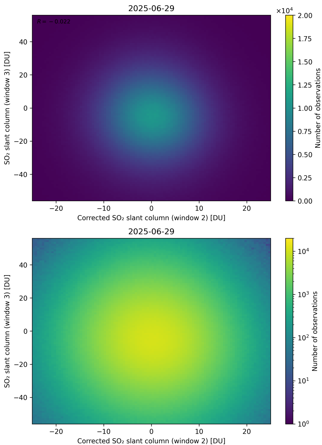
Figure 251: Scatter density plot of “Corrected SO 2 slant column (window 2)” against “SO 2 slant column (window 3)” for 2025-06-28 to 2025-06-30.
