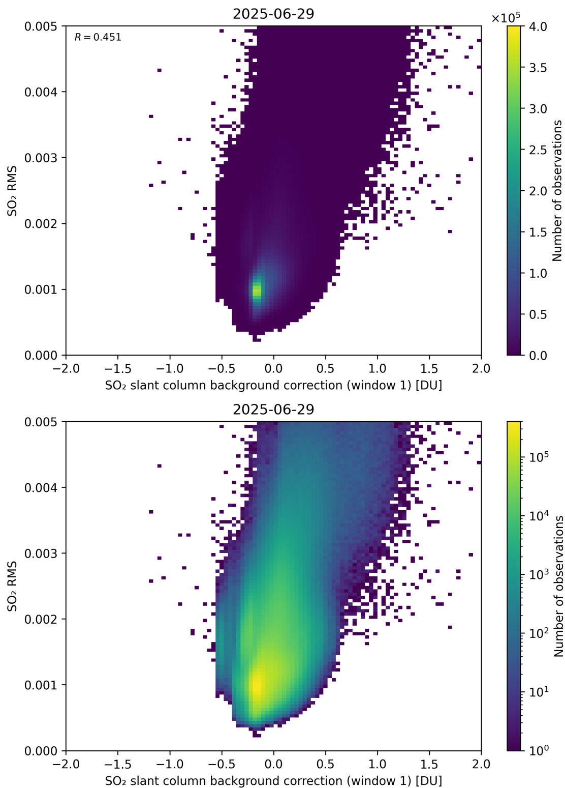
Figure 113: Scatter density plot of “SO 2 slant column background correction (window 1)” against “SO 2 RMS” for 2025-06-28 to 2025-06-30.
