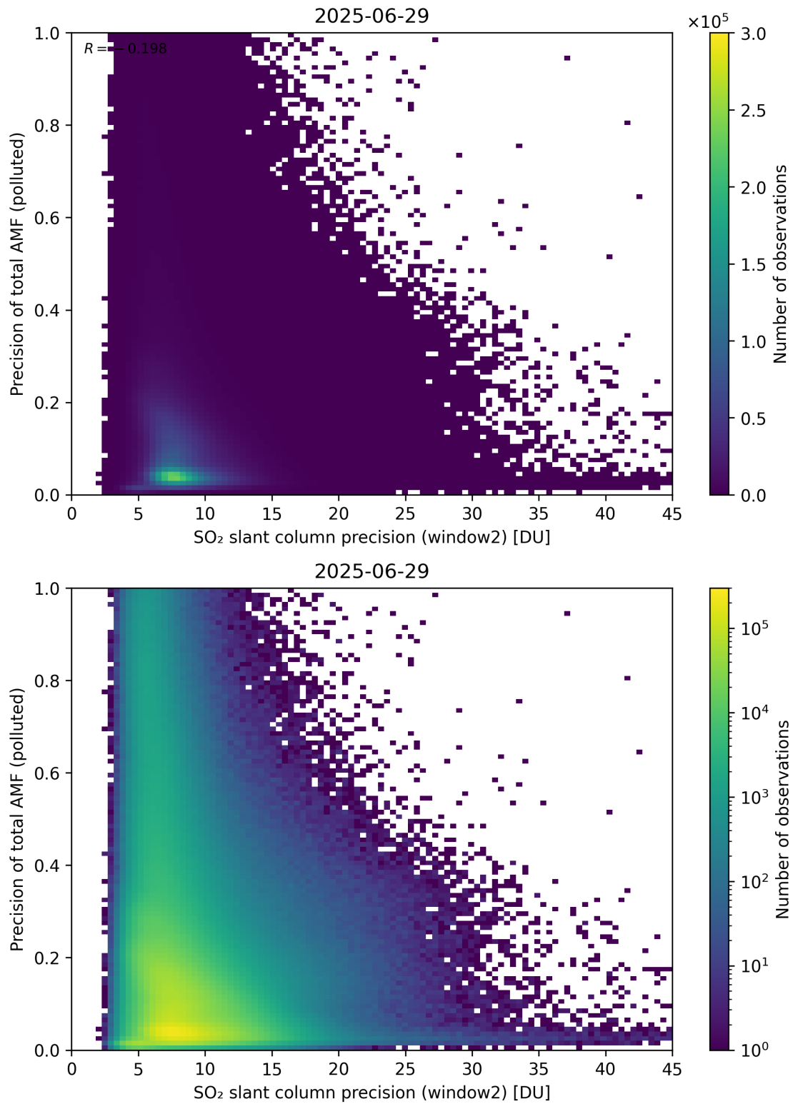
Figure 302: Scatter density plot of “SO 2 slant column precision (window2)” against “Precision of total AMF (polluted)” for 2025-06-28 to 2025-06-30.
