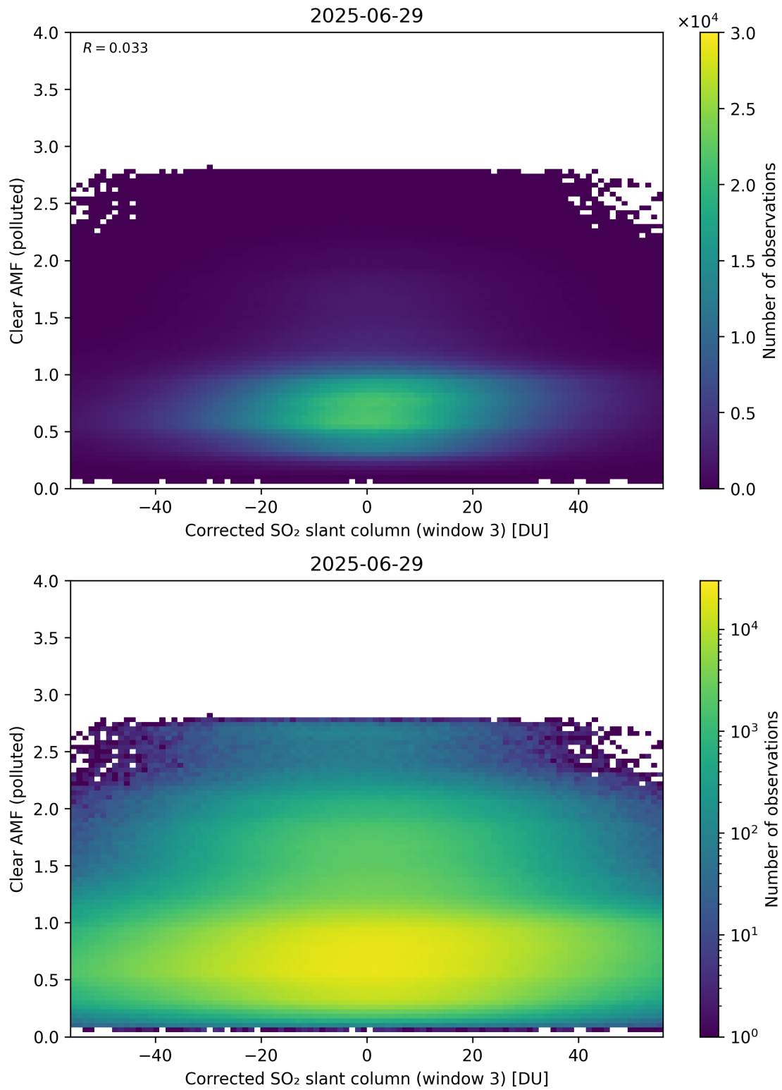
Figure 259: Scatter density plot of “Corrected SO 2 slant column (window 3)” against “Clear AMF (polluted)” for 2025-06-28 to 2025-06-30.
