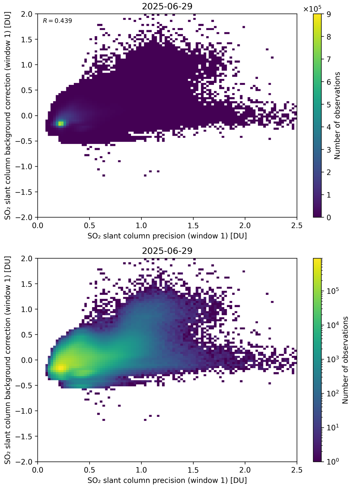
Figure 268: Scatter density plot of “SO 2 slant column precision (window 1)” against “SO 2 slant column background correction (window 1)” for 2025-06-28 to 2025-06-30.
