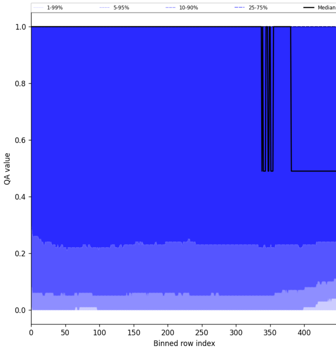
Figure 83: Along track statistics of “QA value” for 2025-06-28 to 2025-06-30
