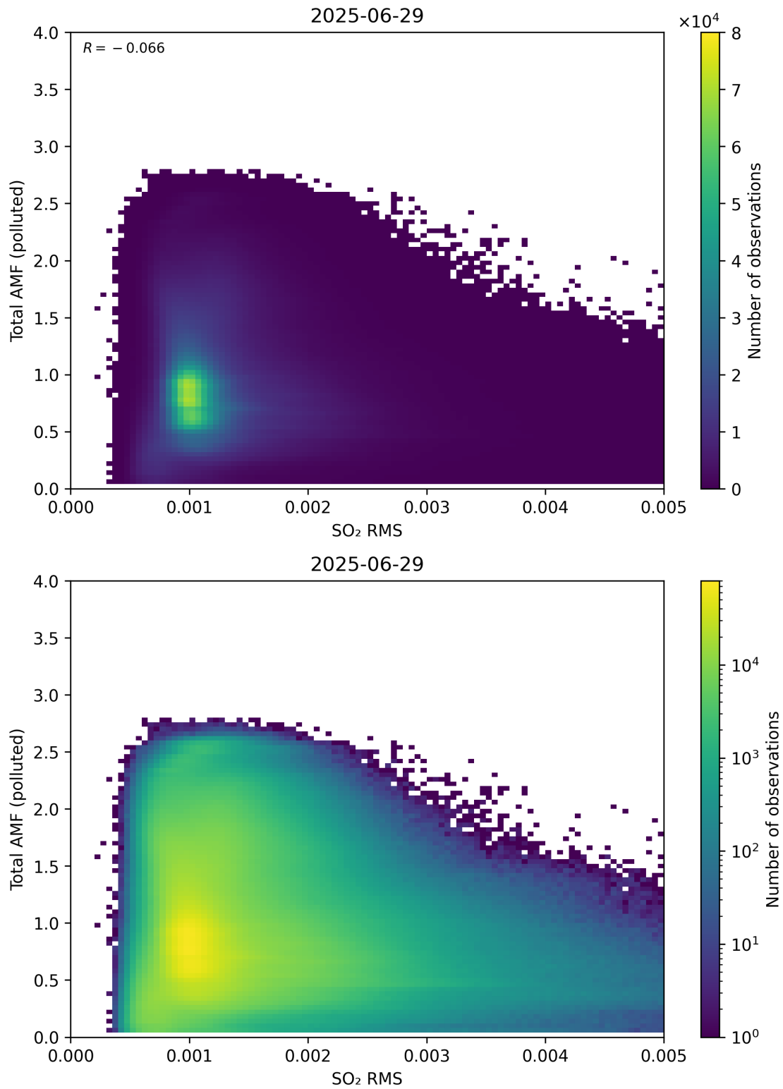
Figure 148: Scatter density plot of “SO 2 RMS” against “Total AMF (polluted)” for 2025-06-28 to 2025-06-30.
