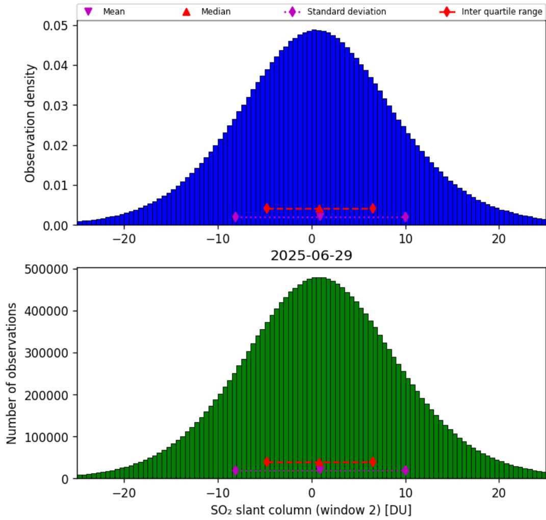
Figure 67: Histogram of “SO 2 slant column (window 2)” for 2025-06-28 to 2025-06-30
