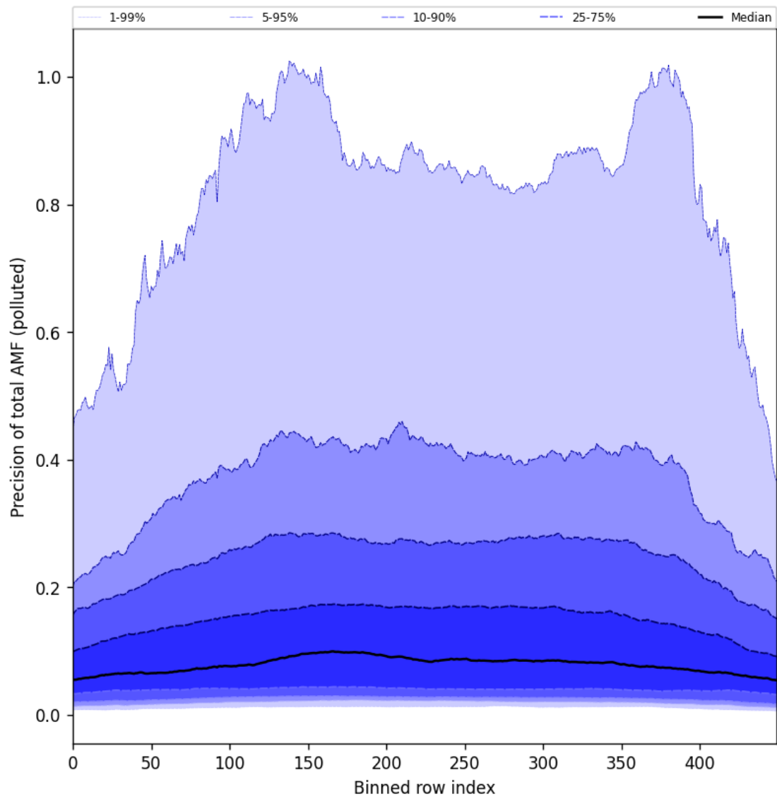
Figure 106: Along track statistics of “Precision of total AMF (polluted)” for 2025-06-28 to 2025-06-30
