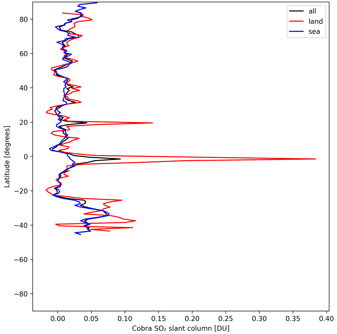
Figure 35: Zonal average of “Cobra SO 2 slant column” for 2025-06-28 to 2025-06-30.
