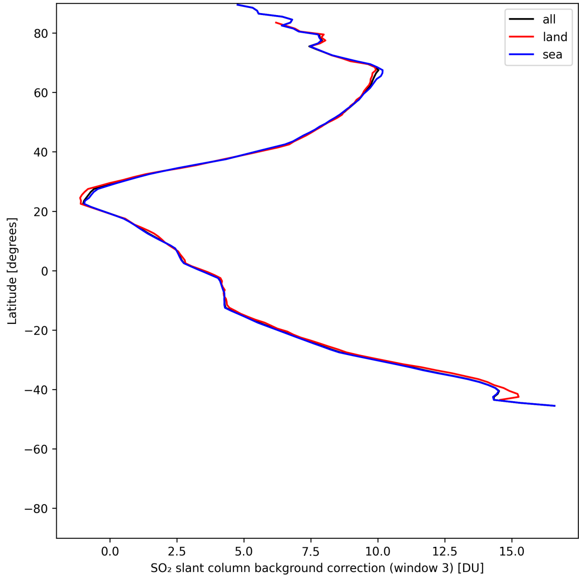
Figure 48: Zonal average of “SO 2 slant column background correction (window 3)” for 2025-06-28 to 2025-06-30.
