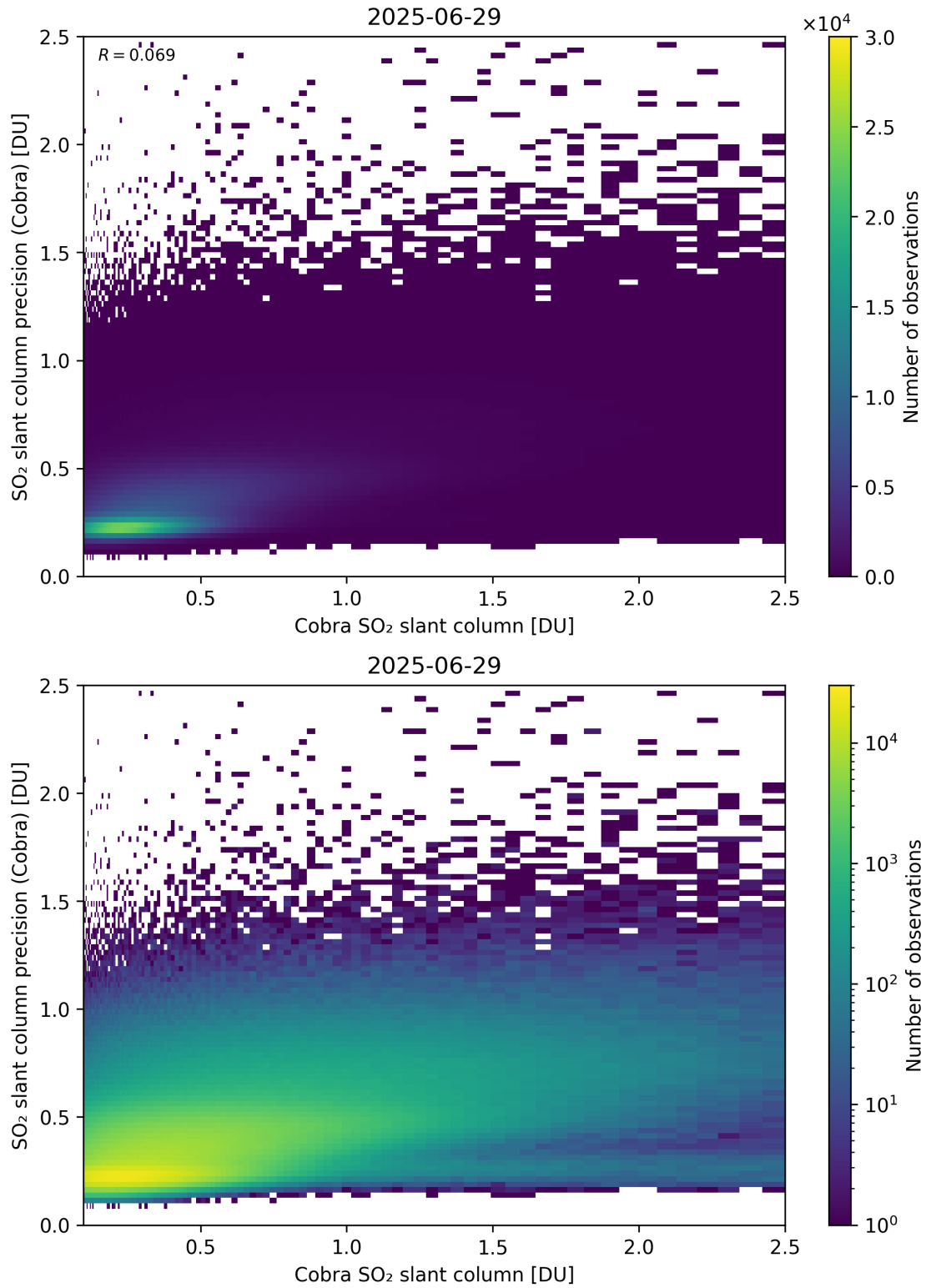
Figure 216: Scatter density plot of “Cobra SO 2 slant column” against “SO 2 slant column precision (Cobra)” for 2025-06-28 to 2025-06-30.
