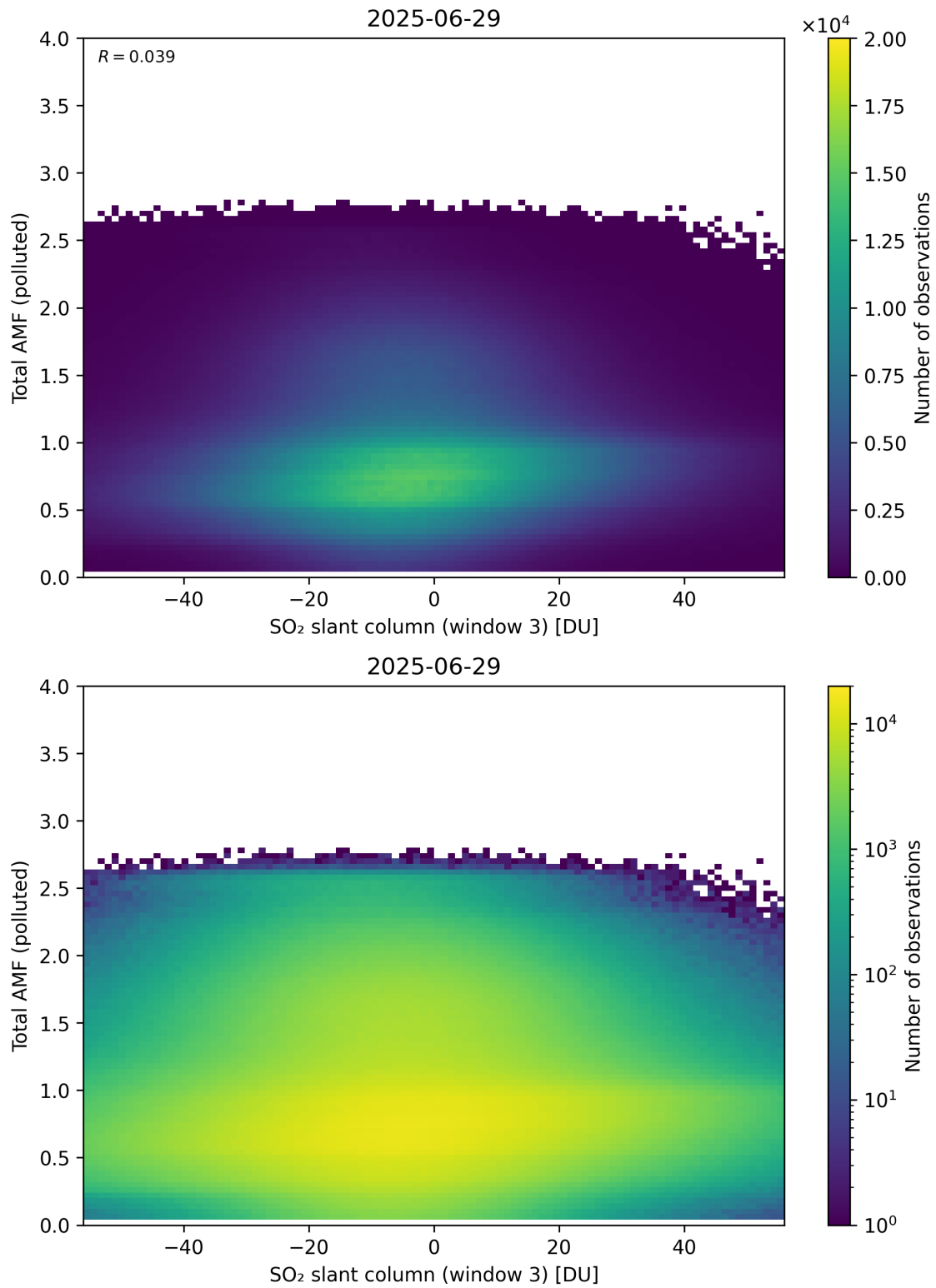
Figure 318: Scatter density plot of “SO 2 slant column (window 3)” against “Total AMF (polluted)” for 2025-06-28 to 2025-06-30.
