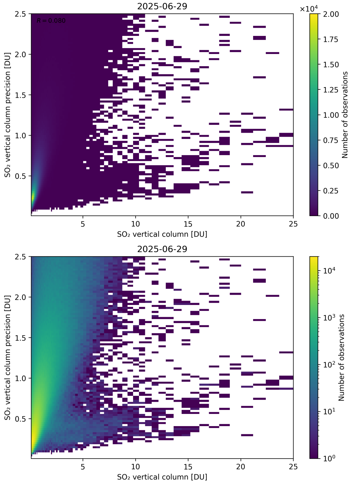
Figure 361: Scatter density plot of “SO 2 vertical column” against “SO 2 vertical column precision” for 2025-06-28 to 2025-06-30.
