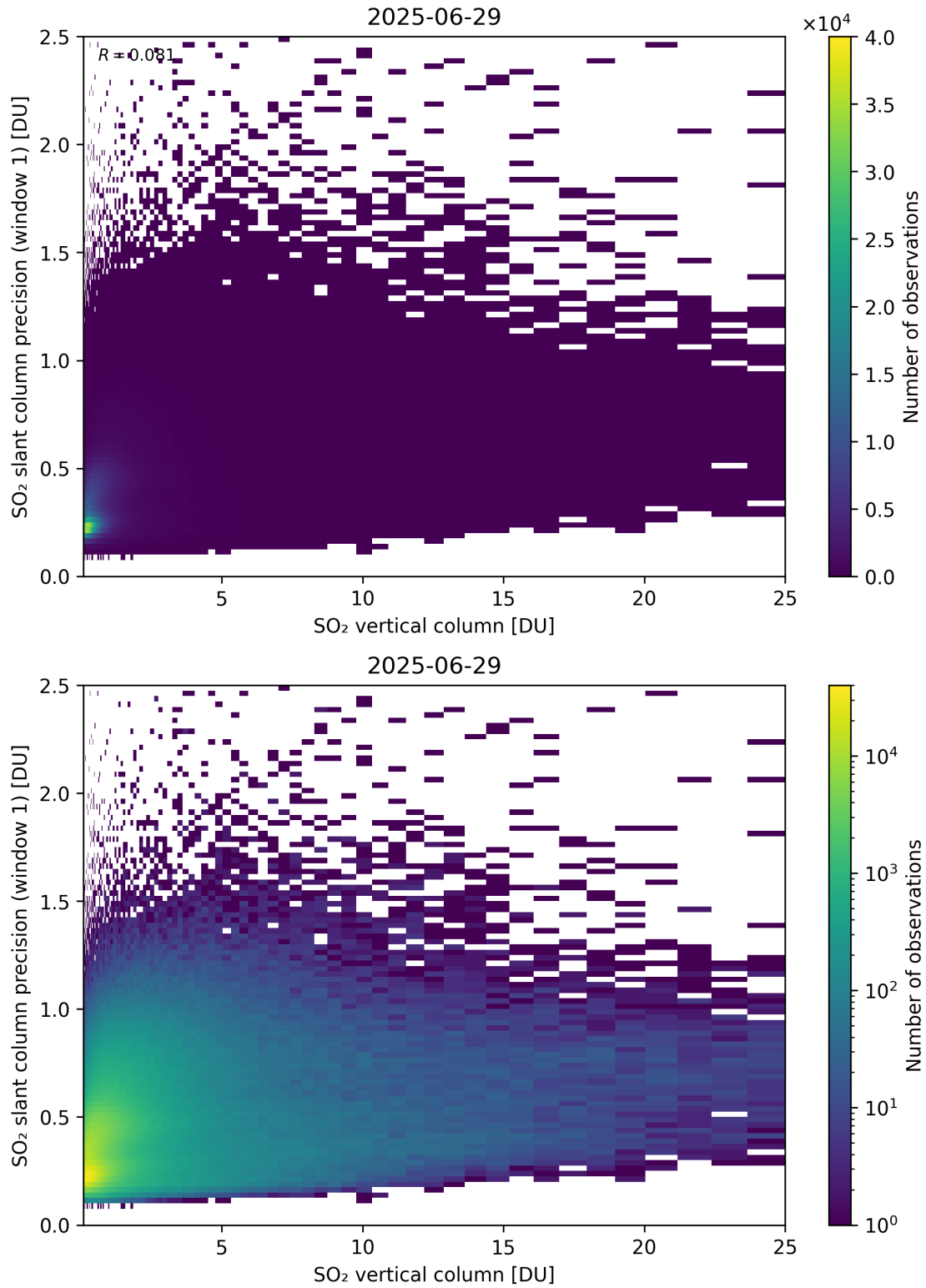
Figure 355: Scatter density plot of “SO 2 vertical column” against “SO 2 slant column precision (window 1)” for 2025-06-28 to 2025-06-30.
