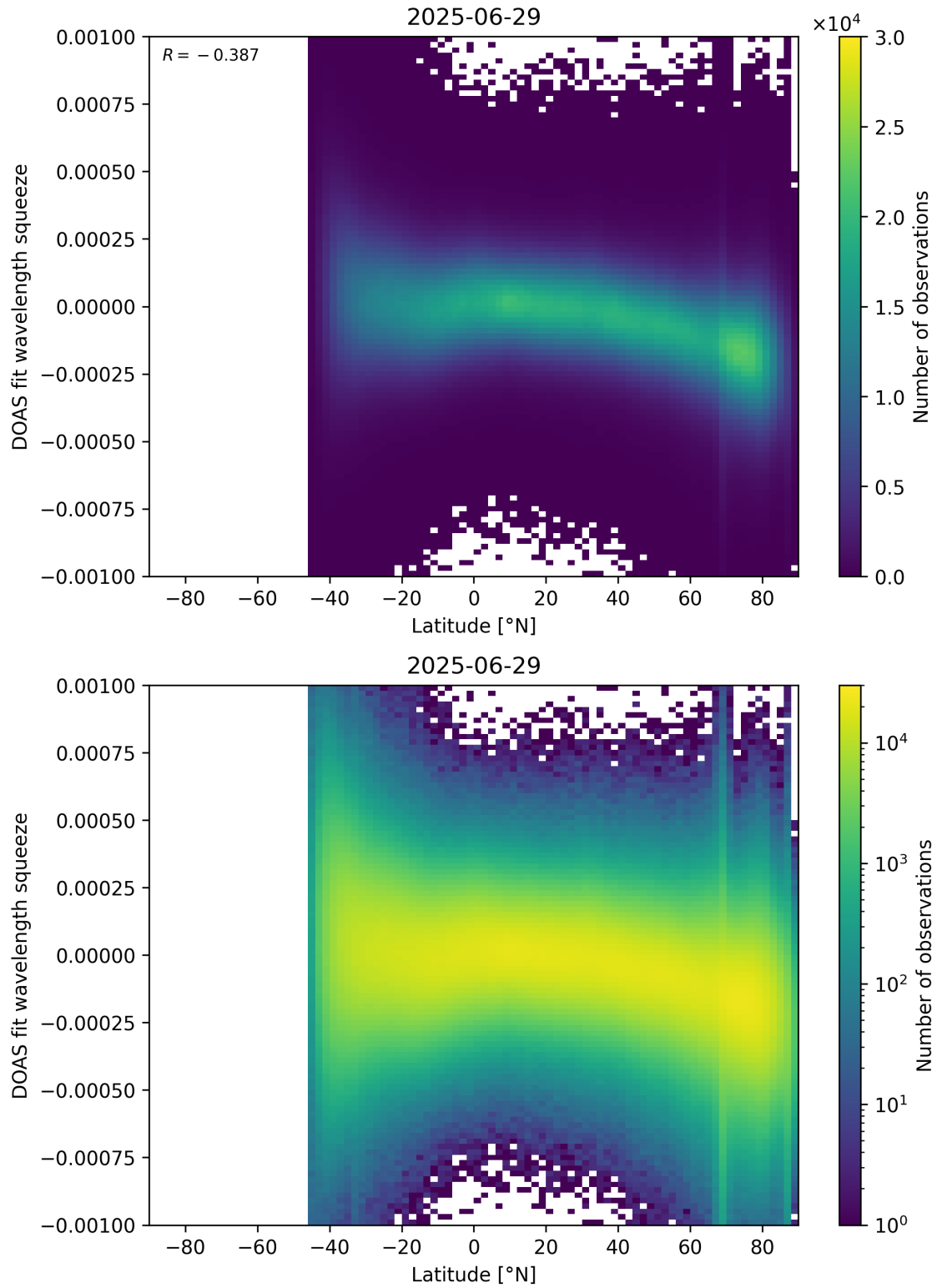
Figure 154: Scatter density plot of “Latitude” against “DOAS fit wavelength squeeze” for 2025-06-28 to 2025-06-30.
