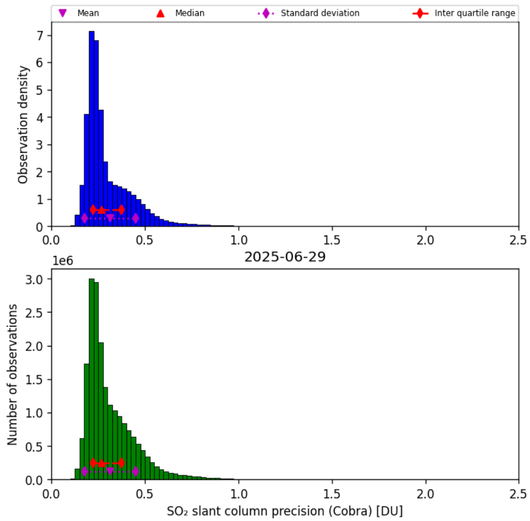
Figure 62: Histogram of “SO 2 slant column precision (Cobra)” for 2025-06-28 to 2025-06-30
