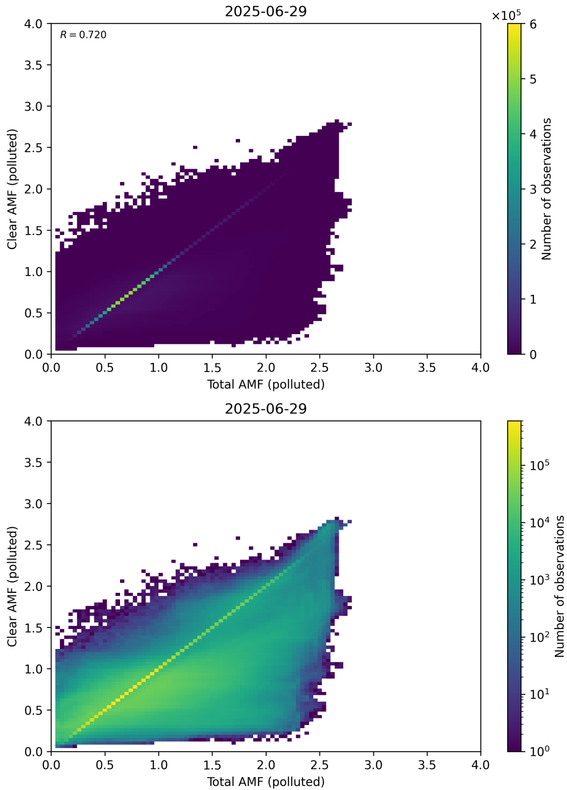
Figure 321: Scatter density plot of “Total AMF (polluted)” against “Clear AMF (polluted)” for 2025-06-28 to 2025-06-30.
