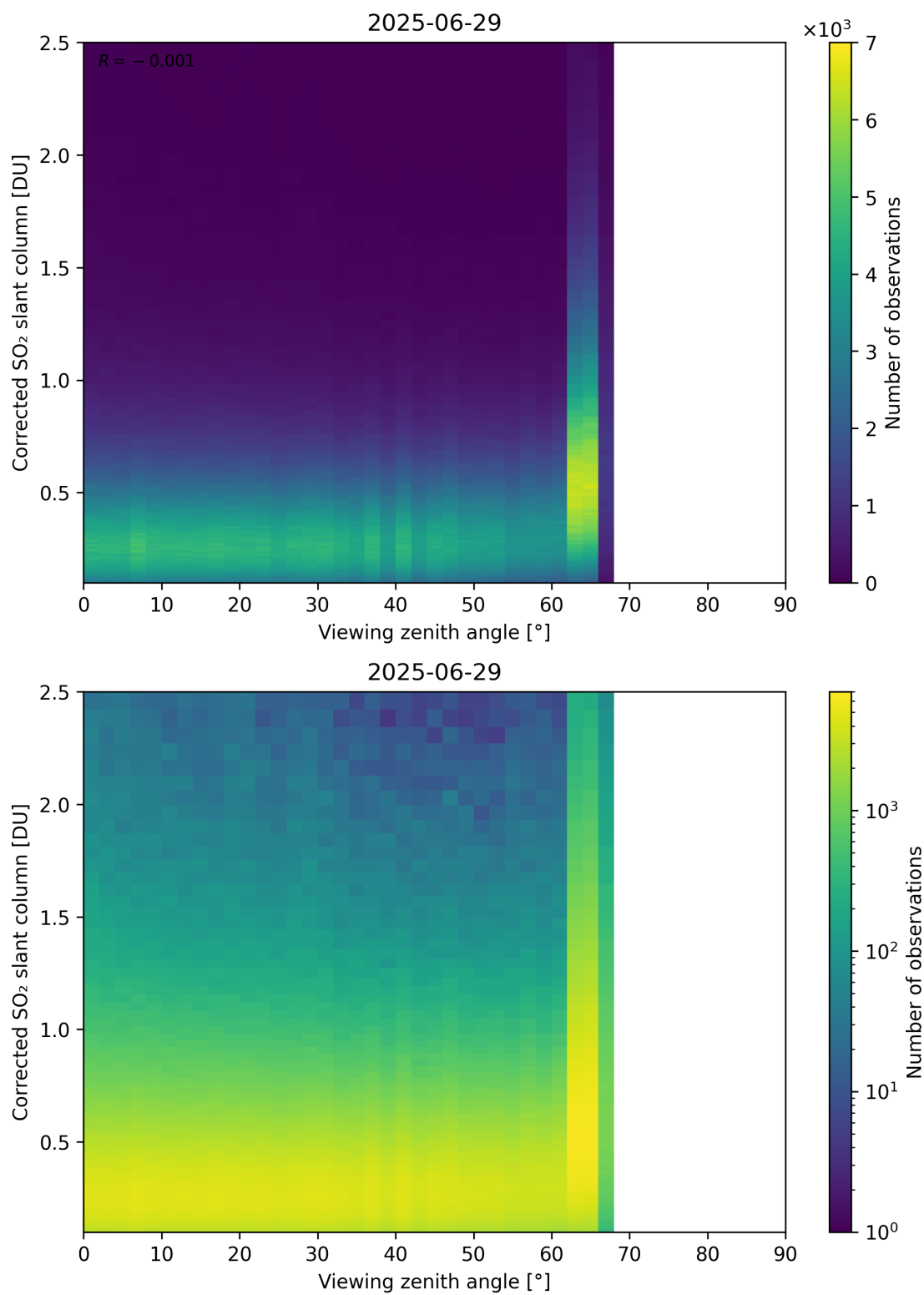
Figure 373: Scatter density plot of “Viewing zenith angle” against “Corrected SO 2 slant column” for 2025-06-28 to 2025-06-30.
