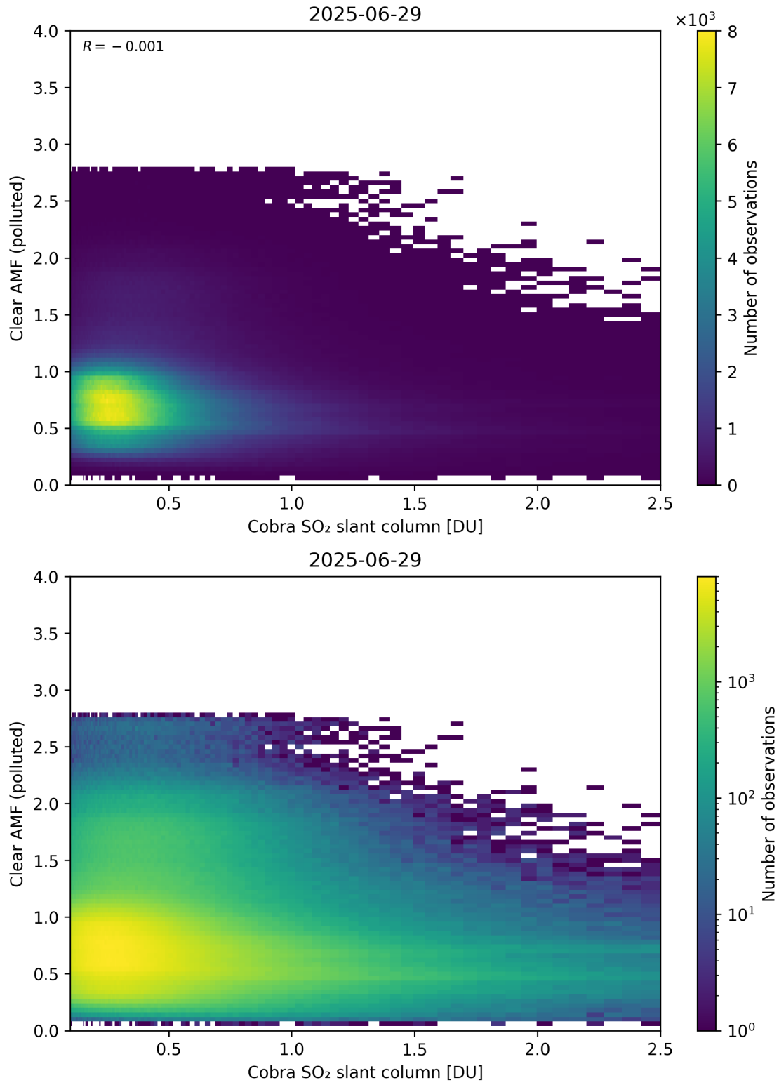
Figure 215: Scatter density plot of “Cobra SO 2 slant column” against “Clear AMF (polluted)” for 2025-06-28 to 2025-06-30.
