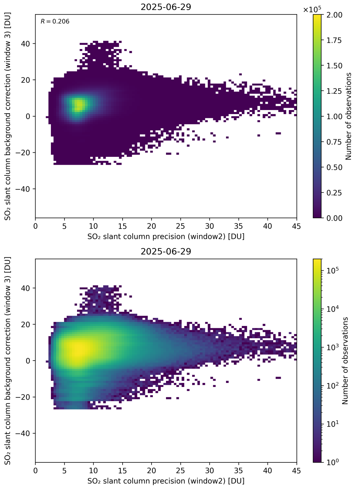
Figure 292: Scatter density plot of “SO 2 slant column precision (window2)” against “SO 2 slant column background correction (window 3)” for 2025-06-28 to 2025-06-30.
