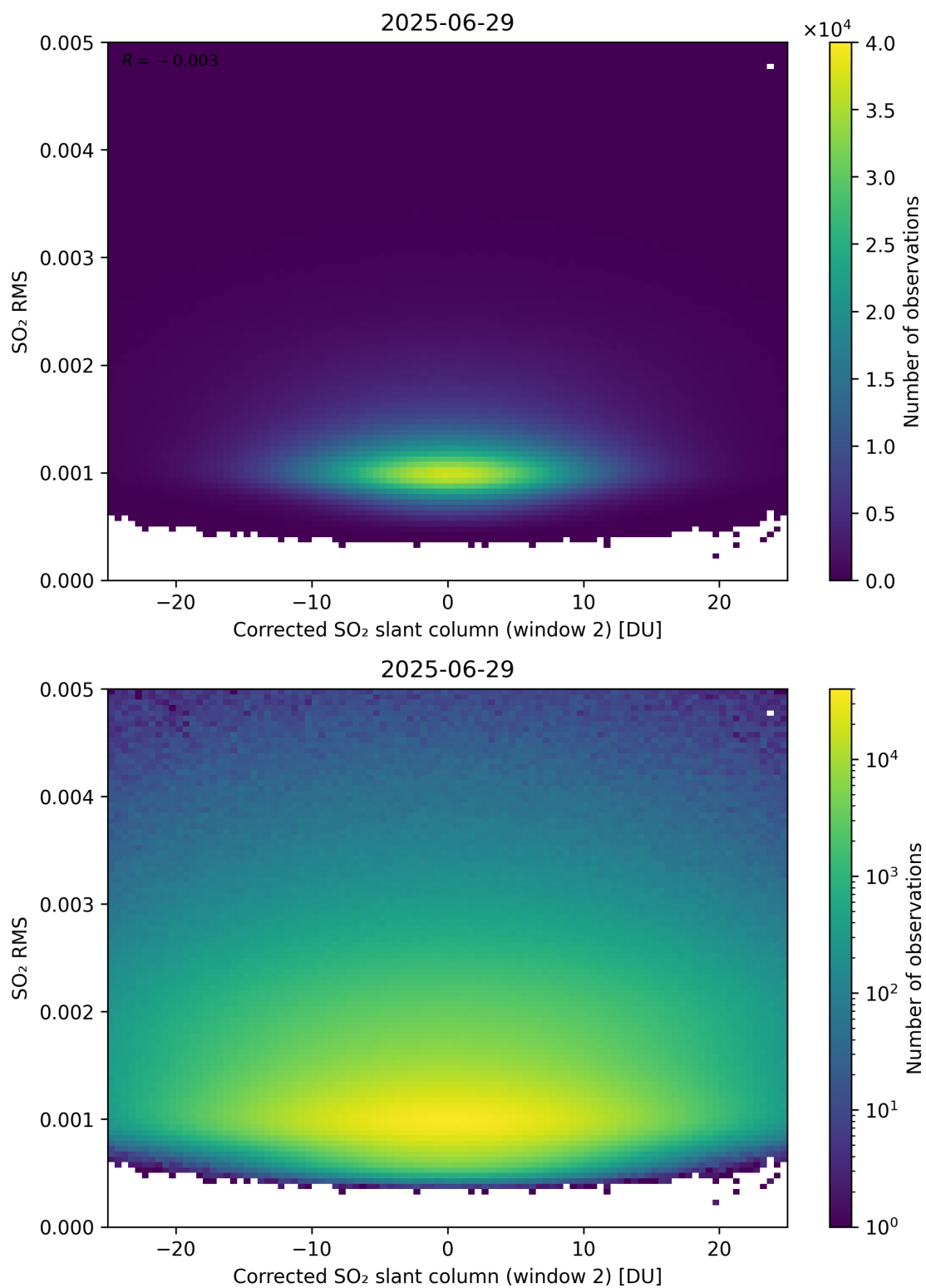
Figure 248: Scatter density plot of “Corrected SO 2 slant column (window 2)” against “SO 2 RMS” for 2025-06-28 to 2025-06-30.
