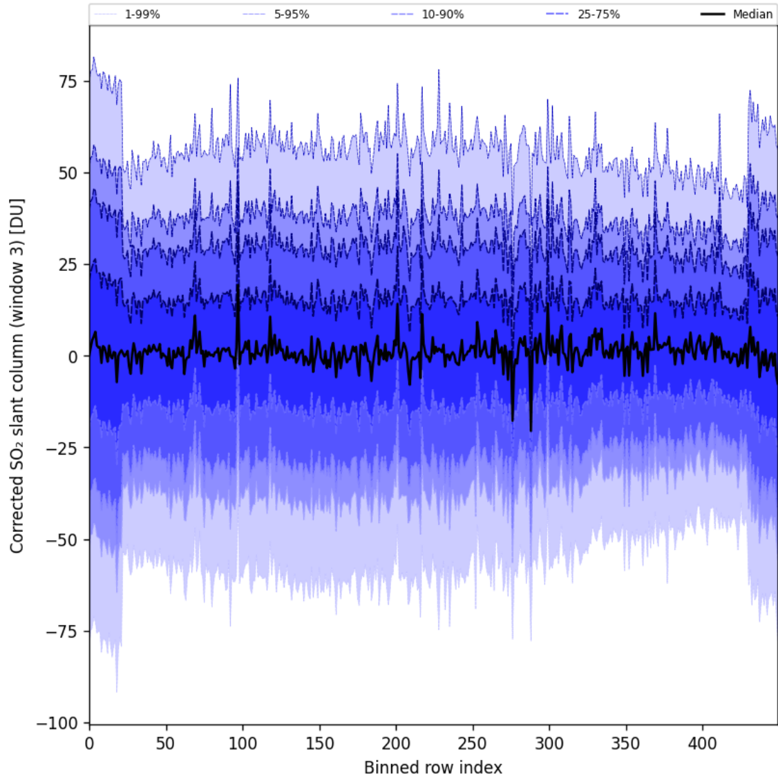
Figure 99: Along track statistics of “Corrected SO 2 slant column (window 3)” for 2025-06-28 to 2025-06-30
