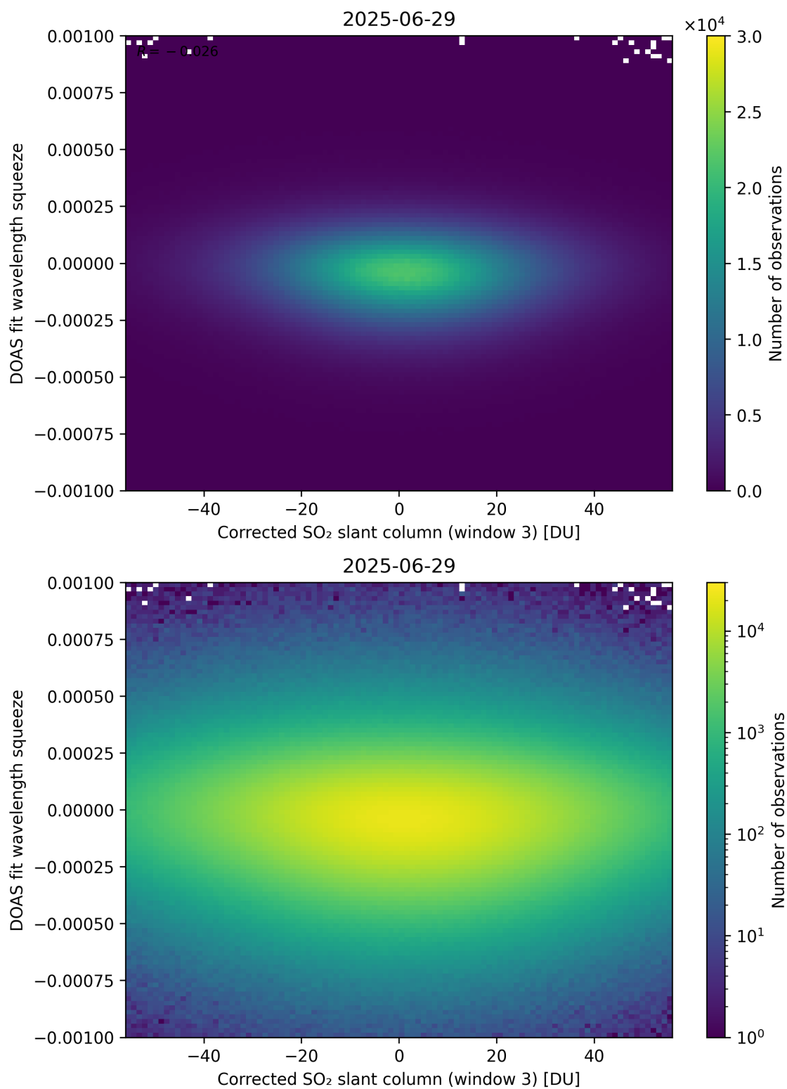
Figure 257: Scatter density plot of “Corrected SO 2 slant column (window 3)” against “DOAS fit wavelength squeeze” for 2025-06-28 to 2025-06-30.
