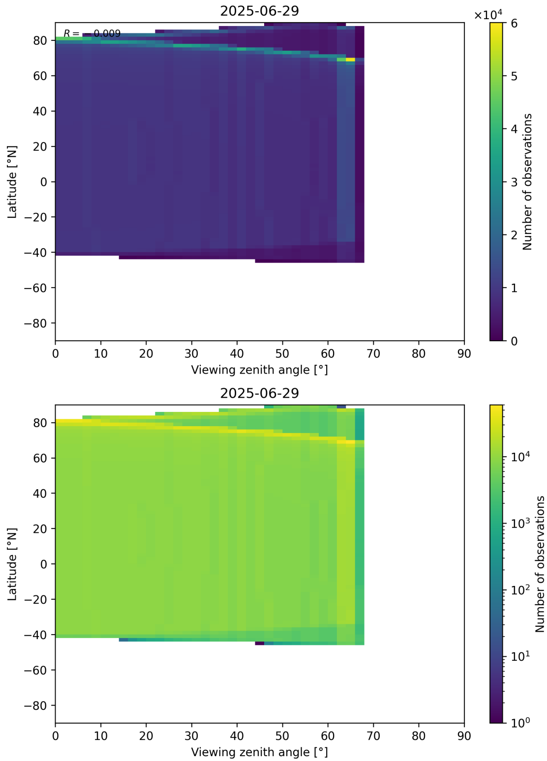
Figure 368: Scatter density plot of “Viewing zenith angle” against “Latitude” for 2025-06-28 to 2025-06-30.
