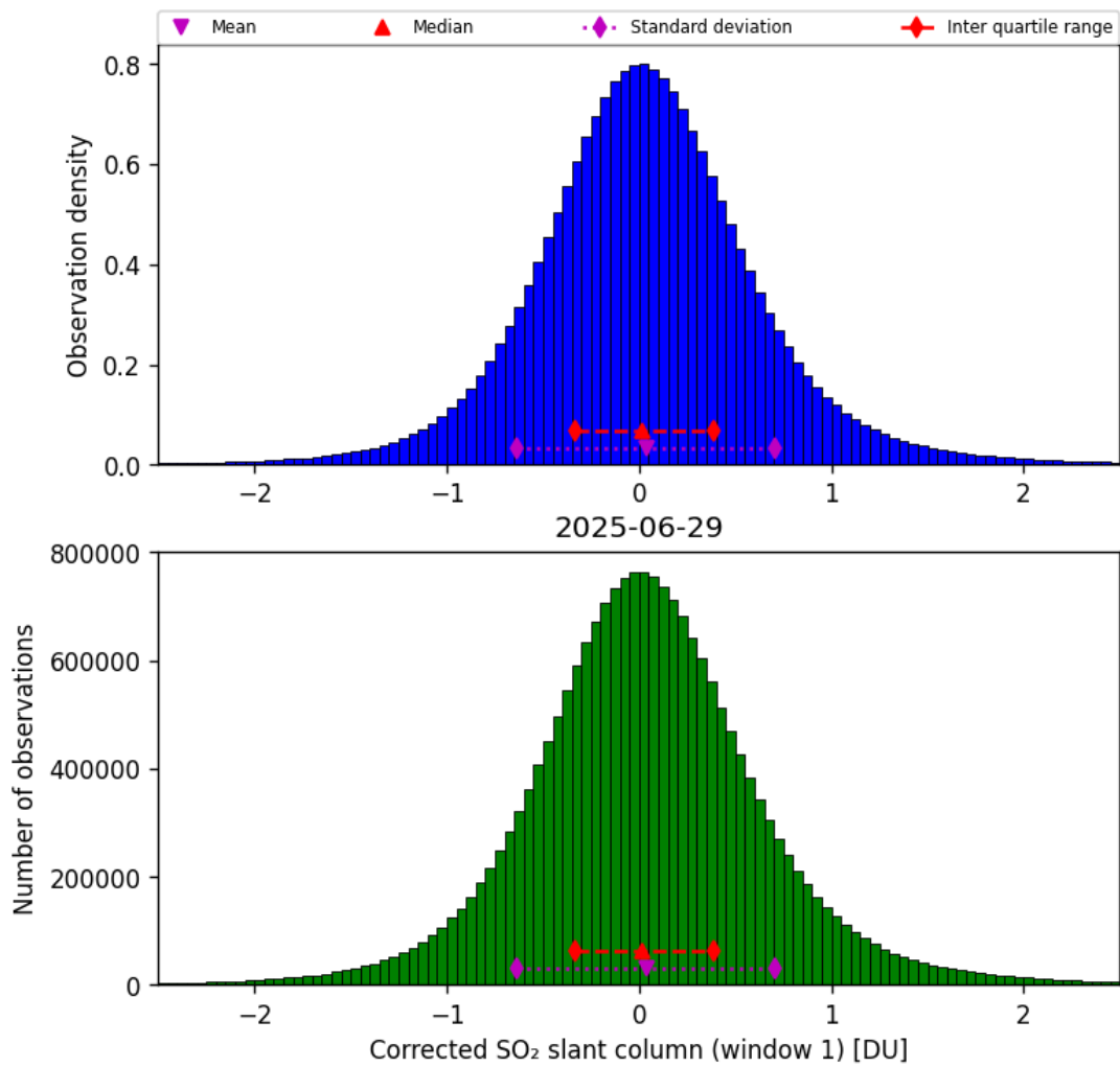
Figure 65: Histogram of “Corrected SO 2 slant column (window 1)” for 2025-06-28 to 2025-06-30
