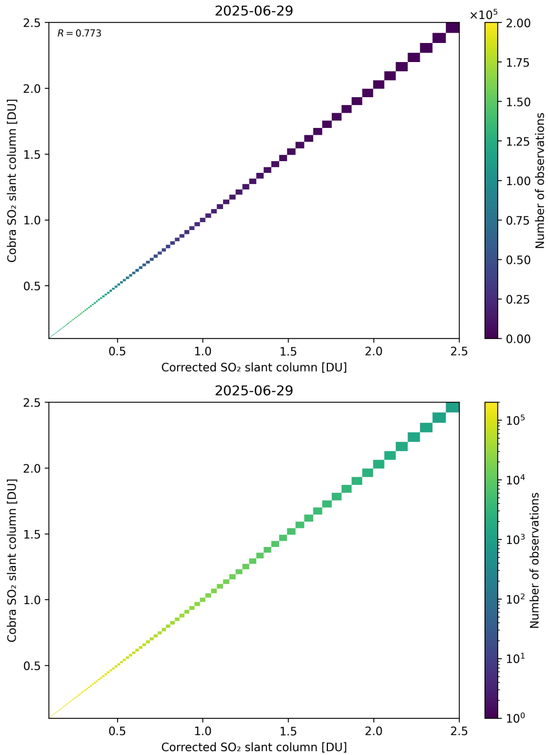
Figure 233: Scatter density plot of “Corrected SO 2 slant column” against “Cobra SO 2 slant column” for 2025-06-28 to 2025-06-30.
