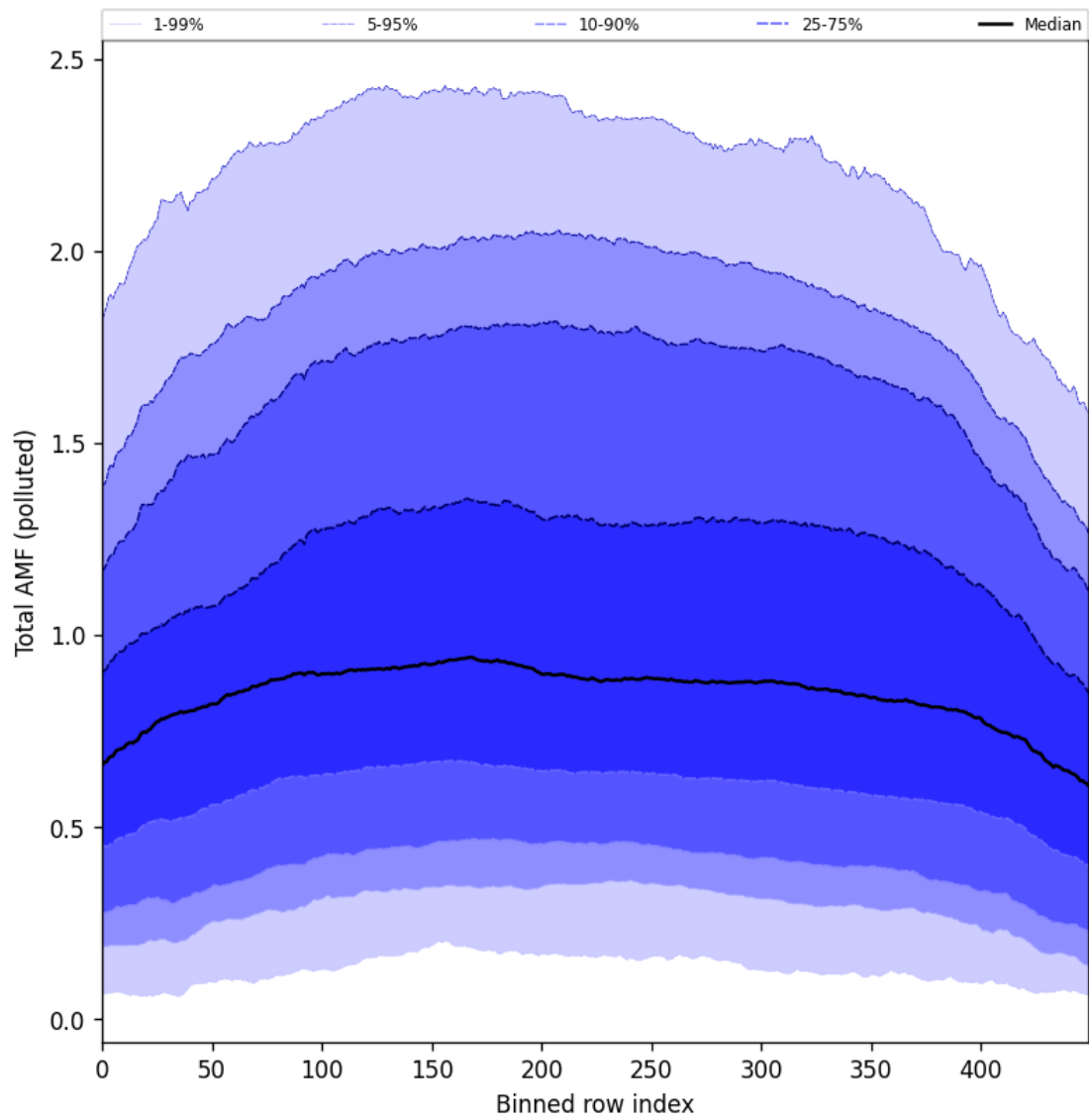
Figure 105: Along track statistics of “Total AMF (polluted)” for 2025-06-28 to 2025-06-30
