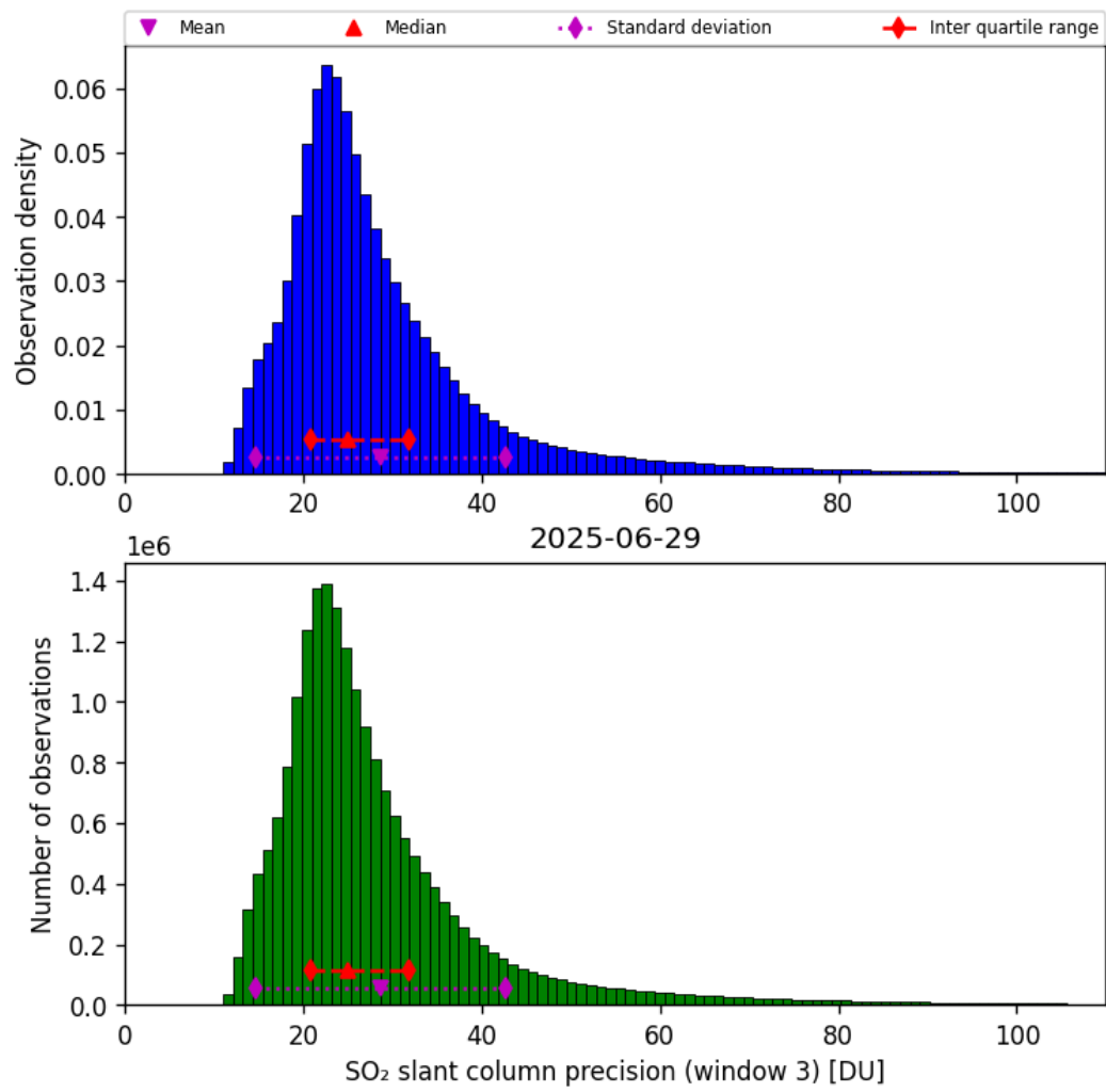
Figure 72: Histogram of “SO 2 slant column precision (window 3)” for 2025-06-28 to 2025-06-30
