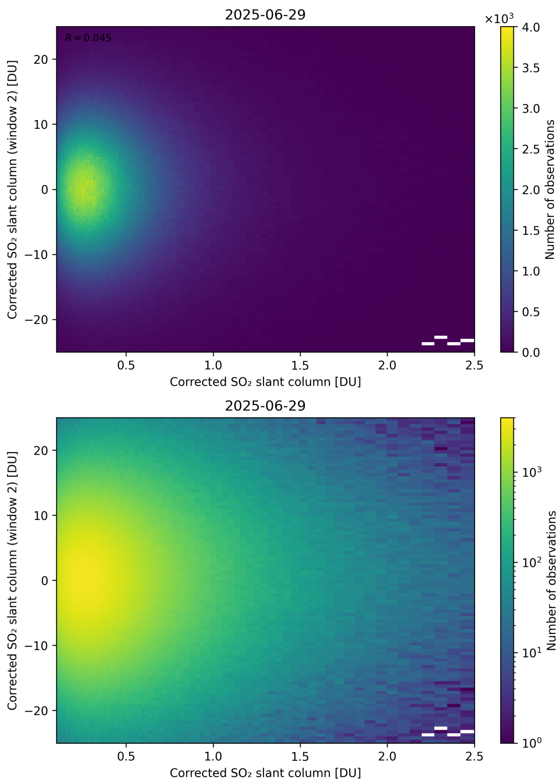
Figure 235: Scatter density plot of “Corrected SO 2 slant column” against “Corrected SO 2 slant column (window 2)” for 2025-06-28 to 2025-06-30.
