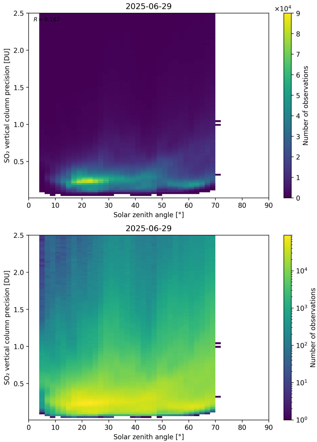
Figure 192: Scatter density plot of “Solar zenith angle” against “SO 2 vertical column precision” for 2025-06-28 to 2025-06-30.
