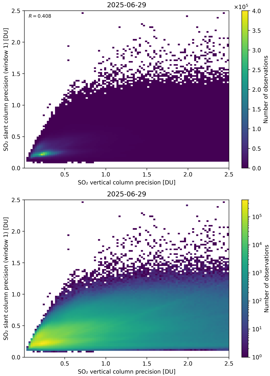
Figure 342: Scatter density plot of “SO 2 vertical column precision” against “SO 2 slant column precision (window 1)” for 2025-06-28 to 2025-06-30.
