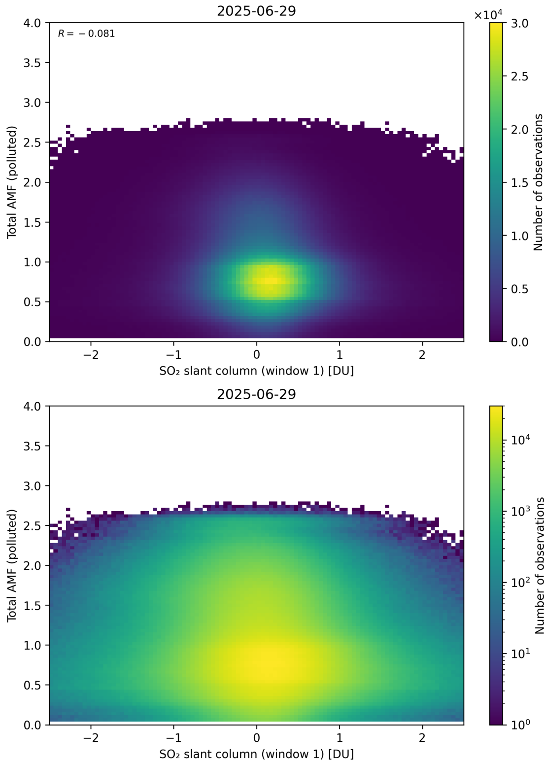
Figure 289: Scatter density plot of “SO 2 slant column (window 1)” against “Total AMF (polluted)” for 2025-06-28 to 2025-06-30.
