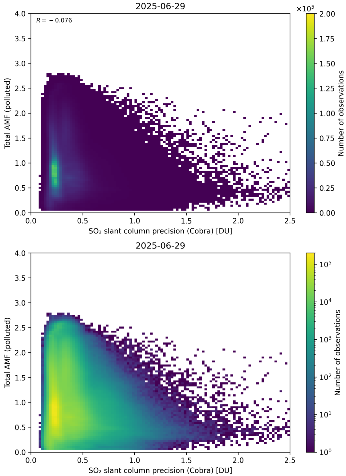
Figure 213: Scatter density plot of “SO 2 slant column precision (Cobra)” against “Total AMF (polluted)” for 2025-06-28 to 2025-06-30.
