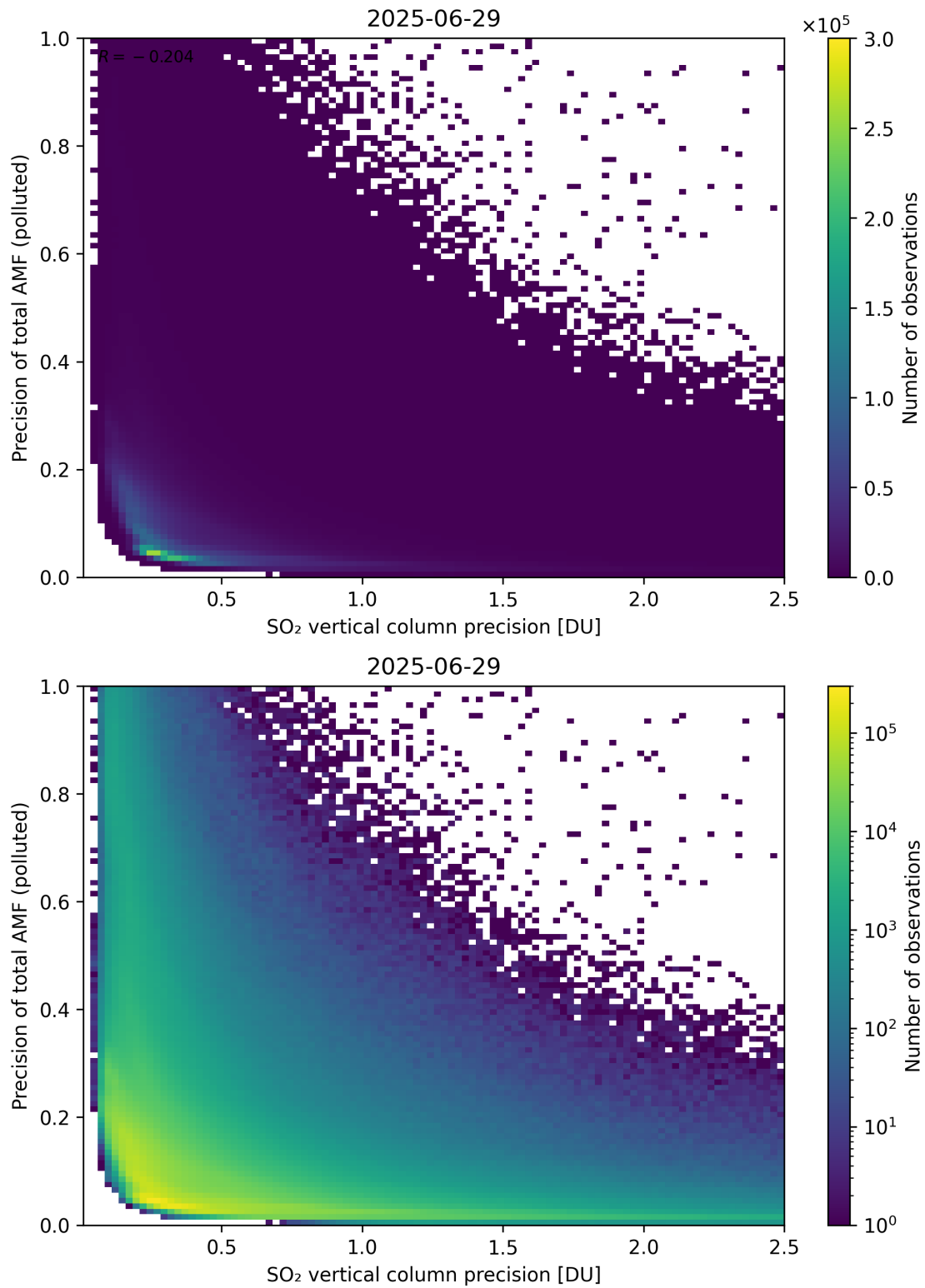
Figure 347: Scatter density plot of “SO 2 vertical column precision” against “Precision of total AMF (polluted)” for 2025-06-28 to 2025-06-30.
