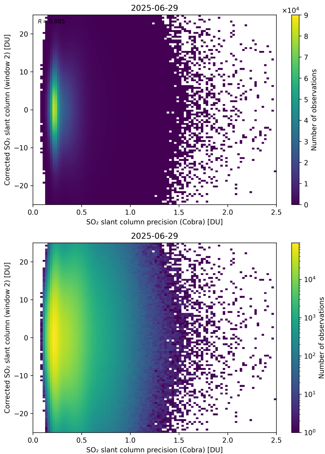
Figure 206: Scatter density plot of “SO 2 slant column precision (Cobra)” against “Corrected SO 2 slant column (window 2)” for 2025-06-28 to 2025-06-30.
