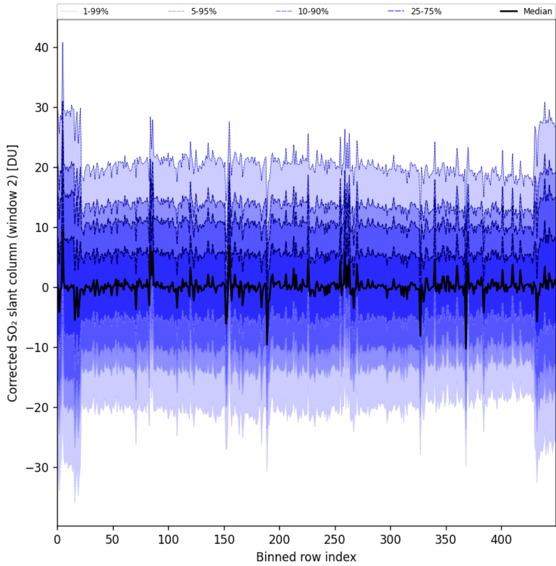
Figure 95: Along track statistics of “Corrected SO 2 slant column (window 2)” for 2025-06-28 to 2025-06-30
