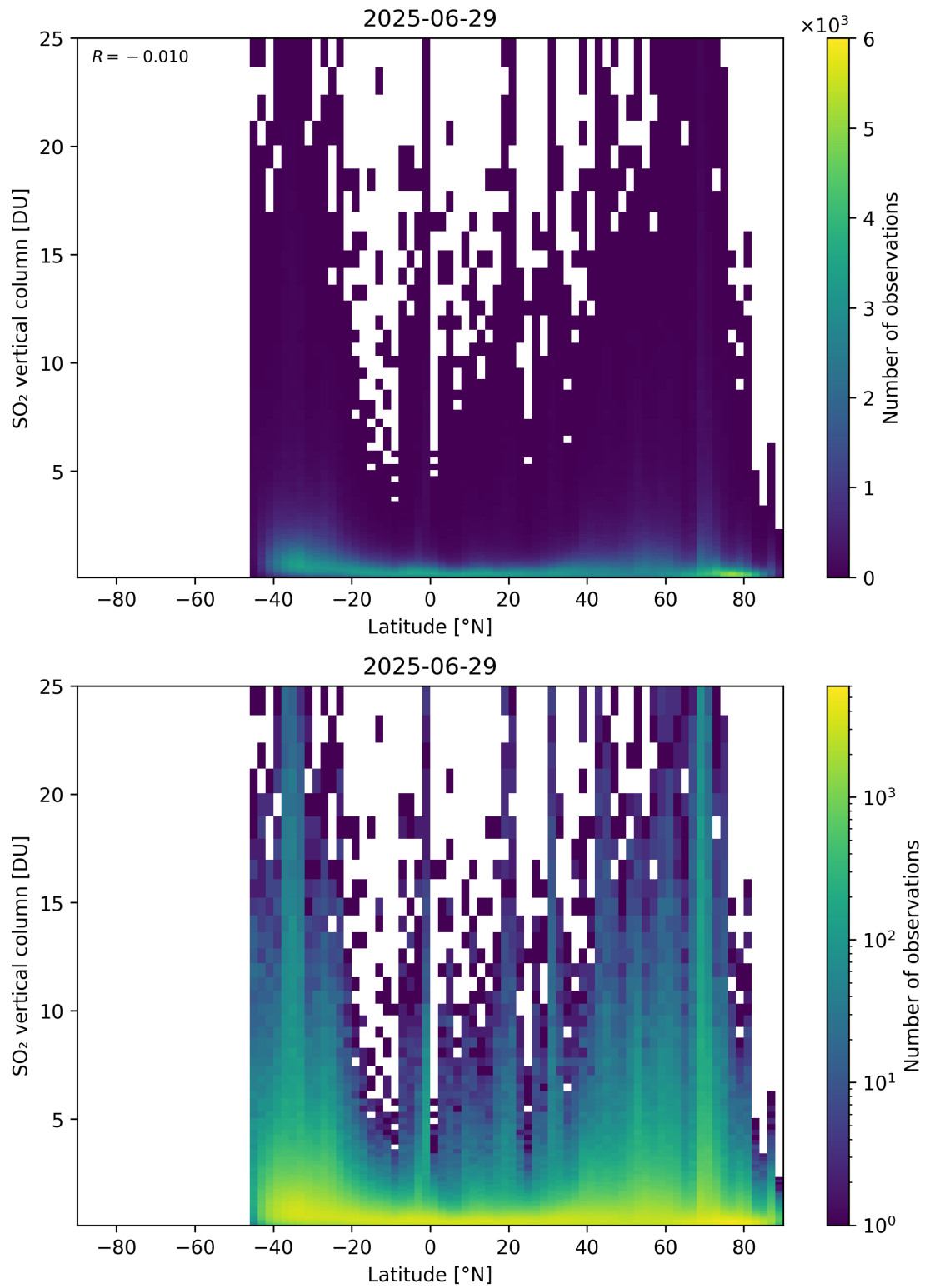
Figure 169: Scatter density plot of “Latitude” against “SO 2 vertical column” for 2025-06-28 to 2025-06-30.
