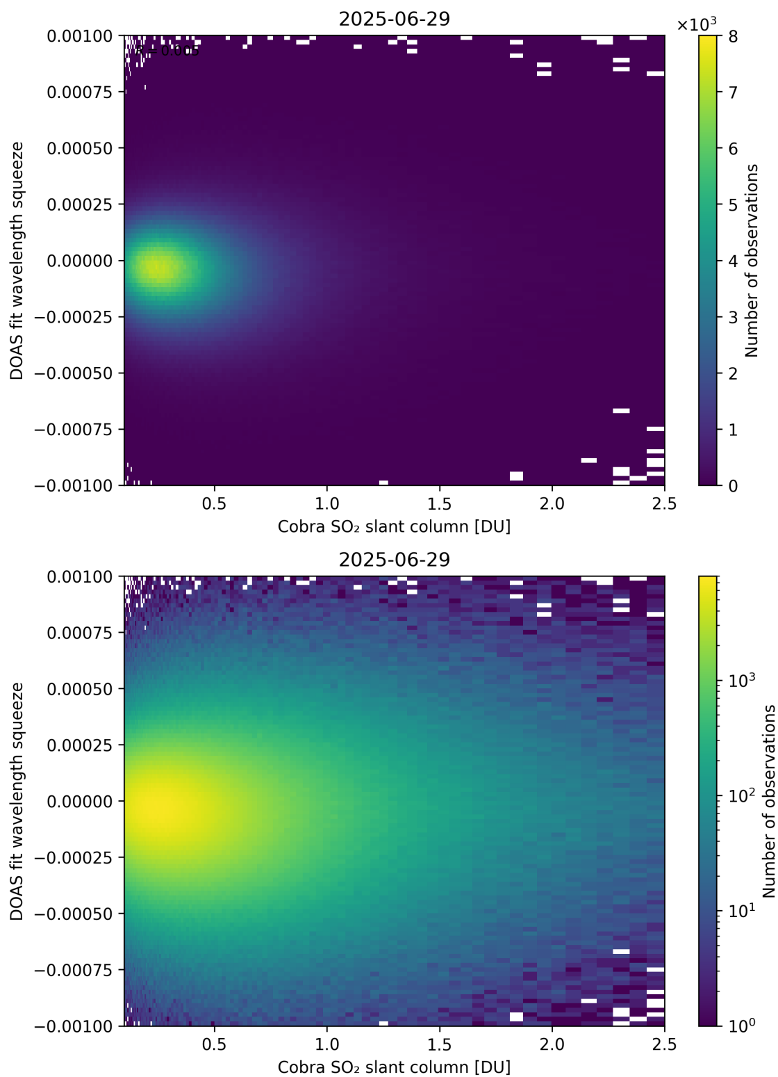
Figure 197: Scatter density plot of “Cobra SO 2 slant column” against “DOAS fit wavelength squeeze” for 2025-06-28 to 2025-06-30.
