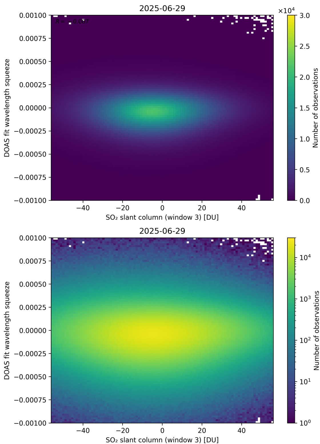
Figure 305: Scatter density plot of “SO 2 slant column (window 3)” against “DOAS fit wavelength squeeze” for 2025-06-28 to 2025-06-30.
