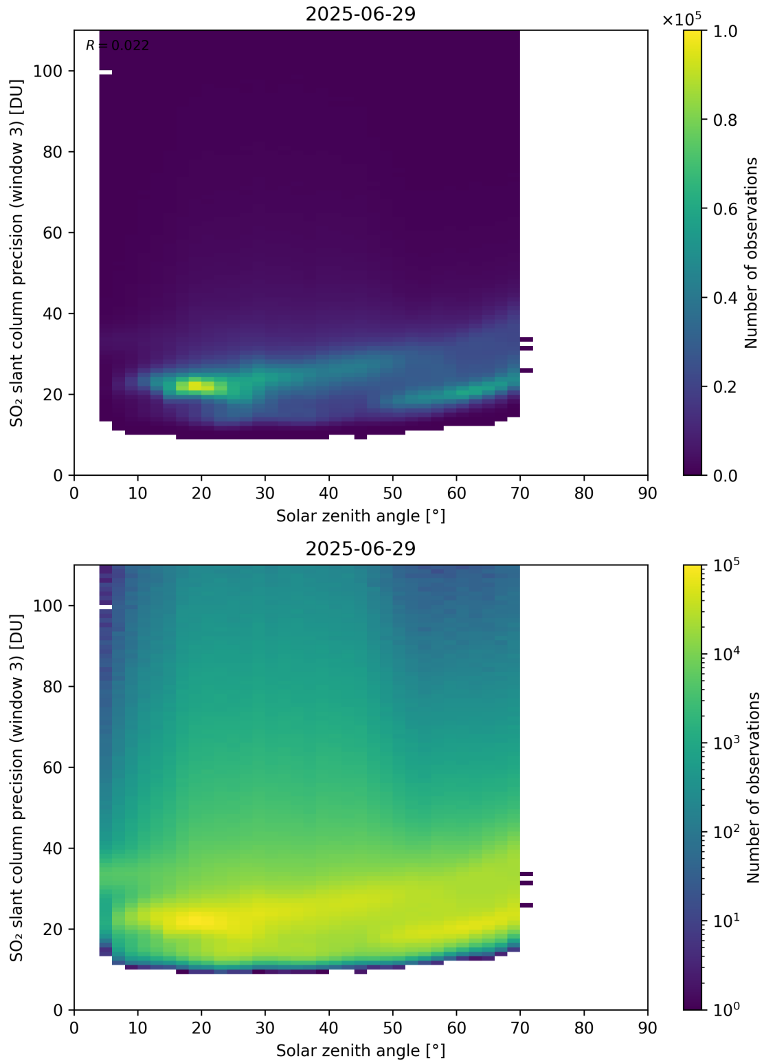
Figure 188: Scatter density plot of “Solar zenith angle” against “SO 2 slant column precision (window 3)” for 2025-06-28 to 2025-06-30.
