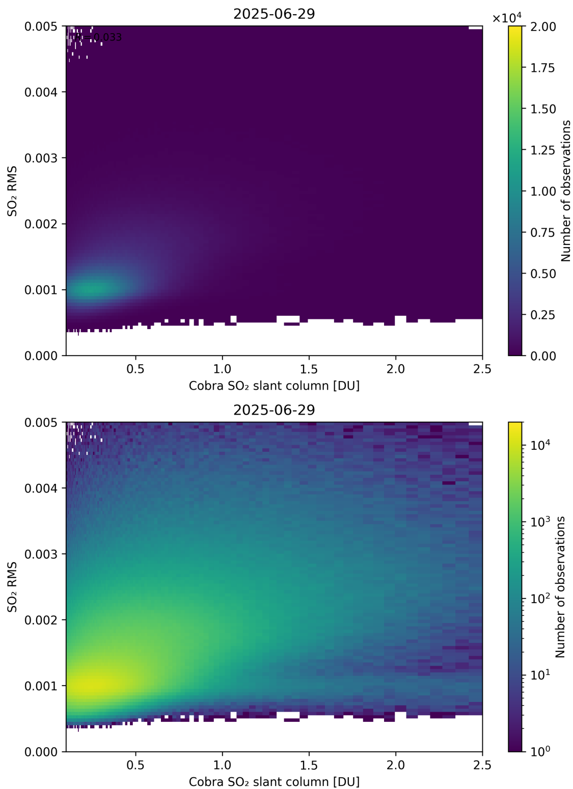
Figure 198: Scatter density plot of “Cobra SO 2 slant column” against “SO 2 RMS” for 2025-06-28 to 2025-06-30.
