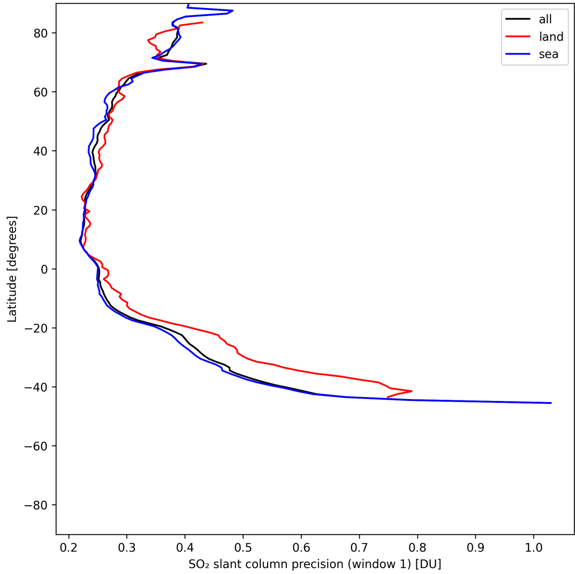
Figure 38: Zonal average of “SO 2 slant column precision (window 1)” for 2025-06-28 to 2025-06-30.
