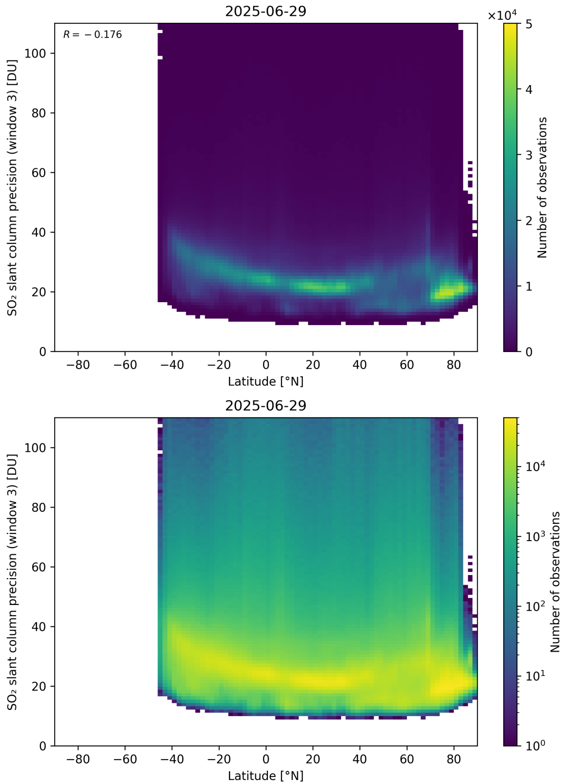
Figure 166: Scatter density plot of “Latitude” against “SO 2 slant column precision (window 3)” for 2025-06-28 to 2025-06-30.
