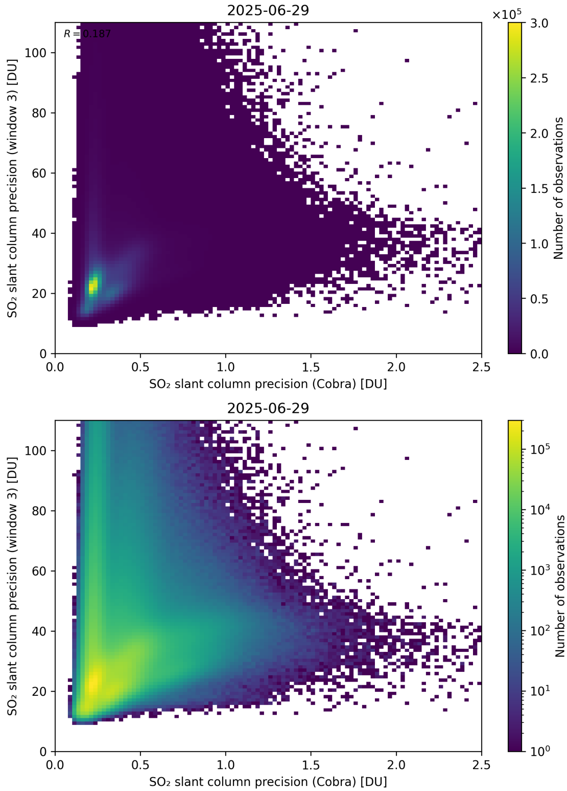
Figure 212: Scatter density plot of “SO 2 slant column precision (Cobra)” against “SO 2 slant column precision (window 3)” for 2025-06-28 to 2025-06-30.
