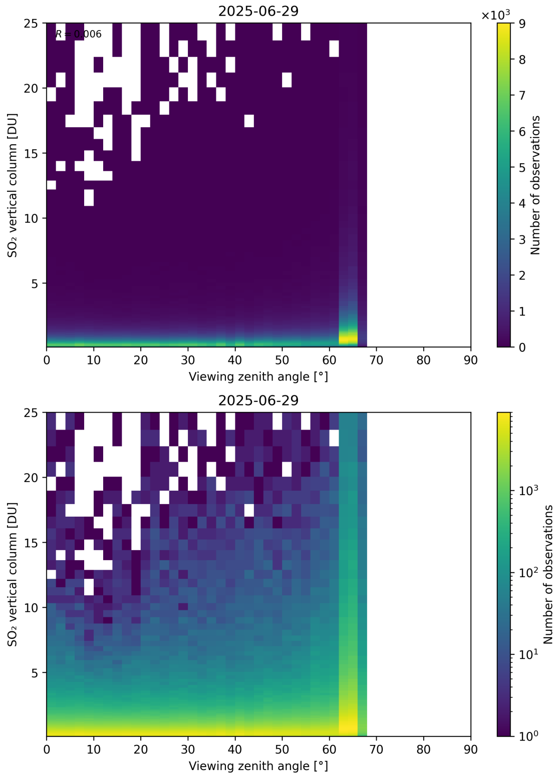
Figure 383: Scatter density plot of “Viewing zenith angle” against “SO 2 vertical column” for 2025-06-28 to 2025-06-30.
