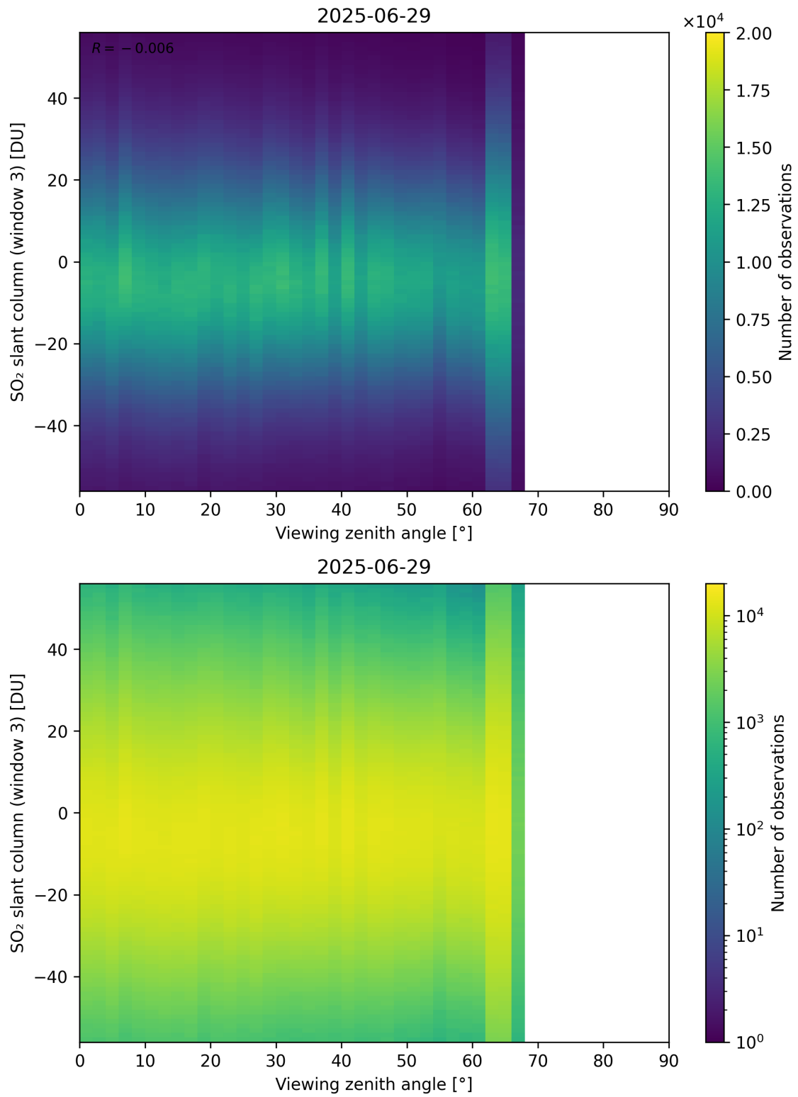
Figure 379: Scatter density plot of “Viewing zenith angle” against “SO 2 slant column (window 3)” for 2025-06-28 to 2025-06-30.
