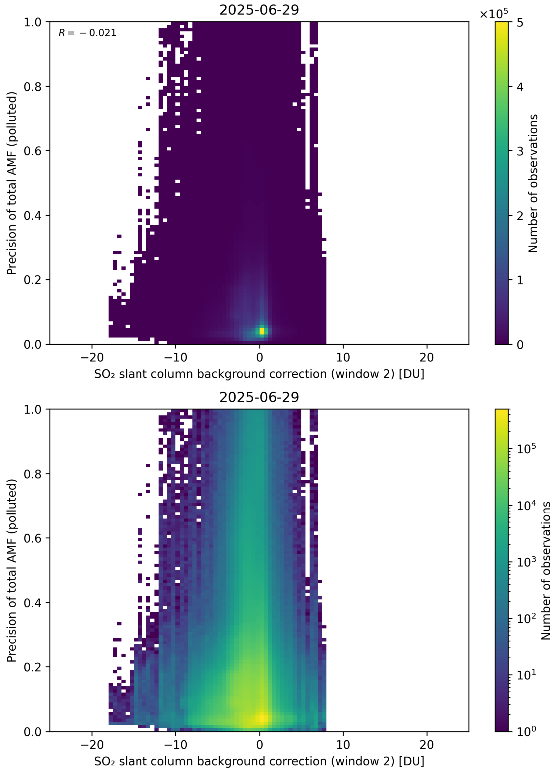
Figure 131: Scatter density plot of “SO 2 slant column background correction (window 2)” against “Precision of total AMF (polluted)” for 2025-06-28 to 2025-06-30.
