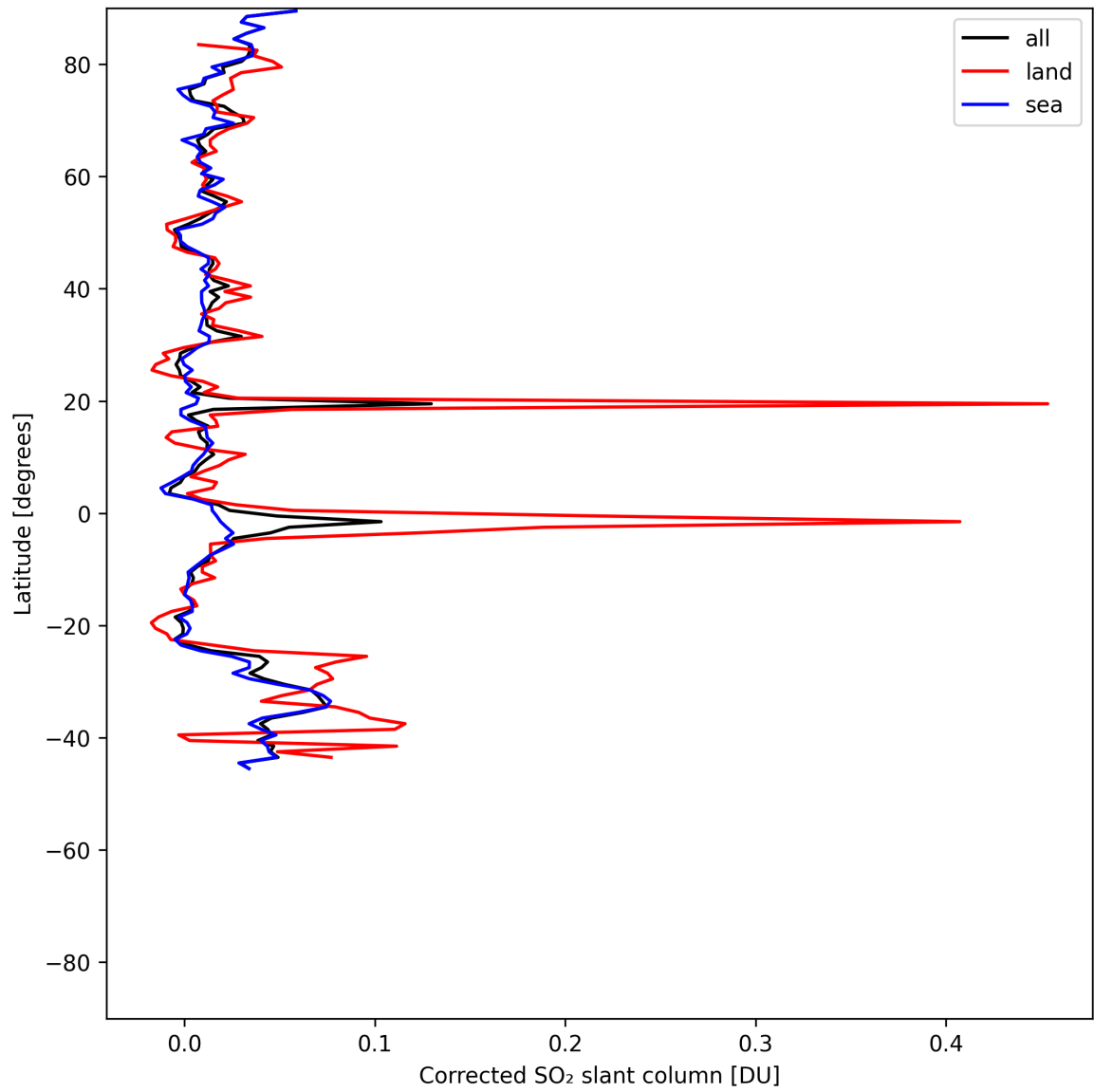
Figure 34: Zonal average of “Corrected SO 2 slant column” for 2025-06-28 to 2025-06-30.
