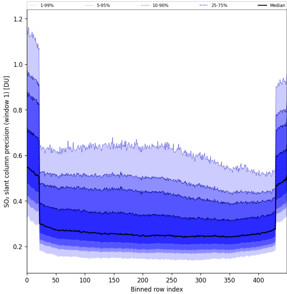
Figure 90: Along track statistics of “SO 2 slant column precision (window 1)” for 2025-06-28 to 2025-06-30
