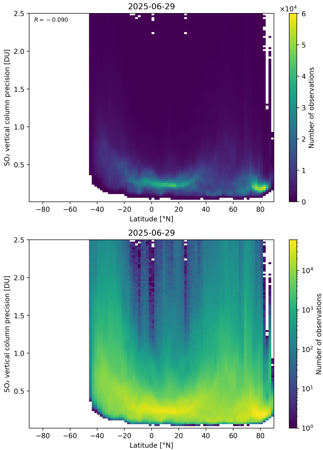
Figure 170: Scatter density plot of “Latitude” against “SO 2 vertical column precision” for 2025-06-28 to 2025-06-30.
