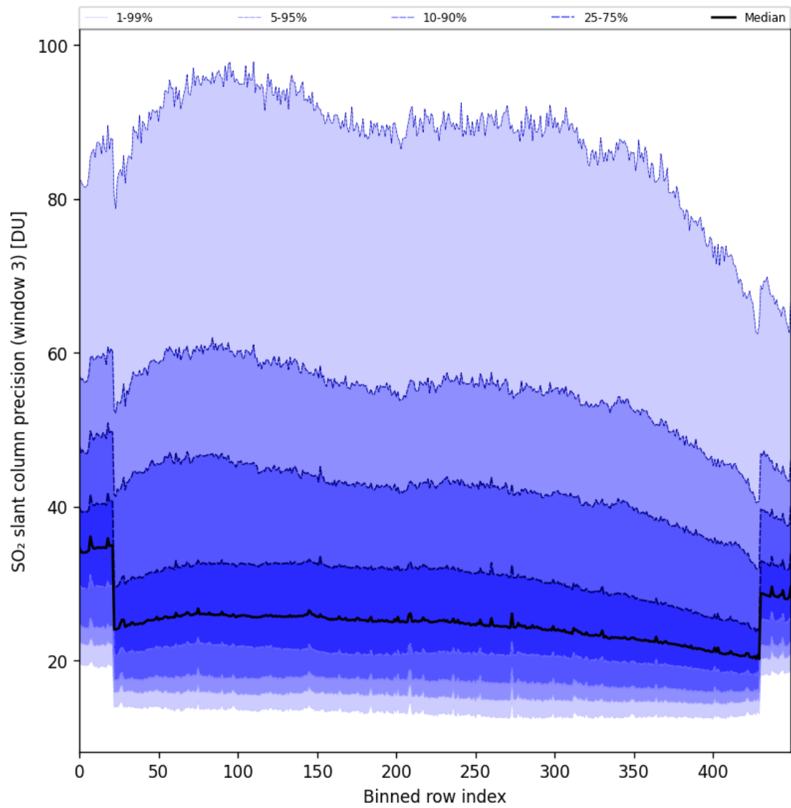
Figure 98: Along track statistics of “SO 2 slant column precision (window 3)” for 2025-06-28 to 2025-06-30
