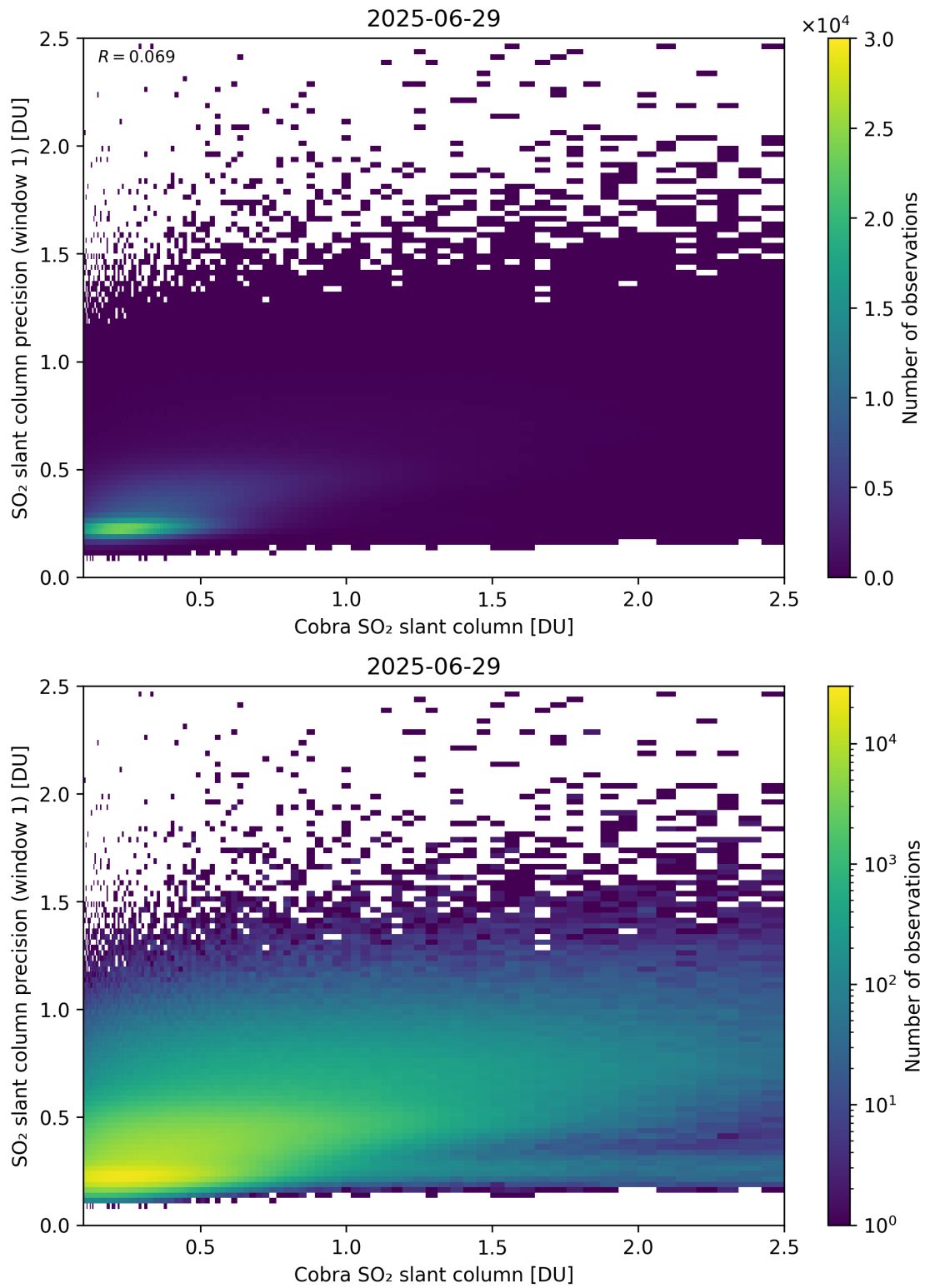
Figure 220: Scatter density plot of “Cobra SO 2 slant column” against “SO 2 slant column precision (window 1)” for 2025-06-28 to 2025-06-30.
