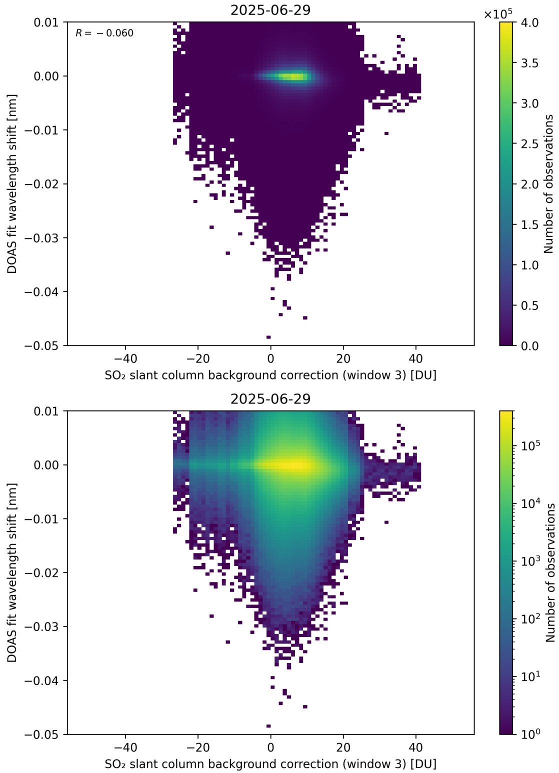
Figure 132: Scatter density plot of “SO 2 slant column background correction (window 3)” against “DOAS fit wavelength shift” for 2025-06-28 to 2025-06-30.
