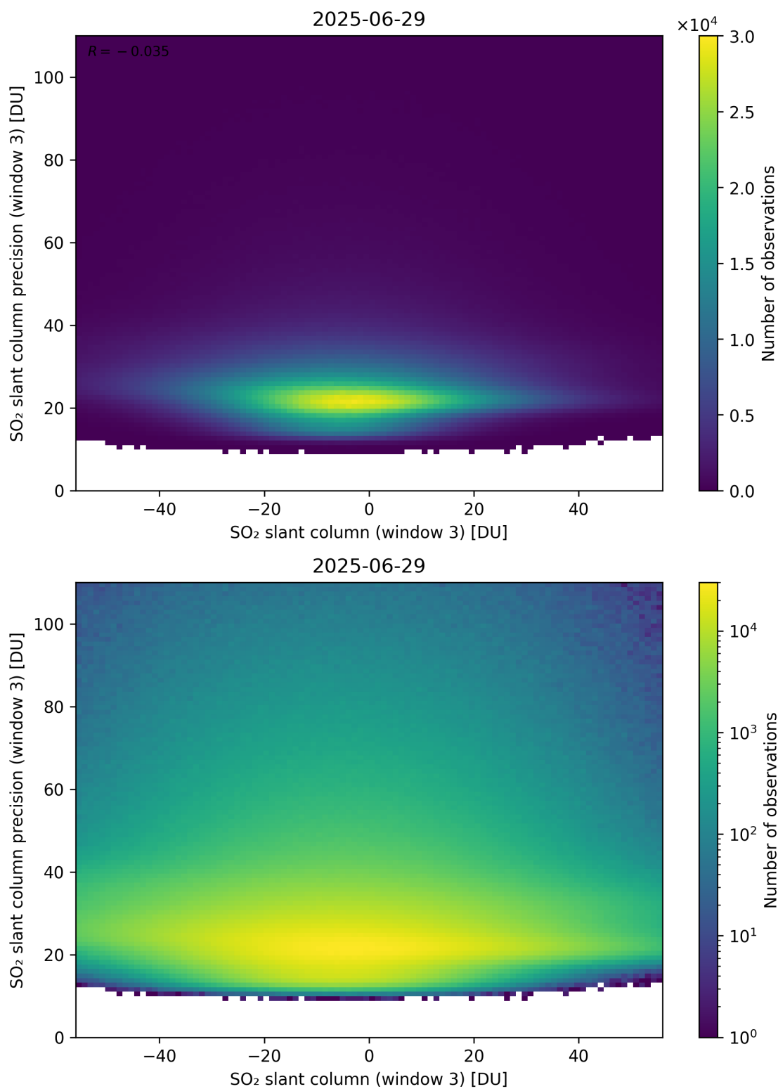
Figure 317: Scatter density plot of “SO 2 slant column (window 3)” against “SO 2 slant column precision (window 3)” for 2025-06-28 to 2025-06-30.
