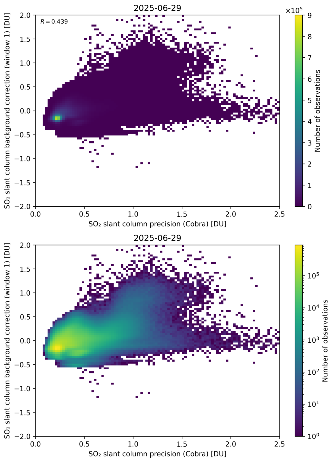
Figure 199: Scatter density plot of “SO 2 slant column precision (Cobra)” against “SO 2 slant column background correction (window 1)” for 2025-06-28 to 2025-06-30.
