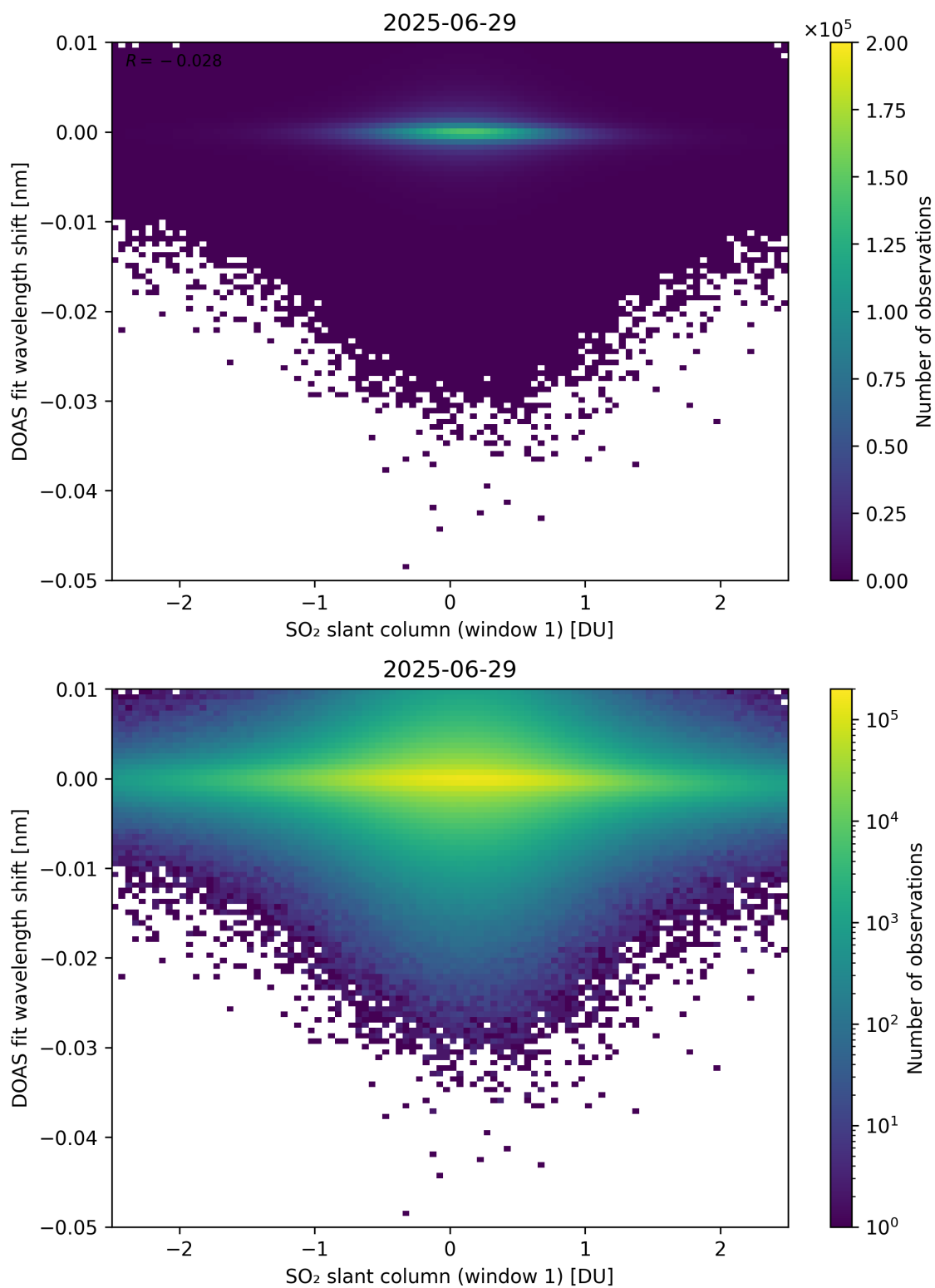
Figure 265: Scatter density plot of “SO 2 slant column (window 1)” against “DOAS fit wavelength shift” for 2025-06-28 to 2025-06-30.
