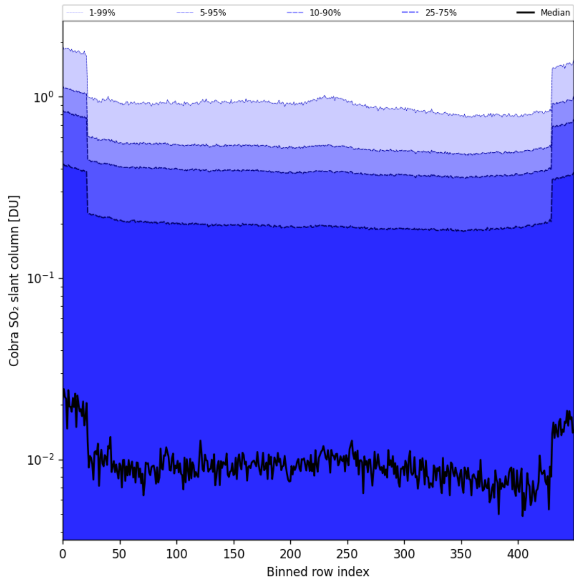
Figure 87: Along track statistics of "Cobra SO 2 slant column" for 2025-06-28 to 2025-06-30
