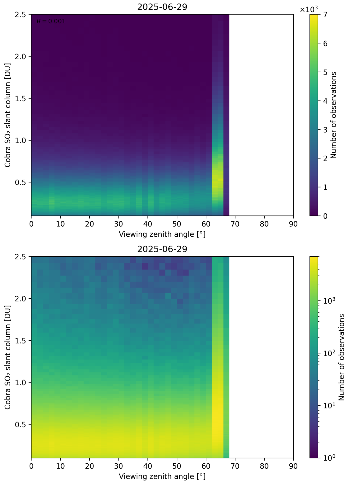
Figure 371: Scatter density plot of “Viewing zenith angle” against “Cobra SO 2 slant column” for 2025-06-28 to 2025-06-30.
