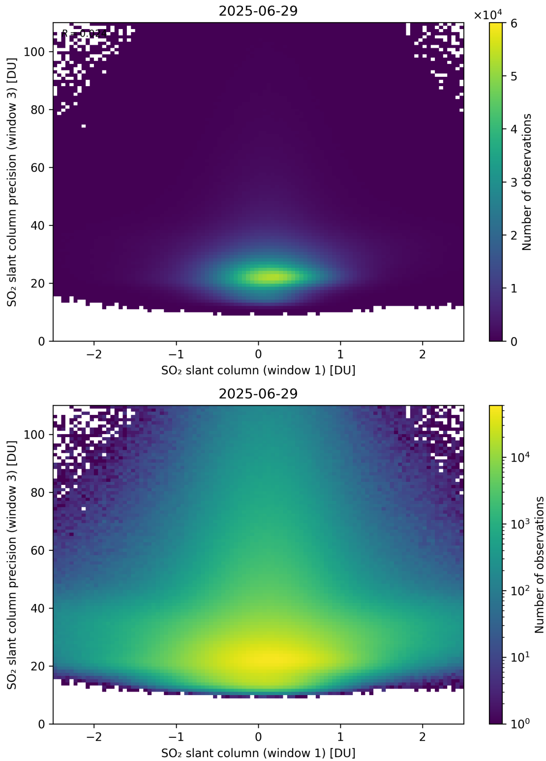
Figure 288: Scatter density plot of “SO 2 slant column (window 1)” against “SO 2 slant column precision (window 3)” for 2025-06-28 to 2025-06-30.
