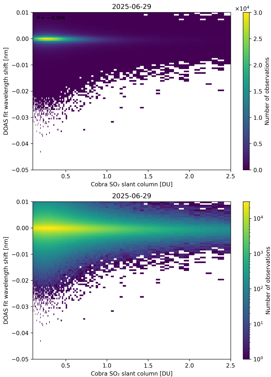
Figure 196: Scatter density plot of “Cobra SO 2 slant column” against “DOAS fit wavelength shift” for 2025-06-28 to 2025-06-30.
