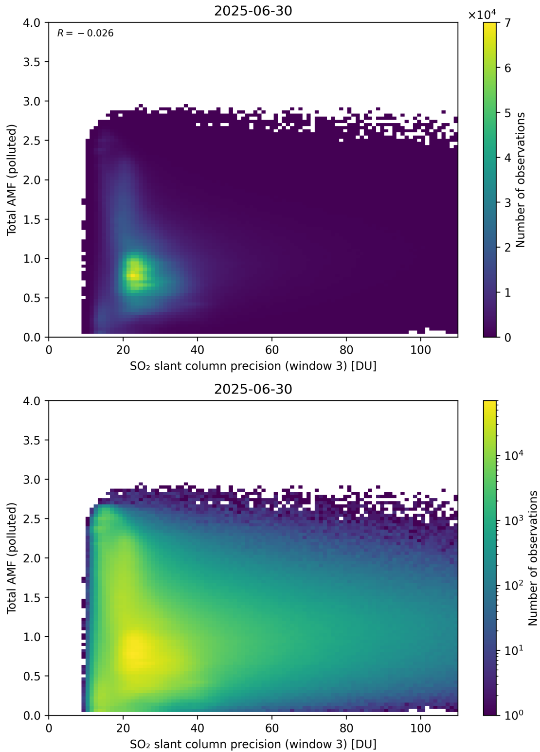
Figure 313: Scatter density plot of “SO 2 slant column precision (window 3)” against “Total AMF (polluted)” for 2025-06-29 to 2025-07-01.
