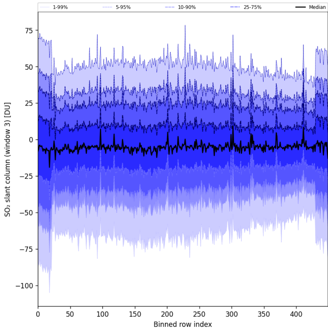
Figure 97: Along track statistics of “SO 2 slant column (window 3)” for 2025-06-29 to 2025-07-01
