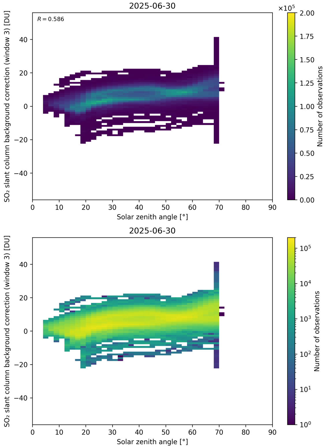
Figure 173: Scatter density plot of “Solar zenith angle” against “SO 2 slant column background correction (window 3)” for 2025-06-29 to 2025-07-01.
