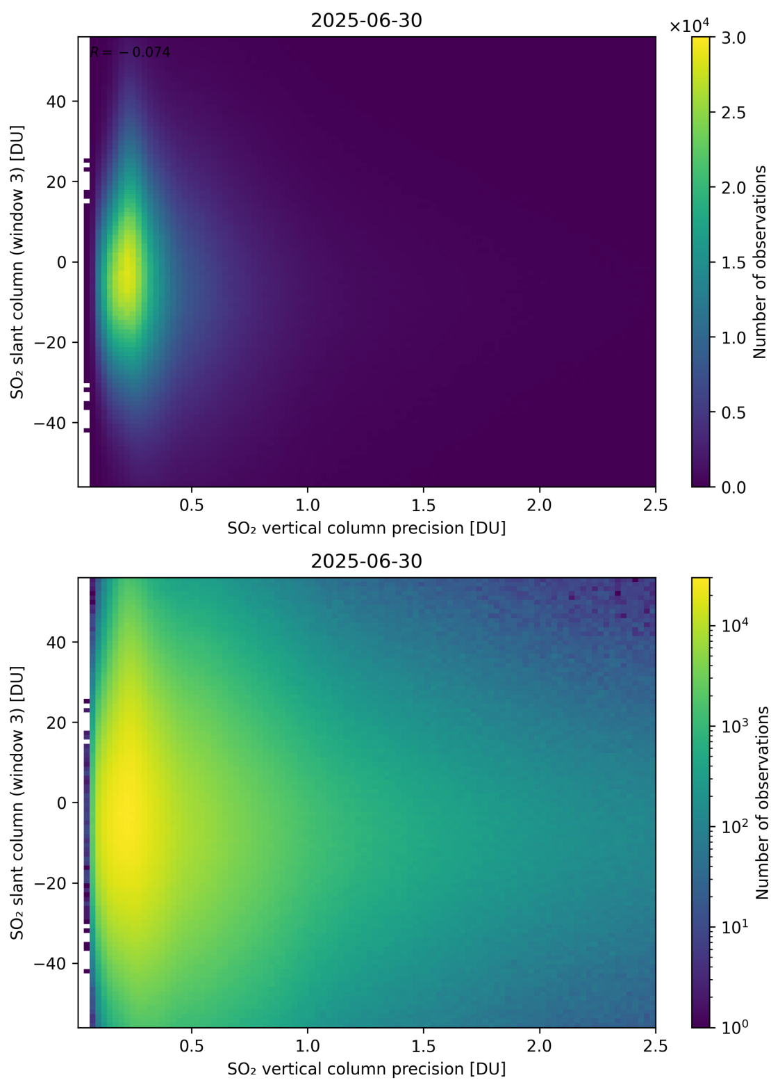
Figure 344: Scatter density plot of “SO 2 vertical column precision” against “SO 2 slant column (window 3)” for 2025-06-29 to 2025-07-01.
