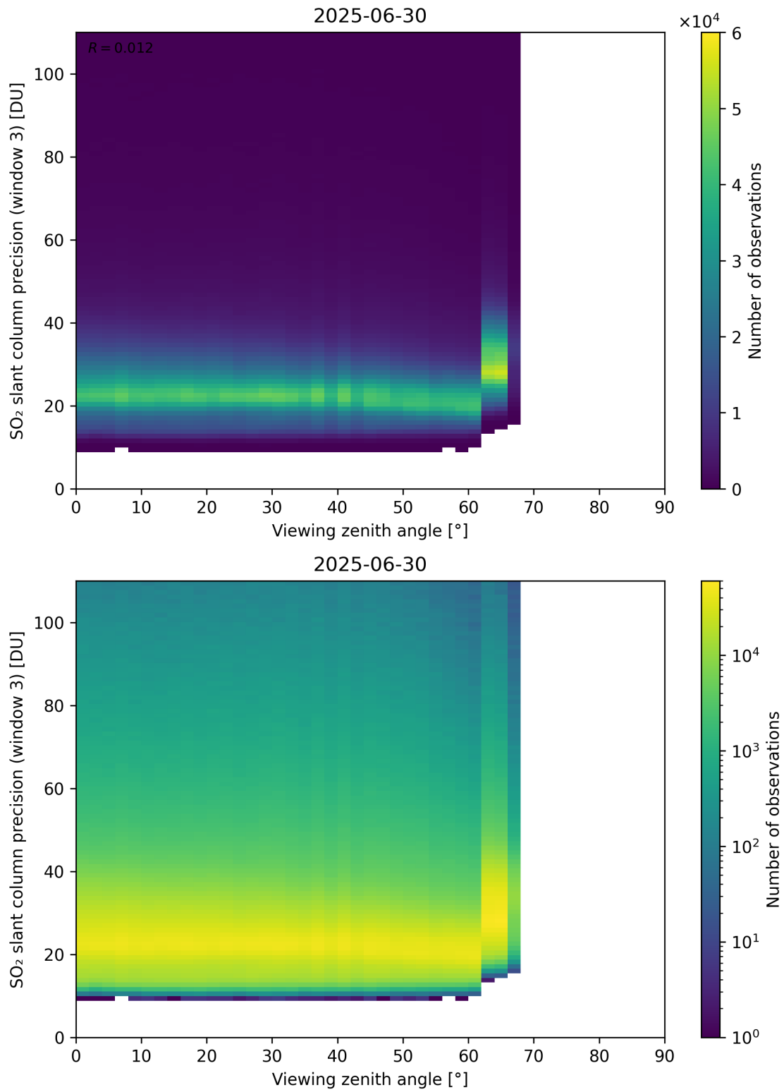
Figure 380: Scatter density plot of “Viewing zenith angle” against “SO 2 slant column precision (window 3)” for 2025-06-29 to 2025-07-01.
