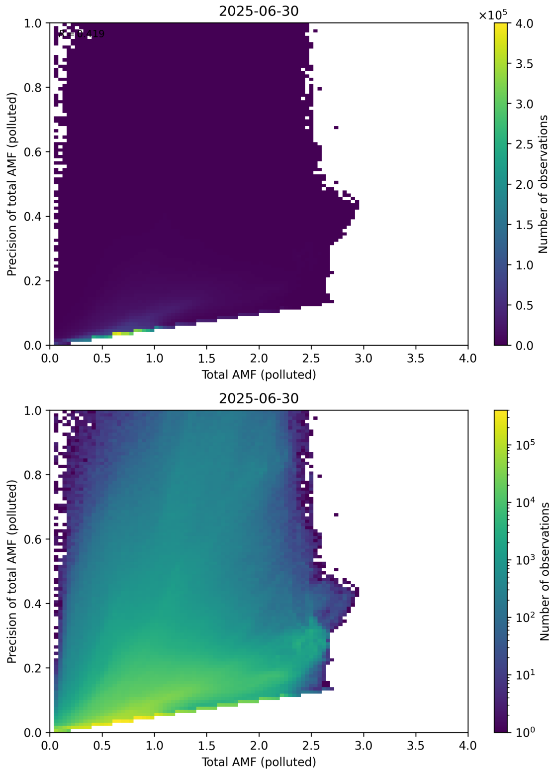
Figure 322: Scatter density plot of “Total AMF (polluted)” against “Precision of total AMF (polluted)” for 2025-06-29 to 2025-07-01.
