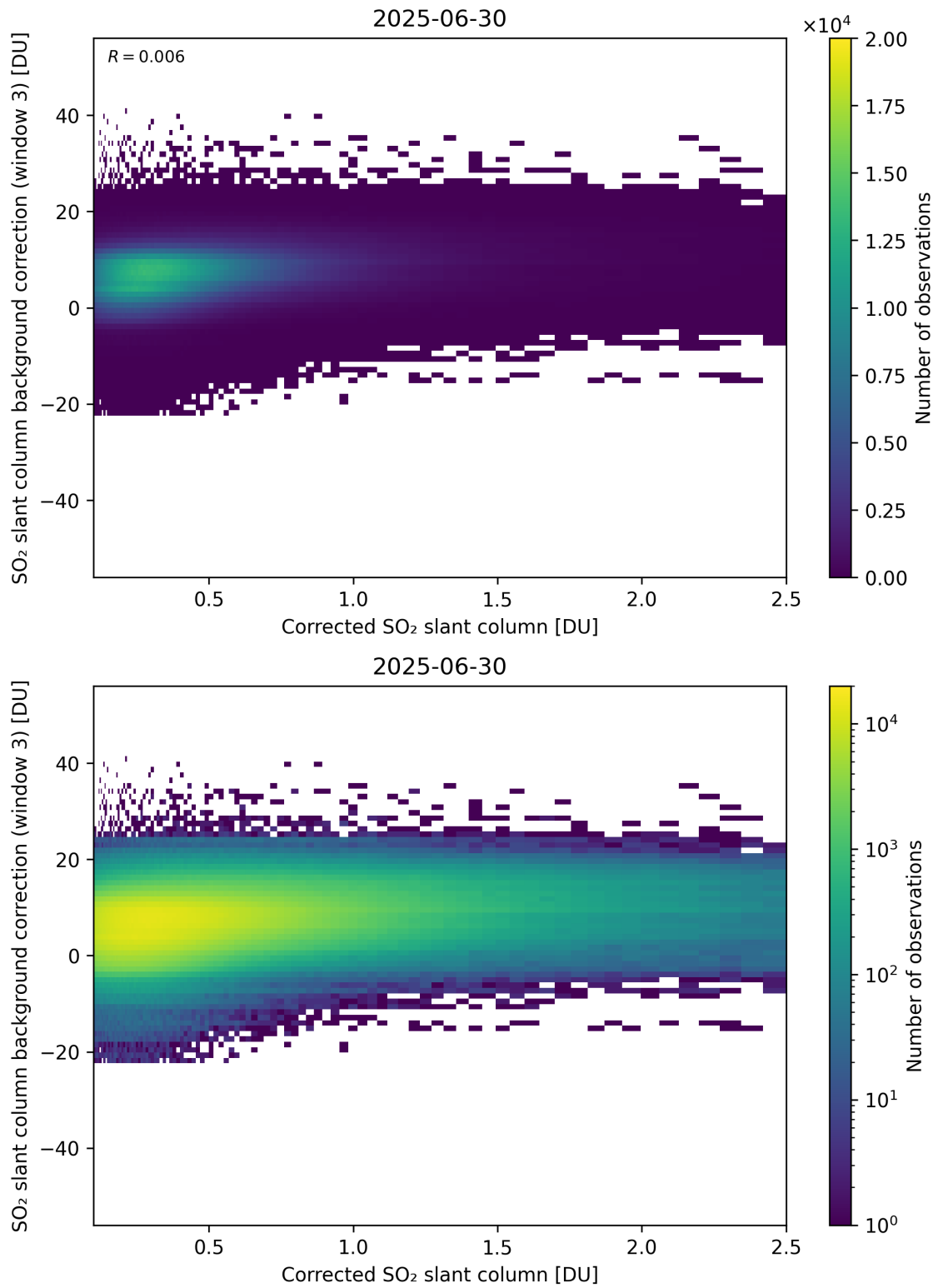
Figure 228: Scatter density plot of “Corrected SO 2 slant column” against “SO 2 slant column background correction (window 3)” for 2025-06-29 to 2025-07-01.
