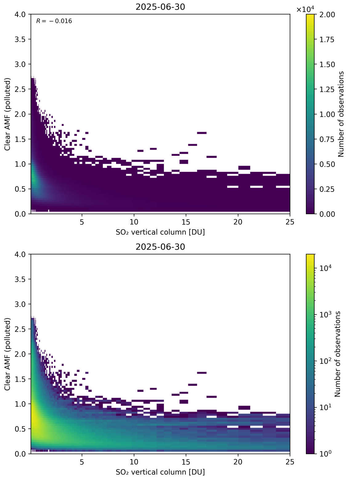
Figure 348: Scatter density plot of “SO 2 vertical column” against “Clear AMF (polluted)” for 2025-06-29 to 2025-07-01.
