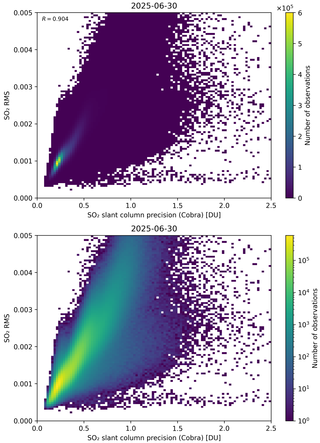
Figure 204: Scatter density plot of “SO 2 slant column precision (Cobra)” against “SO 2 RMS” for 2025-06-29 to 2025-07-01.
