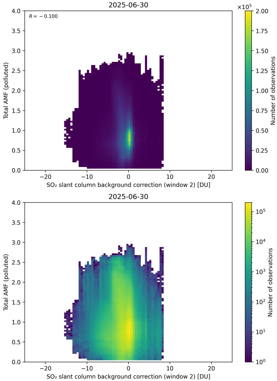
Figure 130: Scatter density plot of “SO 2 slant column background correction (window 2)” against “Total AMF (polluted)” for 2025-06-29 to 2025-07-01.
