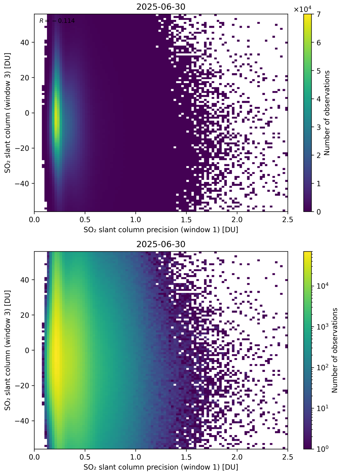
Figure 278: Scatter density plot of “SO 2 slant column precision (window 1)” against “SO 2 slant column (window 3)” for 2025-06-29 to 2025-07-01.
