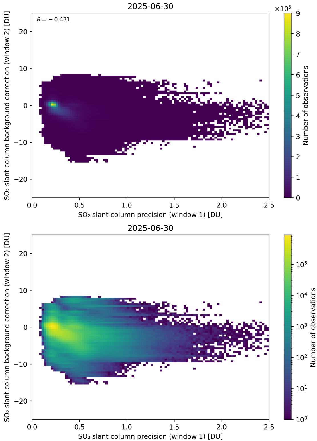
Figure 269: Scatter density plot of “SO 2 slant column precision (window 1)” against “SO 2 slant column background correction (window 2)” for 2025-06-29 to 2025-07-01.
