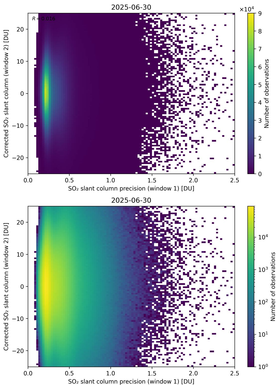
Figure 275: Scatter density plot of “SO 2 slant column precision (window 1)” against “Corrected SO 2 slant column (window 2)” for 2025-06-29 to 2025-07-01.
