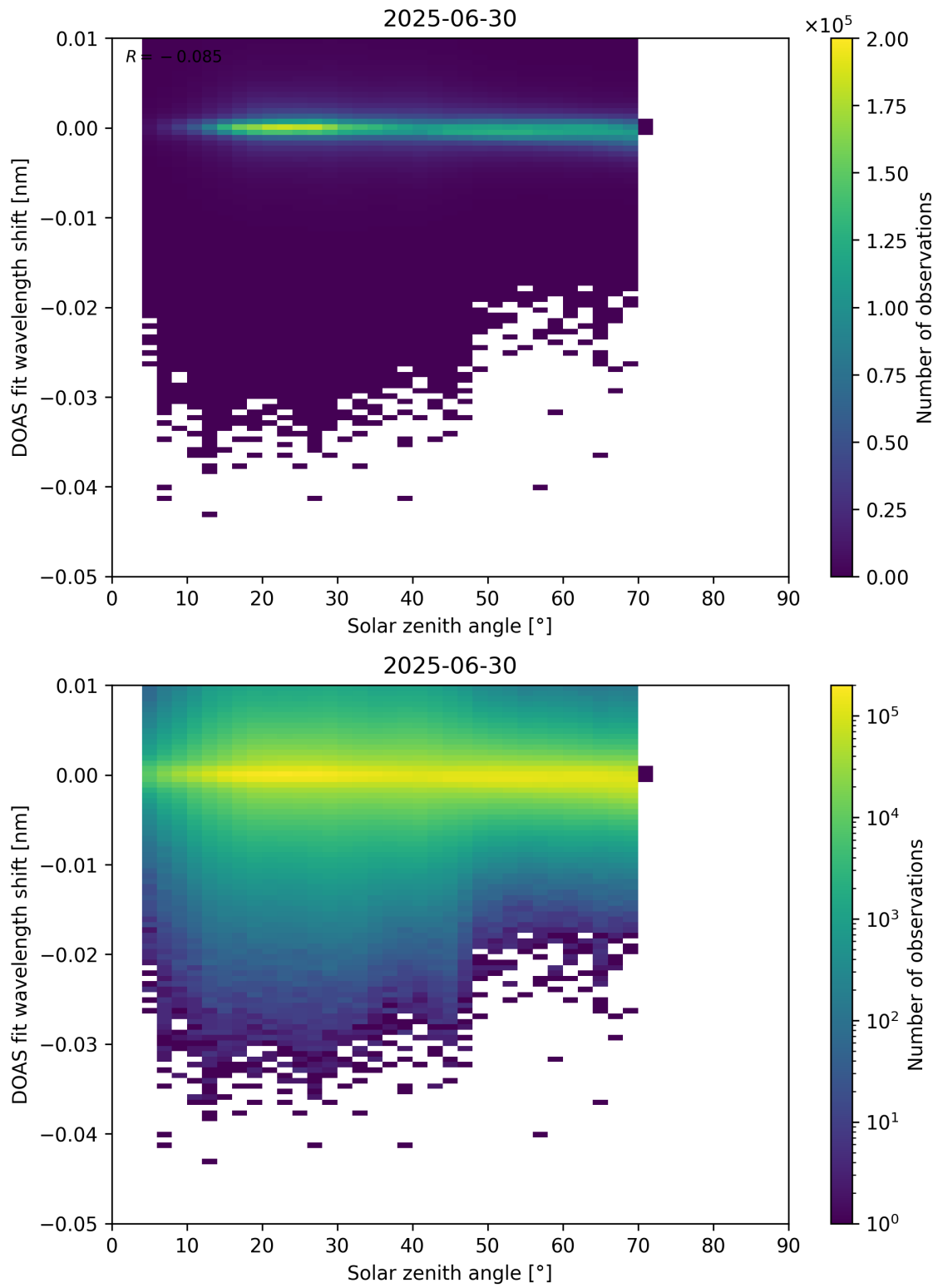
Figure 174: Scatter density plot of “Solar zenith angle” against “DOAS fit wavelength shift” for 2025-06-29 to 2025-07-01.
