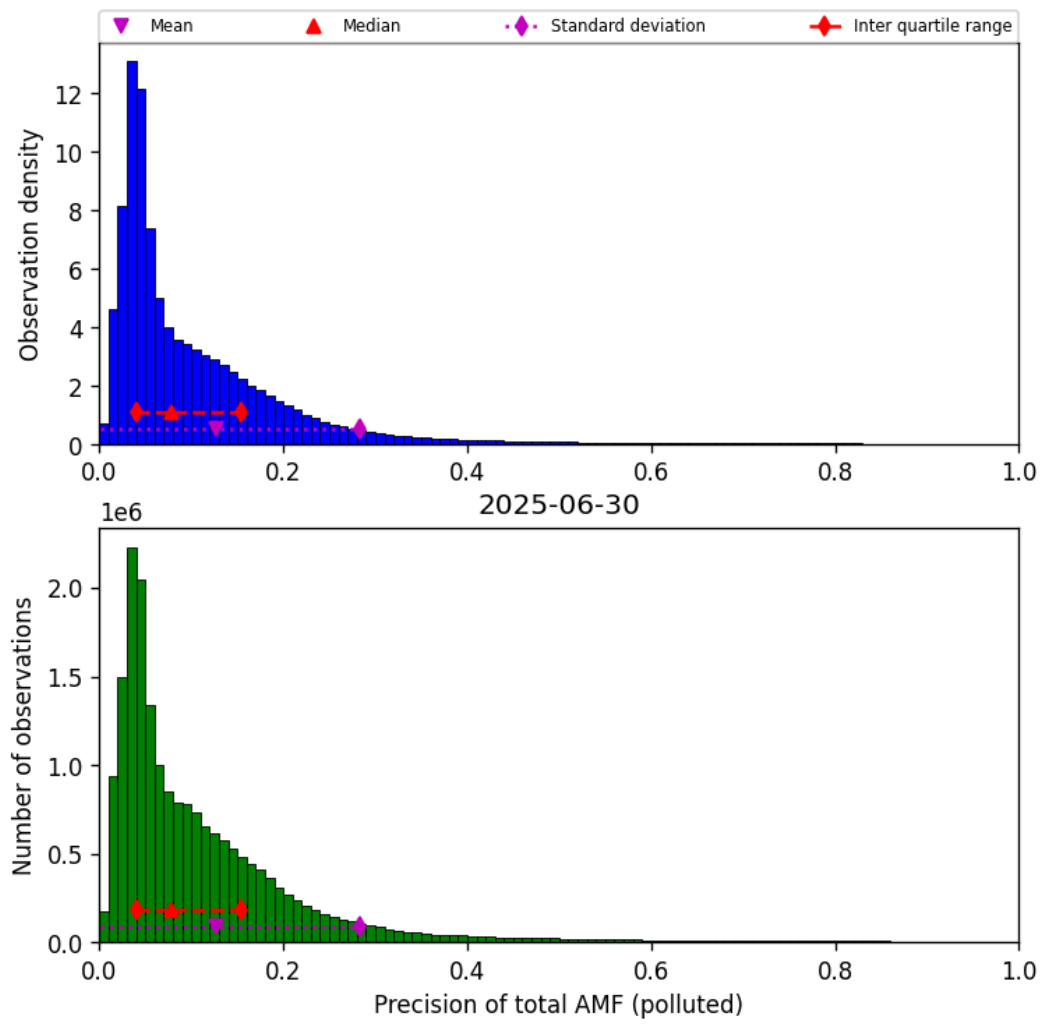
Figure 80: Histogram of “Precision of total AMF (polluted)” for 2025-06-29 to 2025-07-01
