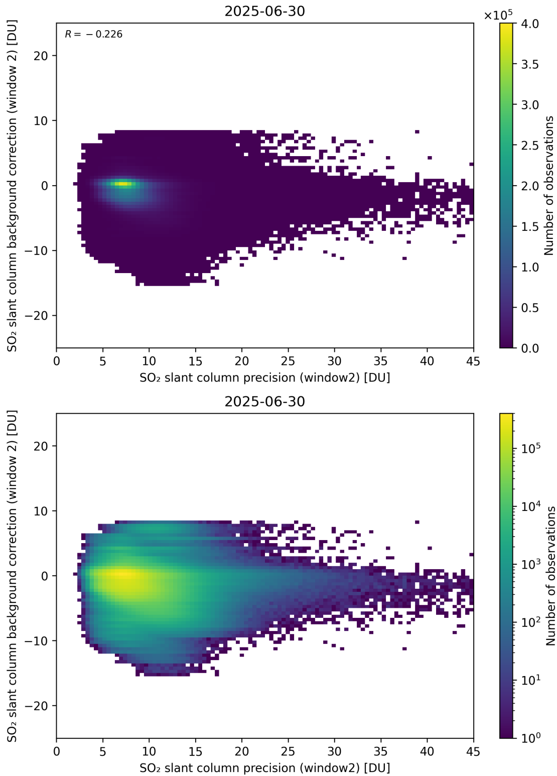
Figure 291: Scatter density plot of “SO 2 slant column precision (window2)” against “SO 2 slant column background correction (window 2)” for 2025-06-29 to 2025-07-01.
