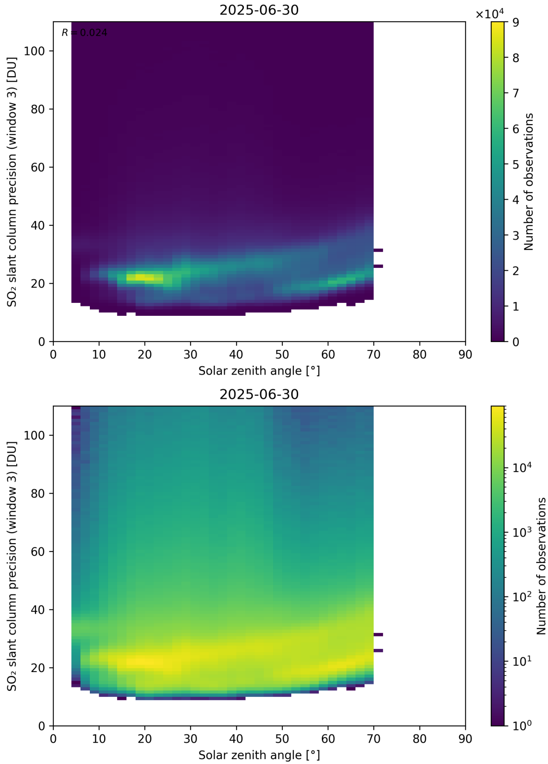
Figure 188: Scatter density plot of “Solar zenith angle” against “SO 2 slant column precision (window 3)” for 2025-06-29 to 2025-07-01.
