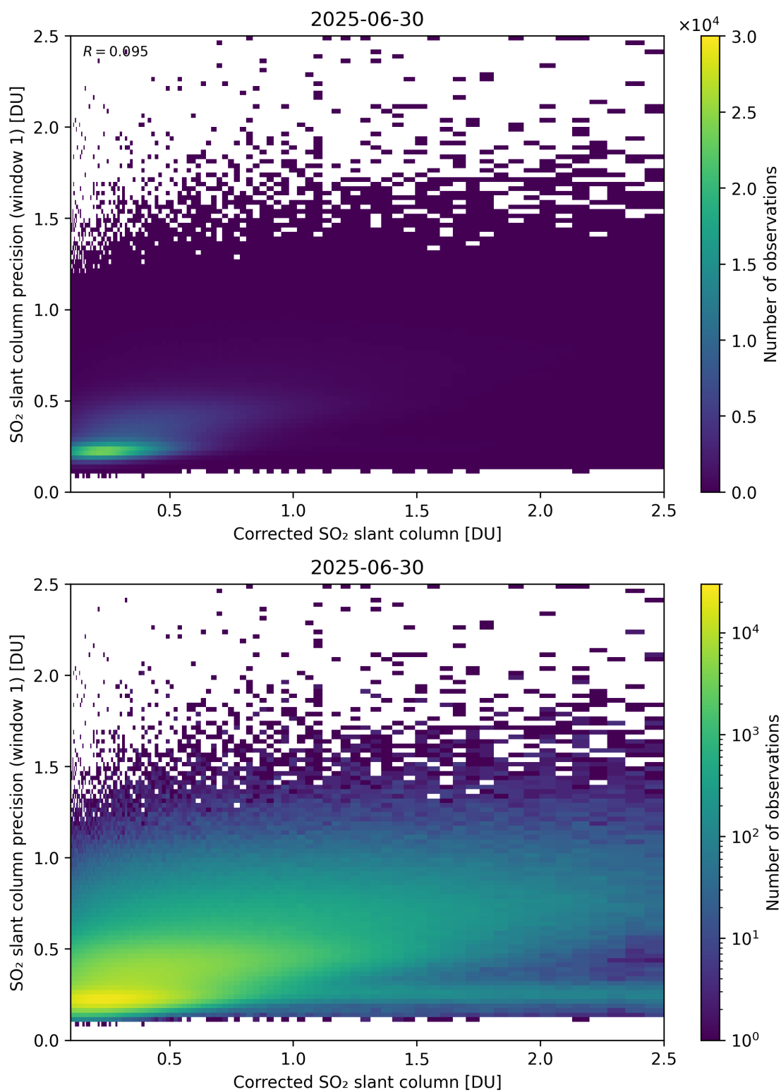
Figure 238: Scatter density plot of “Corrected SO 2 slant column” against “SO 2 slant column precision (window 1)” for 2025-06-29 to 2025-07-01.
