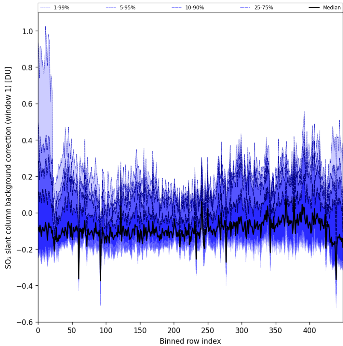
Figure 92: Along track statistics of “SO 2 slant column background correction (window 1)” for 2025-06-29 to 2025-07-01
