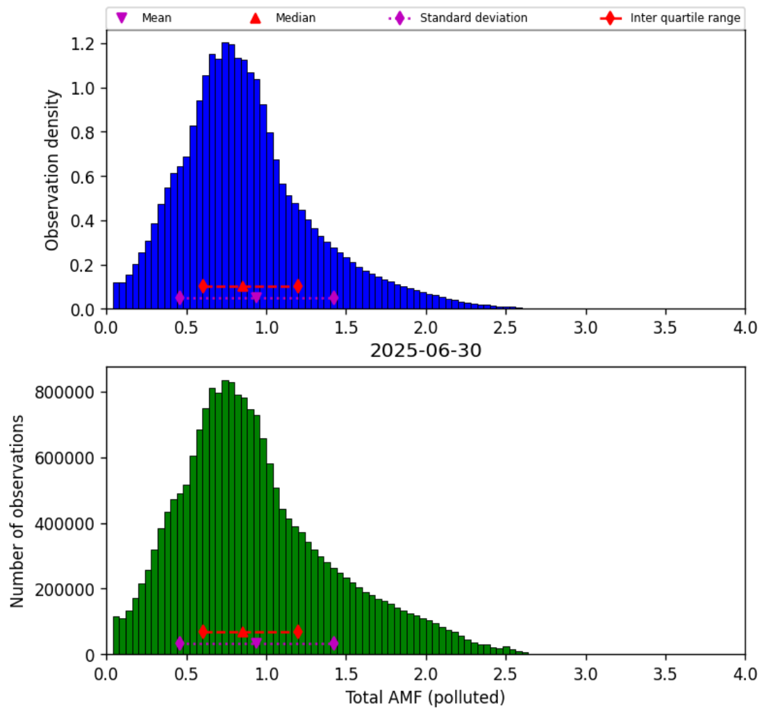
Figure 79: Histogram of “Total AMF (polluted)” for 2025-06-29 to 2025-07-01
