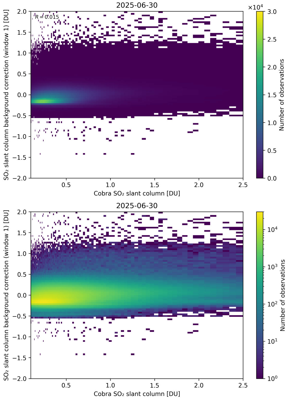
Figure 193: Scatter density plot of “Cobra SO 2 slant column” against “SO 2 slant column background correction (window 1)” for 2025-06-29 to 2025-07-01.
