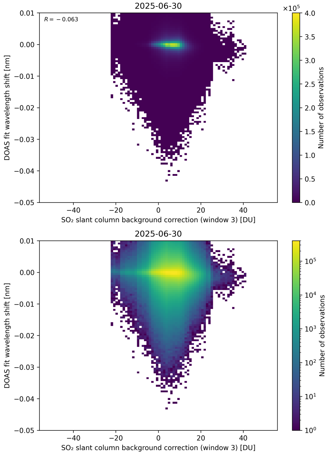
Figure 132: Scatter density plot of “SO 2 slant column background correction (window 3)” against “DOAS fit wavelength shift” for 2025-06-29 to 2025-07-01.
