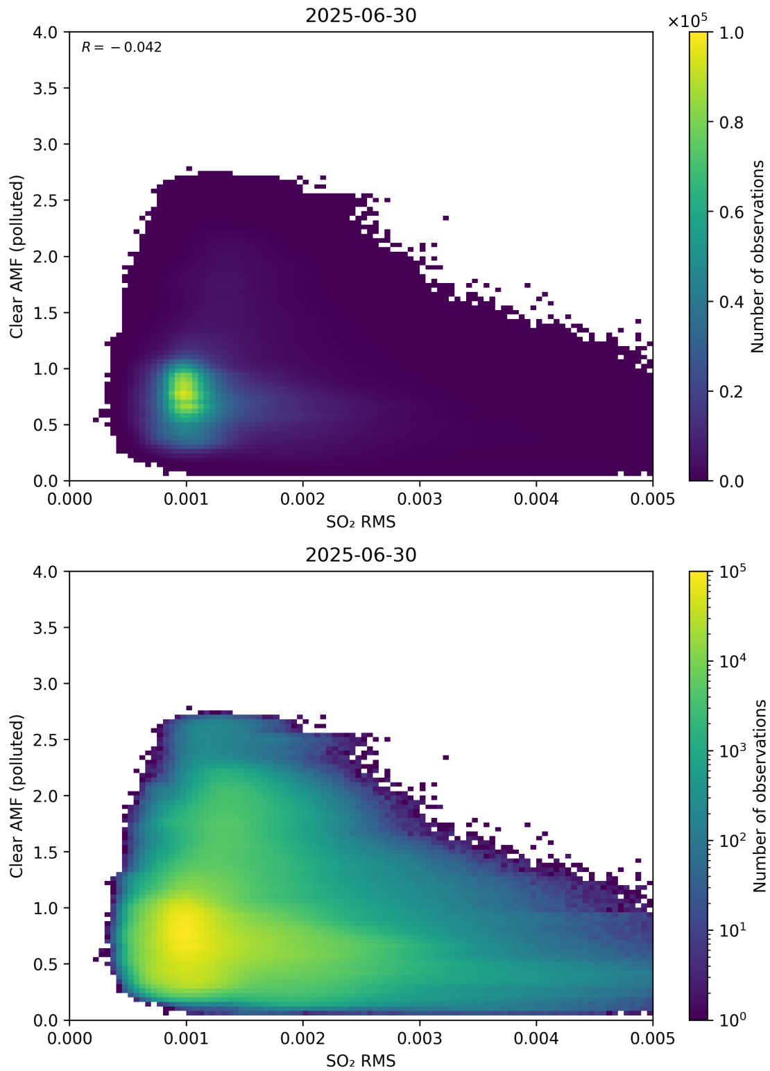
Figure 147: Scatter density plot of “SO 2 RMS” against “Clear AMF (polluted)” for 2025-06-29 to 2025-07-01.
