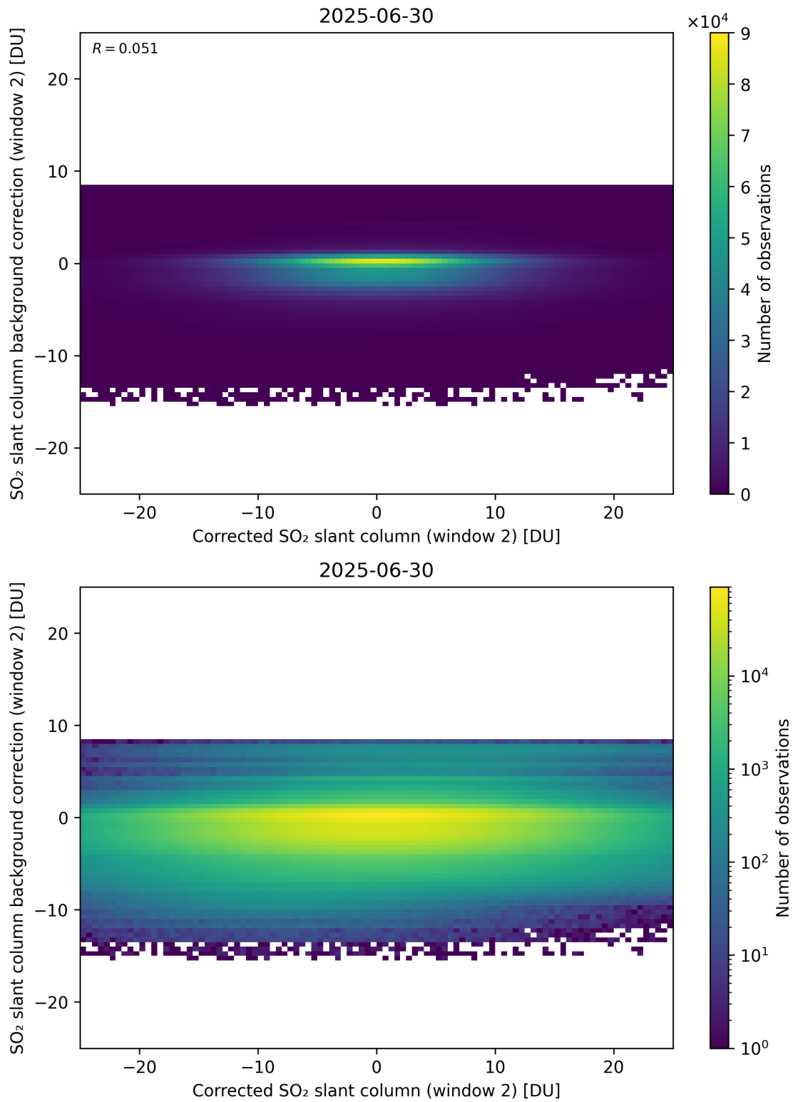
Figure 244: Scatter density plot of “Corrected SO 2 slant column (window 2)” against “SO 2 slant column background correction (window 2)” for 2025-06-29 to 2025-07-01.
