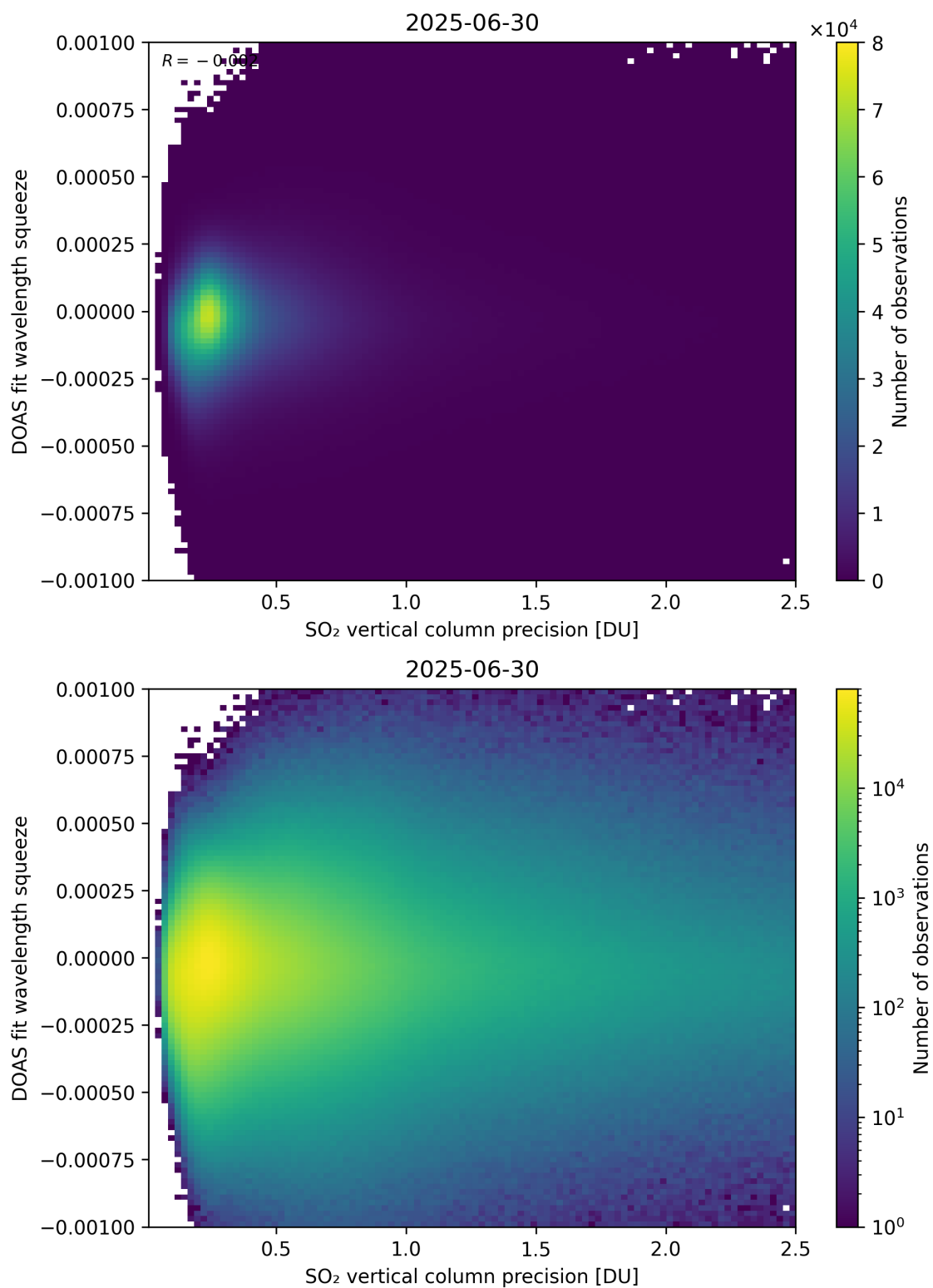
Figure 333: Scatter density plot of “SO 2 vertical column precision” against “DOAS fit wavelength squeeze” for 2025-06-29 to 2025-07-01.
