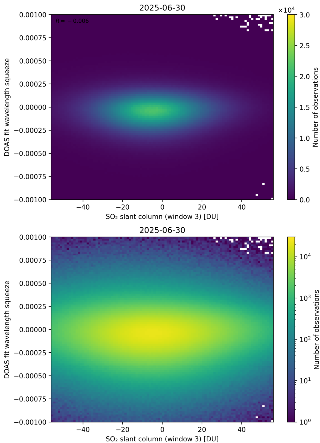
Figure 305: Scatter density plot of “SO 2 slant column (window 3)” against “DOAS fit wavelength squeeze” for 2025-06-29 to 2025-07-01.
