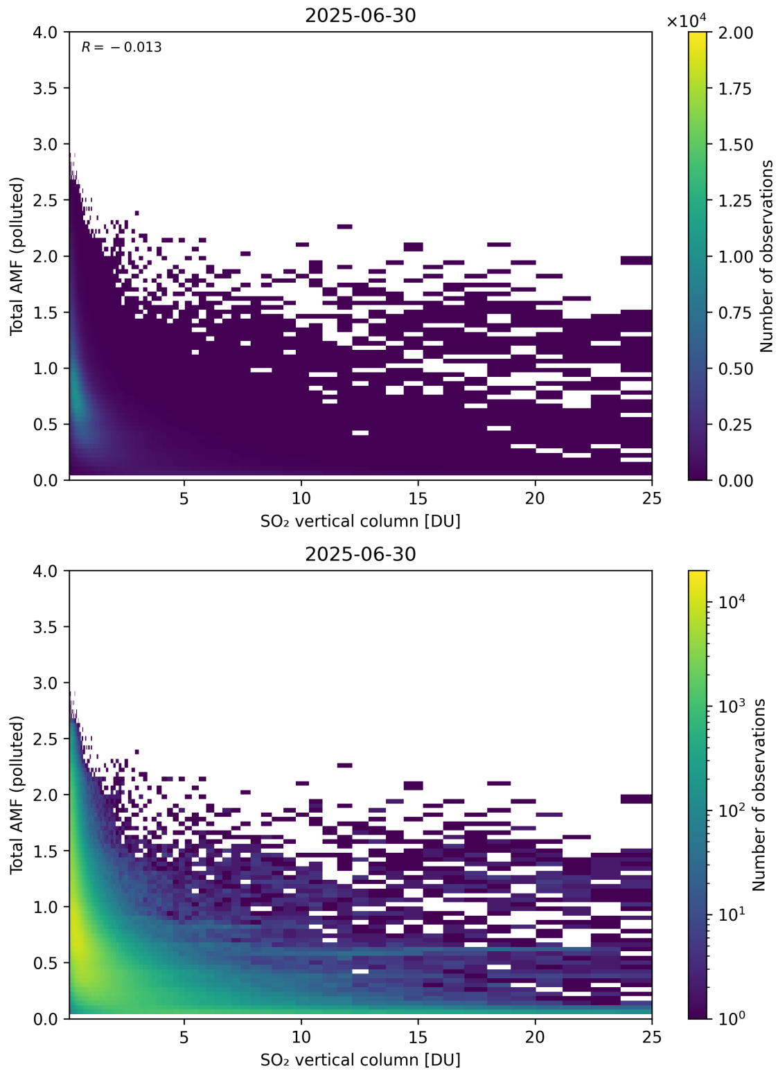
Figure 359: Scatter density plot of “SO 2 vertical column” against “Total AMF (polluted)” for 2025-06-29 to 2025-07-01.
