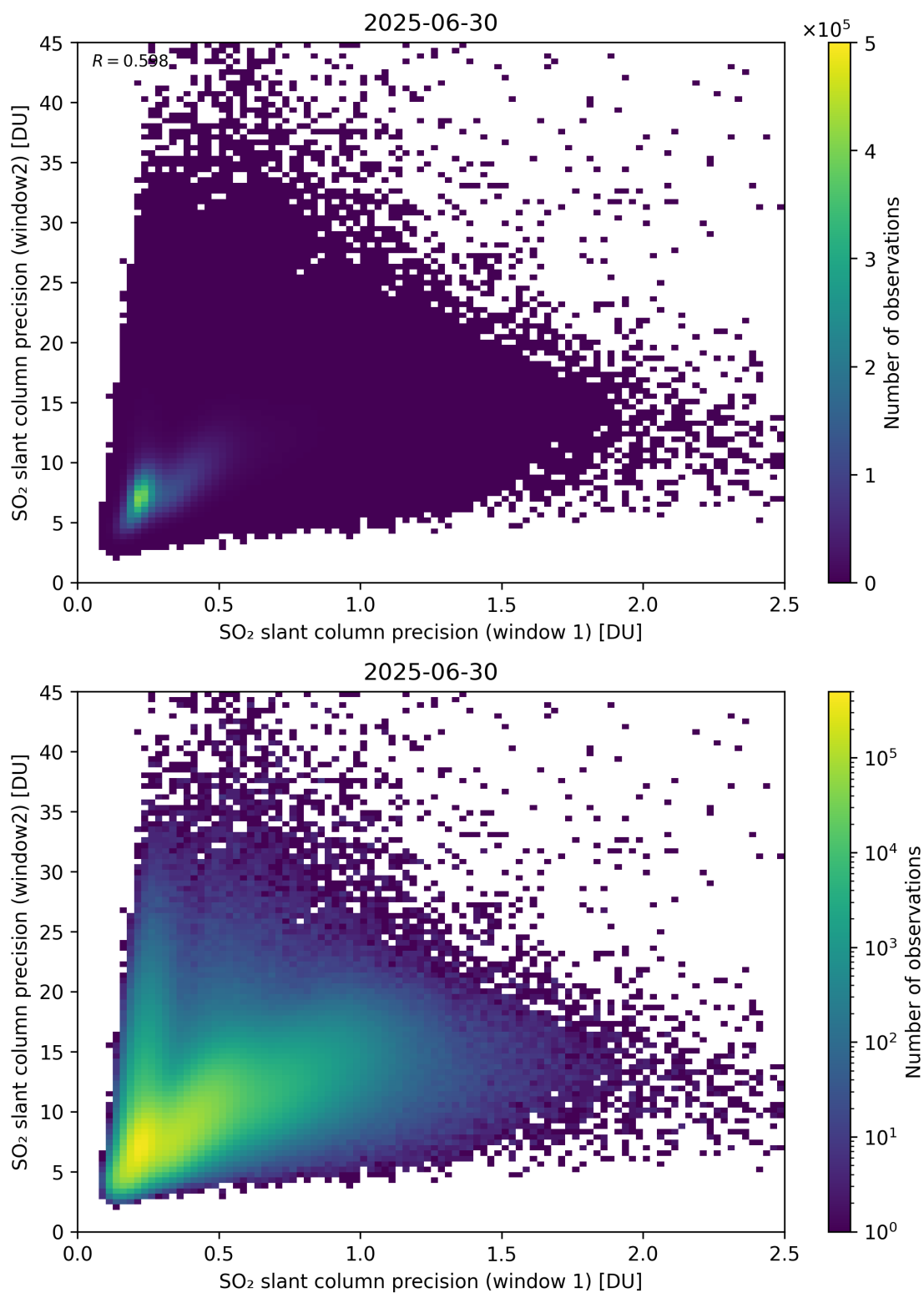
Figure 277: Scatter density plot of “SO 2 slant column precision (window 1)” against “SO 2 slant column precision (window2)” for 2025-06-29 to 2025-07-01.
