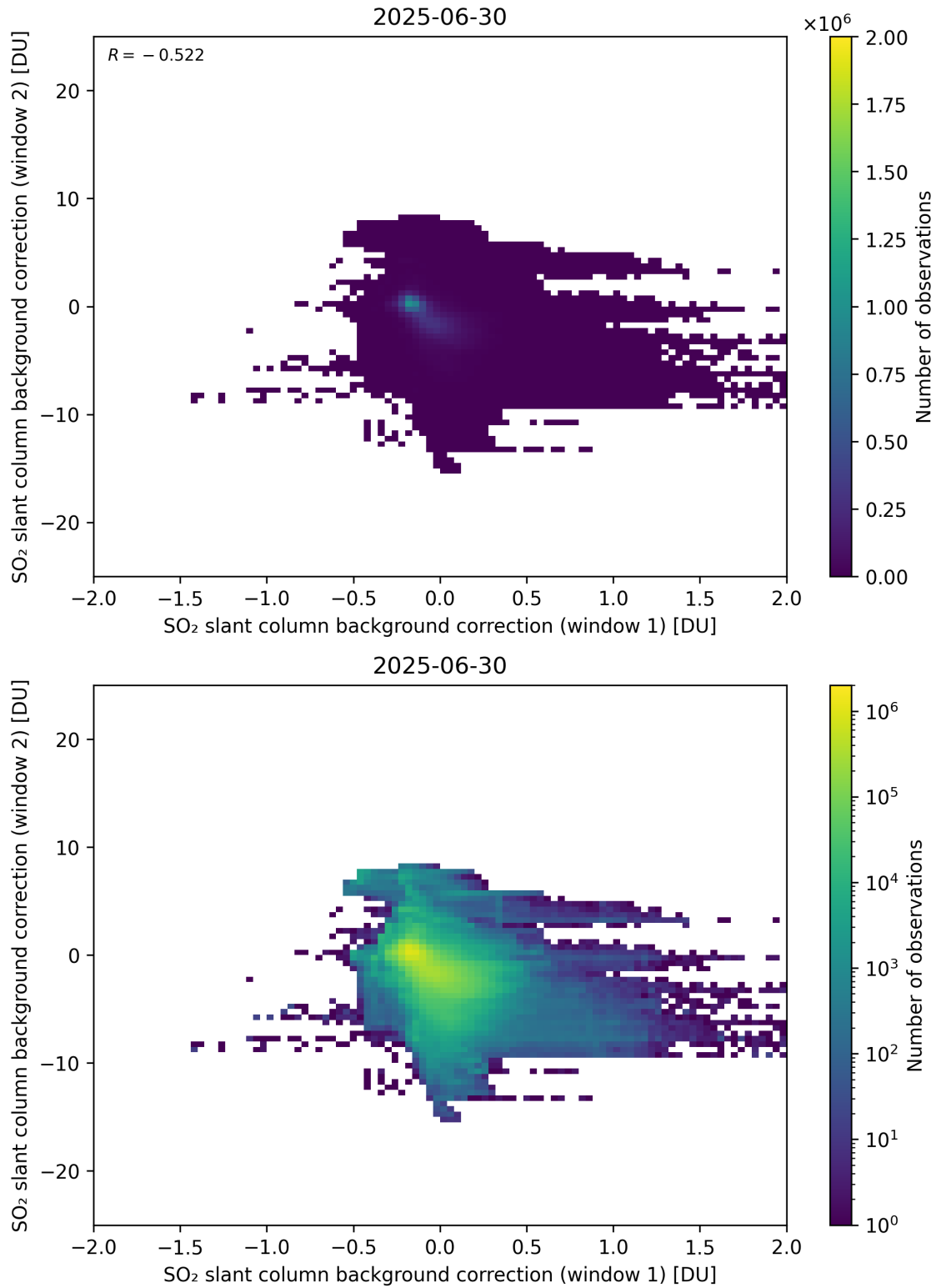
Figure 109: Scatter density plot of “SO 2 slant column background correction (window 1)” against “SO 2 slant column background correction (window 2)” for 2025-06-29 to 2025-07-01.
