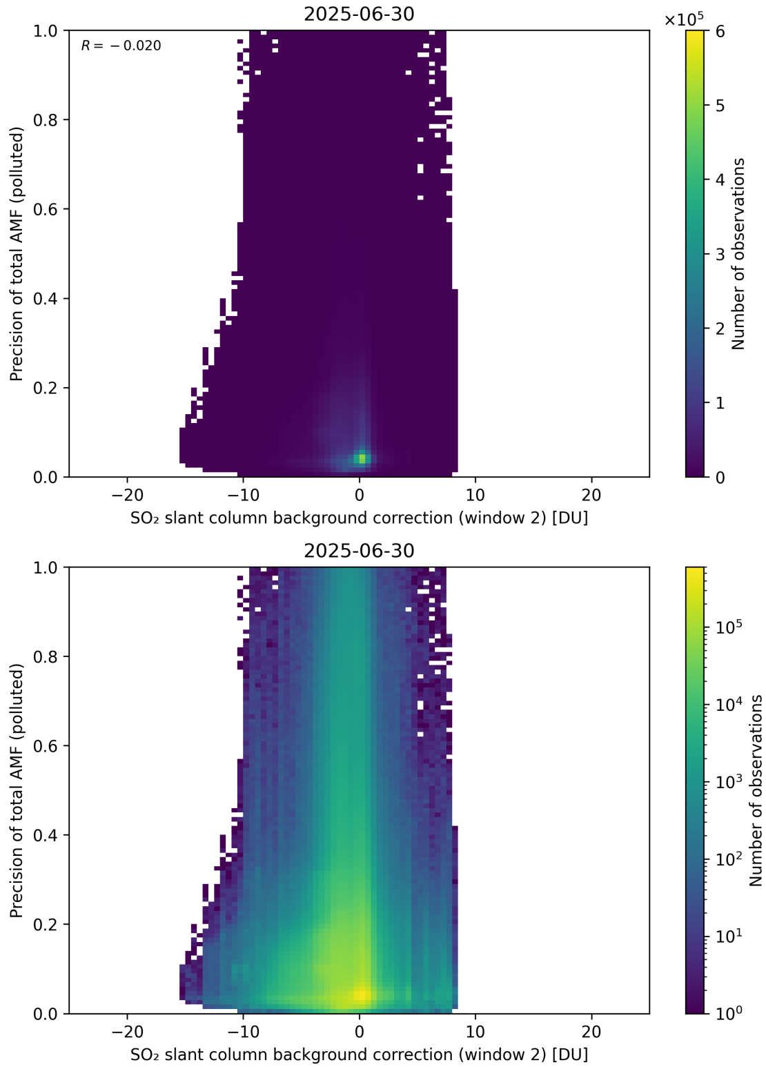
Figure 131: Scatter density plot of “SO 2 slant column background correction (window 2)” against “Precision of total AMF (polluted)” for 2025-06-29 to 2025-07-01.
