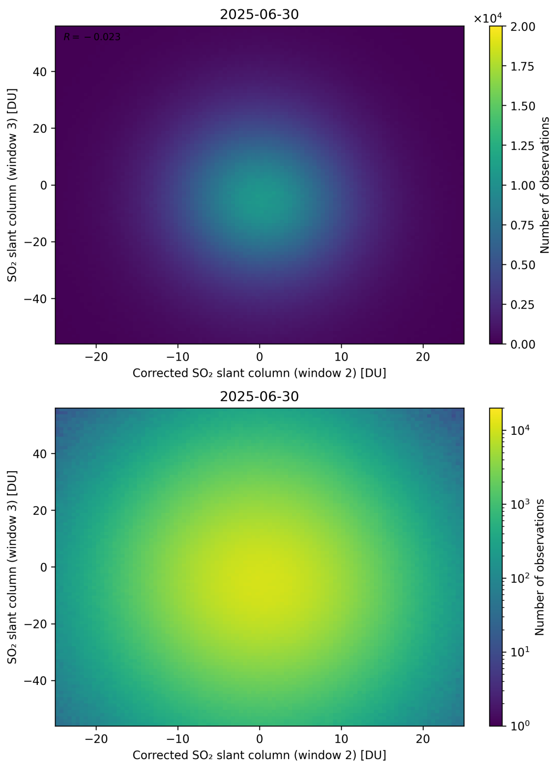
Figure 251: Scatter density plot of “Corrected SO 2 slant column (window 2)” against “SO 2 slant column (window 3)” for 2025-06-29 to 2025-07-01.
