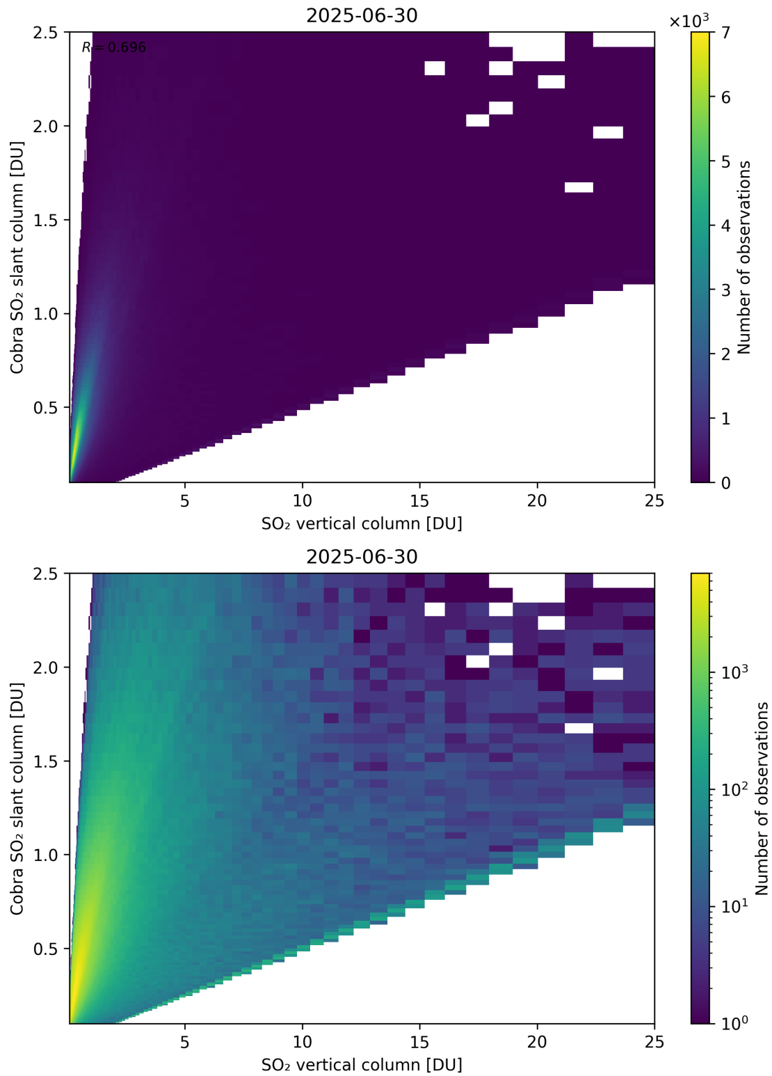
Figure 349: Scatter density plot of “SO 2 vertical column” against “Cobra SO 2 slant column” for 2025-06-29 to 2025-07-01.
