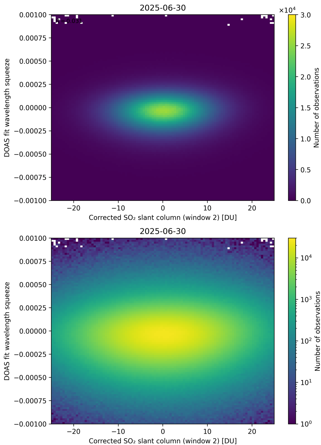
Figure 247: Scatter density plot of “Corrected SO 2 slant column (window 2)” against “DOAS fit wavelength squeeze” for 2025-06-29 to 2025-07-01.
