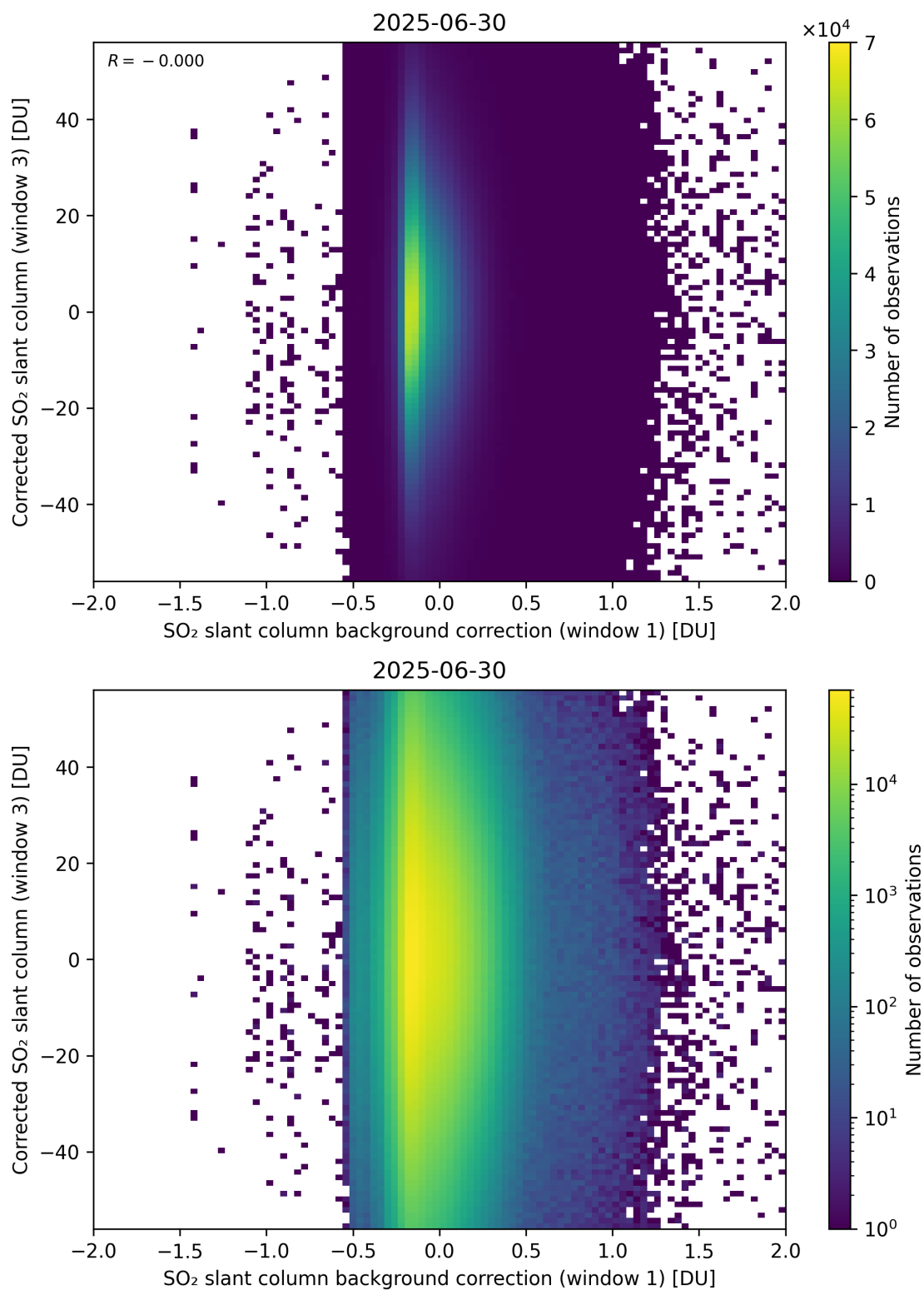
Figure 116: Scatter density plot of “SO 2 slant column background correction (window 1)” against “Corrected SO 2 slant column (window 3)” for 2025-06-29 to 2025-07-01.
