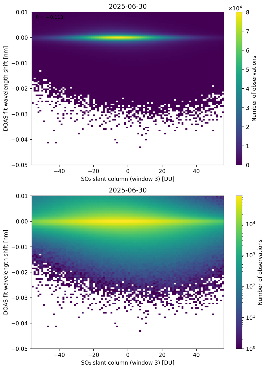
Figure 304: Scatter density plot of “SO 2 slant column (window 3)” against “DOAS fit wavelength shift” for 2025-06-29 to 2025-07-01.
