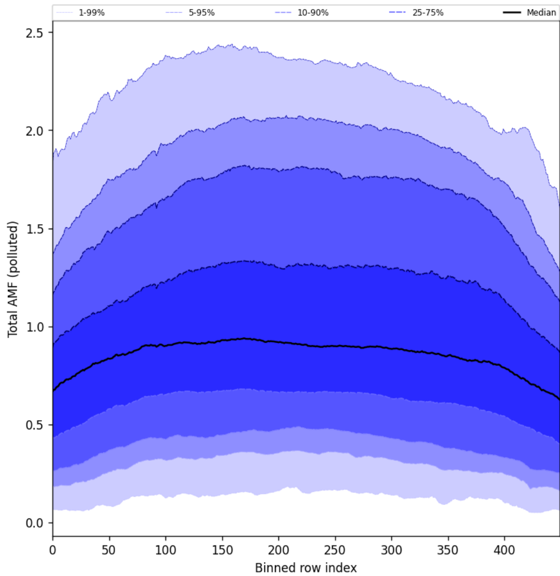
Figure 105: Along track statistics of “Total AMF (polluted)” for 2025-06-29 to 2025-07-01
