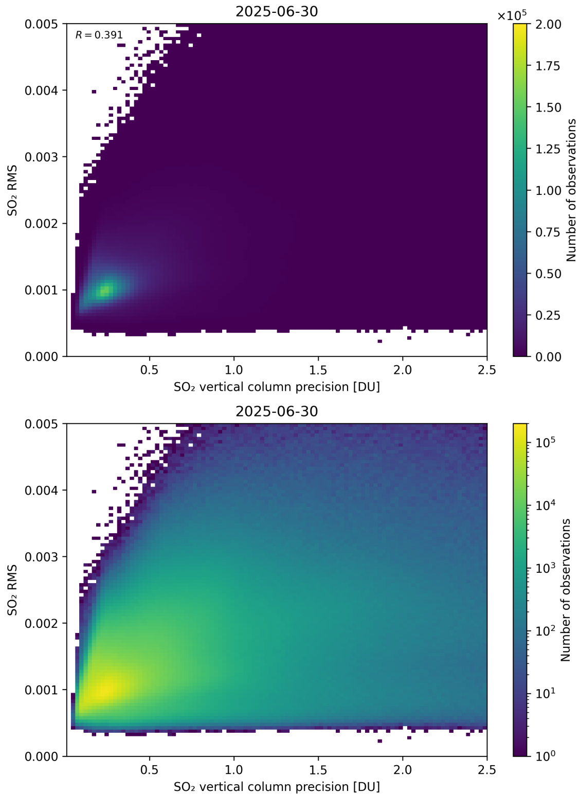
Figure 334: Scatter density plot of “SO 2 vertical column precision” against “SO 2 RMS” for 2025-06-29 to 2025-07-01.
