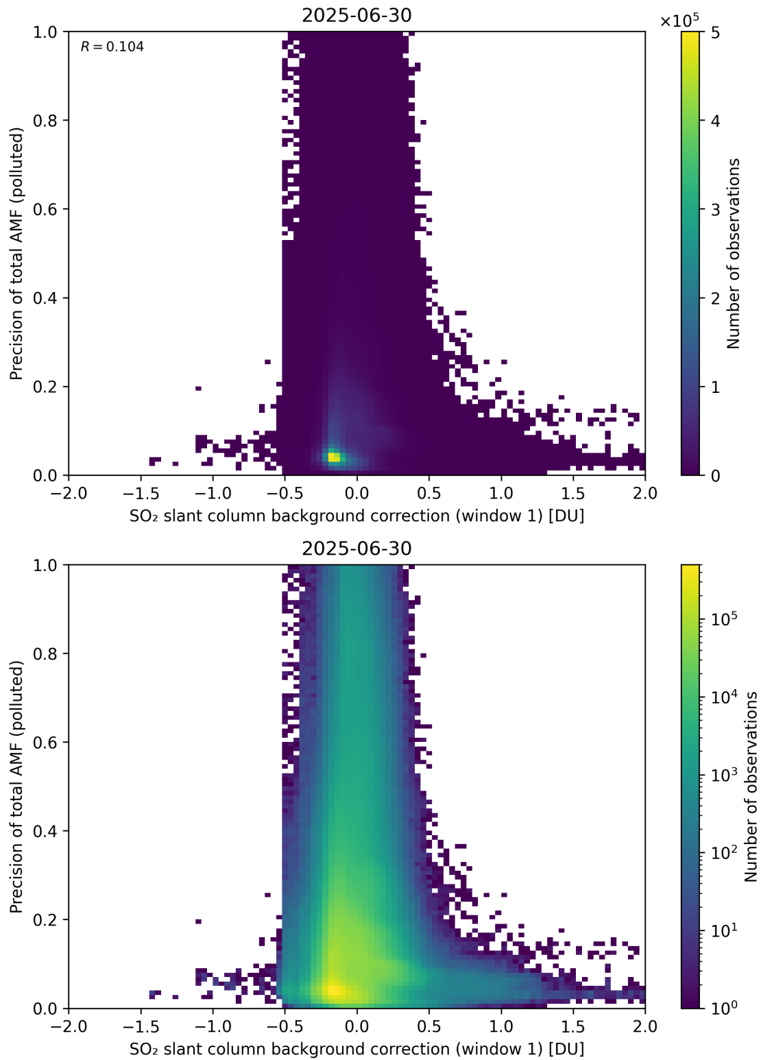
Figure 121: Scatter density plot of “SO 2 slant column background correction (window 1)” against “Precision of total AMF (polluted)” for 2025-06-29 to 2025-07-01.
