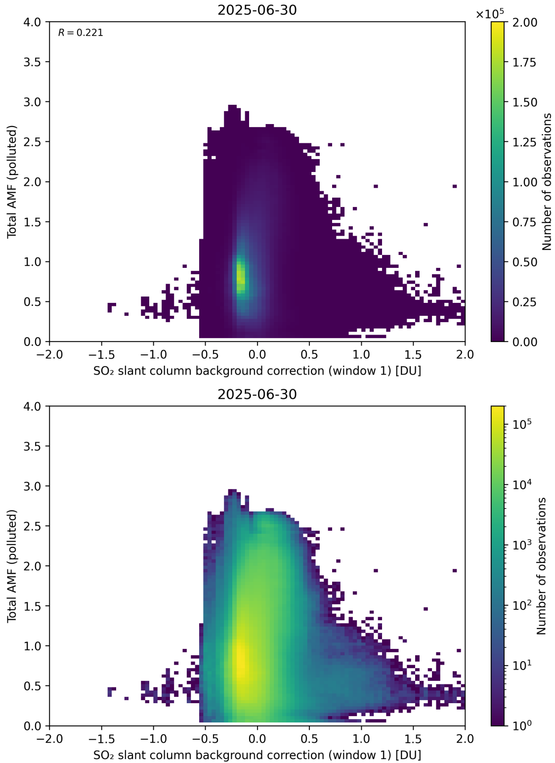
Figure 120: Scatter density plot of “SO 2 slant column background correction (window 1)” against “Total AMF (polluted)” for 2025-06-29 to 2025-07-01.
