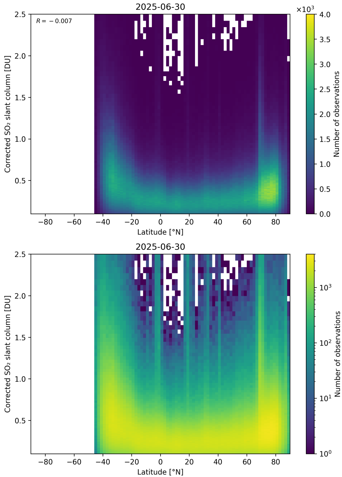
Figure 159: Scatter density plot of “Latitude” against “Corrected SO 2 slant column” for 2025-06-29 to 2025-07-01.
