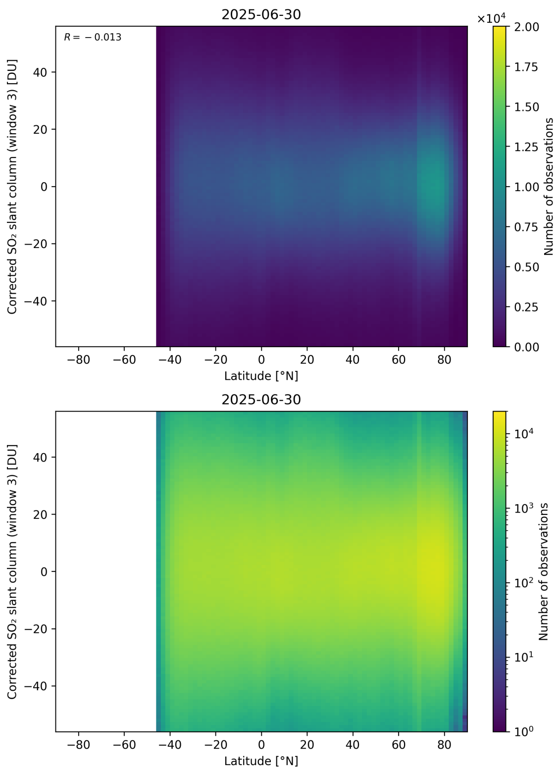
Figure 161: Scatter density plot of “Latitude” against “Corrected SO 2 slant column (window 3)” for 2025-06-29 to 2025-07-01.
