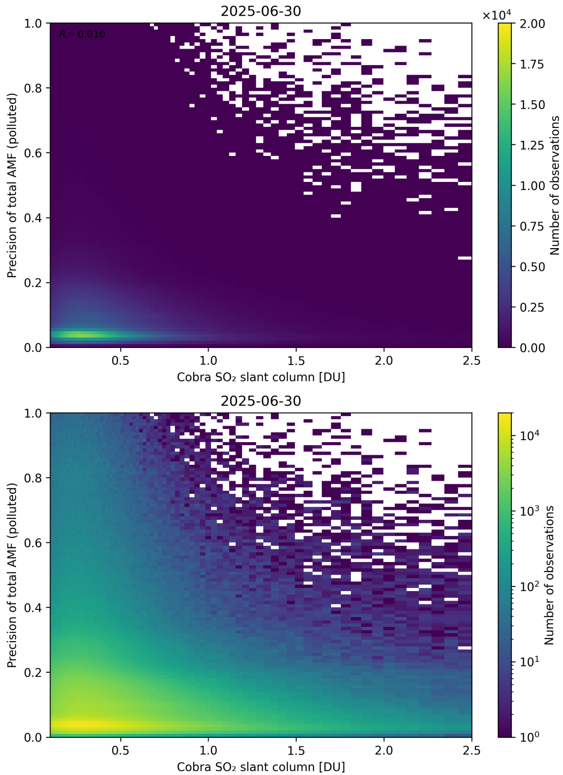
Figure 225: Scatter density plot of “Cobra SO 2 slant column” against “Precision of total AMF (polluted)” for 2025-06-29 to 2025-07-01.
