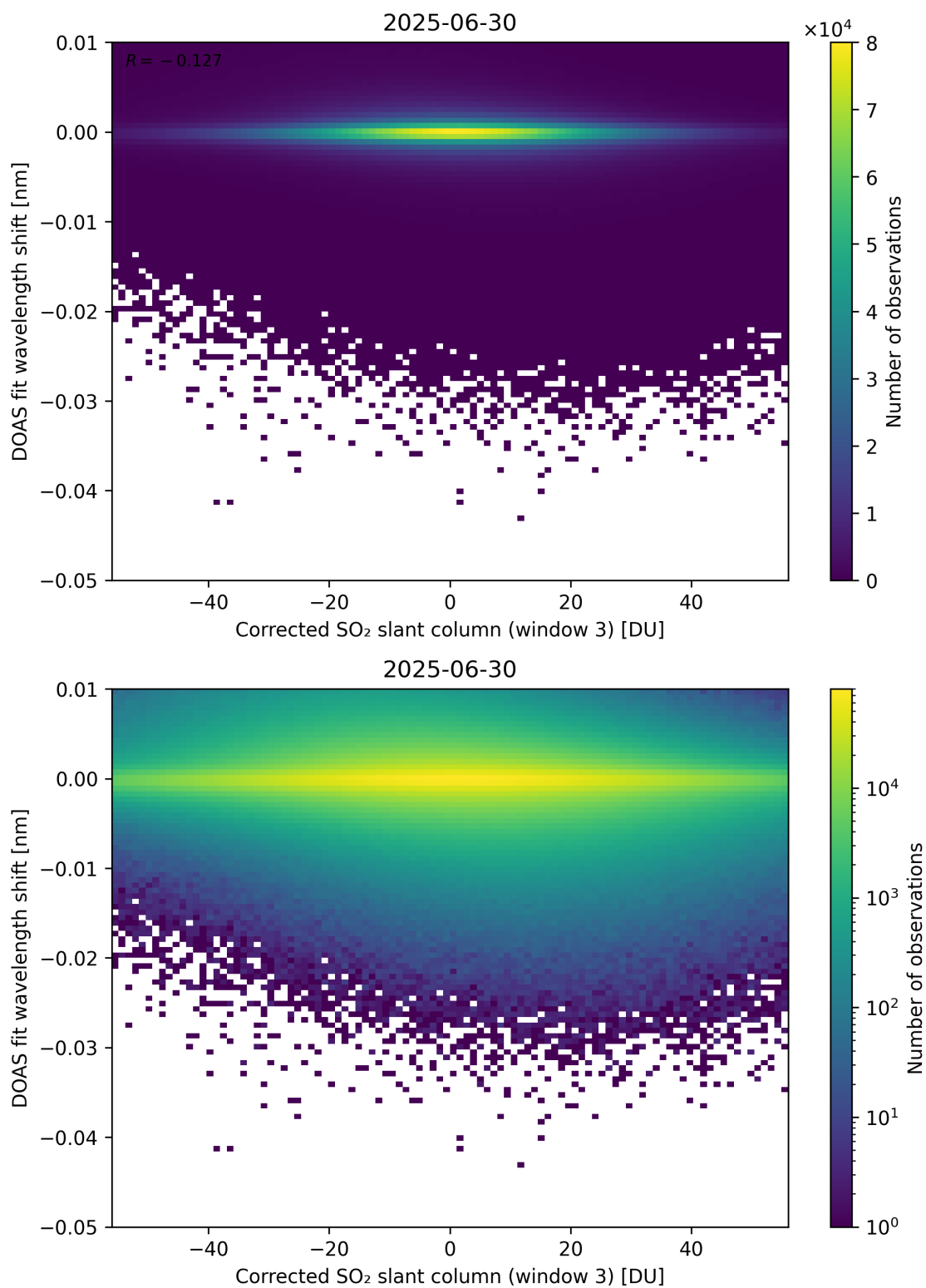
Figure 256: Scatter density plot of “Corrected SO 2 slant column (window 3)” against “DOAS fit wavelength shift” for 2025-06-29 to 2025-07-01.
