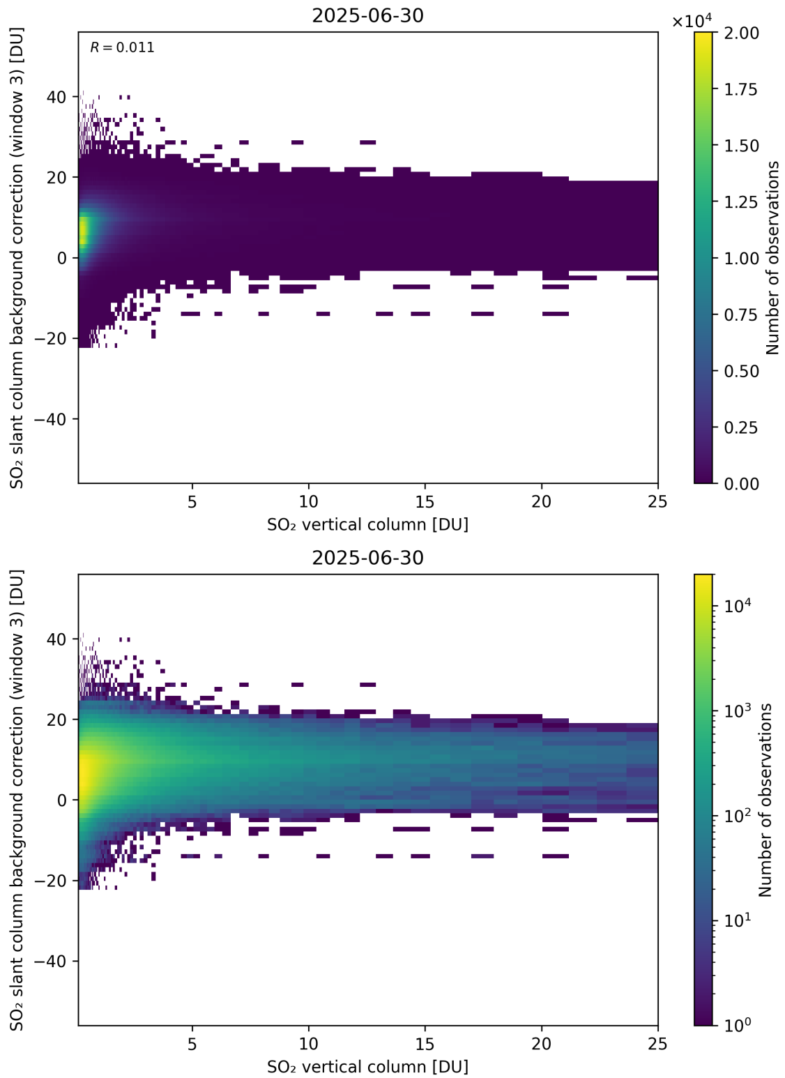
Figure 325: Scatter density plot of “SO 2 vertical column” against “SO 2 slant column background correction (window 3)” for 2025-06-29 to 2025-07-01.
