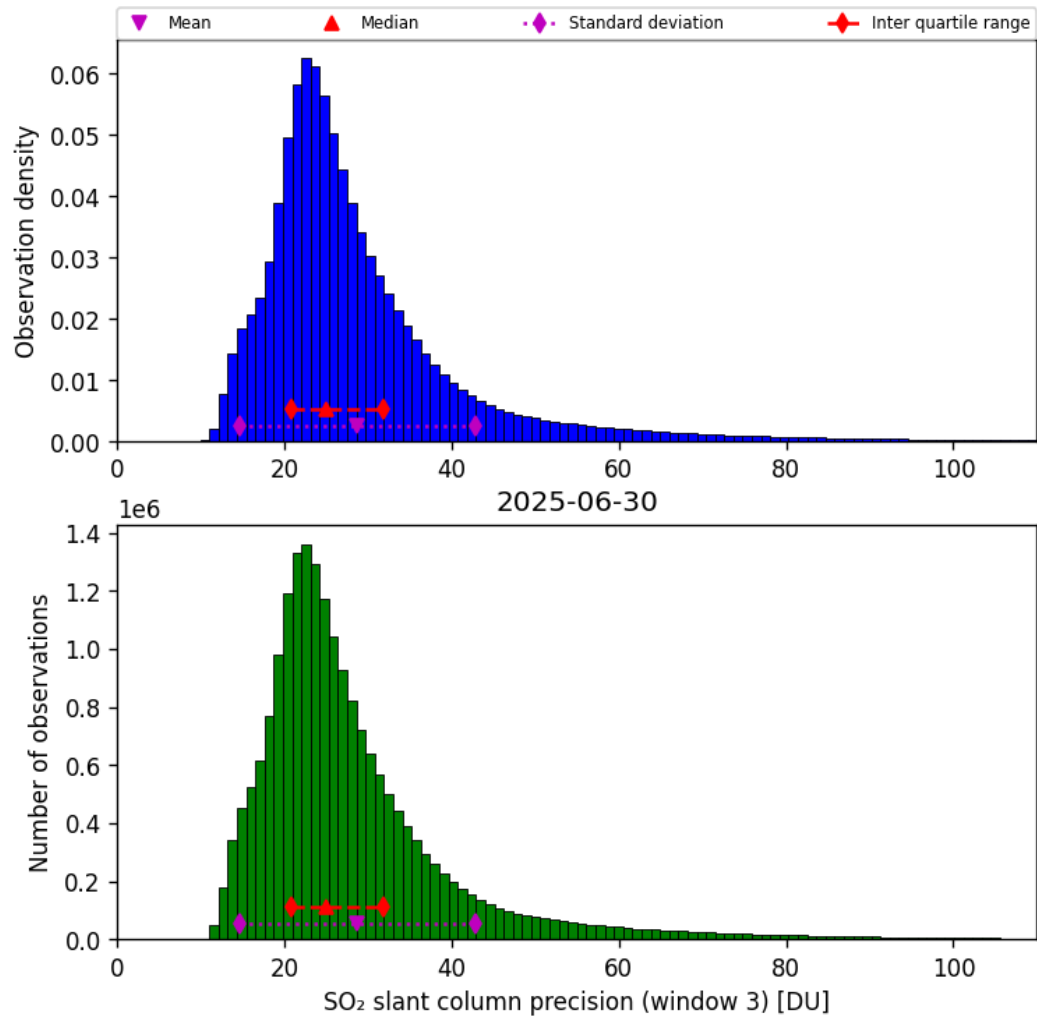
Figure 72: Histogram of “SO 2 slant column precision (window 3)” for 2025-06-29 to 2025-07-01
