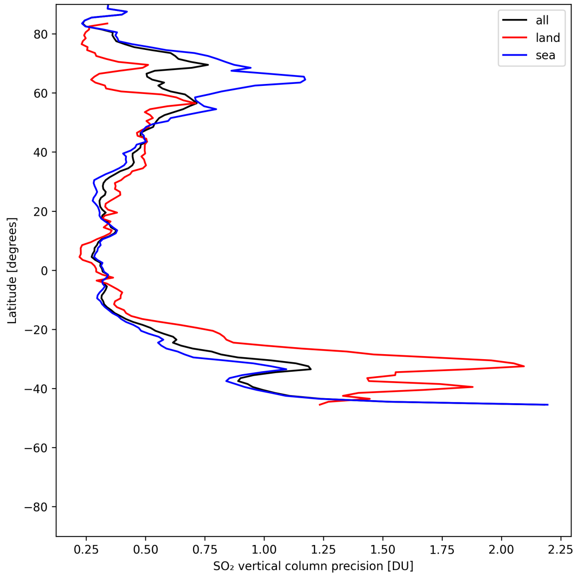
Figure 33: Zonal average of “SO 2 vertical column precision” for 2025-06-29 to 2025-07-01.
