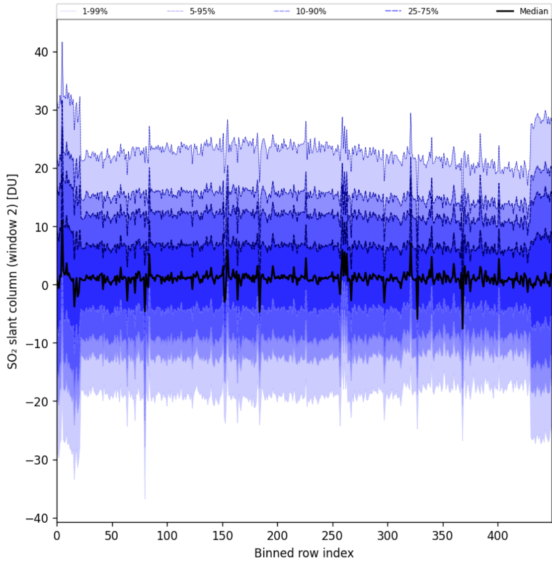
Figure 93: Along track statistics of “SO 2 slant column (window 2)” for 2025-06-29 to 2025-07-01
