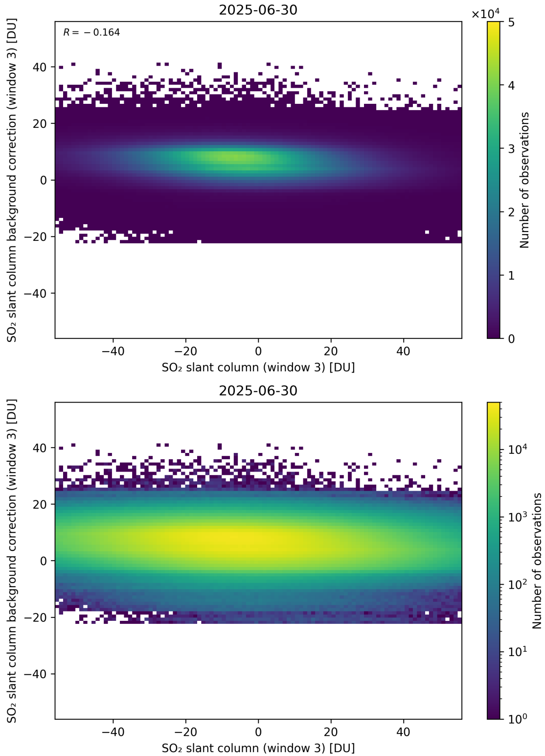
Figure 303: Scatter density plot of “SO 2 slant column (window 3)” against “SO 2 slant column background correction (window 3)” for 2025-06-29 to 2025-07-01.
