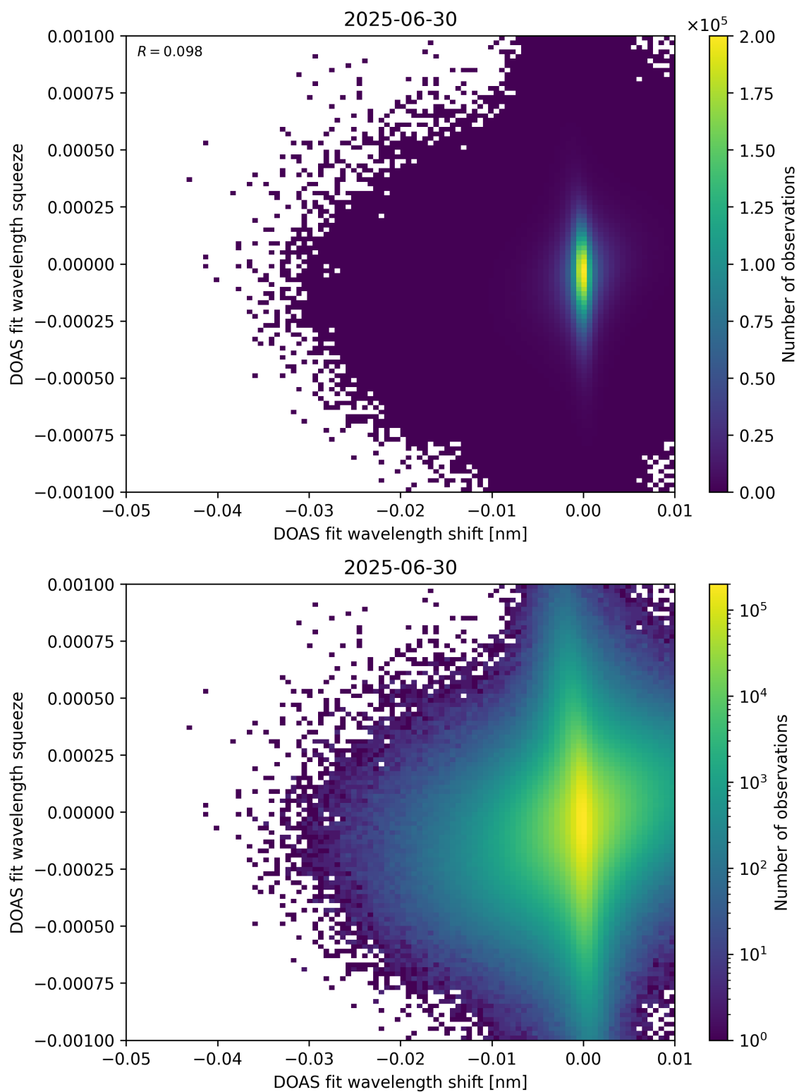
Figure 138: Scatter density plot of “DOAS fit wavelength shift” against “DOAS fit wavelength squeeze” for 2025-06-29 to 2025-07-01.
