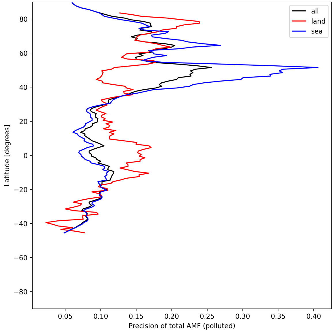
Figure 54: Zonal average of “Precision of total AMF (polluted)” for 2025-06-29 to 2025-07-01.
