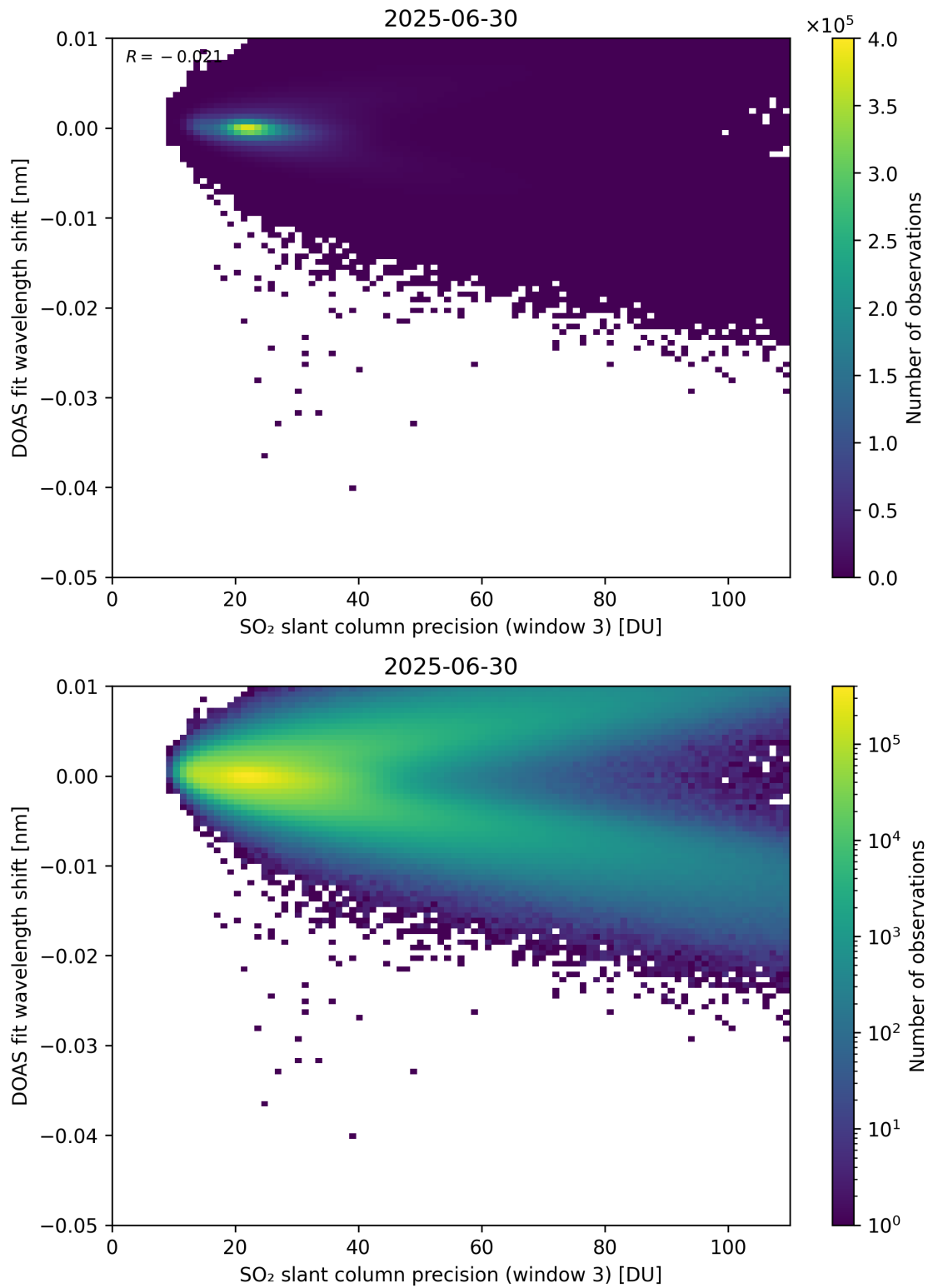
Figure 308: Scatter density plot of “SO 2 slant column precision (window 3)” against “DOAS fit wavelength shift” for 2025-06-29 to 2025-07-01.
