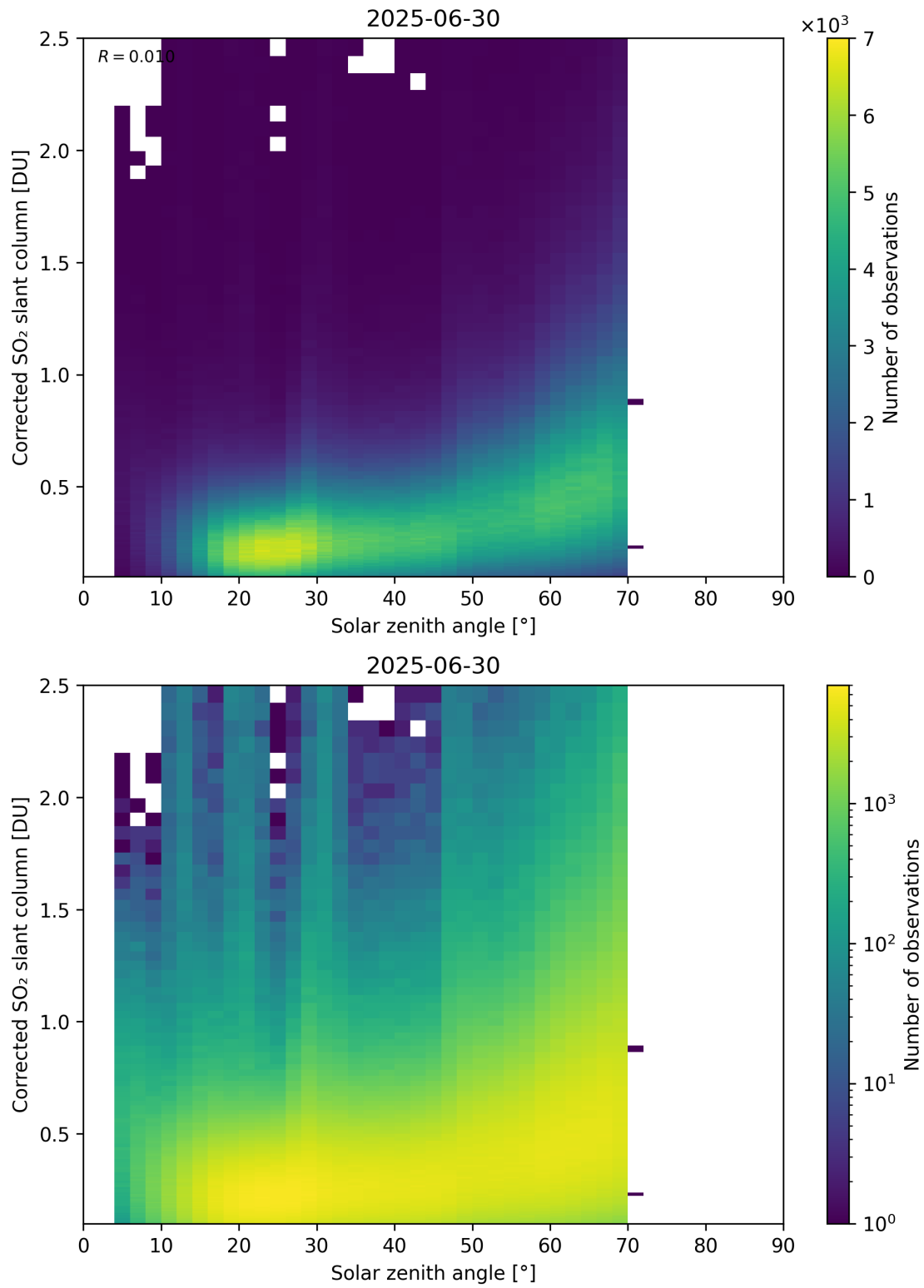
Figure 181: Scatter density plot of “Solar zenith angle” against “Corrected SO 2 slant column” for 2025-06-29 to 2025-07-01.
