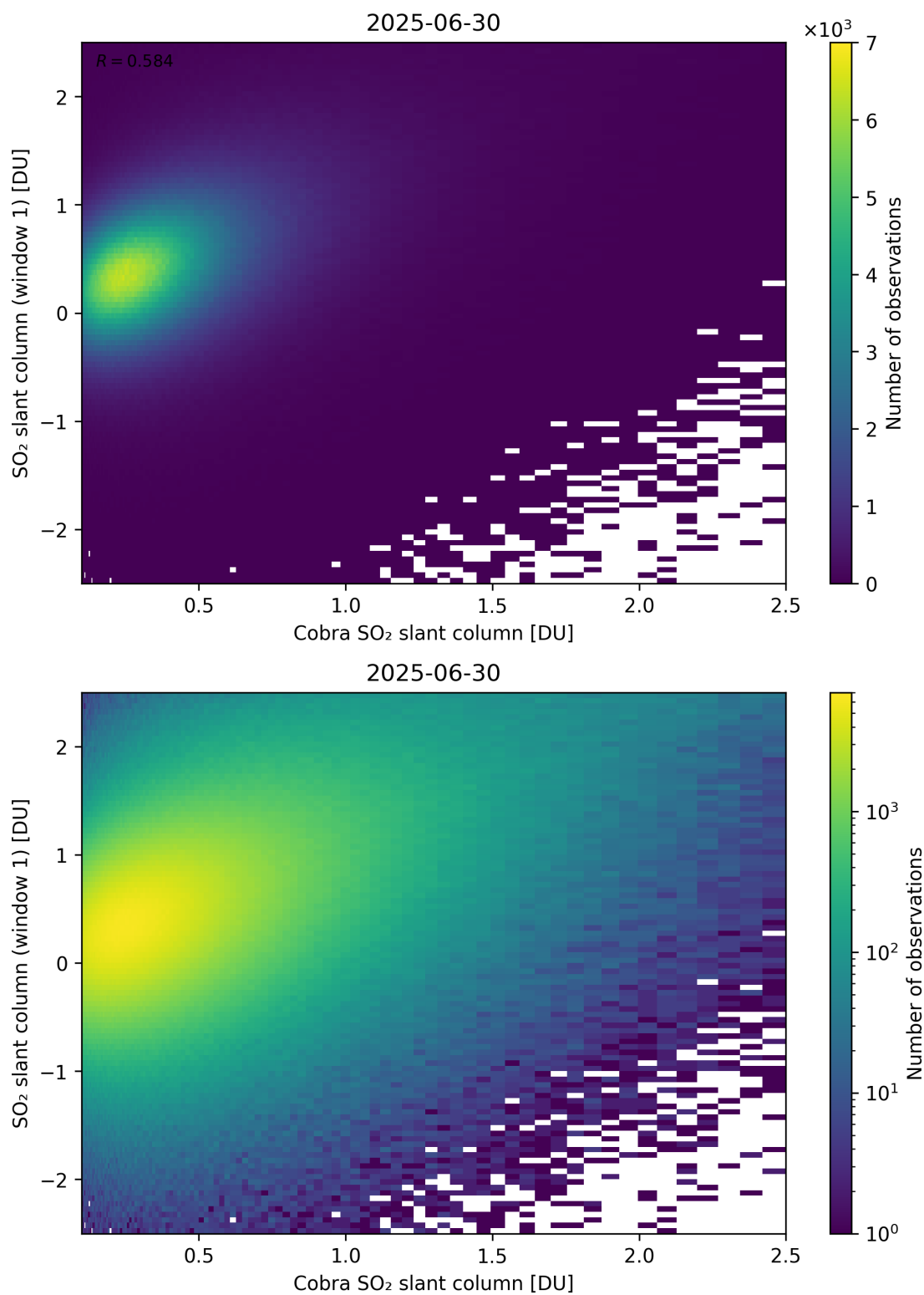
Figure 219: Scatter density plot of “Cobra SO 2 slant column” against “SO 2 slant column (window 1)” for 2025-06-29 to 2025-07-01.
