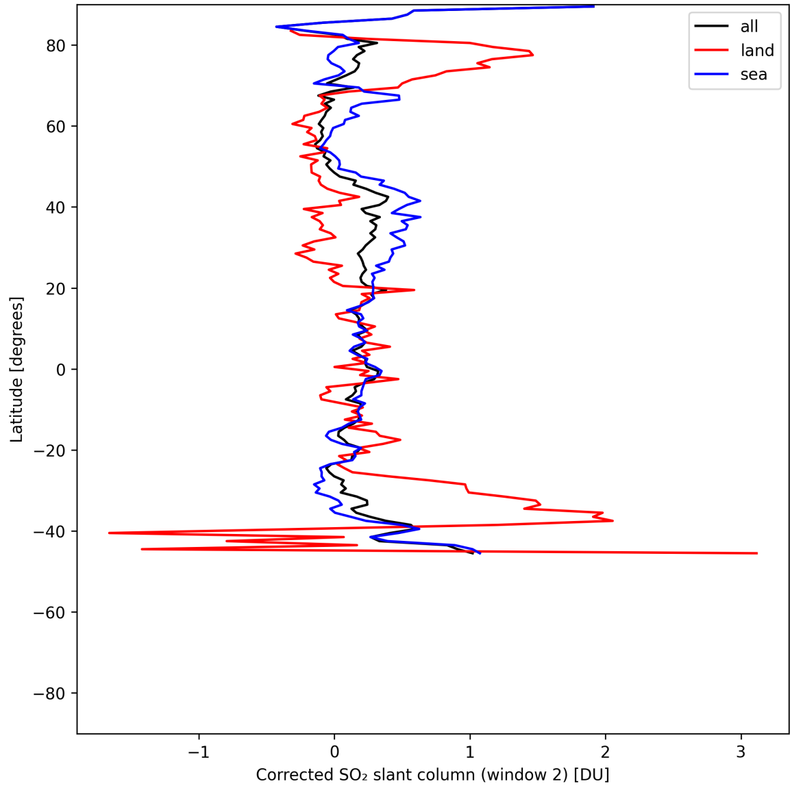
Figure 43: Zonal average of “Corrected SO 2 slant column (window 2)” for 2025-06-29 to 2025-07-01.
