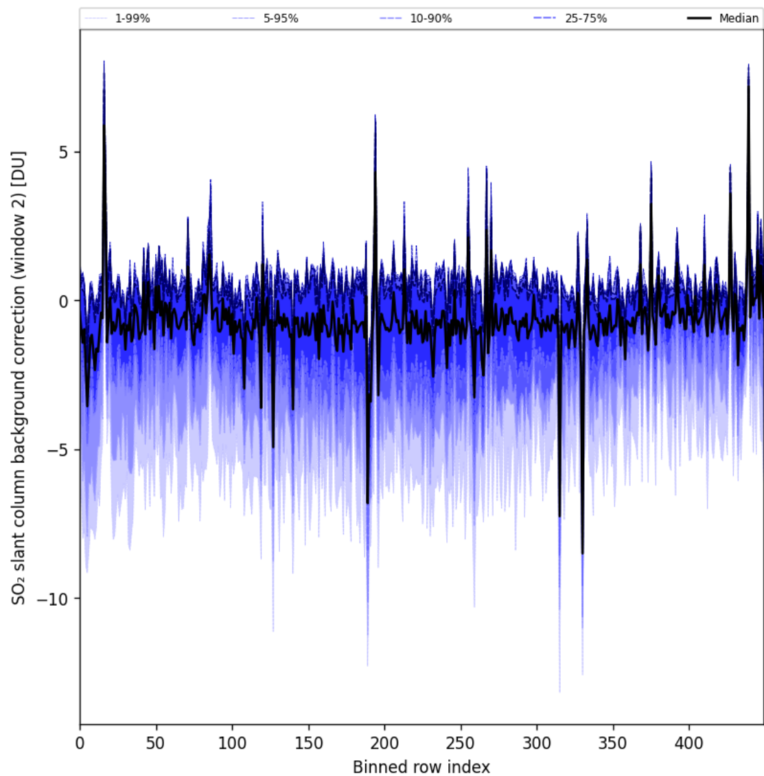
Figure 96: Along track statistics of “SO 2 slant column background correction (window 2)” for 2025-06-29 to 2025-07-01
