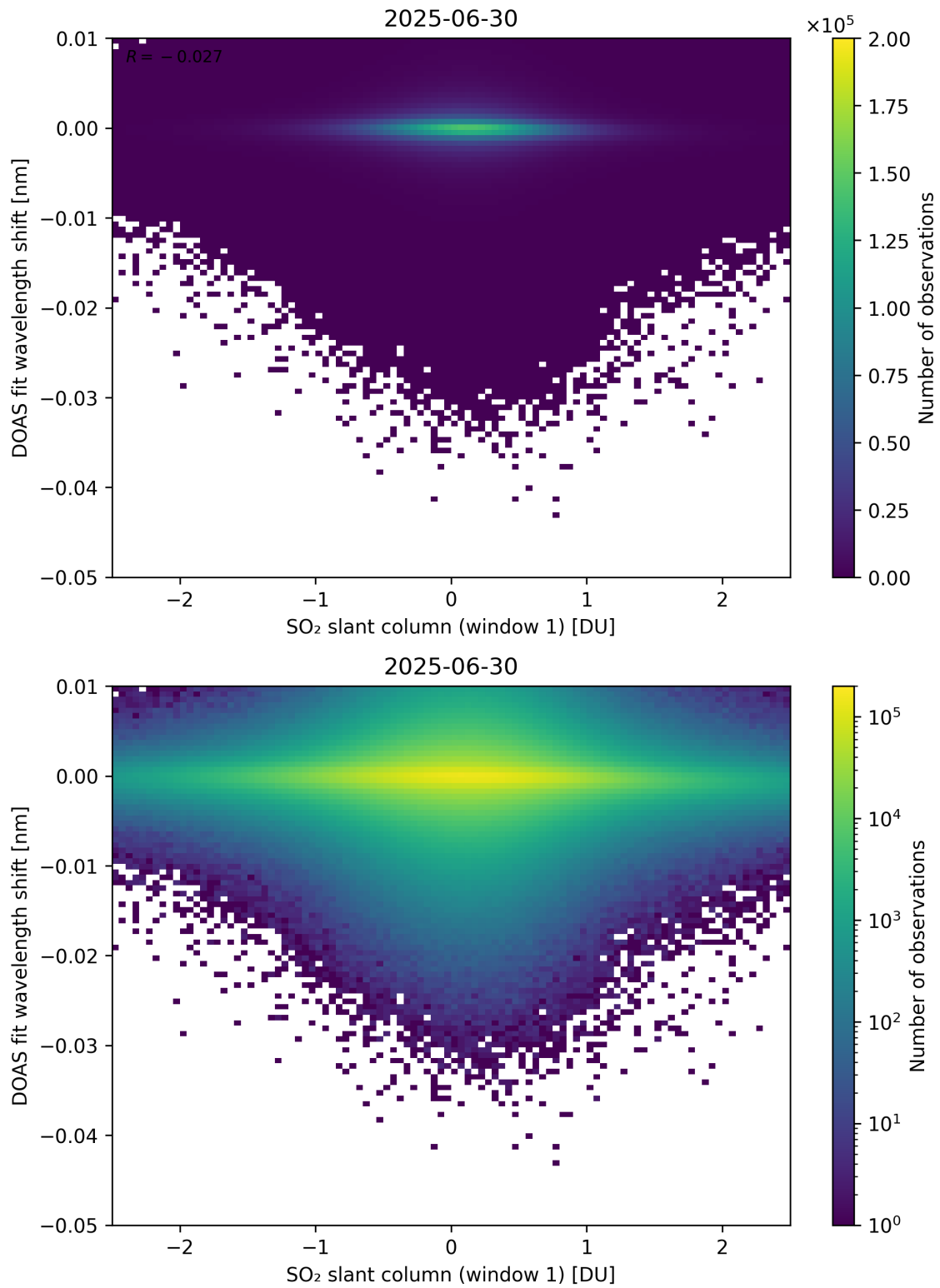
Figure 265: Scatter density plot of “SO 2 slant column (window 1)” against “DOAS fit wavelength shift” for 2025-06-29 to 2025-07-01.
