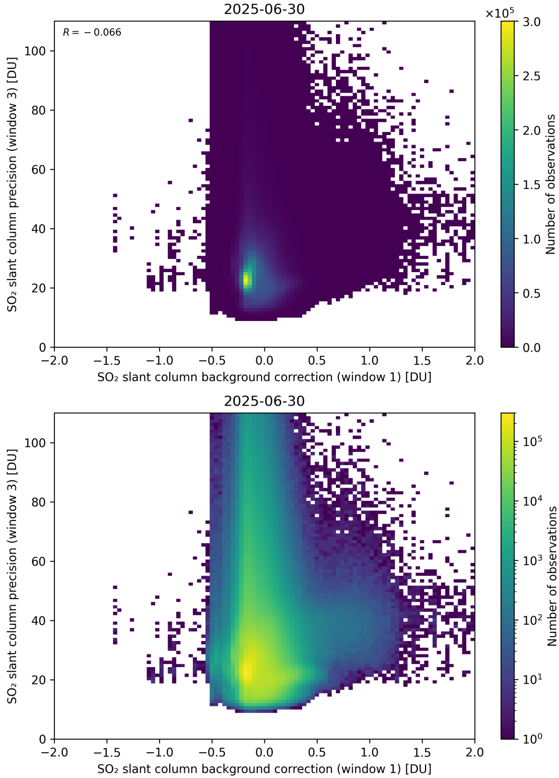
Figure 119: Scatter density plot of “SO 2 slant column background correction (window 1)” against “SO 2 slant column precision (window 3)” for 2025-06-29 to 2025-07-01.
