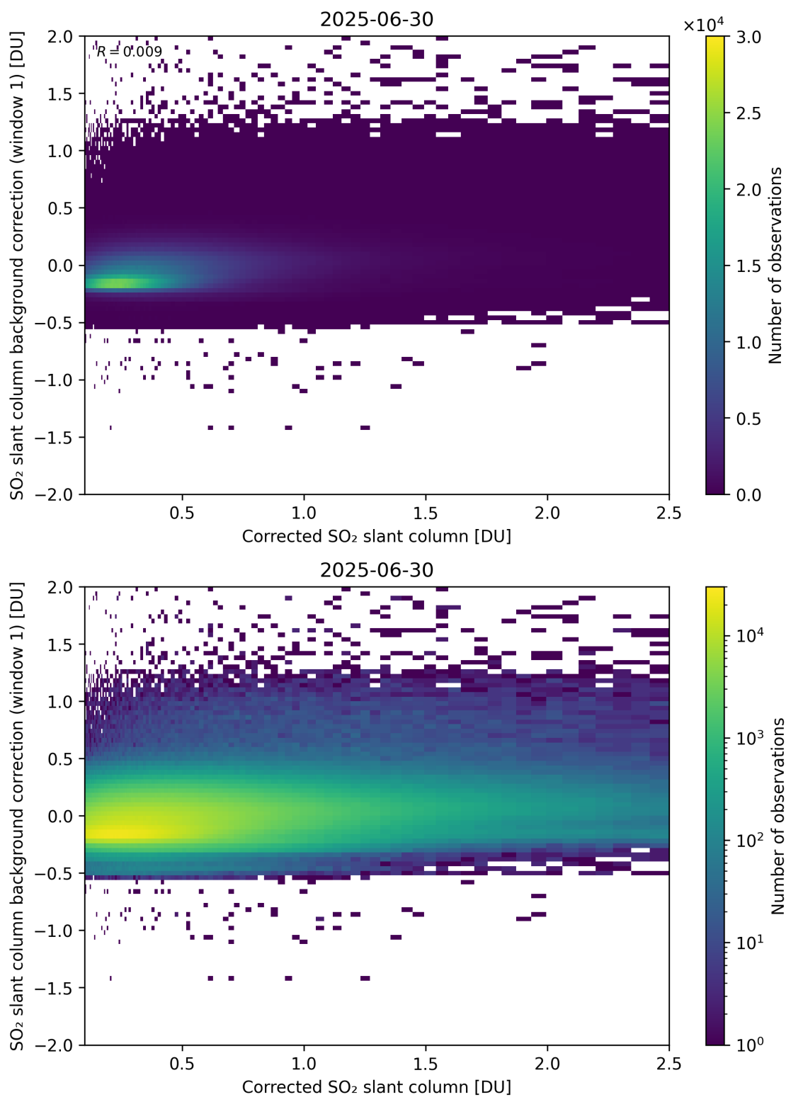
Figure 226: Scatter density plot of “Corrected SO 2 slant column” against “SO 2 slant column background correction (window 1)” for 2025-06-29 to 2025-07-01.
