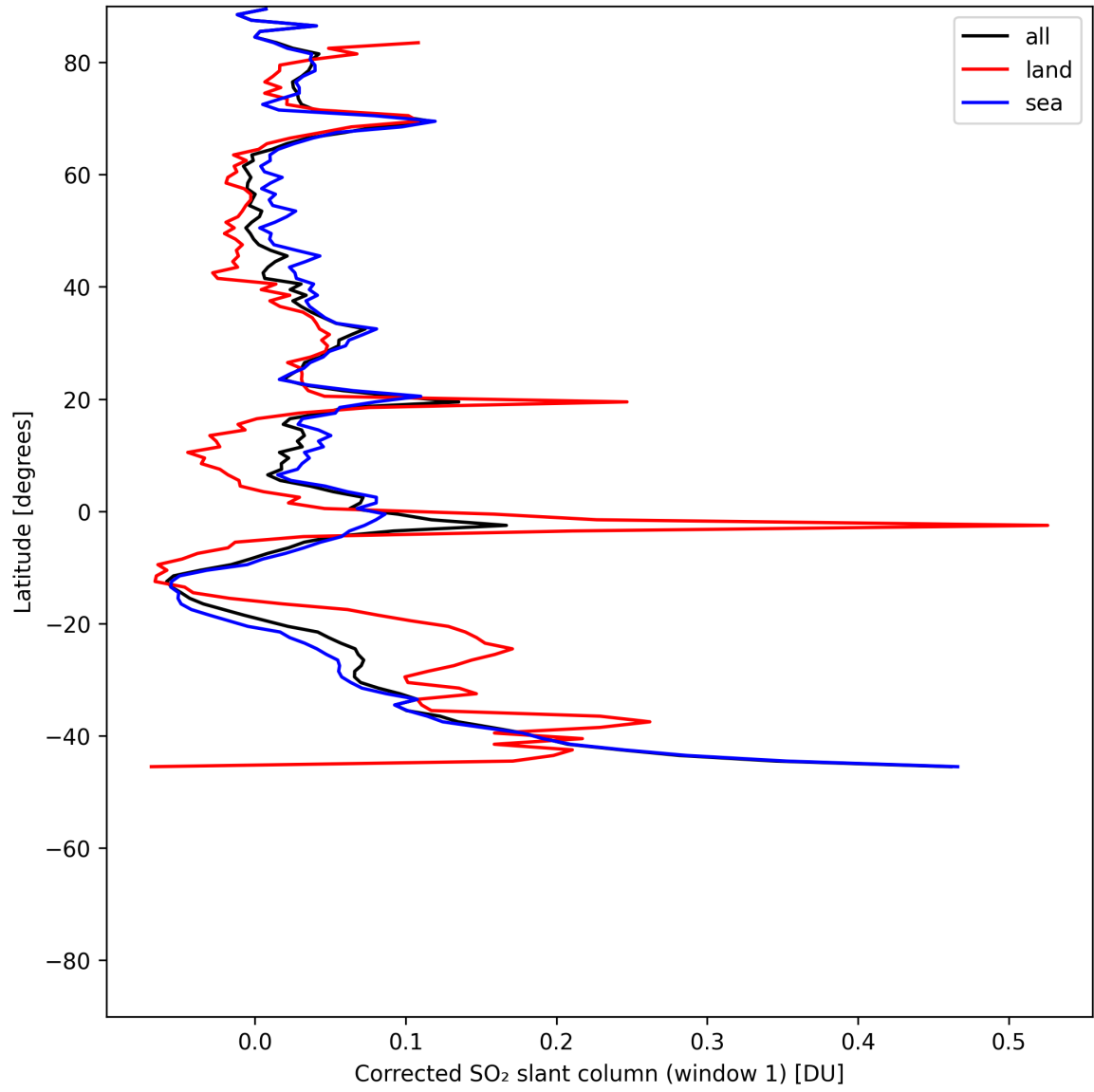
Figure 39: Zonal average of “Corrected SO 2 slant column (window 1)” for 2025-06-29 to 2025-07-01.
