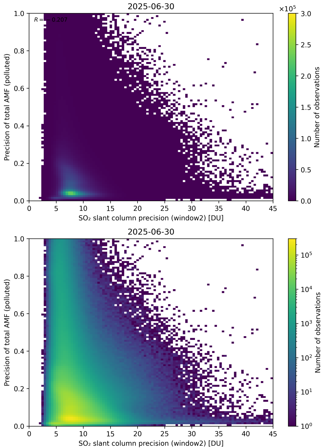
Figure 302: Scatter density plot of “SO 2 slant column precision (window2)” against “Precision of total AMF (polluted)” for 2025-06-29 to 2025-07-01.
