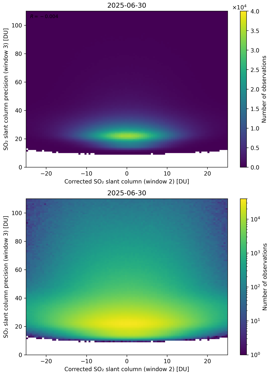
Figure 252: Scatter density plot of “Corrected SO 2 slant column (window 2)” against “SO 2 slant column precision (window 3)” for 2025-06-29 to 2025-07-01.
