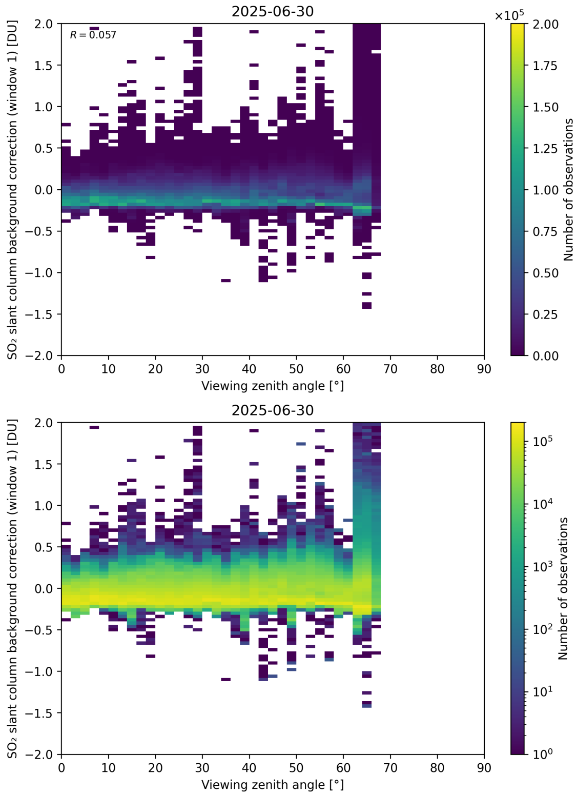
Figure 362: Scatter density plot of “Viewing zenith angle” against “SO 2 slant column background correction (window 1)” for 2025-06-29 to 2025-07-01.
