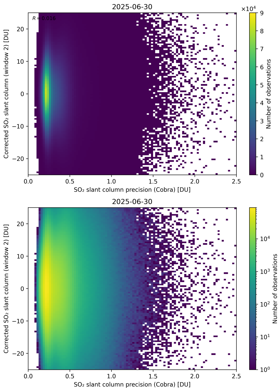
Figure 206: Scatter density plot of “SO 2 slant column precision (Cobra)” against “Corrected SO 2 slant column (window 2)” for 2025-06-29 to 2025-07-01.
