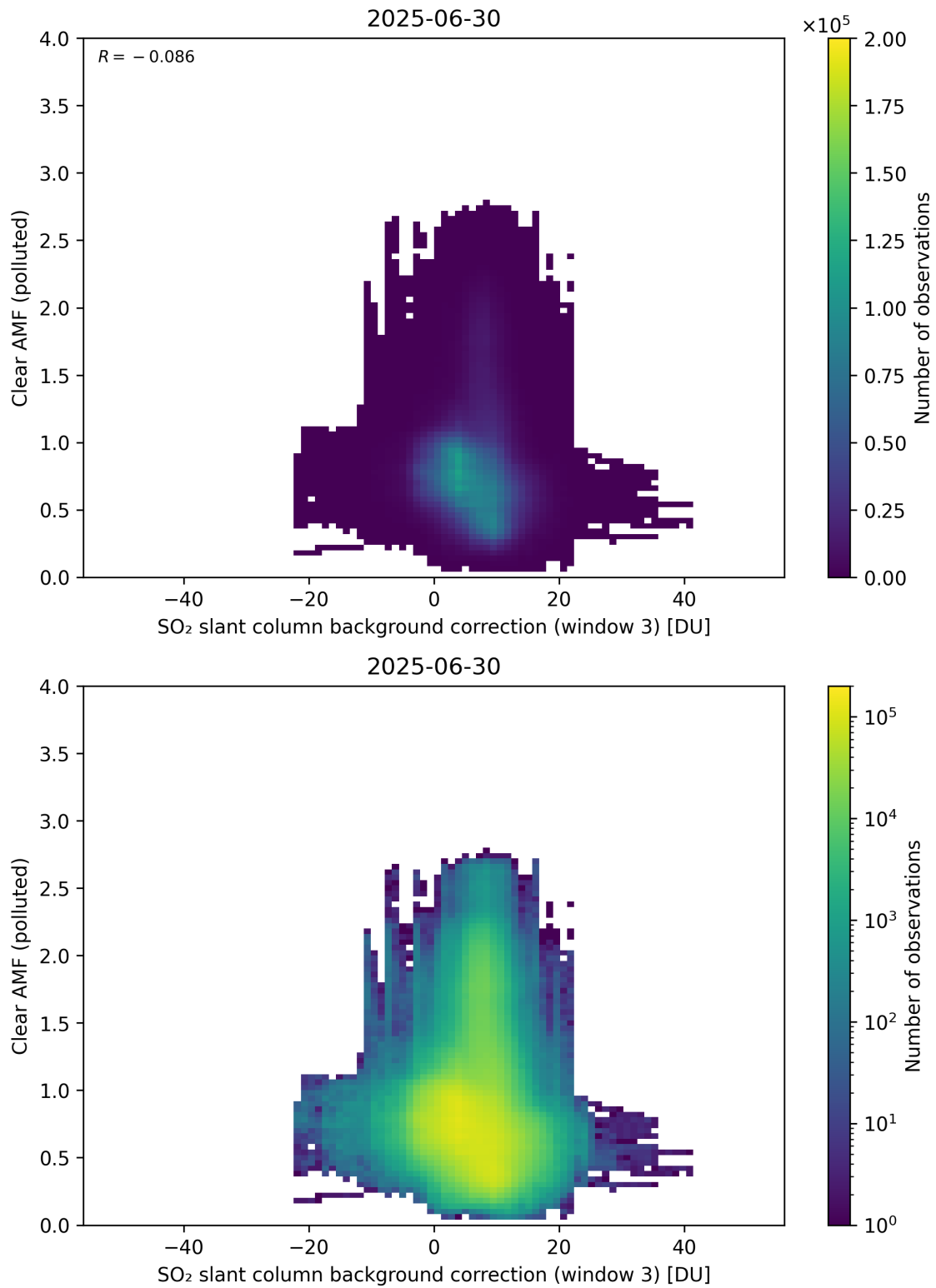
Figure 135: Scatter density plot of “SO 2 slant column background correction (window 3)” against “Clear AMF (polluted)” for 2025-06-29 to 2025-07-01.
