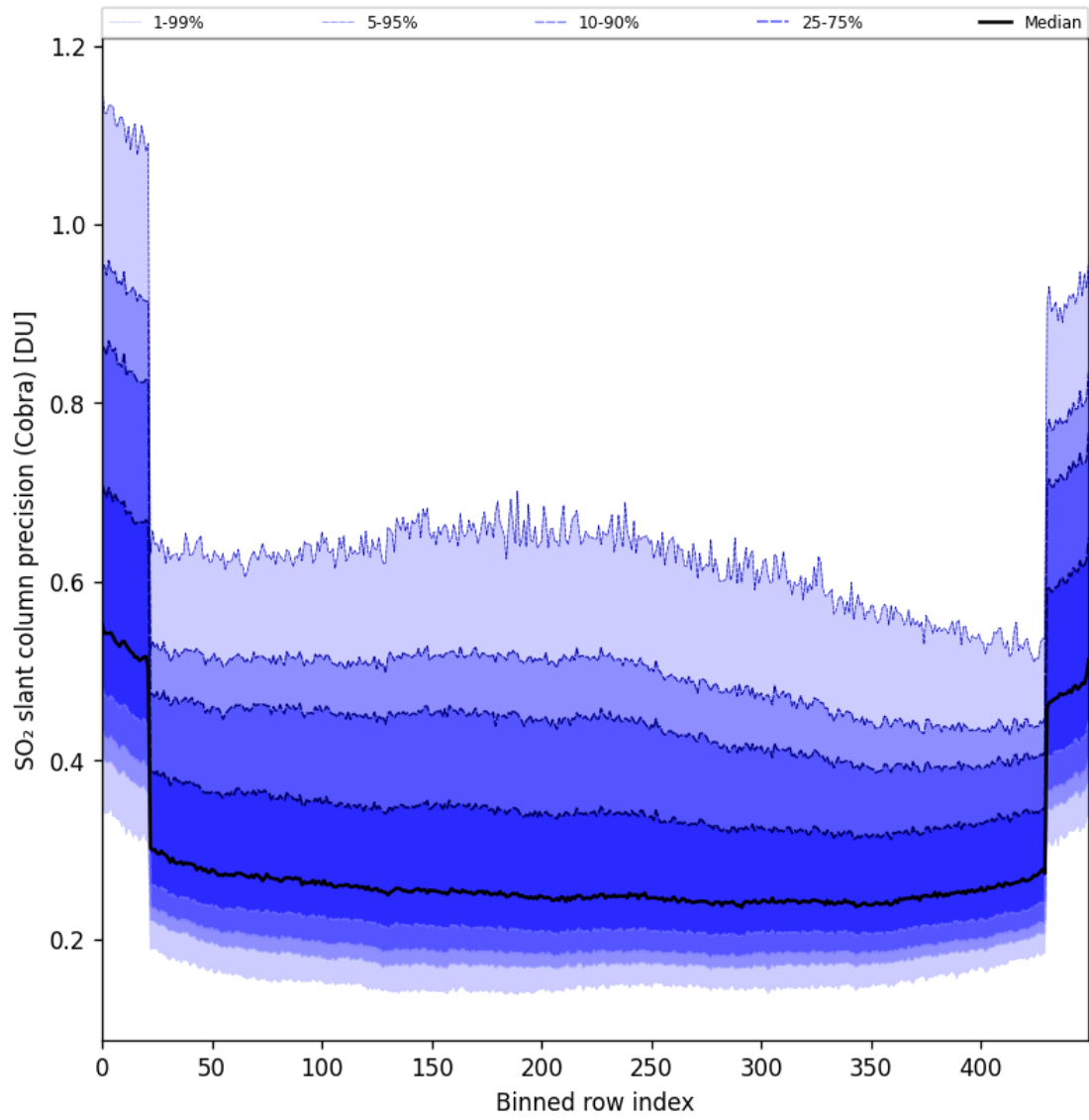
Figure 88: Along track statistics of “SO 2 slant column precision (Cobra)” for 2025-06-29 to 2025-07-01
