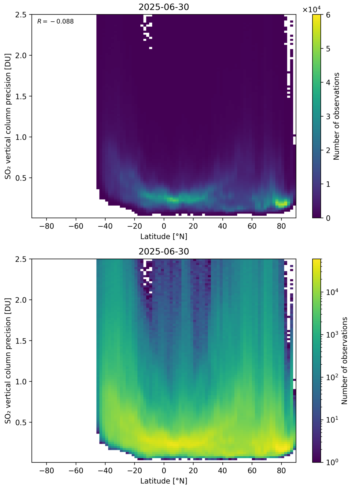
Figure 170: Scatter density plot of “Latitude” against “SO 2 vertical column precision” for 2025-06-29 to 2025-07-01.
