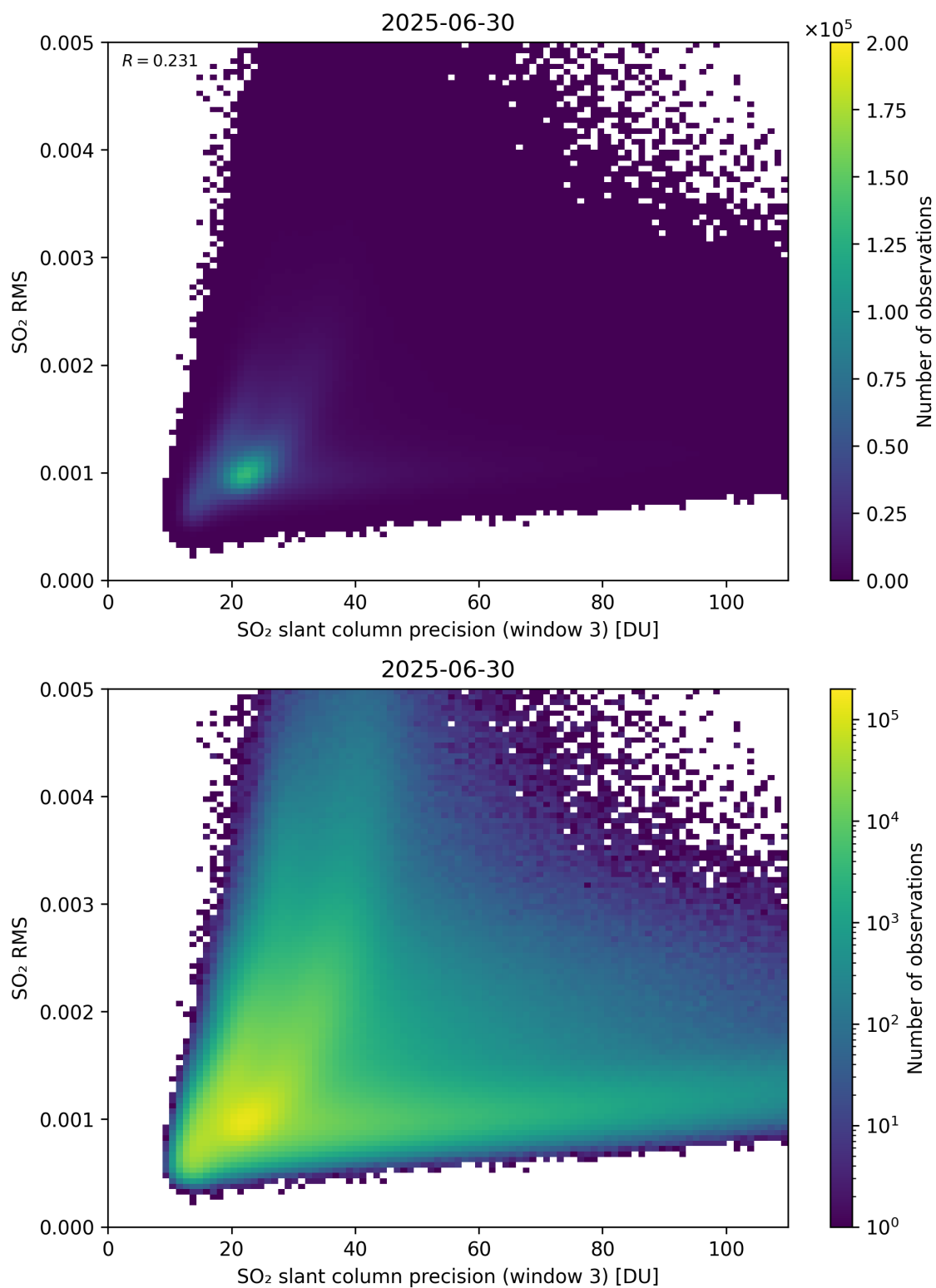
Figure 310: Scatter density plot of “SO 2 slant column precision (window 3)” against “SO 2 RMS” for 2025-06-29 to 2025-07-01.
