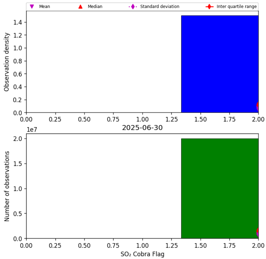
Figure 75: Histogram of “SO 2 Cobra Flag” for 2025-06-29 to 2025-07-01
