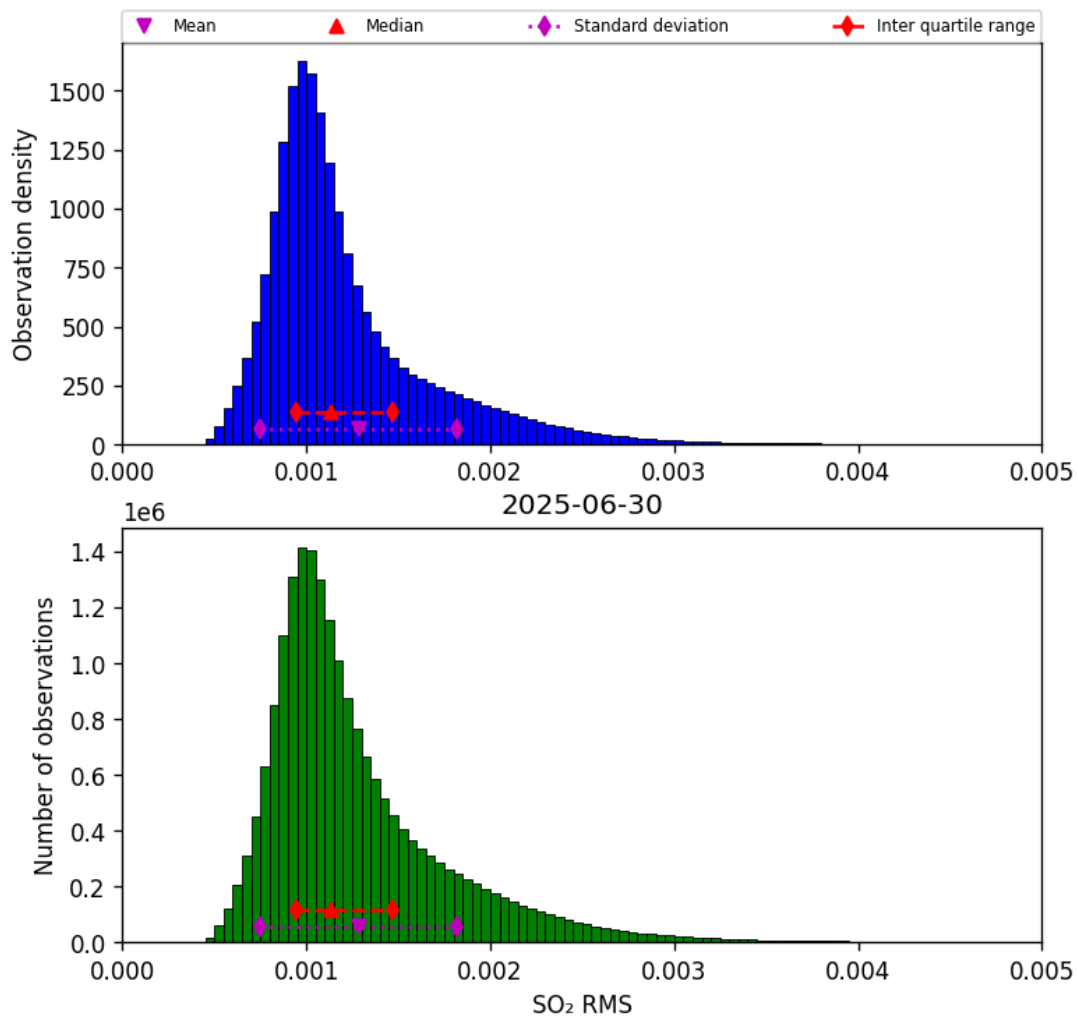
Figure 78: Histogram of “SO 2 RMS” for 2025-06-29 to 2025-07-01
