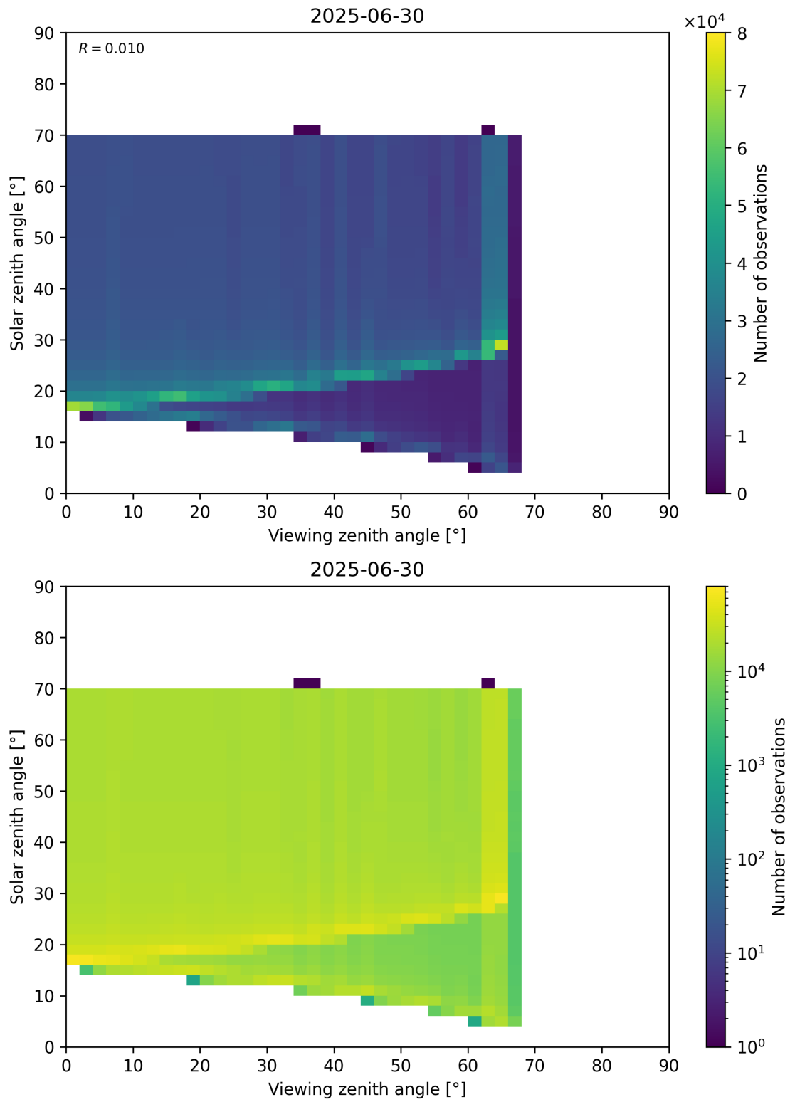
Figure 369: Scatter density plot of “Viewing zenith angle” against “Solar zenith angle” for 2025-06-29 to 2025-07-01.
