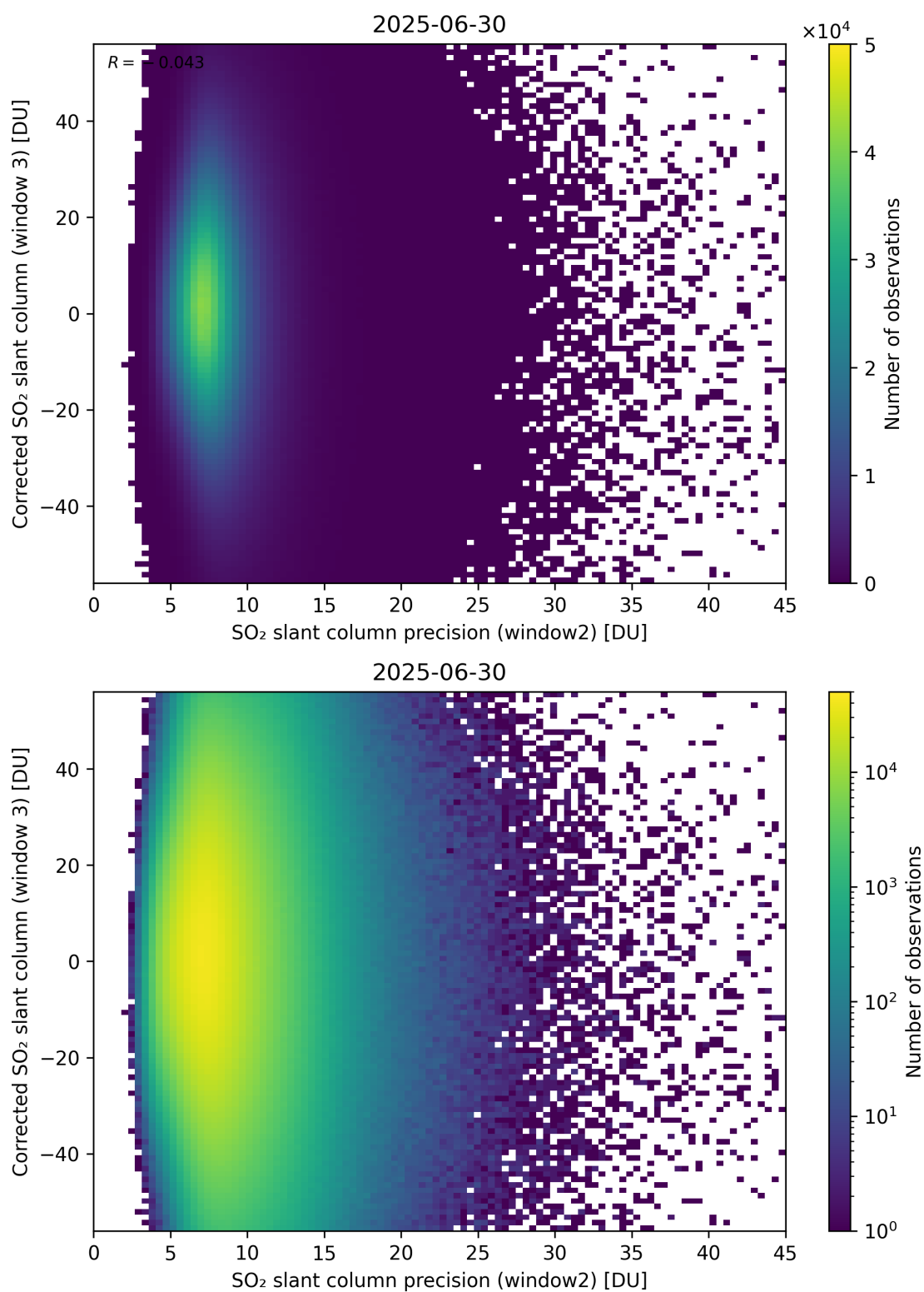
Figure 298: Scatter density plot of “SO 2 slant column precision (window2)” against “Corrected SO 2 slant column (window 3)” for 2025-06-29 to 2025-07-01.
