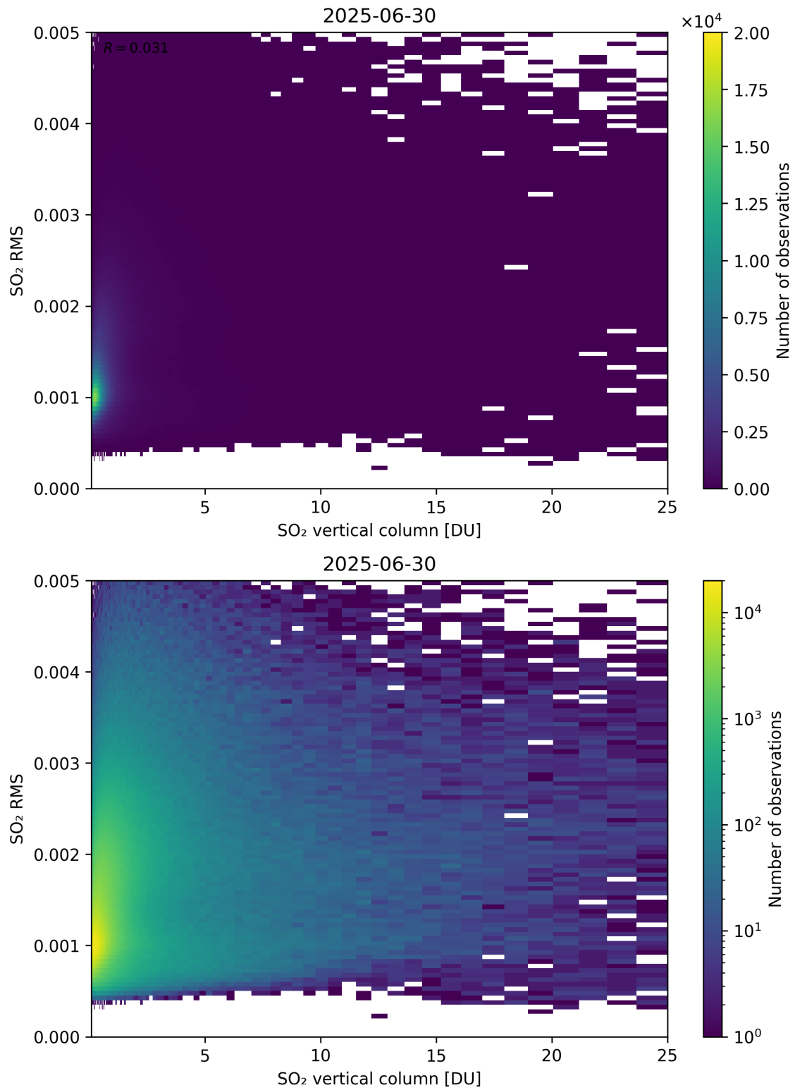
Figure 328: Scatter density plot of “SO 2 vertical column” against “SO 2 RMS” for 2025-06-29 to 2025-07-01.
