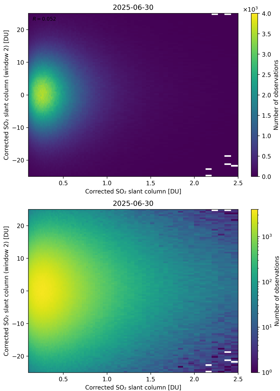
Figure 235: Scatter density plot of “Corrected SO 2 slant column” against “Corrected SO 2 slant column (window 2)” for 2025-06-29 to 2025-07-01.
