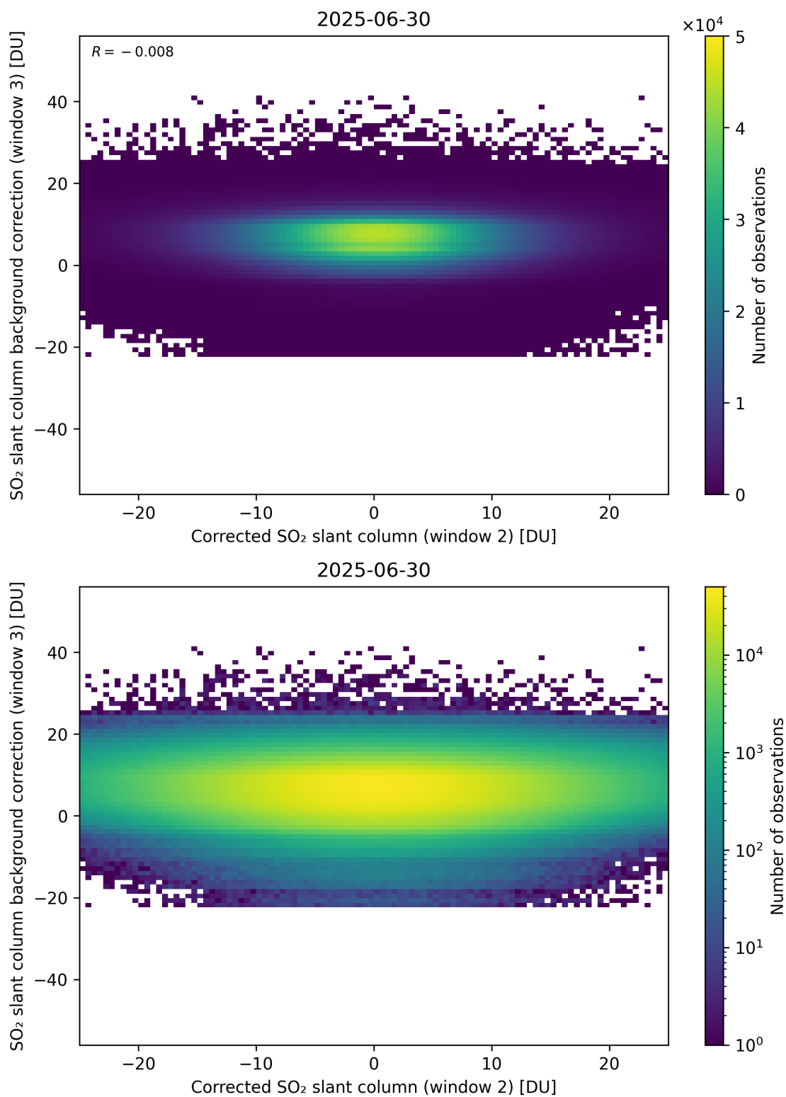
Figure 245: Scatter density plot of “Corrected SO 2 slant column (window 2)” against “SO 2 slant column background correction (window 3)” for 2025-06-29 to 2025-07-01.
