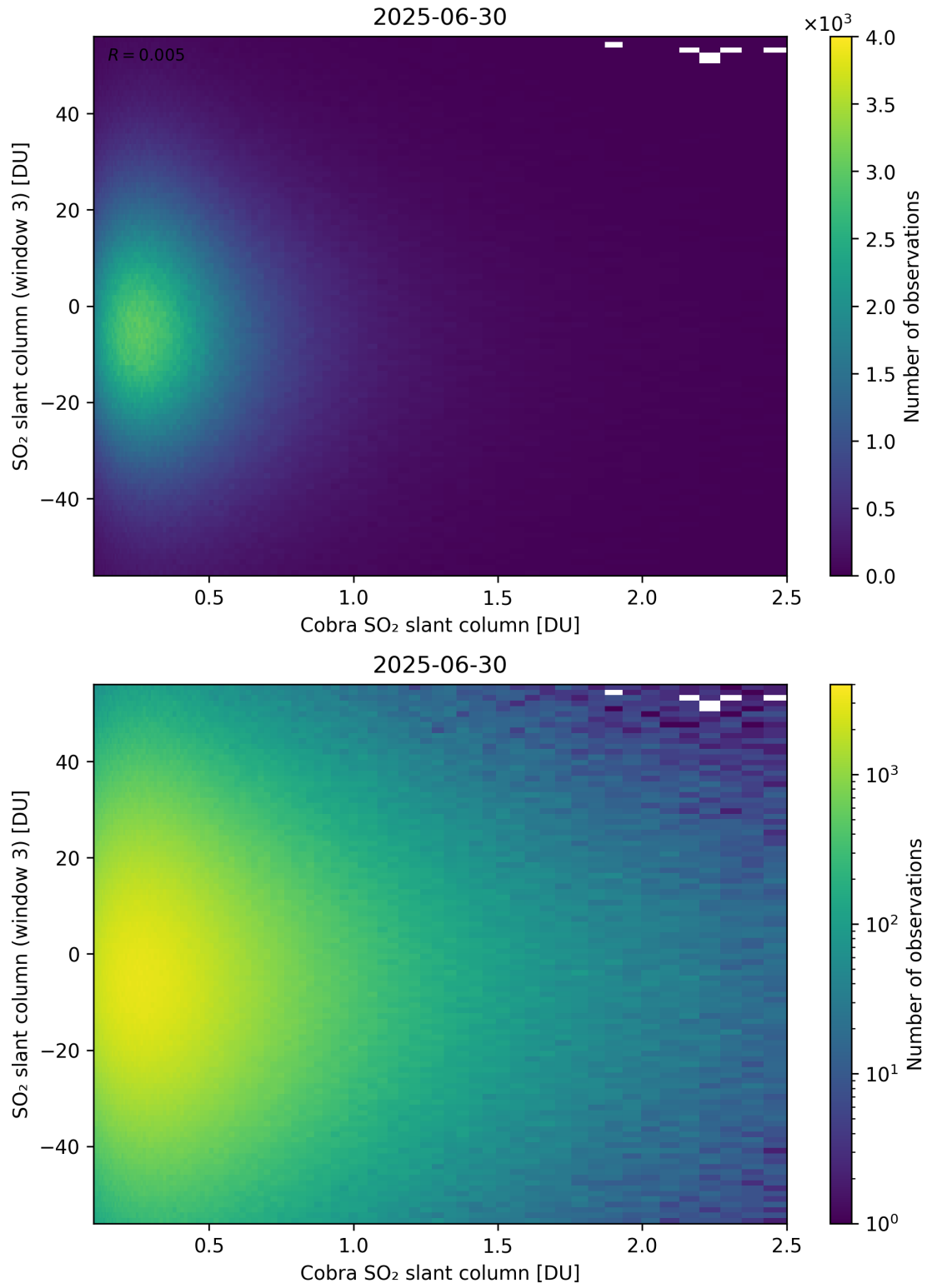
Figure 222: Scatter density plot of “Cobra SO 2 slant column” against “SO 2 slant column (window 3)” for 2025-06-29 to 2025-07-01.
