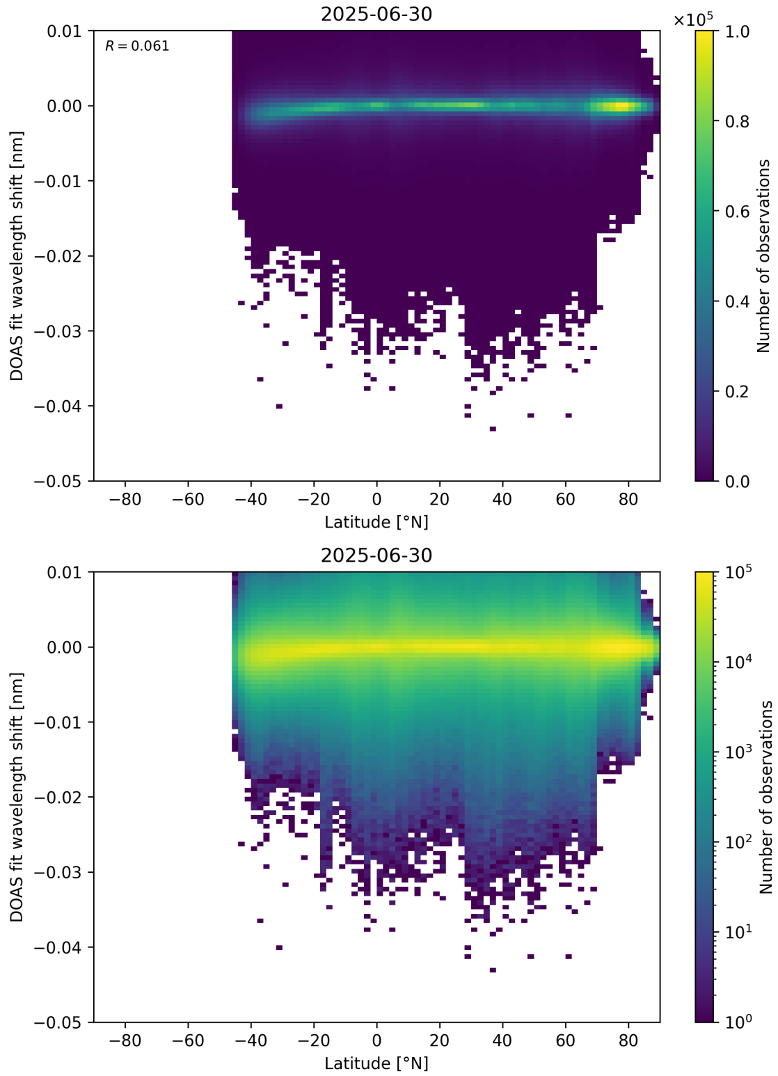
Figure 153: Scatter density plot of “Latitude” against “DOAS fit wavelength shift” for 2025-06-29 to 2025-07-01.
