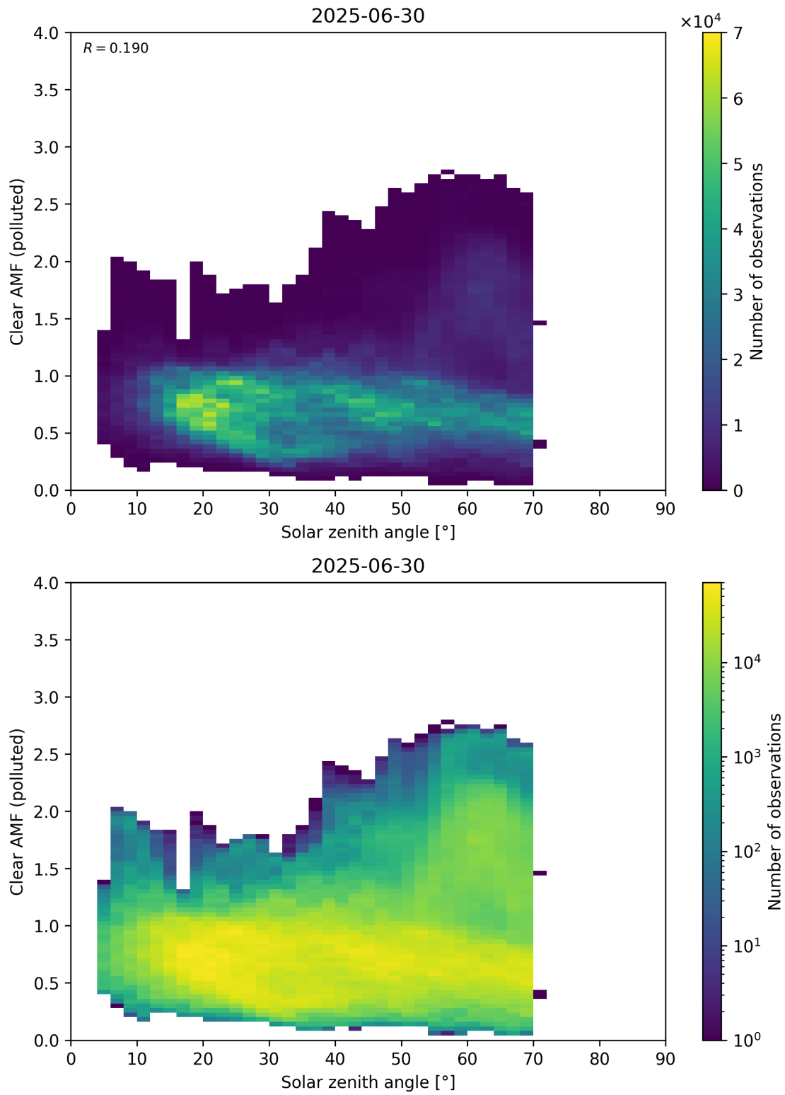
Figure 178: Scatter density plot of “Solar zenith angle” against “Clear AMF (polluted)” for 2025-06-29 to 2025-07-01.
