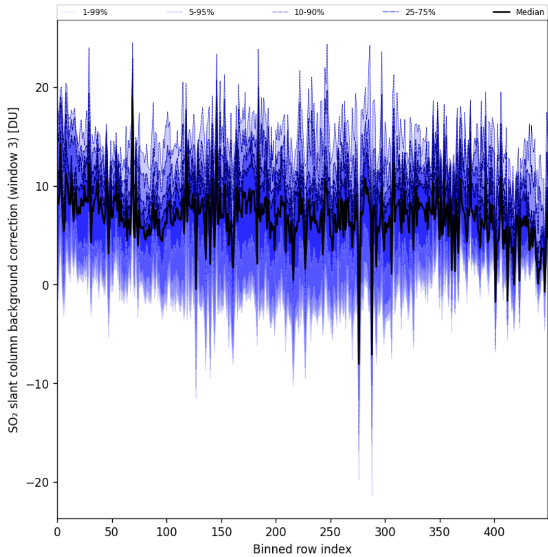
Figure 100: Along track statistics of “SO 2 slant column background correction (window 3)” for 2025-06-29 to 2025-07-01
