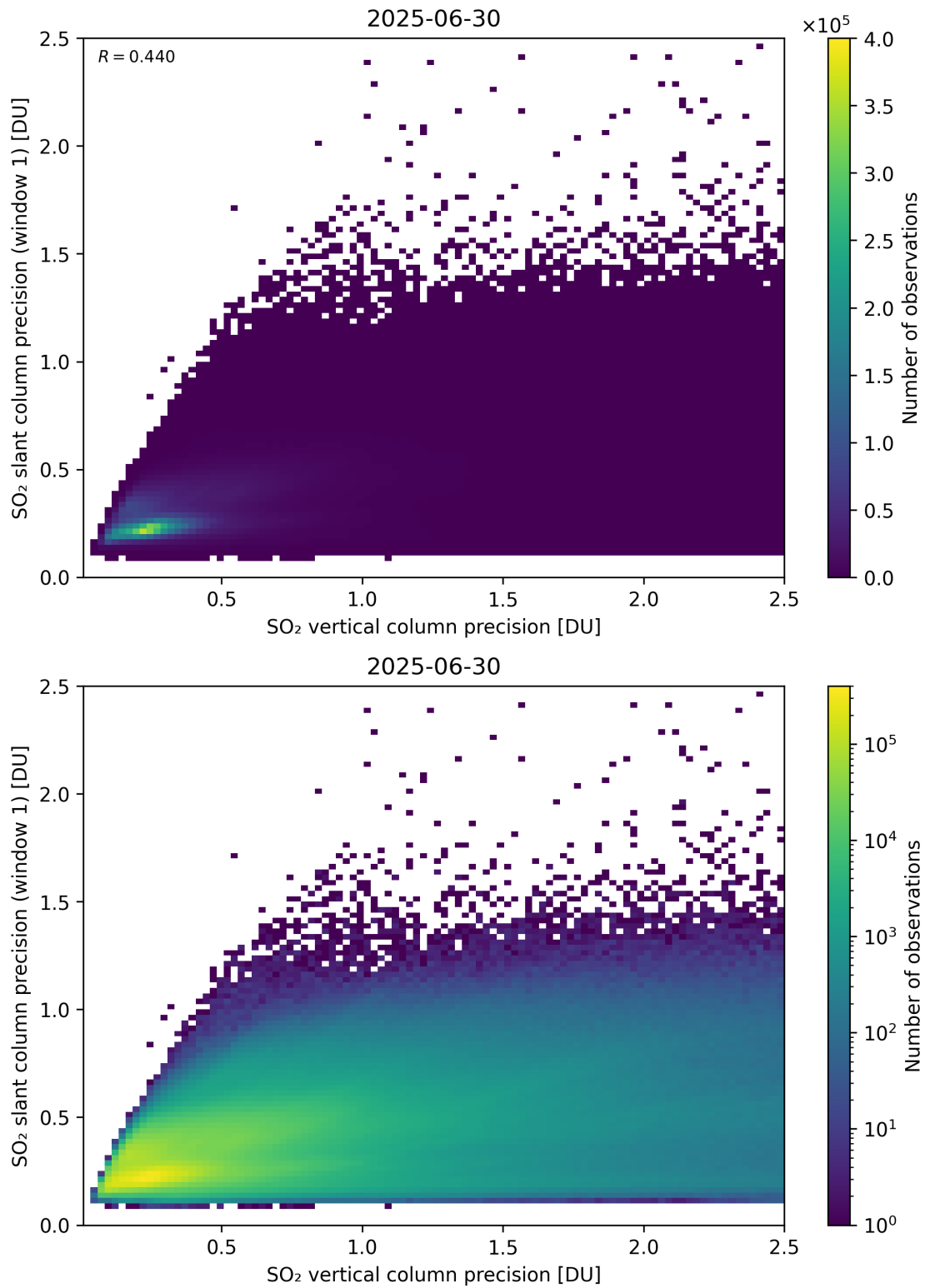
Figure 342: Scatter density plot of “SO 2 vertical column precision” against “SO 2 slant column precision (window 1)” for 2025-06-29 to 2025-07-01.
