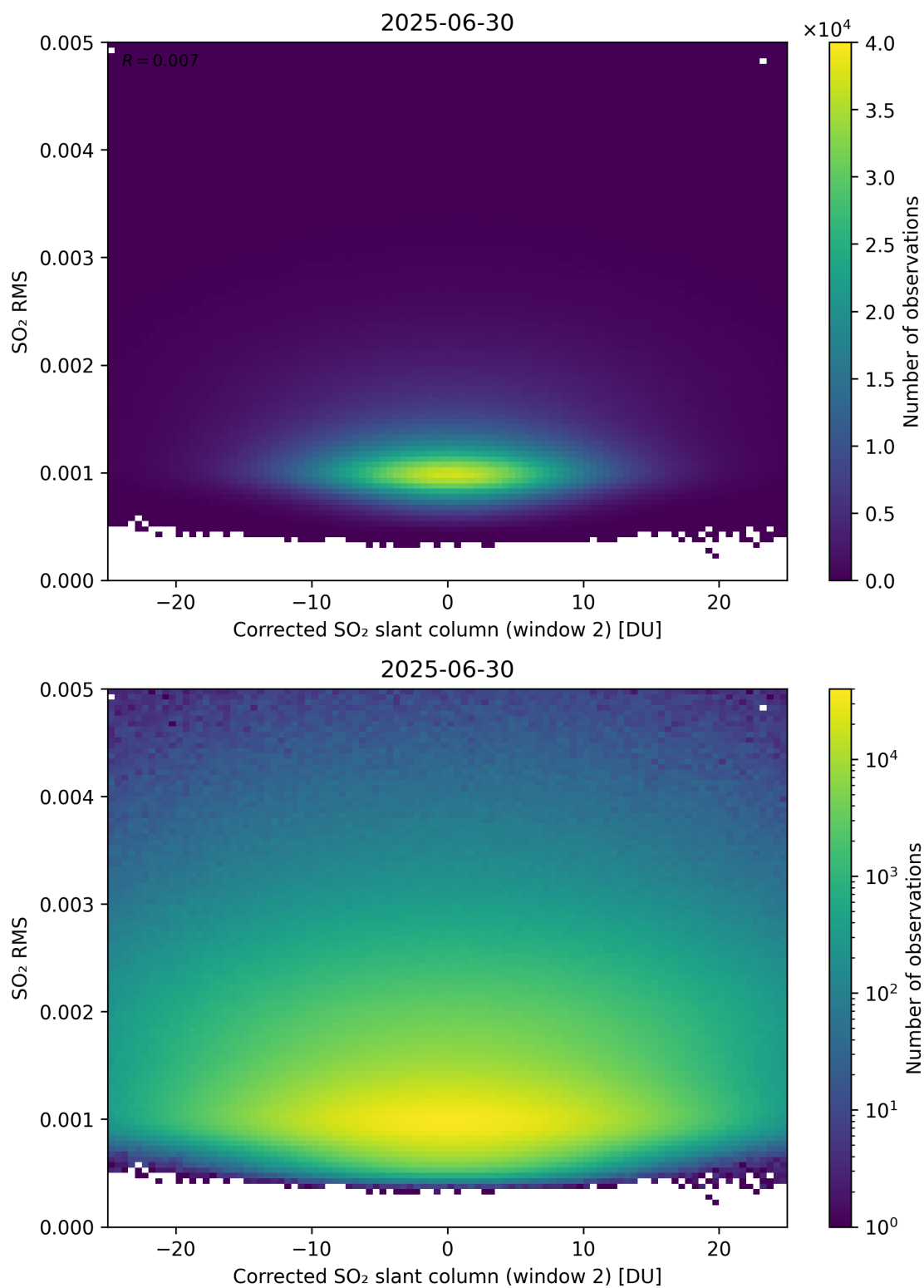
Figure 248: Scatter density plot of “Corrected SO 2 slant column (window 2)” against “SO 2 RMS” for 2025-06-29 to 2025-07-01.
