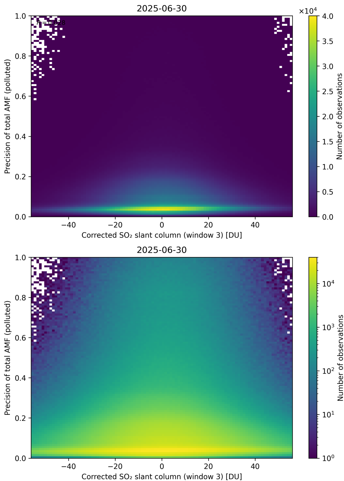
Figure 261: Scatter density plot of “Corrected SO 2 slant column (window 3)” against “Precision of total AMF (polluted)” for 2025-06-29 to 2025-07-01.
