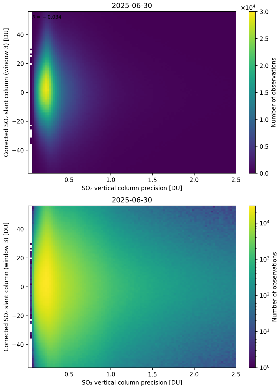
Figure 340: Scatter density plot of “SO 2 vertical column precision” against “Corrected SO 2 slant column (window 3)” for 2025-06-29 to 2025-07-01.
