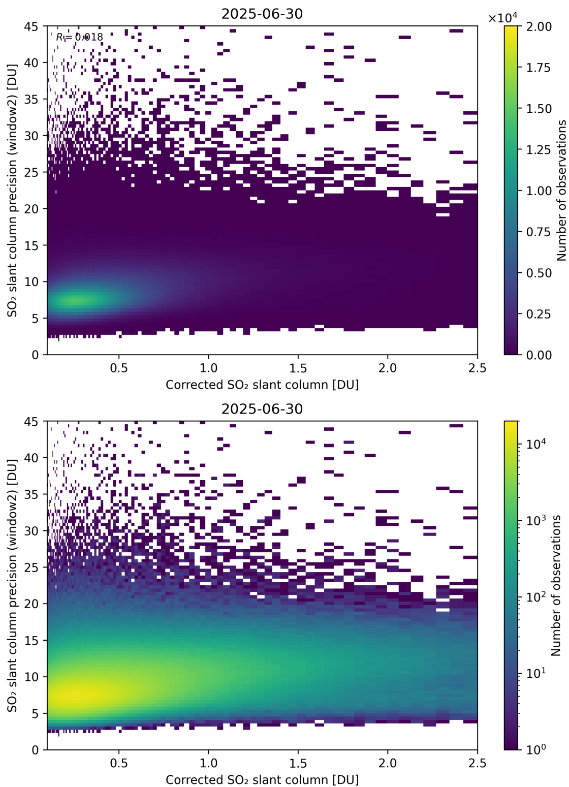
Figure 239: Scatter density plot of “Corrected SO 2 slant column” against “SO 2 slant column precision (window2)” for 2025-06-29 to 2025-07-01.
