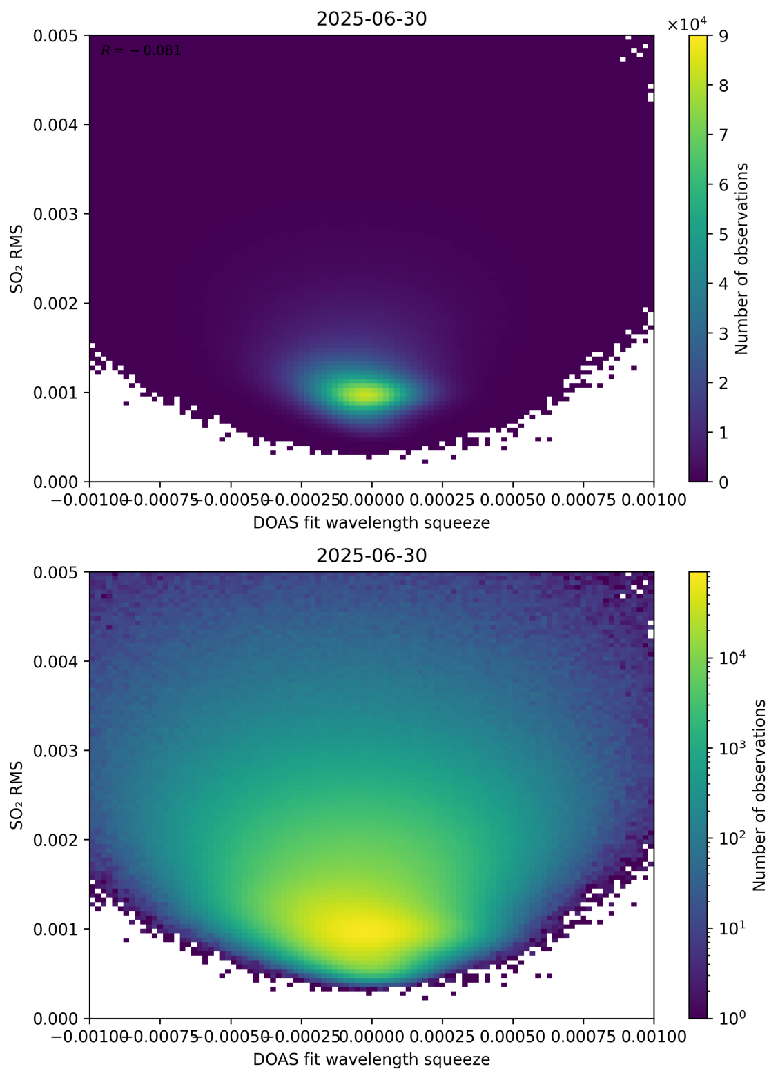
Figure 143: Scatter density plot of “DOAS fit wavelength squeeze” against “SO 2 RMS” for 2025-06-29 to 2025-07-01.
