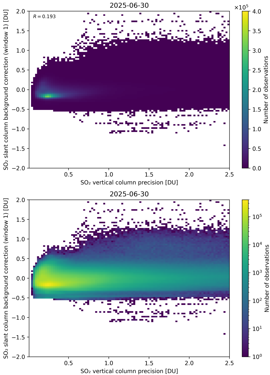
Figure 329: Scatter density plot of “SO 2 vertical column precision” against “SO 2 slant column background correction (window 1)” for 2025-06-29 to 2025-07-01.
