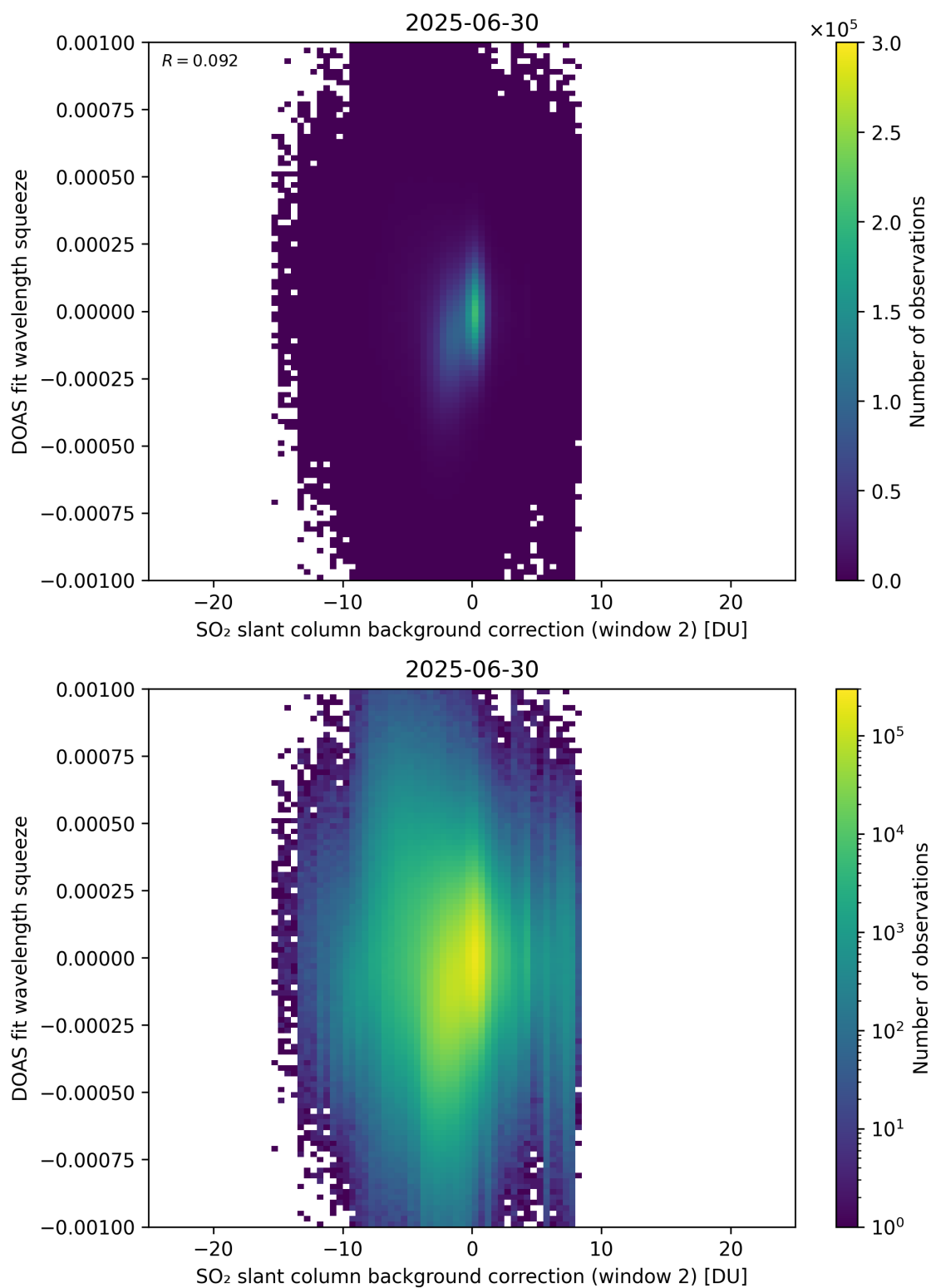
Figure 124: Scatter density plot of “SO 2 slant column background correction (window 2)” against “DOAS fit wavelength squeeze” for 2025-06-29 to 2025-07-01.
