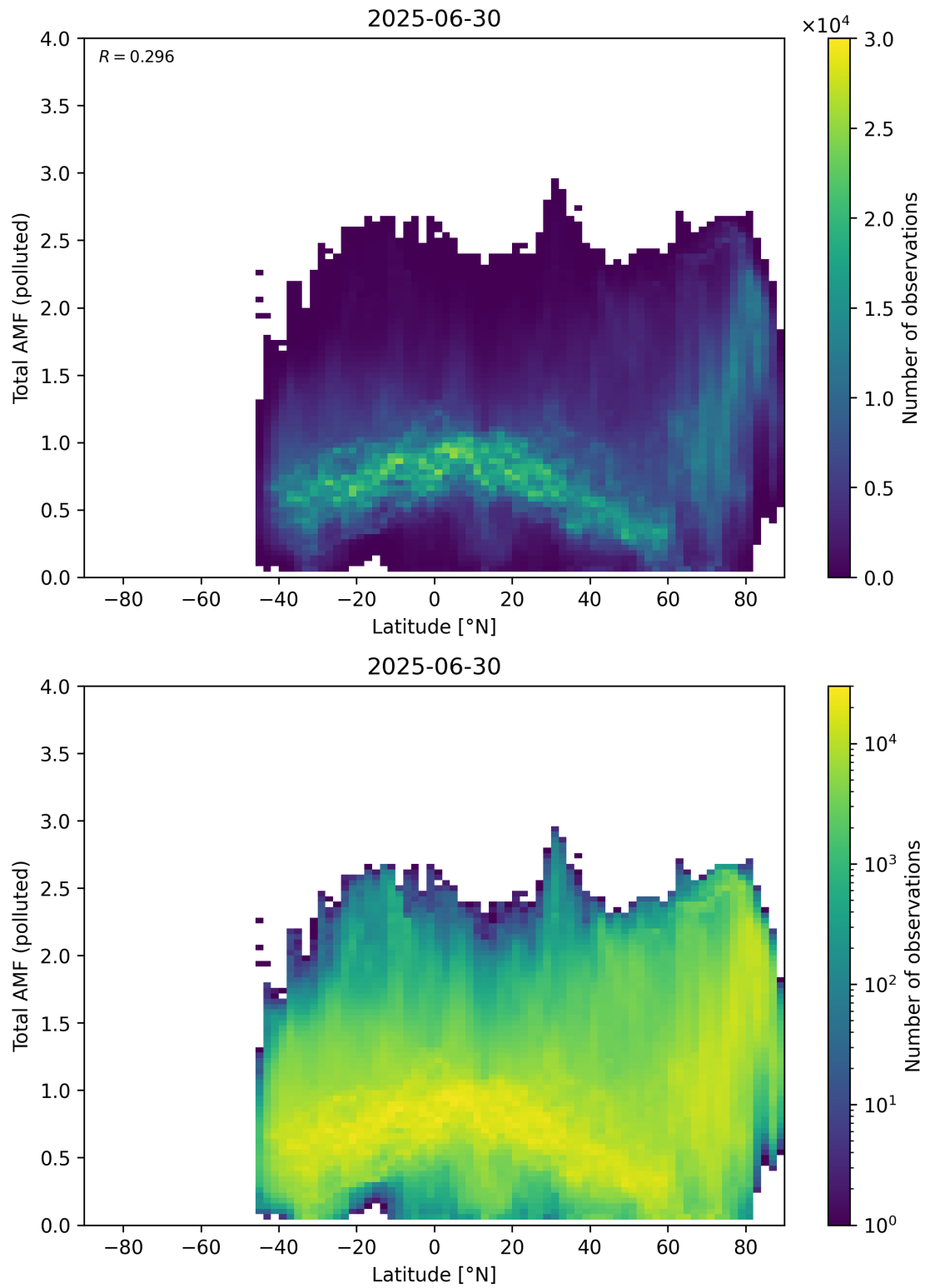
Figure 167: Scatter density plot of “Latitude” against “Total AMF (polluted)” for 2025-06-29 to 2025-07-01.
