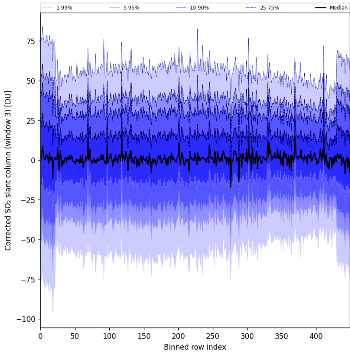
Figure 99: Along track statistics of “Corrected SO 2 slant column (window 3)” for 2025-06-29 to 2025-07-01
