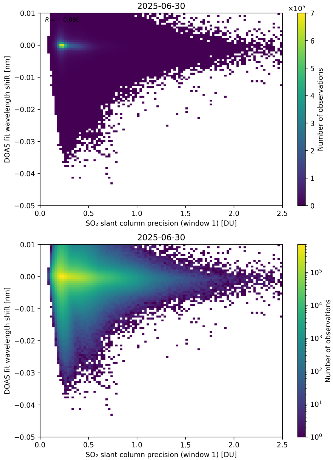
Figure 271: Scatter density plot of “SO 2 slant column precision (window 1)” against “DOAS fit wavelength shift” for 2025-06-29 to 2025-07-01.
