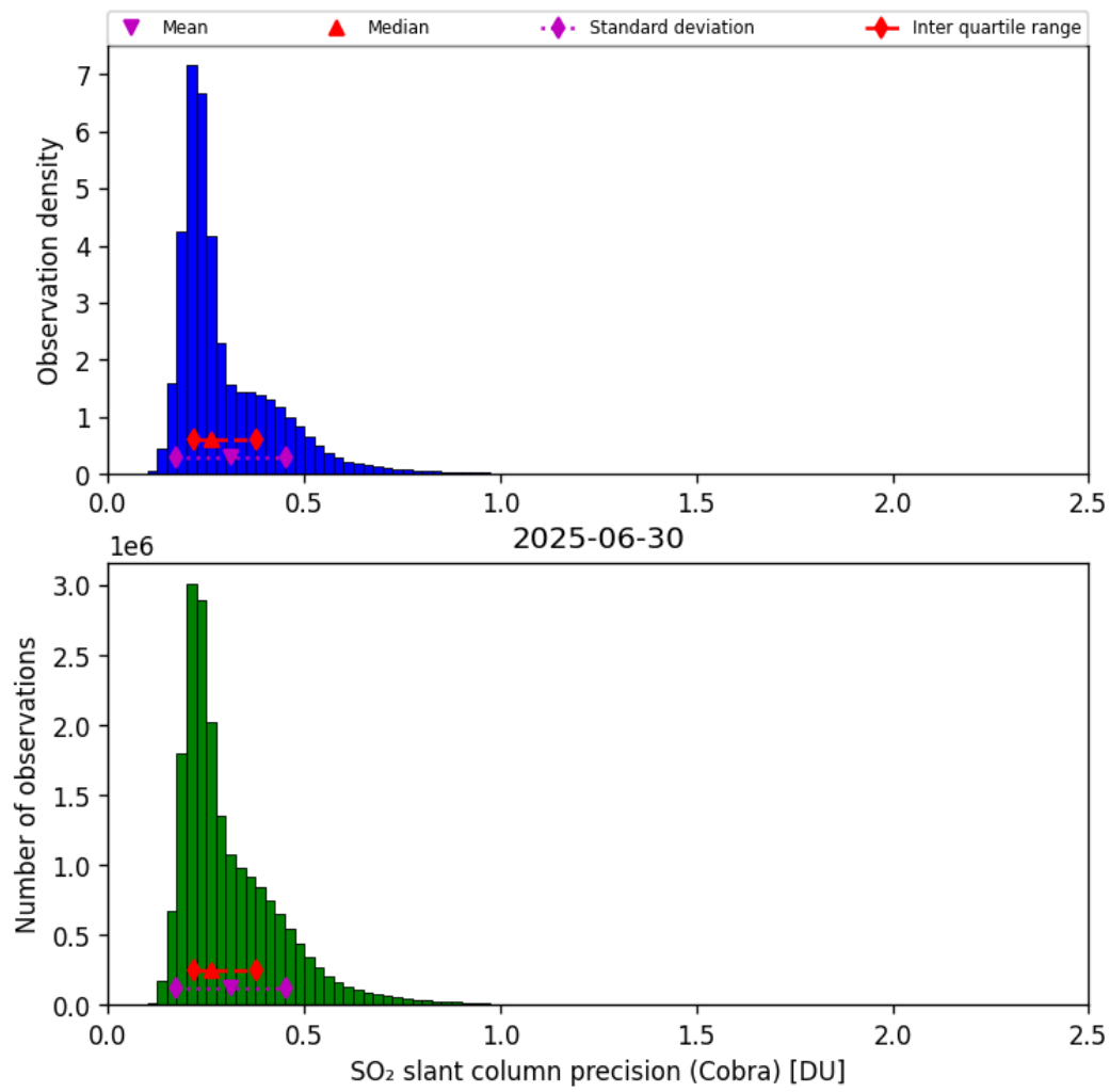
Figure 62: Histogram of “SO 2 slant column precision (Cobra)” for 2025-06-29 to 2025-07-01
