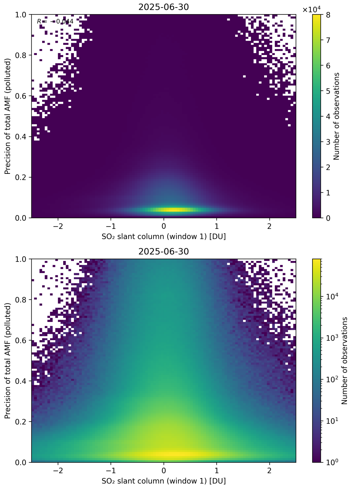
Figure 290: Scatter density plot of “SO 2 slant column (window 1)” against “Precision of total AMF (polluted)” for 2025-06-29 to 2025-07-01.
