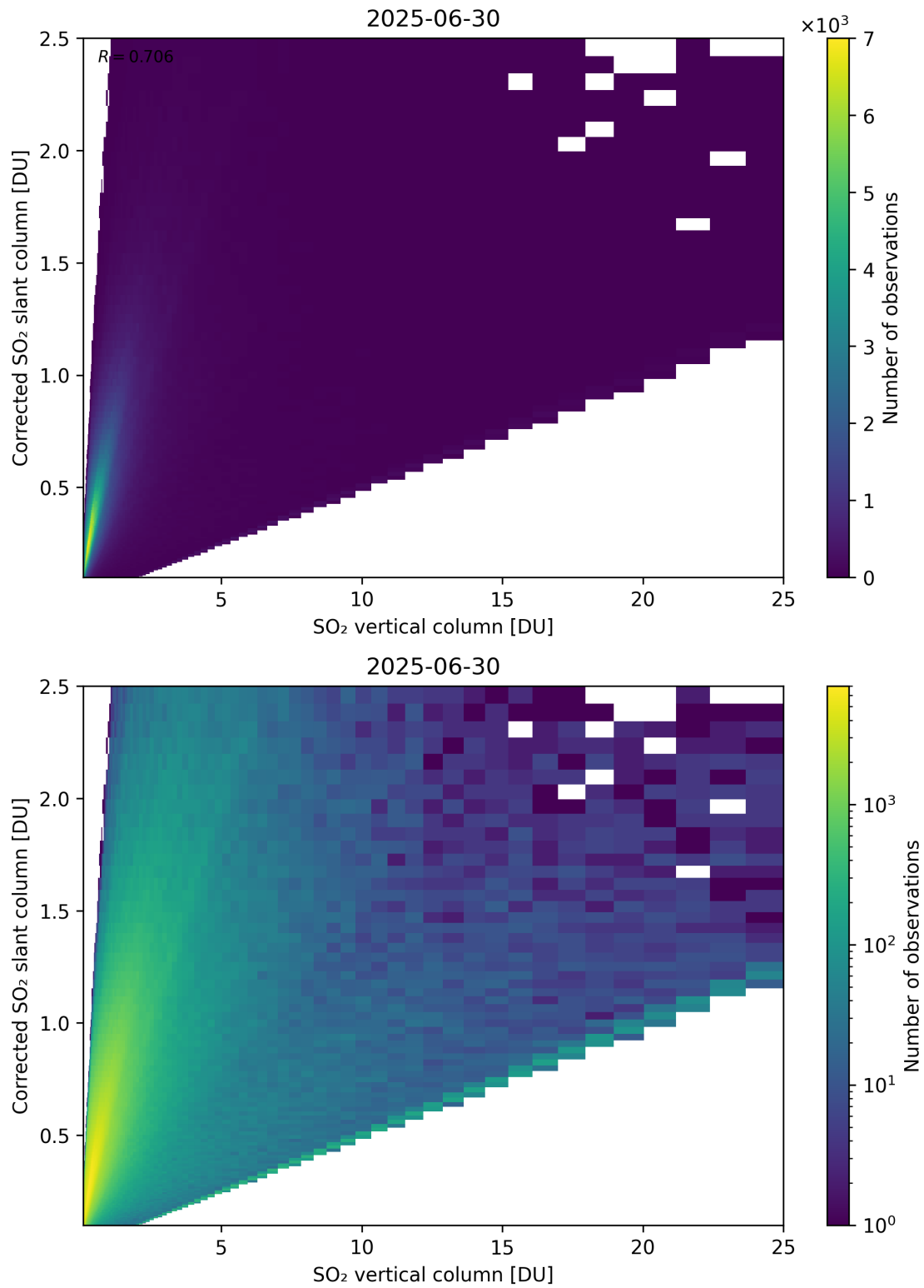
Figure 351: Scatter density plot of “SO 2 vertical column” against “Corrected SO 2 slant column” for 2025-06-29 to 2025-07-01.
