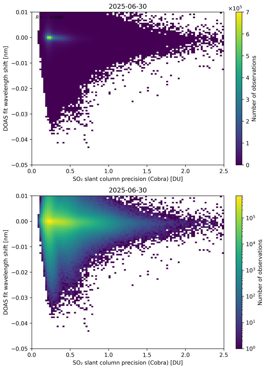
Figure 202: Scatter density plot of “SO 2 slant column precision (Cobra)” against “DOAS fit wavelength shift” for 2025-06-29 to 2025-07-01.
