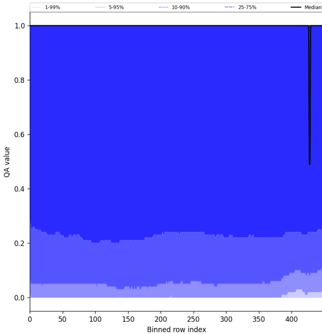
Figure 83: Along track statistics of “QA value” for 2025-06-29 to 2025-07-01
