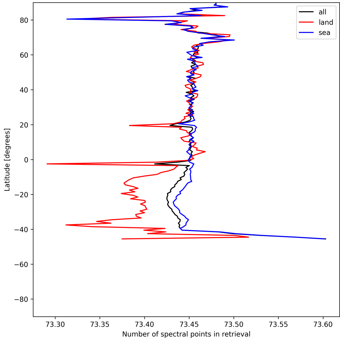
Figure 56: Zonal average of “Number of spectral points in retrieval” for 2025-06-29 to 2025-07-01.
