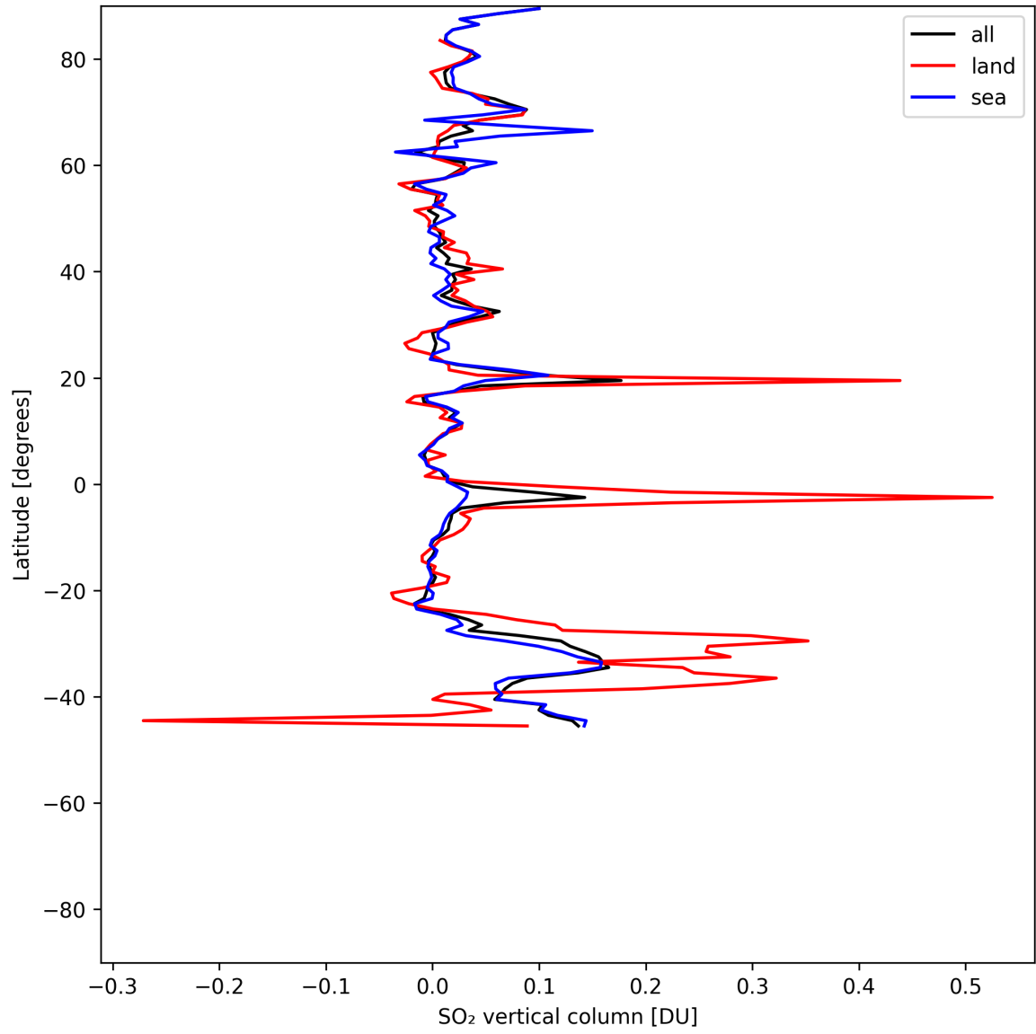
Figure 32: Zonal average of “SO 2 vertical column” for 2025-06-29 to 2025-07-01.
