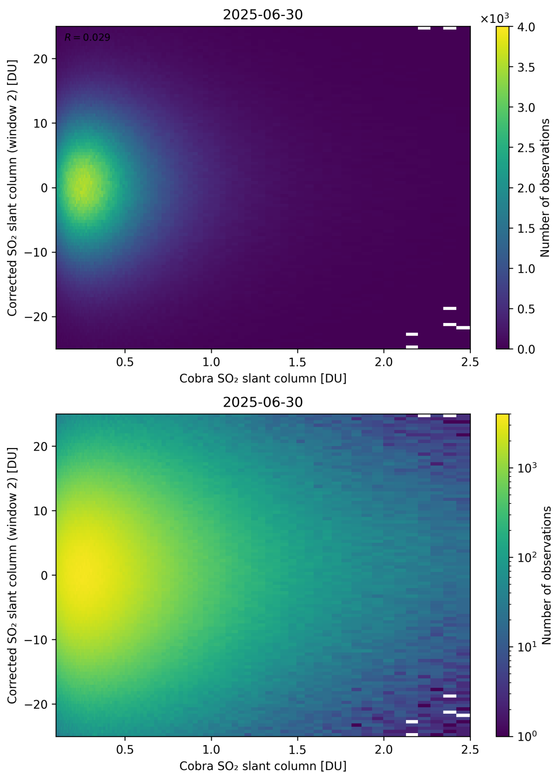
Figure 217: Scatter density plot of “Cobra SO 2 slant column” against “Corrected SO 2 slant column (window 2)” for 2025-06-29 to 2025-07-01.
