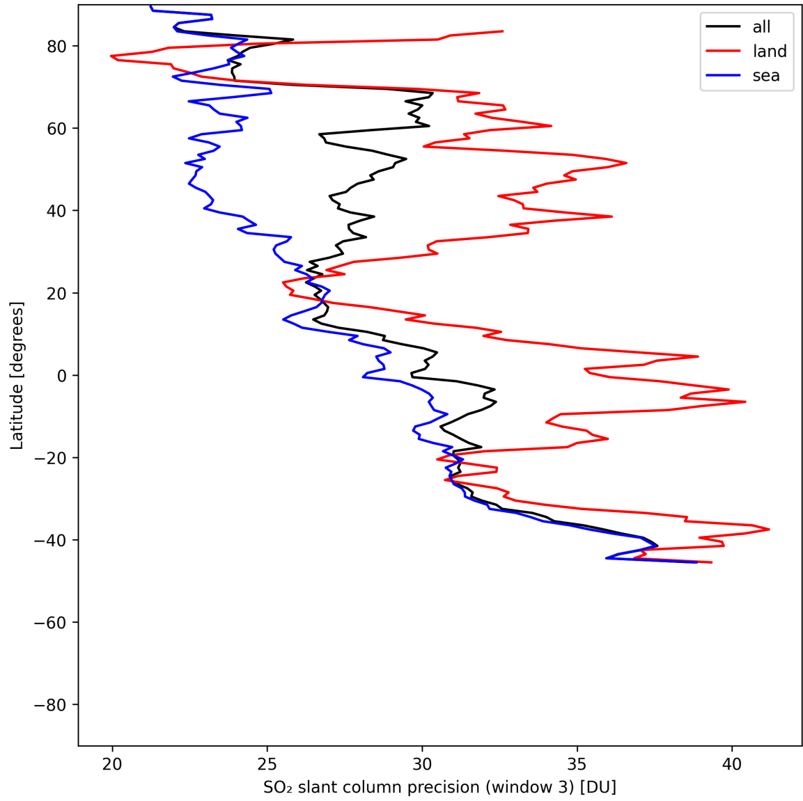
Figure 46: Zonal average of “SO 2 slant column precision (window 3)” for 2025-06-29 to 2025-07-01.
