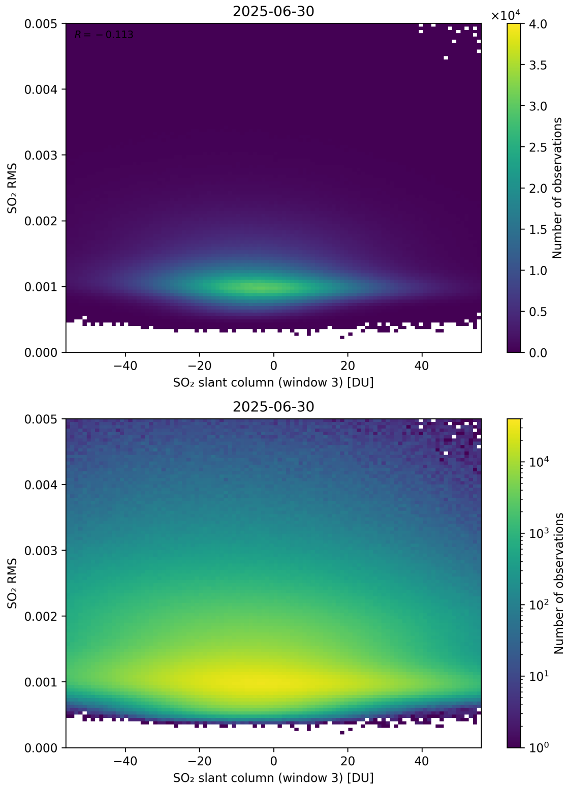
Figure 306: Scatter density plot of “SO 2 slant column (window 3)” against “SO 2 RMS” for 2025-06-29 to 2025-07-01.
