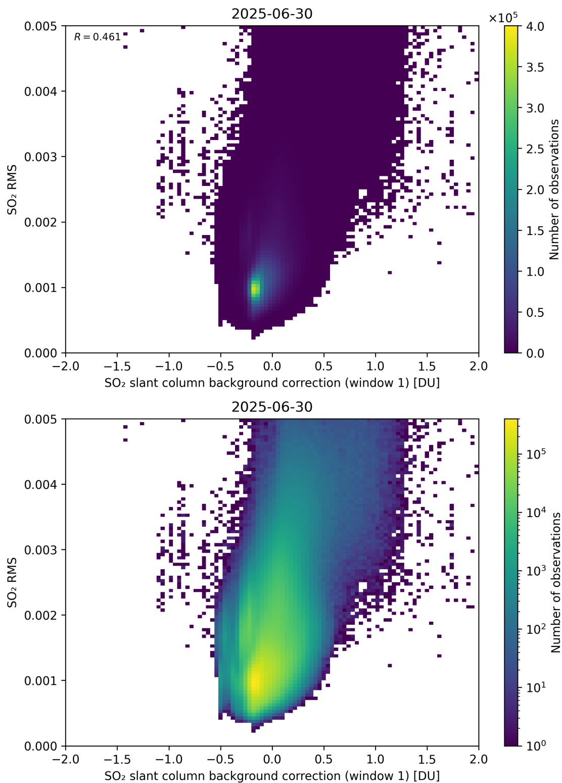
Figure 113: Scatter density plot of “SO 2 slant column background correction (window 1)” against “SO 2 RMS” for 2025-06-29 to 2025-07-01.
