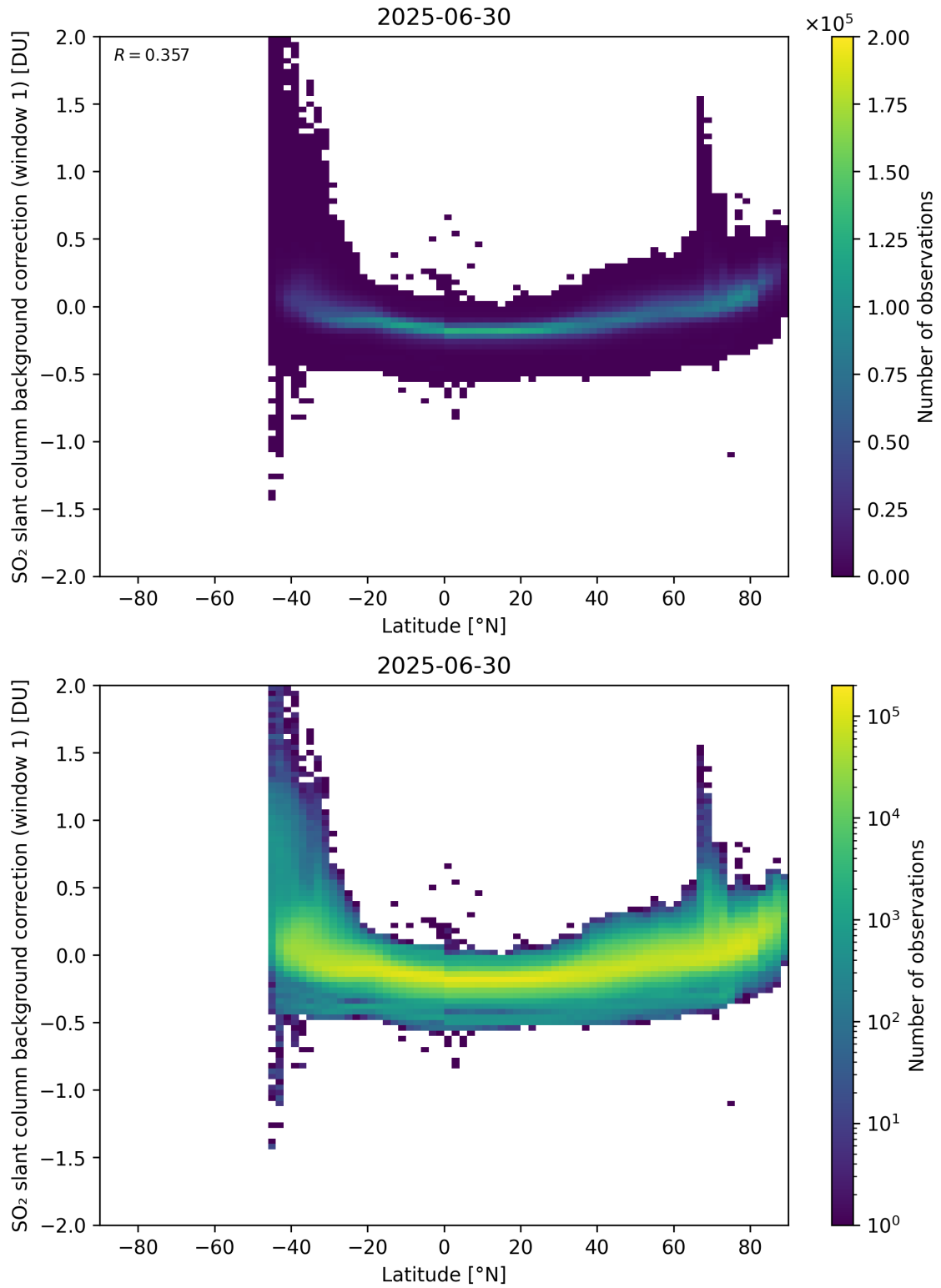
Figure 150: Scatter density plot of “Latitude” against “SO 2 slant column background correction (window 1)” for 2025-06-29 to 2025-07-01.
