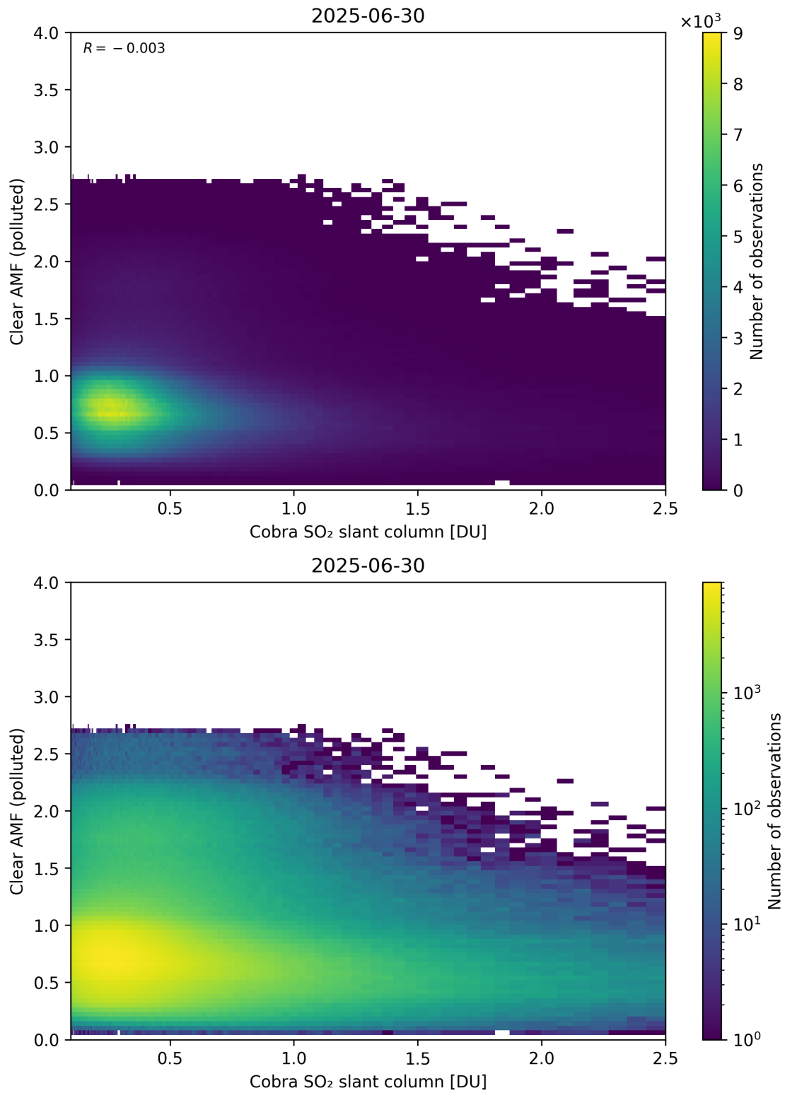
Figure 215: Scatter density plot of “Cobra SO 2 slant column” against “Clear AMF (polluted)” for 2025-06-29 to 2025-07-01.
