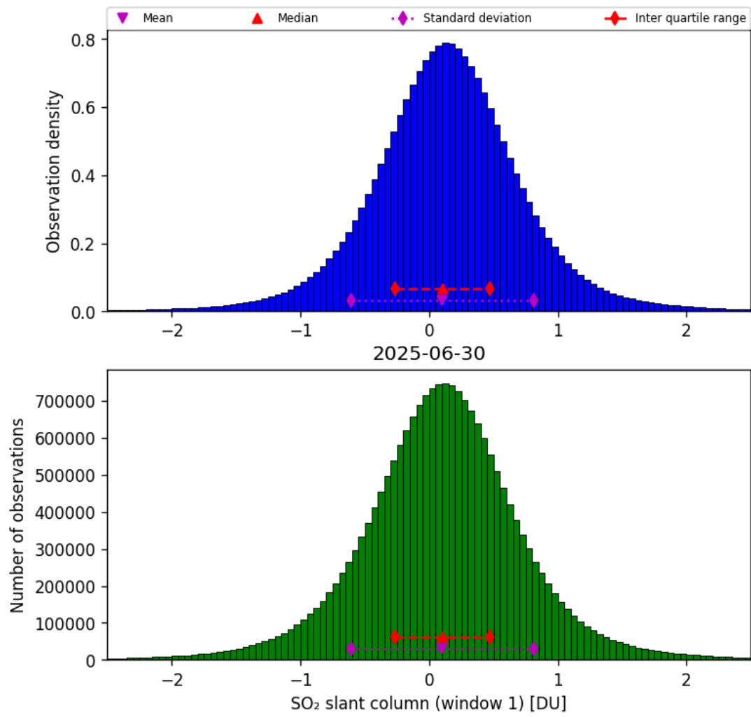
Figure 63: Histogram of “SO 2 slant column (window 1)” for 2025-06-29 to 2025-07-01
