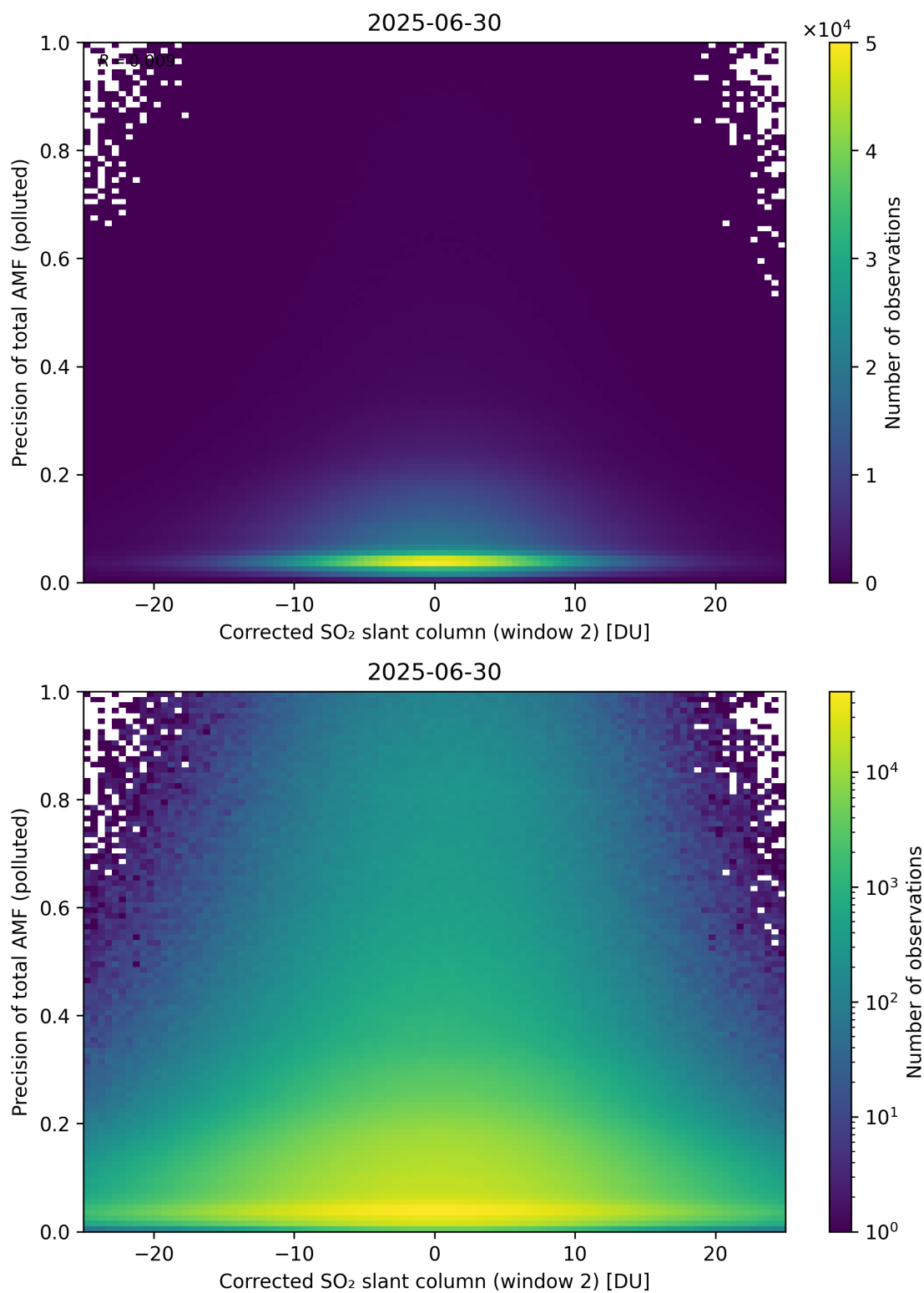
Figure 254: Scatter density plot of “Corrected SO 2 slant column (window 2)” against “Precision of total AMF (polluted)” for 2025-06-29 to 2025-07-01.
