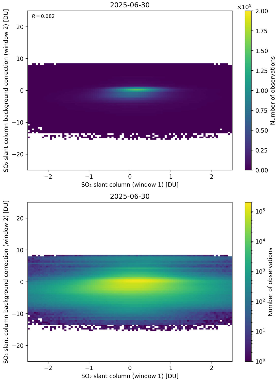
Figure 263: Scatter density plot of “SO 2 slant column (window 1)” against “SO 2 slant column background correction (window 2)” for 2025-06-29 to 2025-07-01.
