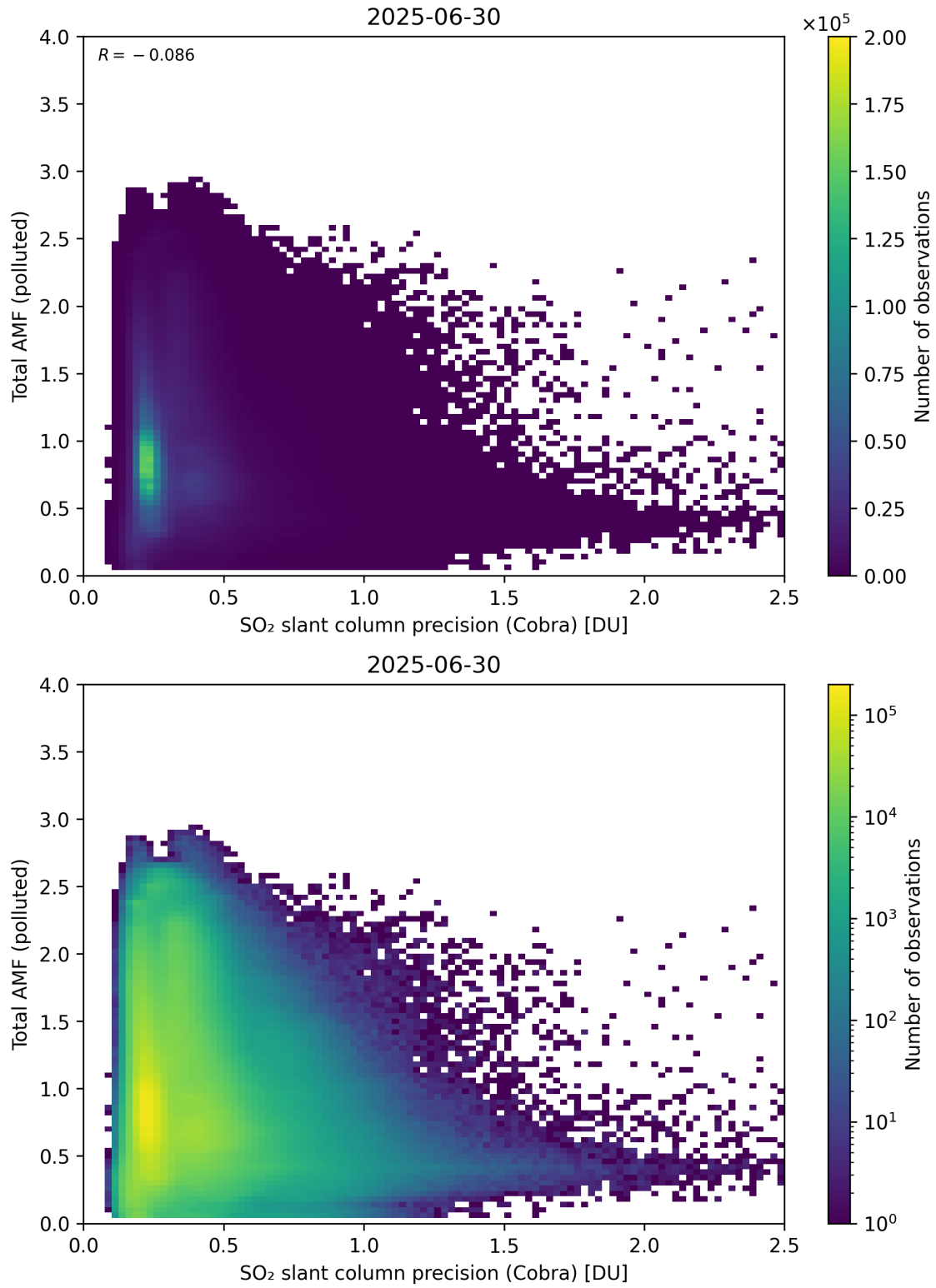
Figure 213: Scatter density plot of “SO 2 slant column precision (Cobra)” against “Total AMF (polluted)” for 2025-06-29 to 2025-07-01.
