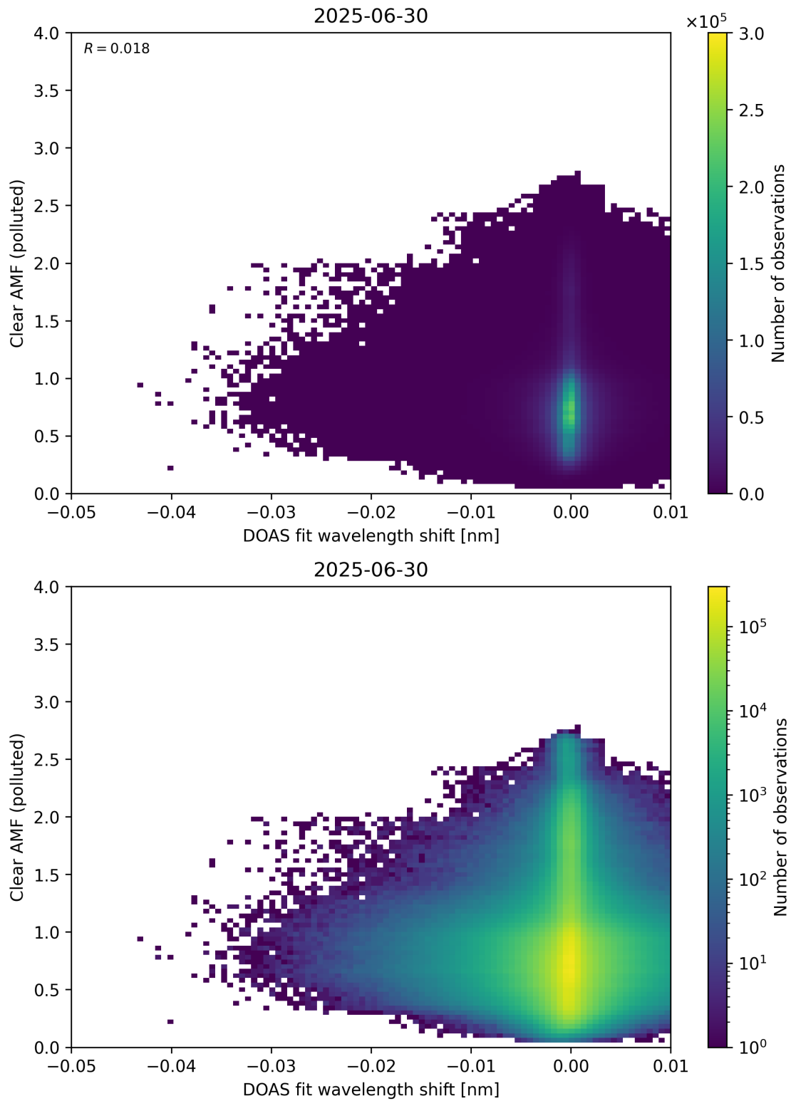
Figure 140: Scatter density plot of “DOAS fit wavelength shift” against “Clear AMF (polluted)” for 2025-06-29 to 2025-07-01.
