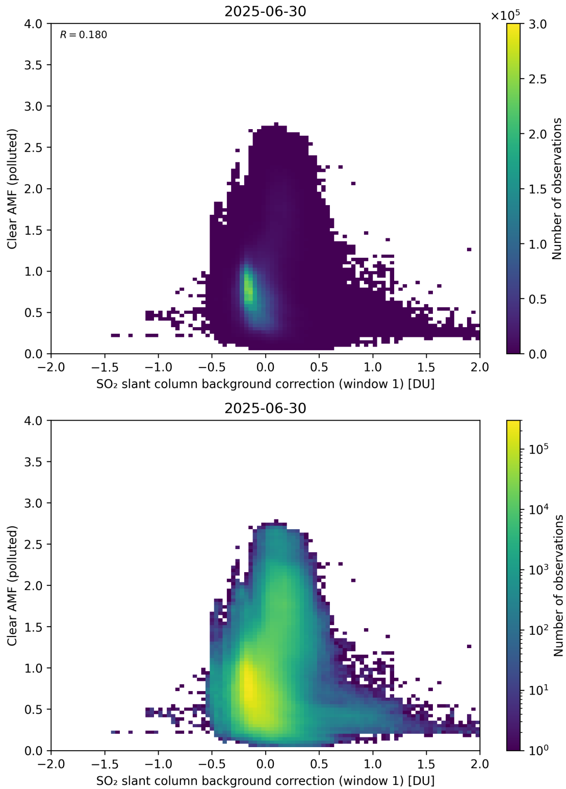
Figure 114: Scatter density plot of “SO 2 slant column background correction (window 1)” against “Clear AMF (polluted)” for 2025-06-29 to 2025-07-01.
