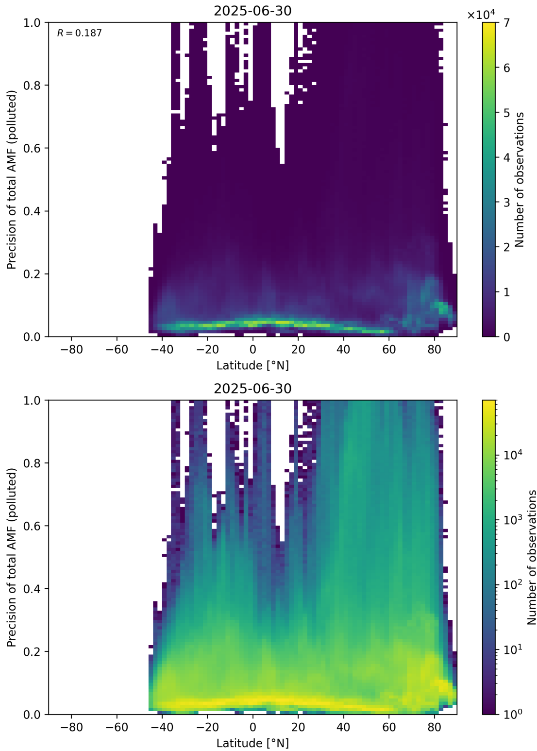
Figure 168: Scatter density plot of “Latitude” against “Precision of total AMF (polluted)” for 2025-06-29 to 2025-07-01.
