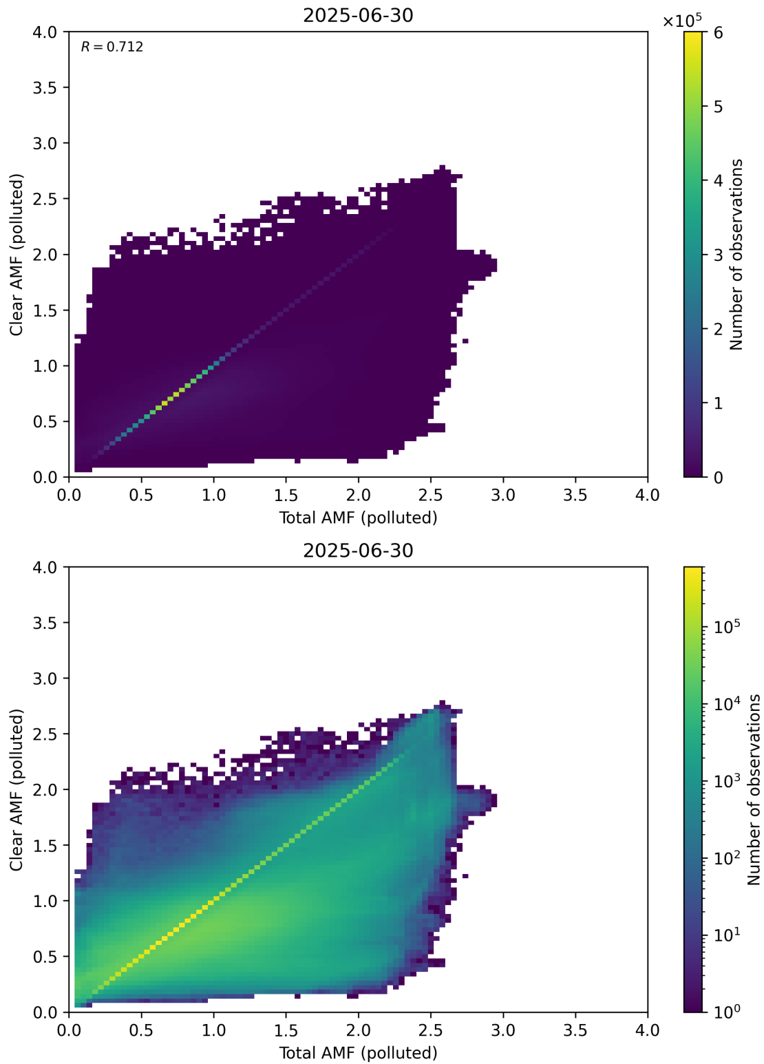
Figure 321: Scatter density plot of “Total AMF (polluted)” against “Clear AMF (polluted)” for 2025-06-29 to 2025-07-01.
