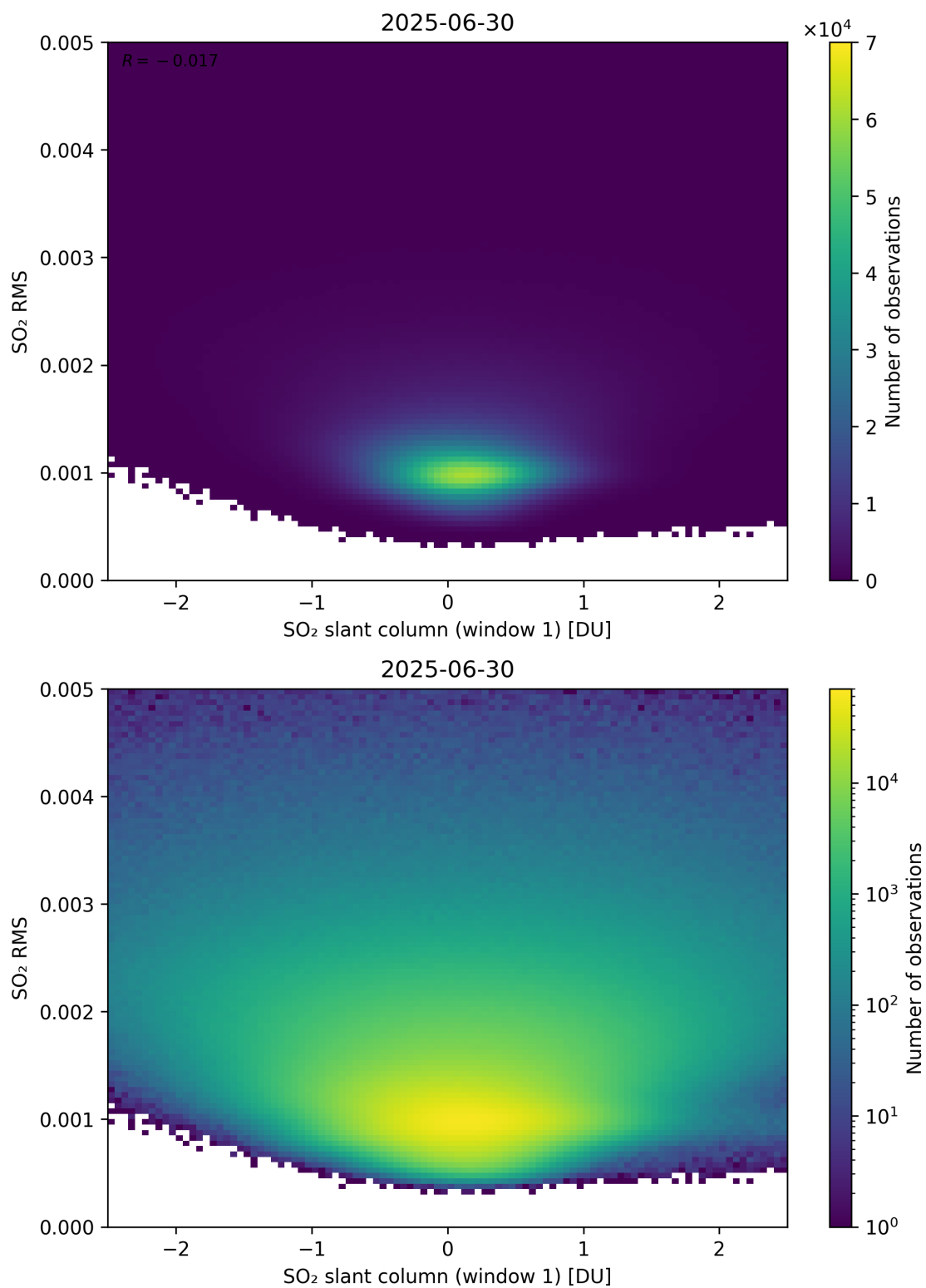
Figure 267: Scatter density plot of “SO 2 slant column (window 1)” against “SO 2 RMS” for 2025-06-29 to 2025-07-01.
