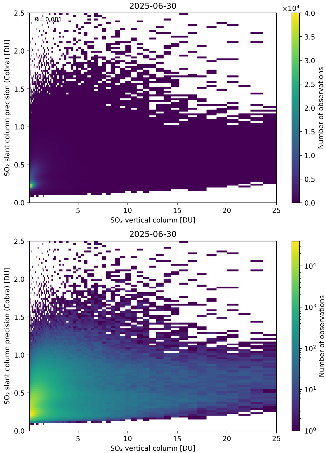
Figure 350: Scatter density plot of “SO 2 vertical column” against “SO 2 slant column precision (Cobra)” for 2025-06-29 to 2025-07-01.
