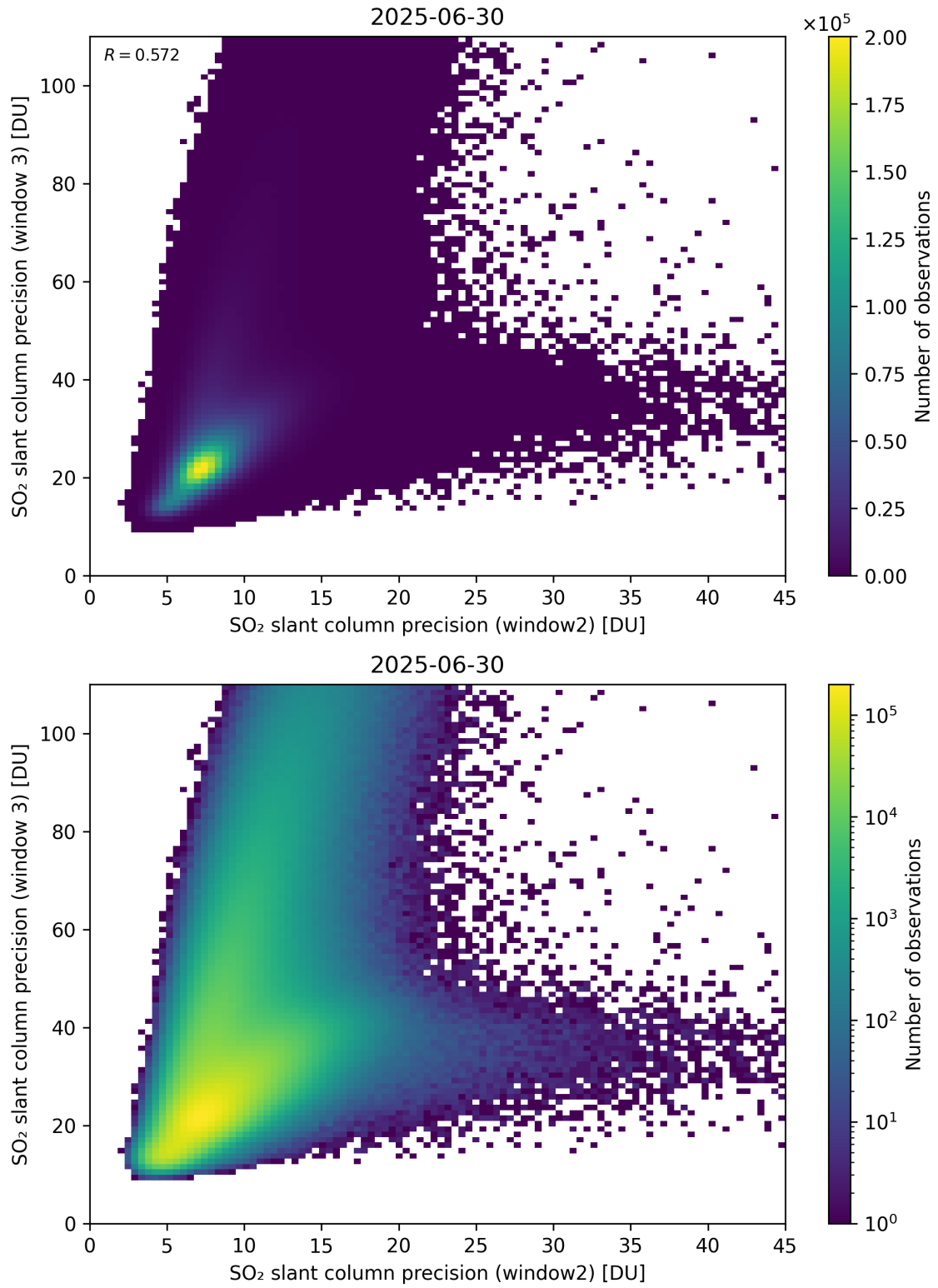
Figure 300: Scatter density plot of “SO 2 slant column precision (window2)” against “SO 2 slant column precision (window 3)” for 2025-06-29 to 2025-07-01.
