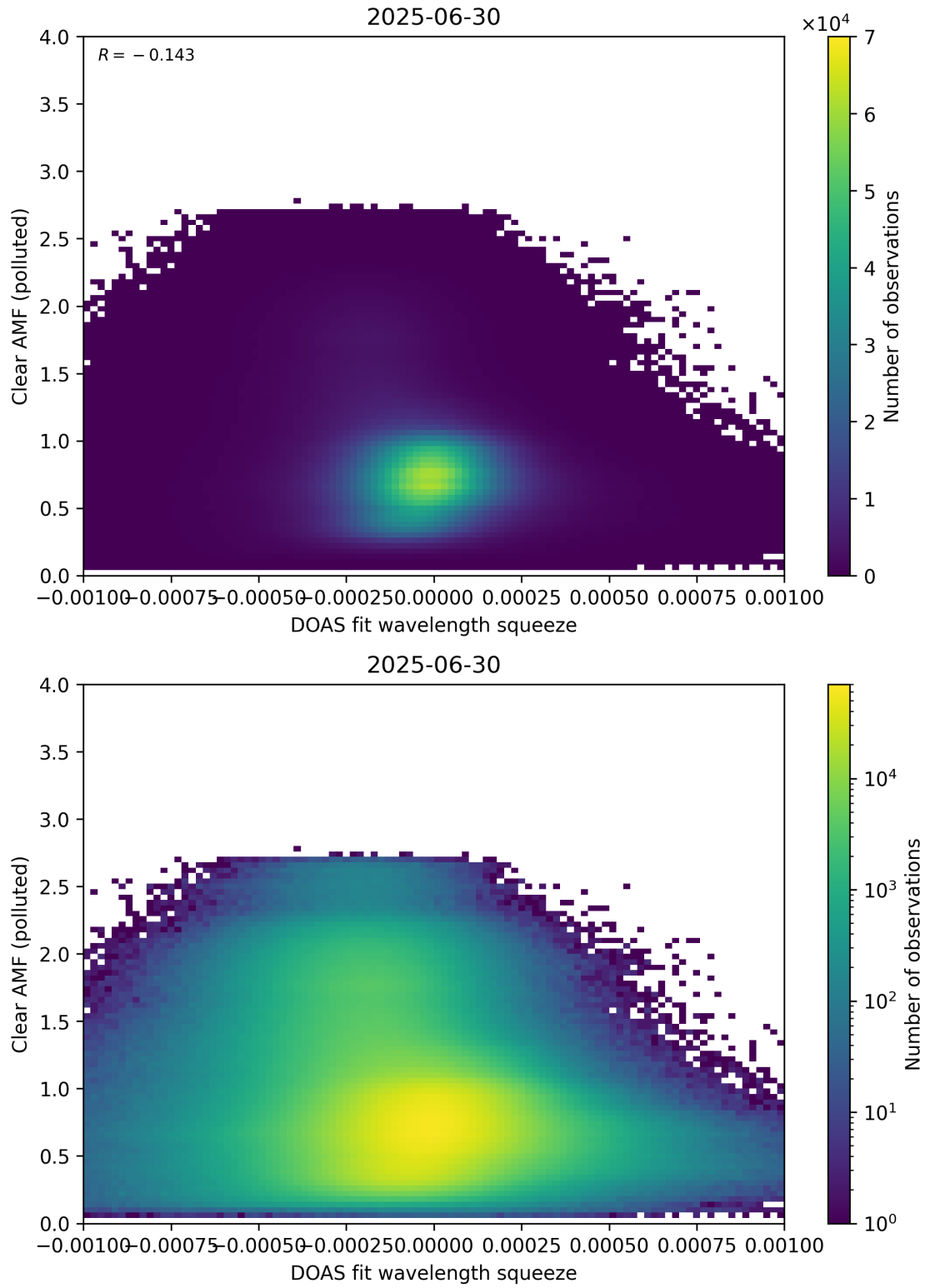
Figure 144: Scatter density plot of “DOAS fit wavelength squeeze” against “Clear AMF (polluted)” for 2025-06-29 to 2025-07-01.
