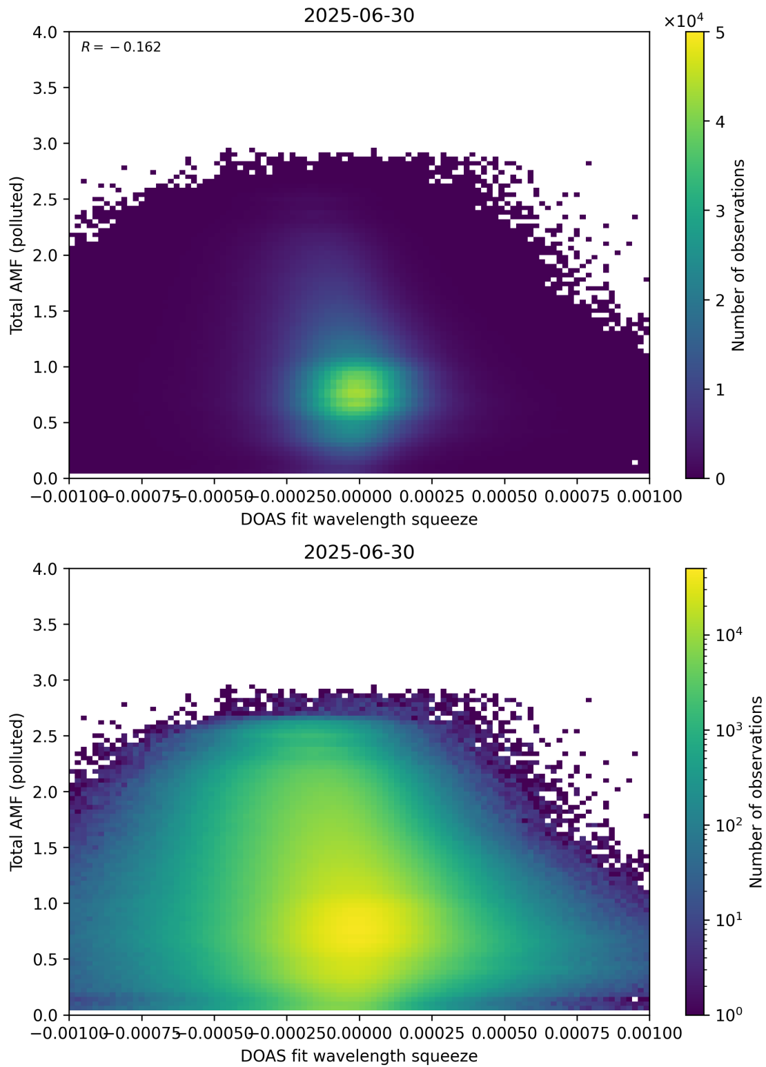
Figure 145: Scatter density plot of “DOAS fit wavelength squeeze” against “Total AMF (polluted)” for 2025-06-29 to 2025-07-01.
