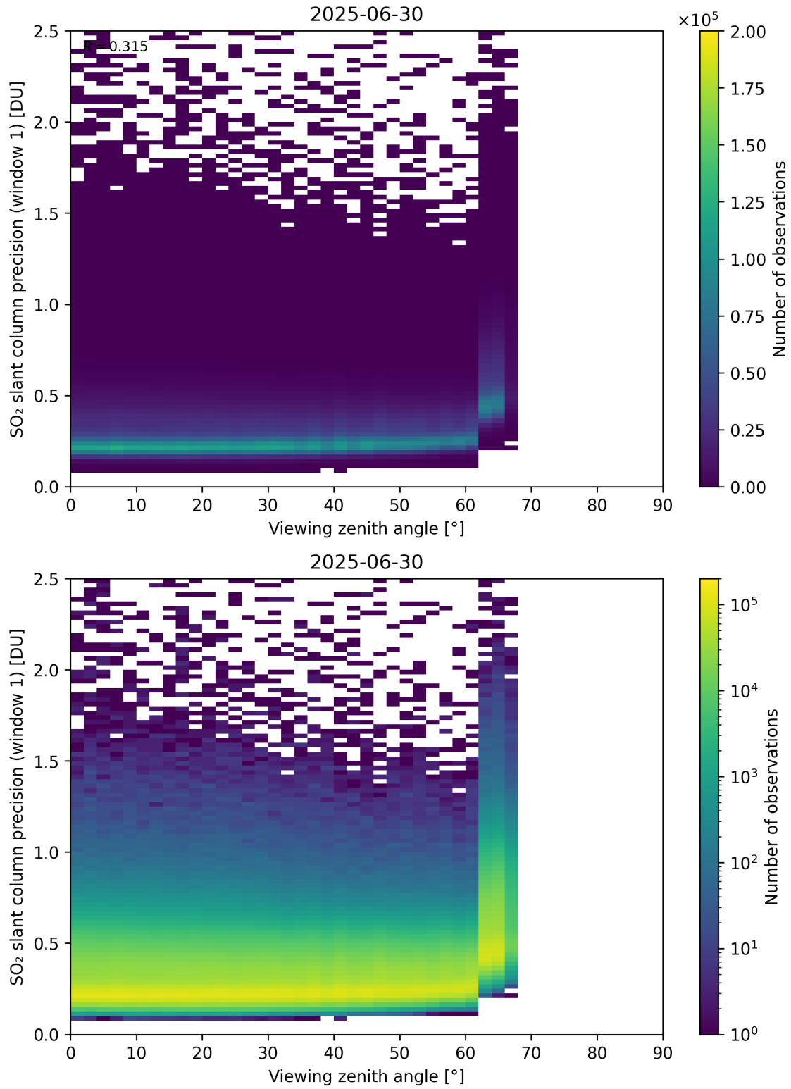
Figure 377: Scatter density plot of “Viewing zenith angle” against “SO 2 slant column precision (window 1)” for 2025-06-29 to 2025-07-01.
