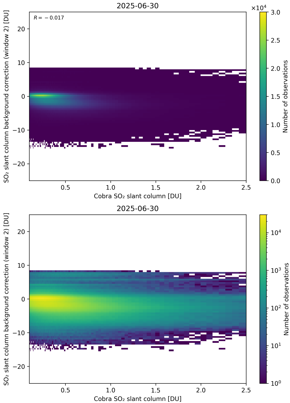
Figure 194: Scatter density plot of “Cobra SO 2 slant column” against “SO 2 slant column background correction (window 2)” for 2025-06-29 to 2025-07-01.
