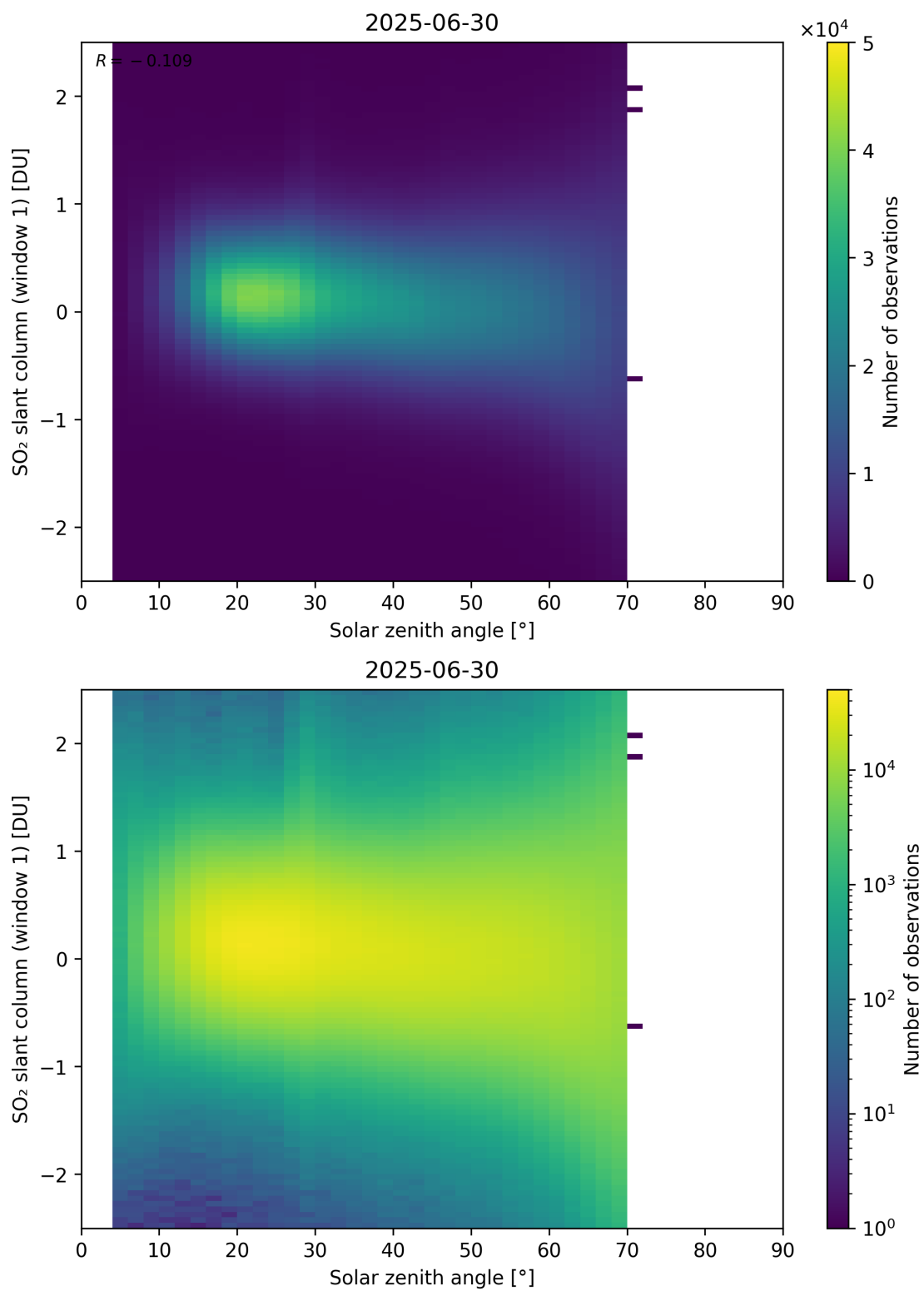
Figure 184: Scatter density plot of “Solar zenith angle” against “SO 2 slant column (window 1)” for 2025-06-29 to 2025-07-01.
