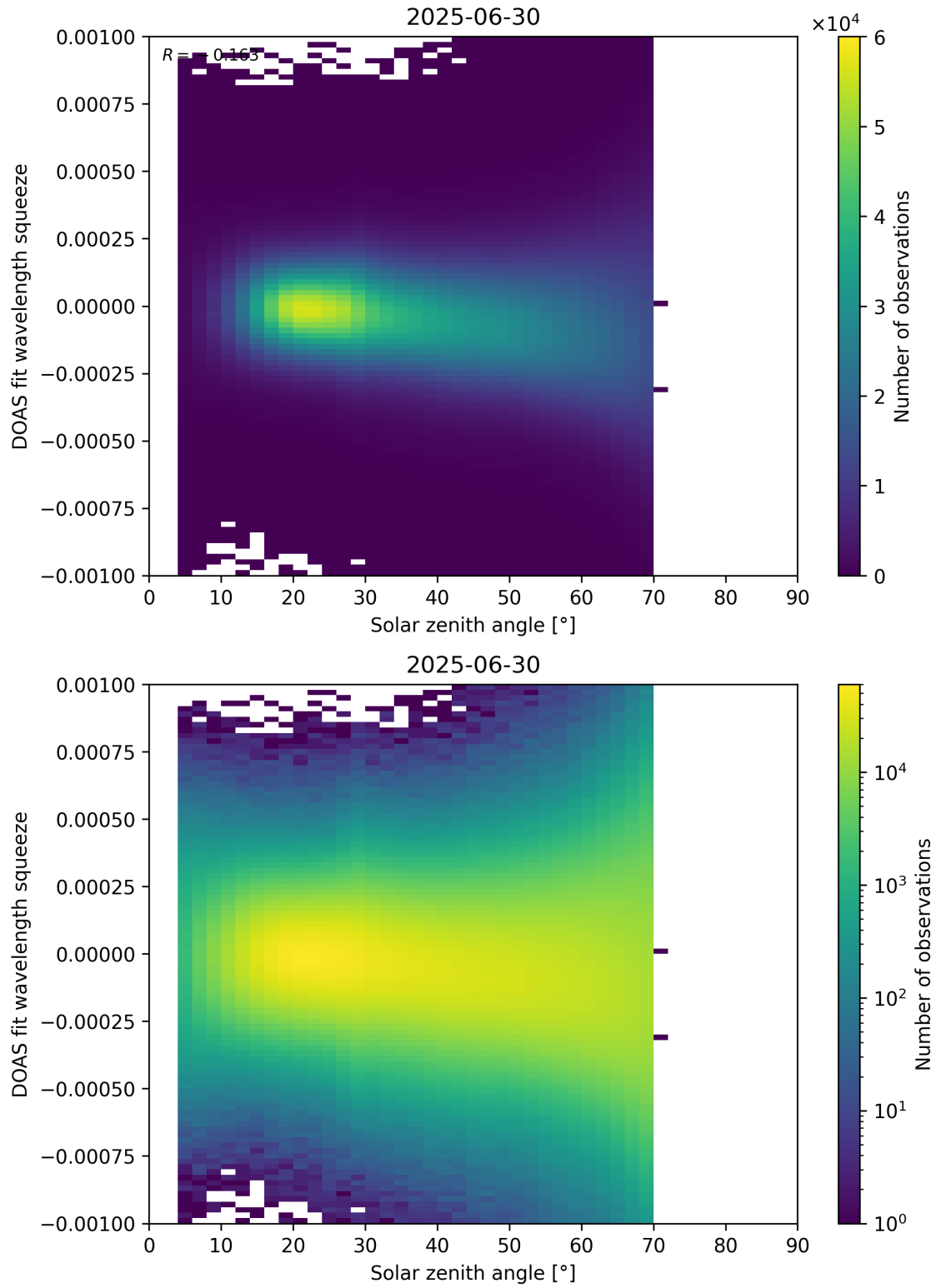
Figure 175: Scatter density plot of “Solar zenith angle” against “DOAS fit wavelength squeeze” for 2025-06-29 to 2025-07-01.
