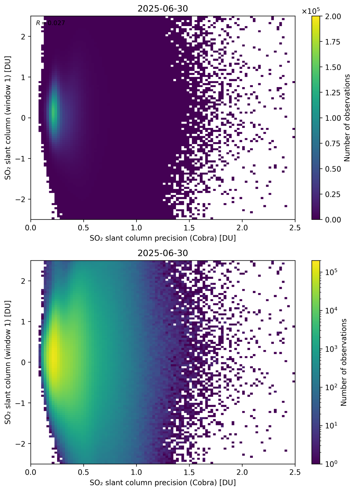
Figure 208: Scatter density plot of “SO 2 slant column precision (Cobra)” against “SO 2 slant column (window 1)” for 2025-06-29 to 2025-07-01.
