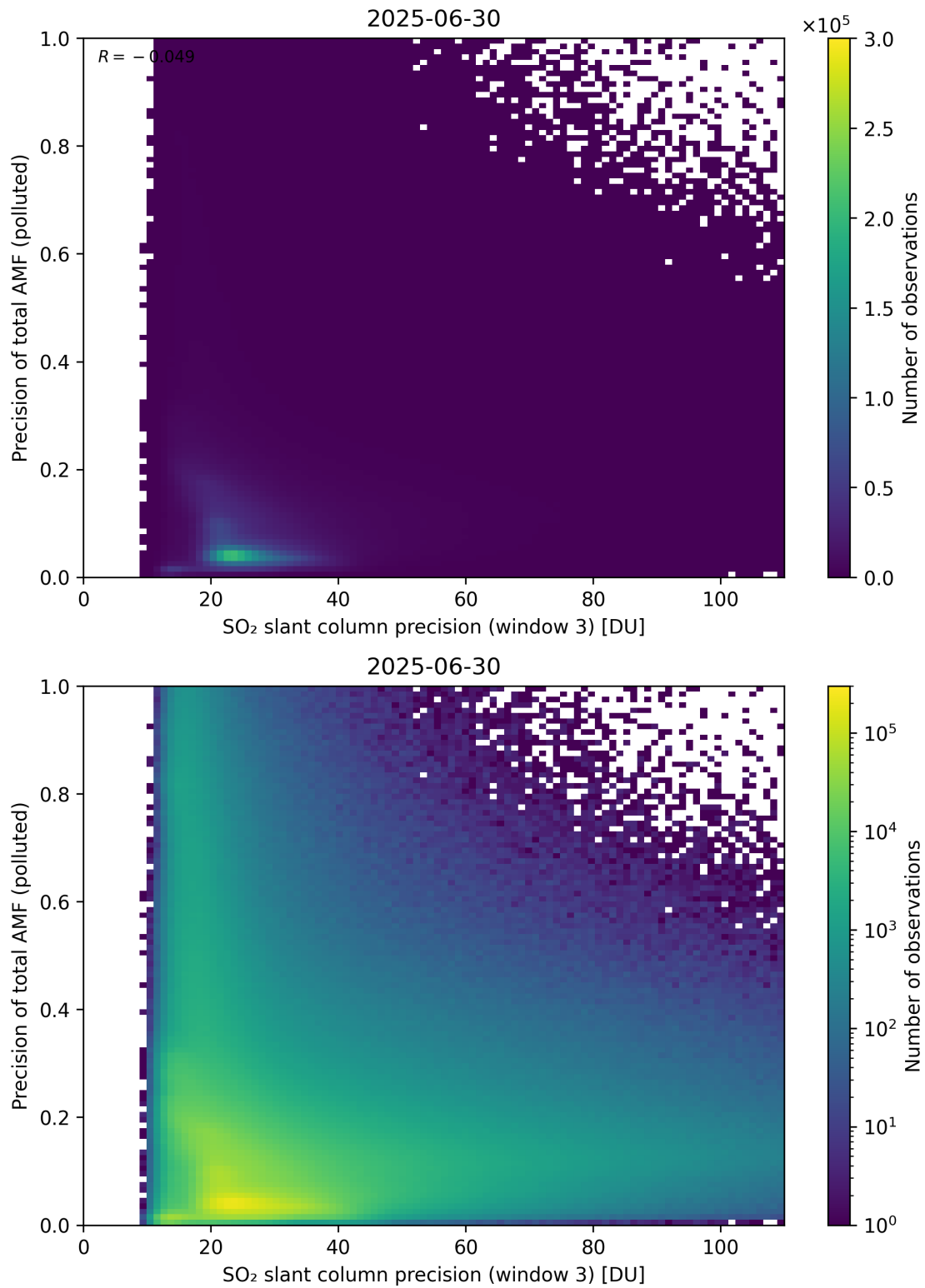
Figure 314: Scatter density plot of “SO 2 slant column precision (window 3)” against “Precision of total AMF (polluted)” for 2025-06-29 to 2025-07-01.
