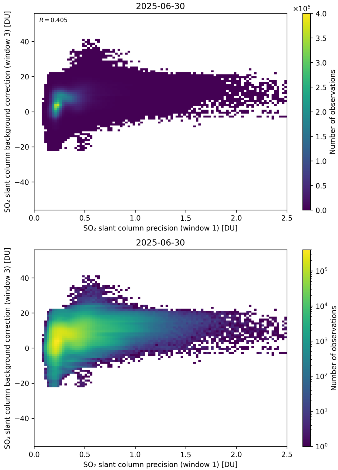
Figure 270: Scatter density plot of “SO 2 slant column precision (window 1)” against “SO 2 slant column background correction (window 3)” for 2025-06-29 to 2025-07-01.
