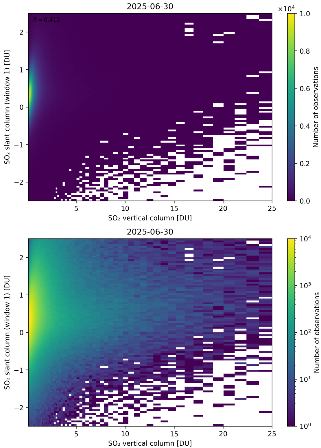
Figure 354: Scatter density plot of “SO 2 vertical column” against “SO 2 slant column (window 1)” for 2025-06-29 to 2025-07-01.
