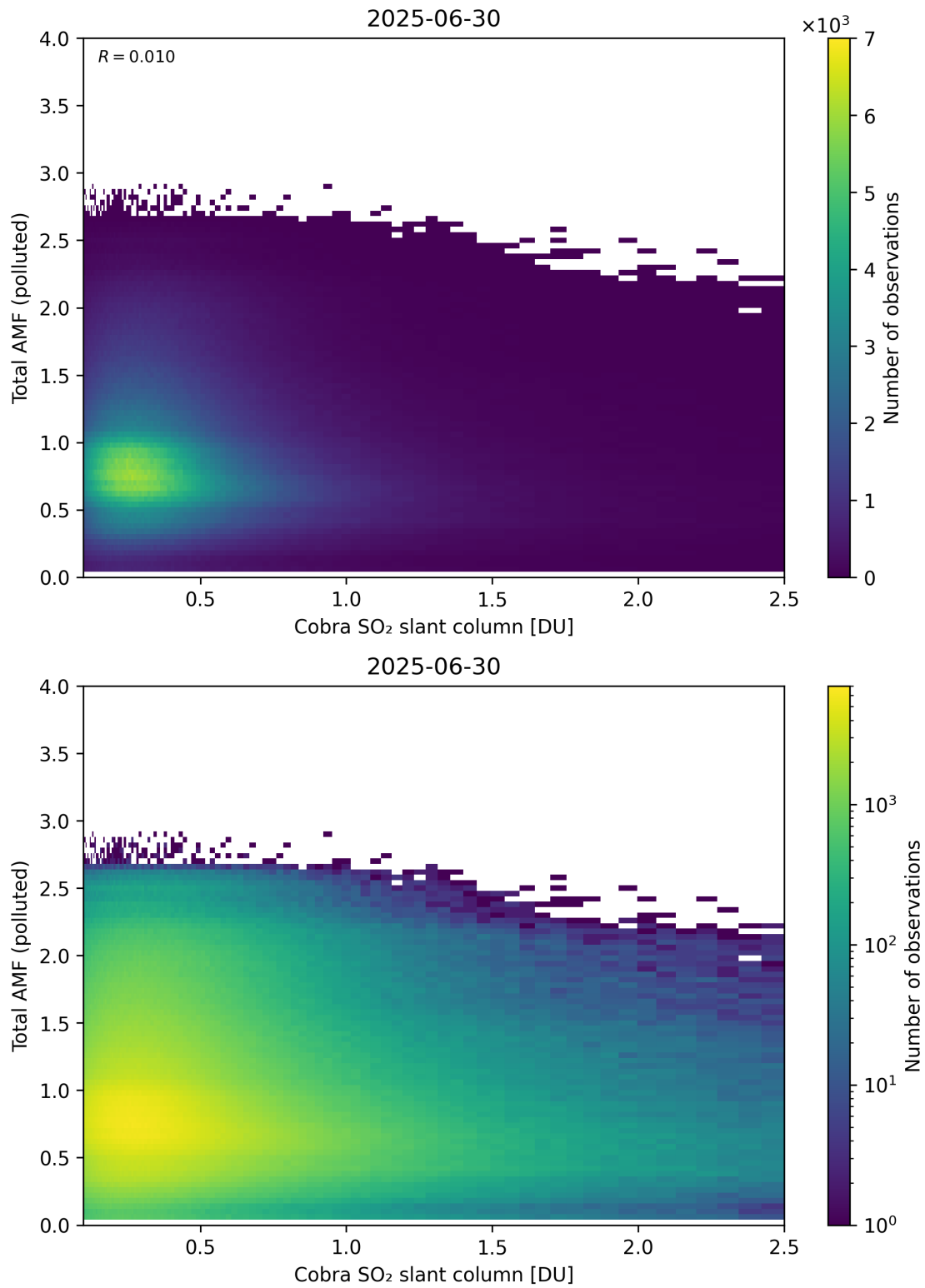
Figure 224: Scatter density plot of “Cobra SO 2 slant column” against “Total AMF (polluted)” for 2025-06-29 to 2025-07-01.
