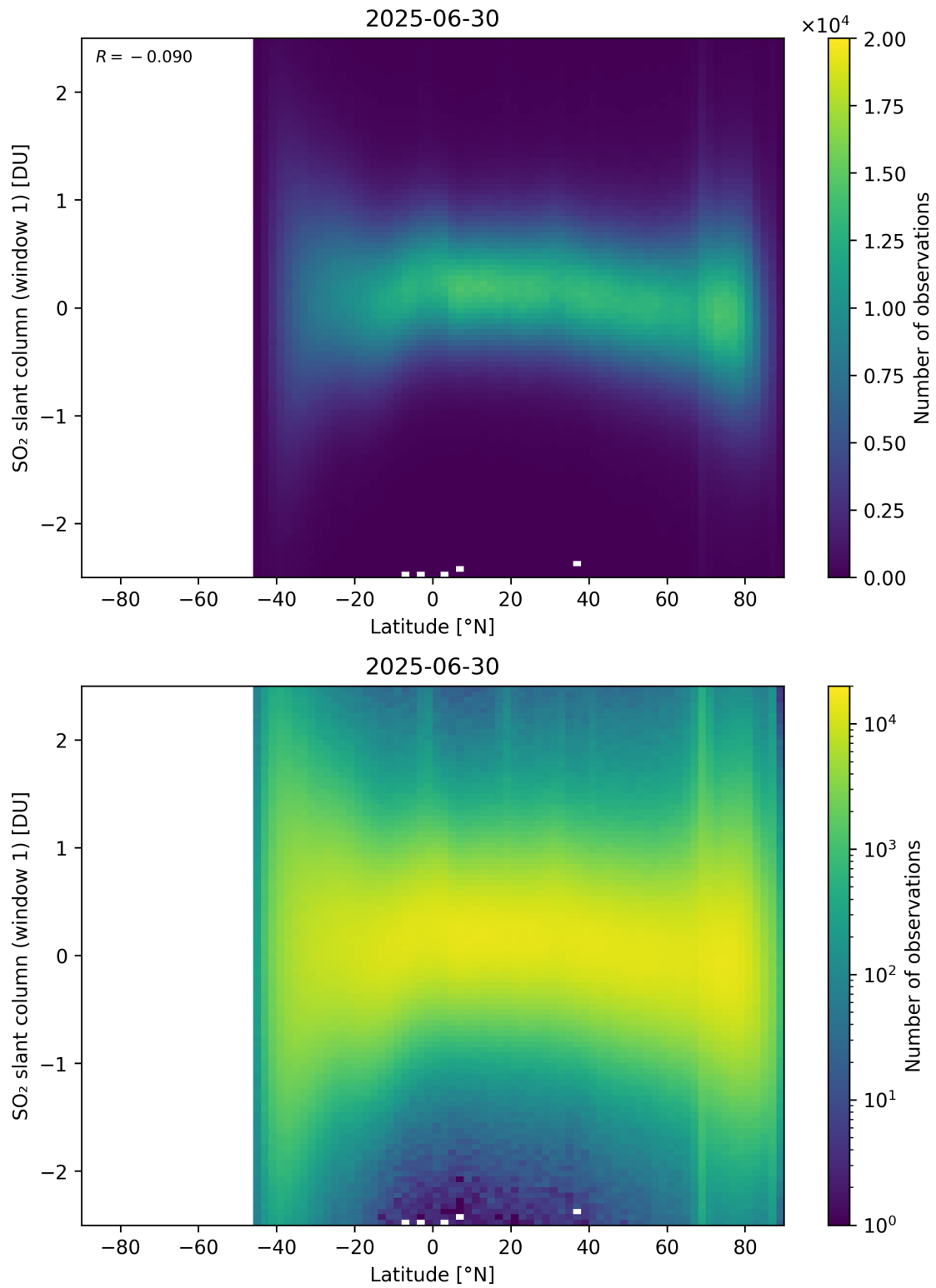
Figure 162: Scatter density plot of “Latitude” against “SO 2 slant column (window 1)” for 2025-06-29 to 2025-07-01.
