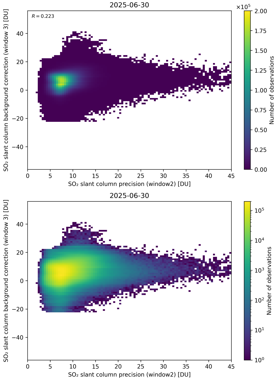
Figure 292: Scatter density plot of “SO 2 slant column precision (window2)” against “SO 2 slant column background correction (window 3)” for 2025-06-29 to 2025-07-01.
