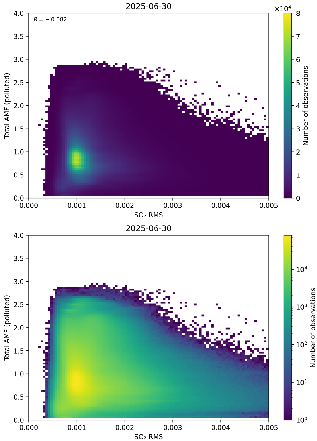
Figure 148: Scatter density plot of “SO 2 RMS” against “Total AMF (polluted)” for 2025-06-29 to 2025-07-01.
