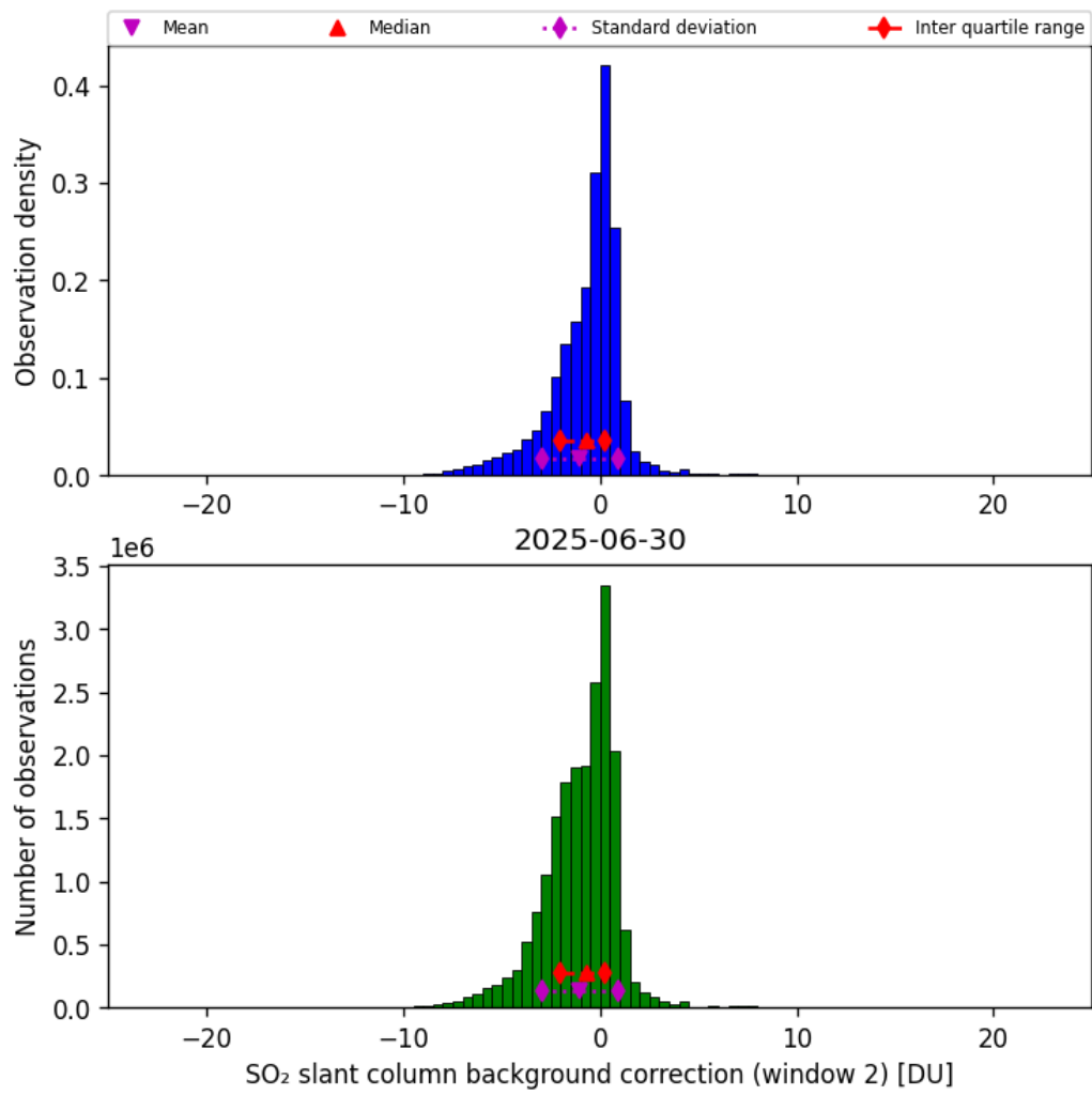
Figure 70: Histogram of “SO 2 slant column background correction (window 2)” for 2025-06-29 to 2025-07-01
