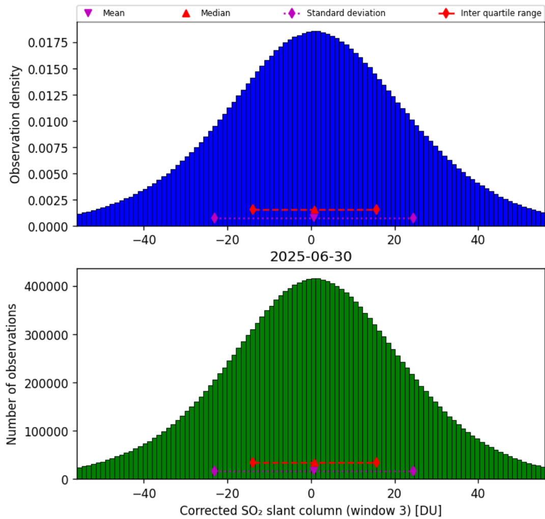
Figure 73: Histogram of “Corrected SO 2 slant column (window 3)” for 2025-06-29 to 2025-07-01
