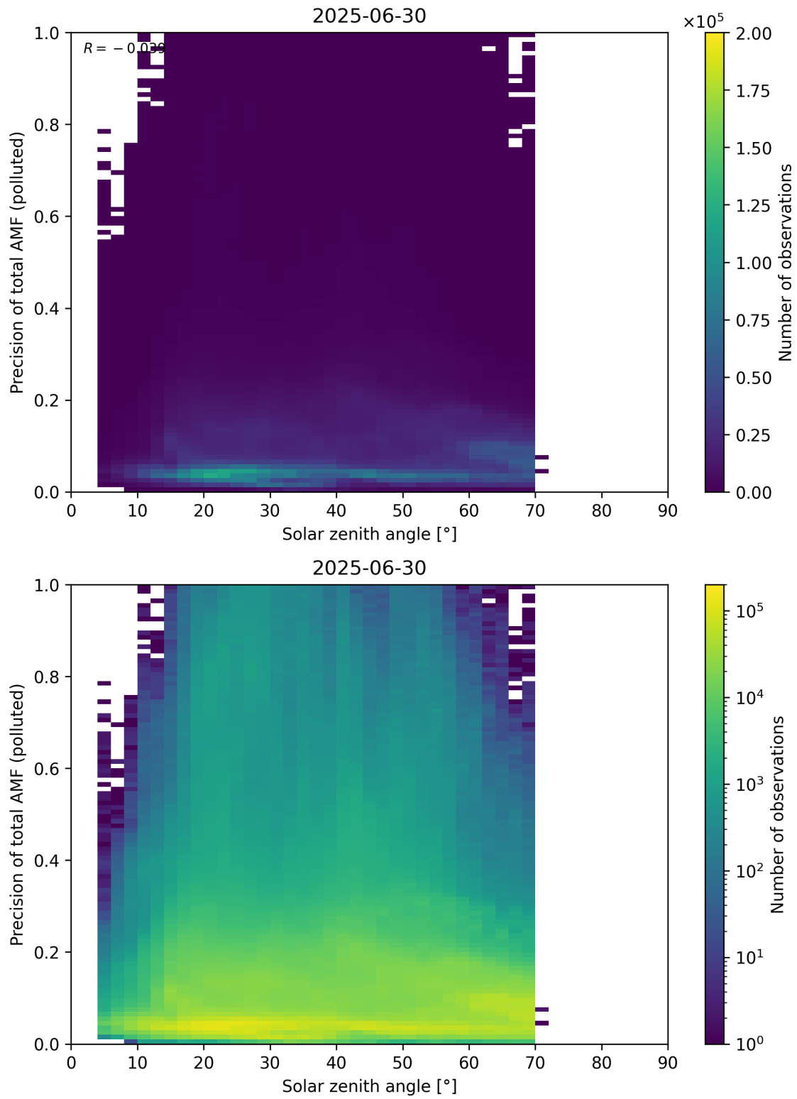
Figure 190: Scatter density plot of “Solar zenith angle” against “Precision of total AMF (polluted)” for 2025-06-29 to 2025-07-01.
