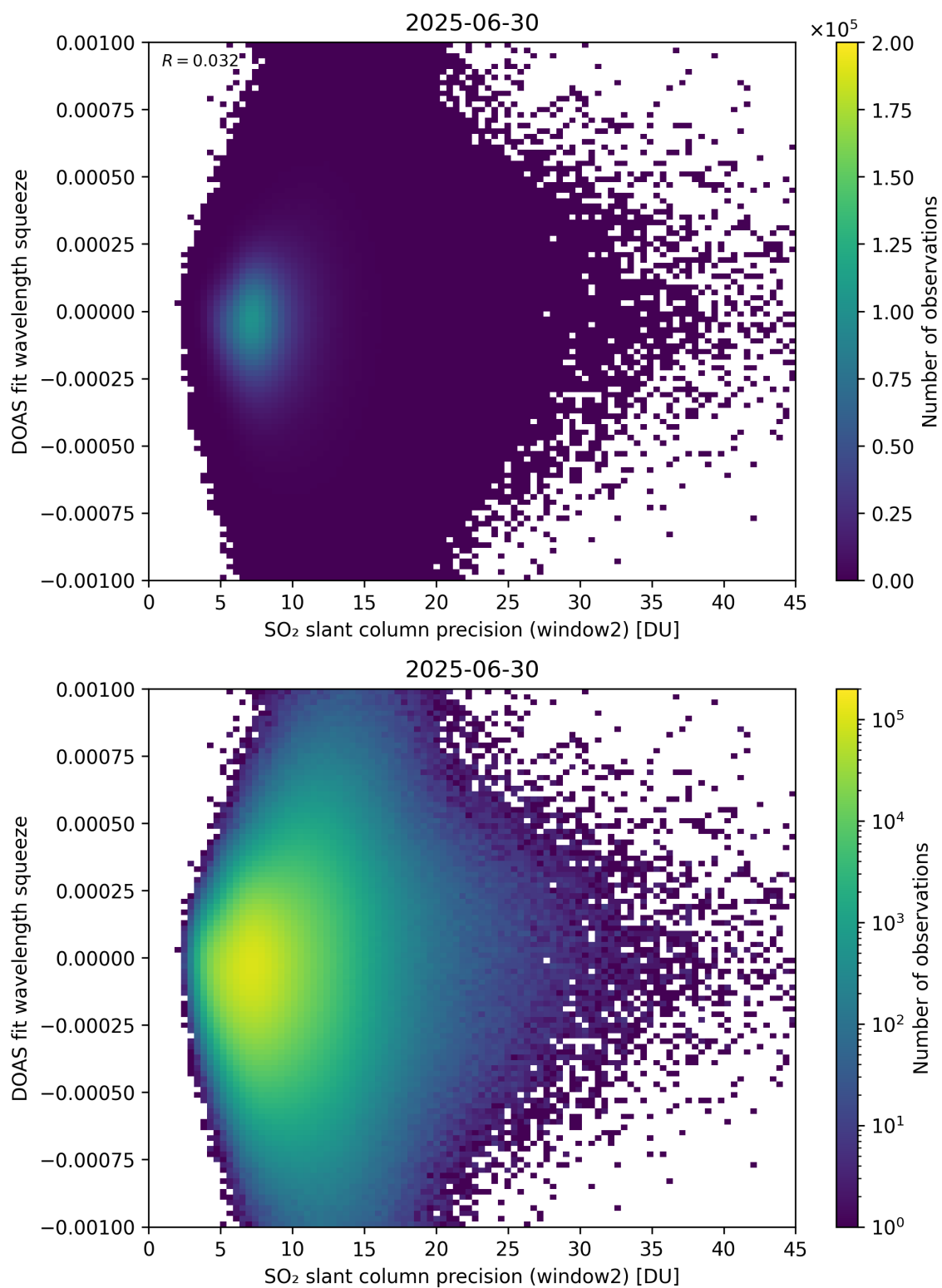
Figure 294: Scatter density plot of “SO 2 slant column precision (window2)” against “DOAS fit wavelength squeeze” for 2025-06-29 to 2025-07-01.
