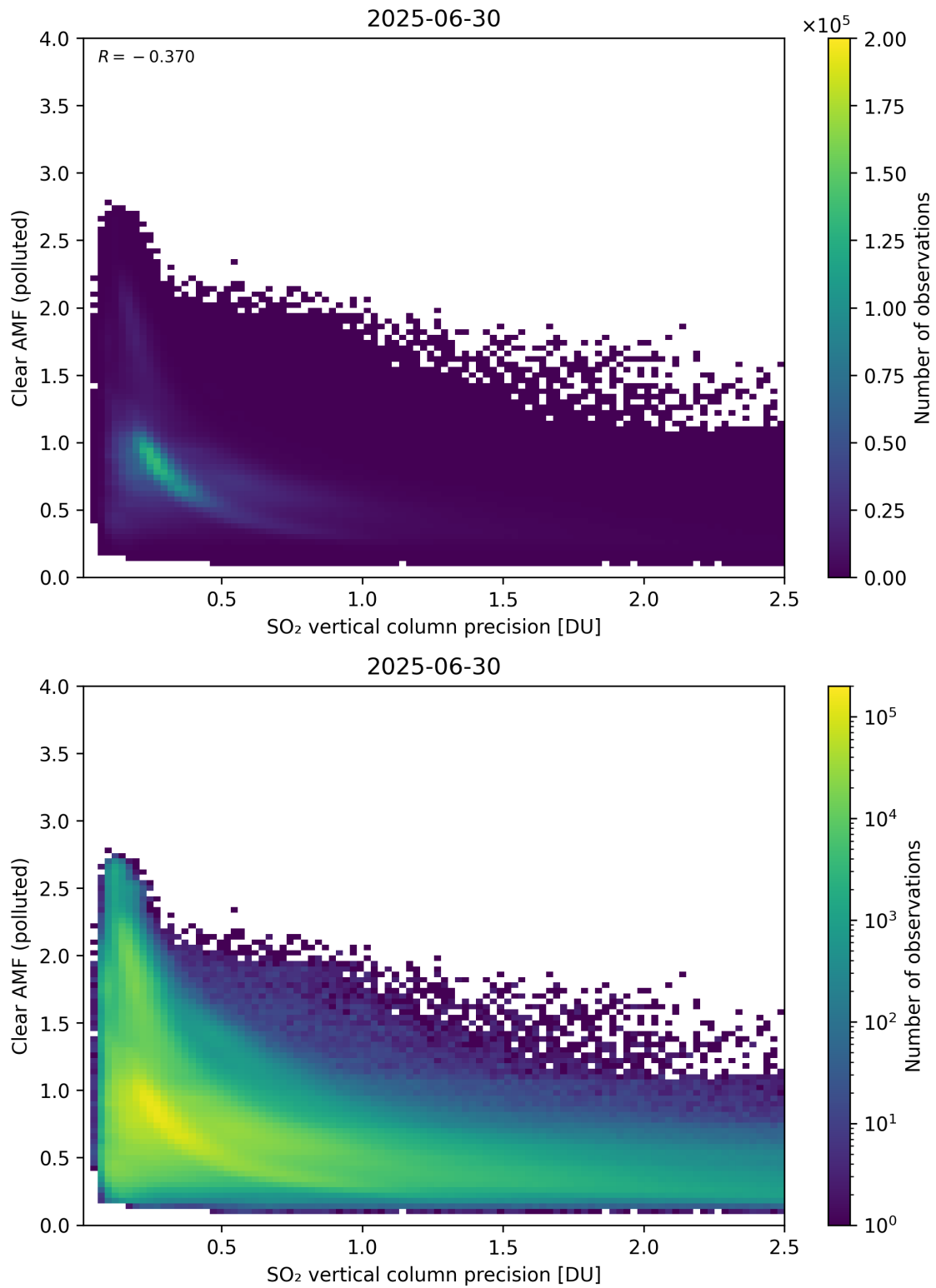
Figure 335: Scatter density plot of “SO 2 vertical column precision” against “Clear AMF (polluted)” for 2025-06-29 to 2025-07-01.
