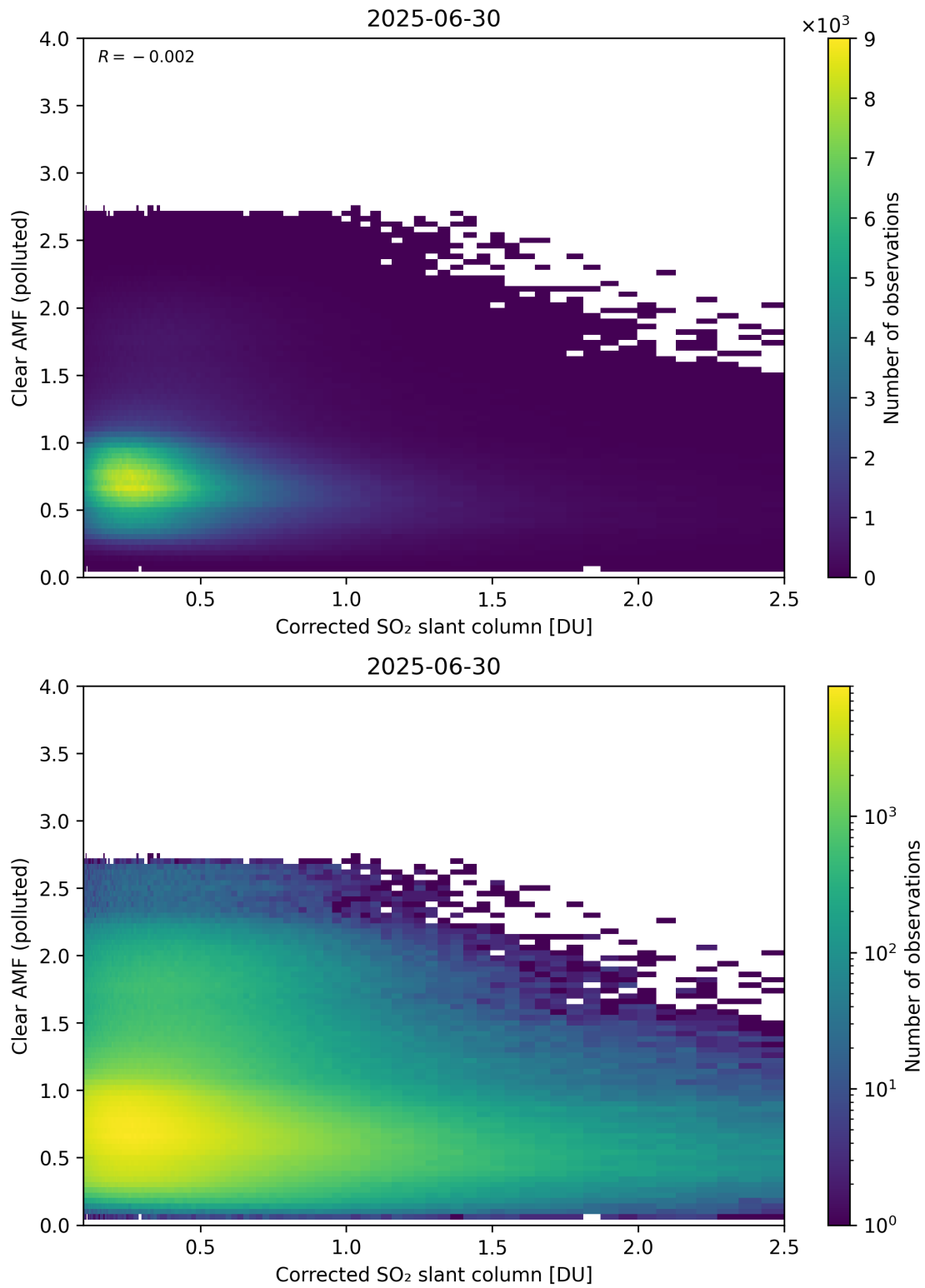
Figure 232: Scatter density plot of “Corrected SO 2 slant column” against “Clear AMF (polluted)” for 2025-06-29 to 2025-07-01.
