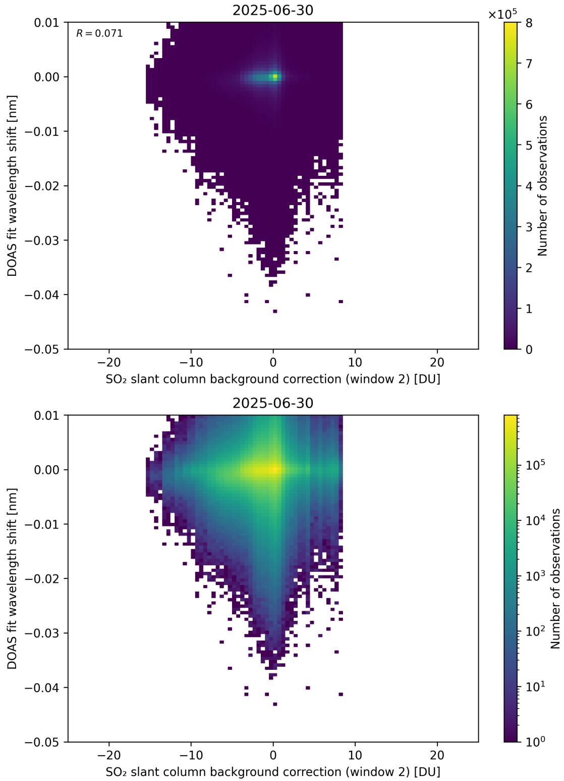
Figure 123: Scatter density plot of “SO 2 slant column background correction (window 2)” against “DOAS fit wavelength shift” for 2025-06-29 to 2025-07-01.
