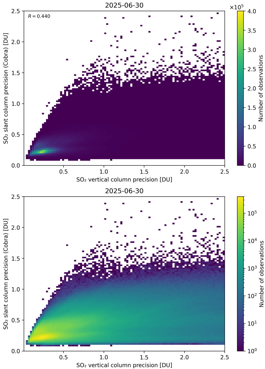
Figure 337: Scatter density plot of “SO 2 vertical column precision” against “SO 2 slant column precision (Cobra)” for 2025-06-29 to 2025-07-01.
