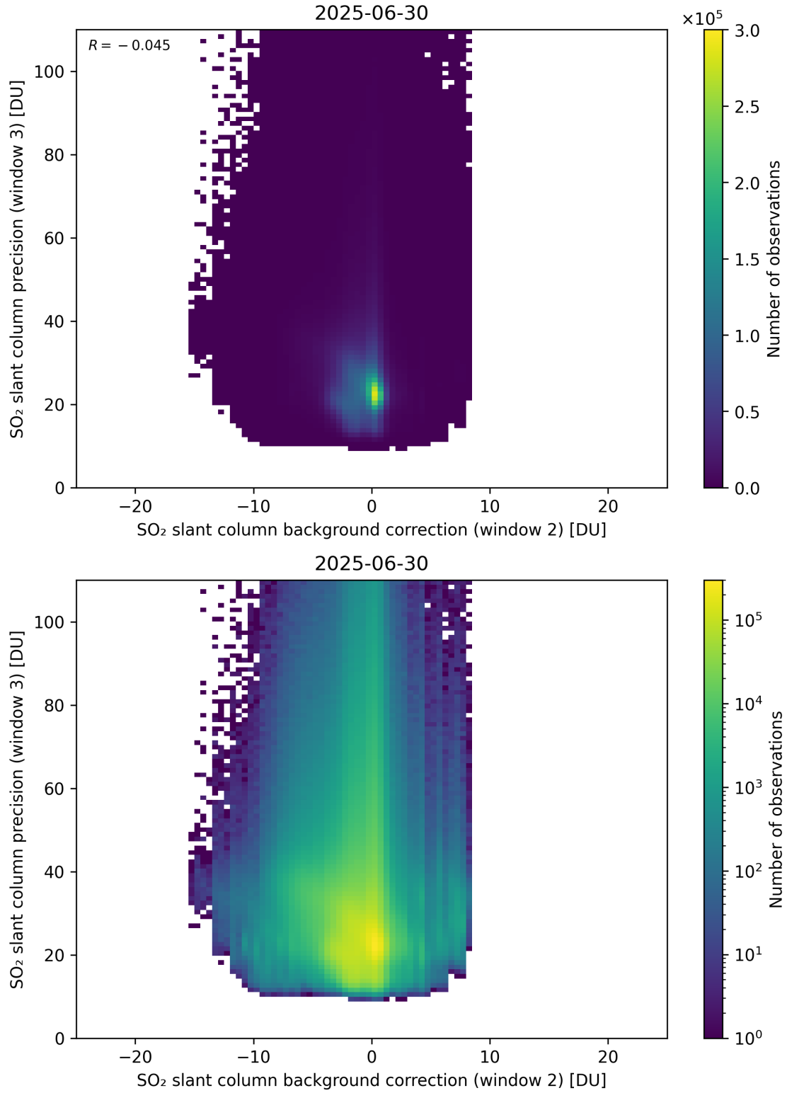
Figure 129: Scatter density plot of “SO 2 slant column background correction (window 2)” against “SO 2 slant column precision (window 3)” for 2025-06-29 to 2025-07-01.
