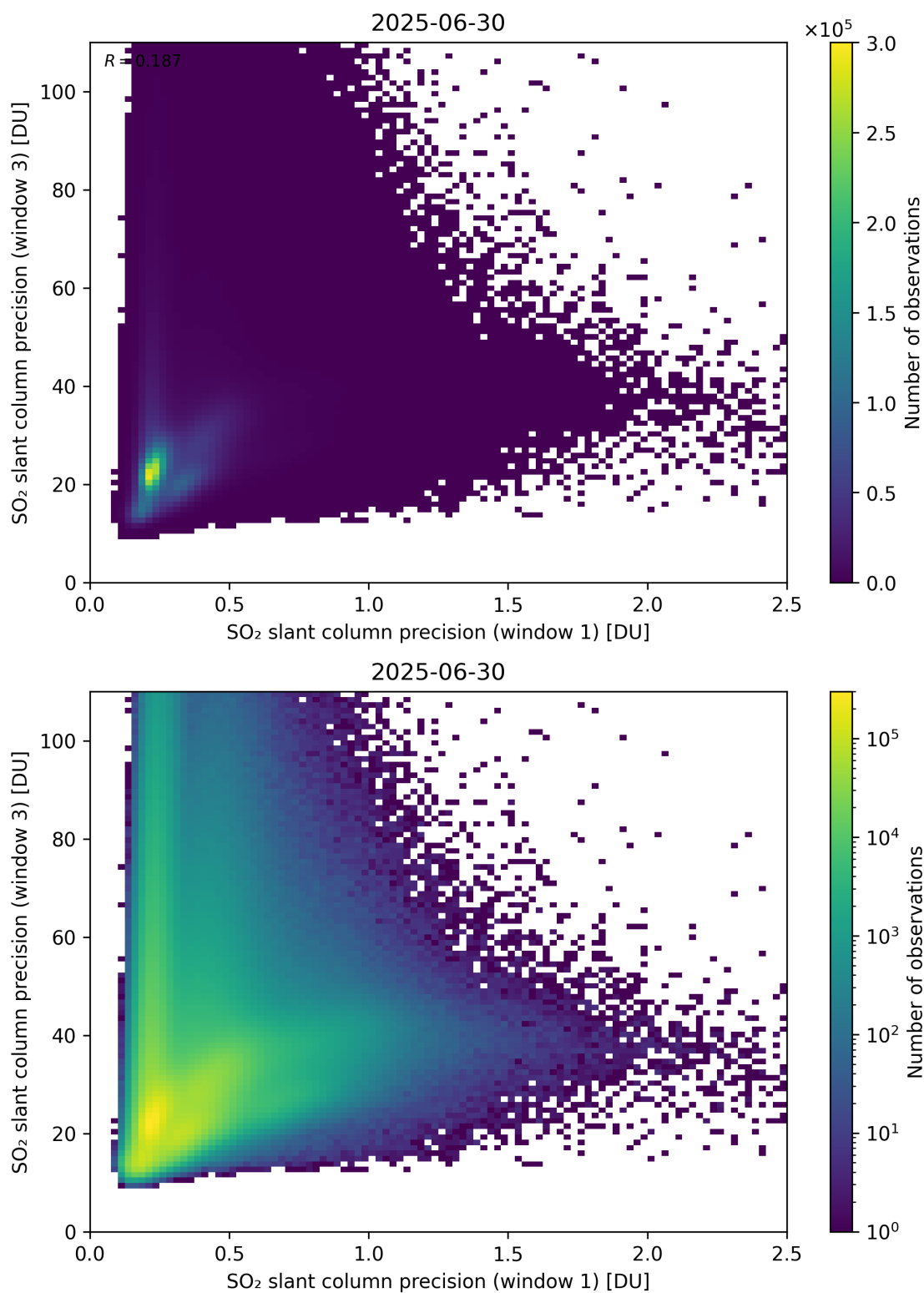
Figure 279: Scatter density plot of “SO 2 slant column precision (window 1)” against “SO 2 slant column precision (window 3)” for 2025-06-29 to 2025-07-01.
