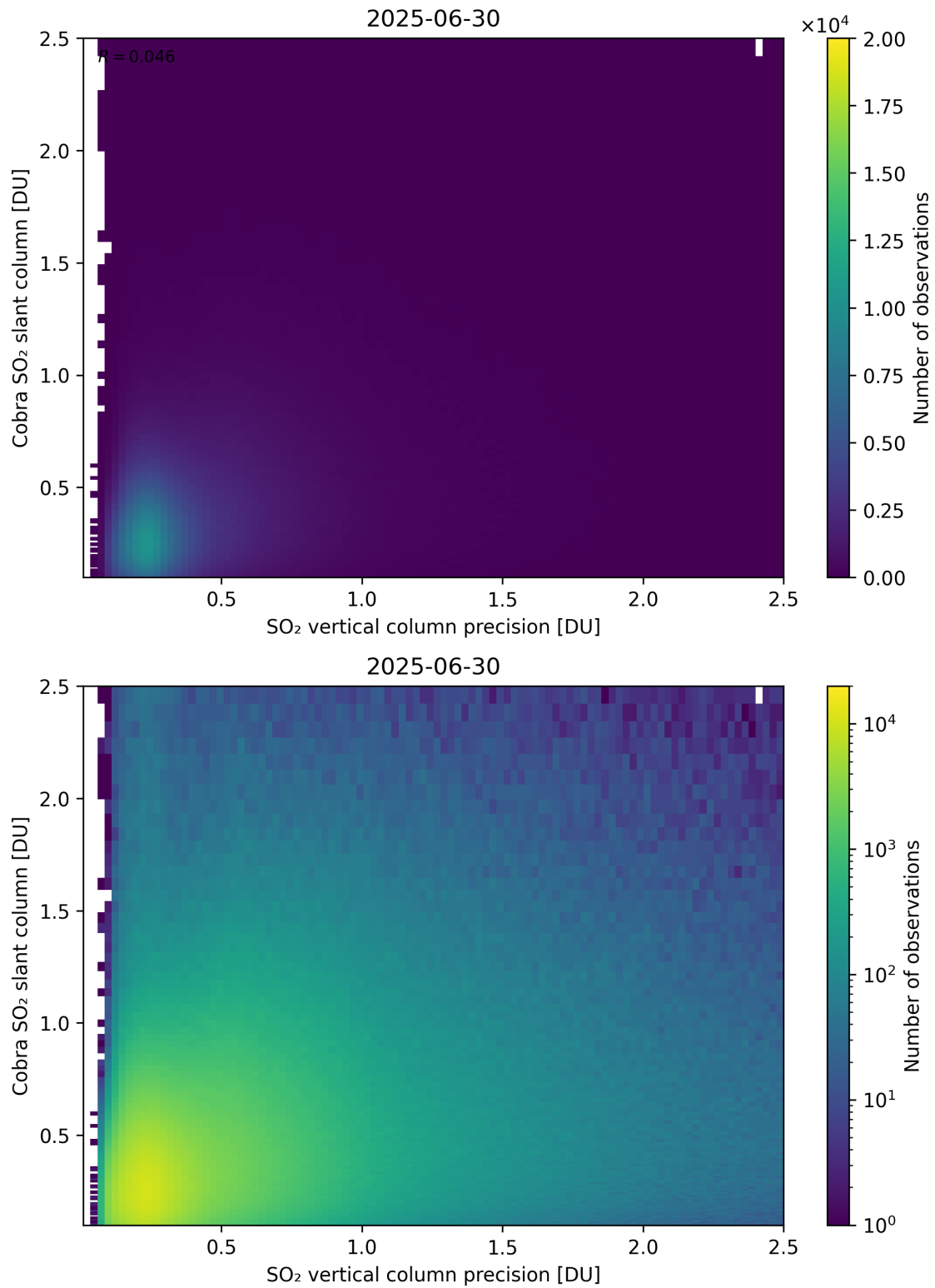
Figure 336: Scatter density plot of “SO 2 vertical column precision” against “Cobra SO 2 slant column” for 2025-06-29 to 2025-07-01.
