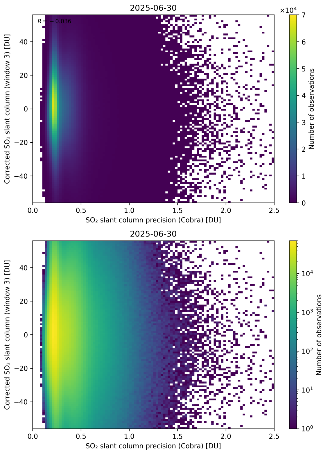
Figure 207: Scatter density plot of “SO 2 slant column precision (Cobra)” against “Corrected SO 2 slant column (window 3)” for 2025-06-29 to 2025-07-01.
