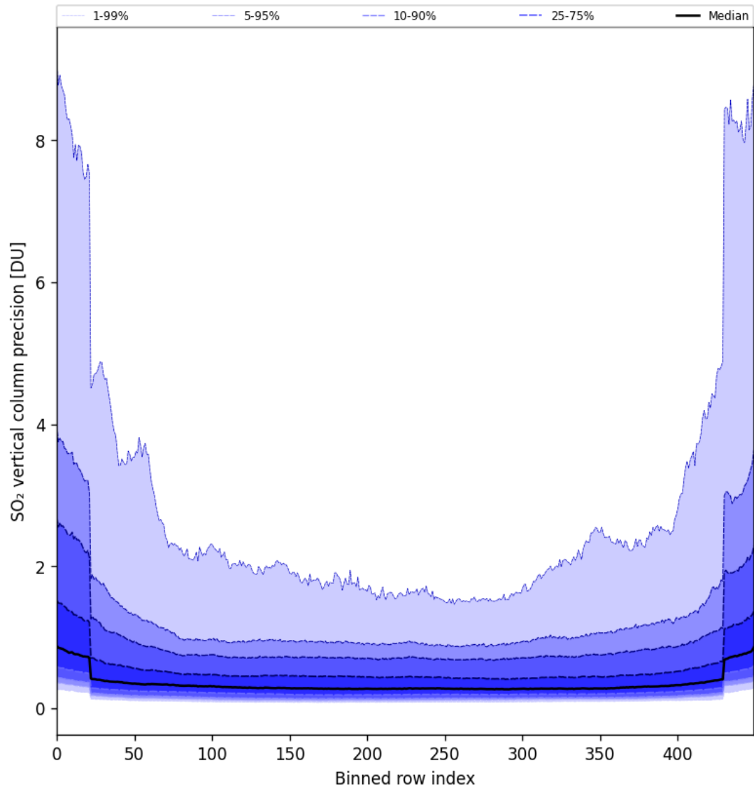
Figure 85: Along track statistics of “SO 2 vertical column precision” for 2025-06-29 to 2025-07-01
