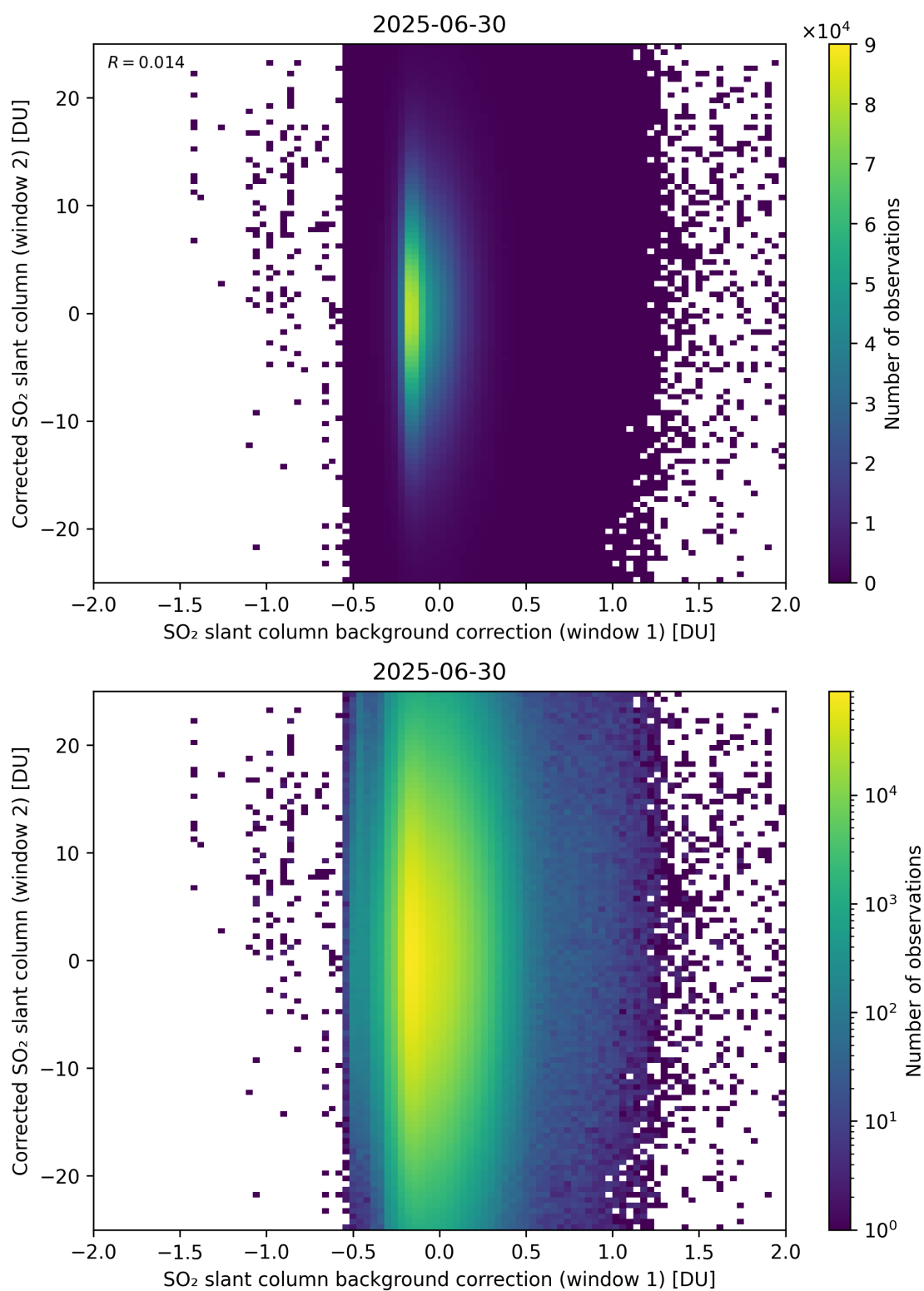
Figure 115: Scatter density plot of “SO 2 slant column background correction (window 1)” against “Corrected SO 2 slant column (window 2)” for 2025-06-29 to 2025-07-01.
