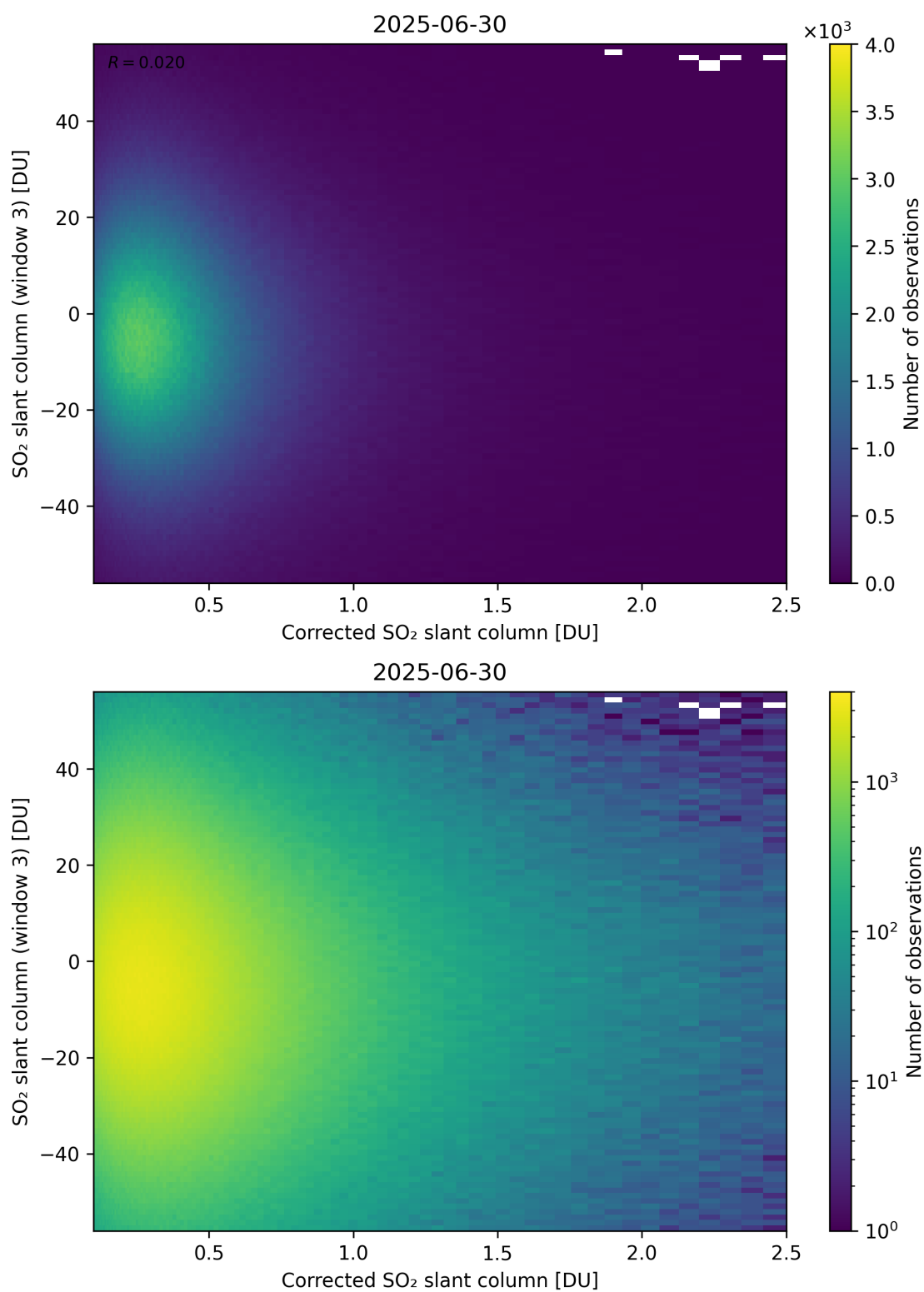
Figure 240: Scatter density plot of “Corrected SO 2 slant column” against “SO 2 slant column (window 3)” for 2025-06-29 to 2025-07-01.
