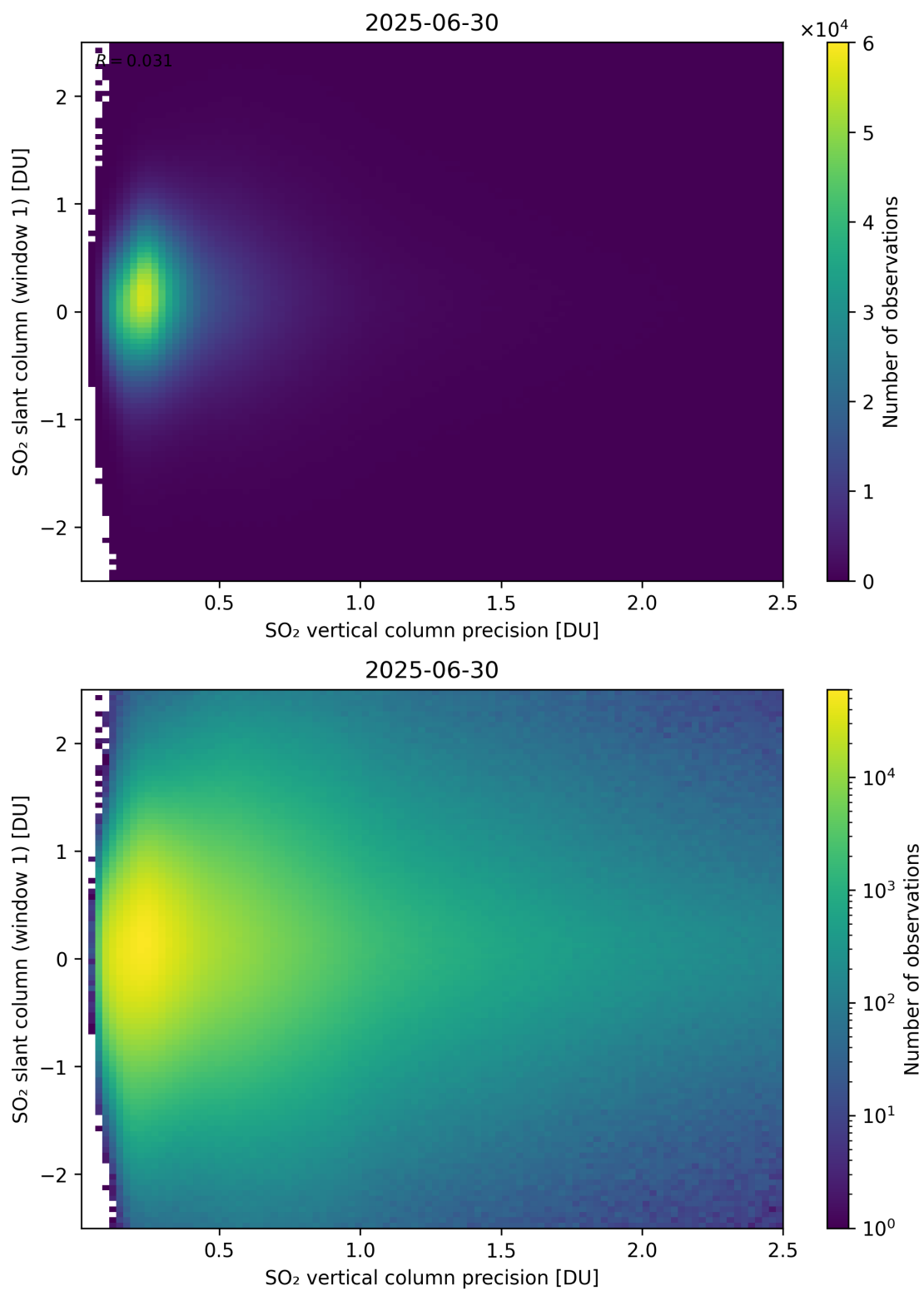
Figure 341: Scatter density plot of “SO 2 vertical column precision” against “SO 2 slant column (window 1)” for 2025-06-29 to 2025-07-01.
