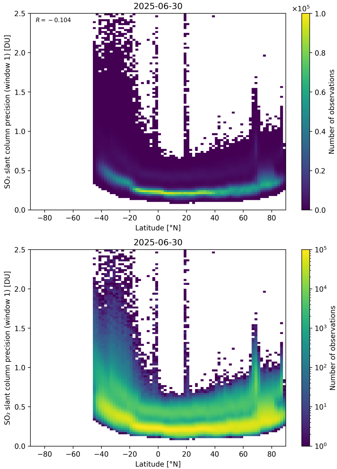
Figure 163: Scatter density plot of “Latitude” against “SO 2 slant column precision (window 1)” for 2025-06-29 to 2025-07-01.
