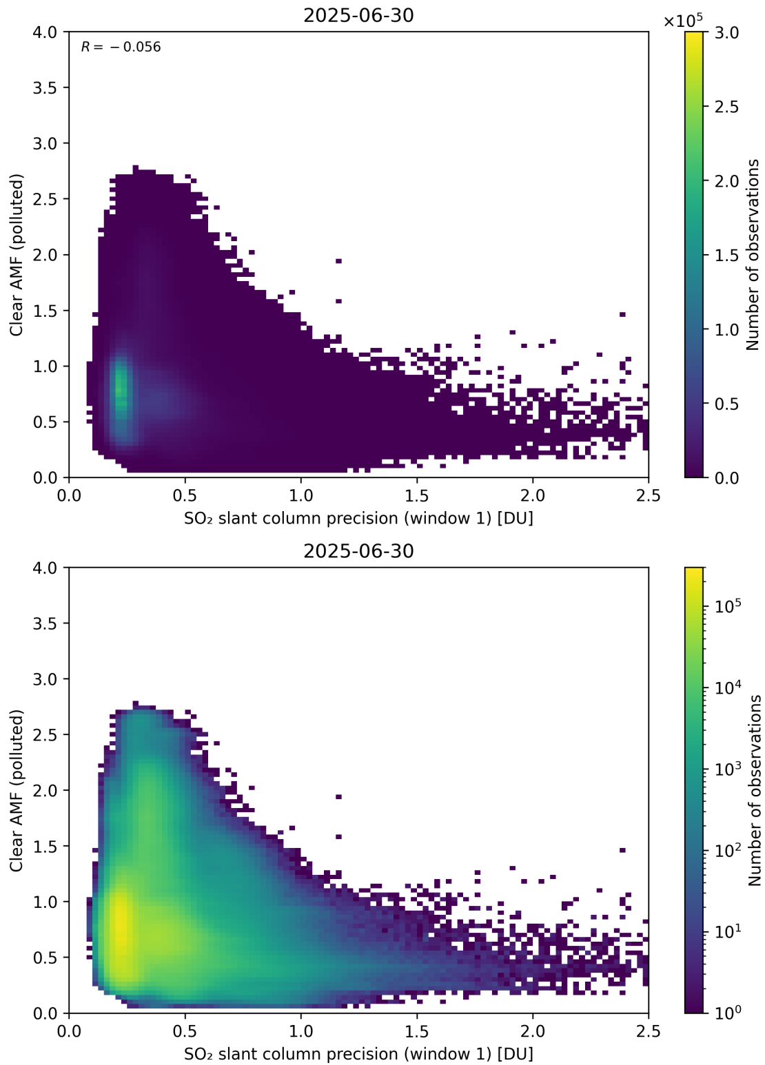
Figure 274: Scatter density plot of “SO 2 slant column precision (window 1)” against “Clear AMF (polluted)” for 2025-06-29 to 2025-07-01.
