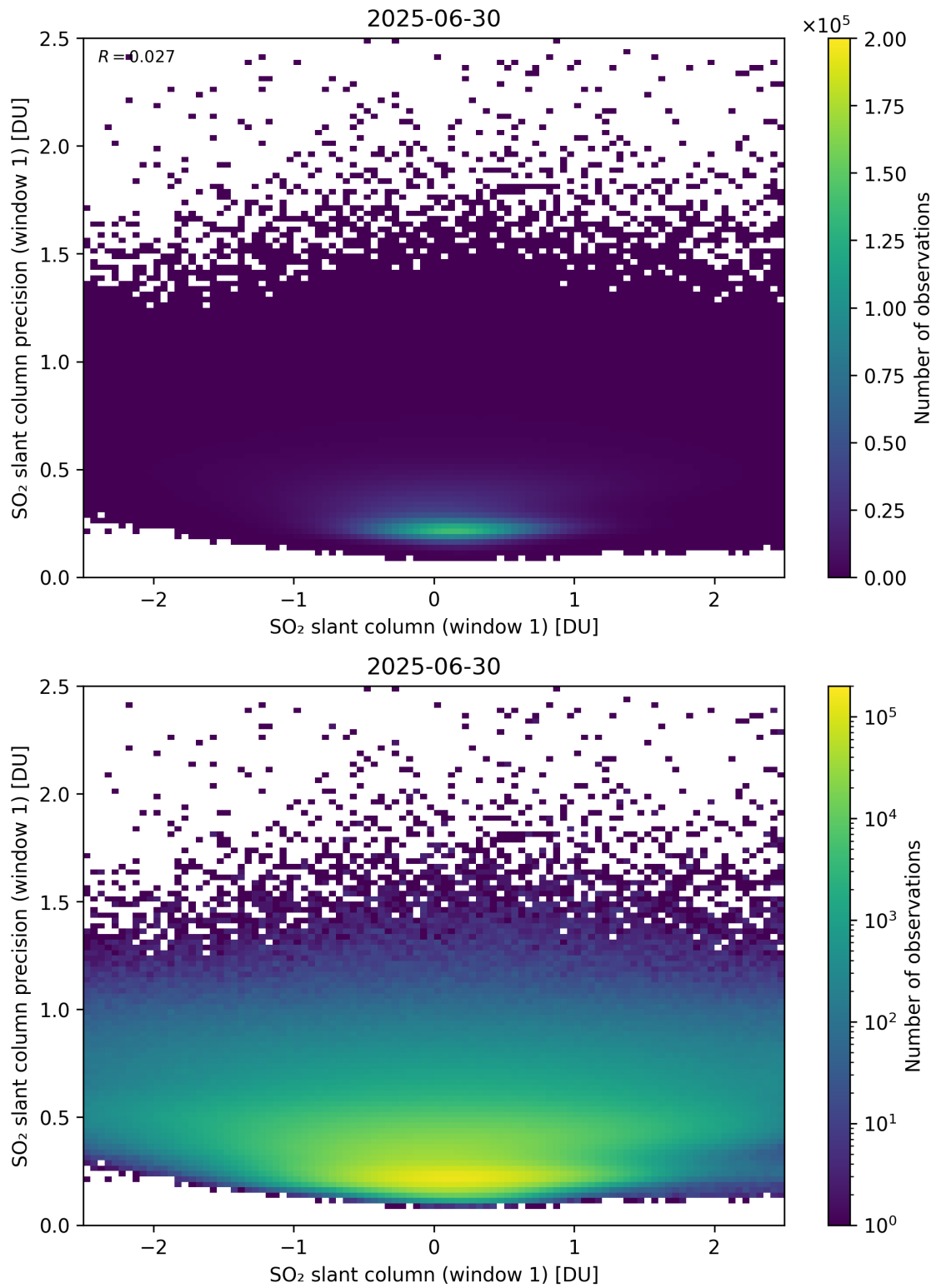
Figure 285: Scatter density plot of “SO 2 slant column (window 1)” against “SO 2 slant column precision (window 1)” for 2025-06-29 to 2025-07-01.
