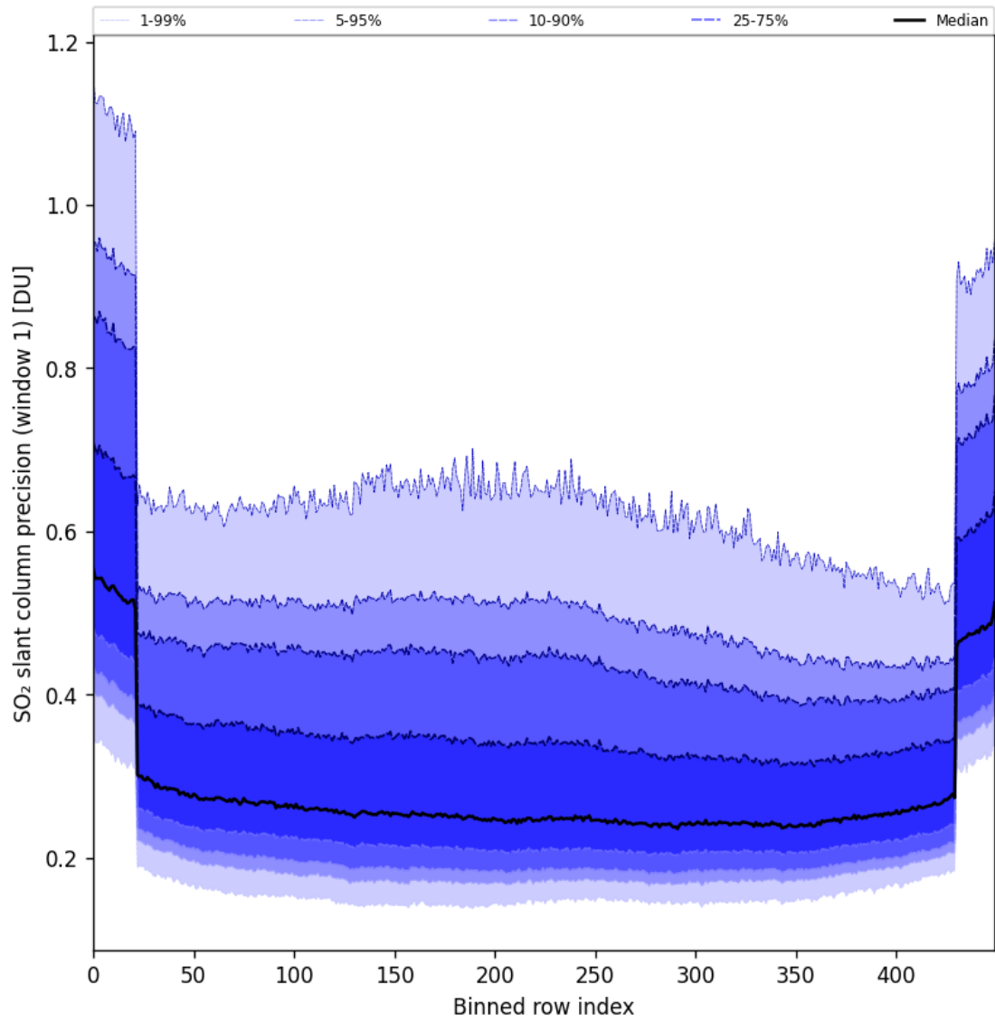
Figure 90: Along track statistics of “SO 2 slant column precision (window 1)” for 2025-06-29 to 2025-07-01
