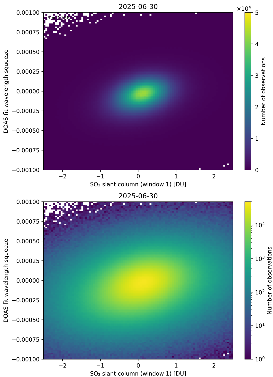
Figure 266: Scatter density plot of “SO 2 slant column (window 1)” against “DOAS fit wavelength squeeze” for 2025-06-29 to 2025-07-01.
