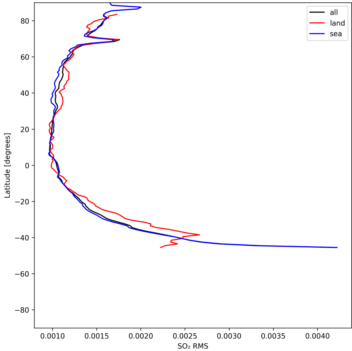
Figure 52: Zonal average of “SO 2 RMS” for 2025-06-29 to 2025-07-01.
