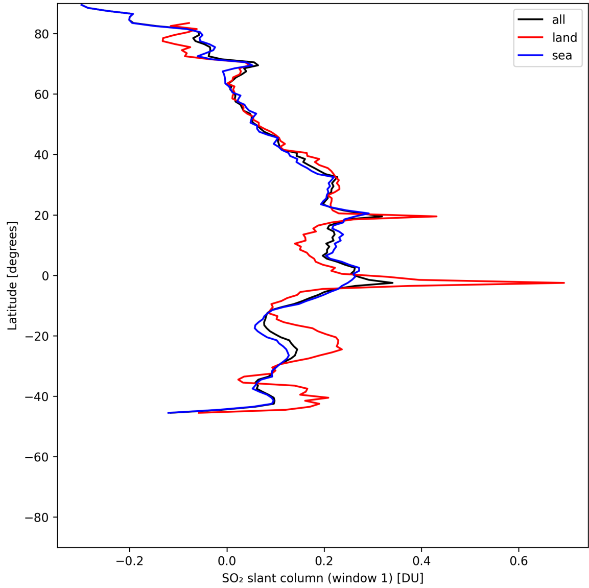
Figure 37: Zonal average of “SO 2 slant column (window 1)” for 2025-06-29 to 2025-07-01.
