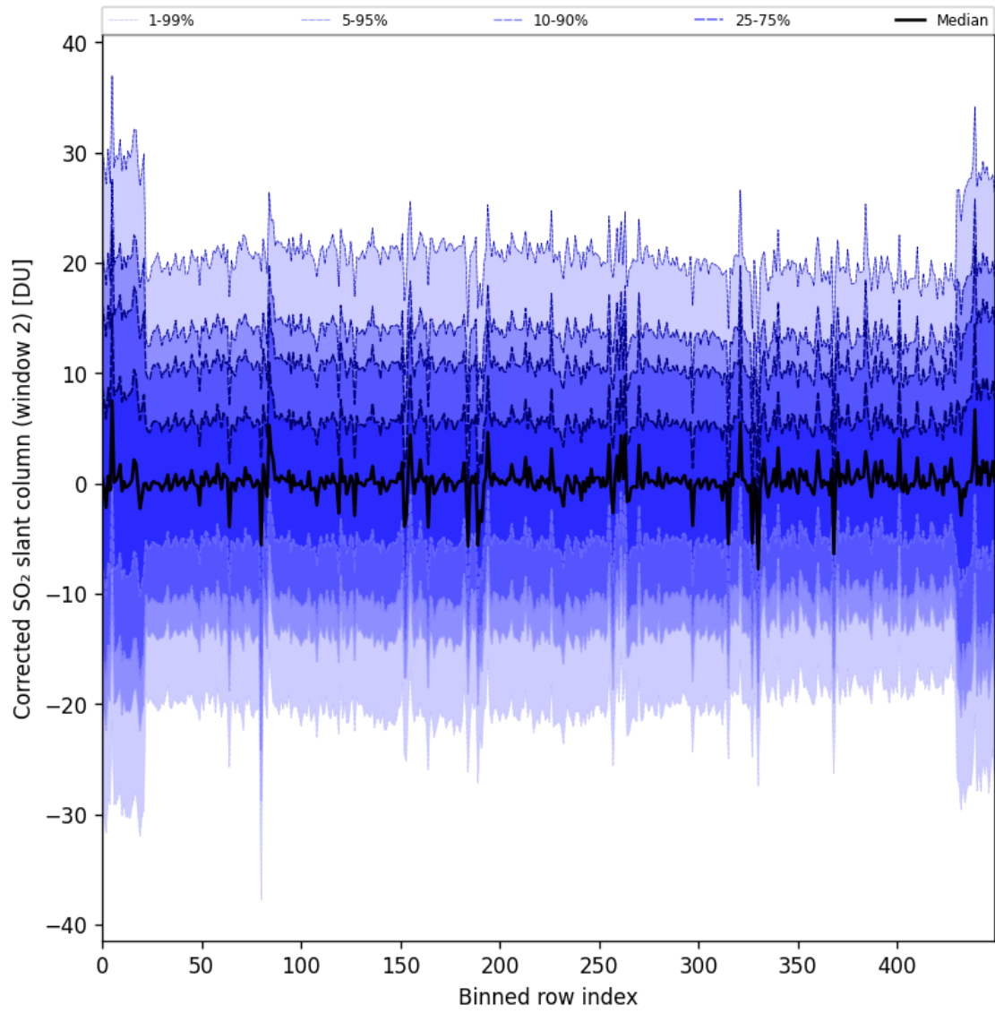
Figure 95: Along track statistics of “Corrected SO 2 slant column (window 2)” for 2025-06-29 to 2025-07-01
