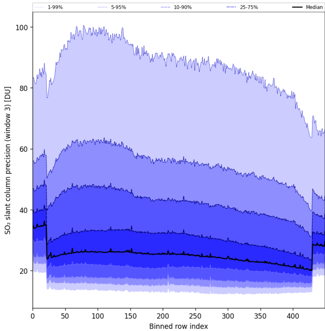
Figure 98: Along track statistics of “SO 2 slant column precision (window 3)” for 2025-06-29 to 2025-07-01
