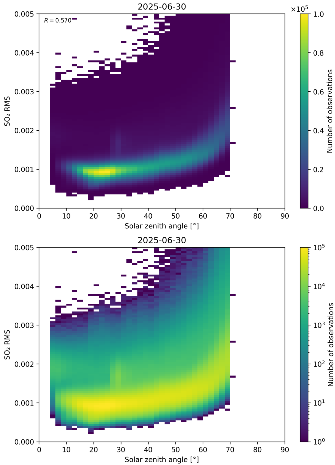
Figure 176: Scatter density plot of “Solar zenith angle” against “SO 2 RMS” for 2025-06-29 to 2025-07-01.
