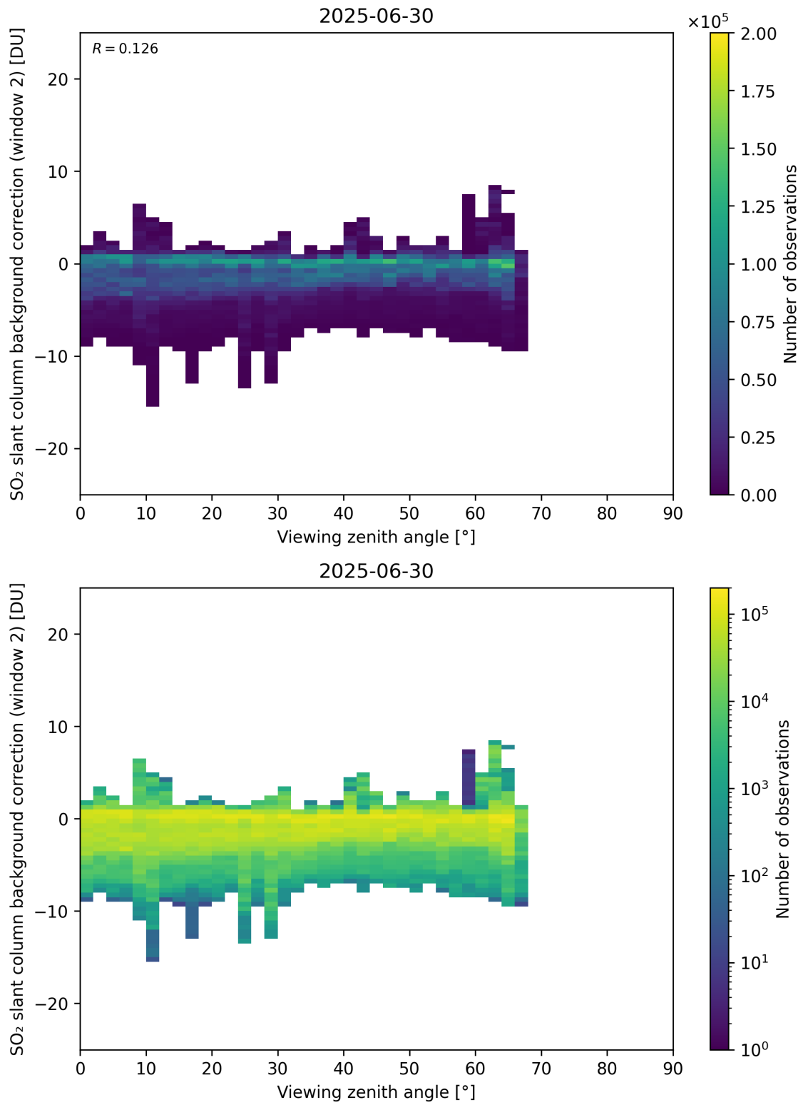
Figure 363: Scatter density plot of “Viewing zenith angle” against “SO 2 slant column background correction (window 2)” for 2025-06-29 to 2025-07-01.
