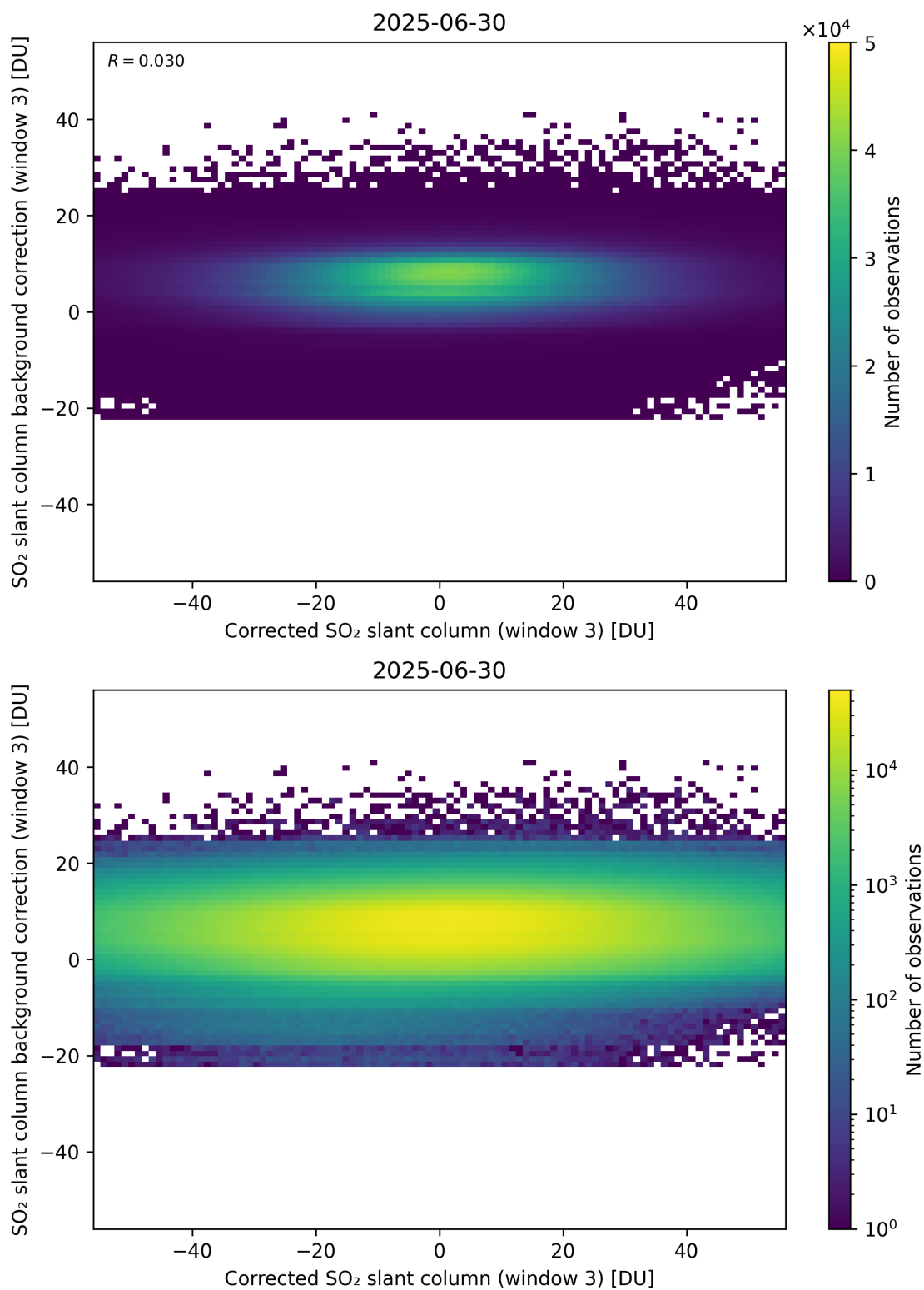
Figure 255: Scatter density plot of “Corrected SO 2 slant column (window 3)” against “SO 2 slant column background correction (window 3)” for 2025-06-29 to 2025-07-01.
