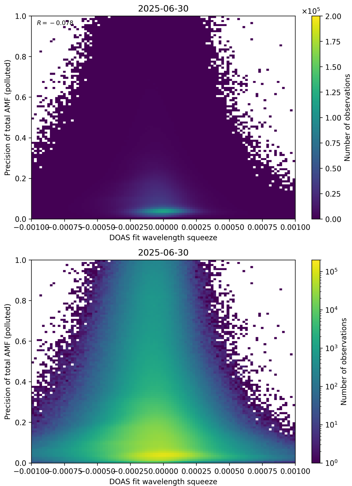
Figure 146: Scatter density plot of “DOAS fit wavelength squeeze” against “Precision of total AMF (polluted)” for 2025-06-29 to 2025-07-01.
