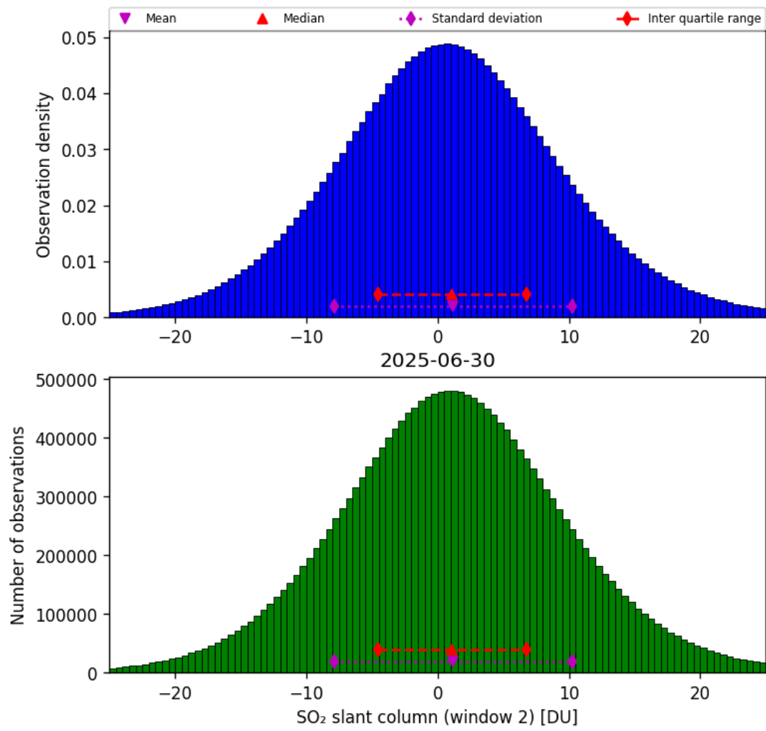
Figure 67: Histogram of “SO 2 slant column (window 2)” for 2025-06-29 to 2025-07-01
