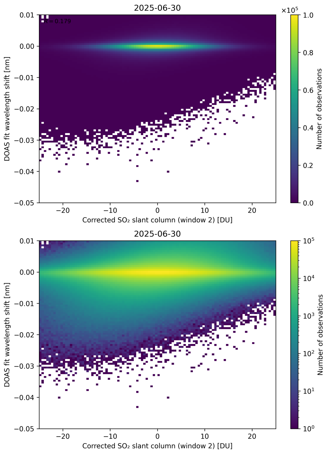
Figure 246: Scatter density plot of “Corrected SO 2 slant column (window 2)” against “DOAS fit wavelength shift” for 2025-06-29 to 2025-07-01.
