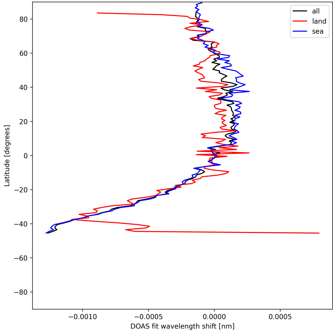
Figure 50: Zonal average of “DOAS fit wavelength shift” for 2025-06-29 to 2025-07-01.
