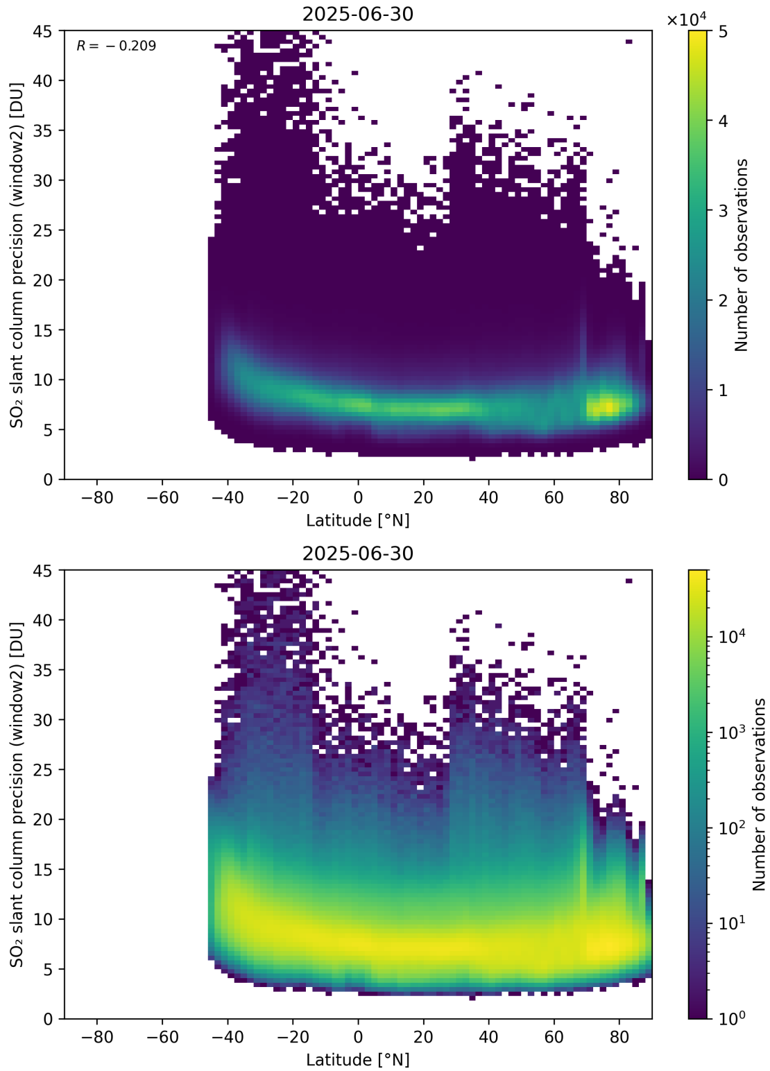
Figure 164: Scatter density plot of “Latitude” against “SO 2 slant column precision (window2)” for 2025-06-29 to 2025-07-01.
