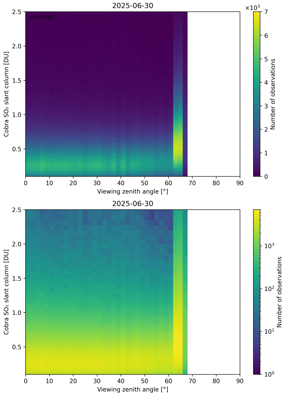
Figure 371: Scatter density plot of “Viewing zenith angle” against “Cobra SO 2 slant column” for 2025-06-29 to 2025-07-01.
