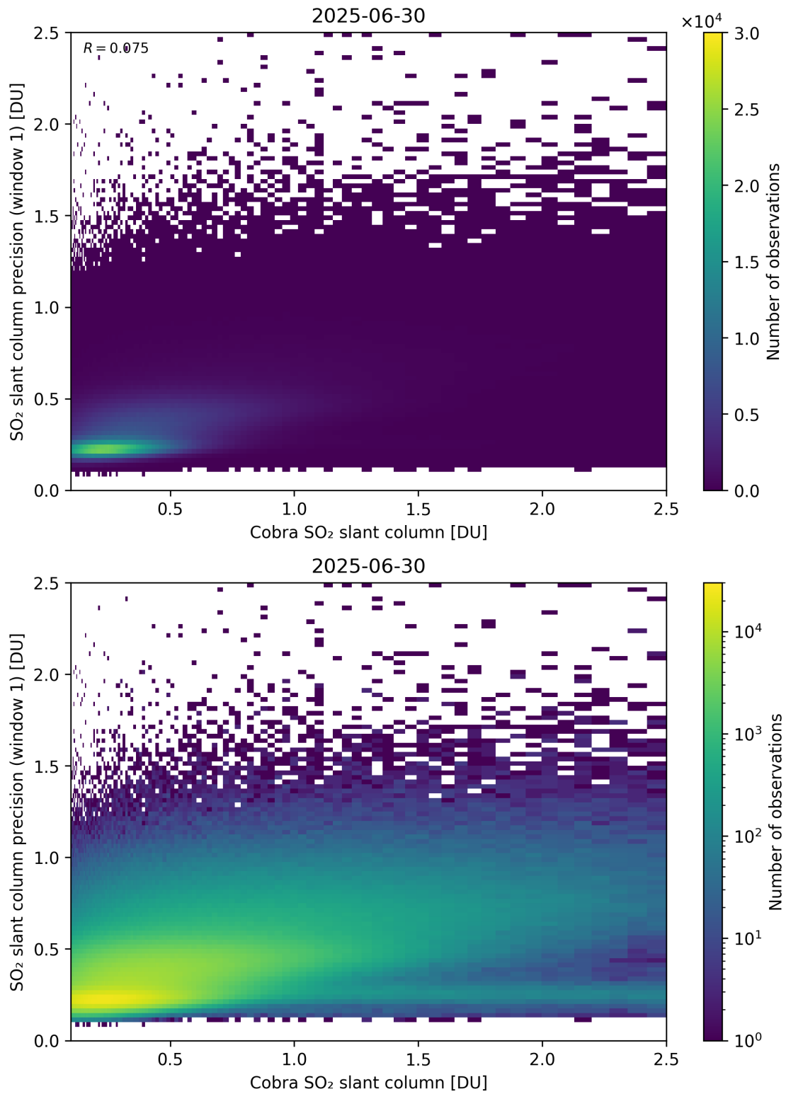
Figure 220: Scatter density plot of “Cobra SO 2 slant column” against “SO 2 slant column precision (window 1)” for 2025-06-29 to 2025-07-01.
