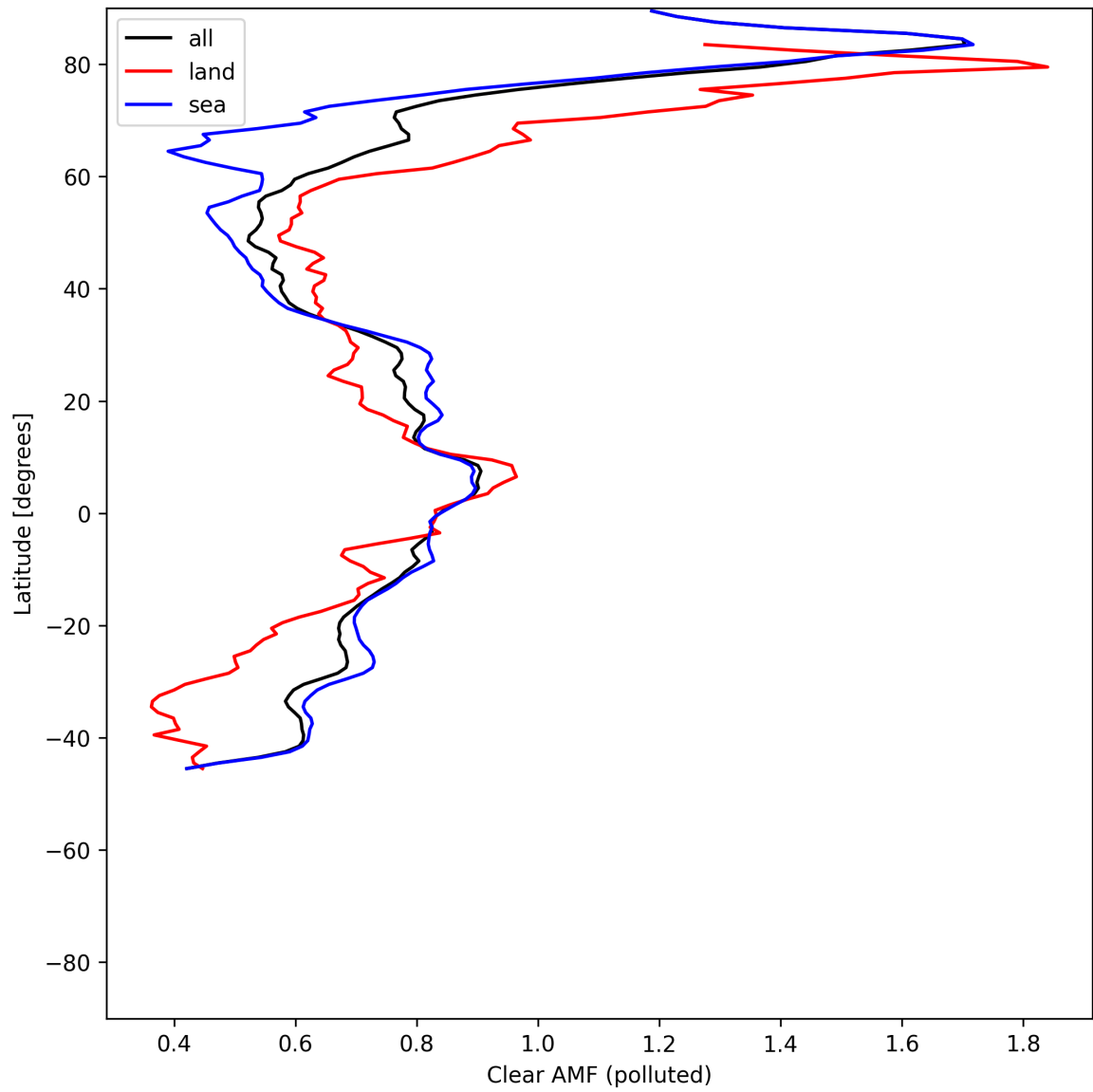
Figure 55: Zonal average of “Clear AMF (polluted)” for 2025-06-29 to 2025-07-01.
