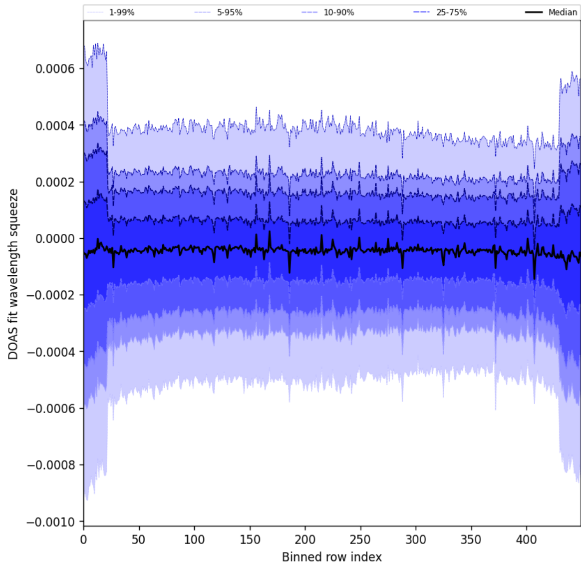
Figure 103: Along track statistics of “DOAS fit wavelength squeeze” for 2025-06-29 to 2025-07-01
