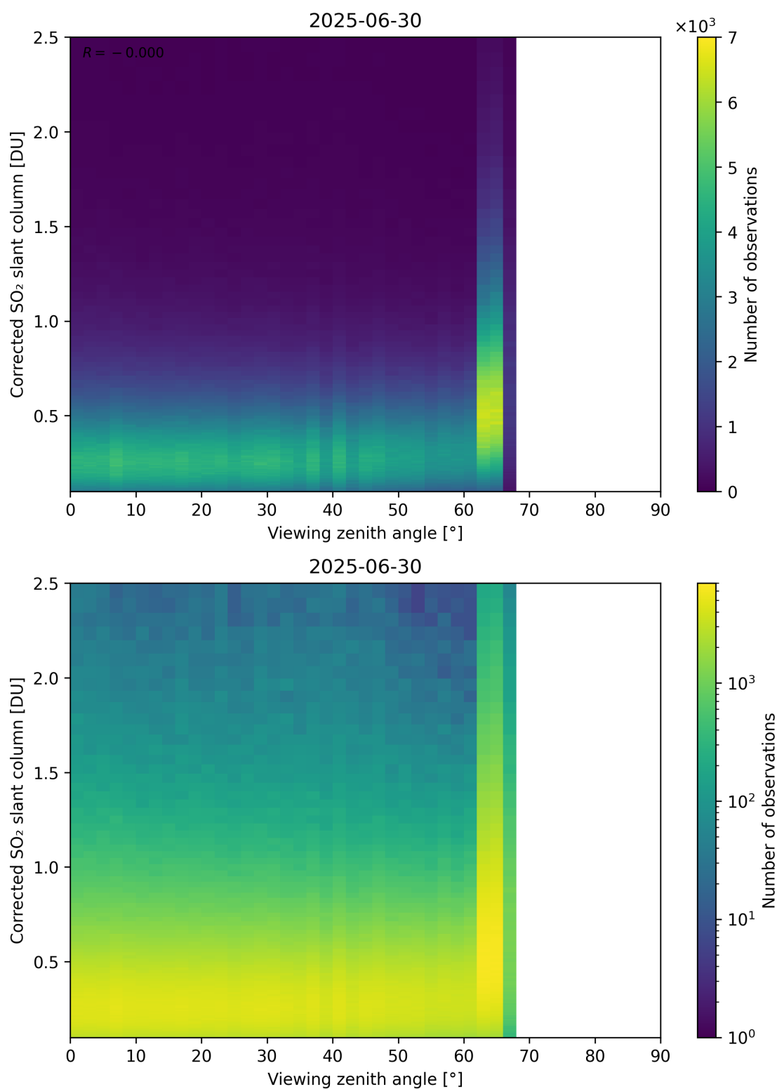
Figure 373: Scatter density plot of “Viewing zenith angle” against “Corrected SO 2 slant column” for 2025-06-29 to 2025-07-01.
