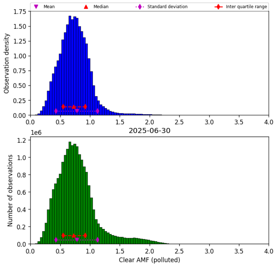
Figure 81: Histogram of “Clear AMF (polluted)” for 2025-06-29 to 2025-07-01
