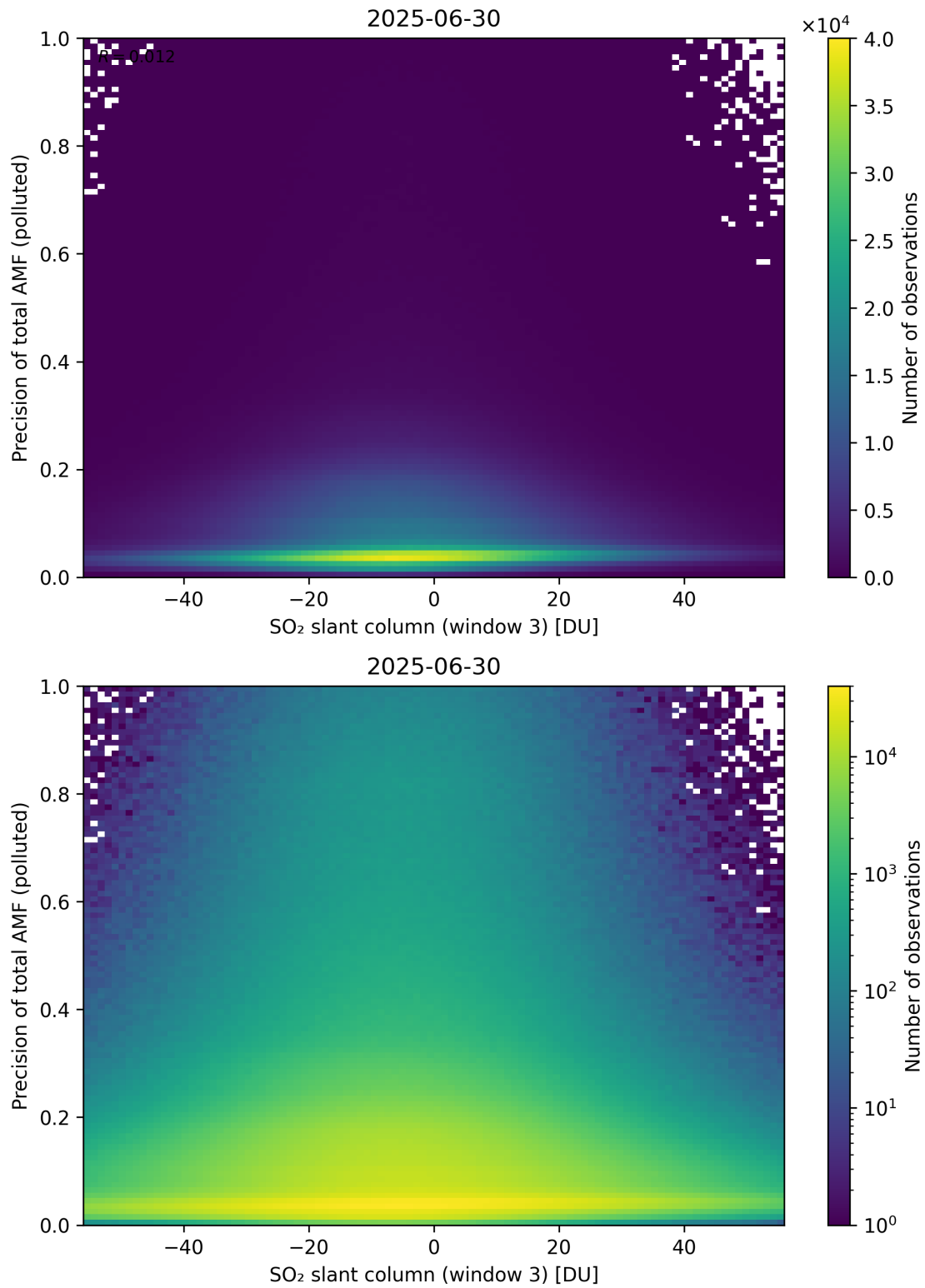
Figure 319: Scatter density plot of “SO 2 slant column (window 3)” against “Precision of total AMF (polluted)” for 2025-06-29 to 2025-07-01.
