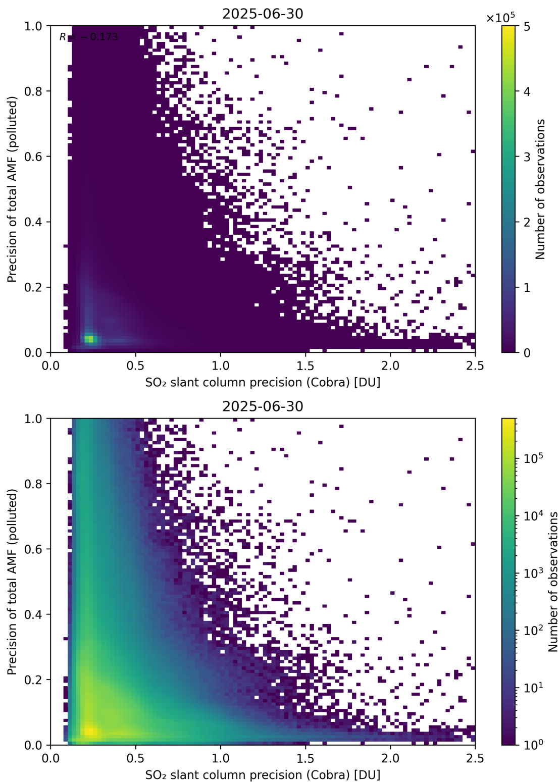
Figure 214: Scatter density plot of “SO 2 slant column precision (Cobra)” against “Precision of total AMF (polluted)” for 2025-06-29 to 2025-07-01.
