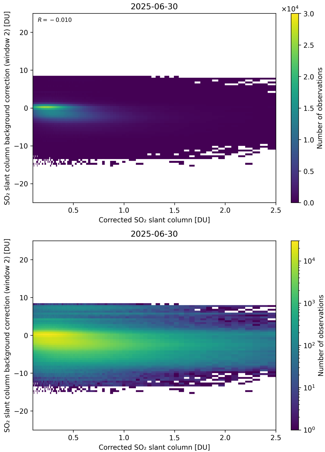
Figure 227: Scatter density plot of “Corrected SO 2 slant column” against “SO 2 slant column background correction (window 2)” for 2025-06-29 to 2025-07-01.
