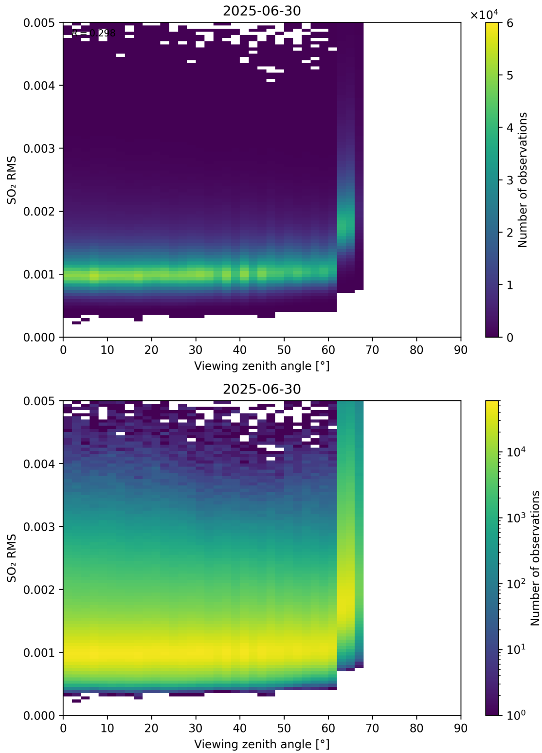
Figure 367: Scatter density plot of “Viewing zenith angle” against “SO 2 RMS” for 2025-06-29 to 2025-07-01.
