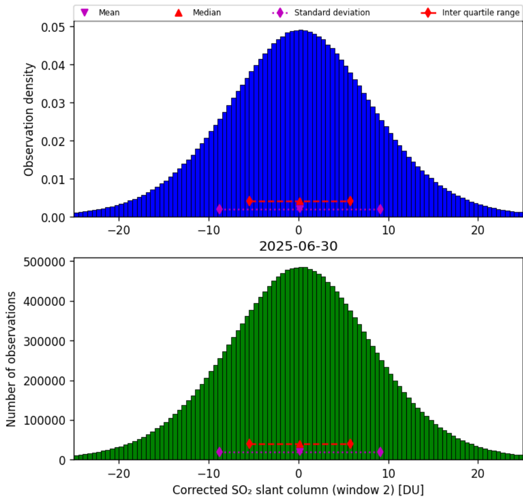
Figure 69: Histogram of “Corrected SO 2 slant column (window 2)” for 2025-06-29 to 2025-07-01
