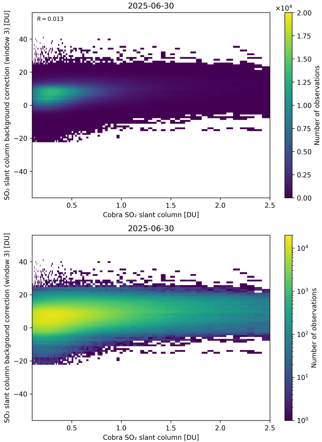
Figure 195: Scatter density plot of “Cobra SO 2 slant column” against “SO 2 slant column background correction (window 3)” for 2025-06-29 to 2025-07-01.
