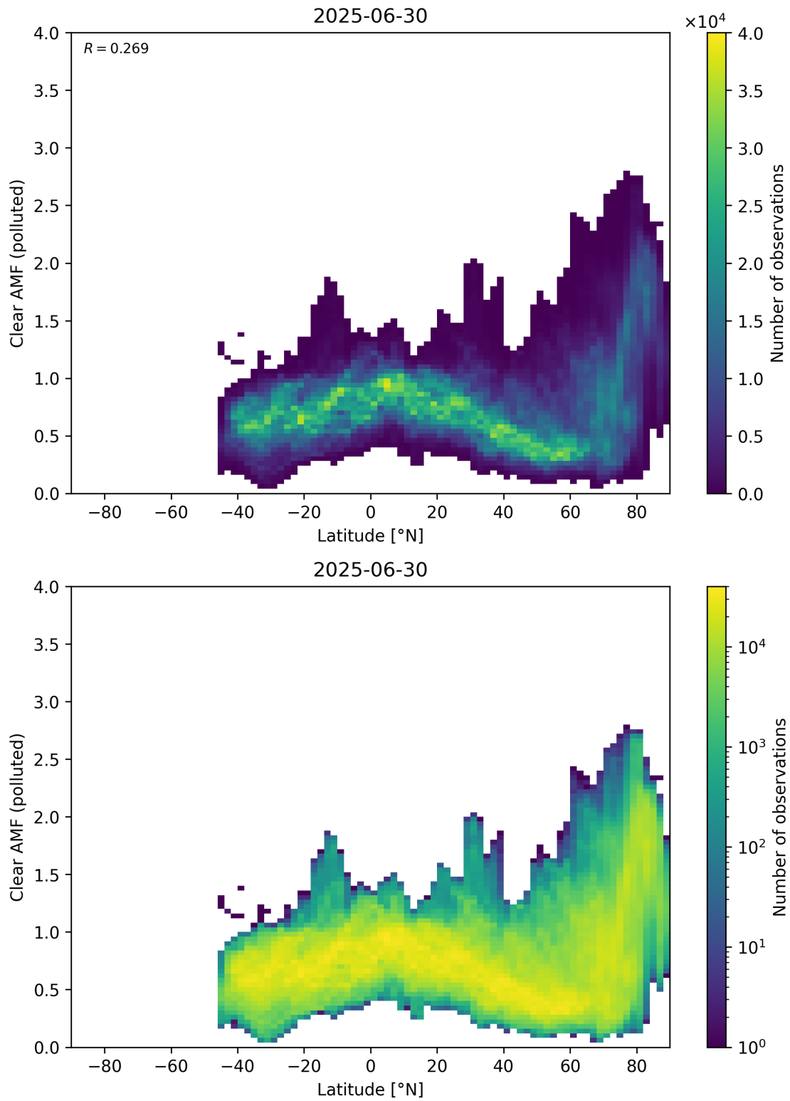
Figure 156: Scatter density plot of “Latitude” against “Clear AMF (polluted)” for 2025-06-29 to 2025-07-01.
