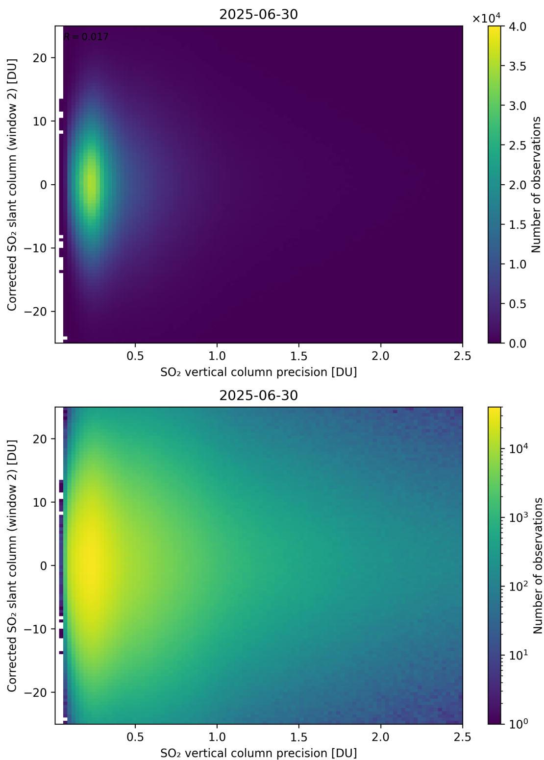
Figure 339: Scatter density plot of “SO 2 vertical column precision” against “Corrected SO 2 slant column (window 2)” for 2025-06-29 to 2025-07-01.
