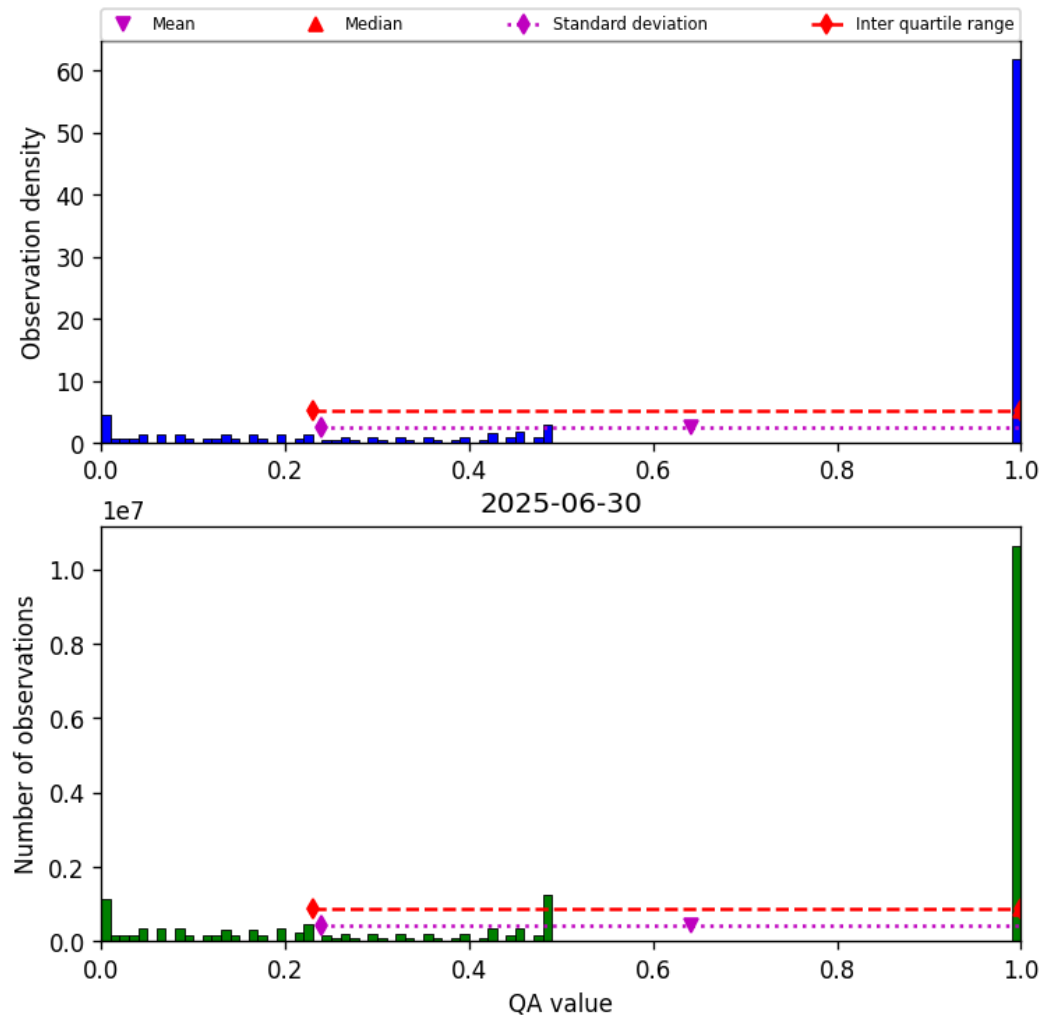
Figure 57: Histogram of “QA value” for 2025-06-29 to 2025-07-01
