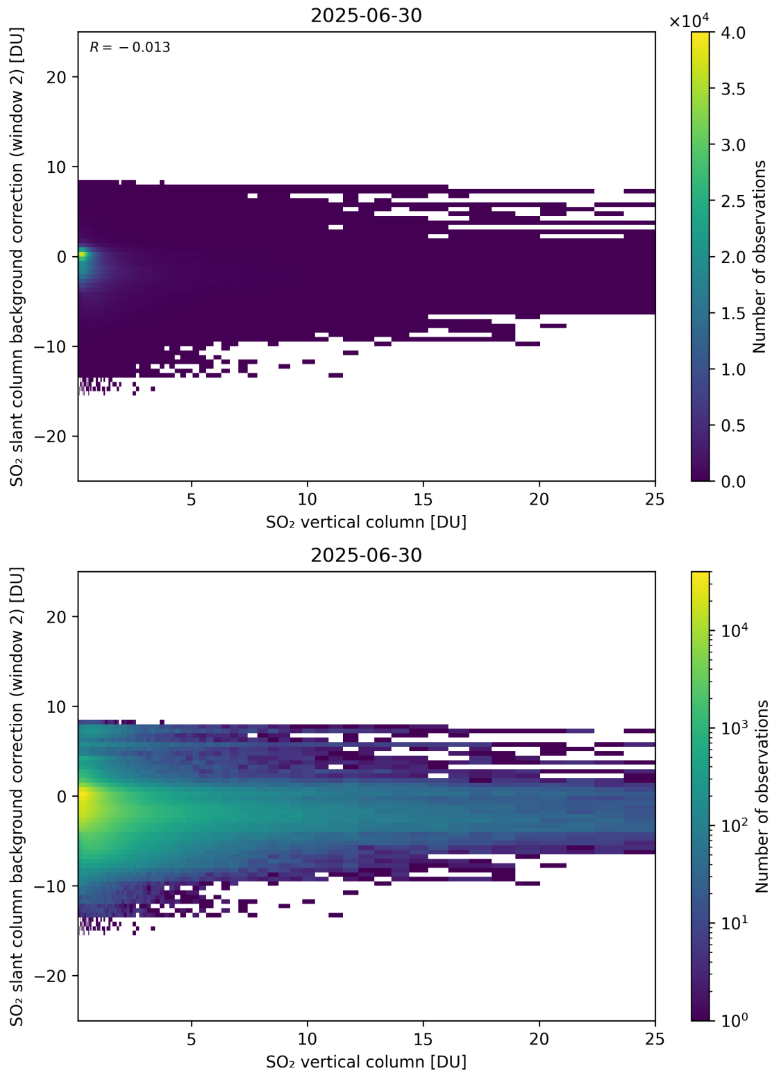
Figure 324: Scatter density plot of “SO 2 vertical column” against “SO 2 slant column background correction (window 2)” for 2025-06-29 to 2025-07-01.
