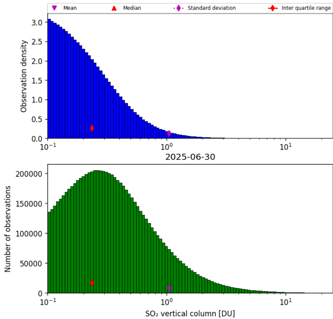
Figure 58: Histogram of “SO 2 vertical column” for 2025-06-29 to 2025-07-01
