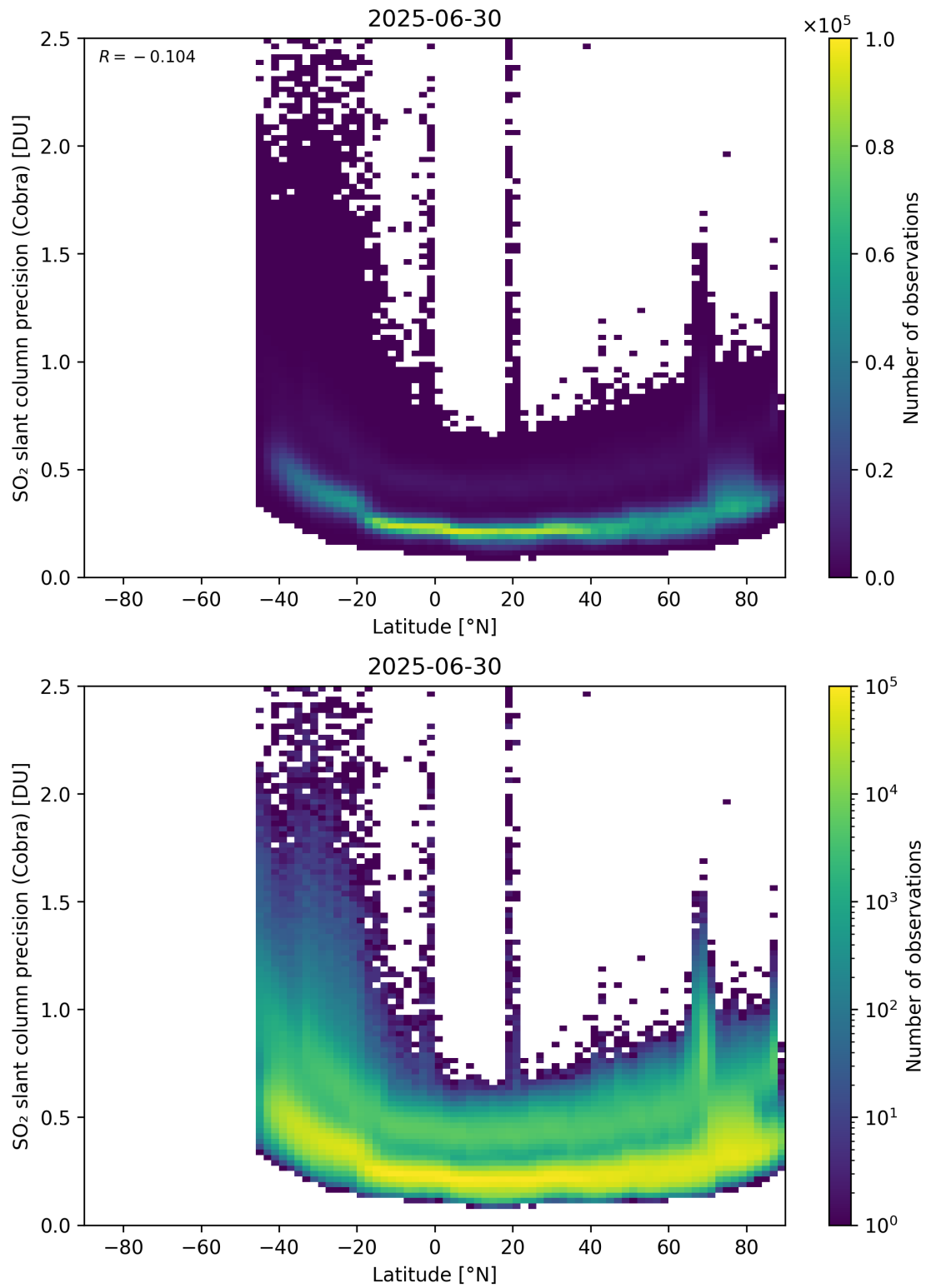
Figure 158: Scatter density plot of “Latitude” against “SO 2 slant column precision (Cobra)” for 2025-06-29 to 2025-07-01.
