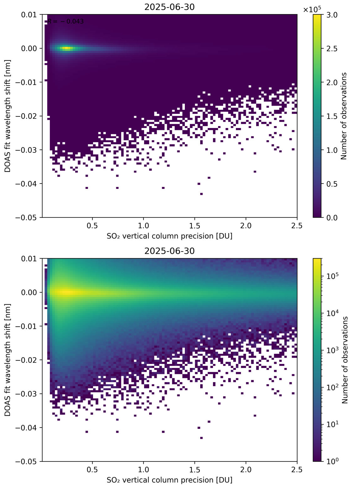
Figure 332: Scatter density plot of “SO 2 vertical column precision” against “DOAS fit wavelength shift” for 2025-06-29 to 2025-07-01.
