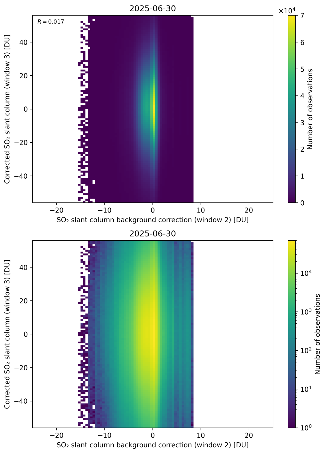
Figure 127: Scatter density plot of “SO 2 slant column background correction (window 2)” against “Corrected SO 2 slant column (window 3)” for 2025-06-29 to 2025-07-01.
