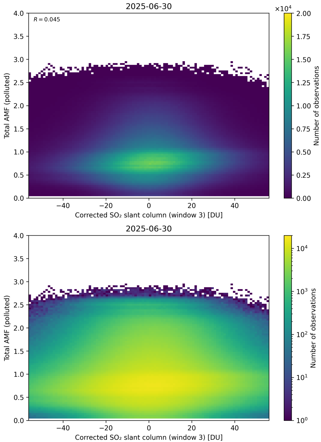
Figure 260: Scatter density plot of “Corrected SO 2 slant column (window 3)” against “Total AMF (polluted)” for 2025-06-29 to 2025-07-01.
