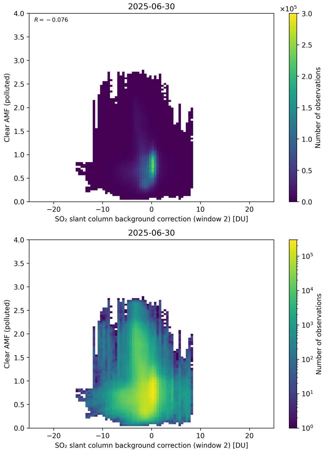
Figure 126: Scatter density plot of “SO 2 slant column background correction (window 2)” against “Clear AMF (polluted)” for 2025-06-29 to 2025-07-01.
