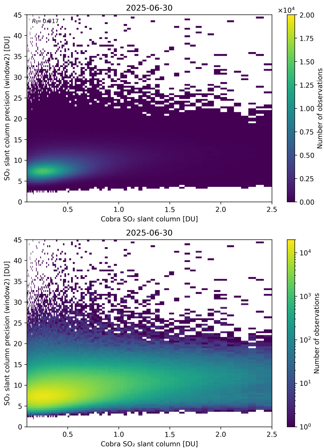
Figure 221: Scatter density plot of “Cobra SO 2 slant column” against “SO 2 slant column precision (window2)” for 2025-06-29 to 2025-07-01.
