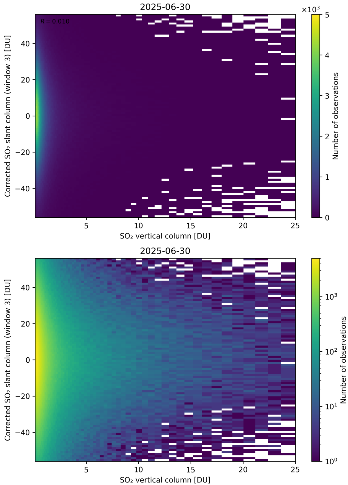
Figure 353: Scatter density plot of “SO 2 vertical column” against “Corrected SO 2 slant column (window 3)” for 2025-06-29 to 2025-07-01.
