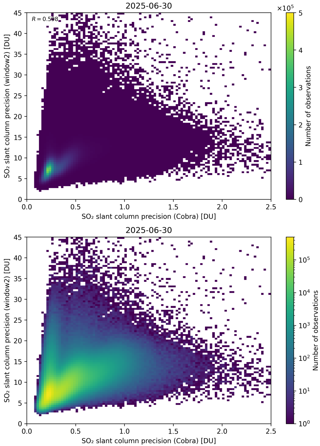
Figure 210: Scatter density plot of “SO 2 slant column precision (Cobra)” against “SO 2 slant column precision (window2)” for 2025-06-29 to 2025-07-01.
