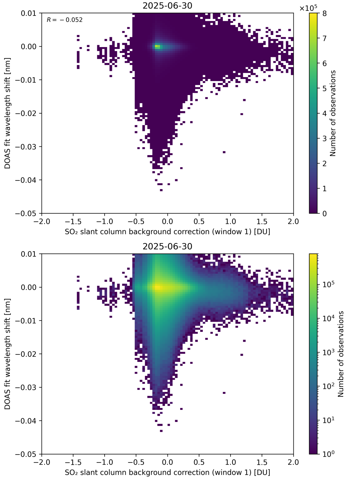
Figure 111: Scatter density plot of “SO 2 slant column background correction (window 1)” against “DOAS fit wavelength shift” for 2025-06-29 to 2025-07-01.
