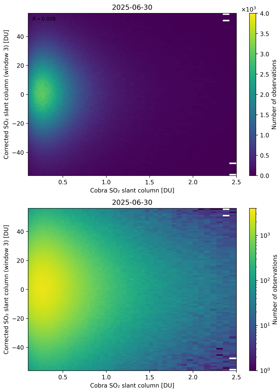
Figure 218: Scatter density plot of “Cobra SO 2 slant column” against “Corrected SO 2 slant column (window 3)” for 2025-06-29 to 2025-07-01.
