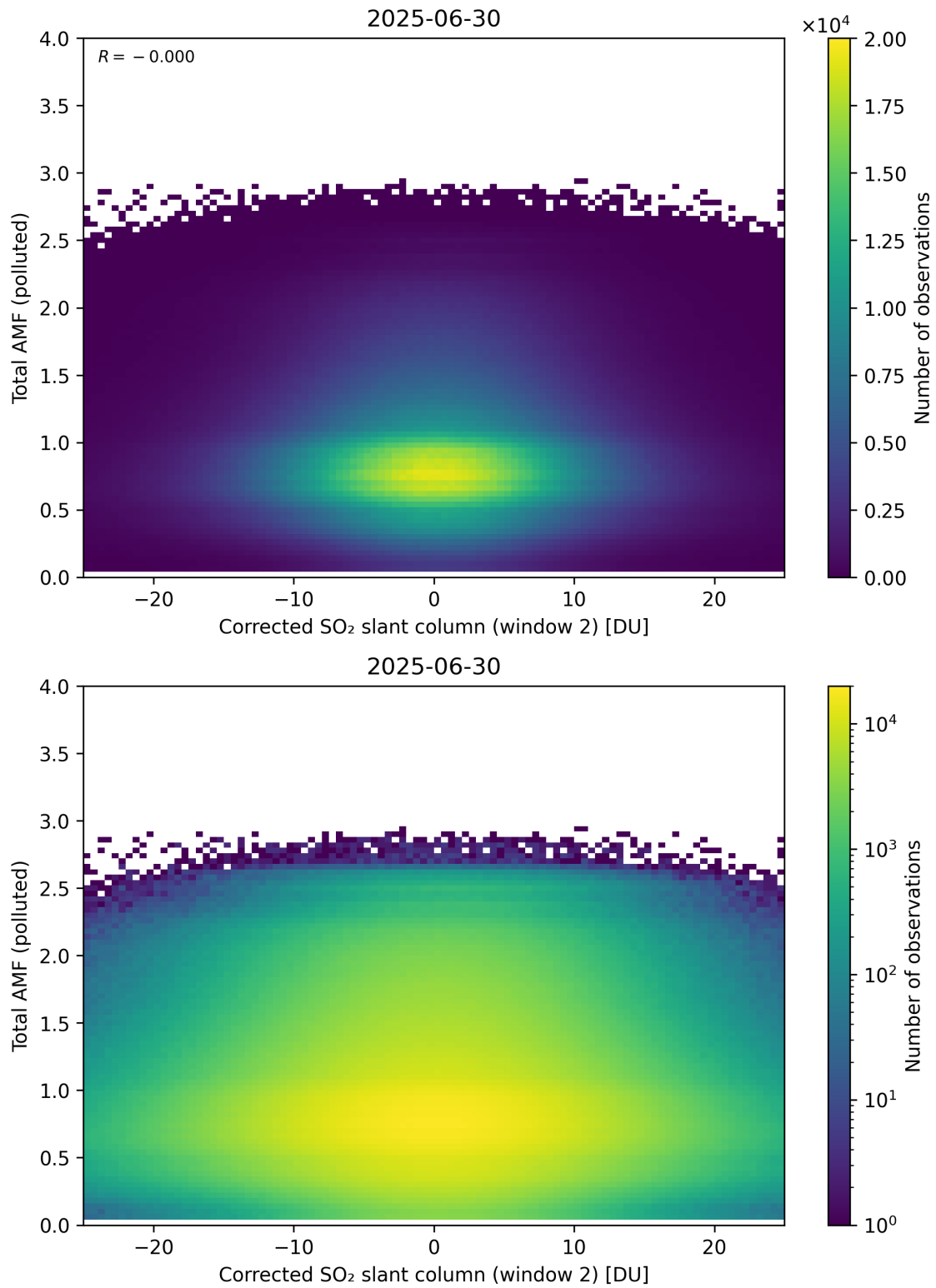
Figure 253: Scatter density plot of “Corrected SO 2 slant column (window 2)” against “Total AMF (polluted)” for 2025-06-29 to 2025-07-01.
