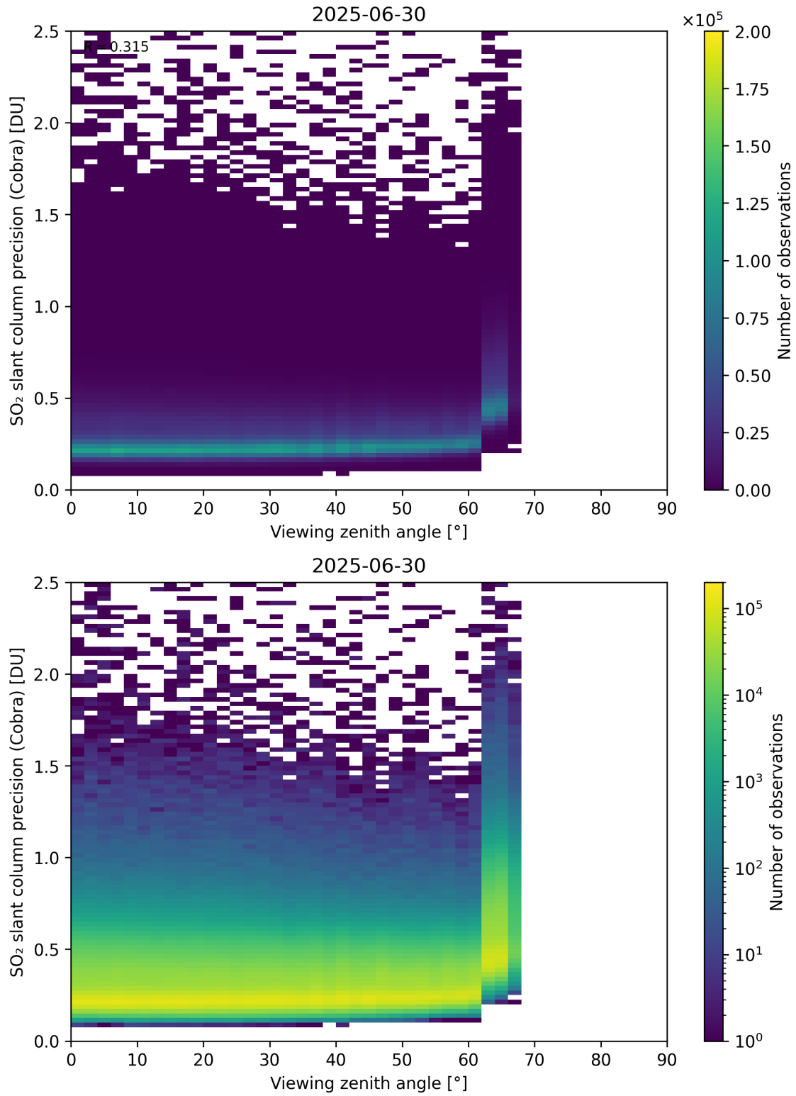
Figure 372: Scatter density plot of “Viewing zenith angle” against “SO 2 slant column precision (Cobra)” for 2025-06-29 to 2025-07-01.
