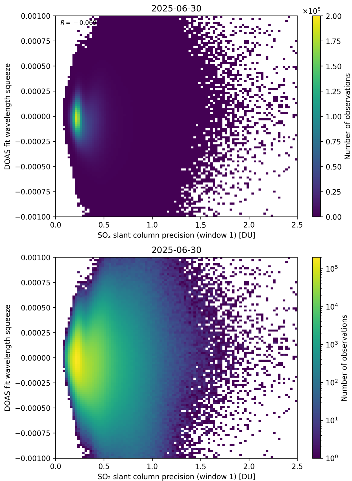
Figure 272: Scatter density plot of “SO 2 slant column precision (window 1)” against “DOAS fit wavelength squeeze” for 2025-06-29 to 2025-07-01.
