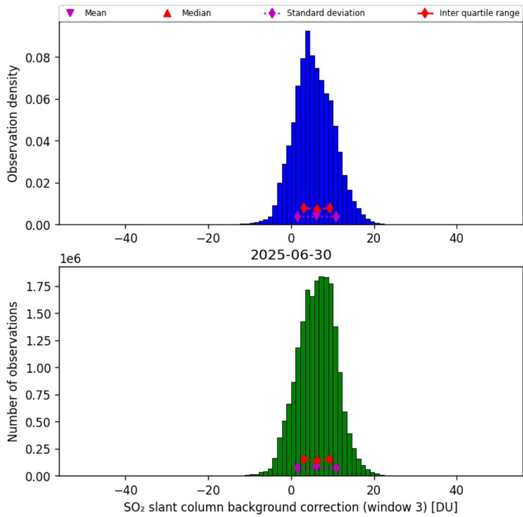
Figure 74: Histogram of “SO 2 slant column background correction (window 3)” for 2025-06-29 to 2025-07-01
