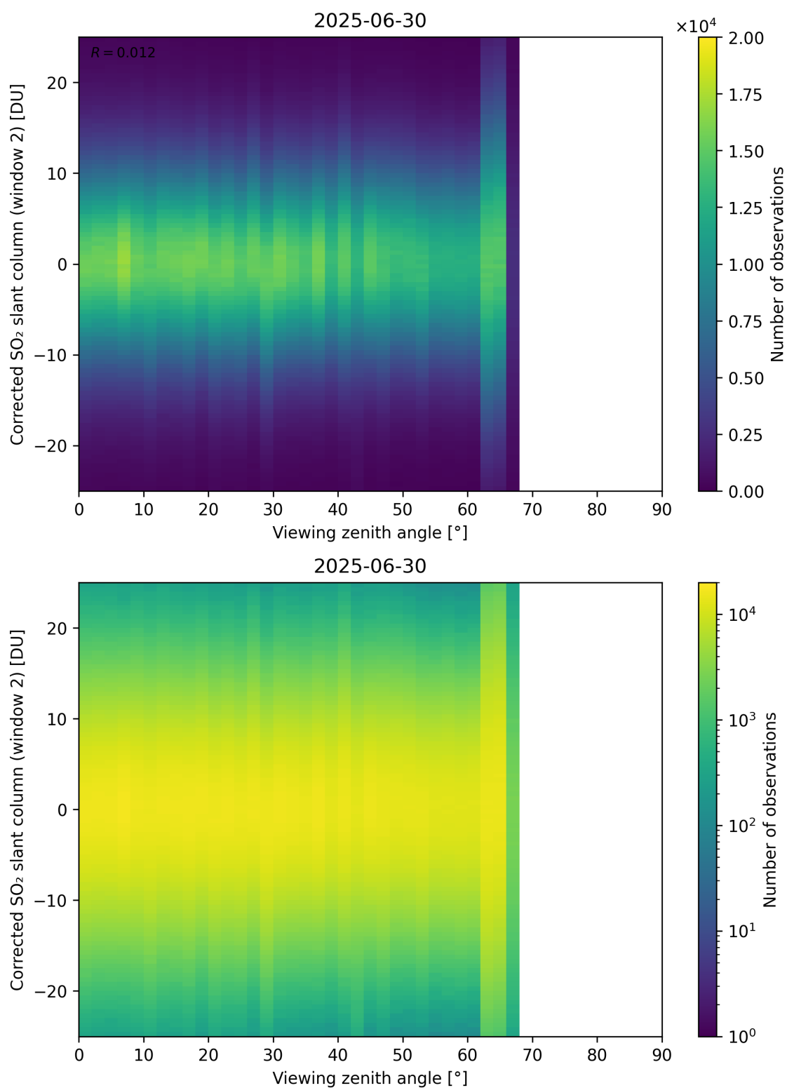
Figure 374: Scatter density plot of “Viewing zenith angle” against “Corrected SO 2 slant column (window 2)” for 2025-06-29 to 2025-07-01.
