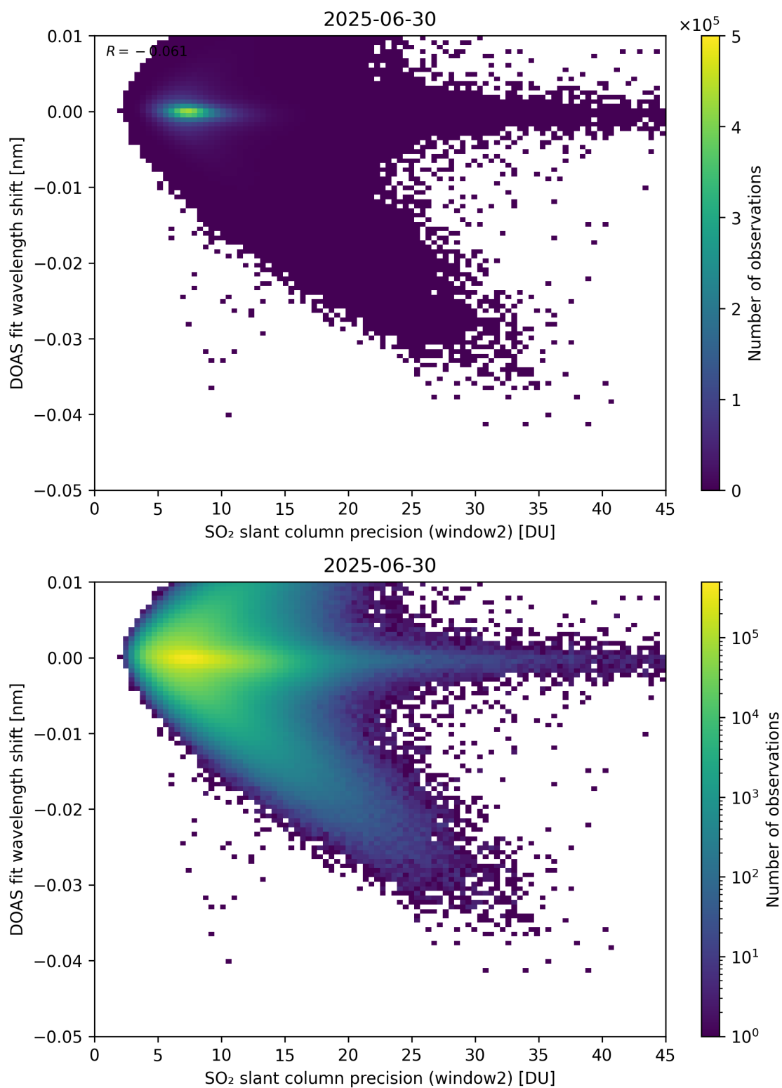
Figure 293: Scatter density plot of “SO 2 slant column precision (window2)” against “DOAS fit wavelength shift” for 2025-06-29 to 2025-07-01.
