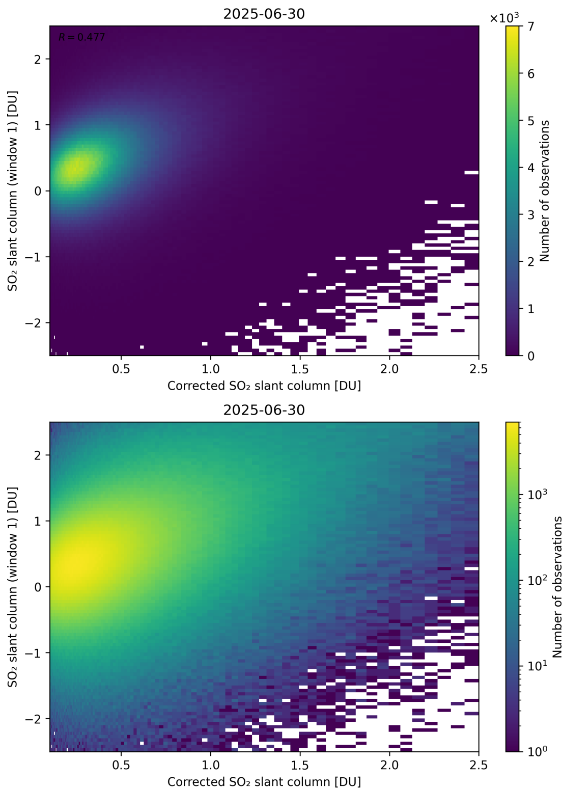
Figure 237: Scatter density plot of “Corrected SO 2 slant column” against “SO 2 slant column (window 1)” for 2025-06-29 to 2025-07-01.
