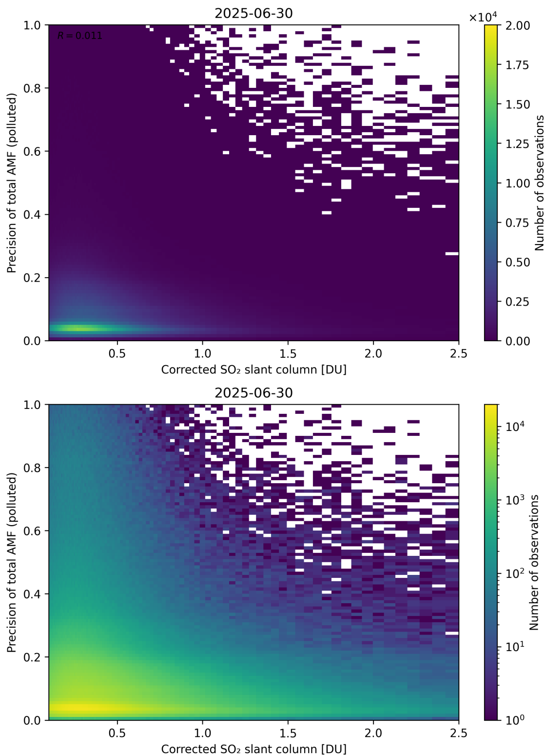
Figure 243: Scatter density plot of “Corrected SO 2 slant column” against “Precision of total AMF (polluted)” for 2025-06-29 to 2025-07-01.
