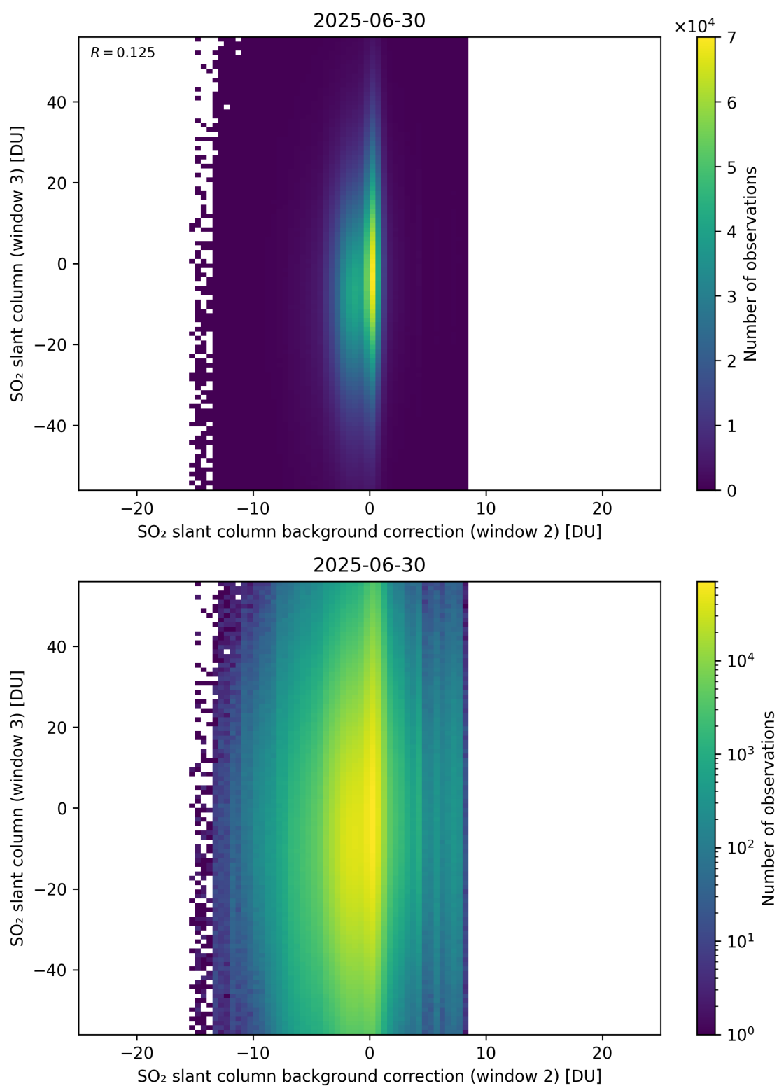
Figure 128: Scatter density plot of “SO 2 slant column background correction (window 2)” against “SO 2 slant column (window 3)” for 2025-06-29 to 2025-07-01.
