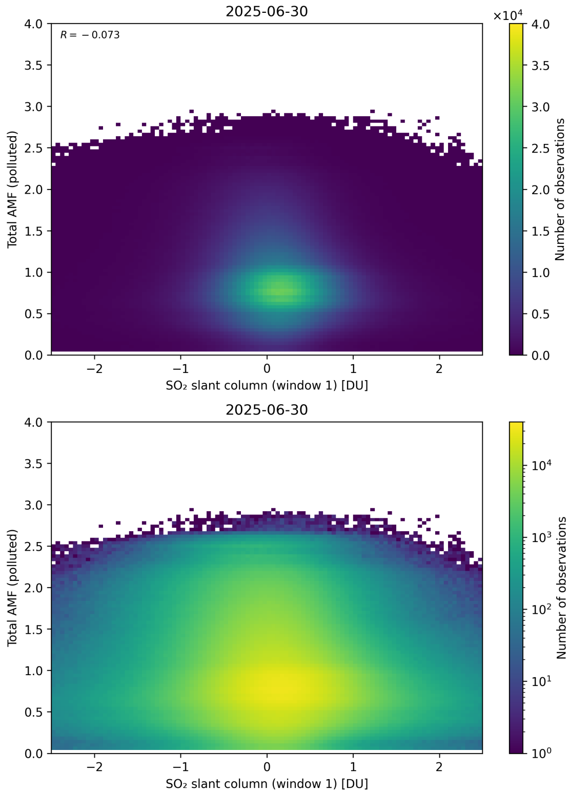
Figure 289: Scatter density plot of “SO 2 slant column (window 1)” against “Total AMF (polluted)” for 2025-06-29 to 2025-07-01.
