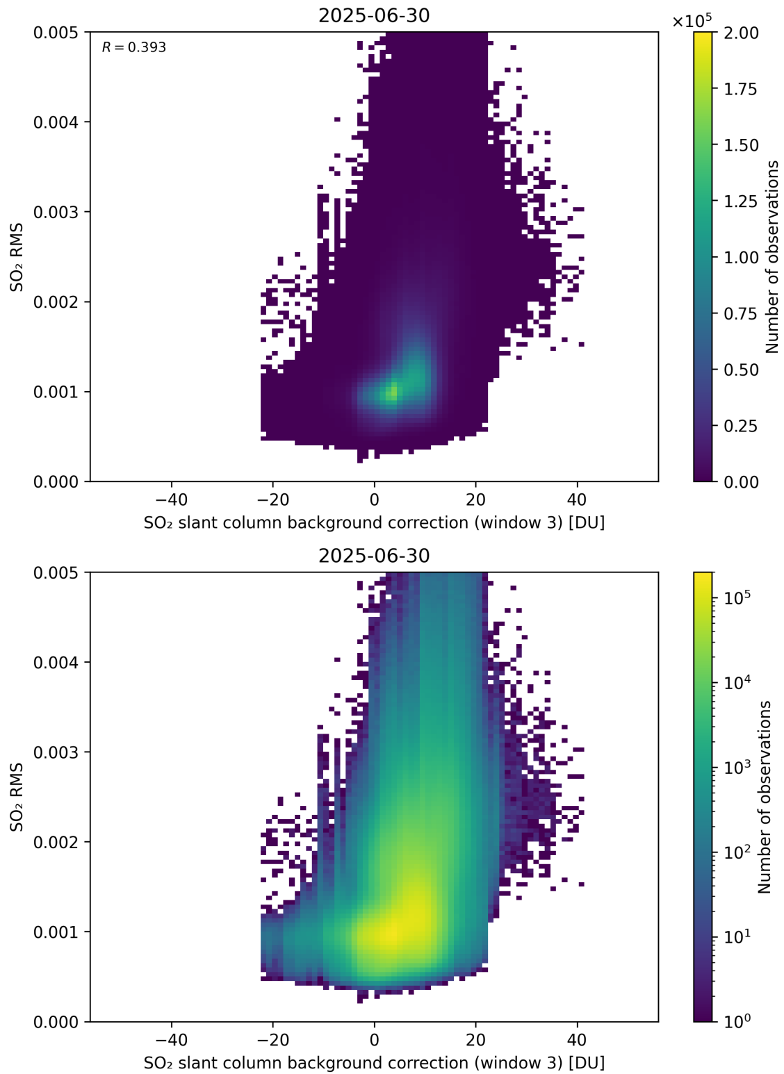
Figure 134: Scatter density plot of “SO 2 slant column background correction (window 3)” against “SO 2 RMS” for 2025-06-29 to 2025-07-01.
