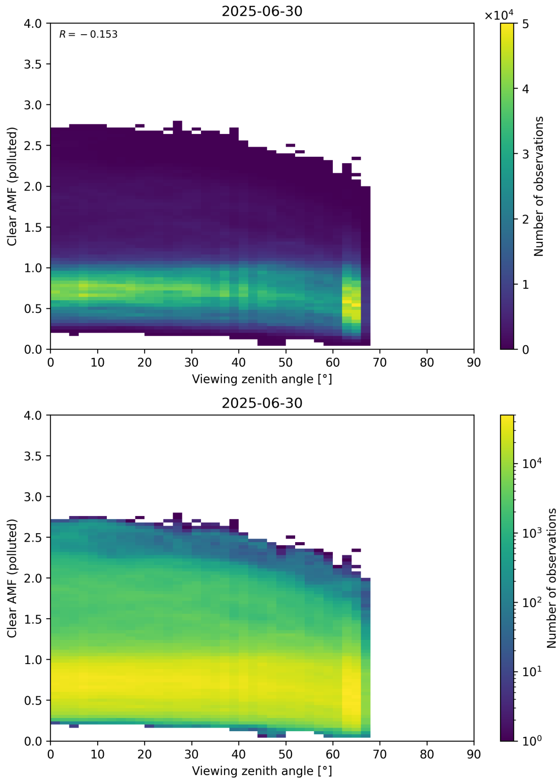
Figure 370: Scatter density plot of “Viewing zenith angle” against “Clear AMF (polluted)” for 2025-06-29 to 2025-07-01.
