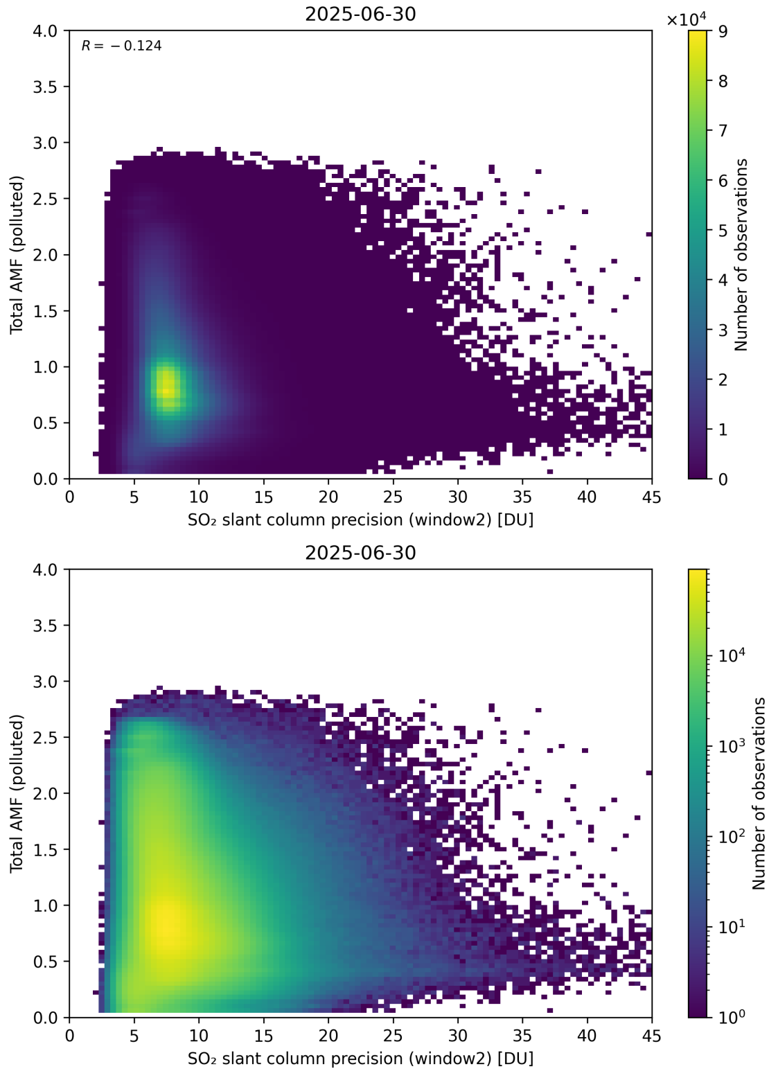
Figure 301: Scatter density plot of “SO 2 slant column precision (window2)” against “Total AMF (polluted)” for 2025-06-29 to 2025-07-01.
