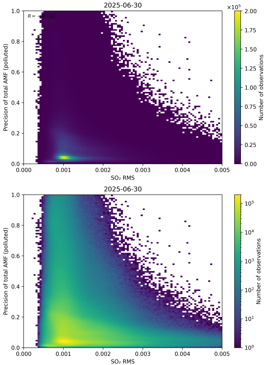
Figure 149: Scatter density plot of “SO 2 RMS” against “Precision of total AMF (polluted)” for 2025-06-29 to 2025-07-01.
