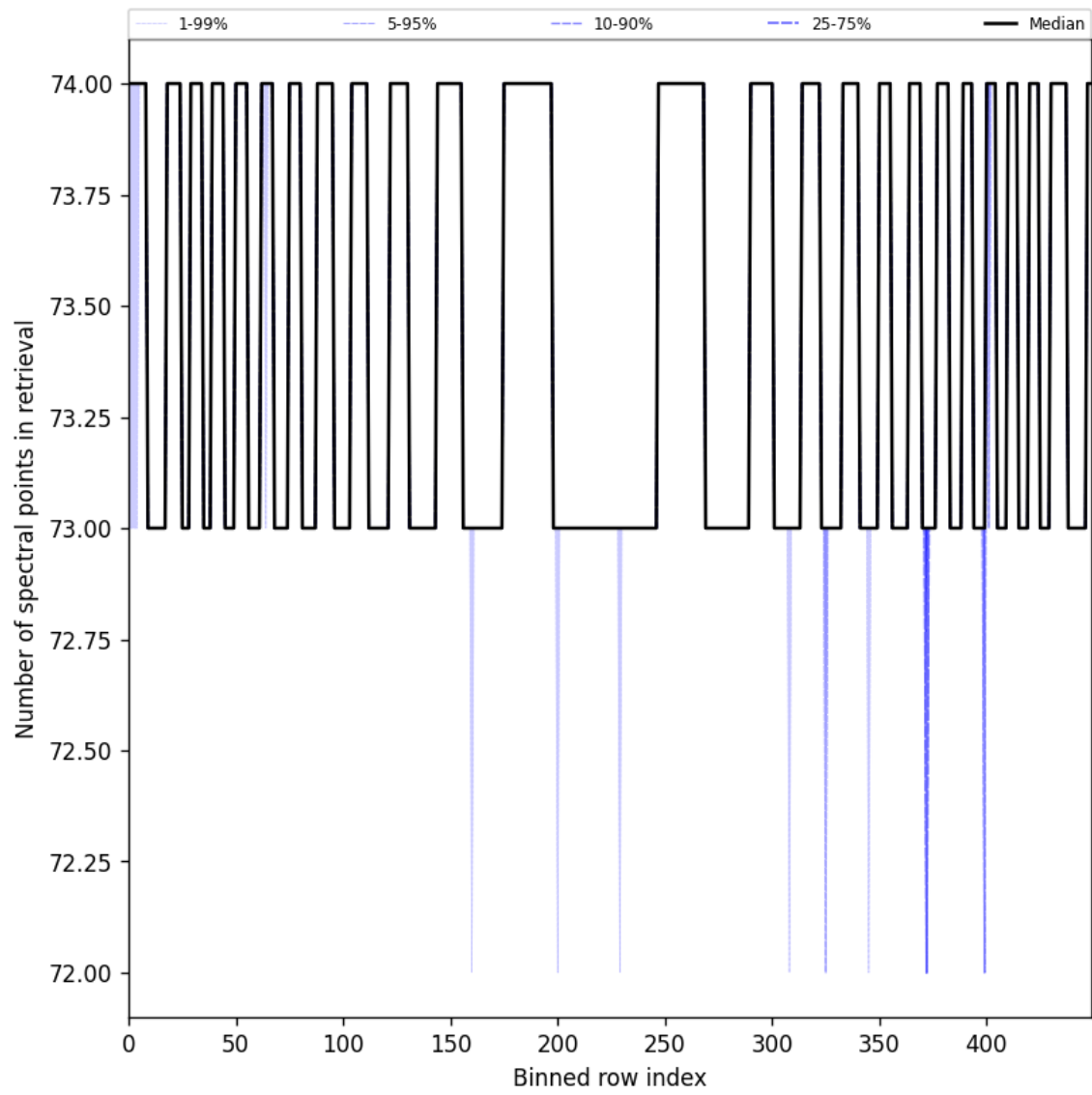
Figure 108: Along track statistics of “Number of spectral points in retrieval” for 2025-06-29 to 2025-07-01
