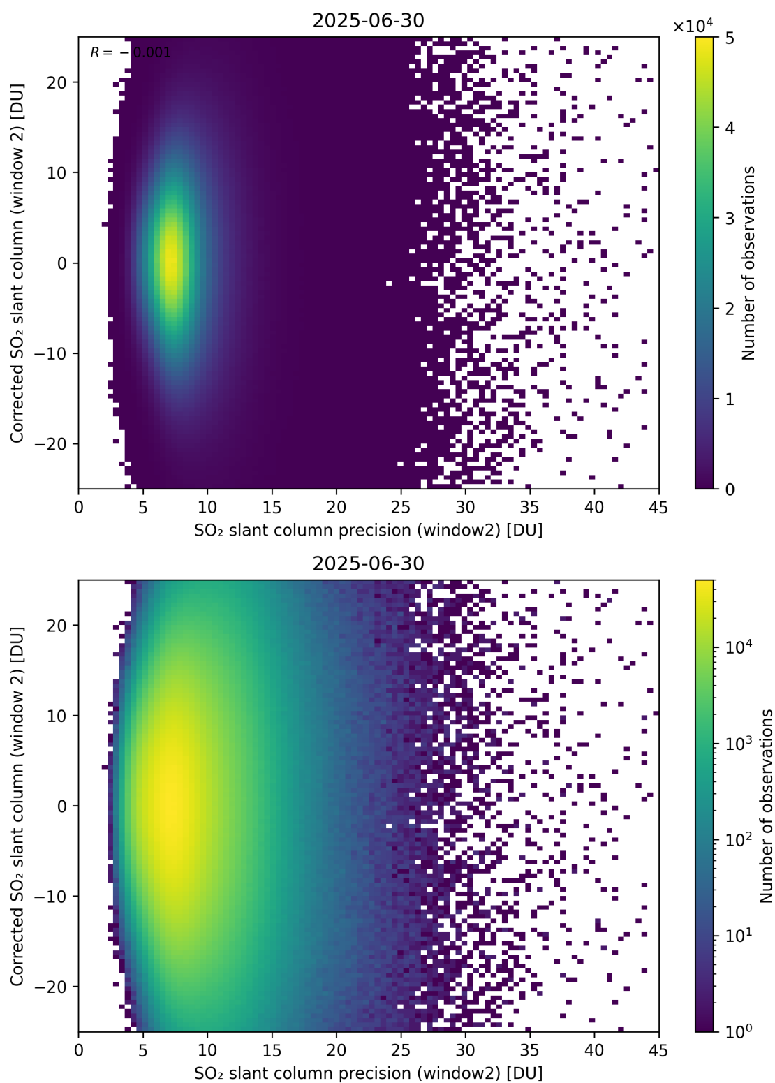
Figure 297: Scatter density plot of “SO 2 slant column precision (window2)” against “Corrected SO 2 slant column (window 2)” for 2025-06-29 to 2025-07-01.
