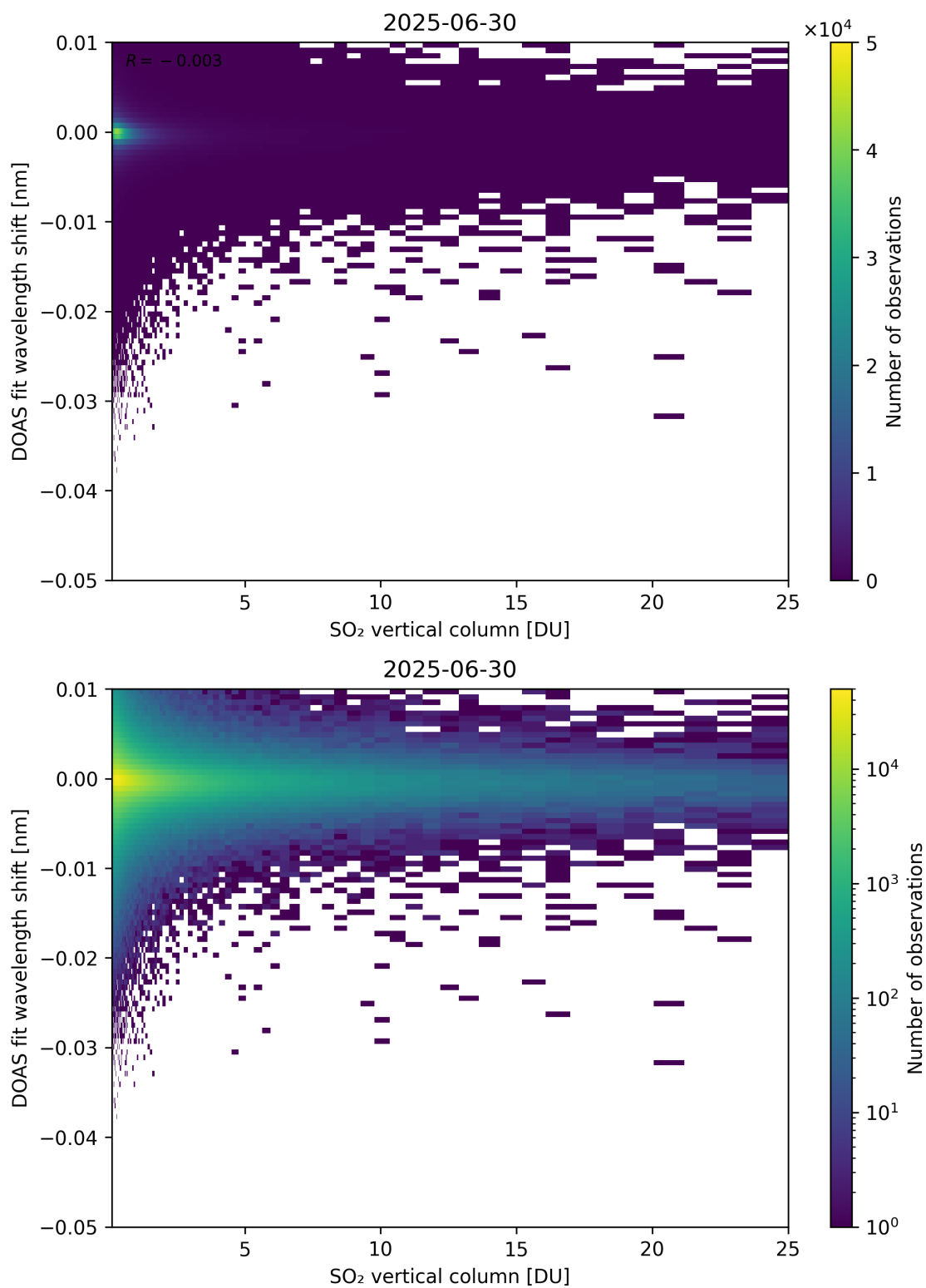
Figure 326: Scatter density plot of “SO 2 vertical column” against “DOAS fit wavelength shift” for 2025-06-29 to 2025-07-01.
