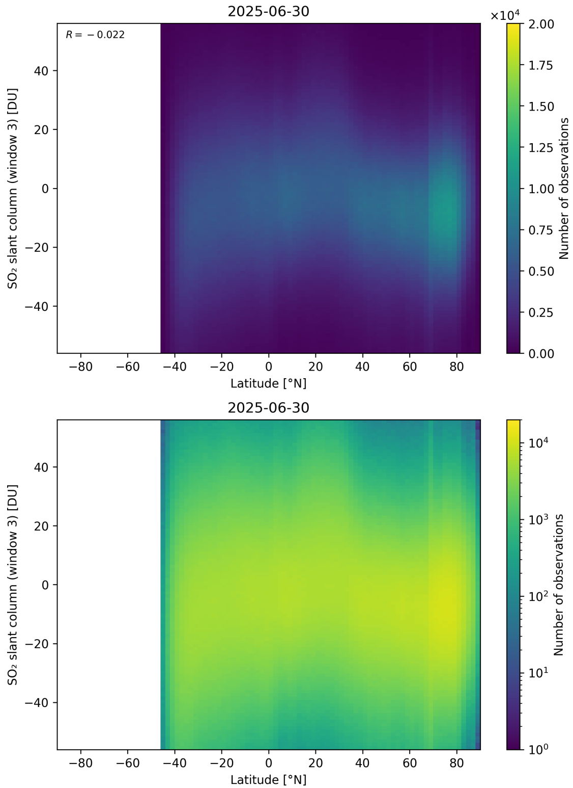
Figure 165: Scatter density plot of “Latitude” against “SO 2 slant column (window 3)” for 2025-06-29 to 2025-07-01.
