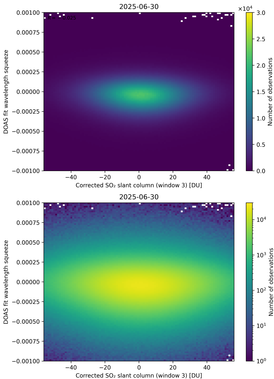
Figure 257: Scatter density plot of “Corrected SO 2 slant column (window 3)” against “DOAS fit wavelength squeeze” for 2025-06-29 to 2025-07-01.
