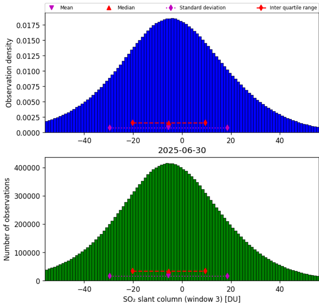
Figure 71: Histogram of “SO 2 slant column (window 3)” for 2025-06-29 to 2025-07-01
