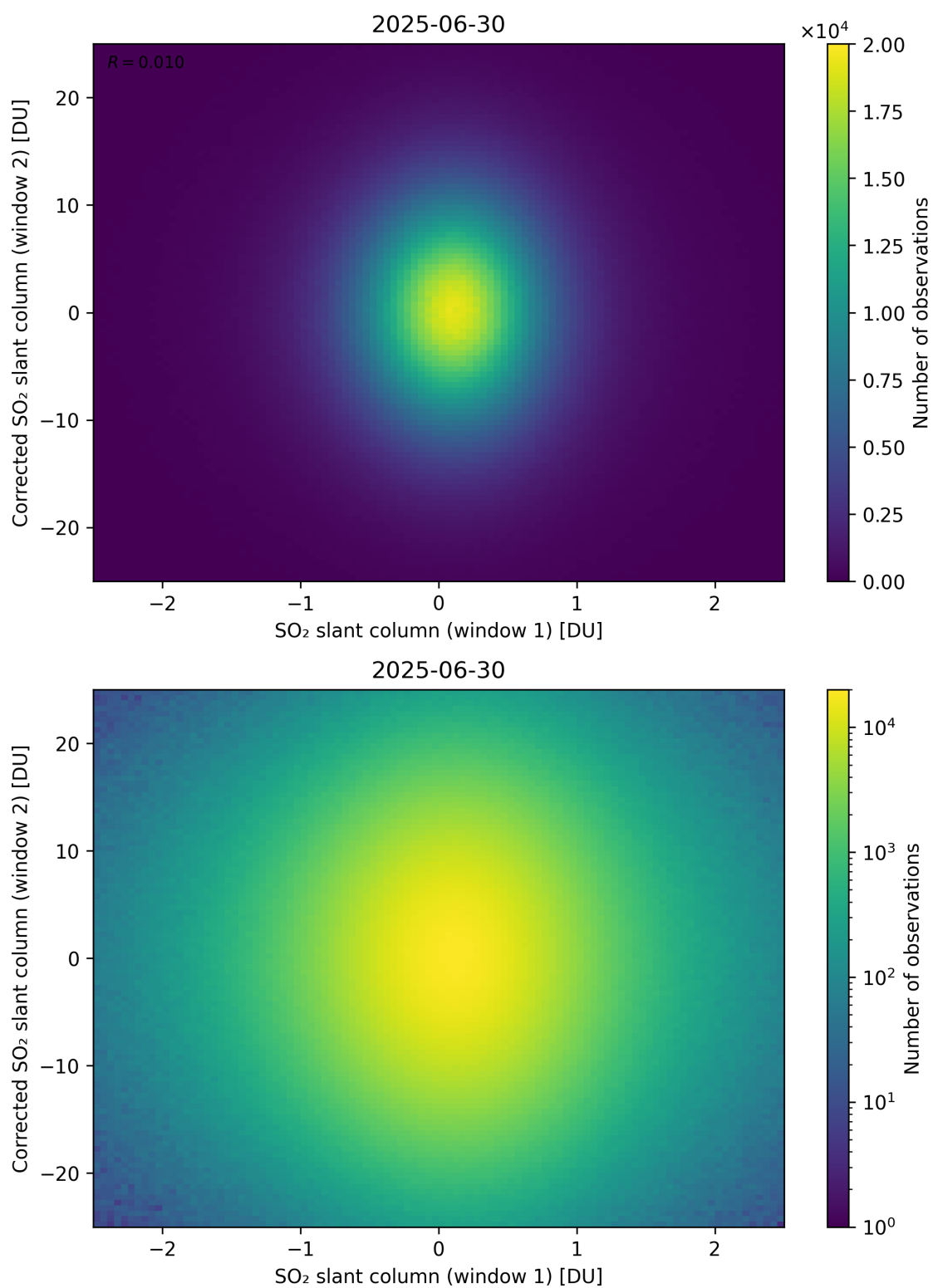
Figure 283: Scatter density plot of “SO 2 slant column (window 1)” against “Corrected SO 2 slant column (window 2)” for 2025-06-29 to 2025-07-01.
