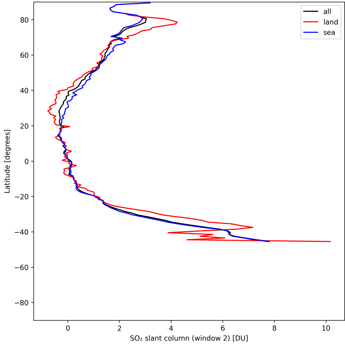
Figure 41: Zonal average of “SO 2 slant column (window 2)” for 2025-06-29 to 2025-07-01.
