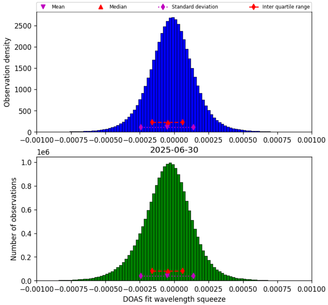
Figure 77: Histogram of “DOAS fit wavelength squeeze” for 2025-06-29 to 2025-07-01
