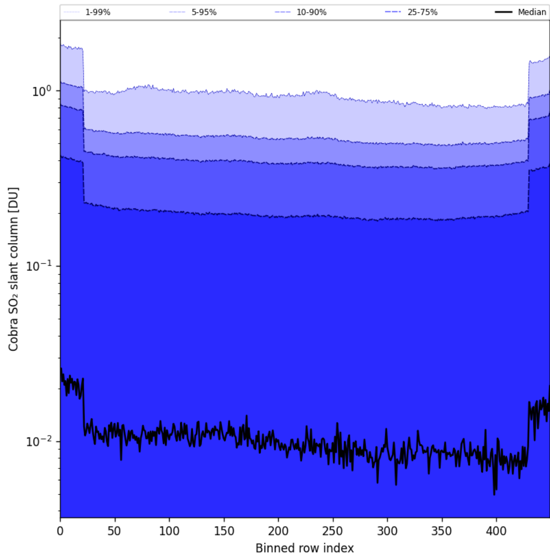
Figure 87: Along track statistics of "Cobra SO 2 slant column" for 2025-06-29 to 2025-07-01
