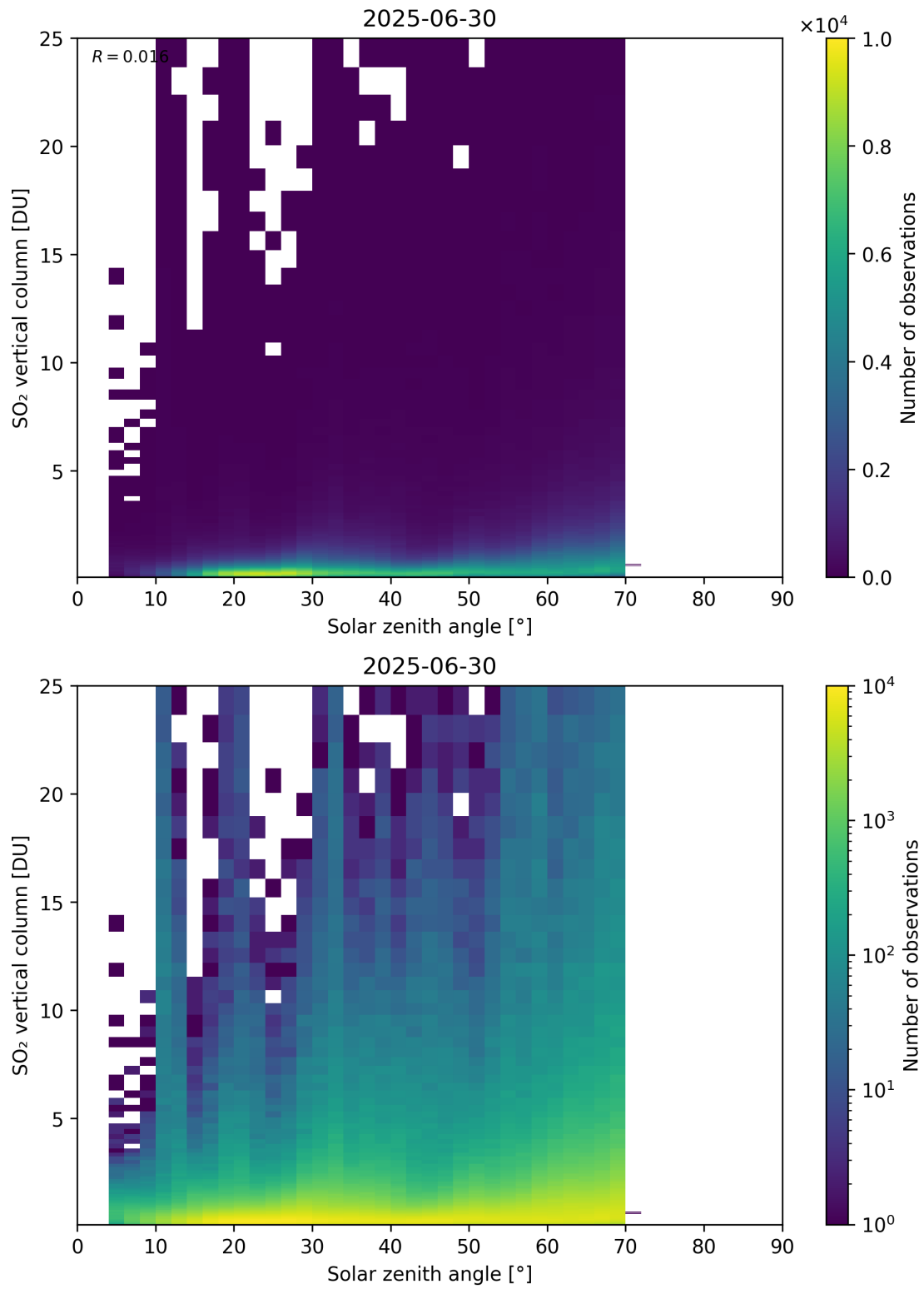
Figure 191: Scatter density plot of “Solar zenith angle” against “SO 2 vertical column” for 2025-06-29 to 2025-07-01.
