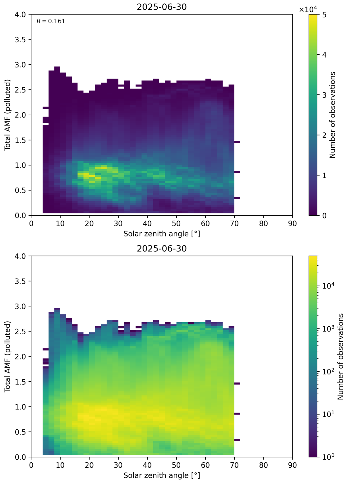
Figure 189: Scatter density plot of “Solar zenith angle” against “Total AMF (polluted)” for 2025-06-29 to 2025-07-01.
