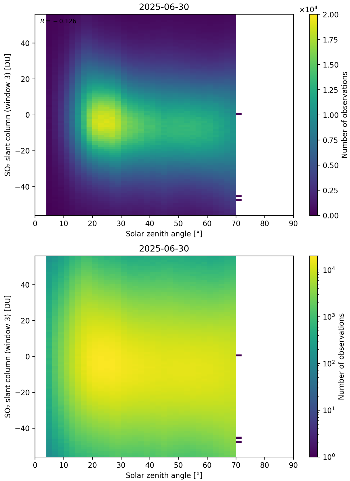
Figure 187: Scatter density plot of “Solar zenith angle” against “SO 2 slant column (window 3)” for 2025-06-29 to 2025-07-01.
