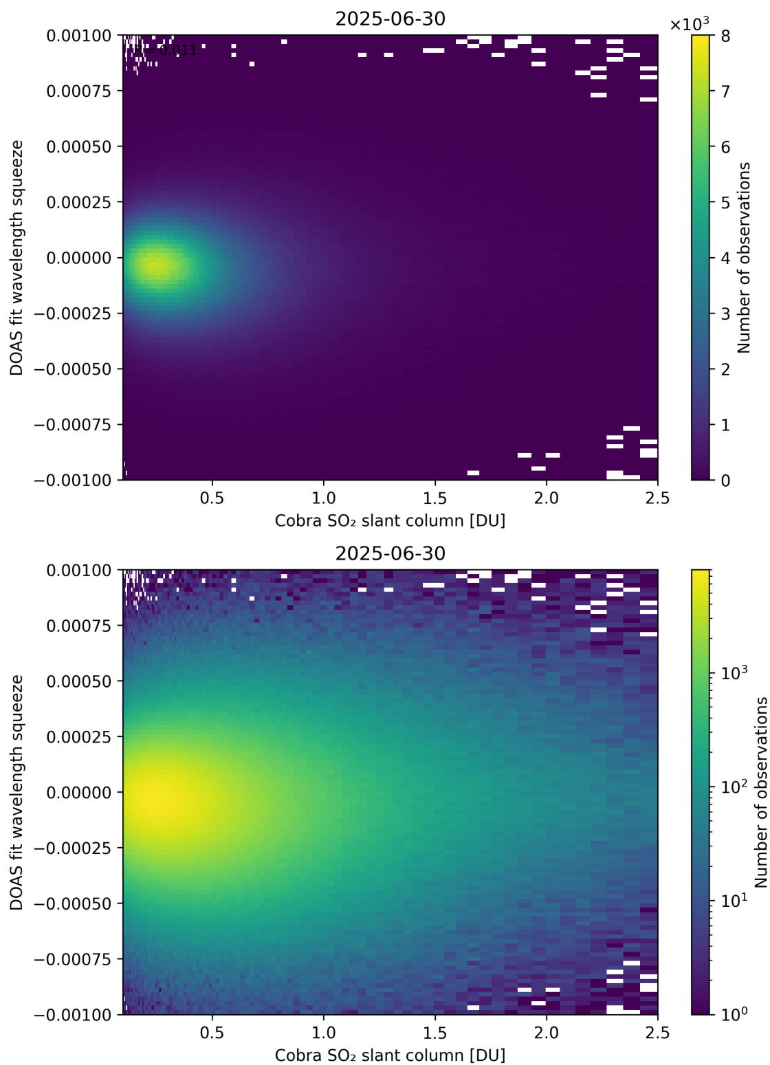
Figure 197: Scatter density plot of “Cobra SO 2 slant column” against “DOAS fit wavelength squeeze” for 2025-06-29 to 2025-07-01.
