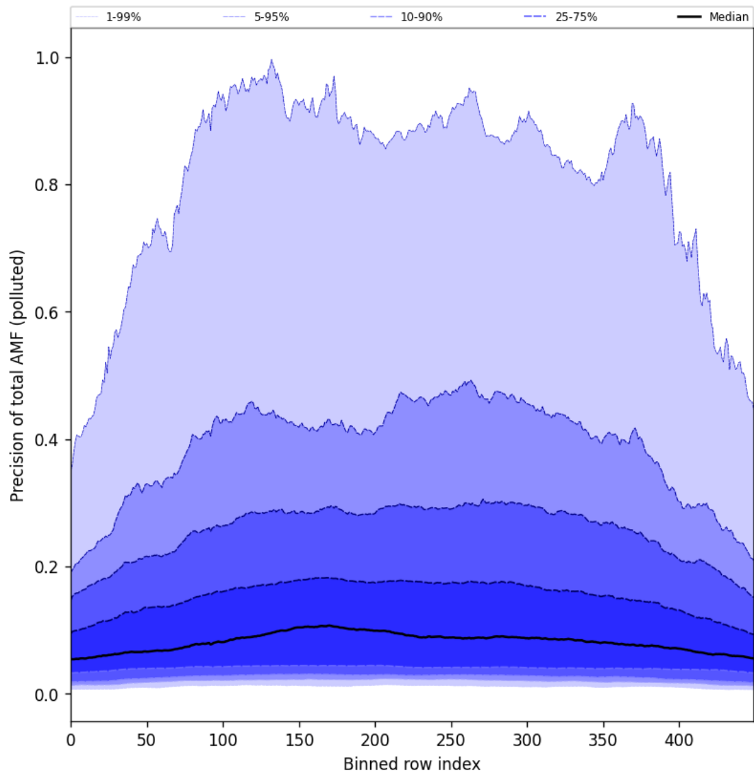
Figure 106: Along track statistics of “Precision of total AMF (polluted)” for 2025-06-29 to 2025-07-01
