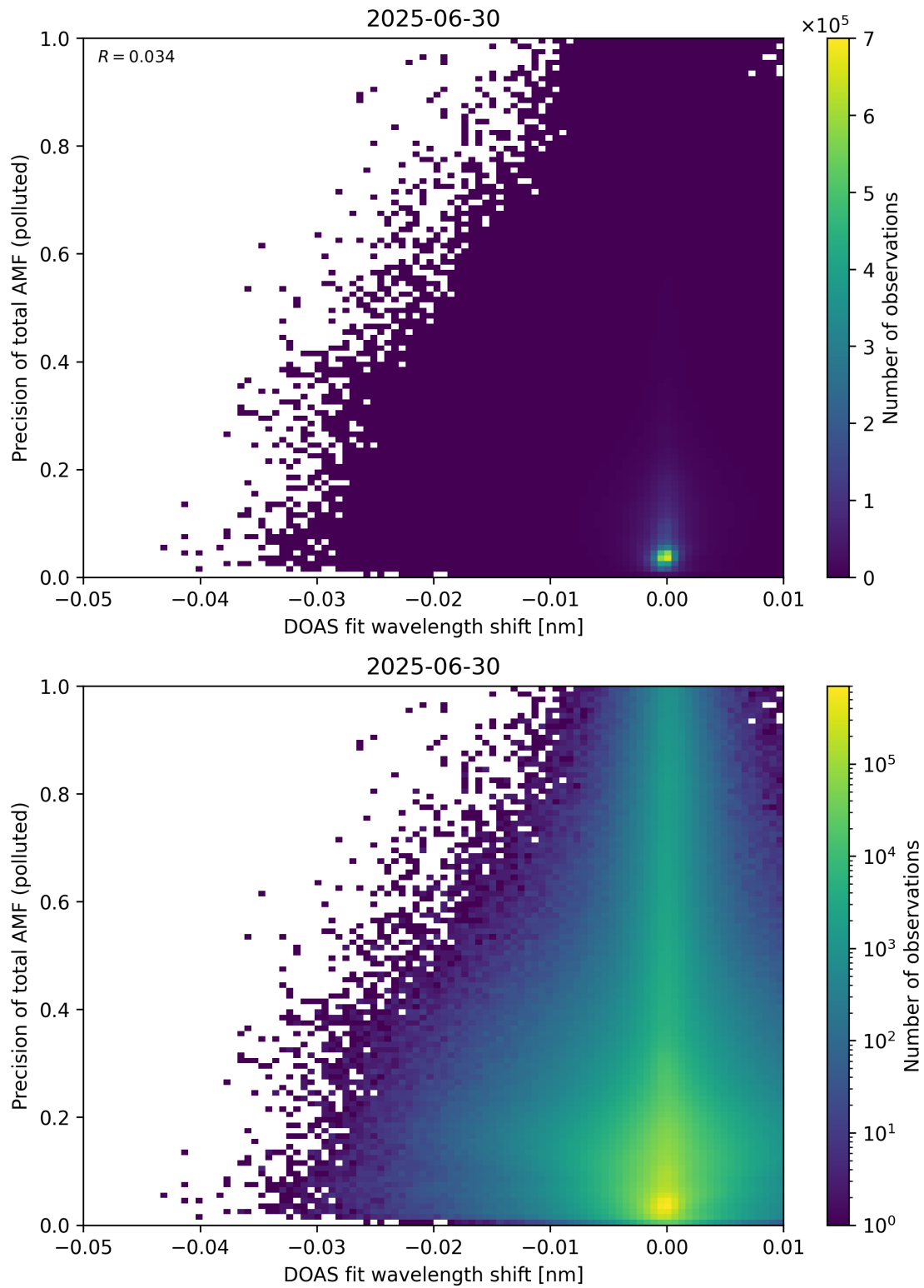
Figure 142: Scatter density plot of “DOAS fit wavelength shift” against “Precision of total AMF (polluted)” for 2025-06-29 to 2025-07-01.
