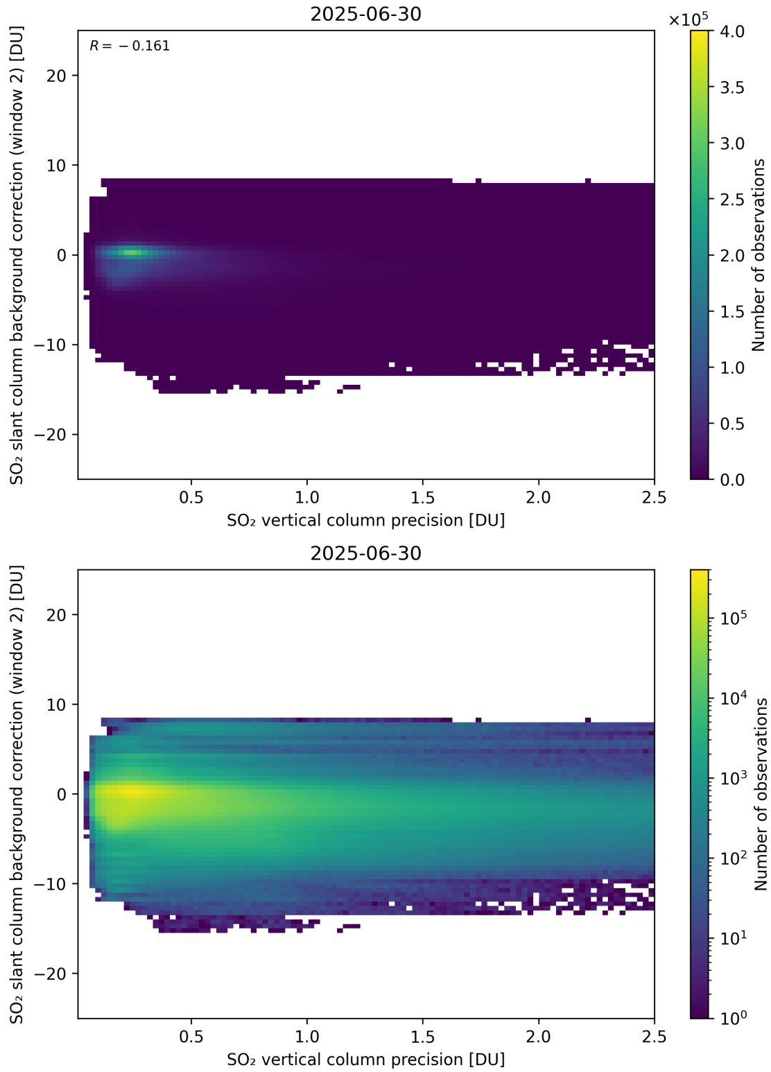
Figure 330: Scatter density plot of “SO 2 vertical column precision” against “SO 2 slant column background correction (window 2)” for 2025-06-29 to 2025-07-01.
