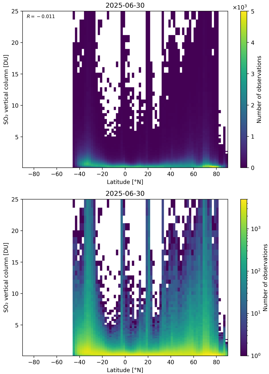
Figure 169: Scatter density plot of “Latitude” against “SO 2 vertical column” for 2025-06-29 to 2025-07-01.
