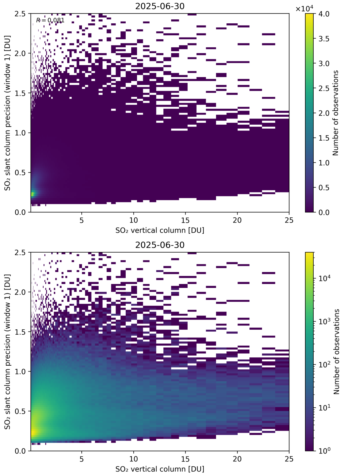
Figure 355: Scatter density plot of “SO 2 vertical column” against “SO 2 slant column precision (window 1)” for 2025-06-29 to 2025-07-01.
