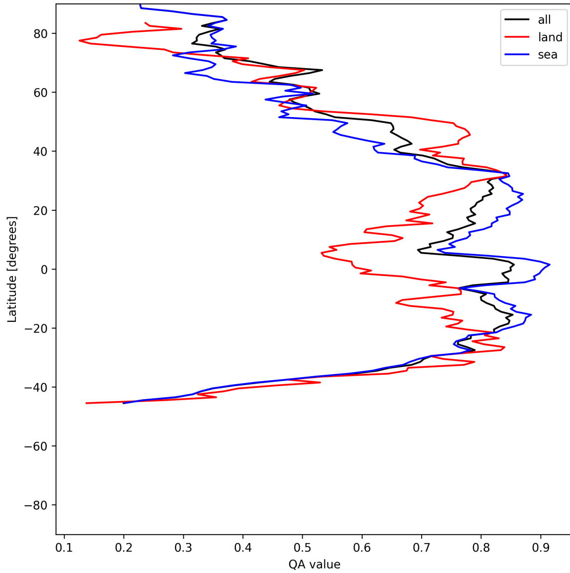
Figure 31: Zonal average of “QA value” for 2025-06-29 to 2025-07-01.
