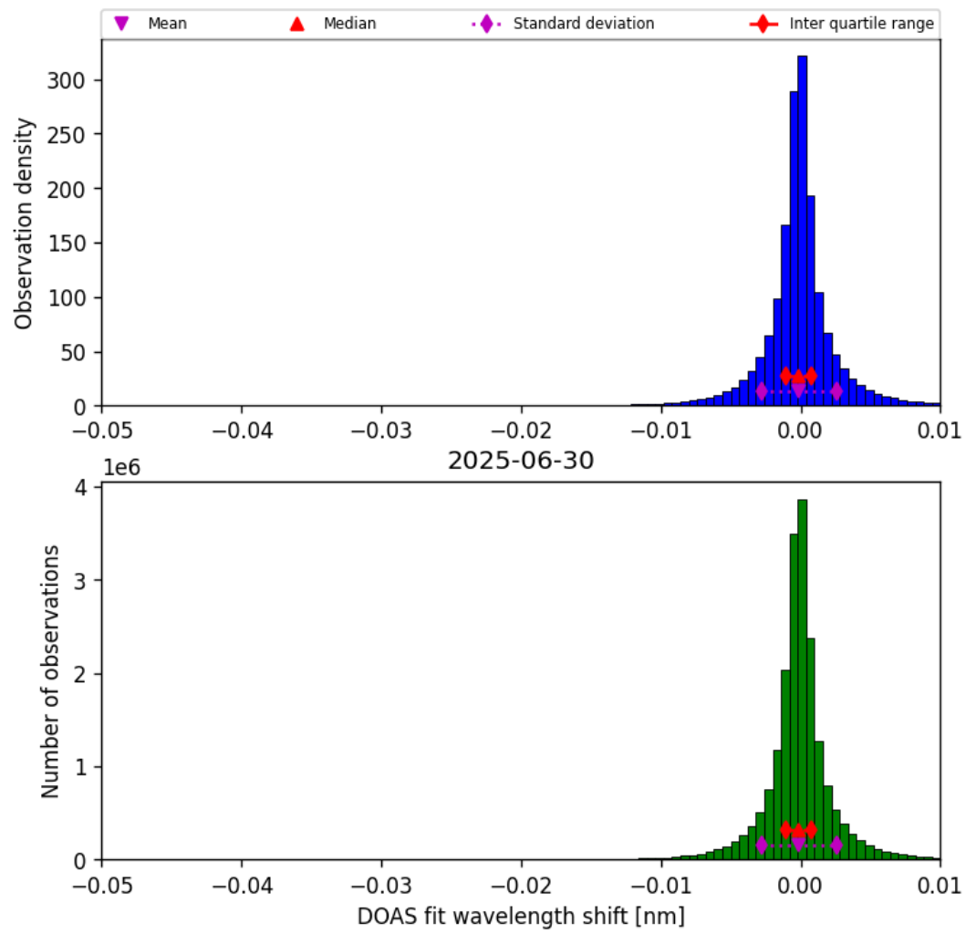
Figure 76: Histogram of “DOAS fit wavelength shift” for 2025-06-29 to 2025-07-01
