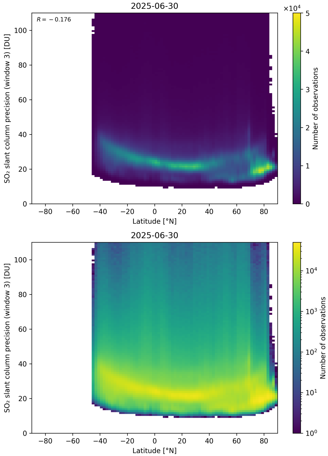
Figure 166: Scatter density plot of “Latitude” against “SO 2 slant column precision (window 3)” for 2025-06-29 to 2025-07-01.
