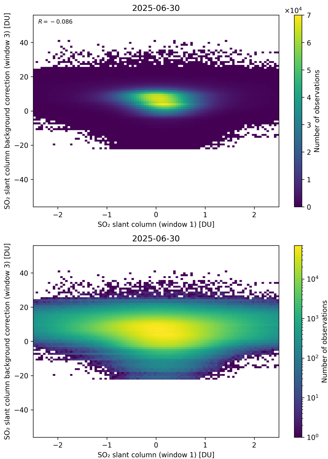
Figure 264: Scatter density plot of “SO 2 slant column (window 1)” against “SO 2 slant column background correction (window 3)” for 2025-06-29 to 2025-07-01.
