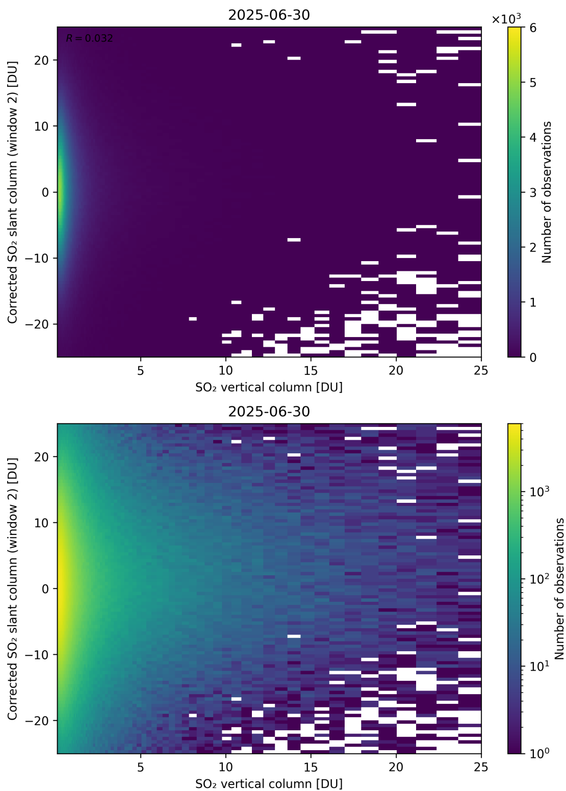
Figure 352: Scatter density plot of “SO 2 vertical column” against “Corrected SO 2 slant column (window 2)” for 2025-06-29 to 2025-07-01.
