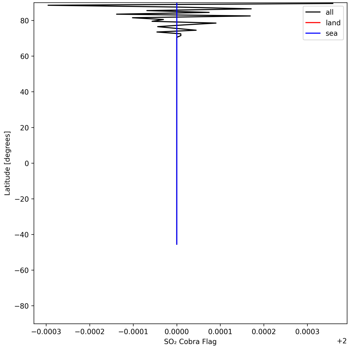
Figure 49: Zonal average of “SO 2 Cobra Flag” for 2025-06-29 to 2025-07-01.
