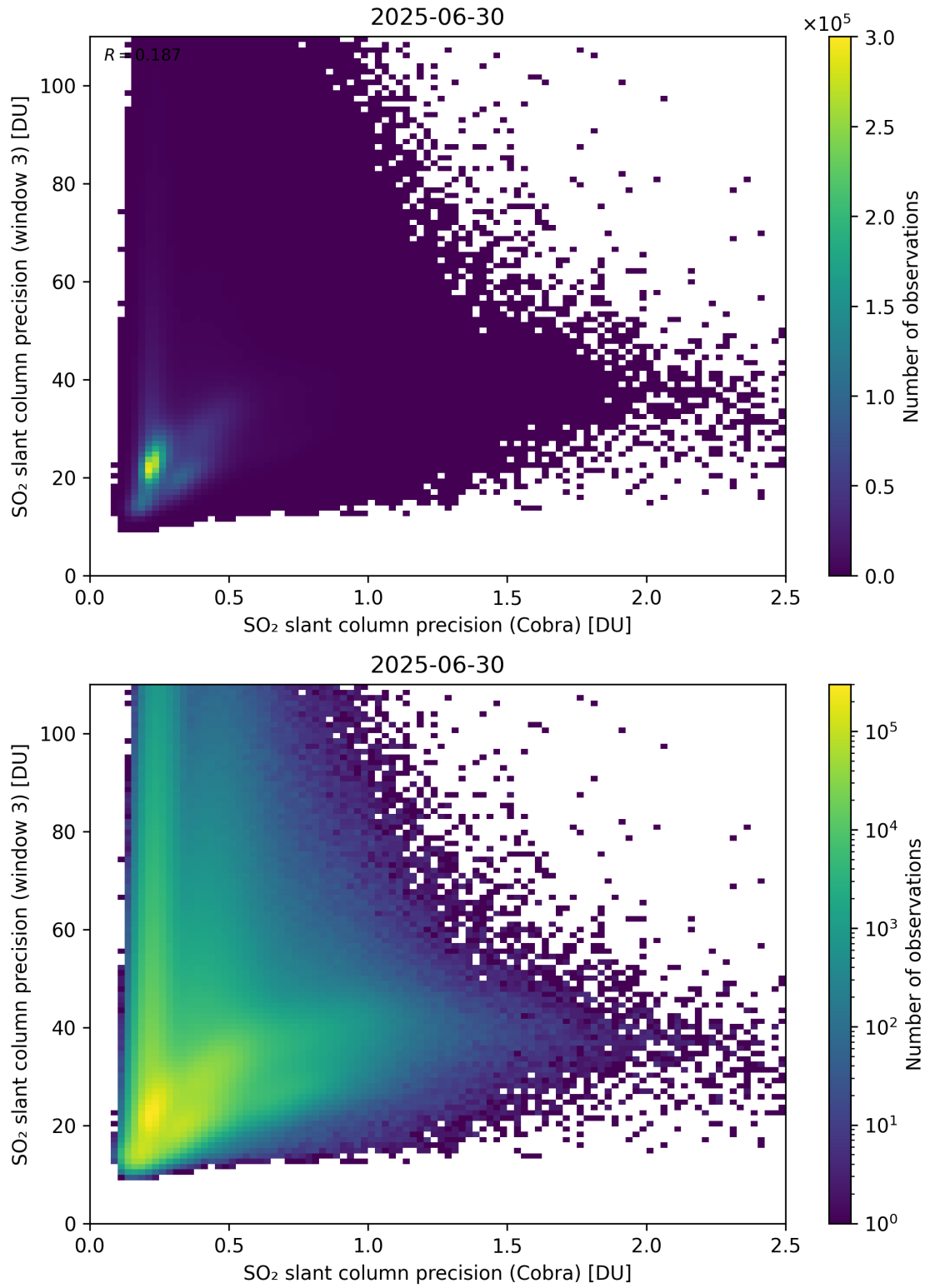
Figure 212: Scatter density plot of “SO 2 slant column precision (Cobra)” against “SO 2 slant column precision (window 3)” for 2025-06-29 to 2025-07-01.
