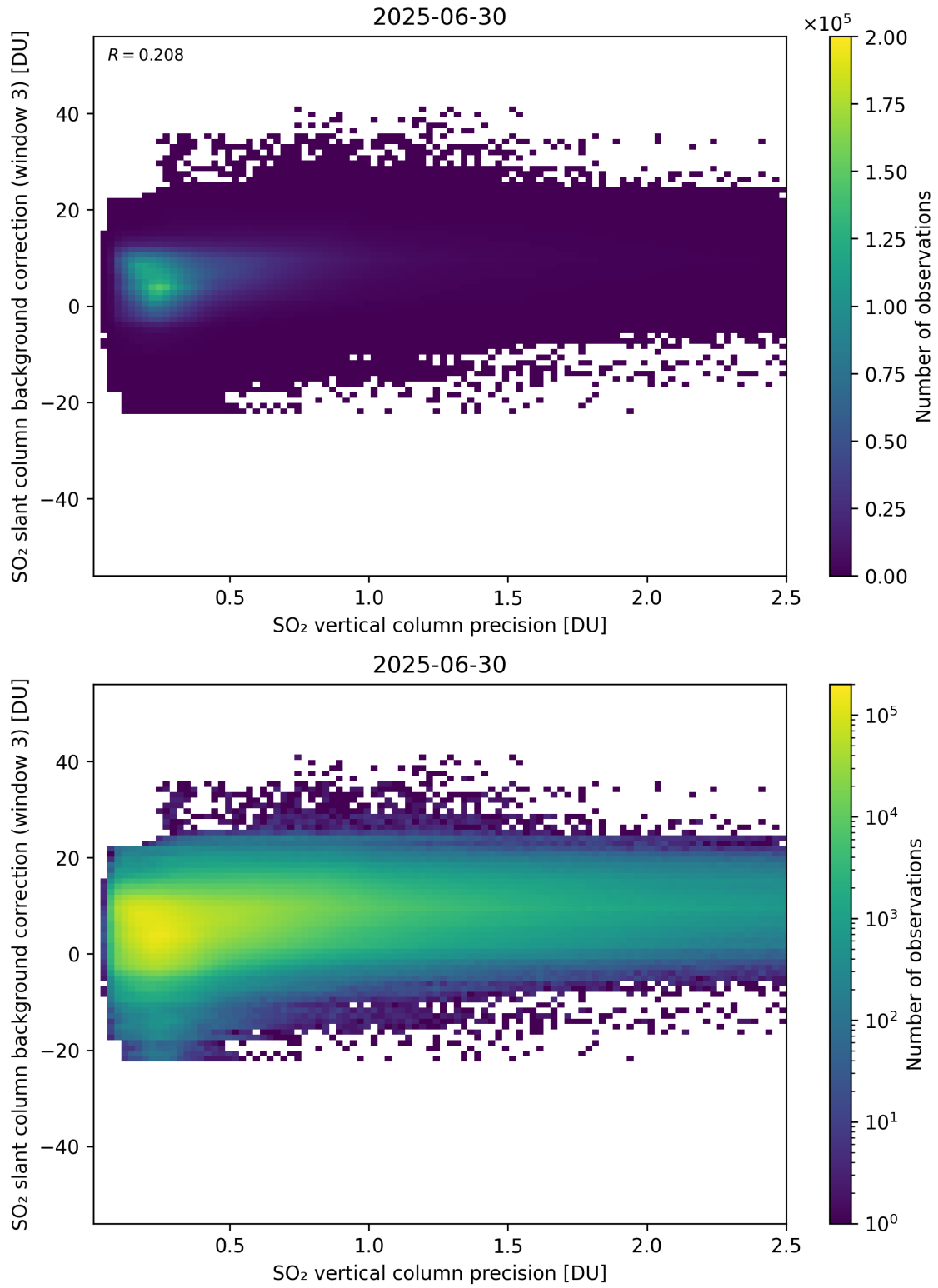
Figure 331: Scatter density plot of “SO 2 vertical column precision” against “SO 2 slant column background correction (window 3)” for 2025-06-29 to 2025-07-01.
