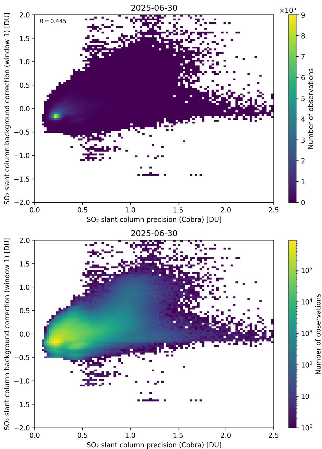
Figure 199: Scatter density plot of “SO 2 slant column precision (Cobra)” against “SO 2 slant column background correction (window 1)” for 2025-06-29 to 2025-07-01.
