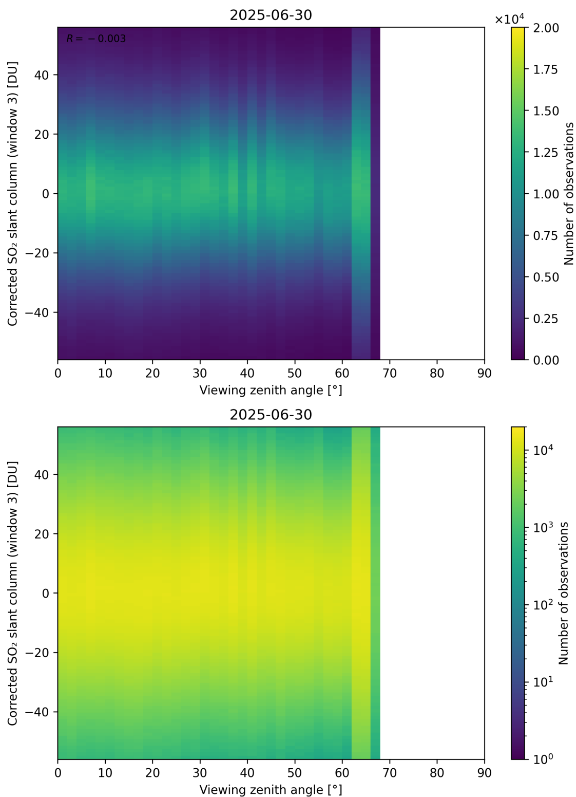
Figure 375: Scatter density plot of “Viewing zenith angle” against “Corrected SO 2 slant column (window 3)” for 2025-06-29 to 2025-07-01.
