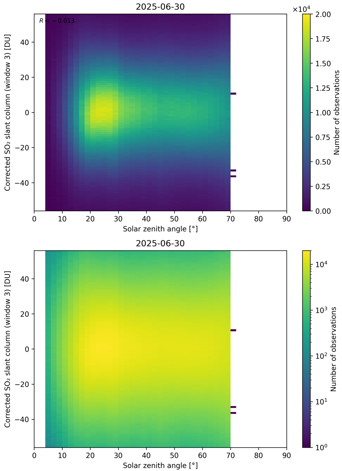
Figure 183: Scatter density plot of “Solar zenith angle” against “Corrected SO 2 slant column (window 3)” for 2025-06-29 to 2025-07-01.
