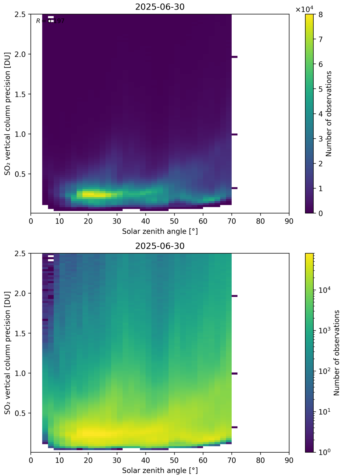
Figure 192: Scatter density plot of “Solar zenith angle” against “SO 2 vertical column precision” for 2025-06-29 to 2025-07-01.
