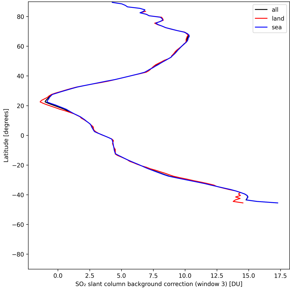
Figure 48: Zonal average of “SO 2 slant column background correction (window 3)” for 2025-06-29 to 2025-07-01.
