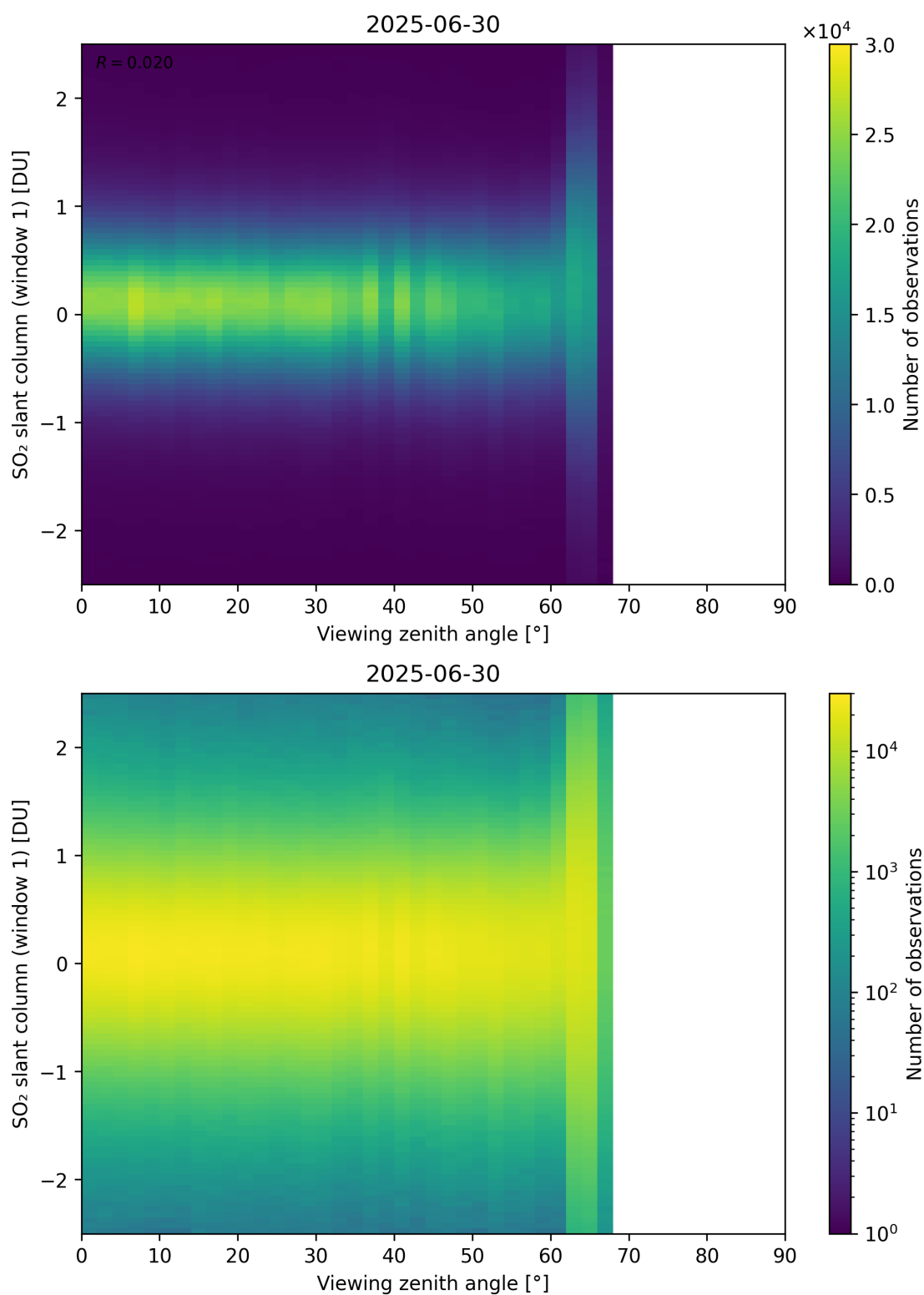
Figure 376: Scatter density plot of “Viewing zenith angle” against “SO 2 slant column (window 1)” for 2025-06-29 to 2025-07-01.
