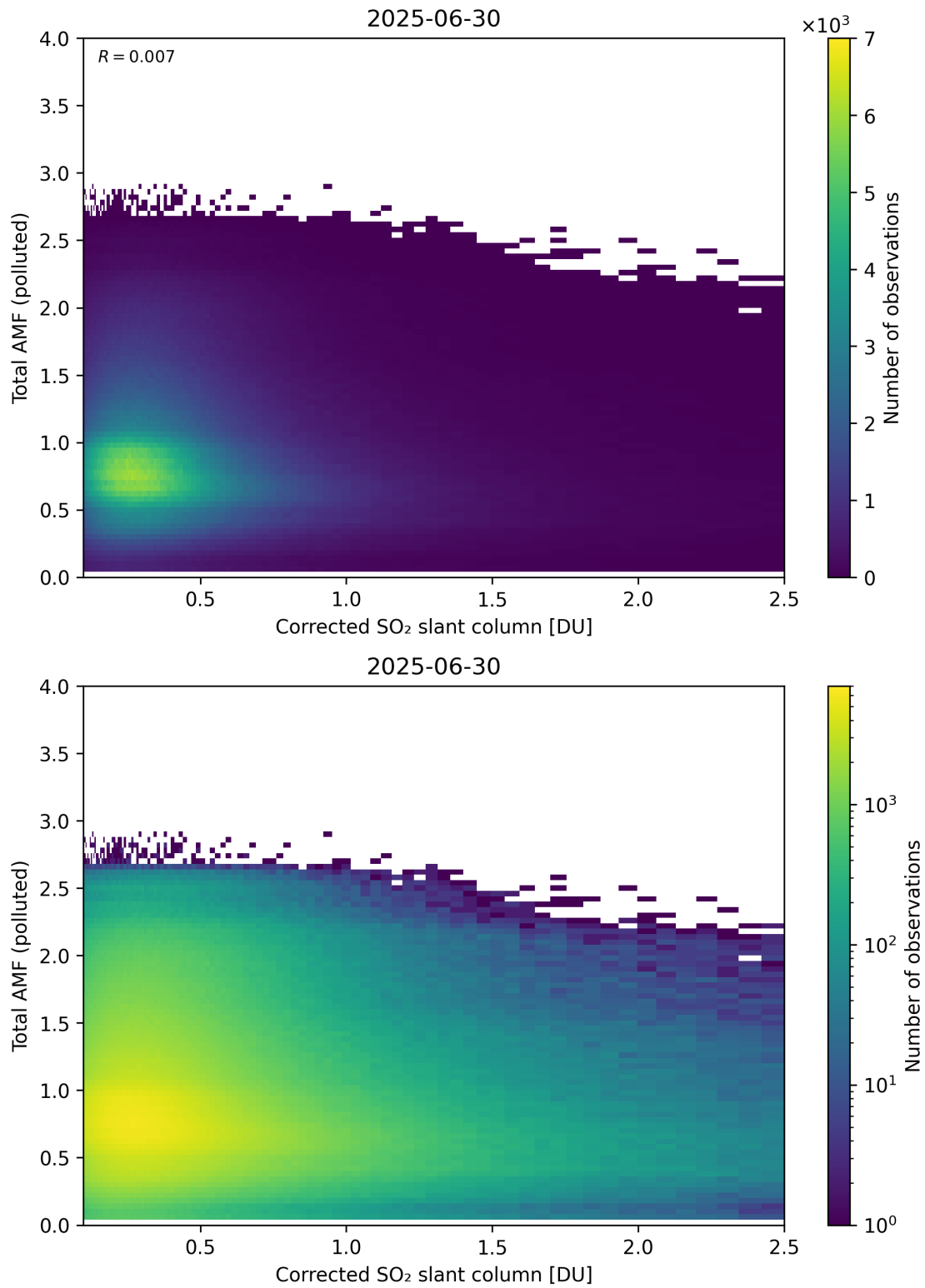
Figure 242: Scatter density plot of “Corrected SO 2 slant column” against “Total AMF (polluted)” for 2025-06-29 to 2025-07-01.
