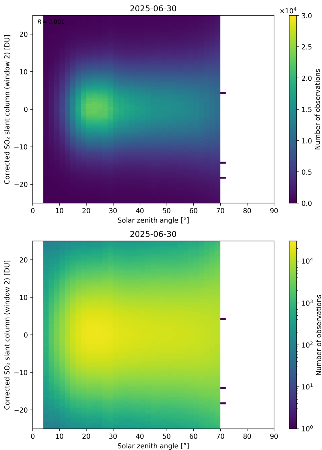
Figure 182: Scatter density plot of “Solar zenith angle” against “Corrected SO 2 slant column (window 2)” for 2025-06-29 to 2025-07-01.
