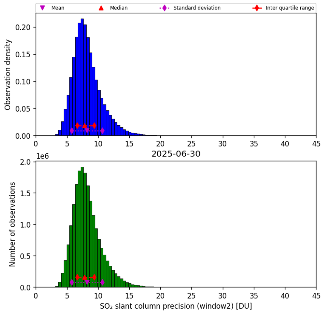
Figure 68: Histogram of “SO 2 slant column precision (window2)” for 2025-06-29 to 2025-07-01
