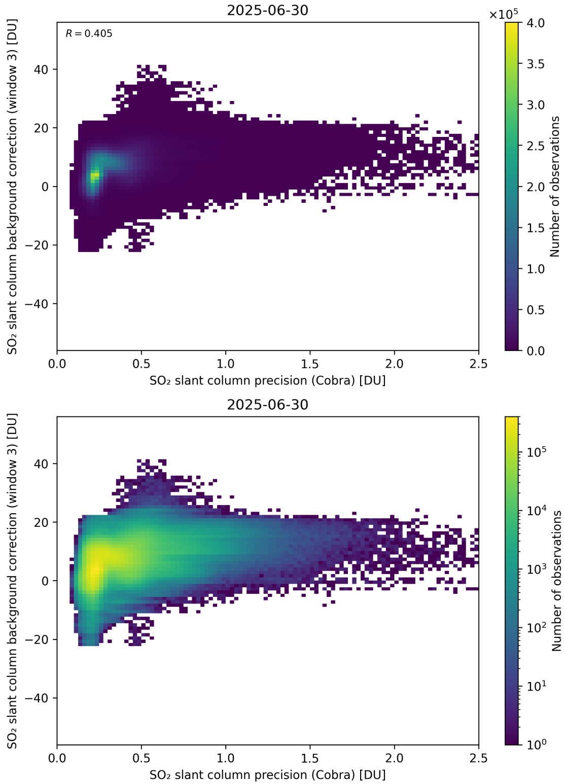
Figure 201: Scatter density plot of “SO 2 slant column precision (Cobra)” against “SO 2 slant column background correction (window 3)” for 2025-06-29 to 2025-07-01.
