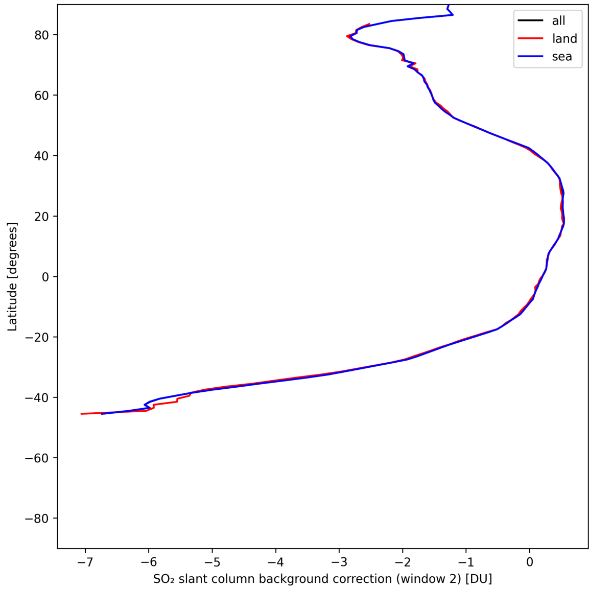
Figure 44: Zonal average of “SO 2 slant column background correction (window 2)” for 2025-06-29 to 2025-07-01.
