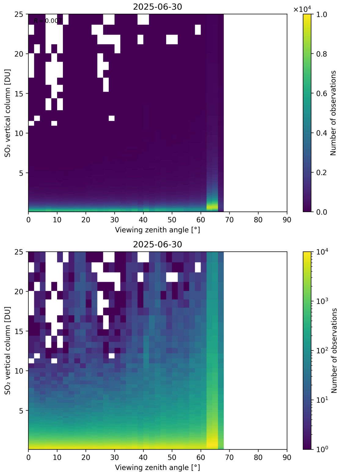
Figure 383: Scatter density plot of “Viewing zenith angle” against “SO 2 vertical column” for 2025-06-29 to 2025-07-01.
