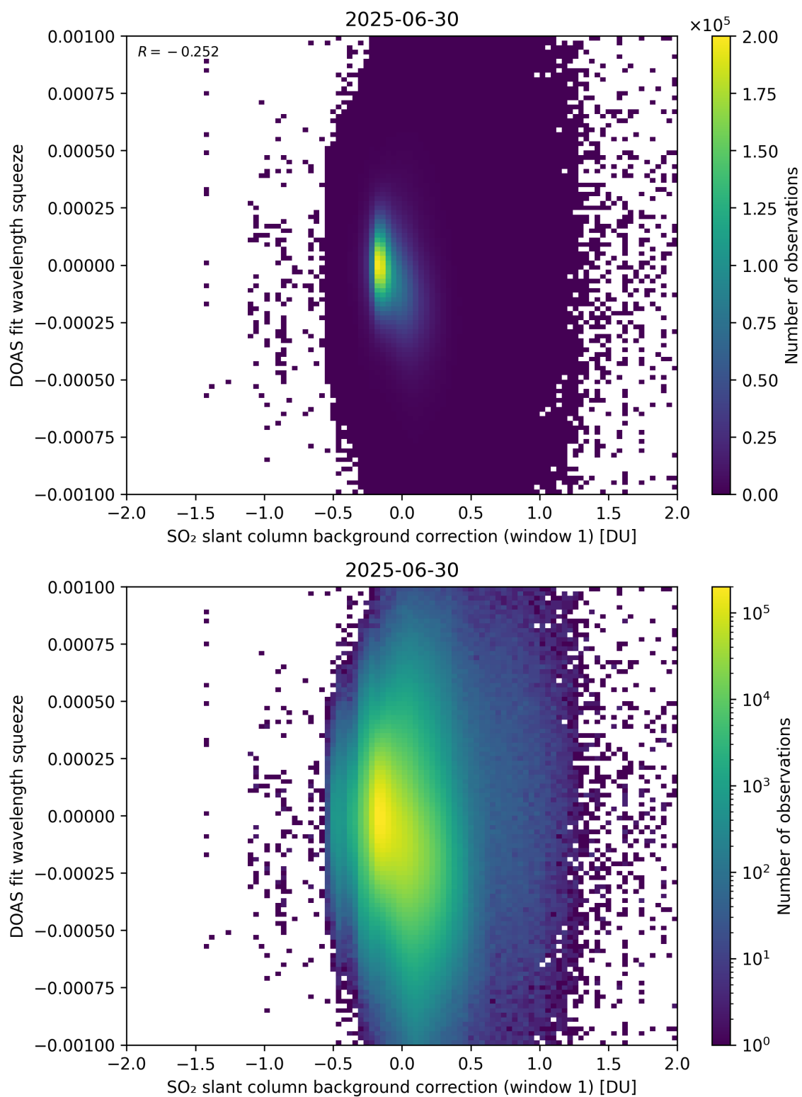
Figure 112: Scatter density plot of “SO 2 slant column background correction (window 1)” against “DOAS fit wavelength squeeze” for 2025-06-29 to 2025-07-01.
