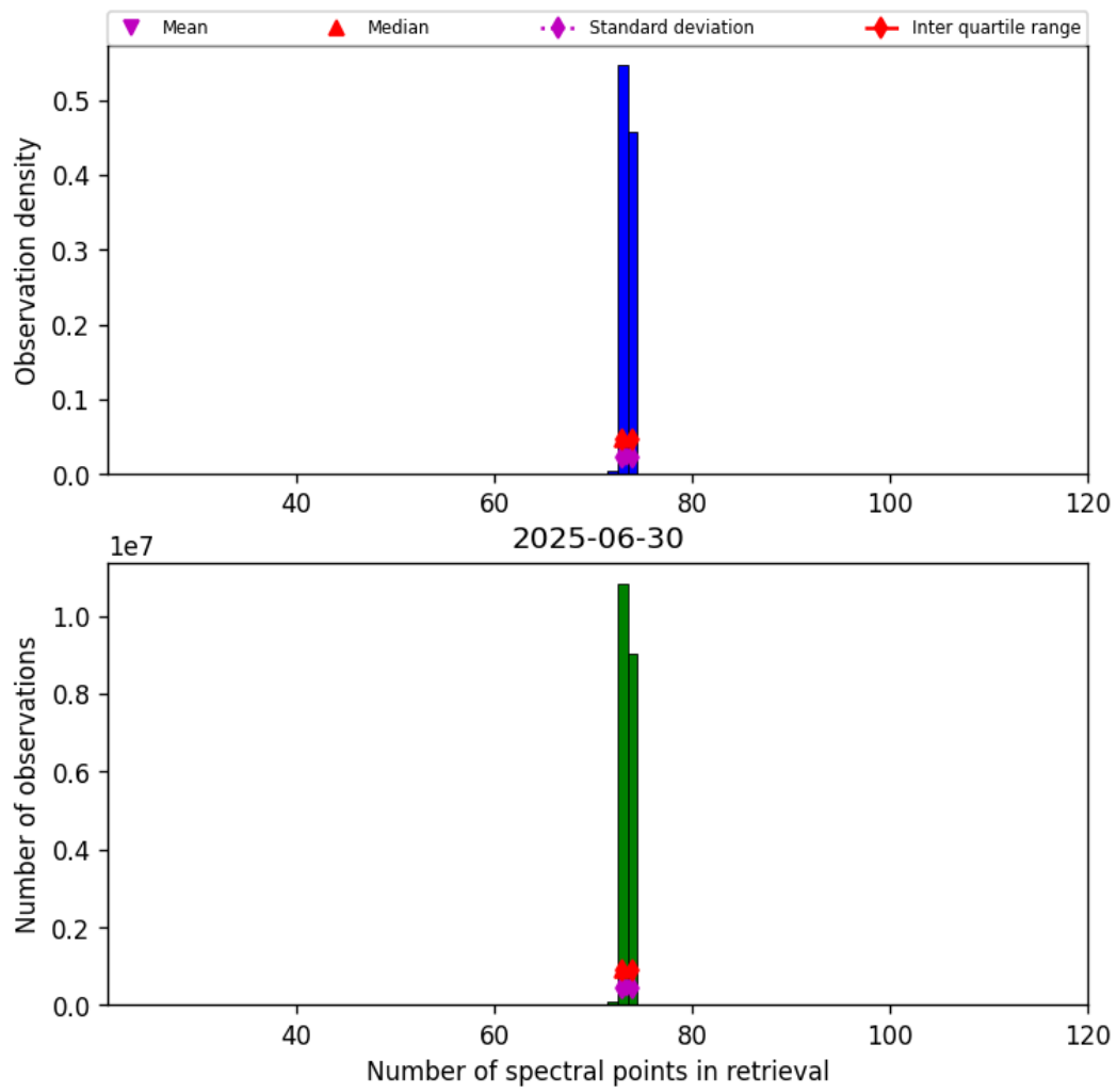
Figure 82: Histogram of “Number of spectral points in retrieval” for 2025-06-29 to 2025-07-01
