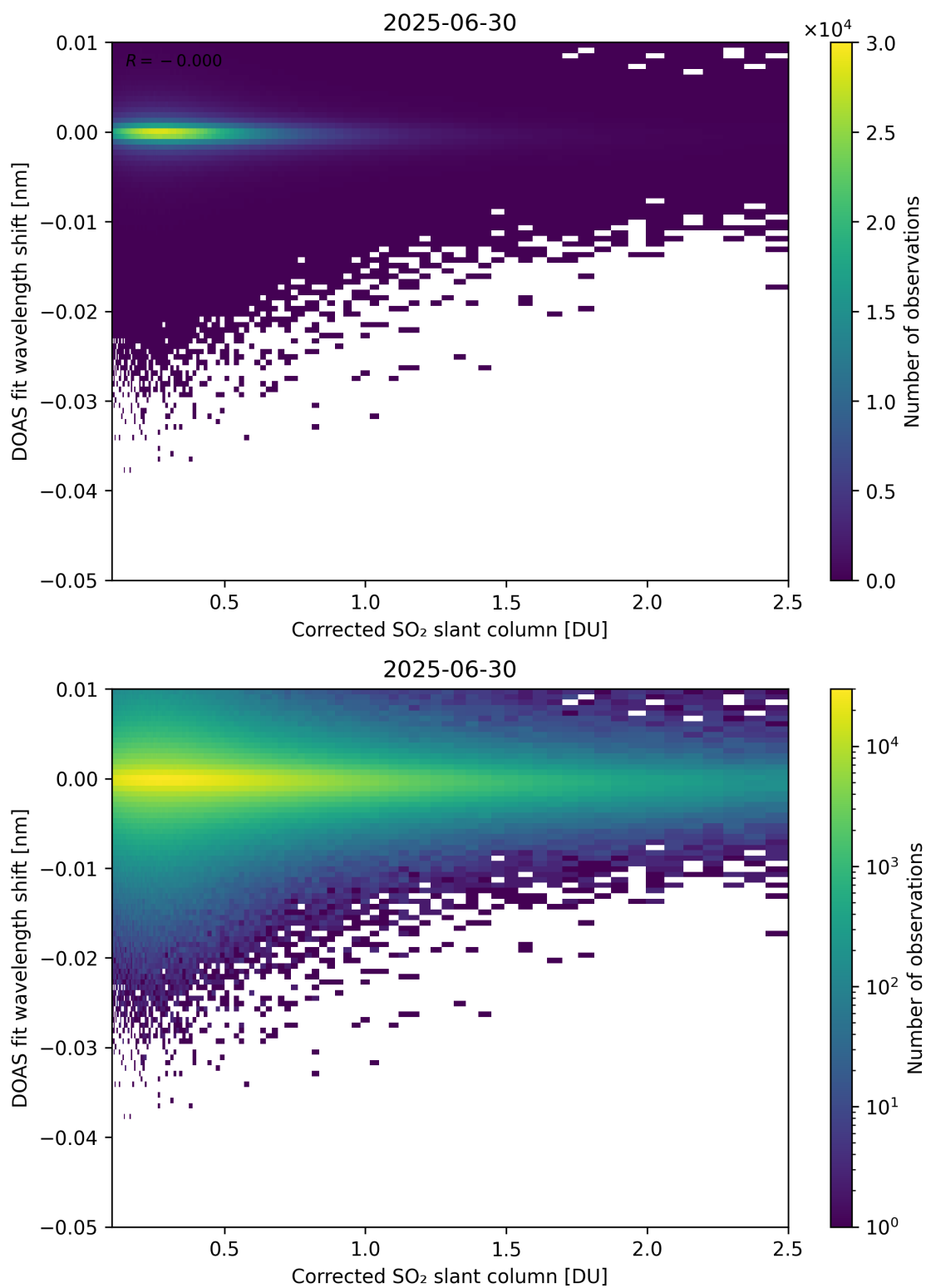
Figure 229: Scatter density plot of “Corrected SO 2 slant column” against “DOAS fit wavelength shift” for 2025-06-29 to 2025-07-01.
