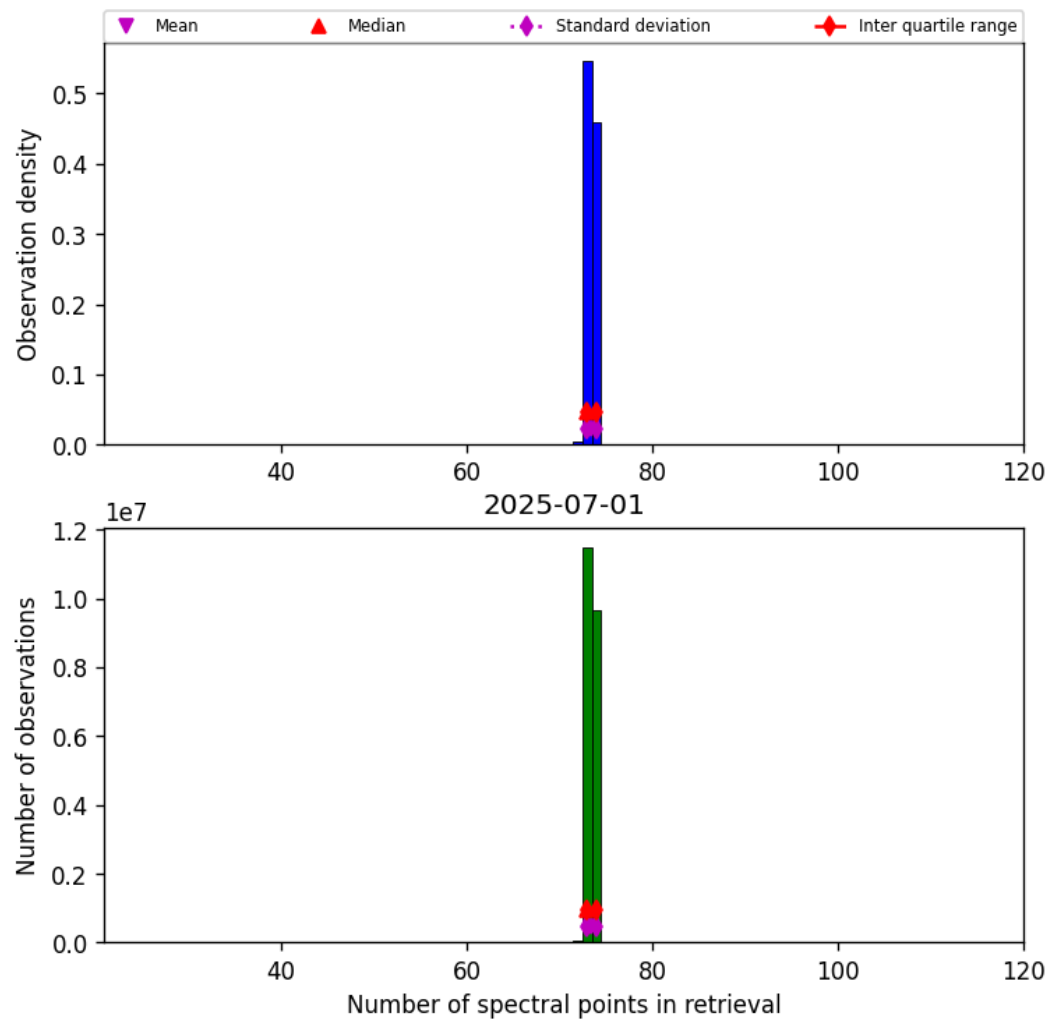
Figure 82: Histogram of "Number of spectral points in retrieval" for 2025-06-30 to 2025-07-02
