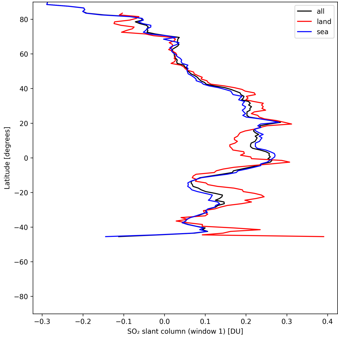
Figure 37: Zonal average of “SO 2 slant column (window 1)” for 2025-06-30 to 2025-07-02.
