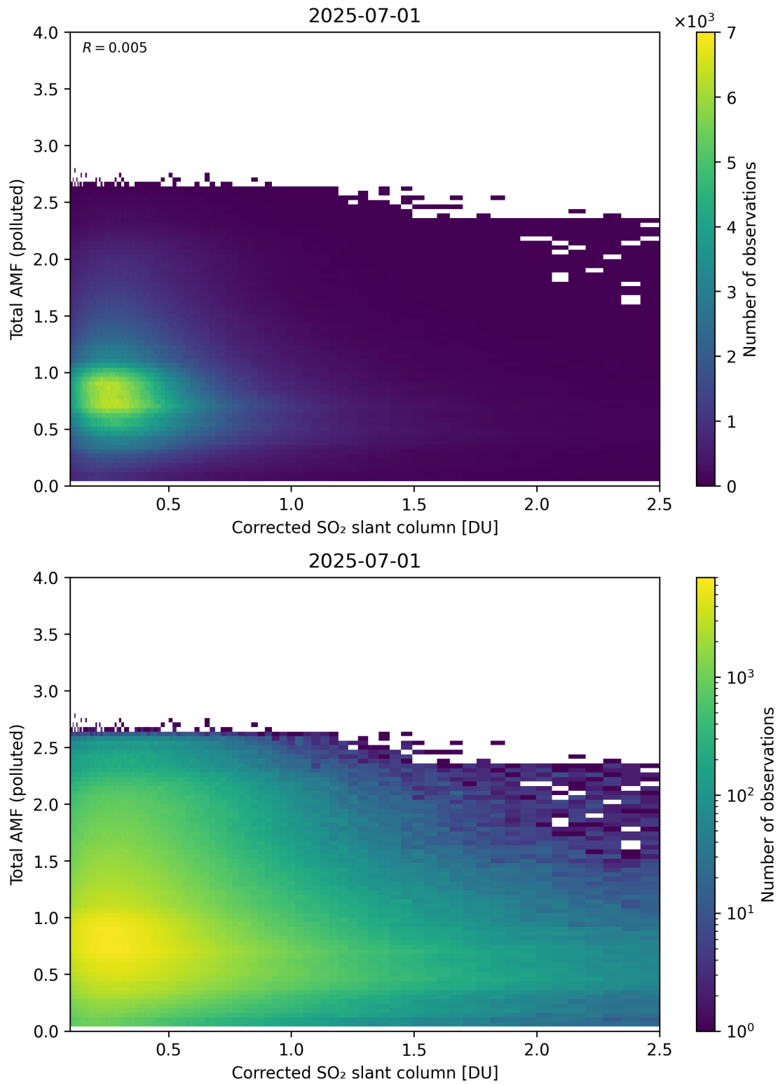
Figure 242: Scatter density plot of “Corrected SO 2 slant column” against “Total AMF (polluted)” for 2025-06-30 to 2025-07-02.
