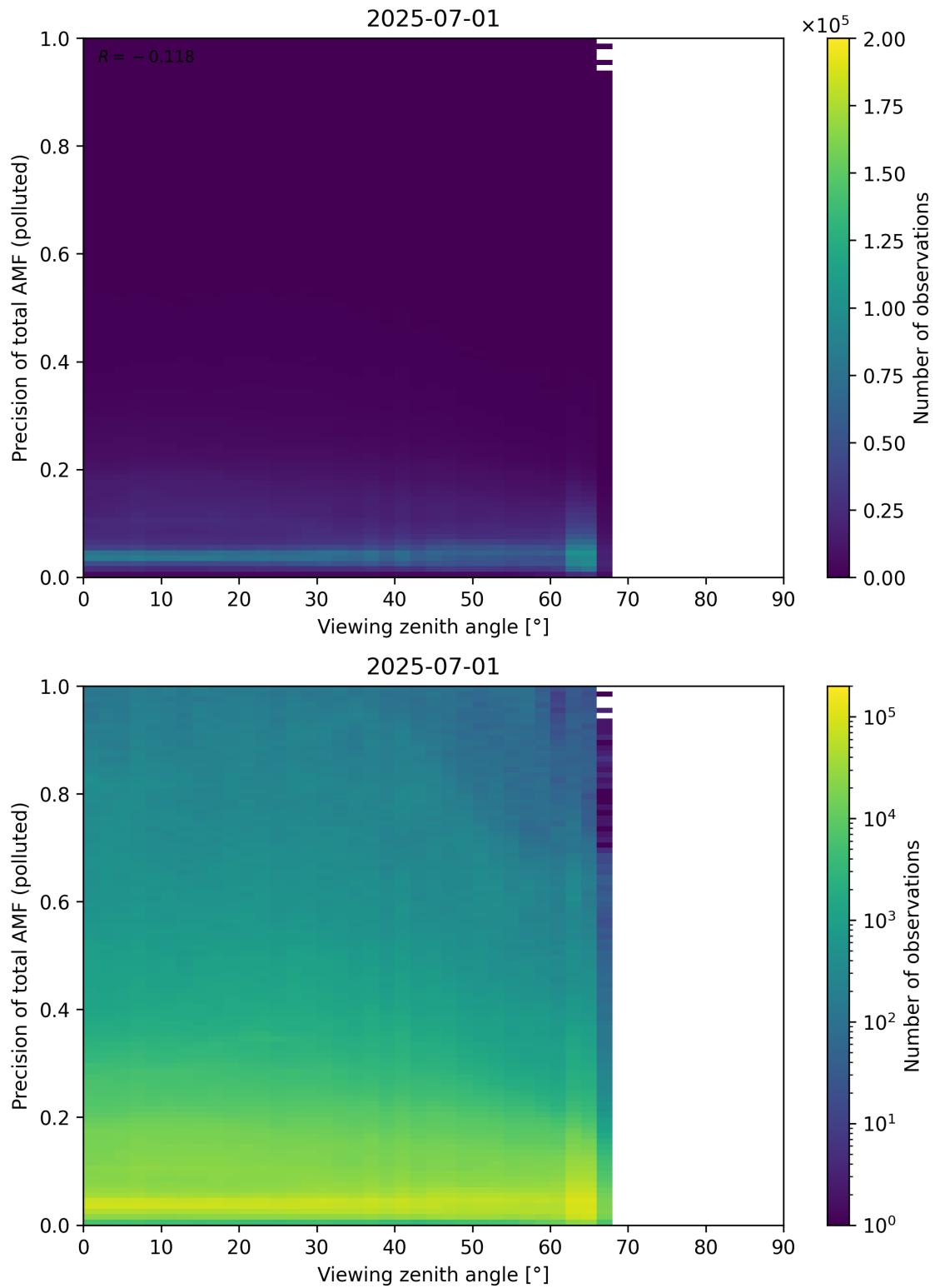
Figure 382: Scatter density plot of “Viewing zenith angle” against “Precision of total AMF (polluted)” for 2025-06-30 to 2025-07-02.
