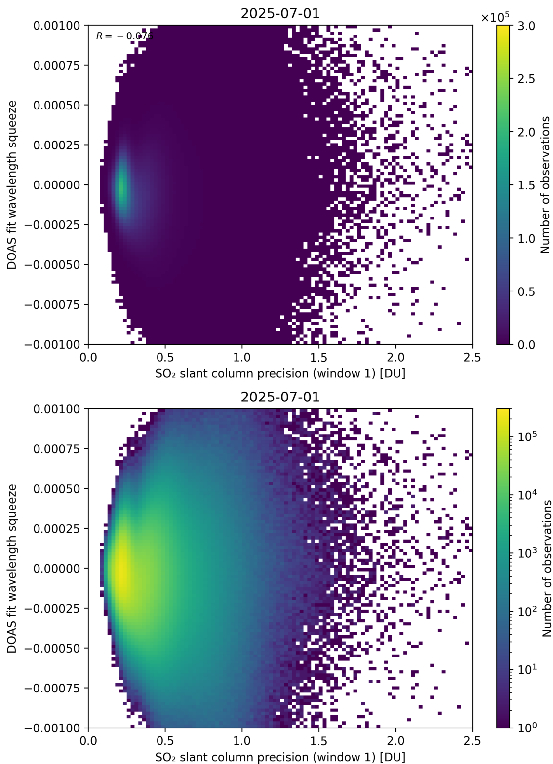
Figure 272: Scatter density plot of “SO 2 slant column precision (window 1)” against “DOAS fit wavelength squeeze” for 2025-06-30 to 2025-07-02.
