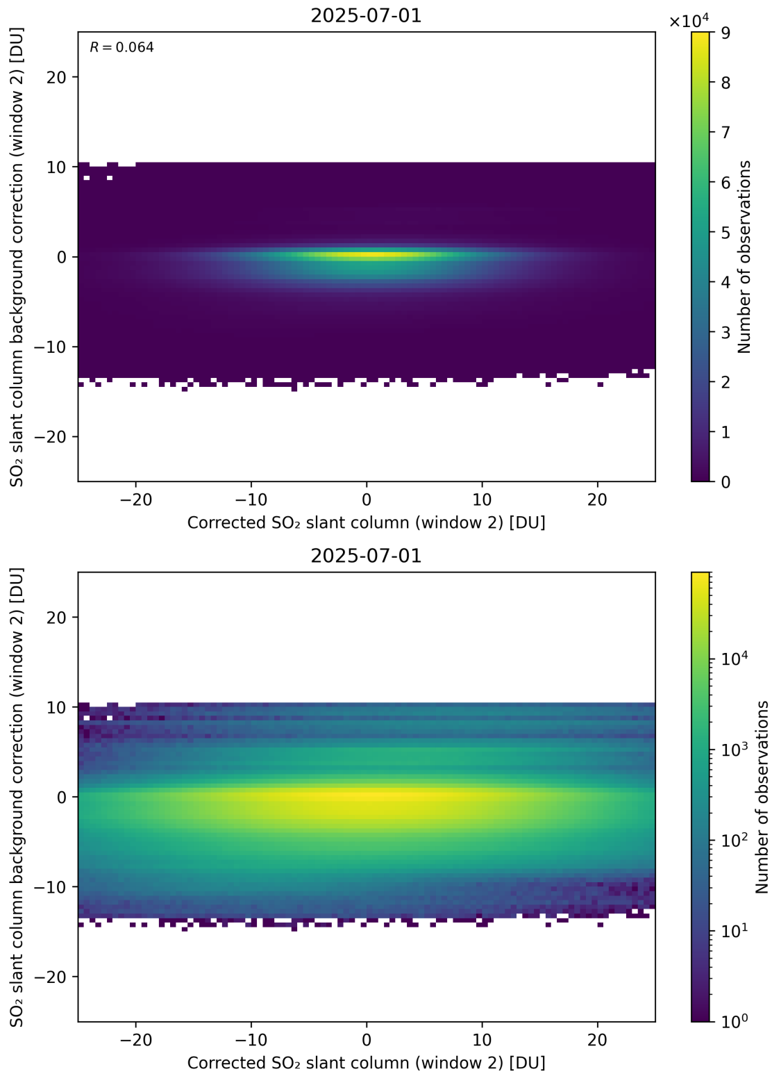
Figure 244: Scatter density plot of “Corrected SO 2 slant column (window 2)” against “SO 2 slant column background correction (window 2)” for 2025-06-30 to 2025-07-02.
