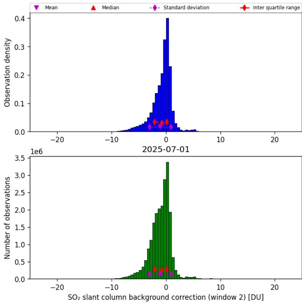
Figure 70: Histogram of “SO 2 slant column background correction (window 2)” for 2025-06-30 to 2025-07-02
