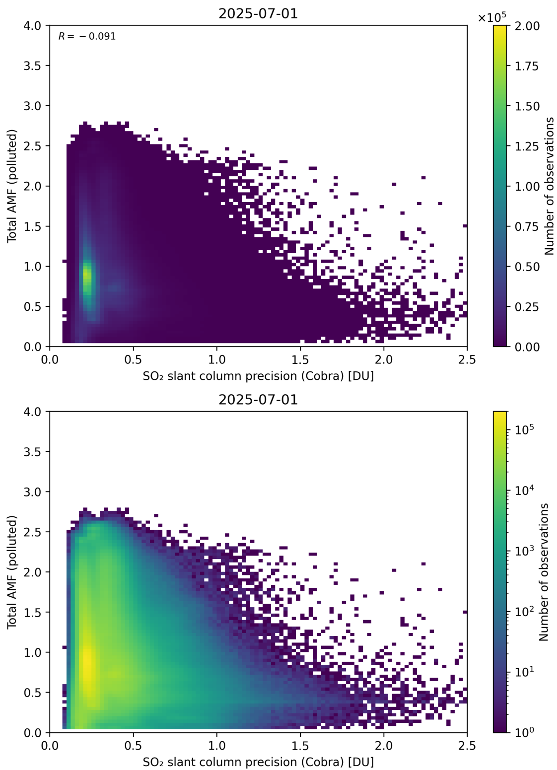
Figure 213: Scatter density plot of “SO 2 slant column precision (Cobra)” against “Total AMF (polluted)” for 2025-06-30 to 2025-07-02.
