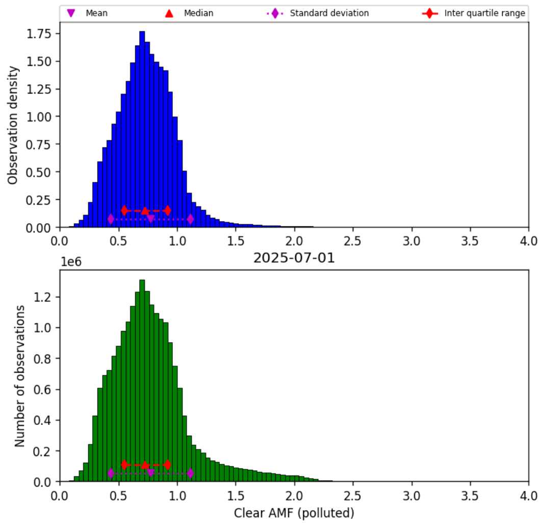
Figure 81: Histogram of “Clear AMF (polluted)” for 2025-06-30 to 2025-07-02
