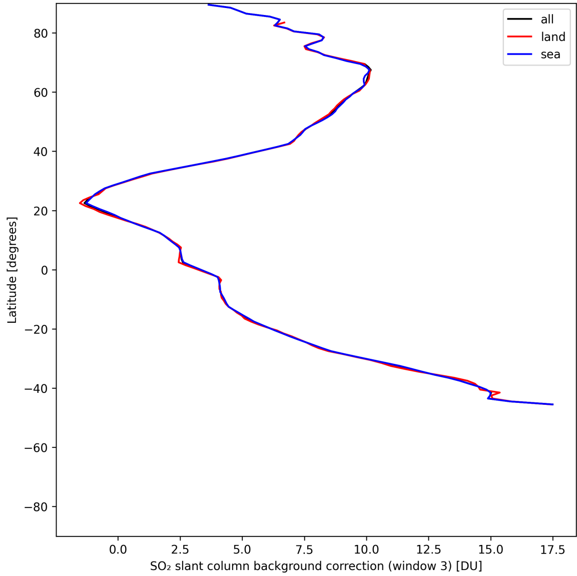
Figure 48: Zonal average of “SO 2 slant column background correction (window 3)” for 2025-06-30 to 2025-07-02.
