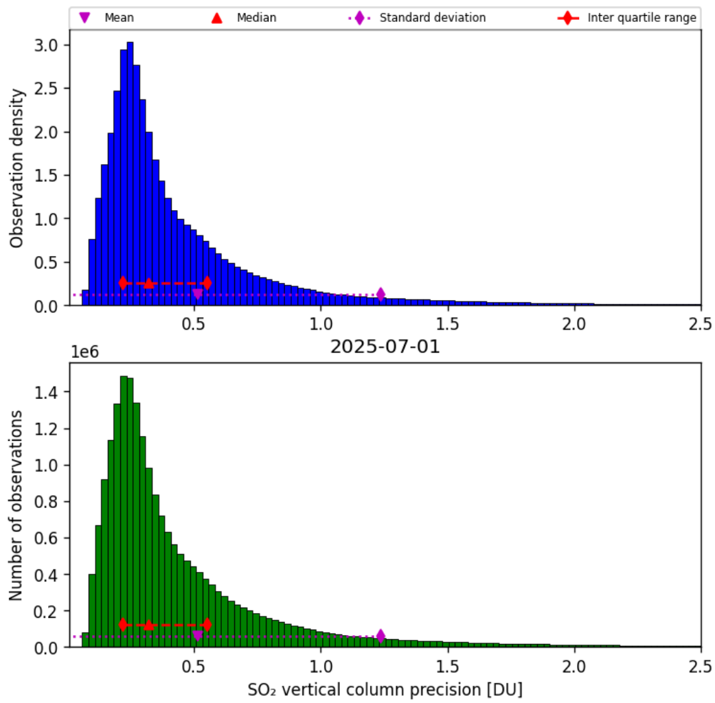
Figure 59: Histogram of “SO 2 vertical column precision” for 2025-06-30 to 2025-07-02
