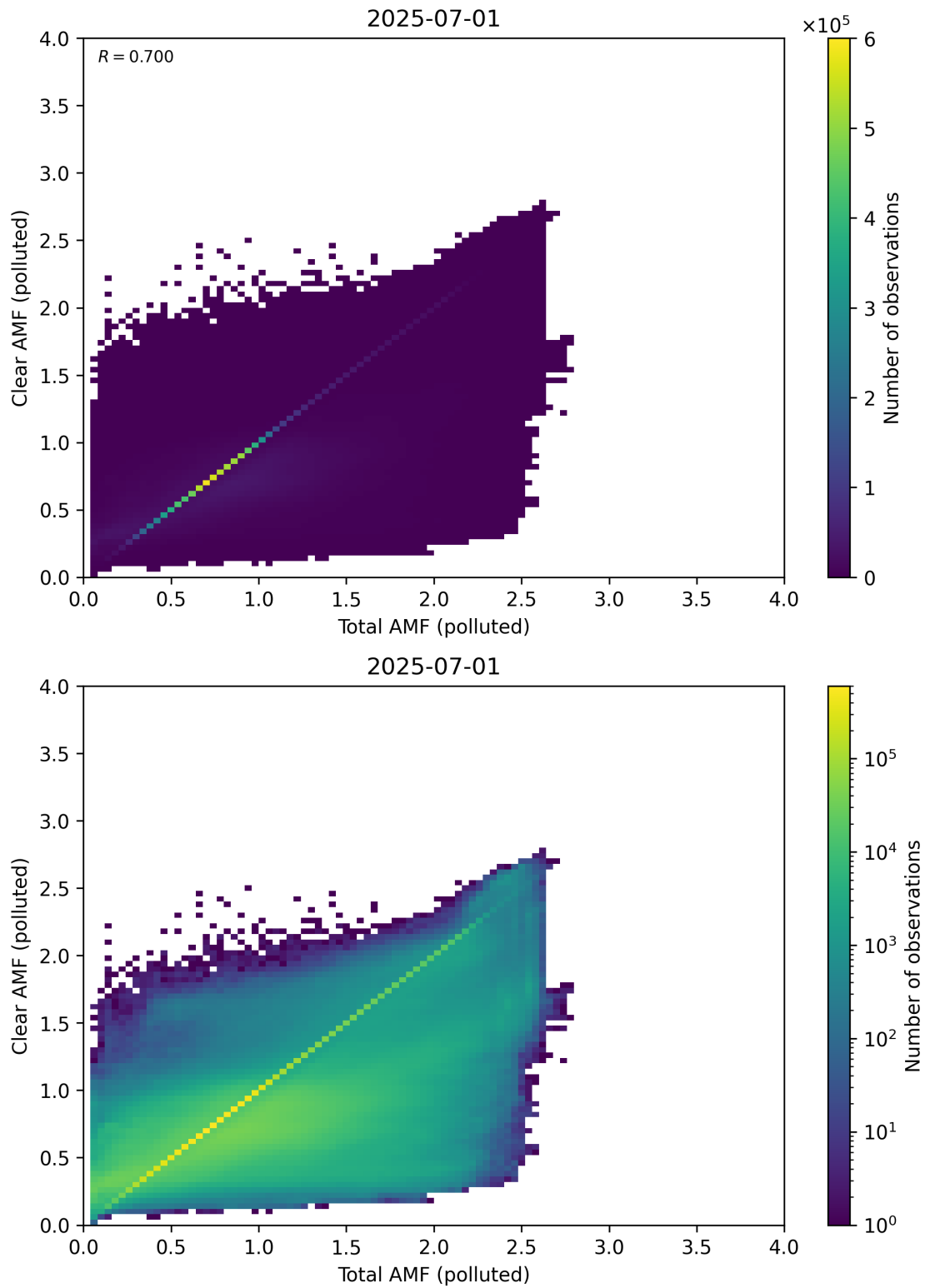
Figure 321: Scatter density plot of “Total AMF (polluted)” against “Clear AMF (polluted)” for 2025-06-30 to 2025-07-02.
