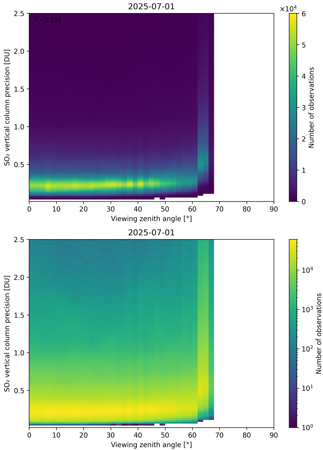
Figure 384: Scatter density plot of “Viewing zenith angle” against “SO 2 vertical column precision” for 2025-06-30 to 2025-07-02.
