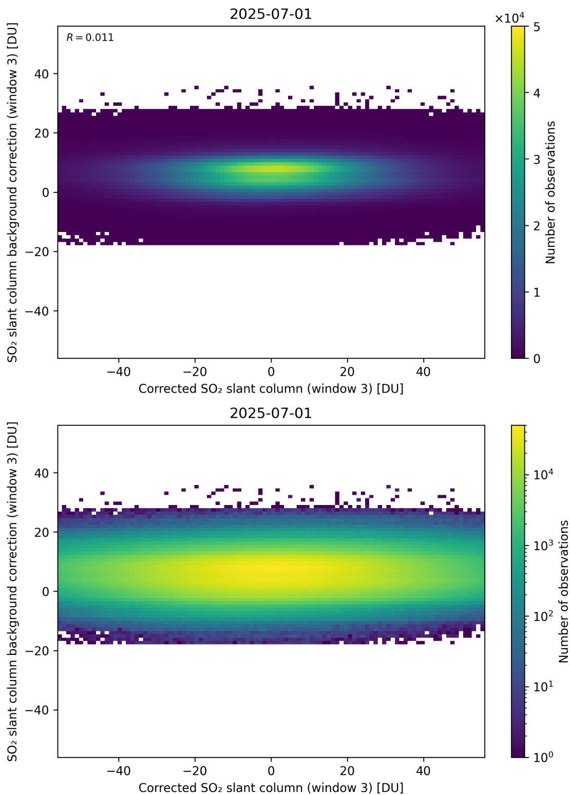
Figure 255: Scatter density plot of “Corrected SO 2 slant column (window 3)” against “SO 2 slant column background correction (window 3)” for 2025-06-30 to 2025-07-02.
