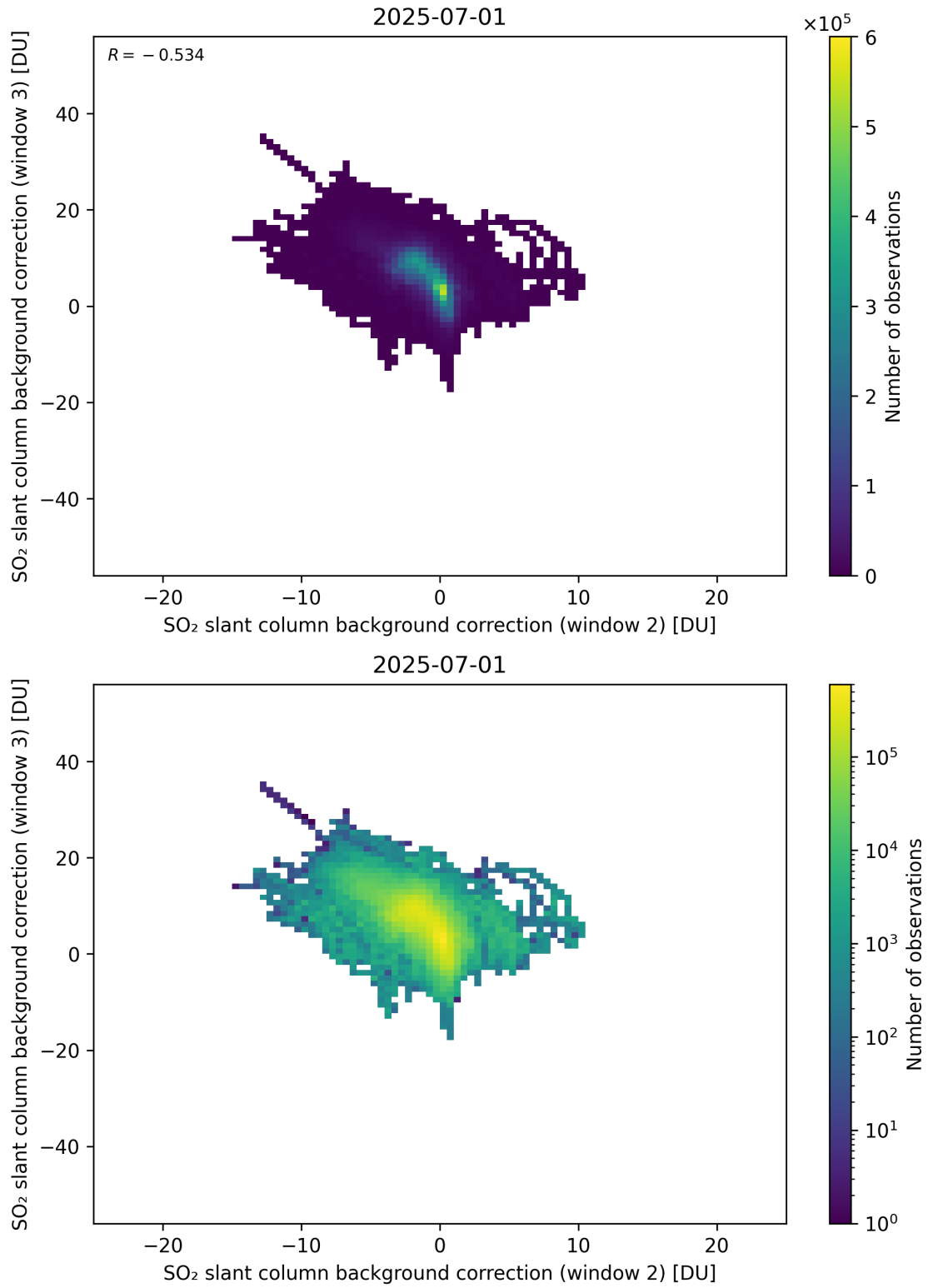
Figure 122: Scatter density plot of “SO 2 slant column background correction (window 2)” against “SO 2 slant column background correction (window 3)” for 2025-06-30 to 2025-07-02.
