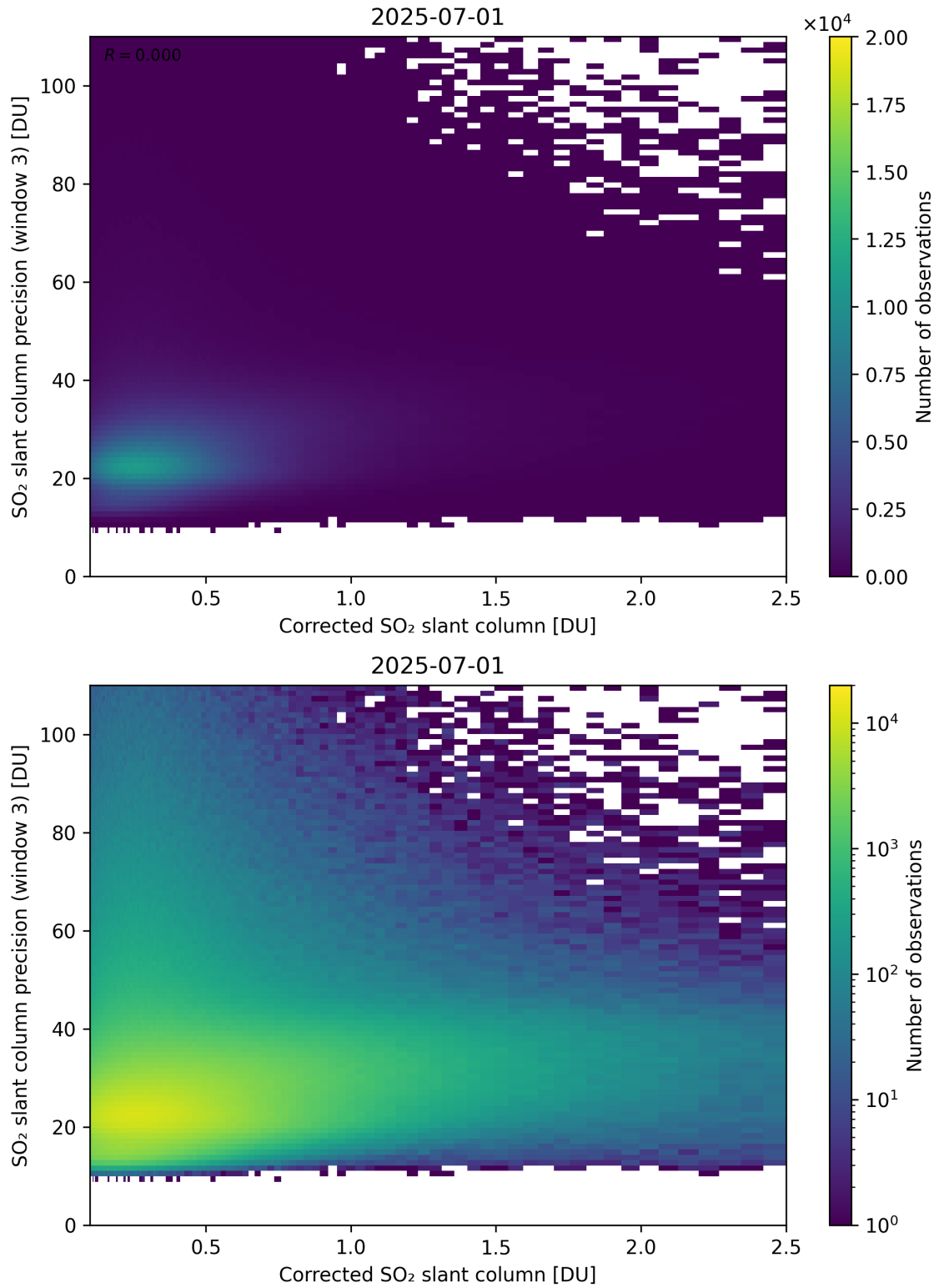
Figure 241: Scatter density plot of “Corrected SO 2 slant column” against “SO 2 slant column precision (window 3)” for 2025-06-30 to 2025-07-02.
