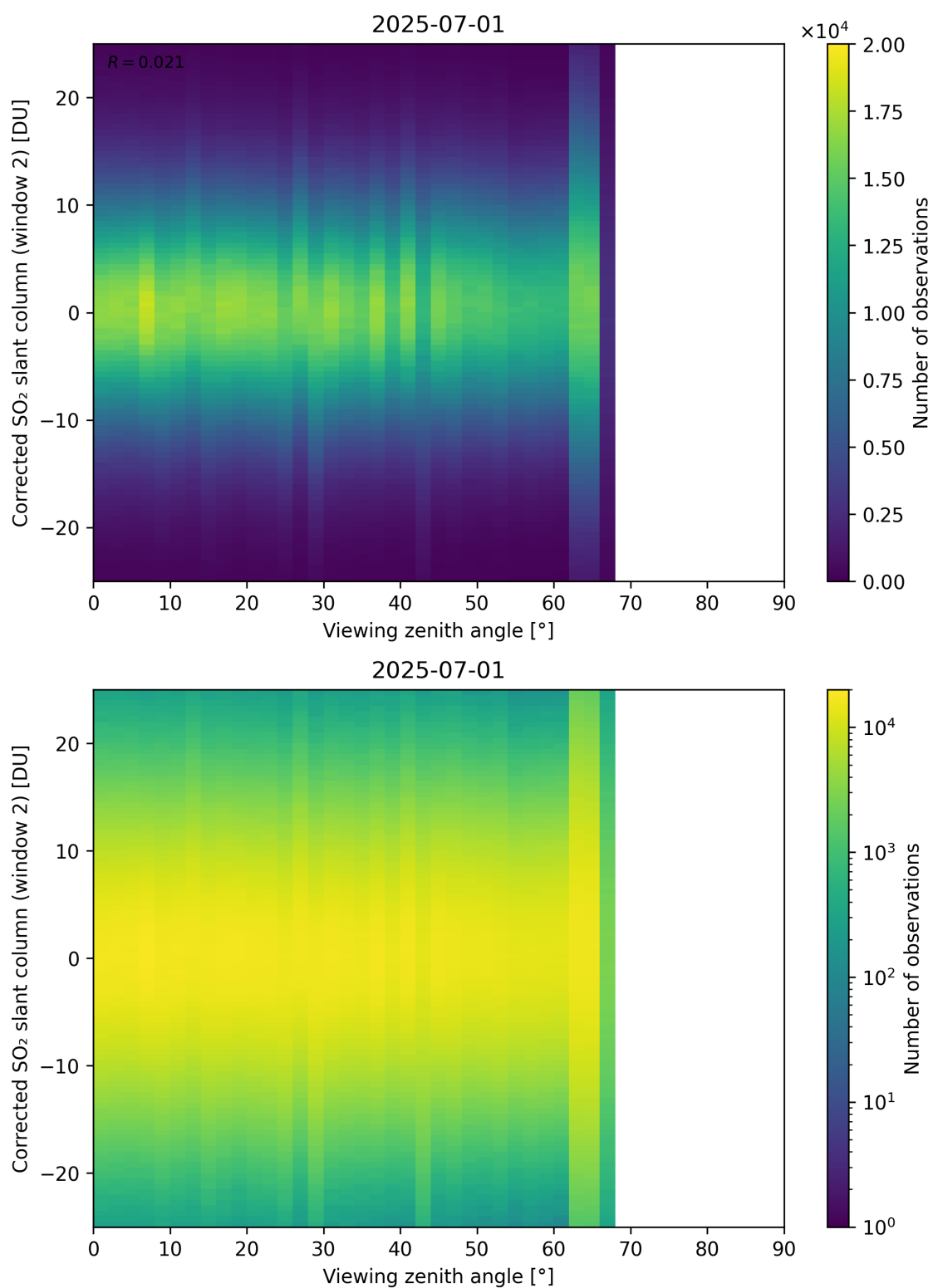
Figure 374: Scatter density plot of “Viewing zenith angle” against “Corrected SO 2 slant column (window 2)” for 2025-06-30 to 2025-07-02.
