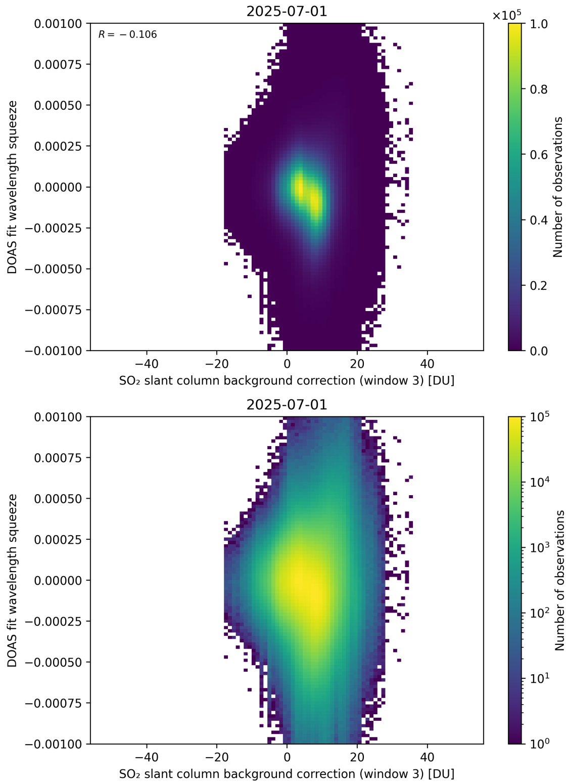
Figure 133: Scatter density plot of “SO 2 slant column background correction (window 3)” against “DOAS fit wavelength squeeze” for 2025-06-30 to 2025-07-02.
