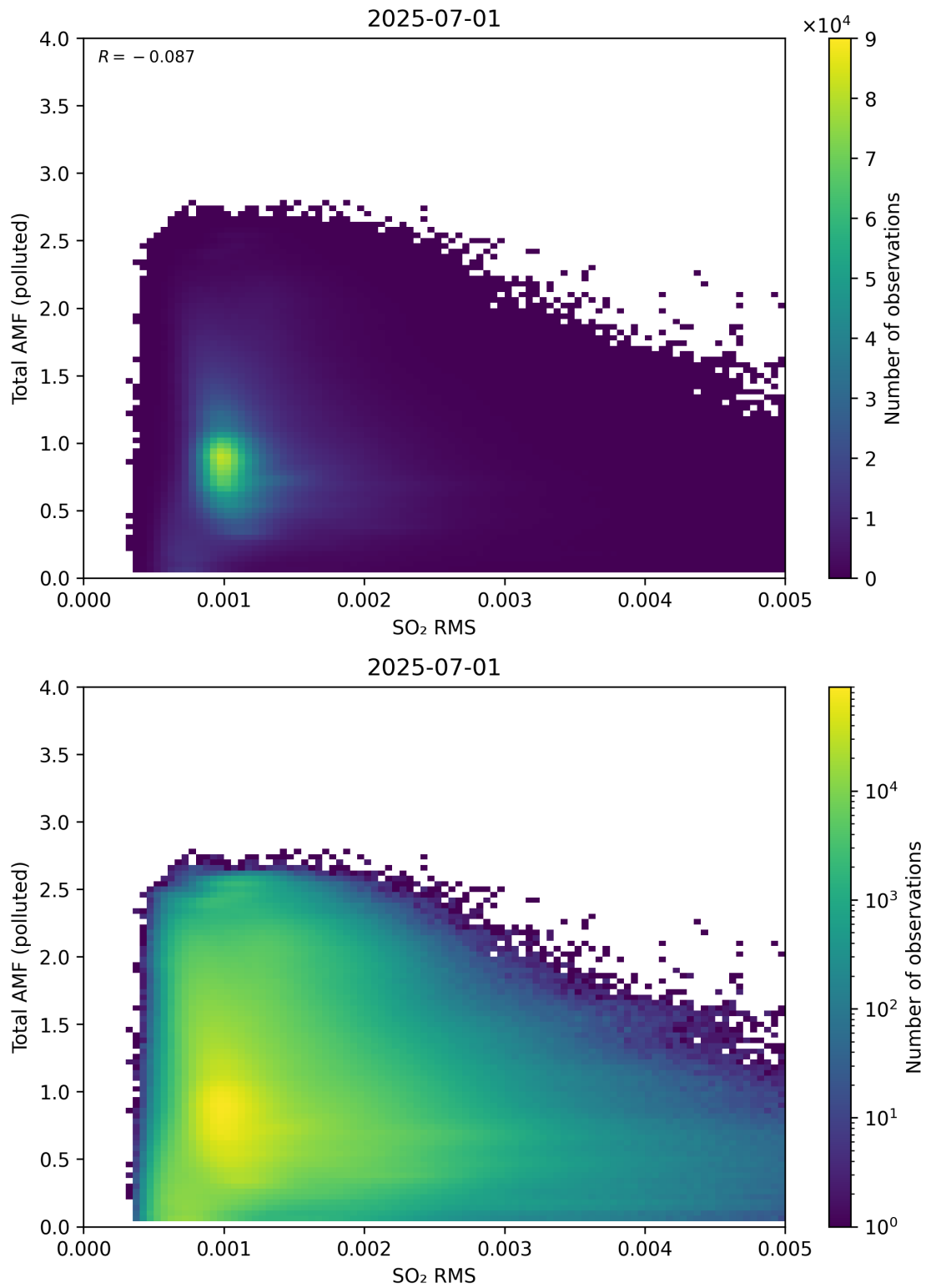
Figure 148: Scatter density plot of “SO 2 RMS” against “Total AMF (polluted)” for 2025-06-30 to 2025-07-02.
