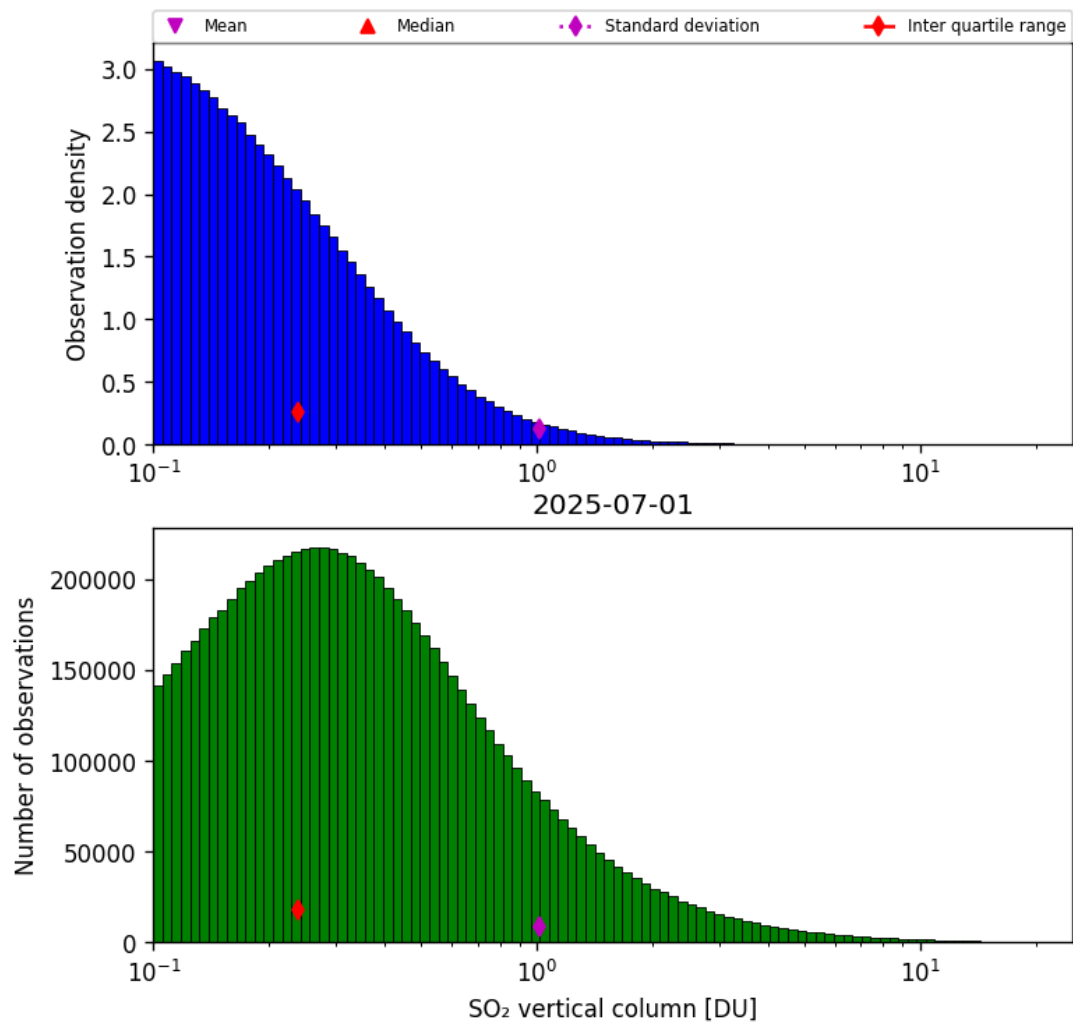
Figure 58: Histogram of “SO 2 vertical column” for 2025-06-30 to 2025-07-02
