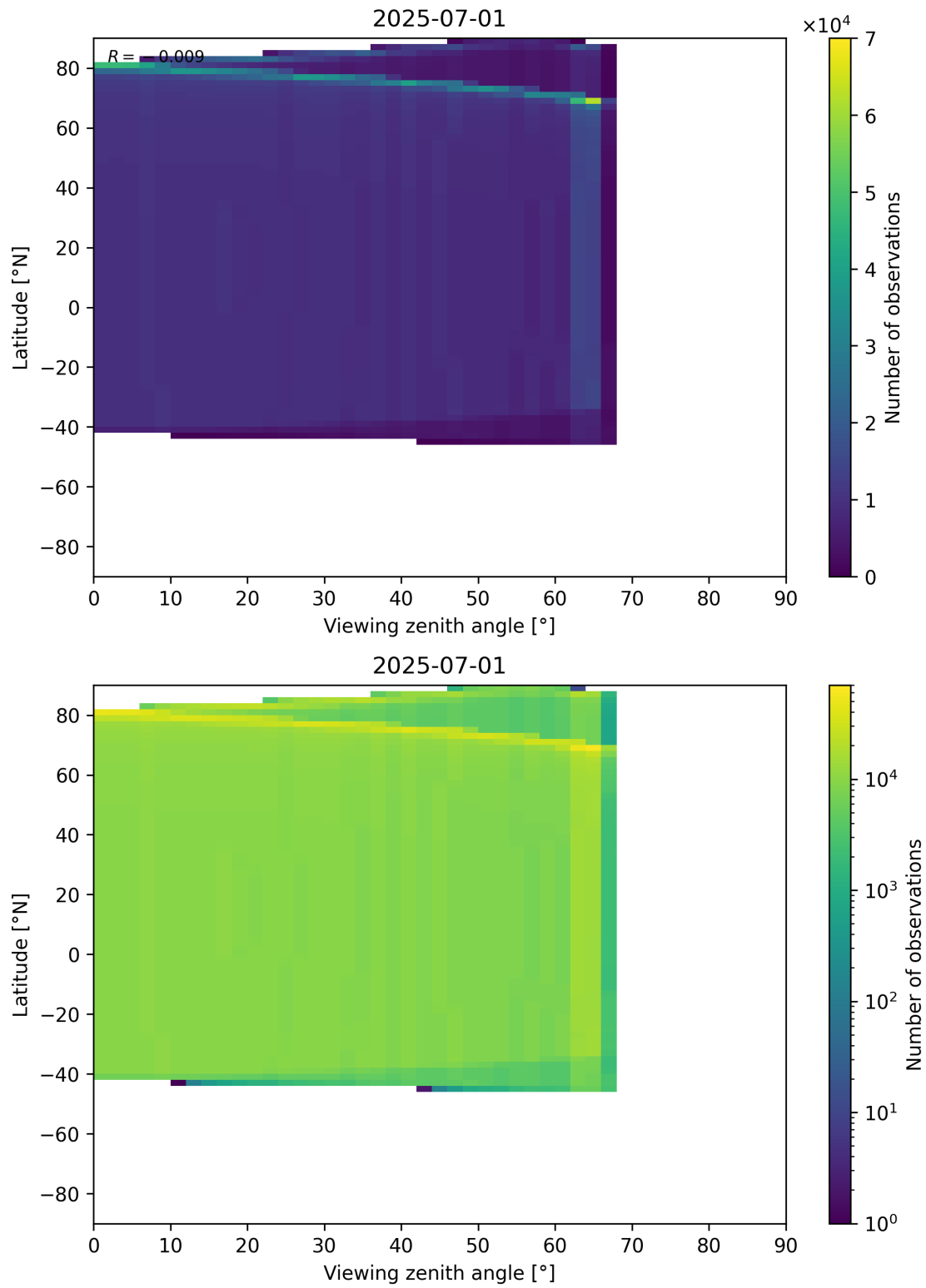
Figure 368: Scatter density plot of “Viewing zenith angle” against “Latitude” for 2025-06-30 to 2025-07-02.
