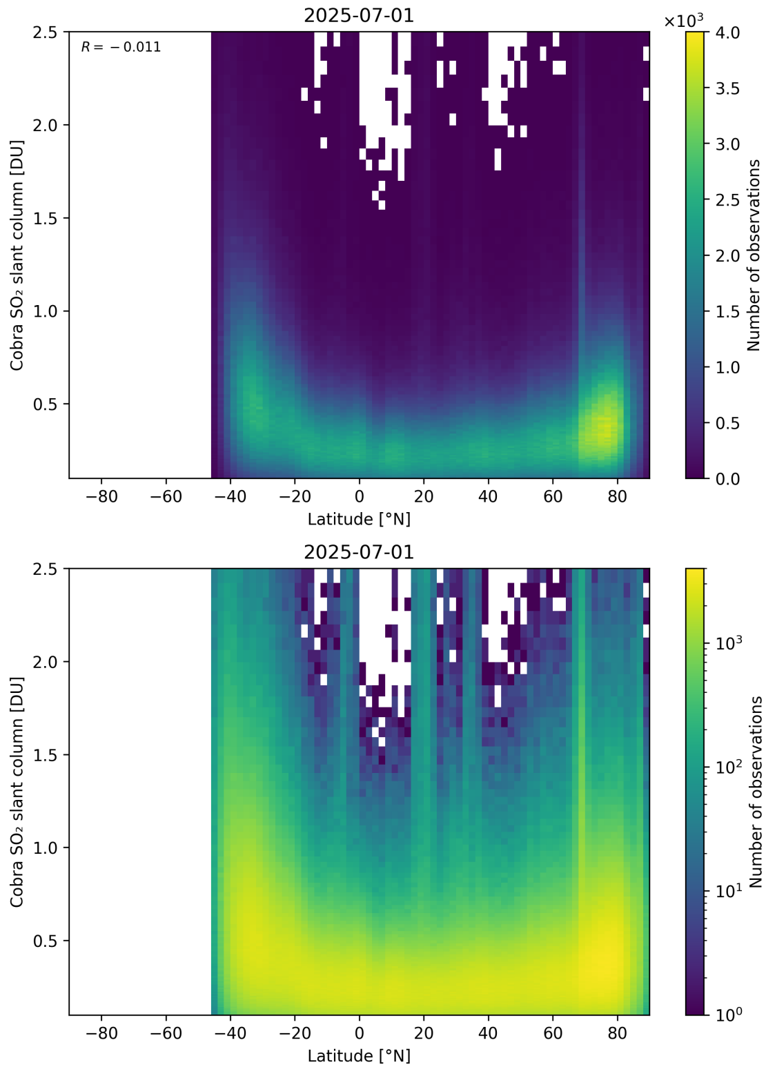
Figure 157: Scatter density plot of “Latitude” against “Cobra SO 2 slant column” for 2025-06-30 to 2025-07-02.
