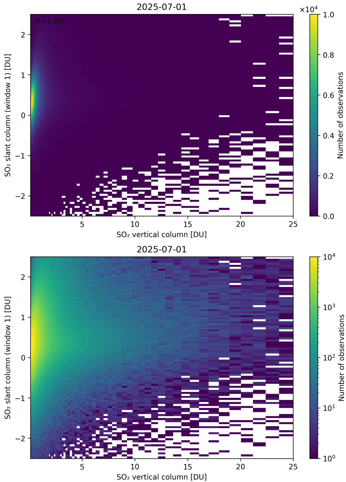
Figure 354: Scatter density plot of “SO 2 vertical column” against “SO 2 slant column (window 1)” for 2025-06-30 to 2025-07-02.
