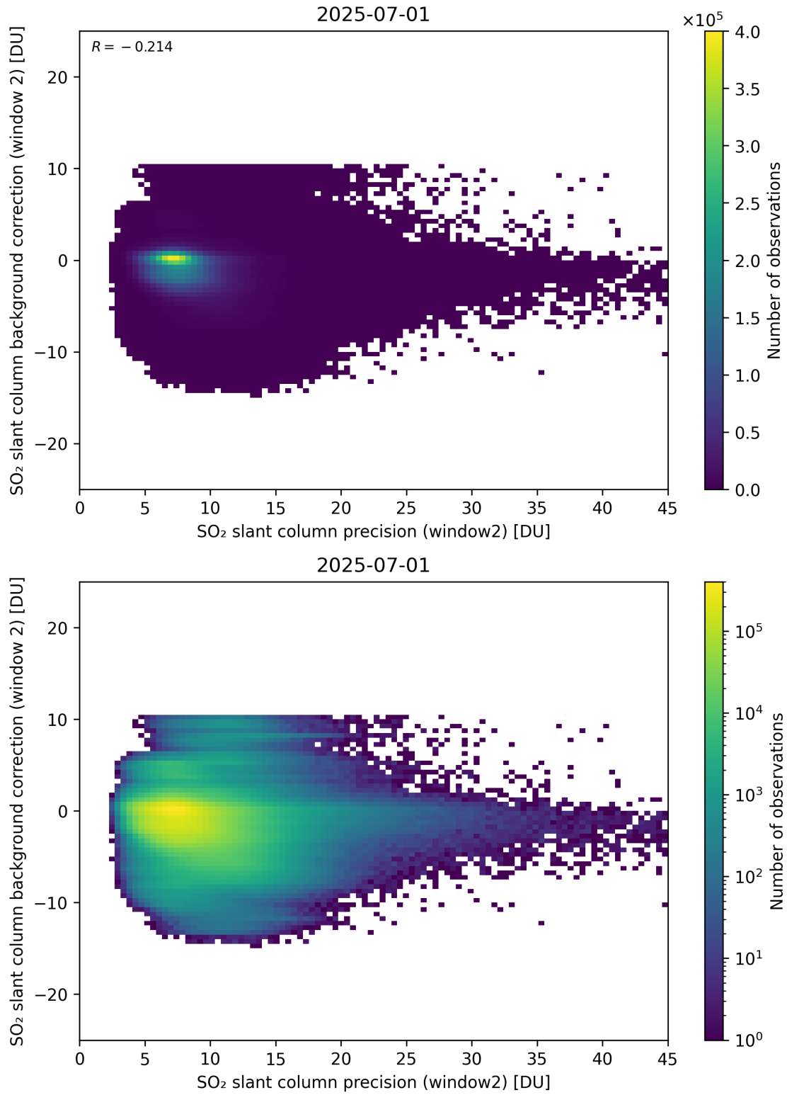
Figure 291: Scatter density plot of “SO 2 slant column precision (window2)” against “SO 2 slant column background correction (window 2)” for 2025-06-30 to 2025-07-02.
