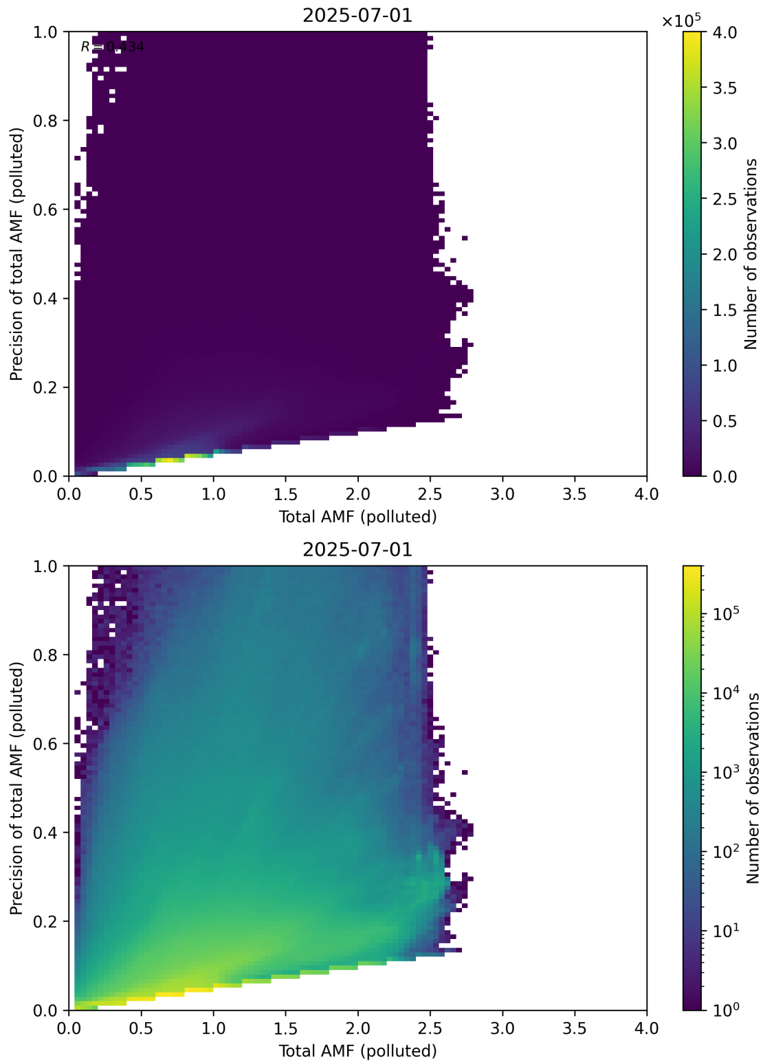
Figure 322: Scatter density plot of “Total AMF (polluted)” against “Precision of total AMF (polluted)” for 2025-06-30 to 2025-07-02.
