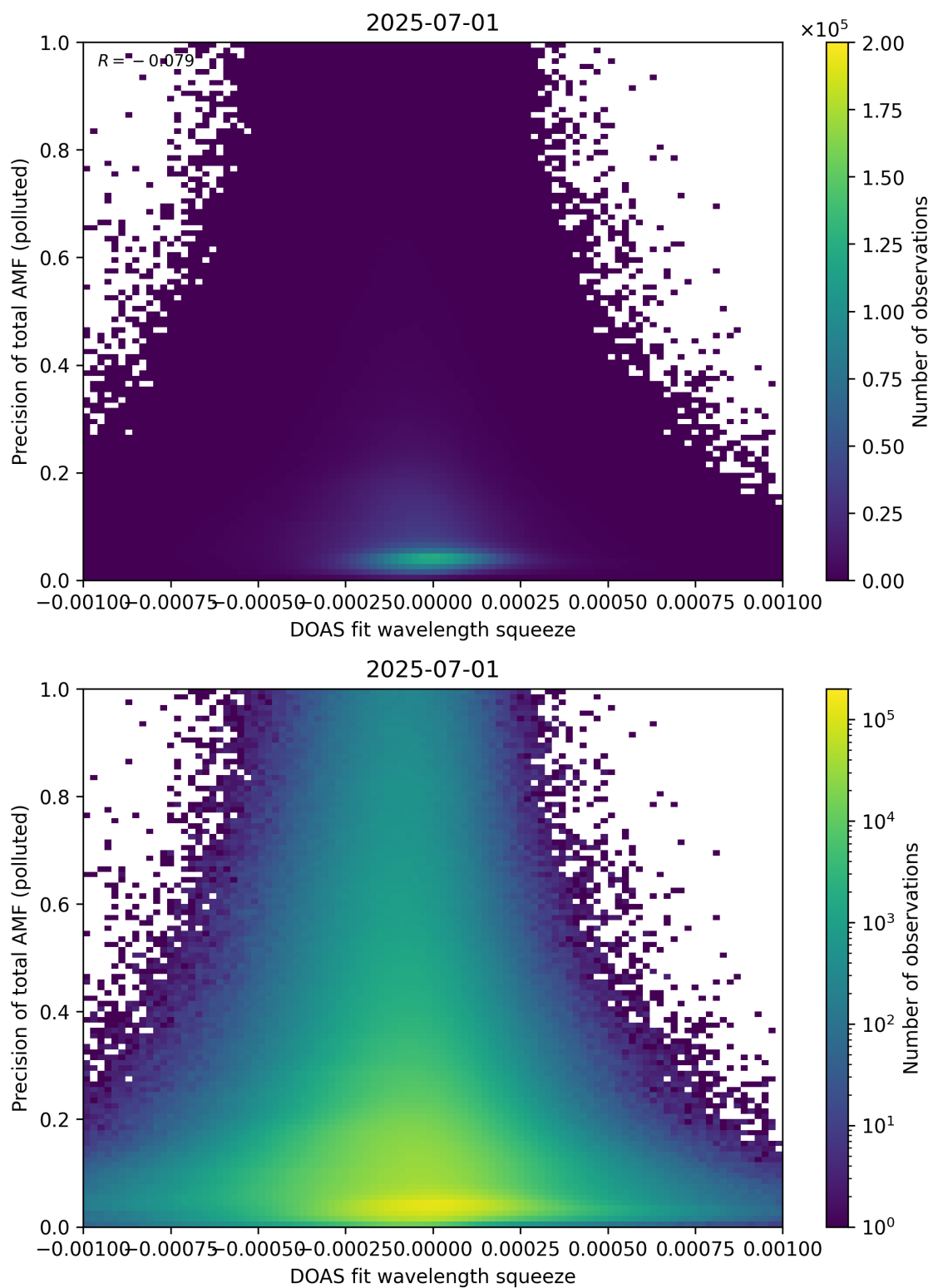
Figure 146: Scatter density plot of “DOAS fit wavelength squeeze” against “Precision of total AMF (polluted)” for 2025-06-30 to 2025-07-02.
