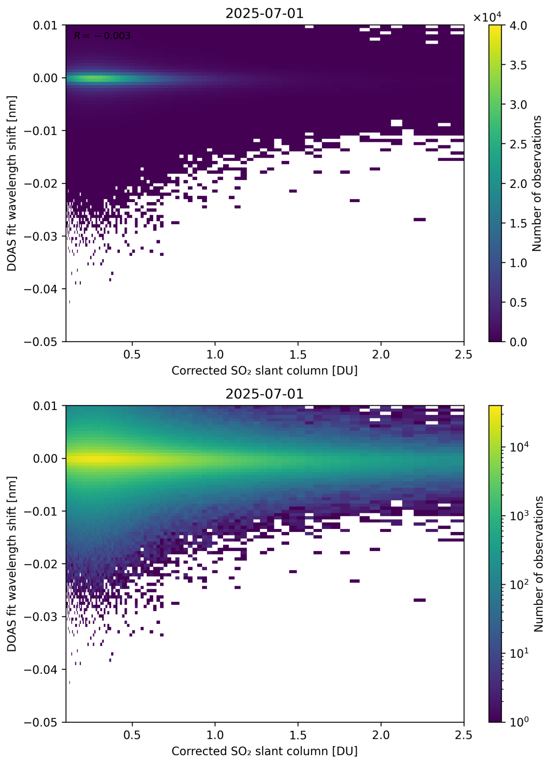
Figure 229: Scatter density plot of “Corrected SO 2 slant column” against “DOAS fit wavelength shift” for 2025-06-30 to 2025-07-02.
