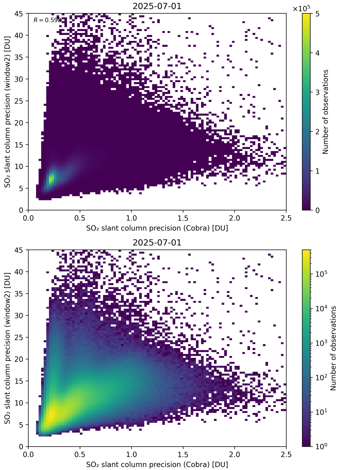
Figure 210: Scatter density plot of “SO 2 slant column precision (Cobra)” against “SO 2 slant column precision (window2)” for 2025-06-30 to 2025-07-02.
