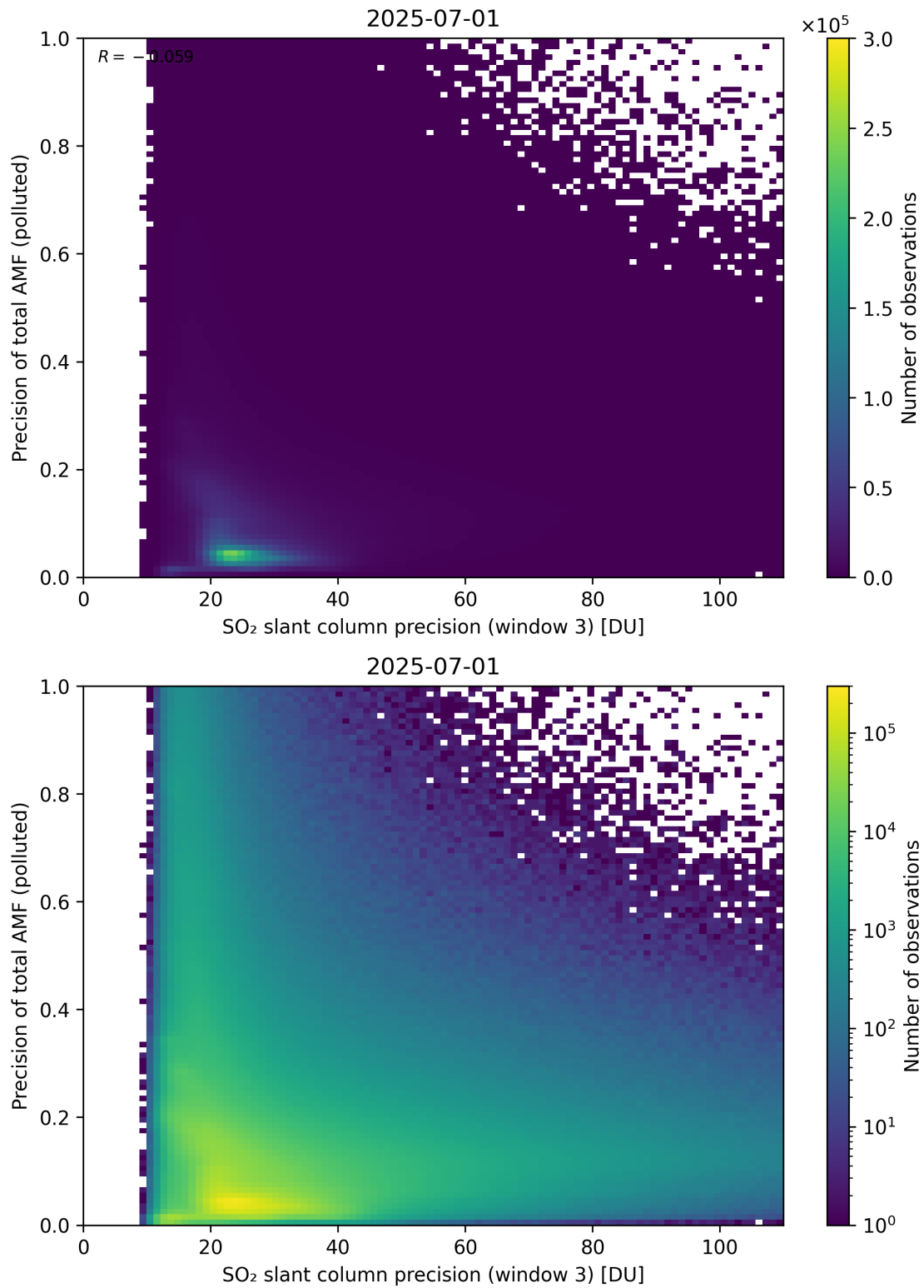
Figure 314: Scatter density plot of “SO 2 slant column precision (window 3)” against “Precision of total AMF (polluted)” for 2025-06-30 to 2025-07-02.
