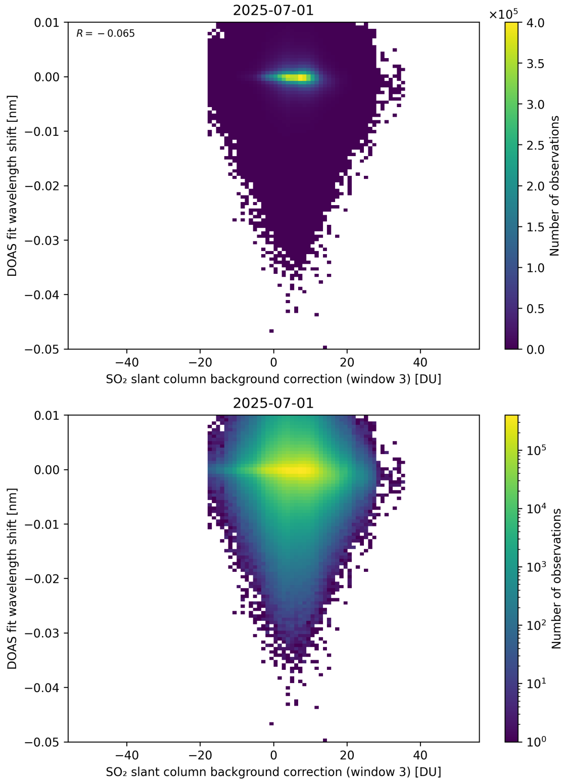
Figure 132: Scatter density plot of “SO 2 slant column background correction (window 3)” against “DOAS fit wavelength shift” for 2025-06-30 to 2025-07-02.
