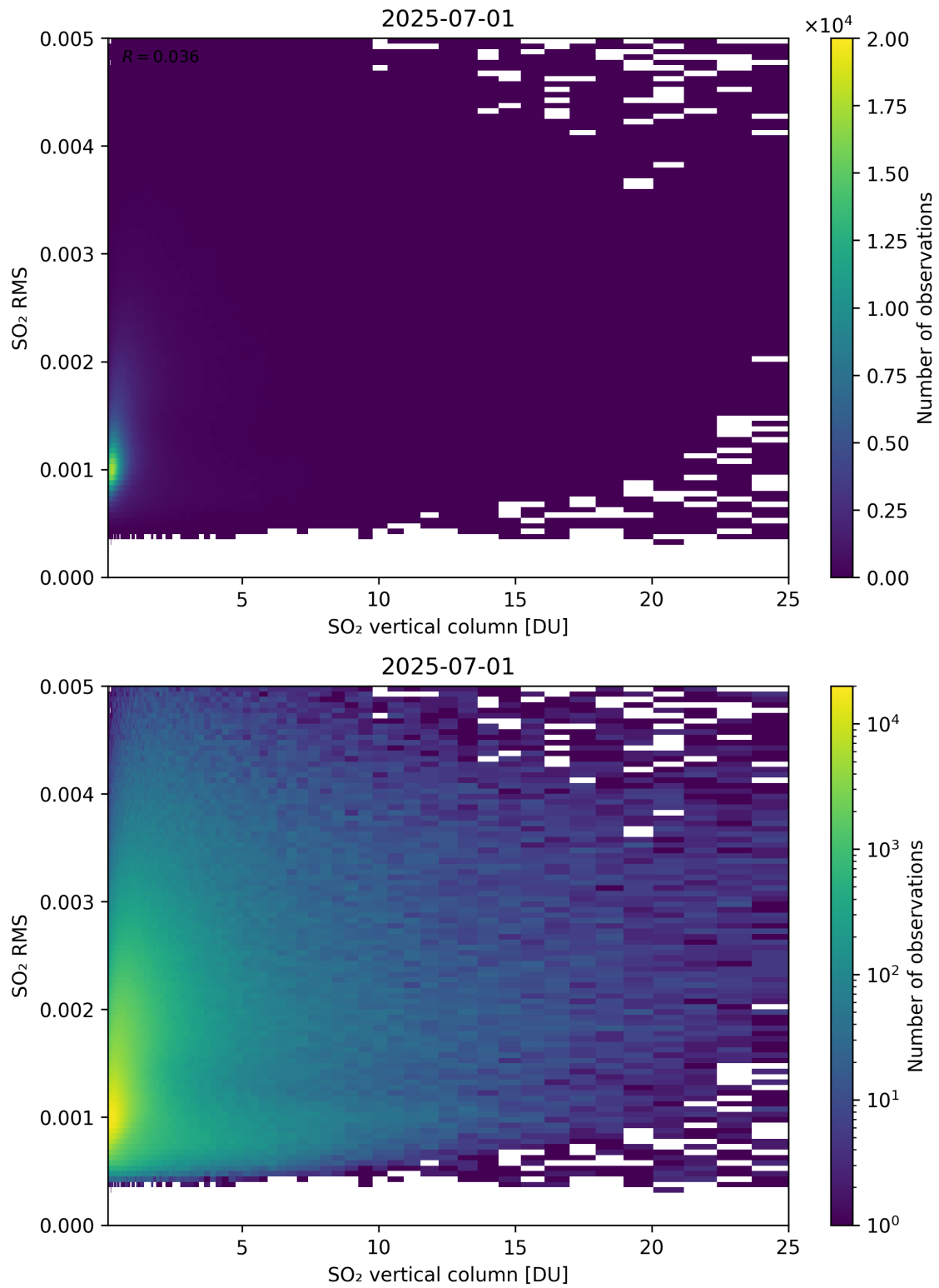
Figure 328: Scatter density plot of “SO 2 vertical column” against “SO 2 RMS” for 2025-06-30 to 2025-07-02.
