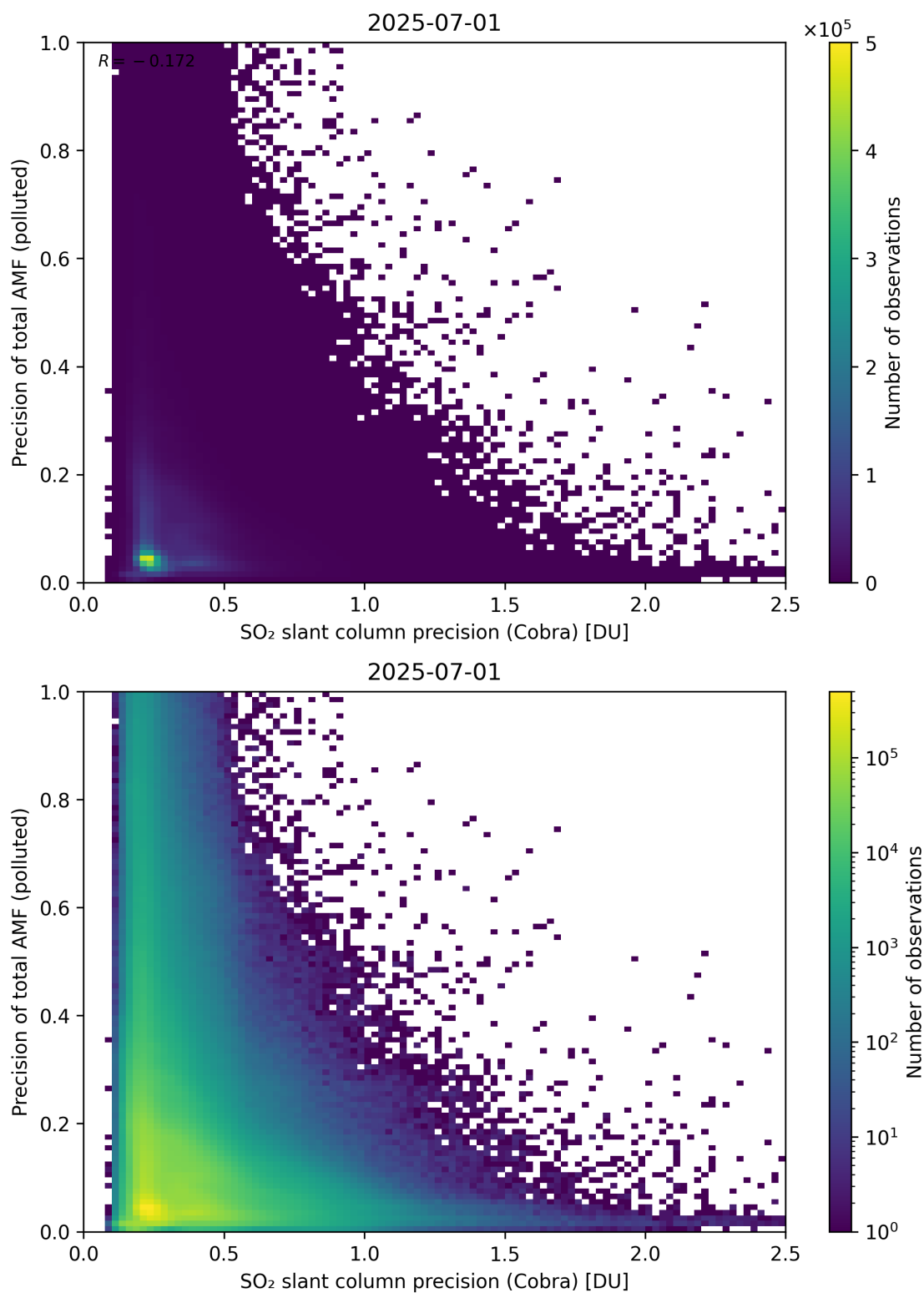
Figure 214: Scatter density plot of “SO 2 slant column precision (Cobra)” against “Precision of total AMF (polluted)” for 2025-06-30 to 2025-07-02.
