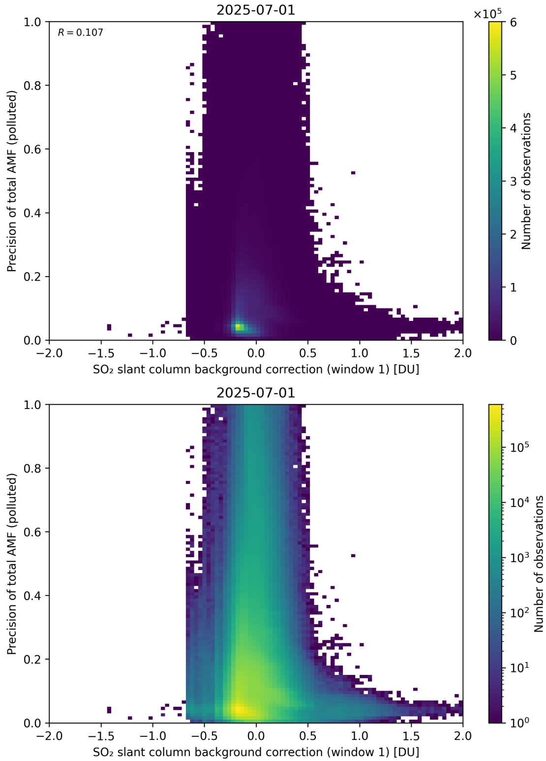
Figure 121: Scatter density plot of “SO 2 slant column background correction (window 1)” against “Precision of total AMF (polluted)” for 2025-06-30 to 2025-07-02.
