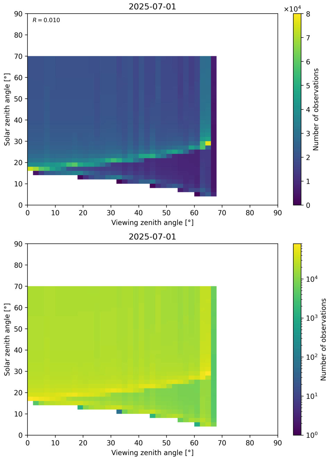
Figure 369: Scatter density plot of “Viewing zenith angle” against “Solar zenith angle” for 2025-06-30 to 2025-07-02.
