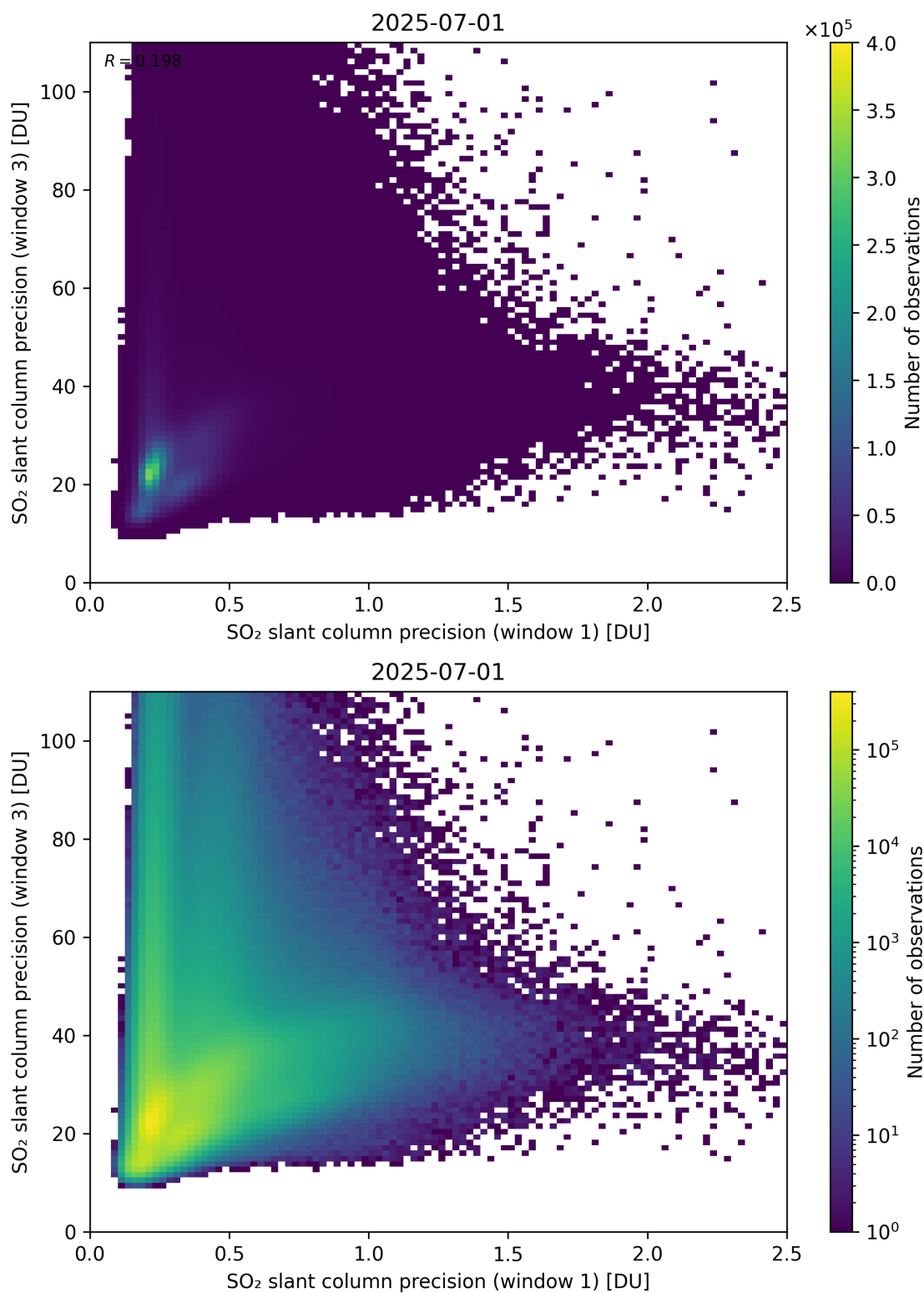
Figure 279: Scatter density plot of “SO 2 slant column precision (window 1)” against “SO 2 slant column precision (window 3)” for 2025-06-30 to 2025-07-02.
