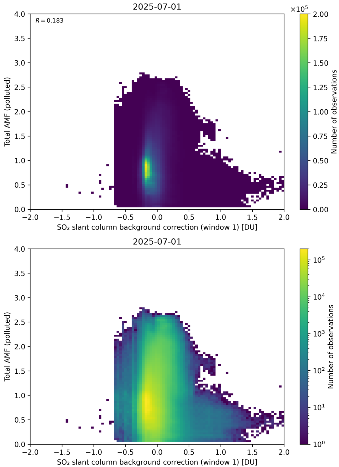
Figure 120: Scatter density plot of “SO 2 slant column background correction (window 1)” against “Total AMF (polluted)” for 2025-06-30 to 2025-07-02.
