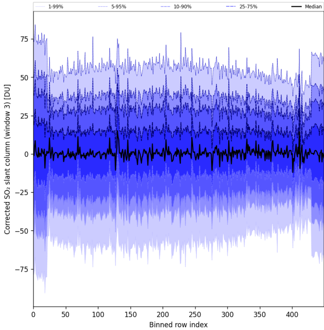
Figure 99: Along track statistics of “Corrected SO 2 slant column (window 3)” for 2025-06-30 to 2025-07-02
