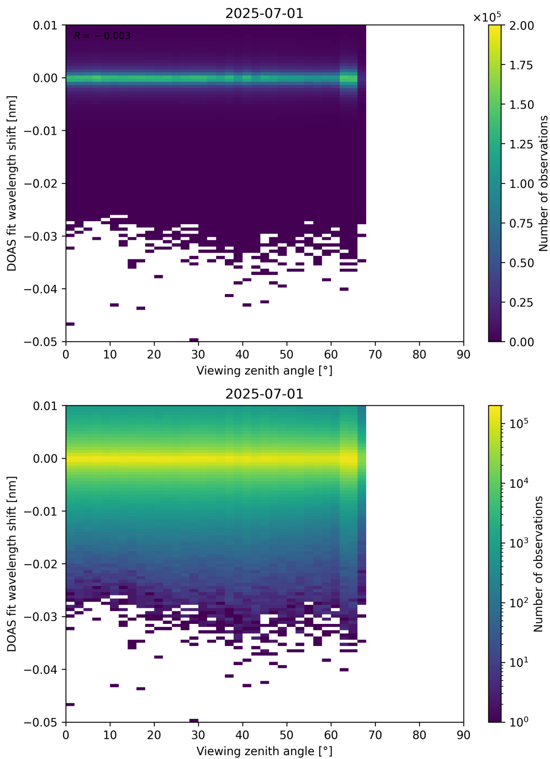
Figure 365: Scatter density plot of “Viewing zenith angle” against “DOAS fit wavelength shift” for 2025-06-30 to 2025-07-02.
