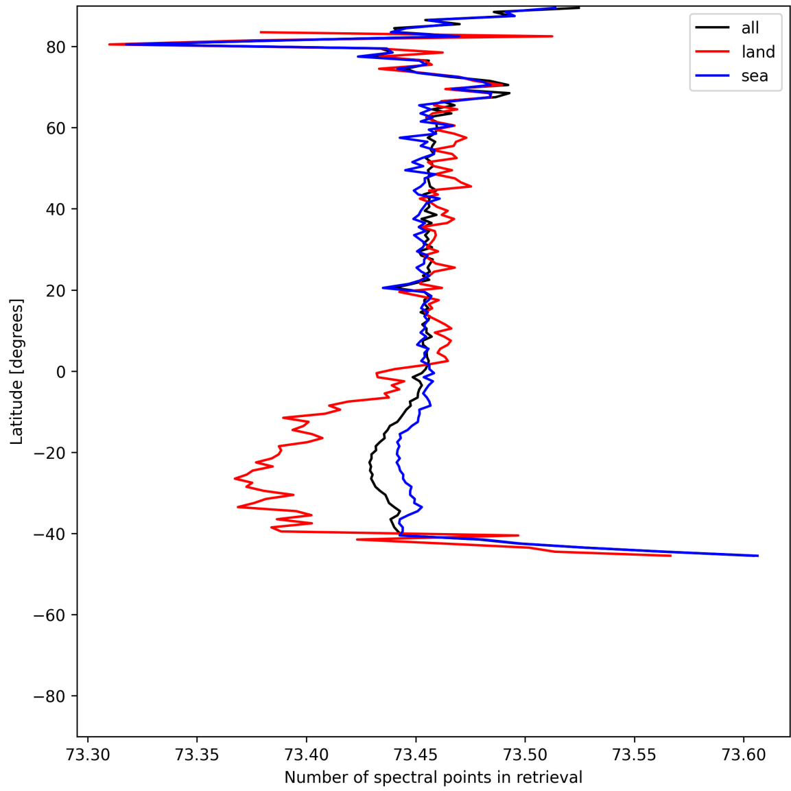
Figure 56: Zonal average of “Number of spectral points in retrieval” for 2025-06-30 to 2025-07-02.
