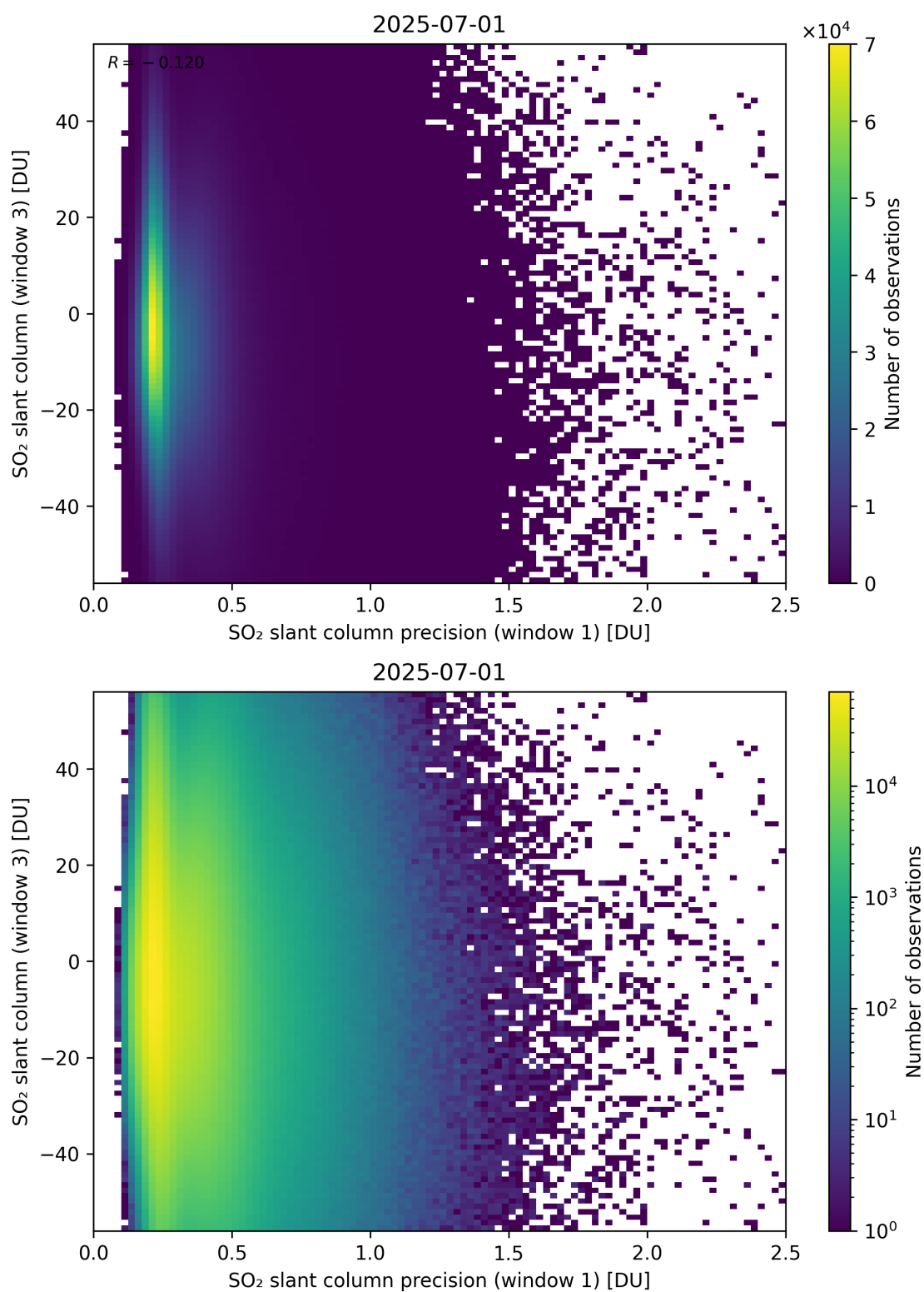
Figure 278: Scatter density plot of “SO 2 slant column precision (window 1)” against “SO 2 slant column (window 3)” for 2025-06-30 to 2025-07-02.
