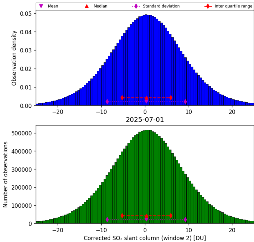
Figure 69: Histogram of “Corrected SO 2 slant column (window 2)” for 2025-06-30 to 2025-07-02
