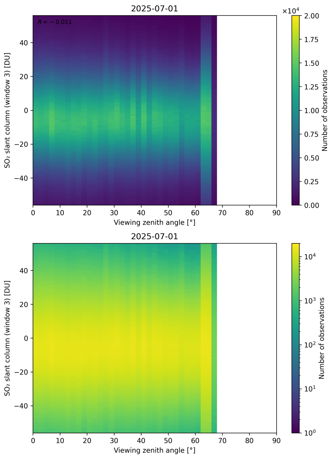
Figure 379: Scatter density plot of “Viewing zenith angle” against “SO 2 slant column (window 3)” for 2025-06-30 to 2025-07-02.
