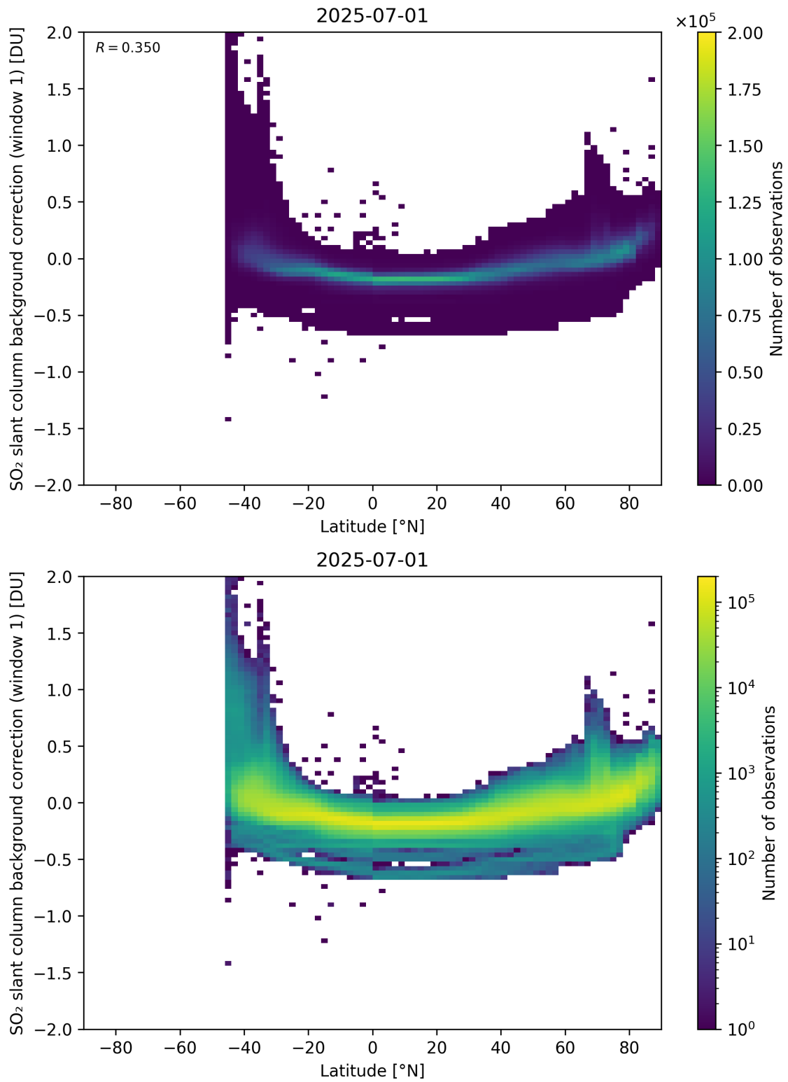
Figure 150: Scatter density plot of “Latitude” against “SO 2 slant column background correction (window 1)” for 2025-06-30 to 2025-07-02.
