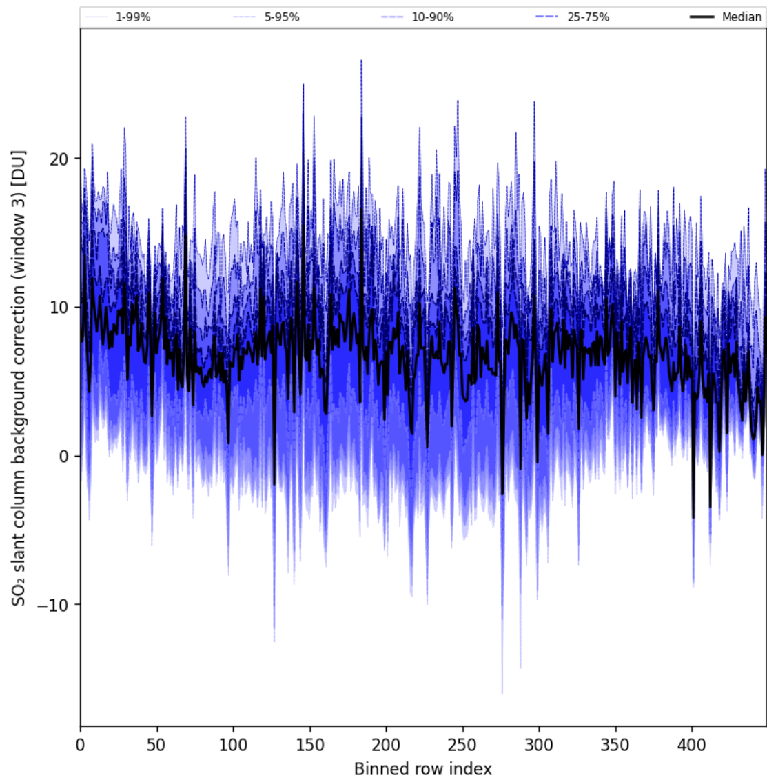
Figure 100: Along track statistics of “SO 2 slant column background correction (window 3)” for 2025-06-30 to 2025-07-02
