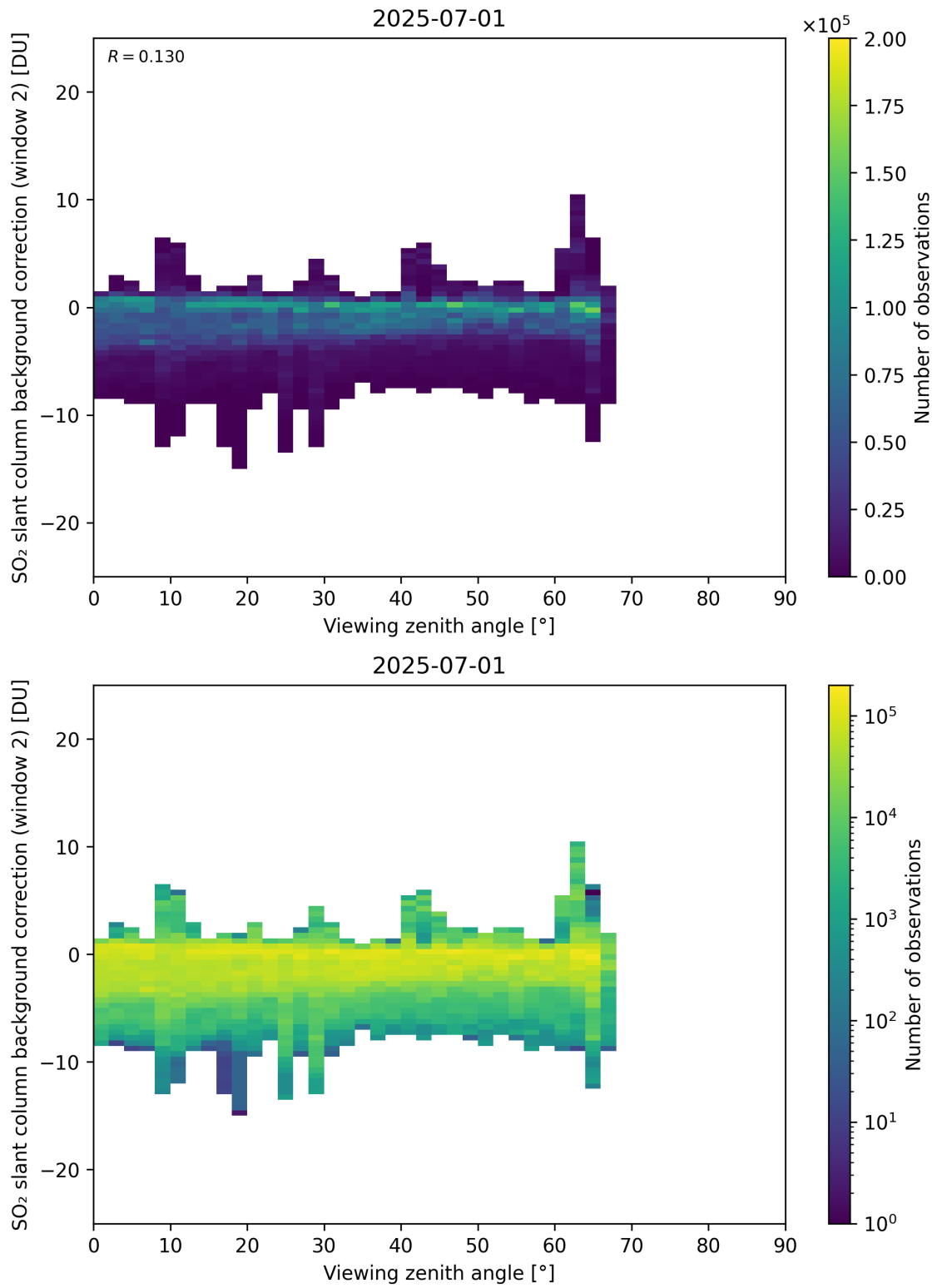
Figure 363: Scatter density plot of “Viewing zenith angle” against “SO 2 slant column background correction (window 2)” for 2025-06-30 to 2025-07-02.
