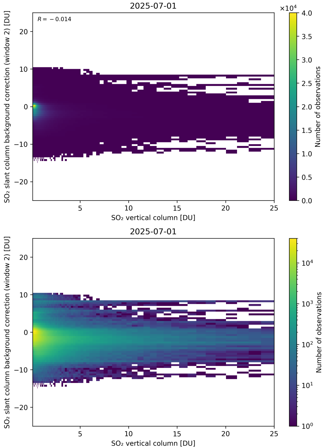
Figure 324: Scatter density plot of “SO 2 vertical column” against “SO 2 slant column background correction (window 2)” for 2025-06-30 to 2025-07-02.
