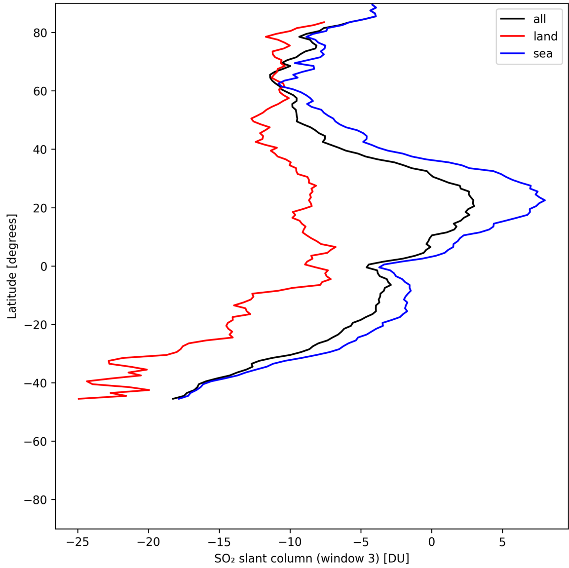
Figure 45: Zonal average of “SO 2 slant column (window 3)” for 2025-06-30 to 2025-07-02.
