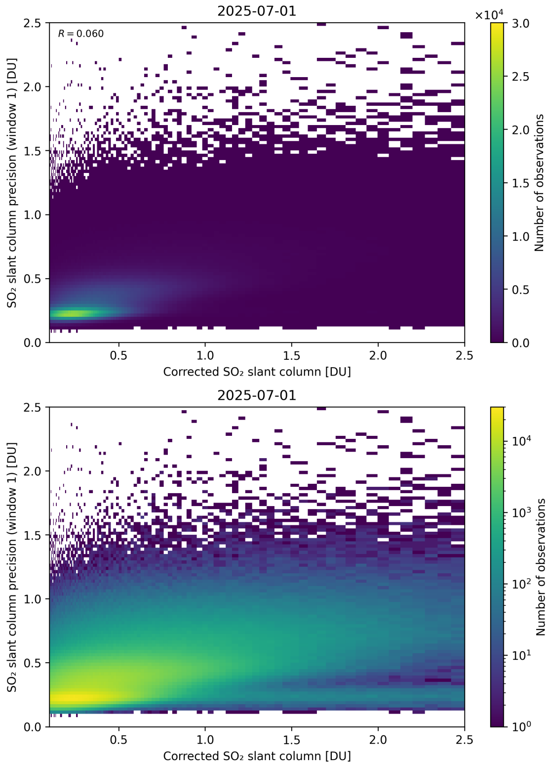
Figure 238: Scatter density plot of “Corrected SO 2 slant column” against “SO 2 slant column precision (window 1)” for 2025-06-30 to 2025-07-02.
