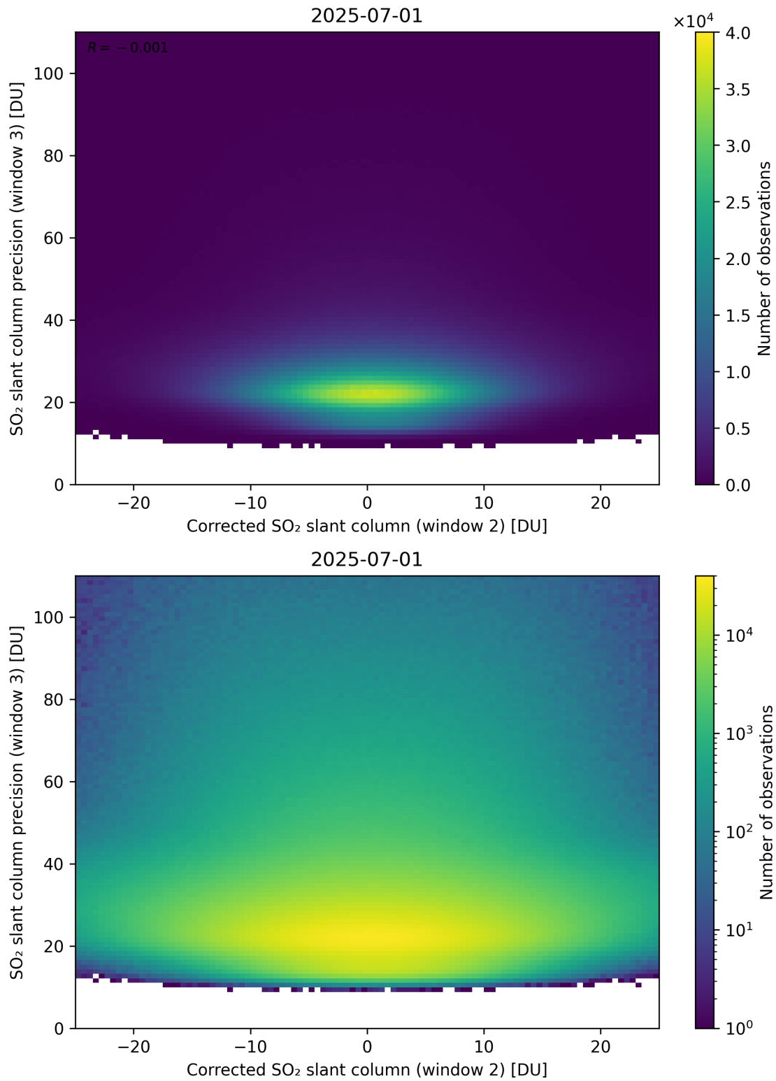
Figure 252: Scatter density plot of “Corrected SO 2 slant column (window 2)” against “SO 2 slant column precision (window 3)” for 2025-06-30 to 2025-07-02.
