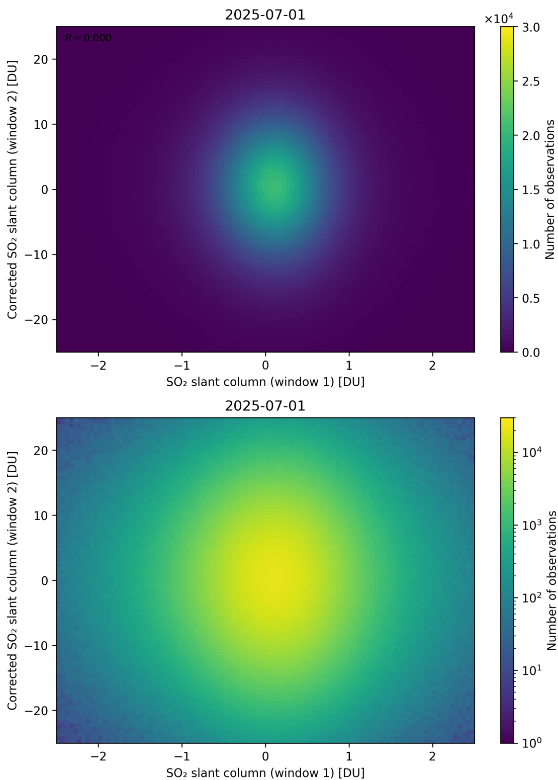
Figure 283: Scatter density plot of “SO 2 slant column (window 1)” against “Corrected SO 2 slant column (window 2)” for 2025-06-30 to 2025-07-02.
