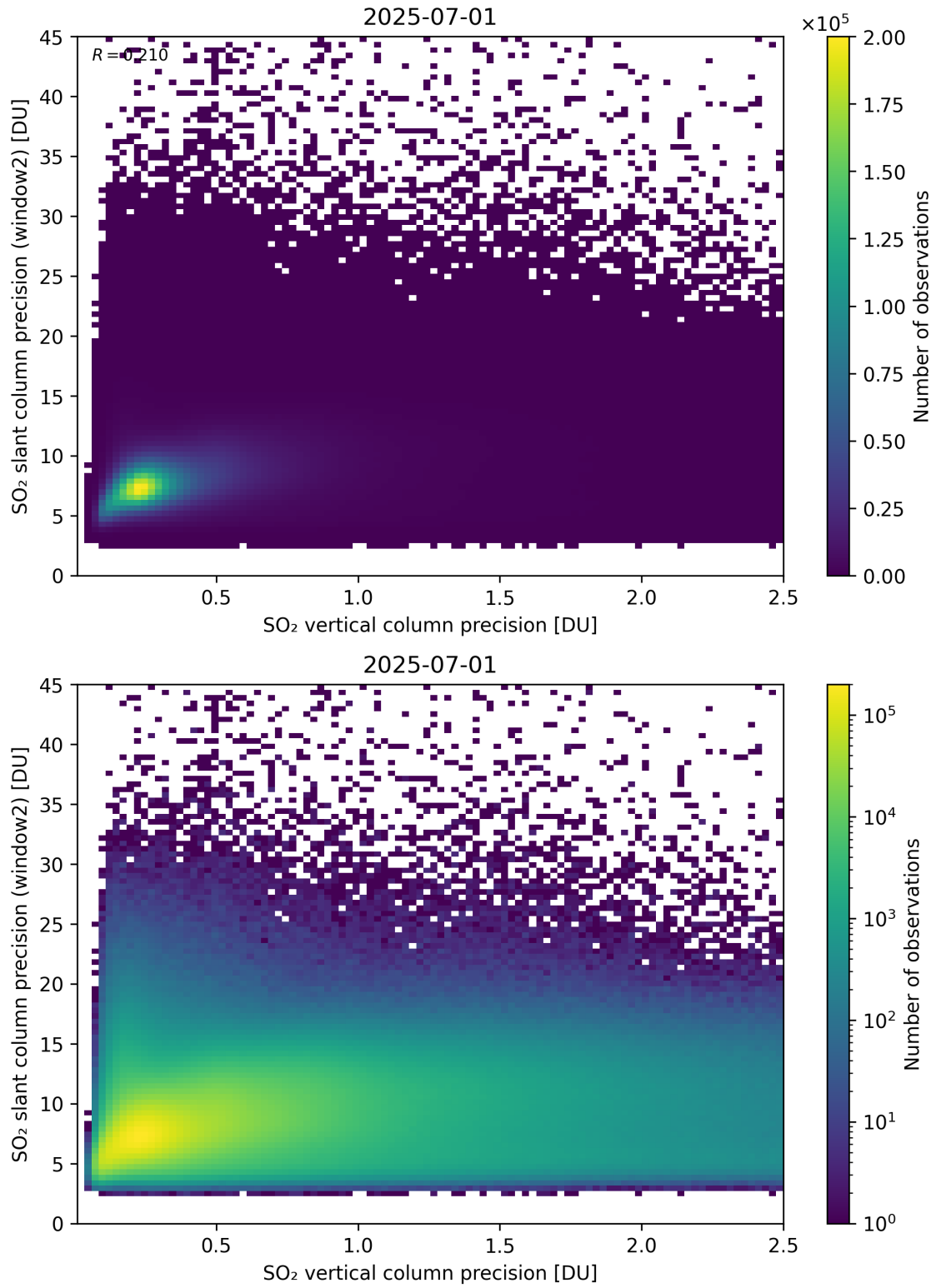
Figure 343: Scatter density plot of “SO 2 vertical column precision” against “SO 2 slant column precision (window2)” for 2025-06-30 to 2025-07-02.
