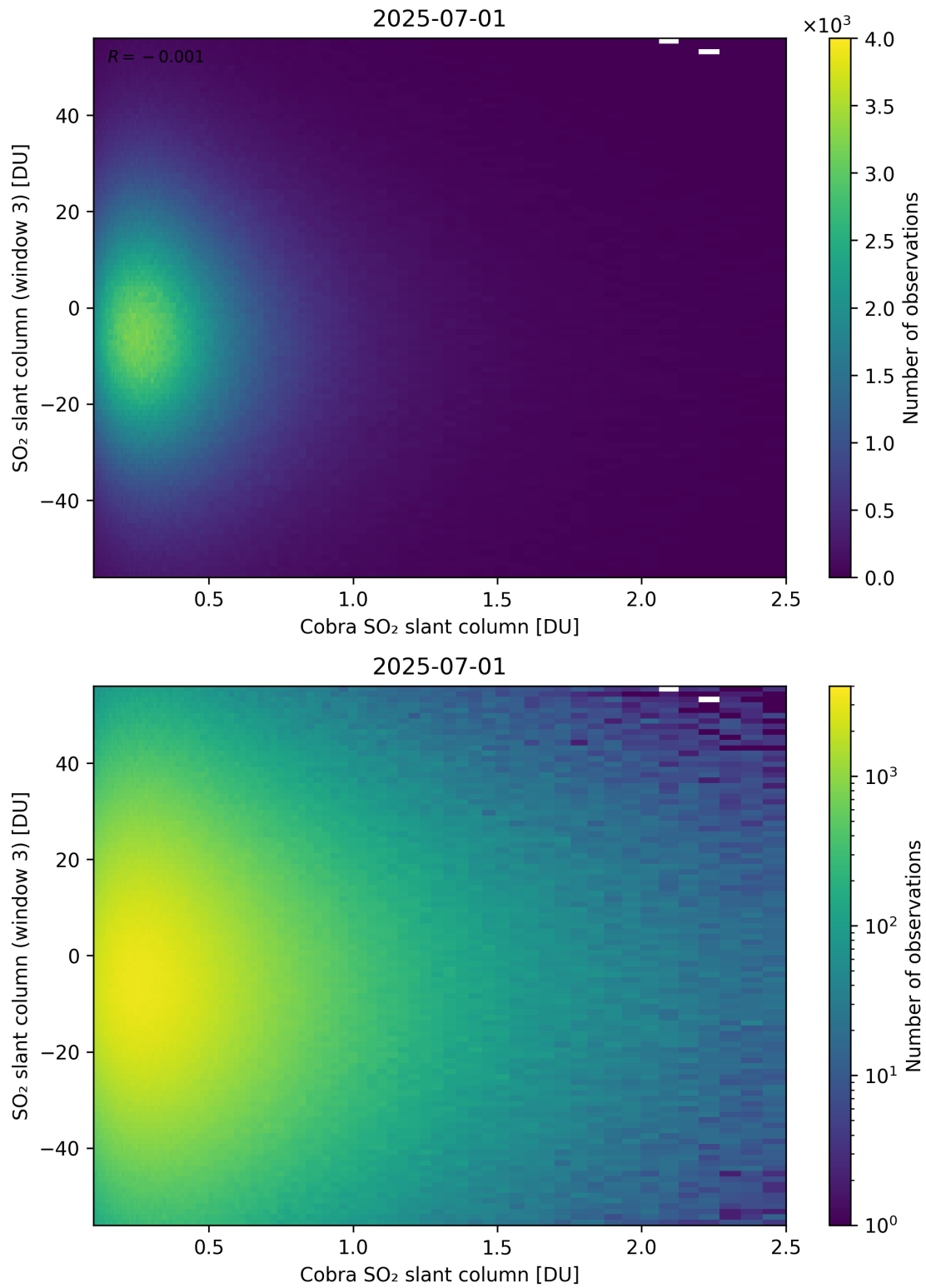
Figure 222: Scatter density plot of “Cobra SO 2 slant column” against “SO 2 slant column (window 3)” for 2025-06-30 to 2025-07-02.
