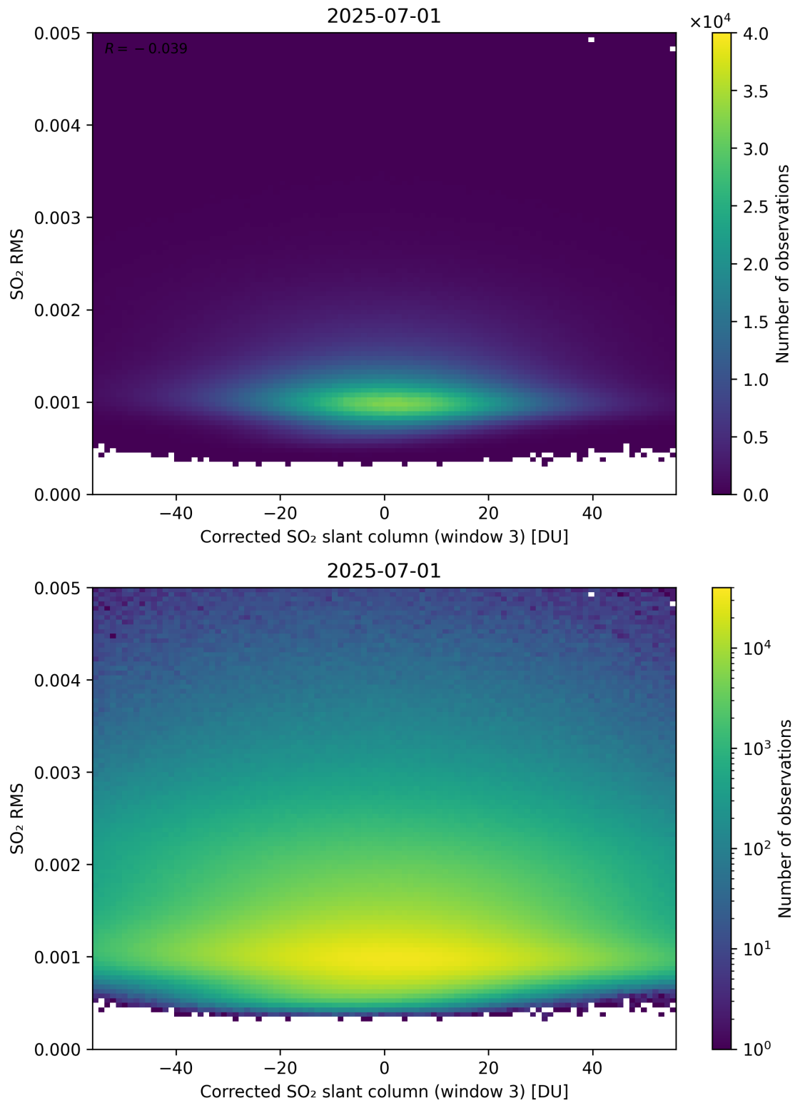
Figure 258: Scatter density plot of “Corrected SO 2 slant column (window 3)” against “SO 2 RMS” for 2025-06-30 to 2025-07-02.
