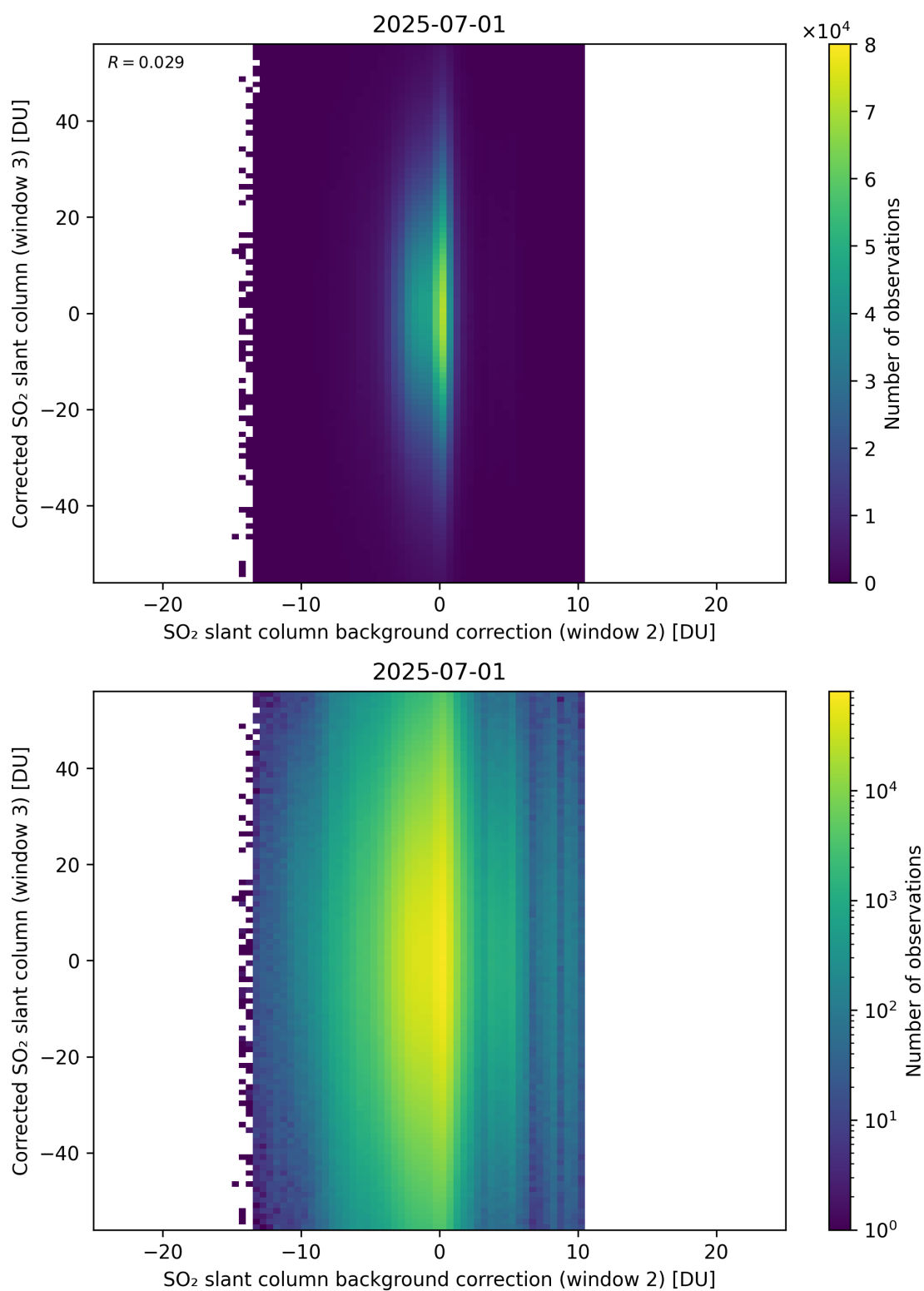
Figure 127: Scatter density plot of “SO 2 slant column background correction (window 2)” against “Corrected SO 2 slant column (window 3)” for 2025-06-30 to 2025-07-02.
