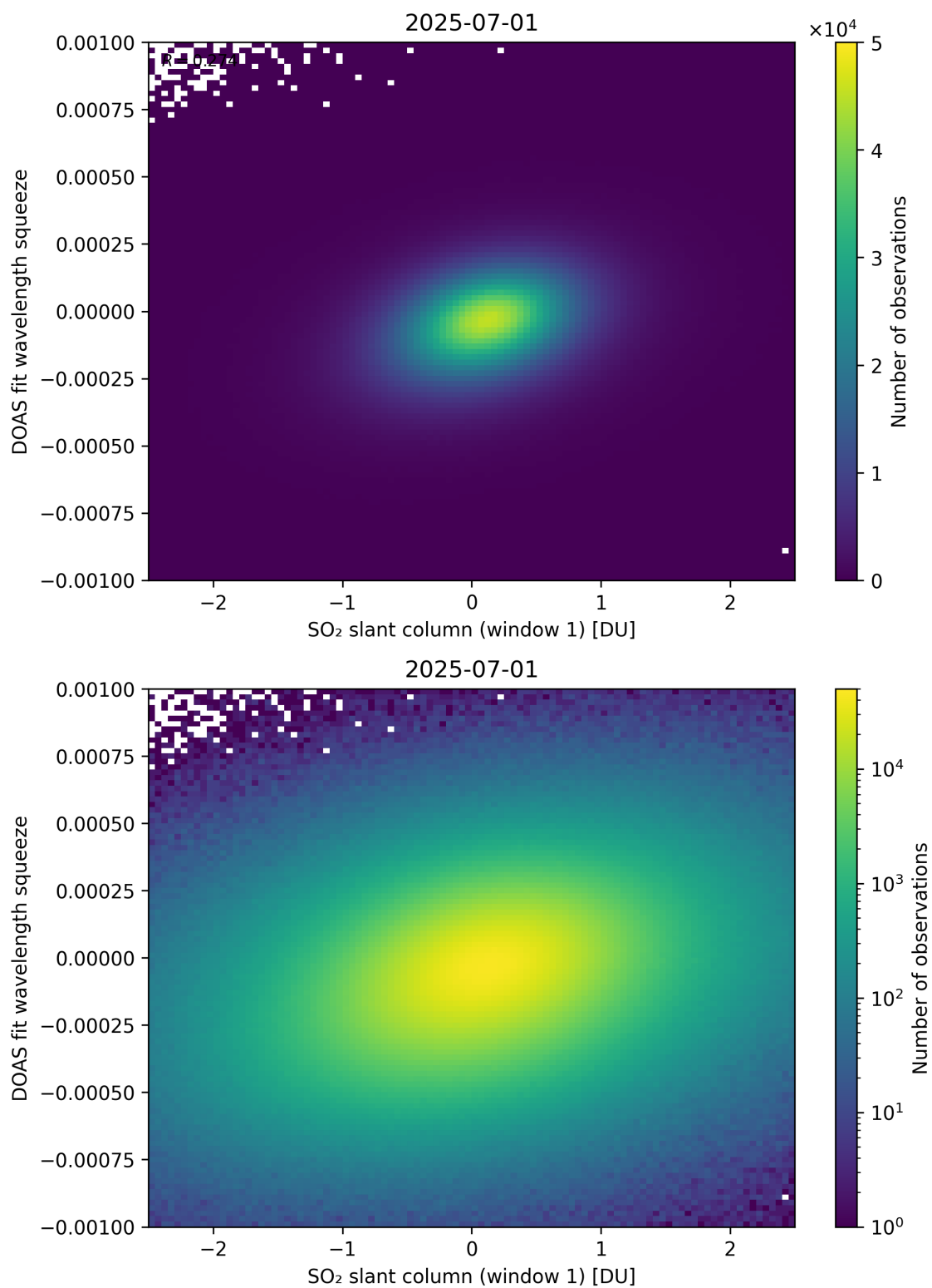
Figure 266: Scatter density plot of “SO 2 slant column (window 1)” against “DOAS fit wavelength squeeze” for 2025-06-30 to 2025-07-02.
