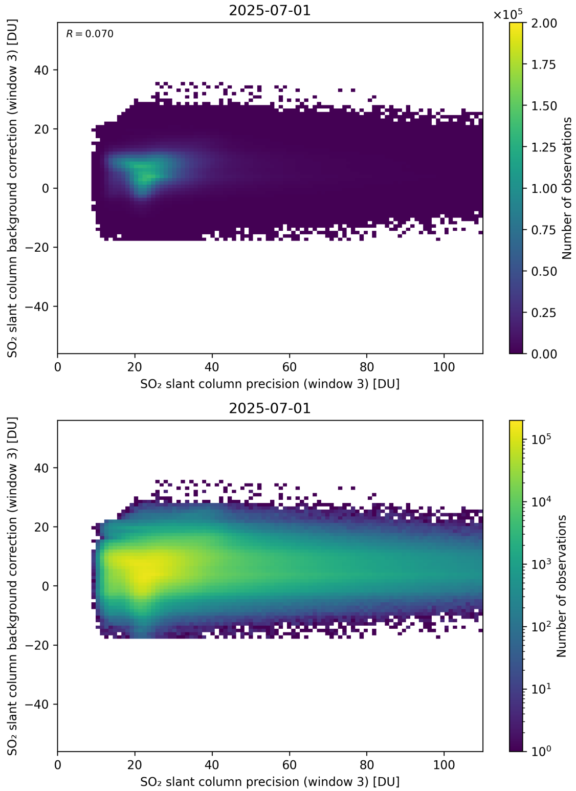
Figure 307: Scatter density plot of “SO 2 slant column precision (window 3)” against “SO 2 slant column background correction (window 3)” for 2025-06-30 to 2025-07-02.
