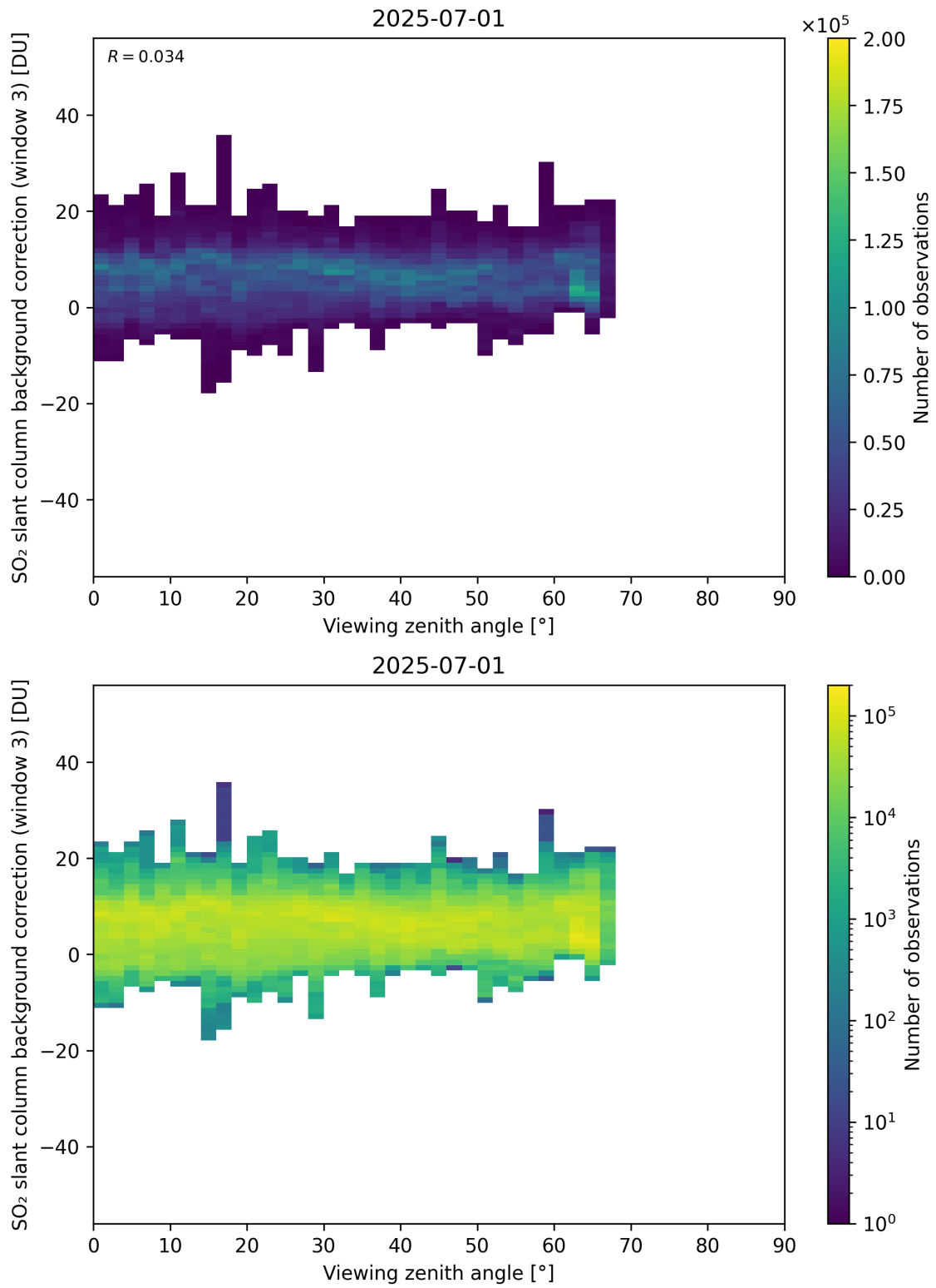
Figure 364: Scatter density plot of “Viewing zenith angle” against “SO 2 slant column background correction (window 3)” for 2025-06-30 to 2025-07-02.
