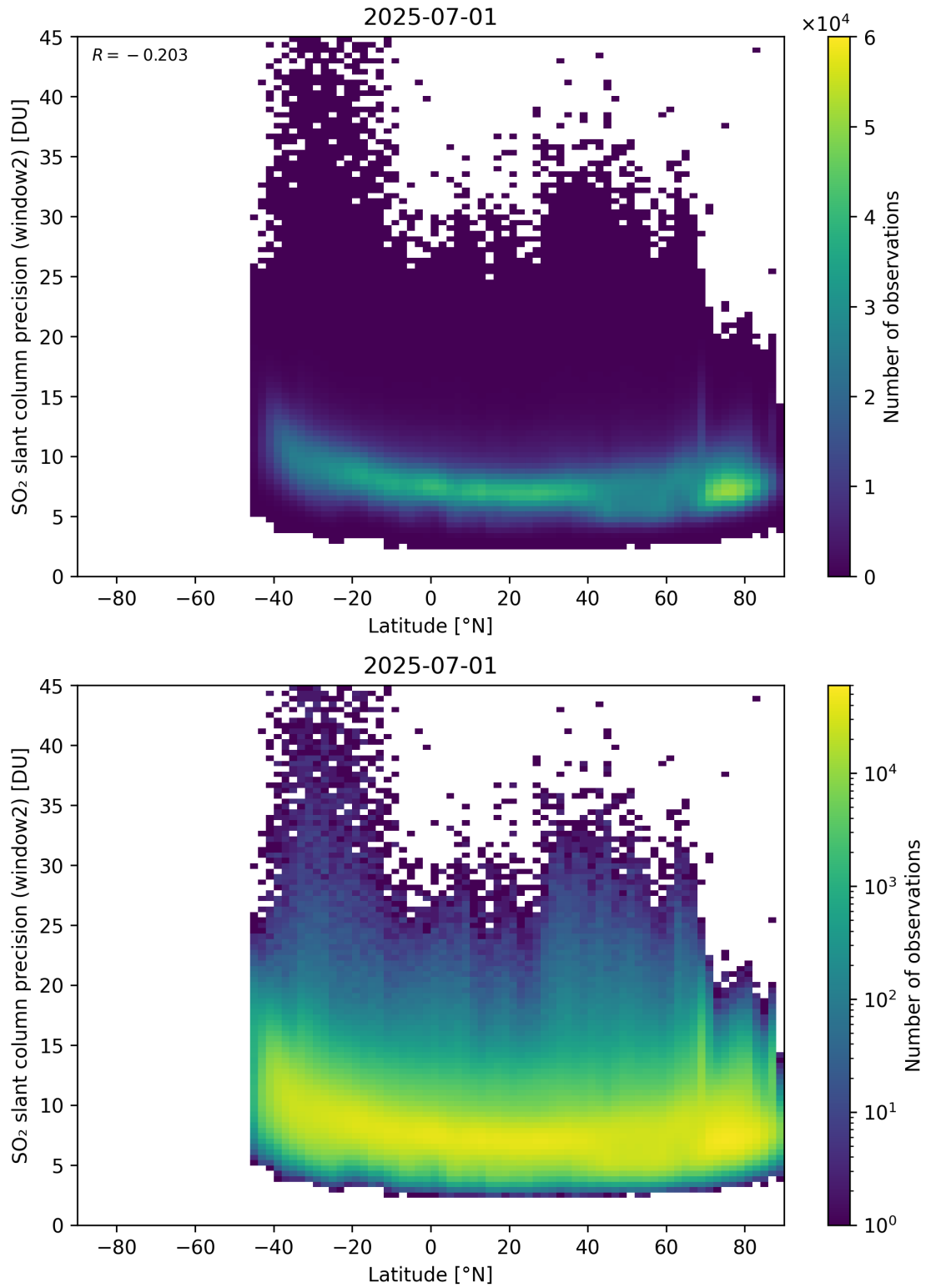
Figure 164: Scatter density plot of “Latitude” against “SO 2 slant column precision (window2)” for 2025-06-30 to 2025-07-02.
