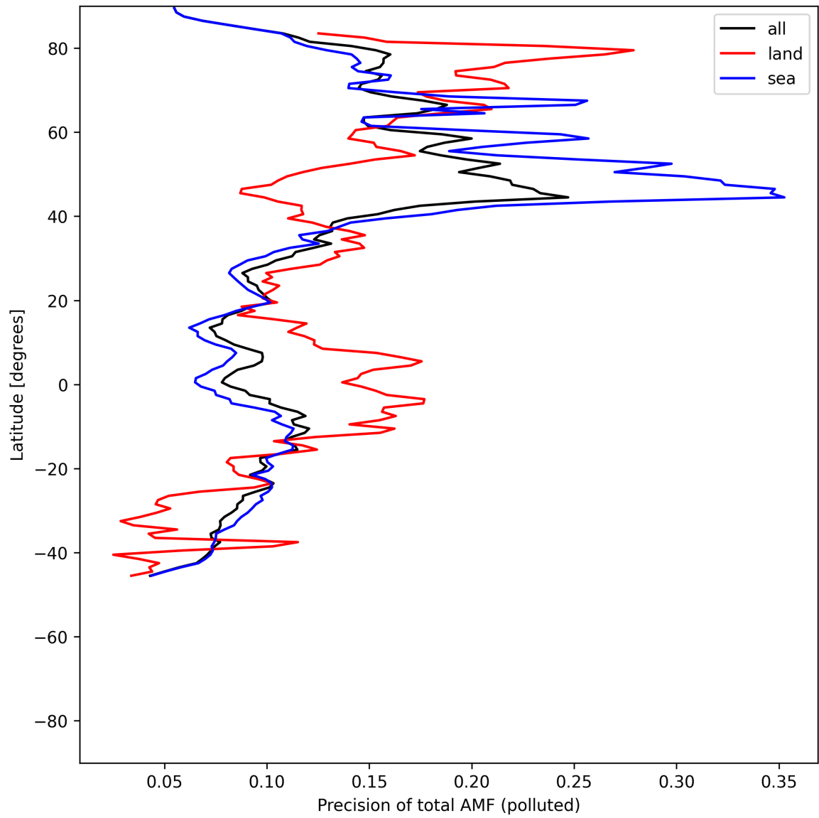
Figure 54: Zonal average of “Precision of total AMF (polluted)” for 2025-06-30 to 2025-07-02.
