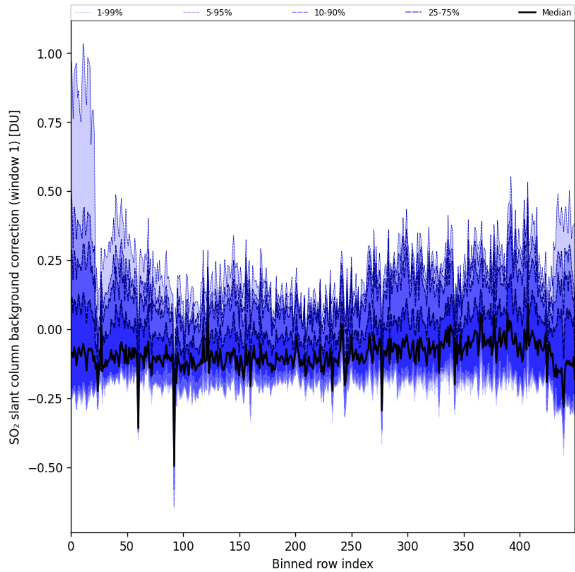
Figure 92: Along track statistics of “SO 2 slant column background correction (window 1)” for 2025-06-30 to 2025-07-02
