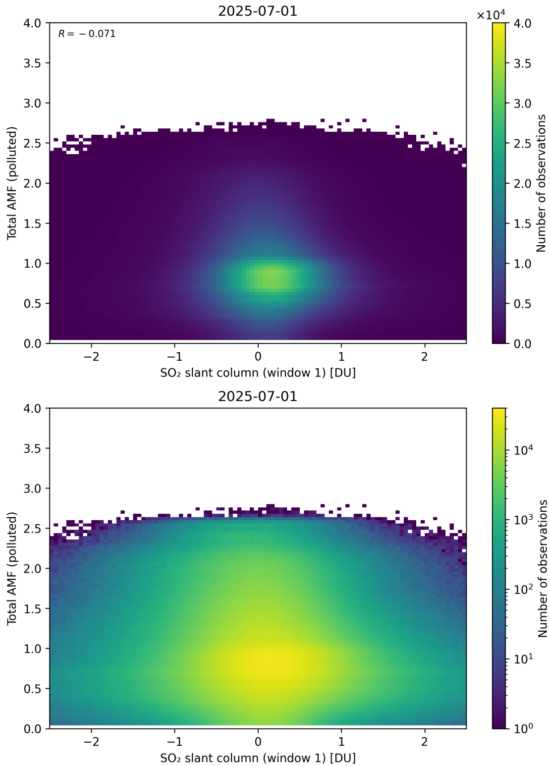
Figure 289: Scatter density plot of “SO 2 slant column (window 1)” against “Total AMF (polluted)” for 2025-06-30 to 2025-07-02.
