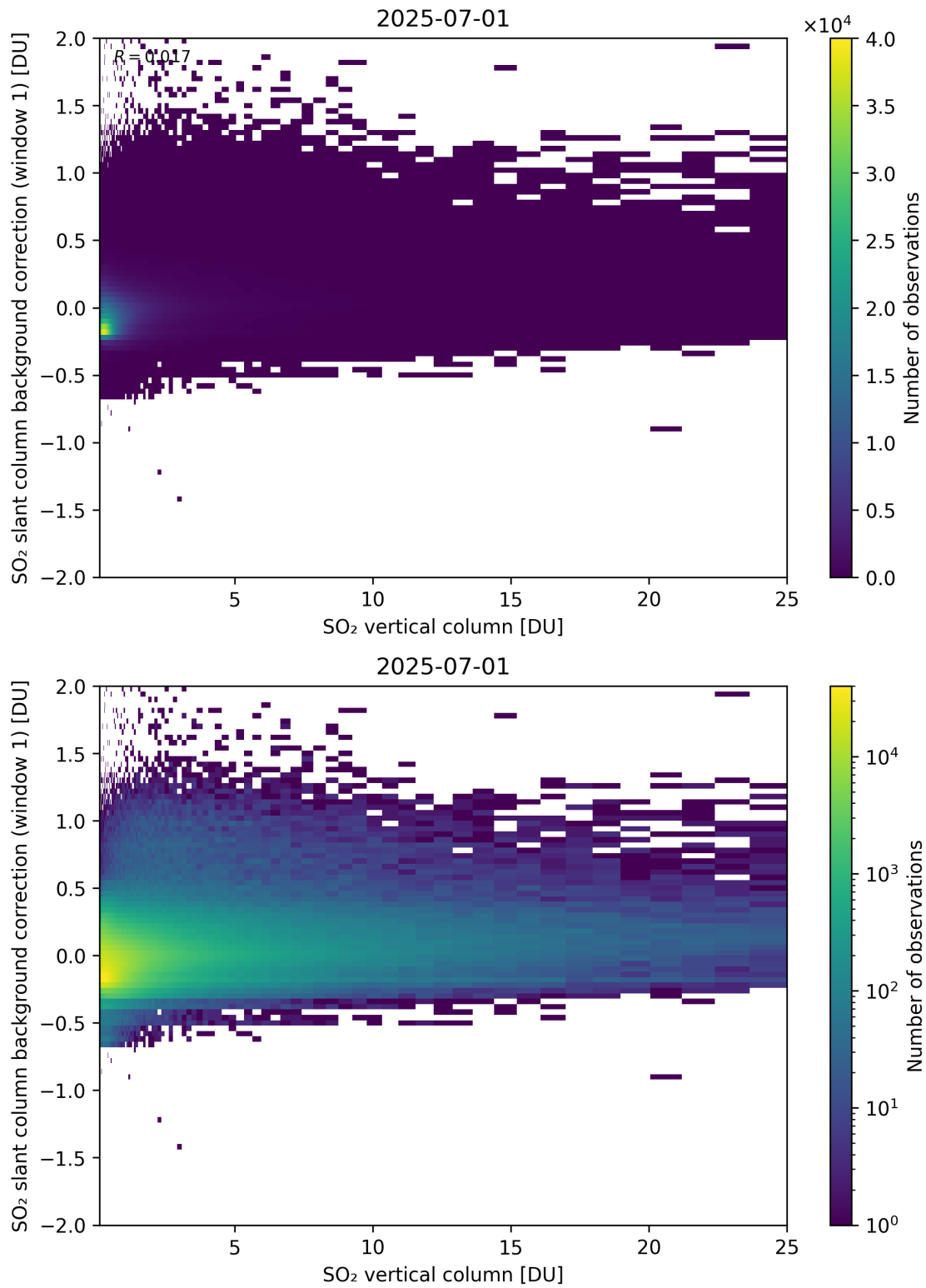
Figure 323: Scatter density plot of “SO 2 vertical column” against “SO 2 slant column background correction (window 1)” for 2025-06-30 to 2025-07-02.
