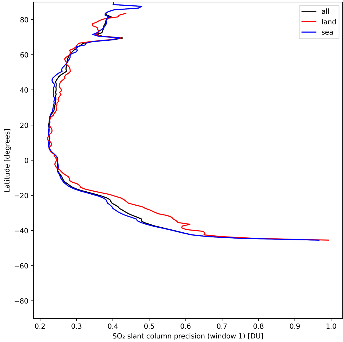
Figure 38: Zonal average of “SO 2 slant column precision (window 1)” for 2025-06-30 to 2025-07-02.
