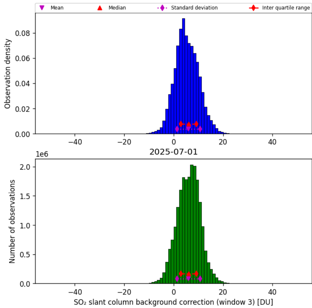
Figure 74: Histogram of “SO 2 slant column background correction (window 3)” for 2025-06-30 to 2025-07-02
