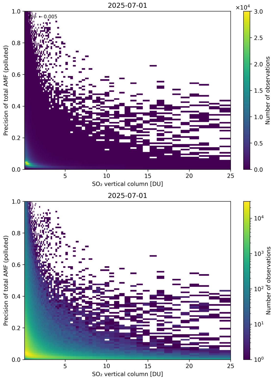
Figure 360: Scatter density plot of “SO 2 vertical column” against “Precision of total AMF (polluted)” for 2025-06-30 to 2025-07-02.
