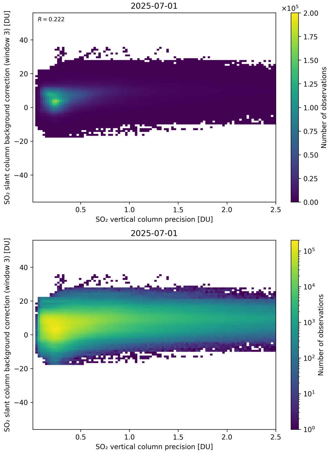
Figure 331: Scatter density plot of “SO 2 vertical column precision” against “SO 2 slant column background correction (window 3)” for 2025-06-30 to 2025-07-02.
