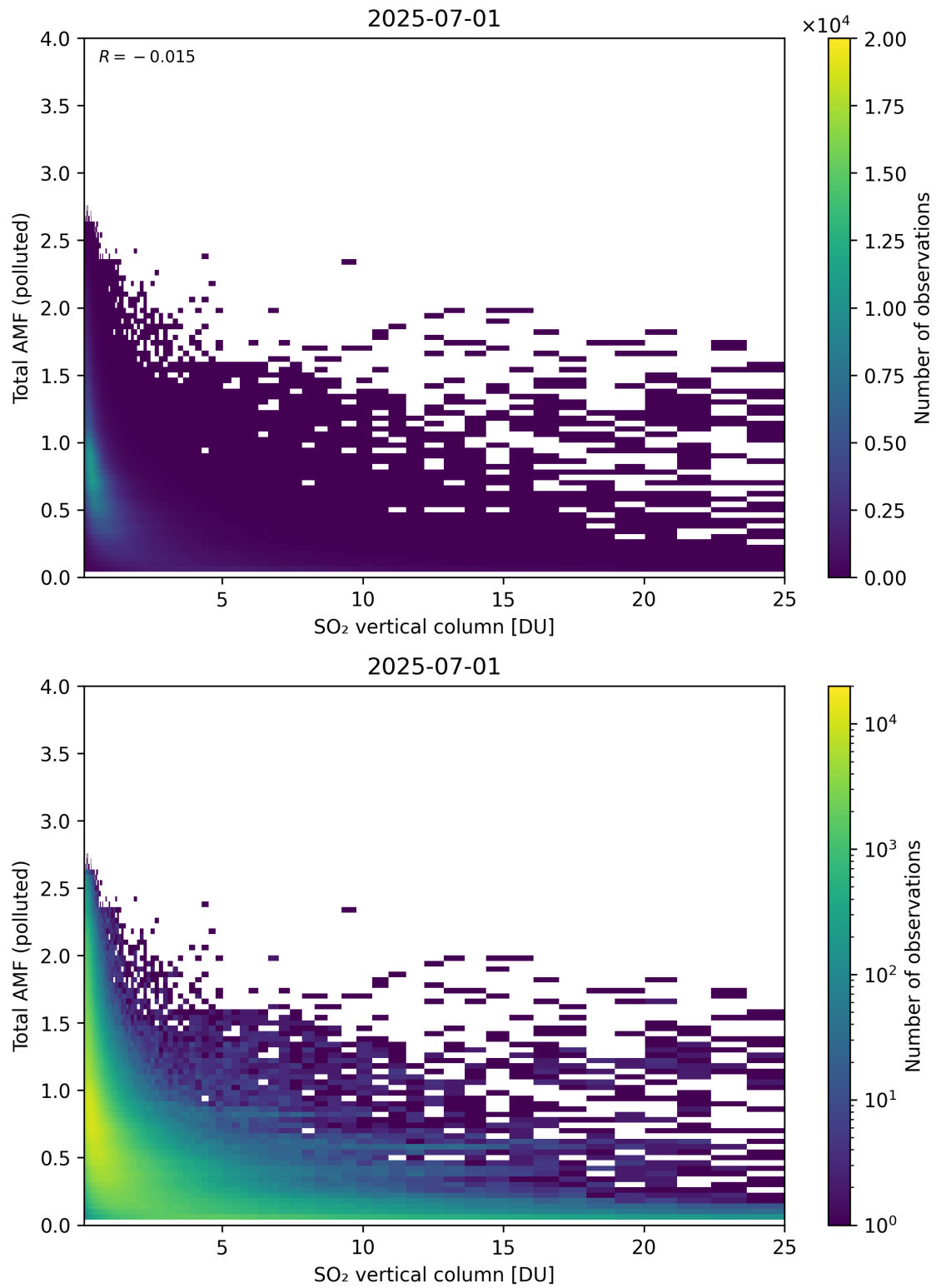
Figure 359: Scatter density plot of “SO 2 vertical column” against “Total AMF (polluted)” for 2025-06-30 to 2025-07-02.
