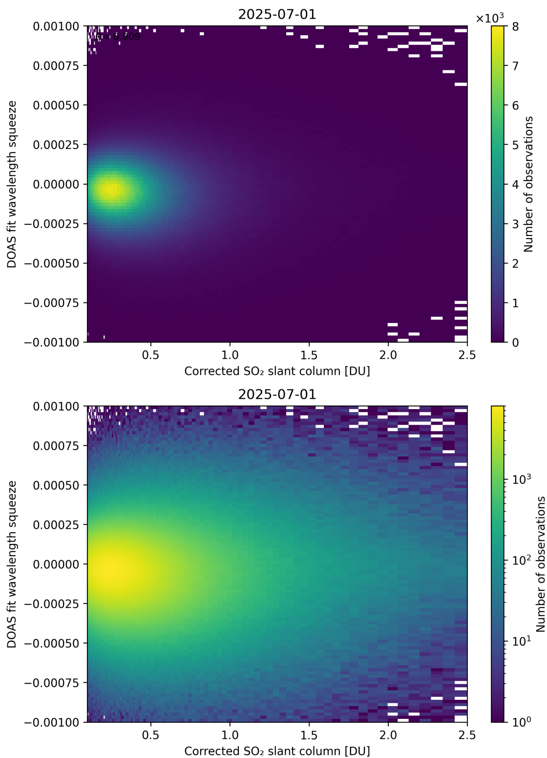
Figure 230: Scatter density plot of “Corrected SO 2 slant column” against “DOAS fit wavelength squeeze” for 2025-06-30 to 2025-07-02.
