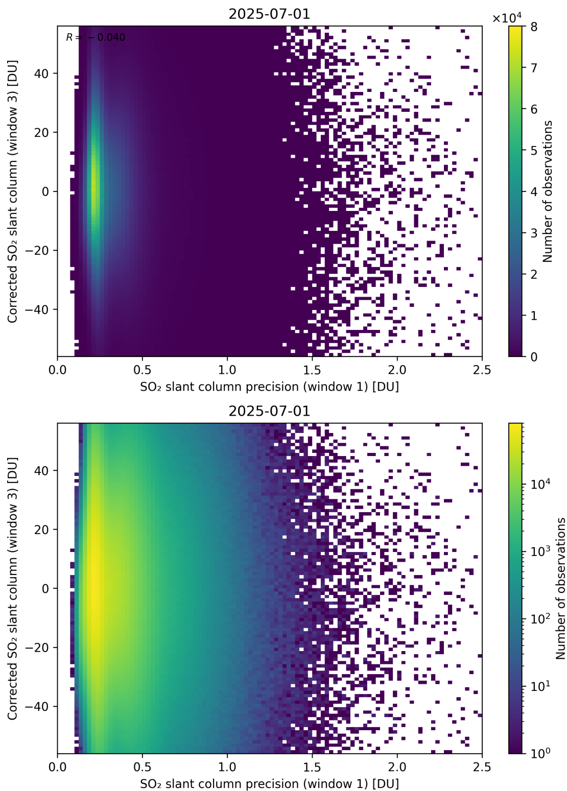
Figure 276: Scatter density plot of “SO 2 slant column precision (window 1)” against “Corrected SO 2 slant column (window 3)” for 2025-06-30 to 2025-07-02.
