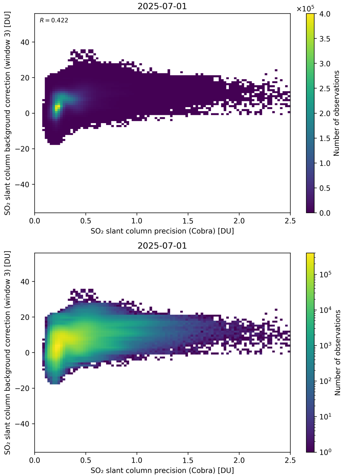
Figure 201: Scatter density plot of “SO 2 slant column precision (Cobra)” against “SO 2 slant column background correction (window 3)” for 2025-06-30 to 2025-07-02.
