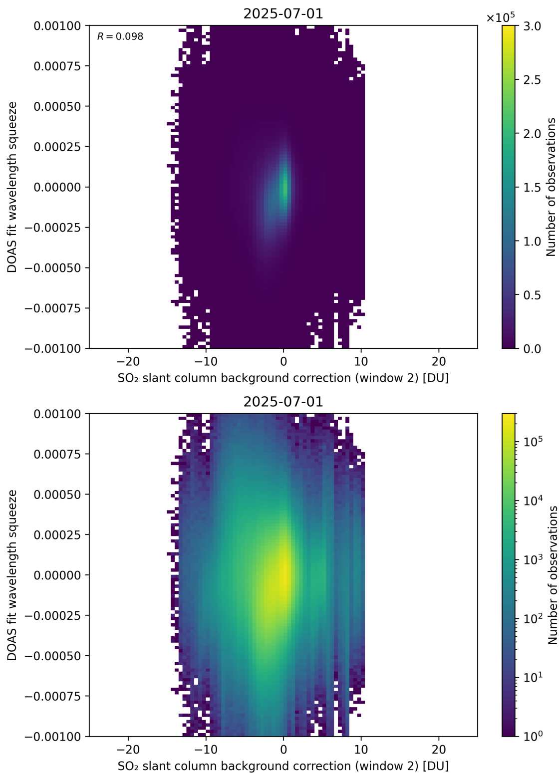
Figure 124: Scatter density plot of “SO 2 slant column background correction (window 2)” against “DOAS fit wavelength squeeze” for 2025-06-30 to 2025-07-02.
