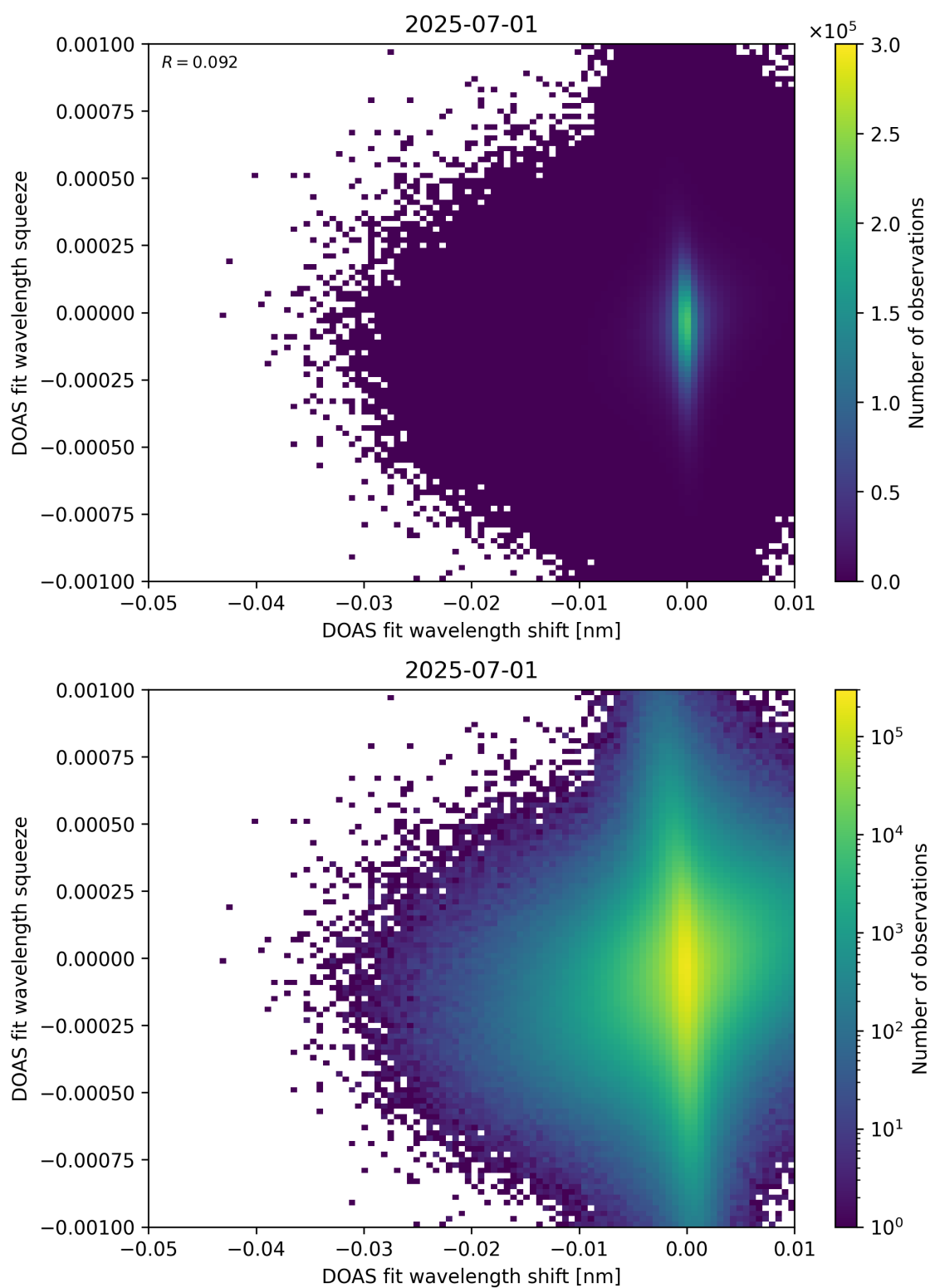
Figure 138: Scatter density plot of “DOAS fit wavelength shift” against “DOAS fit wavelength squeeze” for 2025-06-30 to 2025-07-02.
