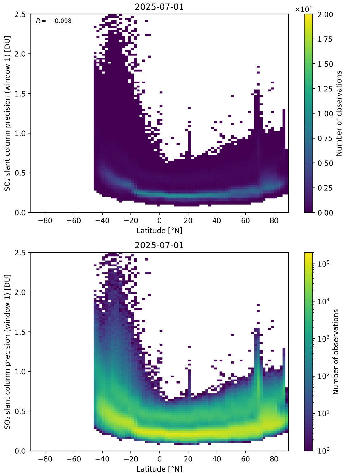
Figure 163: Scatter density plot of “Latitude” against “SO 2 slant column precision (window 1)” for 2025-06-30 to 2025-07-02.
