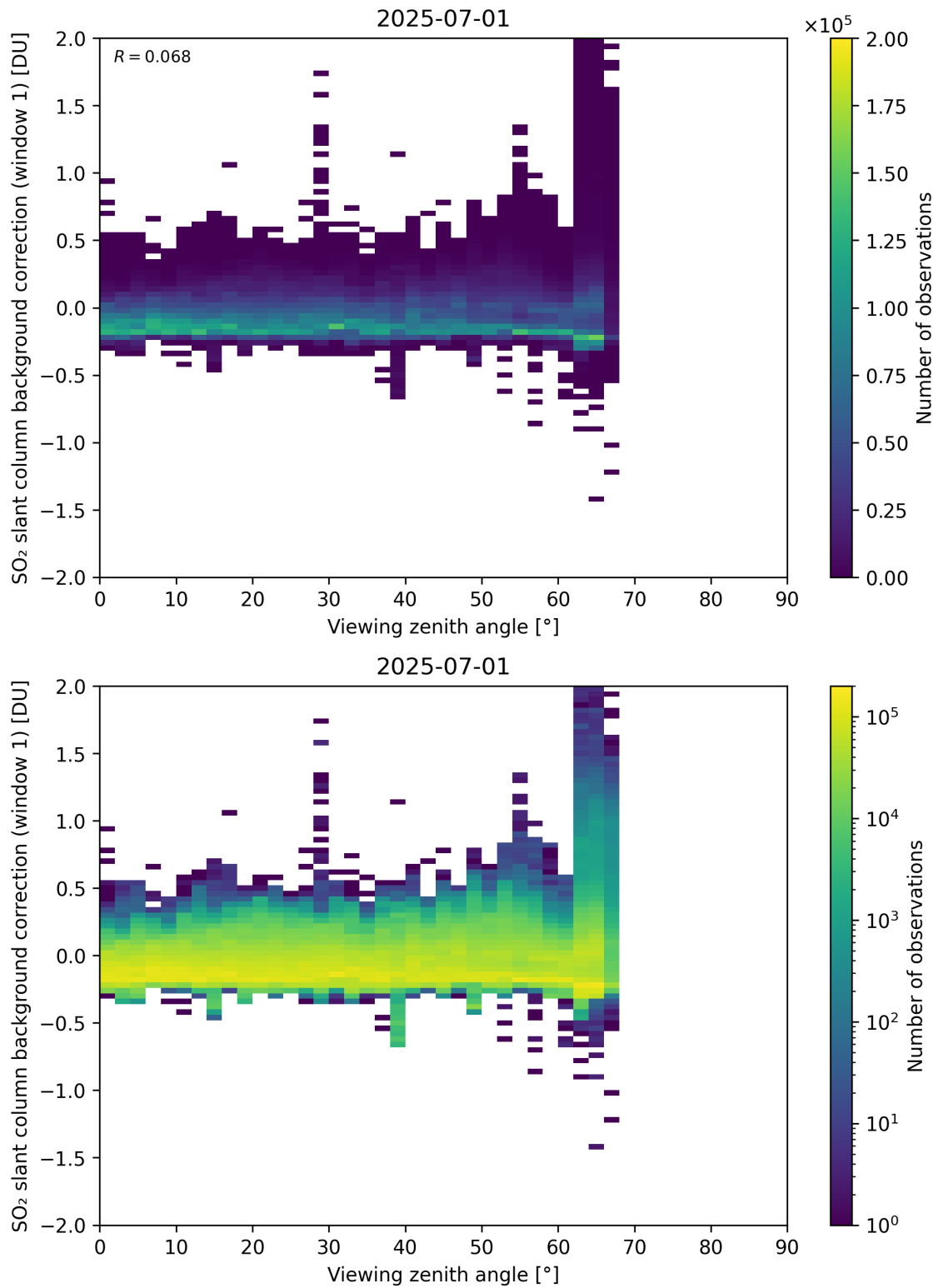
Figure 362: Scatter density plot of “Viewing zenith angle” against “SO 2 slant column background correction (window 1)” for 2025-06-30 to 2025-07-02.
