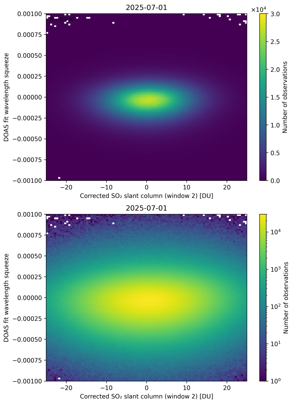
Figure 247: Scatter density plot of “Corrected SO 2 slant column (window 2)” against “DOAS fit wavelength squeeze” for 2025-06-30 to 2025-07-02.
