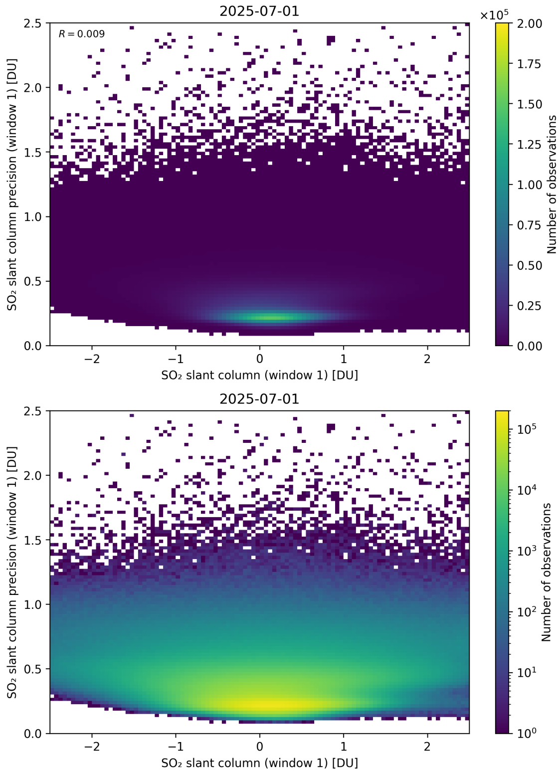
Figure 285: Scatter density plot of “SO 2 slant column (window 1)” against “SO 2 slant column precision (window 1)” for 2025-06-30 to 2025-07-02.
