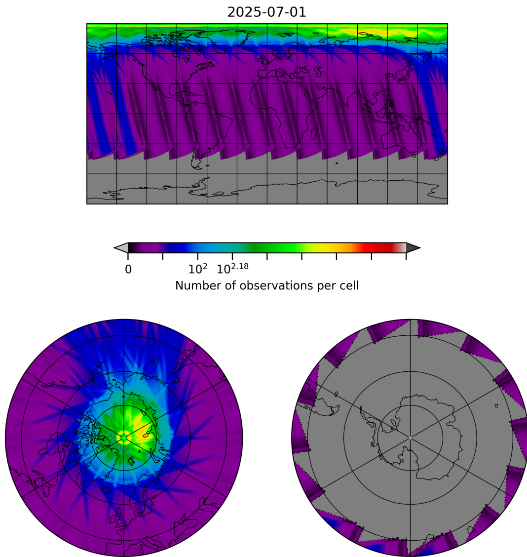
Figure 30: Map of the number of observations for 2025-06-30 to 2025-07-02
