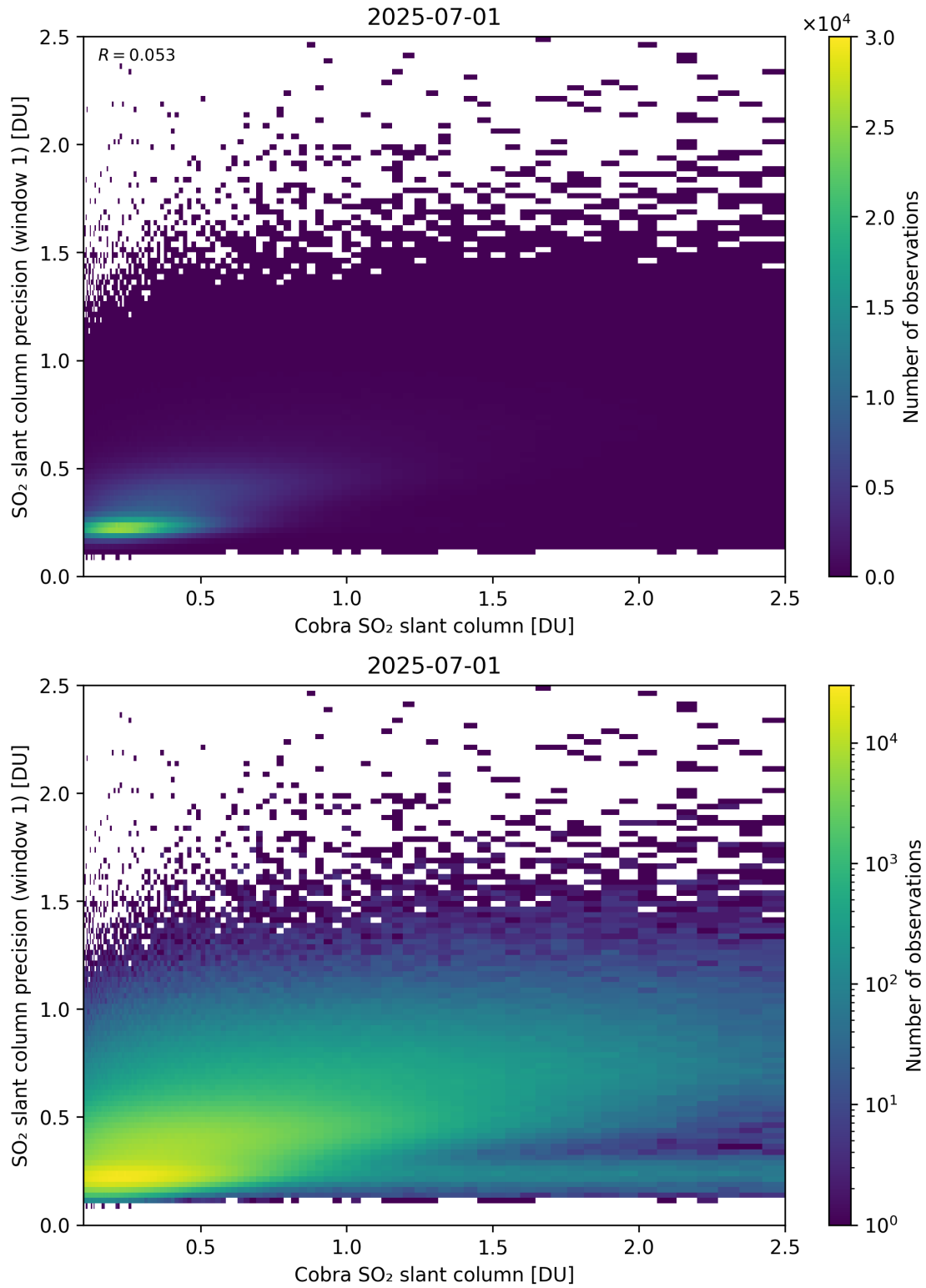
Figure 220: Scatter density plot of “Cobra SO 2 slant column” against “SO 2 slant column precision (window 1)” for 2025-06-30 to 2025-07-02.
