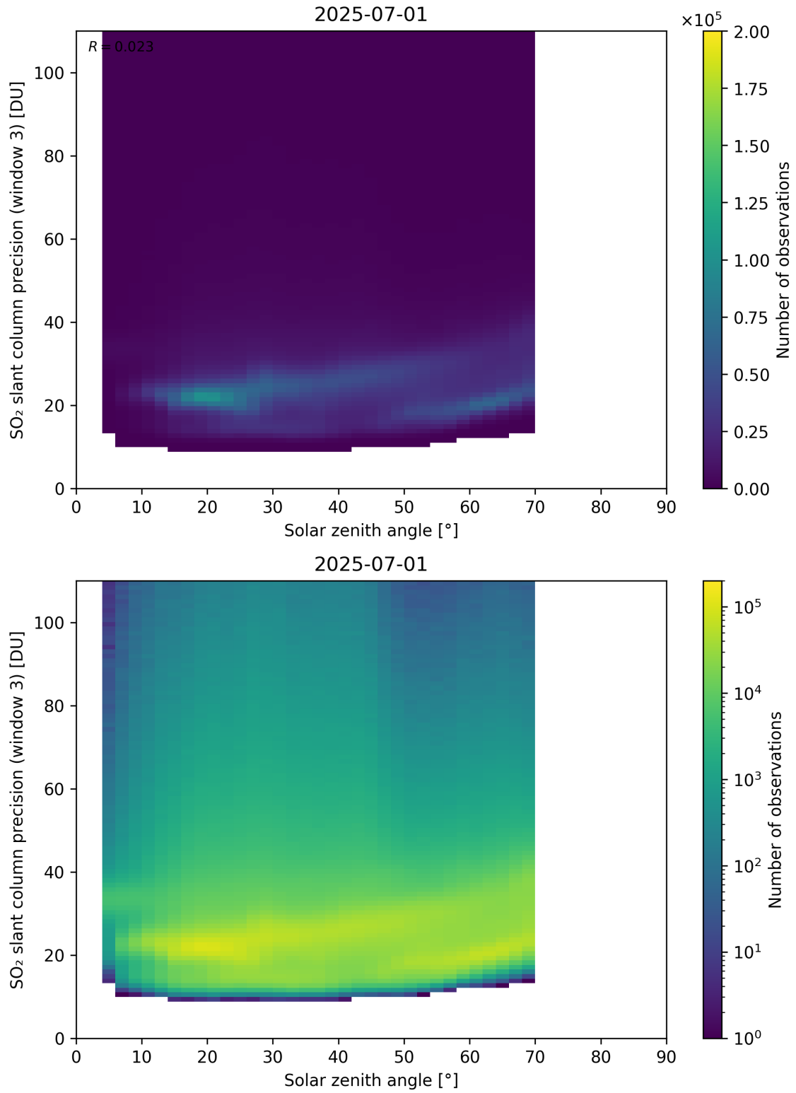
Figure 188: Scatter density plot of “Solar zenith angle” against “SO 2 slant column precision (window 3)” for 2025-06-30 to 2025-07-02.
