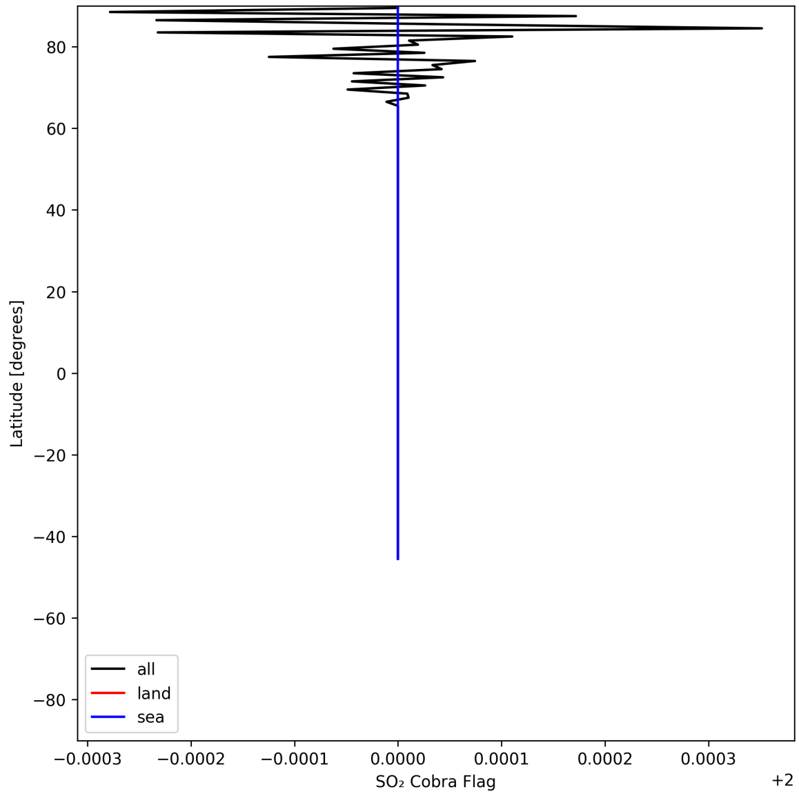
Figure 49: Zonal average of “SO 2 Cobra Flag” for 2025-06-30 to 2025-07-02.
