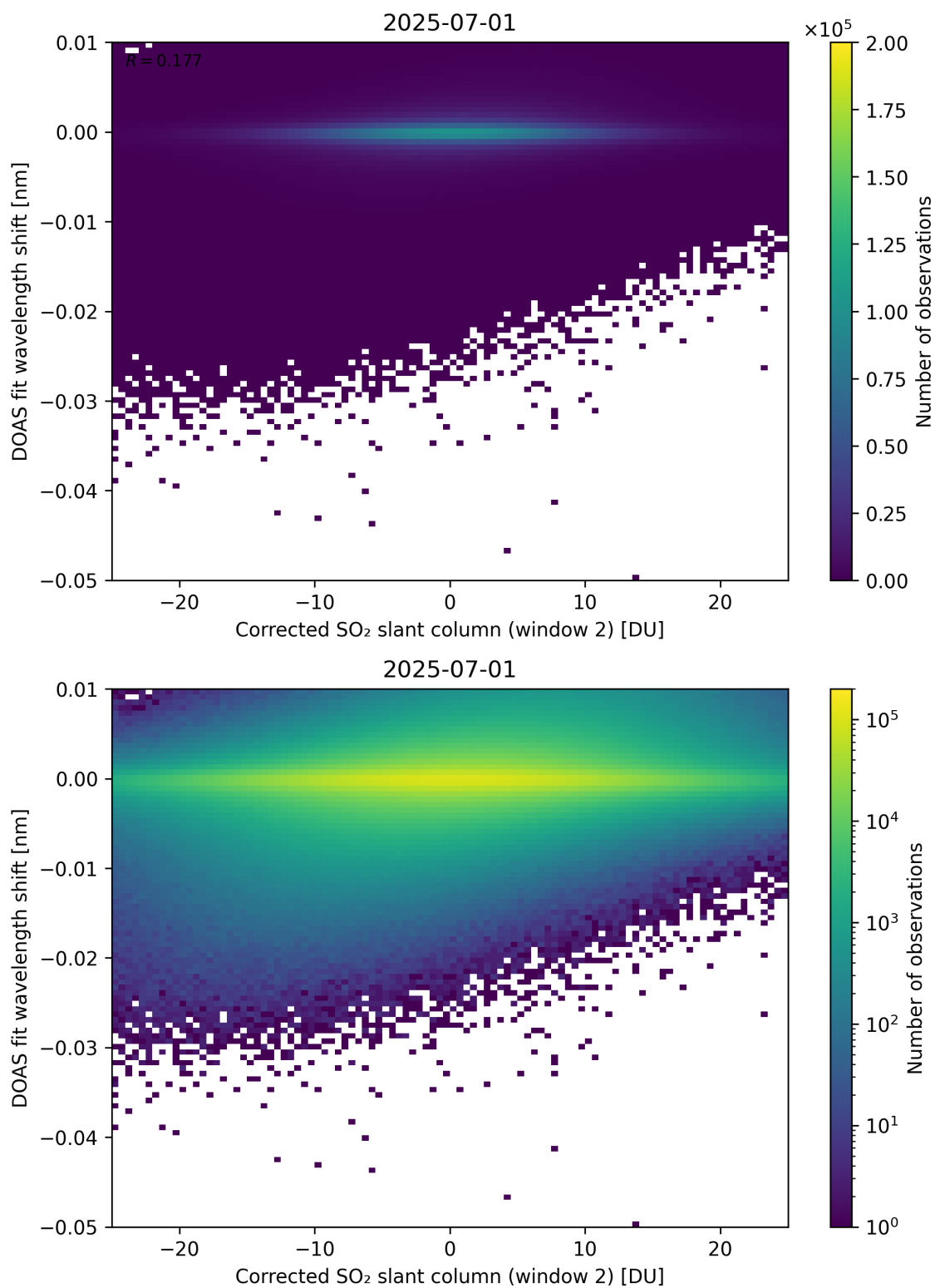
Figure 246: Scatter density plot of “Corrected SO 2 slant column (window 2)” against “DOAS fit wavelength shift” for 2025-06-30 to 2025-07-02.
