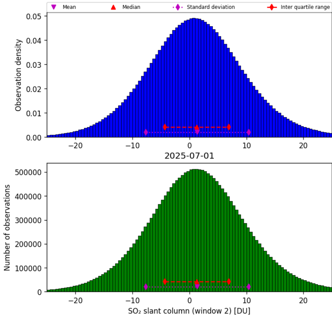
Figure 67: Histogram of “SO 2 slant column (window 2)” for 2025-06-30 to 2025-07-02
