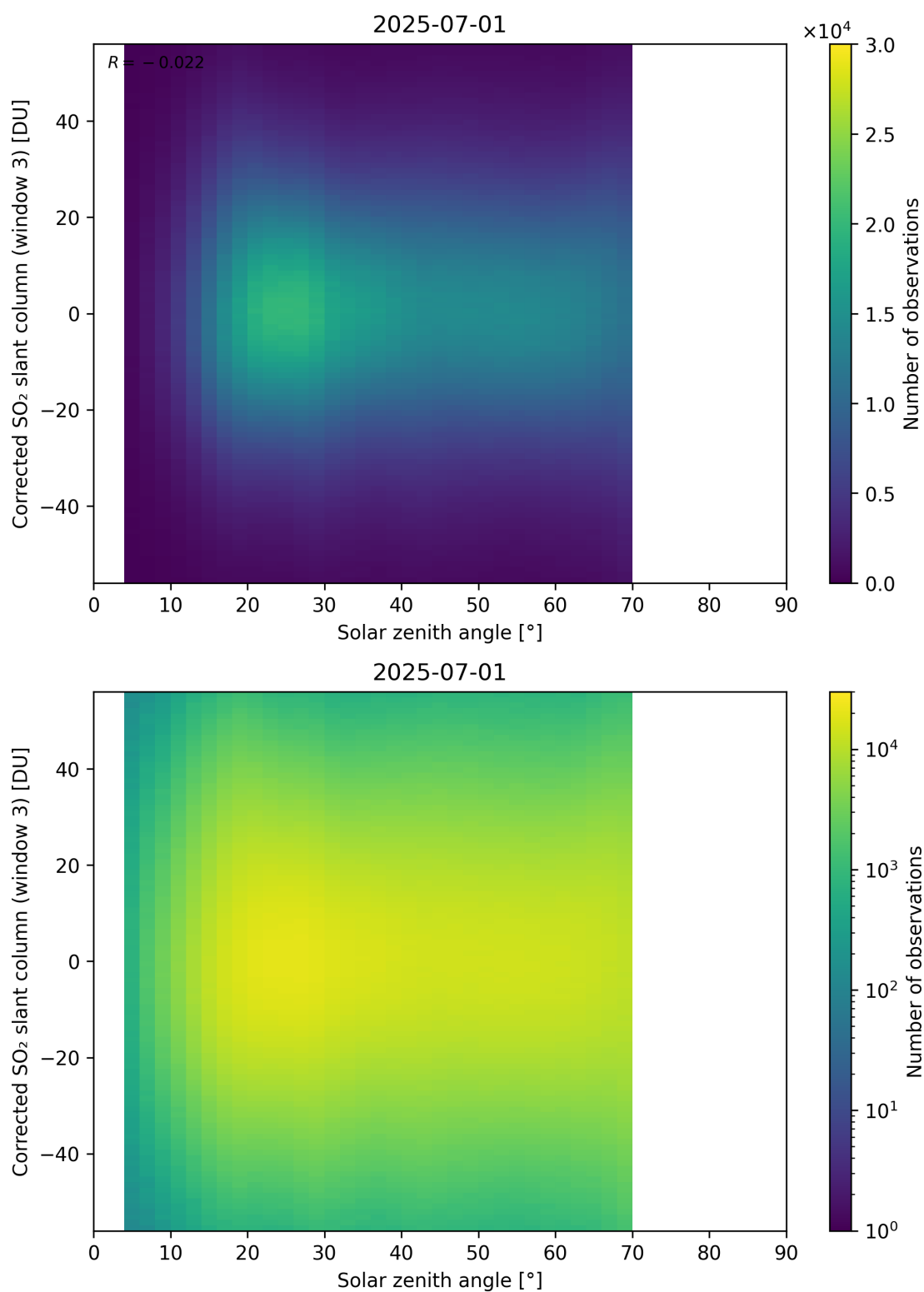
Figure 183: Scatter density plot of “Solar zenith angle” against “Corrected SO 2 slant column (window 3)” for 2025-06-30 to 2025-07-02.
