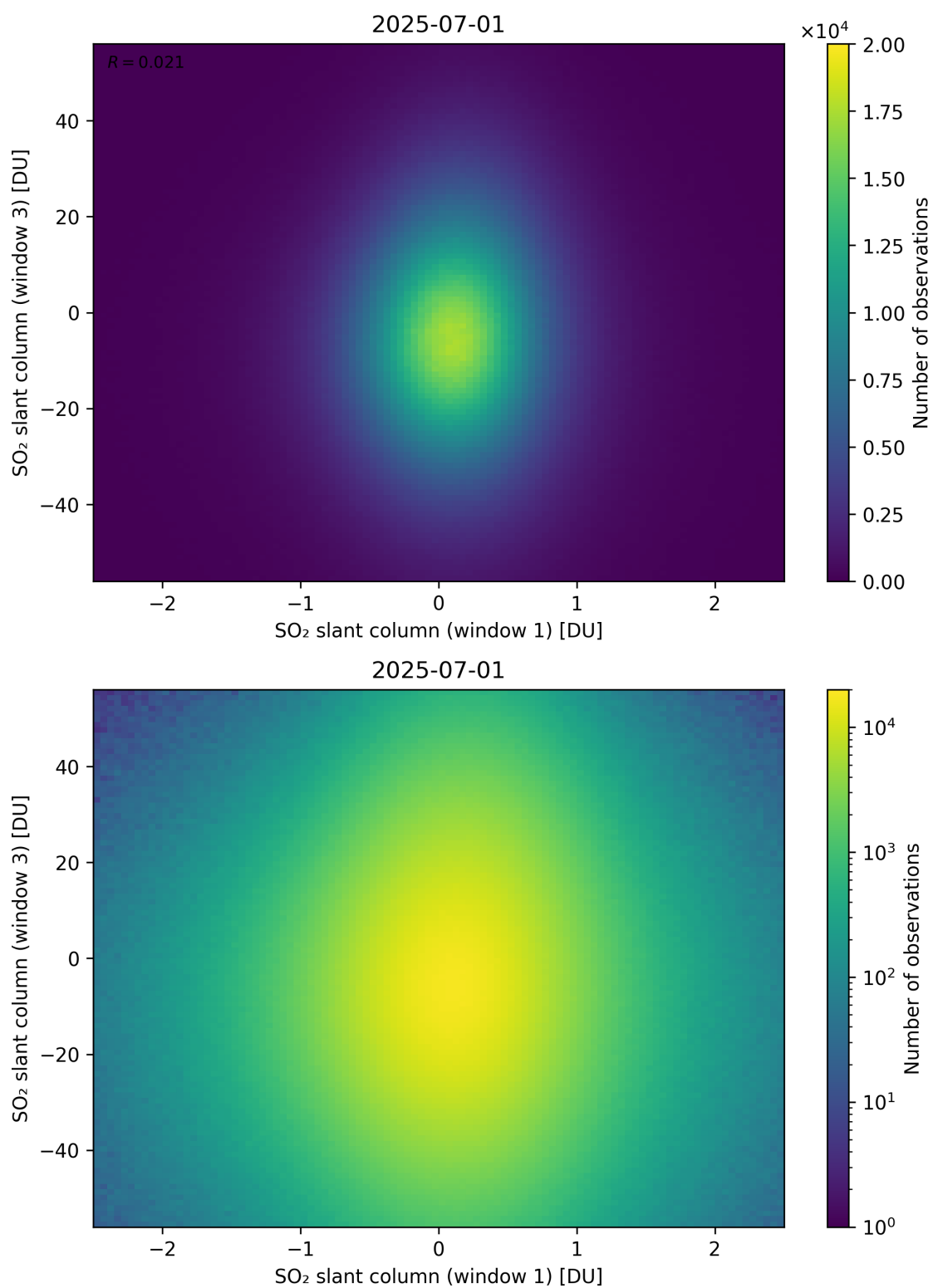
Figure 287: Scatter density plot of “SO 2 slant column (window 1)” against “SO 2 slant column (window 3)” for 2025-06-30 to 2025-07-02.
