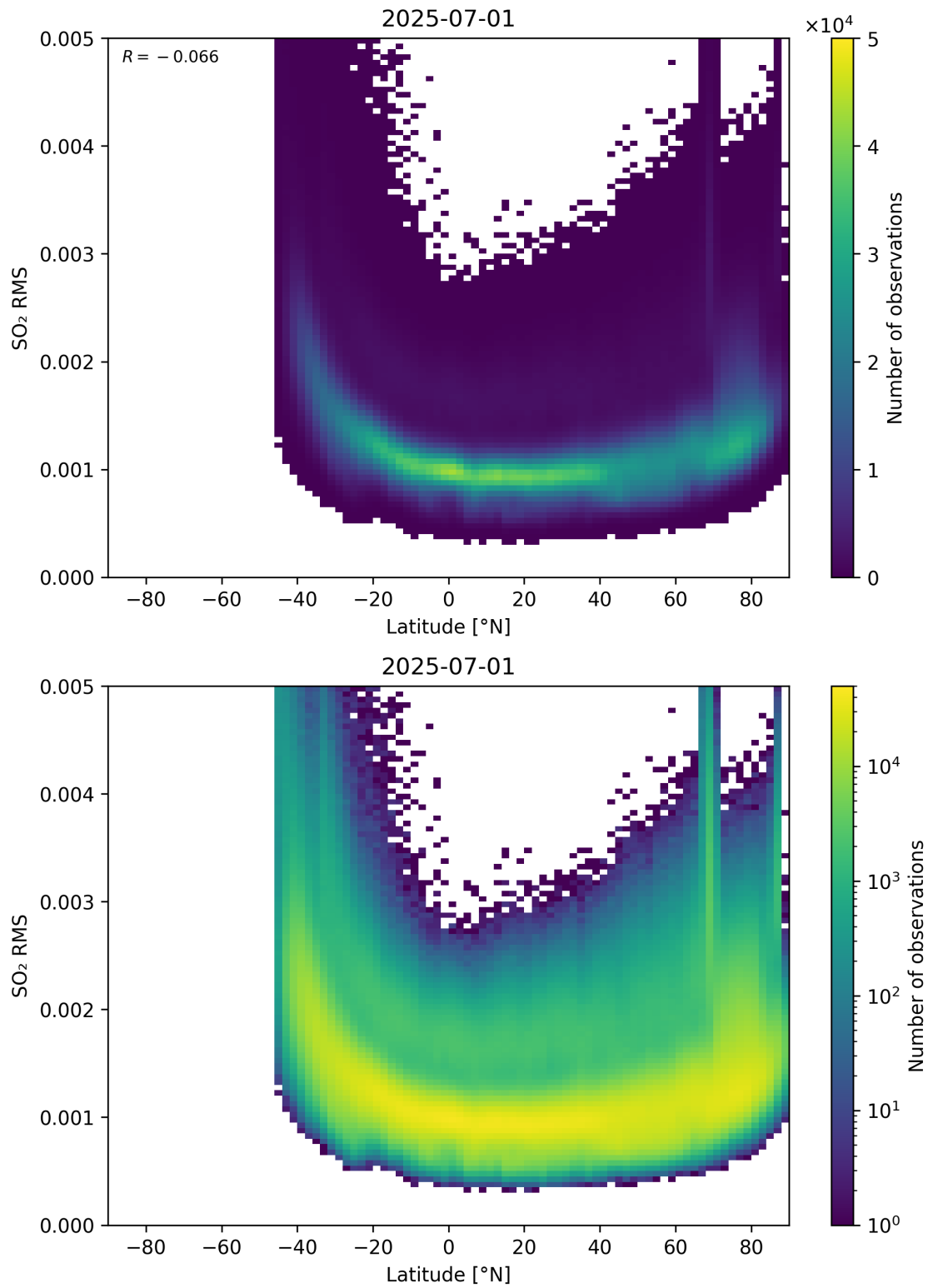
Figure 155: Scatter density plot of “Latitude” against “SO 2 RMS” for 2025-06-30 to 2025-07-02.
