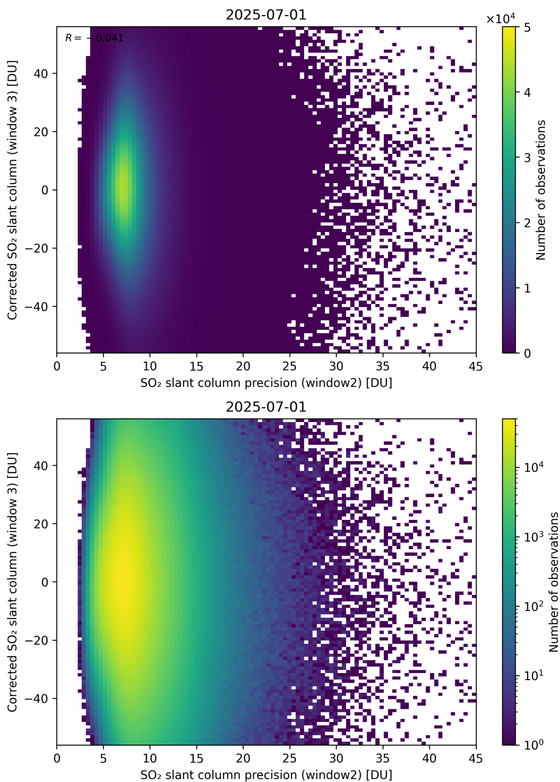
Figure 298: Scatter density plot of “SO 2 slant column precision (window2)” against “Corrected SO 2 slant column (window 3)” for 2025-06-30 to 2025-07-02.
