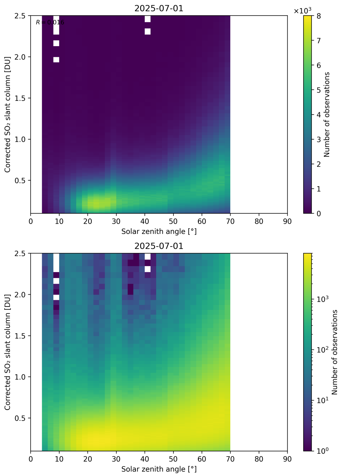
Figure 181: Scatter density plot of “Solar zenith angle” against “Corrected SO 2 slant column” for 2025-06-30 to 2025-07-02.
