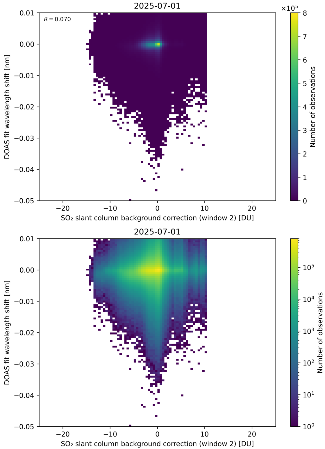
Figure 123: Scatter density plot of “SO 2 slant column background correction (window 2)” against “DOAS fit wavelength shift” for 2025-06-30 to 2025-07-02.
