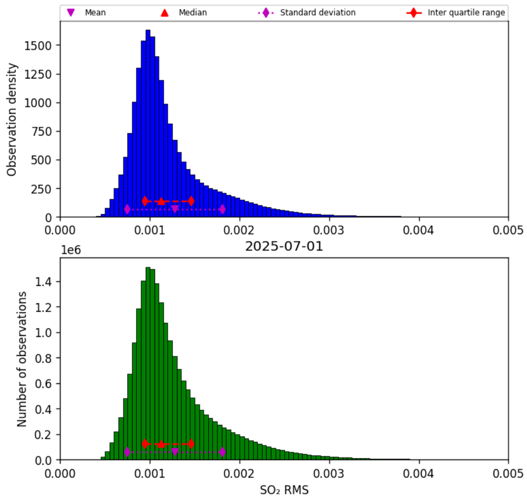
Figure 78: Histogram of “SO 2 RMS” for 2025-06-30 to 2025-07-02
