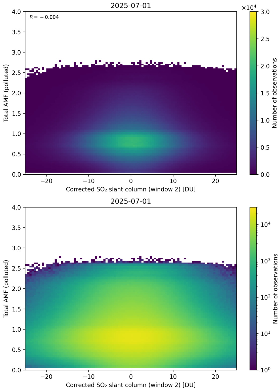
Figure 253: Scatter density plot of “Corrected SO 2 slant column (window 2)” against “Total AMF (polluted)” for 2025-06-30 to 2025-07-02.
