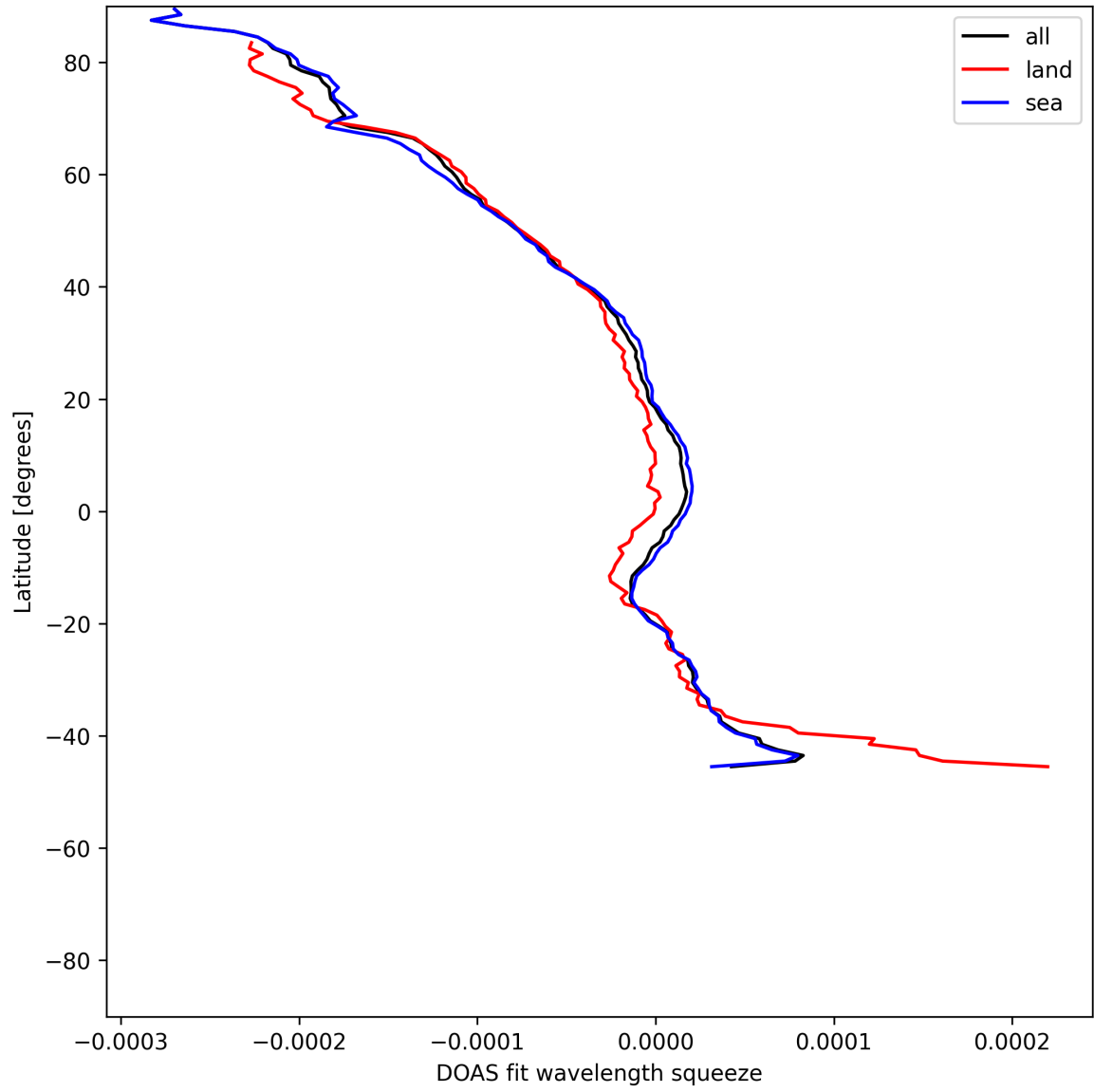
Figure 51: Zonal average of “DOAS fit wavelength squeeze” for 2025-06-30 to 2025-07-02.
