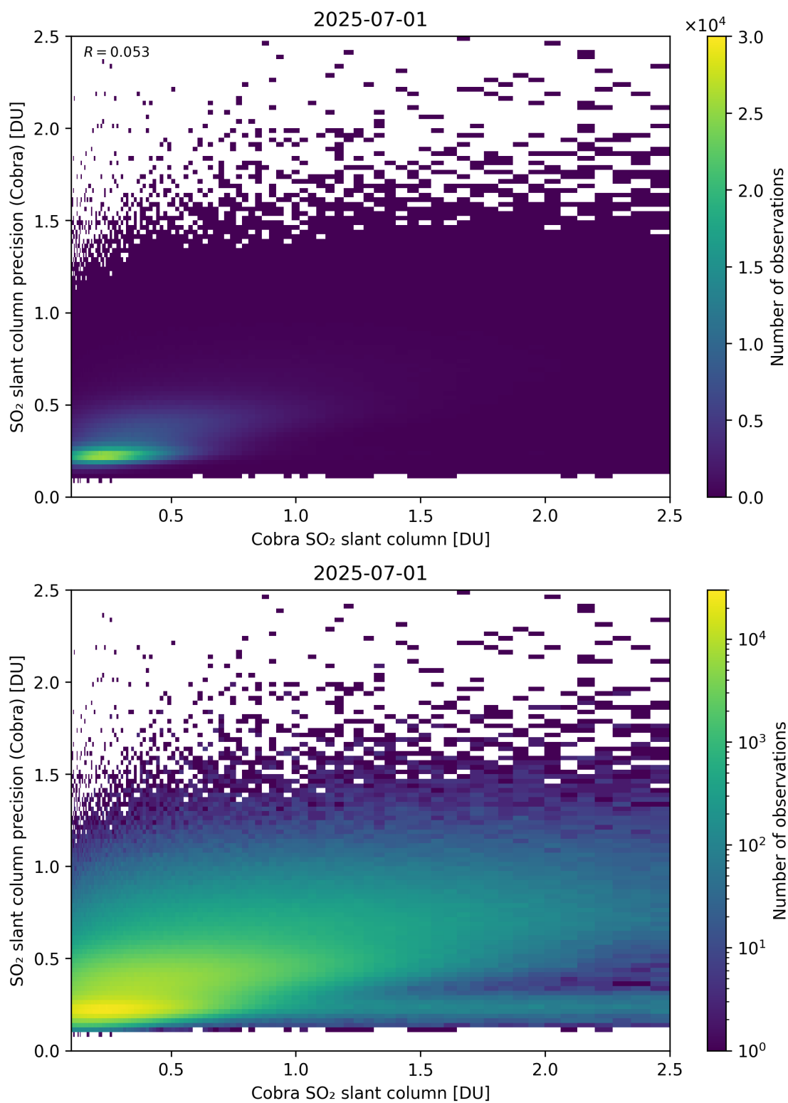
Figure 216: Scatter density plot of “Cobra SO 2 slant column” against “SO 2 slant column precision (Cobra)” for 2025-06-30 to 2025-07-02.
