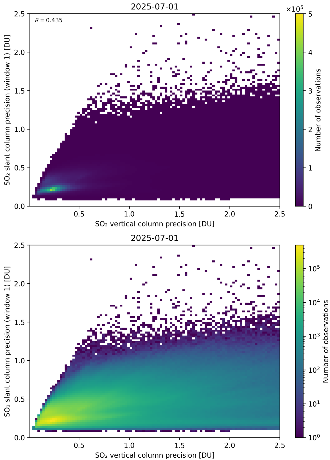
Figure 342: Scatter density plot of “SO 2 vertical column precision” against “SO 2 slant column precision (window 1)” for 2025-06-30 to 2025-07-02.
