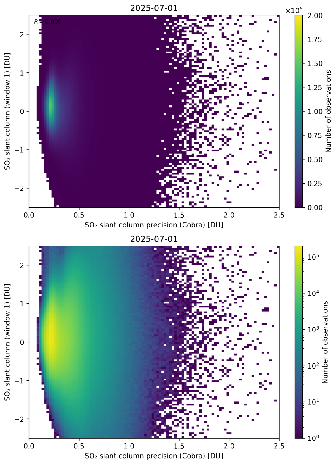
Figure 208: Scatter density plot of “SO 2 slant column precision (Cobra)” against “SO 2 slant column (window 1)” for 2025-06-30 to 2025-07-02.
