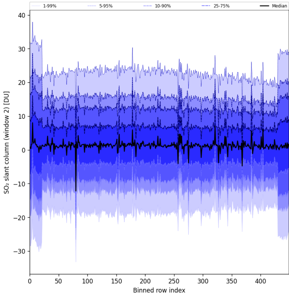
Figure 93: Along track statistics of “SO 2 slant column (window 2)” for 2025-06-30 to 2025-07-02
