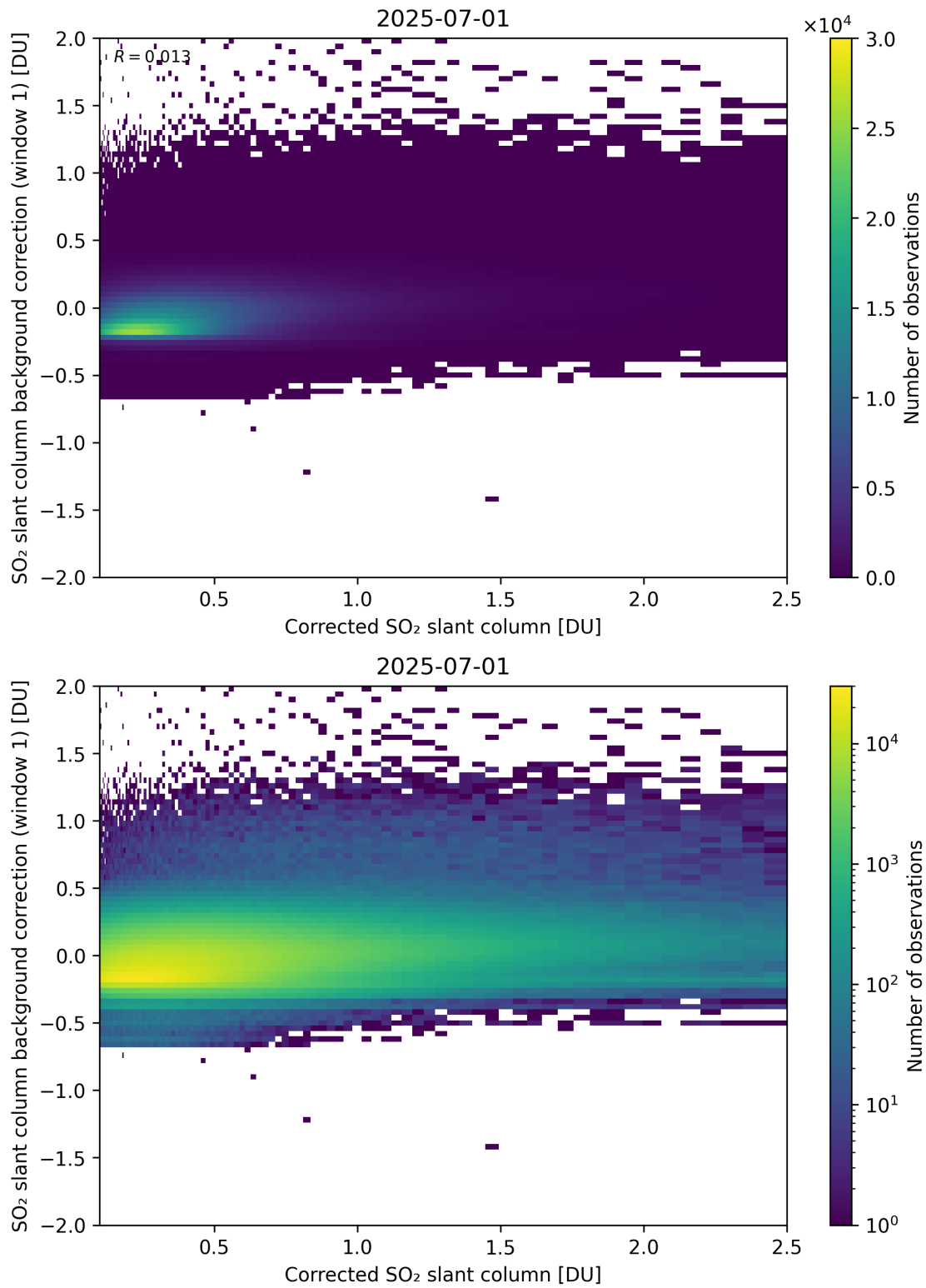
Figure 226: Scatter density plot of “Corrected SO 2 slant column” against “SO 2 slant column background correction (window 1)” for 2025-06-30 to 2025-07-02.
