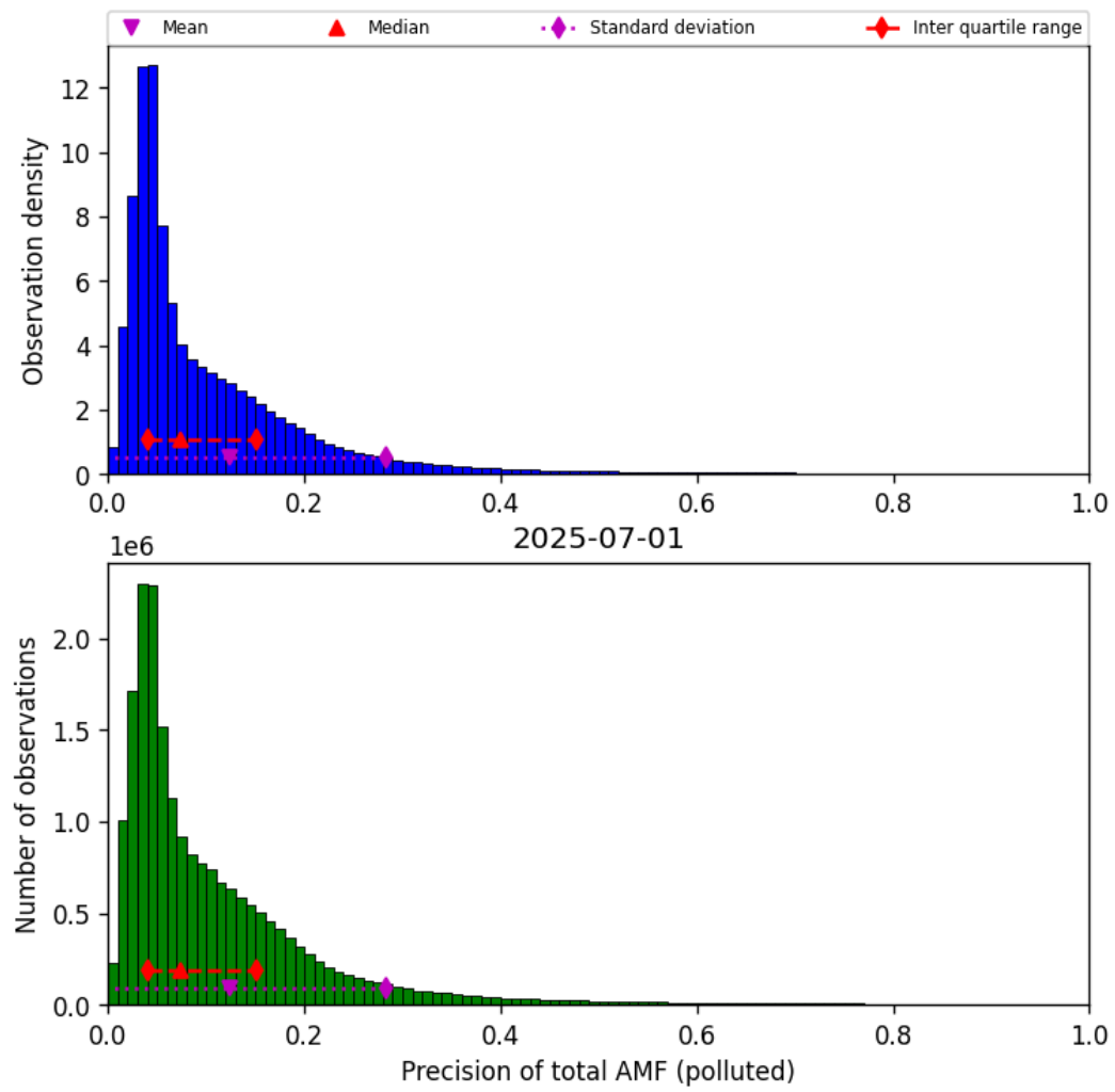
Figure 80: Histogram of “Precision of total AMF (polluted)” for 2025-06-30 to 2025-07-02
