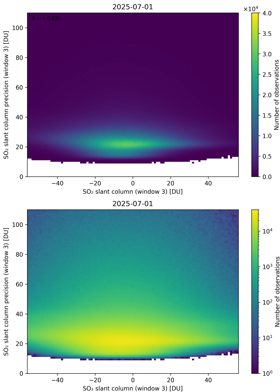
Figure 317: Scatter density plot of “SO 2 slant column (window 3)” against “SO 2 slant column precision (window 3)” for 2025-06-30 to 2025-07-02.
