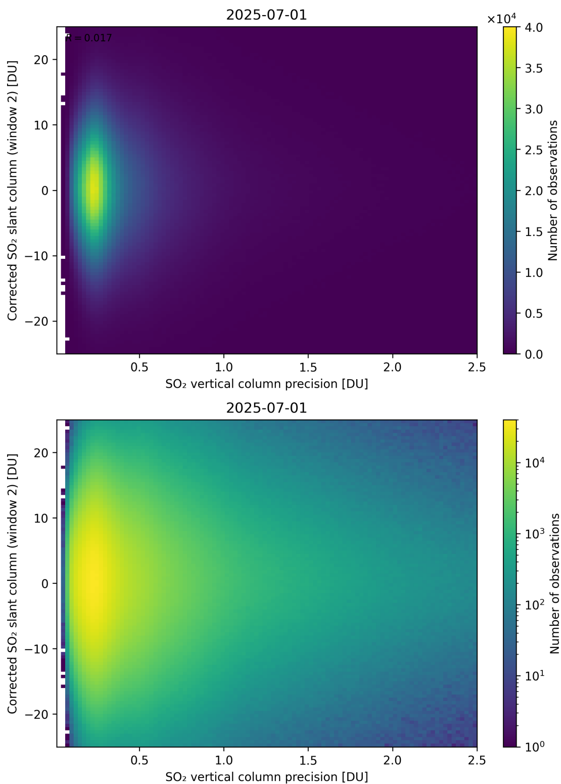
Figure 339: Scatter density plot of “SO 2 vertical column precision” against “Corrected SO 2 slant column (window 2)” for 2025-06-30 to 2025-07-02.
