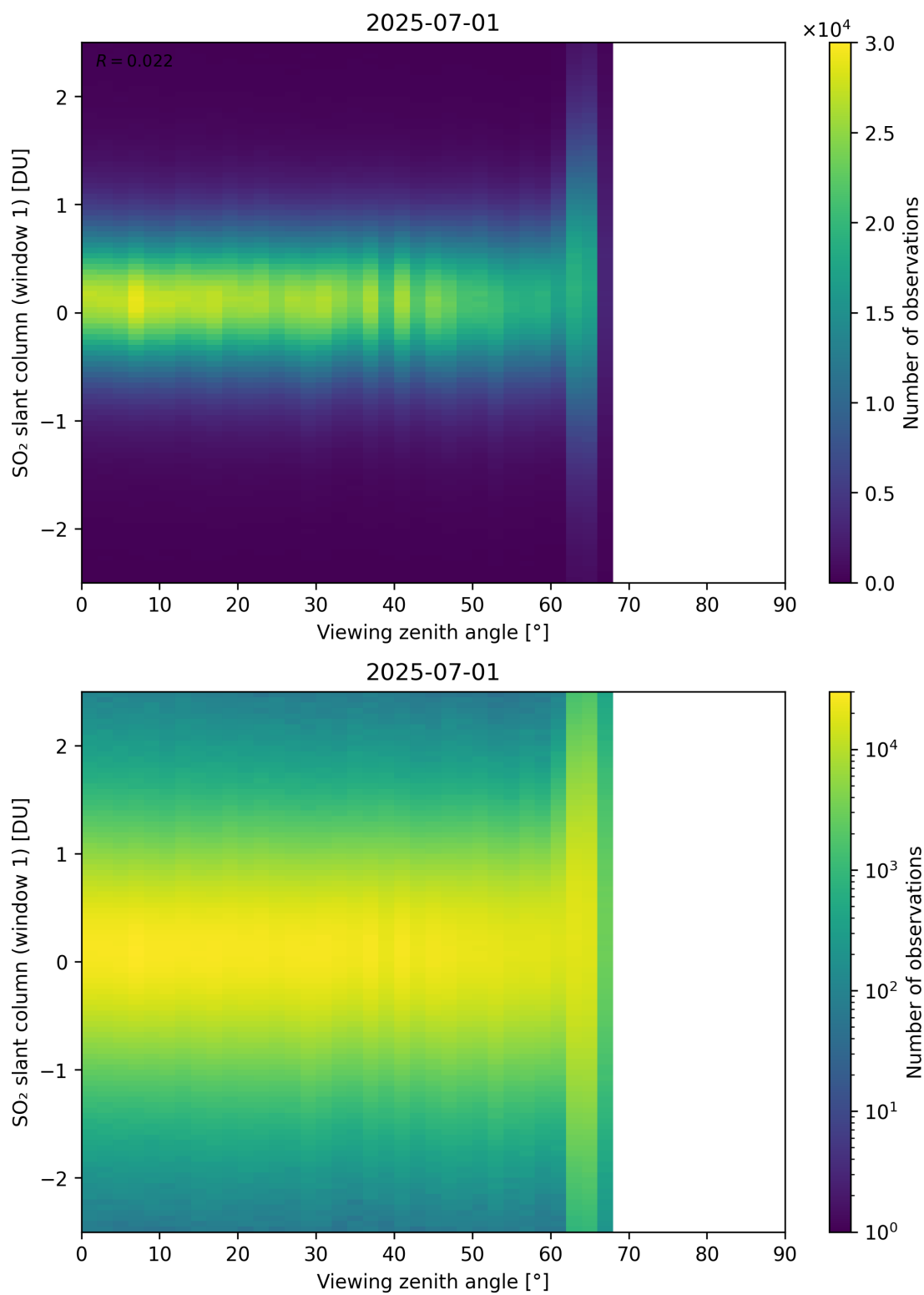
Figure 376: Scatter density plot of “Viewing zenith angle” against “SO 2 slant column (window 1)” for 2025-06-30 to 2025-07-02.
