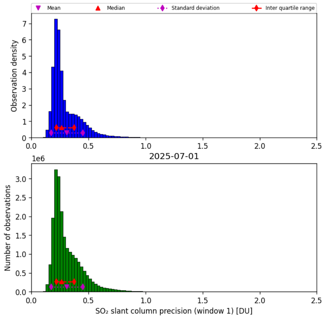
Figure 64: Histogram of “SO 2 slant column precision (window 1)” for 2025-06-30 to 2025-07-02
