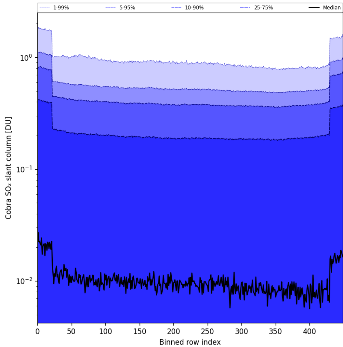
Figure 87: Along track statistics of “Cobra SO 2 slant column” for 2025-06-30 to 2025-07-02
