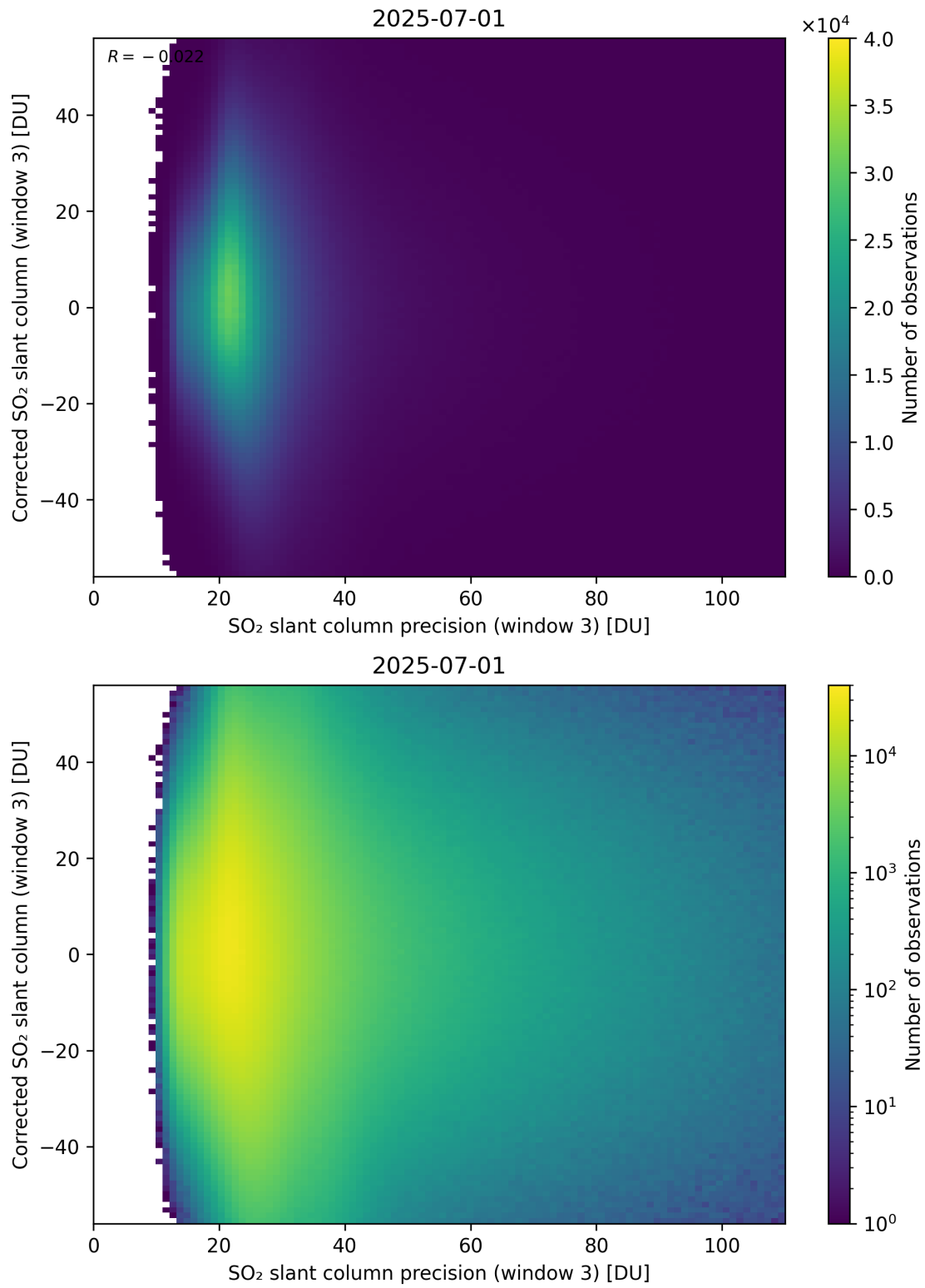
Figure 312: Scatter density plot of “SO 2 slant column precision (window 3)” against “Corrected SO 2 slant column (window 3)” for 2025-06-30 to 2025-07-02.
