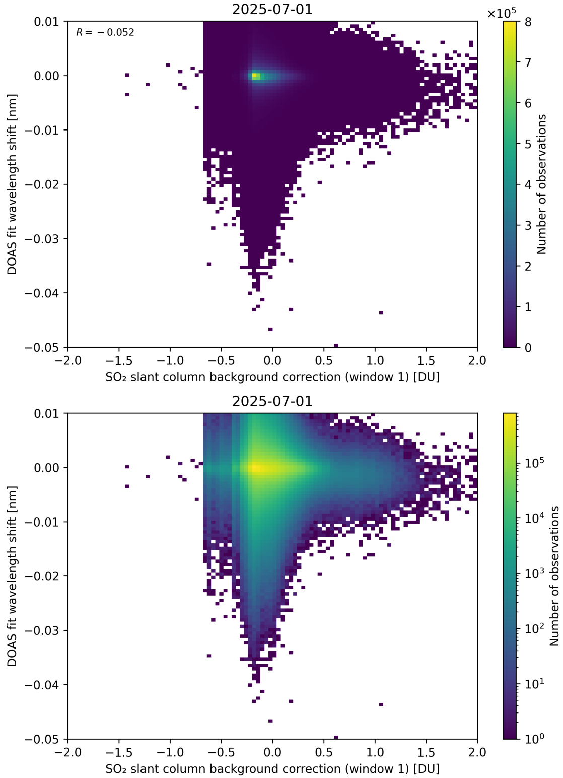
Figure 111: Scatter density plot of “SO 2 slant column background correction (window 1)” against “DOAS fit wavelength shift” for 2025-06-30 to 2025-07-02.
