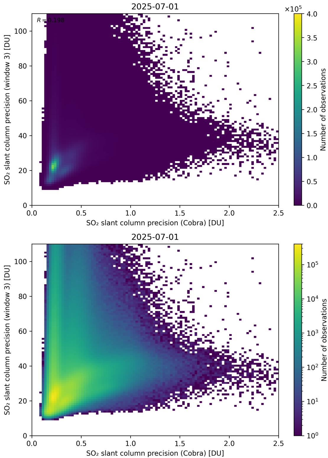
Figure 212: Scatter density plot of “SO 2 slant column precision (Cobra)” against “SO 2 slant column precision (window 3)” for 2025-06-30 to 2025-07-02.
