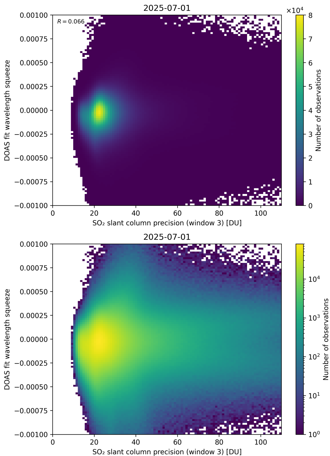
Figure 309: Scatter density plot of “SO 2 slant column precision (window 3)” against “DOAS fit wavelength squeeze” for 2025-06-30 to 2025-07-02.
