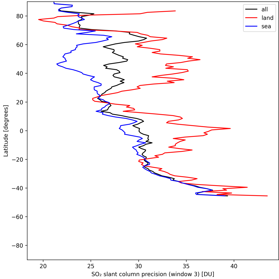
Figure 46: Zonal average of “SO 2 slant column precision (window 3)” for 2025-06-30 to 2025-07-02.
