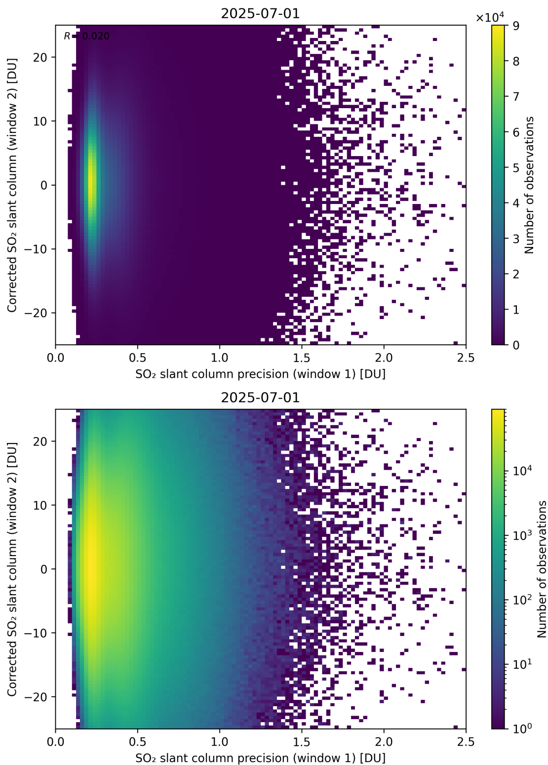
Figure 275: Scatter density plot of “SO 2 slant column precision (window 1)” against “Corrected SO 2 slant column (window 2)” for 2025-06-30 to 2025-07-02.
