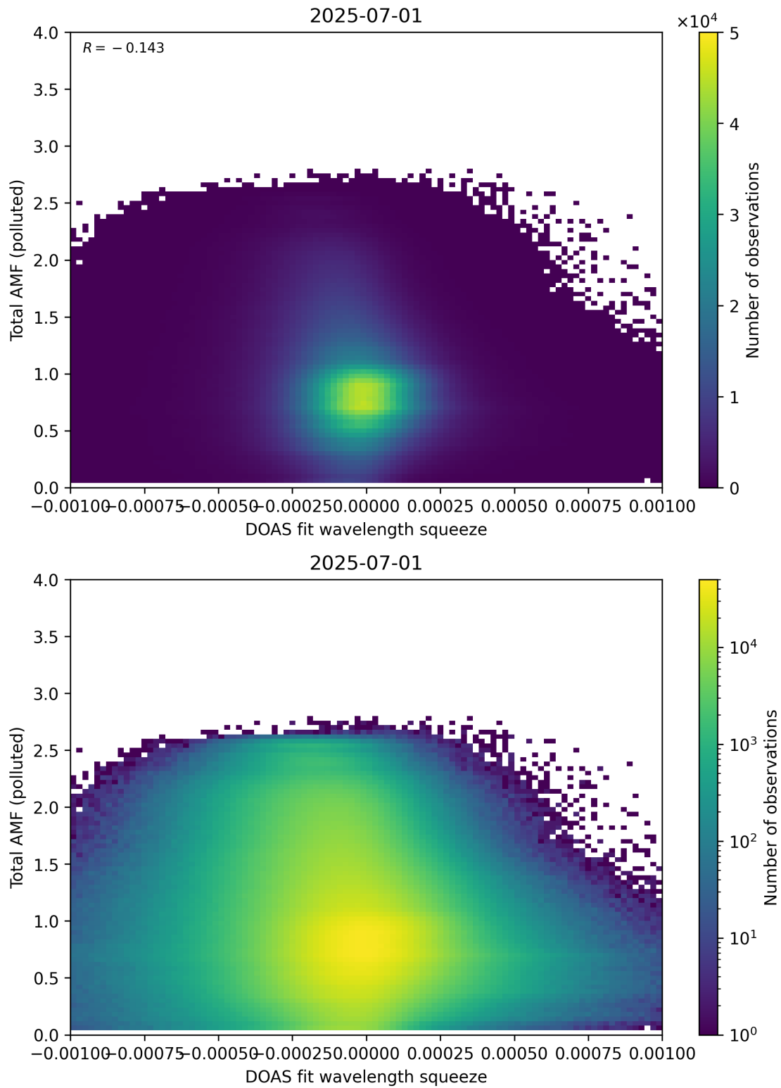
Figure 145: Scatter density plot of “DOAS fit wavelength squeeze” against “Total AMF (polluted)” for 2025-06-30 to 2025-07-02.
