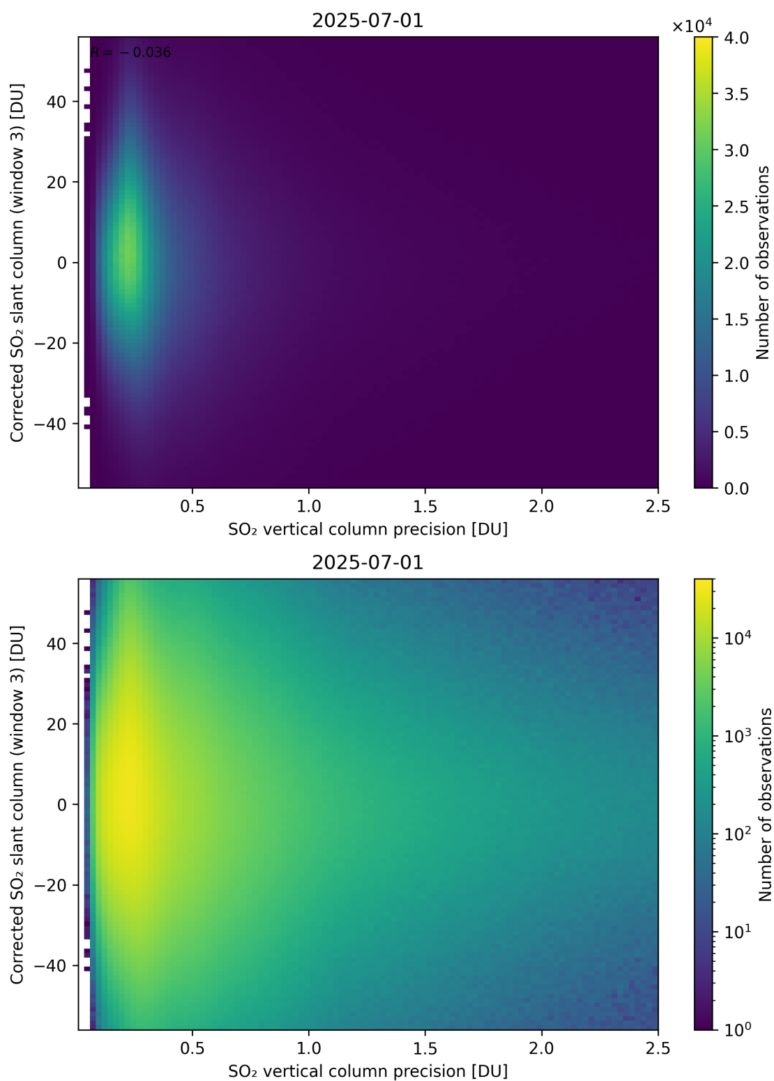
Figure 340: Scatter density plot of “SO 2 vertical column precision” against “Corrected SO 2 slant column (window 3)” for 2025-06-30 to 2025-07-02.
