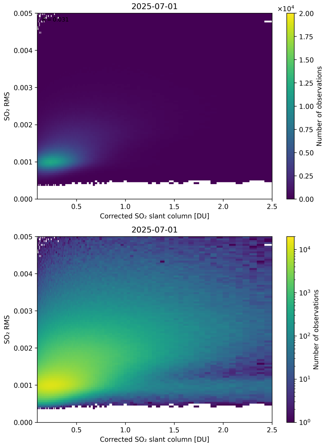
Figure 231: Scatter density plot of “Corrected SO 2 slant column” against “SO 2 RMS” for 2025-06-30 to 2025-07-02.
