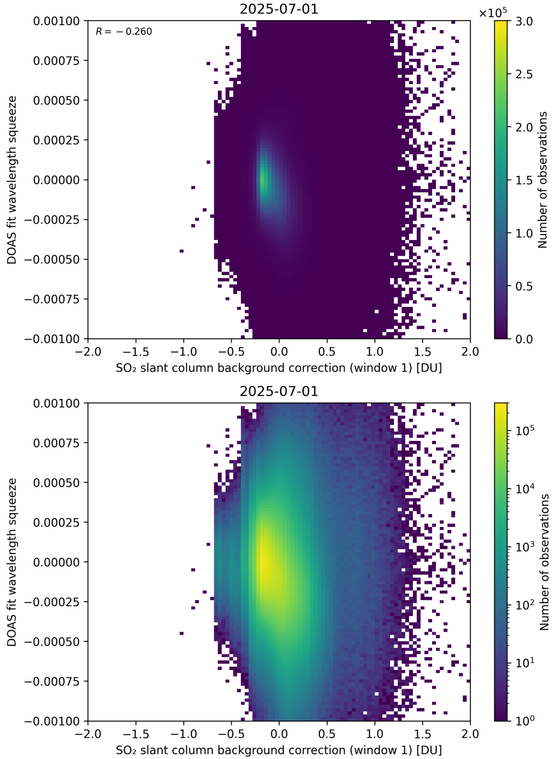
Figure 112: Scatter density plot of “SO 2 slant column background correction (window 1)” against “DOAS fit wavelength squeeze” for 2025-06-30 to 2025-07-02.
