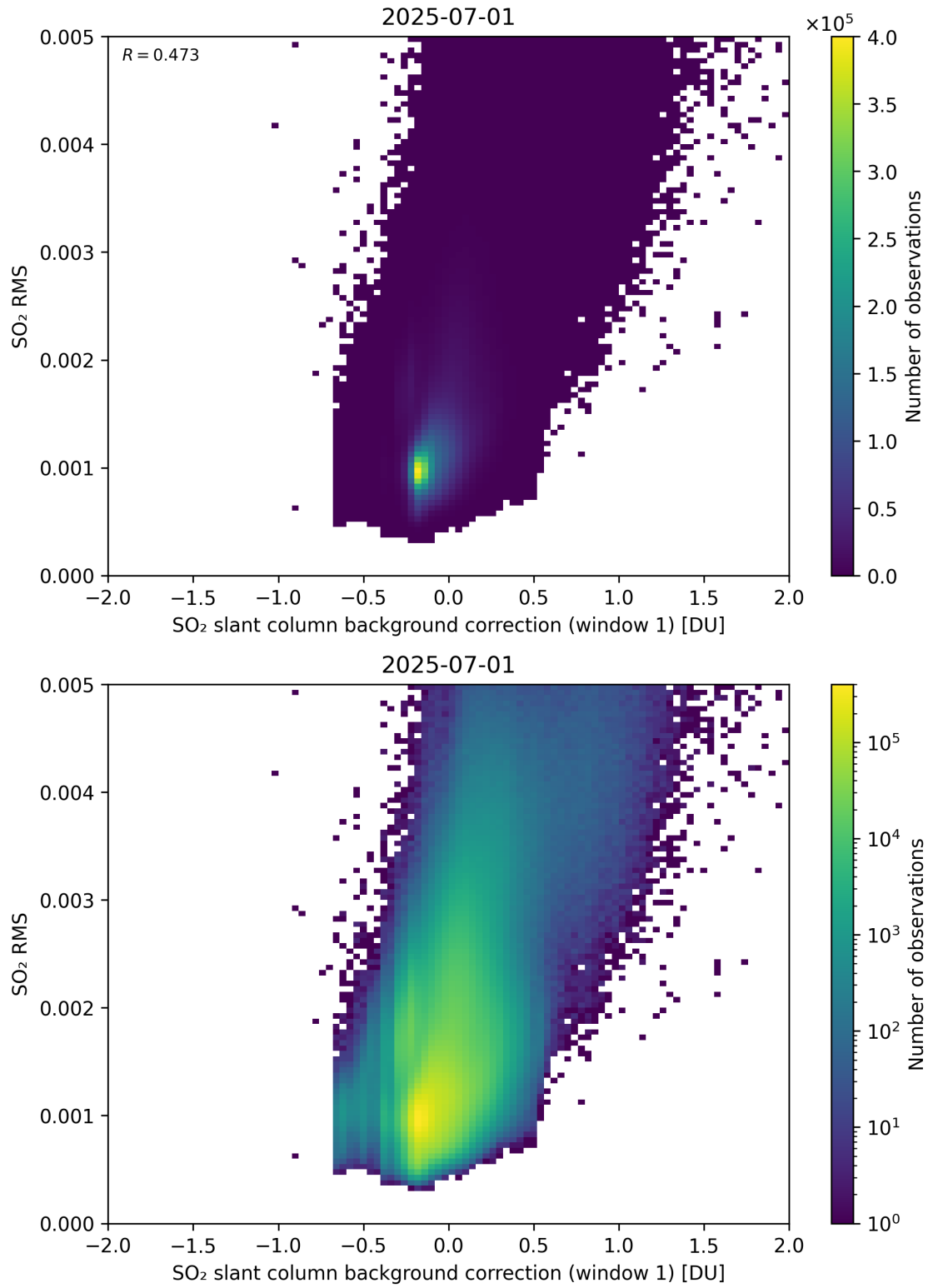
Figure 113: Scatter density plot of “SO 2 slant column background correction (window 1)” against “SO 2 RMS” for 2025-06-30 to 2025-07-02.
