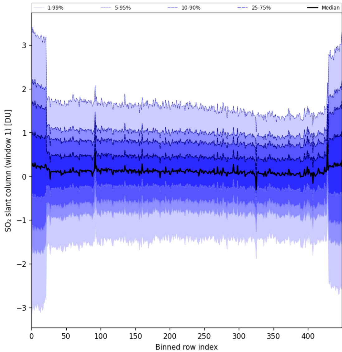
Figure 89: Along track statistics of “SO 2 slant column (window 1)” for 2025-06-30 to 2025-07-02
