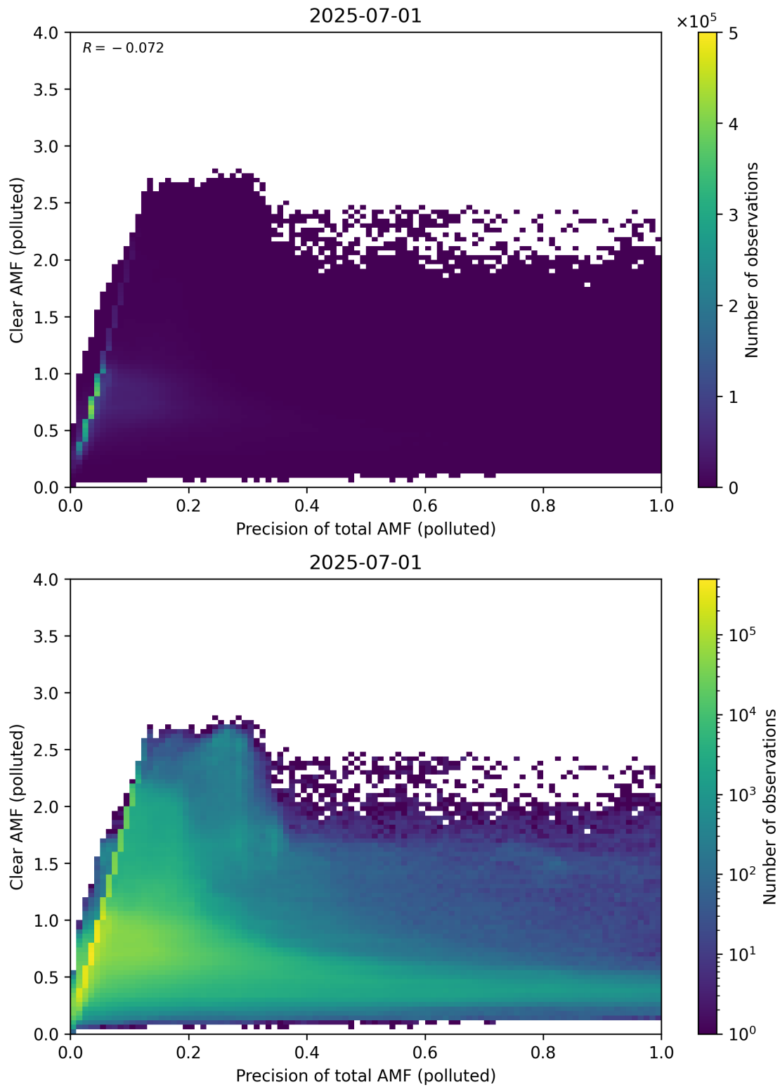
Figure 320: Scatter density plot of “Precision of total AMF (polluted)” against “Clear AMF (polluted)” for 2025-06-30 to 2025-07-02.
