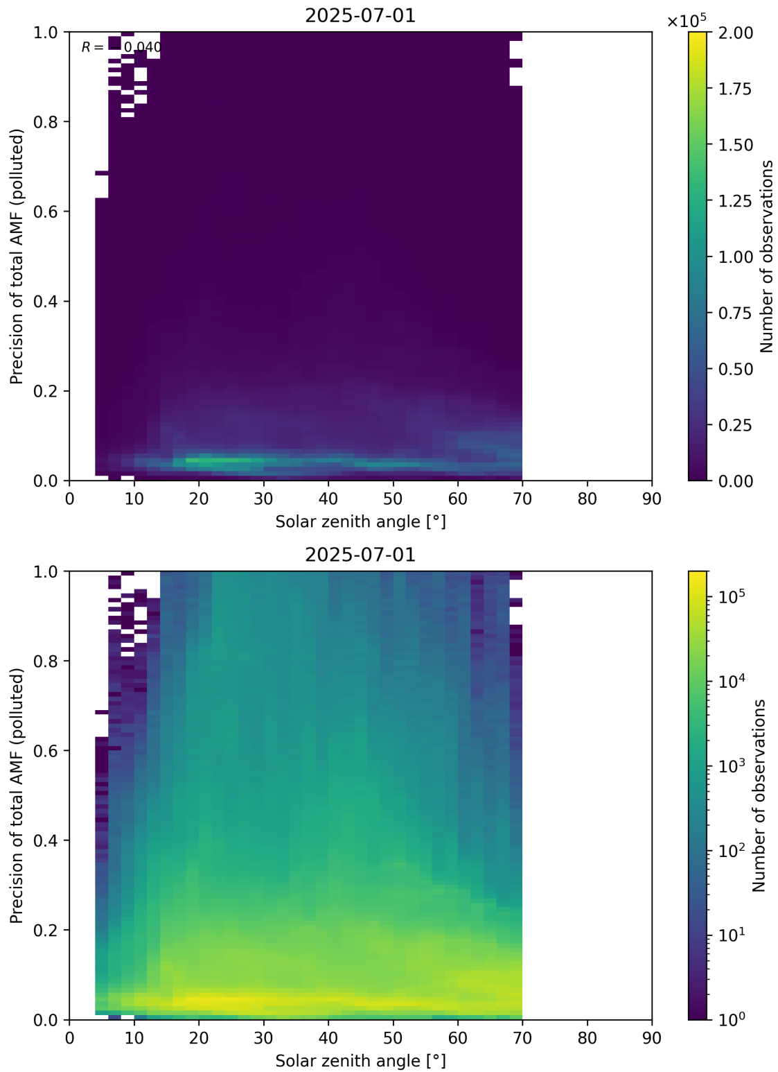
Figure 190: Scatter density plot of “Solar zenith angle” against “Precision of total AMF (polluted)” for 2025-06-30 to 2025-07-02.
