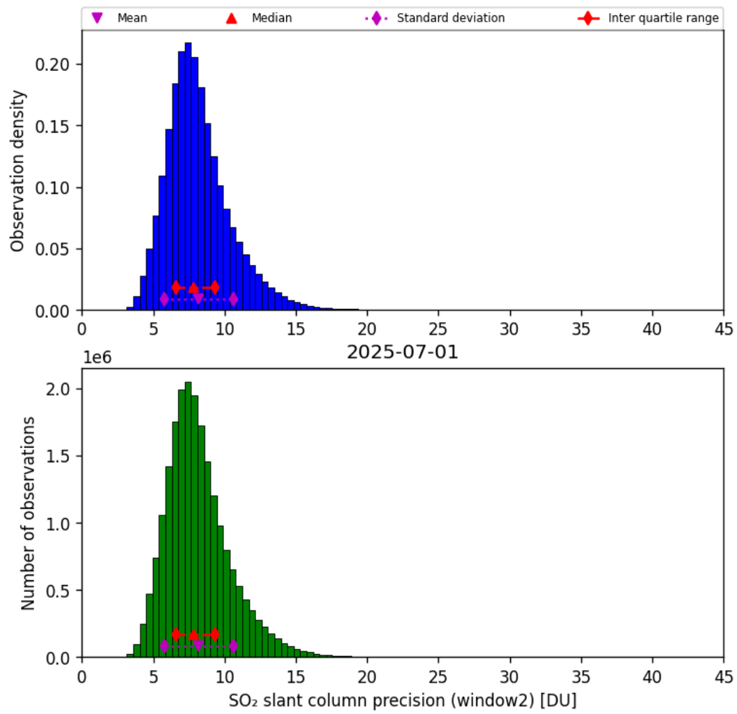
Figure 68: Histogram of “SO 2 slant column precision (window2)” for 2025-06-30 to 2025-07-02
