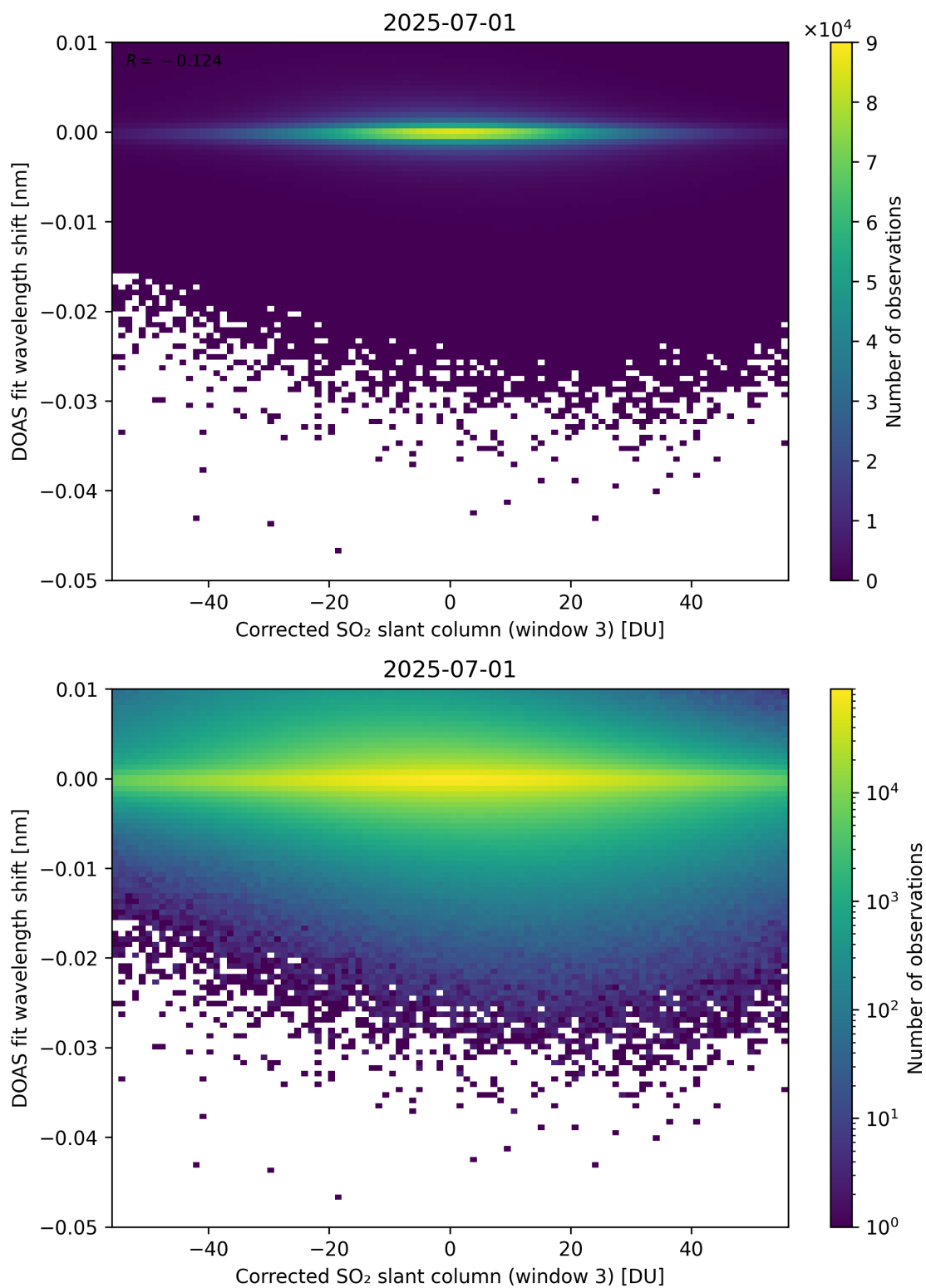
Figure 256: Scatter density plot of “Corrected SO 2 slant column (window 3)” against “DOAS fit wavelength shift” for 2025-06-30 to 2025-07-02.
