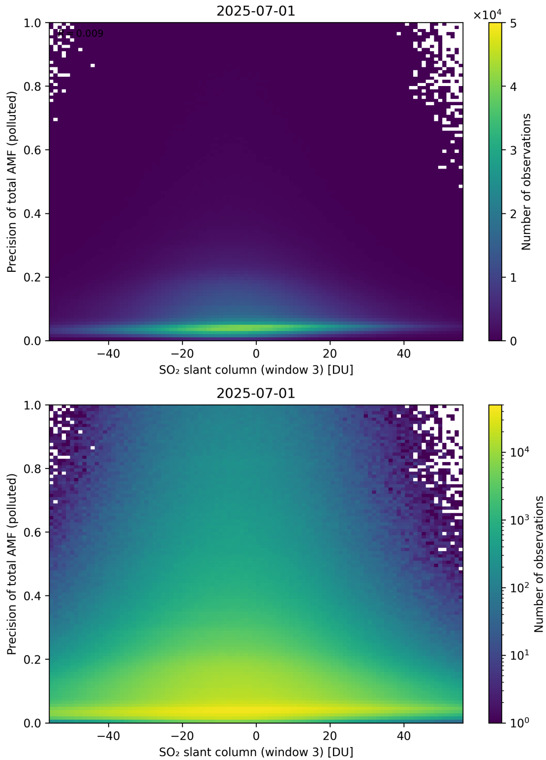
Figure 319: Scatter density plot of “SO 2 slant column (window 3)” against “Precision of total AMF (polluted)” for 2025-06-30 to 2025-07-02.
