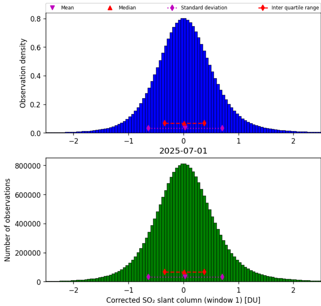
Figure 65: Histogram of “Corrected SO 2 slant column (window 1)” for 2025-06-30 to 2025-07-02
