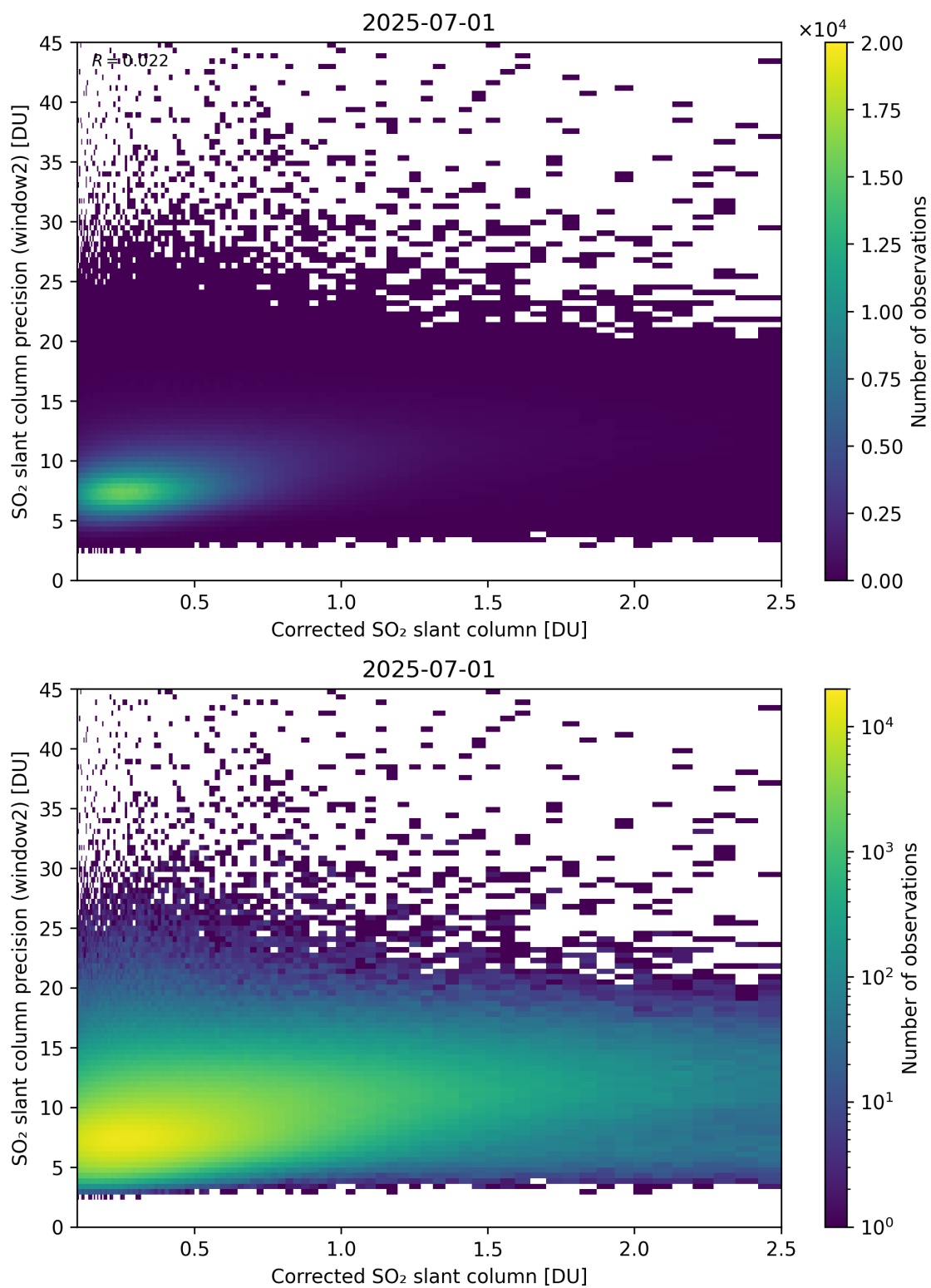
Figure 239: Scatter density plot of “Corrected SO 2 slant column” against “SO 2 slant column precision (window2)” for 2025-06-30 to 2025-07-02.
