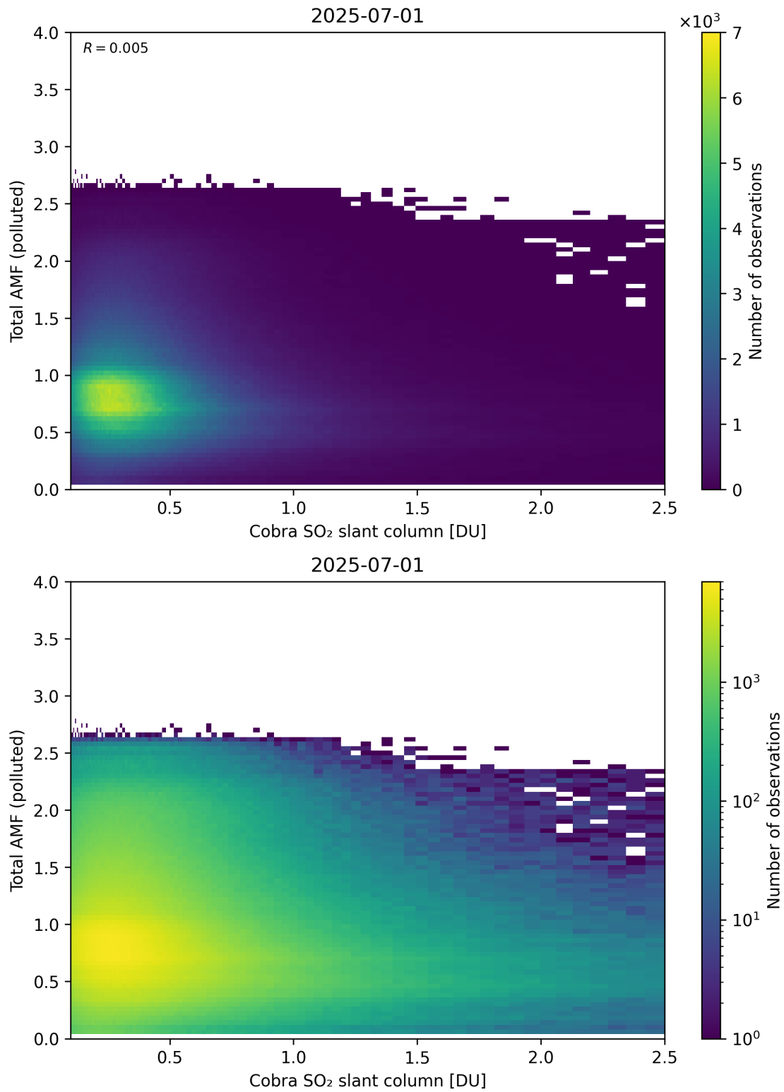
Figure 224: Scatter density plot of “Cobra SO 2 slant column” against “Total AMF (polluted)” for 2025-06-30 to 2025-07-02.
