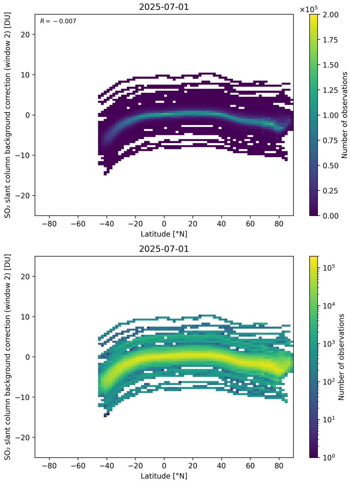
Figure 151: Scatter density plot of “Latitude” against “SO 2 slant column background correction (window 2)” for 2025-06-30 to 2025-07-02.
