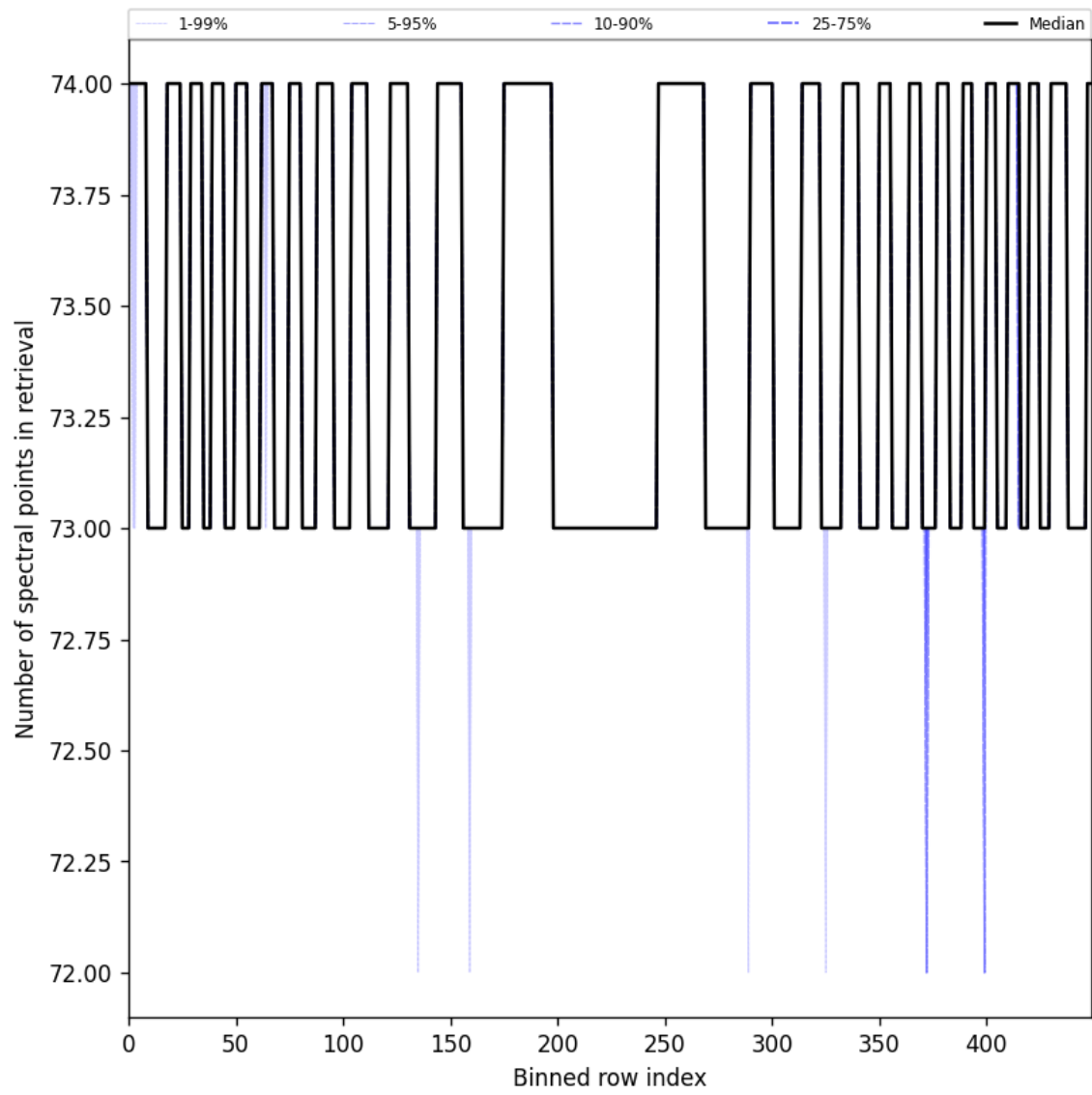
Figure 108: Along track statistics of “Number of spectral points in retrieval” for 2025-06-30 to 2025-07-02
