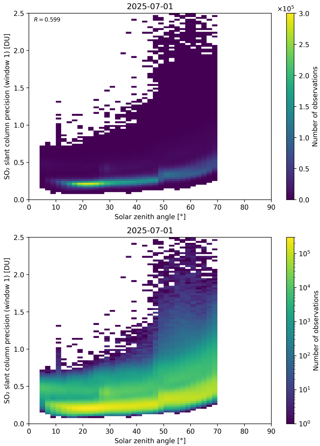
Figure 185: Scatter density plot of “Solar zenith angle” against “SO 2 slant column precision (window 1)” for 2025-06-30 to 2025-07-02.
