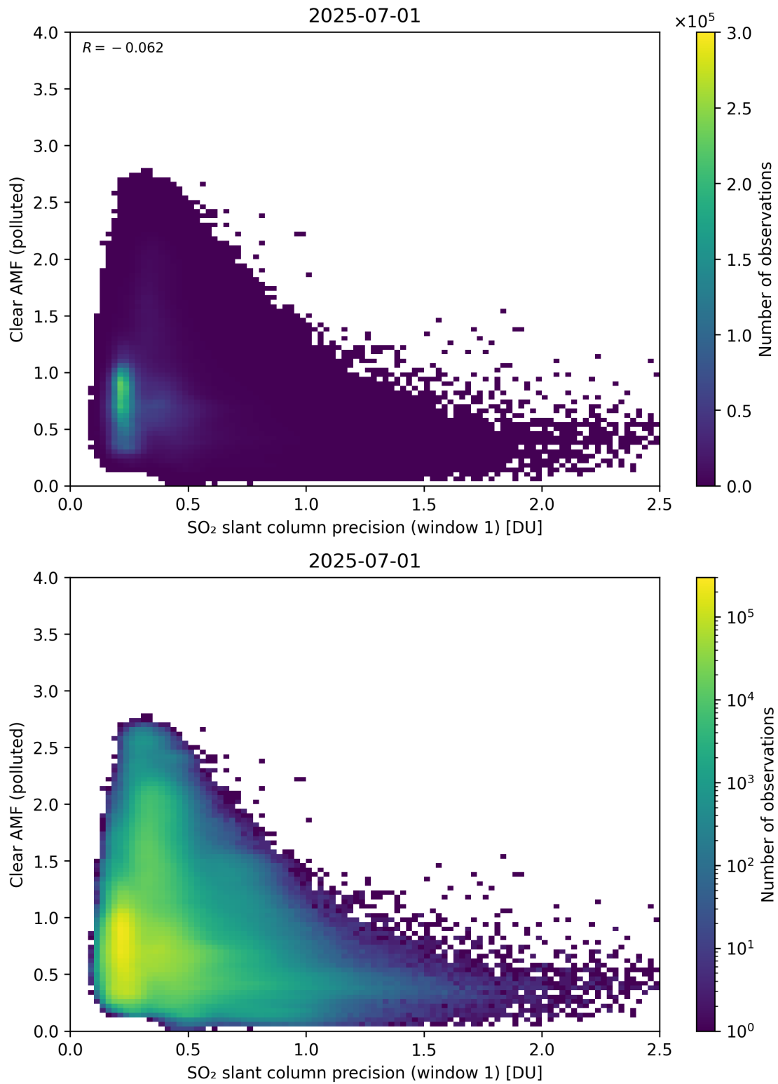
Figure 274: Scatter density plot of “SO 2 slant column precision (window 1)” against “Clear AMF (polluted)” for 2025-06-30 to 2025-07-02.
