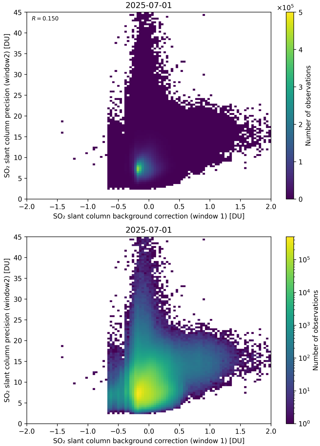
Figure 117: Scatter density plot of “SO 2 slant column background correction (window 1)” against “SO 2 slant column precision (window2)” for 2025-06-30 to 2025-07-02.
