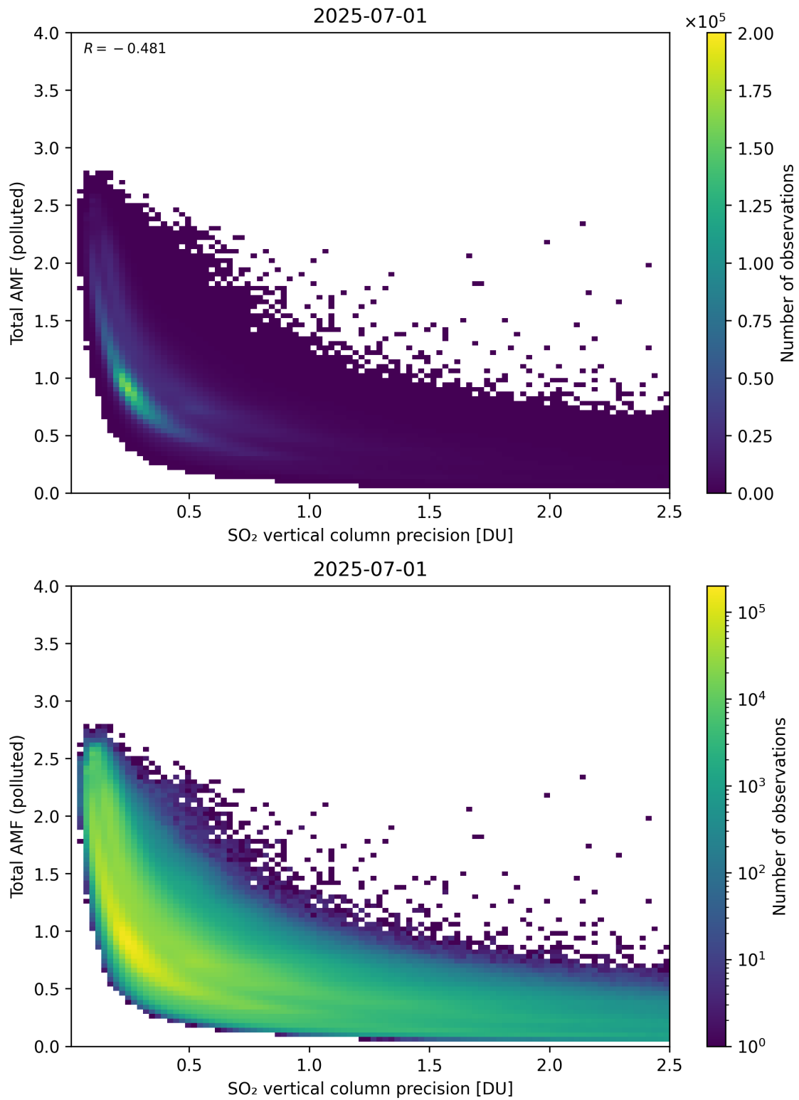
Figure 346: Scatter density plot of “SO 2 vertical column precision” against “Total AMF (polluted)” for 2025-06-30 to 2025-07-02.
