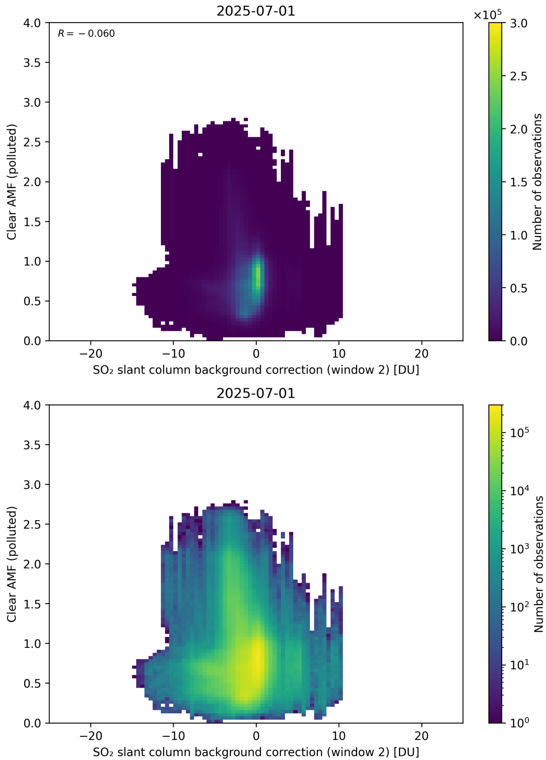
Figure 126: Scatter density plot of “SO 2 slant column background correction (window 2)” against “Clear AMF (polluted)” for 2025-06-30 to 2025-07-02.
