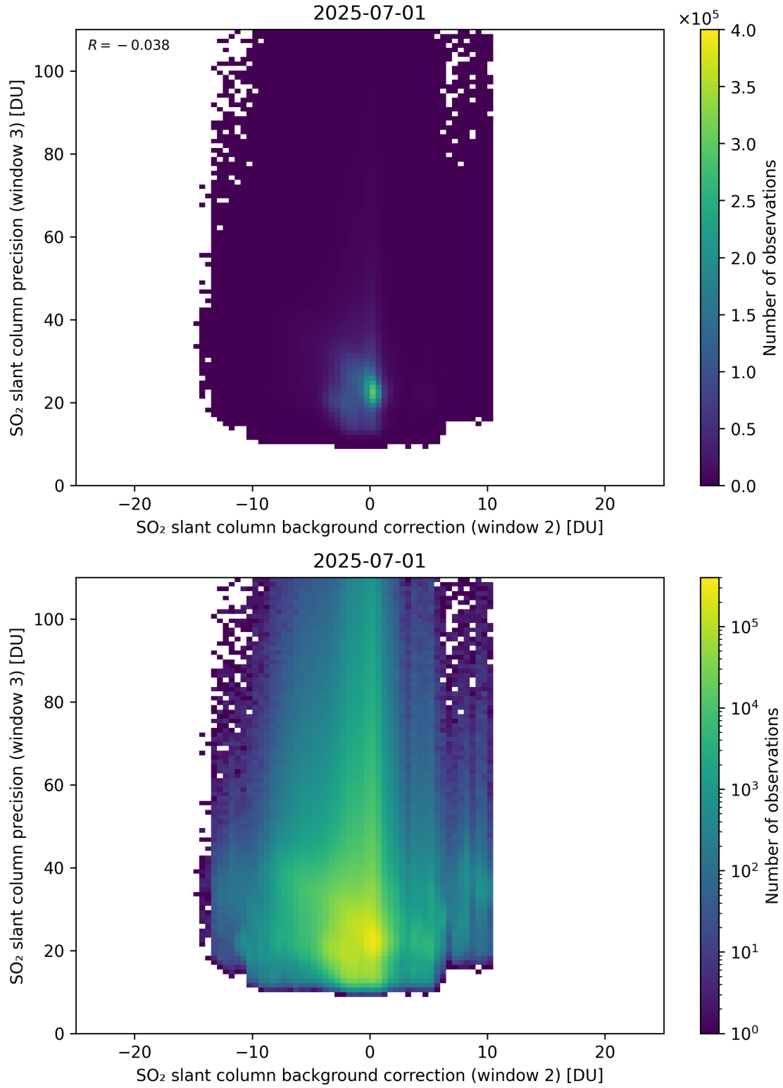
Figure 129: Scatter density plot of “SO 2 slant column background correction (window 2)” against “SO 2 slant column precision (window 3)” for 2025-06-30 to 2025-07-02.
