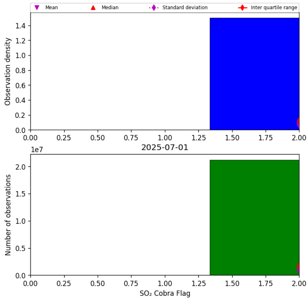
Figure 75: Histogram of “SO 2 Cobra Flag” for 2025-06-30 to 2025-07-02
