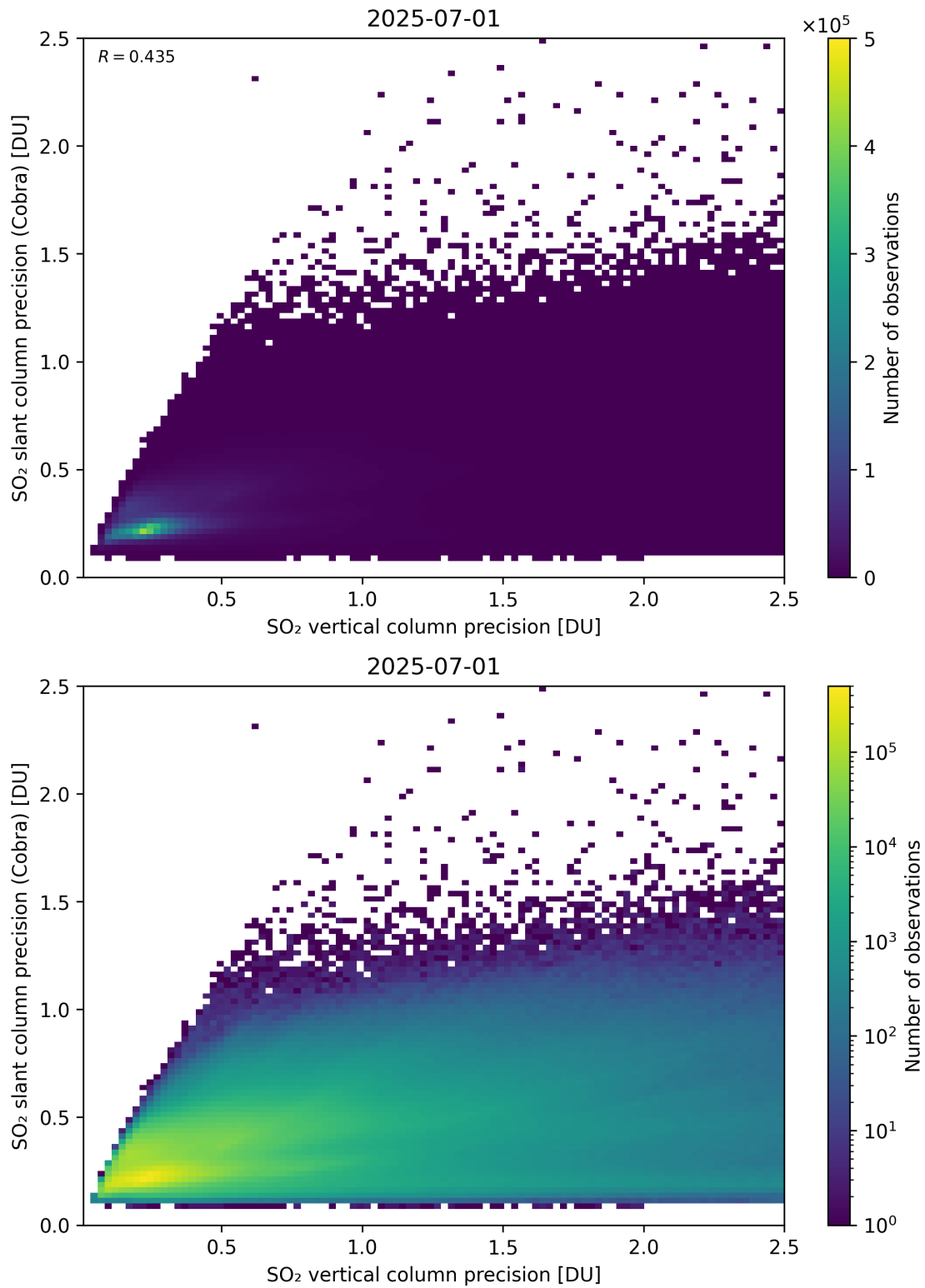
Figure 337: Scatter density plot of “SO 2 vertical column precision” against “SO 2 slant column precision (Cobra)” for 2025-06-30 to 2025-07-02.
