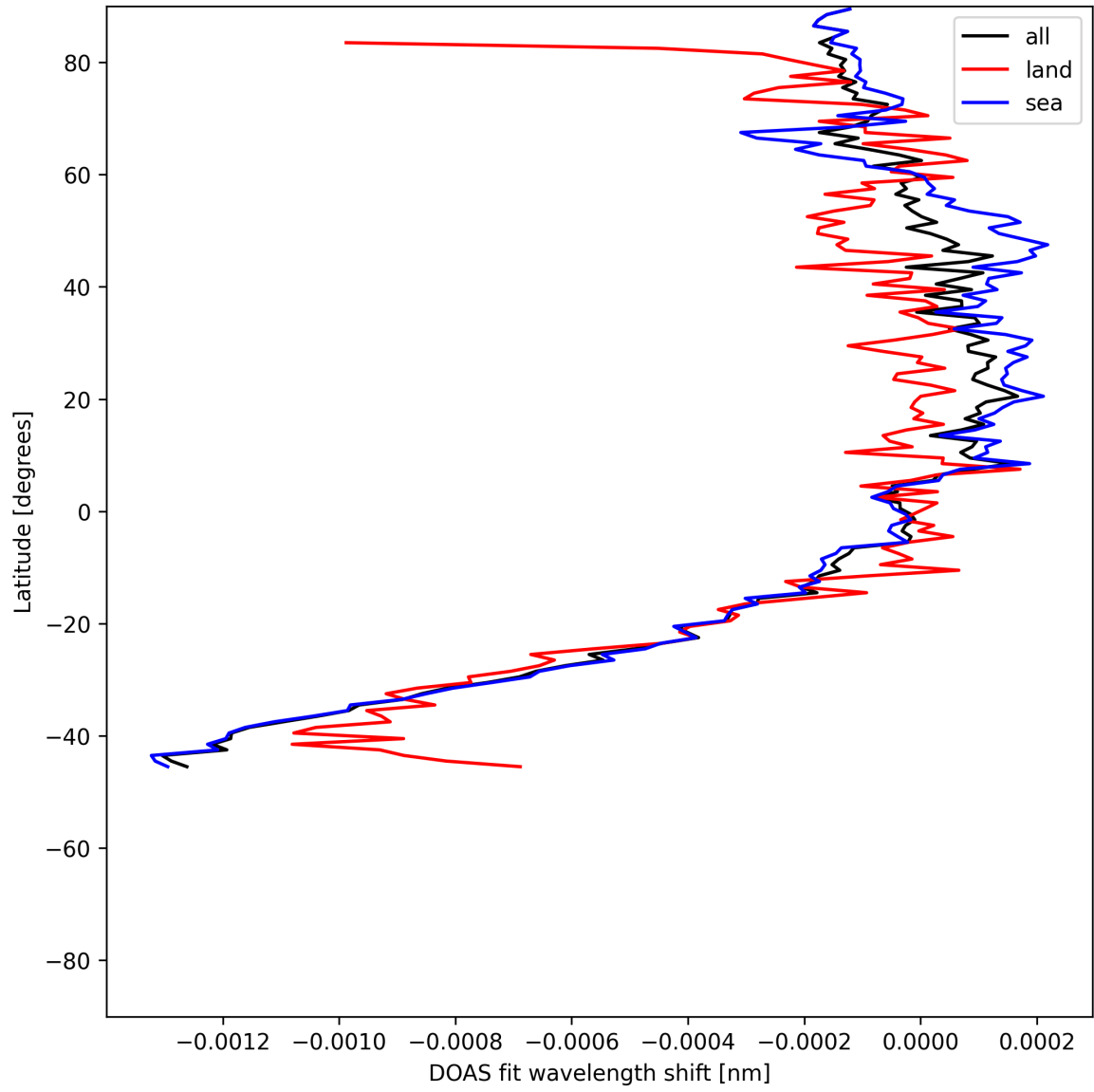
Figure 50: Zonal average of “DOAS fit wavelength shift” for 2025-06-30 to 2025-07-02.
