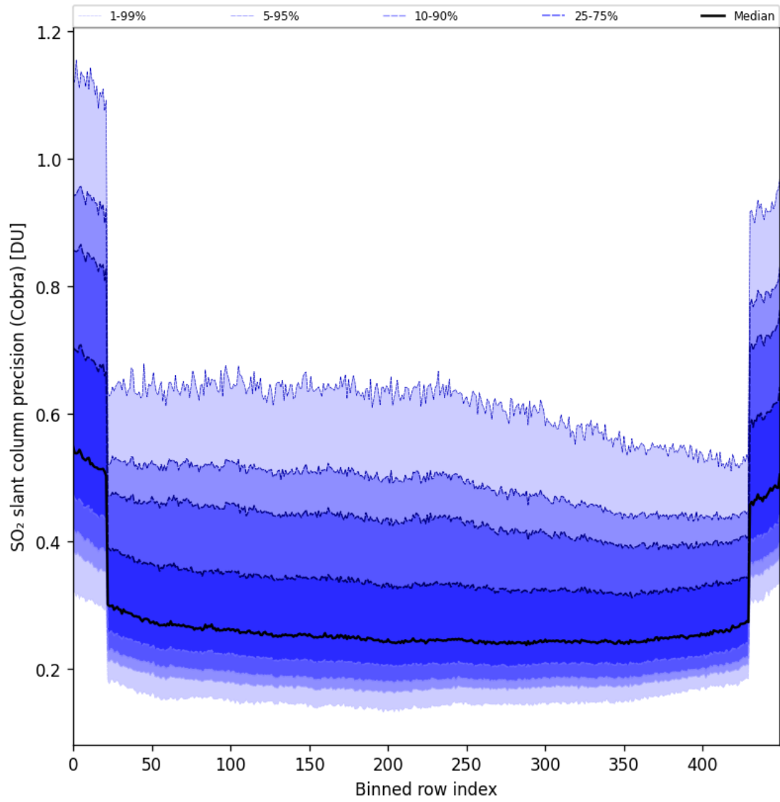
Figure 88: Along track statistics of “SO 2 slant column precision (Cobra)” for 2025-06-30 to 2025-07-02
