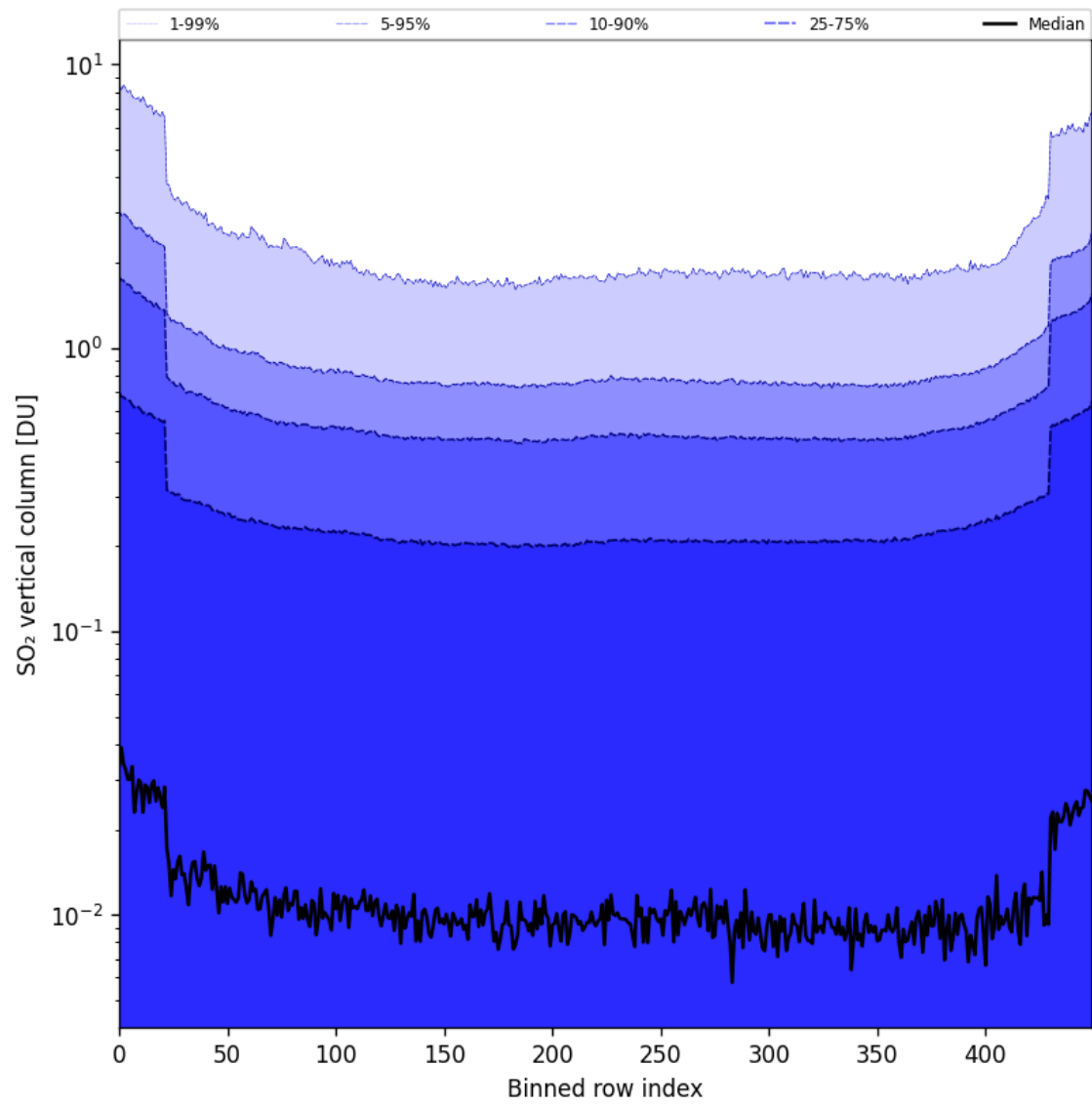
Figure 84: Along track statistics of “SO 2 vertical column” for 2025-06-30 to 2025-07-02
