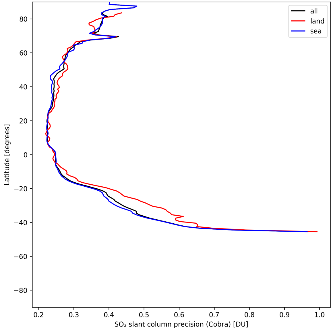
Figure 36: Zonal average of “SO 2 slant column precision (Cobra)” for 2025-06-30 to 2025-07-02.
