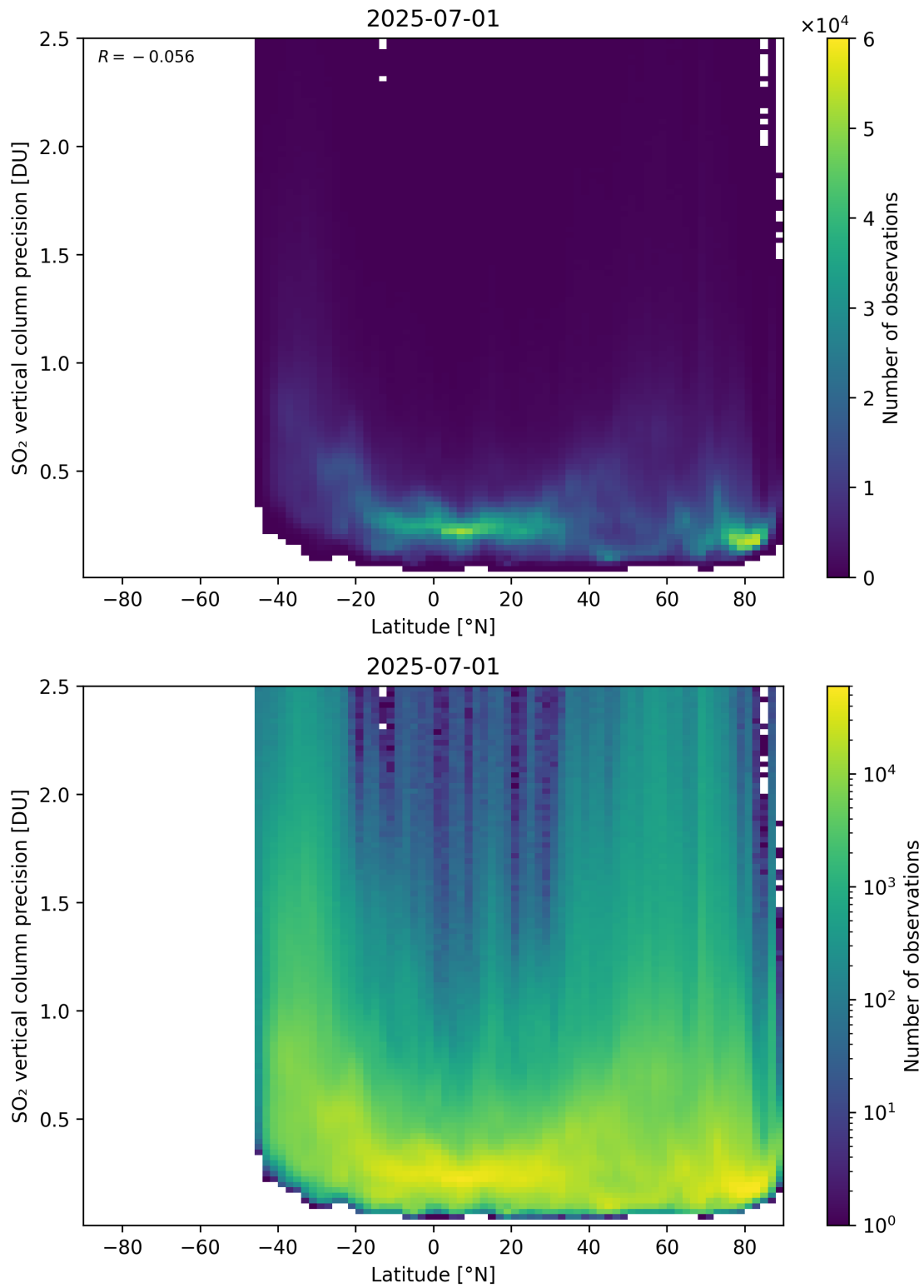
Figure 170: Scatter density plot of “Latitude” against “SO 2 vertical column precision” for 2025-06-30 to 2025-07-02.
