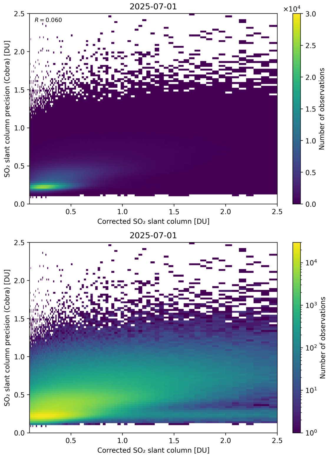
Figure 234: Scatter density plot of “Corrected SO 2 slant column” against “SO 2 slant column precision (Cobra)” for 2025-06-30 to 2025-07-02.
