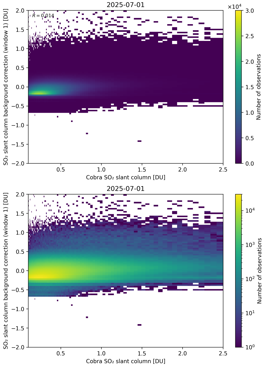
Figure 193: Scatter density plot of “Cobra SO 2 slant column” against “SO 2 slant column background correction (window 1)” for 2025-06-30 to 2025-07-02.
