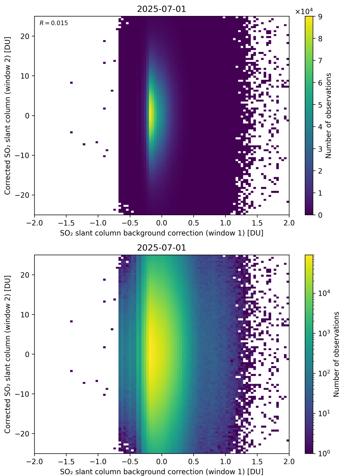
Figure 115: Scatter density plot of “SO 2 slant column background correction (window 1)” against “Corrected SO 2 slant column (window 2)” for 2025-06-30 to 2025-07-02.
