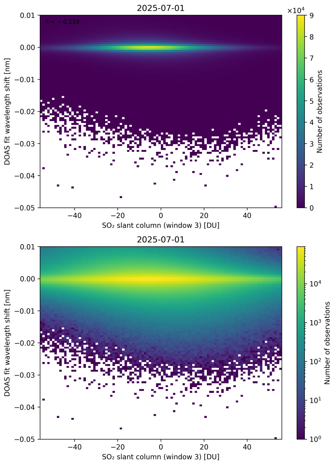
Figure 304: Scatter density plot of “SO 2 slant column (window 3)” against “DOAS fit wavelength shift” for 2025-06-30 to 2025-07-02.
