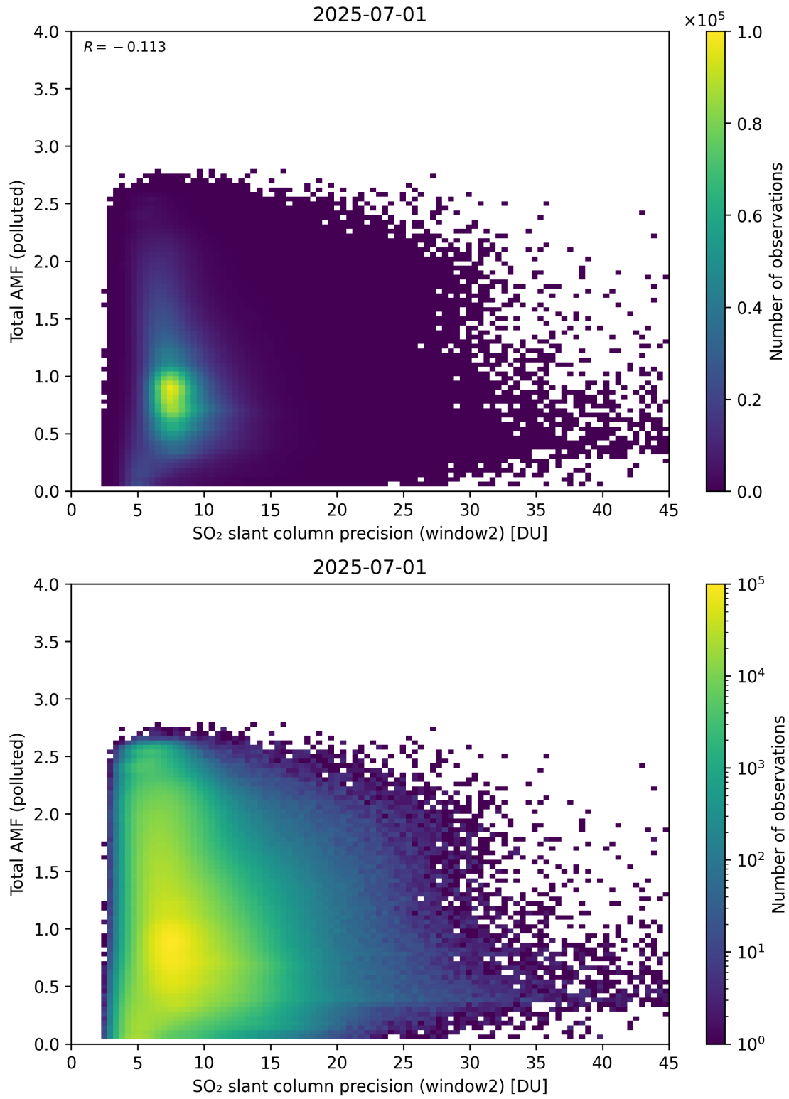
Figure 301: Scatter density plot of “SO 2 slant column precision (window2)” against “Total AMF (polluted)” for 2025-06-30 to 2025-07-02.
