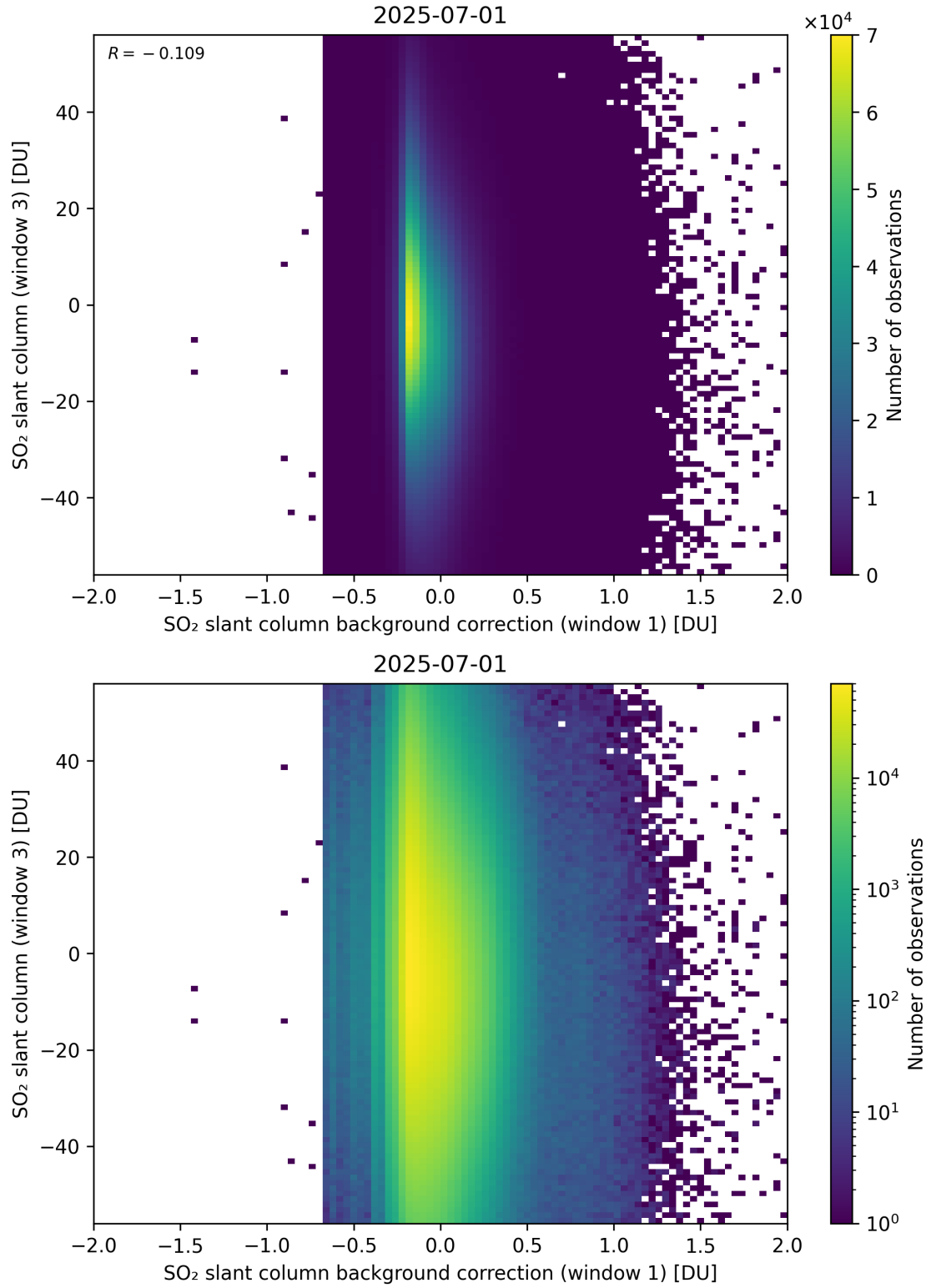
Figure 118: Scatter density plot of “SO 2 slant column background correction (window 1)” against “SO 2 slant column (window 3)” for 2025-06-30 to 2025-07-02.
