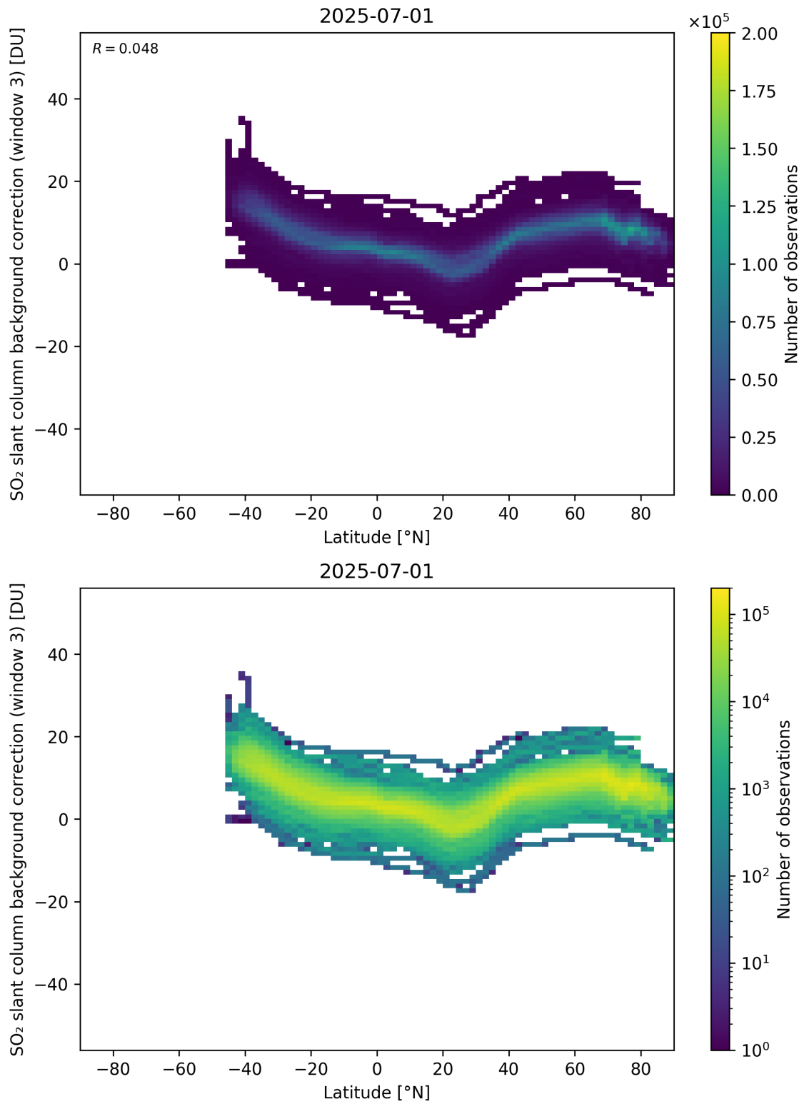
Figure 152: Scatter density plot of “Latitude” against “SO 2 slant column background correction (window 3)” for 2025-06-30 to 2025-07-02.
