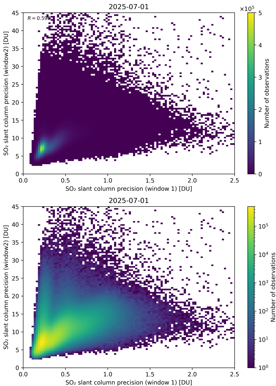
Figure 277: Scatter density plot of “SO 2 slant column precision (window 1)” against “SO 2 slant column precision (window2)” for 2025-06-30 to 2025-07-02.
