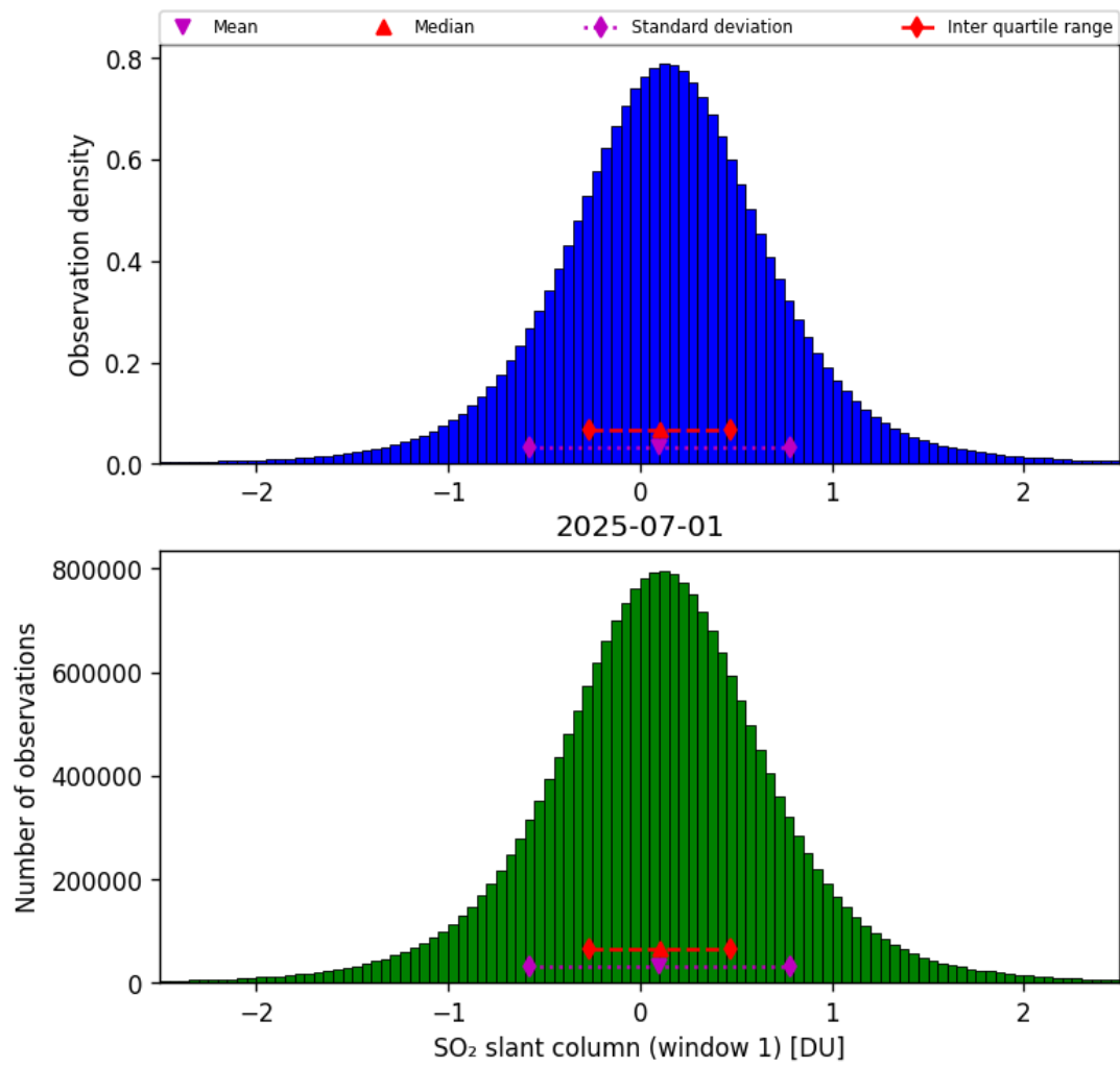
Figure 63: Histogram of “SO 2 slant column (window 1)” for 2025-06-30 to 2025-07-02
