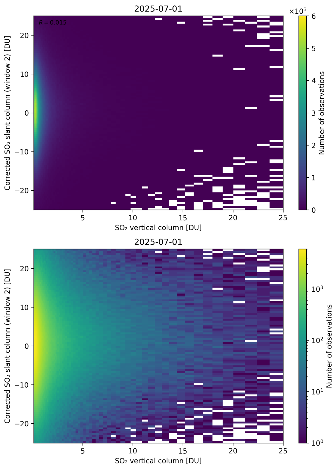
Figure 352: Scatter density plot of “SO 2 vertical column” against “Corrected SO 2 slant column (window 2)” for 2025-06-30 to 2025-07-02.
