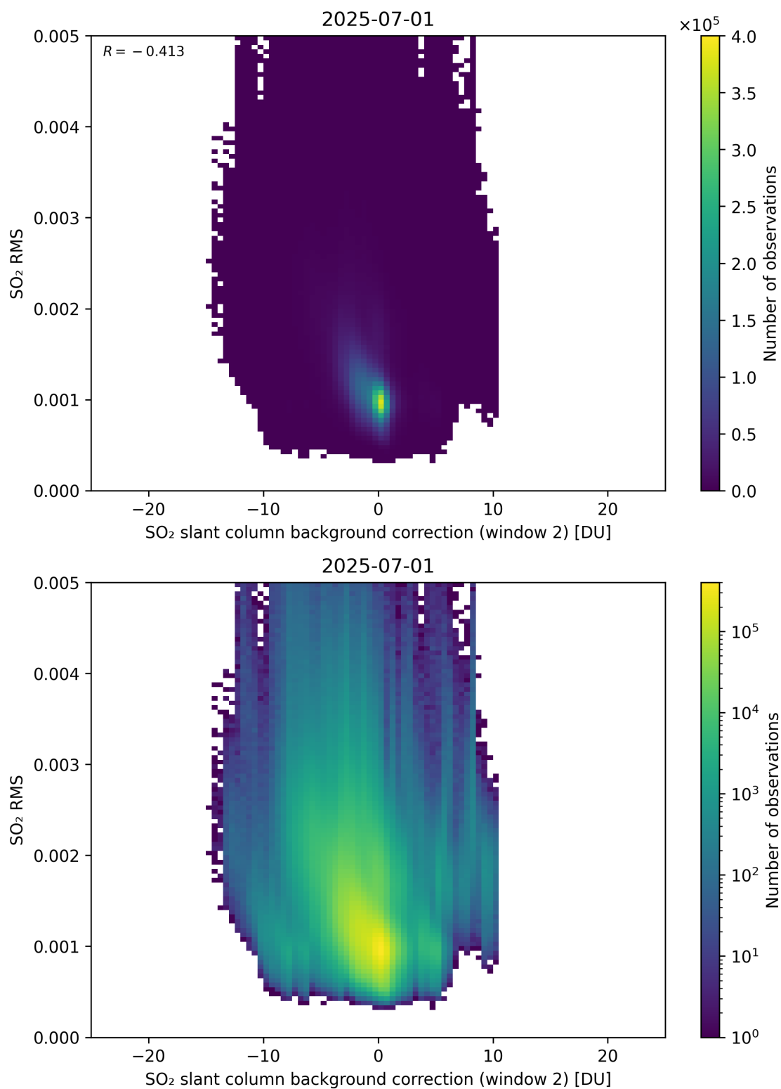
Figure 125: Scatter density plot of “SO 2 slant column background correction (window 2)” against “SO 2 RMS” for 2025-06-30 to 2025-07-02.
