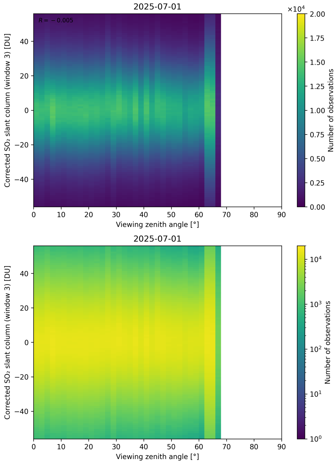
Figure 375: Scatter density plot of “Viewing zenith angle” against “Corrected SO 2 slant column (window 3)” for 2025-06-30 to 2025-07-02.
