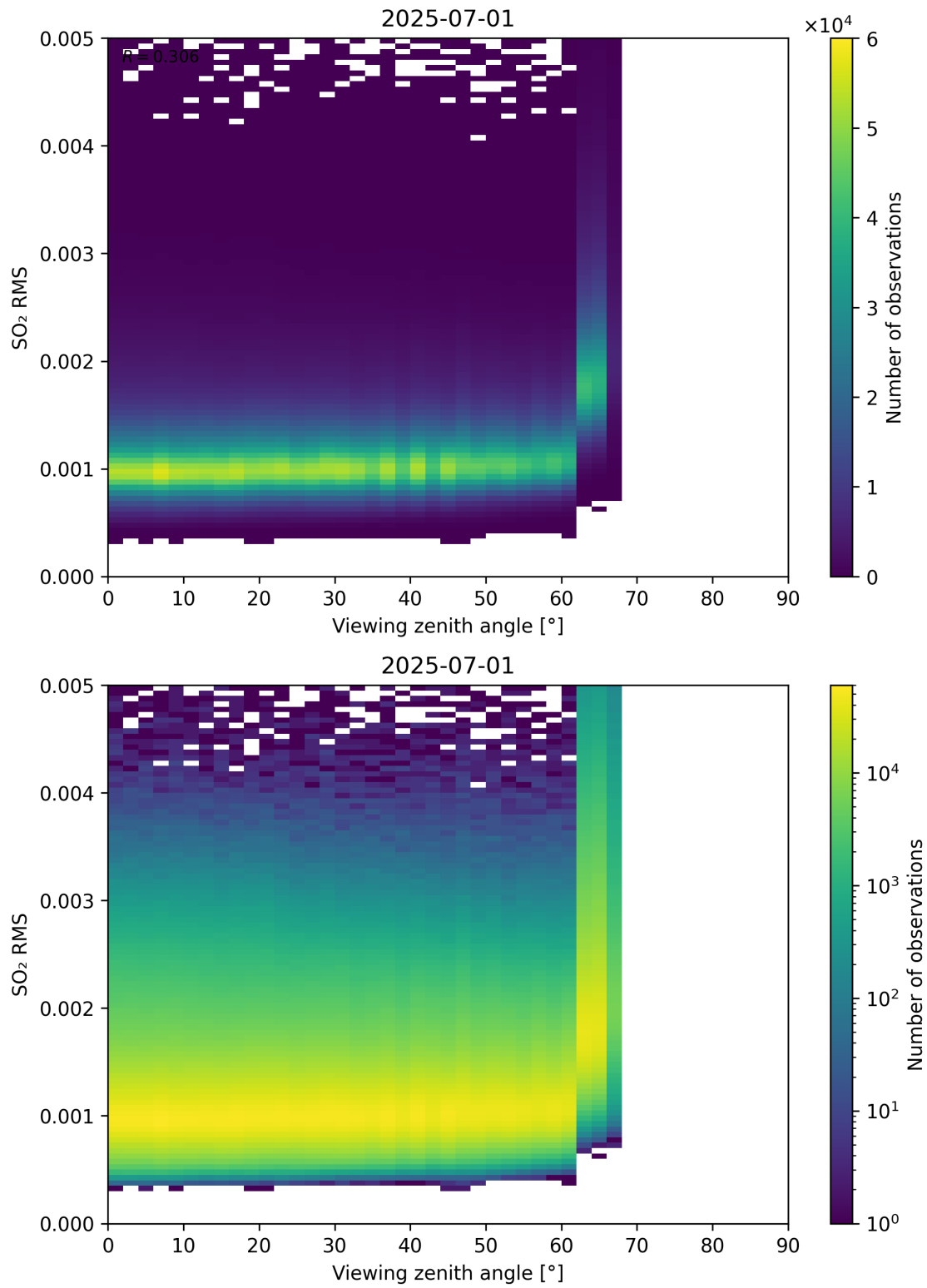
Figure 367: Scatter density plot of “Viewing zenith angle” against “SO 2 RMS” for 2025-06-30 to 2025-07-02.
