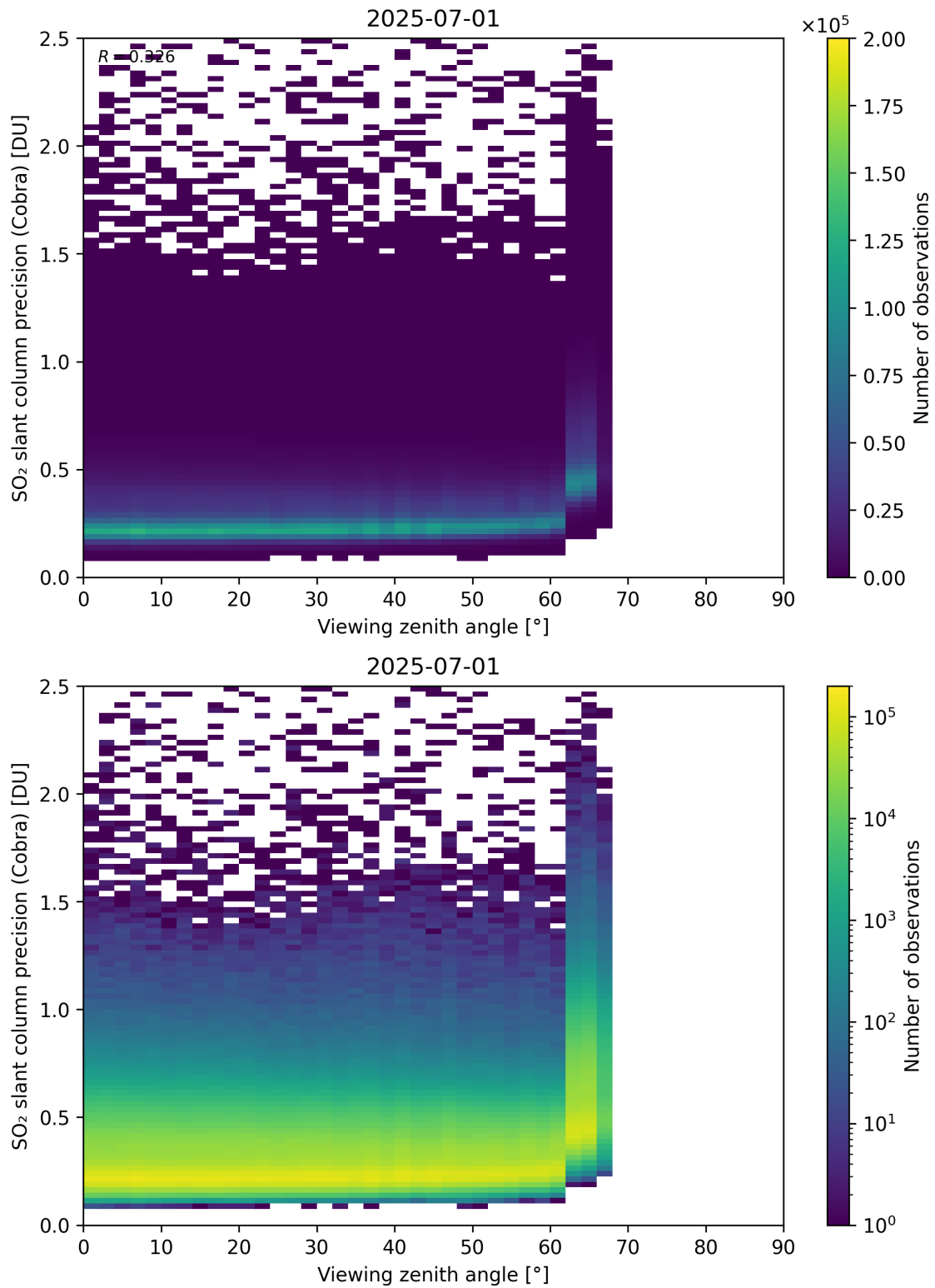
Figure 372: Scatter density plot of “Viewing zenith angle” against “SO 2 slant column precision (Cobra)” for 2025-06-30 to 2025-07-02.
