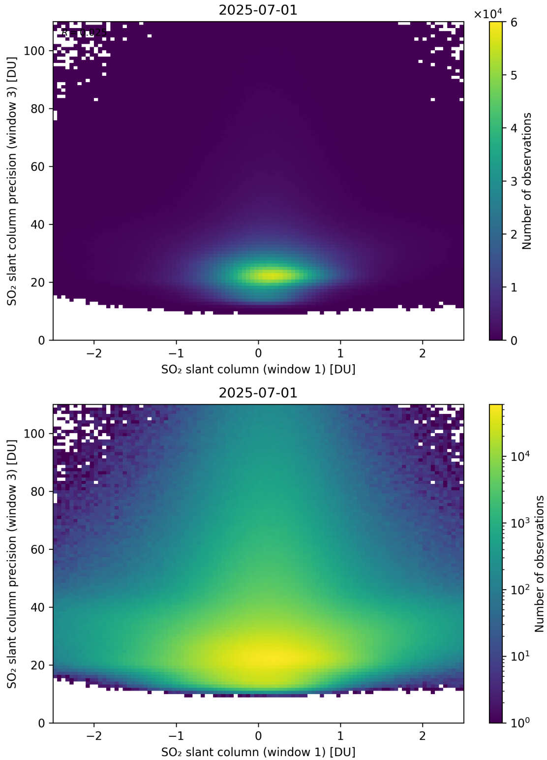
Figure 288: Scatter density plot of “SO 2 slant column (window 1)” against “SO 2 slant column precision (window 3)” for 2025-06-30 to 2025-07-02.
