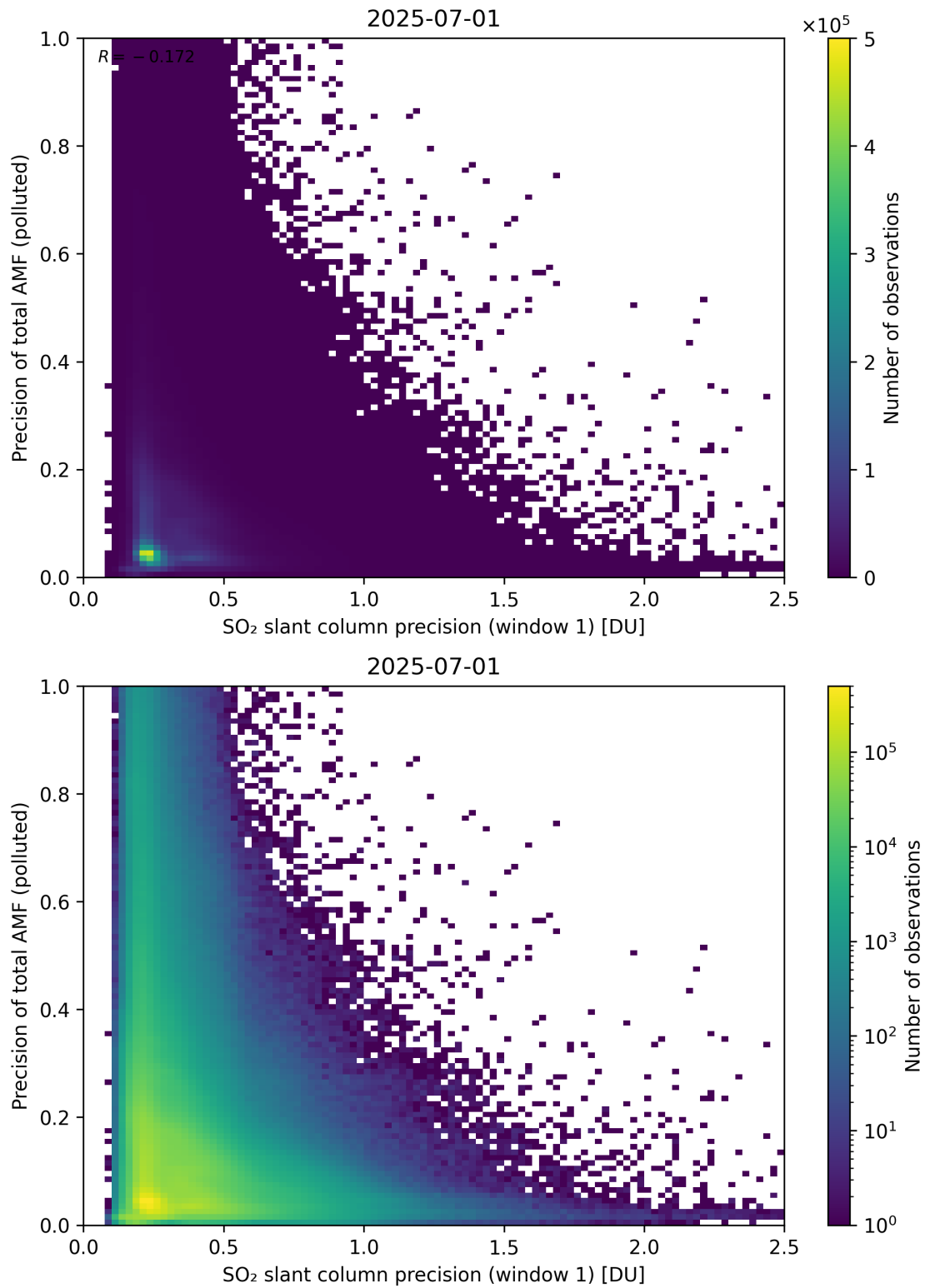
Figure 281: Scatter density plot of “SO 2 slant column precision (window 1)” against “Precision of total AMF (polluted)” for 2025-06-30 to 2025-07-02.
