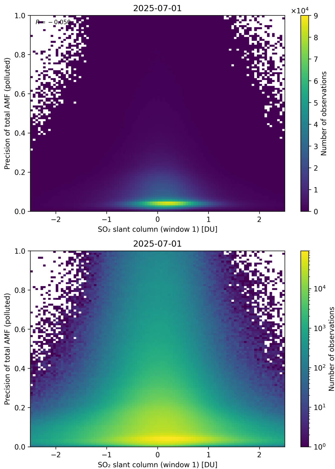
Figure 290: Scatter density plot of “SO 2 slant column (window 1)” against “Precision of total AMF (polluted)” for 2025-06-30 to 2025-07-02.
