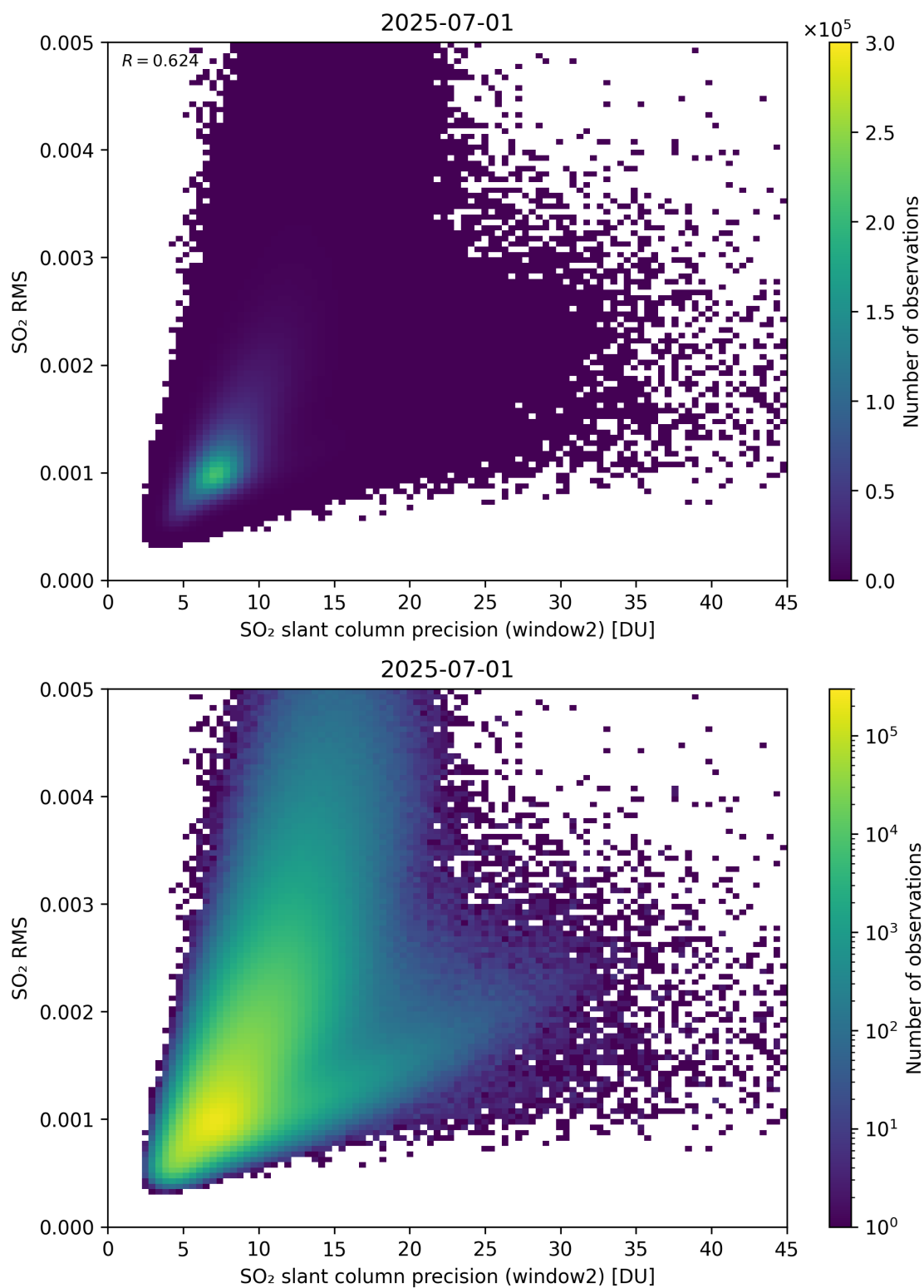
Figure 295: Scatter density plot of “SO 2 slant column precision (window2)” against “SO 2 RMS” for 2025-06-30 to 2025-07-02.
