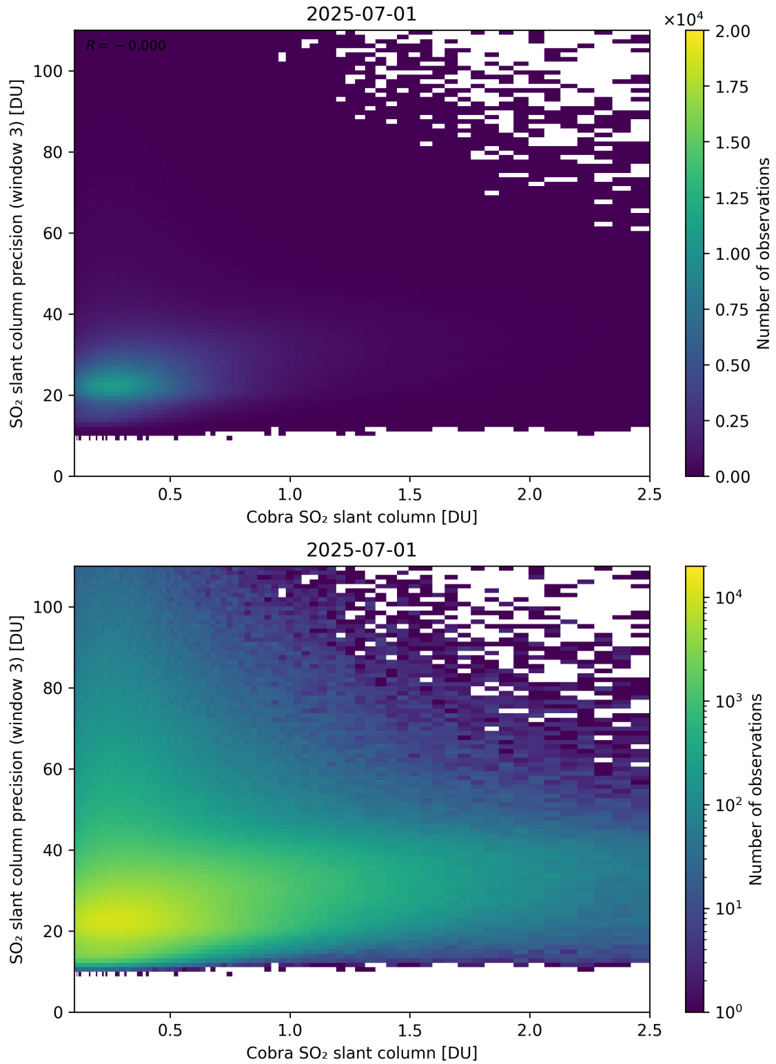
Figure 223: Scatter density plot of “Cobra SO 2 slant column” against “SO 2 slant column precision (window 3)” for 2025-06-30 to 2025-07-02.
