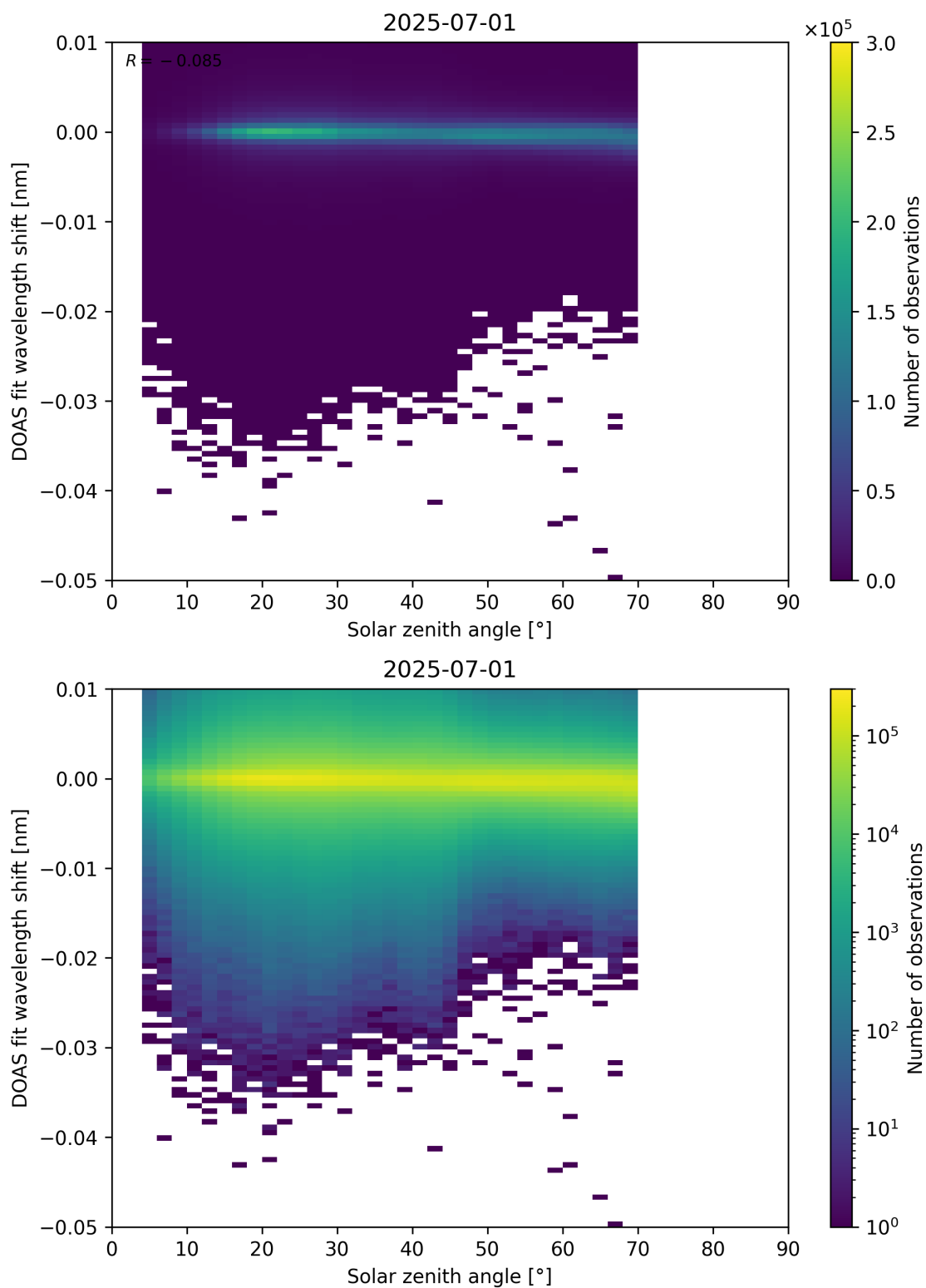
Figure 174: Scatter density plot of “Solar zenith angle” against “DOAS fit wavelength shift” for 2025-06-30 to 2025-07-02.
