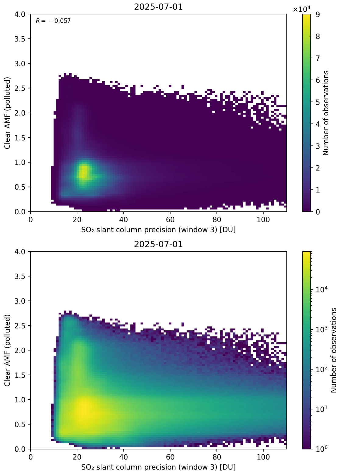
Figure 311: Scatter density plot of “SO 2 slant column precision (window 3)” against “Clear AMF (polluted)” for 2025-06-30 to 2025-07-02.
