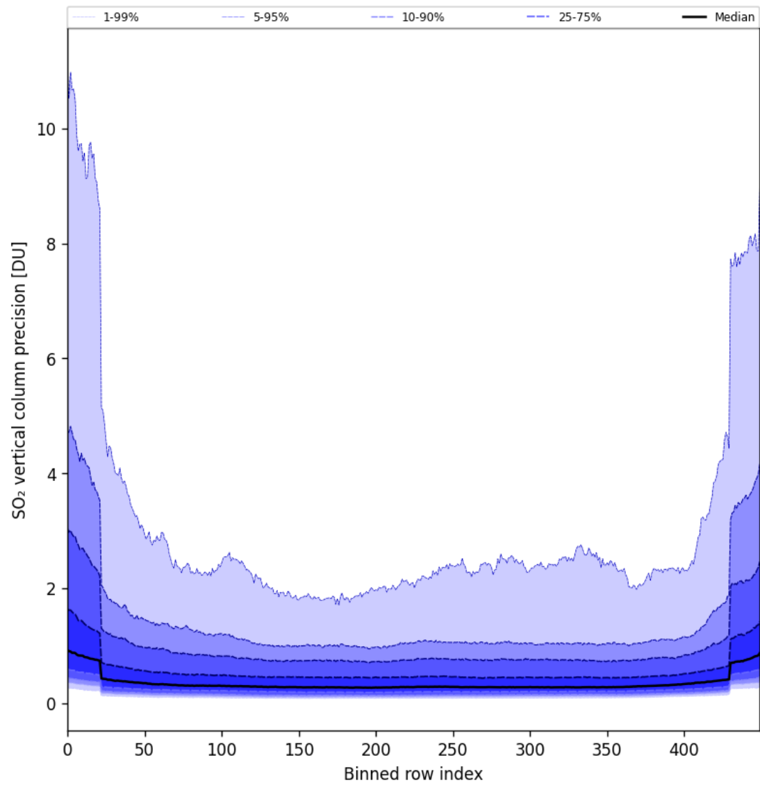
Figure 85: Along track statistics of “SO 2 vertical column precision” for 2025-06-30 to 2025-07-02
