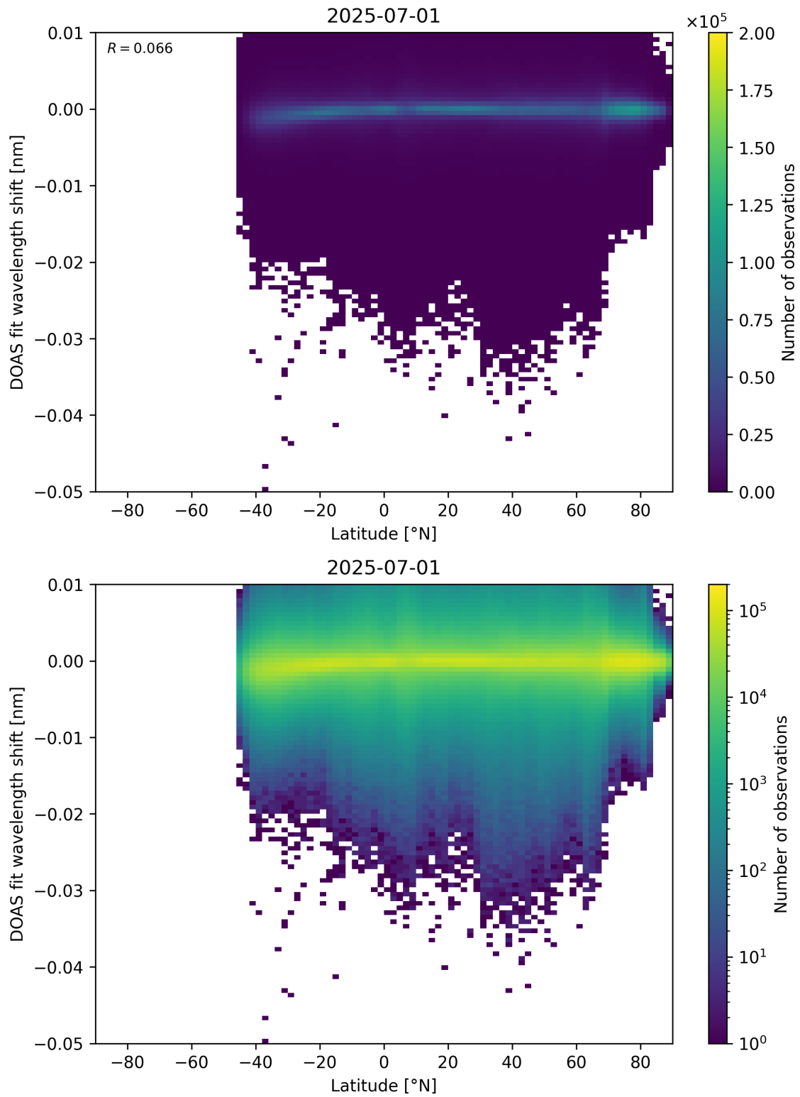
Figure 153: Scatter density plot of “Latitude” against “DOAS fit wavelength shift” for 2025-06-30 to 2025-07-02.
