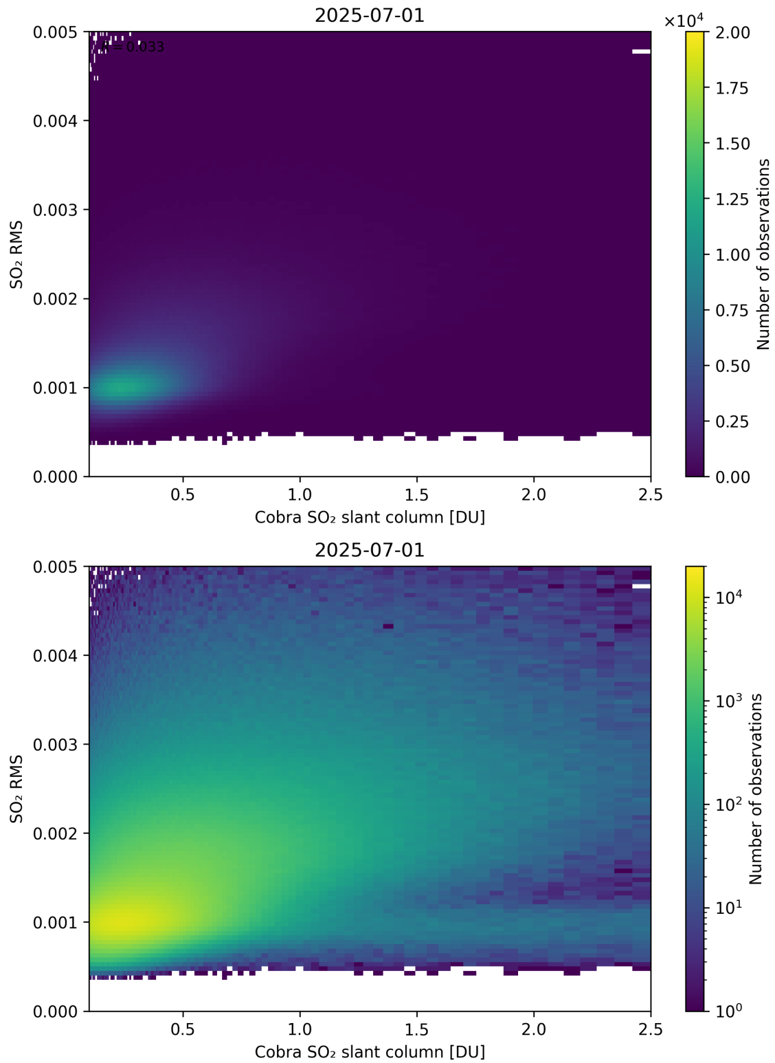
Figure 198: Scatter density plot of “Cobra SO 2 slant column” against “SO 2 RMS” for 2025-06-30 to 2025-07-02.
