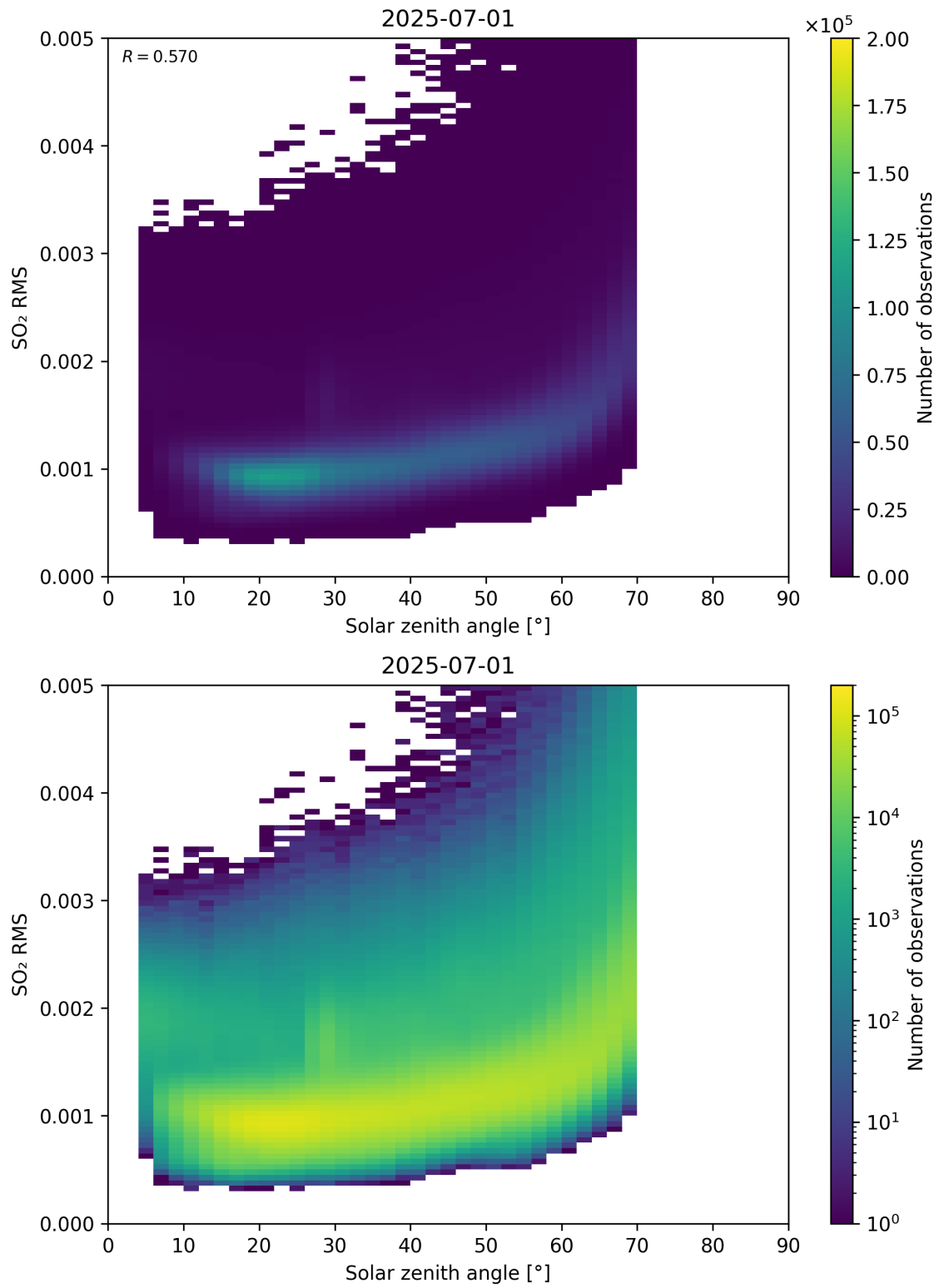
Figure 176: Scatter density plot of “Solar zenith angle” against “SO 2 RMS” for 2025-06-30 to 2025-07-02.
