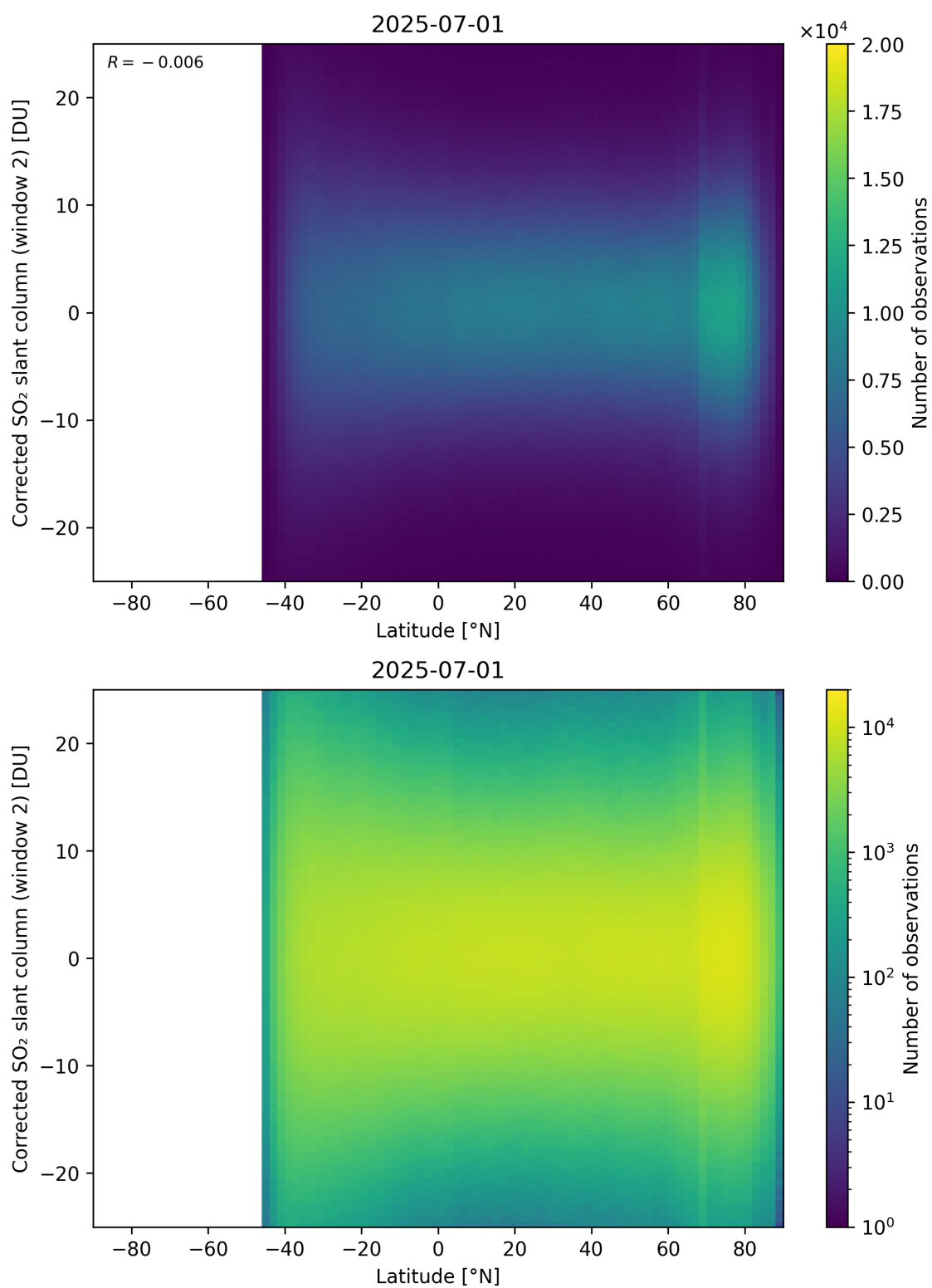
Figure 160: Scatter density plot of “Latitude” against “Corrected SO 2 slant column (window 2)” for 2025-06-30 to 2025-07-02.
