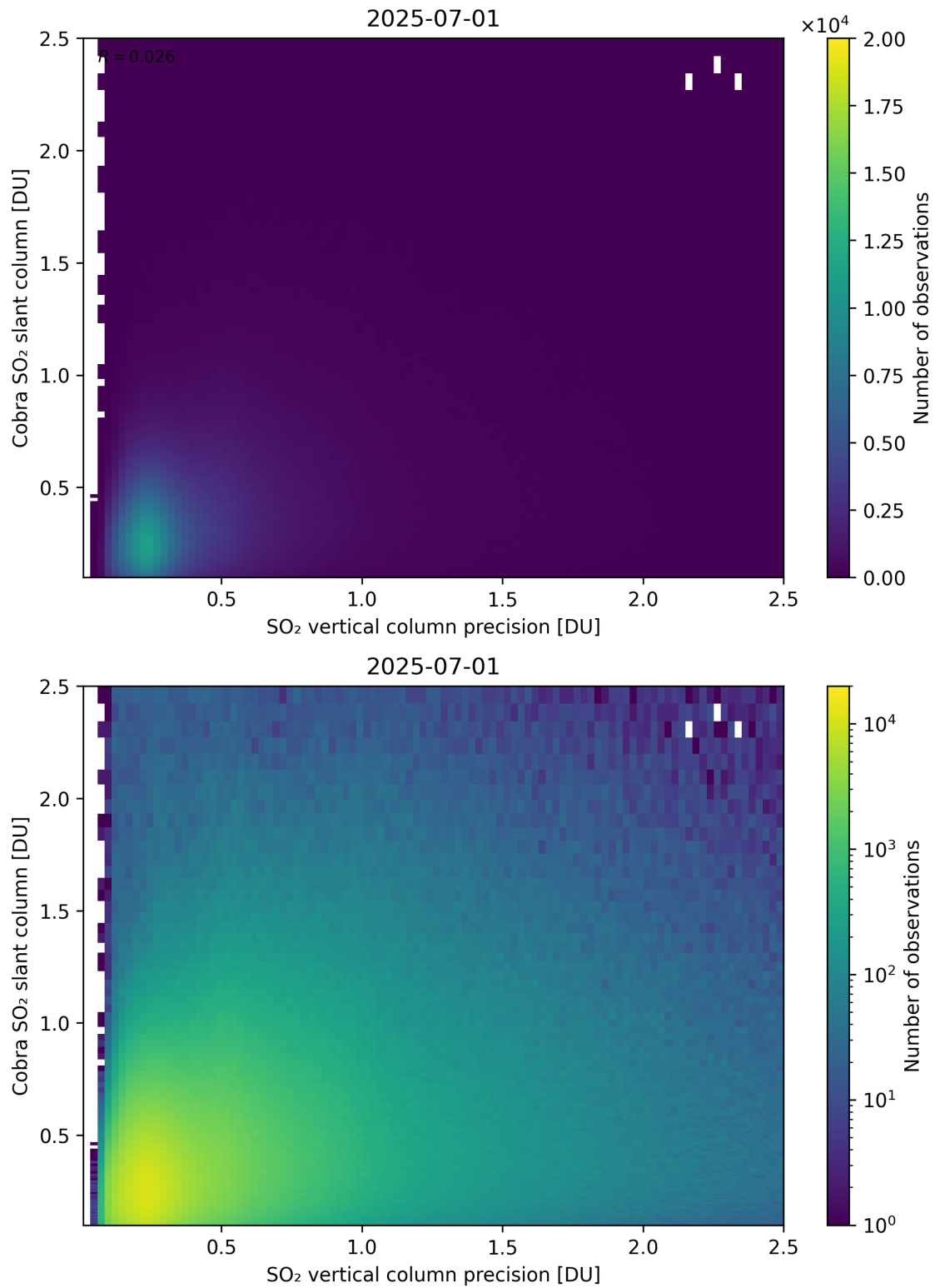
Figure 336: Scatter density plot of “SO 2 vertical column precision” against “Cobra SO 2 slant column” for 2025-06-30 to 2025-07-02.
