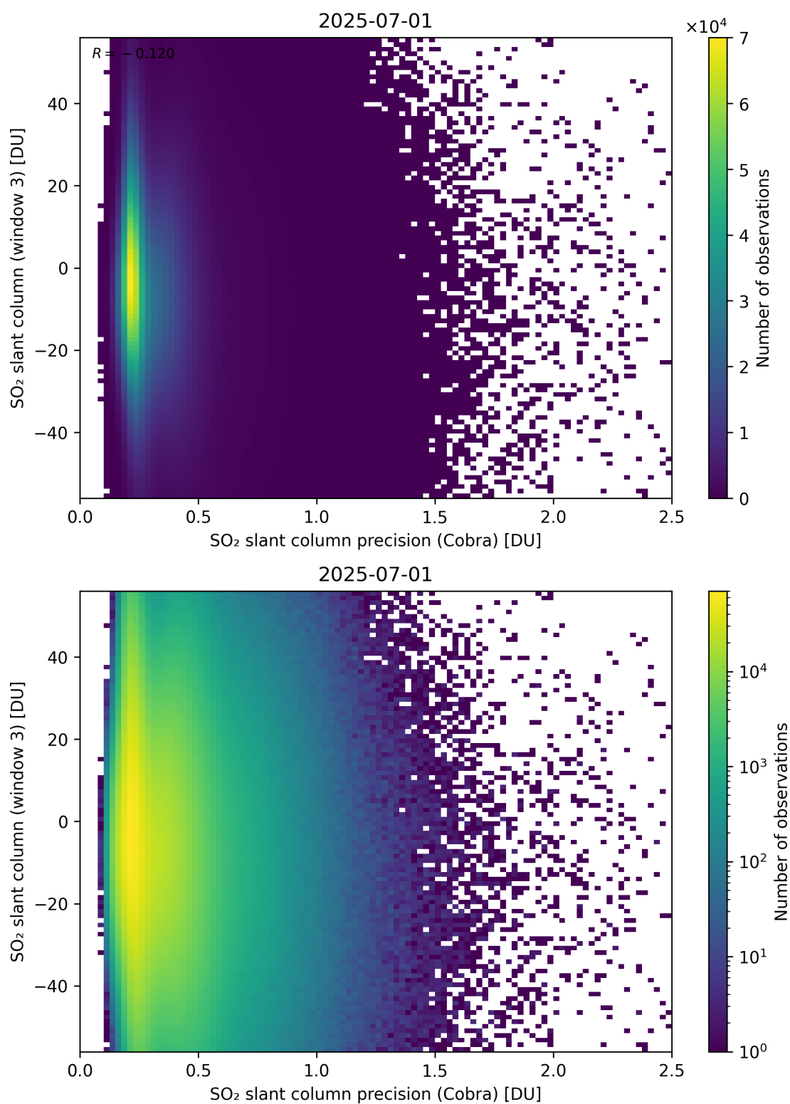
Figure 211: Scatter density plot of “SO 2 slant column precision (Cobra)” against “SO 2 slant column (window 3)” for 2025-06-30 to 2025-07-02.
