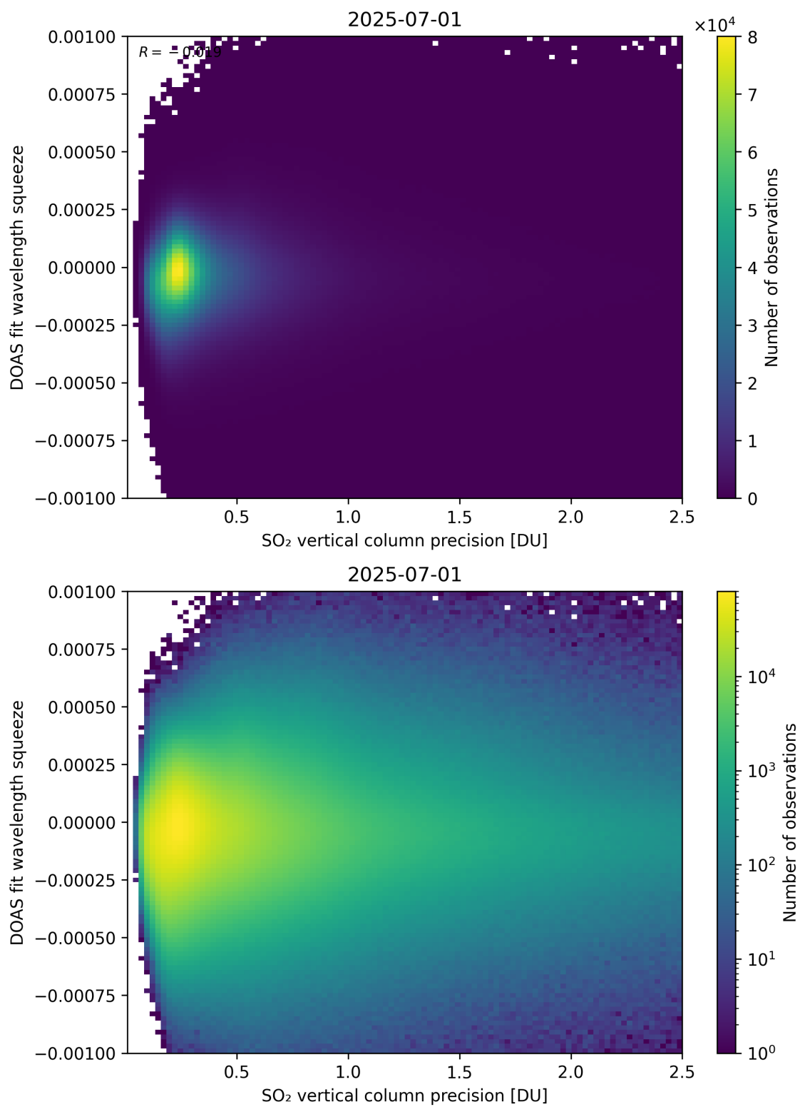
Figure 333: Scatter density plot of “SO 2 vertical column precision” against “DOAS fit wavelength squeeze” for 2025-06-30 to 2025-07-02.
