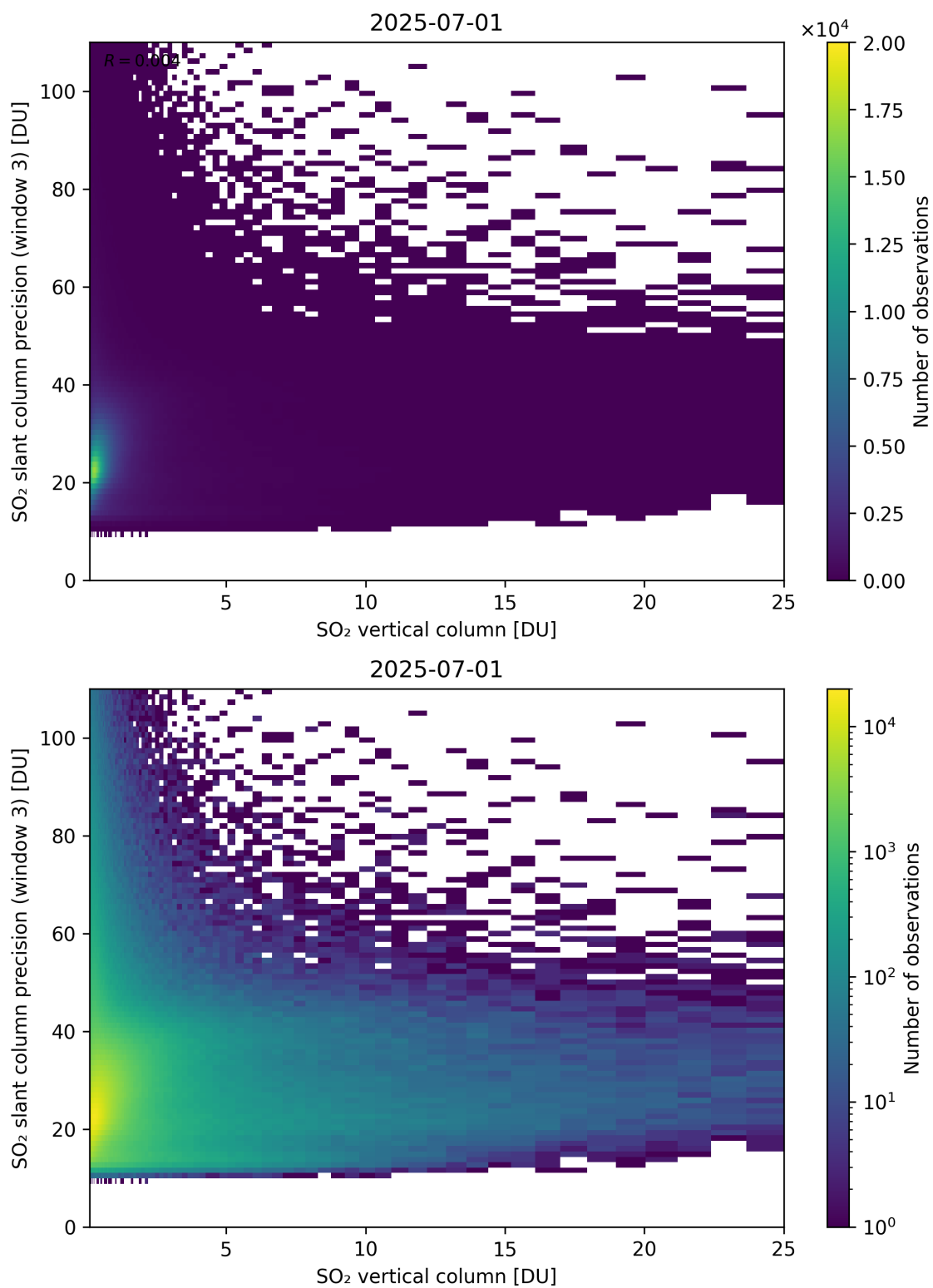
Figure 358: Scatter density plot of “SO 2 vertical column” against “SO 2 slant column precision (window 3)” for 2025-06-30 to 2025-07-02.
