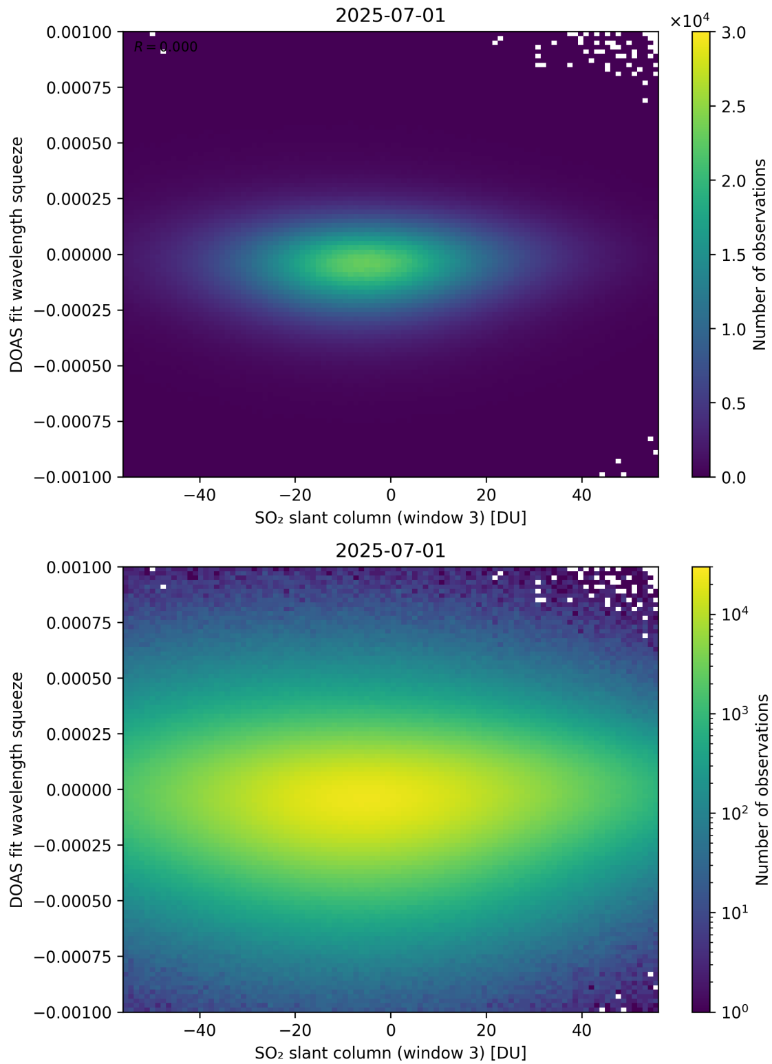
Figure 305: Scatter density plot of “SO 2 slant column (window 3)” against “DOAS fit wavelength squeeze” for 2025-06-30 to 2025-07-02.
