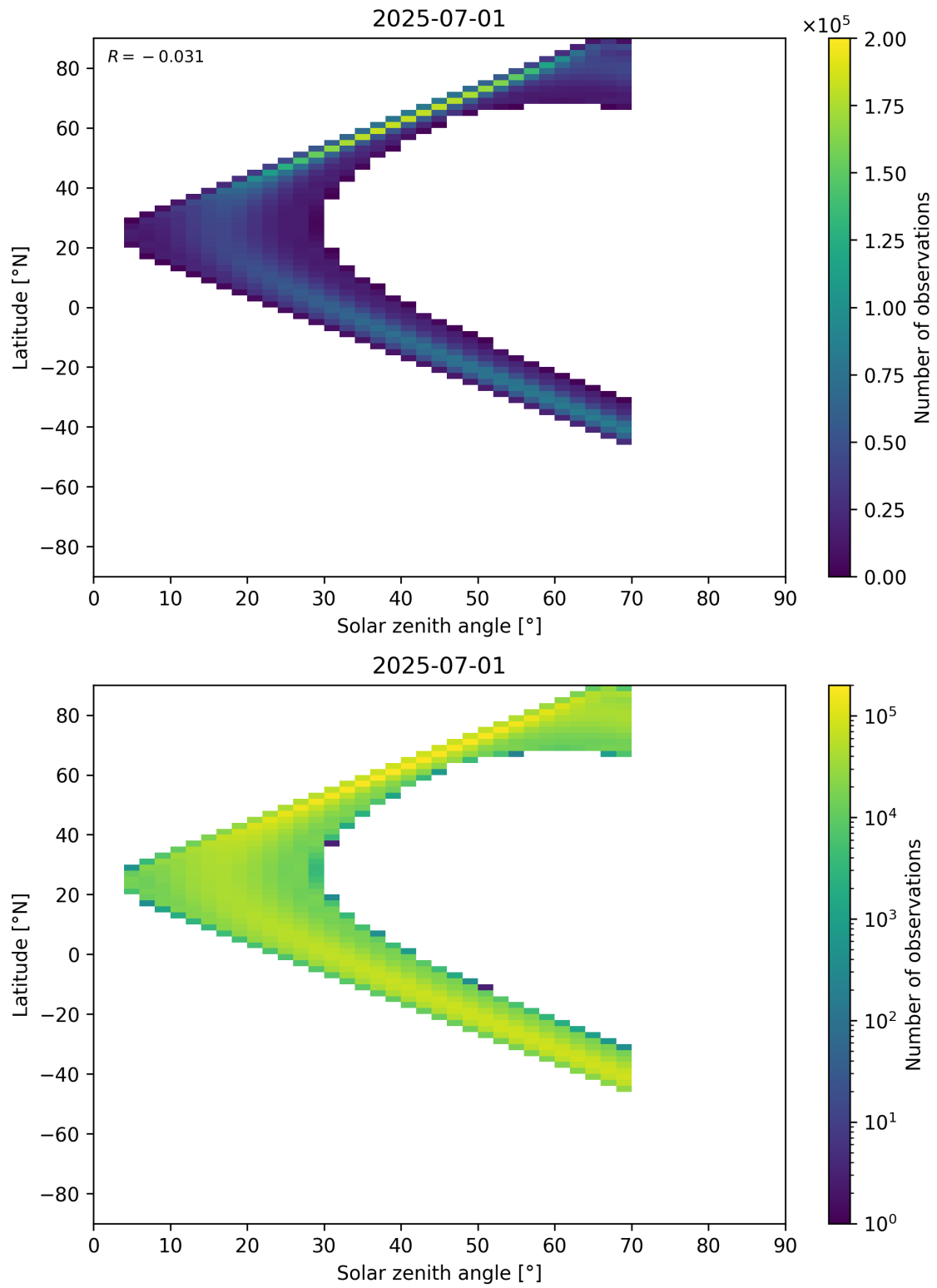
Figure 177: Scatter density plot of “Solar zenith angle” against “Latitude” for 2025-06-30 to 2025-07-02.
