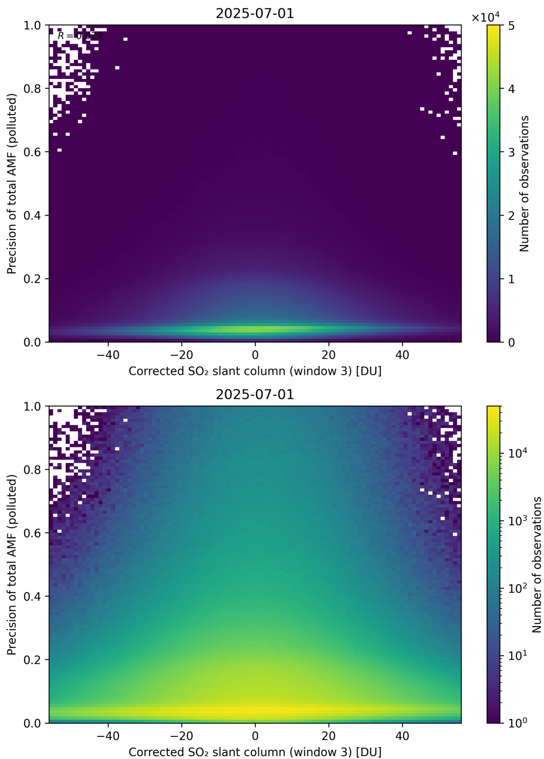
Figure 261: Scatter density plot of “Corrected SO 2 slant column (window 3)” against “Precision of total AMF (polluted)” for 2025-06-30 to 2025-07-02.
