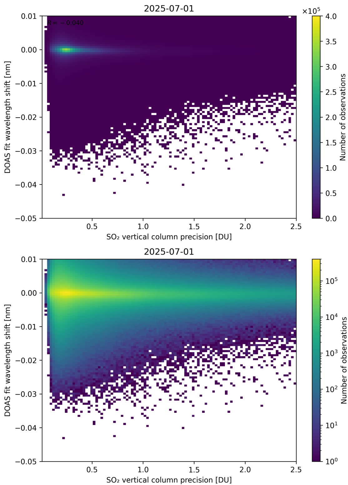
Figure 332: Scatter density plot of “SO 2 vertical column precision” against “DOAS fit wavelength shift” for 2025-06-30 to 2025-07-02.
