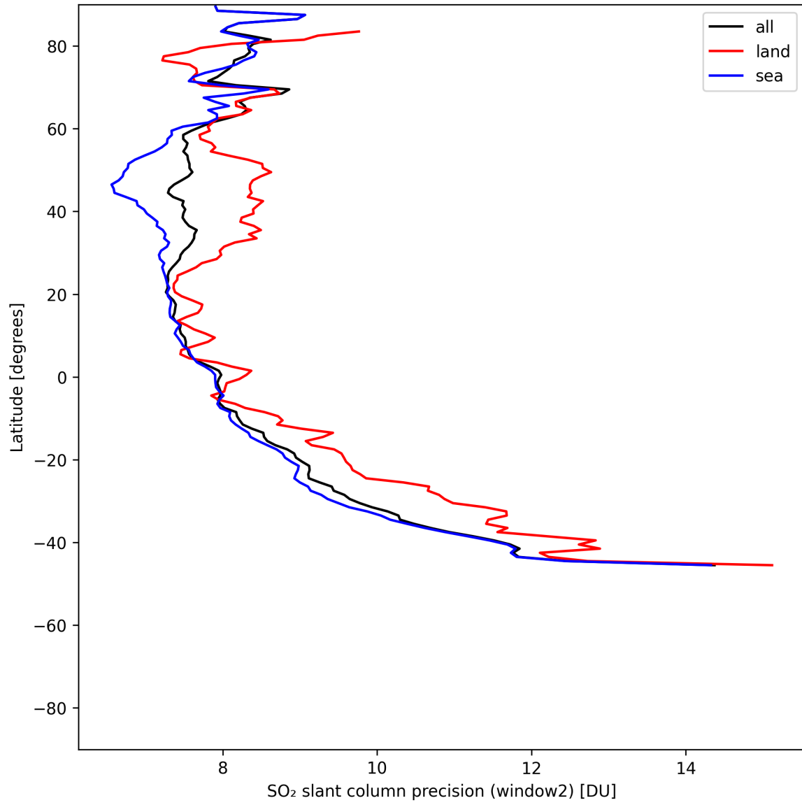
Figure 42: Zonal average of “SO 2 slant column precision (window2)” for 2025-06-30 to 2025-07-02.
