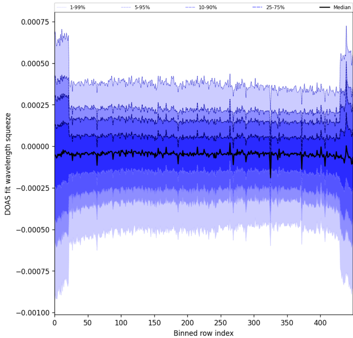
Figure 103: Along track statistics of “DOAS fit wavelength squeeze” for 2025-06-30 to 2025-07-02
