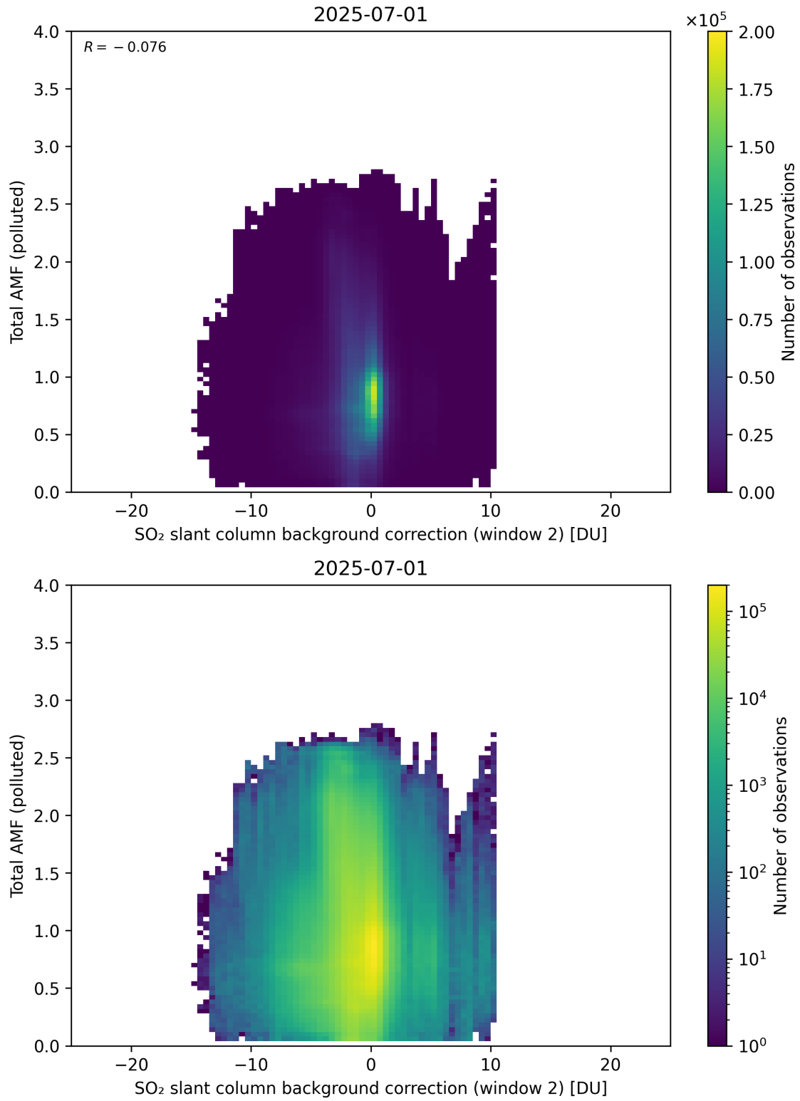
Figure 130: Scatter density plot of “SO 2 slant column background correction (window 2)” against “Total AMF (polluted)” for 2025-06-30 to 2025-07-02.
