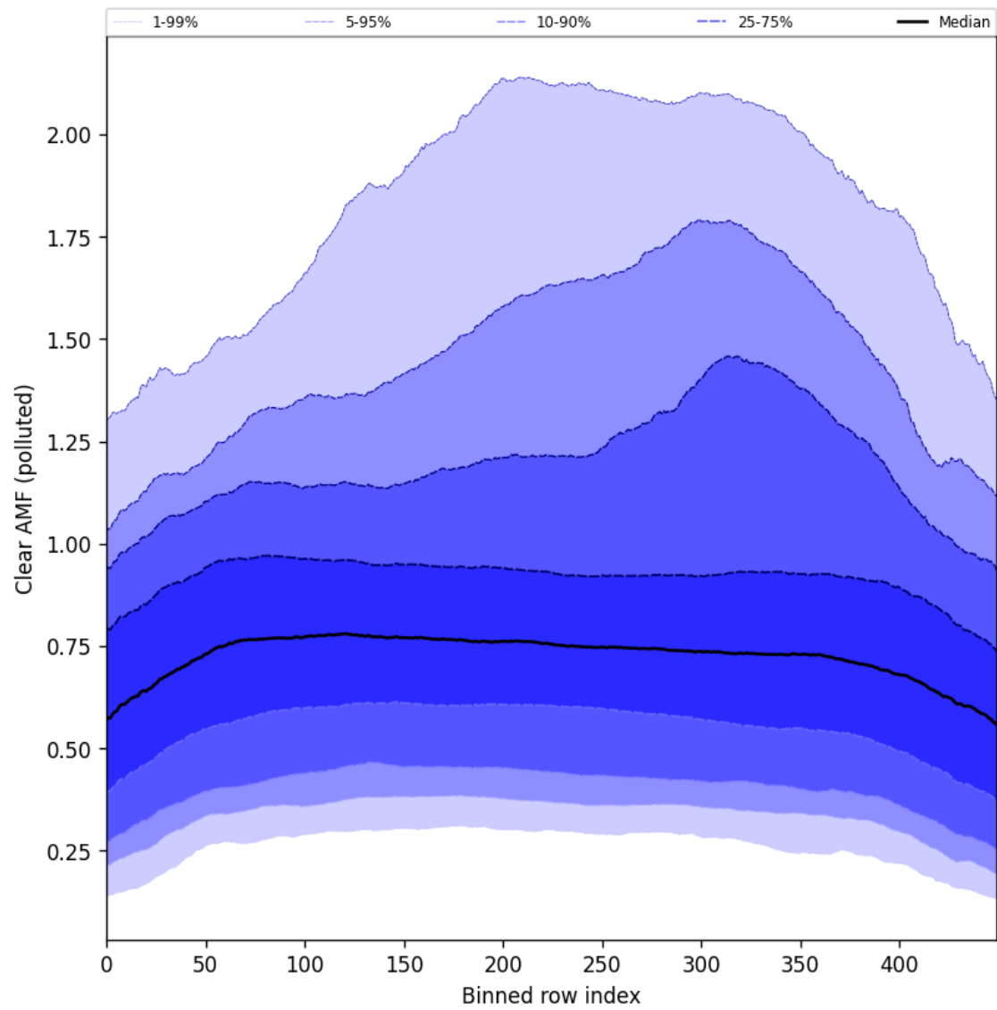
Figure 107: Along track statistics of “Clear AMF (polluted)” for 2025-06-30 to 2025-07-02
