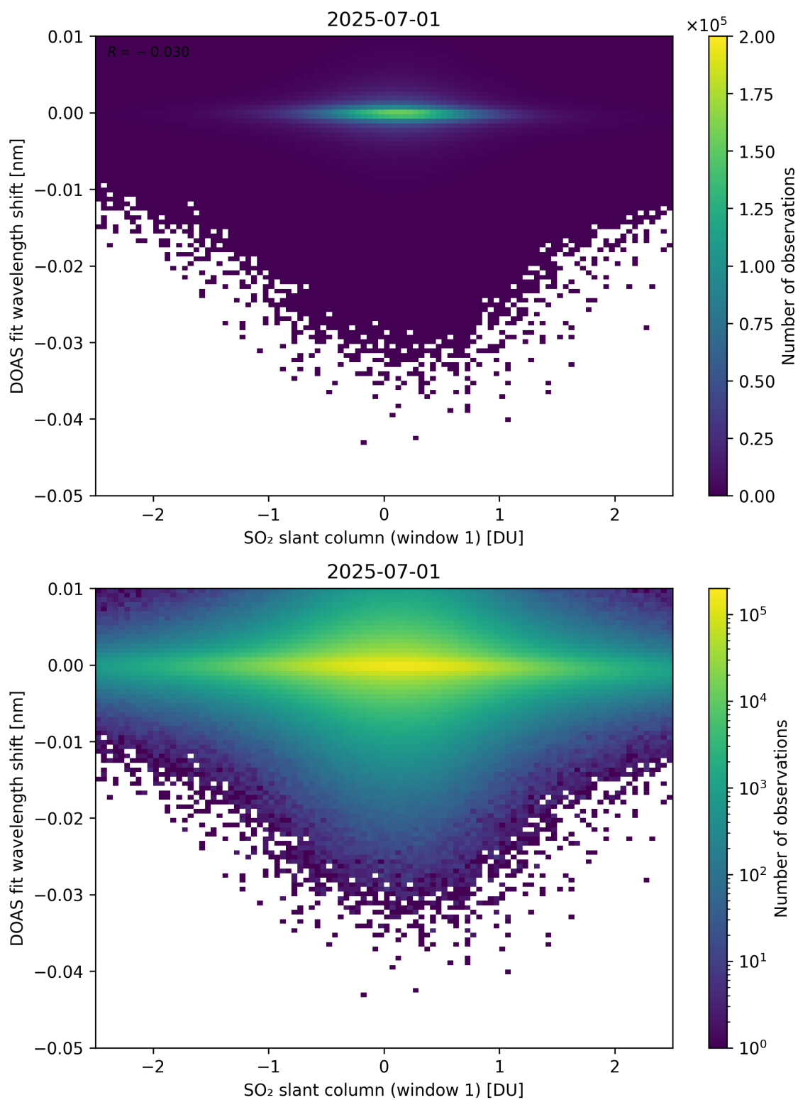
Figure 265: Scatter density plot of “SO 2 slant column (window 1)” against “DOAS fit wavelength shift” for 2025-06-30 to 2025-07-02.
