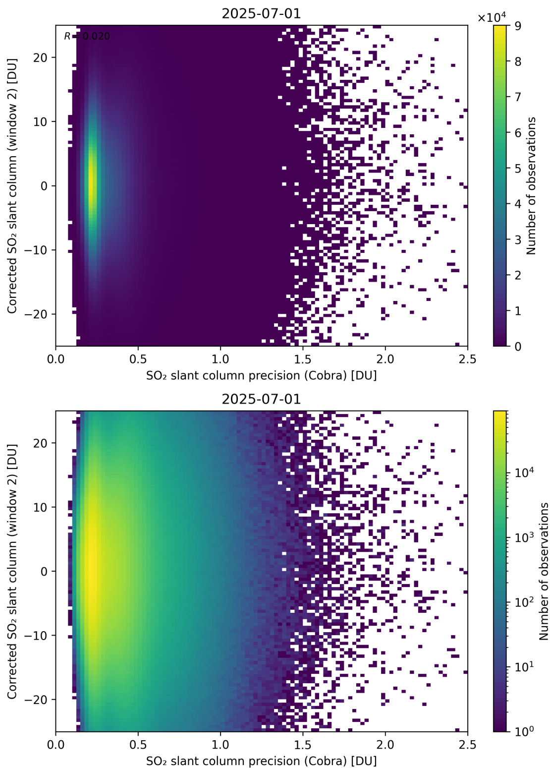
Figure 206: Scatter density plot of “SO 2 slant column precision (Cobra)” against “Corrected SO 2 slant column (window 2)” for 2025-06-30 to 2025-07-02.
