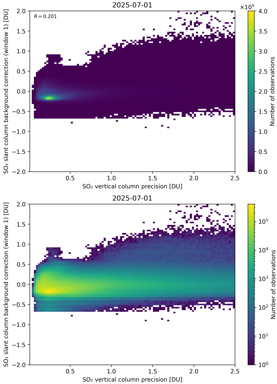
Figure 329: Scatter density plot of “SO 2 vertical column precision” against “SO 2 slant column background correction (window 1)” for 2025-06-30 to 2025-07-02.
