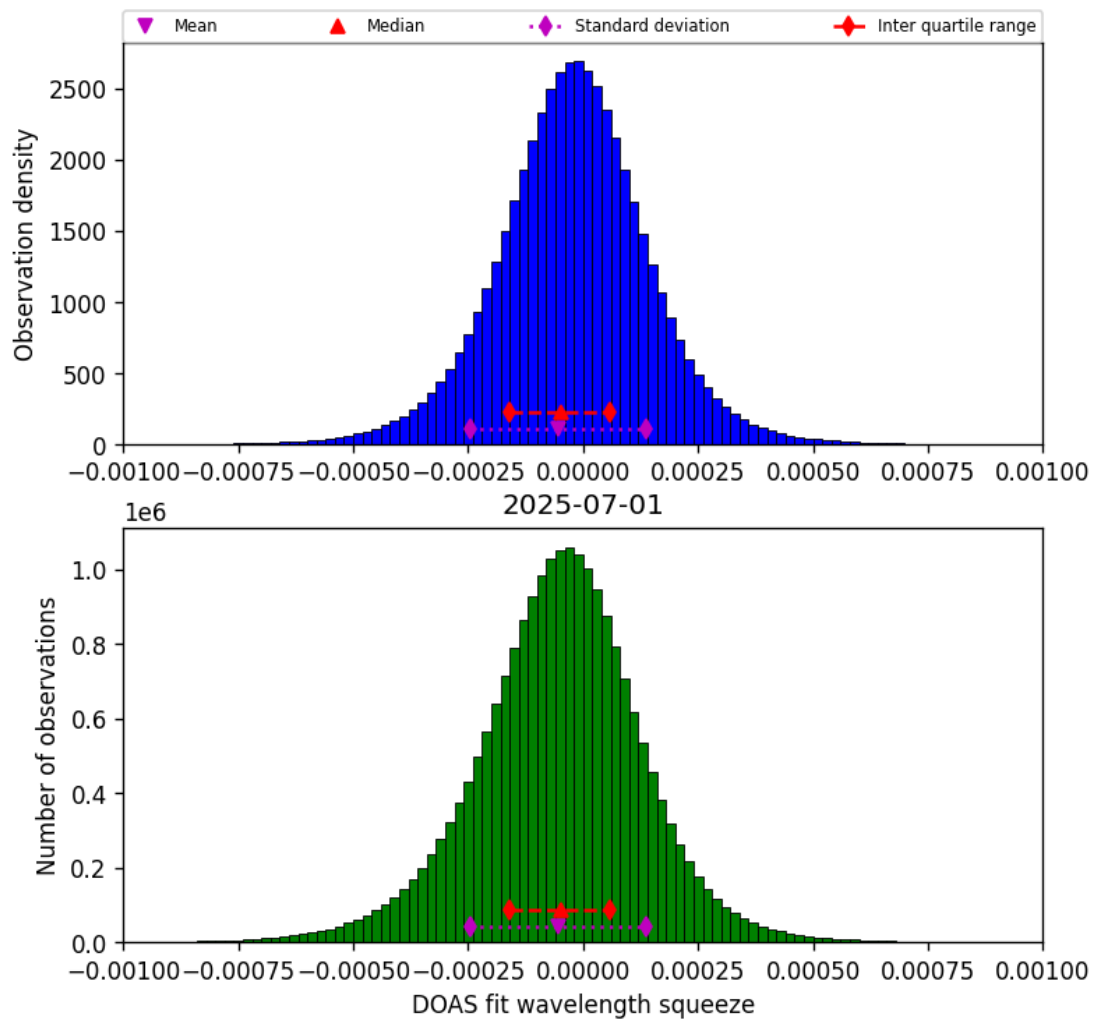
Figure 77: Histogram of “DOAS fit wavelength squeeze” for 2025-06-30 to 2025-07-02
