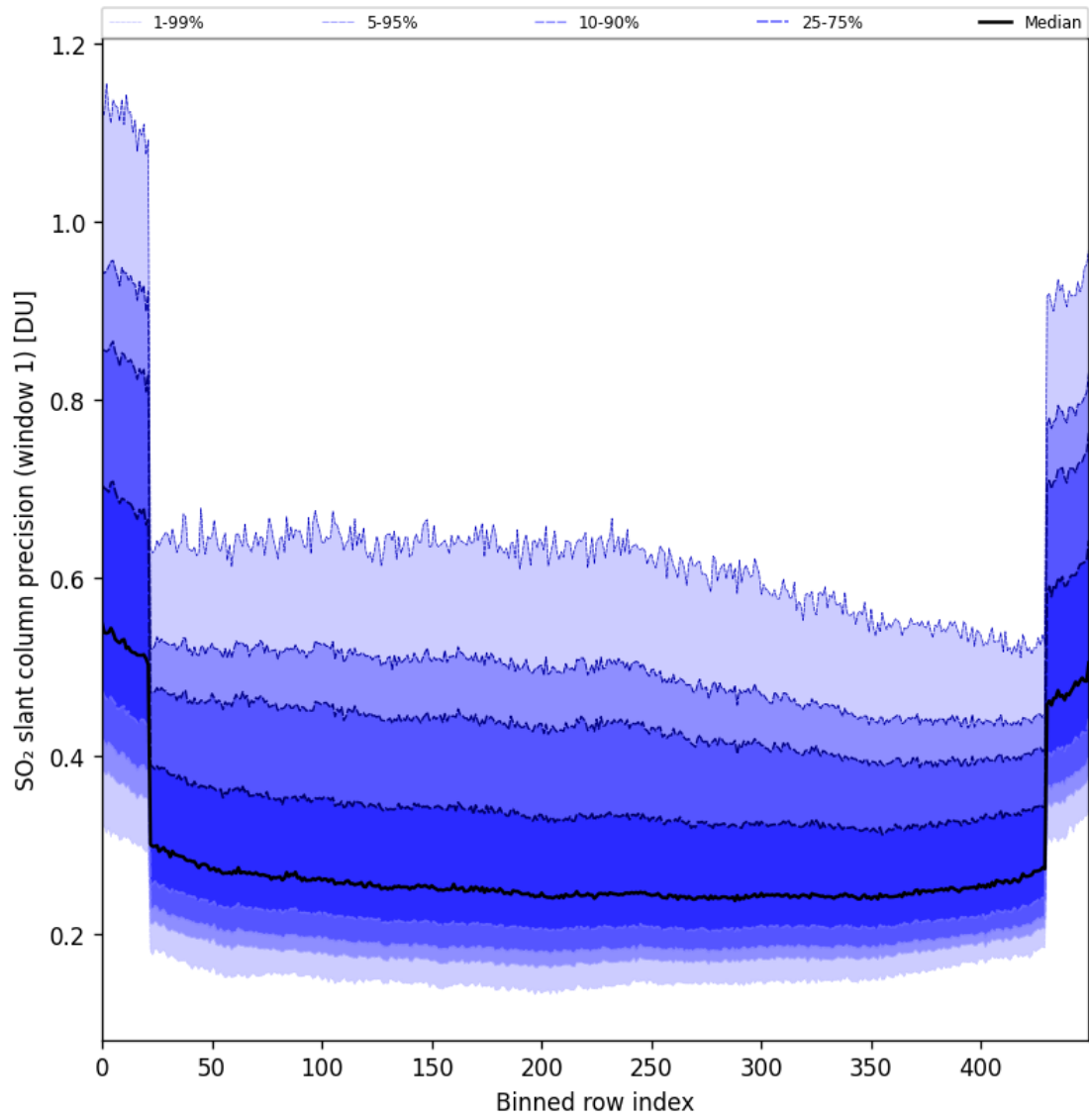
Figure 90: Along track statistics of “SO 2 slant column precision (window 1)” for 2025-06-30 to 2025-07-02
