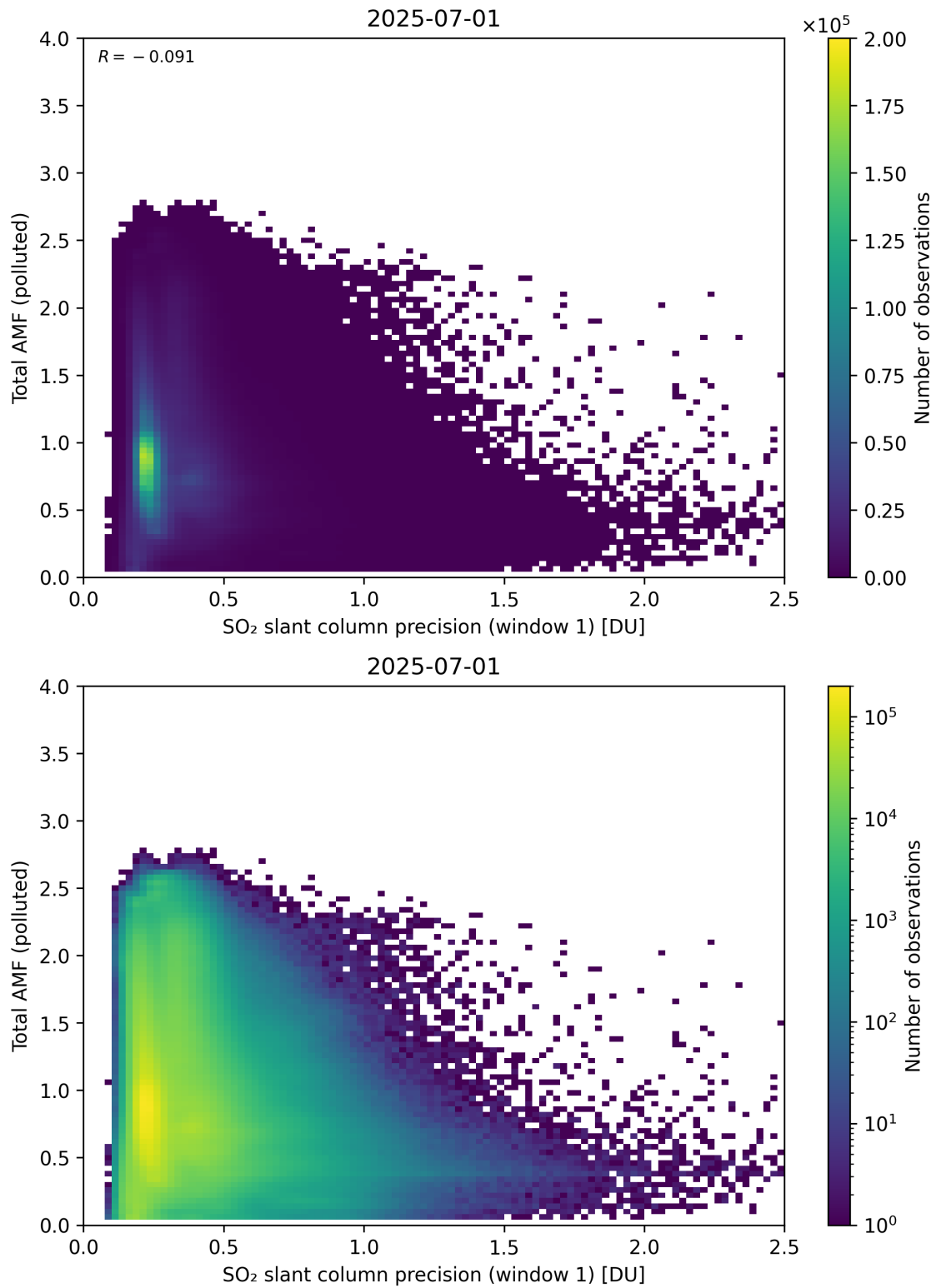
Figure 280: Scatter density plot of “SO 2 slant column precision (window 1)” against “Total AMF (polluted)” for 2025-06-30 to 2025-07-02.
