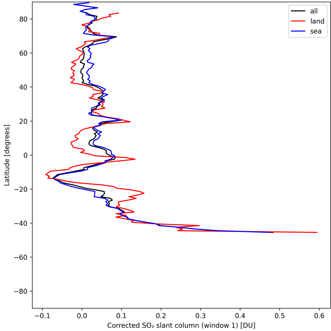
Figure 39: Zonal average of “Corrected SO 2 slant column (window 1)” for 2025-06-30 to 2025-07-02.
