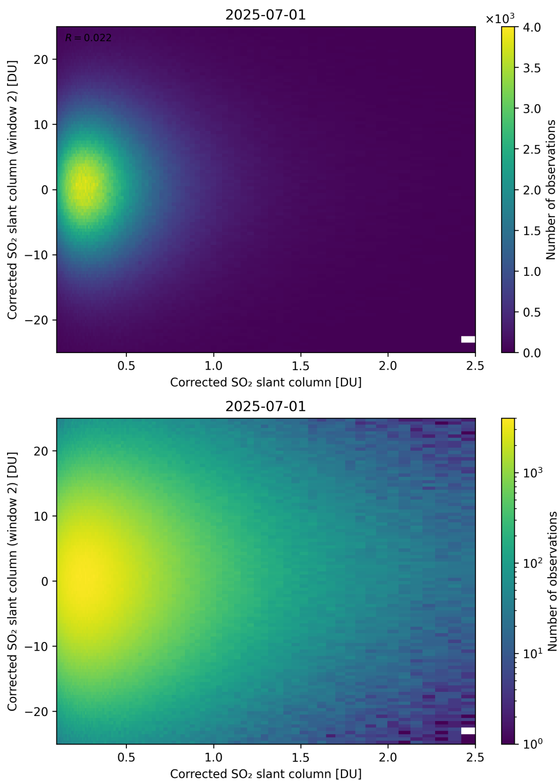
Figure 235: Scatter density plot of “Corrected SO 2 slant column” against “Corrected SO 2 slant column (window 2)” for 2025-06-30 to 2025-07-02.
