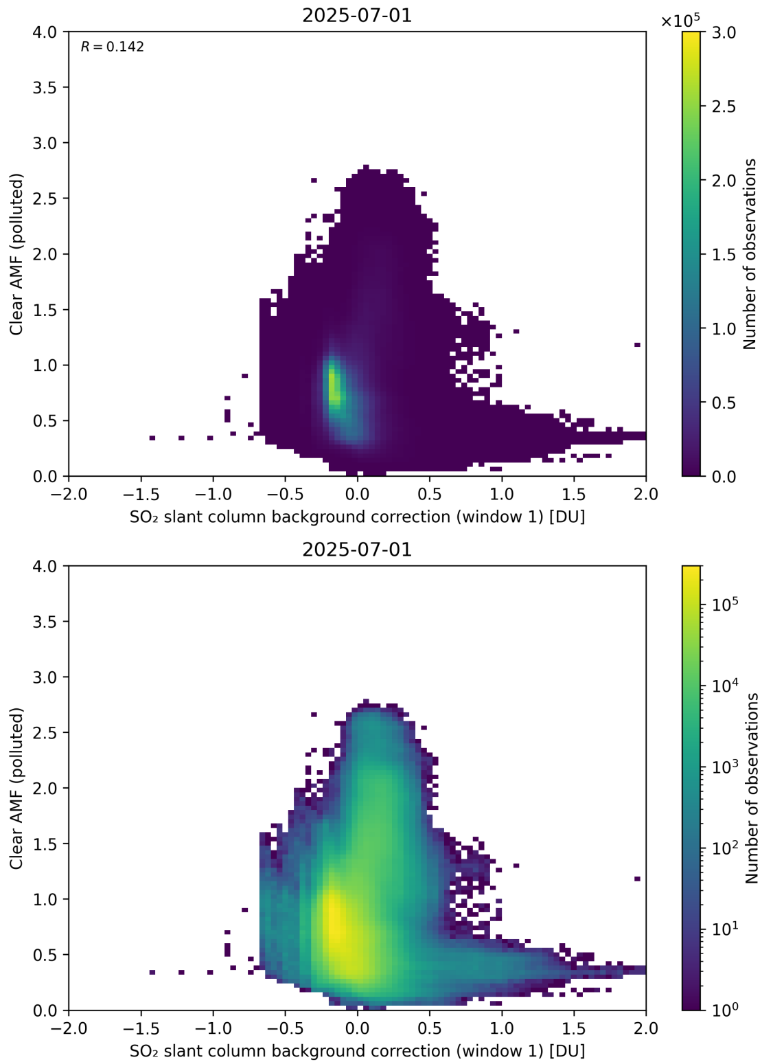
Figure 114: Scatter density plot of “SO 2 slant column background correction (window 1)” against “Clear AMF (polluted)” for 2025-06-30 to 2025-07-02.
