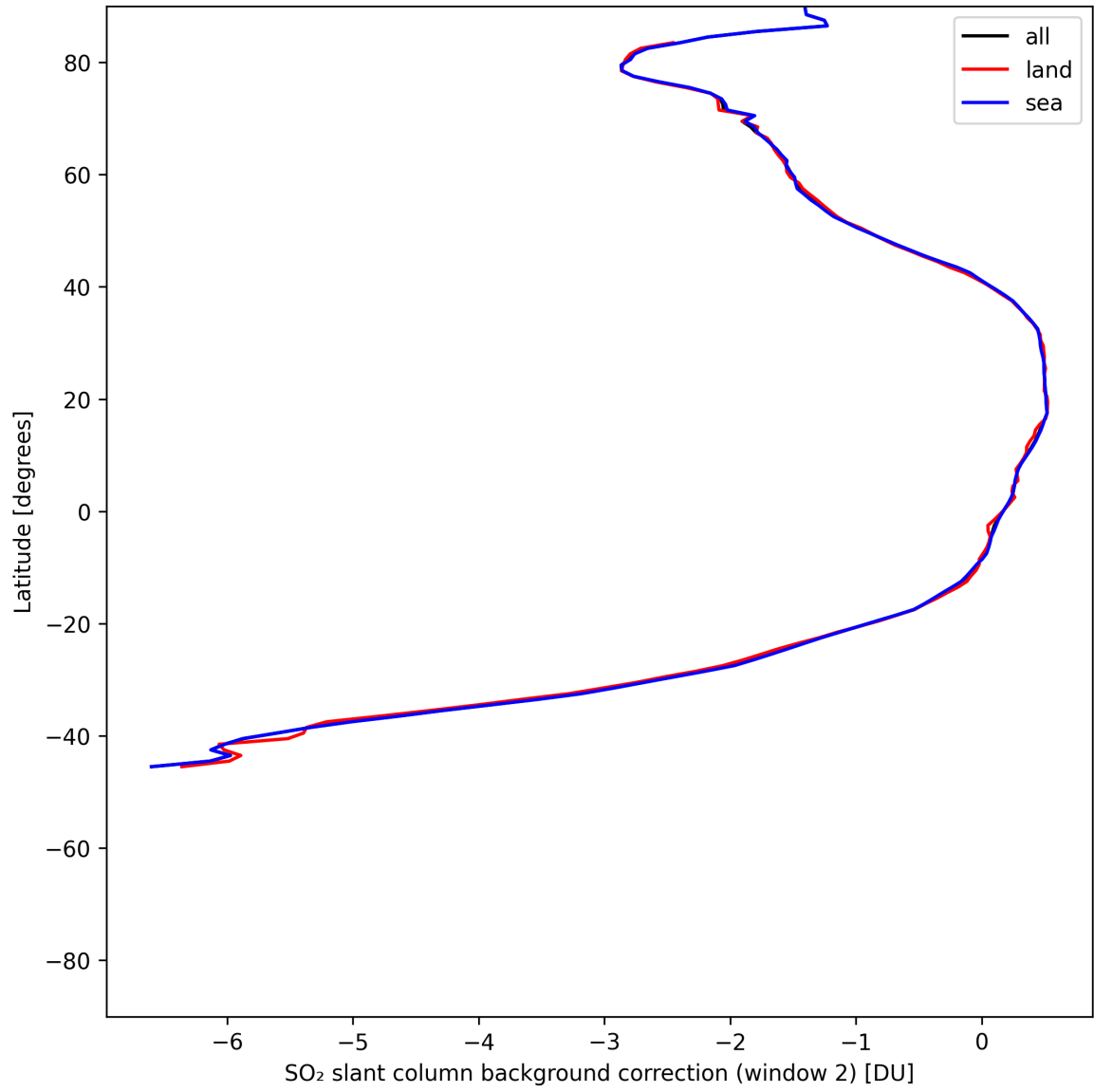
Figure 44: Zonal average of “SO 2 slant column background correction (window 2)” for 2025-06-30 to 2025-07-02.
