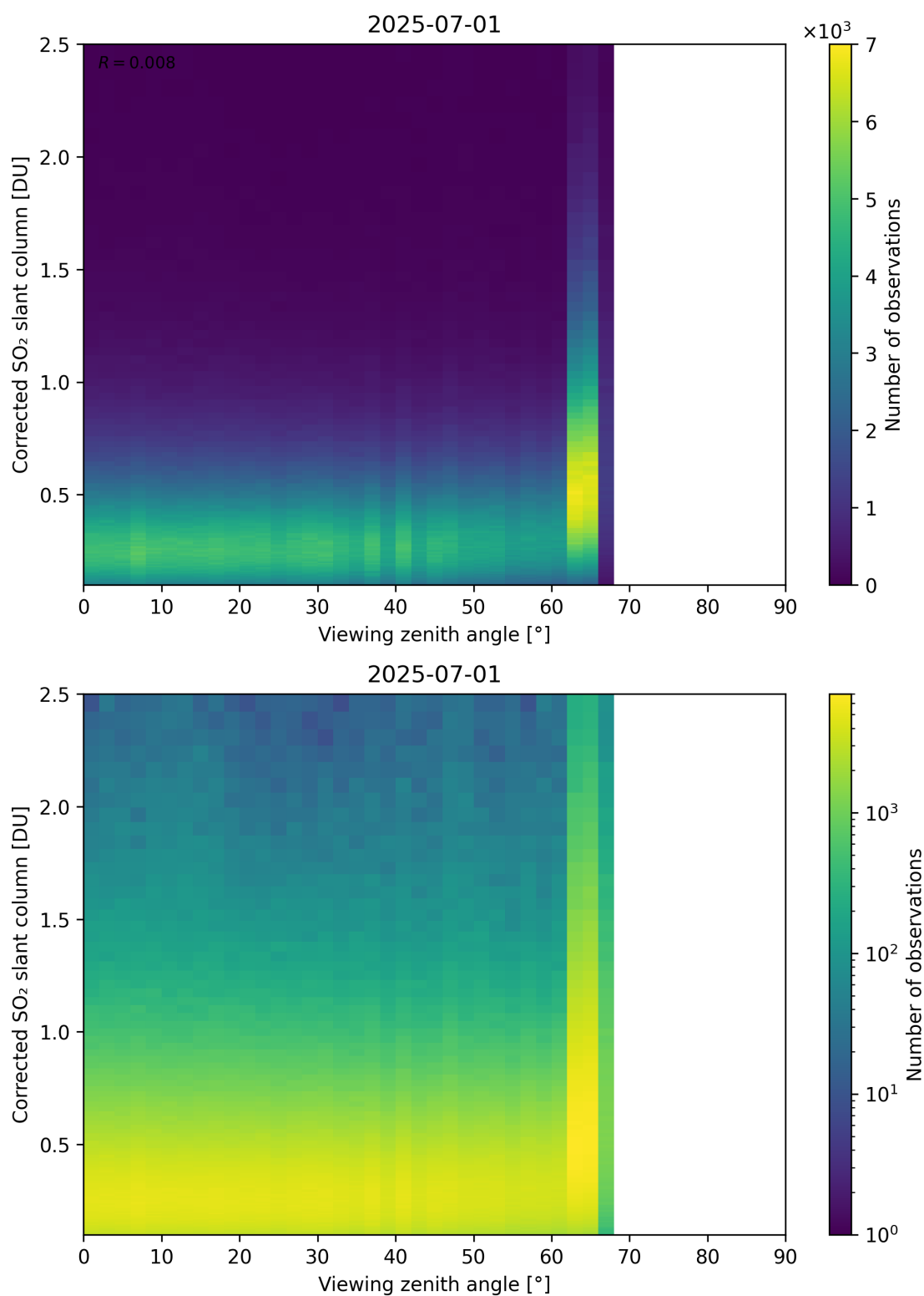
Figure 373: Scatter density plot of “Viewing zenith angle” against “Corrected SO 2 slant column” for 2025-06-30 to 2025-07-02.
