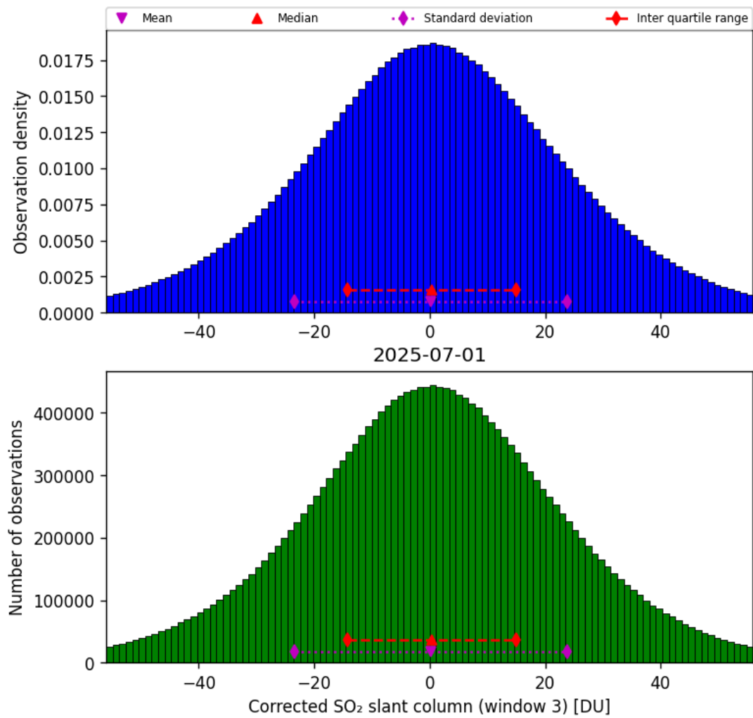
Figure 73: Histogram of “Corrected SO 2 slant column (window 3)” for 2025-06-30 to 2025-07-02
