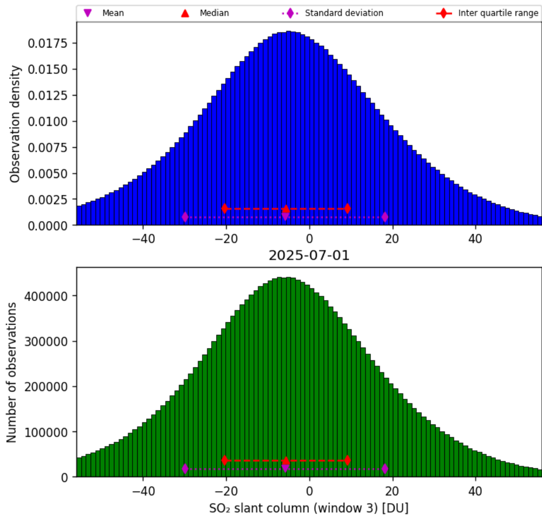
Figure 71: Histogram of “SO 2 slant column (window 3)” for 2025-06-30 to 2025-07-02
