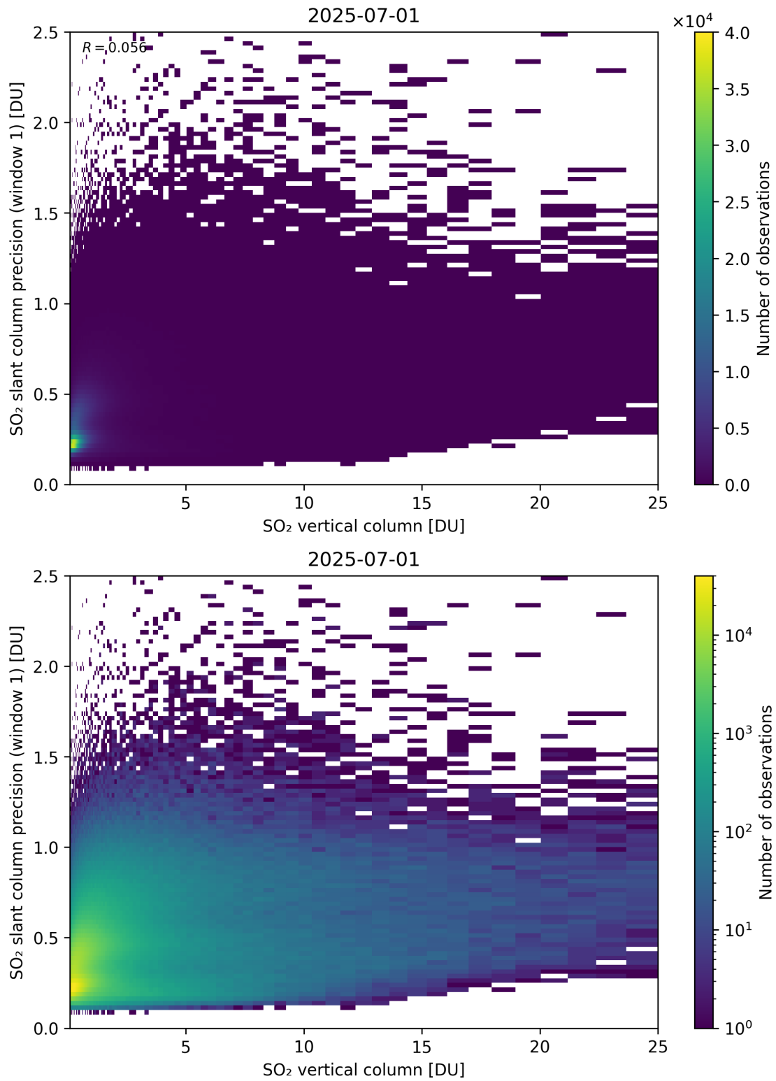
Figure 355: Scatter density plot of “SO 2 vertical column” against “SO 2 slant column precision (window 1)” for 2025-06-30 to 2025-07-02.
