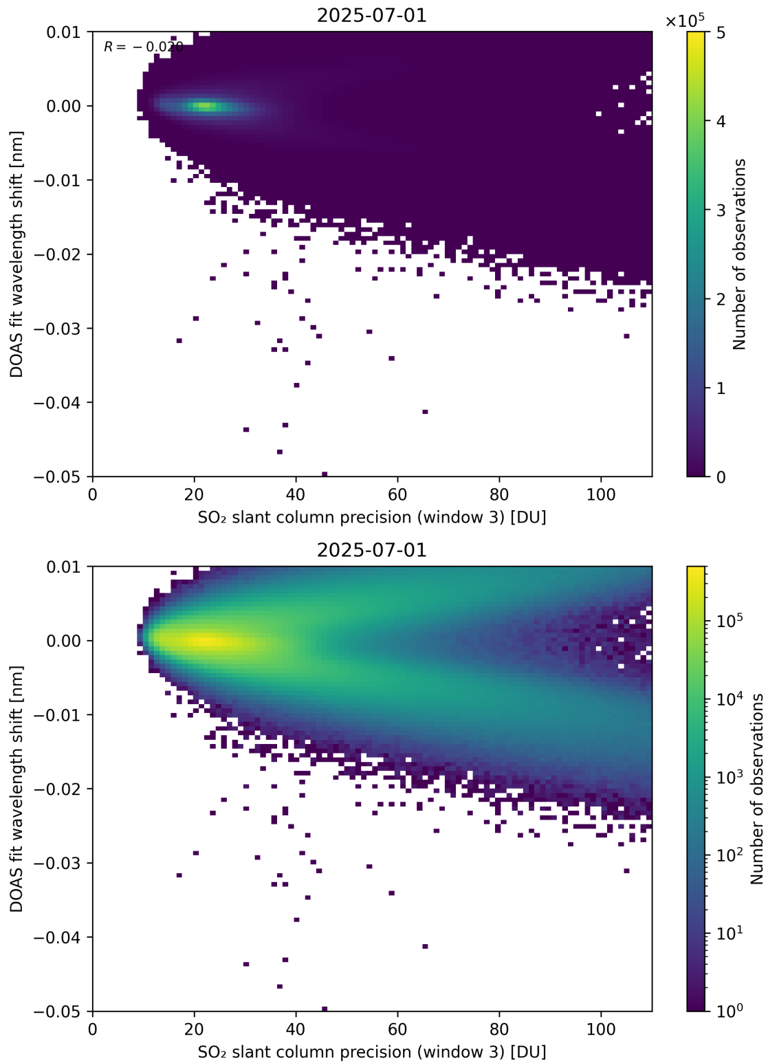
Figure 308: Scatter density plot of “SO 2 slant column precision (window 3)” against “DOAS fit wavelength shift” for 2025-06-30 to 2025-07-02.
