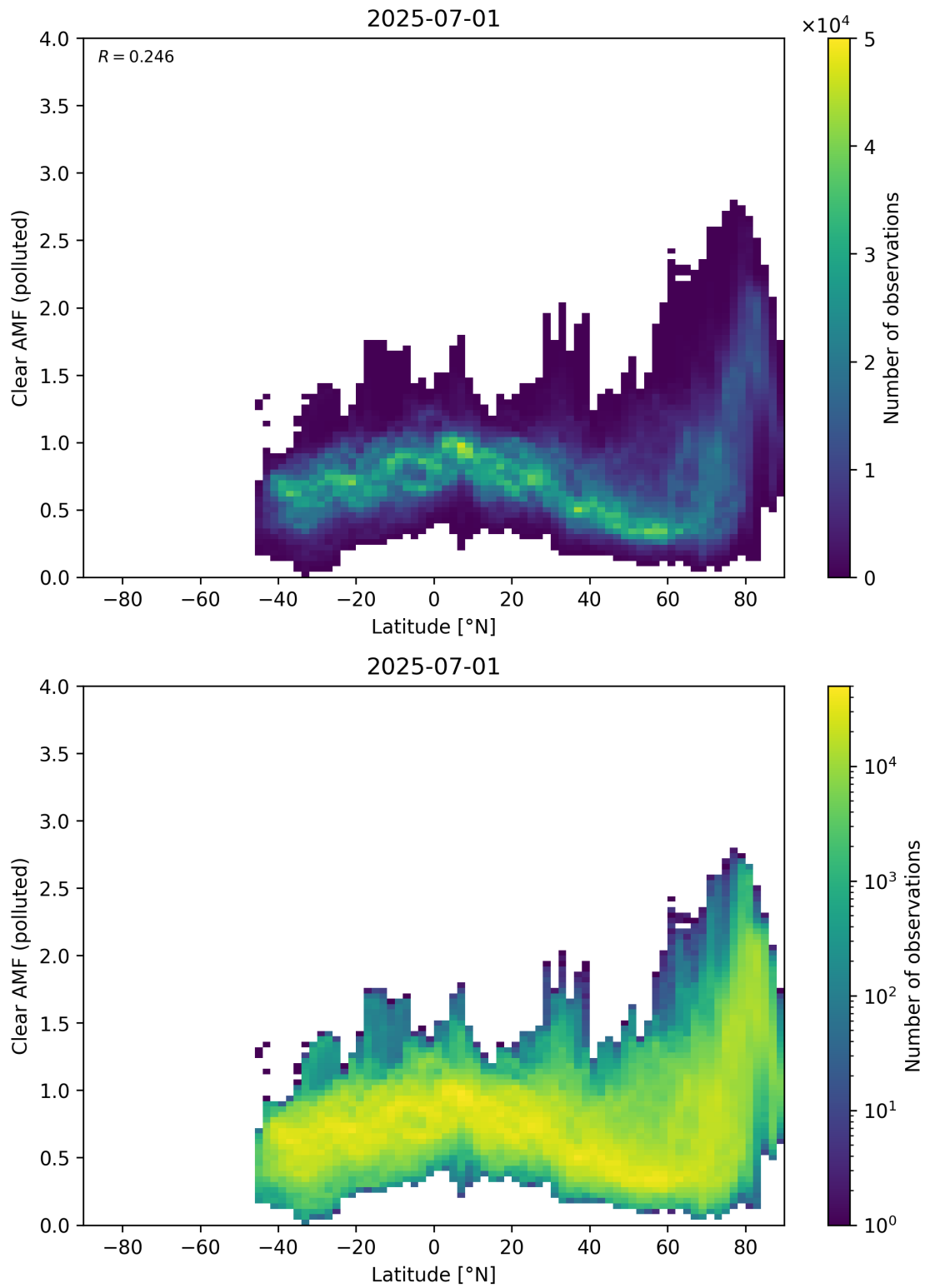
Figure 156: Scatter density plot of “Latitude” against “Clear AMF (polluted)” for 2025-06-30 to 2025-07-02.
