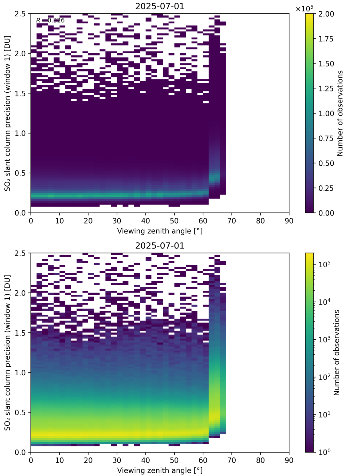
Figure 377: Scatter density plot of “Viewing zenith angle” against “SO 2 slant column precision (window 1)” for 2025-06-30 to 2025-07-02.
