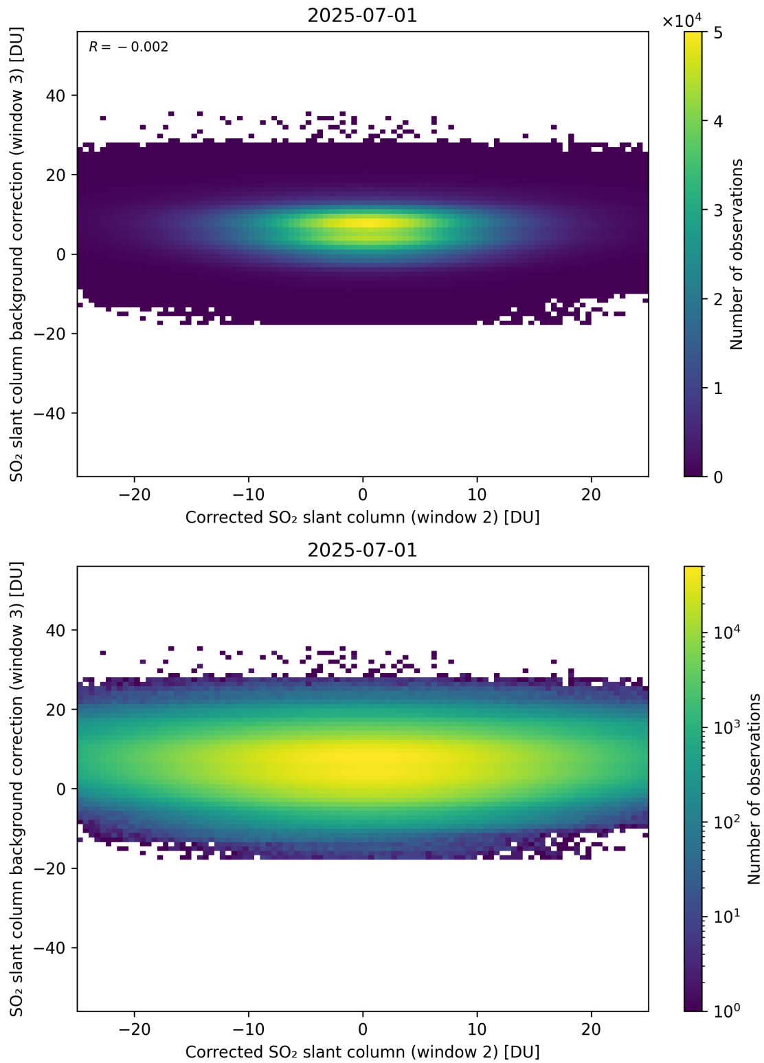
Figure 245: Scatter density plot of “Corrected SO 2 slant column (window 2)” against “SO 2 slant column background correction (window 3)” for 2025-06-30 to 2025-07-02.
