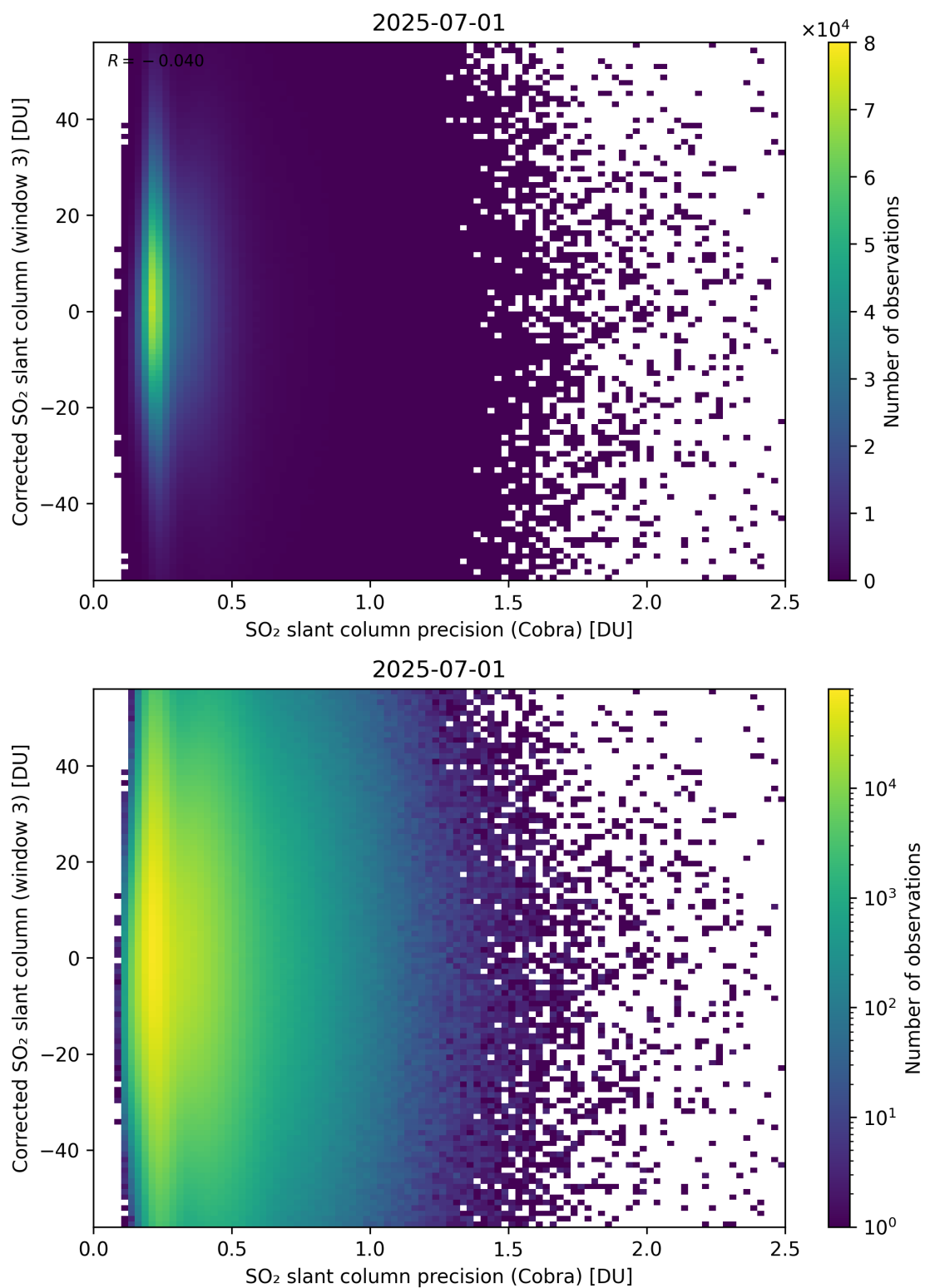
Figure 207: Scatter density plot of “SO 2 slant column precision (Cobra)” against “Corrected SO 2 slant column (window 3)” for 2025-06-30 to 2025-07-02.
