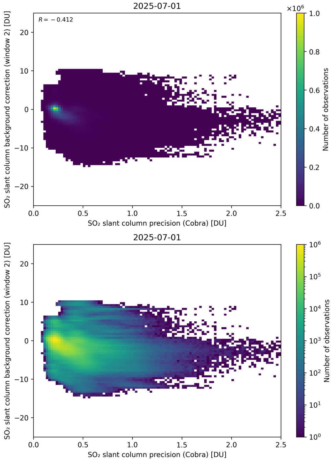
Figure 200: Scatter density plot of “SO 2 slant column precision (Cobra)” against “SO 2 slant column background correction (window 2)” for 2025-06-30 to 2025-07-02.
