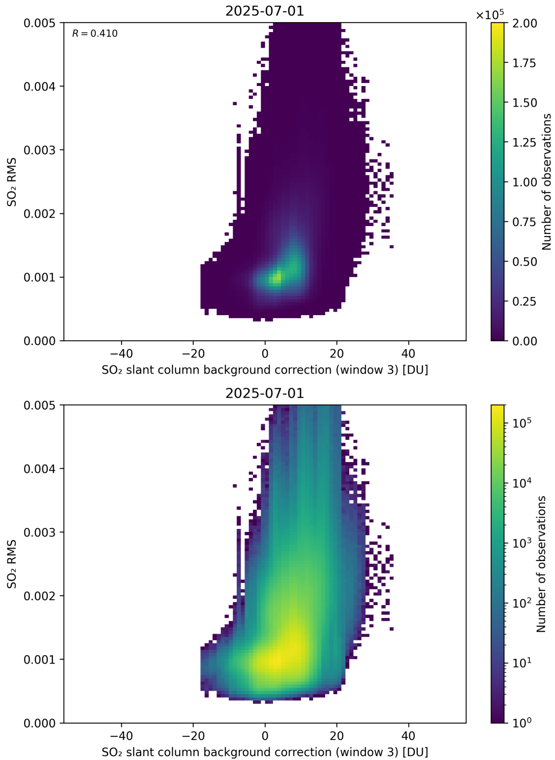
Figure 134: Scatter density plot of “SO 2 slant column background correction (window 3)” against “SO 2 RMS” for 2025-06-30 to 2025-07-02.
