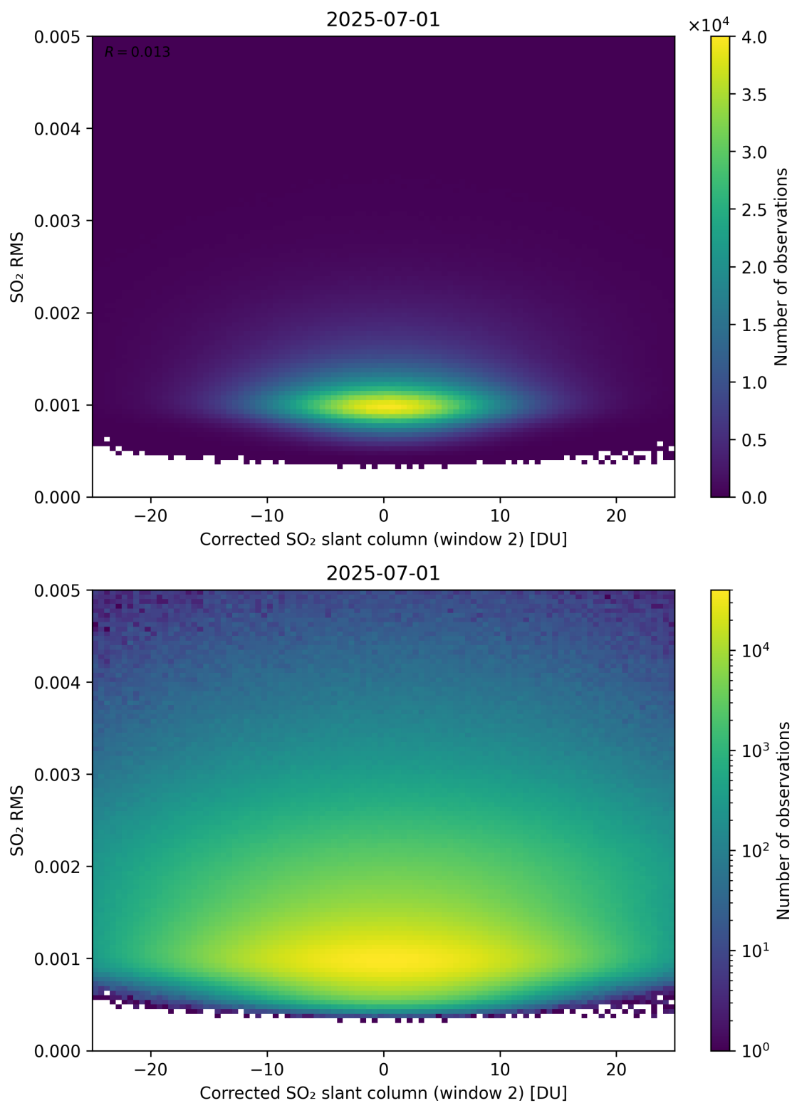
Figure 248: Scatter density plot of “Corrected SO 2 slant column (window 2)” against “SO 2 RMS” for 2025-06-30 to 2025-07-02.
