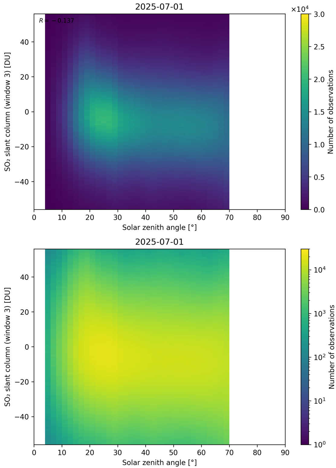
Figure 187: Scatter density plot of “Solar zenith angle” against “SO 2 slant column (window 3)” for 2025-06-30 to 2025-07-02.
