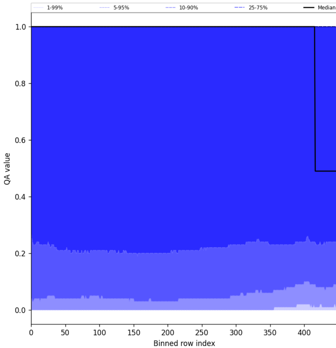
Figure 83: Along track statistics of “QA value” for 2025-06-30 to 2025-07-02
