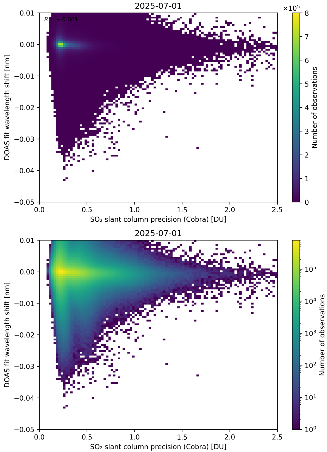
Figure 202: Scatter density plot of “SO 2 slant column precision (Cobra)” against “DOAS fit wavelength shift” for 2025-06-30 to 2025-07-02.
