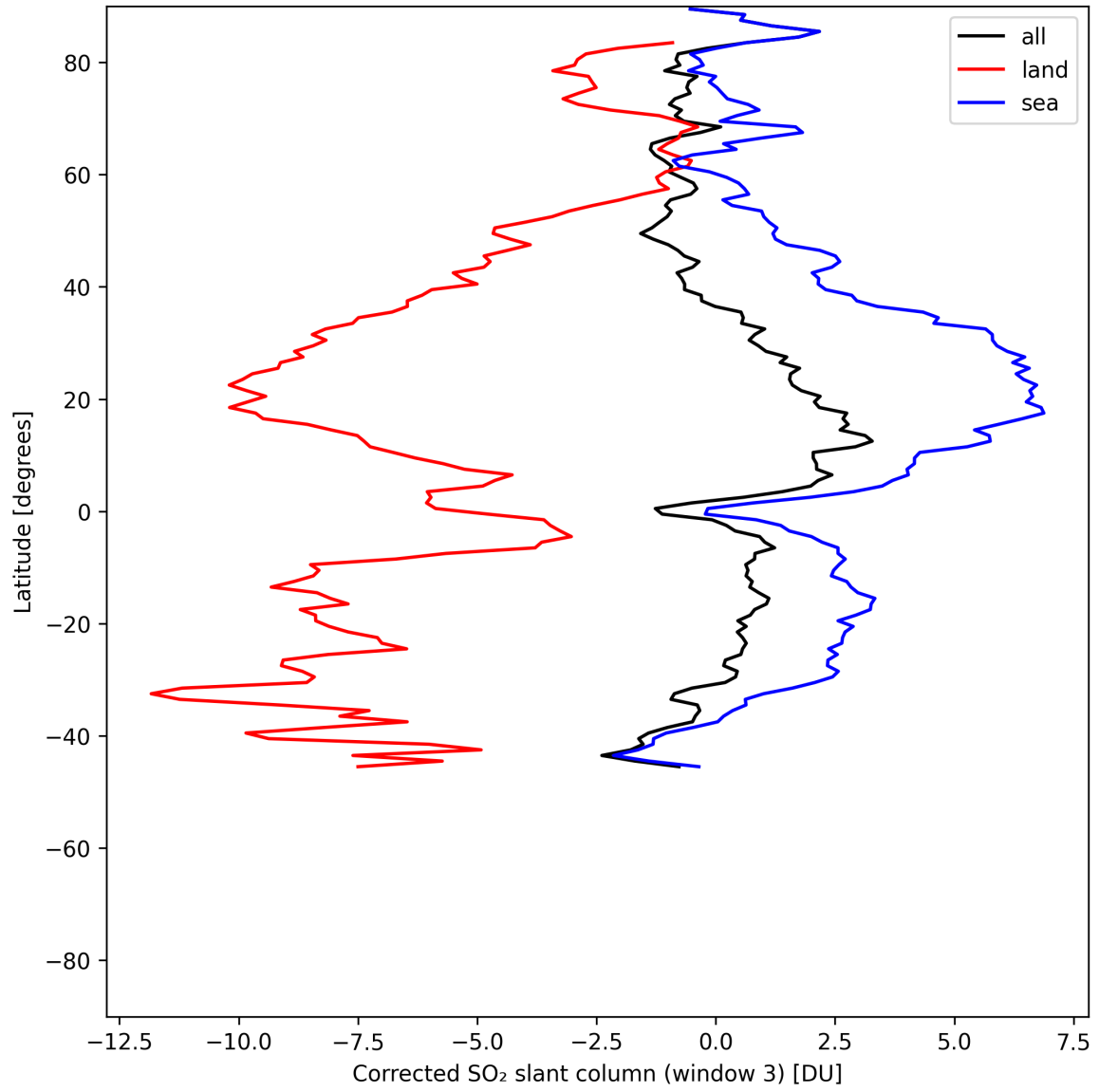
Figure 47: Zonal average of “Corrected SO 2 slant column (window 3)” for 2025-06-30 to 2025-07-02.
