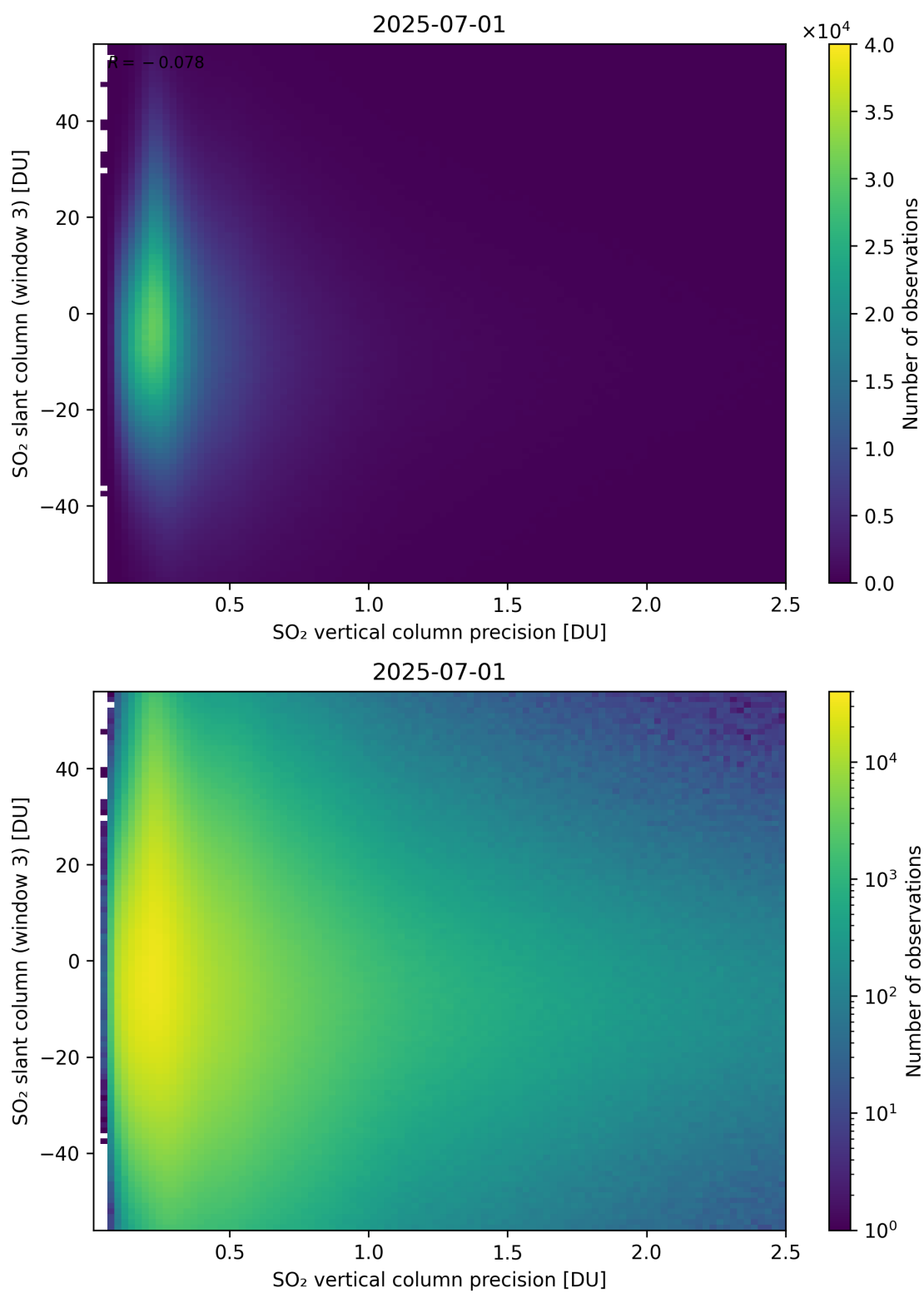
Figure 344: Scatter density plot of “SO 2 vertical column precision” against “SO 2 slant column (window 3)” for 2025-06-30 to 2025-07-02.
