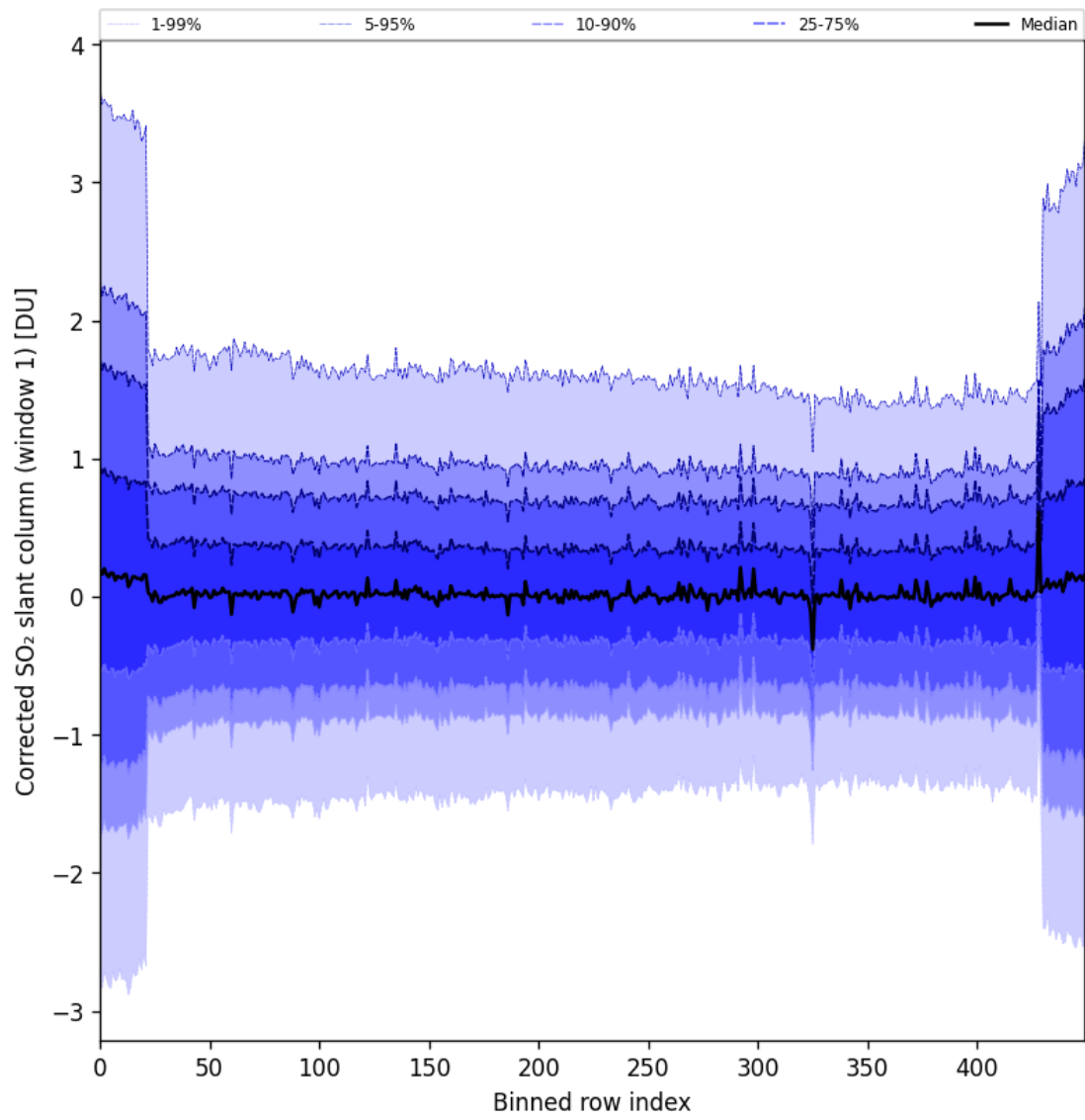
Figure 91: Along track statistics of “Corrected SO 2 slant column (window 1)” for 2025-06-30 to 2025-07-02
