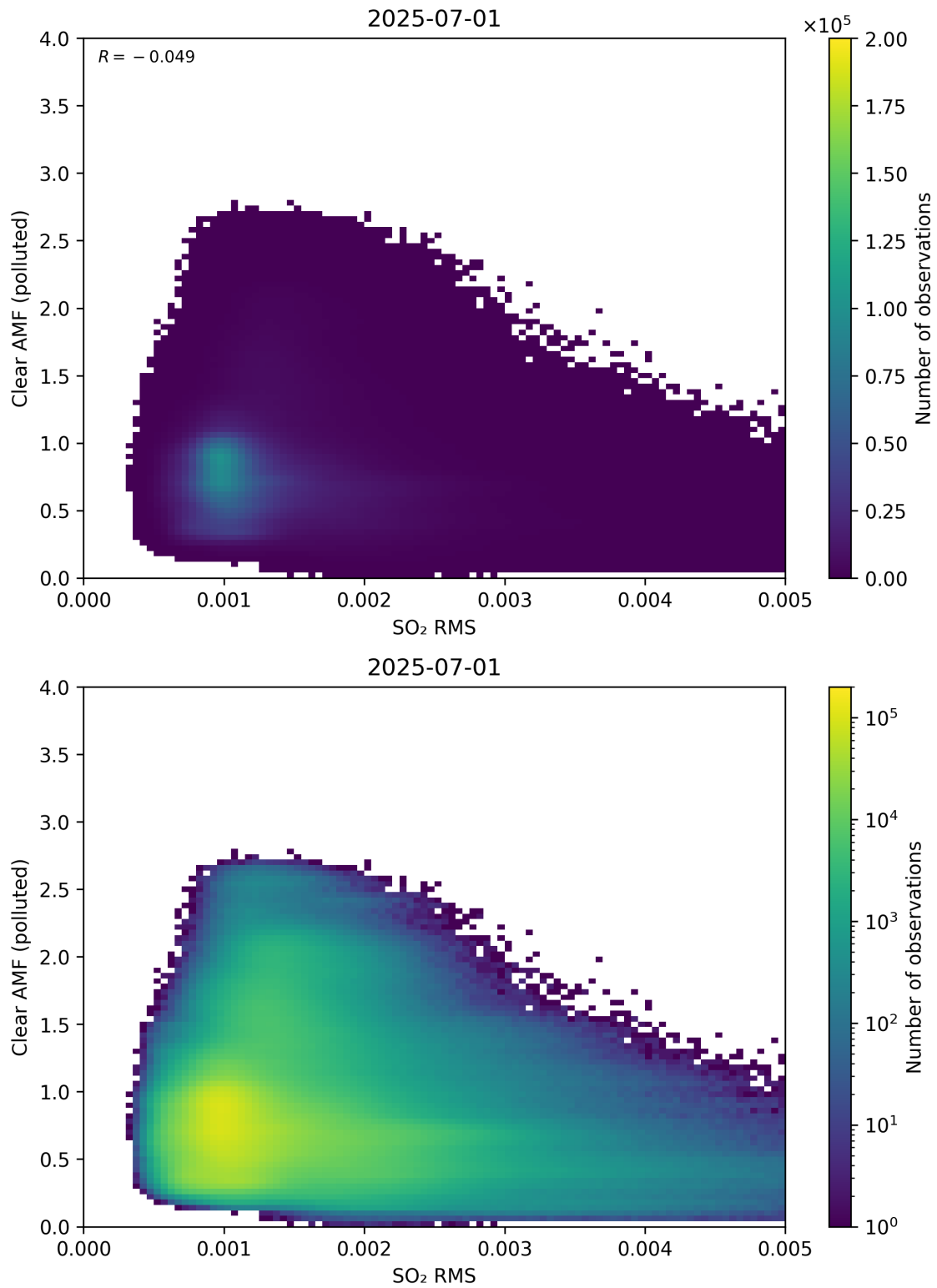
Figure 147: Scatter density plot of “SO 2 RMS” against “Clear AMF (polluted)” for 2025-06-30 to 2025-07-02.
