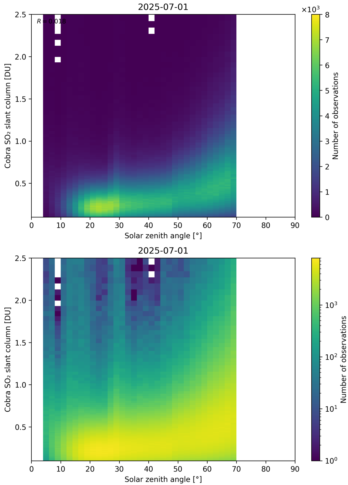
Figure 179: Scatter density plot of “Solar zenith angle” against “Cobra SO 2 slant column” for 2025-06-30 to 2025-07-02.
