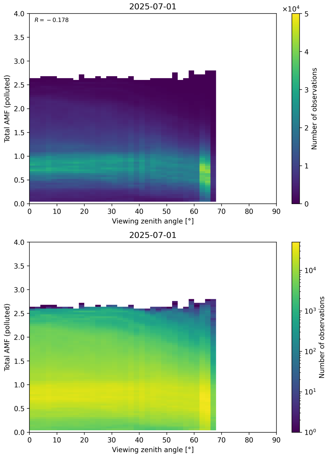
Figure 381: Scatter density plot of “Viewing zenith angle” against “Total AMF (polluted)” for 2025-06-30 to 2025-07-02.
