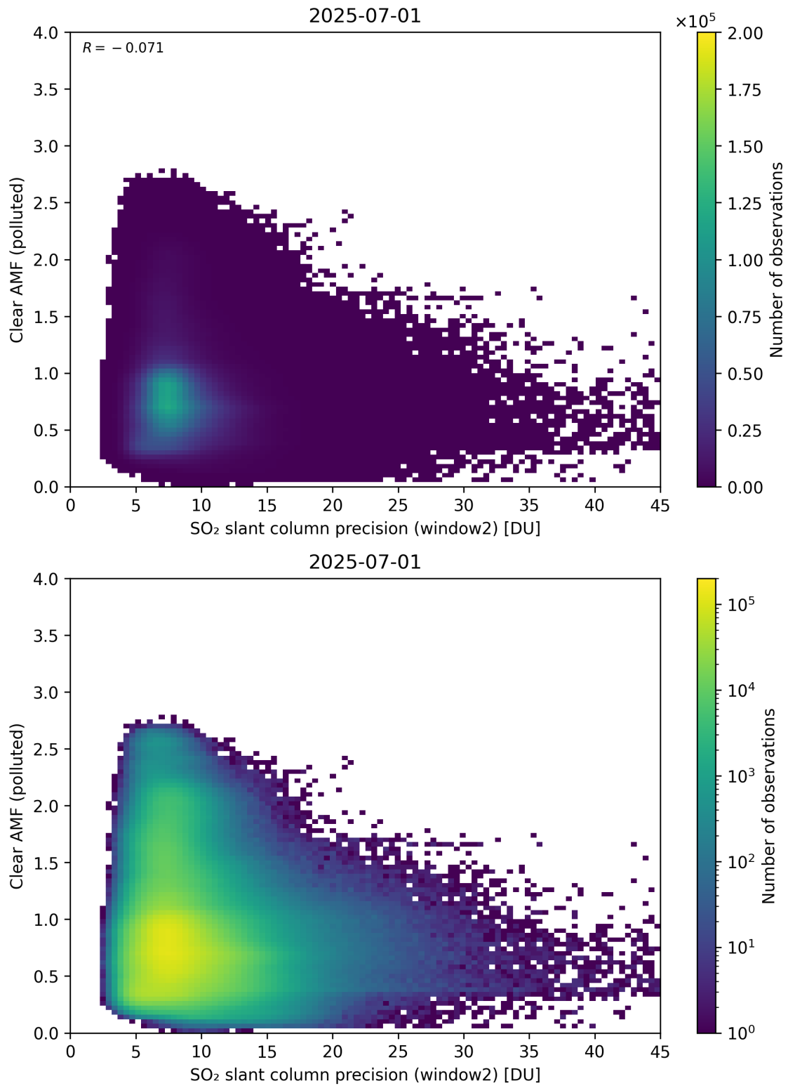
Figure 296: Scatter density plot of “SO 2 slant column precision (window2)” against “Clear AMF (polluted)” for 2025-06-30 to 2025-07-02.
