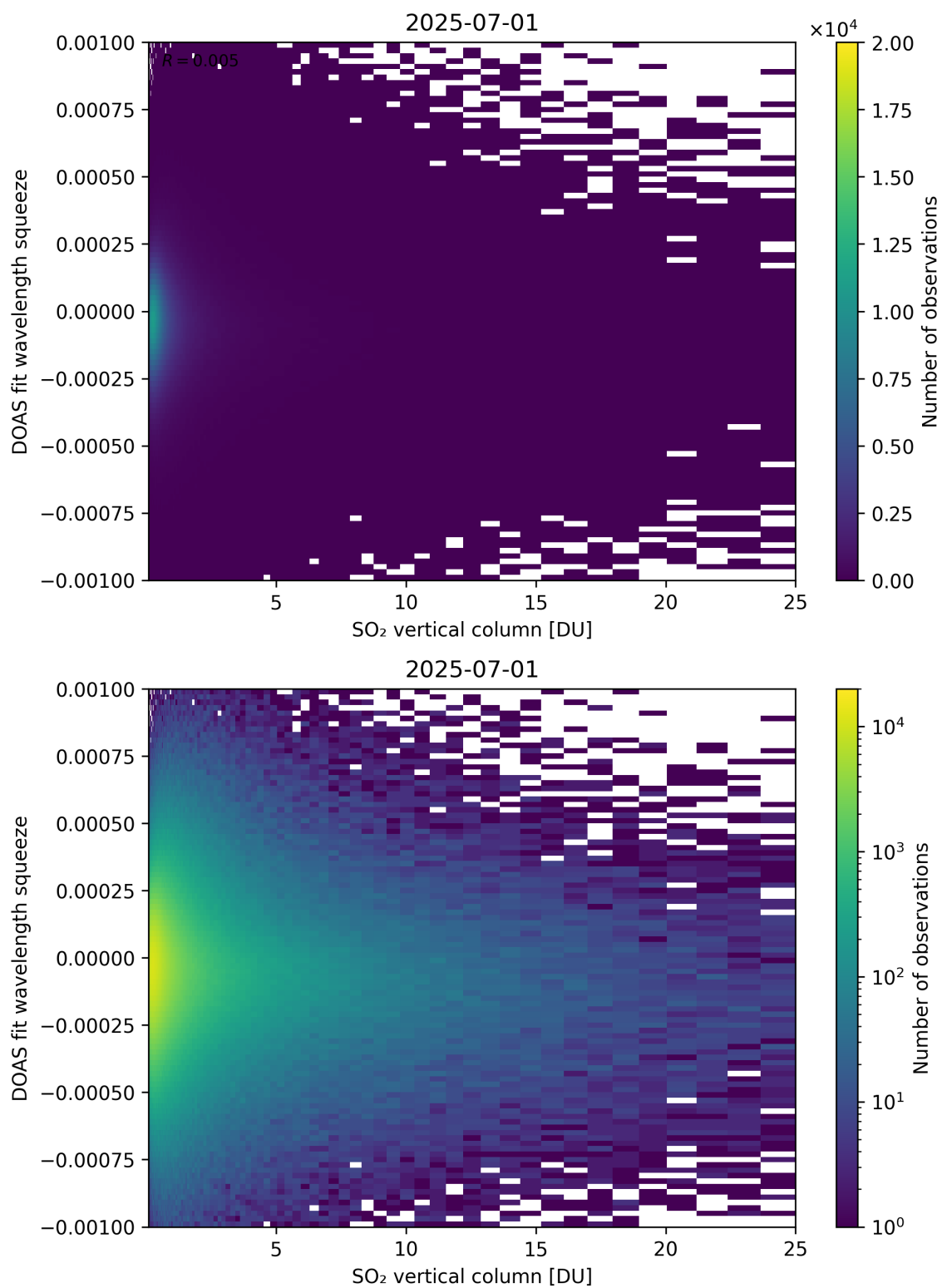
Figure 327: Scatter density plot of “SO 2 vertical column” against “DOAS fit wavelength squeeze” for 2025-06-30 to 2025-07-02.
