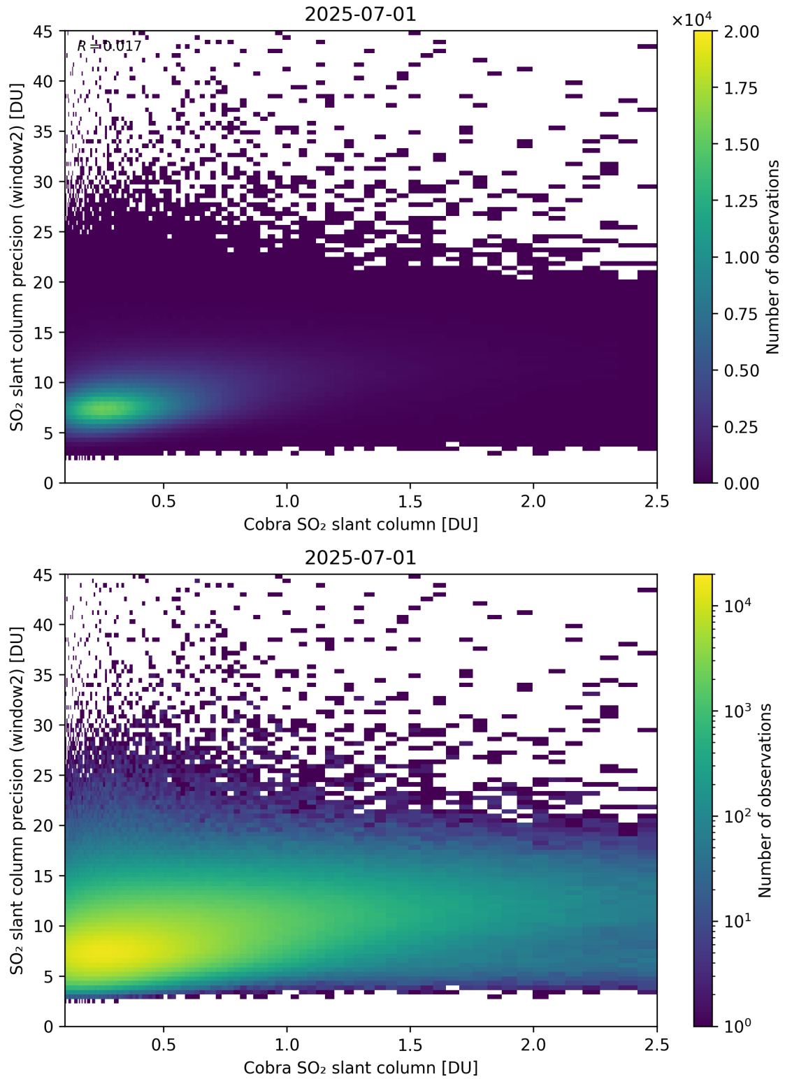
Figure 221: Scatter density plot of “Cobra SO 2 slant column” against “SO 2 slant column precision (window2)” for 2025-06-30 to 2025-07-02.
