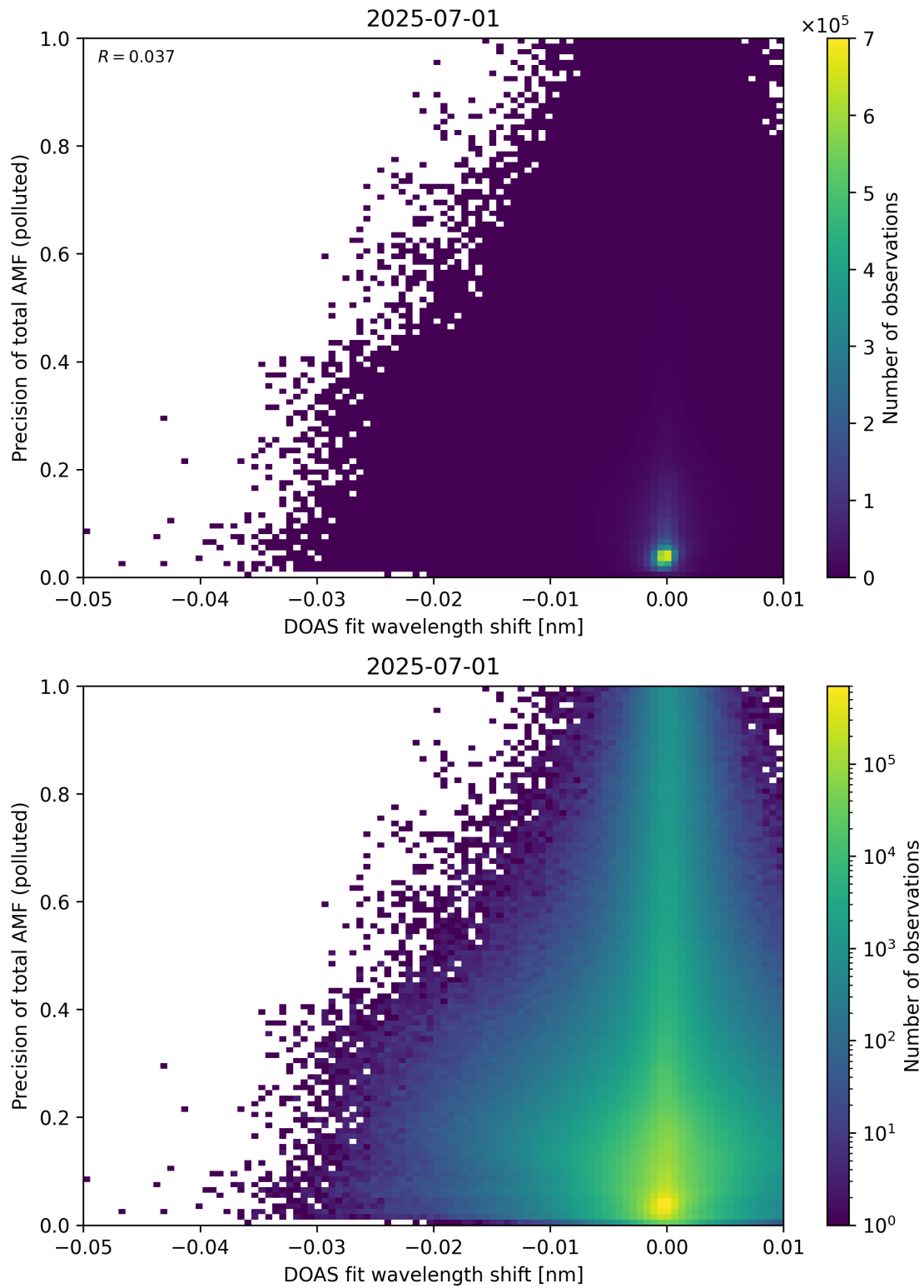
Figure 142: Scatter density plot of “DOAS fit wavelength shift” against “Precision of total AMF (polluted)” for 2025-06-30 to 2025-07-02.
