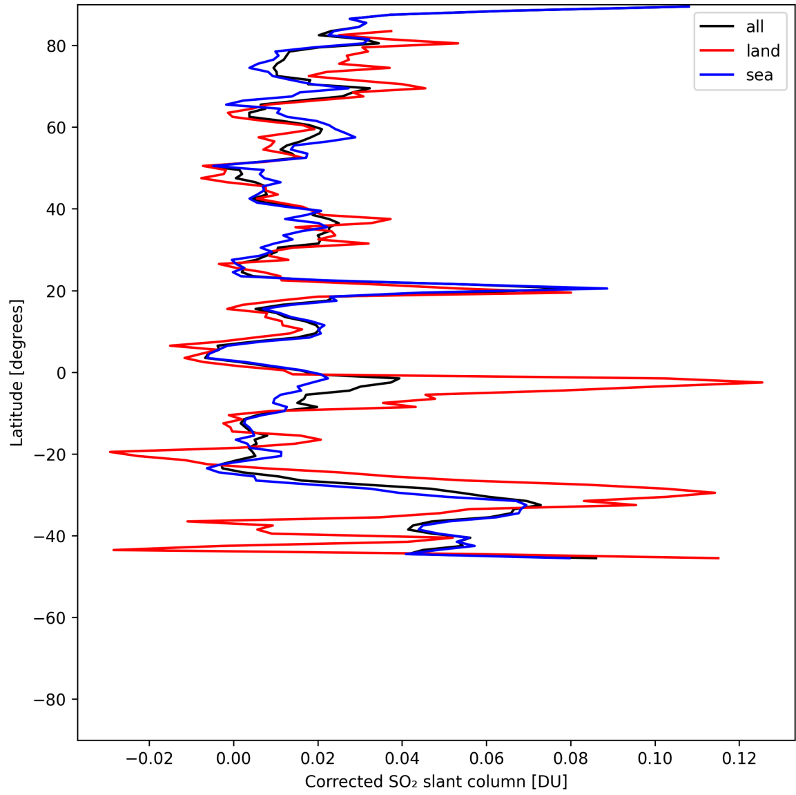
Figure 34: Zonal average of “Corrected SO 2 slant column” for 2025-06-30 to 2025-07-02.
