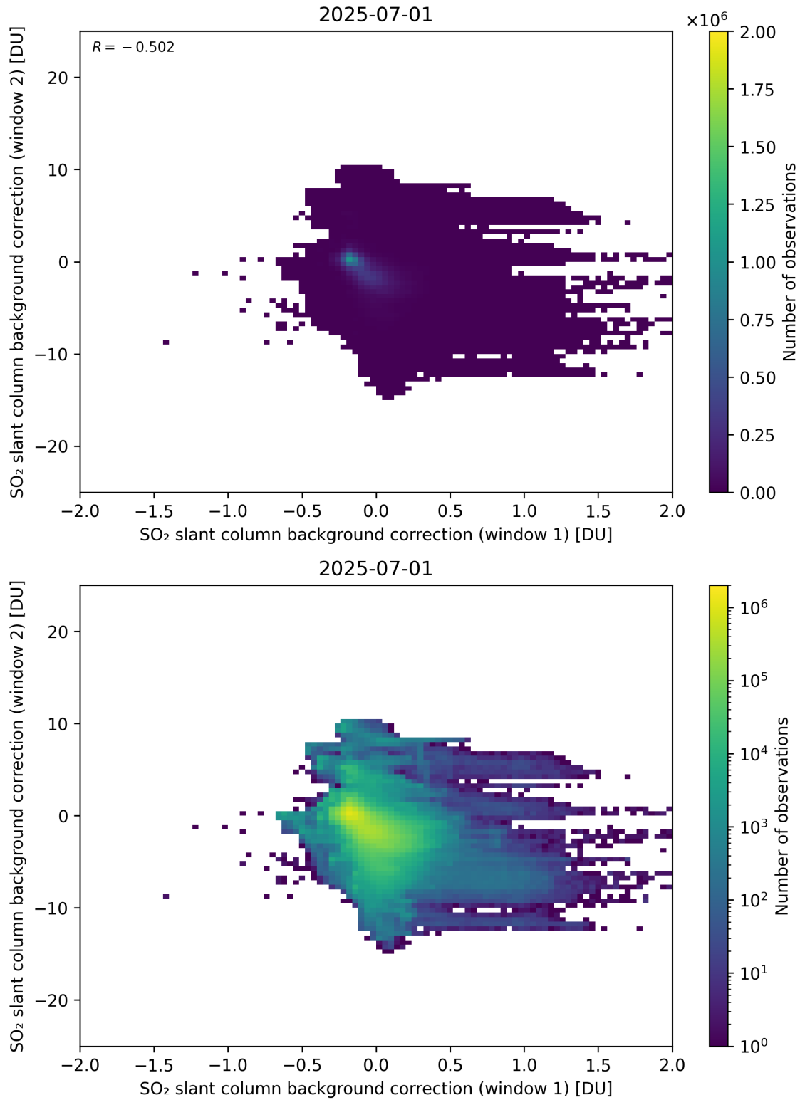
Figure 109: Scatter density plot of “SO 2 slant column background correction (window 1)” against “SO 2 slant column background correction (window 2)” for 2025-06-30 to 2025-07-02.
