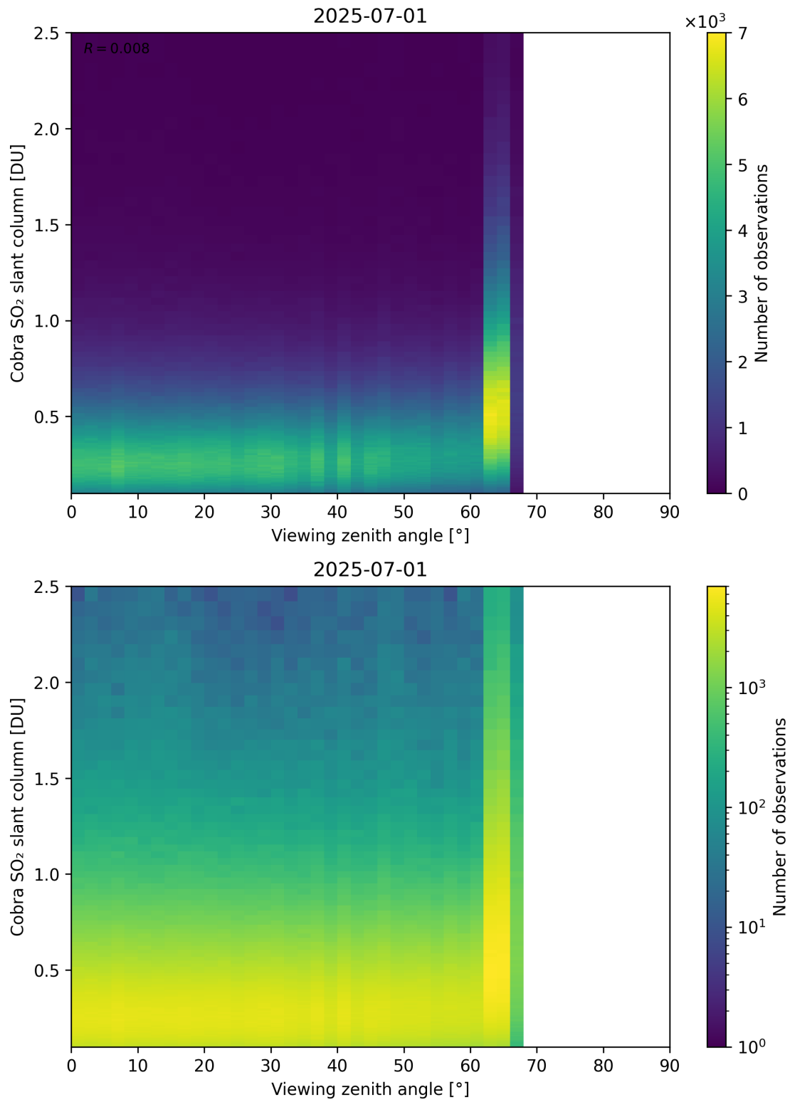
Figure 371: Scatter density plot of “Viewing zenith angle” against “Cobra SO 2 slant column” for 2025-06-30 to 2025-07-02.
