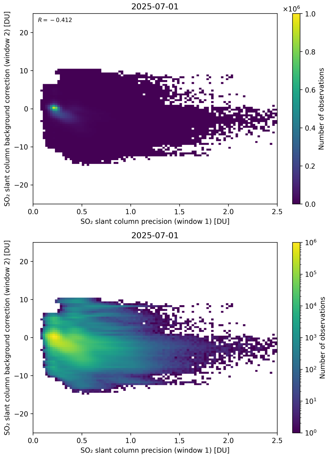
Figure 269: Scatter density plot of “SO 2 slant column precision (window 1)” against “SO 2 slant column background correction (window 2)” for 2025-06-30 to 2025-07-02.
