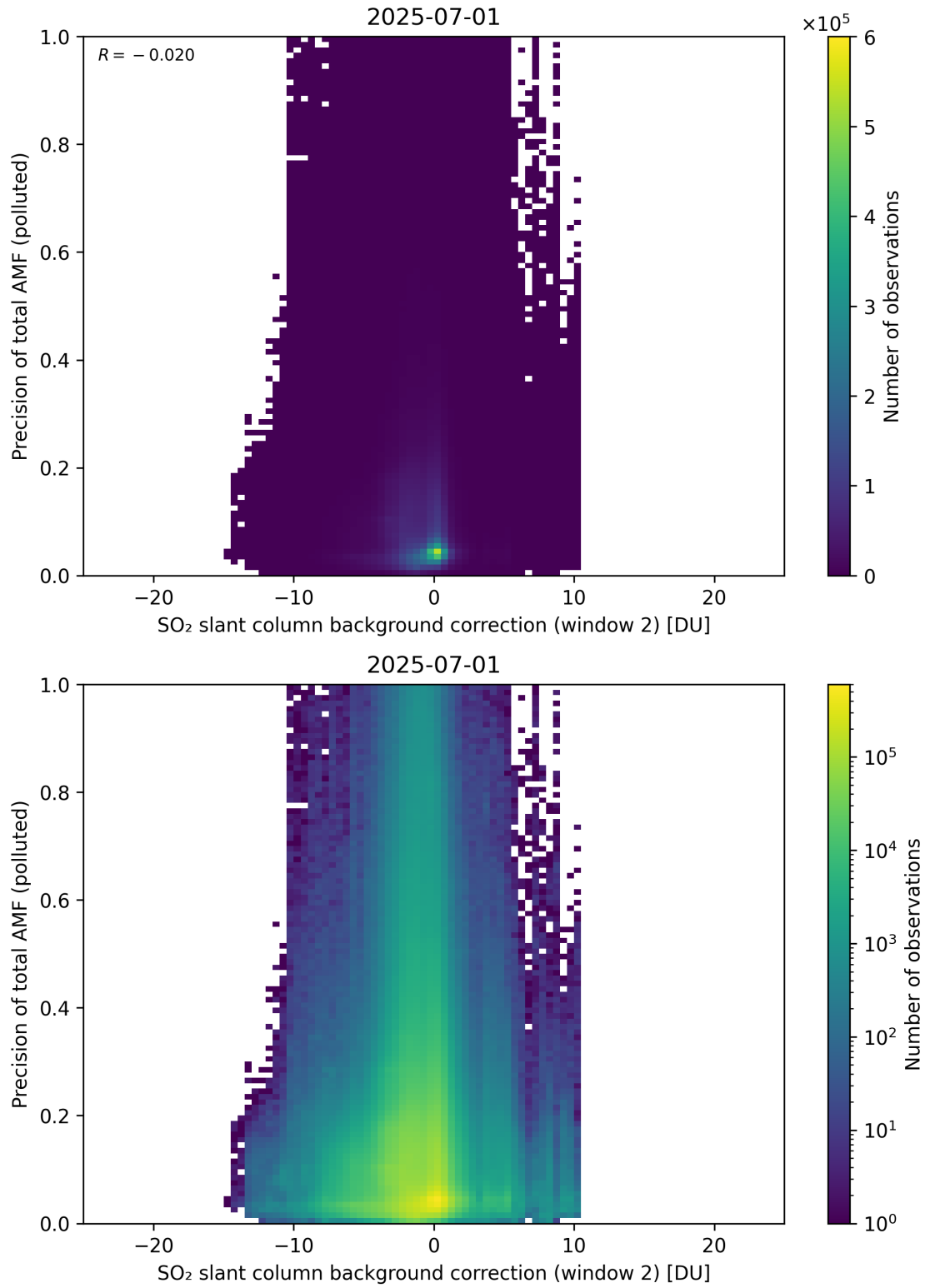
Figure 131: Scatter density plot of “SO 2 slant column background correction (window 2)” against “Precision of total AMF (polluted)” for 2025-06-30 to 2025-07-02.
