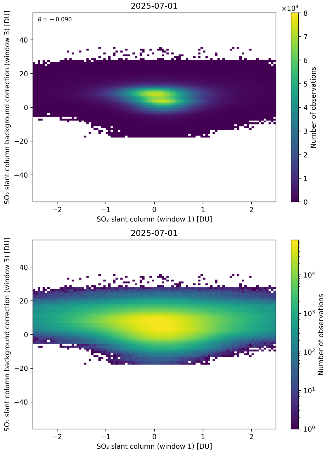
Figure 264: Scatter density plot of “SO 2 slant column (window 1)” against “SO 2 slant column background correction (window 3)” for 2025-06-30 to 2025-07-02.
