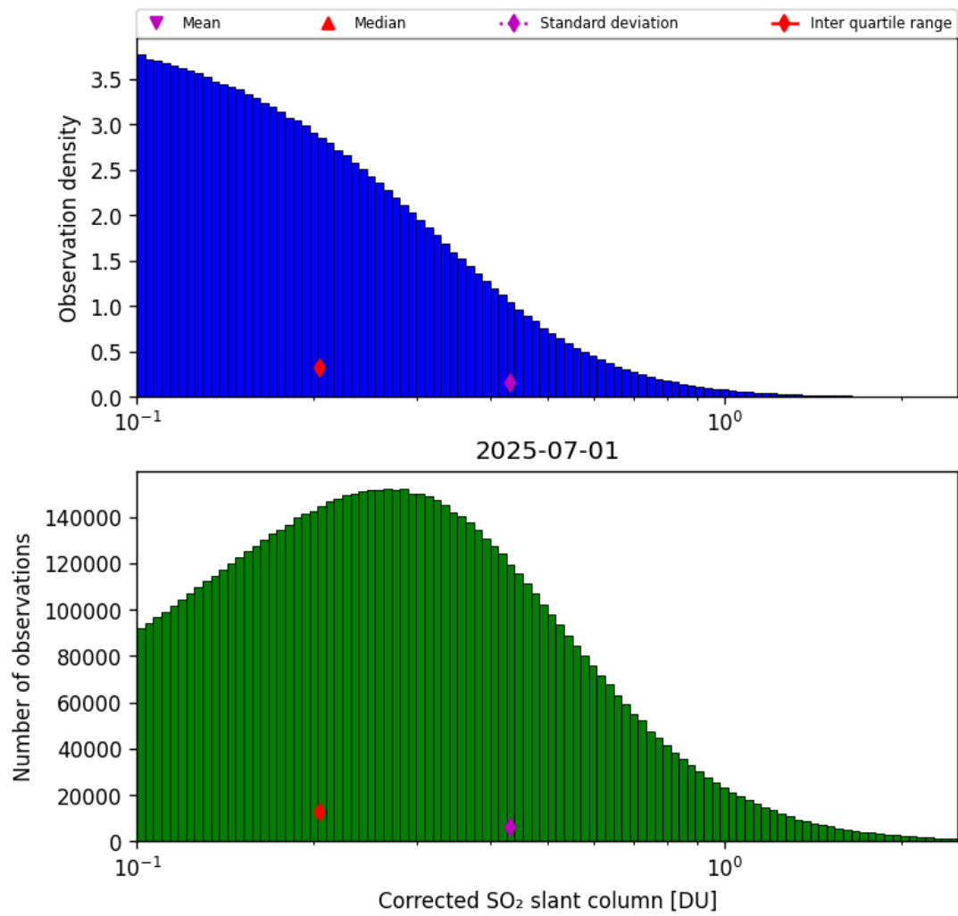
Figure 60: Histogram of “Corrected SO 2 slant column” for 2025-06-30 to 2025-07-02
