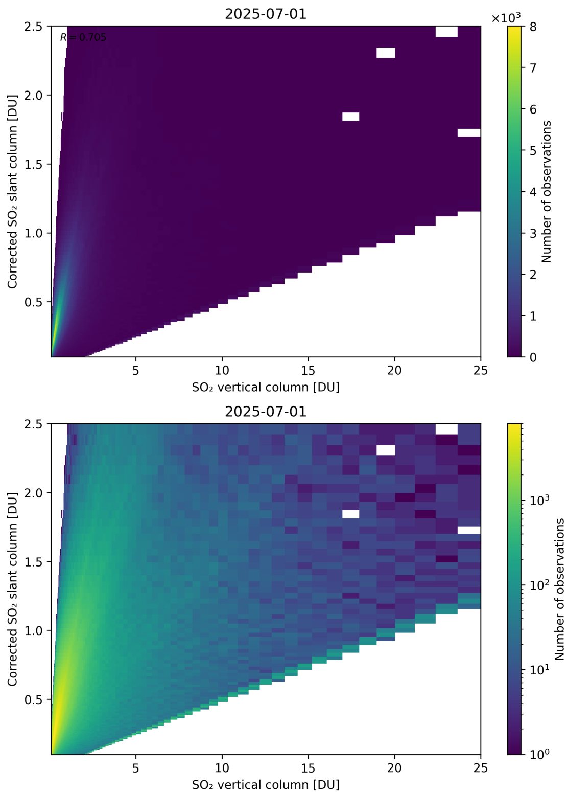
Figure 351: Scatter density plot of “SO 2 vertical column” against “Corrected SO 2 slant column” for 2025-06-30 to 2025-07-02.
