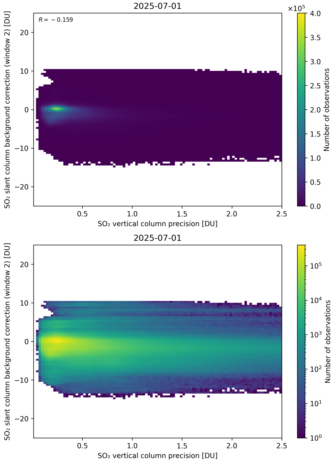
Figure 330: Scatter density plot of “SO 2 vertical column precision” against “SO 2 slant column background correction (window 2)” for 2025-06-30 to 2025-07-02.
