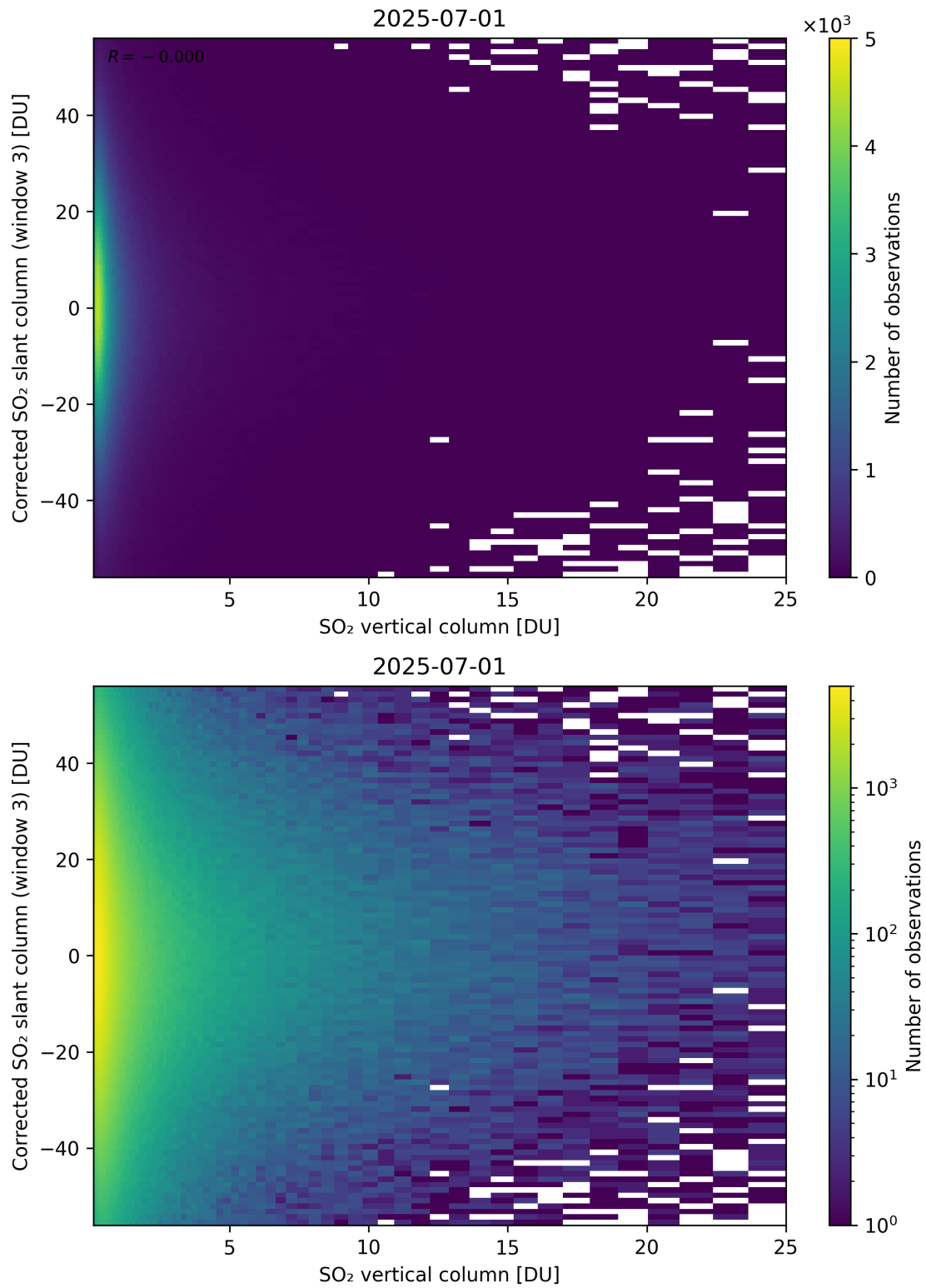
Figure 353: Scatter density plot of “SO 2 vertical column” against “Corrected SO 2 slant column (window 3)” for 2025-06-30 to 2025-07-02.
