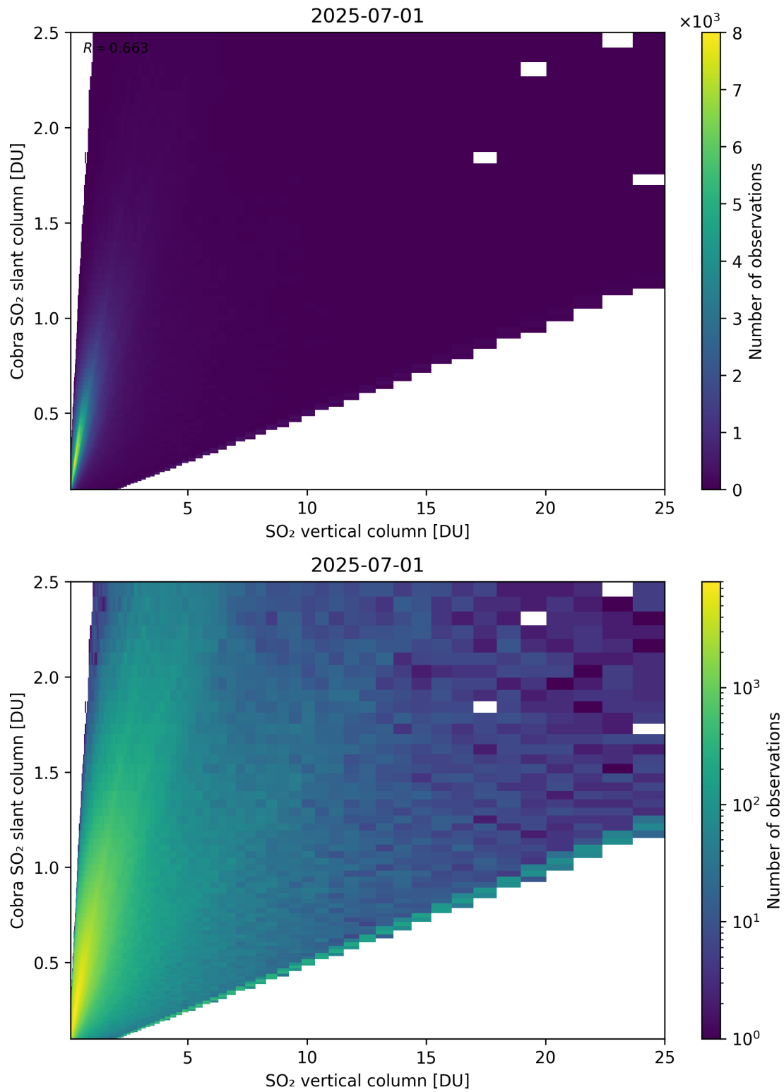
Figure 349: Scatter density plot of “SO 2 vertical column” against “Cobra SO 2 slant column” for 2025-06-30 to 2025-07-02.
