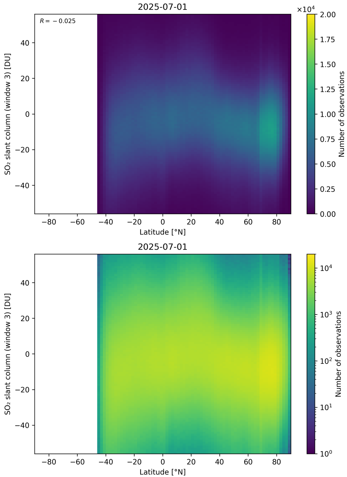
Figure 165: Scatter density plot of “Latitude” against “SO 2 slant column (window 3)” for 2025-06-30 to 2025-07-02.
