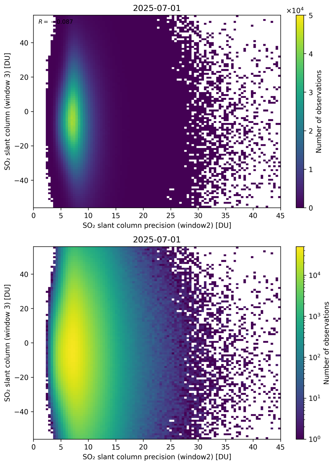
Figure 299: Scatter density plot of “SO 2 slant column precision (window2)” against “SO 2 slant column (window 3)” for 2025-06-30 to 2025-07-02.
