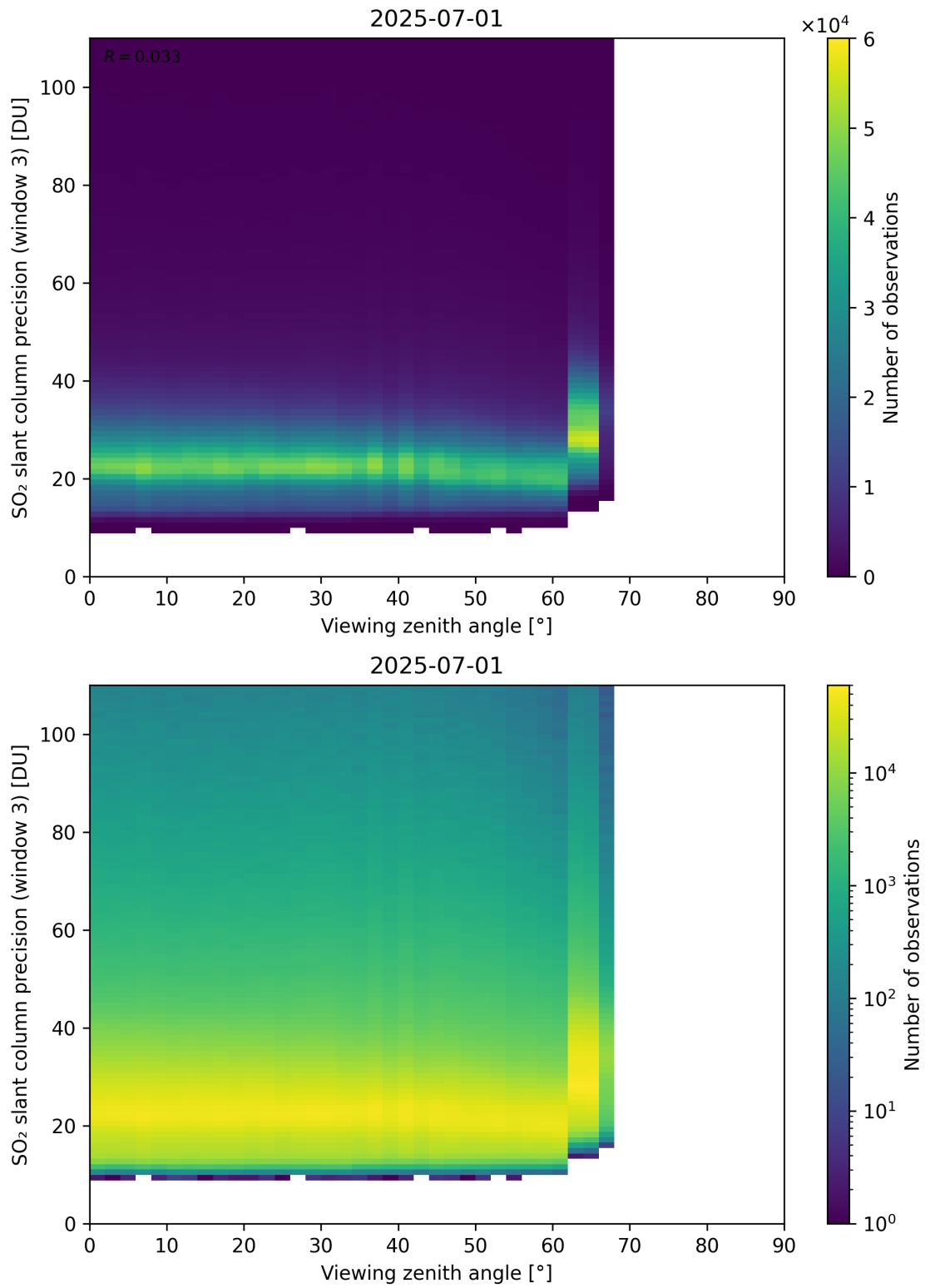
Figure 380: Scatter density plot of “Viewing zenith angle” against “SO 2 slant column precision (window 3)” for 2025-06-30 to 2025-07-02.
