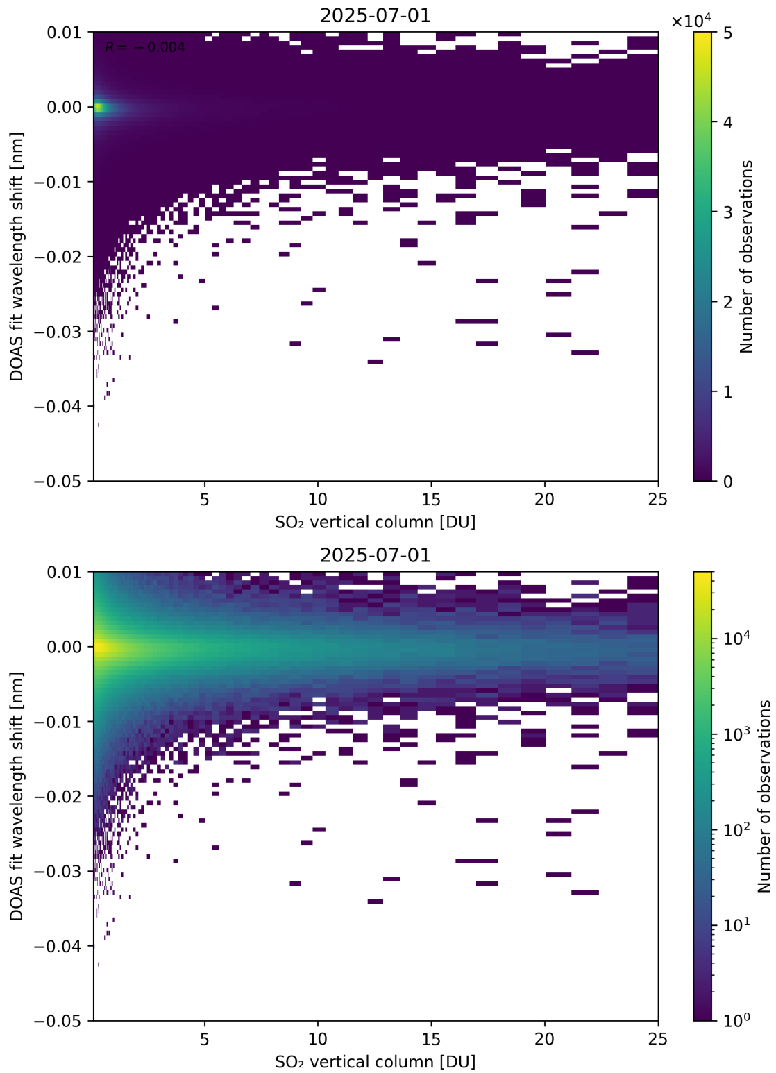
Figure 326: Scatter density plot of “SO 2 vertical column” against “DOAS fit wavelength shift” for 2025-06-30 to 2025-07-02.
