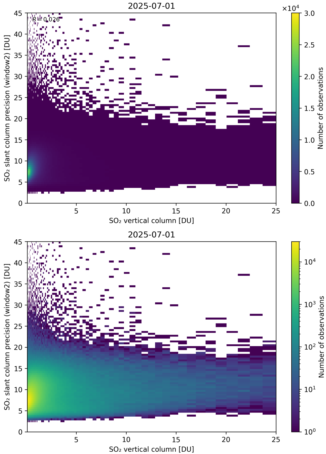
Figure 356: Scatter density plot of “SO 2 vertical column” against “SO 2 slant column precision (window2)” for 2025-06-30 to 2025-07-02.
