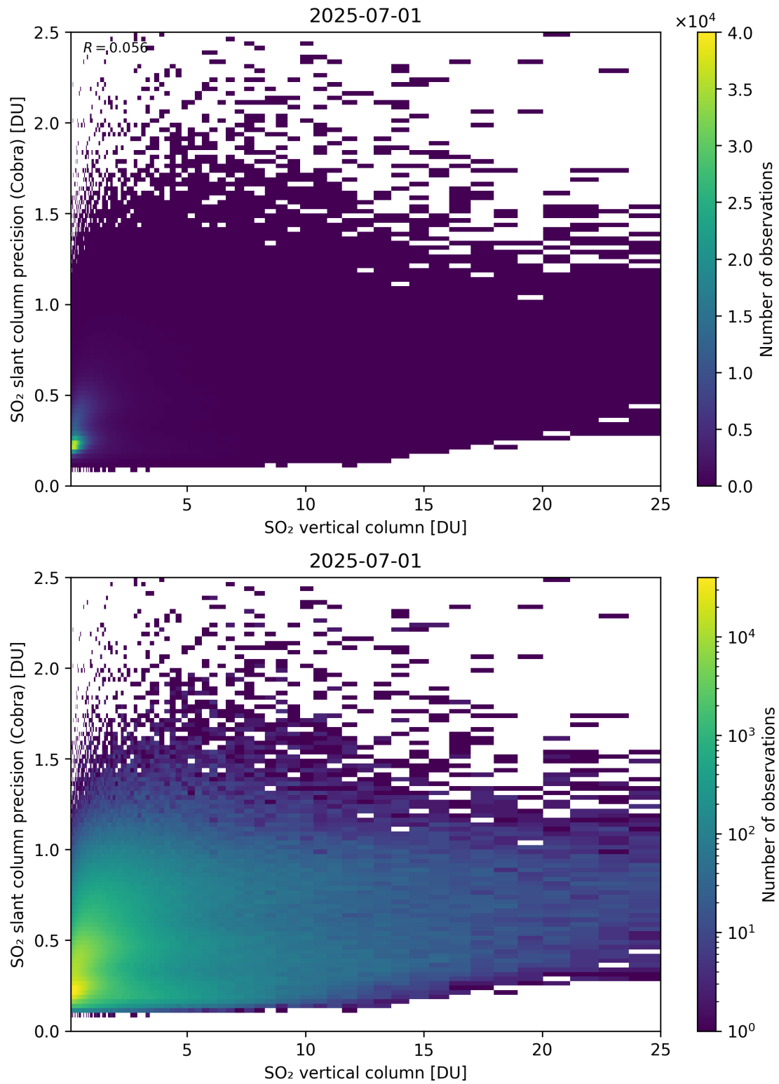
Figure 350: Scatter density plot of “SO 2 vertical column” against “SO 2 slant column precision (Cobra)” for 2025-06-30 to 2025-07-02.
