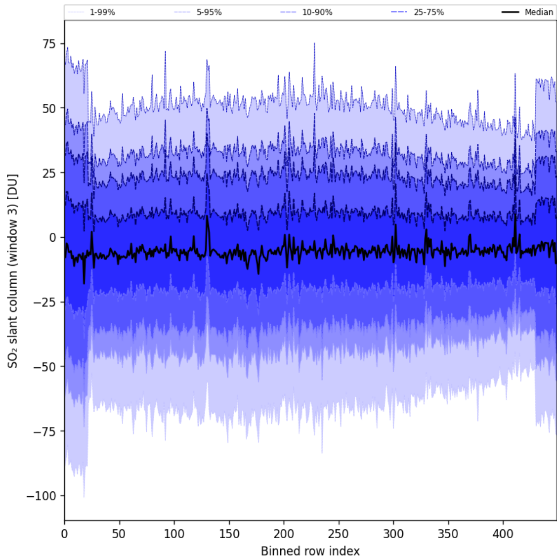
Figure 97: Along track statistics of “SO 2 slant column (window 3)” for 2025-06-30 to 2025-07-02
