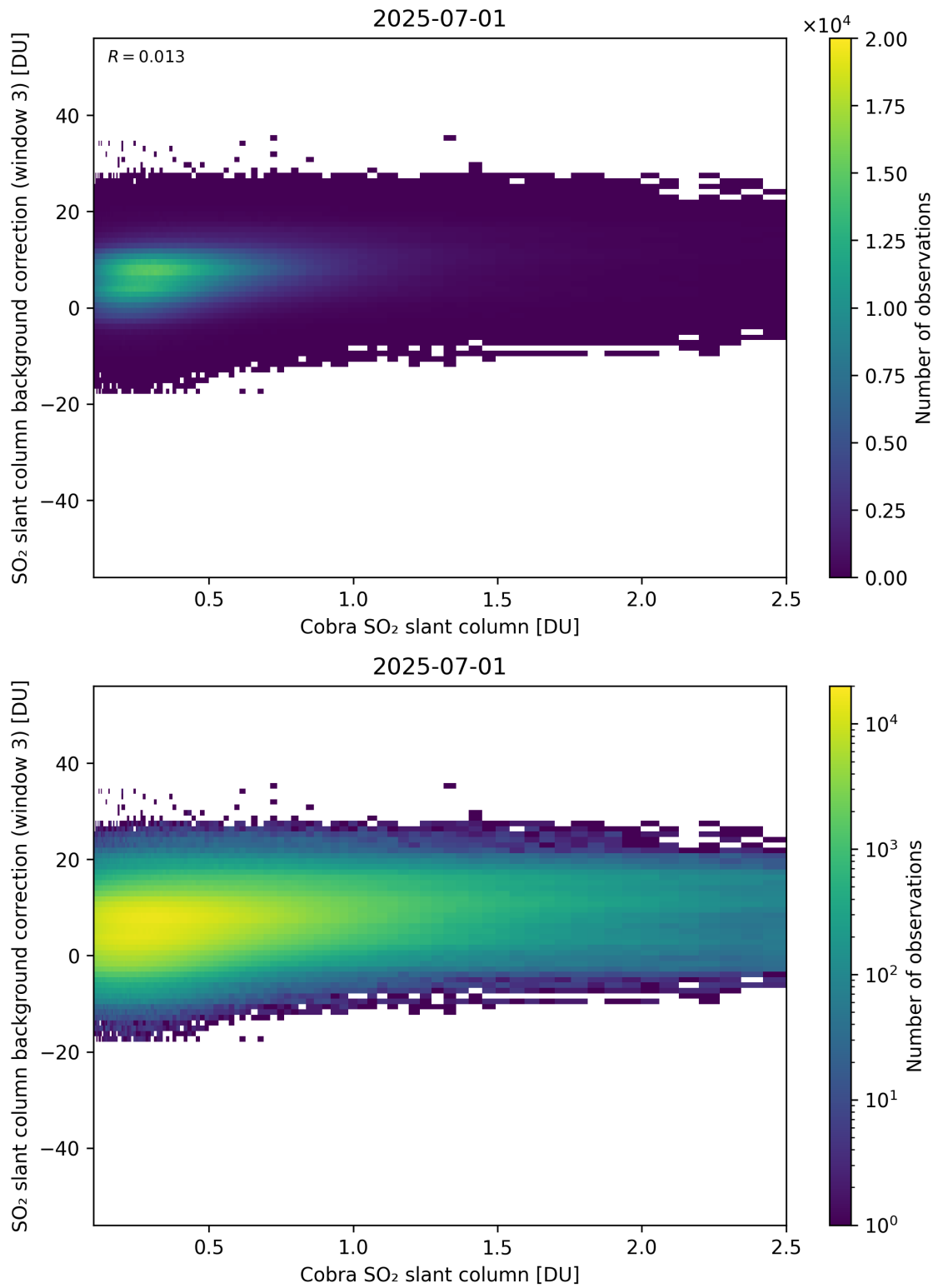
Figure 195: Scatter density plot of “Cobra SO 2 slant column” against “SO 2 slant column background correction (window 3)” for 2025-06-30 to 2025-07-02.
