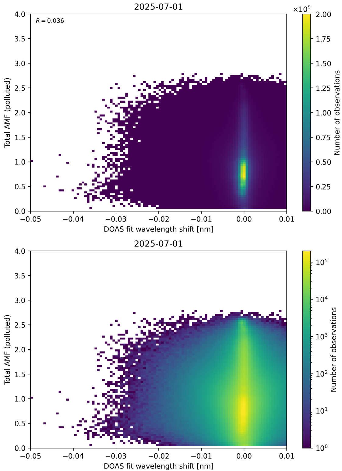
Figure 141: Scatter density plot of “DOAS fit wavelength shift” against “Total AMF (polluted)” for 2025-06-30 to 2025-07-02.
