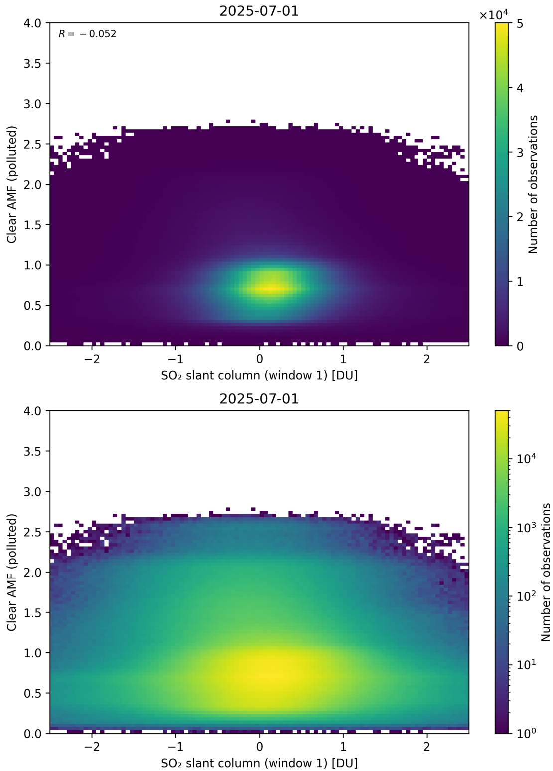
Figure 282: Scatter density plot of “SO 2 slant column (window 1)” against “Clear AMF (polluted)” for 2025-06-30 to 2025-07-02.
