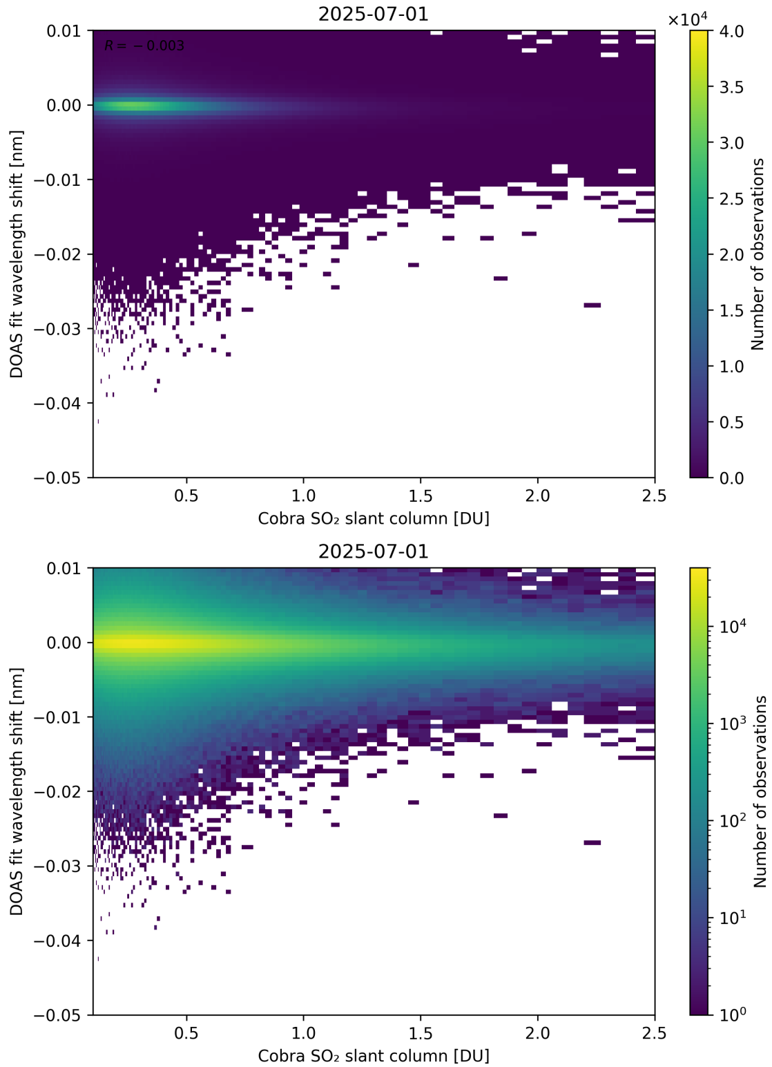
Figure 196: Scatter density plot of “Cobra SO 2 slant column” against “DOAS fit wavelength shift” for 2025-06-30 to 2025-07-02.
