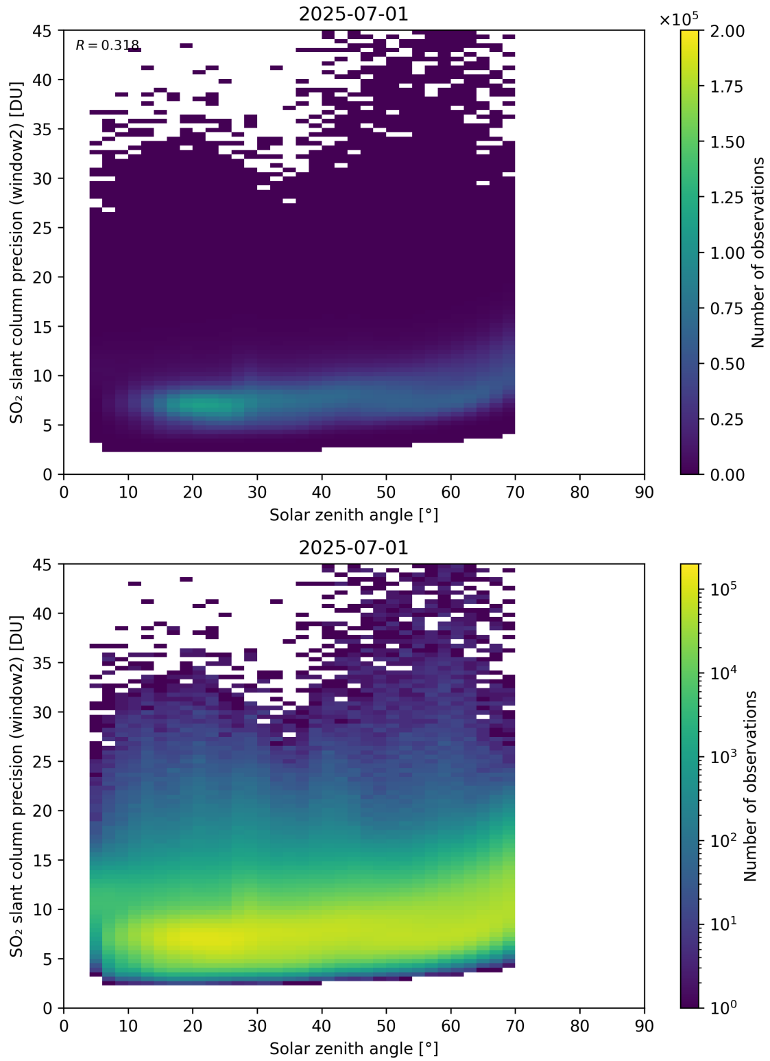
Figure 186: Scatter density plot of “Solar zenith angle” against “SO 2 slant column precision (window2)” for 2025-06-30 to 2025-07-02.
