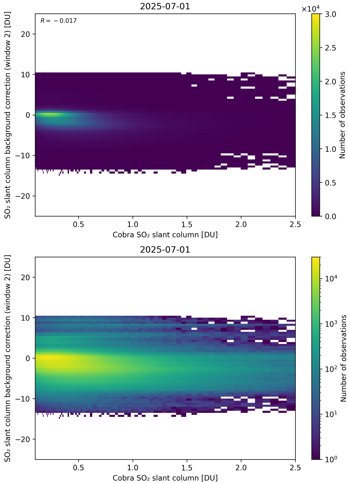
Figure 194: Scatter density plot of “Cobra SO 2 slant column” against “SO 2 slant column background correction (window 2)” for 2025-06-30 to 2025-07-02.
