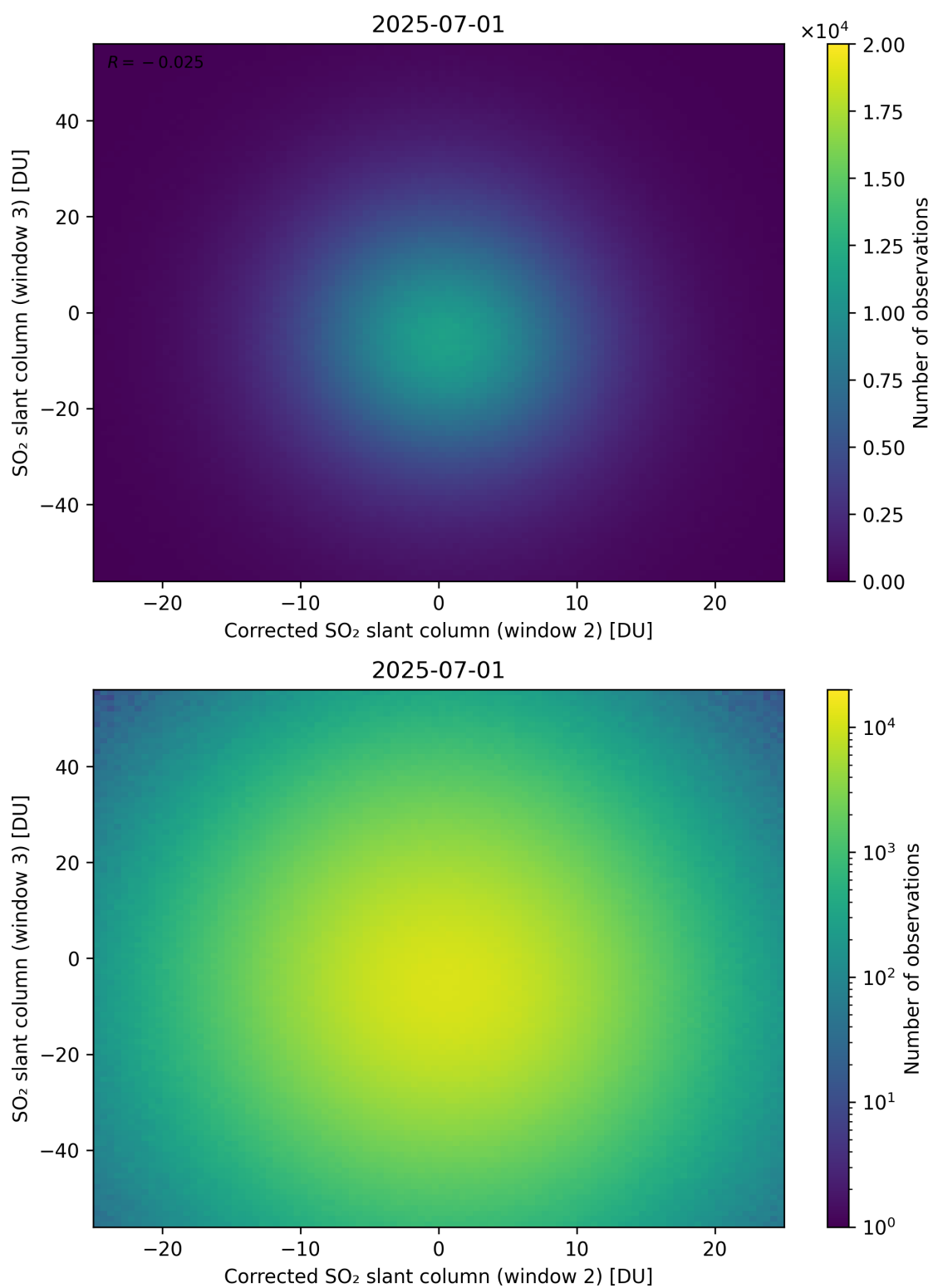
Figure 251: Scatter density plot of “Corrected SO 2 slant column (window 2)” against “SO 2 slant column (window 3)” for 2025-06-30 to 2025-07-02.
