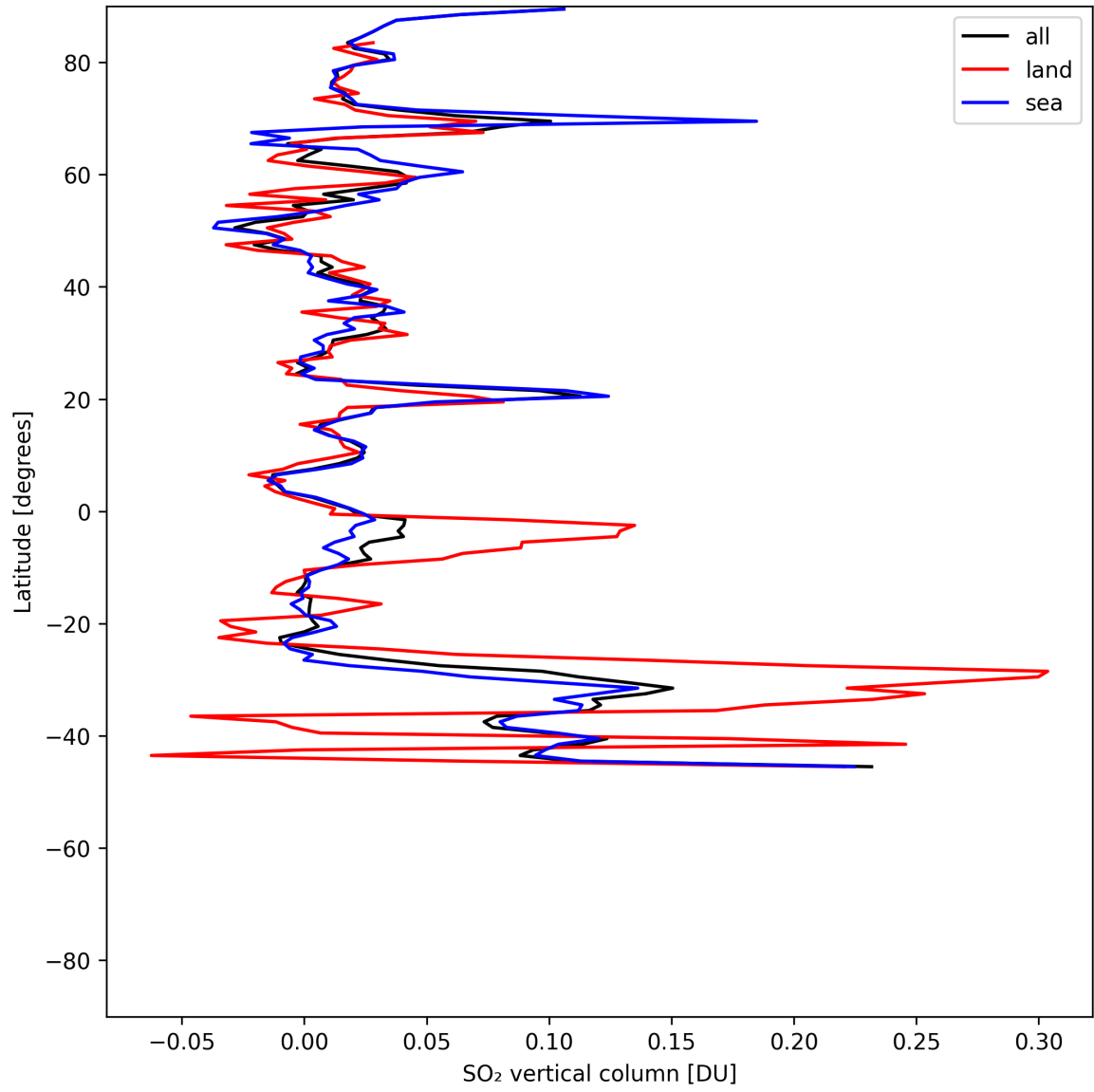
Figure 32: Zonal average of “SO 2 vertical column” for 2025-06-30 to 2025-07-02.
