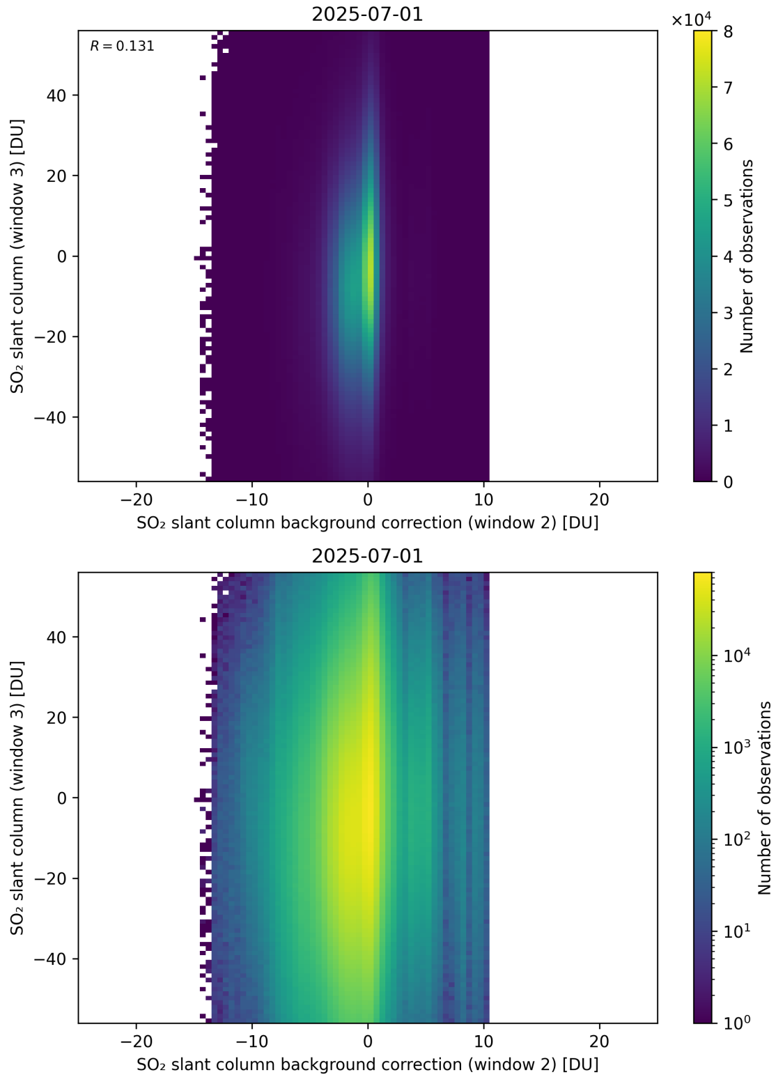
Figure 128: Scatter density plot of “SO 2 slant column background correction (window 2)” against “SO 2 slant column (window 3)” for 2025-06-30 to 2025-07-02.
