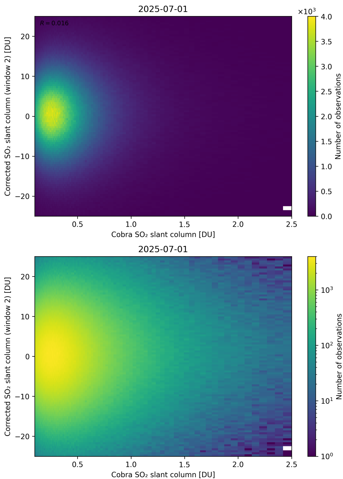
Figure 217: Scatter density plot of “Cobra SO 2 slant column” against “Corrected SO 2 slant column (window 2)” for 2025-06-30 to 2025-07-02.
