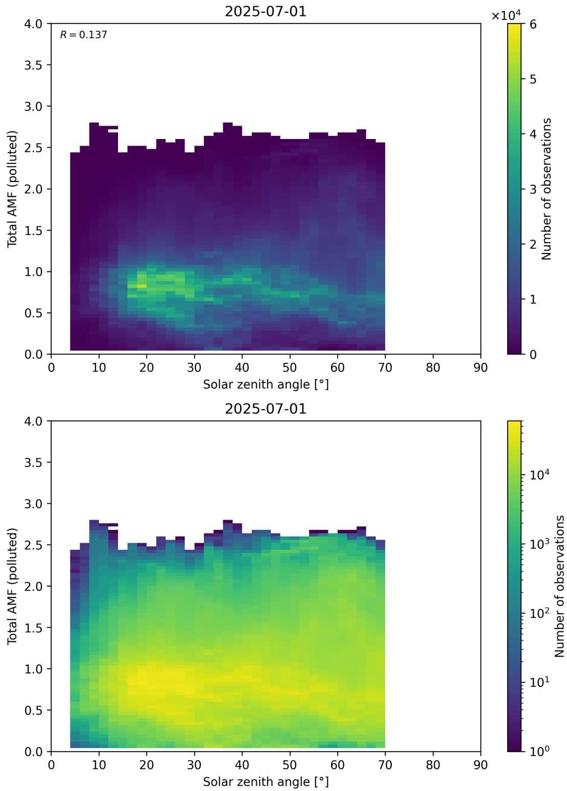
Figure 189: Scatter density plot of “Solar zenith angle” against “Total AMF (polluted)” for 2025-06-30 to 2025-07-02.
