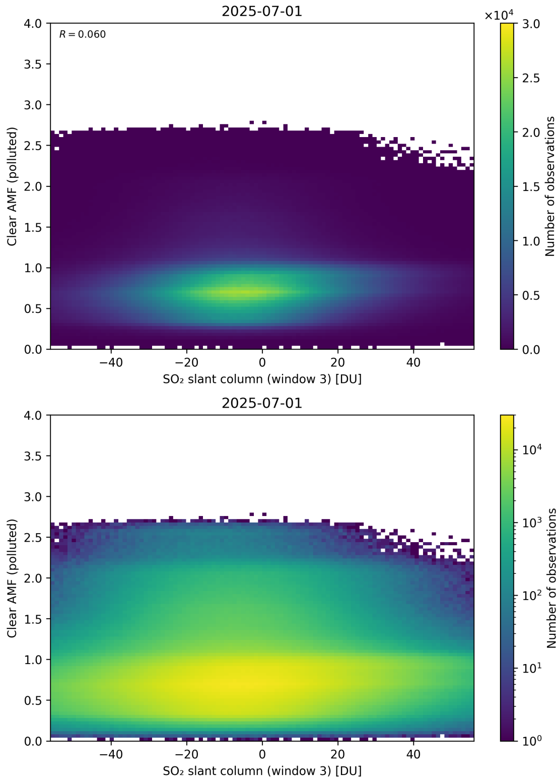
Figure 315: Scatter density plot of “SO 2 slant column (window 3)” against “Clear AMF (polluted)” for 2025-06-30 to 2025-07-02.
