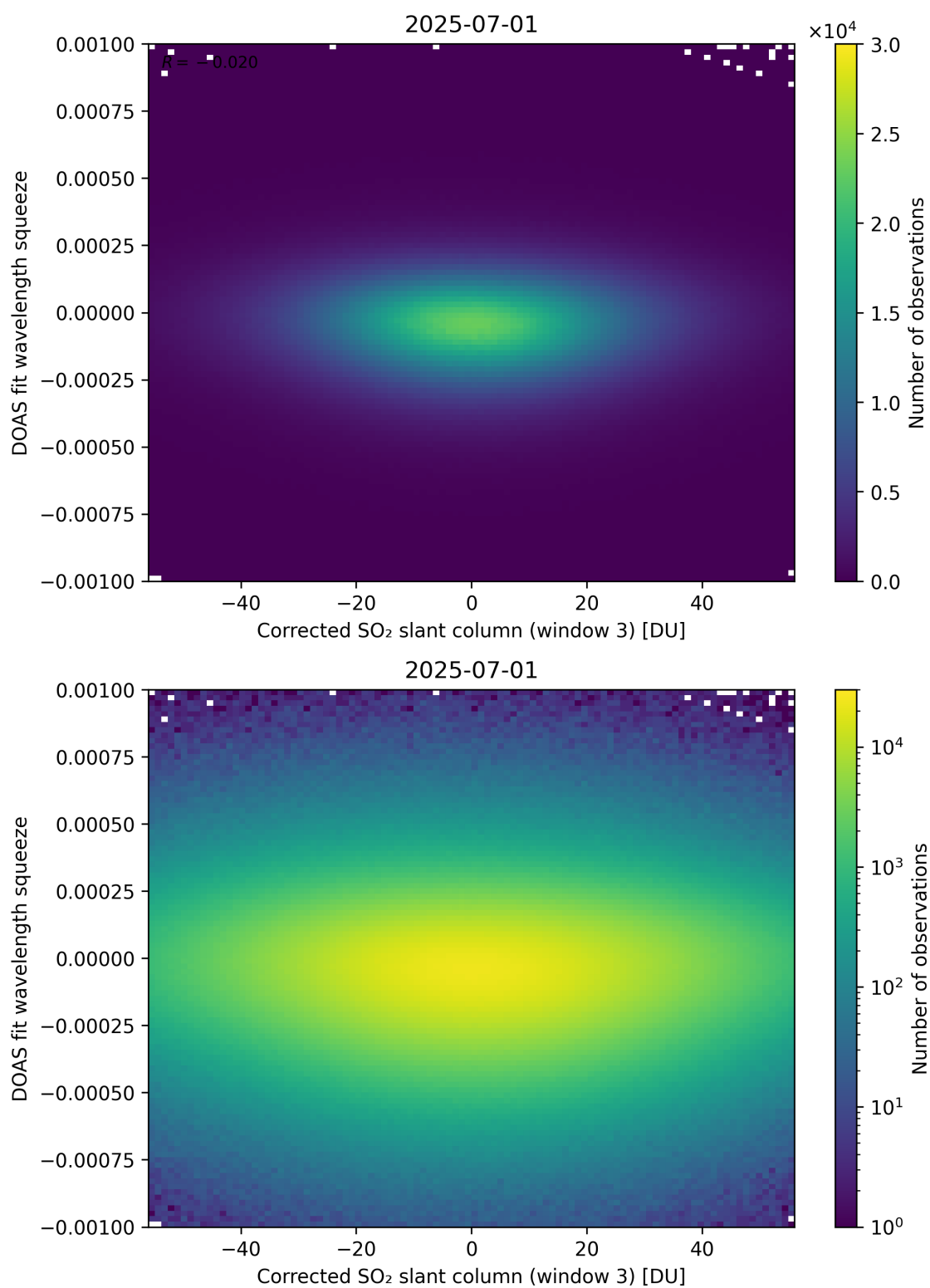
Figure 257: Scatter density plot of “Corrected SO 2 slant column (window 3)” against “DOAS fit wavelength squeeze” for 2025-06-30 to 2025-07-02.
