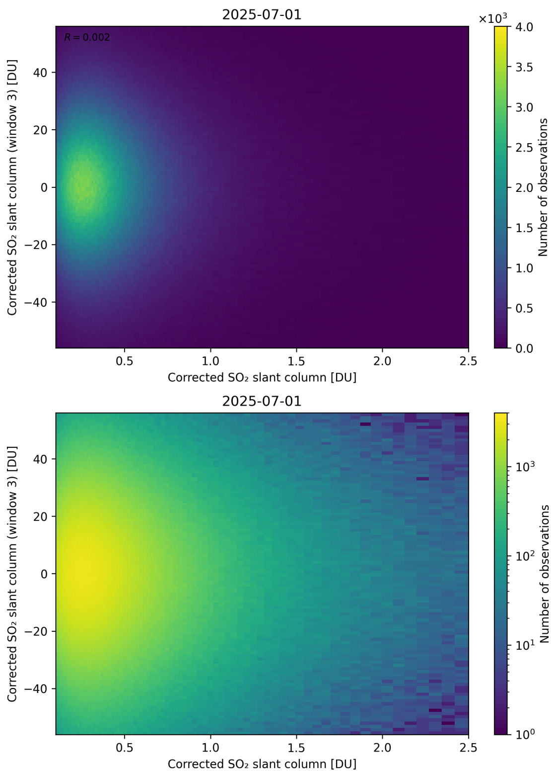
Figure 236: Scatter density plot of “Corrected SO 2 slant column” against “Corrected SO 2 slant column (window 3)” for 2025-06-30 to 2025-07-02.
