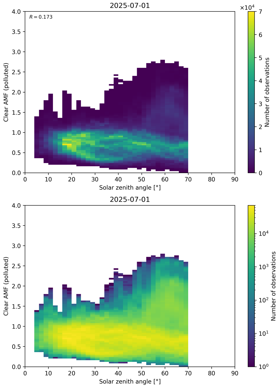
Figure 178: Scatter density plot of “Solar zenith angle” against “Clear AMF (polluted)” for 2025-06-30 to 2025-07-02.
