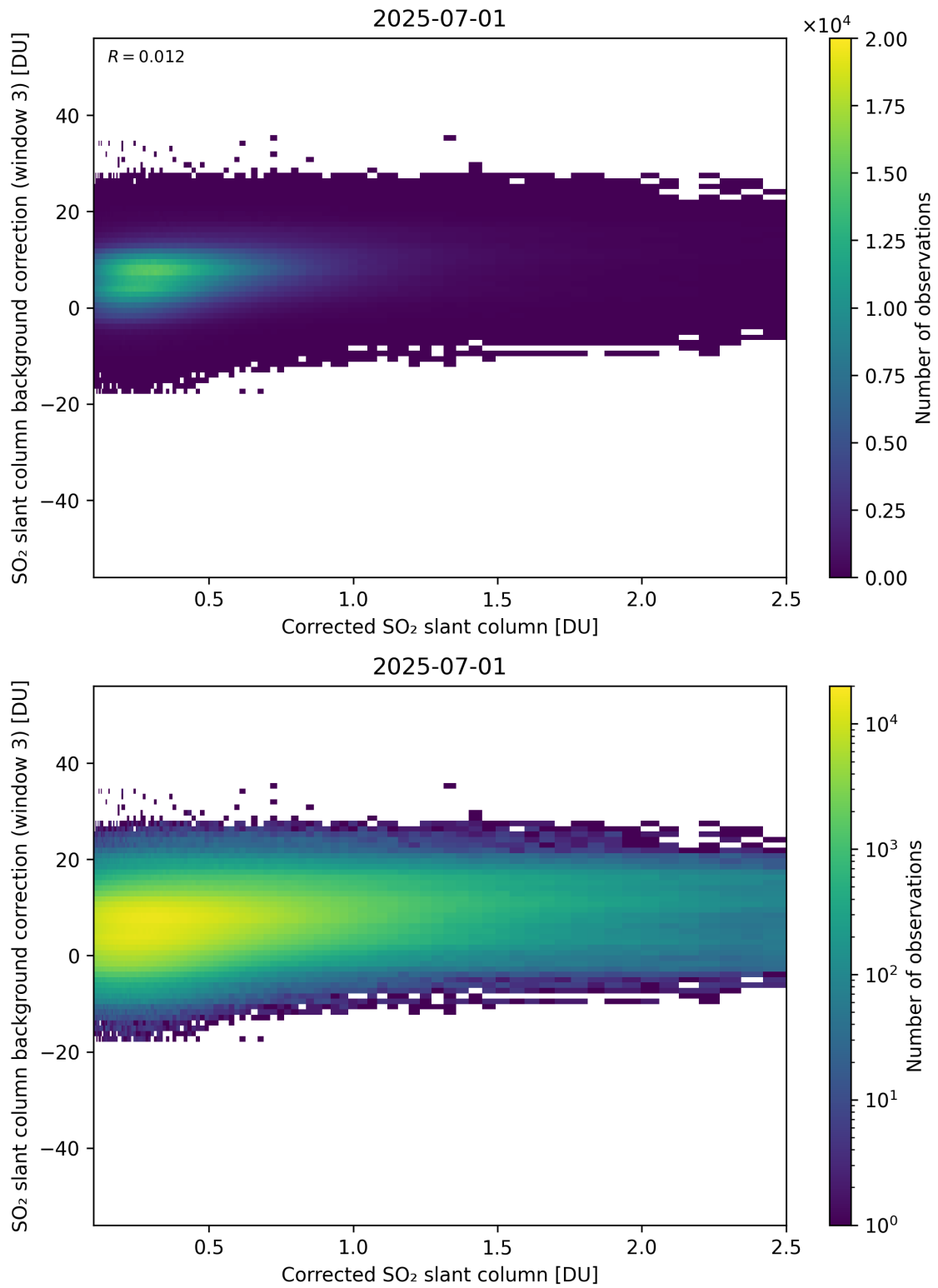
Figure 228: Scatter density plot of “Corrected SO 2 slant column” against “SO 2 slant column background correction (window 3)” for 2025-06-30 to 2025-07-02.
