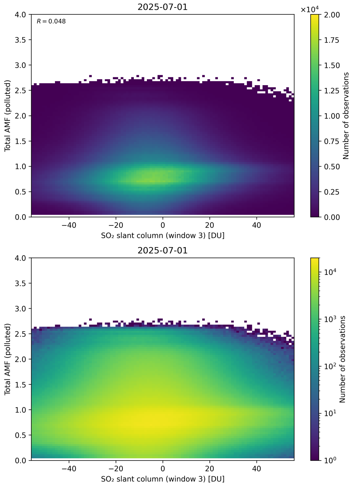
Figure 318: Scatter density plot of “SO 2 slant column (window 3)” against “Total AMF (polluted)” for 2025-06-30 to 2025-07-02.
