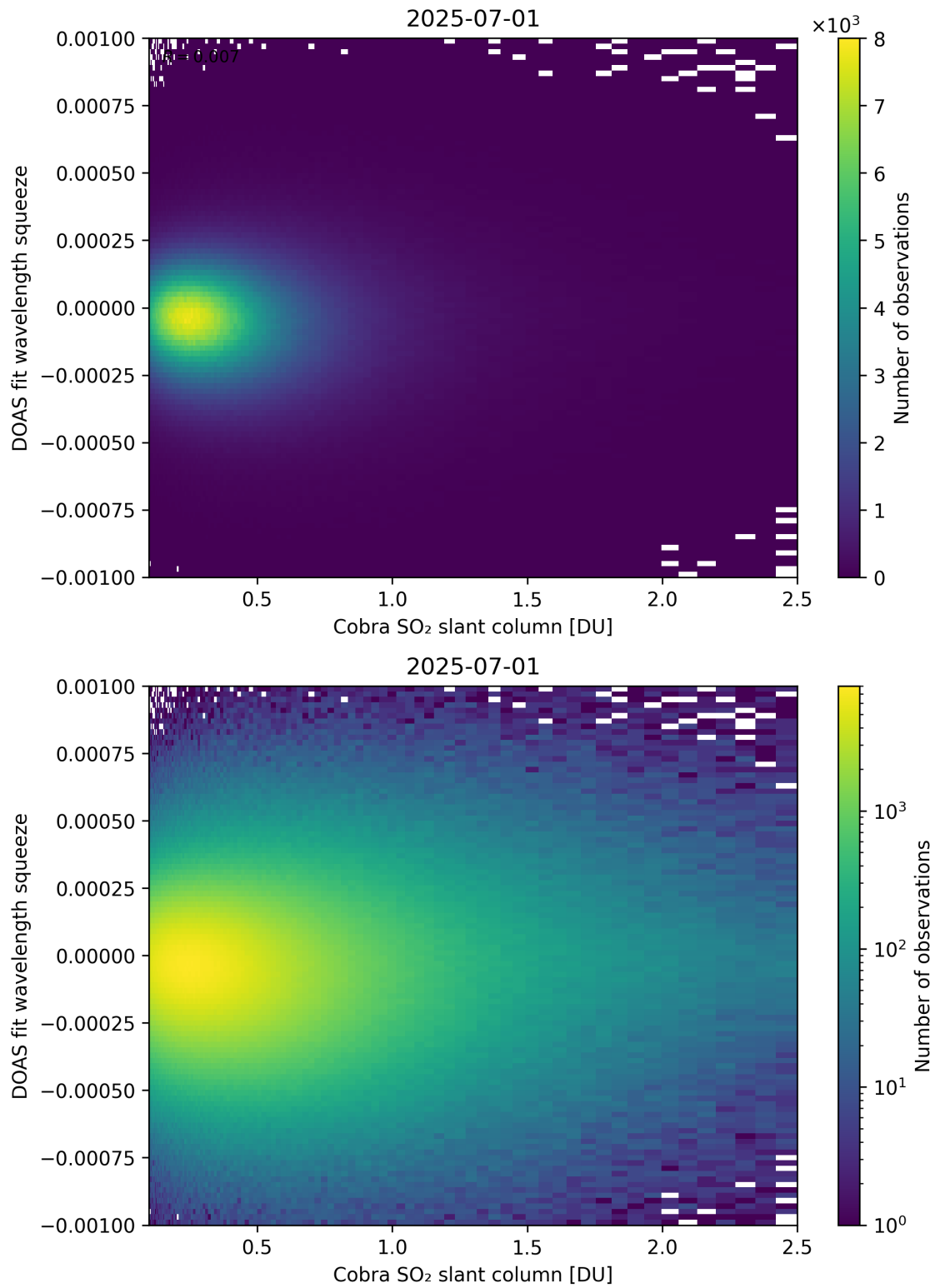
Figure 197: Scatter density plot of “Cobra SO 2 slant column” against “DOAS fit wavelength squeeze” for 2025-06-30 to 2025-07-02.
