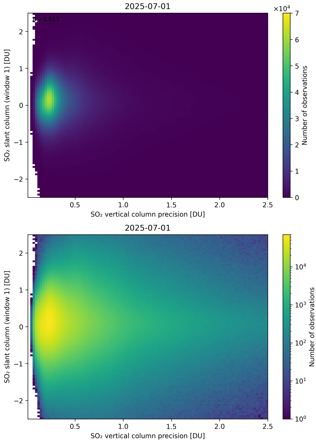
Figure 341: Scatter density plot of “SO 2 vertical column precision” against “SO 2 slant column (window 1)” for 2025-06-30 to 2025-07-02.
