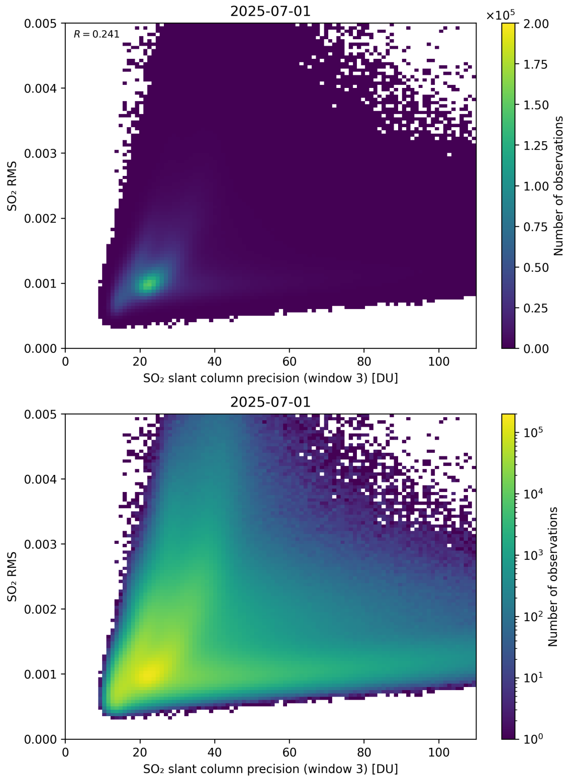
Figure 310: Scatter density plot of “SO 2 slant column precision (window 3)” against “SO 2 RMS” for 2025-06-30 to 2025-07-02.
