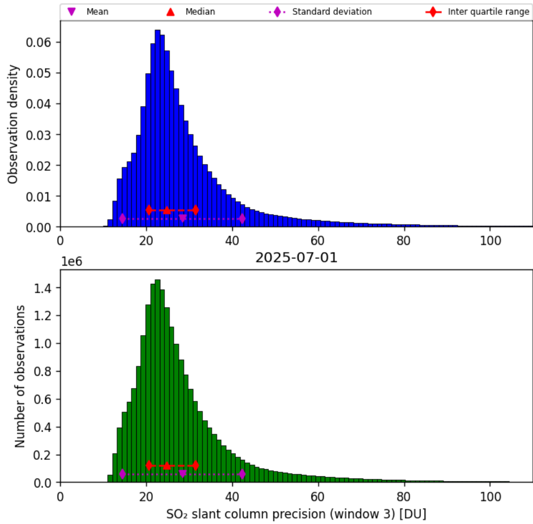
Figure 72: Histogram of “SO 2 slant column precision (window 3)” for 2025-06-30 to 2025-07-02
