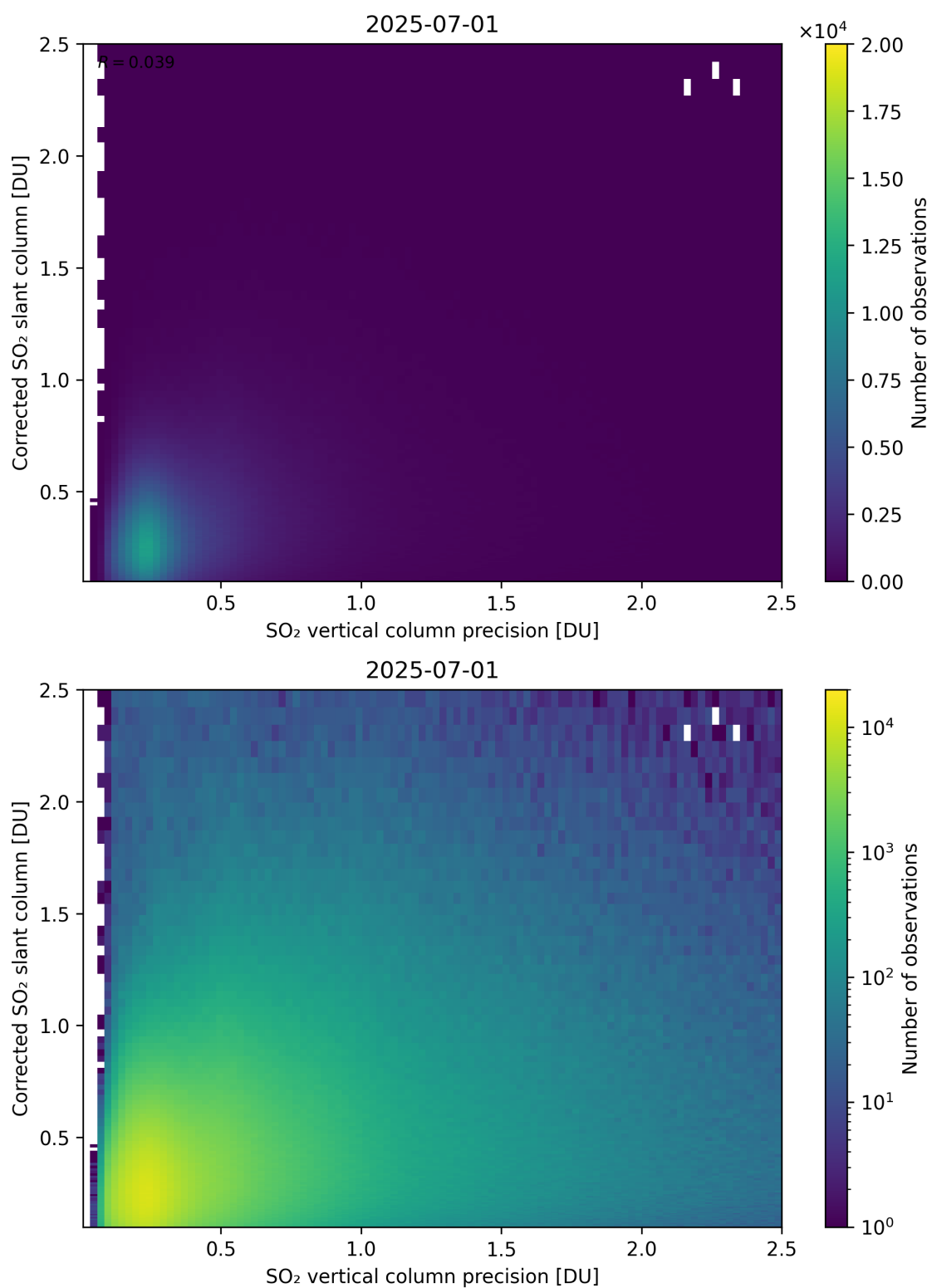
Figure 338: Scatter density plot of “SO 2 vertical column precision” against “Corrected SO 2 slant column” for 2025-06-30 to 2025-07-02.
