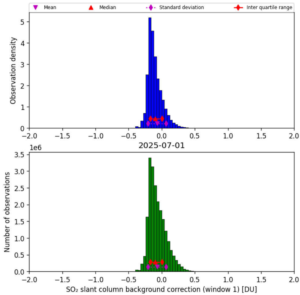
Figure 66: Histogram of “SO 2 slant column background correction (window 1)” for 2025-06-30 to 2025-07-02
