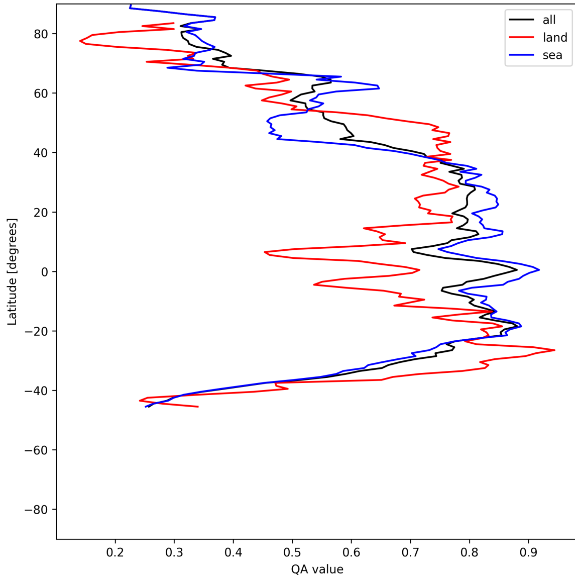
Figure 31: Zonal average of “QA value” for 2025-06-30 to 2025-07-02.
