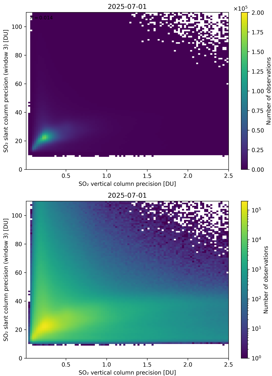
Figure 345: Scatter density plot of “SO 2 vertical column precision” against “SO 2 slant column precision (window 3)” for 2025-06-30 to 2025-07-02.
