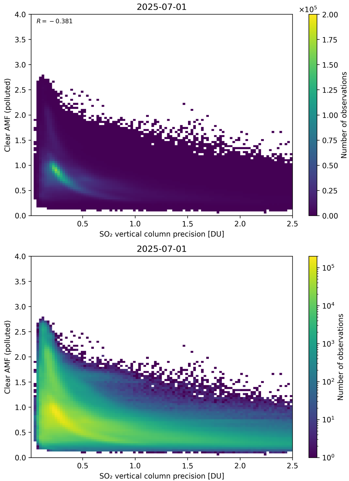
Figure 335: Scatter density plot of “SO 2 vertical column precision” against “Clear AMF (polluted)” for 2025-06-30 to 2025-07-02.
