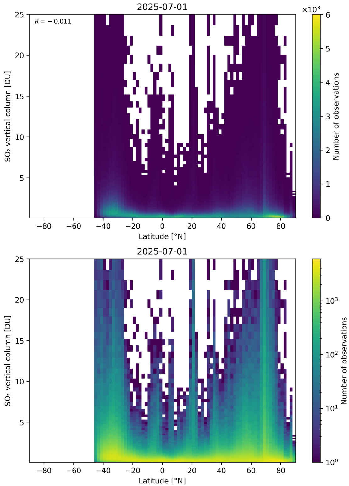
Figure 169: Scatter density plot of “Latitude” against “SO 2 vertical column” for 2025-06-30 to 2025-07-02.
