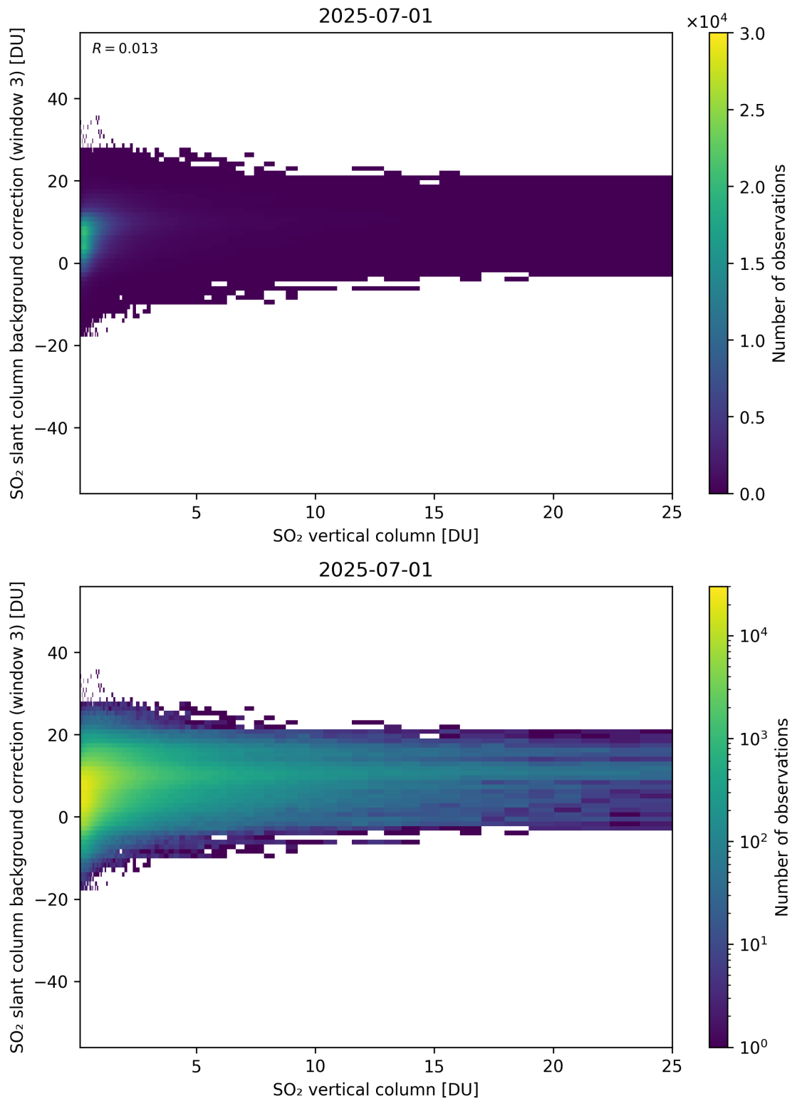
Figure 325: Scatter density plot of “SO 2 vertical column” against “SO 2 slant column background correction (window 3)” for 2025-06-30 to 2025-07-02.
