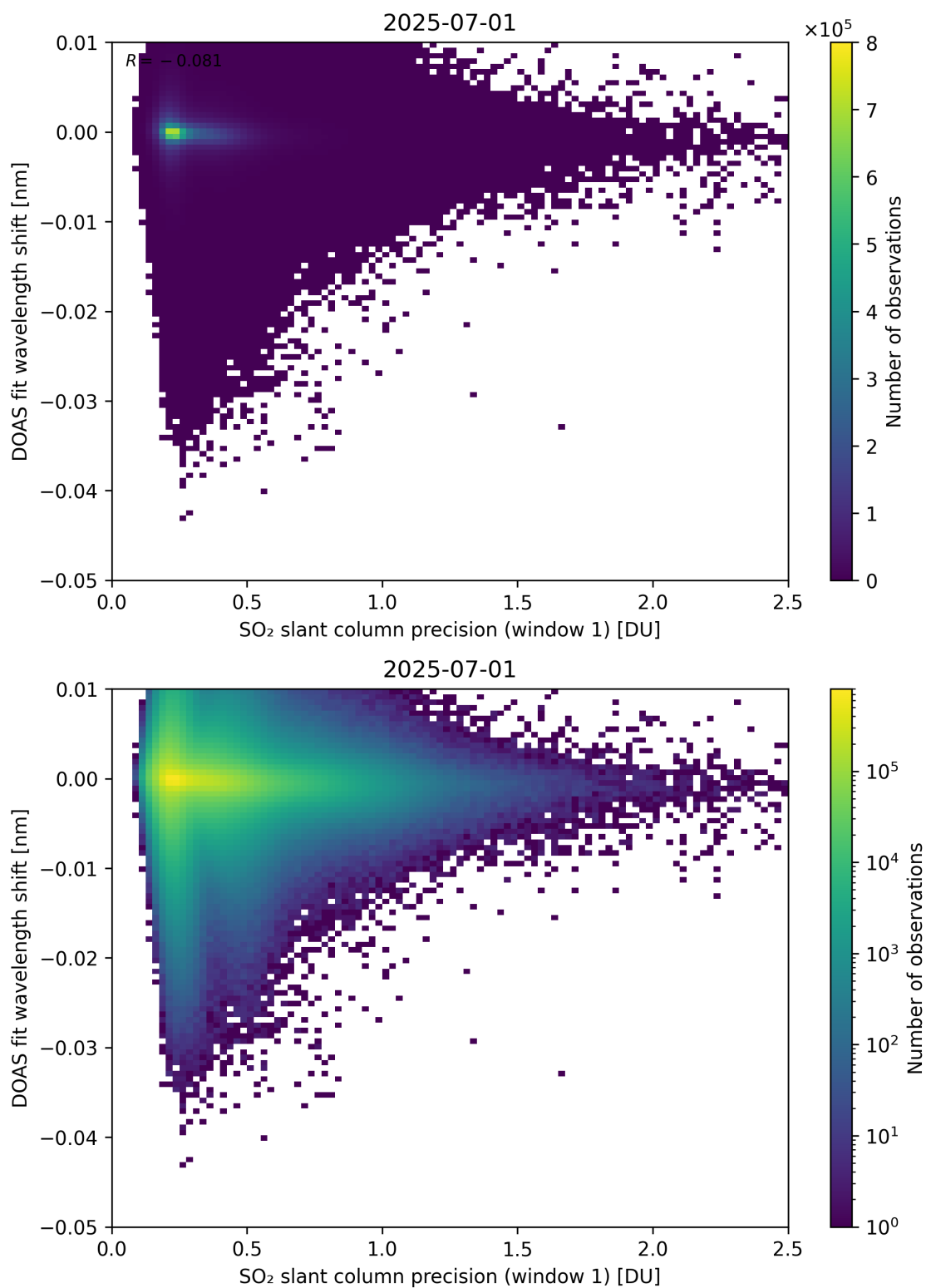
Figure 271: Scatter density plot of “SO 2 slant column precision (window 1)” against “DOAS fit wavelength shift” for 2025-06-30 to 2025-07-02.
