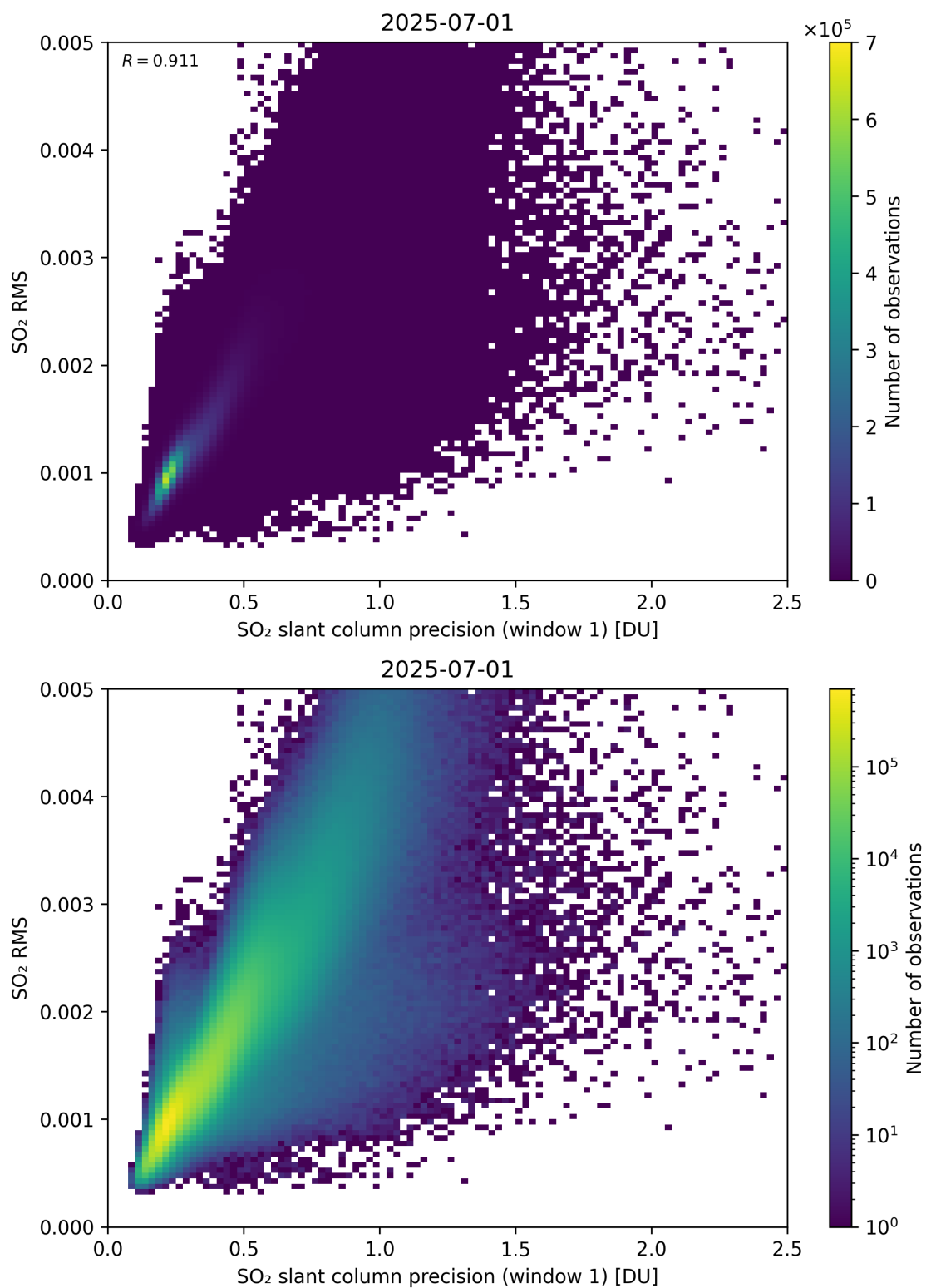
Figure 273: Scatter density plot of “SO 2 slant column precision (window 1)” against “SO 2 RMS” for 2025-06-30 to 2025-07-02.
