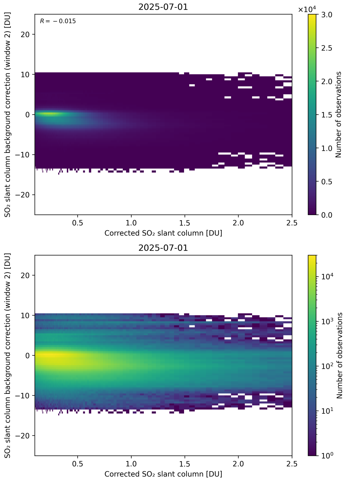
Figure 227: Scatter density plot of “Corrected SO 2 slant column” against “SO 2 slant column background correction (window 2)” for 2025-06-30 to 2025-07-02.
