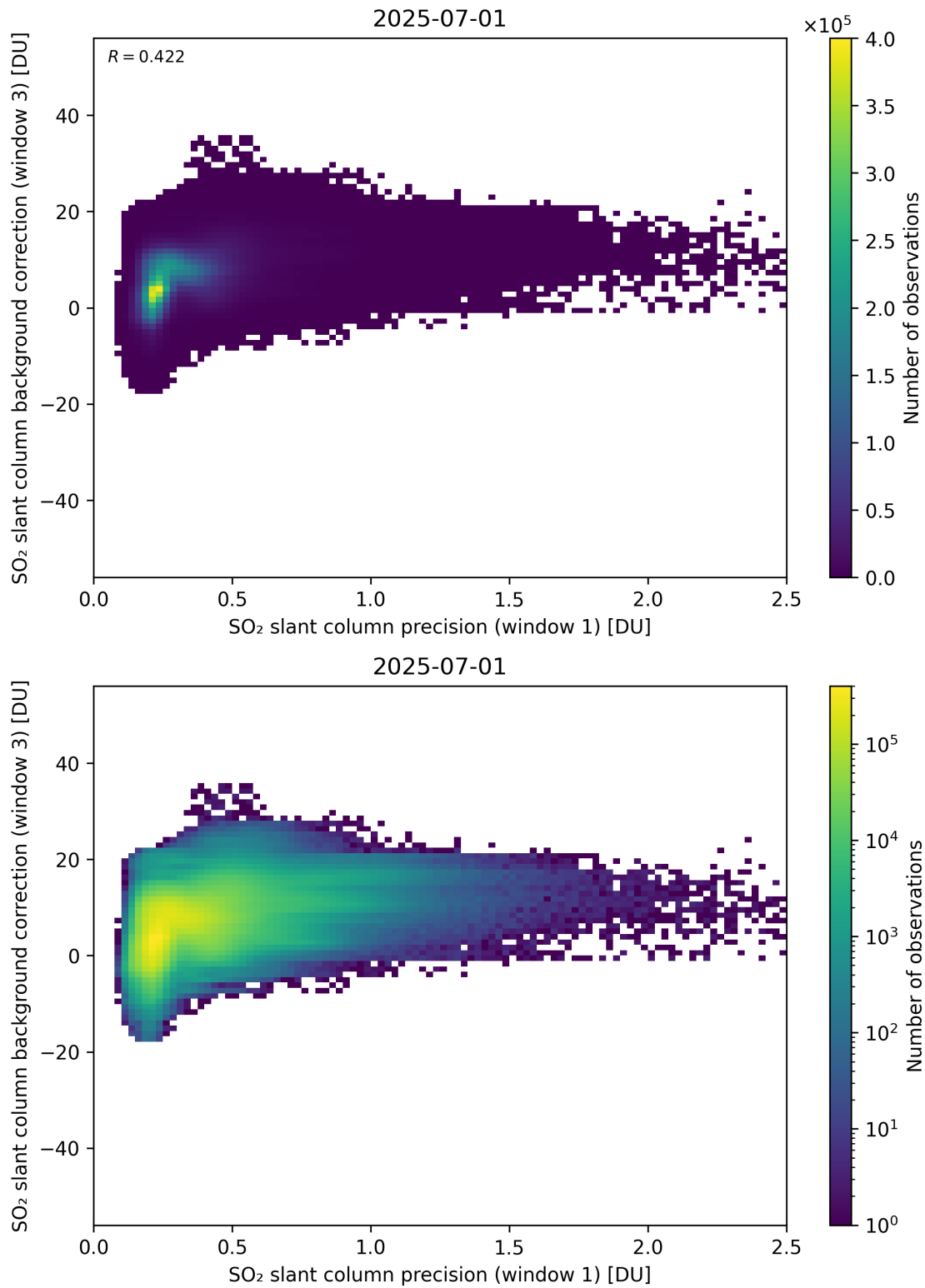
Figure 270: Scatter density plot of “SO 2 slant column precision (window 1)” against “SO 2 slant column background correction (window 3)” for 2025-06-30 to 2025-07-02.
