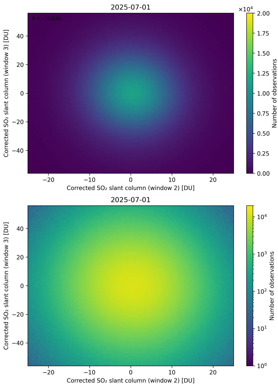
Figure 250: Scatter density plot of “Corrected SO 2 slant column (window 2)” against “Corrected SO 2 slant column (window 3)” for 2025-06-30 to 2025-07-02.
