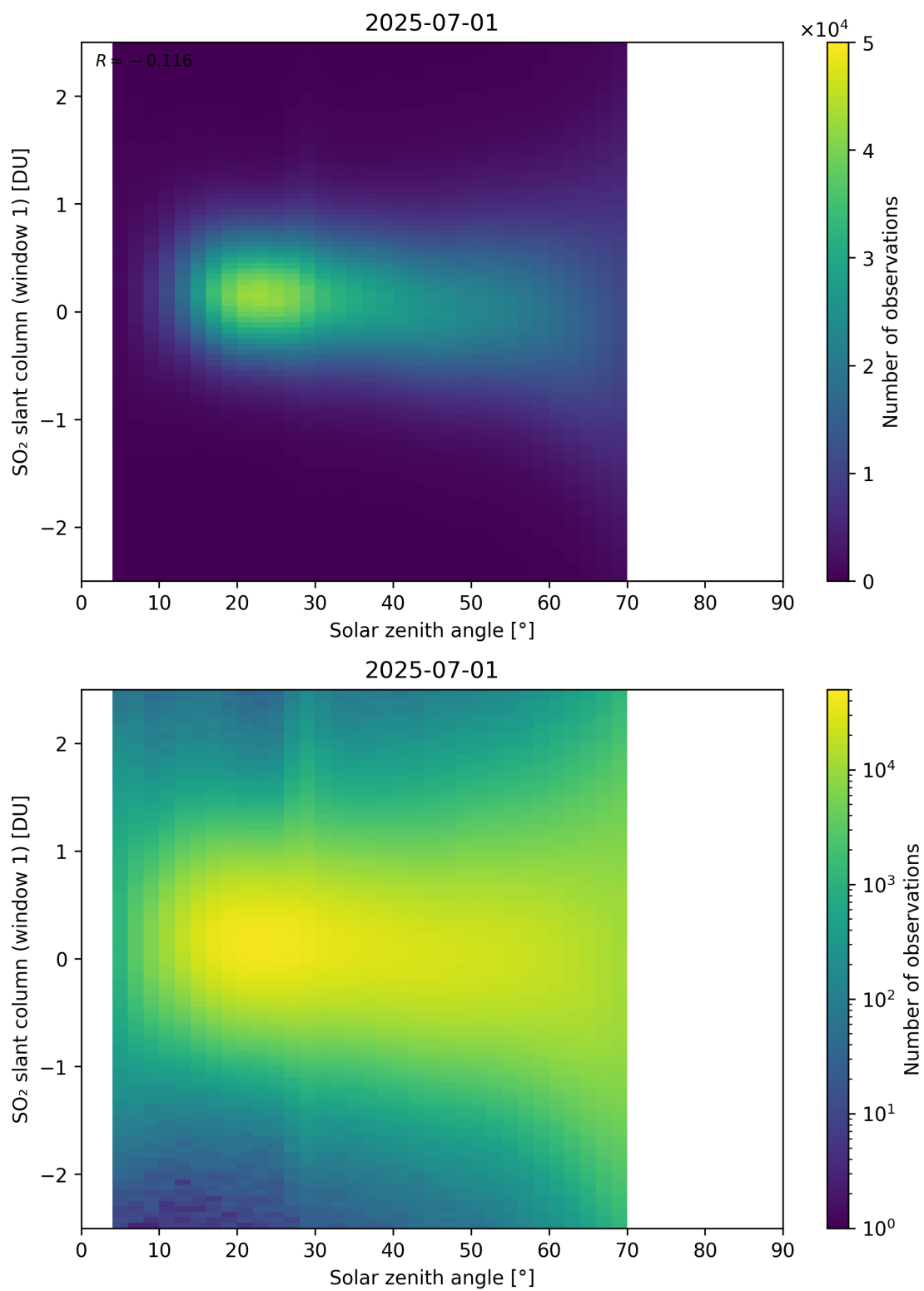
Figure 184: Scatter density plot of “Solar zenith angle” against “SO 2 slant column (window 1)” for 2025-06-30 to 2025-07-02.
