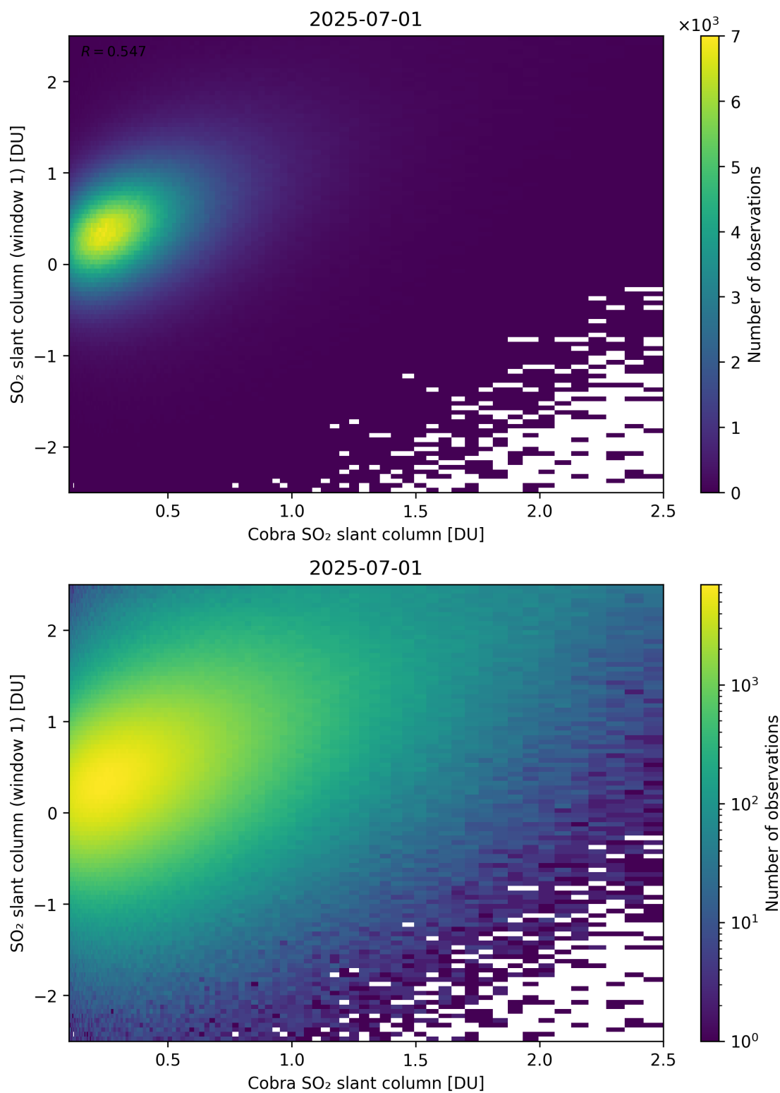
Figure 219: Scatter density plot of “Cobra SO 2 slant column” against “SO 2 slant column (window 1)” for 2025-06-30 to 2025-07-02.
