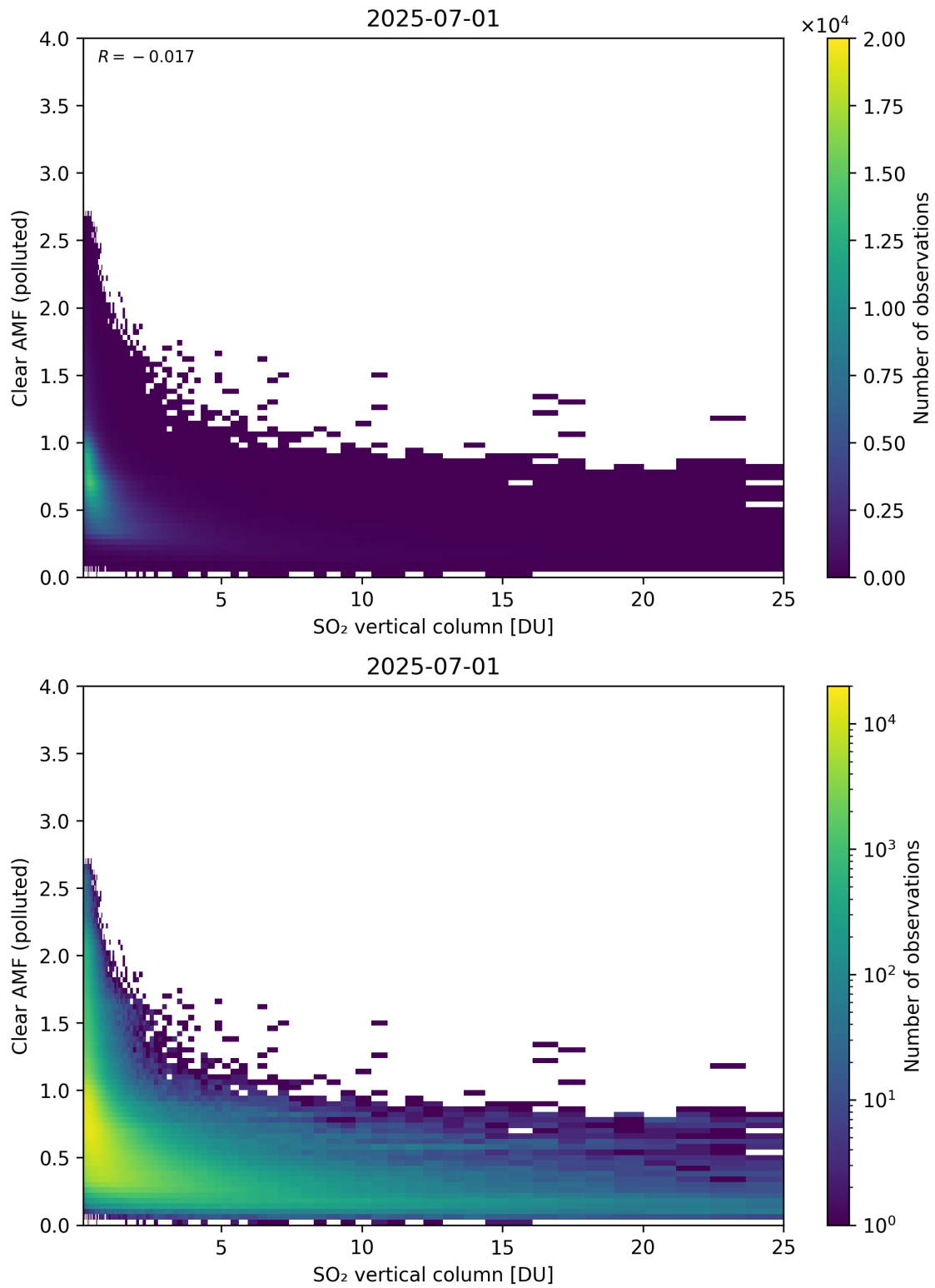
Figure 348: Scatter density plot of “SO 2 vertical column” against “Clear AMF (polluted)” for 2025-06-30 to 2025-07-02.
