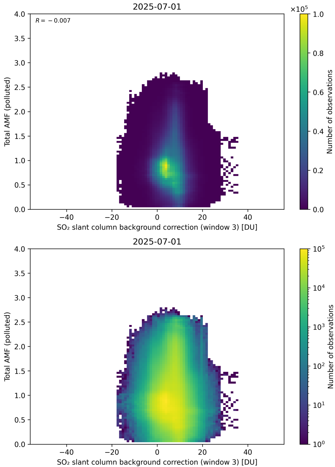
Figure 136: Scatter density plot of “SO 2 slant column background correction (window 3)” against “Total AMF (polluted)” for 2025-06-30 to 2025-07-02.
