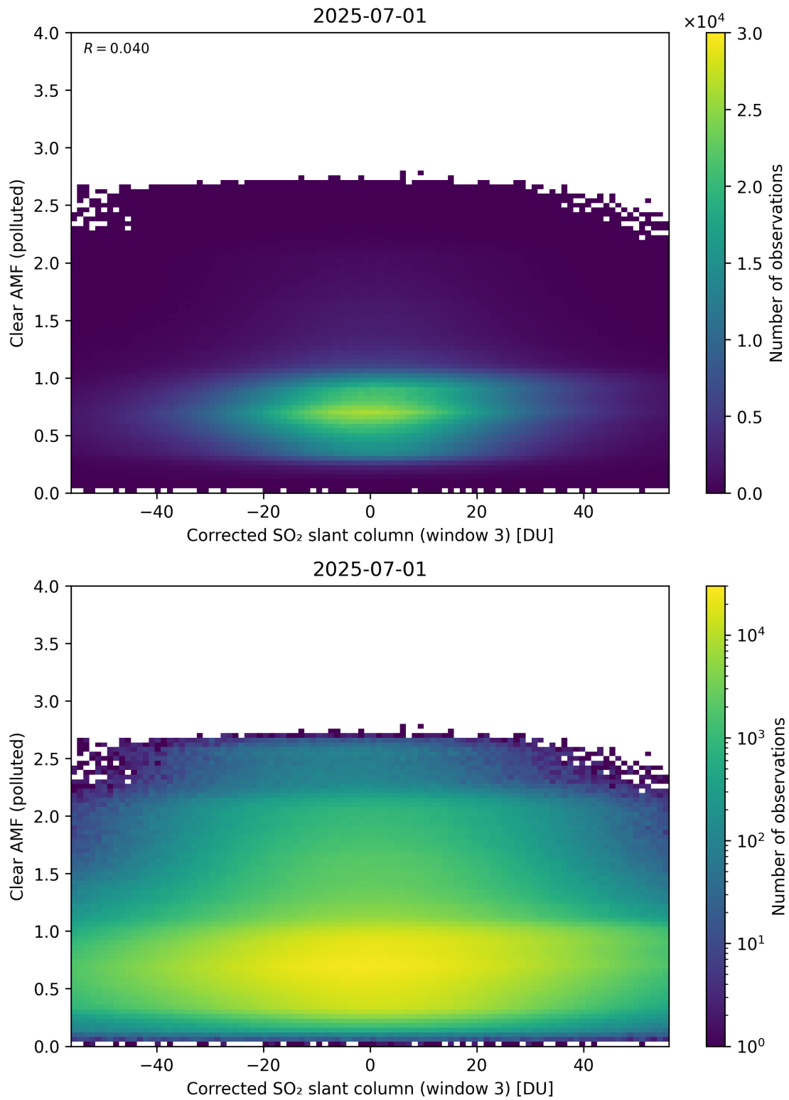
Figure 259: Scatter density plot of “Corrected SO 2 slant column (window 3)” against “Clear AMF (polluted)” for 2025-06-30 to 2025-07-02.
