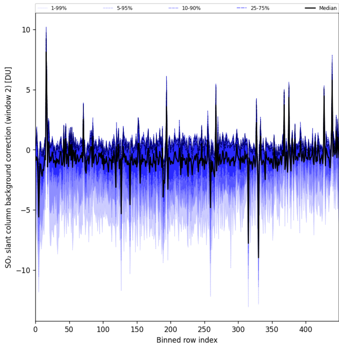
Figure 96: Along track statistics of “SO 2 slant column background correction (window 2)” for 2025-06-30 to 2025-07-02
