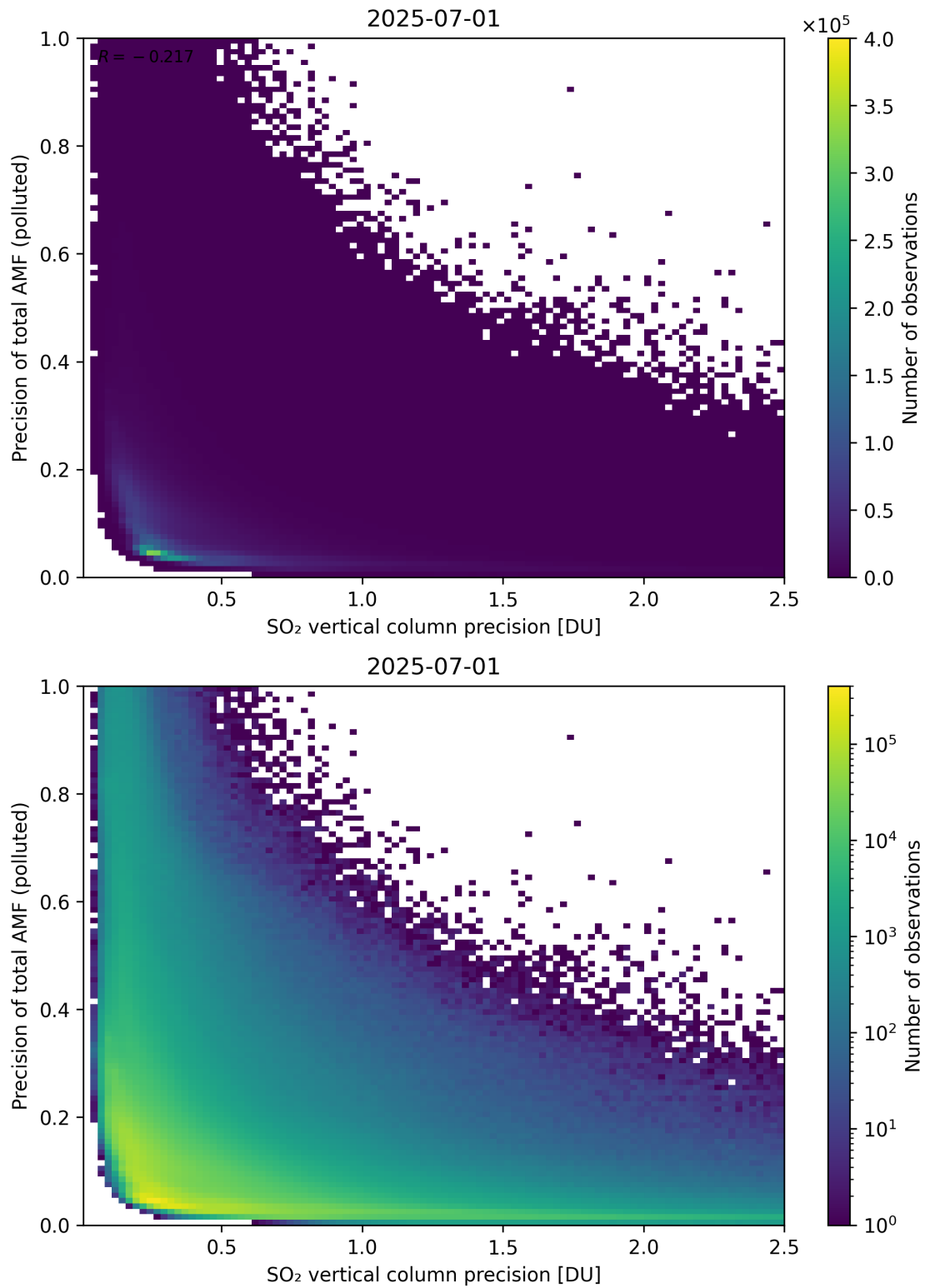
Figure 347: Scatter density plot of “SO 2 vertical column precision” against “Precision of total AMF (polluted)” for 2025-06-30 to 2025-07-02.
