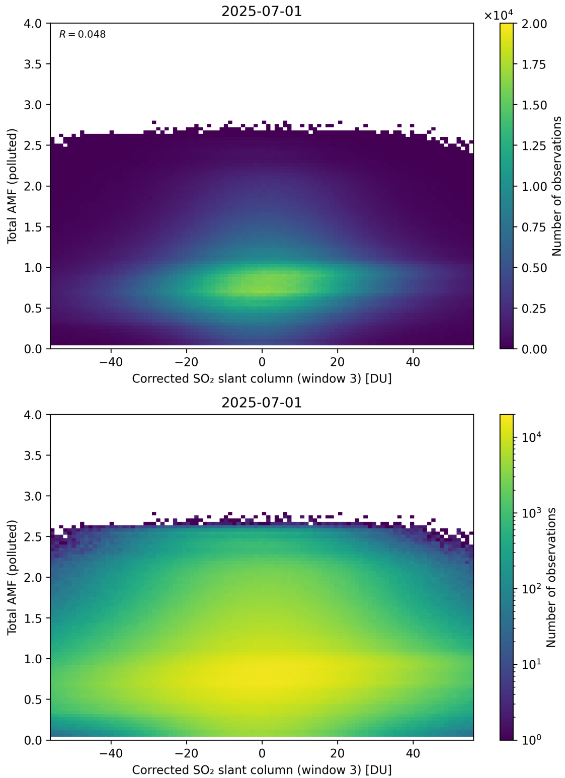
Figure 260: Scatter density plot of “Corrected SO 2 slant column (window 3)” against “Total AMF (polluted)” for 2025-06-30 to 2025-07-02.
