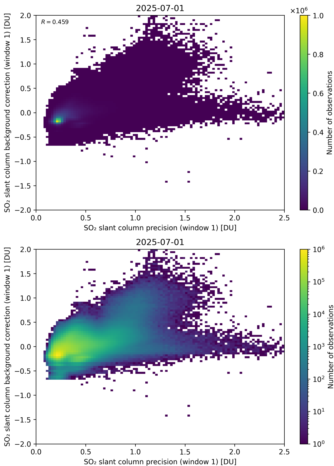
Figure 268: Scatter density plot of “SO 2 slant column precision (window 1)” against “SO 2 slant column background correction (window 1)” for 2025-06-30 to 2025-07-02.
