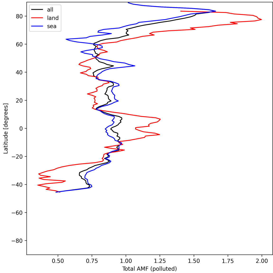
Figure 53: Zonal average of “Total AMF (polluted)” for 2025-06-30 to 2025-07-02.
