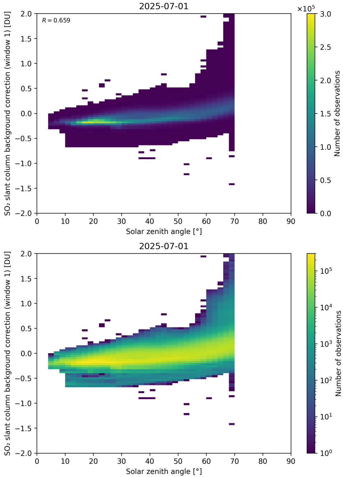
Figure 171: Scatter density plot of “Solar zenith angle” against “SO 2 slant column background correction (window 1)” for 2025-06-30 to 2025-07-02.
