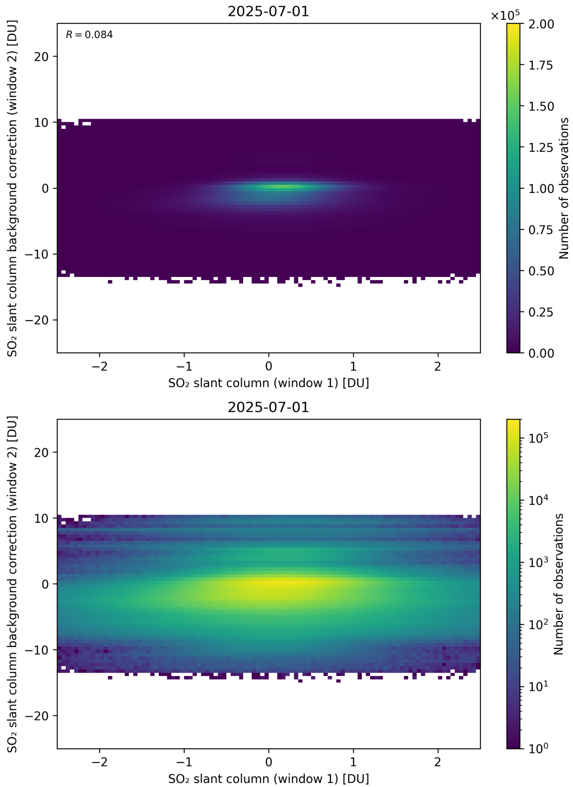
Figure 263: Scatter density plot of “SO 2 slant column (window 1)” against “SO 2 slant column background correction (window 2)” for 2025-06-30 to 2025-07-02.
