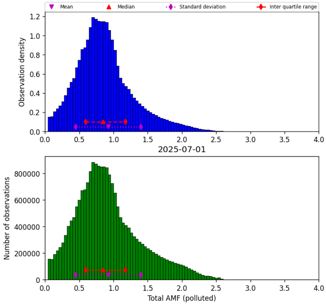
Figure 79: Histogram of “Total AMF (polluted)” for 2025-06-30 to 2025-07-02
