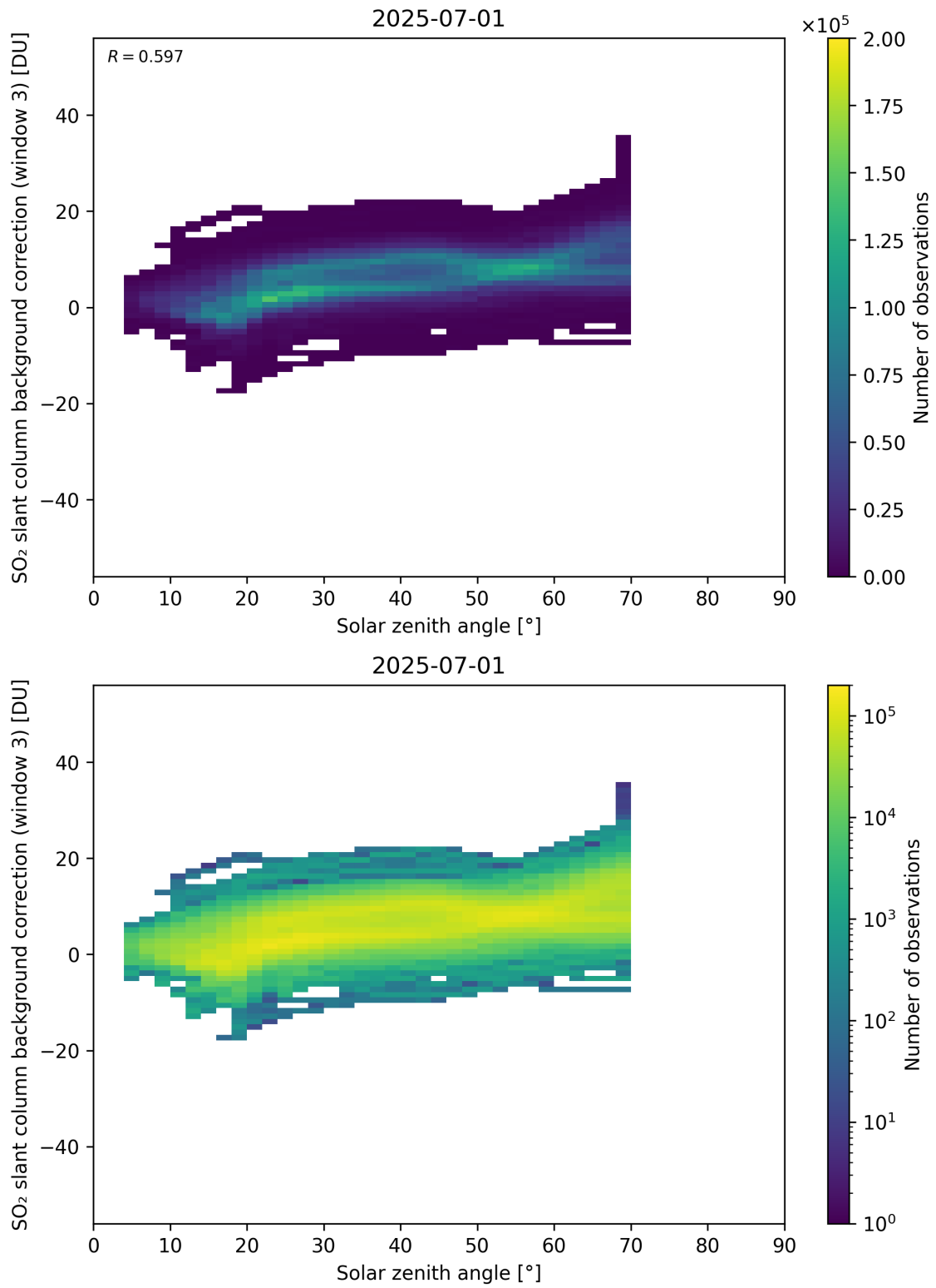
Figure 173: Scatter density plot of “Solar zenith angle” against “SO 2 slant column background correction (window 3)” for 2025-06-30 to 2025-07-02.
