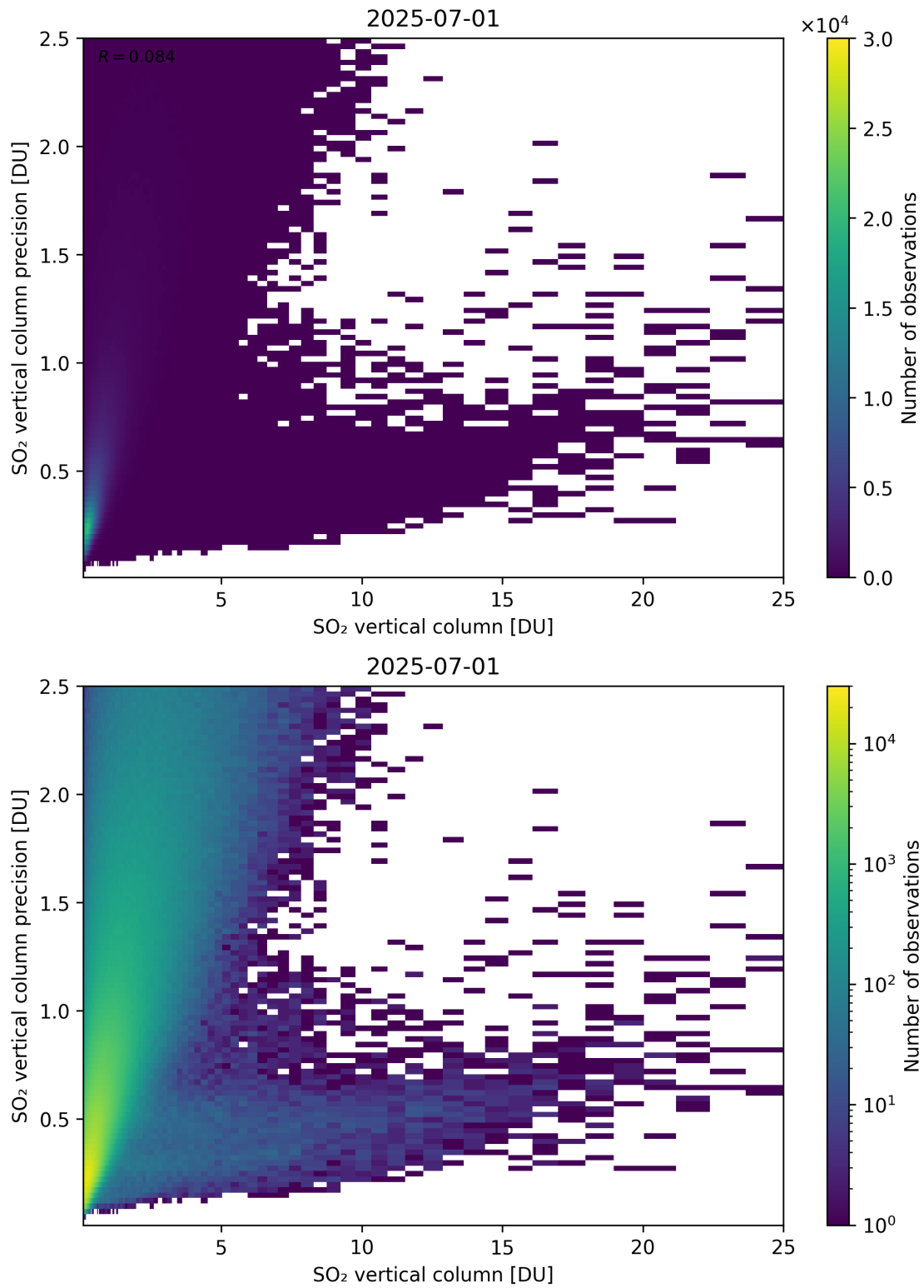
Figure 361: Scatter density plot of “SO 2 vertical column” against “SO 2 vertical column precision” for 2025-06-30 to 2025-07-02.
