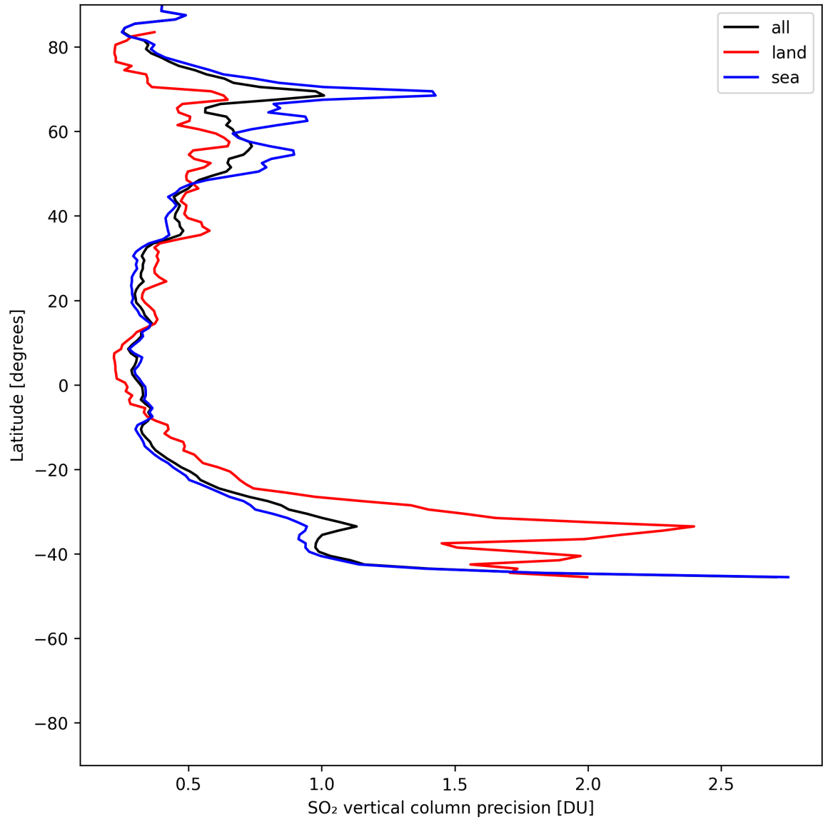
Figure 33: Zonal average of “SO 2 vertical column precision” for 2025-06-30 to 2025-07-02.
