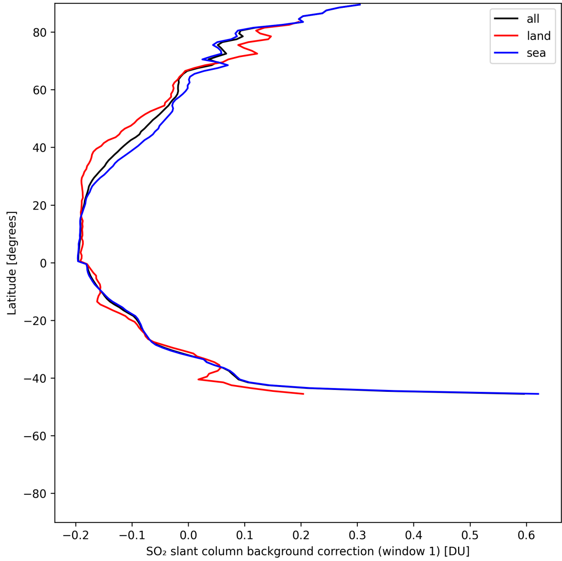
Figure 40: Zonal average of "SO 2 slant column background correction (window 1)" for 2025-06-30 to 2025-07-02.
