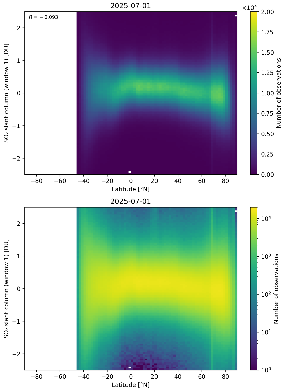
Figure 162: Scatter density plot of “Latitude” against “SO 2 slant column (window 1)” for 2025-06-30 to 2025-07-02.
