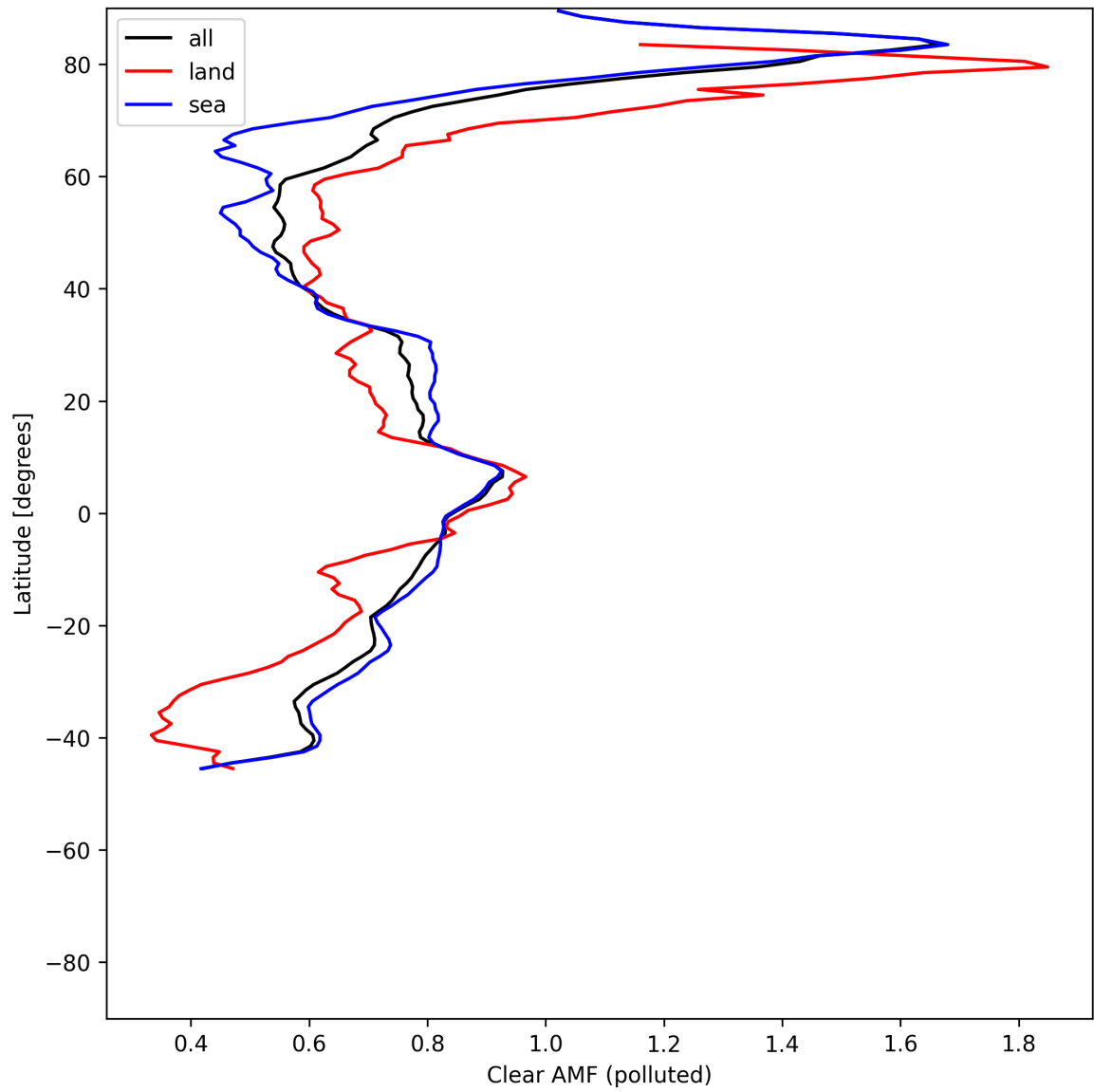
Figure 55: Zonal average of “Clear AMF (polluted)” for 2025-06-30 to 2025-07-02.
