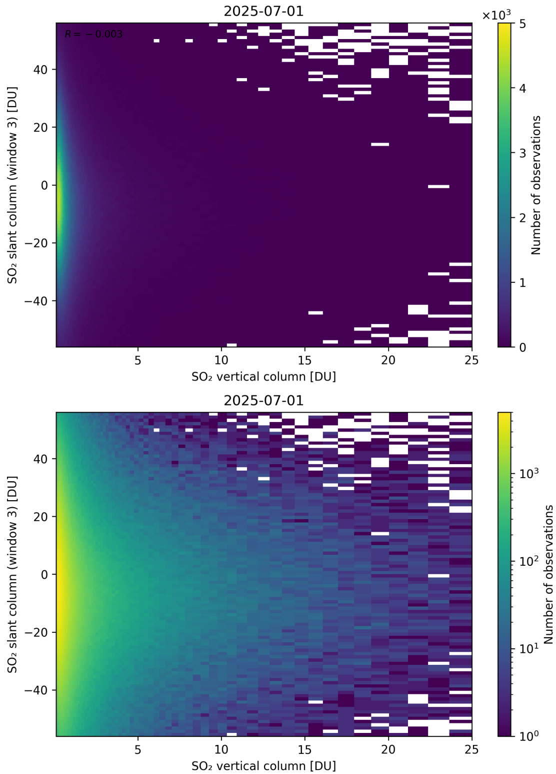
Figure 357: Scatter density plot of “SO 2 vertical column” against “SO 2 slant column (window 3)” for 2025-06-30 to 2025-07-02.
