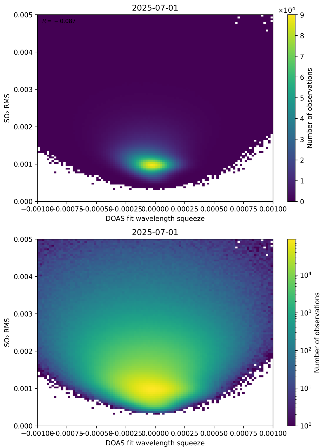
Figure 143: Scatter density plot of “DOAS fit wavelength squeeze” against “SO 2 RMS” for 2025-06-30 to 2025-07-02.
