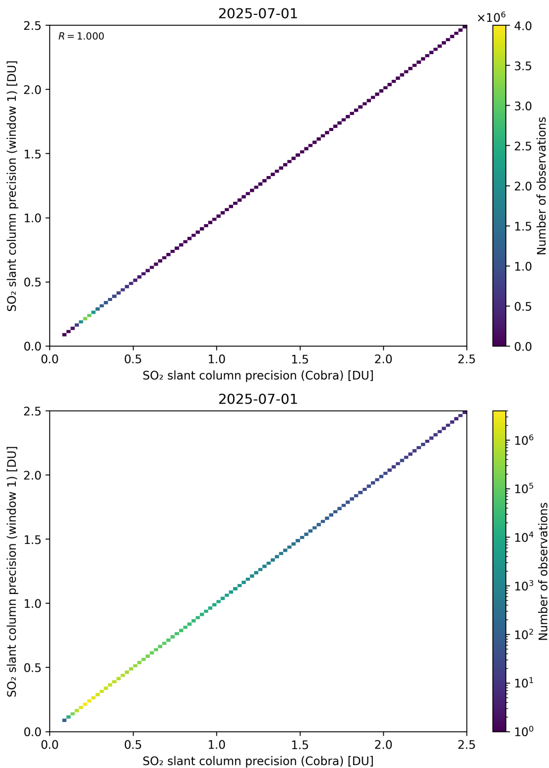
Figure 209: Scatter density plot of “SO 2 slant column precision (Cobra)” against “SO 2 slant column precision (window 1)” for 2025-06-30 to 2025-07-02.
