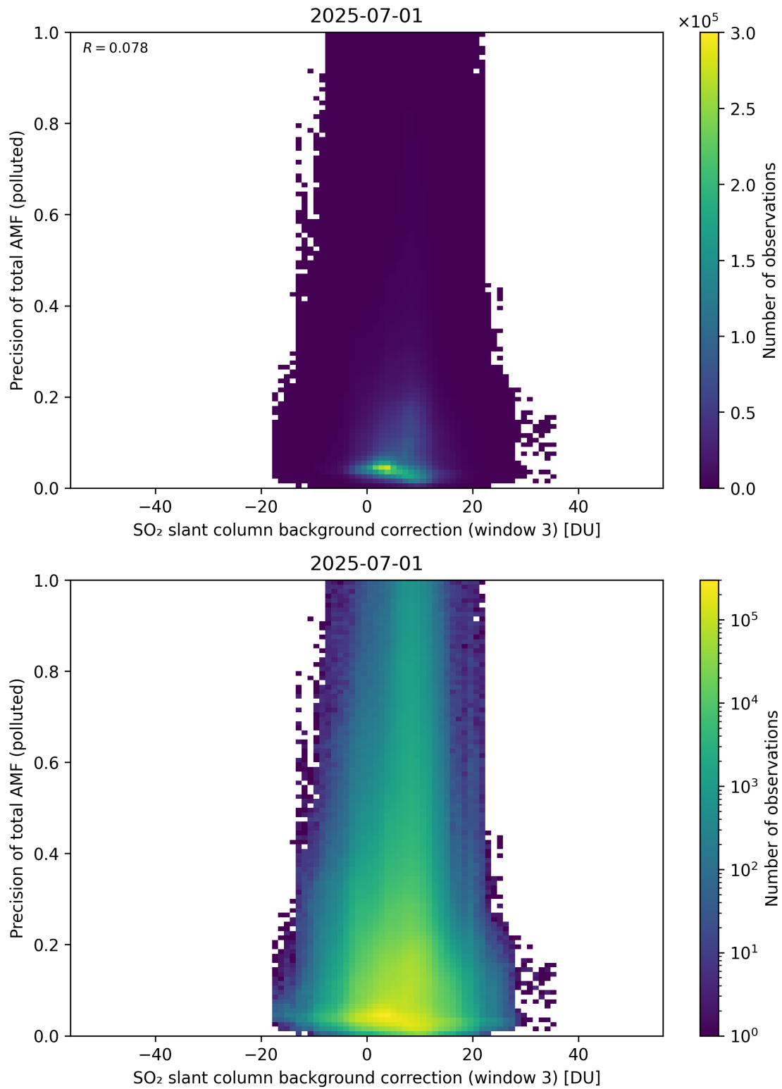
Figure 137: Scatter density plot of “SO 2 slant column background correction (window 3)” against “Precision of total AMF (polluted)” for 2025-06-30 to 2025-07-02.
