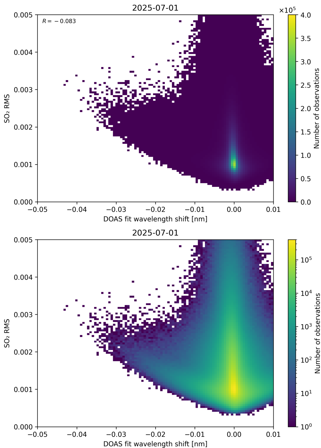
Figure 139: Scatter density plot of “DOAS fit wavelength shift” against “SO 2 RMS” for 2025-06-30 to 2025-07-02.
