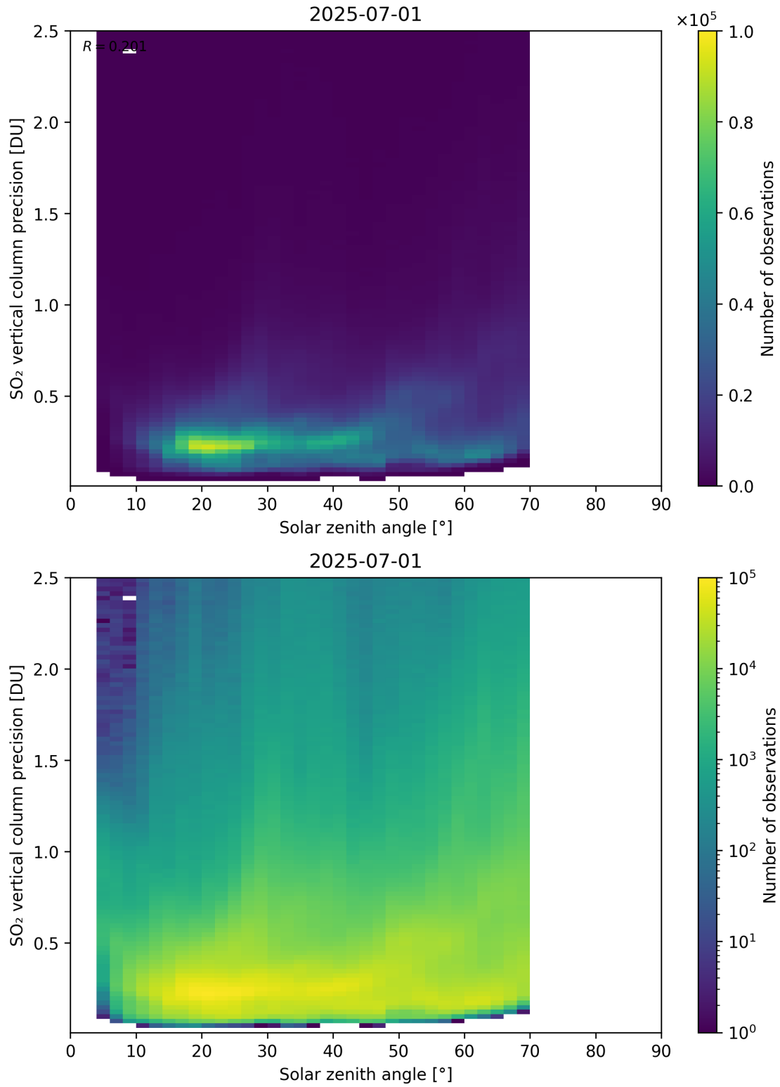
Figure 192: Scatter density plot of “Solar zenith angle” against “SO 2 vertical column precision” for 2025-06-30 to 2025-07-02.
