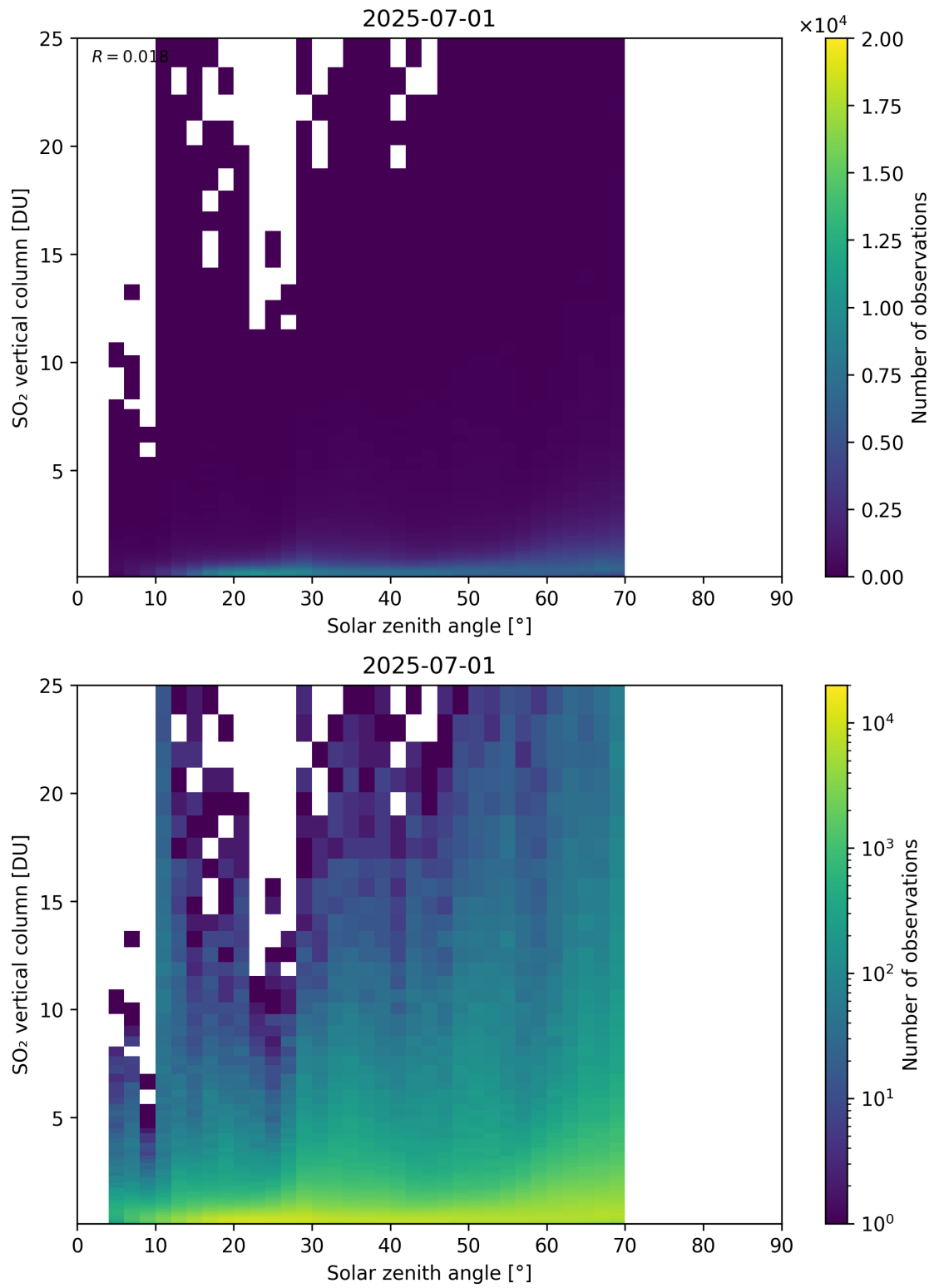
Figure 191: Scatter density plot of “Solar zenith angle” against “SO 2 vertical column” for 2025-06-30 to 2025-07-02.
