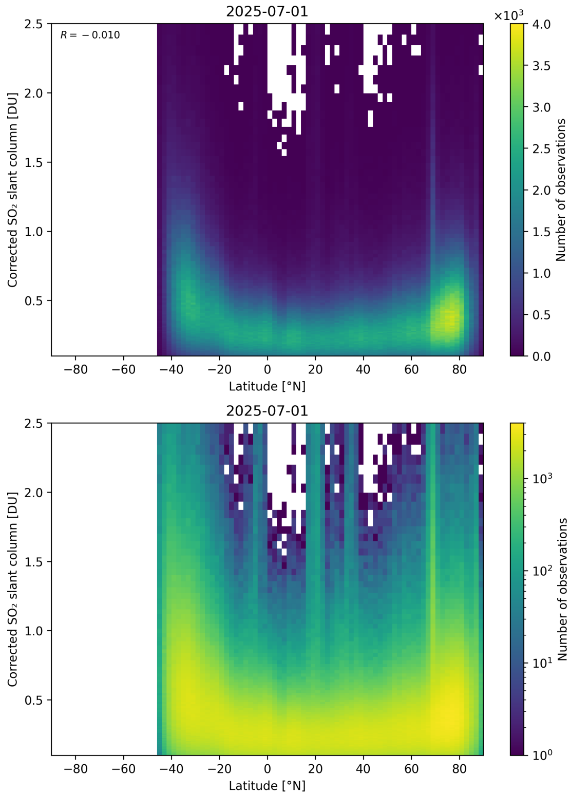
Figure 159: Scatter density plot of “Latitude” against “Corrected SO 2 slant column” for 2025-06-30 to 2025-07-02.
