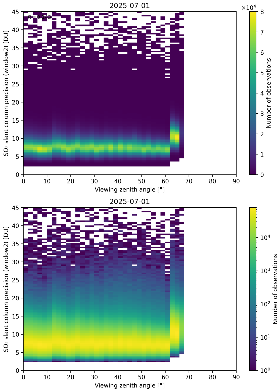
Figure 378: Scatter density plot of “Viewing zenith angle” against “SO 2 slant column precision (window2)” for 2025-06-30 to 2025-07-02.
