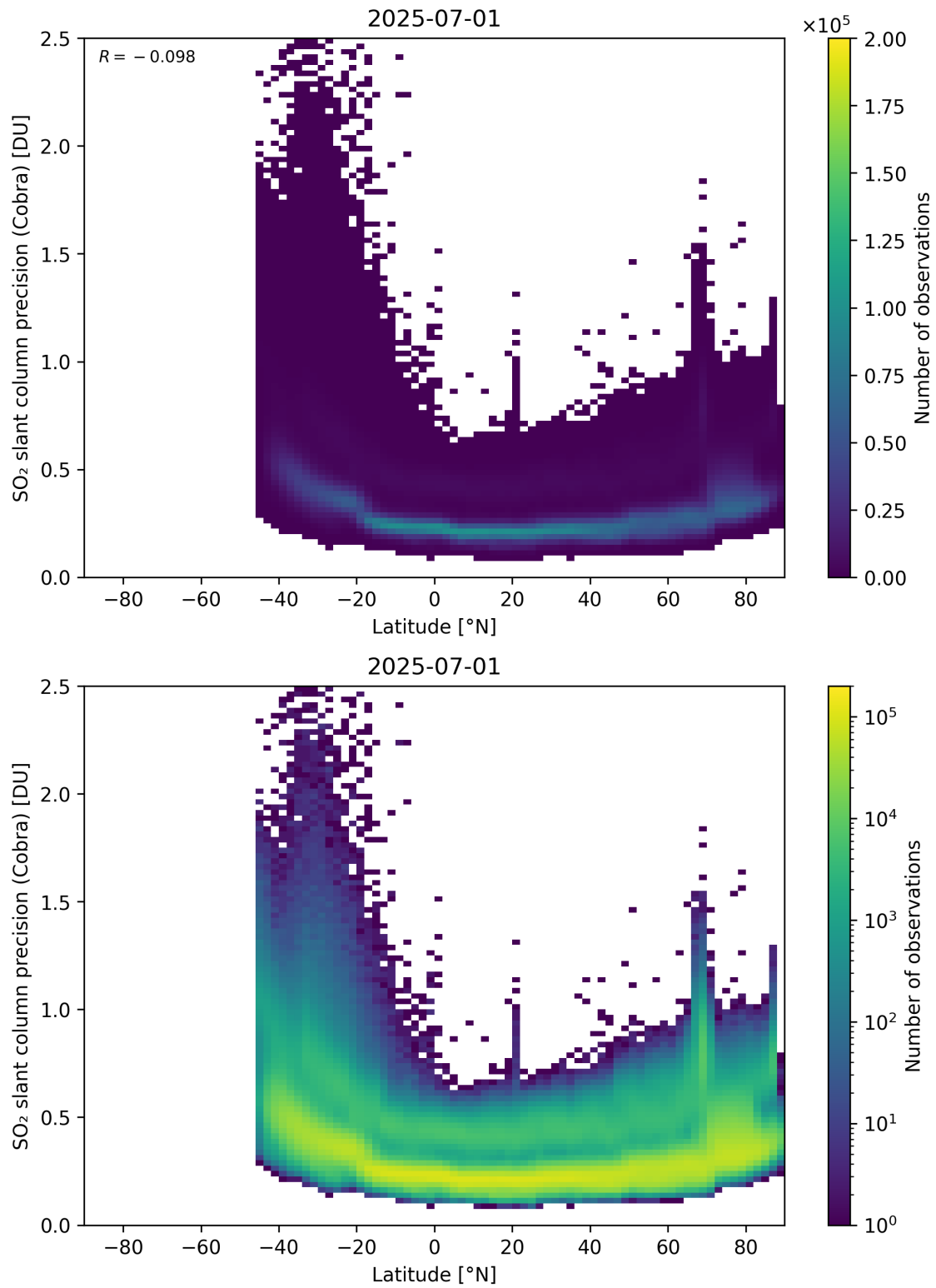
Figure 158: Scatter density plot of “Latitude” against “SO 2 slant column precision (Cobra)” for 2025-06-30 to 2025-07-02.
