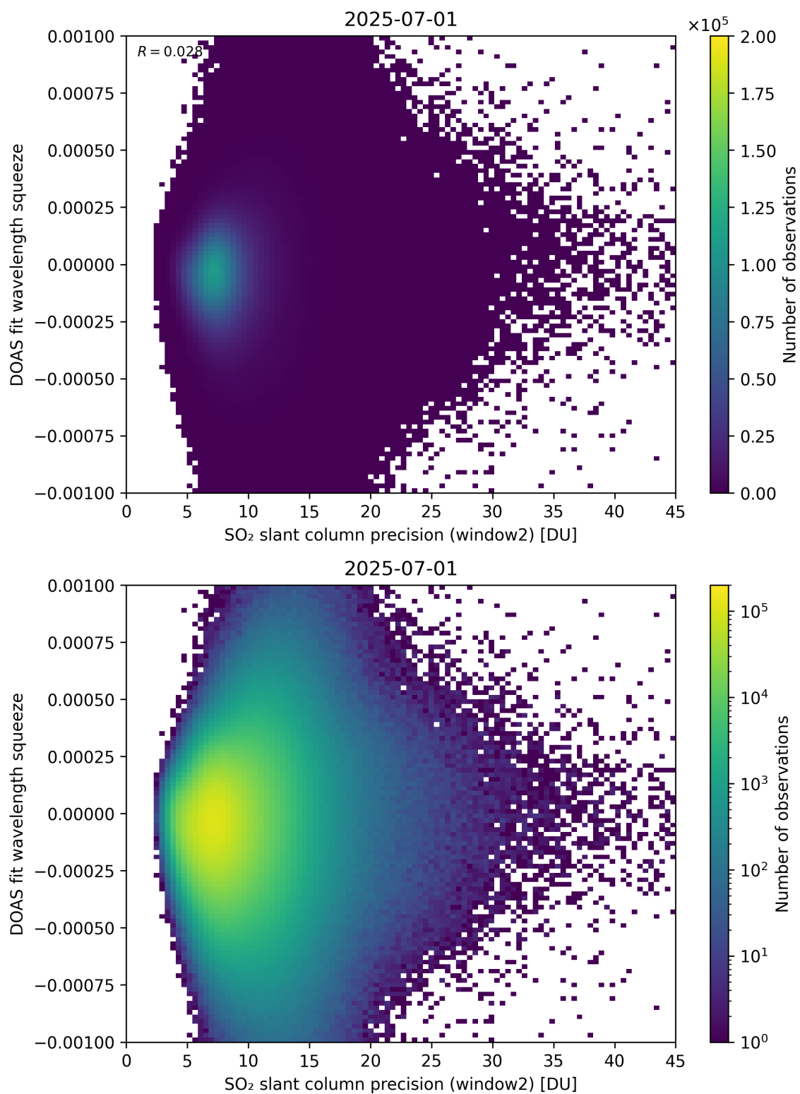
Figure 294: Scatter density plot of “SO 2 slant column precision (window2)” against “DOAS fit wavelength squeeze” for 2025-06-30 to 2025-07-02.
