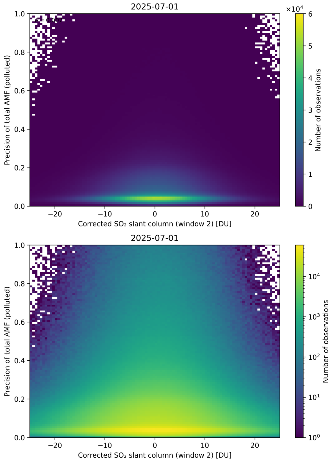
Figure 254: Scatter density plot of “Corrected SO 2 slant column (window 2)” against “Precision of total AMF (polluted)” for 2025-06-30 to 2025-07-02.
