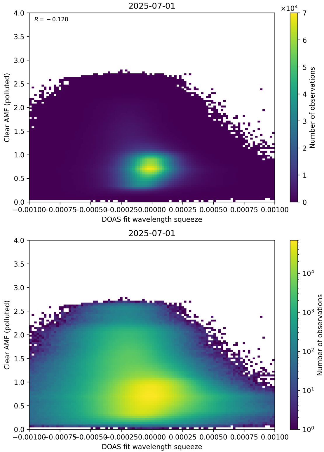
Figure 144: Scatter density plot of “DOAS fit wavelength squeeze” against “Clear AMF (polluted)” for 2025-06-30 to 2025-07-02.
