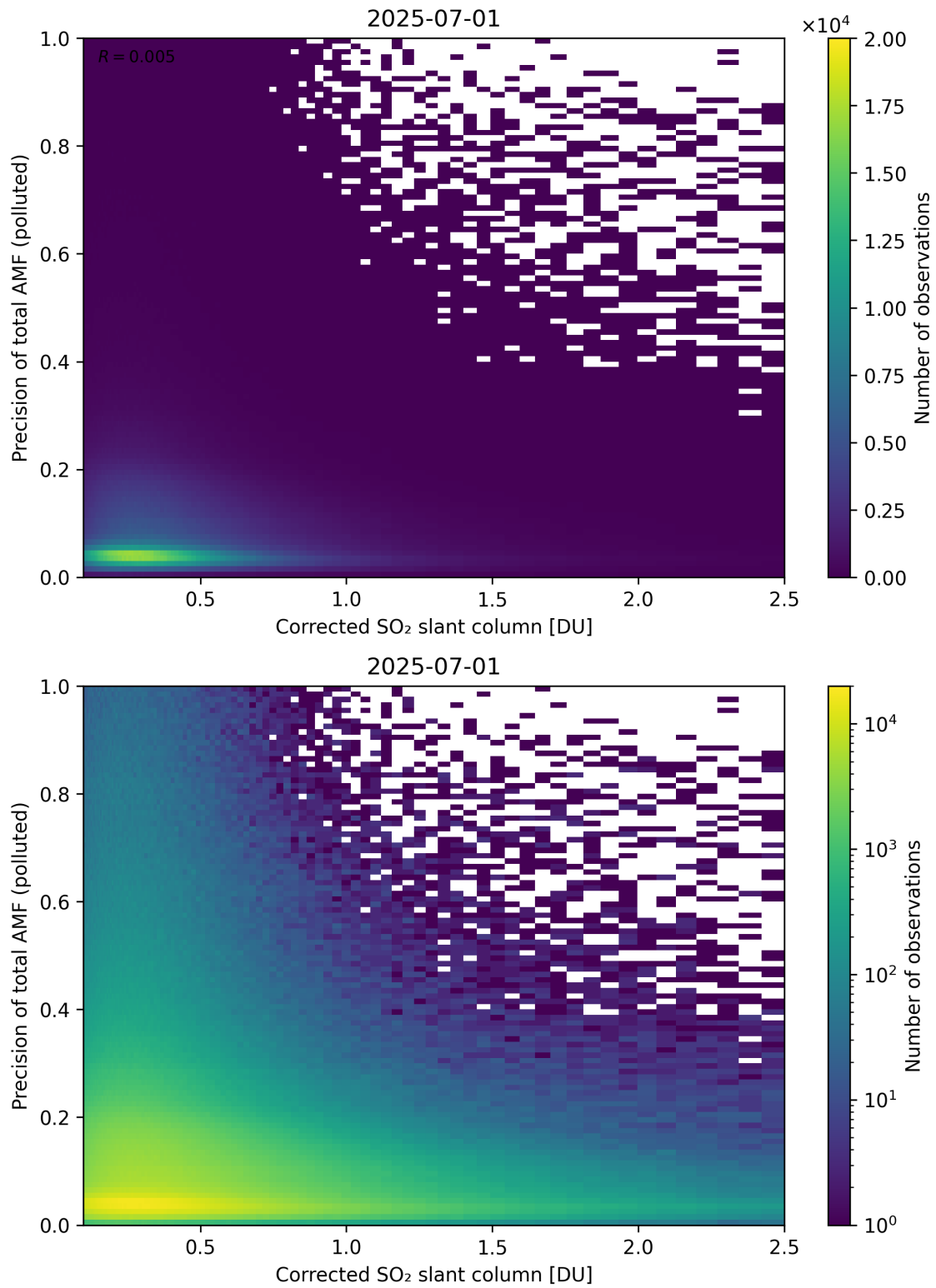
Figure 243: Scatter density plot of “Corrected SO 2 slant column” against “Precision of total AMF (polluted)” for 2025-06-30 to 2025-07-02.
