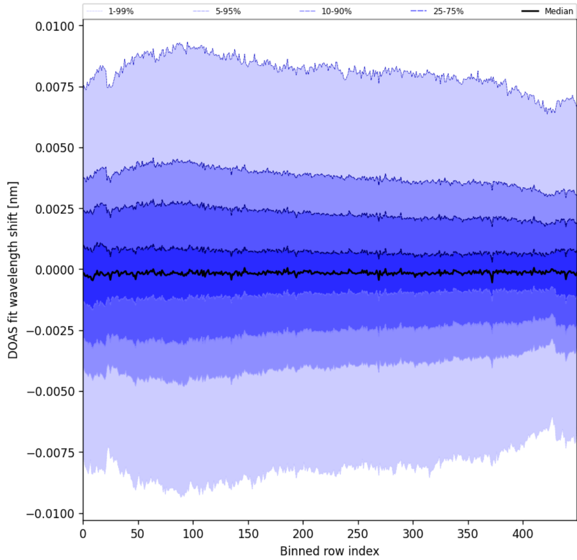
Figure 102: Along track statistics of “DOAS fit wavelength shift” for 2025-06-30 to 2025-07-02
