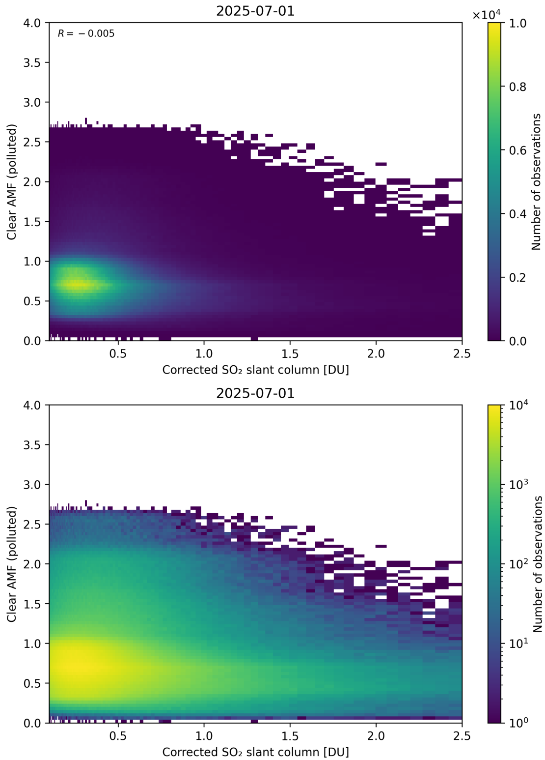
Figure 232: Scatter density plot of “Corrected SO 2 slant column” against “Clear AMF (polluted)” for 2025-06-30 to 2025-07-02.
