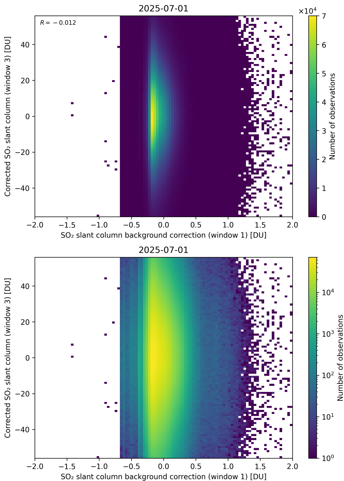
Figure 116: Scatter density plot of “SO 2 slant column background correction (window 1)” against “Corrected SO 2 slant column (window 3)” for 2025-06-30 to 2025-07-02.
