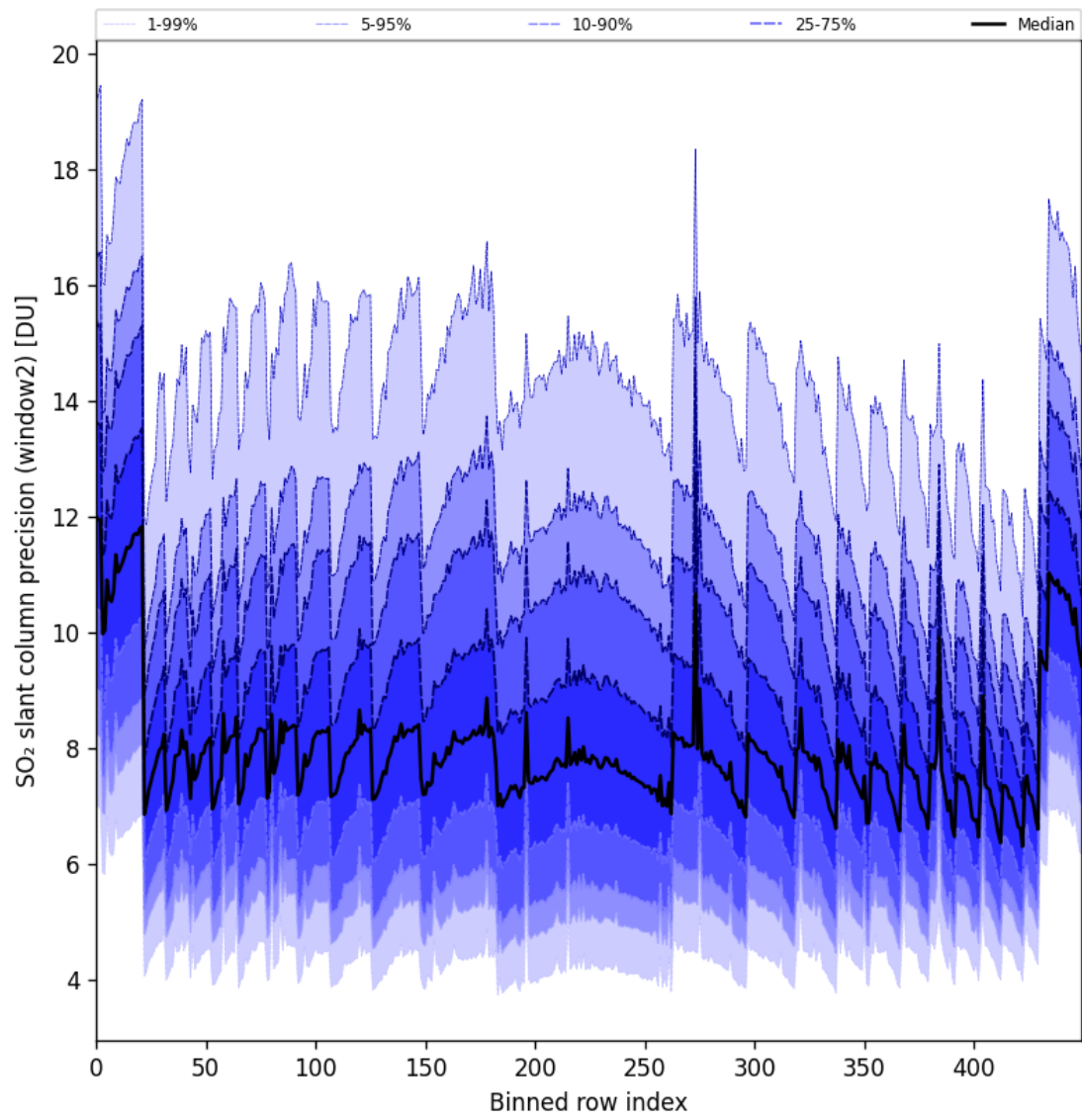
Figure 94: Along track statistics of “SO 2 slant column precision (window2)” for 2025-06-30 to 2025-07-02
