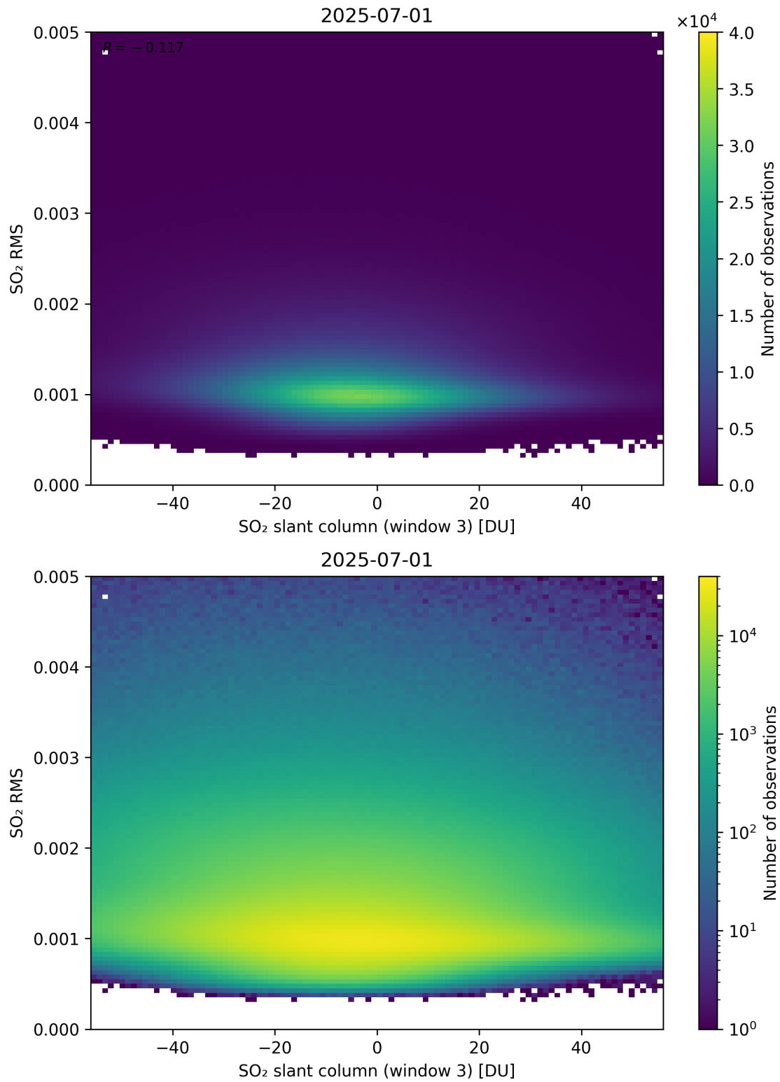
Figure 306: Scatter density plot of “SO 2 slant column (window 3)” against “SO 2 RMS” for 2025-06-30 to 2025-07-02.
