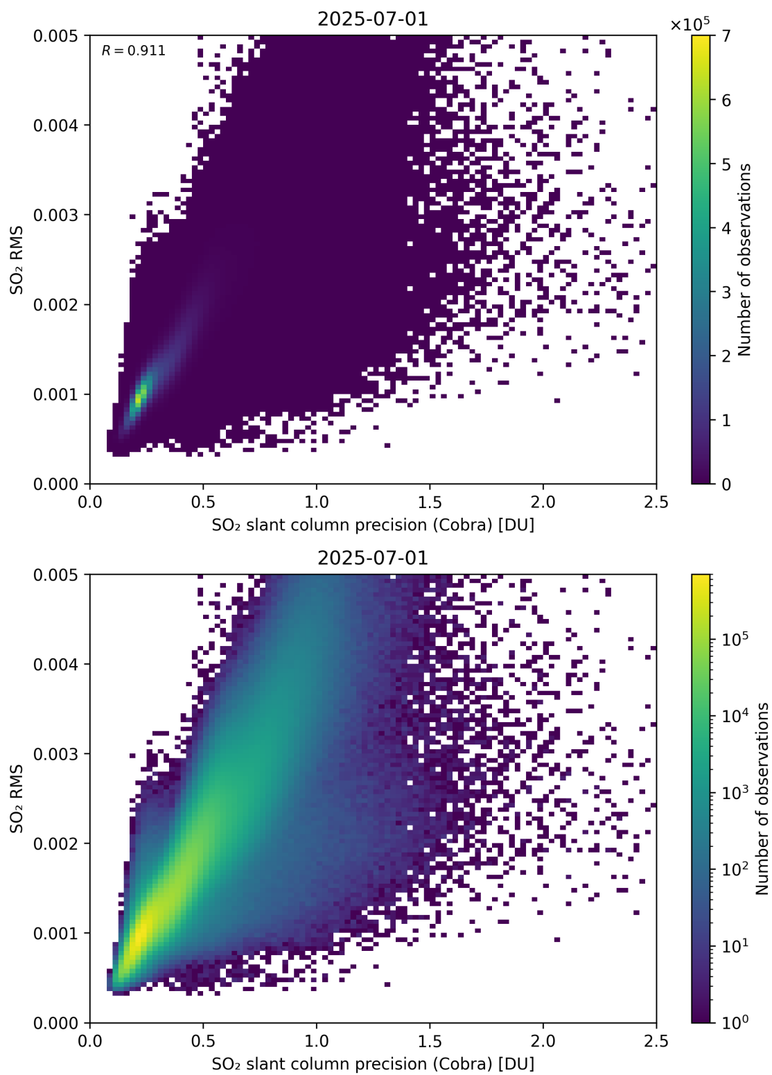
Figure 204: Scatter density plot of “SO 2 slant column precision (Cobra)” against “SO 2 RMS” for 2025-06-30 to 2025-07-02.
