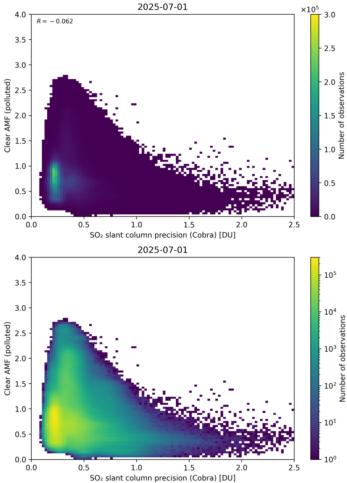
Figure 205: Scatter density plot of “SO 2 slant column precision (Cobra)” against “Clear AMF (polluted)” for 2025-06-30 to 2025-07-02.
