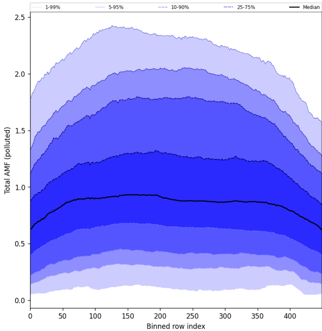
Figure 105: Along track statistics of “Total AMF (polluted)” for 2025-06-30 to 2025-07-02
