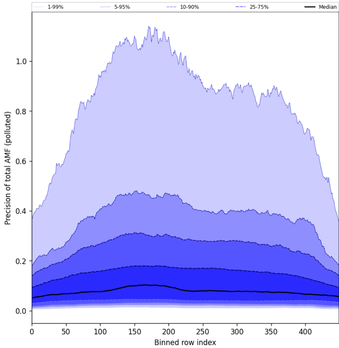
Figure 106: Along track statistics of “Precision of total AMF (polluted)” for 2025-06-30 to 2025-07-02
