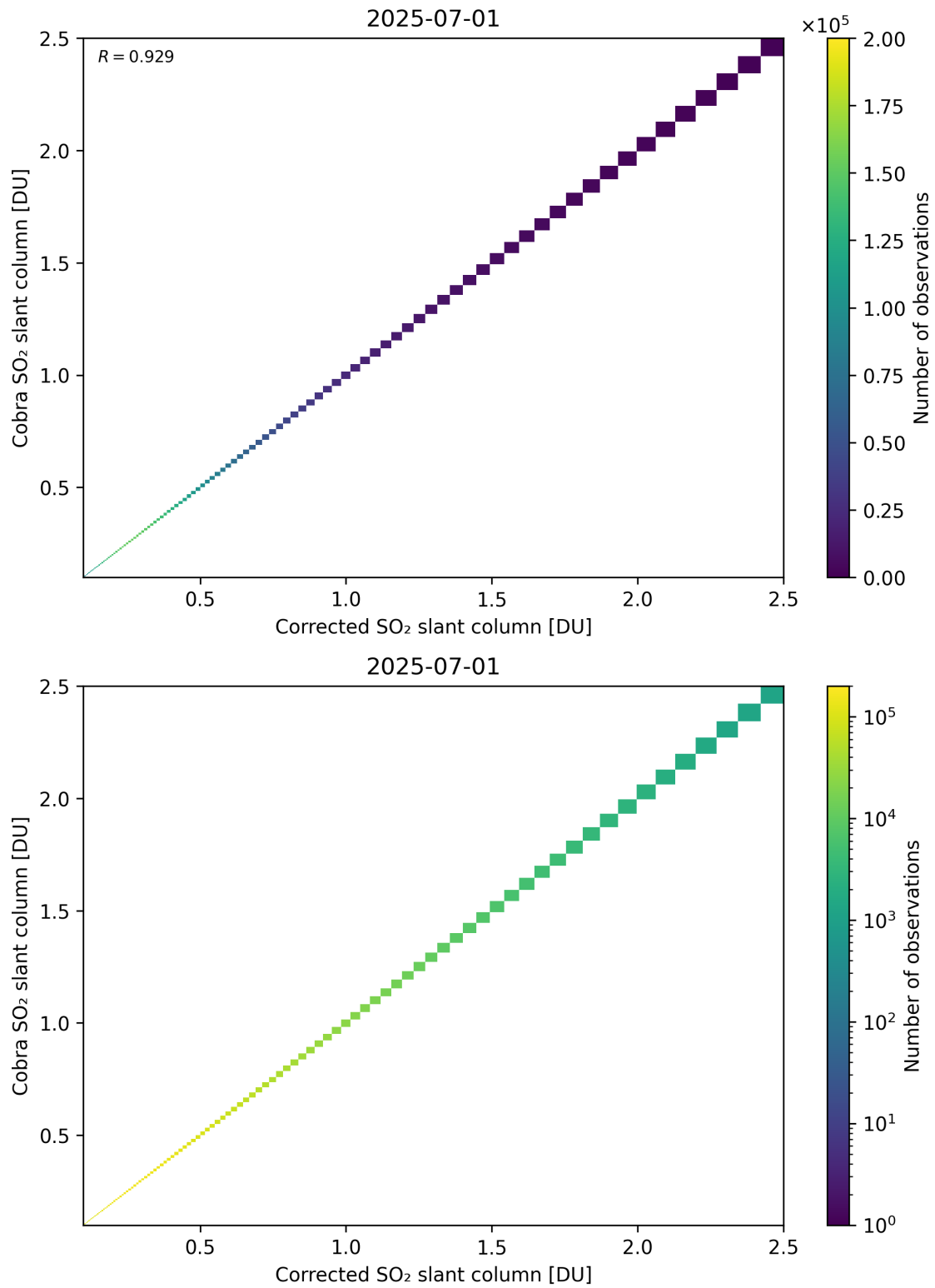
Figure 233: Scatter density plot of “Corrected SO 2 slant column” against “Cobra SO 2 slant column” for 2025-06-30 to 2025-07-02.
