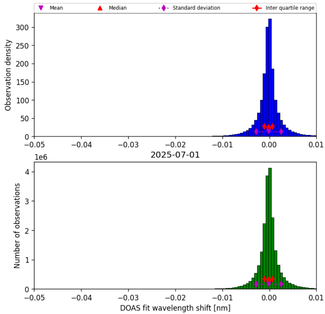
Figure 76: Histogram of “DOAS fit wavelength shift” for 2025-06-30 to 2025-07-02
