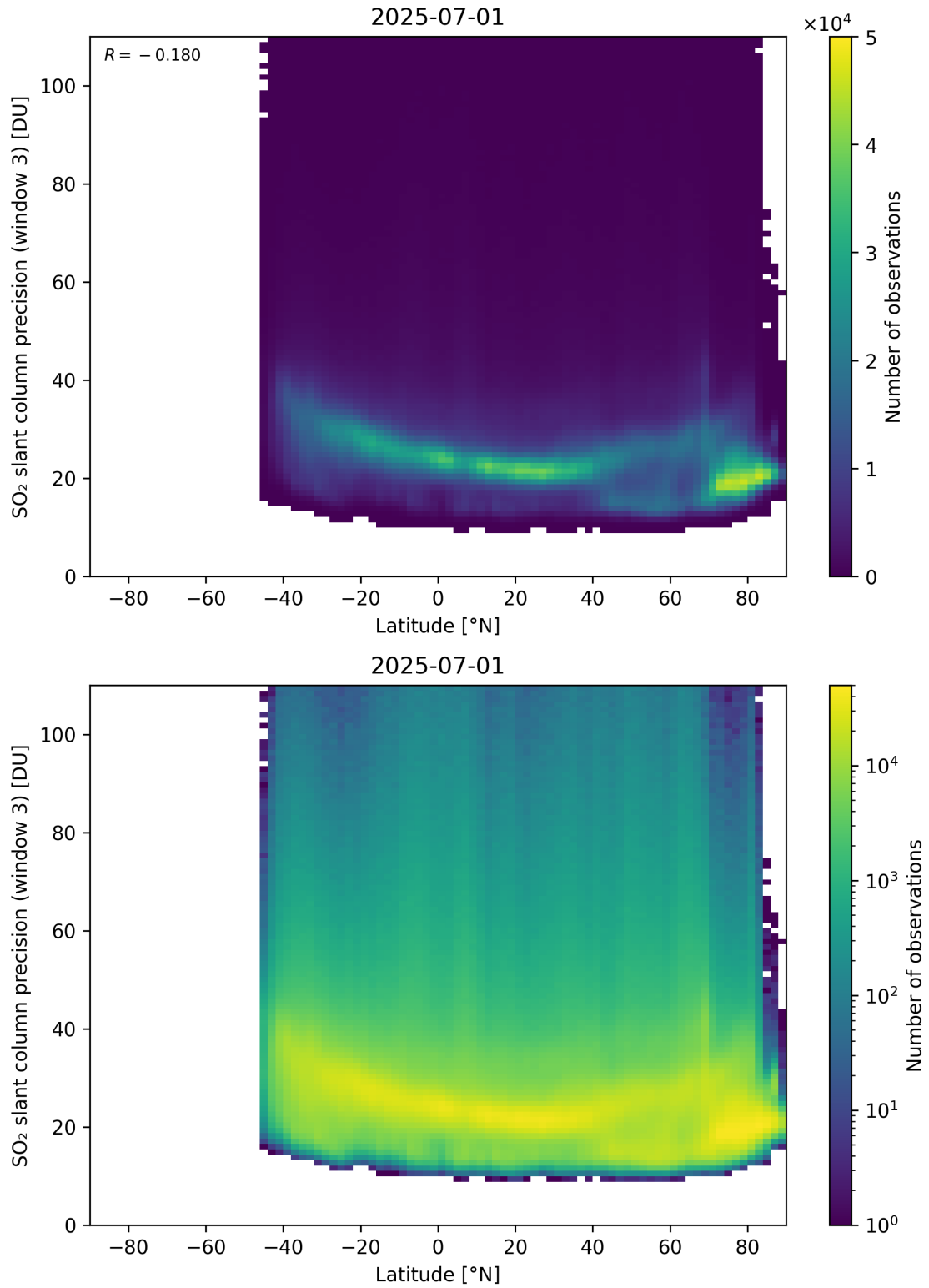
Figure 166: Scatter density plot of “Latitude” against “SO 2 slant column precision (window 3)” for 2025-06-30 to 2025-07-02.
