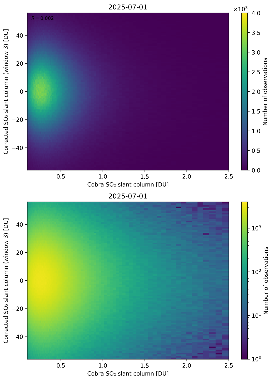
Figure 218: Scatter density plot of “Cobra SO 2 slant column” against “Corrected SO 2 slant column (window 3)” for 2025-06-30 to 2025-07-02.
