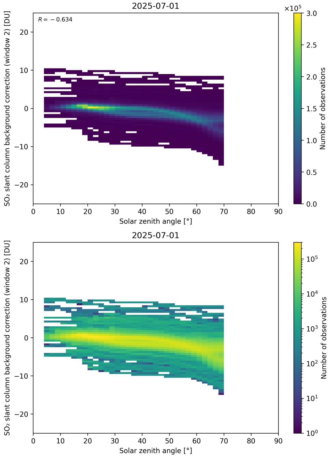
Figure 172: Scatter density plot of “Solar zenith angle” against “SO 2 slant column background correction (window 2)” for 2025-06-30 to 2025-07-02.
