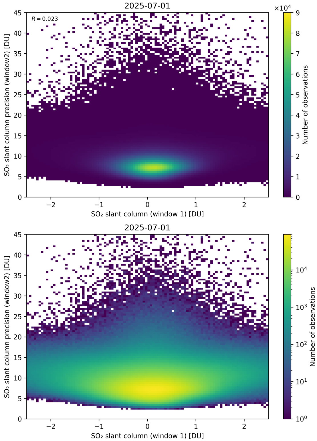
Figure 286: Scatter density plot of “SO 2 slant column (window 1)” against “SO 2 slant column precision (window2)” for 2025-06-30 to 2025-07-02.
