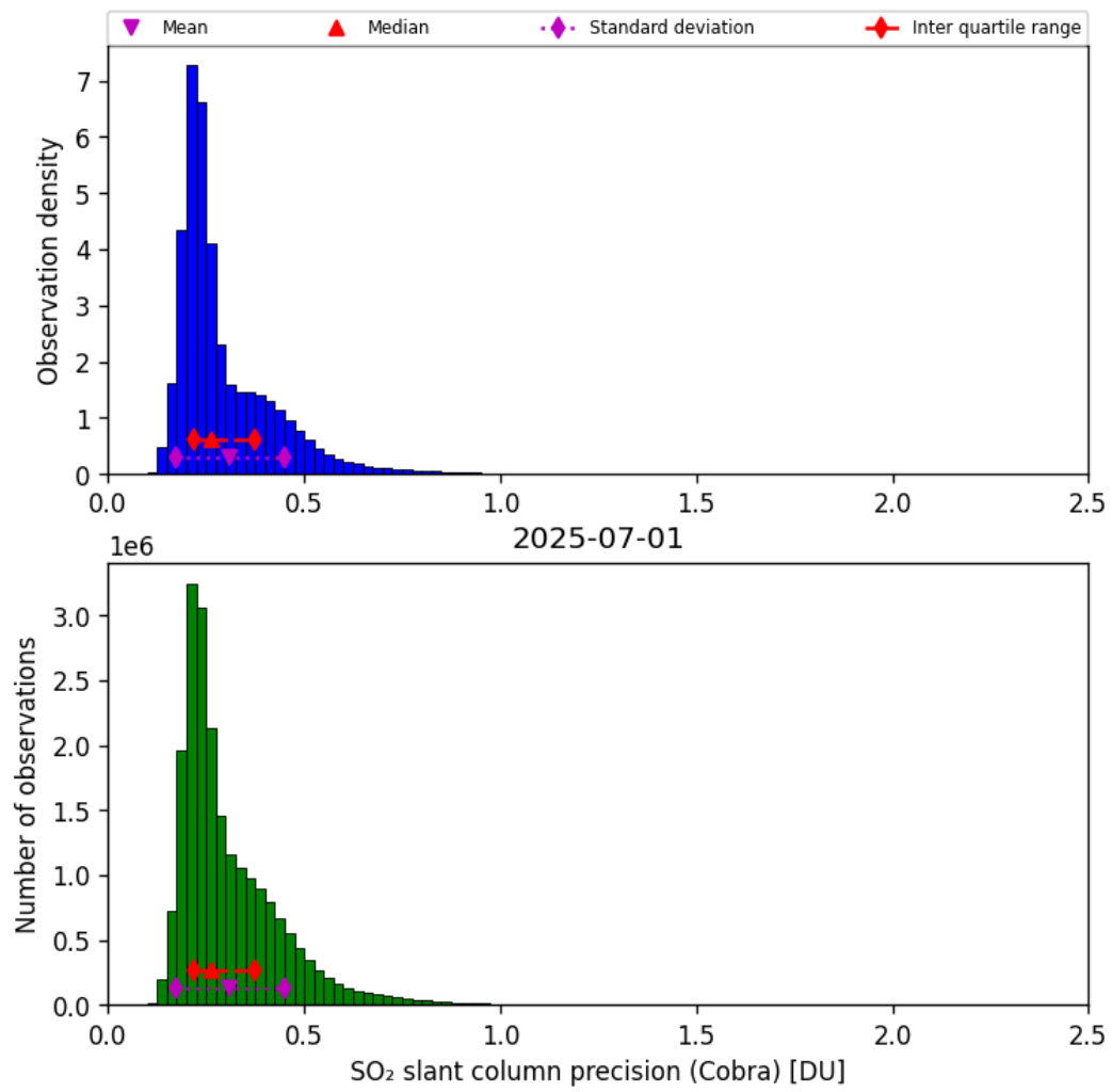
Figure 62: Histogram of “SO 2 slant column precision (Cobra)” for 2025-06-30 to 2025-07-02
