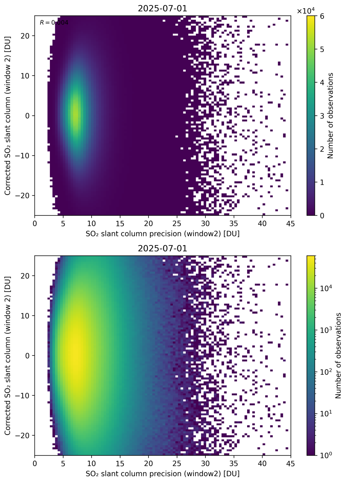
Figure 297: Scatter density plot of “SO 2 slant column precision (window2)” against “Corrected SO 2 slant column (window 2)” for 2025-06-30 to 2025-07-02.
