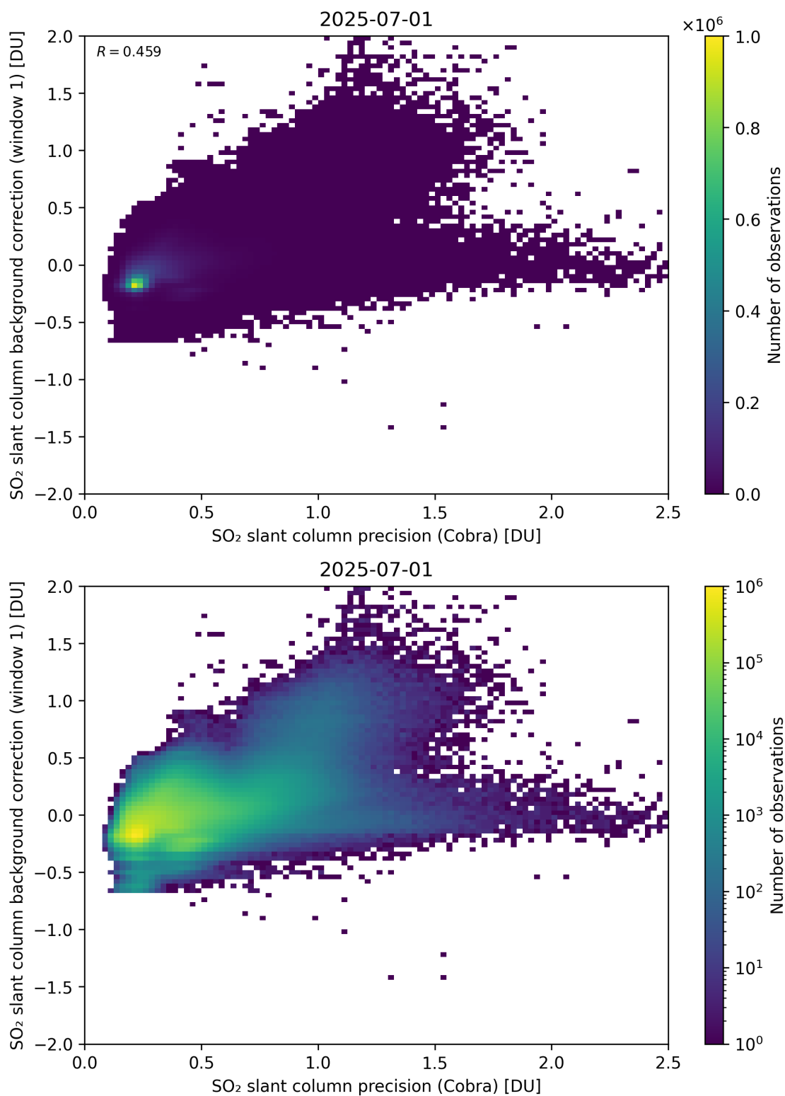
Figure 199: Scatter density plot of “SO 2 slant column precision (Cobra)” against “SO 2 slant column background correction (window 1)” for 2025-06-30 to 2025-07-02.
