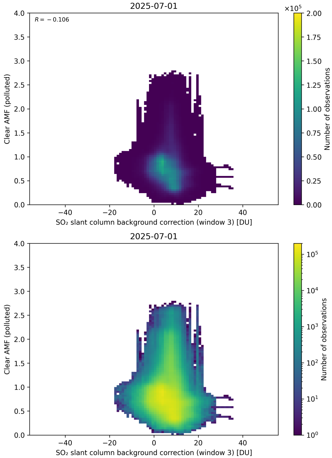
Figure 135: Scatter density plot of “SO 2 slant column background correction (window 3)” against “Clear AMF (polluted)” for 2025-06-30 to 2025-07-02.
