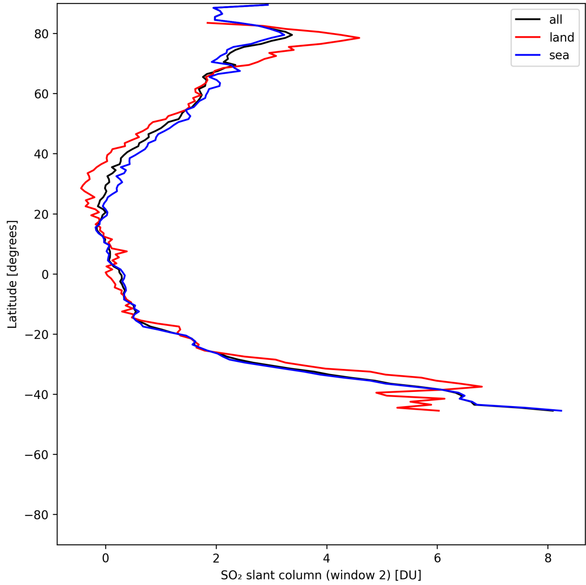
Figure 41: Zonal average of “SO 2 slant column (window 2)” for 2025-06-30 to 2025-07-02.
