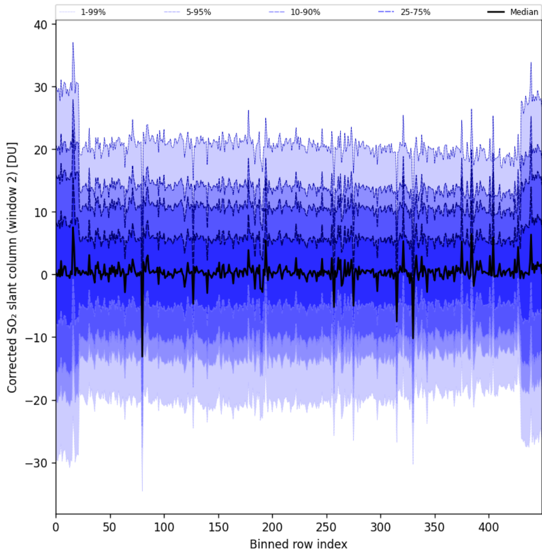
Figure 95: Along track statistics of “Corrected SO 2 slant column (window 2)” for 2025-06-30 to 2025-07-02
