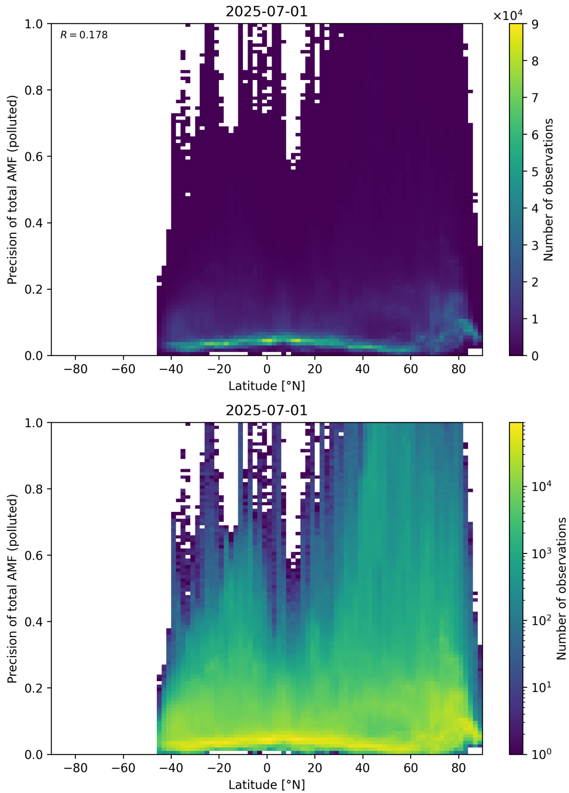
Figure 168: Scatter density plot of “Latitude” against “Precision of total AMF (polluted)” for 2025-06-30 to 2025-07-02.
