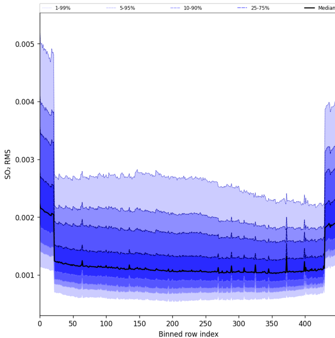
Figure 104: Along track statistics of “SO 2 RMS” for 2025-06-30 to 2025-07-02
