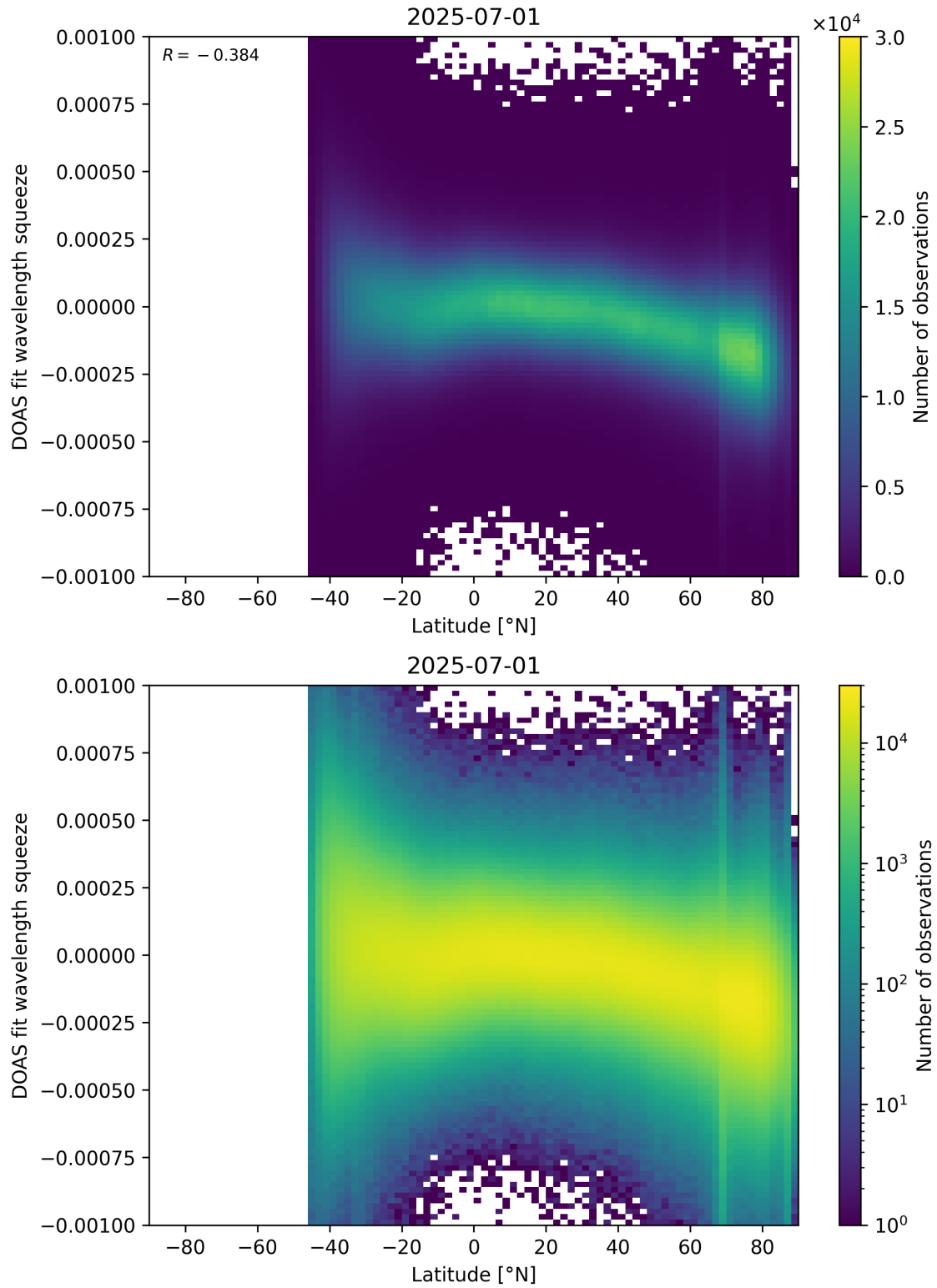
Figure 154: Scatter density plot of “Latitude” against “DOAS fit wavelength squeeze” for 2025-06-30 to 2025-07-02.
