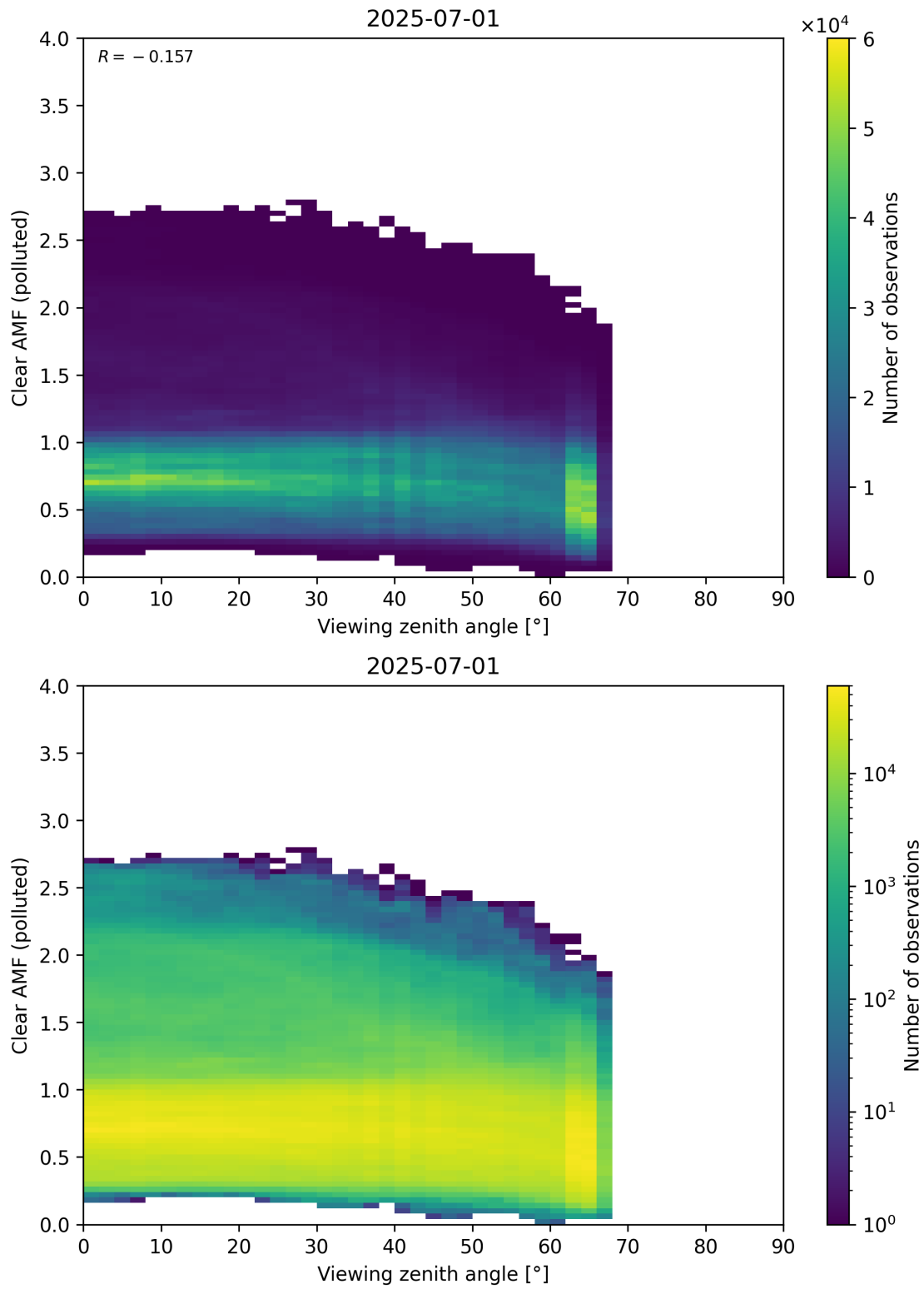
Figure 370: Scatter density plot of “Viewing zenith angle” against “Clear AMF (polluted)” for 2025-06-30 to 2025-07-02.
