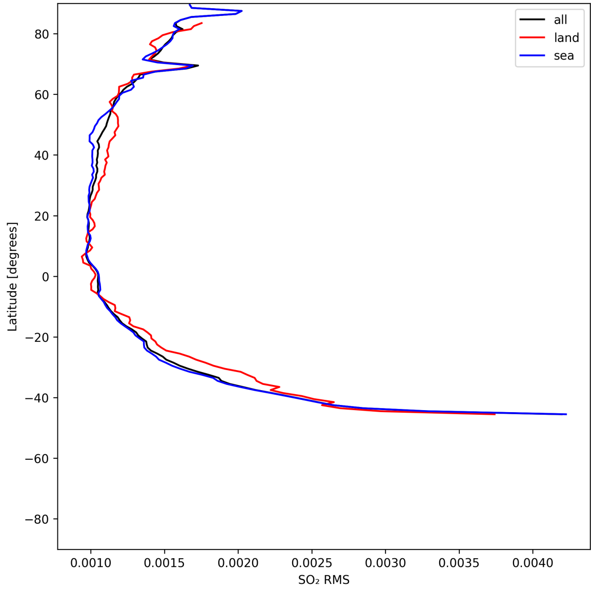
Figure 52: Zonal average of “SO 2 RMS” for 2025-06-30 to 2025-07-02.
