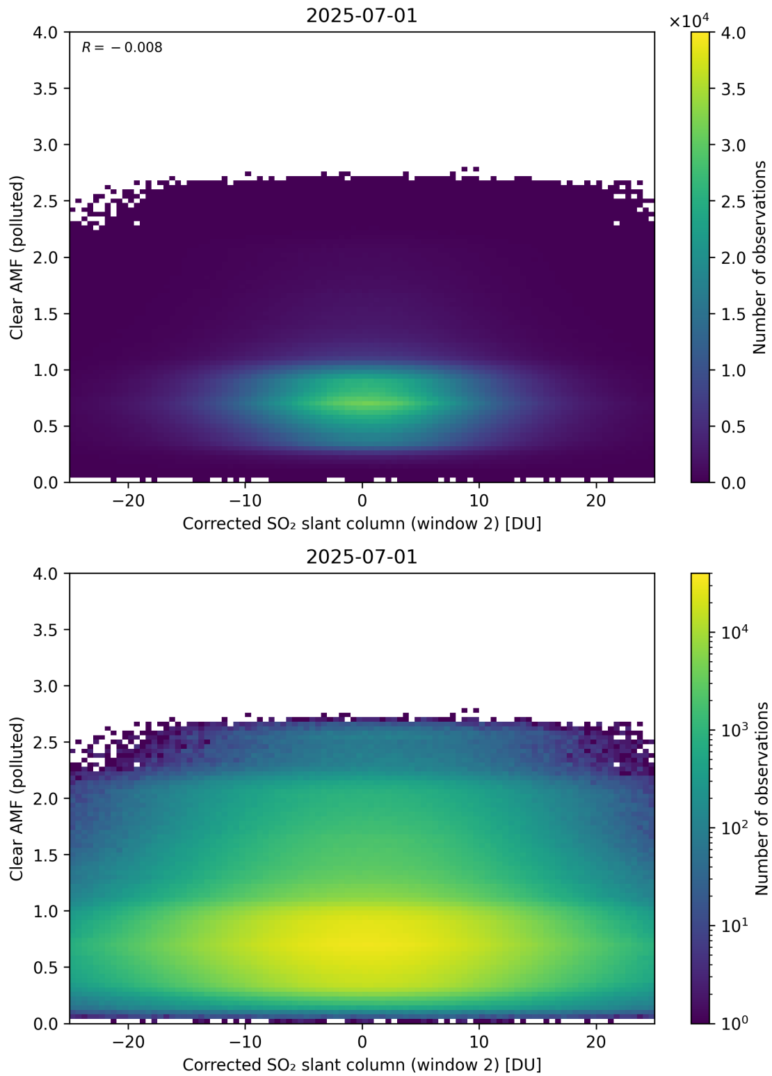
Figure 249: Scatter density plot of “Corrected SO 2 slant column (window 2)” against “Clear AMF (polluted)” for 2025-06-30 to 2025-07-02.
