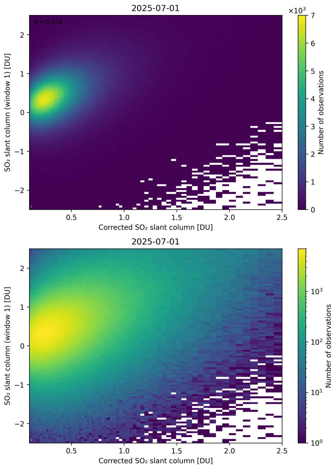
Figure 237: Scatter density plot of “Corrected SO 2 slant column” against “SO 2 slant column (window 1)” for 2025-06-30 to 2025-07-02.
