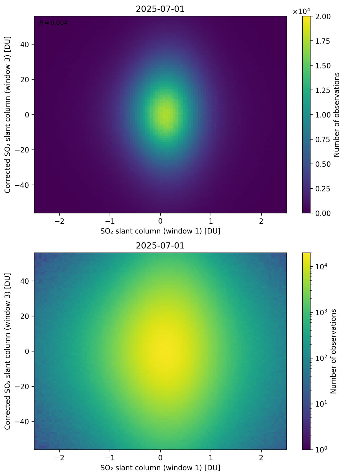
Figure 284: Scatter density plot of “SO 2 slant column (window 1)” against “Corrected SO 2 slant column (window 3)” for 2025-06-30 to 2025-07-02.
