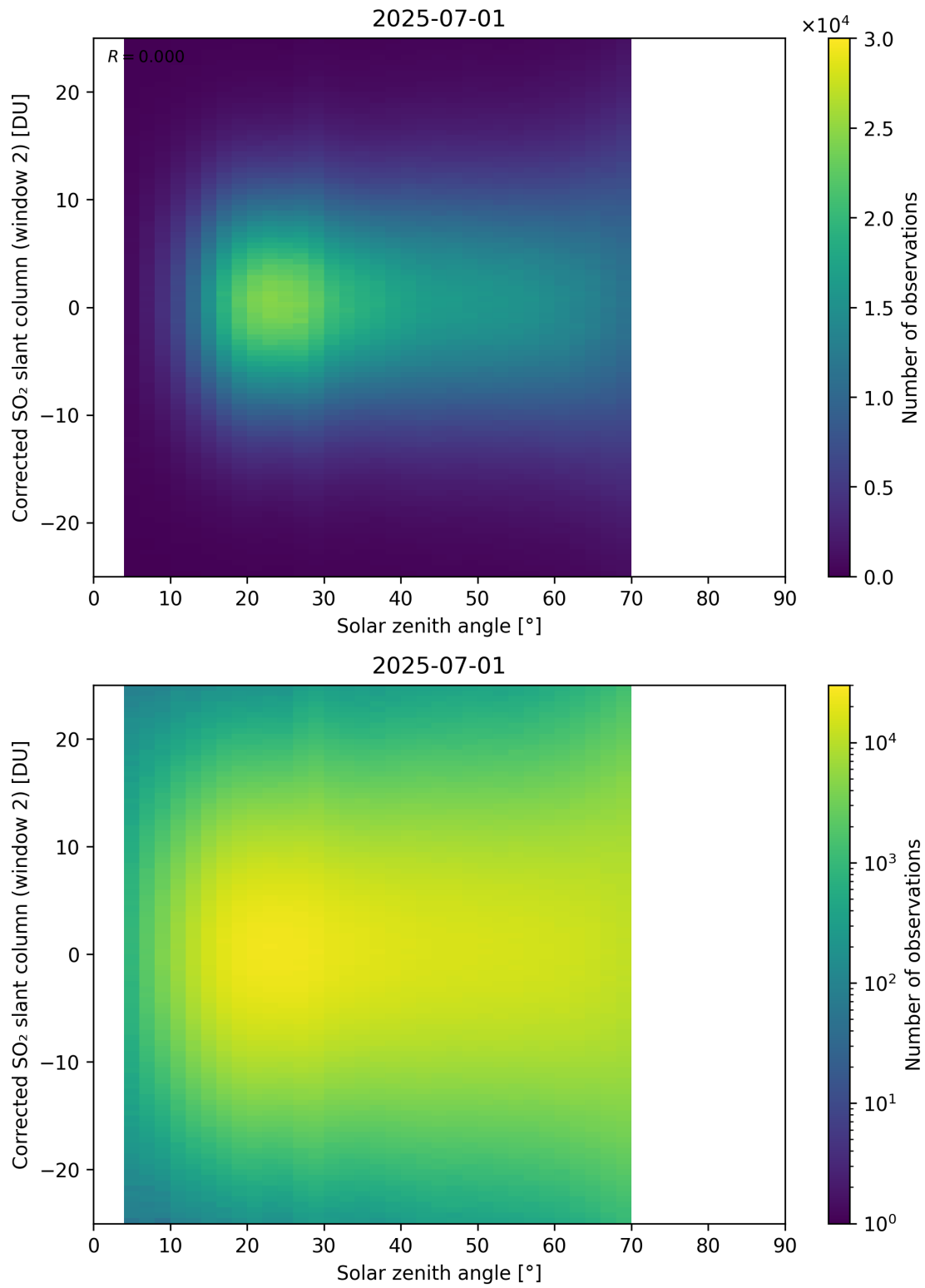
Figure 182: Scatter density plot of “Solar zenith angle” against “Corrected SO 2 slant column (window 2)” for 2025-06-30 to 2025-07-02.
