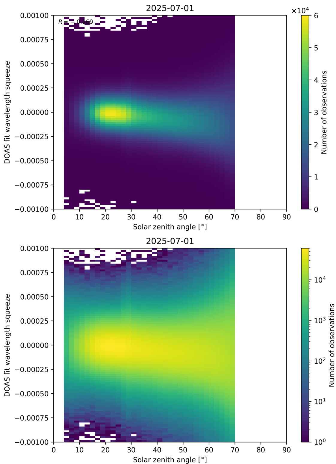
Figure 175: Scatter density plot of “Solar zenith angle” against “DOAS fit wavelength squeeze” for 2025-06-30 to 2025-07-02.
