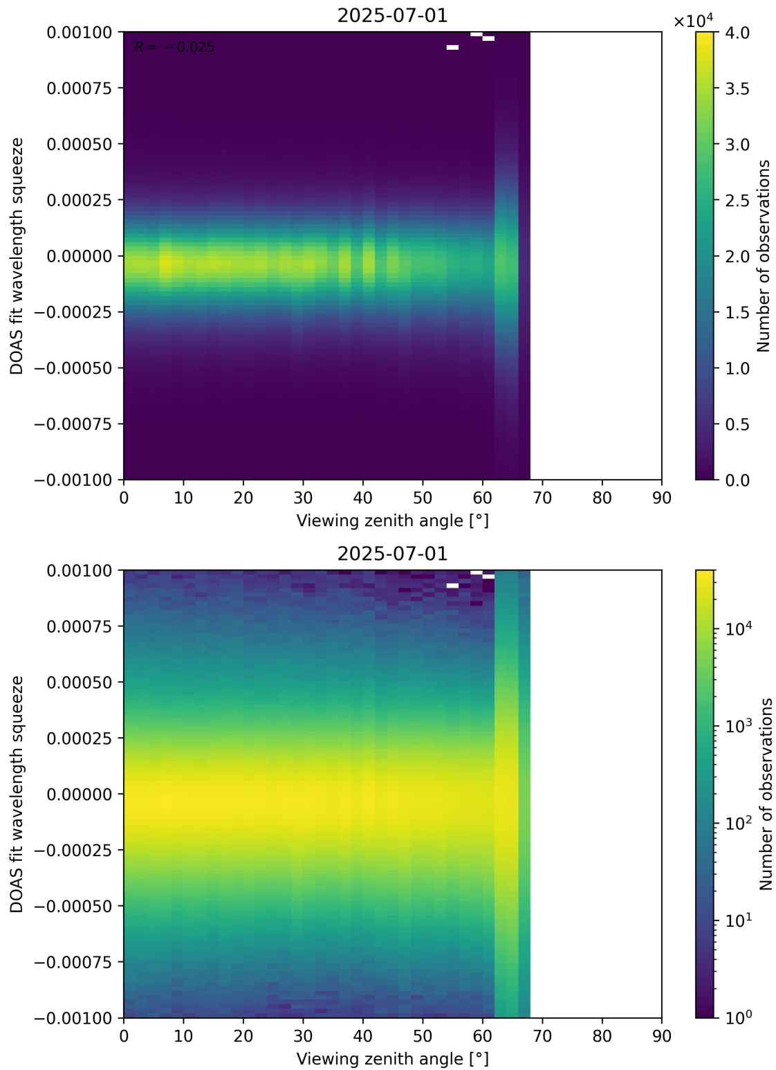
Figure 366: Scatter density plot of “Viewing zenith angle” against “DOAS fit wavelength squeeze” for 2025-06-30 to 2025-07-02.
