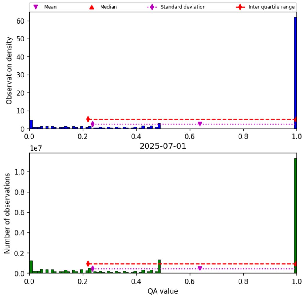
Figure 57: Histogram of “QA value” for 2025-06-30 to 2025-07-02
