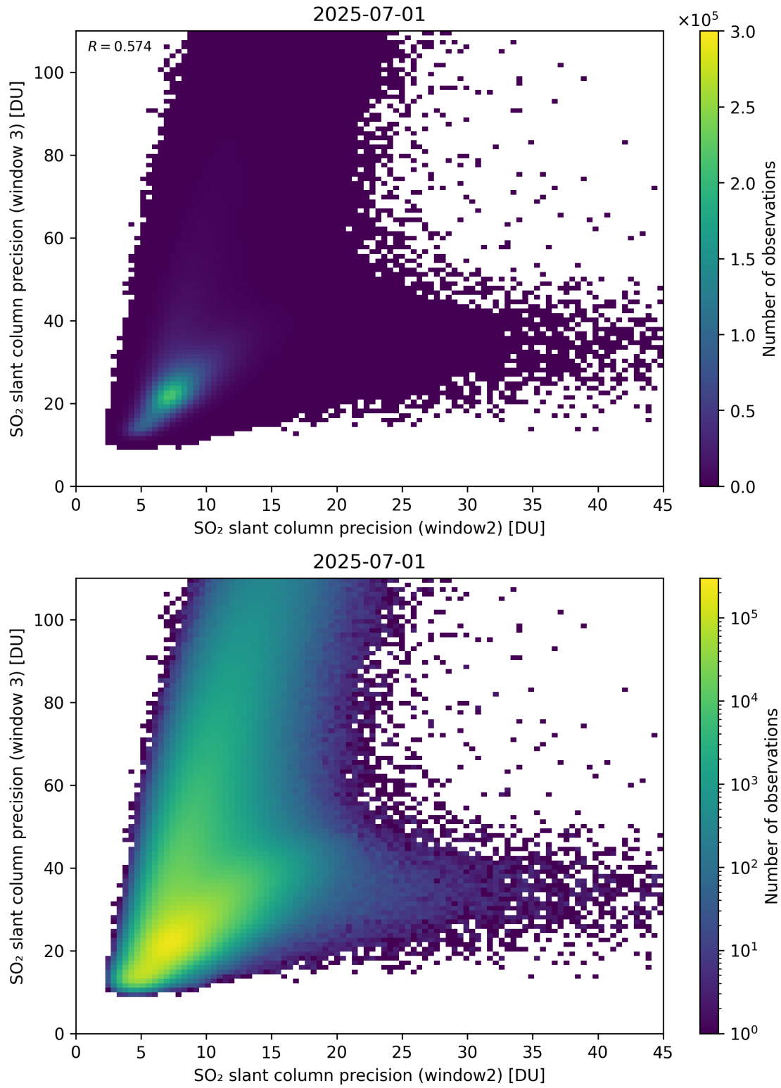
Figure 300: Scatter density plot of “SO 2 slant column precision (window2)” against “SO 2 slant column precision (window 3)” for 2025-06-30 to 2025-07-02.
