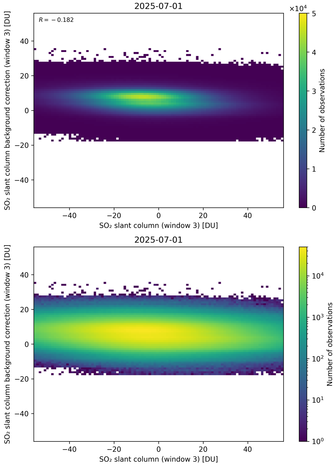
Figure 303: Scatter density plot of “SO 2 slant column (window 3)” against “SO 2 slant column background correction (window 3)” for 2025-06-30 to 2025-07-02.
