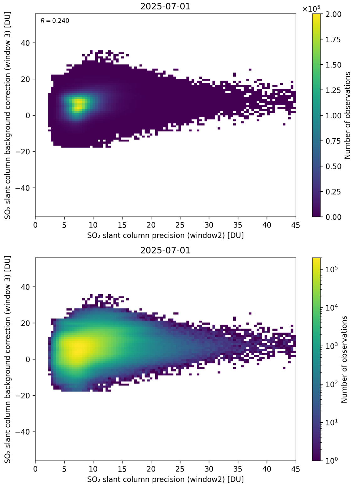
Figure 292: Scatter density plot of “SO 2 slant column precision (window2)” against “SO 2 slant column background correction (window 3)” for 2025-06-30 to 2025-07-02.
