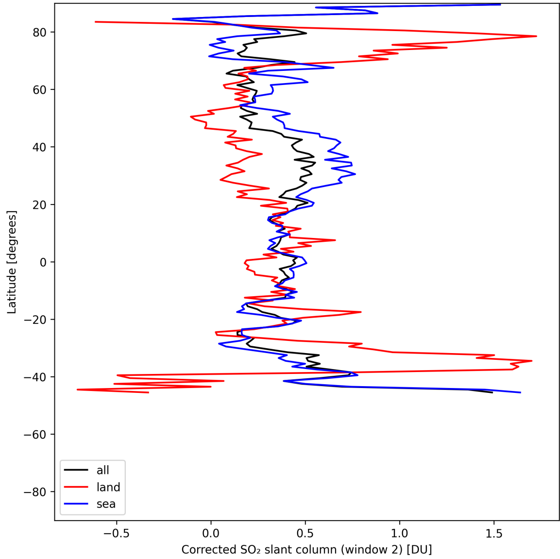
Figure 43: Zonal average of “Corrected SO 2 slant column (window 2)” for 2025-06-30 to 2025-07-02.
