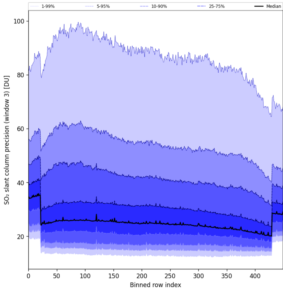
Figure 98: Along track statistics of “SO 2 slant column precision (window 3)” for 2025-06-30 to 2025-07-02
