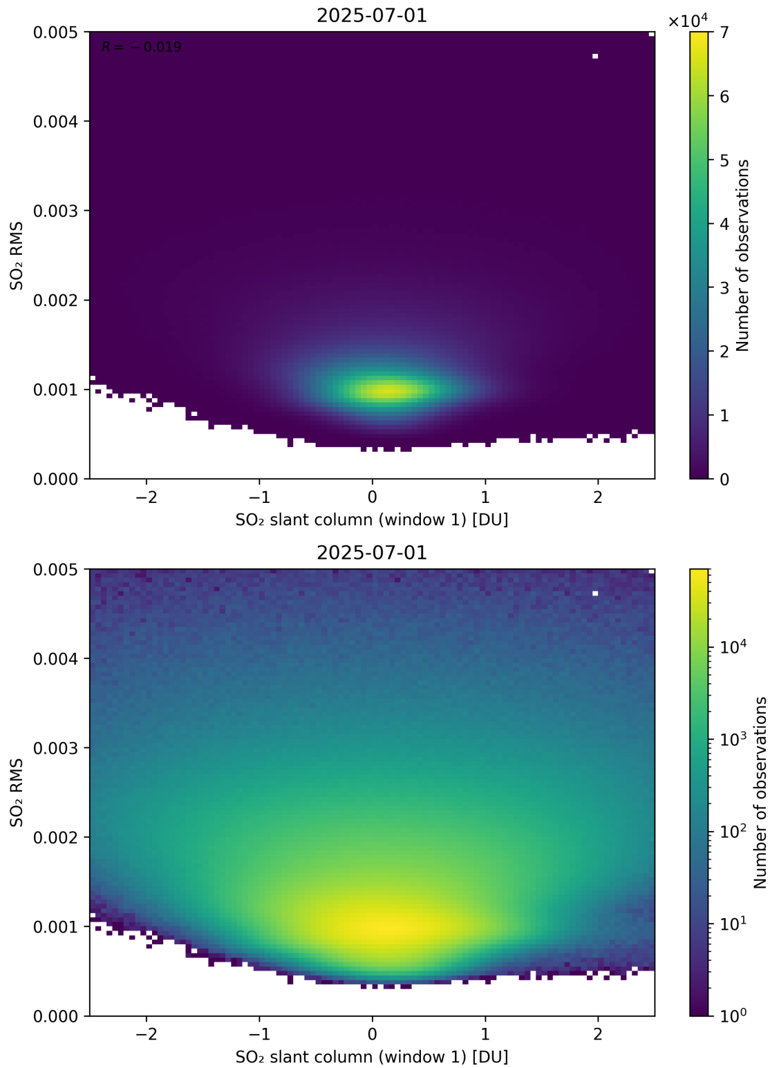
Figure 267: Scatter density plot of “SO 2 slant column (window 1)” against “SO 2 RMS” for 2025-06-30 to 2025-07-02.
