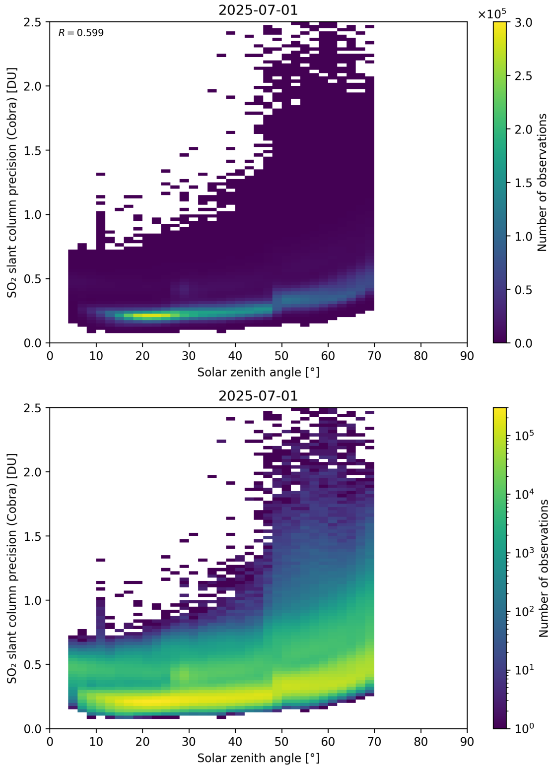
Figure 180: Scatter density plot of “Solar zenith angle” against “SO 2 slant column precision (Cobra)” for 2025-06-30 to 2025-07-02.
