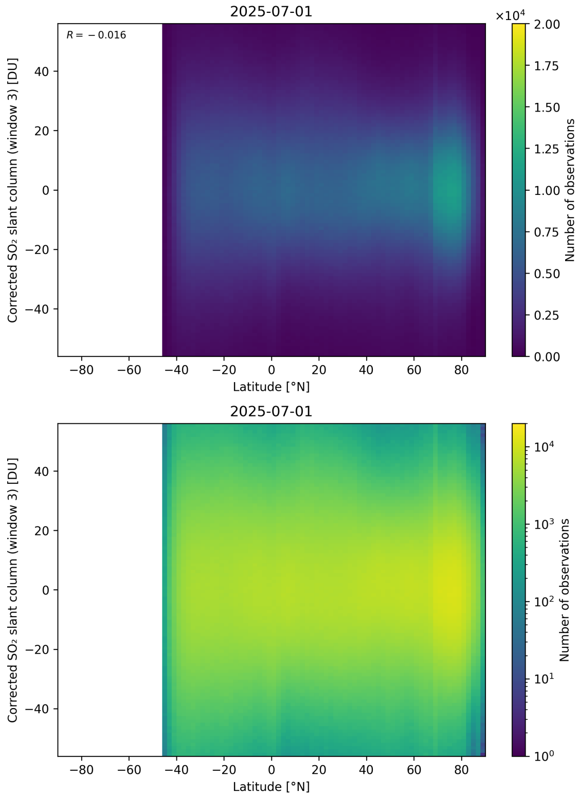
Figure 161: Scatter density plot of “Latitude” against “Corrected SO 2 slant column (window 3)” for 2025-06-30 to 2025-07-02.
