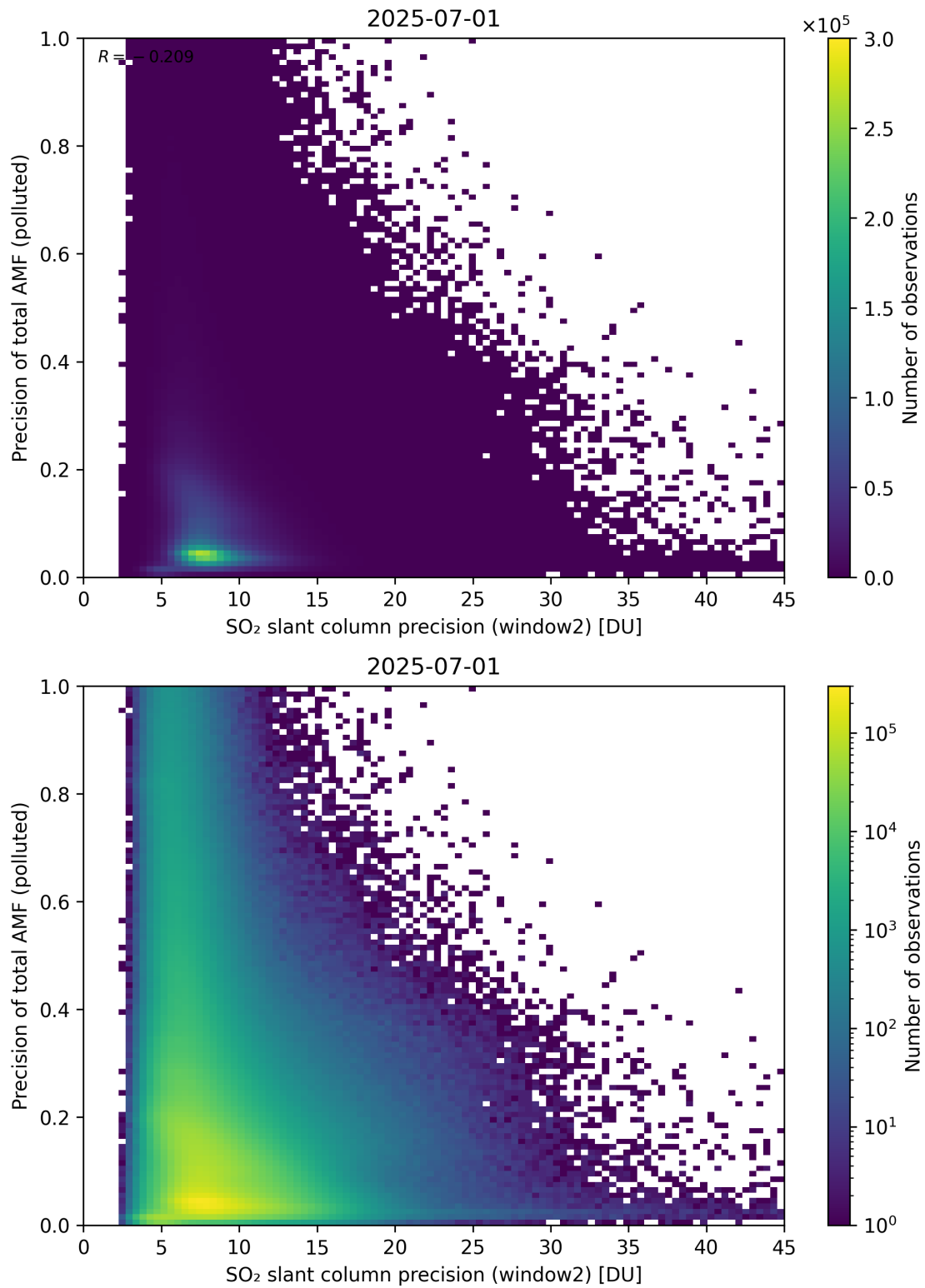
Figure 302: Scatter density plot of “SO 2 slant column precision (window2)” against “Precision of total AMF (polluted)” for 2025-06-30 to 2025-07-02.
