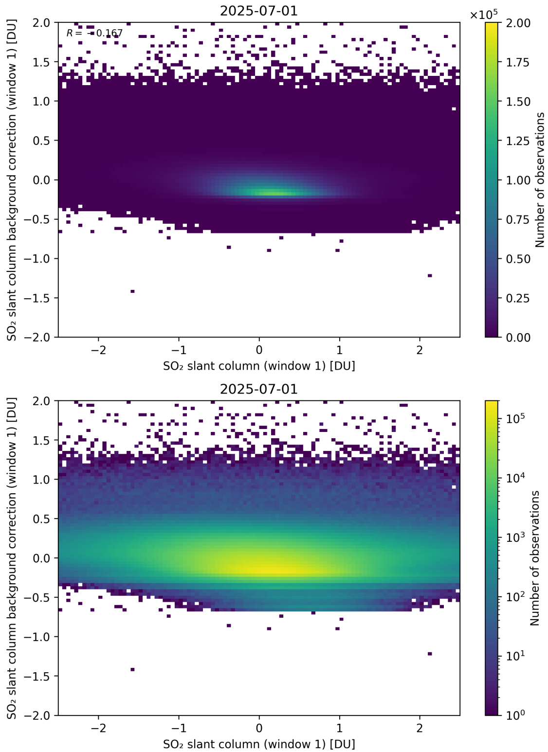
Figure 262: Scatter density plot of “SO 2 slant column (window 1)” against “SO 2 slant column background correction (window 1)” for 2025-06-30 to 2025-07-02.
