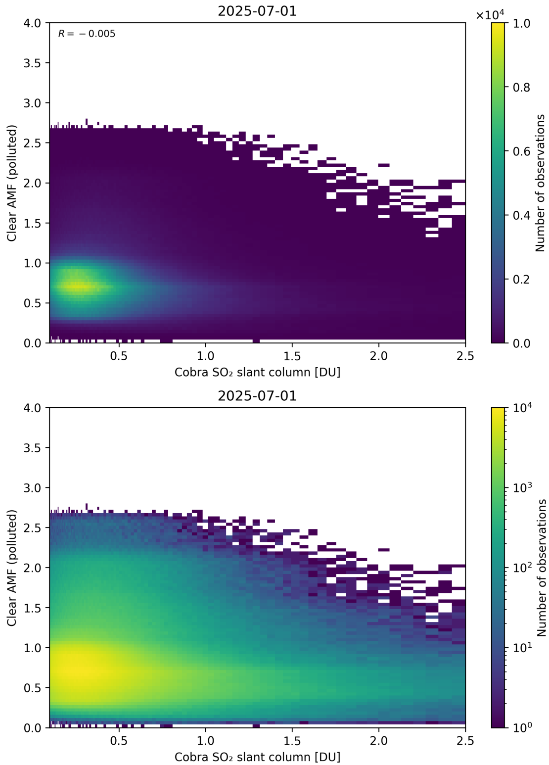
Figure 215: Scatter density plot of “Cobra SO 2 slant column” against “Clear AMF (polluted)” for 2025-06-30 to 2025-07-02.
