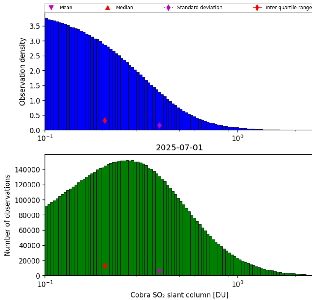
Figure 61: Histogram of “Cobra SO 2 slant column” for 2025-06-30 to 2025-07-02
