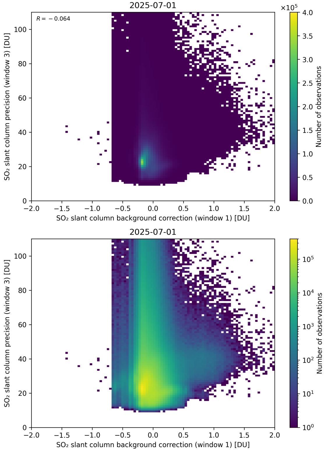
Figure 119: Scatter density plot of “SO 2 slant column background correction (window 1)” against “SO 2 slant column precision (window 3)” for 2025-06-30 to 2025-07-02.
