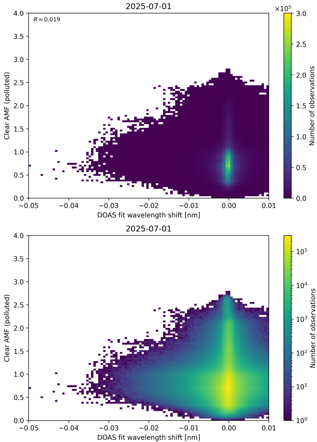
Figure 140: Scatter density plot of “DOAS fit wavelength shift” against “Clear AMF (polluted)” for 2025-06-30 to 2025-07-02.
