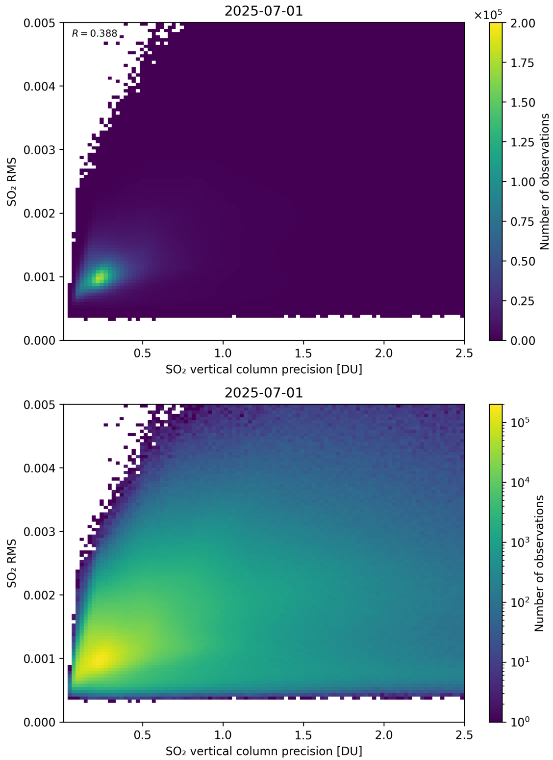
Figure 334: Scatter density plot of “SO 2 vertical column precision” against “SO 2 RMS” for 2025-06-30 to 2025-07-02.
