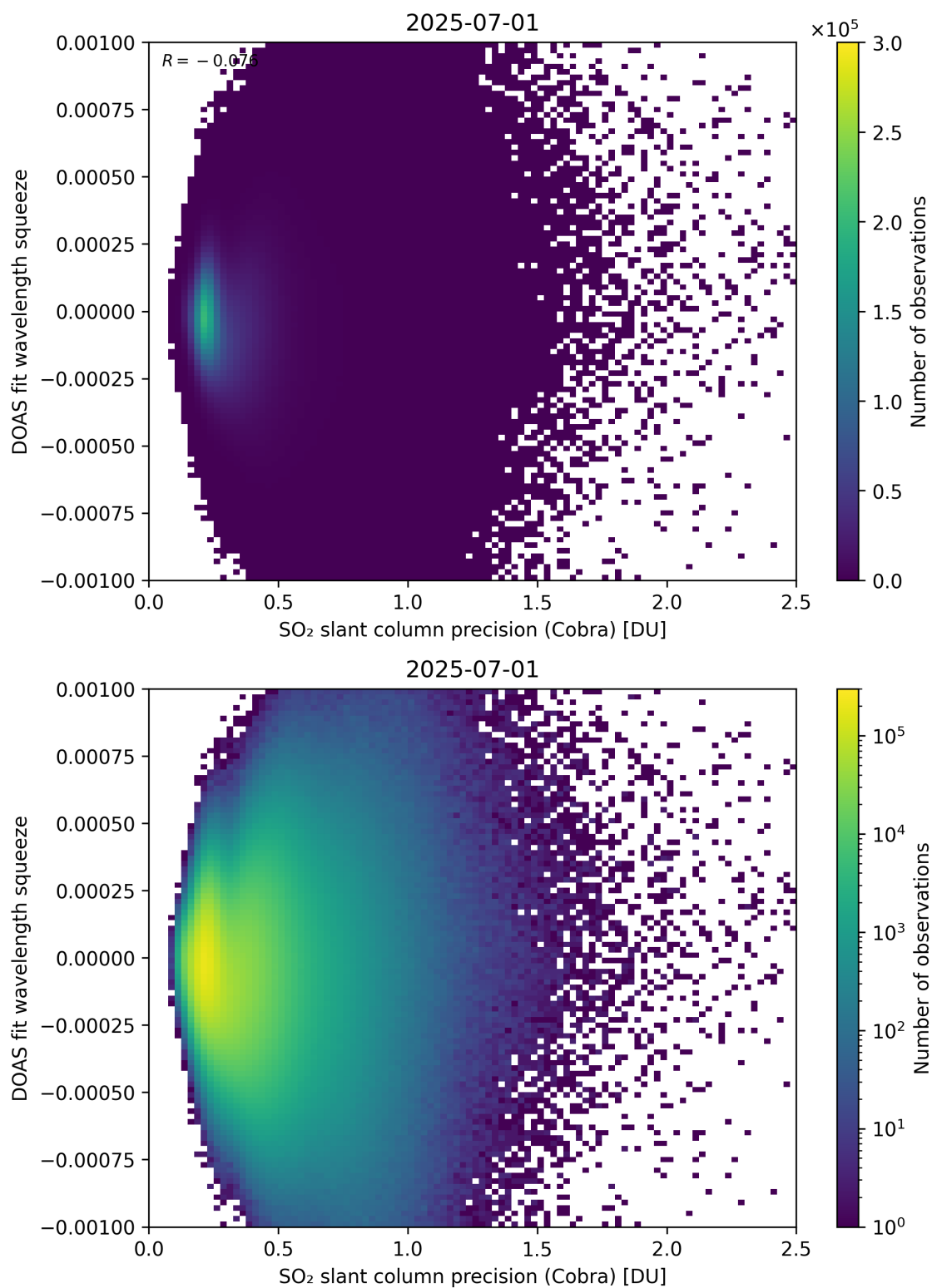
Figure 203: Scatter density plot of “SO 2 slant column precision (Cobra)” against “DOAS fit wavelength squeeze” for 2025-06-30 to 2025-07-02.
