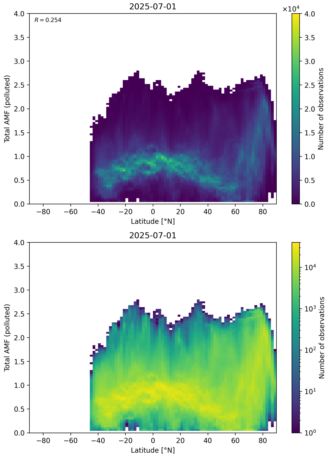
Figure 167: Scatter density plot of “Latitude” against “Total AMF (polluted)” for 2025-06-30 to 2025-07-02.
