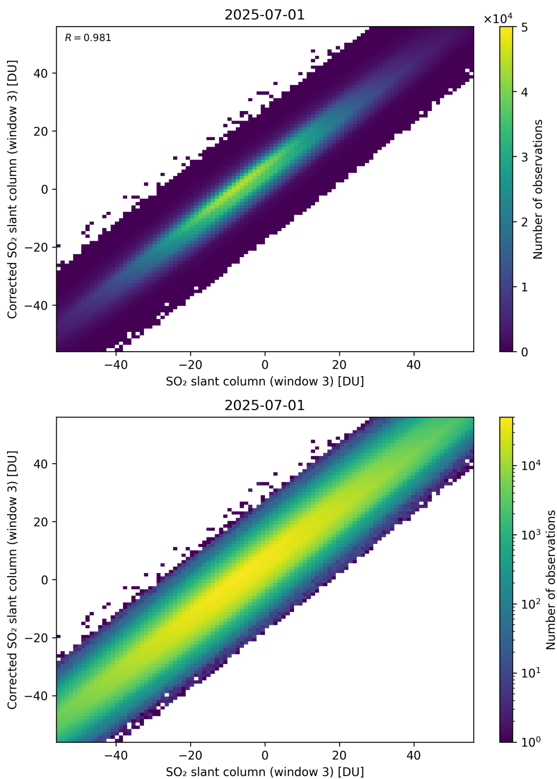
Figure 316: Scatter density plot of “SO 2 slant column (window 3)” against “Corrected SO 2 slant column (window 3)” for 2025-06-30 to 2025-07-02.
