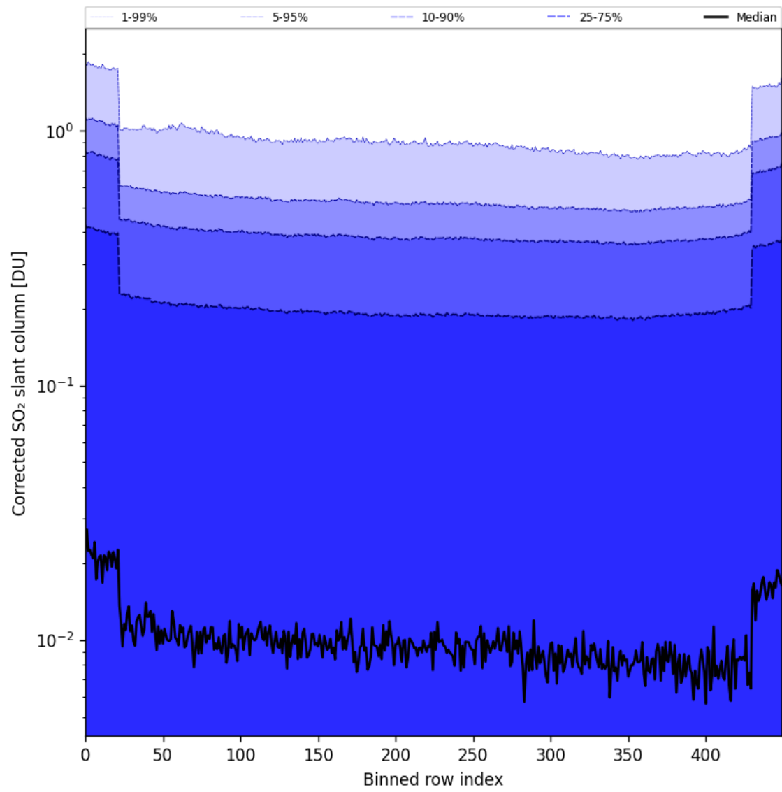
Figure 86: Along track statistics of "Corrected SO 2 slant column" for 2025-06-30 to 2025-07-02
