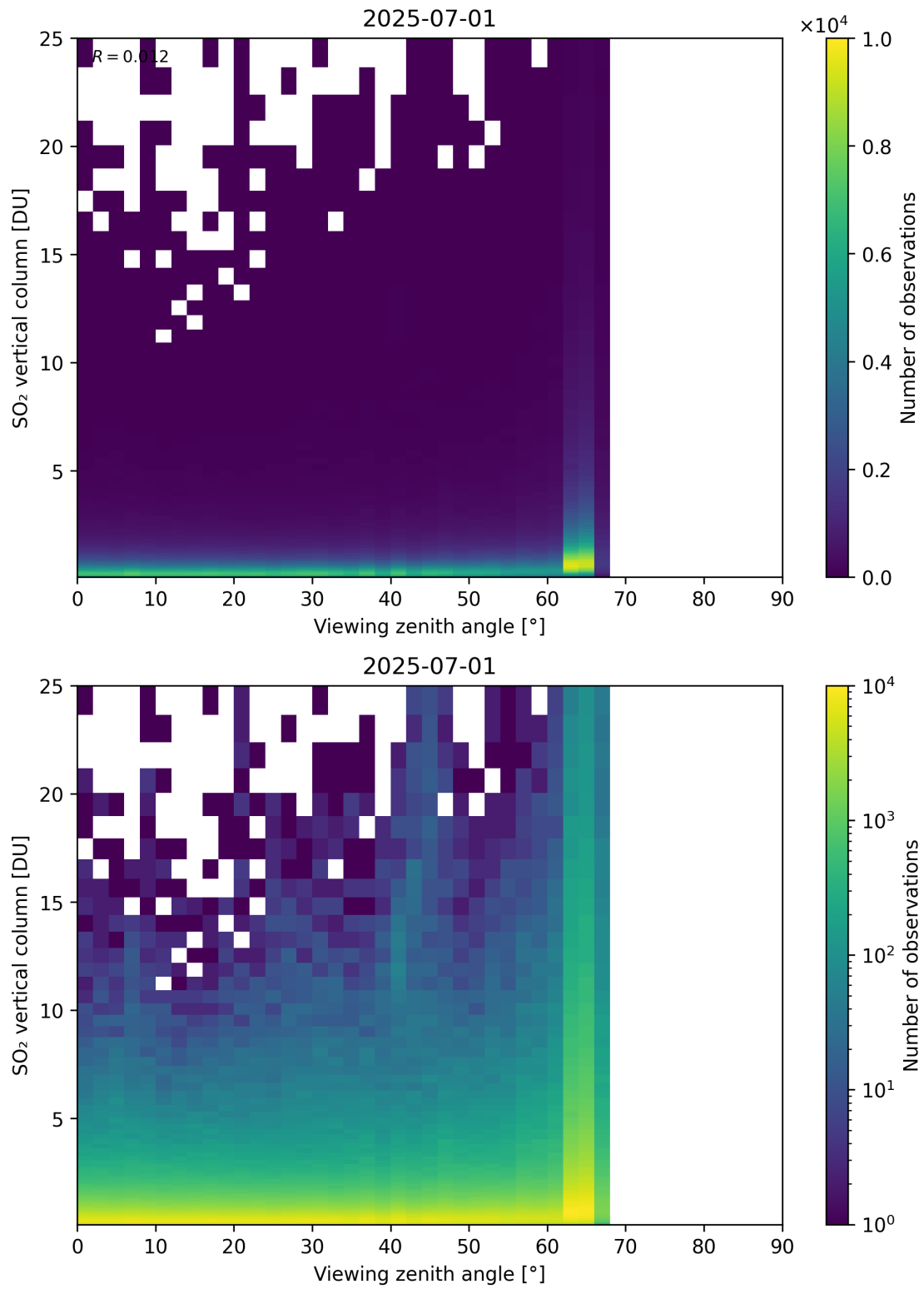
Figure 383: Scatter density plot of “Viewing zenith angle” against “SO 2 vertical column” for 2025-06-30 to 2025-07-02.
