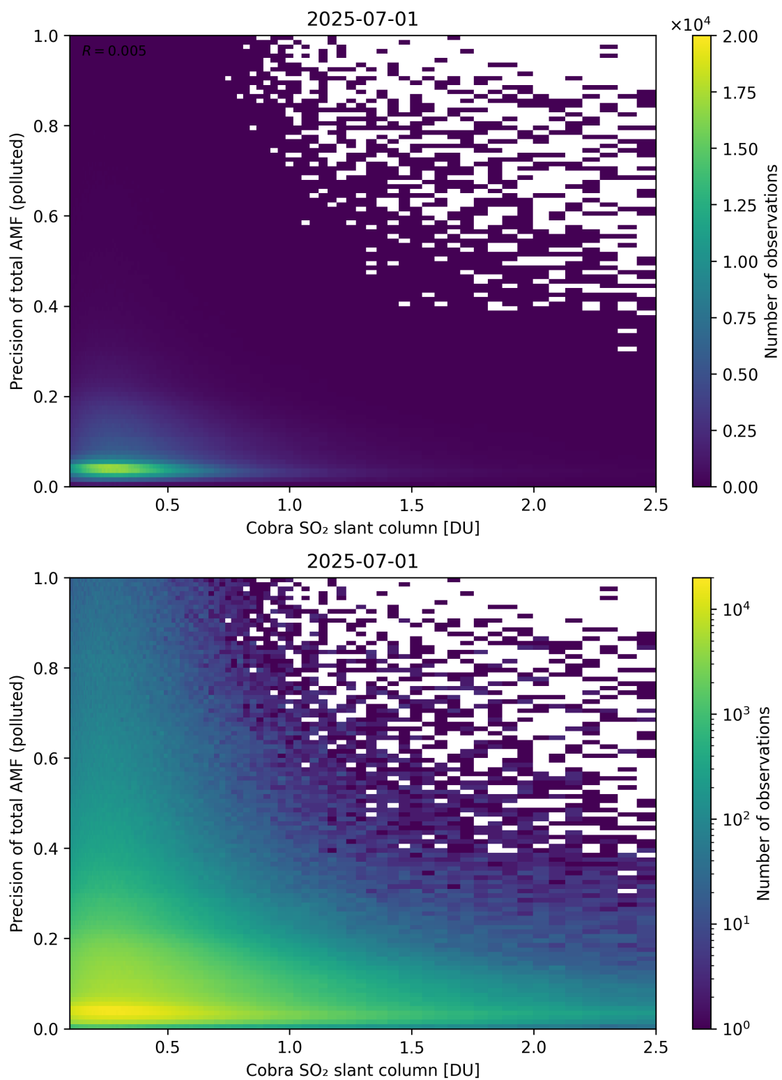
Figure 225: Scatter density plot of “Cobra SO 2 slant column” against “Precision of total AMF (polluted)” for 2025-06-30 to 2025-07-02.
