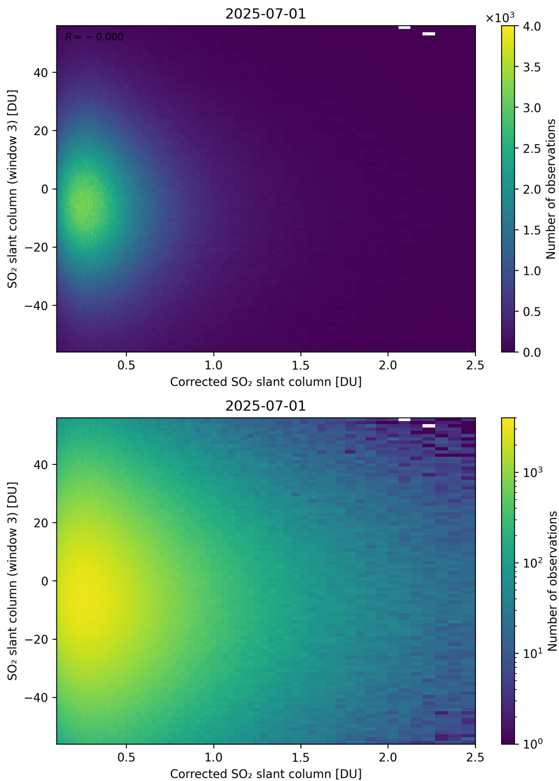
Figure 240: Scatter density plot of “Corrected SO 2 slant column” against “SO 2 slant column (window 3)” for 2025-06-30 to 2025-07-02.
