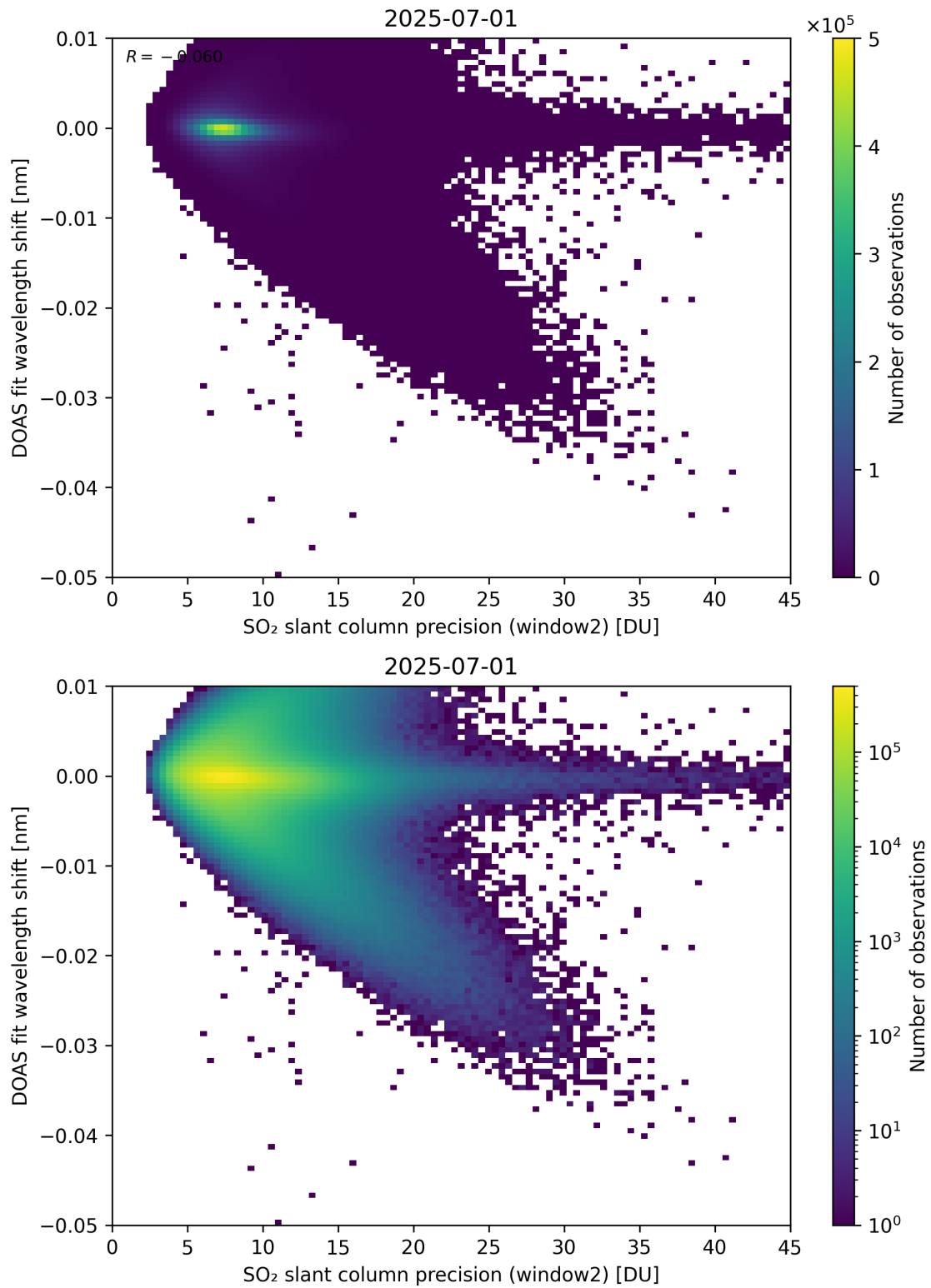
Figure 293: Scatter density plot of “SO 2 slant column precision (window2)” against “DOAS fit wavelength shift” for 2025-06-30 to 2025-07-02.
