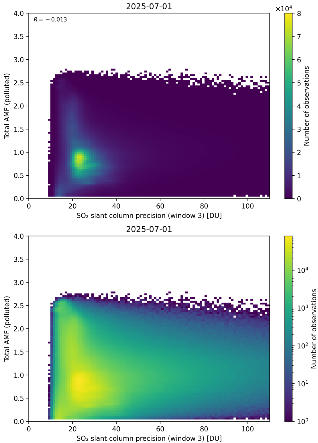
Figure 313: Scatter density plot of “SO 2 slant column precision (window 3)” against “Total AMF (polluted)” for 2025-06-30 to 2025-07-02.
