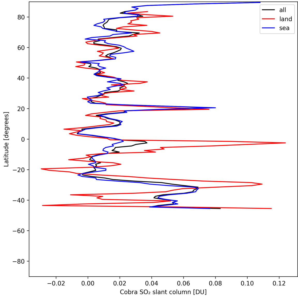
Figure 35: Zonal average of “Cobra SO 2 slant column” for 2025-06-30 to 2025-07-02.
