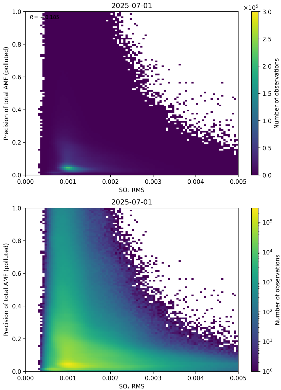
Figure 149: Scatter density plot of “SO 2 RMS” against “Precision of total AMF (polluted)” for 2025-06-30 to 2025-07-02.
