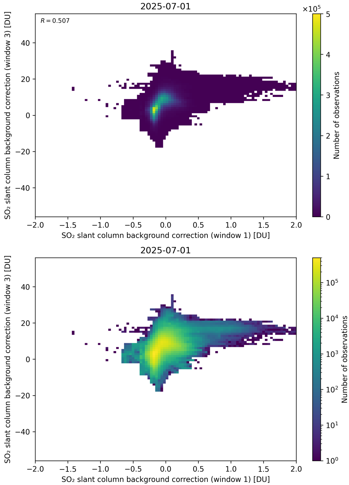
Figure 110: Scatter density plot of “SO 2 slant column background correction (window 1)” against “SO 2 slant column background correction (window 3)” for 2025-06-30 to 2025-07-02.
