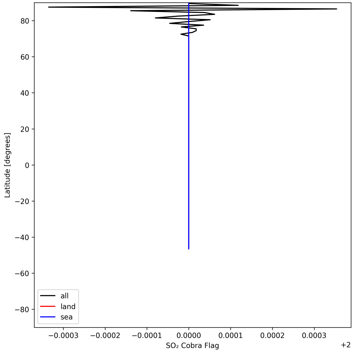
Figure 49: Zonal average of “SO 2 Cobra Flag” for 2025-07-02 to 2025-07-03.
