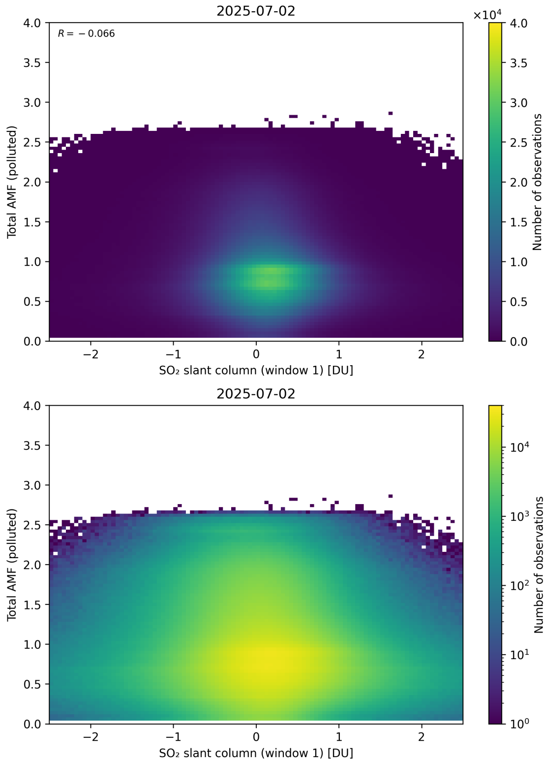
Figure 289: Scatter density plot of “SO 2 slant column (window 1)” against “Total AMF (polluted)” for 2025-07-02 to 2025-07-03.
