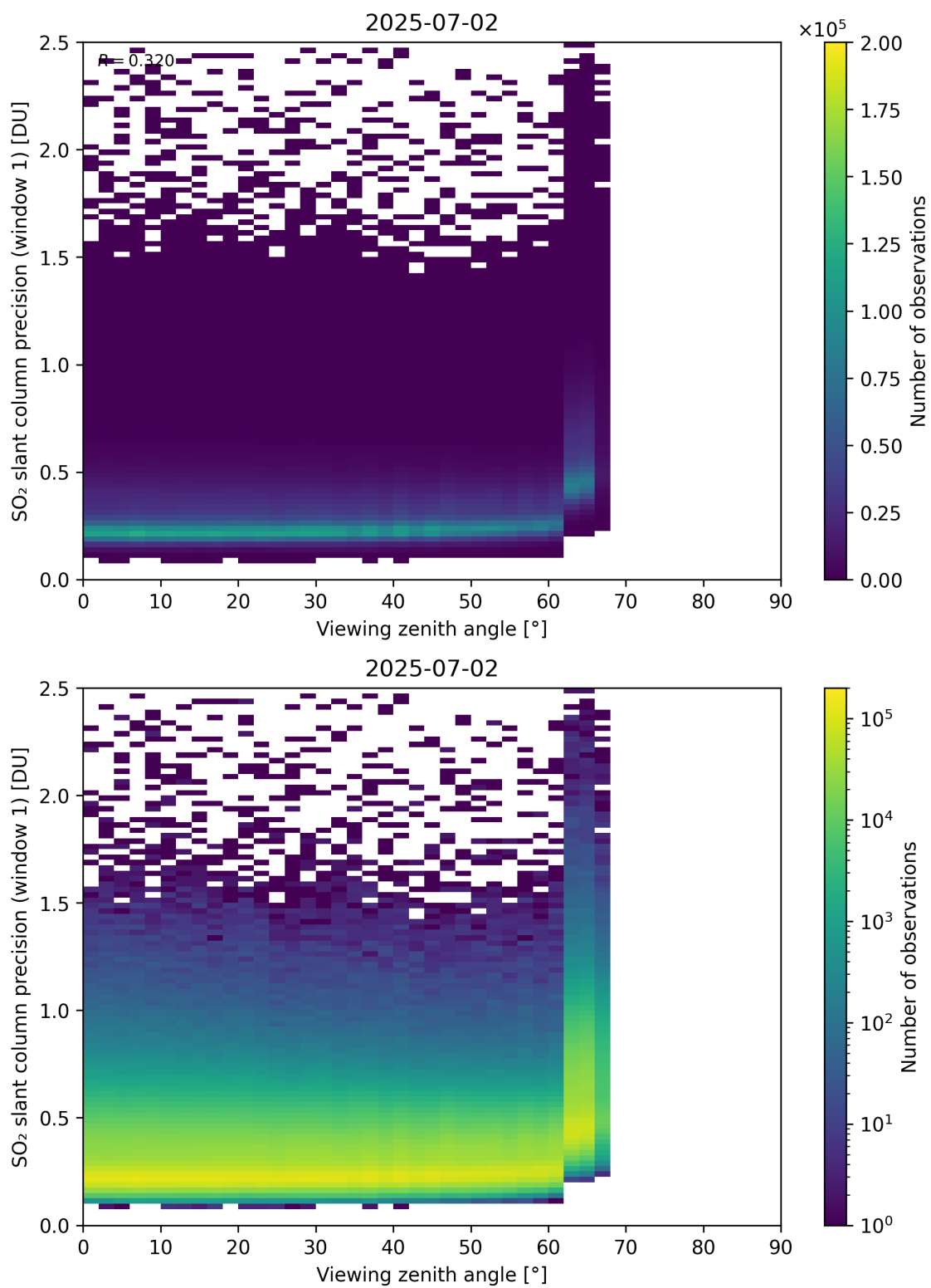
Figure 377: Scatter density plot of “Viewing zenith angle” against “SO 2 slant column precision (window 1)” for 2025-07-02 to 2025-07-03.
