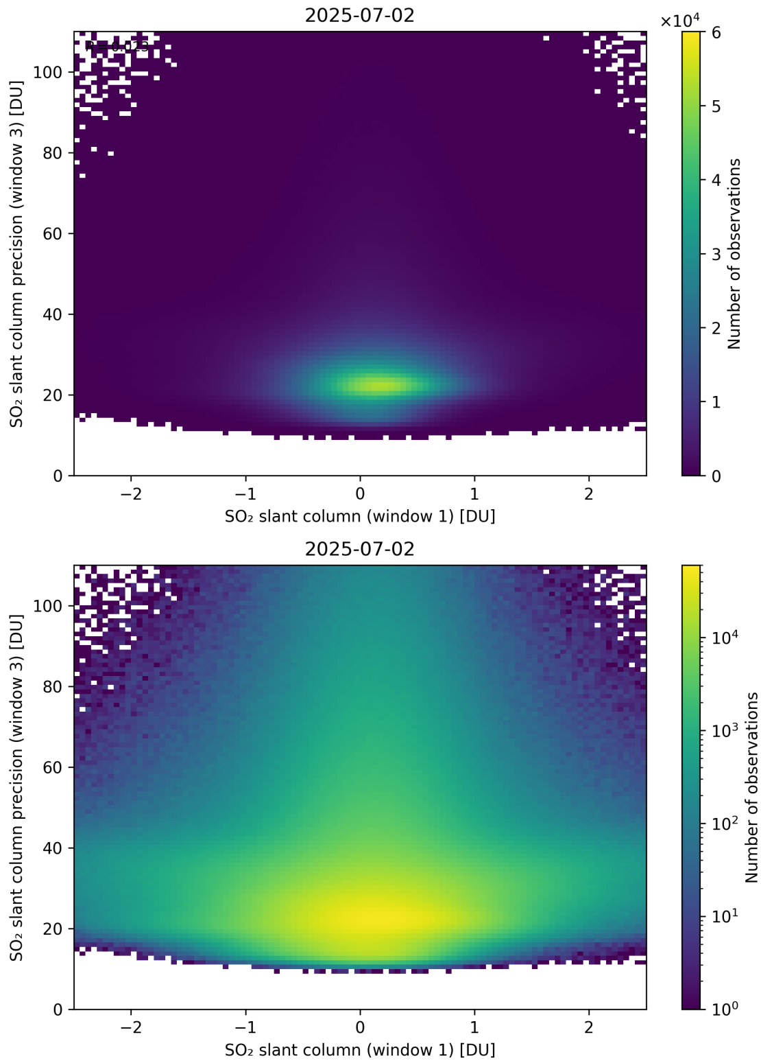
Figure 288: Scatter density plot of “SO 2 slant column (window 1)” against “SO 2 slant column precision (window 3)” for 2025-07-02 to 2025-07-03.
