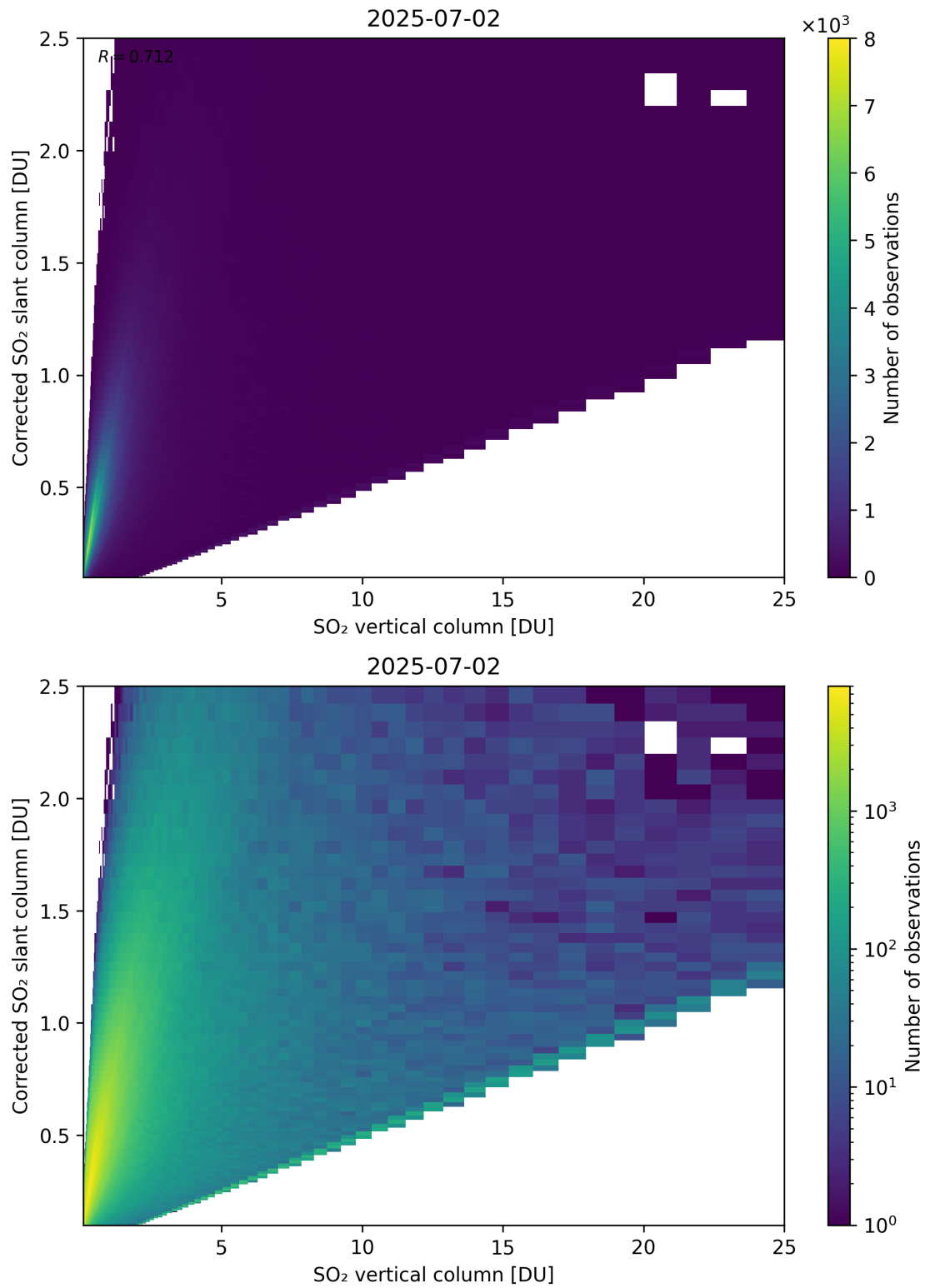
Figure 351: Scatter density plot of “SO 2 vertical column” against “Corrected SO 2 slant column” for 2025-07-02 to 2025-07-03.
