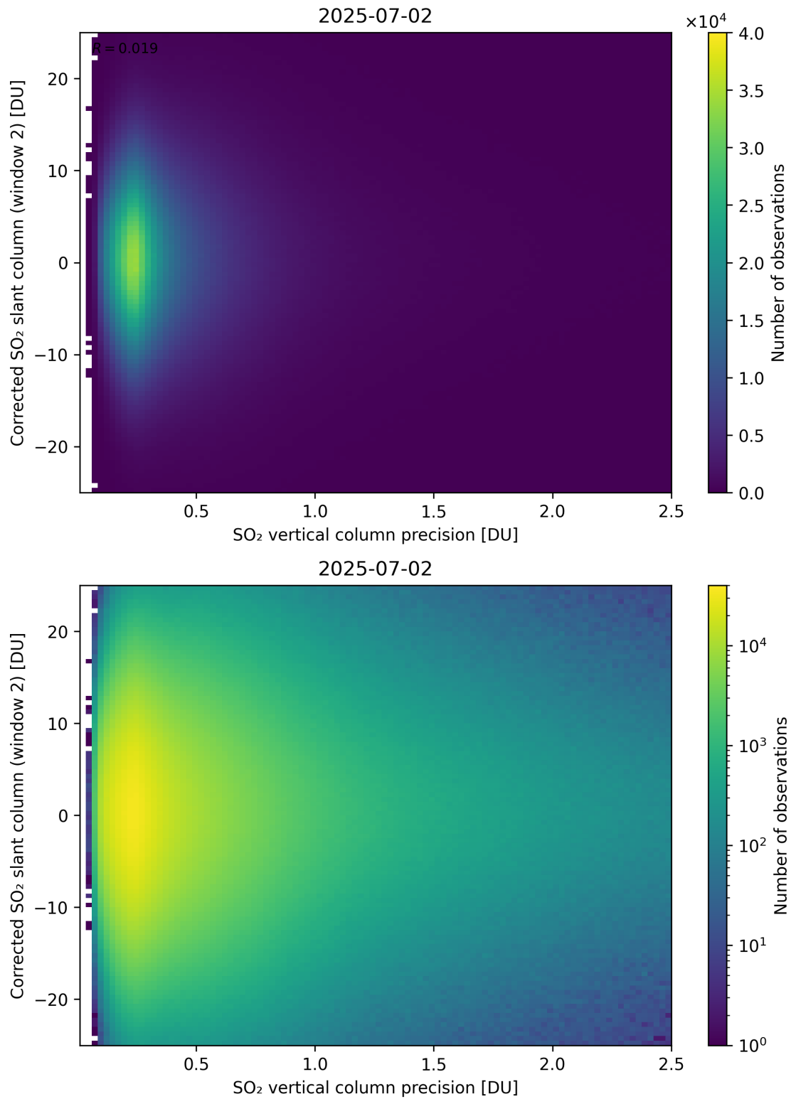
Figure 339: Scatter density plot of “SO 2 vertical column precision” against “Corrected SO 2 slant column (window 2)” for 2025-07-02 to 2025-07-03.
