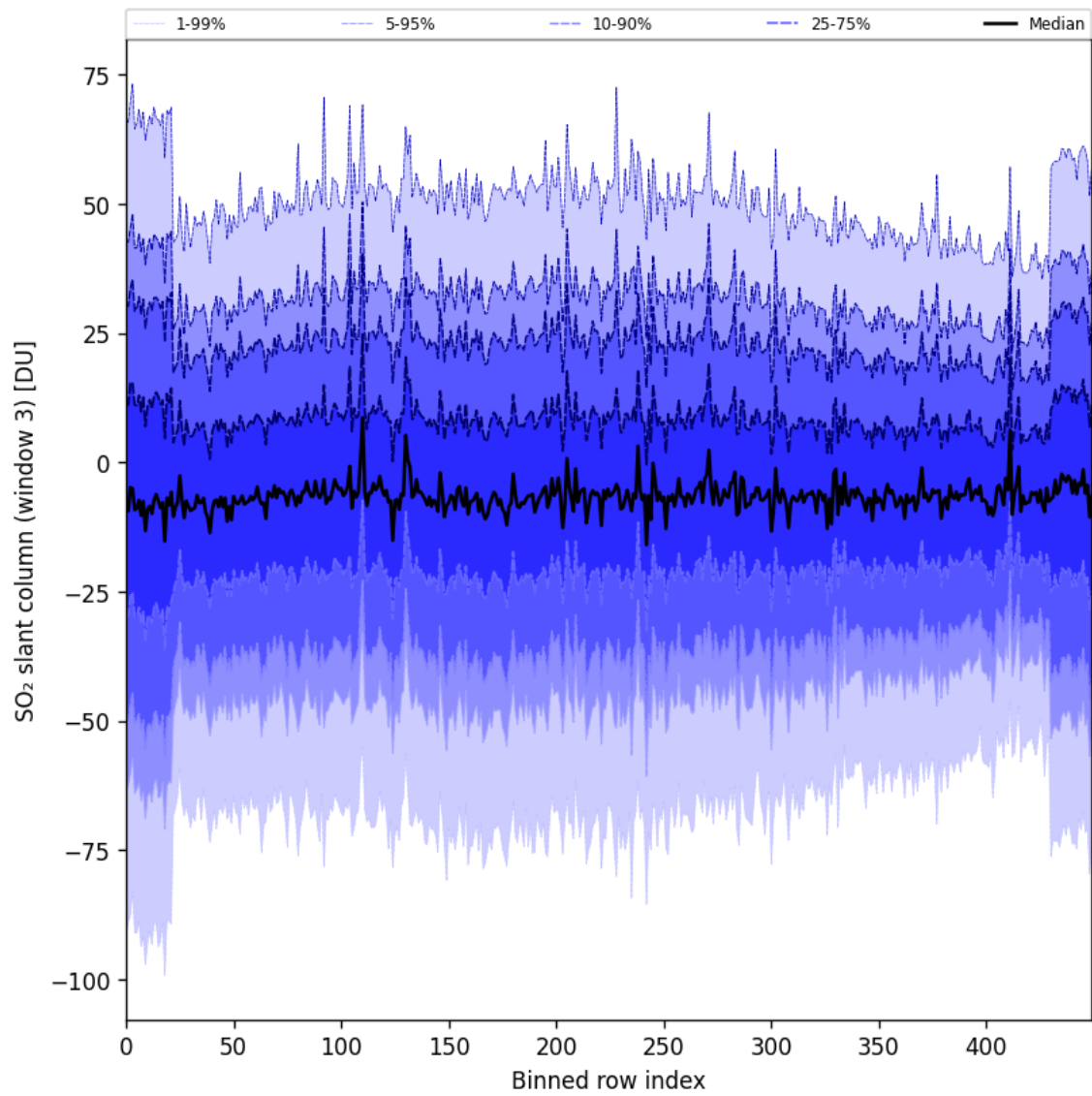
Figure 97: Along track statistics of “SO 2 slant column (window 3)” for 2025-07-02 to 2025-07-03
