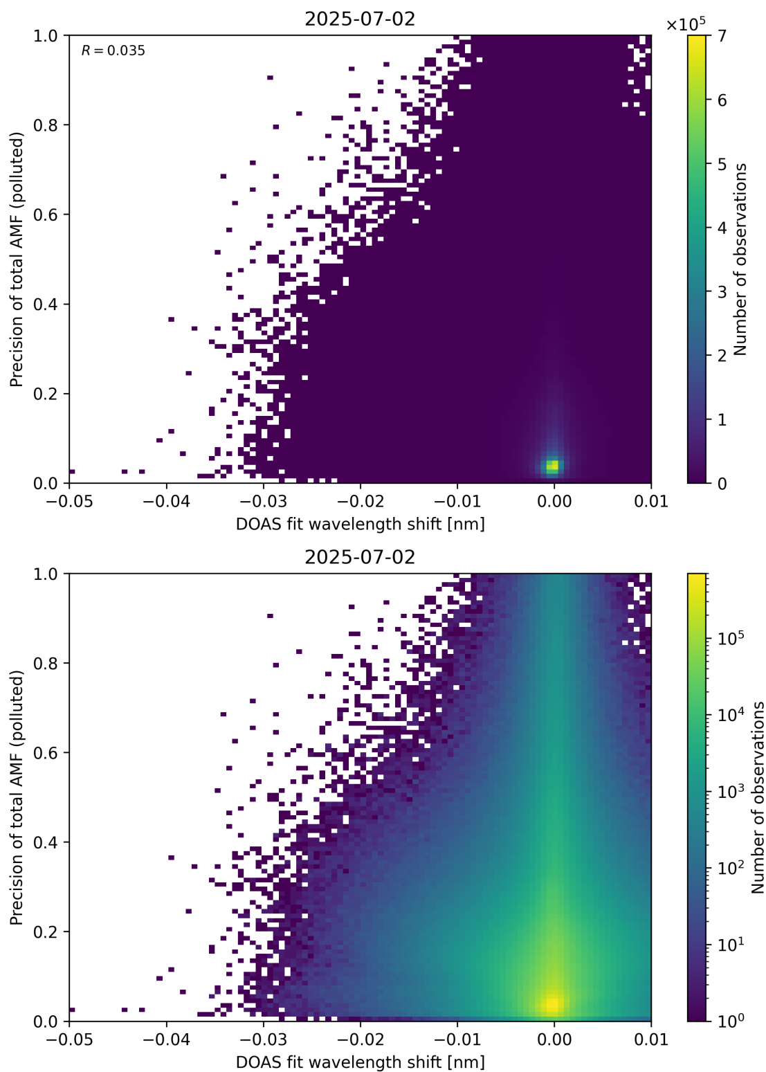
Figure 142: Scatter density plot of “DOAS fit wavelength shift” against “Precision of total AMF (polluted)” for 2025-07-02 to 2025-07-03.
