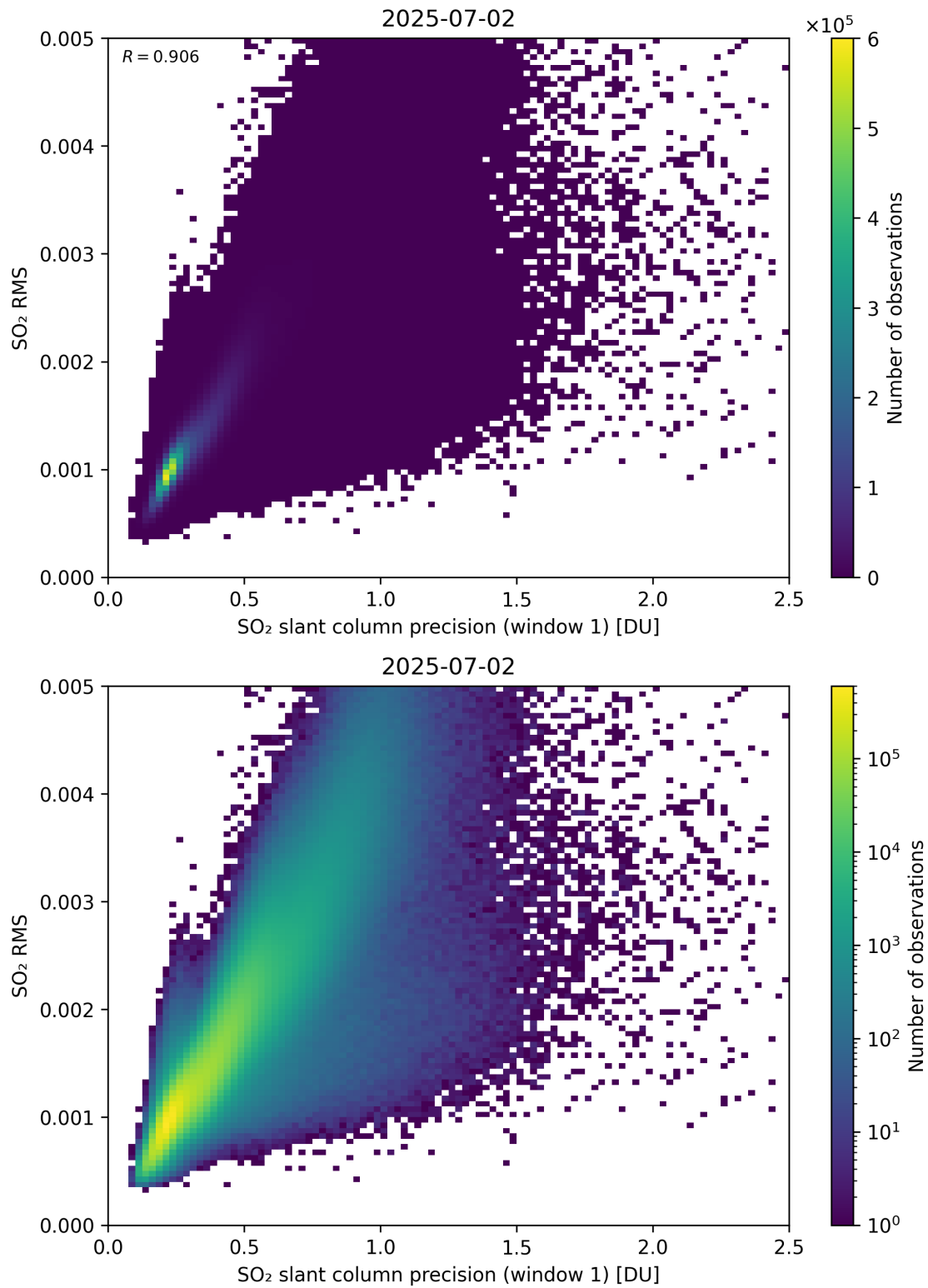
Figure 273: Scatter density plot of “SO 2 slant column precision (window 1)” against “SO 2 RMS” for 2025-07-02 to 2025-07-03.
