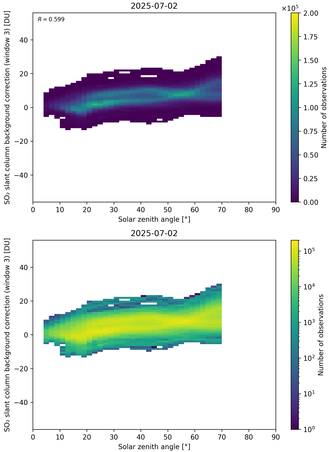
Figure 173: Scatter density plot of “Solar zenith angle” against “SO 2 slant column background correction (window 3)” for 2025-07-02 to 2025-07-03.
