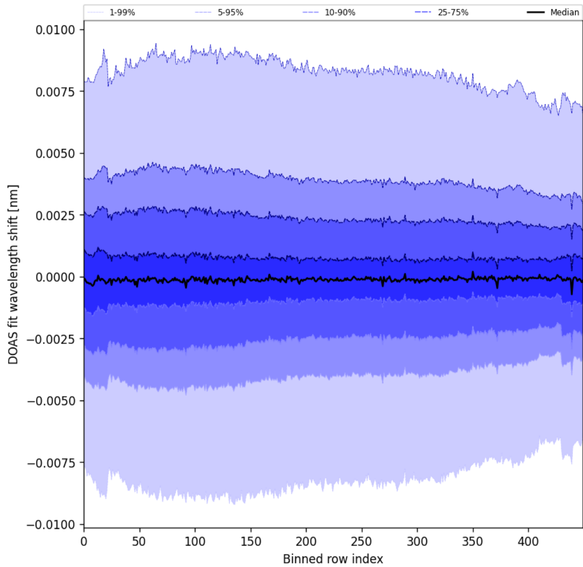
Figure 102: Along track statistics of “DOAS fit wavelength shift” for 2025-07-02 to 2025-07-03
