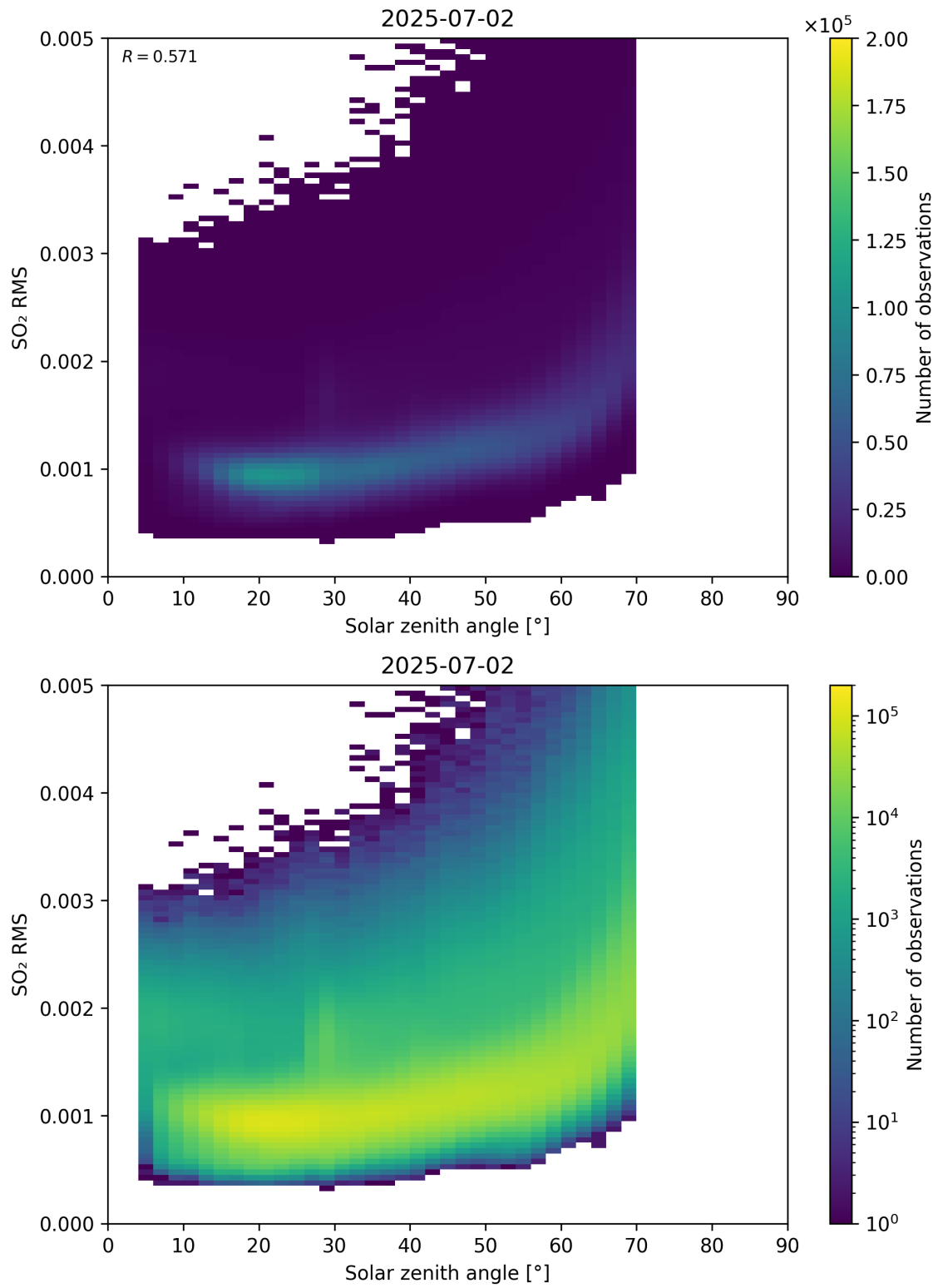
Figure 176: Scatter density plot of “Solar zenith angle” against “SO 2 RMS” for 2025-07-02 to 2025-07-03.
