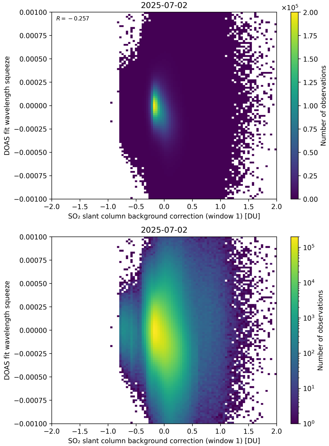
Figure 112: Scatter density plot of “SO 2 slant column background correction (window 1)” against “DOAS fit wavelength squeeze” for 2025-07-02 to 2025-07-03.
