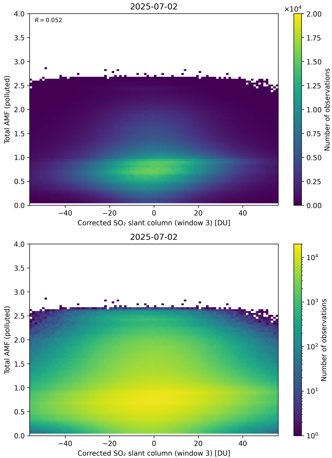
Figure 260: Scatter density plot of “Corrected SO 2 slant column (window 3)” against “Total AMF (polluted)” for 2025-07-02 to 2025-07-03.
