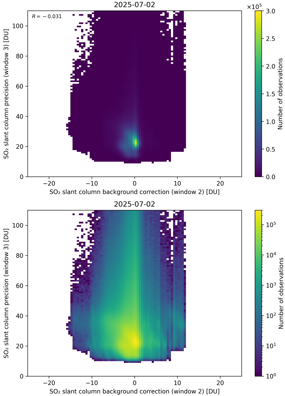
Figure 129: Scatter density plot of “SO 2 slant column background correction (window 2)” against “SO 2 slant column precision (window 3)” for 2025-07-02 to 2025-07-03.
