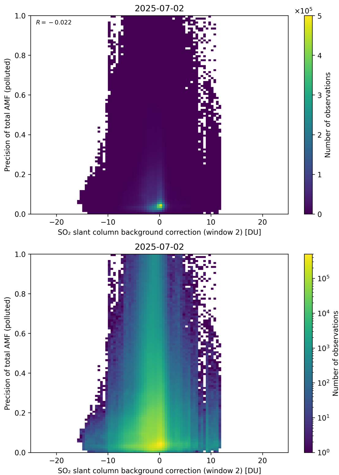
Figure 131: Scatter density plot of “SO 2 slant column background correction (window 2)” against “Precision of total AMF (polluted)” for 2025-07-02 to 2025-07-03.
