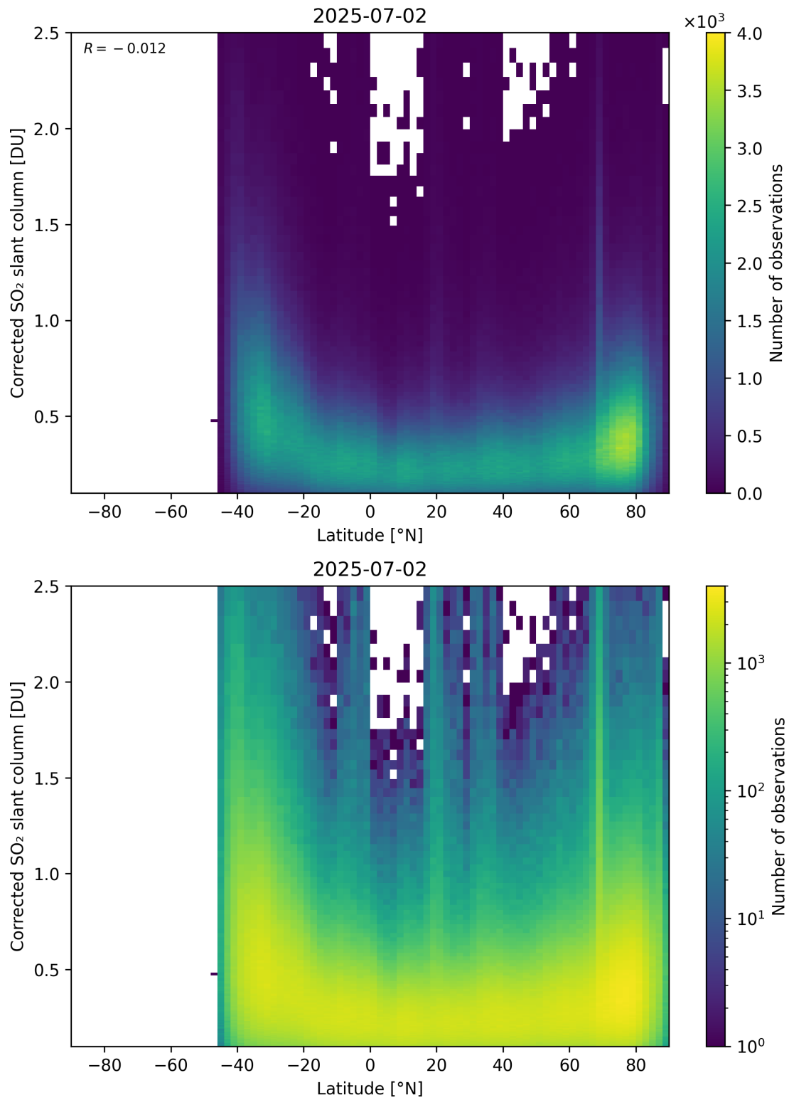
Figure 159: Scatter density plot of “Latitude” against “Corrected SO 2 slant column” for 2025-07-02 to 2025-07-03.
