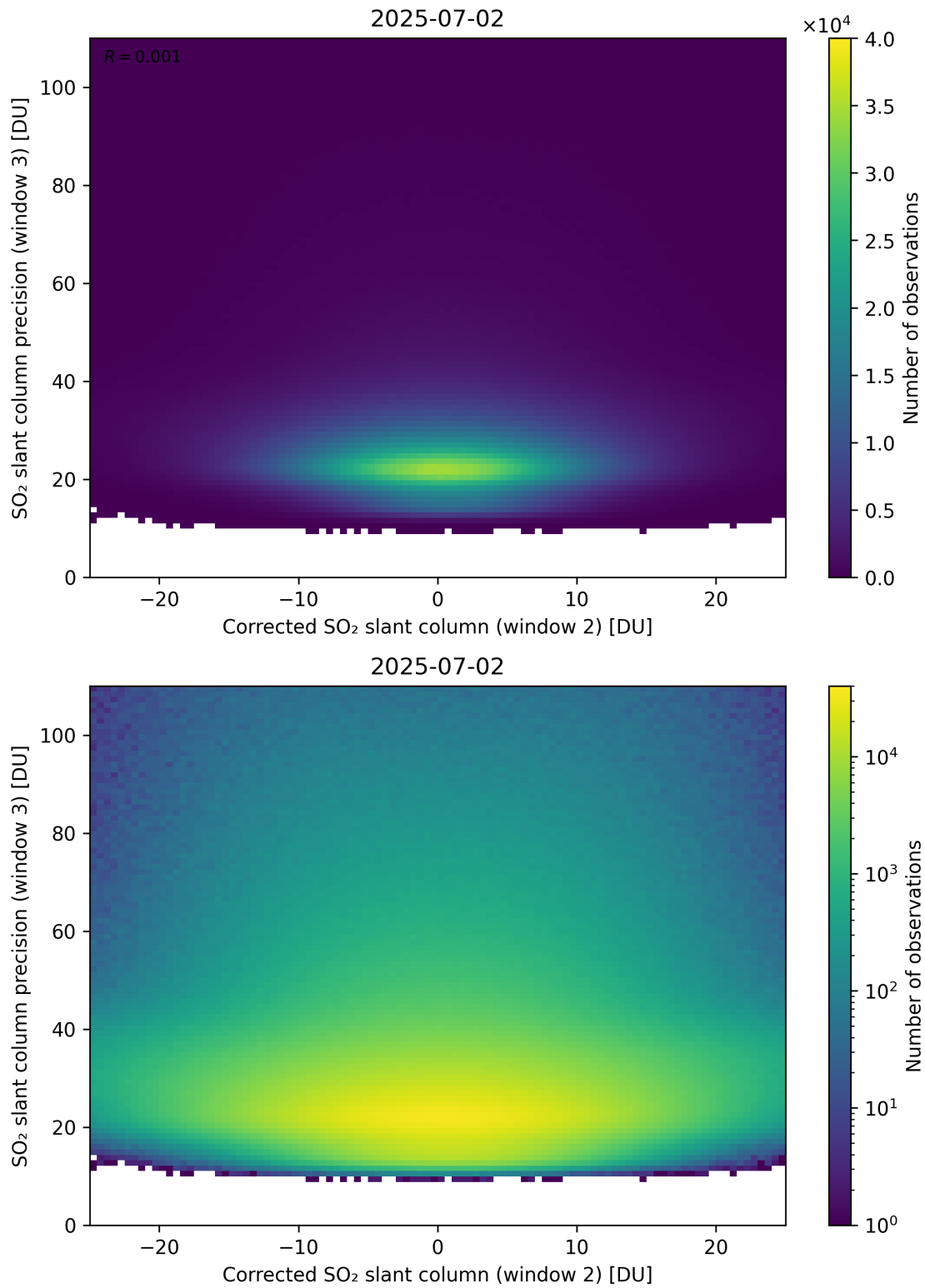
Figure 252: Scatter density plot of “Corrected SO 2 slant column (window 2)” against “SO 2 slant column precision (window 3)” for 2025-07-02 to 2025-07-03.
