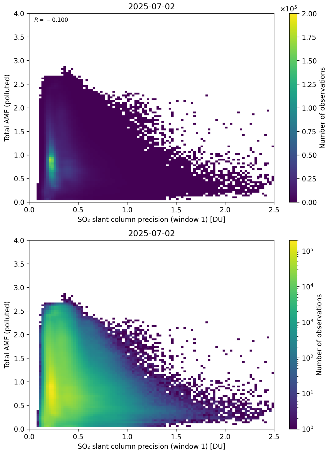
Figure 280: Scatter density plot of “SO 2 slant column precision (window 1)” against “Total AMF (polluted)” for 2025-07-02 to 2025-07-03.
