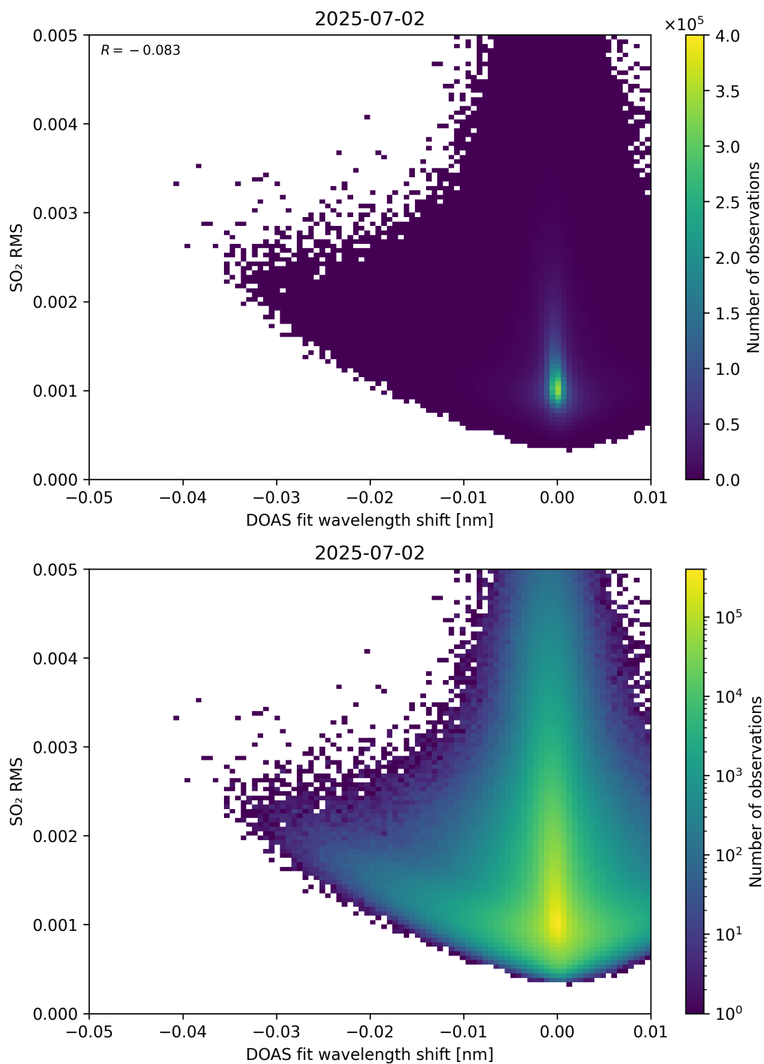
Figure 139: Scatter density plot of “DOAS fit wavelength shift” against “SO 2 RMS” for 2025-07-02 to 2025-07-03.
