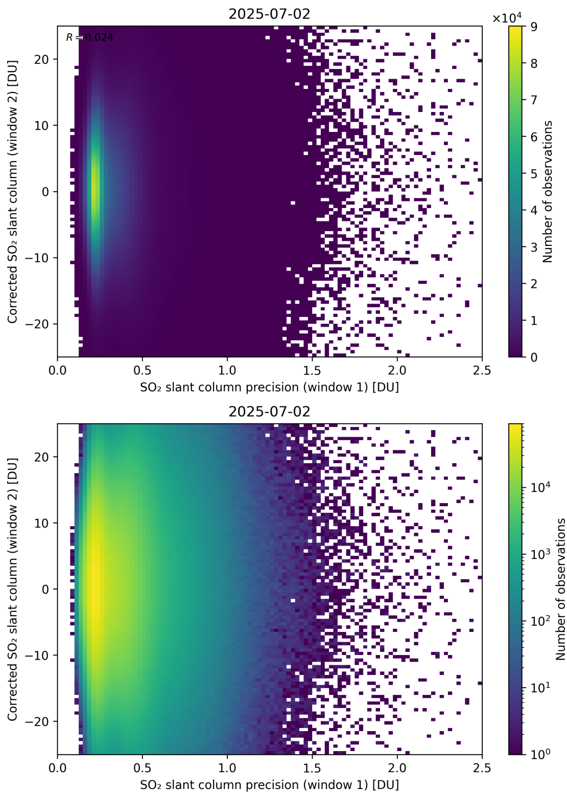
Figure 275: Scatter density plot of “SO 2 slant column precision (window 1)” against “Corrected SO 2 slant column (window 2)” for 2025-07-02 to 2025-07-03.
