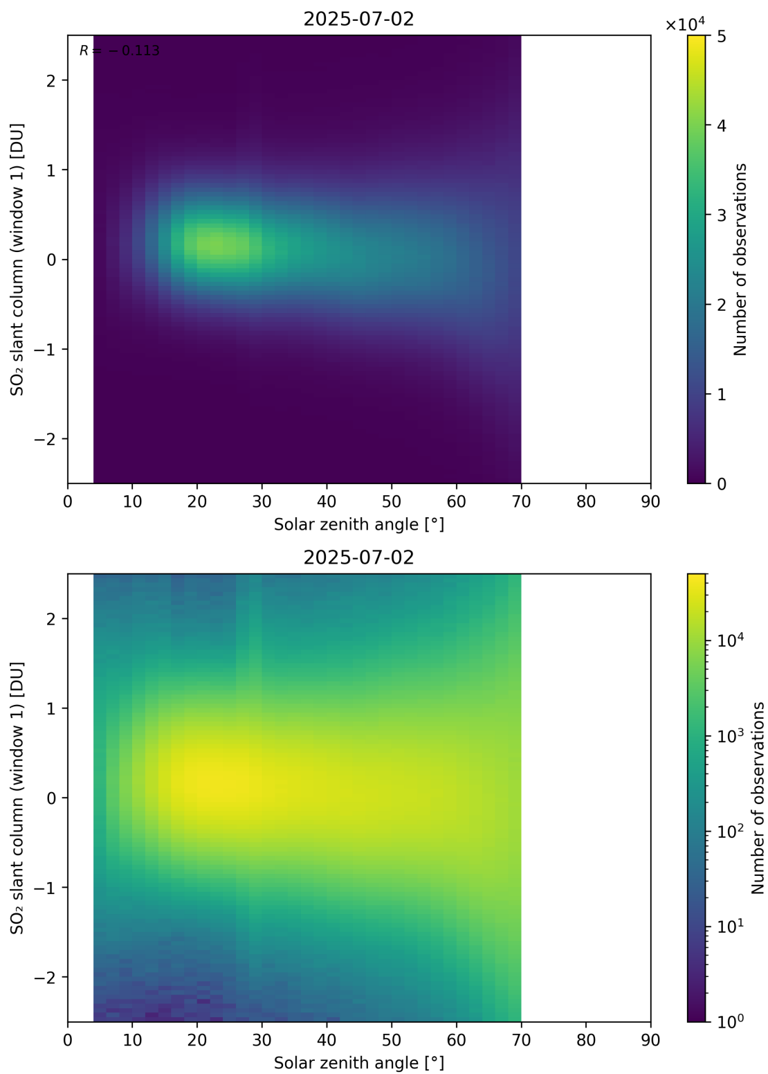
Figure 184: Scatter density plot of “Solar zenith angle” against “SO 2 slant column (window 1)” for 2025-07-02 to 2025-07-03.
