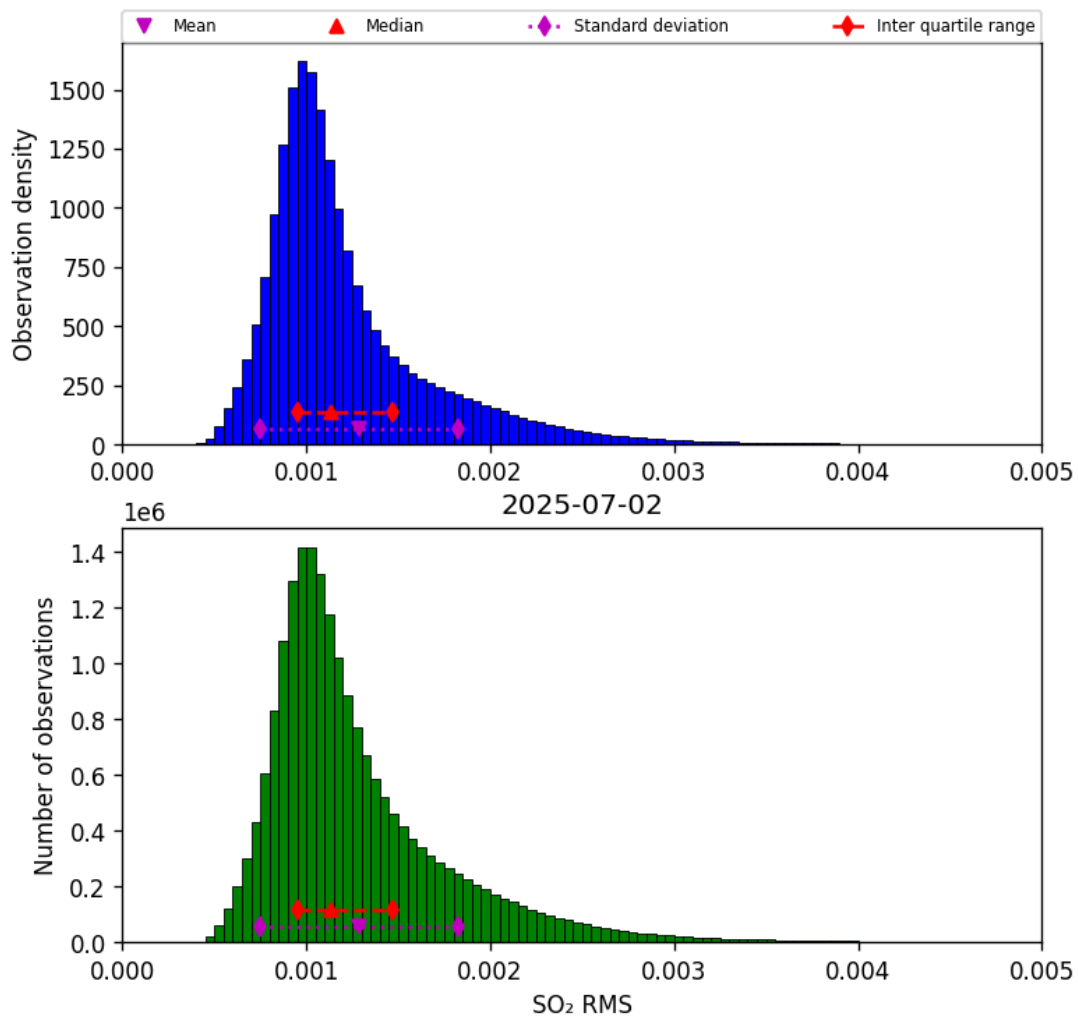
Figure 78: Histogram of “SO 2 RMS” for 2025-07-02 to 2025-07-03
