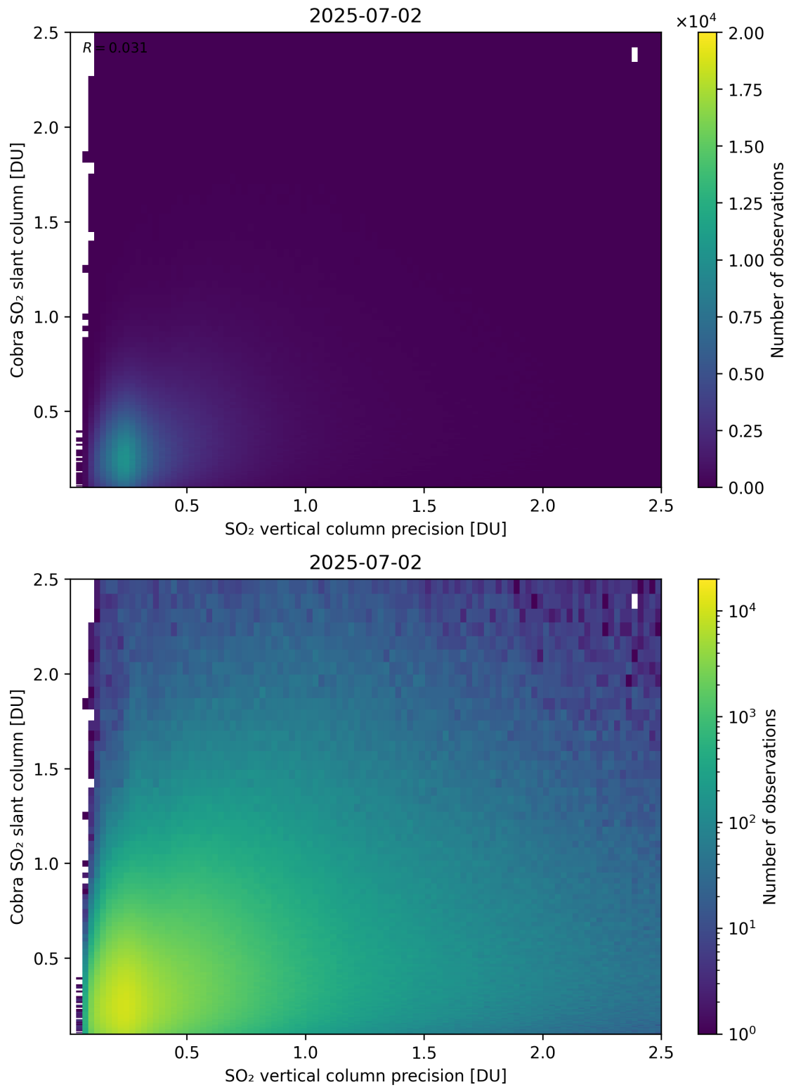
Figure 336: Scatter density plot of “SO 2 vertical column precision” against “Cobra SO 2 slant column” for 2025-07-02 to 2025-07-03.
