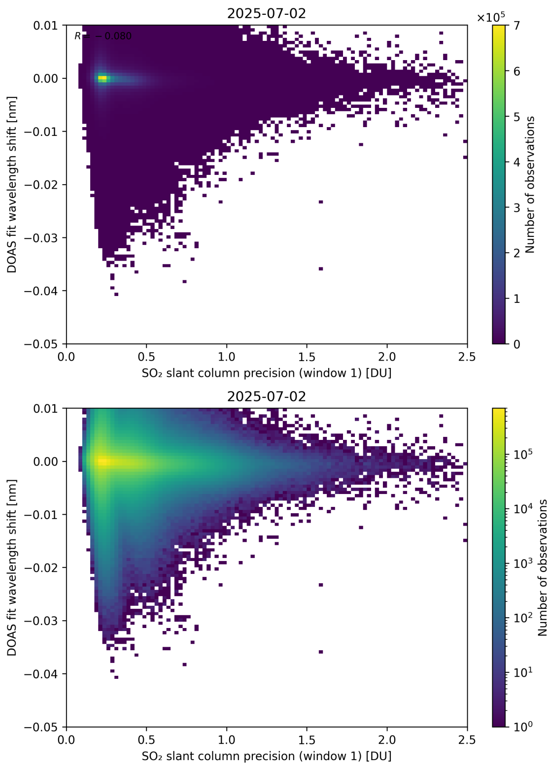
Figure 271: Scatter density plot of “SO 2 slant column precision (window 1)” against “DOAS fit wavelength shift” for 2025-07-02 to 2025-07-03.
