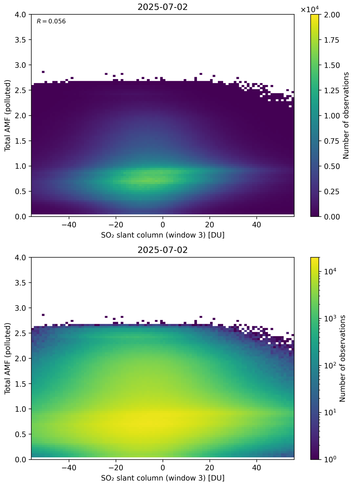
Figure 318: Scatter density plot of “SO 2 slant column (window 3)” against “Total AMF (polluted)” for 2025-07-02 to 2025-07-03.
