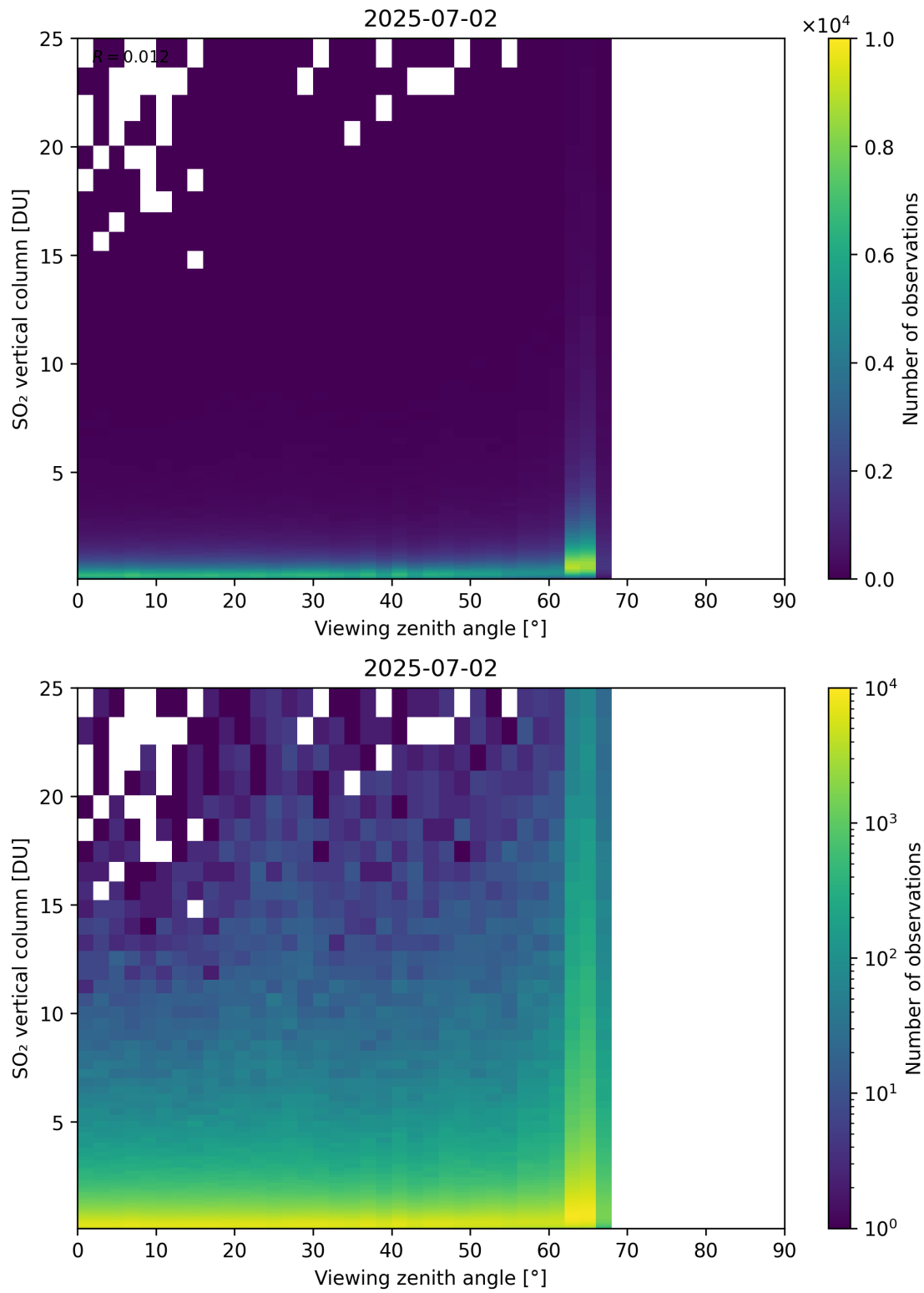
Figure 383: Scatter density plot of “Viewing zenith angle” against “SO 2 vertical column” for 2025-07-02 to 2025-07-03.
