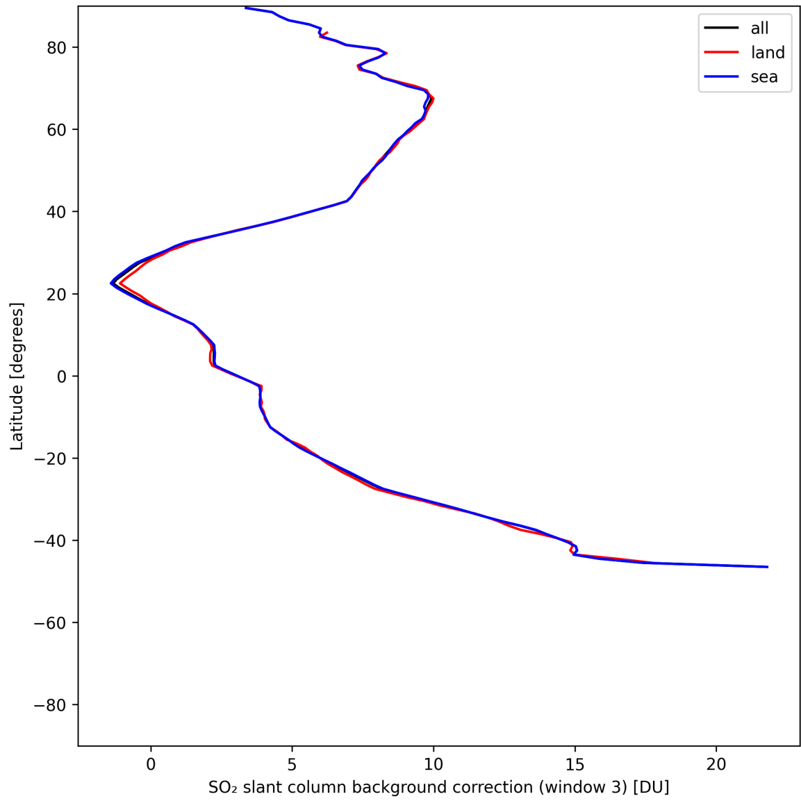
Figure 48: Zonal average of “SO 2 slant column background correction (window 3)” for 2025-07-02 to 2025-07-03.
