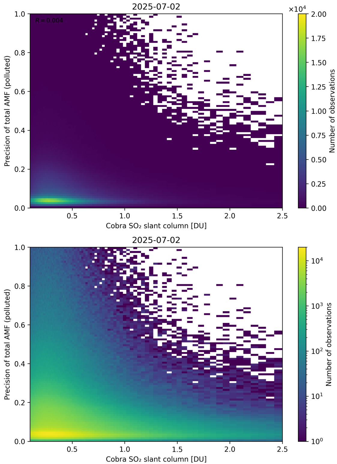
Figure 225: Scatter density plot of “Cobra SO 2 slant column” against “Precision of total AMF (polluted)” for 2025-07-02 to 2025-07-03.
