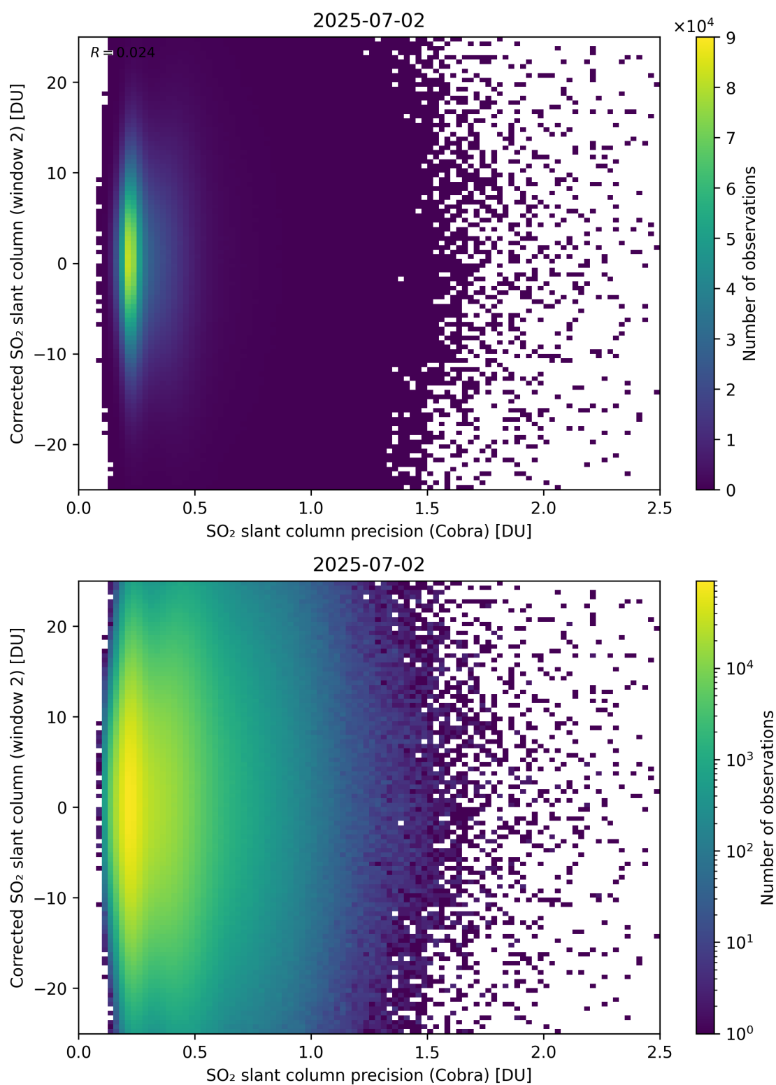
Figure 206: Scatter density plot of “SO 2 slant column precision (Cobra)” against “Corrected SO 2 slant column (window 2)” for 2025-07-02 to 2025-07-03.
