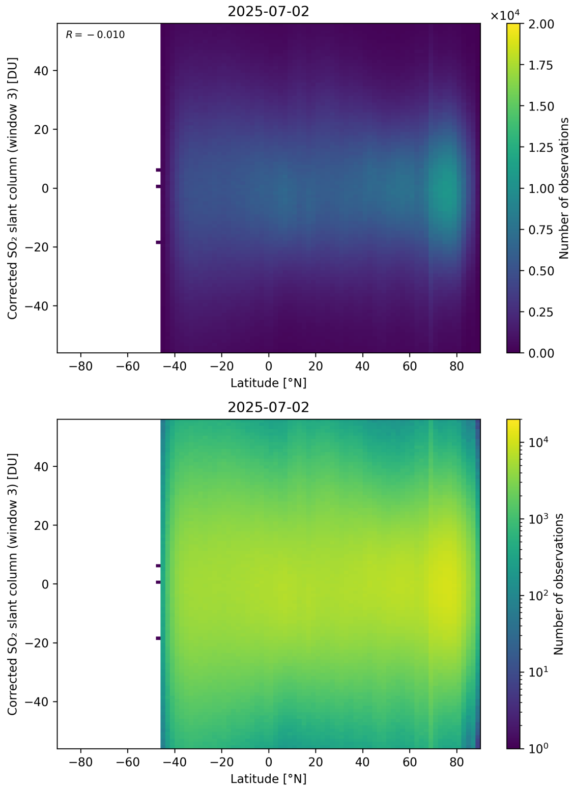
Figure 161: Scatter density plot of “Latitude” against “Corrected SO 2 slant column (window 3)” for 2025-07-02 to 2025-07-03.
