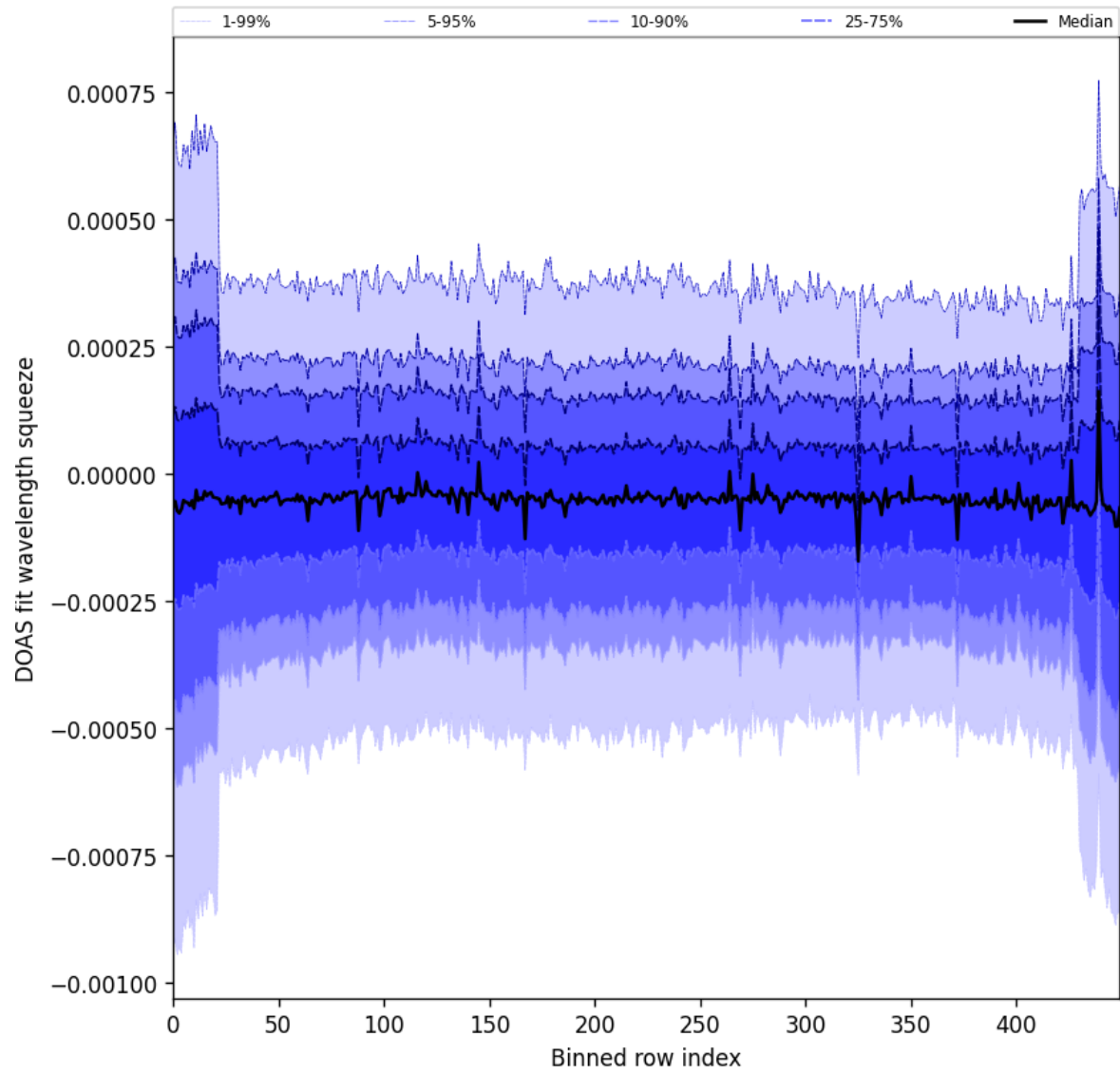
Figure 103: Along track statistics of “DOAS fit wavelength squeeze” for 2025-07-02 to 2025-07-03
