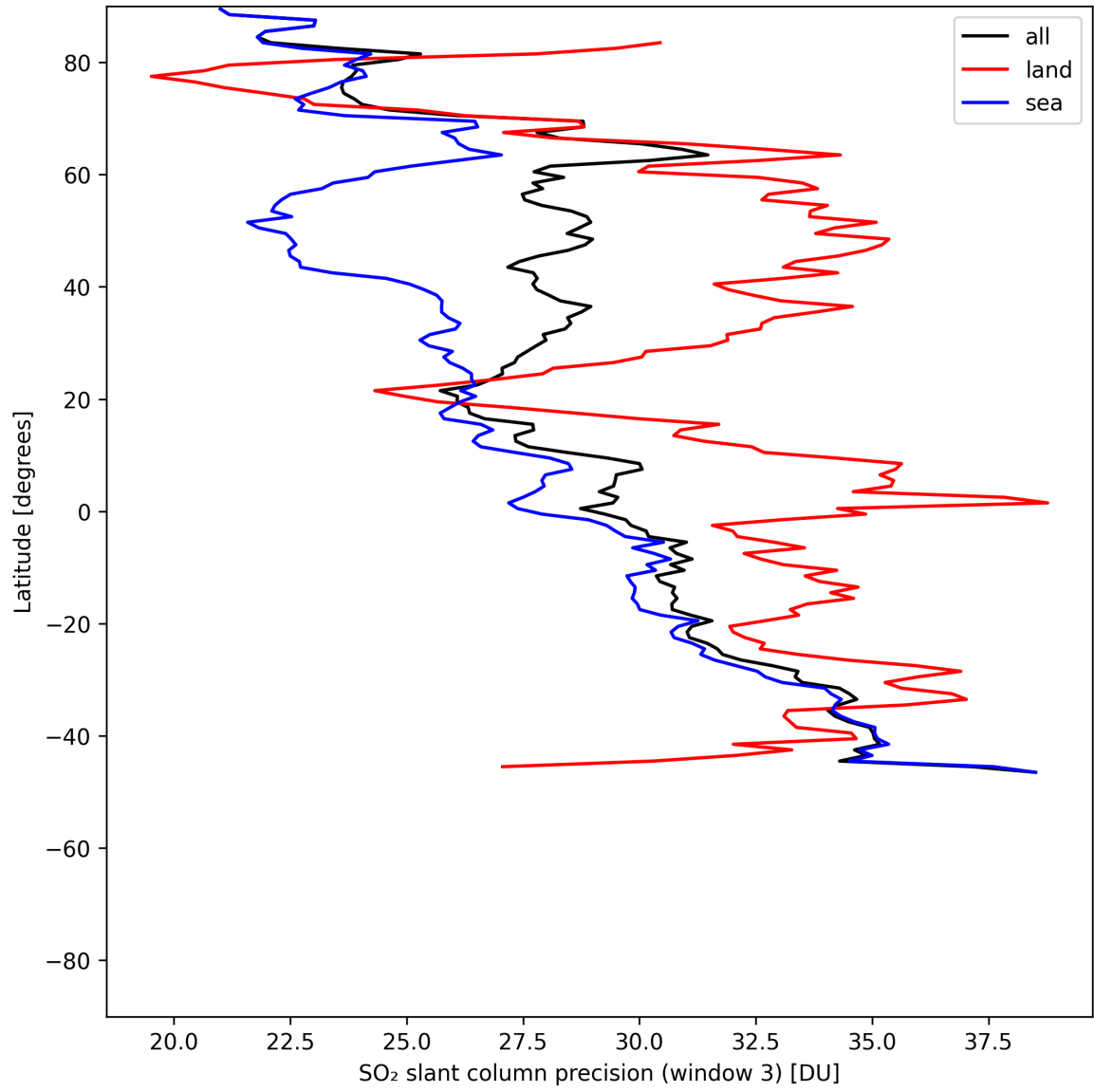
Figure 46: Zonal average of “SO 2 slant column precision (window 3)” for 2025-07-02 to 2025-07-03.
