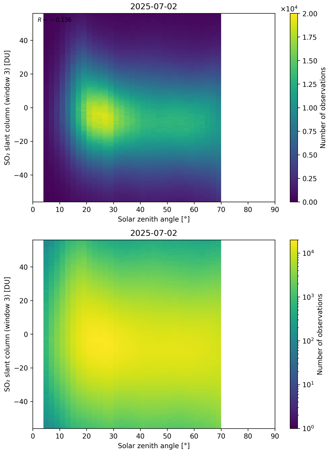
Figure 187: Scatter density plot of “Solar zenith angle” against “SO 2 slant column (window 3)” for 2025-07-02 to 2025-07-03.
