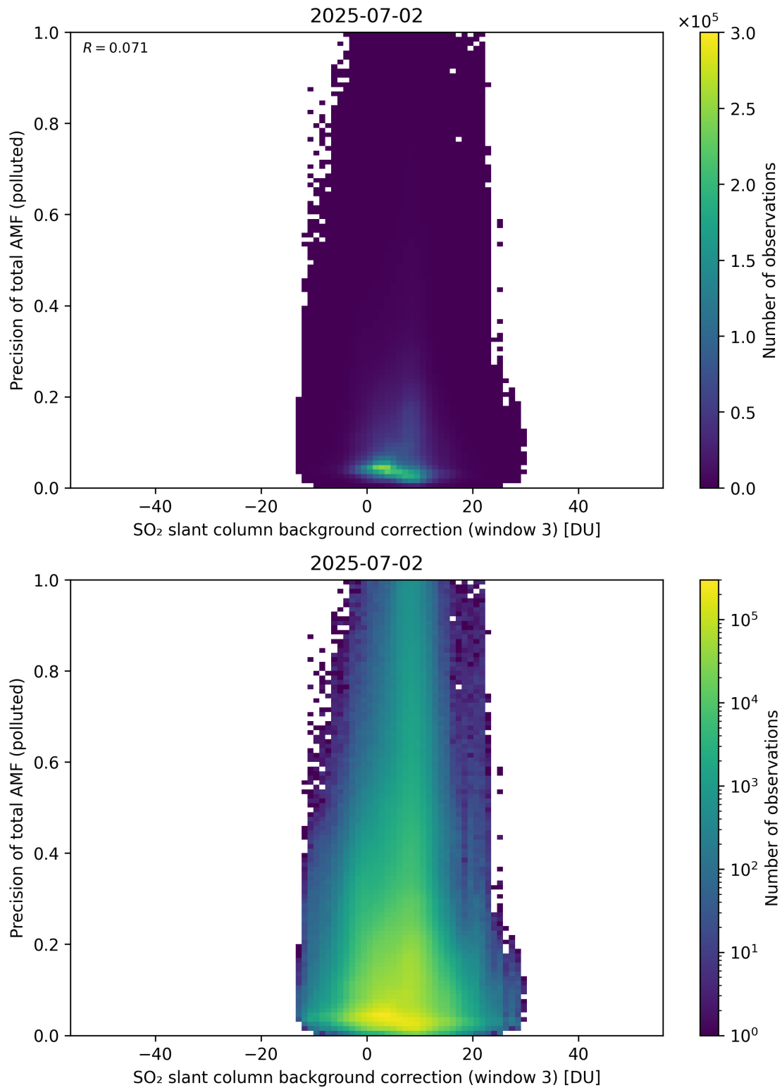
Figure 137: Scatter density plot of “SO 2 slant column background correction (window 3)” against “Precision of total AMF (polluted)” for 2025-07-02 to 2025-07-03.
