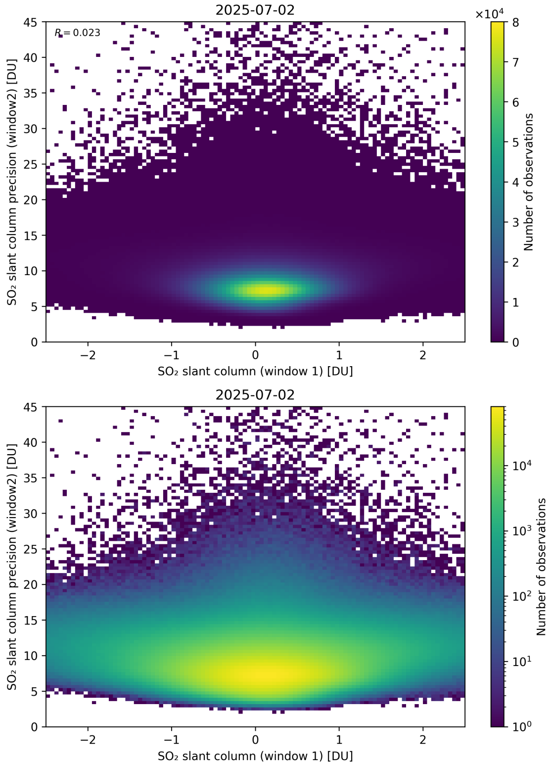
Figure 286: Scatter density plot of “SO 2 slant column (window 1)” against “SO 2 slant column precision (window2)” for 2025-07-02 to 2025-07-03.
