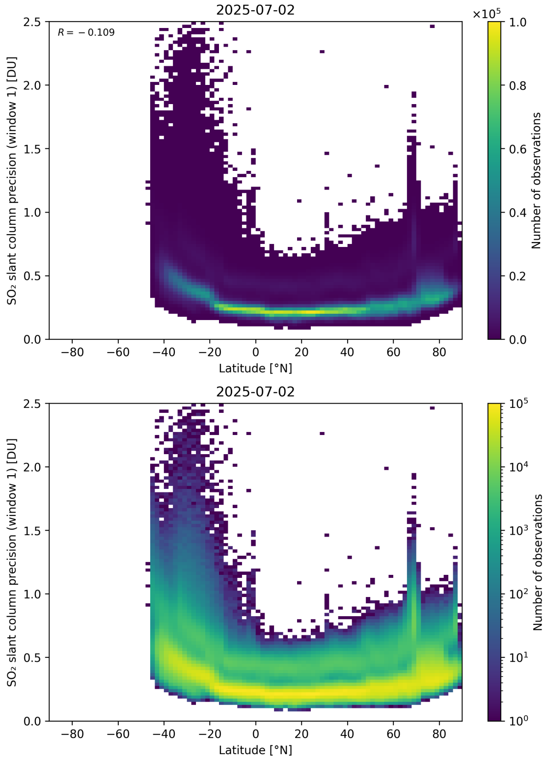
Figure 163: Scatter density plot of “Latitude” against “SO 2 slant column precision (window 1)” for 2025-07-02 to 2025-07-03.
