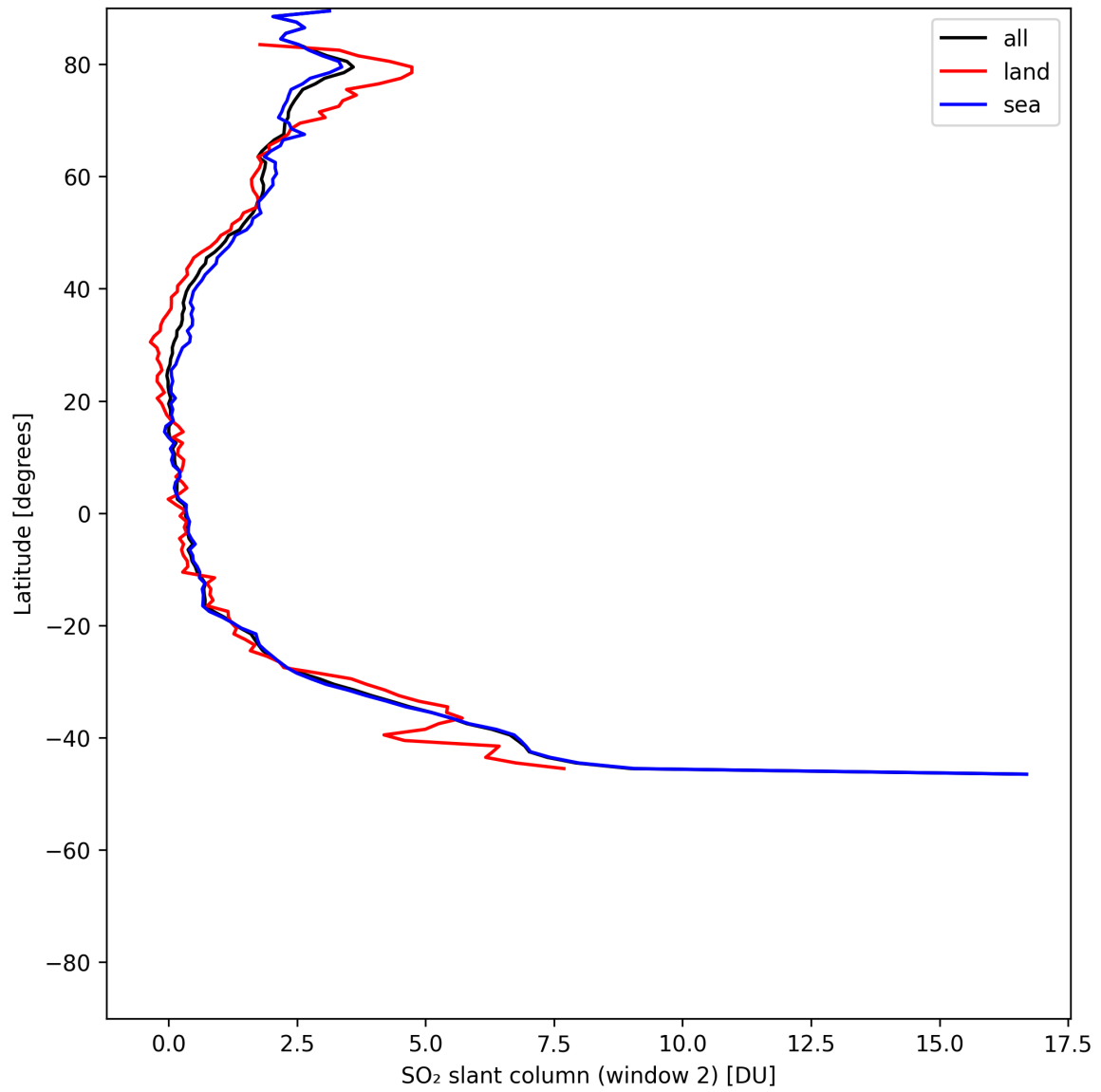
Figure 41: Zonal average of “SO 2 slant column (window 2)” for 2025-07-02 to 2025-07-03.
