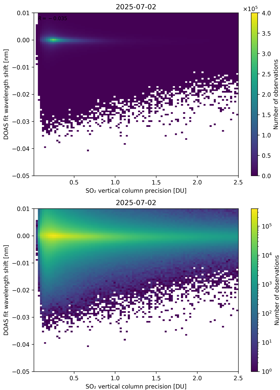
Figure 332: Scatter density plot of “SO 2 vertical column precision” against “DOAS fit wavelength shift” for 2025-07-02 to 2025-07-03.
