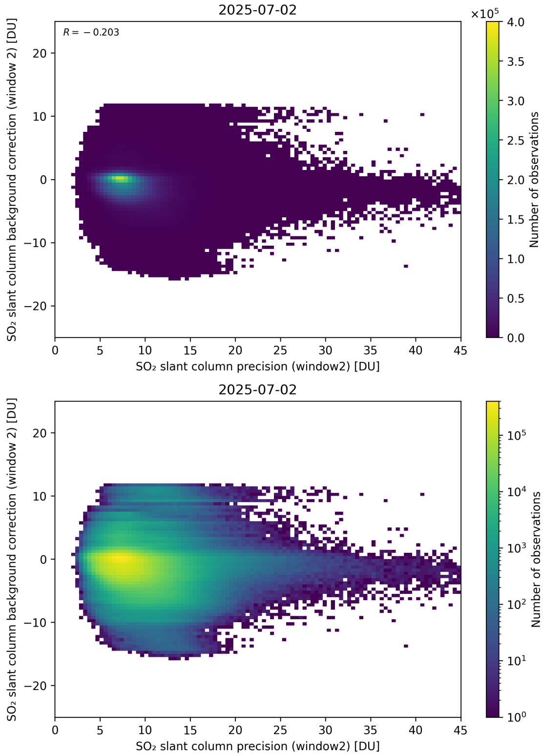
Figure 291: Scatter density plot of “SO 2 slant column precision (window2)” against “SO 2 slant column background correction (window 2)” for 2025-07-02 to 2025-07-03.
