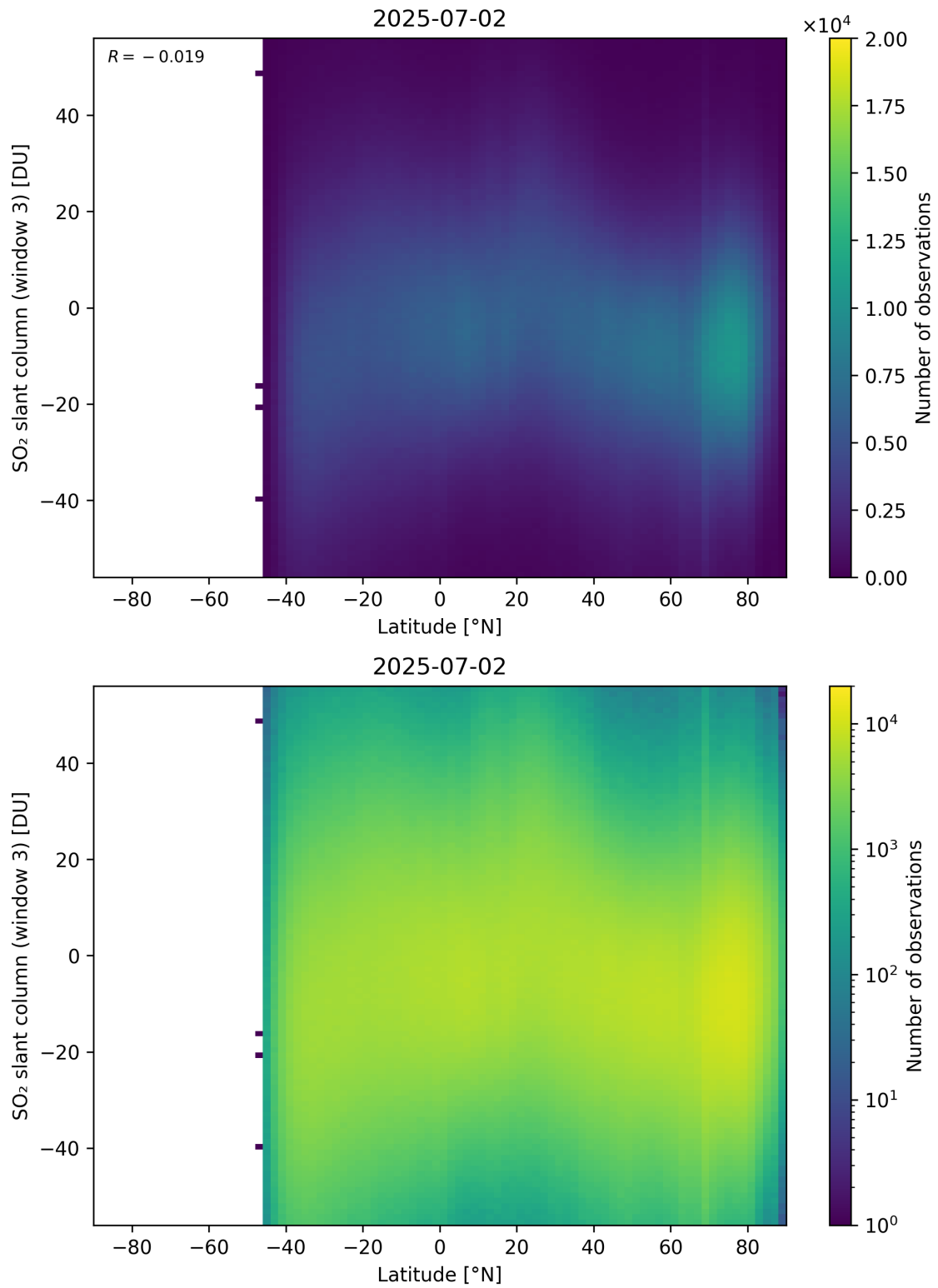
Figure 165: Scatter density plot of “Latitude” against “SO 2 slant column (window 3)” for 2025-07-02 to 2025-07-03.
