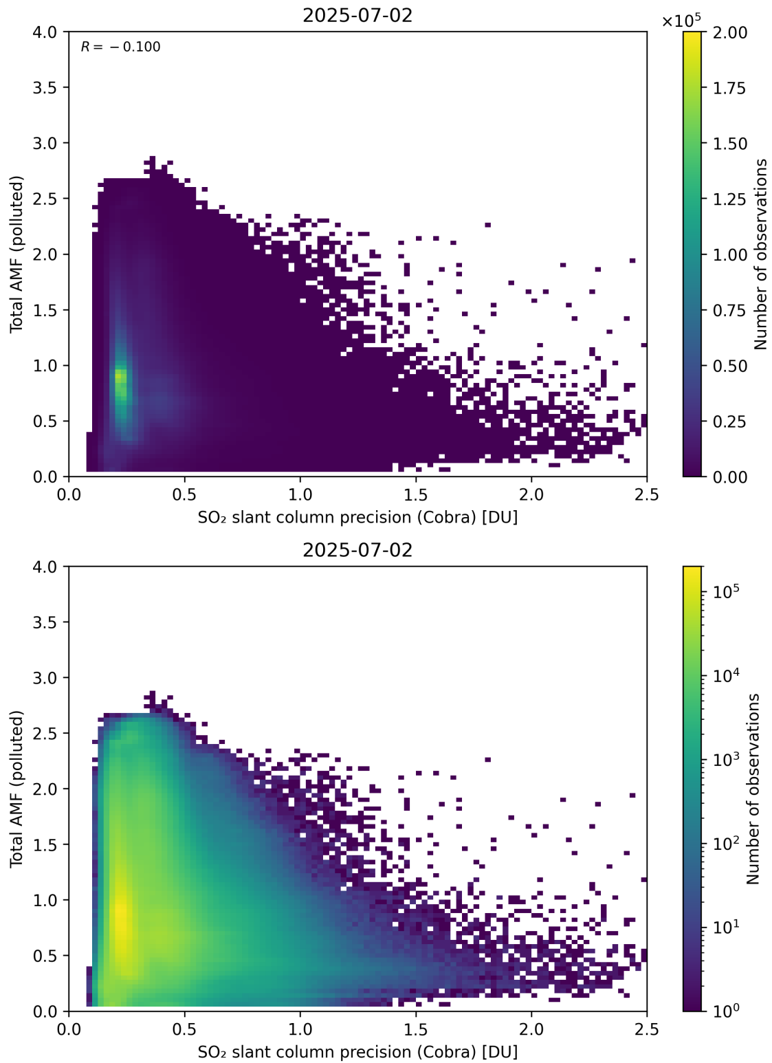
Figure 213: Scatter density plot of “SO 2 slant column precision (Cobra)” against “Total AMF (polluted)” for 2025-07-02 to 2025-07-03.
