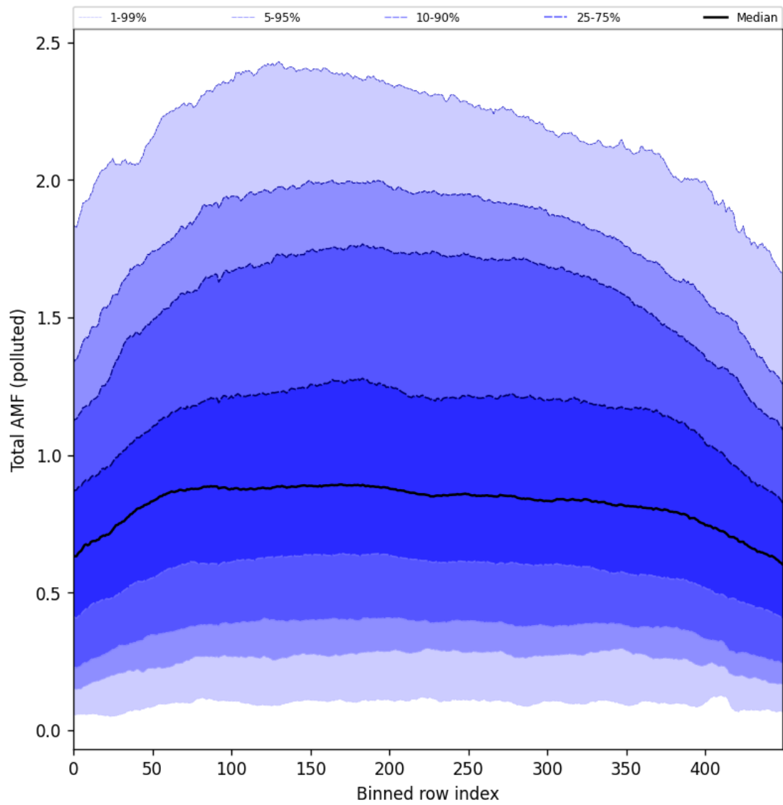
Figure 105: Along track statistics of “Total AMF (polluted)” for 2025-07-02 to 2025-07-03
