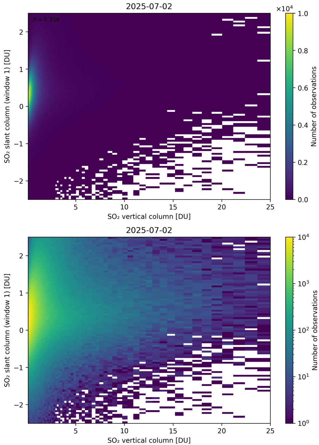
Figure 354: Scatter density plot of “SO 2 vertical column” against “SO 2 slant column (window 1)” for 2025-07-02 to 2025-07-03.
