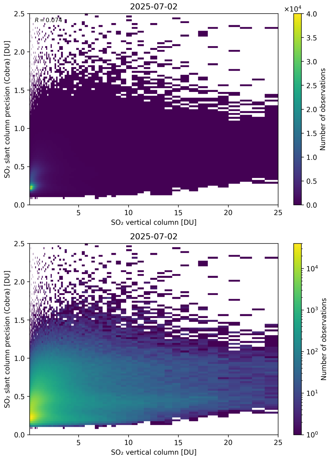
Figure 350: Scatter density plot of “SO 2 vertical column” against “SO 2 slant column precision (Cobra)” for 2025-07-02 to 2025-07-03.
