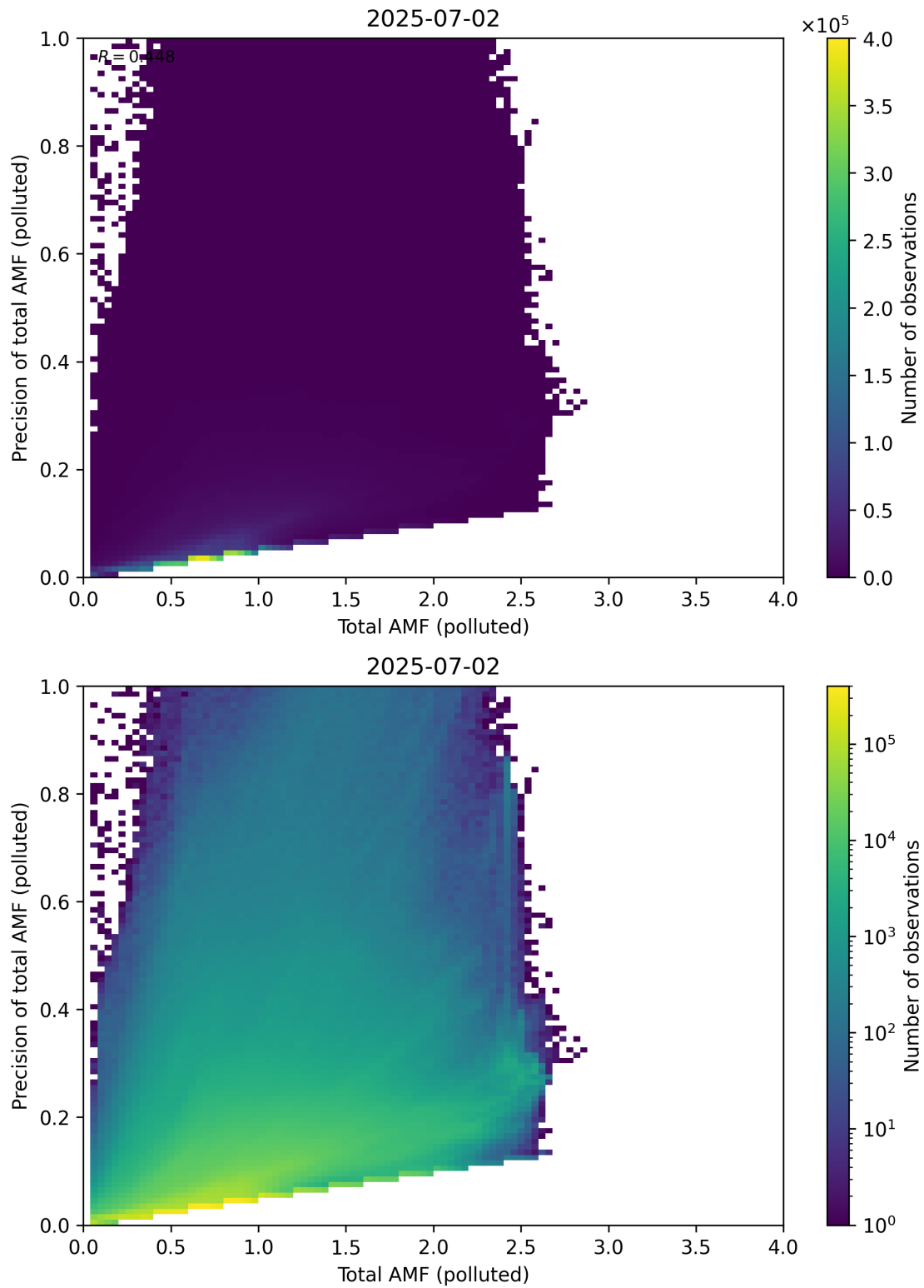
Figure 322: Scatter density plot of “Total AMF (polluted)” against “Precision of total AMF (polluted)” for 2025-07-02 to 2025-07-03.
