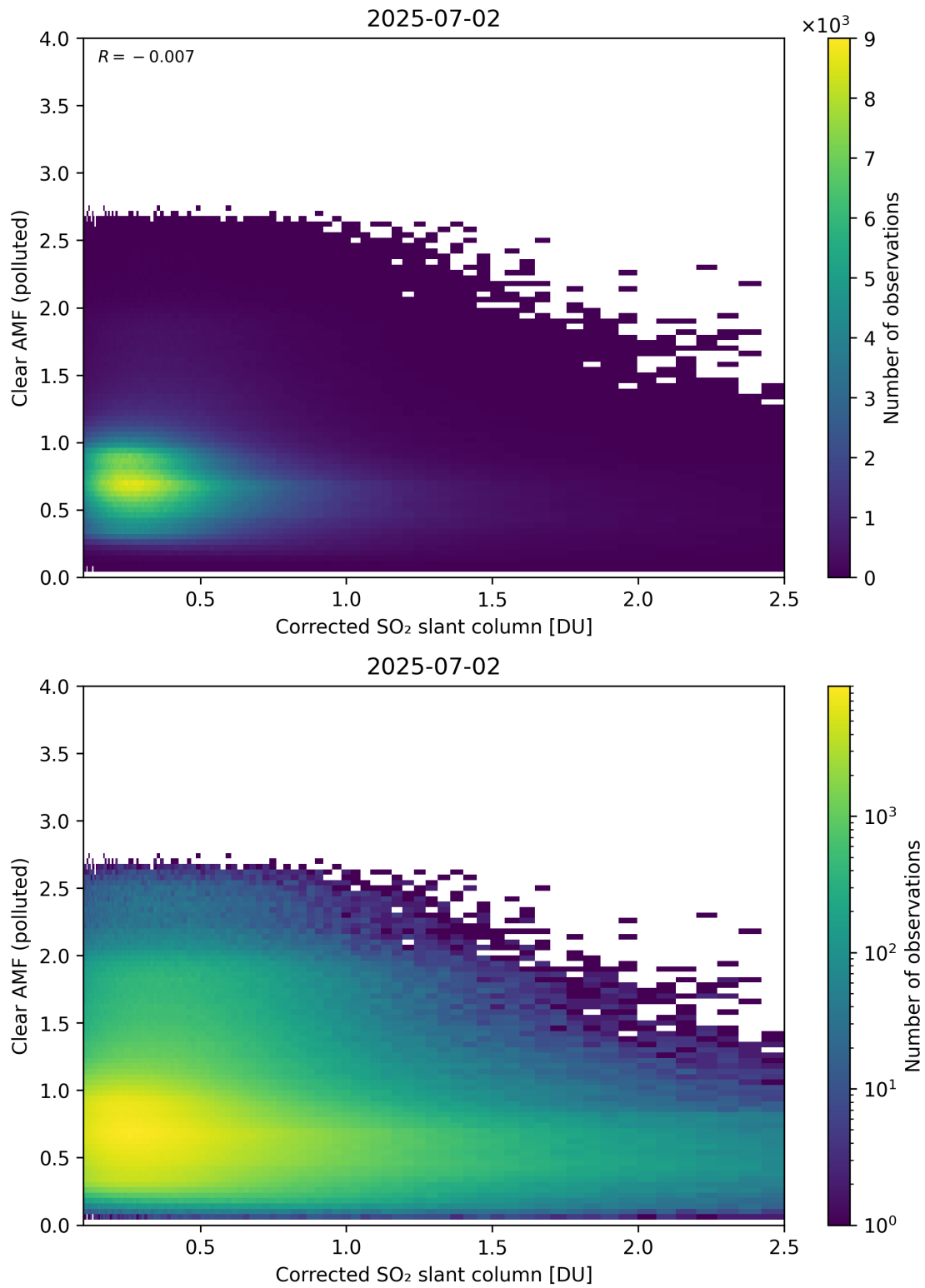
Figure 232: Scatter density plot of “Corrected SO 2 slant column” against “Clear AMF (polluted)” for 2025-07-02 to 2025-07-03.
