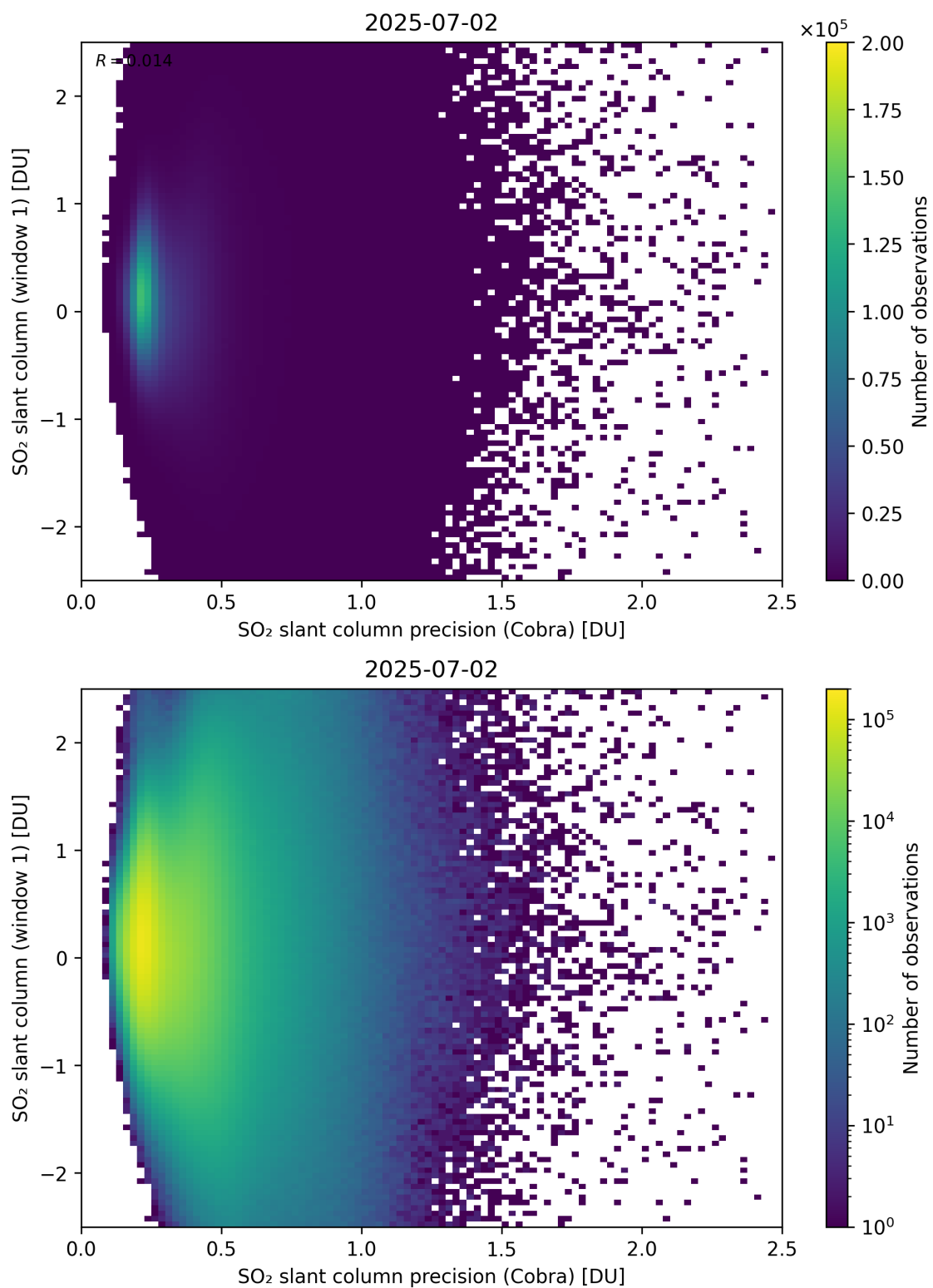
Figure 208: Scatter density plot of “SO 2 slant column precision (Cobra)” against “SO 2 slant column (window 1)” for 2025-07-02 to 2025-07-03.
