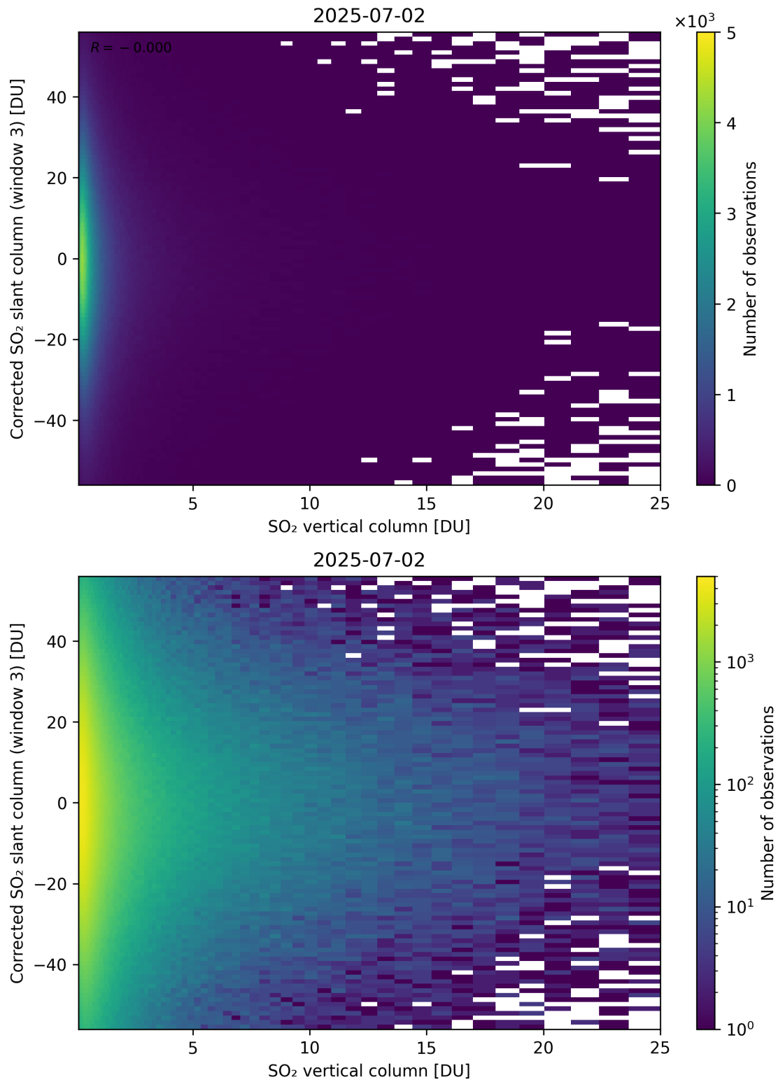
Figure 353: Scatter density plot of “SO 2 vertical column” against “Corrected SO 2 slant column (window 3)” for 2025-07-02 to 2025-07-03.
