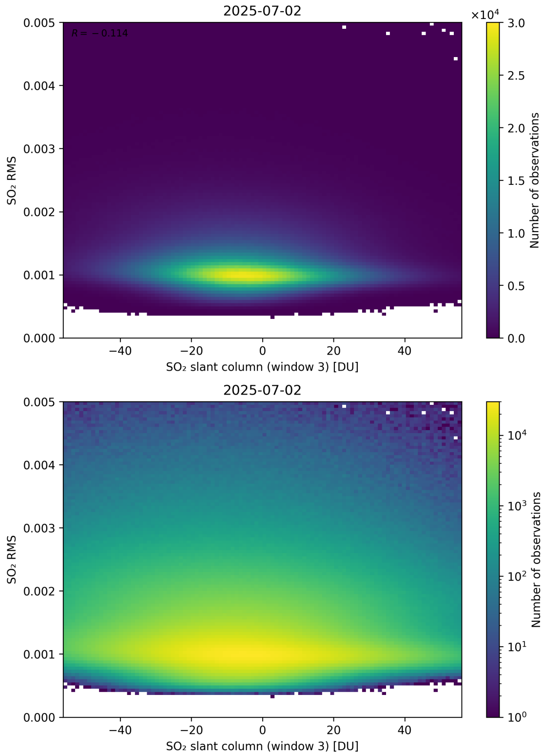
Figure 306: Scatter density plot of “SO 2 slant column (window 3)” against “SO 2 RMS” for 2025-07-02 to 2025-07-03.
