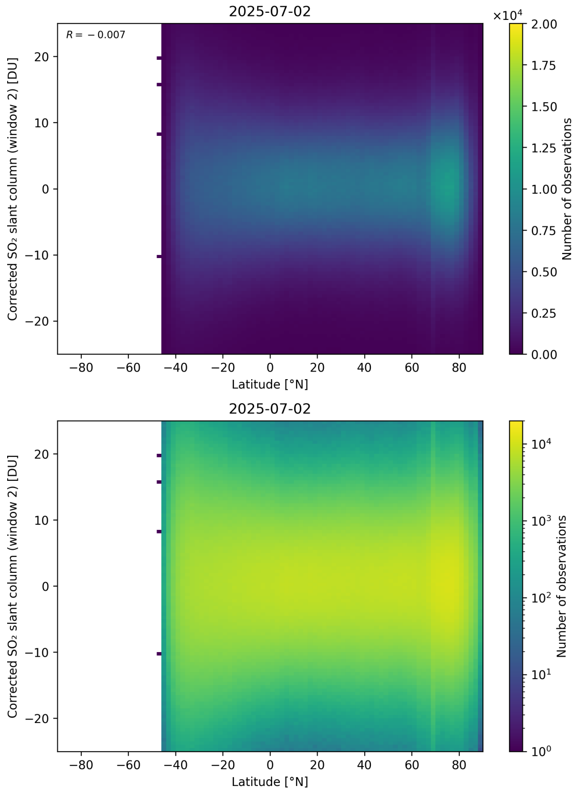
Figure 160: Scatter density plot of “Latitude” against “Corrected SO 2 slant column (window 2)” for 2025-07-02 to 2025-07-03.
