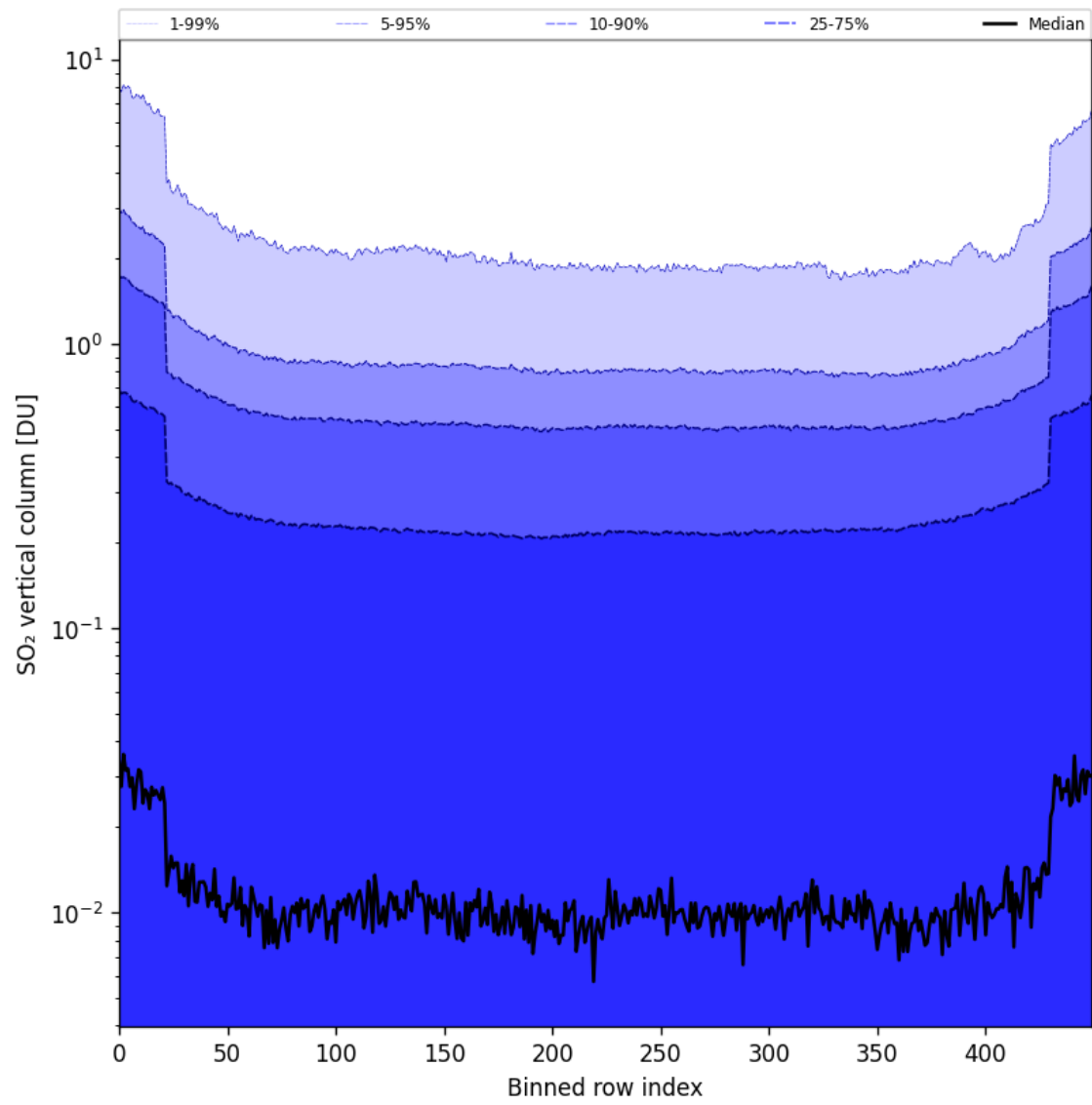
Figure 84: Along track statistics of “SO 2 vertical column” for 2025-07-02 to 2025-07-03
