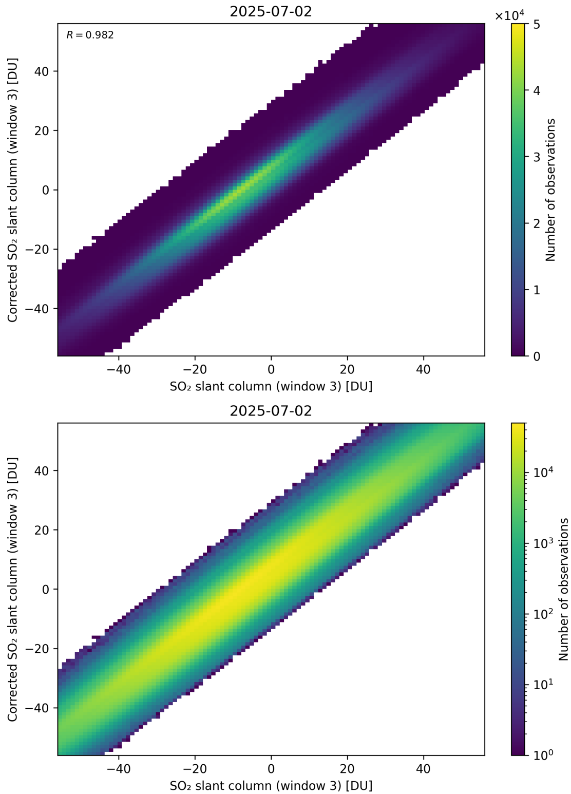
Figure 316: Scatter density plot of “SO 2 slant column (window 3)” against “Corrected SO 2 slant column (window 3)” for 2025-07-02 to 2025-07-03.
