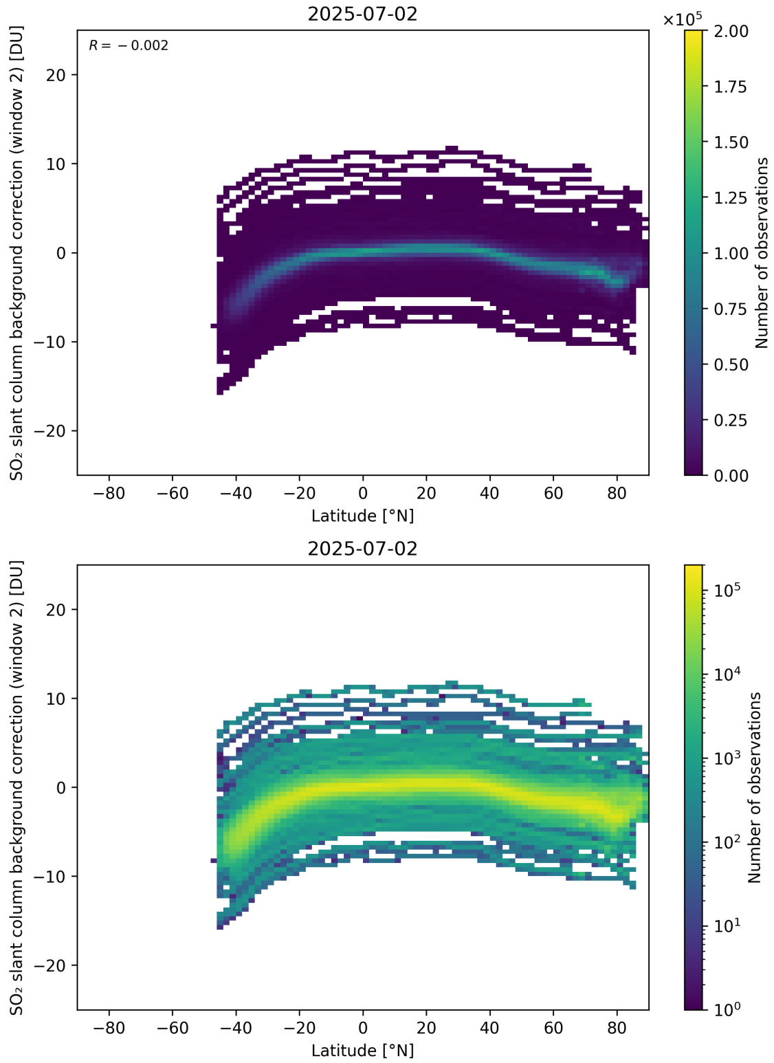
Figure 151: Scatter density plot of “Latitude” against “SO 2 slant column background correction (window 2)” for 2025-07-02 to 2025-07-03.
