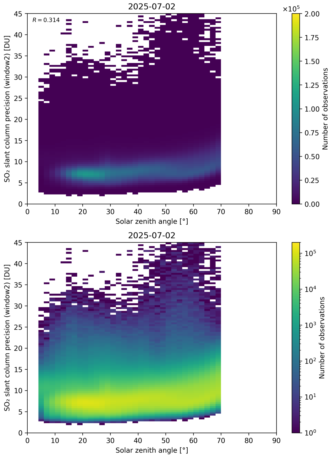
Figure 186: Scatter density plot of “Solar zenith angle” against “SO 2 slant column precision (window2)” for 2025-07-02 to 2025-07-03.
