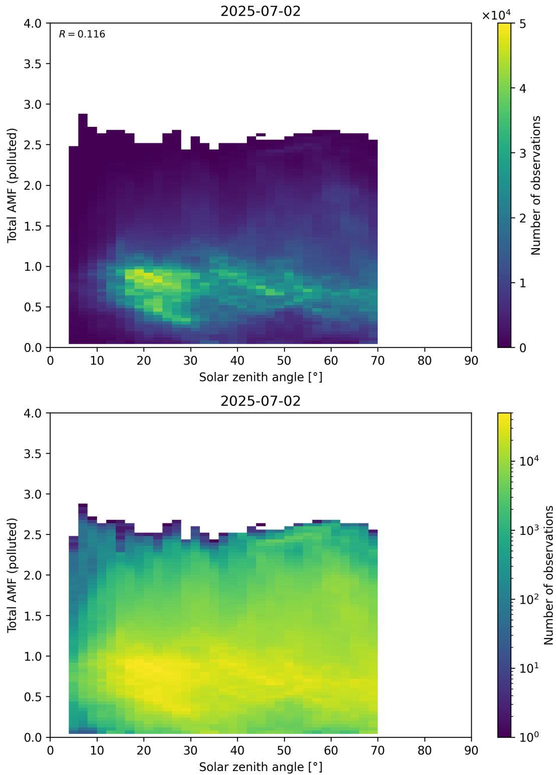
Figure 189: Scatter density plot of “Solar zenith angle” against “Total AMF (polluted)” for 2025-07-02 to 2025-07-03.
