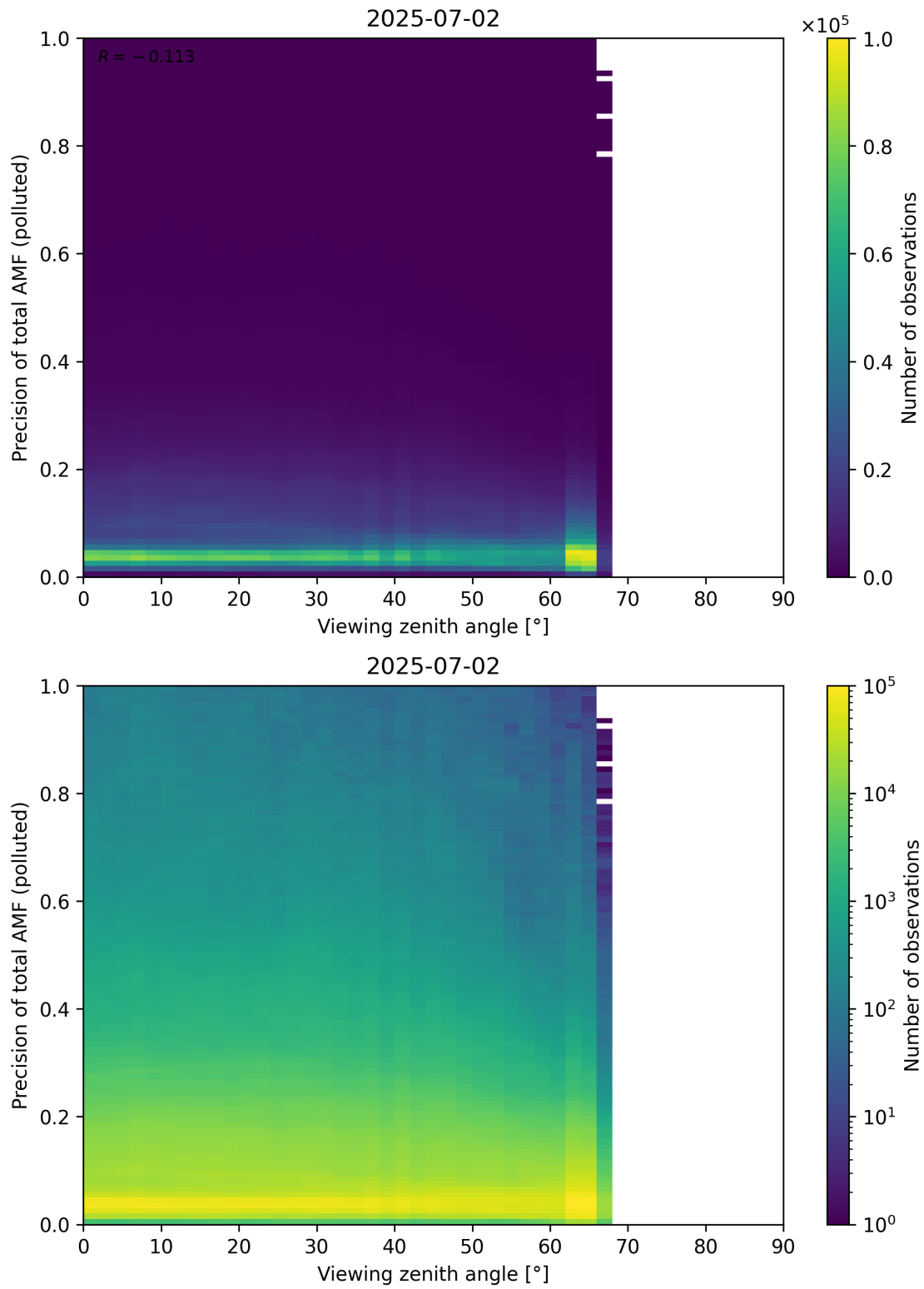
Figure 382: Scatter density plot of “Viewing zenith angle” against “Precision of total AMF (polluted)” for 2025-07-02 to 2025-07-03.
