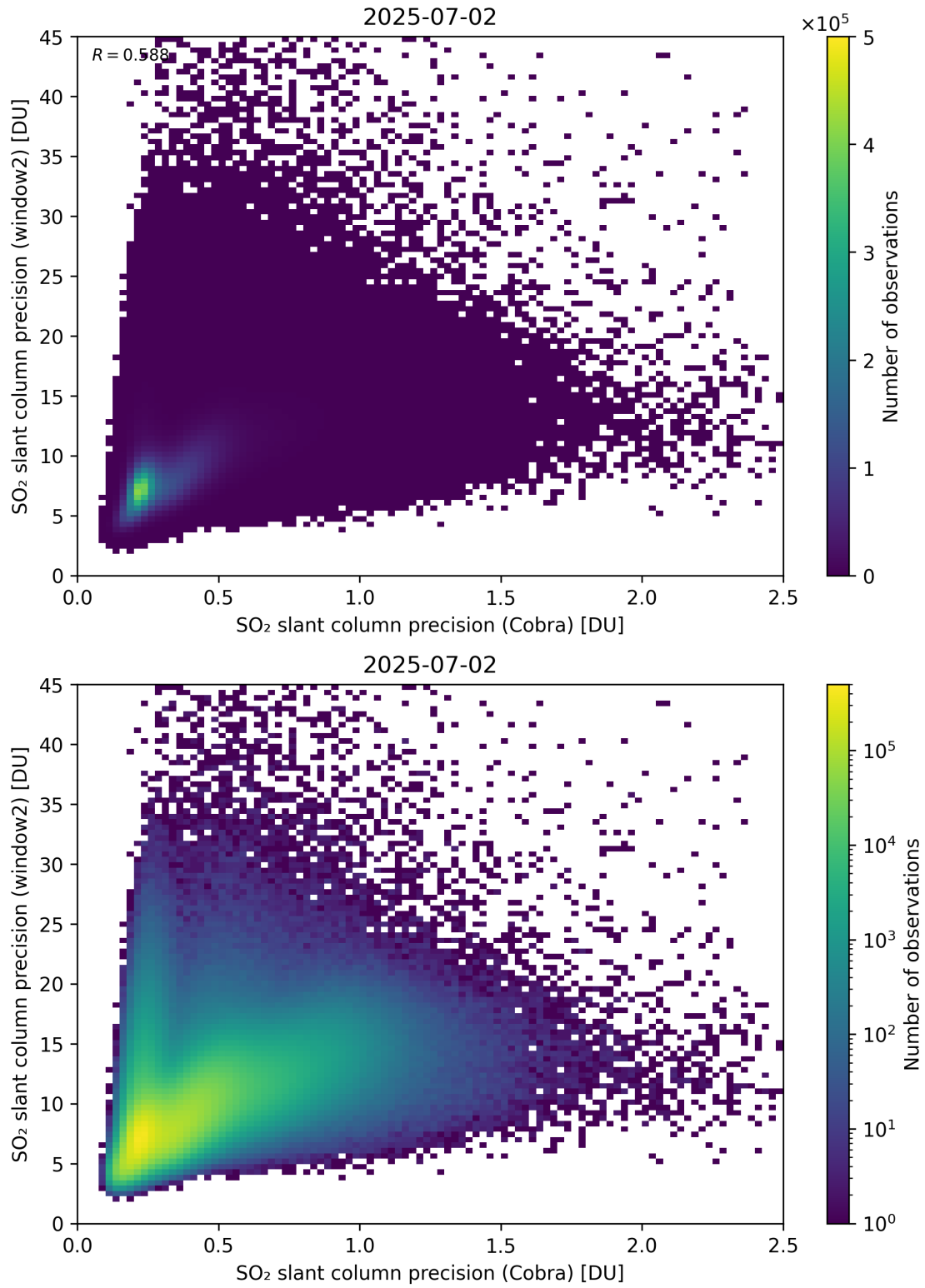
Figure 210: Scatter density plot of “SO 2 slant column precision (Cobra)” against “SO 2 slant column precision (window2)” for 2025-07-02 to 2025-07-03.
