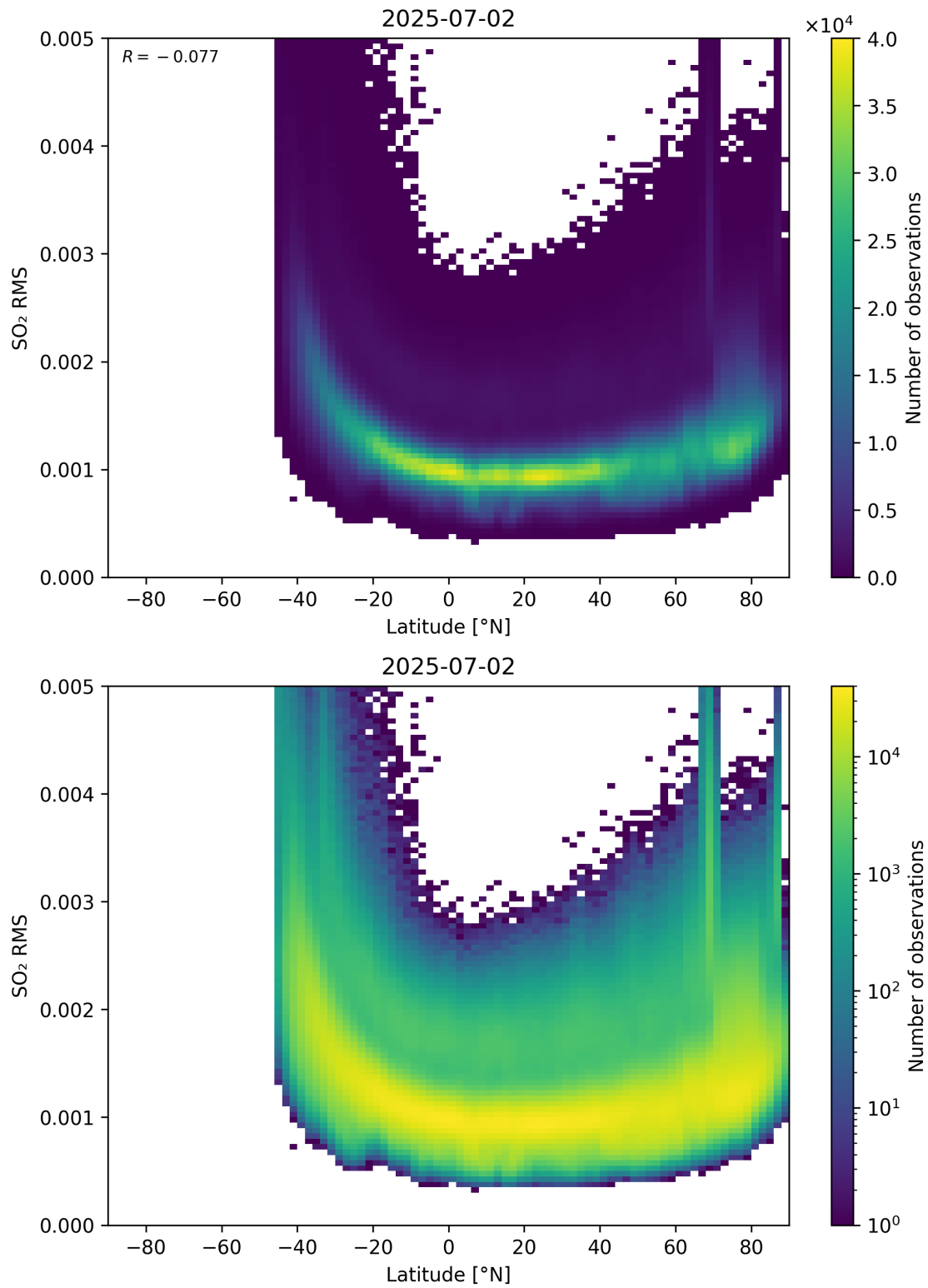
Figure 155: Scatter density plot of “Latitude” against “SO 2 RMS” for 2025-07-02 to 2025-07-03.
