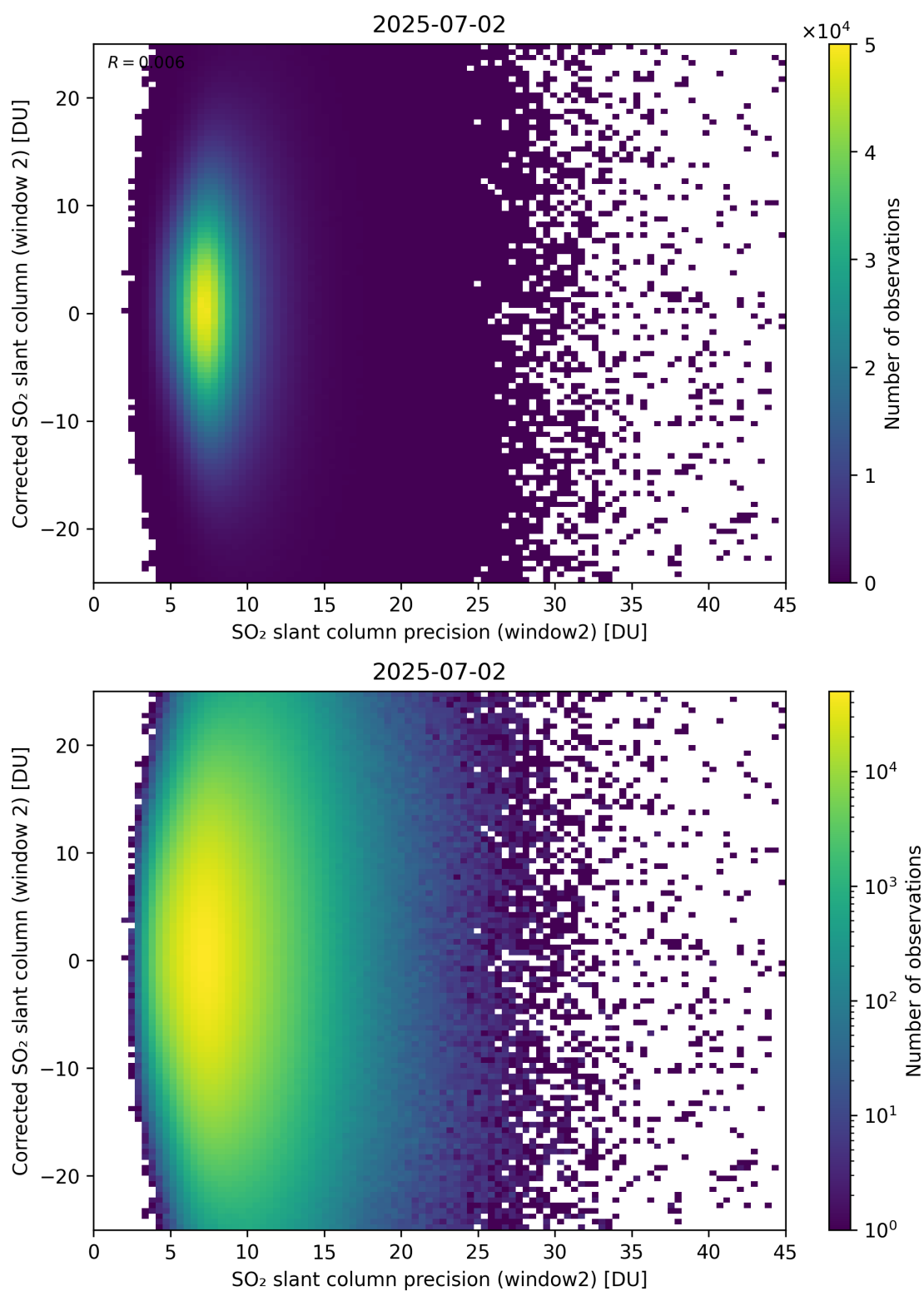
Figure 297: Scatter density plot of “SO 2 slant column precision (window2)” against “Corrected SO 2 slant column (window 2)” for 2025-07-02 to 2025-07-03.
