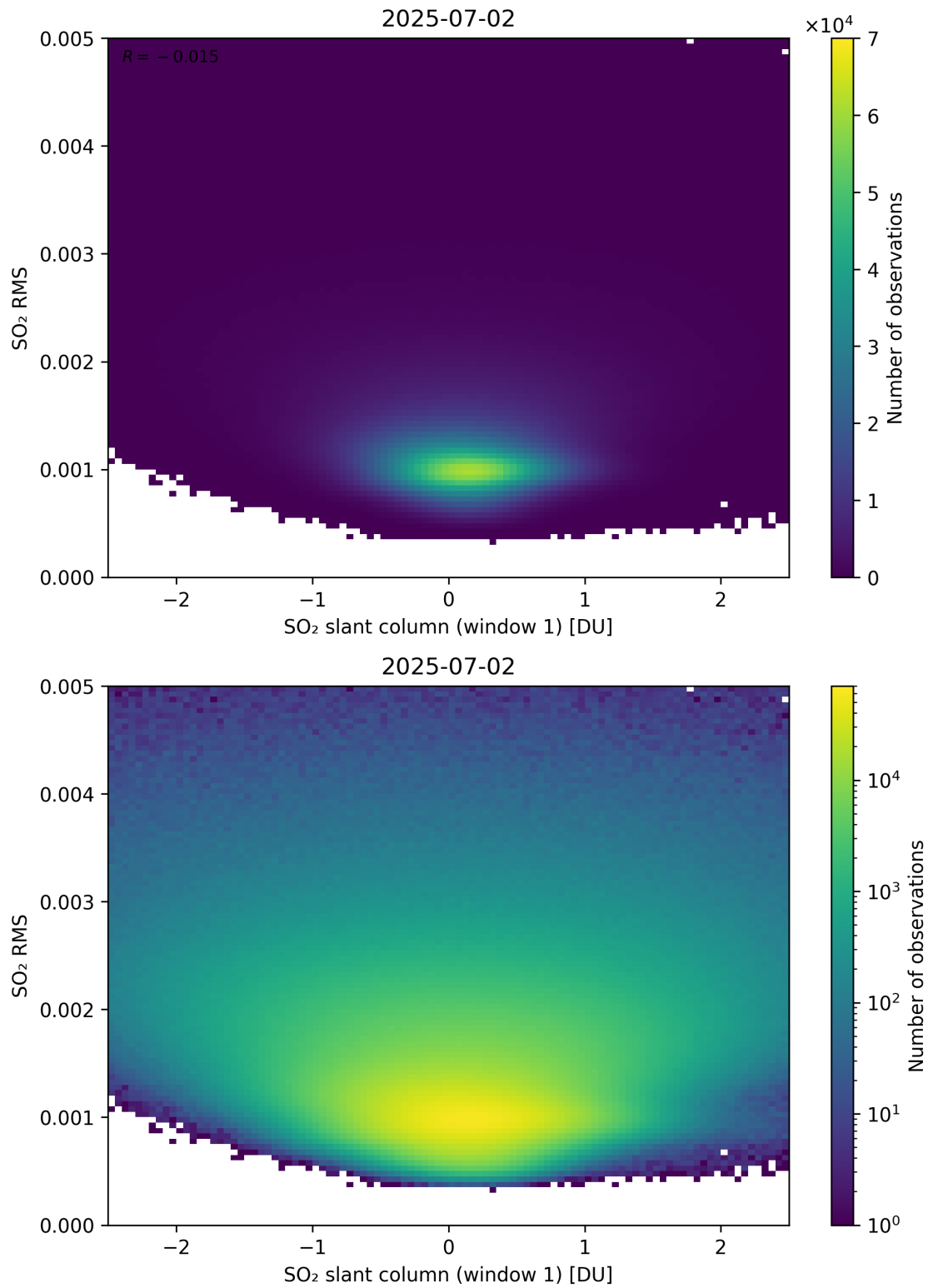
Figure 267: Scatter density plot of “SO 2 slant column (window 1)” against “SO 2 RMS” for 2025-07-02 to 2025-07-03.
