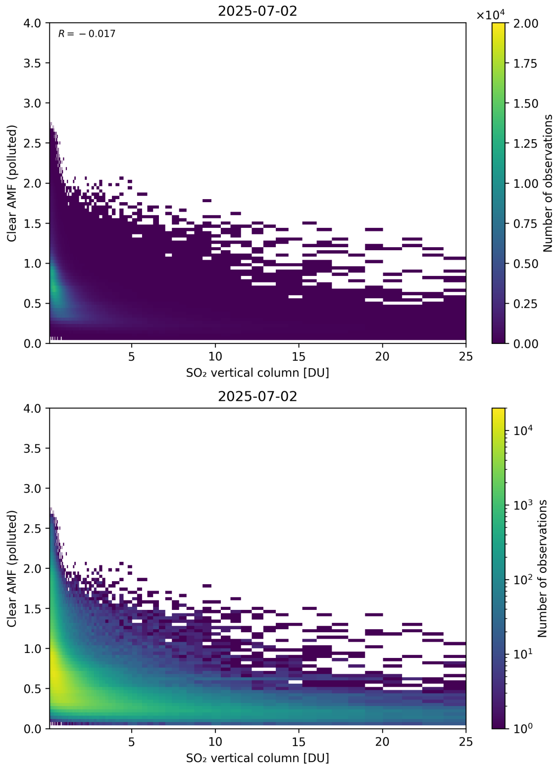
Figure 348: Scatter density plot of “SO 2 vertical column” against “Clear AMF (polluted)” for 2025-07-02 to 2025-07-03.
