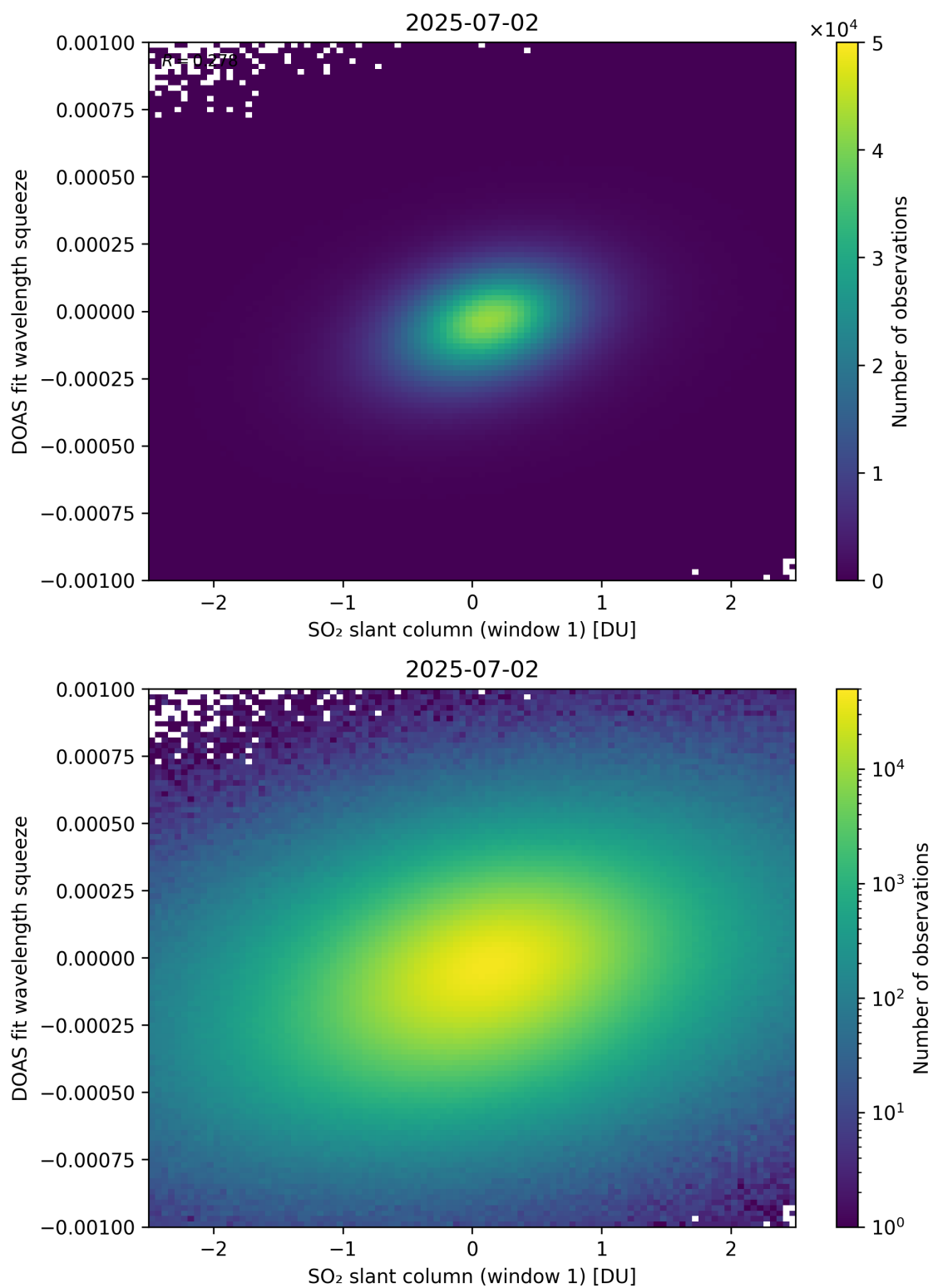
Figure 266: Scatter density plot of “SO 2 slant column (window 1)” against “DOAS fit wavelength squeeze” for 2025-07-02 to 2025-07-03.
