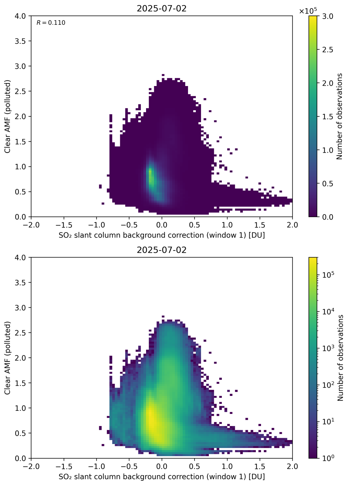
Figure 114: Scatter density plot of “SO 2 slant column background correction (window 1)” against “Clear AMF (polluted)” for 2025-07-02 to 2025-07-03.
