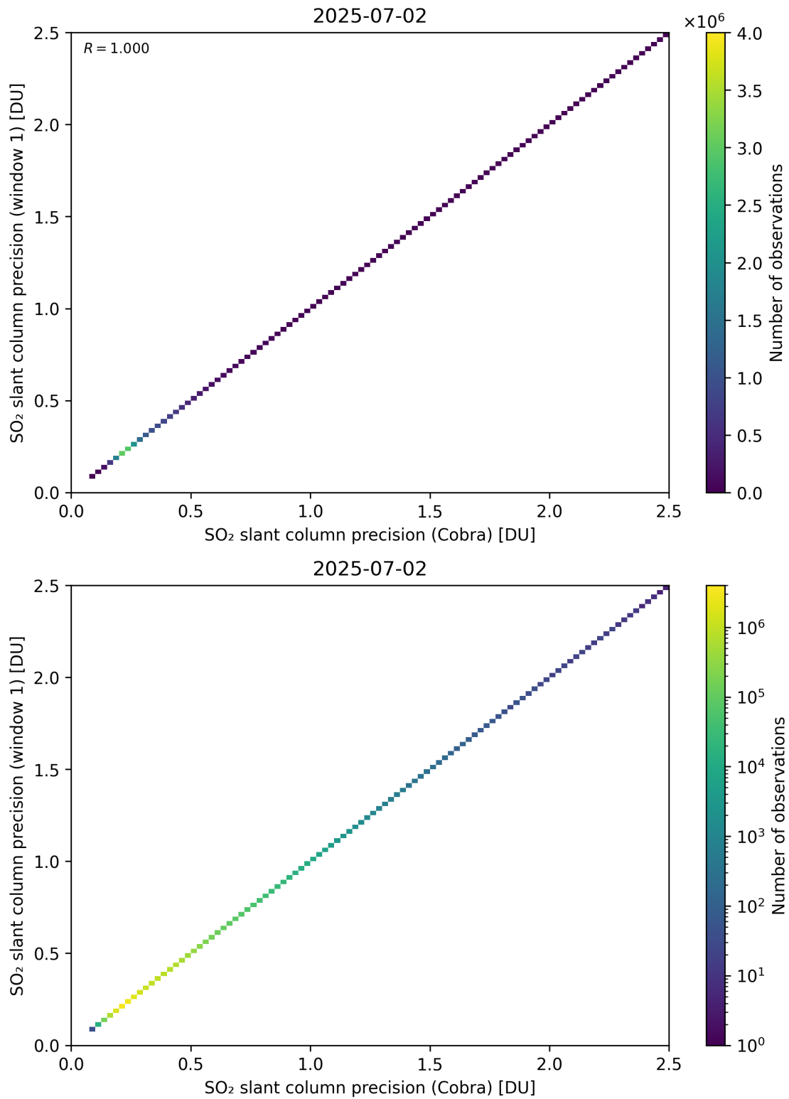
Figure 209: Scatter density plot of “SO 2 slant column precision (Cobra)” against “SO 2 slant column precision (window 1)” for 2025-07-02 to 2025-07-03.
