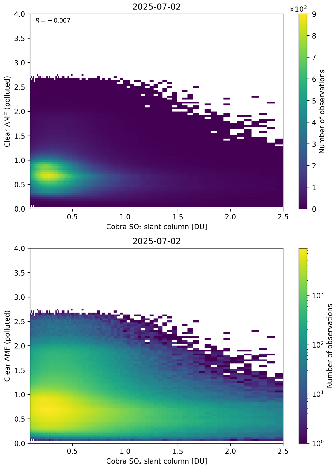
Figure 215: Scatter density plot of “Cobra SO 2 slant column” against “Clear AMF (polluted)” for 2025-07-02 to 2025-07-03.
