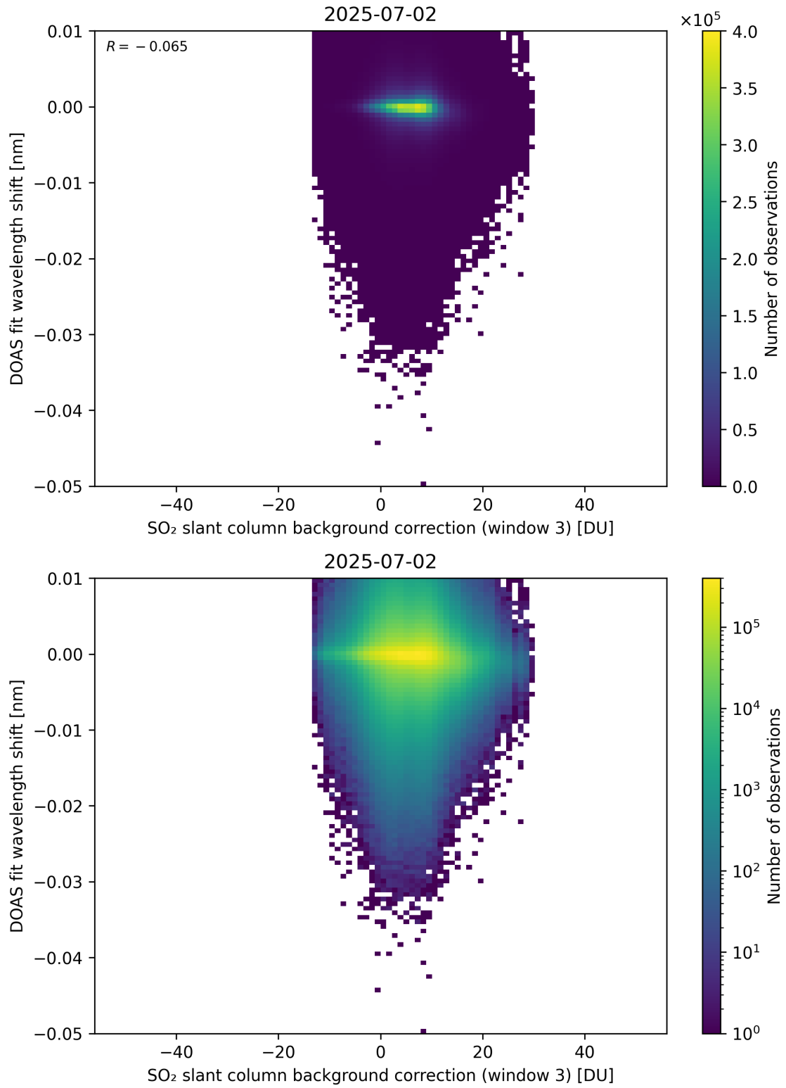
Figure 132: Scatter density plot of “SO 2 slant column background correction (window 3)” against “DOAS fit wavelength shift” for 2025-07-02 to 2025-07-03.
