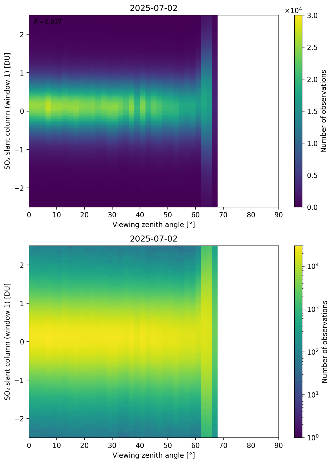
Figure 376: Scatter density plot of “Viewing zenith angle” against “SO 2 slant column (window 1)” for 2025-07-02 to 2025-07-03.
