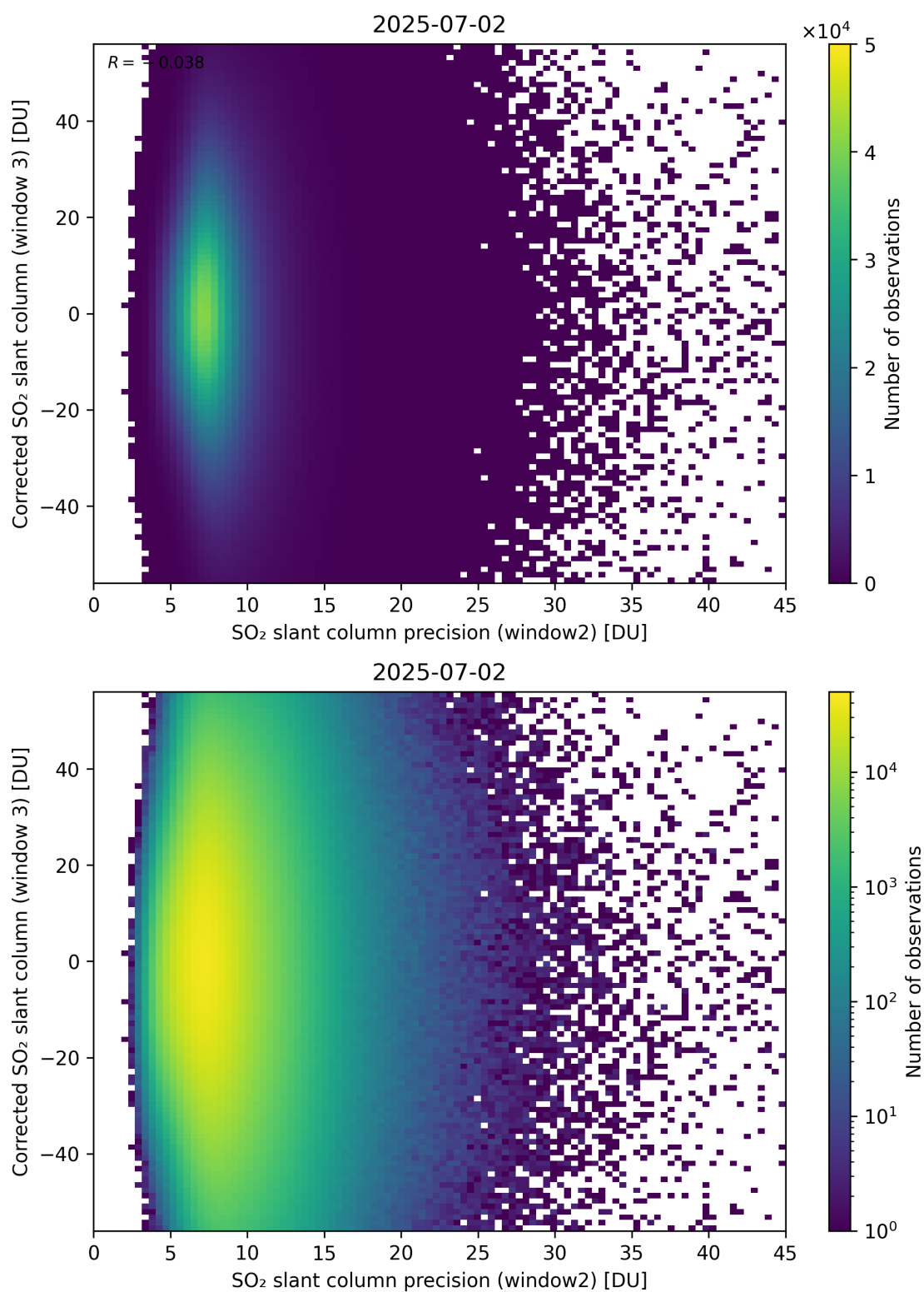
Figure 298: Scatter density plot of “SO 2 slant column precision (window2)” against “Corrected SO 2 slant column (window 3)” for 2025-07-02 to 2025-07-03.
