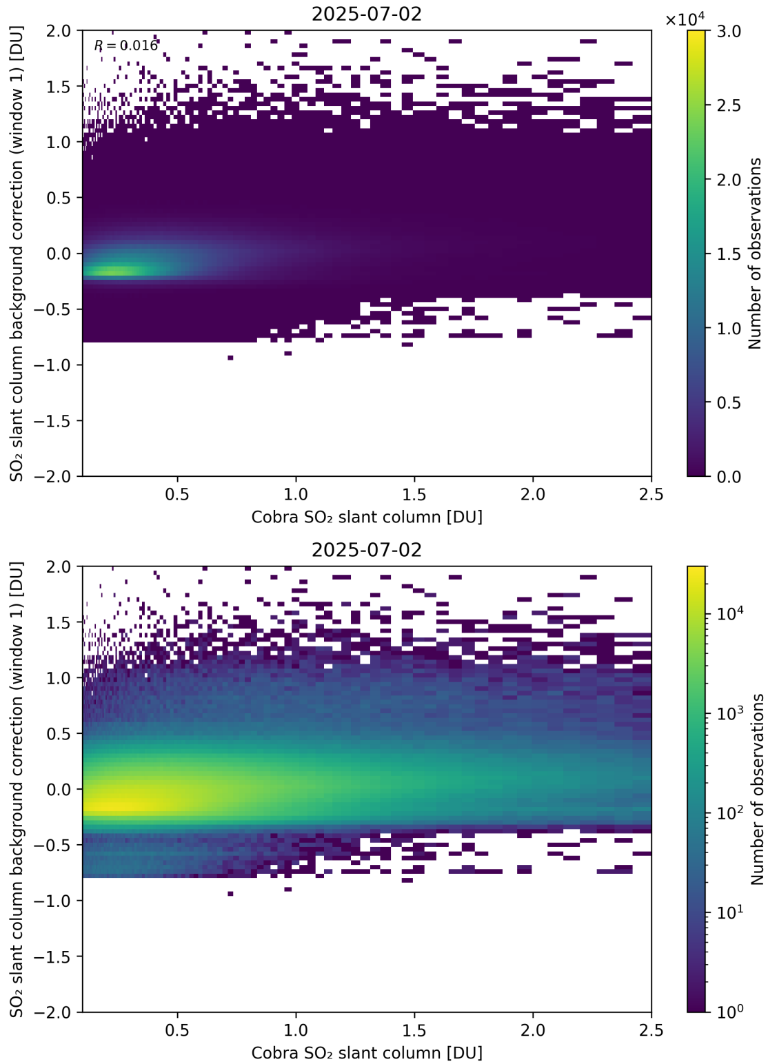
Figure 193: Scatter density plot of “Cobra SO 2 slant column” against “SO 2 slant column background correction (window 1)” for 2025-07-02 to 2025-07-03.
