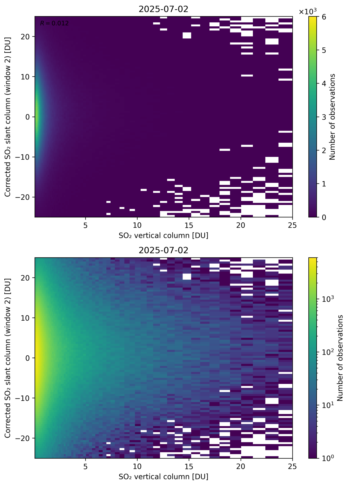
Figure 352: Scatter density plot of “SO 2 vertical column” against “Corrected SO 2 slant column (window 2)” for 2025-07-02 to 2025-07-03.
