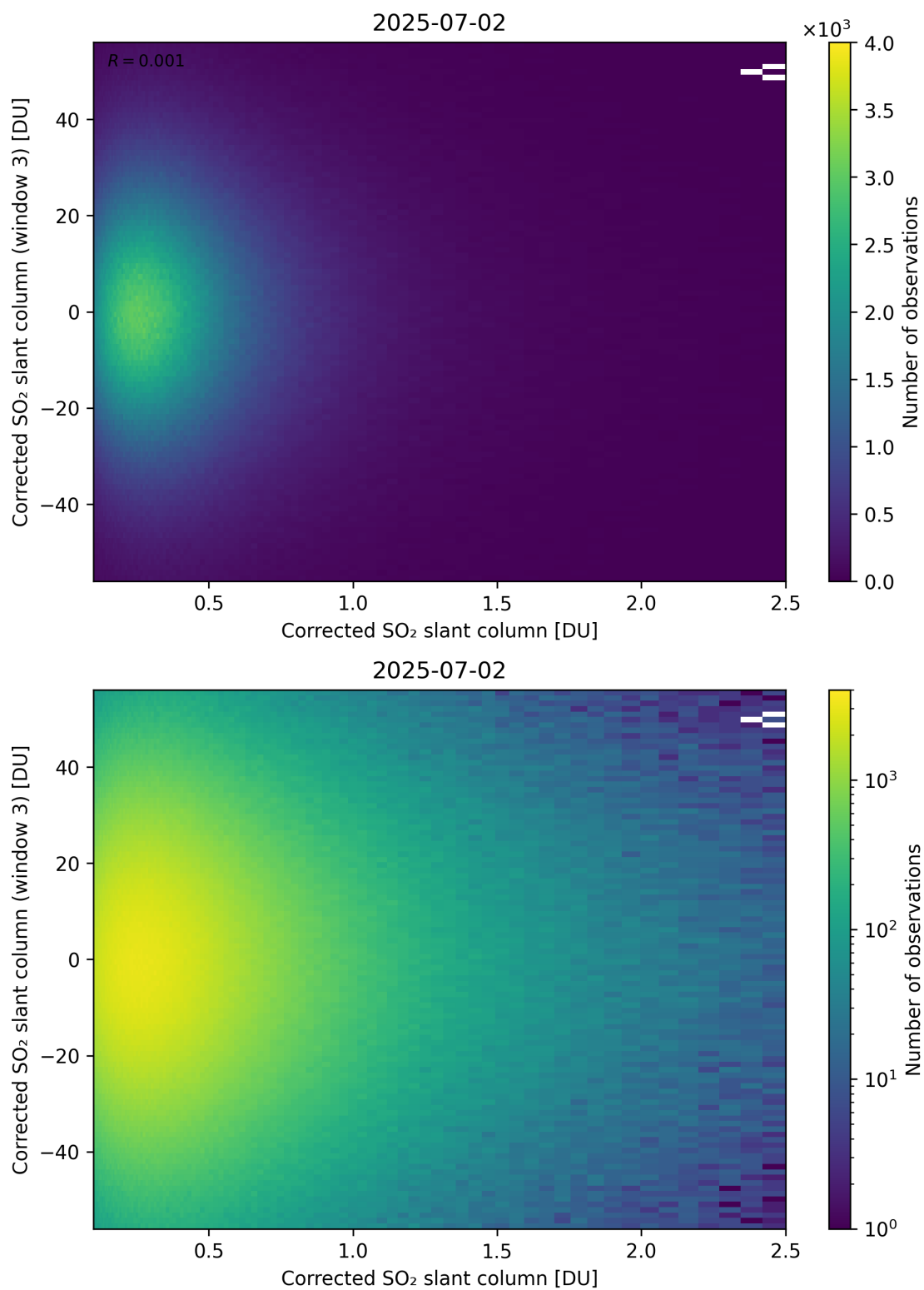
Figure 236: Scatter density plot of “Corrected SO 2 slant column” against “Corrected SO 2 slant column (window 3)” for 2025-07-02 to 2025-07-03.
