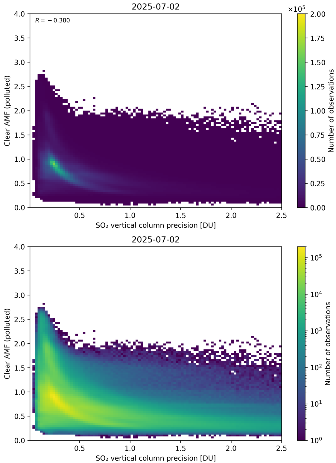
Figure 335: Scatter density plot of “SO 2 vertical column precision” against “Clear AMF (polluted)” for 2025-07-02 to 2025-07-03.
