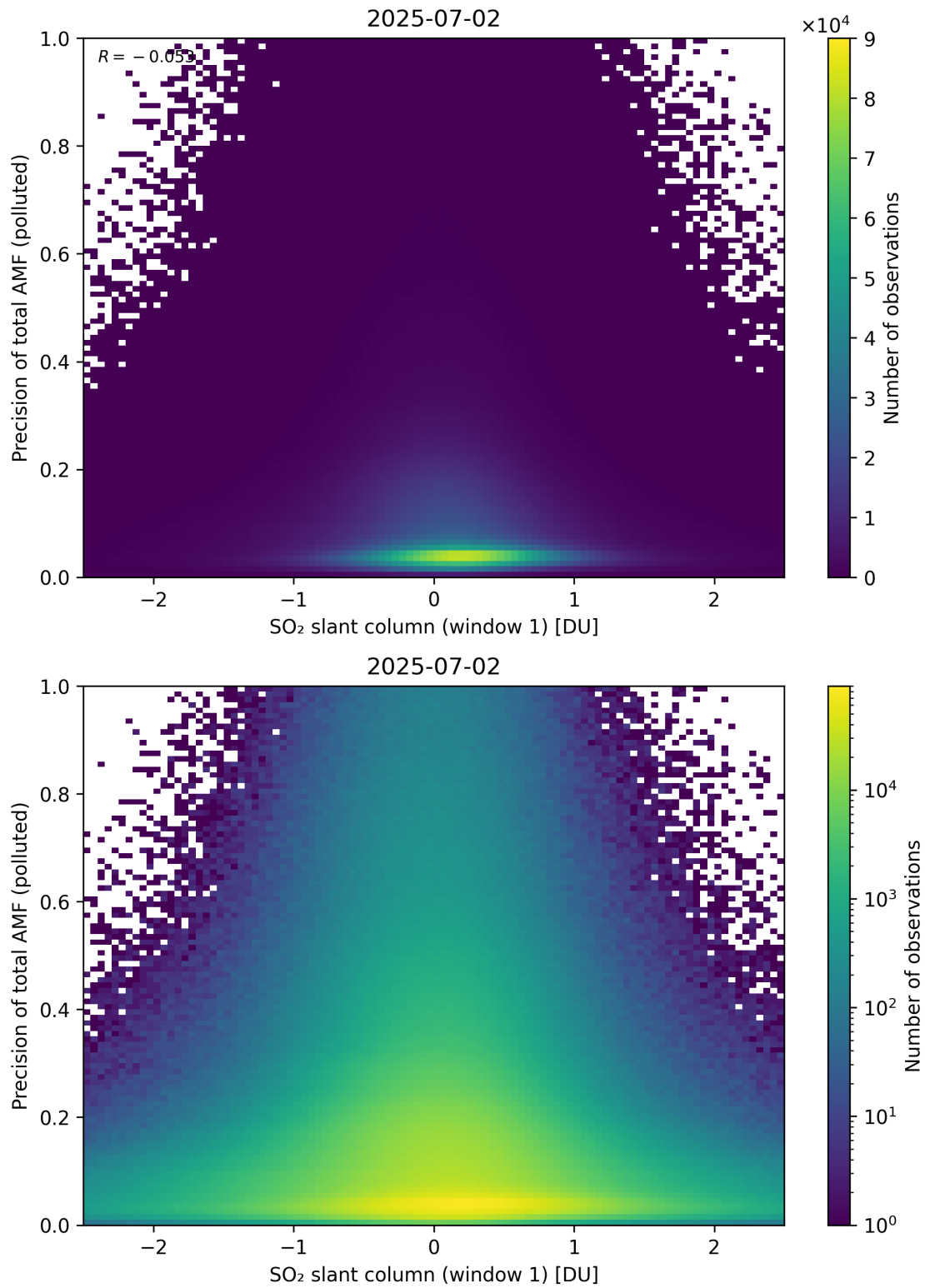
Figure 290: Scatter density plot of “SO 2 slant column (window 1)” against “Precision of total AMF (polluted)” for 2025-07-02 to 2025-07-03.
