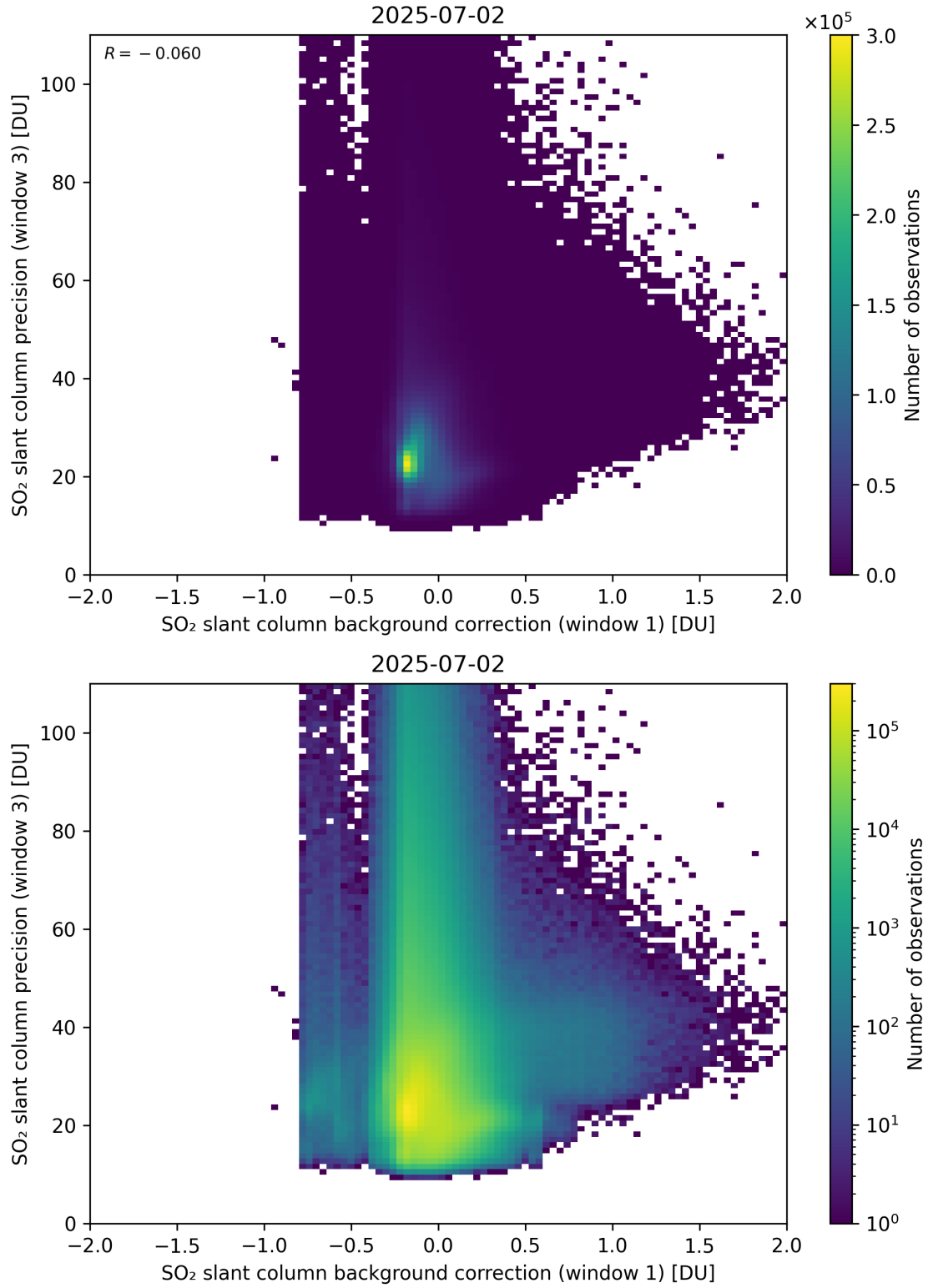
Figure 119: Scatter density plot of “SO 2 slant column background correction (window 1)” against “SO 2 slant column precision (window 3)” for 2025-07-02 to 2025-07-03.
