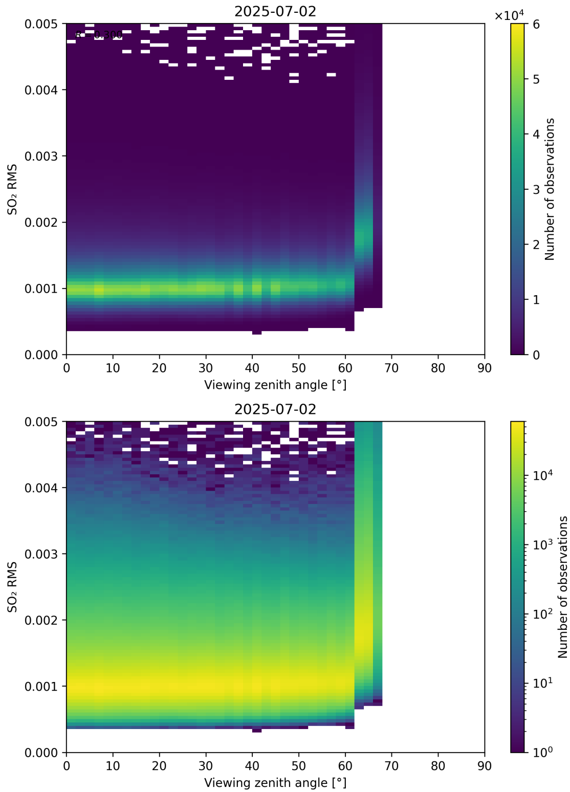
Figure 367: Scatter density plot of “Viewing zenith angle” against “SO 2 RMS” for 2025-07-02 to 2025-07-03.
