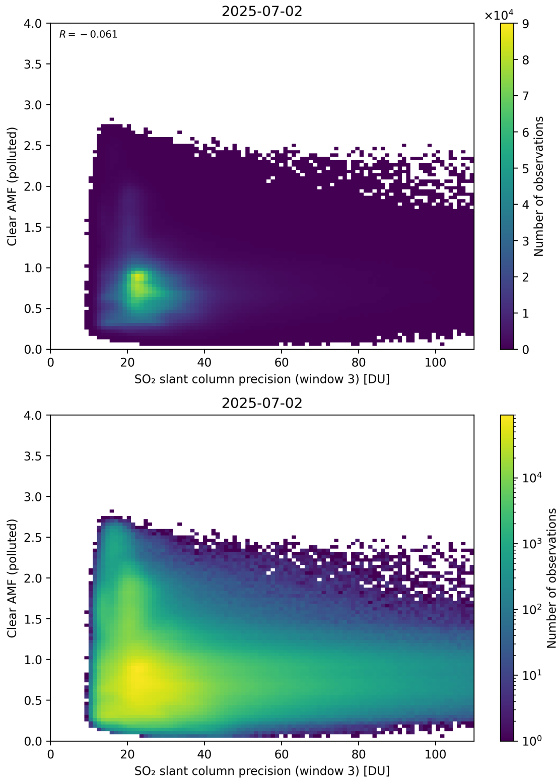
Figure 311: Scatter density plot of “SO 2 slant column precision (window 3)” against “Clear AMF (polluted)” for 2025-07-02 to 2025-07-03.
