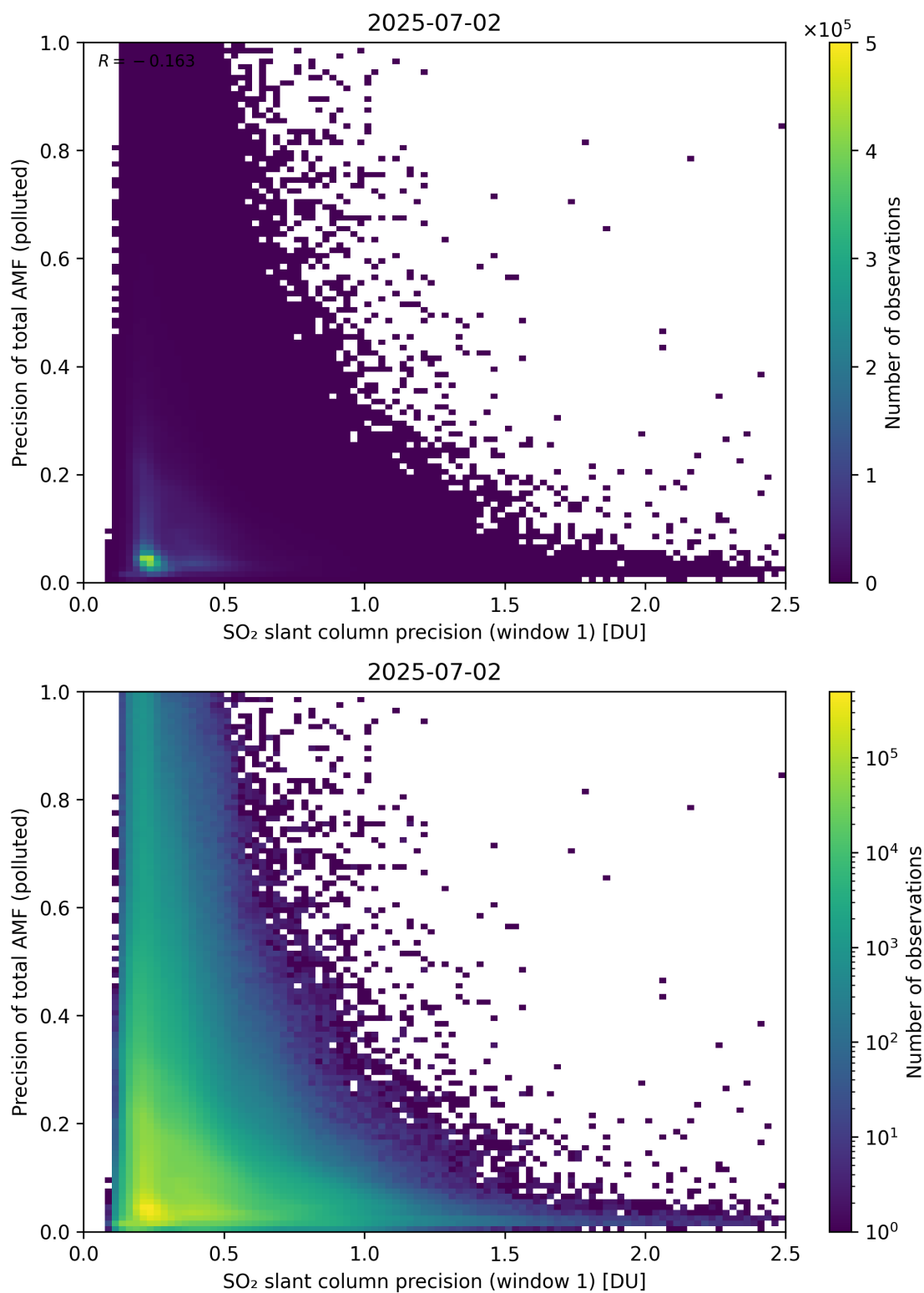
Figure 281: Scatter density plot of “SO 2 slant column precision (window 1)” against “Precision of total AMF (polluted)” for 2025-07-02 to 2025-07-03.
