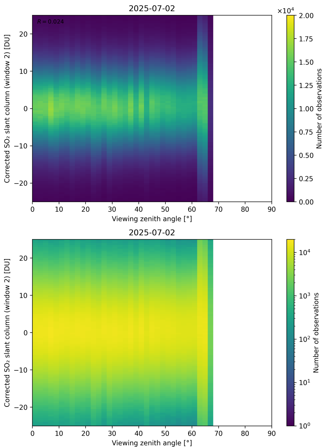
Figure 374: Scatter density plot of “Viewing zenith angle” against “Corrected SO 2 slant column (window 2)” for 2025-07-02 to 2025-07-03.
