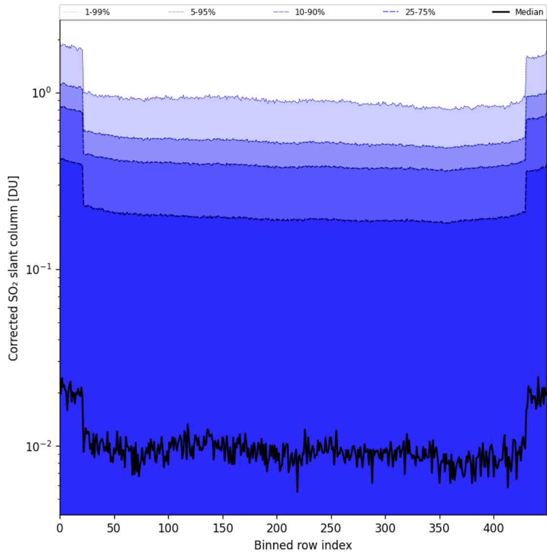
Figure 86: Along track statistics of “Corrected SO 2 slant column” for 2025-07-02 to 2025-07-03
