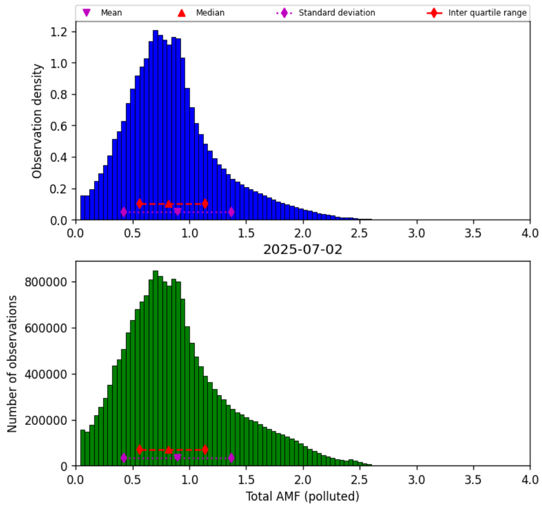
Figure 79: Histogram of “Total AMF (polluted)” for 2025-07-02 to 2025-07-03
