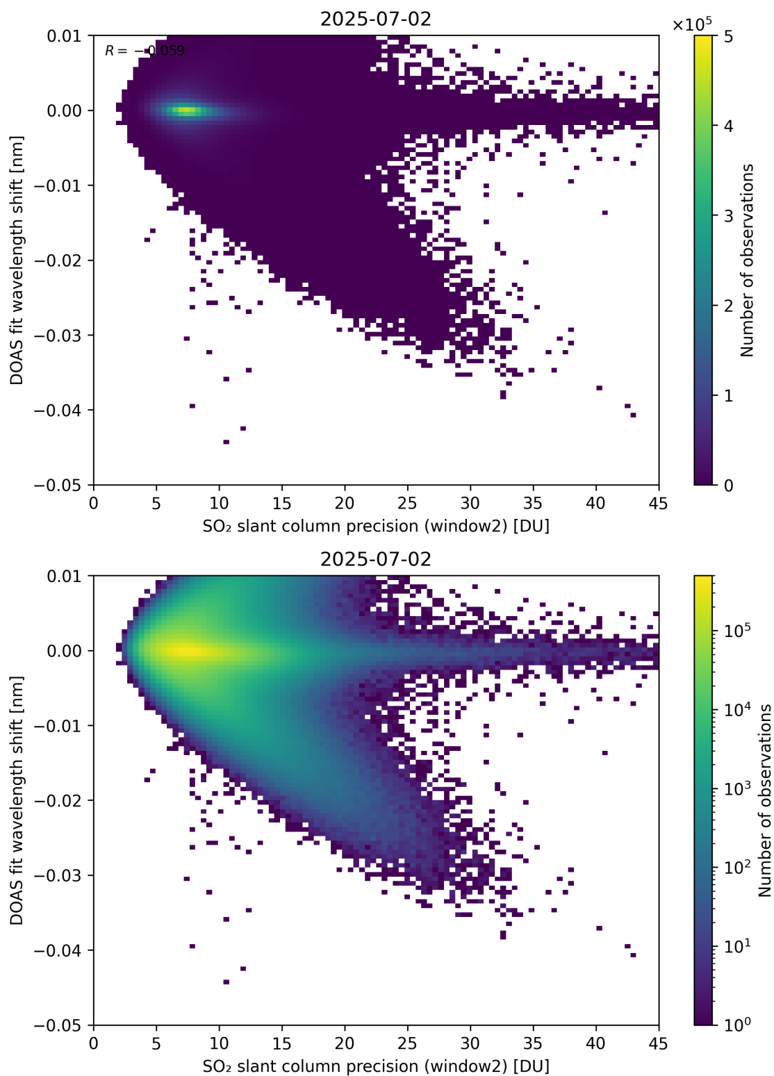
Figure 293: Scatter density plot of “SO 2 slant column precision (window2)” against “DOAS fit wavelength shift” for 2025-07-02 to 2025-07-03.
