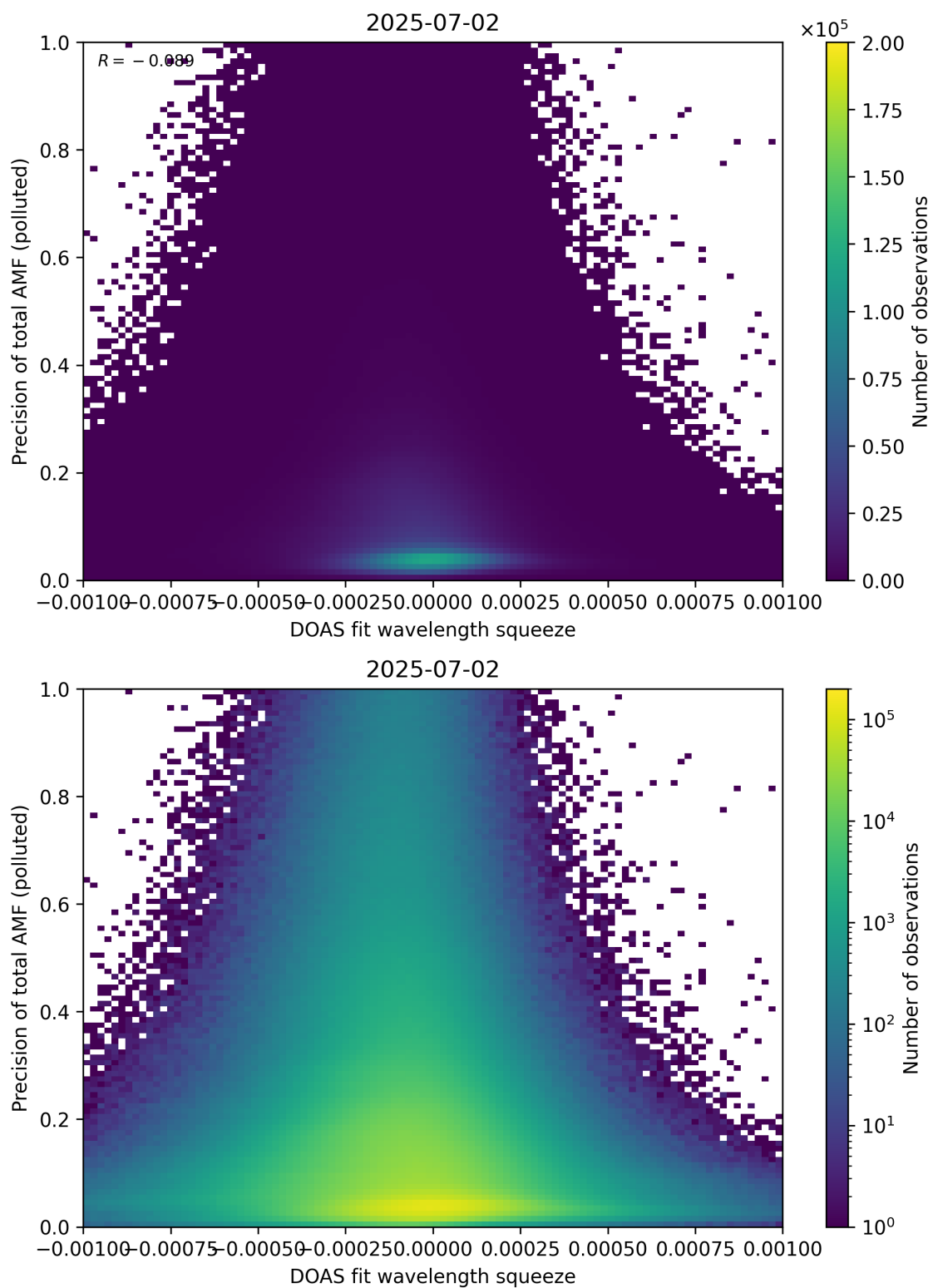
Figure 146: Scatter density plot of “DOAS fit wavelength squeeze” against “Precision of total AMF (polluted)” for 2025-07-02 to 2025-07-03.
