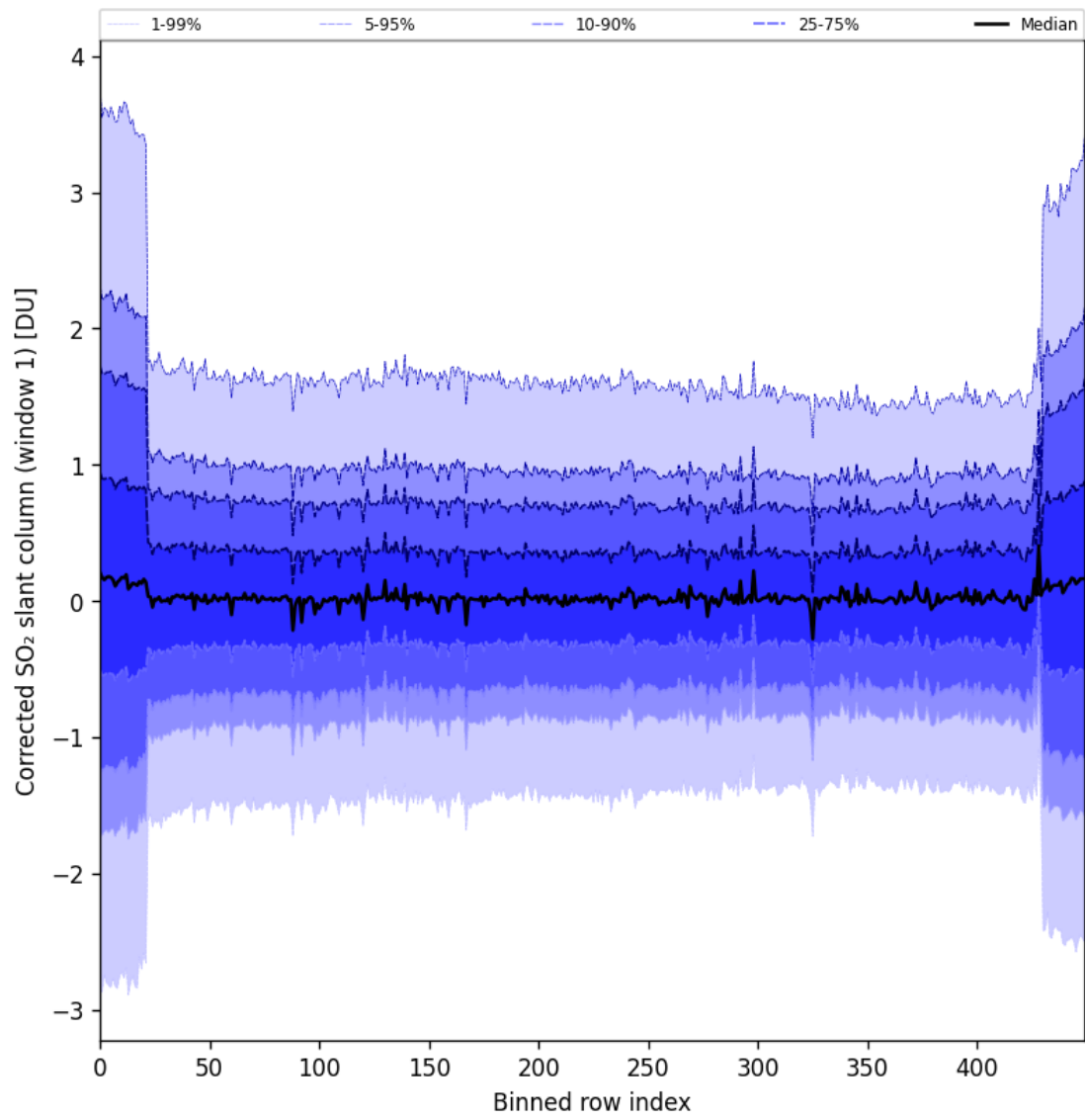
Figure 91: Along track statistics of “Corrected SO 2 slant column (window 1)” for 2025-07-02 to 2025-07-03
