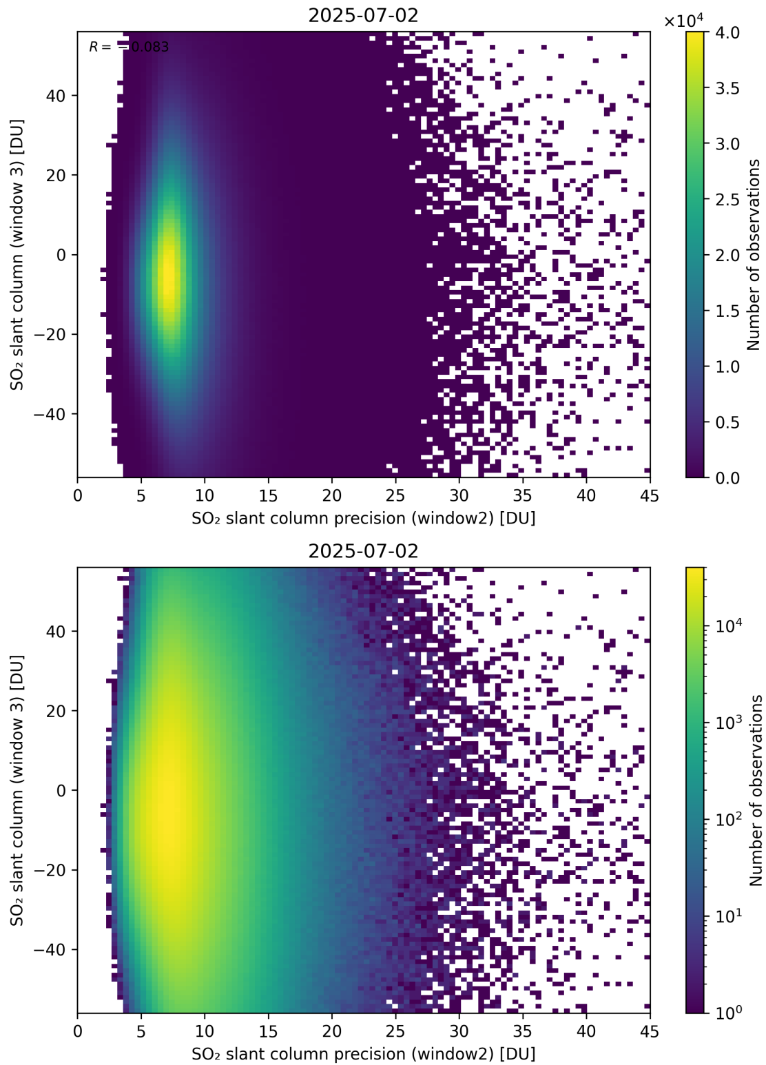
Figure 299: Scatter density plot of “SO 2 slant column precision (window2)” against “SO 2 slant column (window 3)” for 2025-07-02 to 2025-07-03.
