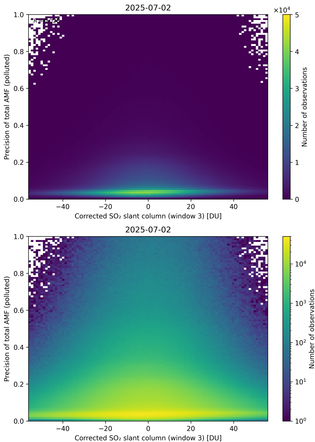
Figure 261: Scatter density plot of “Corrected SO 2 slant column (window 3)” against “Precision of total AMF (polluted)” for 2025-07-02 to 2025-07-03.
