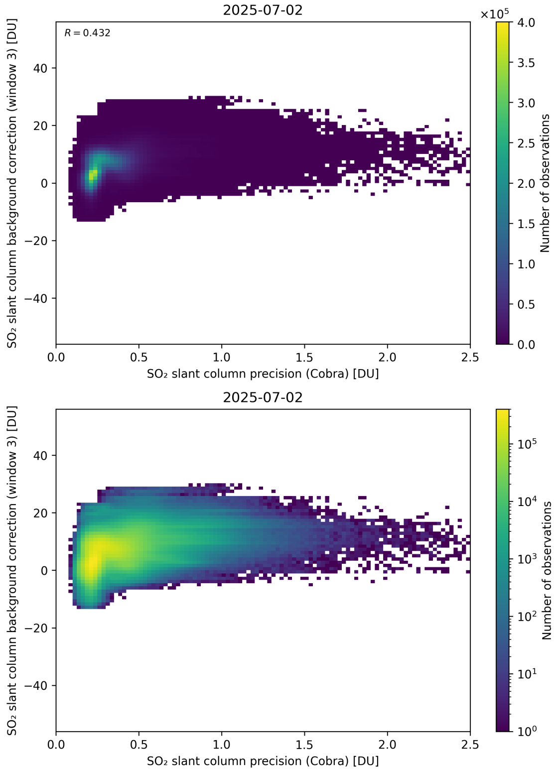
Figure 201: Scatter density plot of “SO 2 slant column precision (Cobra)” against “SO 2 slant column background correction (window 3)” for 2025-07-02 to 2025-07-03.
