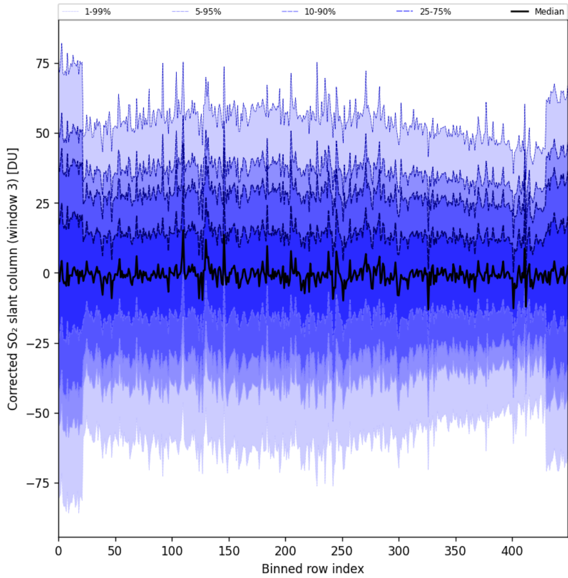
Figure 99: Along track statistics of “Corrected SO 2 slant column (window 3)” for 2025-07-02 to 2025-07-03
