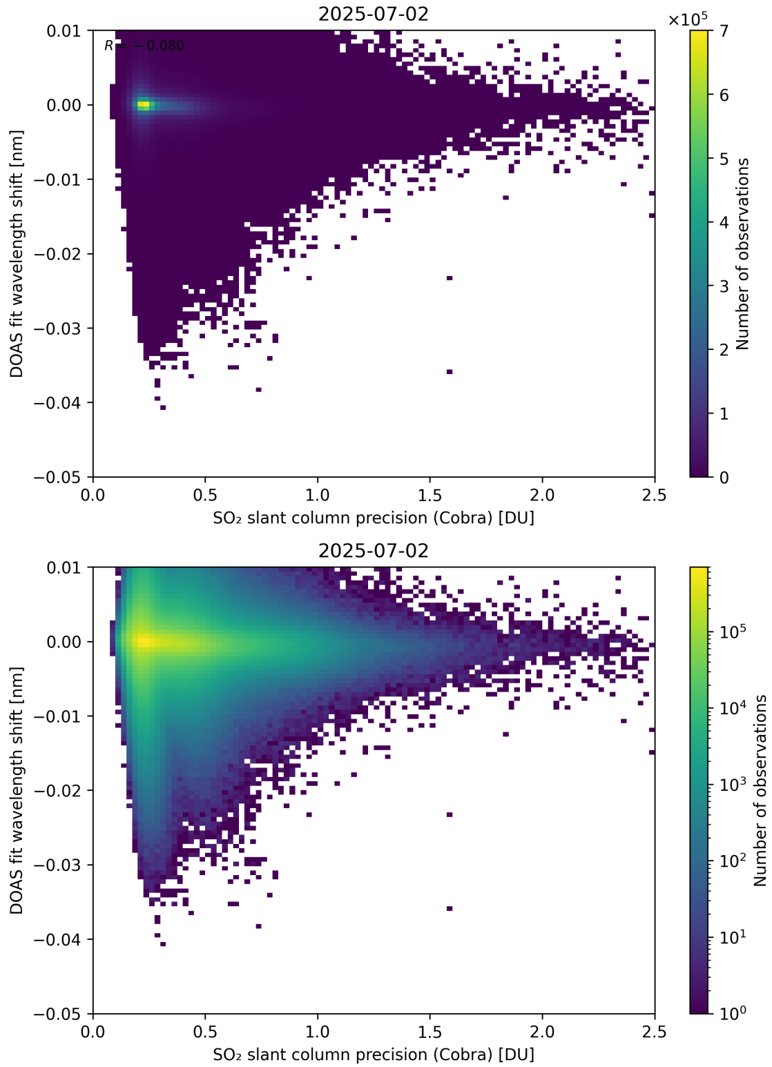
Figure 202: Scatter density plot of “SO 2 slant column precision (Cobra)” against “DOAS fit wavelength shift” for 2025-07-02 to 2025-07-03.
