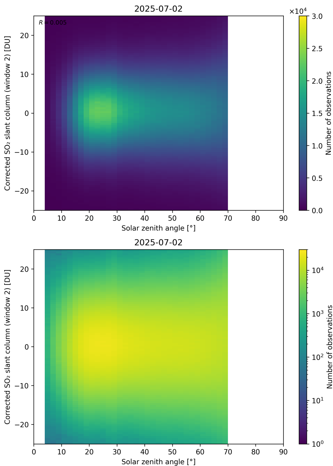
Figure 182: Scatter density plot of “Solar zenith angle” against “Corrected SO 2 slant column (window 2)” for 2025-07-02 to 2025-07-03.
