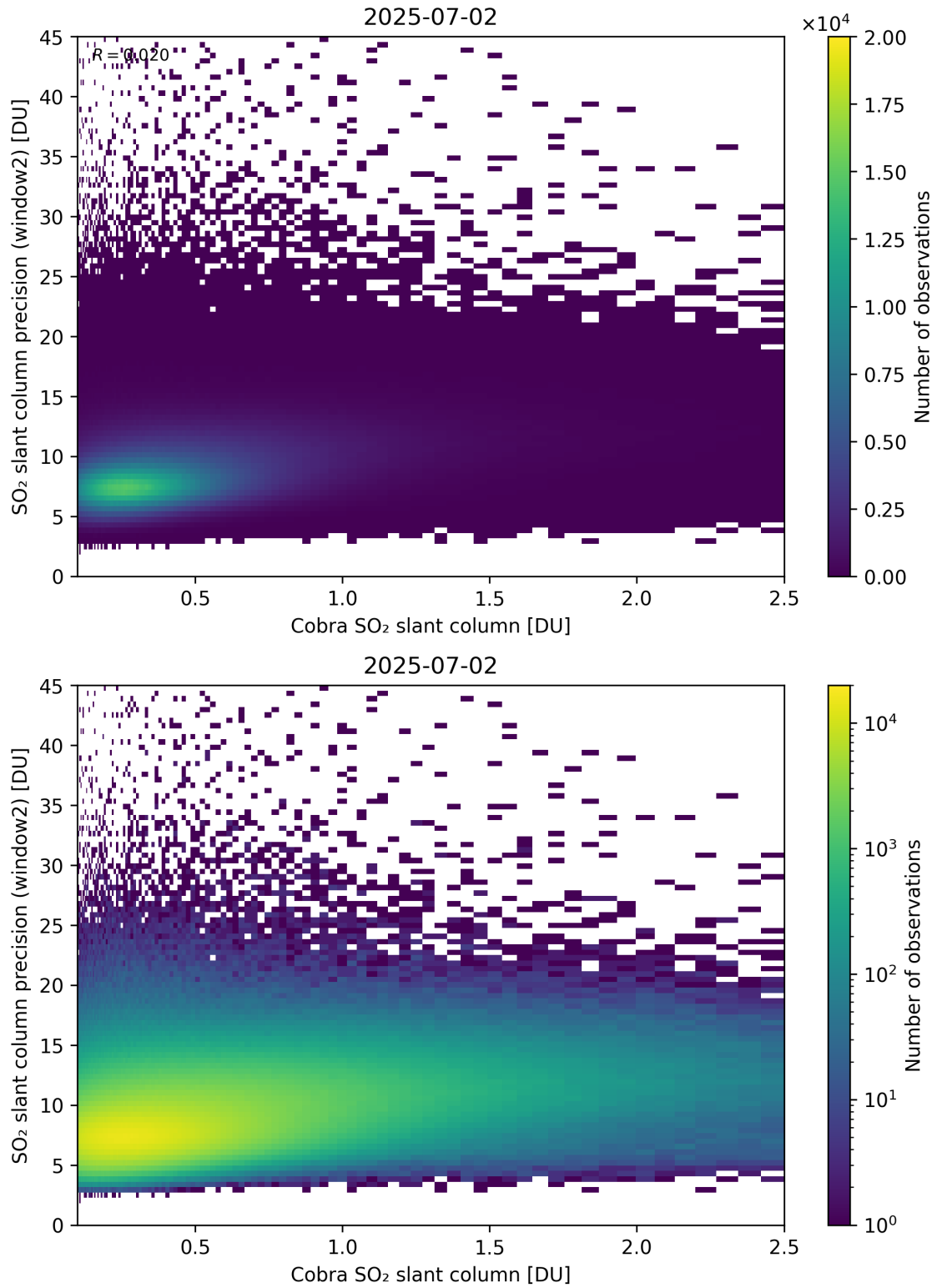
Figure 221: Scatter density plot of “Cobra SO 2 slant column” against “SO 2 slant column precision (window2)” for 2025-07-02 to 2025-07-03.
