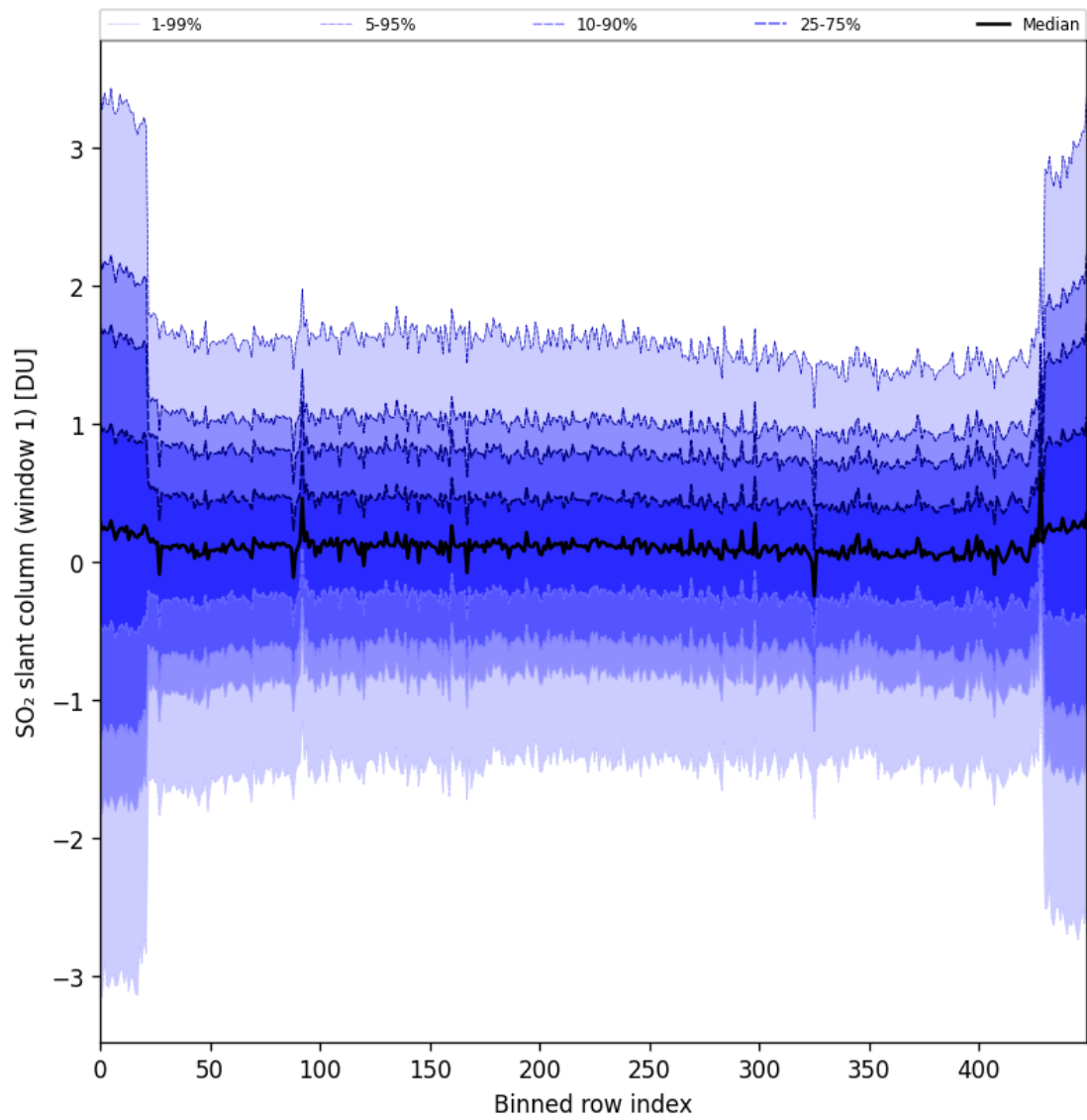
Figure 89: Along track statistics of “SO 2 slant column (window 1)” for 2025-07-02 to 2025-07-03
