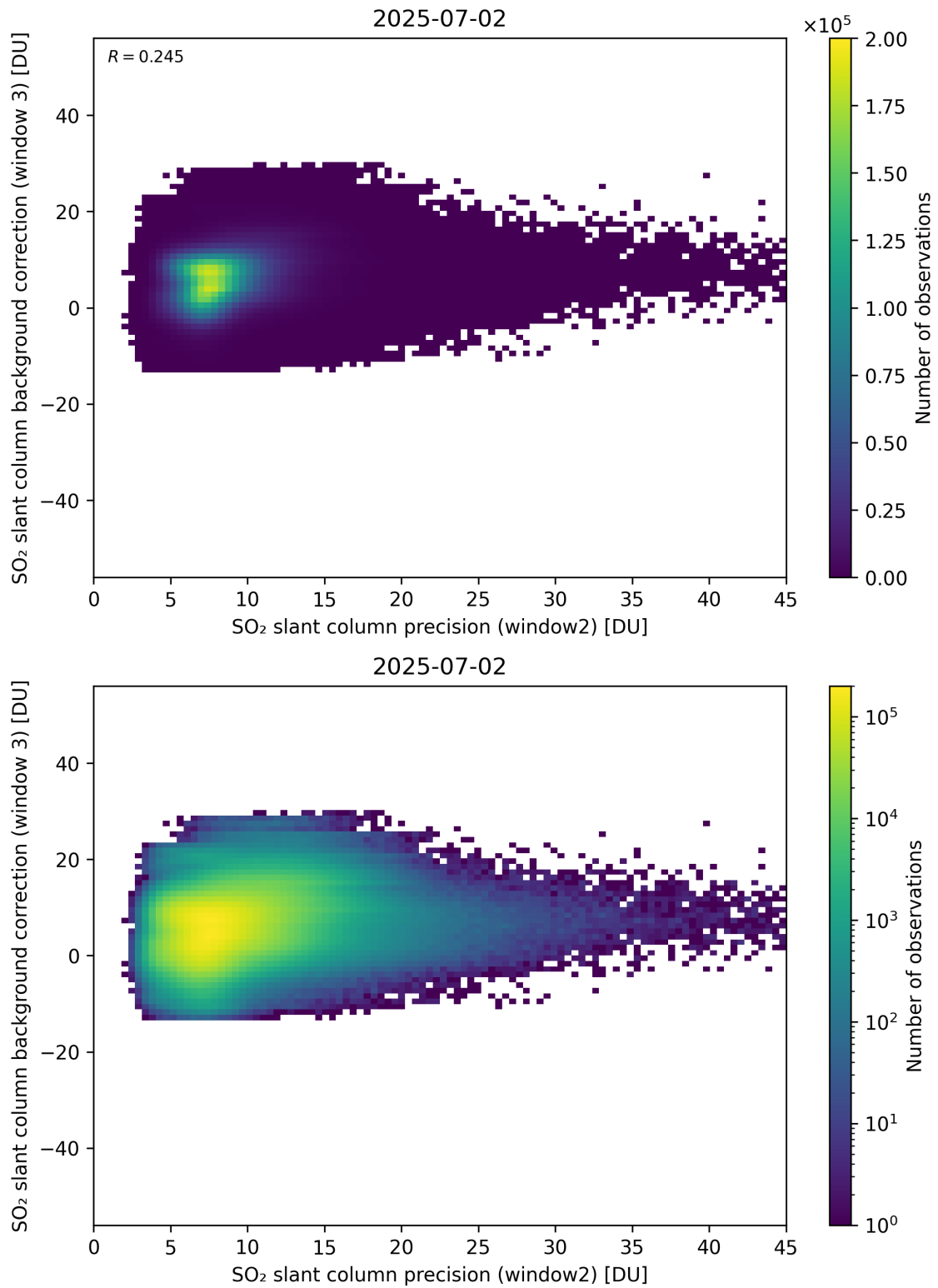
Figure 292: Scatter density plot of “SO 2 slant column precision (window2)” against “SO 2 slant column background correction (window 3)” for 2025-07-02 to 2025-07-03.
