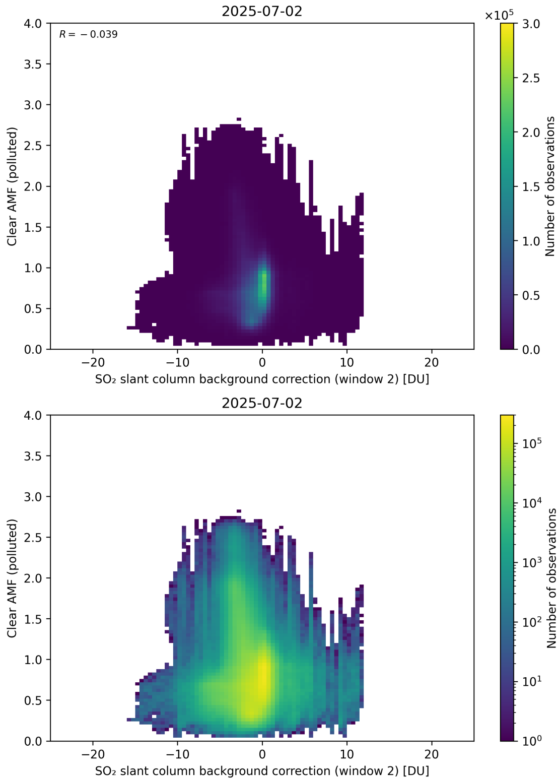
Figure 126: Scatter density plot of “SO 2 slant column background correction (window 2)” against “Clear AMF (polluted)” for 2025-07-02 to 2025-07-03.
