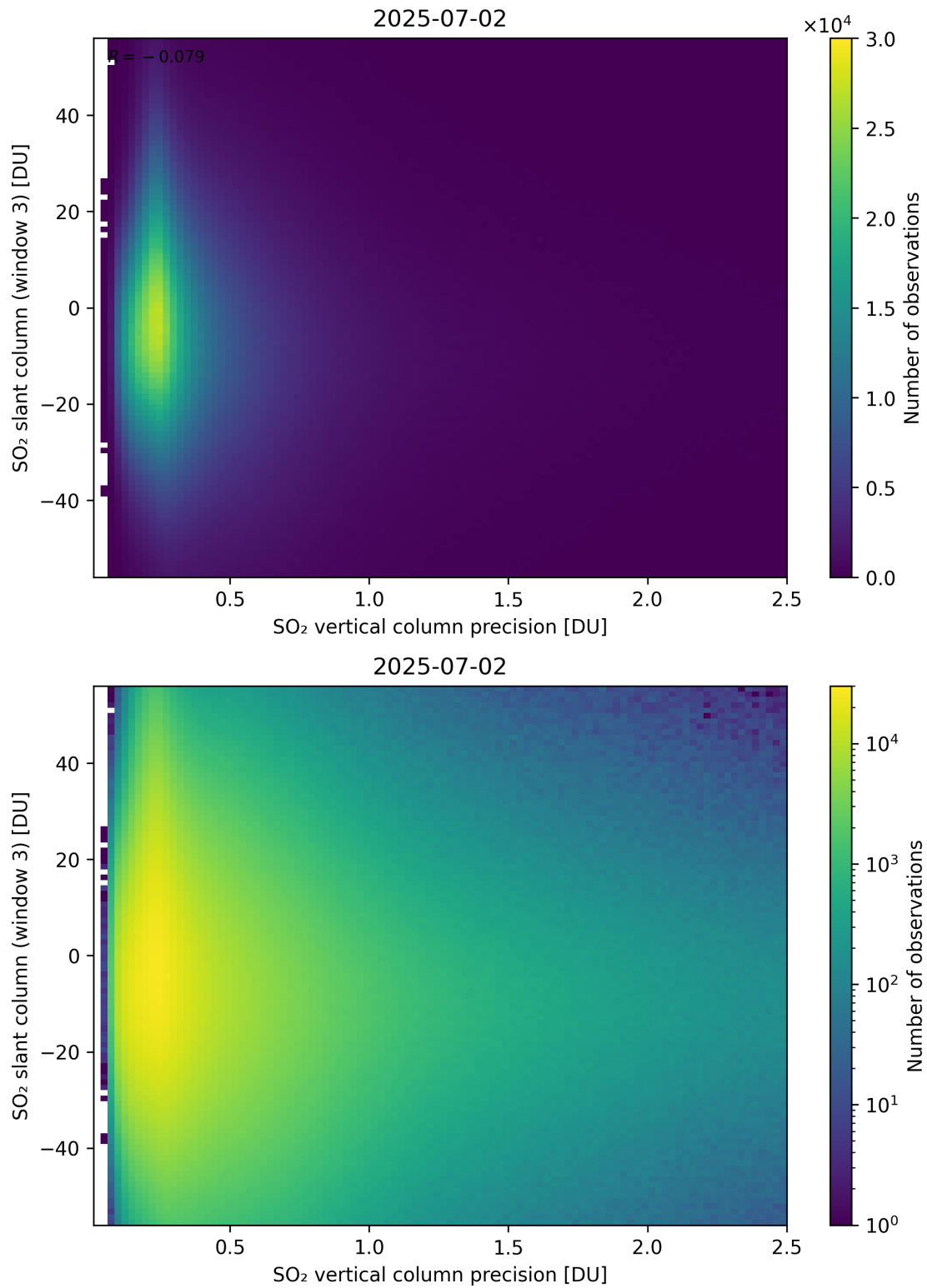
Figure 344: Scatter density plot of “SO 2 vertical column precision” against “SO 2 slant column (window 3)” for 2025-07-02 to 2025-07-03.
