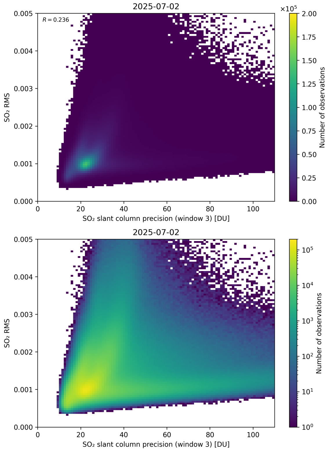
Figure 310: Scatter density plot of “SO 2 slant column precision (window 3)” against “SO 2 RMS” for 2025-07-02 to 2025-07-03.
