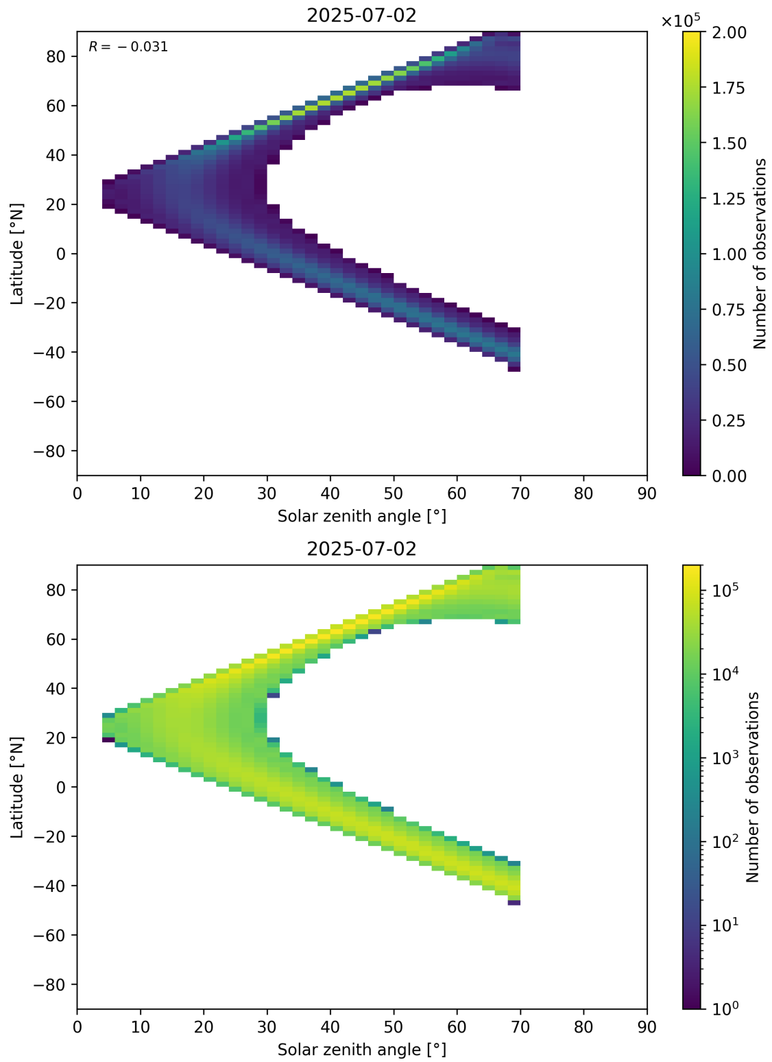
Figure 177: Scatter density plot of “Solar zenith angle” against “Latitude” for 2025-07-02 to 2025-07-03.
