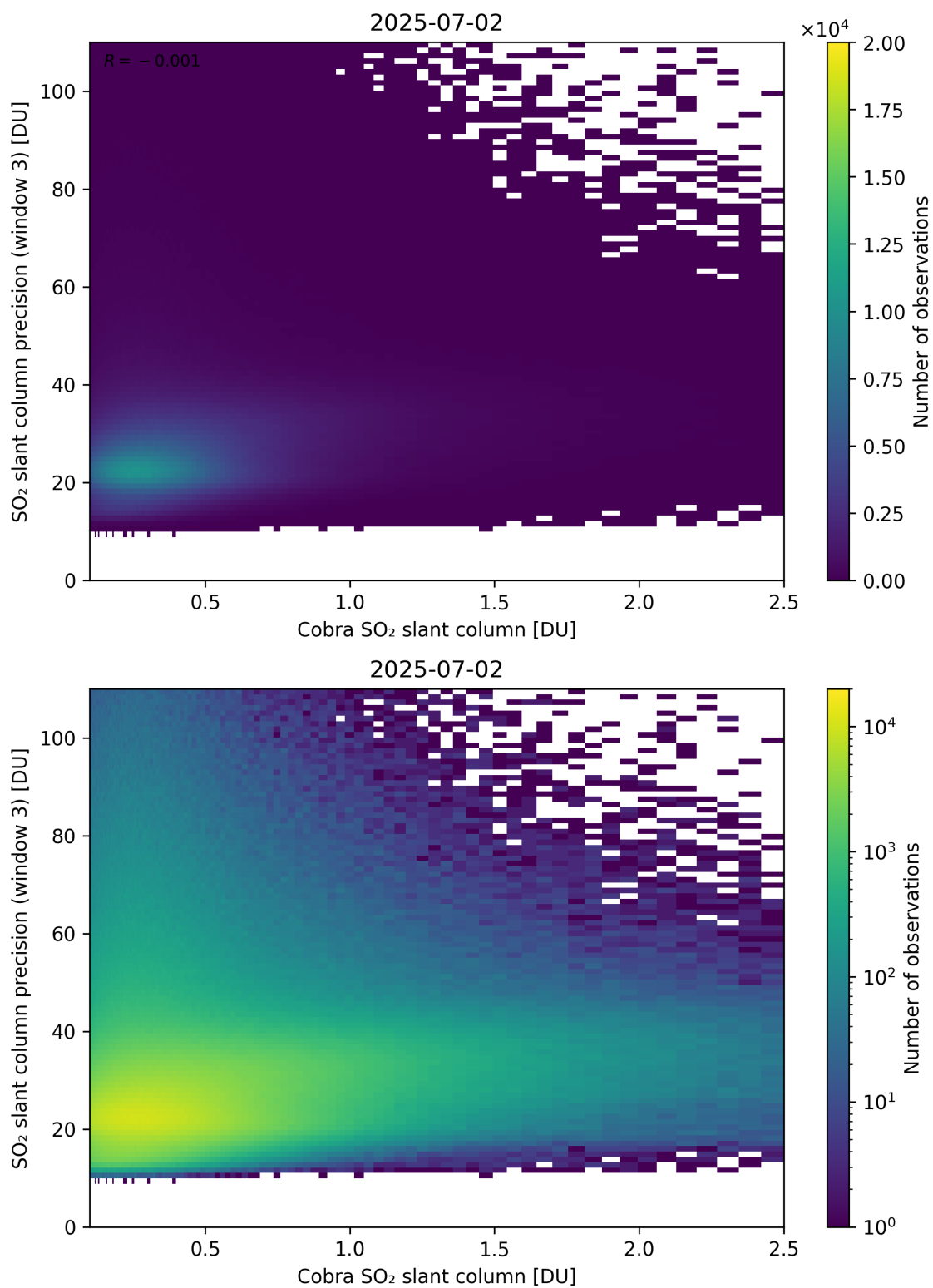
Figure 223: Scatter density plot of “Cobra SO 2 slant column” against “SO 2 slant column precision (window 3)” for 2025-07-02 to 2025-07-03.
