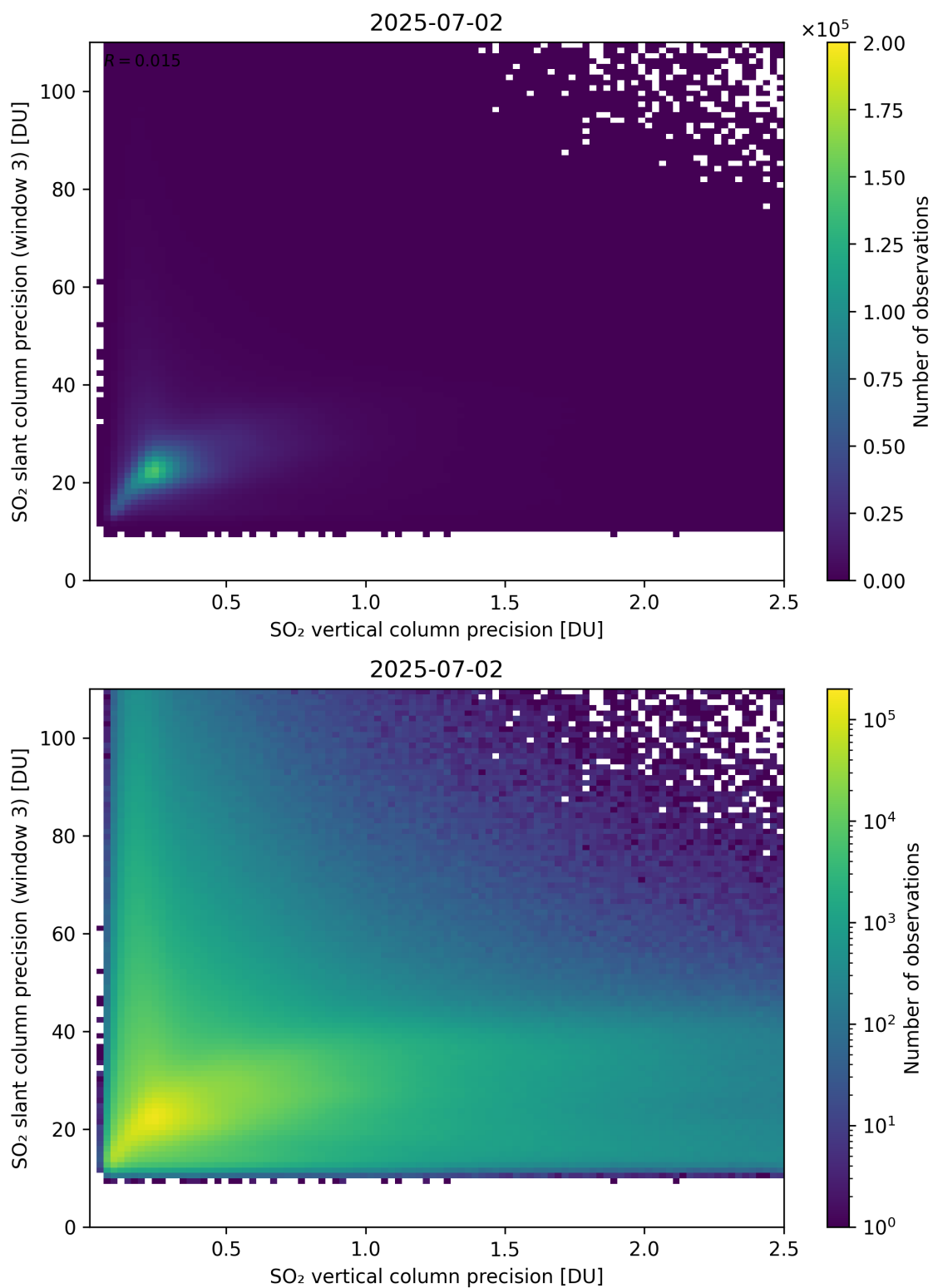
Figure 345: Scatter density plot of “SO 2 vertical column precision” against “SO 2 slant column precision (window 3)” for 2025-07-02 to 2025-07-03.
