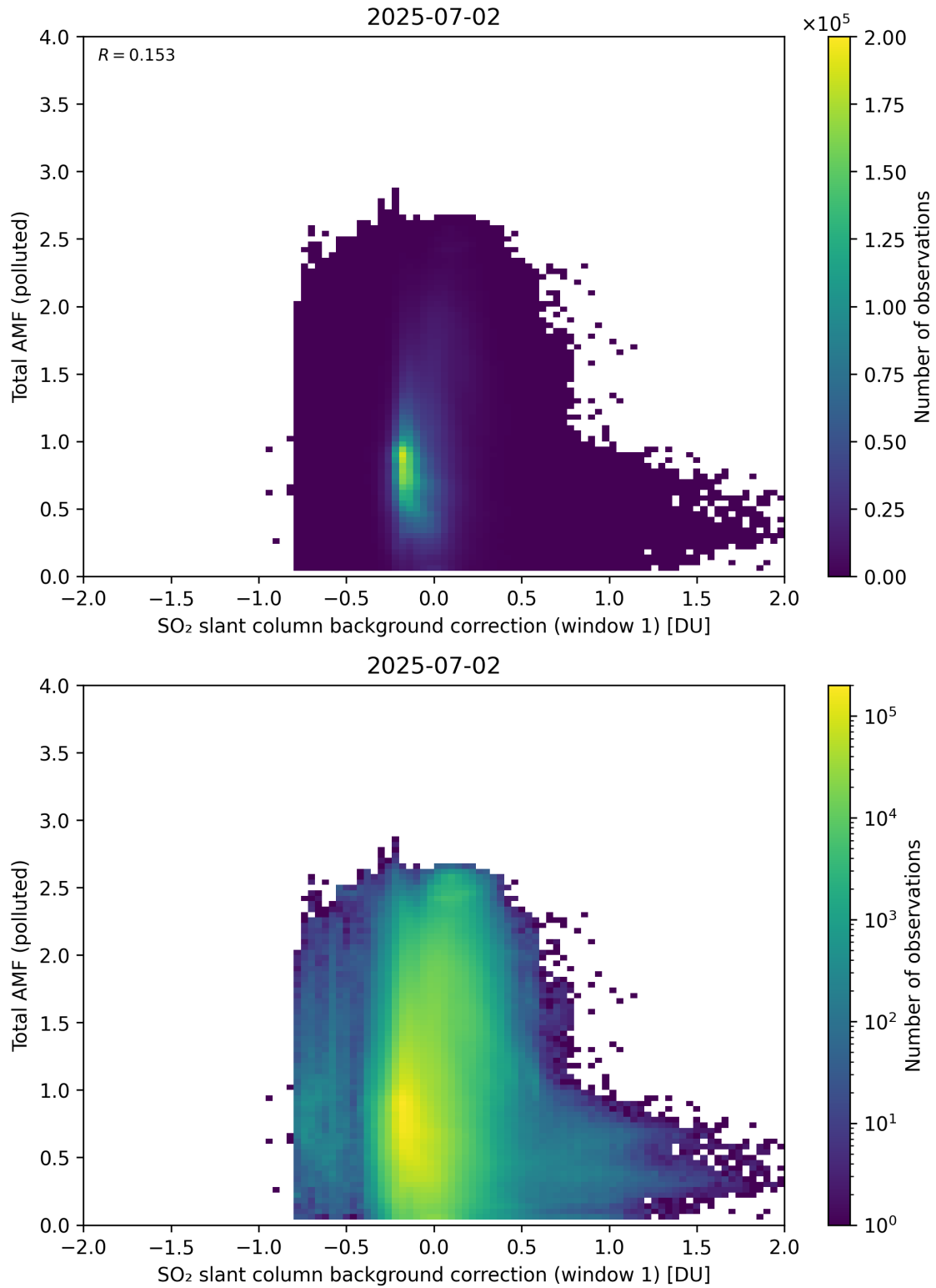
Figure 120: Scatter density plot of “SO 2 slant column background correction (window 1)” against “Total AMF (polluted)” for 2025-07-02 to 2025-07-03.
