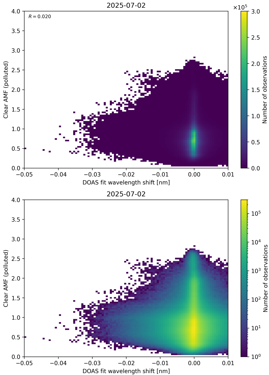
Figure 140: Scatter density plot of “DOAS fit wavelength shift” against “Clear AMF (polluted)” for 2025-07-02 to 2025-07-03.
