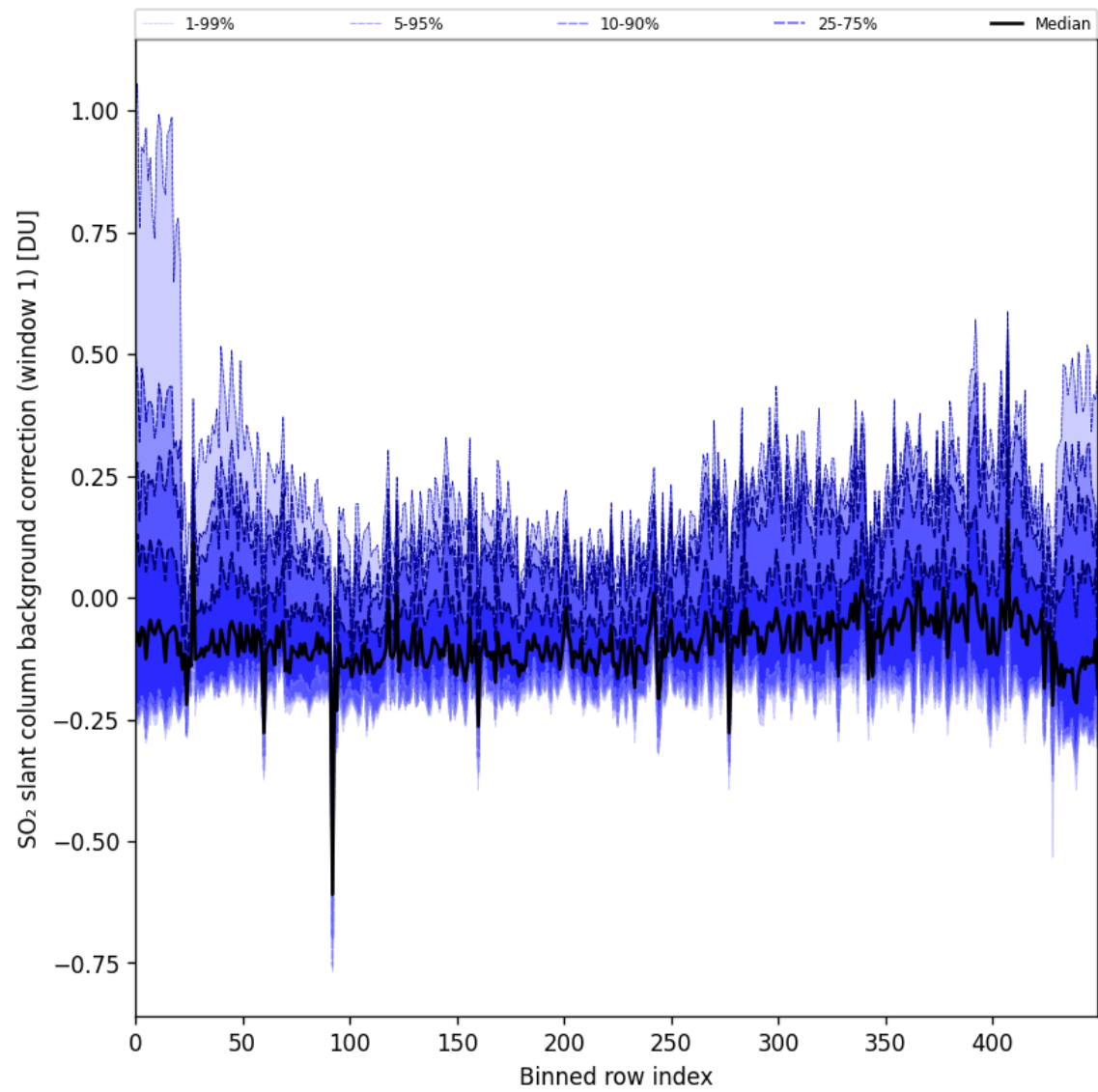
Figure 92: Along track statistics of “SO 2 slant column background correction (window 1)” for 2025-07-02 to 2025-07-03
