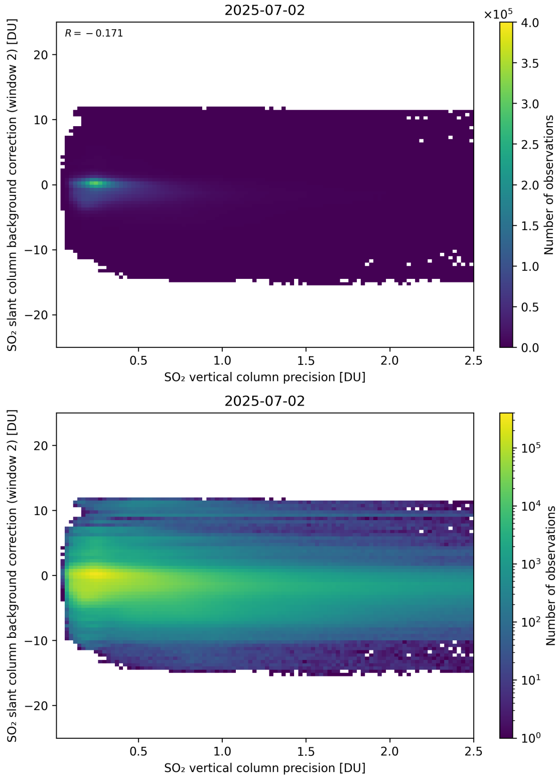
Figure 330: Scatter density plot of “SO 2 vertical column precision” against “SO 2 slant column background correction (window 2)” for 2025-07-02 to 2025-07-03.
