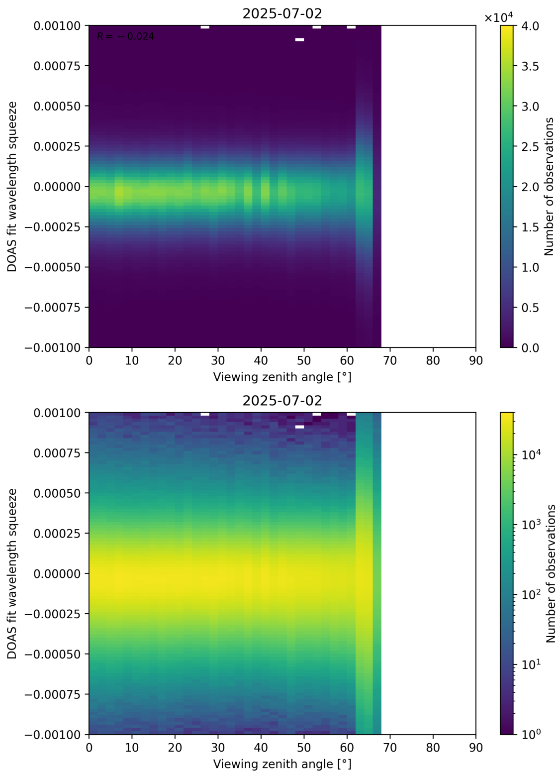
Figure 366: Scatter density plot of “Viewing zenith angle” against “DOAS fit wavelength squeeze” for 2025-07-02 to 2025-07-03.
