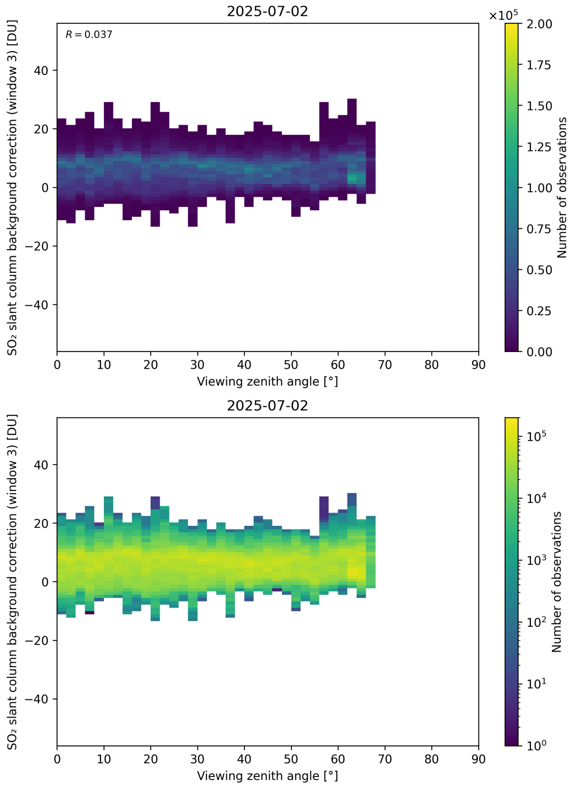
Figure 364: Scatter density plot of “Viewing zenith angle” against “SO 2 slant column background correction (window 3)” for 2025-07-02 to 2025-07-03.
