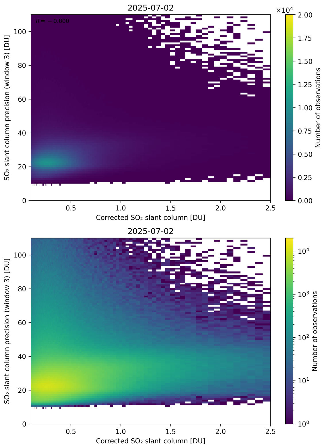
Figure 241: Scatter density plot of “Corrected SO 2 slant column” against “SO 2 slant column precision (window 3)” for 2025-07-02 to 2025-07-03.
