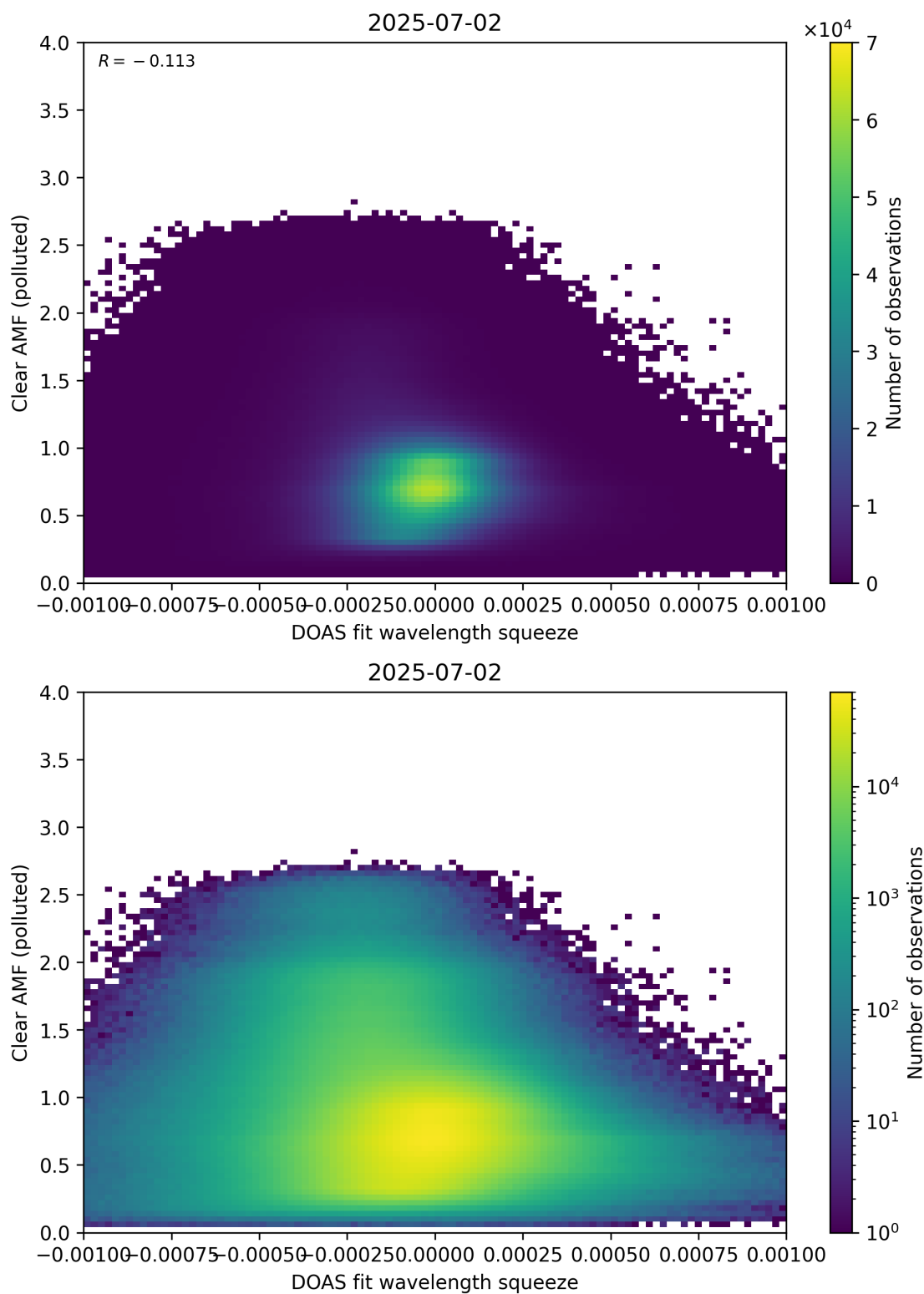
Figure 144: Scatter density plot of “DOAS fit wavelength squeeze” against “Clear AMF (polluted)” for 2025-07-02 to 2025-07-03.
