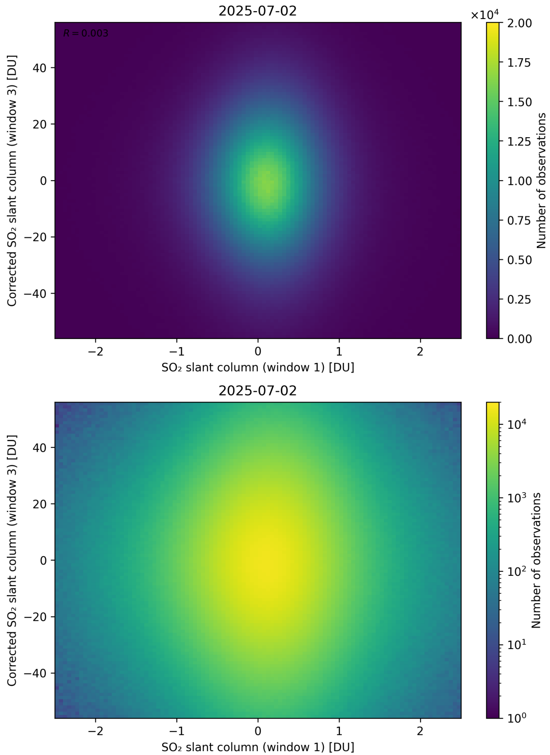
Figure 284: Scatter density plot of “SO 2 slant column (window 1)” against “Corrected SO 2 slant column (window 3)” for 2025-07-02 to 2025-07-03.
