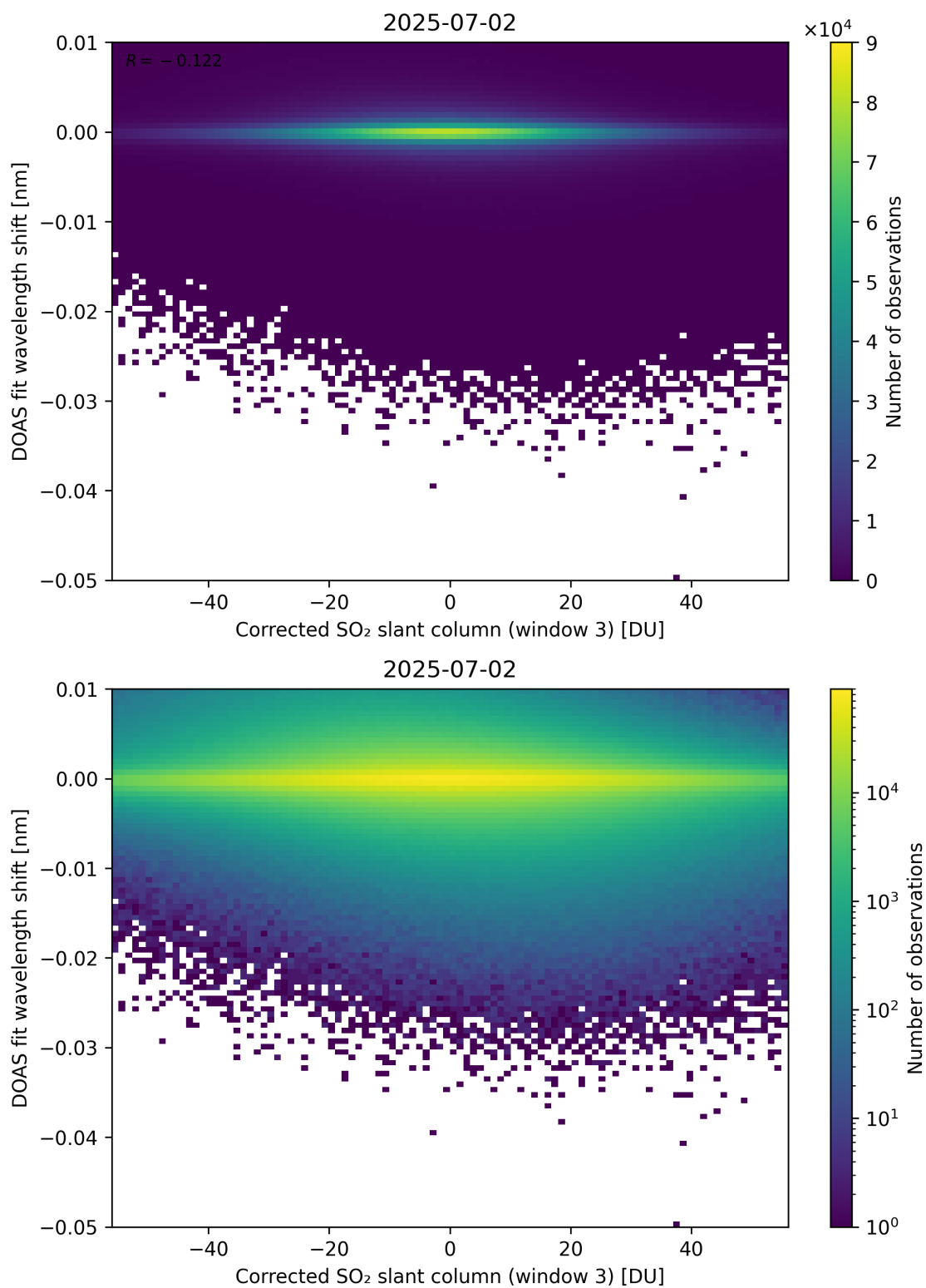
Figure 256: Scatter density plot of “Corrected SO 2 slant column (window 3)” against “DOAS fit wavelength shift” for 2025-07-02 to 2025-07-03.
