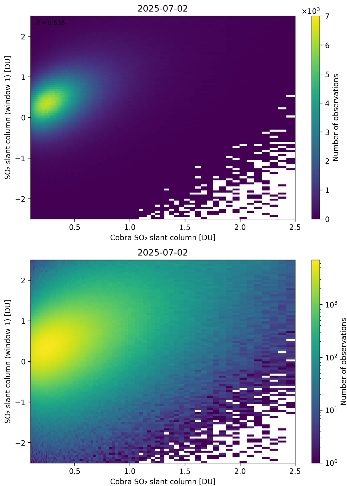
Figure 219: Scatter density plot of “Cobra SO 2 slant column” against “SO 2 slant column (window 1)” for 2025-07-02 to 2025-07-03.
