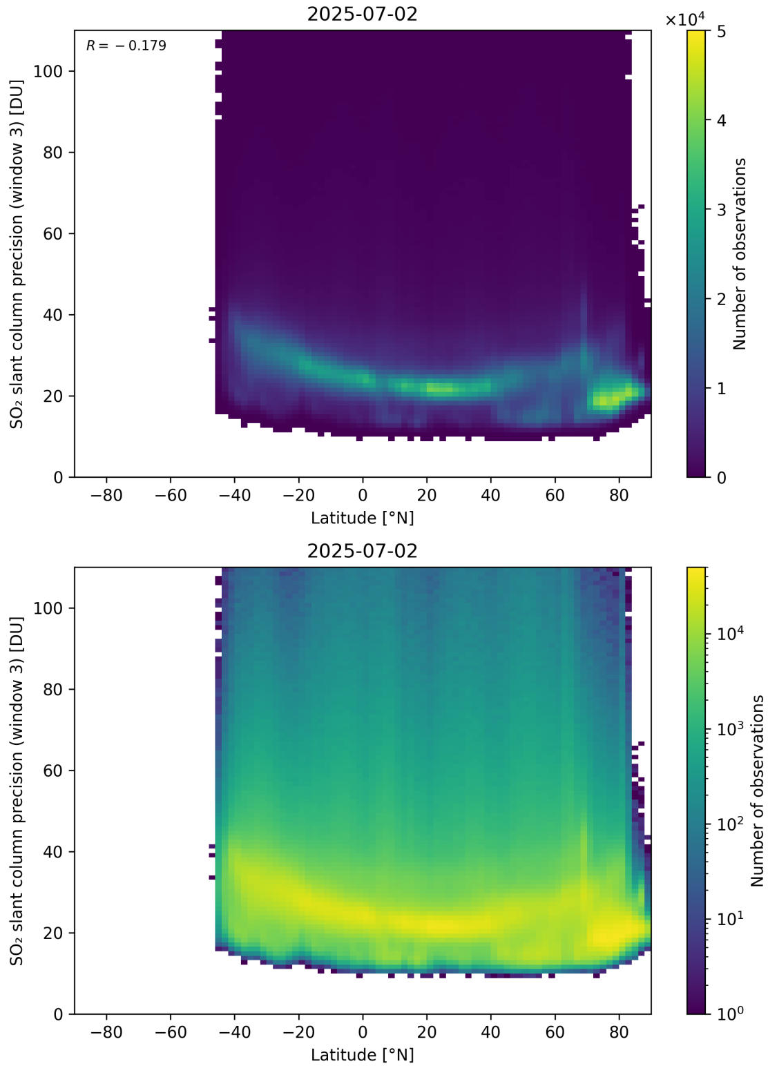
Figure 166: Scatter density plot of “Latitude” against “SO 2 slant column precision (window 3)” for 2025-07-02 to 2025-07-03.
