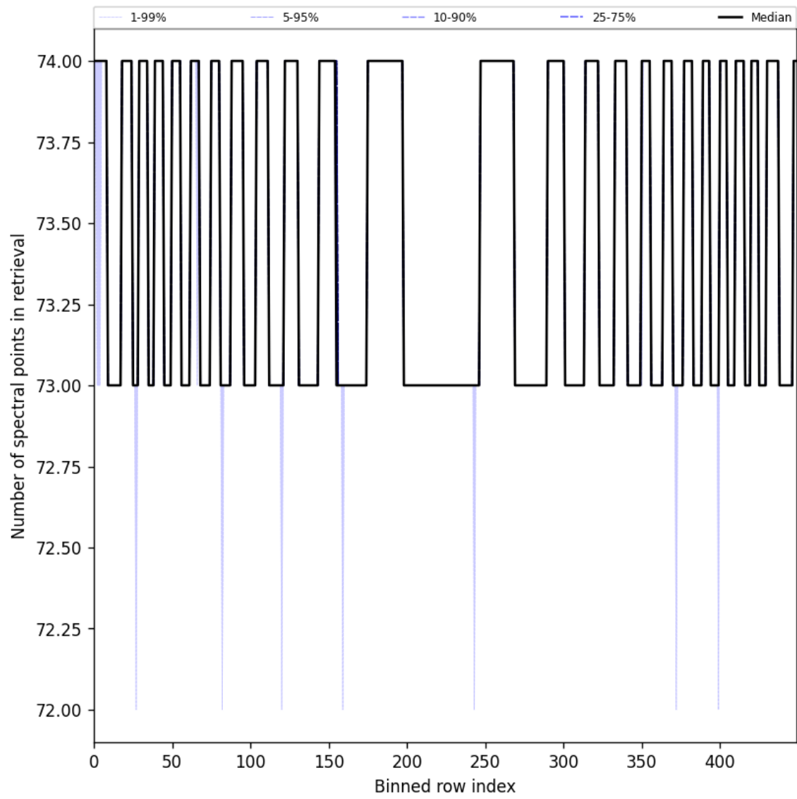
Figure 108: Along track statistics of “Number of spectral points in retrieval” for 2025-07-02 to 2025-07-03
