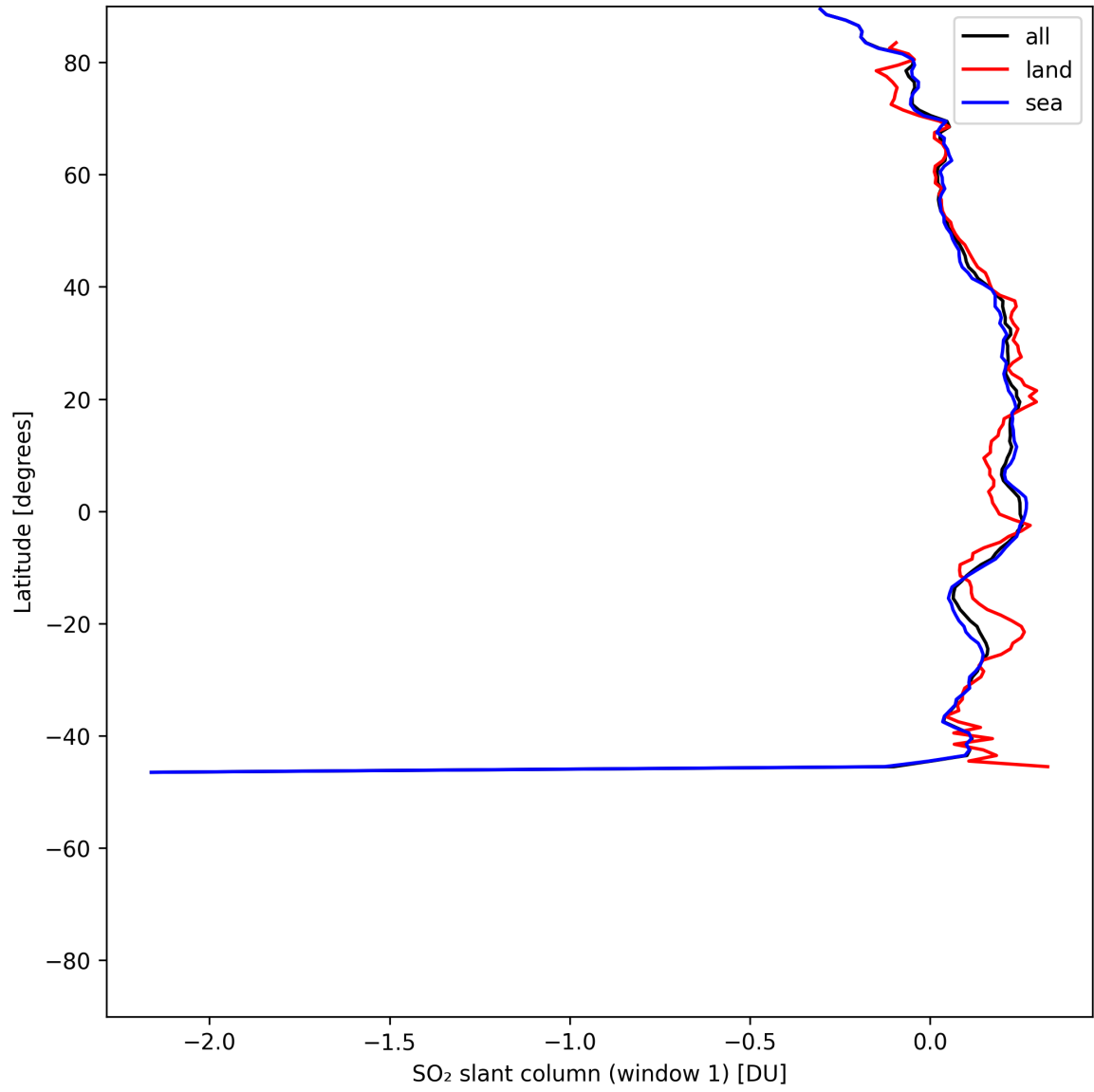
Figure 37: Zonal average of “SO 2 slant column (window 1)” for 2025-07-02 to 2025-07-03.
