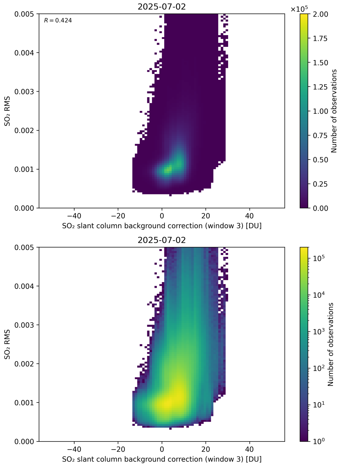
Figure 134: Scatter density plot of “SO 2 slant column background correction (window 3)” against “SO 2 RMS” for 2025-07-02 to 2025-07-03.
