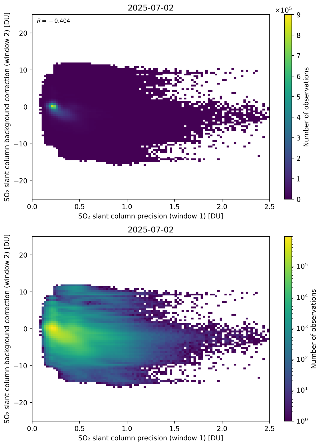
Figure 269: Scatter density plot of “SO 2 slant column precision (window 1)” against “SO 2 slant column background correction (window 2)” for 2025-07-02 to 2025-07-03.
