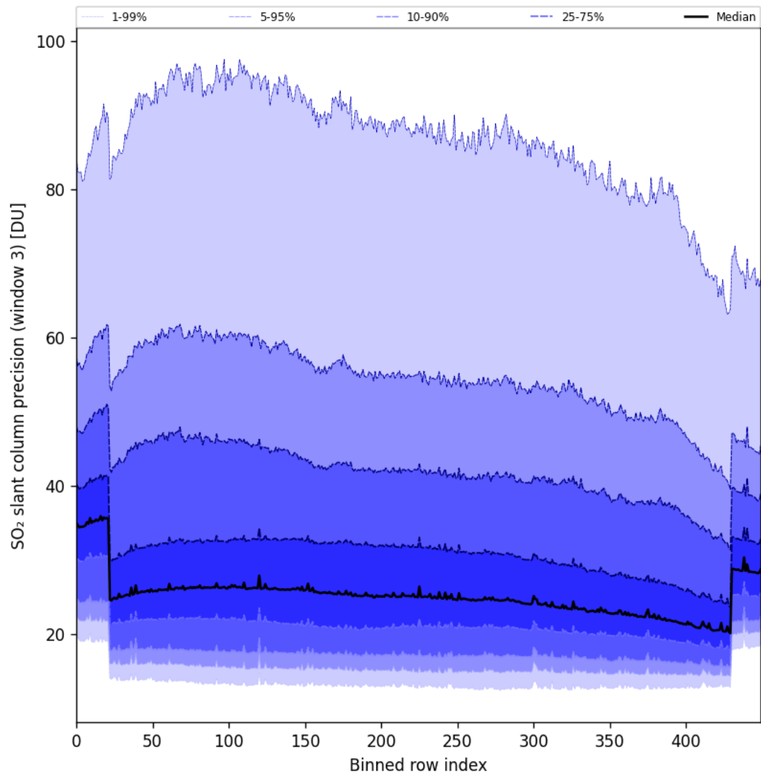
Figure 98: Along track statistics of “SO 2 slant column precision (window 3)” for 2025-07-02 to 2025-07-03
