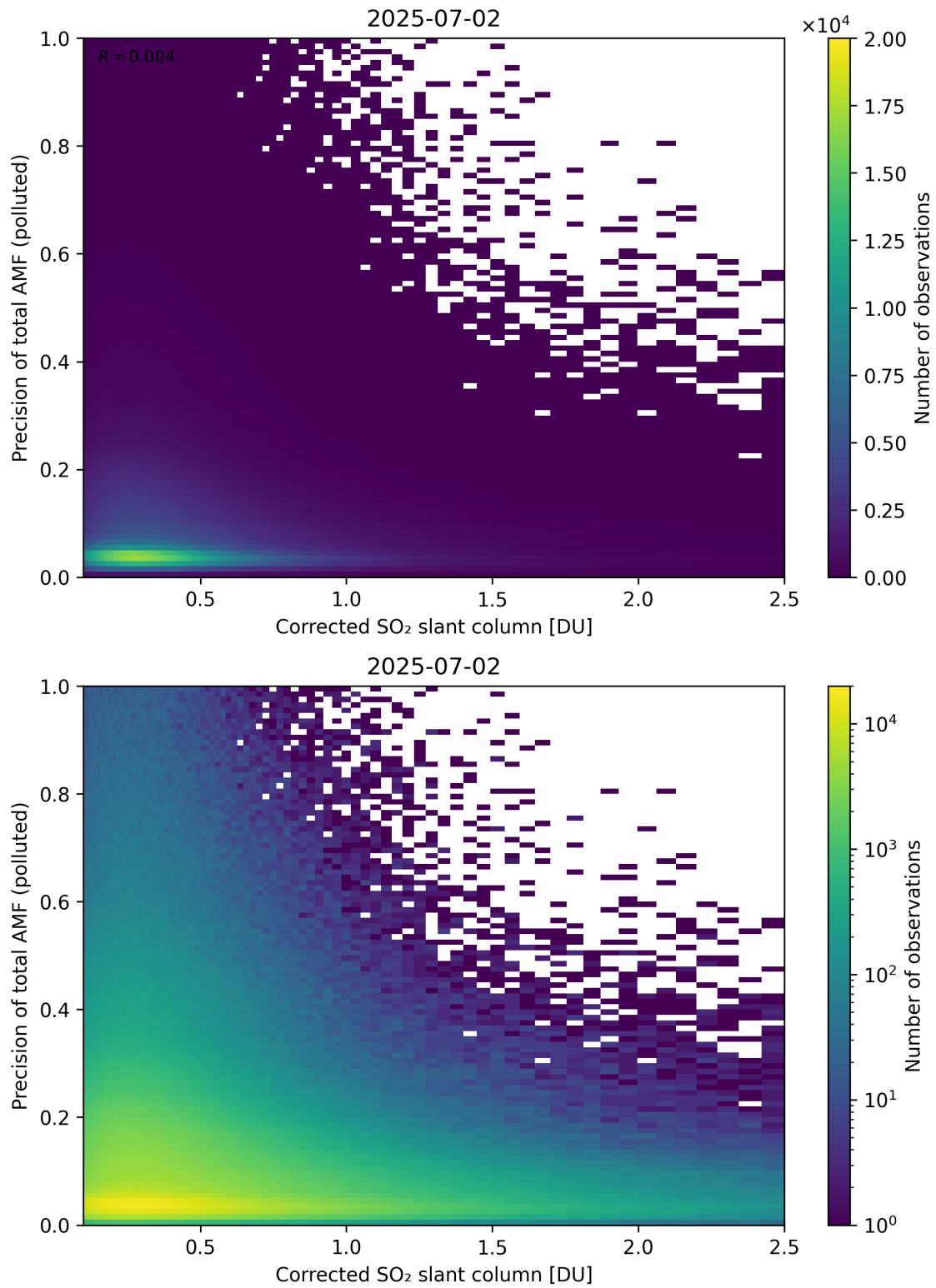
Figure 243: Scatter density plot of “Corrected SO 2 slant column” against “Precision of total AMF (polluted)” for 2025-07-02 to 2025-07-03.
