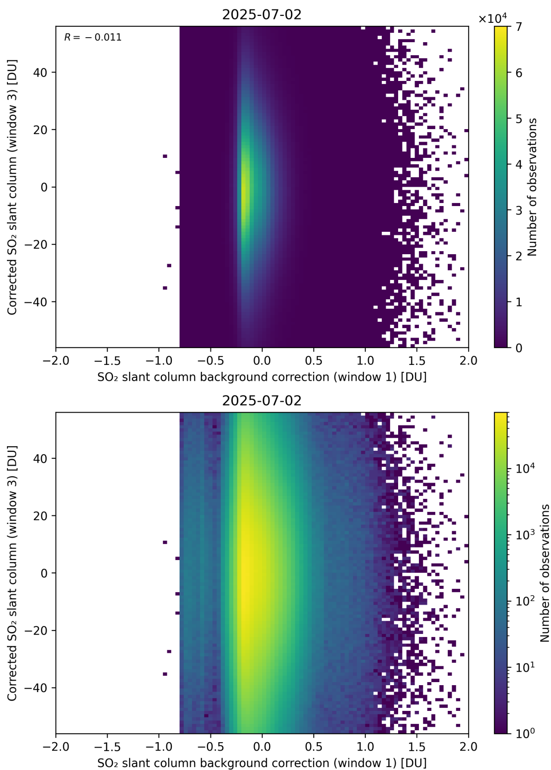
Figure 116: Scatter density plot of “SO 2 slant column background correction (window 1)” against “Corrected SO 2 slant column (window 3)” for 2025-07-02 to 2025-07-03.
