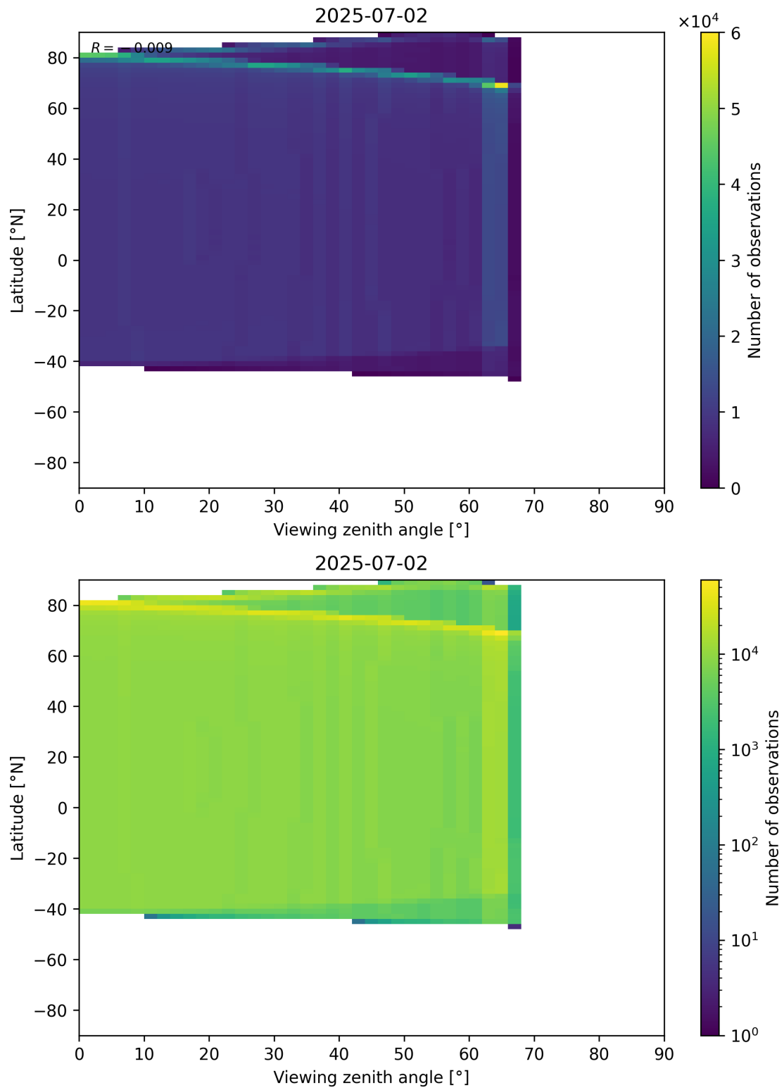
Figure 368: Scatter density plot of “Viewing zenith angle” against “Latitude” for 2025-07-02 to 2025-07-03.
