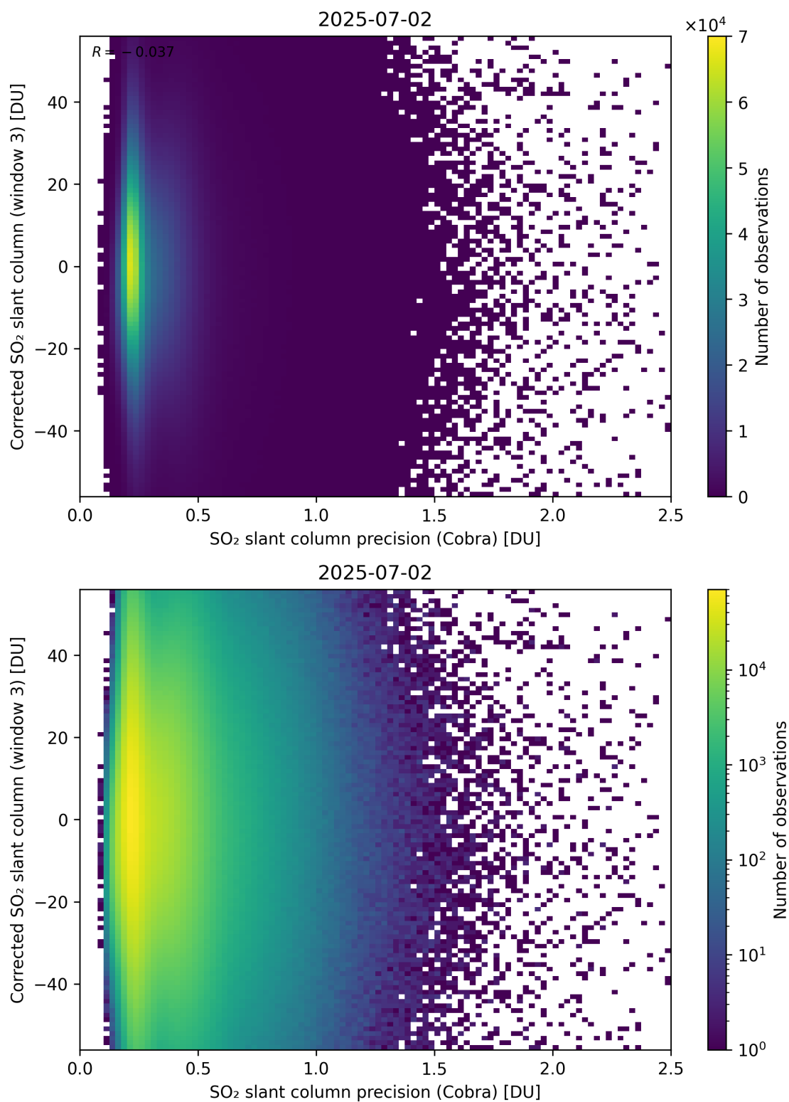
Figure 207: Scatter density plot of “SO 2 slant column precision (Cobra)” against “Corrected SO 2 slant column (window 3)” for 2025-07-02 to 2025-07-03.
