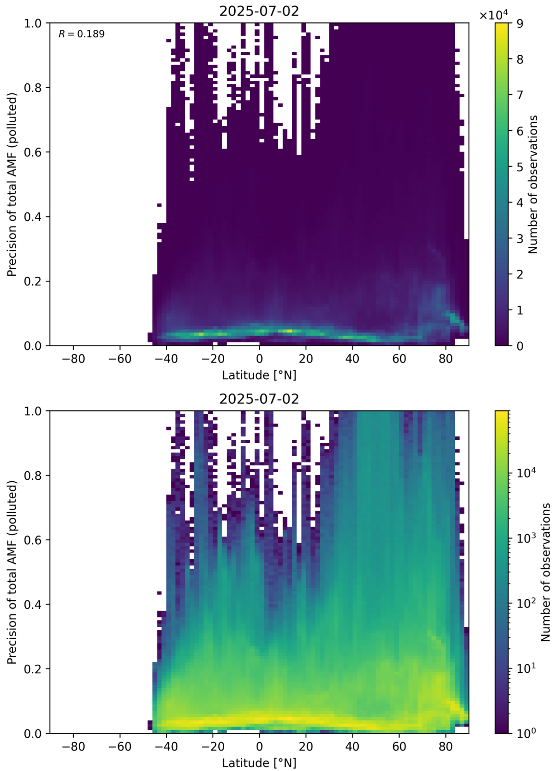
Figure 168: Scatter density plot of “Latitude” against “Precision of total AMF (polluted)” for 2025-07-02 to 2025-07-03.
