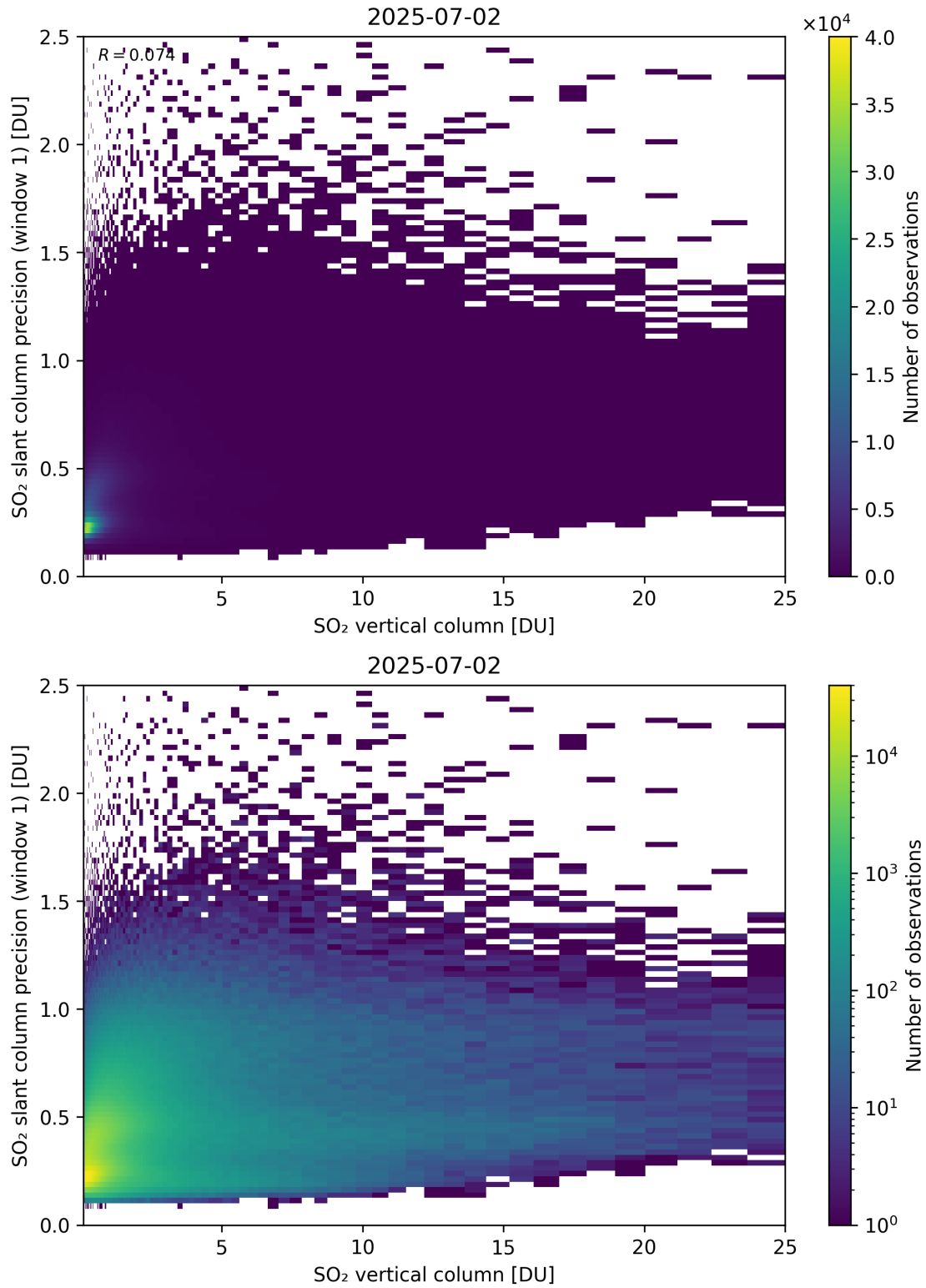
Figure 355: Scatter density plot of “SO 2 vertical column” against “SO 2 slant column precision (window 1)” for 2025-07-02 to 2025-07-03.
