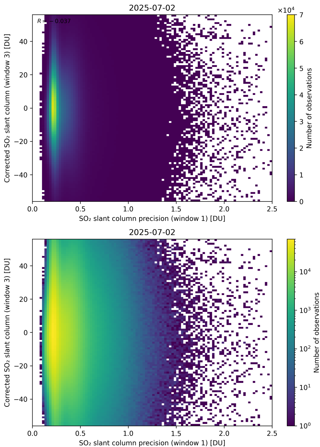
Figure 276: Scatter density plot of “SO 2 slant column precision (window 1)” against “Corrected SO 2 slant column (window 3)” for 2025-07-02 to 2025-07-03.
