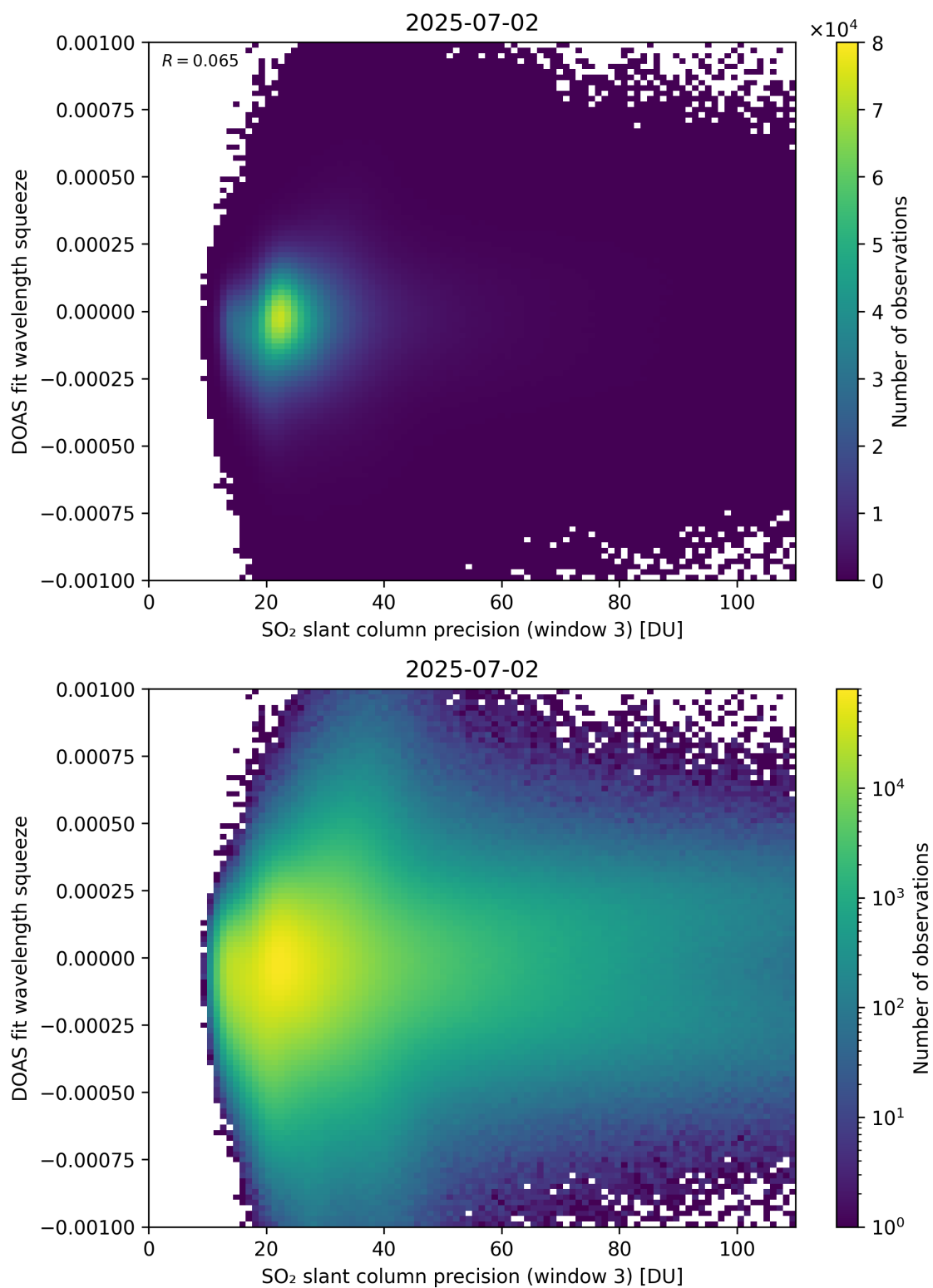
Figure 309: Scatter density plot of “SO 2 slant column precision (window 3)” against “DOAS fit wavelength squeeze” for 2025-07-02 to 2025-07-03.
