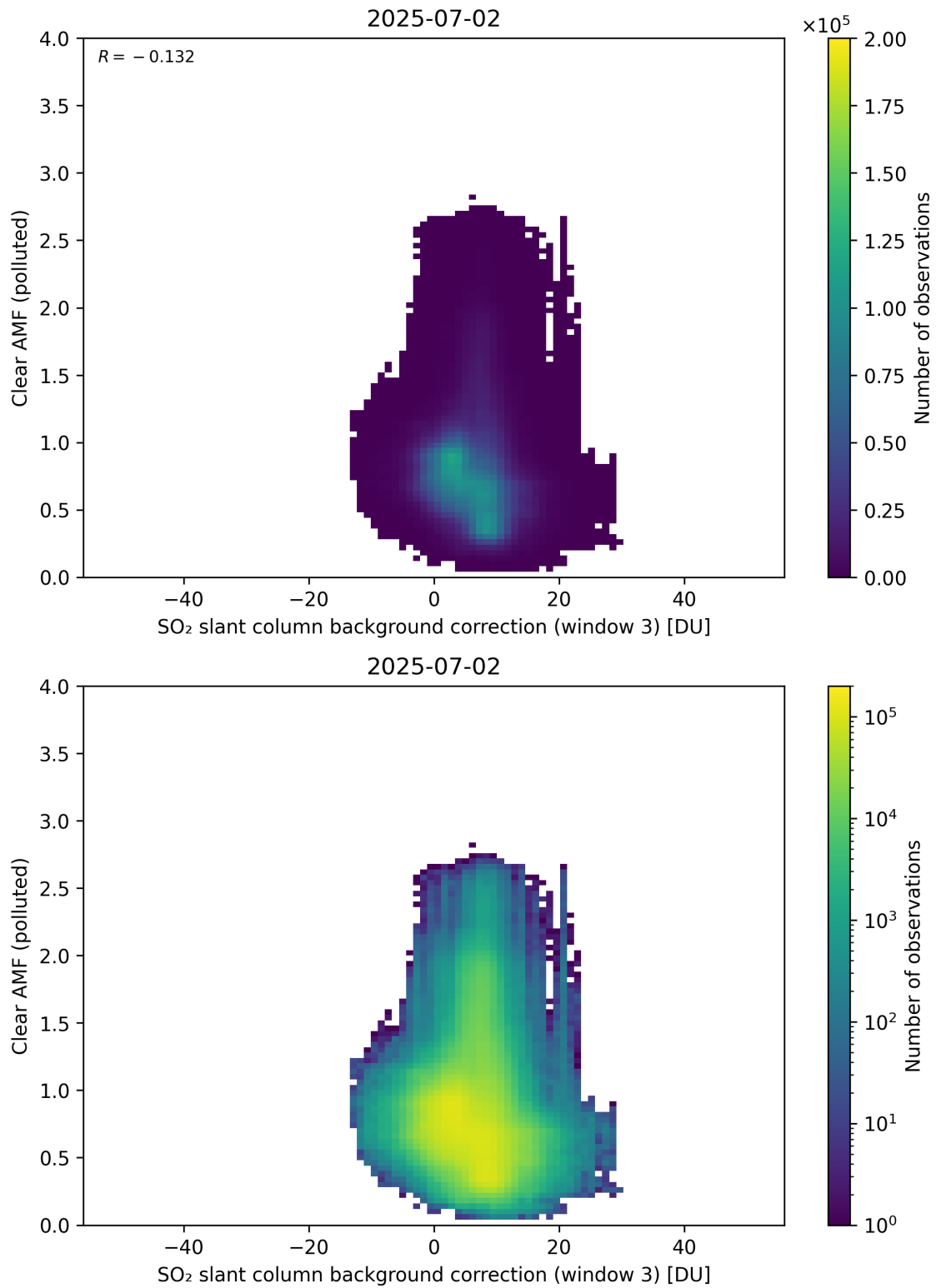
Figure 135: Scatter density plot of “SO 2 slant column background correction (window 3)” against “Clear AMF (polluted)” for 2025-07-02 to 2025-07-03.
