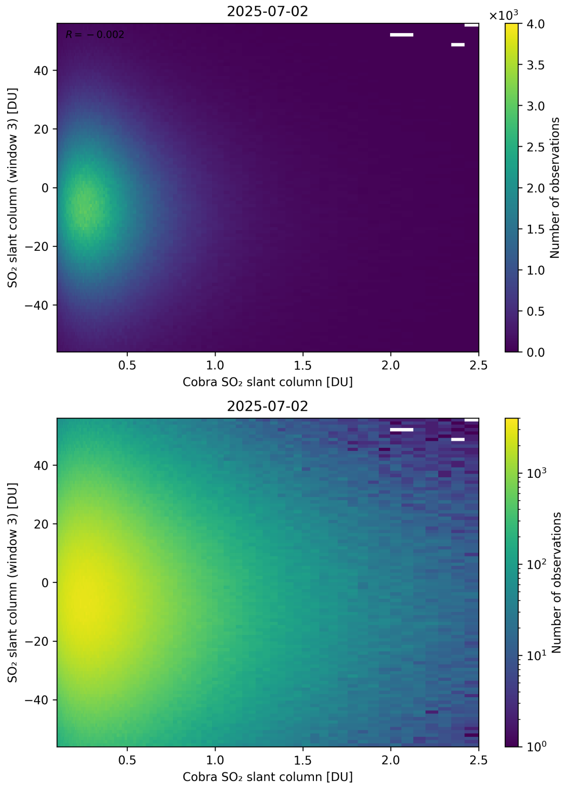
Figure 222: Scatter density plot of “Cobra SO 2 slant column” against “SO 2 slant column (window 3)” for 2025-07-02 to 2025-07-03.
