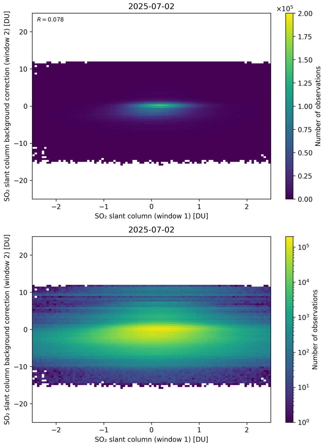
Figure 263: Scatter density plot of “SO 2 slant column (window 1)” against “SO 2 slant column background correction (window 2)” for 2025-07-02 to 2025-07-03.
