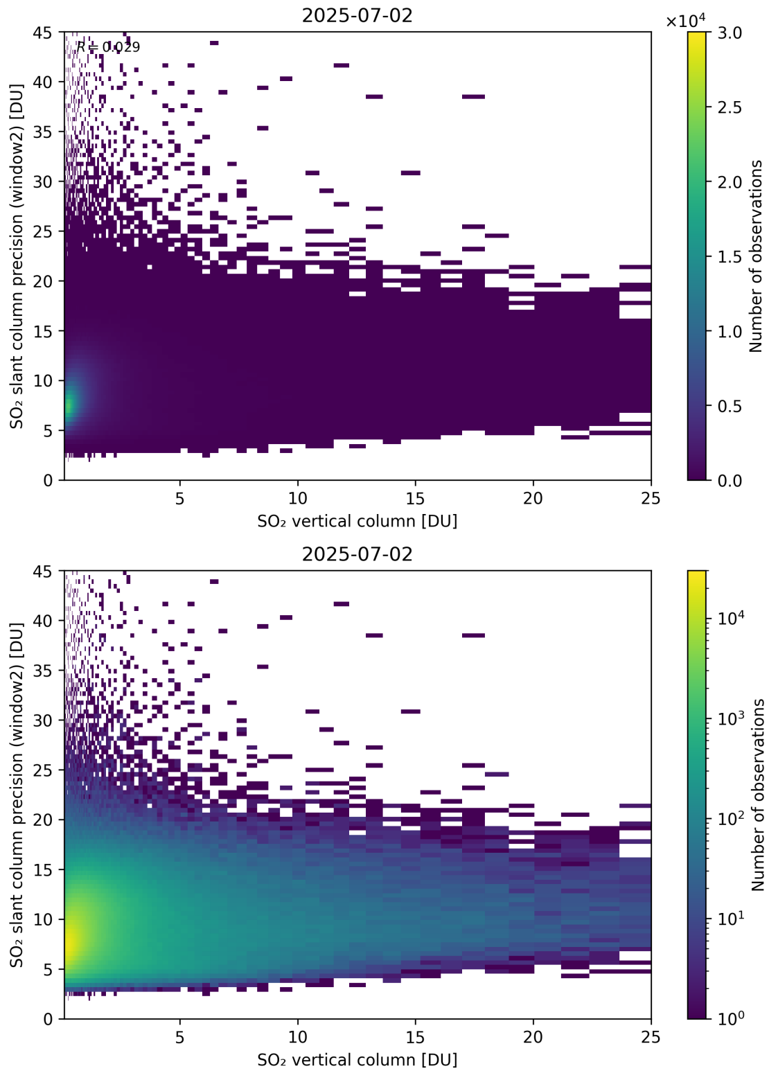
Figure 356: Scatter density plot of “SO 2 vertical column” against “SO 2 slant column precision (window2)” for 2025-07-02 to 2025-07-03.
