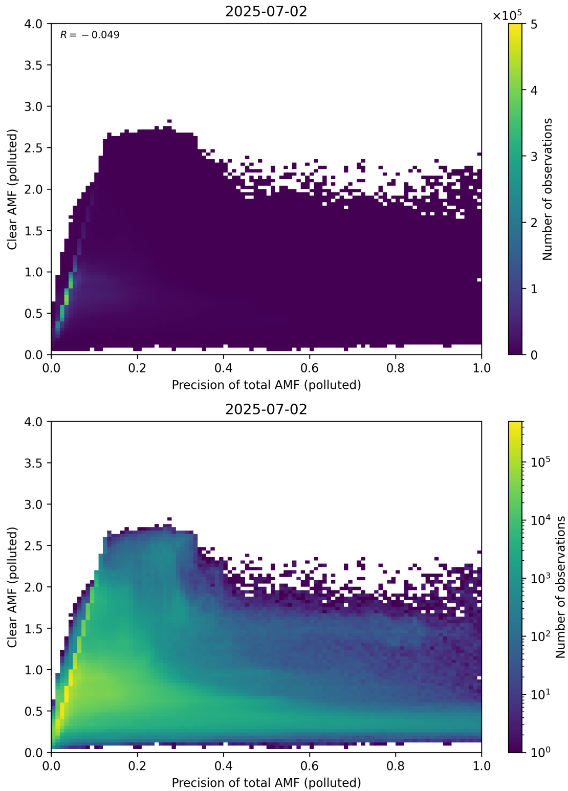
Figure 320: Scatter density plot of “Precision of total AMF (polluted)” against “Clear AMF (polluted)” for 2025-07-02 to 2025-07-03.
