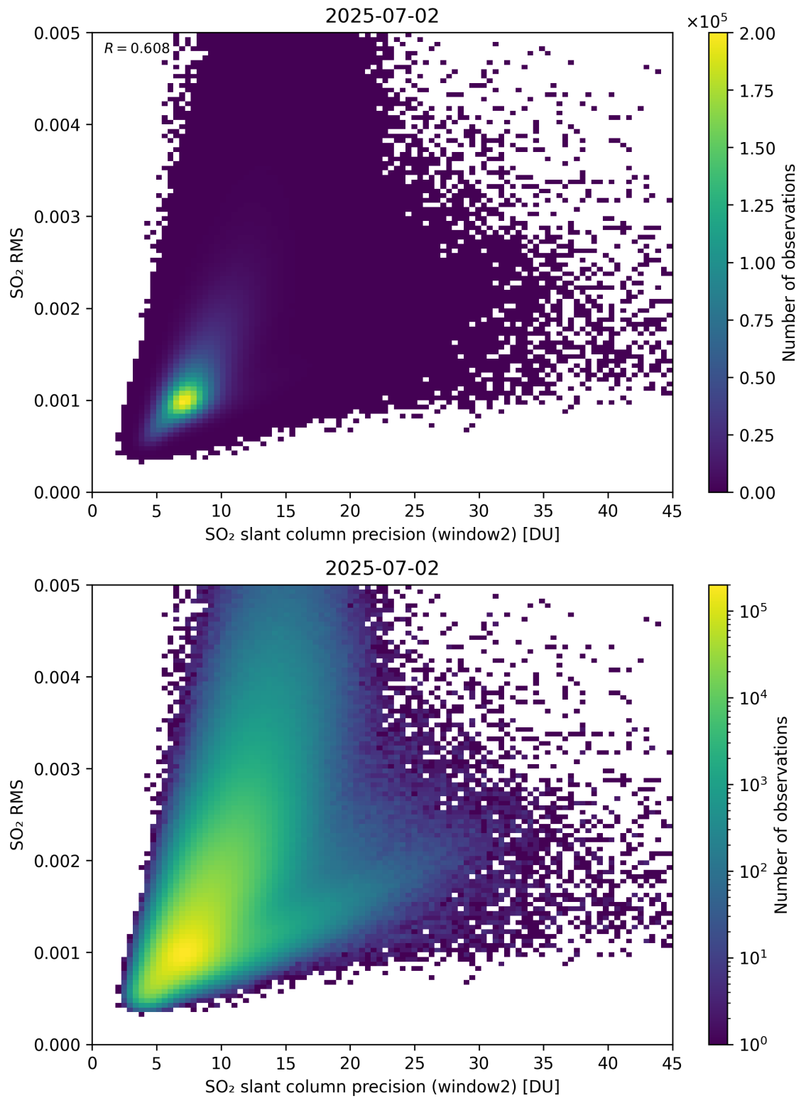
Figure 295: Scatter density plot of “SO 2 slant column precision (window2)” against “SO 2 RMS” for 2025-07-02 to 2025-07-03.
