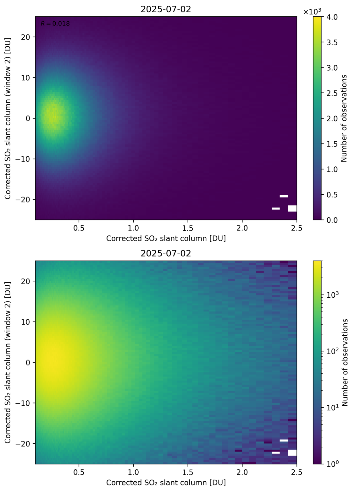
Figure 235: Scatter density plot of “Corrected SO 2 slant column” against “Corrected SO 2 slant column (window 2)” for 2025-07-02 to 2025-07-03.
