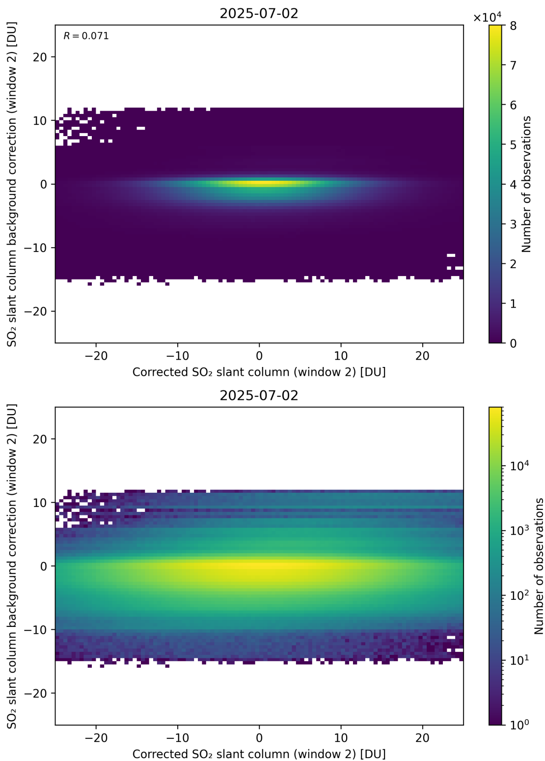
Figure 244: Scatter density plot of “Corrected SO 2 slant column (window 2)” against “SO 2 slant column background correction (window 2)” for 2025-07-02 to 2025-07-03.
