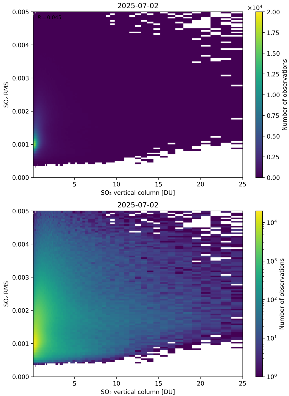
Figure 328: Scatter density plot of “SO 2 vertical column” against “SO 2 RMS” for 2025-07-02 to 2025-07-03.
