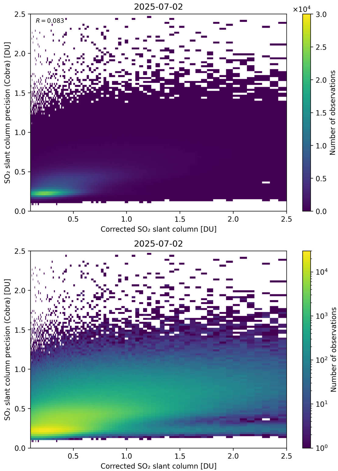
Figure 234: Scatter density plot of “Corrected SO 2 slant column” against “SO 2 slant column precision (Cobra)” for 2025-07-02 to 2025-07-03.
