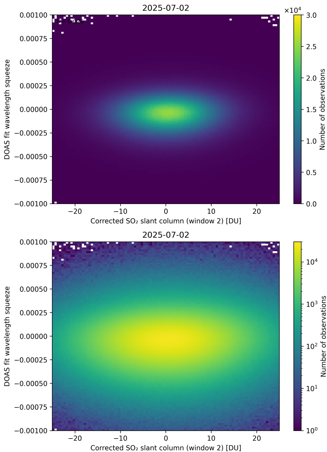
Figure 247: Scatter density plot of “Corrected SO 2 slant column (window 2)” against “DOAS fit wavelength squeeze” for 2025-07-02 to 2025-07-03.
