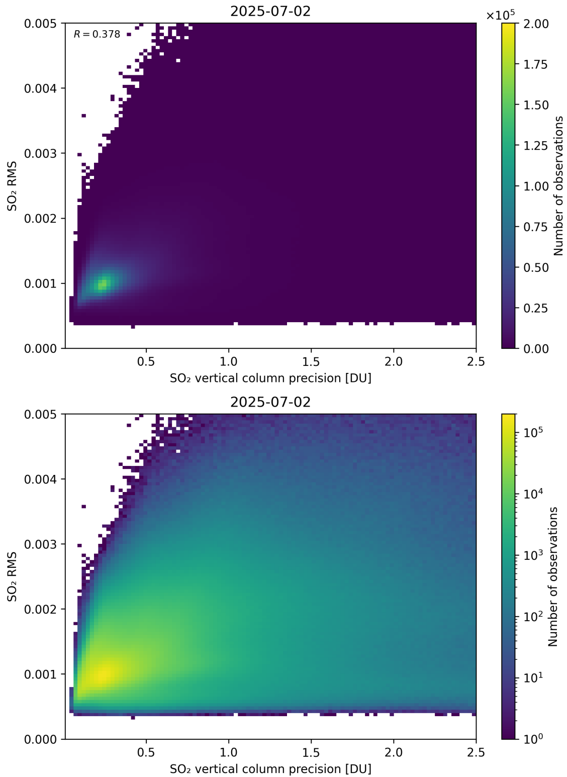
Figure 334: Scatter density plot of “SO 2 vertical column precision” against “SO 2 RMS” for 2025-07-02 to 2025-07-03.
