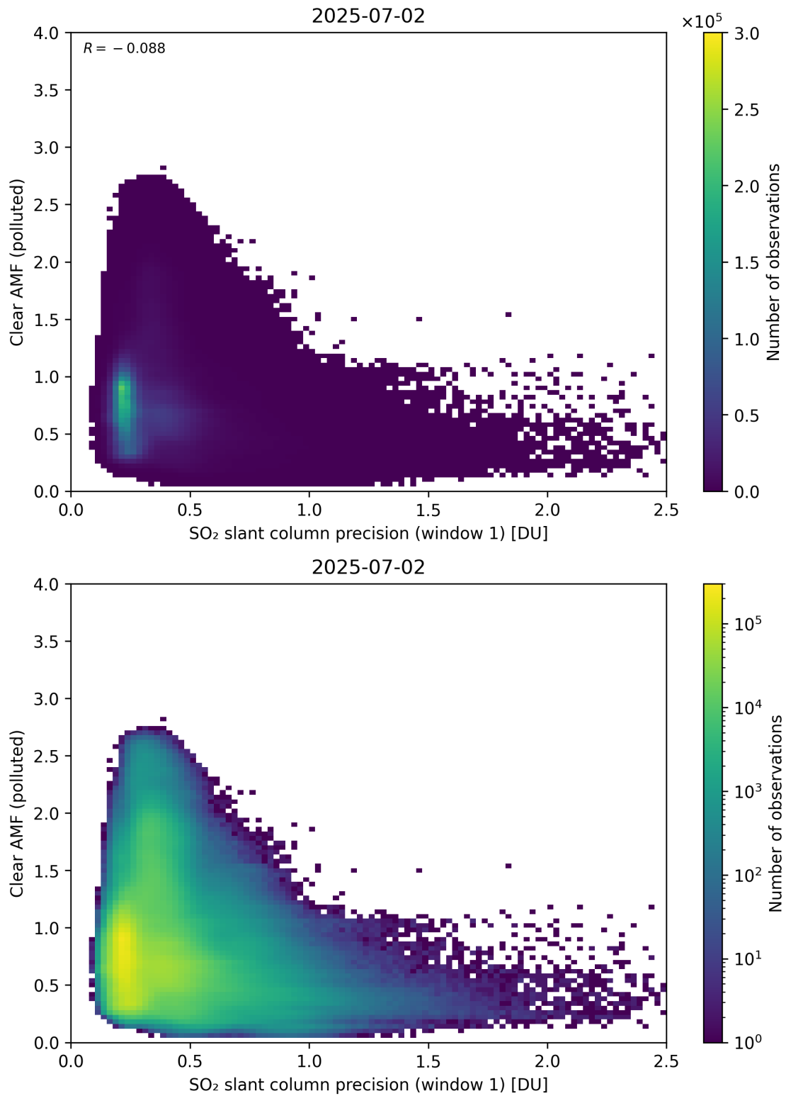
Figure 274: Scatter density plot of “SO 2 slant column precision (window 1)” against “Clear AMF (polluted)” for 2025-07-02 to 2025-07-03.
