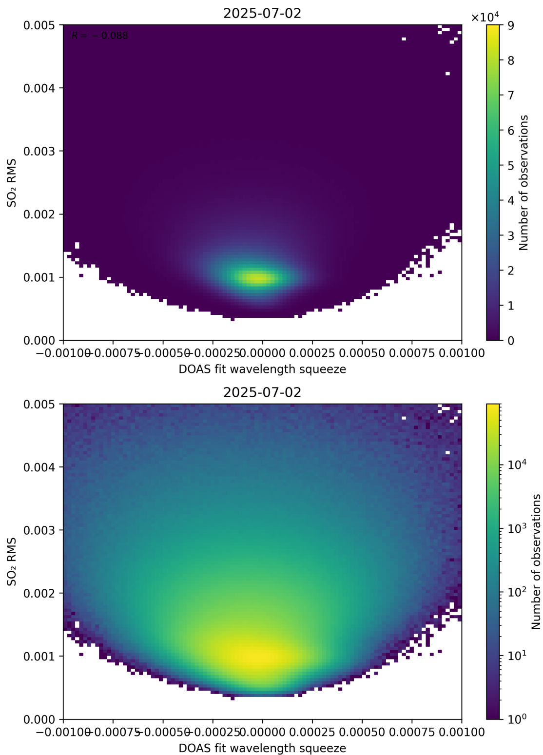
Figure 143: Scatter density plot of “DOAS fit wavelength squeeze” against “SO 2 RMS” for 2025-07-02 to 2025-07-03.
