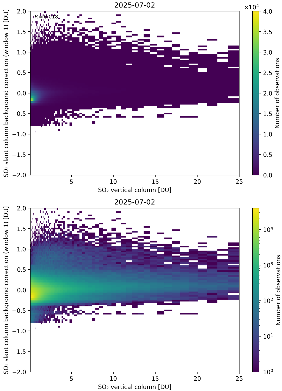
Figure 323: Scatter density plot of “SO 2 vertical column” against “SO 2 slant column background correction (window 1)” for 2025-07-02 to 2025-07-03.
