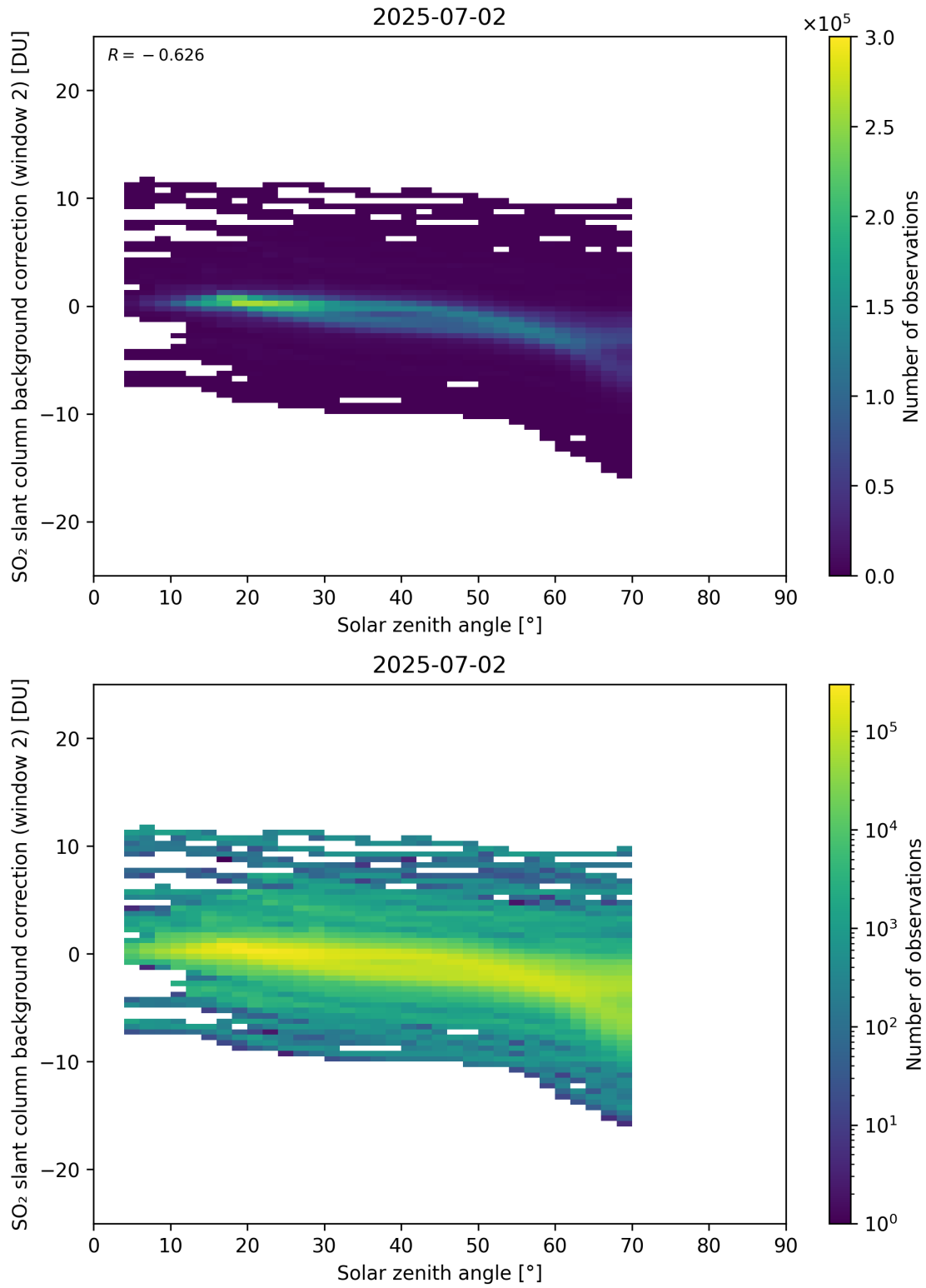
Figure 172: Scatter density plot of “Solar zenith angle” against “SO 2 slant column background correction (window 2)” for 2025-07-02 to 2025-07-03.
