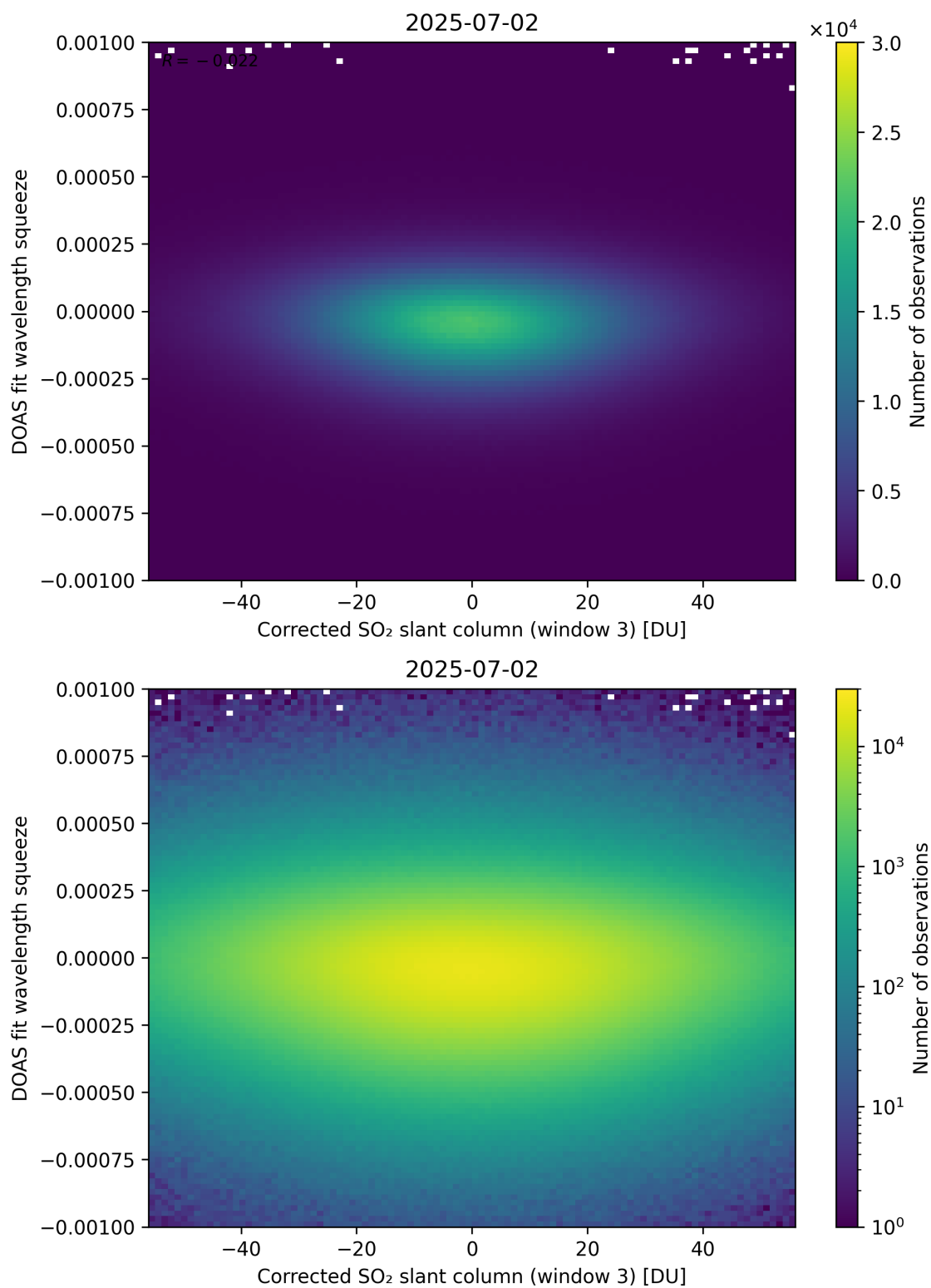
Figure 257: Scatter density plot of “Corrected SO 2 slant column (window 3)” against “DOAS fit wavelength squeeze” for 2025-07-02 to 2025-07-03.
