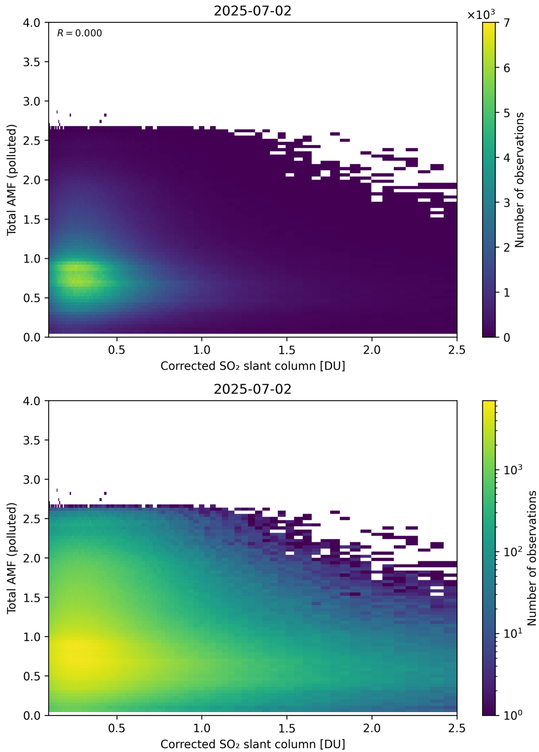
Figure 242: Scatter density plot of “Corrected SO 2 slant column” against “Total AMF (polluted)” for 2025-07-02 to 2025-07-03.
