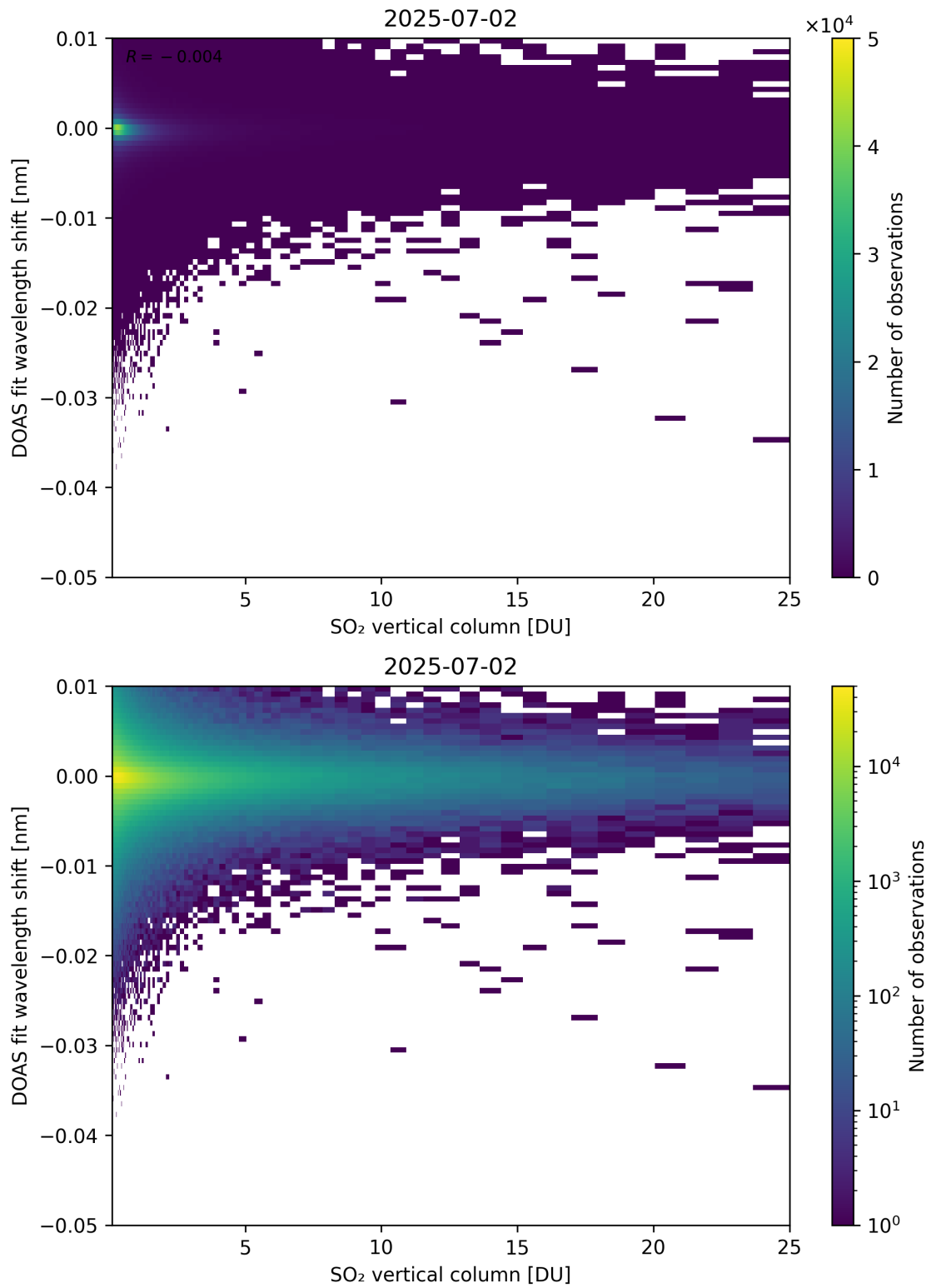
Figure 326: Scatter density plot of “SO 2 vertical column” against “DOAS fit wavelength shift” for 2025-07-02 to 2025-07-03.
