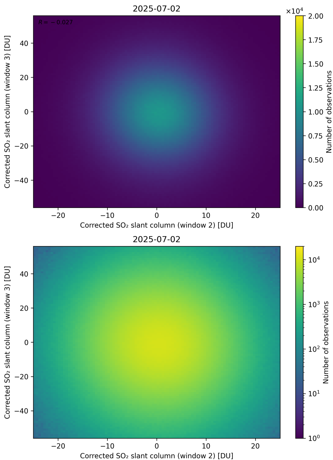
Figure 250: Scatter density plot of “Corrected SO 2 slant column (window 2)” against “Corrected SO 2 slant column (window 3)” for 2025-07-02 to 2025-07-03.
