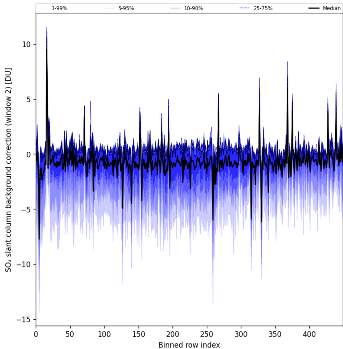
Figure 96: Along track statistics of “SO 2 slant column background correction (window 2)” for 2025-07-02 to 2025-07-03
