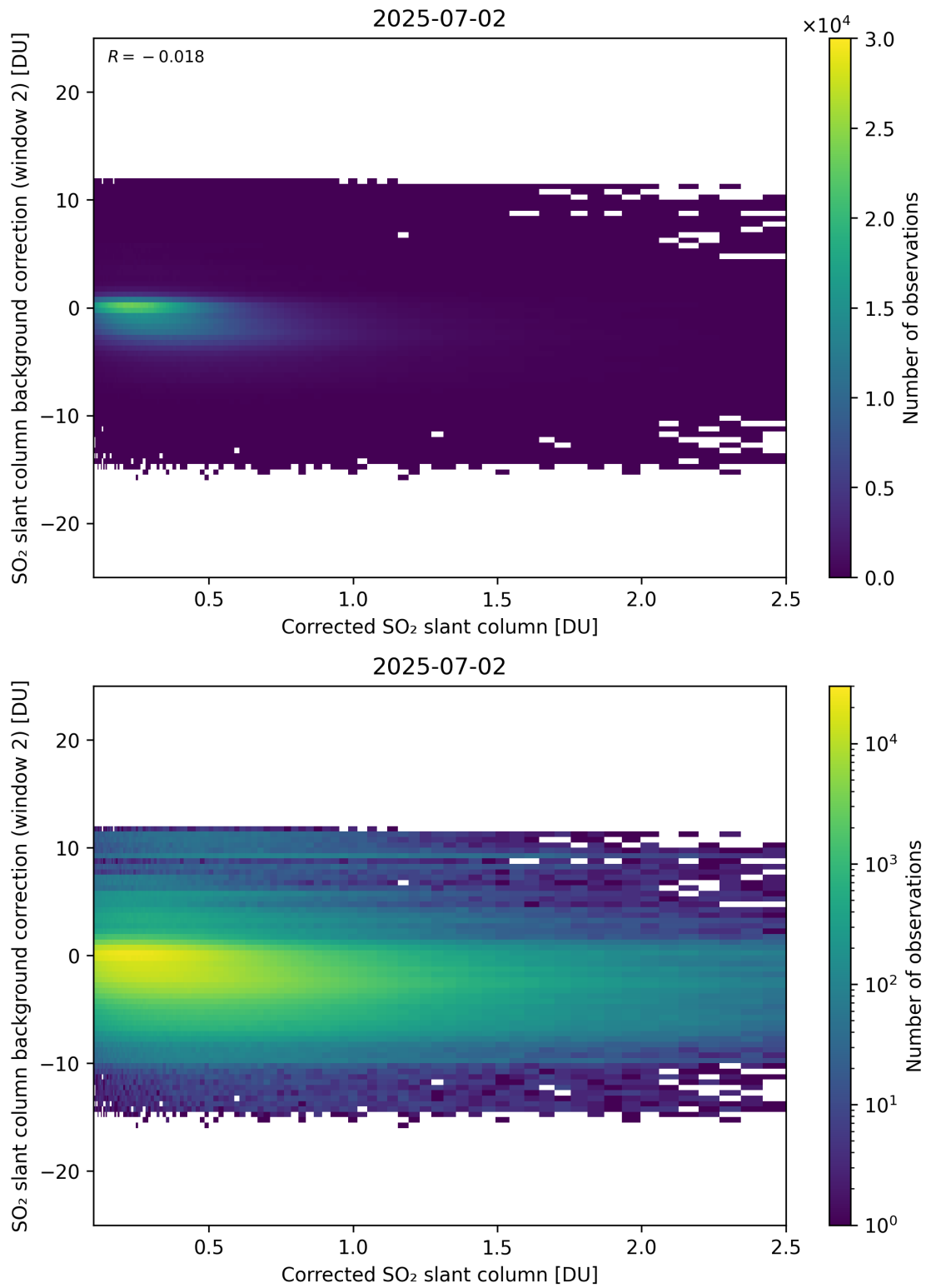
Figure 227: Scatter density plot of “Corrected SO 2 slant column” against “SO 2 slant column background correction (window 2)” for 2025-07-02 to 2025-07-03.
