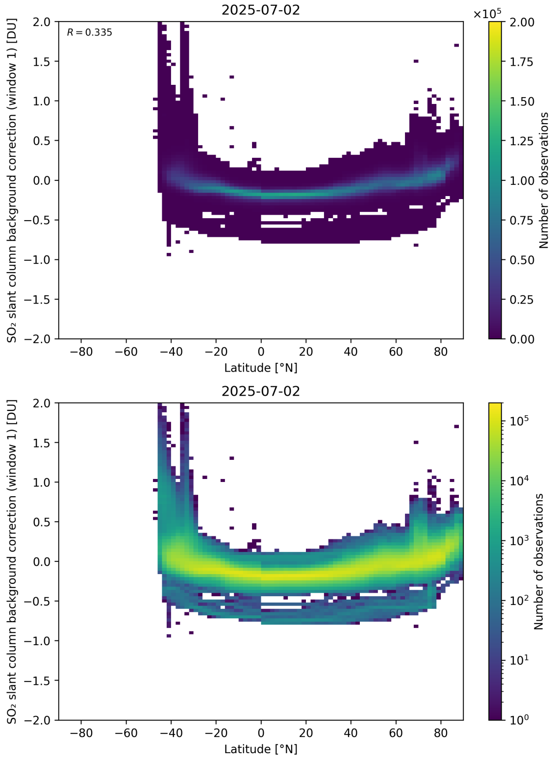
Figure 150: Scatter density plot of “Latitude” against “SO 2 slant column background correction (window 1)” for 2025-07-02 to 2025-07-03.
