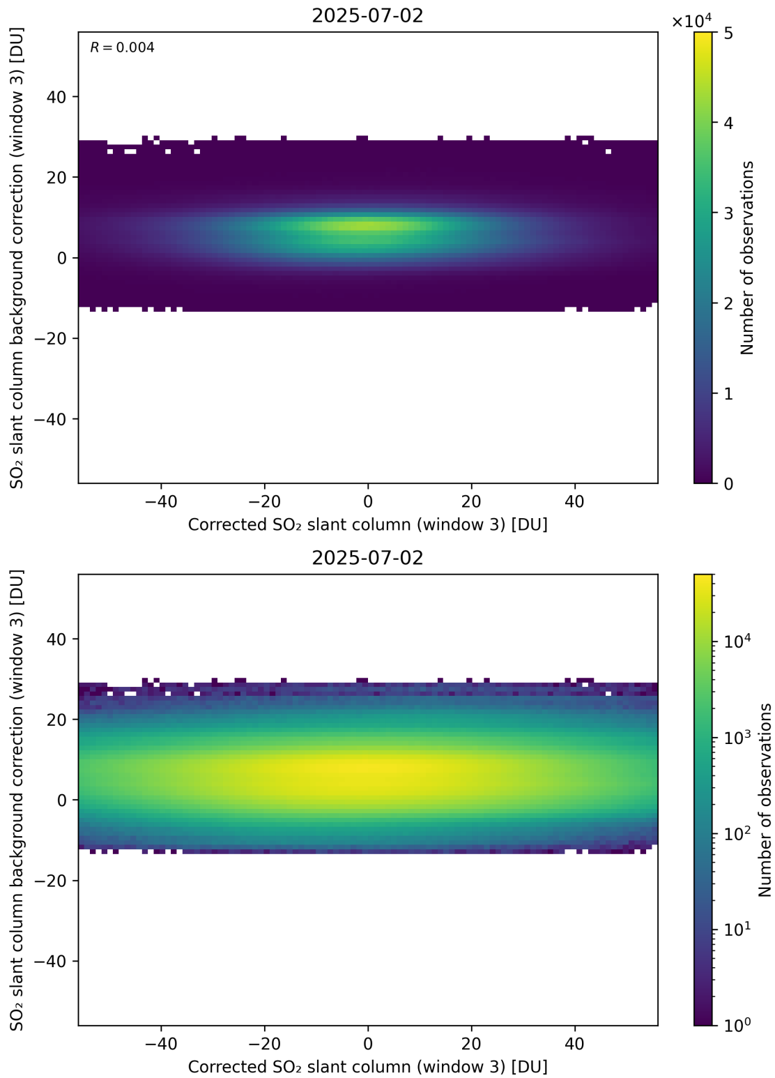
Figure 255: Scatter density plot of “Corrected SO 2 slant column (window 3)” against “SO 2 slant column background correction (window 3)” for 2025-07-02 to 2025-07-03.
