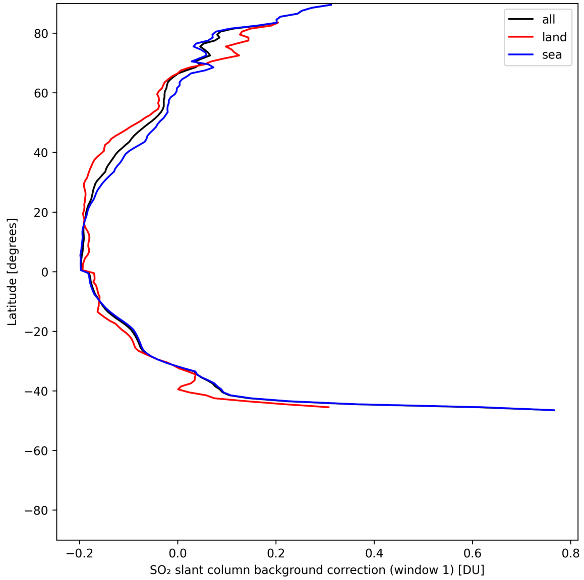
Figure 40: Zonal average of “SO 2 slant column background correction (window 1)” for 2025-07-02 to 2025-07-03.
