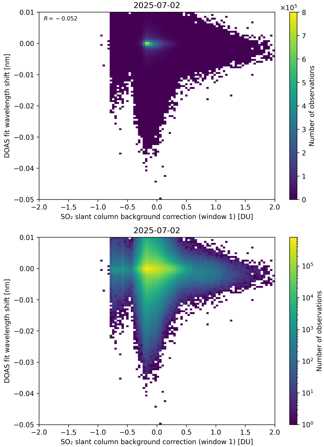
Figure 111: Scatter density plot of “SO 2 slant column background correction (window 1)” against “DOAS fit wavelength shift” for 2025-07-02 to 2025-07-03.
