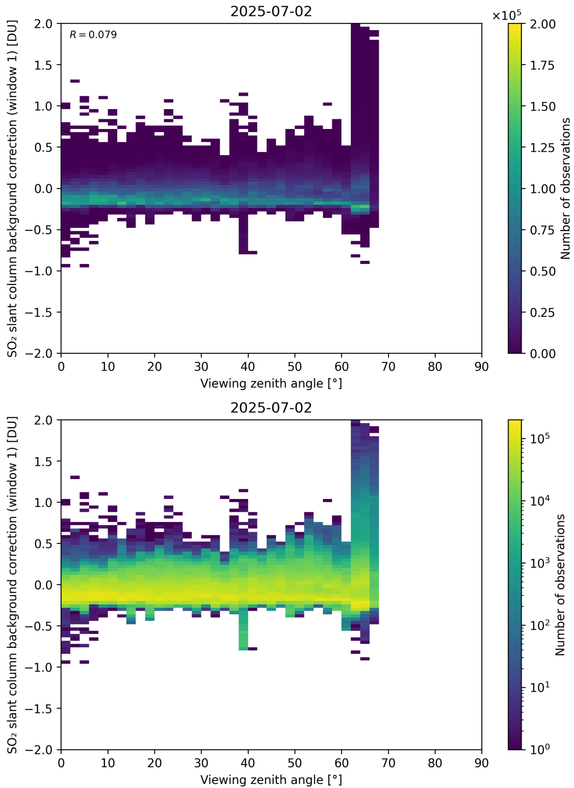
Figure 362: Scatter density plot of “Viewing zenith angle” against “SO 2 slant column background correction (window 1)” for 2025-07-02 to 2025-07-03.
