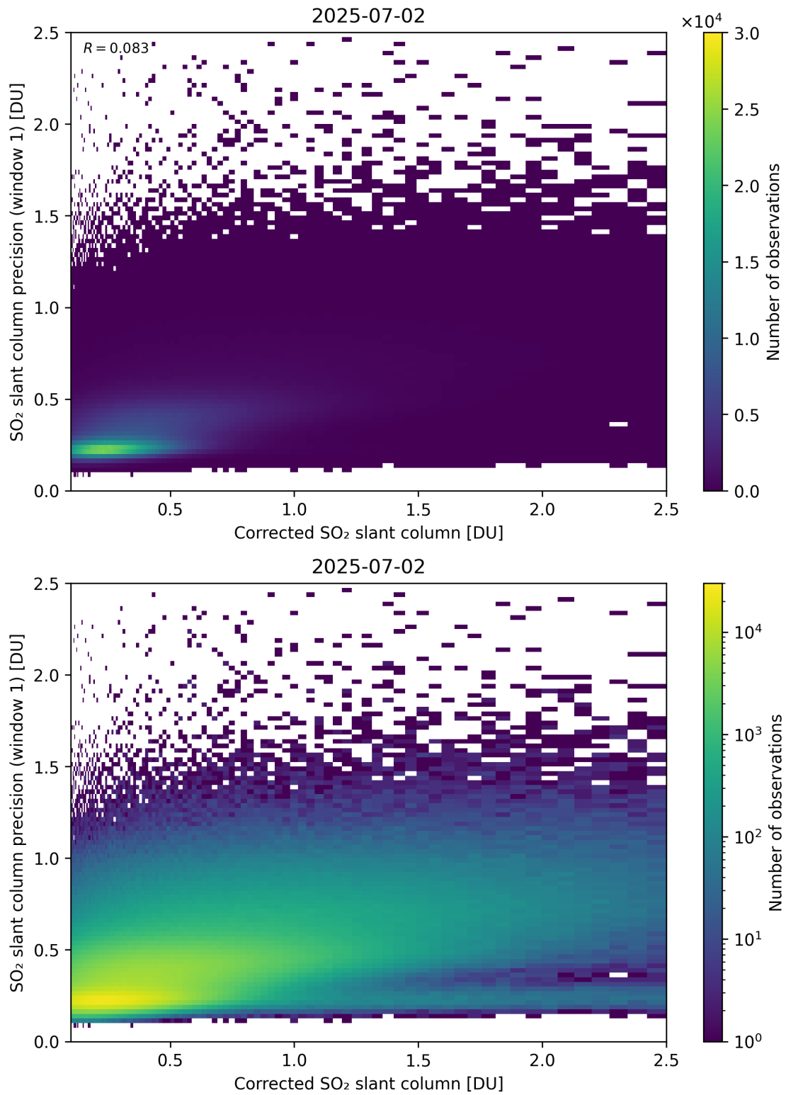
Figure 238: Scatter density plot of “Corrected SO 2 slant column” against “SO 2 slant column precision (window 1)” for 2025-07-02 to 2025-07-03.
