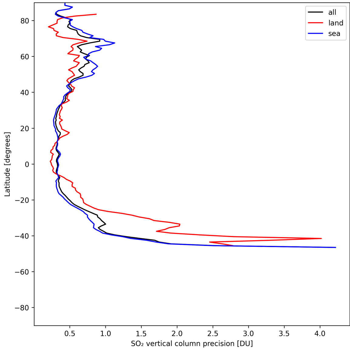
Figure 33: Zonal average of “SO 2 vertical column precision” for 2025-07-02 to 2025-07-03.
