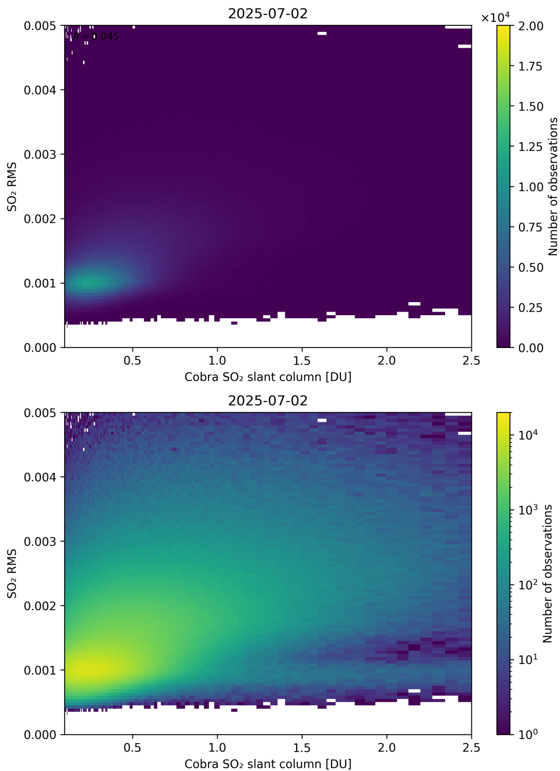
Figure 198: Scatter density plot of “Cobra SO 2 slant column” against “SO 2 RMS” for 2025-07-02 to 2025-07-03.
