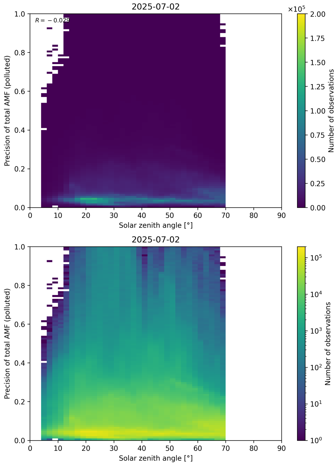
Figure 190: Scatter density plot of “Solar zenith angle” against “Precision of total AMF (polluted)” for 2025-07-02 to 2025-07-03.
