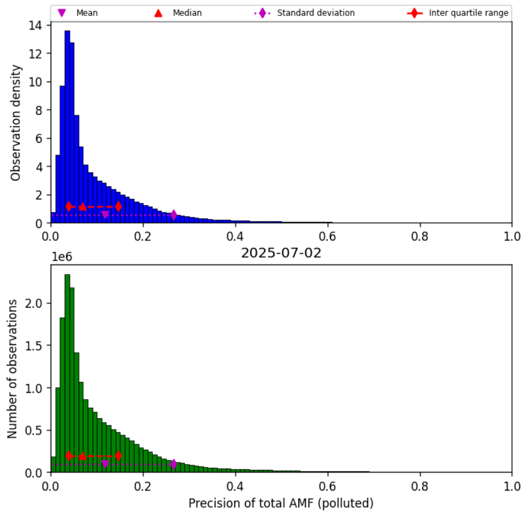
Figure 80: Histogram of “Precision of total AMF (polluted)” for 2025-07-02 to 2025-07-03
