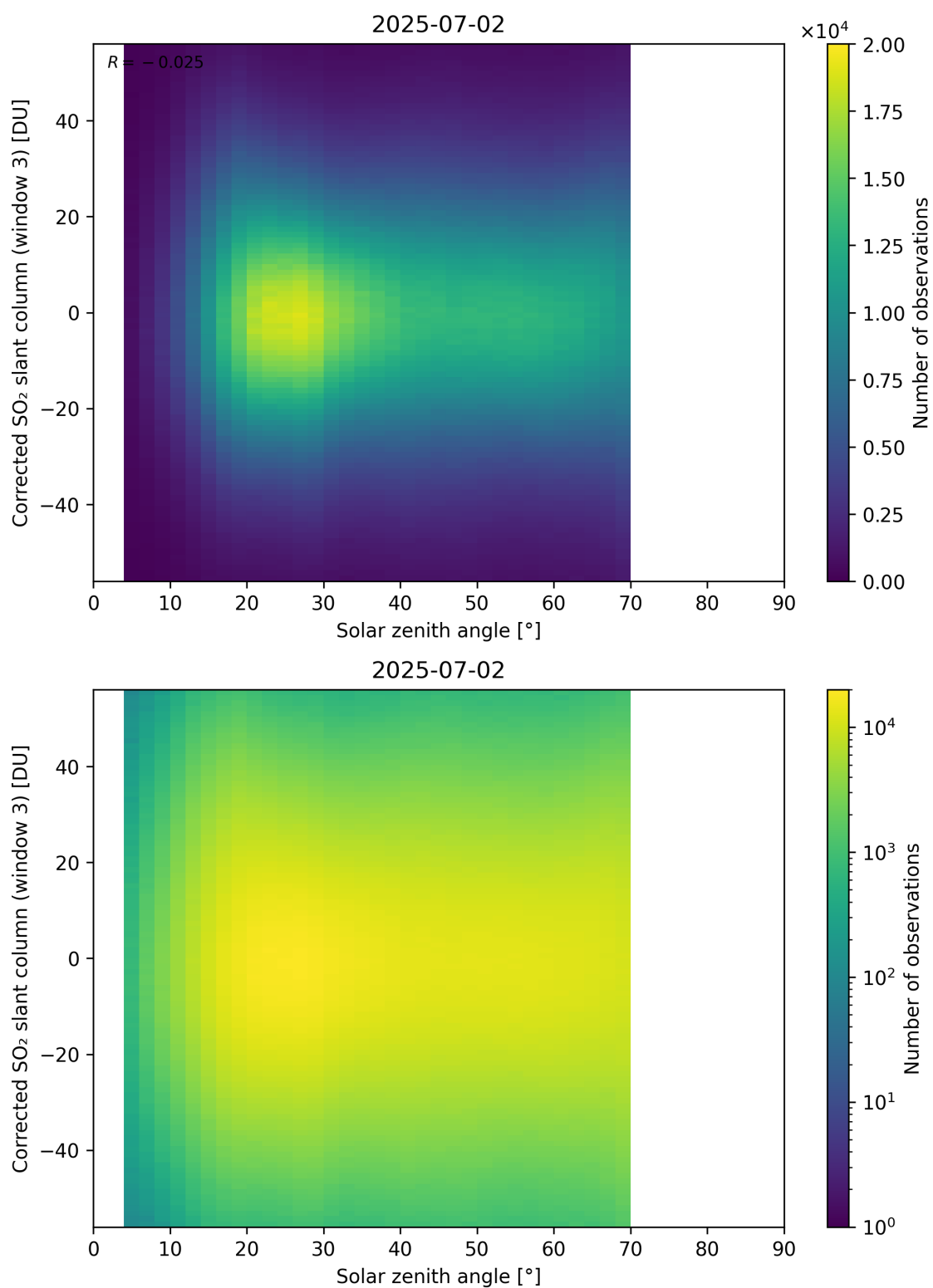
Figure 183: Scatter density plot of “Solar zenith angle” against “Corrected SO 2 slant column (window 3)” for 2025-07-02 to 2025-07-03.
