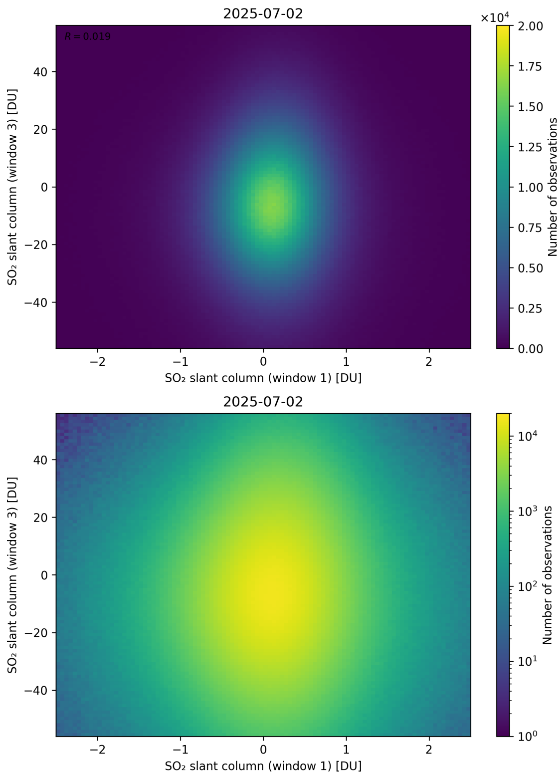
Figure 287: Scatter density plot of “SO 2 slant column (window 1)” against “SO 2 slant column (window 3)” for 2025-07-02 to 2025-07-03.
