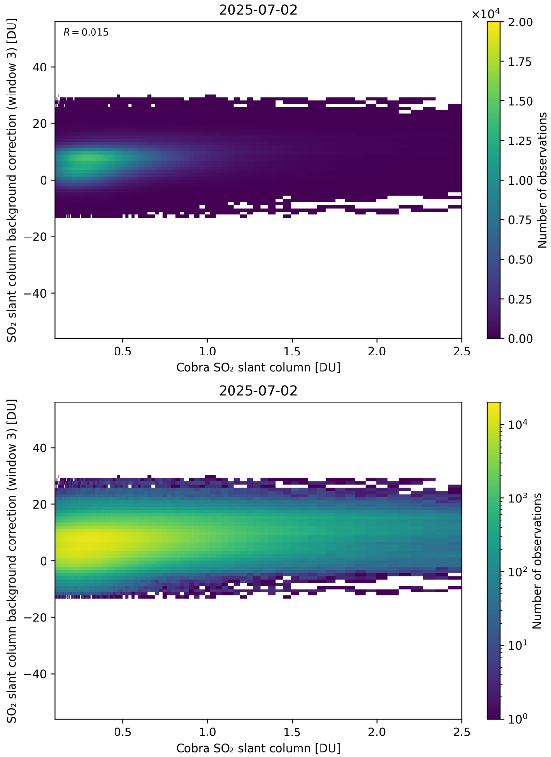
Figure 195: Scatter density plot of “Cobra SO 2 slant column” against “SO 2 slant column background correction (window 3)” for 2025-07-02 to 2025-07-03.
