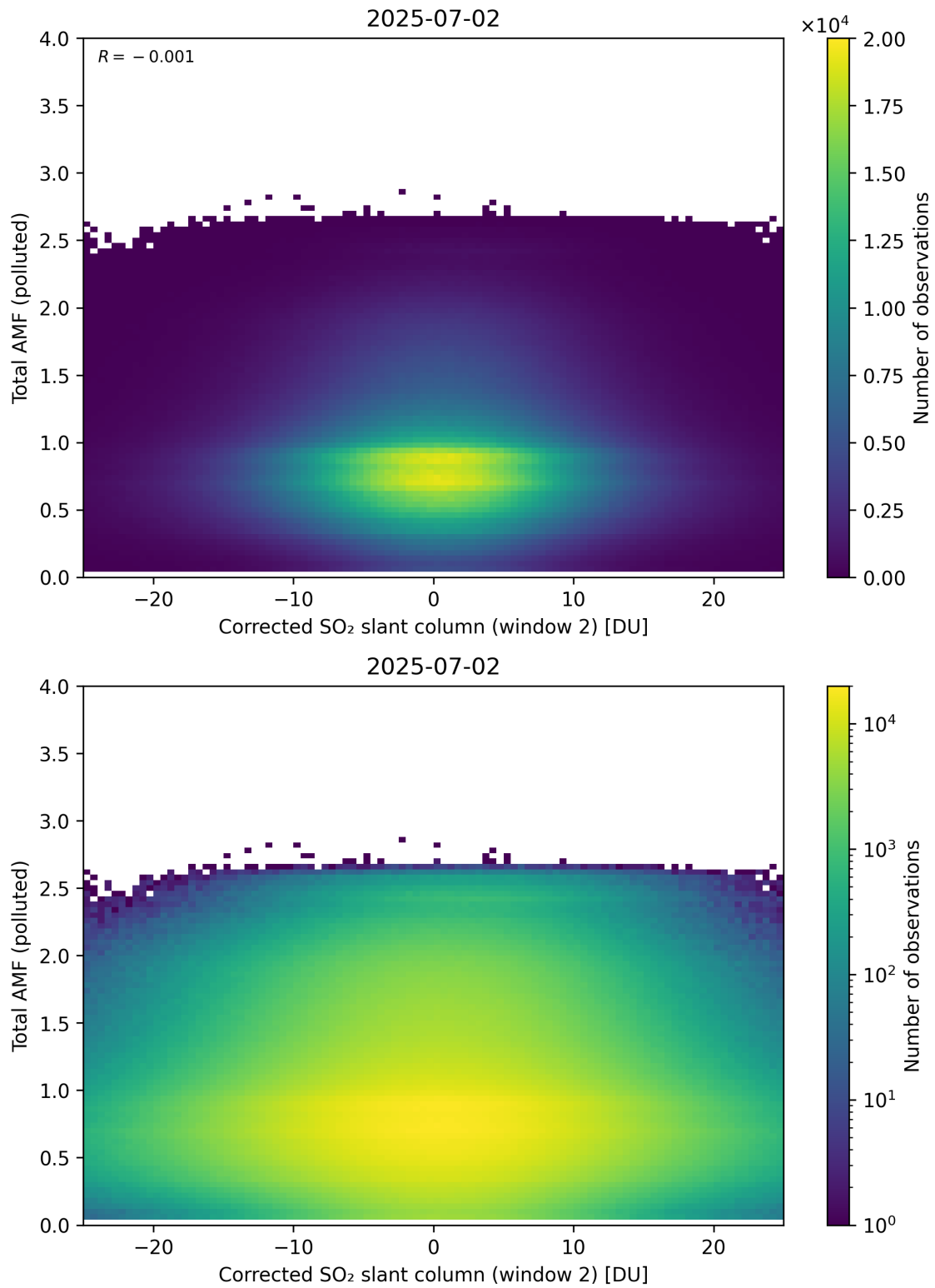
Figure 253: Scatter density plot of “Corrected SO 2 slant column (window 2)” against “Total AMF (polluted)” for 2025-07-02 to 2025-07-03.
