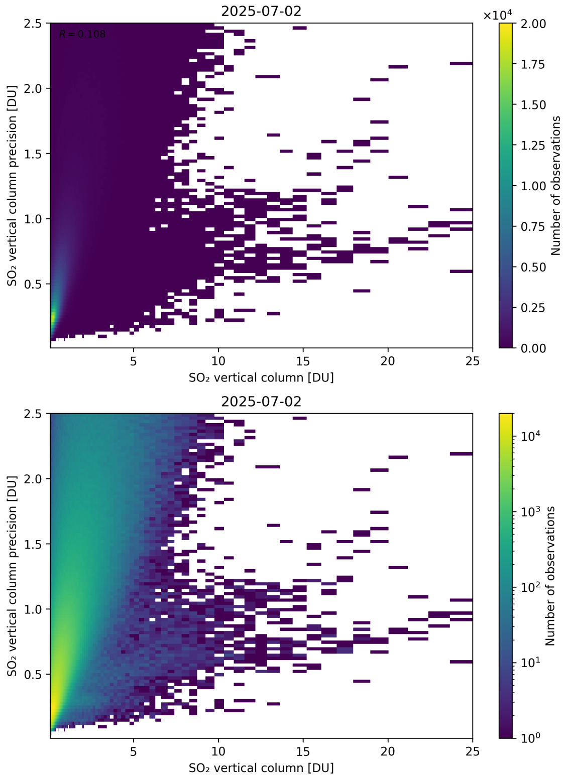
Figure 361: Scatter density plot of “SO 2 vertical column” against “SO 2 vertical column precision” for 2025-07-02 to 2025-07-03.
