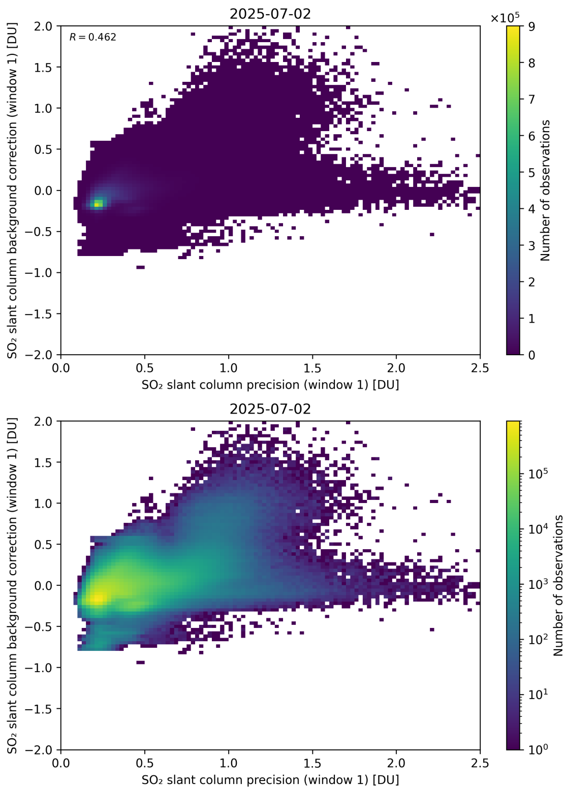
Figure 268: Scatter density plot of “SO 2 slant column precision (window 1)” against “SO 2 slant column background correction (window 1)” for 2025-07-02 to 2025-07-03.
