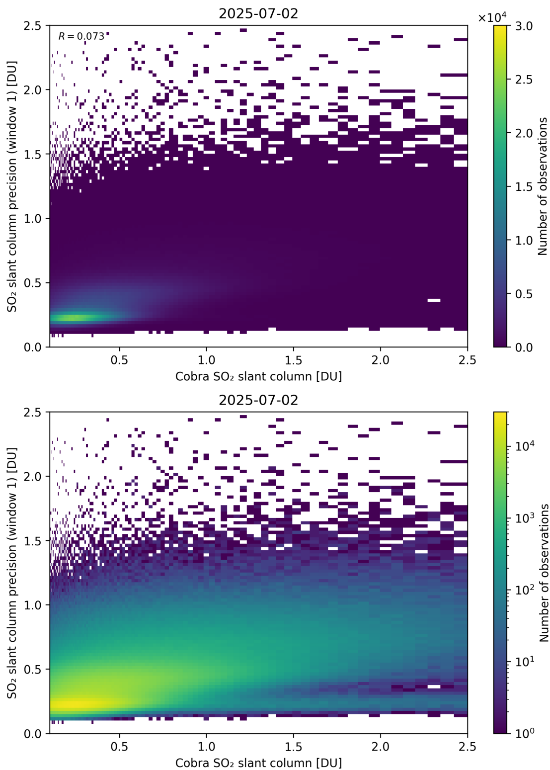
Figure 220: Scatter density plot of “Cobra SO 2 slant column” against “SO 2 slant column precision (window 1)” for 2025-07-02 to 2025-07-03.
