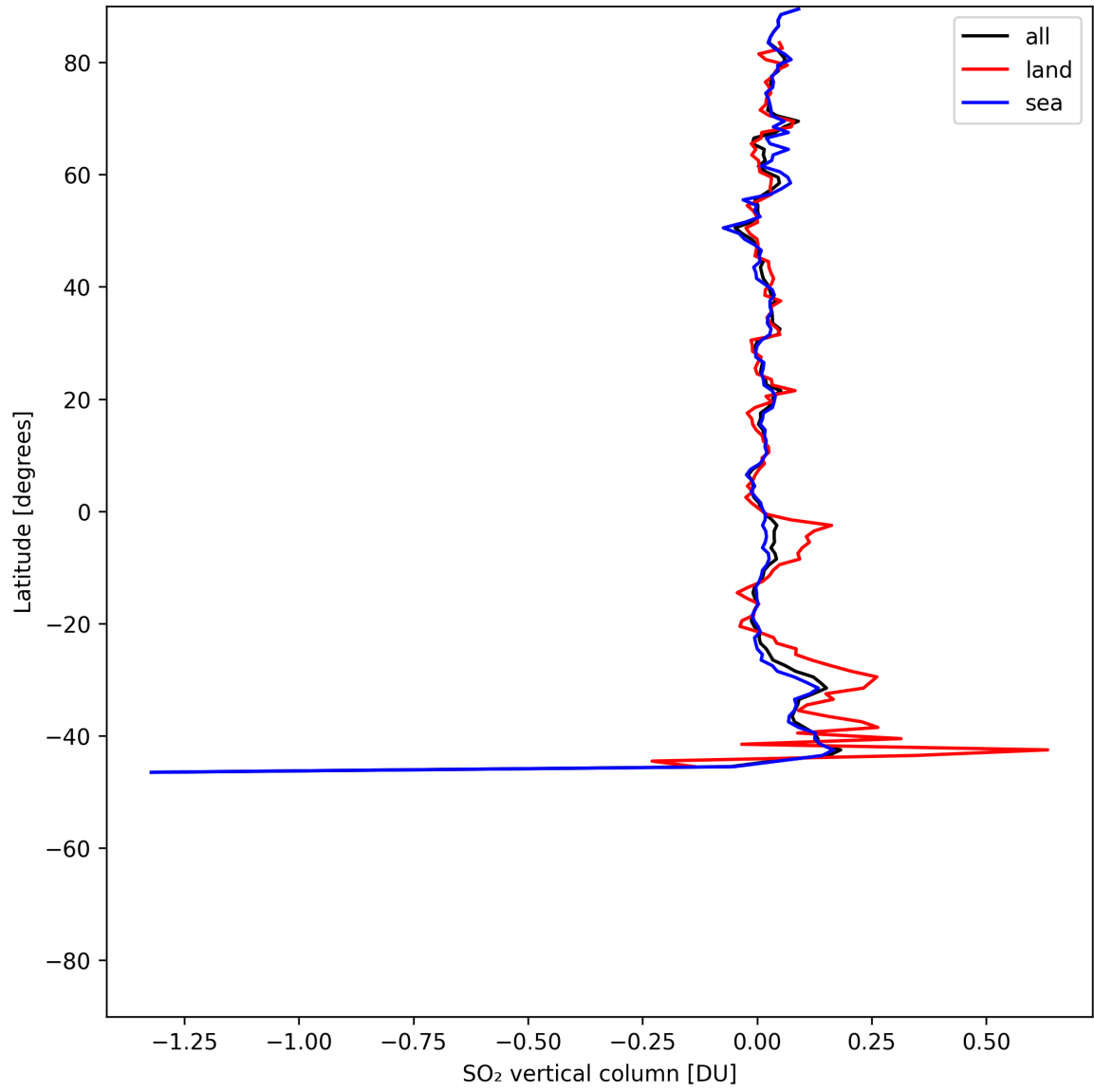
Figure 32: Zonal average of “SO 2 vertical column” for 2025-07-02 to 2025-07-03.
