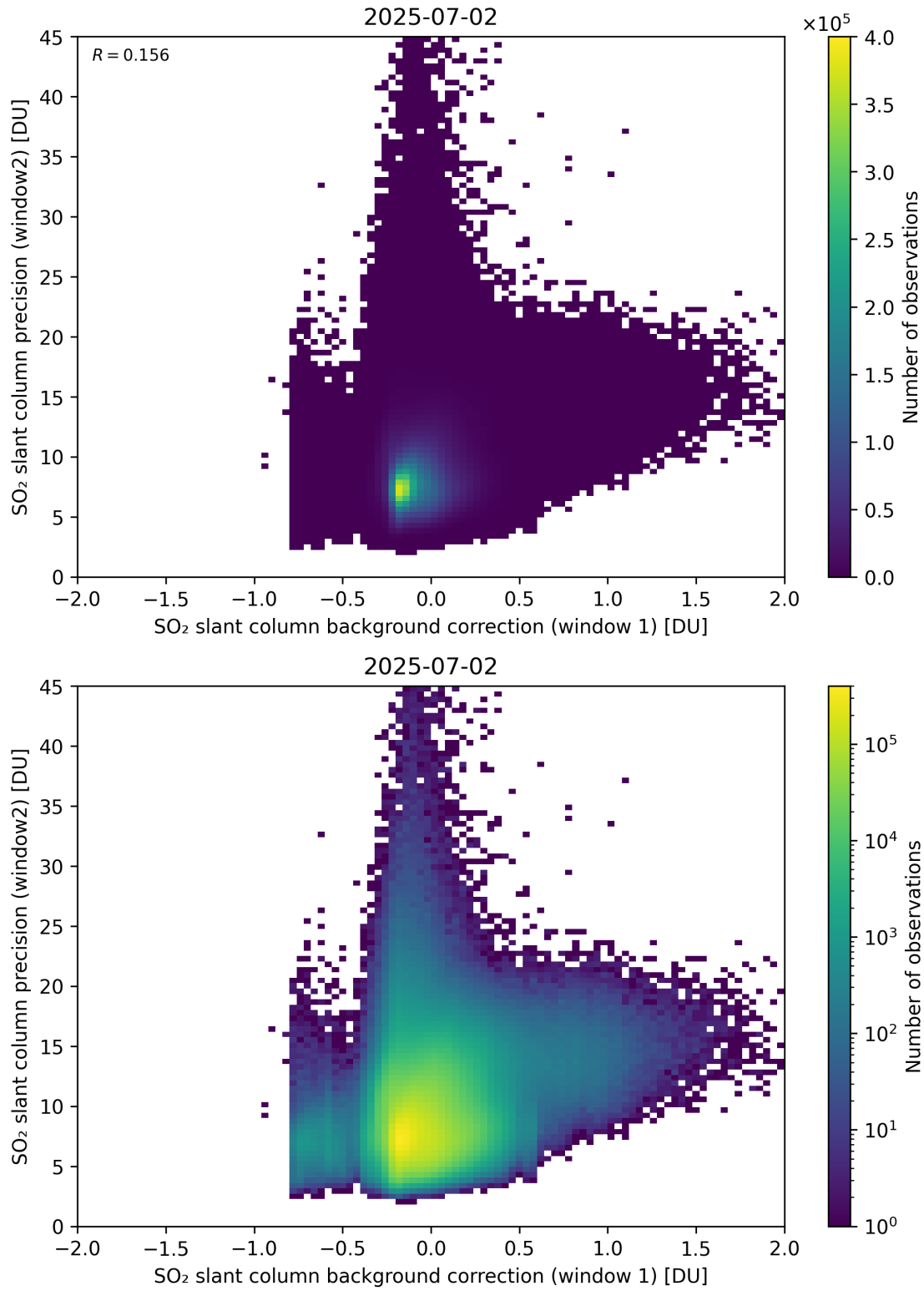
Figure 117: Scatter density plot of “SO 2 slant column background correction (window 1)” against “SO 2 slant column precision (window2)” for 2025-07-02 to 2025-07-03.
