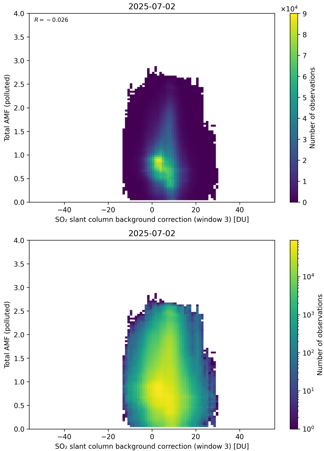
Figure 136: Scatter density plot of “SO 2 slant column background correction (window 3)” against “Total AMF (polluted)” for 2025-07-02 to 2025-07-03.
