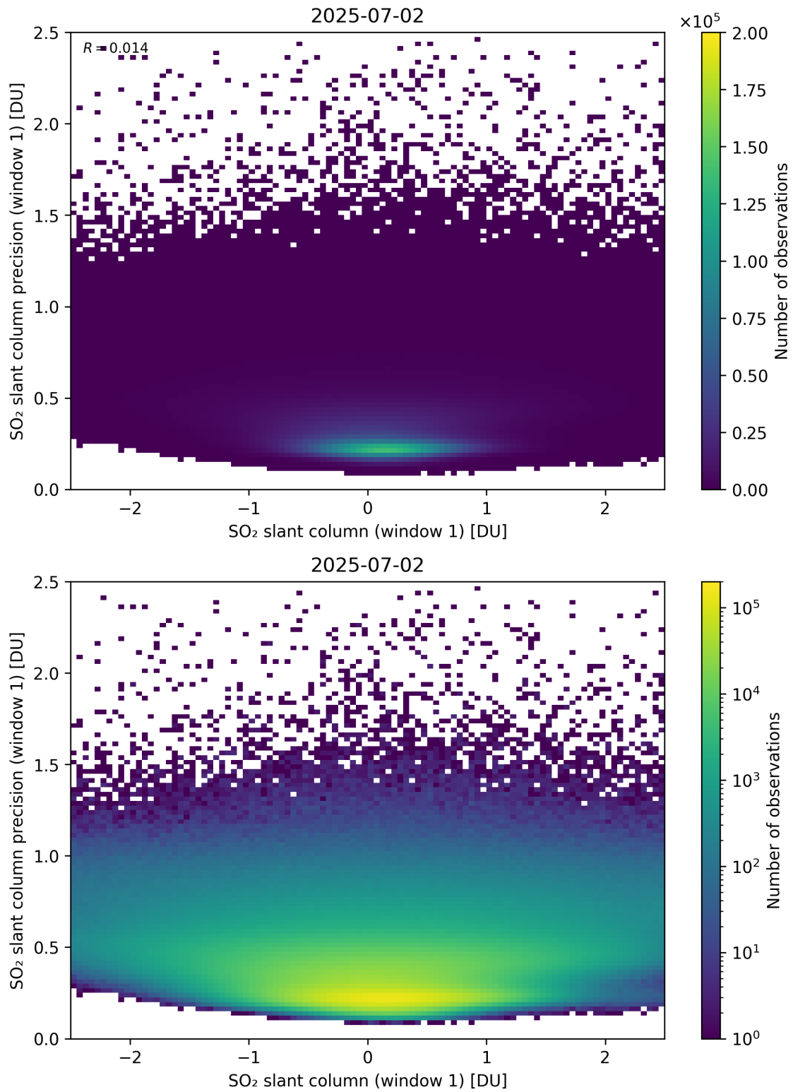
Figure 285: Scatter density plot of “SO 2 slant column (window 1)” against “SO 2 slant column precision (window 1)” for 2025-07-02 to 2025-07-03.
