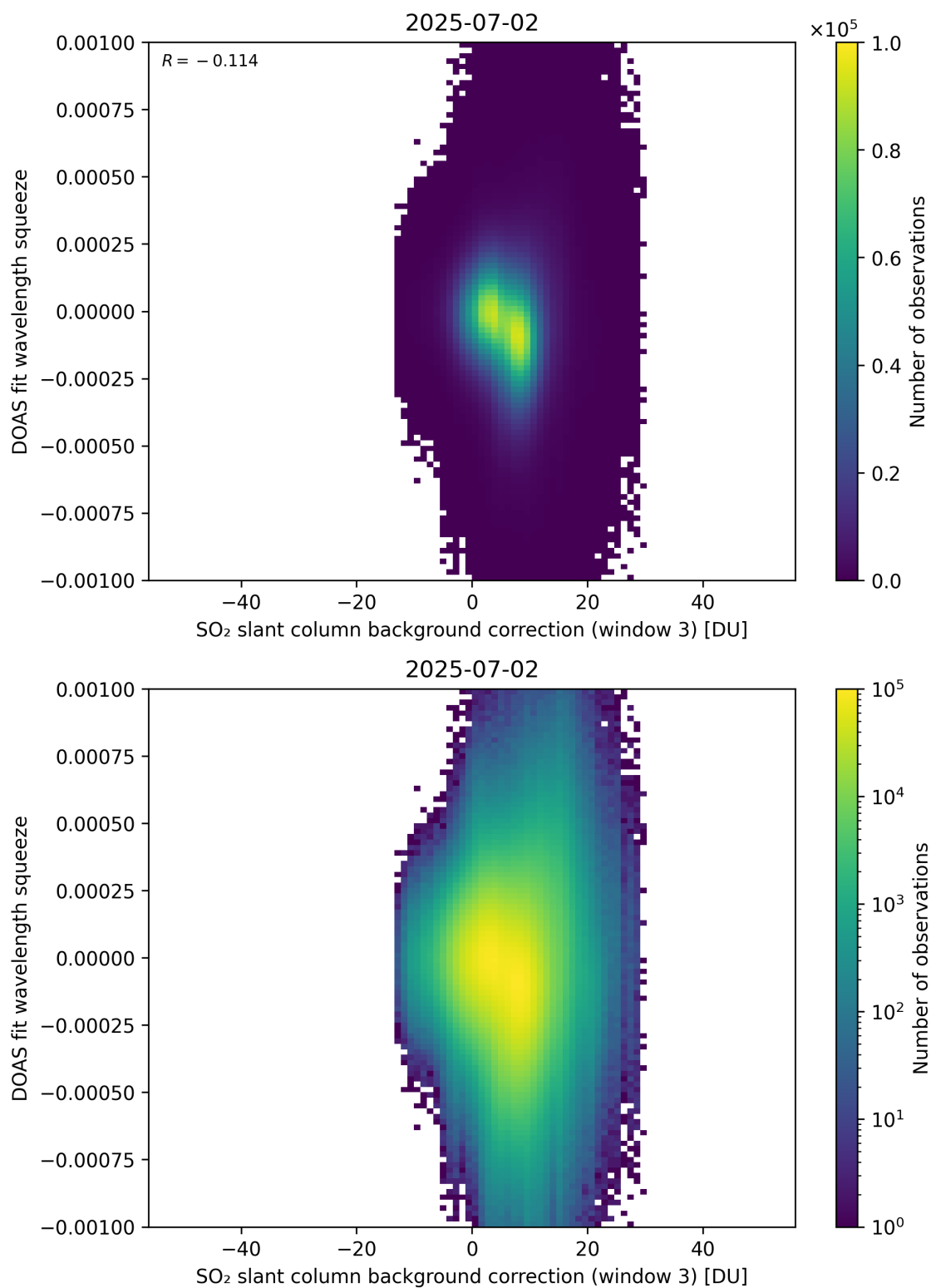
Figure 133: Scatter density plot of “SO 2 slant column background correction (window 3)” against “DOAS fit wavelength squeeze” for 2025-07-02 to 2025-07-03.
