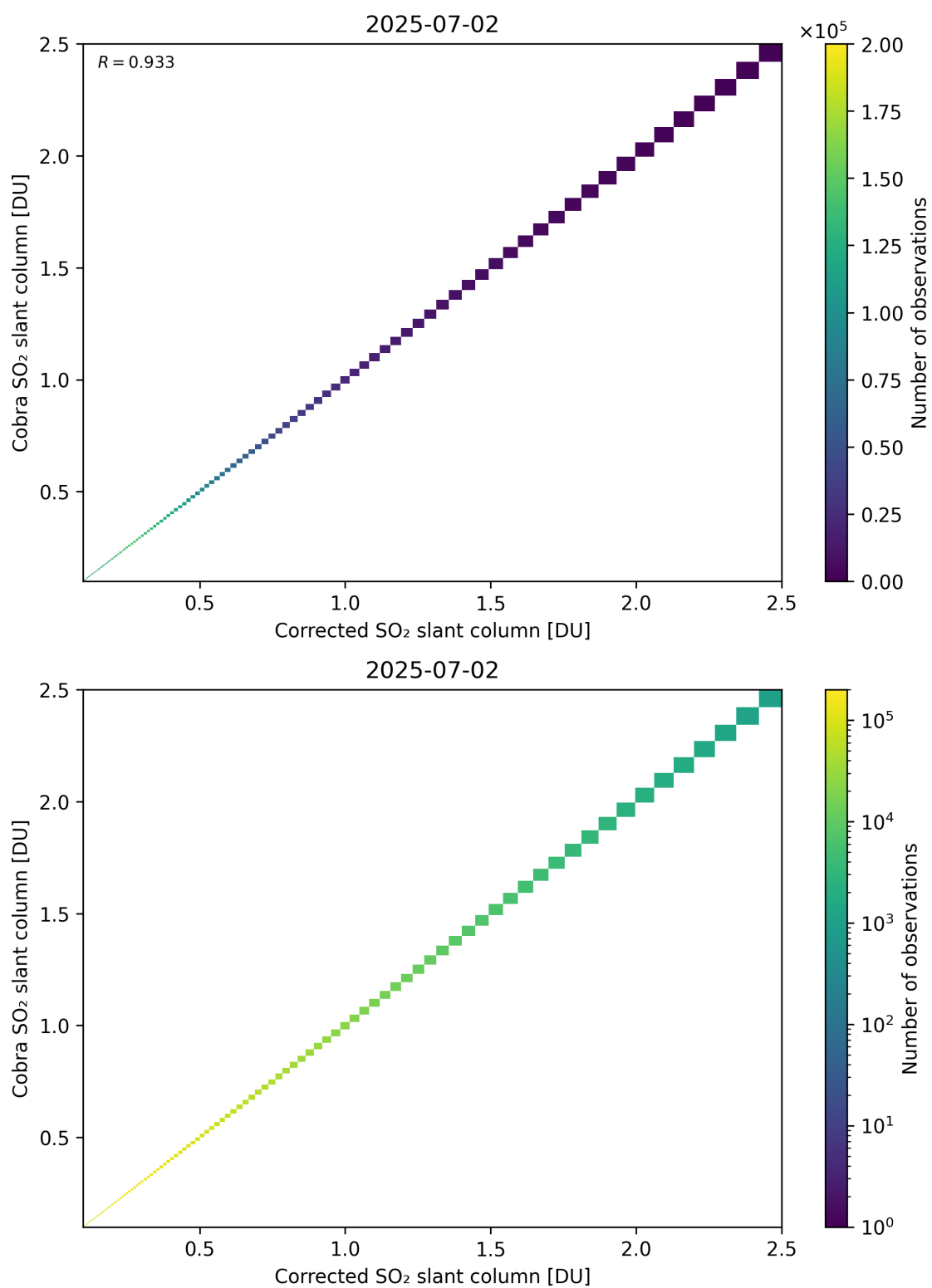
Figure 233: Scatter density plot of “Corrected SO 2 slant column” against “Cobra SO 2 slant column” for 2025-07-02 to 2025-07-03.
