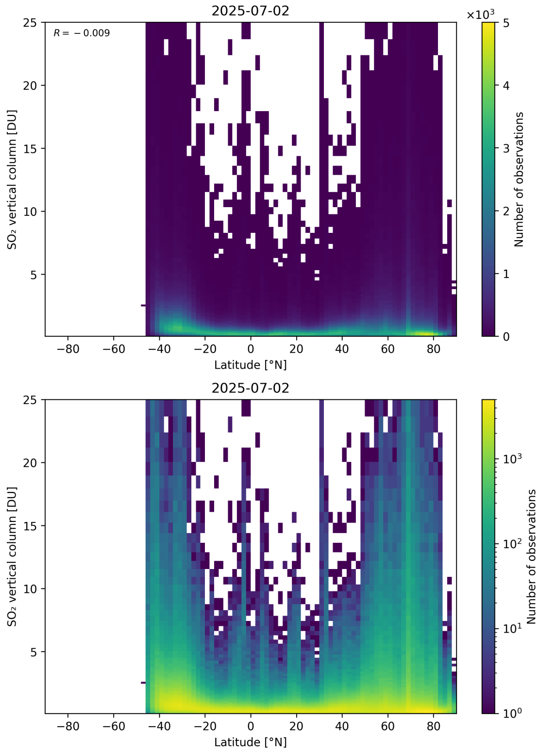
Figure 169: Scatter density plot of “Latitude” against “SO 2 vertical column” for 2025-07-02 to 2025-07-03.
