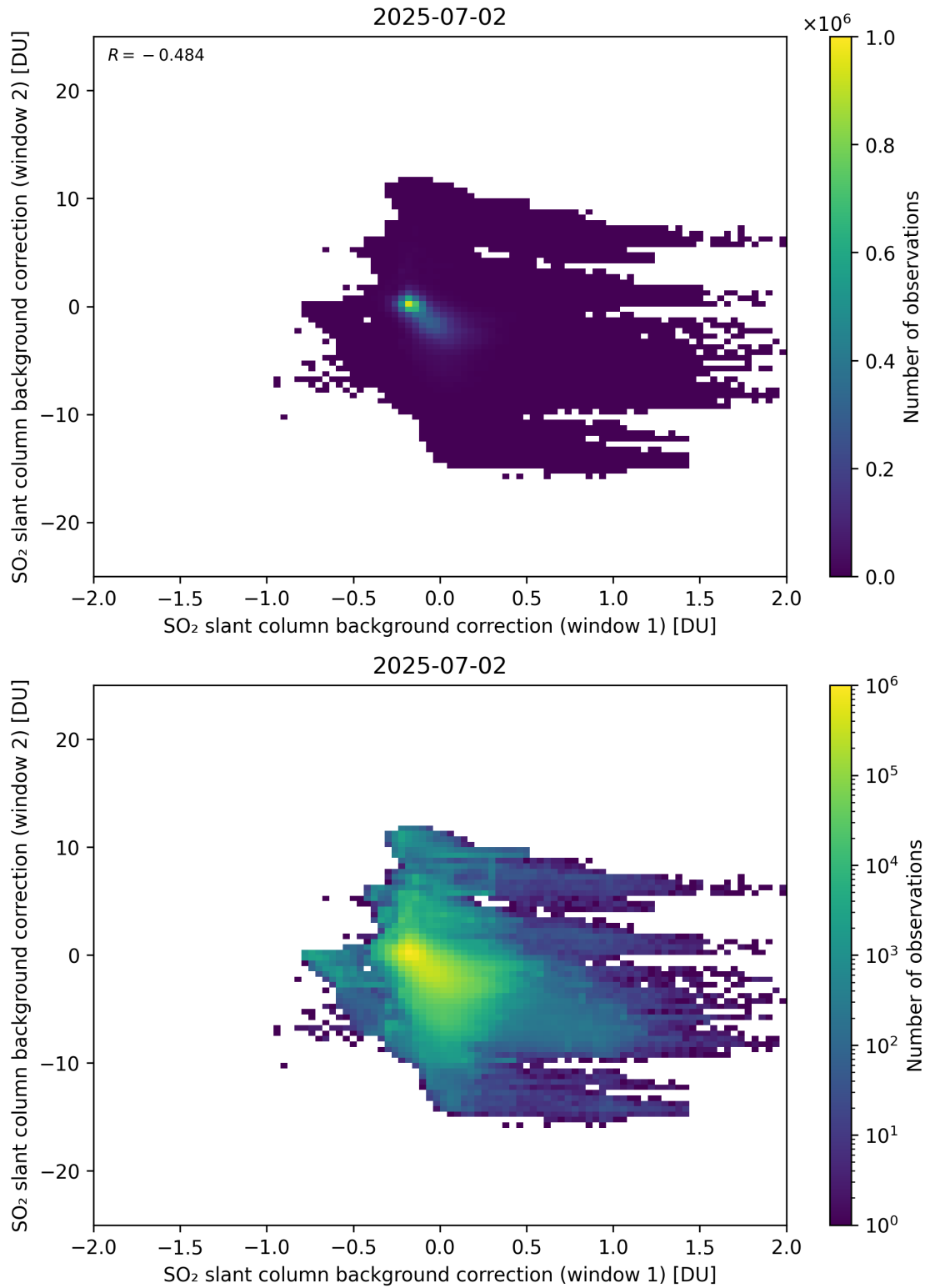
Figure 109: Scatter density plot of “SO 2 slant column background correction (window 1)” against “SO 2 slant column background correction (window 2)” for 2025-07-02 to 2025-07-03.
