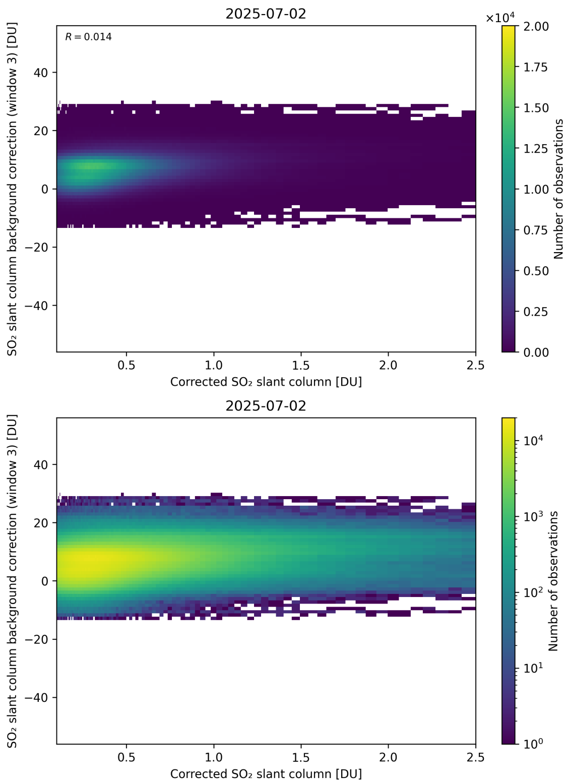
Figure 228: Scatter density plot of “Corrected SO 2 slant column” against “SO 2 slant column background correction (window 3)” for 2025-07-02 to 2025-07-03.
