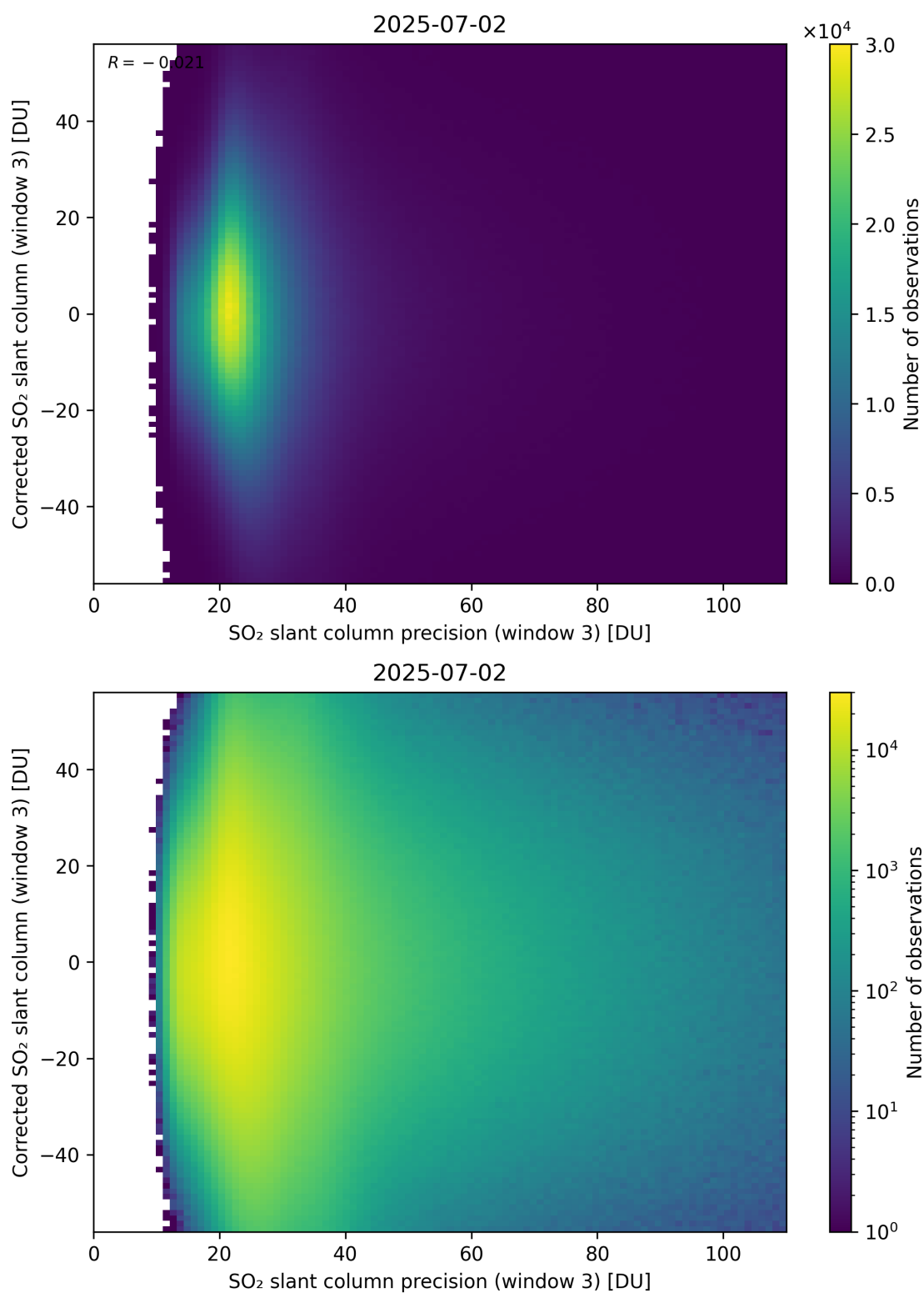
Figure 312: Scatter density plot of “SO 2 slant column precision (window 3)” against “Corrected SO 2 slant column (window 3)” for 2025-07-02 to 2025-07-03.
