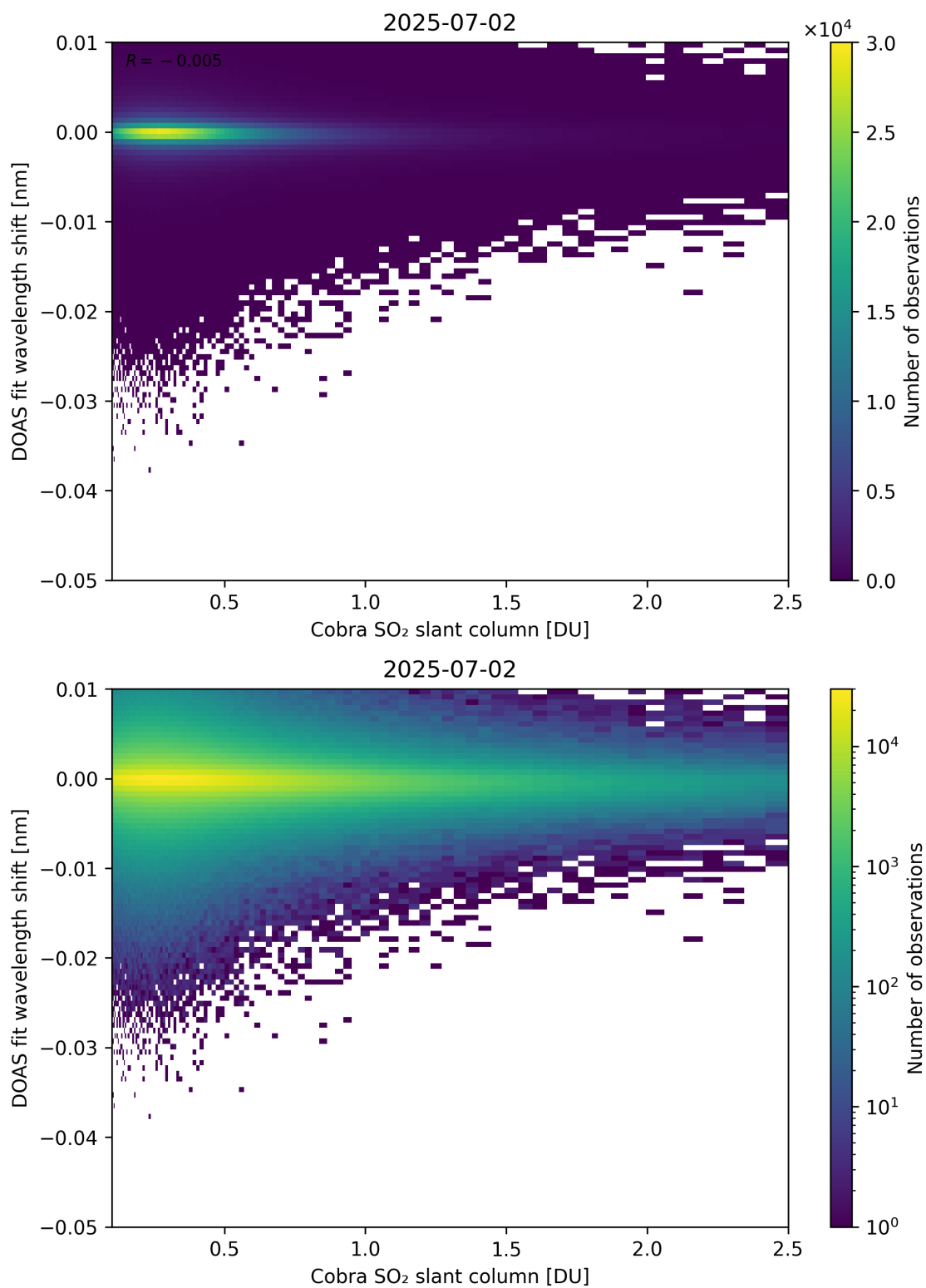
Figure 196: Scatter density plot of “Cobra SO 2 slant column” against “DOAS fit wavelength shift” for 2025-07-02 to 2025-07-03.
