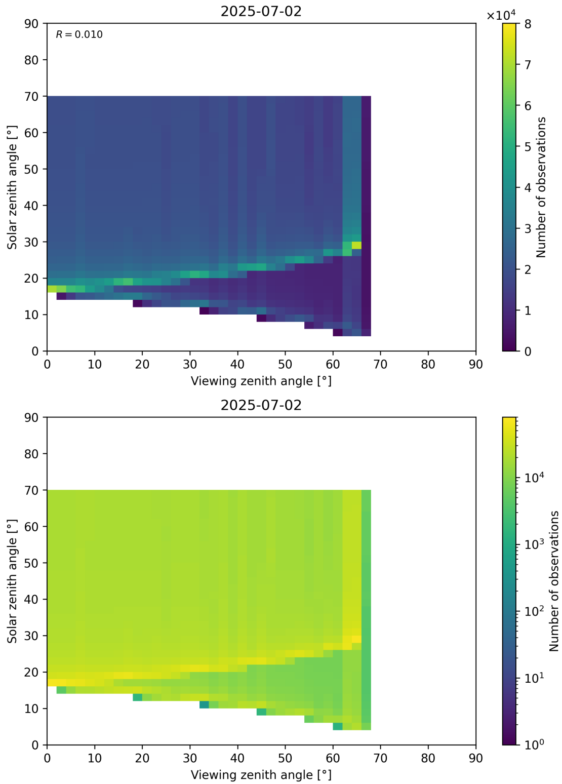
Figure 369: Scatter density plot of “Viewing zenith angle” against “Solar zenith angle” for 2025-07-02 to 2025-07-03.
