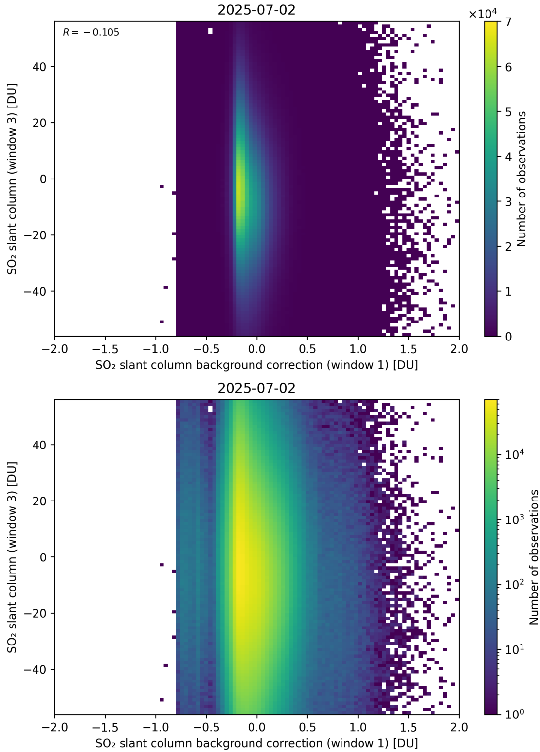
Figure 118: Scatter density plot of “SO 2 slant column background correction (window 1)” against “SO 2 slant column (window 3)” for 2025-07-02 to 2025-07-03.
