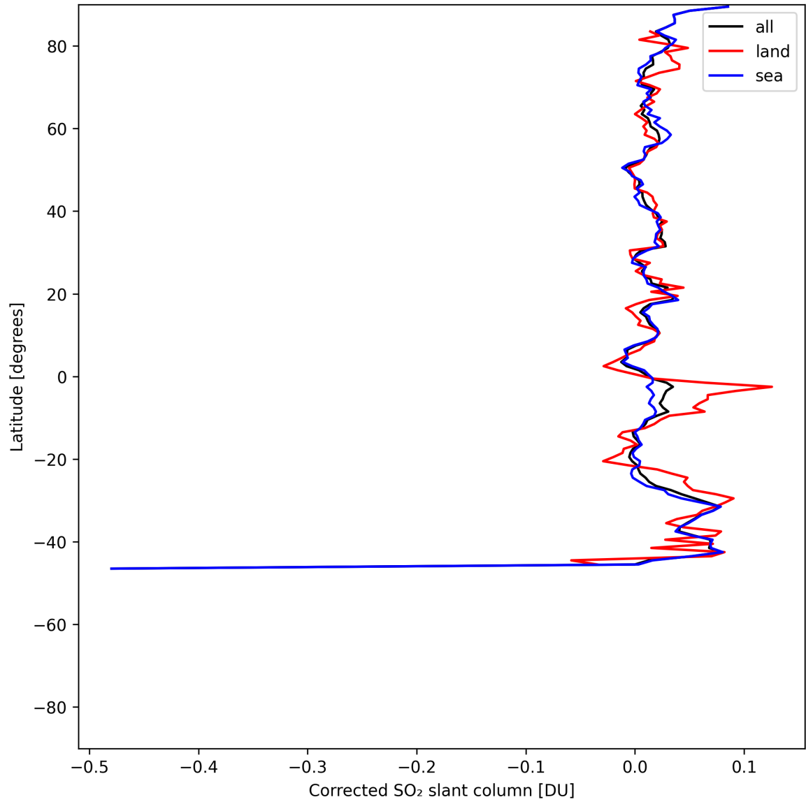
Figure 34: Zonal average of “Corrected SO 2 slant column” for 2025-07-02 to 2025-07-03.
