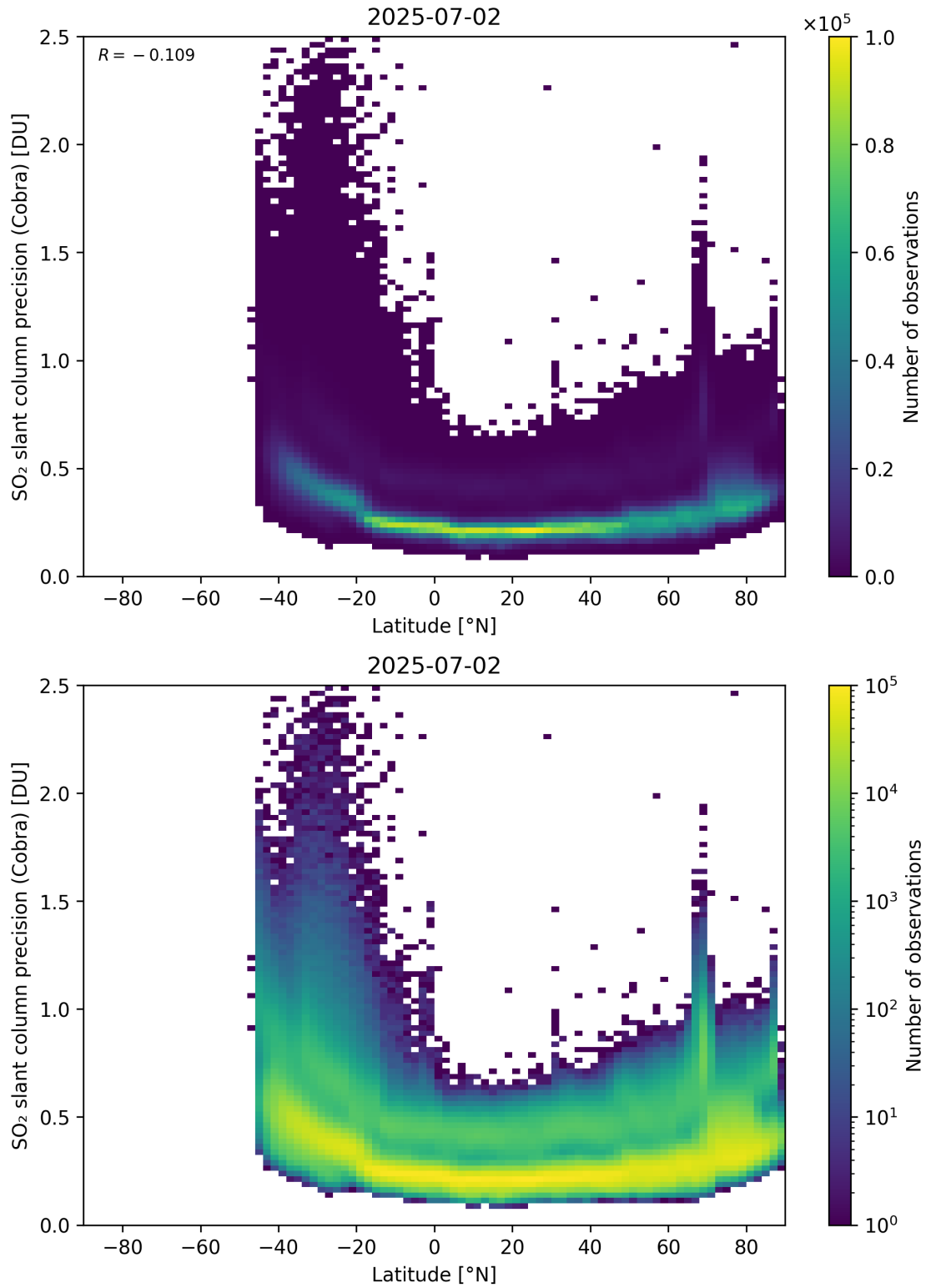
Figure 158: Scatter density plot of “Latitude” against “SO 2 slant column precision (Cobra)” for 2025-07-02 to 2025-07-03.
