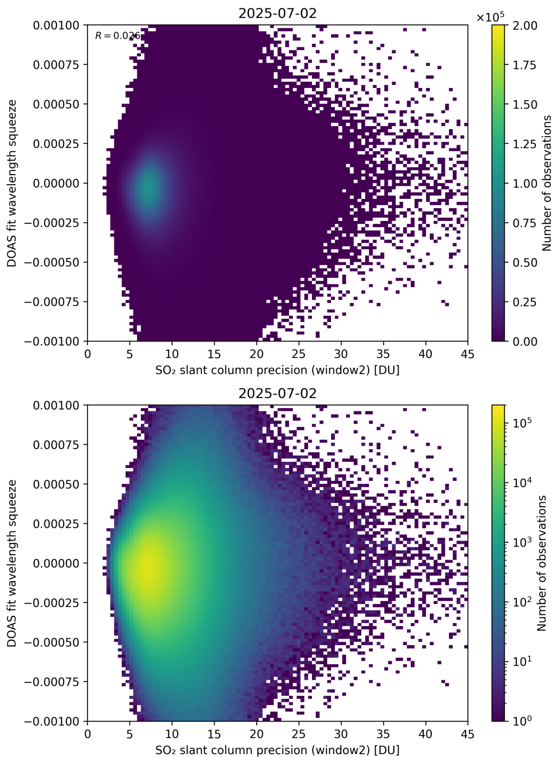
Figure 294: Scatter density plot of “SO 2 slant column precision (window2)” against “DOAS fit wavelength squeeze” for 2025-07-02 to 2025-07-03.
