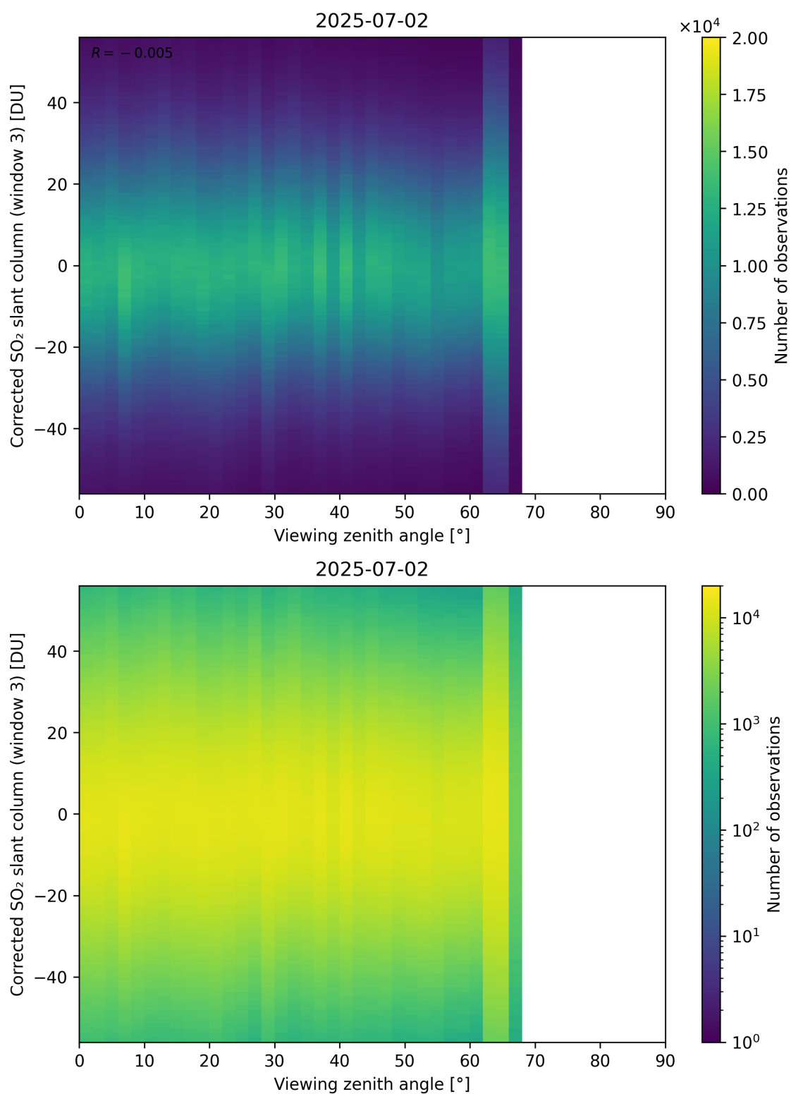
Figure 375: Scatter density plot of “Viewing zenith angle” against “Corrected SO 2 slant column (window 3)” for 2025-07-02 to 2025-07-03.
