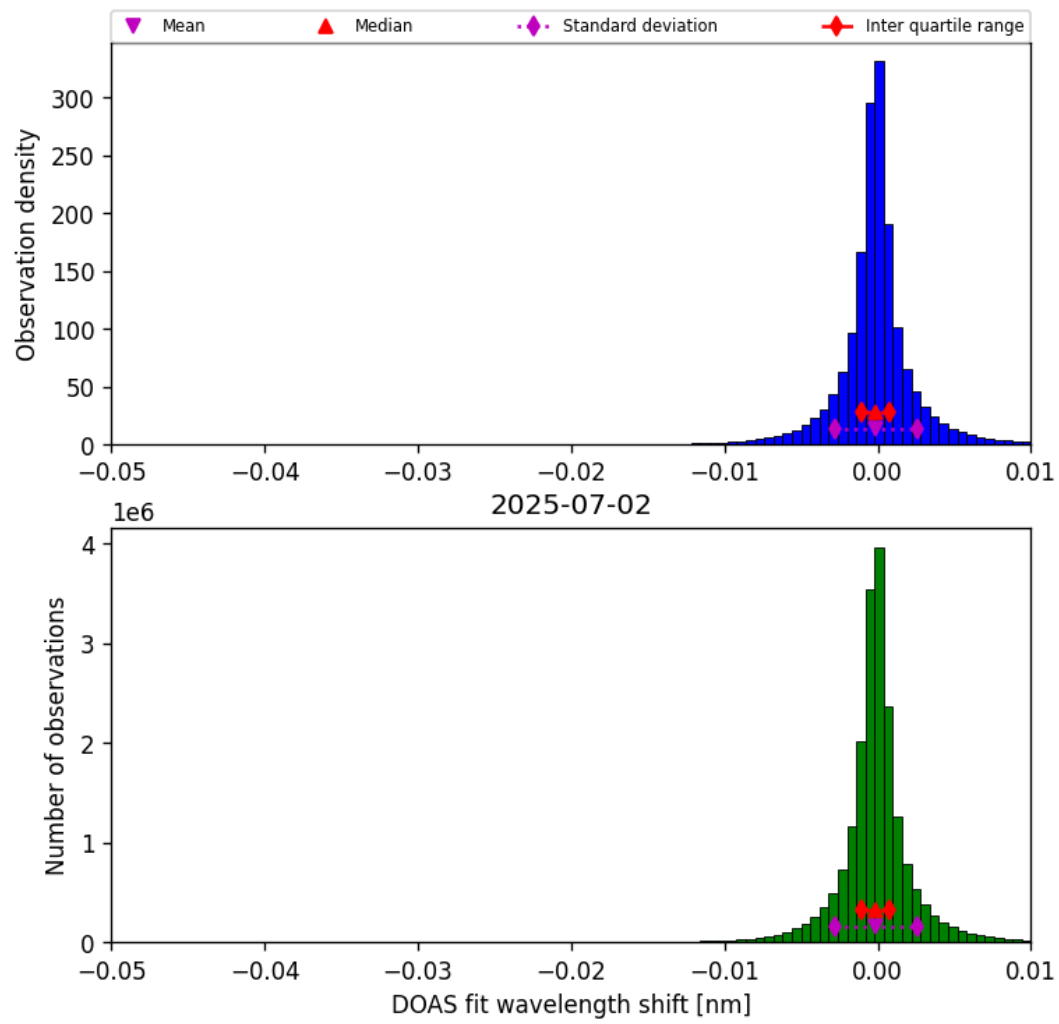
Figure 76: Histogram of “DOAS fit wavelength shift” for 2025-07-02 to 2025-07-03
