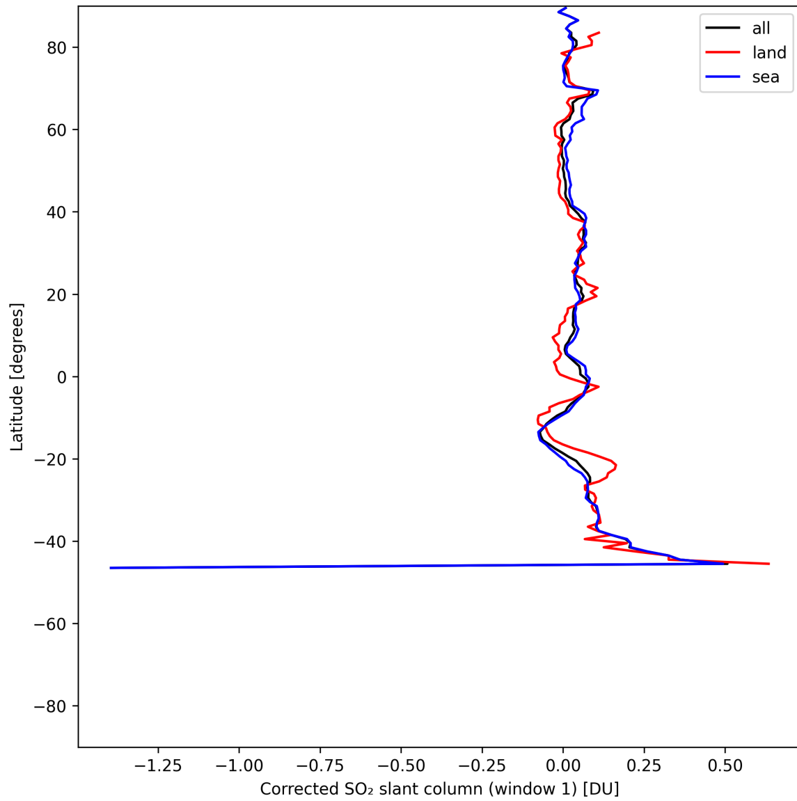
Figure 39: Zonal average of “Corrected SO 2 slant column (window 1)” for 2025-07-02 to 2025-07-03.
