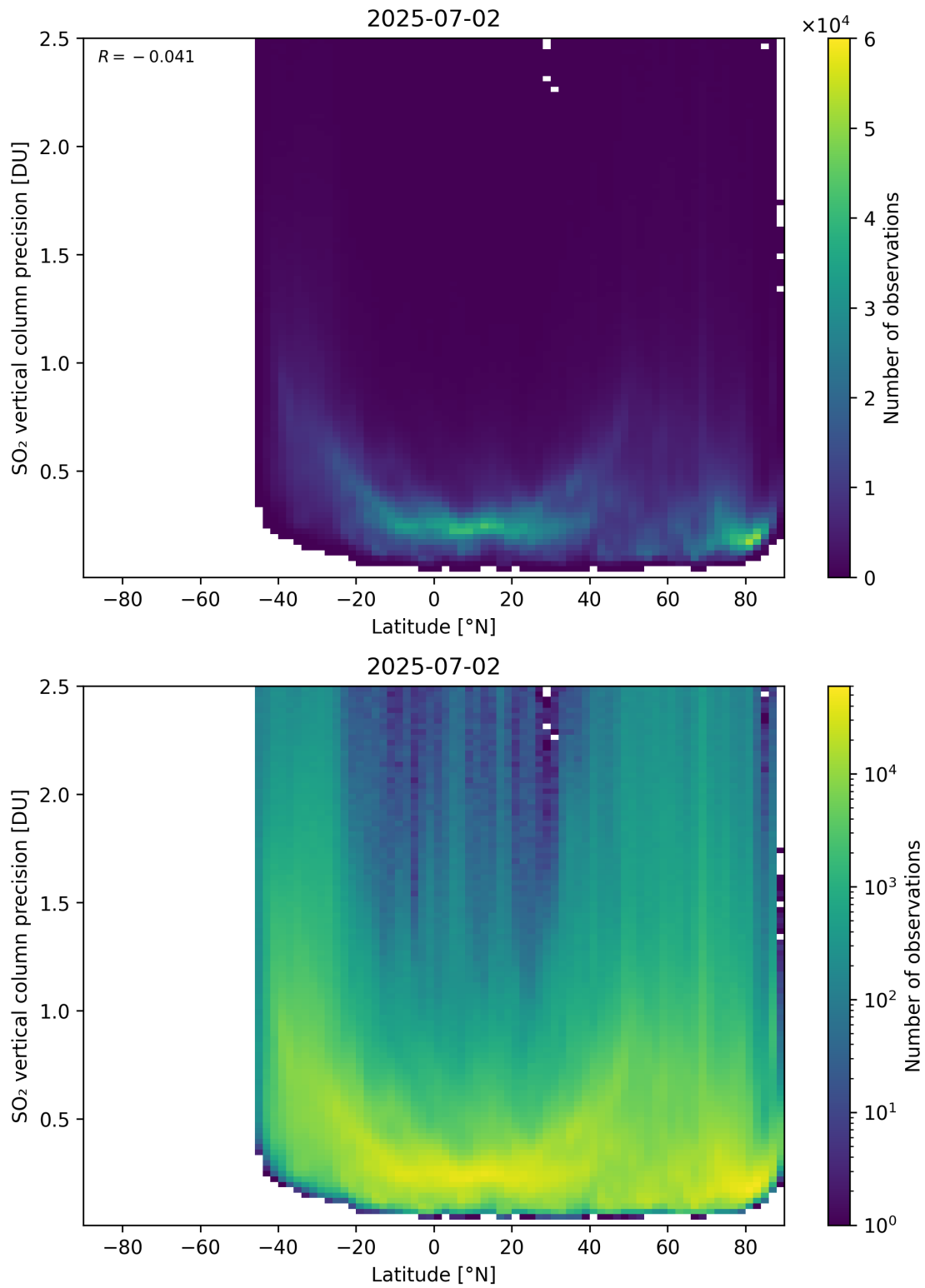
Figure 170: Scatter density plot of “Latitude” against “SO 2 vertical column precision” for 2025-07-02 to 2025-07-03.
