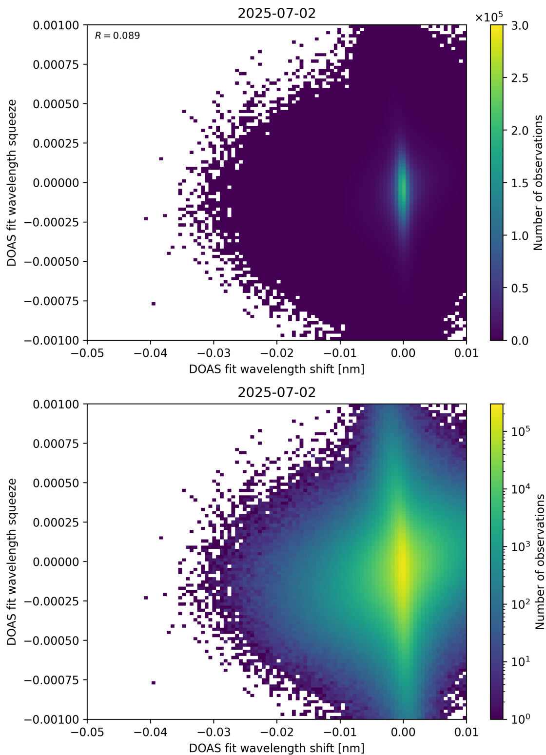
Figure 138: Scatter density plot of “DOAS fit wavelength shift” against “DOAS fit wavelength squeeze” for 2025-07-02 to 2025-07-03.
