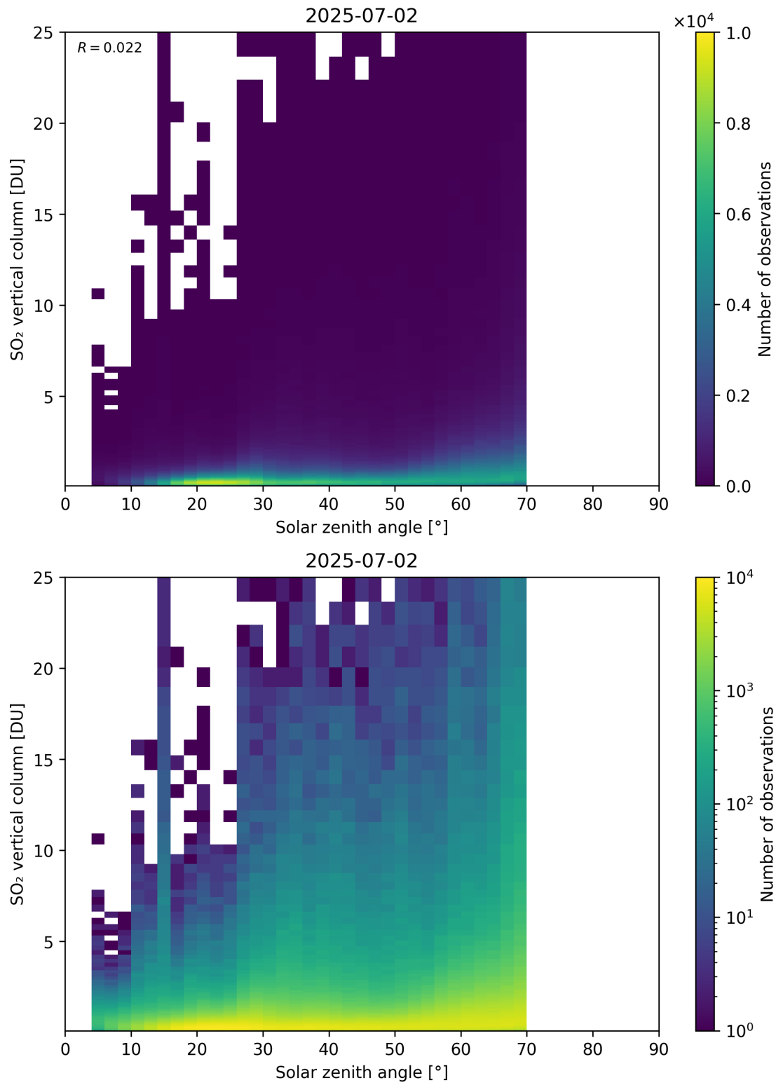
Figure 191: Scatter density plot of “Solar zenith angle” against “SO 2 vertical column” for 2025-07-02 to 2025-07-03.
