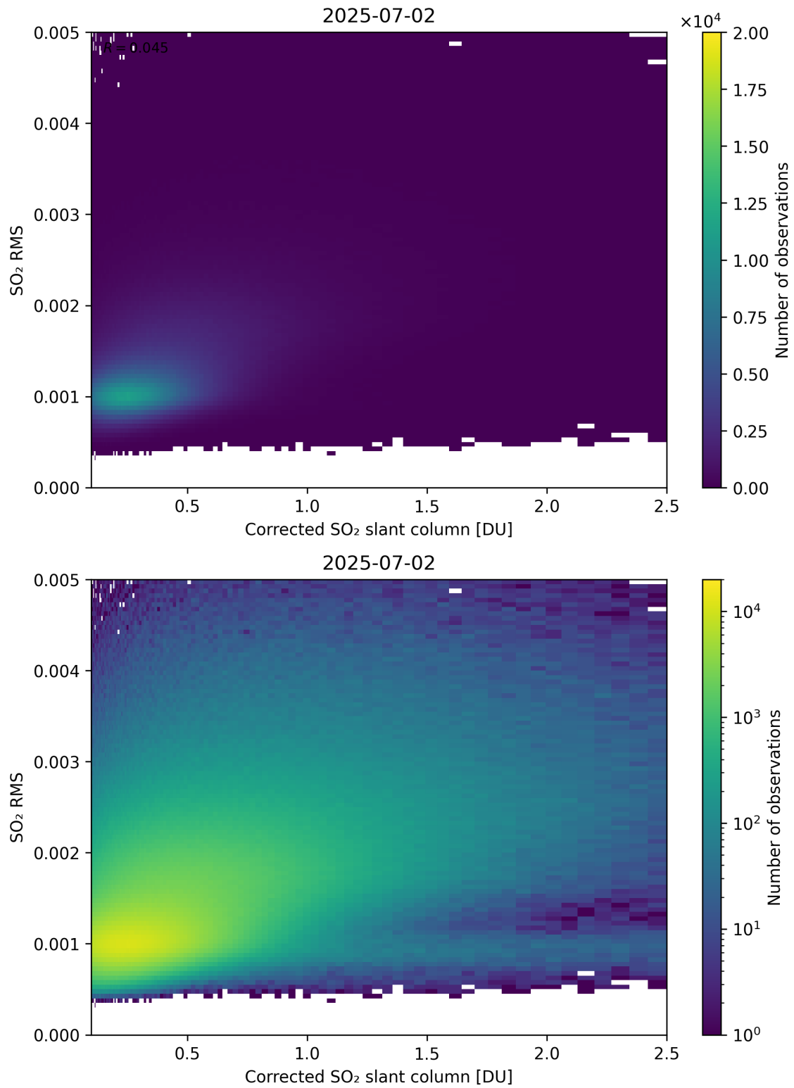
Figure 231: Scatter density plot of “Corrected SO 2 slant column” against “SO 2 RMS” for 2025-07-02 to 2025-07-03.
