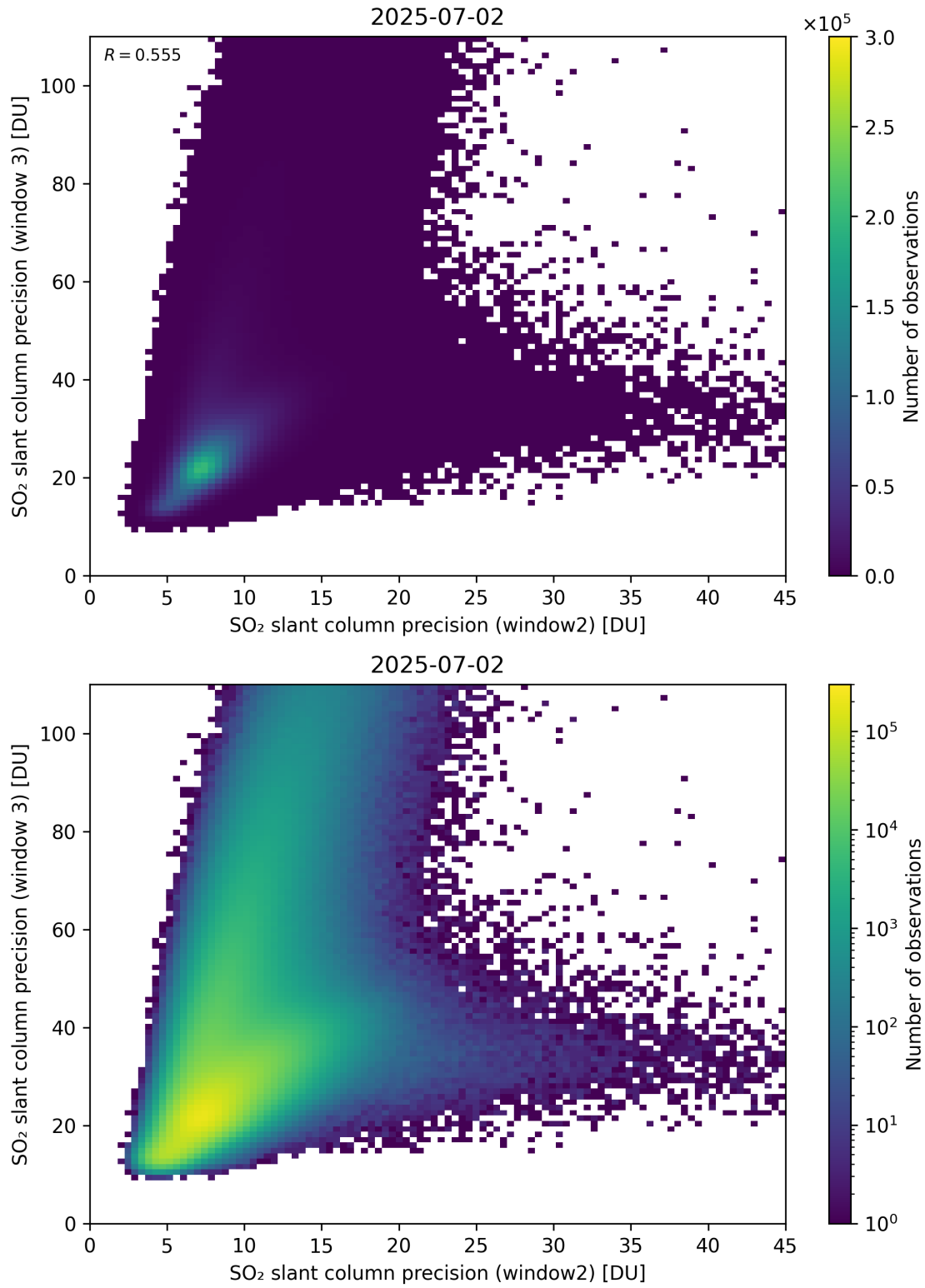
Figure 300: Scatter density plot of “SO 2 slant column precision (window2)” against “SO 2 slant column precision (window 3)” for 2025-07-02 to 2025-07-03.
