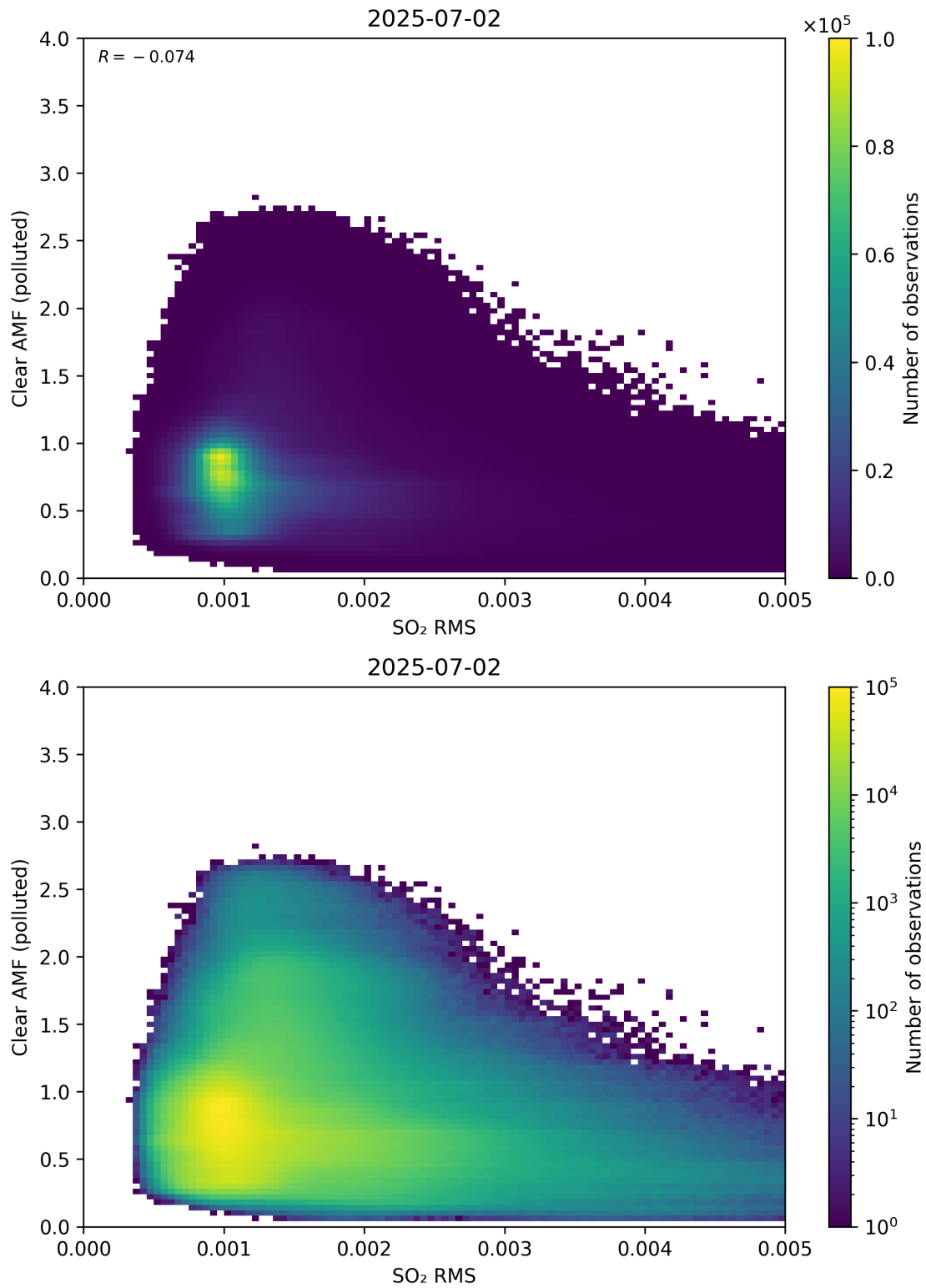
Figure 147: Scatter density plot of “SO 2 RMS” against “Clear AMF (polluted)” for 2025-07-02 to 2025-07-03.
