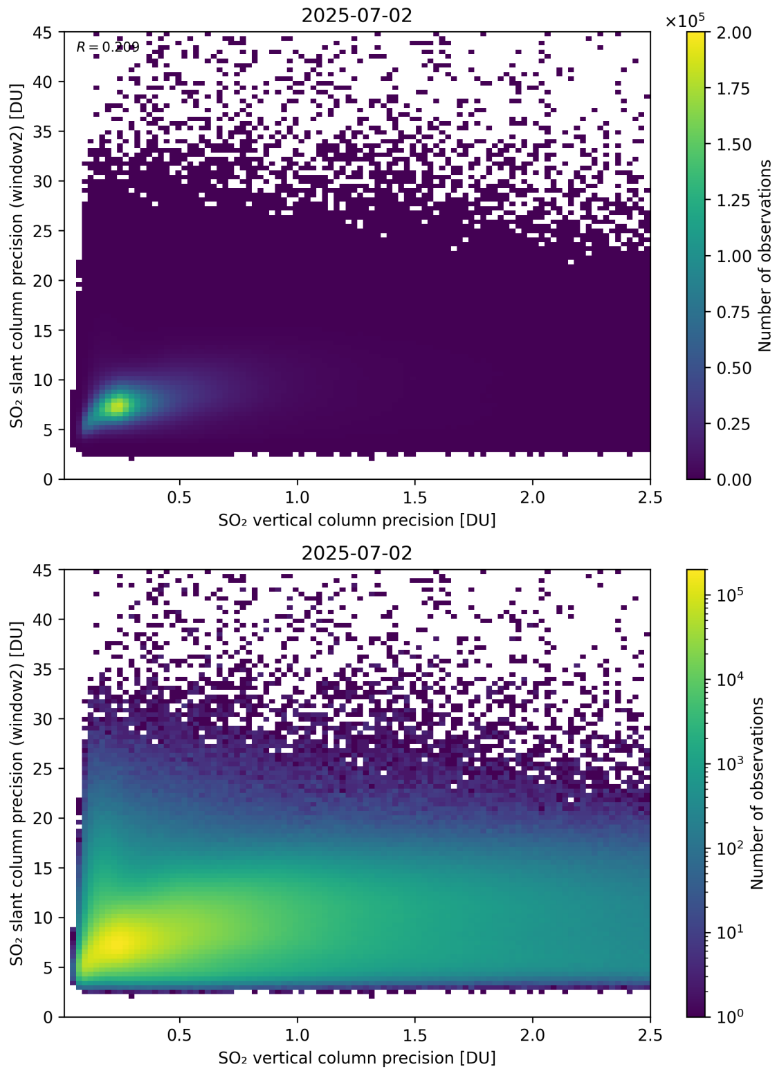
Figure 343: Scatter density plot of “SO 2 vertical column precision” against “SO 2 slant column precision (window2)” for 2025-07-02 to 2025-07-03.
