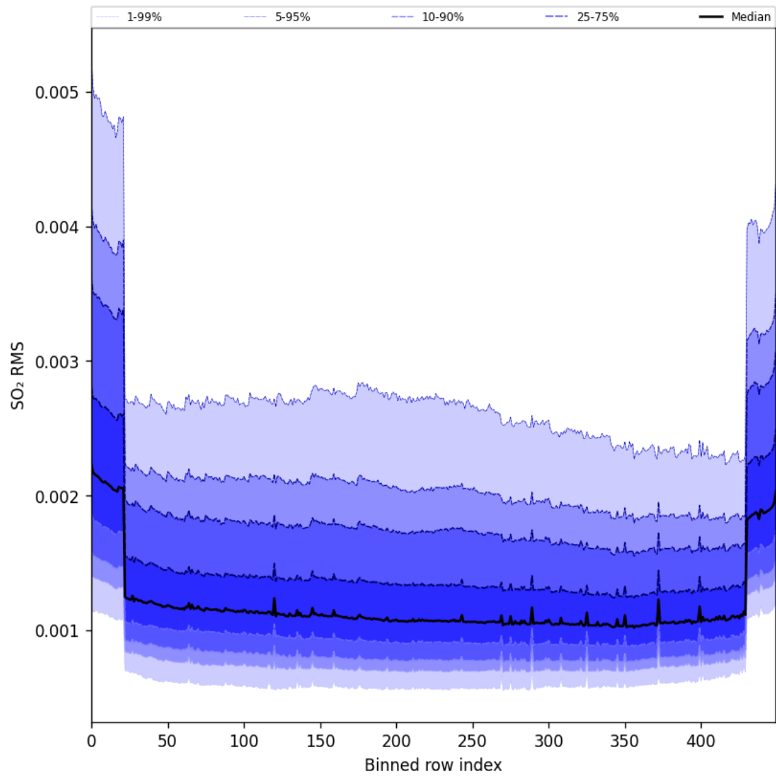
Figure 104: Along track statistics of “SO 2 RMS” for 2025-07-02 to 2025-07-03
