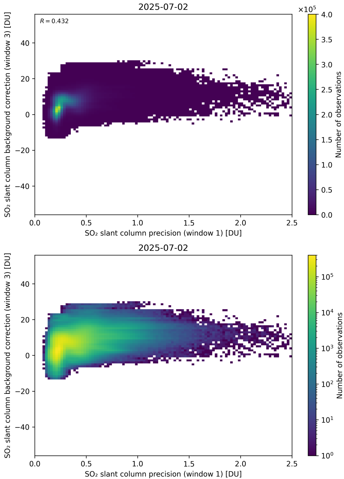
Figure 270: Scatter density plot of “SO 2 slant column precision (window 1)” against “SO 2 slant column background correction (window 3)” for 2025-07-02 to 2025-07-03.
