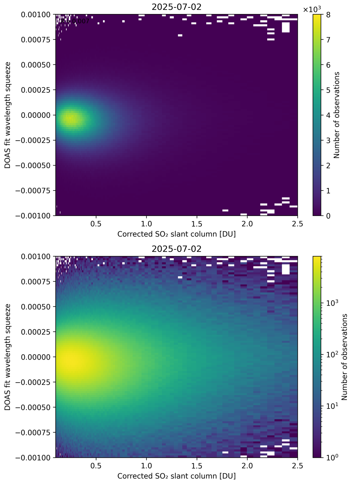
Figure 230: Scatter density plot of “Corrected SO 2 slant column” against “DOAS fit wavelength squeeze” for 2025-07-02 to 2025-07-03.
