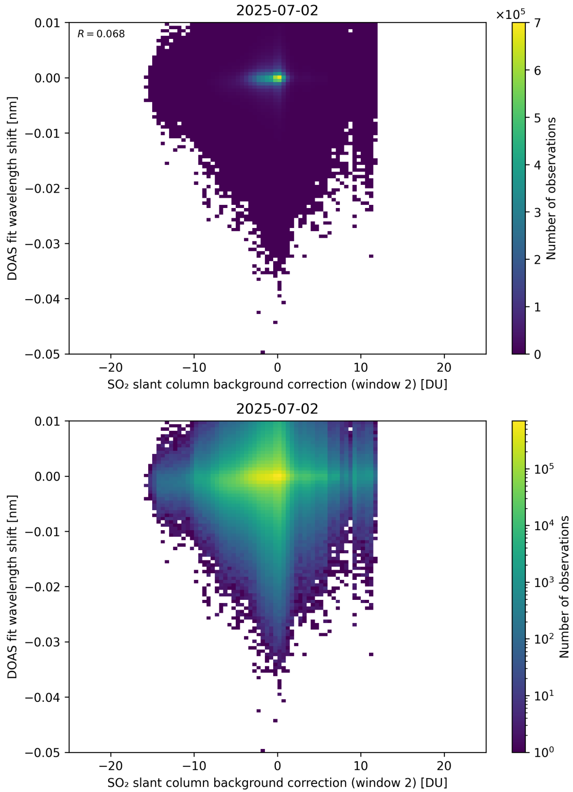
Figure 123: Scatter density plot of “SO 2 slant column background correction (window 2)” against “DOAS fit wavelength shift” for 2025-07-02 to 2025-07-03.
