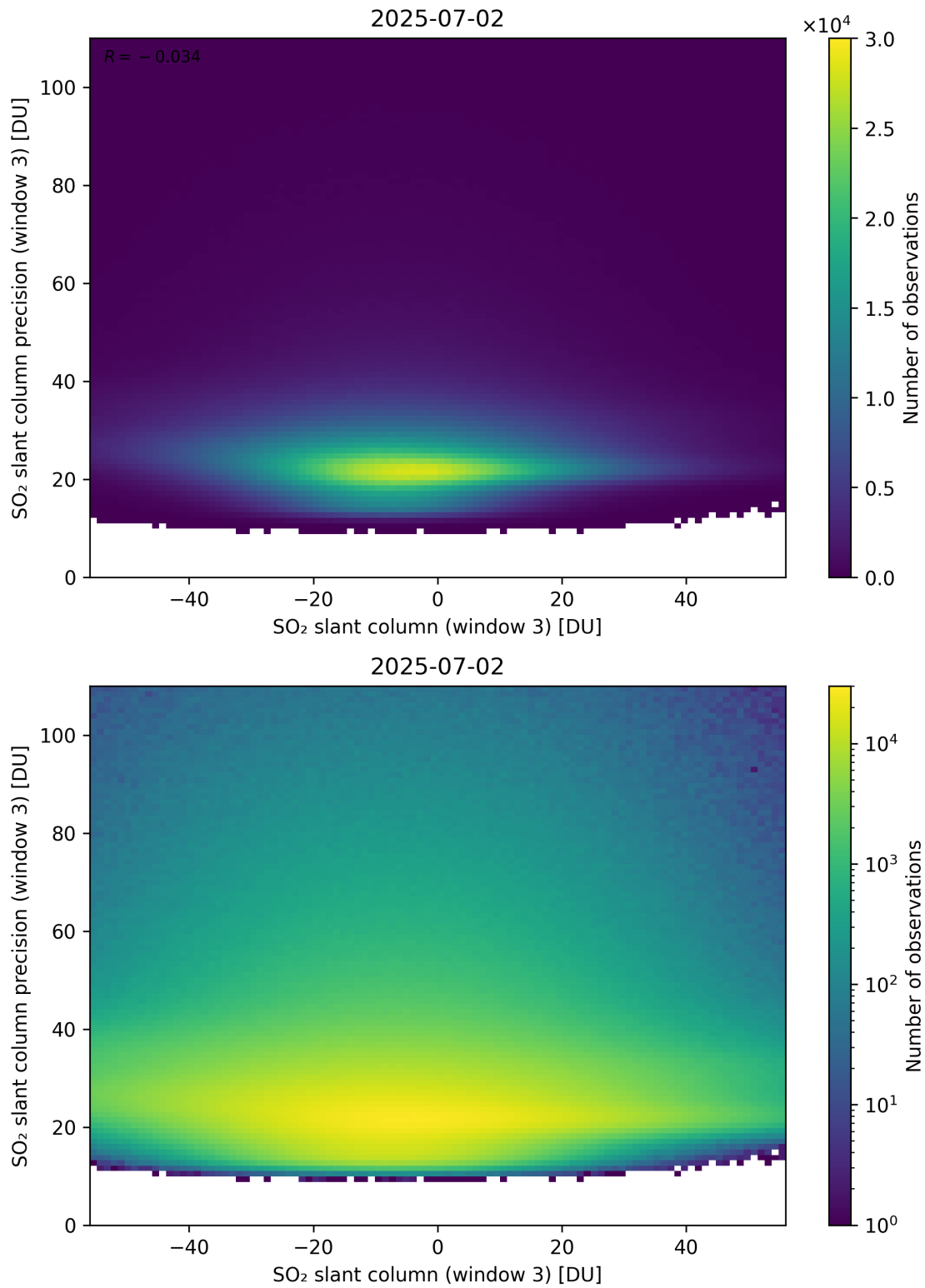
Figure 317: Scatter density plot of “SO 2 slant column (window 3)” against “SO 2 slant column precision (window 3)” for 2025-07-02 to 2025-07-03.
