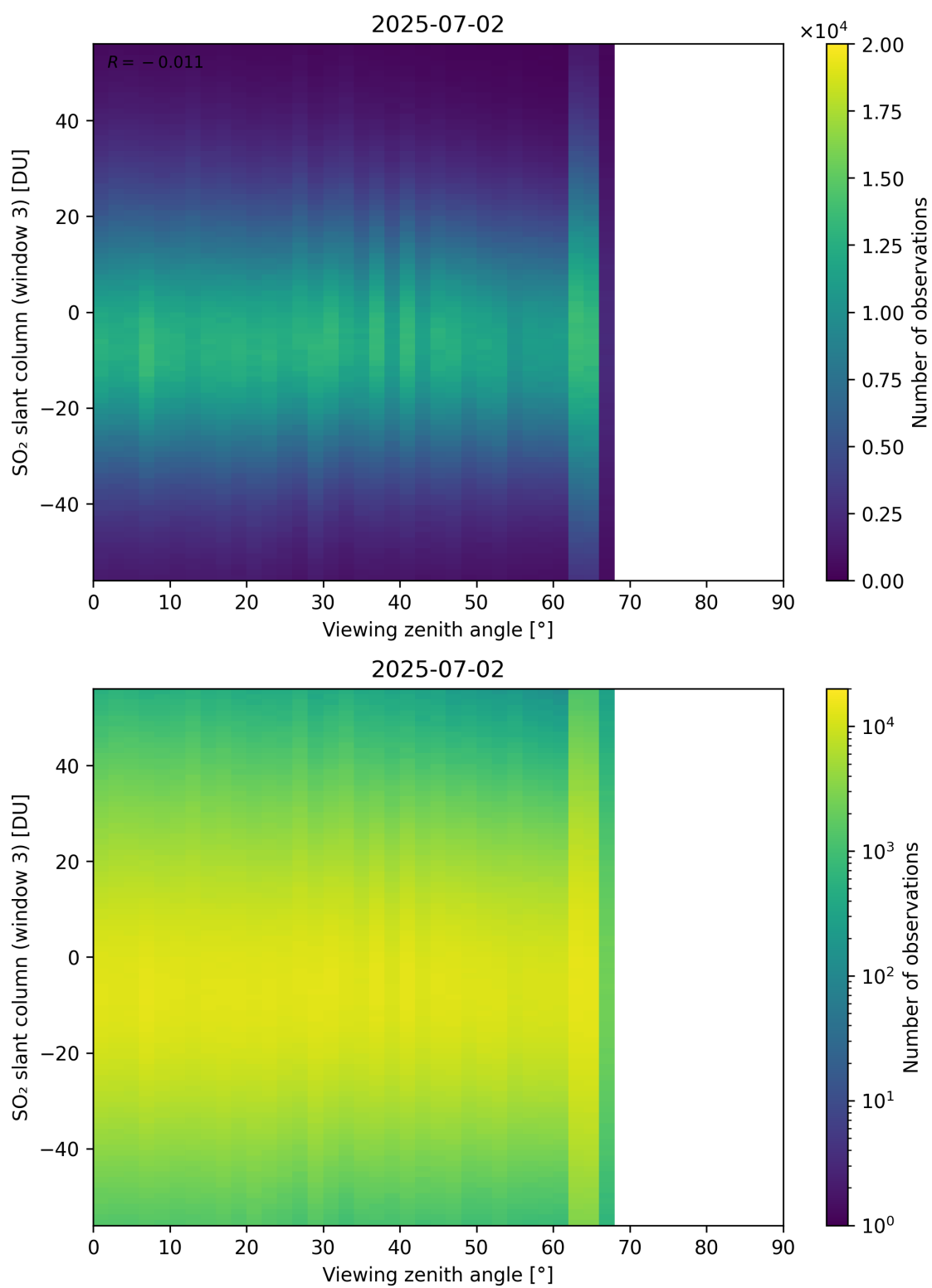
Figure 379: Scatter density plot of “Viewing zenith angle” against “SO 2 slant column (window 3)” for 2025-07-02 to 2025-07-03.
