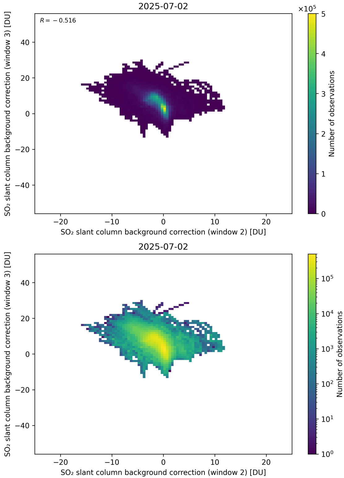
Figure 122: Scatter density plot of “SO 2 slant column background correction (window 2)” against “SO 2 slant column background correction (window 3)” for 2025-07-02 to 2025-07-03.
