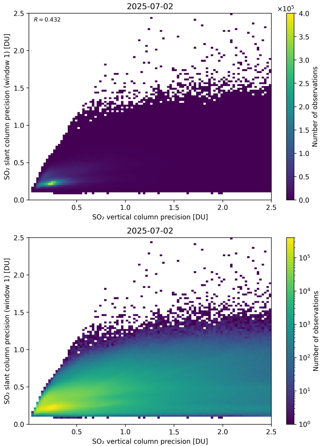
Figure 342: Scatter density plot of “SO 2 vertical column precision” against “SO 2 slant column precision (window 1)” for 2025-07-02 to 2025-07-03.
