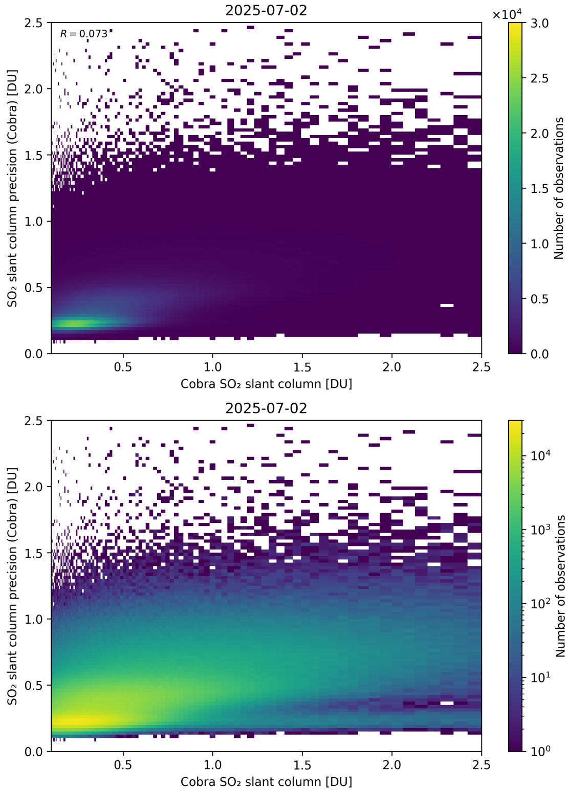
Figure 216: Scatter density plot of “Cobra SO 2 slant column” against “SO 2 slant column precision (Cobra)” for 2025-07-02 to 2025-07-03.
