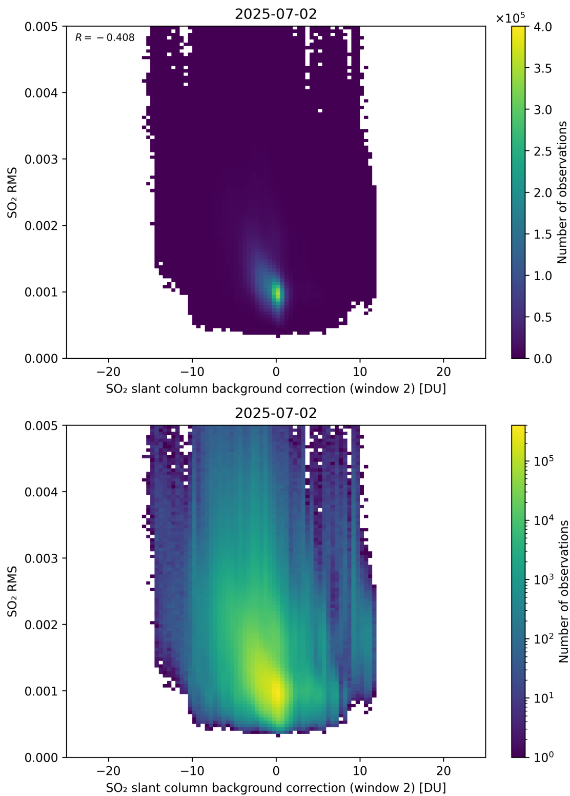
Figure 125: Scatter density plot of “SO 2 slant column background correction (window 2)” against “SO 2 RMS” for 2025-07-02 to 2025-07-03.
