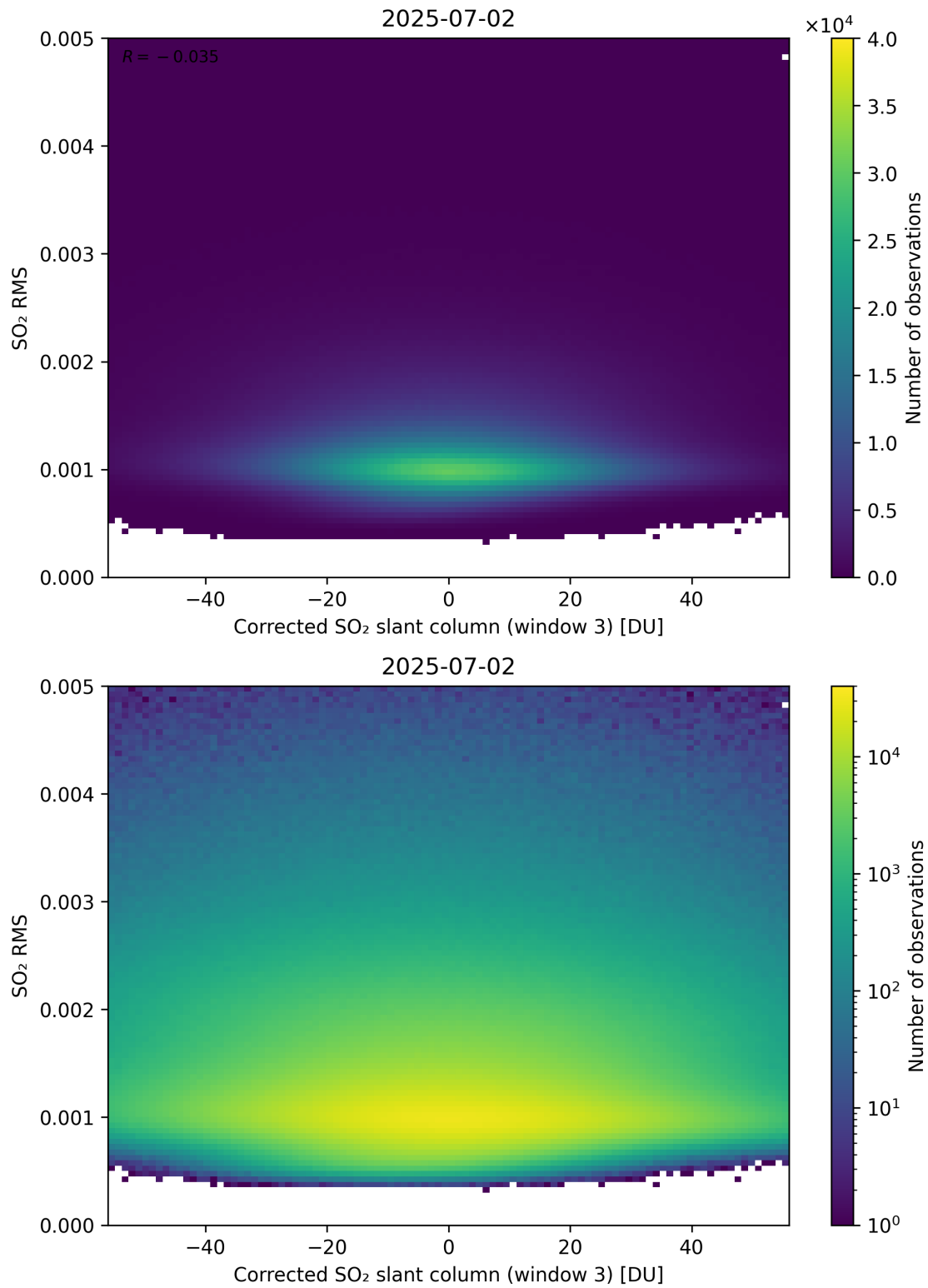
Figure 258: Scatter density plot of “Corrected SO 2 slant column (window 3)” against “SO 2 RMS” for 2025-07-02 to 2025-07-03.
