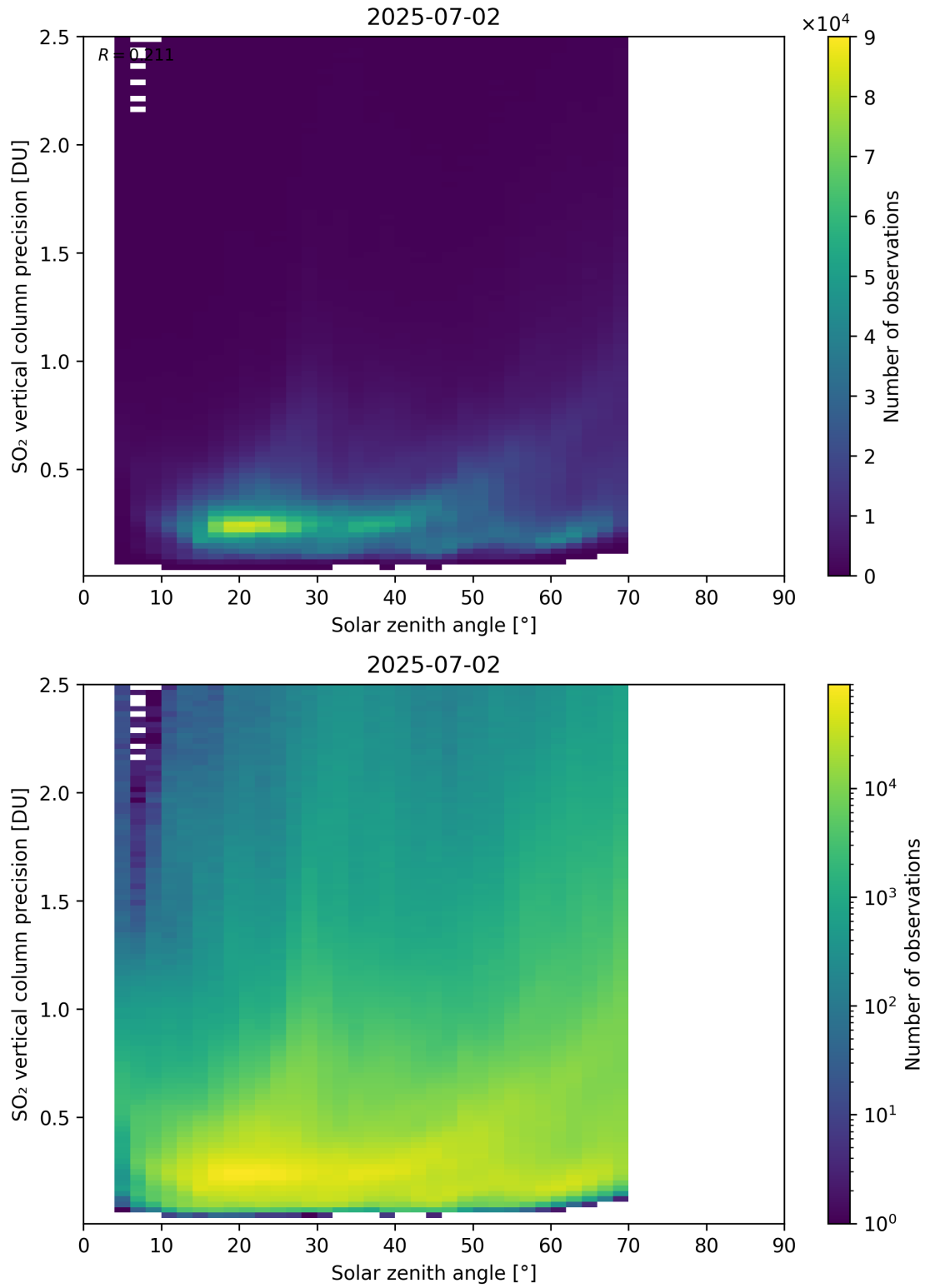
Figure 192: Scatter density plot of “Solar zenith angle” against “SO 2 vertical column precision” for 2025-07-02 to 2025-07-03.
