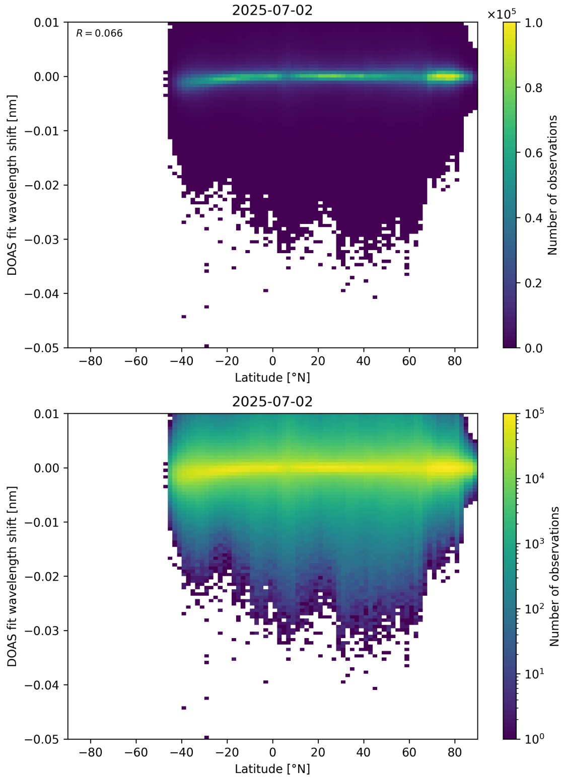
Figure 153: Scatter density plot of “Latitude” against “DOAS fit wavelength shift” for 2025-07-02 to 2025-07-03.
