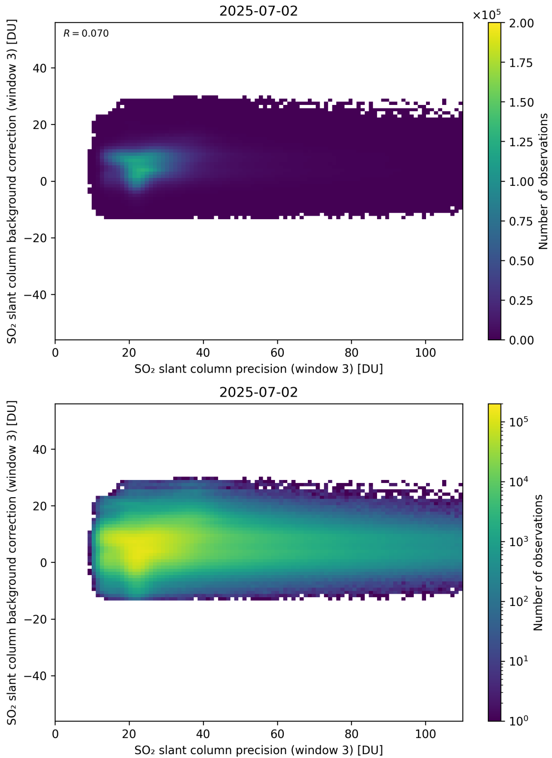
Figure 307: Scatter density plot of “SO 2 slant column precision (window 3)” against “SO 2 slant column background correction (window 3)” for 2025-07-02 to 2025-07-03.
