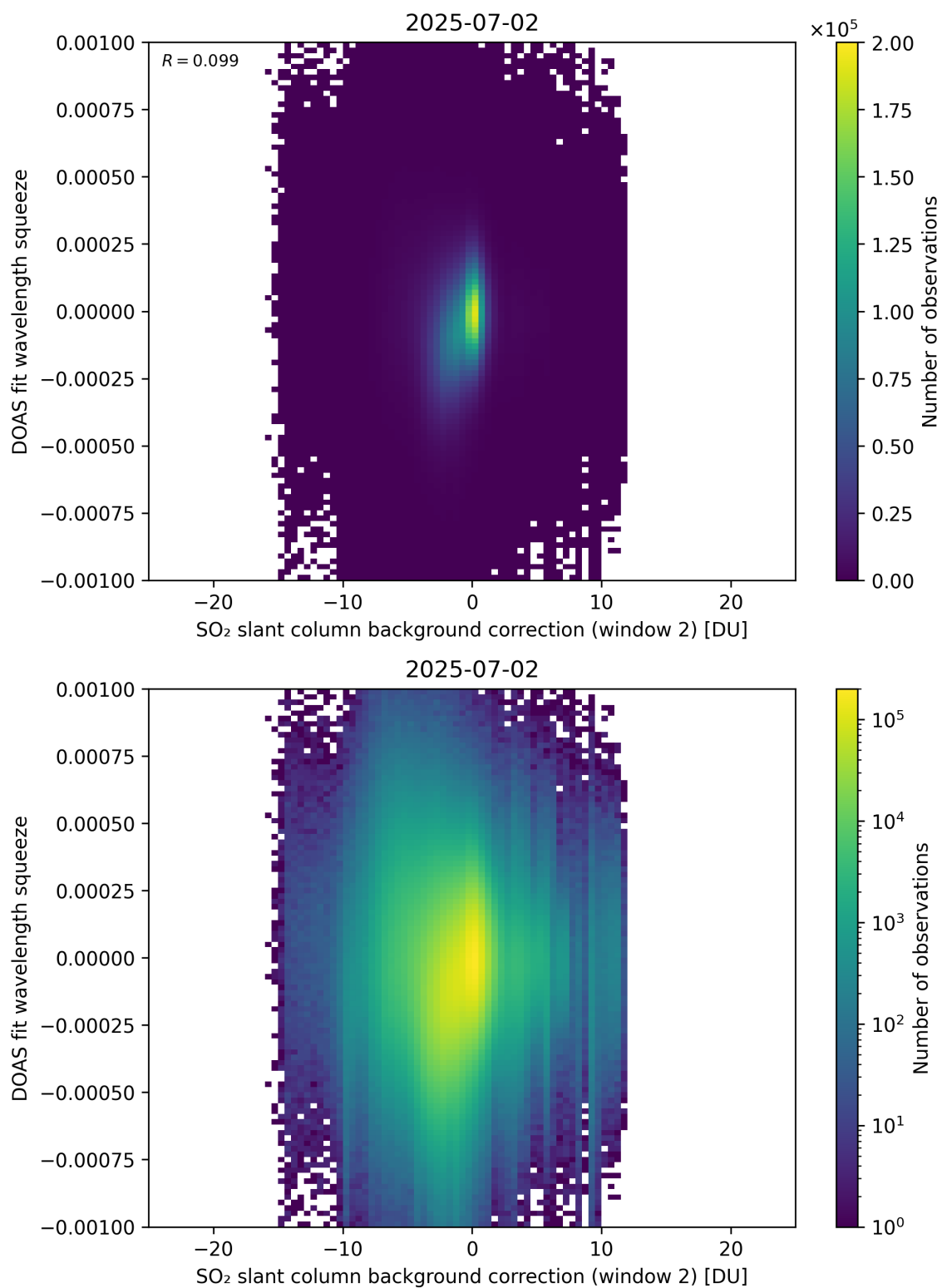
Figure 124: Scatter density plot of “SO 2 slant column background correction (window 2)” against “DOAS fit wavelength squeeze” for 2025-07-02 to 2025-07-03.
