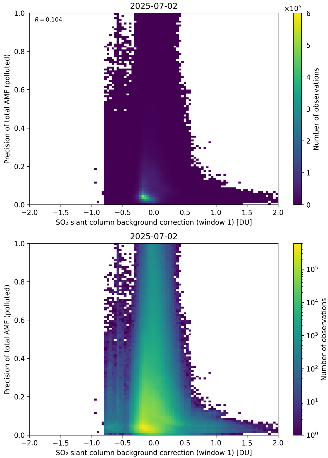
Figure 121: Scatter density plot of “SO 2 slant column background correction (window 1)” against “Precision of total AMF (polluted)” for 2025-07-02 to 2025-07-03.
