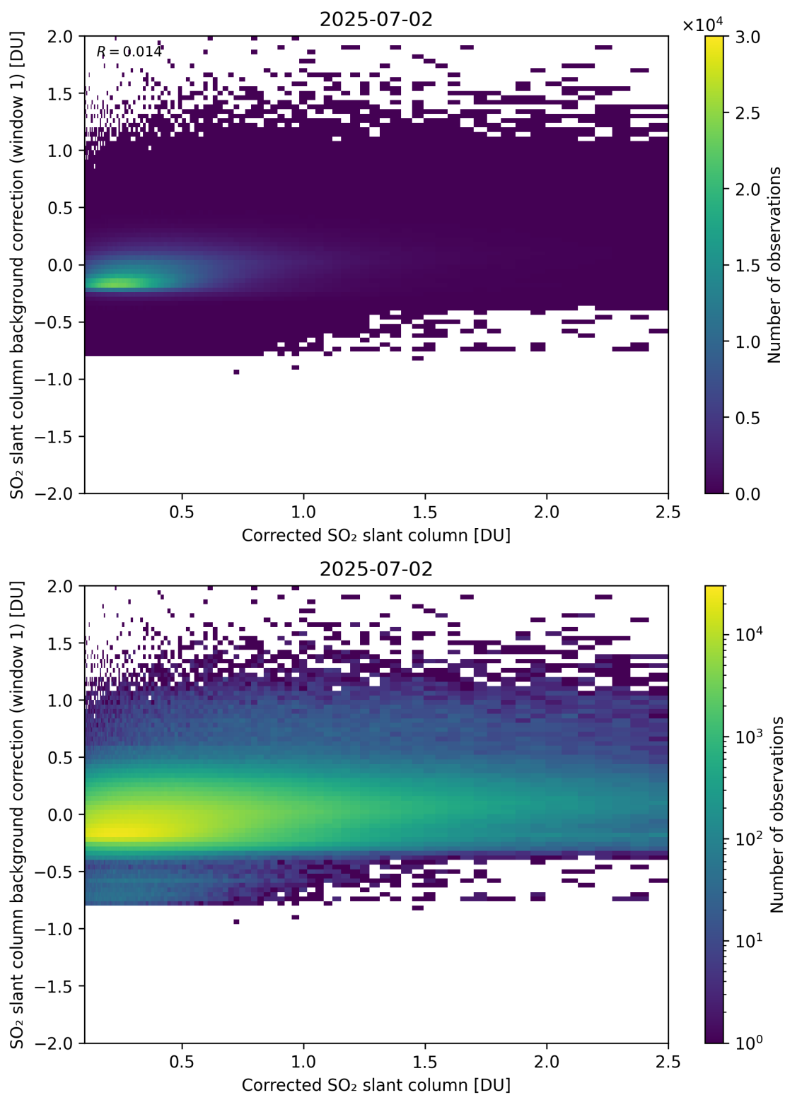
Figure 226: Scatter density plot of “Corrected SO 2 slant column” against “SO 2 slant column background correction (window 1)” for 2025-07-02 to 2025-07-03.
