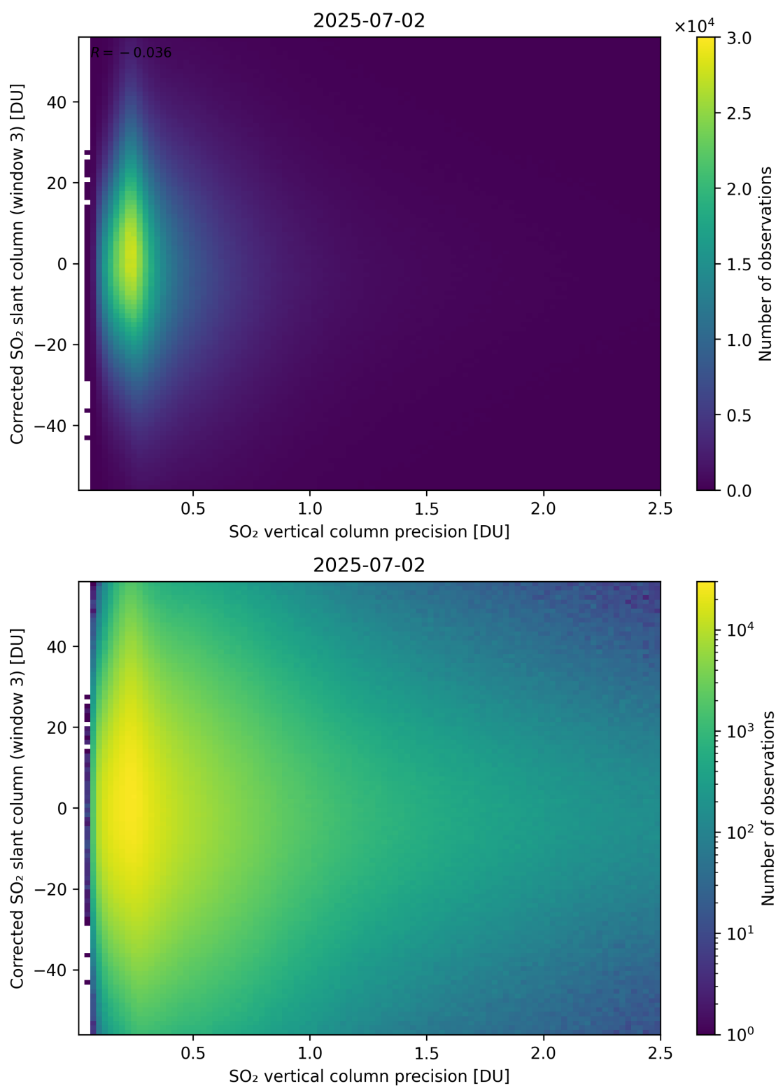
Figure 340: Scatter density plot of “SO 2 vertical column precision” against “Corrected SO 2 slant column (window 3)” for 2025-07-02 to 2025-07-03.
