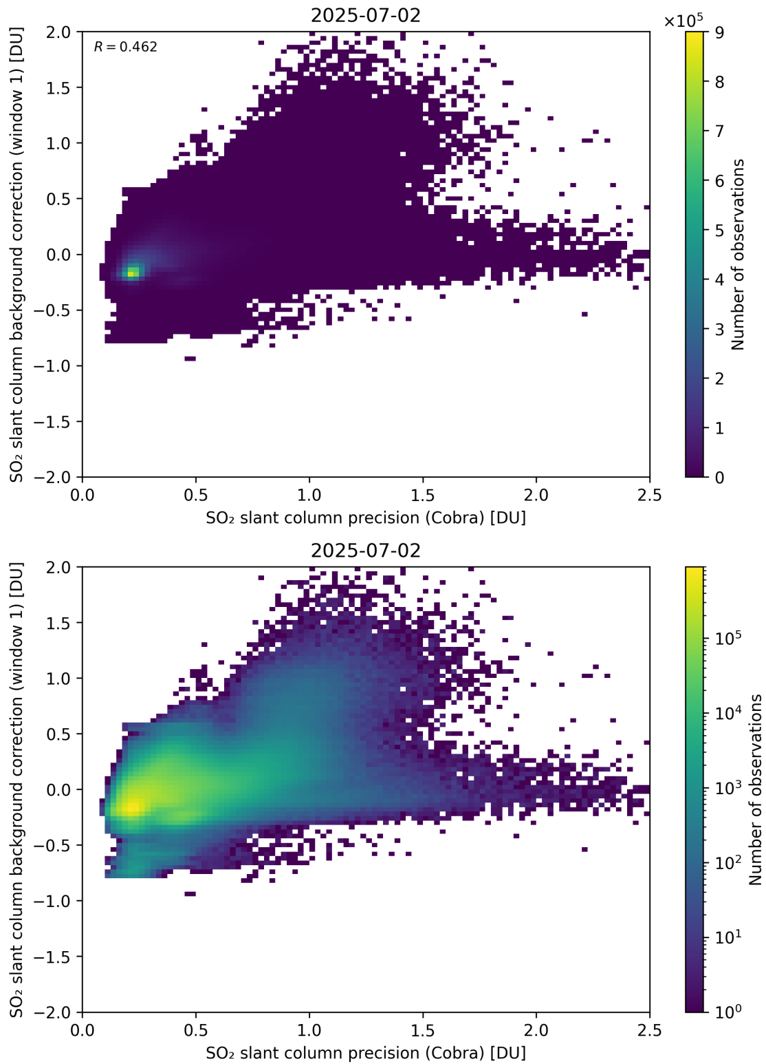
Figure 199: Scatter density plot of “SO 2 slant column precision (Cobra)” against “SO 2 slant column background correction (window 1)” for 2025-07-02 to 2025-07-03.
