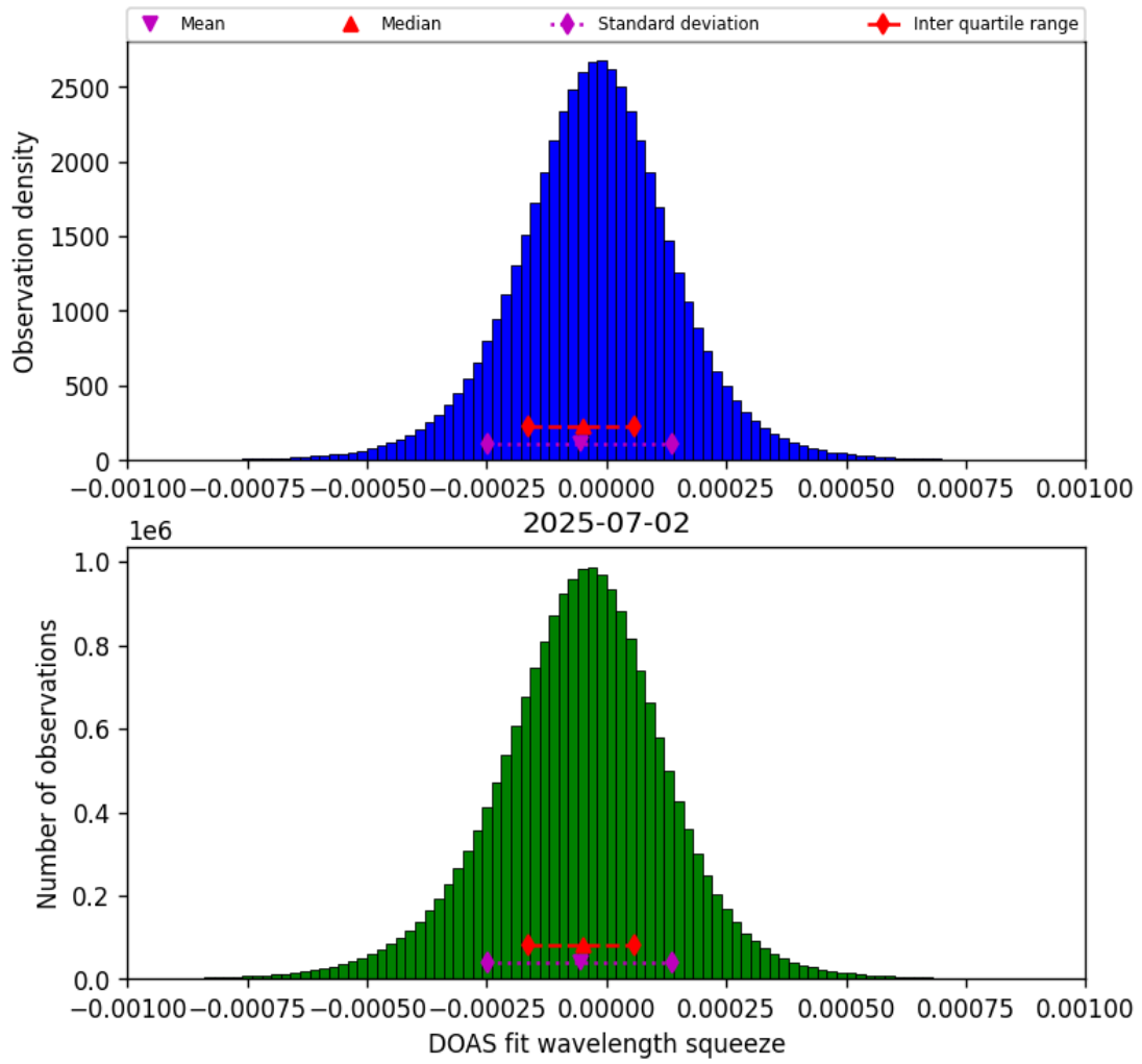
Figure 77: Histogram of “DOAS fit wavelength squeeze” for 2025-07-02 to 2025-07-03
