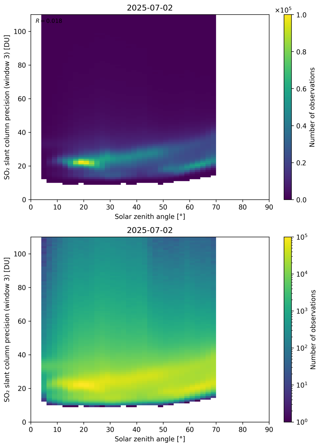
Figure 188: Scatter density plot of “Solar zenith angle” against “SO 2 slant column precision (window 3)” for 2025-07-02 to 2025-07-03.
