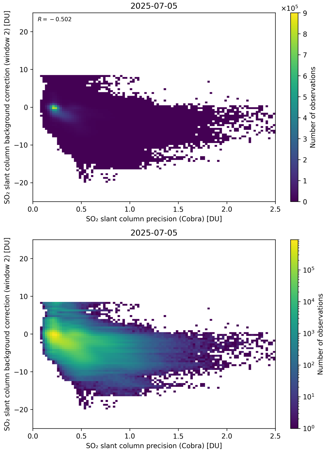
Figure 200: Scatter density plot of “SO 2 slant column precision (Cobra)” against “SO 2 slant column background correction (window 2)” for 2025-07-04 to 2025-07-06.
