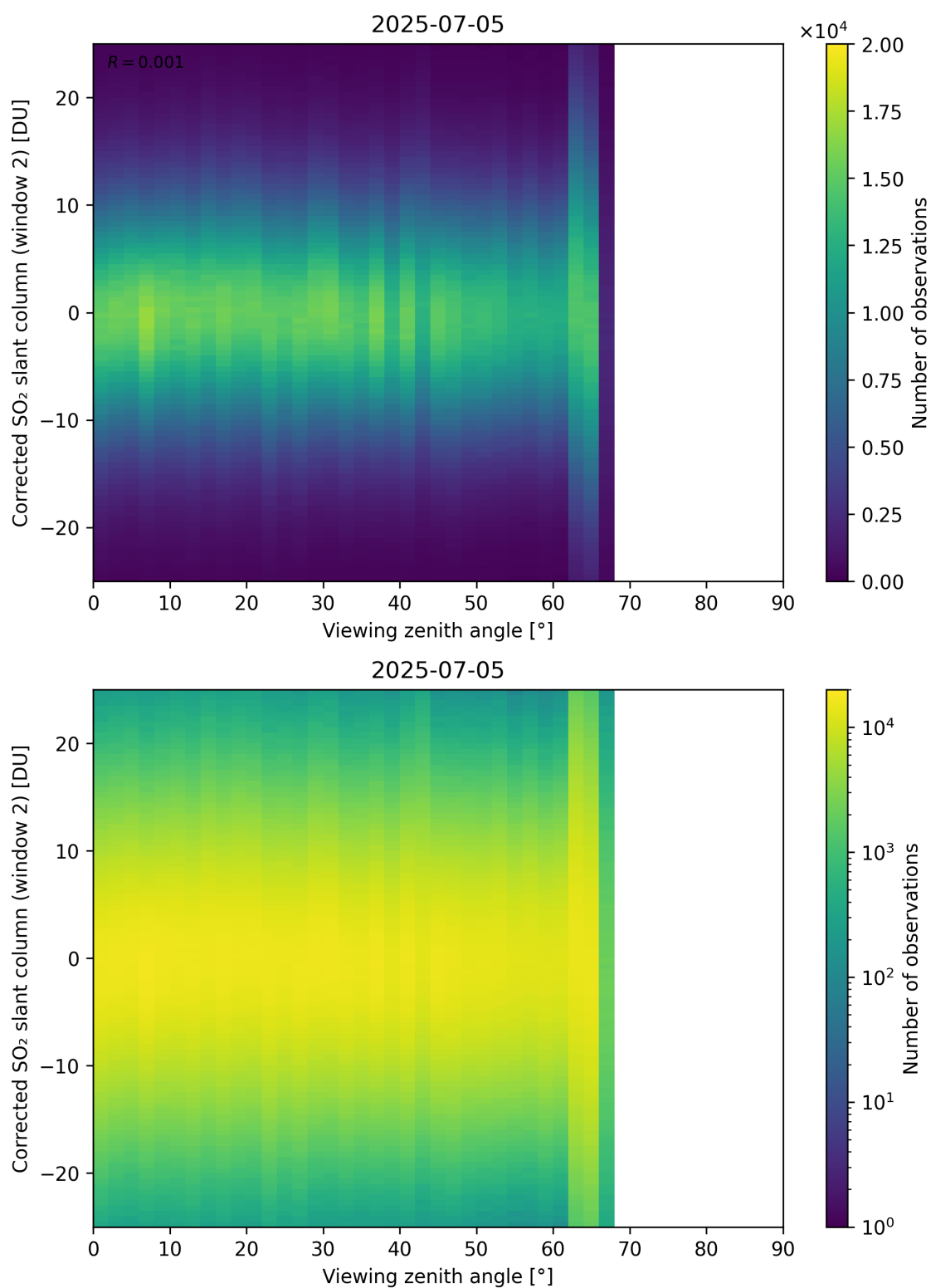
Figure 374: Scatter density plot of “Viewing zenith angle” against “Corrected SO 2 slant column (window 2)” for 2025-07-04 to 2025-07-06.
