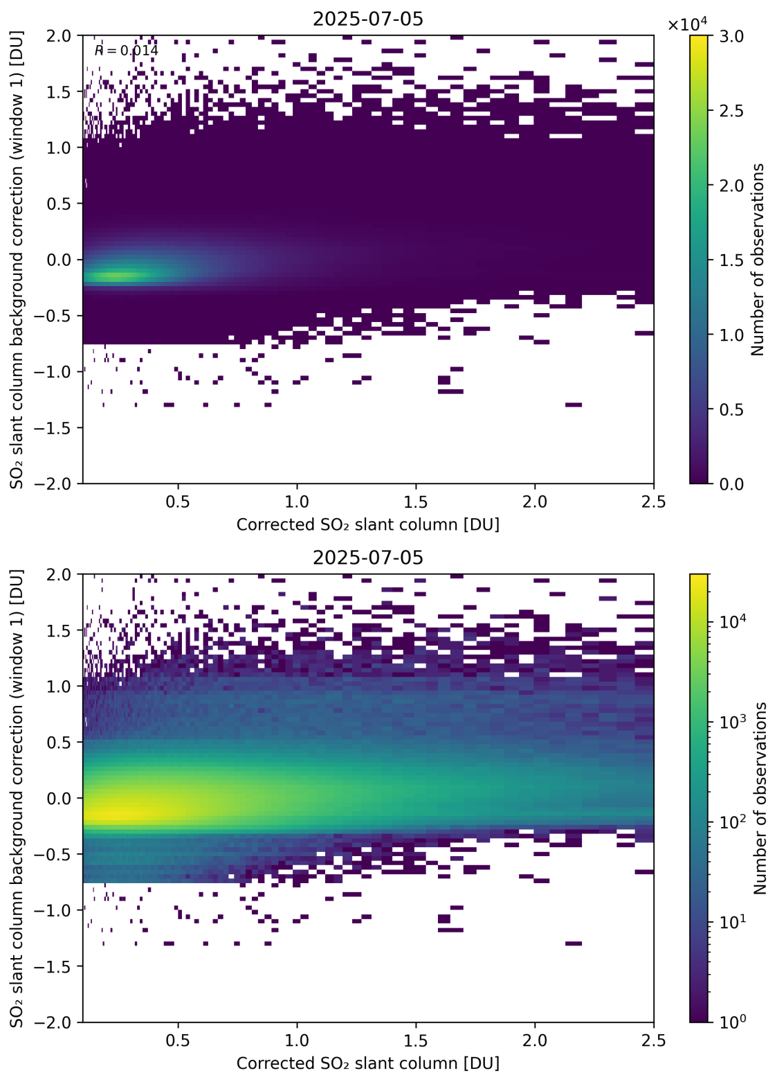
Figure 226: Scatter density plot of “Corrected SO 2 slant column” against “SO 2 slant column background correction (window 1)” for 2025-07-04 to 2025-07-06.
