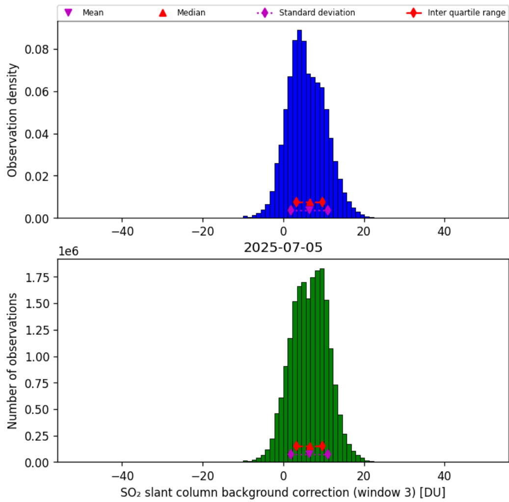
Figure 74: Histogram of “SO 2 slant column background correction (window 3)” for 2025-07-04 to 2025-07-06
