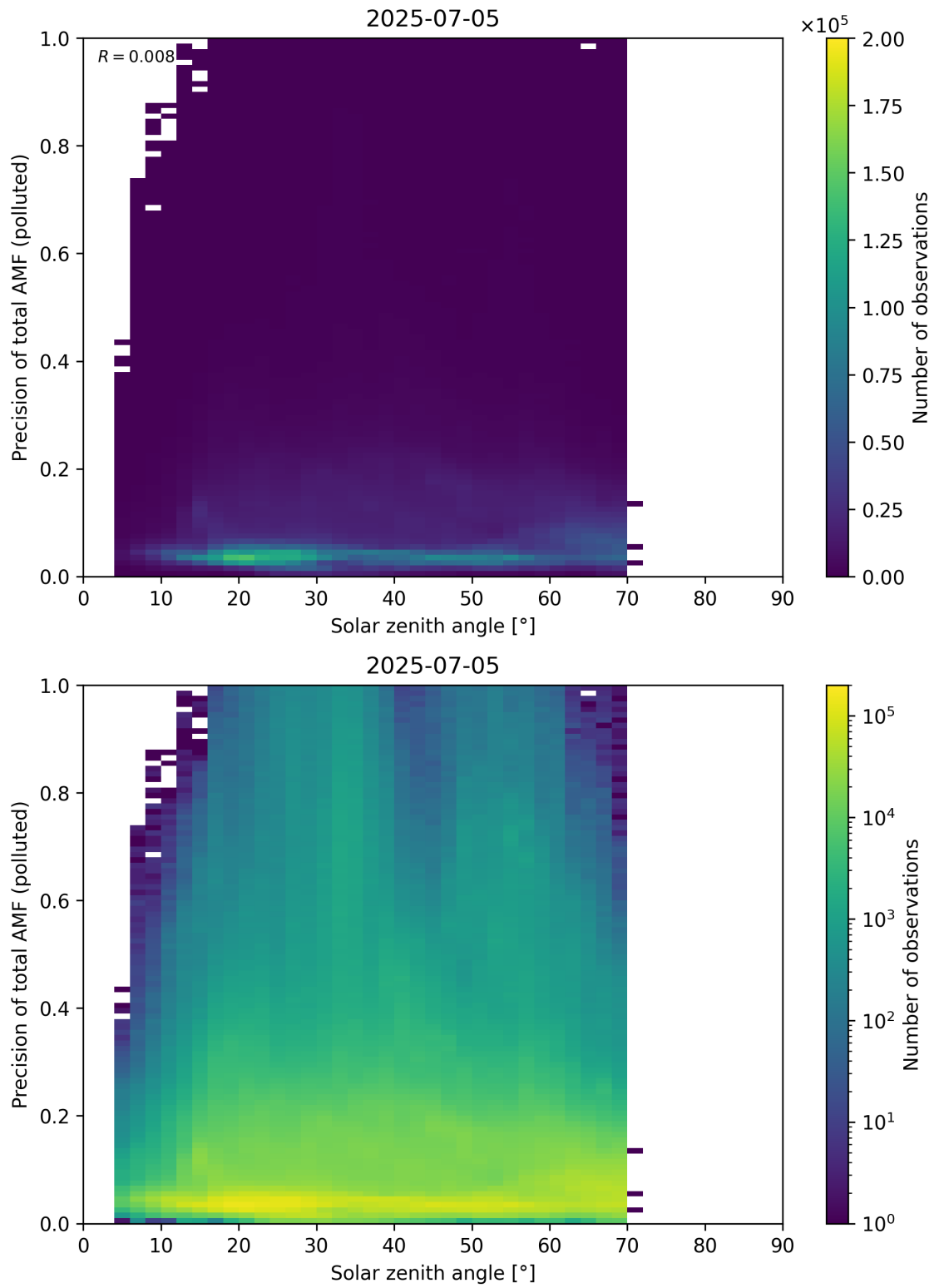
Figure 190: Scatter density plot of “Solar zenith angle” against “Precision of total AMF (polluted)” for 2025-07-04 to 2025-07-06.
