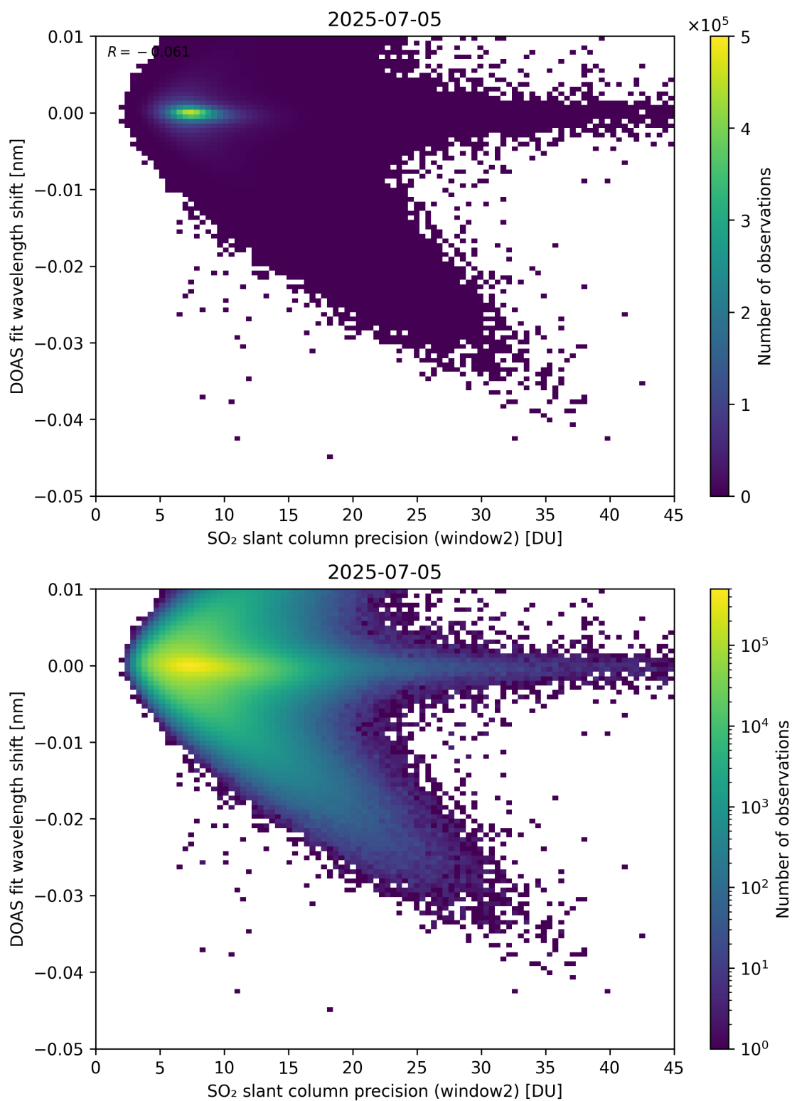
Figure 293: Scatter density plot of “SO 2 slant column precision (window2)” against “DOAS fit wavelength shift” for 2025-07-04 to 2025-07-06.
