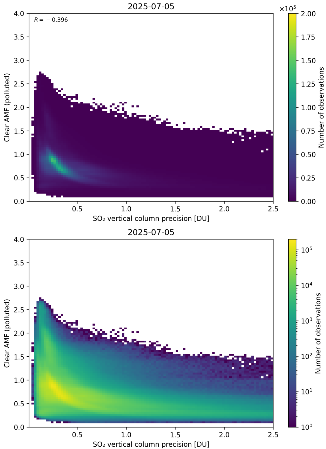
Figure 335: Scatter density plot of “SO 2 vertical column precision” against “Clear AMF (polluted)” for 2025-07-04 to 2025-07-06.
