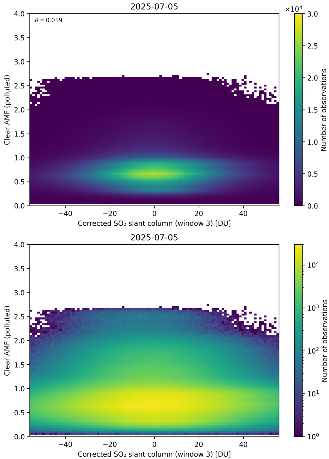
Figure 259: Scatter density plot of “Corrected SO 2 slant column (window 3)” against “Clear AMF (polluted)” for 2025-07-04 to 2025-07-06.
