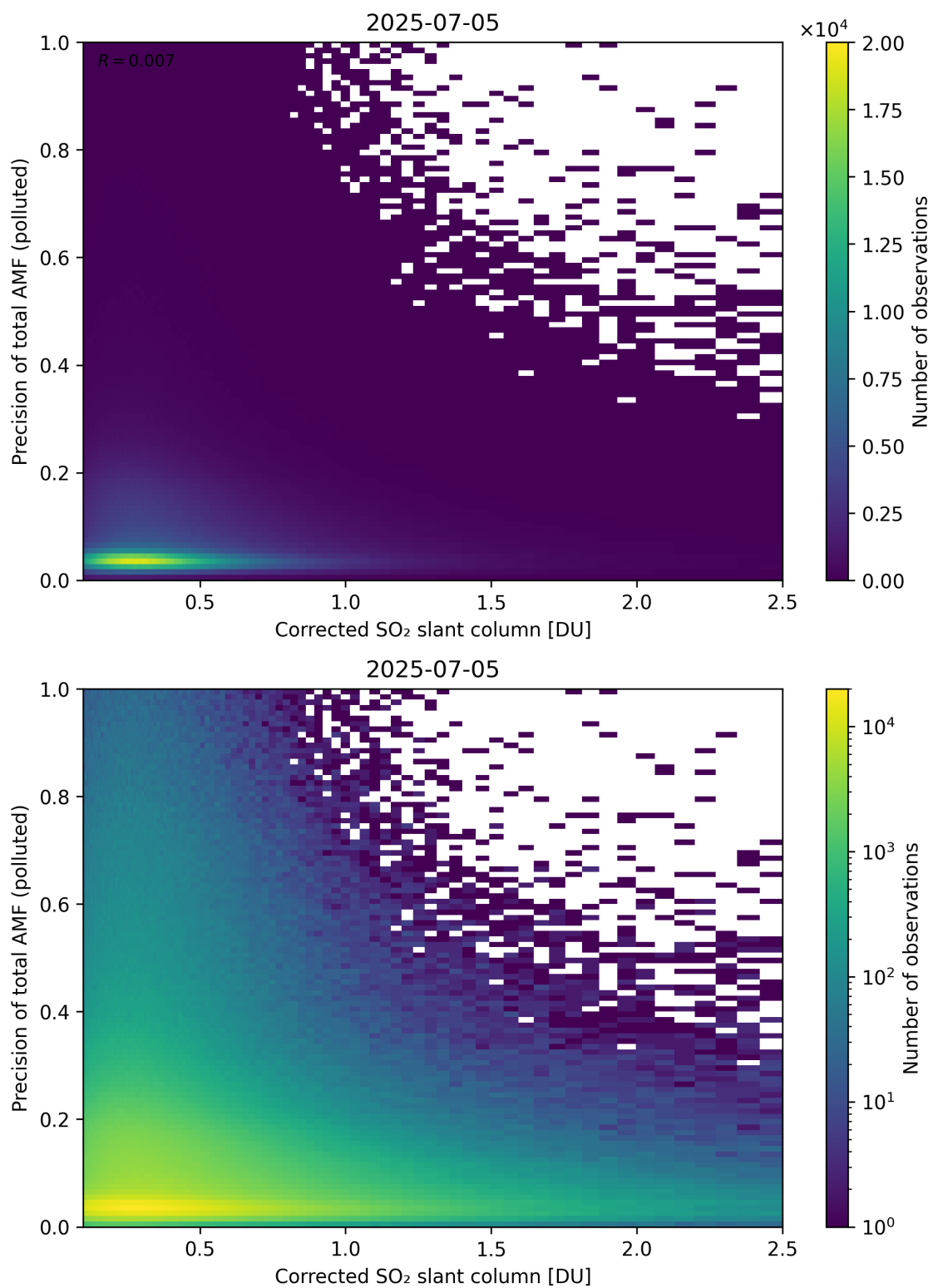
Figure 243: Scatter density plot of “Corrected SO 2 slant column” against “Precision of total AMF (polluted)” for 2025-07-04 to 2025-07-06.
