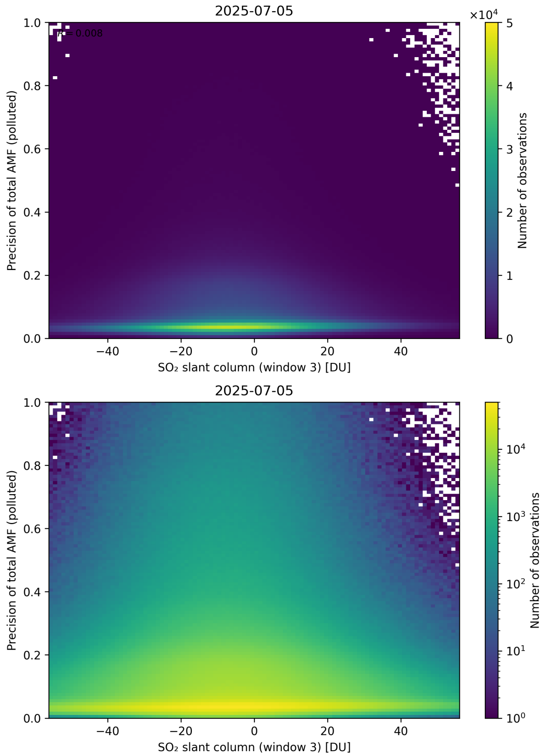
Figure 319: Scatter density plot of “SO 2 slant column (window 3)” against “Precision of total AMF (polluted)” for 2025-07-04 to 2025-07-06.
