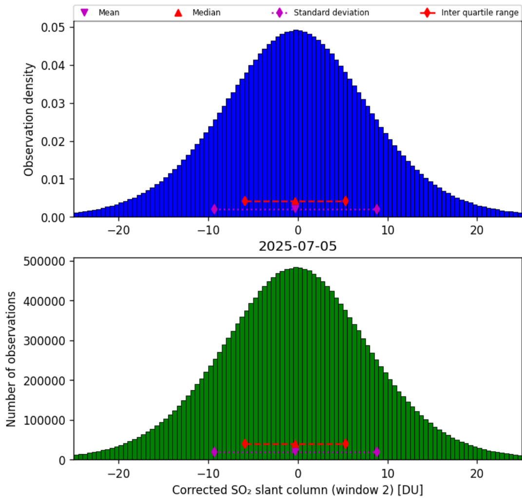
Figure 69: Histogram of “Corrected SO 2 slant column (window 2)” for 2025-07-04 to 2025-07-06
