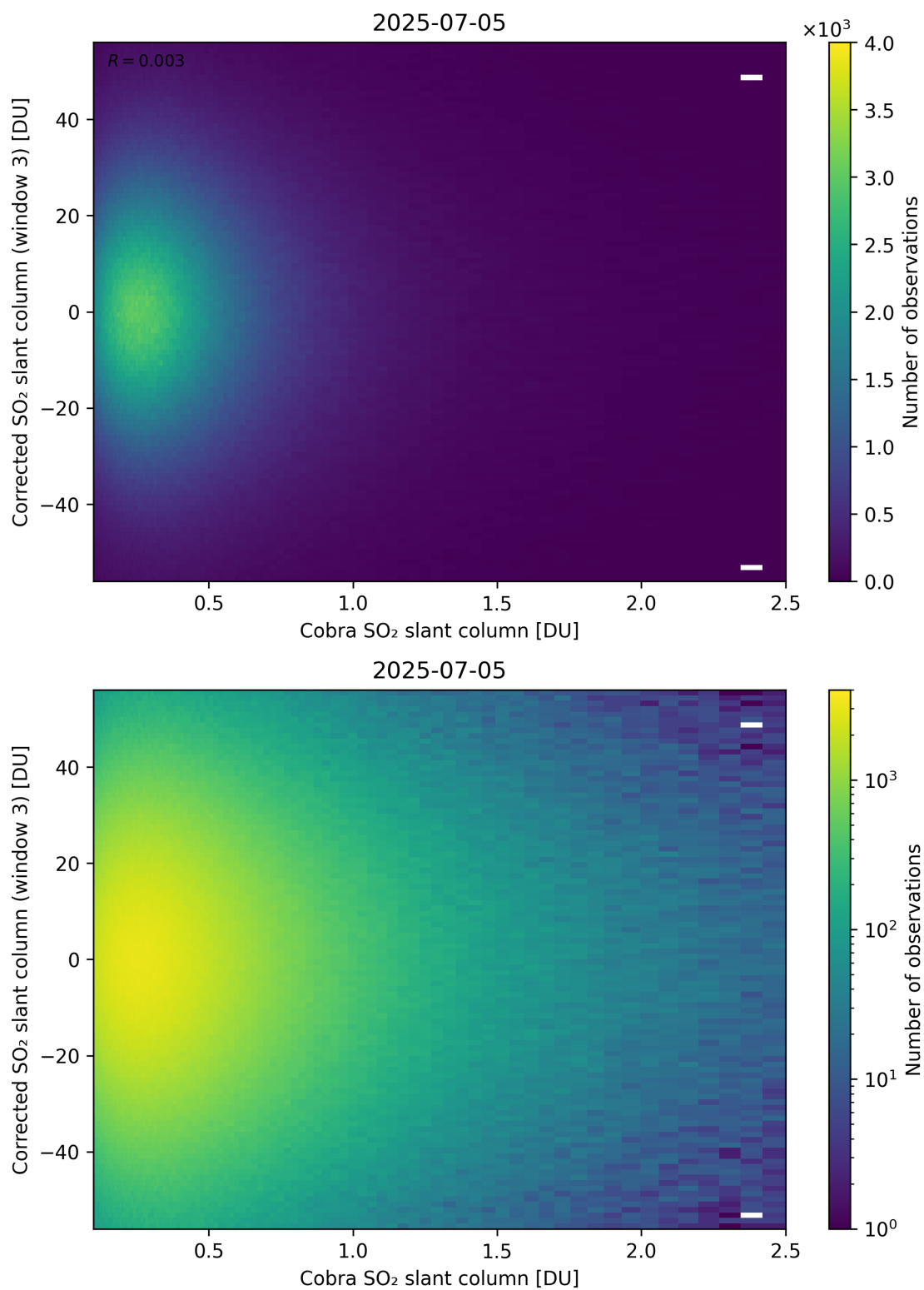
Figure 218: Scatter density plot of “Cobra SO 2 slant column” against “Corrected SO 2 slant column (window 3)” for 2025-07-04 to 2025-07-06.
