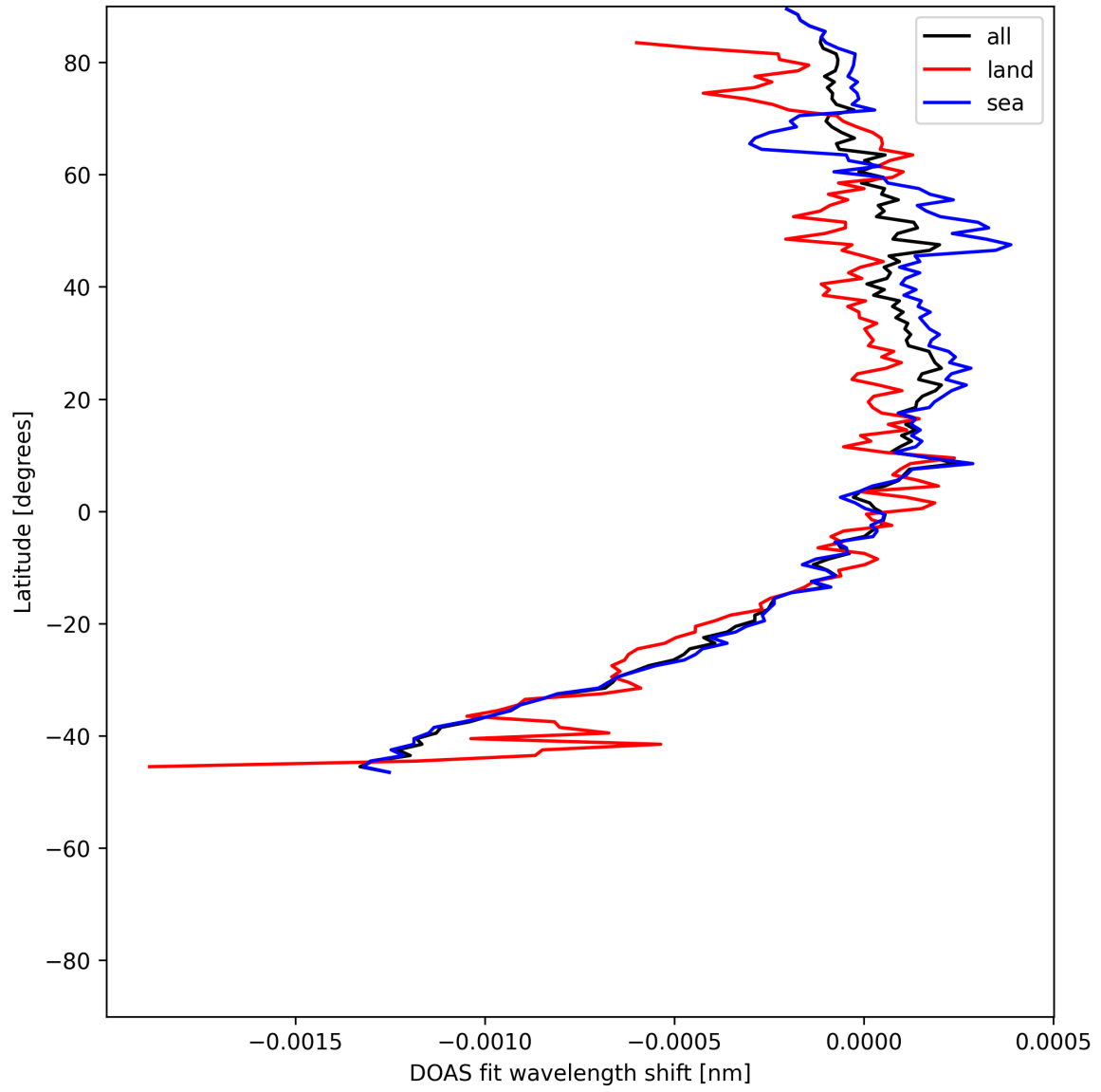
Figure 50: Zonal average of “DOAS fit wavelength shift” for 2025-07-04 to 2025-07-06.
