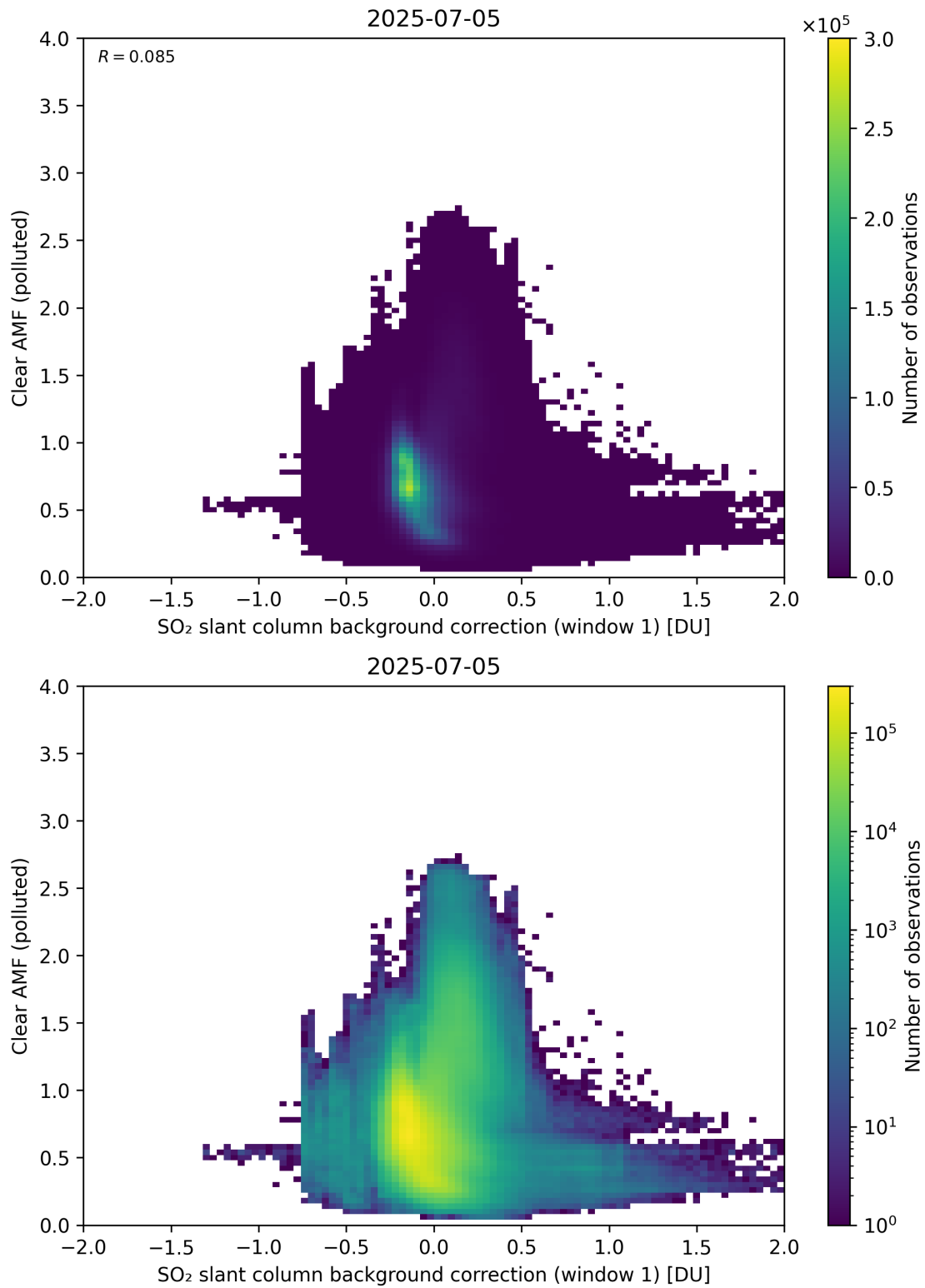
Figure 114: Scatter density plot of “SO 2 slant column background correction (window 1)” against “Clear AMF (polluted)” for 2025-07-04 to 2025-07-06.
