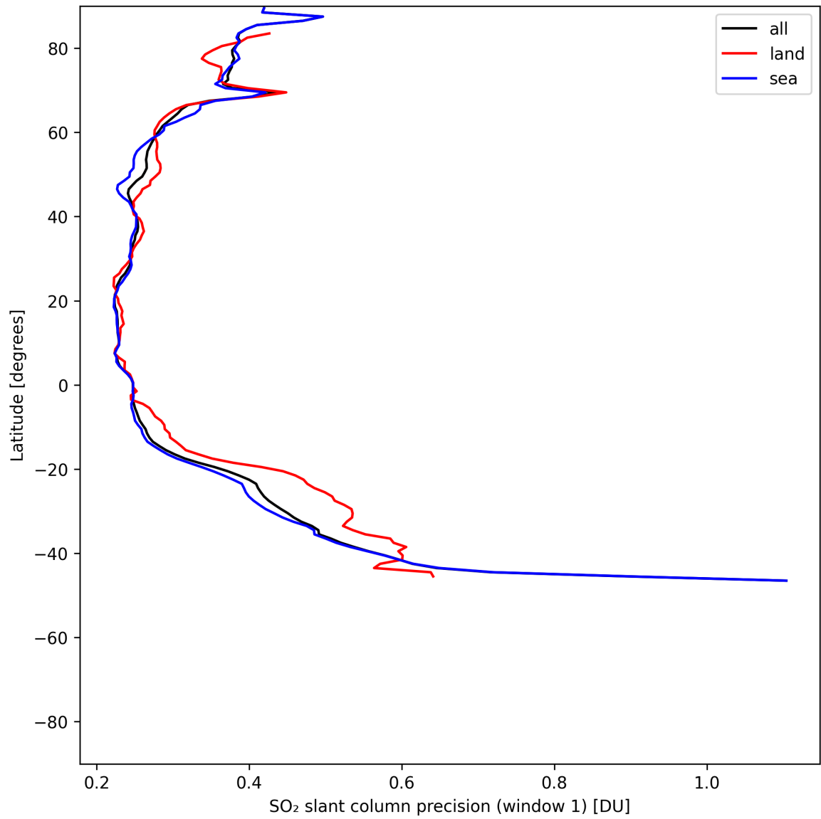
Figure 38: Zonal average of “SO 2 slant column precision (window 1)” for 2025-07-04 to 2025-07-06.
