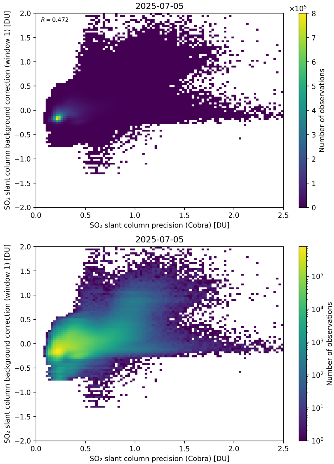
Figure 199: Scatter density plot of “SO 2 slant column precision (Cobra)” against “SO 2 slant column background correction (window 1)” for 2025-07-04 to 2025-07-06.
