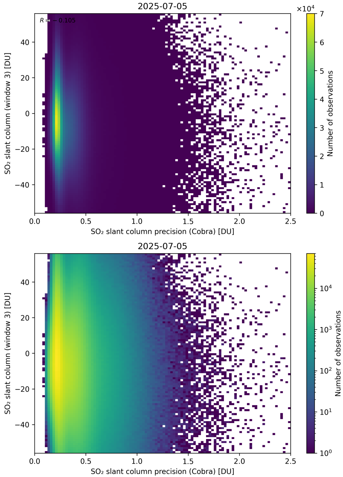
Figure 211: Scatter density plot of “SO 2 slant column precision (Cobra)” against “SO 2 slant column (window 3)” for 2025-07-04 to 2025-07-06.
