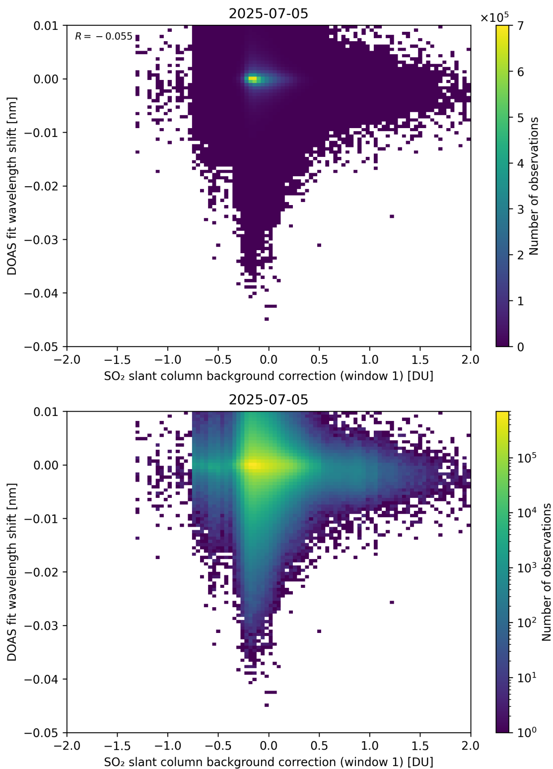
Figure 111: Scatter density plot of “SO 2 slant column background correction (window 1)” against “DOAS fit wavelength shift” for 2025-07-04 to 2025-07-06.
