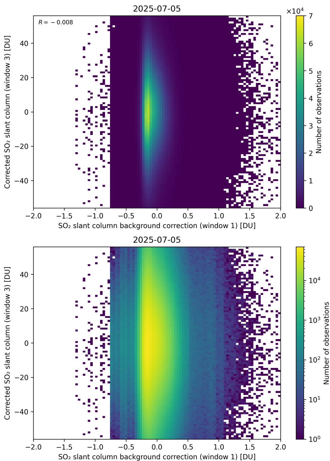
Figure 116: Scatter density plot of “SO 2 slant column background correction (window 1)” against “Corrected SO 2 slant column (window 3)” for 2025-07-04 to 2025-07-06.
