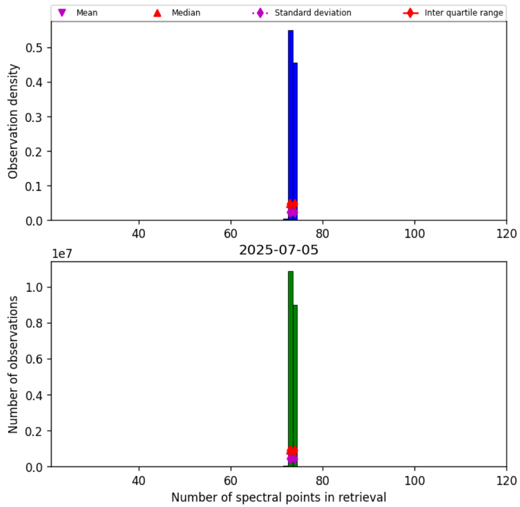
Figure 82: Histogram of “Number of spectral points in retrieval” for 2025-07-04 to 2025-07-06
