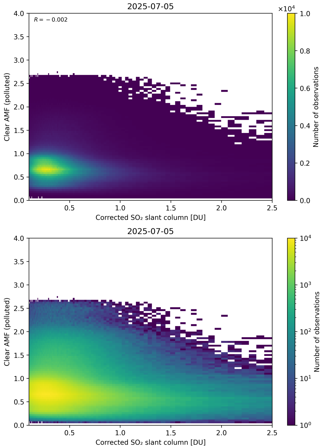
Figure 232: Scatter density plot of “Corrected SO 2 slant column” against “Clear AMF (polluted)” for 2025-07-04 to 2025-07-06.
