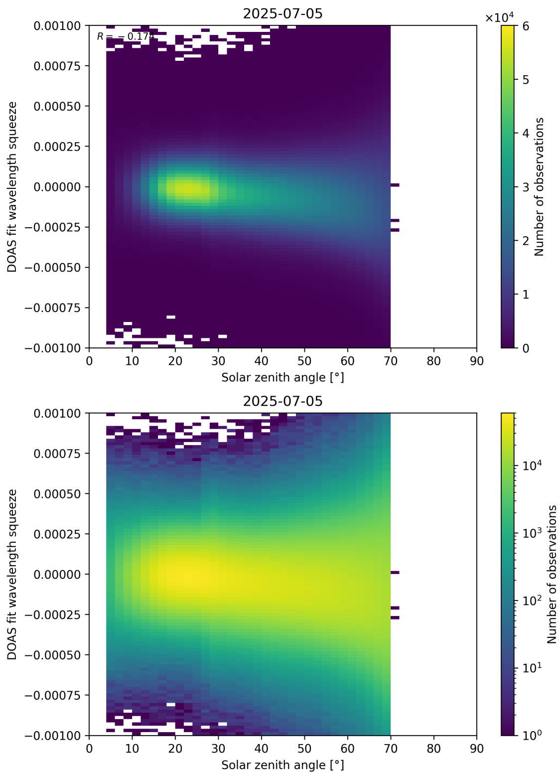
Figure 175: Scatter density plot of “Solar zenith angle” against “DOAS fit wavelength squeeze” for 2025-07-04 to 2025-07-06.
