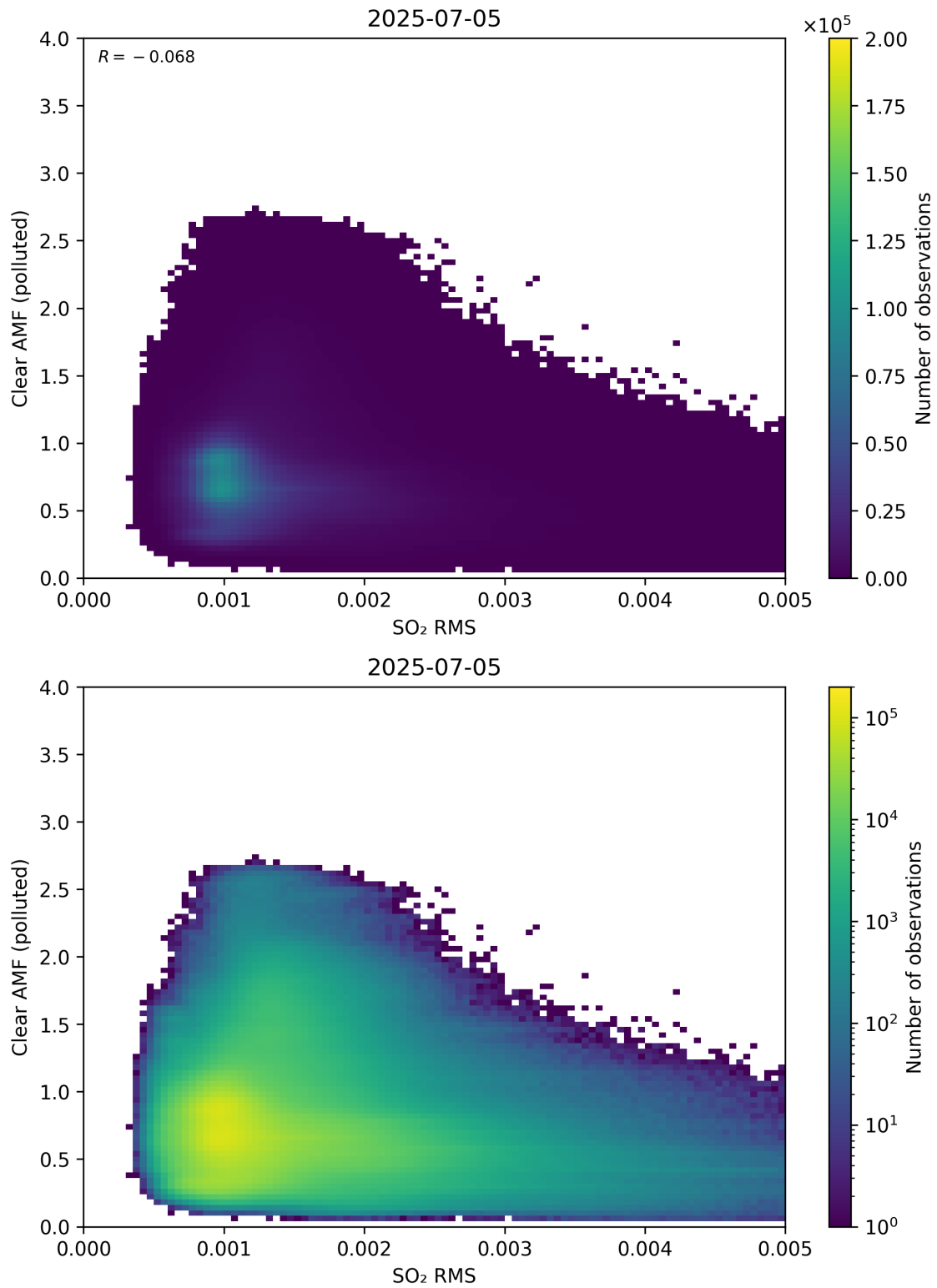
Figure 147: Scatter density plot of “SO 2 RMS” against “Clear AMF (polluted)” for 2025-07-04 to 2025-07-06.
