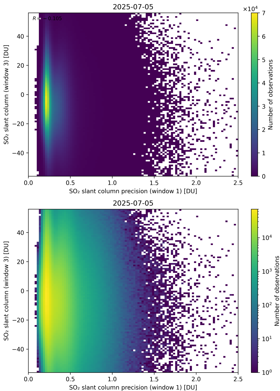
Figure 278: Scatter density plot of “SO 2 slant column precision (window 1)” against “SO 2 slant column (window 3)” for 2025-07-04 to 2025-07-06.
