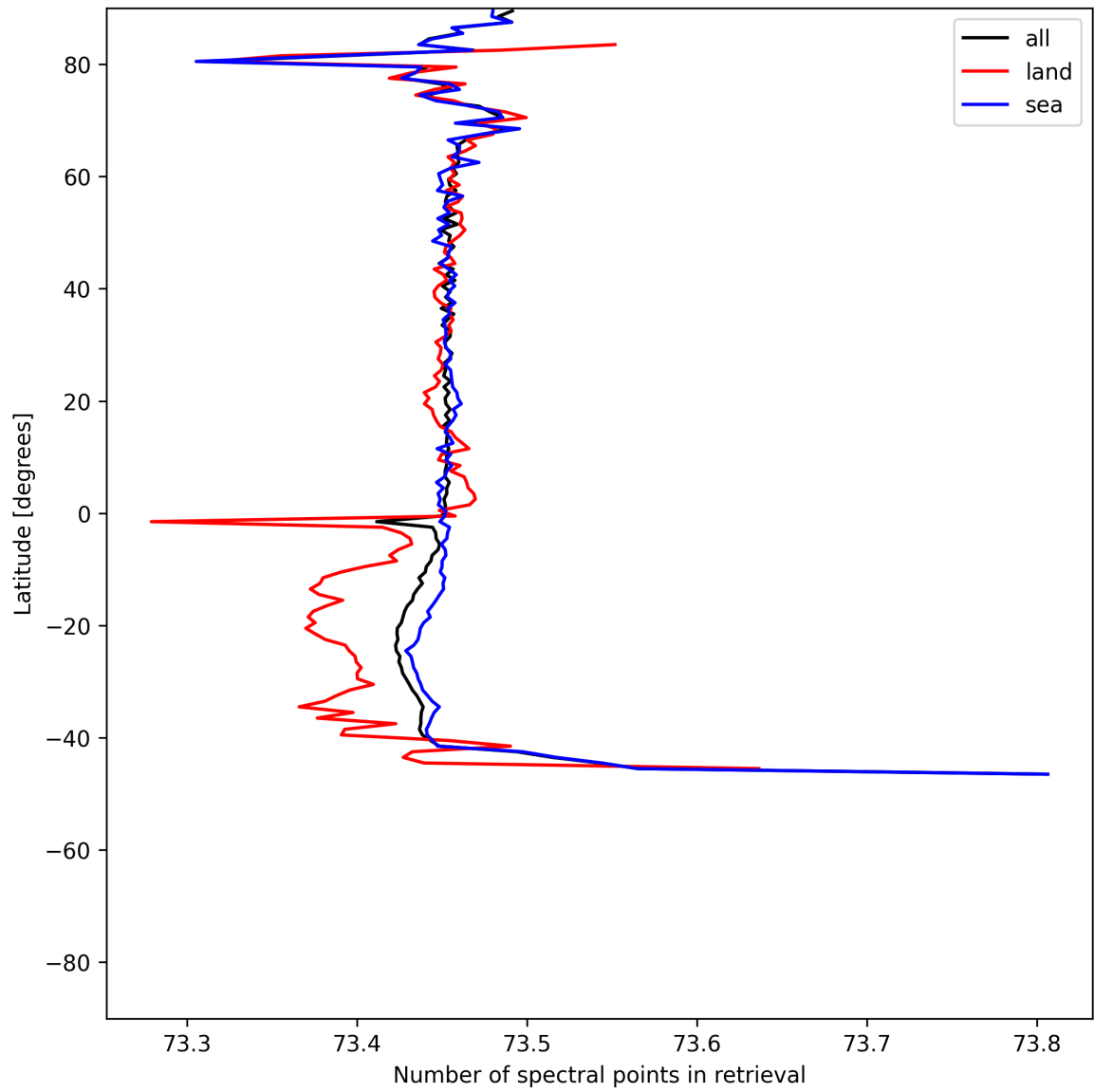
Figure 56: Zonal average of “Number of spectral points in retrieval” for 2025-07-04 to 2025-07-06.
