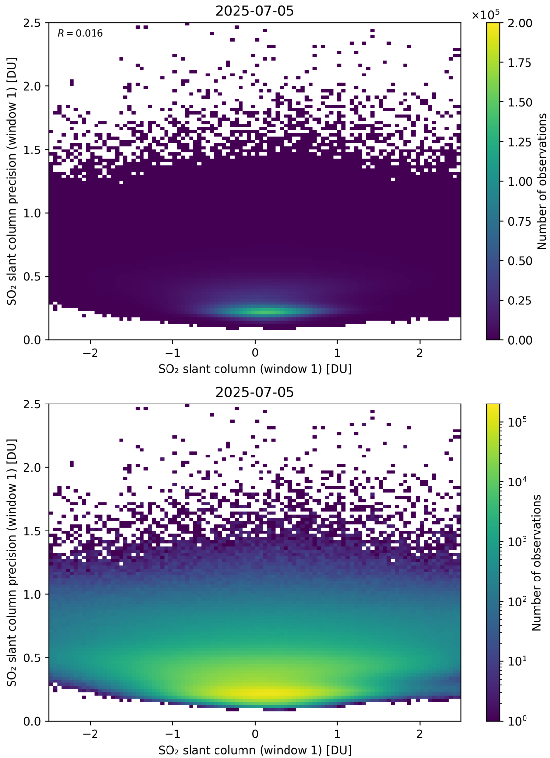
Figure 285: Scatter density plot of “SO 2 slant column (window 1)” against “SO 2 slant column precision (window 1)” for 2025-07-04 to 2025-07-06.
