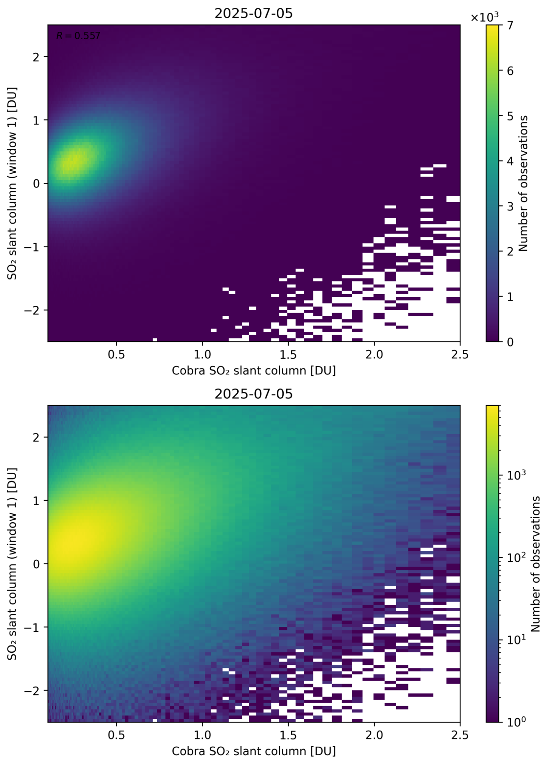
Figure 219: Scatter density plot of “Cobra SO 2 slant column” against “SO 2 slant column (window 1)” for 2025-07-04 to 2025-07-06.
