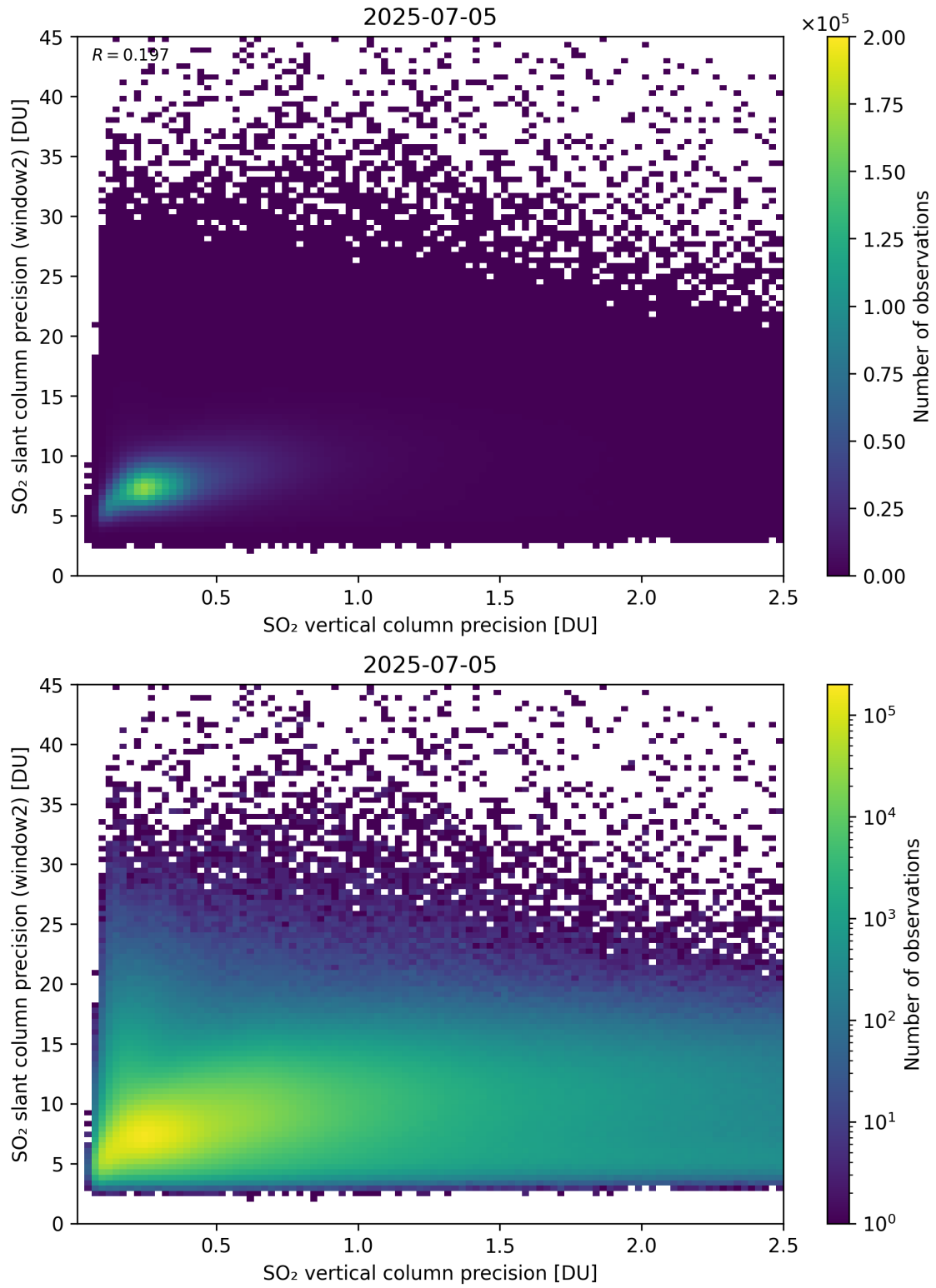
Figure 343: Scatter density plot of “SO 2 vertical column precision” against “SO 2 slant column precision (window2)” for 2025-07-04 to 2025-07-06.
