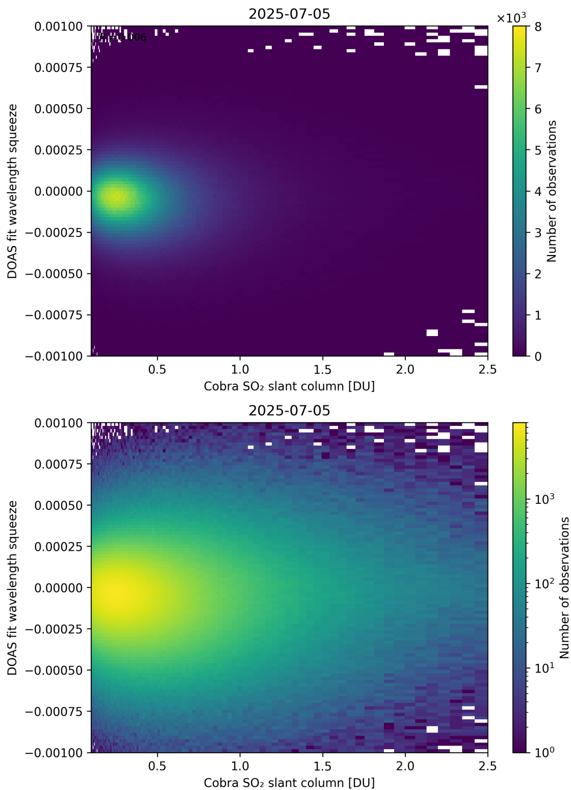
Figure 197: Scatter density plot of “Cobra SO 2 slant column” against “DOAS fit wavelength squeeze” for 2025-07-04 to 2025-07-06.
