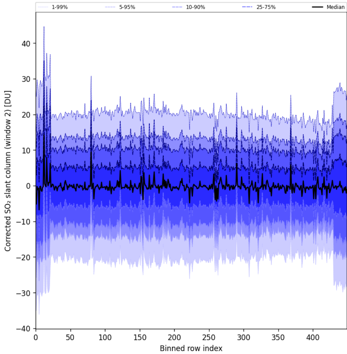
Figure 95: Along track statistics of “Corrected SO 2 slant column (window 2)” for 2025-07-04 to 2025-07-06
