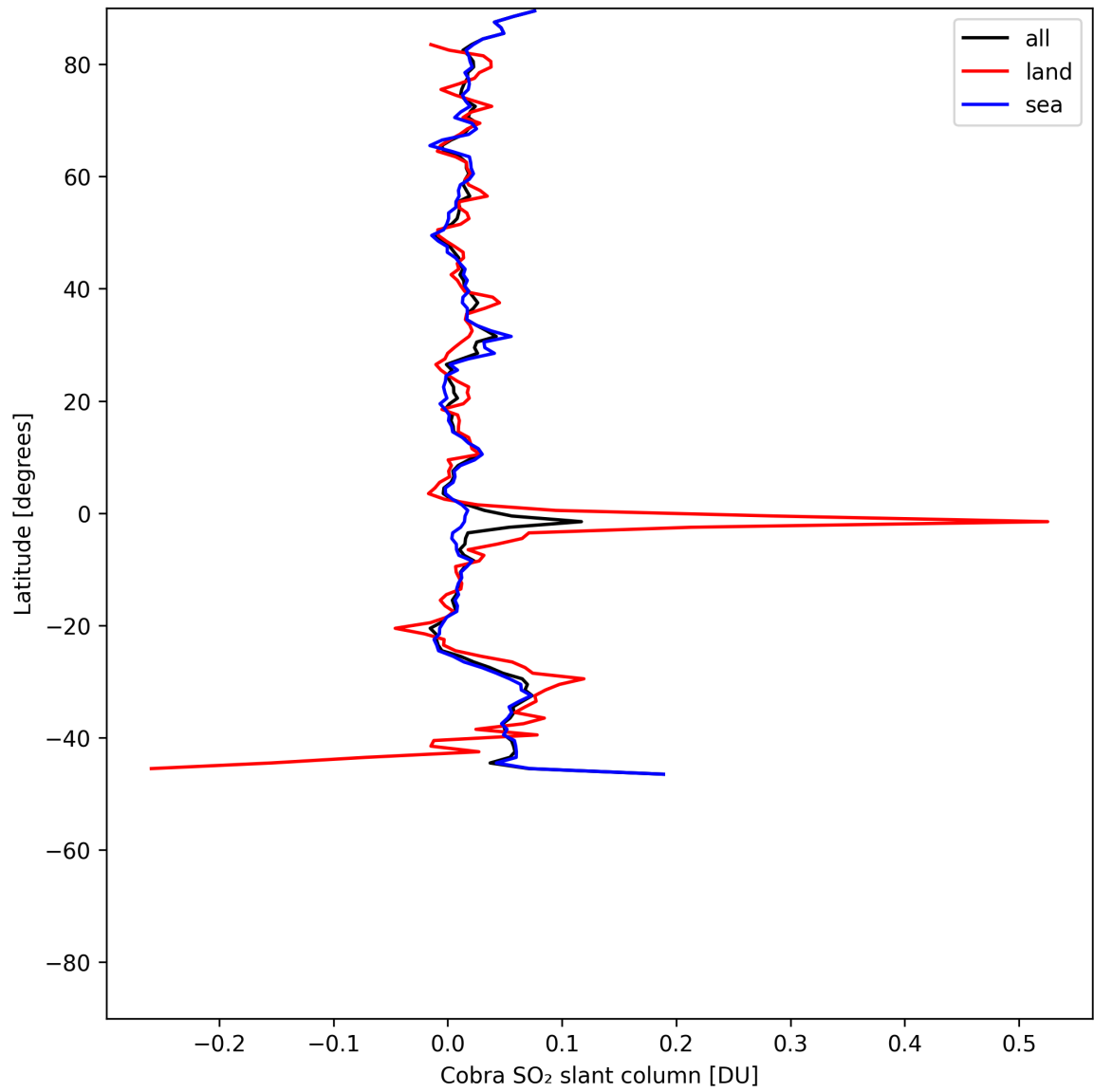
Figure 35: Zonal average of “Cobra SO 2 slant column” for 2025-07-04 to 2025-07-06.
