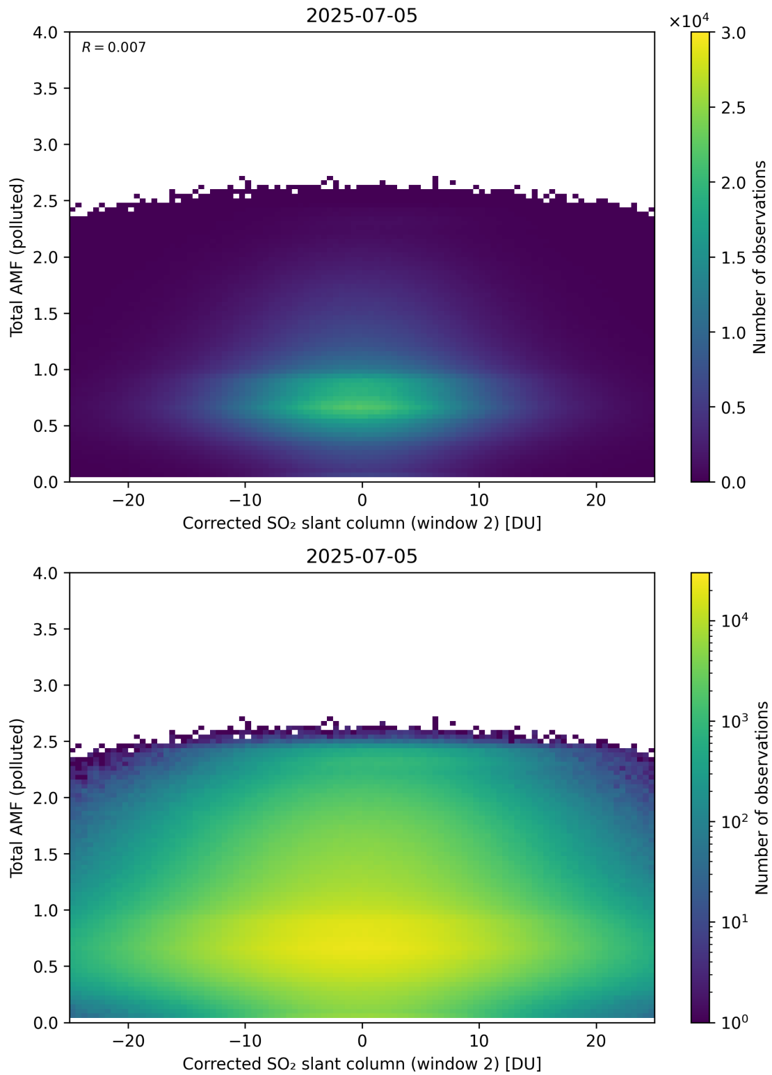
Figure 253: Scatter density plot of “Corrected SO 2 slant column (window 2)” against “Total AMF (polluted)” for 2025-07-04 to 2025-07-06.
