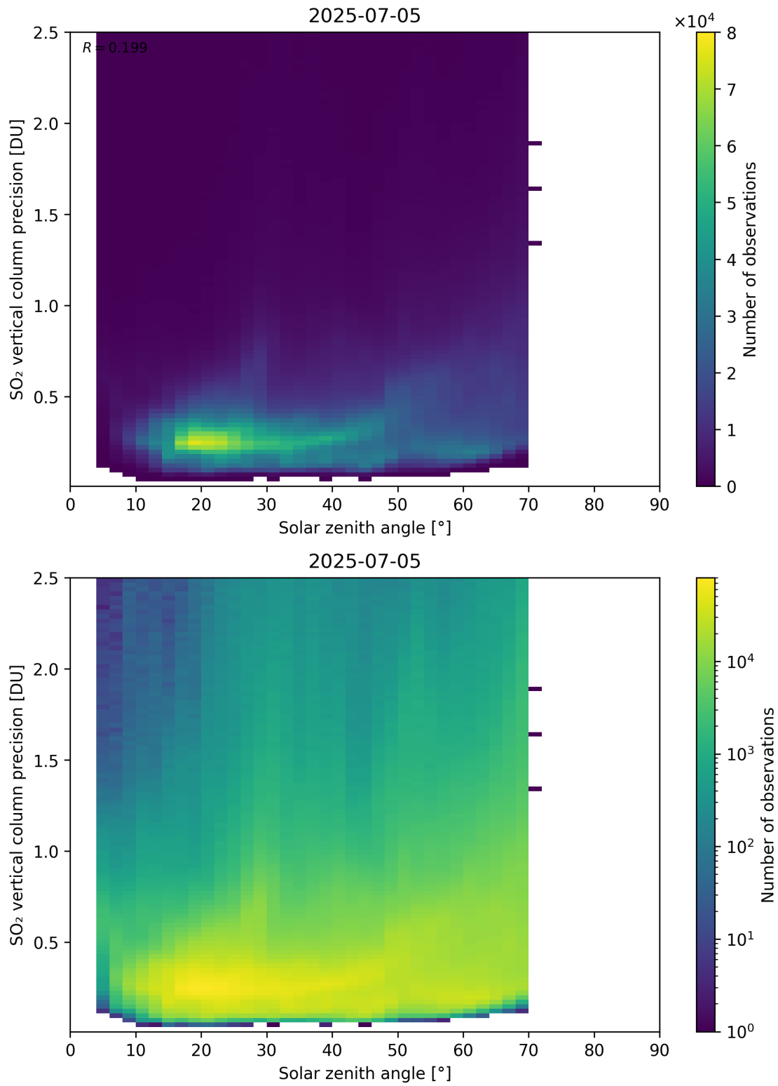
Figure 192: Scatter density plot of “Solar zenith angle” against “SO 2 vertical column precision” for 2025-07-04 to 2025-07-06.
