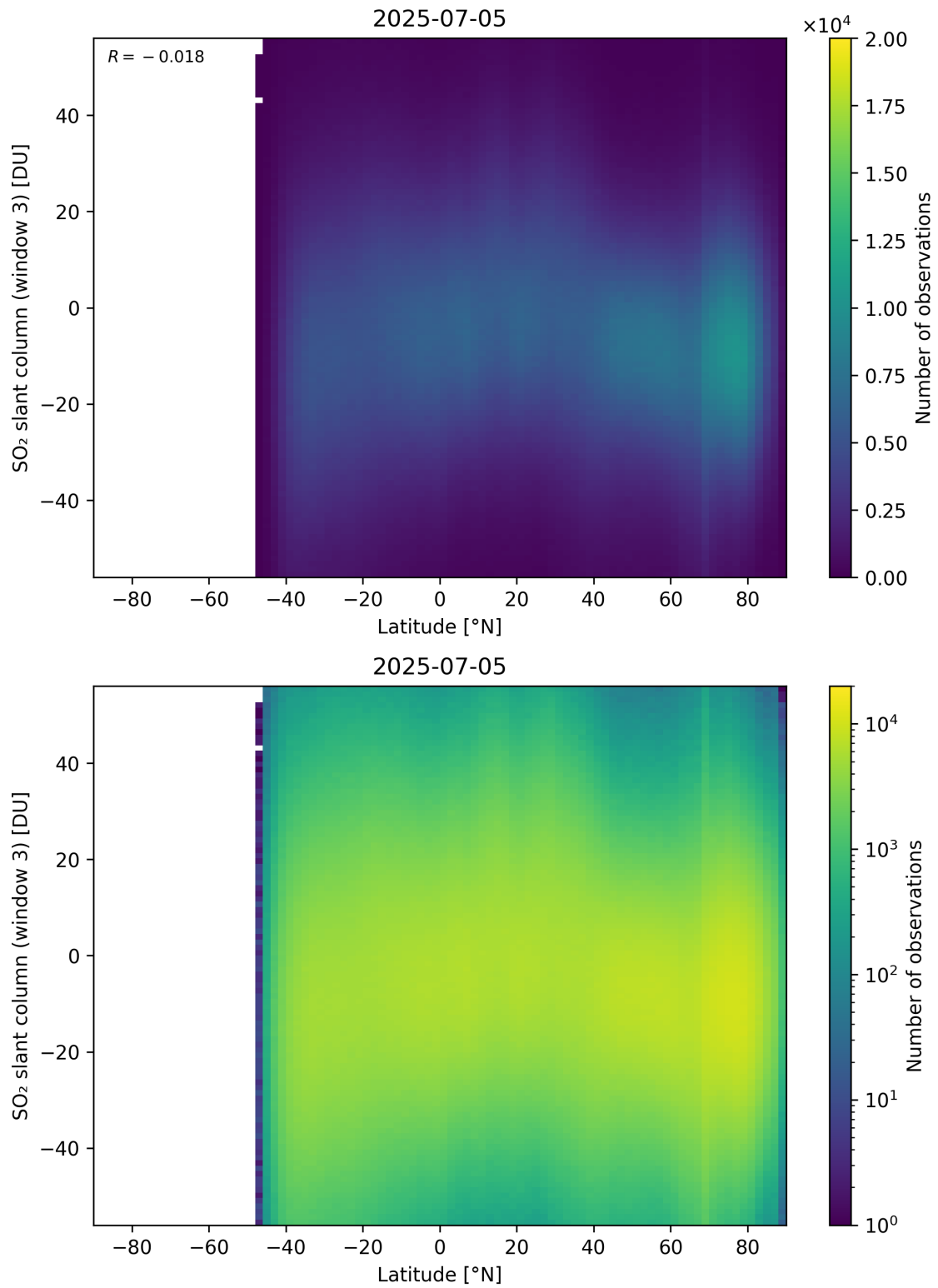
Figure 165: Scatter density plot of “Latitude” against “SO 2 slant column (window 3)” for 2025-07-04 to 2025-07-06.
