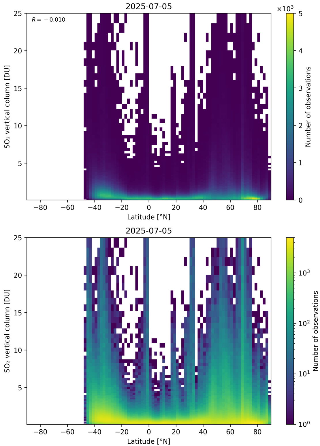
Figure 169: Scatter density plot of “Latitude” against “SO 2 vertical column” for 2025-07-04 to 2025-07-06.
