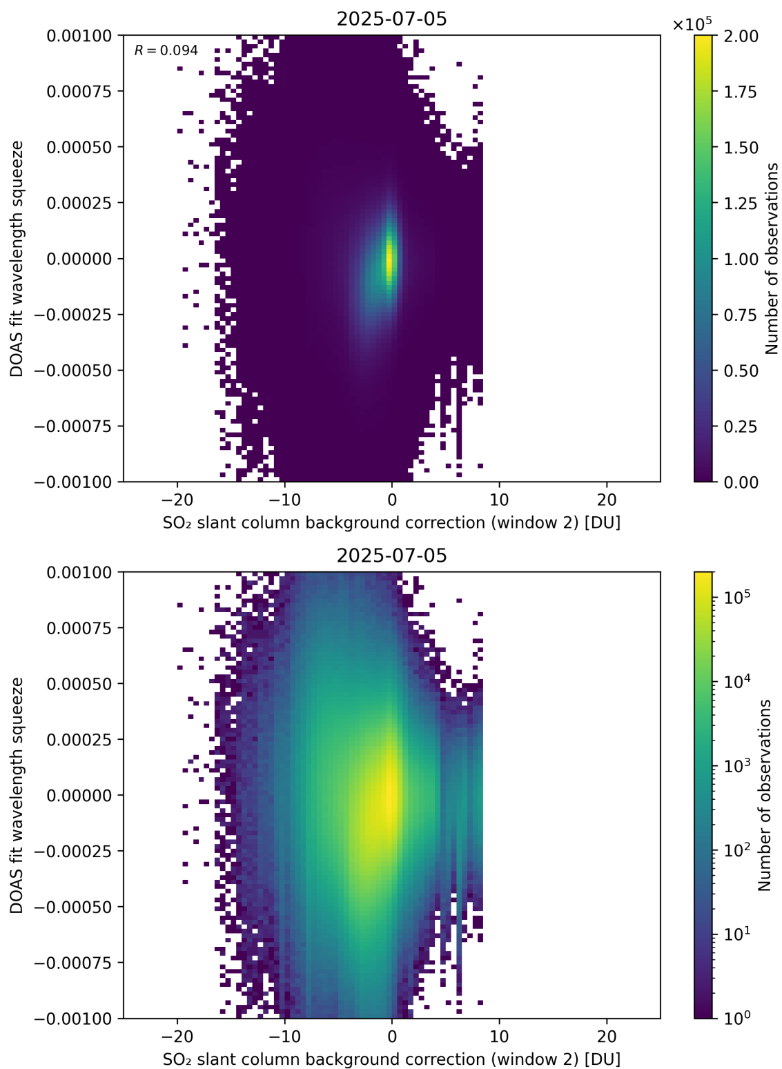
Figure 124: Scatter density plot of “SO 2 slant column background correction (window 2)” against “DOAS fit wavelength squeeze” for 2025-07-04 to 2025-07-06.
