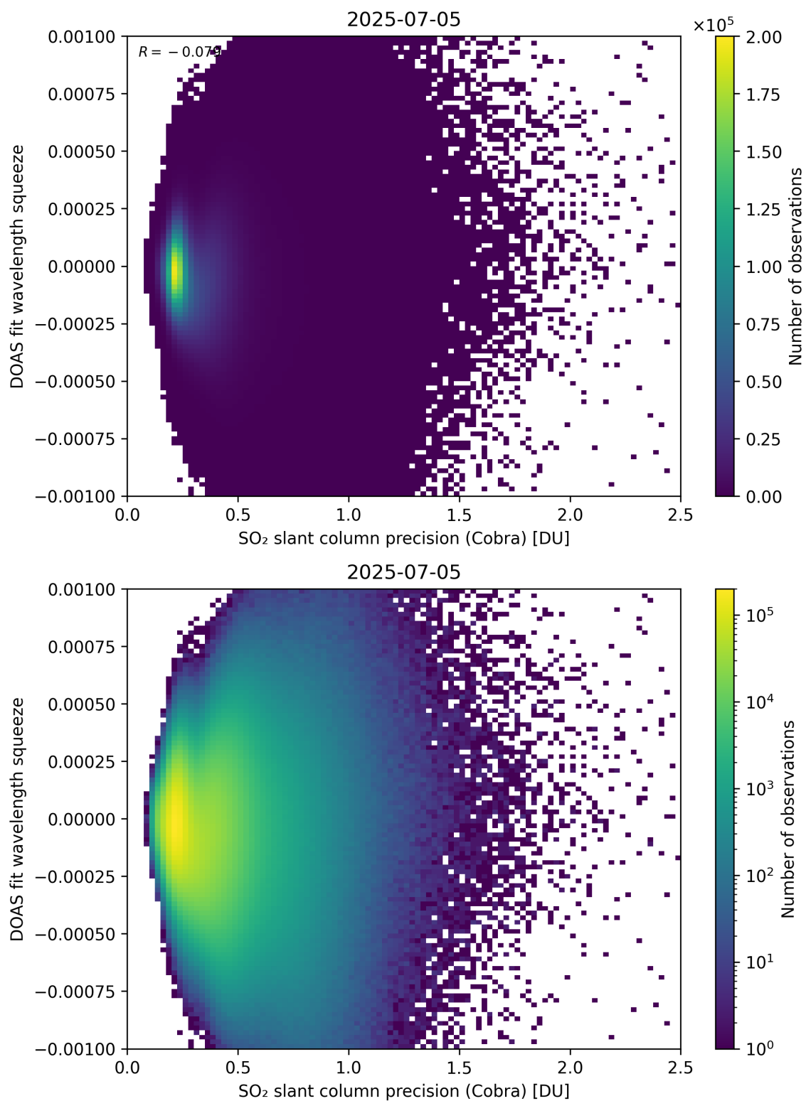
Figure 203: Scatter density plot of “SO 2 slant column precision (Cobra)” against “DOAS fit wavelength squeeze” for 2025-07-04 to 2025-07-06.
