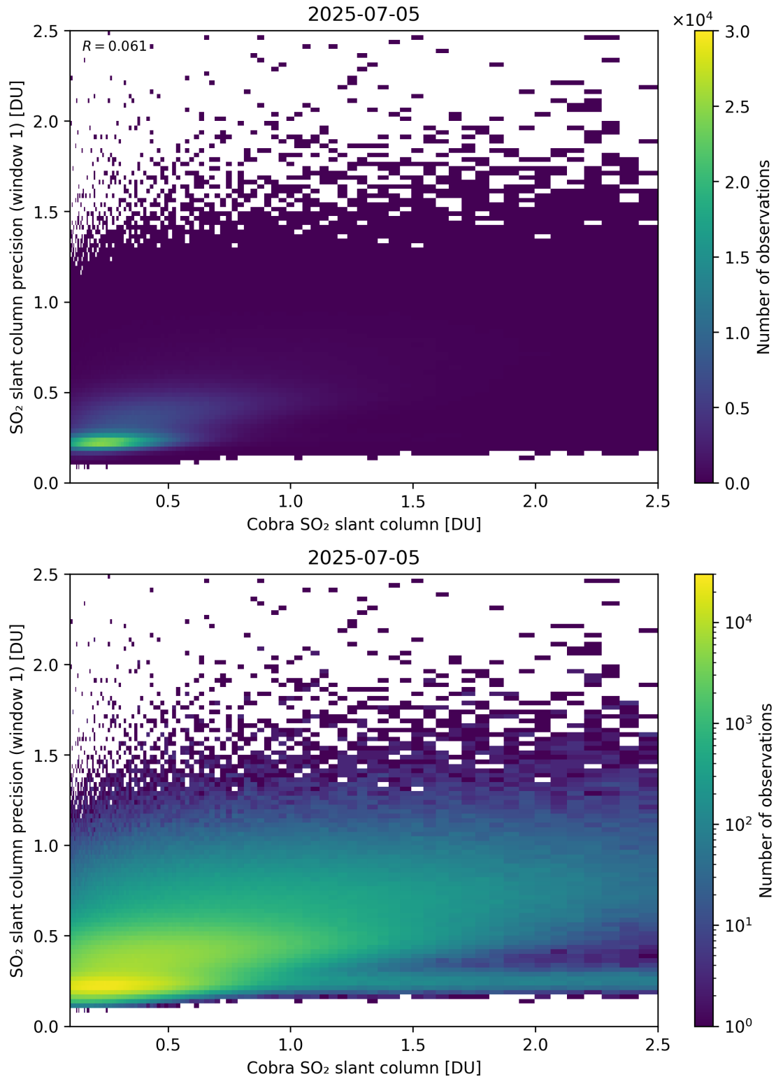
Figure 220: Scatter density plot of “Cobra SO 2 slant column” against “SO 2 slant column precision (window 1)” for 2025-07-04 to 2025-07-06.
