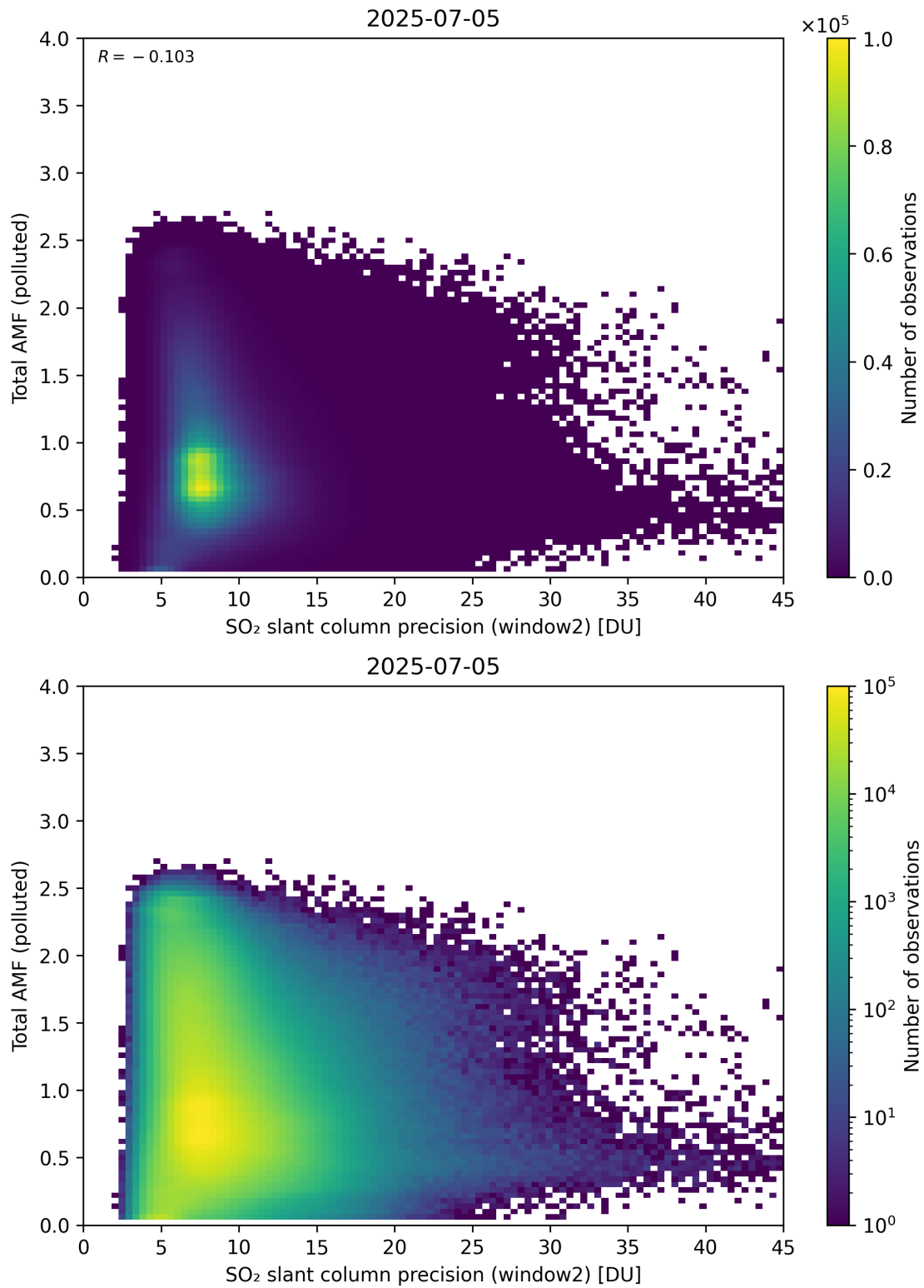
Figure 301: Scatter density plot of “SO 2 slant column precision (window2)” against “Total AMF (polluted)” for 2025-07-04 to 2025-07-06.
