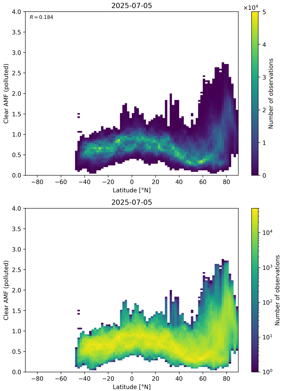
Figure 156: Scatter density plot of “Latitude” against “Clear AMF (polluted)” for 2025-07-04 to 2025-07-06.
