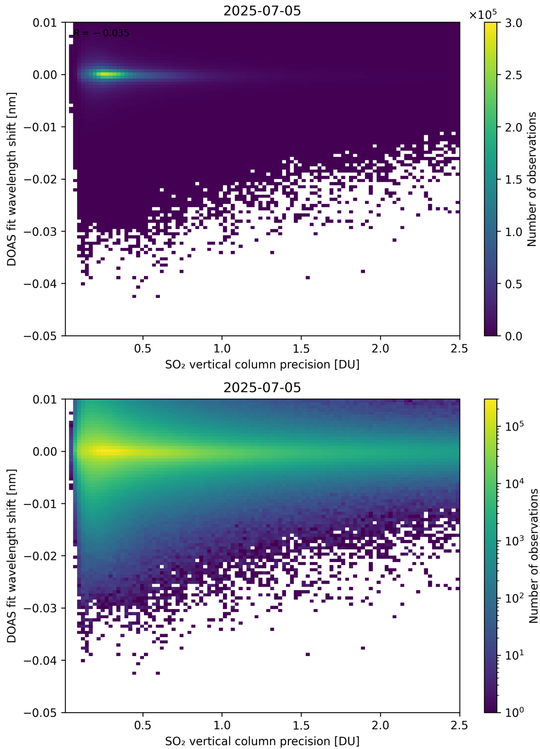
Figure 332: Scatter density plot of “SO 2 vertical column precision” against “DOAS fit wavelength shift” for 2025-07-04 to 2025-07-06.
