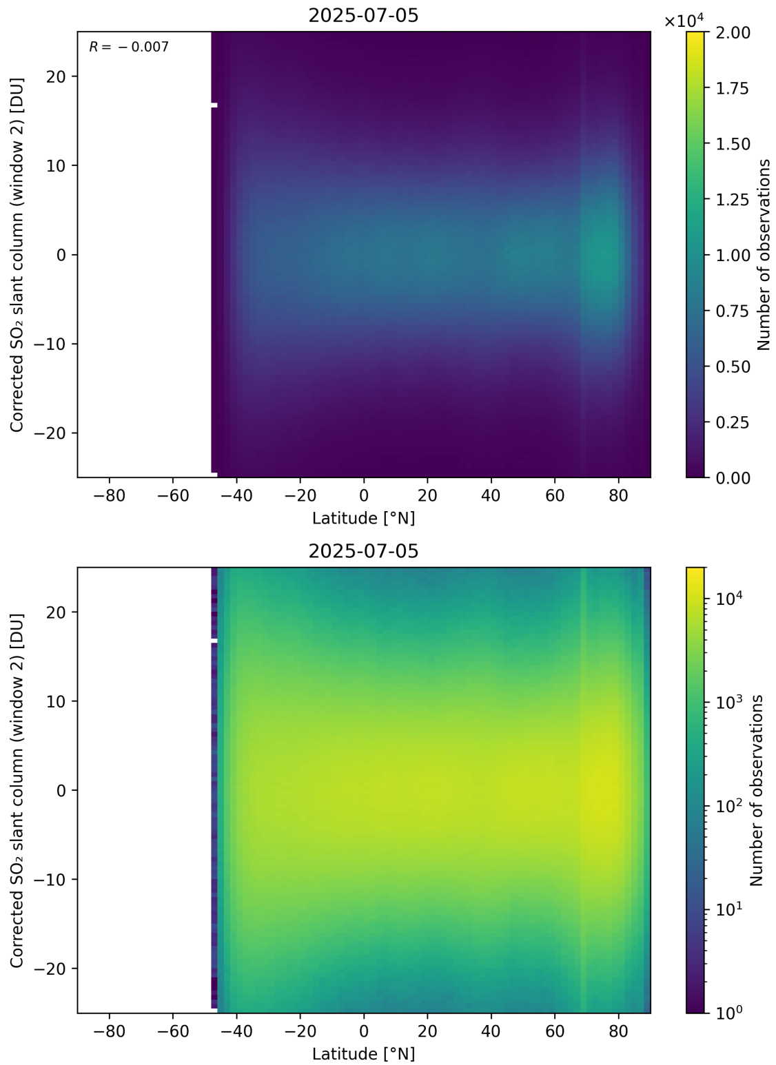
Figure 160: Scatter density plot of “Latitude” against “Corrected SO 2 slant column (window 2)” for 2025-07-04 to 2025-07-06.
