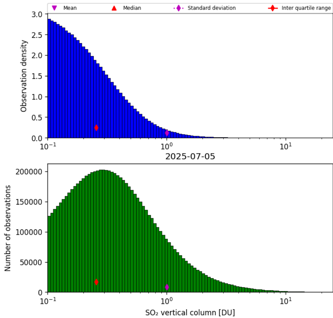
Figure 58: Histogram of “SO 2 vertical column” for 2025-07-04 to 2025-07-06
