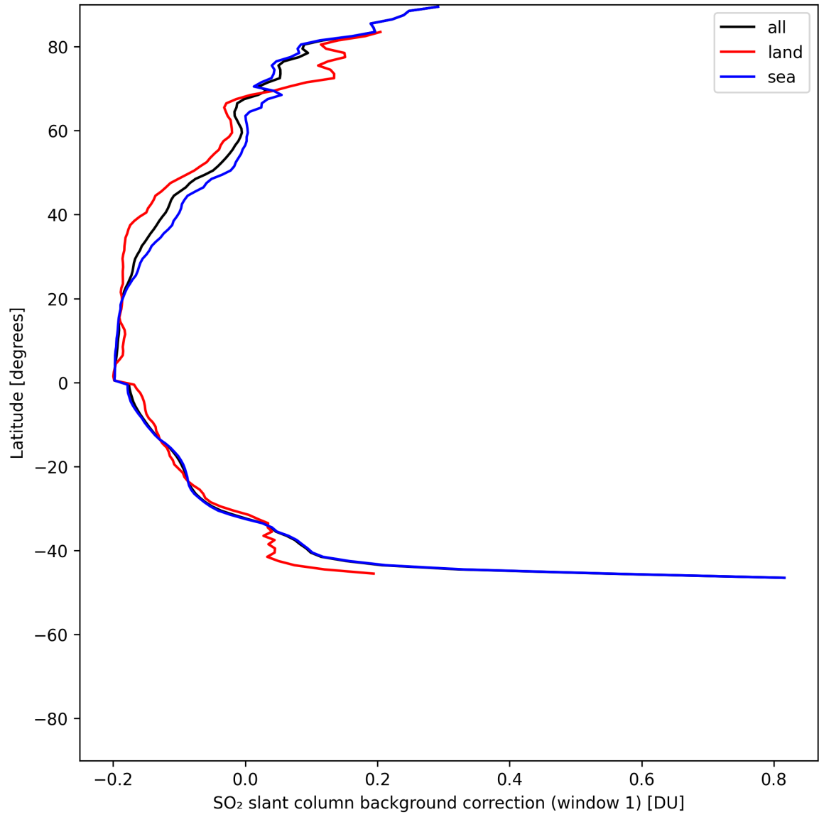
Figure 40: Zonal average of “SO 2 slant column background correction (window 1)” for 2025-07-04 to 2025-07-06.
