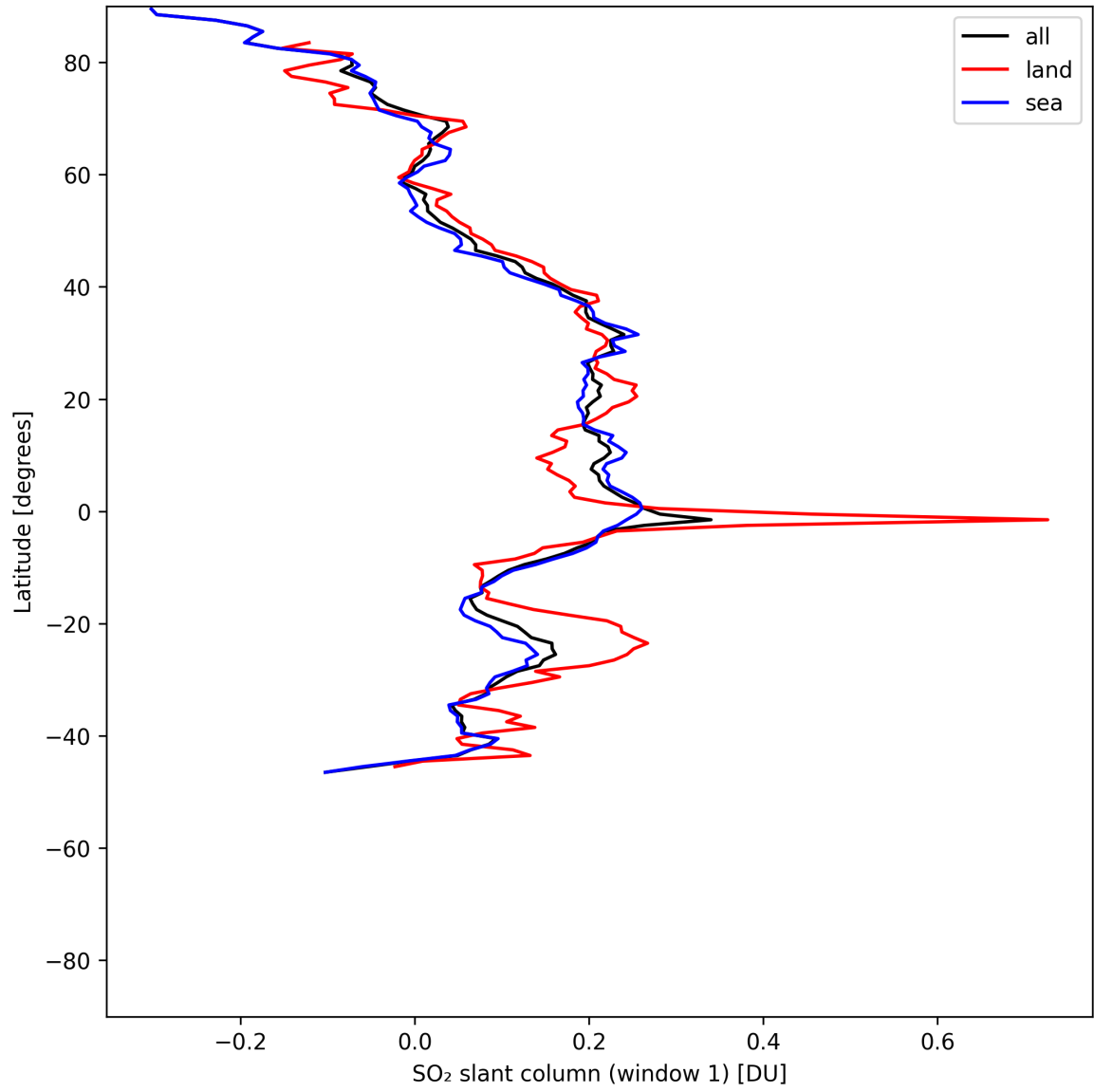
Figure 37: Zonal average of “SO 2 slant column (window 1)” for 2025-07-04 to 2025-07-06.
