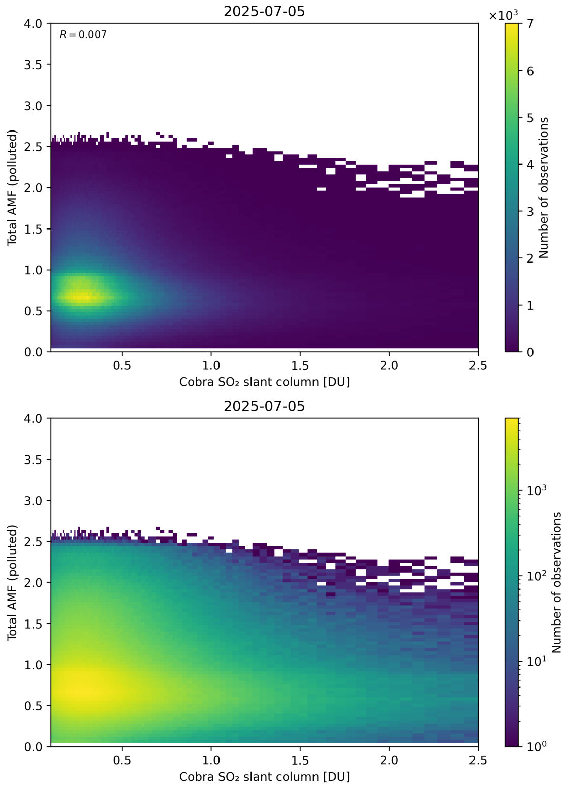
Figure 224: Scatter density plot of “Cobra SO 2 slant column” against “Total AMF (polluted)” for 2025-07-04 to 2025-07-06.
