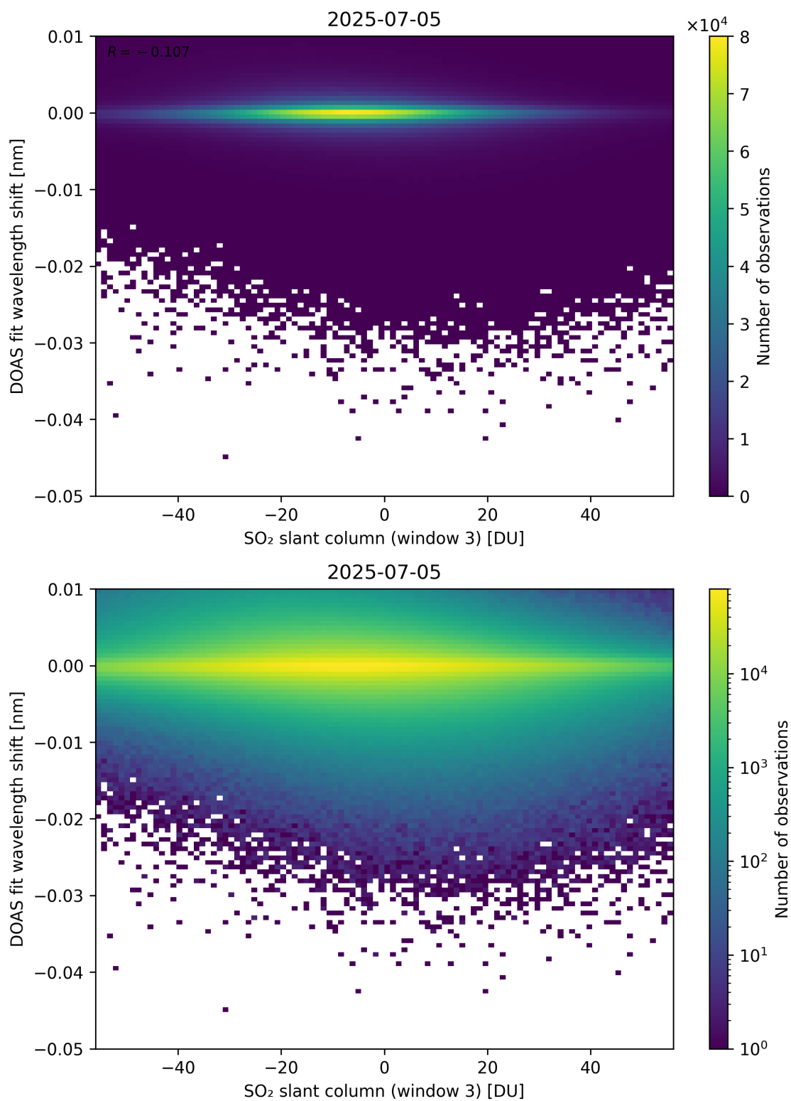
Figure 304: Scatter density plot of “SO 2 slant column (window 3)” against “DOAS fit wavelength shift” for 2025-07-04 to 2025-07-06.
