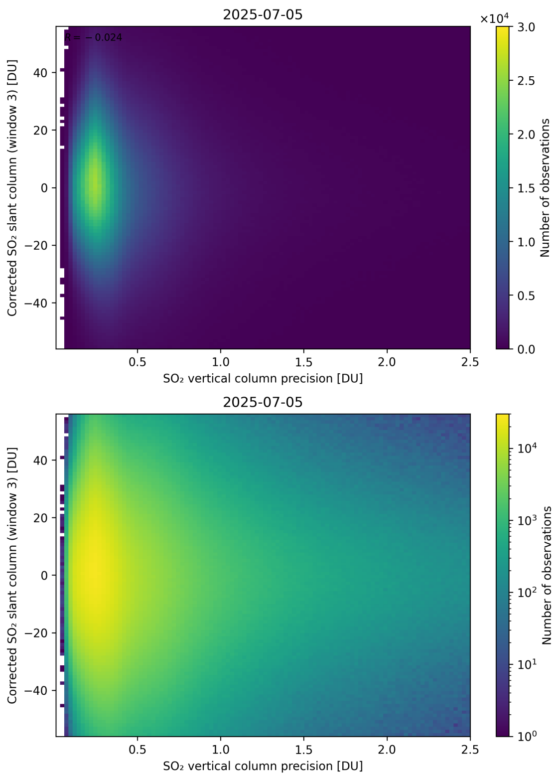
Figure 340: Scatter density plot of “SO 2 vertical column precision” against “Corrected SO 2 slant column (window 3)” for 2025-07-04 to 2025-07-06.
