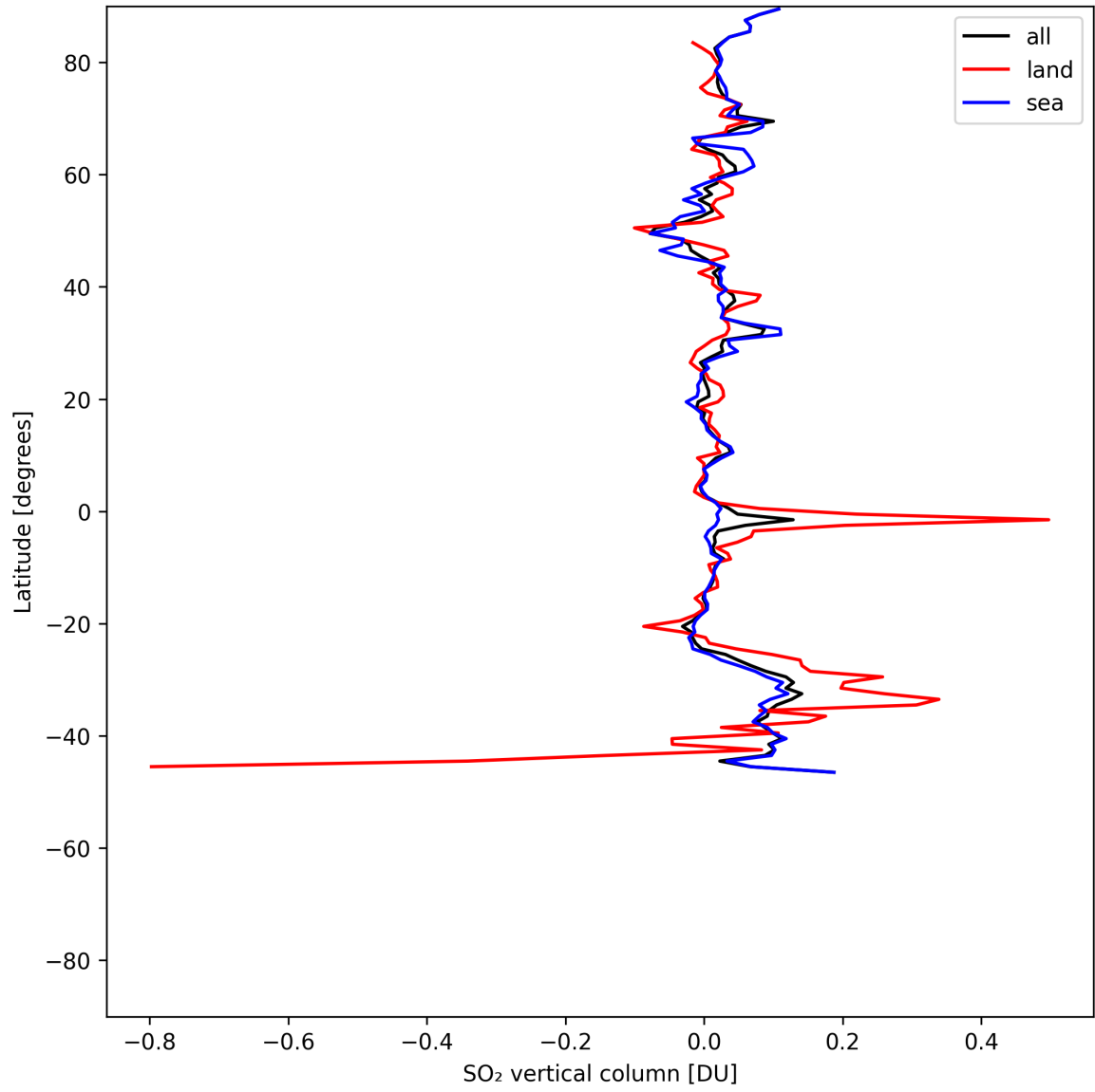
Figure 32: Zonal average of “SO 2 vertical column” for 2025-07-04 to 2025-07-06.
