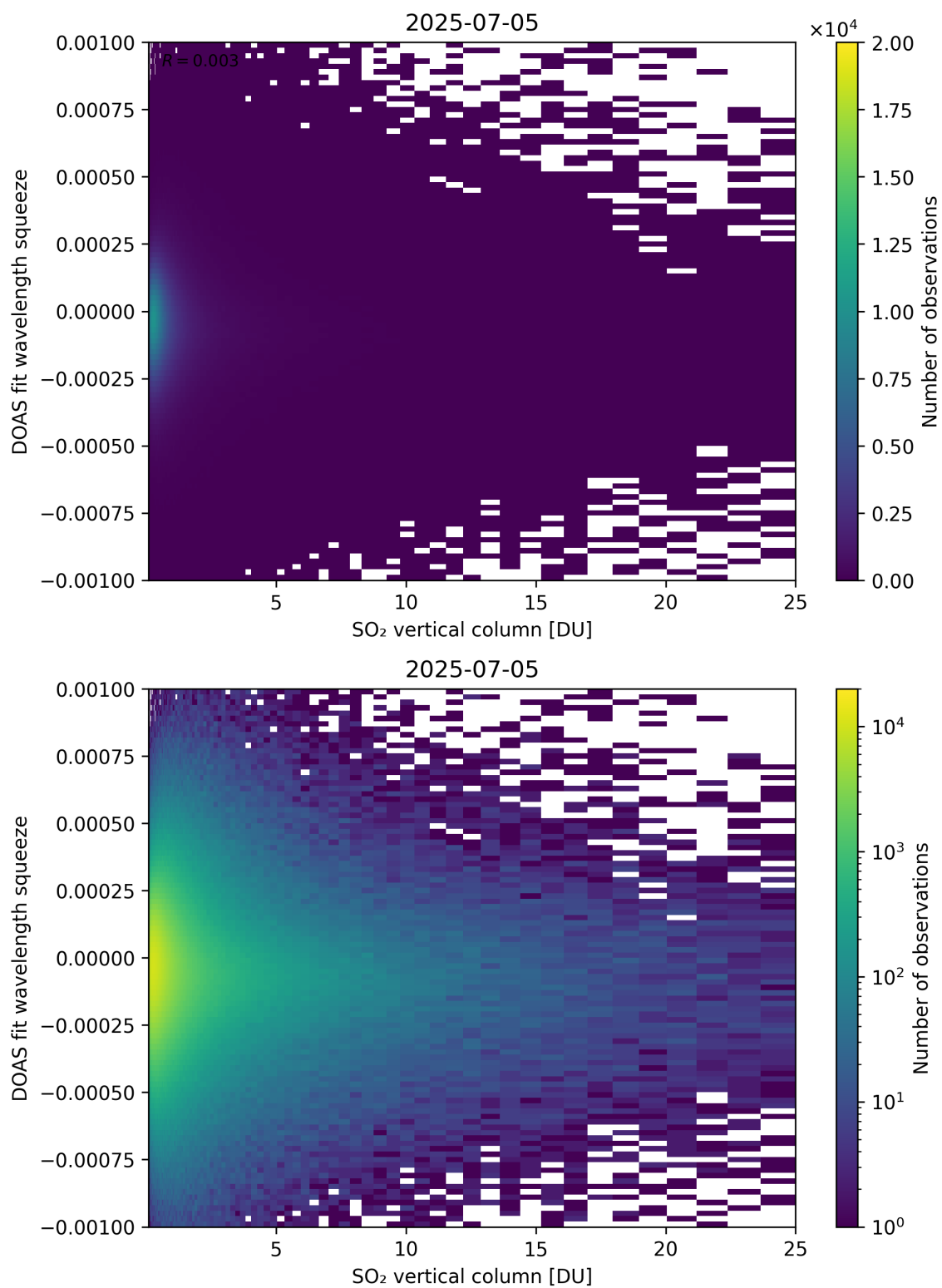
Figure 327: Scatter density plot of “SO 2 vertical column” against “DOAS fit wavelength squeeze” for 2025-07-04 to 2025-07-06.
