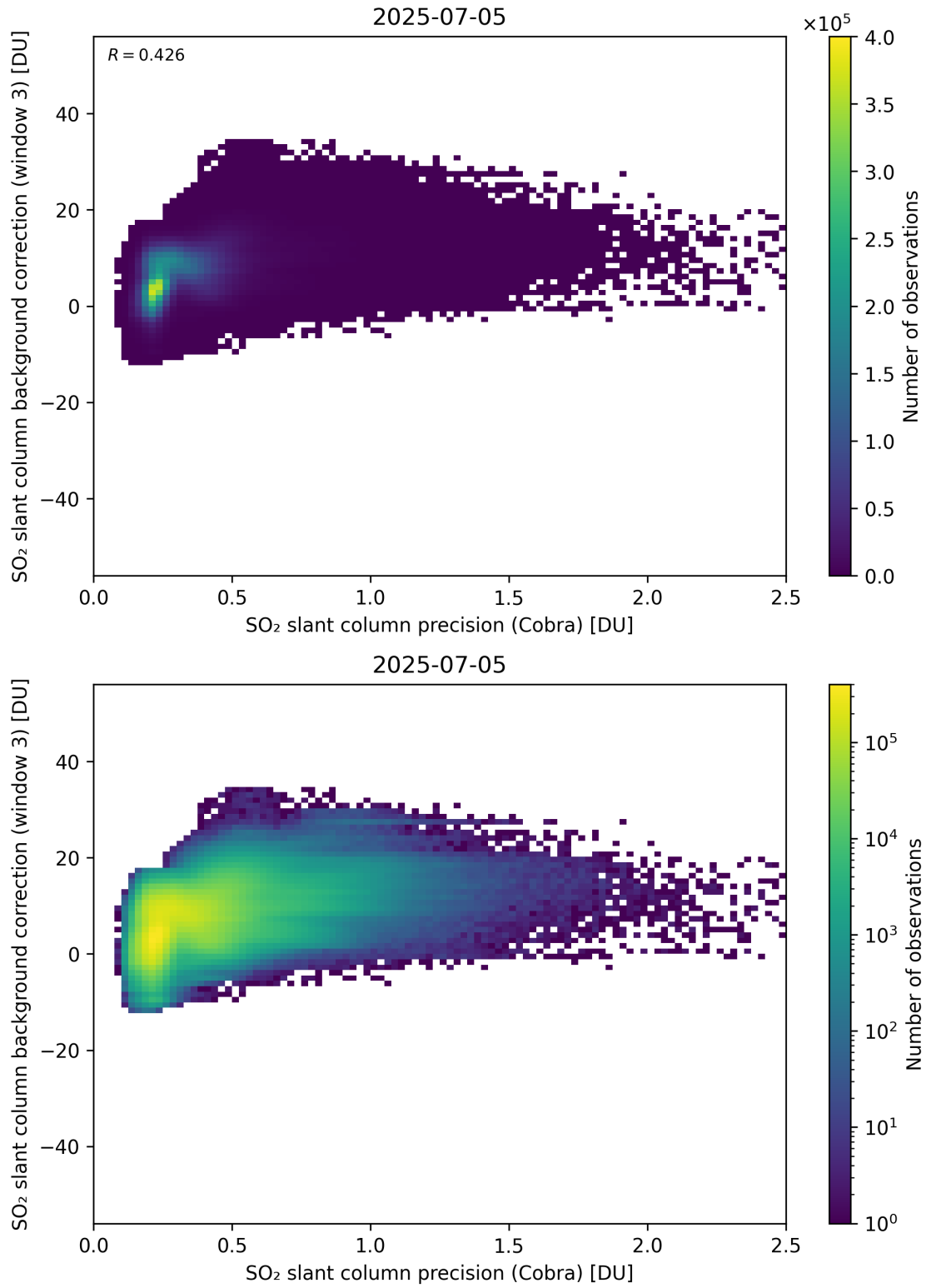
Figure 201: Scatter density plot of “SO 2 slant column precision (Cobra)” against “SO 2 slant column background correction (window 3)” for 2025-07-04 to 2025-07-06.
