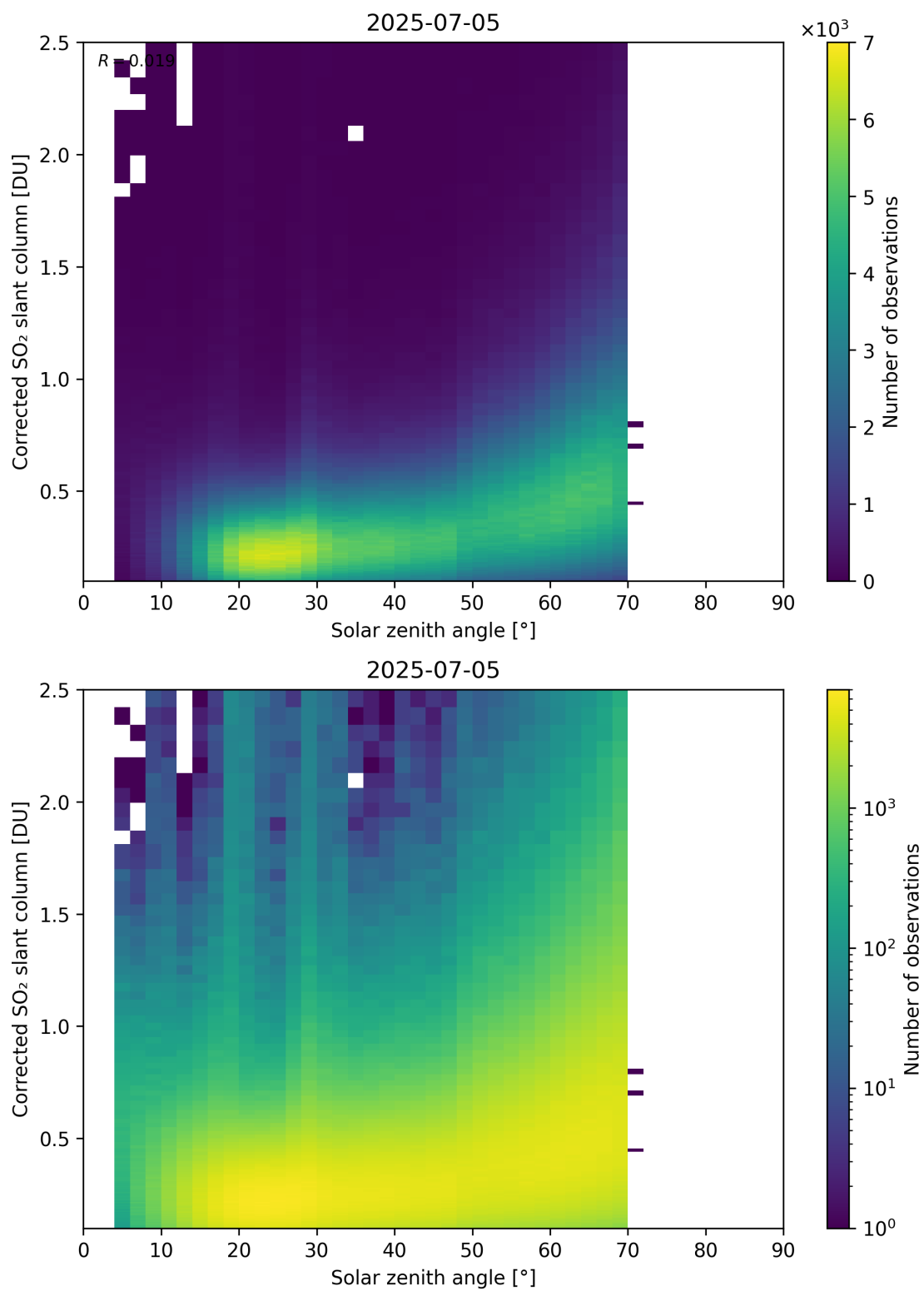
Figure 181: Scatter density plot of “Solar zenith angle” against “Corrected SO 2 slant column” for 2025-07-04 to 2025-07-06.
