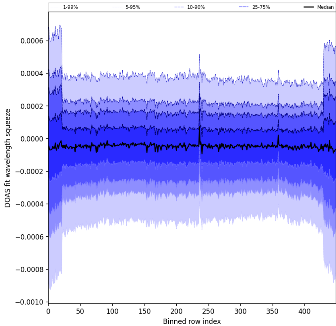
Figure 103: Along track statistics of “DOAS fit wavelength squeeze” for 2025-07-04 to 2025-07-06
