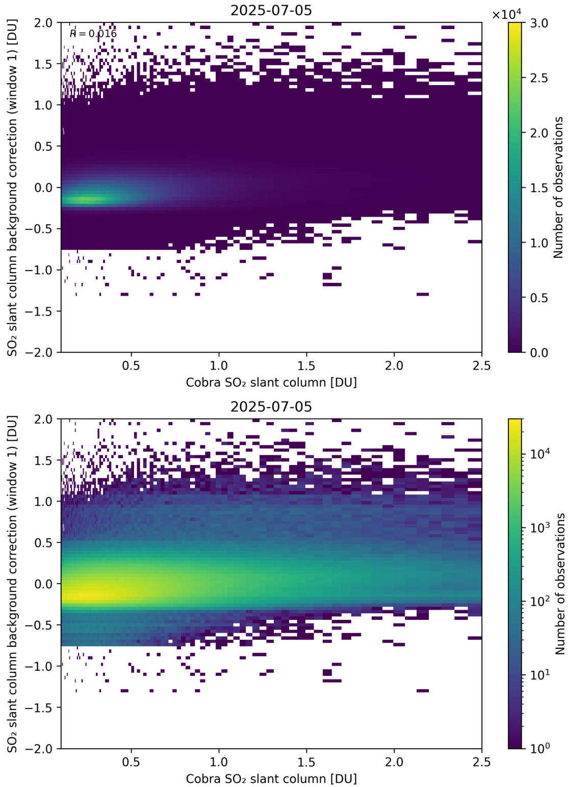
Figure 193: Scatter density plot of “Cobra SO 2 slant column” against “SO 2 slant column background correction (window 1)” for 2025-07-04 to 2025-07-06.
