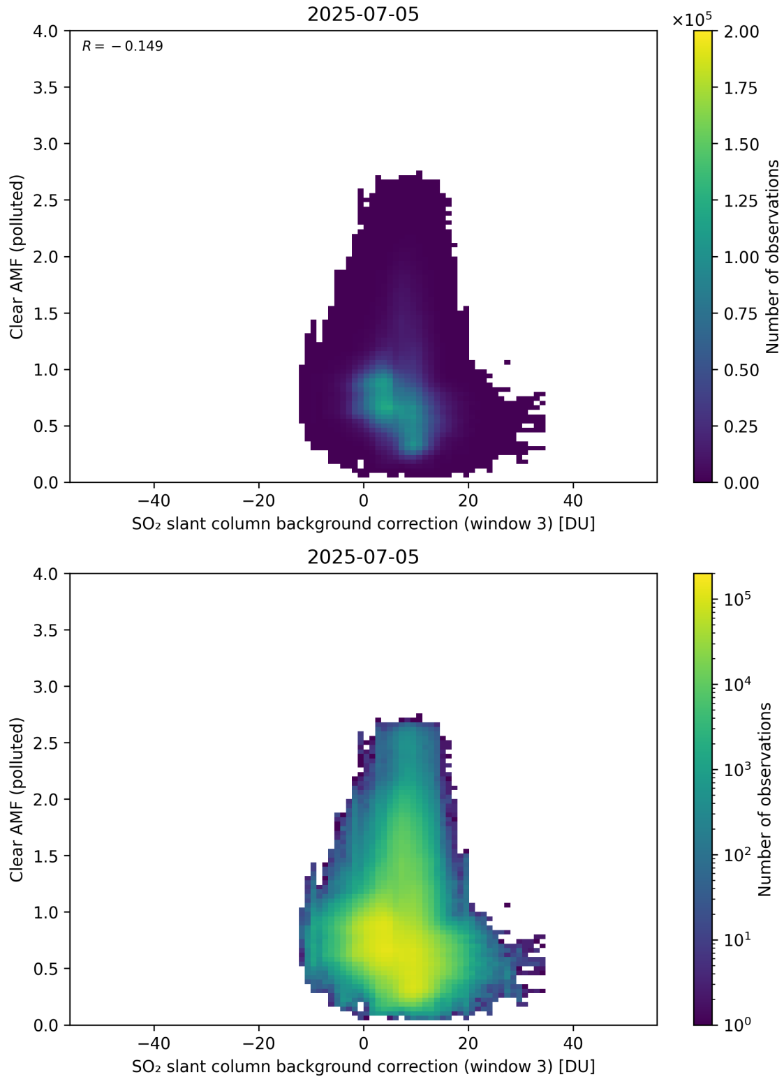
Figure 135: Scatter density plot of “SO 2 slant column background correction (window 3)” against “Clear AMF (polluted)” for 2025-07-04 to 2025-07-06.
