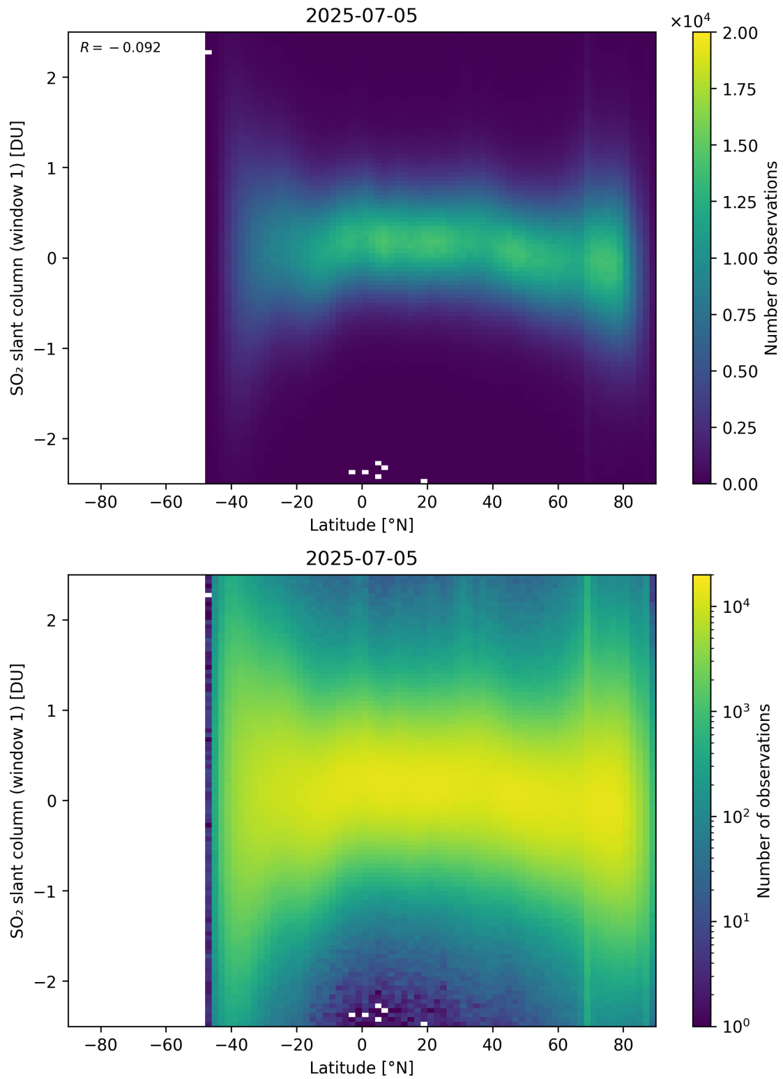
Figure 162: Scatter density plot of “Latitude” against “SO 2 slant column (window 1)” for 2025-07-04 to 2025-07-06.
