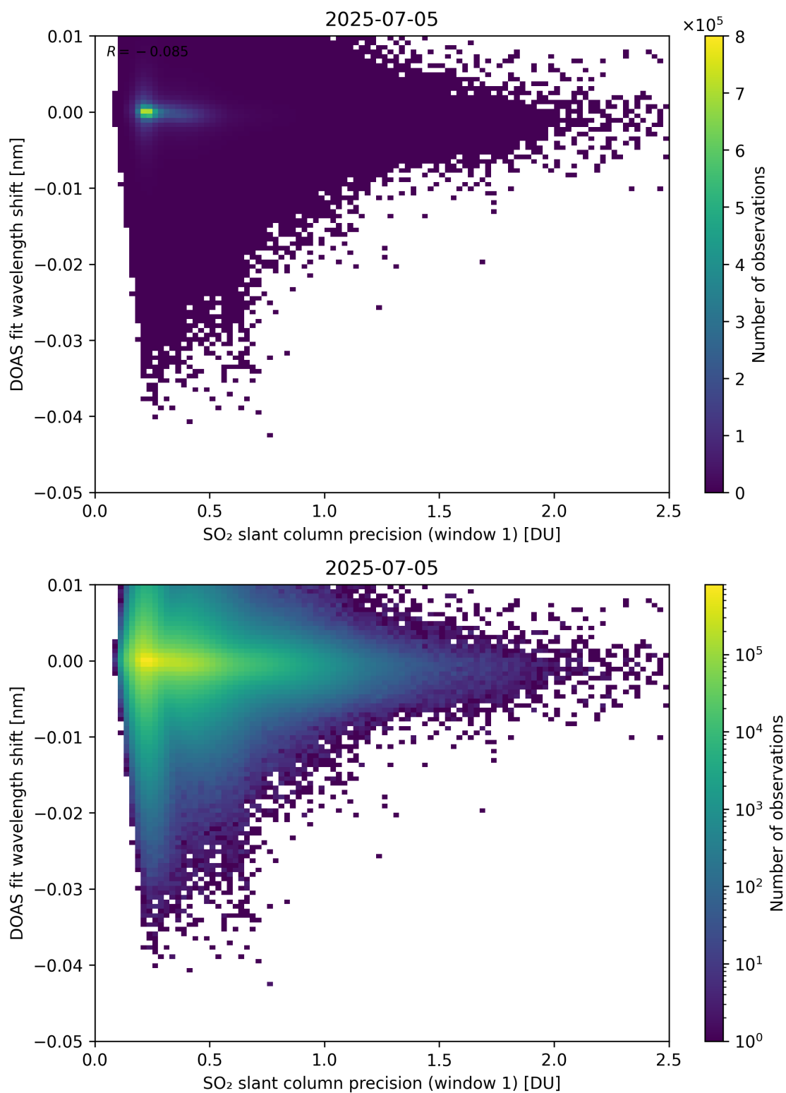
Figure 271: Scatter density plot of “SO 2 slant column precision (window 1)” against “DOAS fit wavelength shift” for 2025-07-04 to 2025-07-06.
