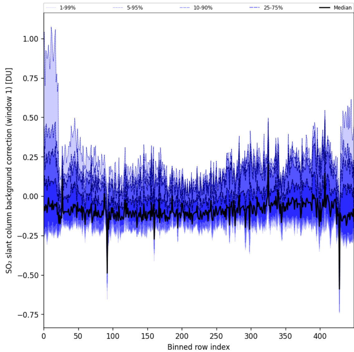
Figure 92: Along track statistics of “SO 2 slant column background correction (window 1)” for 2025-07-04 to 2025-07-06
