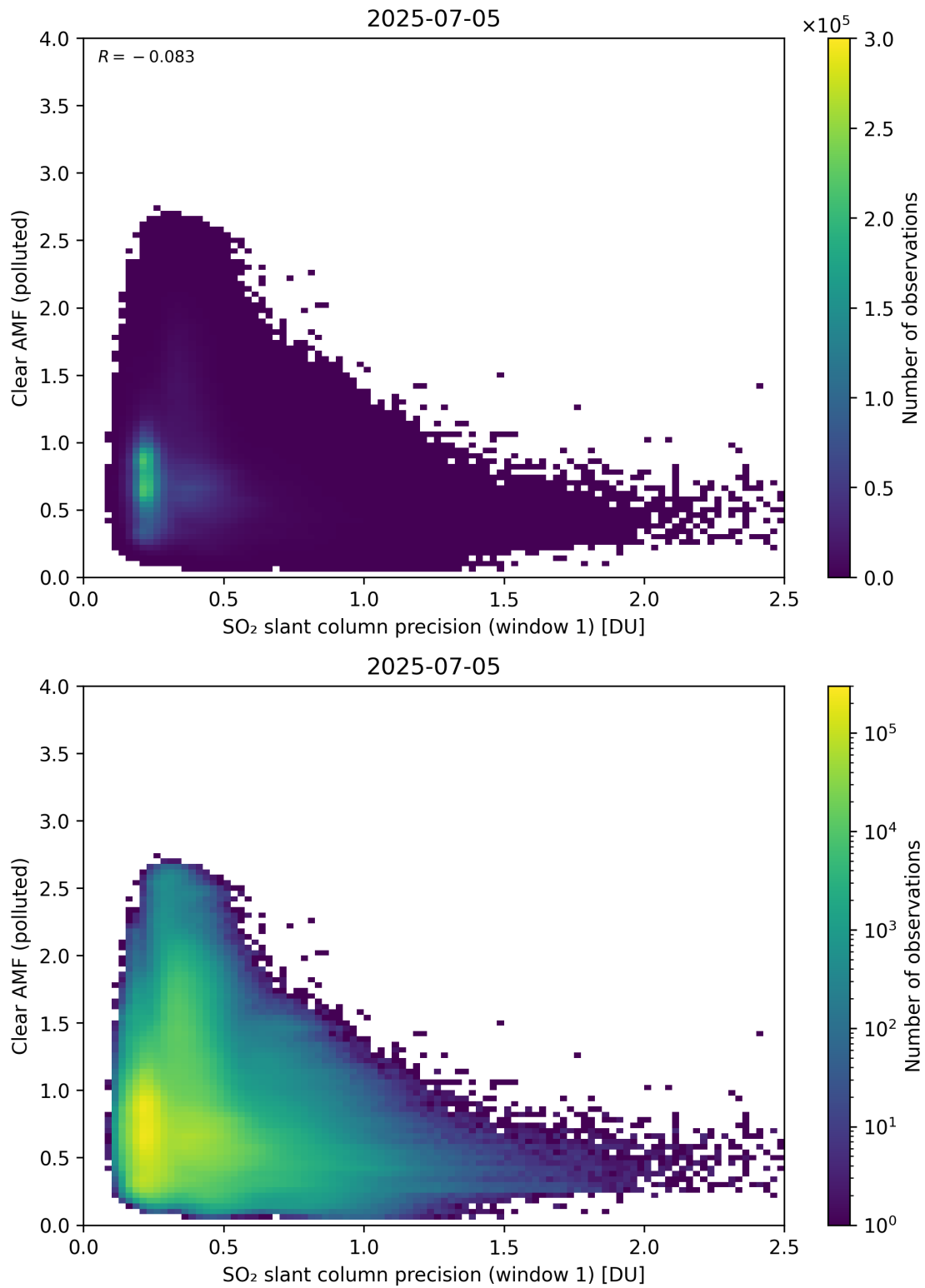
Figure 274: Scatter density plot of “SO 2 slant column precision (window 1)” against “Clear AMF (polluted)” for 2025-07-04 to 2025-07-06.
