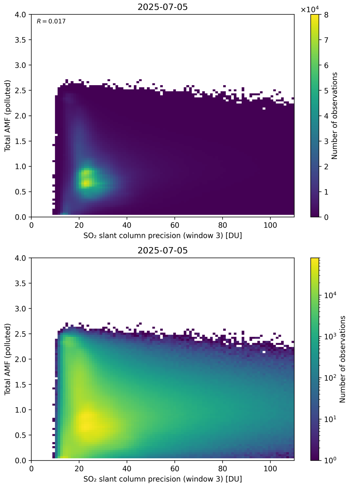
Figure 313: Scatter density plot of “SO 2 slant column precision (window 3)” against “Total AMF (polluted)” for 2025-07-04 to 2025-07-06.
