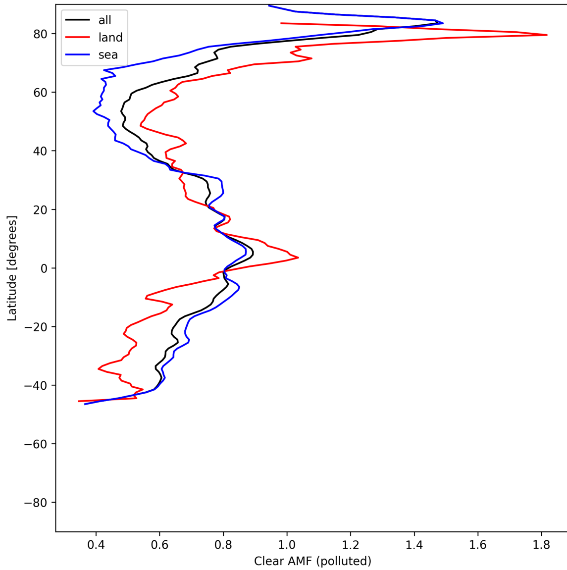
Figure 55: Zonal average of “Clear AMF (polluted)” for 2025-07-04 to 2025-07-06.
