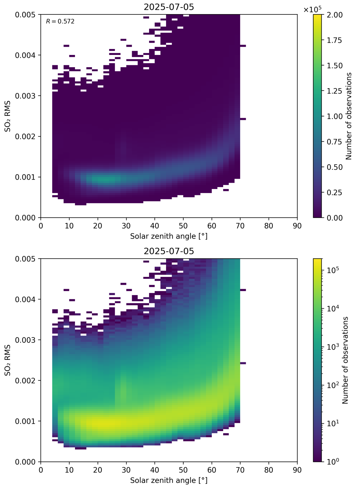
Figure 176: Scatter density plot of “Solar zenith angle” against “SO 2 RMS” for 2025-07-04 to 2025-07-06.
