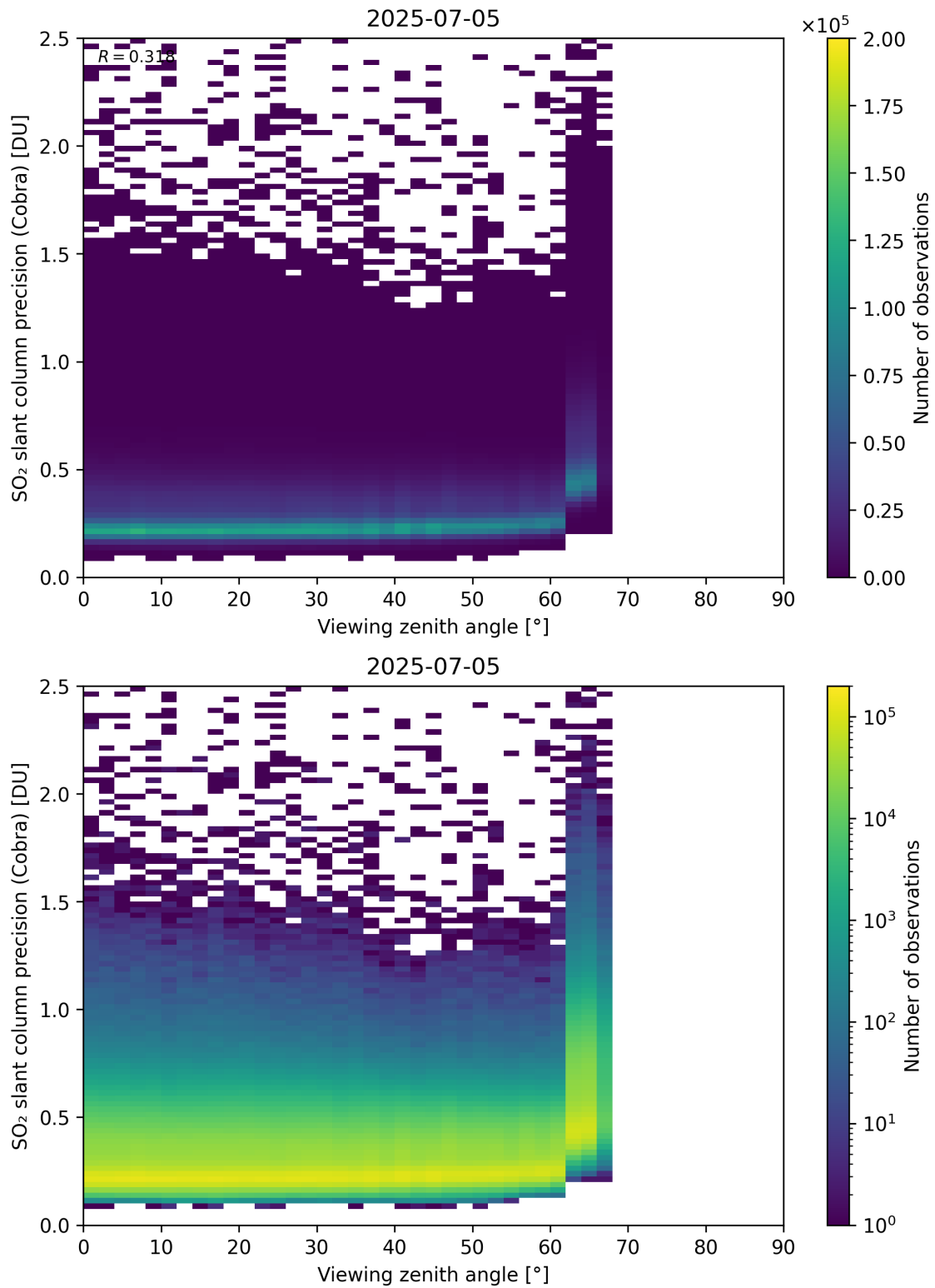
Figure 372: Scatter density plot of “Viewing zenith angle” against “SO 2 slant column precision (Cobra)” for 2025-07-04 to 2025-07-06.
