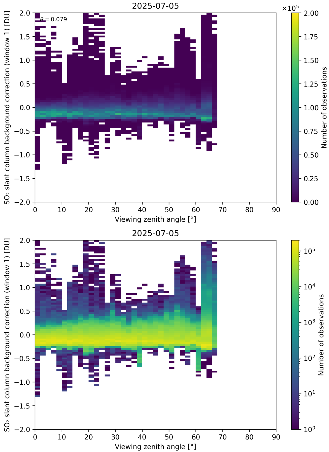
Figure 362: Scatter density plot of “Viewing zenith angle” against “SO 2 slant column background correction (window 1)” for 2025-07-04 to 2025-07-06.
