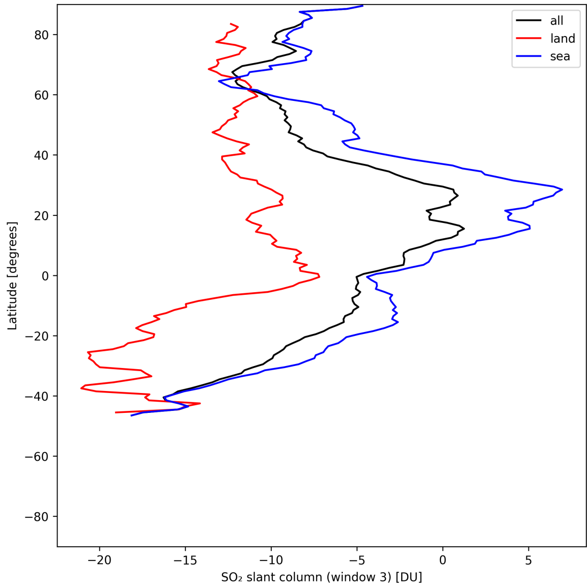
Figure 45: Zonal average of “SO 2 slant column (window 3)” for 2025-07-04 to 2025-07-06.
