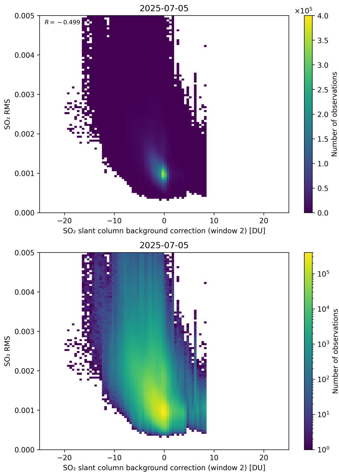
Figure 125: Scatter density plot of “SO 2 slant column background correction (window 2)” against “SO 2 RMS” for 2025-07-04 to 2025-07-06.
