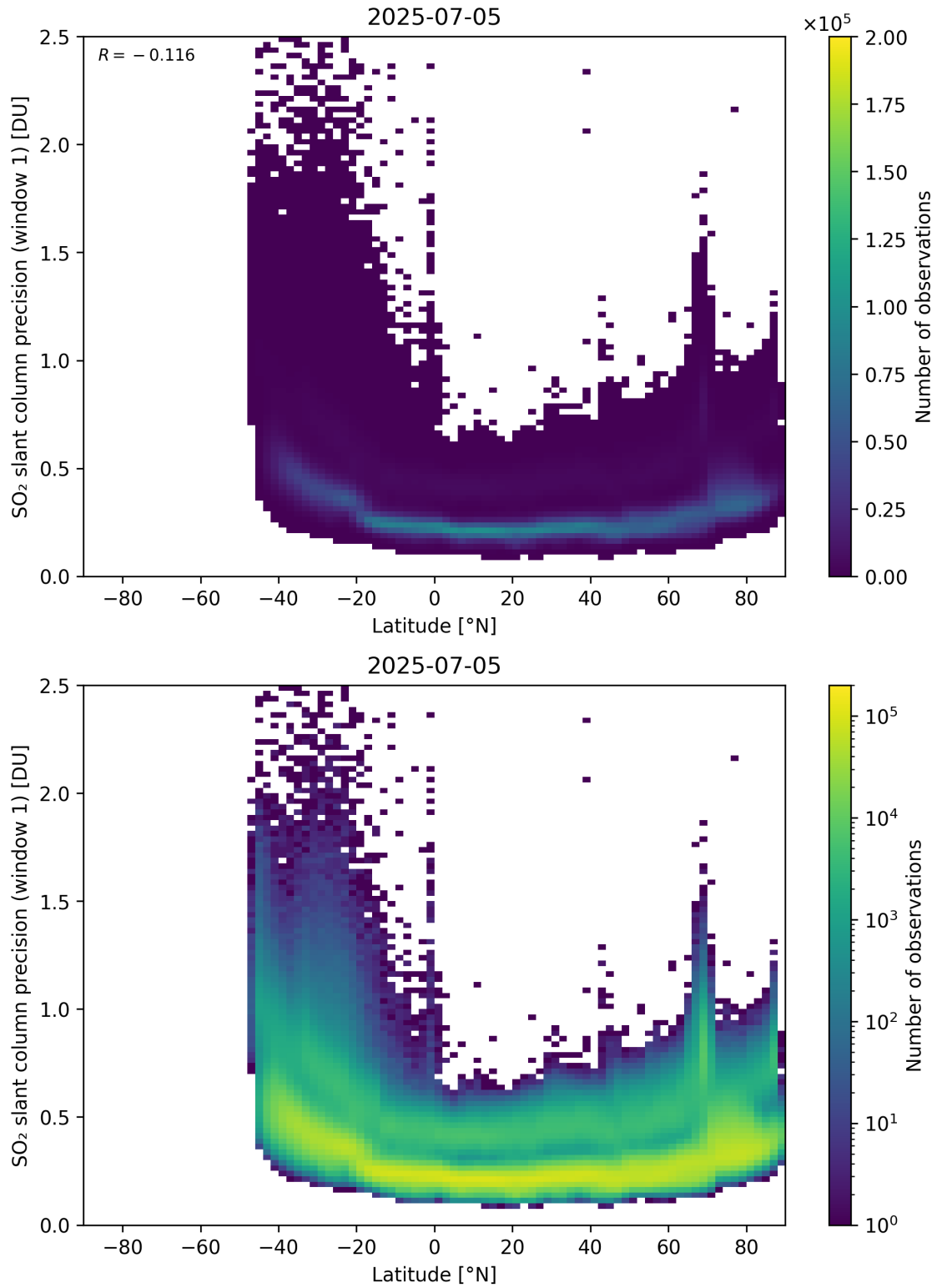
Figure 163: Scatter density plot of “Latitude” against “SO 2 slant column precision (window 1)” for 2025-07-04 to 2025-07-06.
