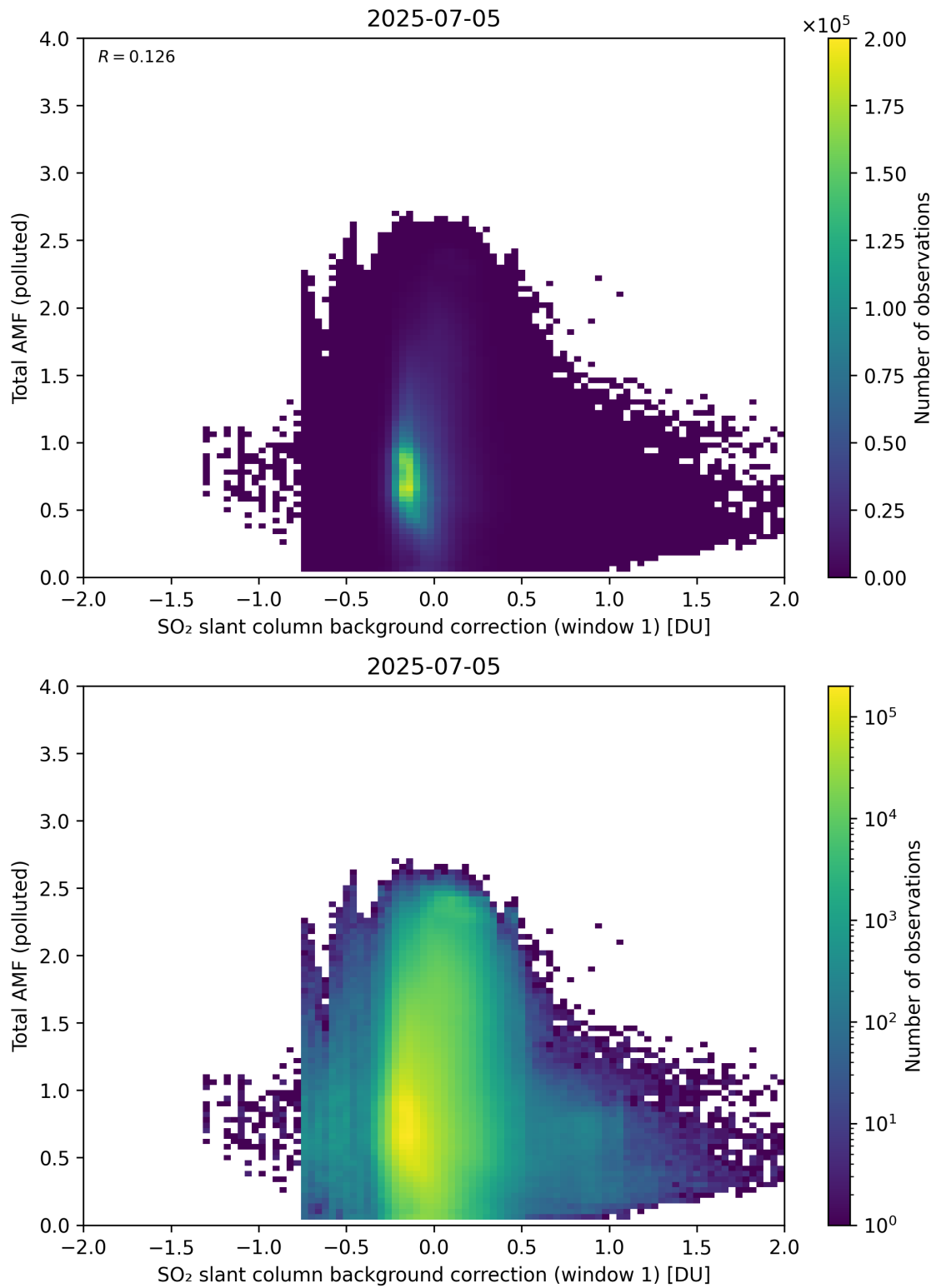
Figure 120: Scatter density plot of “SO 2 slant column background correction (window 1)” against “Total AMF (polluted)” for 2025-07-04 to 2025-07-06.
