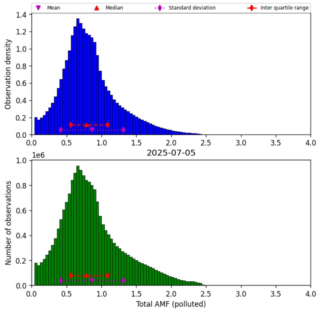
Figure 79: Histogram of “Total AMF (polluted)” for 2025-07-04 to 2025-07-06
