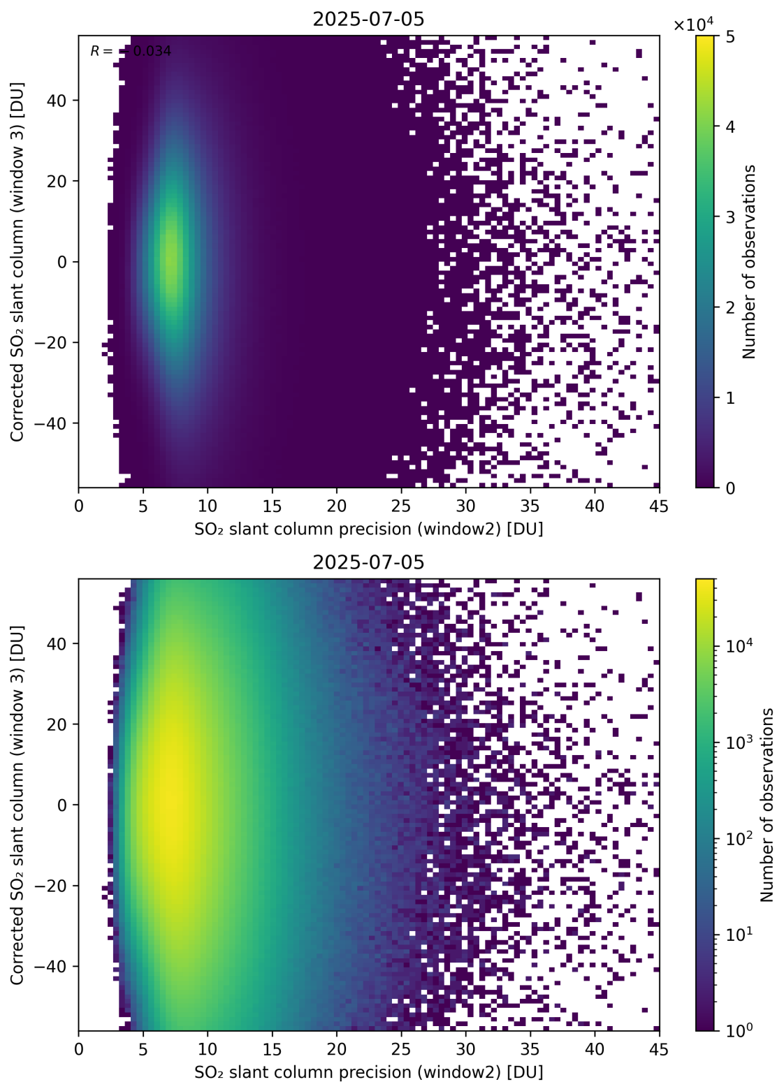
Figure 298: Scatter density plot of “SO 2 slant column precision (window2)” against “Corrected SO 2 slant column (window 3)” for 2025-07-04 to 2025-07-06.
