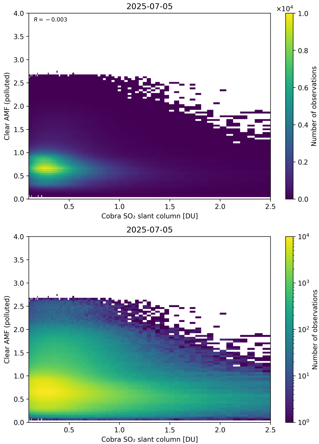
Figure 215: Scatter density plot of “Cobra SO 2 slant column” against “Clear AMF (polluted)” for 2025-07-04 to 2025-07-06.
