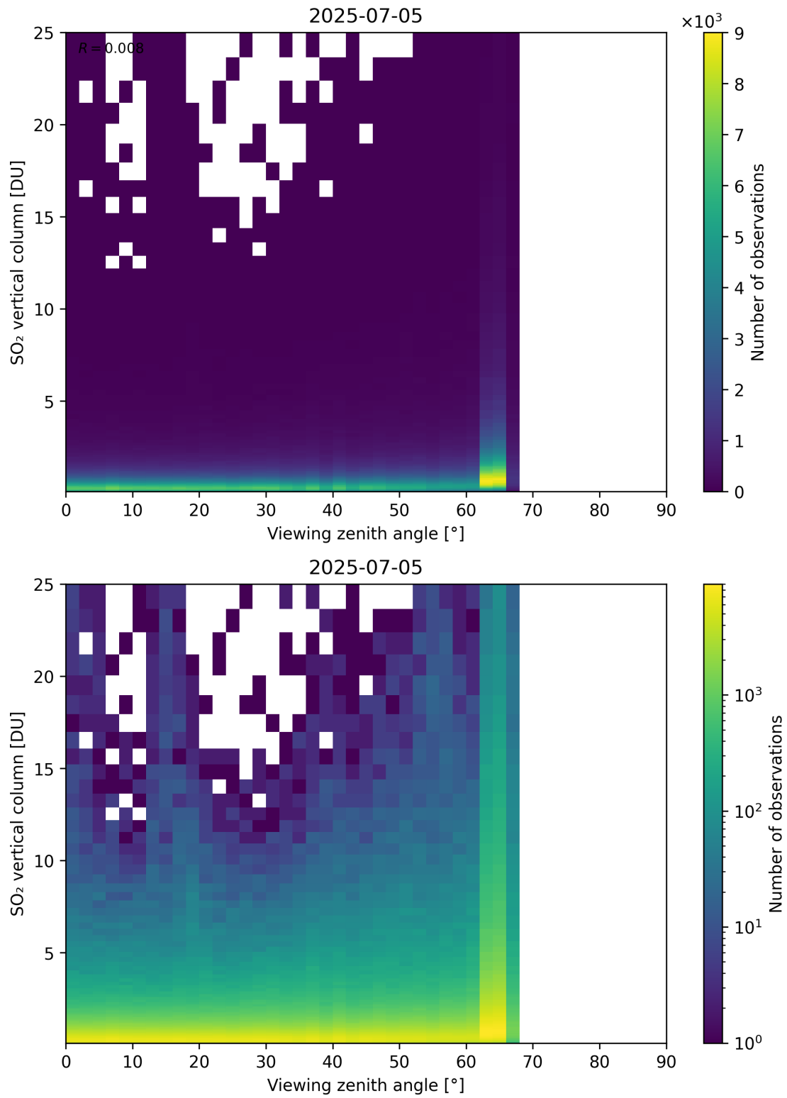
Figure 383: Scatter density plot of “Viewing zenith angle” against “SO 2 vertical column” for 2025-07-04 to 2025-07-06.
