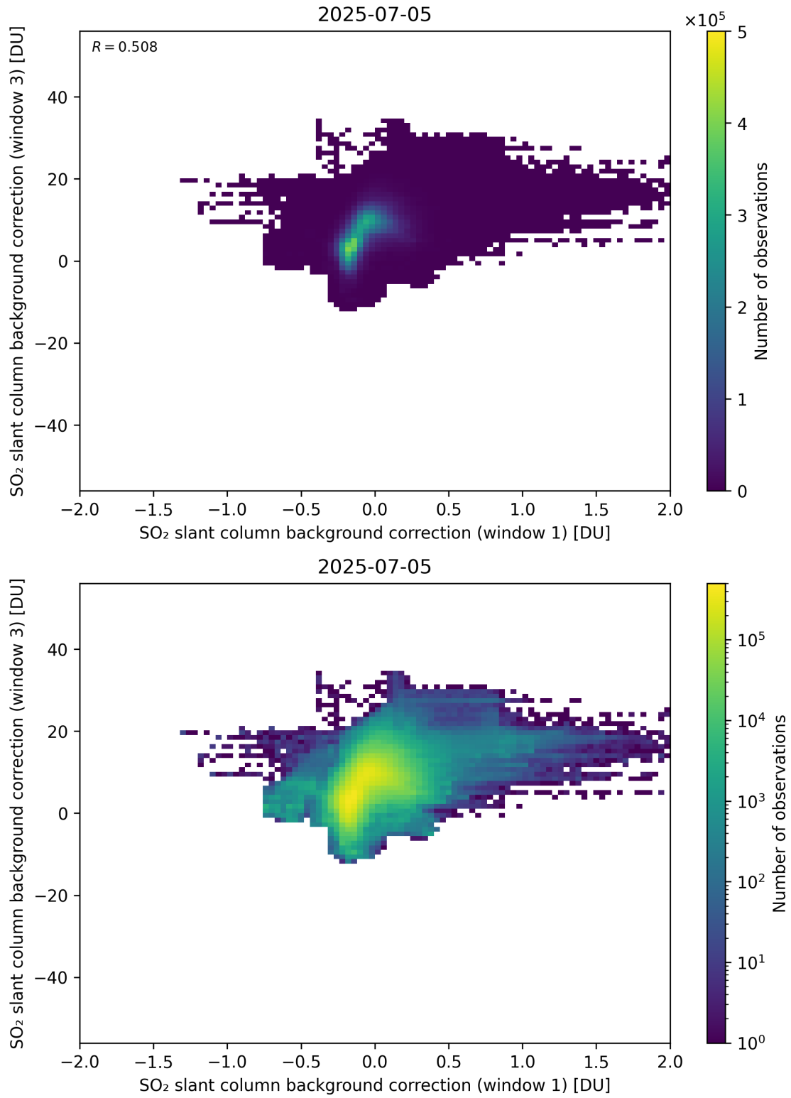
Figure 110: Scatter density plot of “SO 2 slant column background correction (window 1)” against “SO 2 slant column background correction (window 3)” for 2025-07-04 to 2025-07-06.
