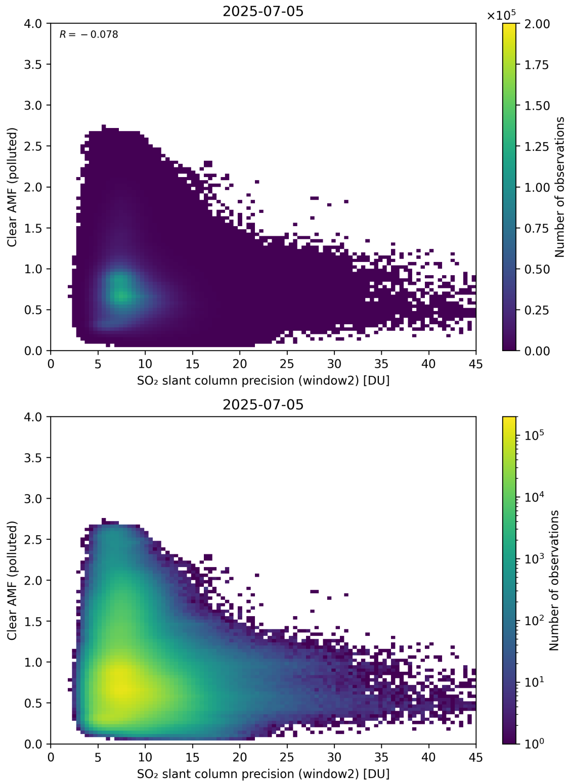
Figure 296: Scatter density plot of “SO 2 slant column precision (window2)” against “Clear AMF (polluted)” for 2025-07-04 to 2025-07-06.
