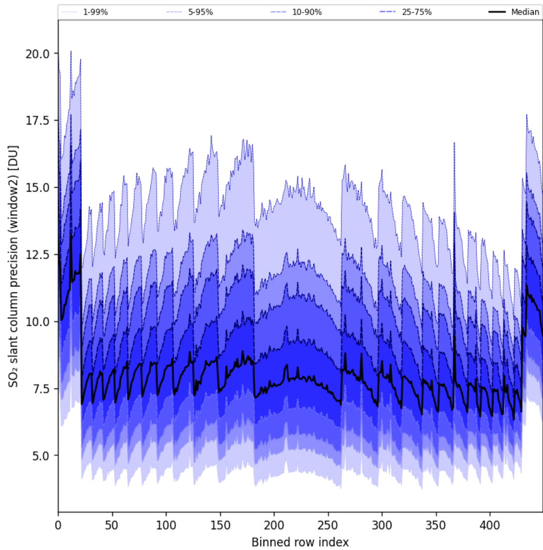
Figure 94: Along track statistics of “SO 2 slant column precision (window2)” for 2025-07-04 to 2025-07-06
