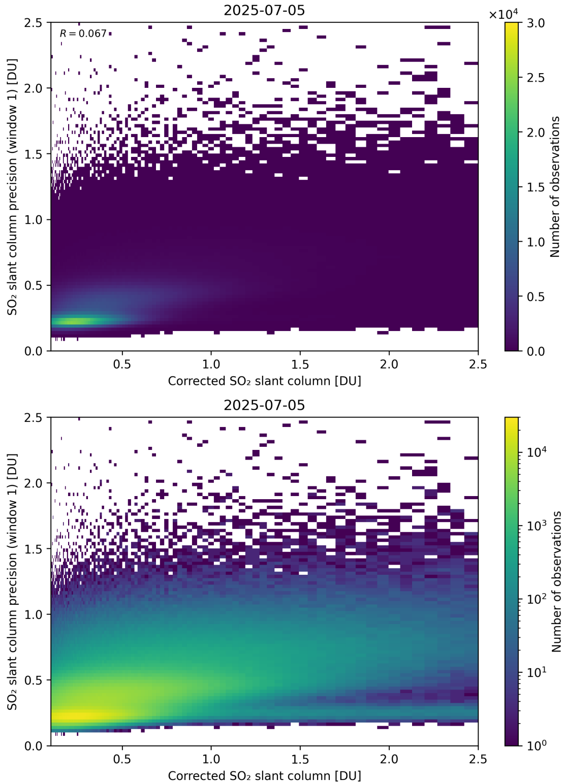
Figure 238: Scatter density plot of “Corrected SO 2 slant column” against “SO 2 slant column precision (window 1)” for 2025-07-04 to 2025-07-06.
