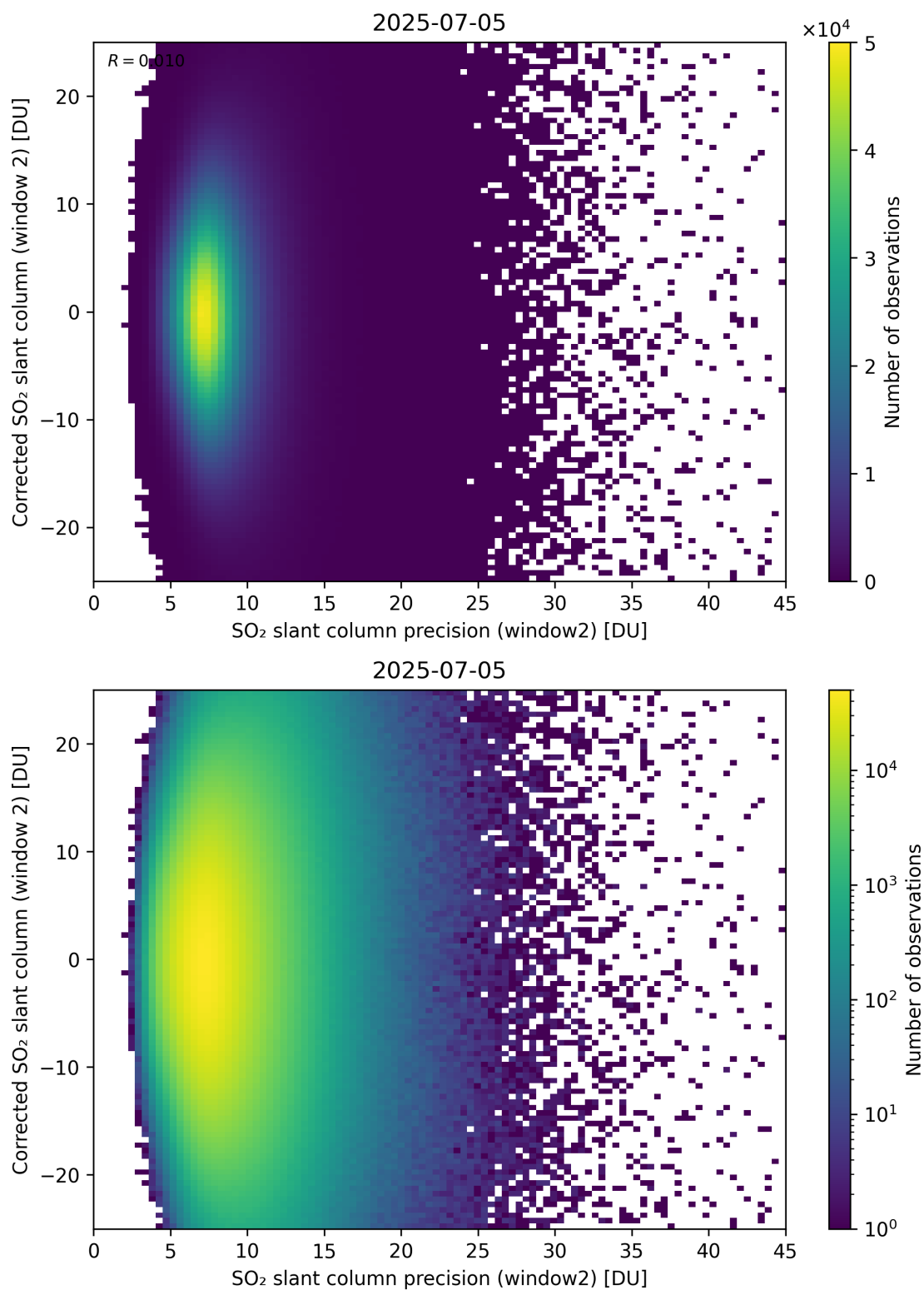
Figure 297: Scatter density plot of “SO 2 slant column precision (window2)” against “Corrected SO 2 slant column (window 2)” for 2025-07-04 to 2025-07-06.
