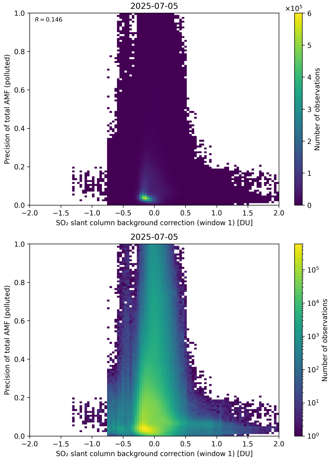
Figure 121: Scatter density plot of “SO 2 slant column background correction (window 1)” against “Precision of total AMF (polluted)” for 2025-07-04 to 2025-07-06.
