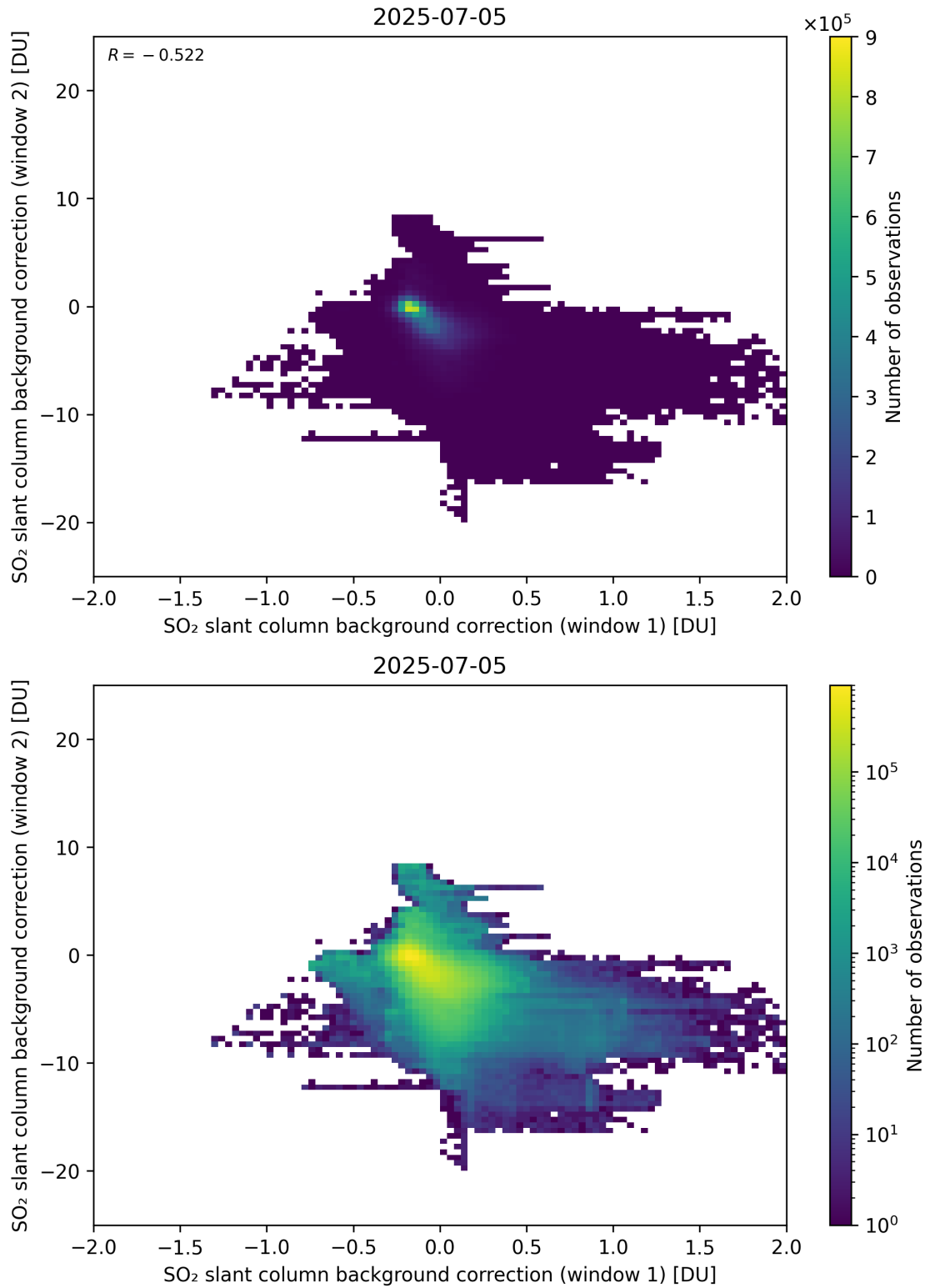
Figure 109: Scatter density plot of “SO 2 slant column background correction (window 1)” against “SO 2 slant column background correction (window 2)” for 2025-07-04 to 2025-07-06.
