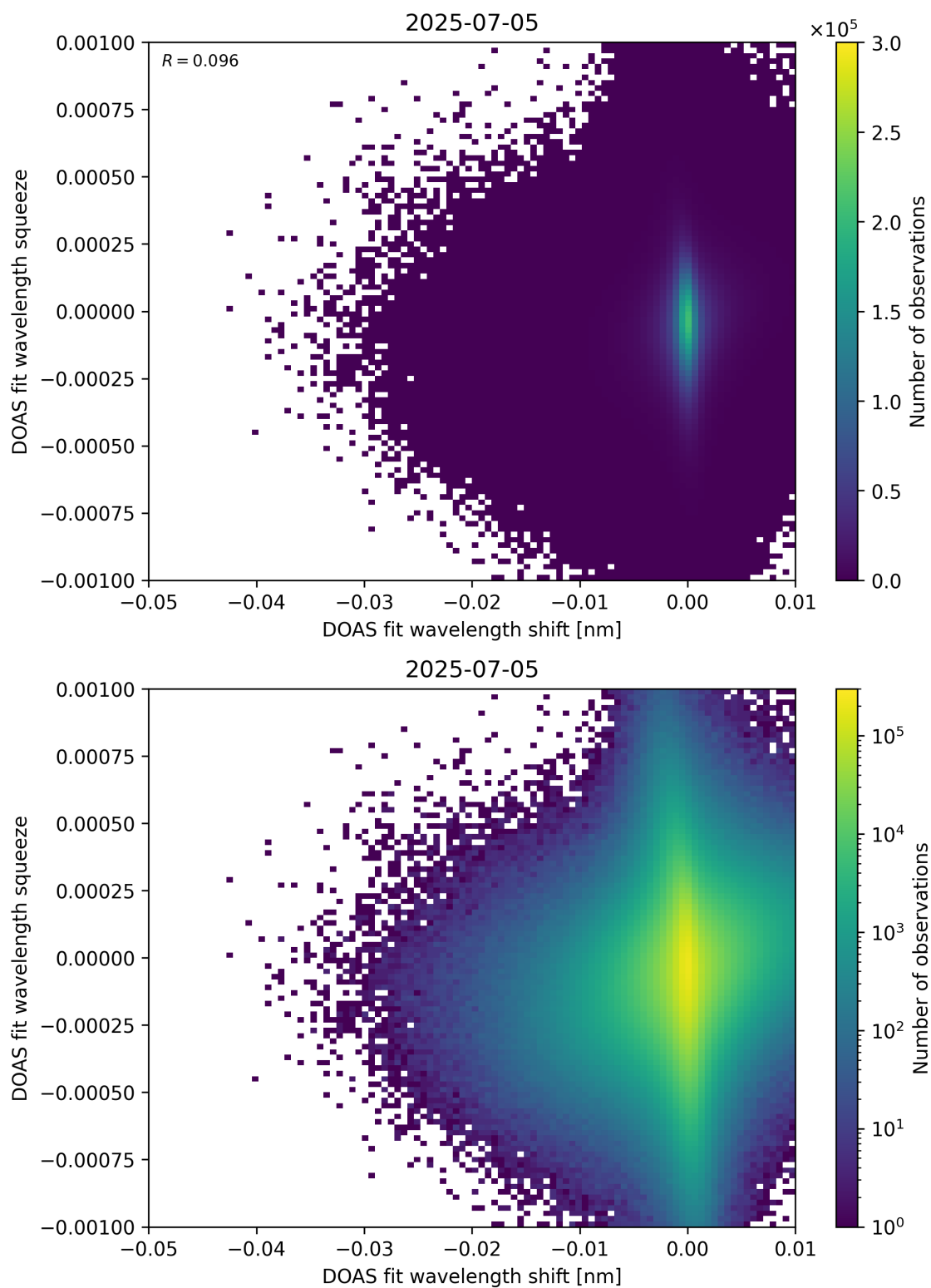
Figure 138: Scatter density plot of “DOAS fit wavelength shift” against “DOAS fit wavelength squeeze” for 2025-07-04 to 2025-07-06.
