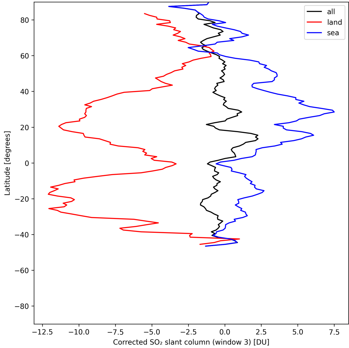
Figure 47: Zonal average of “Corrected SO 2 slant column (window 3)” for 2025-07-04 to 2025-07-06.
