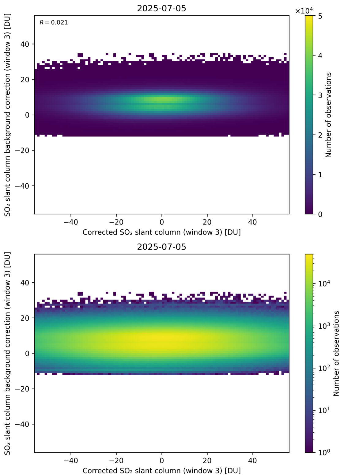
Figure 255: Scatter density plot of “Corrected SO 2 slant column (window 3)” against “SO 2 slant column background correction (window 3)” for 2025-07-04 to 2025-07-06.
