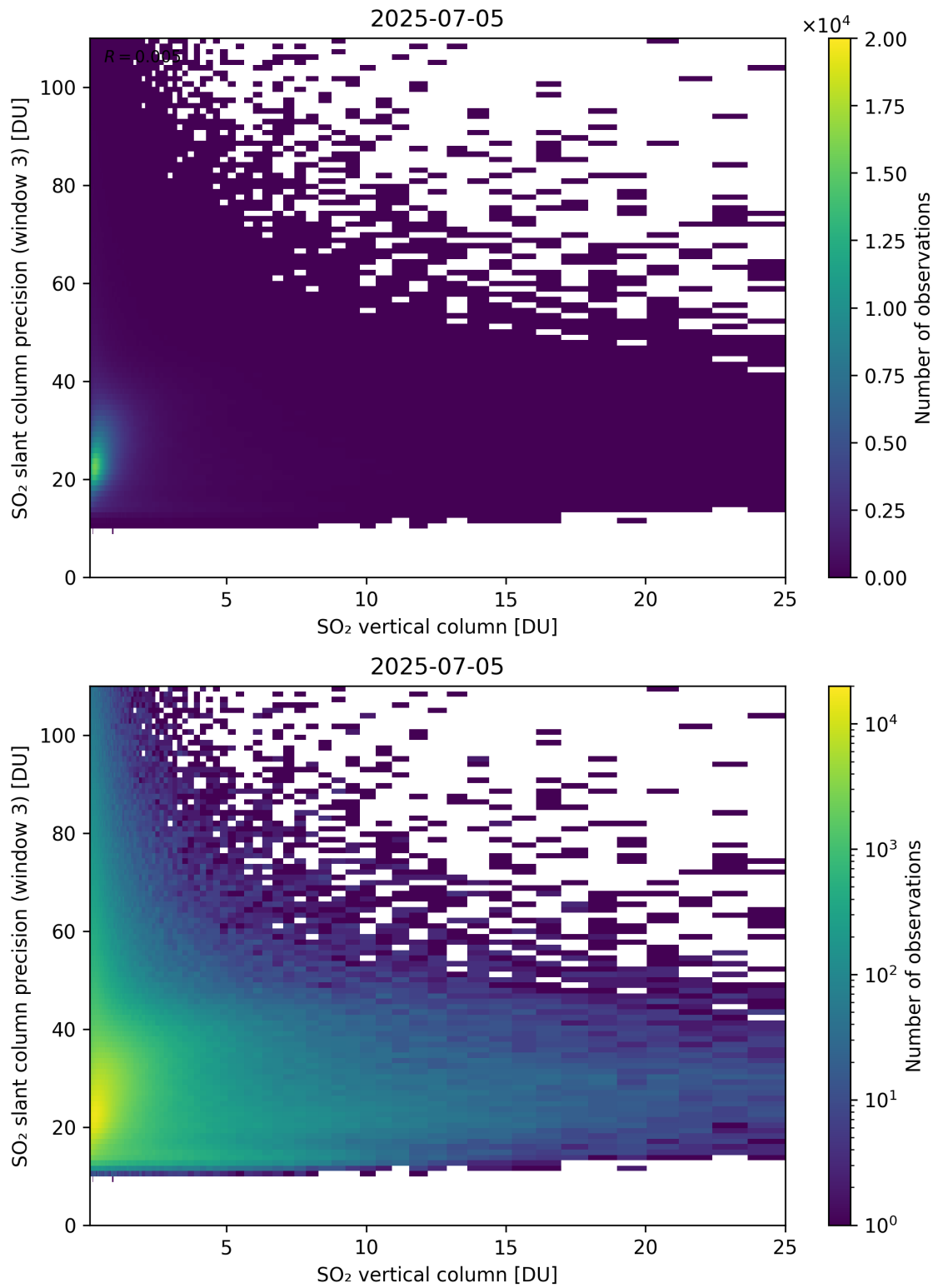
Figure 358: Scatter density plot of “SO 2 vertical column” against “SO 2 slant column precision (window 3)” for 2025-07-04 to 2025-07-06.
