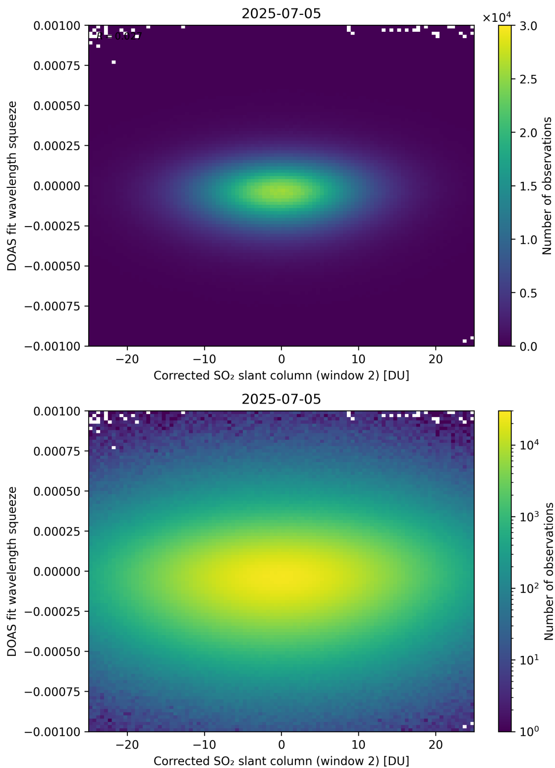
Figure 247: Scatter density plot of “Corrected SO 2 slant column (window 2)” against “DOAS fit wavelength squeeze” for 2025-07-04 to 2025-07-06.
