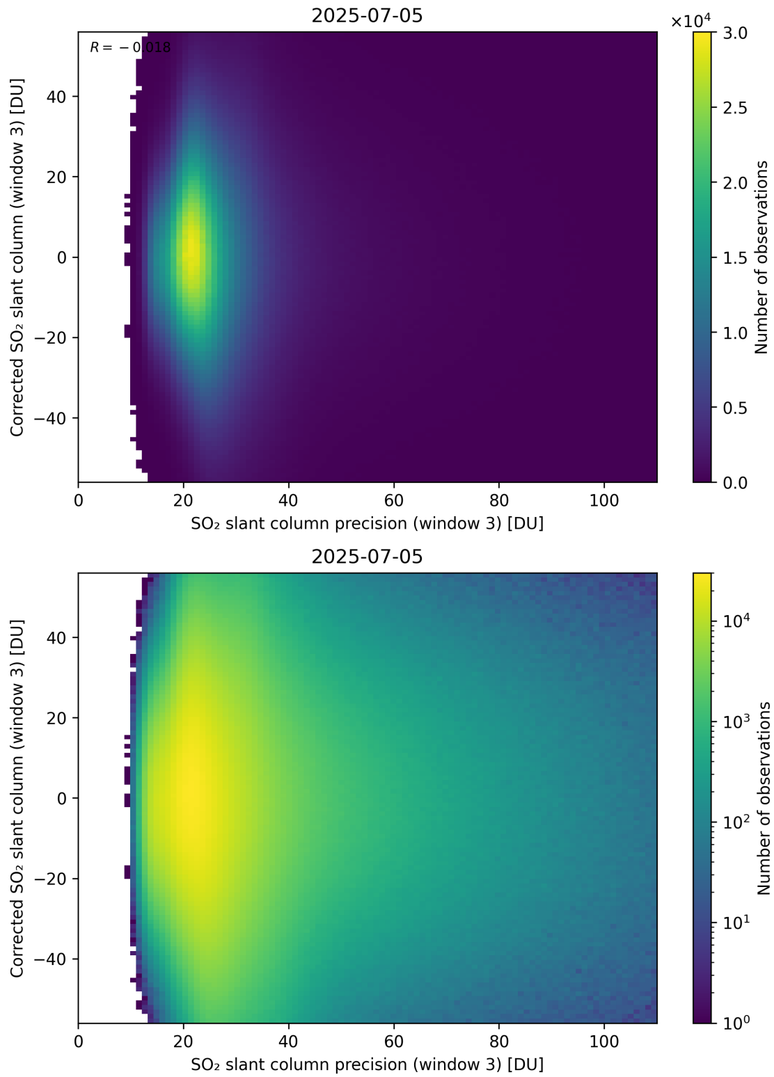
Figure 312: Scatter density plot of “SO 2 slant column precision (window 3)” against “Corrected SO 2 slant column (window 3)” for 2025-07-04 to 2025-07-06.
