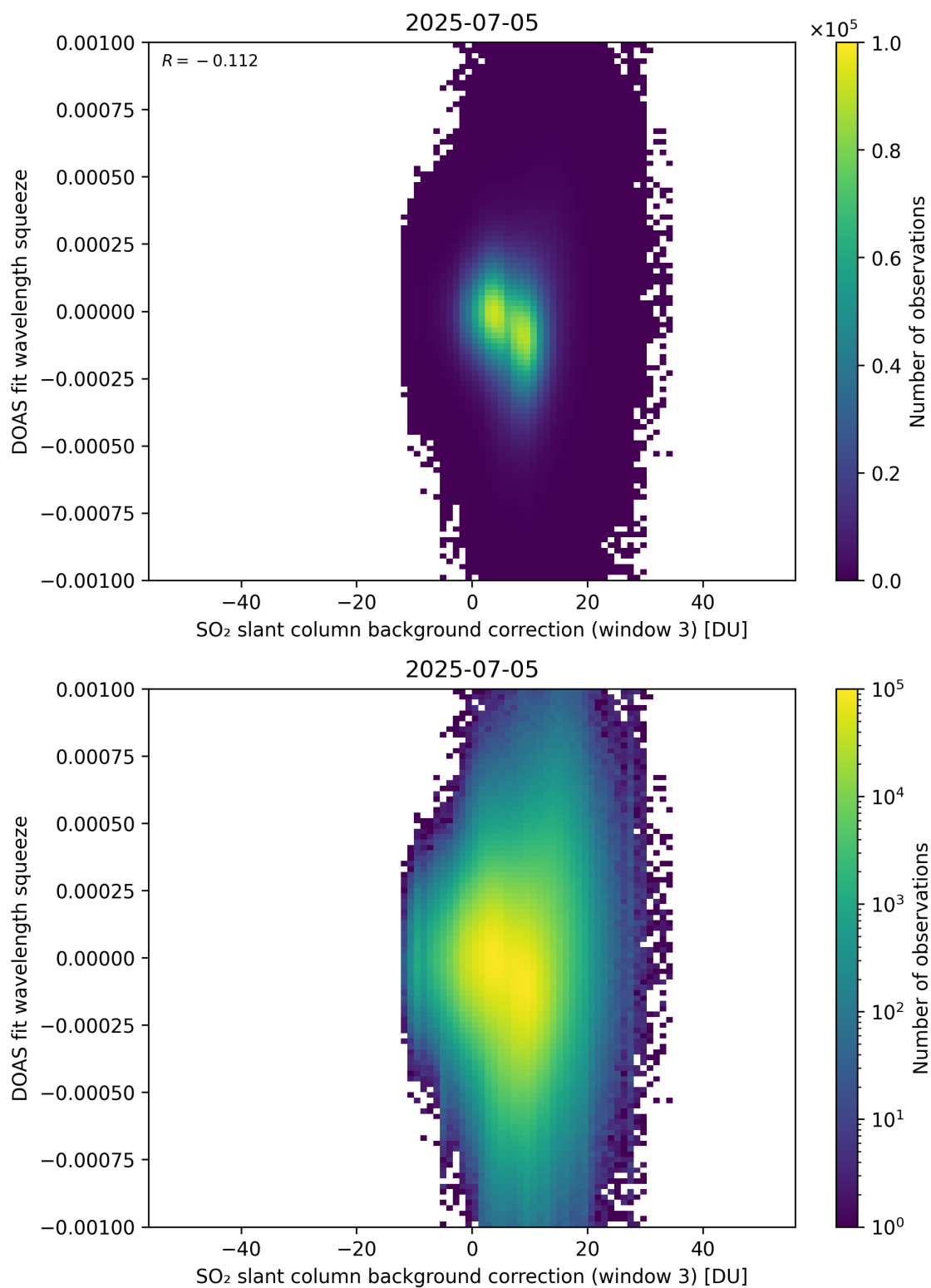
Figure 133: Scatter density plot of “SO 2 slant column background correction (window 3)” against “DOAS fit wavelength squeeze” for 2025-07-04 to 2025-07-06.
