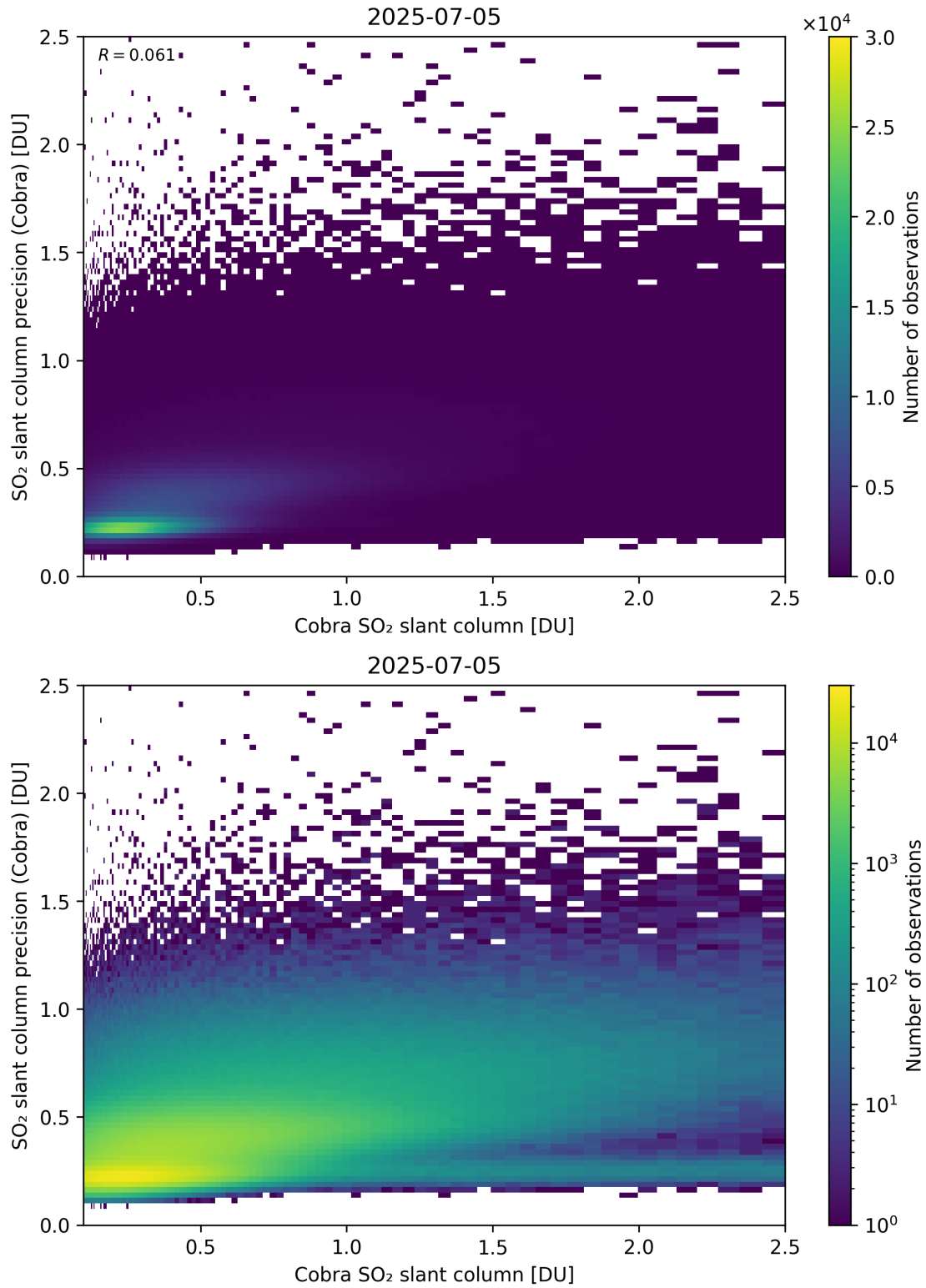
Figure 216: Scatter density plot of “Cobra SO 2 slant column” against “SO 2 slant column precision (Cobra)” for 2025-07-04 to 2025-07-06.
