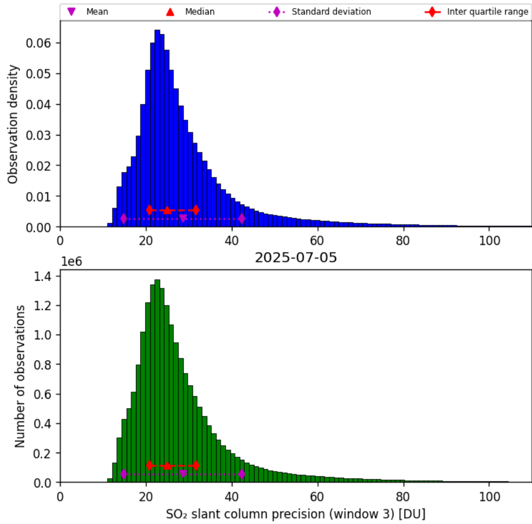
Figure 72: Histogram of “SO 2 slant column precision (window 3)” for 2025-07-04 to 2025-07-06
