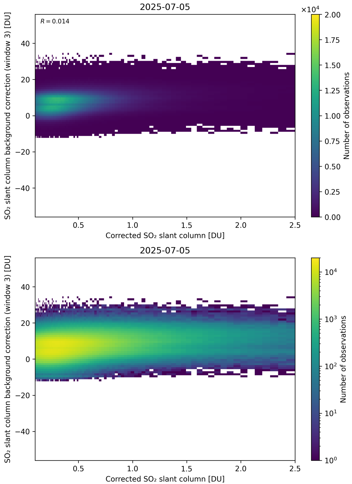
Figure 228: Scatter density plot of “Corrected SO 2 slant column” against “SO 2 slant column background correction (window 3)” for 2025-07-04 to 2025-07-06.
