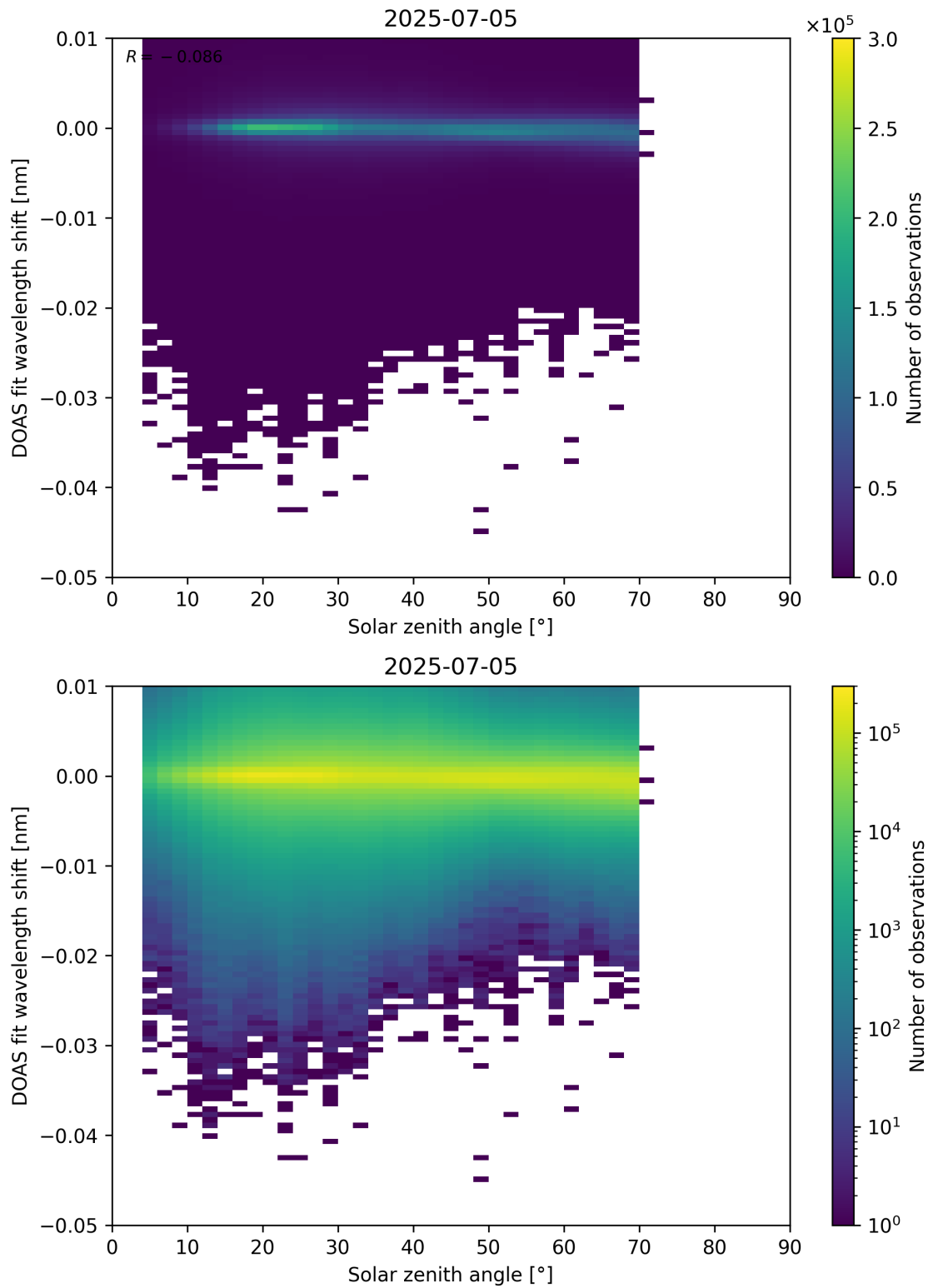
Figure 174: Scatter density plot of “Solar zenith angle” against “DOAS fit wavelength shift” for 2025-07-04 to 2025-07-06.
