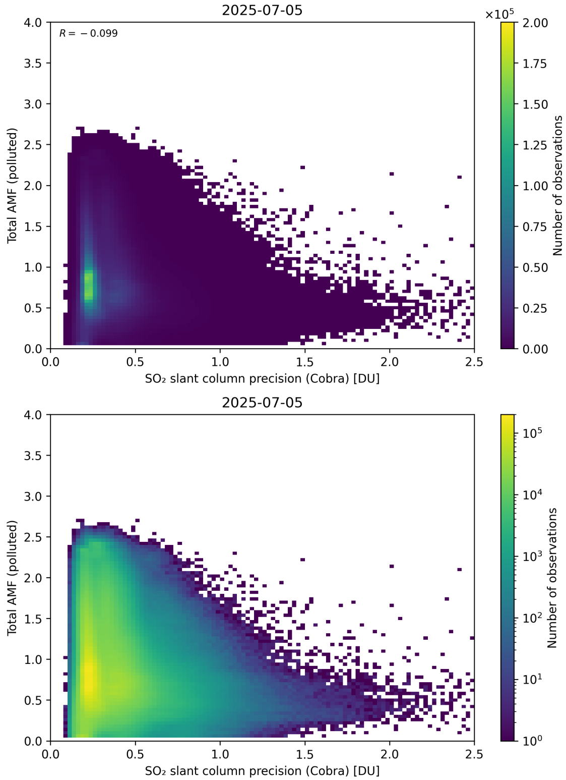
Figure 213: Scatter density plot of “SO 2 slant column precision (Cobra)” against “Total AMF (polluted)” for 2025-07-04 to 2025-07-06.
