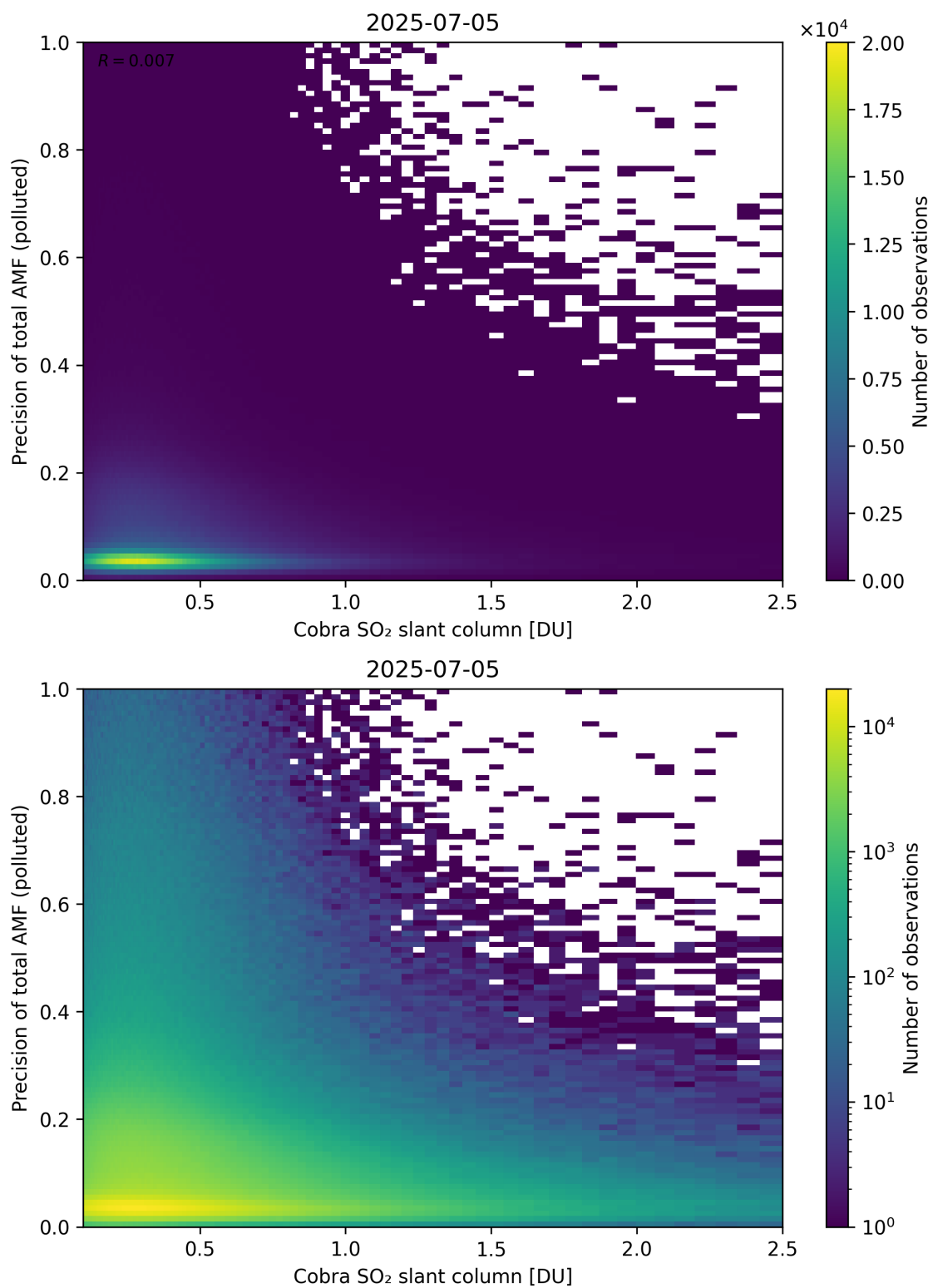
Figure 225: Scatter density plot of “Cobra SO 2 slant column” against “Precision of total AMF (polluted)” for 2025-07-04 to 2025-07-06.
