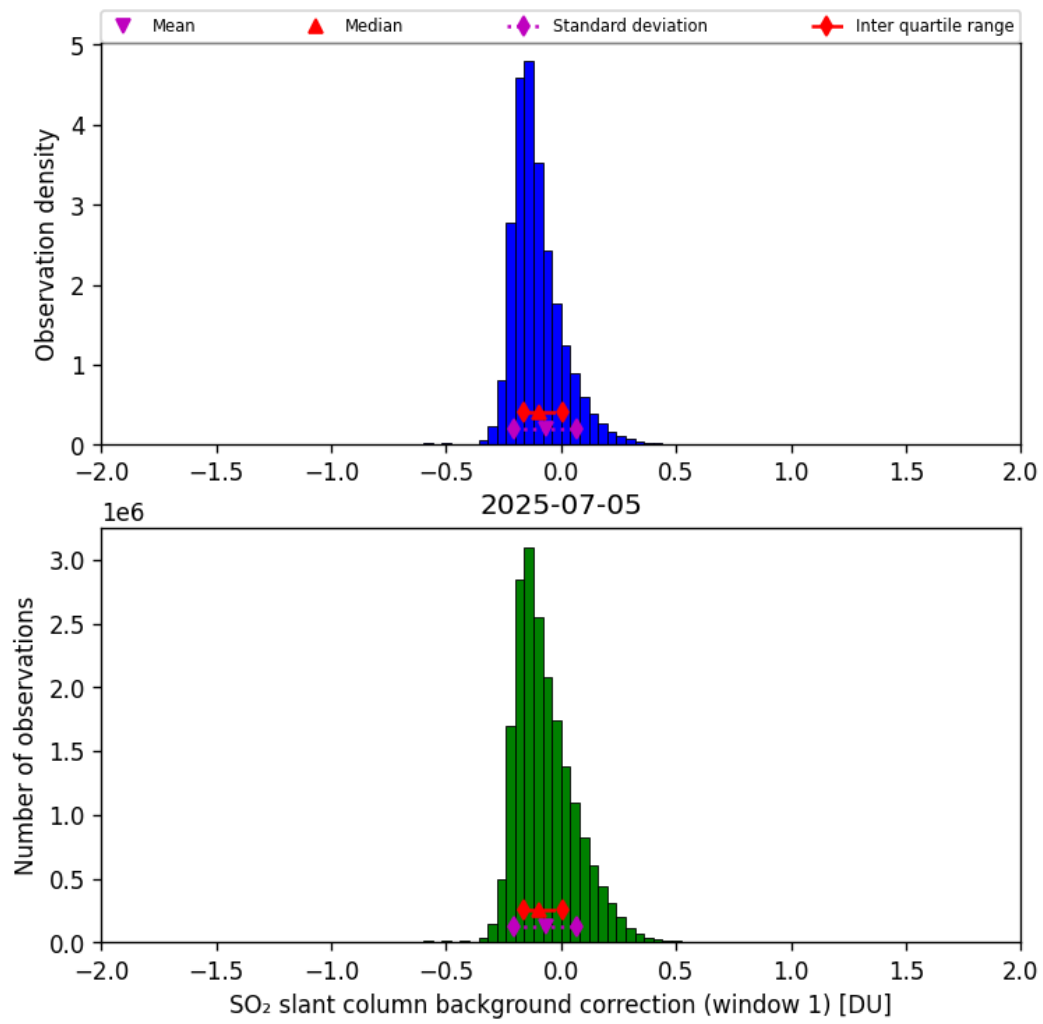
Figure 66: Histogram of “SO 2 slant column background correction (window 1)” for 2025-07-04 to 2025-07-06
