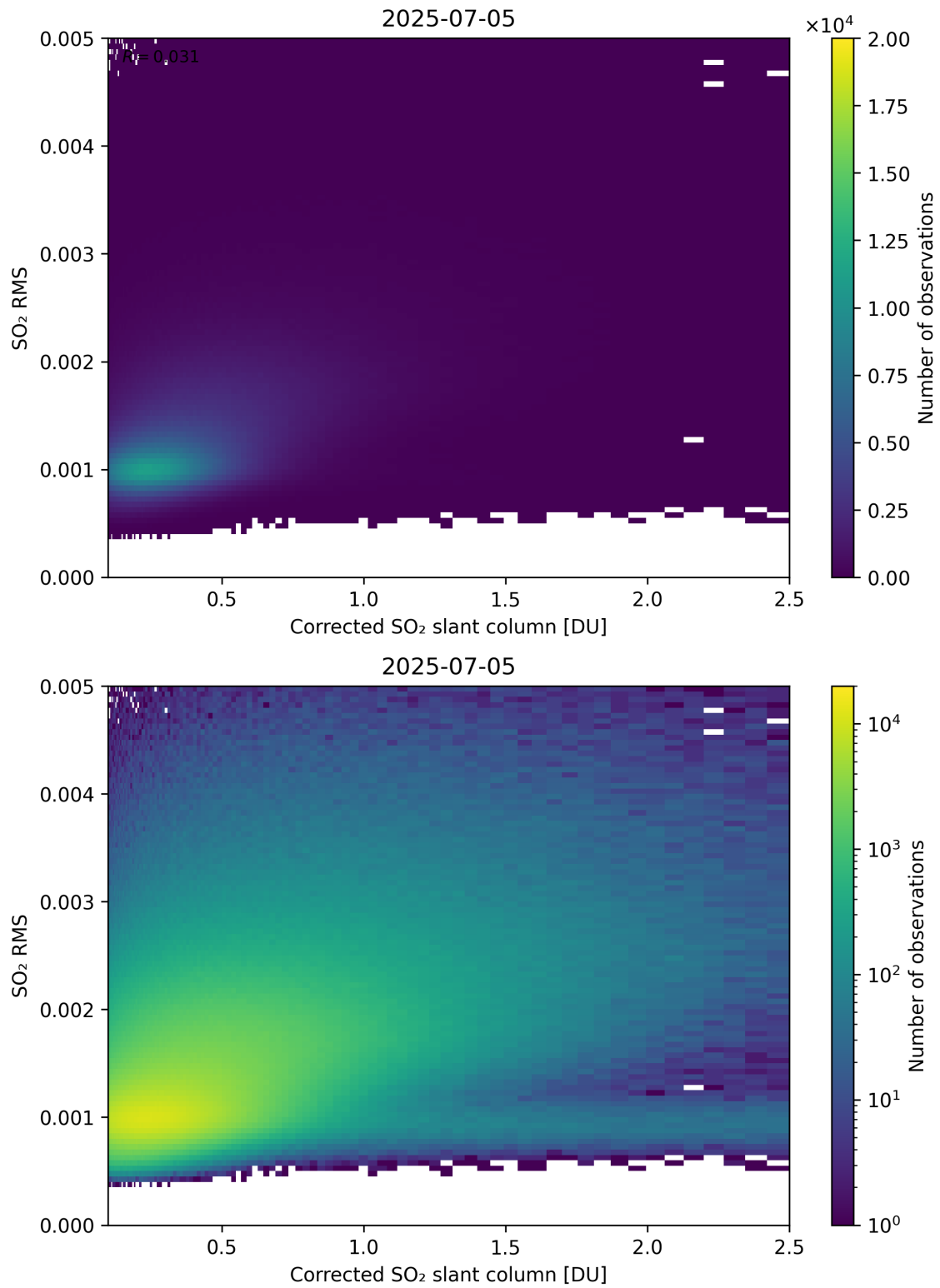
Figure 231: Scatter density plot of “Corrected SO 2 slant column” against “SO 2 RMS” for 2025-07-04 to 2025-07-06.
