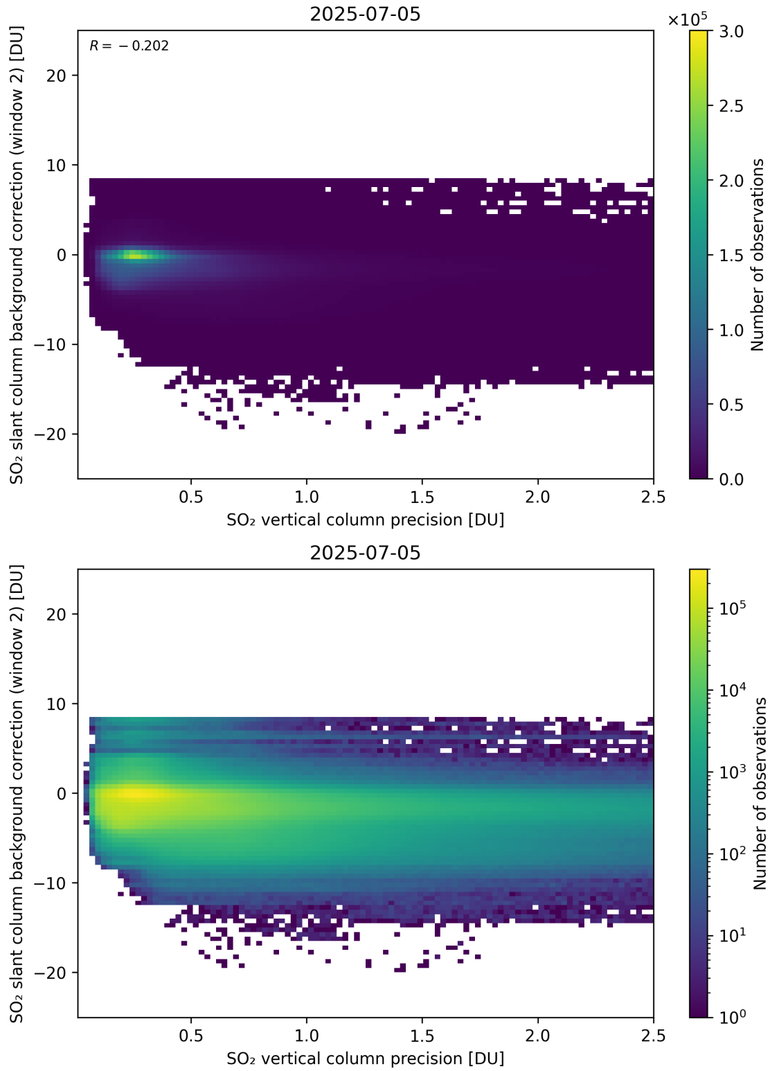
Figure 330: Scatter density plot of “SO 2 vertical column precision” against “SO 2 slant column background correction (window 2)” for 2025-07-04 to 2025-07-06.
