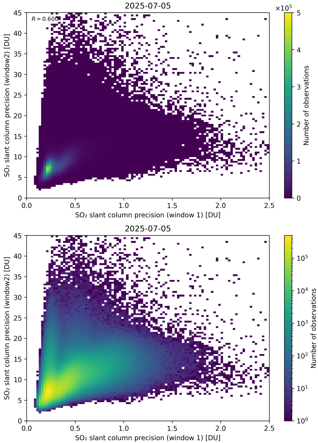
Figure 277: Scatter density plot of “SO 2 slant column precision (window 1)” against “SO 2 slant column precision (window2)” for 2025-07-04 to 2025-07-06.
