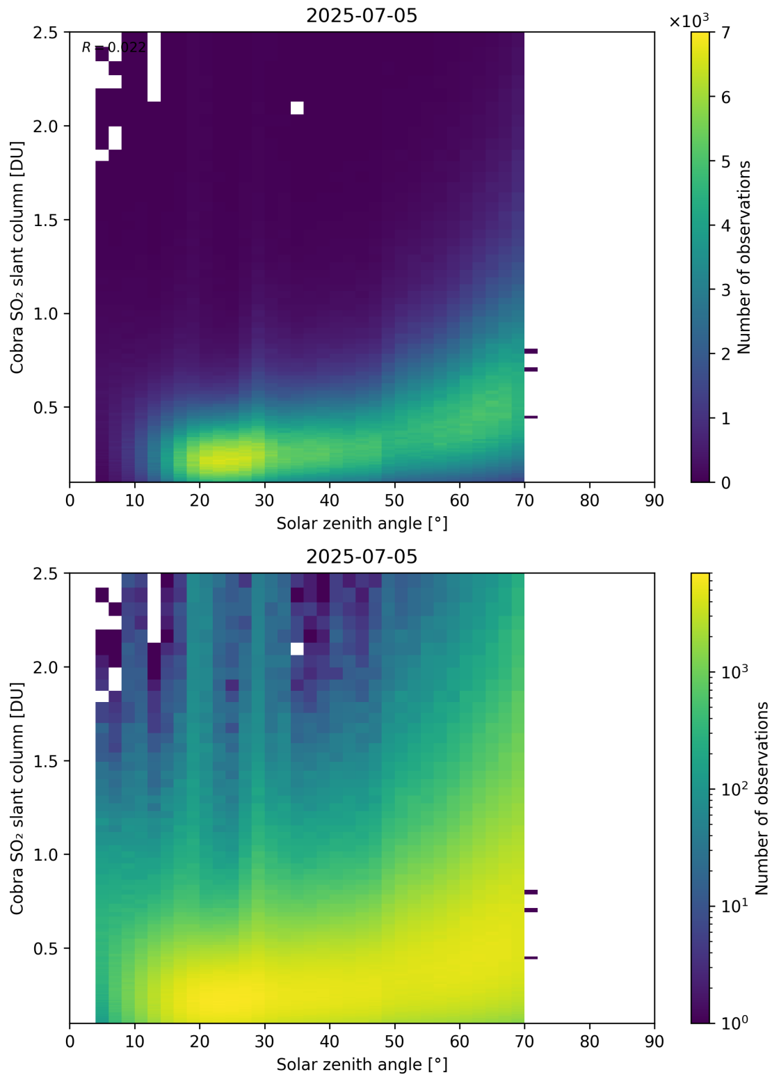
Figure 179: Scatter density plot of “Solar zenith angle” against “Cobra SO 2 slant column” for 2025-07-04 to 2025-07-06.
