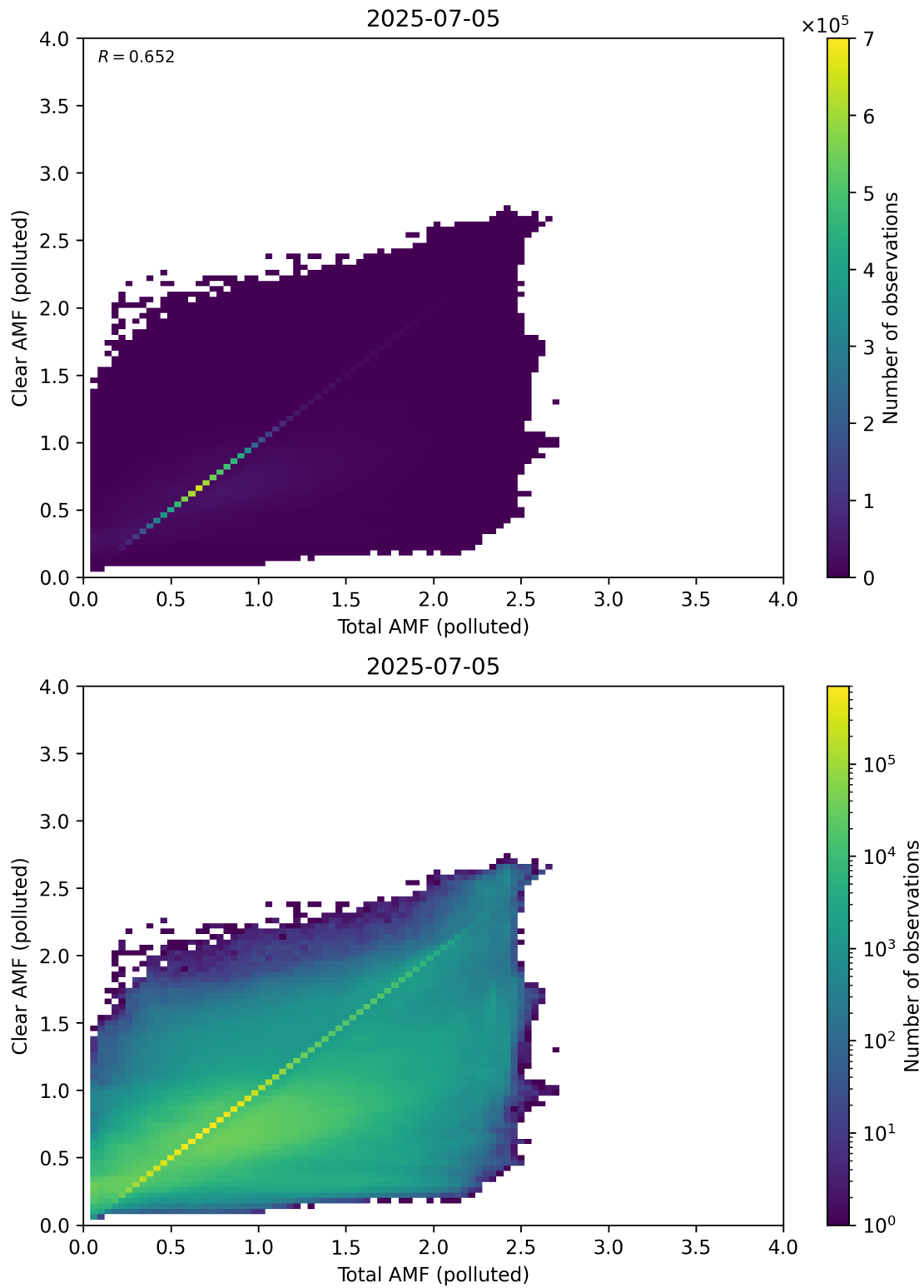
Figure 321: Scatter density plot of “Total AMF (polluted)” against “Clear AMF (polluted)” for 2025-07-04 to 2025-07-06.
