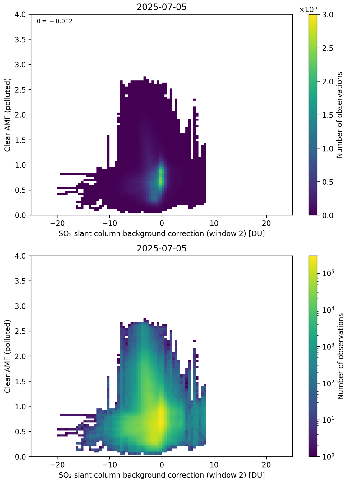
Figure 126: Scatter density plot of “SO 2 slant column background correction (window 2)” against “Clear AMF (polluted)” for 2025-07-04 to 2025-07-06.
