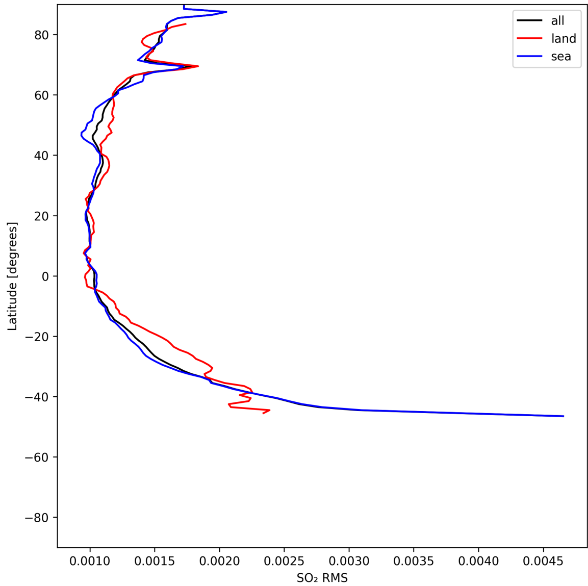
Figure 52: Zonal average of “SO 2 RMS” for 2025-07-04 to 2025-07-06.
