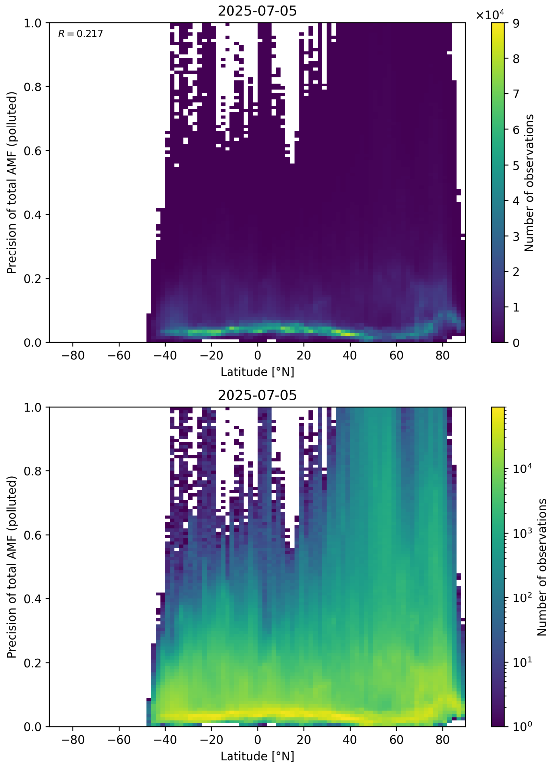
Figure 168: Scatter density plot of “Latitude” against “Precision of total AMF (polluted)” for 2025-07-04 to 2025-07-06.
