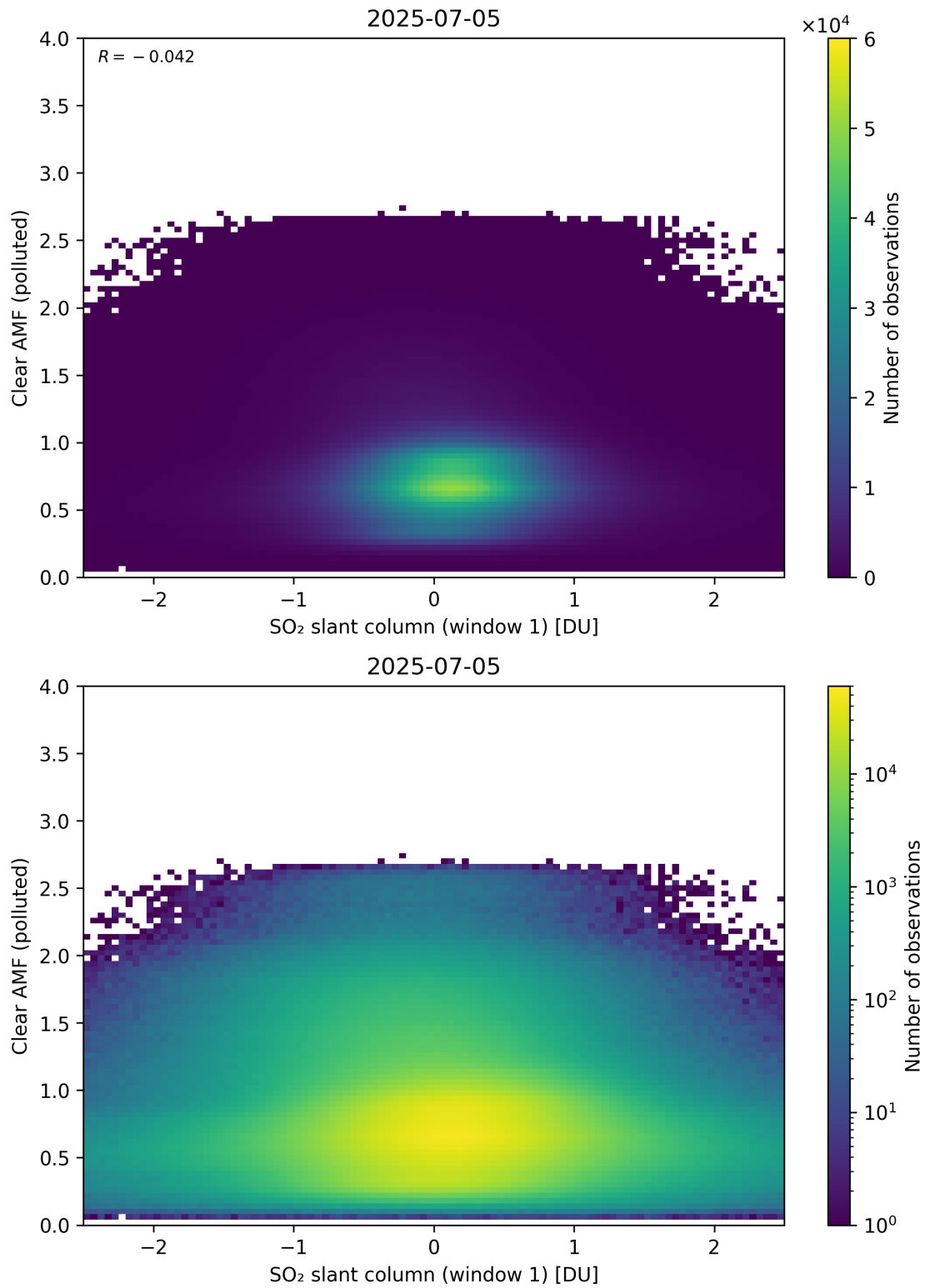
Figure 282: Scatter density plot of “SO 2 slant column (window 1)” against “Clear AMF (polluted)” for 2025-07-04 to 2025-07-06.
