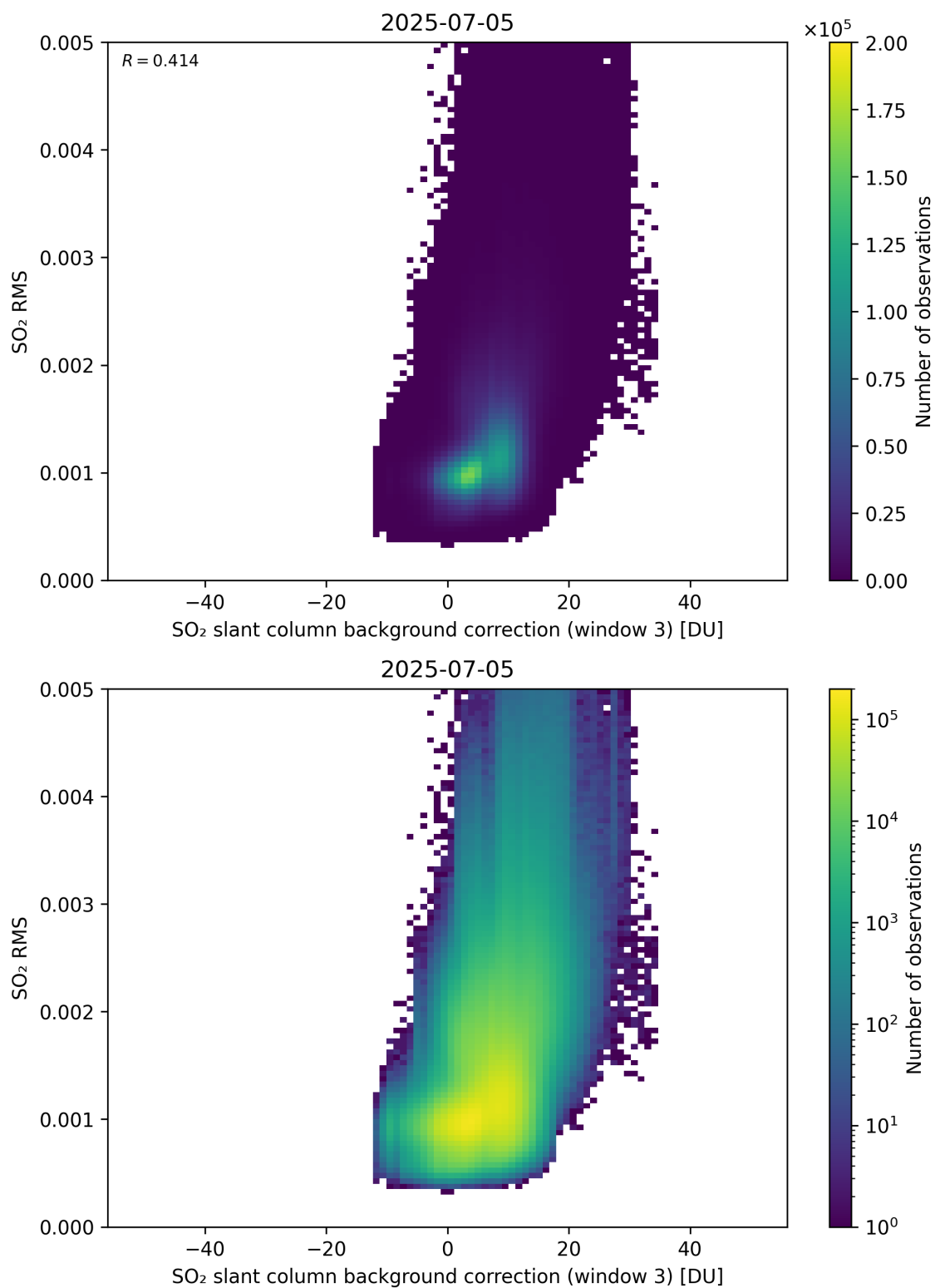
Figure 134: Scatter density plot of “SO 2 slant column background correction (window 3)” against “SO 2 RMS” for 2025-07-04 to 2025-07-06.
