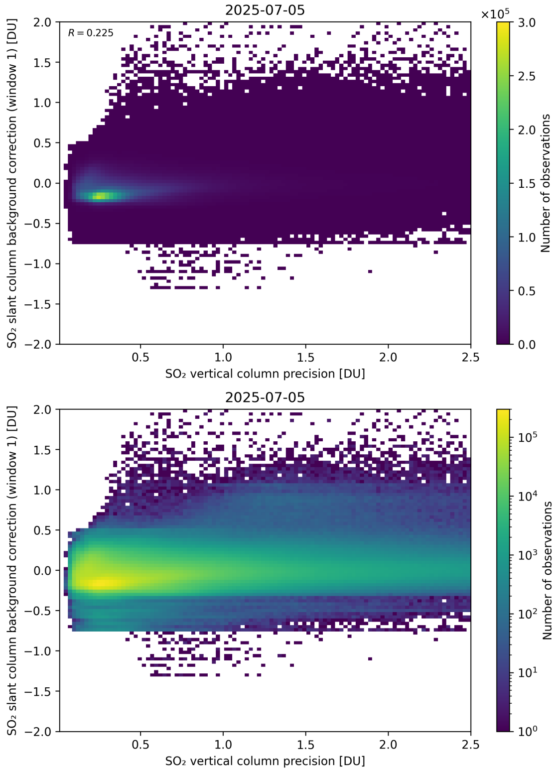
Figure 329: Scatter density plot of “SO 2 vertical column precision” against “SO 2 slant column background correction (window 1)” for 2025-07-04 to 2025-07-06.
