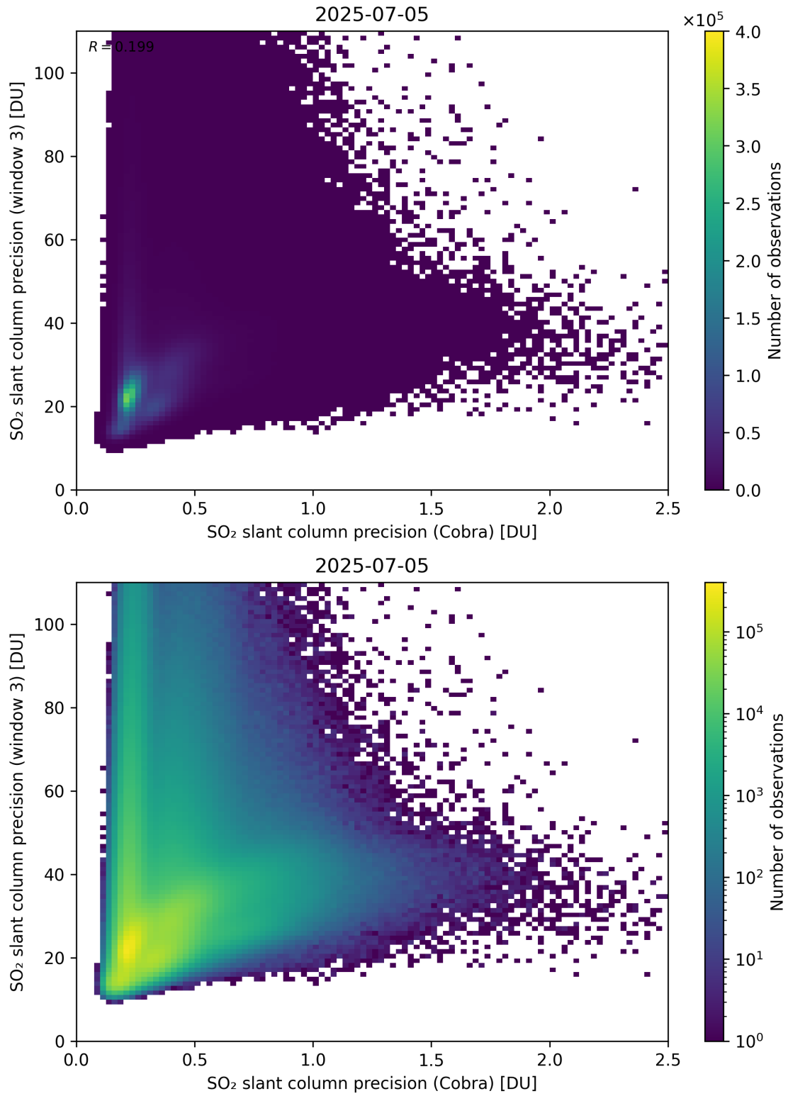
Figure 212: Scatter density plot of “SO 2 slant column precision (Cobra)” against “SO 2 slant column precision (window 3)” for 2025-07-04 to 2025-07-06.
