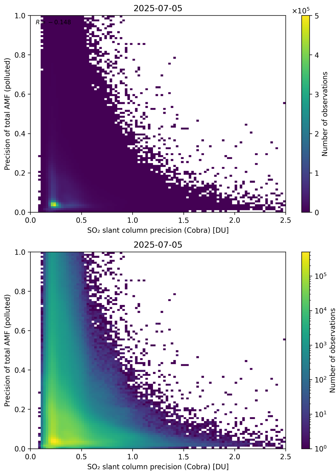
Figure 214: Scatter density plot of “SO 2 slant column precision (Cobra)” against “Precision of total AMF (polluted)” for 2025-07-04 to 2025-07-06.
