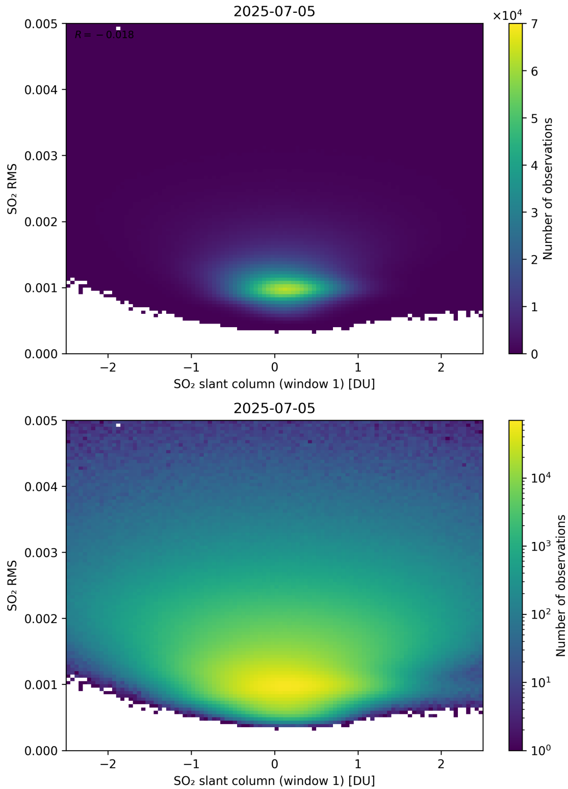
Figure 267: Scatter density plot of “SO 2 slant column (window 1)” against “SO 2 RMS” for 2025-07-04 to 2025-07-06.
