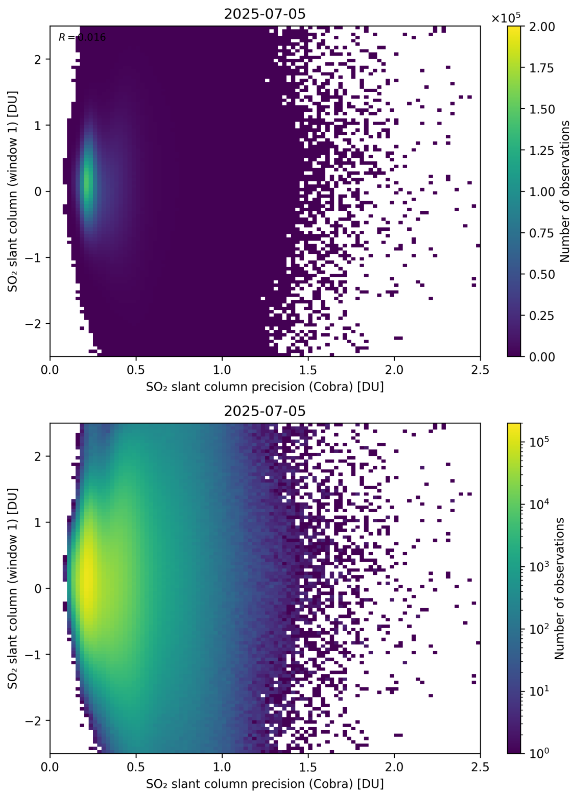
Figure 208: Scatter density plot of “SO 2 slant column precision (Cobra)” against “SO 2 slant column (window 1)” for 2025-07-04 to 2025-07-06.
