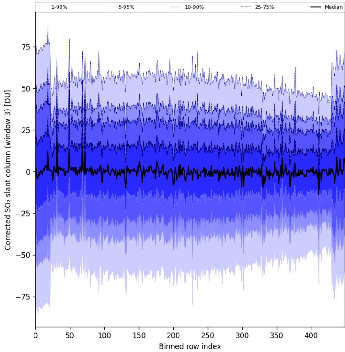
Figure 99: Along track statistics of “Corrected SO 2 slant column (window 3)” for 2025-07-04 to 2025-07-06
