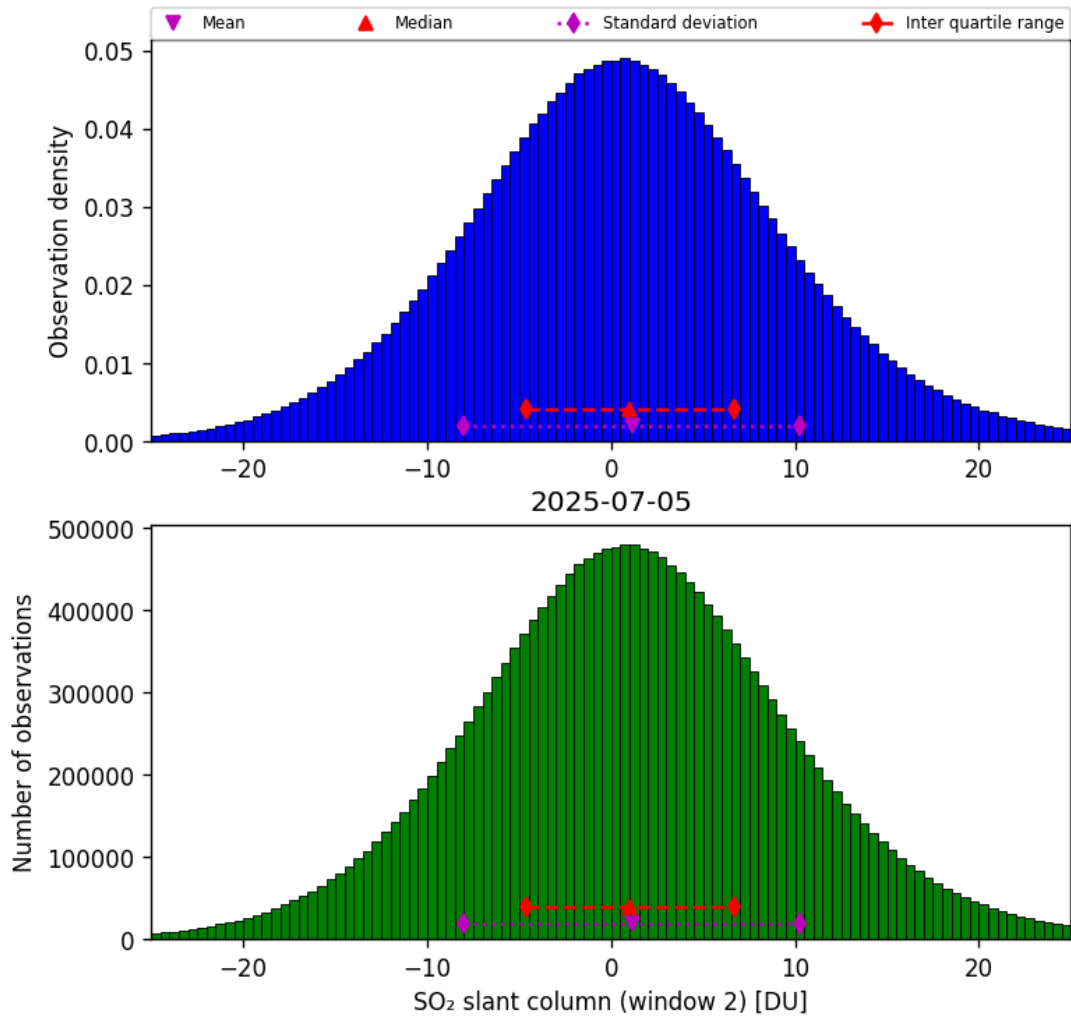
Figure 67: Histogram of “SO 2 slant column (window 2)” for 2025-07-04 to 2025-07-06
