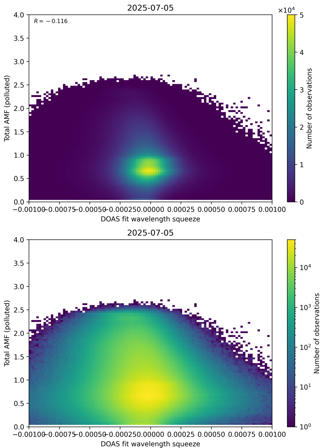
Figure 145: Scatter density plot of “DOAS fit wavelength squeeze” against “Total AMF (polluted)” for 2025-07-04 to 2025-07-06.
