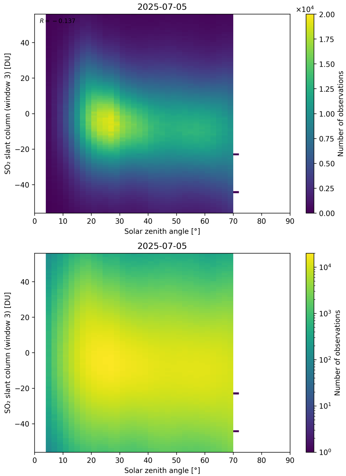
Figure 187: Scatter density plot of “Solar zenith angle” against “SO 2 slant column (window 3)” for 2025-07-04 to 2025-07-06.
