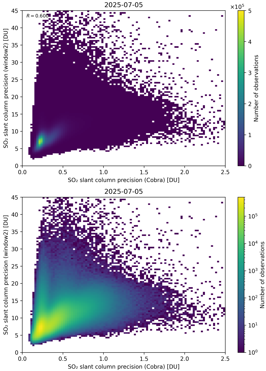
Figure 210: Scatter density plot of “SO 2 slant column precision (Cobra)” against “SO 2 slant column precision (window2)” for 2025-07-04 to 2025-07-06.
