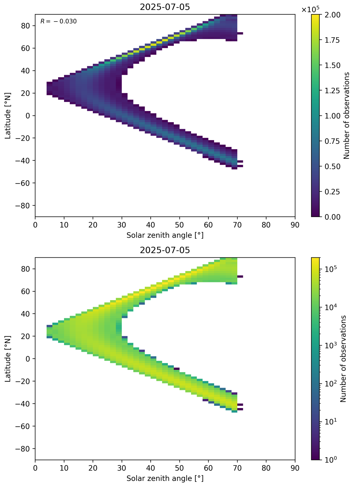
Figure 177: Scatter density plot of “Solar zenith angle” against “Latitude” for 2025-07-04 to 2025-07-06.
