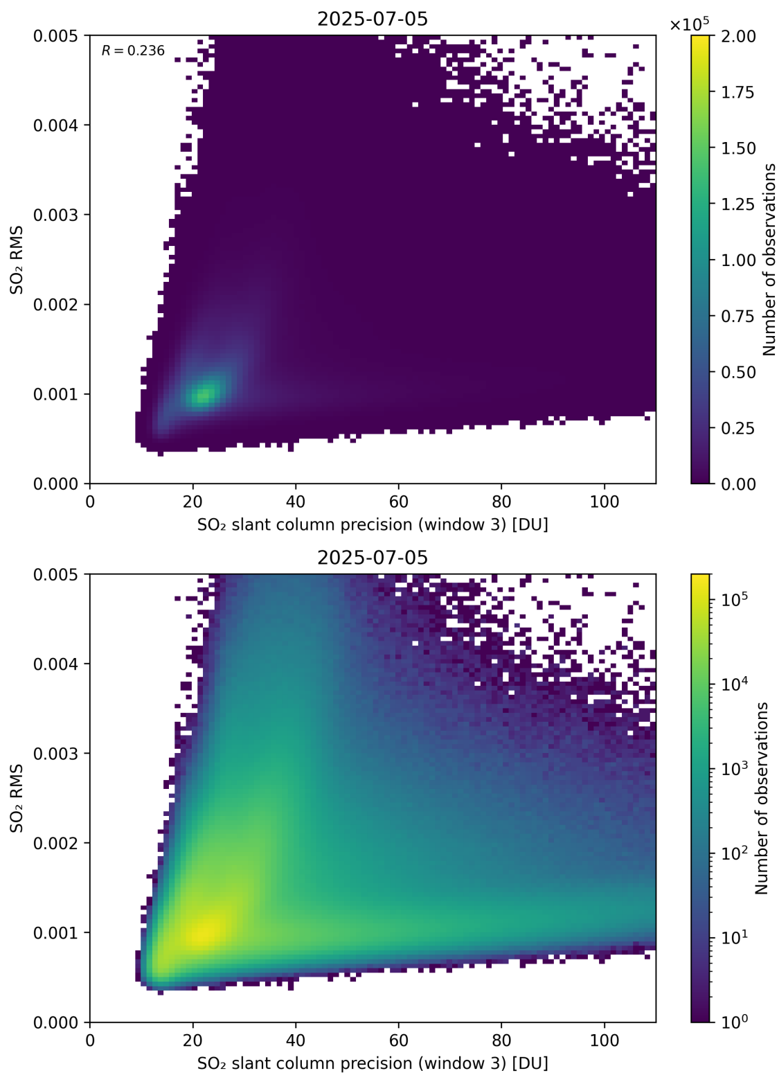
Figure 310: Scatter density plot of “SO 2 slant column precision (window 3)” against “SO 2 RMS” for 2025-07-04 to 2025-07-06.
