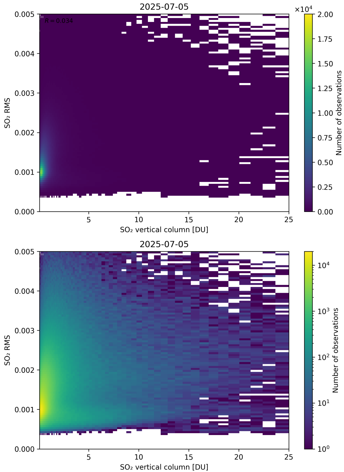
Figure 328: Scatter density plot of “SO 2 vertical column” against “SO 2 RMS” for 2025-07-04 to 2025-07-06.
