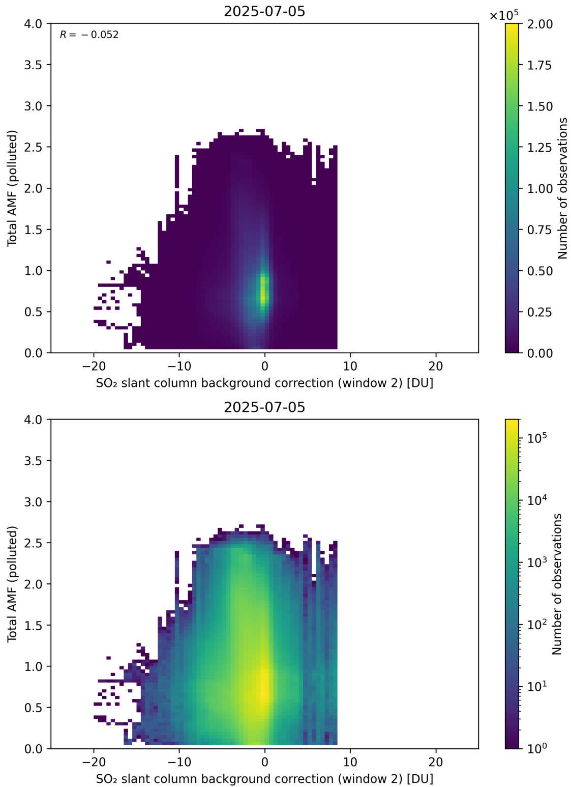
Figure 130: Scatter density plot of “SO 2 slant column background correction (window 2)” against “Total AMF (polluted)” for 2025-07-04 to 2025-07-06.
