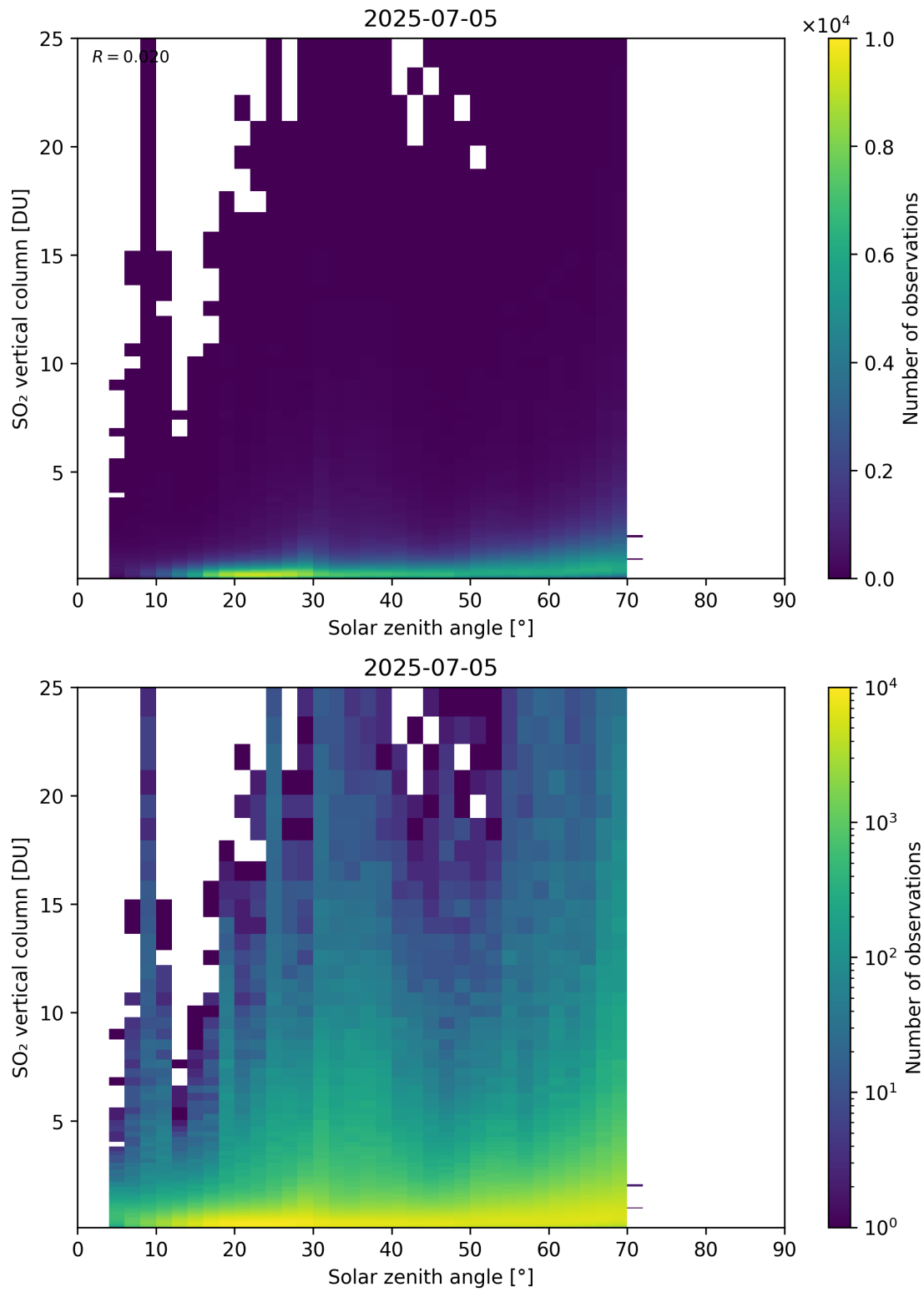
Figure 191: Scatter density plot of “Solar zenith angle” against “SO 2 vertical column” for 2025-07-04 to 2025-07-06.
