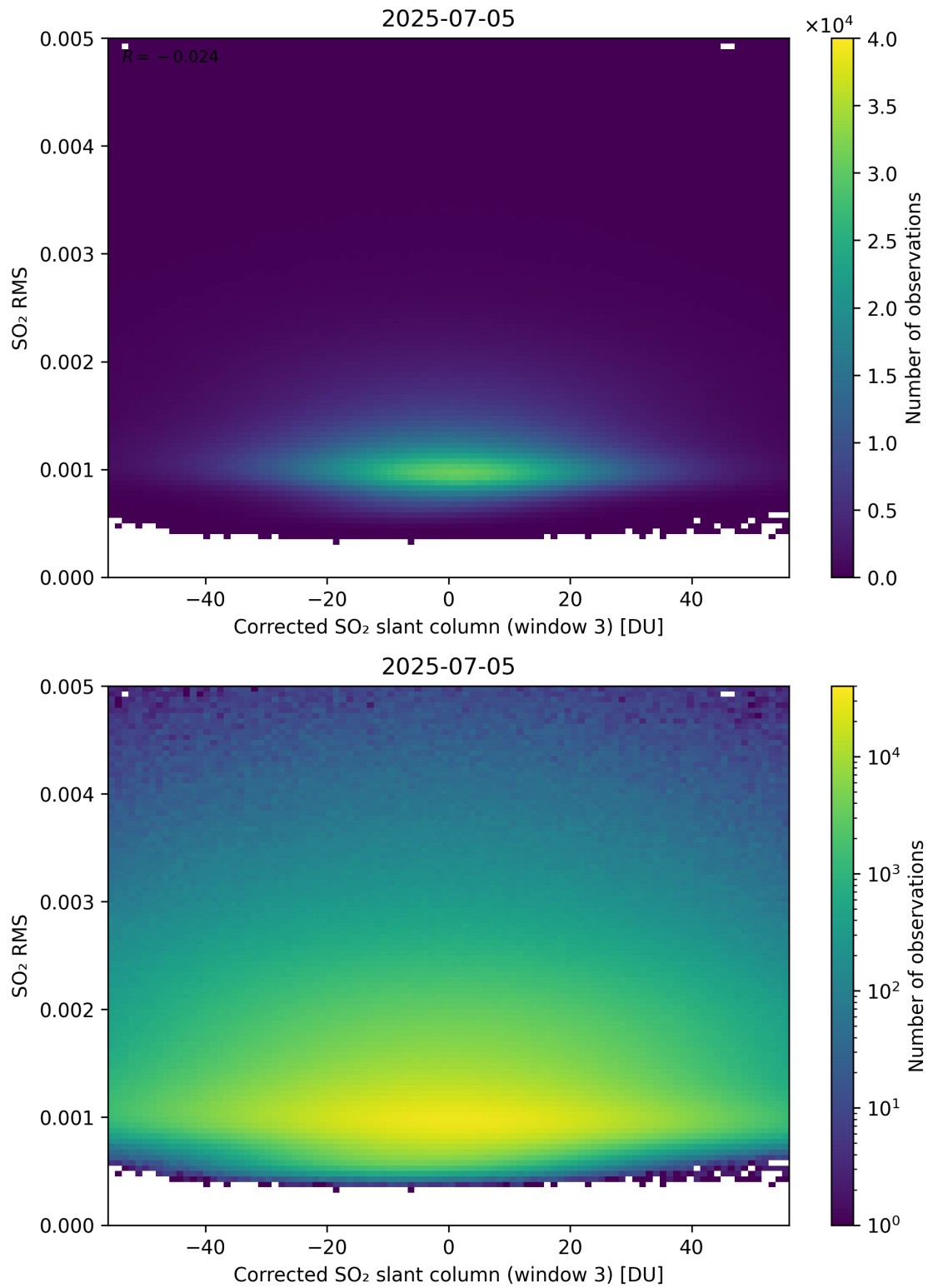
Figure 258: Scatter density plot of “Corrected SO 2 slant column (window 3)” against “SO 2 RMS” for 2025-07-04 to 2025-07-06.
