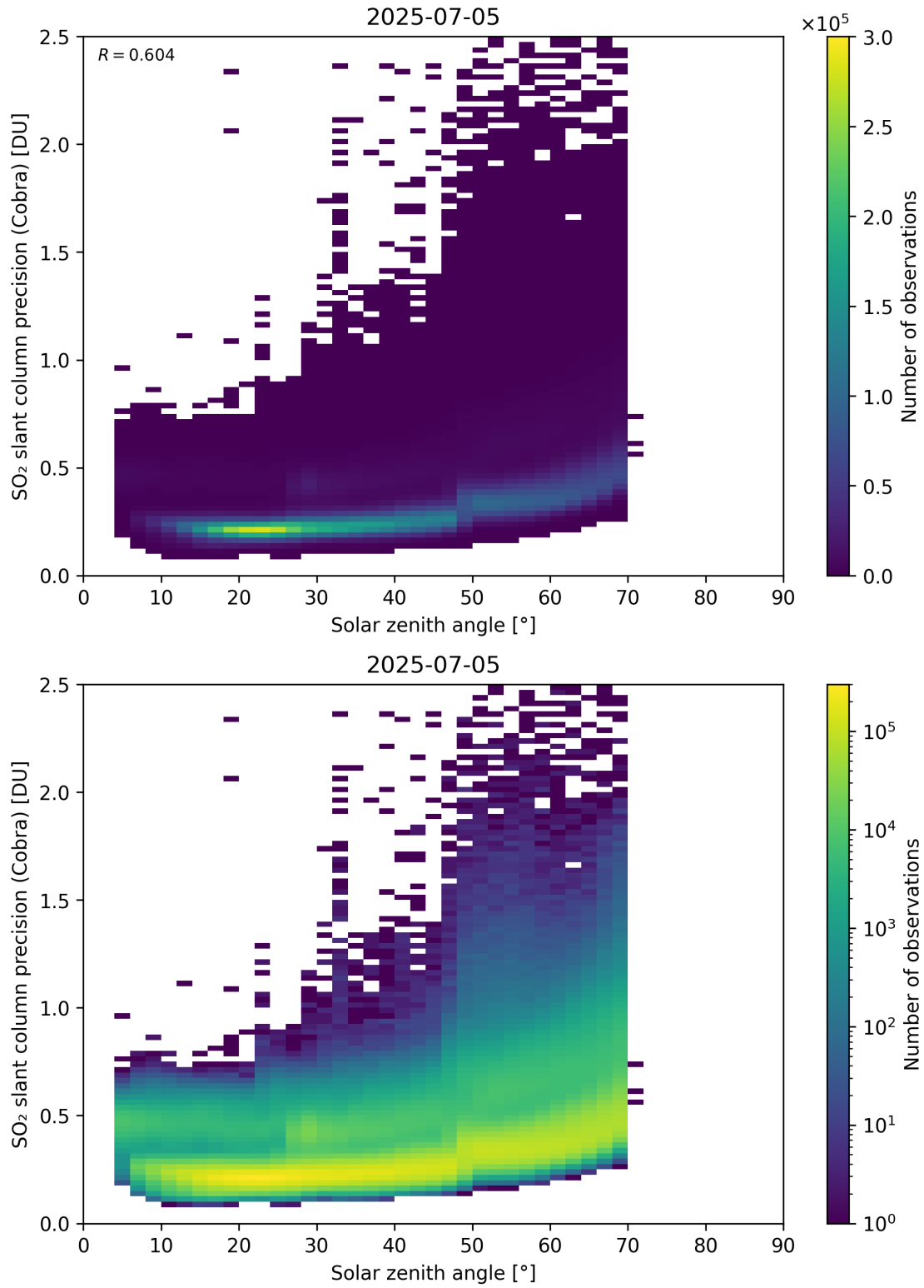
Figure 180: Scatter density plot of “Solar zenith angle” against “SO 2 slant column precision (Cobra)” for 2025-07-04 to 2025-07-06.
