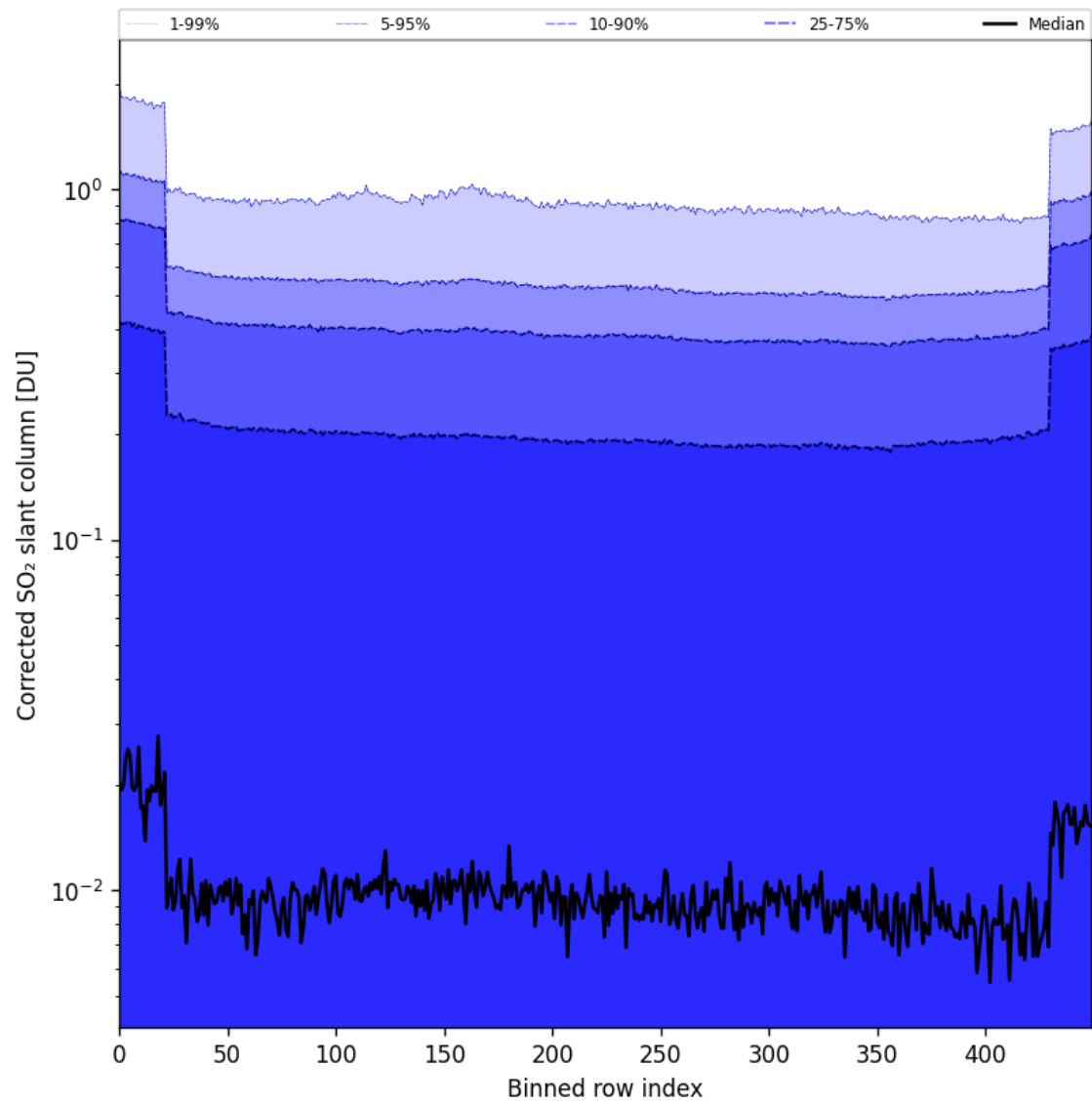
Figure 86: Along track statistics of “Corrected SO 2 slant column” for 2025-07-04 to 2025-07-06
