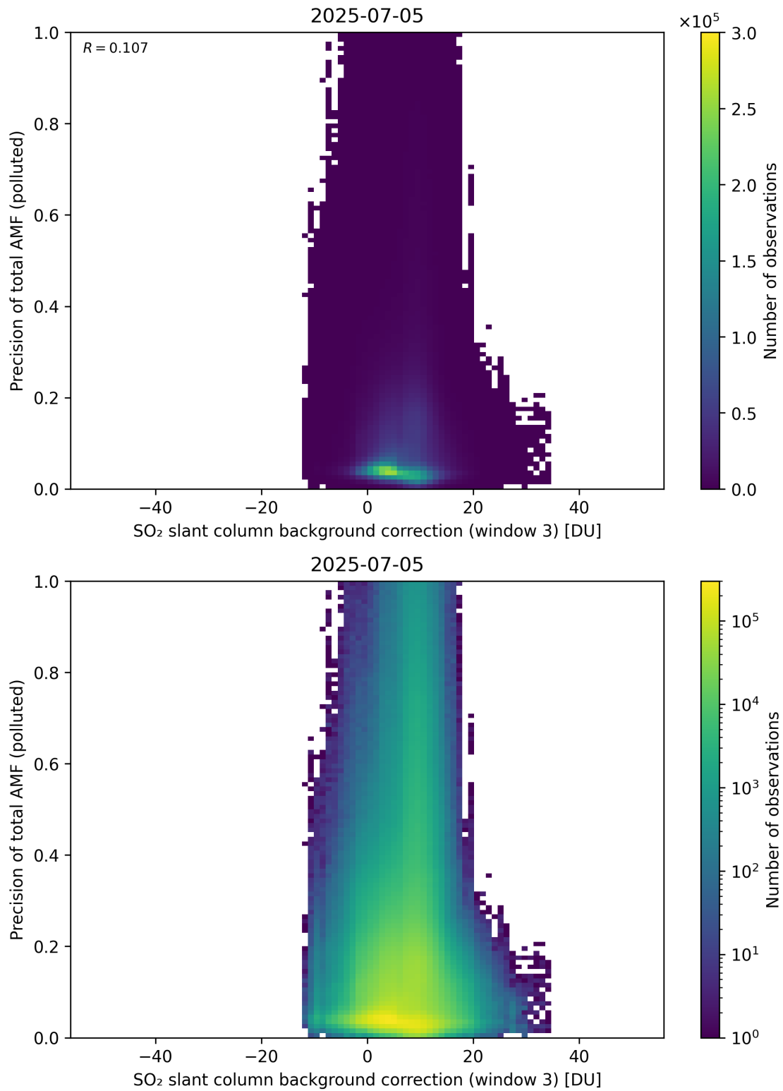
Figure 137: Scatter density plot of “SO 2 slant column background correction (window 3)” against “Precision of total AMF (polluted)” for 2025-07-04 to 2025-07-06.
