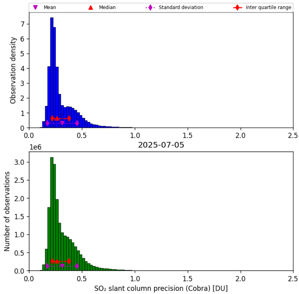
Figure 62: Histogram of “SO 2 slant column precision (Cobra)” for 2025-07-04 to 2025-07-06
