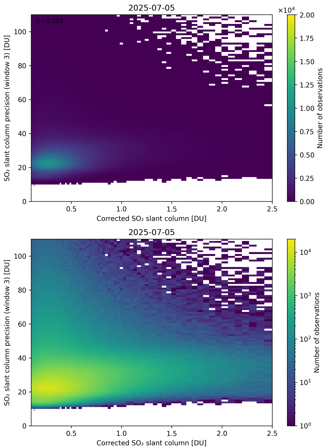
Figure 241: Scatter density plot of “Corrected SO 2 slant column” against “SO 2 slant column precision (window 3)” for 2025-07-04 to 2025-07-06.
