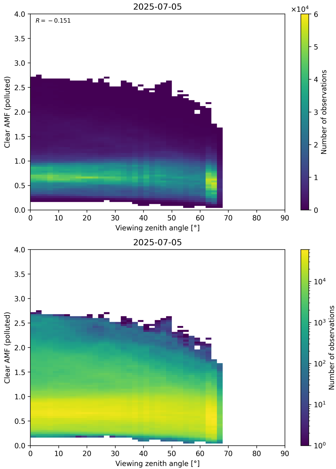
Figure 370: Scatter density plot of “Viewing zenith angle” against “Clear AMF (polluted)” for 2025-07-04 to 2025-07-06.
