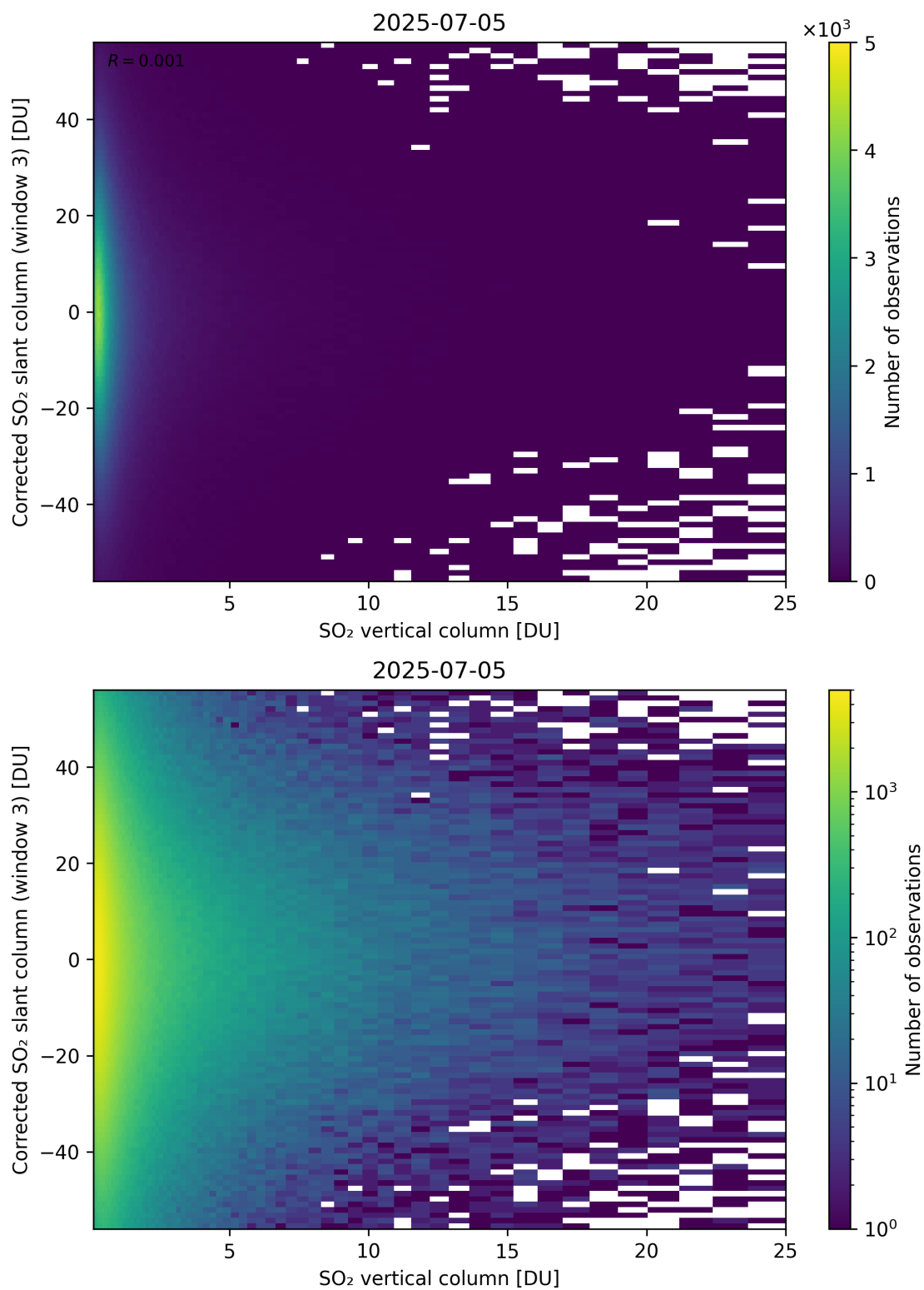
Figure 353: Scatter density plot of “SO 2 vertical column” against “Corrected SO 2 slant column (window 3)” for 2025-07-04 to 2025-07-06.
