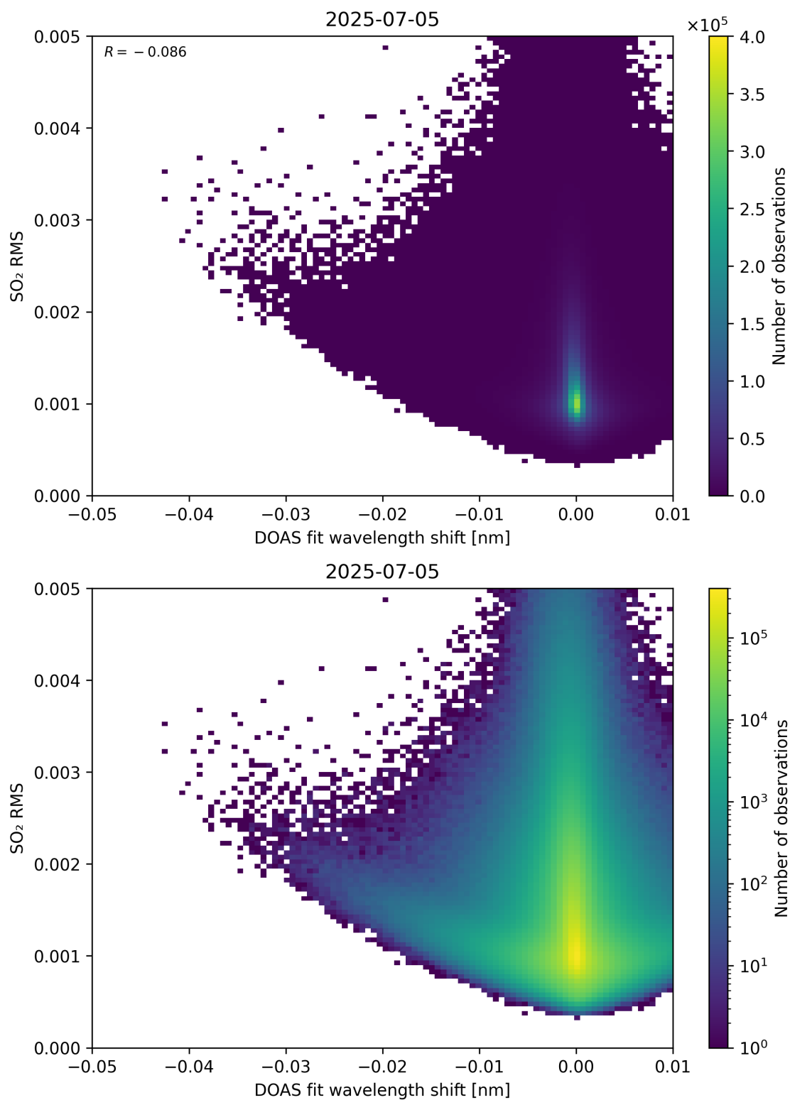
Figure 139: Scatter density plot of “DOAS fit wavelength shift” against “SO 2 RMS” for 2025-07-04 to 2025-07-06.
