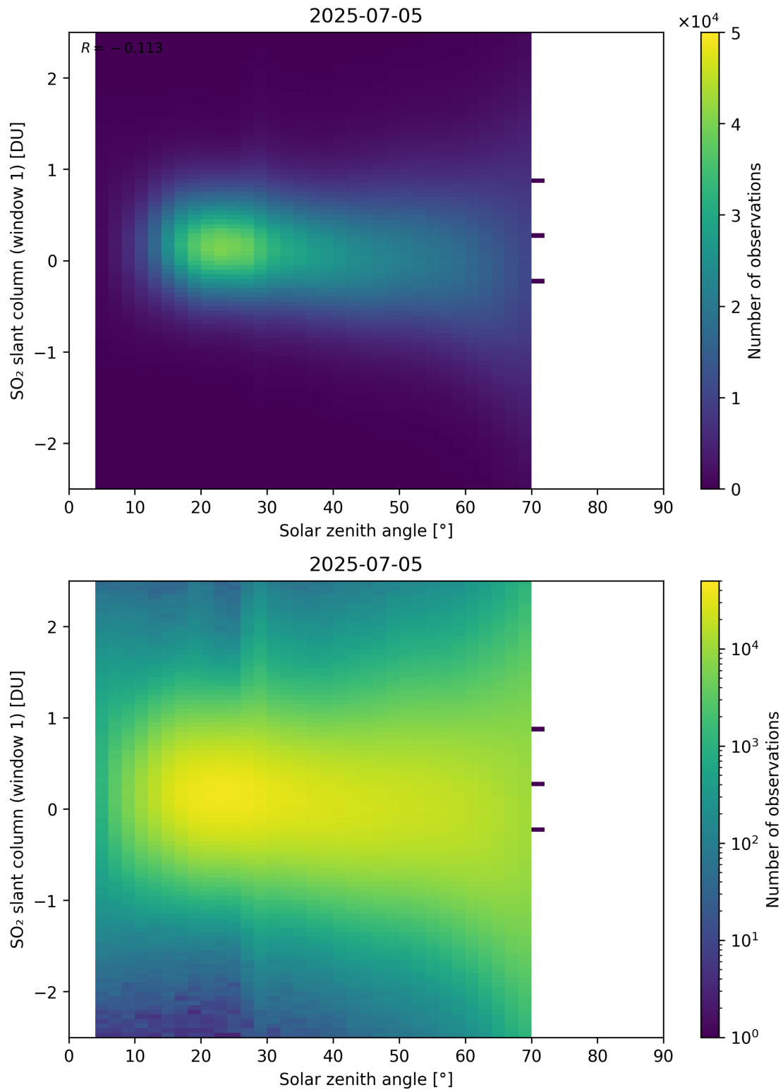
Figure 184: Scatter density plot of “Solar zenith angle” against “SO 2 slant column (window 1)” for 2025-07-04 to 2025-07-06.
