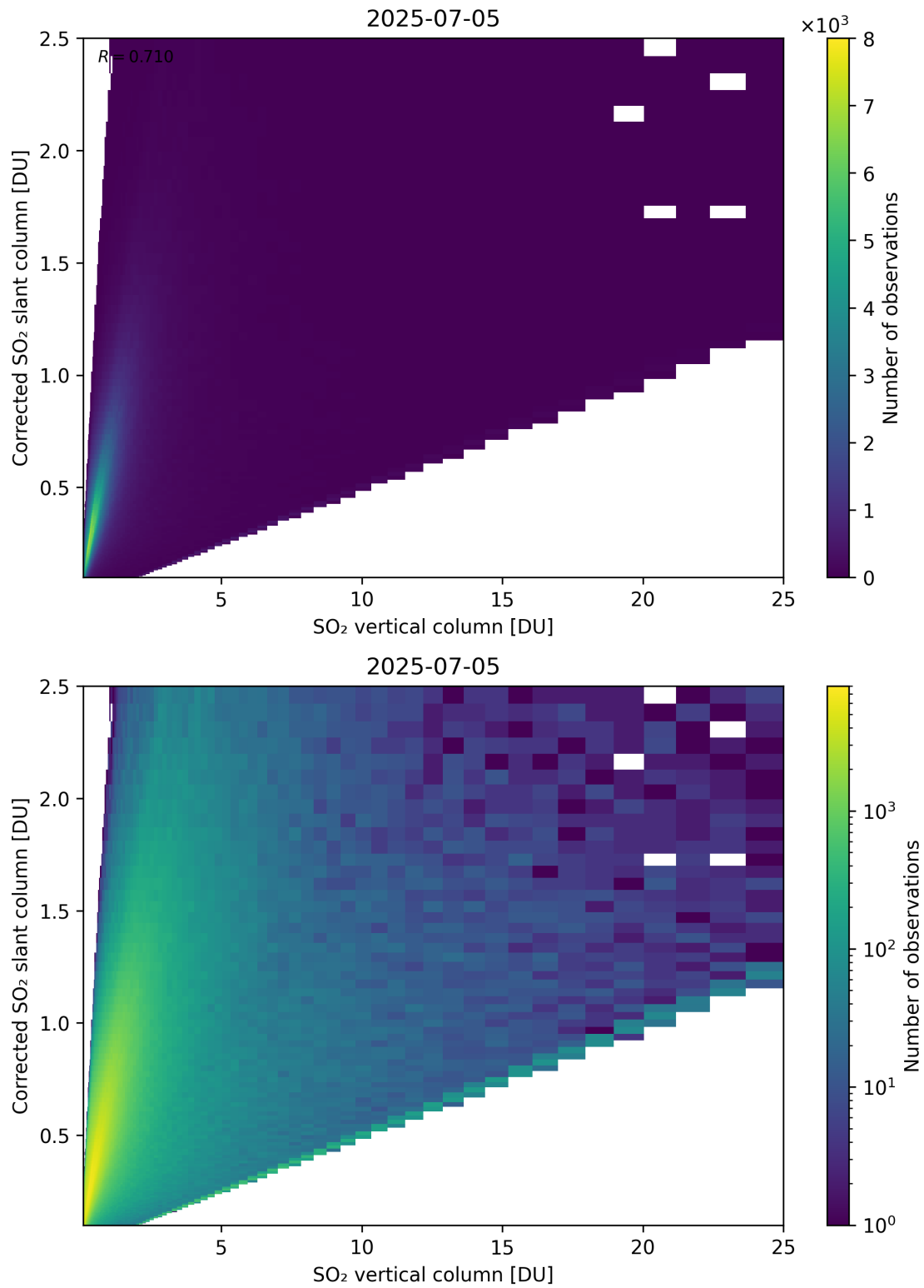
Figure 351: Scatter density plot of “SO 2 vertical column” against “Corrected SO 2 slant column” for 2025-07-04 to 2025-07-06.
