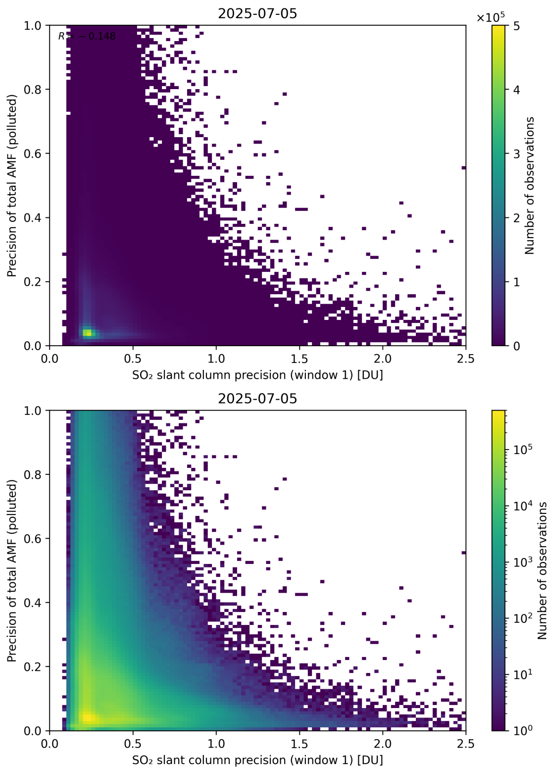
Figure 281: Scatter density plot of “SO 2 slant column precision (window 1)” against “Precision of total AMF (polluted)” for 2025-07-04 to 2025-07-06.
