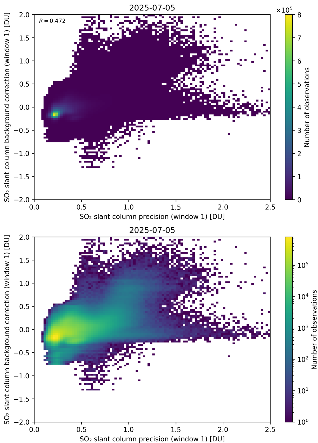
Figure 268: Scatter density plot of “SO 2 slant column precision (window 1)” against “SO 2 slant column background correction (window 1)” for 2025-07-04 to 2025-07-06.
