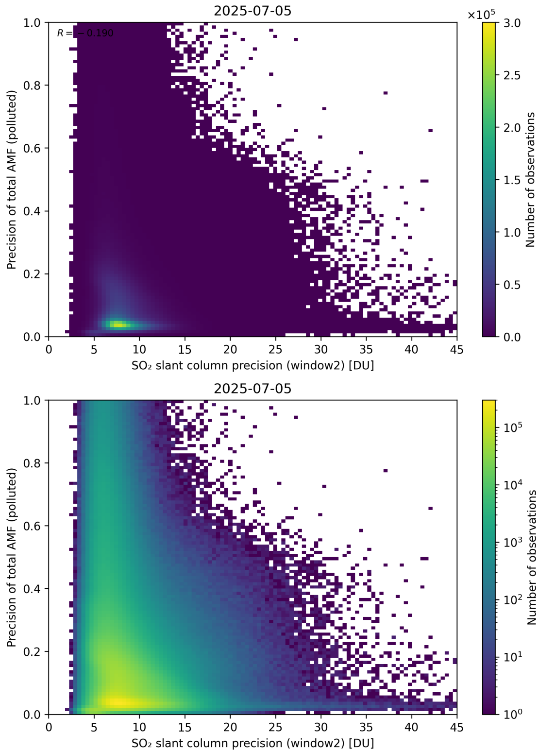
Figure 302: Scatter density plot of “SO 2 slant column precision (window2)” against “Precision of total AMF (polluted)” for 2025-07-04 to 2025-07-06.
