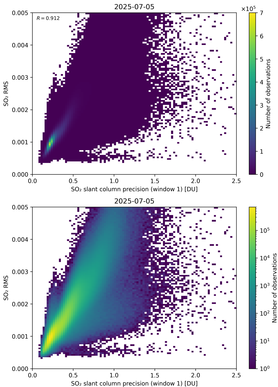
Figure 273: Scatter density plot of “SO 2 slant column precision (window 1)” against “SO 2 RMS” for 2025-07-04 to 2025-07-06.
