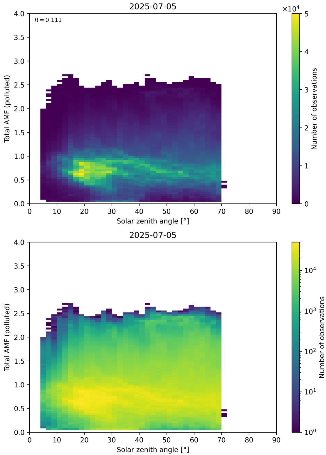
Figure 189: Scatter density plot of “Solar zenith angle” against “Total AMF (polluted)” for 2025-07-04 to 2025-07-06.
