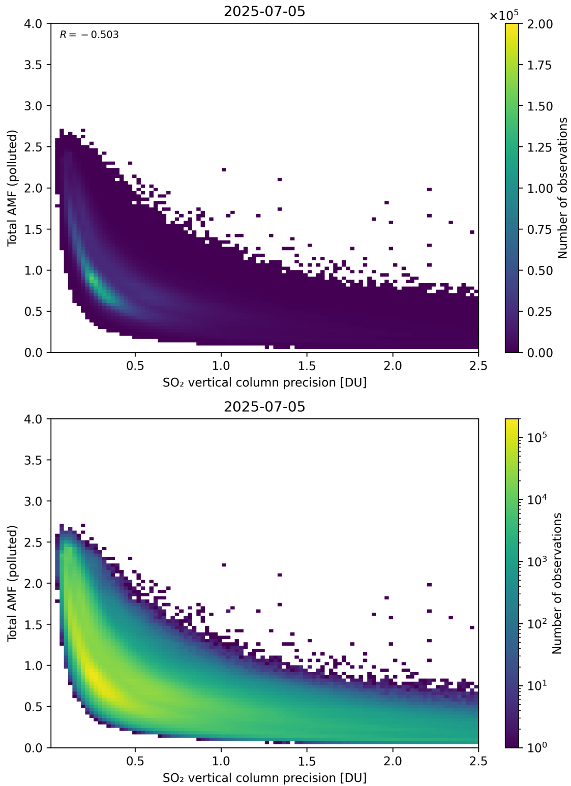
Figure 346: Scatter density plot of “SO 2 vertical column precision” against “Total AMF (polluted)” for 2025-07-04 to 2025-07-06.
