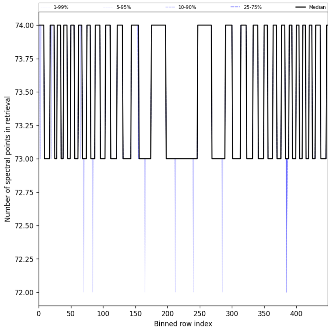
Figure 108: Along track statistics of “Number of spectral points in retrieval” for 2025-07-04 to 2025-07-06
