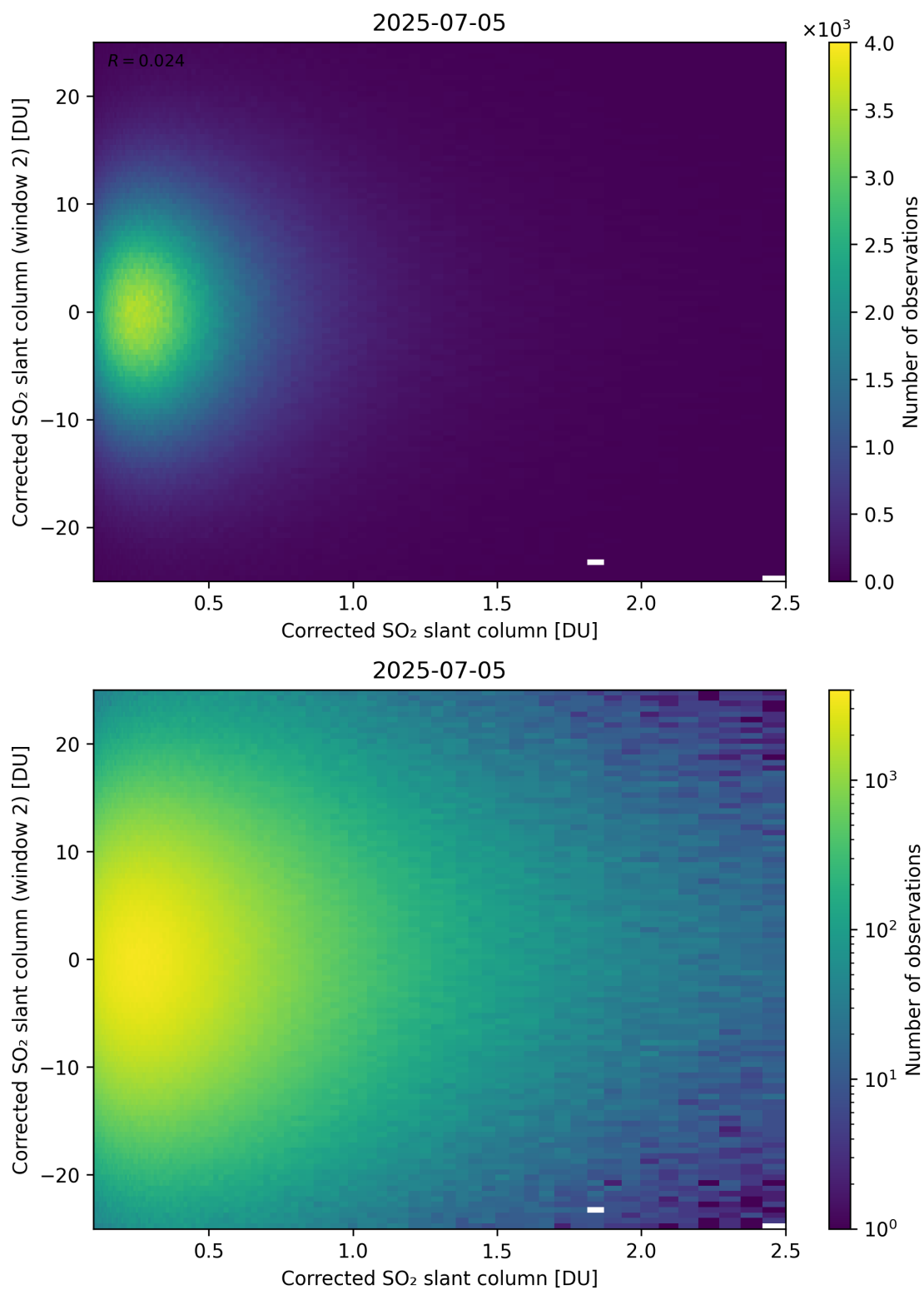
Figure 235: Scatter density plot of “Corrected SO 2 slant column” against “Corrected SO 2 slant column (window 2)” for 2025-07-04 to 2025-07-06.
