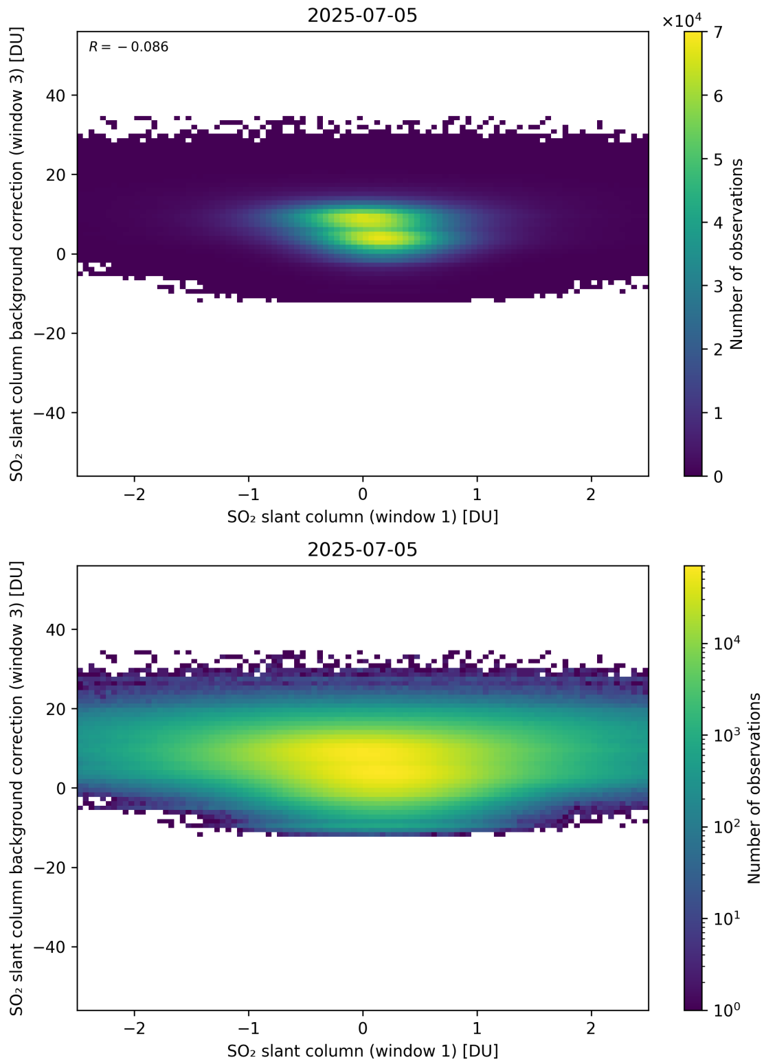
Figure 264: Scatter density plot of “SO 2 slant column (window 1)” against “SO 2 slant column background correction (window 3)” for 2025-07-04 to 2025-07-06.
