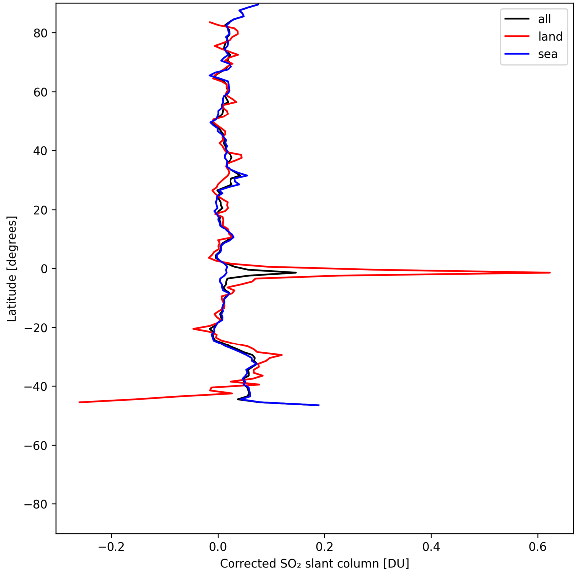
Figure 34: Zonal average of “Corrected SO 2 slant column” for 2025-07-04 to 2025-07-06.
