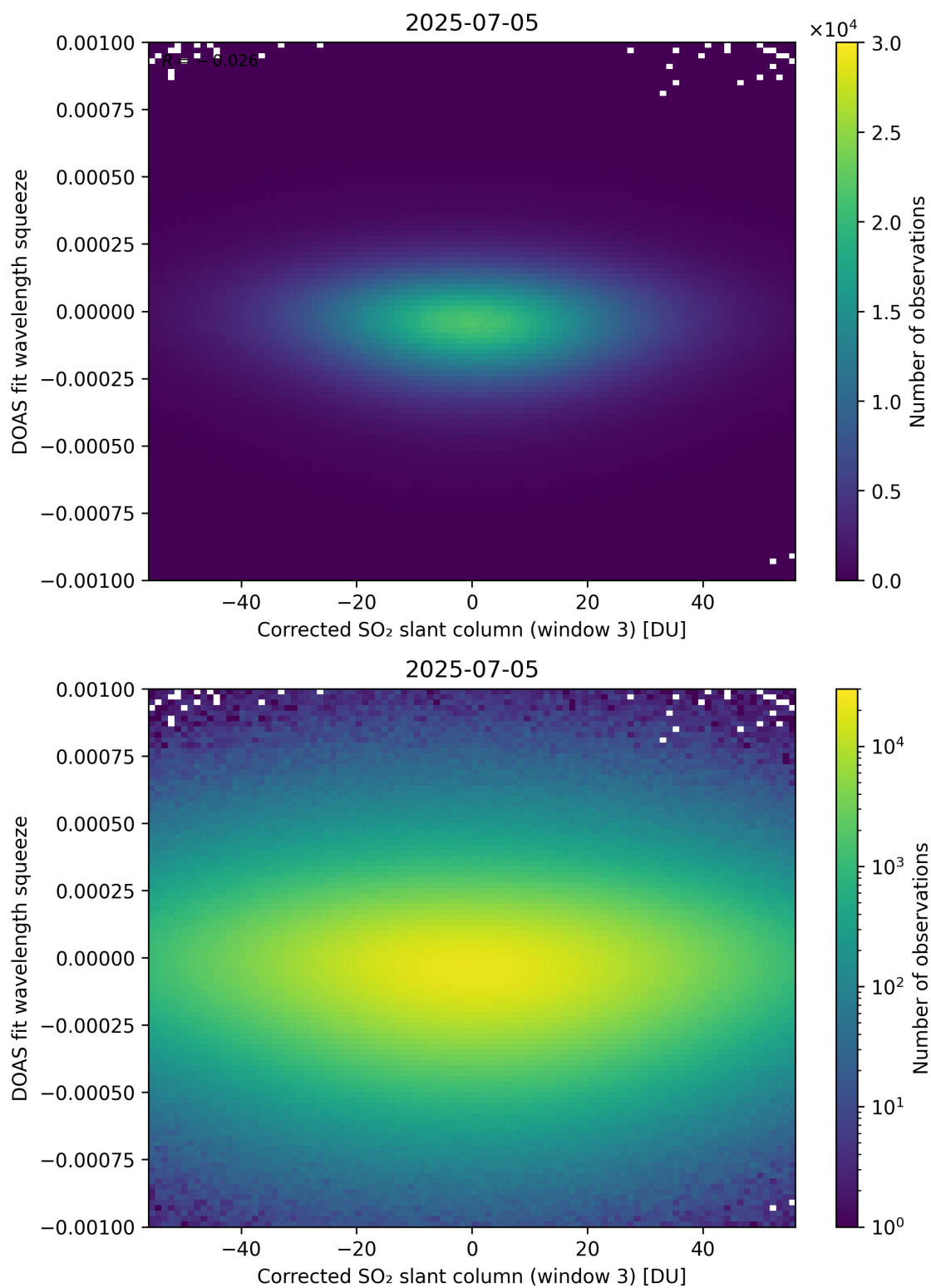
Figure 257: Scatter density plot of “Corrected SO 2 slant column (window 3)” against “DOAS fit wavelength squeeze” for 2025-07-04 to 2025-07-06.
