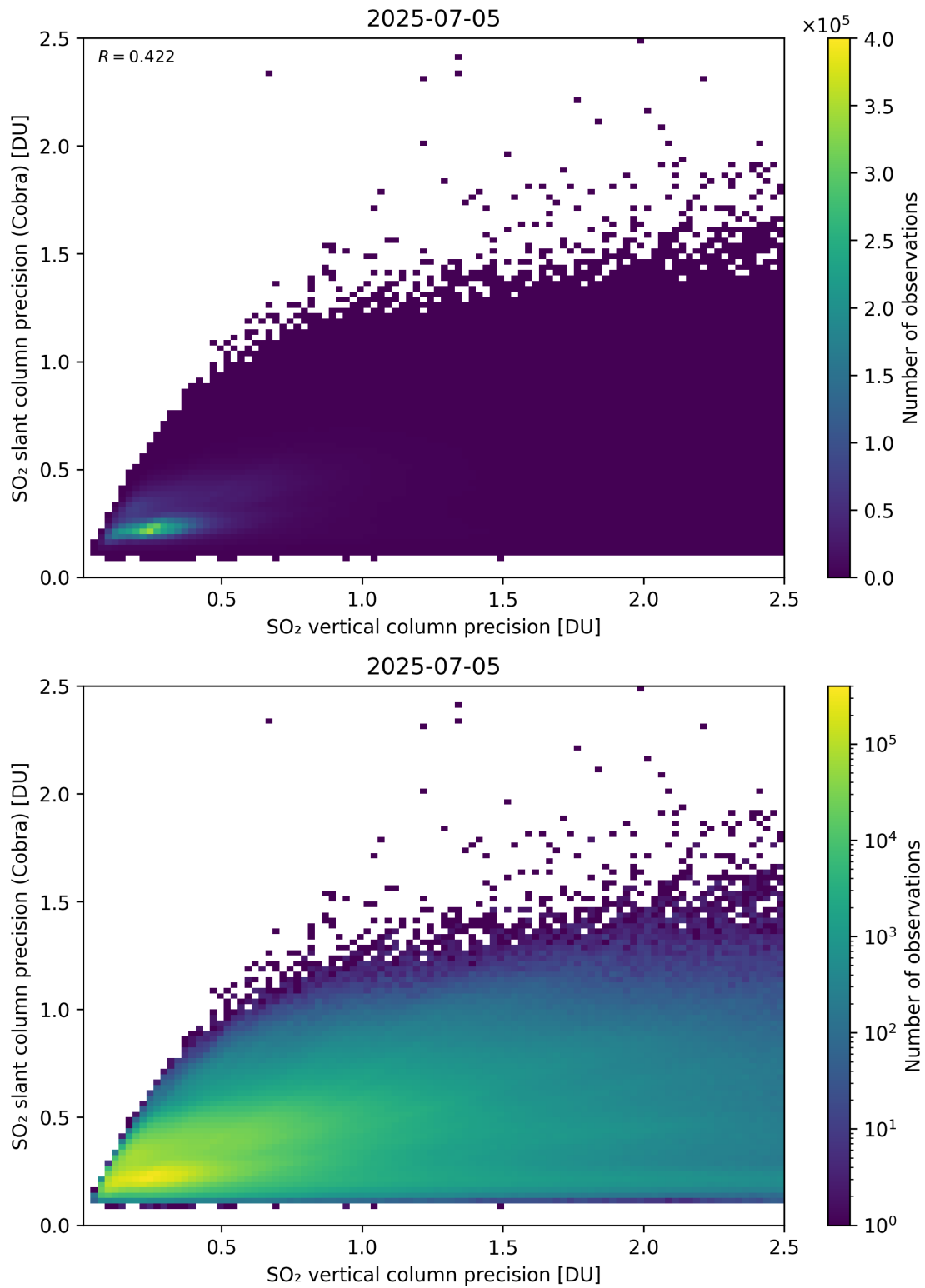
Figure 337: Scatter density plot of “SO 2 vertical column precision” against “SO 2 slant column precision (Cobra)” for 2025-07-04 to 2025-07-06.
