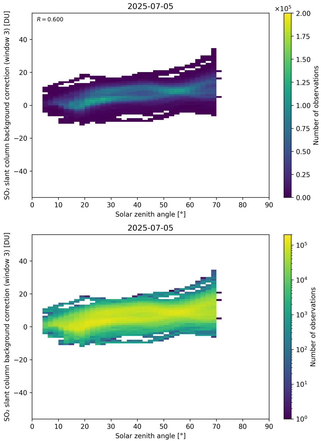
Figure 173: Scatter density plot of “Solar zenith angle” against “SO 2 slant column background correction (window 3)” for 2025-07-04 to 2025-07-06.
