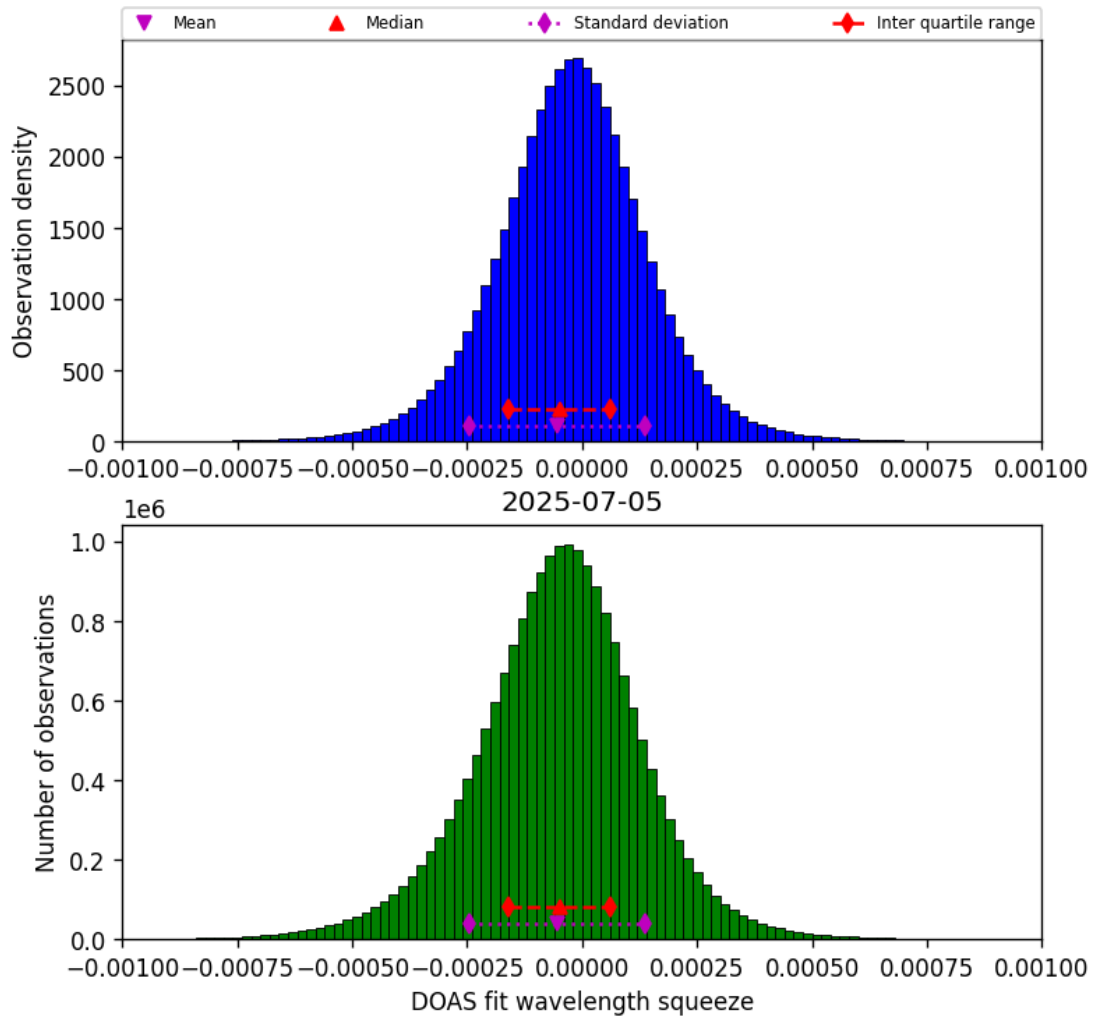
Figure 77: Histogram of “DOAS fit wavelength squeeze” for 2025-07-04 to 2025-07-06
