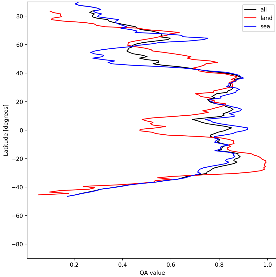
Figure 31: Zonal average of “QA value” for 2025-07-04 to 2025-07-06.
