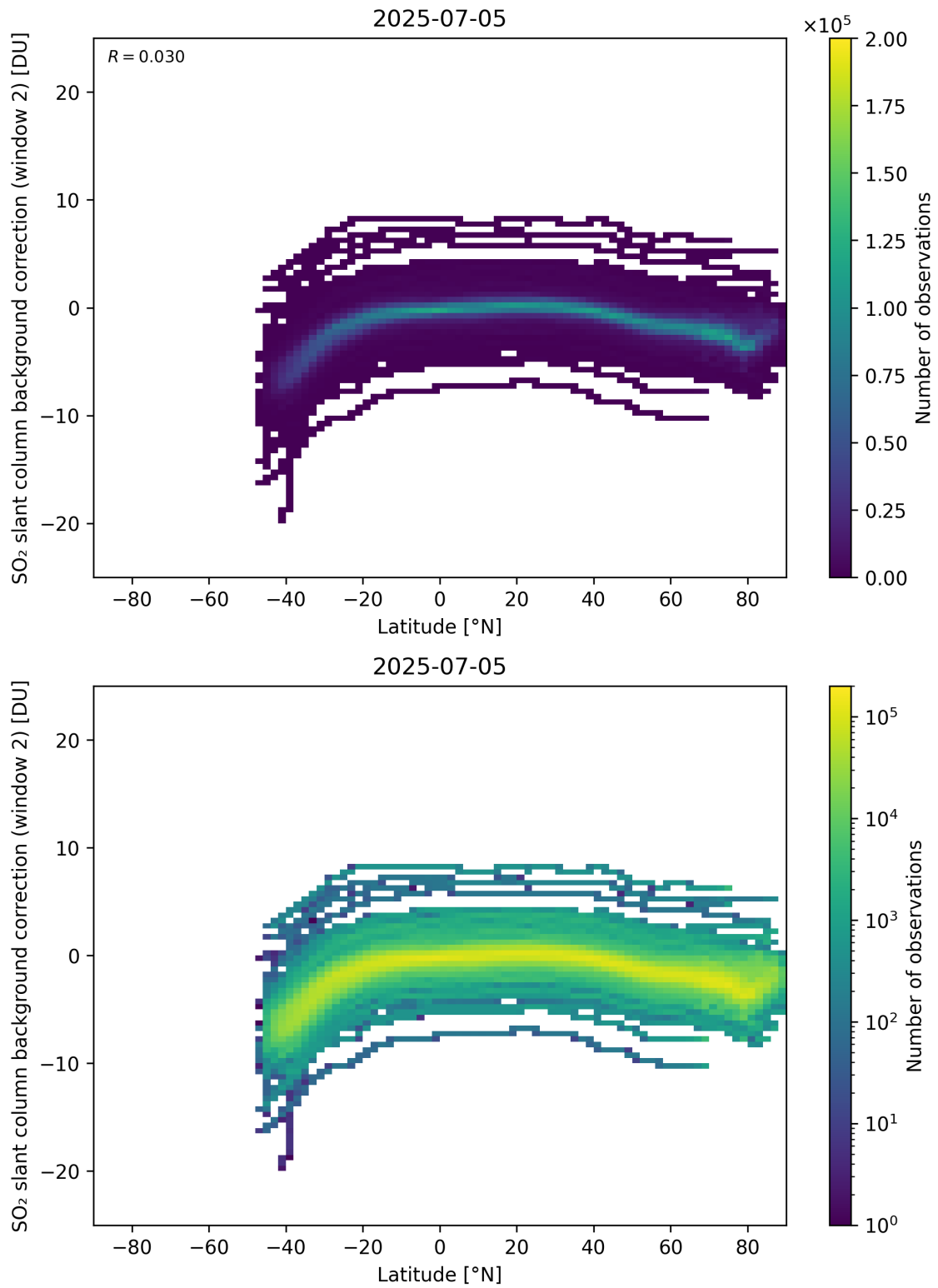
Figure 151: Scatter density plot of “Latitude” against “SO 2 slant column background correction (window 2)” for 2025-07-04 to 2025-07-06.
