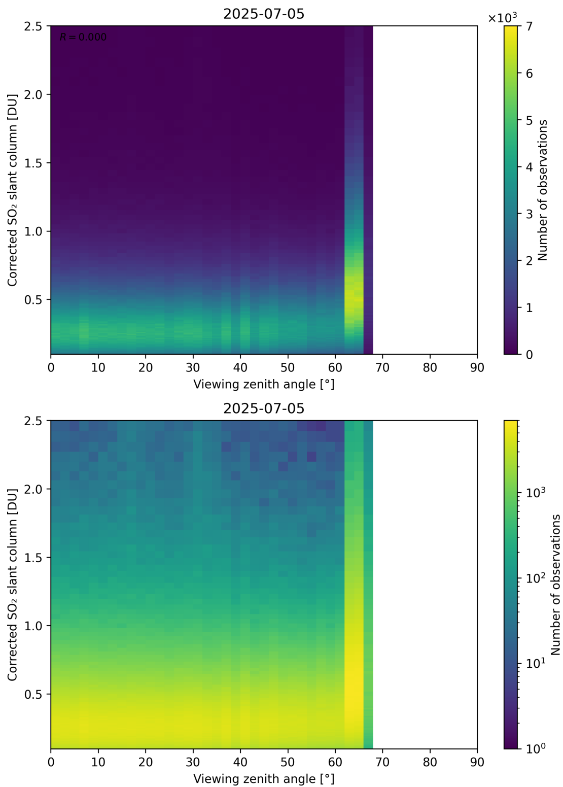
Figure 373: Scatter density plot of “Viewing zenith angle” against “Corrected SO 2 slant column” for 2025-07-04 to 2025-07-06.
