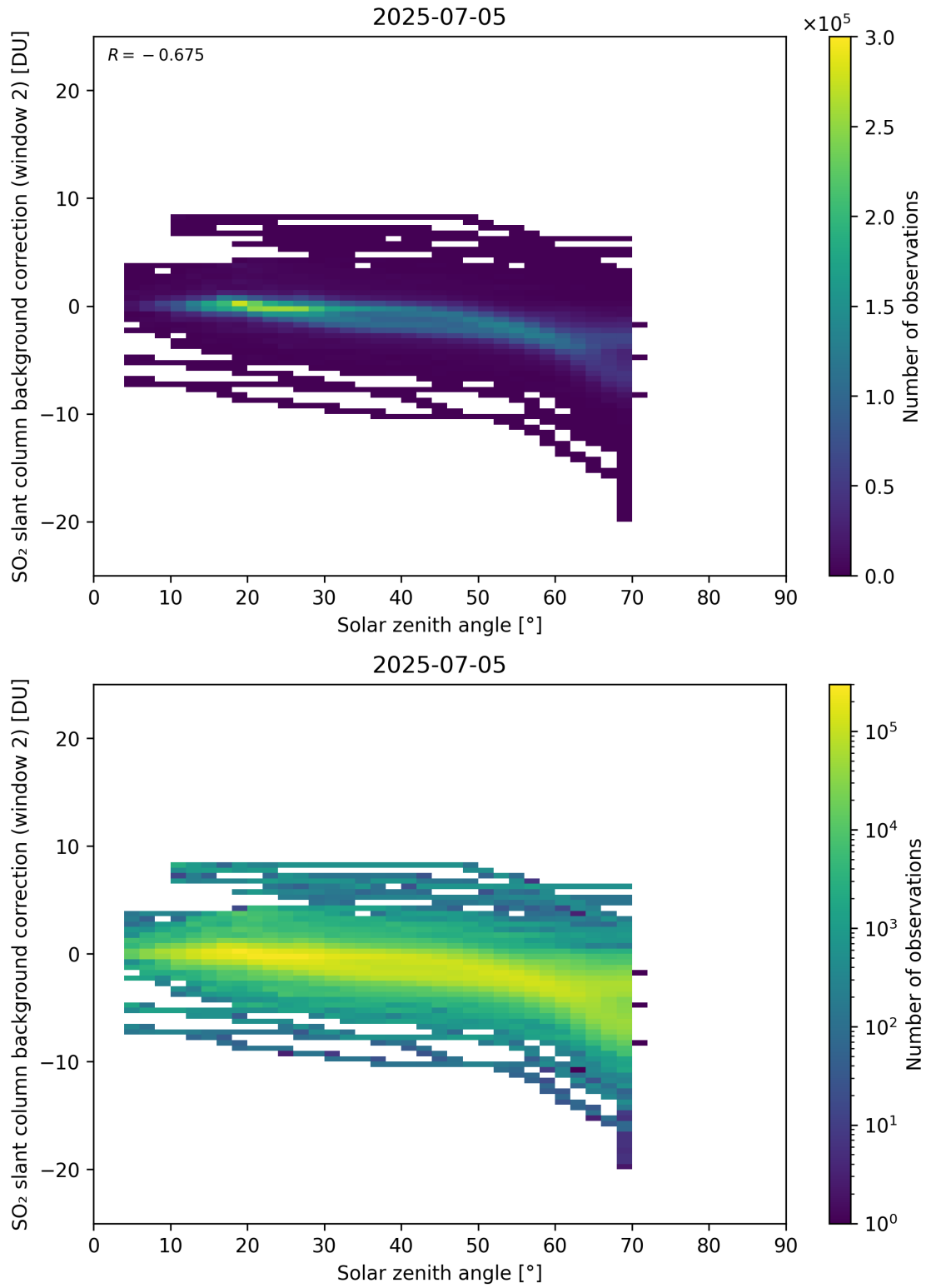
Figure 172: Scatter density plot of “Solar zenith angle” against “SO 2 slant column background correction (window 2)” for 2025-07-04 to 2025-07-06.
