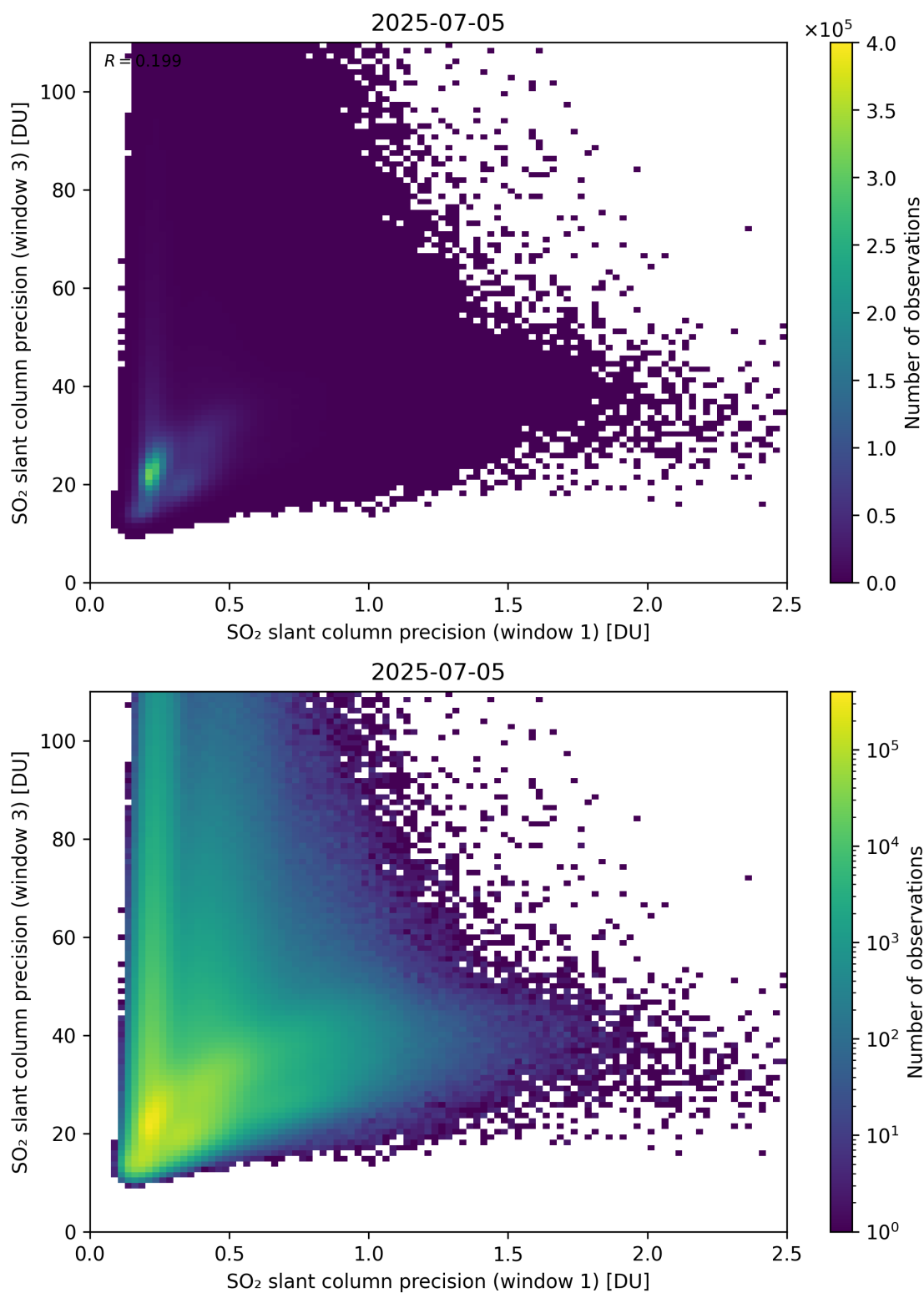
Figure 279: Scatter density plot of “SO 2 slant column precision (window 1)” against “SO 2 slant column precision (window 3)” for 2025-07-04 to 2025-07-06.
