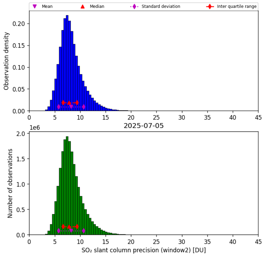
Figure 68: Histogram of “SO 2 slant column precision (window2)” for 2025-07-04 to 2025-07-06
