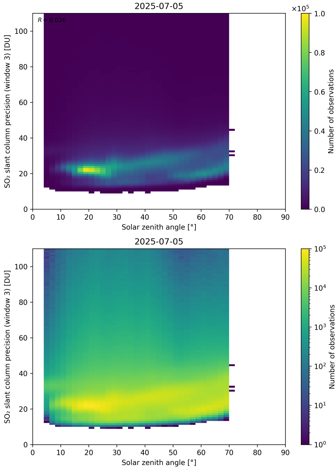
Figure 188: Scatter density plot of “Solar zenith angle” against “SO 2 slant column precision (window 3)” for 2025-07-04 to 2025-07-06.
