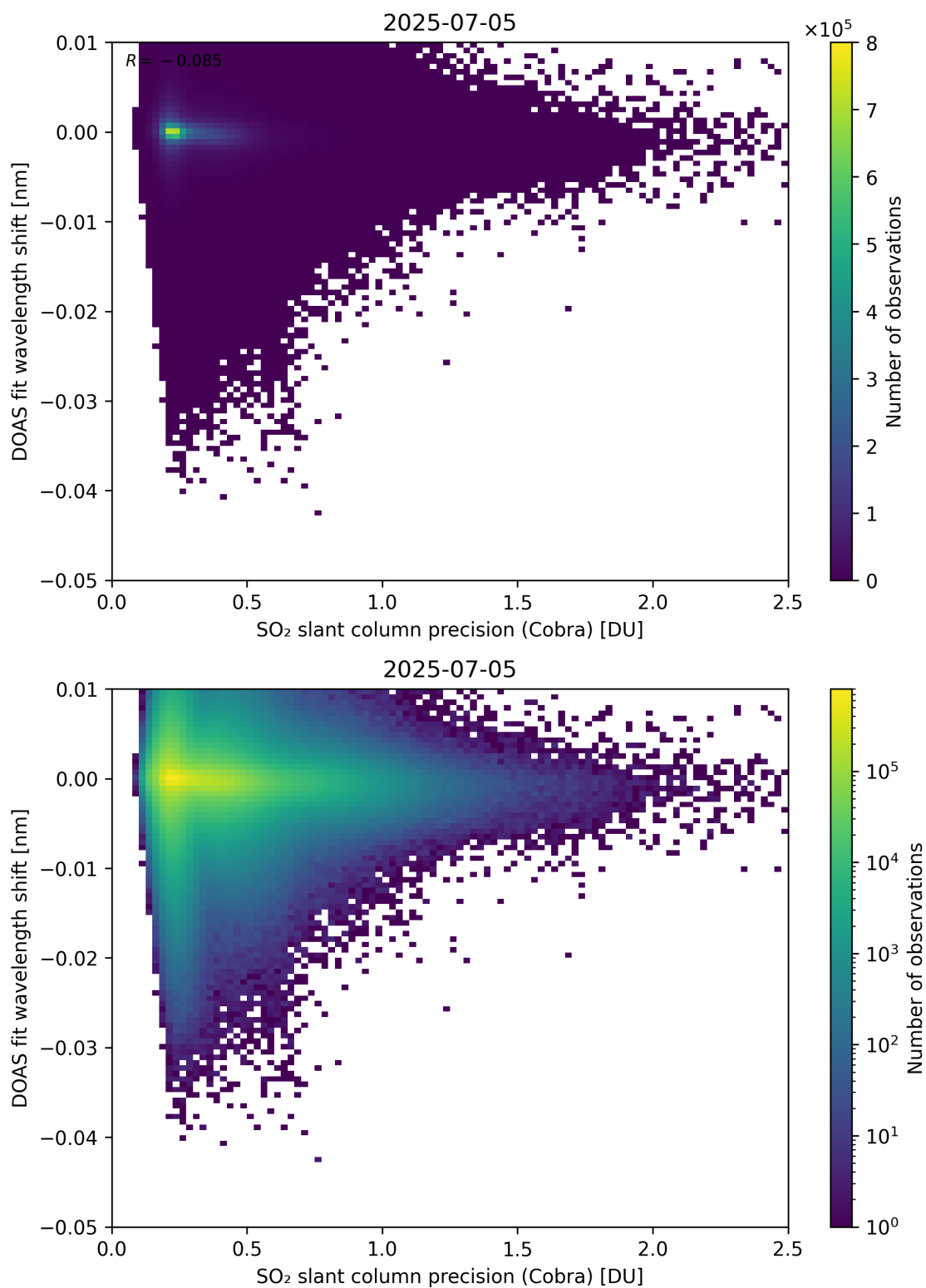
Figure 202: Scatter density plot of “SO 2 slant column precision (Cobra)” against “DOAS fit wavelength shift” for 2025-07-04 to 2025-07-06.
