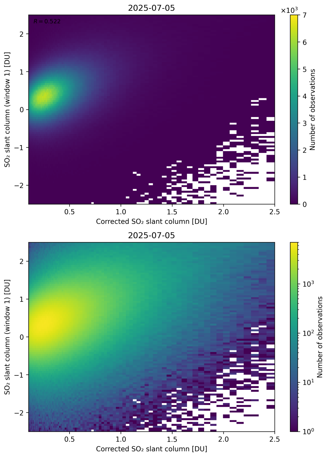
Figure 237: Scatter density plot of “Corrected SO 2 slant column” against “SO 2 slant column (window 1)” for 2025-07-04 to 2025-07-06.
