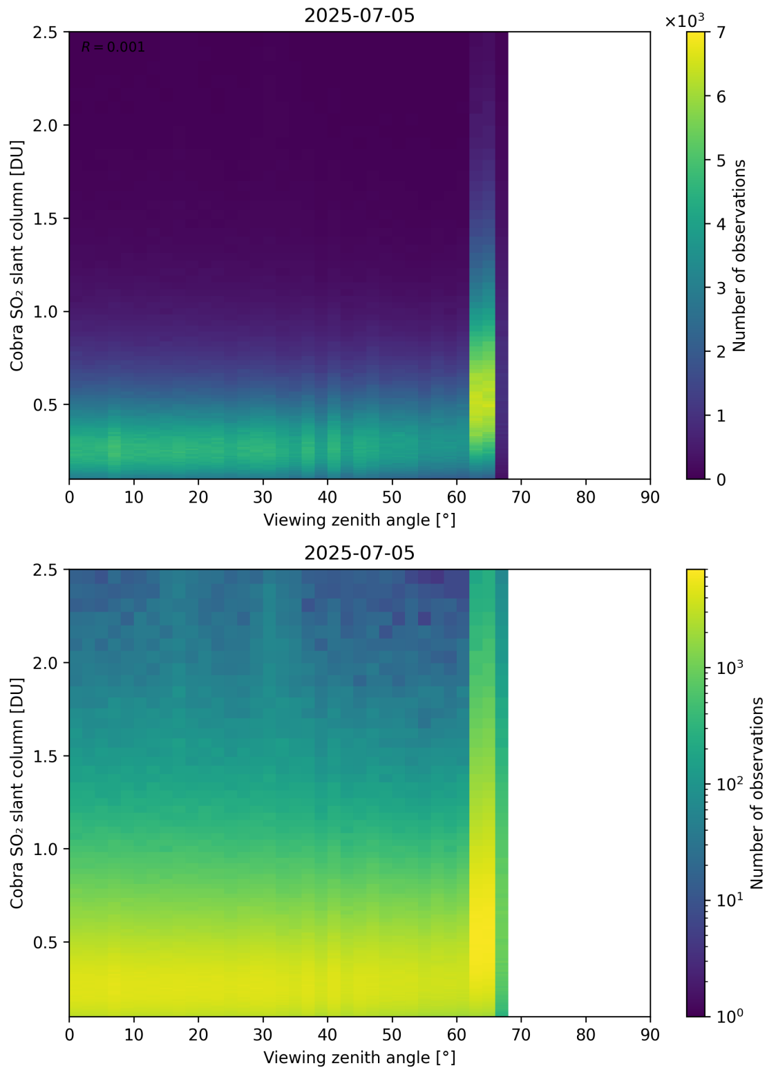
Figure 371: Scatter density plot of “Viewing zenith angle” against “Cobra SO 2 slant column” for 2025-07-04 to 2025-07-06.
