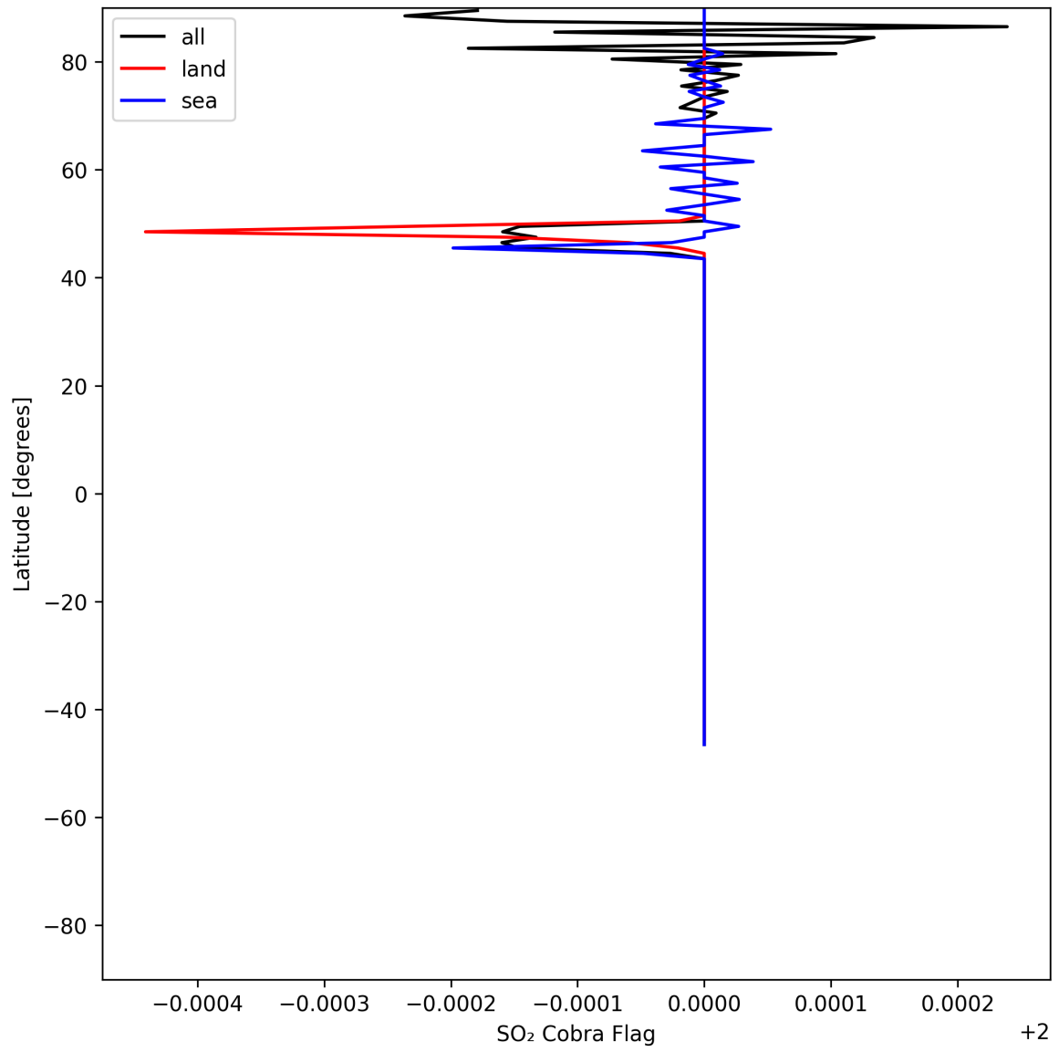
Figure 49: Zonal average of "SO 2 Cobra Flag" for 2025-07-04 to 2025-07-06.
