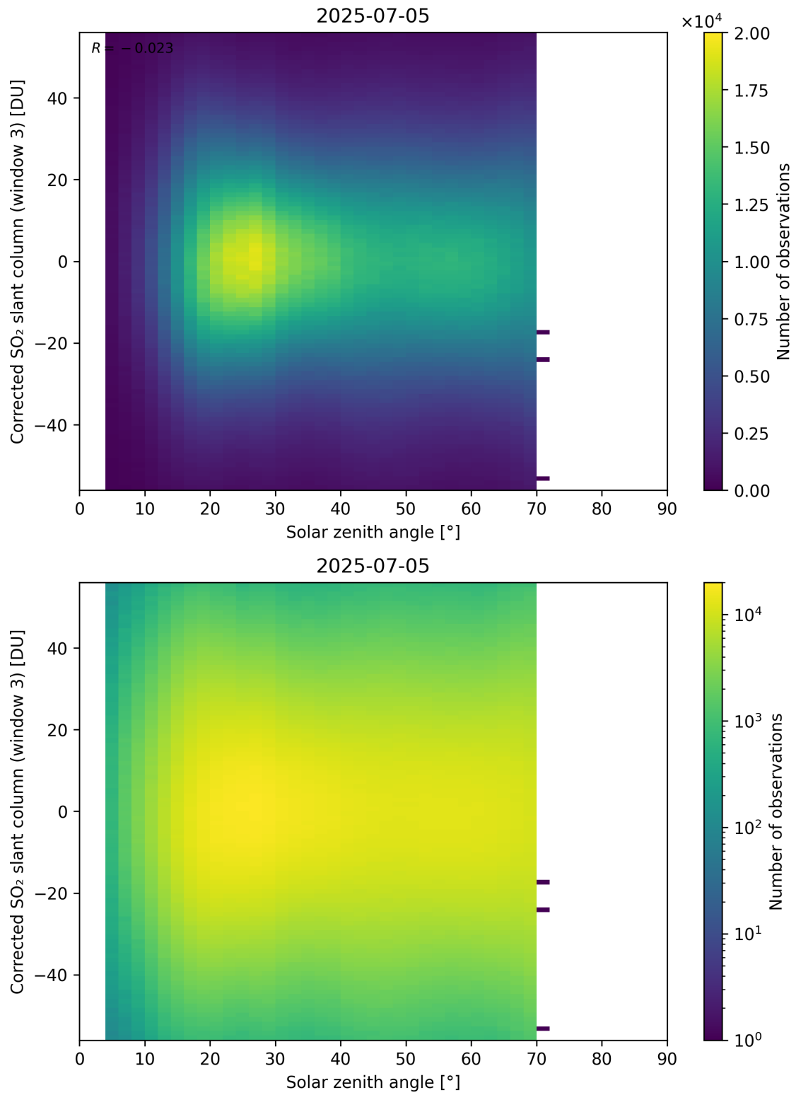
Figure 183: Scatter density plot of “Solar zenith angle” against “Corrected SO 2 slant column (window 3)” for 2025-07-04 to 2025-07-06.
