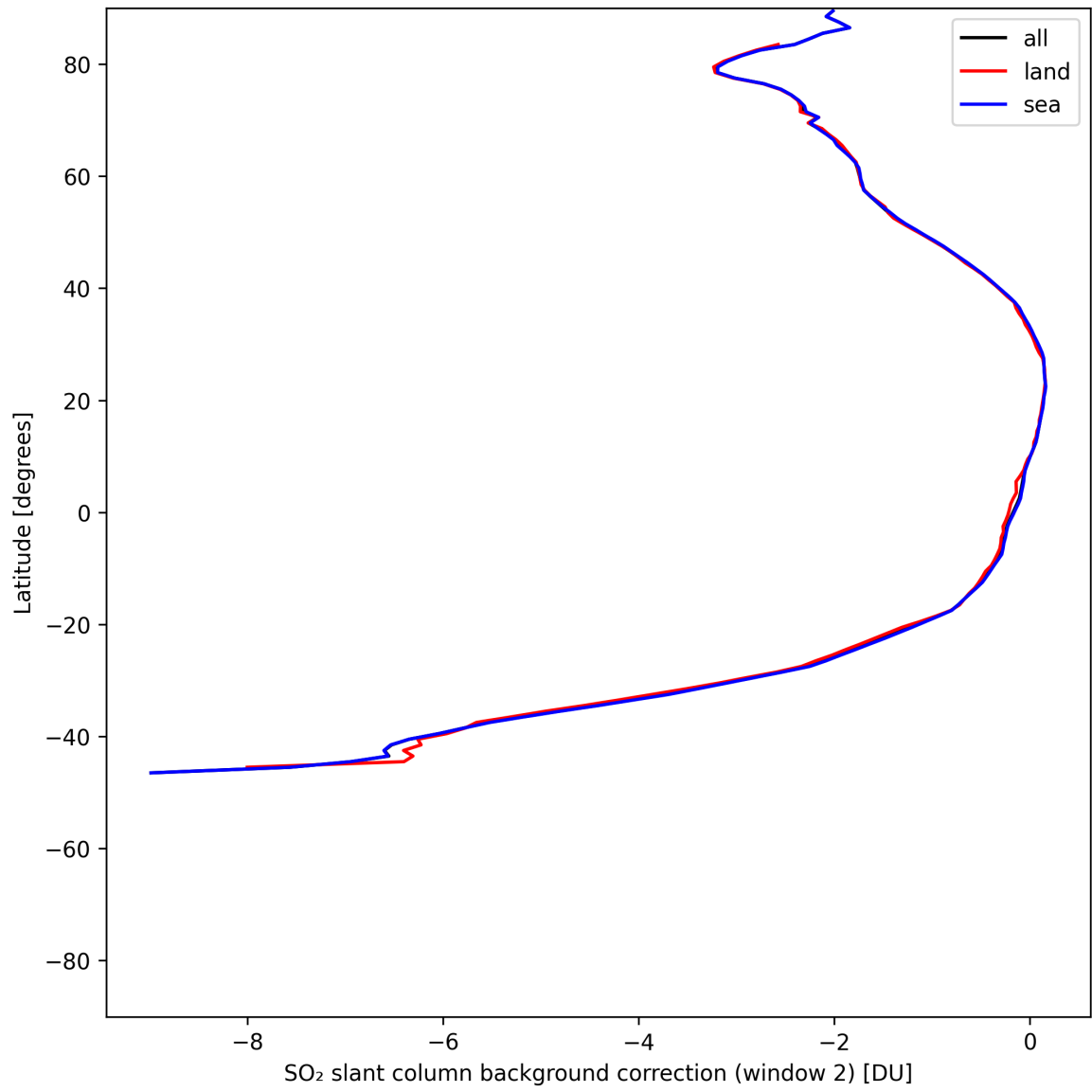
Figure 44: Zonal average of “SO 2 slant column background correction (window 2)” for 2025-07-04 to 2025-07-06.
