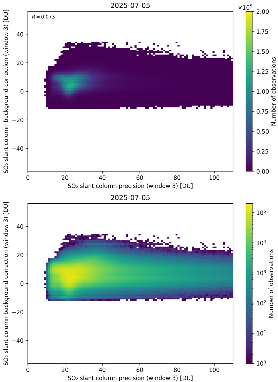
Figure 307: Scatter density plot of “SO 2 slant column precision (window 3)” against “SO 2 slant column background correction (window 3)” for 2025-07-04 to 2025-07-06.
