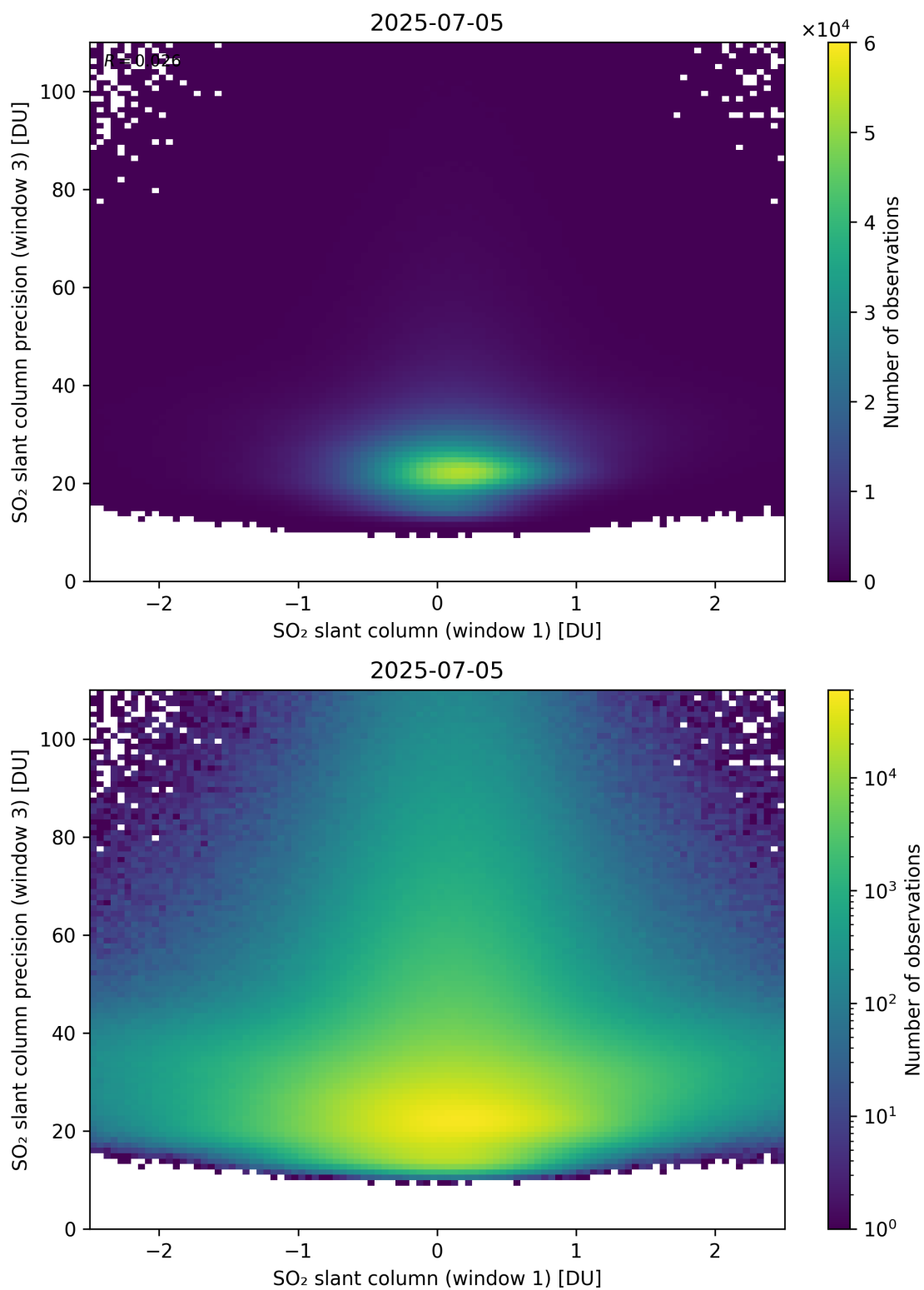
Figure 288: Scatter density plot of “SO 2 slant column (window 1)” against “SO 2 slant column precision (window 3)” for 2025-07-04 to 2025-07-06.
