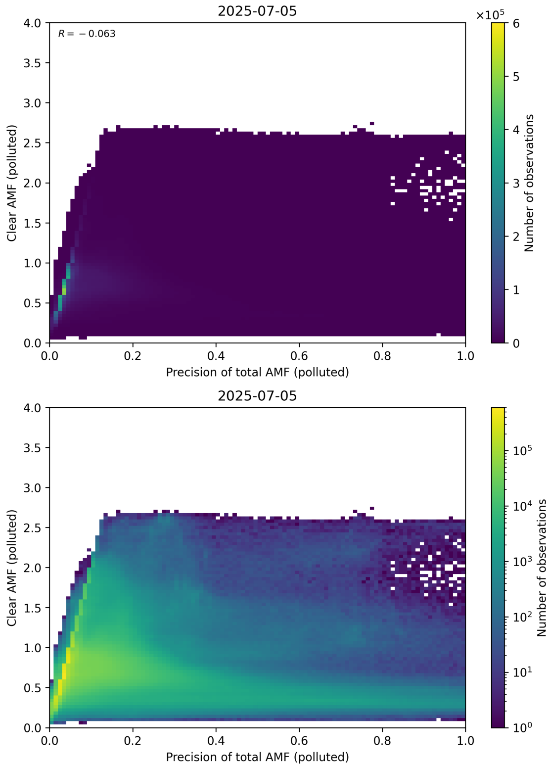
Figure 320: Scatter density plot of “Precision of total AMF (polluted)” against “Clear AMF (polluted)” for 2025-07-04 to 2025-07-06.
