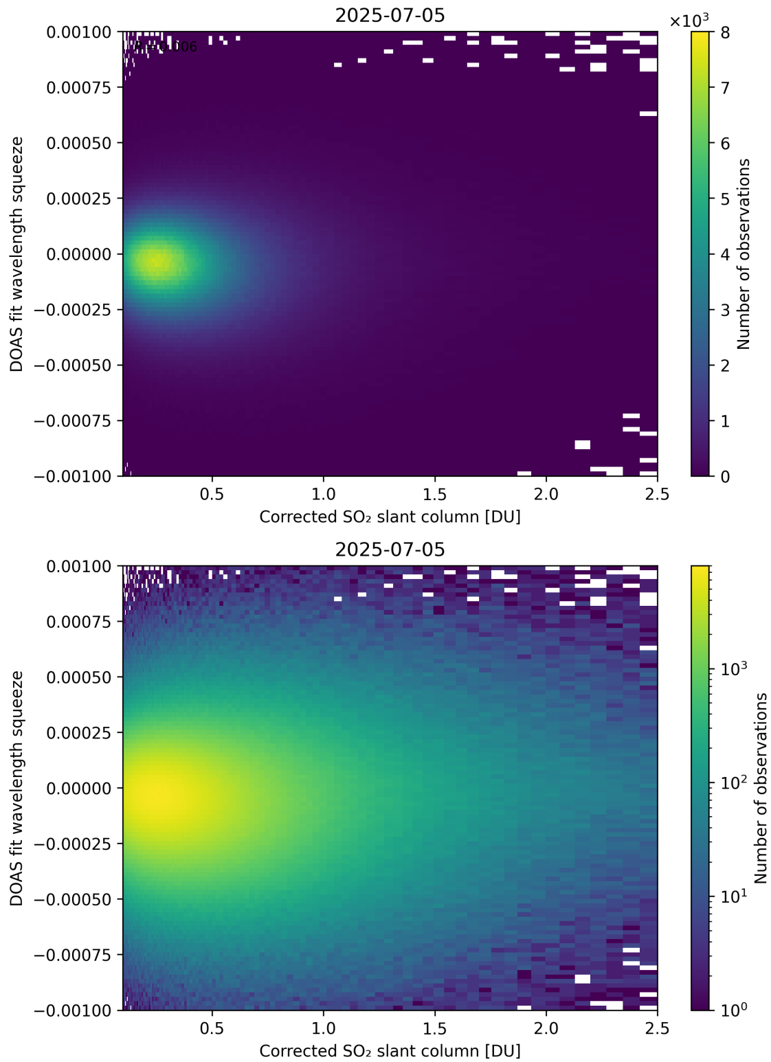
Figure 230: Scatter density plot of "Corrected SO 2 slant column" against "DOAS fit wavelength squeeze" for 2025-07-04 to 2025-07-06.
