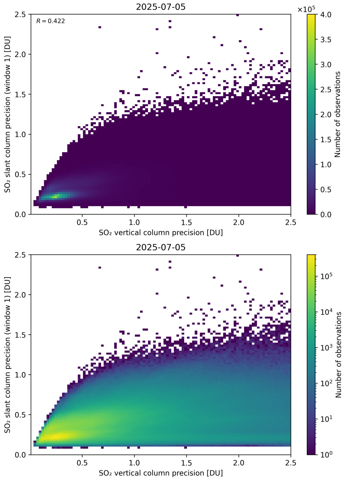
Figure 342: Scatter density plot of “SO 2 vertical column precision” against “SO 2 slant column precision (window 1)” for 2025-07-04 to 2025-07-06.
