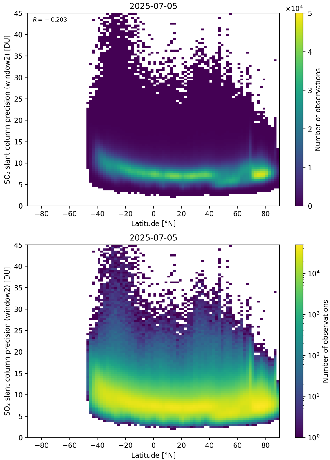
Figure 164: Scatter density plot of “Latitude” against “SO 2 slant column precision (window2)” for 2025-07-04 to 2025-07-06.
