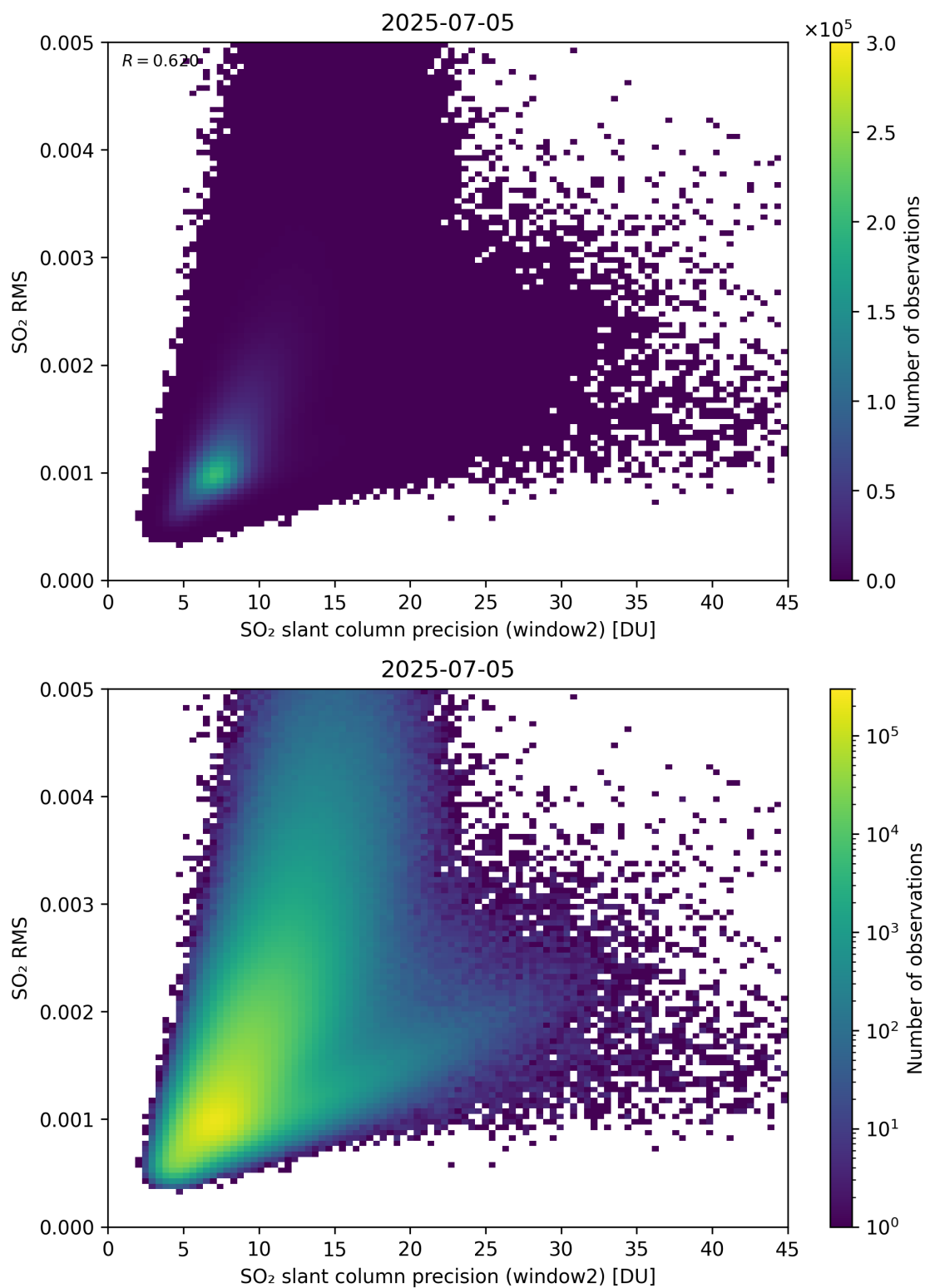
Figure 295: Scatter density plot of “SO 2 slant column precision (window2)” against “SO 2 RMS” for 2025-07-04 to 2025-07-06.
