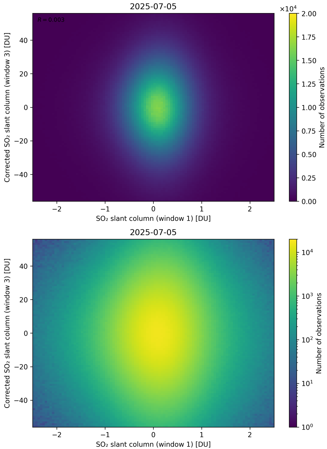
Figure 284: Scatter density plot of “SO 2 slant column (window 1)” against “Corrected SO 2 slant column (window 3)” for 2025-07-04 to 2025-07-06.
