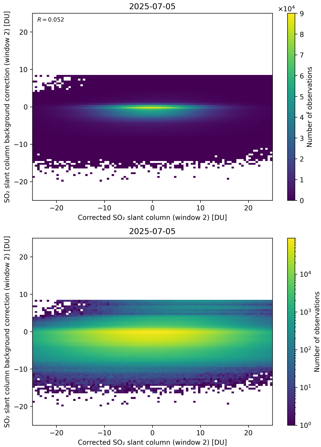
Figure 244: Scatter density plot of “Corrected SO 2 slant column (window 2)” against “SO 2 slant column background correction (window 2)” for 2025-07-04 to 2025-07-06.
