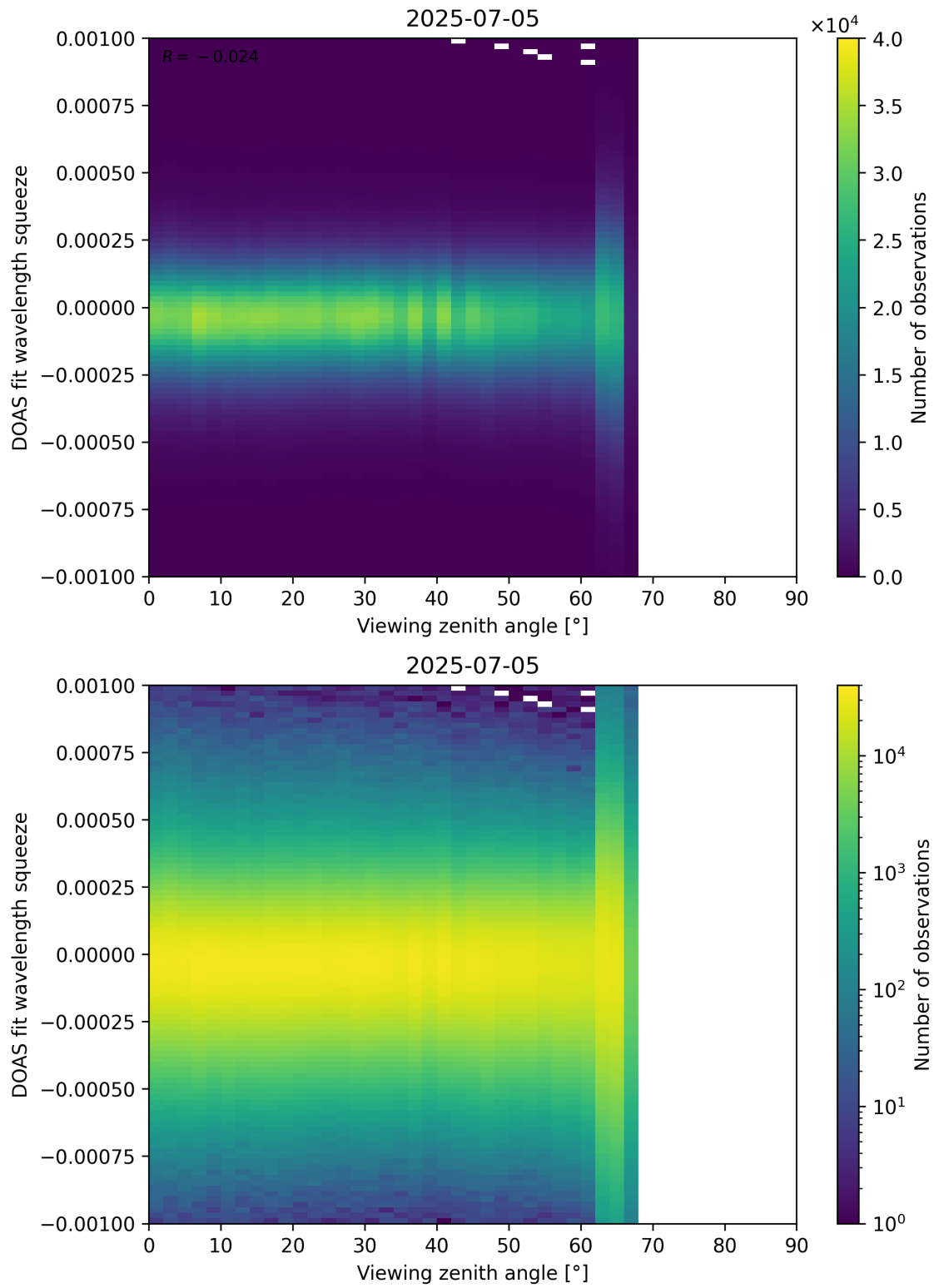
Figure 366: Scatter density plot of “Viewing zenith angle” against “DOAS fit wavelength squeeze” for 2025-07-04 to 2025-07-06.
