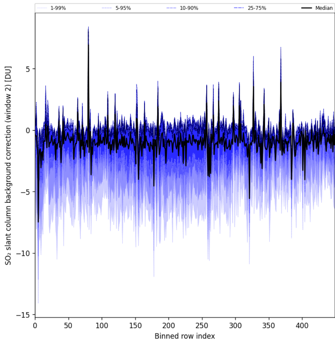
Figure 96: Along track statistics of “SO 2 slant column background correction (window 2)” for 2025-07-04 to 2025-07-06
