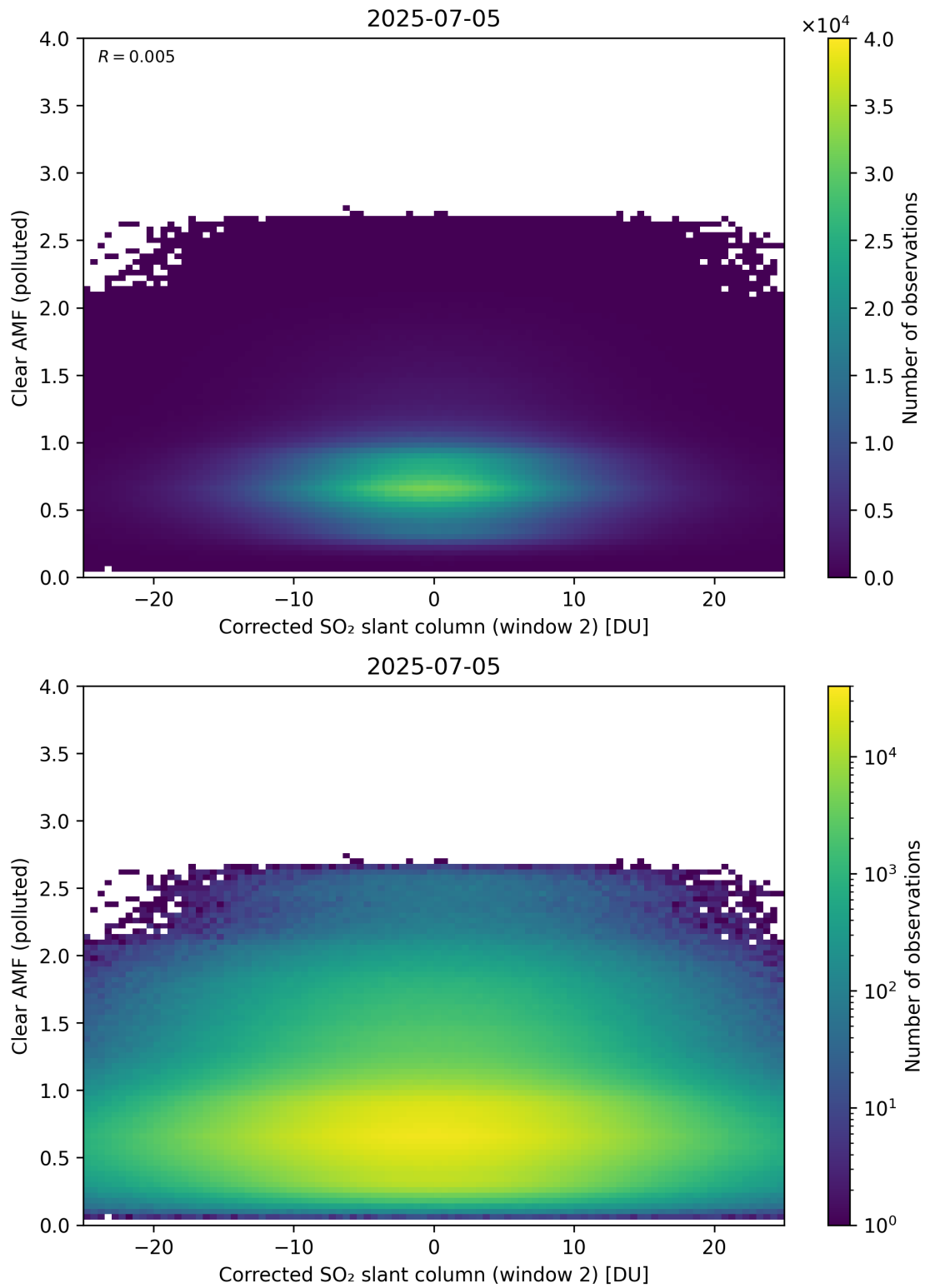
Figure 249: Scatter density plot of “Corrected SO 2 slant column (window 2)” against “Clear AMF (polluted)” for 2025-07-04 to 2025-07-06.
