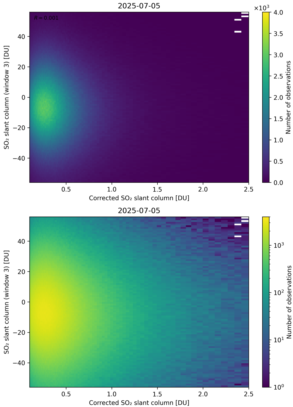
Figure 240: Scatter density plot of “Corrected SO 2 slant column” against “SO 2 slant column (window 3)” for 2025-07-04 to 2025-07-06.
