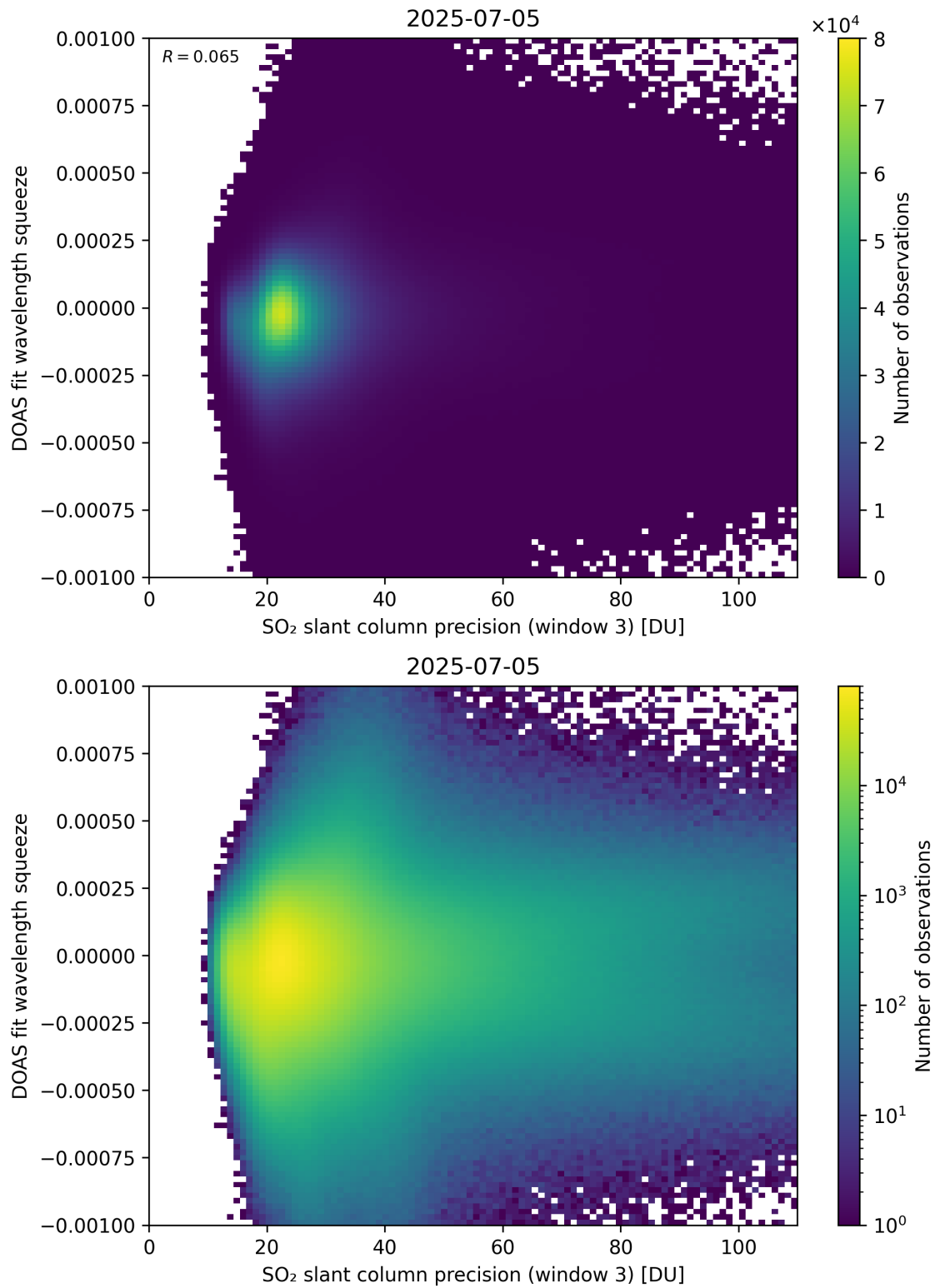
Figure 309: Scatter density plot of “SO 2 slant column precision (window 3)” against “DOAS fit wavelength squeeze” for 2025-07-04 to 2025-07-06.
