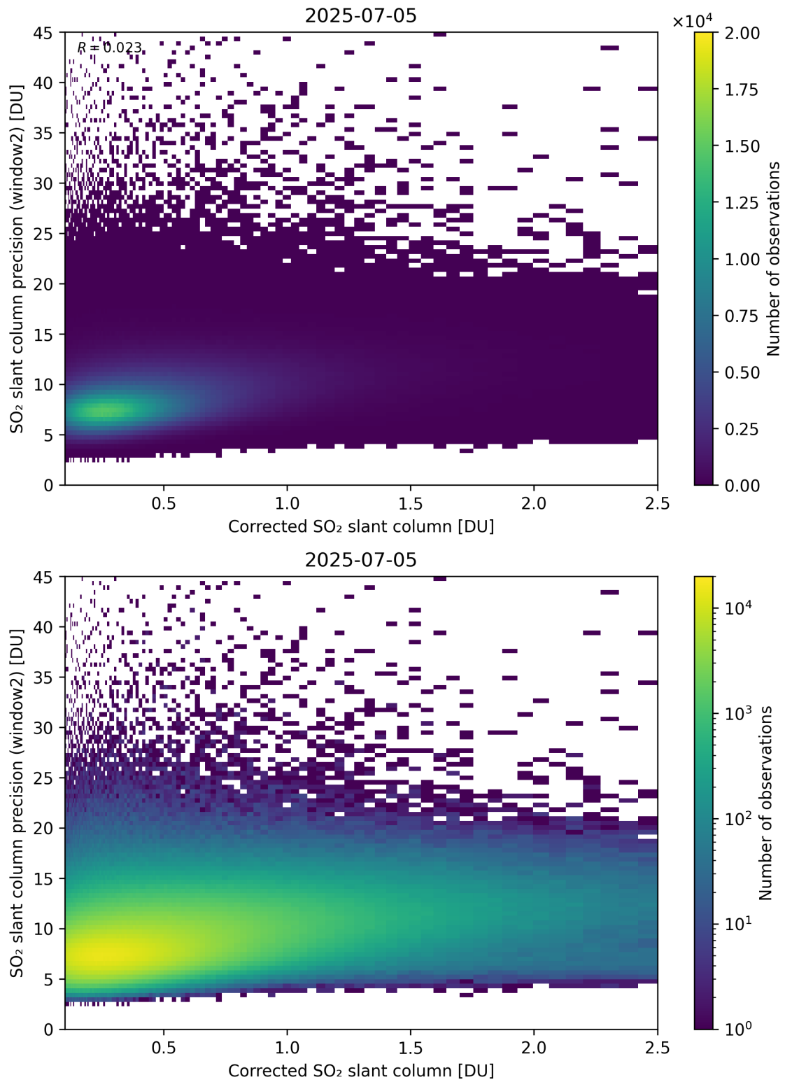
Figure 239: Scatter density plot of “Corrected SO 2 slant column” against “SO 2 slant column precision (window2)” for 2025-07-04 to 2025-07-06.
