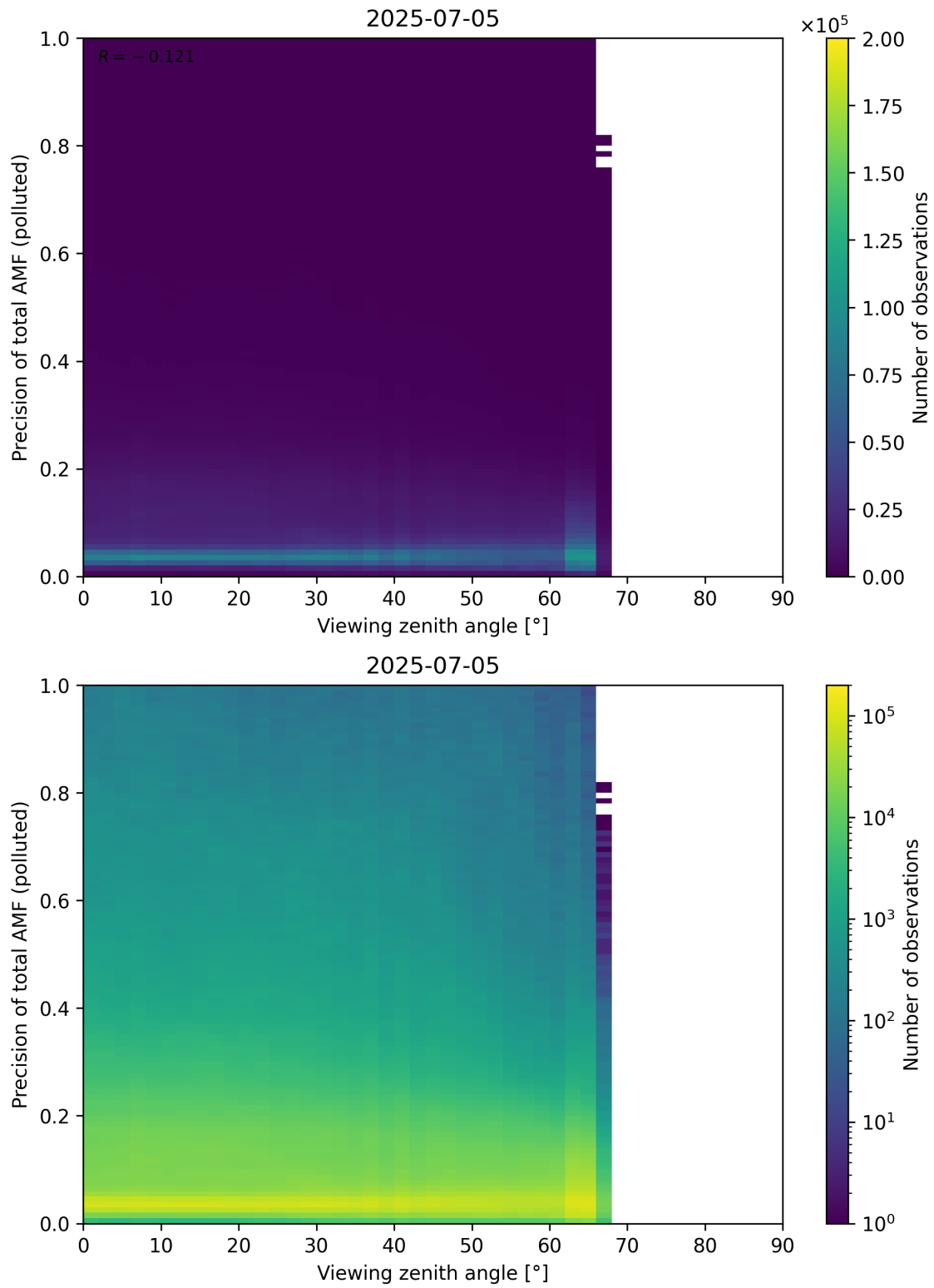
Figure 382: Scatter density plot of “Viewing zenith angle” against “Precision of total AMF (polluted)” for 2025-07-04 to 2025-07-06.
