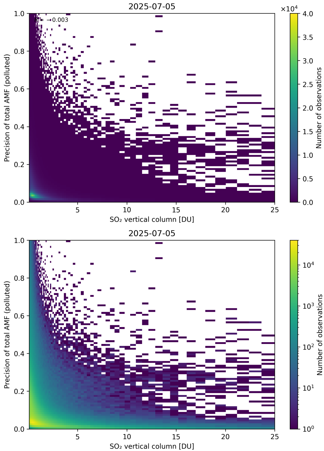
Figure 360: Scatter density plot of “SO 2 vertical column” against “Precision of total AMF (polluted)” for 2025-07-04 to 2025-07-06.
