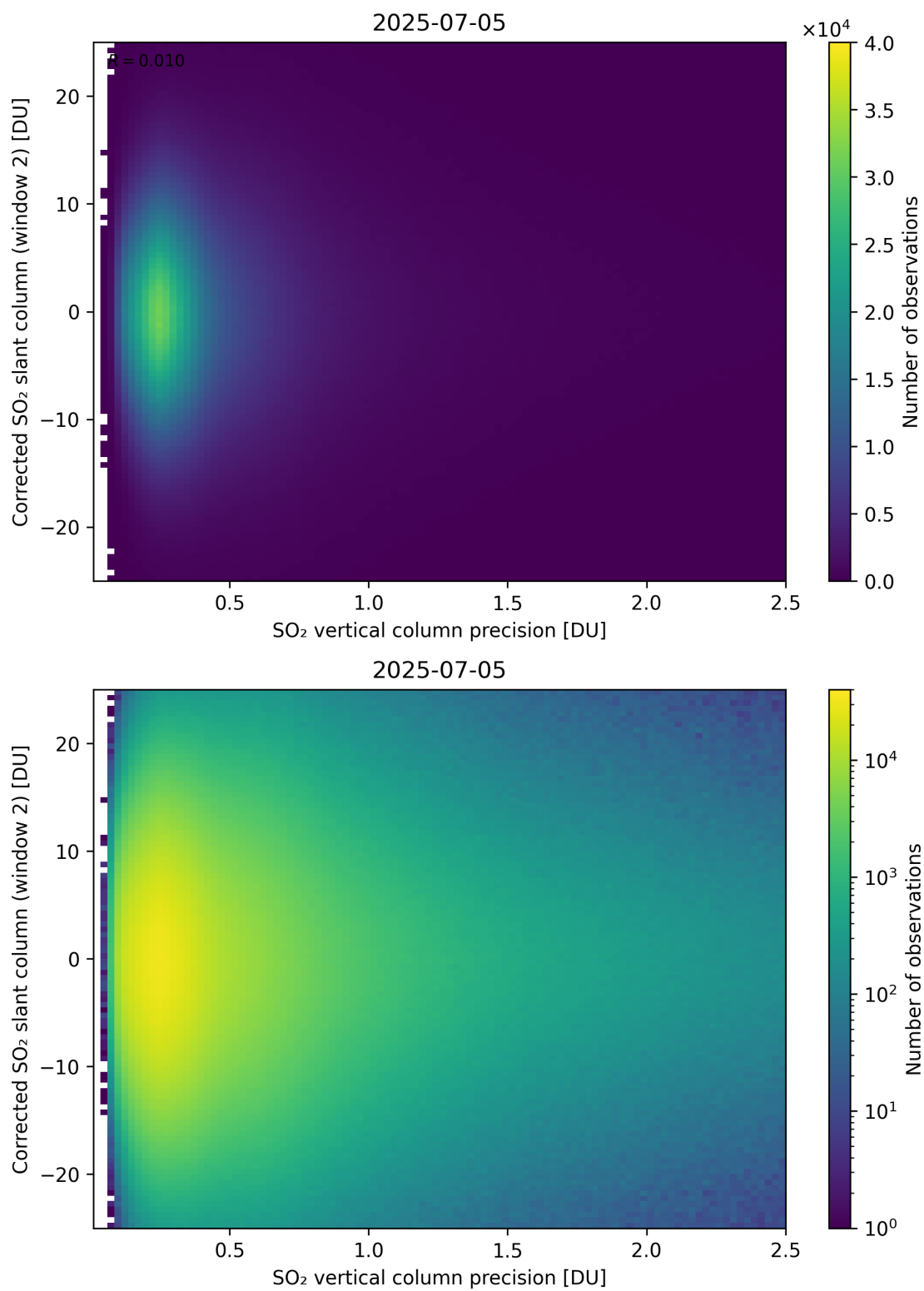
Figure 339: Scatter density plot of “SO 2 vertical column precision” against “Corrected SO 2 slant column (window 2)” for 2025-07-04 to 2025-07-06.
