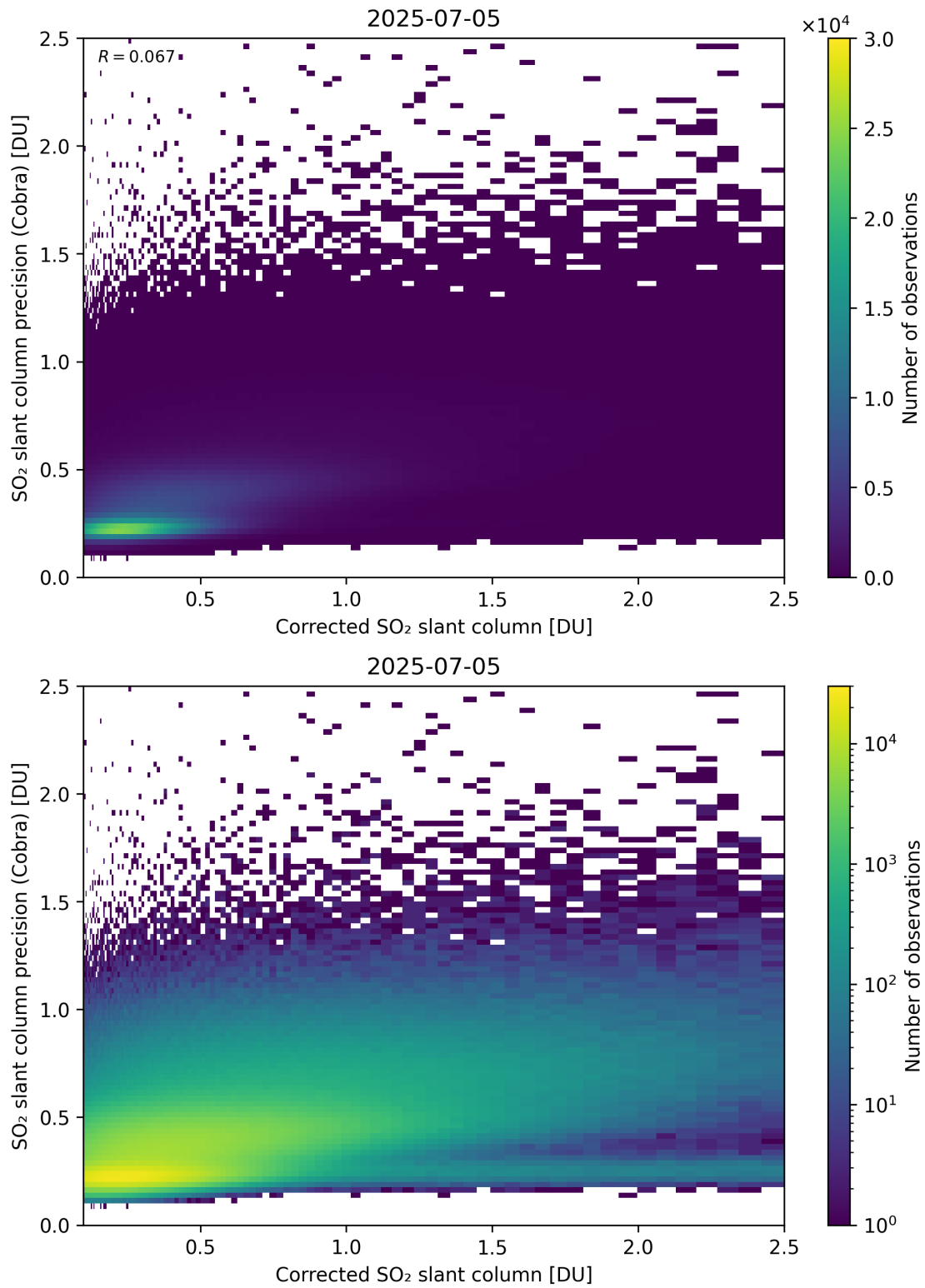
Figure 234: Scatter density plot of “Corrected SO 2 slant column” against “SO 2 slant column precision (Cobra)” for 2025-07-04 to 2025-07-06.
