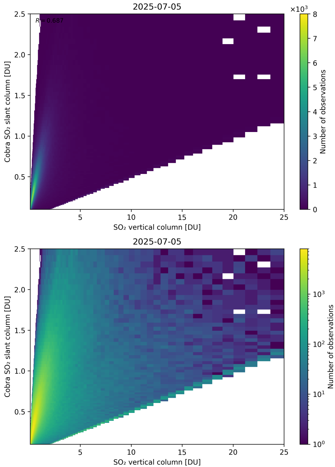
Figure 349: Scatter density plot of “SO 2 vertical column” against “Cobra SO 2 slant column” for 2025-07-04 to 2025-07-06.
