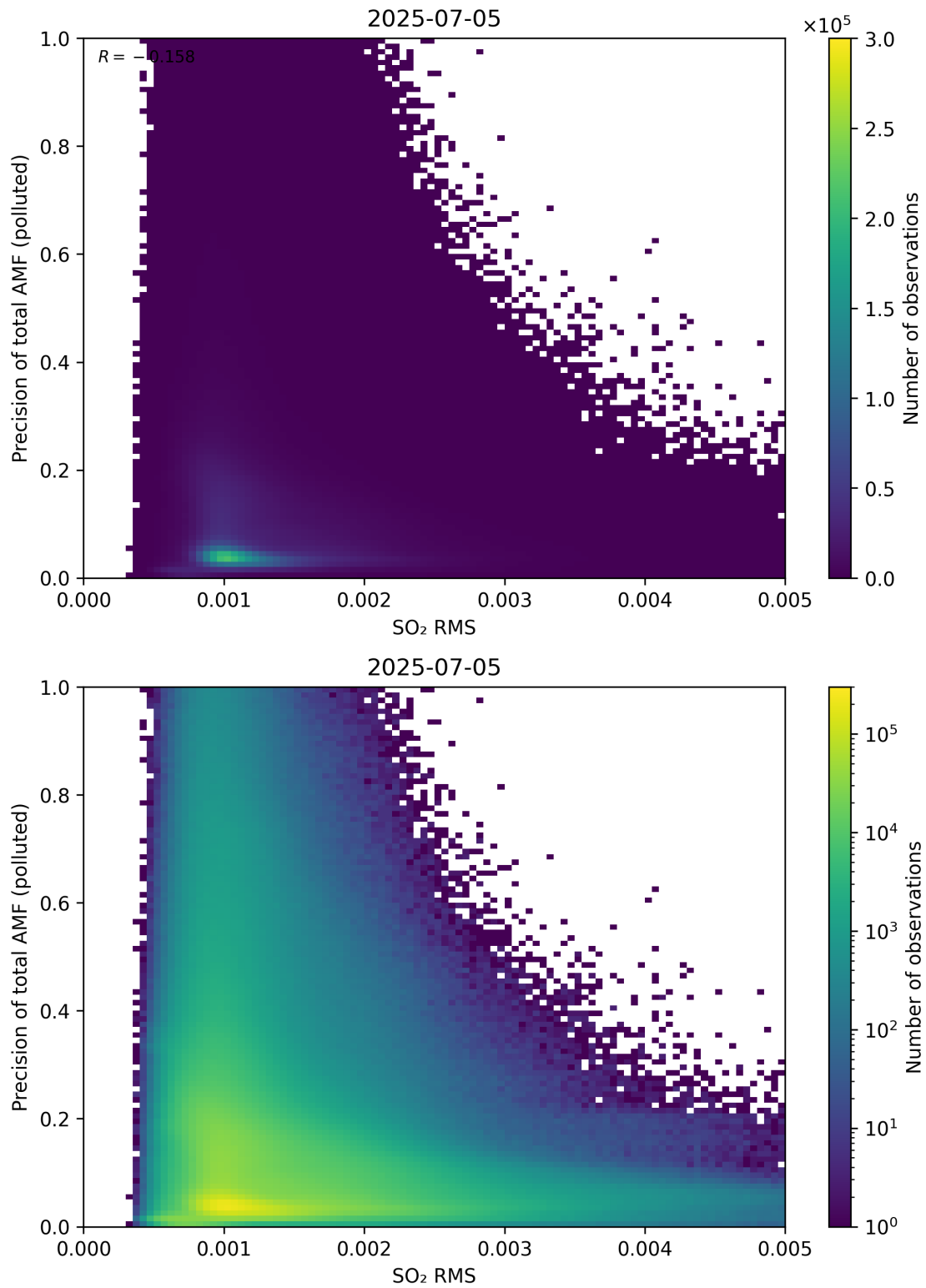
Figure 149: Scatter density plot of “SO 2 RMS” against “Precision of total AMF (polluted)” for 2025-07-04 to 2025-07-06.
