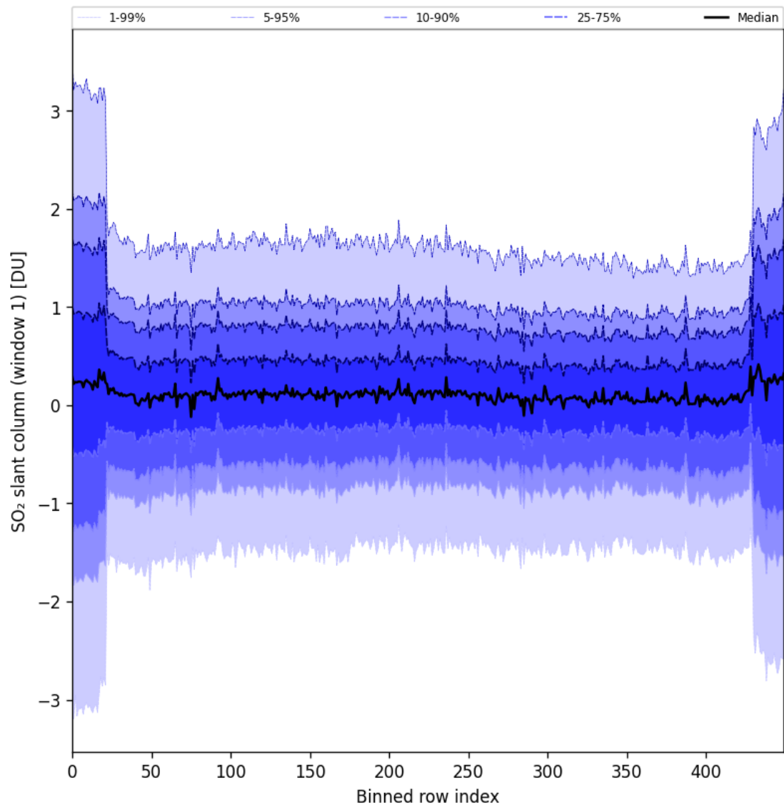
Figure 89: Along track statistics of “SO 2 slant column (window 1)” for 2025-07-04 to 2025-07-06
