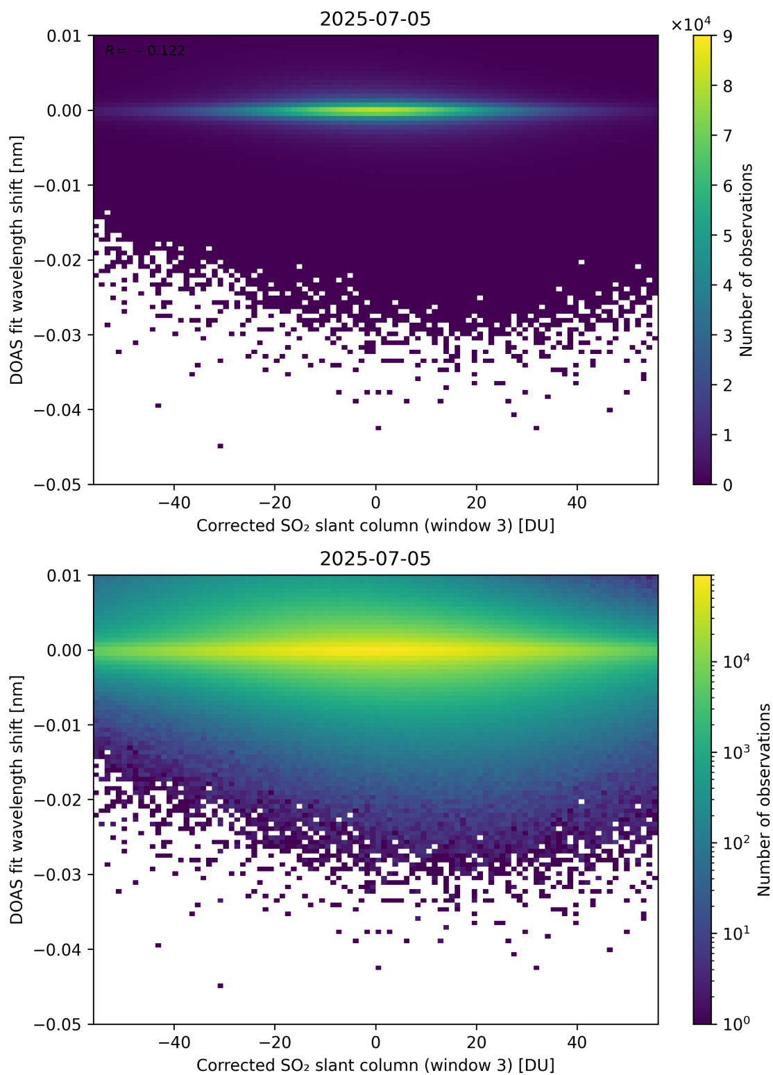
Figure 256: Scatter density plot of “Corrected SO 2 slant column (window 3)” against “DOAS fit wavelength shift” for 2025-07-04 to 2025-07-06.
