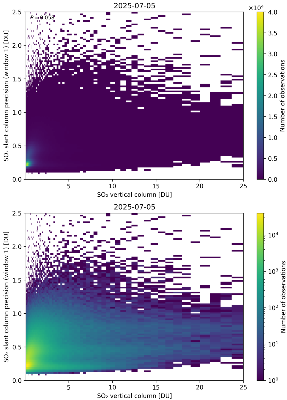
Figure 355: Scatter density plot of “SO 2 vertical column” against “SO 2 slant column precision (window 1)” for 2025-07-04 to 2025-07-06.
