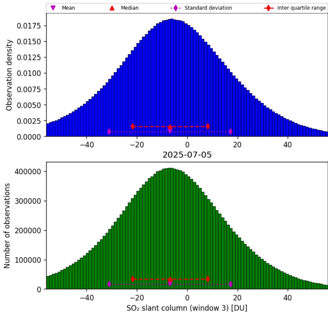
Figure 71: Histogram of “SO 2 slant column (window 3)” for 2025-07-04 to 2025-07-06
