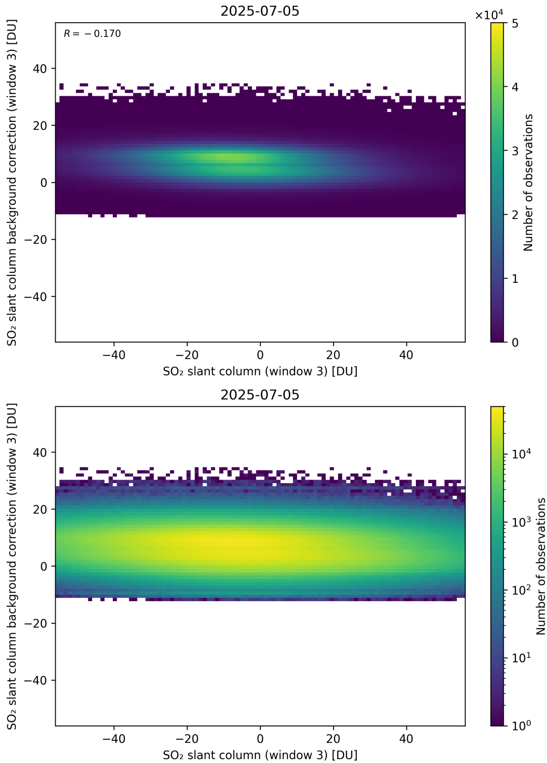
Figure 303: Scatter density plot of “SO 2 slant column (window 3)” against “SO 2 slant column background correction (window 3)” for 2025-07-04 to 2025-07-06.
