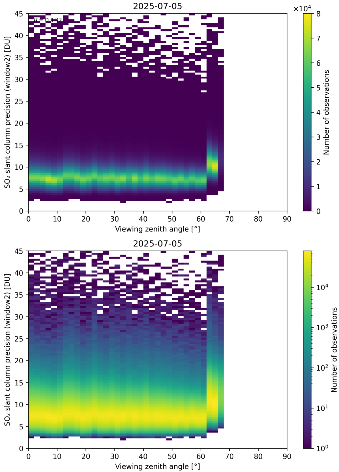
Figure 378: Scatter density plot of “Viewing zenith angle” against “SO 2 slant column precision (window2)” for 2025-07-04 to 2025-07-06.
