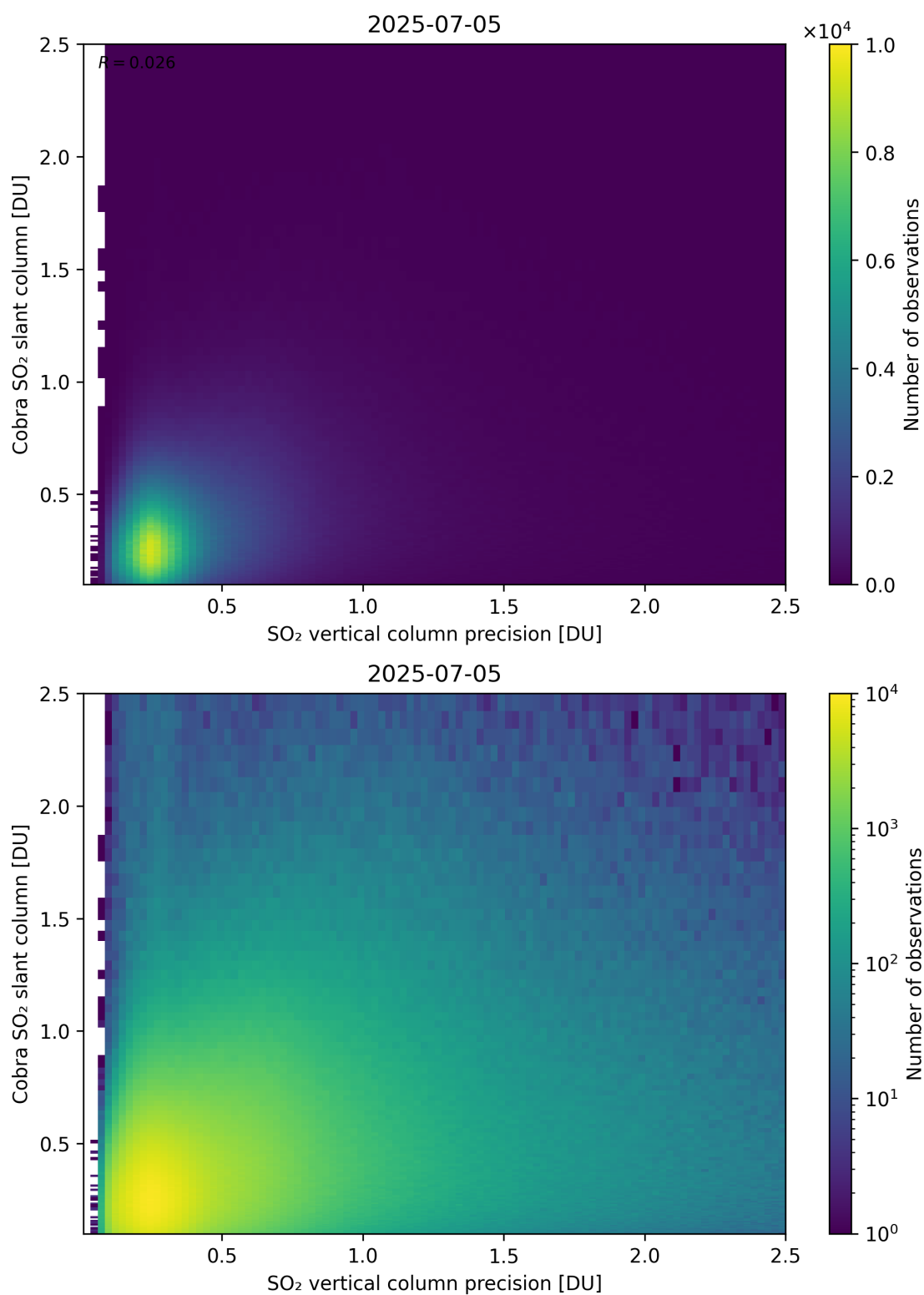
Figure 336: Scatter density plot of “SO 2 vertical column precision” against “Cobra SO 2 slant column” for 2025-07-04 to 2025-07-06.
