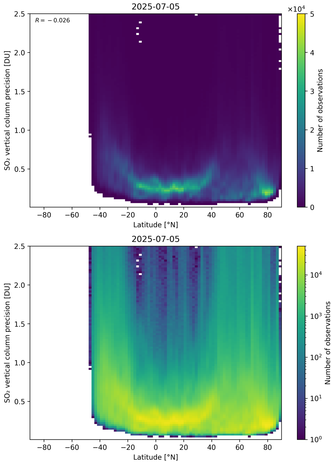
Figure 170: Scatter density plot of “Latitude” against “SO 2 vertical column precision” for 2025-07-04 to 2025-07-06.
