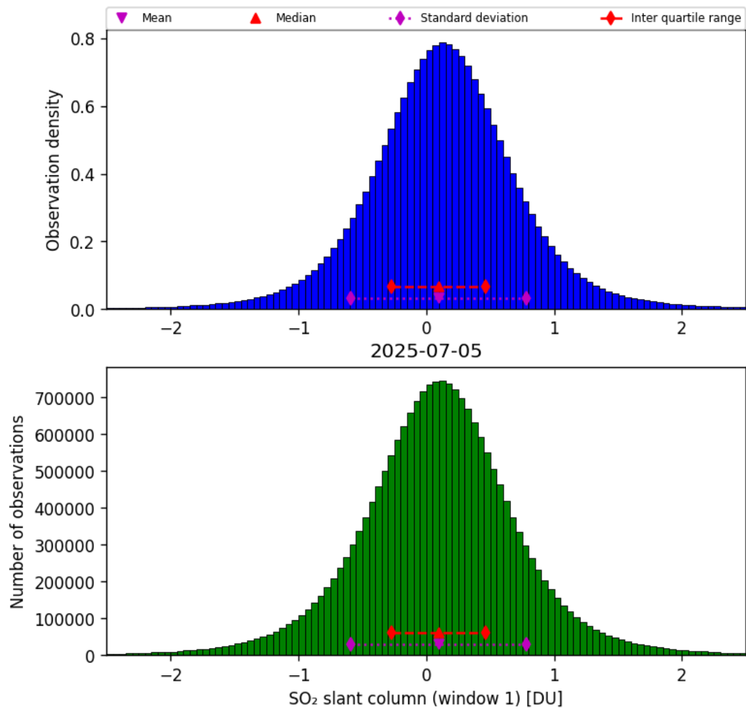
Figure 63: Histogram of “SO 2 slant column (window 1)” for 2025-07-04 to 2025-07-06
