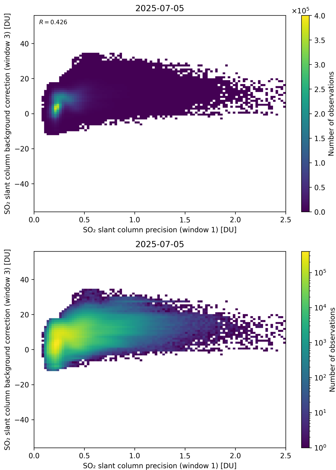
Figure 270: Scatter density plot of “SO 2 slant column precision (window 1)” against “SO 2 slant column background correction (window 3)” for 2025-07-04 to 2025-07-06.
