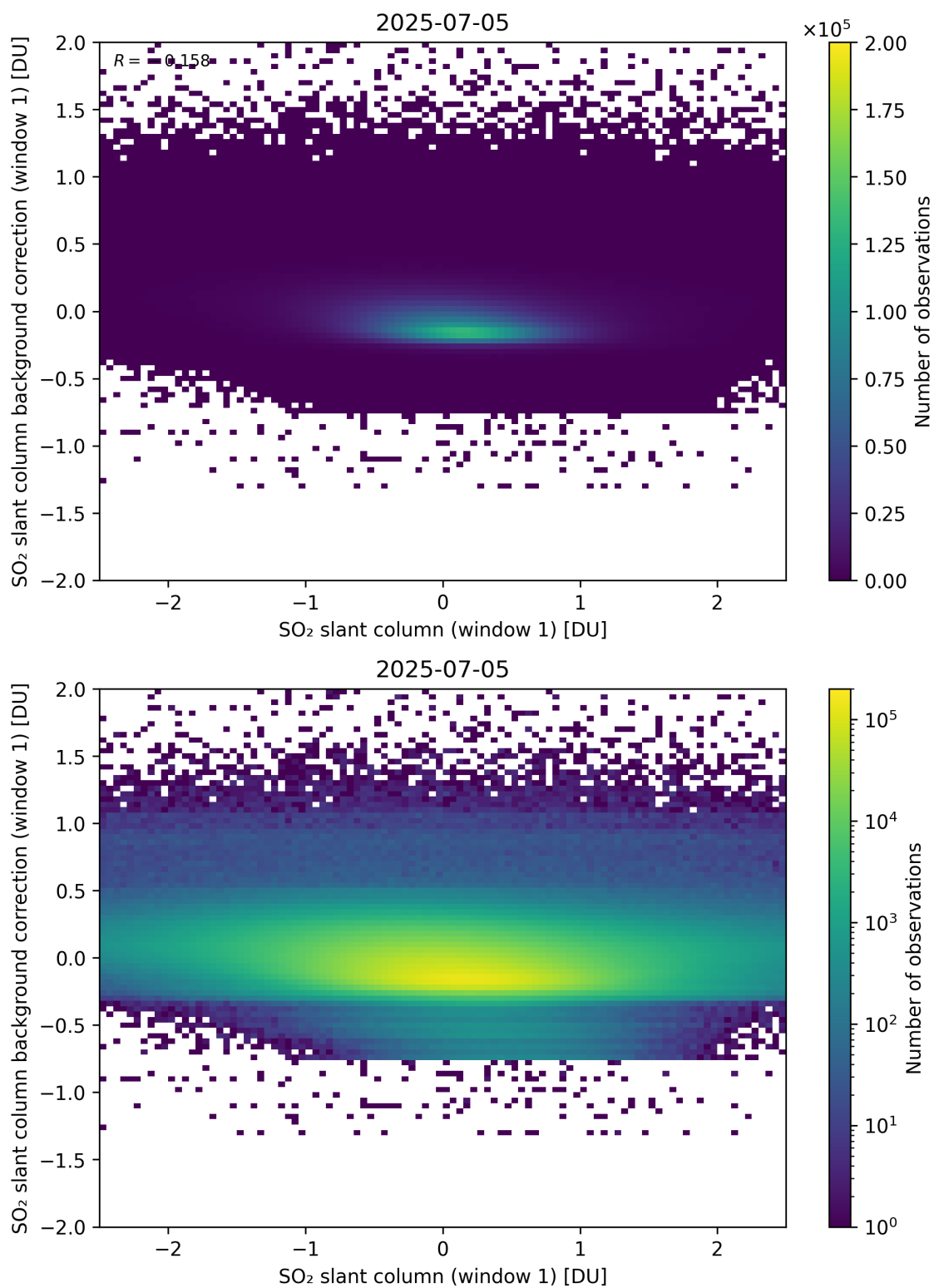
Figure 262: Scatter density plot of “SO 2 slant column (window 1)” against “SO 2 slant column background correction (window 1)” for 2025-07-04 to 2025-07-06.
