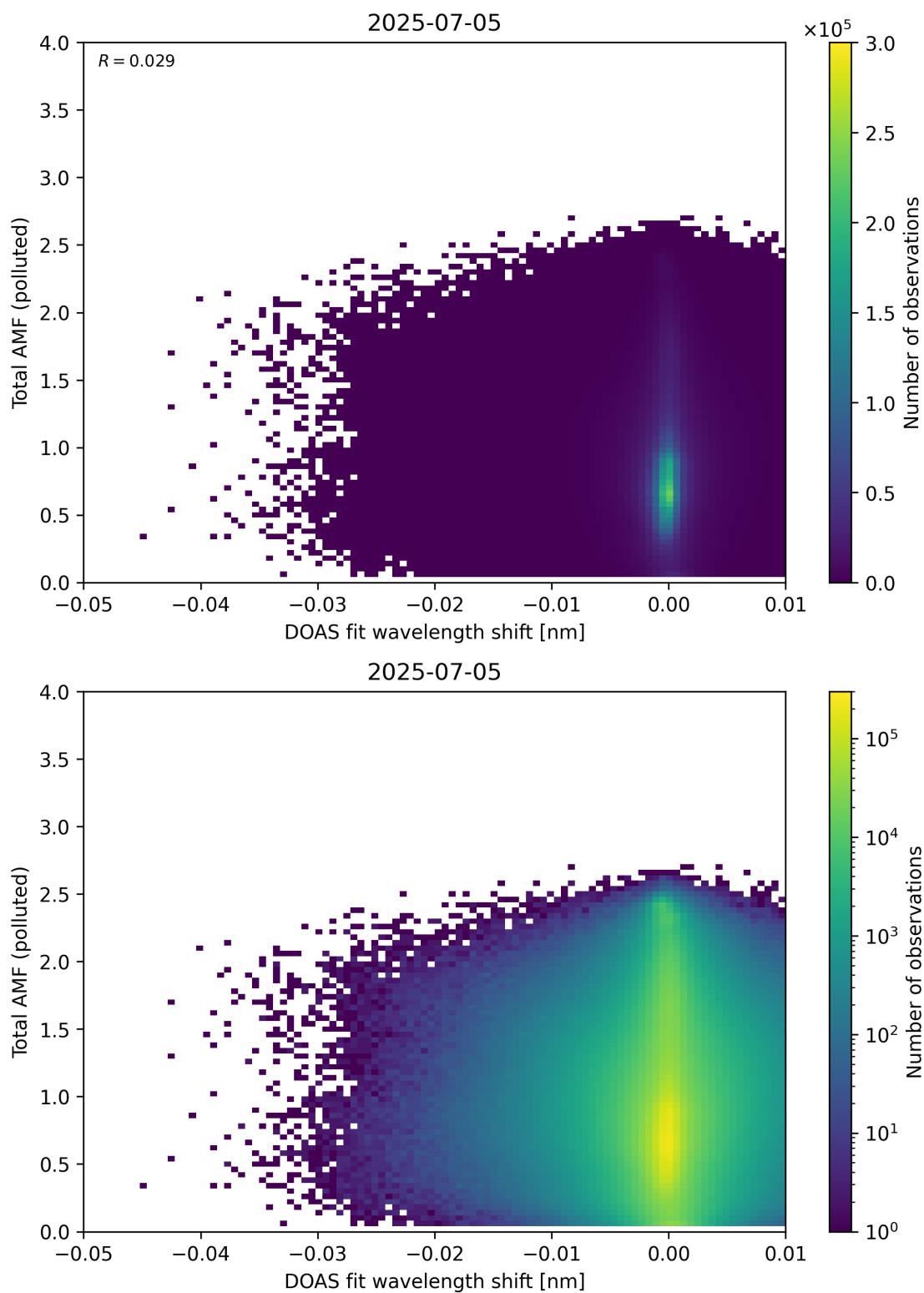
Figure 141: Scatter density plot of “DOAS fit wavelength shift” against “Total AMF (polluted)” for 2025-07-04 to 2025-07-06.
