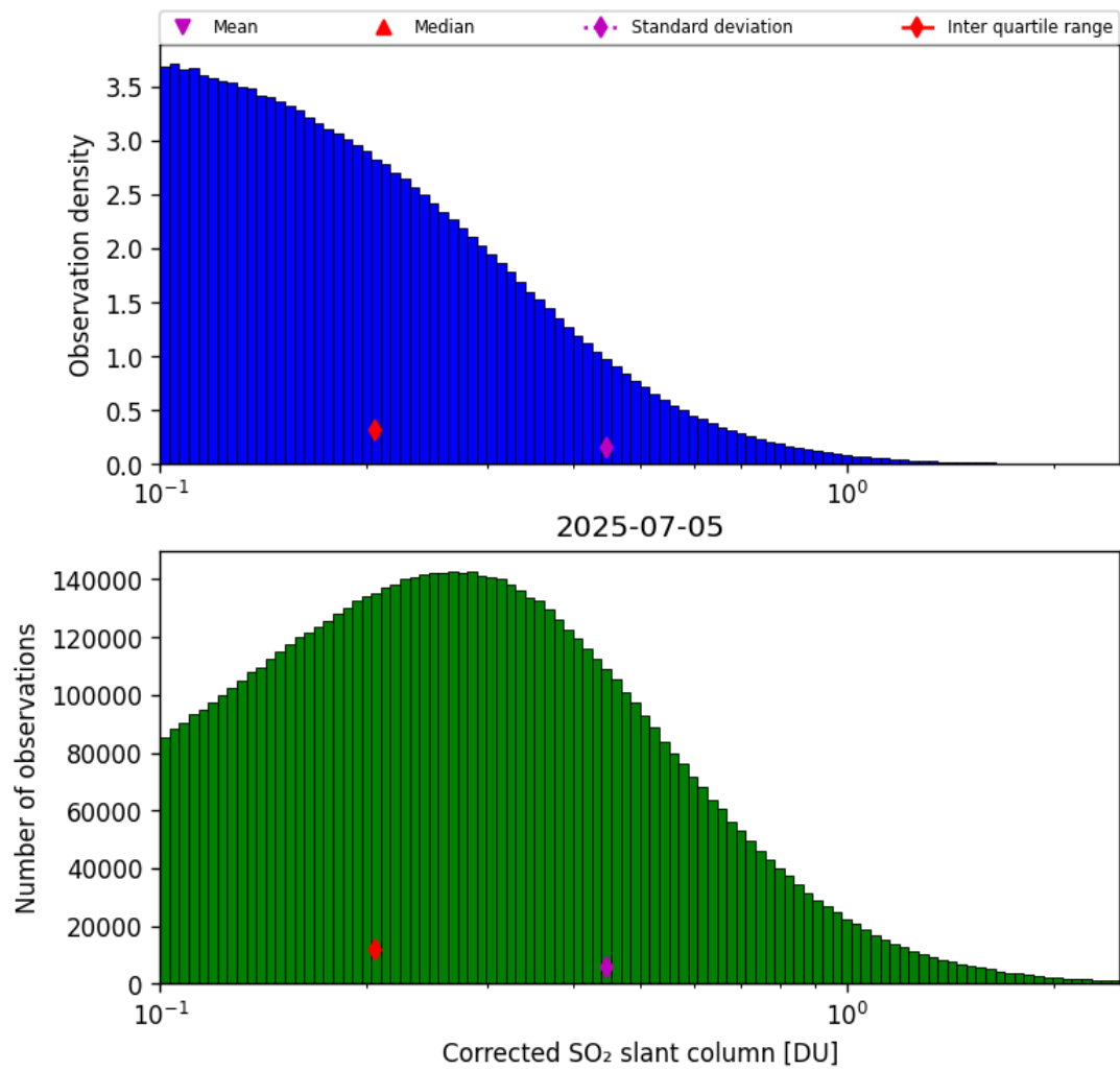
Figure 60: Histogram of “Corrected SO 2 slant column” for 2025-07-04 to 2025-07-06
