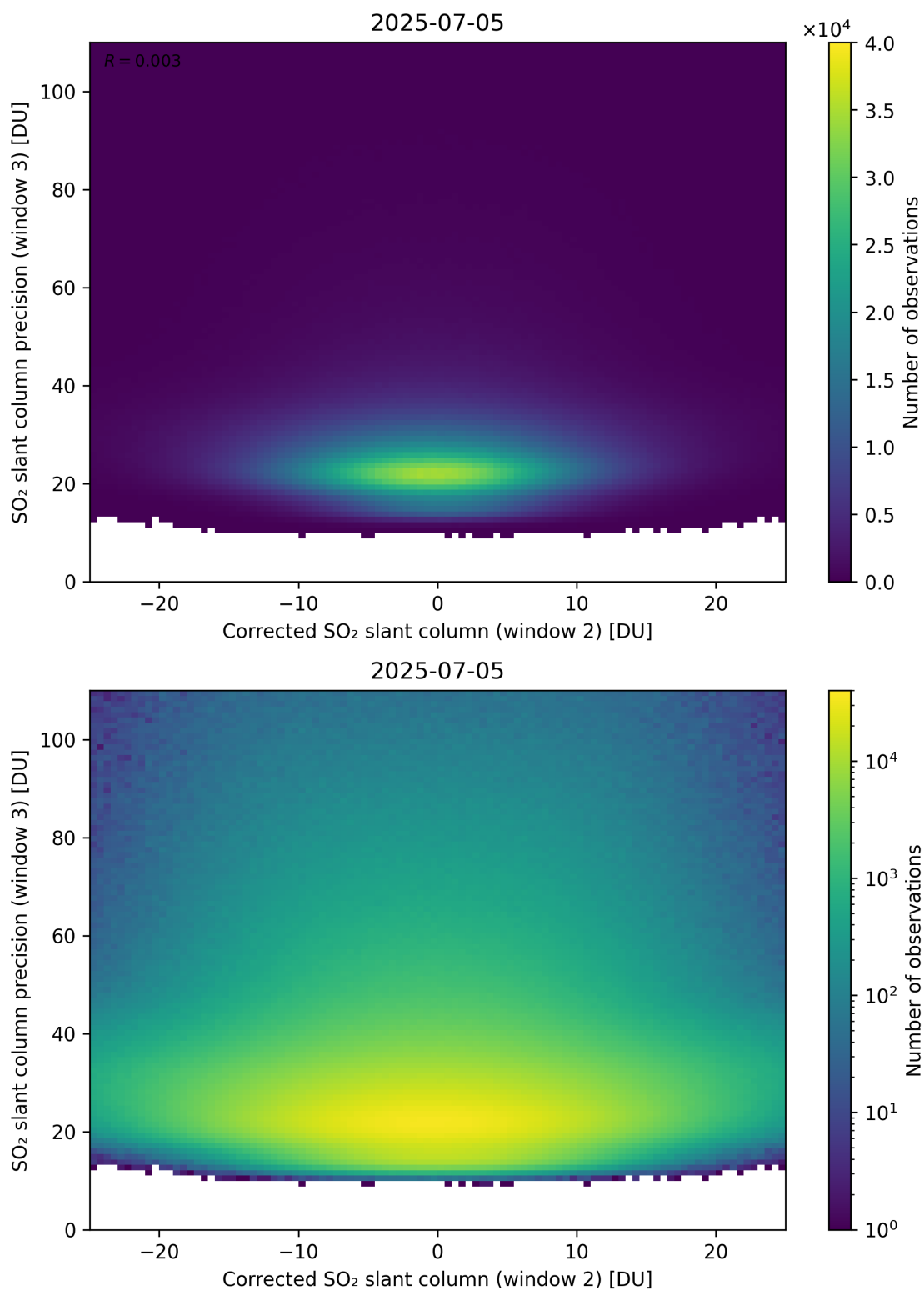
Figure 252: Scatter density plot of “Corrected SO 2 slant column (window 2)” against “SO 2 slant column precision (window 3)” for 2025-07-04 to 2025-07-06.
