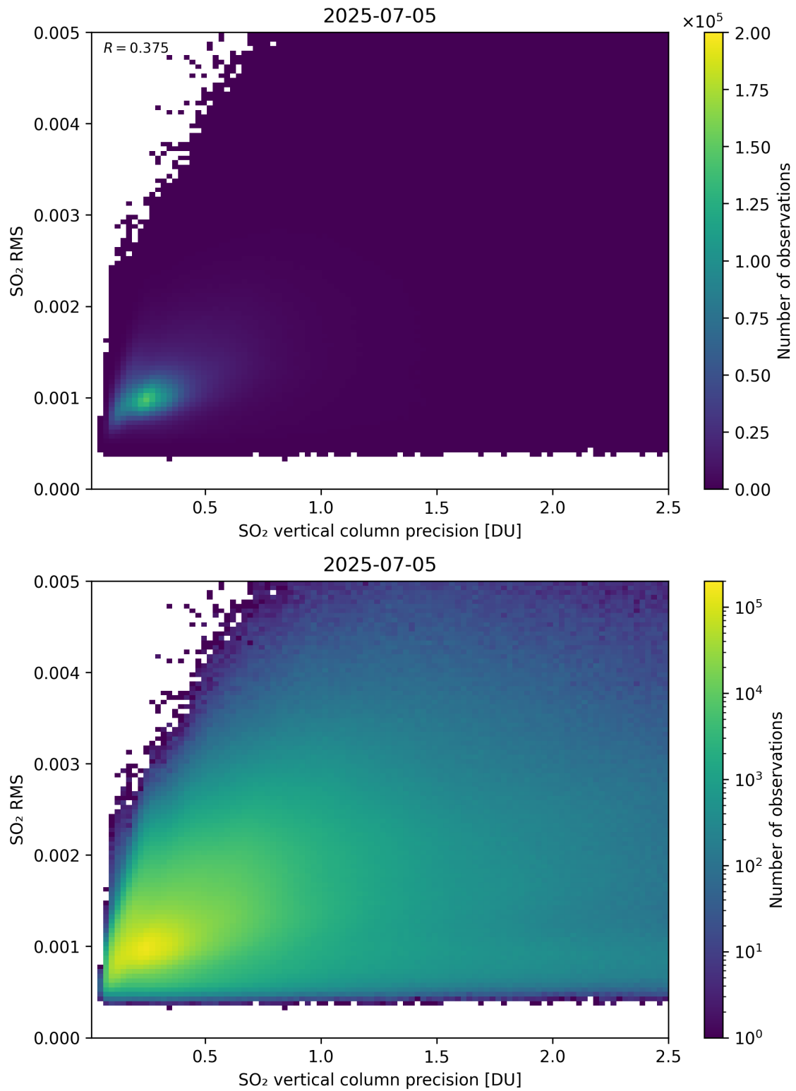
Figure 334: Scatter density plot of “SO 2 vertical column precision” against “SO 2 RMS” for 2025-07-04 to 2025-07-06.
