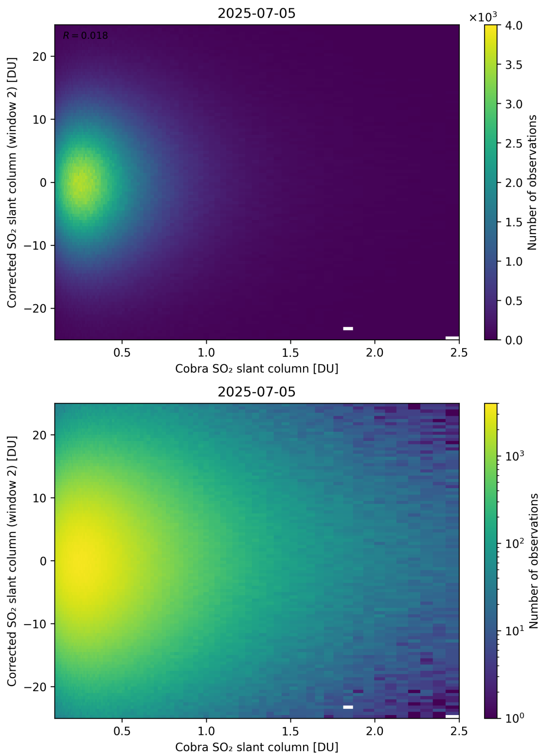
Figure 217: Scatter density plot of “Cobra SO 2 slant column” against “Corrected SO 2 slant column (window 2)” for 2025-07-04 to 2025-07-06.
