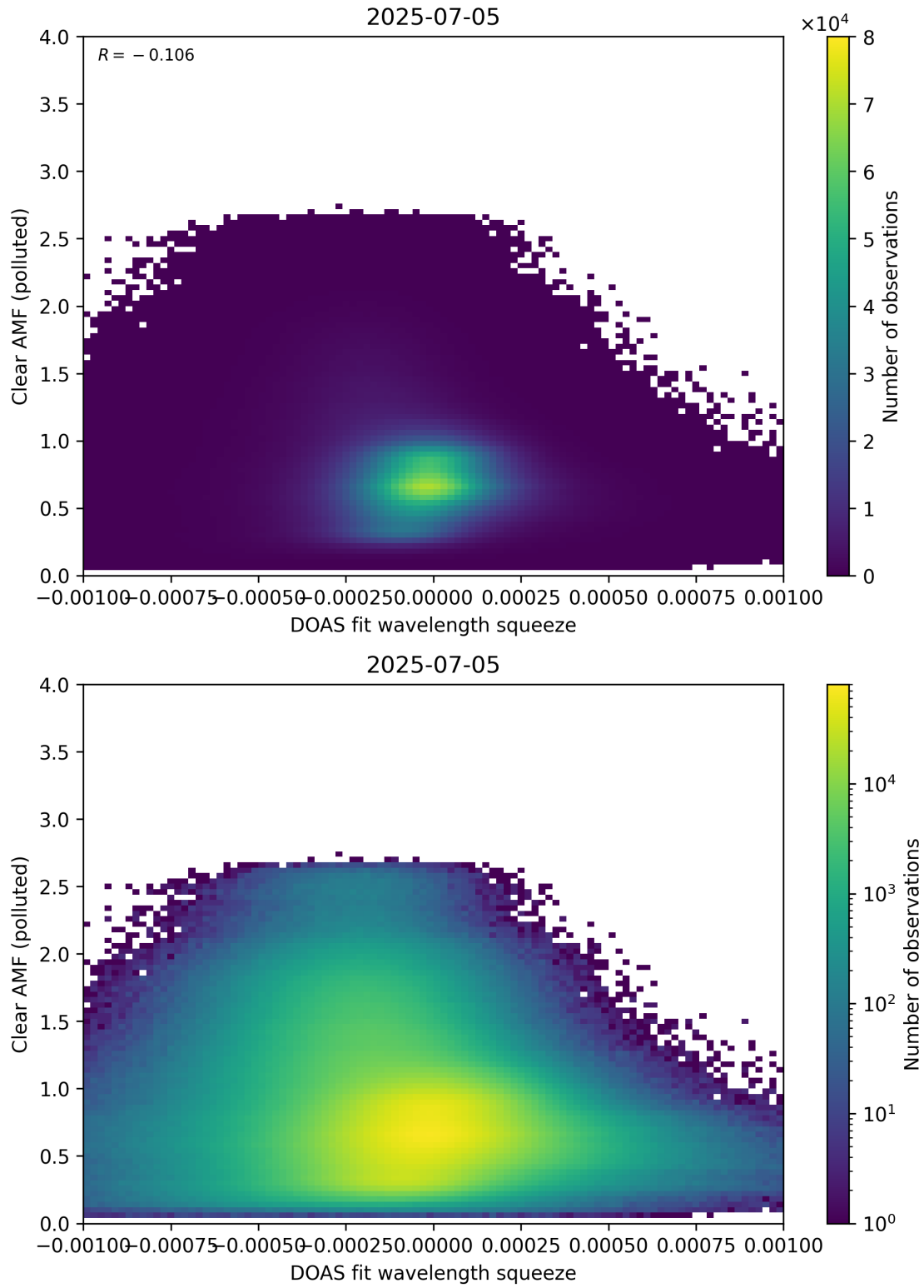
Figure 144: Scatter density plot of “DOAS fit wavelength squeeze” against “Clear AMF (polluted)” for 2025-07-04 to 2025-07-06.
