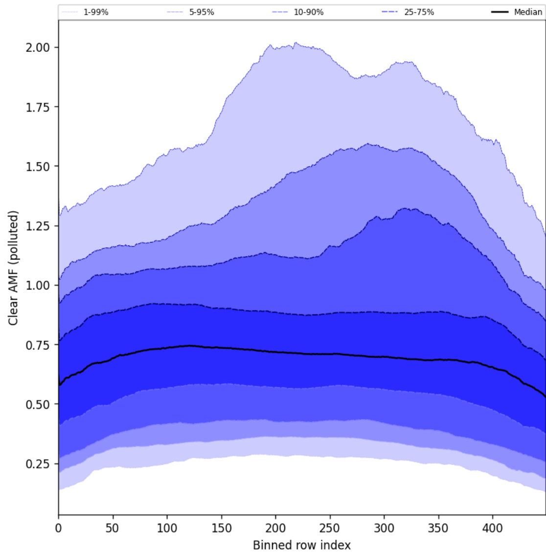
Figure 107: Along track statistics of “Clear AMF (polluted)” for 2025-07-04 to 2025-07-06
