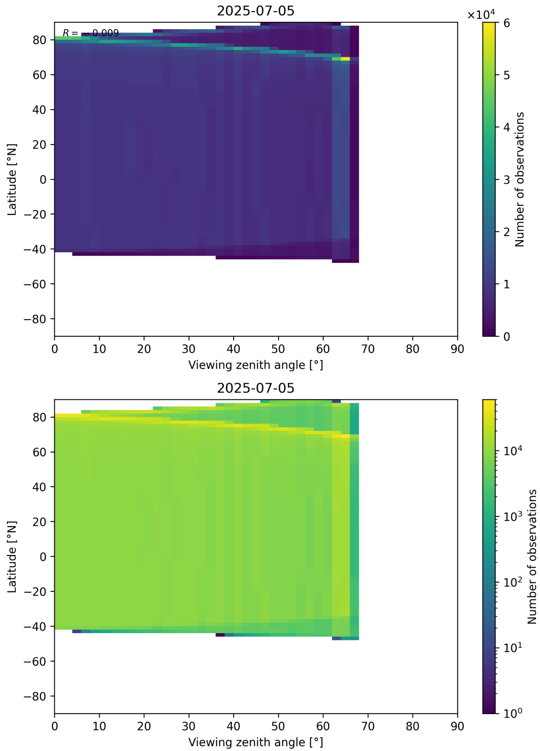
Figure 368: Scatter density plot of “Viewing zenith angle” against “Latitude” for 2025-07-04 to 2025-07-06.
