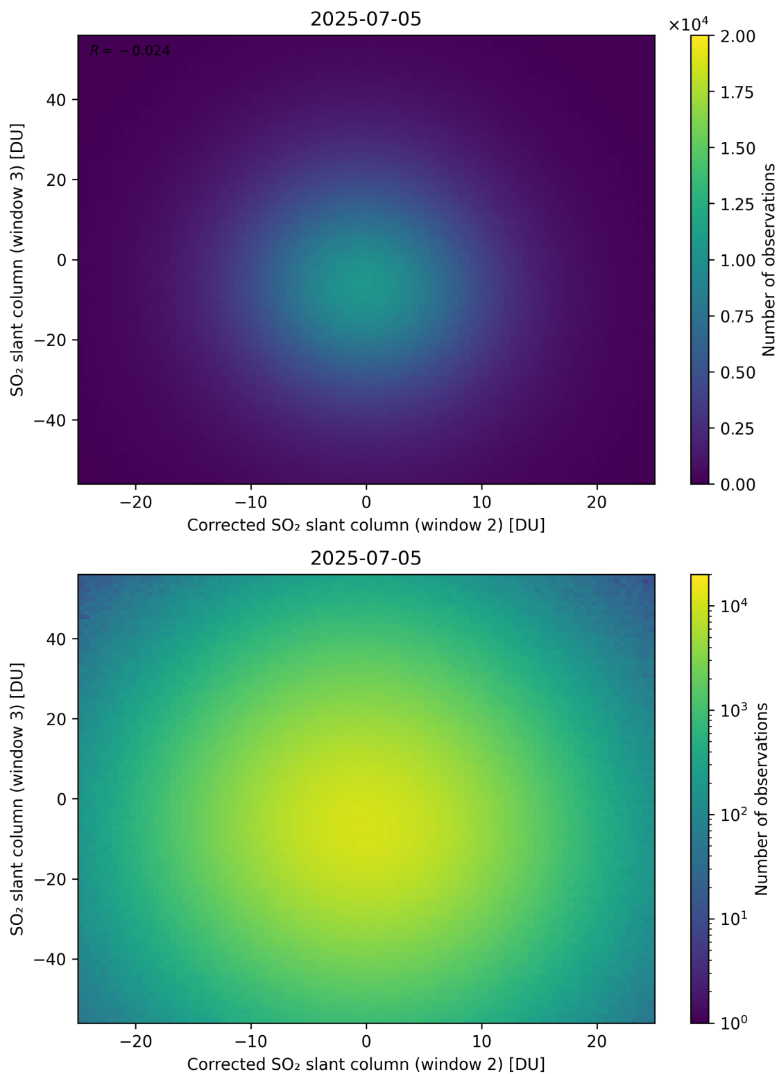
Figure 251: Scatter density plot of “Corrected SO 2 slant column (window 2)” against “SO 2 slant column (window 3)” for 2025-07-04 to 2025-07-06.
