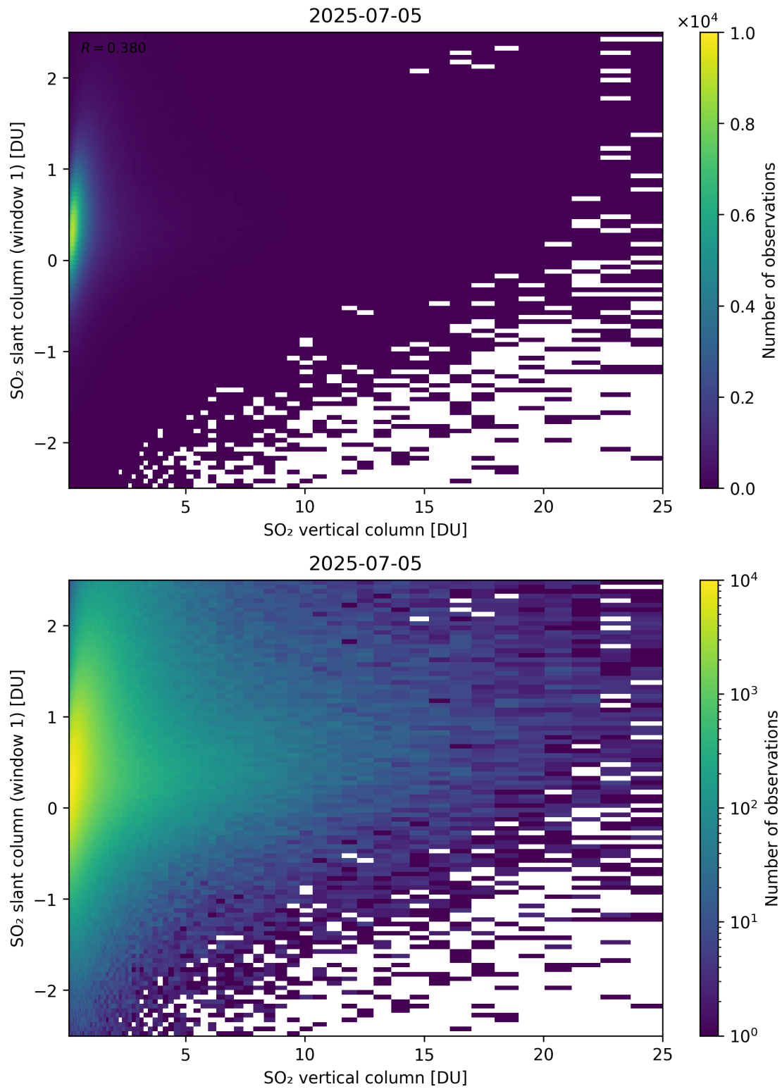
Figure 354: Scatter density plot of “SO 2 vertical column” against “SO 2 slant column (window 1)” for 2025-07-04 to 2025-07-06.
