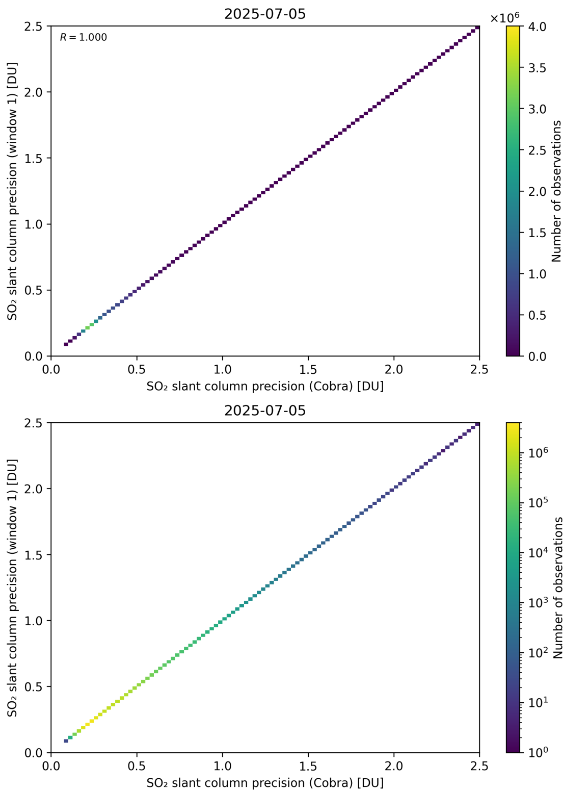
Figure 209: Scatter density plot of “SO 2 slant column precision (Cobra)” against “SO 2 slant column precision (window 1)” for 2025-07-04 to 2025-07-06.
