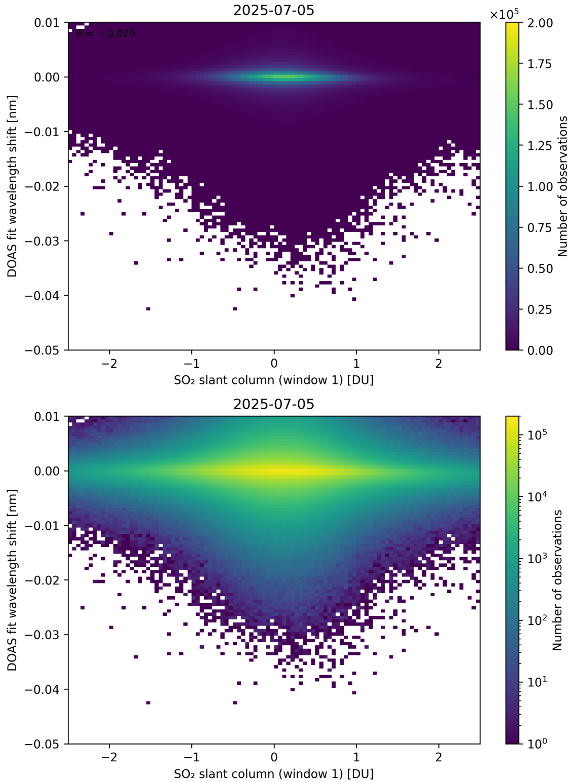
Figure 265: Scatter density plot of “SO 2 slant column (window 1)” against “DOAS fit wavelength shift” for 2025-07-04 to 2025-07-06.
