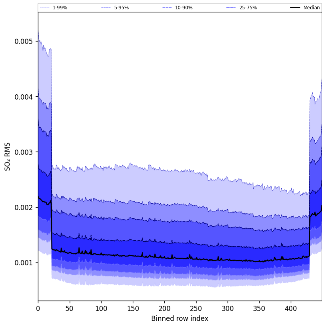
Figure 104: Along track statistics of “SO 2 RMS” for 2025-07-04 to 2025-07-06
