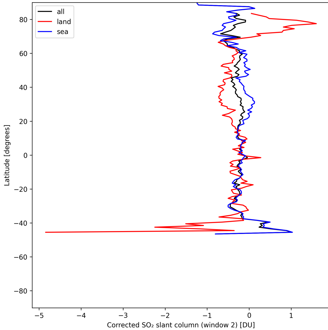
Figure 43: Zonal average of “Corrected SO 2 slant column (window 2)” for 2025-07-04 to 2025-07-06.
