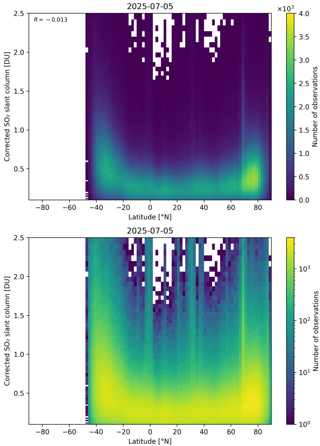
Figure 159: Scatter density plot of “Latitude” against “Corrected SO 2 slant column” for 2025-07-04 to 2025-07-06.
