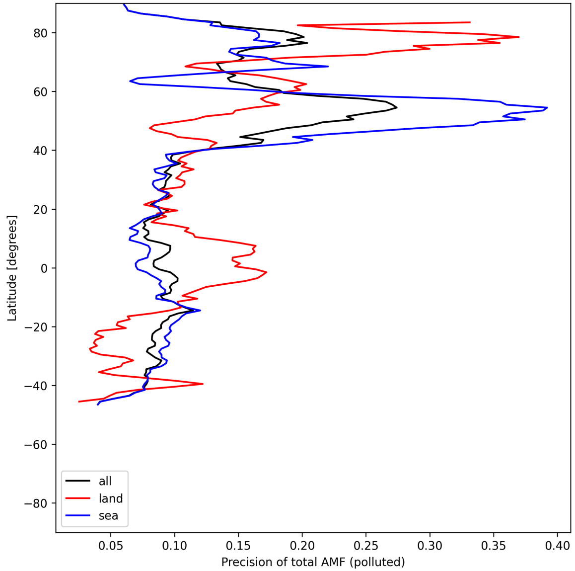
Figure 54: Zonal average of “Precision of total AMF (polluted)” for 2025-07-04 to 2025-07-06.
