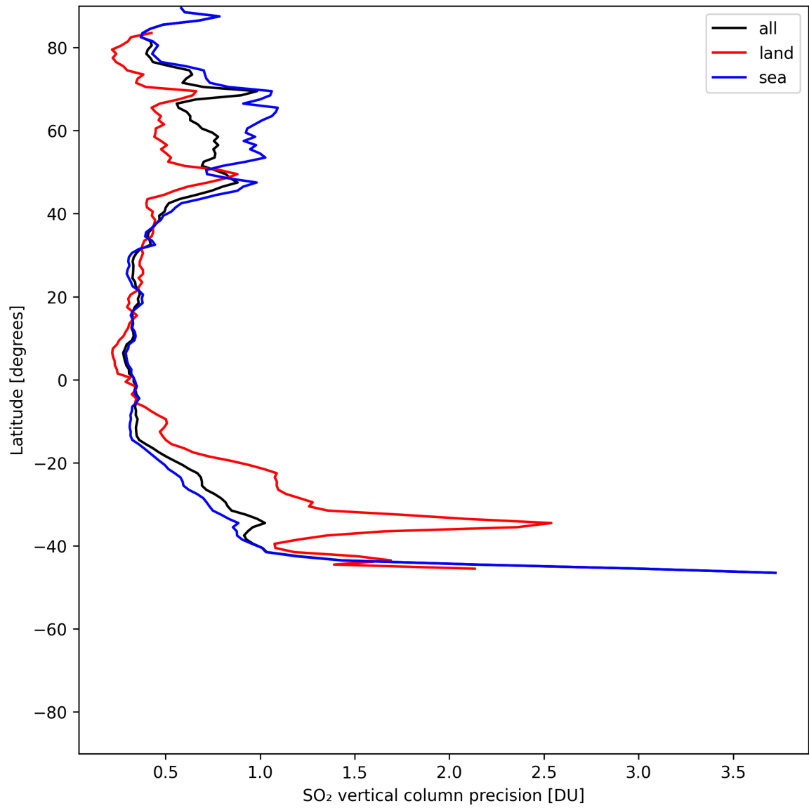
Figure 33: Zonal average of “SO 2 vertical column precision” for 2025-07-04 to 2025-07-06.
