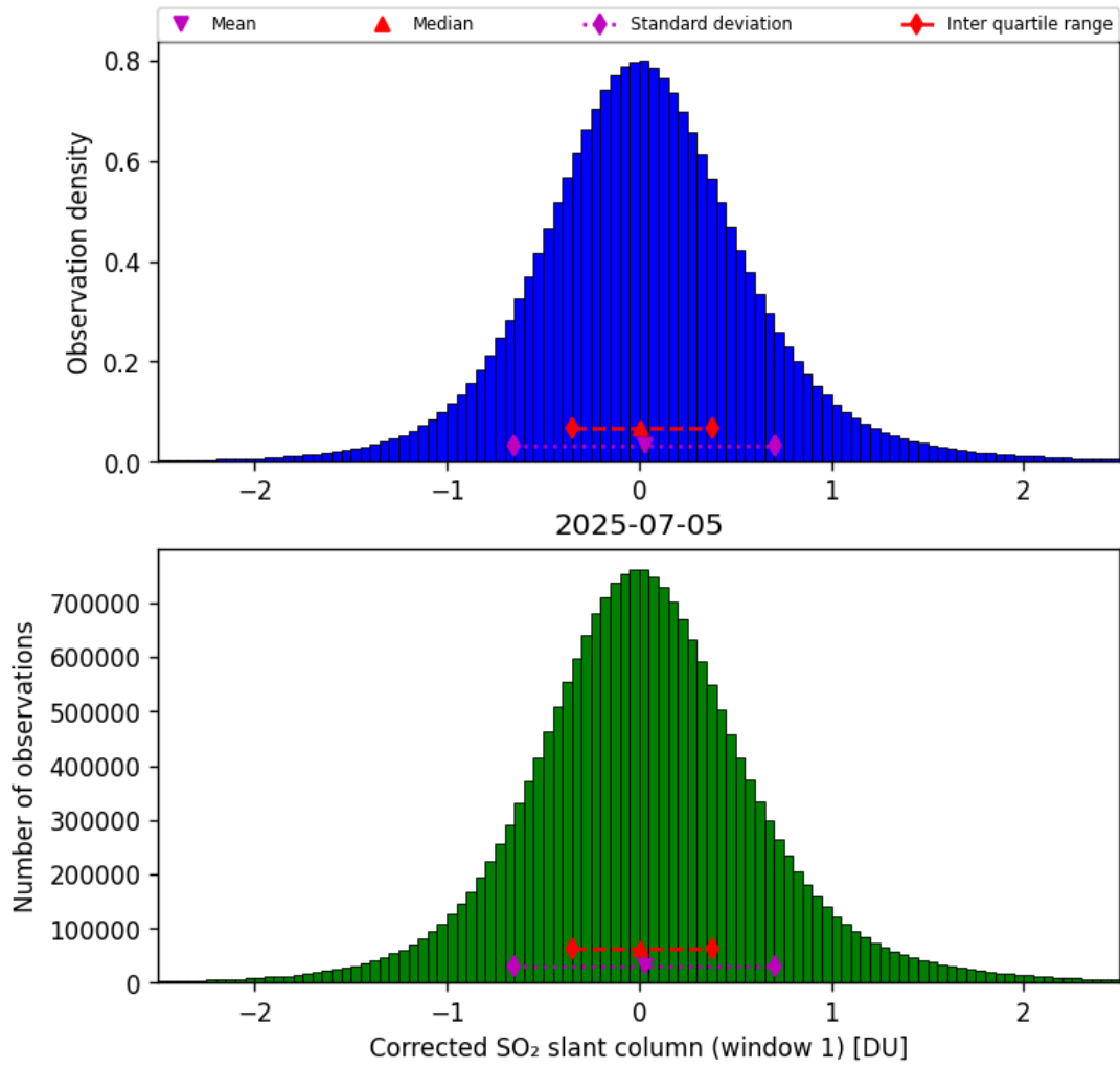
Figure 65: Histogram of “Corrected SO 2 slant column (window 1)” for 2025-07-04 to 2025-07-06
