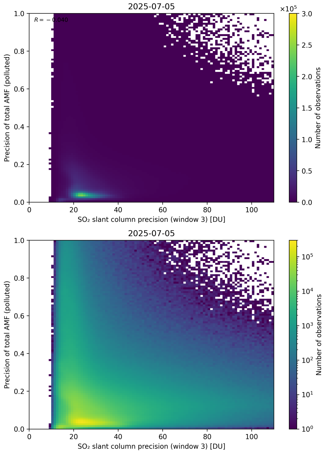
Figure 314: Scatter density plot of “SO 2 slant column precision (window 3)” against “Precision of total AMF (polluted)” for 2025-07-04 to 2025-07-06.
