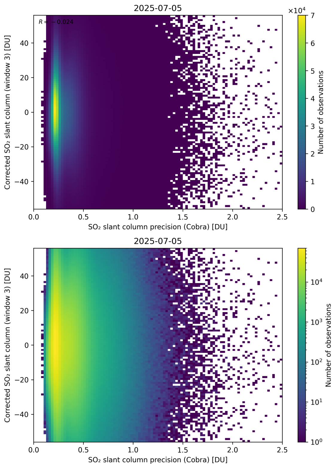
Figure 207: Scatter density plot of “SO 2 slant column precision (Cobra)” against “Corrected SO 2 slant column (window 3)” for 2025-07-04 to 2025-07-06.
