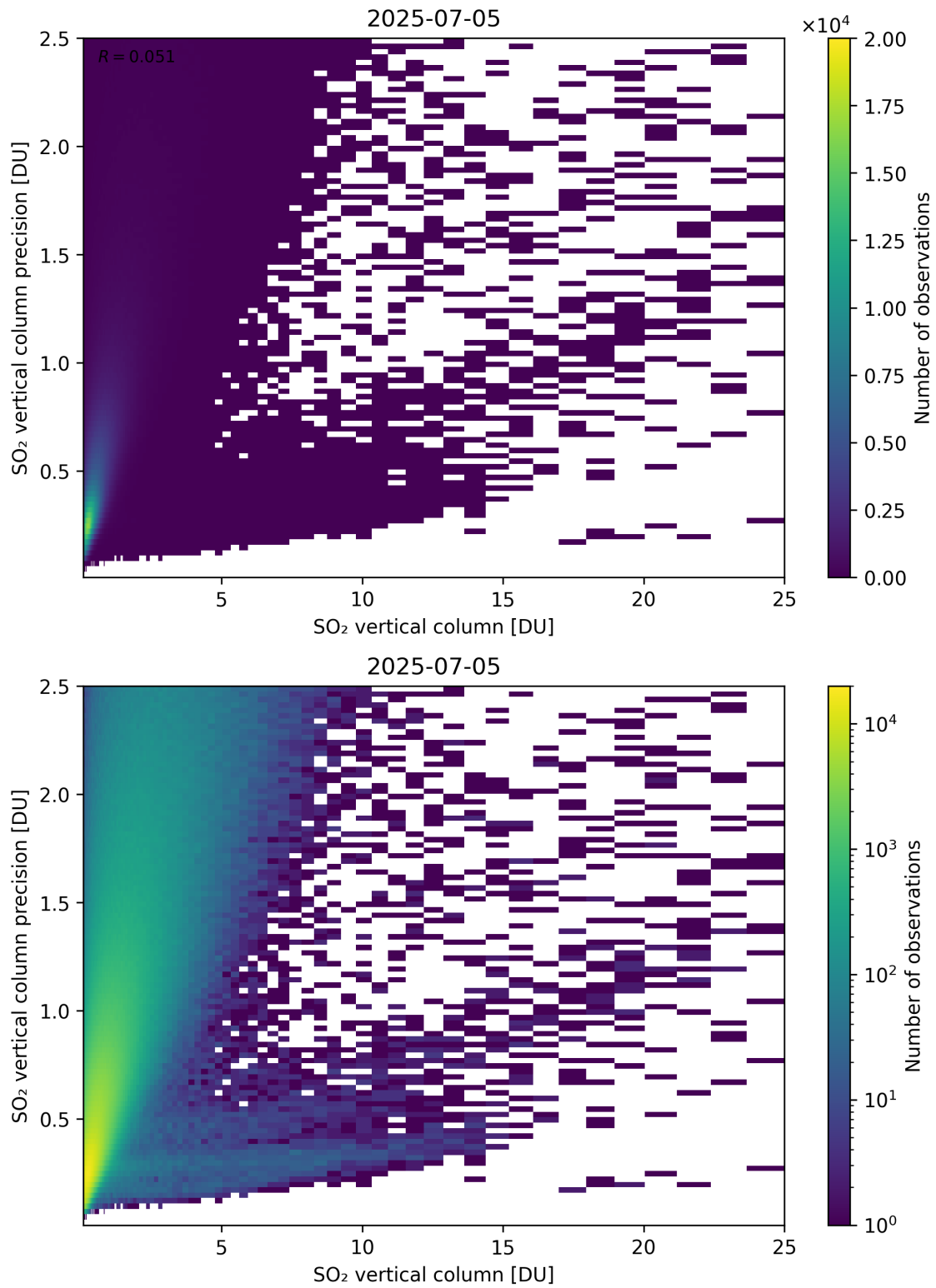
Figure 361: Scatter density plot of “SO 2 vertical column” against “SO 2 vertical column precision” for 2025-07-04 to 2025-07-06.
