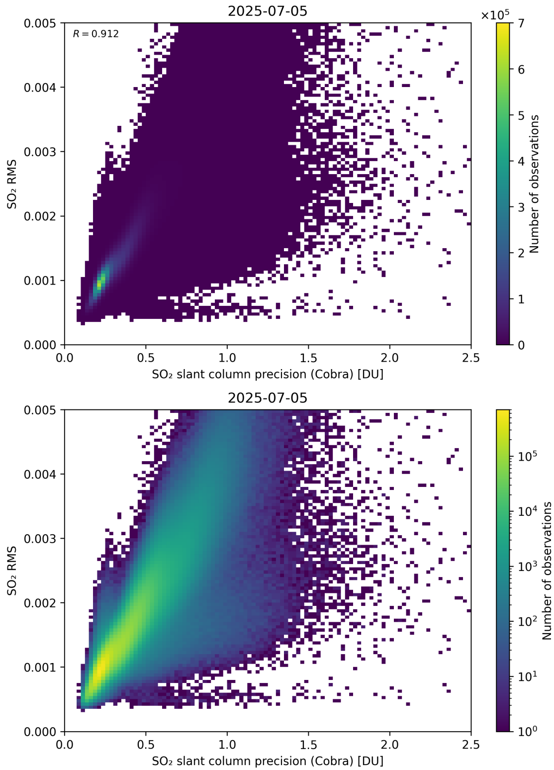
Figure 204: Scatter density plot of “SO 2 slant column precision (Cobra)” against “SO 2 RMS” for 2025-07-04 to 2025-07-06.
