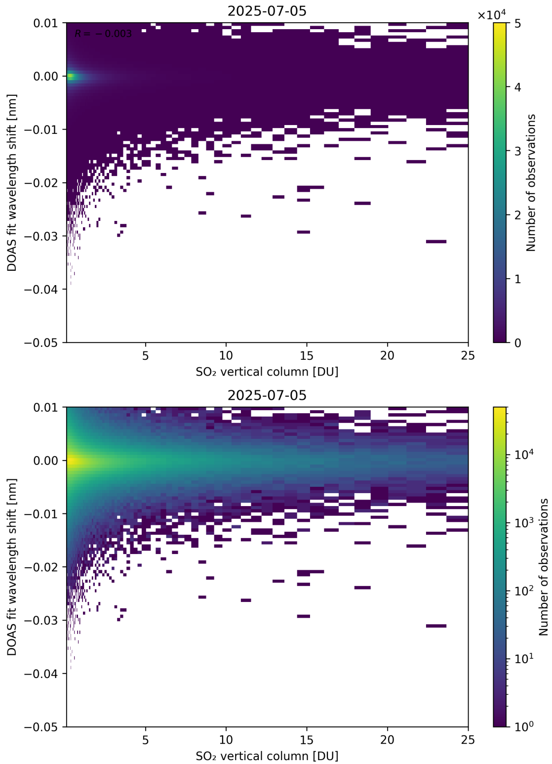
Figure 326: Scatter density plot of “SO 2 vertical column” against “DOAS fit wavelength shift” for 2025-07-04 to 2025-07-06.
