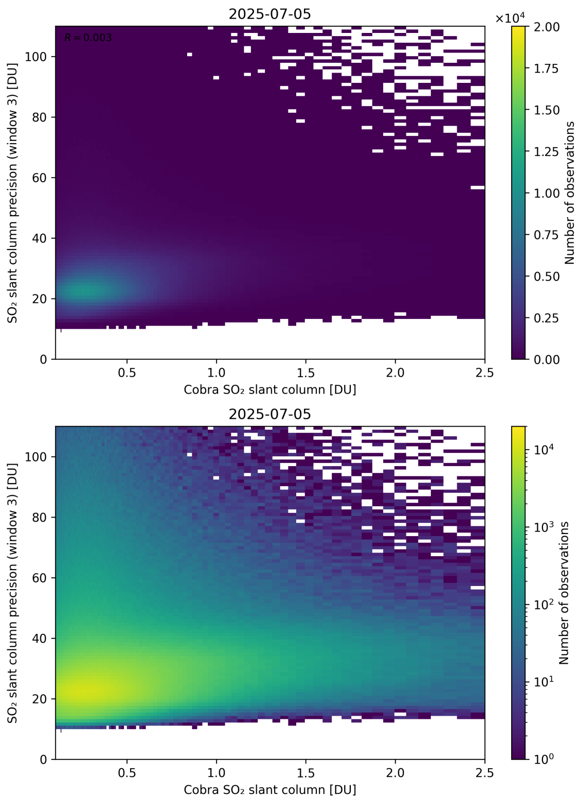
Figure 223: Scatter density plot of “Cobra SO 2 slant column” against “SO 2 slant column precision (window 3)” for 2025-07-04 to 2025-07-06.
