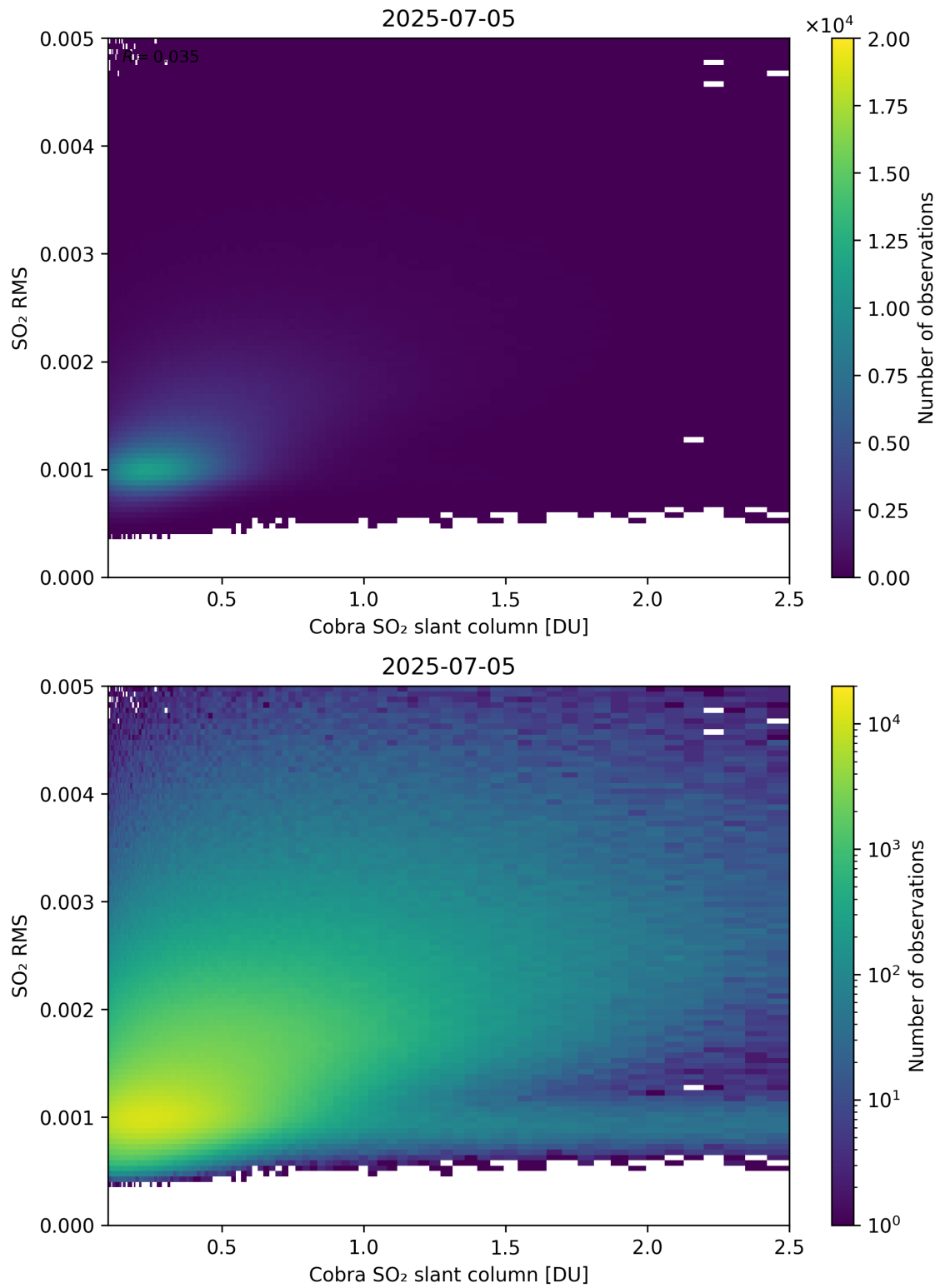
Figure 198: Scatter density plot of “Cobra SO 2 slant column” against “SO 2 RMS” for 2025-07-04 to 2025-07-06.
