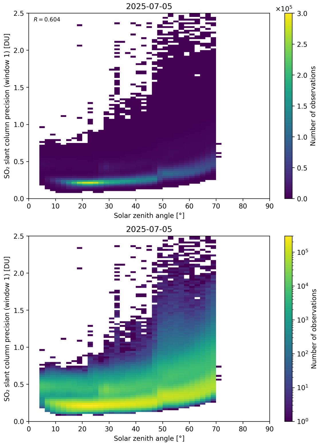
Figure 185: Scatter density plot of “Solar zenith angle” against “SO 2 slant column precision (window 1)” for 2025-07-04 to 2025-07-06.
