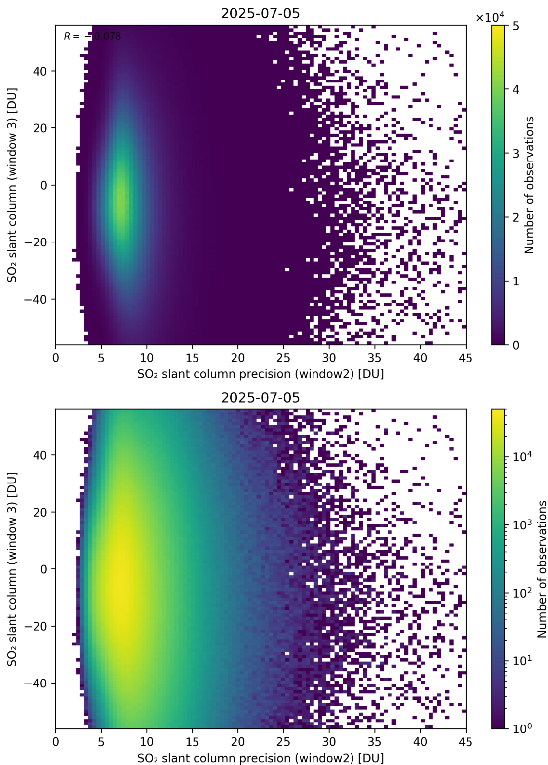
Figure 299: Scatter density plot of “SO 2 slant column precision (window2)” against “SO 2 slant column (window 3)” for 2025-07-04 to 2025-07-06.
