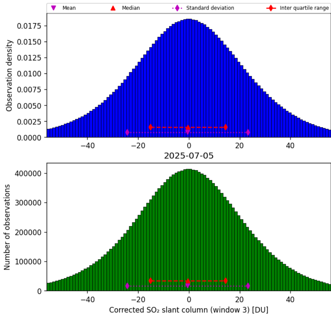
Figure 73: Histogram of “Corrected SO 2 slant column (window 3)” for 2025-07-04 to 2025-07-06
