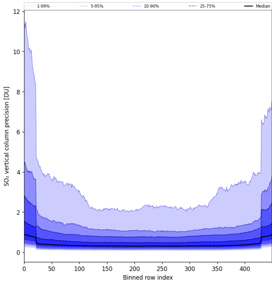
Figure 85: Along track statistics of “SO 2 vertical column precision” for 2025-07-04 to 2025-07-06
