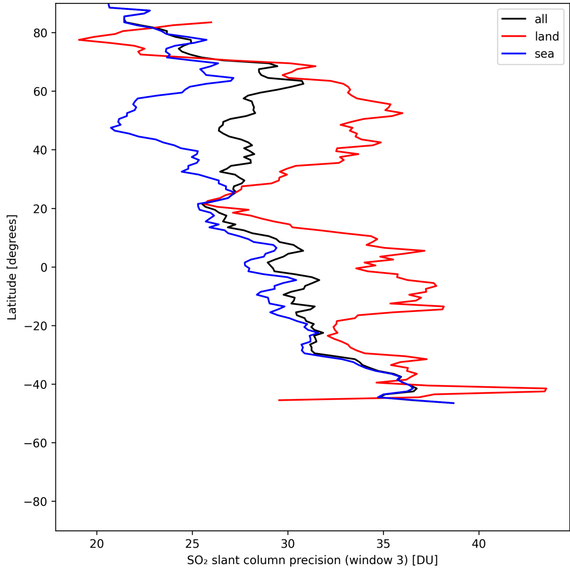
Figure 46: Zonal average of “SO 2 slant column precision (window 3)” for 2025-07-04 to 2025-07-06.
