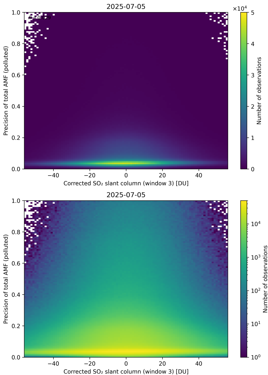
Figure 261: Scatter density plot of “Corrected SO 2 slant column (window 3)” against “Precision of total AMF (polluted)” for 2025-07-04 to 2025-07-06.
