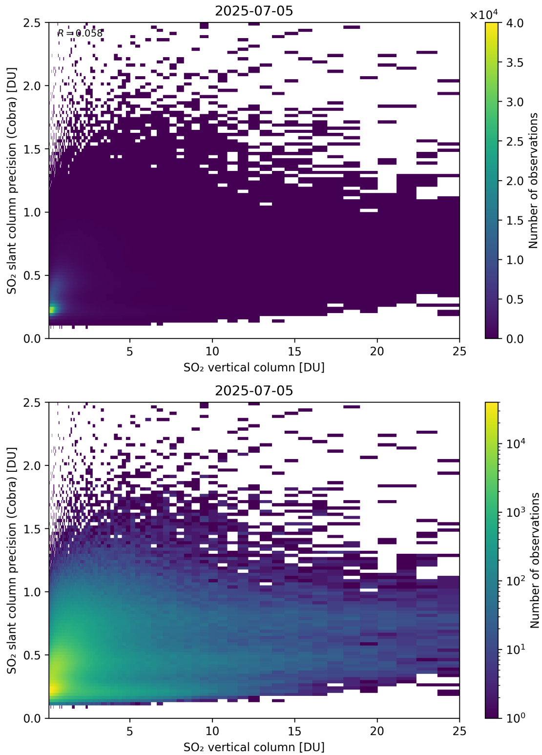
Figure 350: Scatter density plot of “SO 2 vertical column” against “SO 2 slant column precision (Cobra)” for 2025-07-04 to 2025-07-06.
