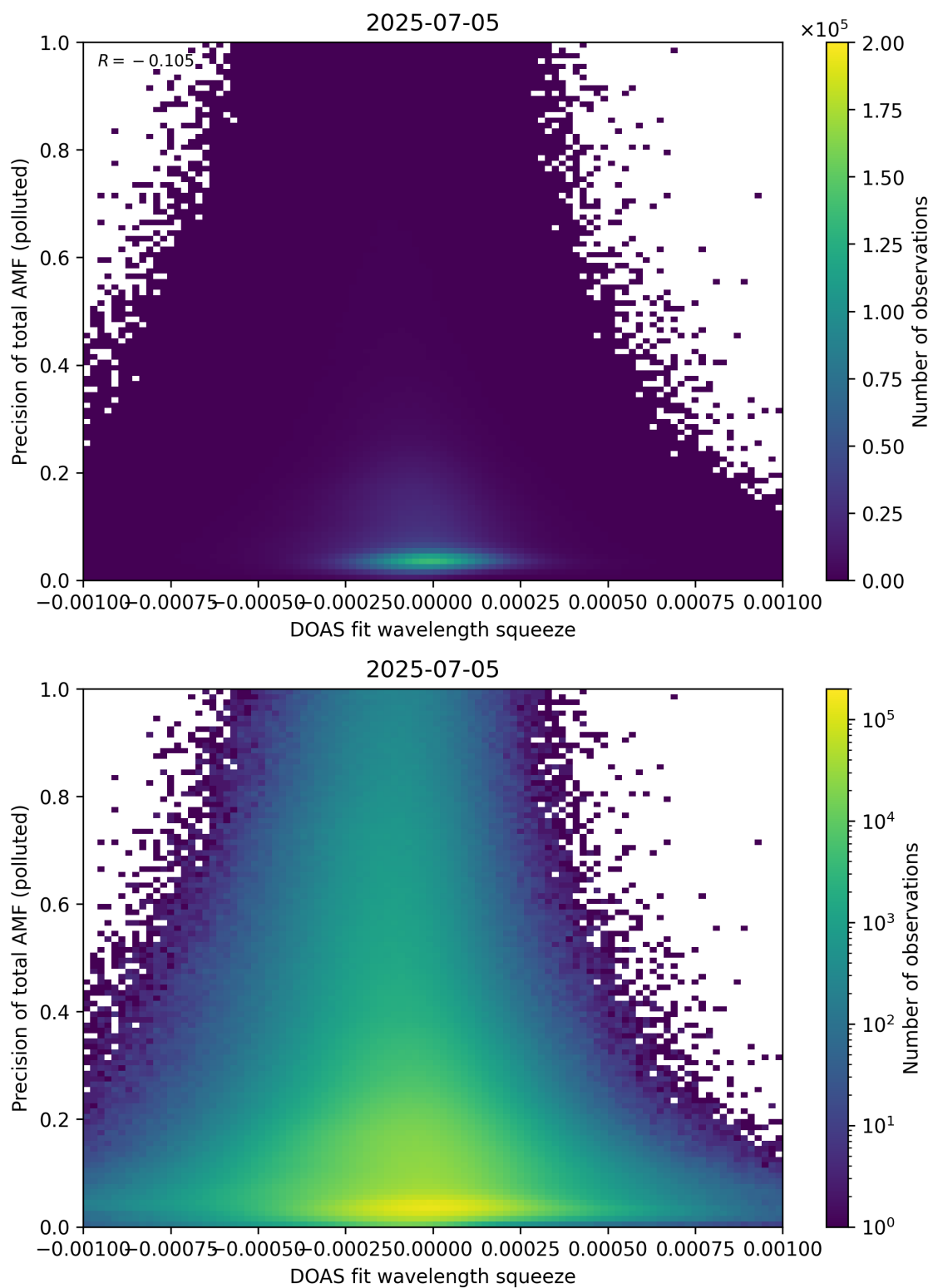
Figure 146: Scatter density plot of “DOAS fit wavelength squeeze” against “Precision of total AMF (polluted)” for 2025-07-04 to 2025-07-06.
