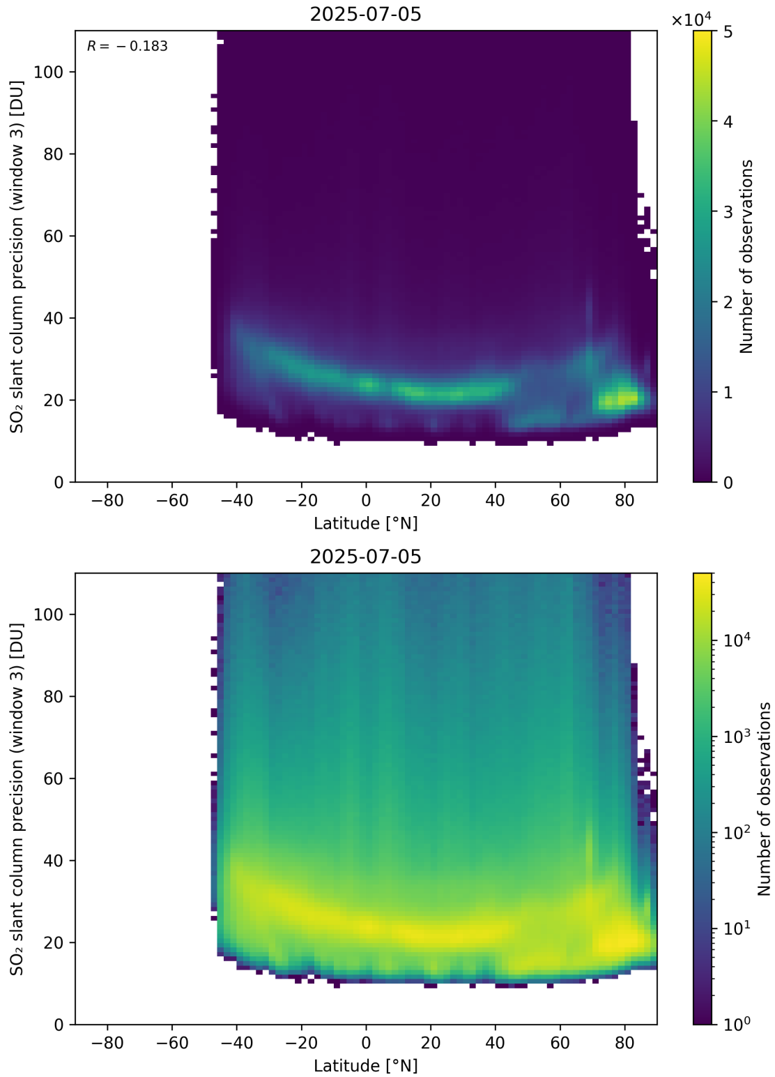
Figure 166: Scatter density plot of “Latitude” against “SO 2 slant column precision (window 3)” for 2025-07-04 to 2025-07-06.
