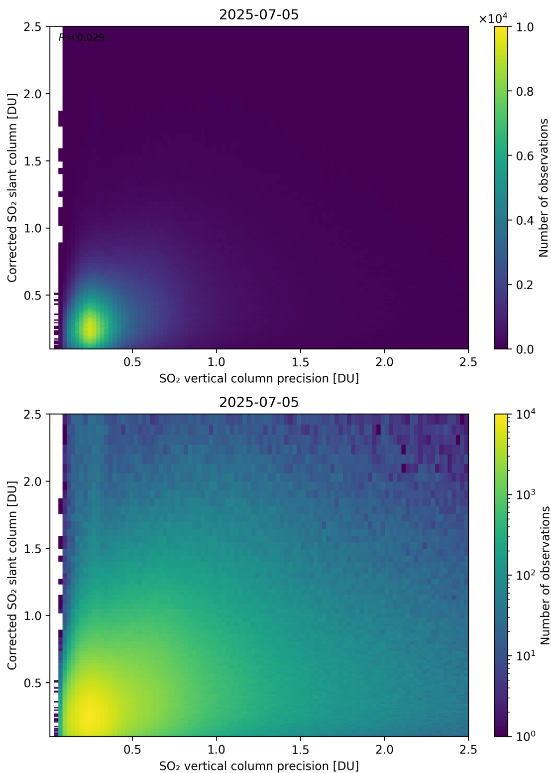
Figure 338: Scatter density plot of “SO 2 vertical column precision” against “Corrected SO 2 slant column” for 2025-07-04 to 2025-07-06.
