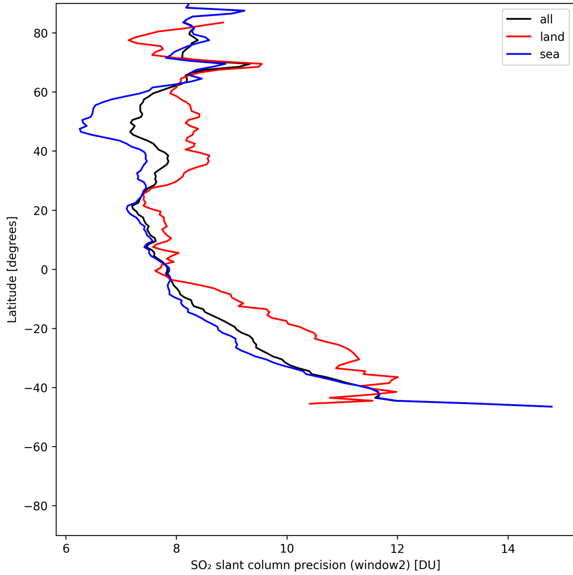
Figure 42: Zonal average of “SO 2 slant column precision (window2)” for 2025-07-04 to 2025-07-06.
