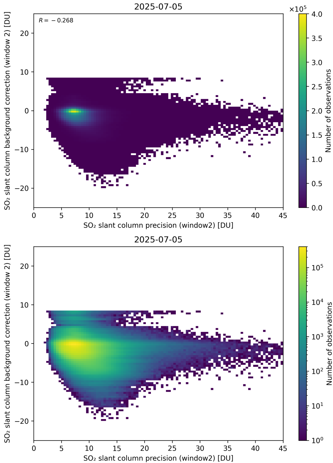
Figure 291: Scatter density plot of “SO 2 slant column precision (window2)” against “SO 2 slant column background correction (window 2)” for 2025-07-04 to 2025-07-06.
