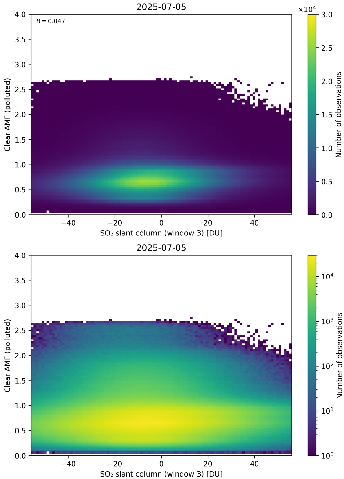
Figure 315: Scatter density plot of “SO 2 slant column (window 3)” against “Clear AMF (polluted)” for 2025-07-04 to 2025-07-06.
