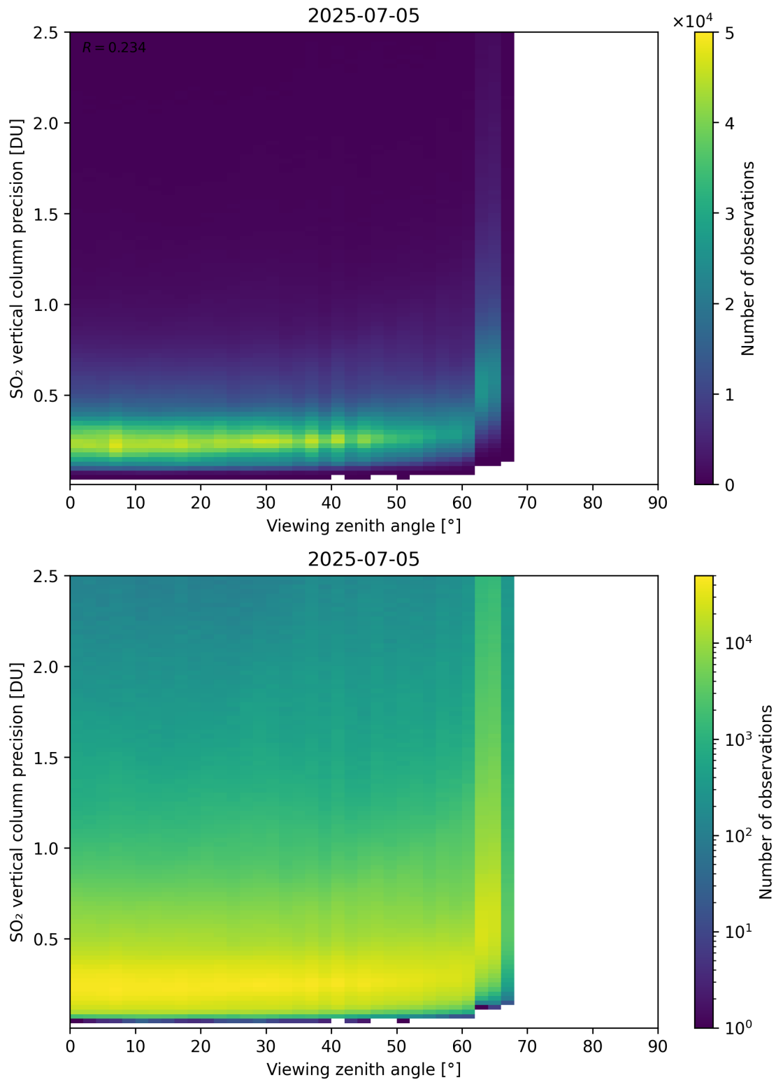
Figure 384: Scatter density plot of “Viewing zenith angle” against “SO 2 vertical column precision” for 2025-07-04 to 2025-07-06.
