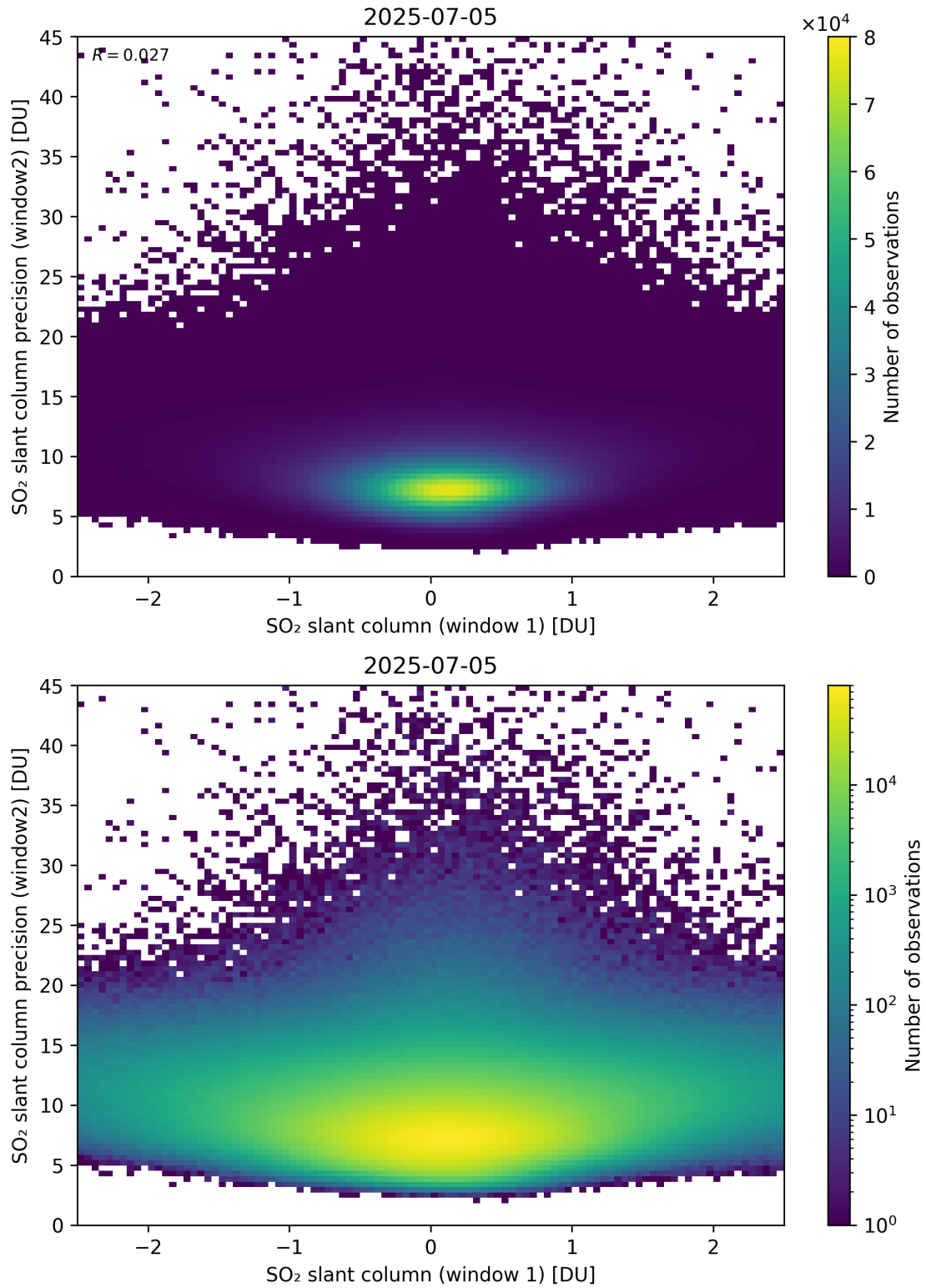
Figure 286: Scatter density plot of “SO 2 slant column (window 1)” against “SO 2 slant column precision (window2)” for 2025-07-04 to 2025-07-06.
