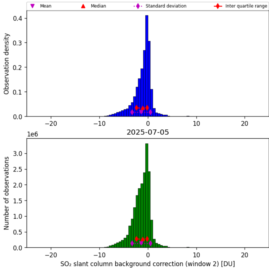
Figure 70: Histogram of “SO 2 slant column background correction (window 2)” for 2025-07-04 to 2025-07-06
