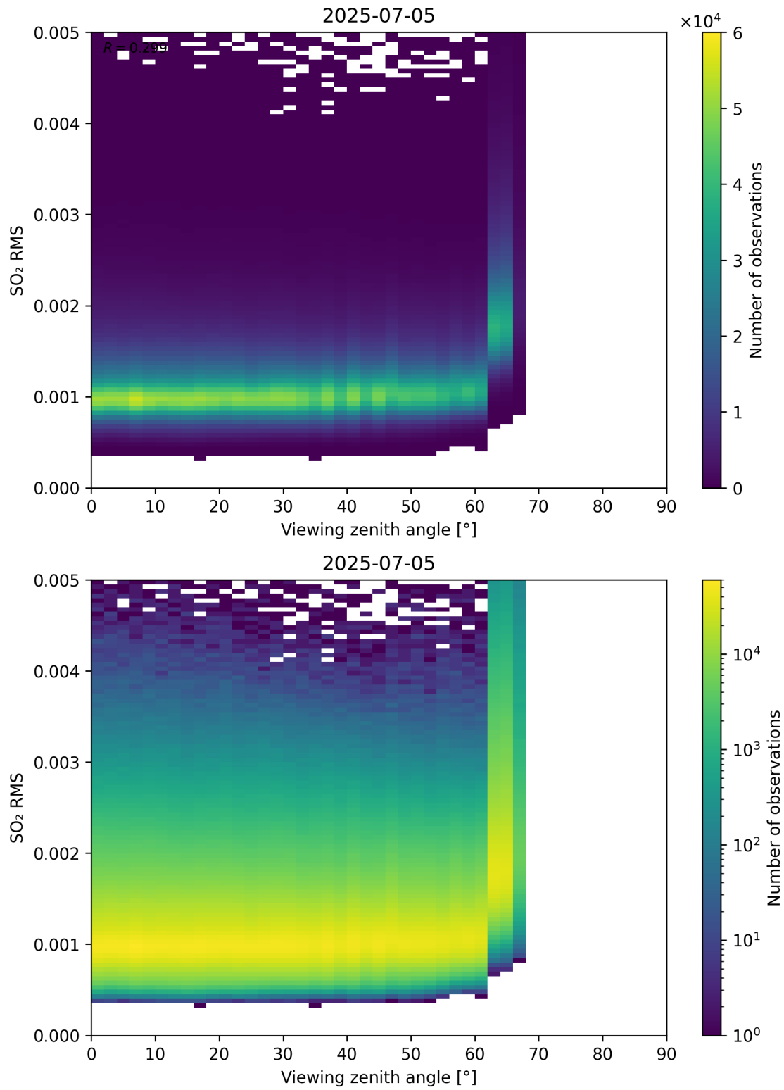
Figure 367: Scatter density plot of “Viewing zenith angle” against “SO 2 RMS” for 2025-07-04 to 2025-07-06.
