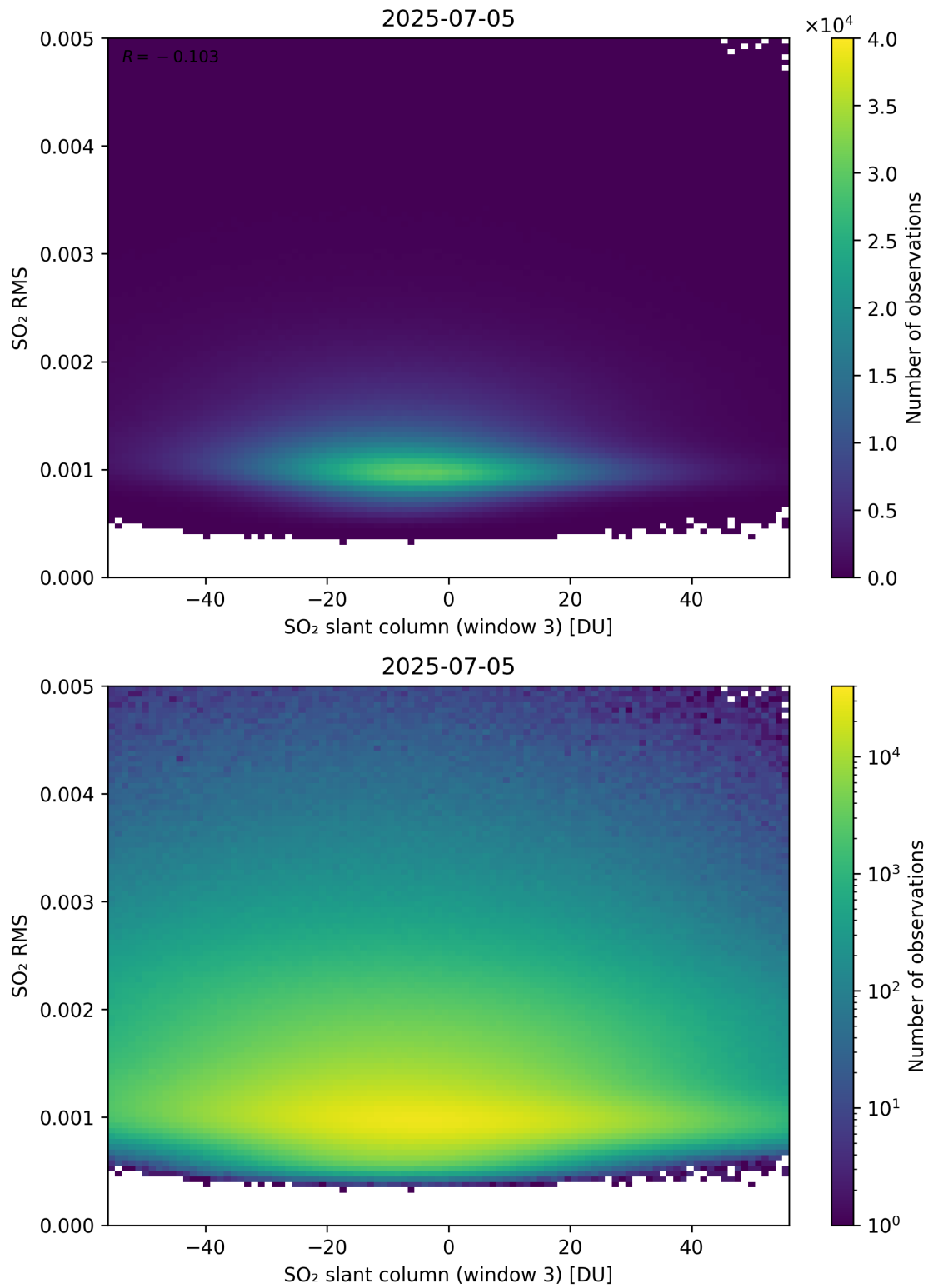
Figure 306: Scatter density plot of “SO 2 slant column (window 3)” against “SO 2 RMS” for 2025-07-04 to 2025-07-06.
