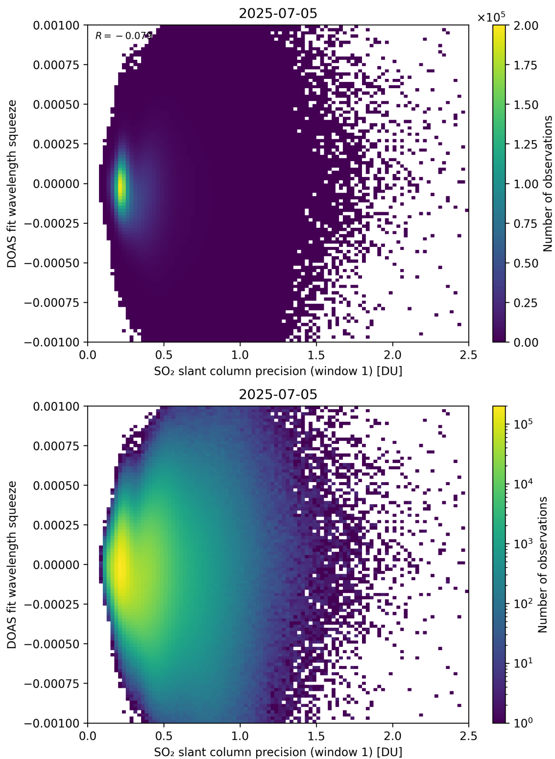
Figure 272: Scatter density plot of “SO 2 slant column precision (window 1)” against “DOAS fit wavelength squeeze” for 2025-07-04 to 2025-07-06.
