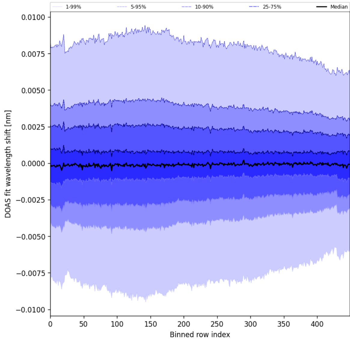
Figure 102: Along track statistics of “DOAS fit wavelength shift” for 2025-07-04 to 2025-07-06
