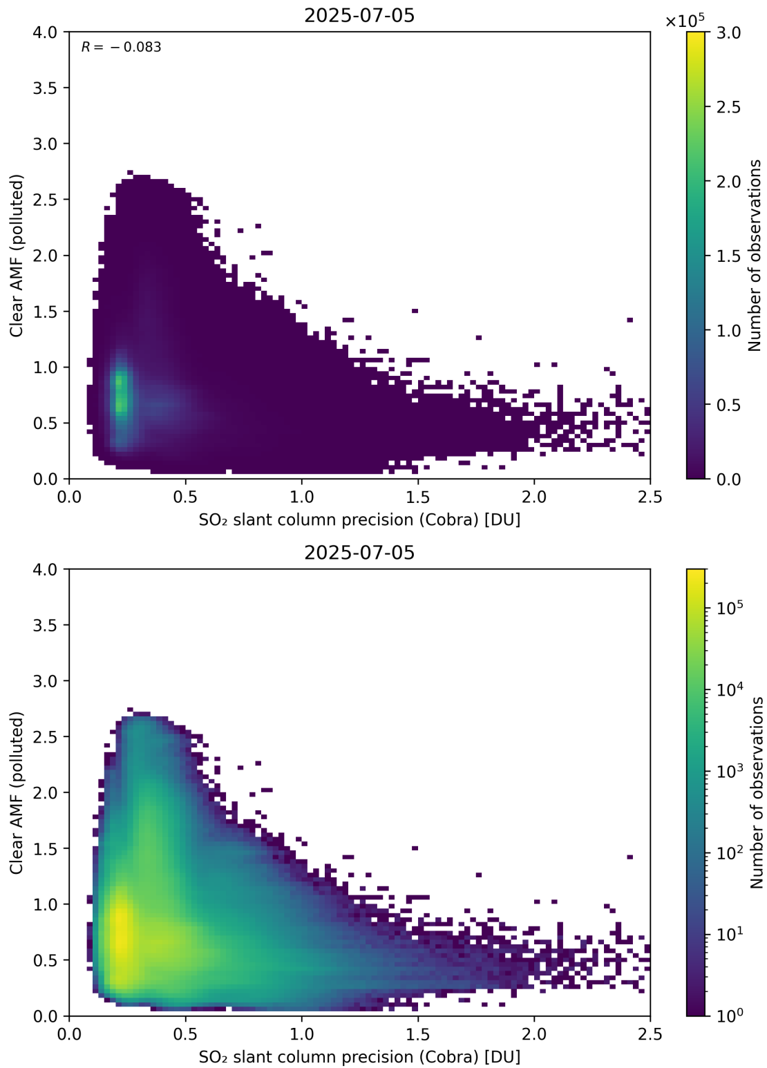
Figure 205: Scatter density plot of “SO 2 slant column precision (Cobra)” against “Clear AMF (polluted)” for 2025-07-04 to 2025-07-06.
