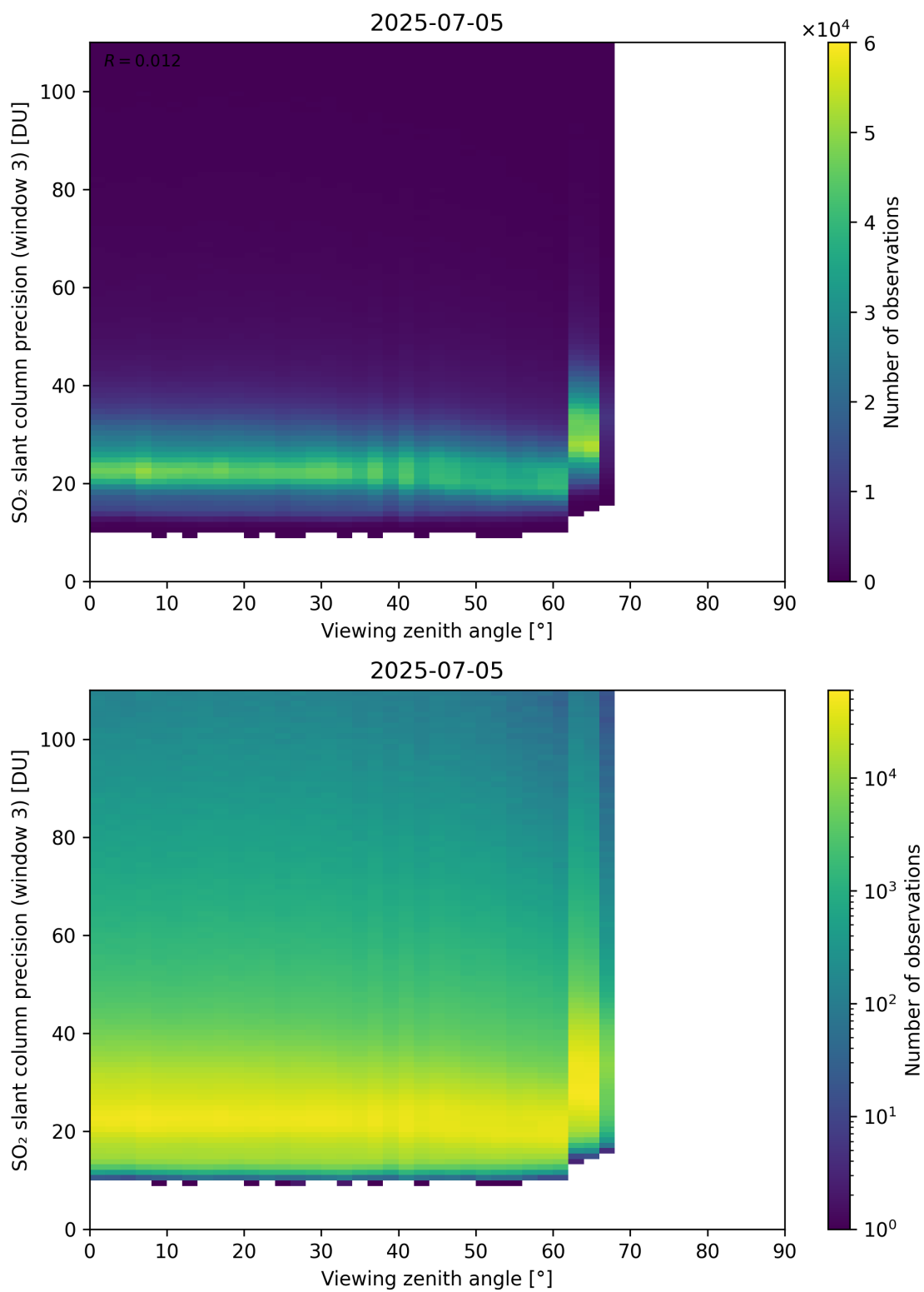
Figure 380: Scatter density plot of “Viewing zenith angle” against “SO 2 slant column precision (window 3)” for 2025-07-04 to 2025-07-06.
