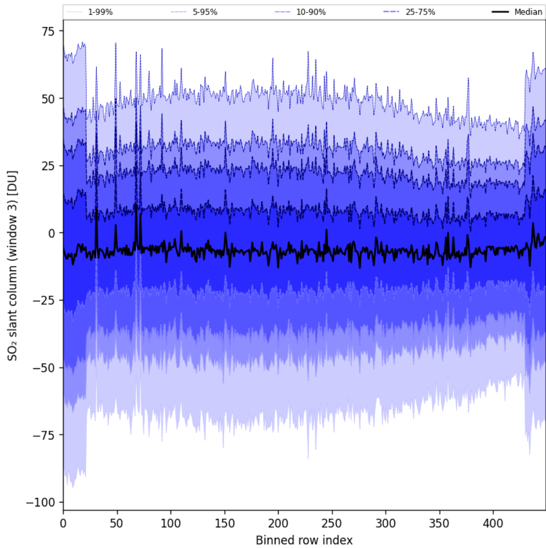
Figure 97: Along track statistics of “SO 2 slant column (window 3)” for 2025-07-04 to 2025-07-06
