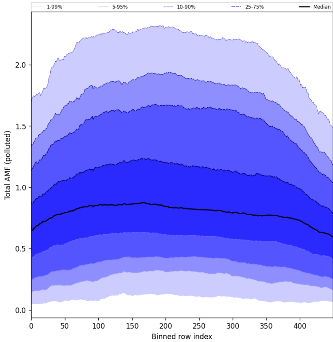
Figure 105: Along track statistics of “Total AMF (polluted)” for 2025-07-04 to 2025-07-06
