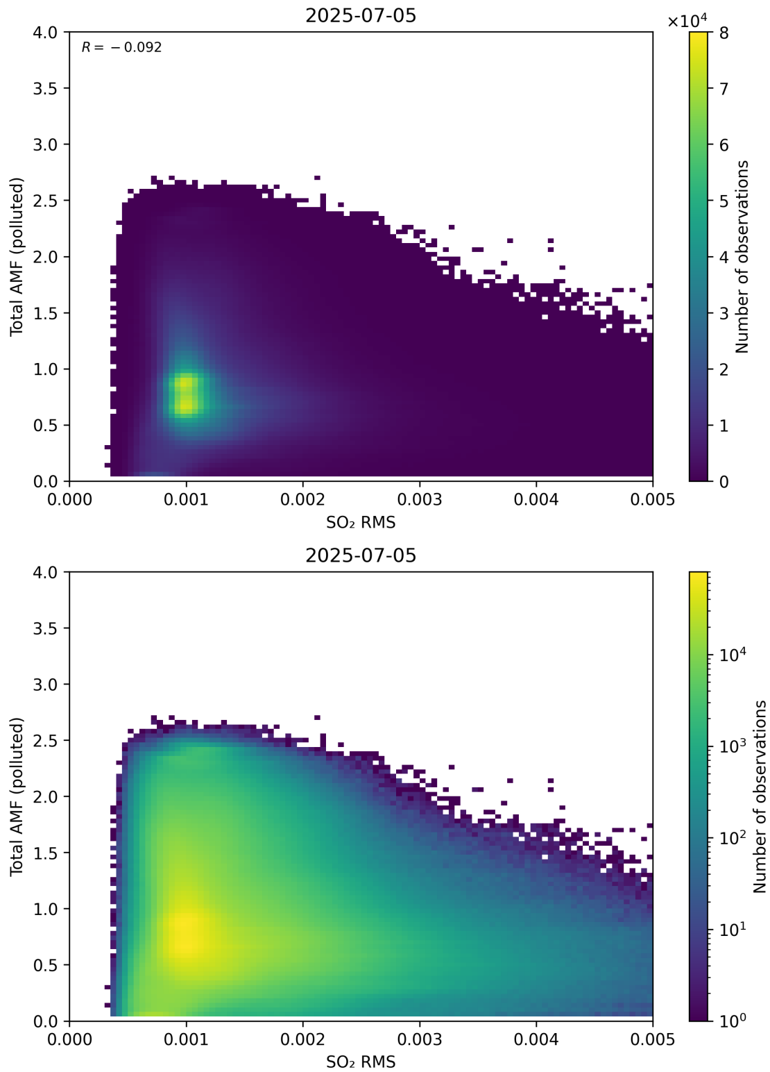
Figure 148: Scatter density plot of “SO 2 RMS” against “Total AMF (polluted)” for 2025-07-04 to 2025-07-06.
