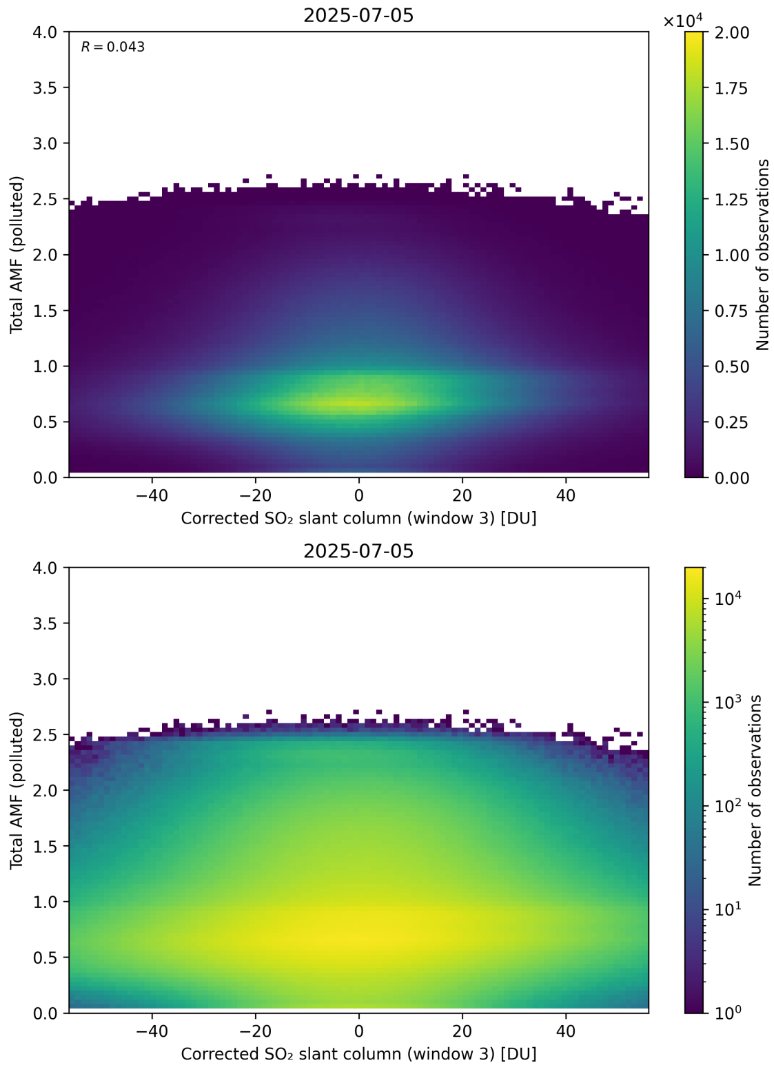
Figure 260: Scatter density plot of “Corrected SO 2 slant column (window 3)” against “Total AMF (polluted)” for 2025-07-04 to 2025-07-06.
