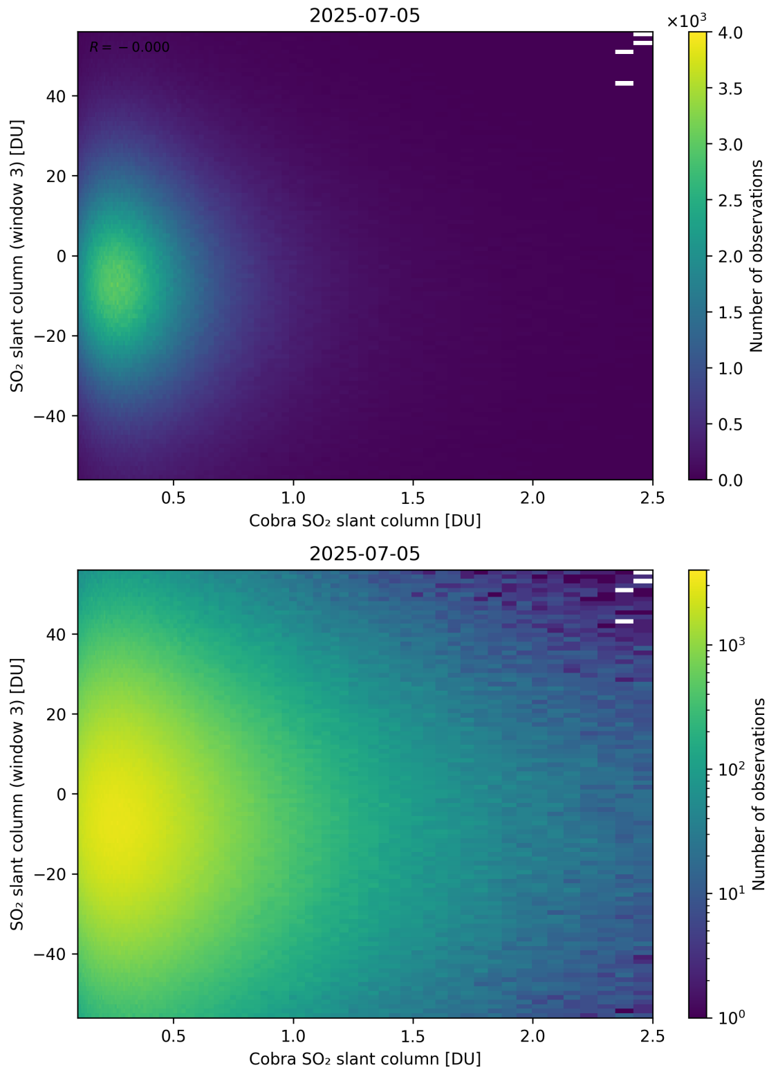
Figure 222: Scatter density plot of “Cobra SO 2 slant column” against “SO 2 slant column (window 3)” for 2025-07-04 to 2025-07-06.
