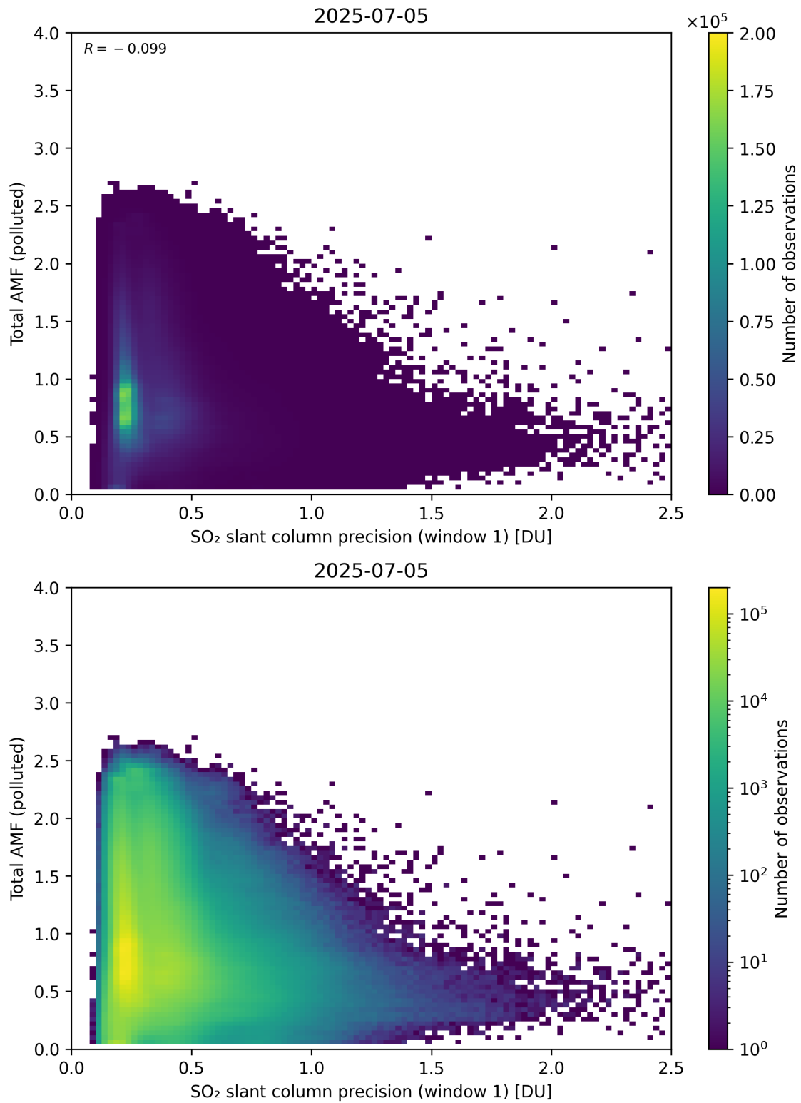
Figure 280: Scatter density plot of “SO 2 slant column precision (window 1)” against “Total AMF (polluted)” for 2025-07-04 to 2025-07-06.
