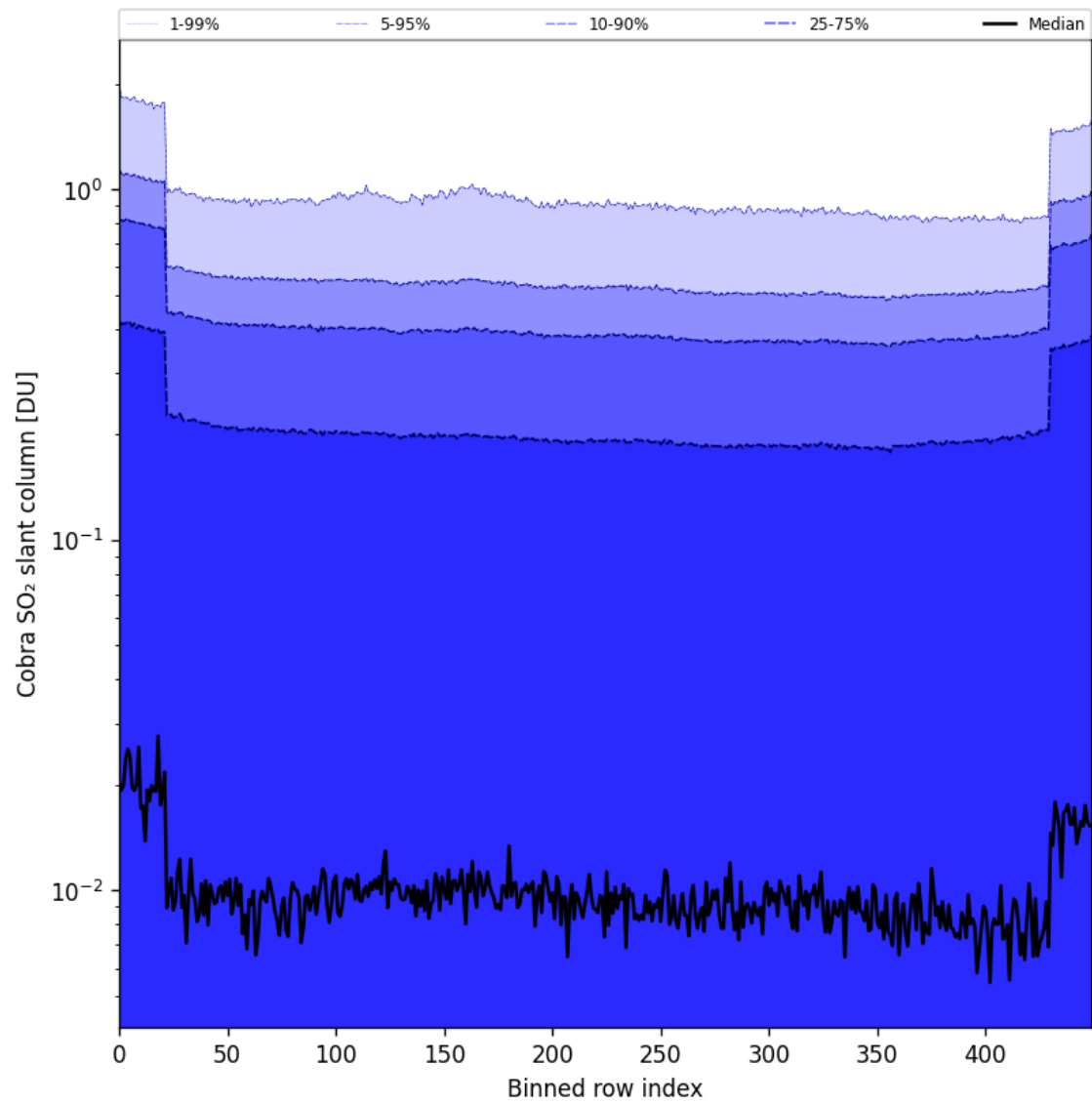
Figure 87: Along track statistics of “Cobra SO 2 slant column” for 2025-07-04 to 2025-07-06
