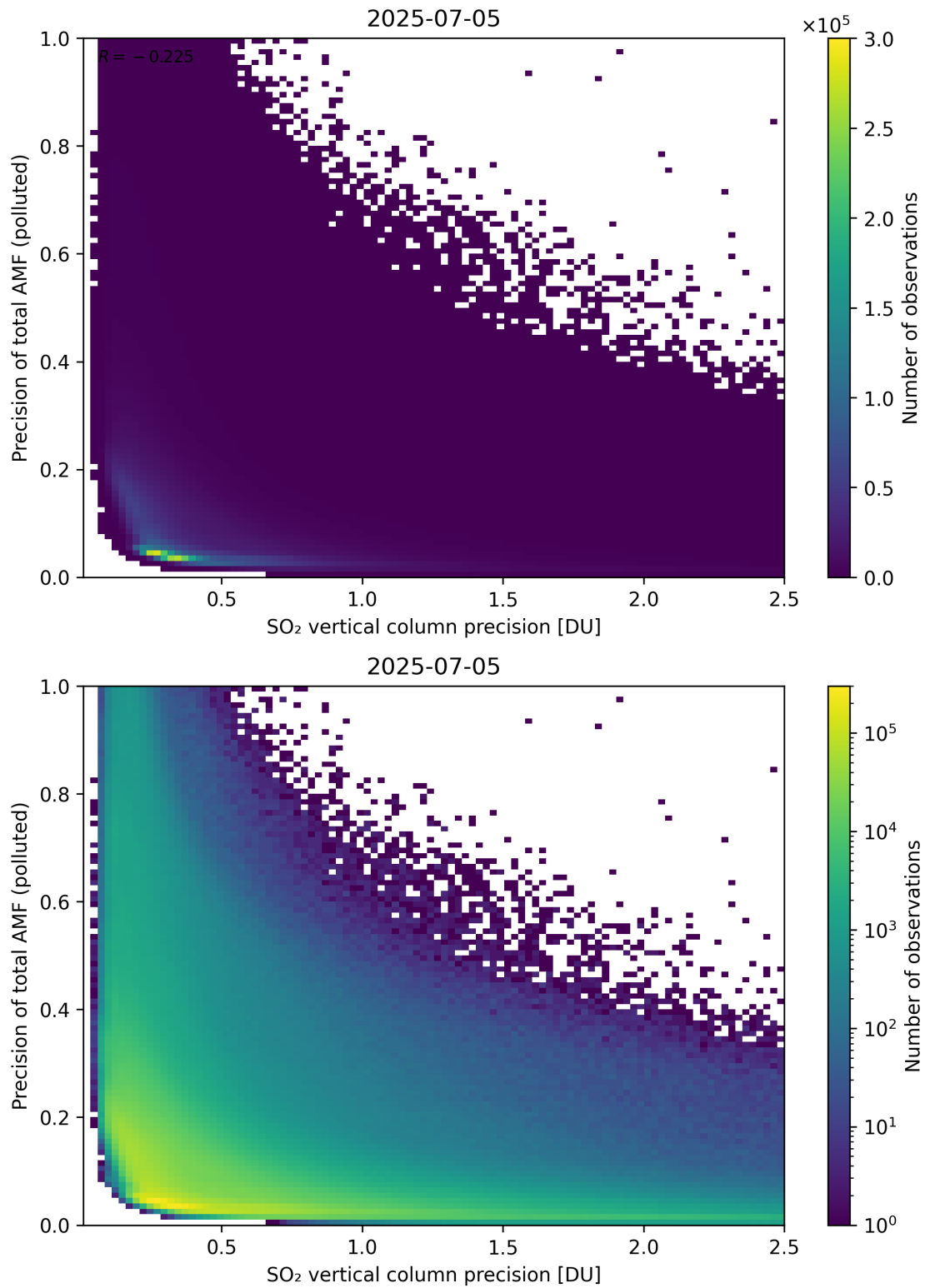
Figure 347: Scatter density plot of “SO 2 vertical column precision” against “Precision of total AMF (polluted)” for 2025-07-04 to 2025-07-06.
