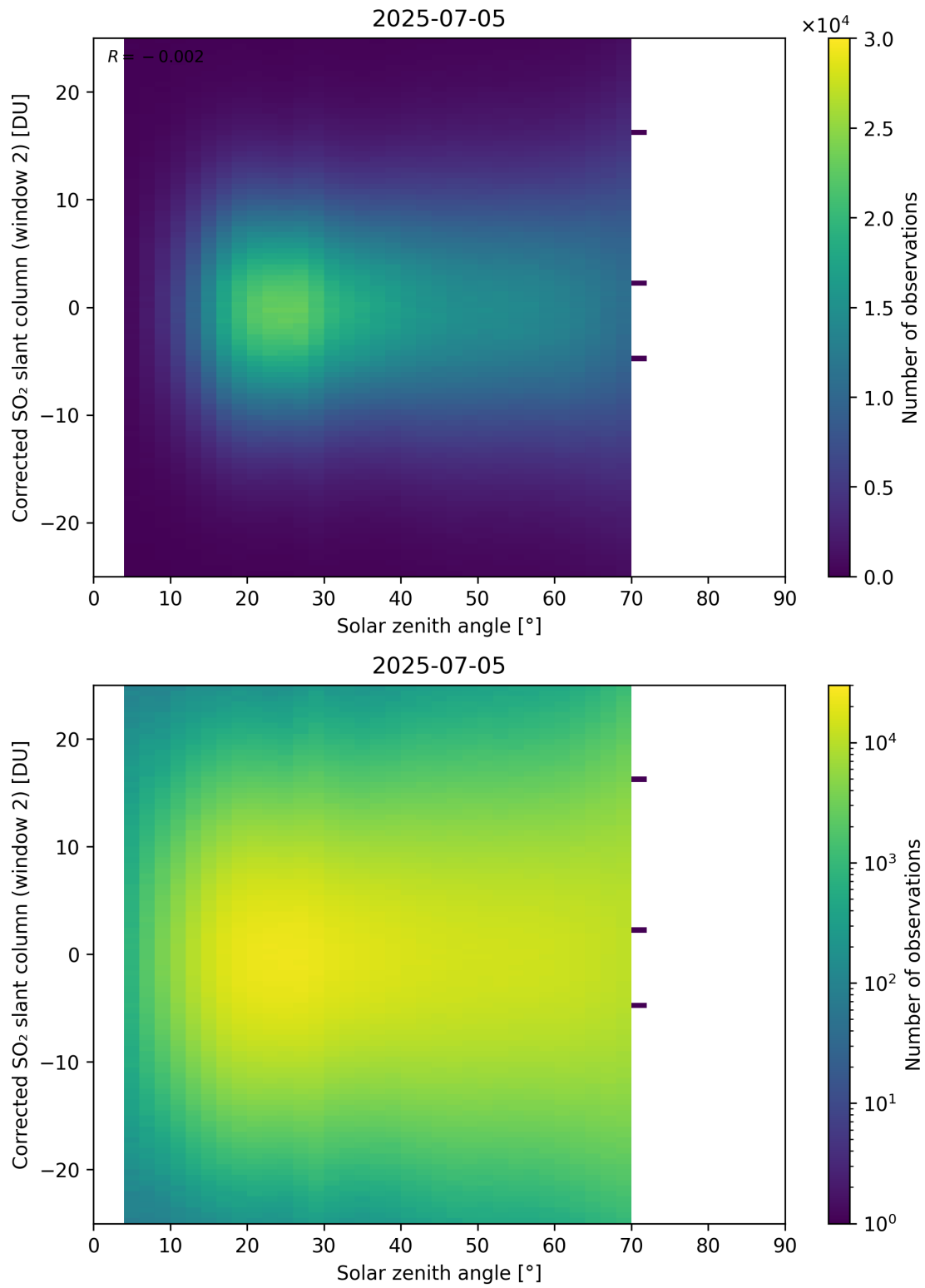
Figure 182: Scatter density plot of “Solar zenith angle” against “Corrected SO 2 slant column (window 2)” for 2025-07-04 to 2025-07-06.
