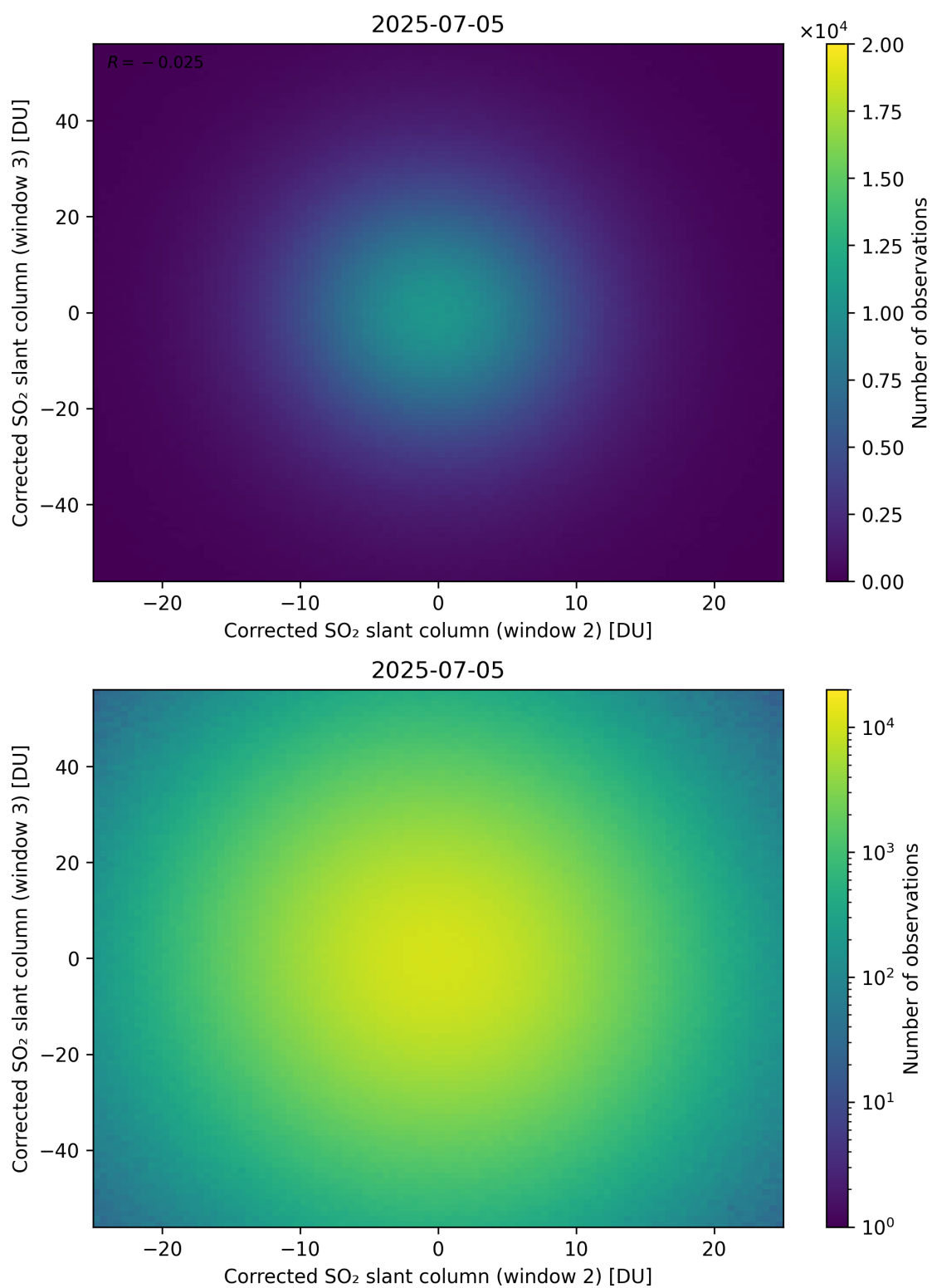
Figure 250: Scatter density plot of “Corrected SO 2 slant column (window 2)” against “Corrected SO 2 slant column (window 3)” for 2025-07-04 to 2025-07-06.
