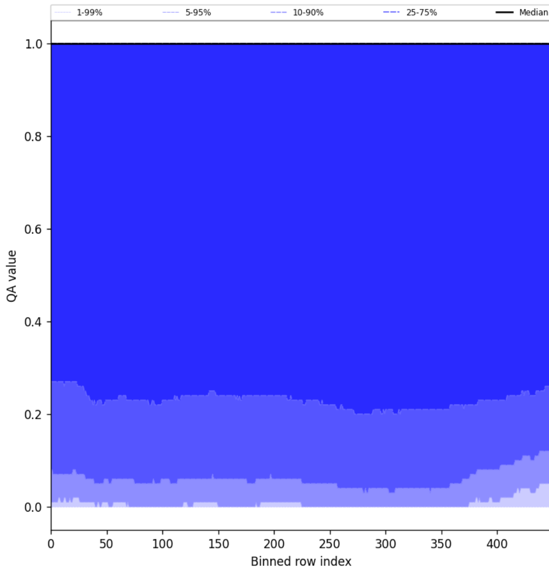
Figure 83: Along track statistics of “QA value” for 2025-07-04 to 2025-07-06
