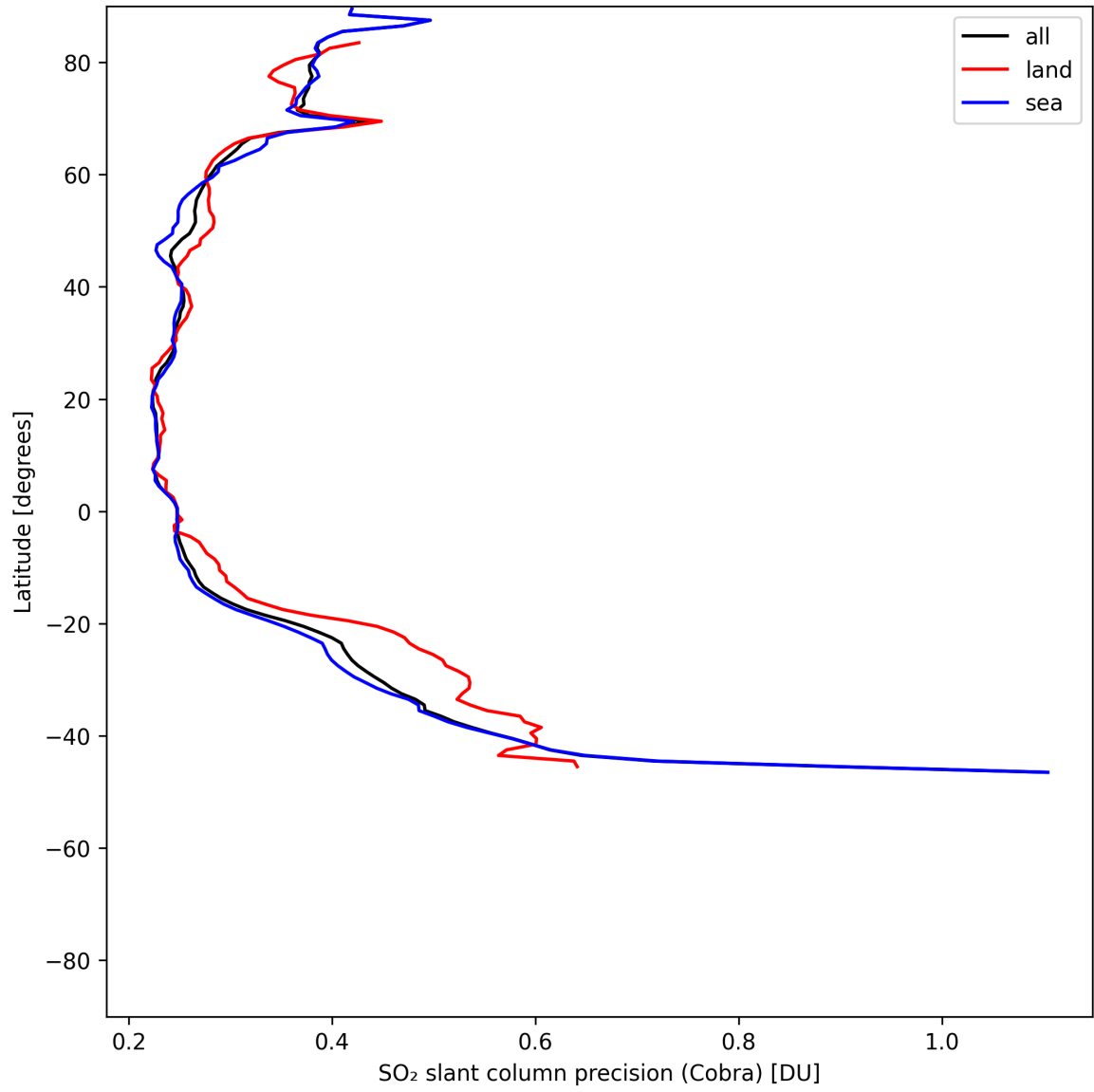
Figure 36: Zonal average of “SO 2 slant column precision (Cobra)” for 2025-07-04 to 2025-07-06.
