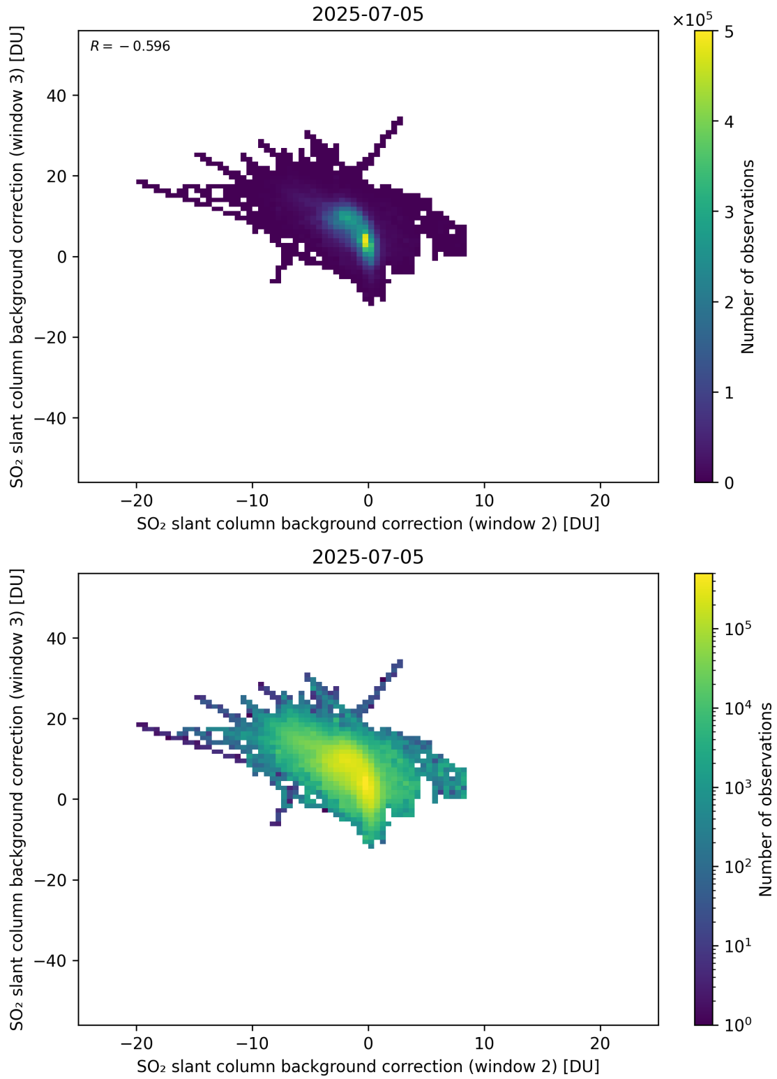
Figure 122: Scatter density plot of “SO 2 slant column background correction (window 2)” against “SO 2 slant column background correction (window 3)” for 2025-07-04 to 2025-07-06.
