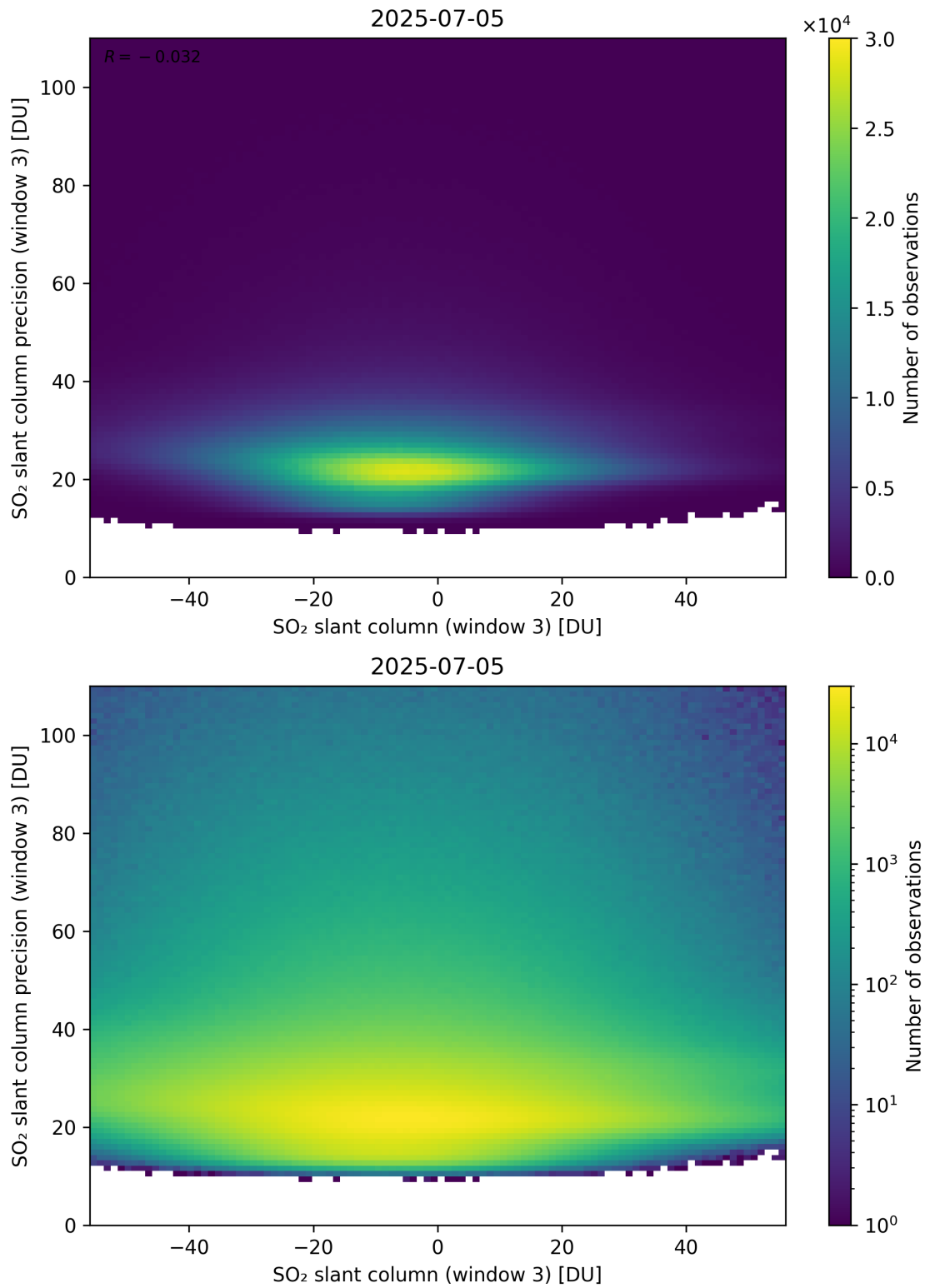
Figure 317: Scatter density plot of “SO 2 slant column (window 3)” against “SO 2 slant column precision (window 3)” for 2025-07-04 to 2025-07-06.
