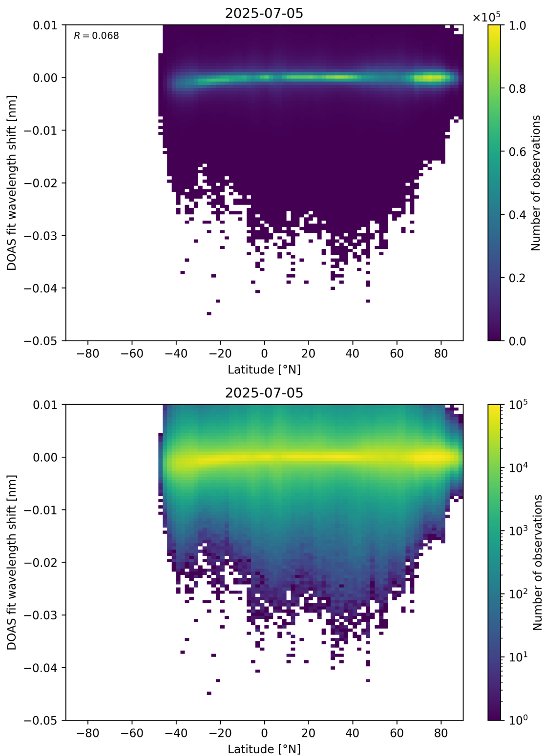
Figure 153: Scatter density plot of “Latitude” against “DOAS fit wavelength shift” for 2025-07-04 to 2025-07-06.
