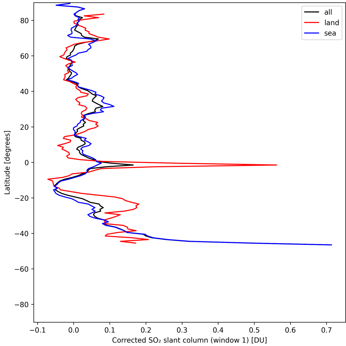
Figure 39: Zonal average of “Corrected SO 2 slant column (window 1)” for 2025-07-04 to 2025-07-06.
