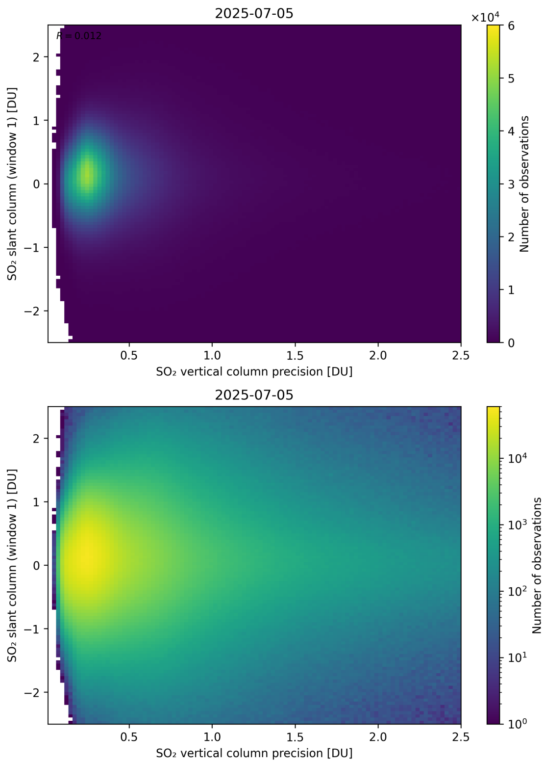
Figure 341: Scatter density plot of “SO 2 vertical column precision” against “SO 2 slant column (window 1)” for 2025-07-04 to 2025-07-06.
