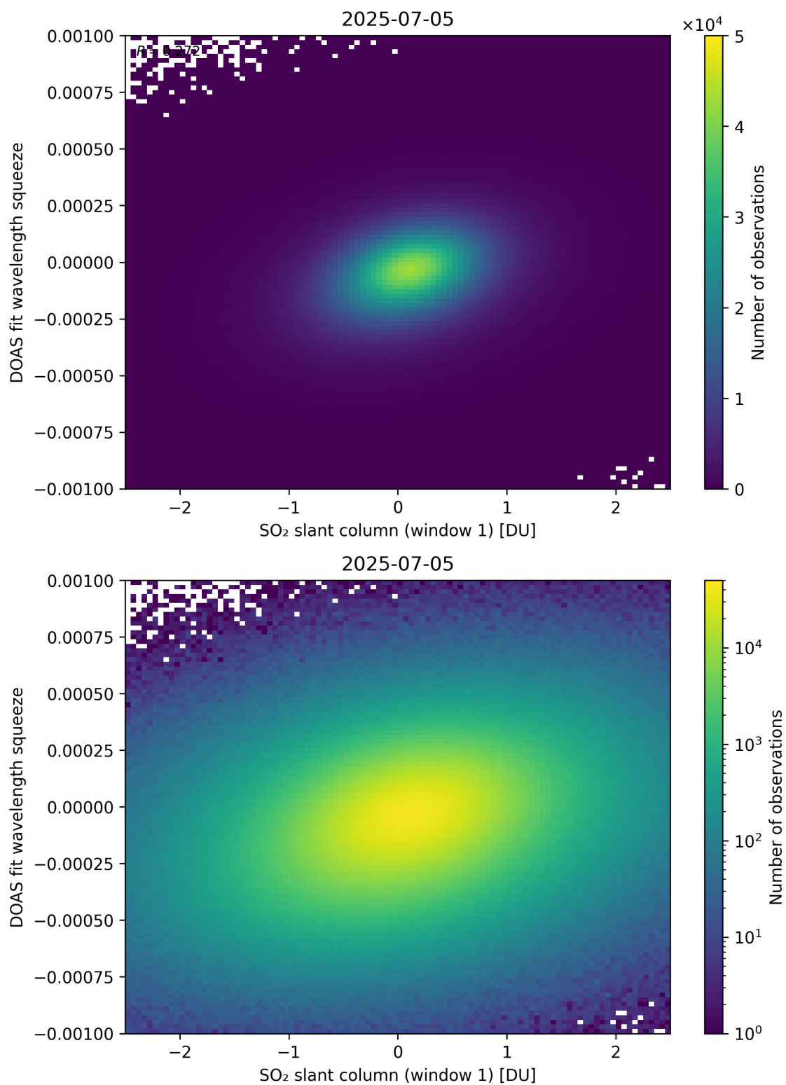
Figure 266: Scatter density plot of “SO 2 slant column (window 1)” against “DOAS fit wavelength squeeze” for 2025-07-04 to 2025-07-06.
