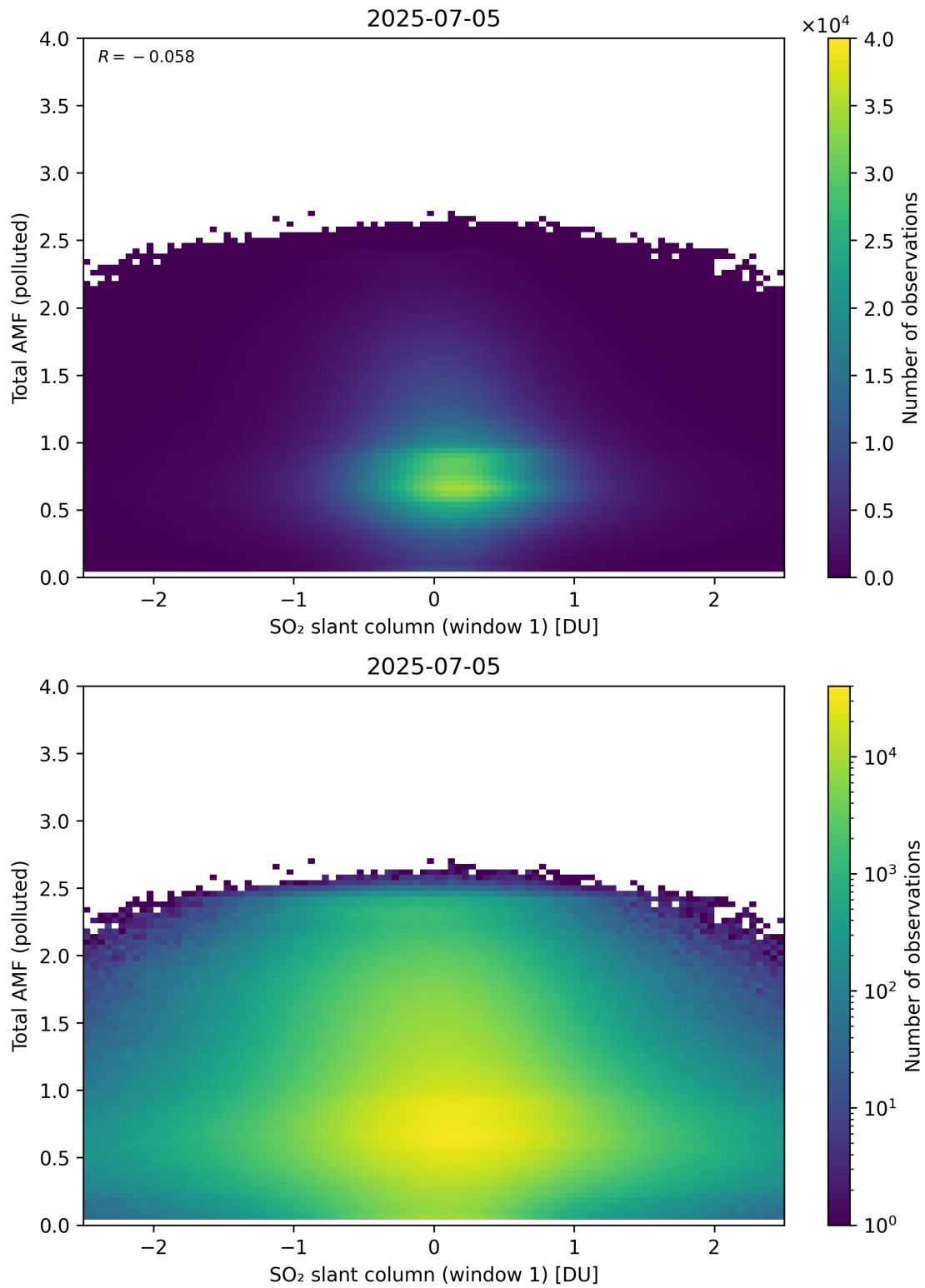
Figure 289: Scatter density plot of “SO 2 slant column (window 1)” against “Total AMF (polluted)” for 2025-07-04 to 2025-07-06.
