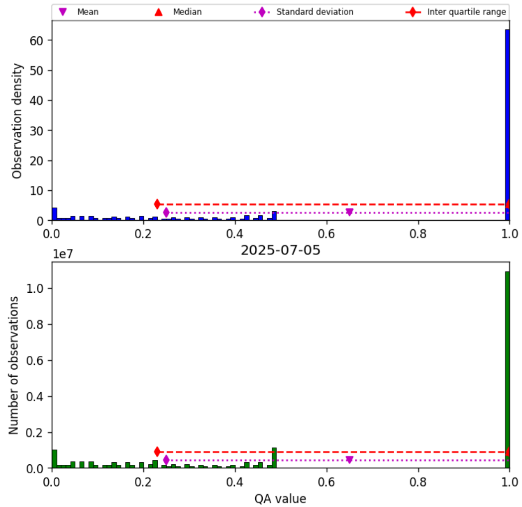
Figure 57: Histogram of “QA value” for 2025-07-04 to 2025-07-06
