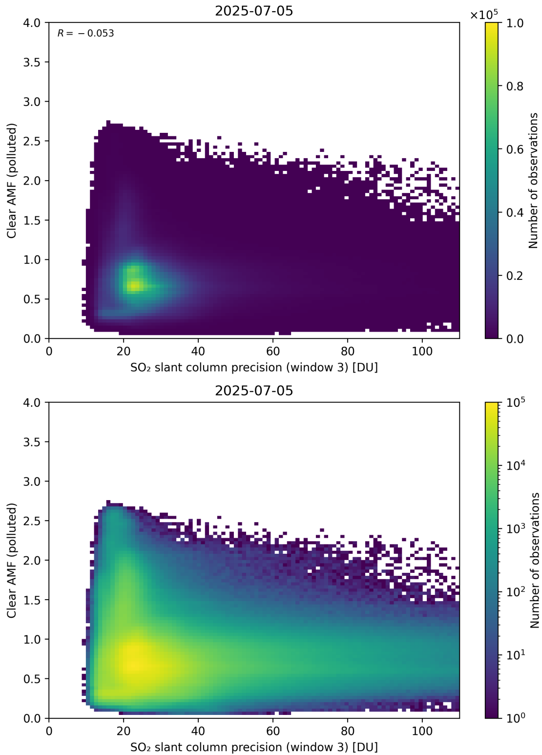
Figure 311: Scatter density plot of “SO 2 slant column precision (window 3)” against “Clear AMF (polluted)” for 2025-07-04 to 2025-07-06.
