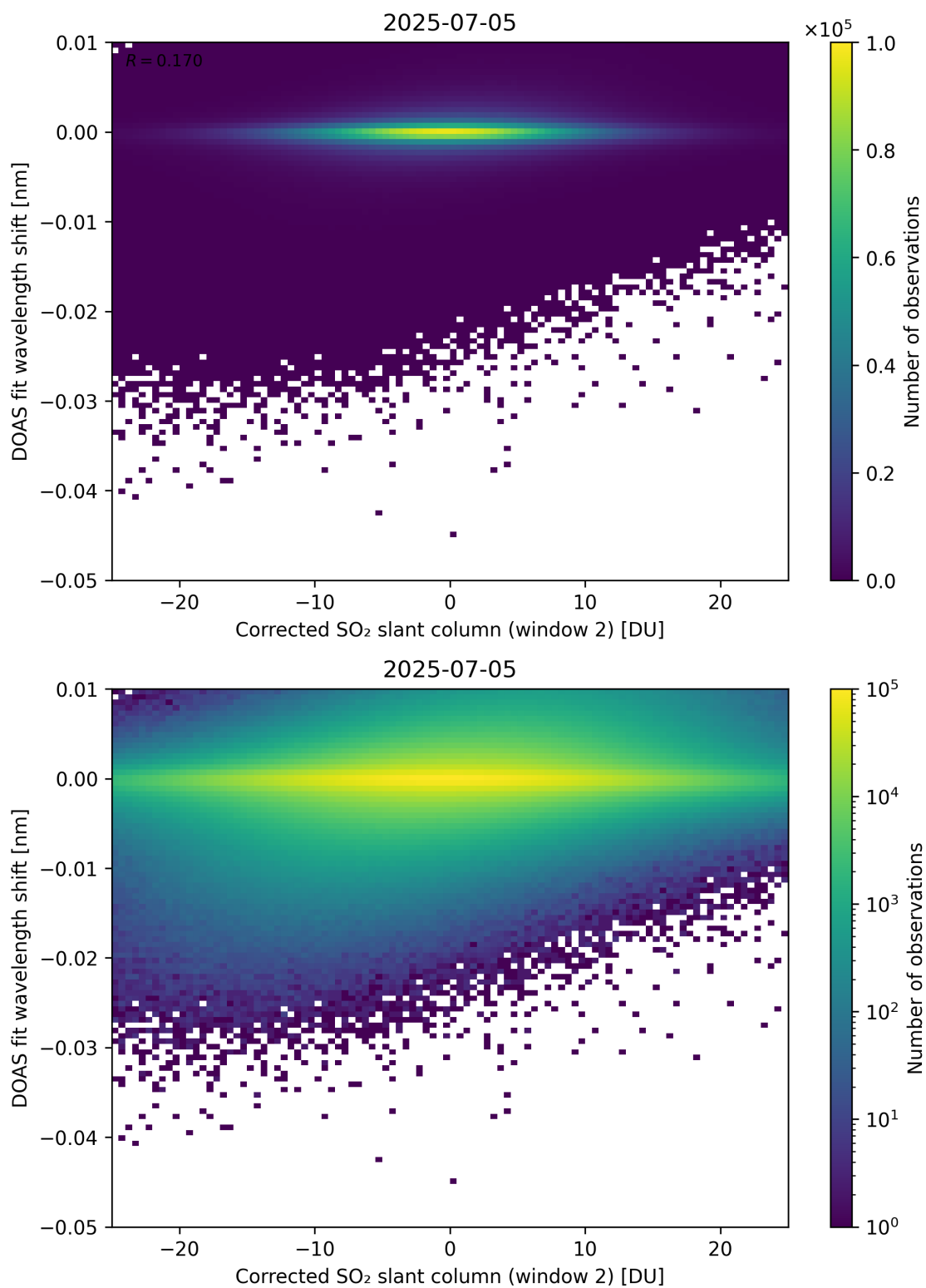
Figure 246: Scatter density plot of “Corrected SO 2 slant column (window 2)” against “DOAS fit wavelength shift” for 2025-07-04 to 2025-07-06.
