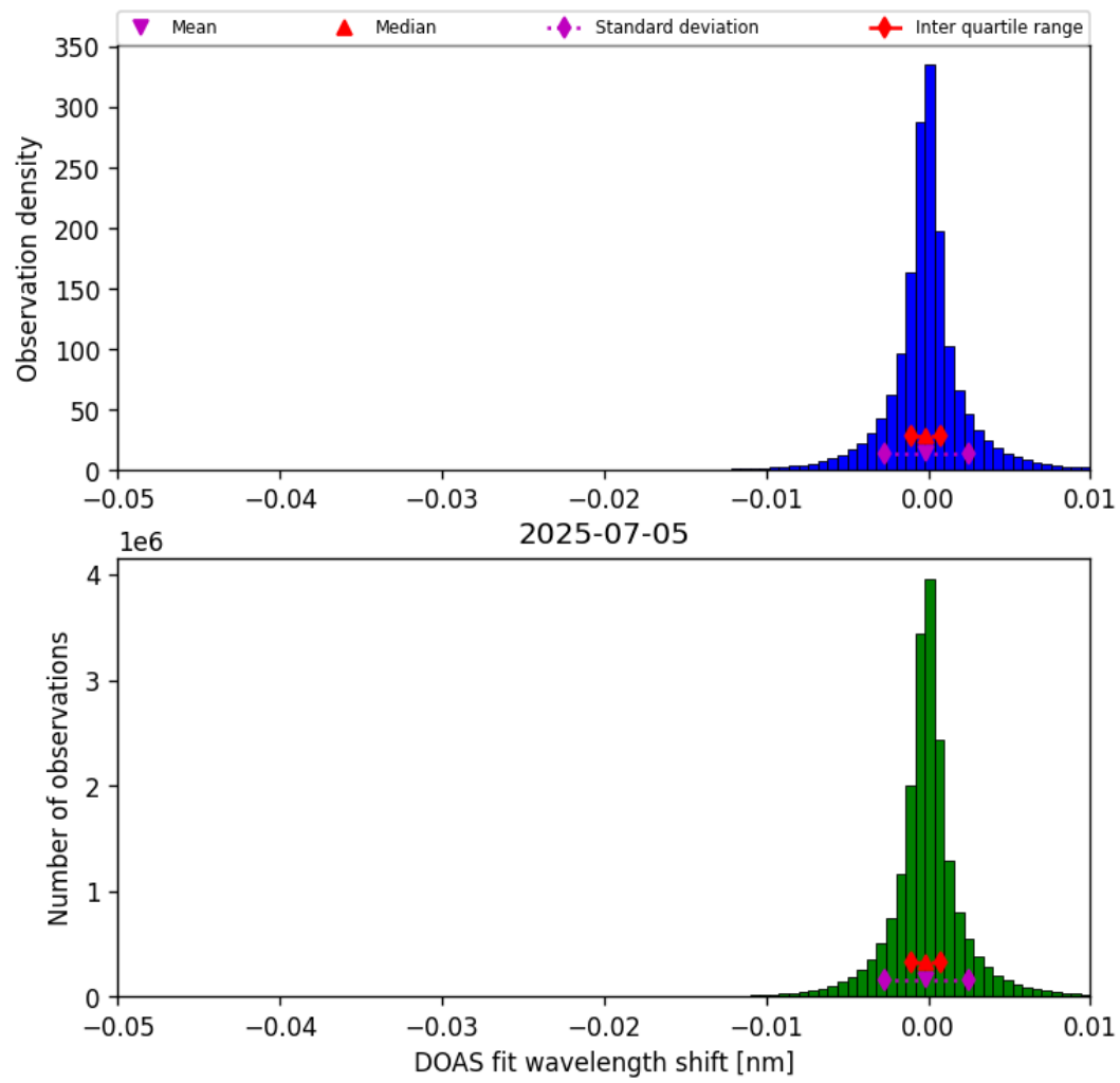
Figure 76: Histogram of “DOAS fit wavelength shift” for 2025-07-04 to 2025-07-06
