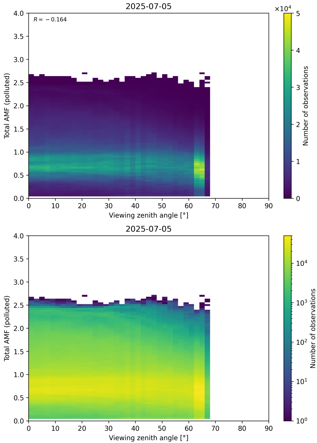
Figure 381: Scatter density plot of “Viewing zenith angle” against “Total AMF (polluted)” for 2025-07-04 to 2025-07-06.
