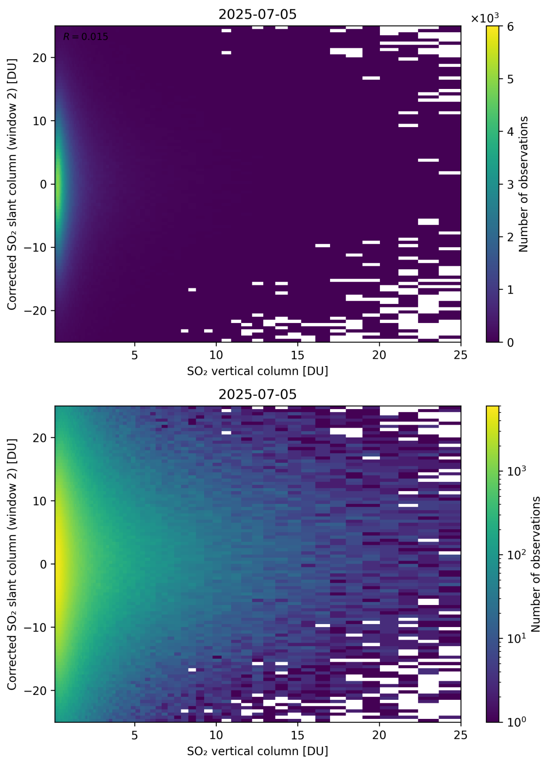
Figure 352: Scatter density plot of “SO 2 vertical column” against “Corrected SO 2 slant column (window 2)” for 2025-07-04 to 2025-07-06.
