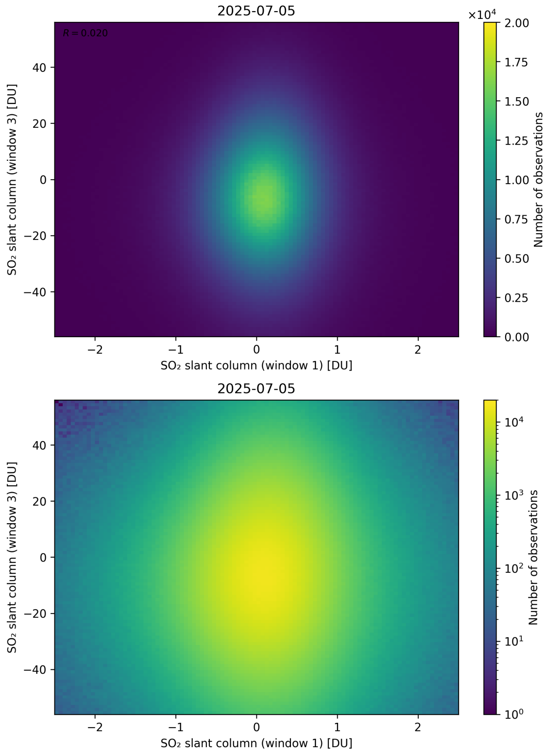
Figure 287: Scatter density plot of “SO 2 slant column (window 1)” against “SO 2 slant column (window 3)” for 2025-07-04 to 2025-07-06.
