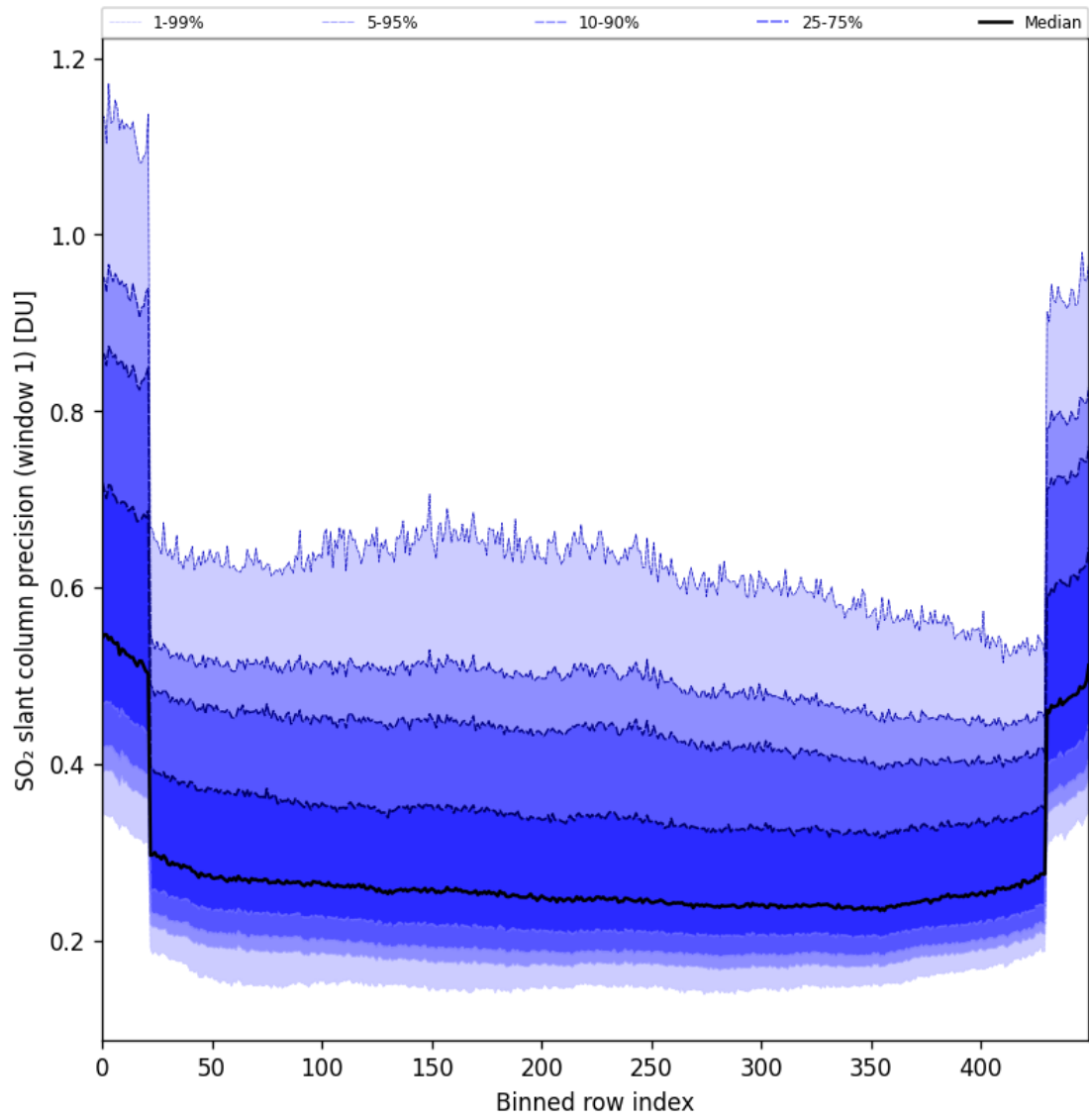
Figure 90: Along track statistics of “SO 2 slant column precision (window 1)” for 2025-07-04 to 2025-07-06
