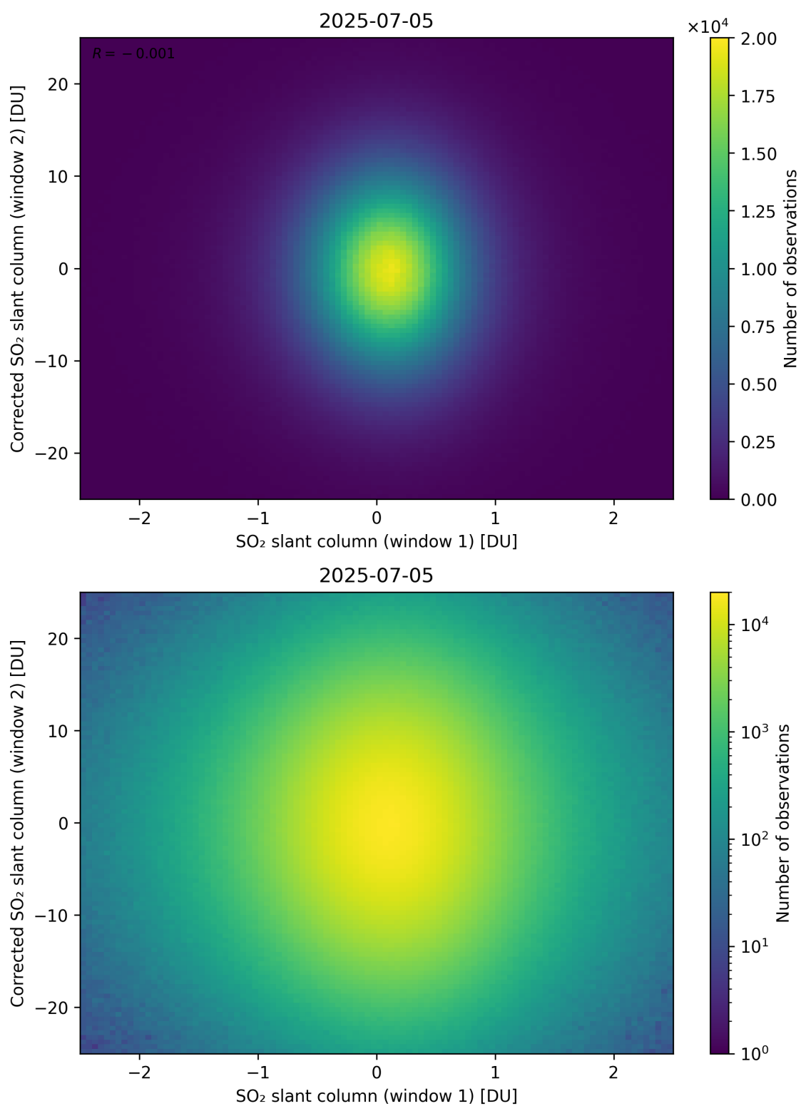
Figure 283: Scatter density plot of “SO 2 slant column (window 1)” against “Corrected SO 2 slant column (window 2)” for 2025-07-04 to 2025-07-06.
