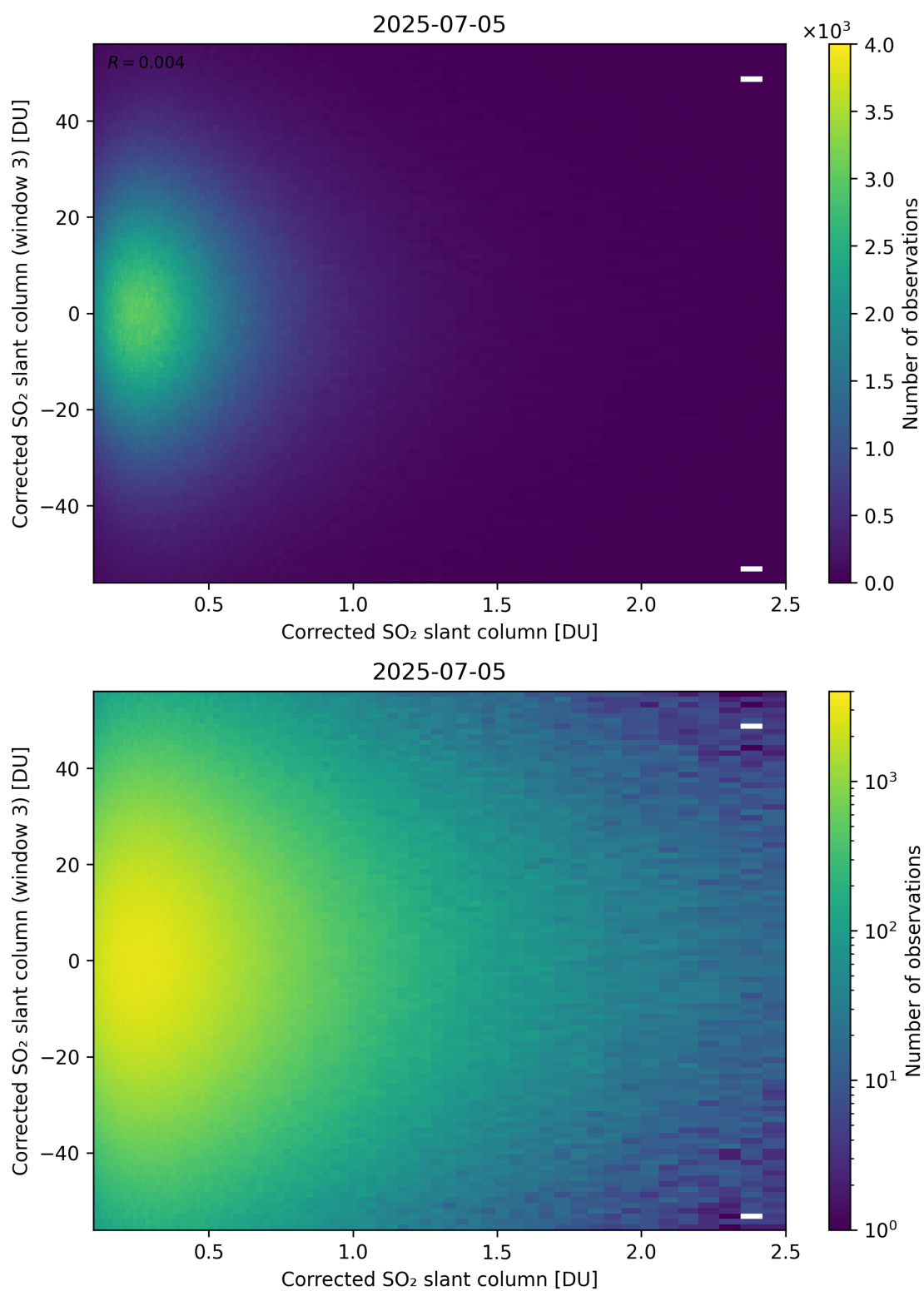
Figure 236: Scatter density plot of “Corrected SO 2 slant column” against “Corrected SO 2 slant column (window 3)” for 2025-07-04 to 2025-07-06.
