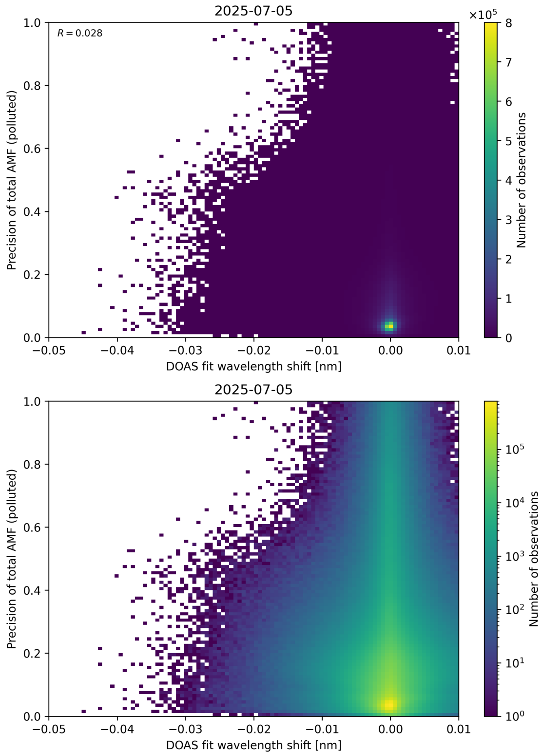
Figure 142: Scatter density plot of “DOAS fit wavelength shift” against “Precision of total AMF (polluted)” for 2025-07-04 to 2025-07-06.
