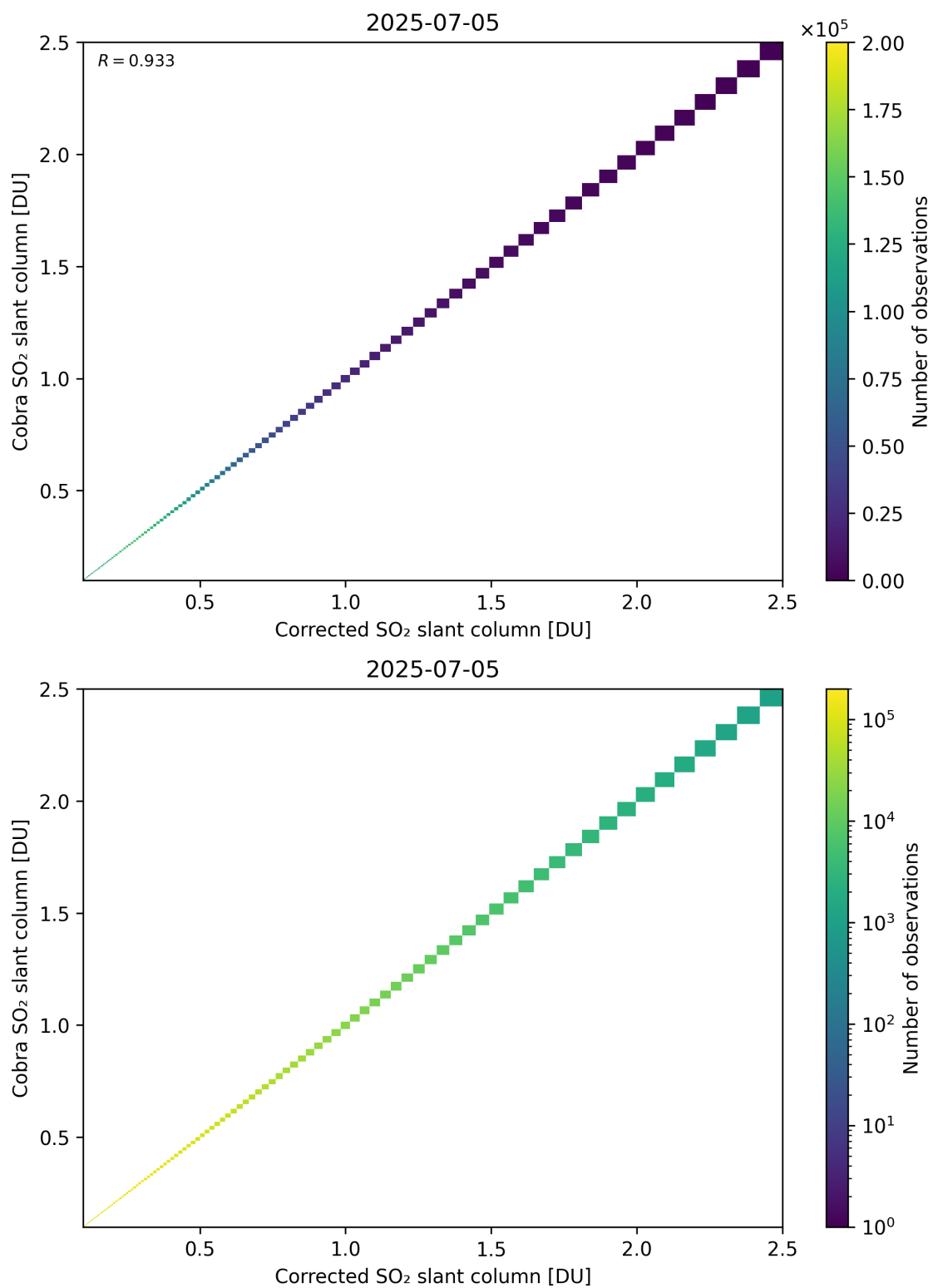
Figure 233: Scatter density plot of “Corrected SO 2 slant column” against “Cobra SO 2 slant column” for 2025-07-04 to 2025-07-06.
