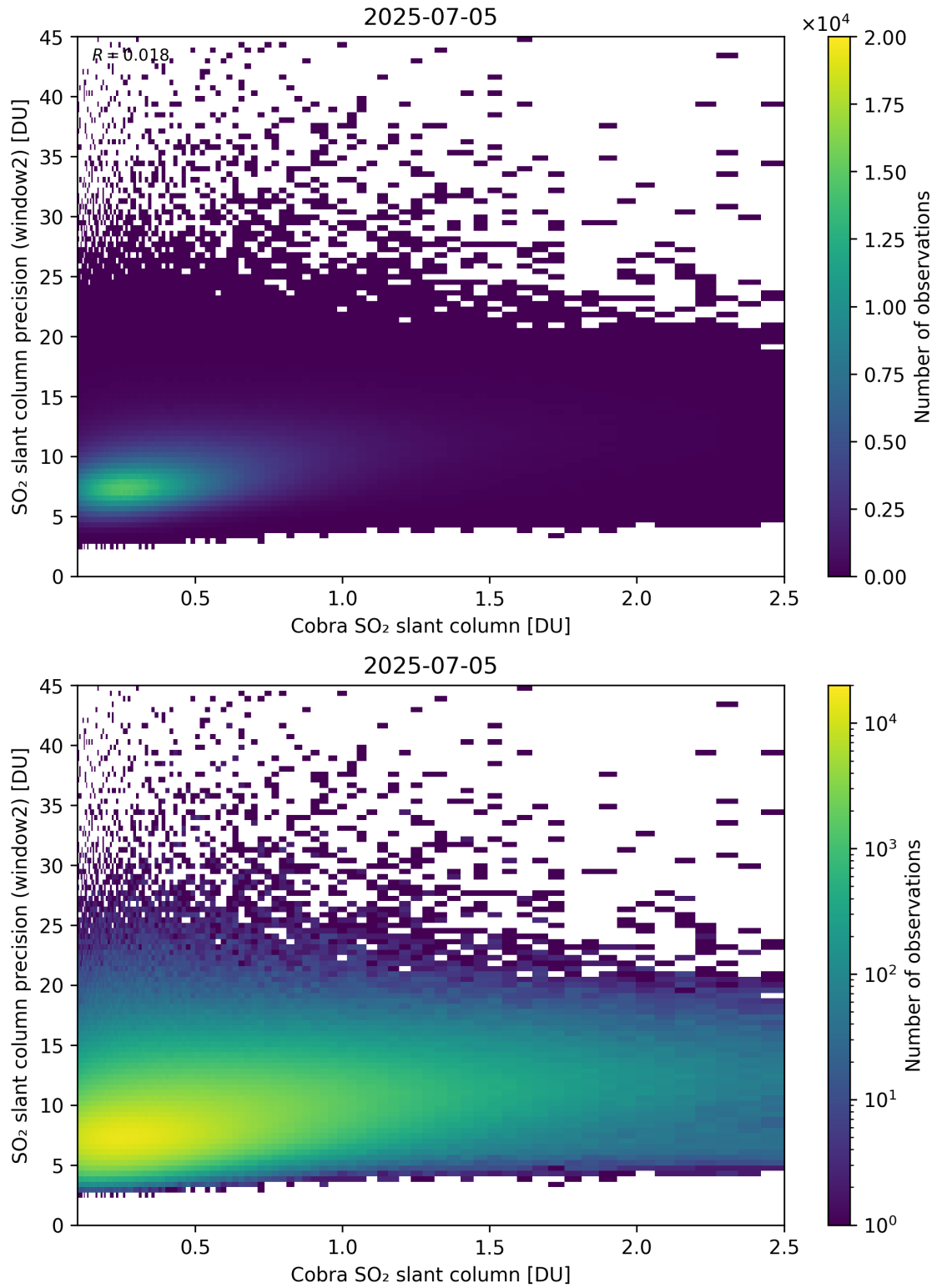
Figure 221: Scatter density plot of “Cobra SO 2 slant column” against “SO 2 slant column precision (window2)” for 2025-07-04 to 2025-07-06.
