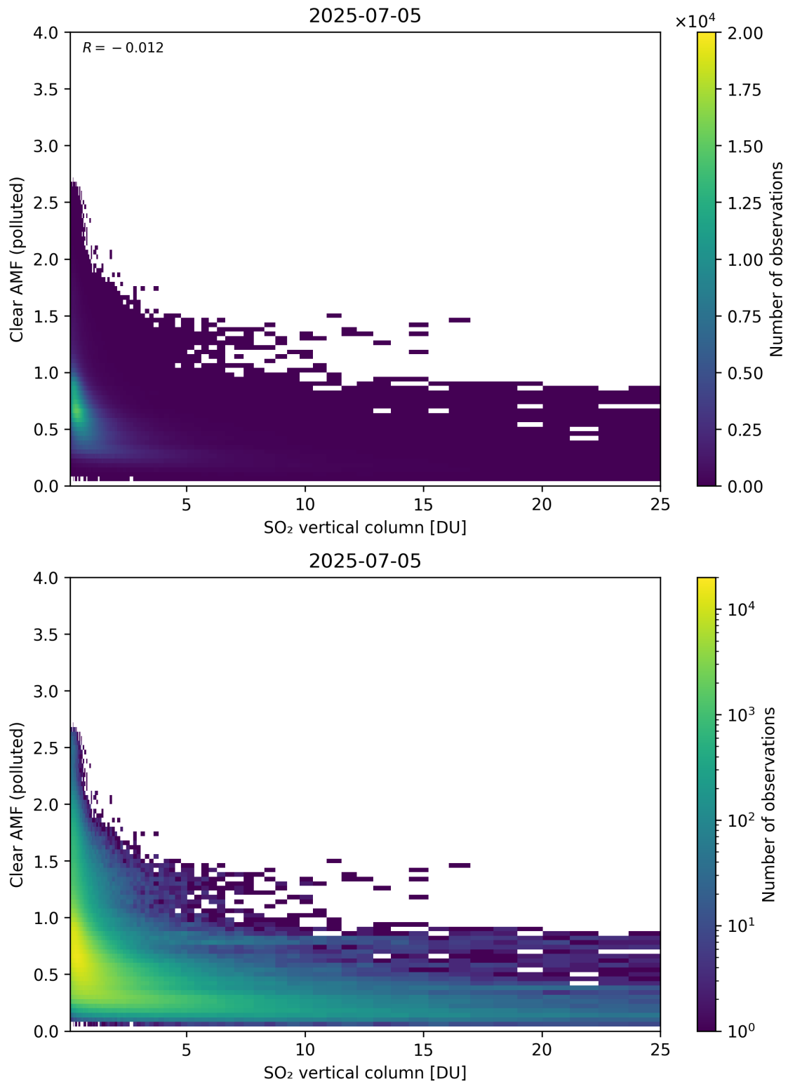
Figure 348: Scatter density plot of “SO 2 vertical column” against “Clear AMF (polluted)” for 2025-07-04 to 2025-07-06.
