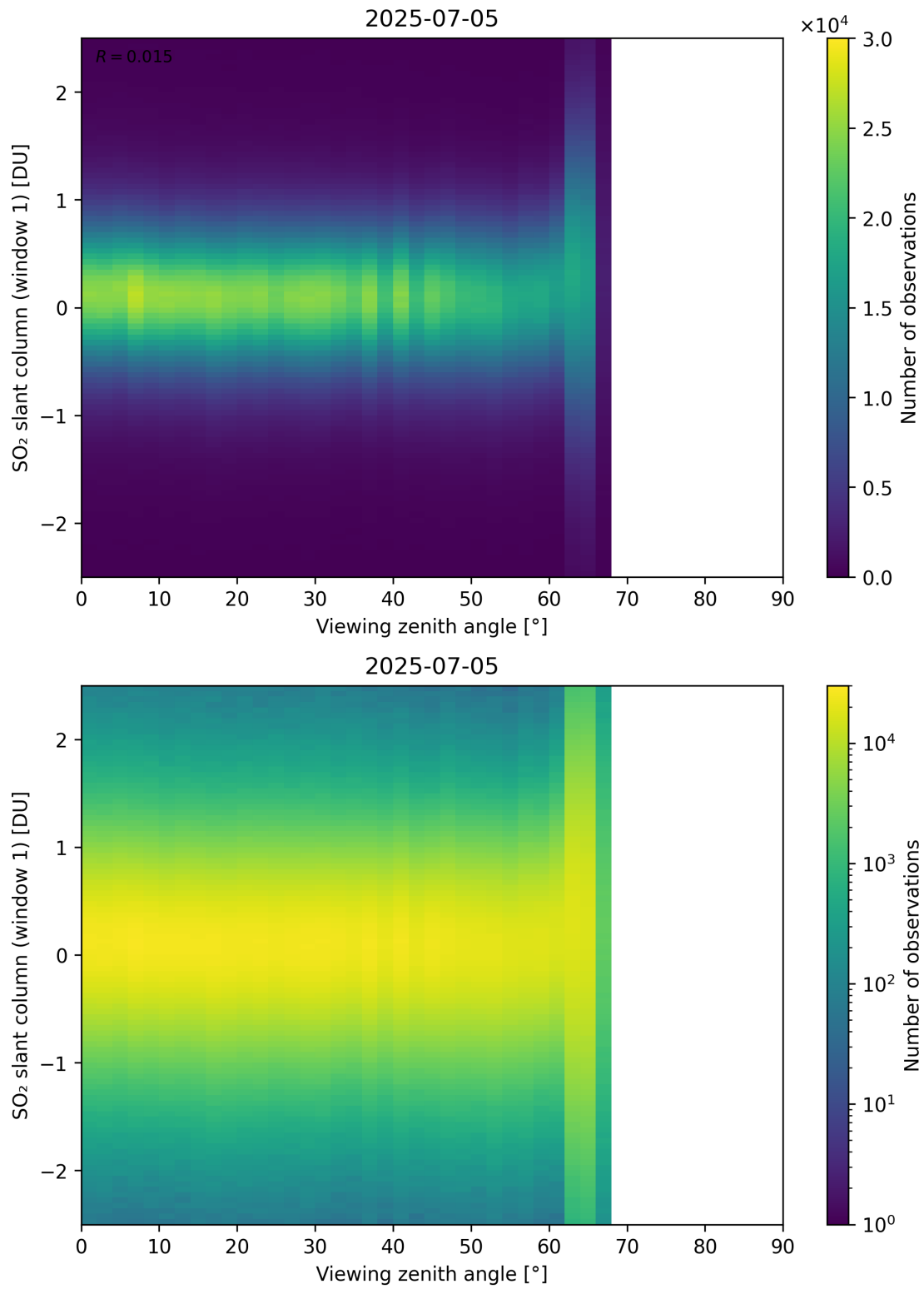
Figure 376: Scatter density plot of “Viewing zenith angle” against “SO 2 slant column (window 1)” for 2025-07-04 to 2025-07-06.
