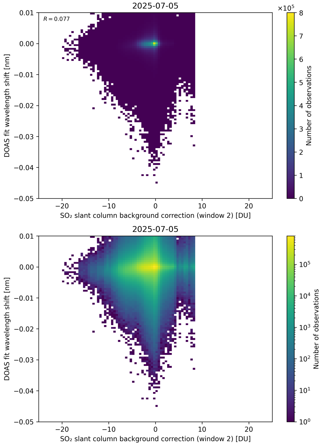
Figure 123: Scatter density plot of “SO 2 slant column background correction (window 2)” against “DOAS fit wavelength shift” for 2025-07-04 to 2025-07-06.
