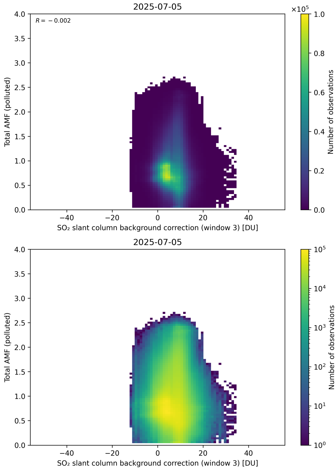
Figure 136: Scatter density plot of “SO 2 slant column background correction (window 3)” against “Total AMF (polluted)” for 2025-07-04 to 2025-07-06.
