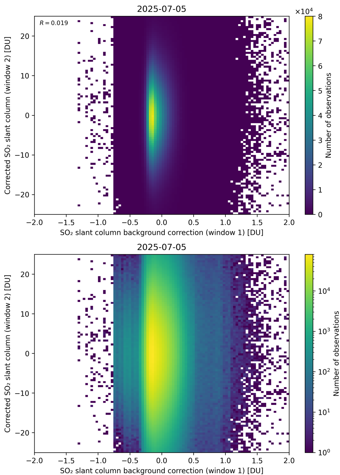
Figure 115: Scatter density plot of “SO 2 slant column background correction (window 1)” against “Corrected SO 2 slant column (window 2)” for 2025-07-04 to 2025-07-06.
