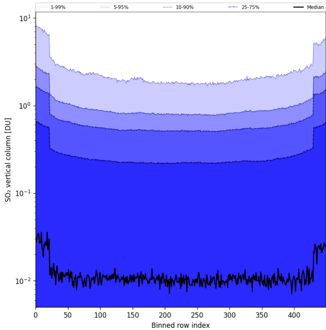
Figure 84: Along track statistics of “SO 2 vertical column” for 2025-07-04 to 2025-07-06
