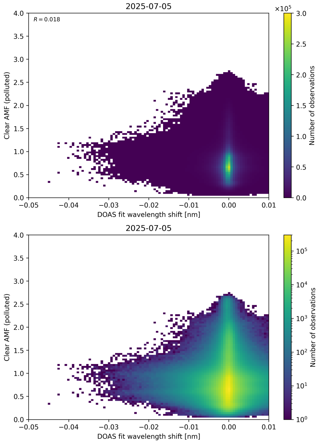
Figure 140: Scatter density plot of “DOAS fit wavelength shift” against “Clear AMF (polluted)” for 2025-07-04 to 2025-07-06.
