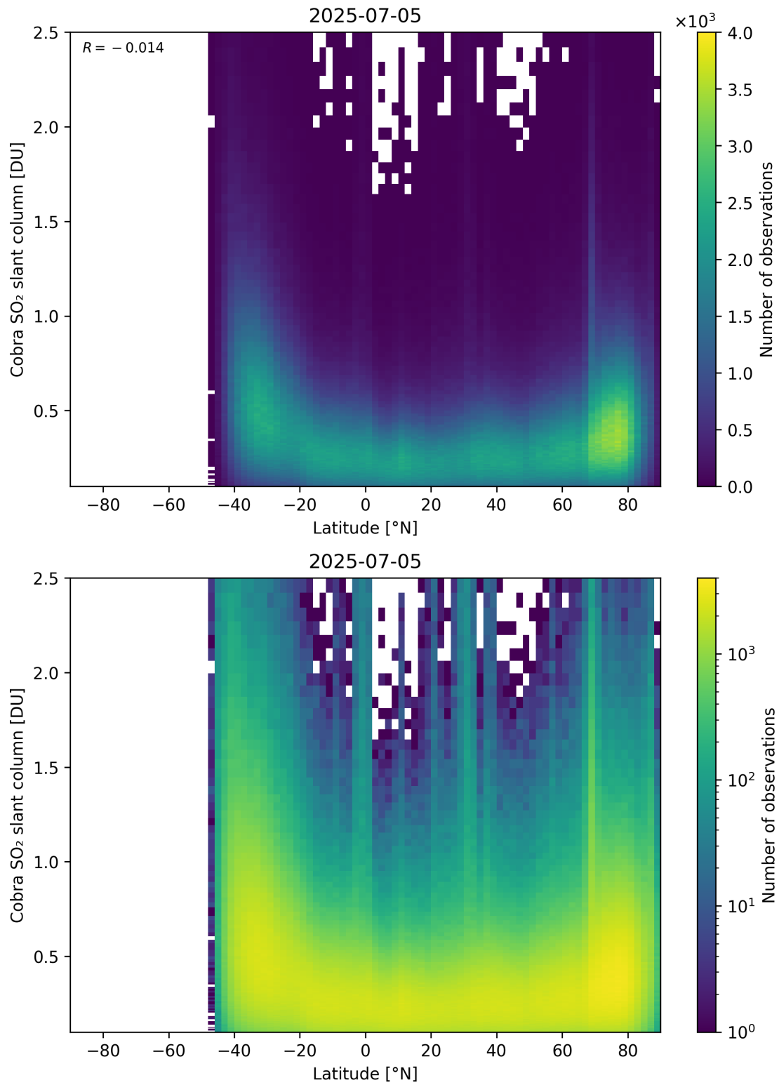
Figure 157: Scatter density plot of “Latitude” against “Cobra SO 2 slant column” for 2025-07-04 to 2025-07-06.
