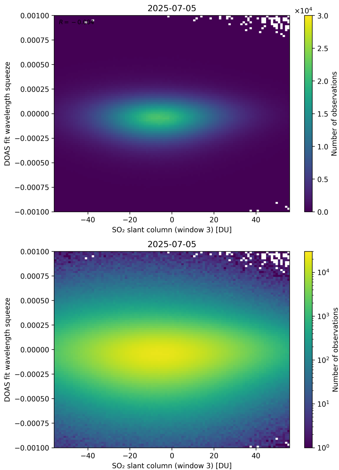
Figure 305: Scatter density plot of “SO 2 slant column (window 3)” against “DOAS fit wavelength squeeze” for 2025-07-04 to 2025-07-06.
