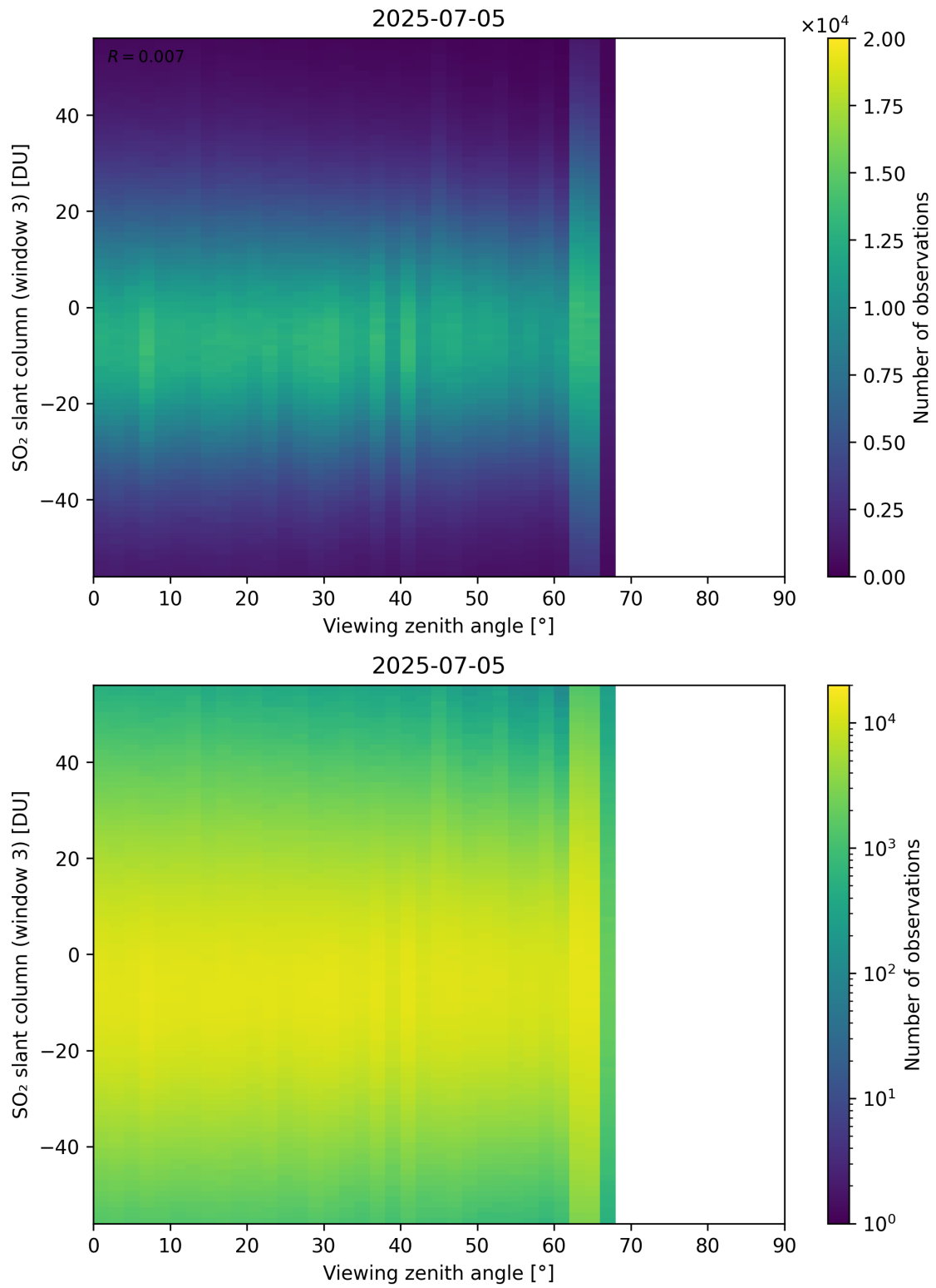
Figure 379: Scatter density plot of “Viewing zenith angle” against “SO 2 slant column (window 3)” for 2025-07-04 to 2025-07-06.
