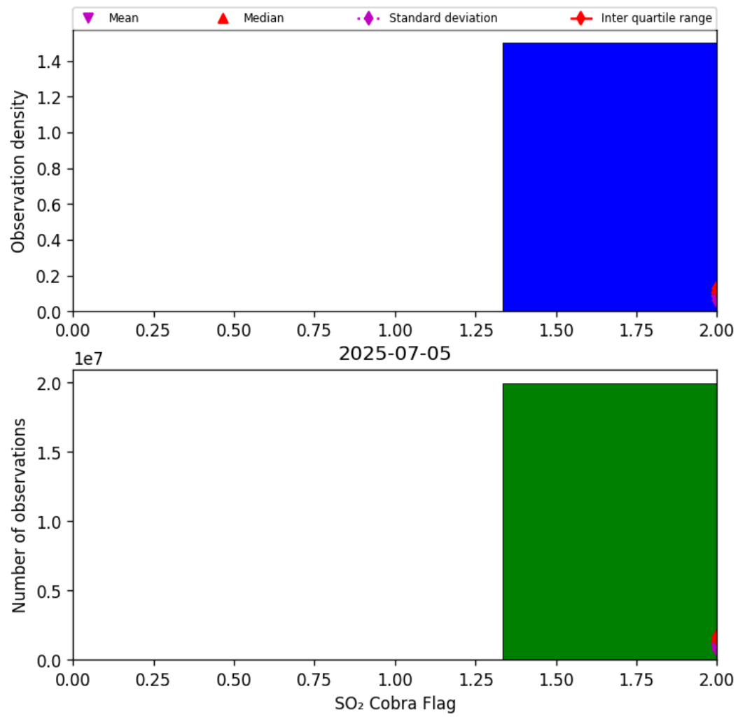
Figure 75: Histogram of “SO 2 Cobra Flag” for 2025-07-04 to 2025-07-06
