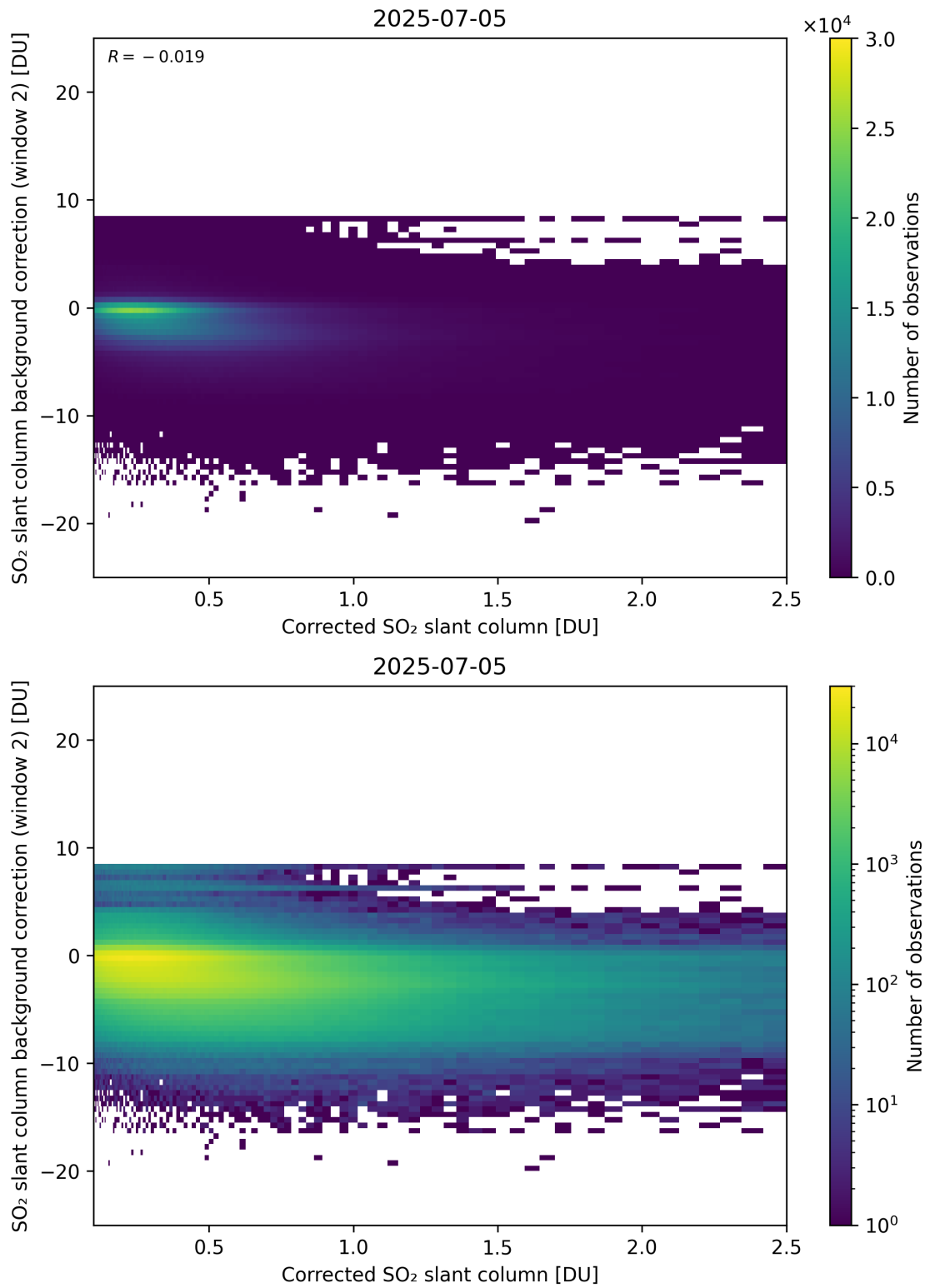
Figure 227: Scatter density plot of “Corrected SO 2 slant column” against “SO 2 slant column background correction (window 2)” for 2025-07-04 to 2025-07-06.
