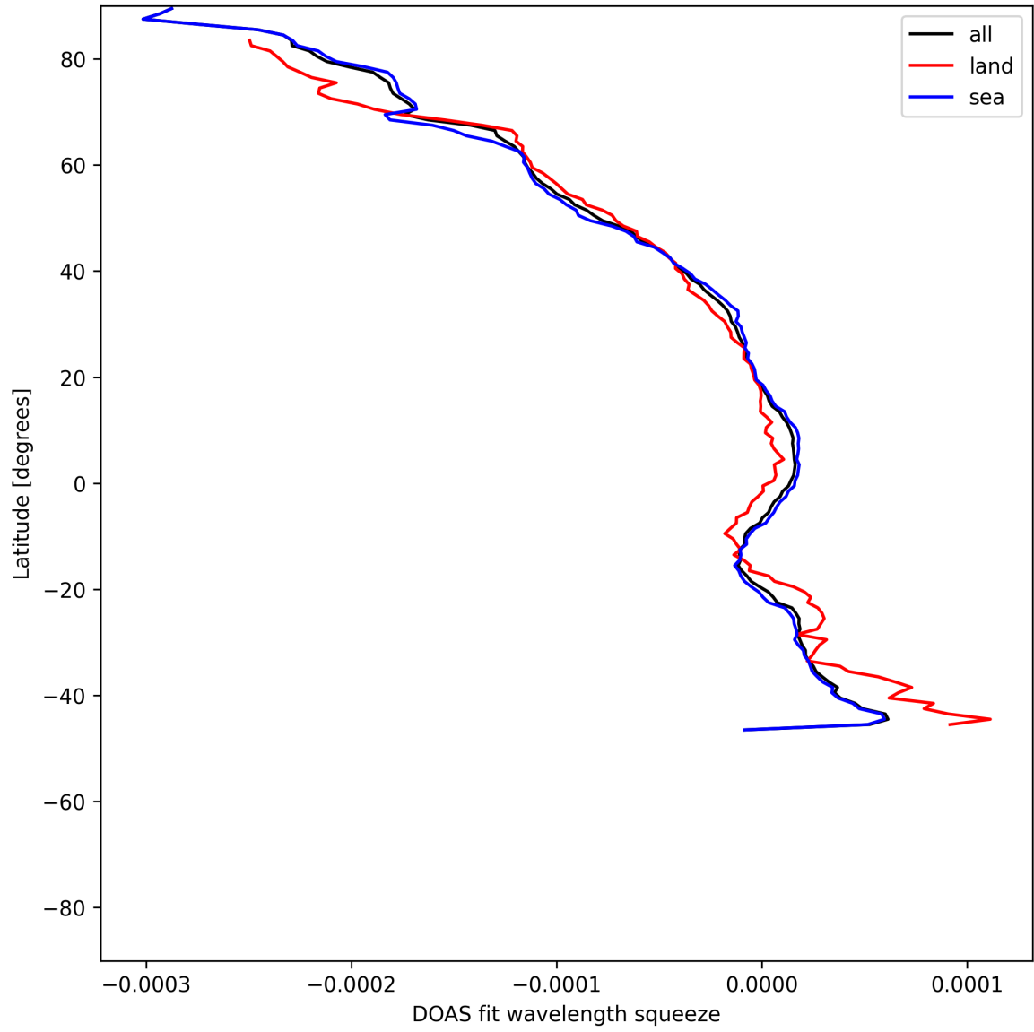
Figure 51: Zonal average of “DOAS fit wavelength squeeze” for 2025-07-04 to 2025-07-06.
