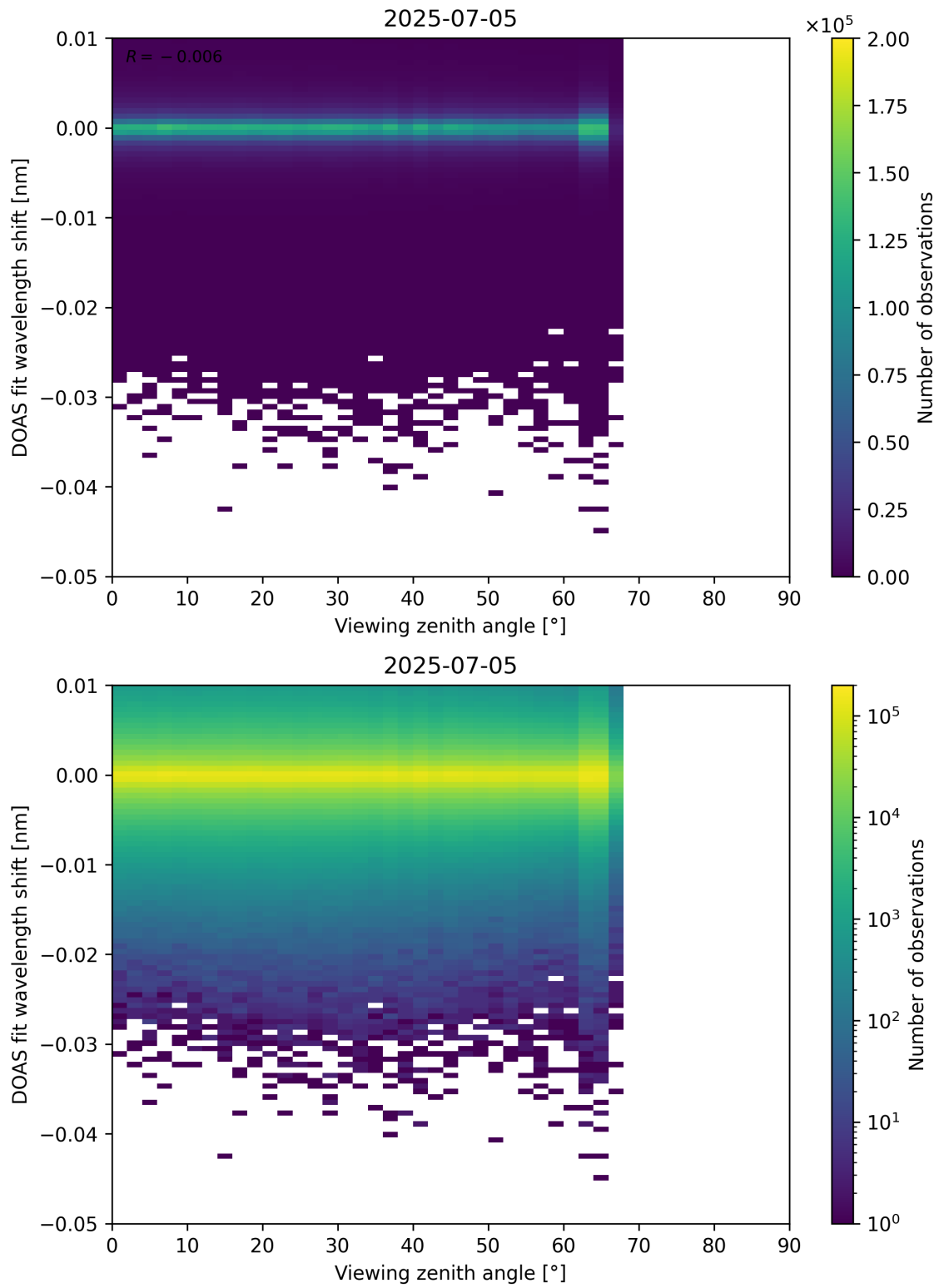
Figure 365: Scatter density plot of “Viewing zenith angle” against “DOAS fit wavelength shift” for 2025-07-04 to 2025-07-06.
