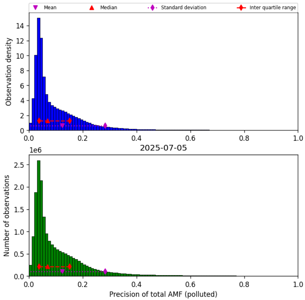
Figure 80: Histogram of “Precision of total AMF (polluted)” for 2025-07-04 to 2025-07-06
