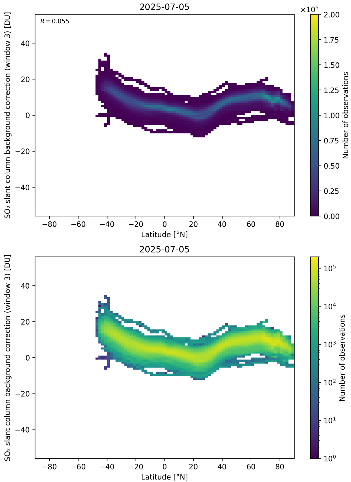
Figure 152: Scatter density plot of “Latitude” against “SO 2 slant column background correction (window 3)” for 2025-07-04 to 2025-07-06.
