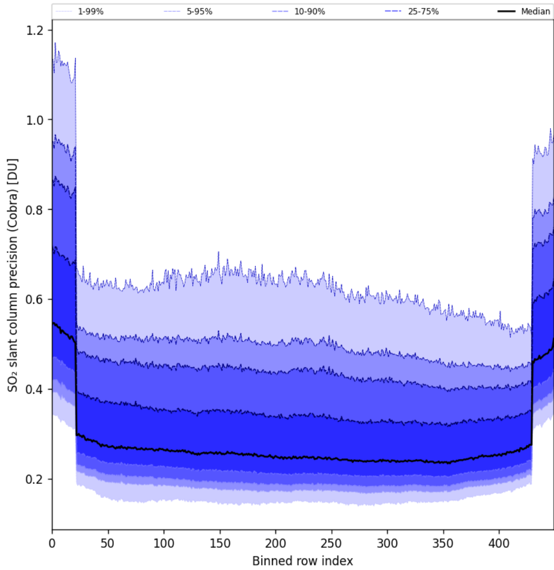
Figure 88: Along track statistics of “SO 2 slant column precision (Cobra)” for 2025-07-04 to 2025-07-06
