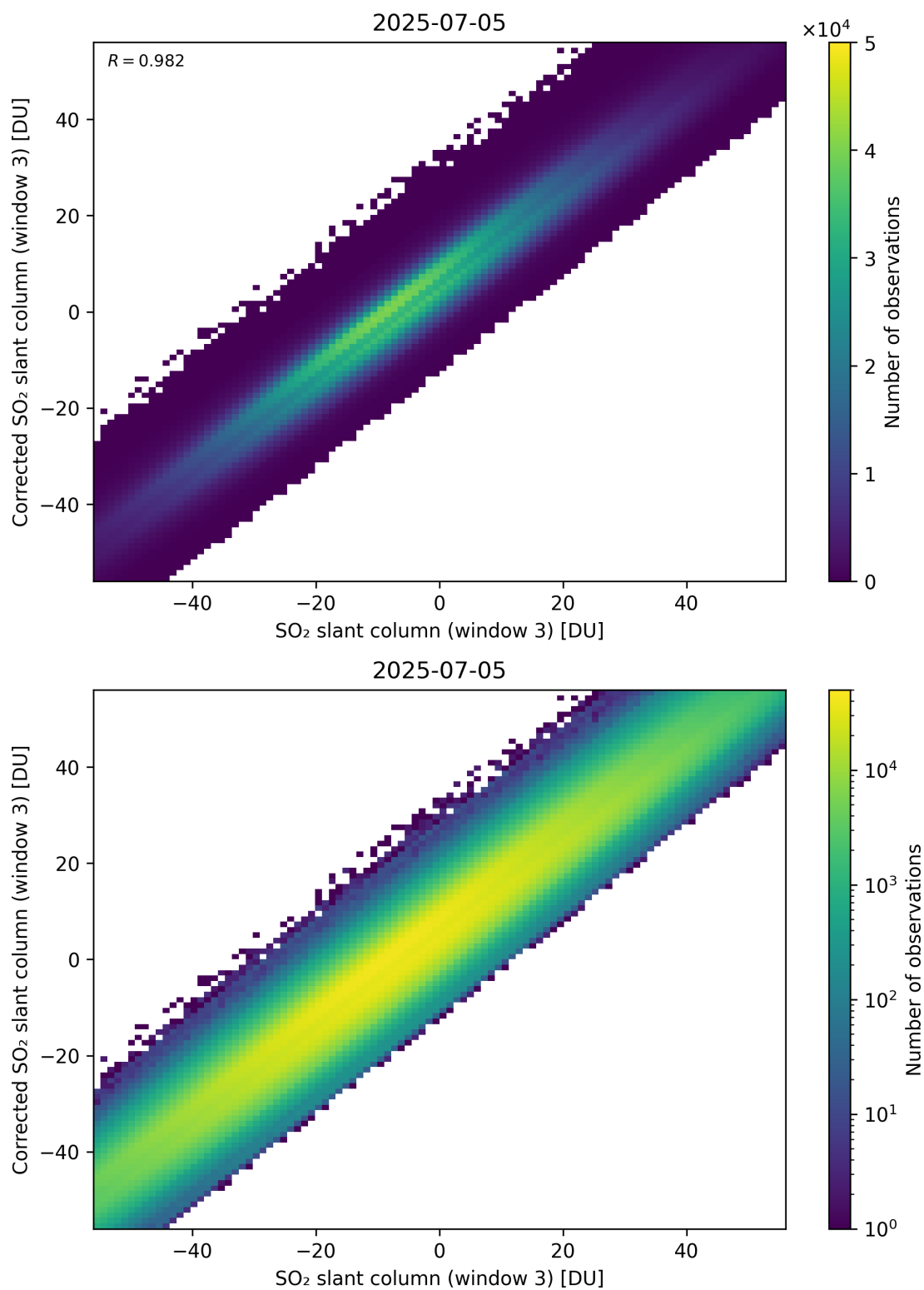
Figure 316: Scatter density plot of “SO 2 slant column (window 3)” against “Corrected SO 2 slant column (window 3)” for 2025-07-04 to 2025-07-06.
