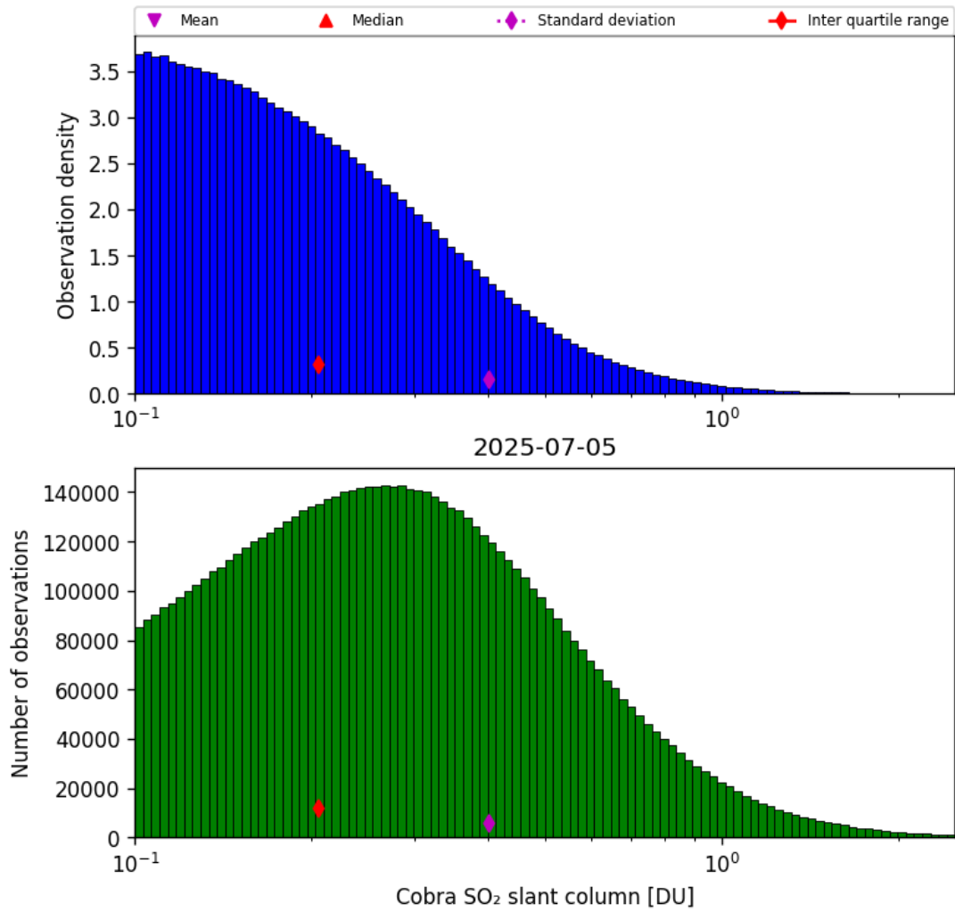
Figure 61: Histogram of “Cobra SO 2 slant column” for 2025-07-04 to 2025-07-06
