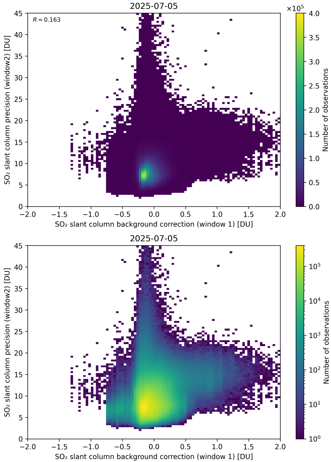
Figure 117: Scatter density plot of “SO 2 slant column background correction (window 1)” against “SO 2 slant column precision (window2)” for 2025-07-04 to 2025-07-06.
