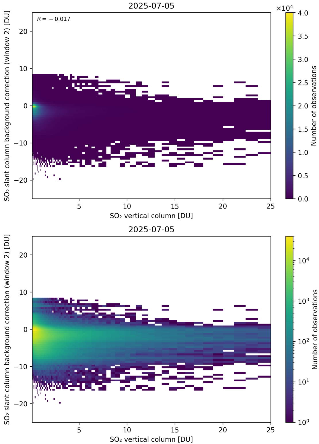
Figure 324: Scatter density plot of “SO 2 vertical column” against “SO 2 slant column background correction (window 2)” for 2025-07-04 to 2025-07-06.
