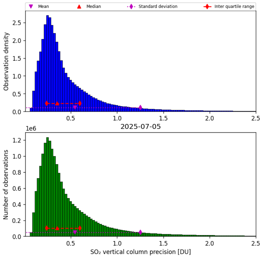
Figure 59: Histogram of “SO 2 vertical column precision” for 2025-07-04 to 2025-07-06
