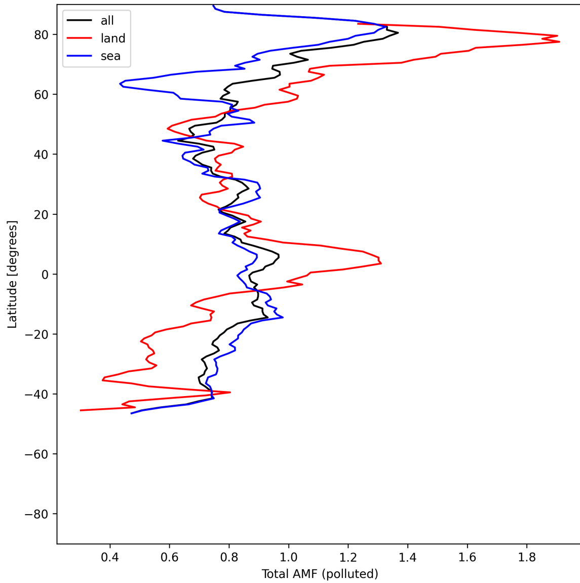
Figure 53: Zonal average of “Total AMF (polluted)” for 2025-07-04 to 2025-07-06.
