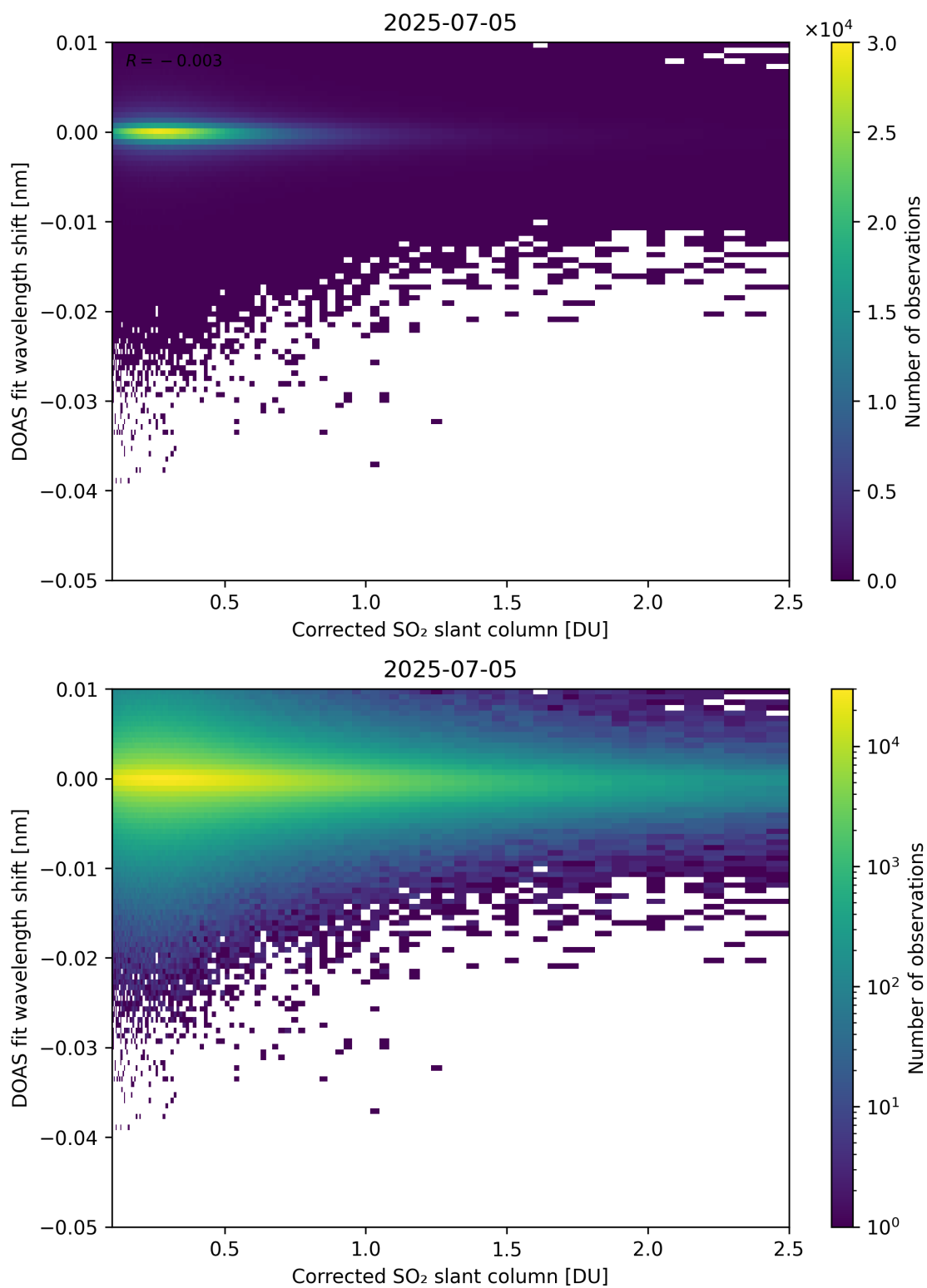
Figure 229: Scatter density plot of “Corrected SO 2 slant column” against “DOAS fit wavelength shift” for 2025-07-04 to 2025-07-06.
