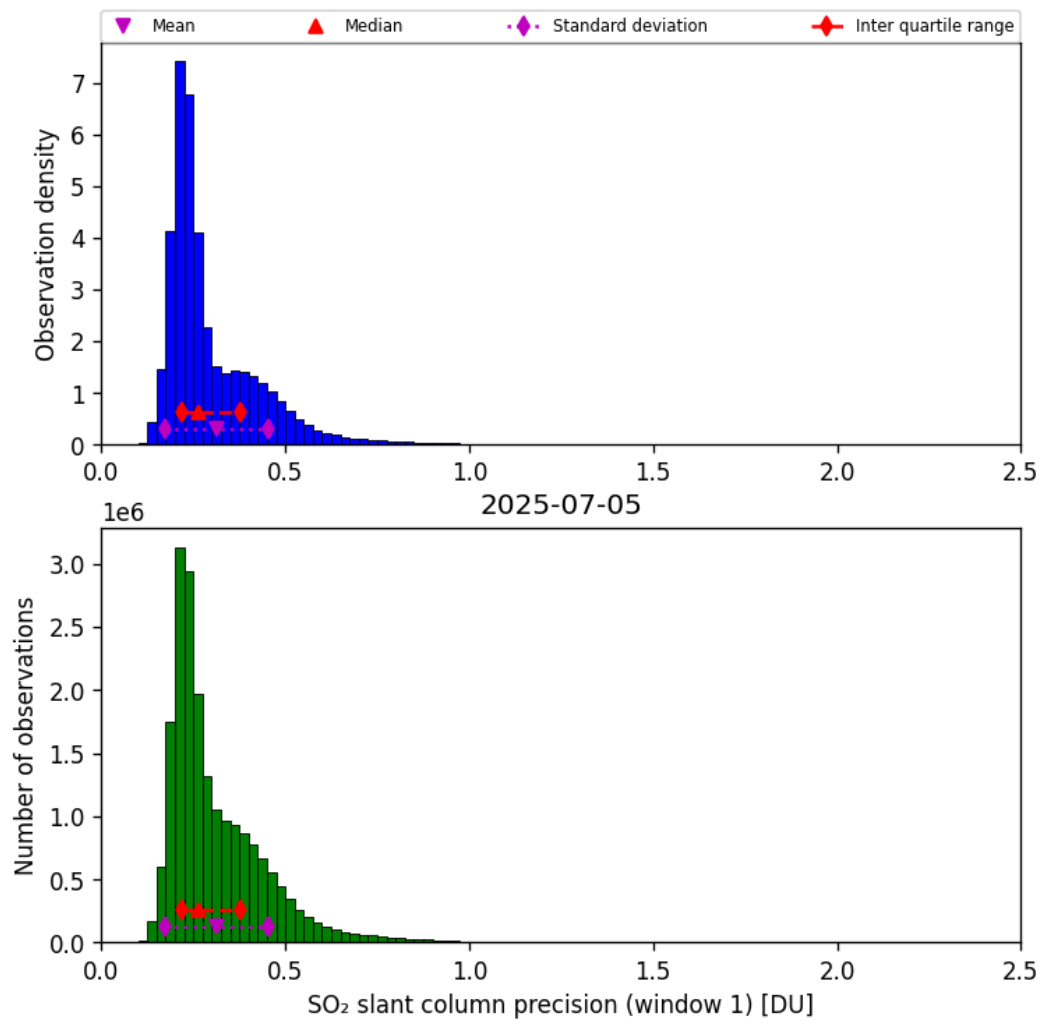
Figure 64: Histogram of “SO 2 slant column precision (window 1)” for 2025-07-04 to 2025-07-06
