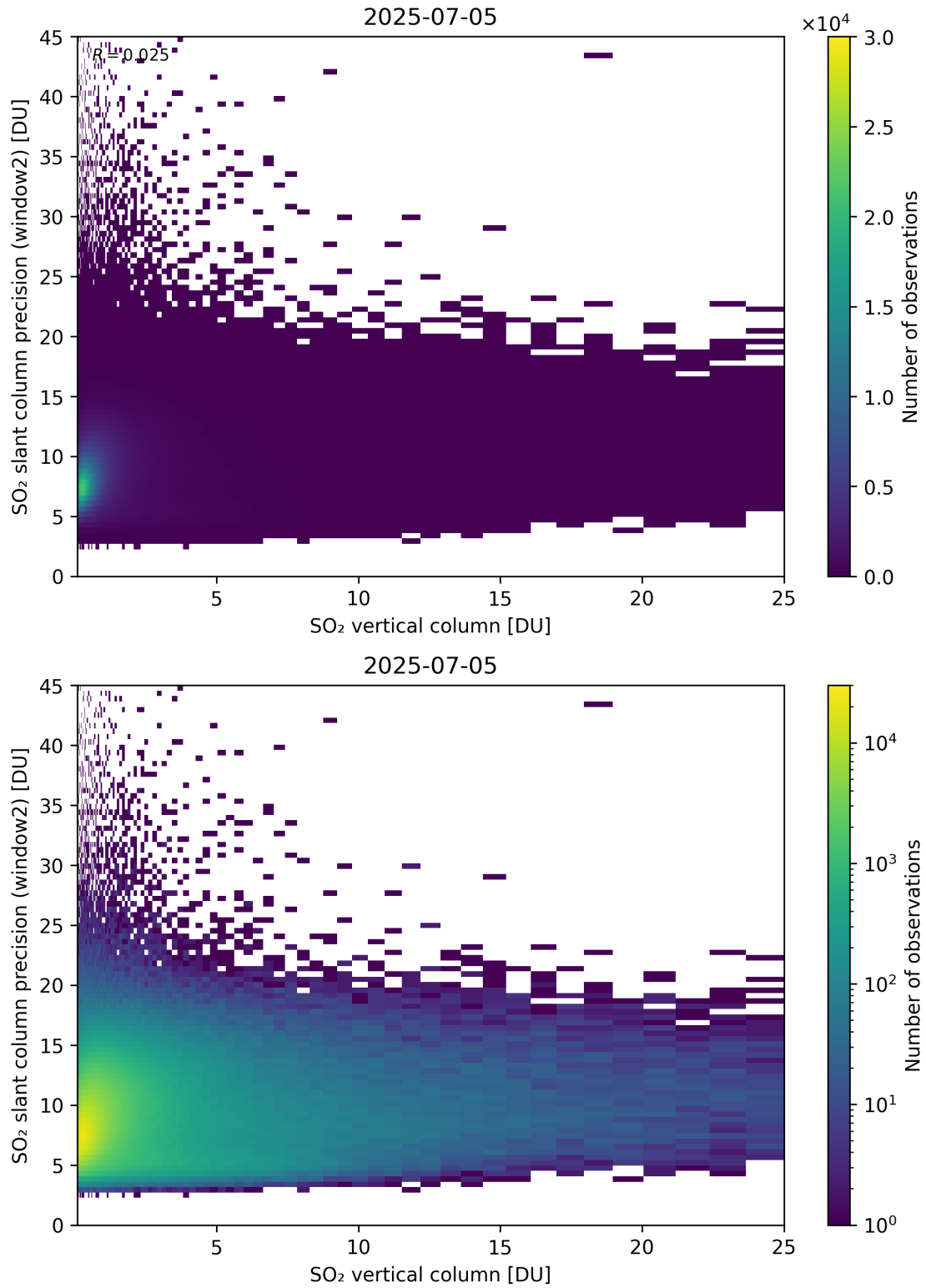
Figure 356: Scatter density plot of “SO 2 vertical column” against “SO 2 slant column precision (window2)” for 2025-07-04 to 2025-07-06.
