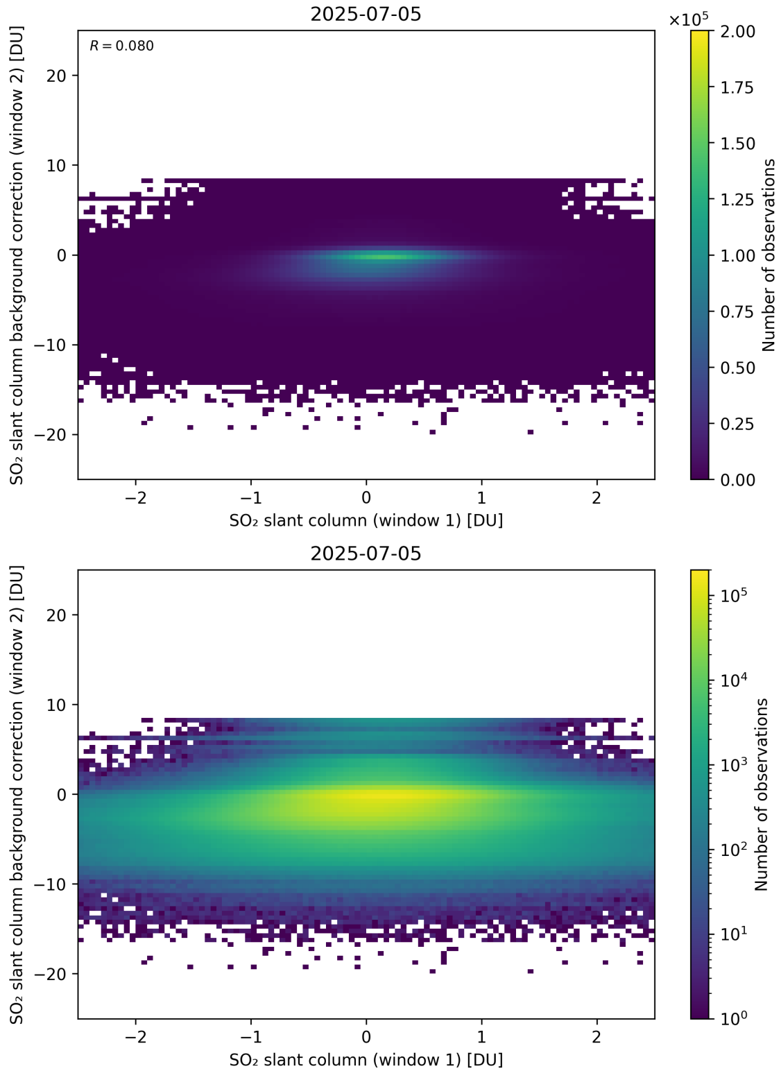
Figure 263: Scatter density plot of “SO 2 slant column (window 1)” against “SO 2 slant column background correction (window 2)” for 2025-07-04 to 2025-07-06.
