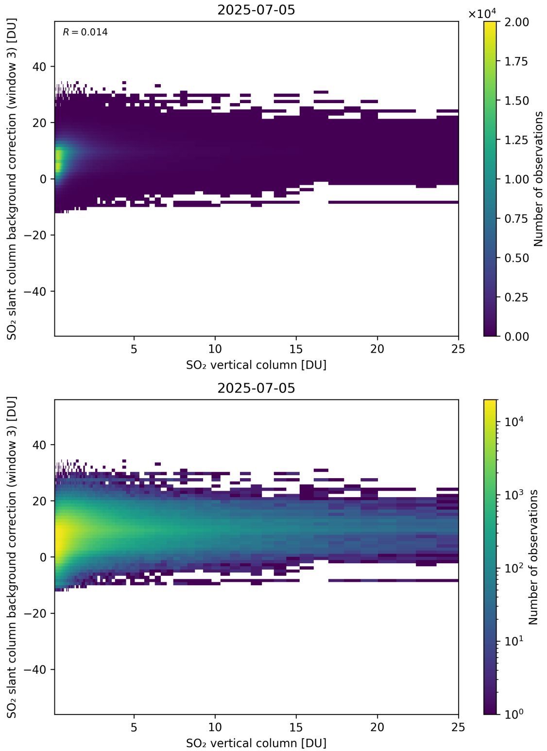
Figure 325: Scatter density plot of “SO 2 vertical column” against “SO 2 slant column background correction (window 3)” for 2025-07-04 to 2025-07-06.
