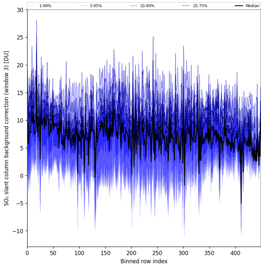
Figure 100: Along track statistics of “SO 2 slant column background correction (window 3)” for 2025-07-04 to 2025-07-06
