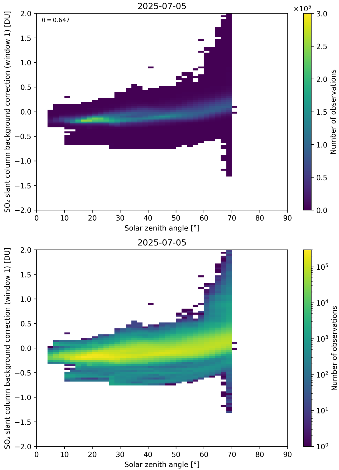
Figure 171: Scatter density plot of “Solar zenith angle” against “SO 2 slant column background correction (window 1)” for 2025-07-04 to 2025-07-06.
