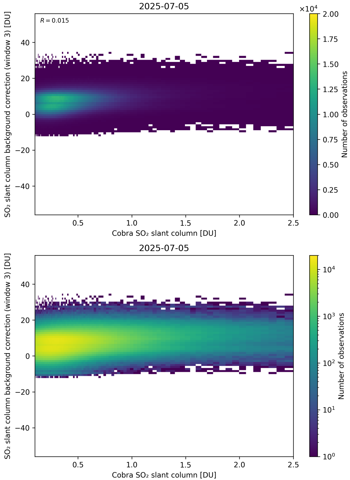
Figure 195: Scatter density plot of “Cobra SO 2 slant column” against “SO 2 slant column background correction (window 3)” for 2025-07-04 to 2025-07-06.
