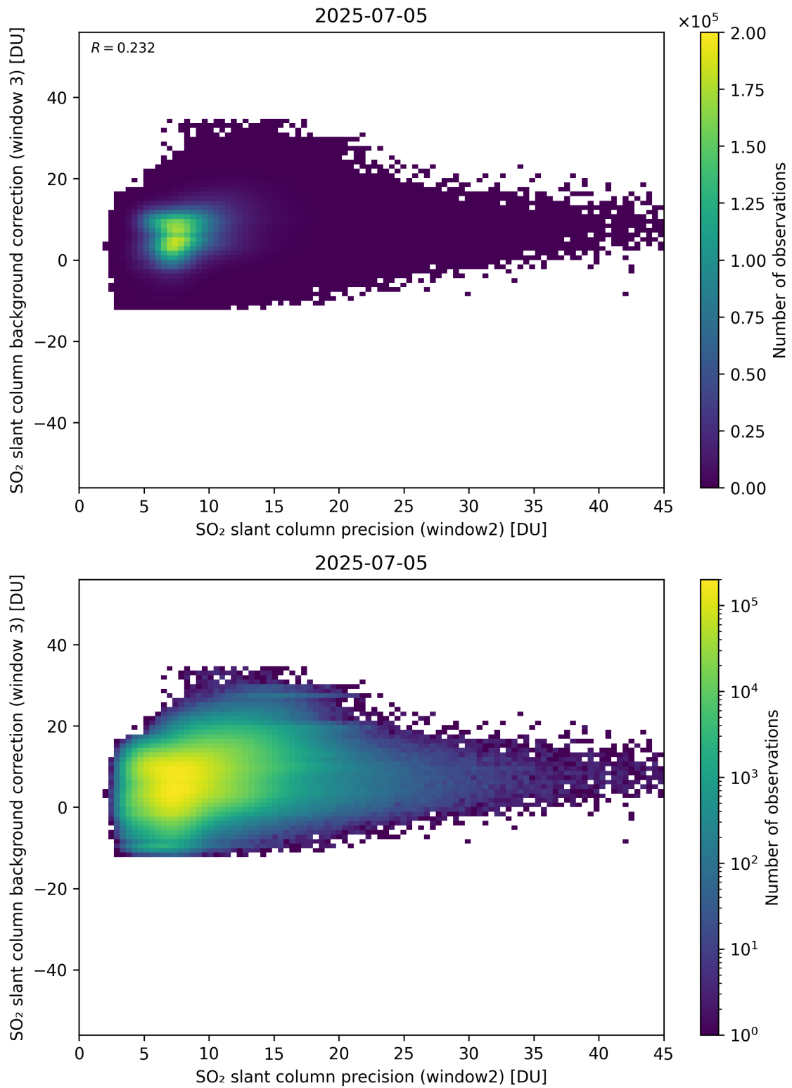
Figure 292: Scatter density plot of “SO 2 slant column precision (window2)” against “SO 2 slant column background correction (window 3)” for 2025-07-04 to 2025-07-06.
