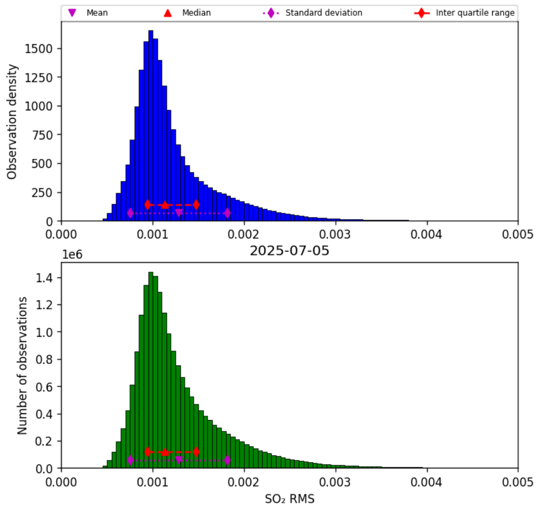
Figure 78: Histogram of “SO 2 RMS” for 2025-07-04 to 2025-07-06
