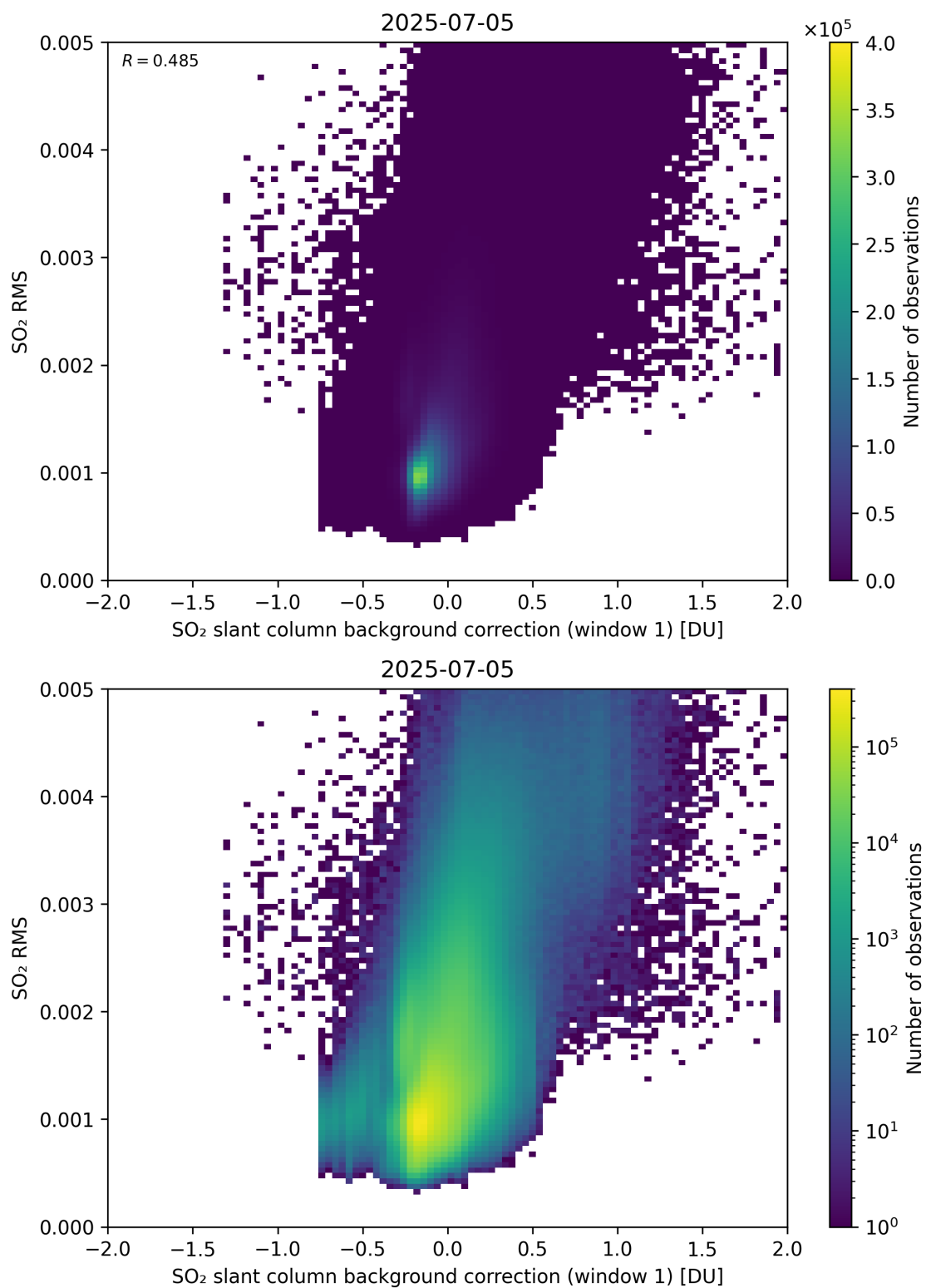
Figure 113: Scatter density plot of “SO 2 slant column background correction (window 1)” against “SO 2 RMS” for 2025-07-04 to 2025-07-06.
