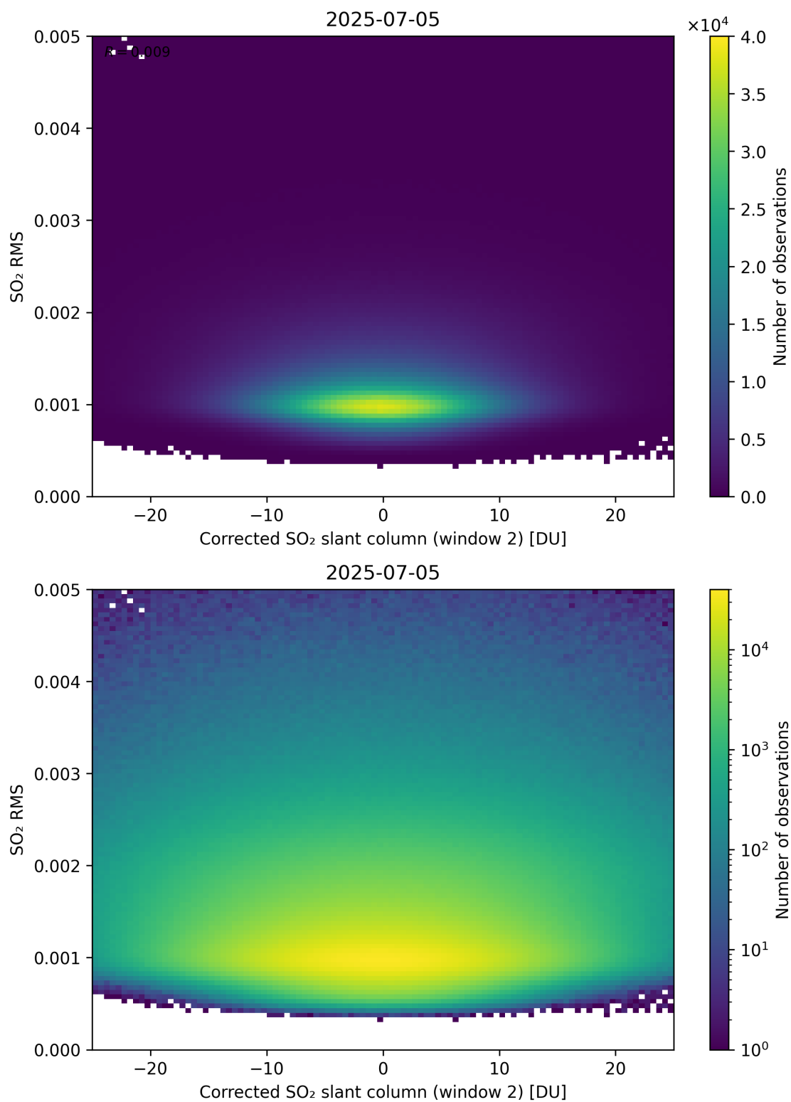
Figure 248: Scatter density plot of “Corrected SO 2 slant column (window 2)” against “SO 2 RMS” for 2025-07-04 to 2025-07-06.
