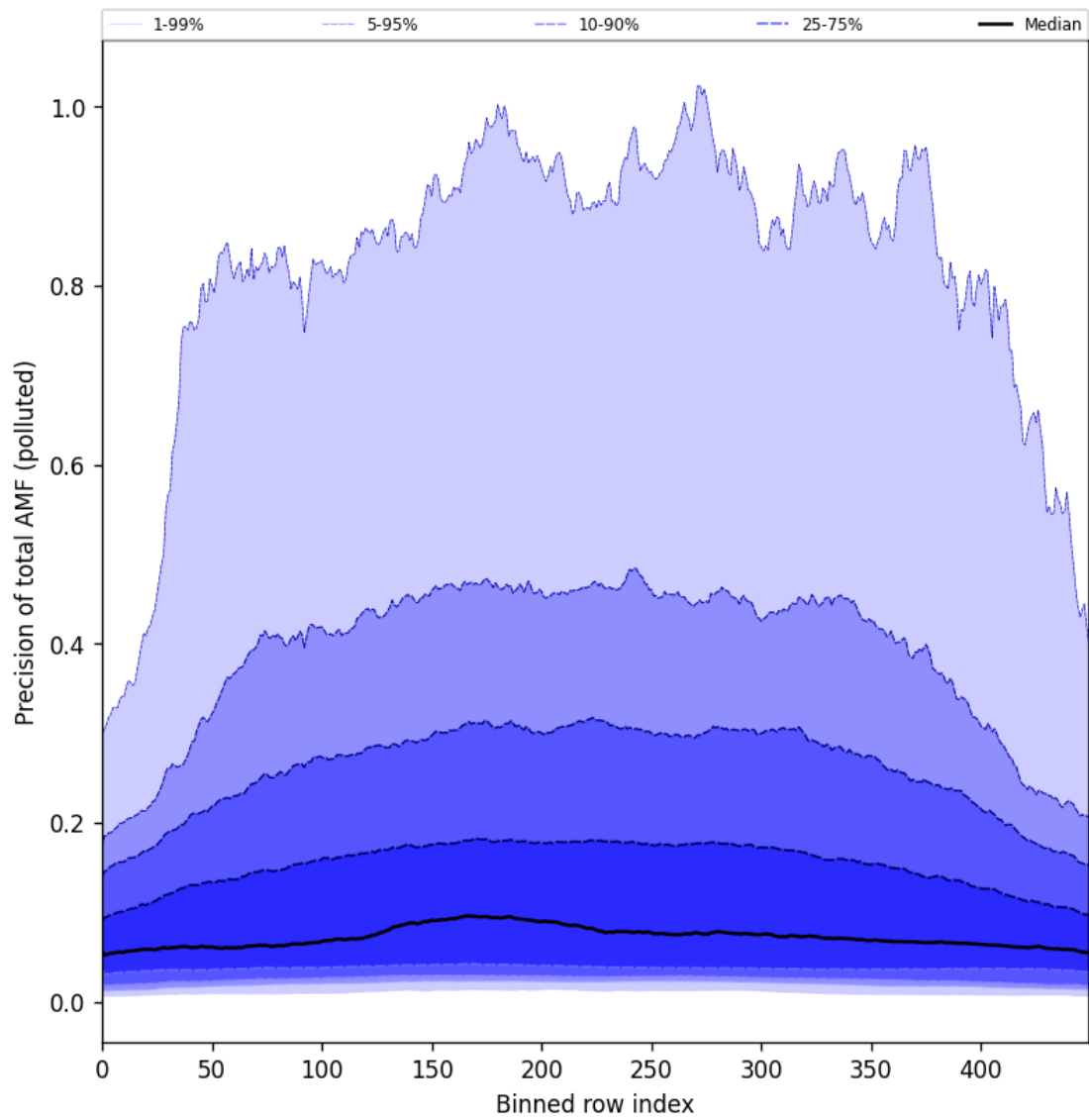
Figure 106: Along track statistics of “Precision of total AMF (polluted)” for 2025-07-04 to 2025-07-06
