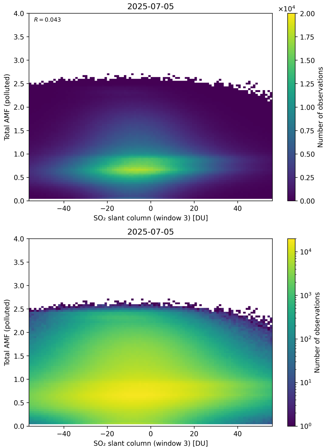
Figure 318: Scatter density plot of “SO 2 slant column (window 3)” against “Total AMF (polluted)” for 2025-07-04 to 2025-07-06.
