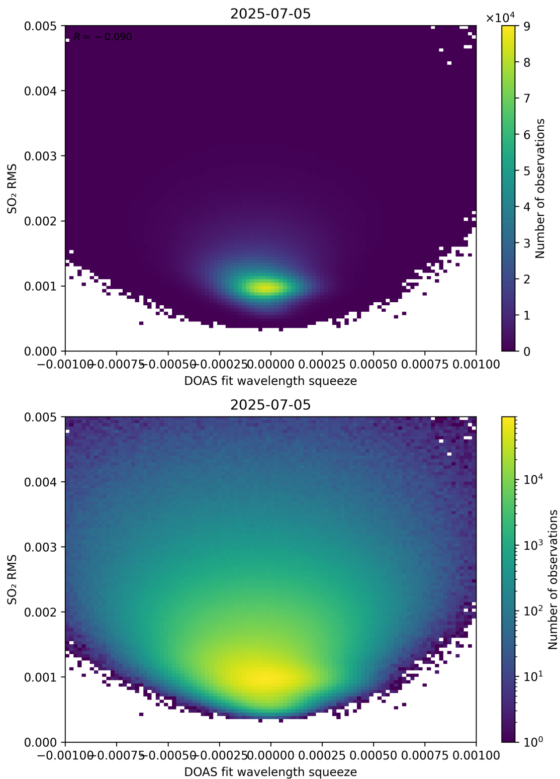
Figure 143: Scatter density plot of “DOAS fit wavelength squeeze” against “SO 2 RMS” for 2025-07-04 to 2025-07-06.
