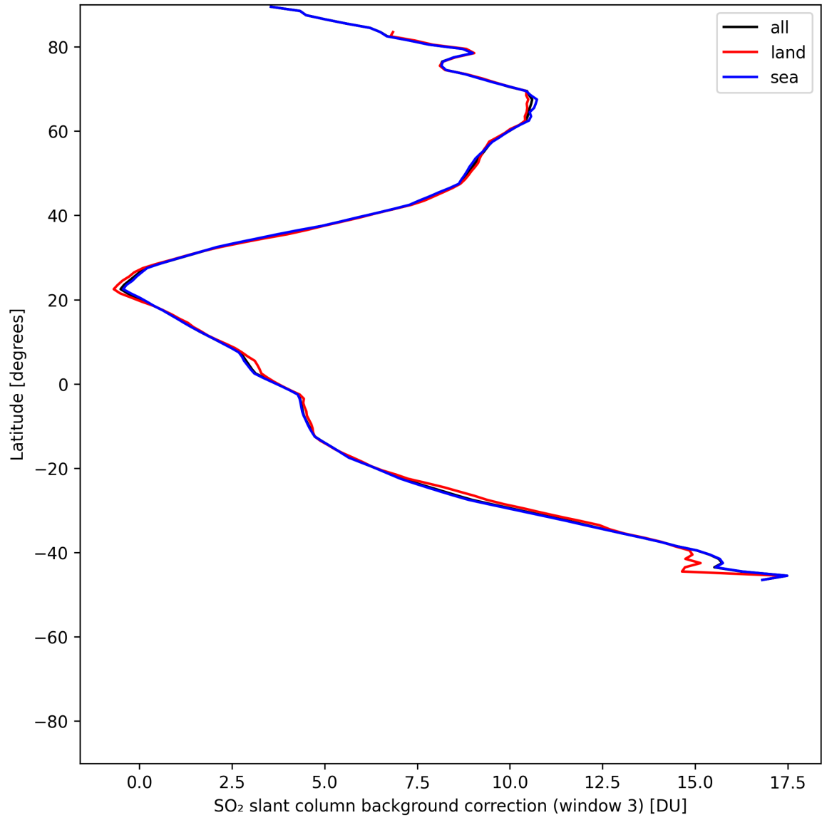
Figure 48: Zonal average of “SO 2 slant column background correction (window 3)” for 2025-07-04 to 2025-07-06.
