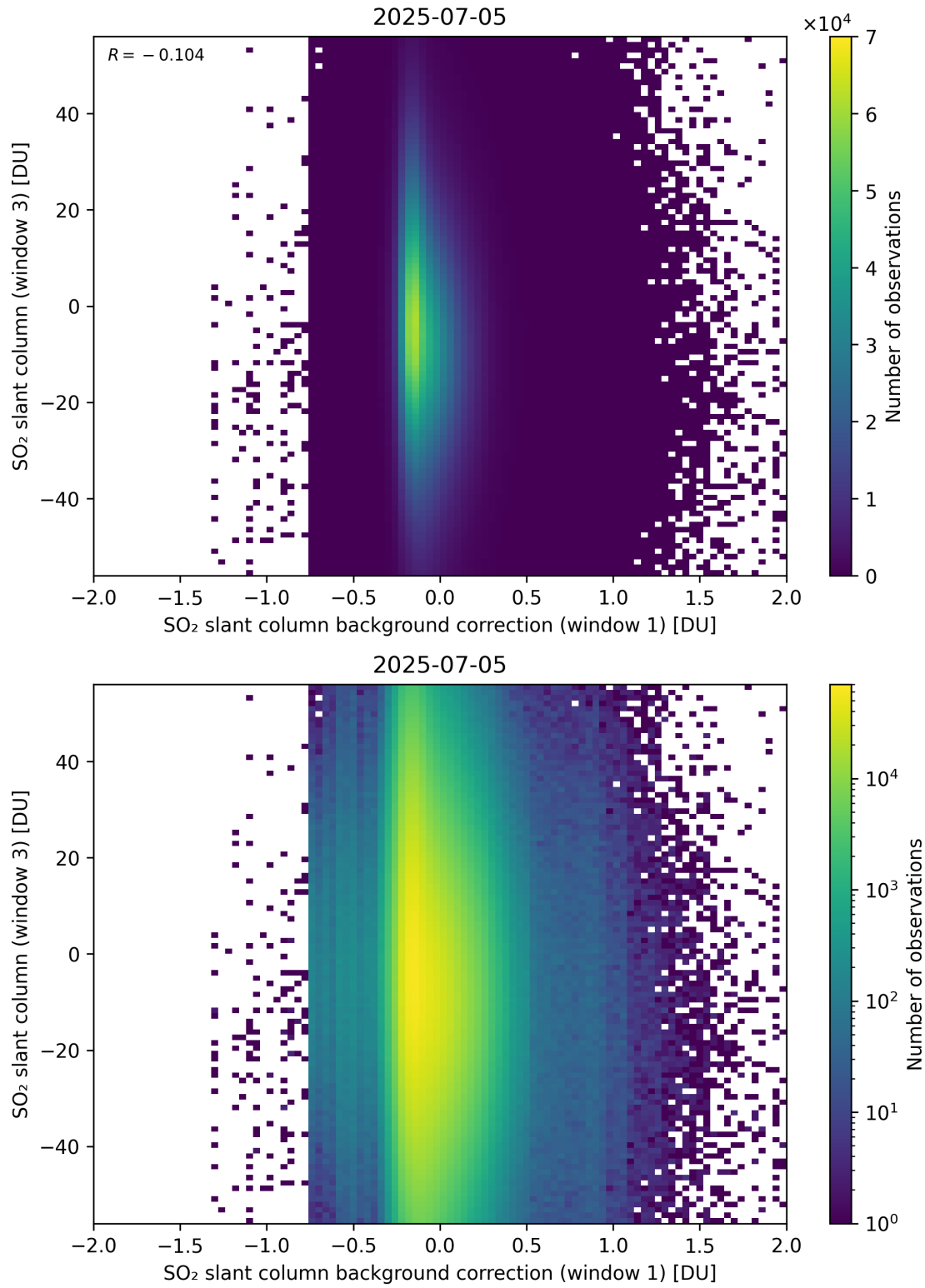
Figure 118: Scatter density plot of “SO 2 slant column background correction (window 1)” against “SO 2 slant column (window 3)” for 2025-07-04 to 2025-07-06.
