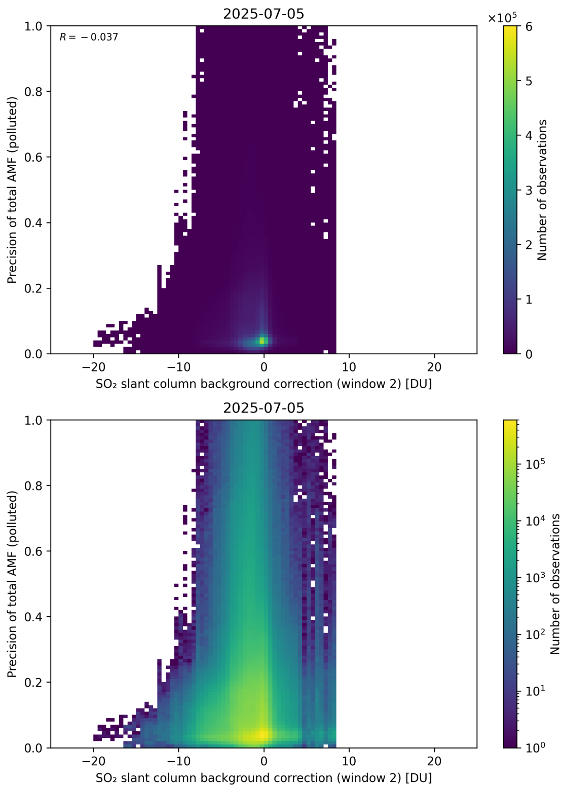
Figure 131: Scatter density plot of “SO 2 slant column background correction (window 2)” against “Precision of total AMF (polluted)” for 2025-07-04 to 2025-07-06.
