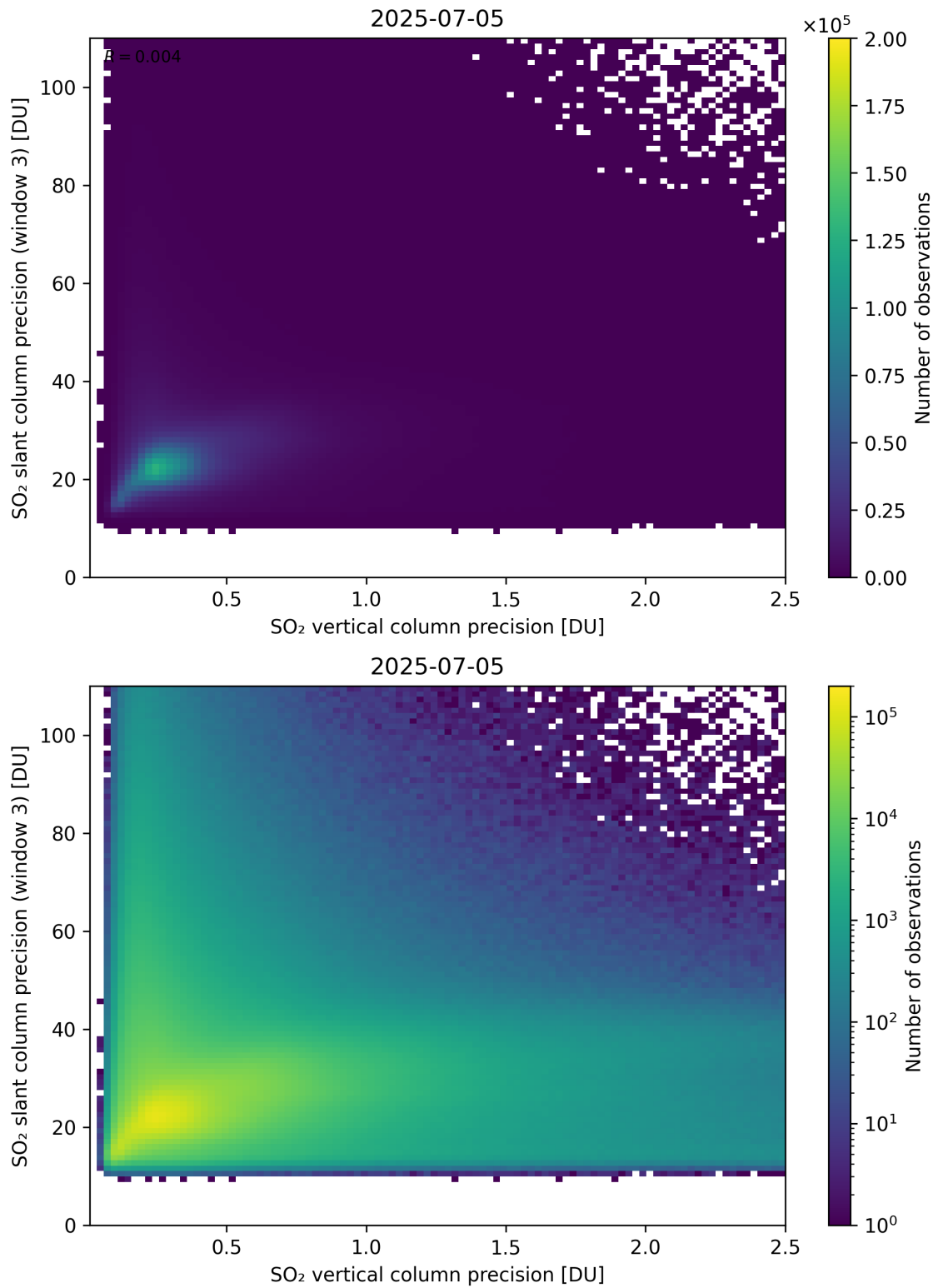
Figure 345: Scatter density plot of “SO 2 vertical column precision” against “SO 2 slant column precision (window 3)” for 2025-07-04 to 2025-07-06.
