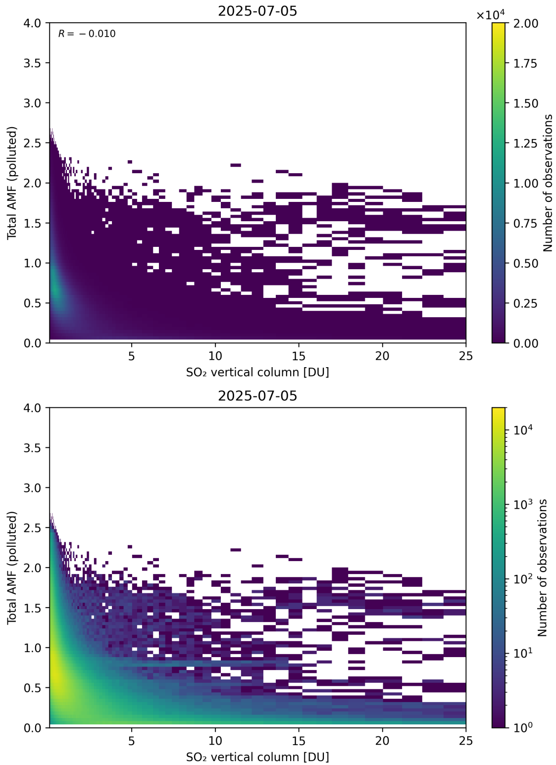
Figure 359: Scatter density plot of “SO 2 vertical column” against “Total AMF (polluted)” for 2025-07-04 to 2025-07-06.
