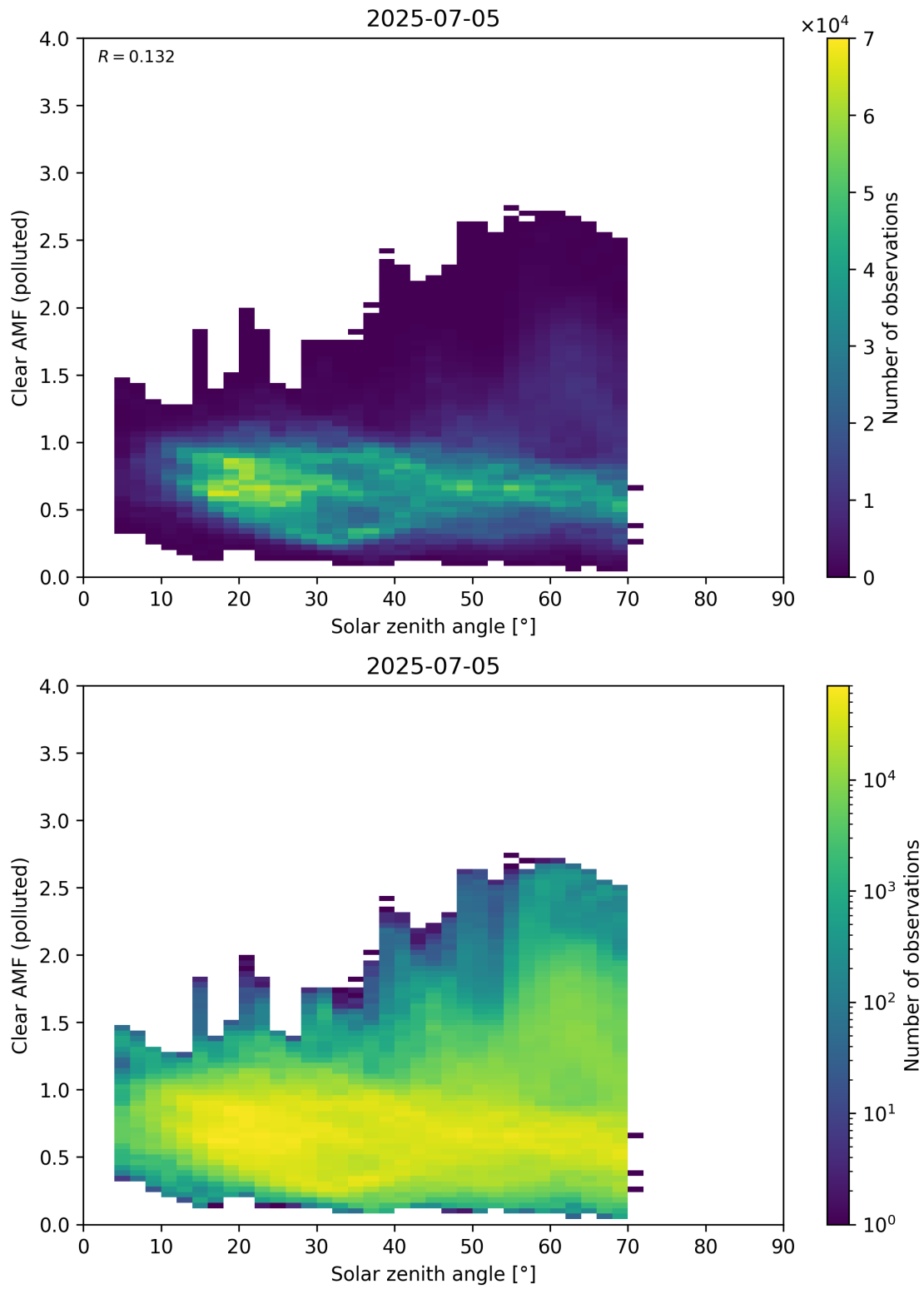
Figure 178: Scatter density plot of “Solar zenith angle” against “Clear AMF (polluted)” for 2025-07-04 to 2025-07-06.
