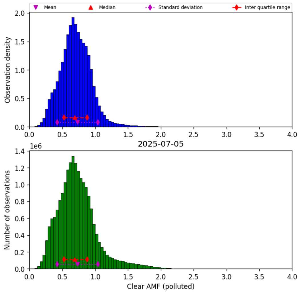
Figure 81: Histogram of “Clear AMF (polluted)” for 2025-07-04 to 2025-07-06
