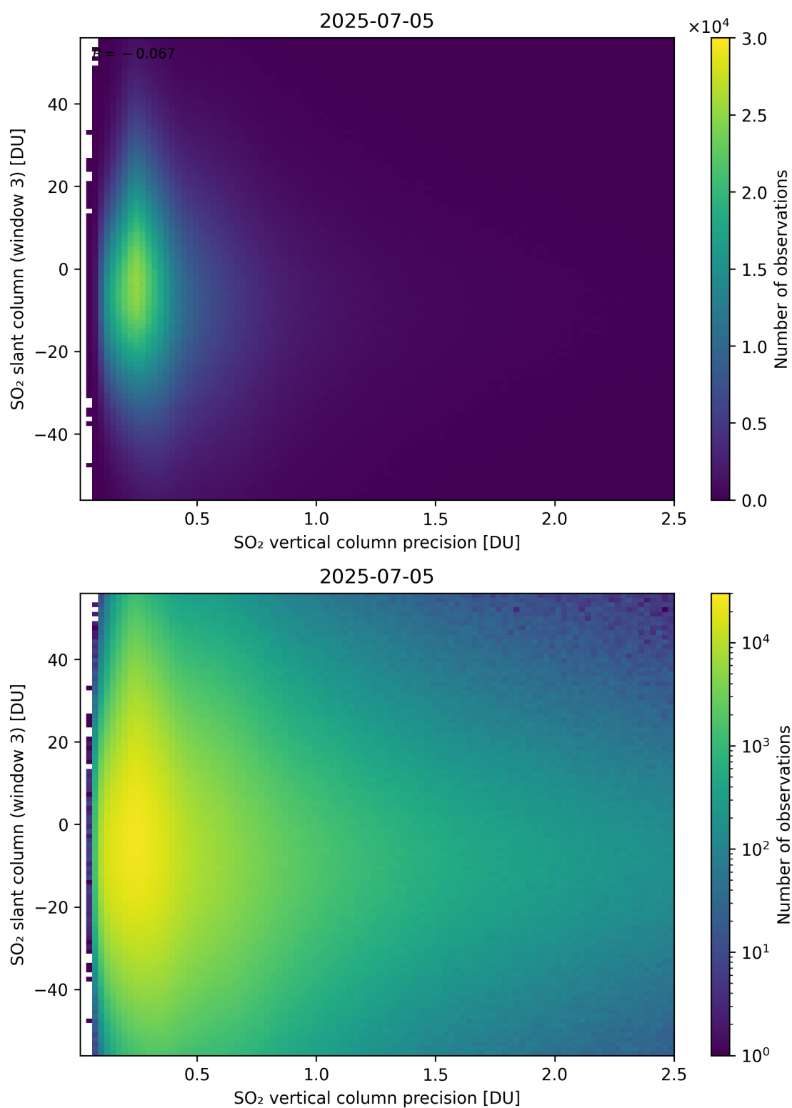
Figure 344: Scatter density plot of “SO 2 vertical column precision” against “SO 2 slant column (window 3)” for 2025-07-04 to 2025-07-06.
