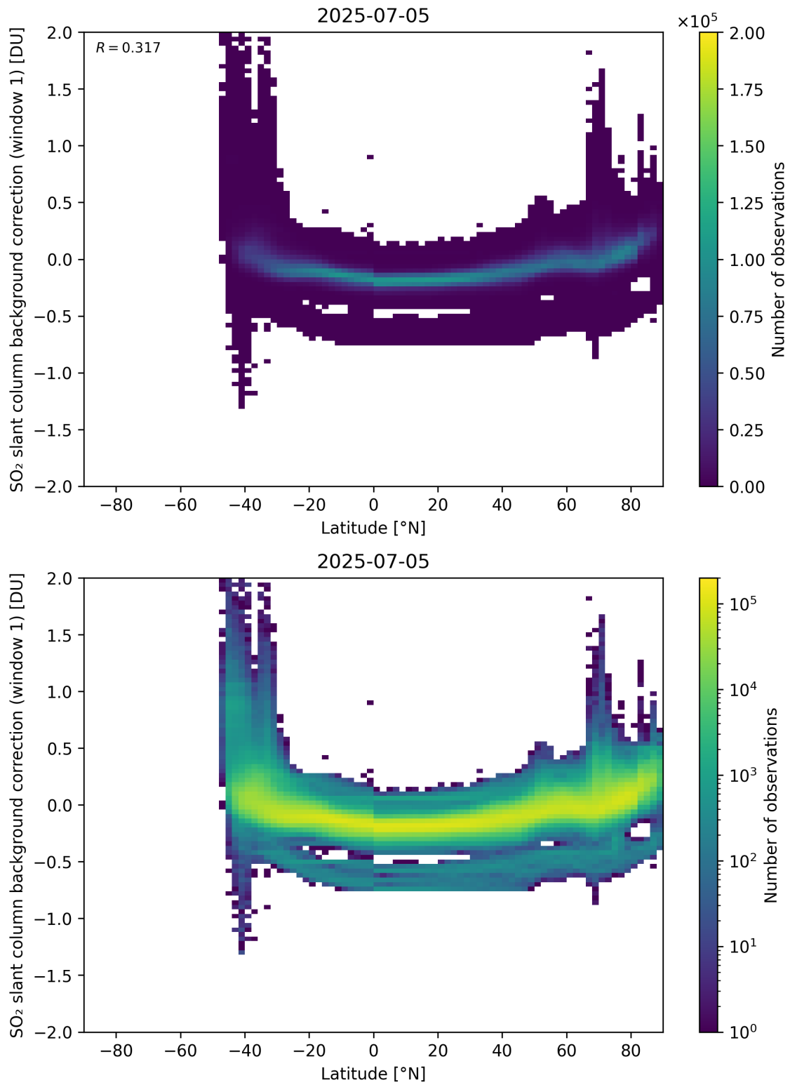
Figure 150: Scatter density plot of “Latitude” against “SO 2 slant column background correction (window 1)” for 2025-07-04 to 2025-07-06.
