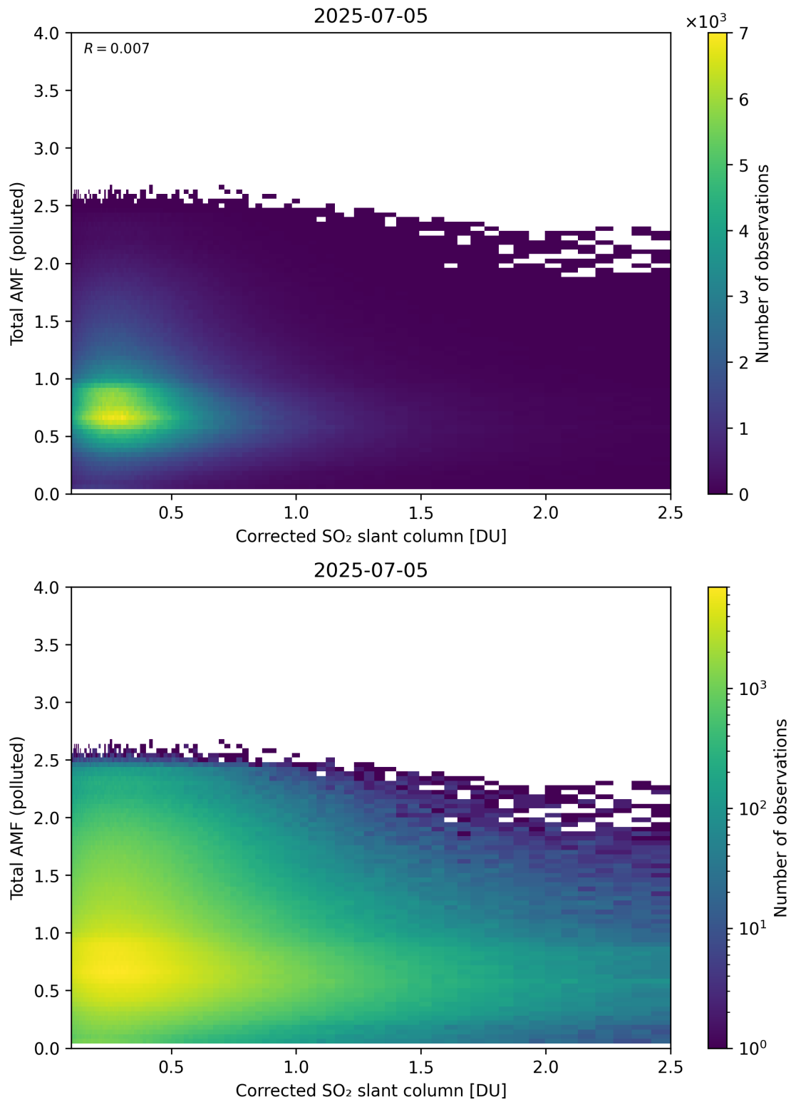
Figure 242: Scatter density plot of “Corrected SO 2 slant column” against “Total AMF (polluted)” for 2025-07-04 to 2025-07-06.
