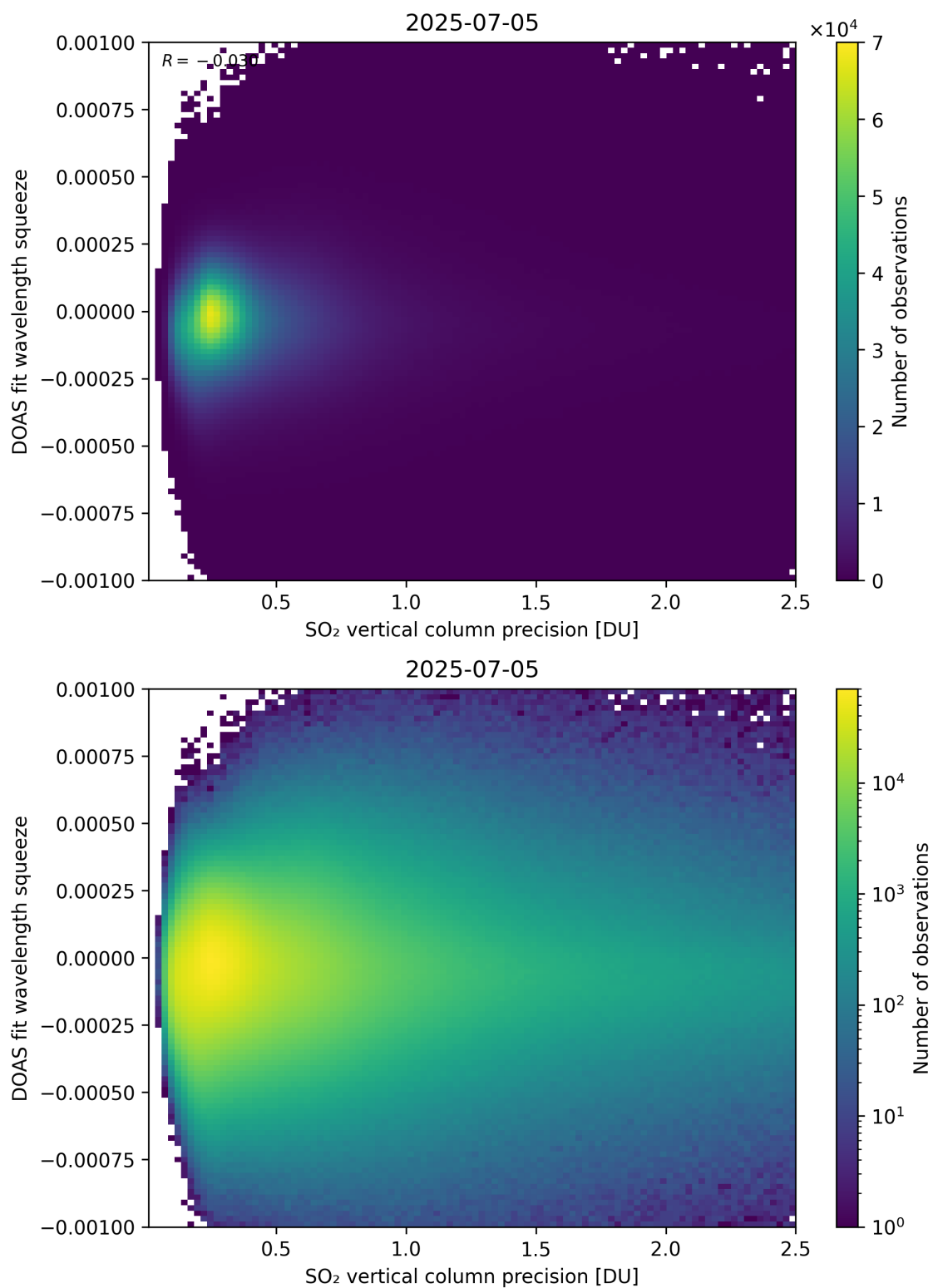
Figure 333: Scatter density plot of “SO 2 vertical column precision” against “DOAS fit wavelength squeeze” for 2025-07-04 to 2025-07-06.
