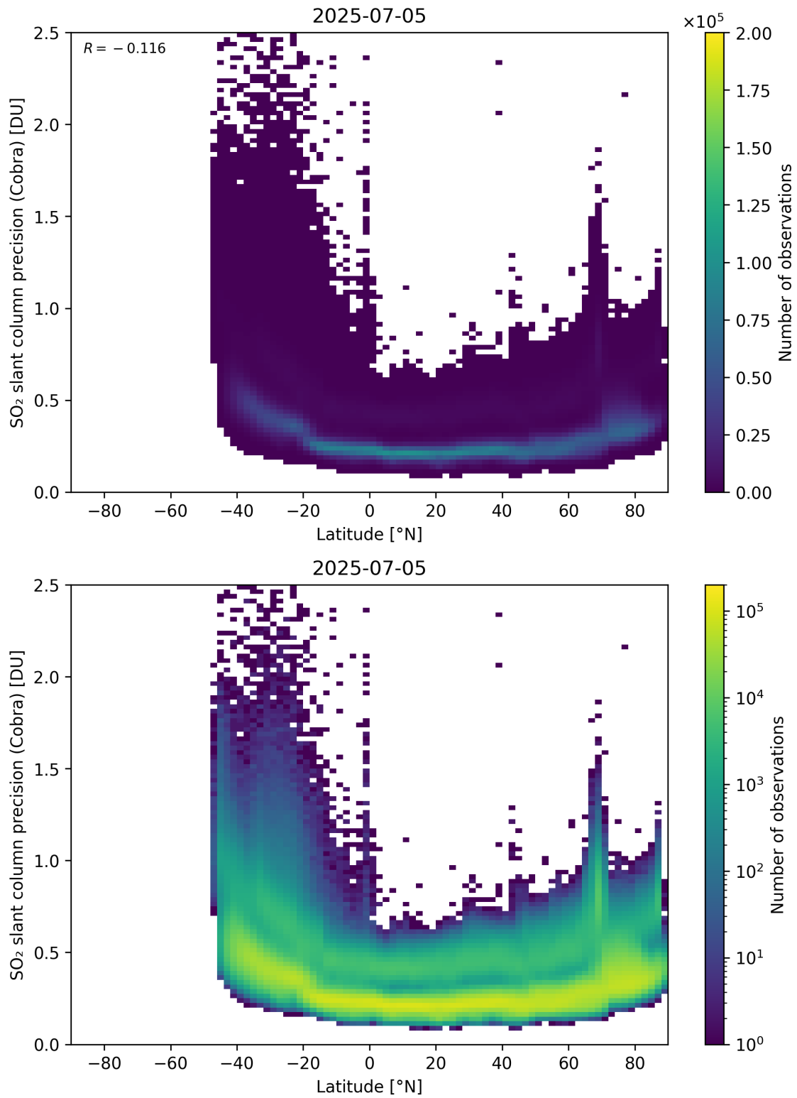
Figure 158: Scatter density plot of “Latitude” against “SO 2 slant column precision (Cobra)” for 2025-07-04 to 2025-07-06.
