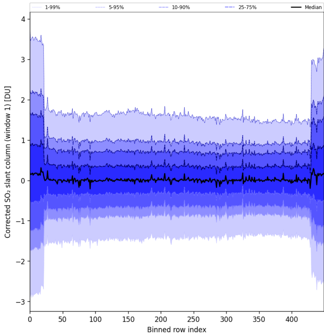
Figure 91: Along track statistics of “Corrected SO 2 slant column (window 1)” for 2025-07-04 to 2025-07-06
