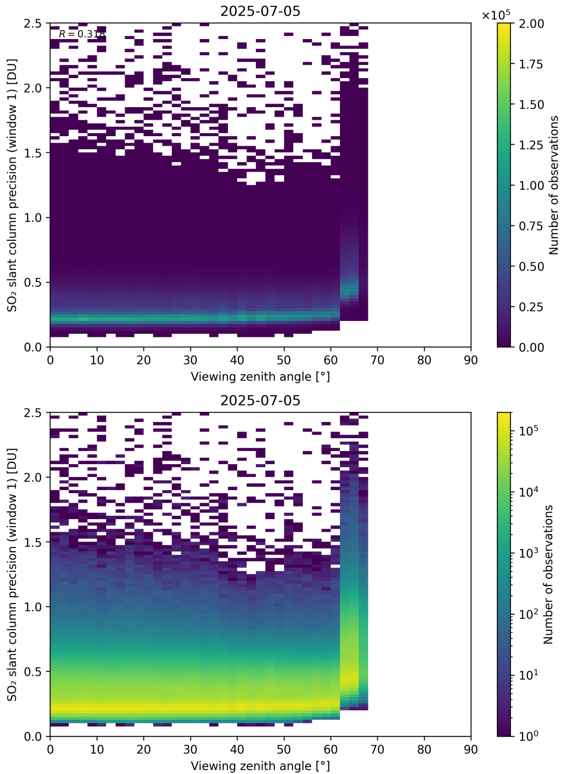
Figure 377: Scatter density plot of “Viewing zenith angle” against “SO 2 slant column precision (window 1)” for 2025-07-04 to 2025-07-06.
