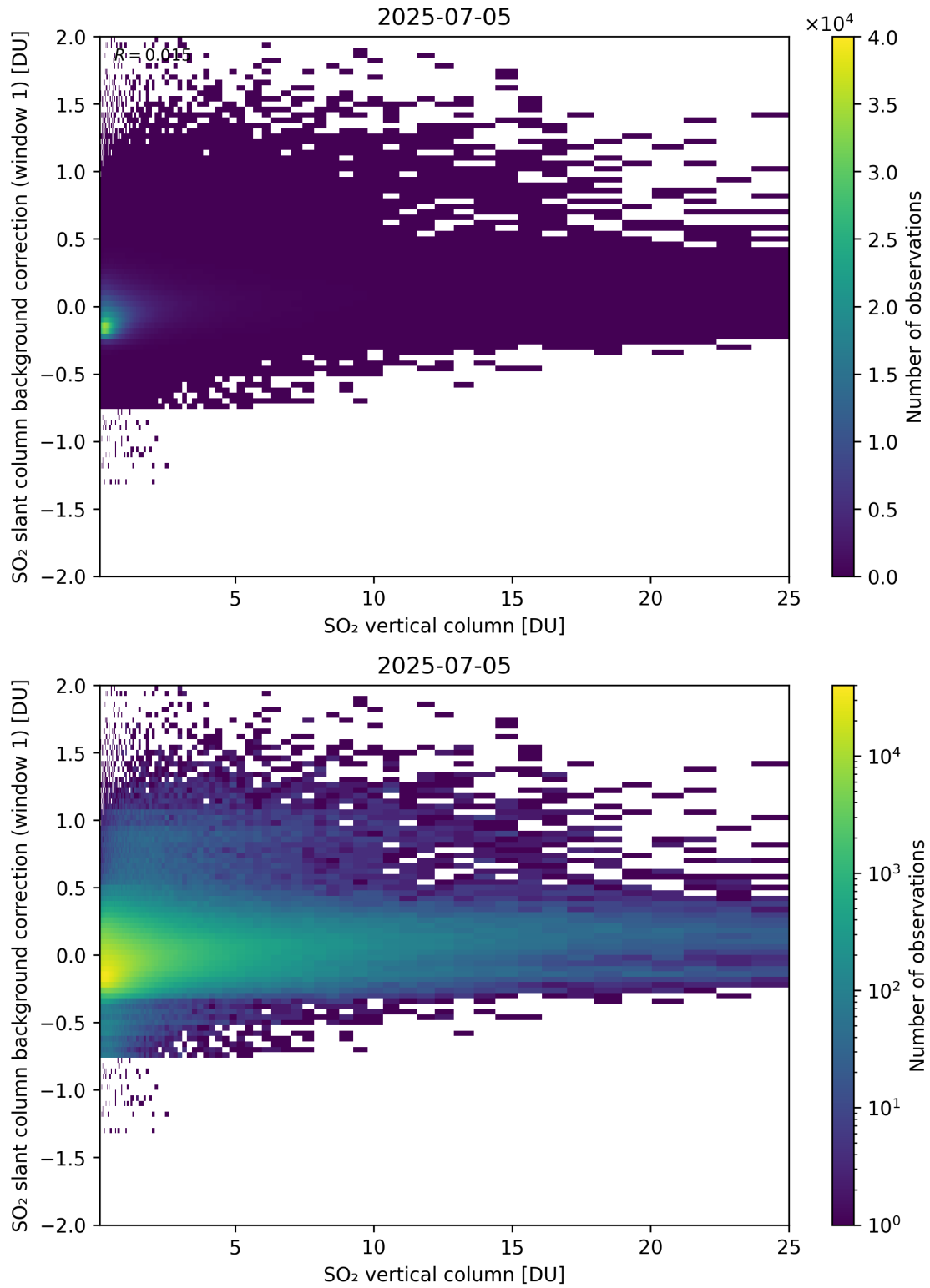
Figure 323: Scatter density plot of “SO 2 vertical column” against “SO 2 slant column background correction (window 1)” for 2025-07-04 to 2025-07-06.
