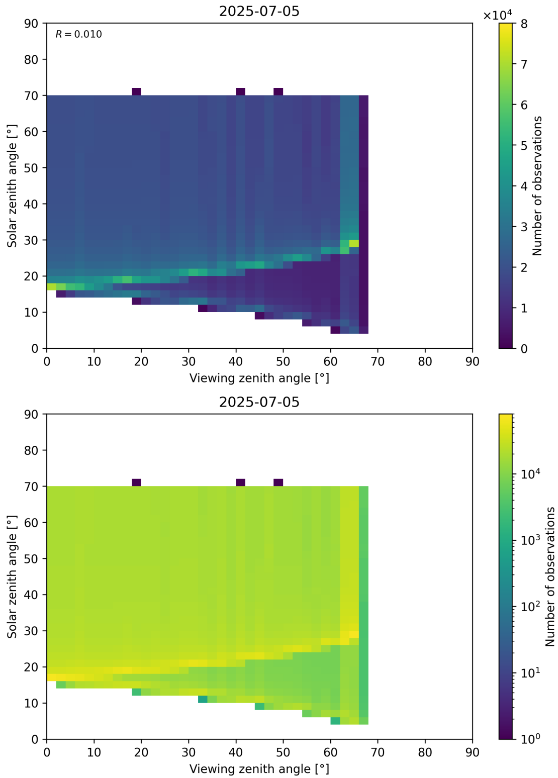
Figure 369: Scatter density plot of “Viewing zenith angle” against “Solar zenith angle” for 2025-07-04 to 2025-07-06.
