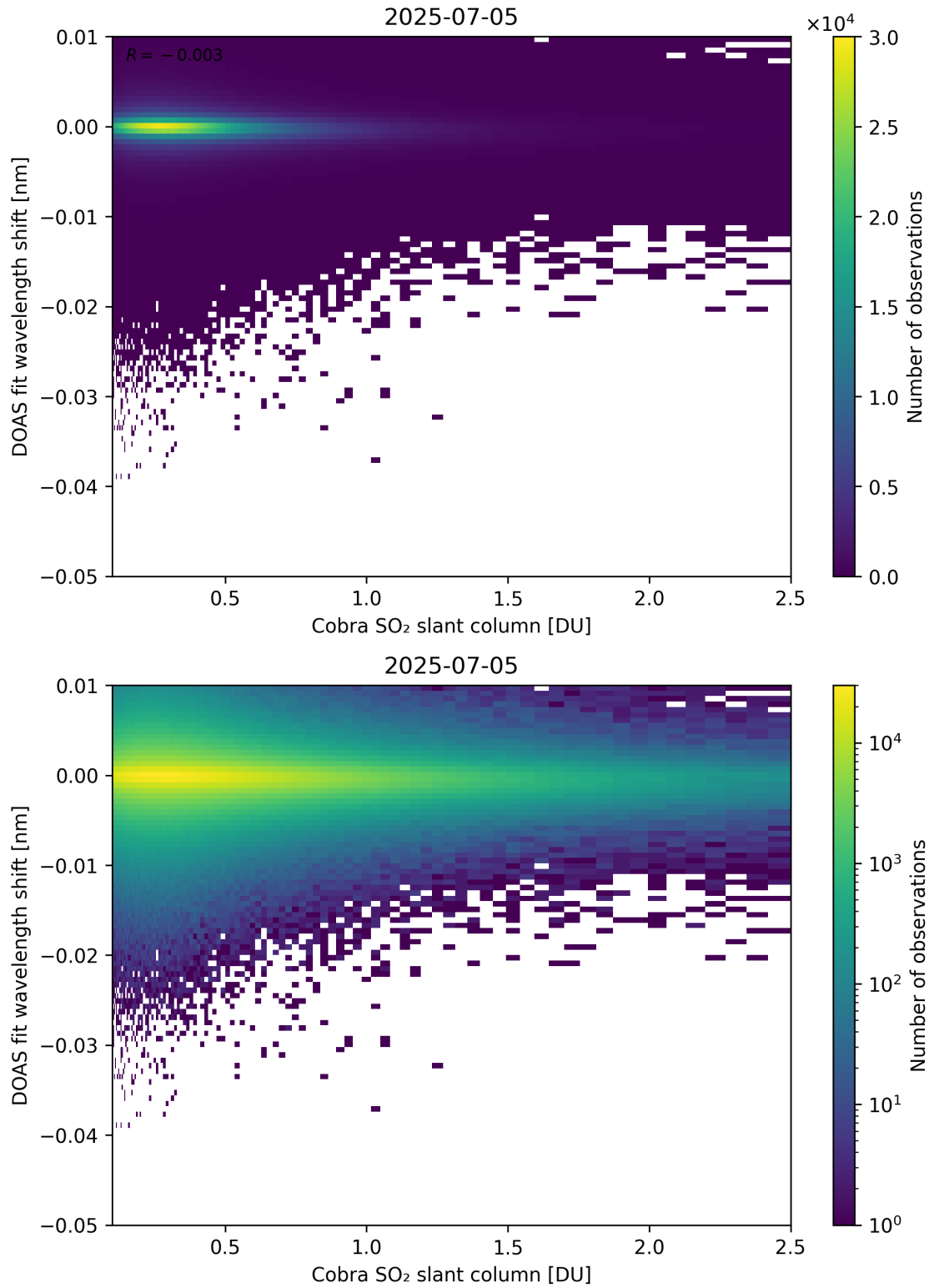
Figure 196: Scatter density plot of “Cobra SO 2 slant column” against “DOAS fit wavelength shift” for 2025-07-04 to 2025-07-06.
