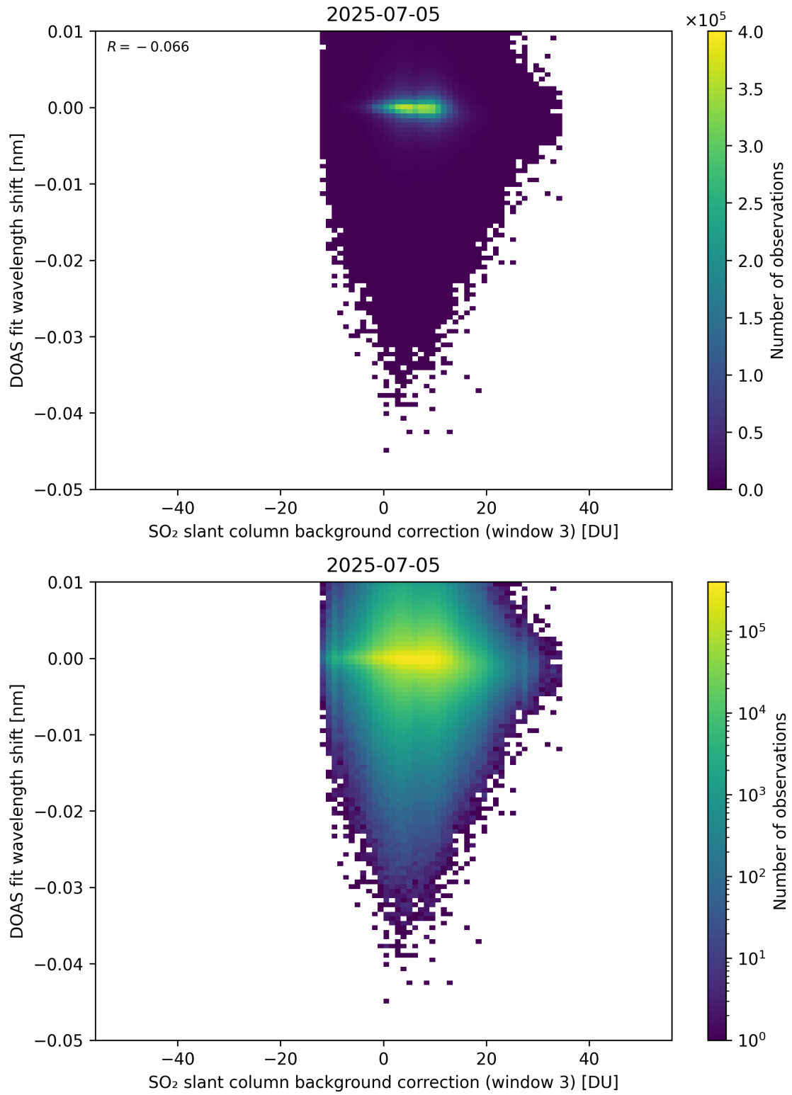
Figure 132: Scatter density plot of “SO 2 slant column background correction (window 3)” against “DOAS fit wavelength shift” for 2025-07-04 to 2025-07-06.
