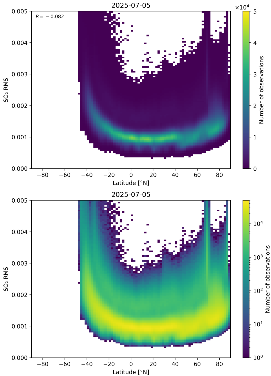
Figure 155: Scatter density plot of “Latitude” against “SO 2 RMS” for 2025-07-04 to 2025-07-06.
