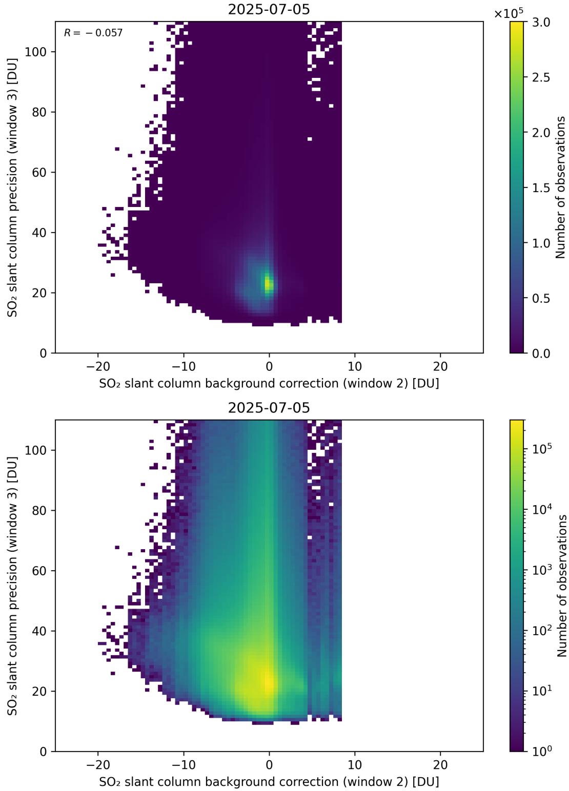
Figure 129: Scatter density plot of “SO 2 slant column background correction (window 2)” against “SO 2 slant column precision (window 3)” for 2025-07-04 to 2025-07-06.
