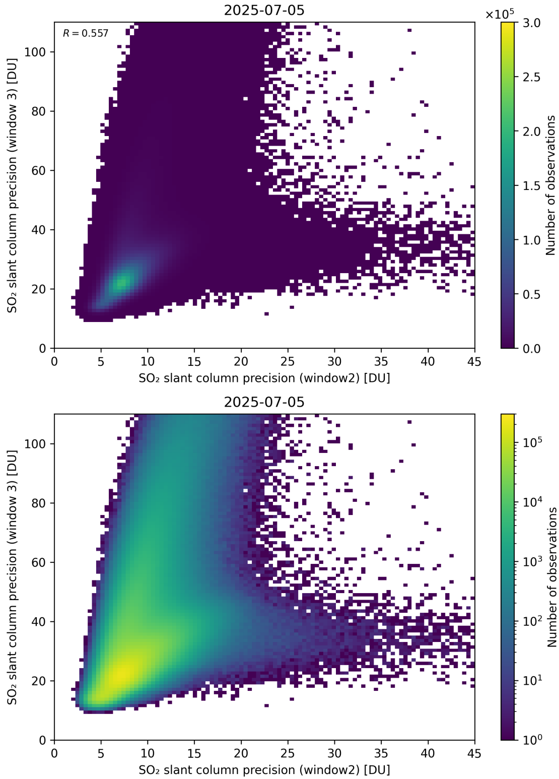
Figure 300: Scatter density plot of “SO 2 slant column precision (window2)” against “SO 2 slant column precision (window 3)” for 2025-07-04 to 2025-07-06.
