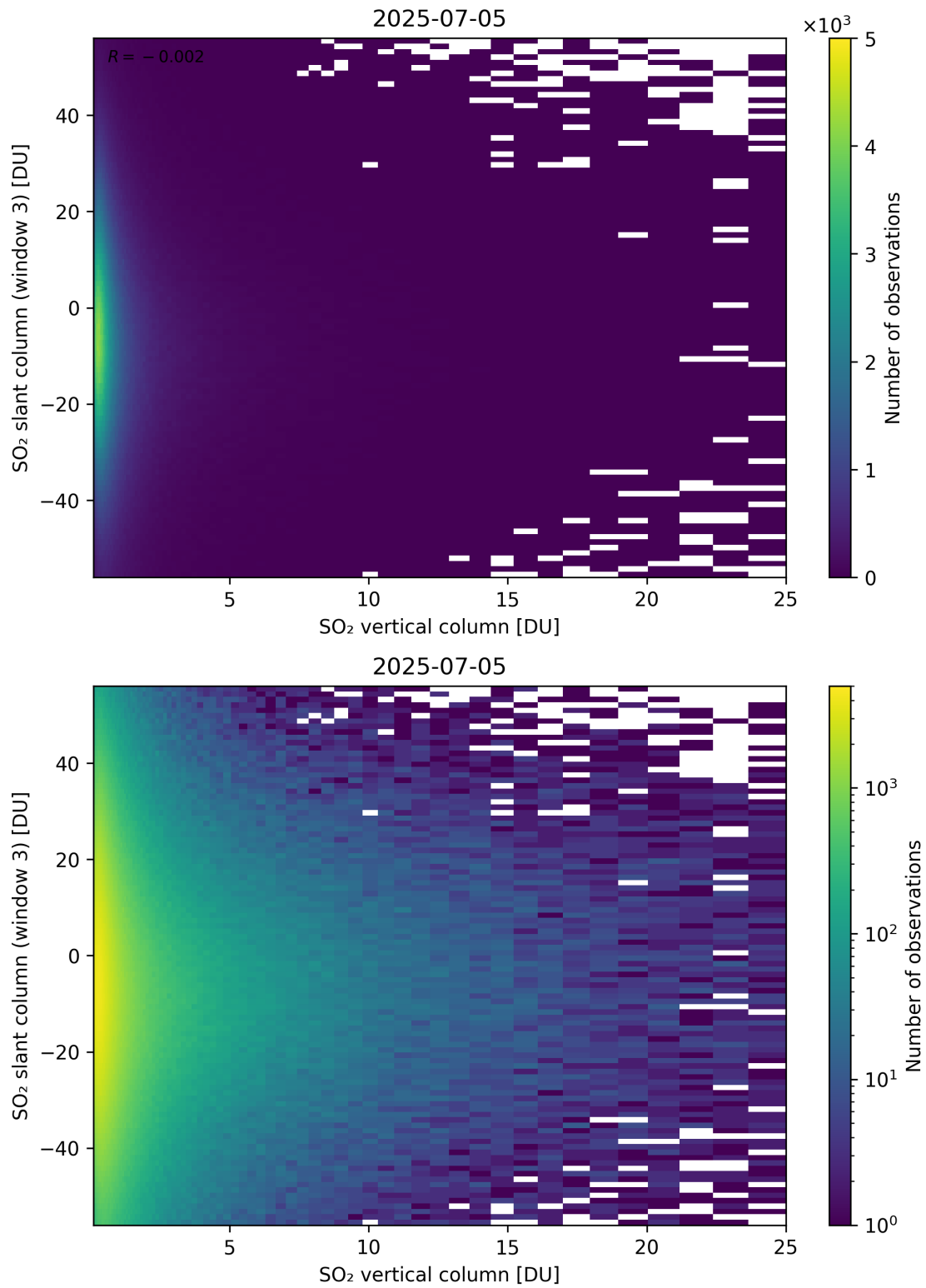
Figure 357: Scatter density plot of “SO 2 vertical column” against “SO 2 slant column (window 3)” for 2025-07-04 to 2025-07-06.
