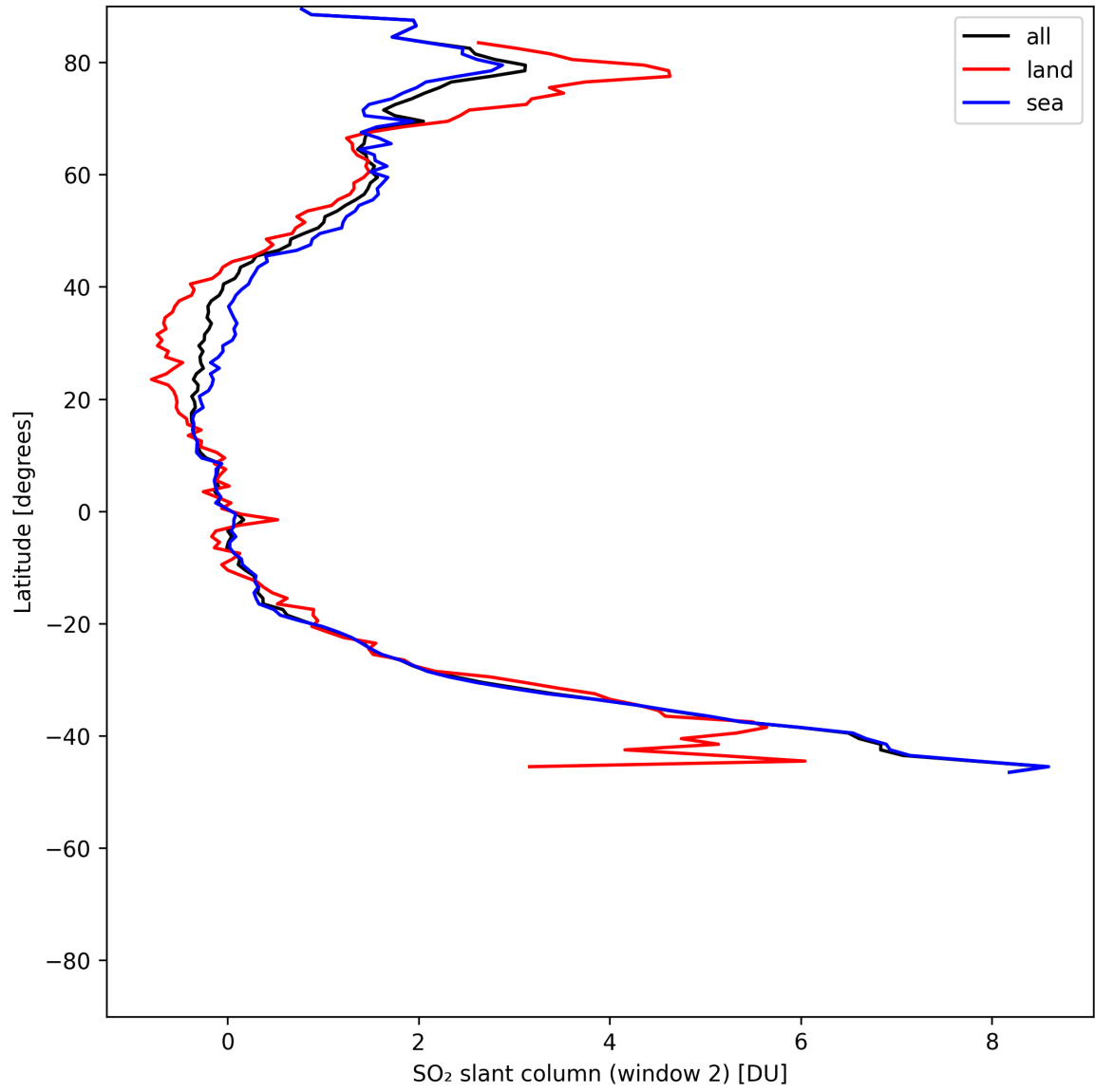
Figure 41: Zonal average of “SO 2 slant column (window 2)” for 2025-07-04 to 2025-07-06.
