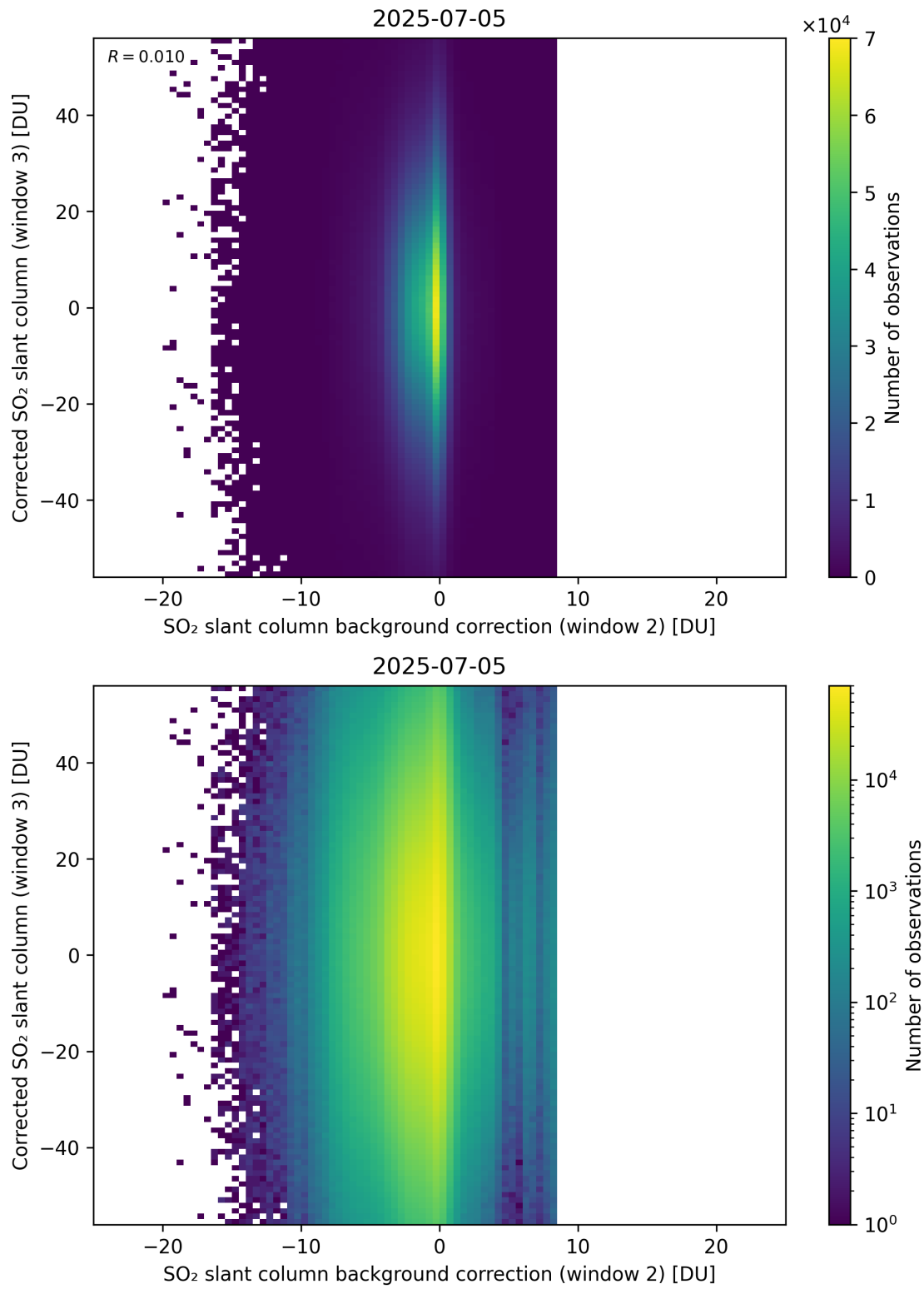
Figure 127: Scatter density plot of “SO 2 slant column background correction (window 2)” against “Corrected SO 2 slant column (window 3)” for 2025-07-04 to 2025-07-06.
