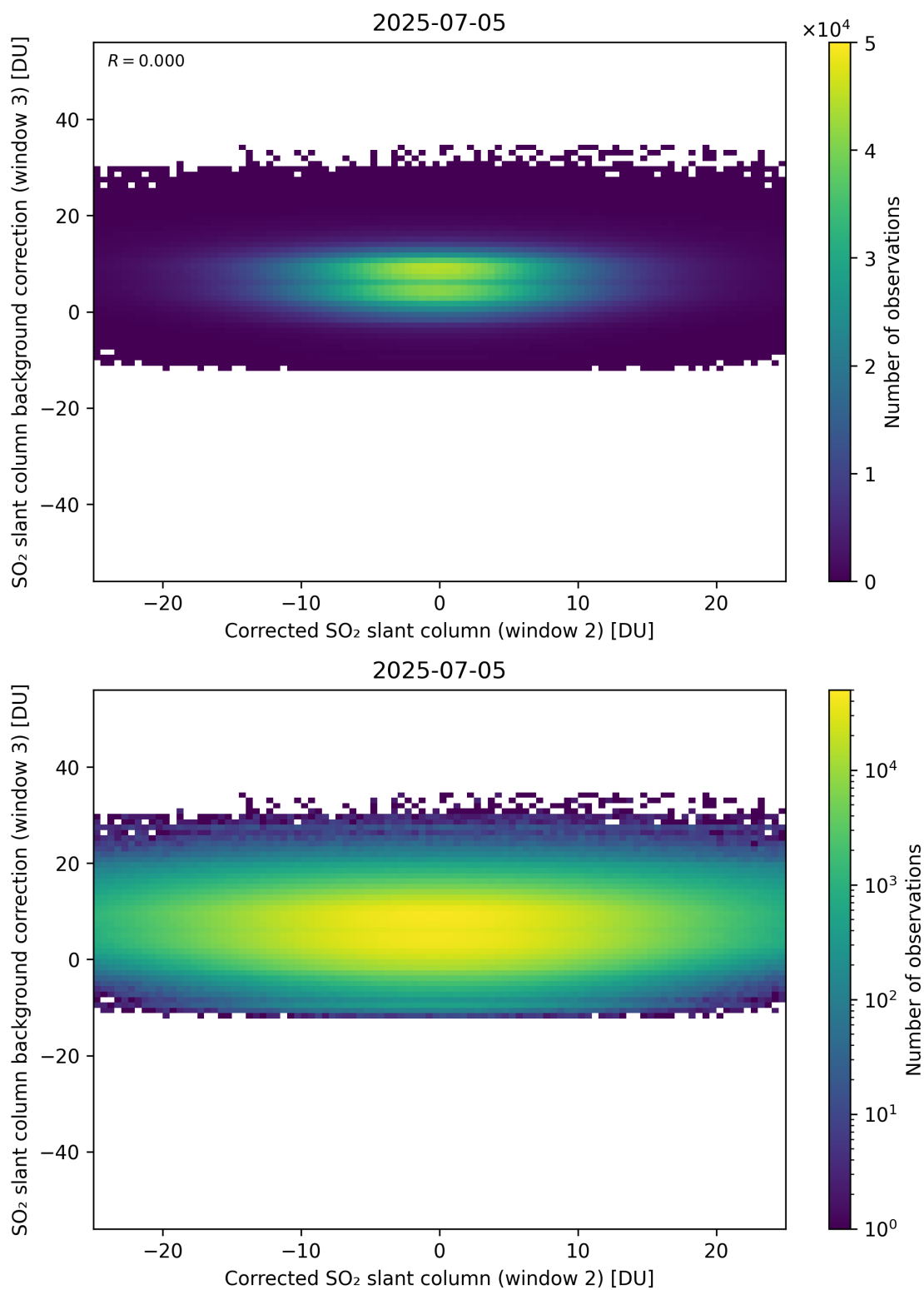
Figure 245: Scatter density plot of “Corrected SO 2 slant column (window 2)” against “SO 2 slant column background correction (window 3)” for 2025-07-04 to 2025-07-06.
