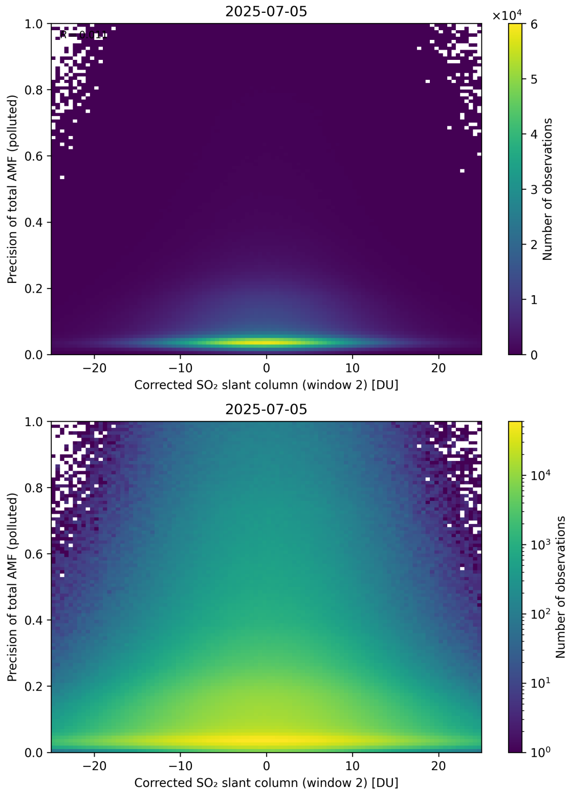
Figure 254: Scatter density plot of “Corrected SO 2 slant column (window 2)” against “Precision of total AMF (polluted)” for 2025-07-04 to 2025-07-06.
