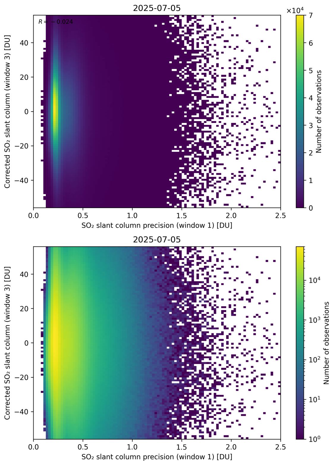
Figure 276: Scatter density plot of “SO 2 slant column precision (window 1)” against “Corrected SO 2 slant column (window 3)” for 2025-07-04 to 2025-07-06.
