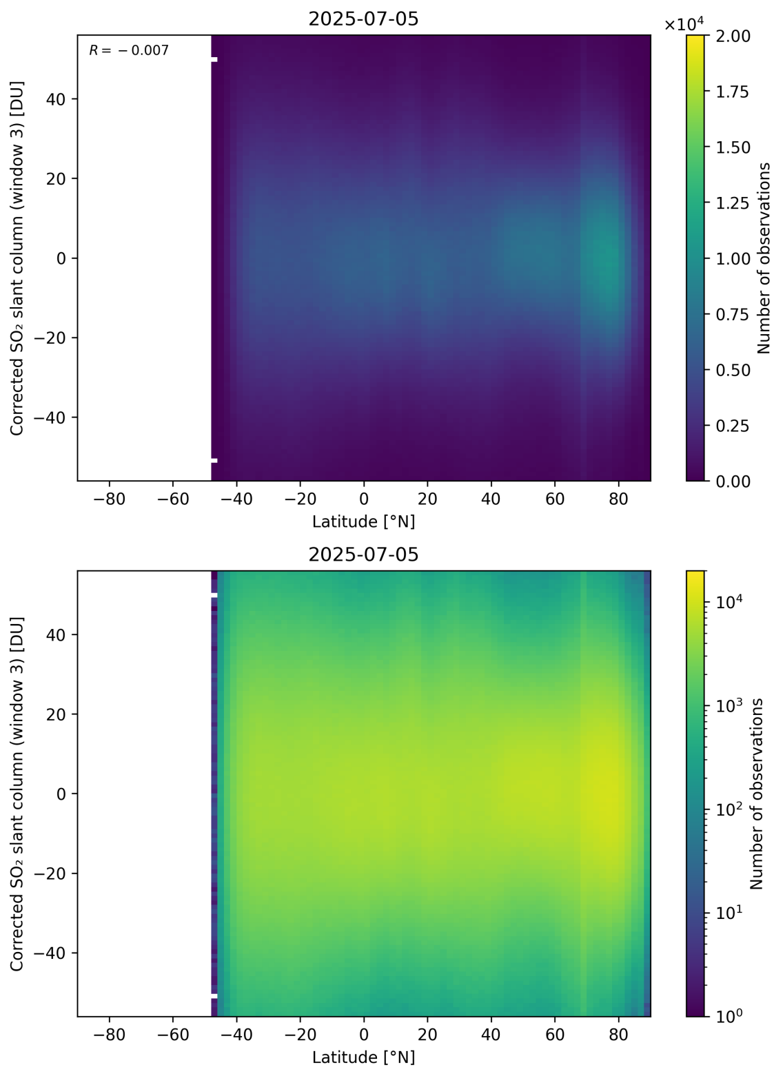
Figure 161: Scatter density plot of “Latitude” against “Corrected SO 2 slant column (window 3)” for 2025-07-04 to 2025-07-06.
