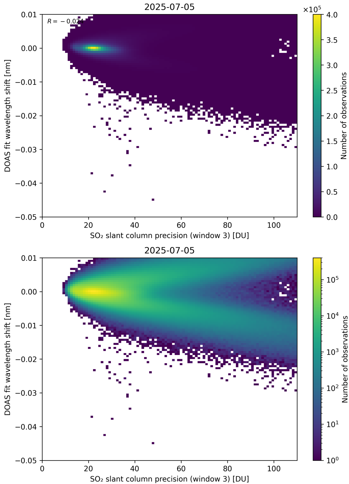
Figure 308: Scatter density plot of “SO 2 slant column precision (window 3)” against “DOAS fit wavelength shift” for 2025-07-04 to 2025-07-06.
