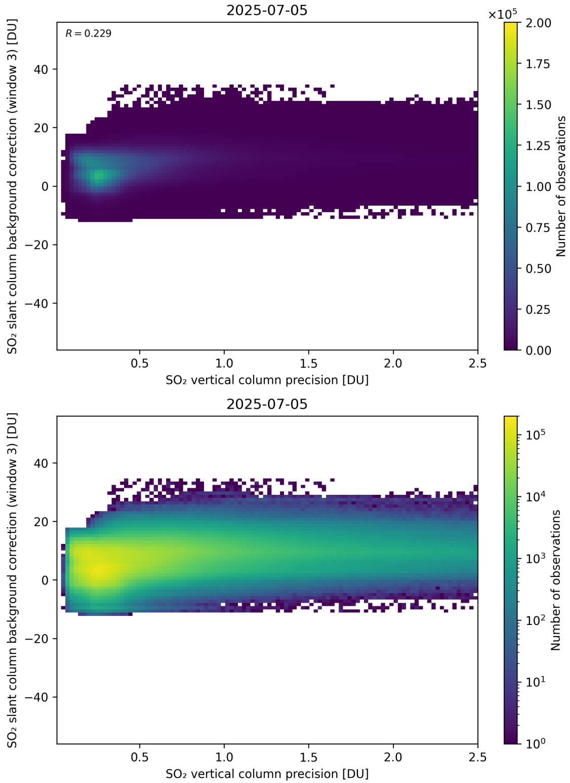
Figure 331: Scatter density plot of “SO 2 vertical column precision” against “SO 2 slant column background correction (window 3)” for 2025-07-04 to 2025-07-06.
