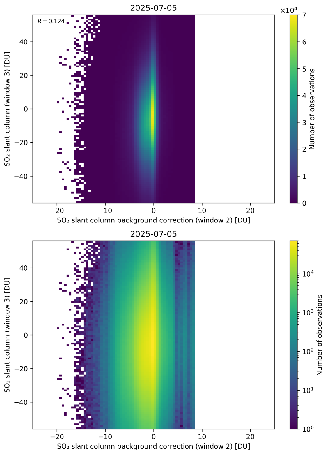
Figure 128: Scatter density plot of “SO 2 slant column background correction (window 2)” against “SO 2 slant column (window 3)” for 2025-07-04 to 2025-07-06.
