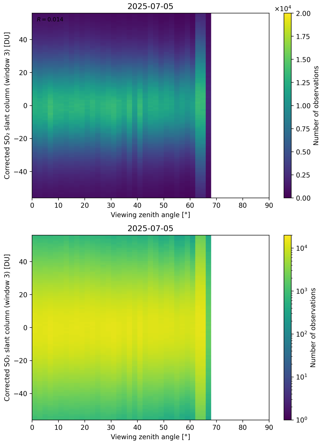
Figure 375: Scatter density plot of “Viewing zenith angle” against “Corrected SO 2 slant column (window 3)” for 2025-07-04 to 2025-07-06.
