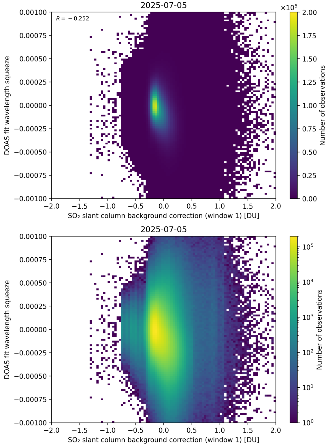
Figure 112: Scatter density plot of “SO 2 slant column background correction (window 1)” against “DOAS fit wavelength squeeze” for 2025-07-04 to 2025-07-06.
