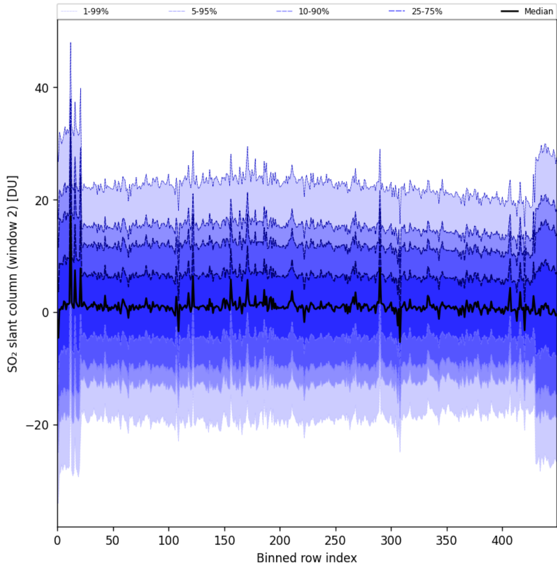
Figure 93: Along track statistics of “SO 2 slant column (window 2)” for 2025-07-04 to 2025-07-06
