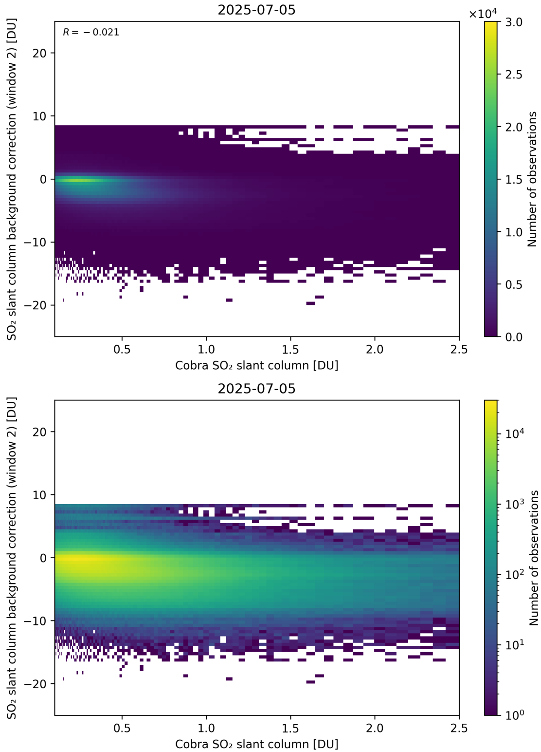
Figure 194: Scatter density plot of “Cobra SO 2 slant column” against “SO 2 slant column background correction (window 2)” for 2025-07-04 to 2025-07-06.
