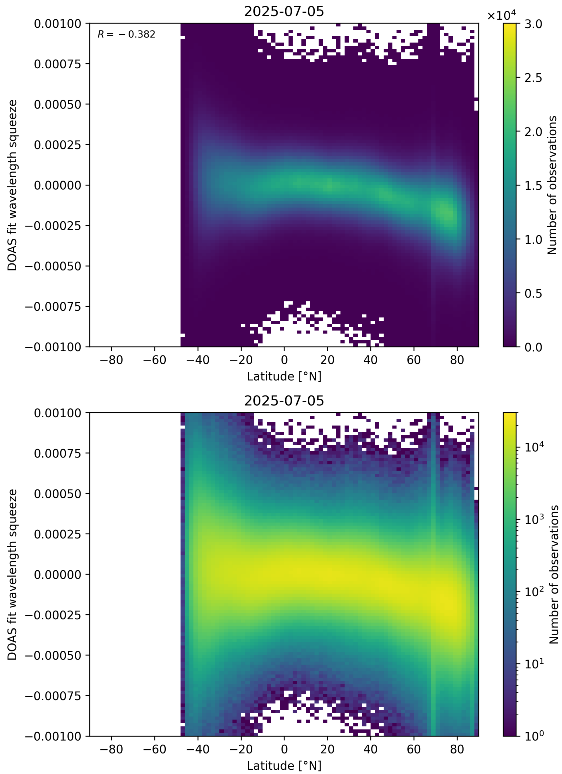
Figure 154: Scatter density plot of “Latitude” against “DOAS fit wavelength squeeze” for 2025-07-04 to 2025-07-06.
