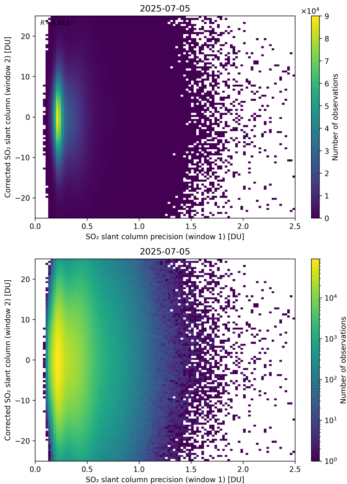
Figure 275: Scatter density plot of “SO 2 slant column precision (window 1)” against “Corrected SO 2 slant column (window 2)” for 2025-07-04 to 2025-07-06.
