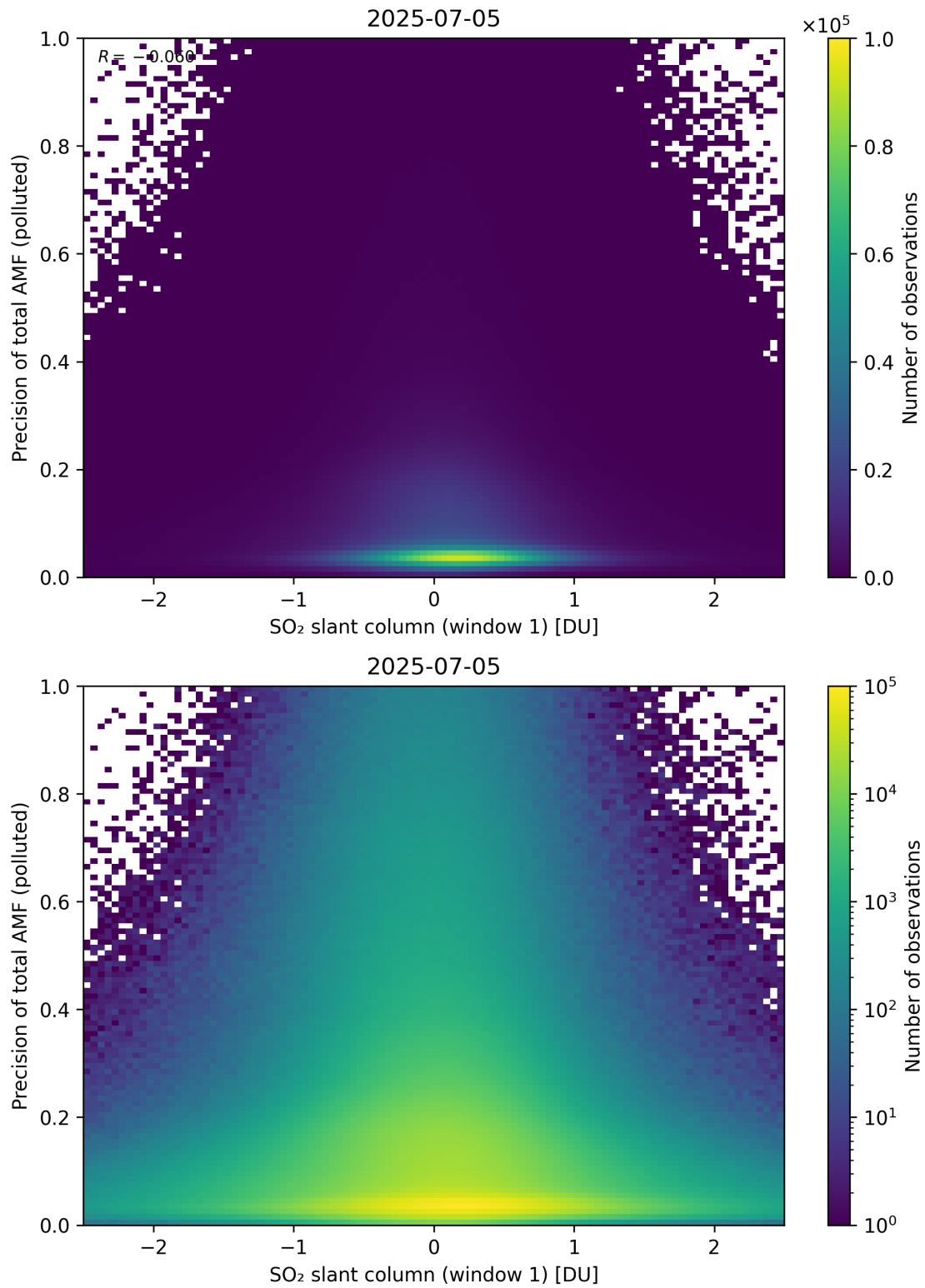
Figure 290: Scatter density plot of “SO 2 slant column (window 1)” against “Precision of total AMF (polluted)” for 2025-07-04 to 2025-07-06.
