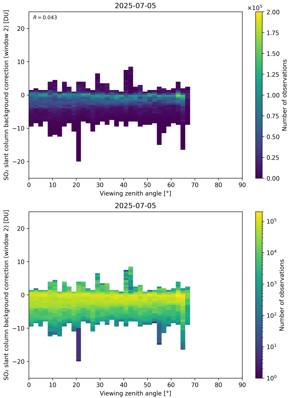
Figure 363: Scatter density plot of “Viewing zenith angle” against “SO 2 slant column background correction (window 2)” for 2025-07-04 to 2025-07-06.
