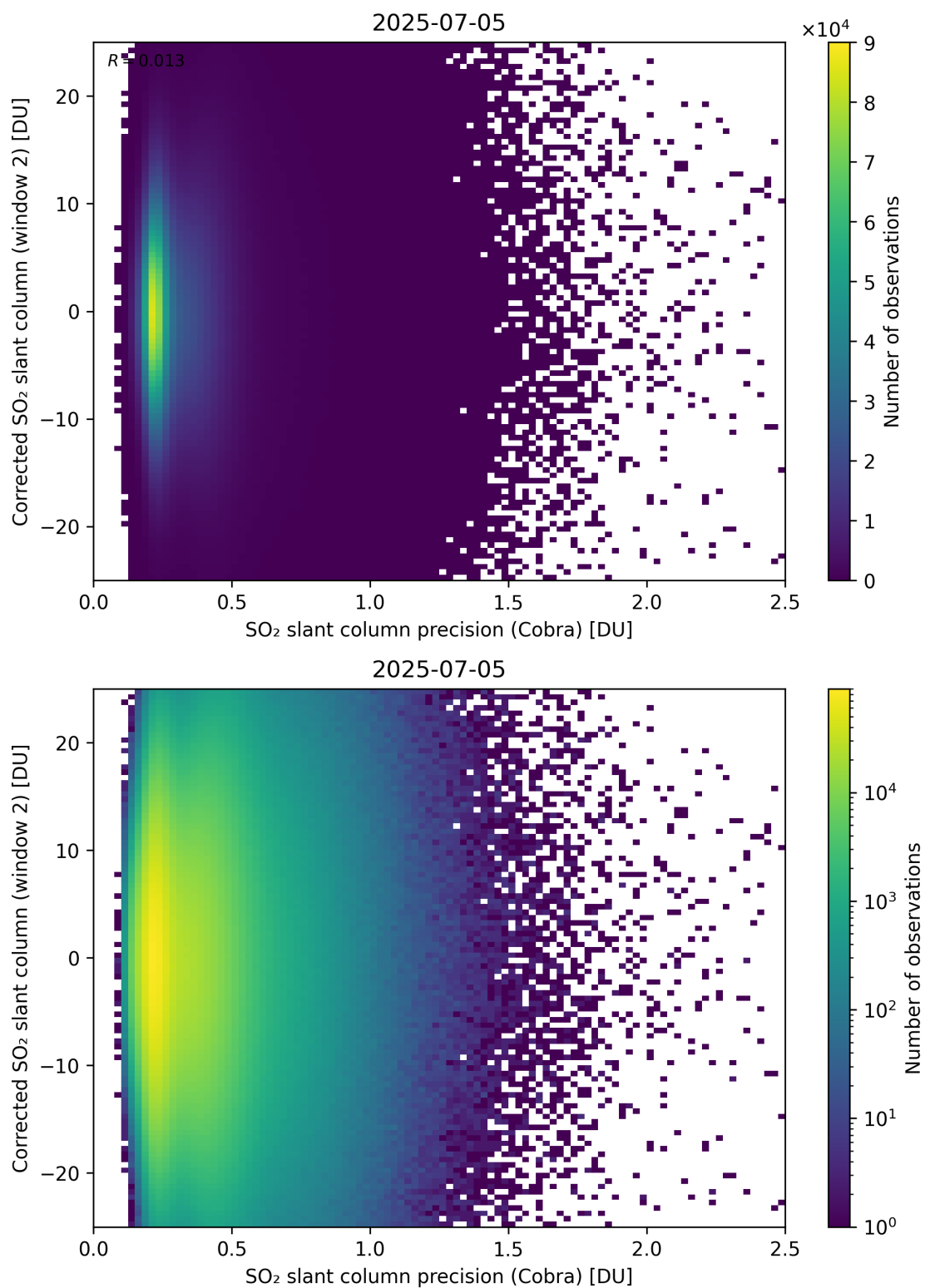
Figure 206: Scatter density plot of “SO 2 slant column precision (Cobra)” against “Corrected SO 2 slant column (window 2)” for 2025-07-04 to 2025-07-06.
