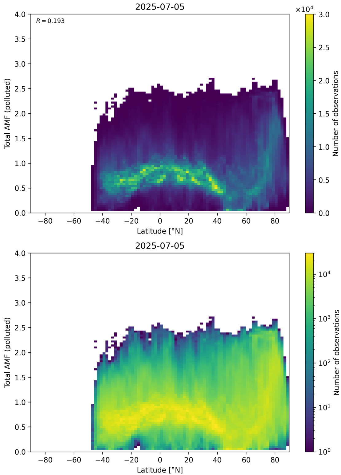
Figure 167: Scatter density plot of “Latitude” against “Total AMF (polluted)” for 2025-07-04 to 2025-07-06.
