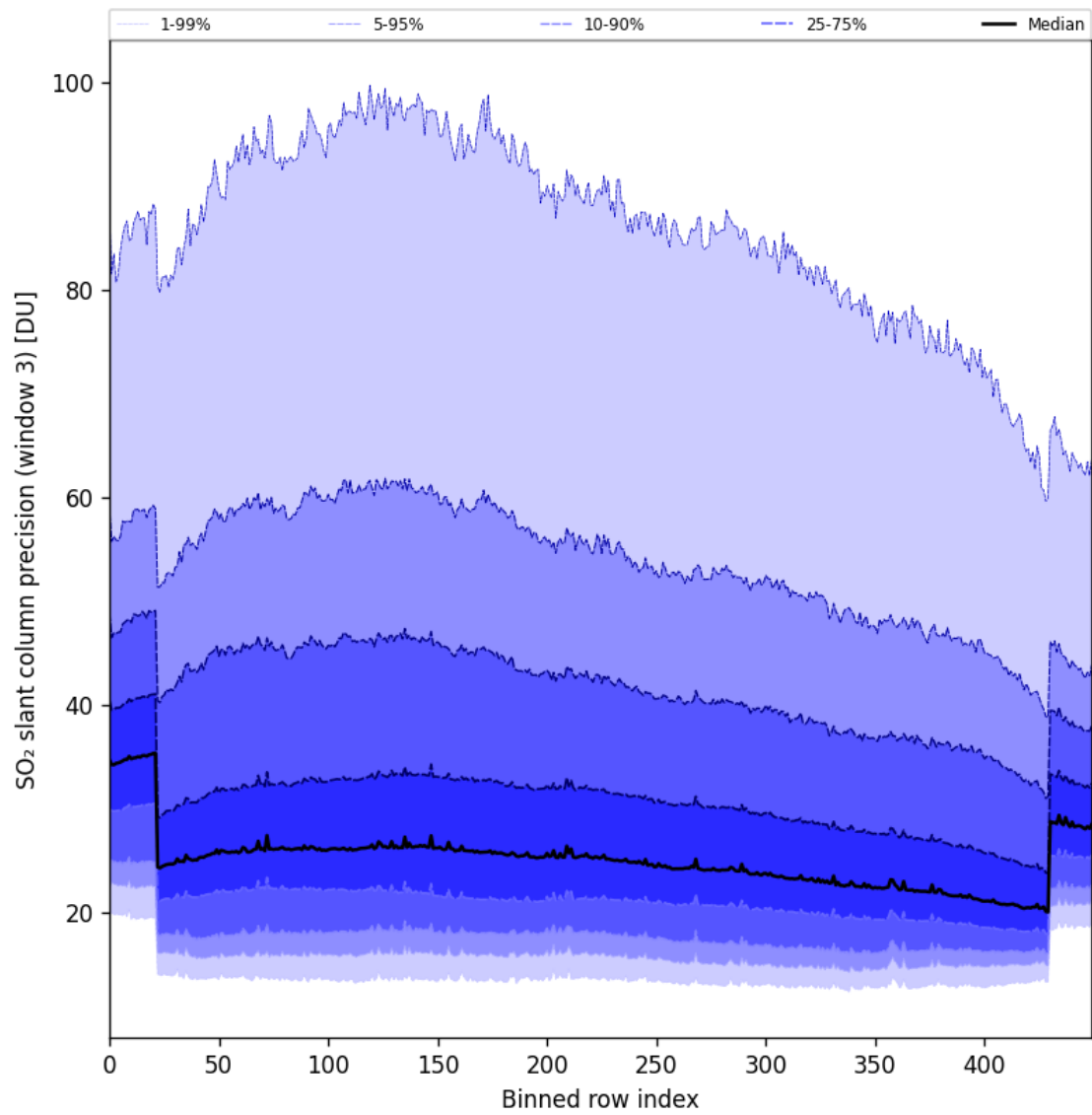
Figure 98: Along track statistics of “SO 2 slant column precision (window 3)” for 2025-07-04 to 2025-07-06
