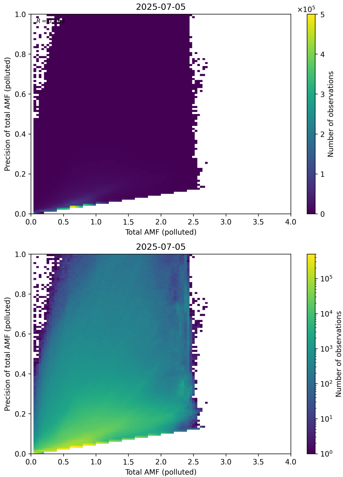
Figure 322: Scatter density plot of “Total AMF (polluted)” against “Precision of total AMF (polluted)” for 2025-07-04 to 2025-07-06.
