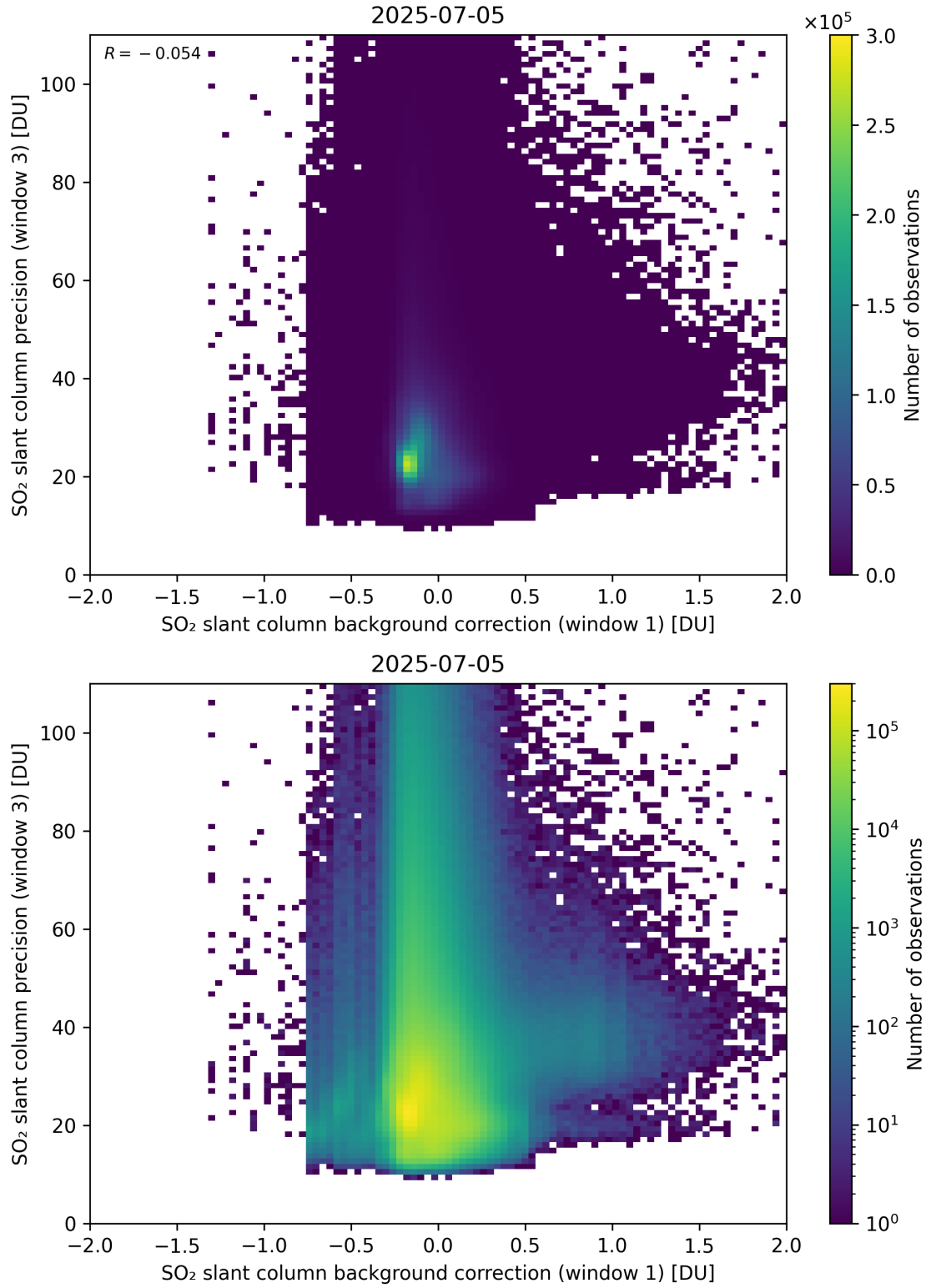
Figure 119: Scatter density plot of “SO 2 slant column background correction (window 1)” against “SO 2 slant column precision (window 3)” for 2025-07-04 to 2025-07-06.
