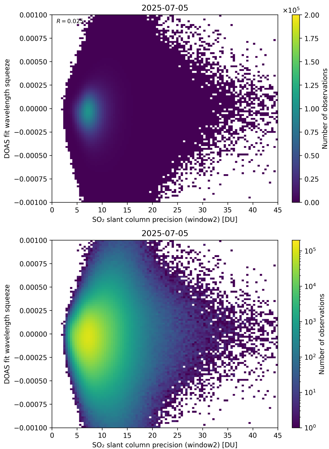
Figure 294: Scatter density plot of “SO 2 slant column precision (window2)” against “DOAS fit wavelength squeeze” for 2025-07-04 to 2025-07-06.
