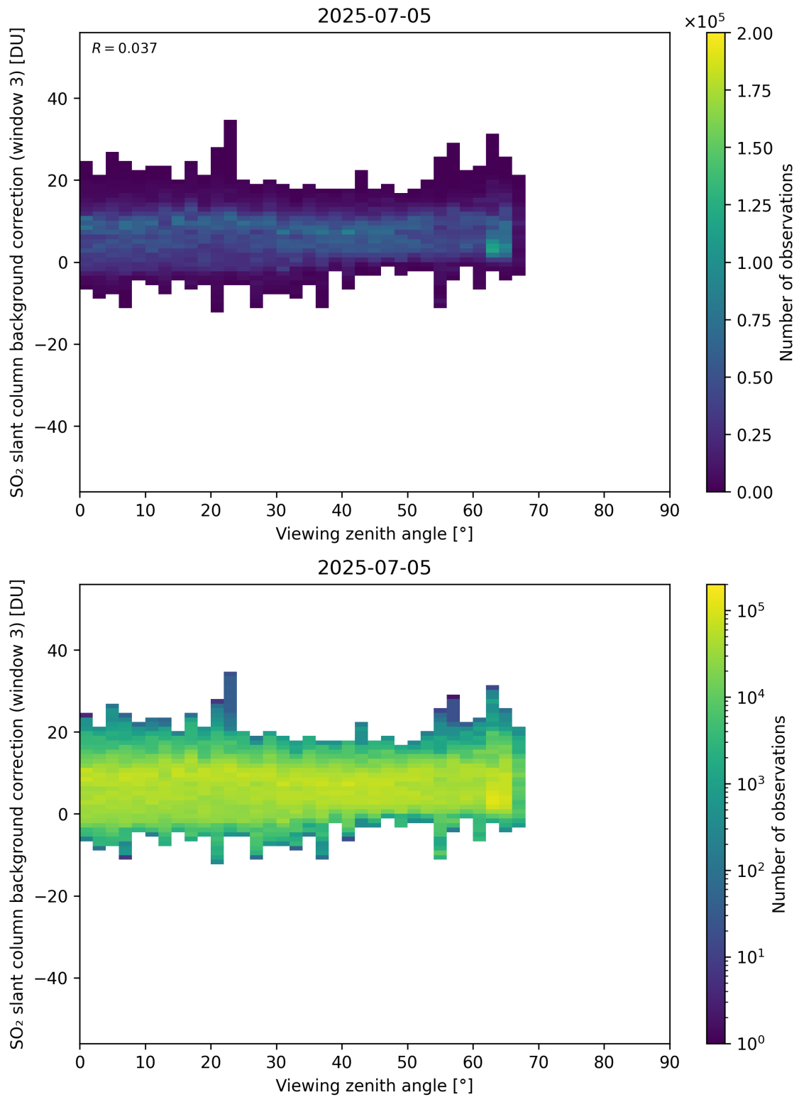
Figure 364: Scatter density plot of “Viewing zenith angle” against “SO 2 slant column background correction (window 3)” for 2025-07-04 to 2025-07-06.
