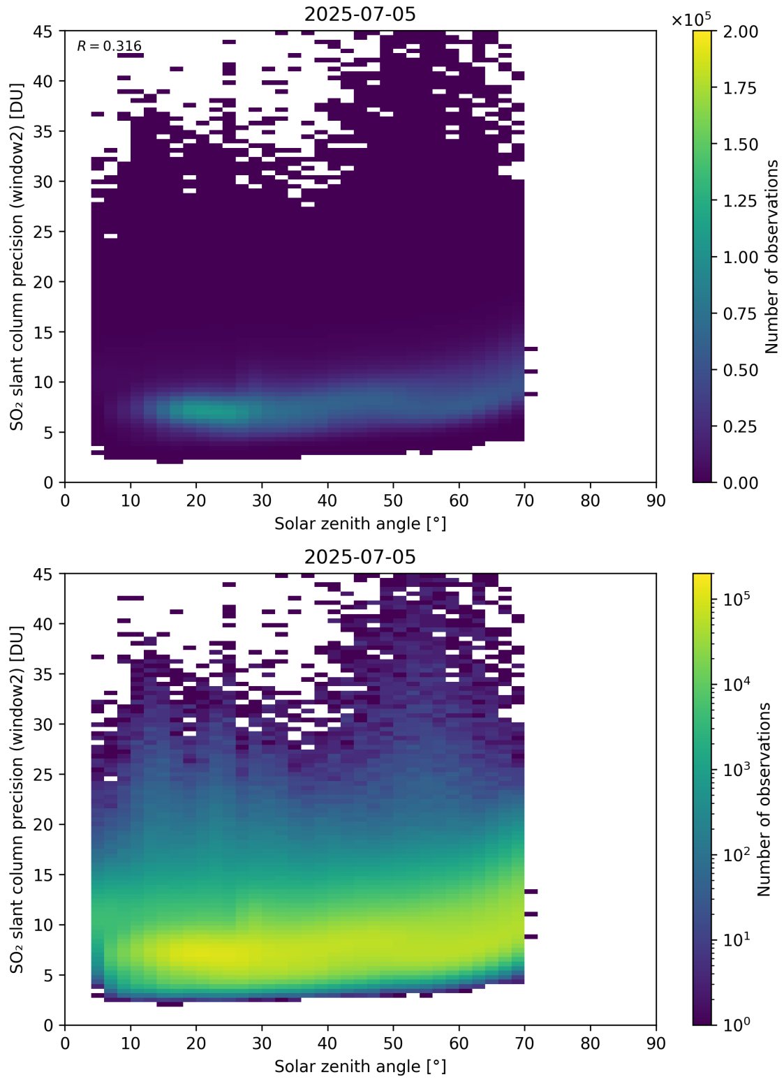
Figure 186: Scatter density plot of “Solar zenith angle” against “SO 2 slant column precision (window2)” for 2025-07-04 to 2025-07-06.
