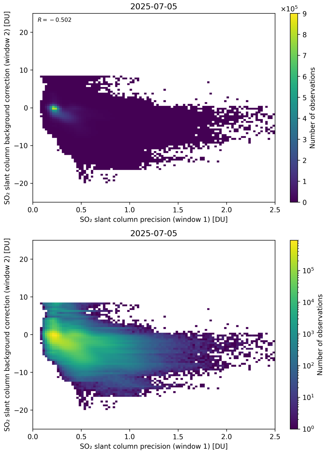
Figure 269: Scatter density plot of “SO 2 slant column precision (window 1)” against “SO 2 slant column background correction (window 2)” for 2025-07-04 to 2025-07-06.
