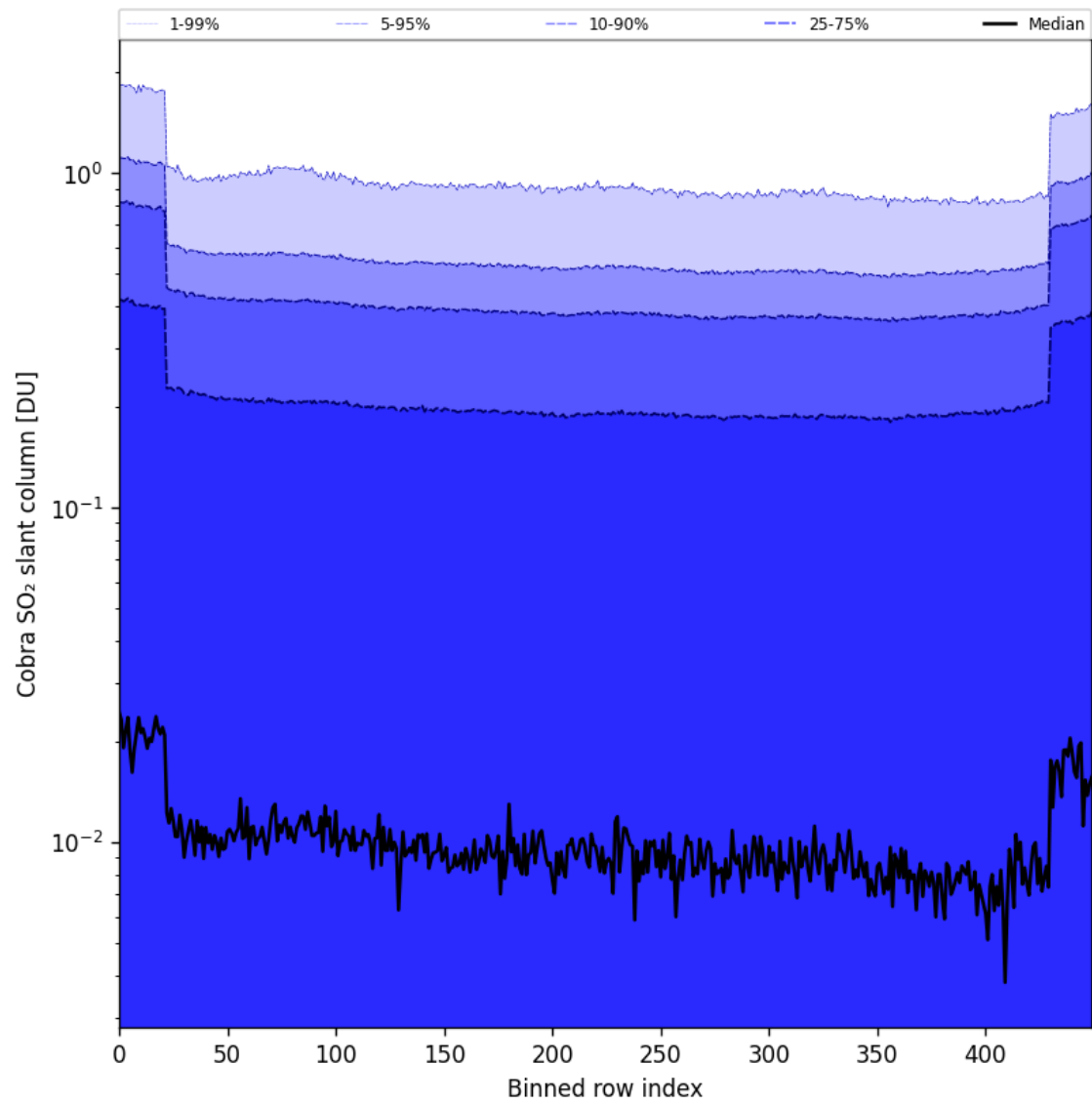
Figure 87: Along track statistics of “Cobra SO 2 slant column” for 2025-07-05 to 2025-07-07
