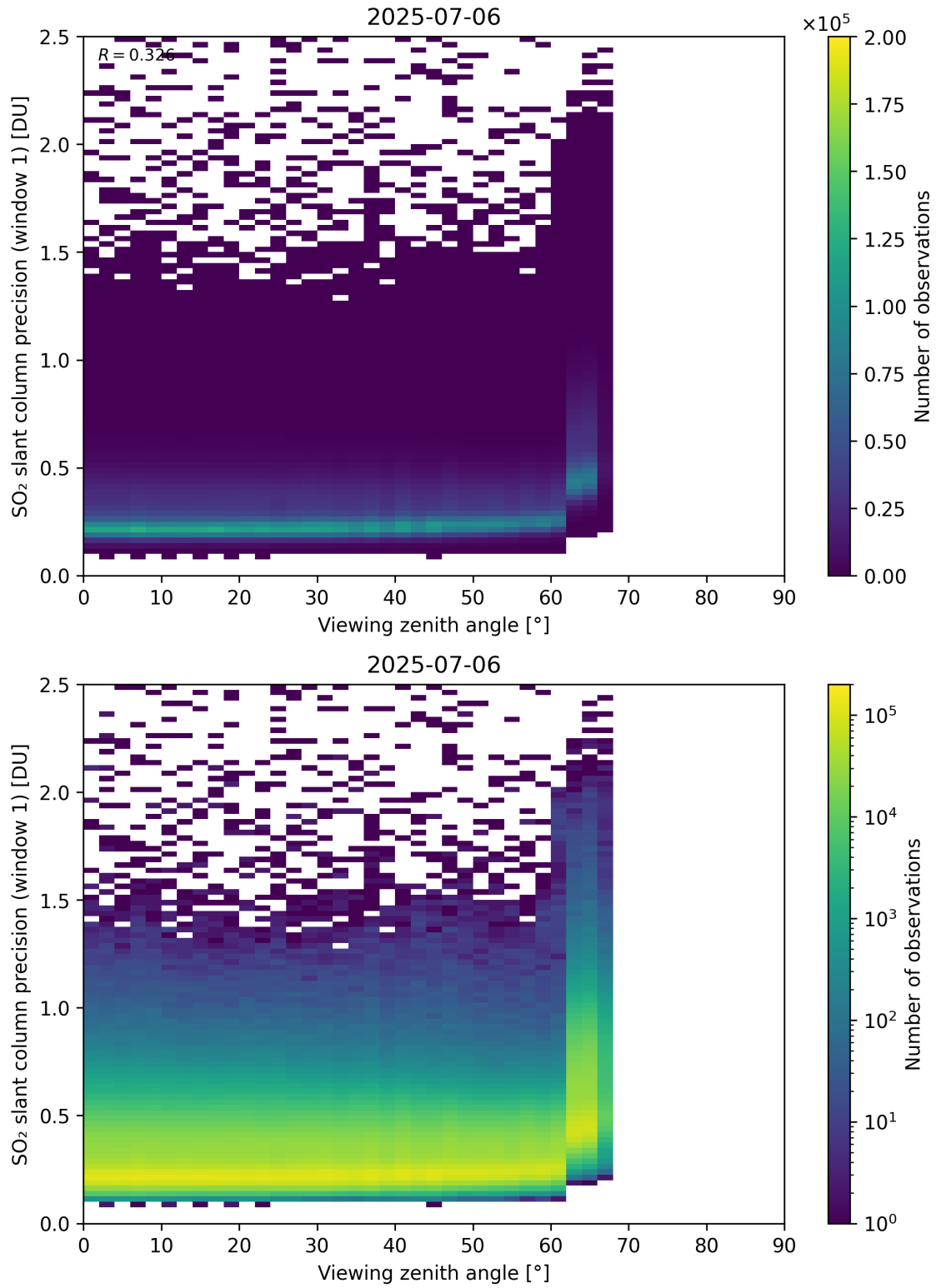
Figure 377: Scatter density plot of “Viewing zenith angle” against “SO 2 slant column precision (window 1)” for 2025-07-05 to 2025-07-07.
