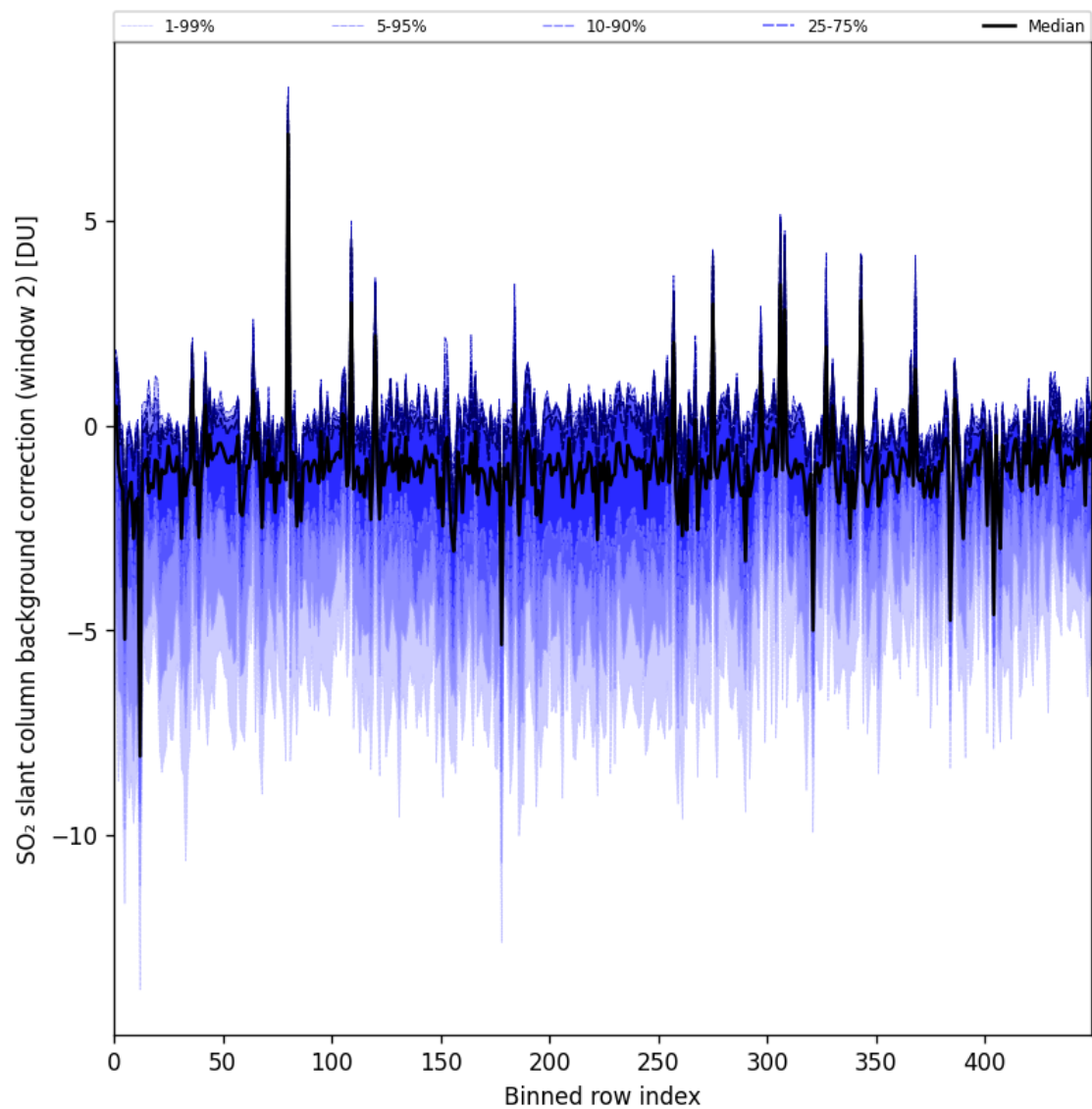
Figure 96: Along track statistics of “SO 2 slant column background correction (window 2)” for 2025-07-05 to 2025-07-07
