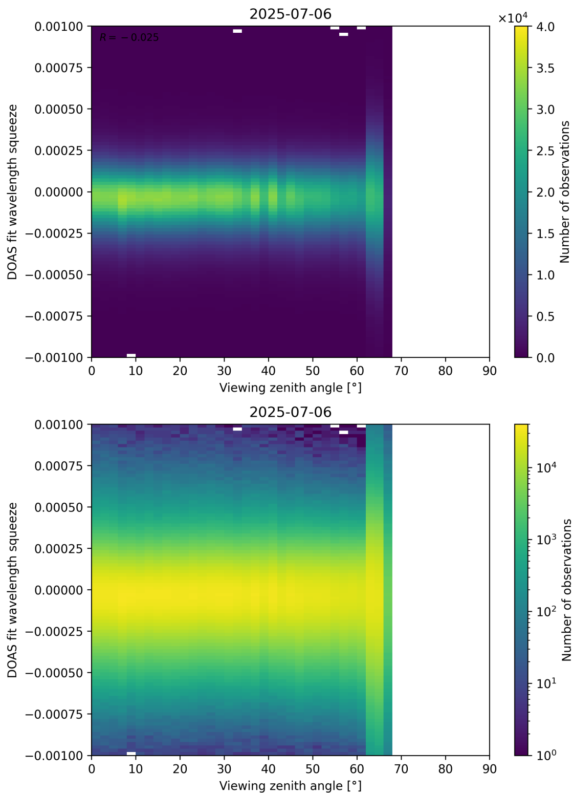
Figure 366: Scatter density plot of “Viewing zenith angle” against “DOAS fit wavelength squeeze” for 2025-07-05 to 2025-07-07.
