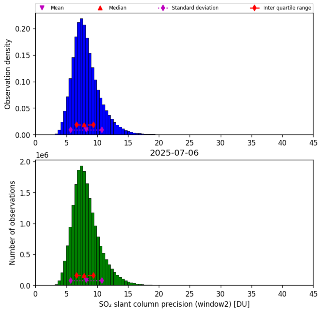
Figure 68: Histogram of “SO 2 slant column precision (window2)” for 2025-07-05 to 2025-07-07
