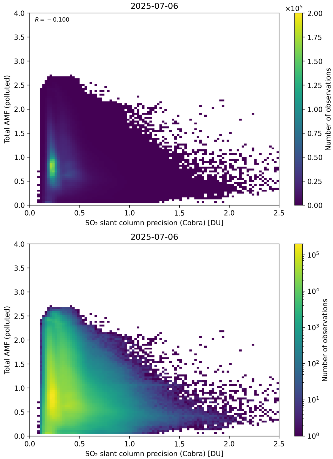
Figure 213: Scatter density plot of “SO 2 slant column precision (Cobra)” against “Total AMF (polluted)” for 2025-07-05 to 2025-07-07.
