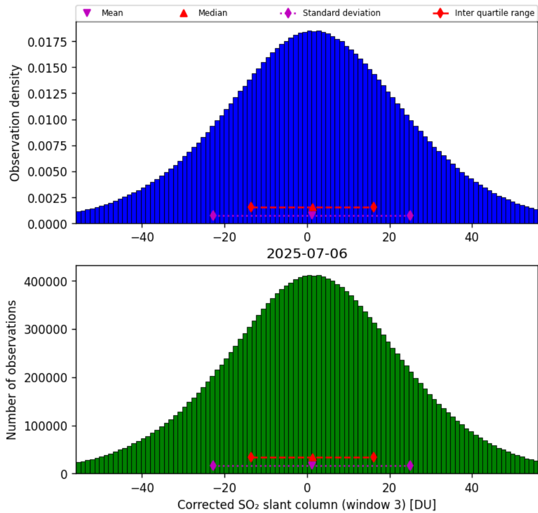
Figure 73: Histogram of “Corrected SO 2 slant column (window 3)” for 2025-07-05 to 2025-07-07
