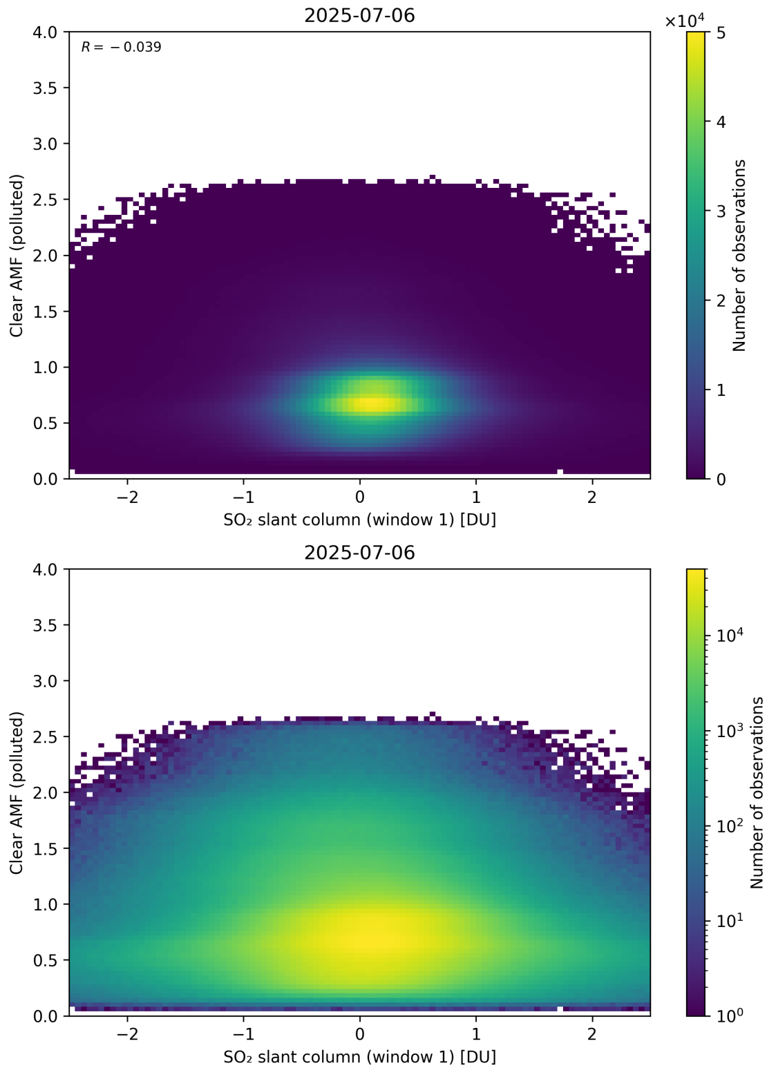
Figure 282: Scatter density plot of “SO 2 slant column (window 1)” against “Clear AMF (polluted)” for 2025-07-05 to 2025-07-07.
