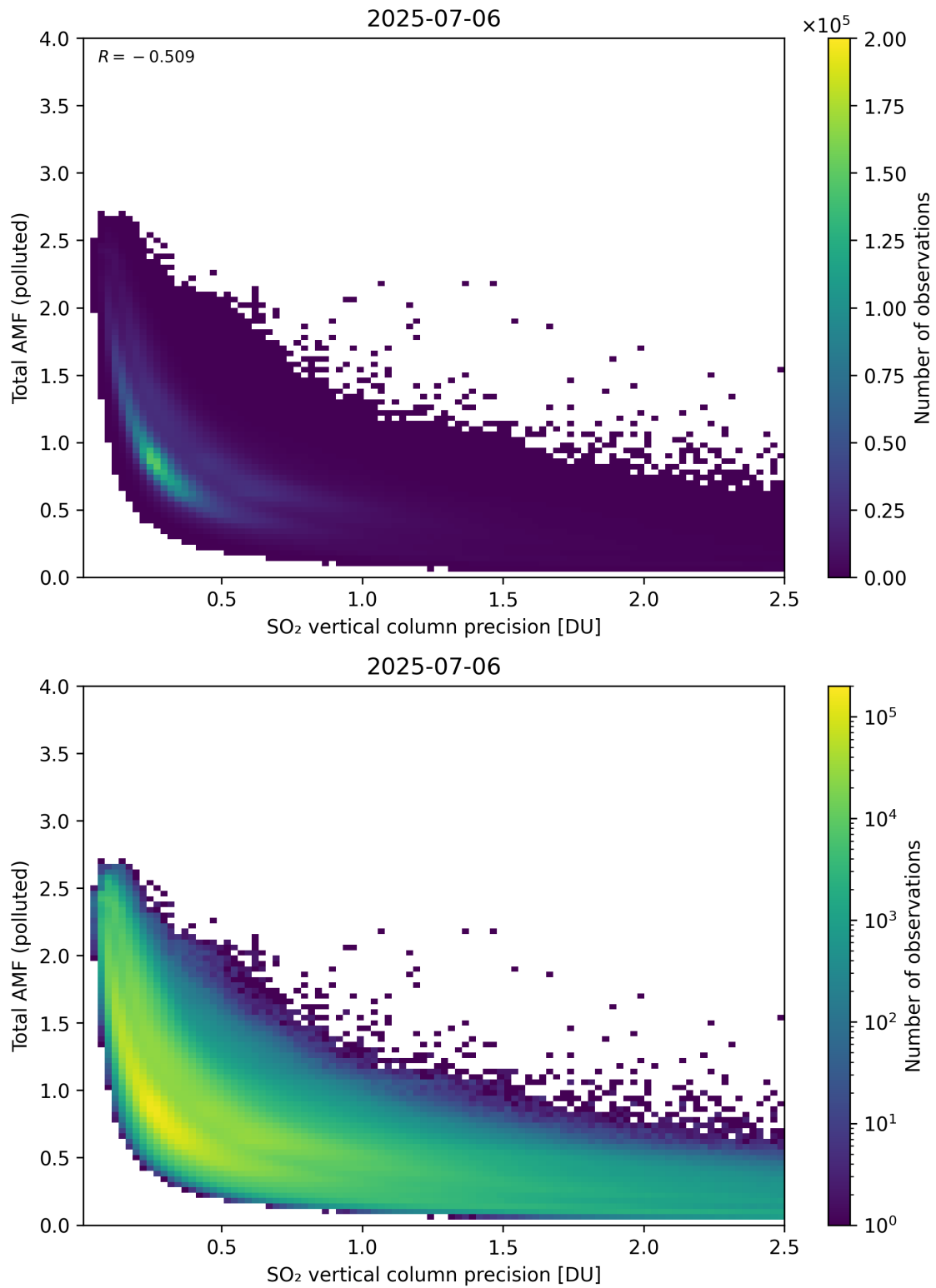
Figure 346: Scatter density plot of “SO 2 vertical column precision” against “Total AMF (polluted)” for 2025-07-05 to 2025-07-07.
