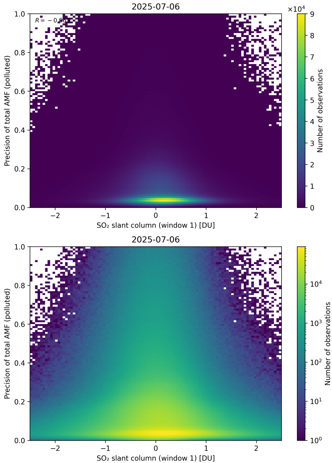
Figure 290: Scatter density plot of “SO 2 slant column (window 1)” against “Precision of total AMF (polluted)” for 2025-07-05 to 2025-07-07.
