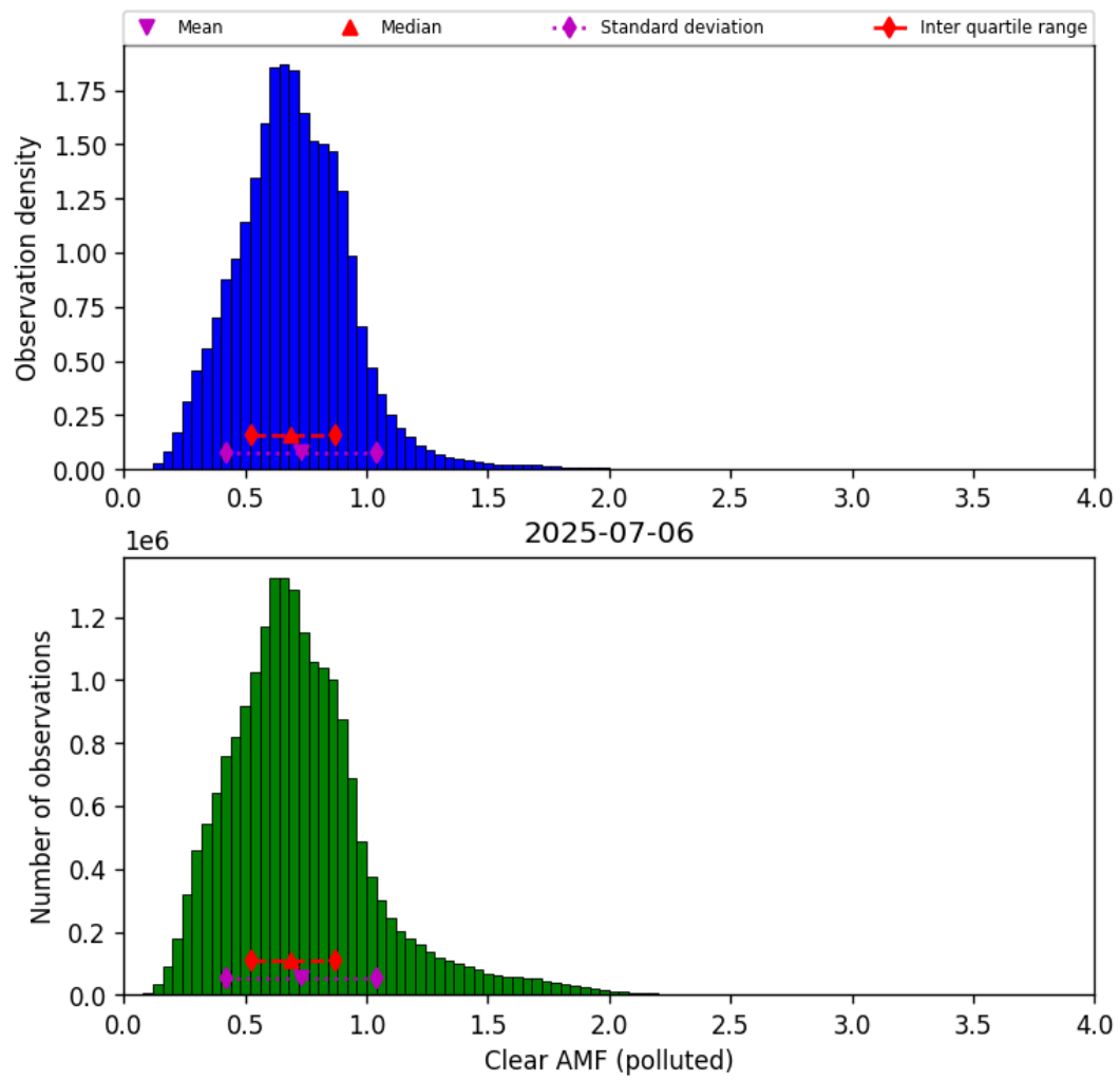
Figure 81: Histogram of “Clear AMF (polluted)” for 2025-07-05 to 2025-07-07
