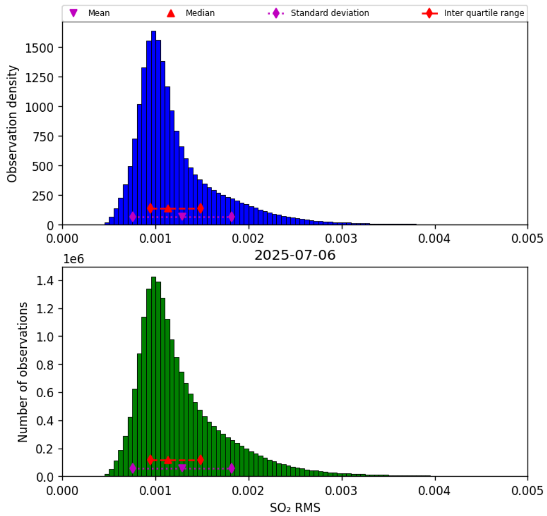
Figure 78: Histogram of “SO 2 RMS” for 2025-07-05 to 2025-07-07
