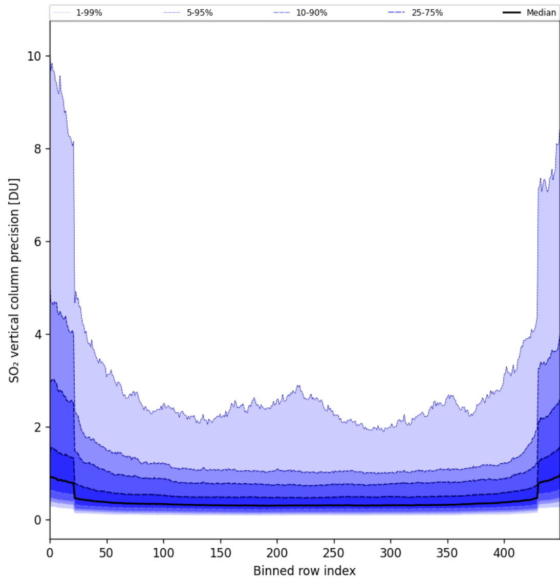
Figure 85: Along track statistics of “SO 2 vertical column precision” for 2025-07-05 to 2025-07-07
