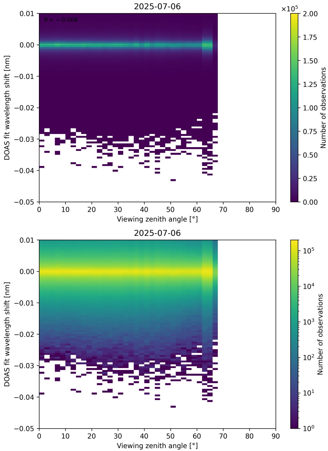
Figure 365: Scatter density plot of “Viewing zenith angle” against “DOAS fit wavelength shift” for 2025-07-05 to 2025-07-07.
