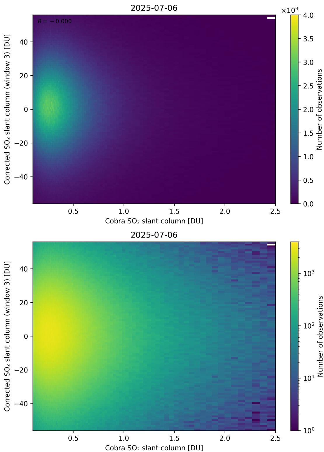
Figure 218: Scatter density plot of “Cobra SO 2 slant column” against “Corrected SO 2 slant column (window 3)” for 2025-07-05 to 2025-07-07.
