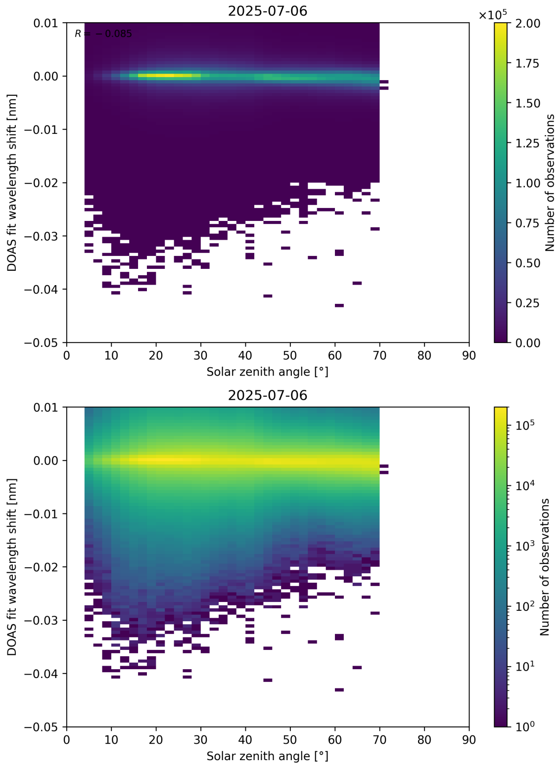
Figure 174: Scatter density plot of “Solar zenith angle” against “DOAS fit wavelength shift” for 2025-07-05 to 2025-07-07.
