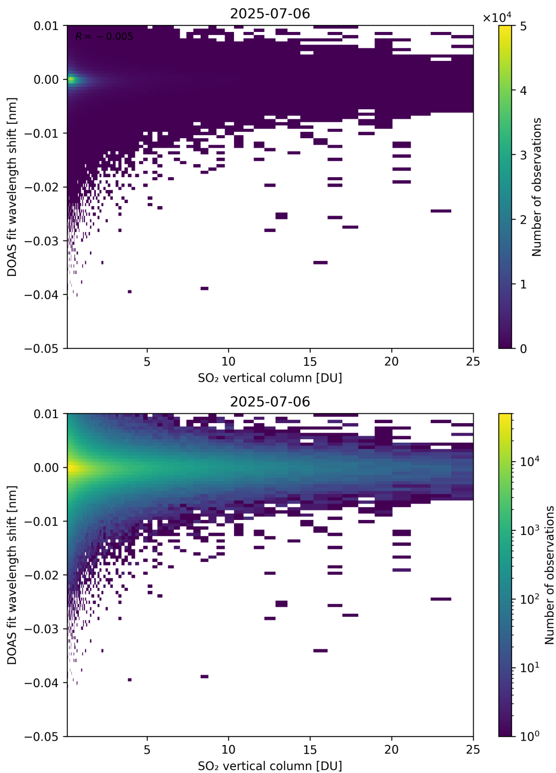
Figure 326: Scatter density plot of “SO 2 vertical column” against “DOAS fit wavelength shift” for 2025-07-05 to 2025-07-07.
