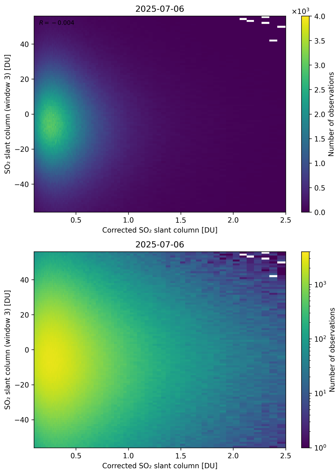
Figure 240: Scatter density plot of “Corrected SO 2 slant column” against “SO 2 slant column (window 3)” for 2025-07-05 to 2025-07-07.
