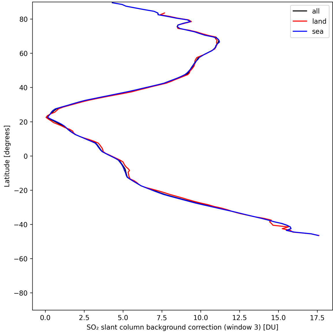
Figure 48: Zonal average of “SO 2 slant column background correction (window 3)” for 2025-07-05 to 2025-07-07.
