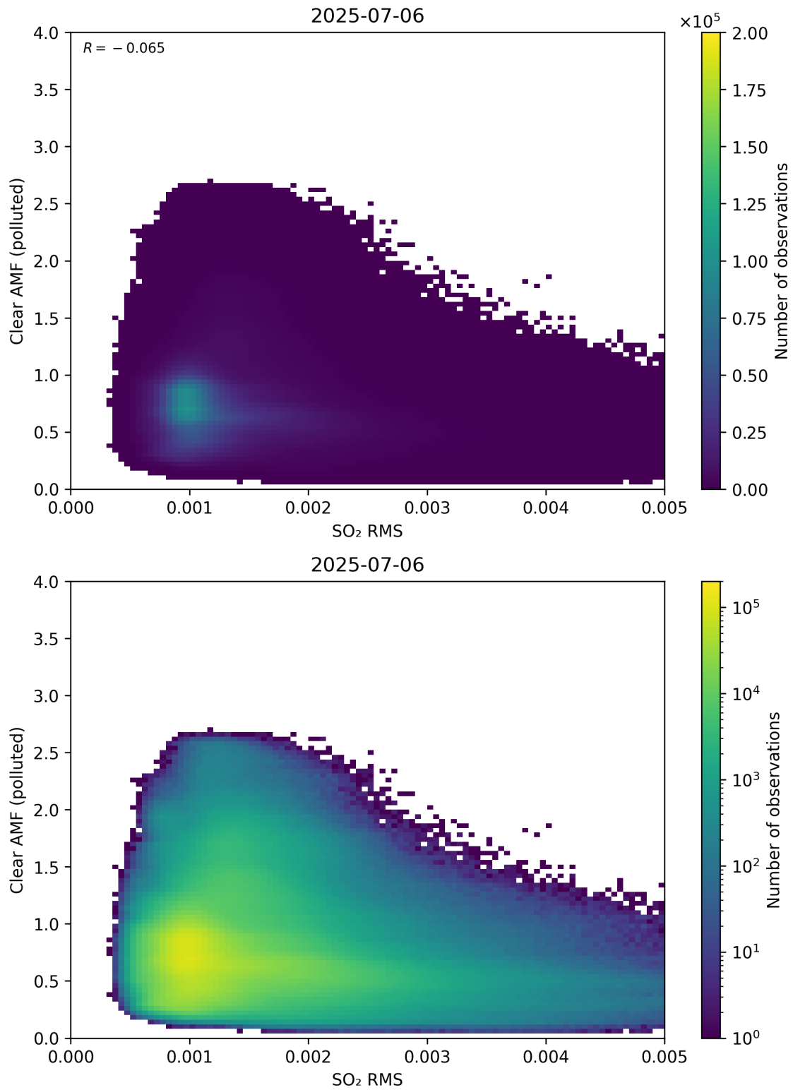
Figure 147: Scatter density plot of “SO 2 RMS” against “Clear AMF (polluted)” for 2025-07-05 to 2025-07-07.
