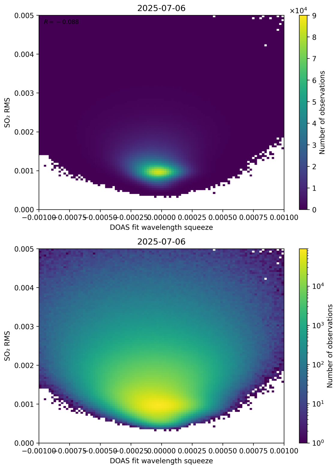
Figure 143: Scatter density plot of “DOAS fit wavelength squeeze” against “SO 2 RMS” for 2025-07-05 to 2025-07-07.
