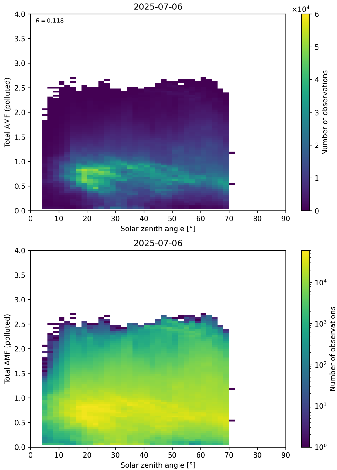
Figure 189: Scatter density plot of “Solar zenith angle” against “Total AMF (polluted)” for 2025-07-05 to 2025-07-07.
