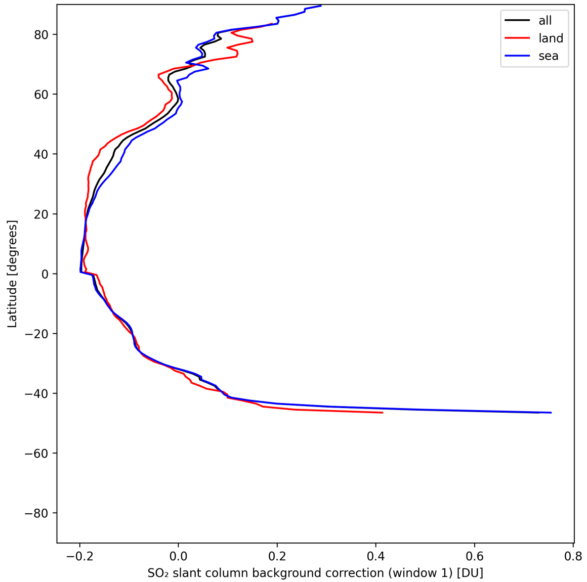
Figure 40: Zonal average of “SO 2 slant column background correction (window 1)” for 2025-07-05 to 2025-07-07.
