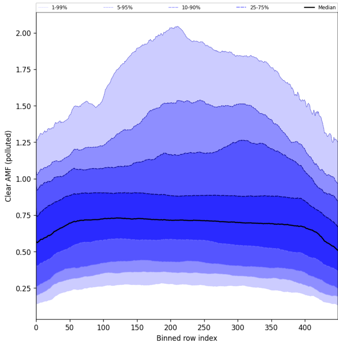
Figure 107: Along track statistics of “Clear AMF (polluted)” for 2025-07-05 to 2025-07-07
