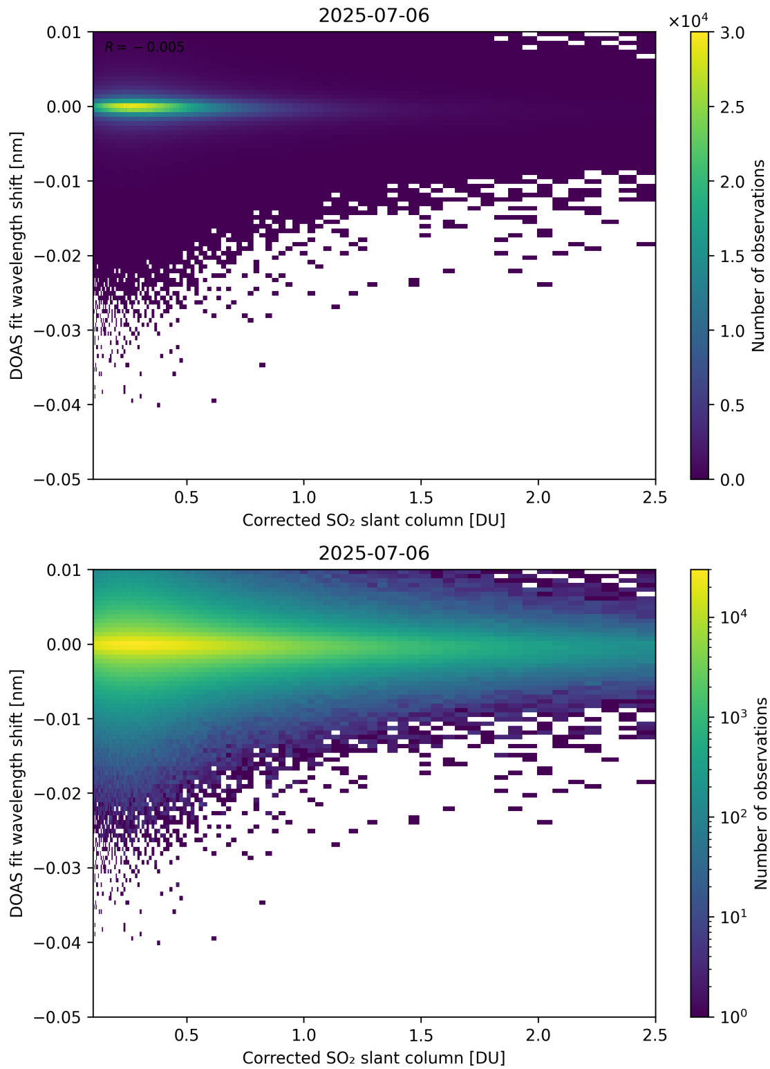
Figure 229: Scatter density plot of “Corrected SO 2 slant column” against “DOAS fit wavelength shift” for 2025-07-05 to 2025-07-07.
