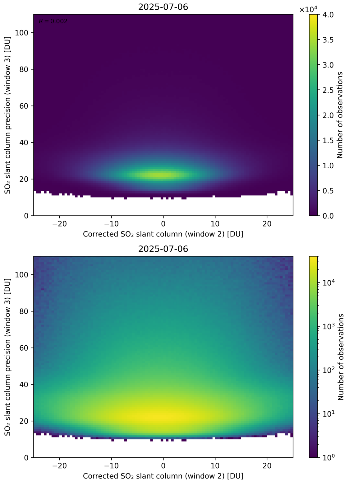
Figure 252: Scatter density plot of “Corrected SO 2 slant column (window 2)” against “SO 2 slant column precision (window 3)” for 2025-07-05 to 2025-07-07.
