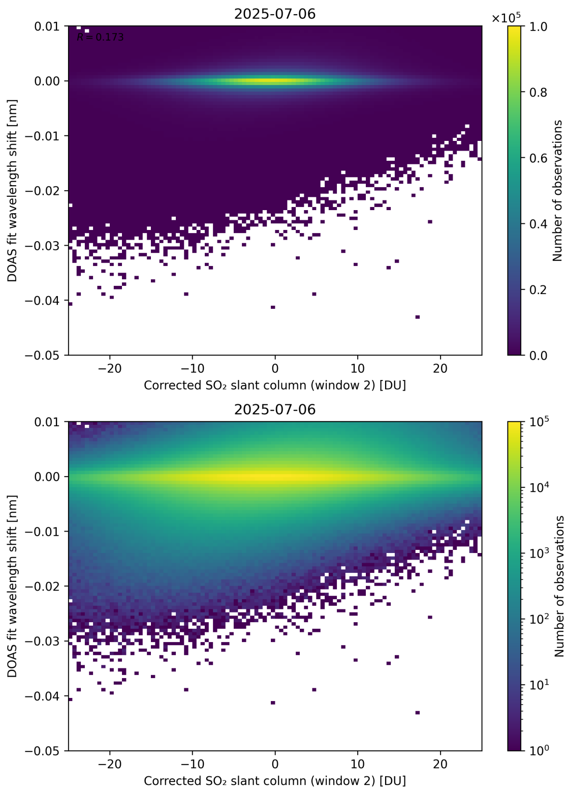
Figure 246: Scatter density plot of “Corrected SO 2 slant column (window 2)” against “DOAS fit wavelength shift” for 2025-07-05 to 2025-07-07.
