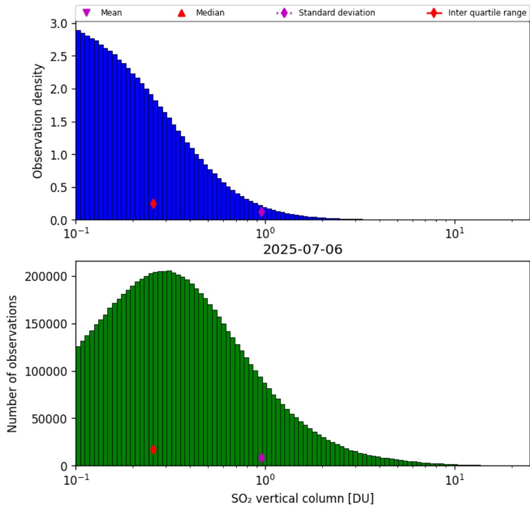
Figure 58: Histogram of “SO 2 vertical column” for 2025-07-05 to 2025-07-07
