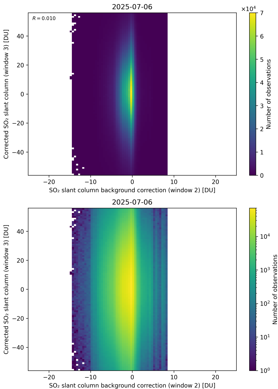
Figure 127: Scatter density plot of “SO 2 slant column background correction (window 2)” against “Corrected SO 2 slant column (window 3)” for 2025-07-05 to 2025-07-07.
