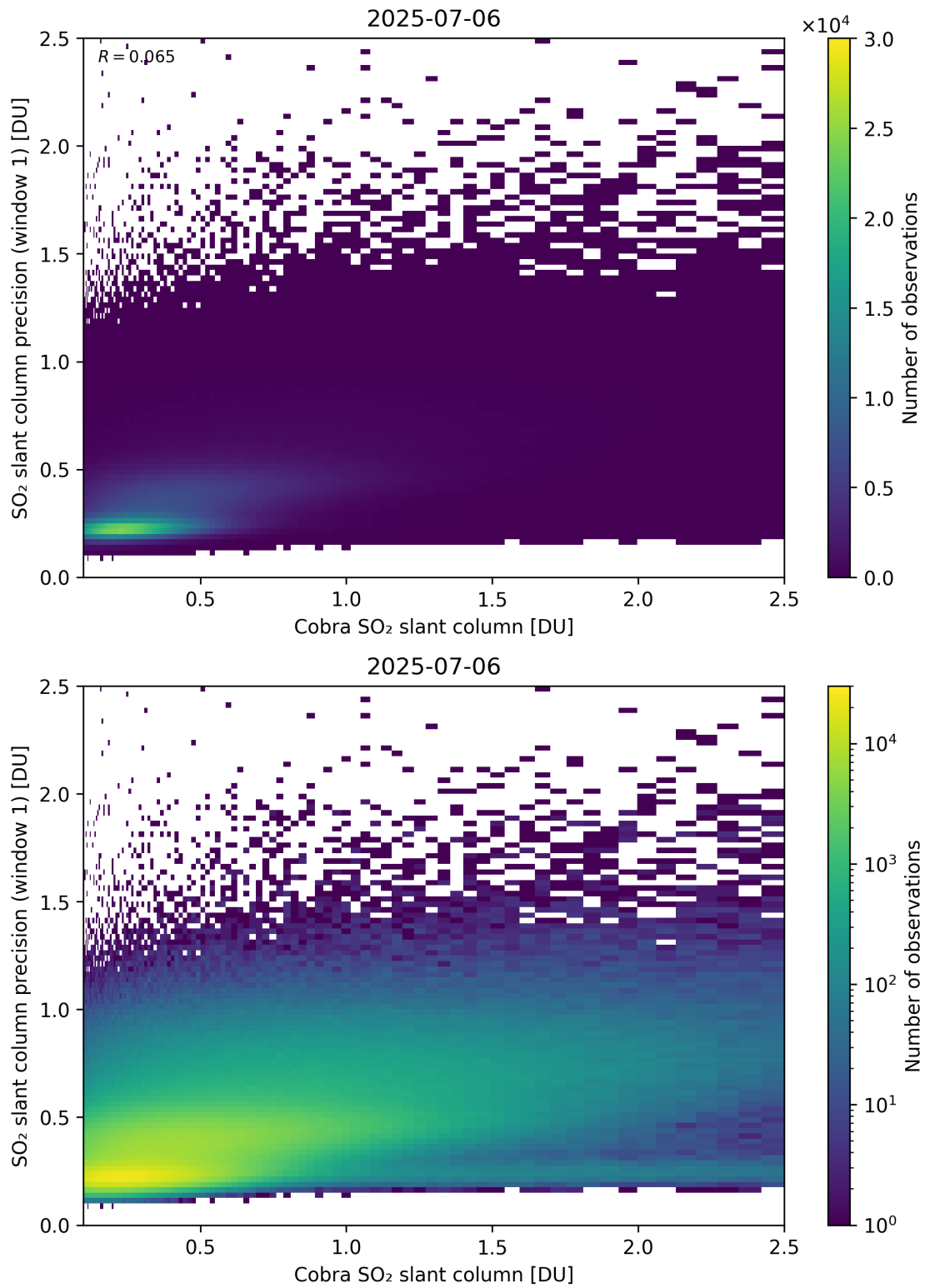
Figure 220: Scatter density plot of “Cobra SO 2 slant column” against “SO 2 slant column precision (window 1)” for 2025-07-05 to 2025-07-07.
