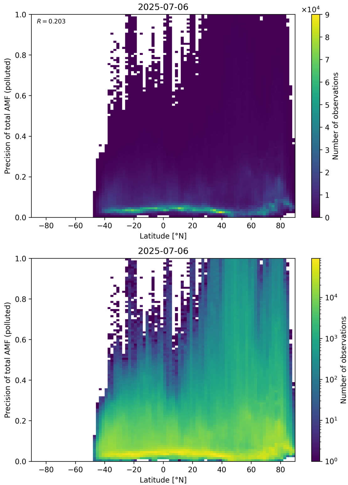
Figure 168: Scatter density plot of “Latitude” against “Precision of total AMF (polluted)” for 2025-07-05 to 2025-07-07.
