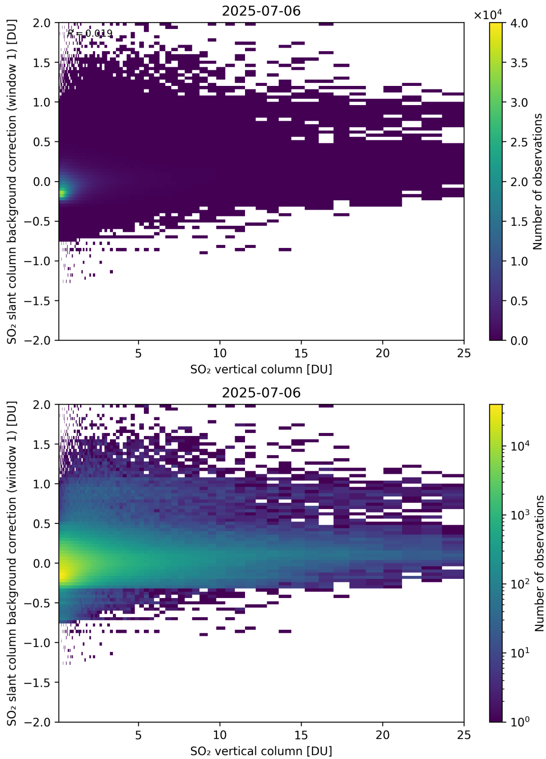
Figure 323: Scatter density plot of “SO 2 vertical column” against “SO 2 slant column background correction (window 1)” for 2025-07-05 to 2025-07-07.
