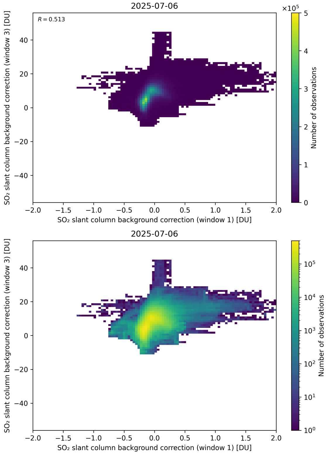
Figure 110: Scatter density plot of “SO 2 slant column background correction (window 1)” against “SO 2 slant column background correction (window 3)” for 2025-07-05 to 2025-07-07.
