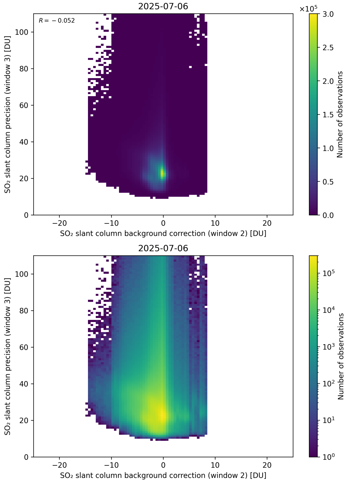
Figure 129: Scatter density plot of “SO 2 slant column background correction (window 2)” against “SO 2 slant column precision (window 3)” for 2025-07-05 to 2025-07-07.
