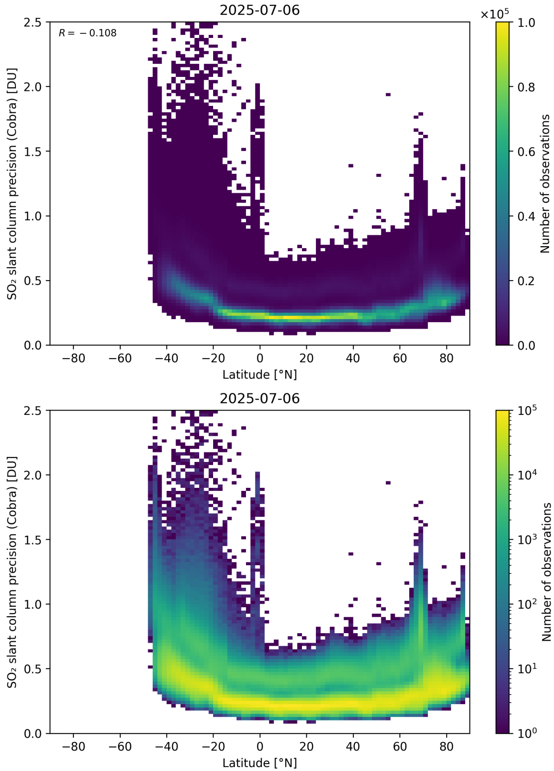
Figure 158: Scatter density plot of “Latitude” against “SO 2 slant column precision (Cobra)” for 2025-07-05 to 2025-07-07.
