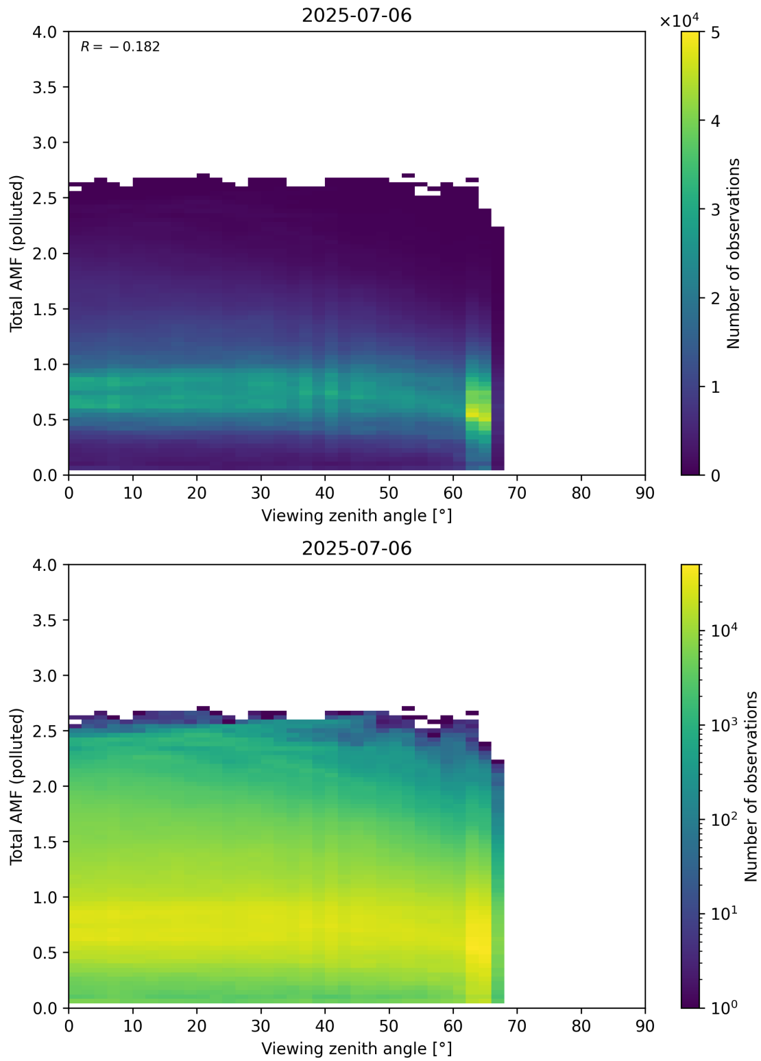
Figure 381: Scatter density plot of “Viewing zenith angle” against “Total AMF (polluted)” for 2025-07-05 to 2025-07-07.
