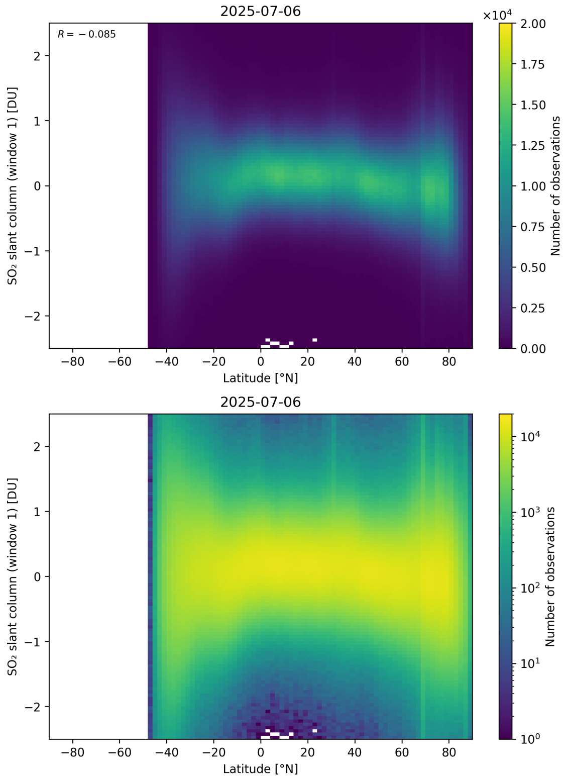
Figure 162: Scatter density plot of “Latitude” against “SO 2 slant column (window 1)” for 2025-07-05 to 2025-07-07.
