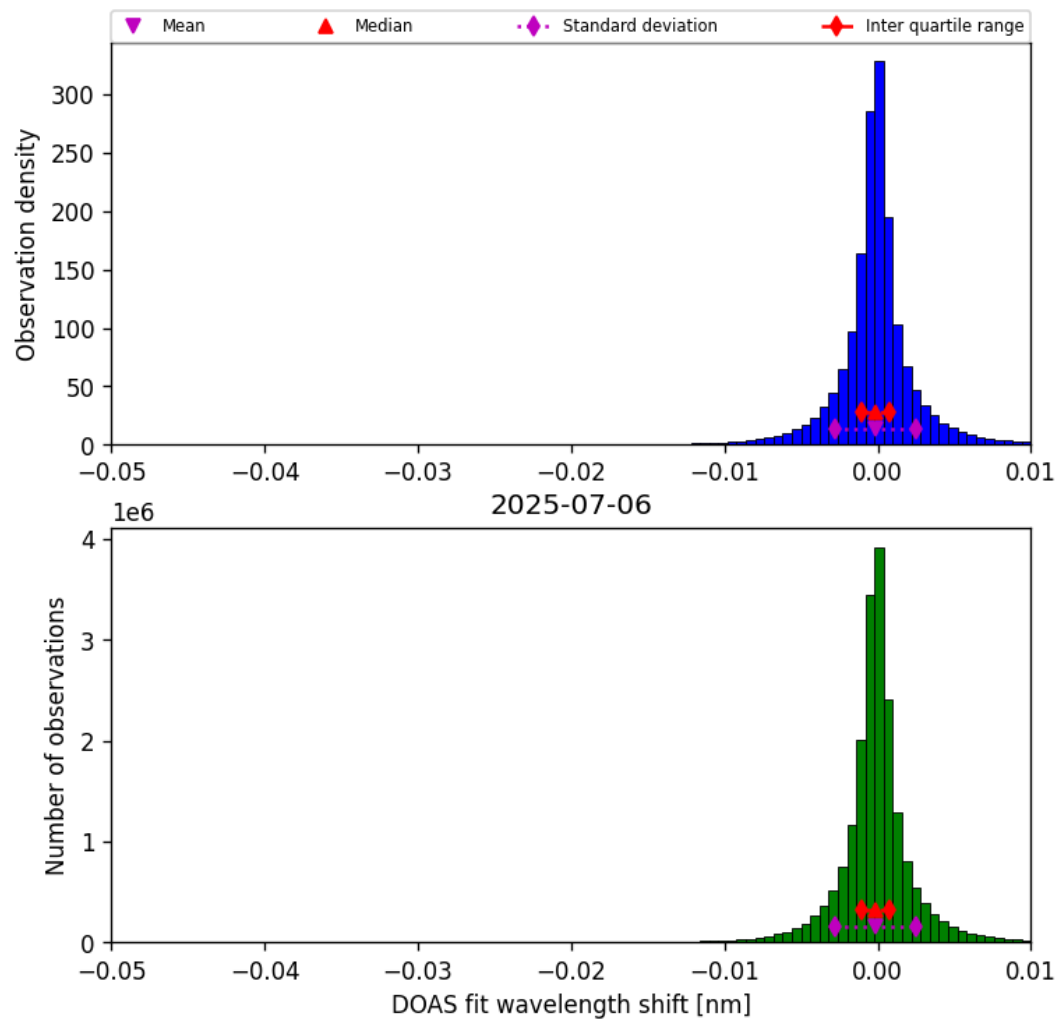
Figure 76: Histogram of “DOAS fit wavelength shift” for 2025-07-05 to 2025-07-07
