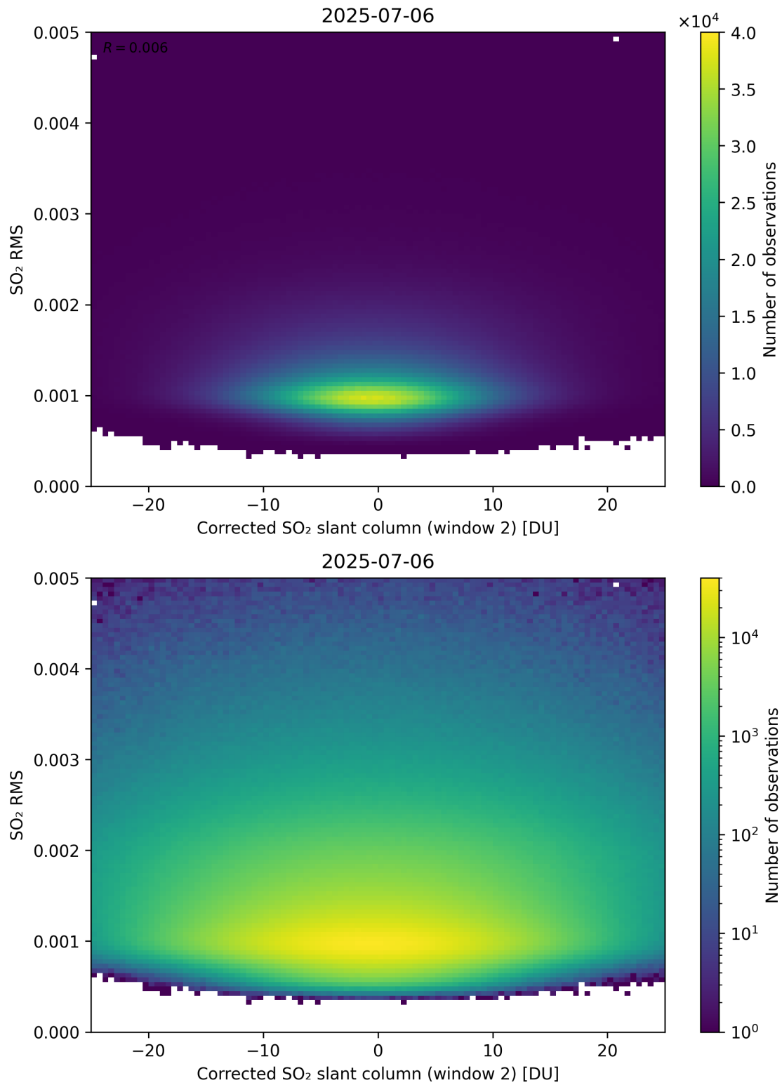
Figure 248: Scatter density plot of “Corrected SO 2 slant column (window 2)” against “SO 2 RMS” for 2025-07-05 to 2025-07-07.
