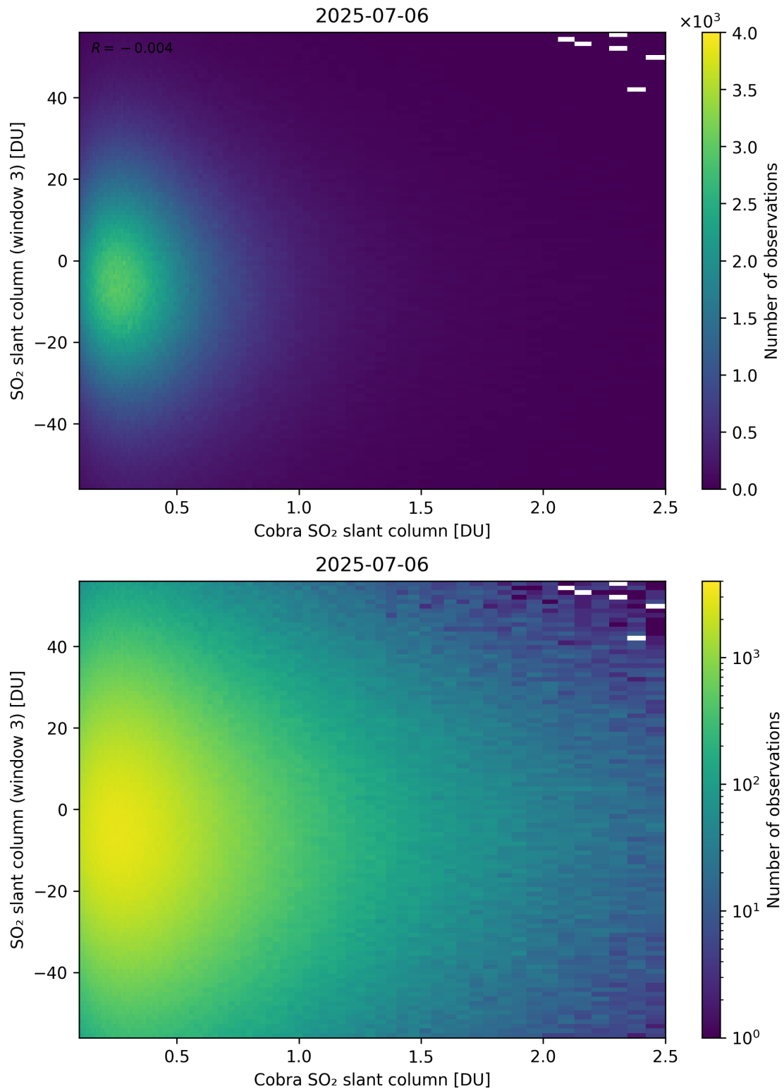
Figure 222: Scatter density plot of “Cobra SO 2 slant column” against “SO 2 slant column (window 3)” for 2025-07-05 to 2025-07-07.
