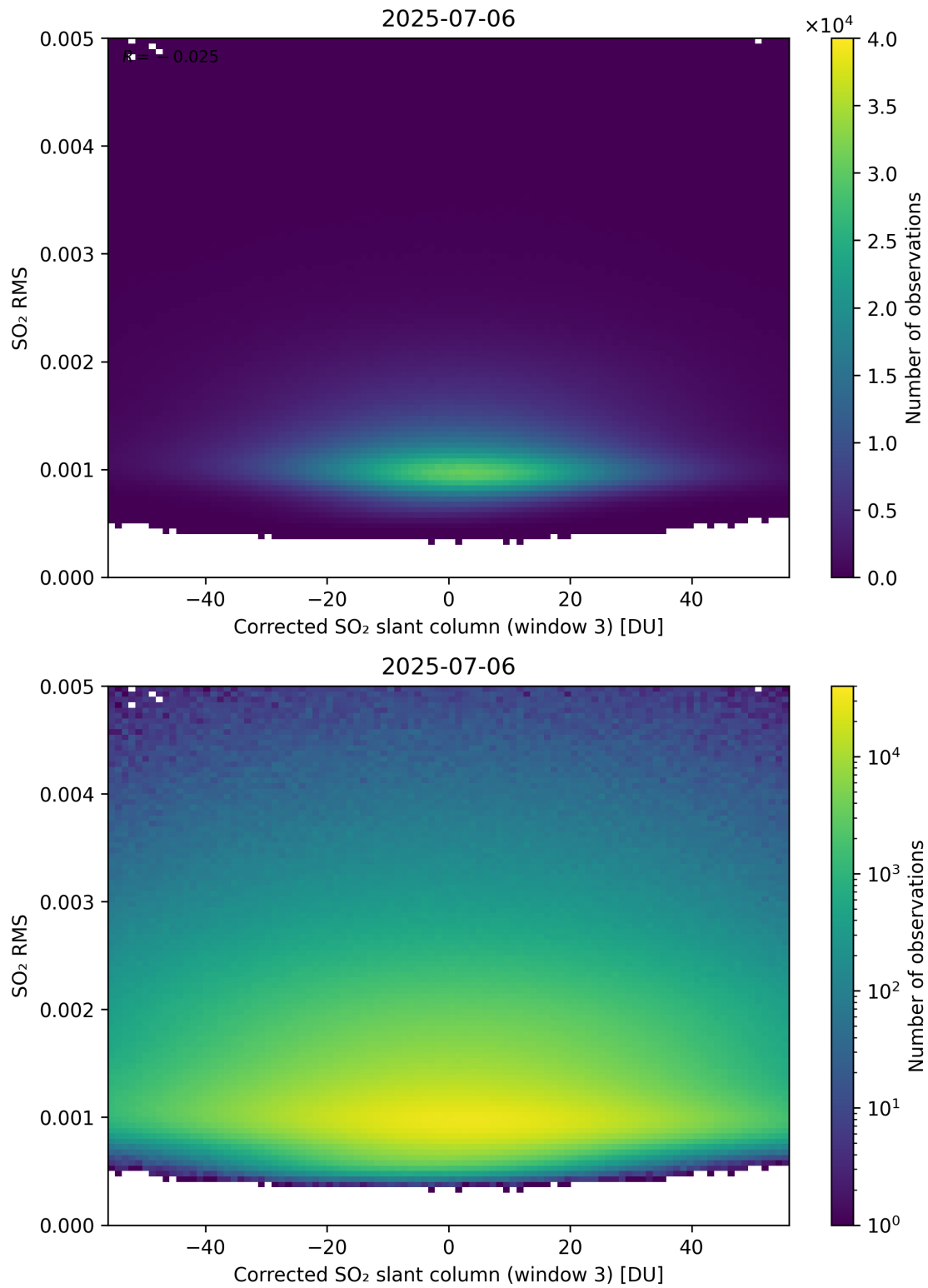
Figure 258: Scatter density plot of “Corrected SO 2 slant column (window 3)” against “SO 2 RMS” for 2025-07-05 to 2025-07-07.
