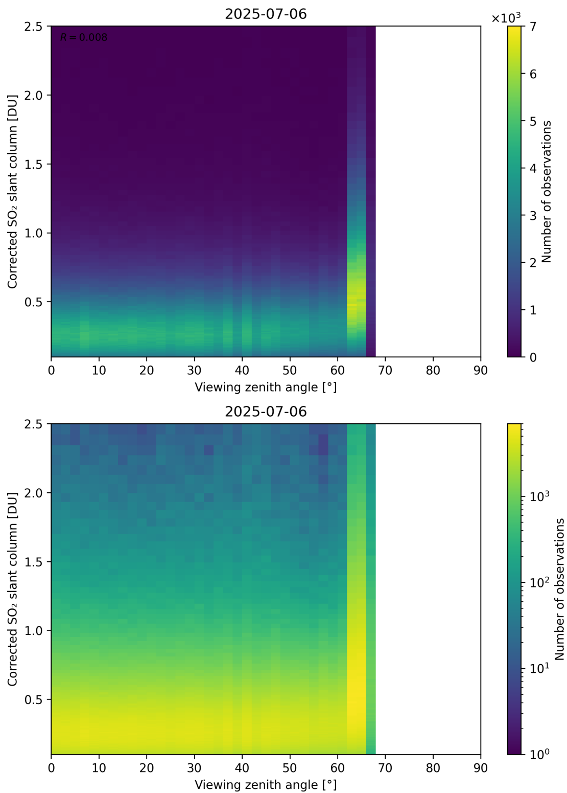
Figure 373: Scatter density plot of “Viewing zenith angle” against “Corrected SO 2 slant column” for 2025-07-05 to 2025-07-07.
