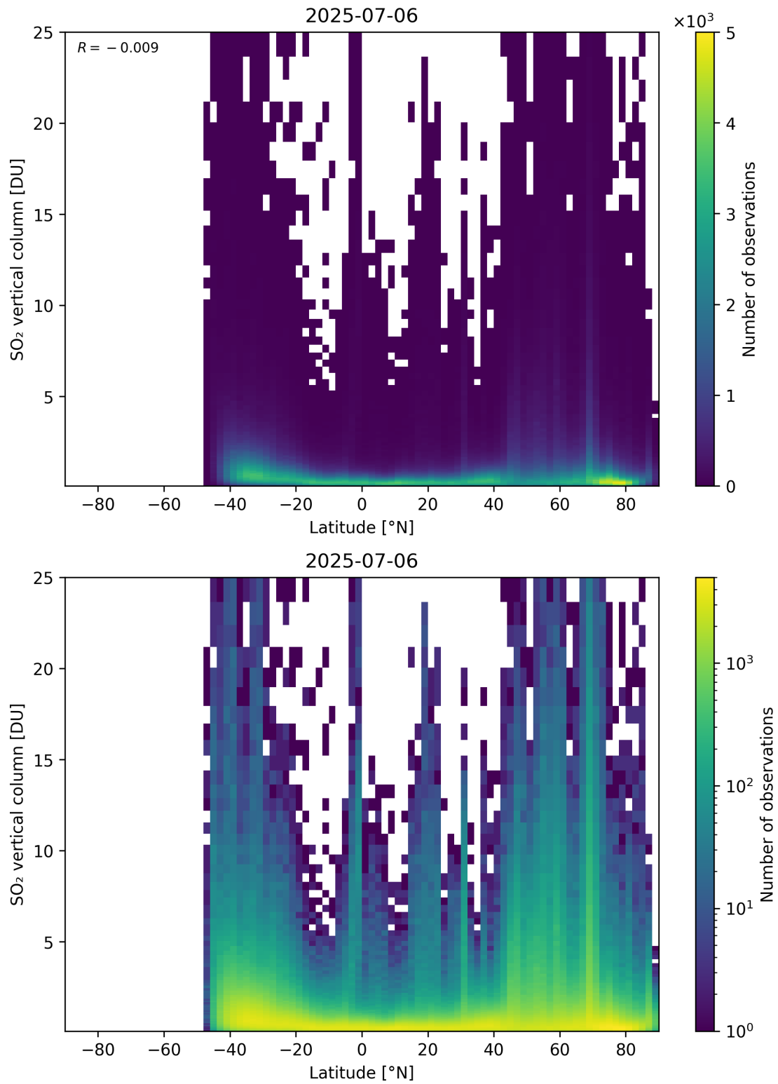
Figure 169: Scatter density plot of “Latitude” against “SO 2 vertical column” for 2025-07-05 to 2025-07-07.
