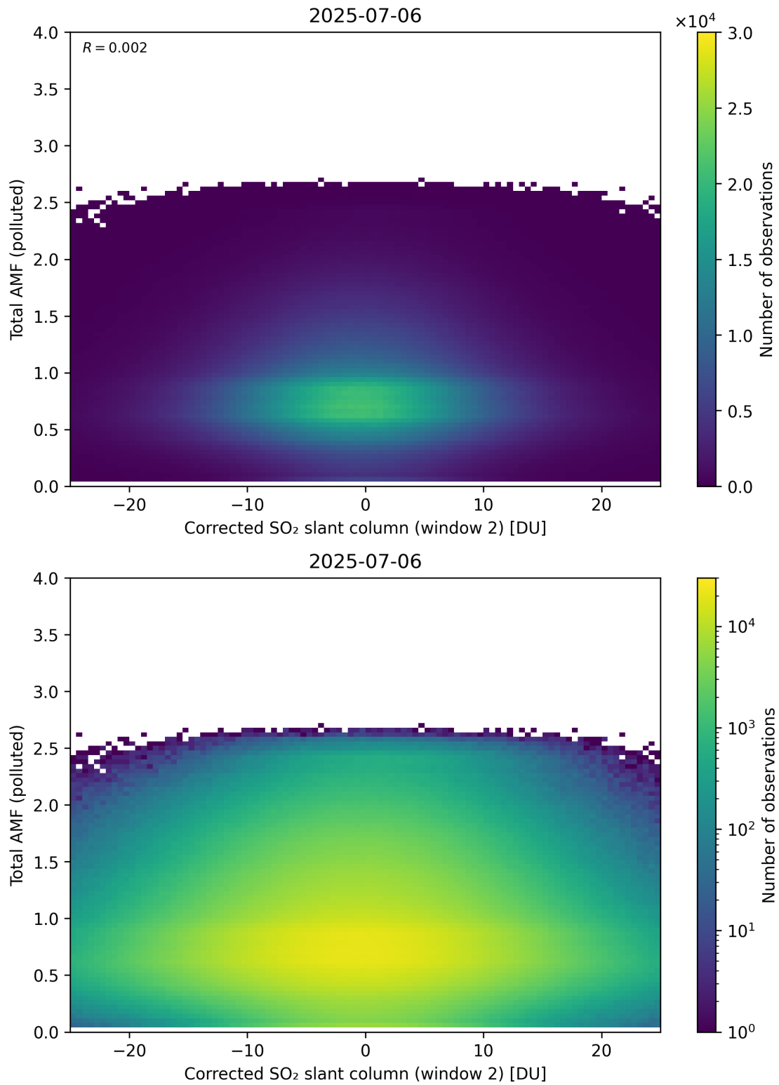
Figure 253: Scatter density plot of “Corrected SO 2 slant column (window 2)” against “Total AMF (polluted)” for 2025-07-05 to 2025-07-07.
