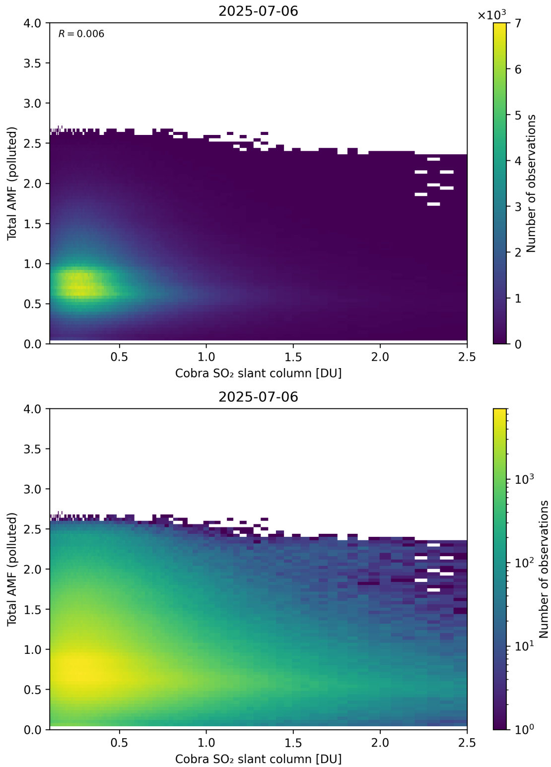
Figure 224: Scatter density plot of “Cobra SO 2 slant column” against “Total AMF (polluted)” for 2025-07-05 to 2025-07-07.
