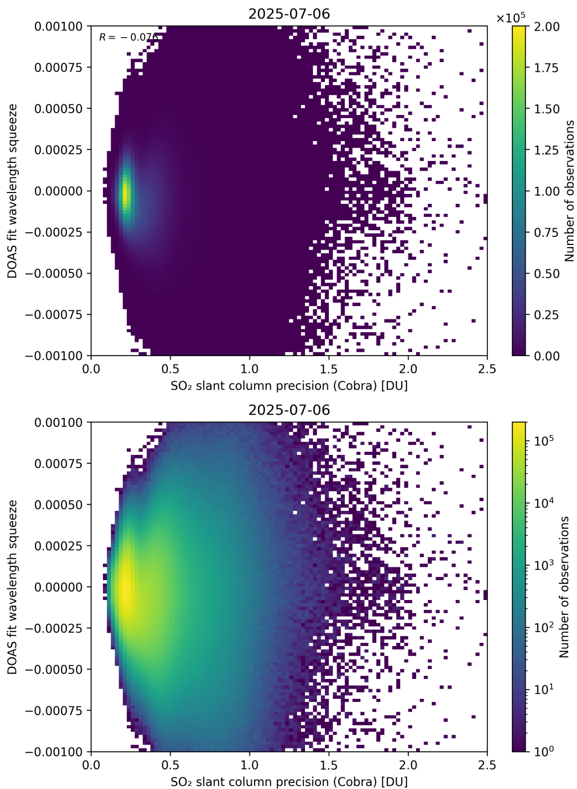
Figure 203: Scatter density plot of “SO 2 slant column precision (Cobra)” against “DOAS fit wavelength squeeze” for 2025-07-05 to 2025-07-07.
