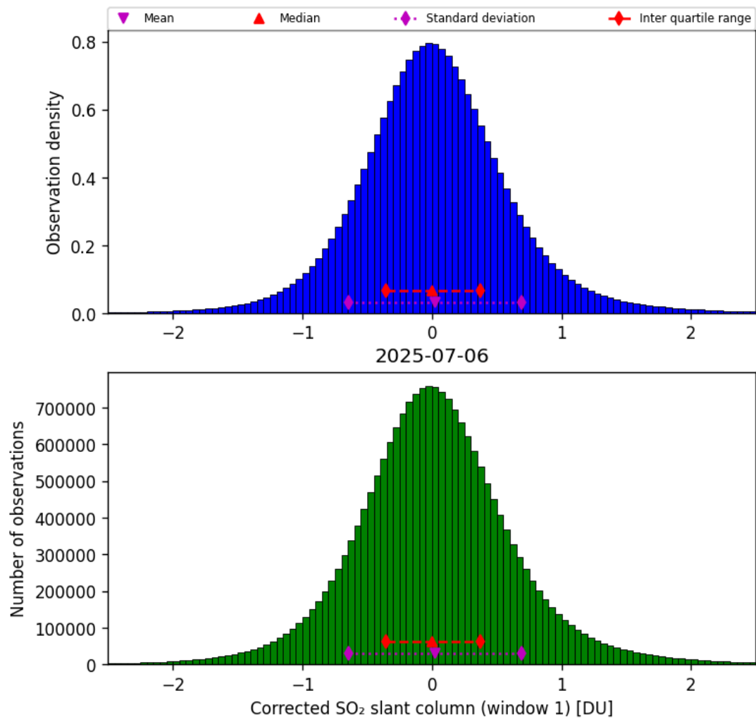
Figure 65: Histogram of “Corrected SO 2 slant column (window 1)” for 2025-07-05 to 2025-07-07
