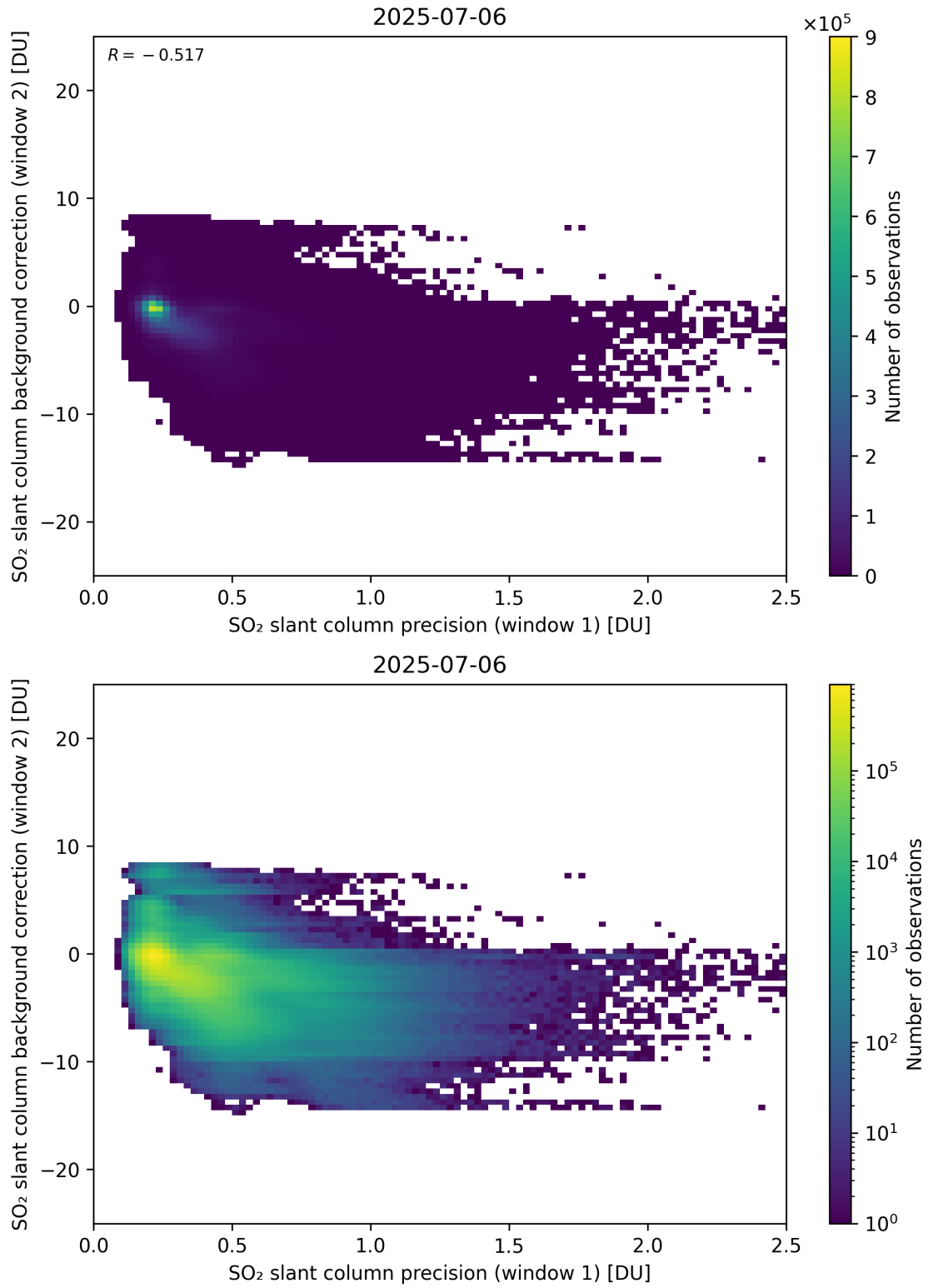
Figure 269: Scatter density plot of “SO 2 slant column precision (window 1)” against “SO 2 slant column background correction (window 2)” for 2025-07-05 to 2025-07-07.
