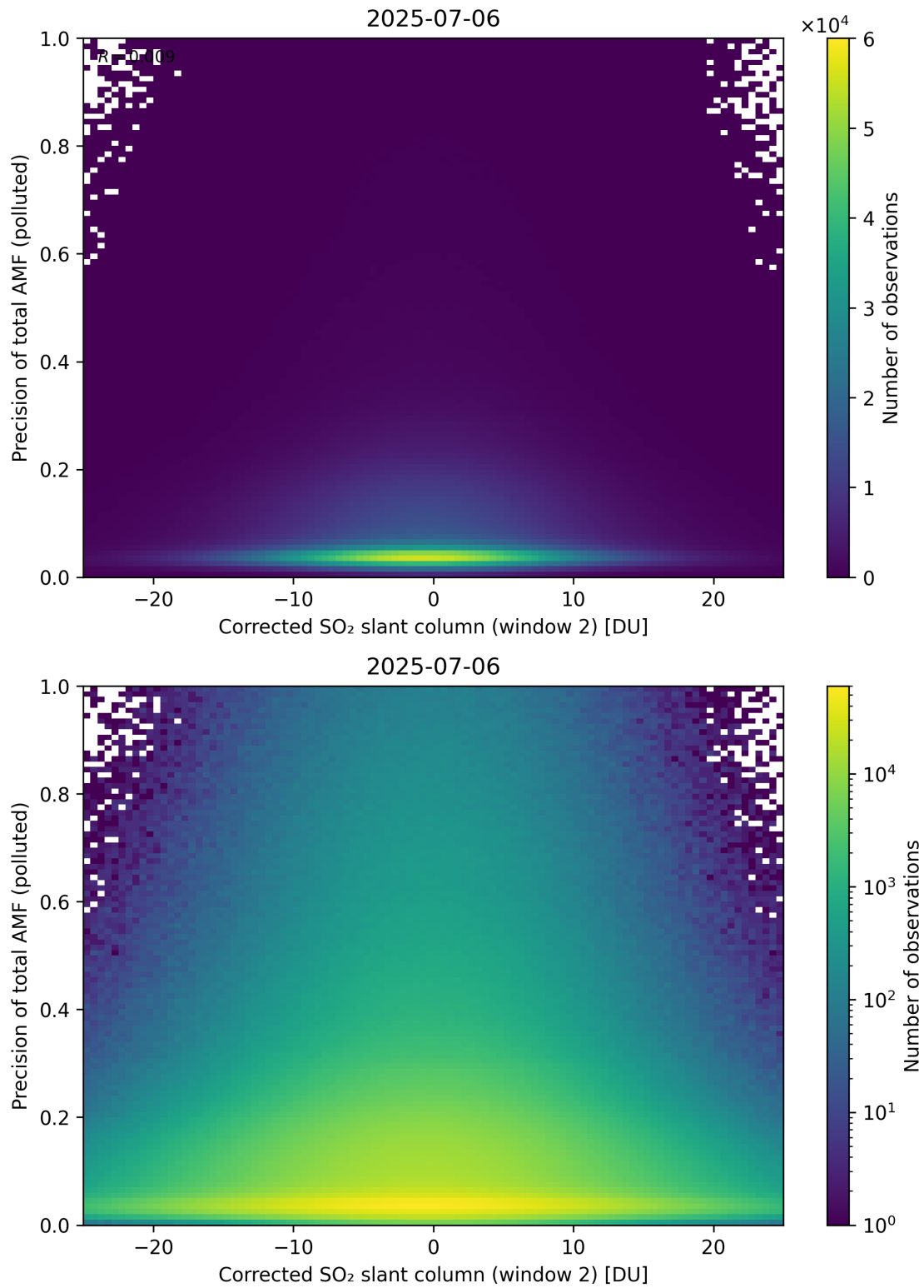
Figure 254: Scatter density plot of “Corrected SO 2 slant column (window 2)” against “Precision of total AMF (polluted)” for 2025-07-05 to 2025-07-07.
