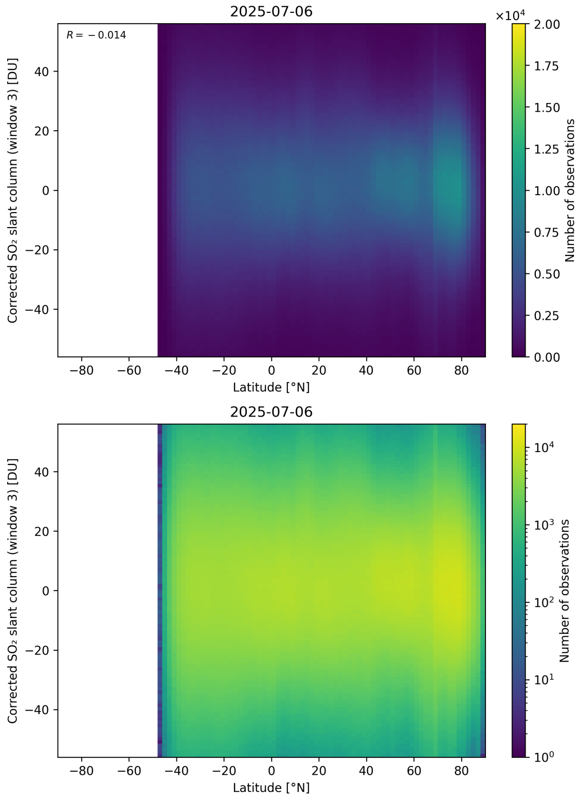
Figure 161: Scatter density plot of “Latitude” against “Corrected SO 2 slant column (window 3)” for 2025-07-05 to 2025-07-07.
