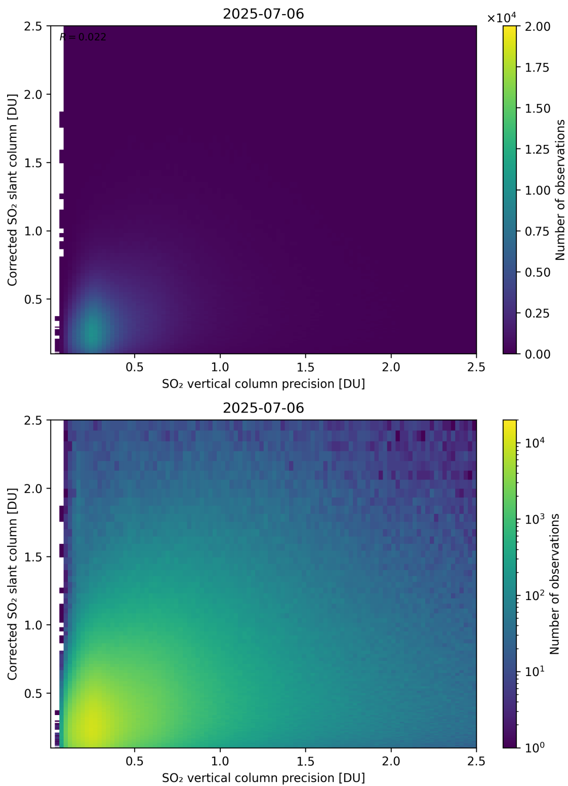
Figure 338: Scatter density plot of “SO 2 vertical column precision” against “Corrected SO 2 slant column” for 2025-07-05 to 2025-07-07.
