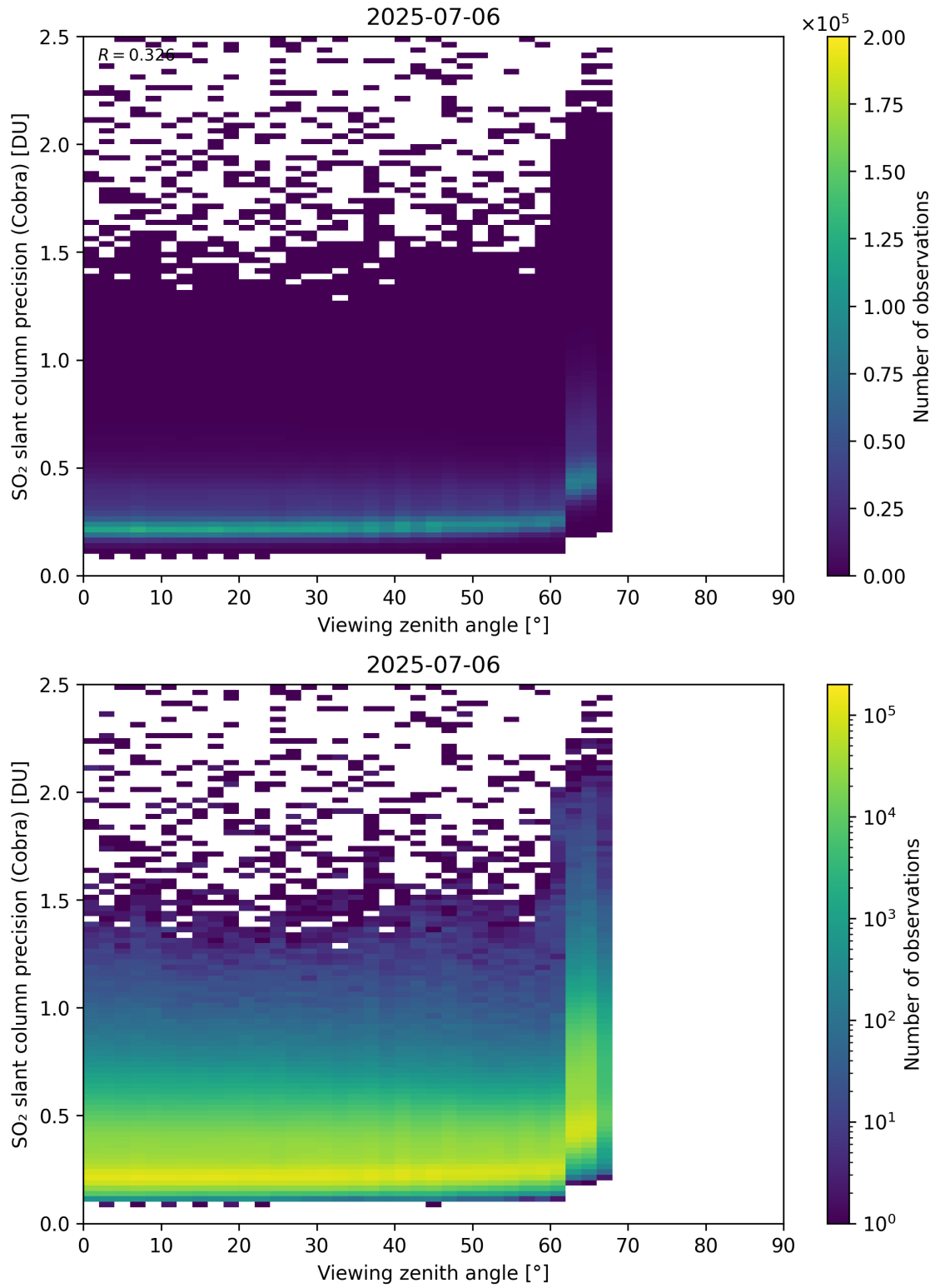
Figure 372: Scatter density plot of “Viewing zenith angle” against “SO 2 slant column precision (Cobra)” for 2025-07-05 to 2025-07-07.
