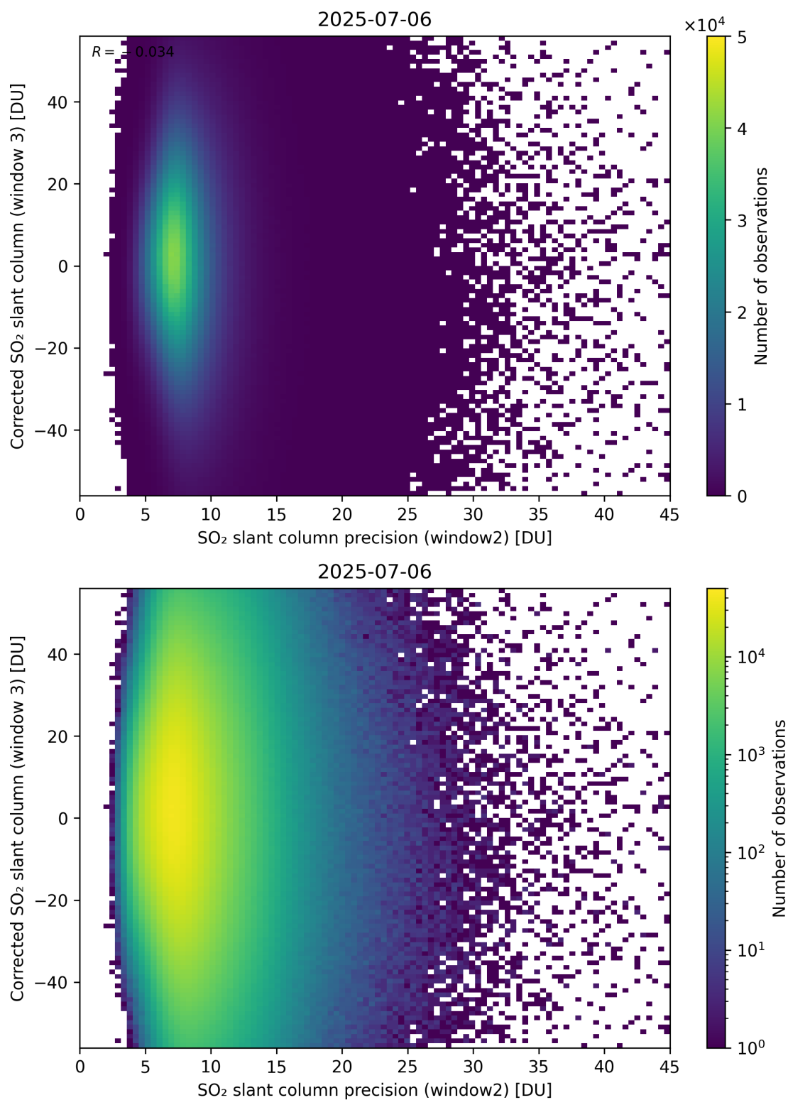
Figure 298: Scatter density plot of “SO 2 slant column precision (window2)” against “Corrected SO 2 slant column (window 3)” for 2025-07-05 to 2025-07-07.
