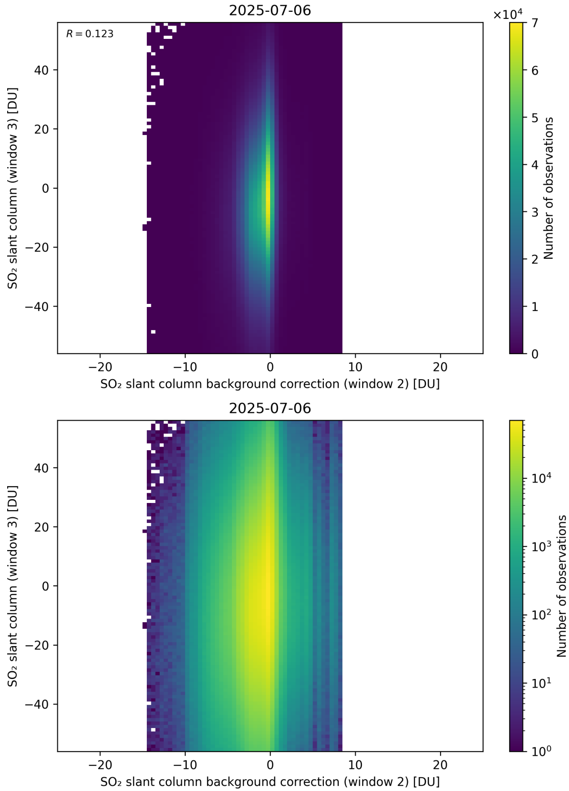
Figure 128: Scatter density plot of “SO 2 slant column background correction (window 2)” against “SO 2 slant column (window 3)” for 2025-07-05 to 2025-07-07.
