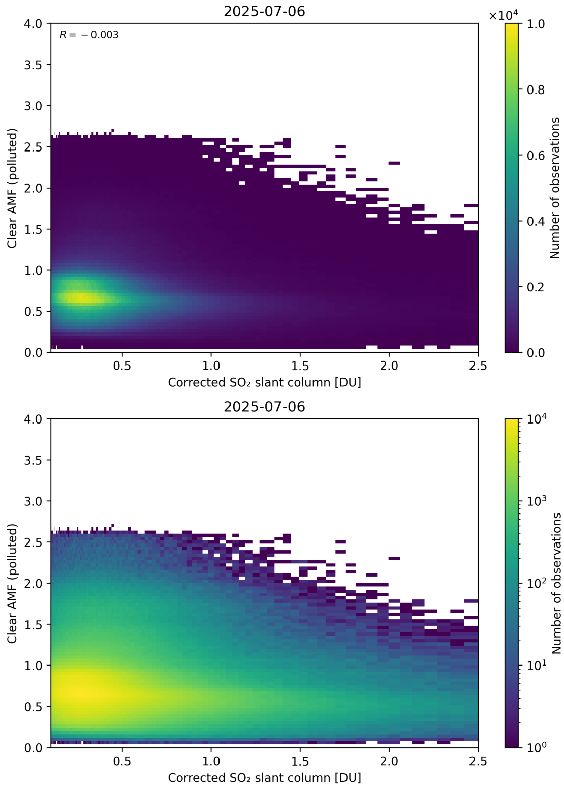
Figure 232: Scatter density plot of “Corrected SO 2 slant column” against “Clear AMF (polluted)” for 2025-07-05 to 2025-07-07.
