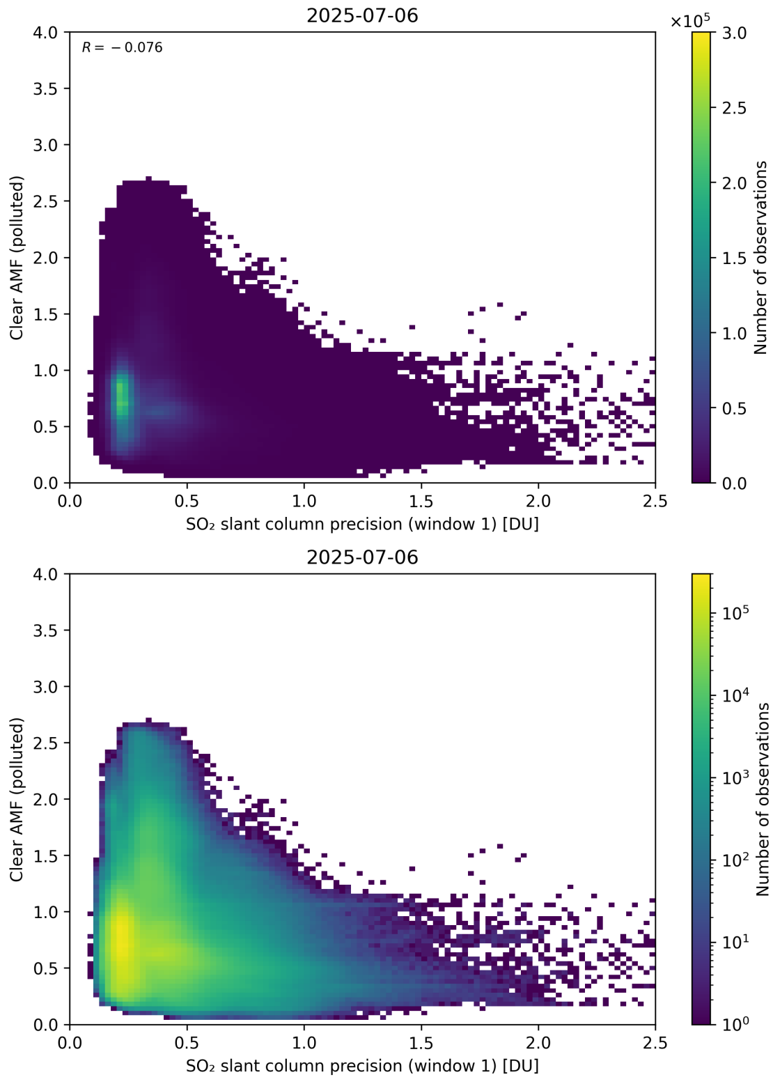
Figure 274: Scatter density plot of “SO 2 slant column precision (window 1)” against “Clear AMF (polluted)” for 2025-07-05 to 2025-07-07.
