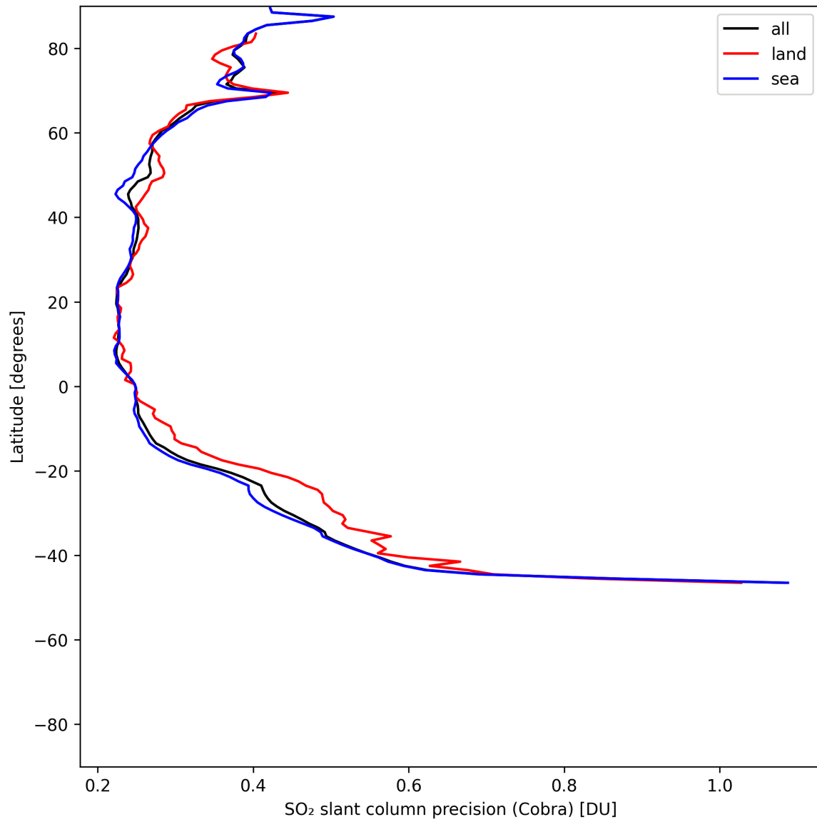
Figure 36: Zonal average of “SO 2 slant column precision (Cobra)” for 2025-07-05 to 2025-07-07.
