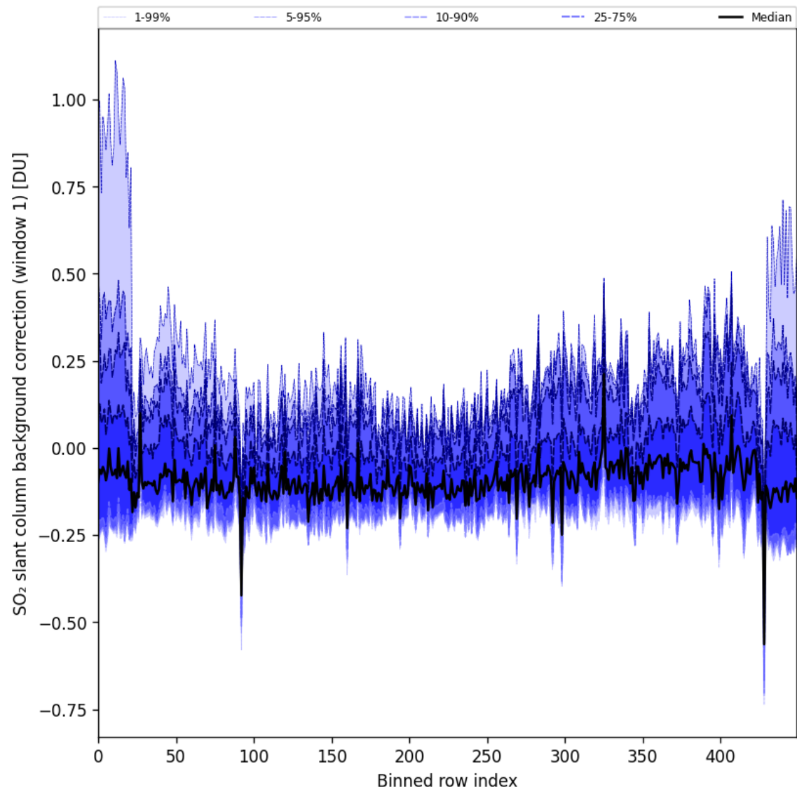
Figure 92: Along track statistics of “SO 2 slant column background correction (window 1)” for 2025-07-05 to 2025-07-07
