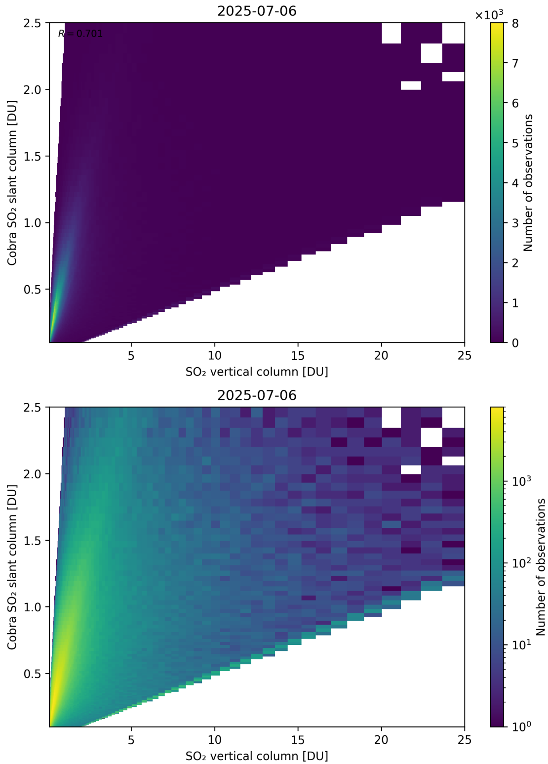
Figure 349: Scatter density plot of “SO 2 vertical column” against “Cobra SO 2 slant column” for 2025-07-05 to 2025-07-07.
