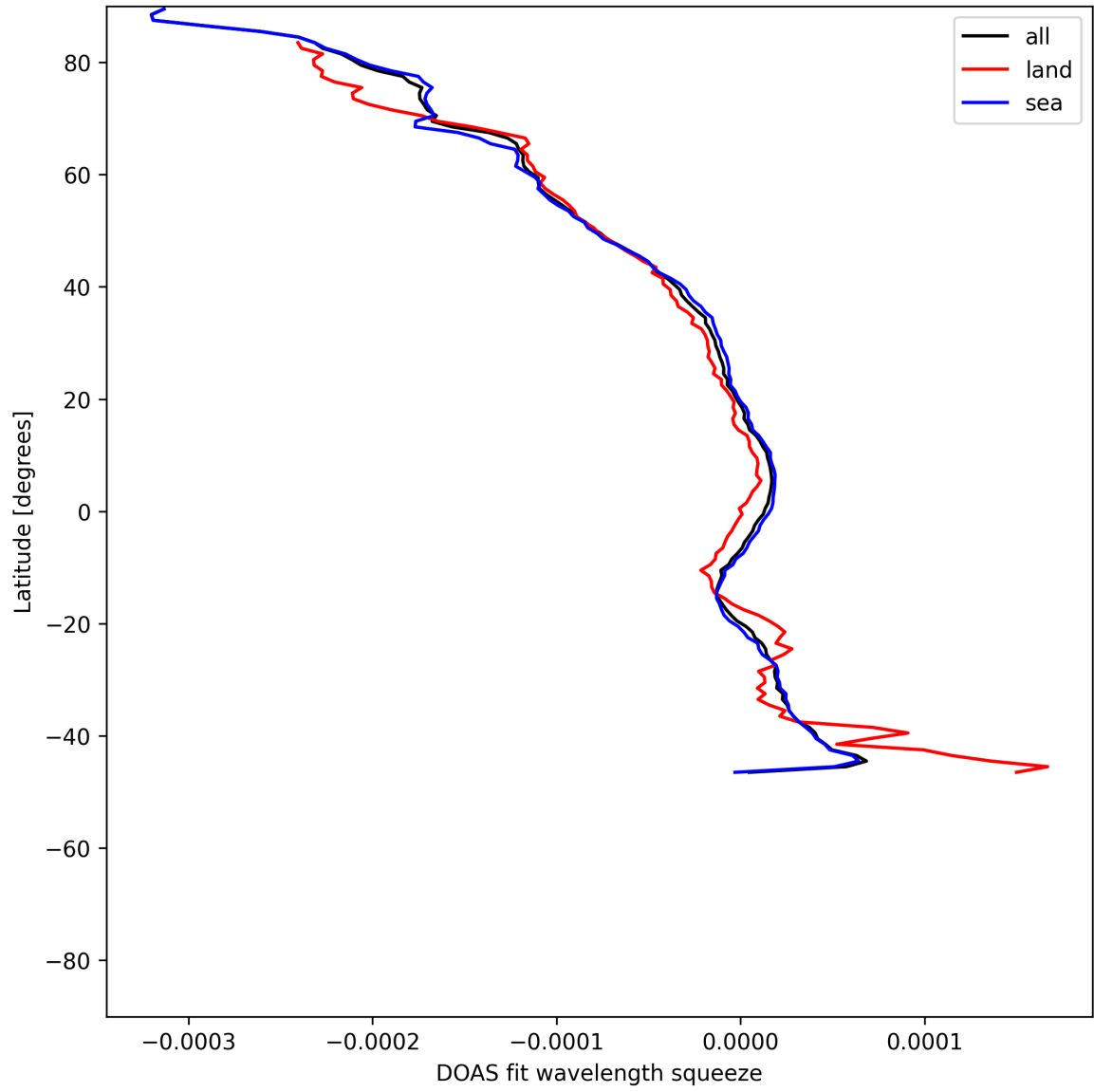
Figure 51: Zonal average of “DOAS fit wavelength squeeze” for 2025-07-05 to 2025-07-07.
