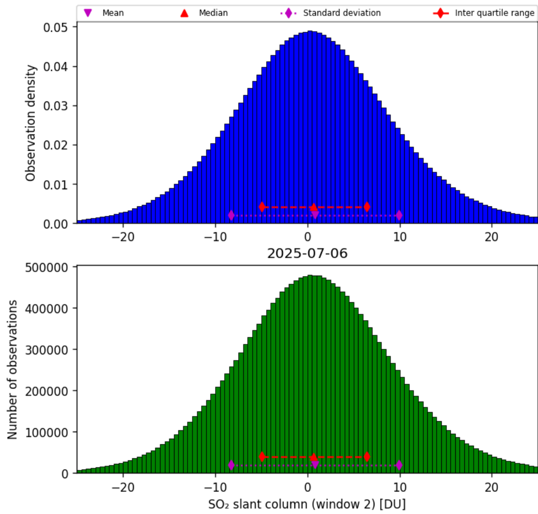
Figure 67: Histogram of “SO 2 slant column (window 2)” for 2025-07-05 to 2025-07-07
