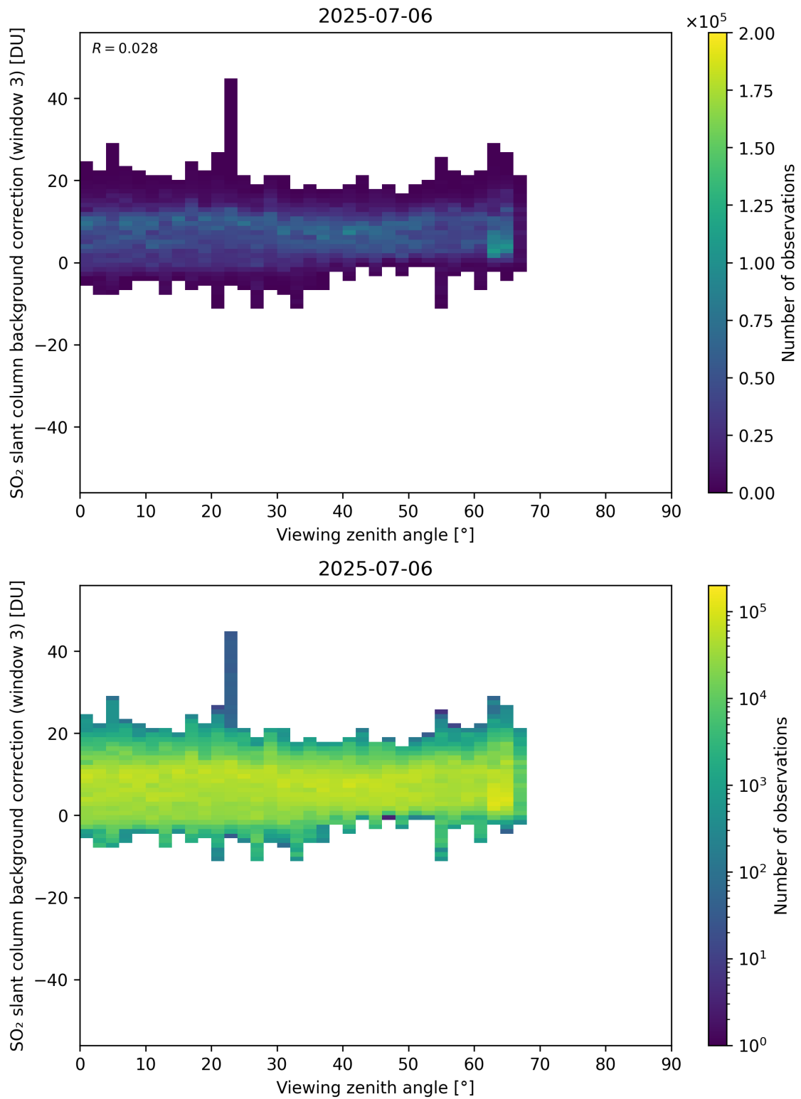
Figure 364: Scatter density plot of “Viewing zenith angle” against “SO 2 slant column background correction (window 3)” for 2025-07-05 to 2025-07-07.
