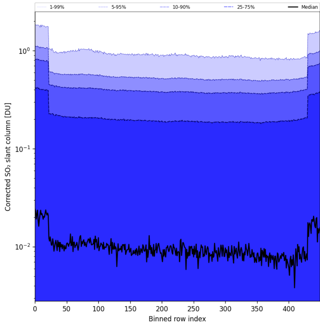
Figure 86: Along track statistics of “Corrected SO 2 slant column” for 2025-07-05 to 2025-07-07
