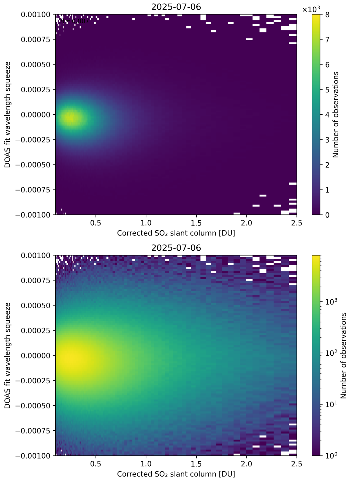
Figure 230: Scatter density plot of "Corrected SO 2 slant column" against "DOAS fit wavelength squeeze" for 2025-07-05 to 2025-07-07.
