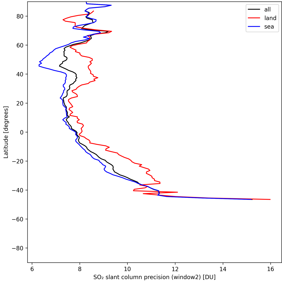
Figure 42: Zonal average of “SO 2 slant column precision (window2)” for 2025-07-05 to 2025-07-07.
