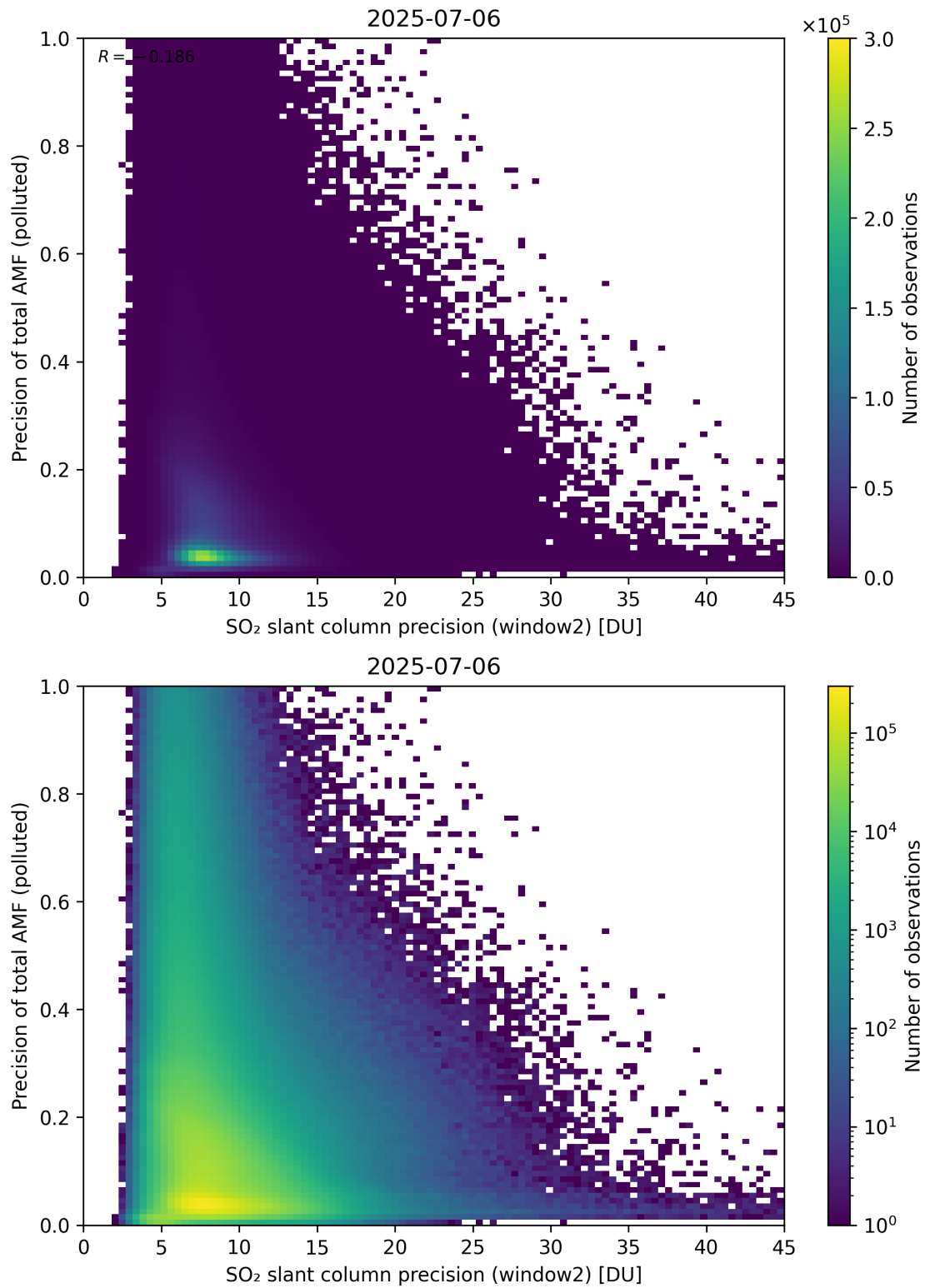
Figure 302: Scatter density plot of “SO 2 slant column precision (window2)” against “Precision of total AMF (polluted)” for 2025-07-05 to 2025-07-07.
