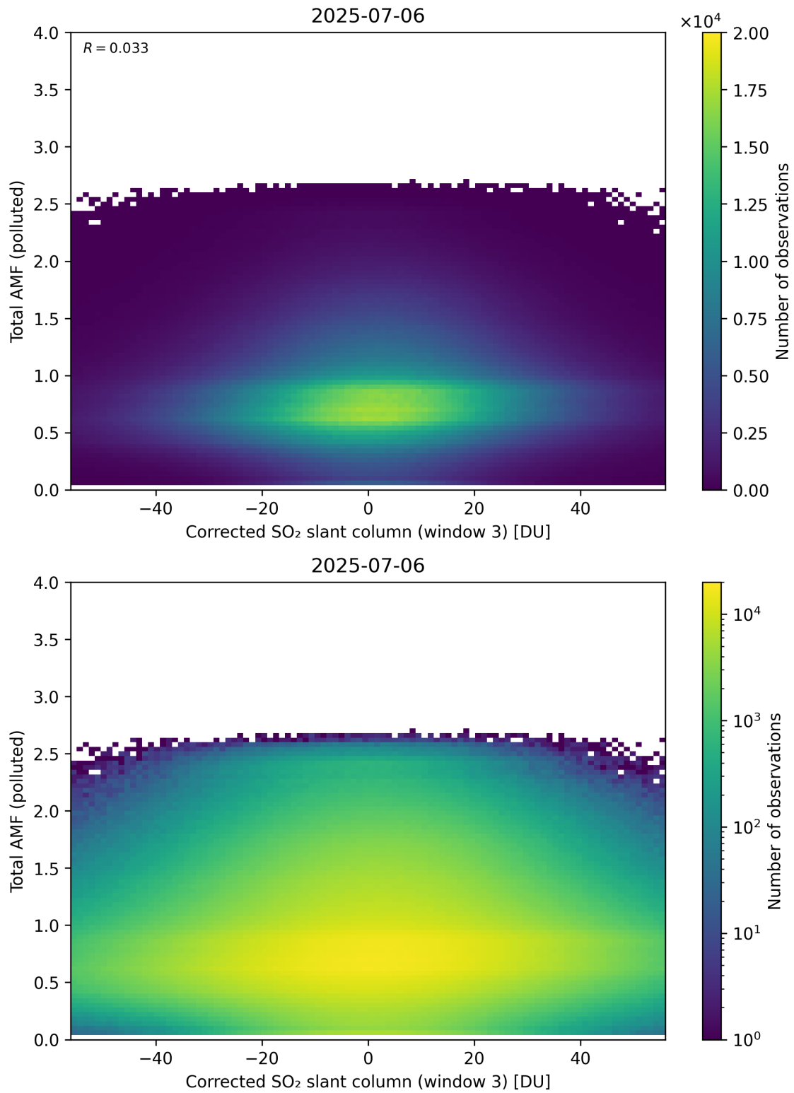
Figure 260: Scatter density plot of “Corrected SO 2 slant column (window 3)” against “Total AMF (polluted)” for 2025-07-05 to 2025-07-07.
