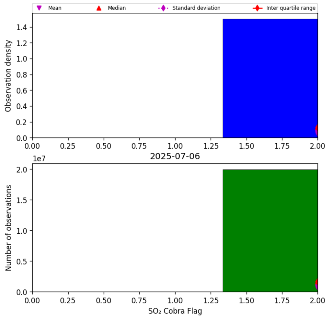
Figure 75: Histogram of “SO 2 Cobra Flag” for 2025-07-05 to 2025-07-07
