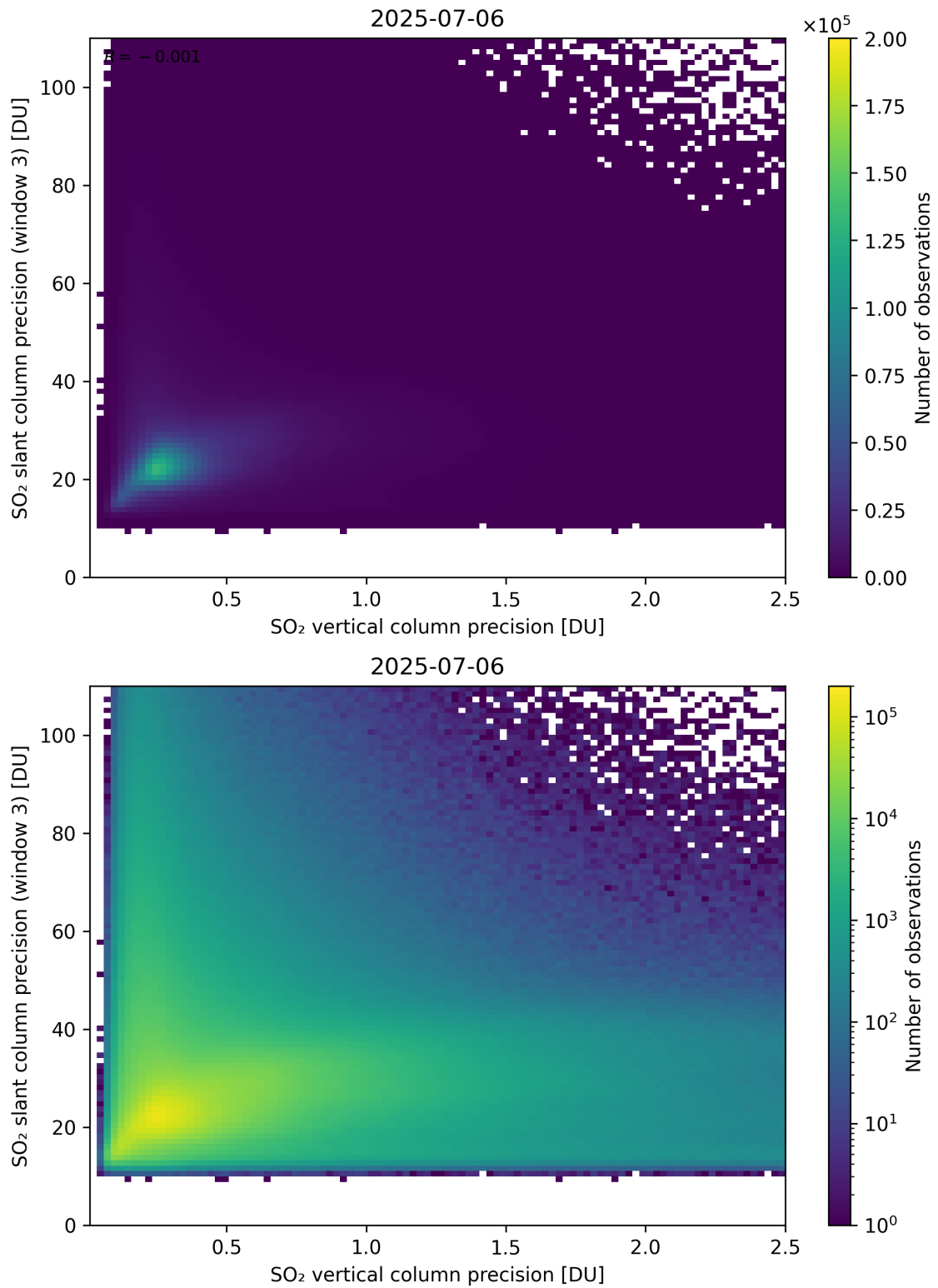
Figure 345: Scatter density plot of “SO 2 vertical column precision” against “SO 2 slant column precision (window 3)” for 2025-07-05 to 2025-07-07.
