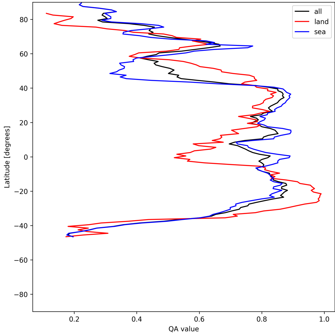
Figure 31: Zonal average of “QA value” for 2025-07-05 to 2025-07-07.
