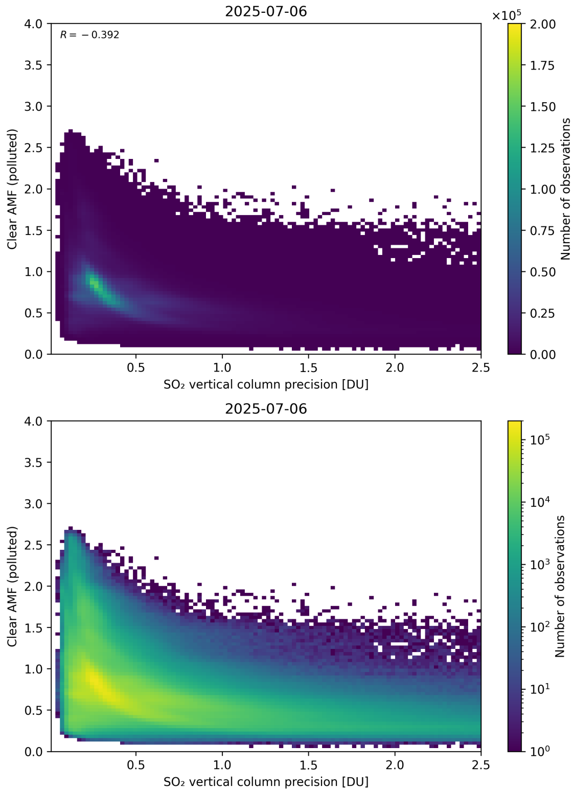
Figure 335: Scatter density plot of “SO 2 vertical column precision” against “Clear AMF (polluted)” for 2025-07-05 to 2025-07-07.
