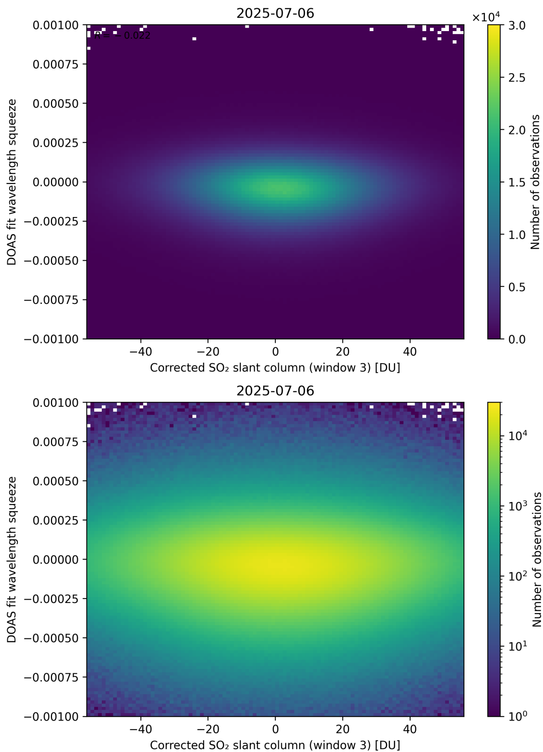
Figure 257: Scatter density plot of “Corrected SO 2 slant column (window 3)” against “DOAS fit wavelength squeeze” for 2025-07-05 to 2025-07-07.
