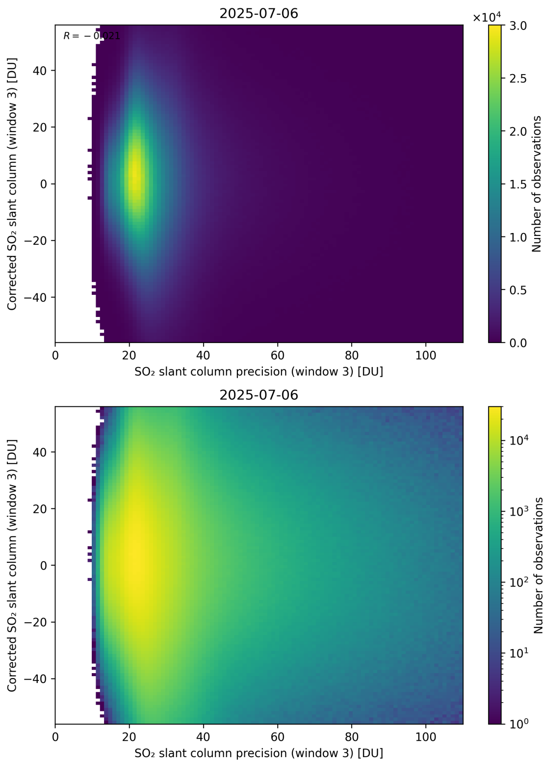
Figure 312: Scatter density plot of “SO 2 slant column precision (window 3)” against “Corrected SO 2 slant column (window 3)” for 2025-07-05 to 2025-07-07.
