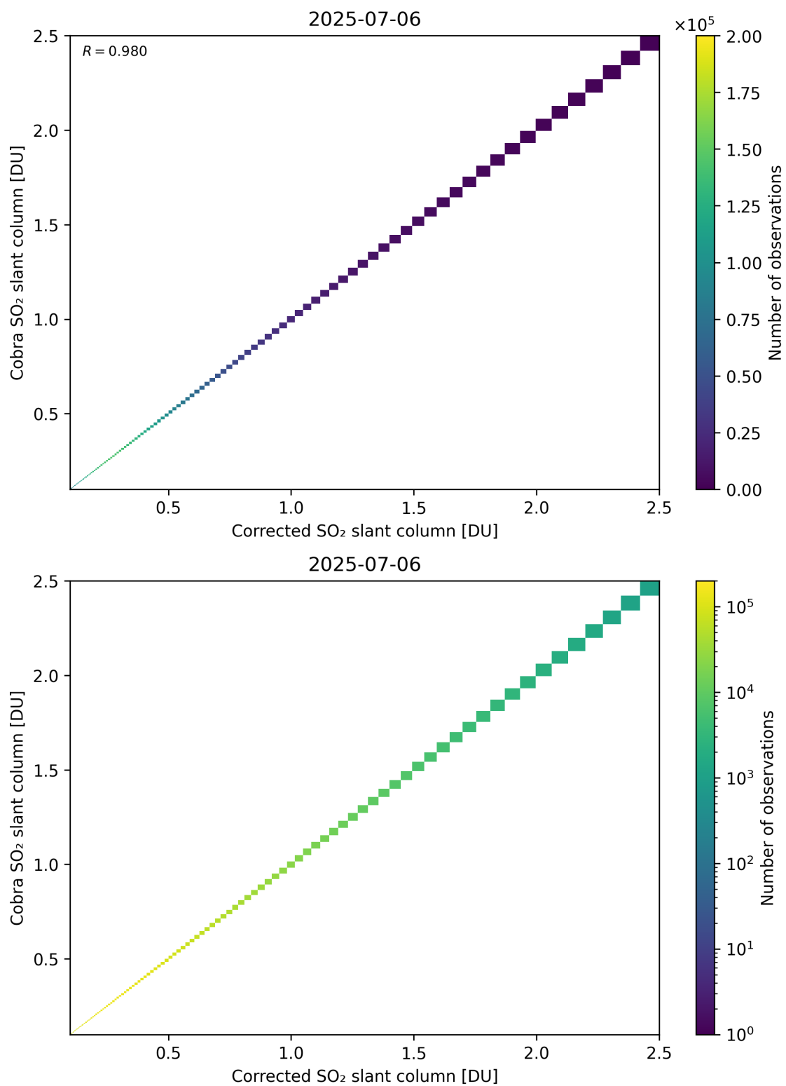
Figure 233: Scatter density plot of “Corrected SO 2 slant column” against “Cobra SO 2 slant column” for 2025-07-05 to 2025-07-07.
