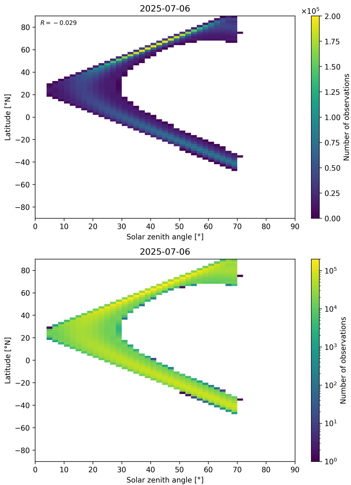
Figure 177: Scatter density plot of “Solar zenith angle” against “Latitude” for 2025-07-05 to 2025-07-07.
