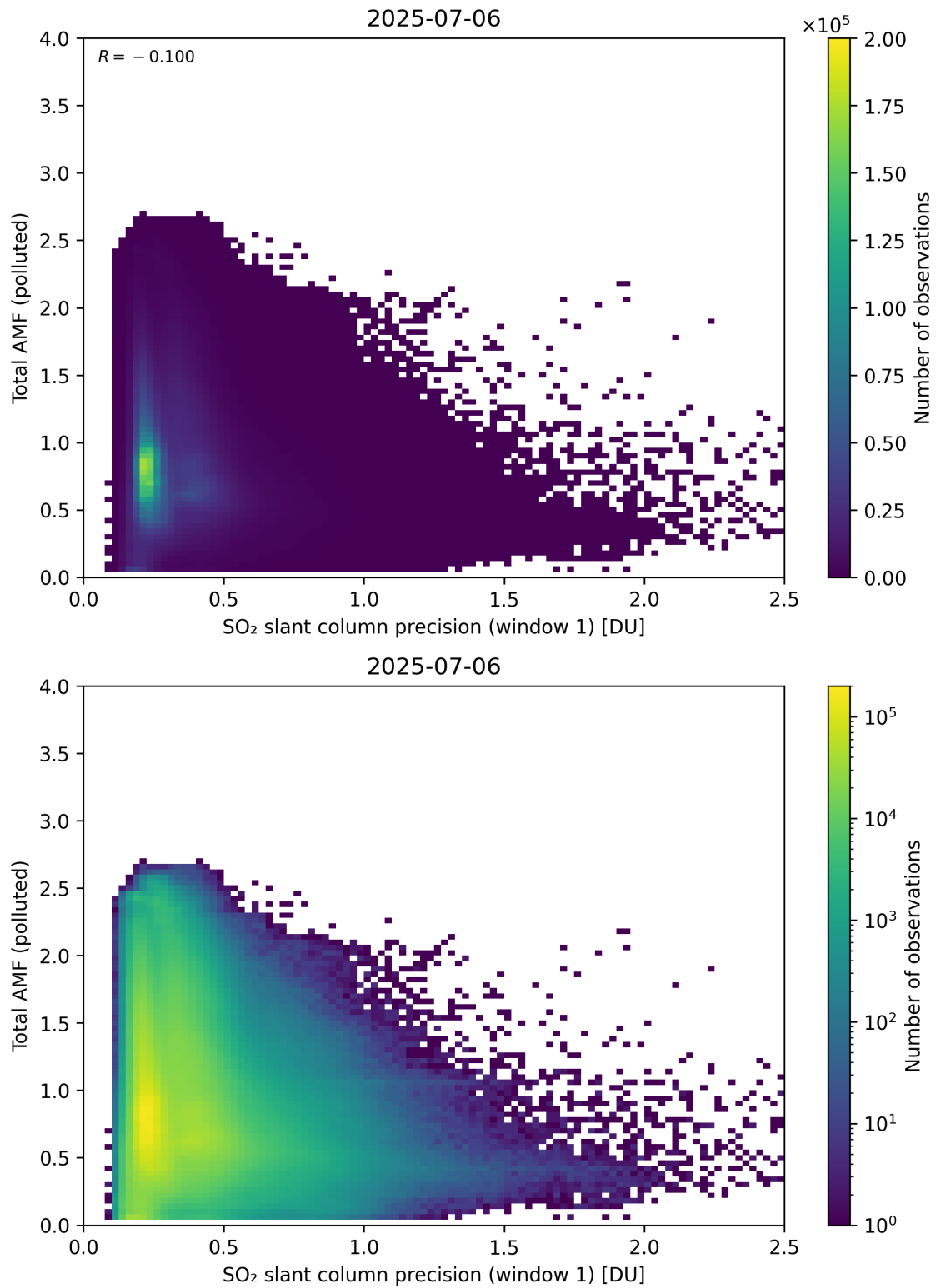
Figure 280: Scatter density plot of “SO 2 slant column precision (window 1)” against “Total AMF (polluted)” for 2025-07-05 to 2025-07-07.
