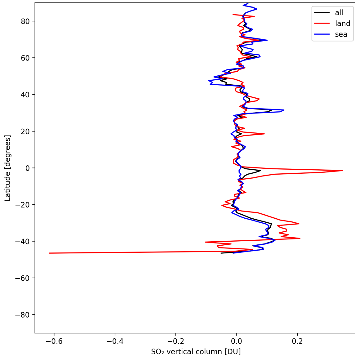
Figure 32: Zonal average of “SO 2 vertical column” for 2025-07-05 to 2025-07-07.
