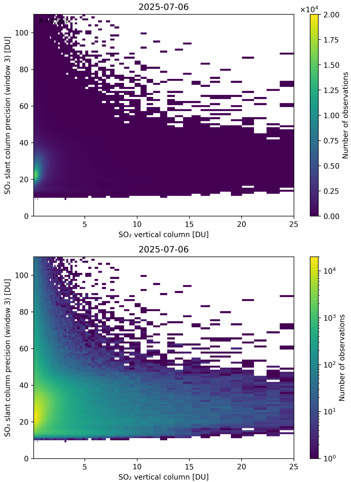
Figure 358: Scatter density plot of “SO 2 vertical column” against “SO 2 slant column precision (window 3)” for 2025-07-05 to 2025-07-07.
