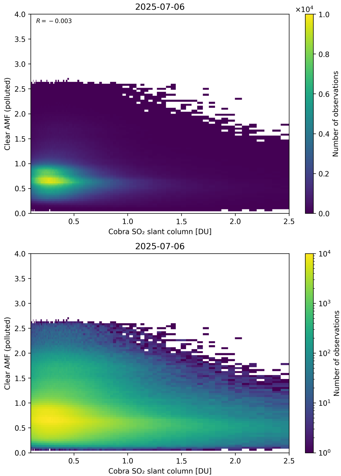
Figure 215: Scatter density plot of “Cobra SO 2 slant column” against “Clear AMF (polluted)” for 2025-07-05 to 2025-07-07.
