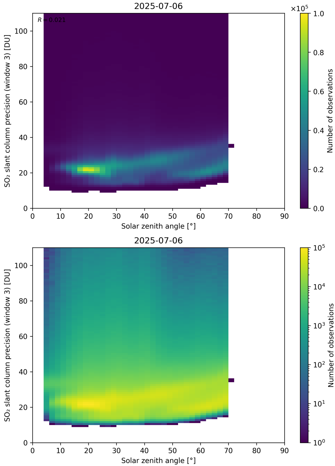
Figure 188: Scatter density plot of “Solar zenith angle” against “SO 2 slant column precision (window 3)” for 2025-07-05 to 2025-07-07.
