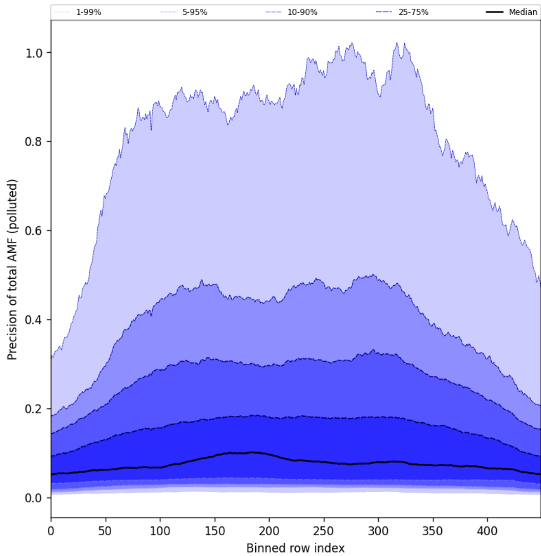
Figure 106: Along track statistics of “Precision of total AMF (polluted)” for 2025-07-05 to 2025-07-07
