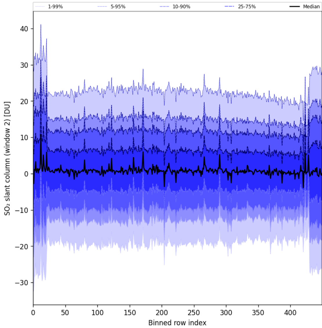
Figure 93: Along track statistics of "SO 2 slant column (window 2)" for 2025-07-05 to 2025-07-07
