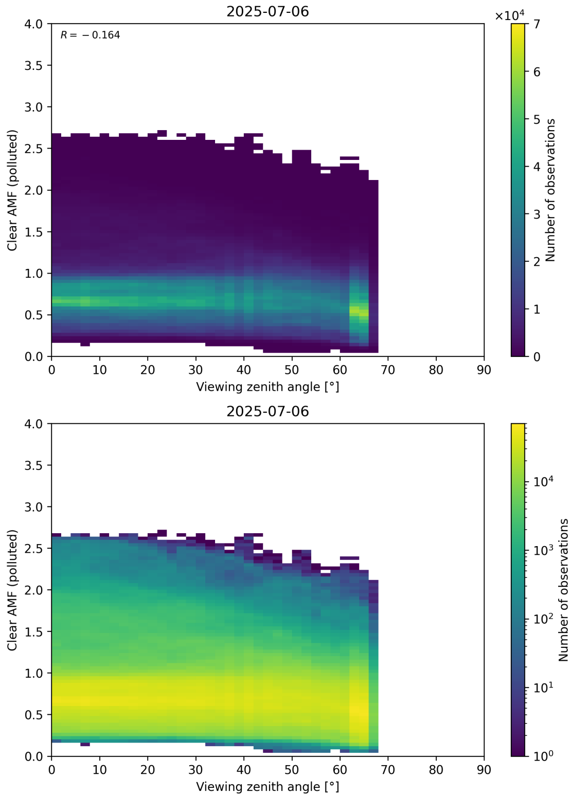
Figure 370: Scatter density plot of “Viewing zenith angle” against “Clear AMF (polluted)” for 2025-07-05 to 2025-07-07.
