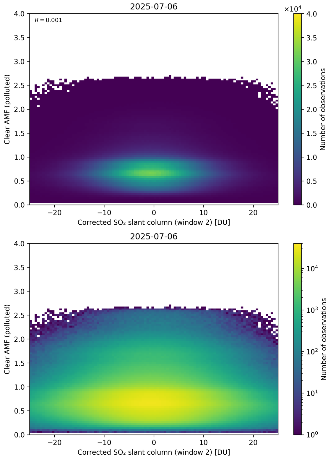
Figure 249: Scatter density plot of “Corrected SO 2 slant column (window 2)” against “Clear AMF (polluted)” for 2025-07-05 to 2025-07-07.
