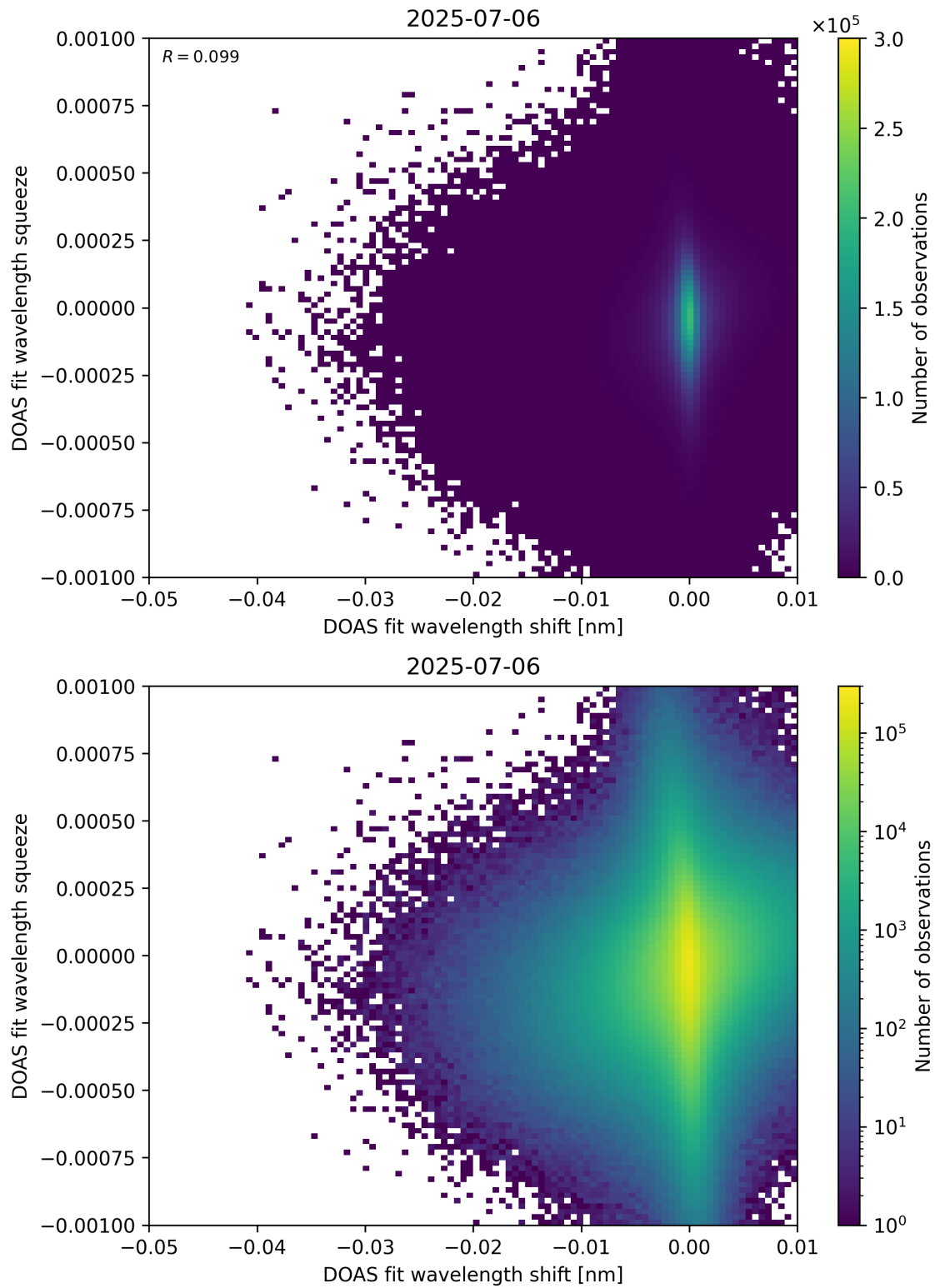
Figure 138: Scatter density plot of “DOAS fit wavelength shift” against “DOAS fit wavelength squeeze” for 2025-07-05 to 2025-07-07.
