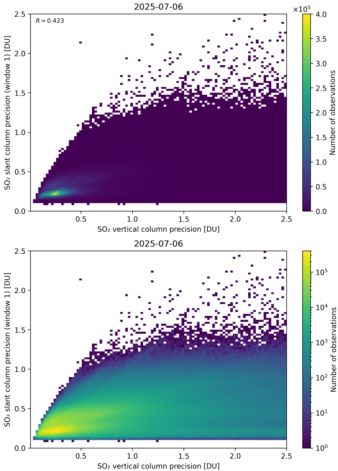
Figure 342: Scatter density plot of “SO 2 vertical column precision” against “SO 2 slant column precision (window 1)” for 2025-07-05 to 2025-07-07.
