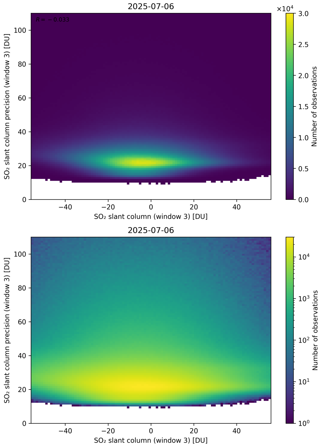
Figure 317: Scatter density plot of “SO 2 slant column (window 3)” against “SO 2 slant column precision (window 3)” for 2025-07-05 to 2025-07-07.
