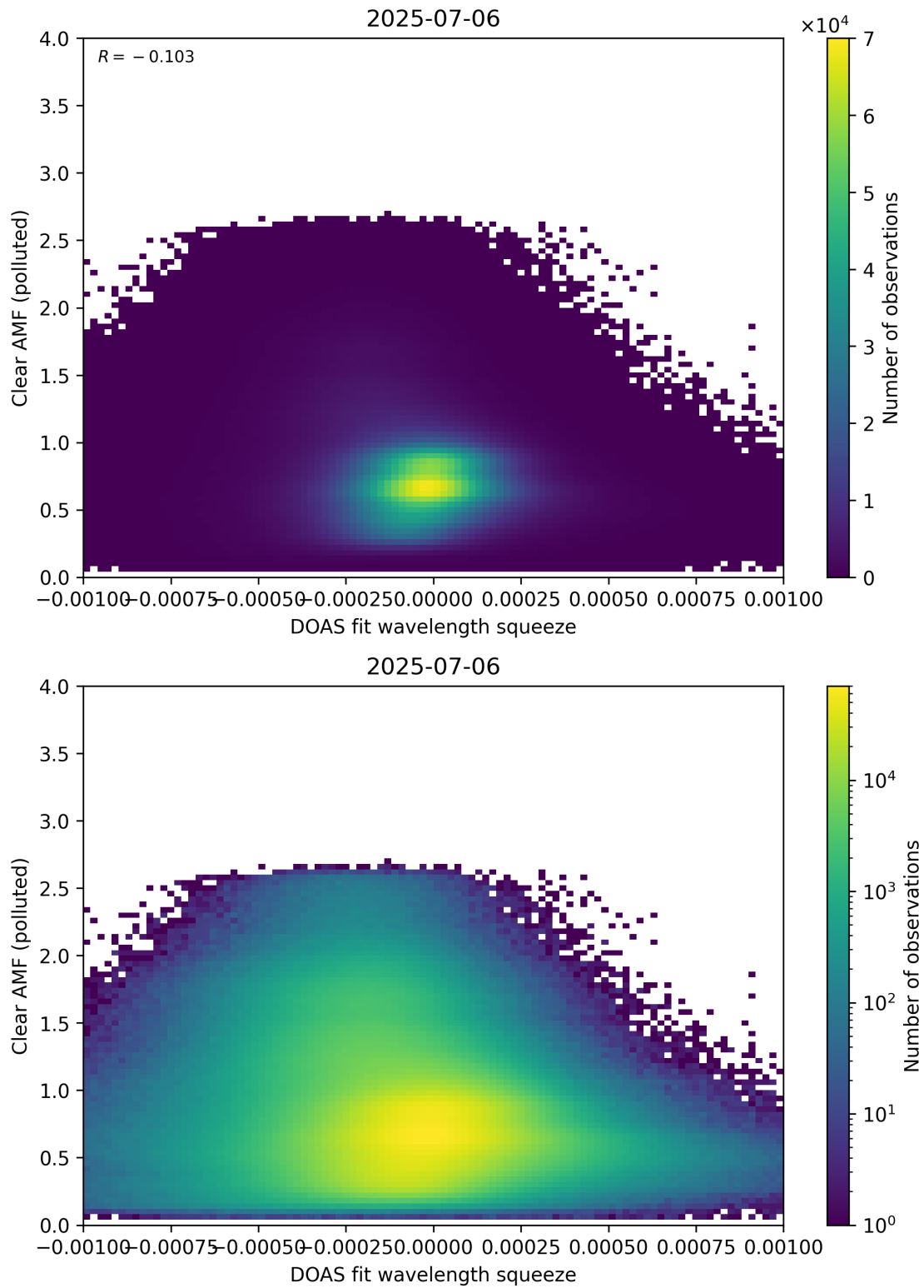
Figure 144: Scatter density plot of “DOAS fit wavelength squeeze” against “Clear AMF (polluted)” for 2025-07-05 to 2025-07-07.
