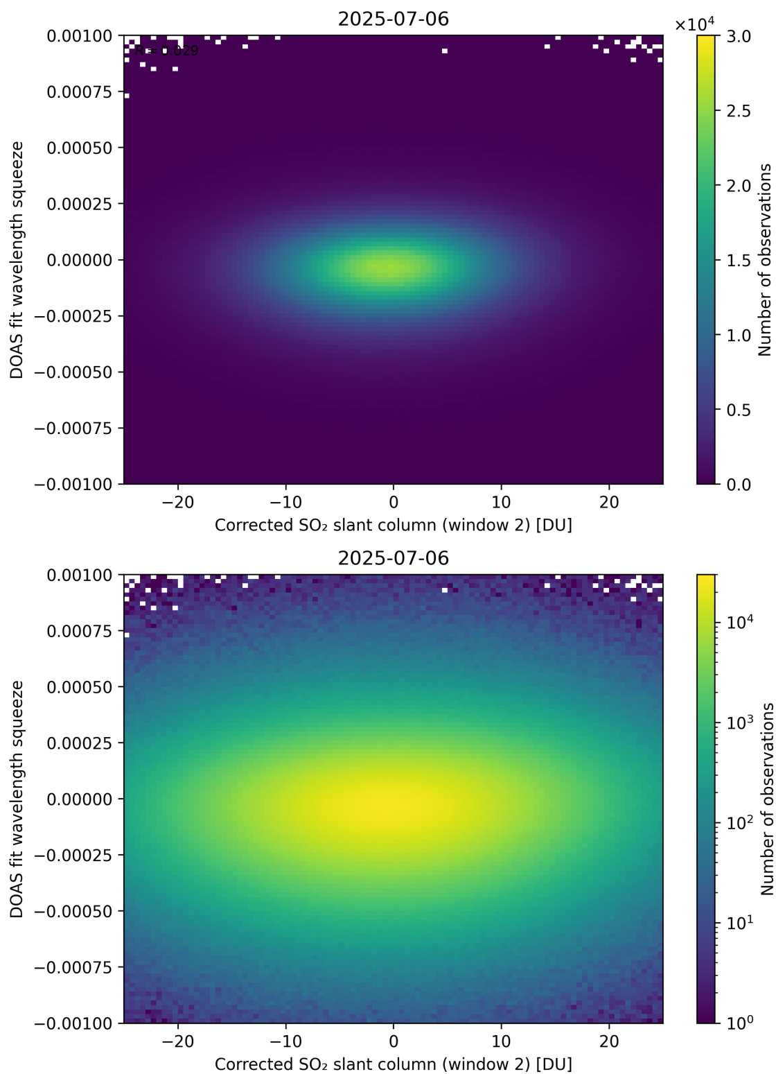
Figure 247: Scatter density plot of “Corrected SO 2 slant column (window 2)” against “DOAS fit wavelength squeeze” for 2025-07-05 to 2025-07-07.
