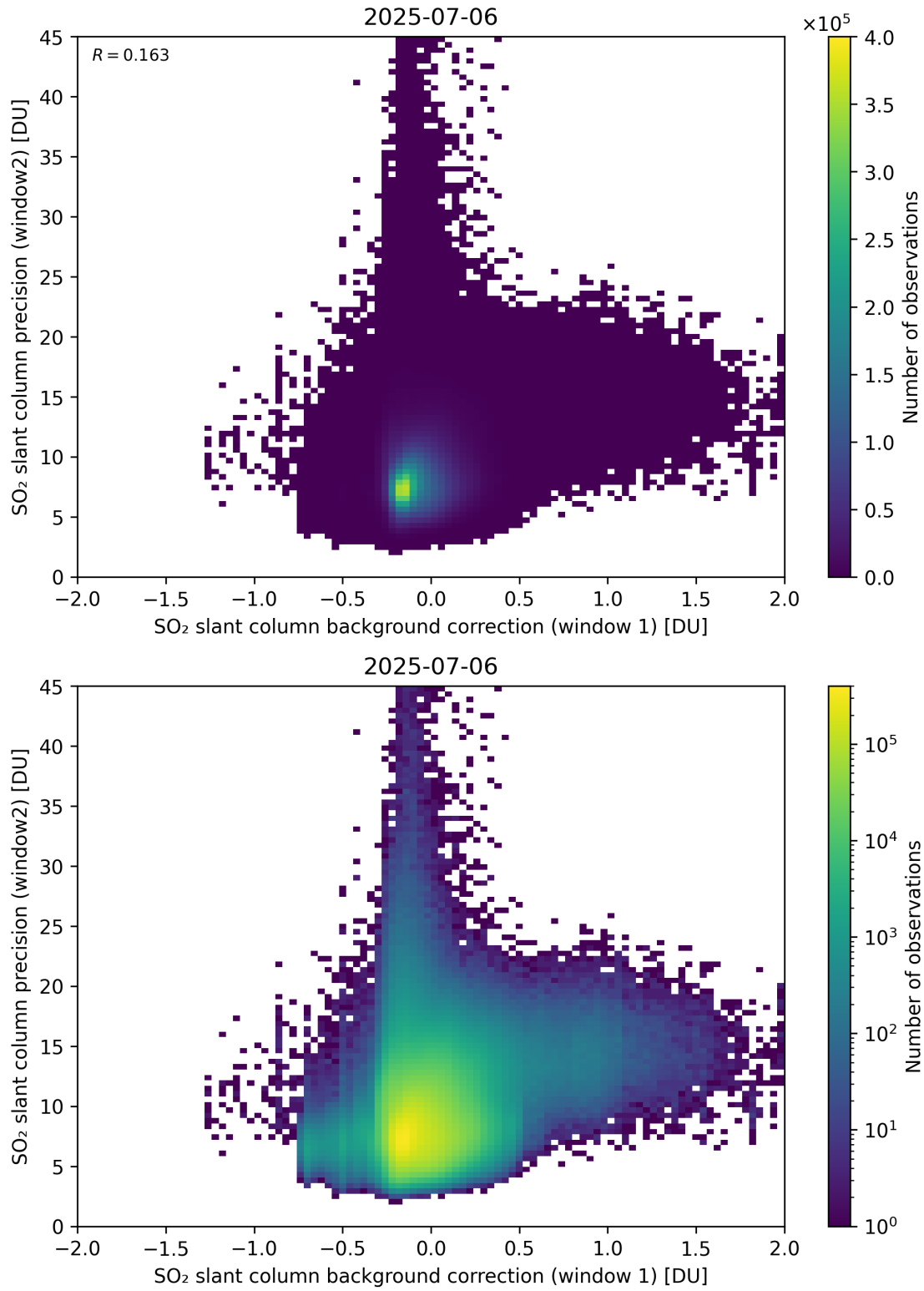
Figure 117: Scatter density plot of “SO 2 slant column background correction (window 1)” against “SO 2 slant column precision (window2)” for 2025-07-05 to 2025-07-07.
