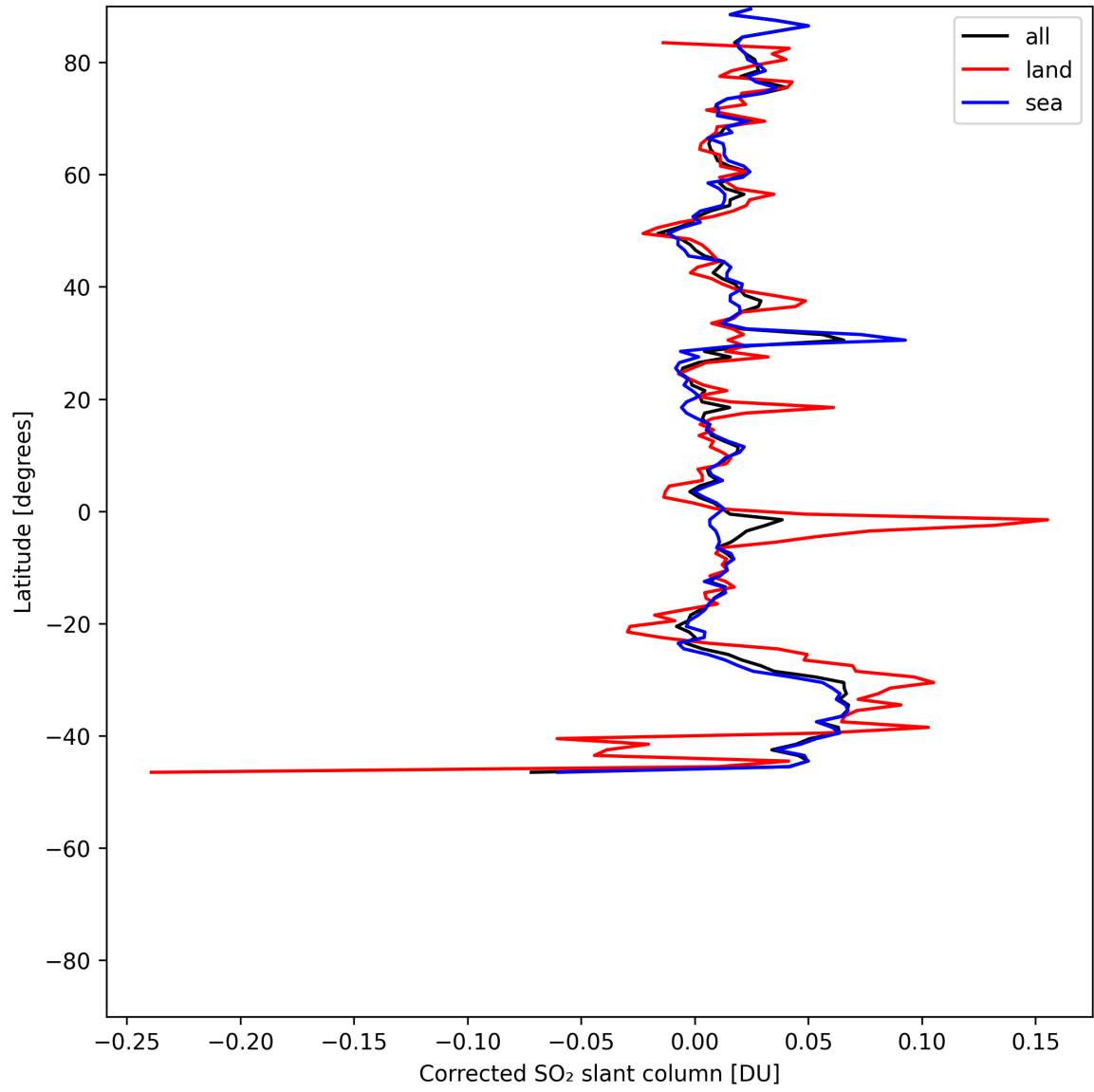
Figure 34: Zonal average of “Corrected SO 2 slant column” for 2025-07-05 to 2025-07-07.
