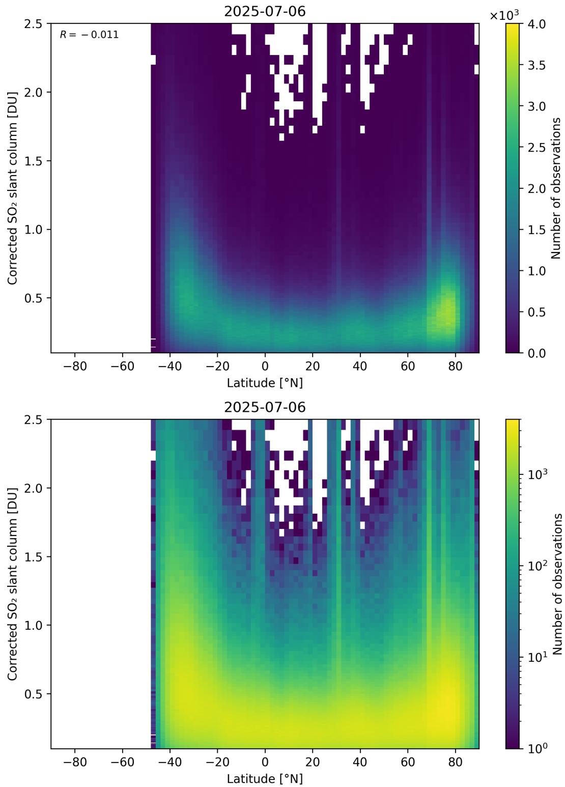
Figure 159: Scatter density plot of “Latitude” against “Corrected SO 2 slant column” for 2025-07-05 to 2025-07-07.
