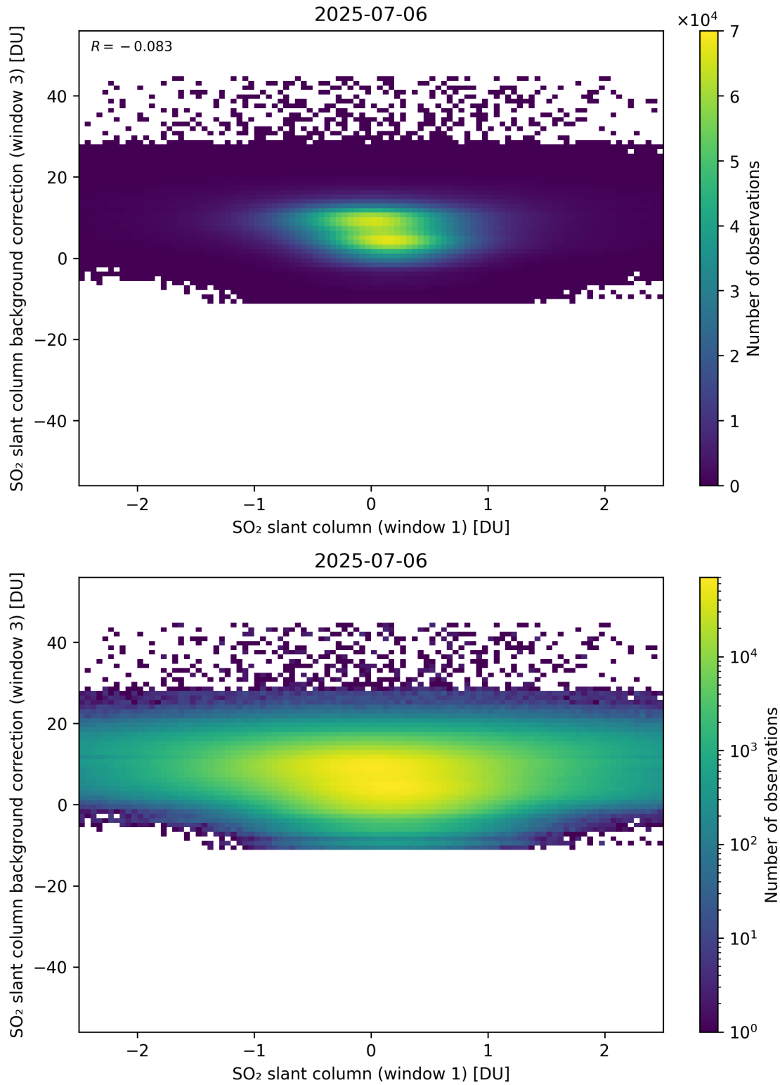
Figure 264: Scatter density plot of “SO 2 slant column (window 1)” against “SO 2 slant column background correction (window 3)” for 2025-07-05 to 2025-07-07.
