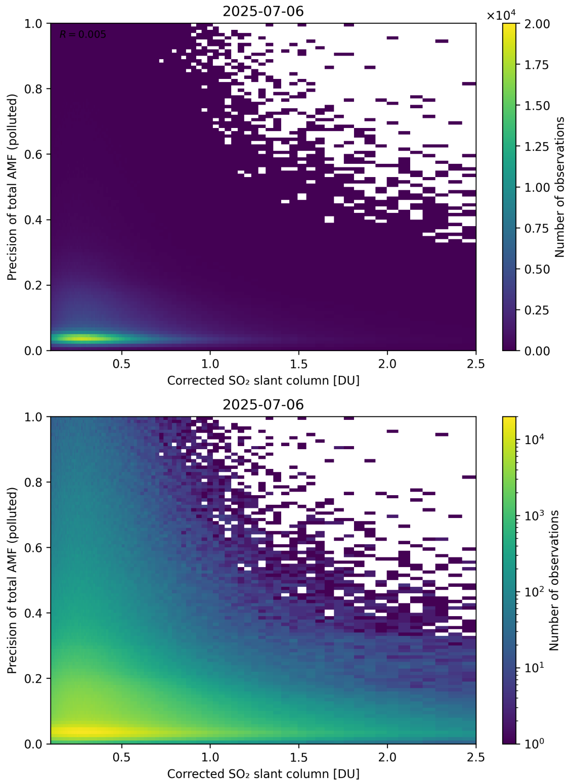
Figure 243: Scatter density plot of “Corrected SO 2 slant column” against “Precision of total AMF (polluted)” for 2025-07-05 to 2025-07-07.
