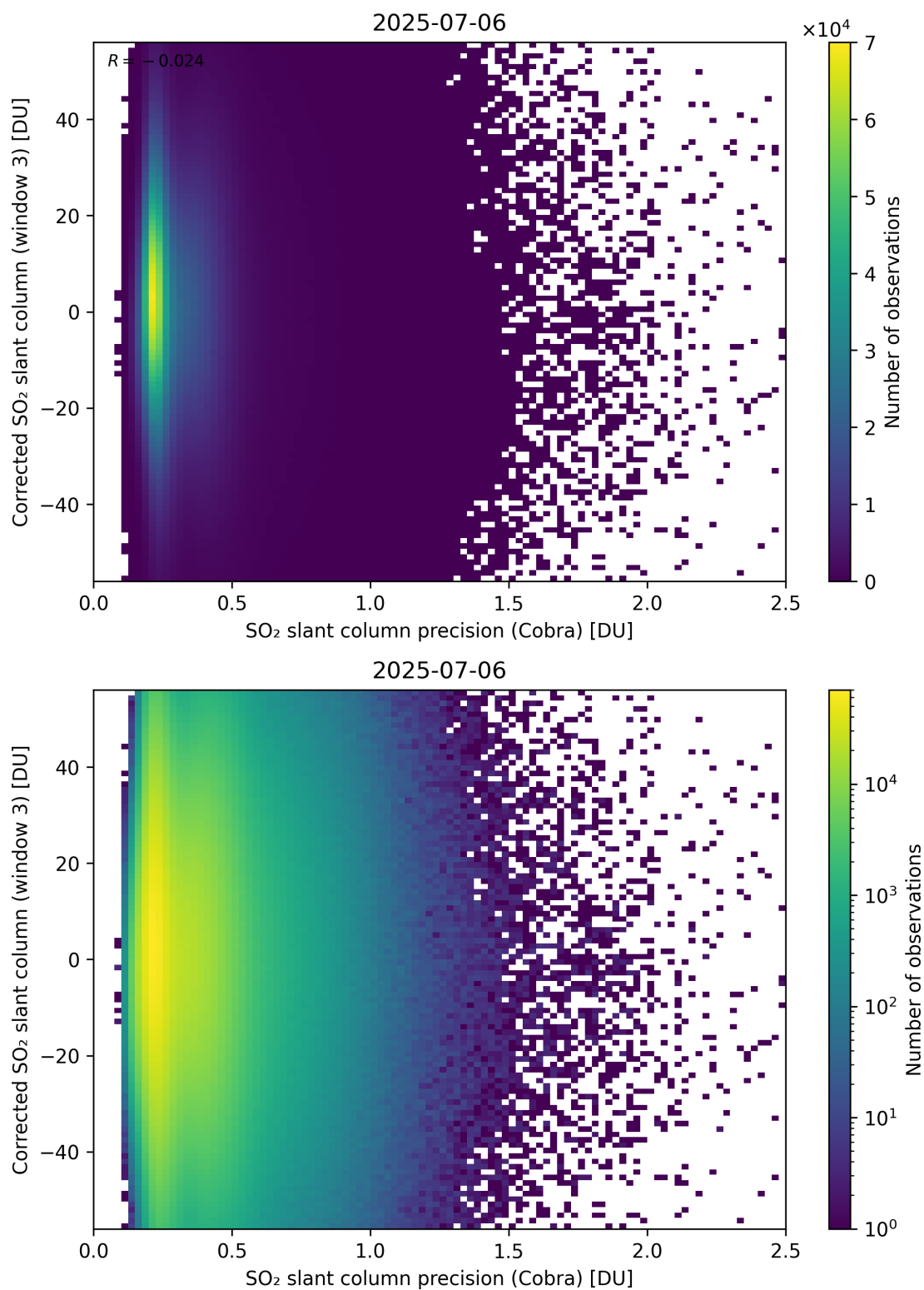
Figure 207: Scatter density plot of “SO 2 slant column precision (Cobra)” against “Corrected SO 2 slant column (window 3)” for 2025-07-05 to 2025-07-07.
