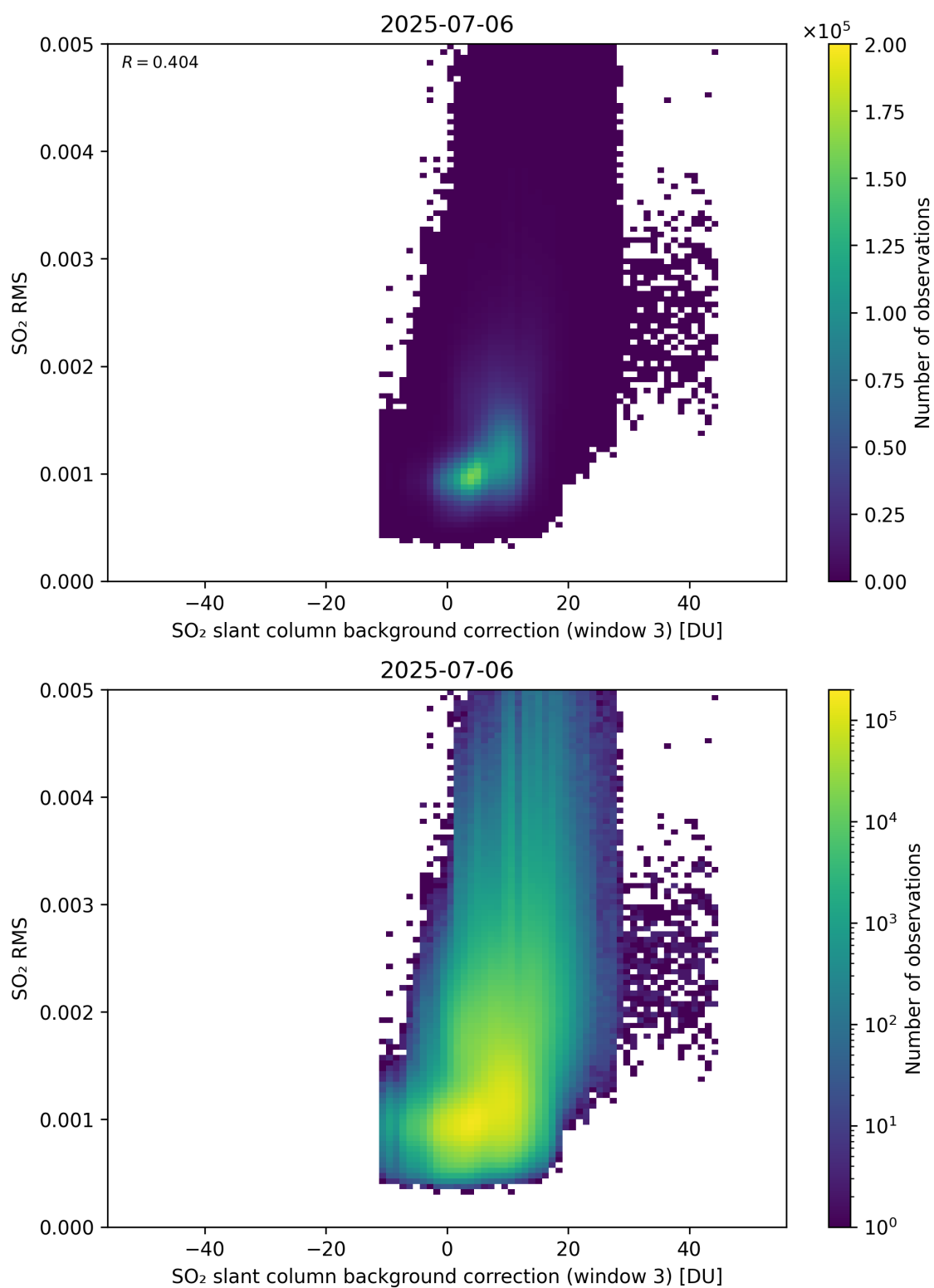
Figure 134: Scatter density plot of “SO 2 slant column background correction (window 3)” against “SO 2 RMS” for 2025-07-05 to 2025-07-07.
