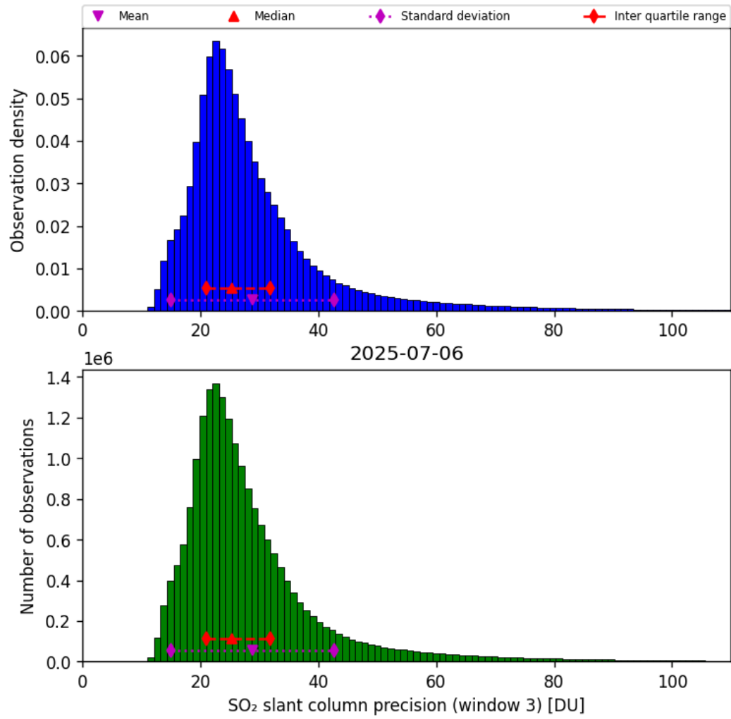
Figure 72: Histogram of “SO 2 slant column precision (window 3)” for 2025-07-05 to 2025-07-07
