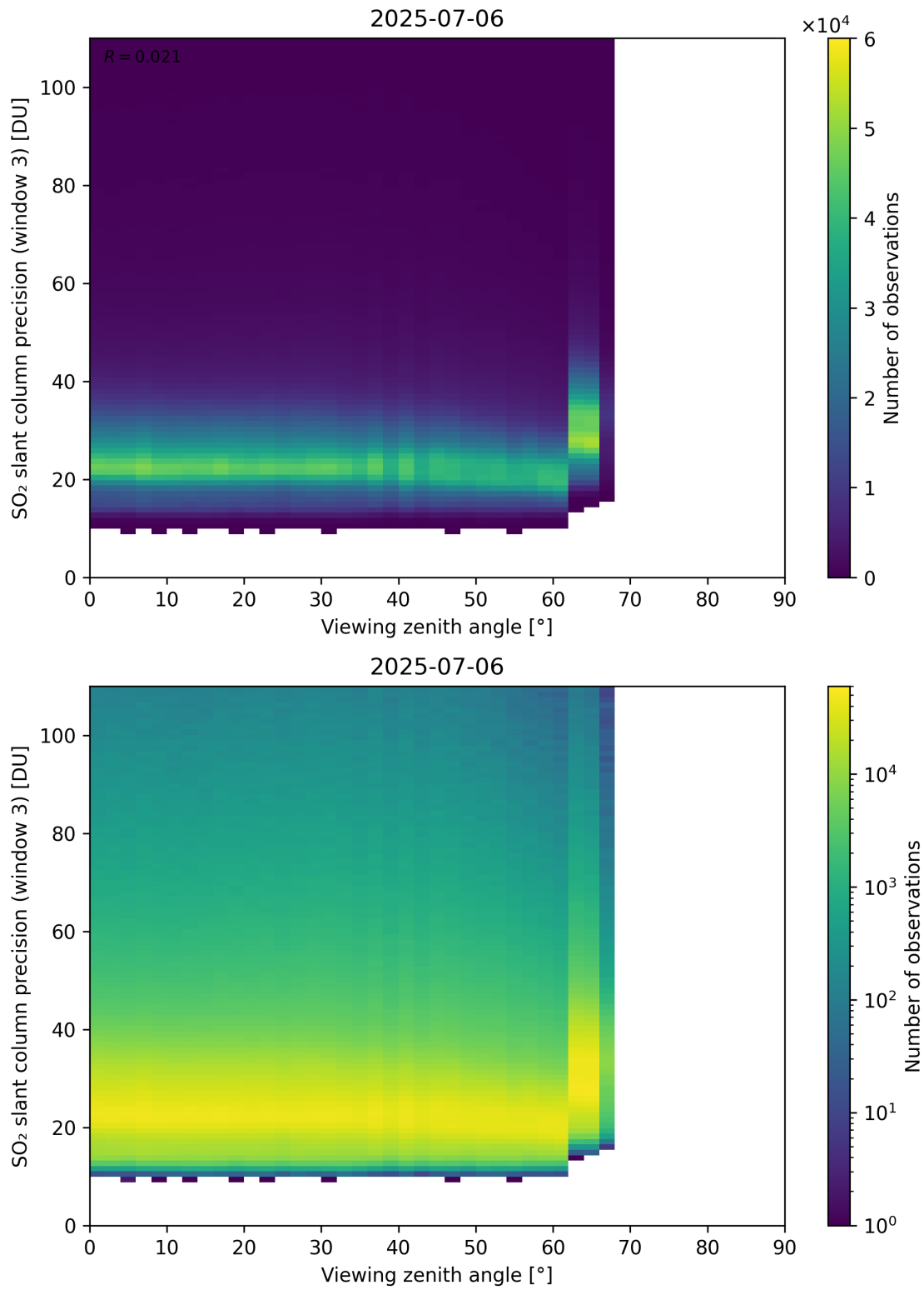
Figure 380: Scatter density plot of “Viewing zenith angle” against “SO 2 slant column precision (window 3)” for 2025-07-05 to 2025-07-07.
