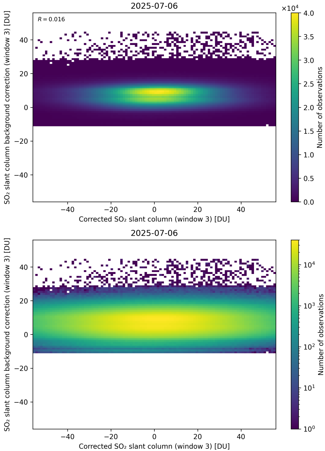
Figure 255: Scatter density plot of “Corrected SO 2 slant column (window 3)” against “SO 2 slant column background correction (window 3)” for 2025-07-05 to 2025-07-07.
