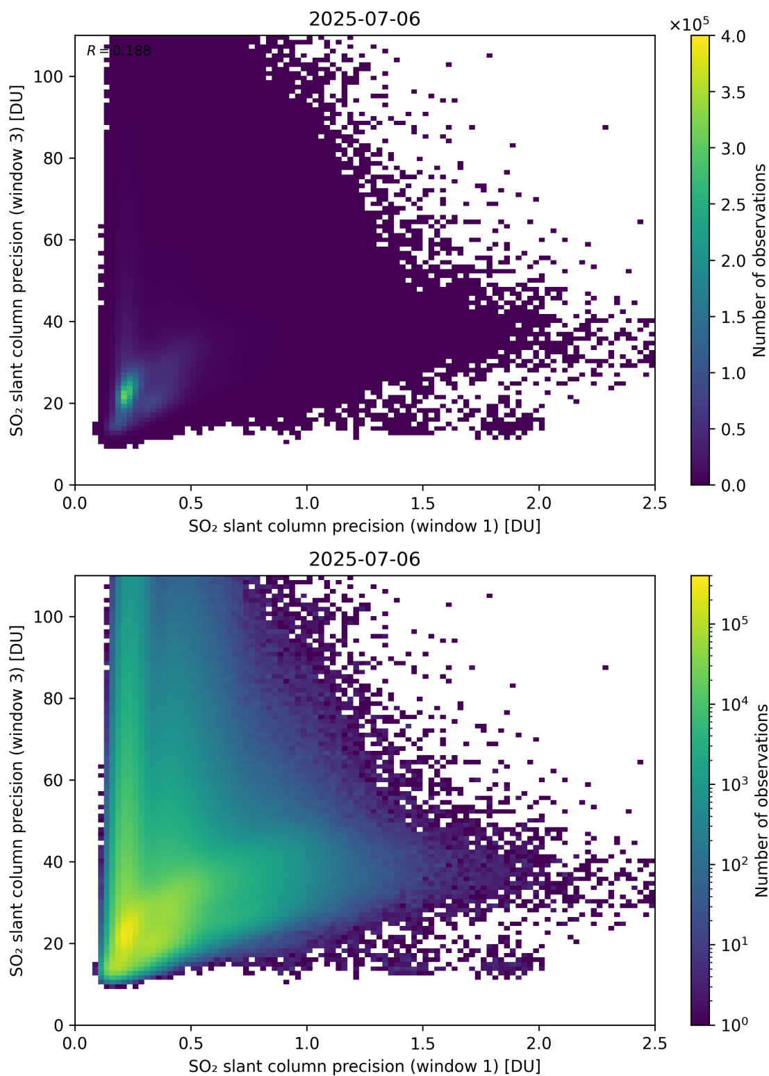
Figure 279: Scatter density plot of “SO 2 slant column precision (window 1)” against “SO 2 slant column precision (window 3)” for 2025-07-05 to 2025-07-07.
