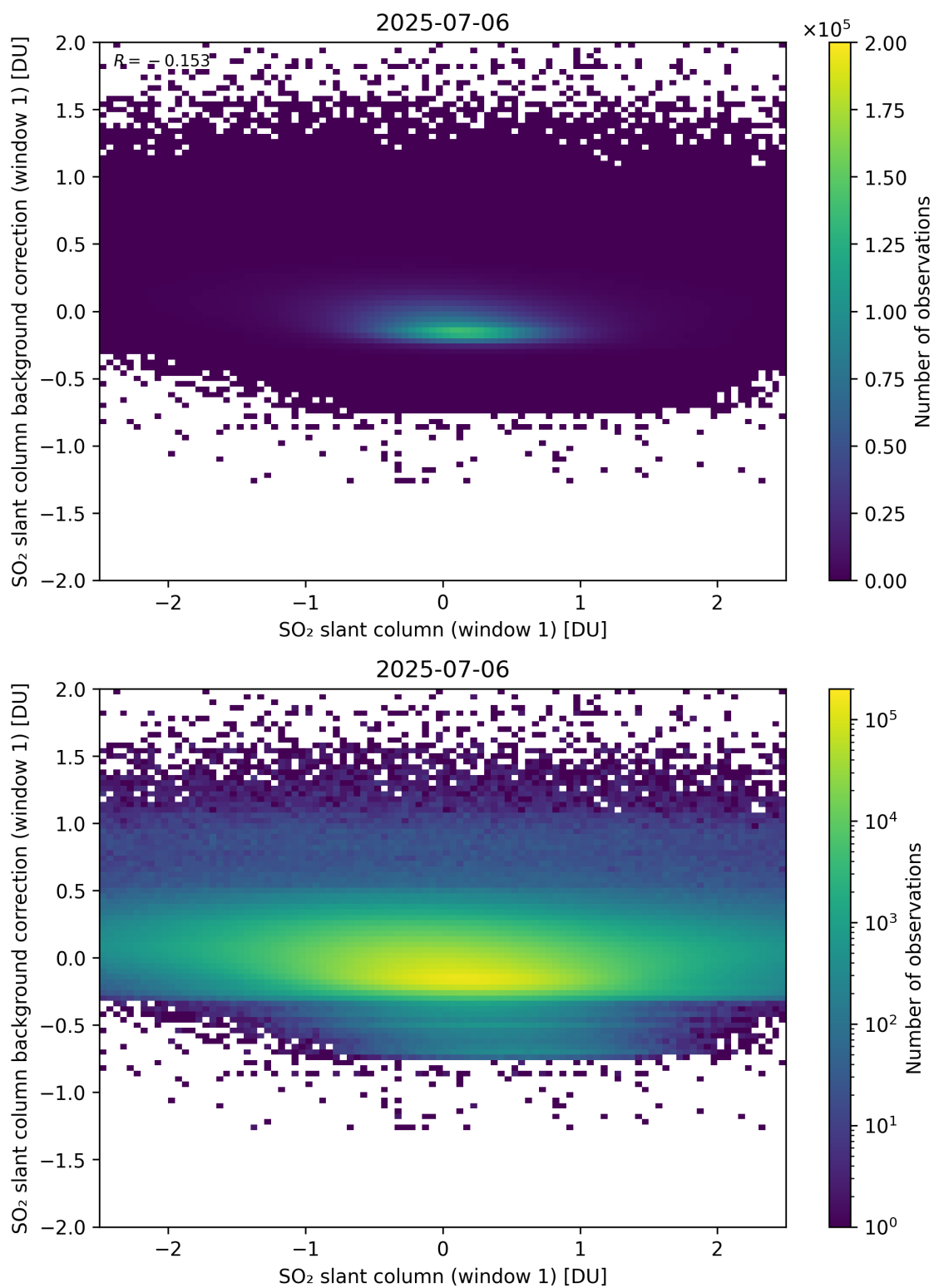
Figure 262: Scatter density plot of “SO 2 slant column (window 1)” against “SO 2 slant column background correction (window 1)” for 2025-07-05 to 2025-07-07.
