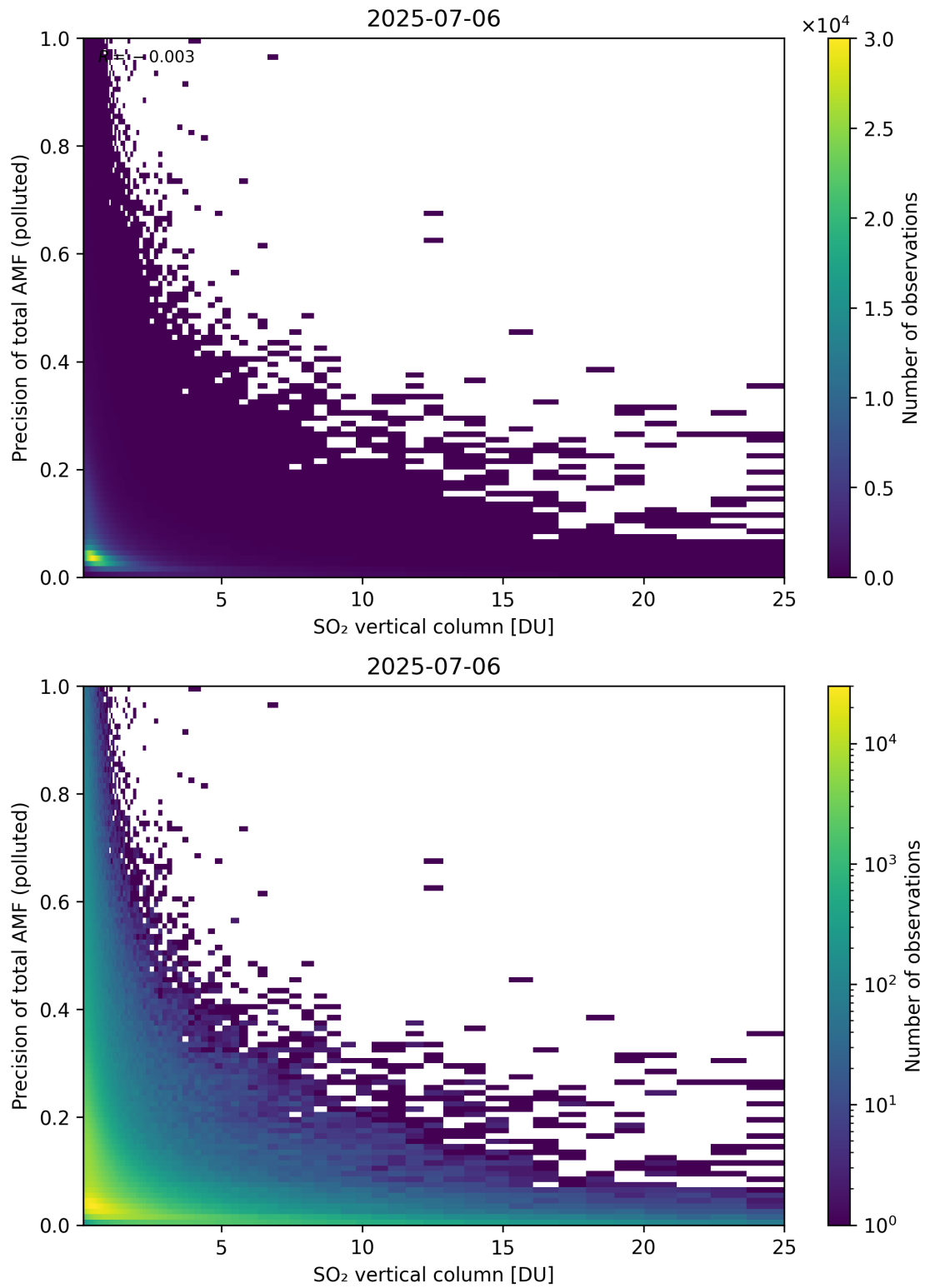
Figure 360: Scatter density plot of “SO 2 vertical column” against “Precision of total AMF (polluted)” for 2025-07-05 to 2025-07-07.
