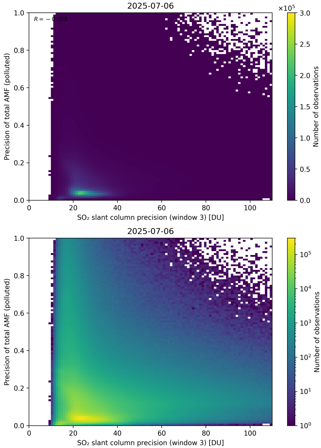
Figure 314: Scatter density plot of “SO 2 slant column precision (window 3)” against “Precision of total AMF (polluted)” for 2025-07-05 to 2025-07-07.
