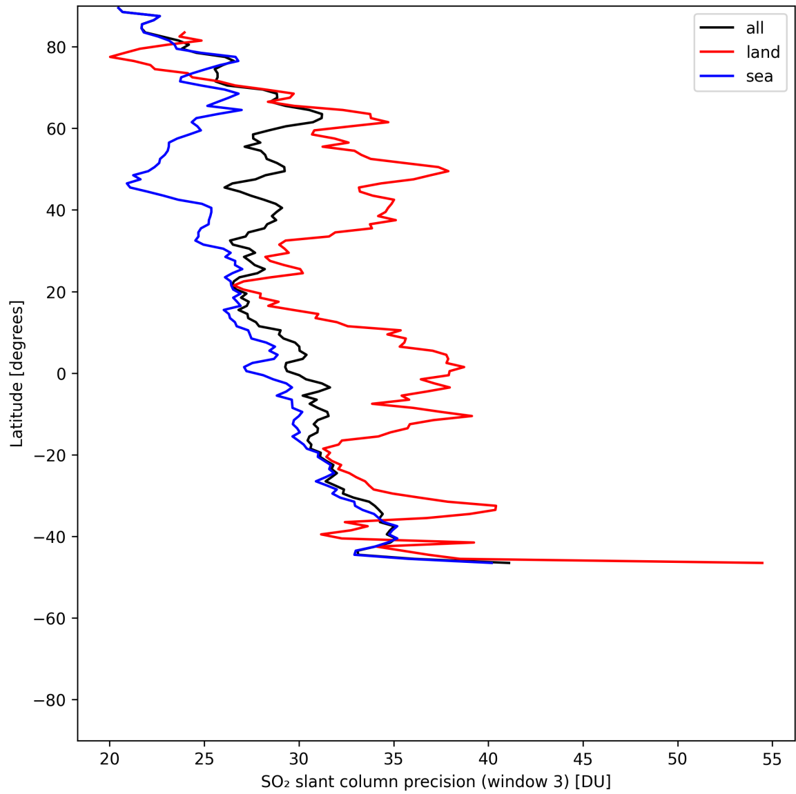
Figure 46: Zonal average of “SO 2 slant column precision (window 3)” for 2025-07-05 to 2025-07-07.
