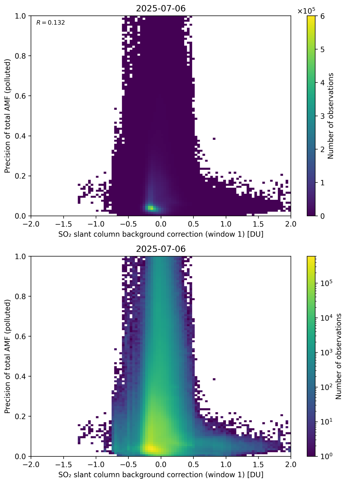
Figure 121: Scatter density plot of “SO 2 slant column background correction (window 1)” against “Precision of total AMF (polluted)” for 2025-07-05 to 2025-07-07.
