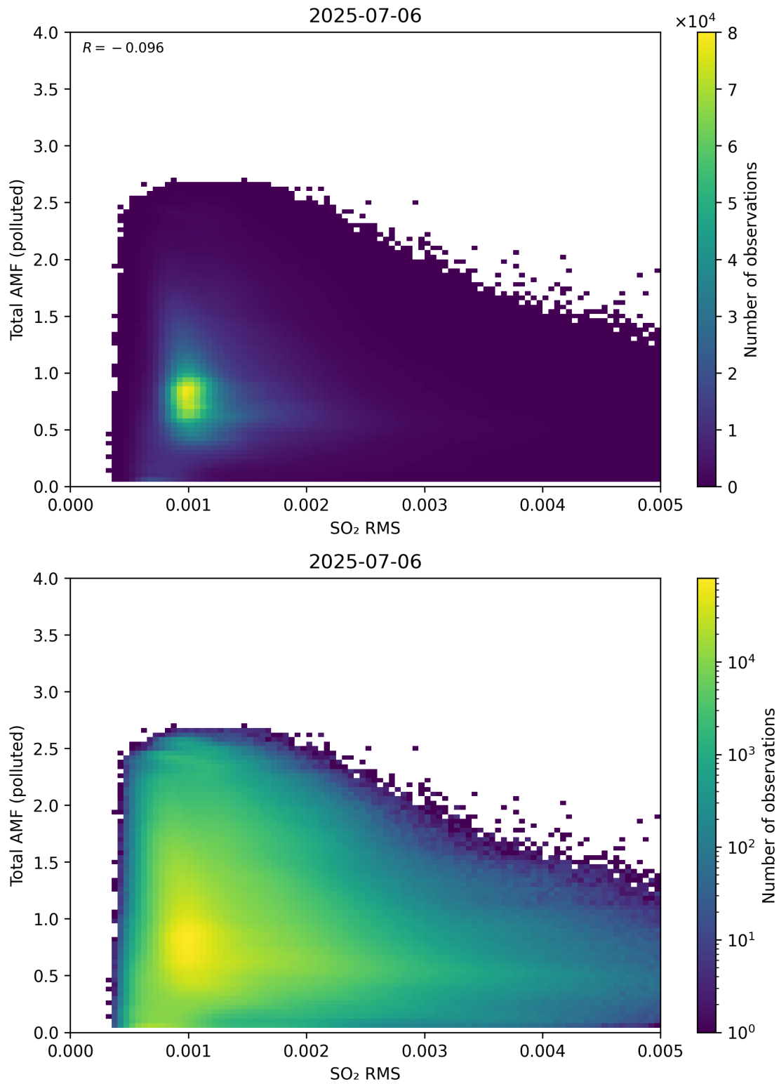
Figure 148: Scatter density plot of “SO 2 RMS” against “Total AMF (polluted)” for 2025-07-05 to 2025-07-07.
