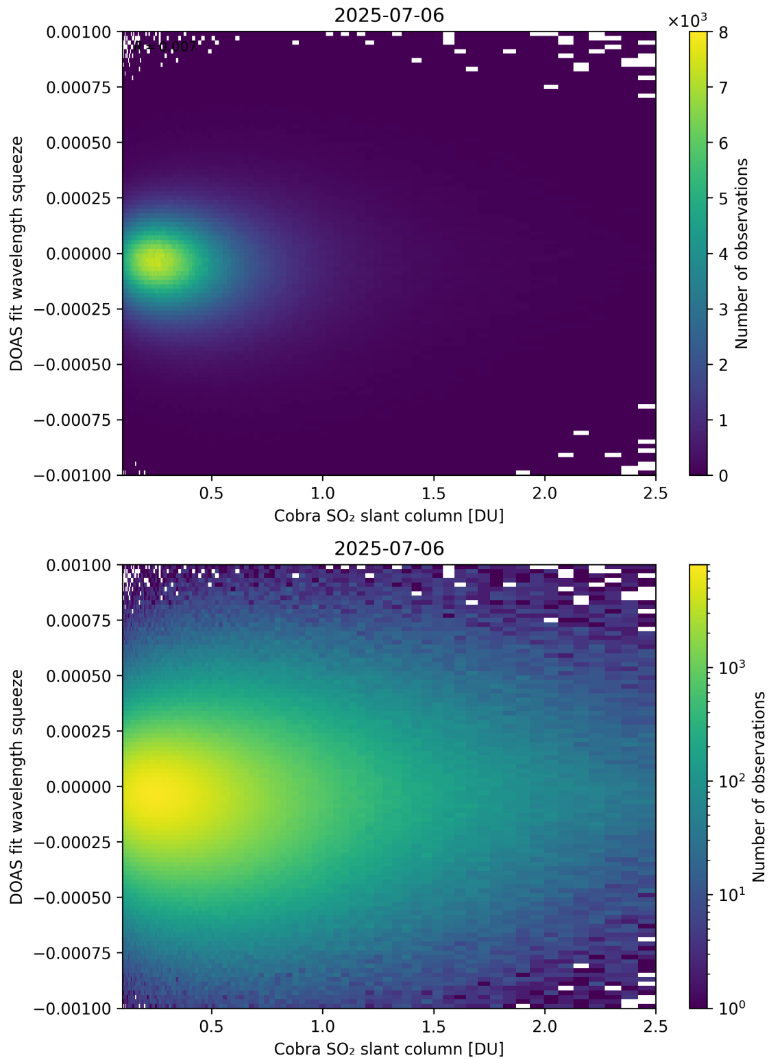
Figure 197: Scatter density plot of “Cobra SO 2 slant column” against “DOAS fit wavelength squeeze” for 2025-07-05 to 2025-07-07.
