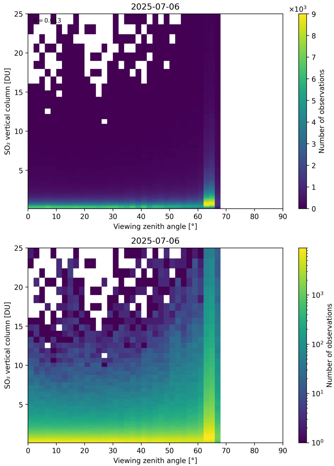
Figure 383: Scatter density plot of “Viewing zenith angle” against “SO 2 vertical column” for 2025-07-05 to 2025-07-07.
