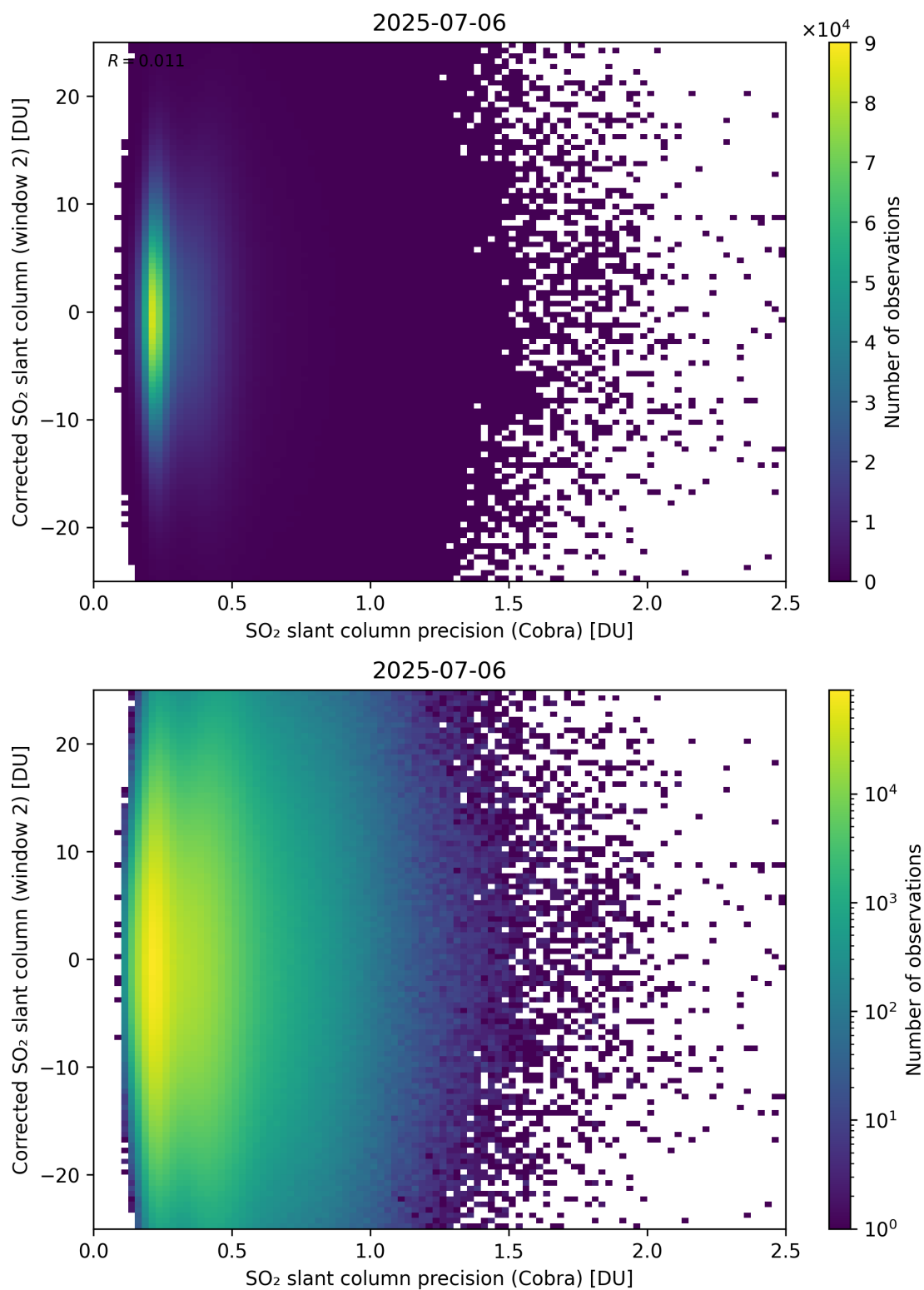
Figure 206: Scatter density plot of “SO 2 slant column precision (Cobra)” against “Corrected SO 2 slant column (window 2)” for 2025-07-05 to 2025-07-07.
