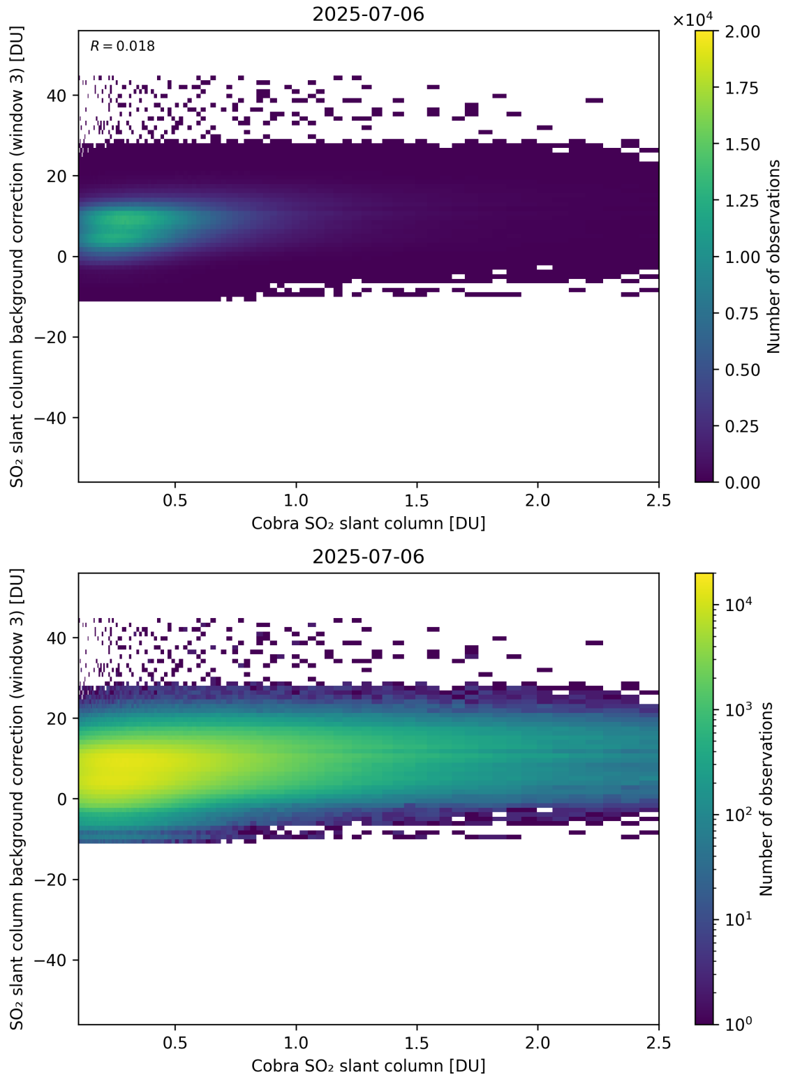
Figure 195: Scatter density plot of “Cobra SO 2 slant column” against “SO 2 slant column background correction (window 3)” for 2025-07-05 to 2025-07-07.
