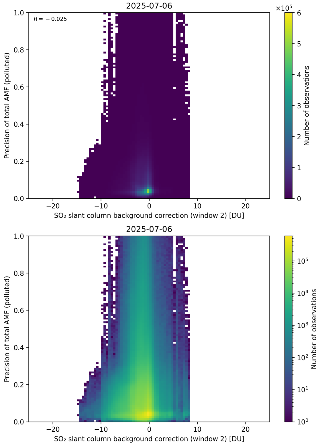
Figure 131: Scatter density plot of “SO 2 slant column background correction (window 2)” against “Precision of total AMF (polluted)” for 2025-07-05 to 2025-07-07.
