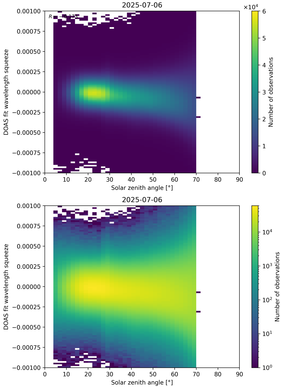
Figure 175: Scatter density plot of “Solar zenith angle” against “DOAS fit wavelength squeeze” for 2025-07-05 to 2025-07-07.
