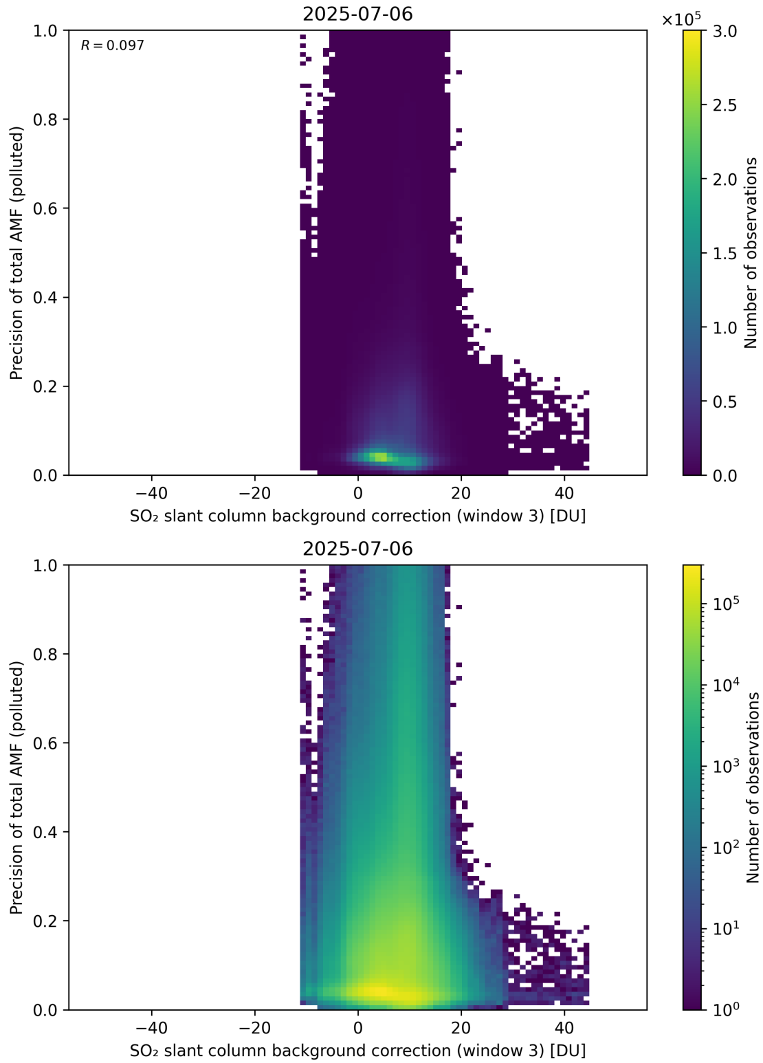
Figure 137: Scatter density plot of “SO 2 slant column background correction (window 3)” against “Precision of total AMF (polluted)” for 2025-07-05 to 2025-07-07.
