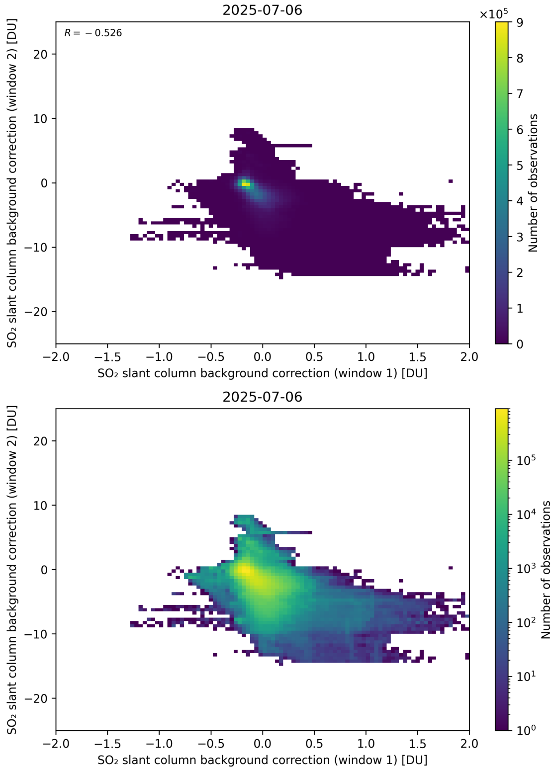
Figure 109: Scatter density plot of “SO 2 slant column background correction (window 1)” against “SO 2 slant column background correction (window 2)” for 2025-07-05 to 2025-07-07.
