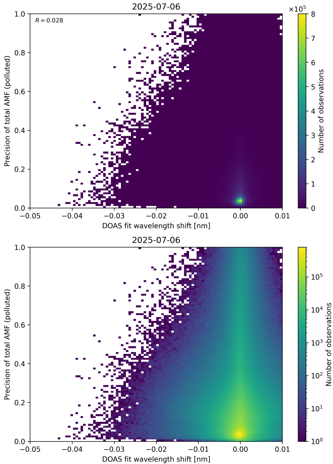
Figure 142: Scatter density plot of “DOAS fit wavelength shift” against “Precision of total AMF (polluted)” for 2025-07-05 to 2025-07-07.
