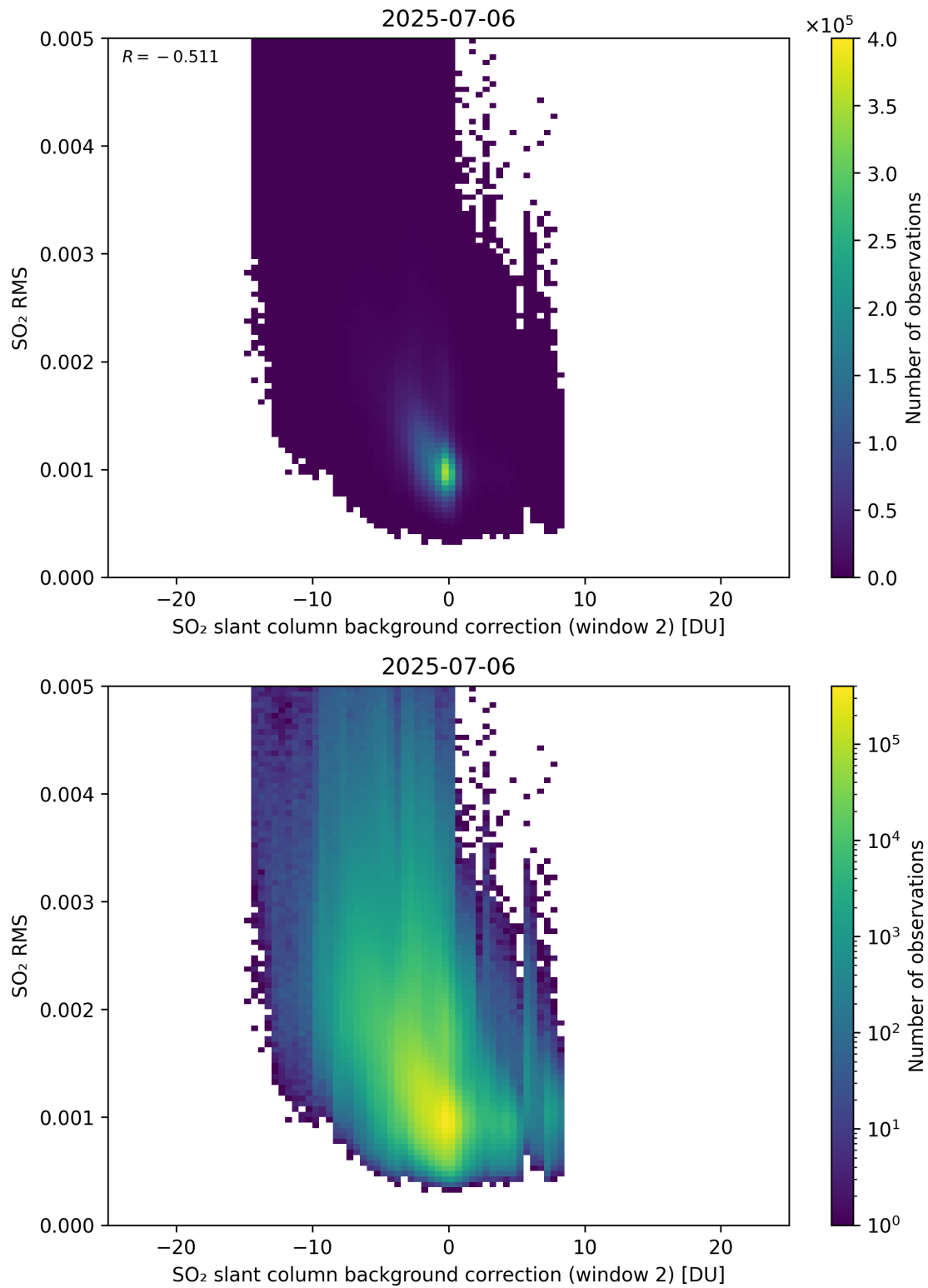
Figure 125: Scatter density plot of “SO 2 slant column background correction (window 2)” against “SO 2 RMS” for 2025-07-05 to 2025-07-07.
