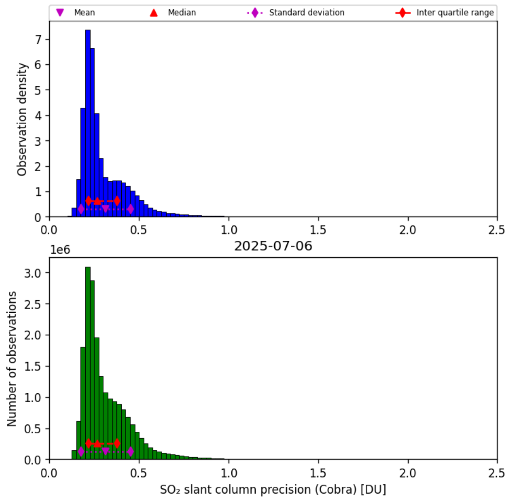
Figure 62: Histogram of “SO 2 slant column precision (Cobra)” for 2025-07-05 to 2025-07-07
