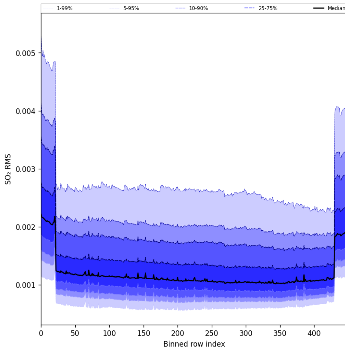
Figure 104: Along track statistics of “SO 2 RMS” for 2025-07-05 to 2025-07-07
