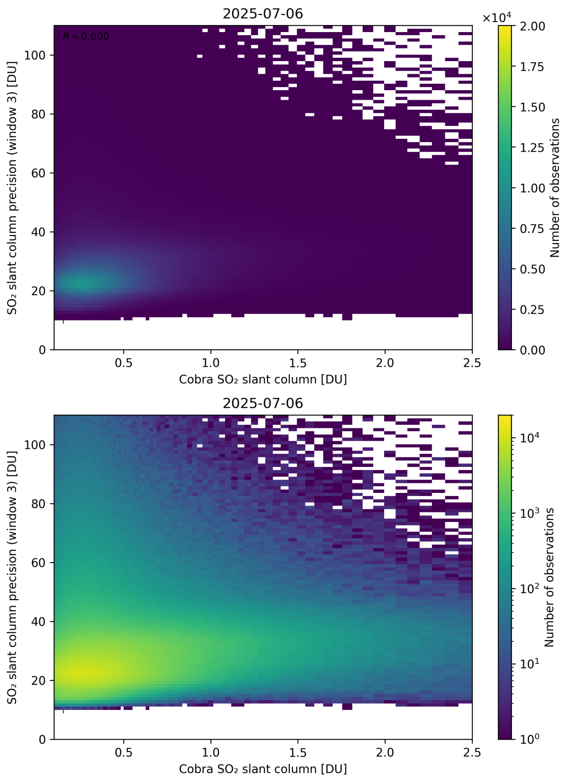
Figure 223: Scatter density plot of “Cobra SO 2 slant column” against “SO 2 slant column precision (window 3)” for 2025-07-05 to 2025-07-07.
