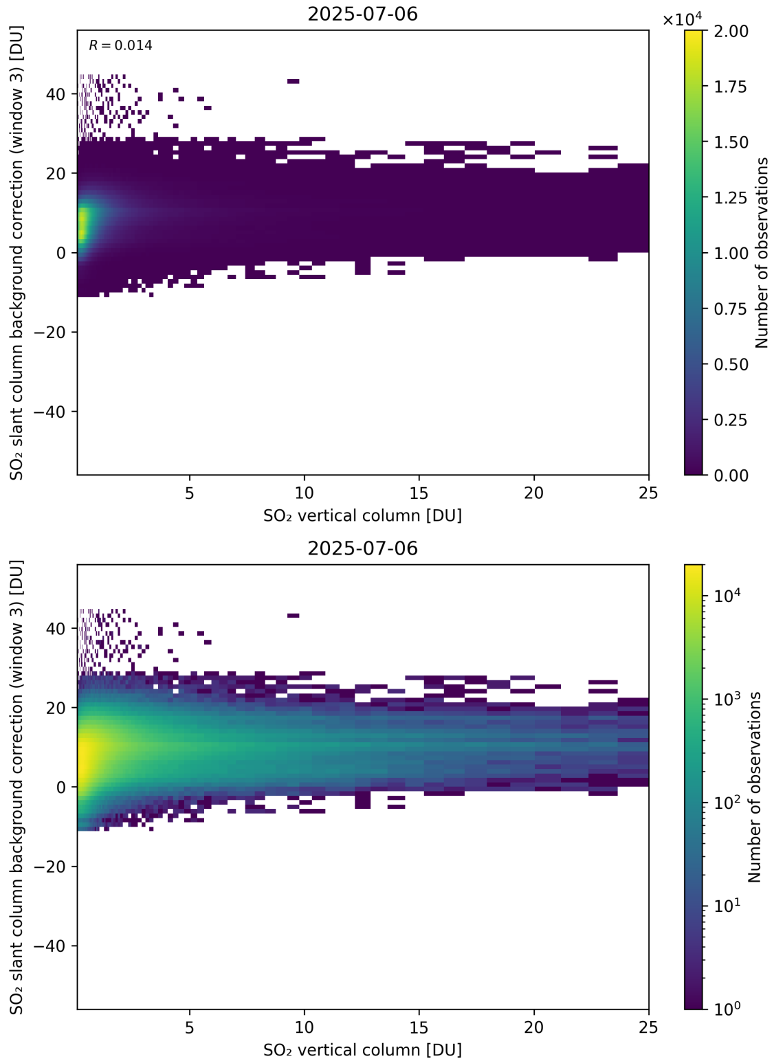
Figure 325: Scatter density plot of “SO 2 vertical column” against “SO 2 slant column background correction (window 3)” for 2025-07-05 to 2025-07-07.
