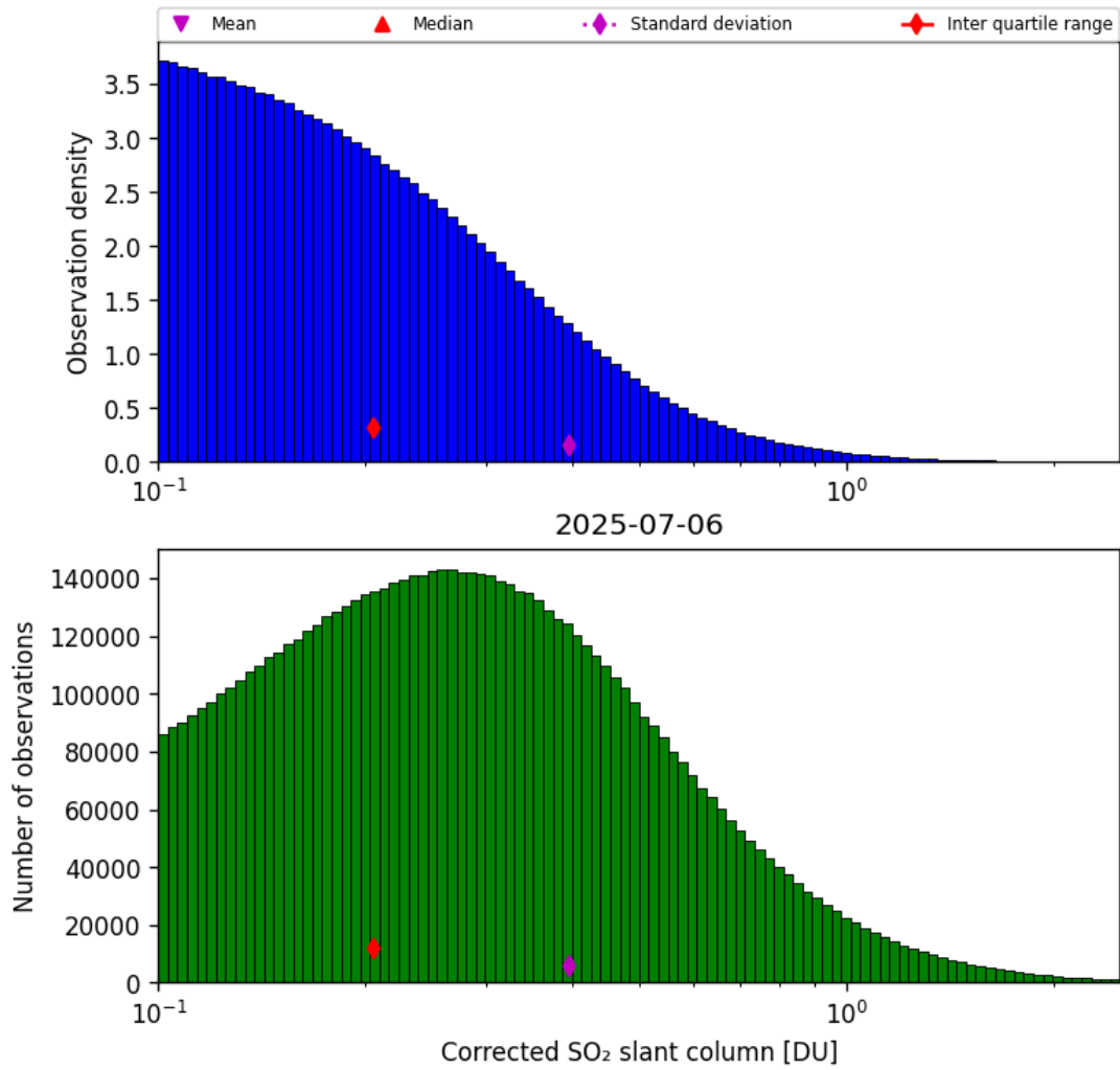
Figure 60: Histogram of “Corrected SO 2 slant column” for 2025-07-05 to 2025-07-07
