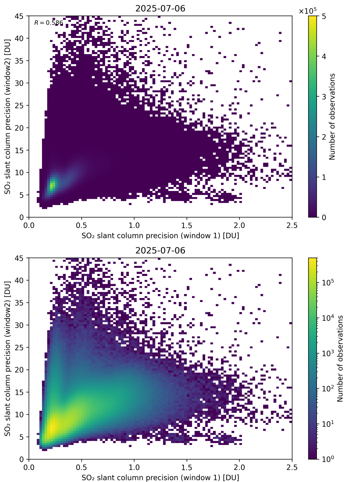
Figure 277: Scatter density plot of “SO 2 slant column precision (window 1)” against “SO 2 slant column precision (window2)” for 2025-07-05 to 2025-07-07.
