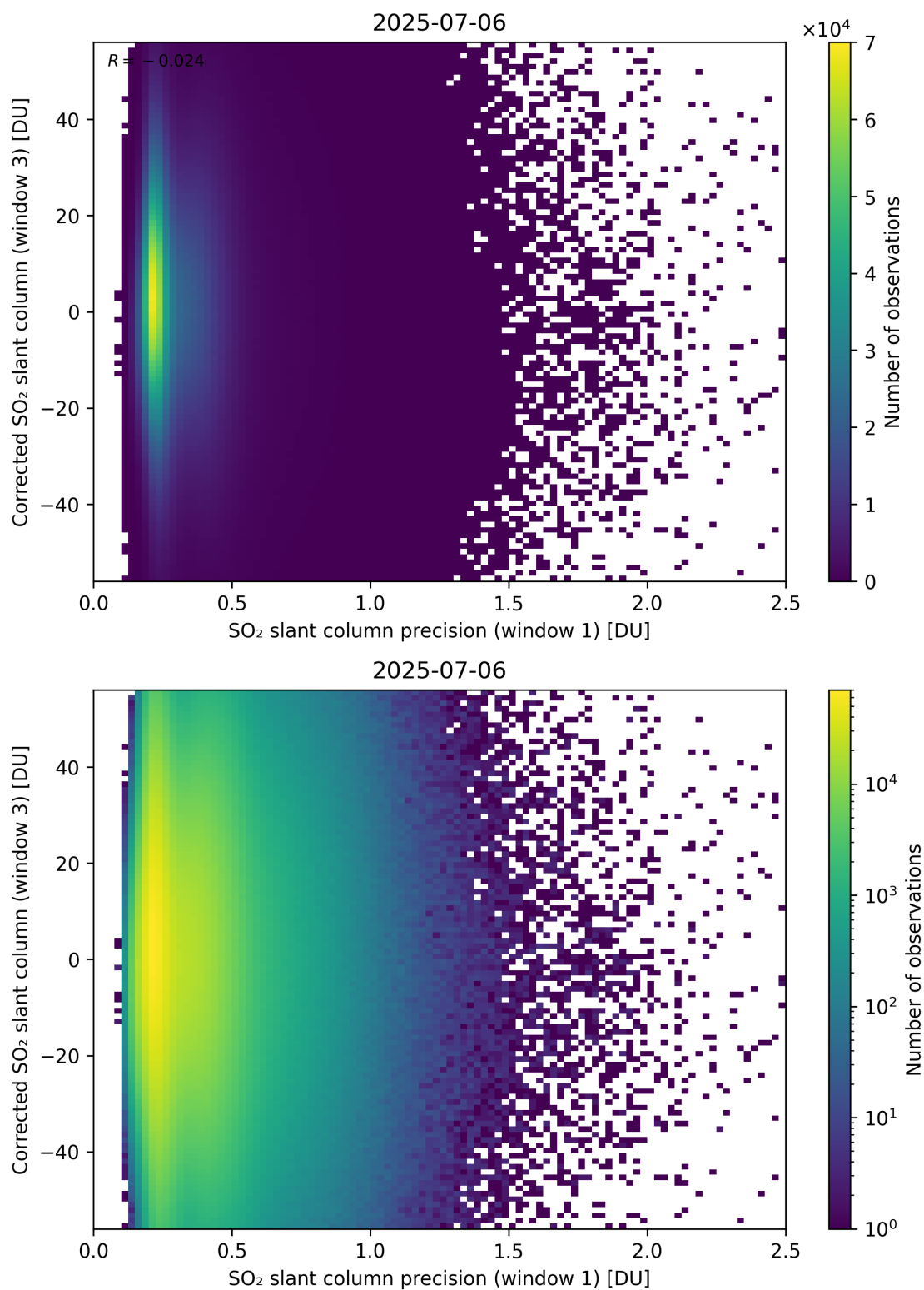
Figure 276: Scatter density plot of “SO 2 slant column precision (window 1)” against “Corrected SO 2 slant column (window 3)” for 2025-07-05 to 2025-07-07.
