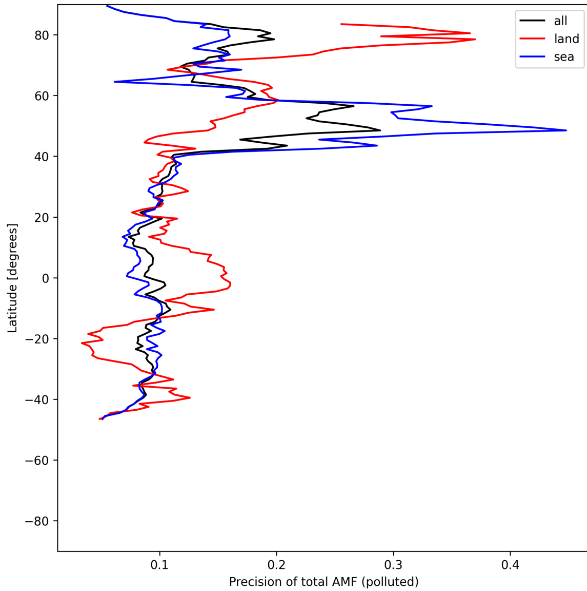
Figure 54: Zonal average of “Precision of total AMF (polluted)” for 2025-07-05 to 2025-07-07.
