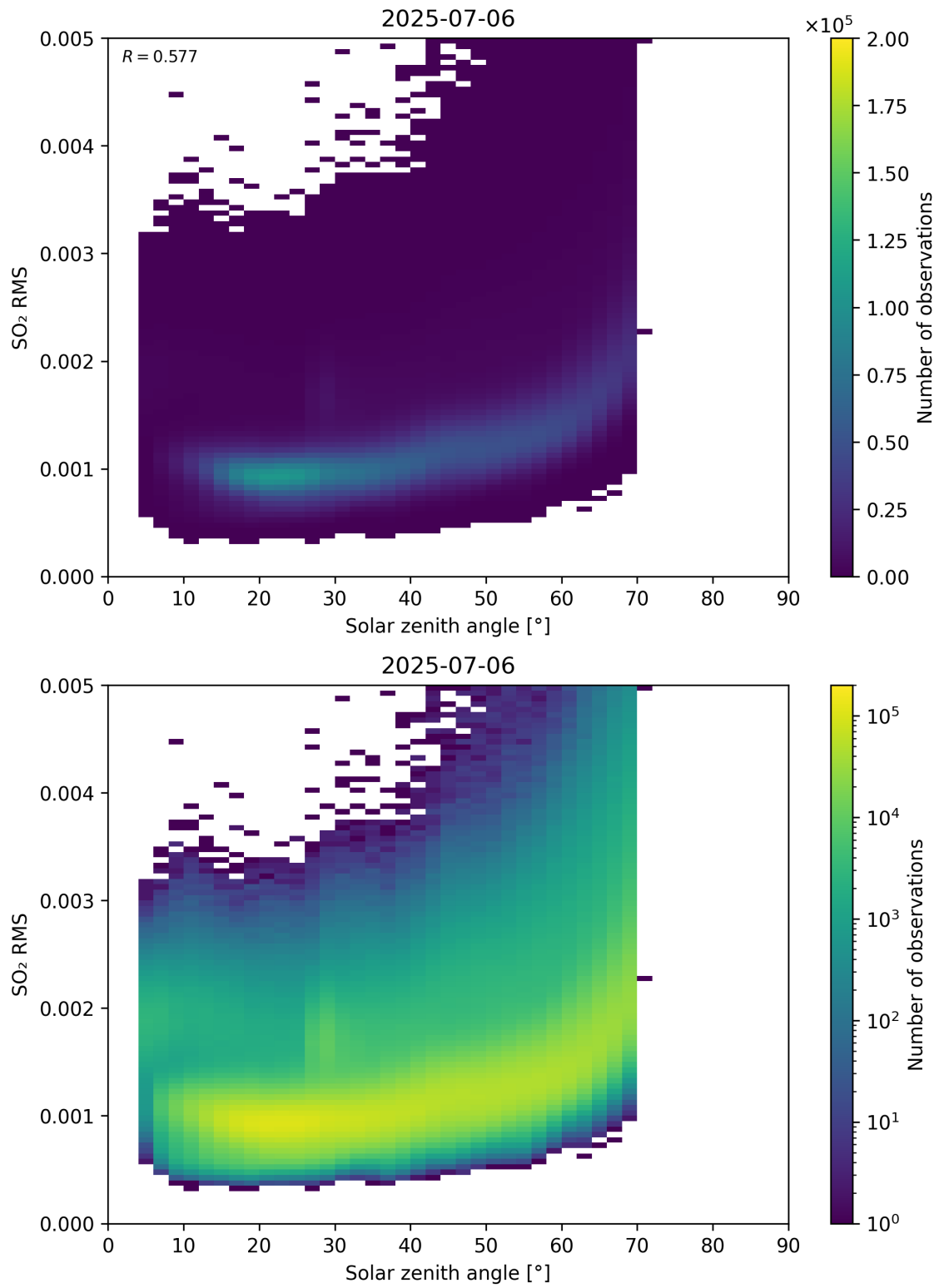
Figure 176: Scatter density plot of “Solar zenith angle” against “SO 2 RMS” for 2025-07-05 to 2025-07-07.
