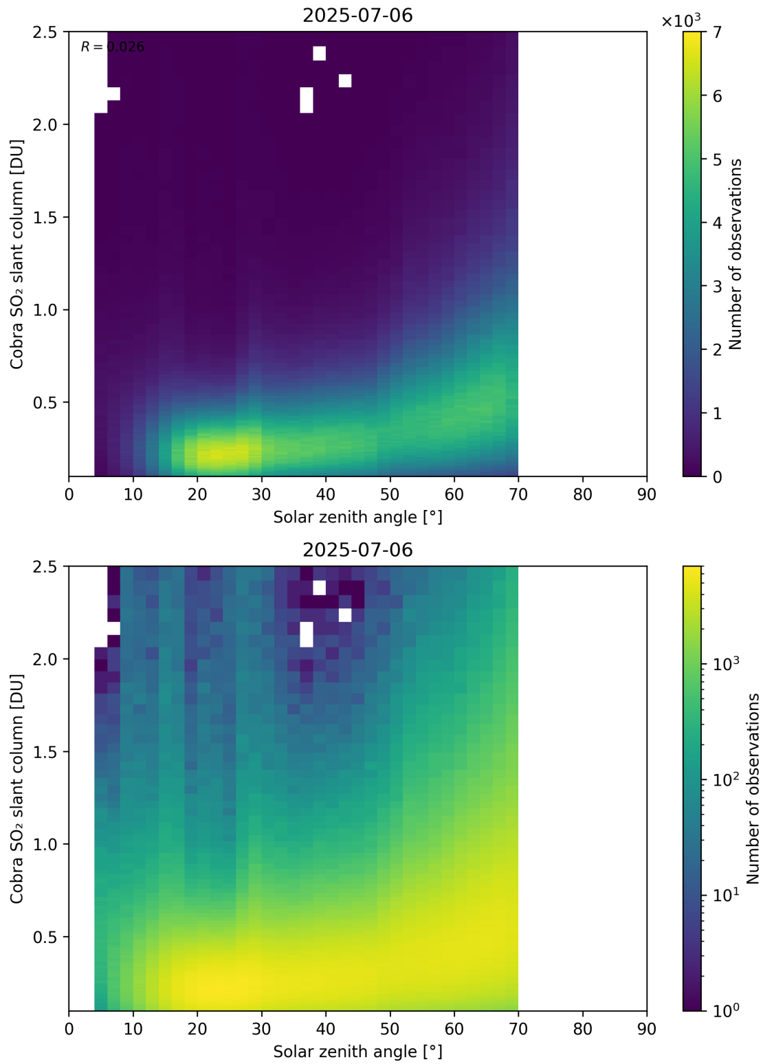
Figure 179: Scatter density plot of “Solar zenith angle” against “Cobra SO 2 slant column” for 2025-07-05 to 2025-07-07.
