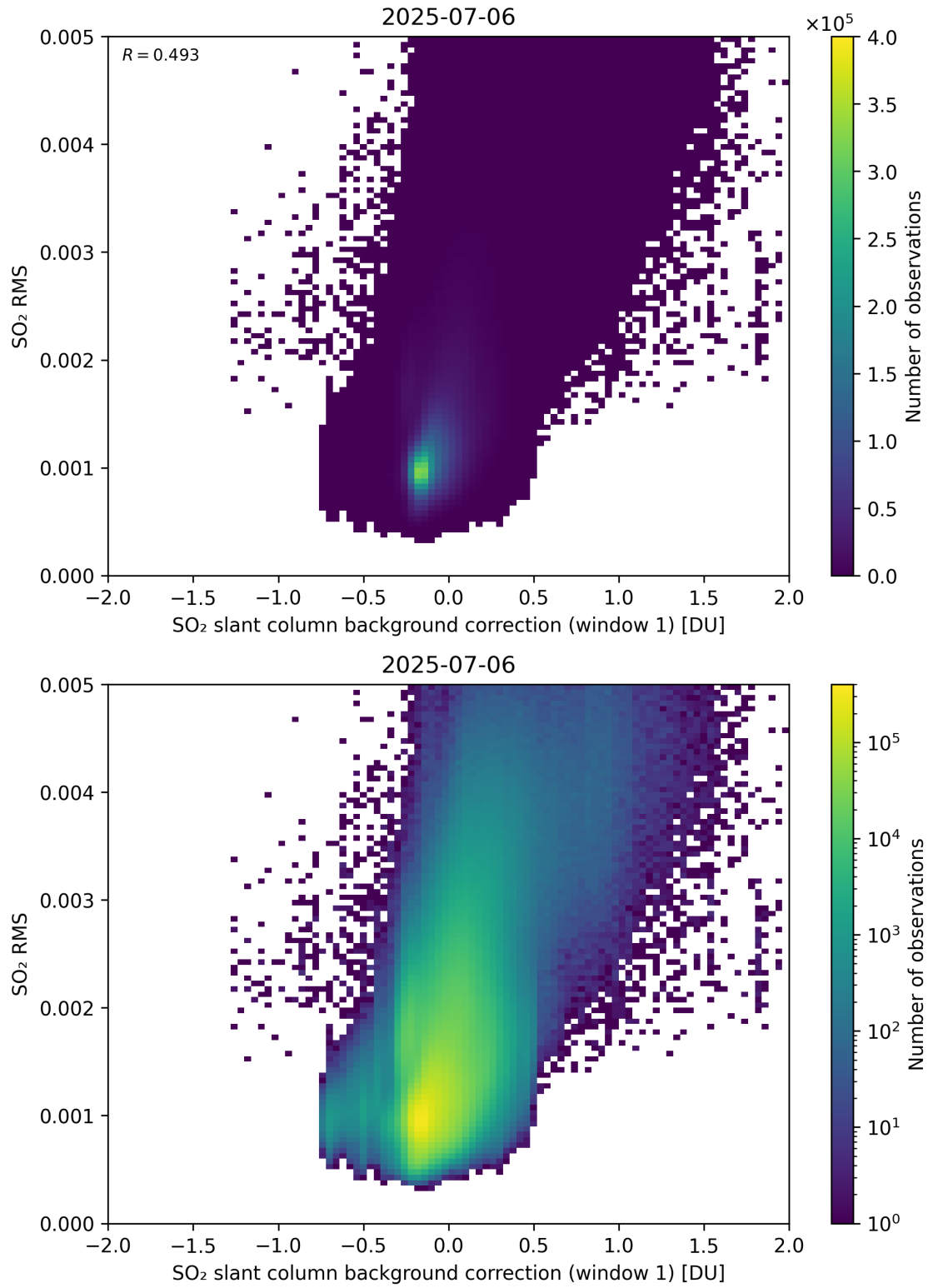
Figure 113: Scatter density plot of “SO 2 slant column background correction (window 1)” against “SO 2 RMS” for 2025-07-05 to 2025-07-07.
