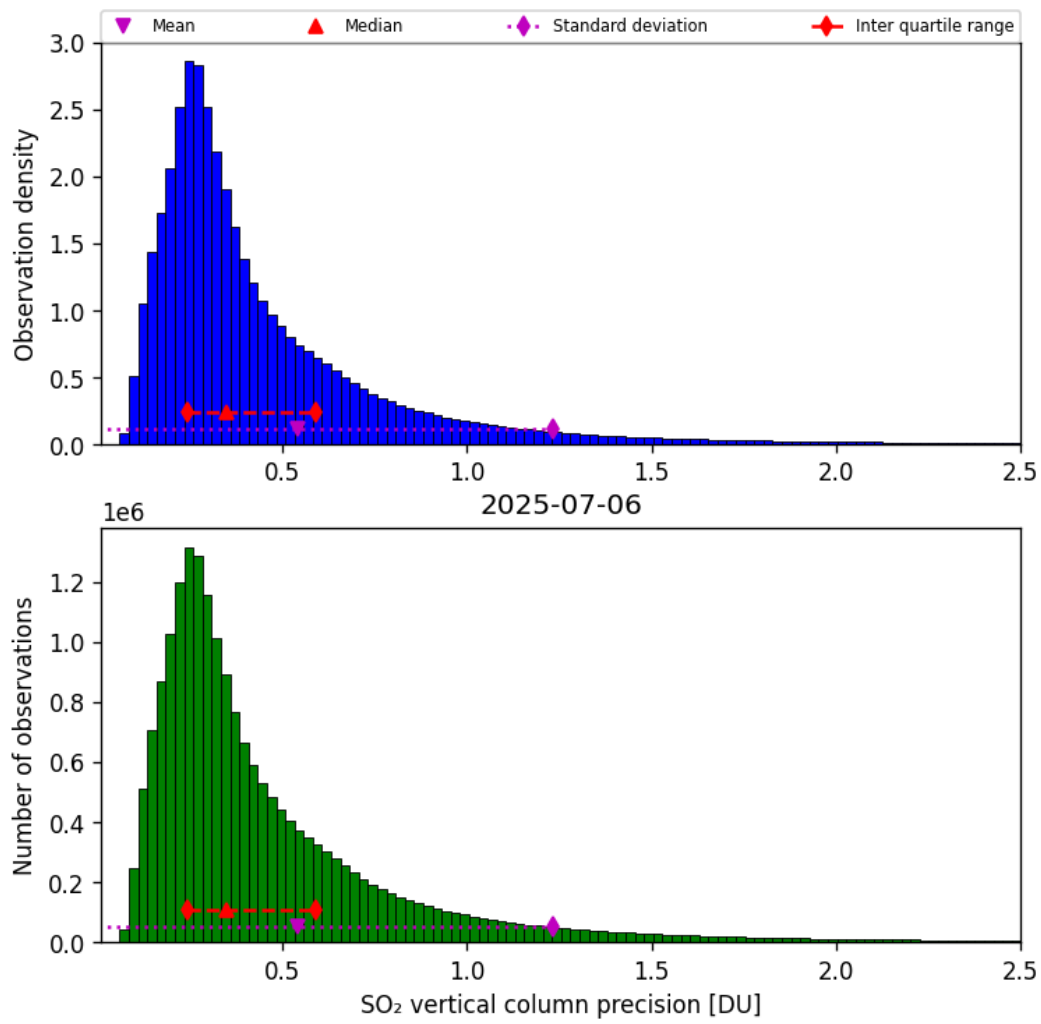
Figure 59: Histogram of “SO 2 vertical column precision” for 2025-07-05 to 2025-07-07
