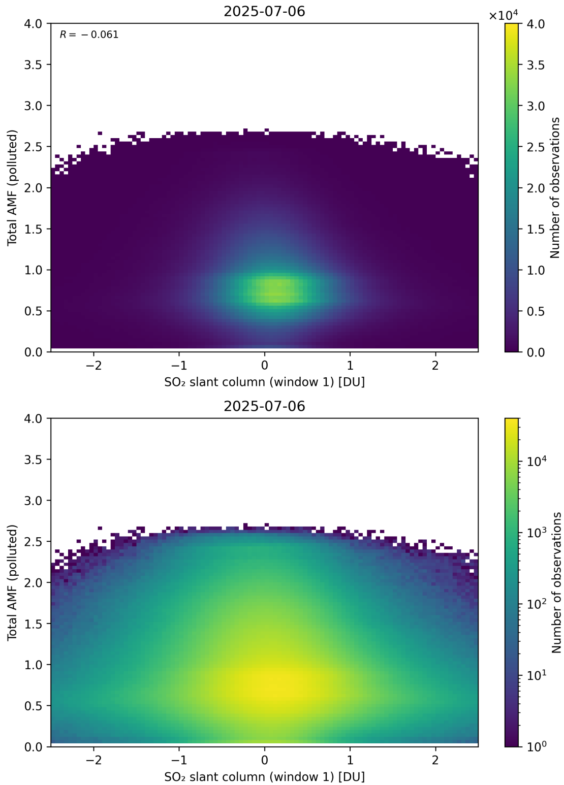
Figure 289: Scatter density plot of “SO 2 slant column (window 1)” against “Total AMF (polluted)” for 2025-07-05 to 2025-07-07.
