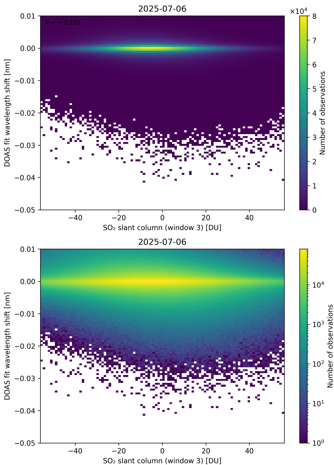
Figure 304: Scatter density plot of “SO 2 slant column (window 3)” against “DOAS fit wavelength shift” for 2025-07-05 to 2025-07-07.
