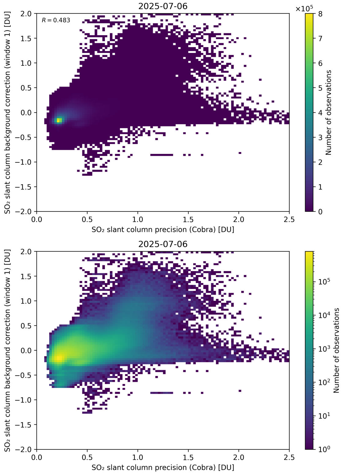
Figure 199: Scatter density plot of “SO 2 slant column precision (Cobra)” against “SO 2 slant column background correction (window 1)” for 2025-07-05 to 2025-07-07.
