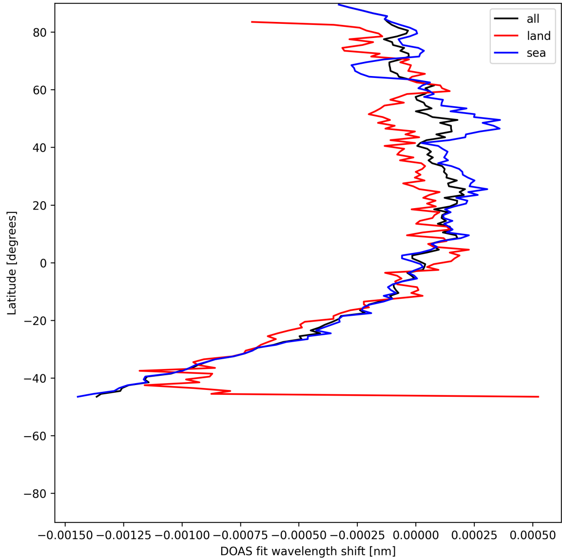
Figure 50: Zonal average of “DOAS fit wavelength shift” for 2025-07-05 to 2025-07-07.
