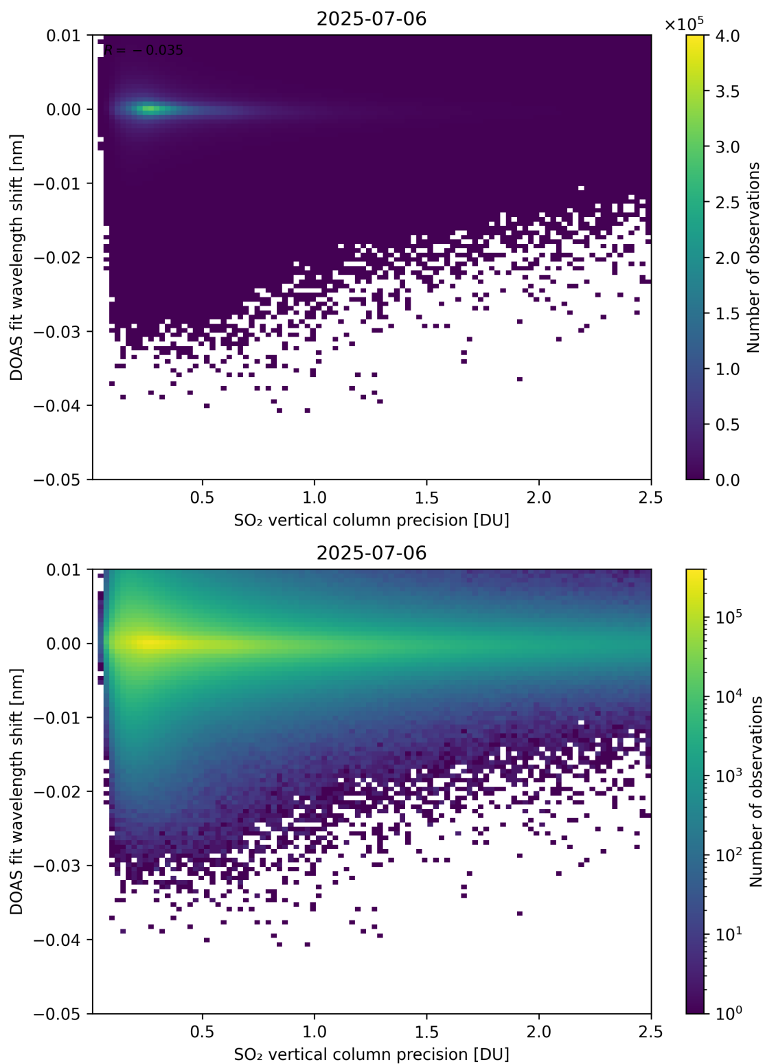
Figure 332: Scatter density plot of “SO 2 vertical column precision” against “DOAS fit wavelength shift” for 2025-07-05 to 2025-07-07.
