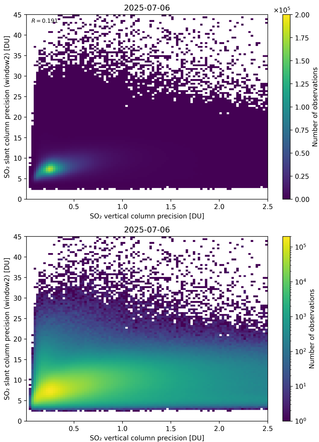
Figure 343: Scatter density plot of “SO 2 vertical column precision” against “SO 2 slant column precision (window2)” for 2025-07-05 to 2025-07-07.
