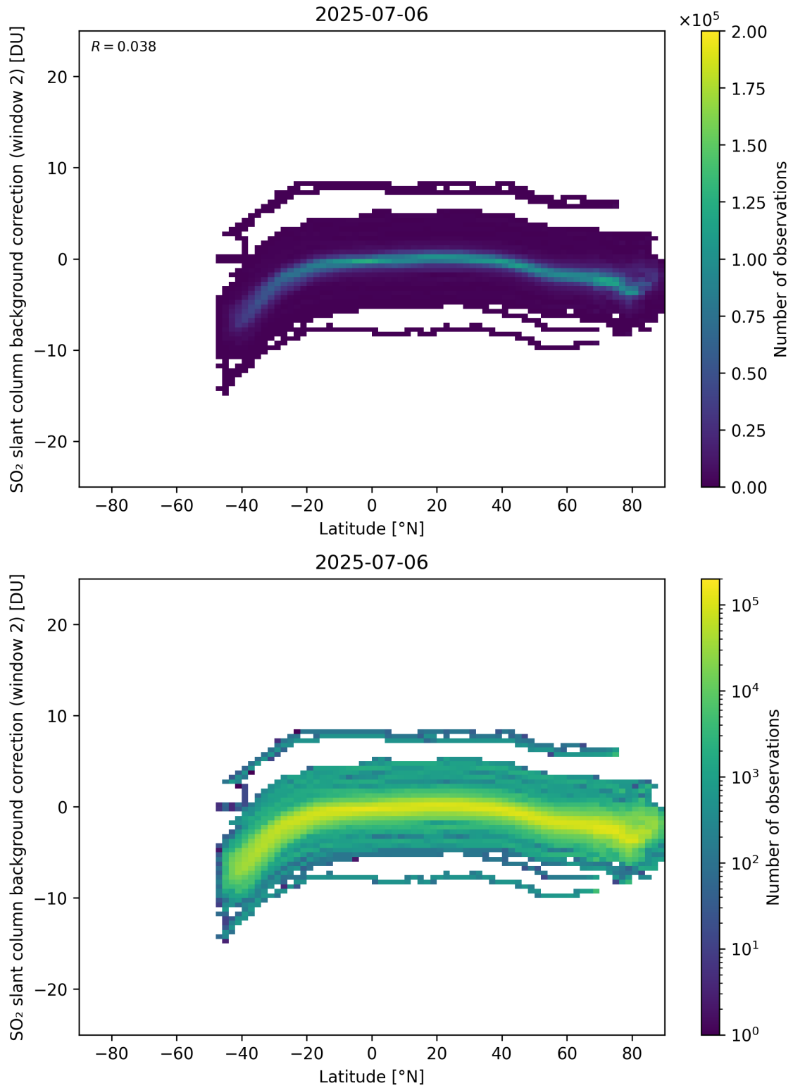
Figure 151: Scatter density plot of “Latitude” against “SO 2 slant column background correction (window 2)” for 2025-07-05 to 2025-07-07.
