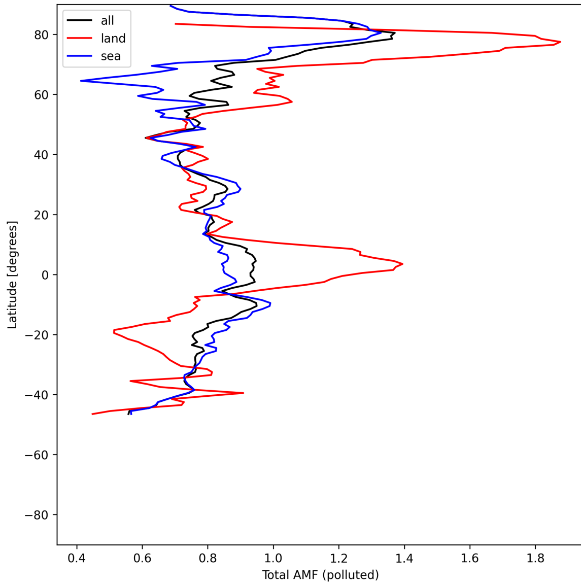
Figure 53: Zonal average of “Total AMF (polluted)” for 2025-07-05 to 2025-07-07.
