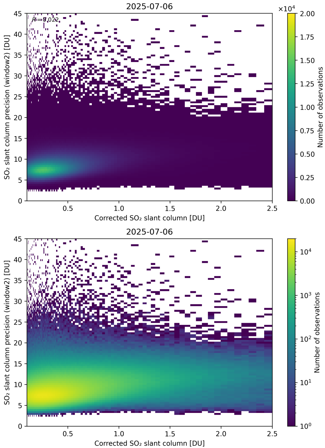
Figure 239: Scatter density plot of “Corrected SO 2 slant column” against “SO 2 slant column precision (window2)” for 2025-07-05 to 2025-07-07.
