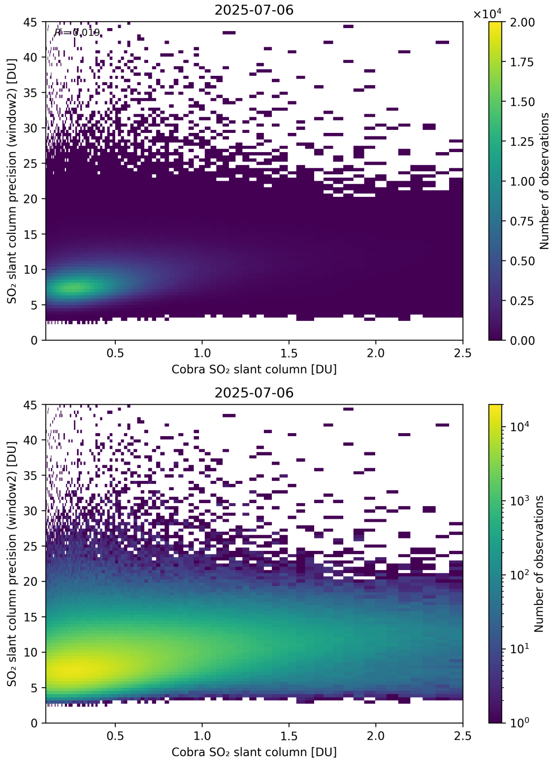
Figure 221: Scatter density plot of “Cobra SO 2 slant column” against “SO 2 slant column precision (window2)” for 2025-07-05 to 2025-07-07.
