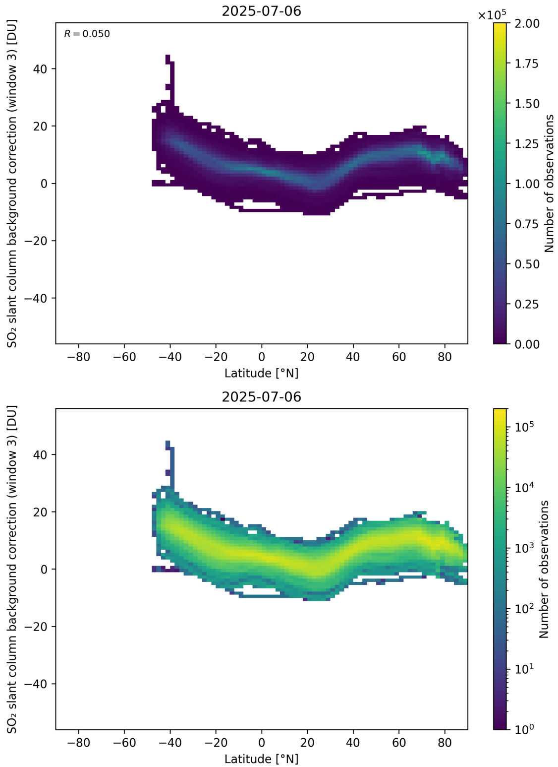
Figure 152: Scatter density plot of “Latitude” against “SO 2 slant column background correction (window 3)” for 2025-07-05 to 2025-07-07.
