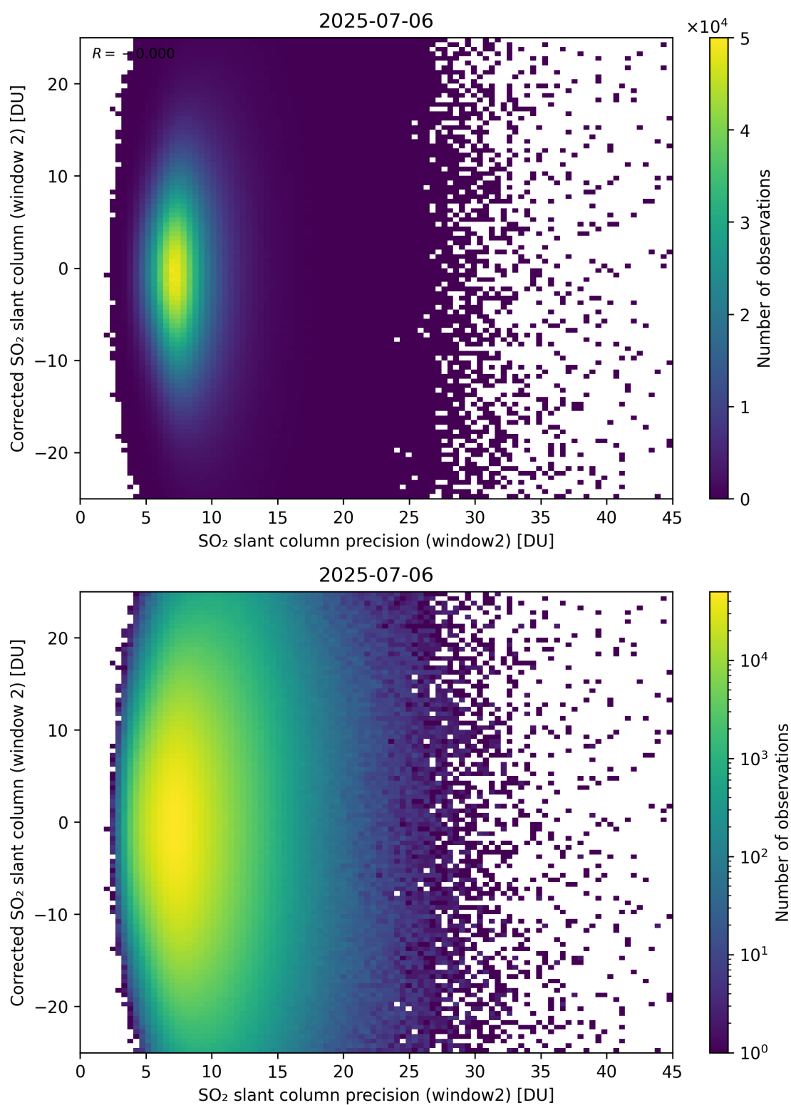
Figure 297: Scatter density plot of “SO 2 slant column precision (window2)” against “Corrected SO 2 slant column (window 2)” for 2025-07-05 to 2025-07-07.
