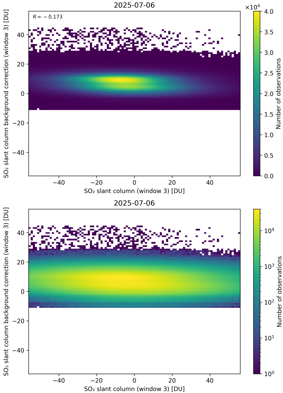
Figure 303: Scatter density plot of “SO 2 slant column (window 3)” against “SO 2 slant column background correction (window 3)” for 2025-07-05 to 2025-07-07.
