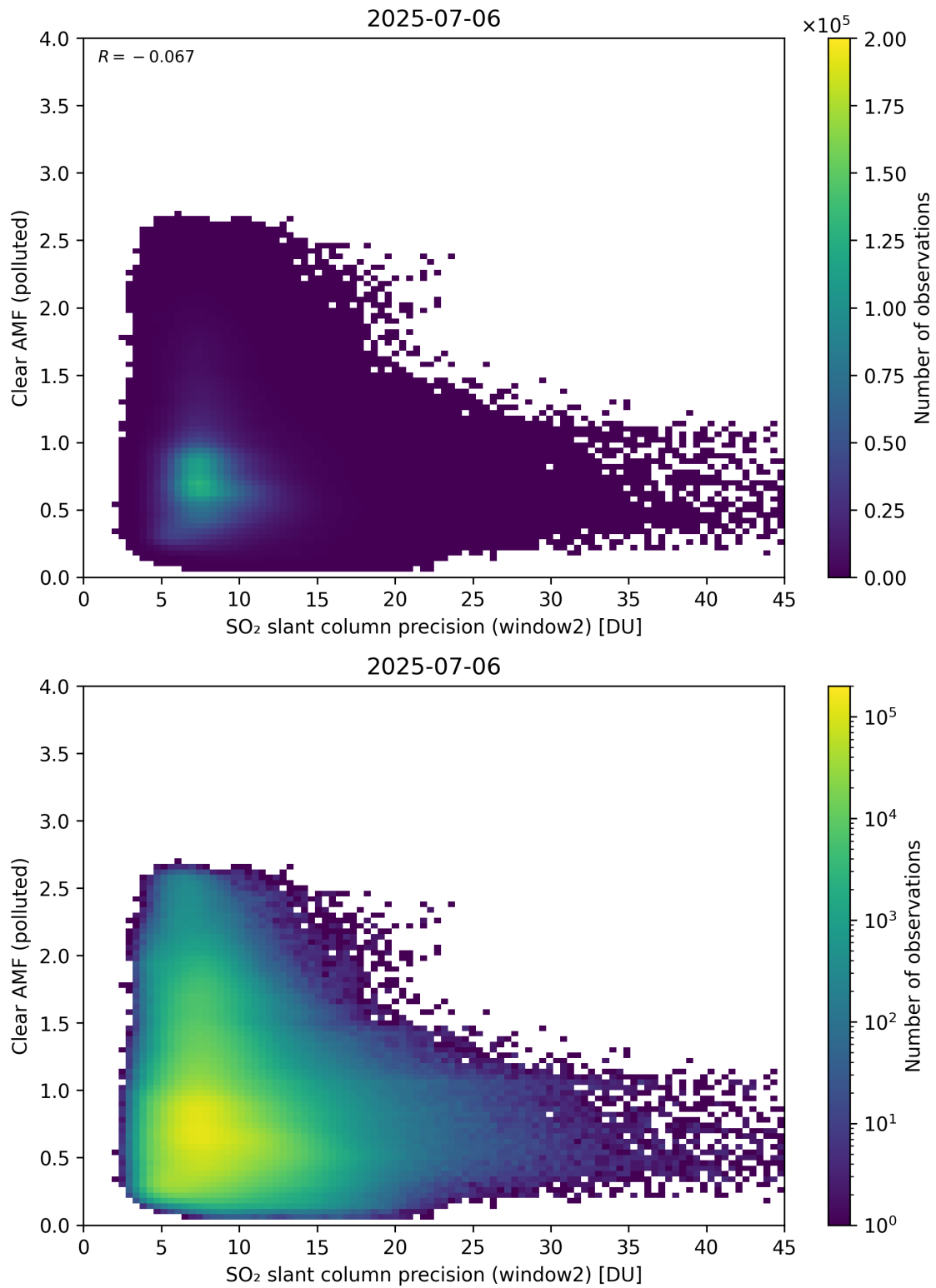
Figure 296: Scatter density plot of “SO 2 slant column precision (window2)” against “Clear AMF (polluted)” for 2025-07-05 to 2025-07-07.
