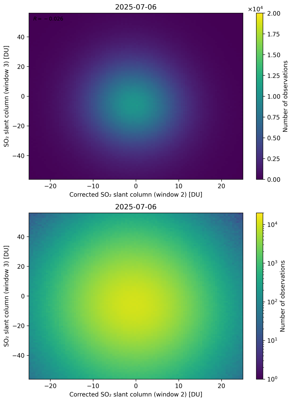
Figure 251: Scatter density plot of “Corrected SO 2 slant column (window 2)” against “SO 2 slant column (window 3)” for 2025-07-05 to 2025-07-07.
