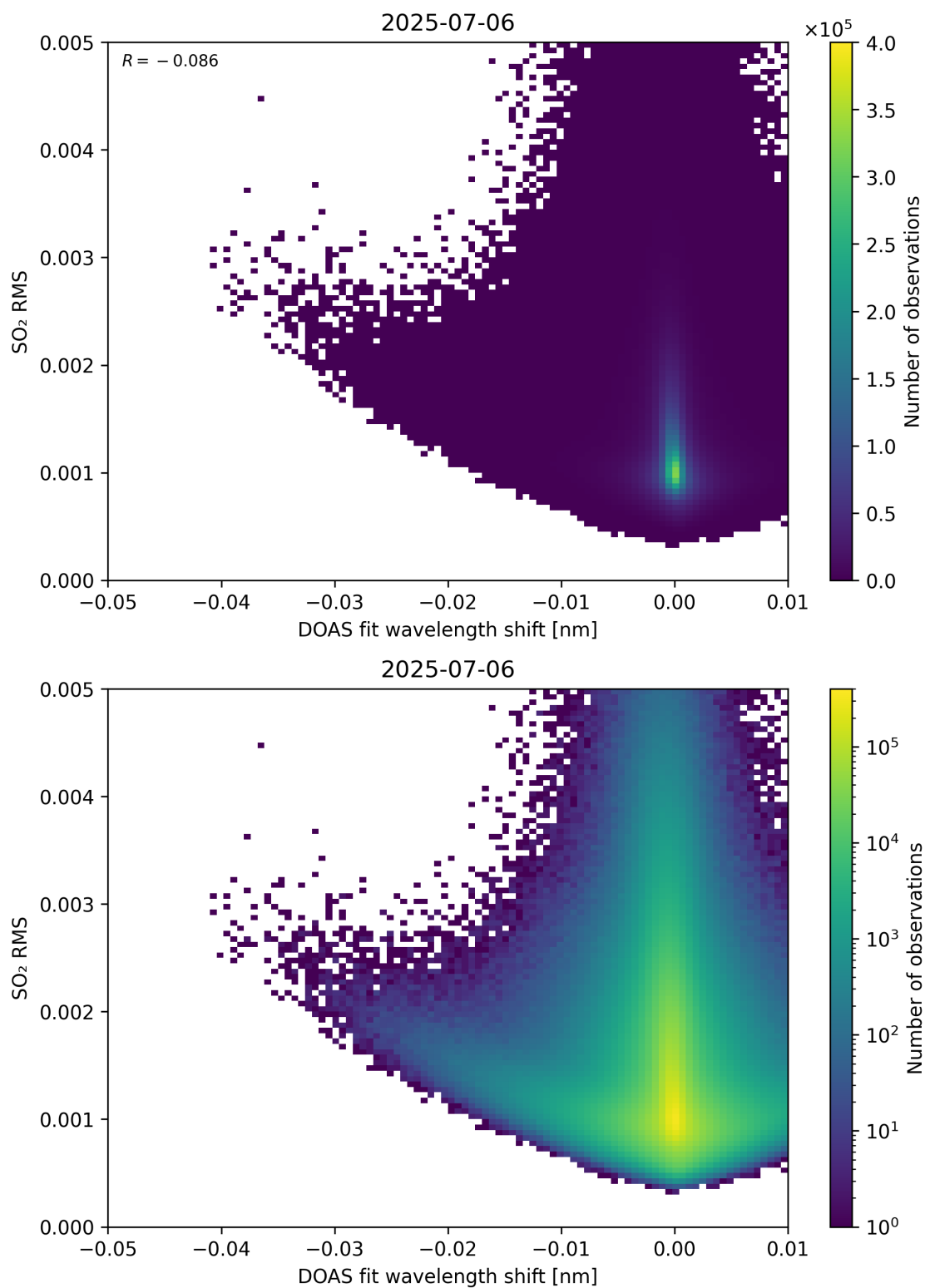
Figure 139: Scatter density plot of “DOAS fit wavelength shift” against “SO 2 RMS” for 2025-07-05 to 2025-07-07.
