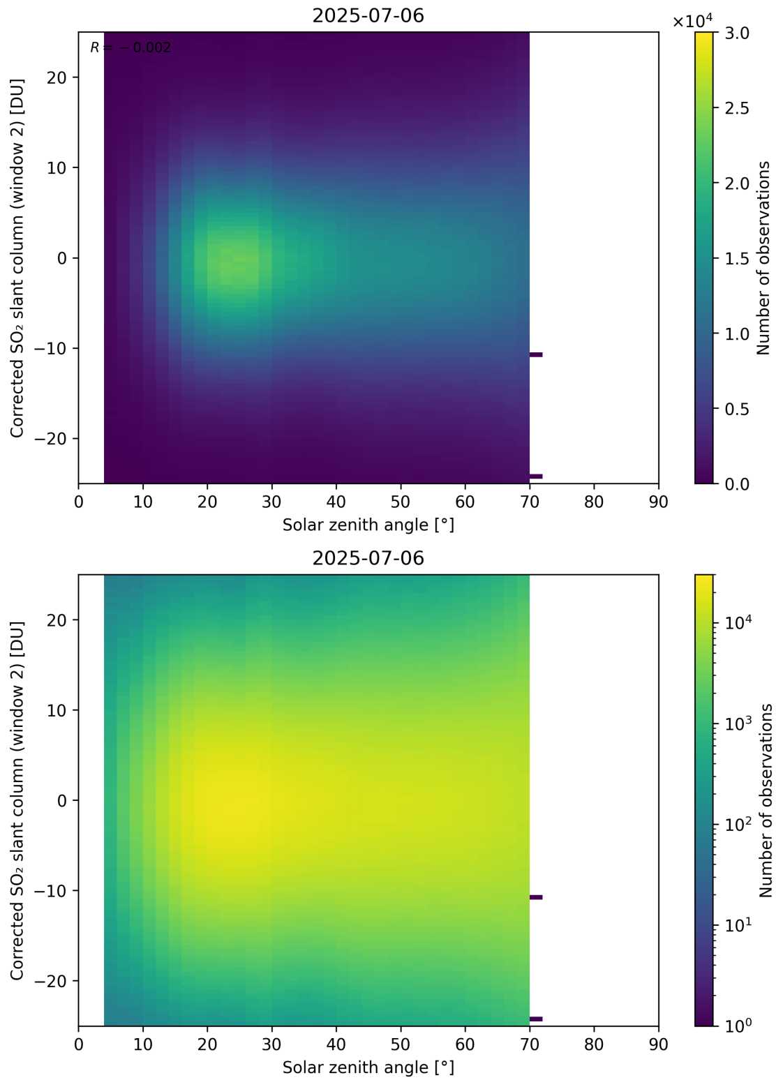
Figure 182: Scatter density plot of “Solar zenith angle” against “Corrected SO 2 slant column (window 2)” for 2025-07-05 to 2025-07-07.
