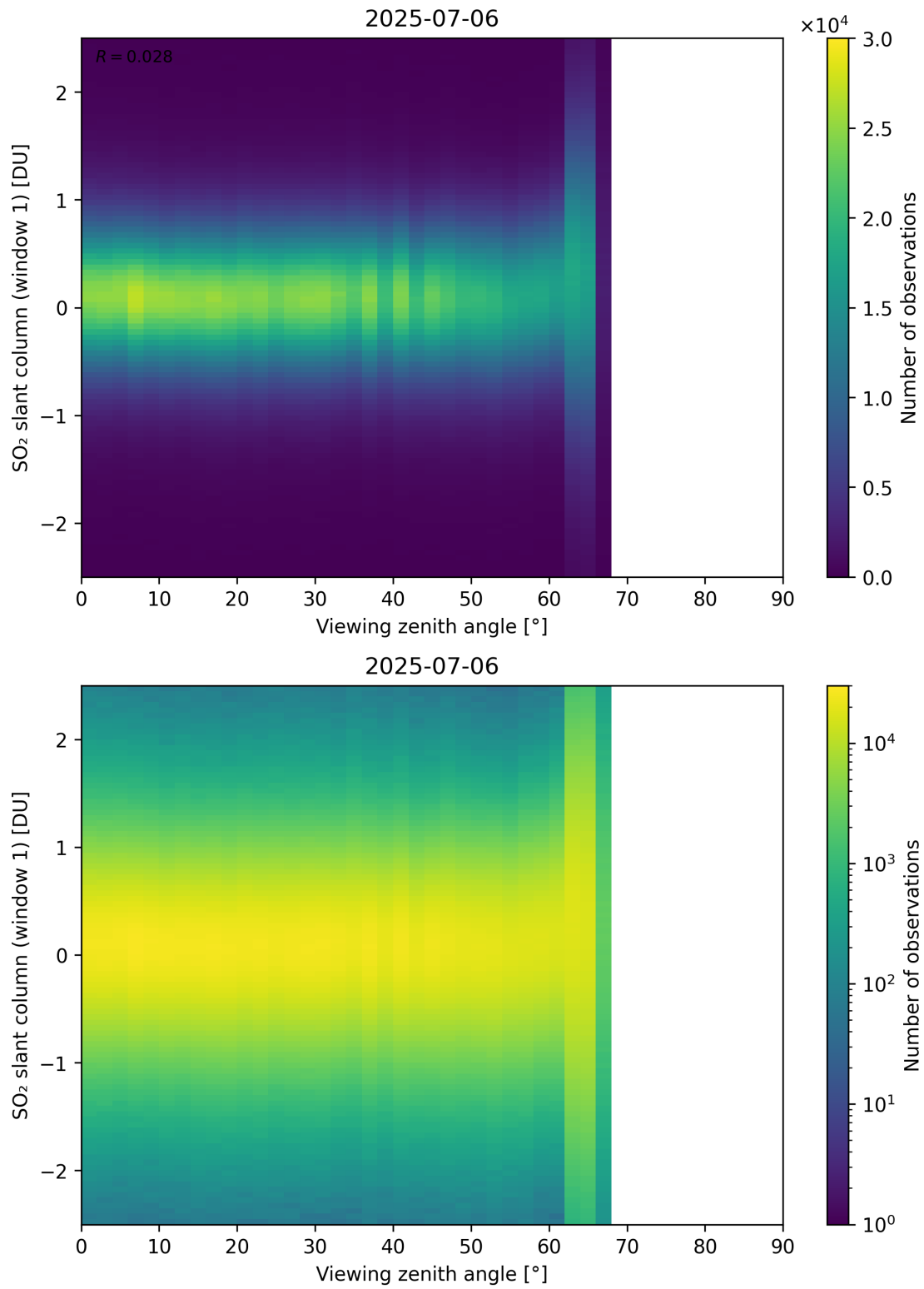
Figure 376: Scatter density plot of “Viewing zenith angle” against “SO 2 slant column (window 1)” for 2025-07-05 to 2025-07-07.
