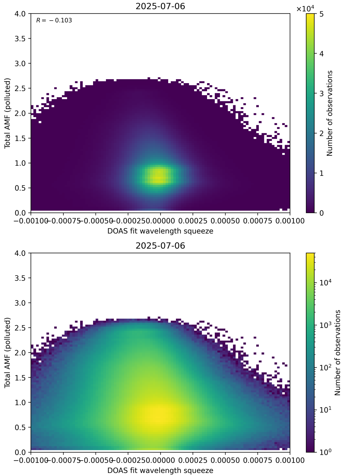
Figure 145: Scatter density plot of “DOAS fit wavelength squeeze” against “Total AMF (polluted)” for 2025-07-05 to 2025-07-07.
