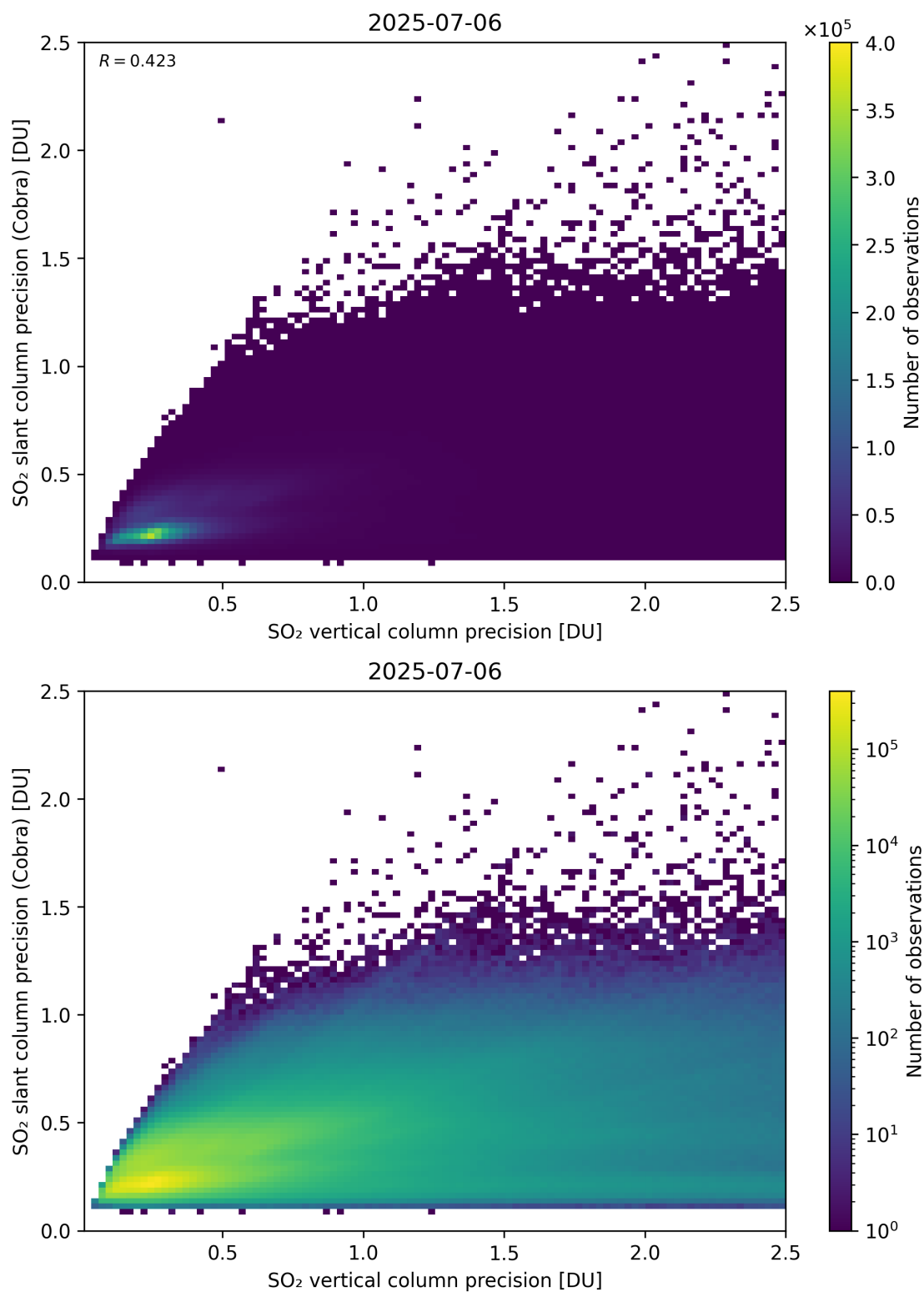
Figure 337: Scatter density plot of “SO 2 vertical column precision” against “SO 2 slant column precision (Cobra)” for 2025-07-05 to 2025-07-07.
