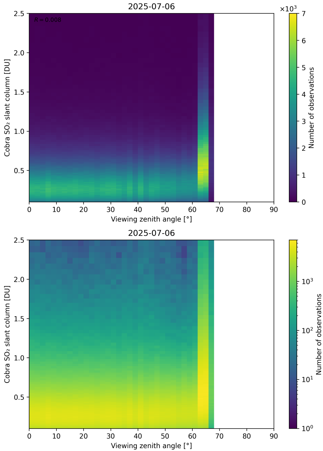
Figure 371: Scatter density plot of “Viewing zenith angle” against “Cobra SO 2 slant column” for 2025-07-05 to 2025-07-07.
