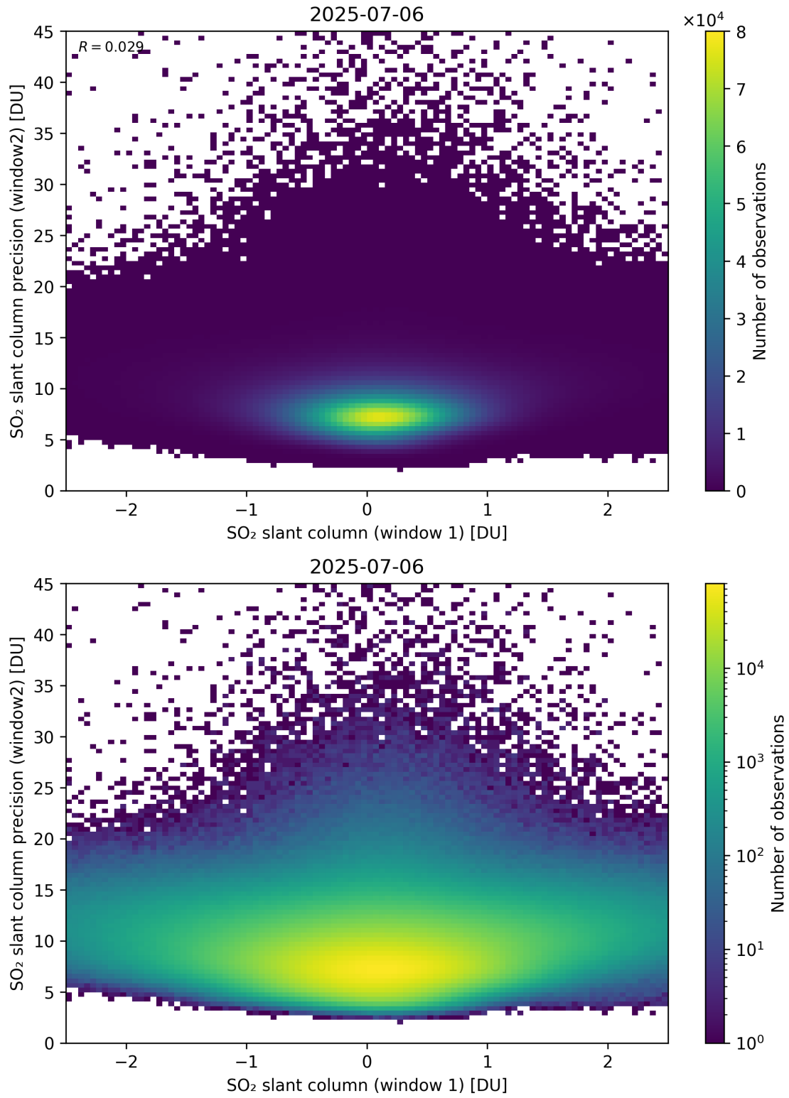
Figure 286: Scatter density plot of “SO 2 slant column (window 1)” against “SO 2 slant column precision (window2)” for 2025-07-05 to 2025-07-07.
