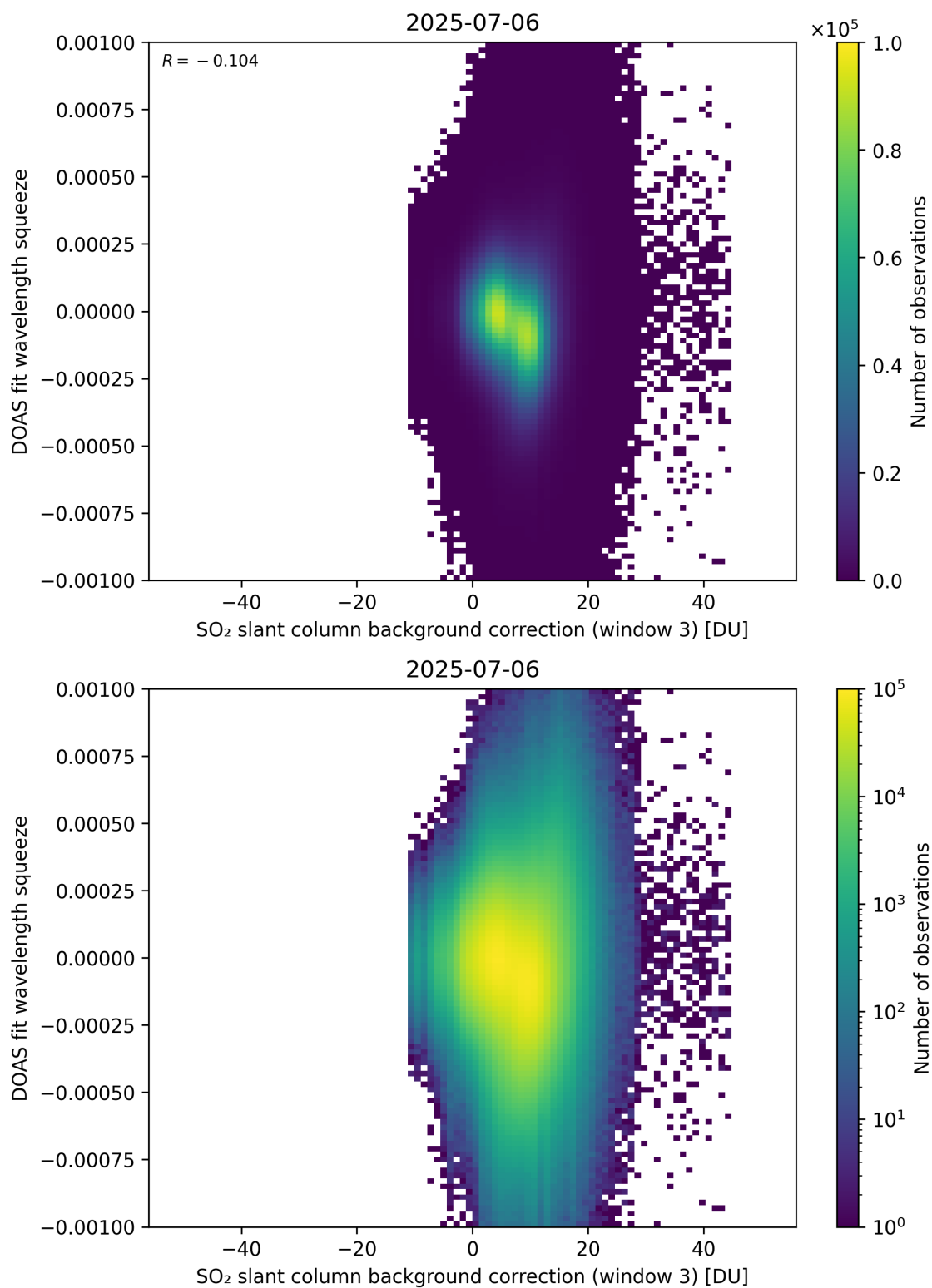
Figure 133: Scatter density plot of “SO 2 slant column background correction (window 3)” against “DOAS fit wavelength squeeze” for 2025-07-05 to 2025-07-07.
