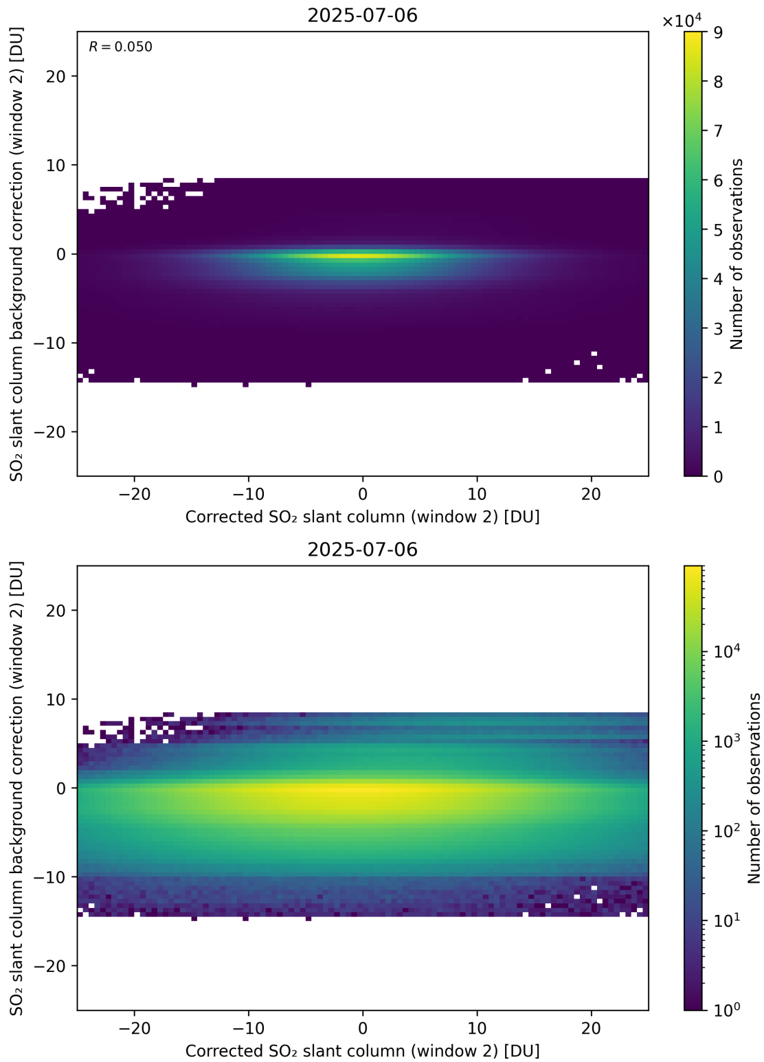
Figure 244: Scatter density plot of “Corrected SO 2 slant column (window 2)” against “SO 2 slant column background correction (window 2)” for 2025-07-05 to 2025-07-07.
