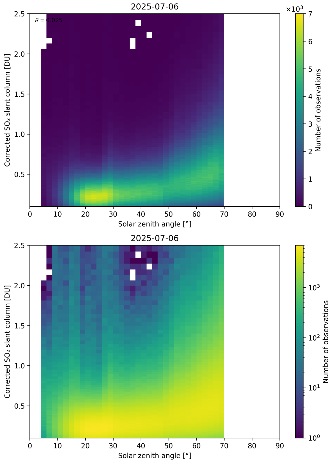
Figure 181: Scatter density plot of “Solar zenith angle” against “Corrected SO 2 slant column” for 2025-07-05 to 2025-07-07.
