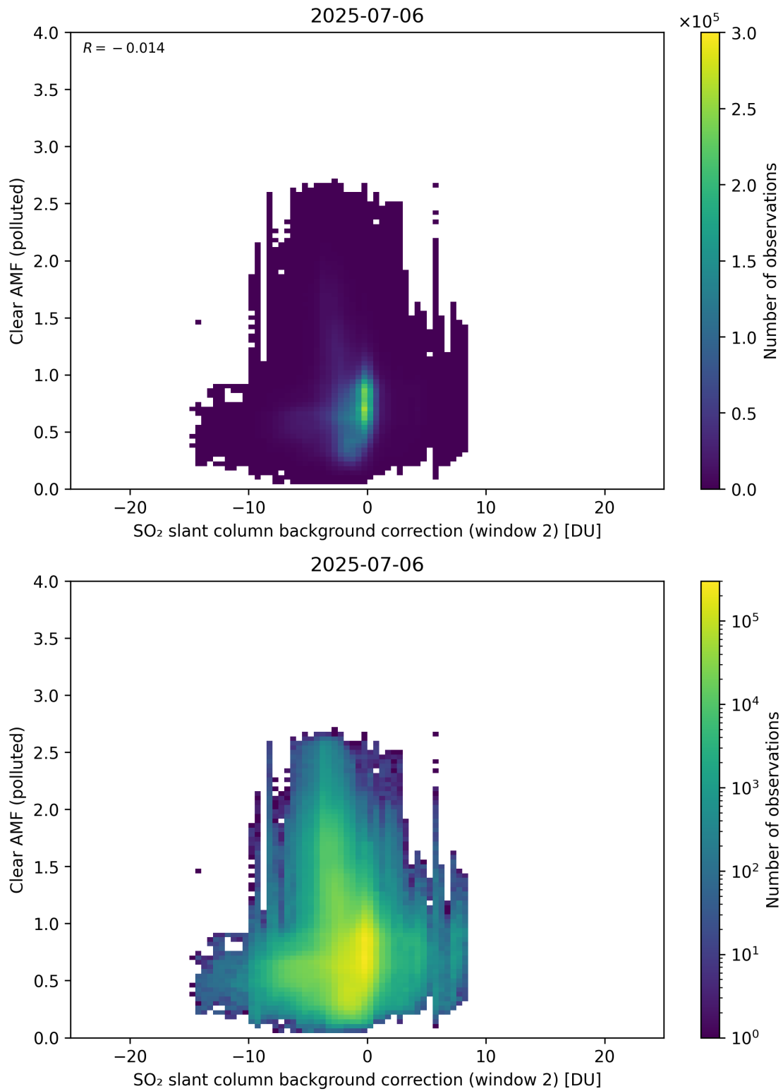
Figure 126: Scatter density plot of “SO 2 slant column background correction (window 2)” against “Clear AMF (polluted)” for 2025-07-05 to 2025-07-07.
