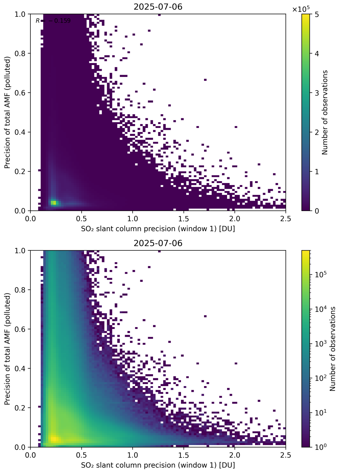
Figure 281: Scatter density plot of “SO 2 slant column precision (window 1)” against “Precision of total AMF (polluted)” for 2025-07-05 to 2025-07-07.
