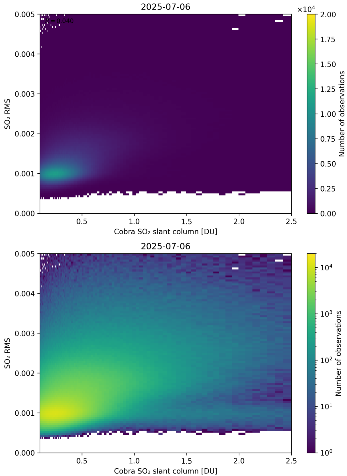
Figure 198: Scatter density plot of “Cobra SO 2 slant column” against “SO 2 RMS” for 2025-07-05 to 2025-07-07.
