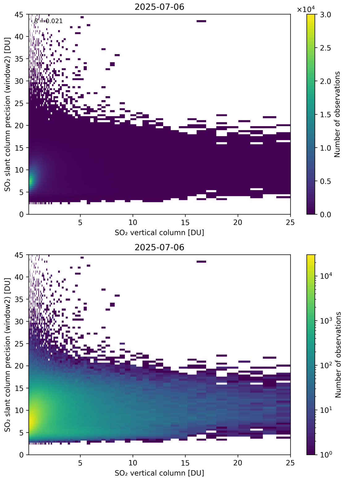
Figure 356: Scatter density plot of “SO 2 vertical column” against “SO 2 slant column precision (window2)” for 2025-07-05 to 2025-07-07.
