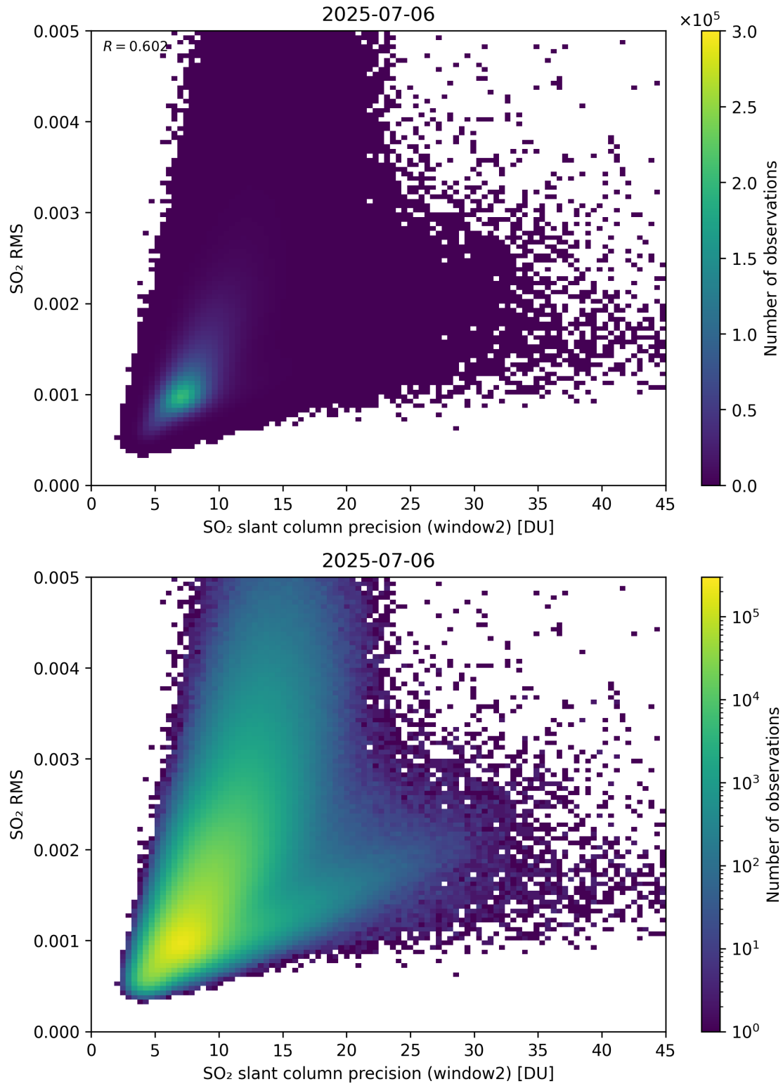
Figure 295: Scatter density plot of “SO 2 slant column precision (window2)” against “SO 2 RMS” for 2025-07-05 to 2025-07-07.
