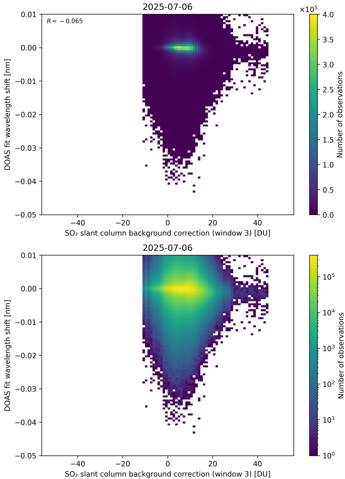
Figure 132: Scatter density plot of “SO 2 slant column background correction (window 3)” against “DOAS fit wavelength shift” for 2025-07-05 to 2025-07-07.
