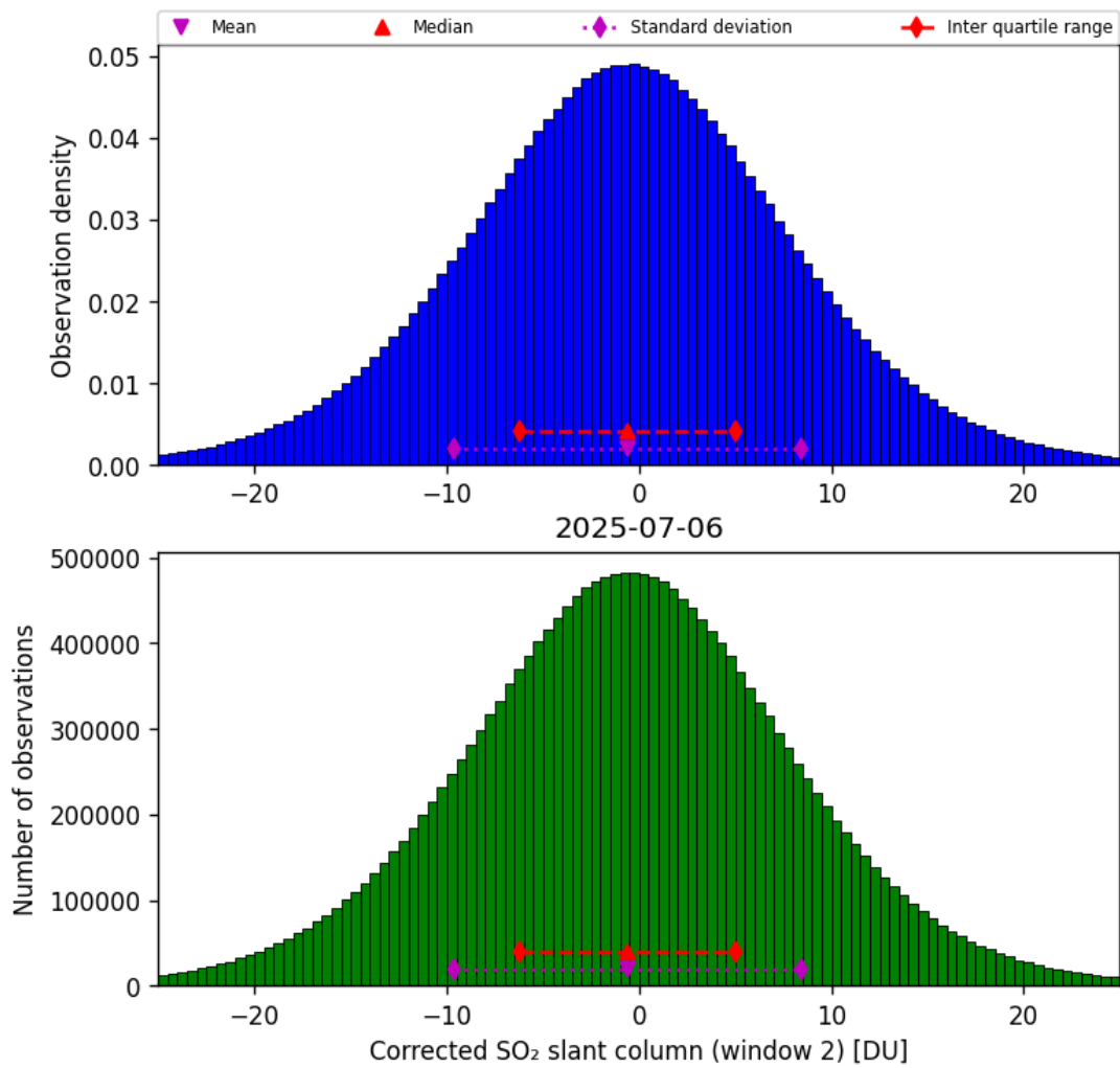
Figure 69: Histogram of “Corrected SO 2 slant column (window 2)” for 2025-07-05 to 2025-07-07
