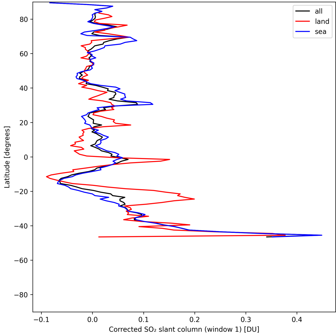
Figure 39: Zonal average of “Corrected SO 2 slant column (window 1)” for 2025-07-05 to 2025-07-07.
