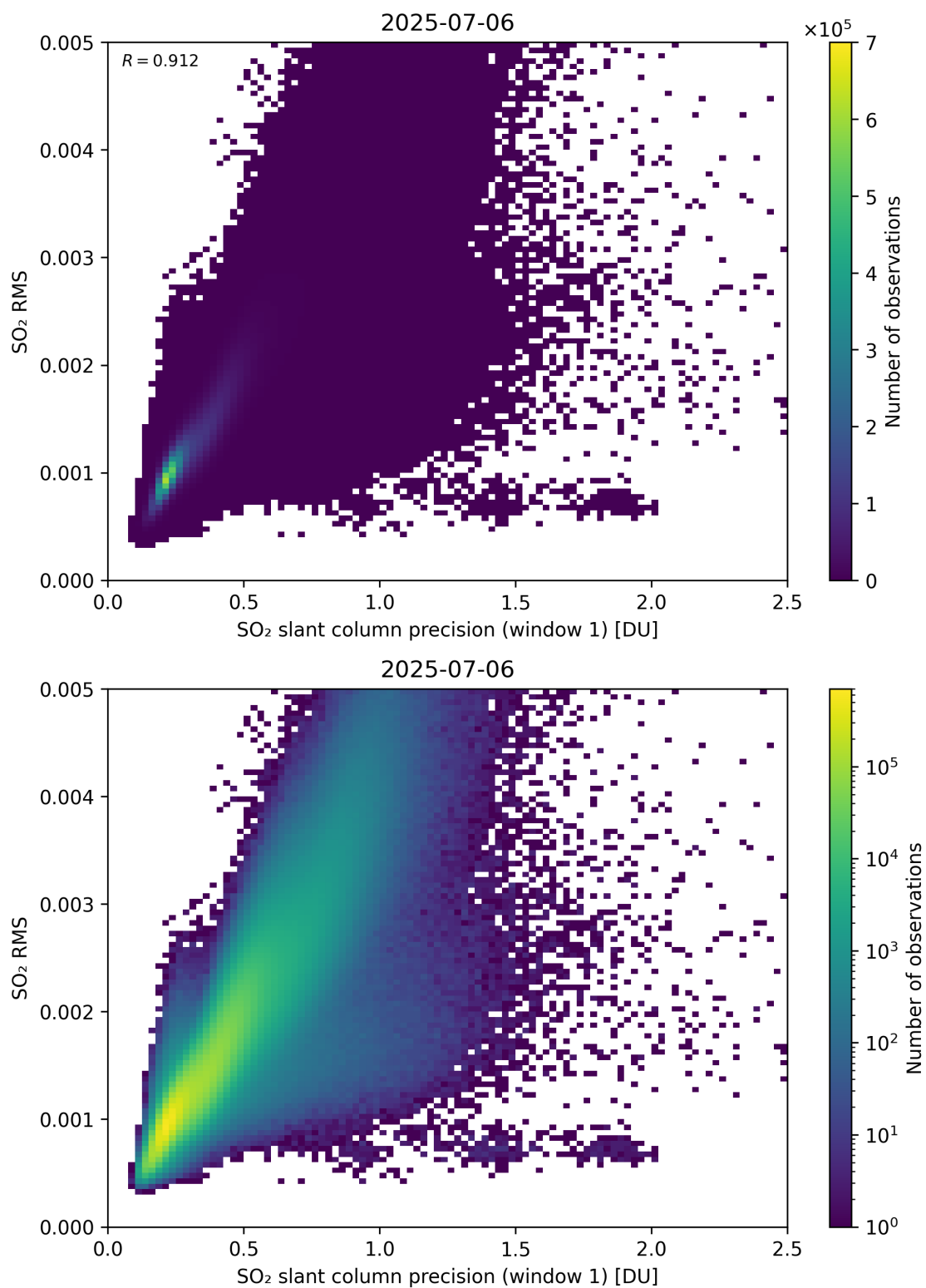
Figure 273: Scatter density plot of “SO 2 slant column precision (window 1)” against “SO 2 RMS” for 2025-07-05 to 2025-07-07.
