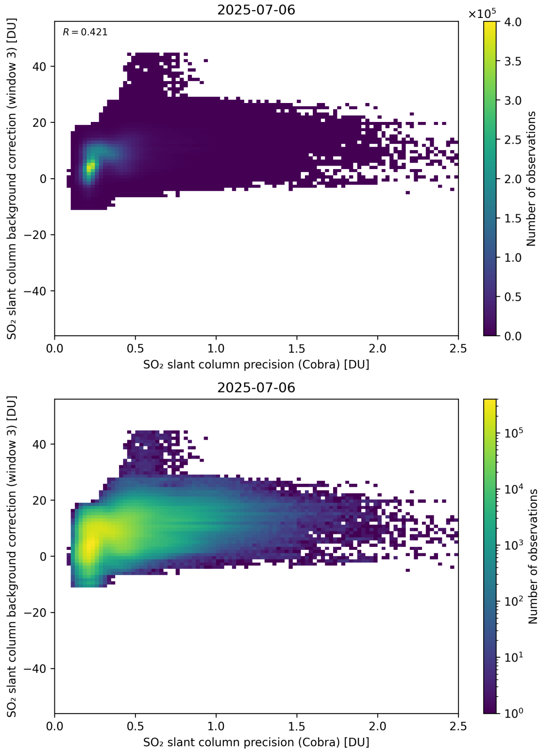
Figure 201: Scatter density plot of “SO 2 slant column precision (Cobra)” against “SO 2 slant column background correction (window 3)” for 2025-07-05 to 2025-07-07.
