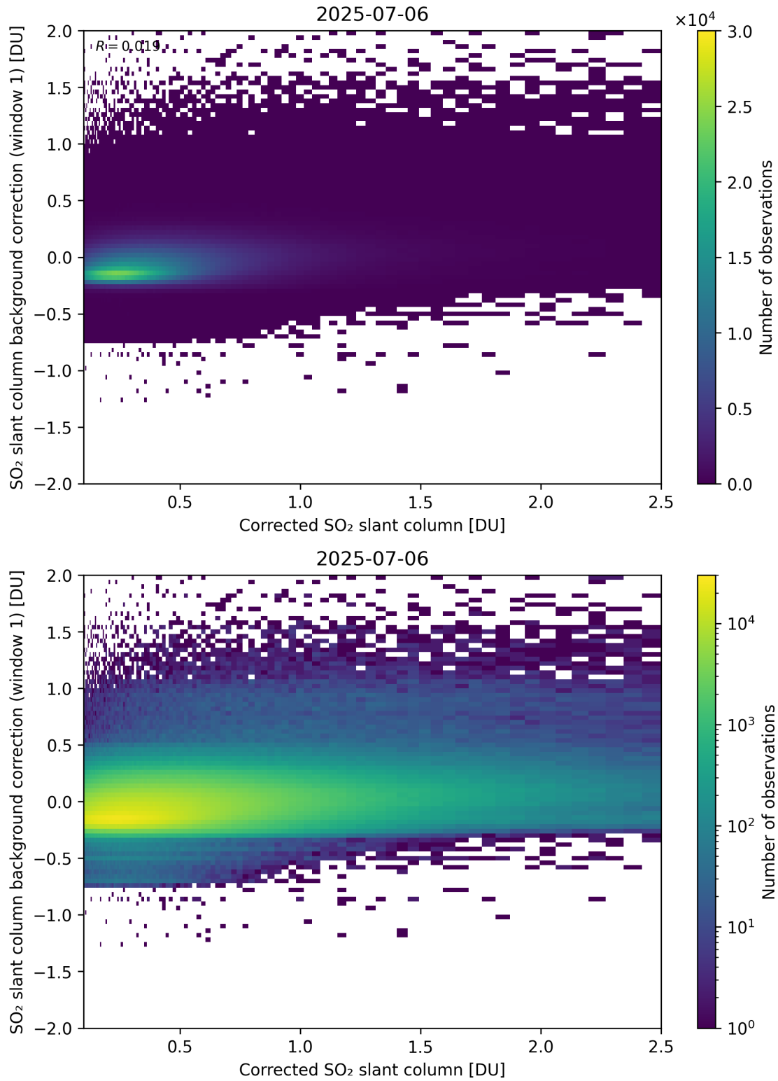
Figure 226: Scatter density plot of “Corrected SO 2 slant column” against “SO 2 slant column background correction (window 1)” for 2025-07-05 to 2025-07-07.
