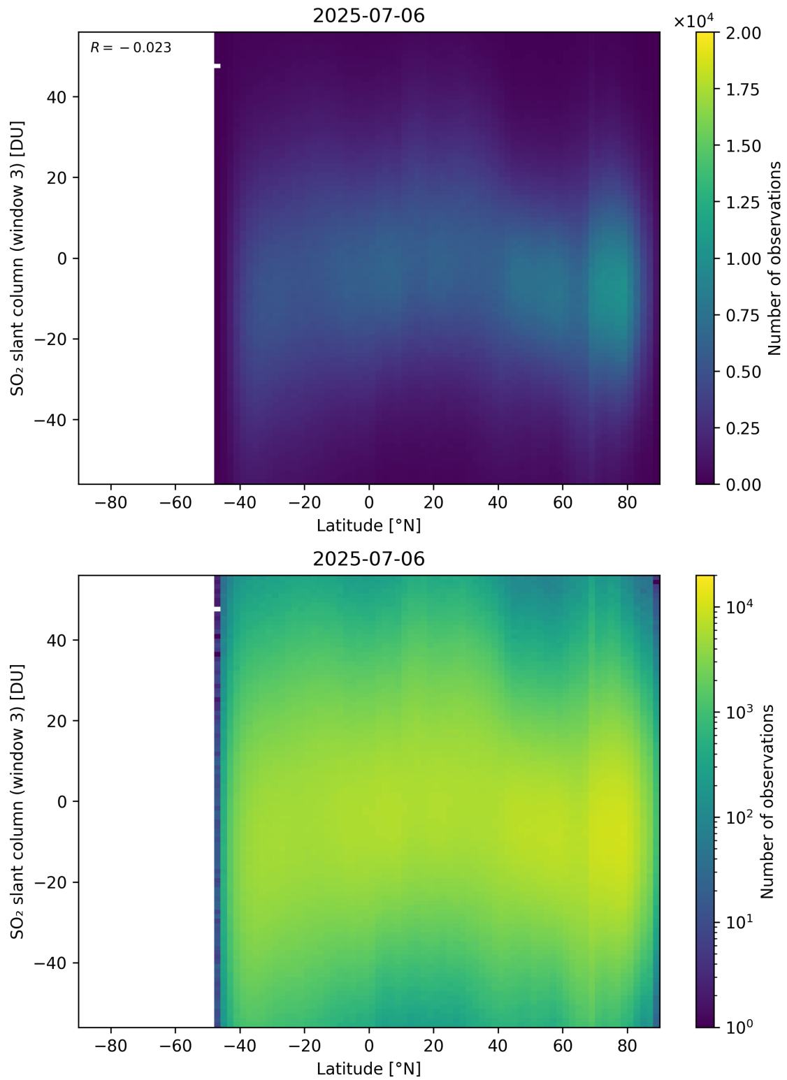
Figure 165: Scatter density plot of “Latitude” against “SO 2 slant column (window 3)” for 2025-07-05 to 2025-07-07.
