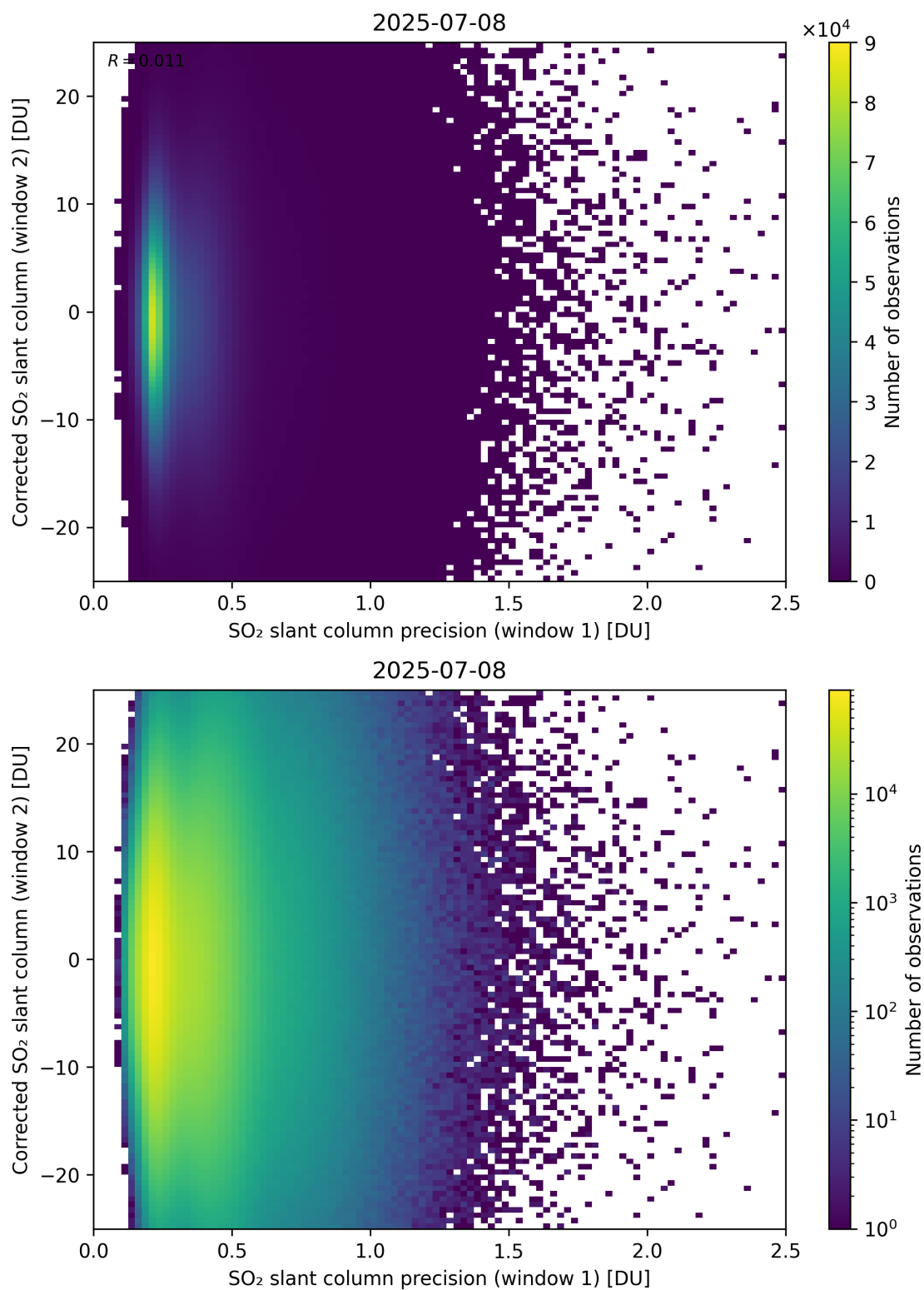
Figure 275: Scatter density plot of “SO 2 slant column precision (window 1)” against “Corrected SO 2 slant column (window 2)” for 2025-07-08 to 2025-07-09.
