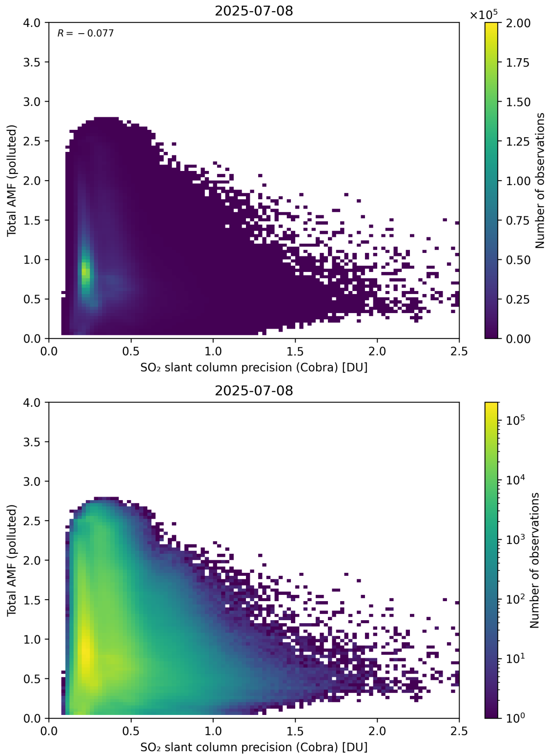
Figure 213: Scatter density plot of “SO 2 slant column precision (Cobra)” against “Total AMF (polluted)” for 2025-07-08 to 2025-07-09.
