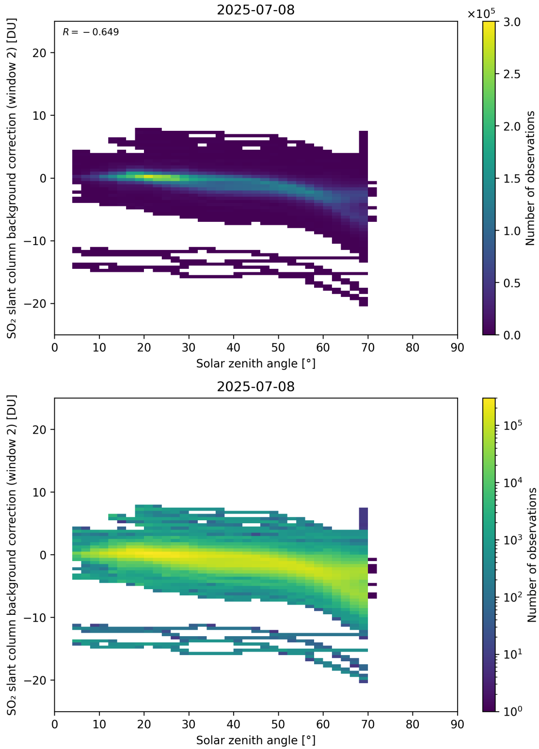
Figure 172: Scatter density plot of “Solar zenith angle” against “SO 2 slant column background correction (window 2)” for 2025-07-08 to 2025-07-09.
