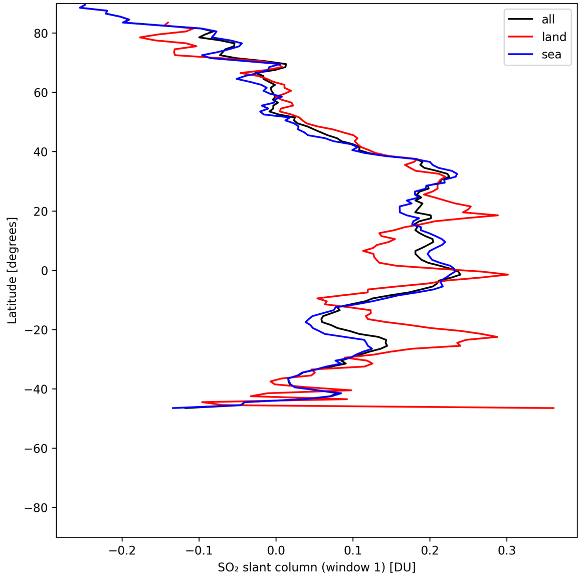
Figure 37: Zonal average of “SO 2 slant column (window 1)” for 2025-07-08 to 2025-07-09.
