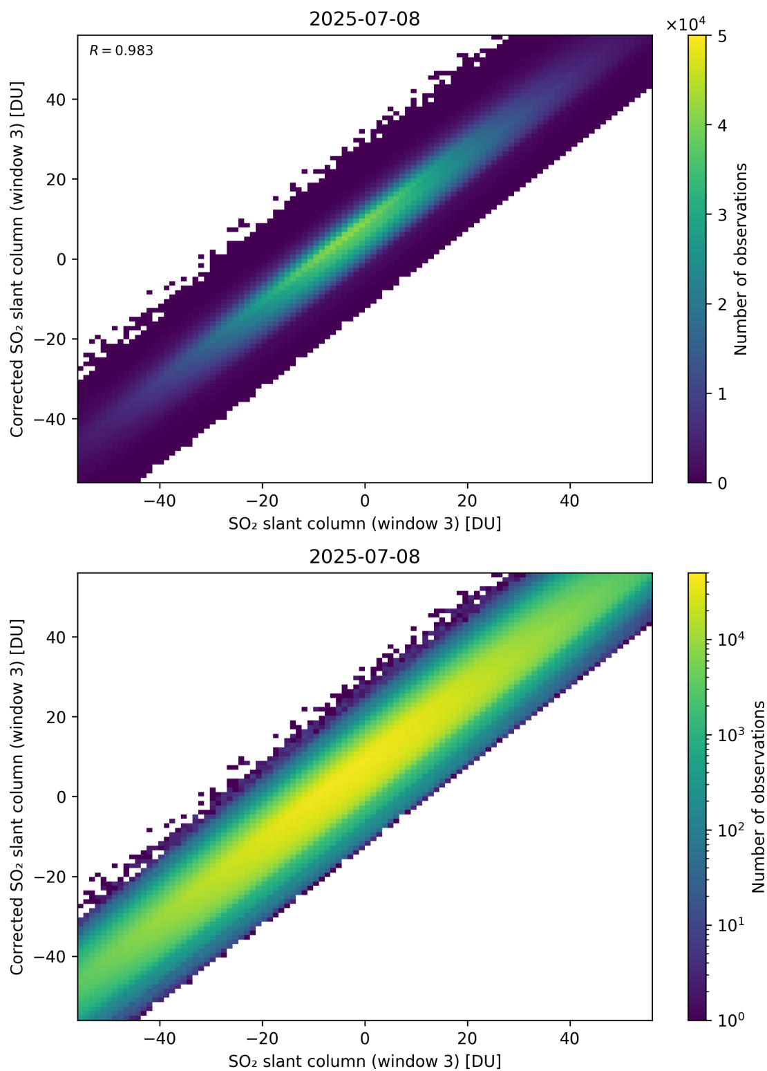
Figure 316: Scatter density plot of “SO 2 slant column (window 3)” against “Corrected SO 2 slant column (window 3)” for 2025-07-08 to 2025-07-09.
