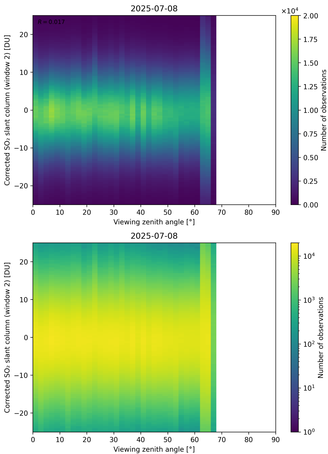
Figure 374: Scatter density plot of “Viewing zenith angle” against “Corrected SO 2 slant column (window 2)” for 2025-07-08 to 2025-07-09.
