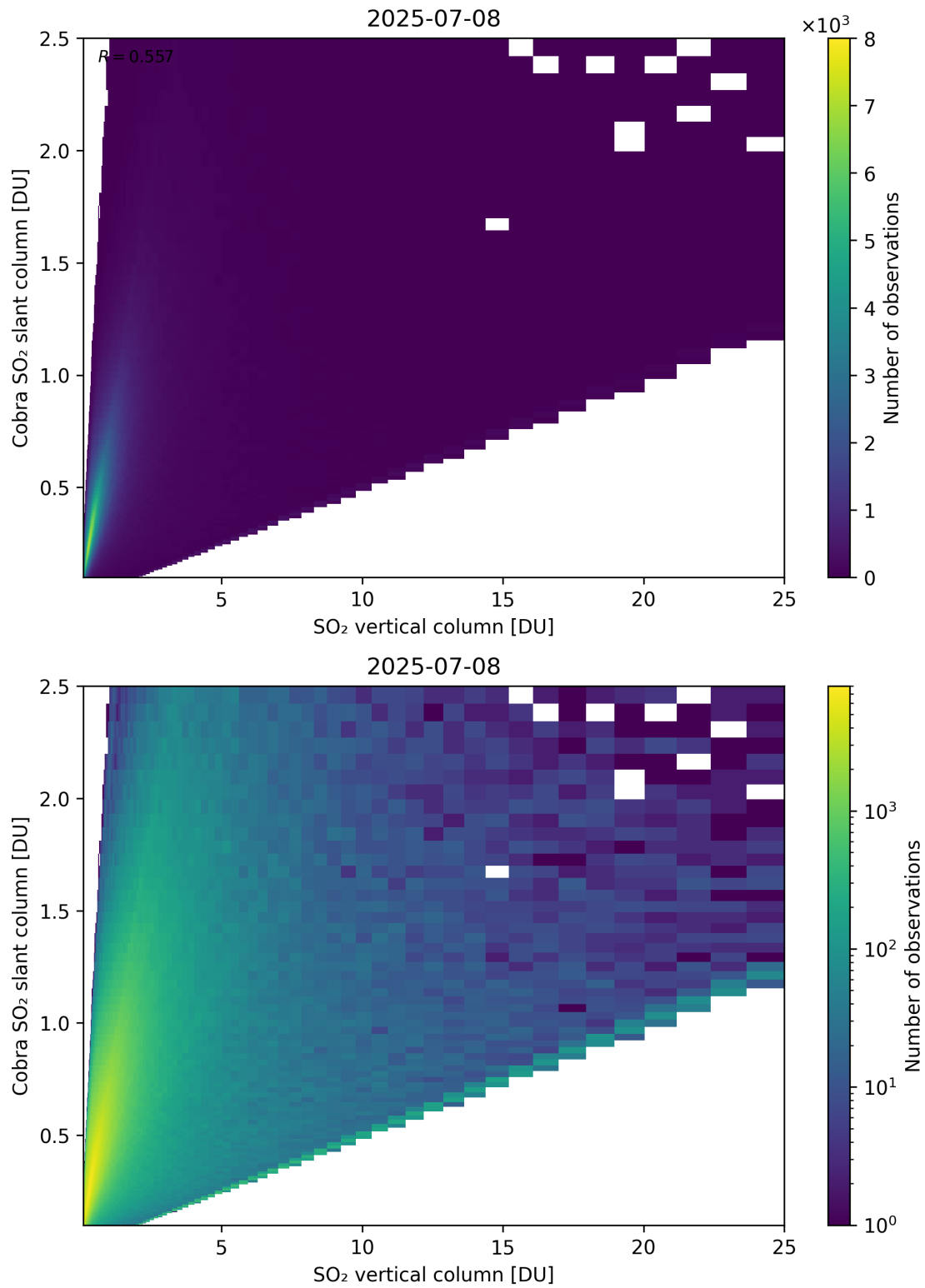
Figure 349: Scatter density plot of “SO 2 vertical column” against “Cobra SO 2 slant column” for 2025-07-08 to 2025-07-09.
