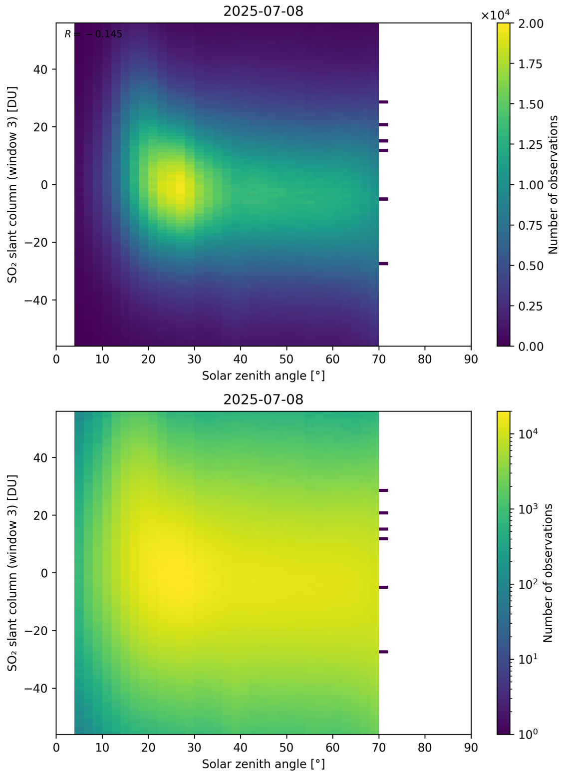
Figure 187: Scatter density plot of “Solar zenith angle” against “SO 2 slant column (window 3)” for 2025-07-08 to 2025-07-09.
