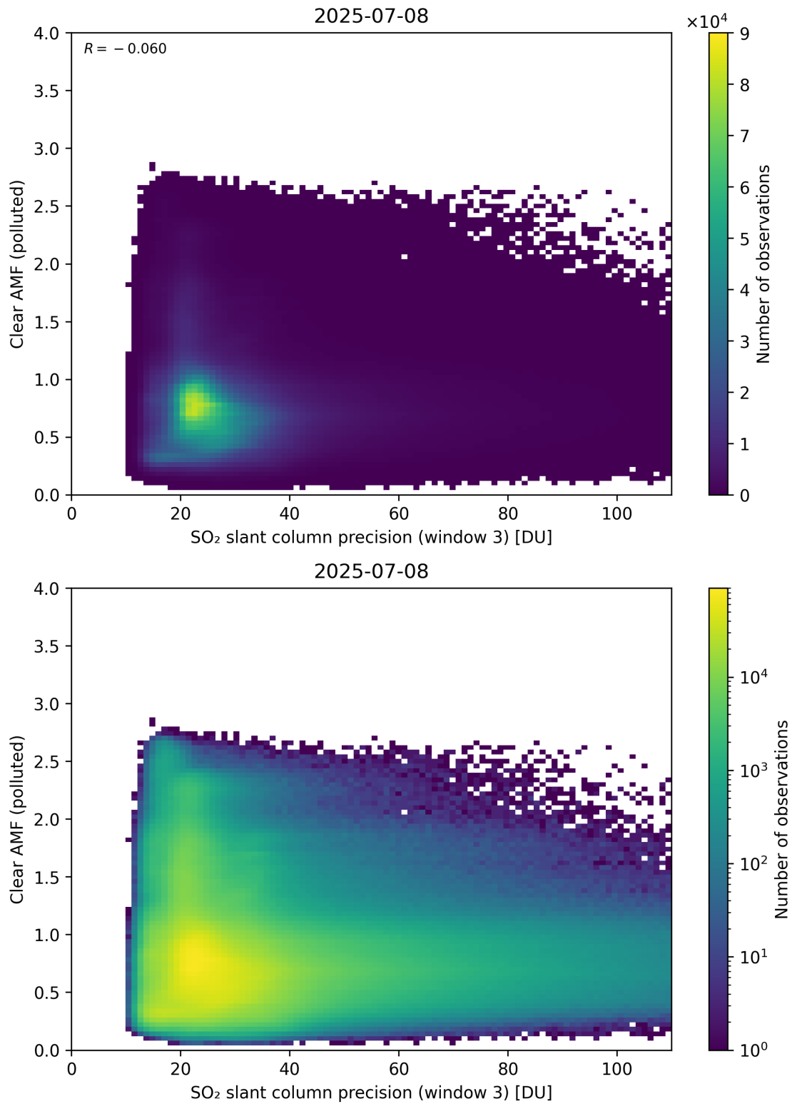
Figure 311: Scatter density plot of “SO 2 slant column precision (window 3)” against “Clear AMF (polluted)” for 2025-07-08 to 2025-07-09.
