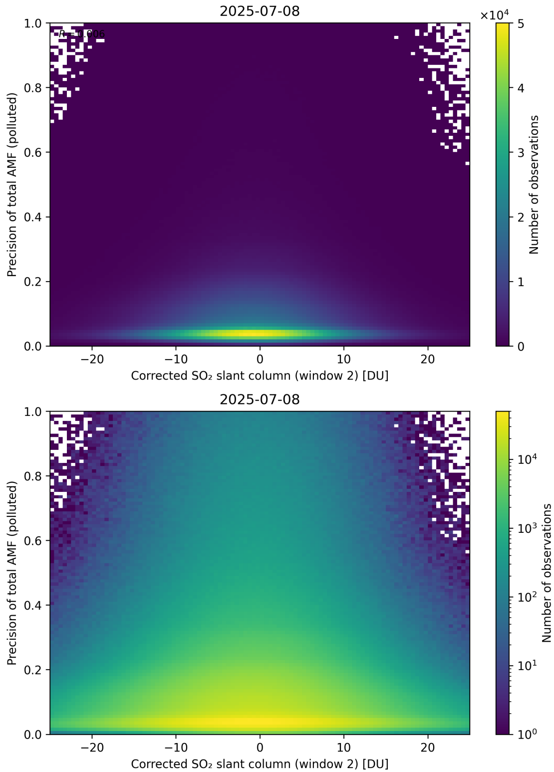
Figure 254: Scatter density plot of “Corrected SO 2 slant column (window 2)” against “Precision of total AMF (polluted)” for 2025-07-08 to 2025-07-09.
