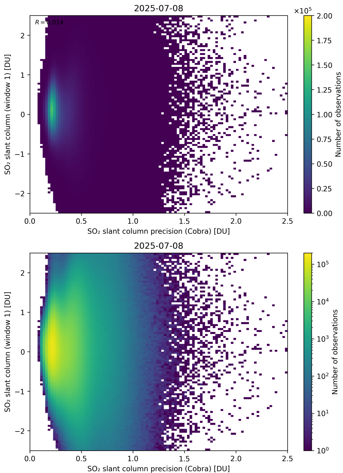
Figure 208: Scatter density plot of “SO 2 slant column precision (Cobra)” against “SO 2 slant column (window 1)” for 2025-07-08 to 2025-07-09.
