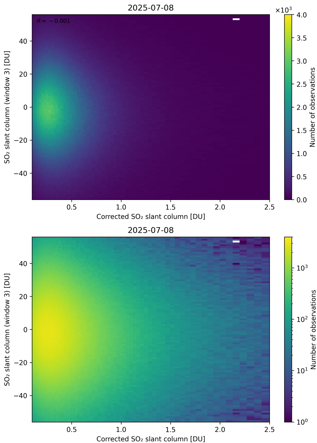
Figure 240: Scatter density plot of “Corrected SO 2 slant column” against “SO 2 slant column (window 3)” for 2025-07-08 to 2025-07-09.
