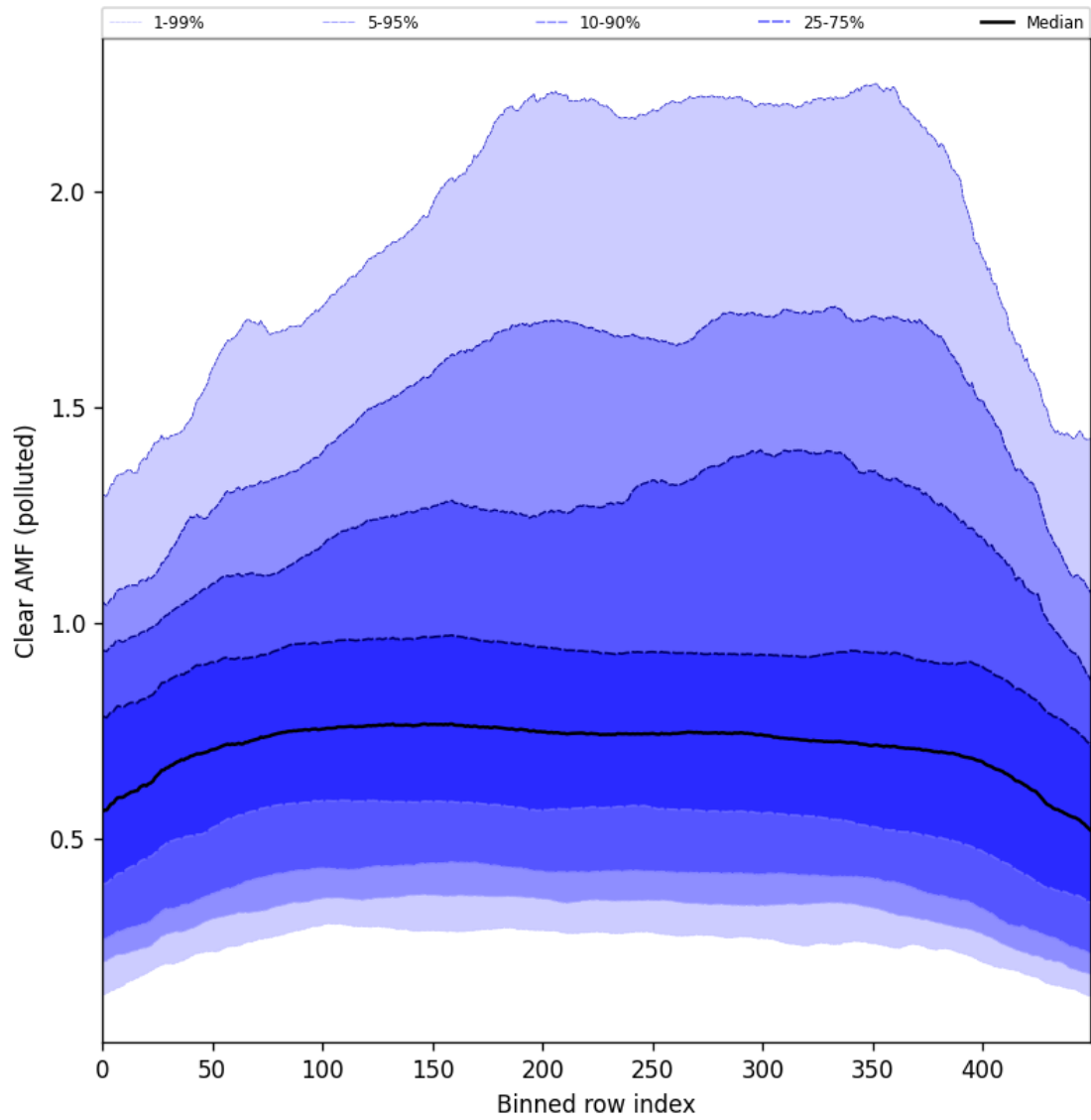
Figure 107: Along track statistics of “Clear AMF (polluted)” for 2025-07-08 to 2025-07-09
