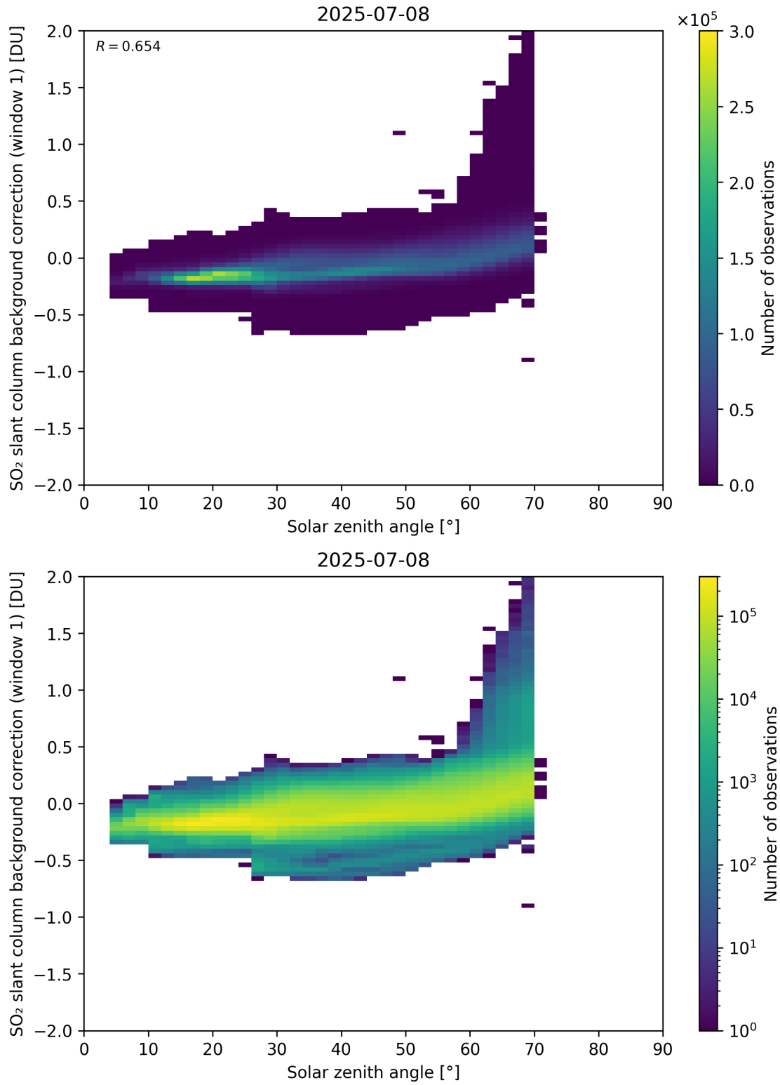
Figure 171: Scatter density plot of “Solar zenith angle” against “SO 2 slant column background correction (window 1)” for 2025-07-08 to 2025-07-09.
