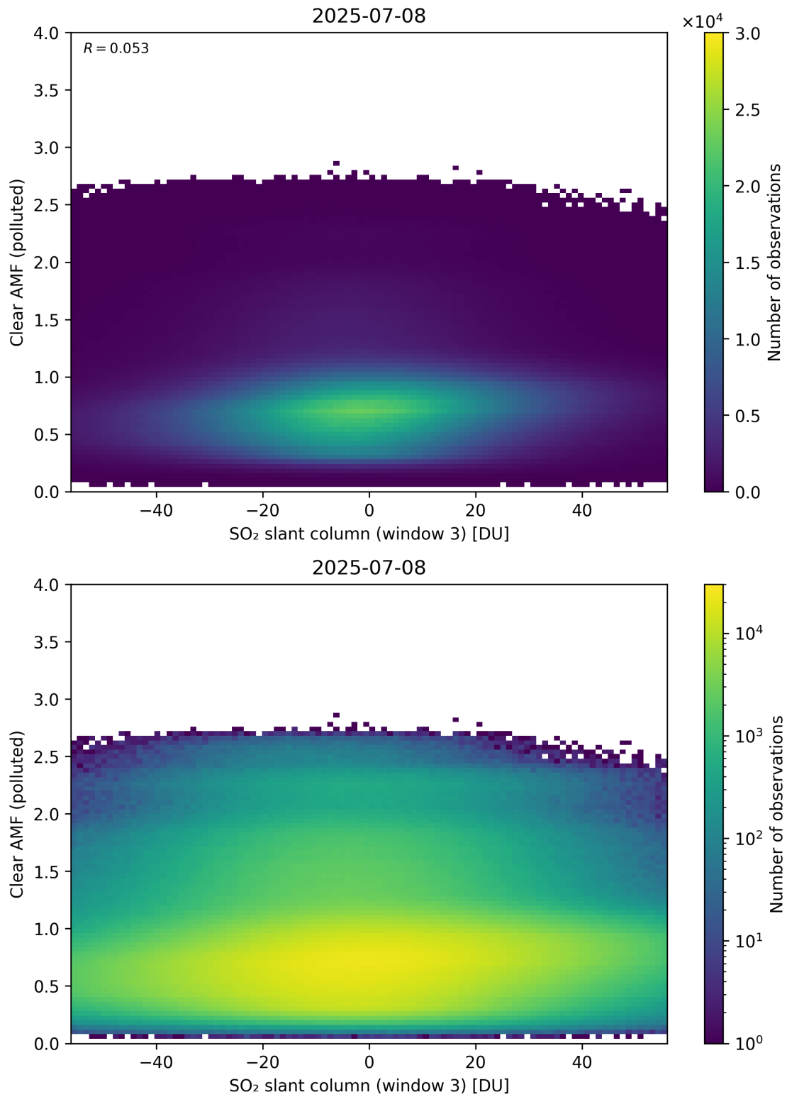
Figure 315: Scatter density plot of “SO 2 slant column (window 3)” against “Clear AMF (polluted)” for 2025-07-08 to 2025-07-09.
