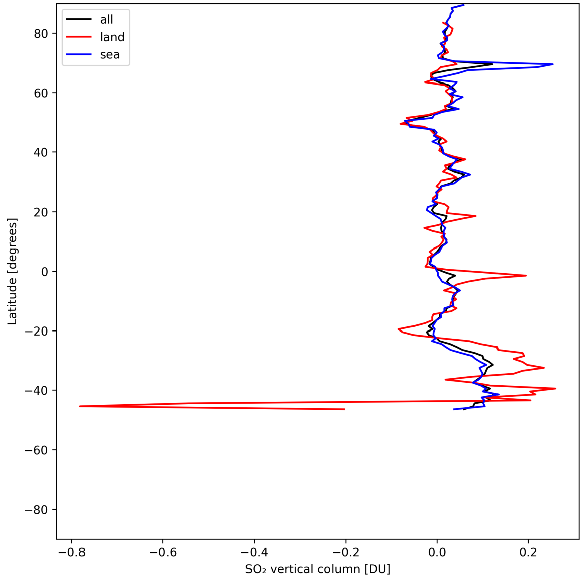
Figure 32: Zonal average of “SO 2 vertical column” for 2025-07-08 to 2025-07-09.
