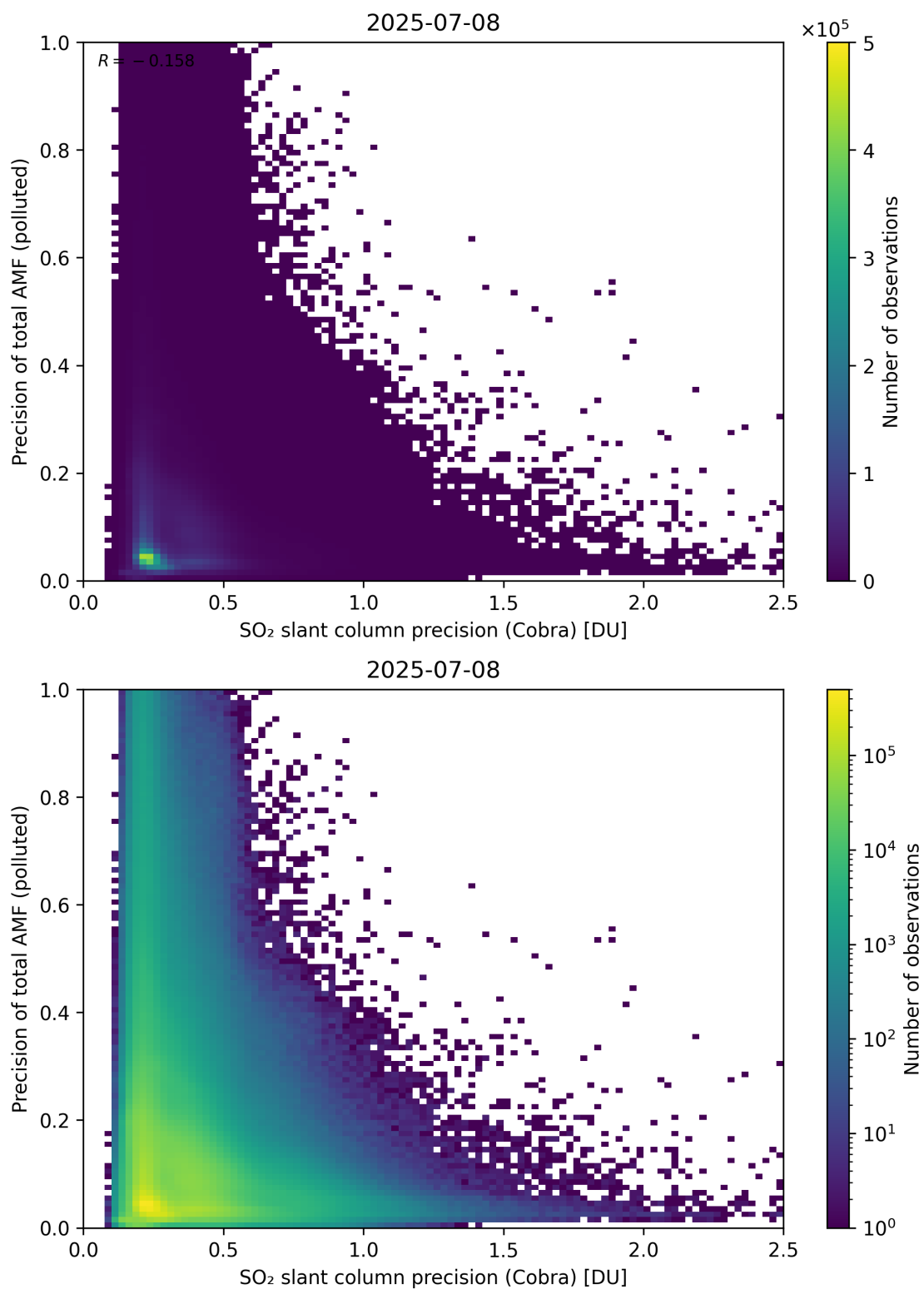
Figure 214: Scatter density plot of “SO 2 slant column precision (Cobra)” against “Precision of total AMF (polluted)” for 2025-07-08 to 2025-07-09.
