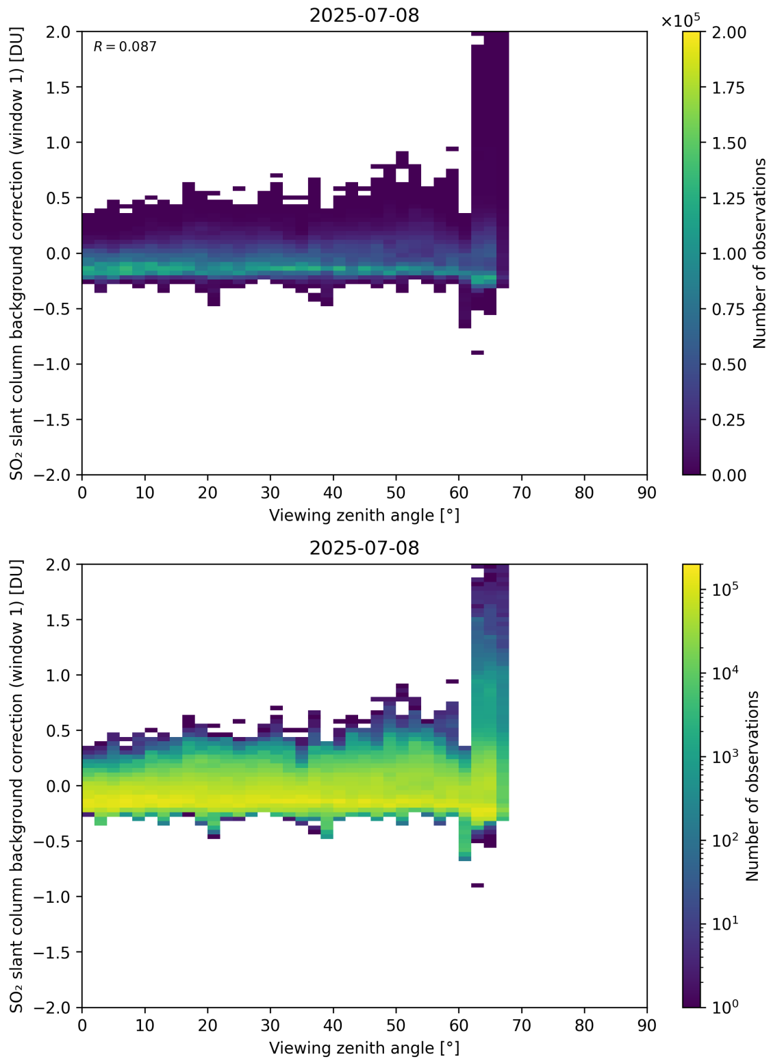
Figure 362: Scatter density plot of “Viewing zenith angle” against “SO 2 slant column background correction (window 1)” for 2025-07-08 to 2025-07-09.
