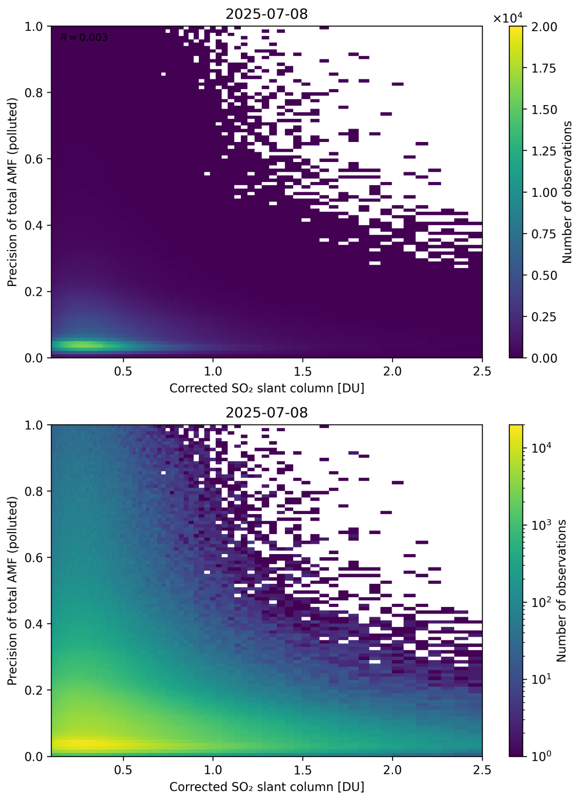
Figure 243: Scatter density plot of “Corrected SO 2 slant column” against “Precision of total AMF (polluted)” for 2025-07-08 to 2025-07-09.
