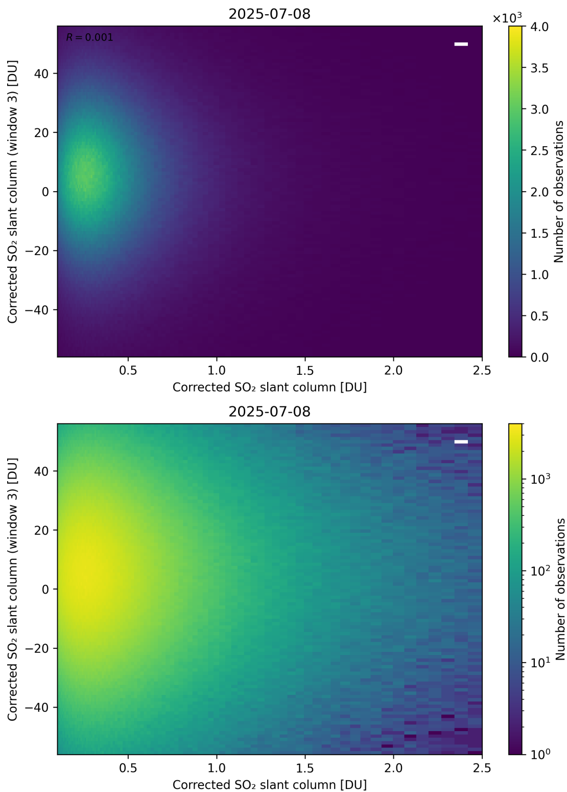
Figure 236: Scatter density plot of “Corrected SO 2 slant column” against “Corrected SO 2 slant column (window 3)” for 2025-07-08 to 2025-07-09.
