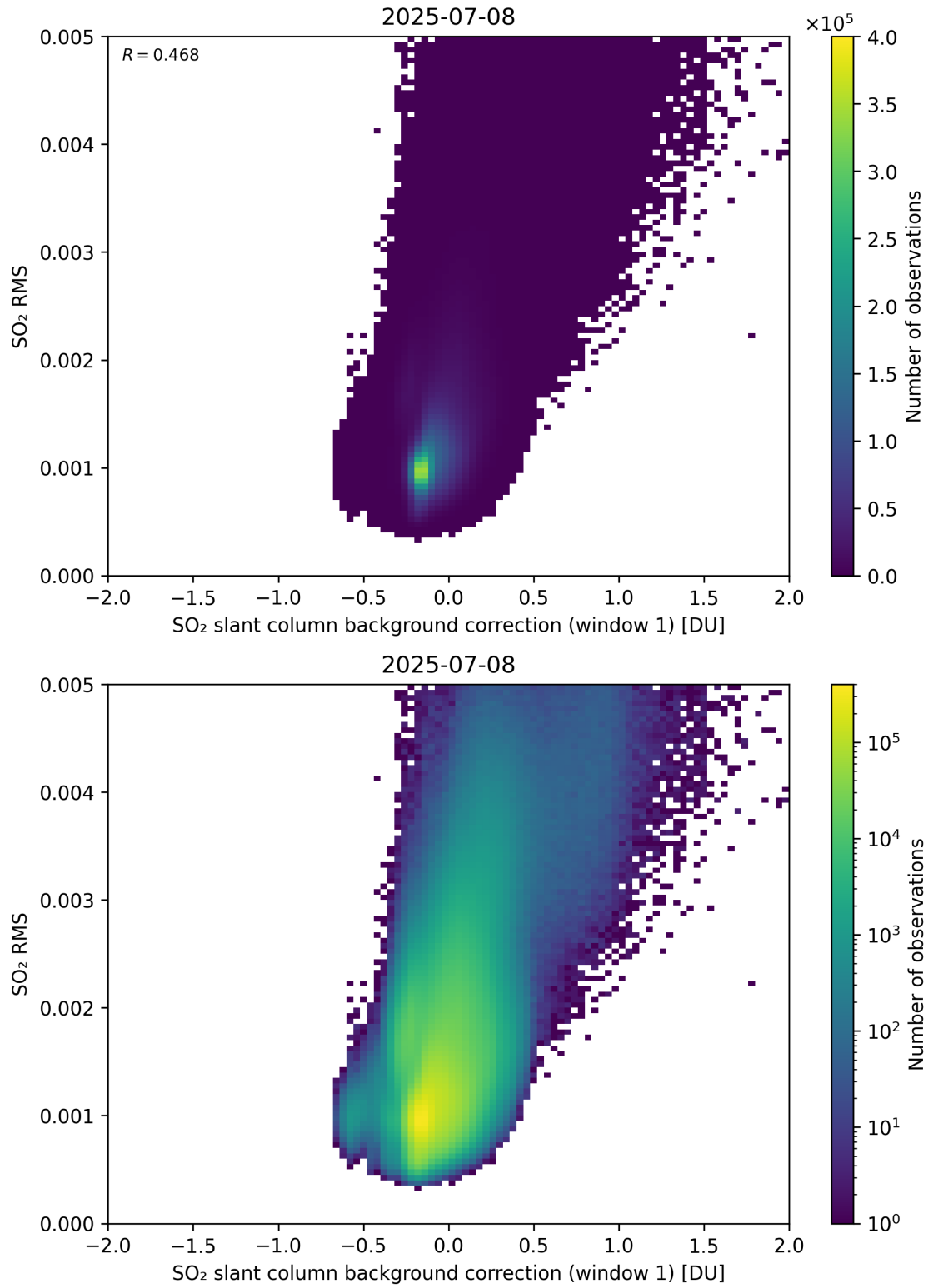
Figure 113: Scatter density plot of “SO 2 slant column background correction (window 1)” against “SO 2 RMS” for 2025-07-08 to 2025-07-09.
