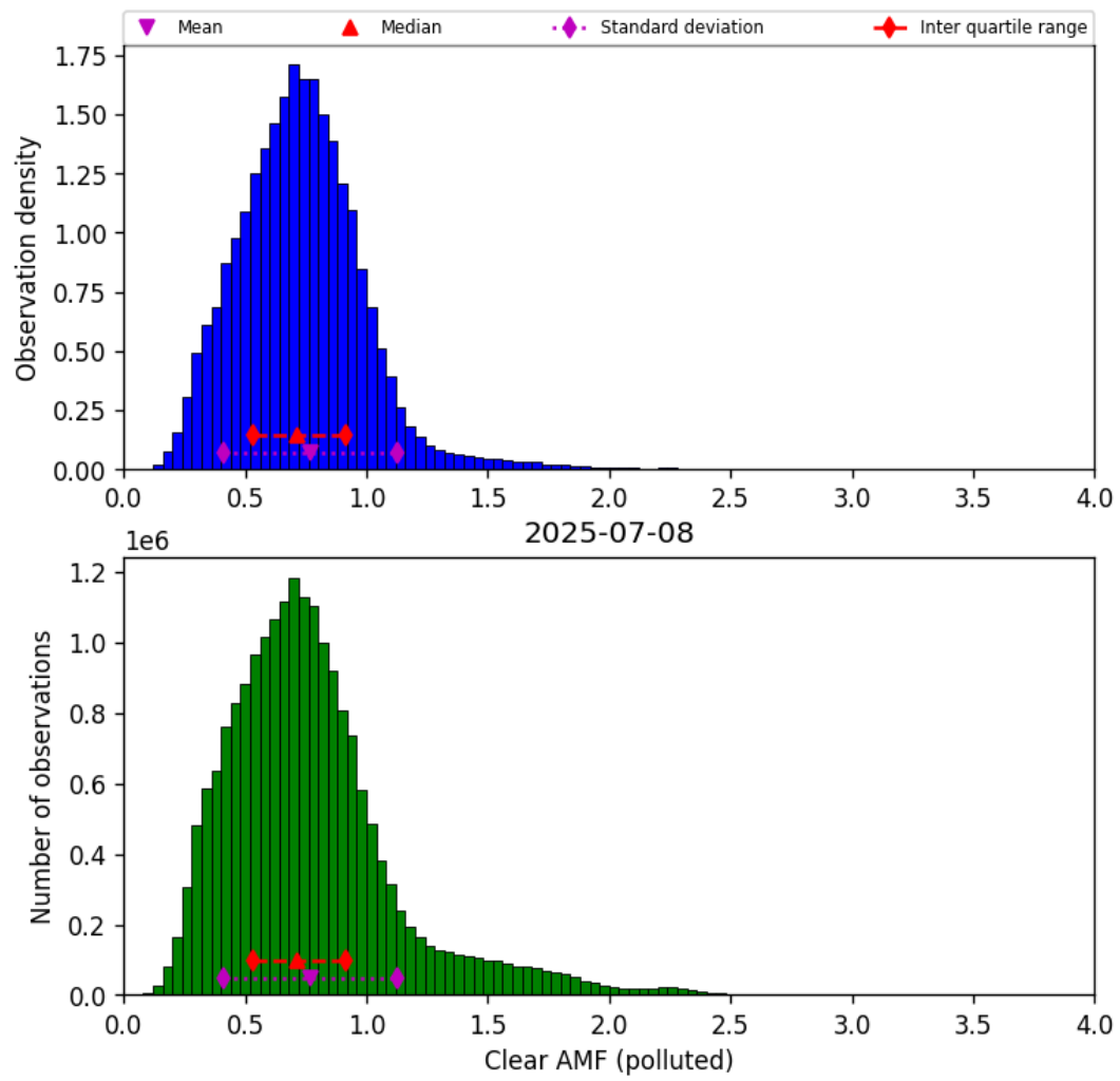
Figure 81: Histogram of “Clear AMF (polluted)” for 2025-07-08 to 2025-07-09
