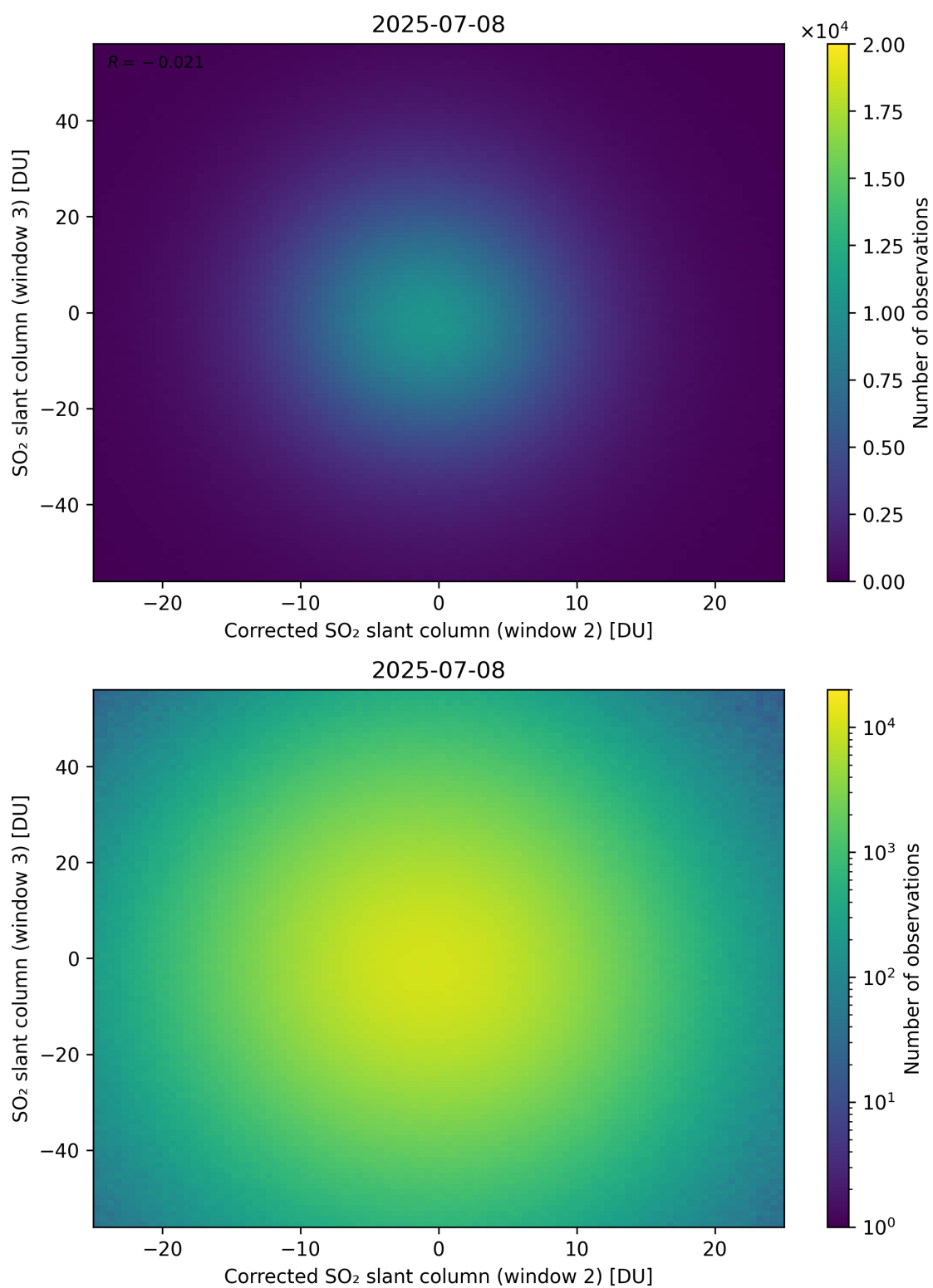
Figure 251: Scatter density plot of “Corrected SO 2 slant column (window 2)” against “SO 2 slant column (window 3)” for 2025-07-08 to 2025-07-09.
