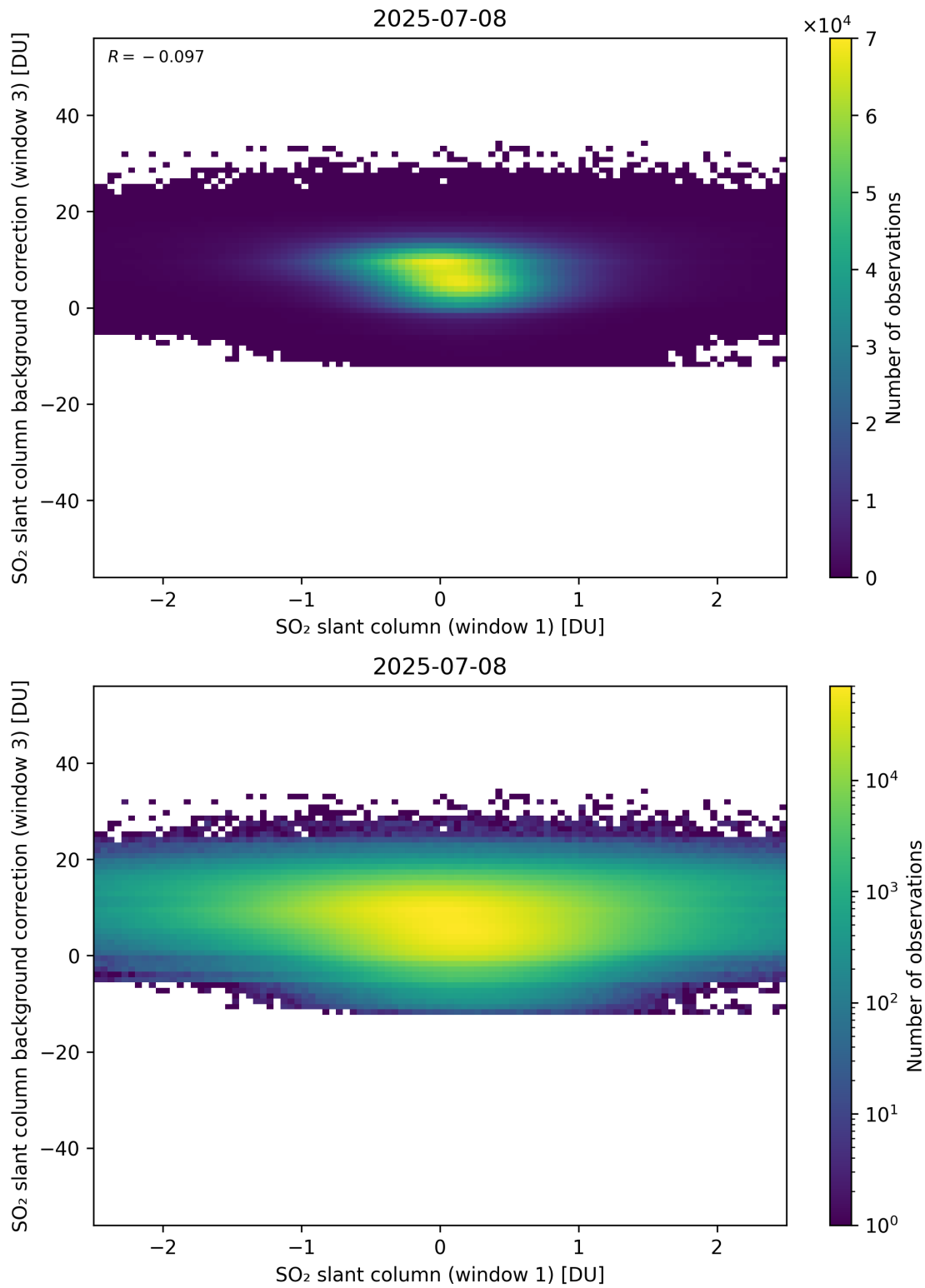
Figure 264: Scatter density plot of “SO 2 slant column (window 1)” against “SO 2 slant column background correction (window 3)” for 2025-07-08 to 2025-07-09.
