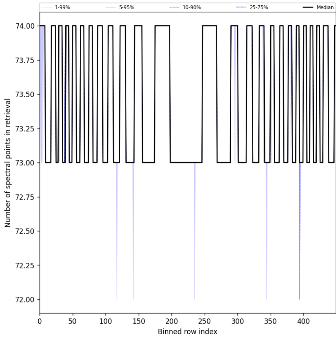
Figure 108: Along track statistics of “Number of spectral points in retrieval” for 2025-07-08 to 2025-07-09
