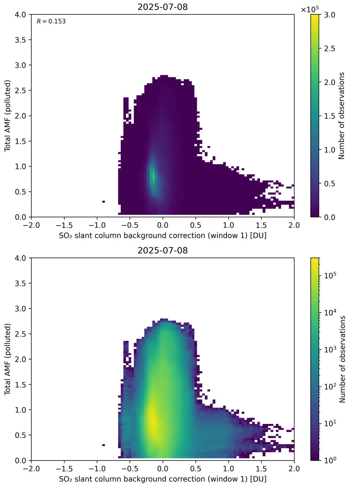
Figure 120: Scatter density plot of “SO 2 slant column background correction (window 1)” against “Total AMF (polluted)” for 2025-07-08 to 2025-07-09.
