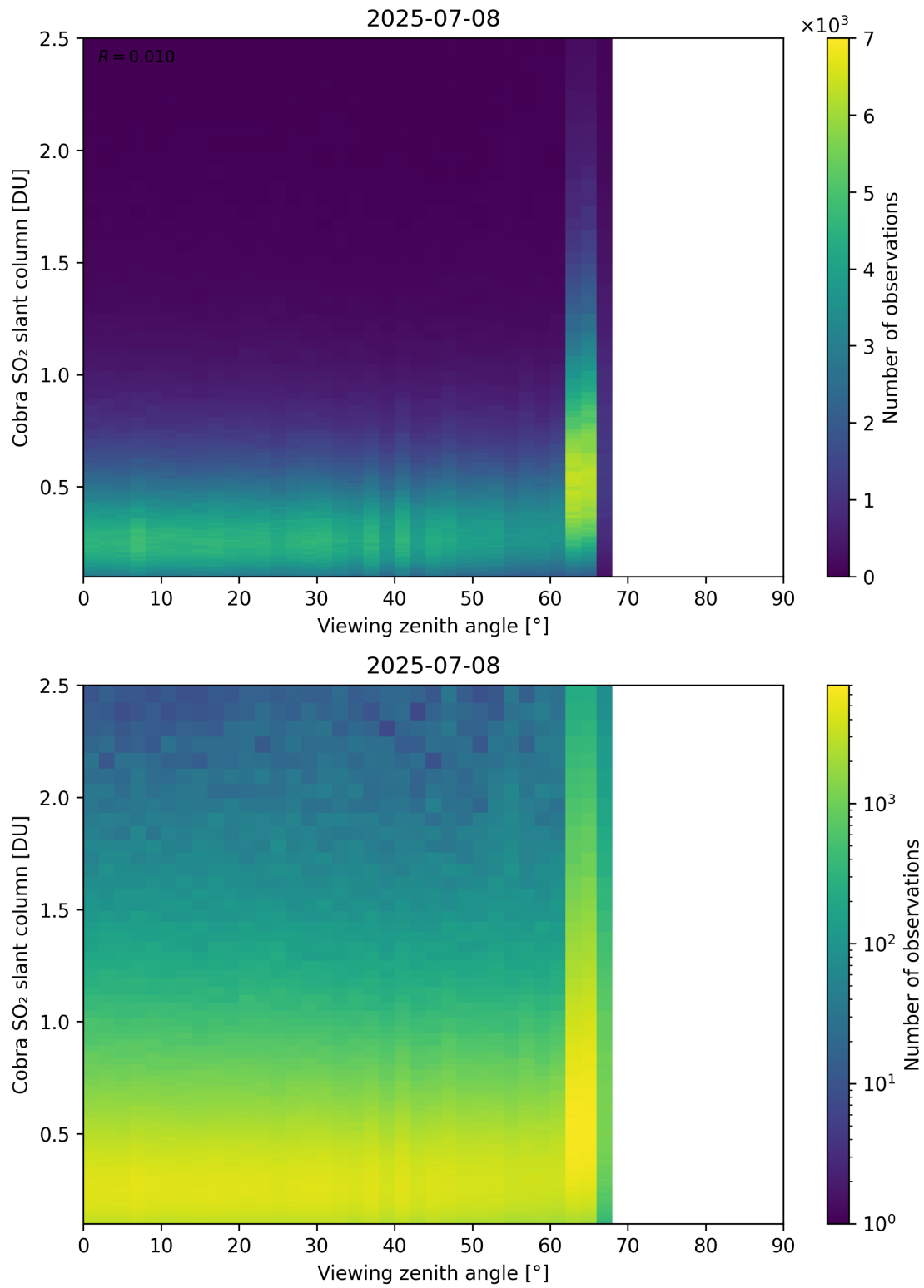
Figure 371: Scatter density plot of “Viewing zenith angle” against “Cobra SO 2 slant column” for 2025-07-08 to 2025-07-09.
