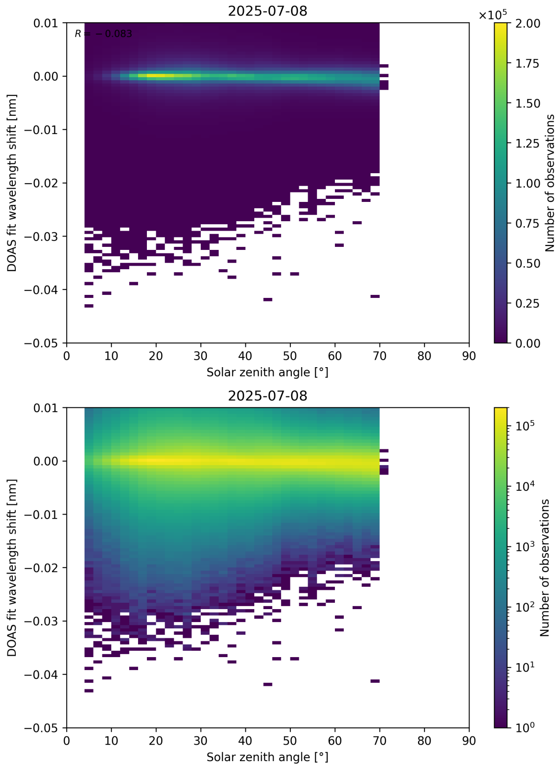
Figure 174: Scatter density plot of “Solar zenith angle” against “DOAS fit wavelength shift” for 2025-07-08 to 2025-07-09.
