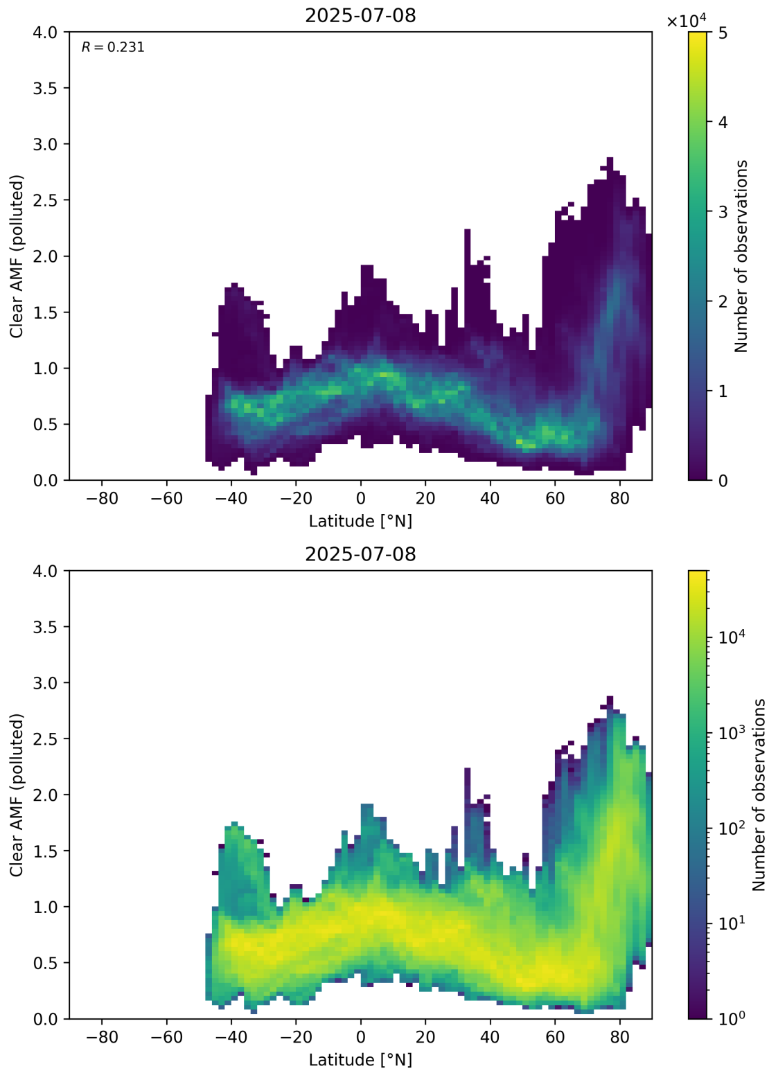
Figure 156: Scatter density plot of “Latitude” against “Clear AMF (polluted)” for 2025-07-08 to 2025-07-09.
