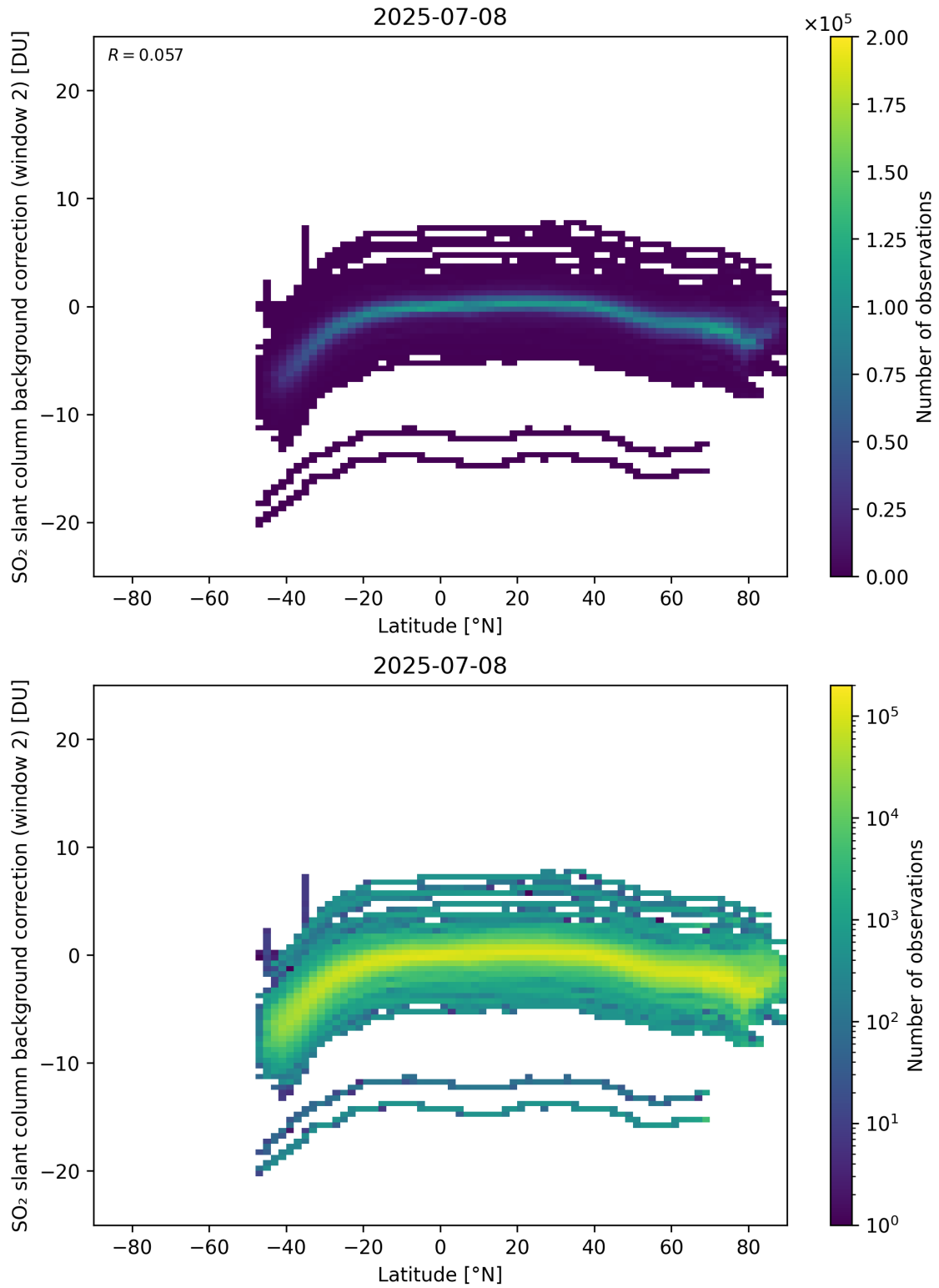
Figure 151: Scatter density plot of “Latitude” against “SO 2 slant column background correction (window 2)” for 2025-07-08 to 2025-07-09.
