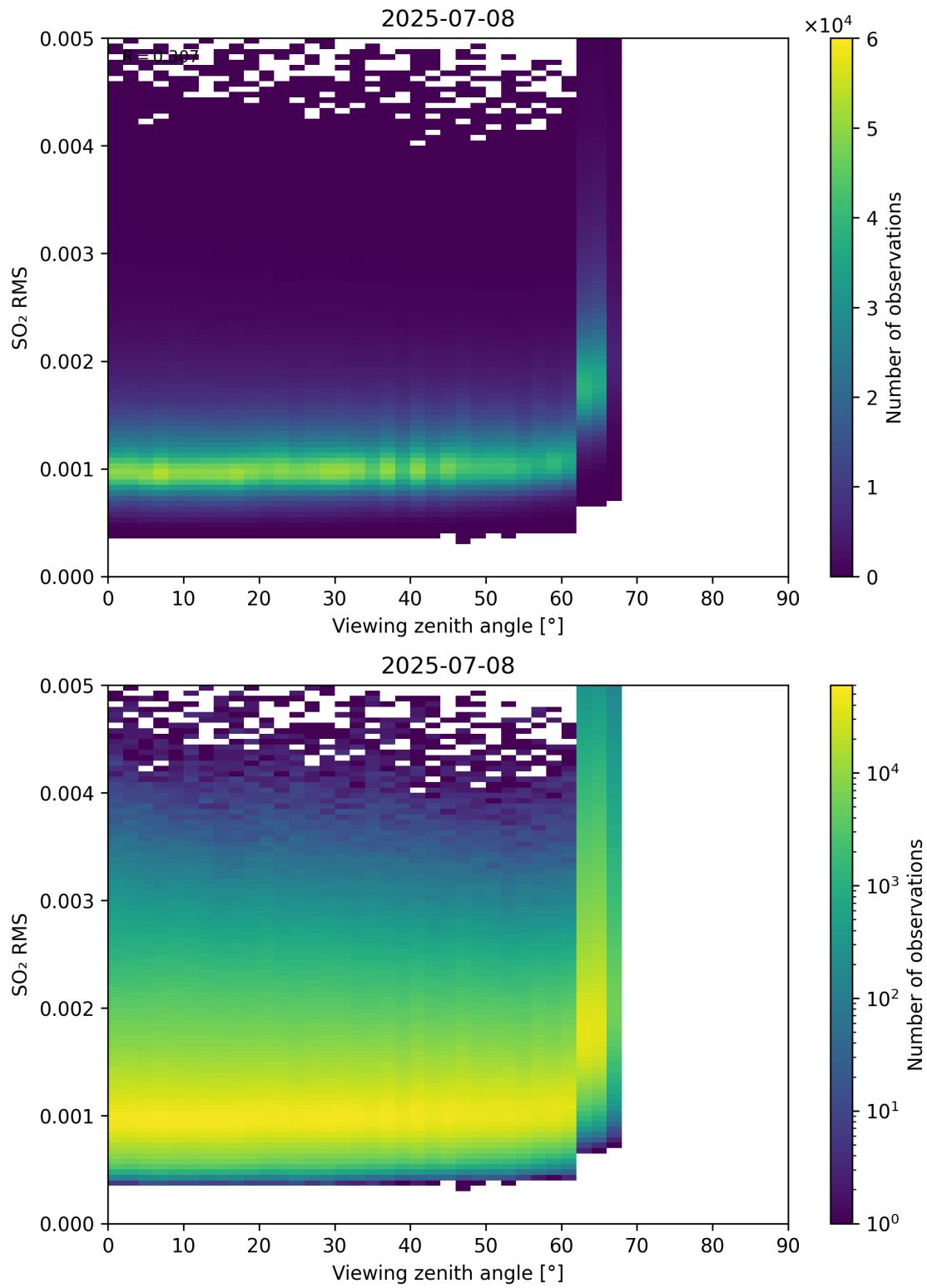
Figure 367: Scatter density plot of “Viewing zenith angle” against “SO 2 RMS” for 2025-07-08 to 2025-07-09.
