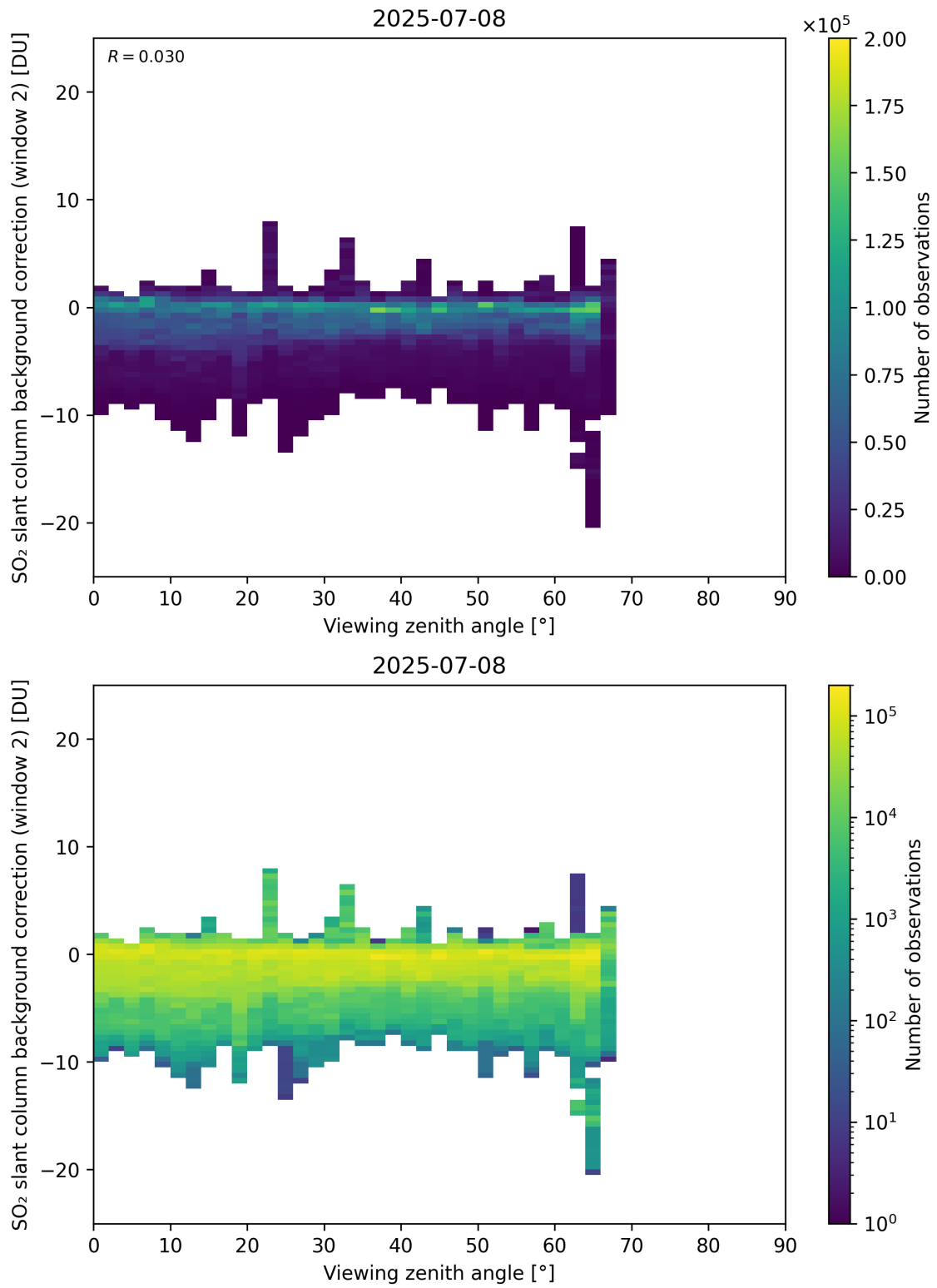
Figure 363: Scatter density plot of “Viewing zenith angle” against “SO 2 slant column background correction (window 2)” for 2025-07-08 to 2025-07-09.
