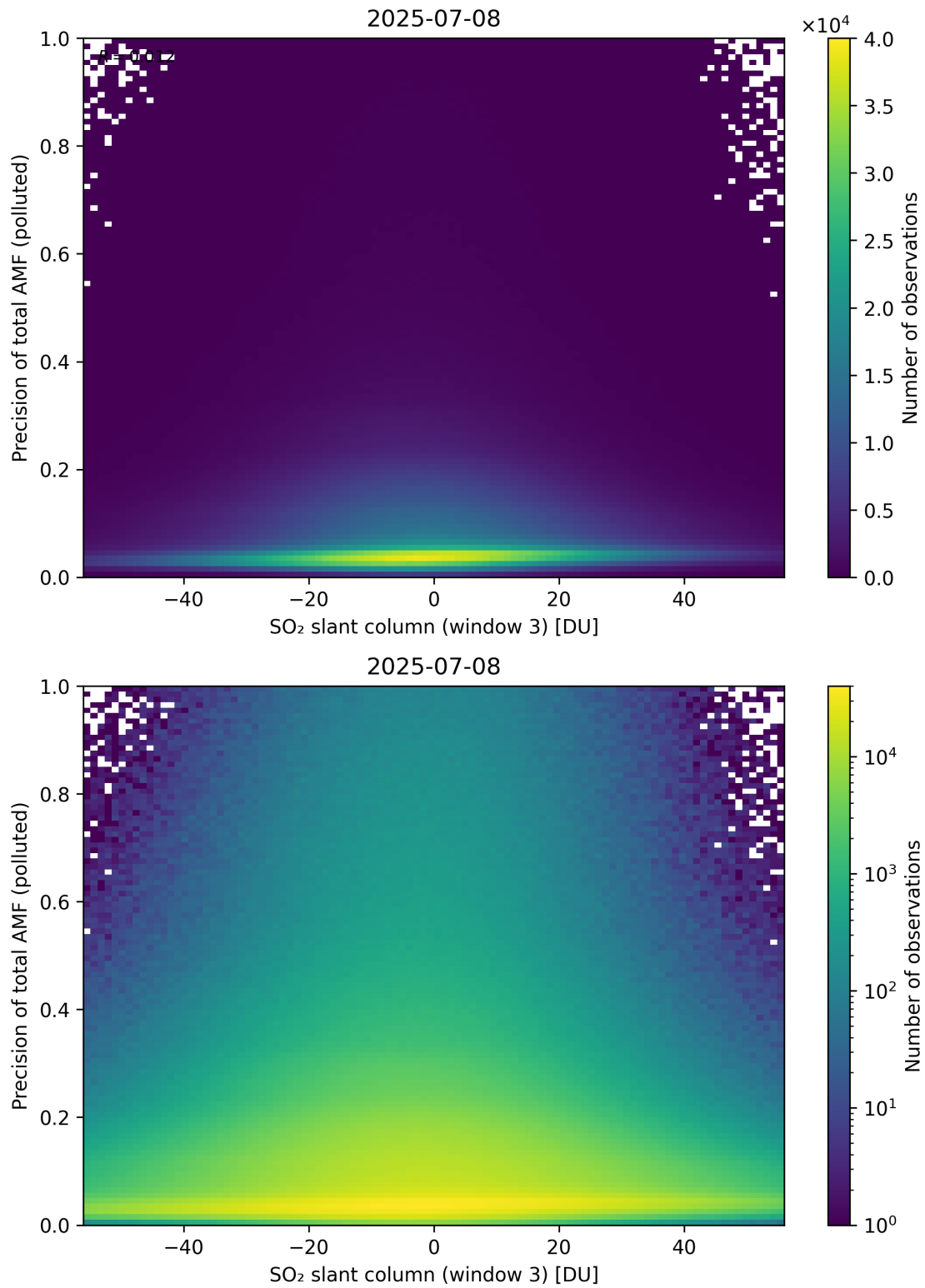
Figure 319: Scatter density plot of “SO 2 slant column (window 3)” against “Precision of total AMF (polluted)” for 2025-07-08 to 2025-07-09.
