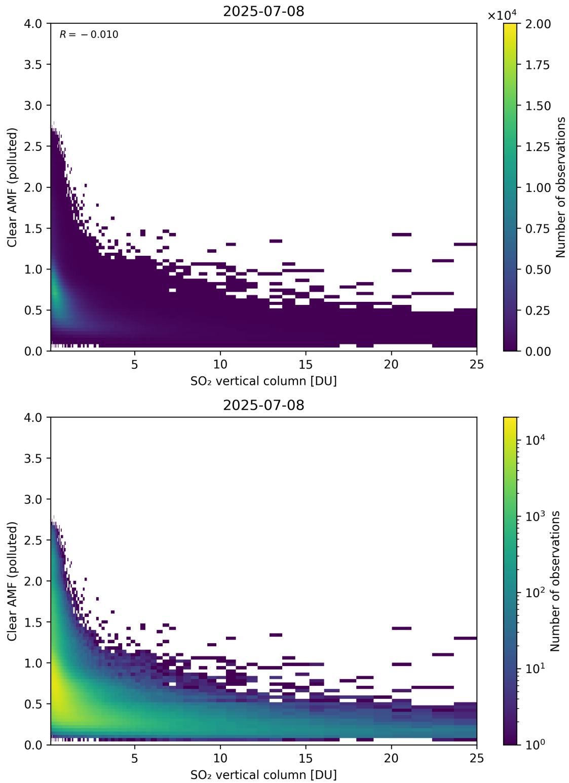
Figure 348: Scatter density plot of “SO 2 vertical column” against “Clear AMF (polluted)” for 2025-07-08 to 2025-07-09.
