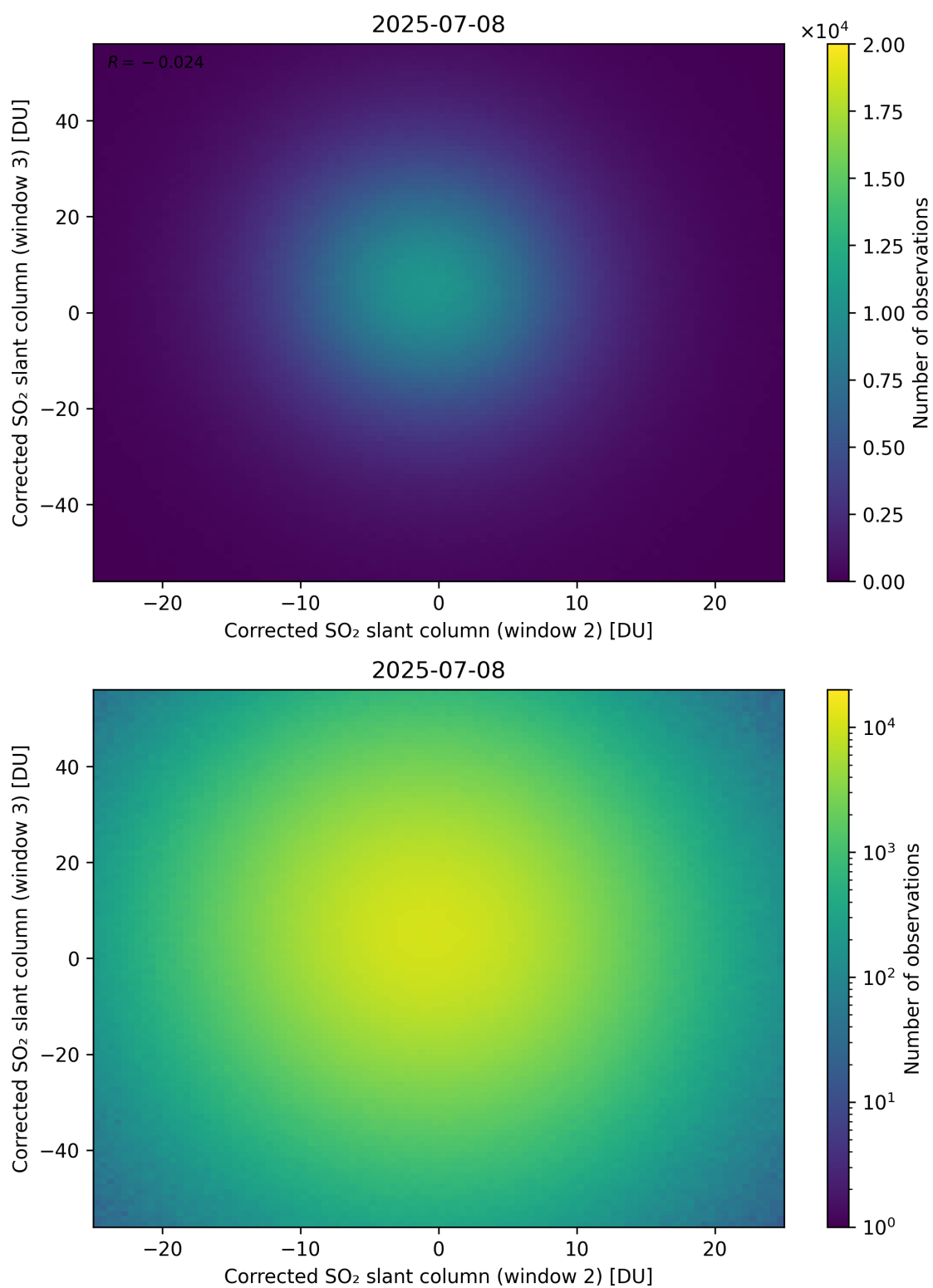
Figure 250: Scatter density plot of “Corrected SO 2 slant column (window 2)” against “Corrected SO 2 slant column (window 3)” for 2025-07-08 to 2025-07-09.
