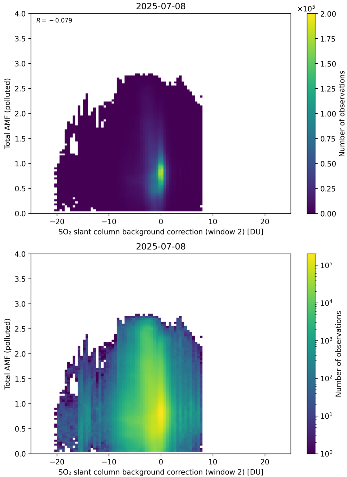
Figure 130: Scatter density plot of “SO 2 slant column background correction (window 2)” against “Total AMF (polluted)” for 2025-07-08 to 2025-07-09.
