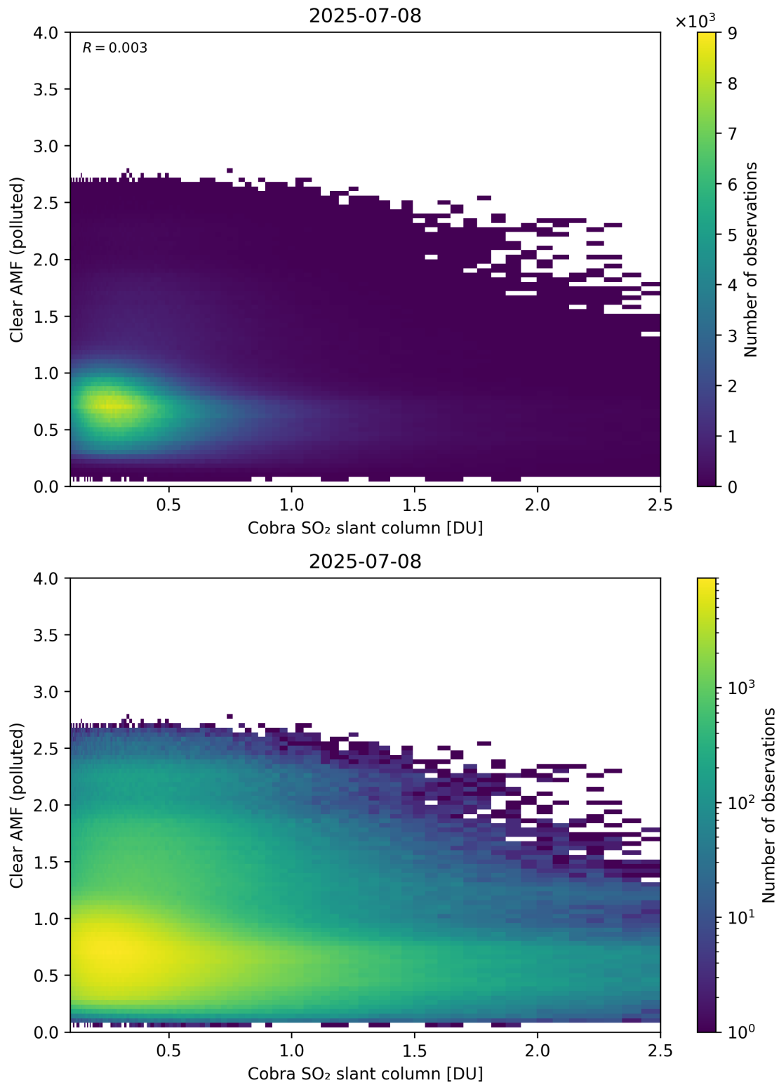
Figure 215: Scatter density plot of “Cobra SO 2 slant column” against “Clear AMF (polluted)” for 2025-07-08 to 2025-07-09.
