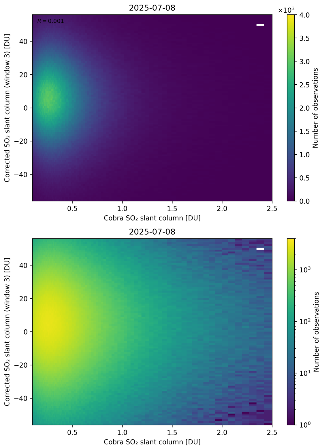
Figure 218: Scatter density plot of “Cobra SO 2 slant column” against “Corrected SO 2 slant column (window 3)” for 2025-07-08 to 2025-07-09.
