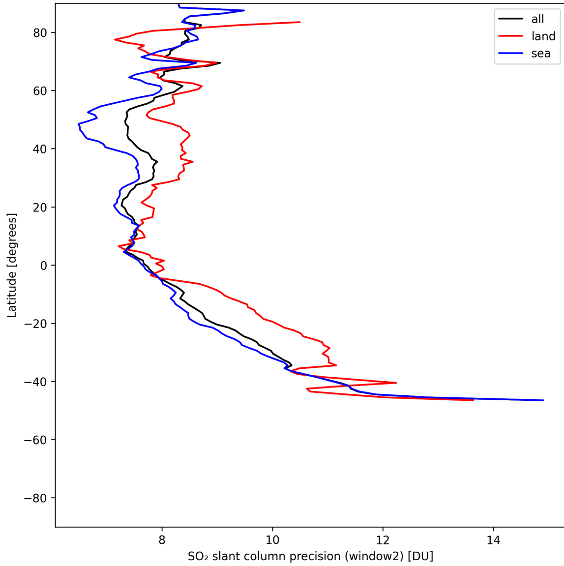
Figure 42: Zonal average of “SO 2 slant column precision (window2)” for 2025-07-08 to 2025-07-09.
