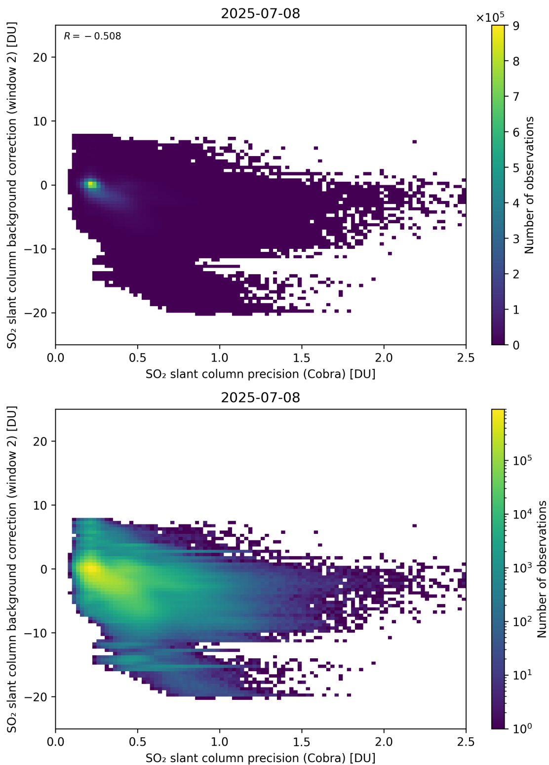
Figure 200: Scatter density plot of “SO 2 slant column precision (Cobra)” against “SO 2 slant column background correction (window 2)” for 2025-07-08 to 2025-07-09.
