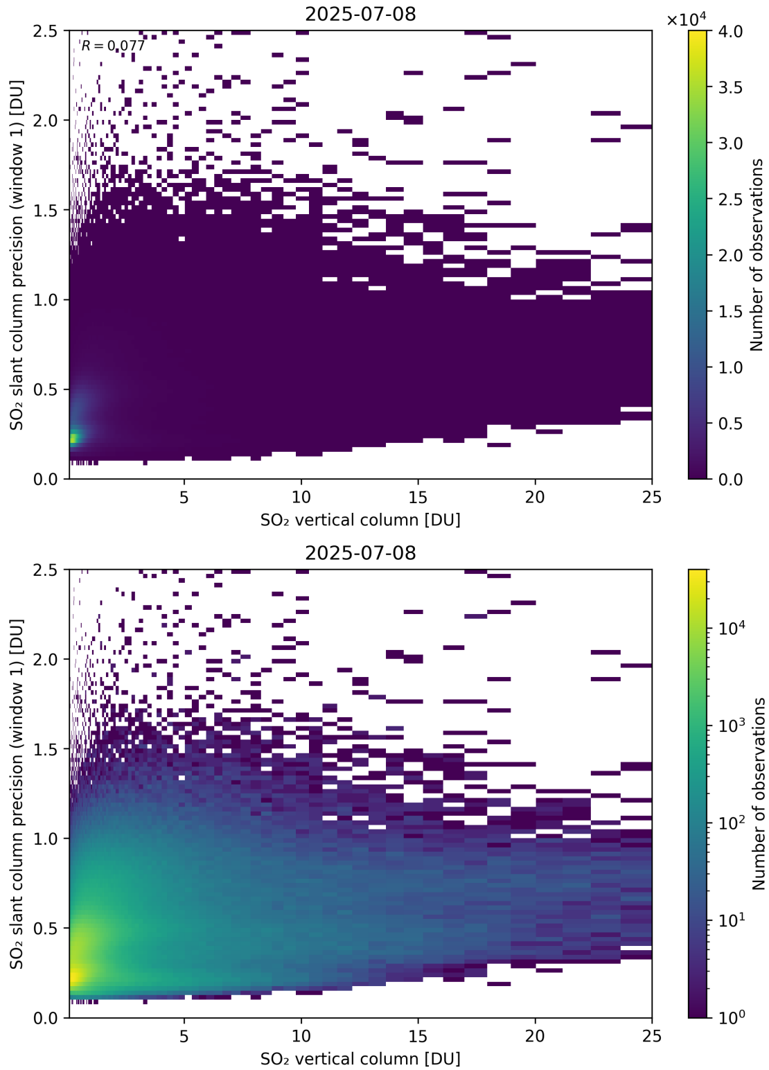
Figure 355: Scatter density plot of “SO 2 vertical column” against “SO 2 slant column precision (window 1)” for 2025-07-08 to 2025-07-09.
