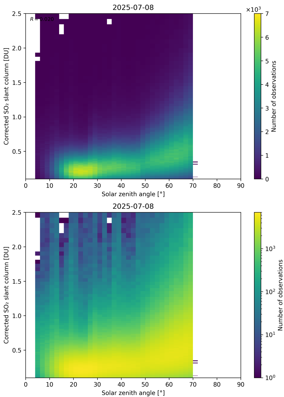
Figure 181: Scatter density plot of “Solar zenith angle” against “Corrected SO 2 slant column” for 2025-07-08 to 2025-07-09.
