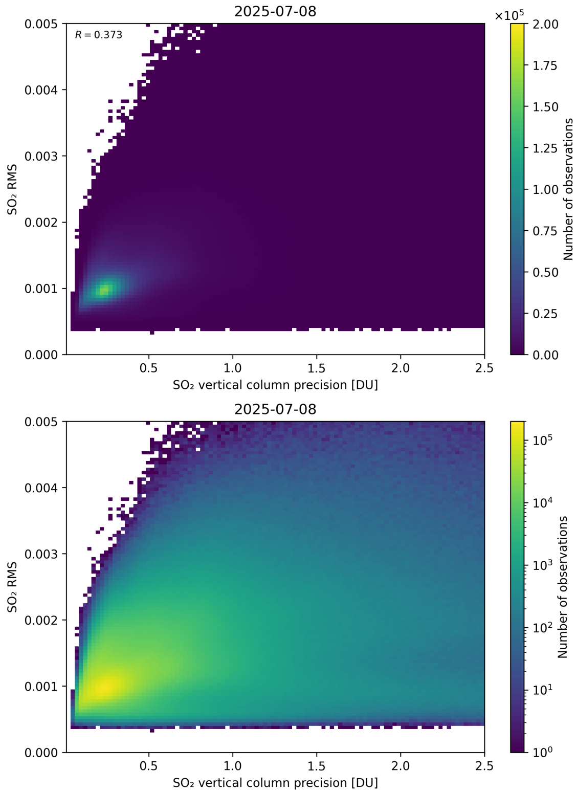
Figure 334: Scatter density plot of “SO 2 vertical column precision” against “SO 2 RMS” for 2025-07-08 to 2025-07-09.
