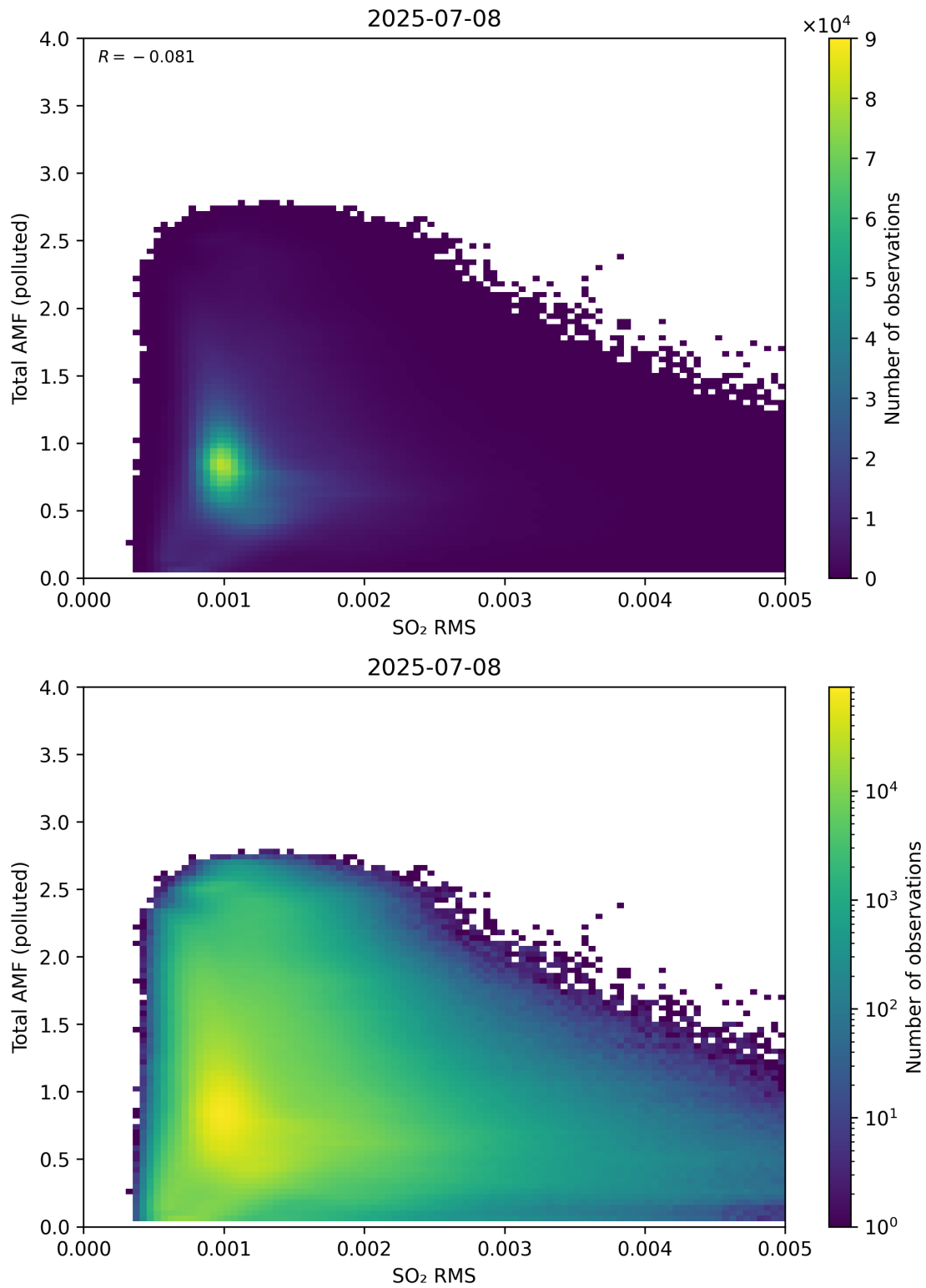
Figure 148: Scatter density plot of “SO 2 RMS” against “Total AMF (polluted)” for 2025-07-08 to 2025-07-09.
