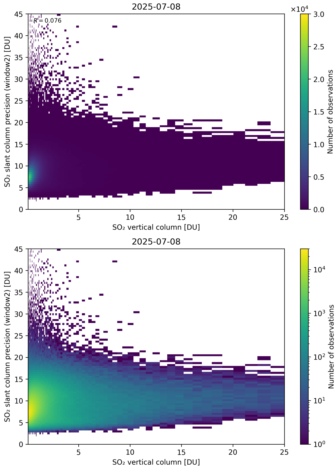
Figure 356: Scatter density plot of “SO 2 vertical column” against “SO 2 slant column precision (window2)” for 2025-07-08 to 2025-07-09.
