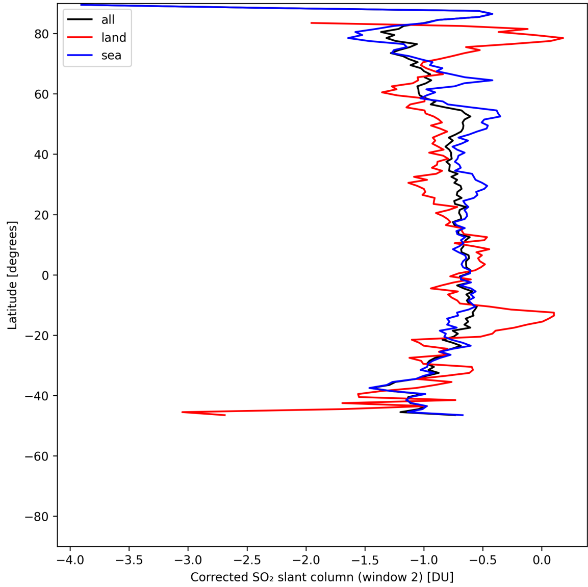
Figure 43: Zonal average of “Corrected SO 2 slant column (window 2)” for 2025-07-08 to 2025-07-09.
