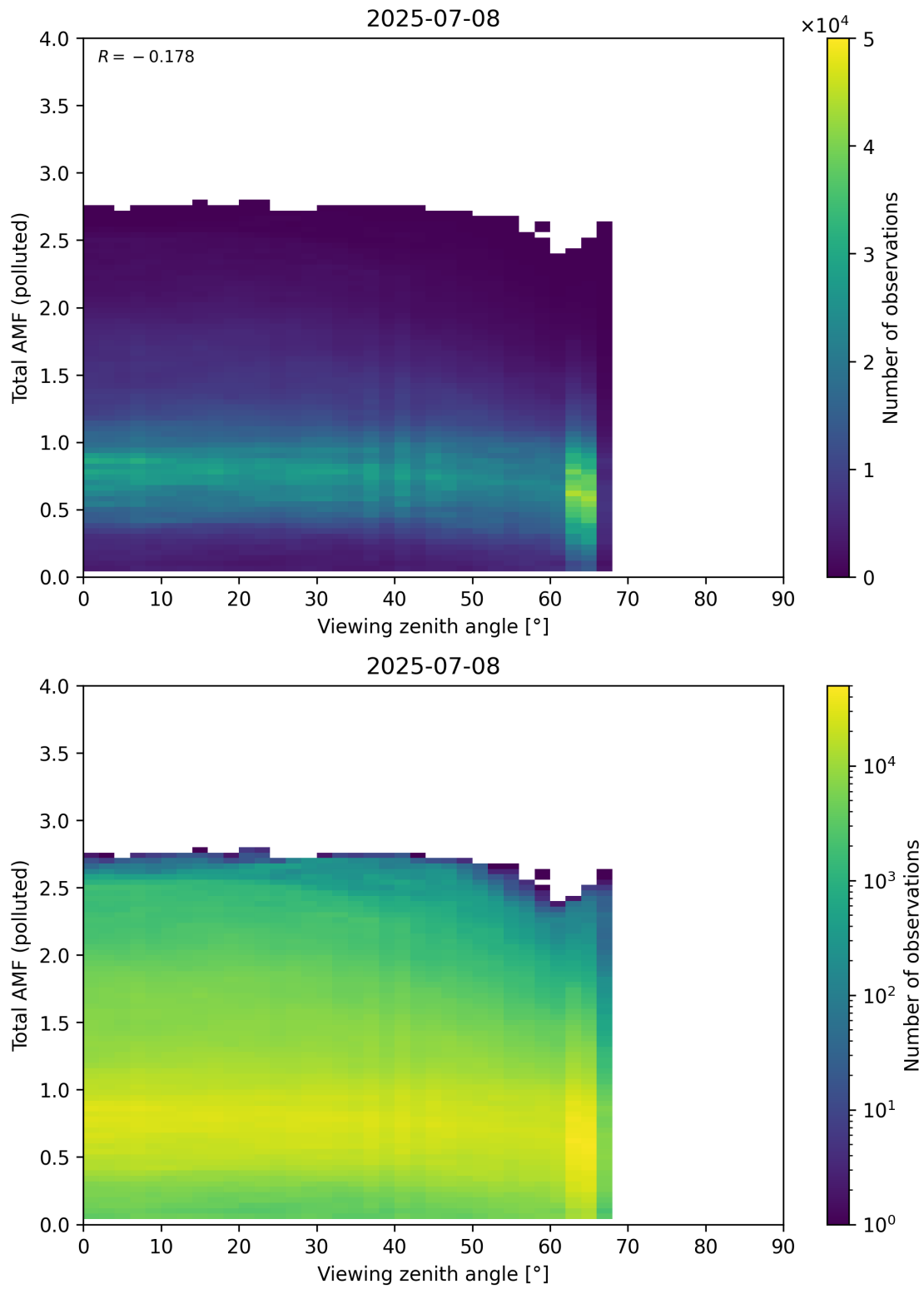
Figure 381: Scatter density plot of “Viewing zenith angle” against “Total AMF (polluted)” for 2025-07-08 to 2025-07-09.
