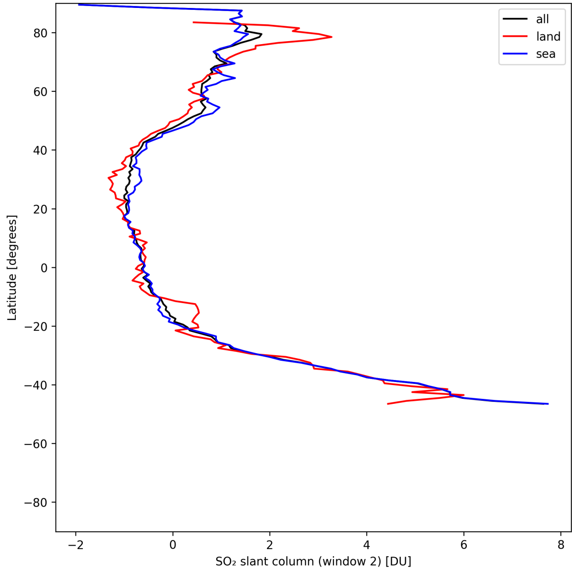
Figure 41: Zonal average of “SO 2 slant column (window 2)” for 2025-07-08 to 2025-07-09.
