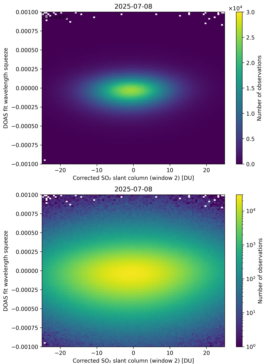
Figure 247: Scatter density plot of “Corrected SO 2 slant column (window 2)” against “DOAS fit wavelength squeeze” for 2025-07-08 to 2025-07-09.
