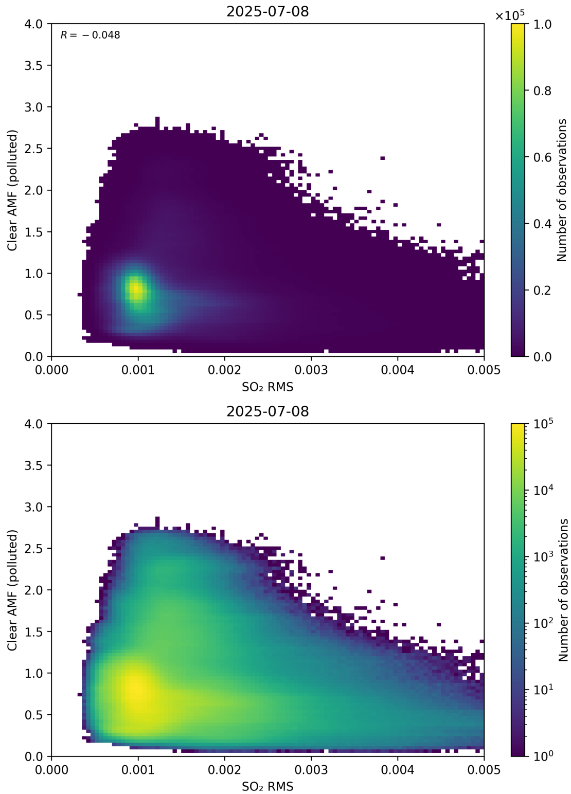
Figure 147: Scatter density plot of “SO 2 RMS” against “Clear AMF (polluted)” for 2025-07-08 to 2025-07-09.
