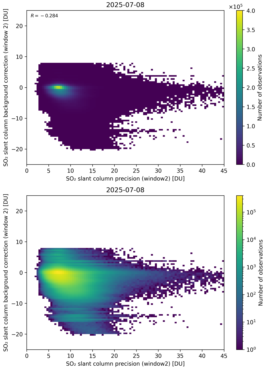
Figure 291: Scatter density plot of “SO 2 slant column precision (window2)” against “SO 2 slant column background correction (window 2)” for 2025-07-08 to 2025-07-09.
