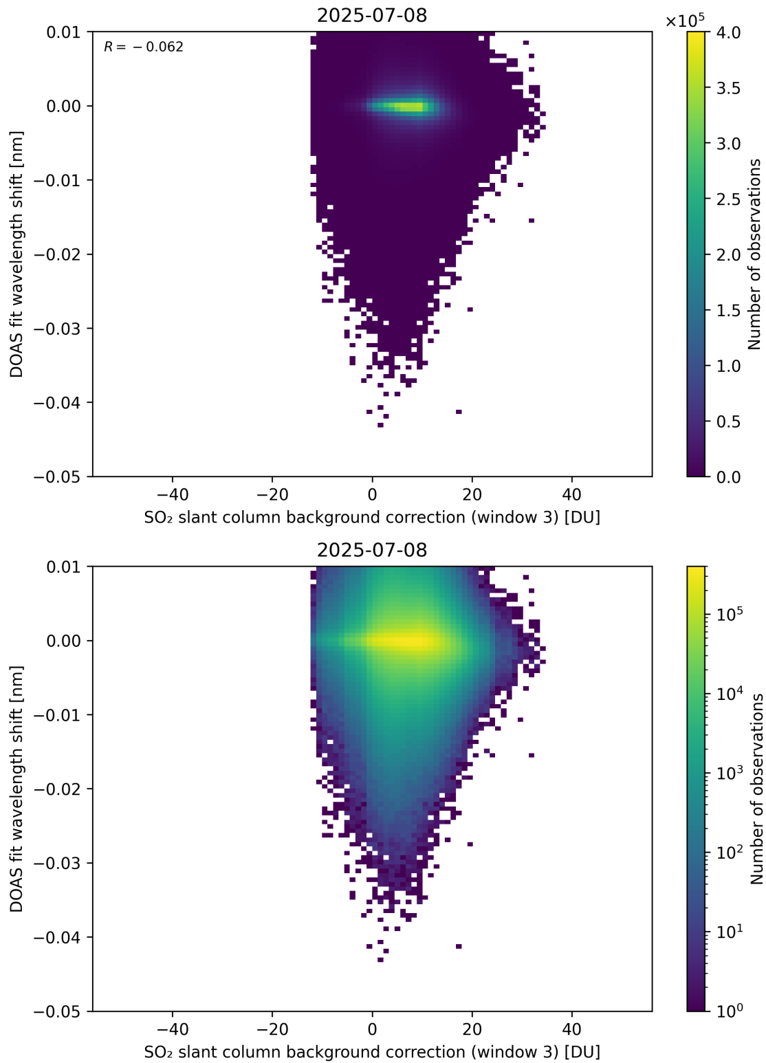
Figure 132: Scatter density plot of “SO 2 slant column background correction (window 3)” against “DOAS fit wavelength shift” for 2025-07-08 to 2025-07-09.
