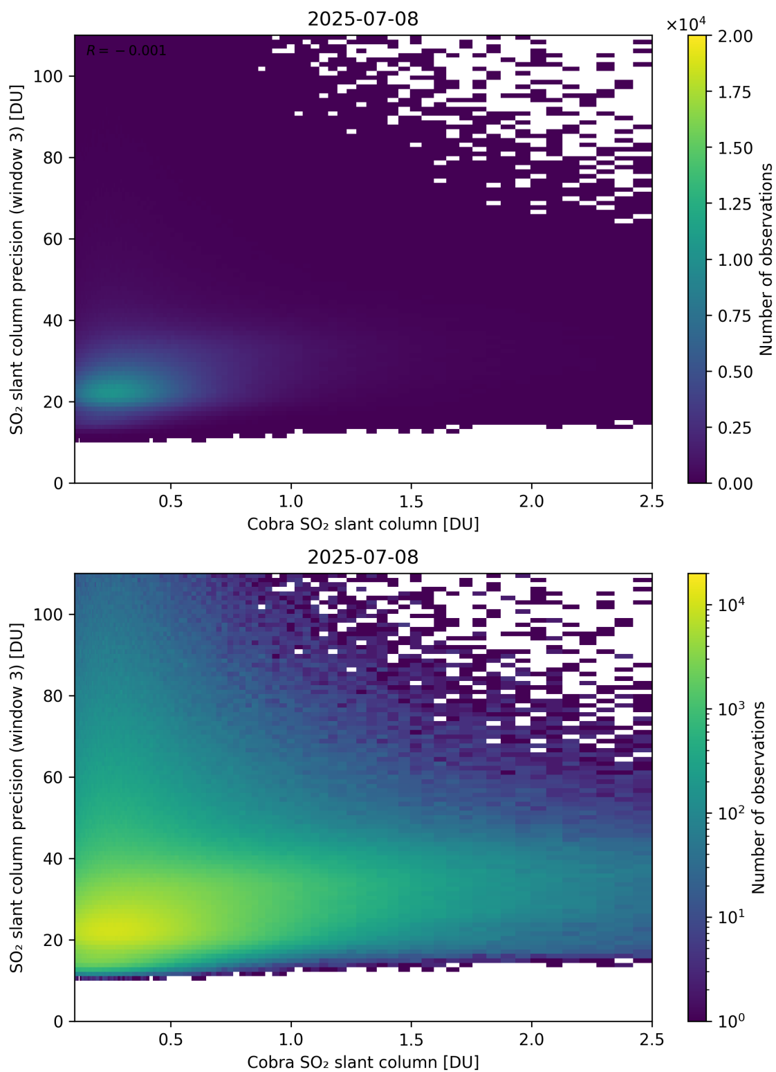
Figure 223: Scatter density plot of “Cobra SO 2 slant column” against “SO 2 slant column precision (window 3)” for 2025-07-08 to 2025-07-09.
