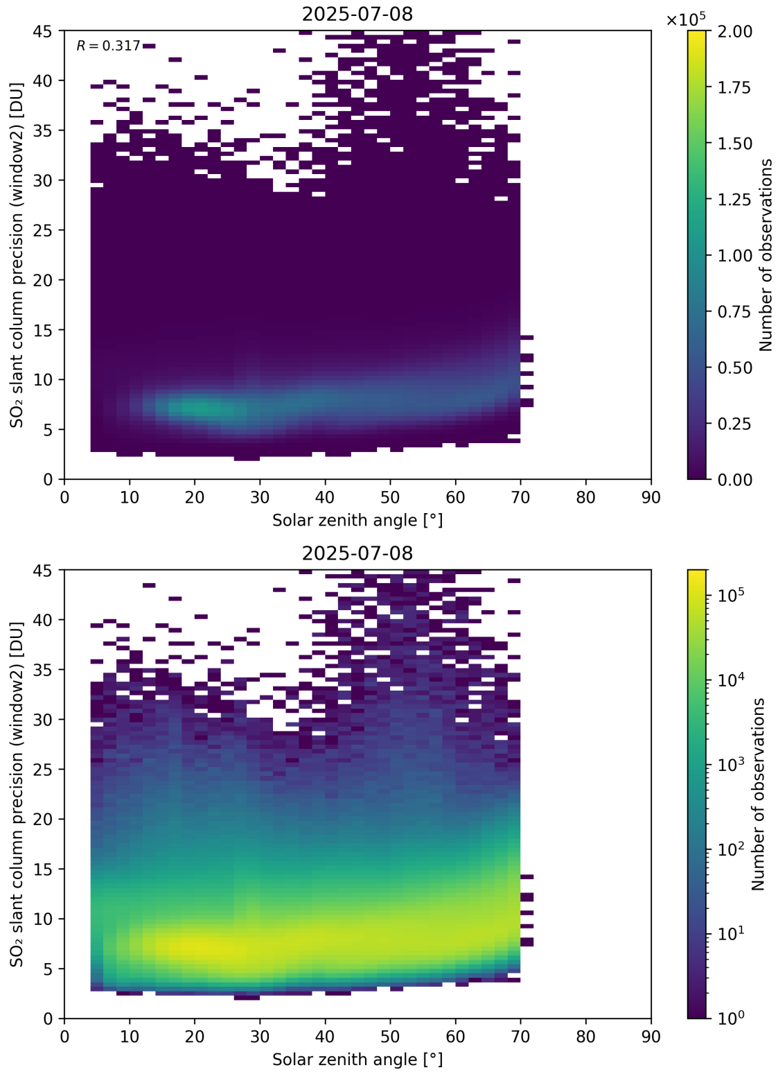
Figure 186: Scatter density plot of “Solar zenith angle” against “SO 2 slant column precision (window2)” for 2025-07-08 to 2025-07-09.
