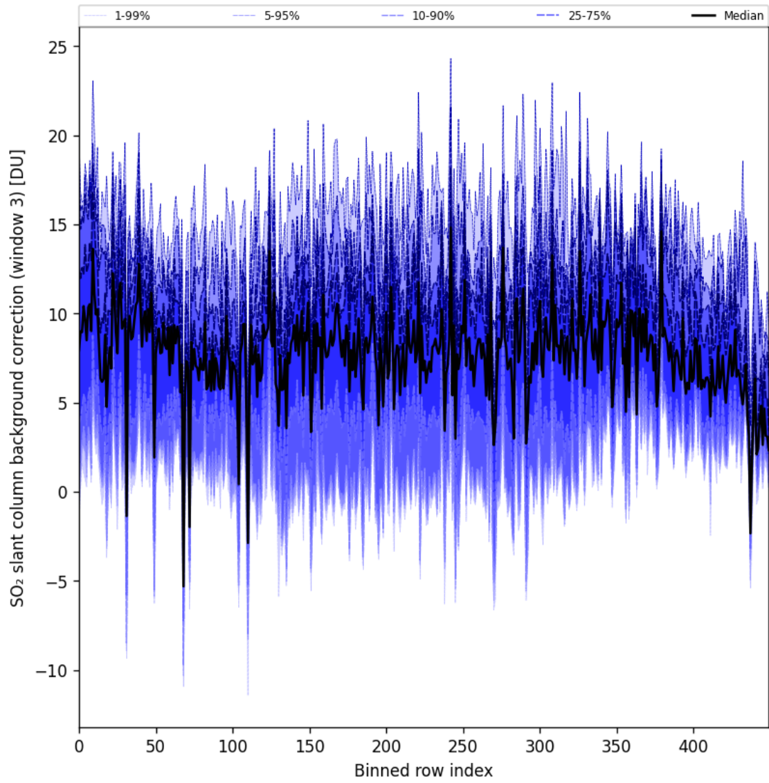
Figure 100: Along track statistics of “SO 2 slant column background correction (window 3)” for 2025-07-08 to 2025-07-09
