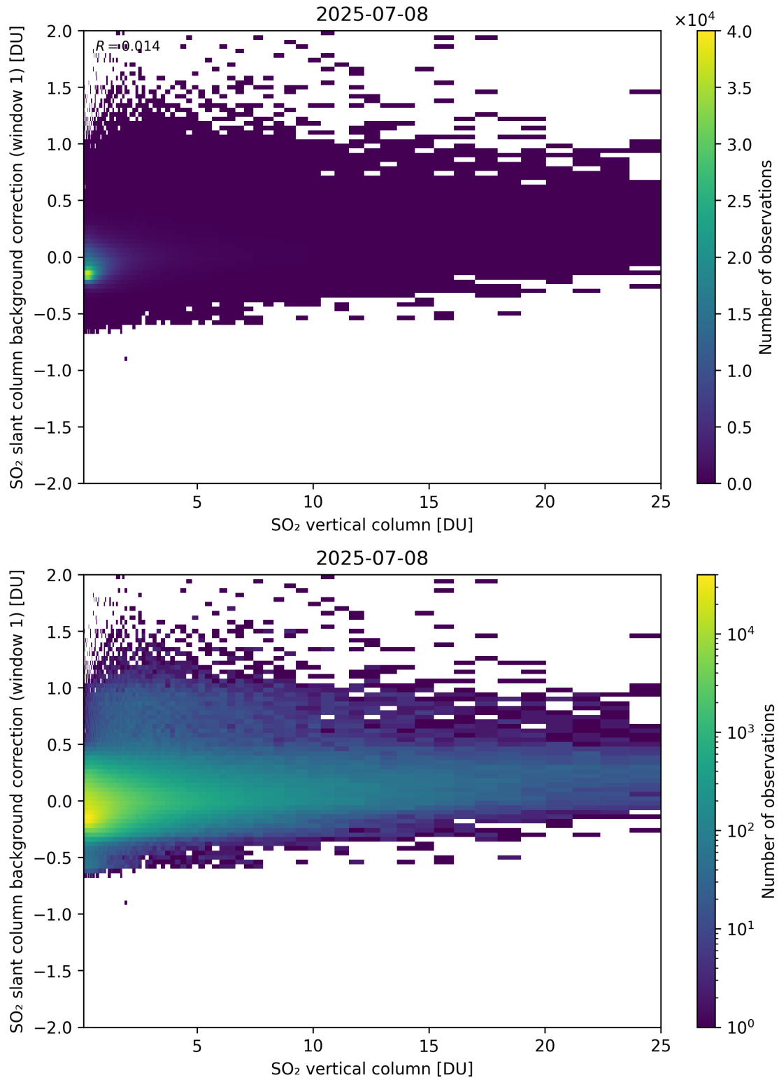
Figure 323: Scatter density plot of “SO 2 vertical column” against “SO 2 slant column background correction (window 1)” for 2025-07-08 to 2025-07-09.
