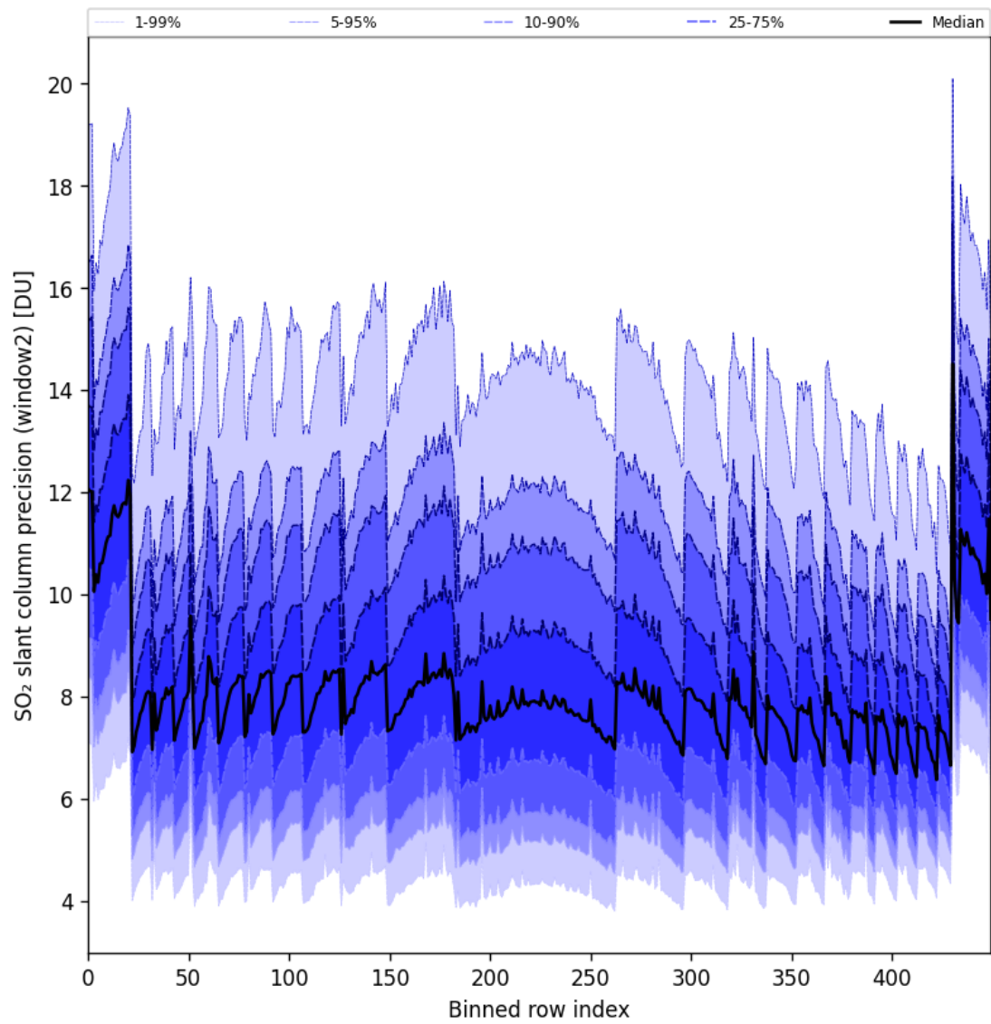
Figure 94: Along track statistics of “SO 2 slant column precision (window2)” for 2025-07-08 to 2025-07-09
