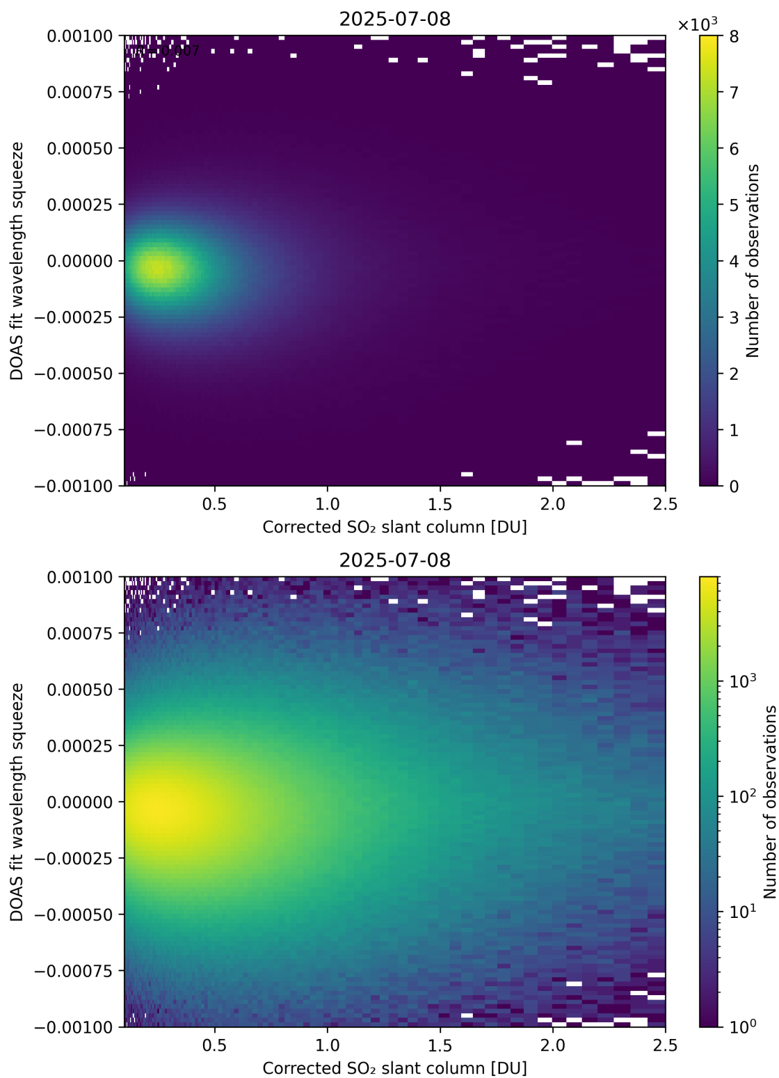
Figure 230: Scatter density plot of “Corrected SO 2 slant column” against “DOAS fit wavelength squeeze” for 2025-07-08 to 2025-07-09.
