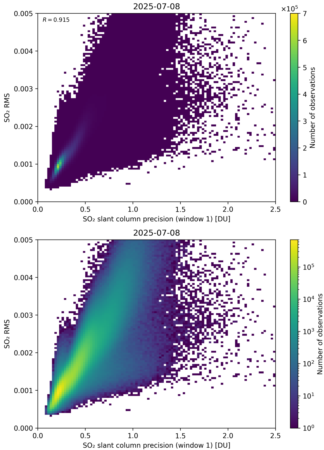
Figure 273: Scatter density plot of “SO 2 slant column precision (window 1)” against “SO 2 RMS” for 2025-07-08 to 2025-07-09.
