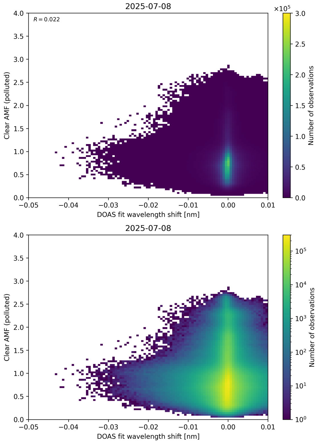
Figure 140: Scatter density plot of “DOAS fit wavelength shift” against “Clear AMF (polluted)” for 2025-07-08 to 2025-07-09.
