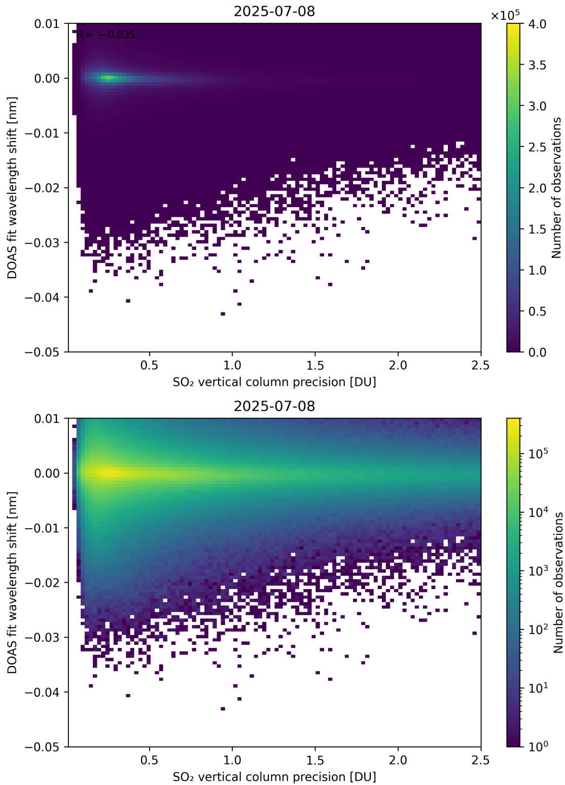
Figure 332: Scatter density plot of “SO 2 vertical column precision” against “DOAS fit wavelength shift” for 2025-07-08 to 2025-07-09.
