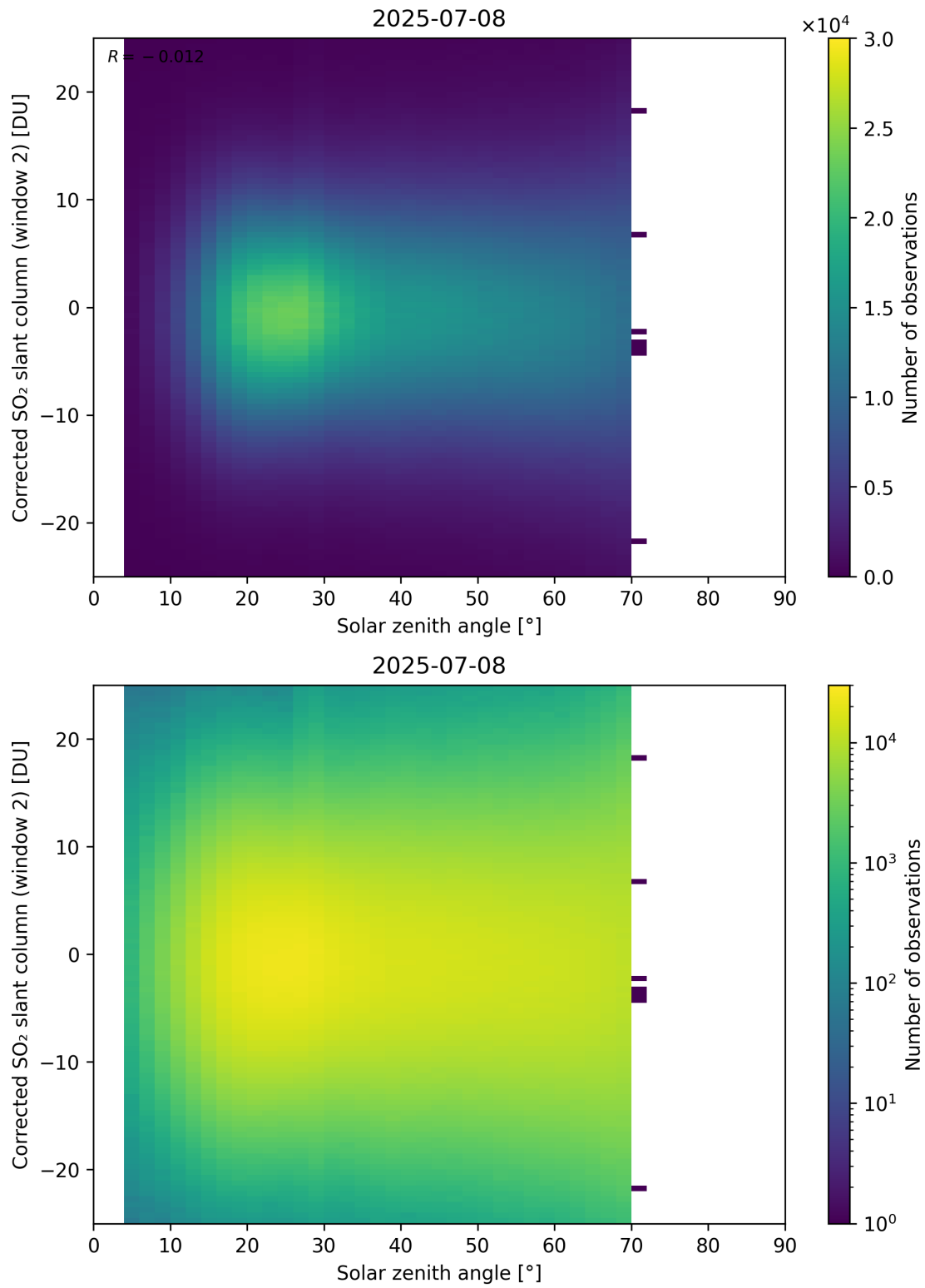
Figure 182: Scatter density plot of “Solar zenith angle” against “Corrected SO 2 slant column (window 2)” for 2025-07-08 to 2025-07-09.
