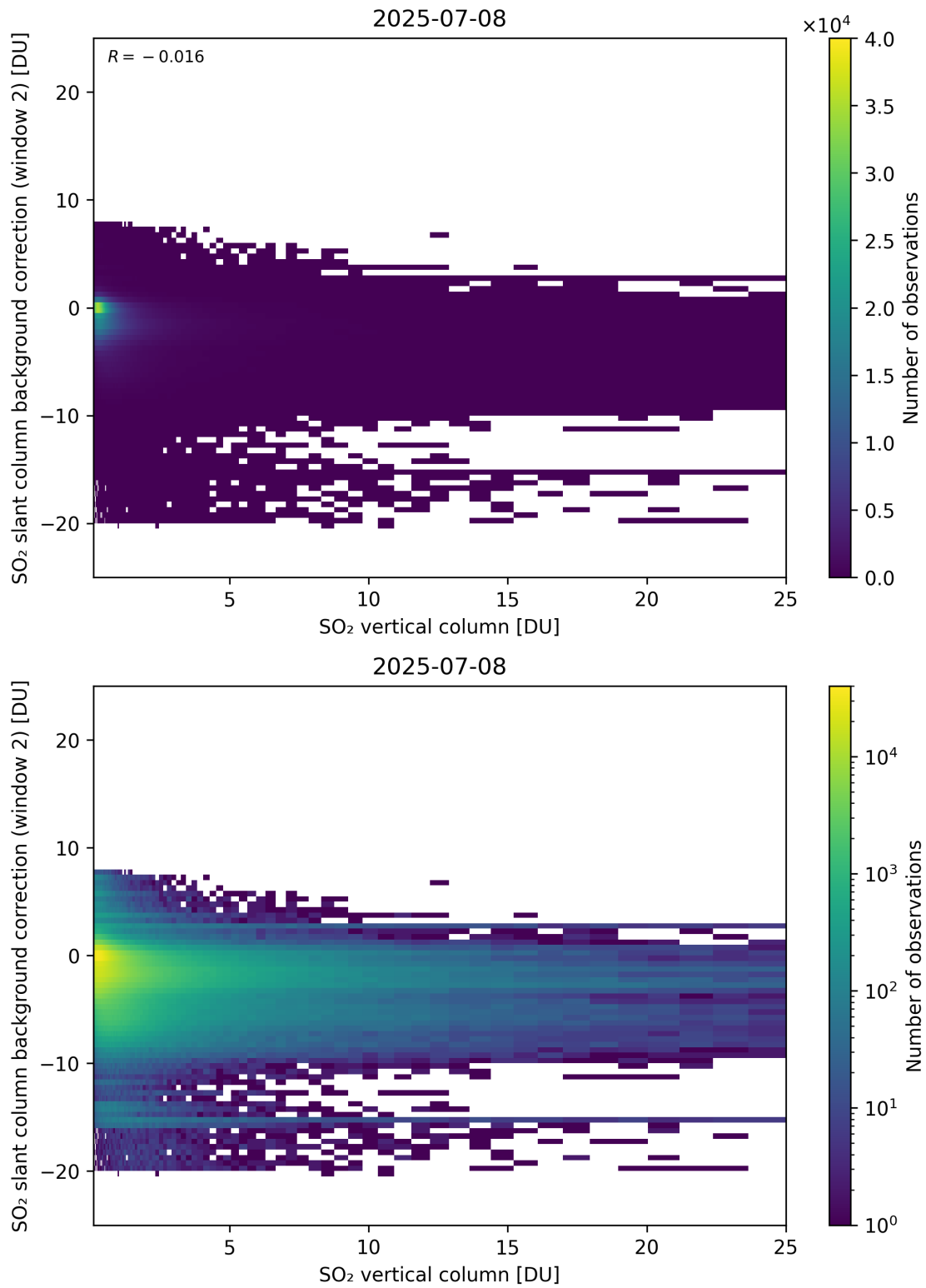
Figure 324: Scatter density plot of “SO 2 vertical column” against “SO 2 slant column background correction (window 2)” for 2025-07-08 to 2025-07-09.
