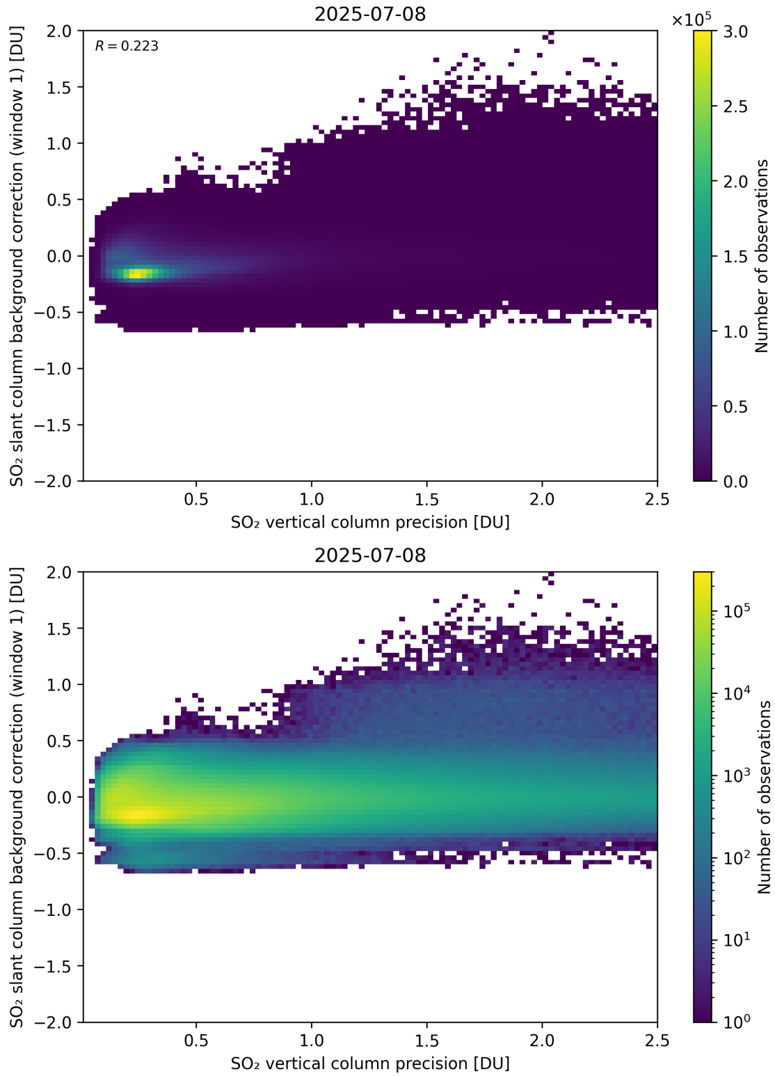
Figure 329: Scatter density plot of “SO 2 vertical column precision” against “SO 2 slant column background correction (window 1)” for 2025-07-08 to 2025-07-09.
