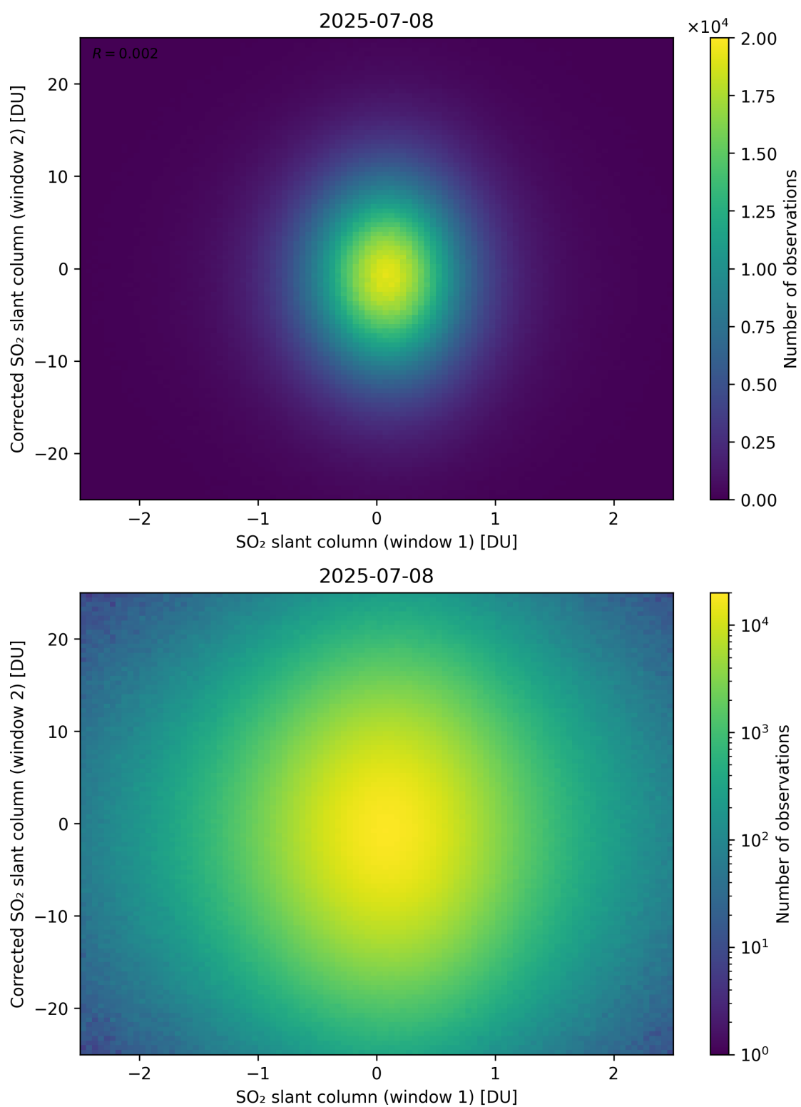
Figure 283: Scatter density plot of “SO 2 slant column (window 1)” against “Corrected SO 2 slant column (window 2)” for 2025-07-08 to 2025-07-09.
