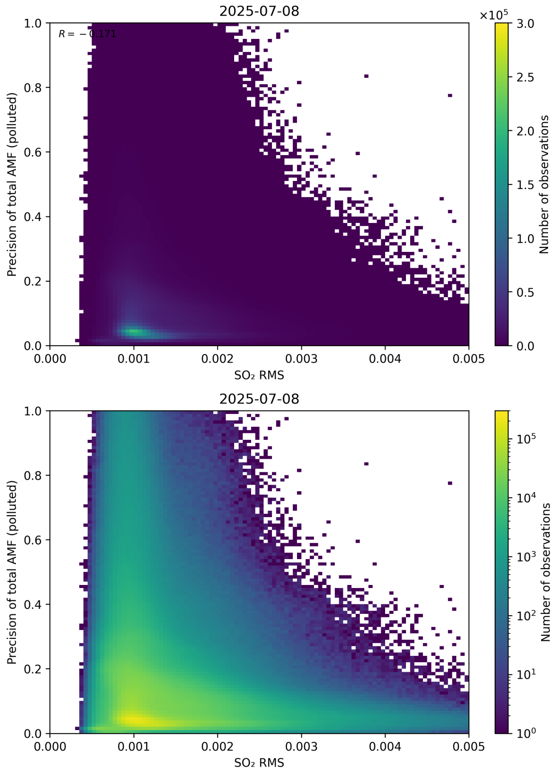
Figure 149: Scatter density plot of “SO 2 RMS” against “Precision of total AMF (polluted)” for 2025-07-08 to 2025-07-09.
