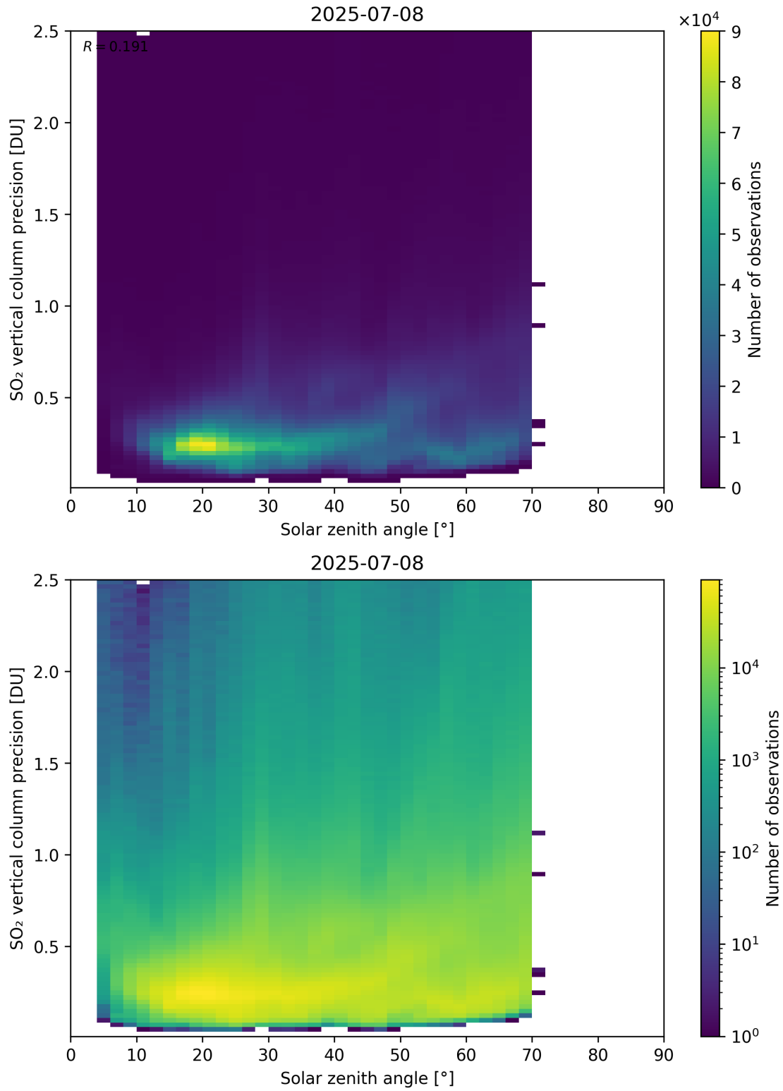
Figure 192: Scatter density plot of “Solar zenith angle” against “SO 2 vertical column precision” for 2025-07-08 to 2025-07-09.
