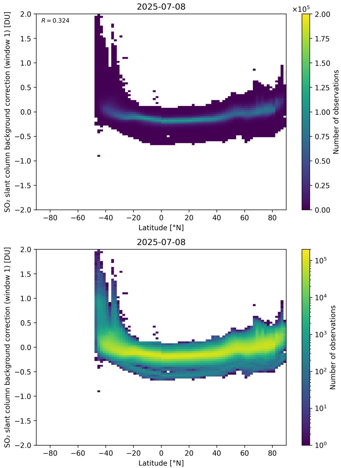
Figure 150: Scatter density plot of “Latitude” against “SO 2 slant column background correction (window 1)” for 2025-07-08 to 2025-07-09.
