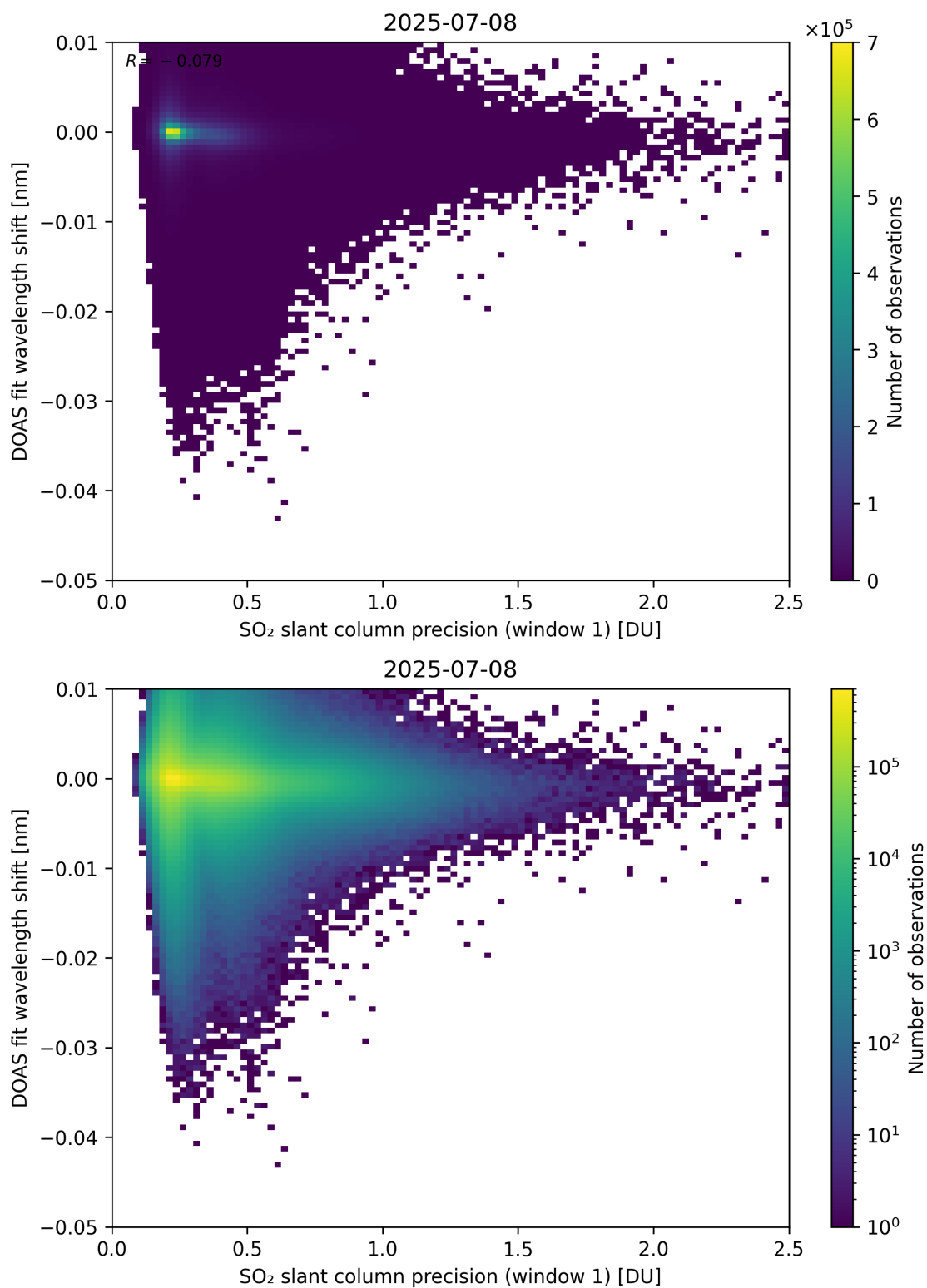
Figure 271: Scatter density plot of “SO 2 slant column precision (window 1)” against “DOAS fit wavelength shift” for 2025-07-08 to 2025-07-09.
