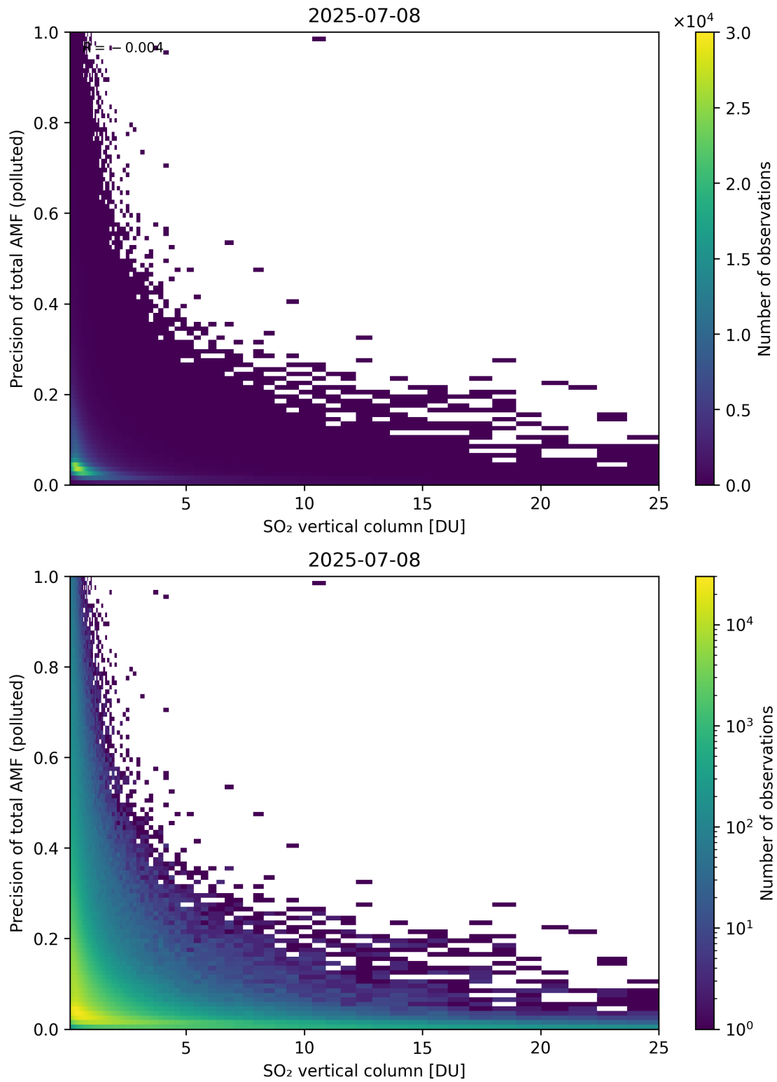
Figure 360: Scatter density plot of “SO 2 vertical column” against “Precision of total AMF (polluted)” for 2025-07-08 to 2025-07-09.
