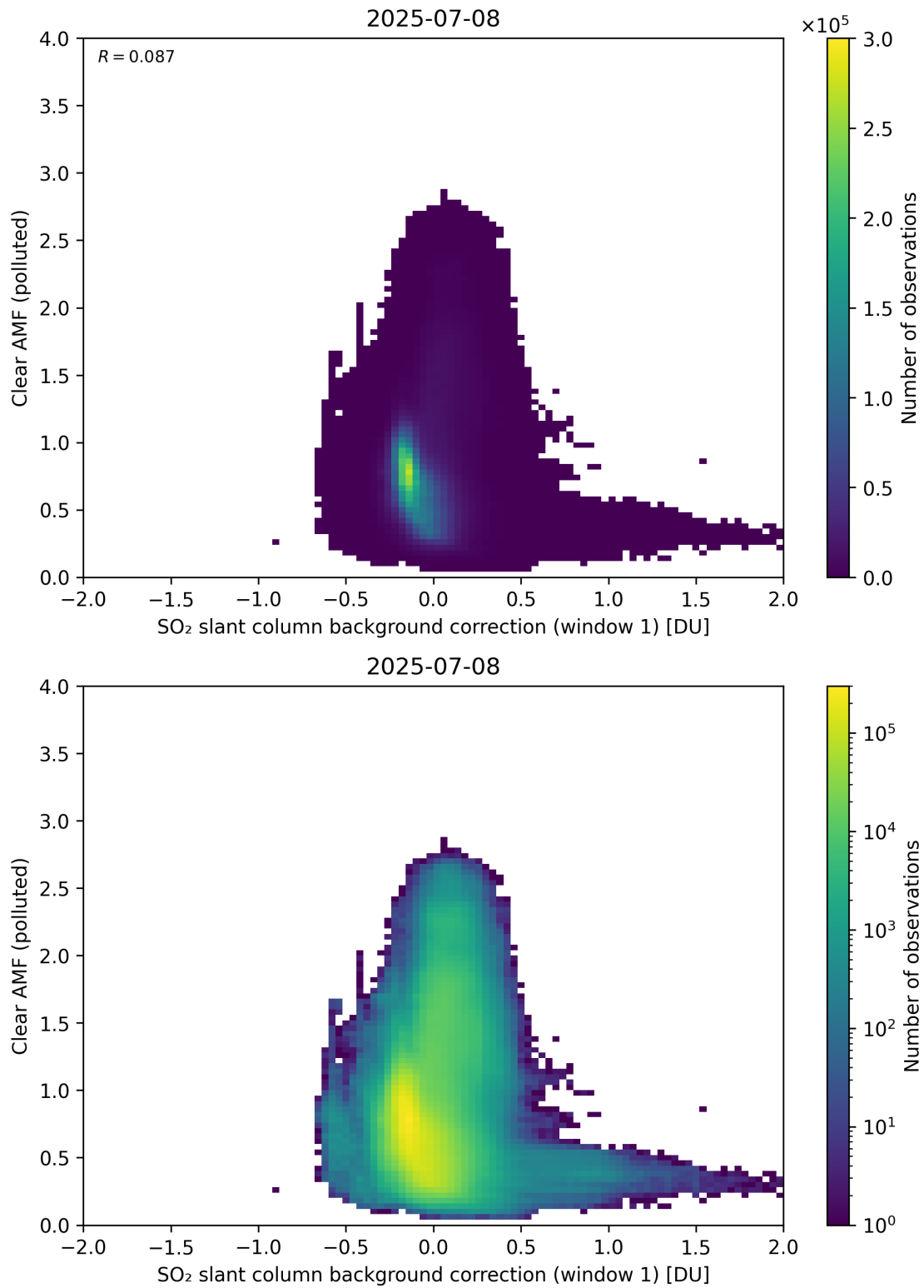
Figure 114: Scatter density plot of “SO 2 slant column background correction (window 1)” against “Clear AMF (polluted)” for 2025-07-08 to 2025-07-09.
