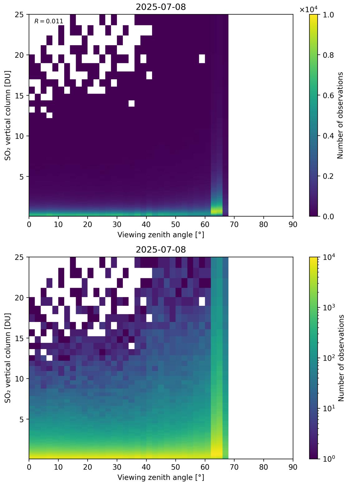
Figure 383: Scatter density plot of “Viewing zenith angle” against “SO 2 vertical column” for 2025-07-08 to 2025-07-09.
