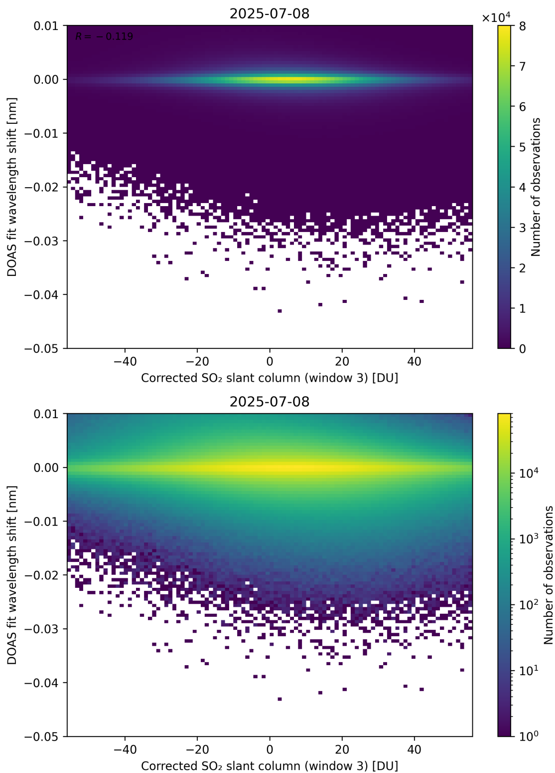
Figure 256: Scatter density plot of “Corrected SO 2 slant column (window 3)” against “DOAS fit wavelength shift” for 2025-07-08 to 2025-07-09.
