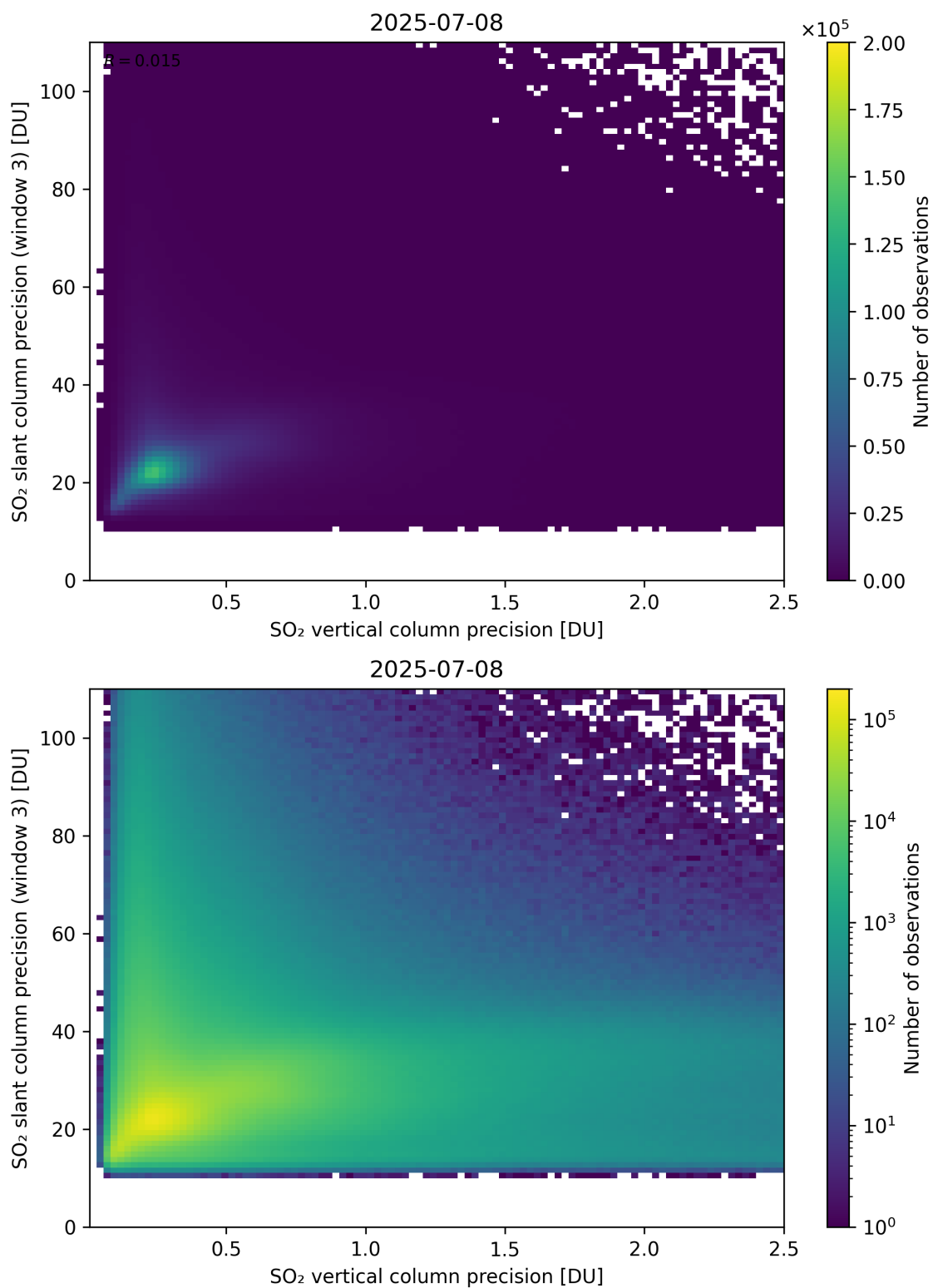
Figure 345: Scatter density plot of “SO 2 vertical column precision” against “SO 2 slant column precision (window 3)” for 2025-07-08 to 2025-07-09.
