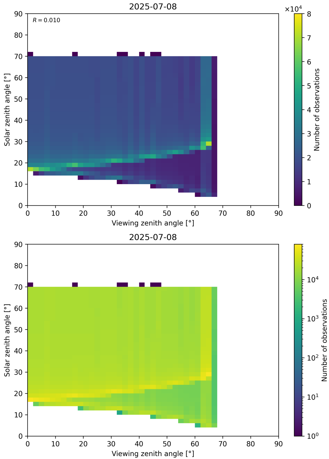
Figure 369: Scatter density plot of “Viewing zenith angle” against “Solar zenith angle” for 2025-07-08 to 2025-07-09.
