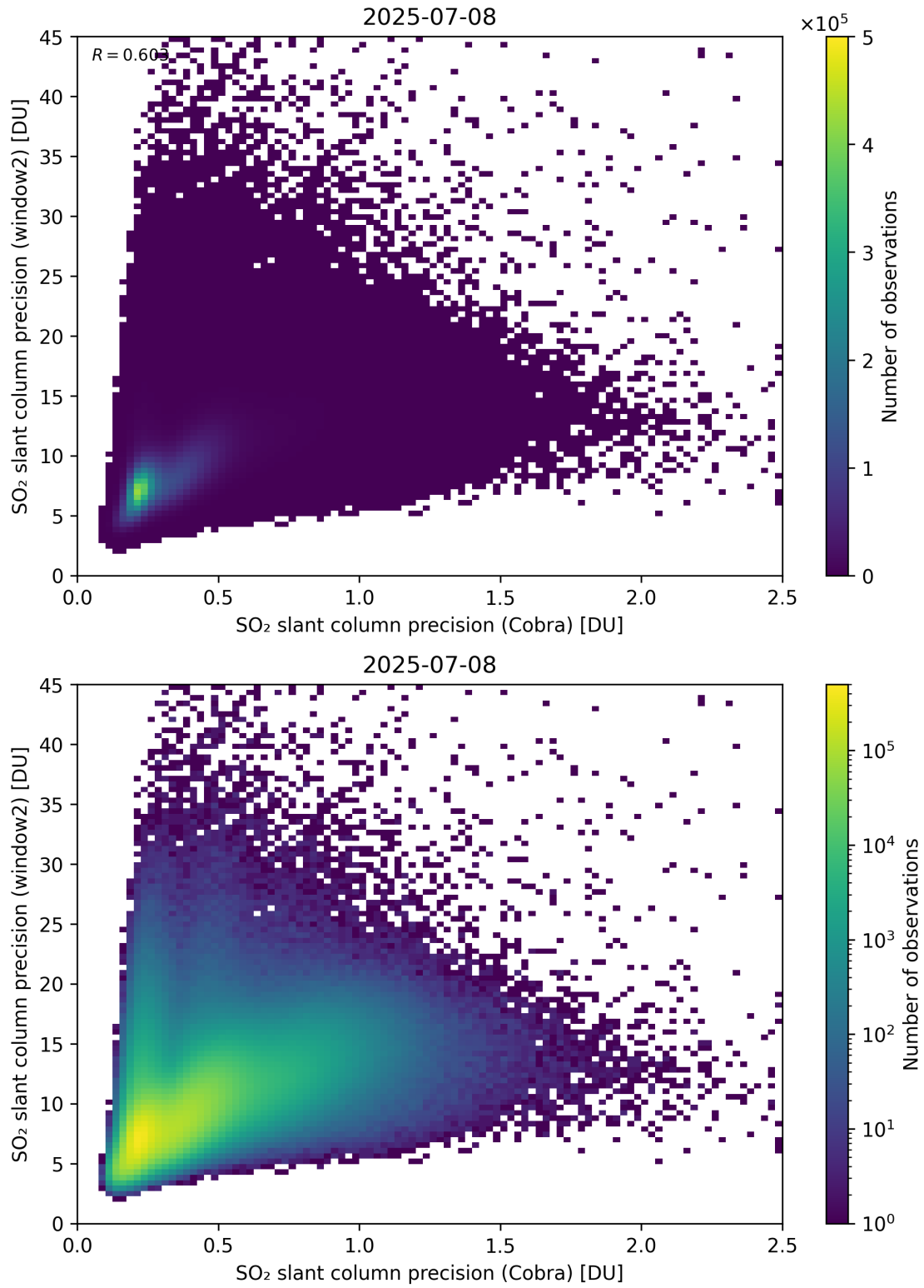
Figure 210: Scatter density plot of “SO 2 slant column precision (Cobra)” against “SO 2 slant column precision (window2)” for 2025-07-08 to 2025-07-09.
