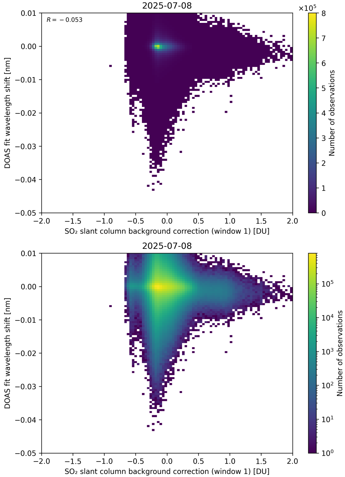
Figure 111: Scatter density plot of “SO 2 slant column background correction (window 1)” against “DOAS fit wavelength shift” for 2025-07-08 to 2025-07-09.
