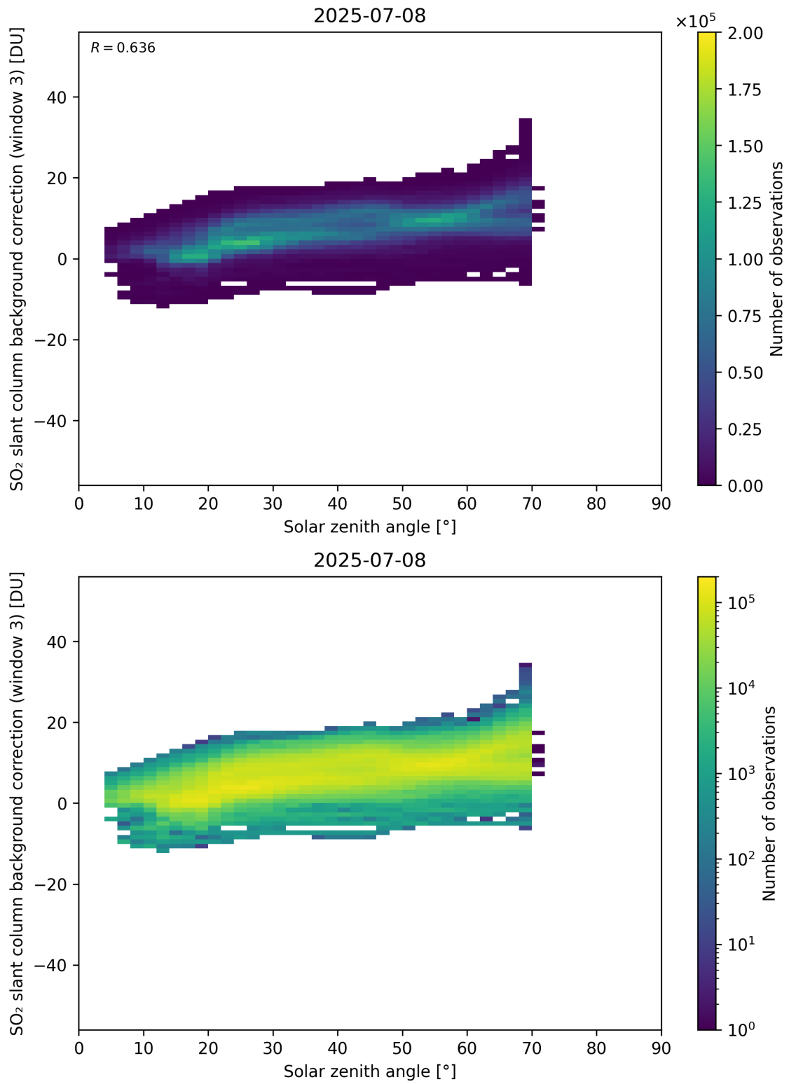
Figure 173: Scatter density plot of “Solar zenith angle” against “SO 2 slant column background correction (window 3)” for 2025-07-08 to 2025-07-09.
