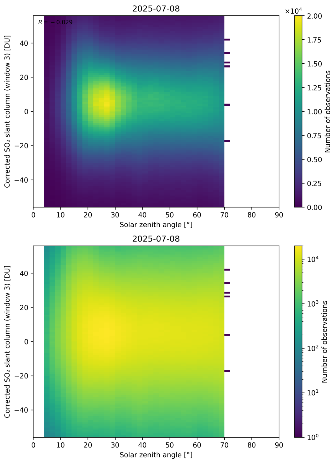
Figure 183: Scatter density plot of “Solar zenith angle” against “Corrected SO 2 slant column (window 3)” for 2025-07-08 to 2025-07-09.
