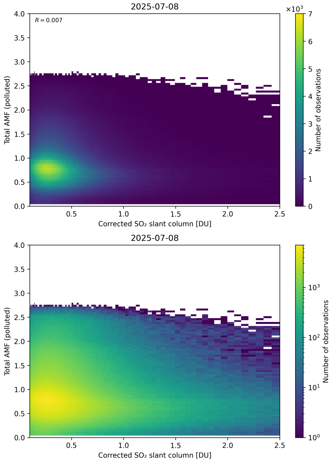
Figure 242: Scatter density plot of “Corrected SO 2 slant column” against “Total AMF (polluted)” for 2025-07-08 to 2025-07-09.
