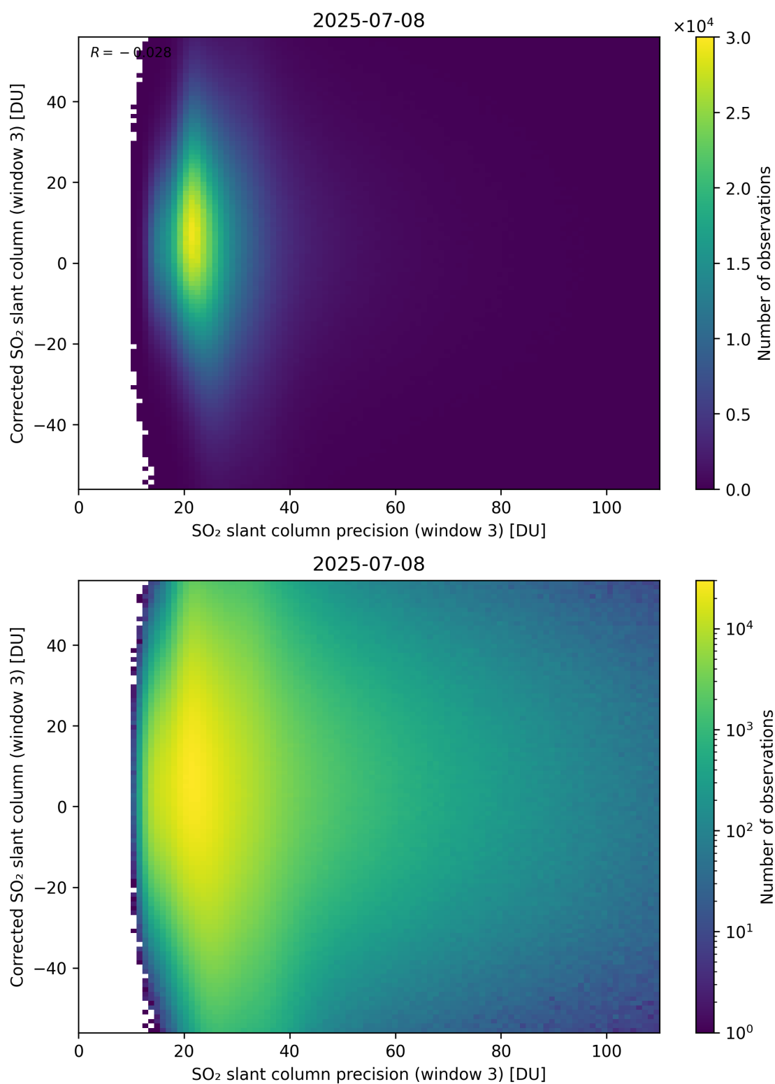
Figure 312: Scatter density plot of “SO 2 slant column precision (window 3)” against “Corrected SO 2 slant column (window 3)” for 2025-07-08 to 2025-07-09.
