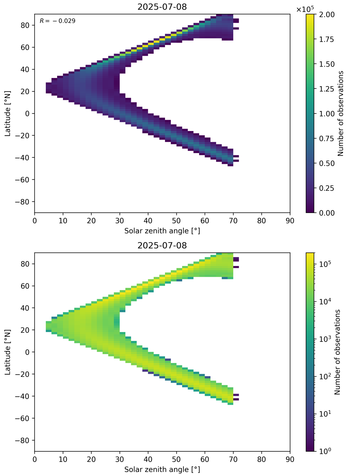
Figure 177: Scatter density plot of “Solar zenith angle” against “Latitude” for 2025-07-08 to 2025-07-09.
