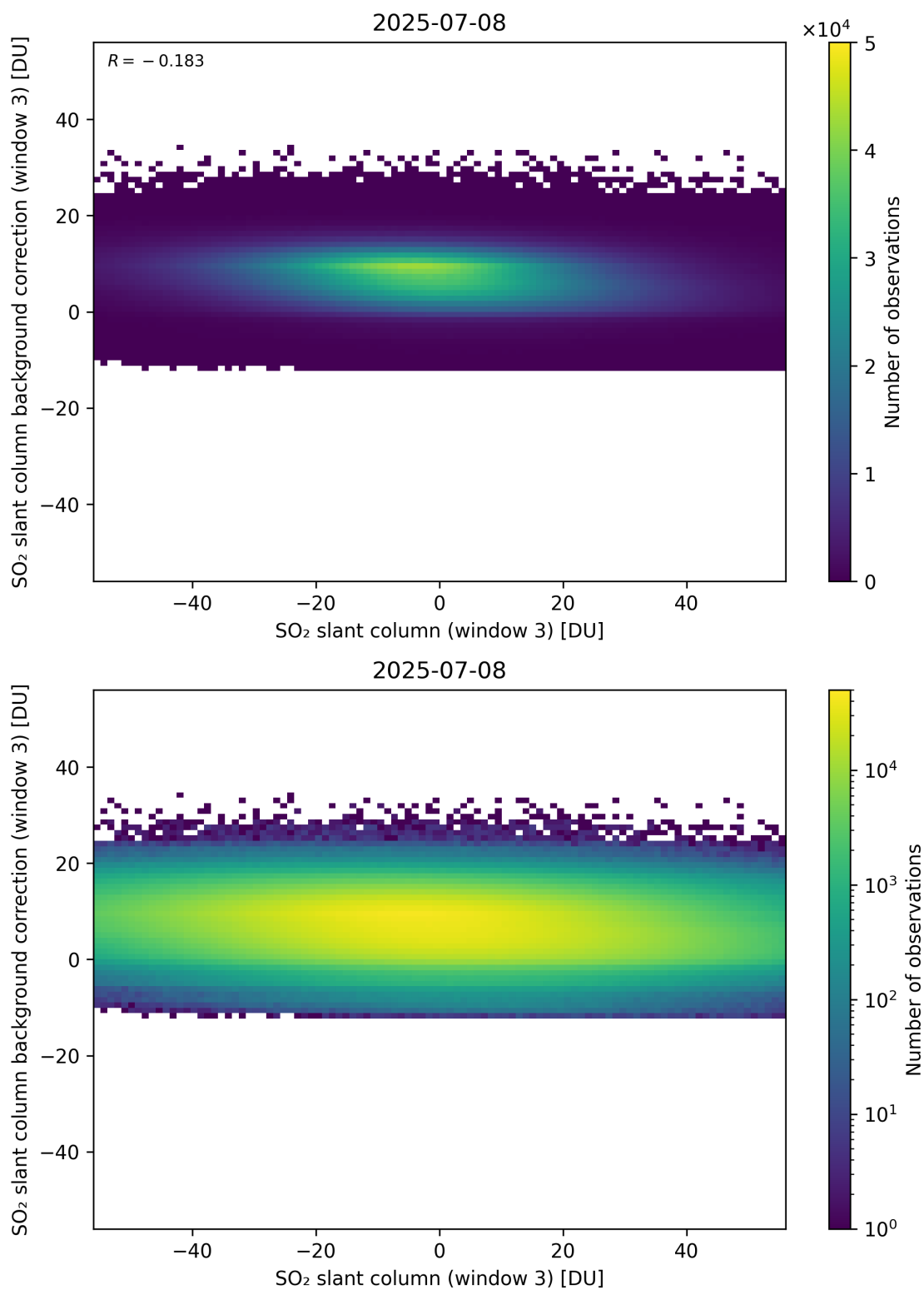
Figure 303: Scatter density plot of “SO 2 slant column (window 3)” against “SO 2 slant column background correction (window 3)” for 2025-07-08 to 2025-07-09.
