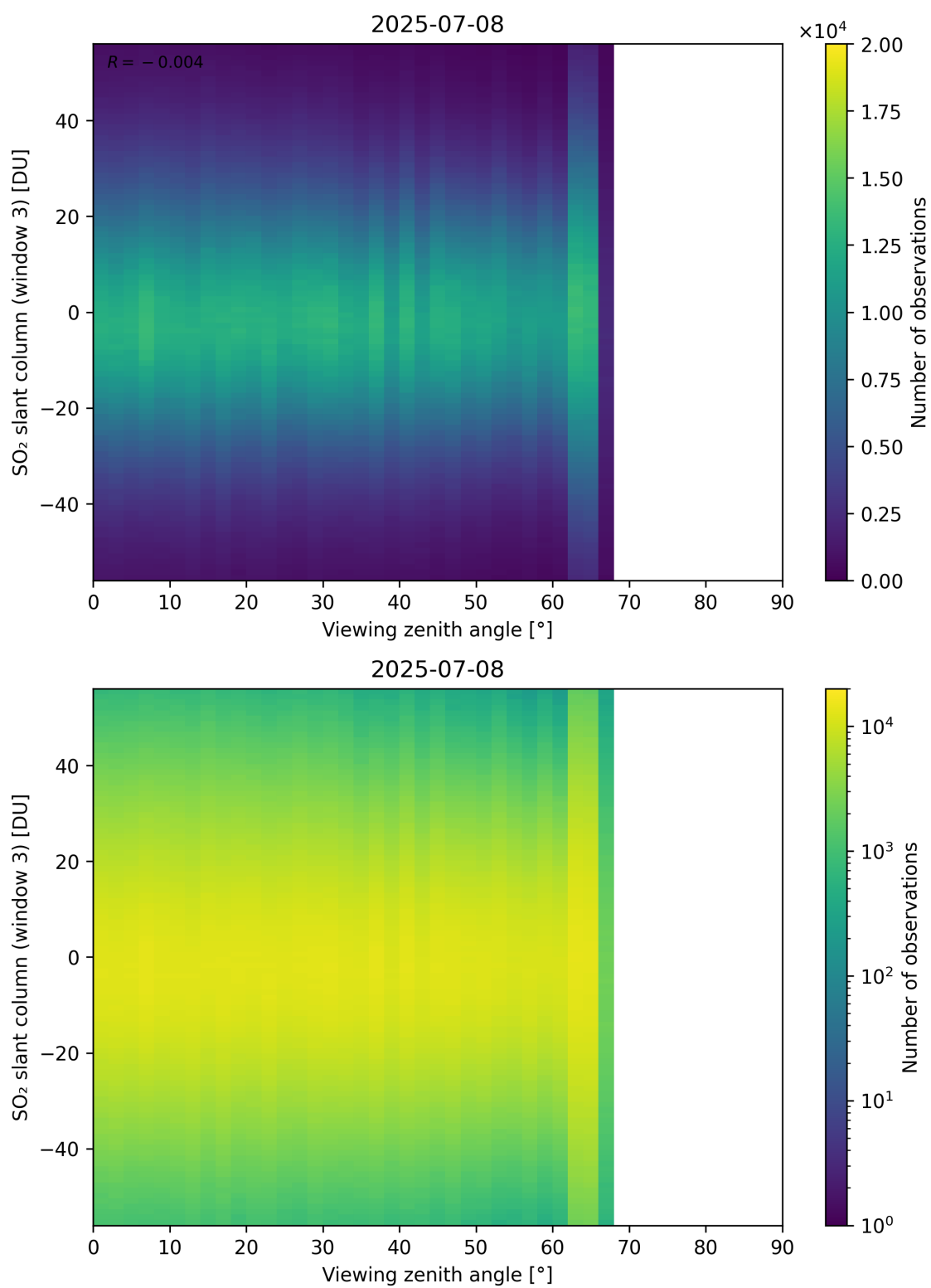
Figure 379: Scatter density plot of “Viewing zenith angle” against “SO 2 slant column (window 3)” for 2025-07-08 to 2025-07-09.
