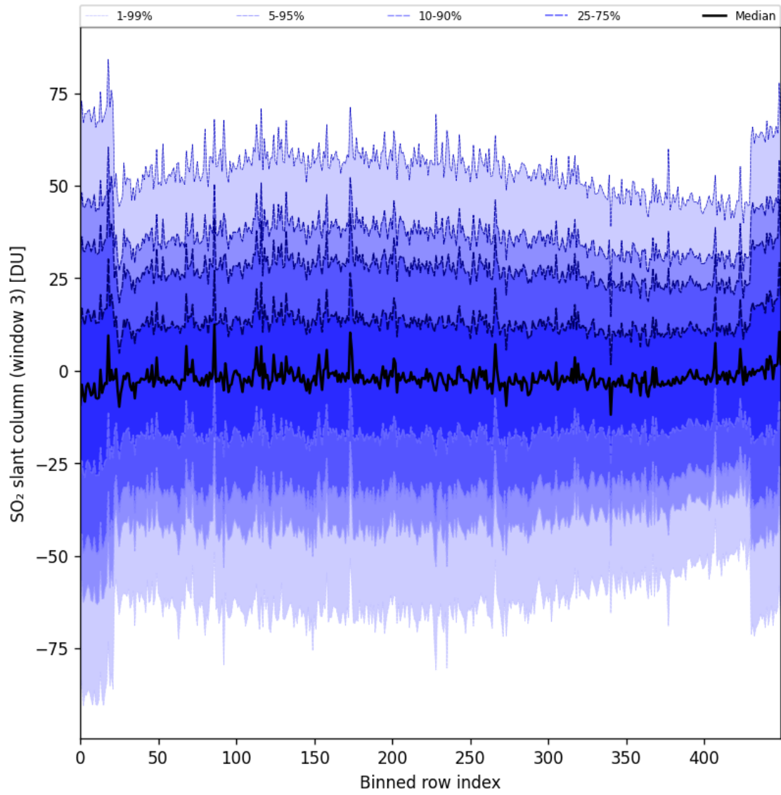
Figure 97: Along track statistics of “SO 2 slant column (window 3)” for 2025-07-08 to 2025-07-09
