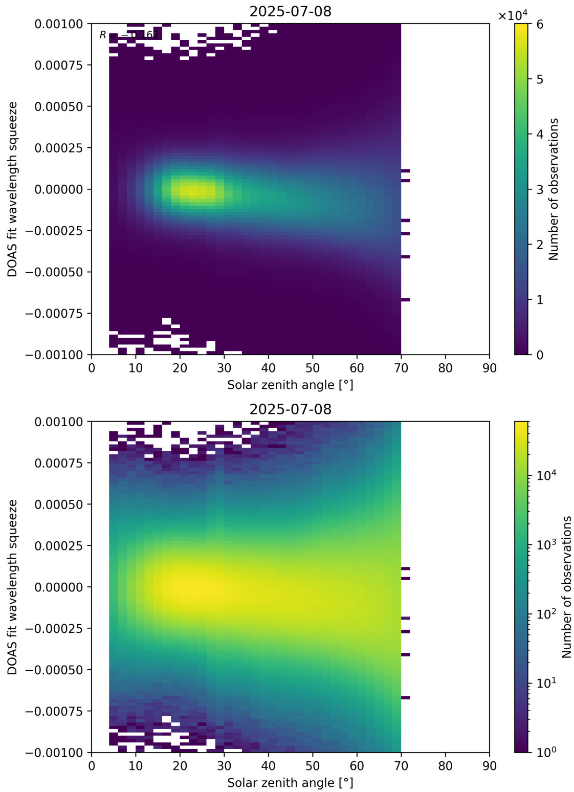
Figure 175: Scatter density plot of “Solar zenith angle” against “DOAS fit wavelength squeeze” for 2025-07-08 to 2025-07-09.
