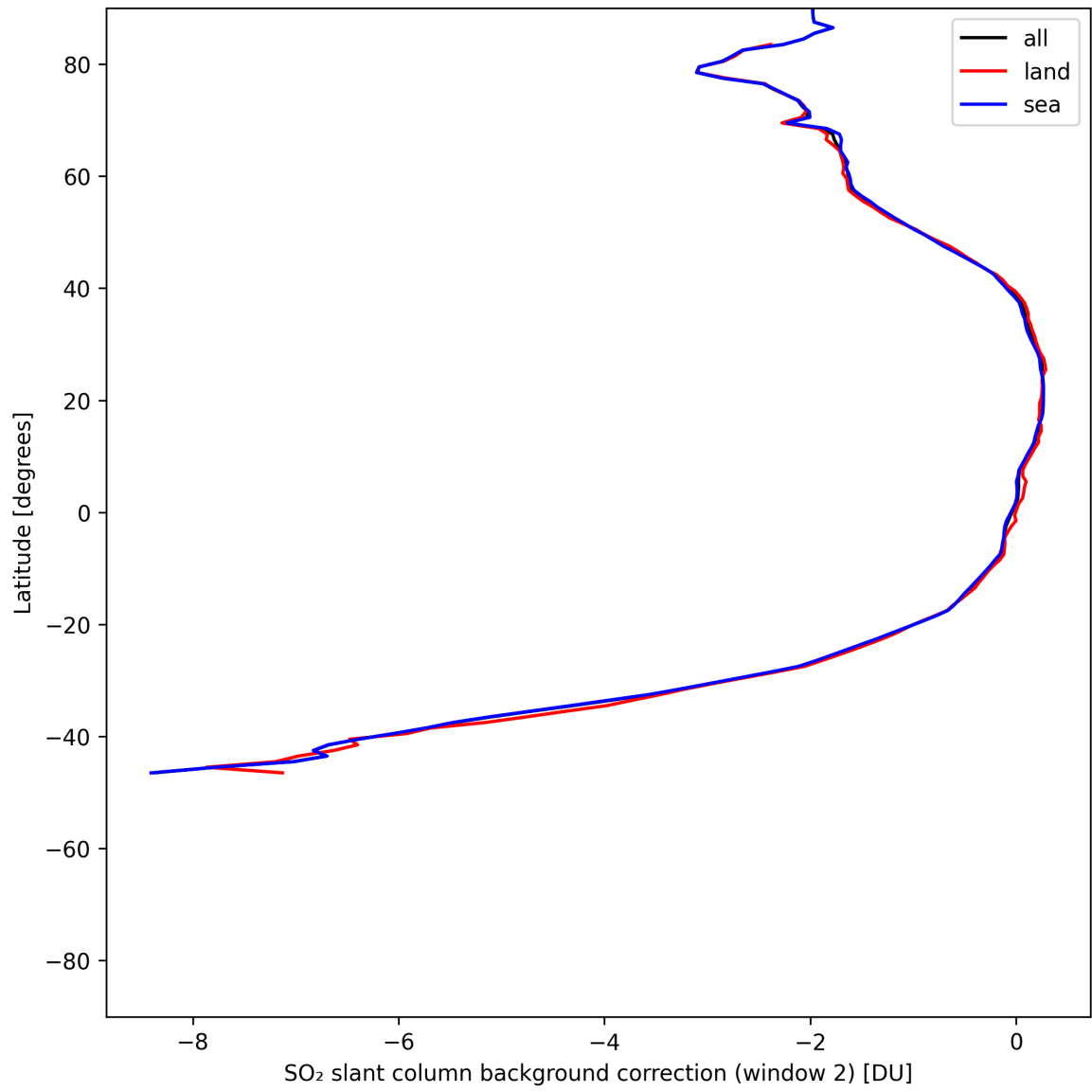
Figure 44: Zonal average of “SO 2 slant column background correction (window 2)” for 2025-07-08 to 2025-07-09.
