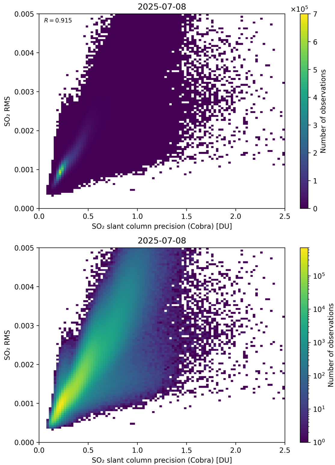
Figure 204: Scatter density plot of “SO 2 slant column precision (Cobra)” against “SO 2 RMS” for 2025-07-08 to 2025-07-09.
