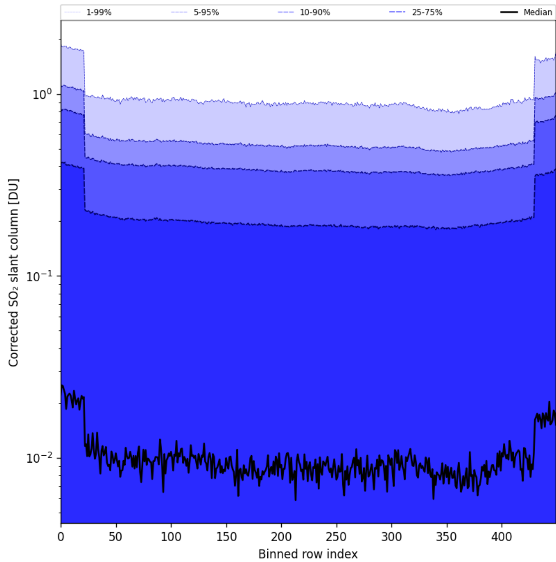
Figure 86: Along track statistics of “Corrected SO 2 slant column” for 2025-07-08 to 2025-07-09
