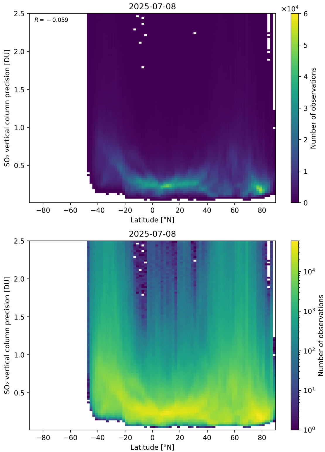
Figure 170: Scatter density plot of “Latitude” against “SO 2 vertical column precision” for 2025-07-08 to 2025-07-09.
