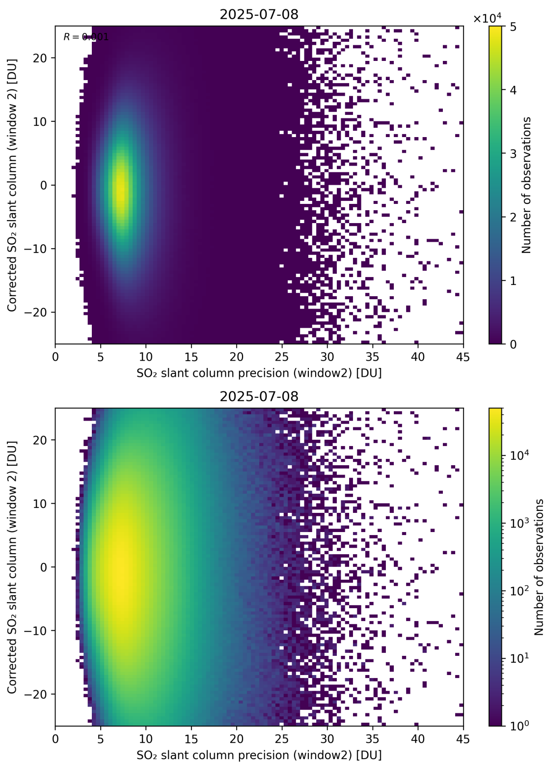
Figure 297: Scatter density plot of “SO 2 slant column precision (window2)” against “Corrected SO 2 slant column (window 2)” for 2025-07-08 to 2025-07-09.
