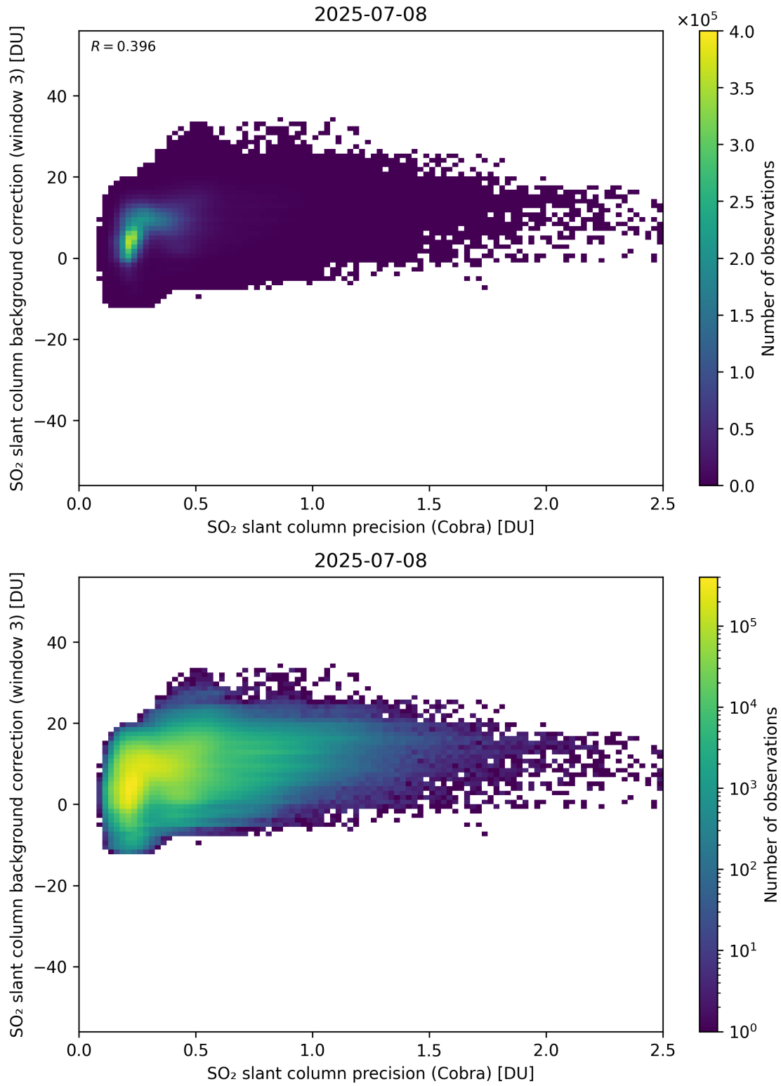
Figure 201: Scatter density plot of “SO 2 slant column precision (Cobra)” against “SO 2 slant column background correction (window 3)” for 2025-07-08 to 2025-07-09.
