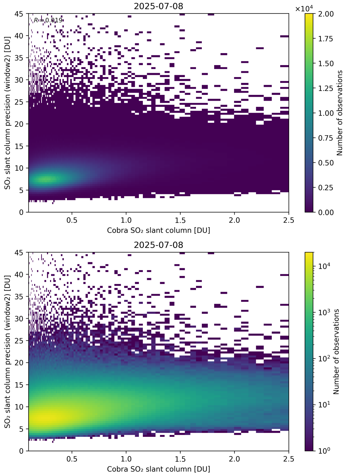
Figure 221: Scatter density plot of “Cobra SO 2 slant column” against “SO 2 slant column precision (window2)” for 2025-07-08 to 2025-07-09.
