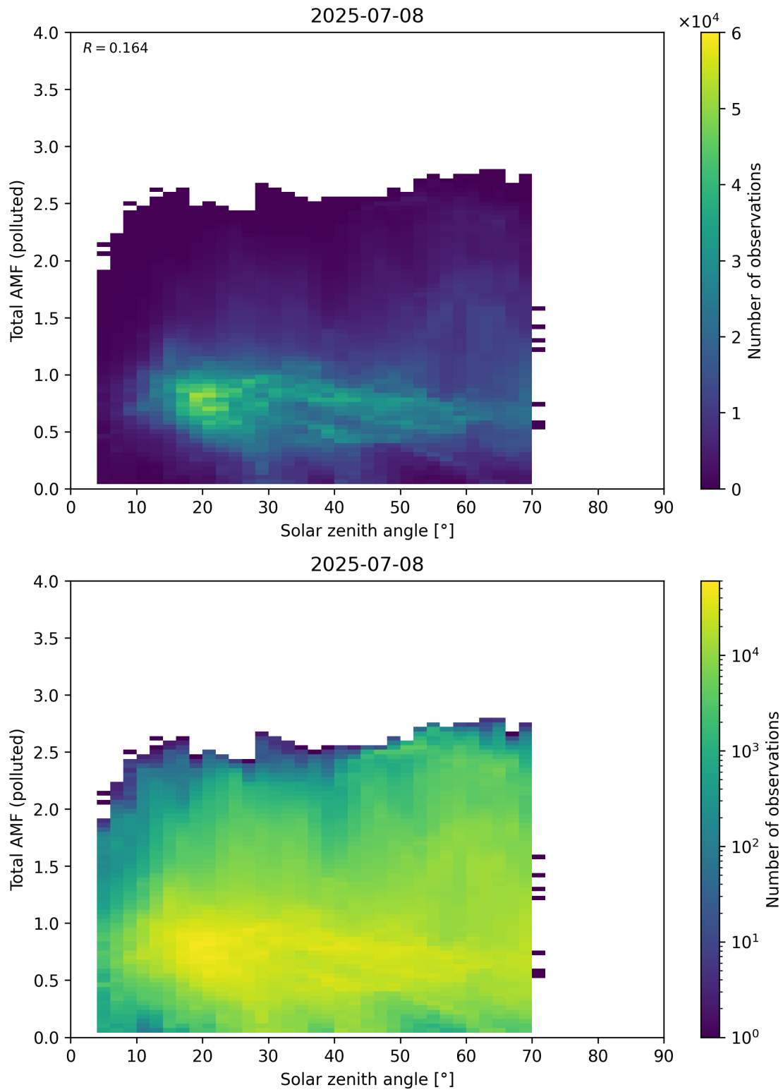
Figure 189: Scatter density plot of “Solar zenith angle” against “Total AMF (polluted)” for 2025-07-08 to 2025-07-09.
