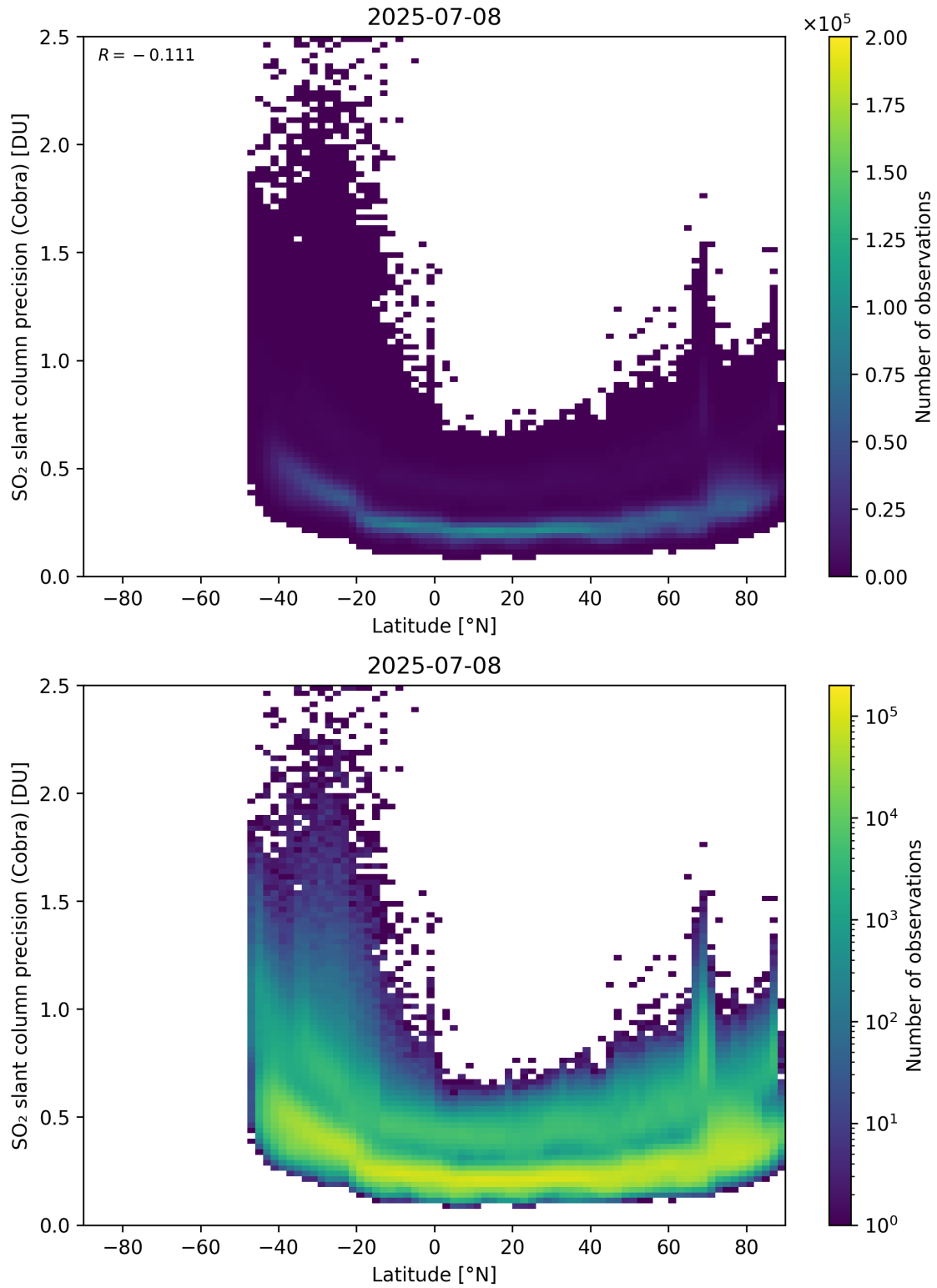
Figure 158: Scatter density plot of “Latitude” against “SO 2 slant column precision (Cobra)” for 2025-07-08 to 2025-07-09.
