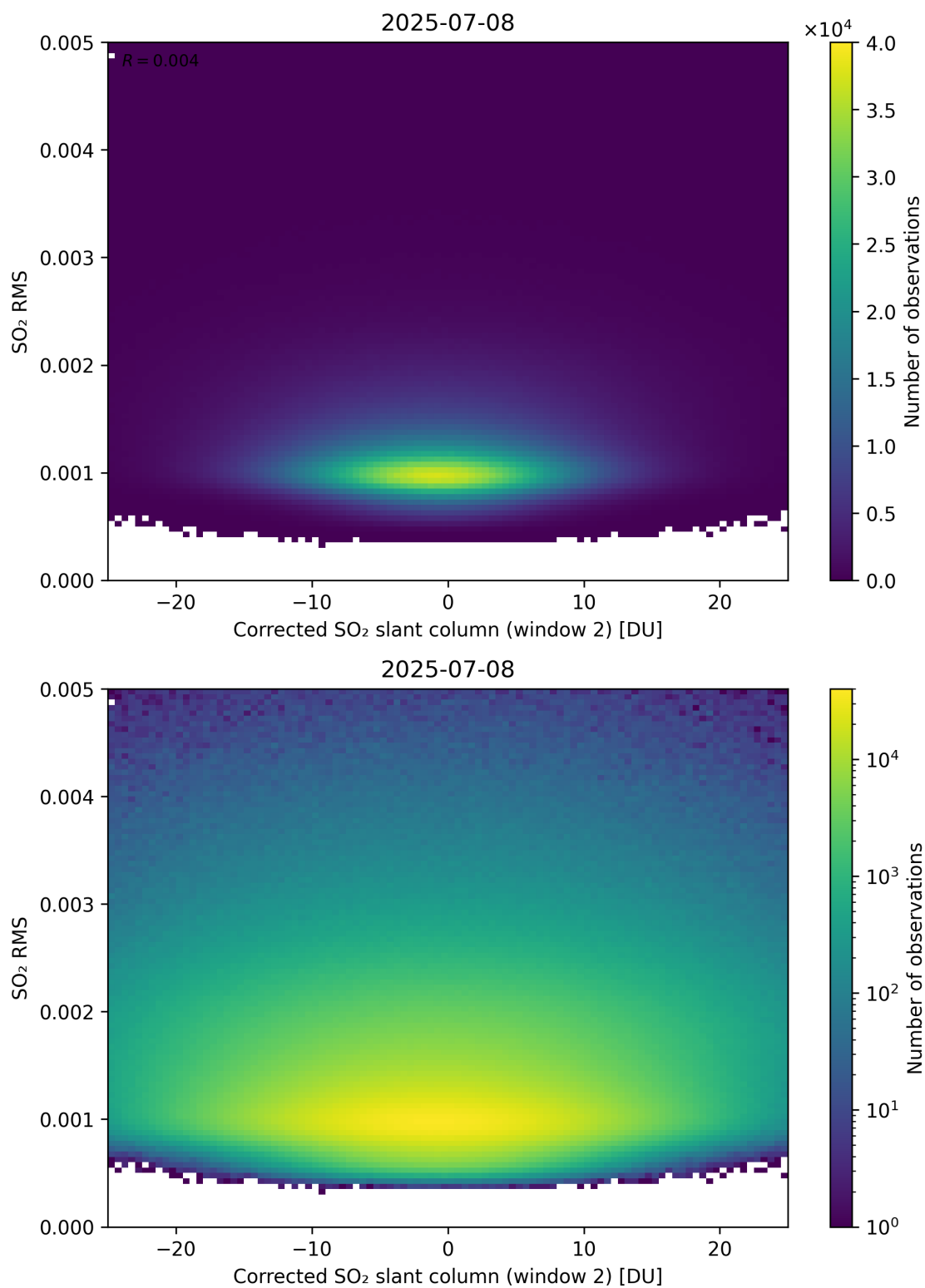
Figure 248: Scatter density plot of “Corrected SO 2 slant column (window 2)” against “SO 2 RMS” for 2025-07-08 to 2025-07-09.
