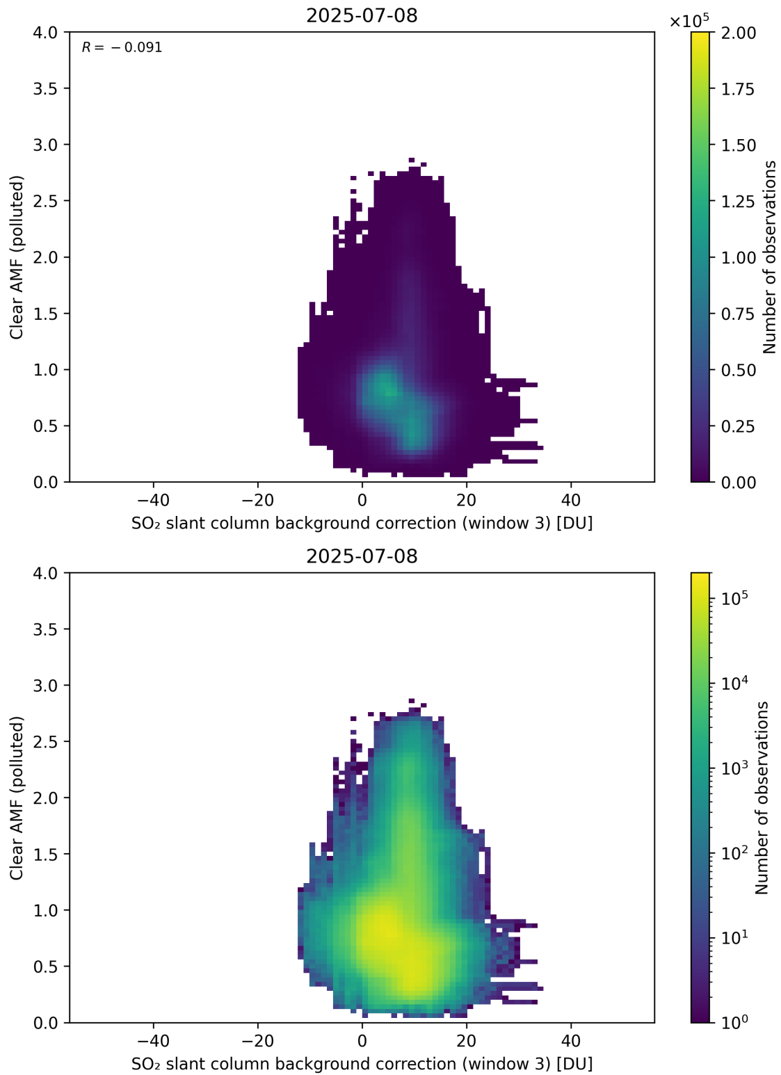
Figure 135: Scatter density plot of “SO 2 slant column background correction (window 3)” against “Clear AMF (polluted)” for 2025-07-08 to 2025-07-09.
