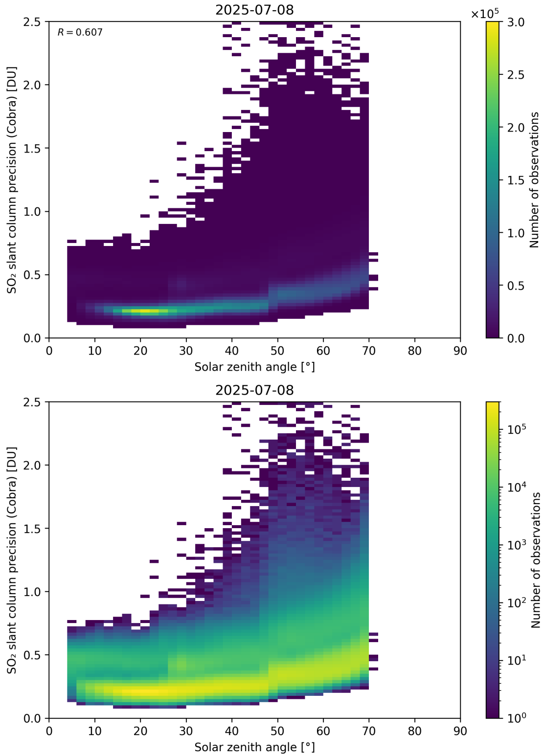
Figure 180: Scatter density plot of “Solar zenith angle” against “SO 2 slant column precision (Cobra)” for 2025-07-08 to 2025-07-09.
