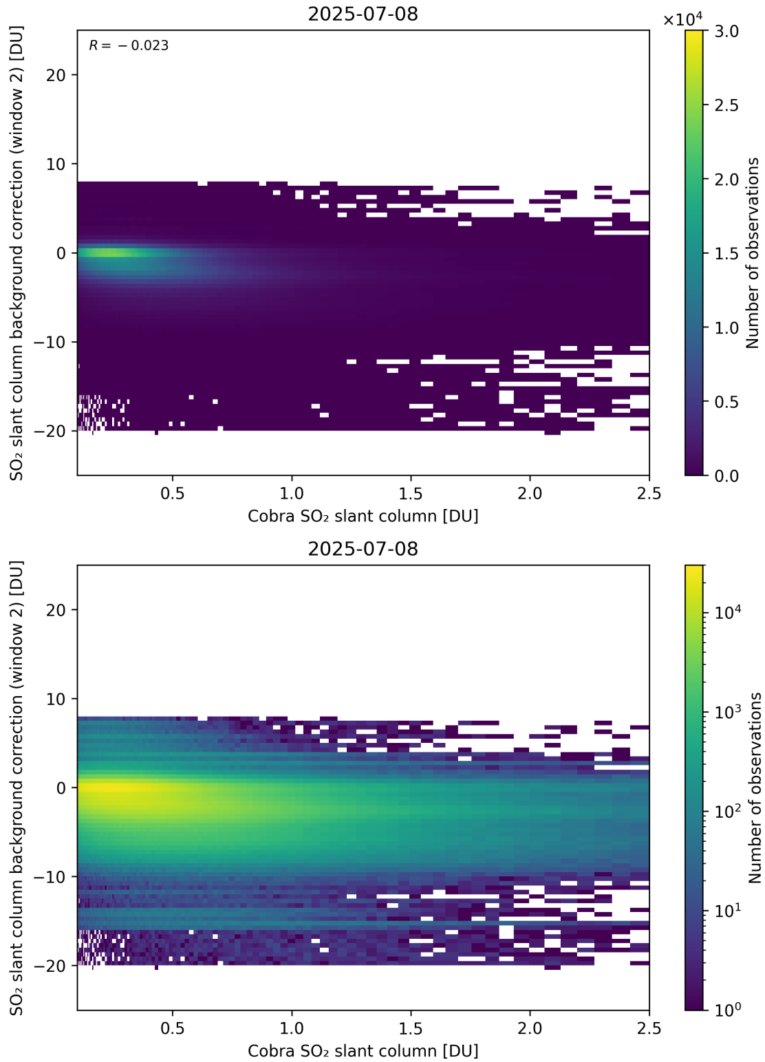
Figure 194: Scatter density plot of “Cobra SO 2 slant column” against “SO 2 slant column background correction (window 2)” for 2025-07-08 to 2025-07-09.
