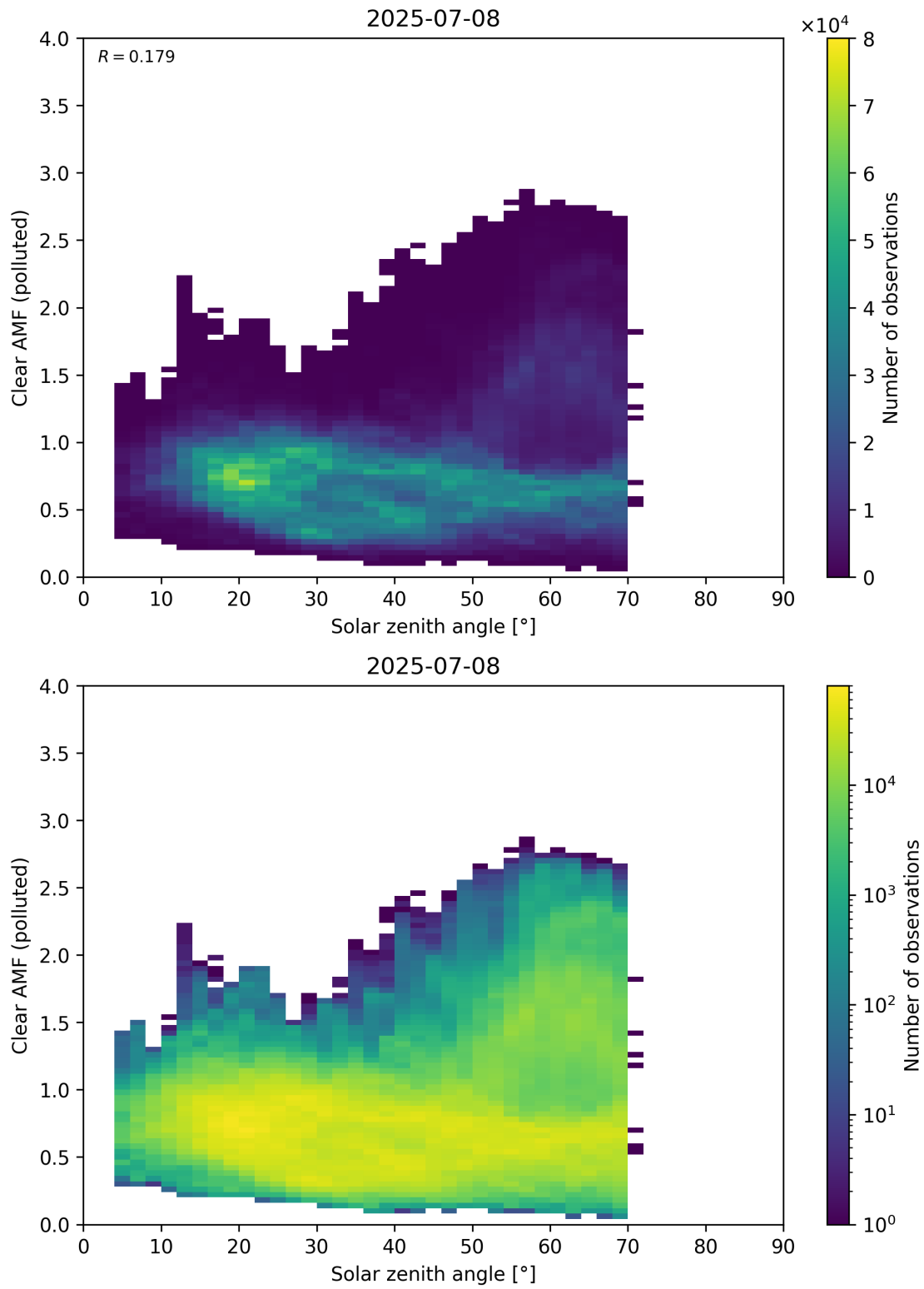
Figure 178: Scatter density plot of “Solar zenith angle” against “Clear AMF (polluted)” for 2025-07-08 to 2025-07-09.
