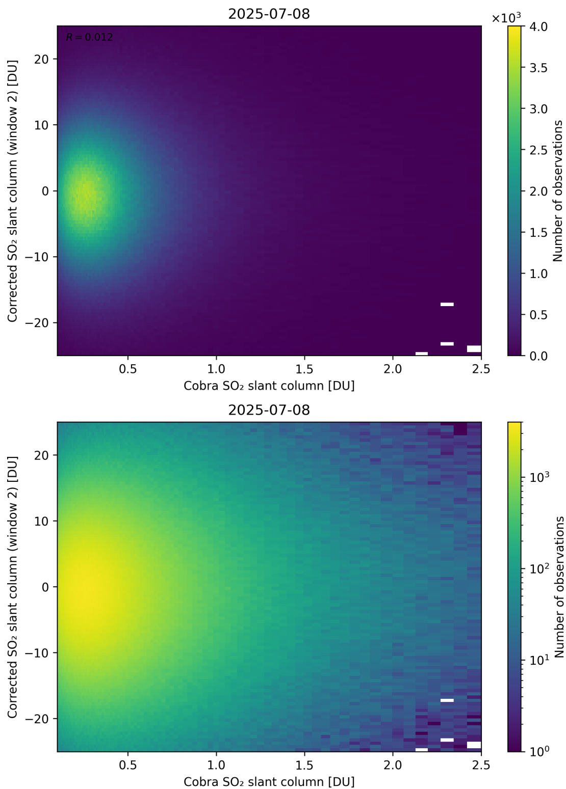
Figure 217: Scatter density plot of “Cobra SO 2 slant column” against “Corrected SO 2 slant column (window 2)” for 2025-07-08 to 2025-07-09.
