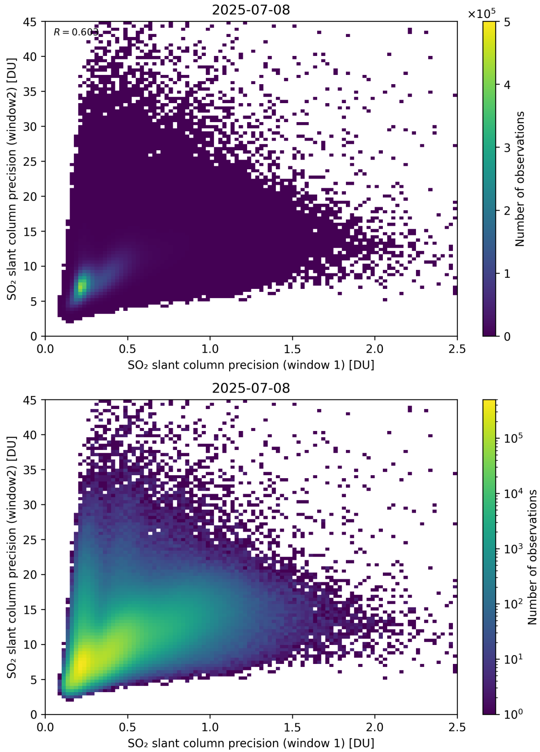
Figure 277: Scatter density plot of “SO 2 slant column precision (window 1)” against “SO 2 slant column precision (window2)” for 2025-07-08 to 2025-07-09.
