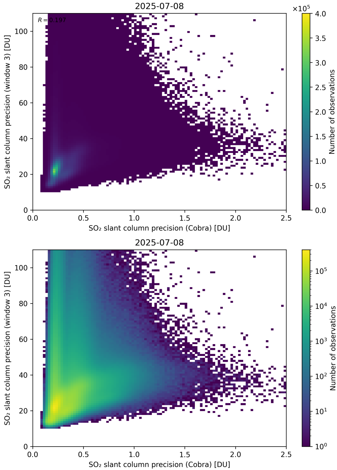
Figure 212: Scatter density plot of “SO 2 slant column precision (Cobra)” against “SO 2 slant column precision (window 3)” for 2025-07-08 to 2025-07-09.
