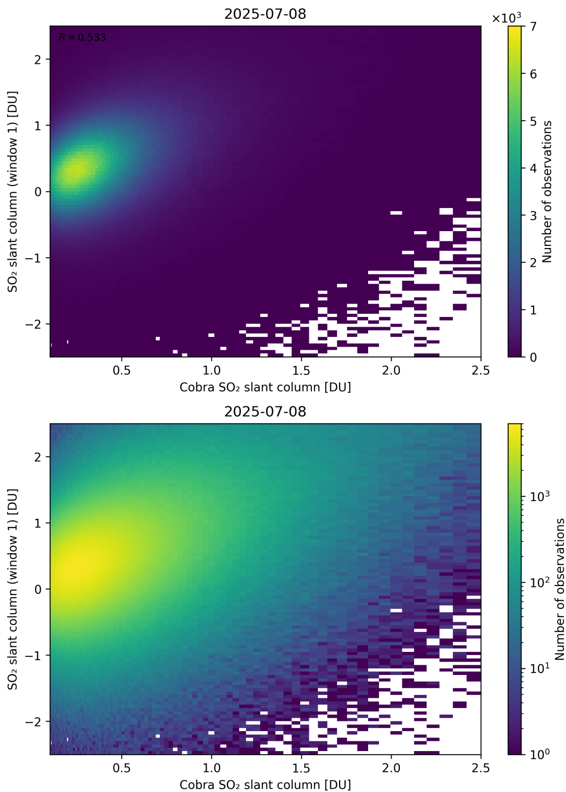
Figure 219: Scatter density plot of “Cobra SO 2 slant column” against “SO 2 slant column (window 1)” for 2025-07-08 to 2025-07-09.
