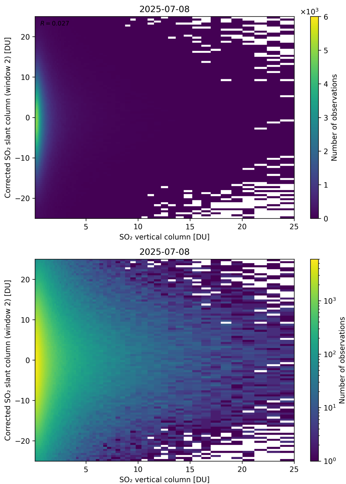
Figure 352: Scatter density plot of “SO 2 vertical column” against “Corrected SO 2 slant column (window 2)” for 2025-07-08 to 2025-07-09.
