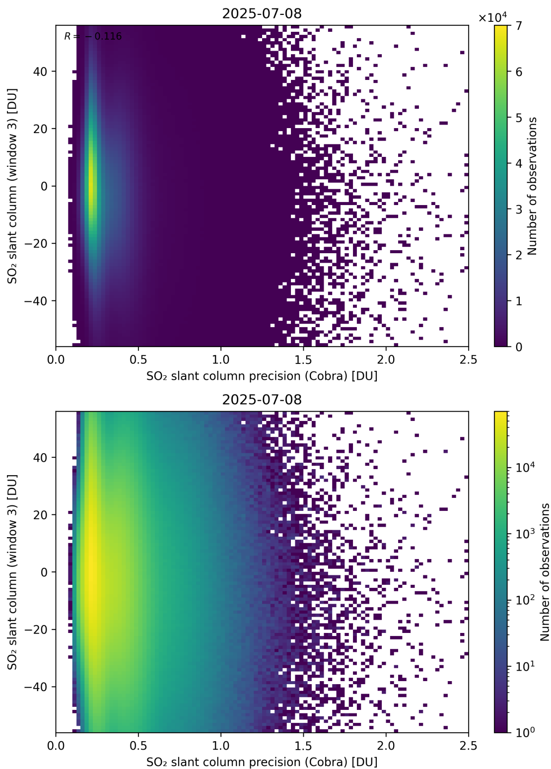
Figure 211: Scatter density plot of “SO 2 slant column precision (Cobra)” against “SO 2 slant column (window 3)” for 2025-07-08 to 2025-07-09.
