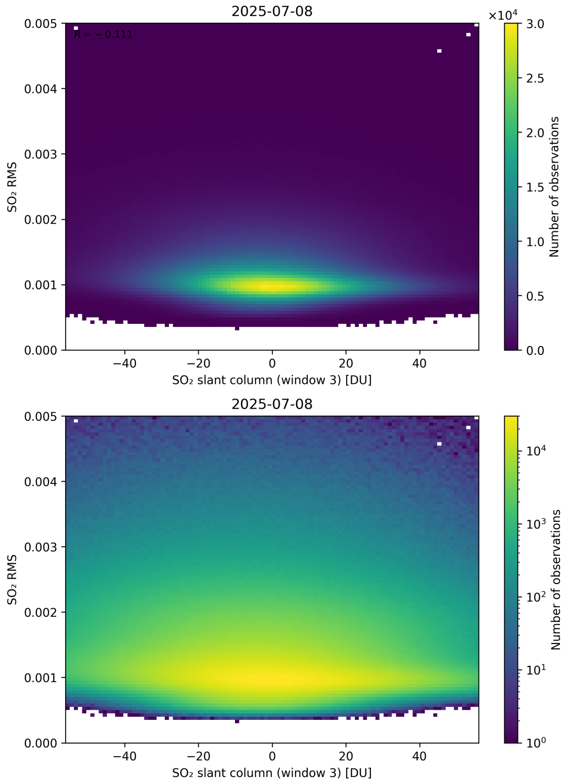
Figure 306: Scatter density plot of “SO 2 slant column (window 3)” against “SO 2 RMS” for 2025-07-08 to 2025-07-09.
