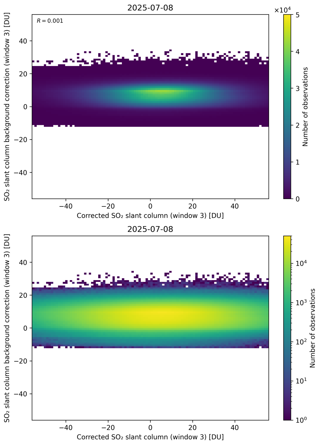
Figure 255: Scatter density plot of “Corrected SO 2 slant column (window 3)” against “SO 2 slant column background correction (window 3)” for 2025-07-08 to 2025-07-09.
