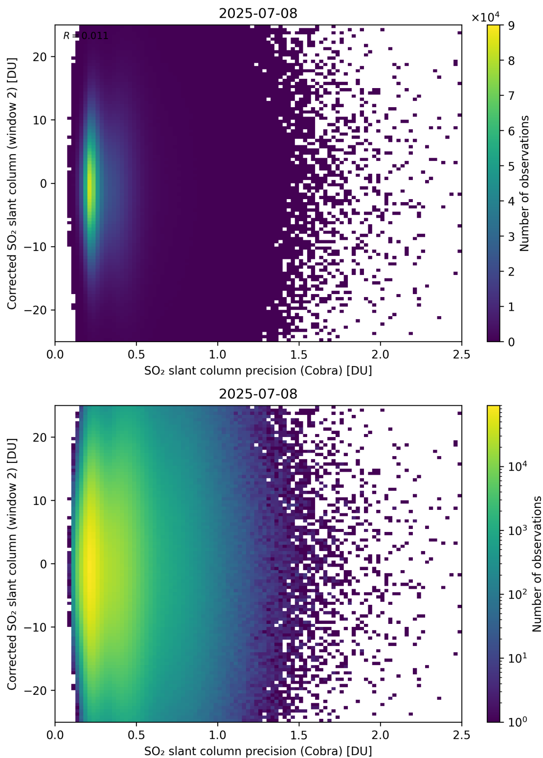
Figure 206: Scatter density plot of “SO 2 slant column precision (Cobra)” against “Corrected SO 2 slant column (window 2)” for 2025-07-08 to 2025-07-09.
