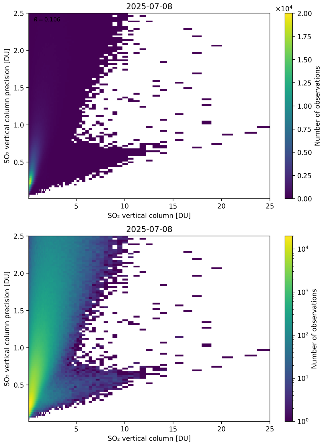
Figure 361: Scatter density plot of “SO 2 vertical column” against “SO 2 vertical column precision” for 2025-07-08 to 2025-07-09.
