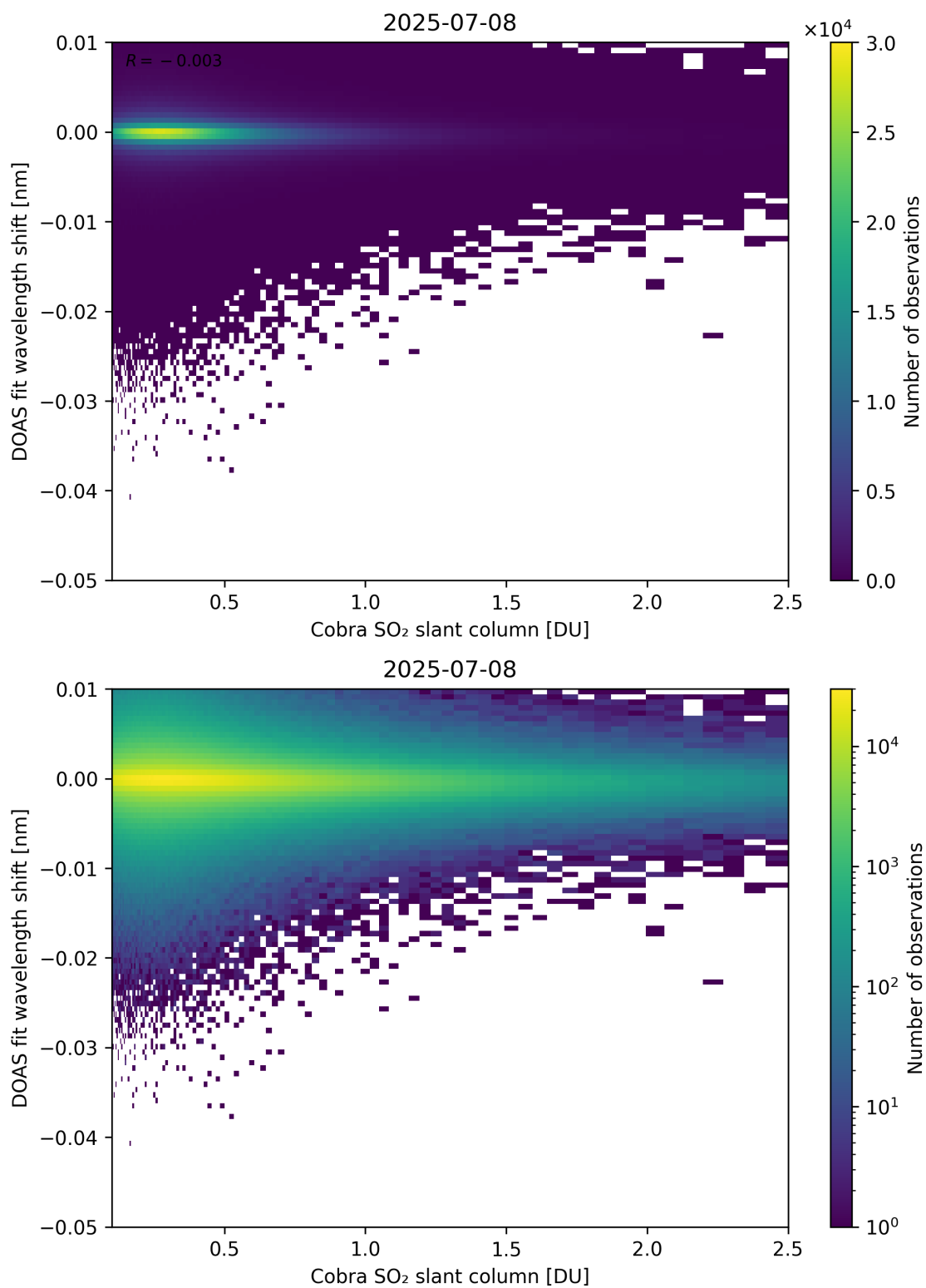
Figure 196: Scatter density plot of “Cobra SO 2 slant column” against “DOAS fit wavelength shift” for 2025-07-08 to 2025-07-09.
