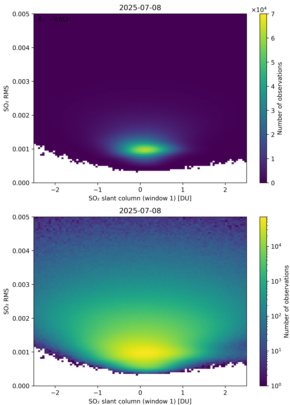
Figure 267: Scatter density plot of “SO 2 slant column (window 1)” against “SO 2 RMS” for 2025-07-08 to 2025-07-09.
