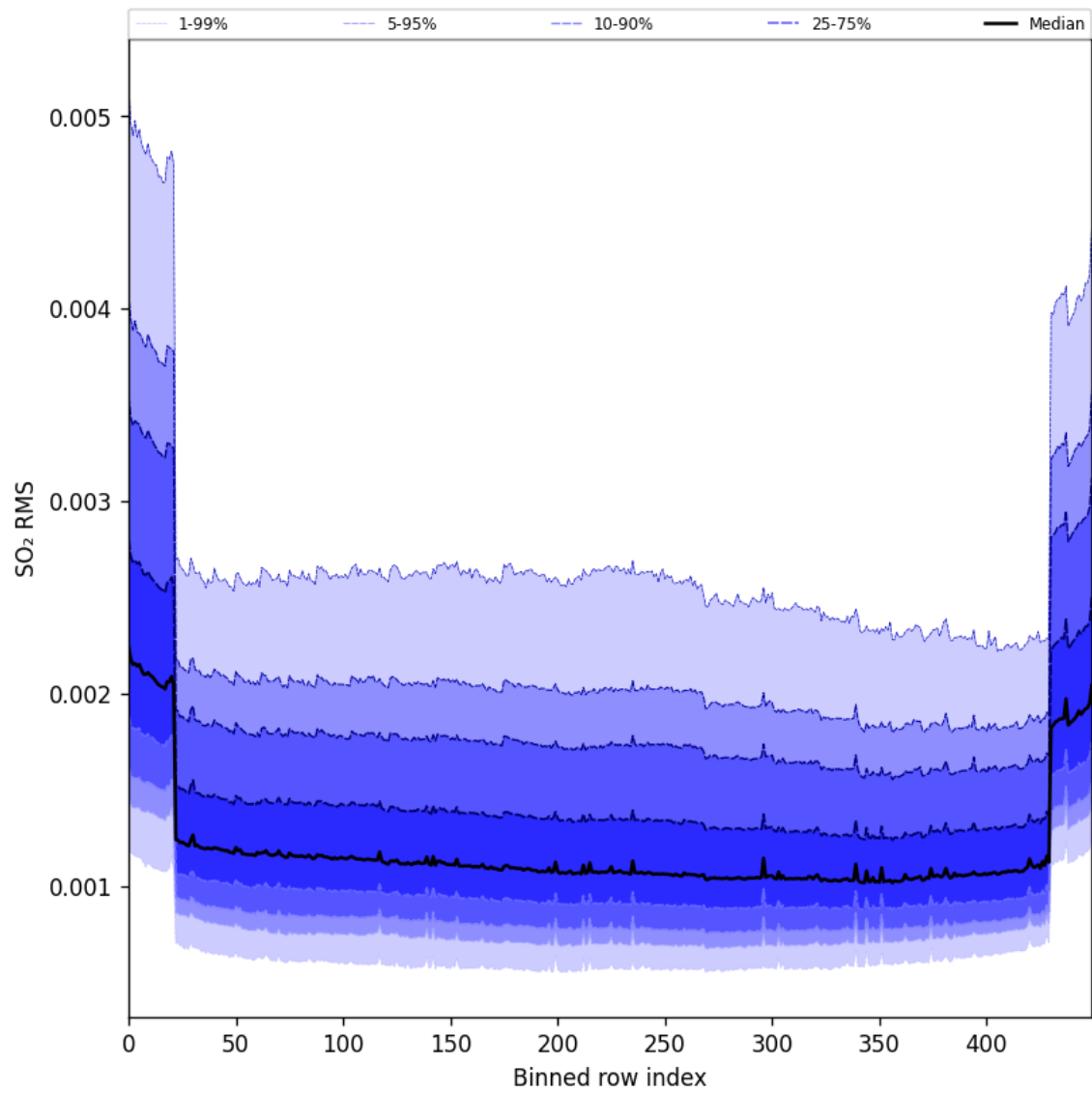
Figure 104: Along track statistics of “SO 2 RMS” for 2025-07-08 to 2025-07-09
