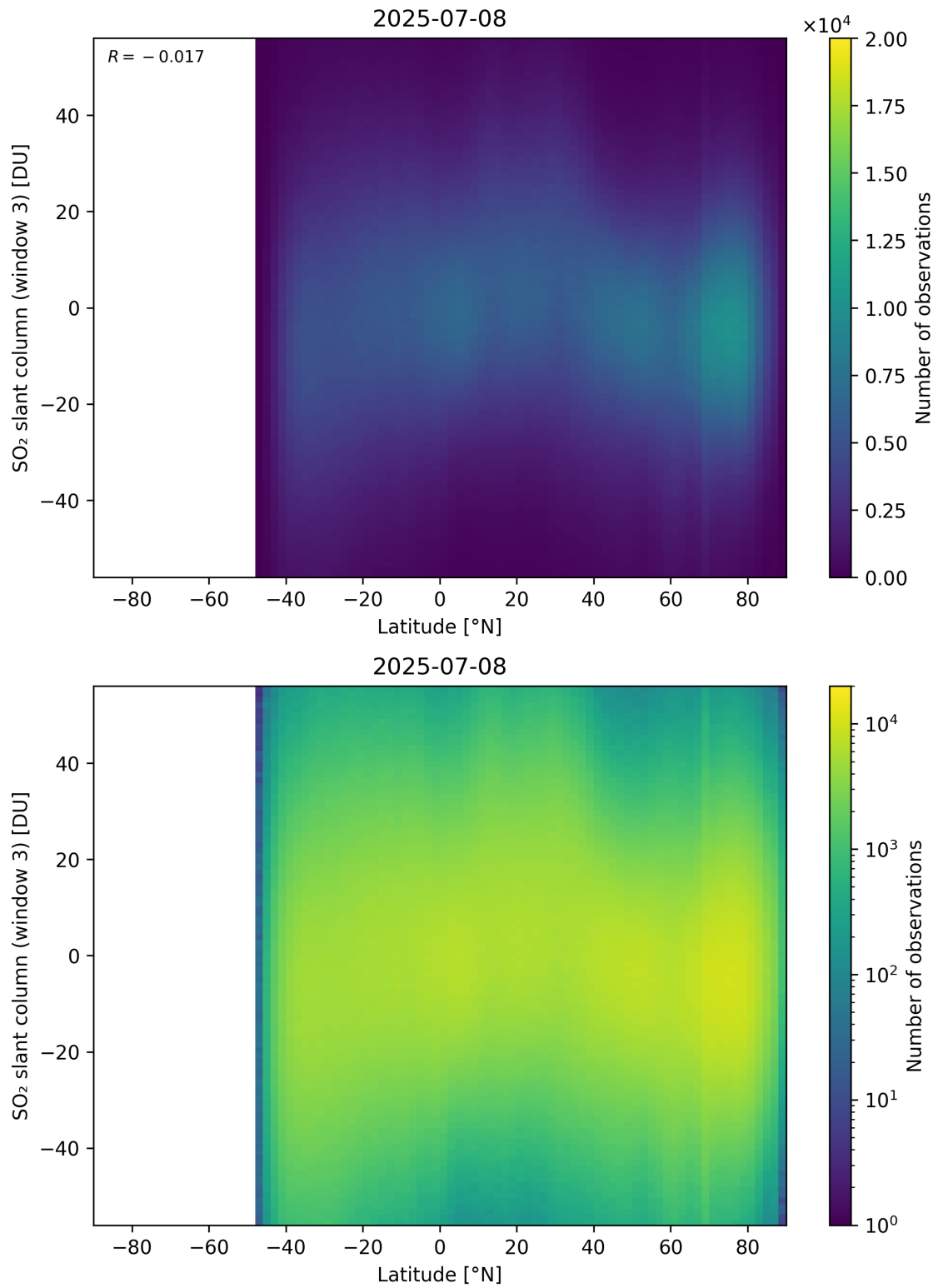
Figure 165: Scatter density plot of “Latitude” against “SO 2 slant column (window 3)” for 2025-07-08 to 2025-07-09.
