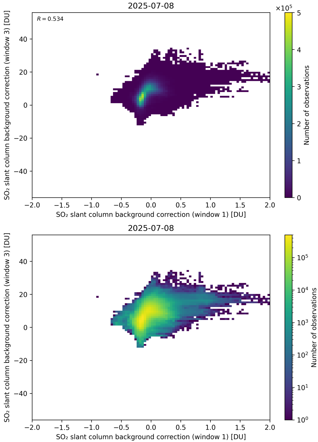
Figure 110: Scatter density plot of “SO 2 slant column background correction (window 1)” against “SO 2 slant column background correction (window 3)” for 2025-07-08 to 2025-07-09.
