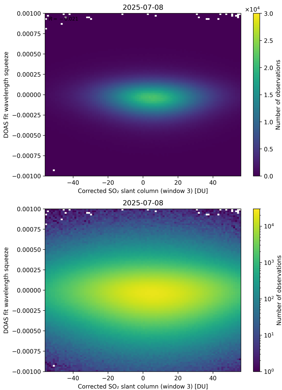
Figure 257: Scatter density plot of “Corrected SO 2 slant column (window 3)” against “DOAS fit wavelength squeeze” for 2025-07-08 to 2025-07-09.
