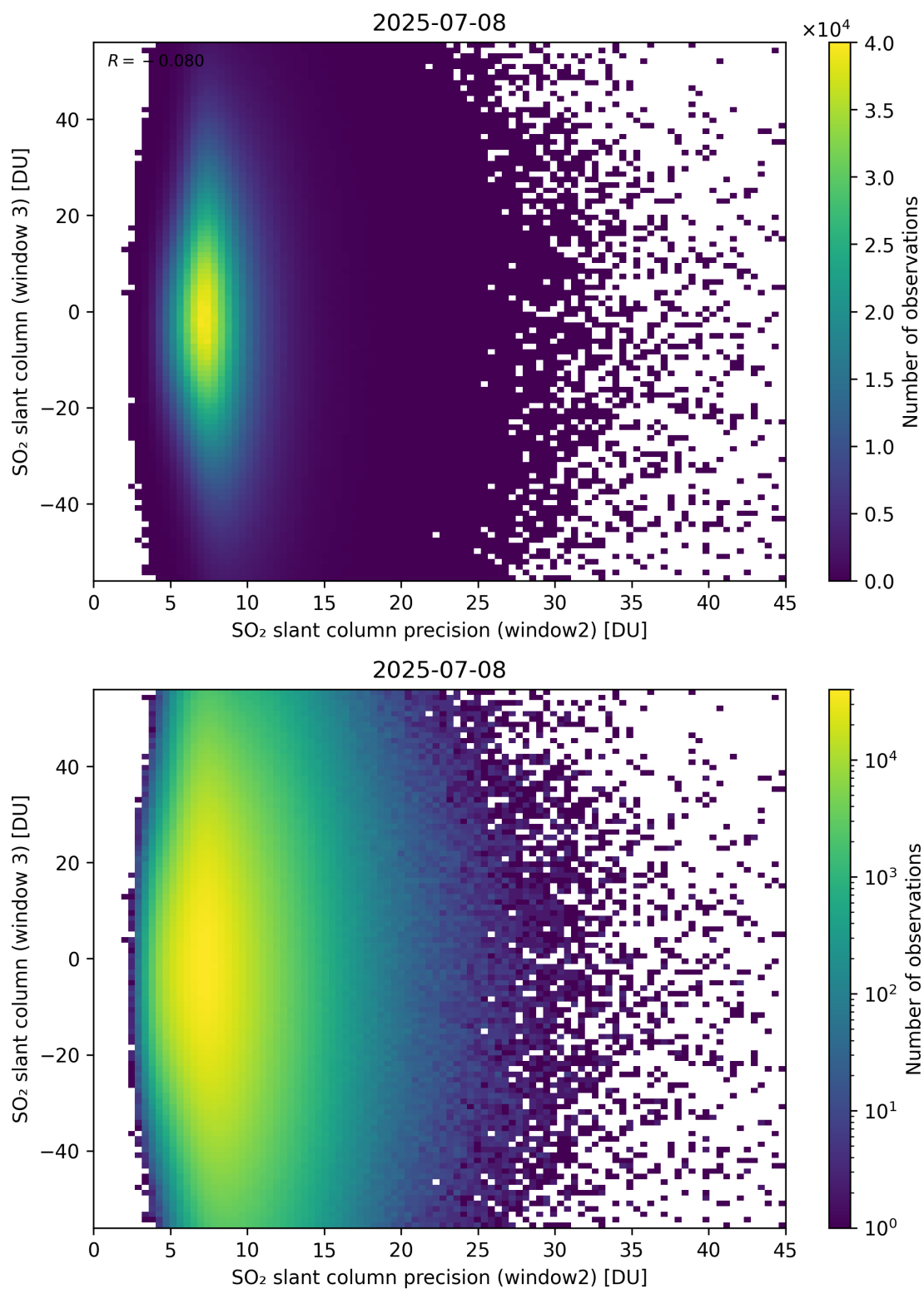
Figure 299: Scatter density plot of “SO 2 slant column precision (window2)” against “SO 2 slant column (window 3)” for 2025-07-08 to 2025-07-09.
