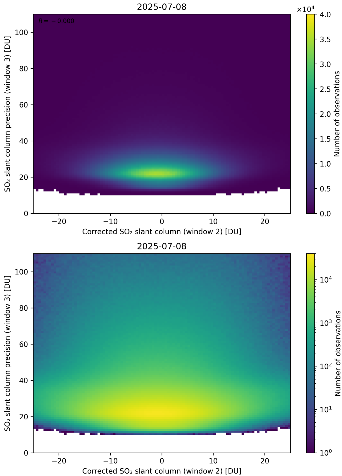
Figure 252: Scatter density plot of “Corrected SO 2 slant column (window 2)” against “SO 2 slant column precision (window 3)” for 2025-07-08 to 2025-07-09.
