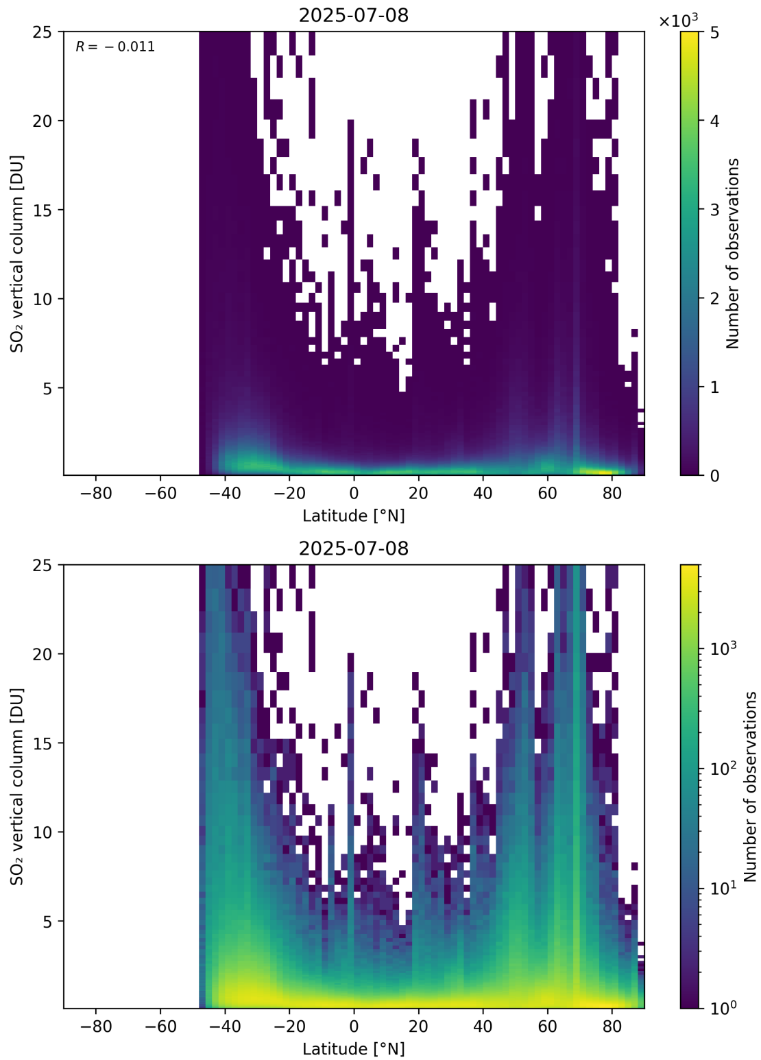
Figure 169: Scatter density plot of “Latitude” against “SO 2 vertical column” for 2025-07-08 to 2025-07-09.
