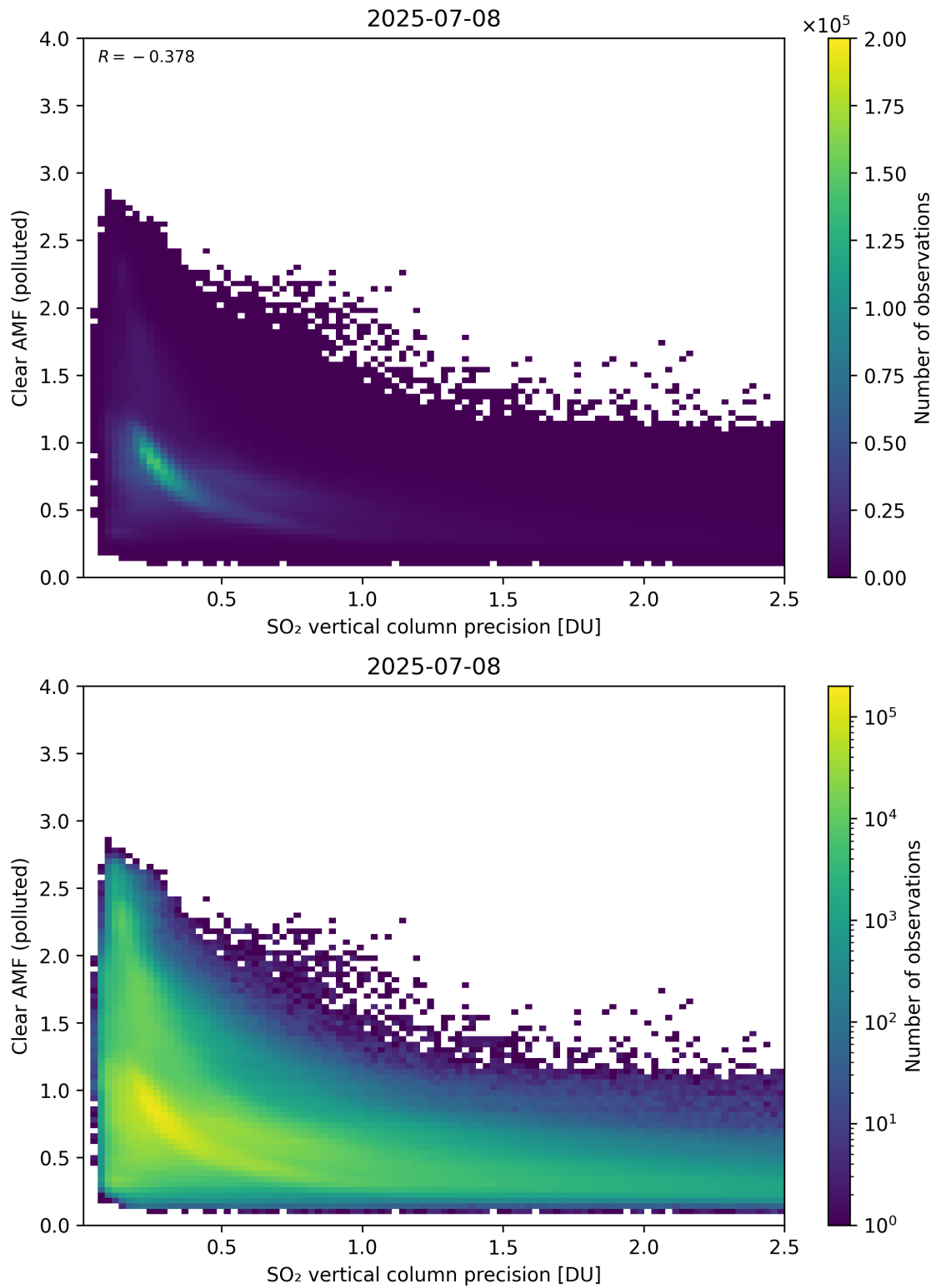
Figure 335: Scatter density plot of “SO 2 vertical column precision” against “Clear AMF (polluted)” for 2025-07-08 to 2025-07-09.
