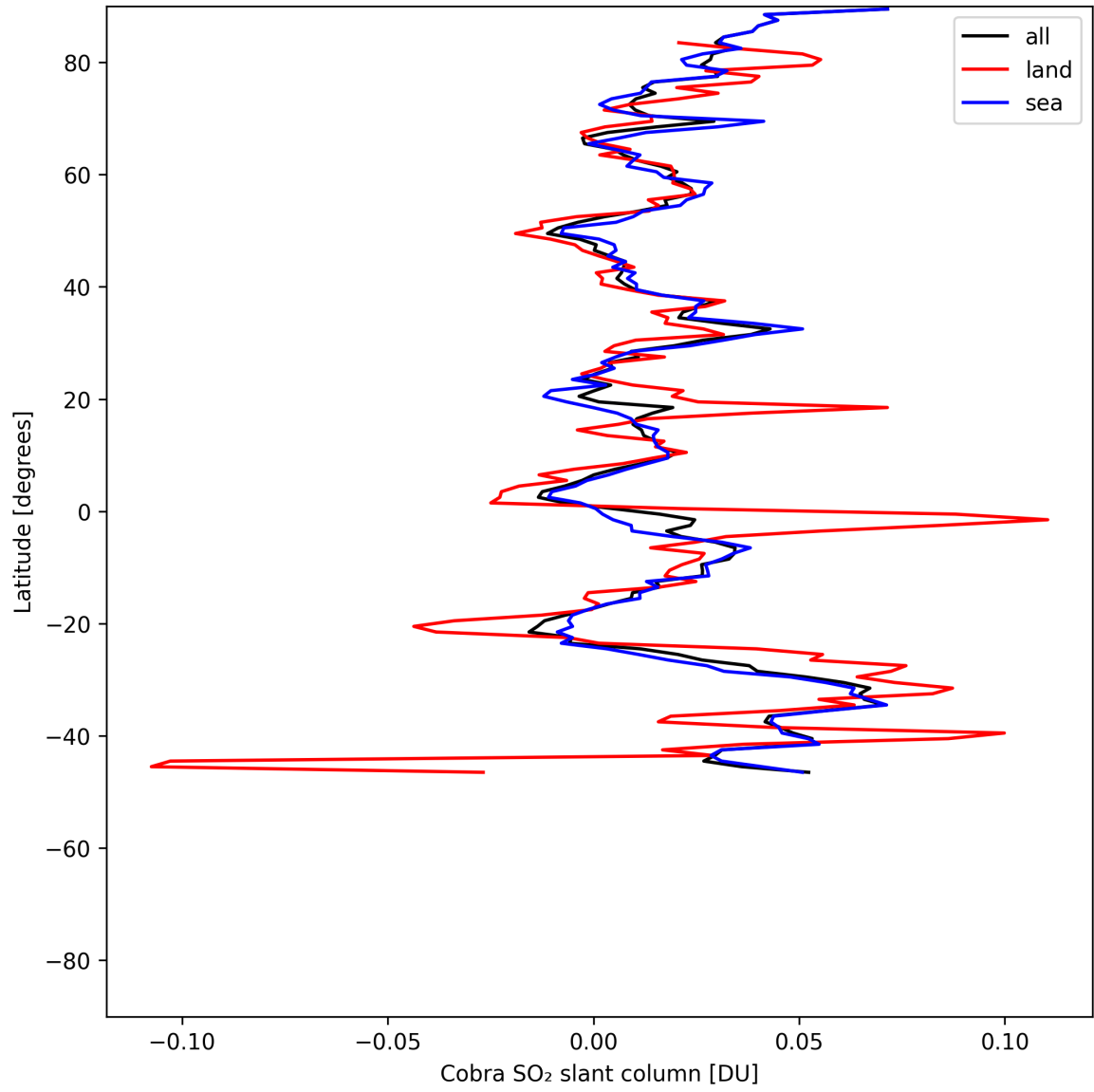
Figure 35: Zonal average of “Cobra SO 2 slant column” for 2025-07-08 to 2025-07-09.
