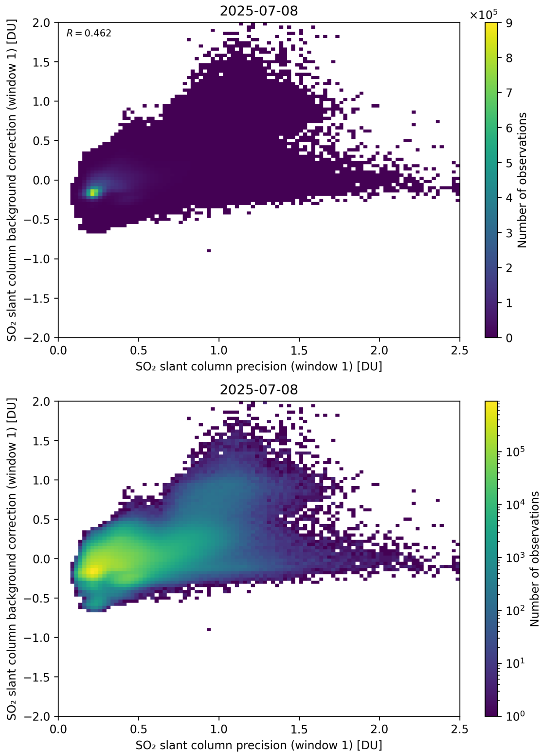
Figure 268: Scatter density plot of “SO 2 slant column precision (window 1)” against “SO 2 slant column background correction (window 1)” for 2025-07-08 to 2025-07-09.
