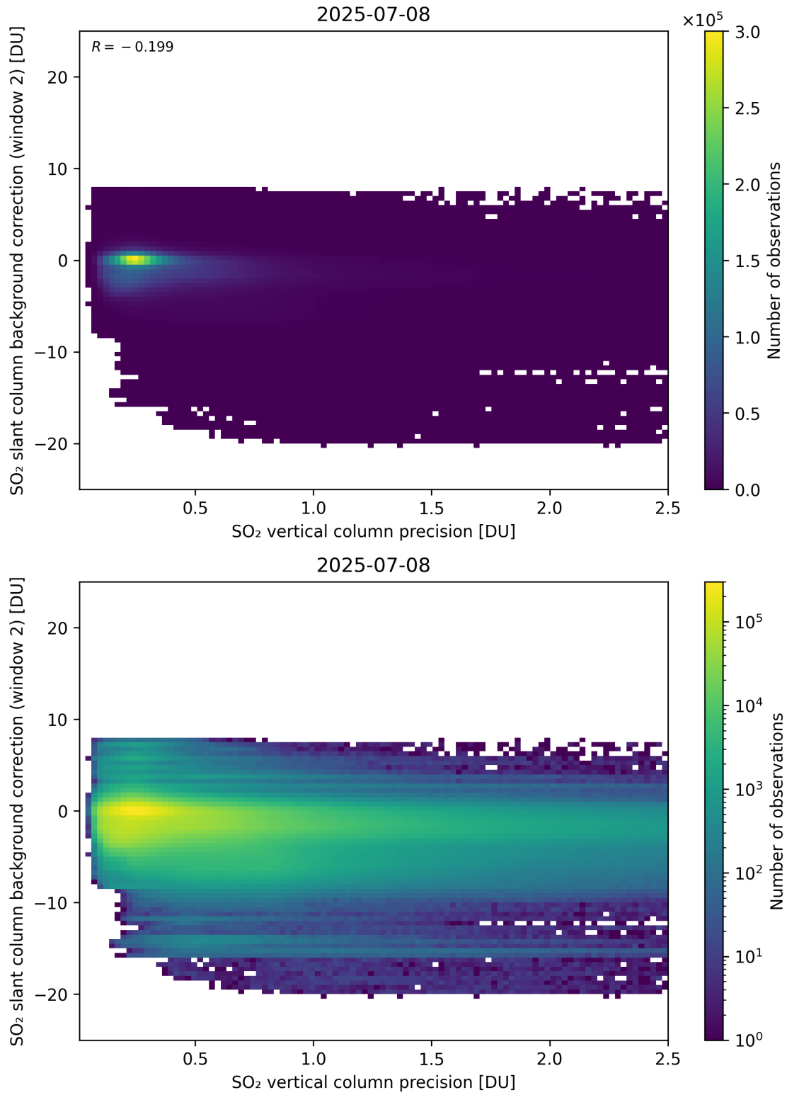
Figure 330: Scatter density plot of “SO 2 vertical column precision” against “SO 2 slant column background correction (window 2)” for 2025-07-08 to 2025-07-09.
