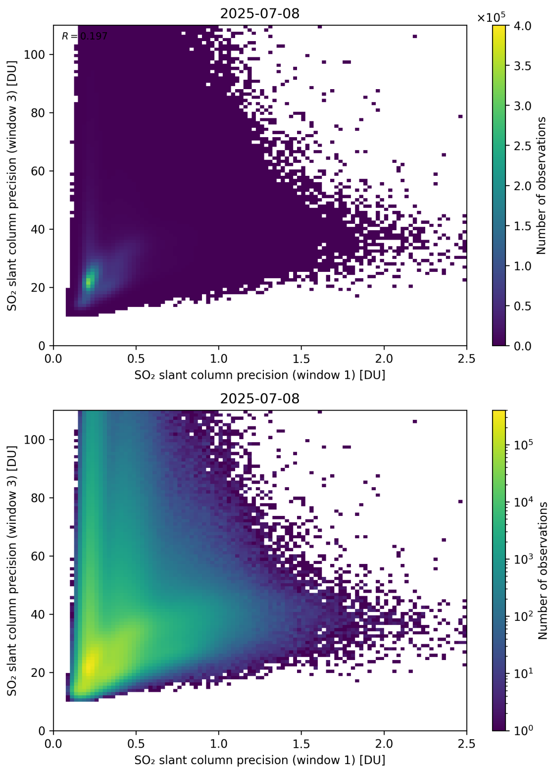
Figure 279: Scatter density plot of “SO 2 slant column precision (window 1)” against “SO 2 slant column precision (window 3)” for 2025-07-08 to 2025-07-09.
