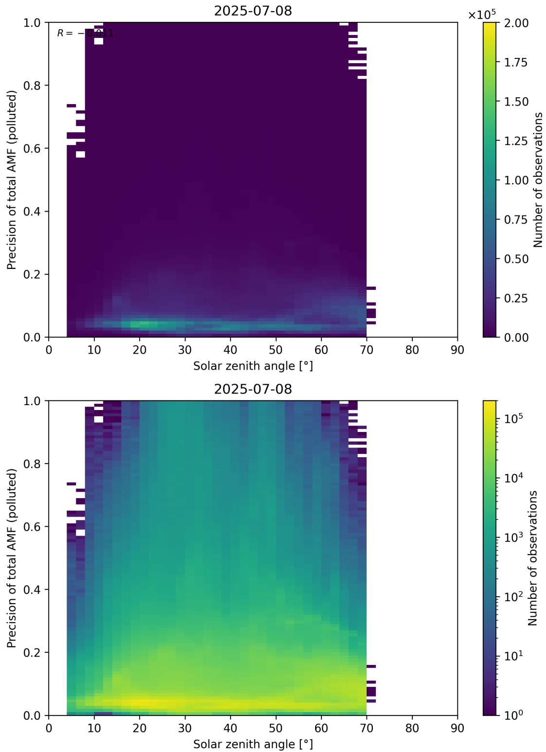
Figure 190: Scatter density plot of “Solar zenith angle” against “Precision of total AMF (polluted)” for 2025-07-08 to 2025-07-09.
