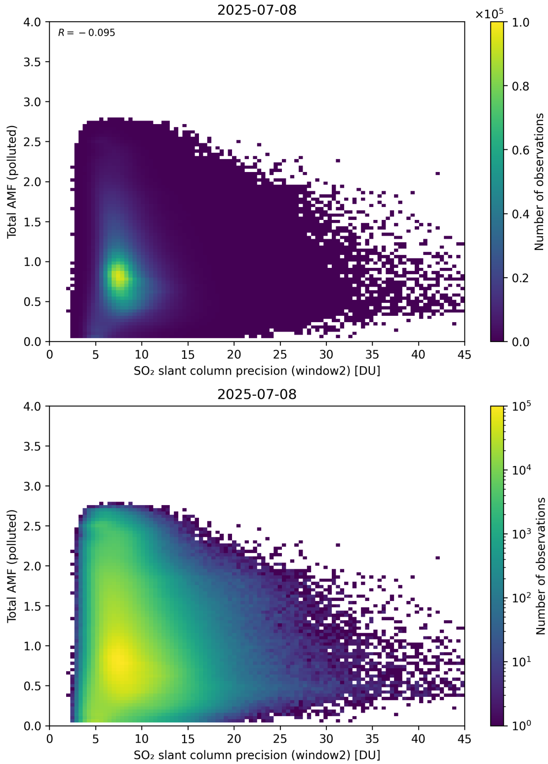
Figure 301: Scatter density plot of “SO 2 slant column precision (window2)” against “Total AMF (polluted)” for 2025-07-08 to 2025-07-09.
