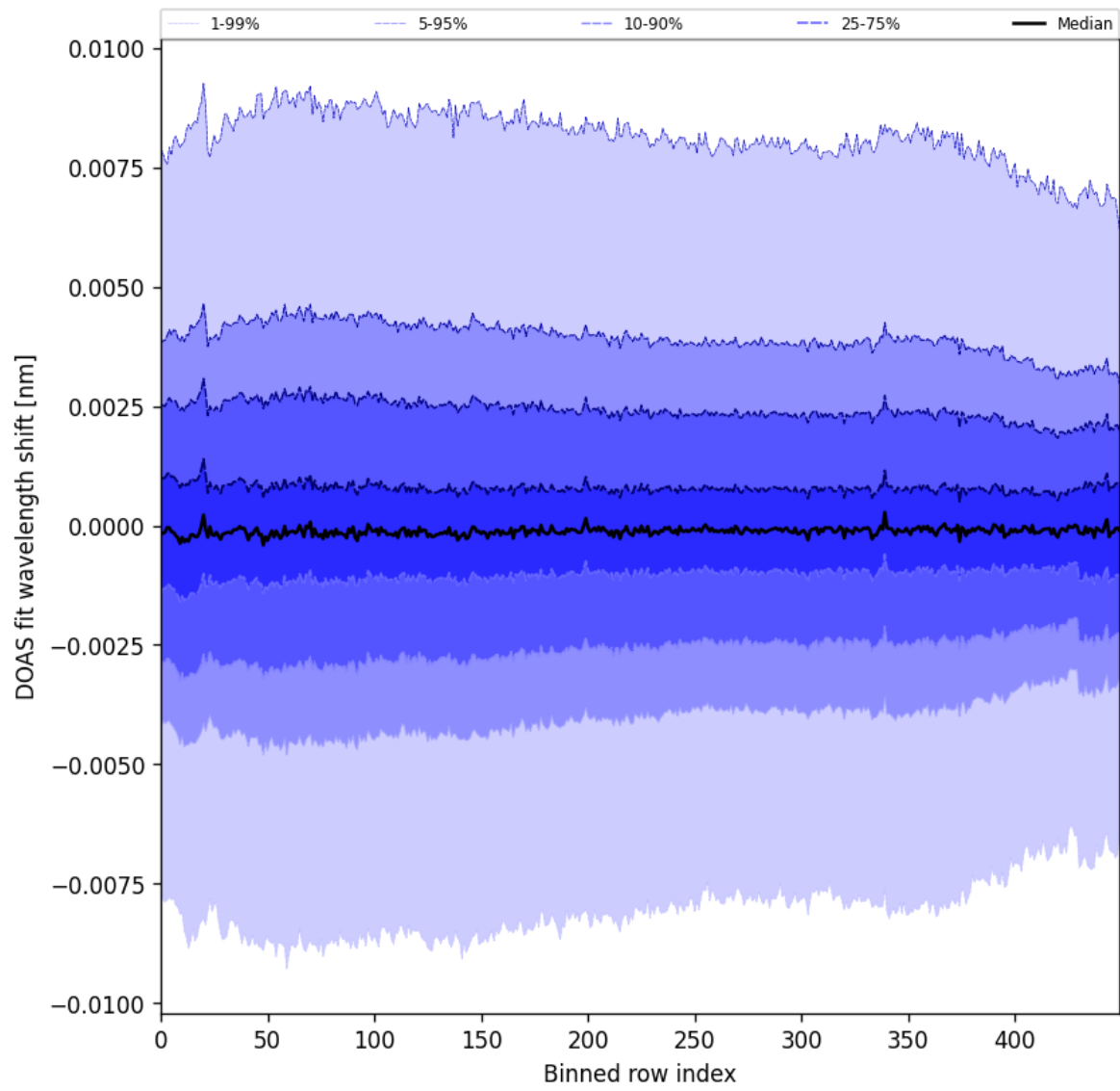
Figure 102: Along track statistics of “DOAS fit wavelength shift” for 2025-07-08 to 2025-07-09
