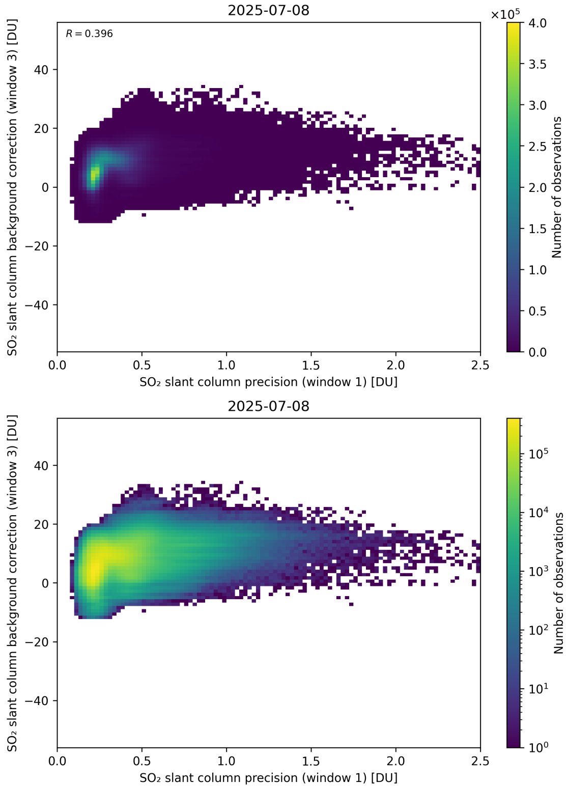
Figure 270: Scatter density plot of “SO 2 slant column precision (window 1)” against “SO 2 slant column background correction (window 3)” for 2025-07-08 to 2025-07-09.
