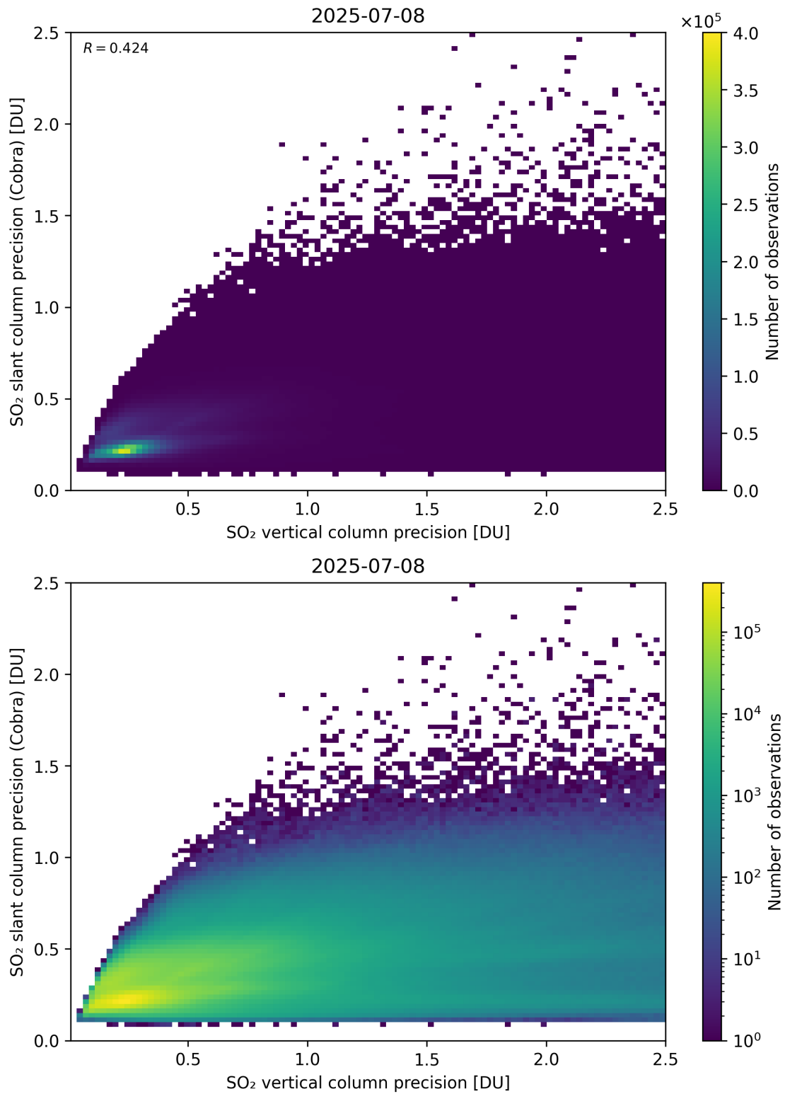
Figure 337: Scatter density plot of “SO 2 vertical column precision” against “SO 2 slant column precision (Cobra)” for 2025-07-08 to 2025-07-09.
