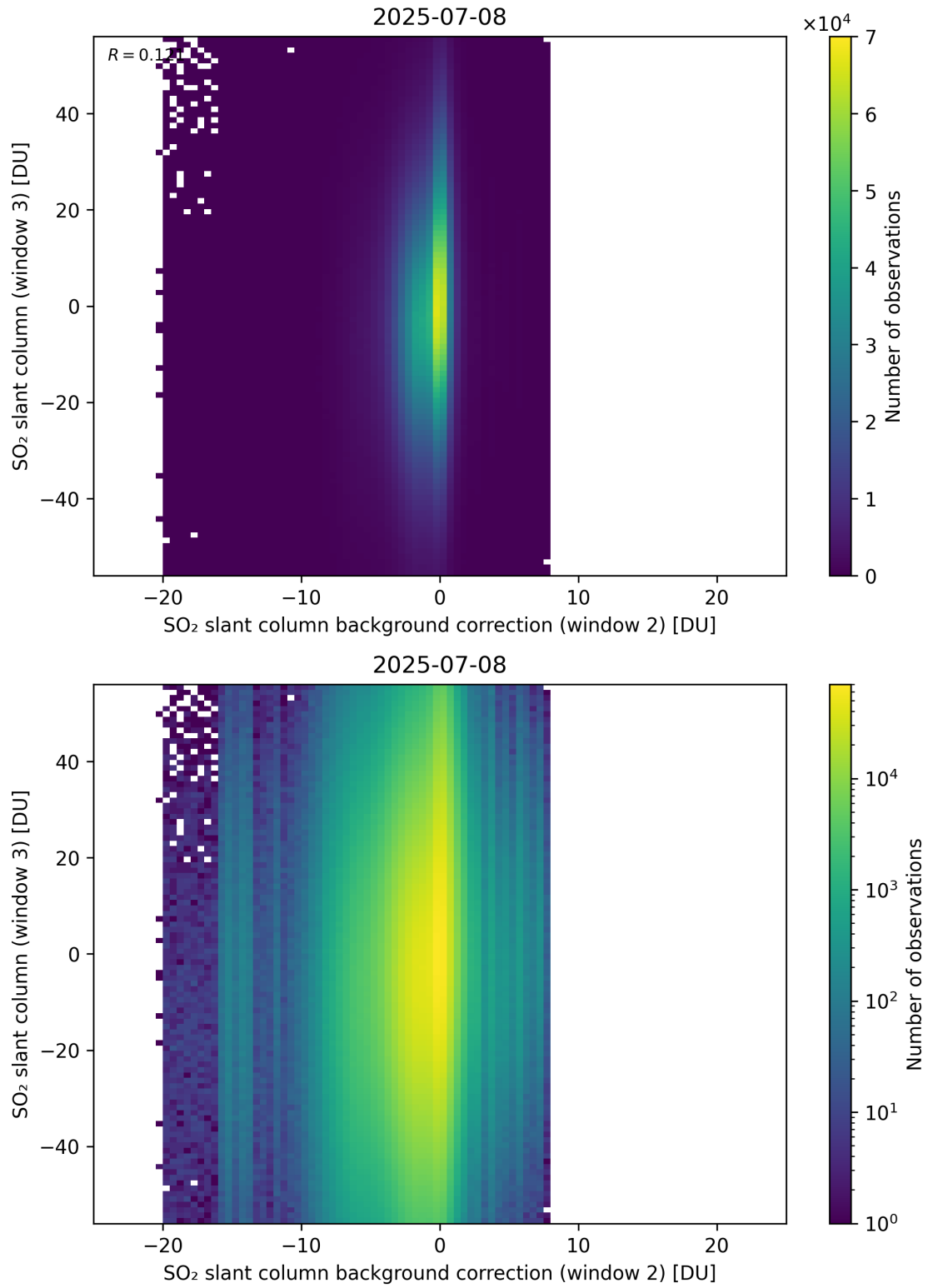
Figure 128: Scatter density plot of “SO 2 slant column background correction (window 2)” against “SO 2 slant column (window 3)” for 2025-07-08 to 2025-07-09.
