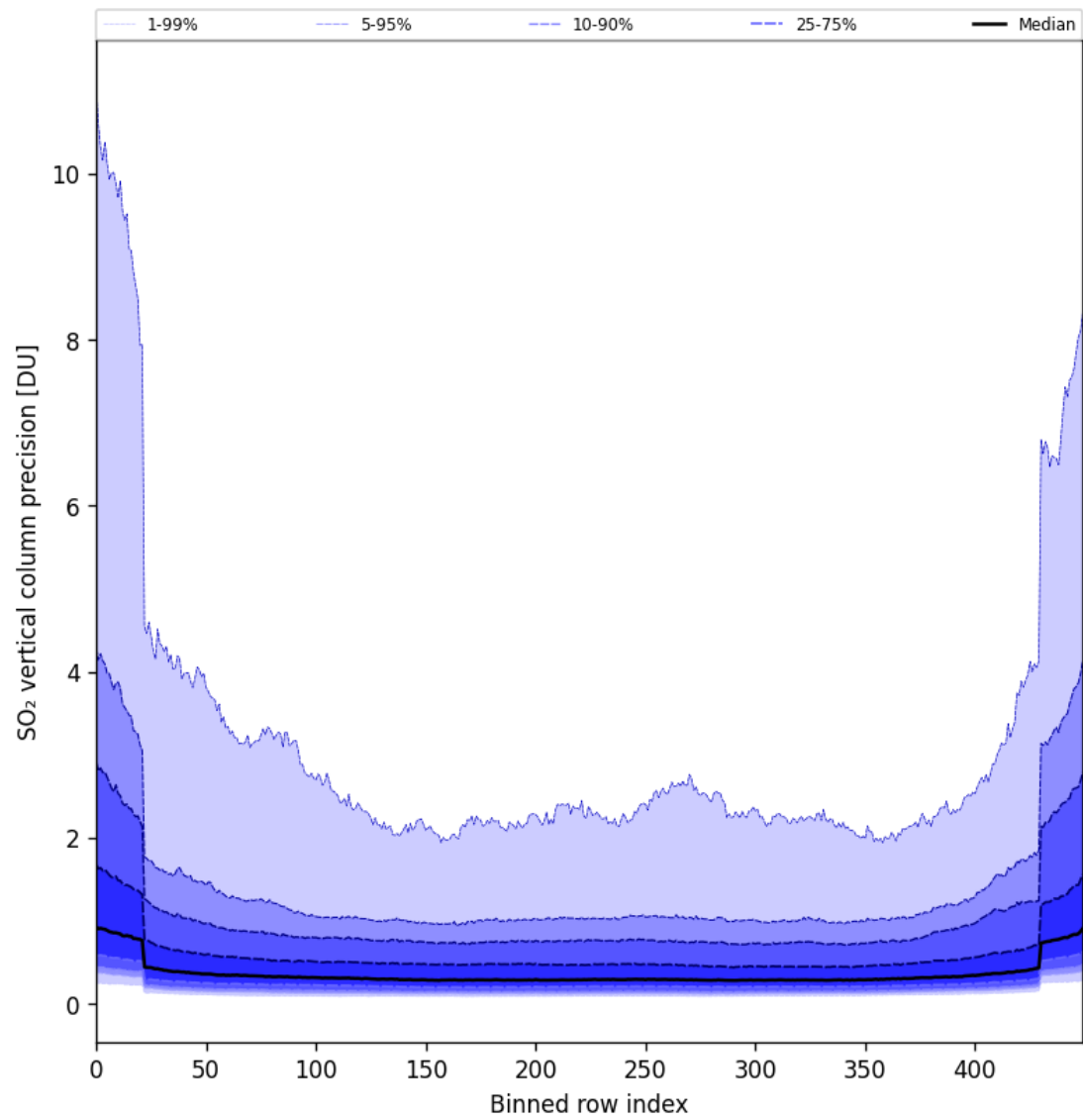
Figure 85: Along track statistics of “SO 2 vertical column precision” for 2025-07-08 to 2025-07-09
