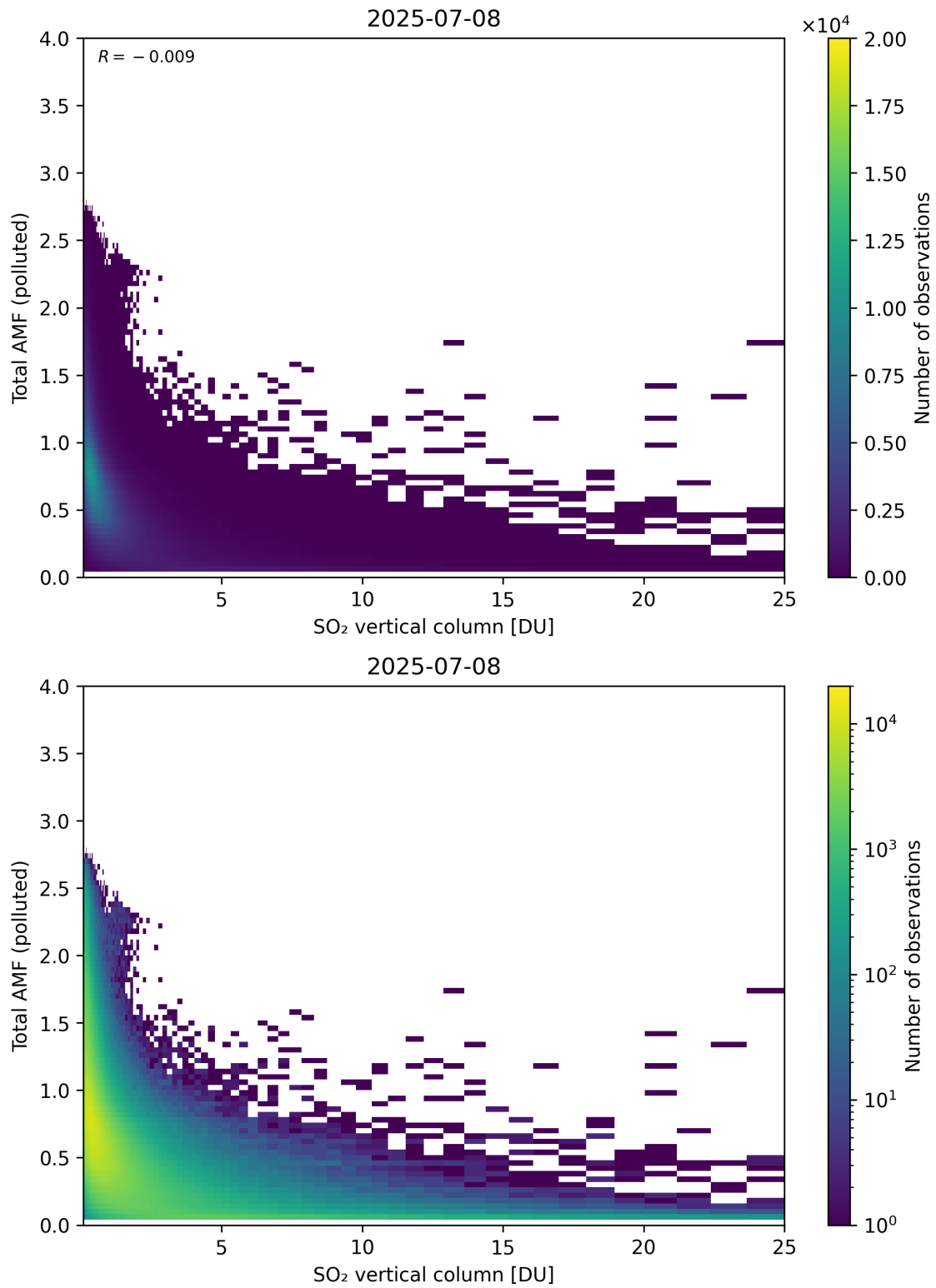
Figure 359: Scatter density plot of “SO 2 vertical column” against “Total AMF (polluted)” for 2025-07-08 to 2025-07-09.
