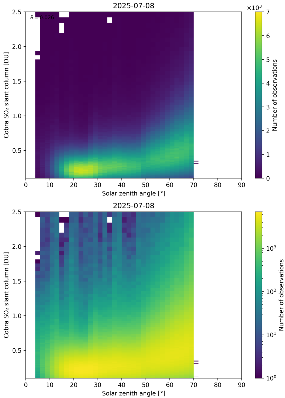
Figure 179: Scatter density plot of “Solar zenith angle” against “Cobra SO 2 slant column” for 2025-07-08 to 2025-07-09.
