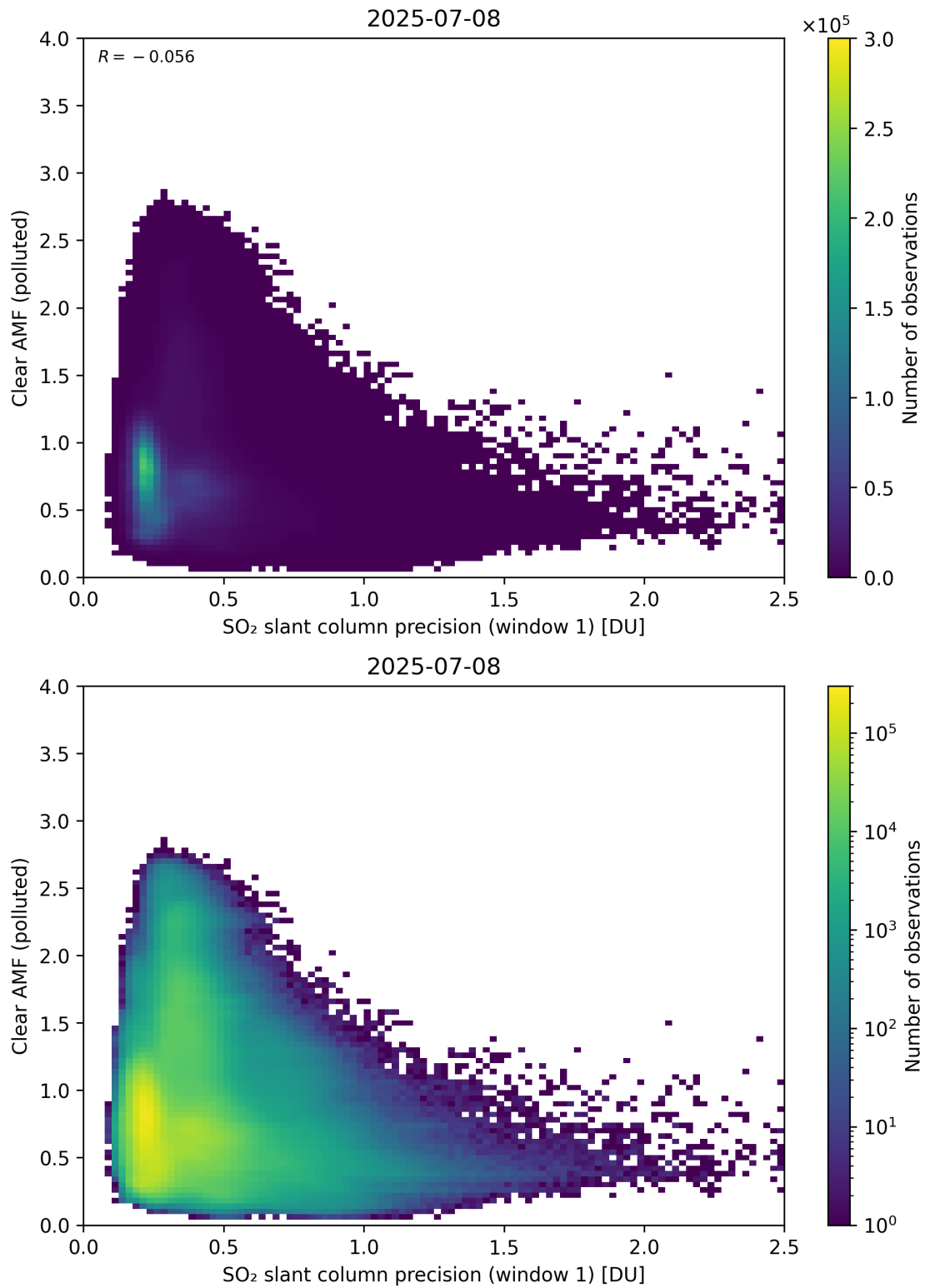
Figure 274: Scatter density plot of “SO 2 slant column precision (window 1)” against “Clear AMF (polluted)” for 2025-07-08 to 2025-07-09.
