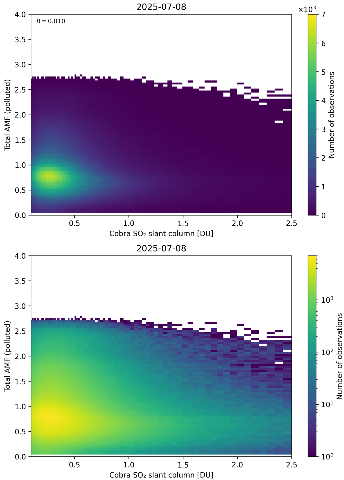
Figure 224: Scatter density plot of “Cobra SO 2 slant column” against “Total AMF (polluted)” for 2025-07-08 to 2025-07-09.
