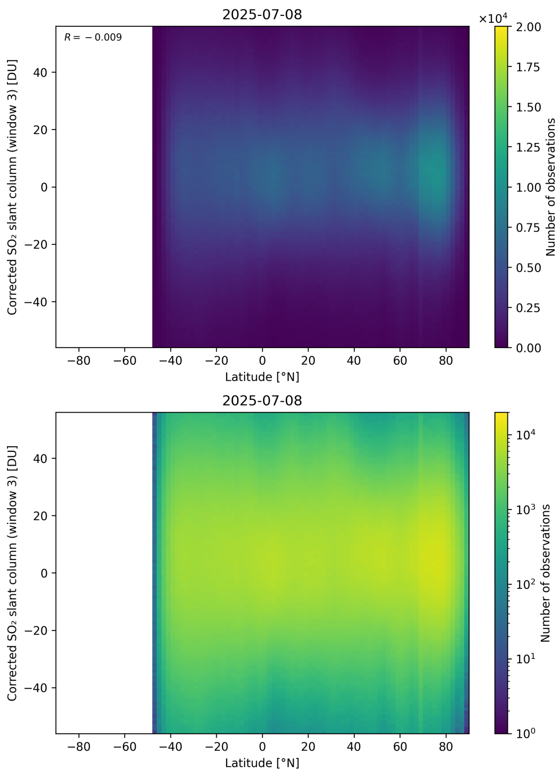
Figure 161: Scatter density plot of “Latitude” against “Corrected SO 2 slant column (window 3)” for 2025-07-08 to 2025-07-09.
