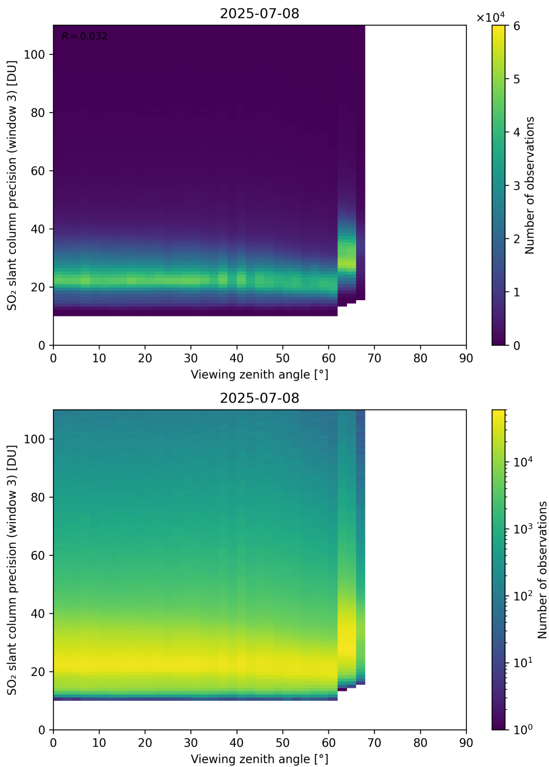
Figure 380: Scatter density plot of “Viewing zenith angle” against “SO 2 slant column precision (window 3)” for 2025-07-08 to 2025-07-09.
