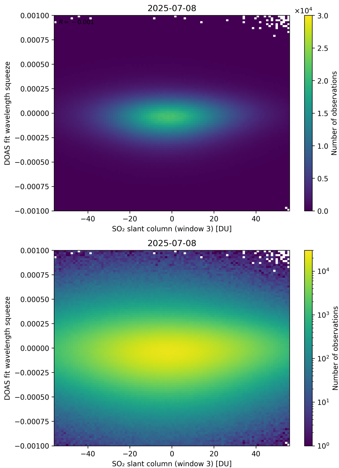
Figure 305: Scatter density plot of “SO 2 slant column (window 3)” against “DOAS fit wavelength squeeze” for 2025-07-08 to 2025-07-09.
