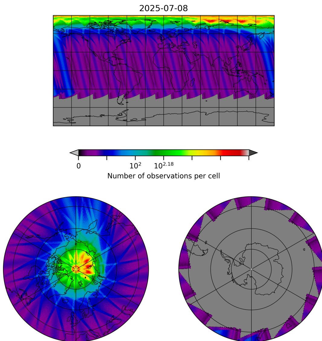
Figure 30: Map of the number of observations for 2025-07-08 to 2025-07-09
