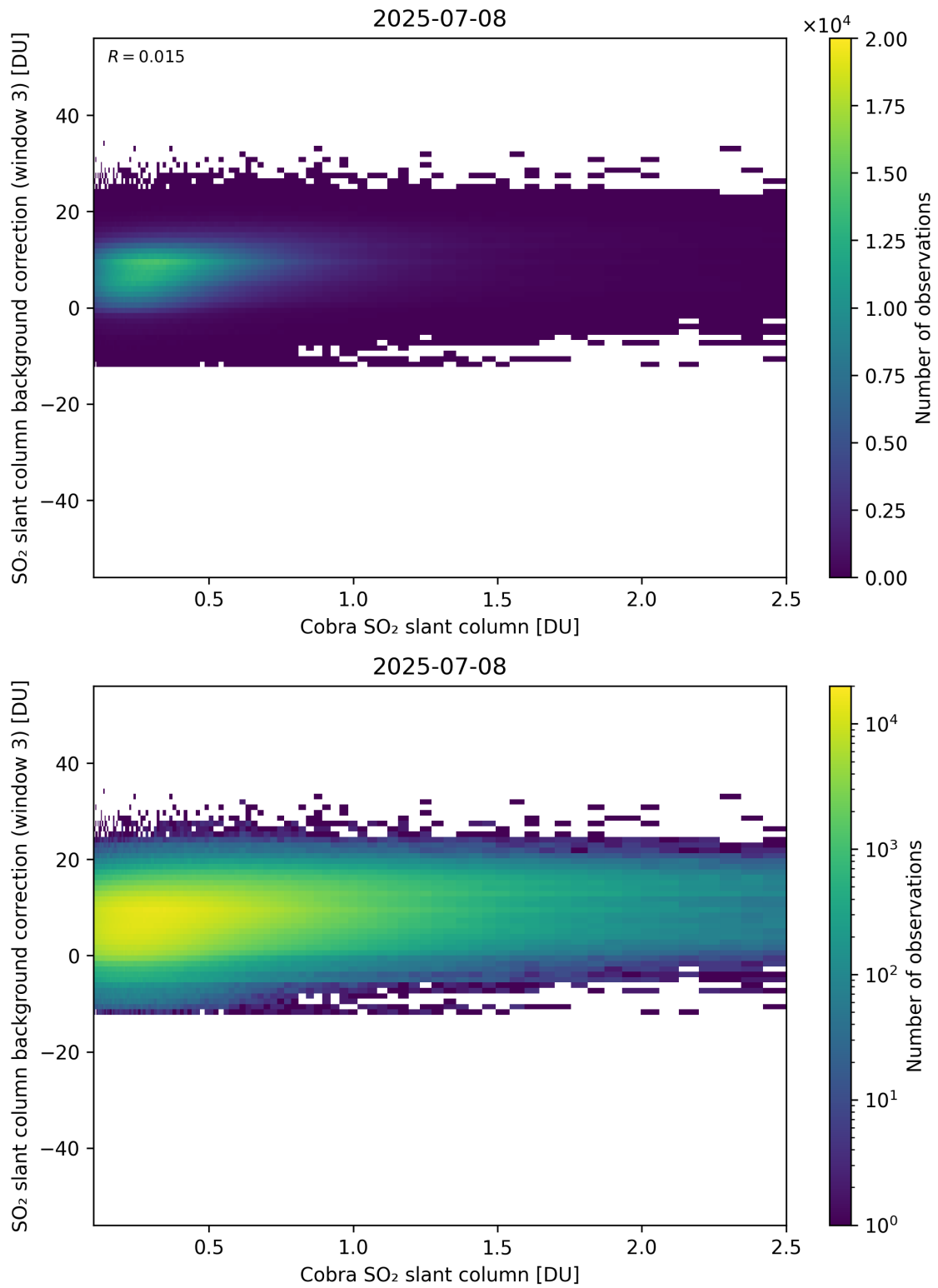
Figure 195: Scatter density plot of “Cobra SO 2 slant column” against “SO 2 slant column background correction (window 3)” for 2025-07-08 to 2025-07-09.
