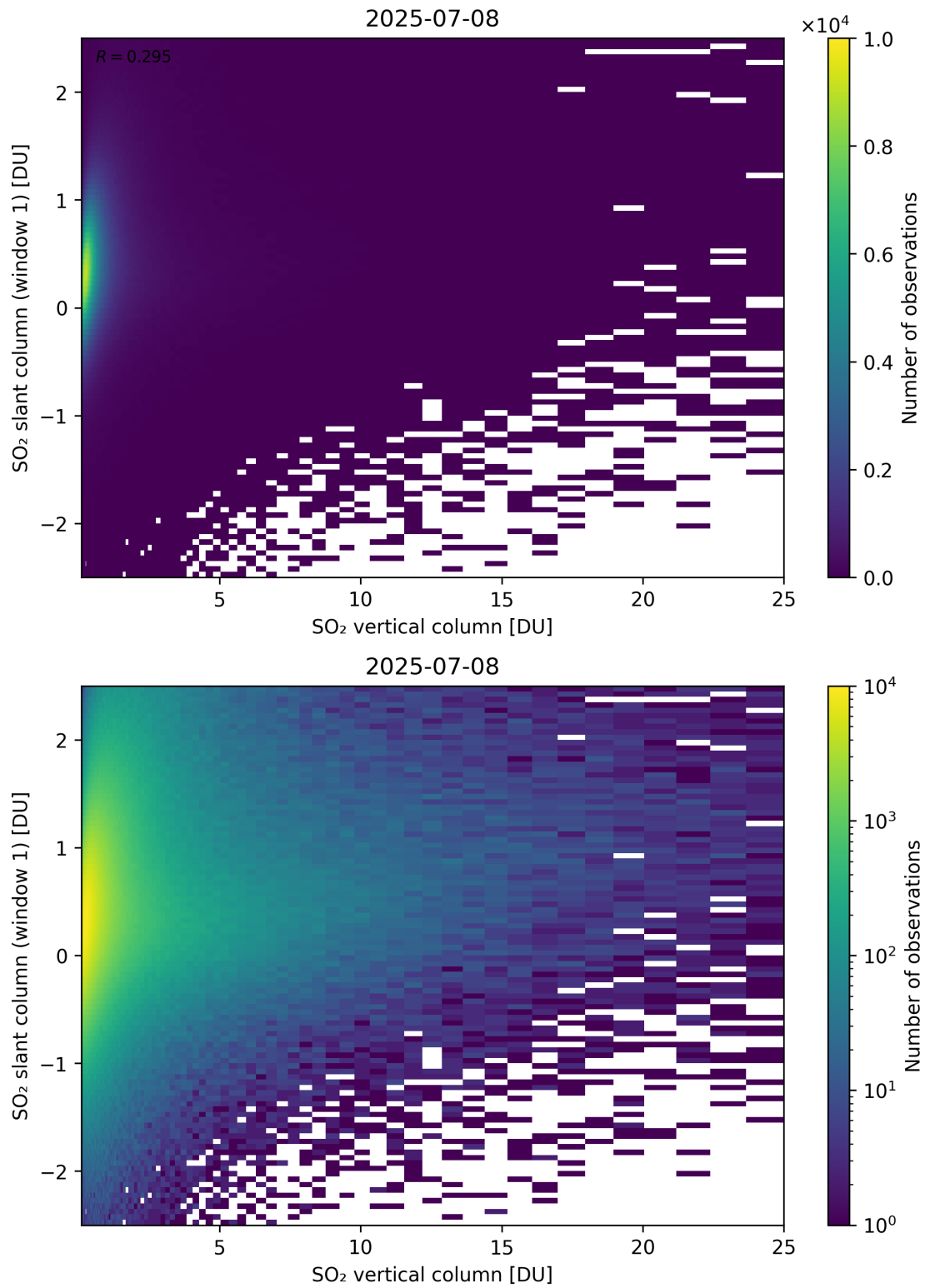
Figure 354: Scatter density plot of “SO 2 vertical column” against “SO 2 slant column (window 1)” for 2025-07-08 to 2025-07-09.
