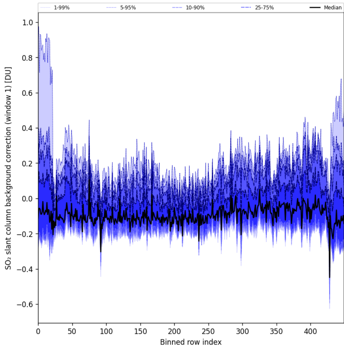
Figure 92: Along track statistics of “SO 2 slant column background correction (window 1)” for 2025-07-08 to 2025-07-09
