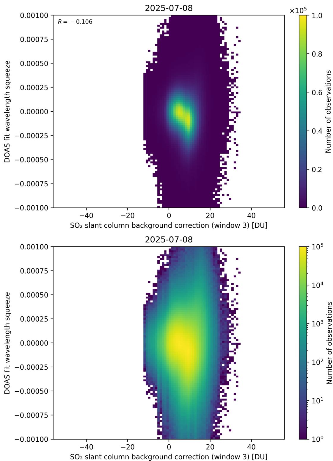
Figure 133: Scatter density plot of “SO 2 slant column background correction (window 3)” against “DOAS fit wavelength squeeze” for 2025-07-08 to 2025-07-09.
