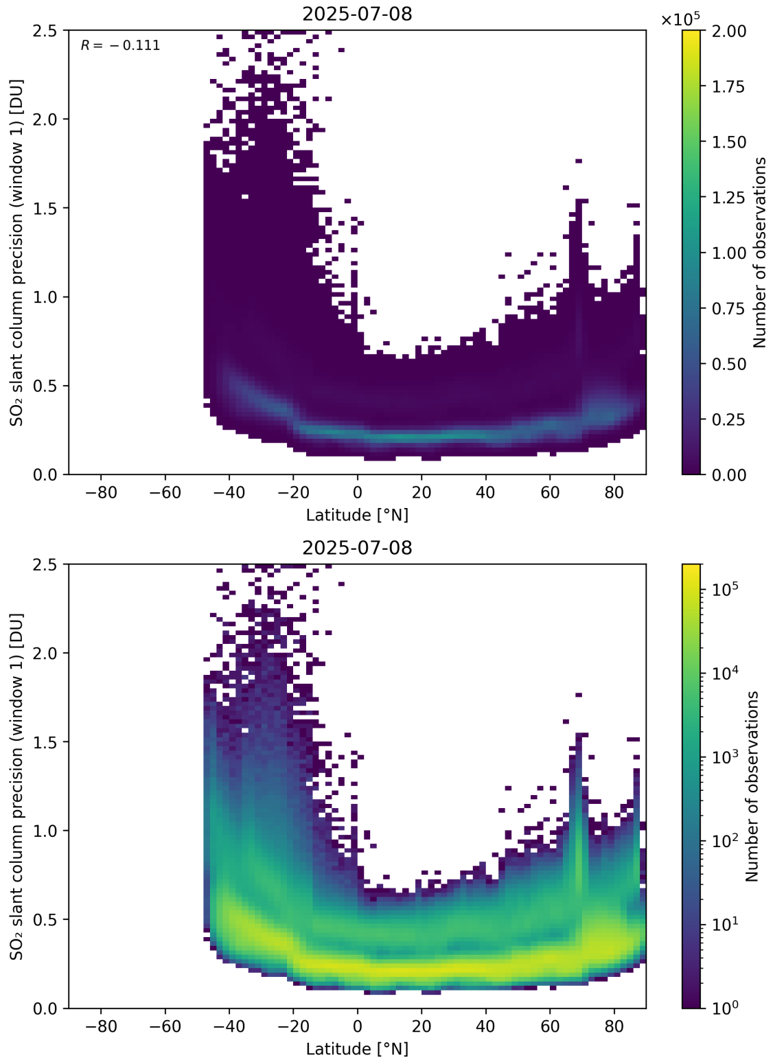
Figure 163: Scatter density plot of “Latitude” against “SO 2 slant column precision (window 1)” for 2025-07-08 to 2025-07-09.
