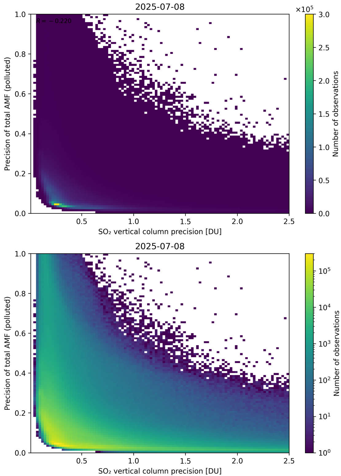
Figure 347: Scatter density plot of “SO 2 vertical column precision” against “Precision of total AMF (polluted)” for 2025-07-08 to 2025-07-09.
