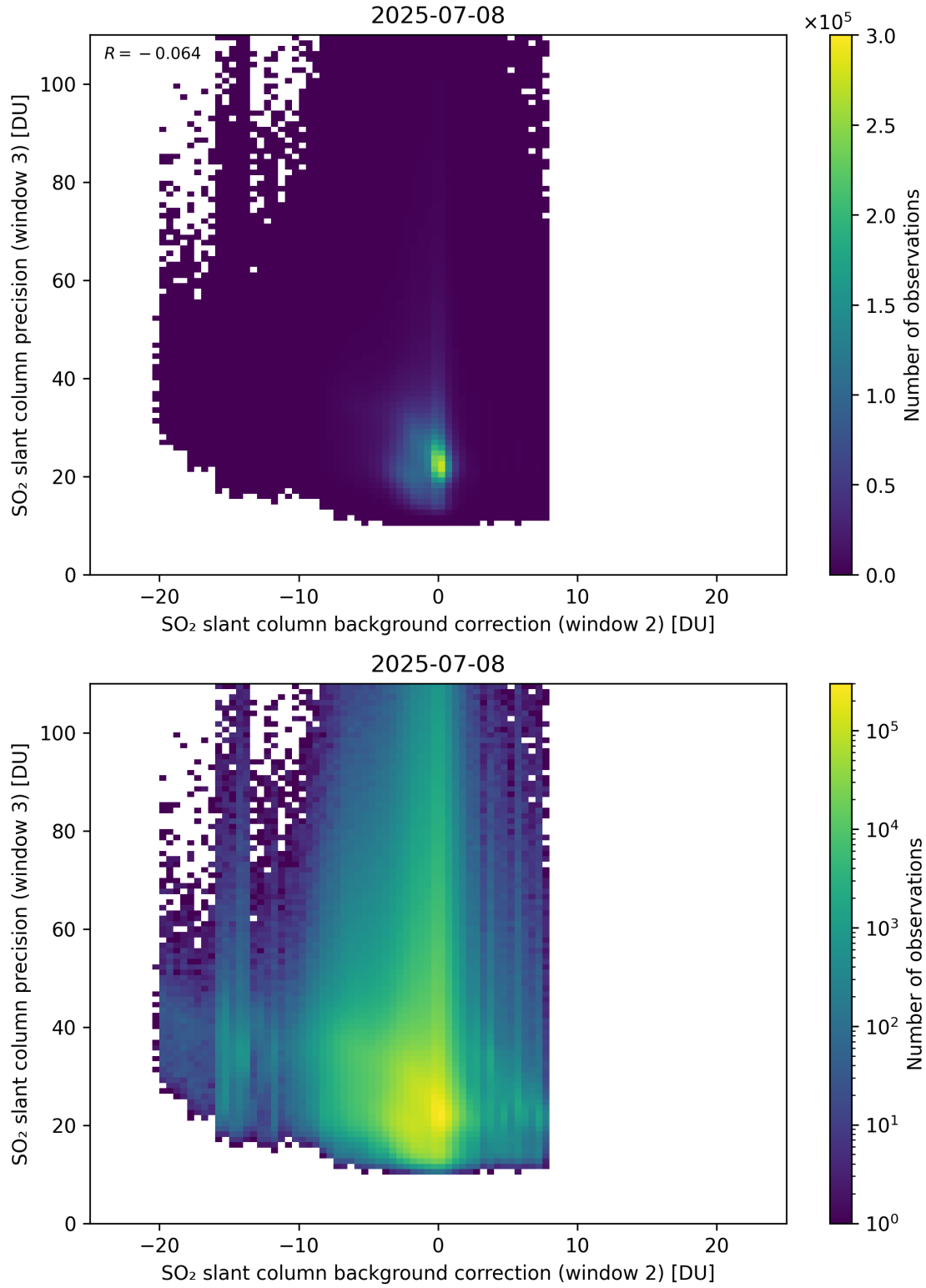
Figure 129: Scatter density plot of “SO 2 slant column background correction (window 2)” against “SO 2 slant column precision (window 3)” for 2025-07-08 to 2025-07-09.
