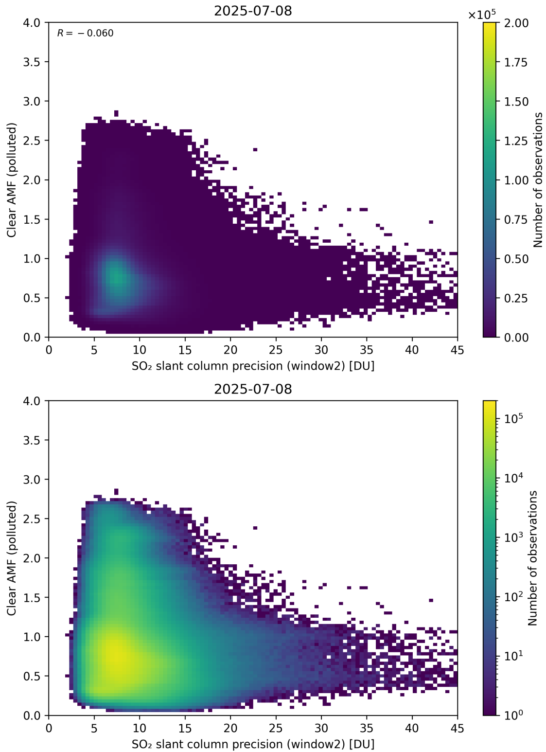
Figure 296: Scatter density plot of “SO 2 slant column precision (window2)” against “Clear AMF (polluted)” for 2025-07-08 to 2025-07-09.
