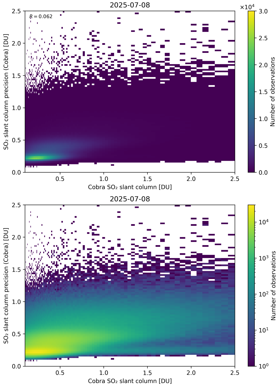
Figure 216: Scatter density plot of “Cobra SO 2 slant column” against “SO 2 slant column precision (Cobra)” for 2025-07-08 to 2025-07-09.
