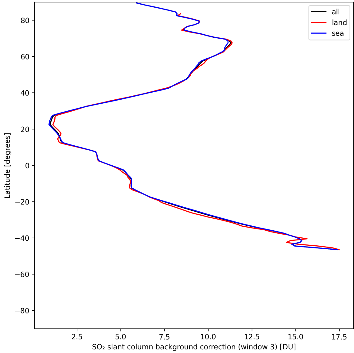
Figure 48: Zonal average of “SO 2 slant column background correction (window 3)” for 2025-07-08 to 2025-07-09.
