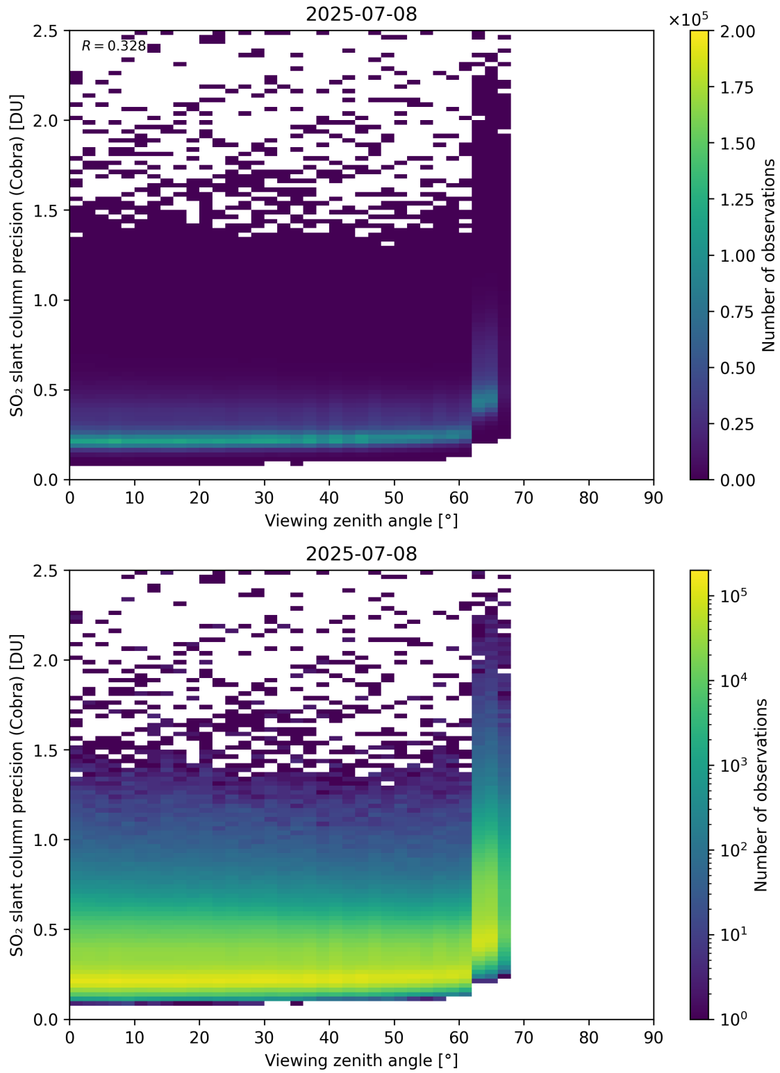
Figure 372: Scatter density plot of “Viewing zenith angle” against “SO 2 slant column precision (Cobra)” for 2025-07-08 to 2025-07-09.
