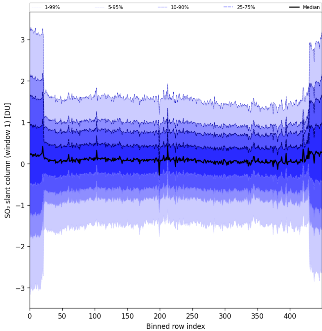
Figure 89: Along track statistics of “SO 2 slant column (window 1)” for 2025-07-08 to 2025-07-09
