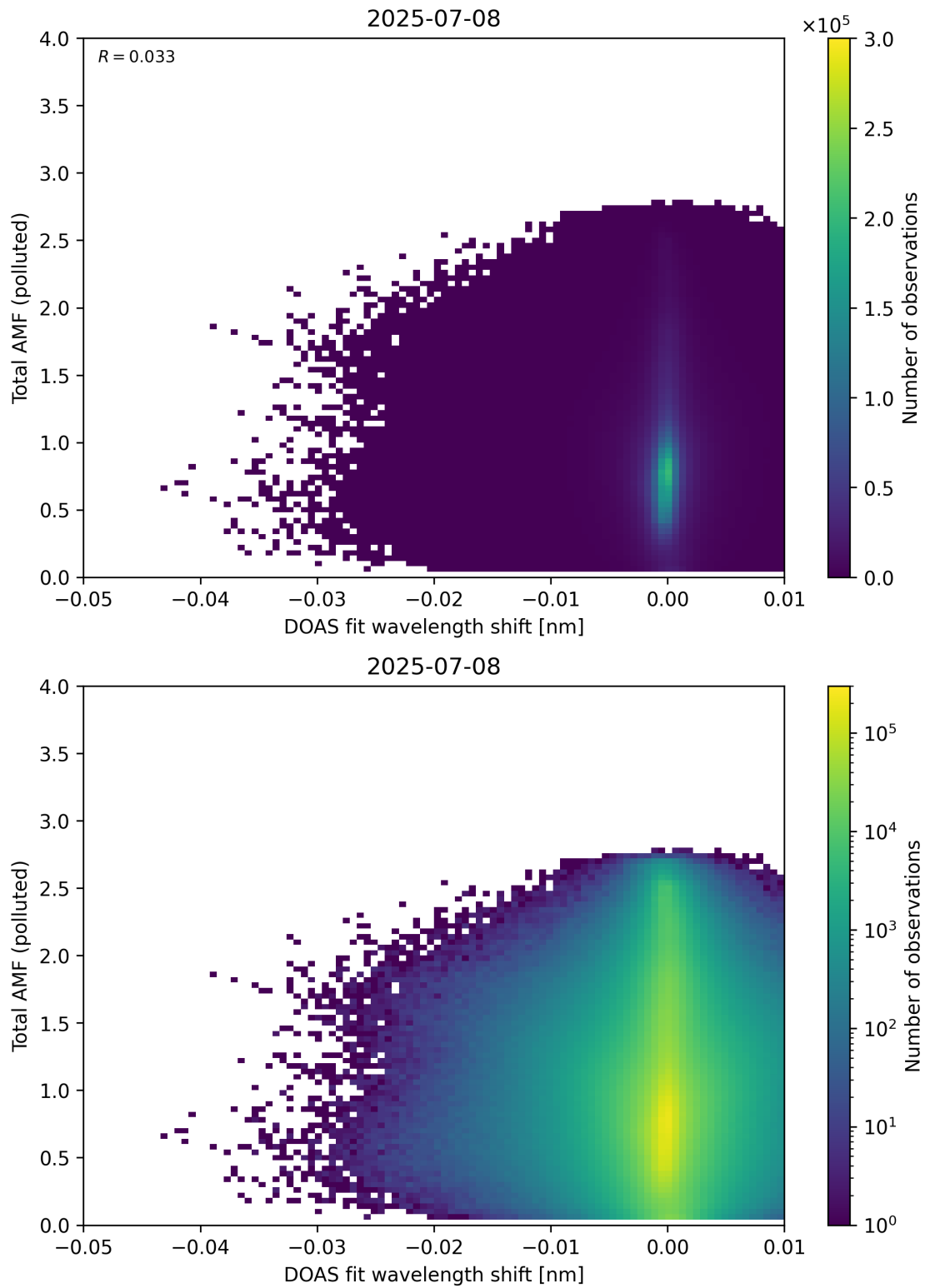
Figure 141: Scatter density plot of “DOAS fit wavelength shift” against “Total AMF (polluted)” for 2025-07-08 to 2025-07-09.
