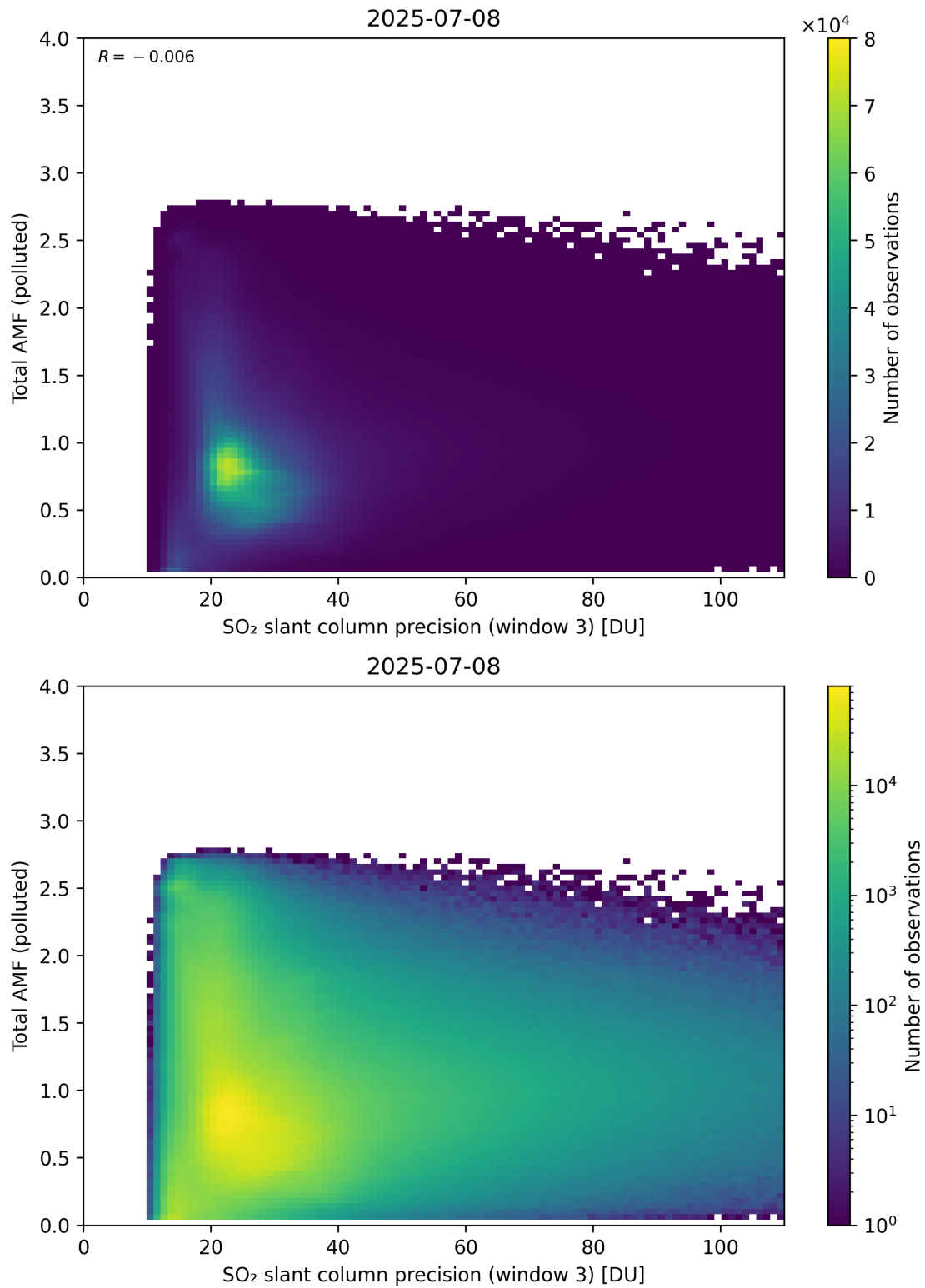
Figure 313: Scatter density plot of “SO 2 slant column precision (window 3)” against “Total AMF (polluted)” for 2025-07-08 to 2025-07-09.
