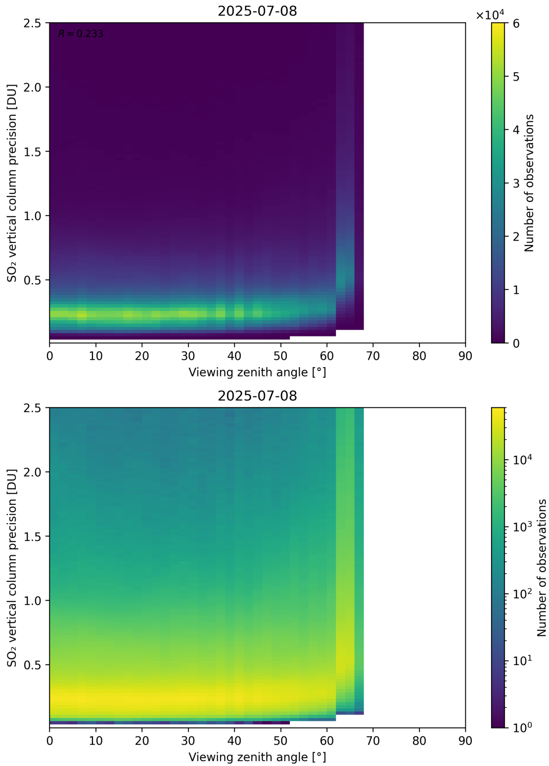
Figure 384: Scatter density plot of “Viewing zenith angle” against “SO 2 vertical column precision” for 2025-07-08 to 2025-07-09.
