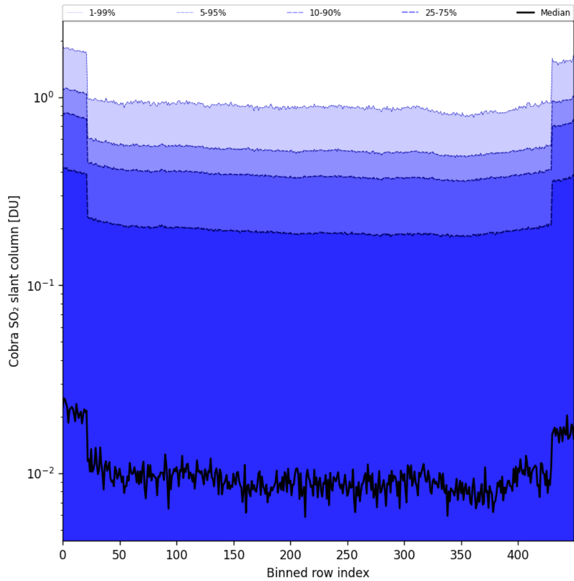
Figure 87: Along track statistics of “Cobra SO 2 slant column” for 2025-07-08 to 2025-07-09
