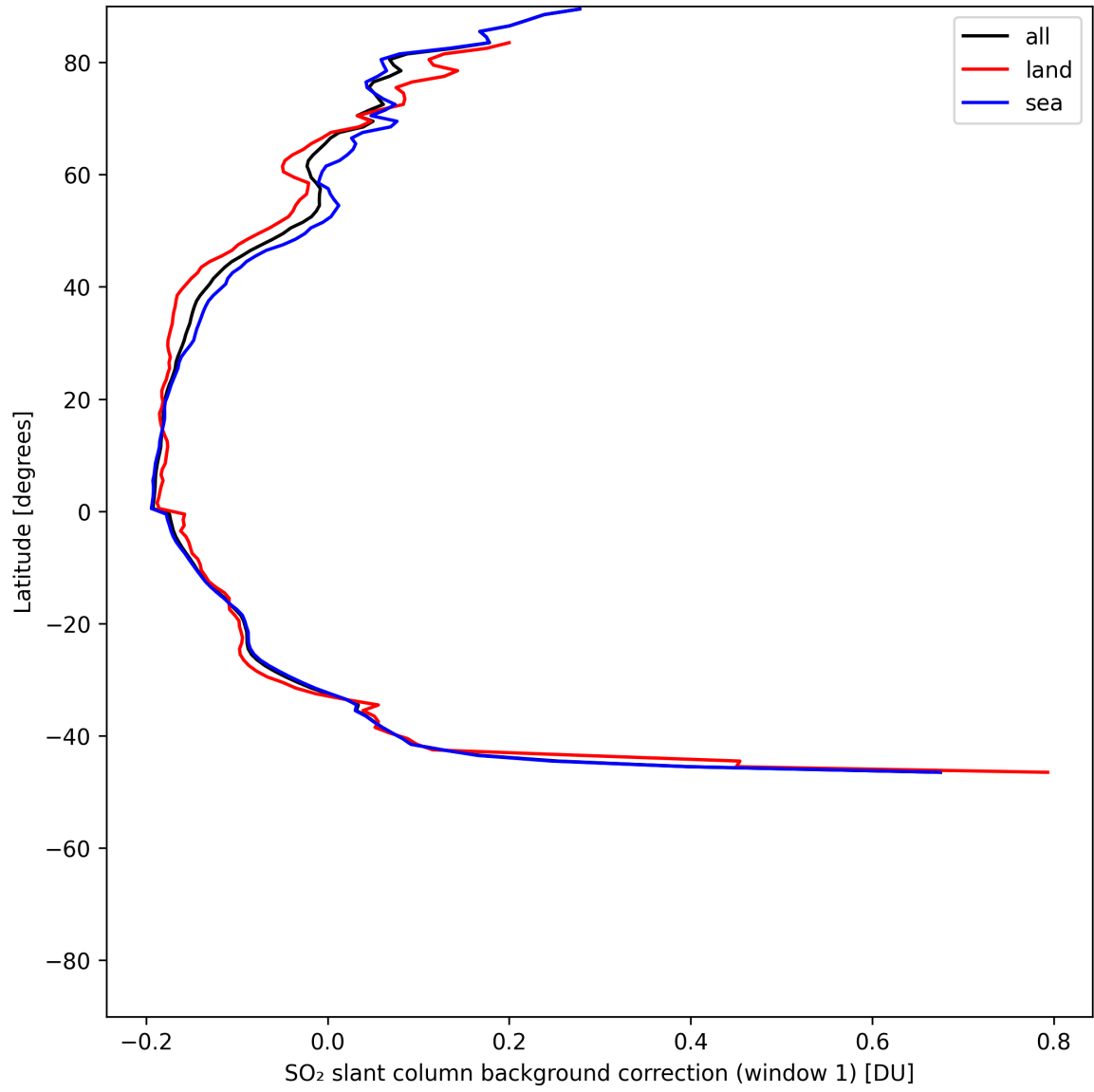
Figure 40: Zonal average of “SO 2 slant column background correction (window 1)” for 2025-07-08 to 2025-07-09.
