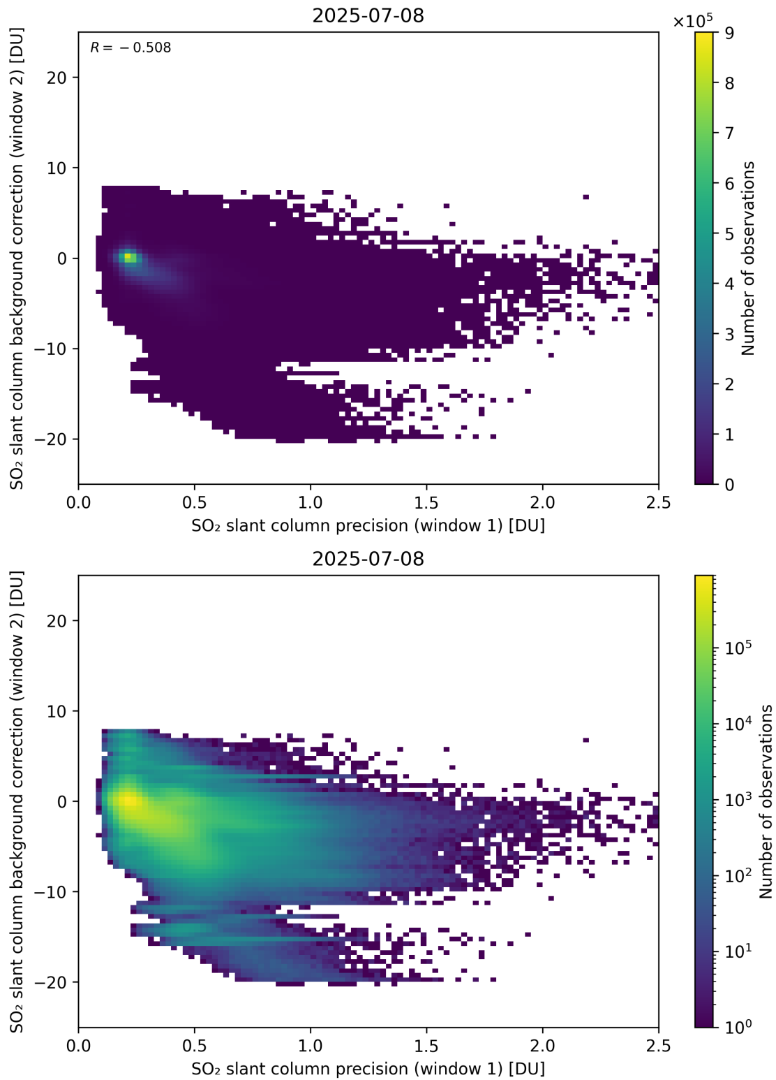
Figure 269: Scatter density plot of “SO 2 slant column precision (window 1)” against “SO 2 slant column background correction (window 2)” for 2025-07-08 to 2025-07-09.
