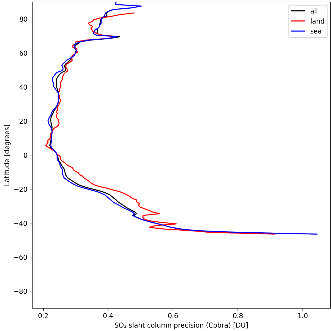
Figure 36: Zonal average of “SO 2 slant column precision (Cobra)” for 2025-07-08 to 2025-07-09.
