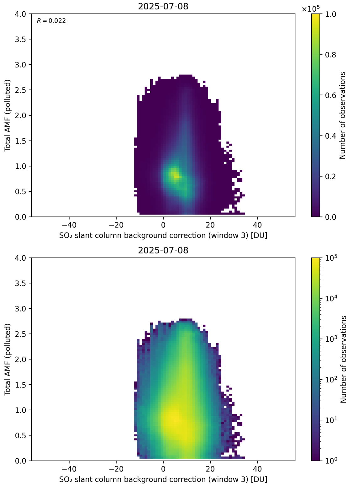
Figure 136: Scatter density plot of “SO 2 slant column background correction (window 3)” against “Total AMF (polluted)” for 2025-07-08 to 2025-07-09.
