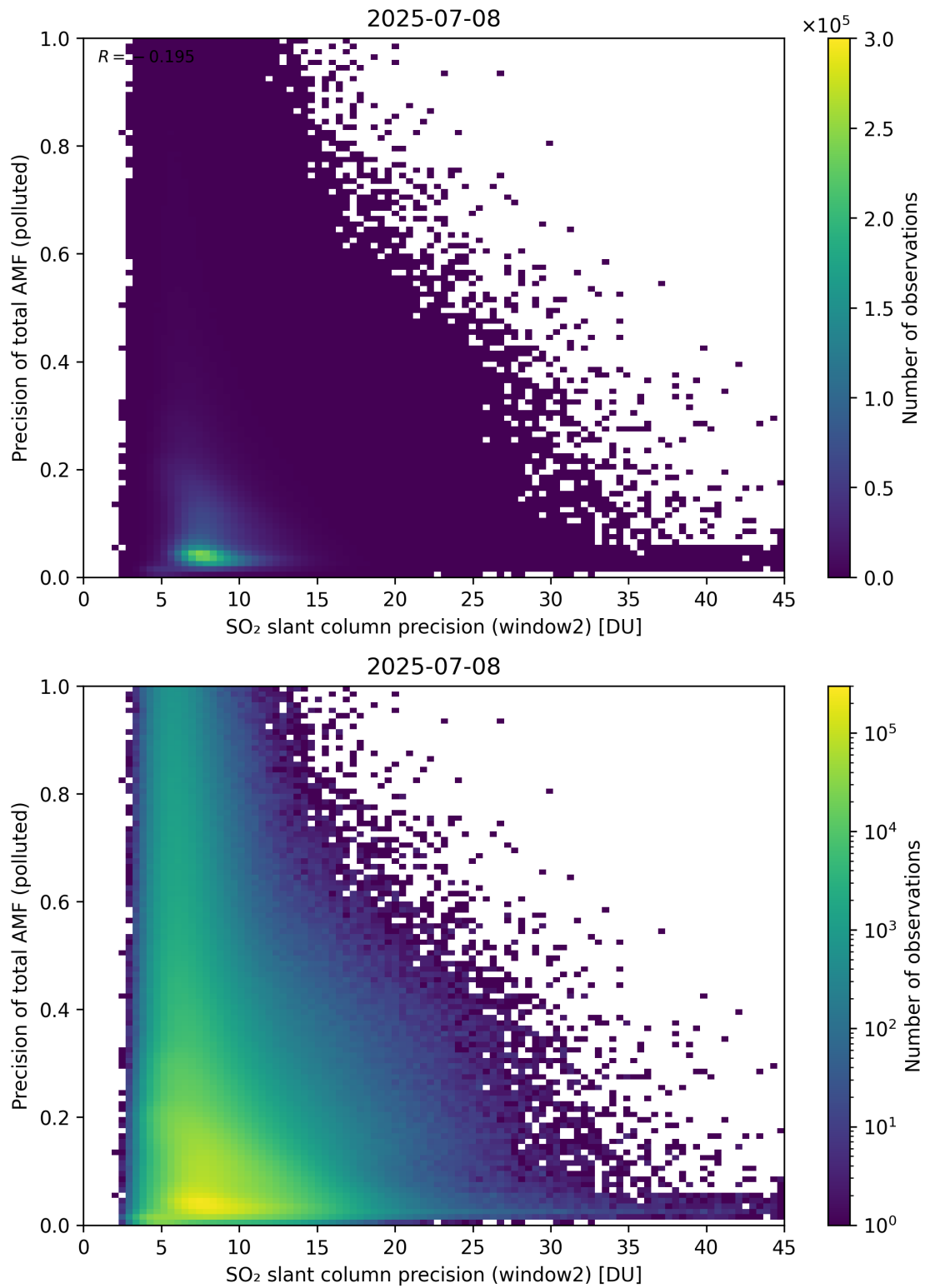
Figure 302: Scatter density plot of “SO 2 slant column precision (window2)” against “Precision of total AMF (polluted)” for 2025-07-08 to 2025-07-09.
