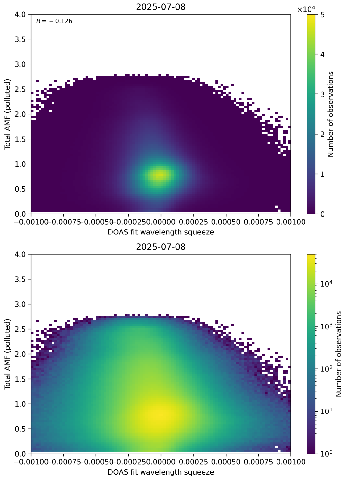
Figure 145: Scatter density plot of “DOAS fit wavelength squeeze” against “Total AMF (polluted)” for 2025-07-08 to 2025-07-09.
