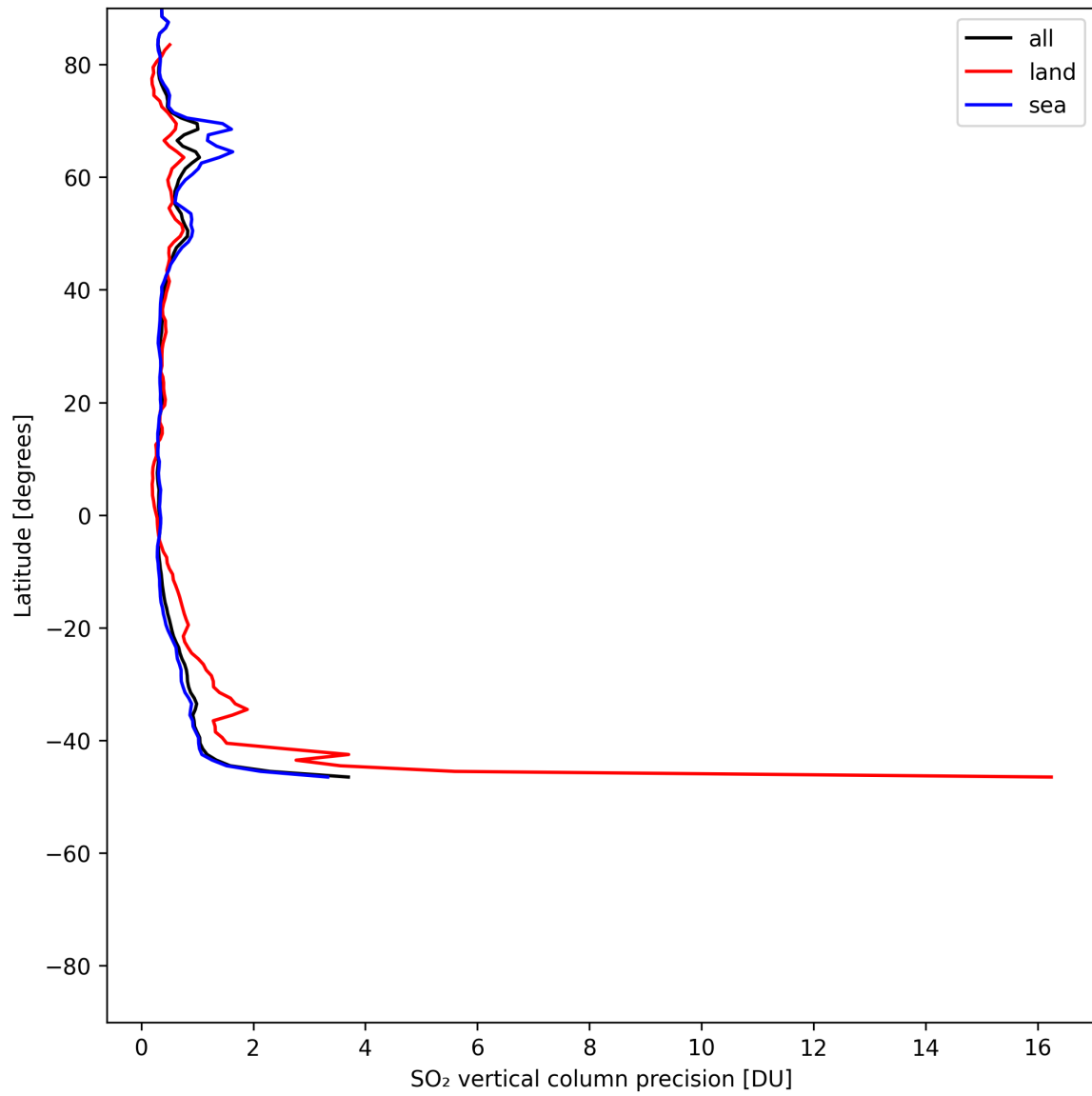
Figure 33: Zonal average of “SO 2 vertical column precision” for 2025-07-08 to 2025-07-09.
