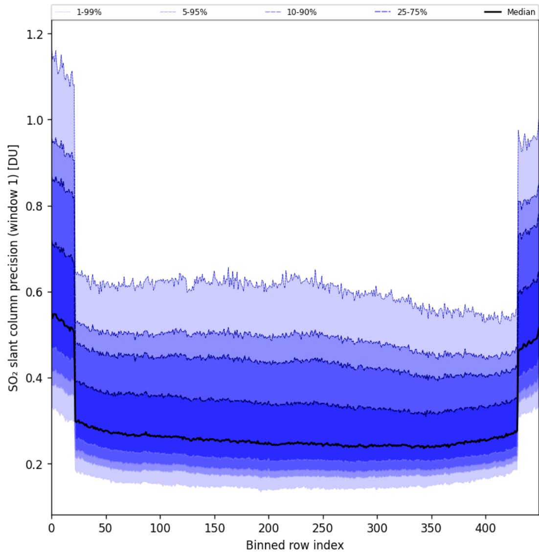
Figure 90: Along track statistics of “SO 2 slant column precision (window 1)” for 2025-07-08 to 2025-07-09
