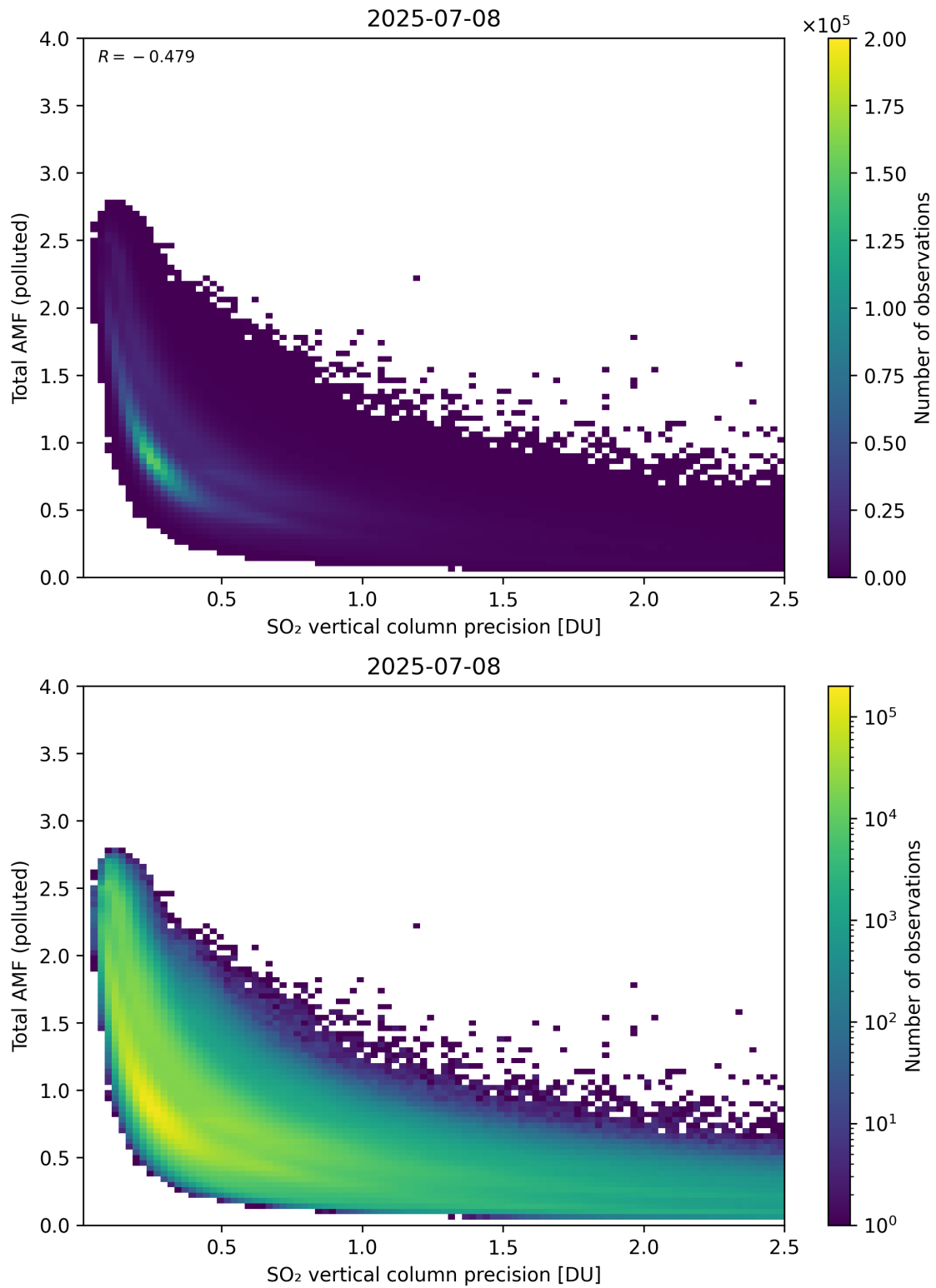
Figure 346: Scatter density plot of “SO 2 vertical column precision” against “Total AMF (polluted)” for 2025-07-08 to 2025-07-09.
