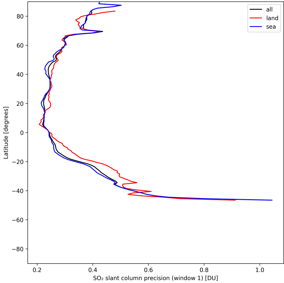
Figure 38: Zonal average of “SO 2 slant column precision (window 1)” for 2025-07-08 to 2025-07-09.
