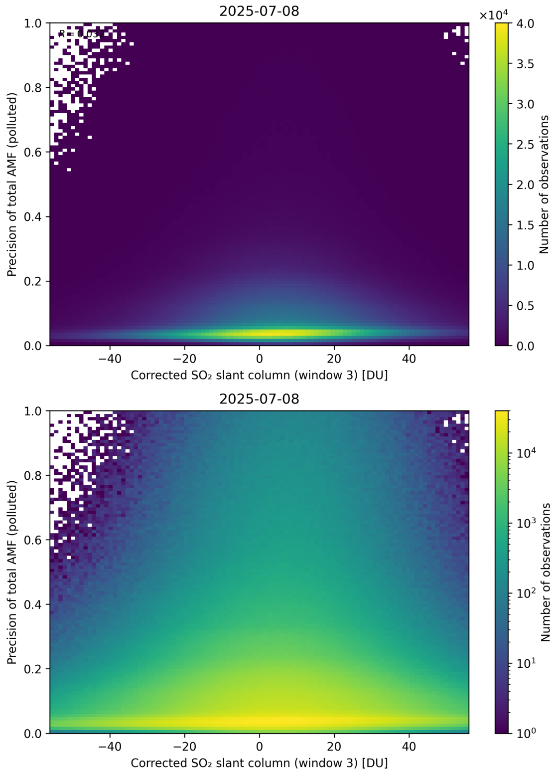
Figure 261: Scatter density plot of “Corrected SO 2 slant column (window 3)” against “Precision of total AMF (polluted)” for 2025-07-08 to 2025-07-09.
