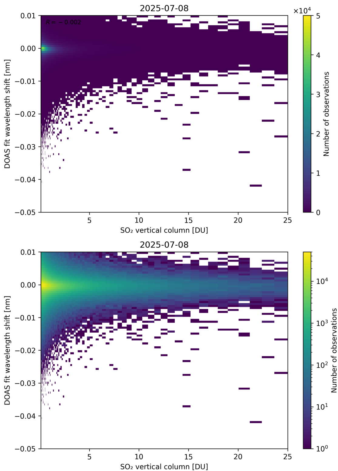
Figure 326: Scatter density plot of “SO 2 vertical column” against “DOAS fit wavelength shift” for 2025-07-08 to 2025-07-09.
