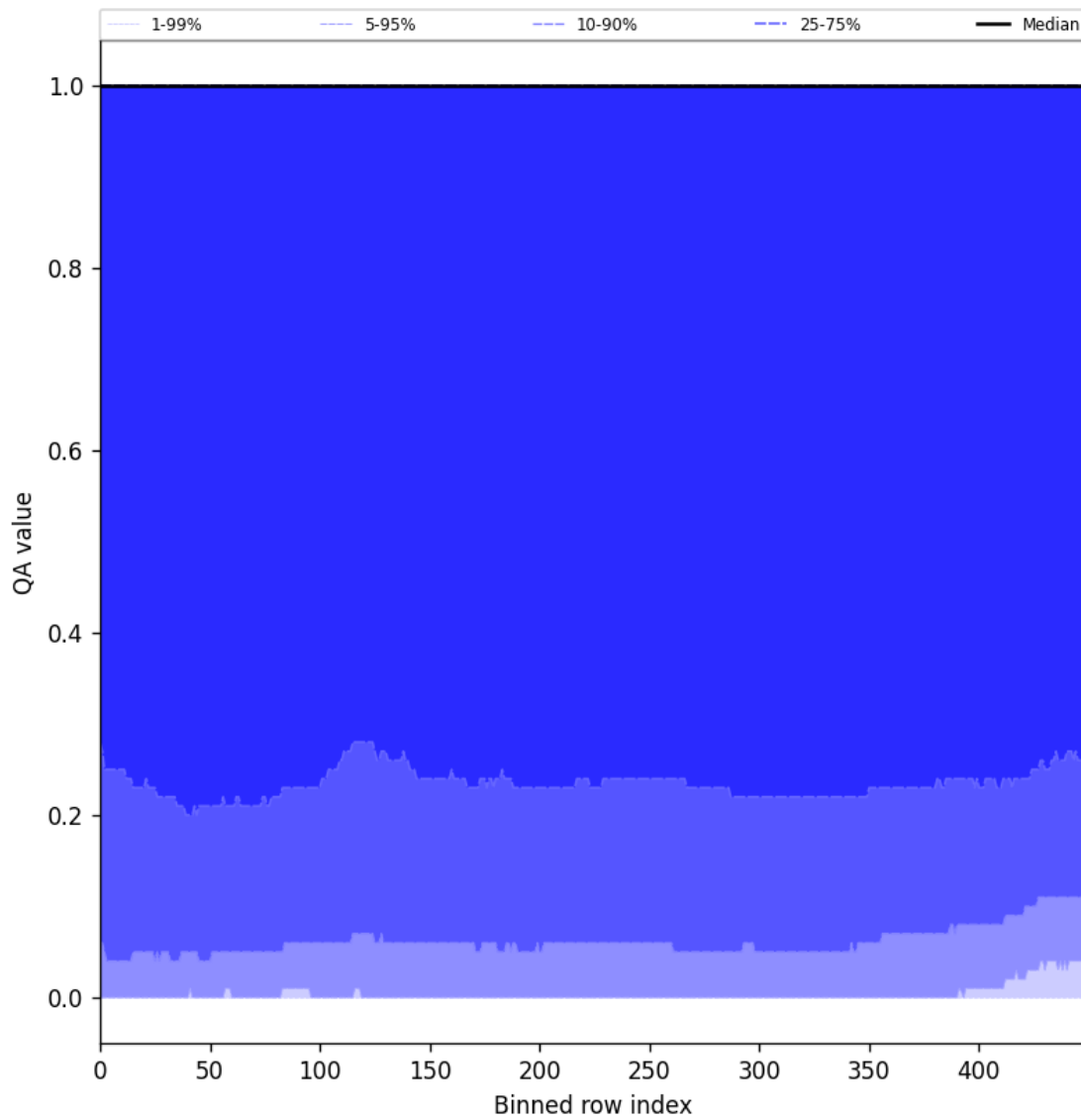
Figure 83: Along track statistics of “QA value” for 2025-07-08 to 2025-07-09
