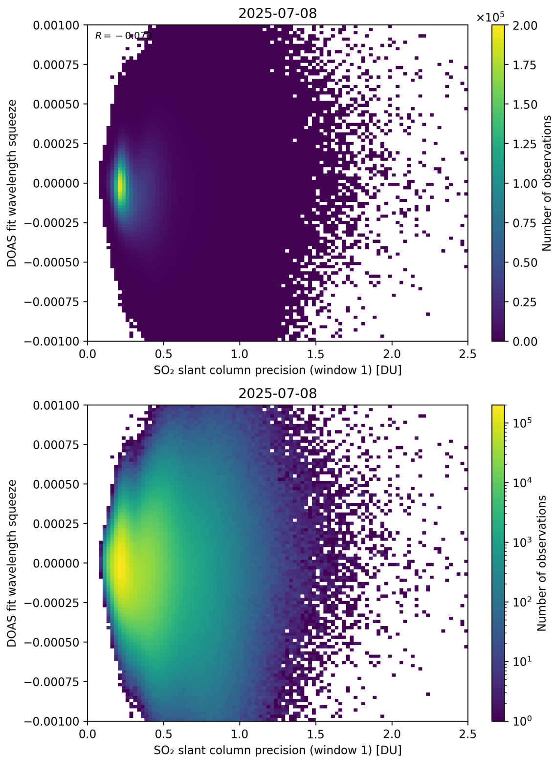
Figure 272: Scatter density plot of “SO 2 slant column precision (window 1)” against “DOAS fit wavelength squeeze” for 2025-07-08 to 2025-07-09.
