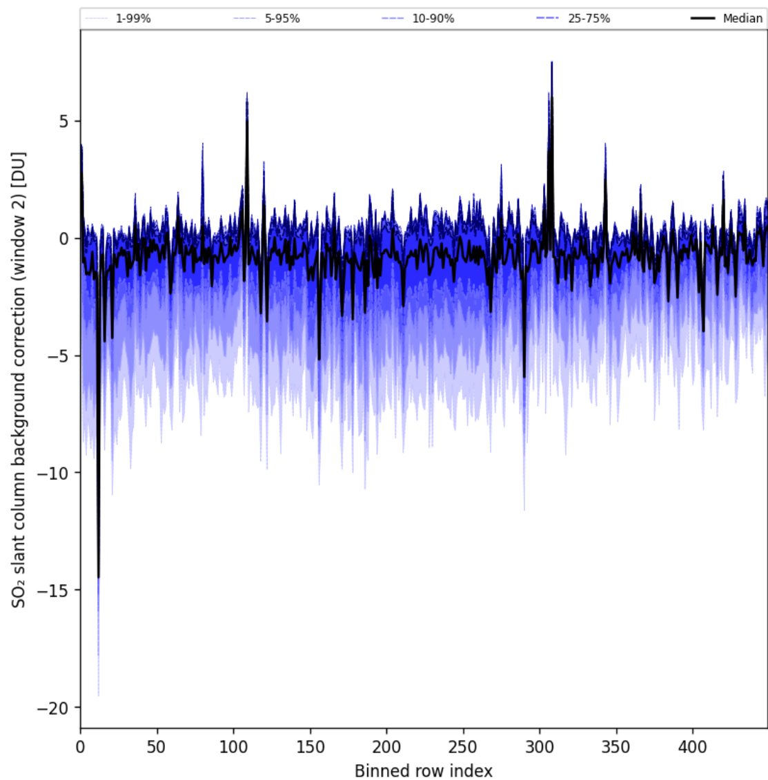
Figure 96: Along track statistics of “SO 2 slant column background correction (window 2)” for 2025-07-08 to 2025-07-09
