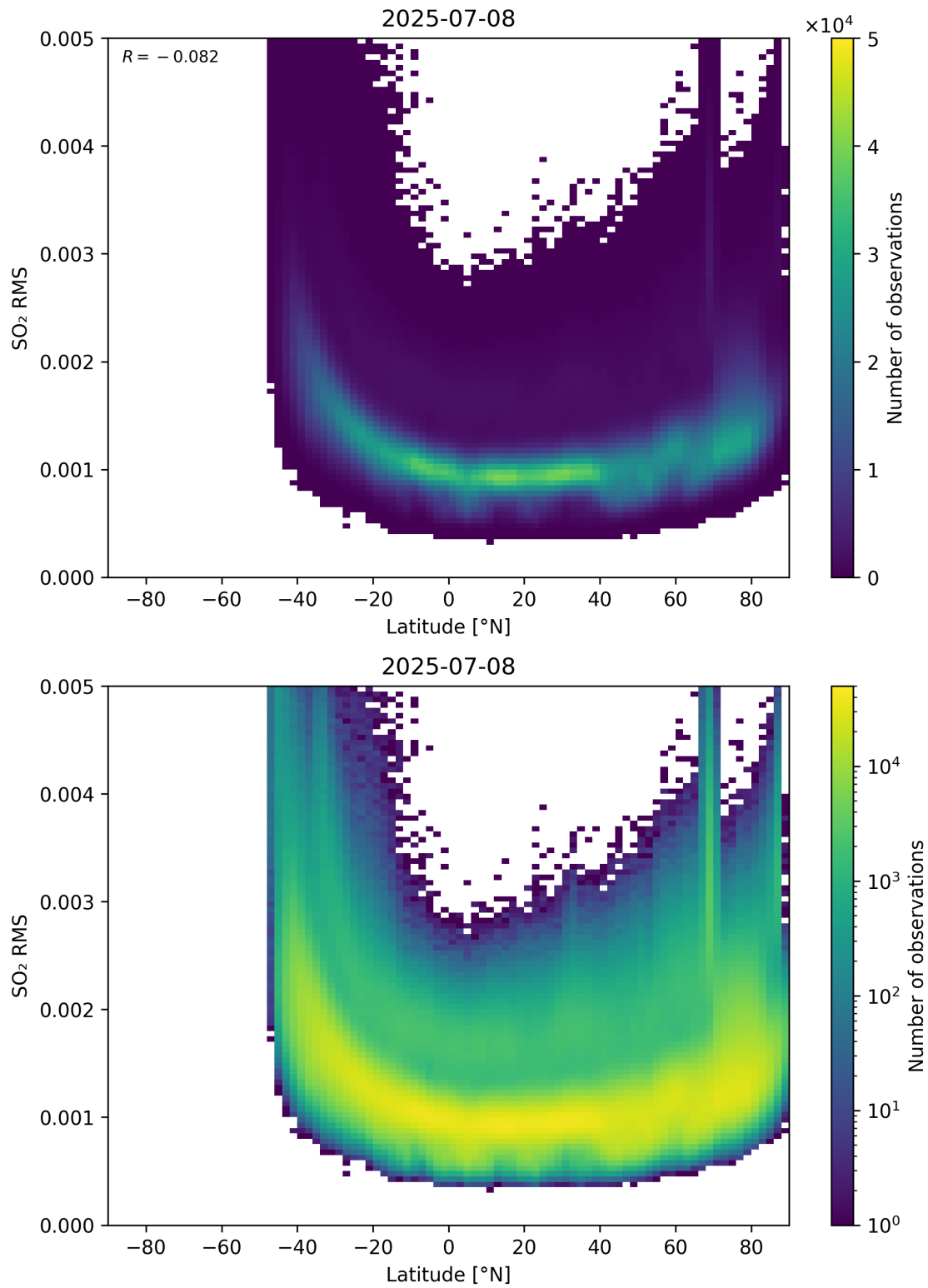
Figure 155: Scatter density plot of “Latitude” against “SO 2 RMS” for 2025-07-08 to 2025-07-09.
