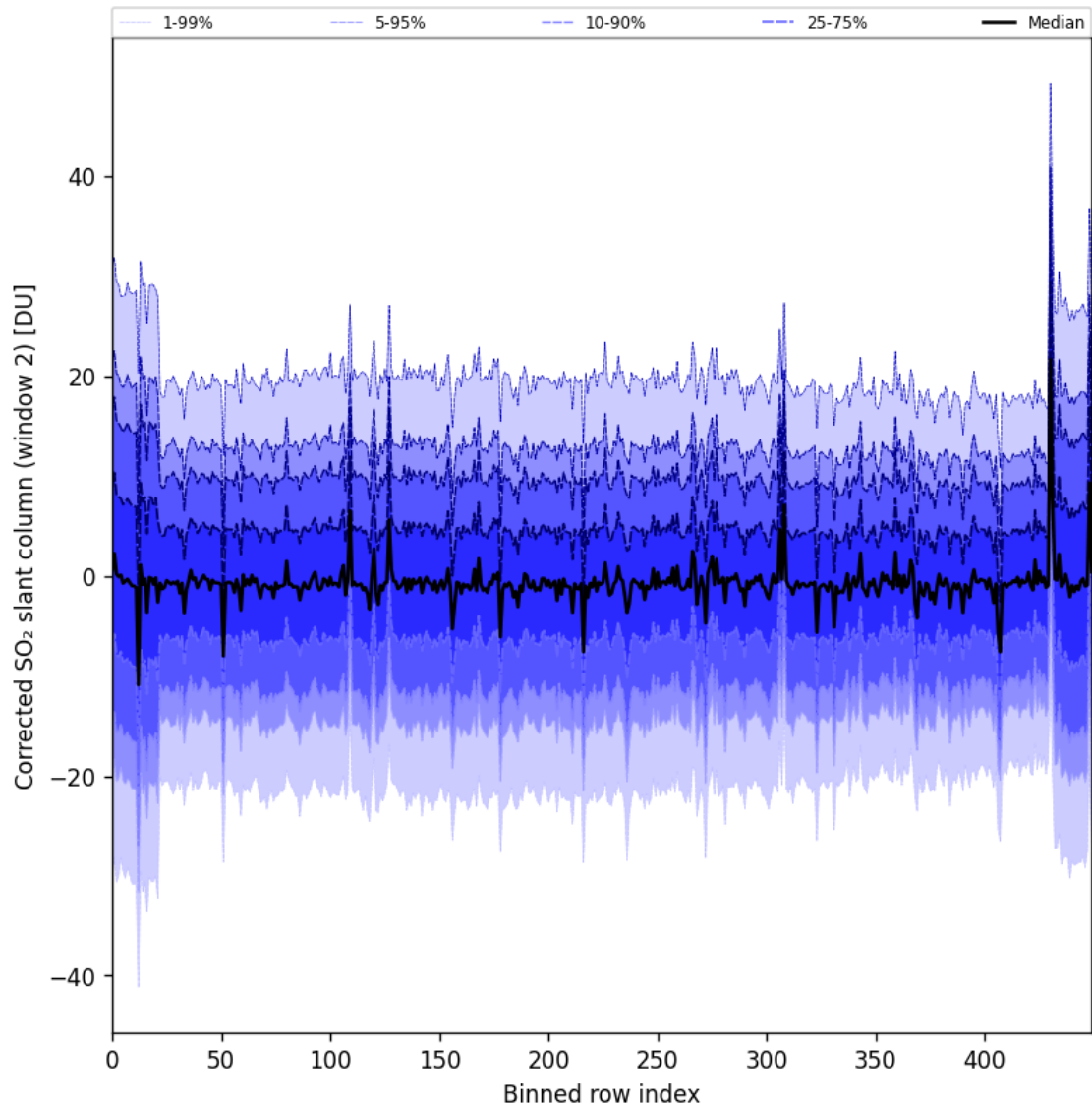
Figure 95: Along track statistics of “Corrected SO 2 slant column (window 2)” for 2025-07-08 to 2025-07-09
