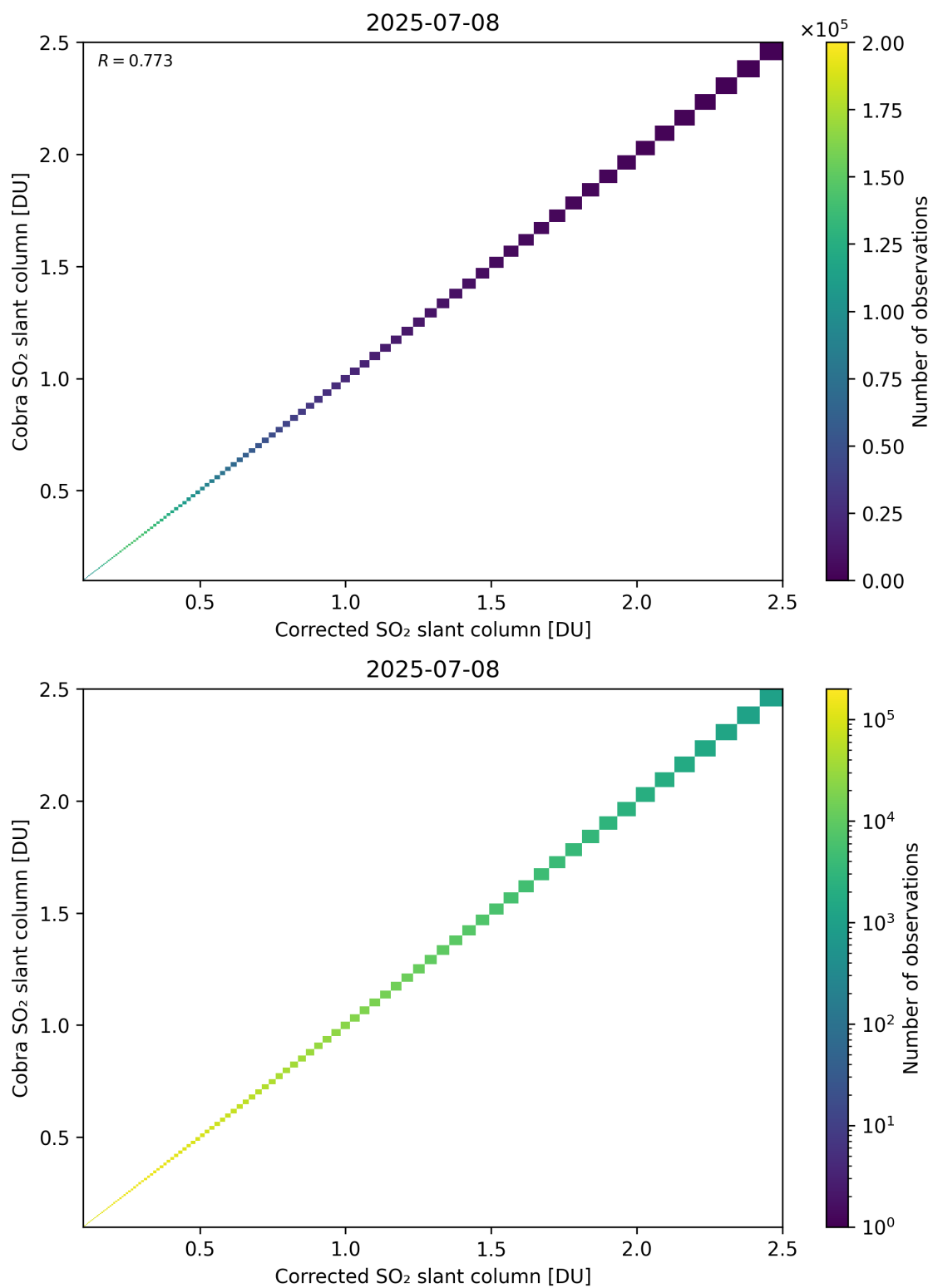
Figure 233: Scatter density plot of “Corrected SO 2 slant column” against “Cobra SO 2 slant column” for 2025-07-08 to 2025-07-09.
