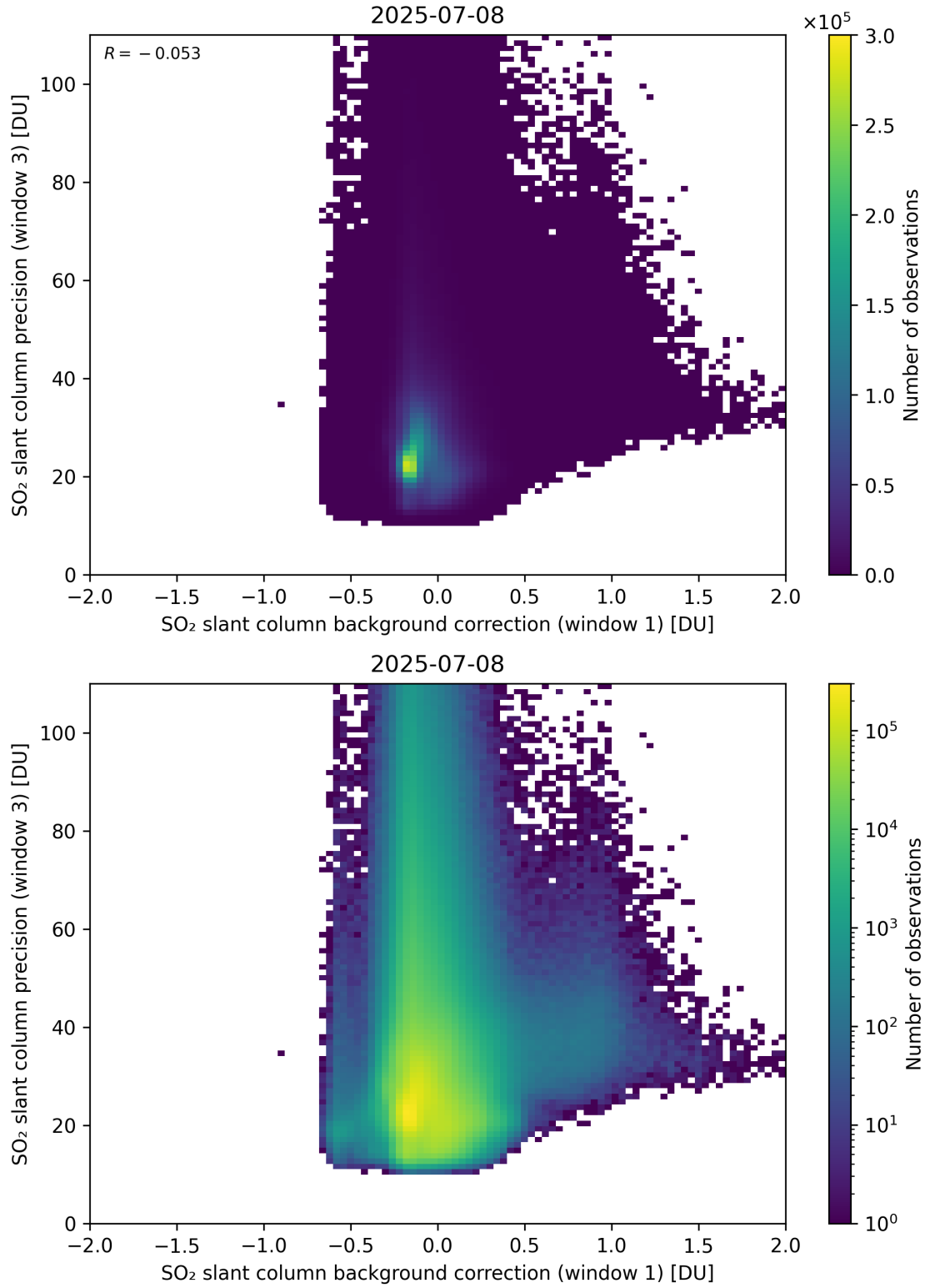
Figure 119: Scatter density plot of “SO 2 slant column background correction (window 1)” against “SO 2 slant column precision (window 3)” for 2025-07-08 to 2025-07-09.
