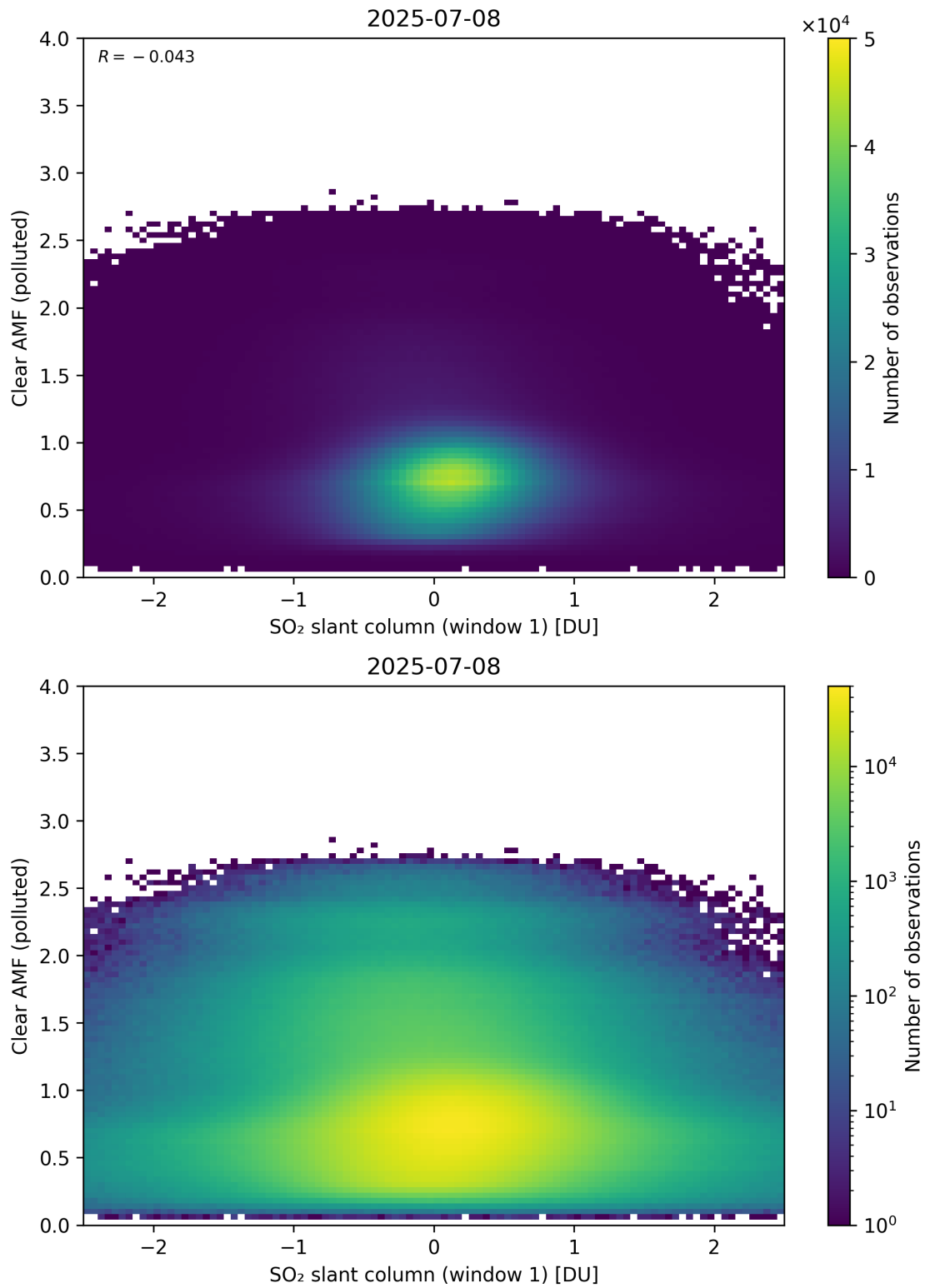
Figure 282: Scatter density plot of “SO 2 slant column (window 1)” against “Clear AMF (polluted)” for 2025-07-08 to 2025-07-09.
