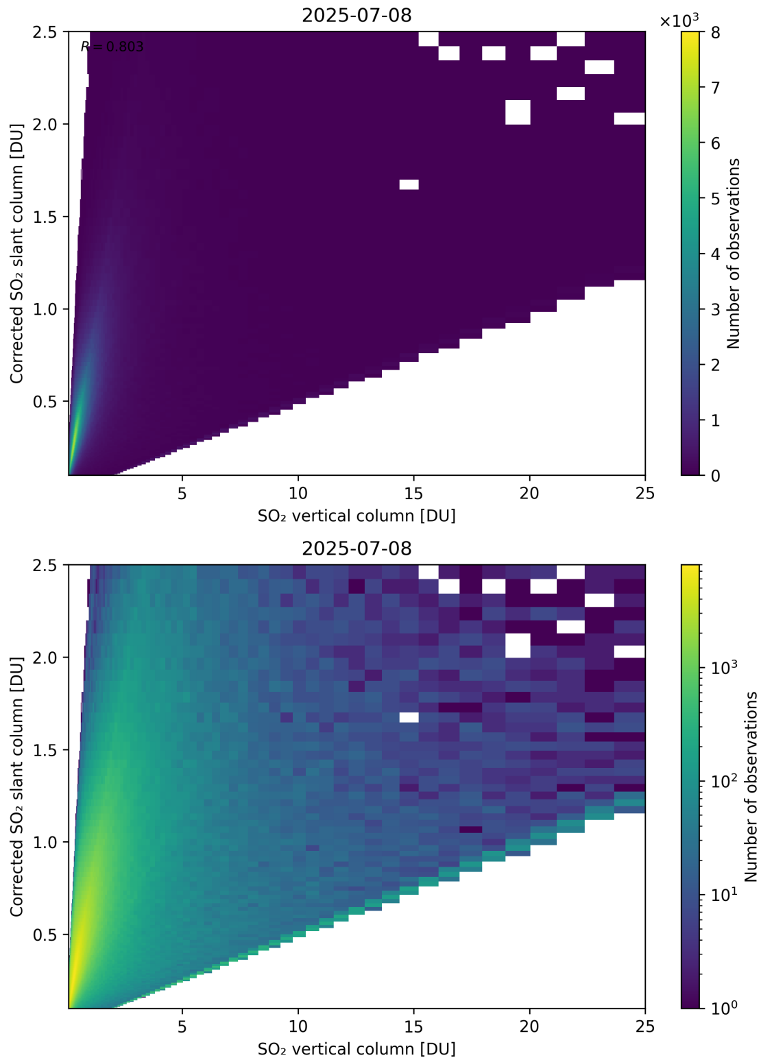
Figure 351: Scatter density plot of “SO 2 vertical column” against “Corrected SO 2 slant column” for 2025-07-08 to 2025-07-09.
