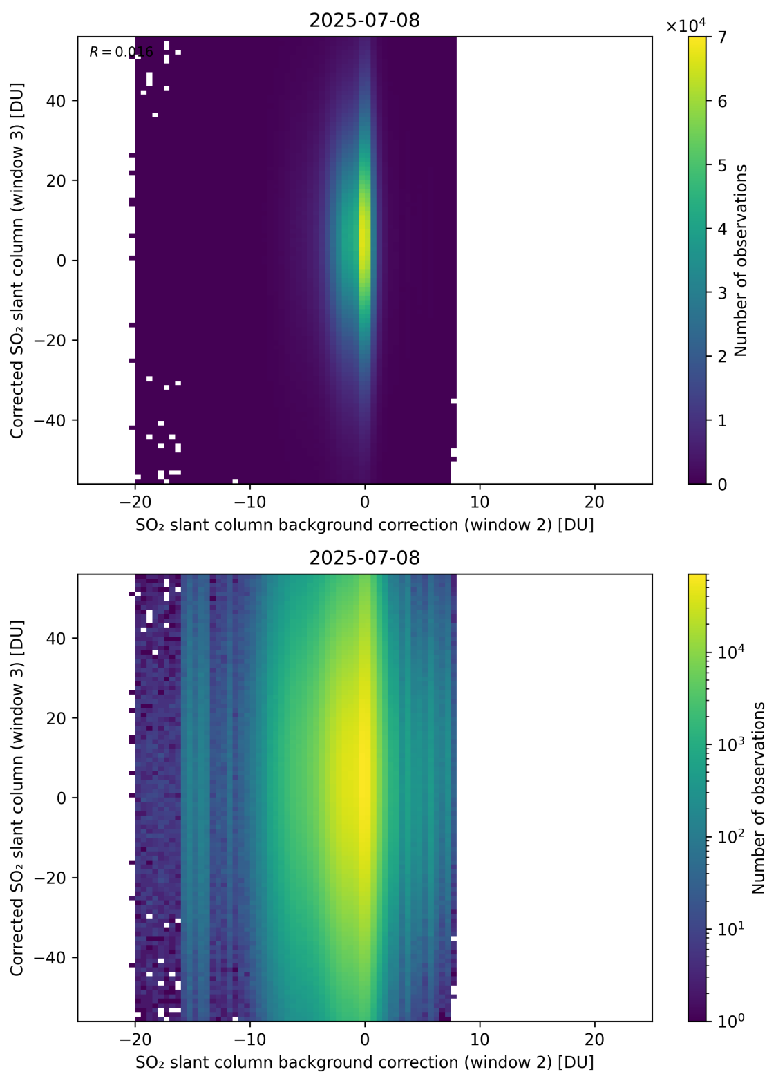
Figure 127: Scatter density plot of “SO 2 slant column background correction (window 2)” against “Corrected SO 2 slant column (window 3)” for 2025-07-08 to 2025-07-09.
