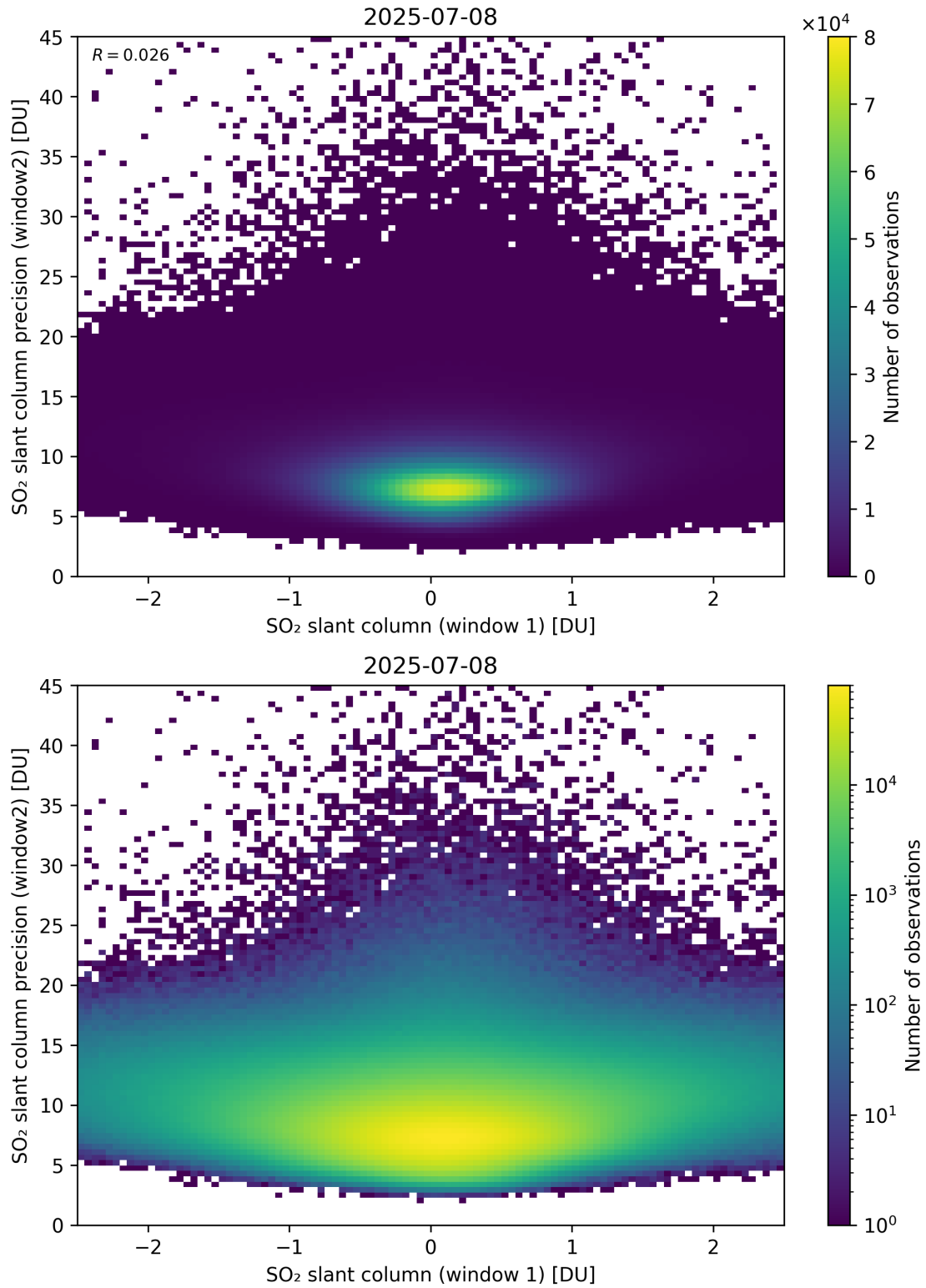
Figure 286: Scatter density plot of “SO 2 slant column (window 1)” against “SO 2 slant column precision (window2)” for 2025-07-08 to 2025-07-09.
