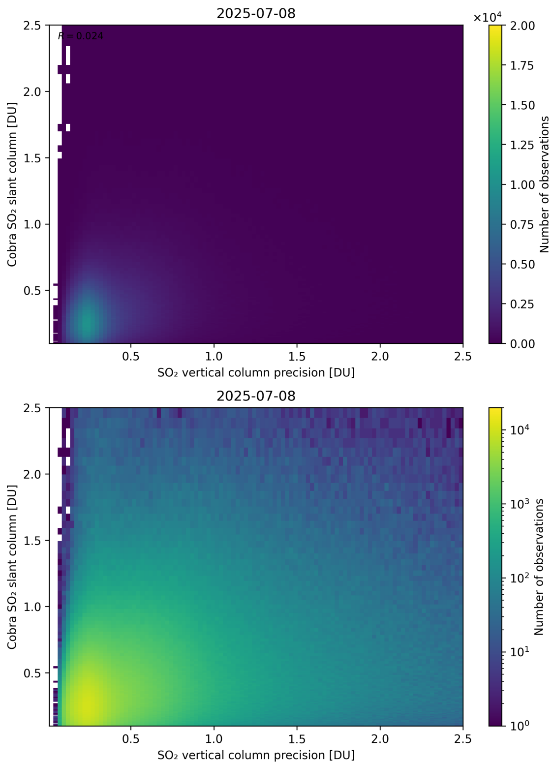
Figure 336: Scatter density plot of “SO 2 vertical column precision” against “Cobra SO 2 slant column” for 2025-07-08 to 2025-07-09.
