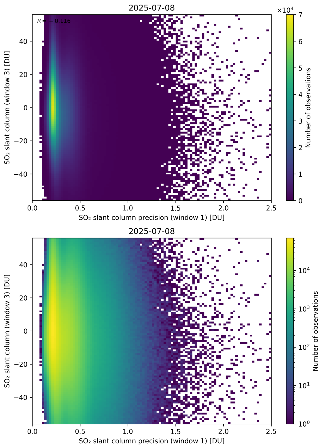
Figure 278: Scatter density plot of “SO 2 slant column precision (window 1)” against “SO 2 slant column (window 3)” for 2025-07-08 to 2025-07-09.
