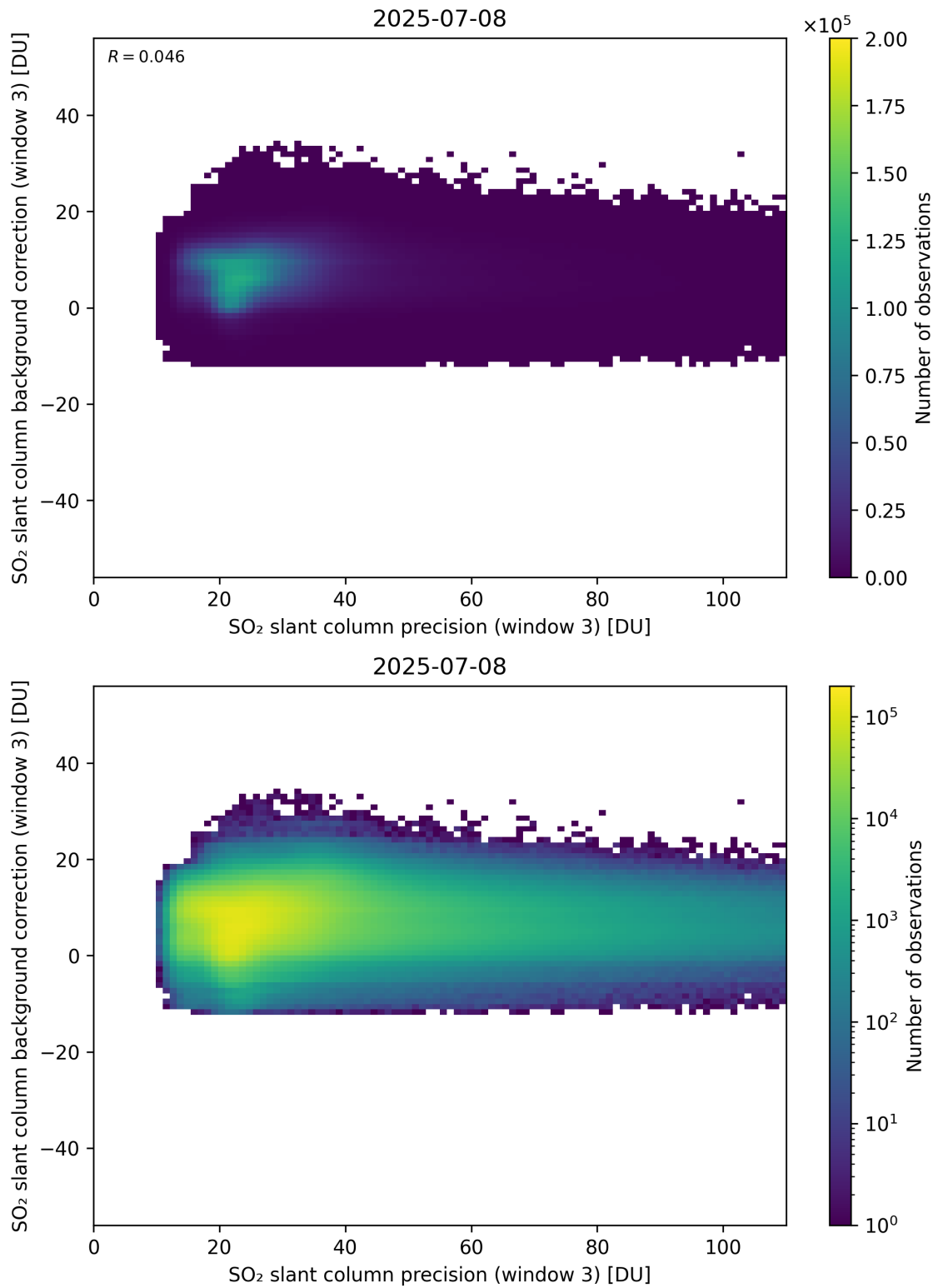
Figure 307: Scatter density plot of “SO 2 slant column precision (window 3)” against “SO 2 slant column background correction (window 3)” for 2025-07-08 to 2025-07-09.
