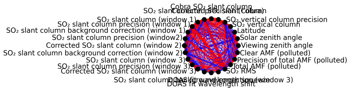
Figure 1: Map of correlation graph for 2025-07-08 to 2025-07-09.
