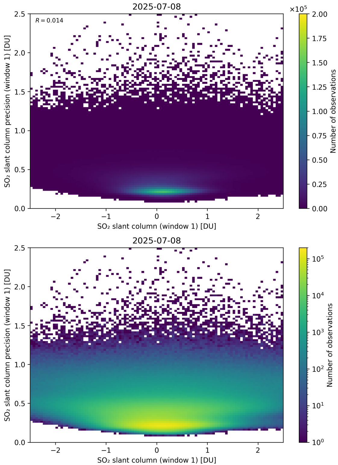
Figure 285: Scatter density plot of “SO 2 slant column (window 1)” against “SO 2 slant column precision (window 1)” for 2025-07-08 to 2025-07-09.
