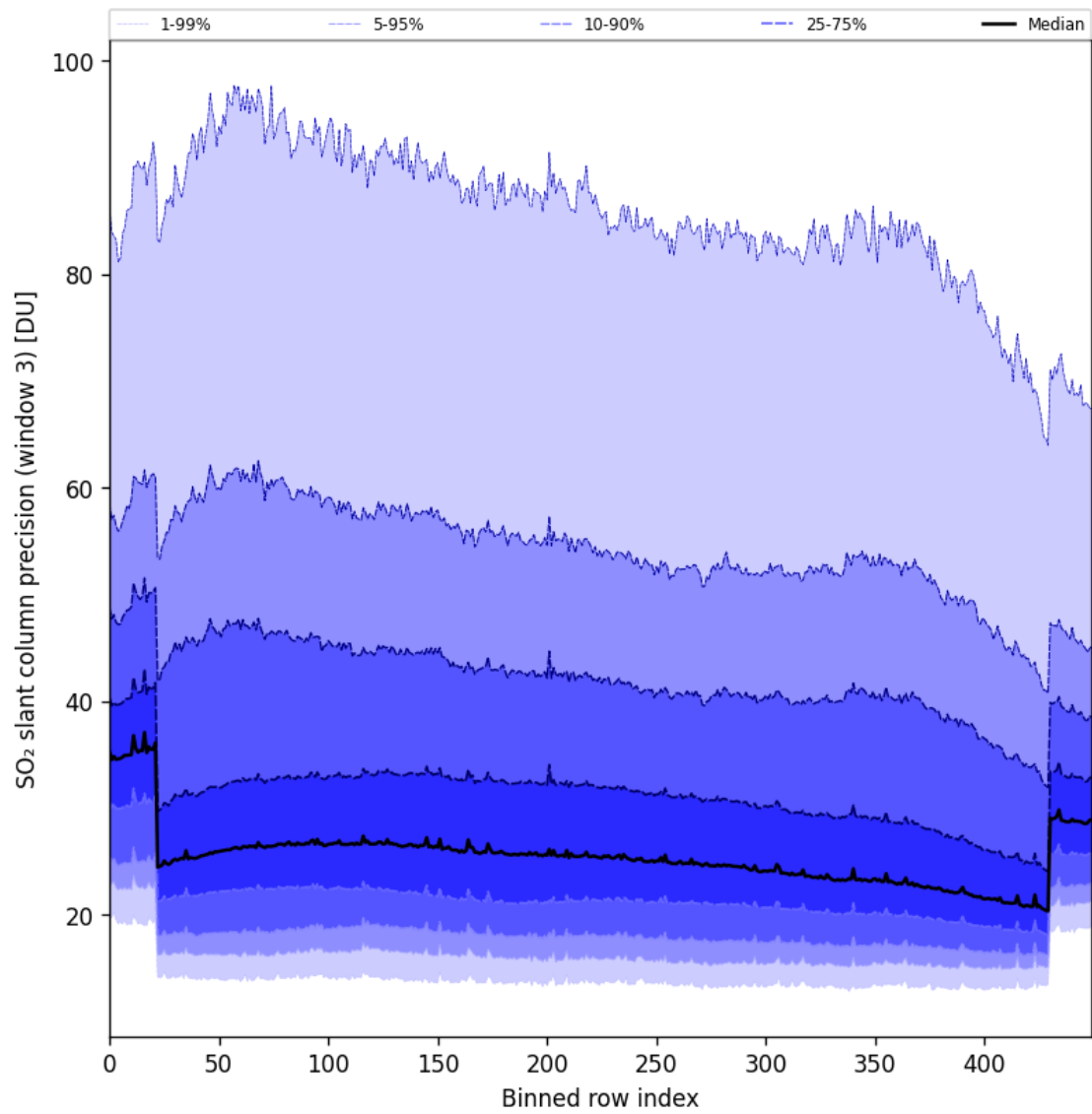
Figure 98: Along track statistics of "SO 2 slant column precision (window 3)" for 2025-07-08 to 2025-07-09
