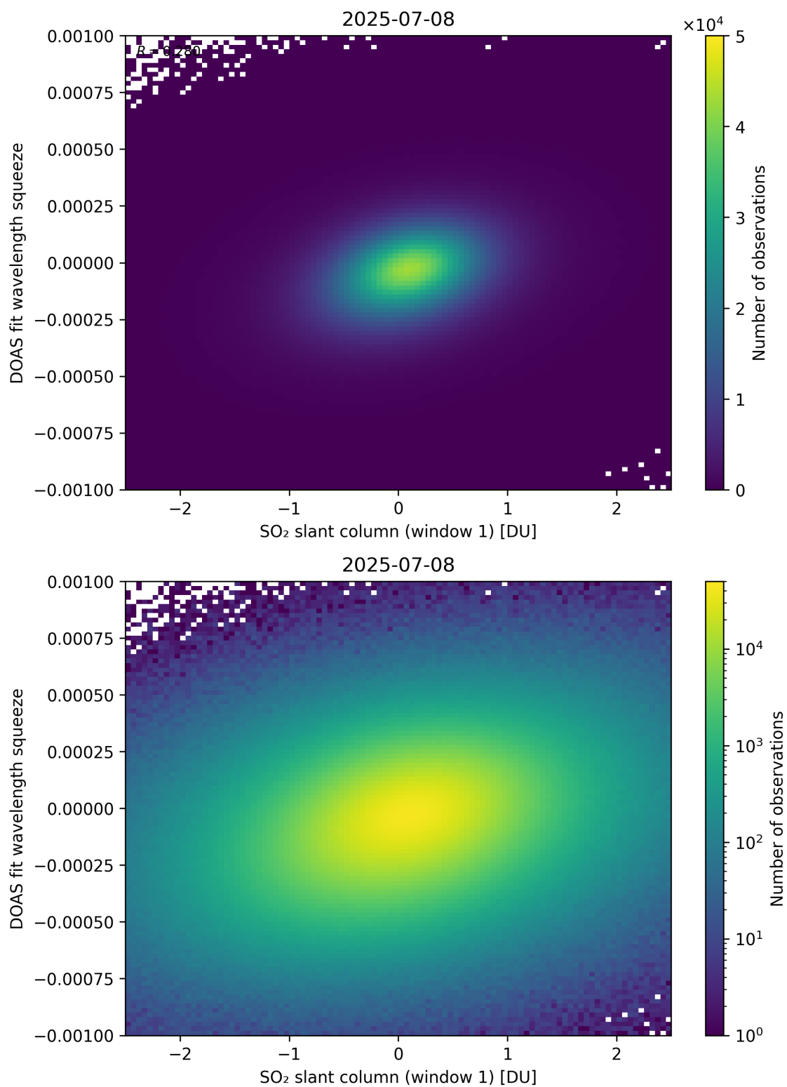
Figure 266: Scatter density plot of “SO 2 slant column (window 1)” against “DOAS fit wavelength squeeze” for 2025-07-08 to 2025-07-09.
