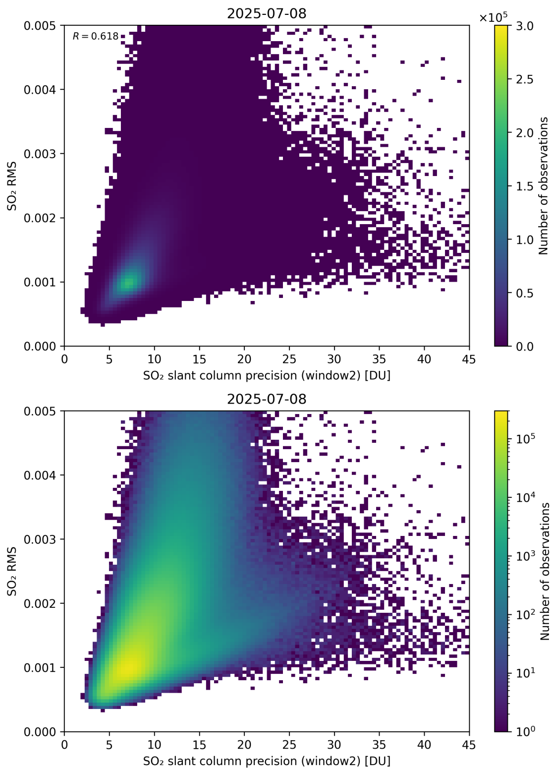
Figure 295: Scatter density plot of “SO 2 slant column precision (window2)” against “SO 2 RMS” for 2025-07-08 to 2025-07-09.
