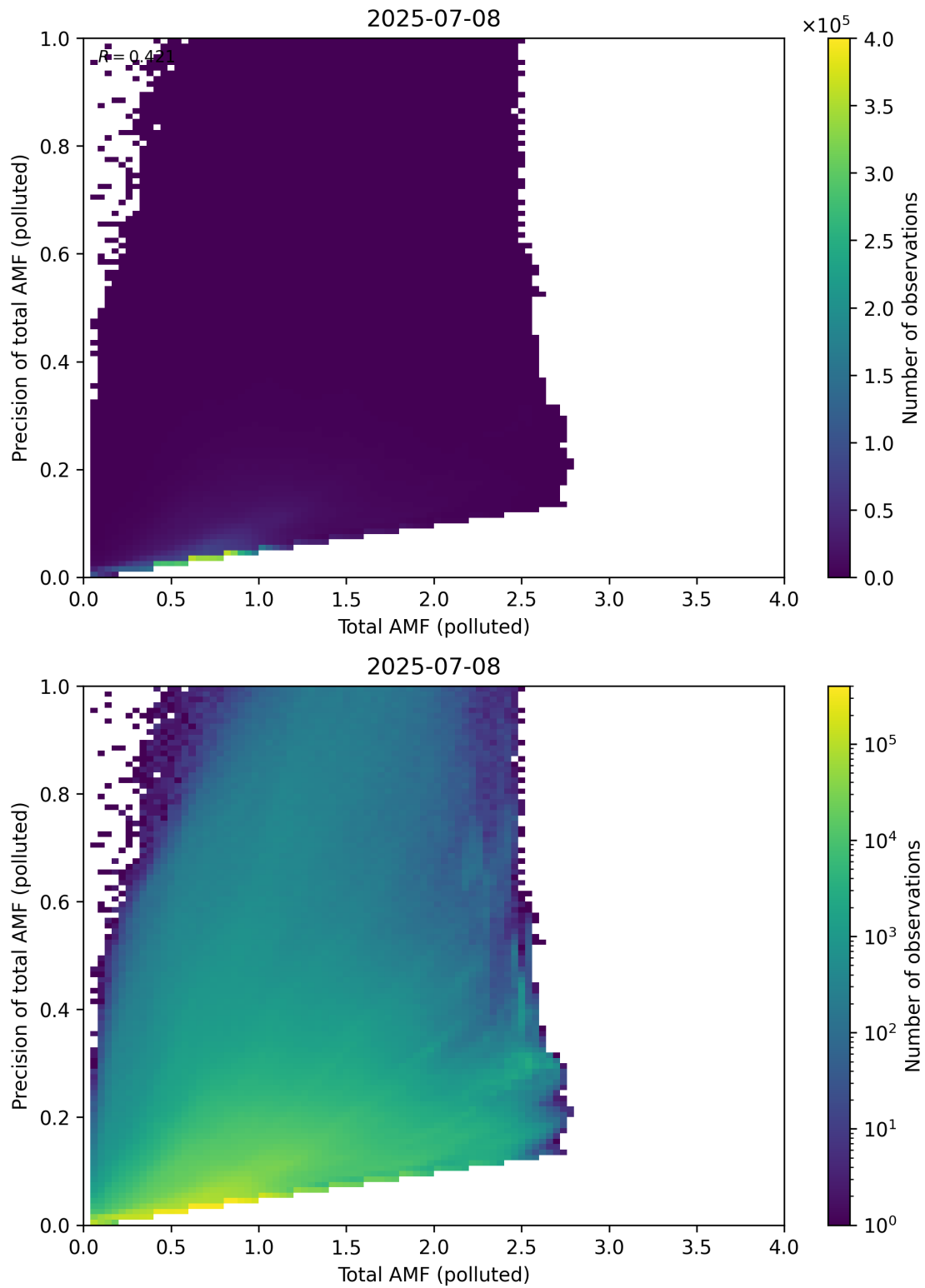
Figure 322: Scatter density plot of “Total AMF (polluted)” against “Precision of total AMF (polluted)” for 2025-07-08 to 2025-07-09.
