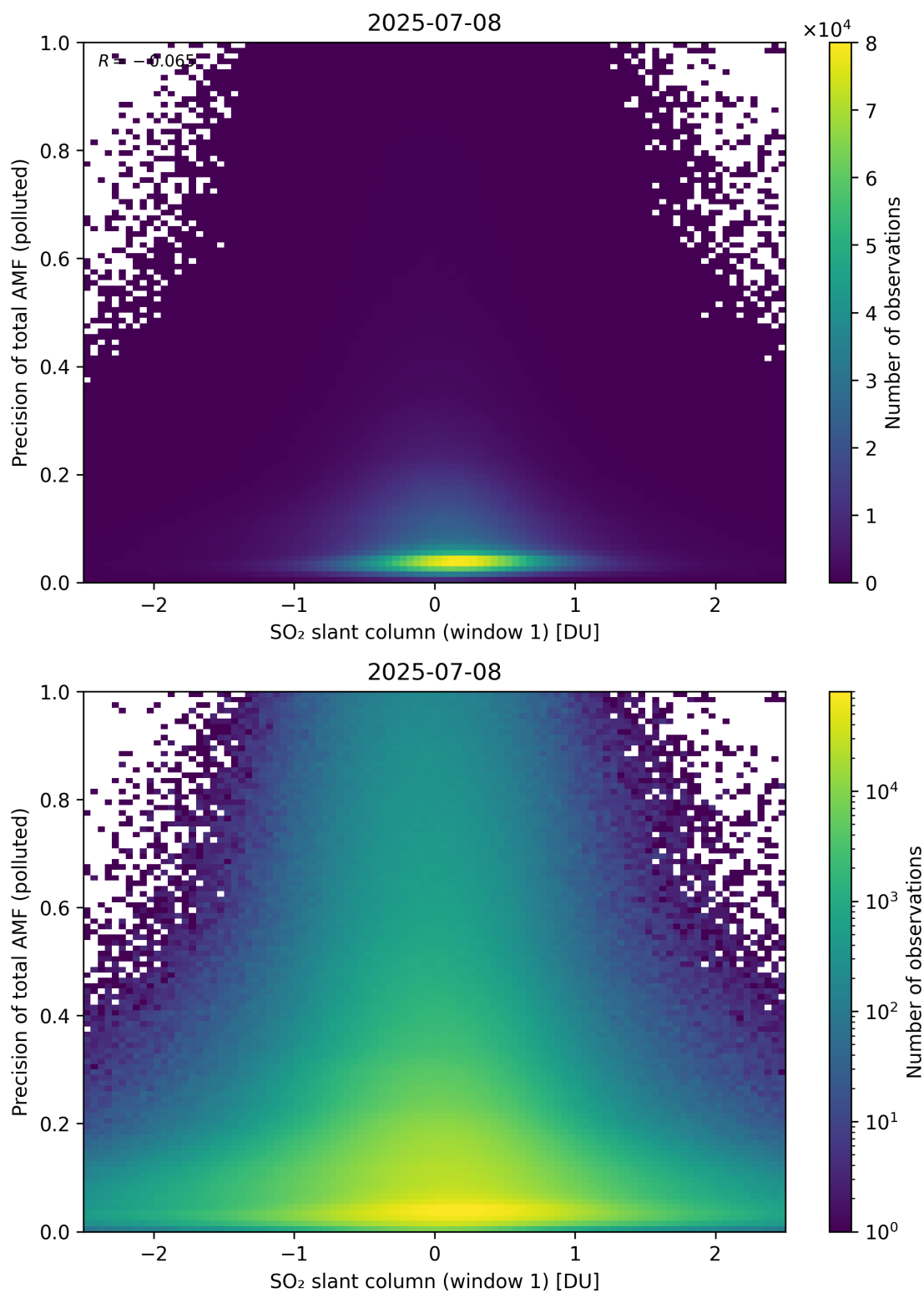
Figure 290: Scatter density plot of “SO 2 slant column (window 1)” against “Precision of total AMF (polluted)” for 2025-07-08 to 2025-07-09.
