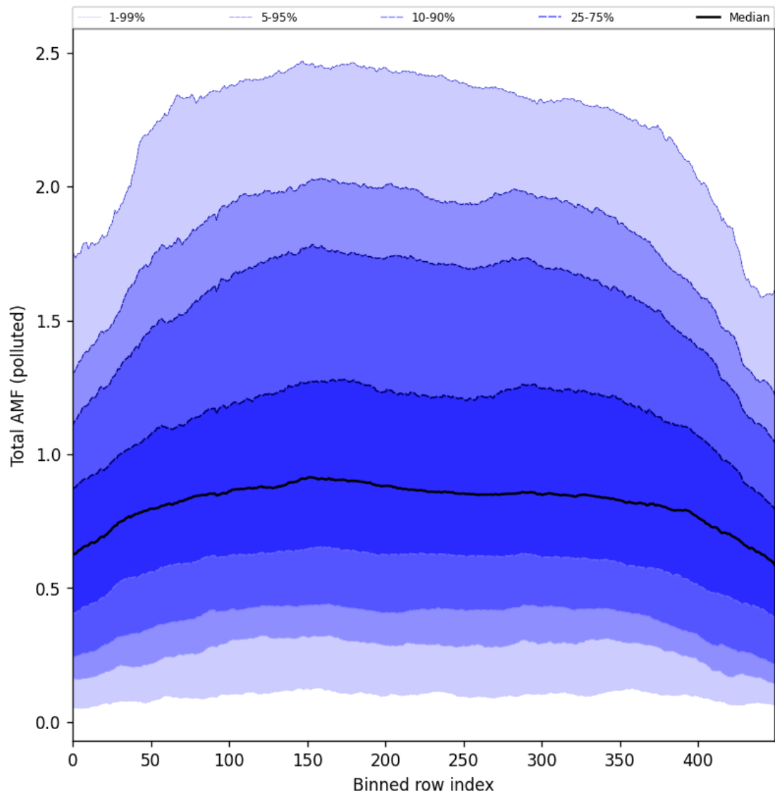
Figure 105: Along track statistics of “Total AMF (polluted)” for 2025-07-08 to 2025-07-09
