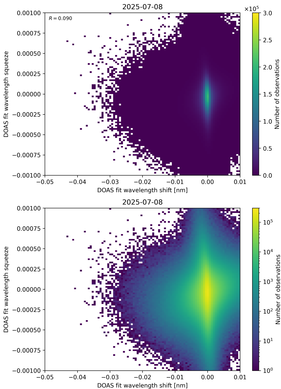
Figure 138: Scatter density plot of “DOAS fit wavelength shift” against “DOAS fit wavelength squeeze” for 2025-07-08 to 2025-07-09.
