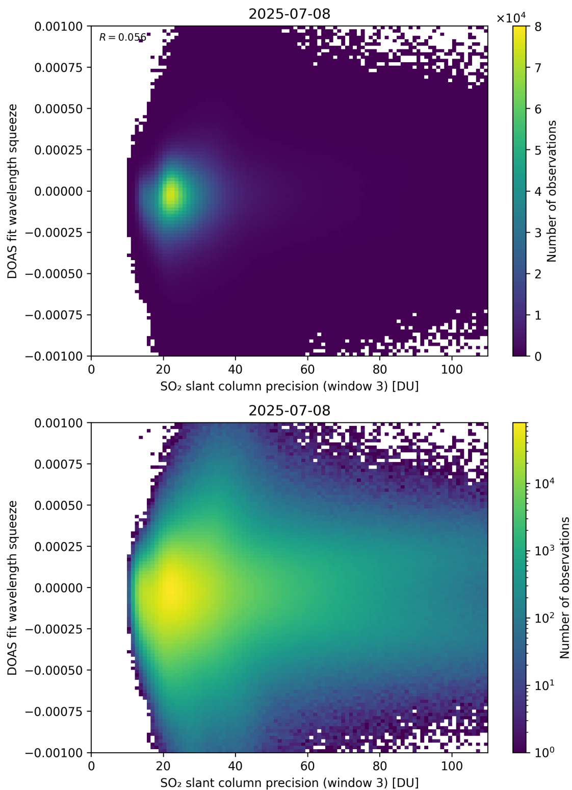
Figure 309: Scatter density plot of “SO 2 slant column precision (window 3)” against “DOAS fit wavelength squeeze” for 2025-07-08 to 2025-07-09.
