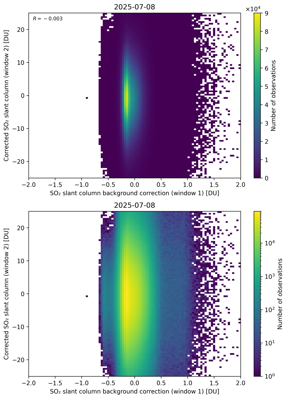
Figure 115: Scatter density plot of “SO 2 slant column background correction (window 1)” against “Corrected SO 2 slant column (window 2)” for 2025-07-08 to 2025-07-09.
