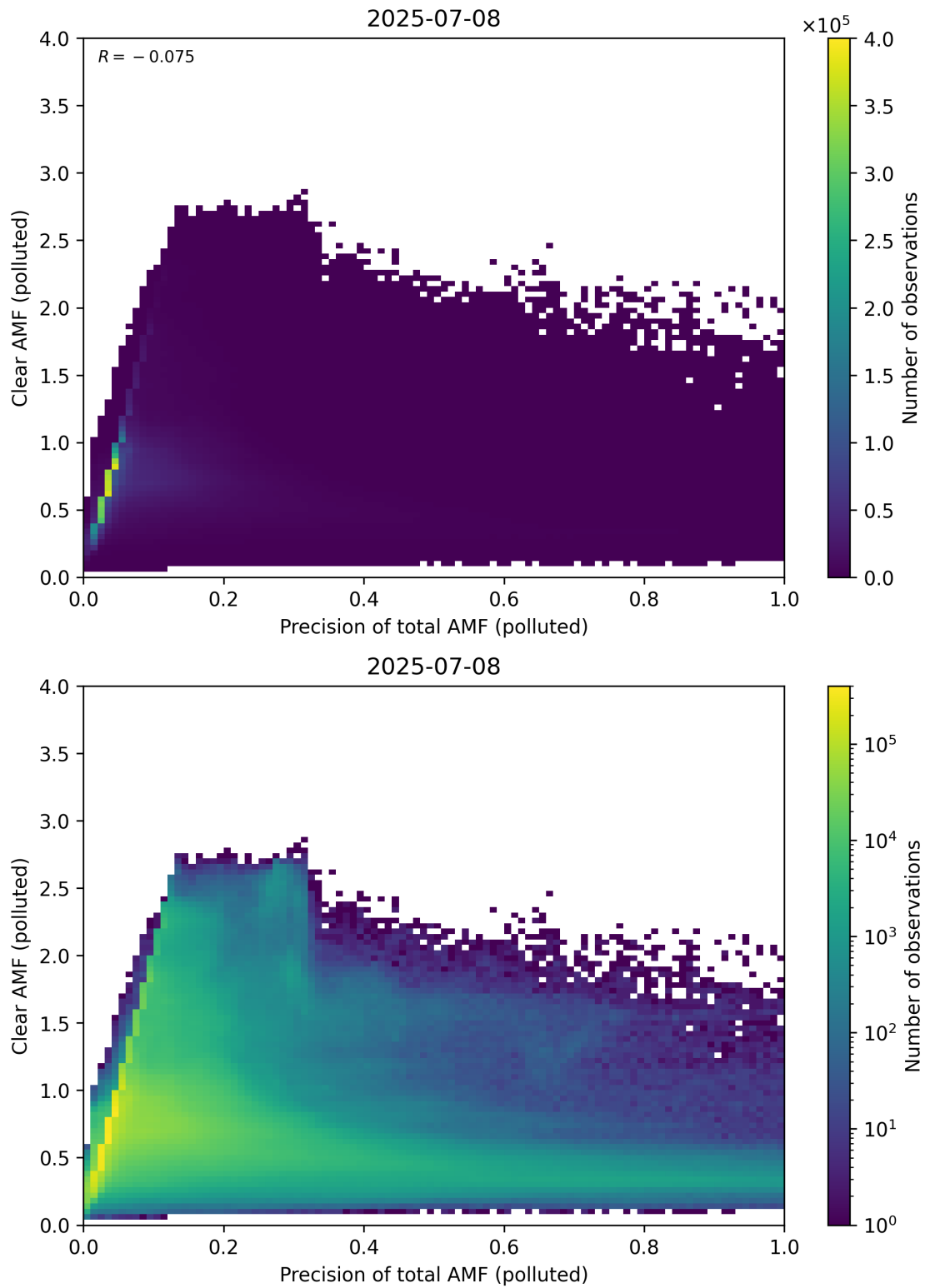
Figure 320: Scatter density plot of “Precision of total AMF (polluted)” against “Clear AMF (polluted)” for 2025-07-08 to 2025-07-09.
