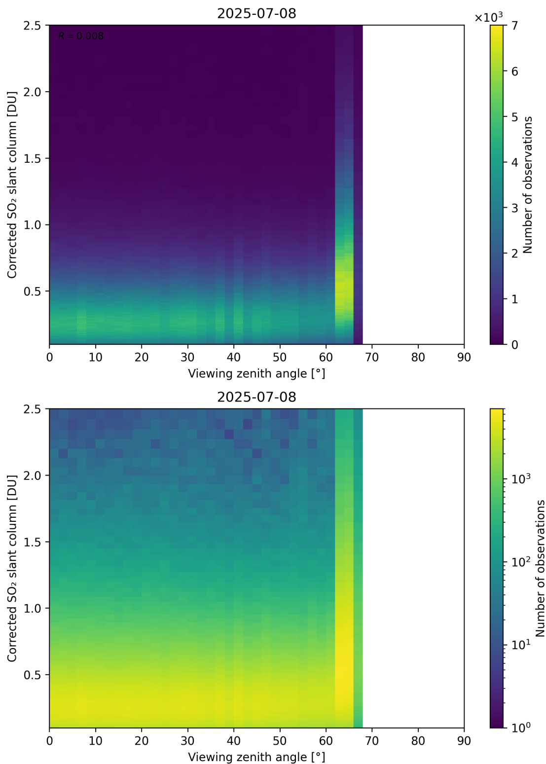
Figure 373: Scatter density plot of “Viewing zenith angle” against “Corrected SO 2 slant column” for 2025-07-08 to 2025-07-09.
