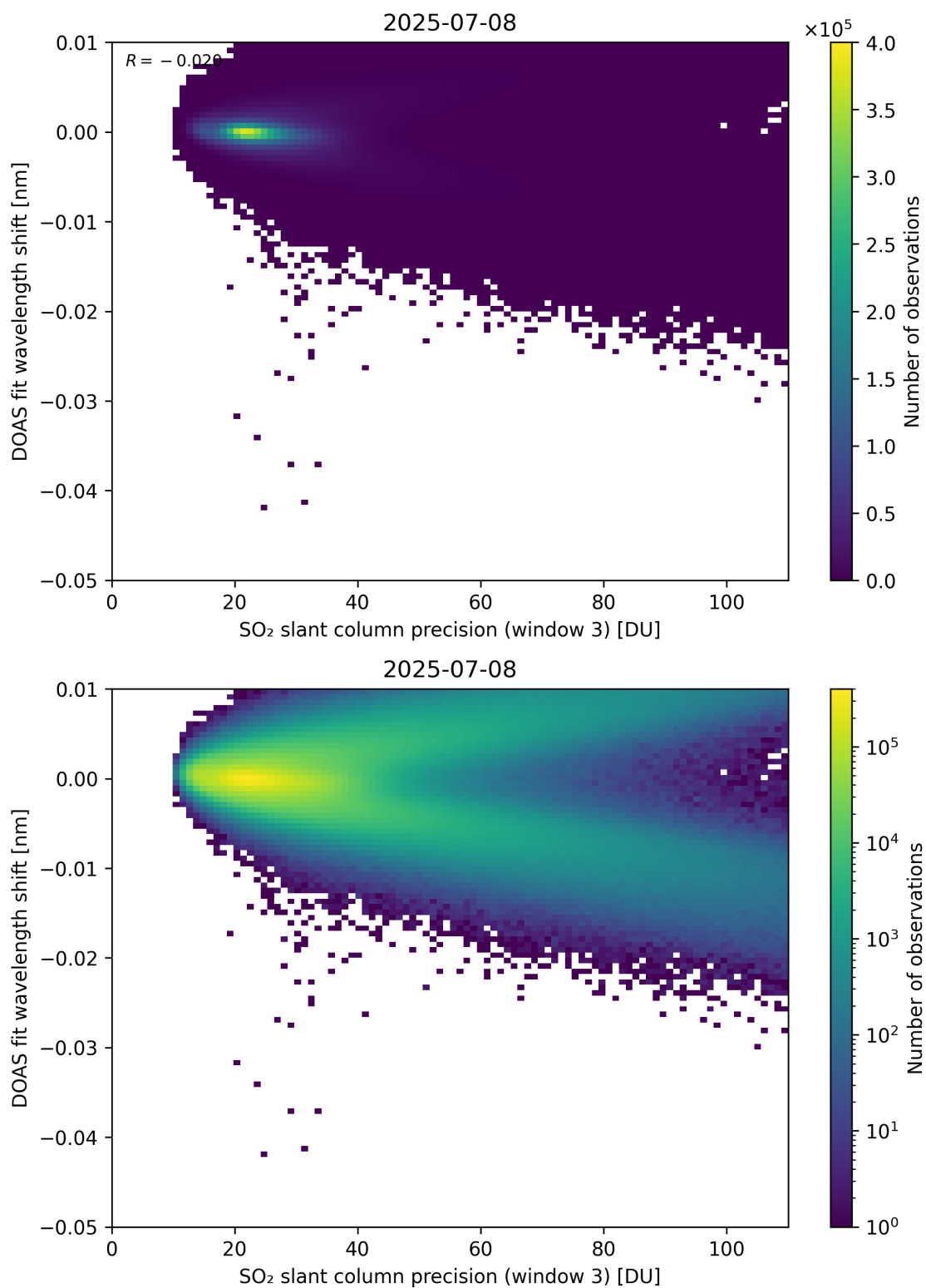
Figure 308: Scatter density plot of “SO 2 slant column precision (window 3)” against “DOAS fit wavelength shift” for 2025-07-08 to 2025-07-09.
