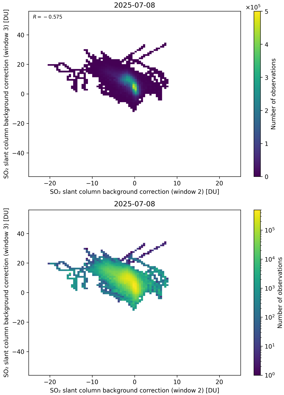
Figure 122: Scatter density plot of “SO 2 slant column background correction (window 2)” against “SO 2 slant column background correction (window 3)” for 2025-07-08 to 2025-07-09.
