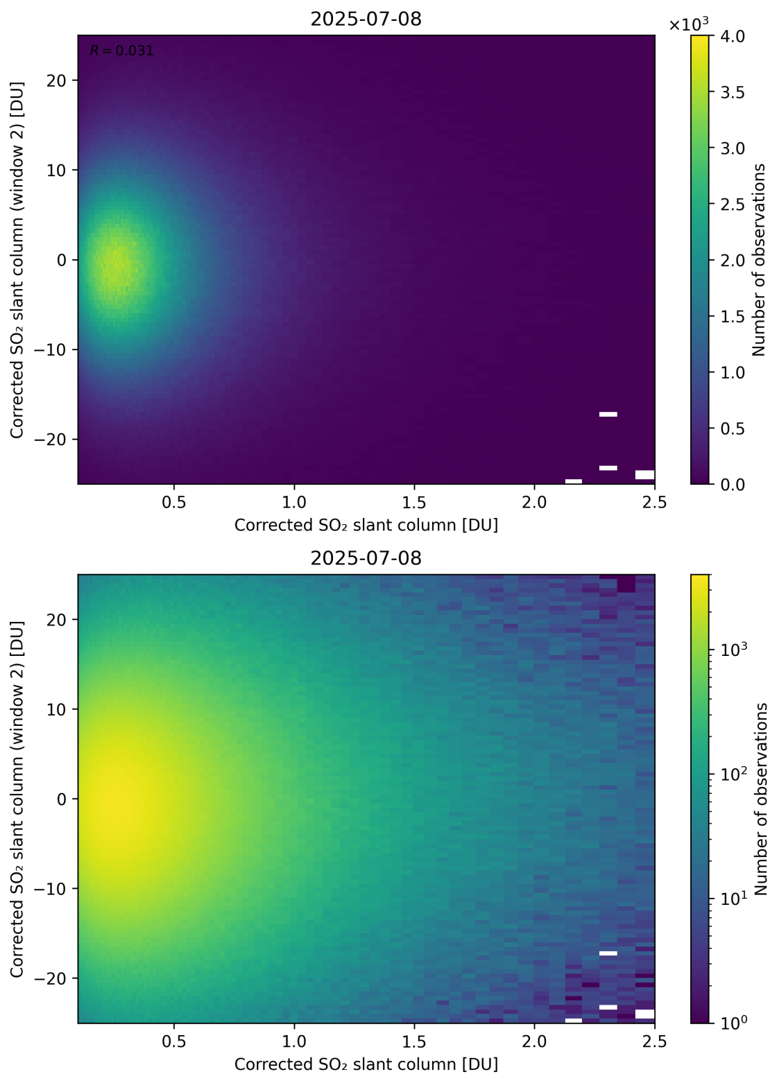
Figure 235: Scatter density plot of “Corrected SO 2 slant column” against “Corrected SO 2 slant column (window 2)” for 2025-07-08 to 2025-07-09.
