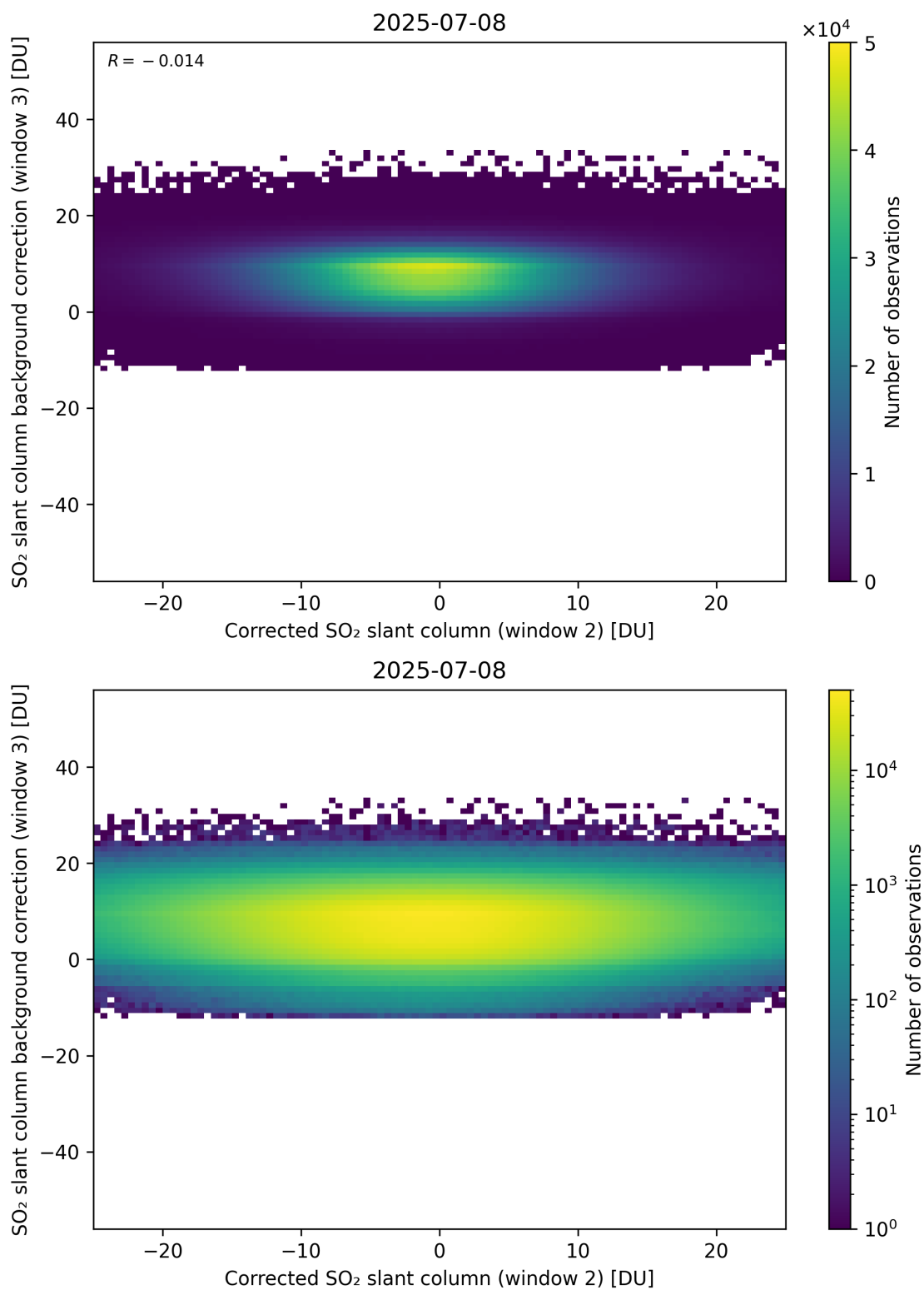
Figure 245: Scatter density plot of “Corrected SO 2 slant column (window 2)” against “SO 2 slant column background correction (window 3)” for 2025-07-08 to 2025-07-09.
