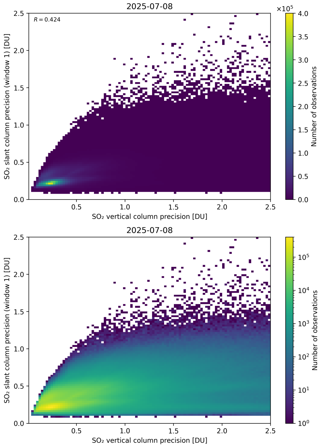
Figure 342: Scatter density plot of “SO 2 vertical column precision” against “SO 2 slant column precision (window 1)” for 2025-07-08 to 2025-07-09.
