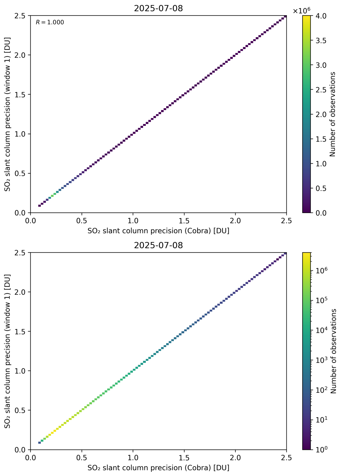
Figure 209: Scatter density plot of “SO 2 slant column precision (Cobra)” against “SO 2 slant column precision (window 1)” for 2025-07-08 to 2025-07-09.
