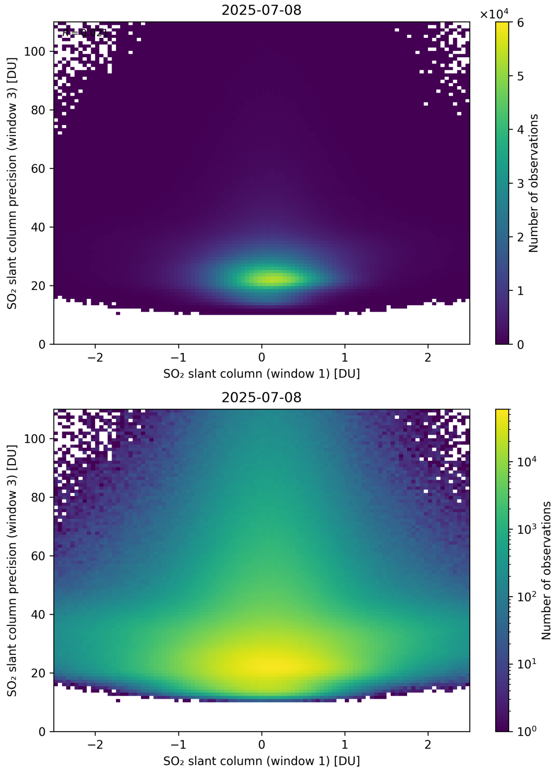
Figure 288: Scatter density plot of “SO 2 slant column (window 1)” against “SO 2 slant column precision (window 3)” for 2025-07-08 to 2025-07-09.
