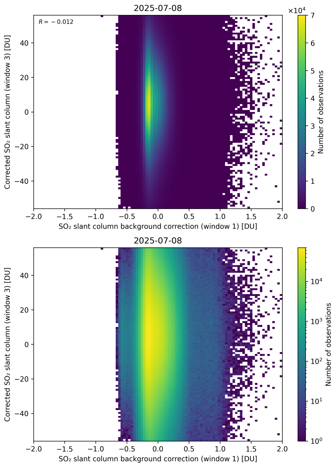
Figure 116: Scatter density plot of “SO 2 slant column background correction (window 1)” against “Corrected SO 2 slant column (window 3)” for 2025-07-08 to 2025-07-09.
