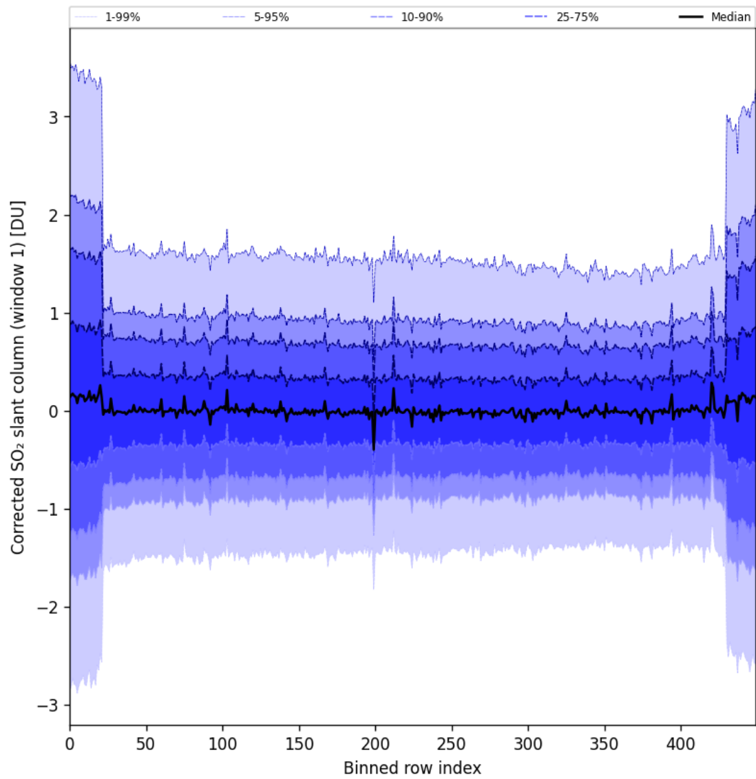
Figure 91: Along track statistics of “Corrected SO 2 slant column (window 1)” for 2025-07-08 to 2025-07-09
