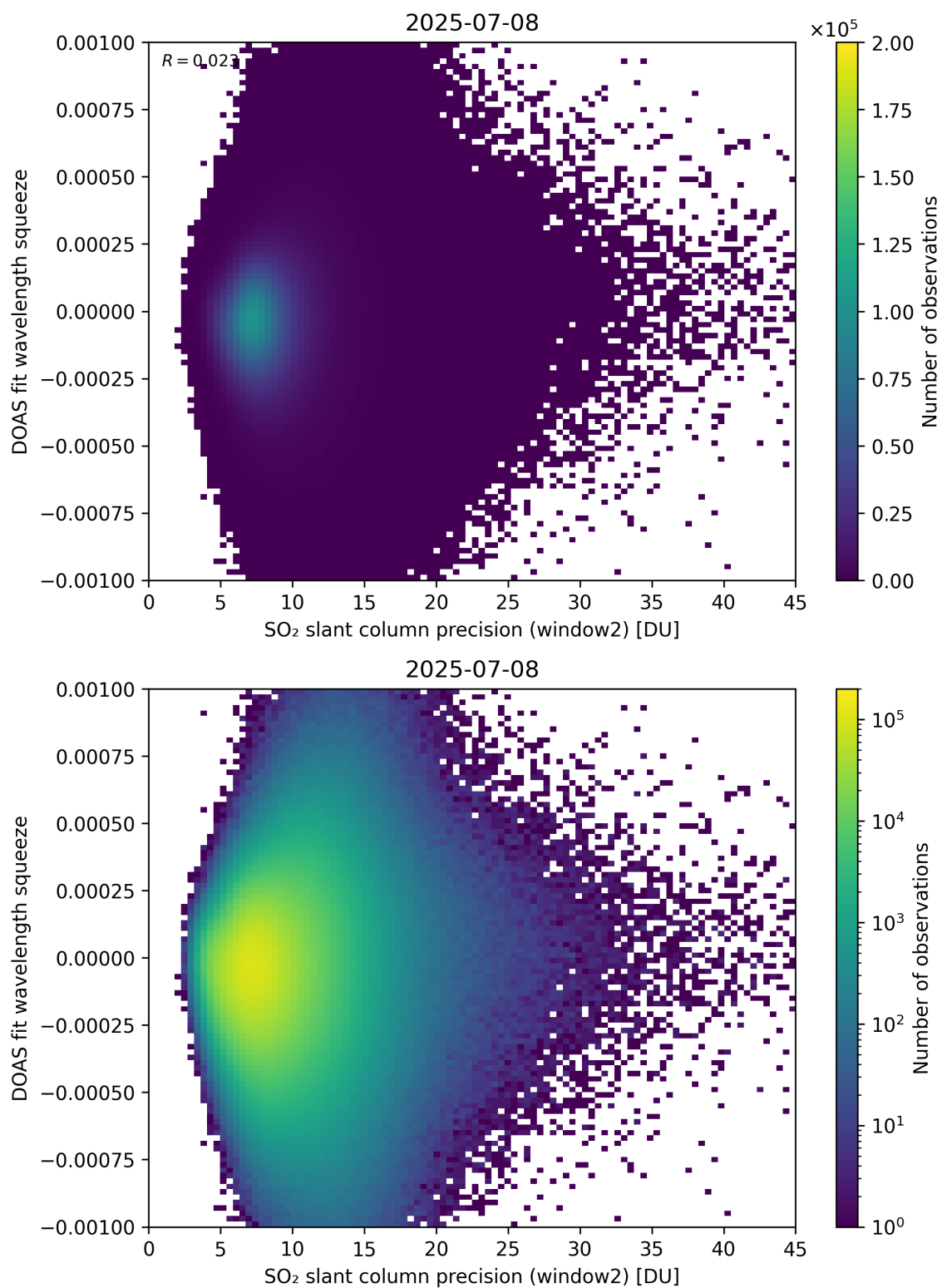
Figure 294: Scatter density plot of “SO 2 slant column precision (window2)” against “DOAS fit wavelength squeeze” for 2025-07-08 to 2025-07-09.
