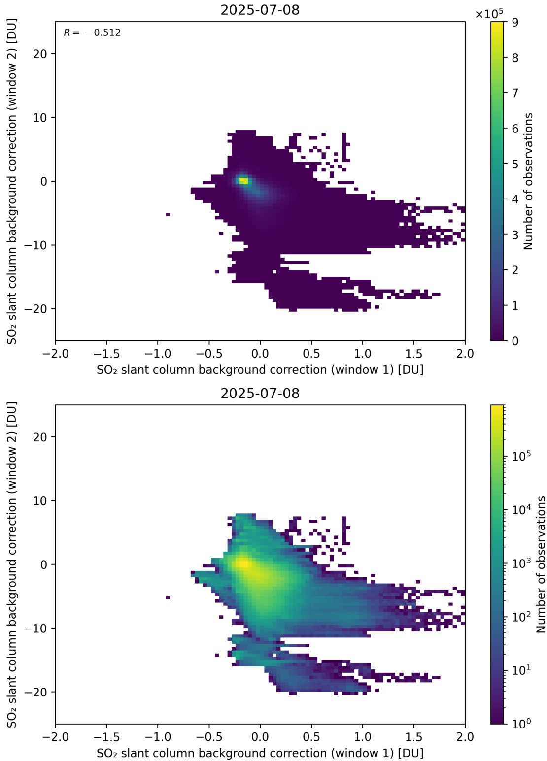
Figure 109: Scatter density plot of “SO 2 slant column background correction (window 1)” against “SO 2 slant column background correction (window 2)” for 2025-07-08 to 2025-07-09.
