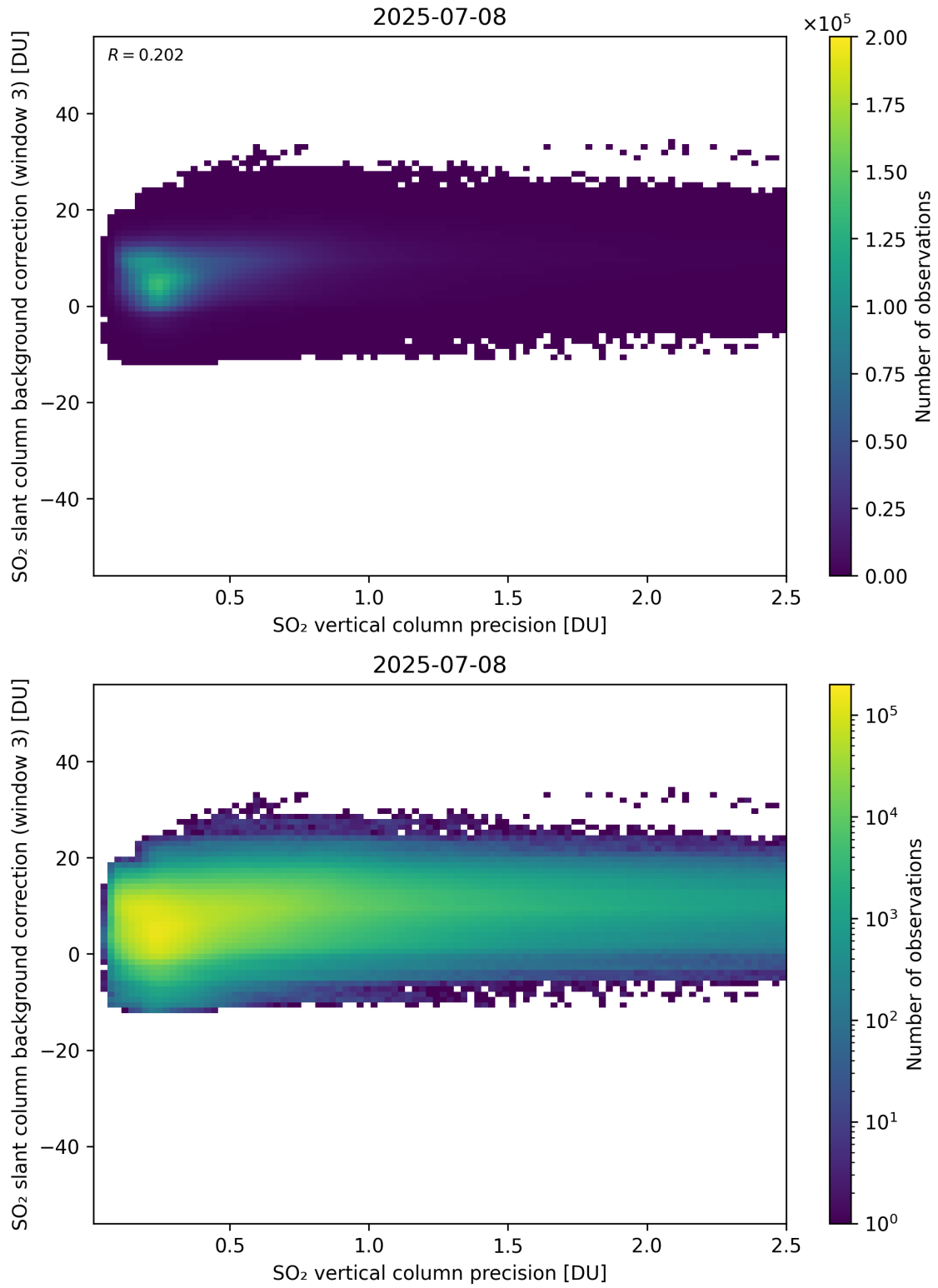
Figure 331: Scatter density plot of “SO 2 vertical column precision” against “SO 2 slant column background correction (window 3)” for 2025-07-08 to 2025-07-09.
