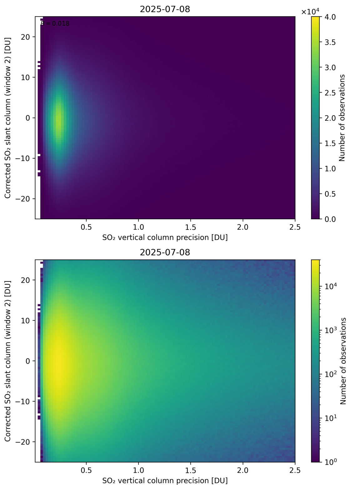
Figure 339: Scatter density plot of “SO 2 vertical column precision” against “Corrected SO 2 slant column (window 2)” for 2025-07-08 to 2025-07-09.
