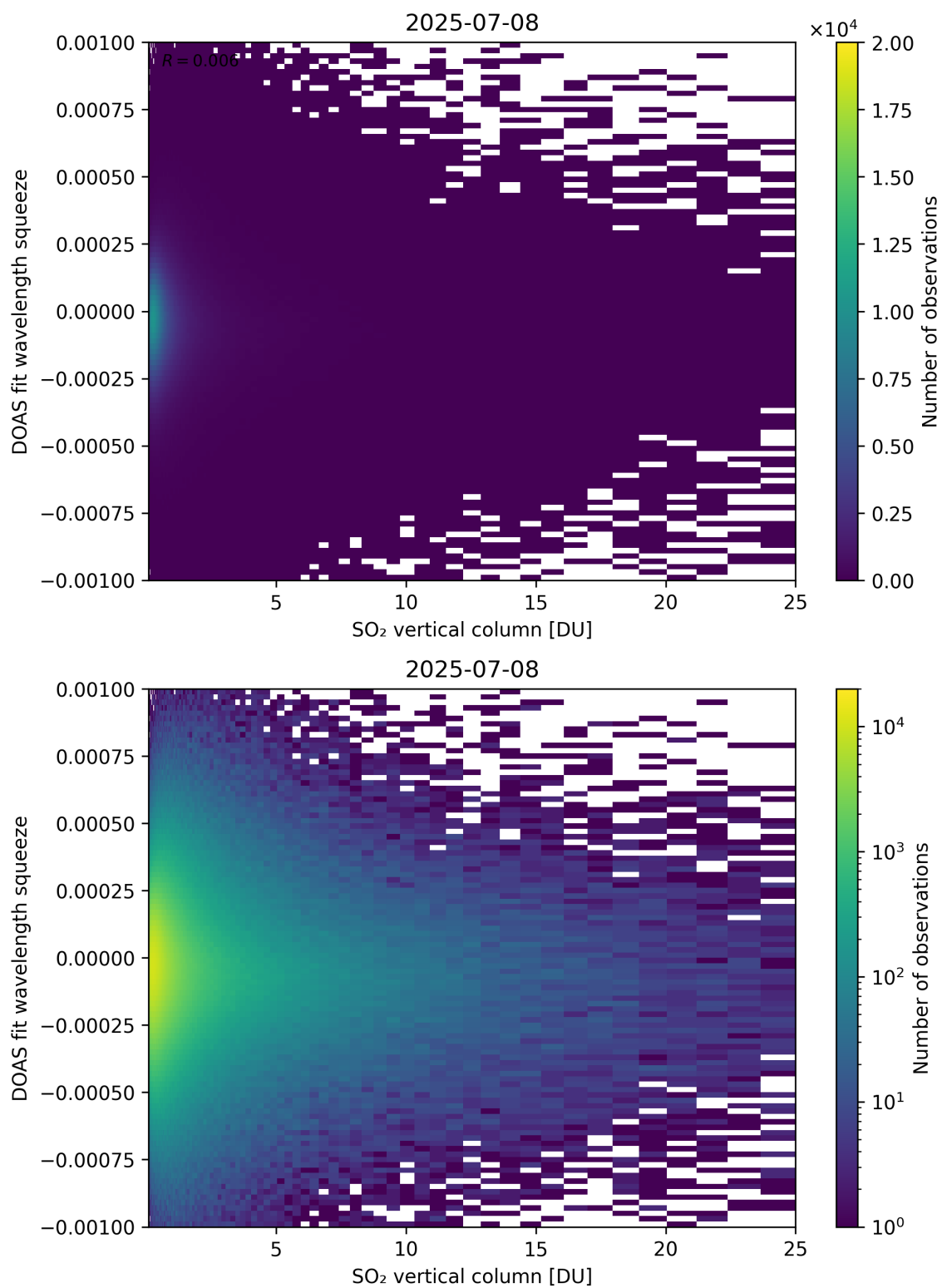
Figure 327: Scatter density plot of “SO 2 vertical column” against “DOAS fit wavelength squeeze” for 2025-07-08 to 2025-07-09.
