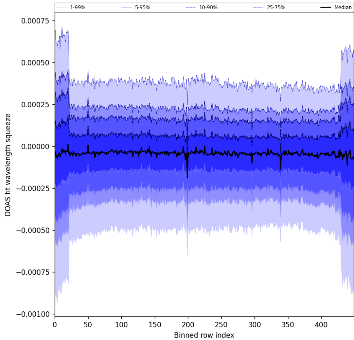
Figure 103: Along track statistics of “DOAS fit wavelength squeeze” for 2025-07-08 to 2025-07-09
