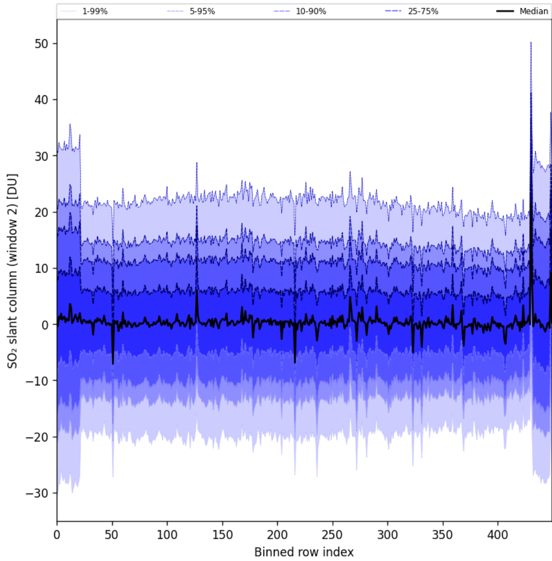
Figure 93: Along track statistics of “SO 2 slant column (window 2)” for 2025-07-08 to 2025-07-09
