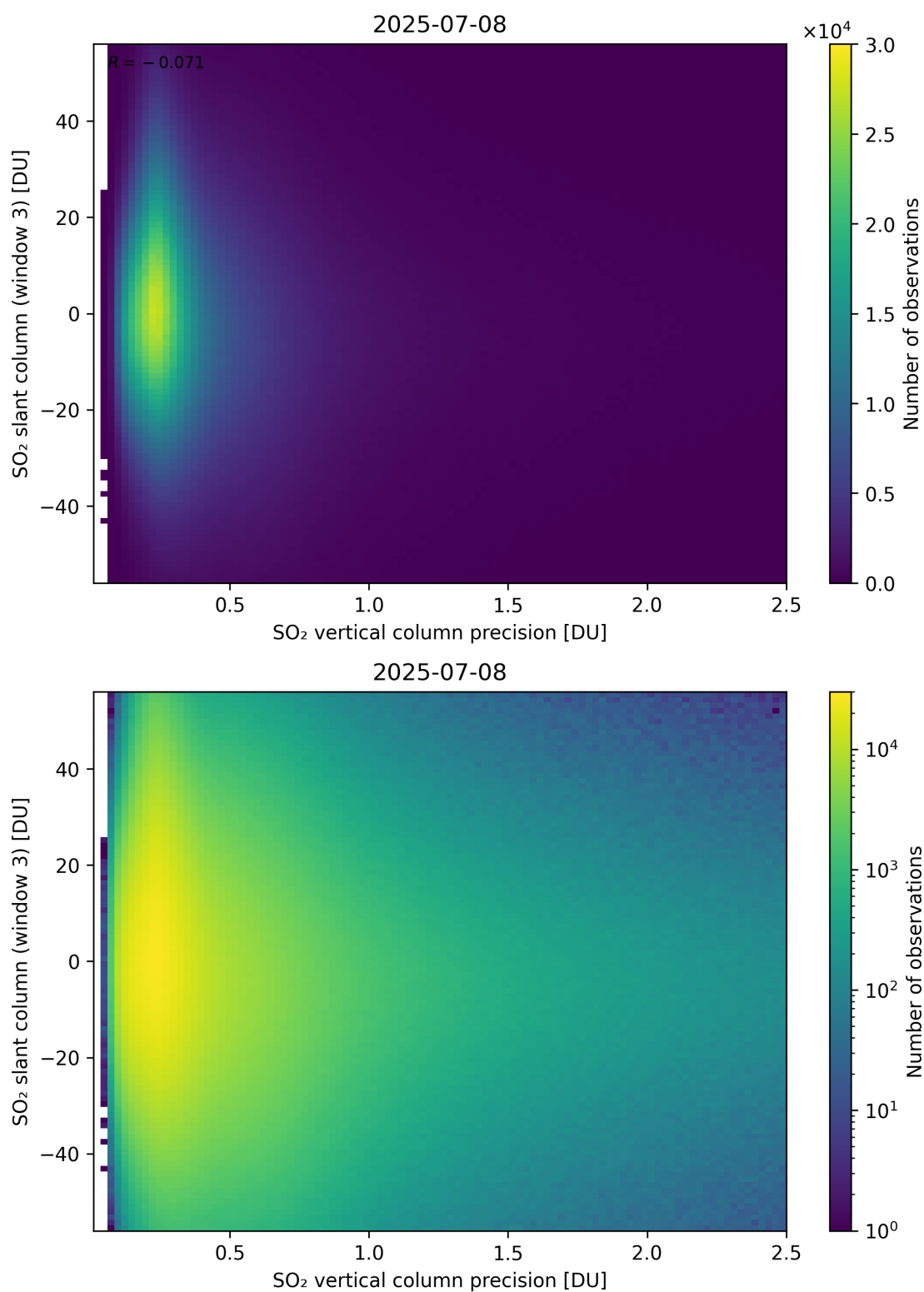
Figure 344: Scatter density plot of “SO 2 vertical column precision” against “SO 2 slant column (window 3)” for 2025-07-08 to 2025-07-09.
