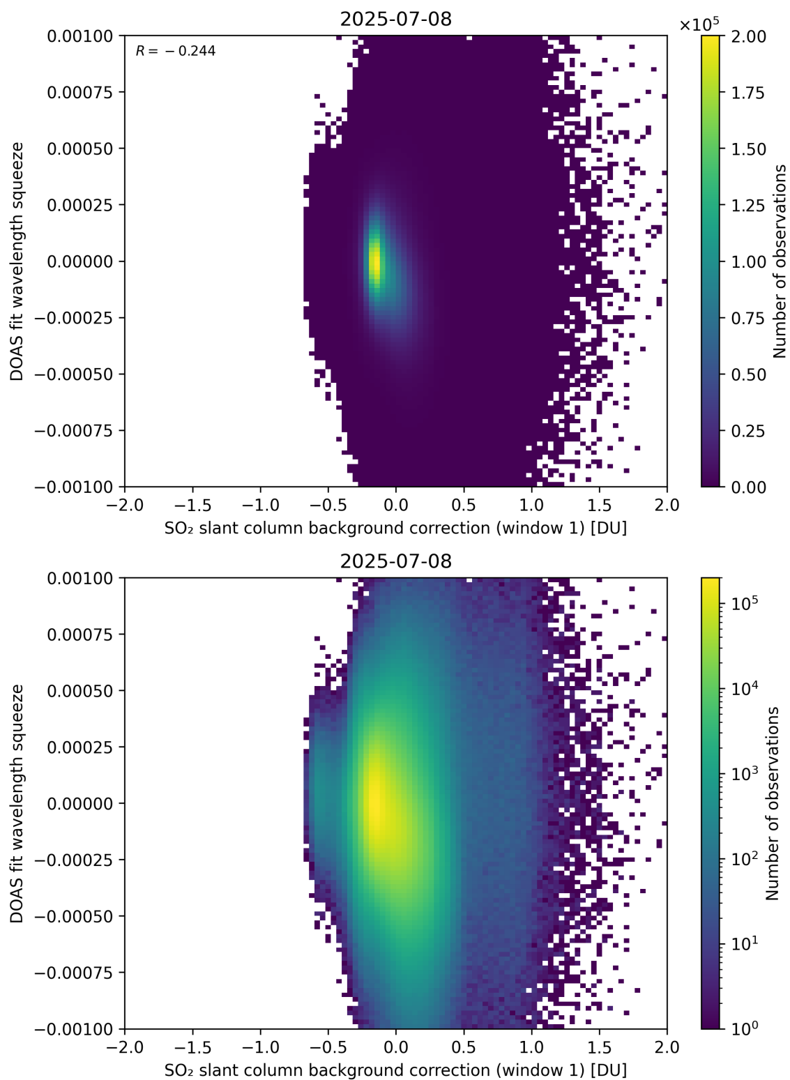
Figure 112: Scatter density plot of “SO 2 slant column background correction (window 1)” against “DOAS fit wavelength squeeze” for 2025-07-08 to 2025-07-09.
