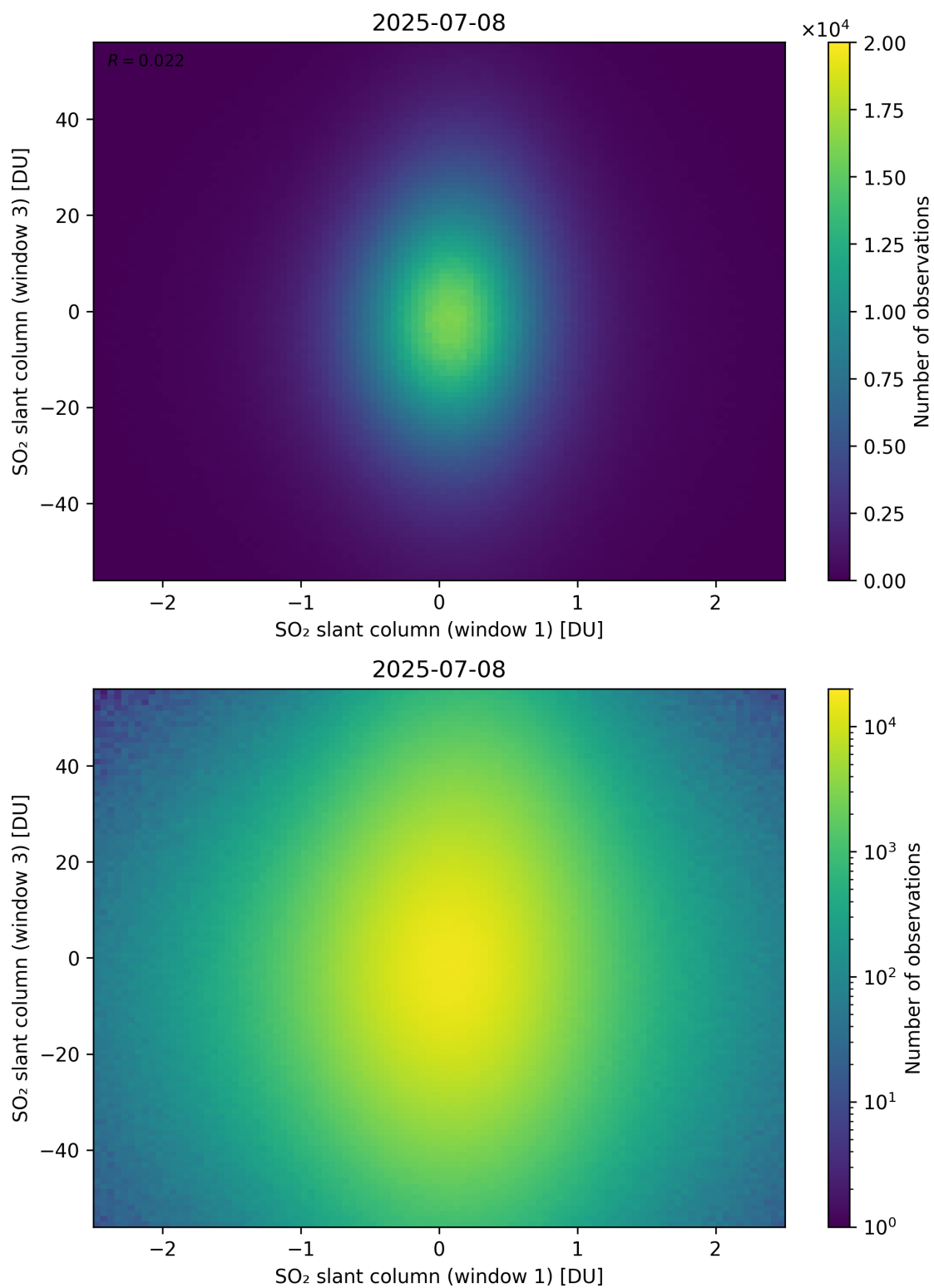
Figure 287: Scatter density plot of “SO 2 slant column (window 1)” against “SO 2 slant column (window 3)” for 2025-07-08 to 2025-07-09.
