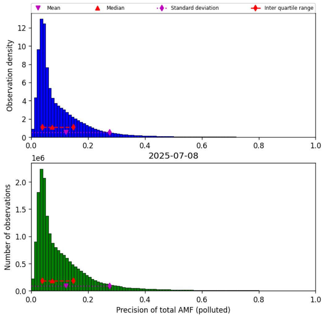
Figure 80: Histogram of “Precision of total AMF (polluted)” for 2025-07-08 to 2025-07-09
