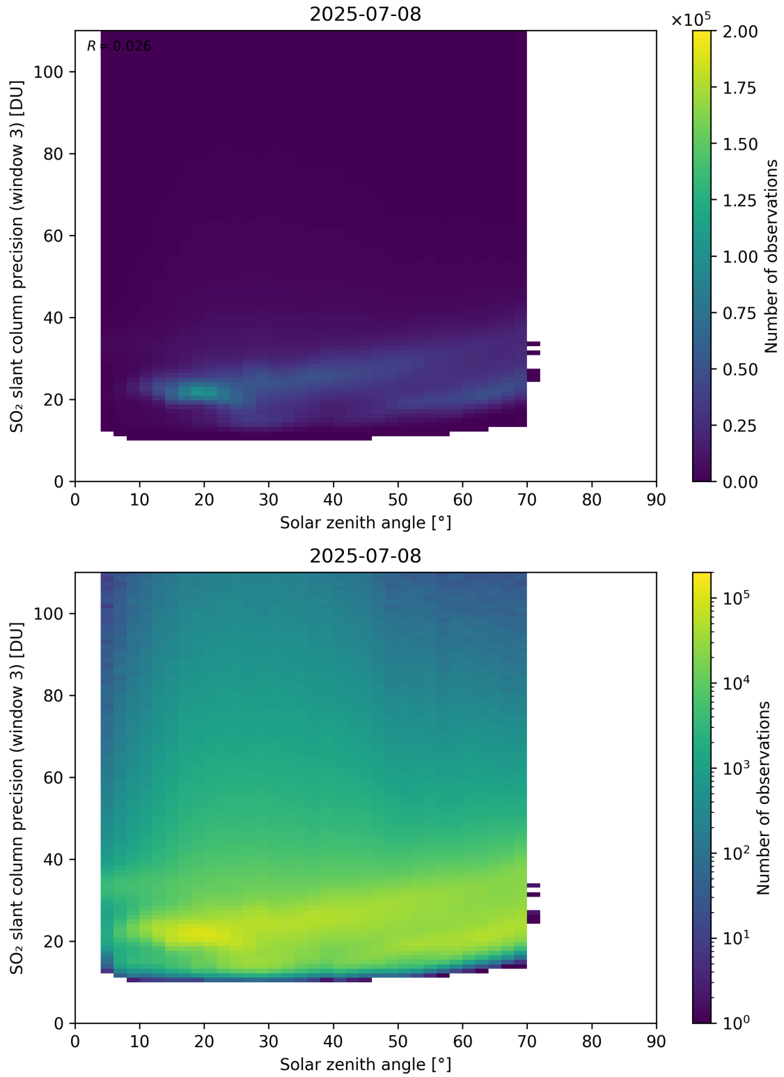
Figure 188: Scatter density plot of “Solar zenith angle” against “SO 2 slant column precision (window 3)” for 2025-07-08 to 2025-07-09.
