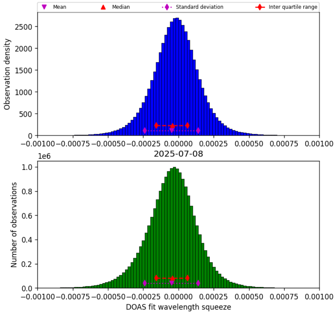
Figure 77: Histogram of “DOAS fit wavelength squeeze” for 2025-07-08 to 2025-07-09
