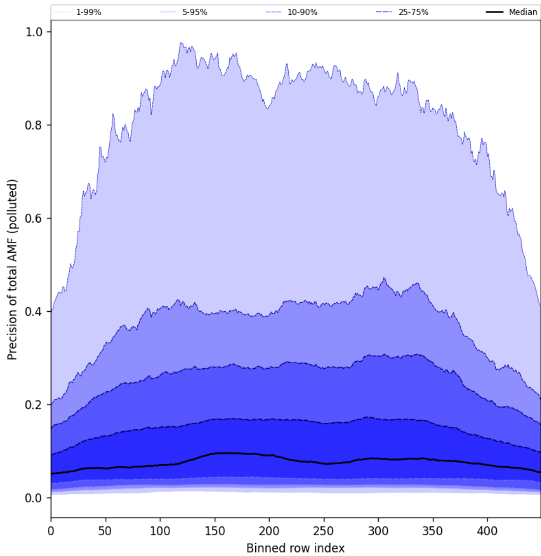
Figure 106: Along track statistics of “Precision of total AMF (polluted)” for 2025-07-08 to 2025-07-09
