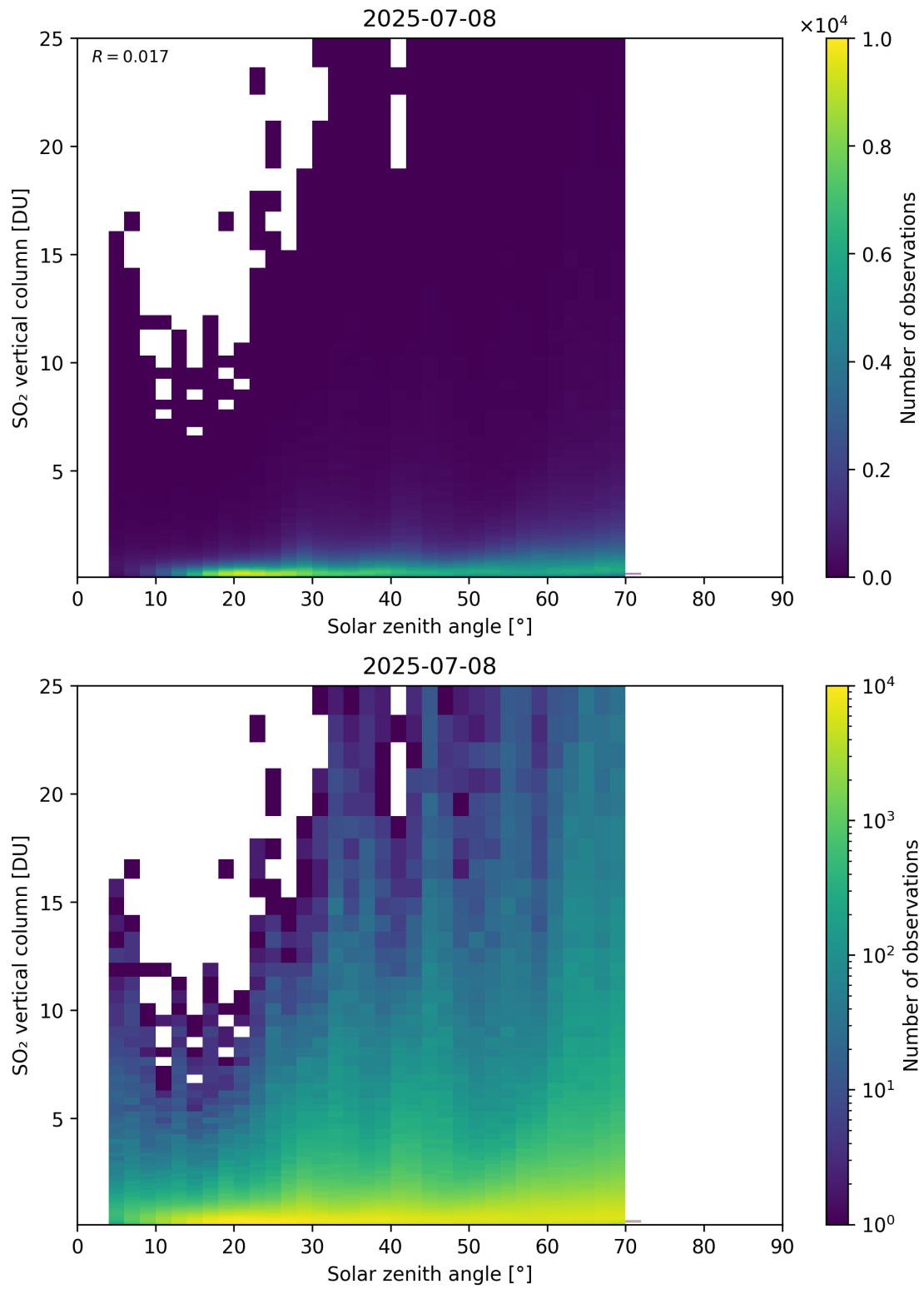
Figure 191: Scatter density plot of “Solar zenith angle” against “SO 2 vertical column” for 2025-07-08 to 2025-07-09.
