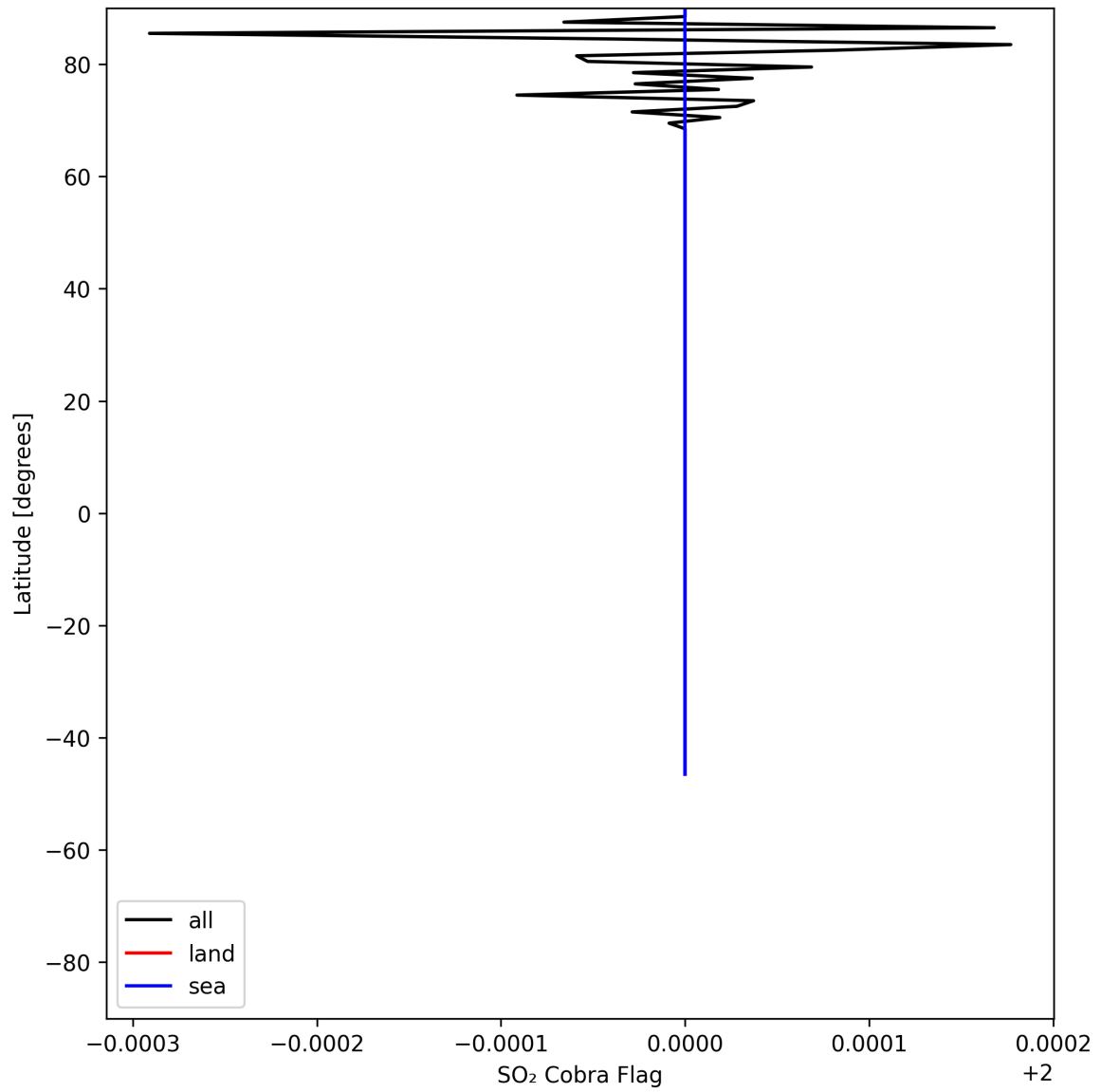
Figure 49: Zonal average of “SO 2 Cobra Flag” for 2025-07-08 to 2025-07-09.
