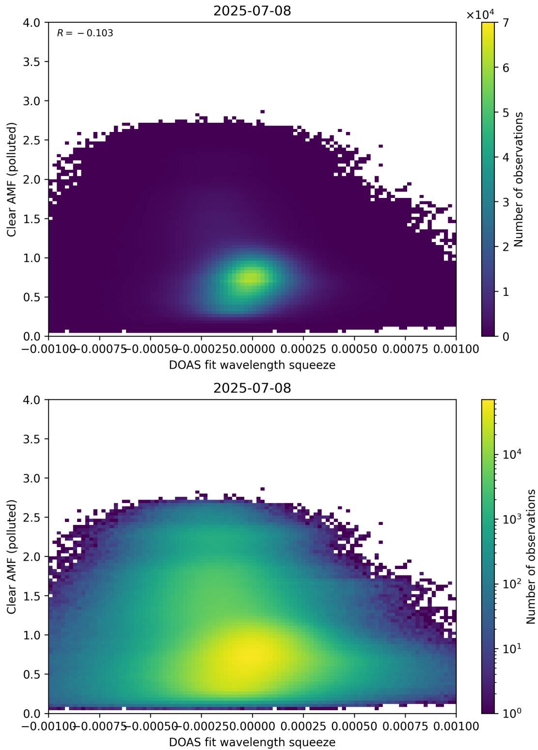
Figure 144: Scatter density plot of “DOAS fit wavelength squeeze” against “Clear AMF (polluted)” for 2025-07-08 to 2025-07-09.
