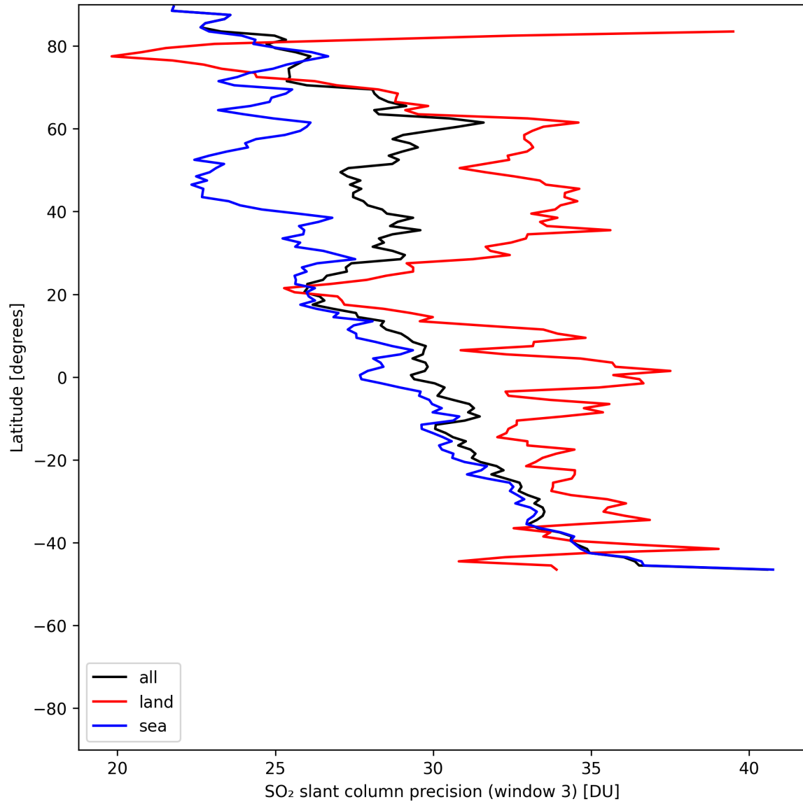
Figure 46: Zonal average of “SO 2 slant column precision (window 3)” for 2025-07-08 to 2025-07-09.
