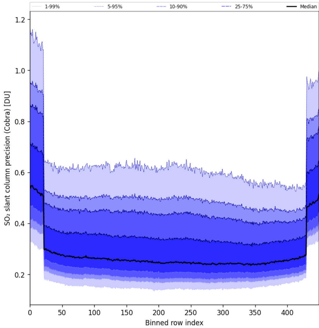
Figure 88: Along track statistics of “SO 2 slant column precision (Cobra)” for 2025-07-08 to 2025-07-09
