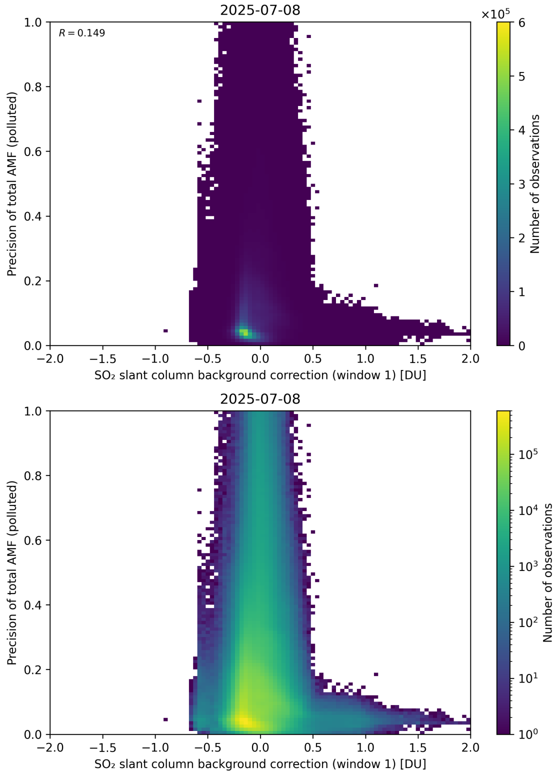
Figure 121: Scatter density plot of “SO 2 slant column background correction (window 1)” against “Precision of total AMF (polluted)” for 2025-07-08 to 2025-07-09.
