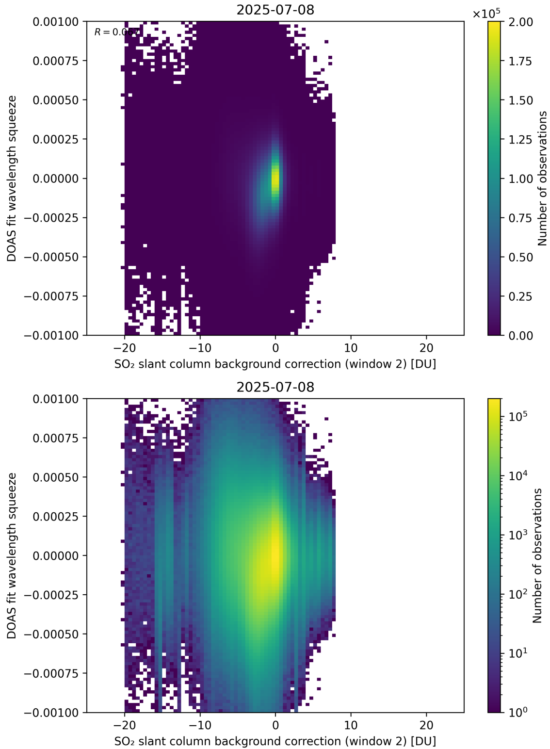
Figure 124: Scatter density plot of “SO 2 slant column background correction (window 2)” against “DOAS fit wavelength squeeze” for 2025-07-08 to 2025-07-09.
