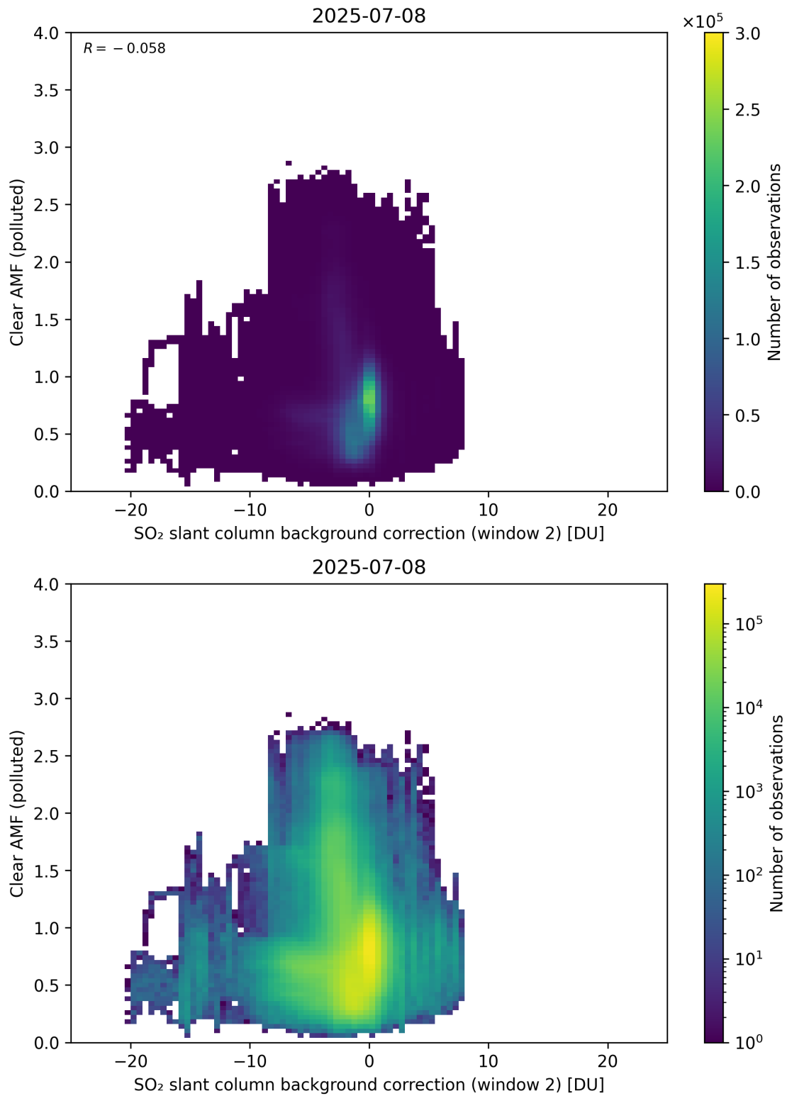
Figure 126: Scatter density plot of “SO 2 slant column background correction (window 2)” against “Clear AMF (polluted)” for 2025-07-08 to 2025-07-09.
