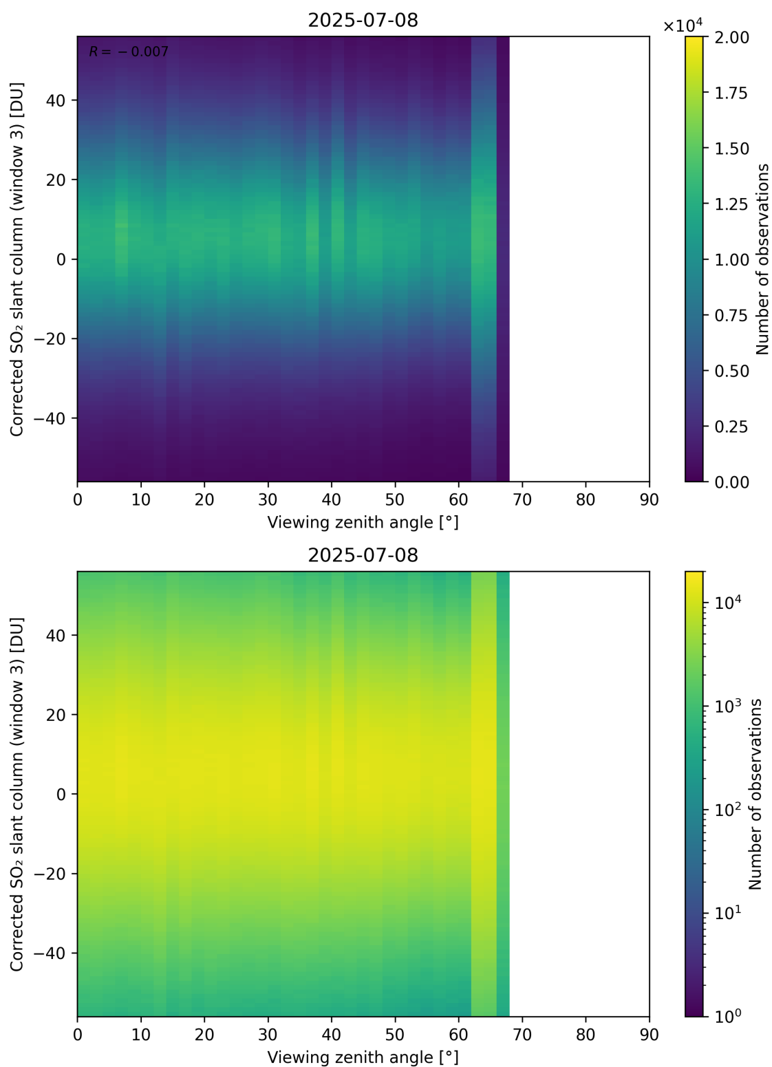
Figure 375: Scatter density plot of “Viewing zenith angle” against “Corrected SO 2 slant column (window 3)” for 2025-07-08 to 2025-07-09.
