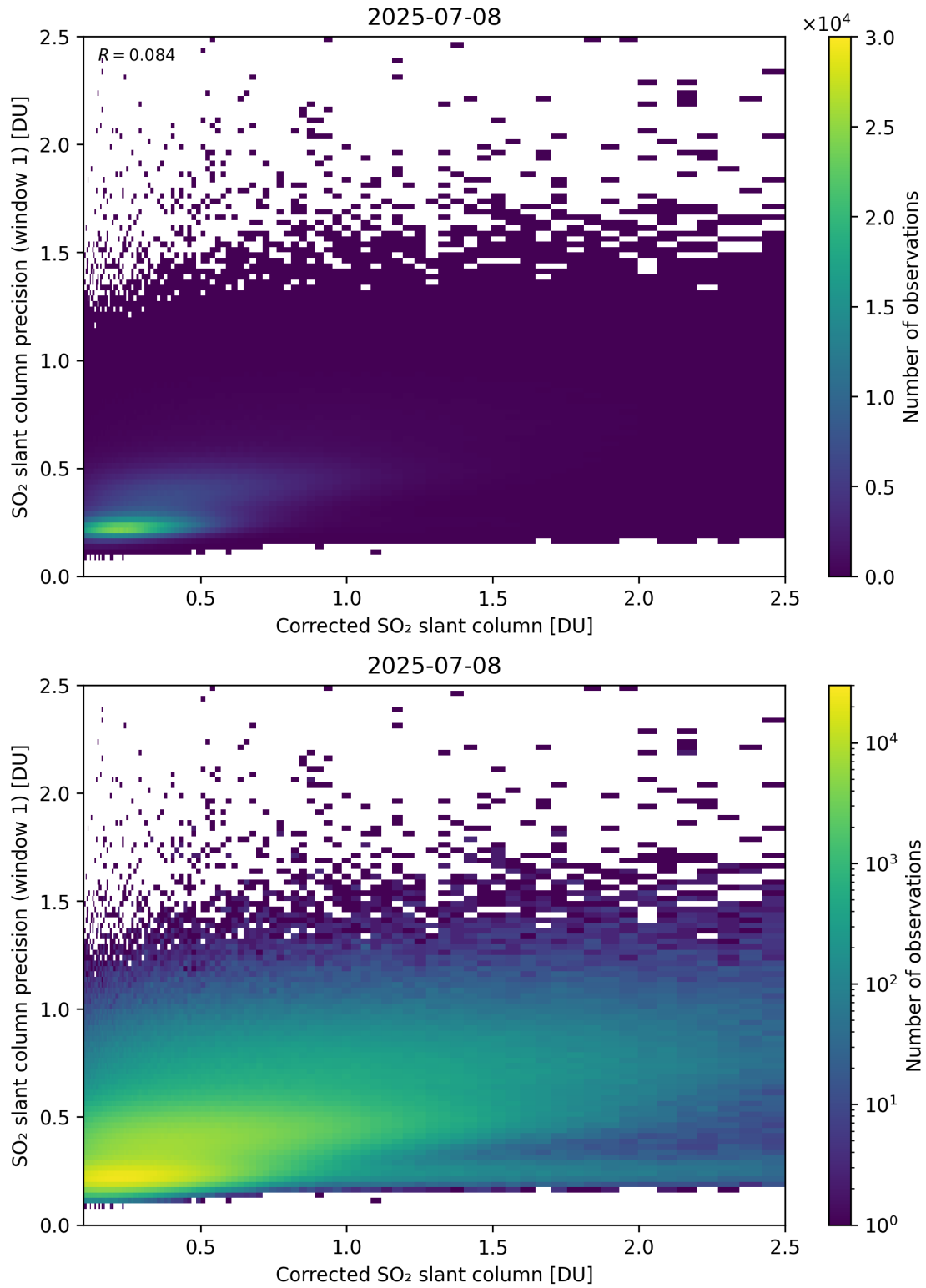
Figure 238: Scatter density plot of “Corrected SO 2 slant column” against “SO 2 slant column precision (window 1)” for 2025-07-08 to 2025-07-09.
