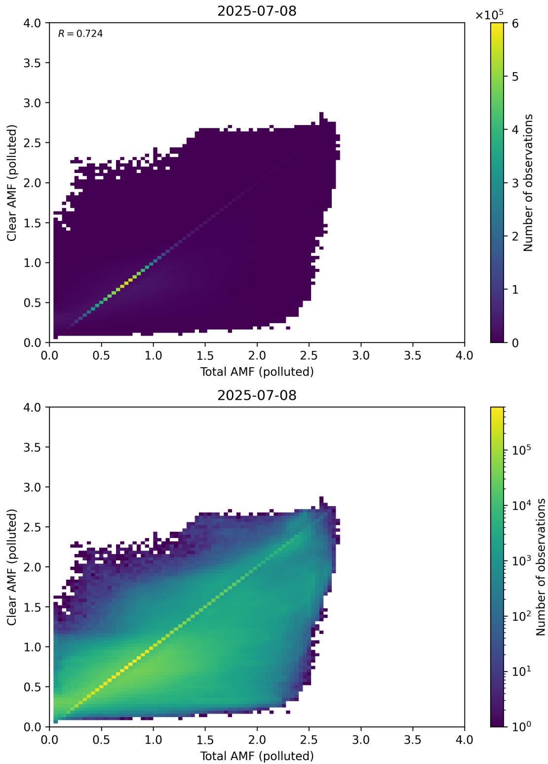
Figure 321: Scatter density plot of “Total AMF (polluted)” against “Clear AMF (polluted)” for 2025-07-08 to 2025-07-09.
