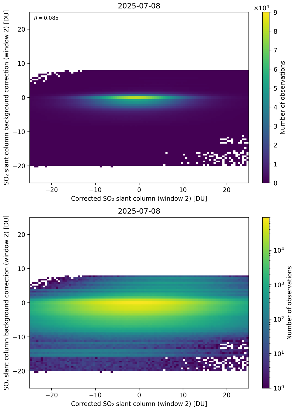
Figure 244: Scatter density plot of “Corrected SO 2 slant column (window 2)” against “SO 2 slant column background correction (window 2)” for 2025-07-08 to 2025-07-09.
