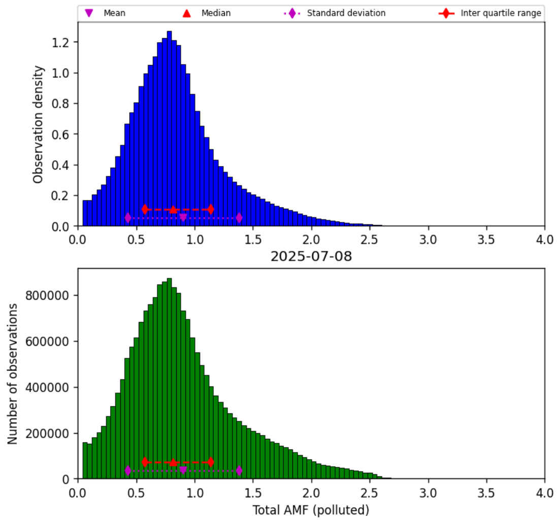
Figure 79: Histogram of “Total AMF (polluted)” for 2025-07-08 to 2025-07-09
