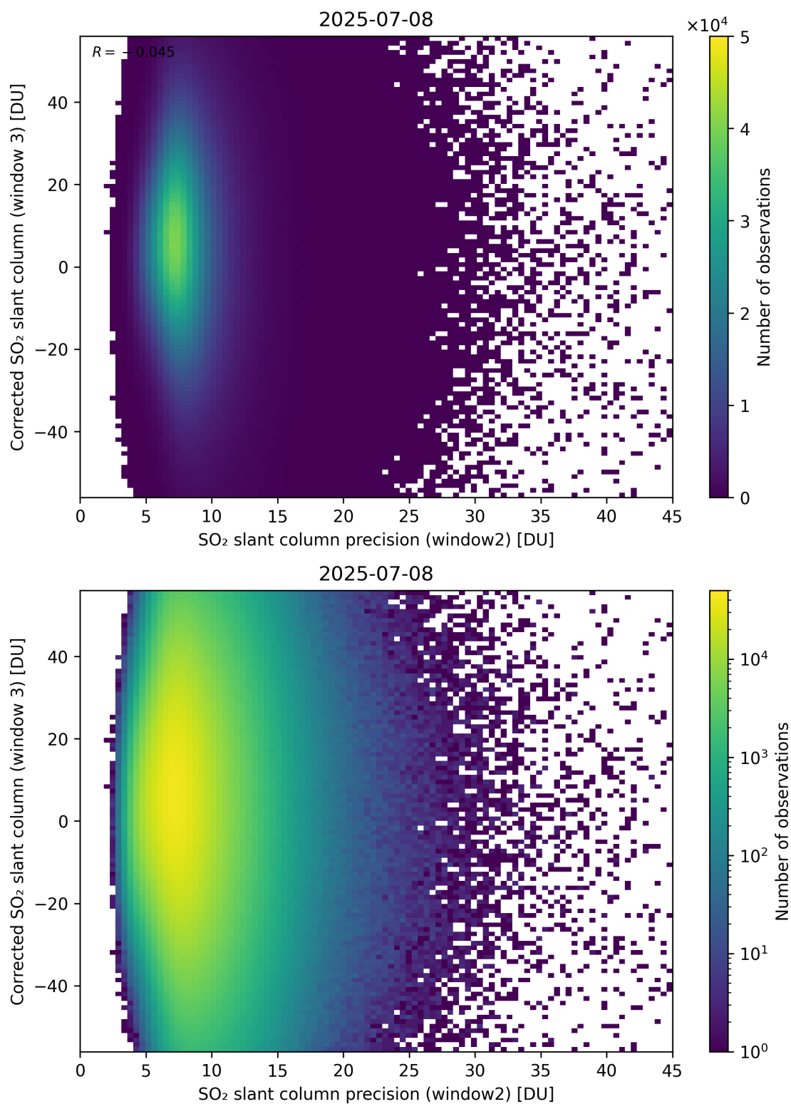
Figure 298: Scatter density plot of “SO 2 slant column precision (window2)” against “Corrected SO 2 slant column (window 3)” for 2025-07-08 to 2025-07-09.
