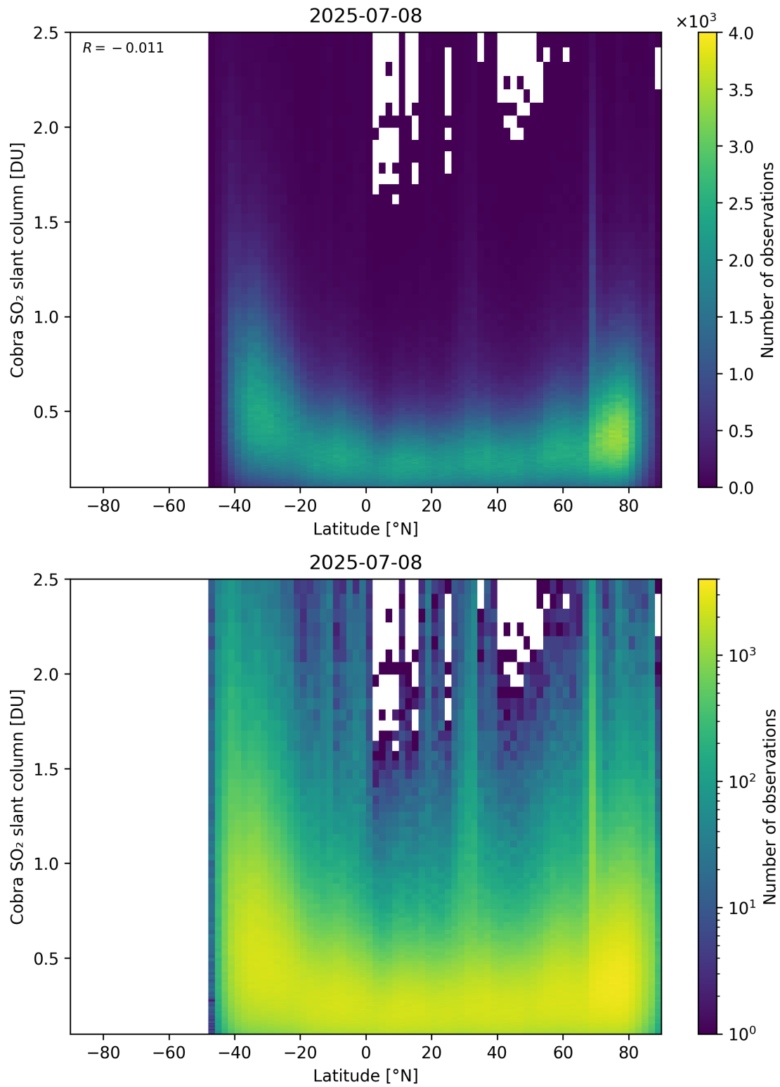
Figure 157: Scatter density plot of “Latitude” against “Cobra SO 2 slant column” for 2025-07-08 to 2025-07-09.
