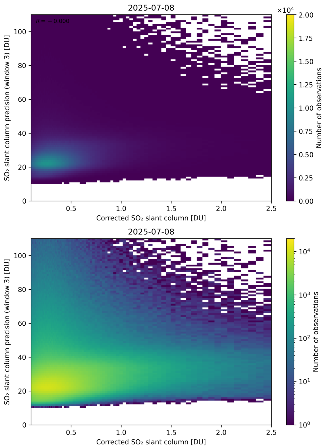
Figure 241: Scatter density plot of “Corrected SO 2 slant column” against “SO 2 slant column precision (window 3)” for 2025-07-08 to 2025-07-09.
