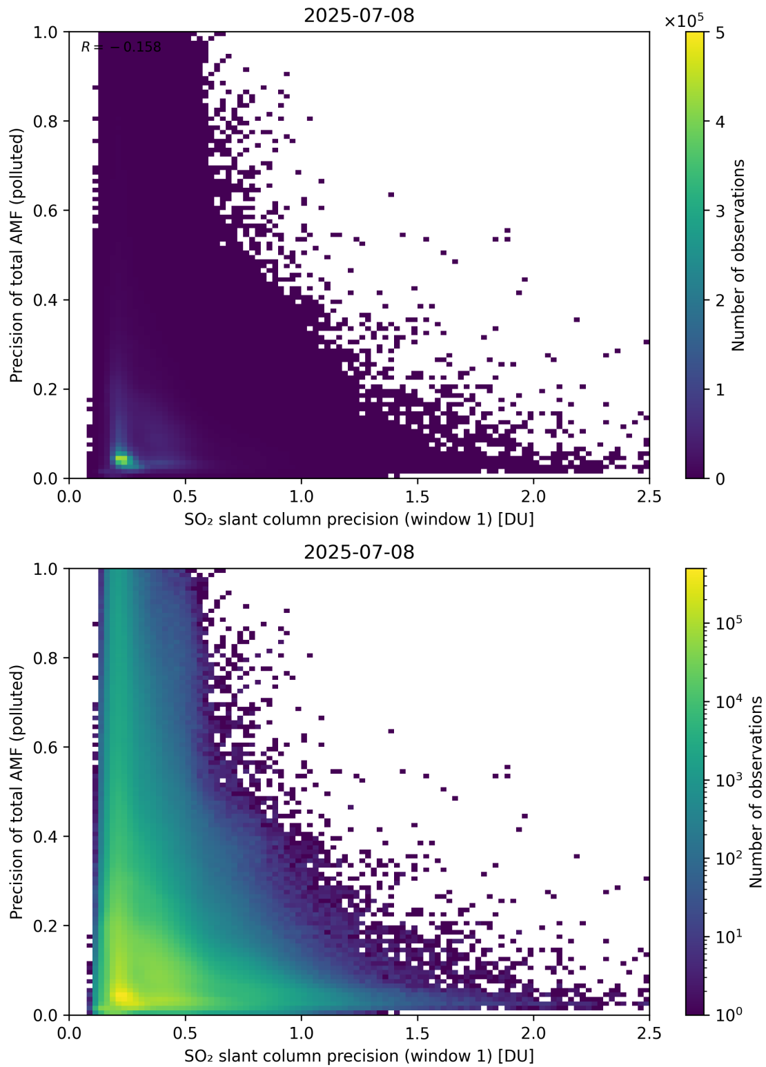
Figure 281: Scatter density plot of “SO 2 slant column precision (window 1)” against “Precision of total AMF (polluted)” for 2025-07-08 to 2025-07-09.
