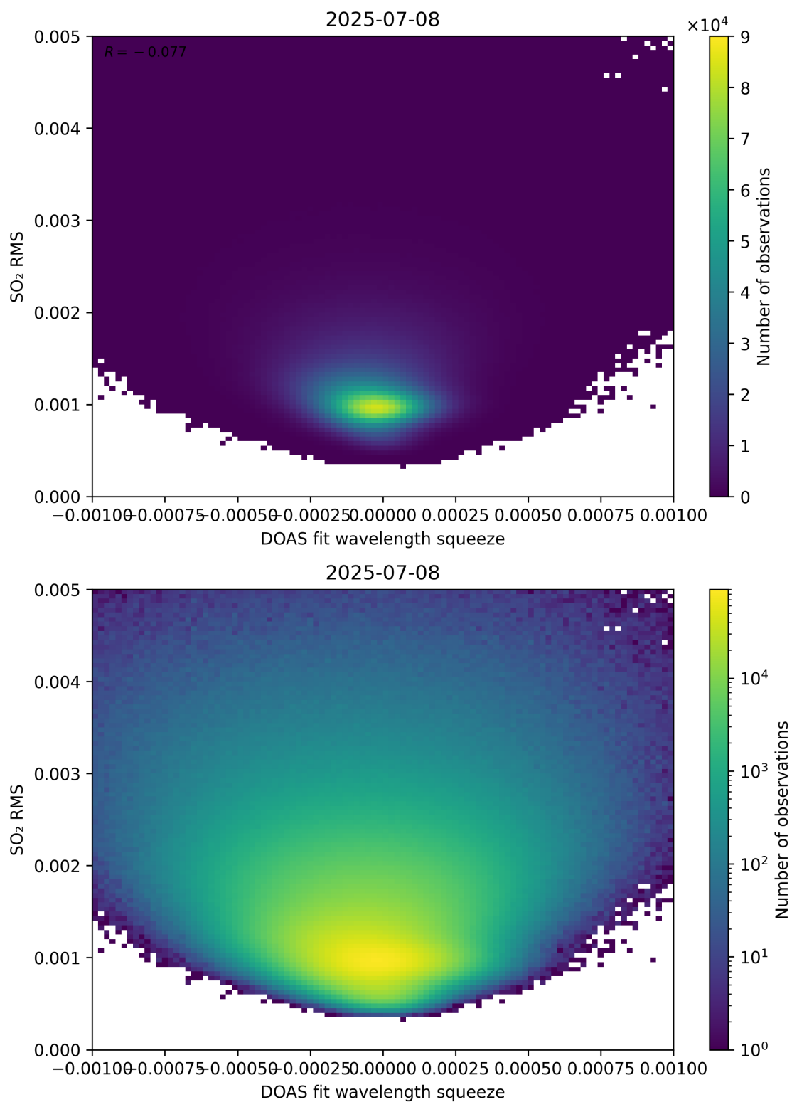
Figure 143: Scatter density plot of “DOAS fit wavelength squeeze” against “SO 2 RMS” for 2025-07-08 to 2025-07-09.
