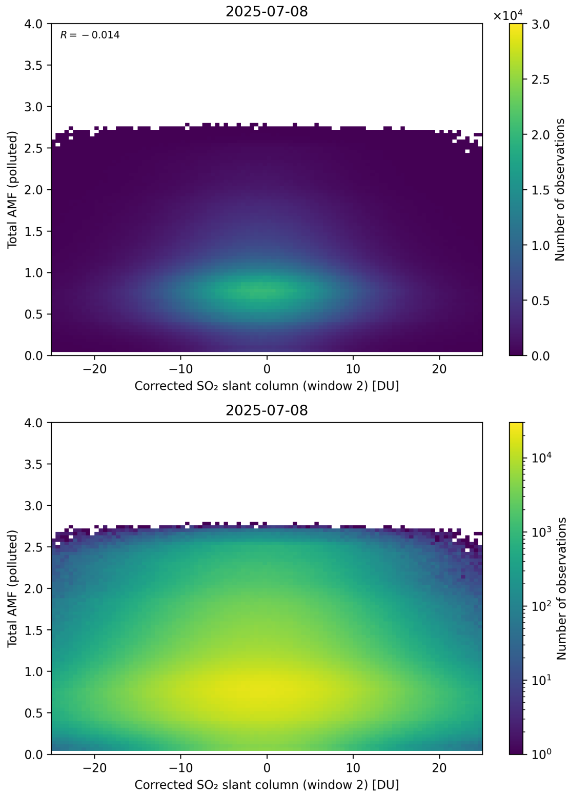
Figure 253: Scatter density plot of “Corrected SO 2 slant column (window 2)” against “Total AMF (polluted)” for 2025-07-08 to 2025-07-09.
