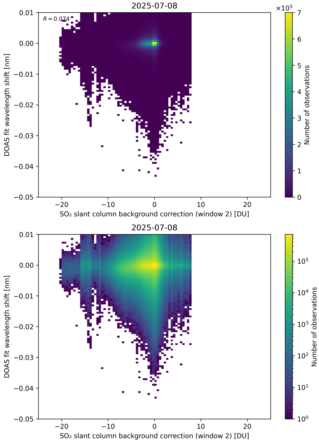
Figure 123: Scatter density plot of “SO 2 slant column background correction (window 2)” against “DOAS fit wavelength shift” for 2025-07-08 to 2025-07-09.
