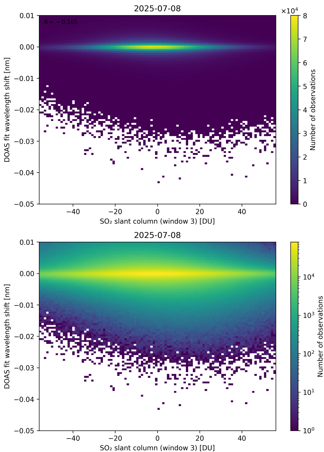
Figure 304: Scatter density plot of “SO 2 slant column (window 3)” against “DOAS fit wavelength shift” for 2025-07-08 to 2025-07-09.
