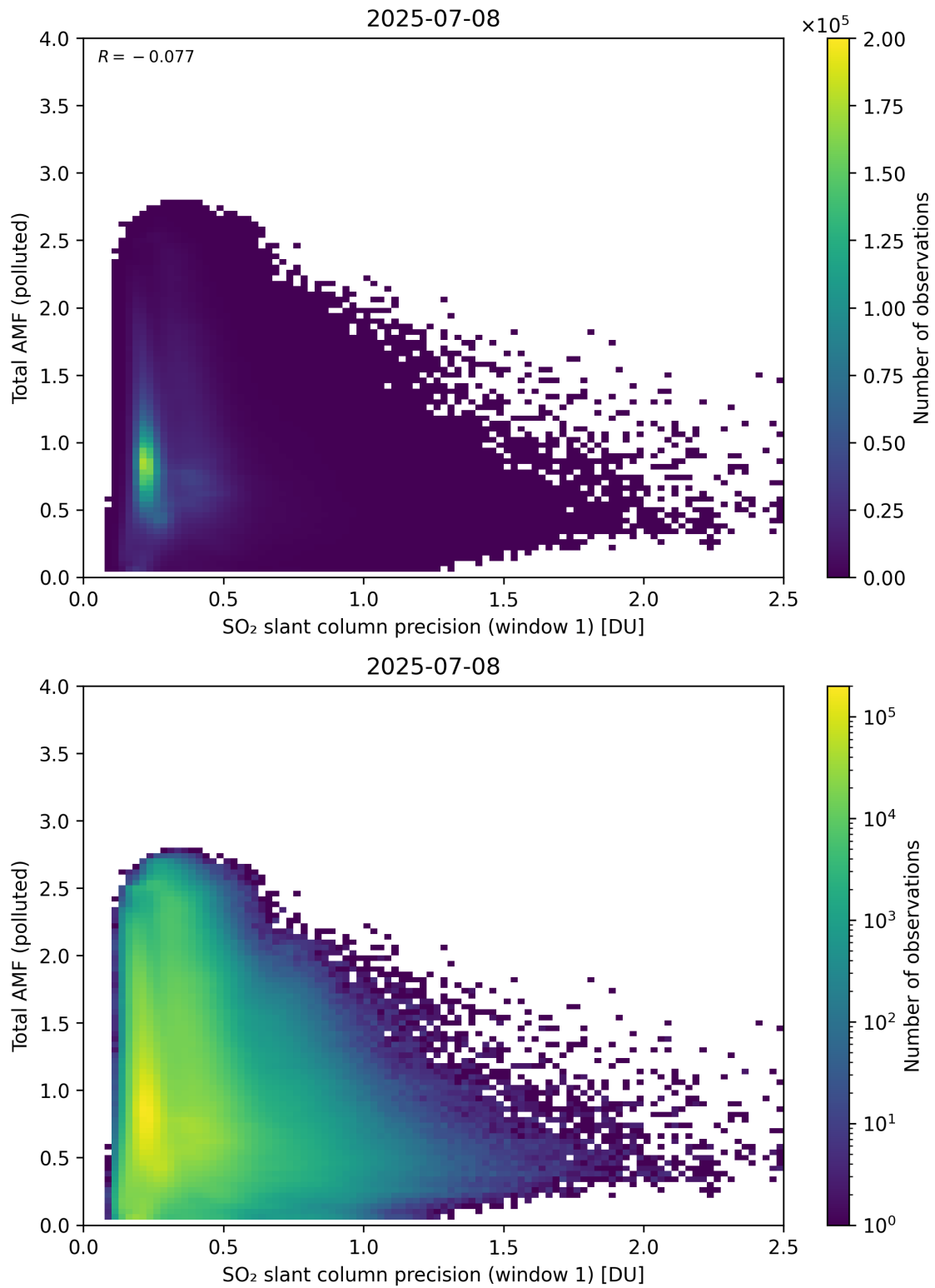
Figure 280: Scatter density plot of “SO 2 slant column precision (window 1)” against “Total AMF (polluted)” for 2025-07-08 to 2025-07-09.
