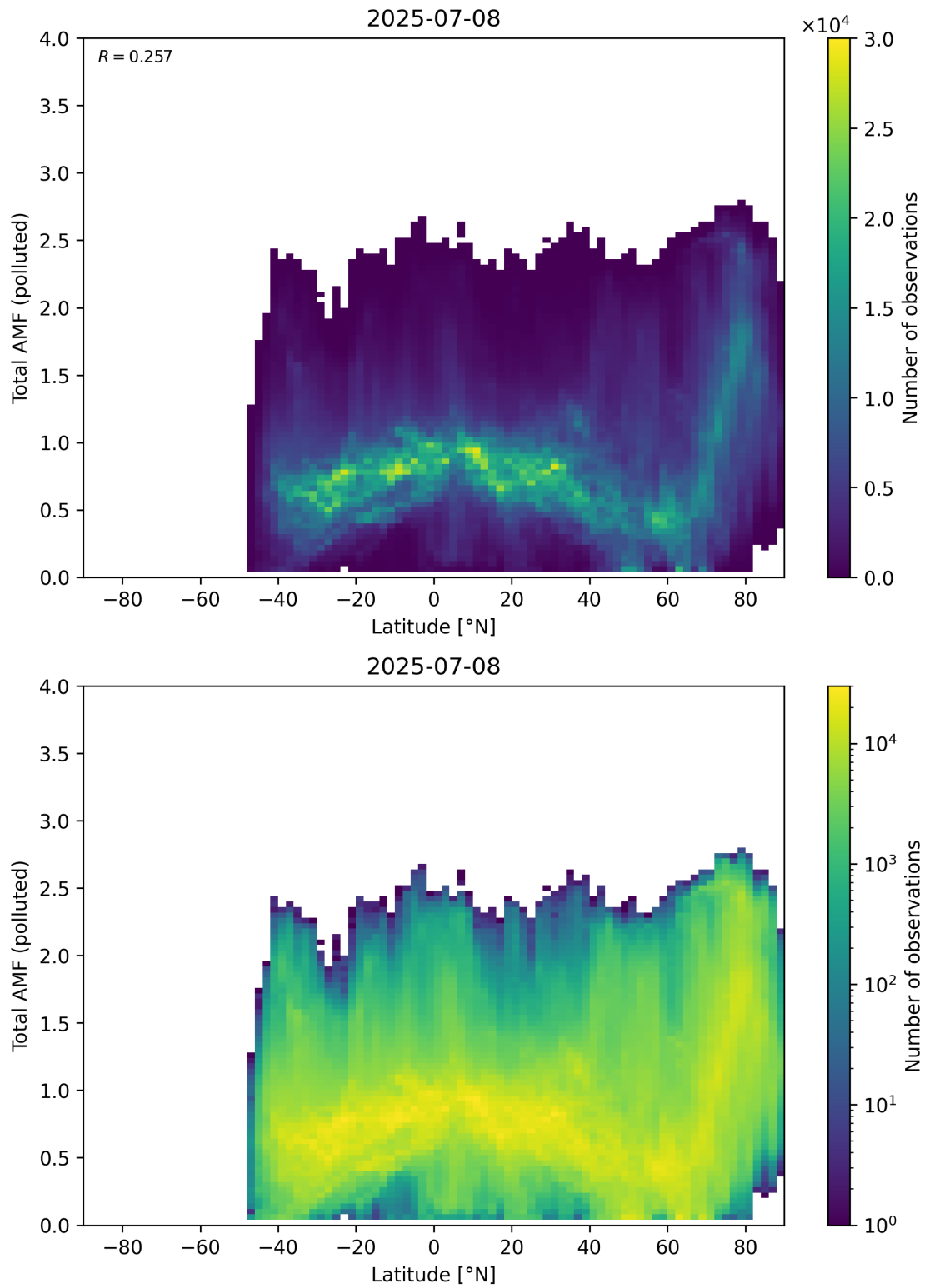
Figure 167: Scatter density plot of “Latitude” against “Total AMF (polluted)” for 2025-07-08 to 2025-07-09.
