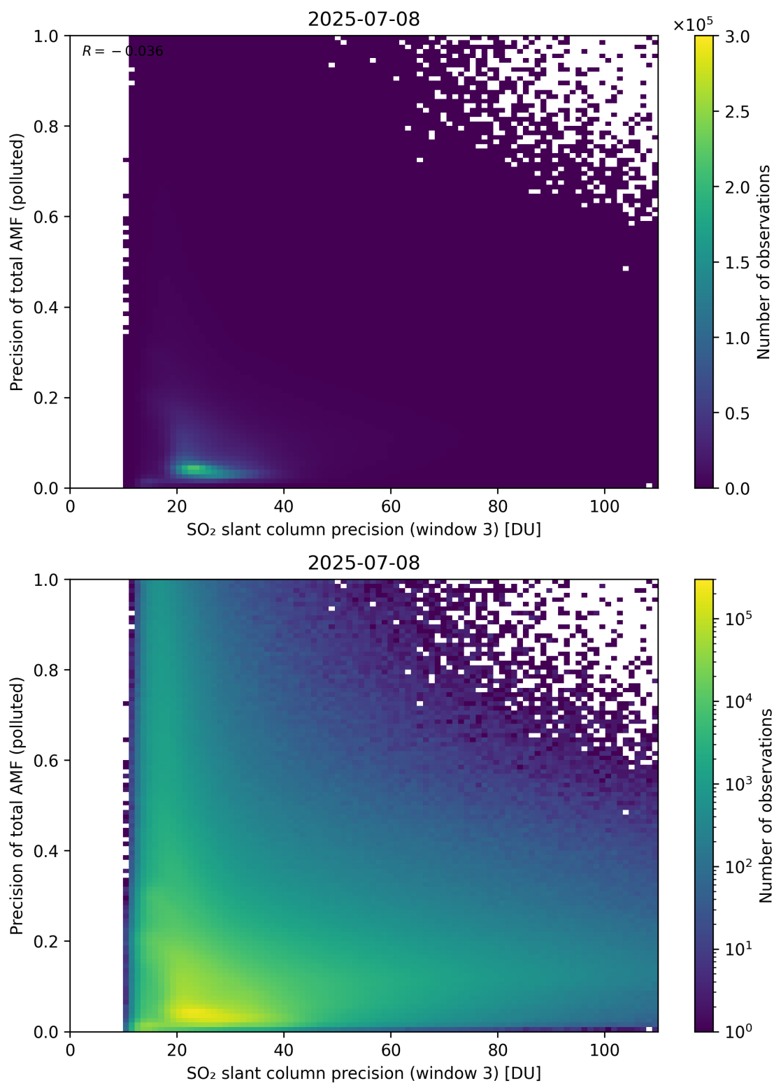
Figure 314: Scatter density plot of “SO 2 slant column precision (window 3)” against “Precision of total AMF (polluted)” for 2025-07-08 to 2025-07-09.
