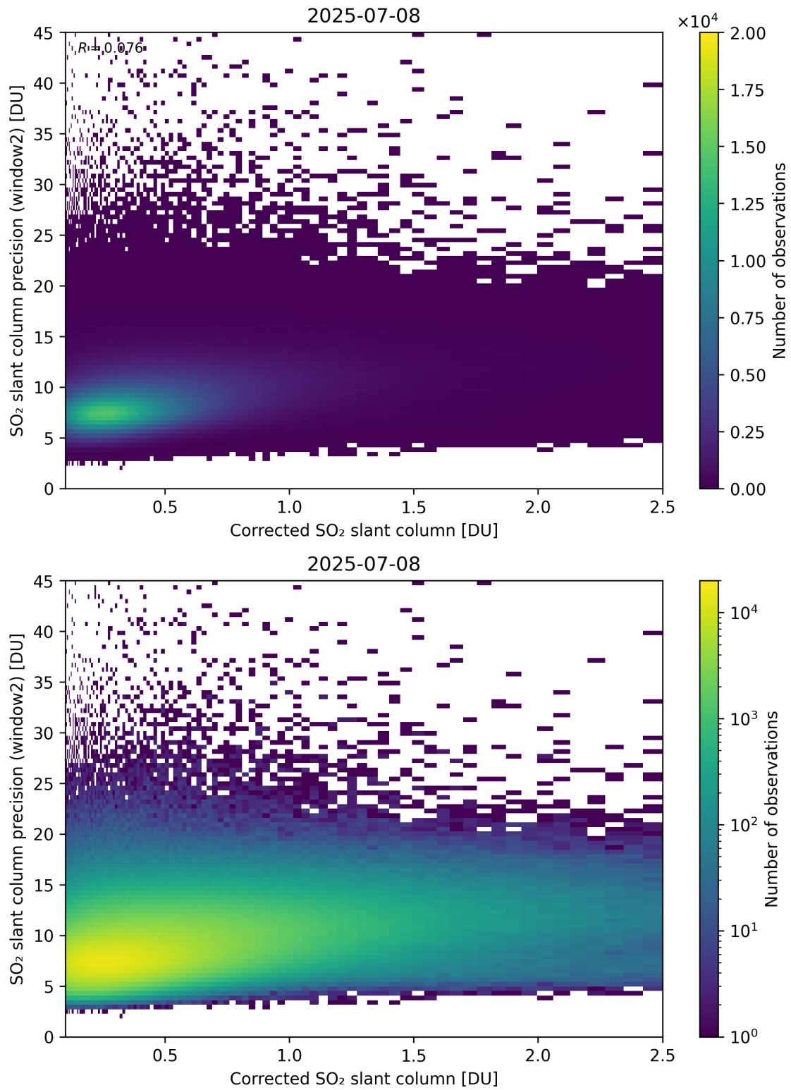
Figure 239: Scatter density plot of “Corrected SO 2 slant column” against “SO 2 slant column precision (window2)” for 2025-07-08 to 2025-07-09.
