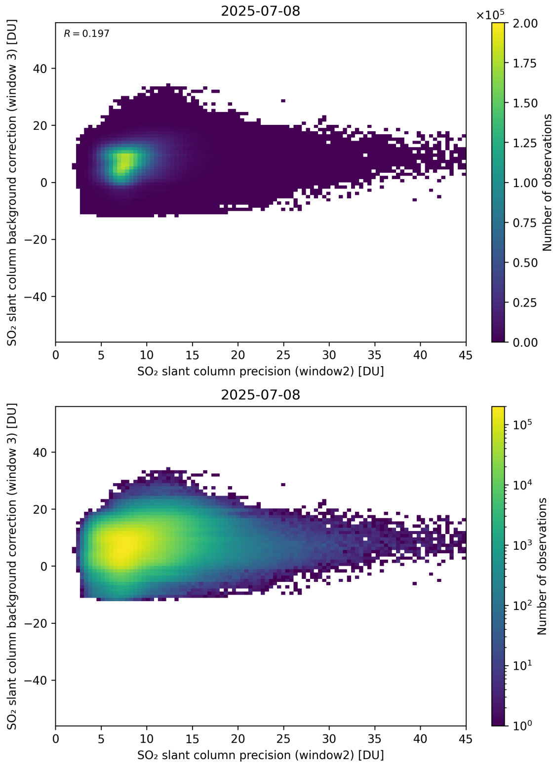
Figure 292: Scatter density plot of “SO 2 slant column precision (window2)” against “SO 2 slant column background correction (window 3)” for 2025-07-08 to 2025-07-09.
