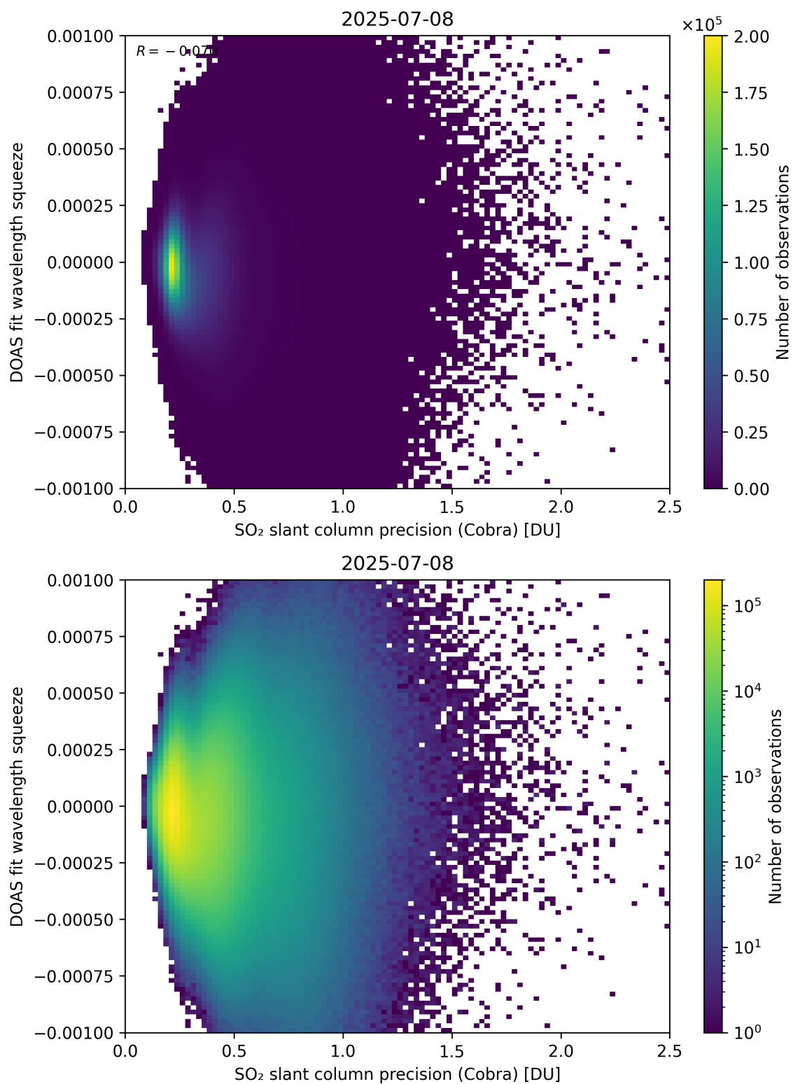
Figure 203: Scatter density plot of “SO 2 slant column precision (Cobra)” against “DOAS fit wavelength squeeze” for 2025-07-08 to 2025-07-09.
