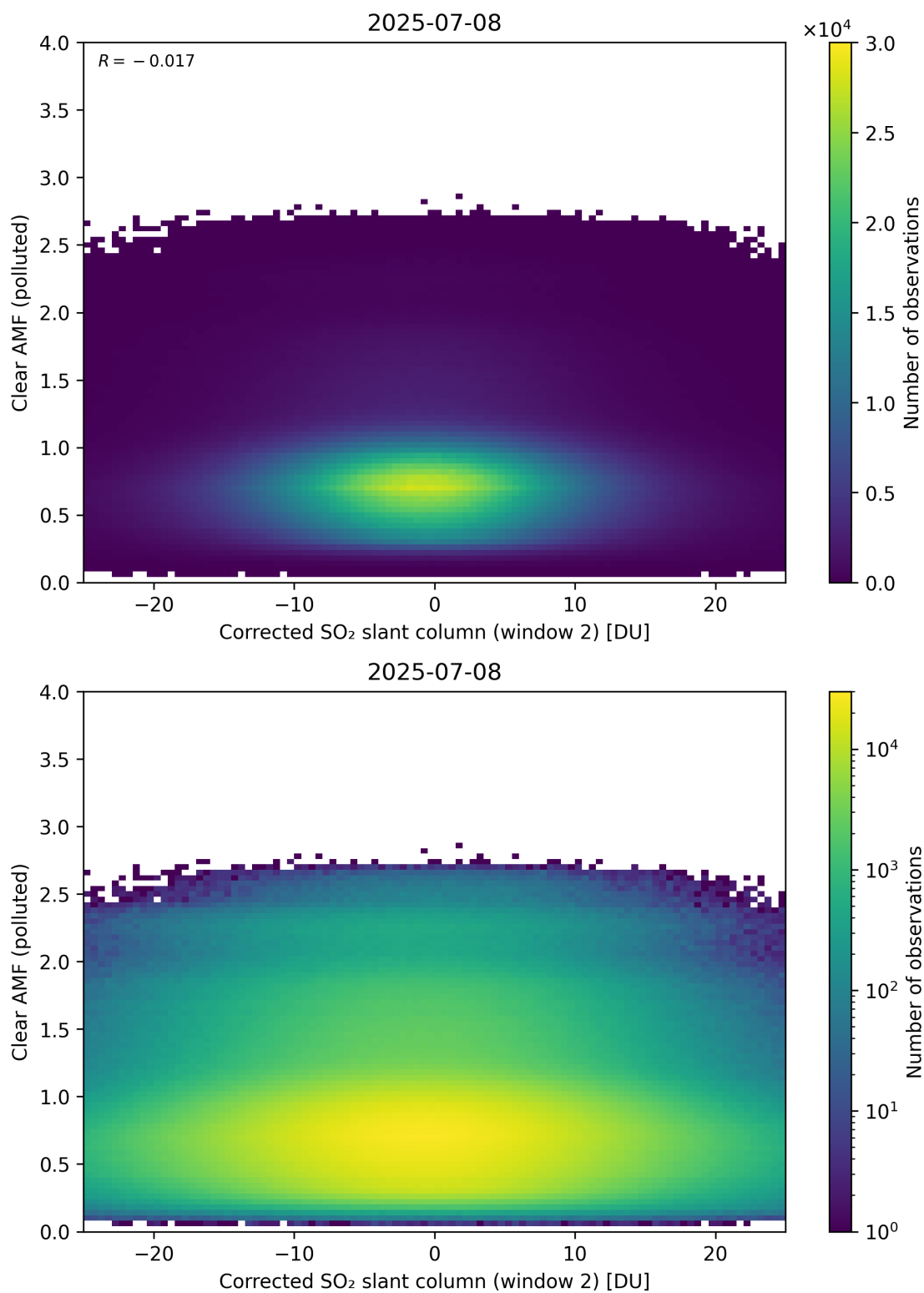
Figure 249: Scatter density plot of “Corrected SO 2 slant column (window 2)” against “Clear AMF (polluted)” for 2025-07-08 to 2025-07-09.
