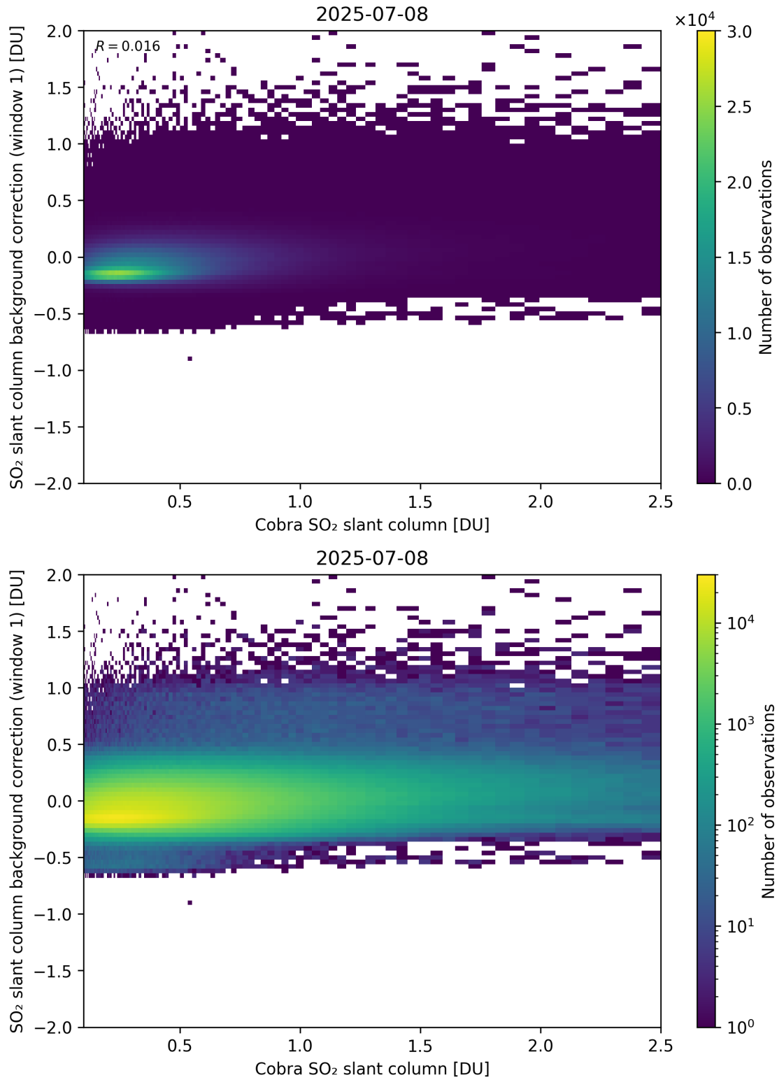
Figure 193: Scatter density plot of “Cobra SO 2 slant column” against “SO 2 slant column background correction (window 1)” for 2025-07-08 to 2025-07-09.
