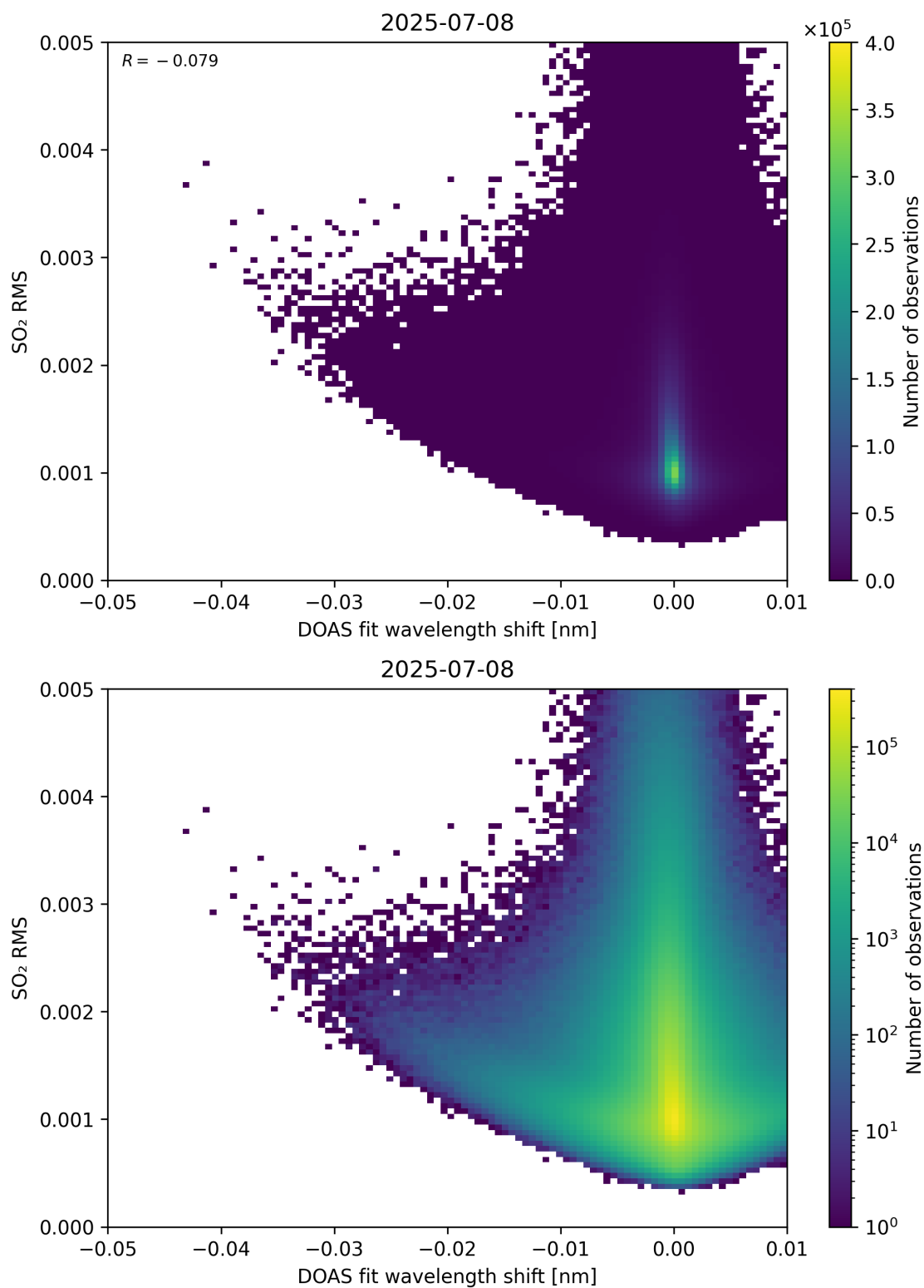
Figure 139: Scatter density plot of “DOAS fit wavelength shift” against “SO 2 RMS” for 2025-07-08 to 2025-07-09.
