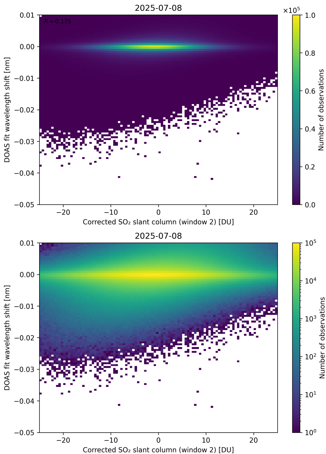
Figure 246: Scatter density plot of “Corrected SO 2 slant column (window 2)” against “DOAS fit wavelength shift” for 2025-07-08 to 2025-07-09.
