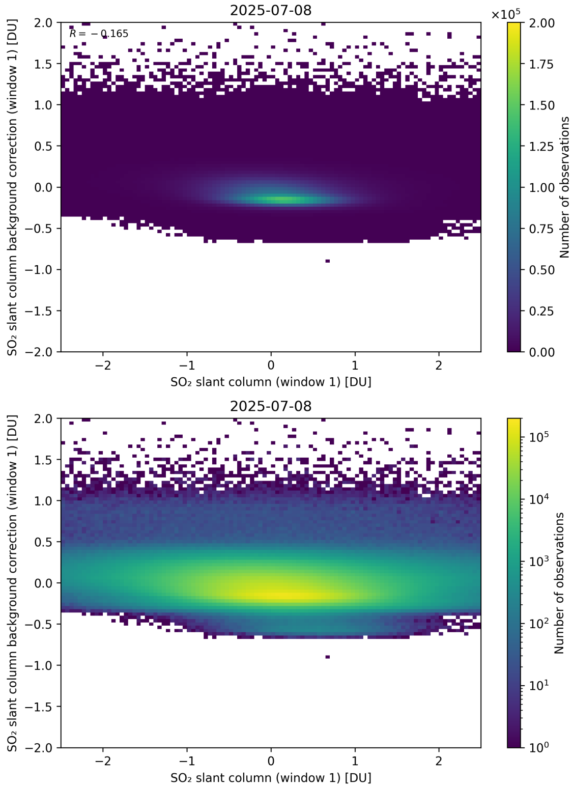
Figure 262: Scatter density plot of “SO 2 slant column (window 1)” against “SO 2 slant column background correction (window 1)” for 2025-07-08 to 2025-07-09.
