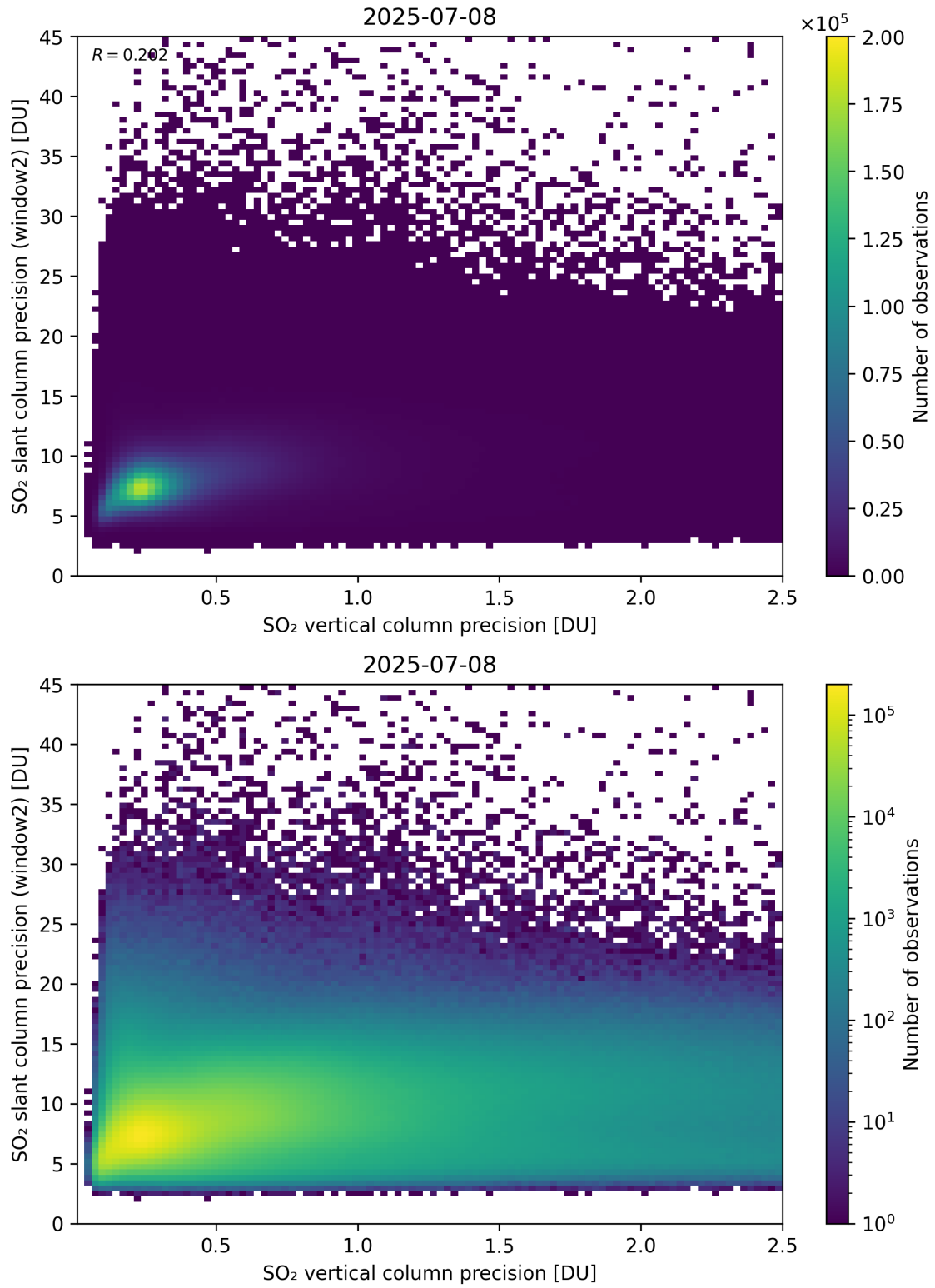
Figure 343: Scatter density plot of “SO 2 vertical column precision” against “SO 2 slant column precision (window2)” for 2025-07-08 to 2025-07-09.
