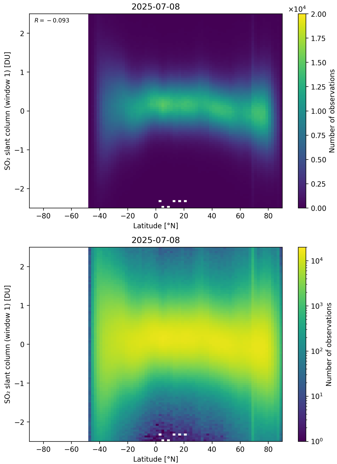
Figure 162: Scatter density plot of “Latitude” against “SO 2 slant column (window 1)” for 2025-07-08 to 2025-07-09.
