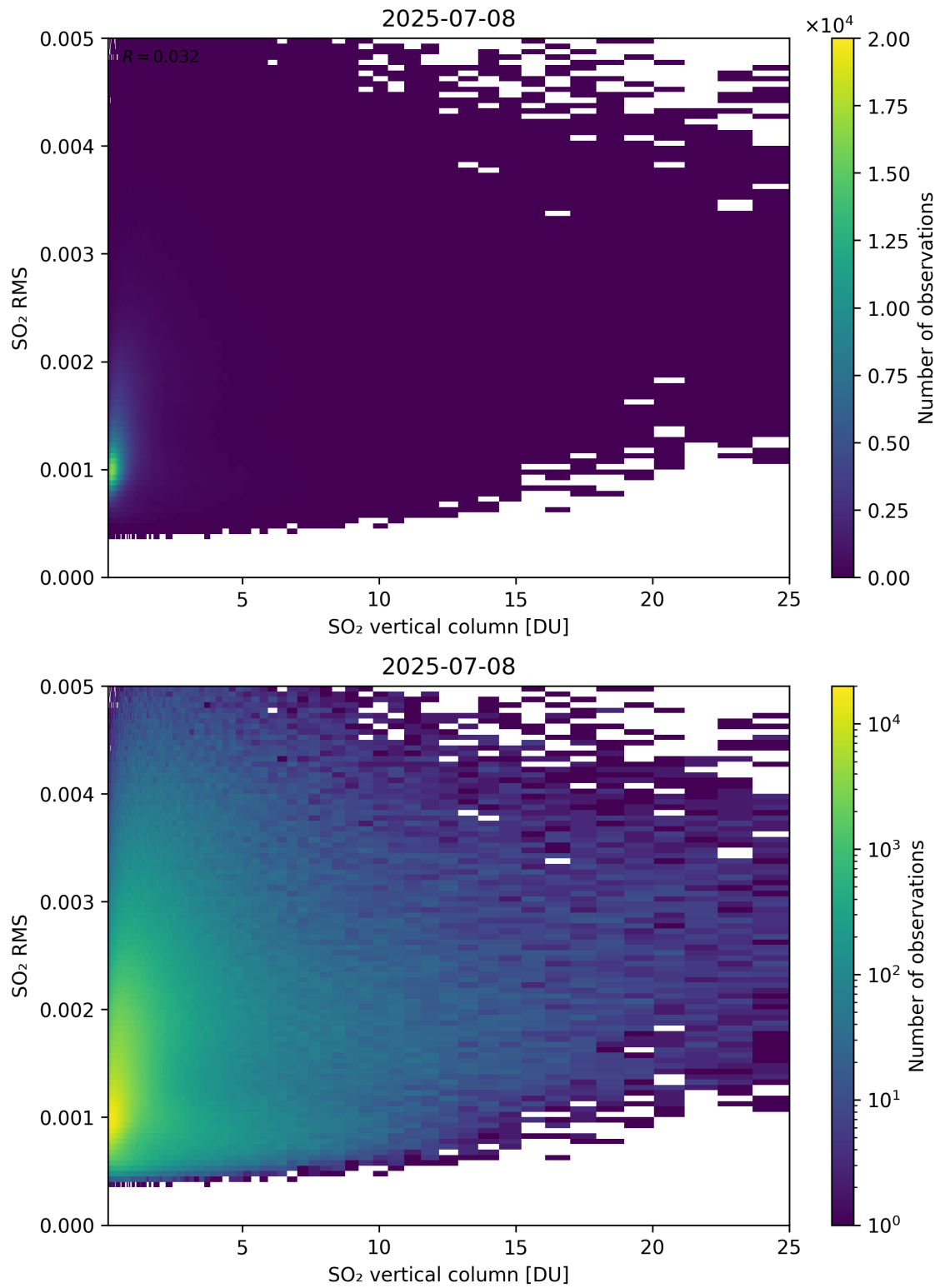
Figure 328: Scatter density plot of “SO 2 vertical column” against “SO 2 RMS” for 2025-07-08 to 2025-07-09.
