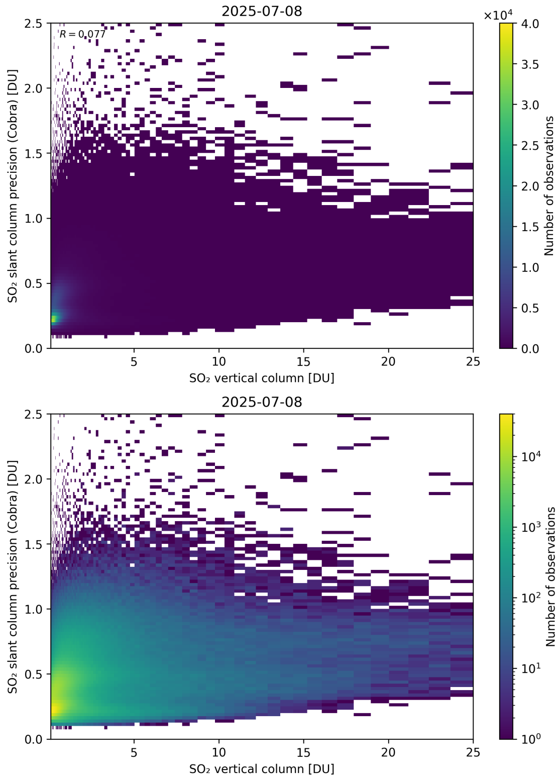
Figure 350: Scatter density plot of “SO 2 vertical column” against “SO 2 slant column precision (Cobra)” for 2025-07-08 to 2025-07-09.
