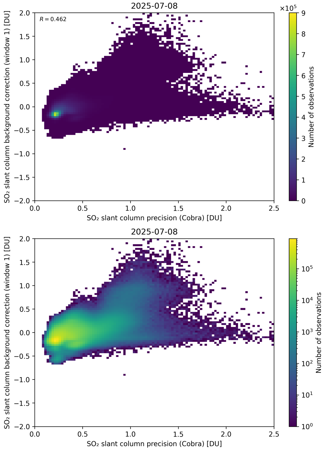
Figure 199: Scatter density plot of “SO 2 slant column precision (Cobra)” against “SO 2 slant column background correction (window 1)” for 2025-07-08 to 2025-07-09.
