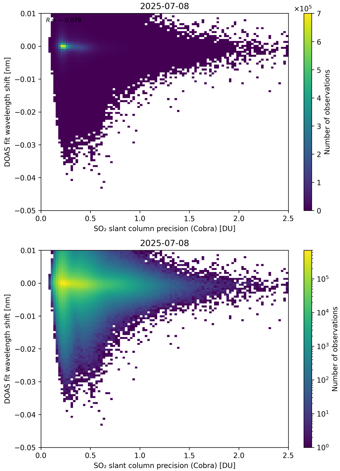
Figure 202: Scatter density plot of “SO 2 slant column precision (Cobra)” against “DOAS fit wavelength shift” for 2025-07-08 to 2025-07-09.
