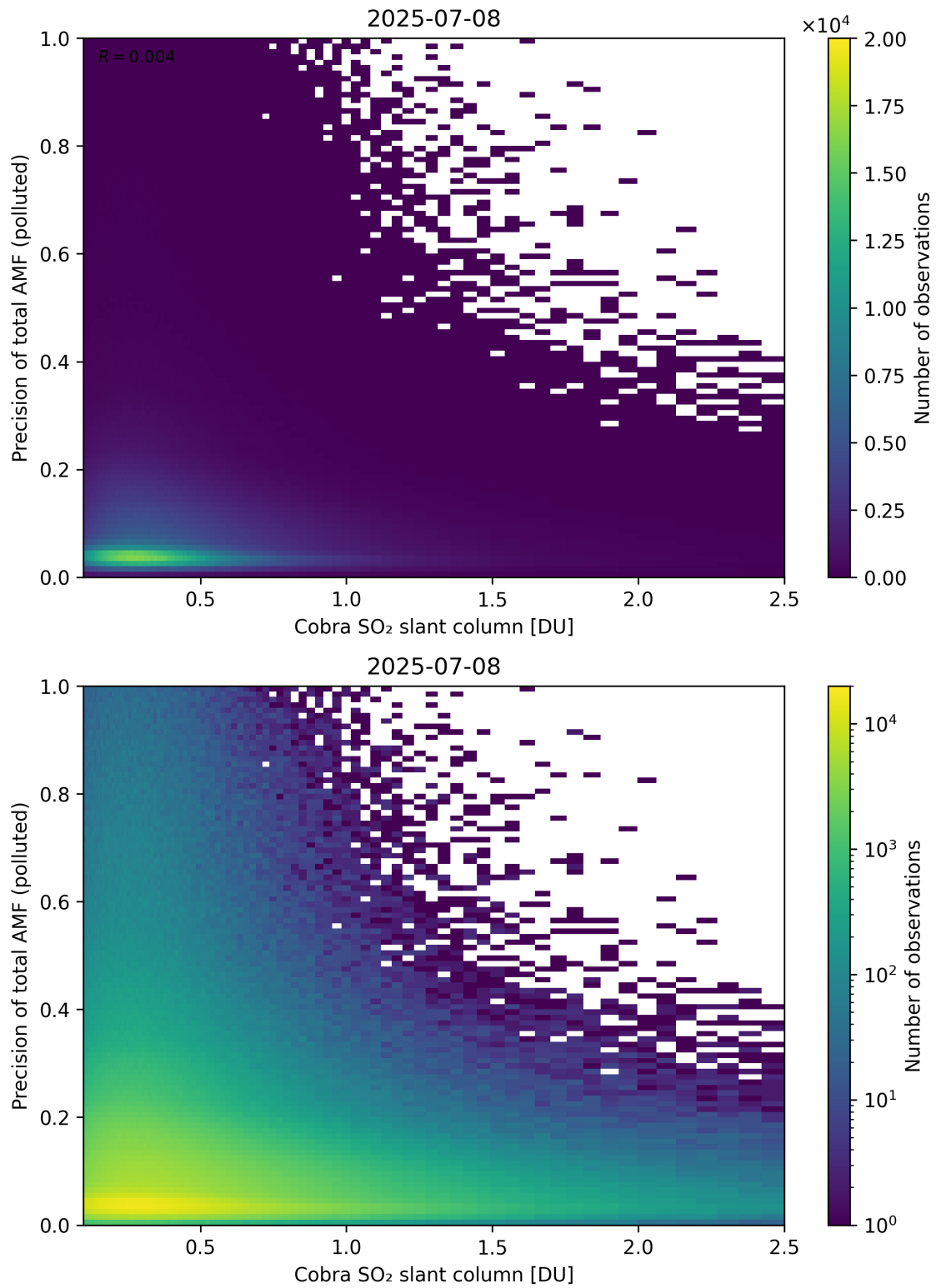
Figure 225: Scatter density plot of “Cobra SO 2 slant column” against “Precision of total AMF (polluted)” for 2025-07-08 to 2025-07-09.
