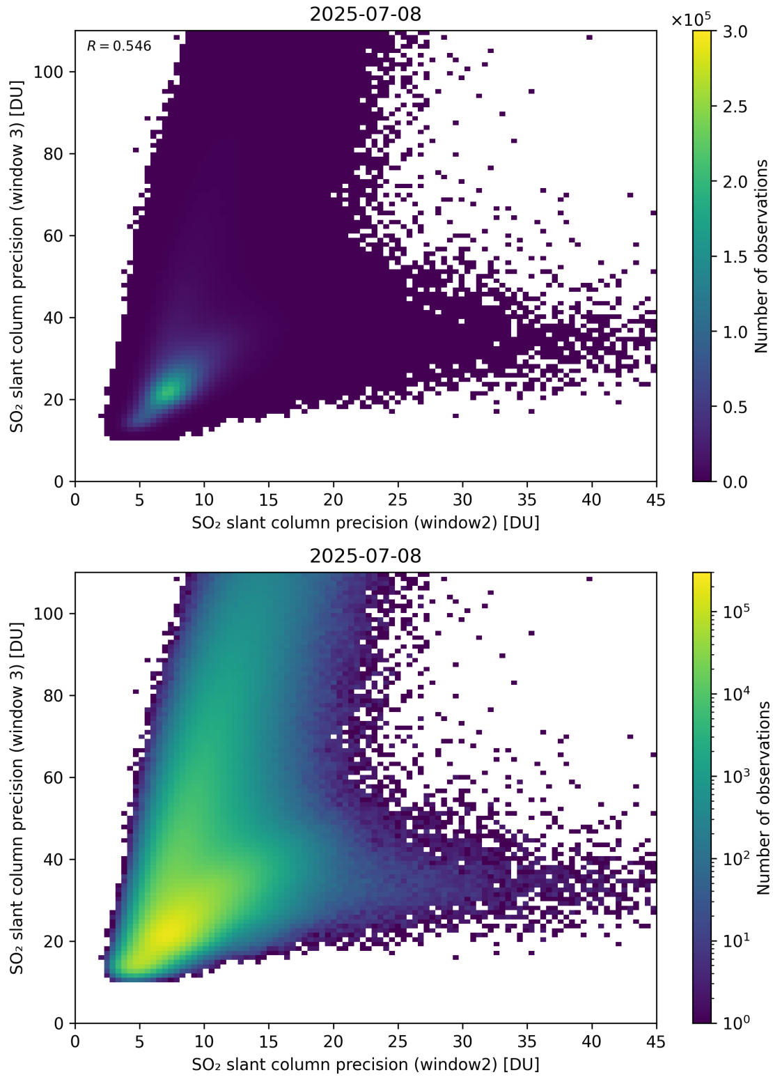
Figure 300: Scatter density plot of “SO 2 slant column precision (window2)” against “SO 2 slant column precision (window 3)” for 2025-07-08 to 2025-07-09.
