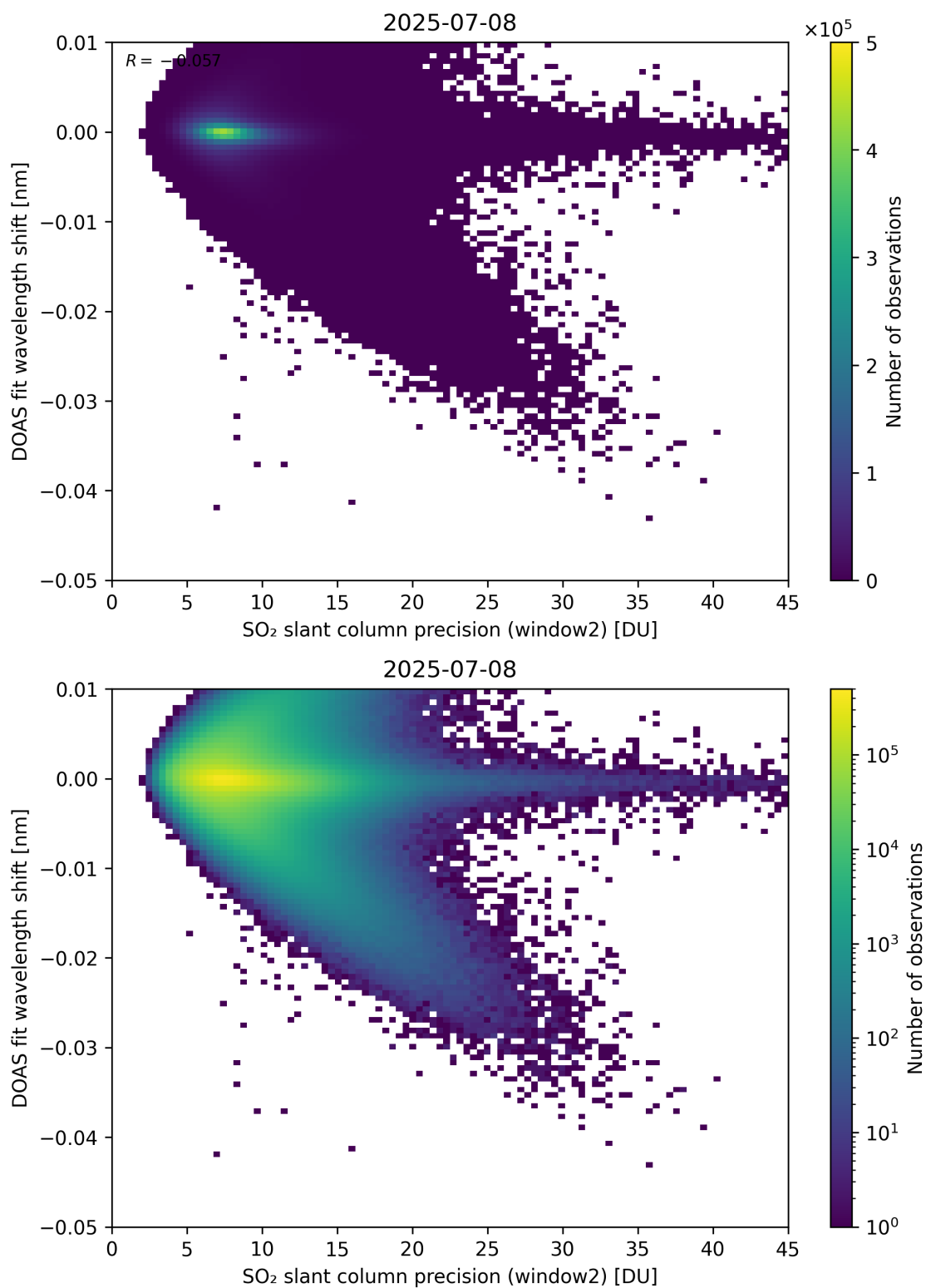
Figure 293: Scatter density plot of “SO 2 slant column precision (window2)” against “DOAS fit wavelength shift” for 2025-07-08 to 2025-07-09.
