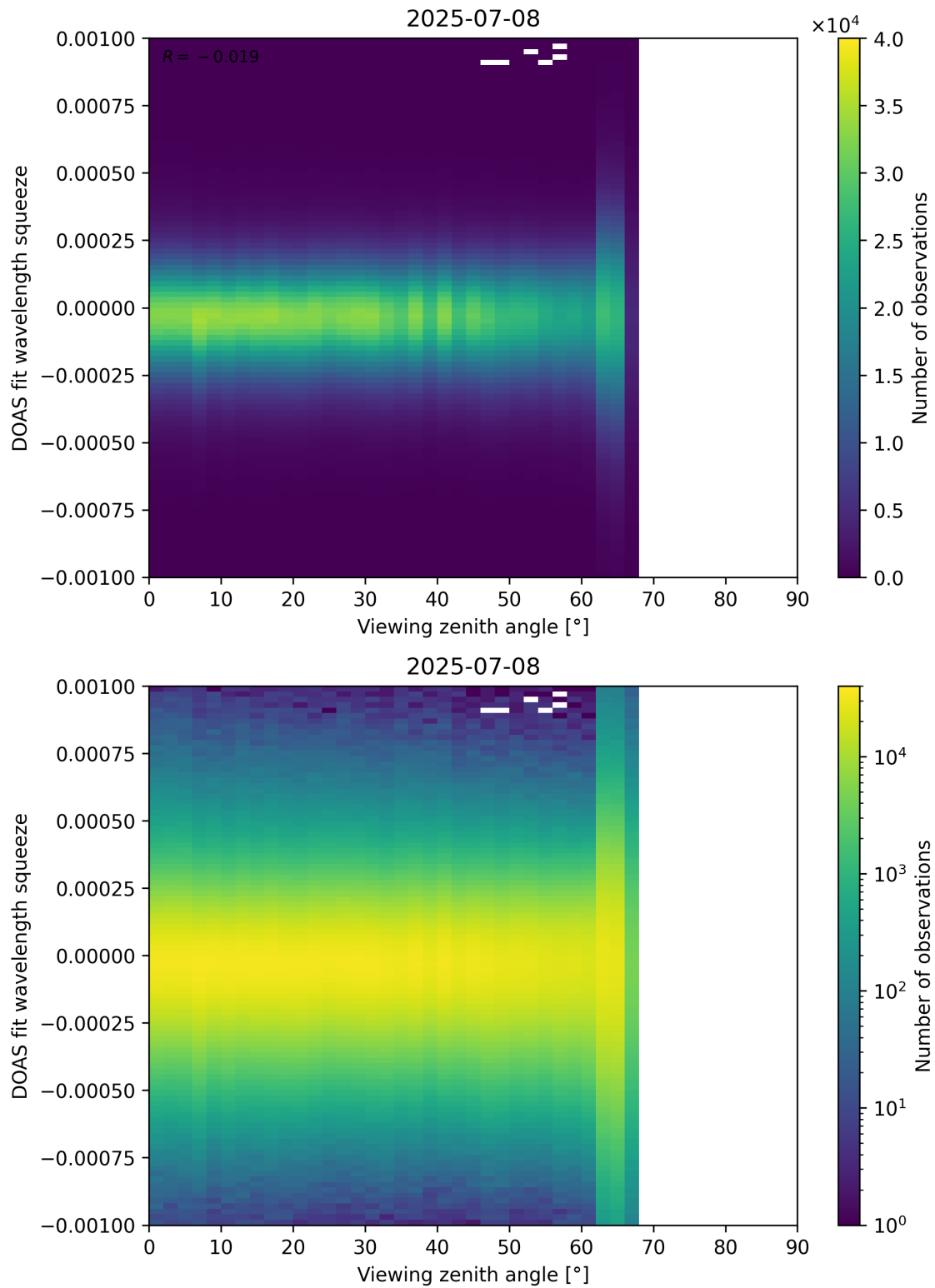
Figure 366: Scatter density plot of “Viewing zenith angle” against “DOAS fit wavelength squeeze” for 2025-07-08 to 2025-07-09.
