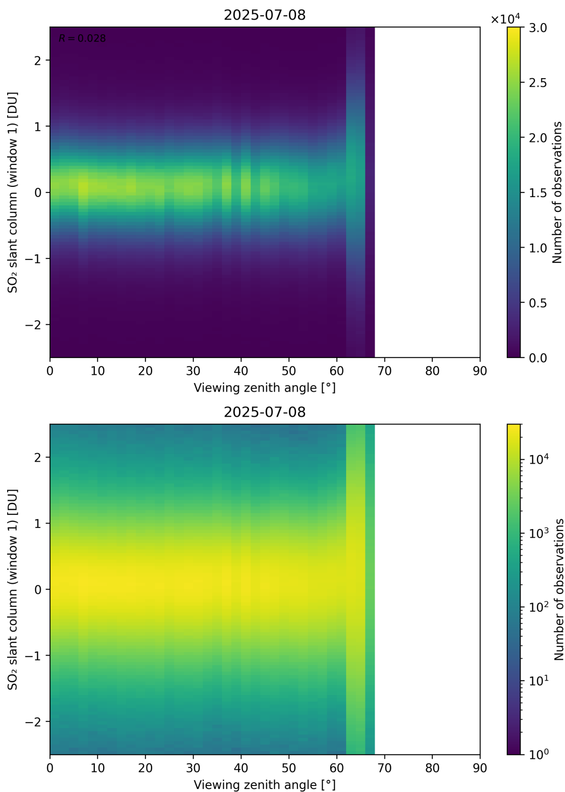
Figure 376: Scatter density plot of “Viewing zenith angle” against “SO 2 slant column (window 1)” for 2025-07-08 to 2025-07-09.
