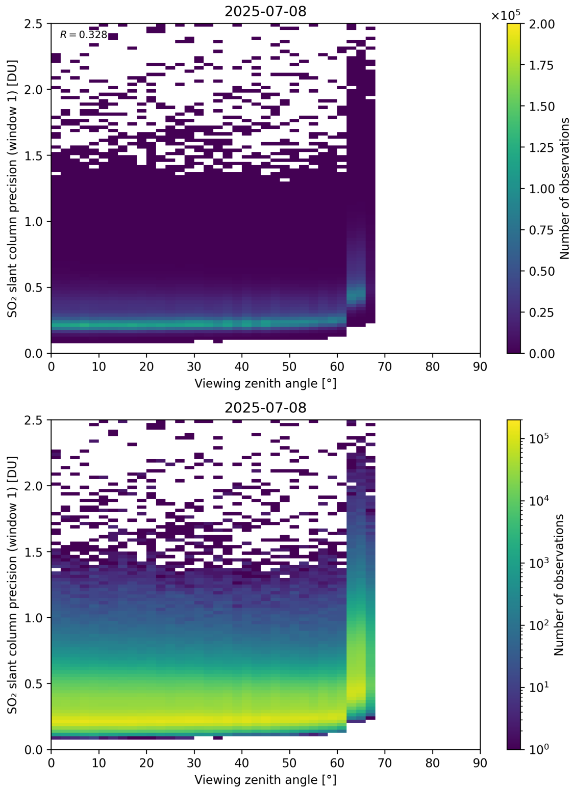
Figure 377: Scatter density plot of “Viewing zenith angle” against “SO 2 slant column precision (window 1)” for 2025-07-08 to 2025-07-09.
