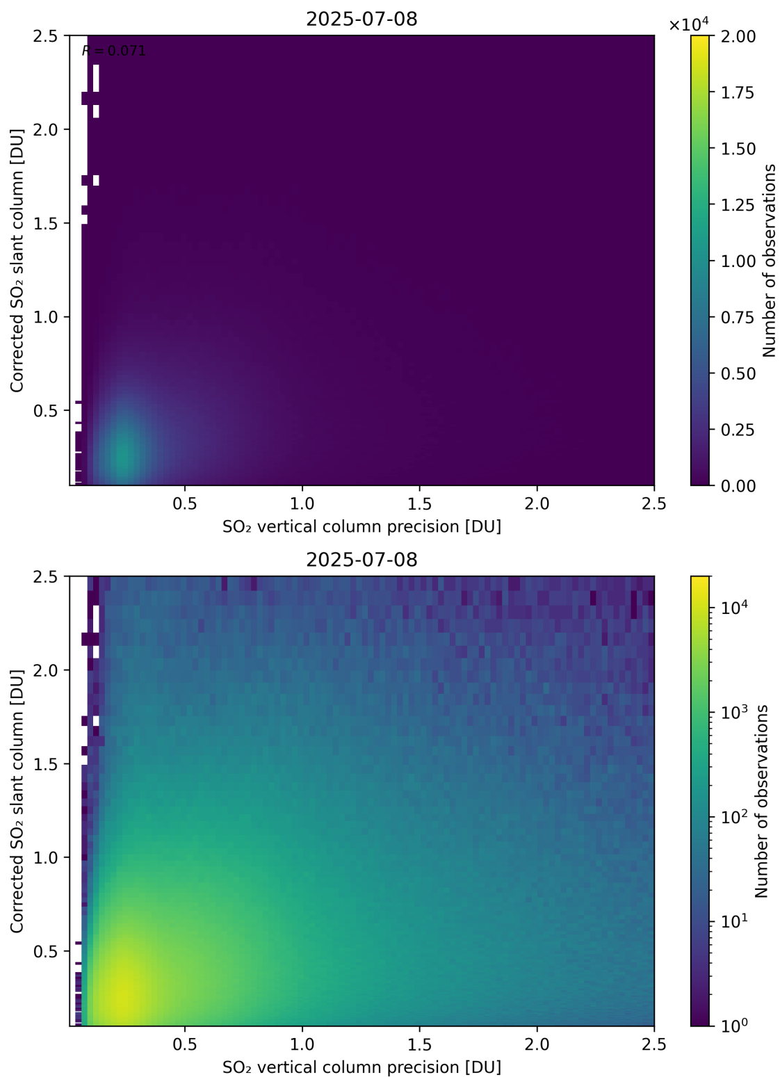
Figure 338: Scatter density plot of “SO 2 vertical column precision” against “Corrected SO 2 slant column” for 2025-07-08 to 2025-07-09.
