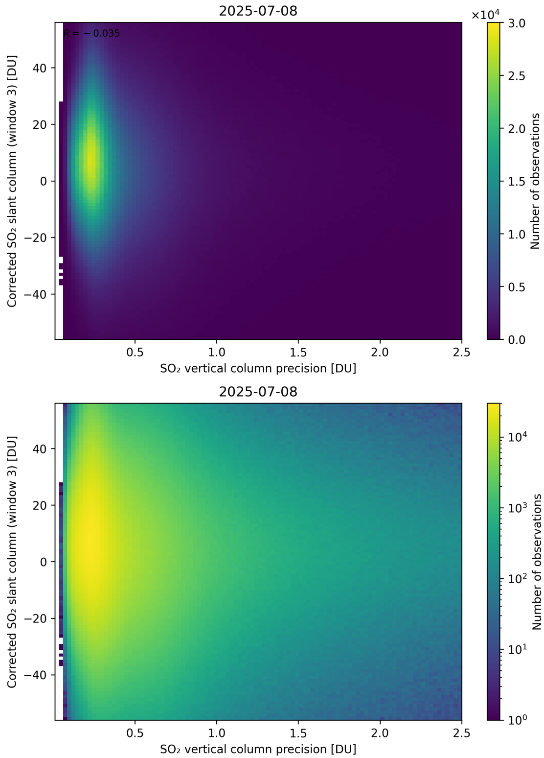
Figure 340: Scatter density plot of “SO 2 vertical column precision” against “Corrected SO 2 slant column (window 3)” for 2025-07-08 to 2025-07-09.
