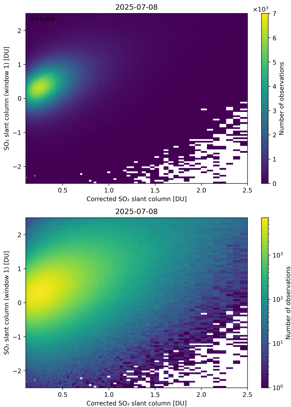
Figure 237: Scatter density plot of “Corrected SO 2 slant column” against “SO 2 slant column (window 1)” for 2025-07-08 to 2025-07-09.
