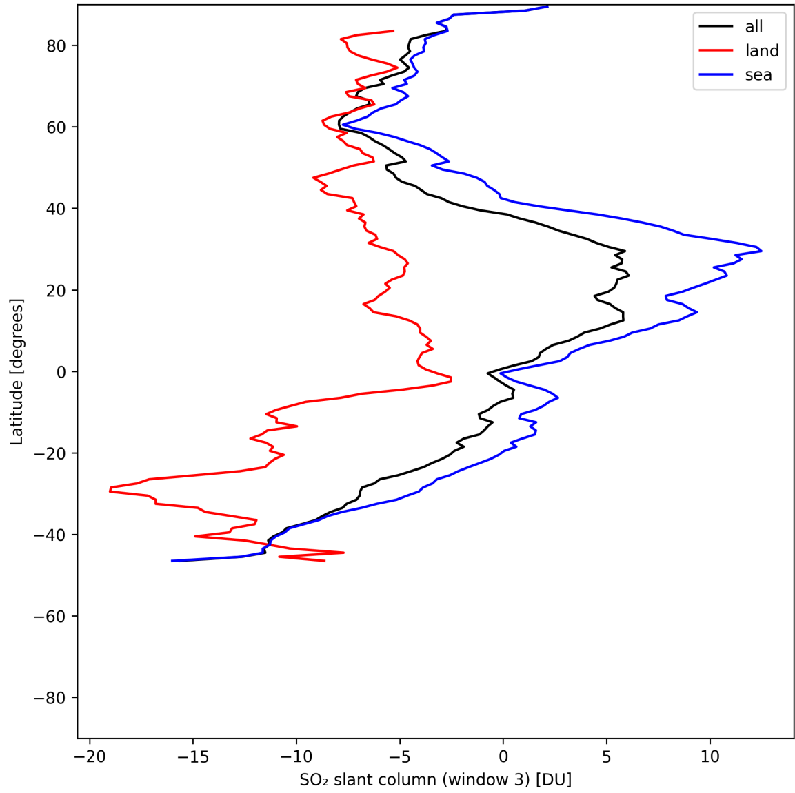
Figure 45: Zonal average of “SO 2 slant column (window 3)” for 2025-07-08 to 2025-07-09.
