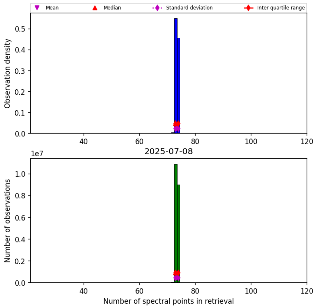
Figure 82: Histogram of “Number of spectral points in retrieval” for 2025-07-08 to 2025-07-09
