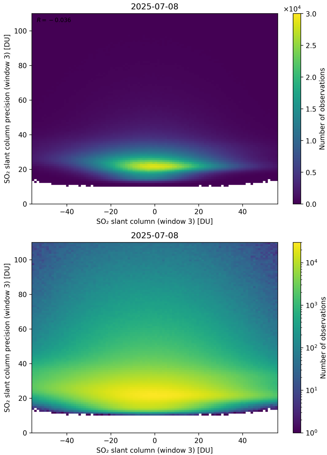
Figure 317: Scatter density plot of “SO 2 slant column (window 3)” against “SO 2 slant column precision (window 3)” for 2025-07-08 to 2025-07-09.
