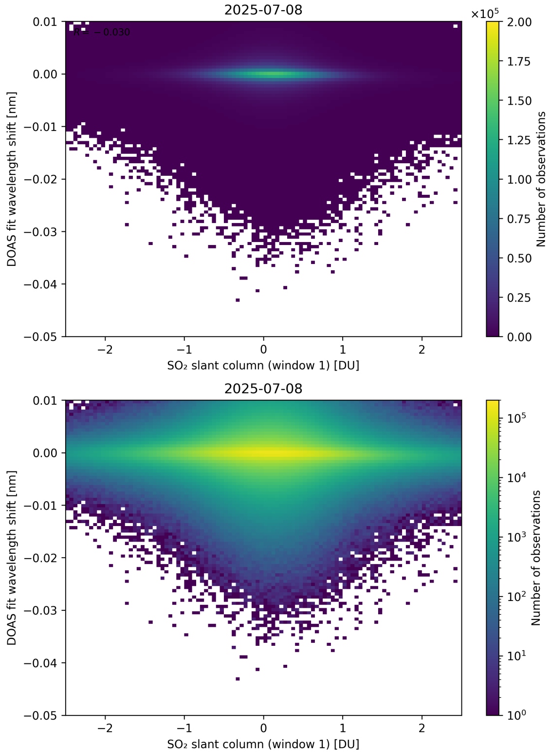
Figure 265: Scatter density plot of “SO 2 slant column (window 1)” against “DOAS fit wavelength shift” for 2025-07-08 to 2025-07-09.
