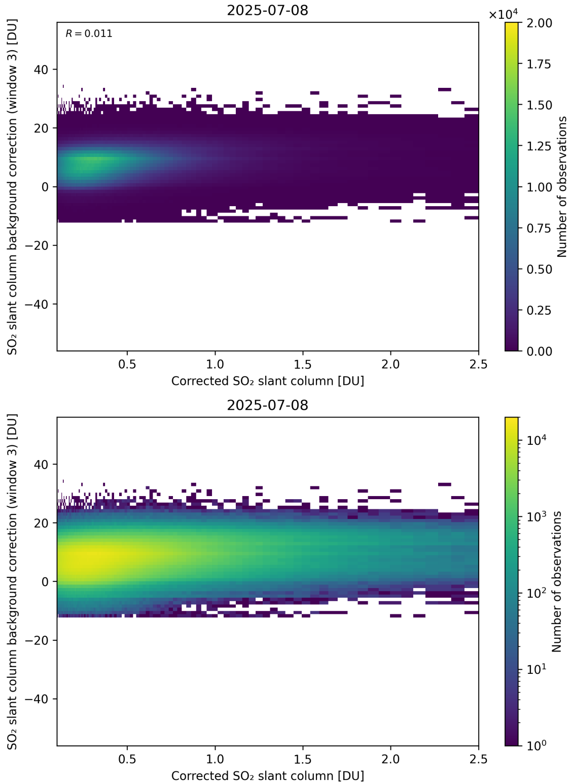
Figure 228: Scatter density plot of “Corrected SO 2 slant column” against “SO 2 slant column background correction (window 3)” for 2025-07-08 to 2025-07-09.
