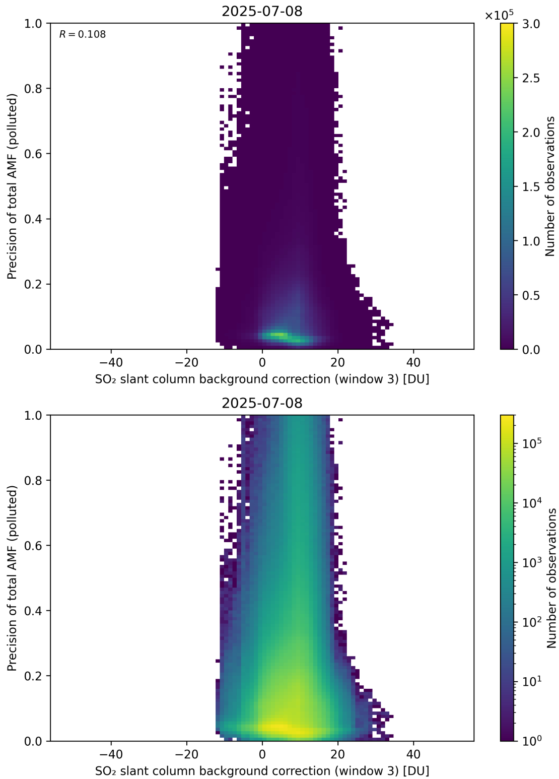
Figure 137: Scatter density plot of “SO 2 slant column background correction (window 3)” against “Precision of total AMF (polluted)” for 2025-07-08 to 2025-07-09.
