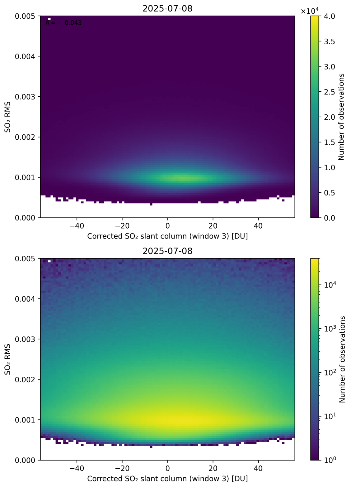
Figure 258: Scatter density plot of “Corrected SO 2 slant column (window 3)” against “SO 2 RMS” for 2025-07-08 to 2025-07-09.
