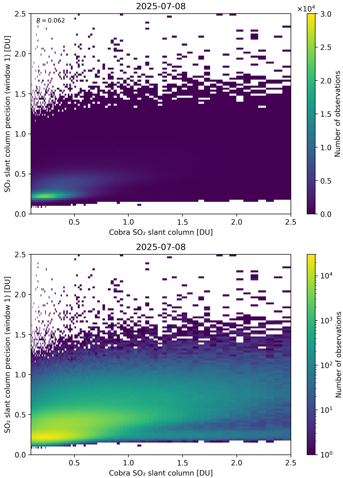
Figure 220: Scatter density plot of “Cobra SO 2 slant column” against “SO 2 slant column precision (window 1)” for 2025-07-08 to 2025-07-09.
