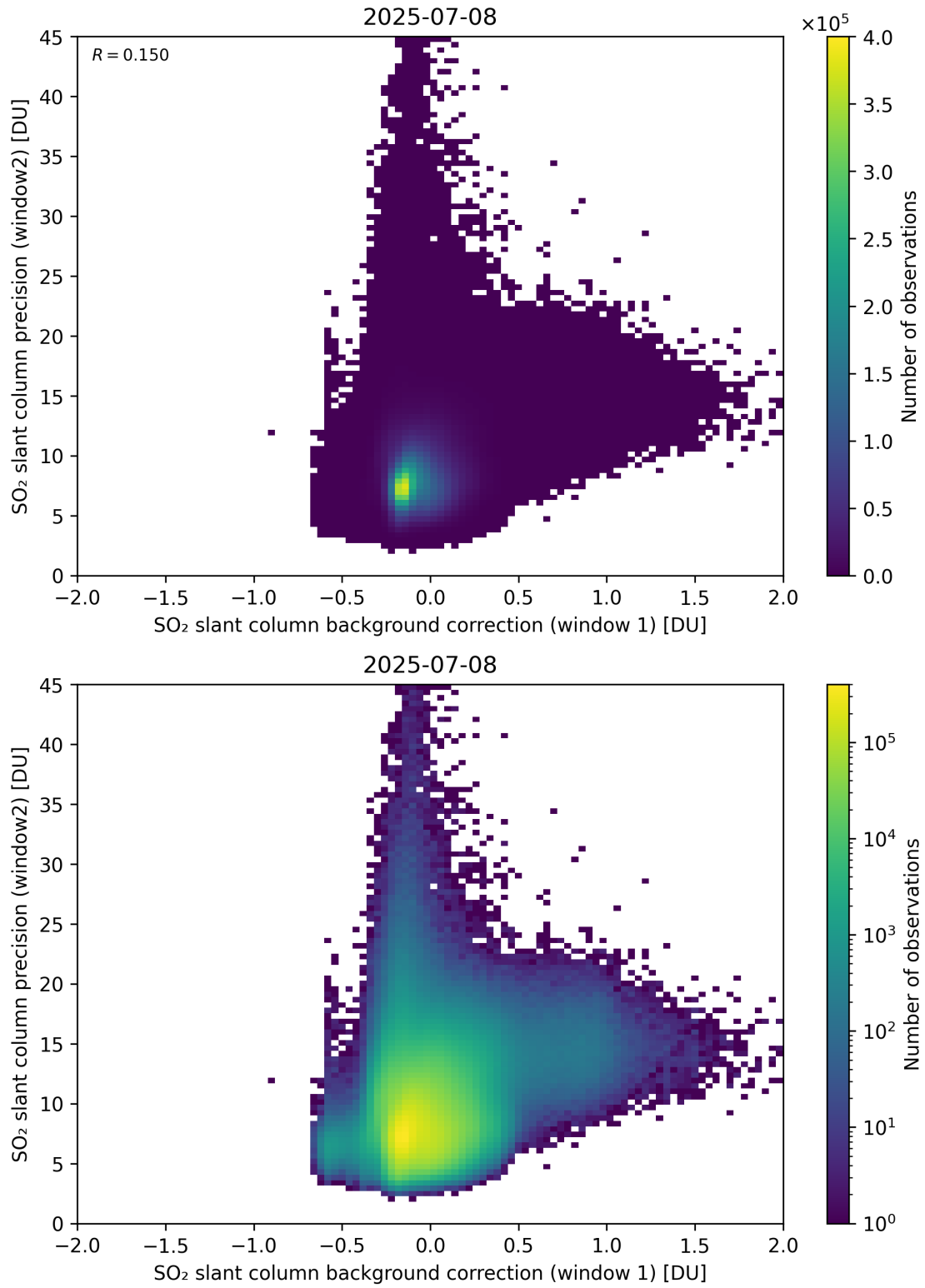
Figure 117: Scatter density plot of “SO 2 slant column background correction (window 1)” against “SO 2 slant column precision (window2)” for 2025-07-08 to 2025-07-09.
