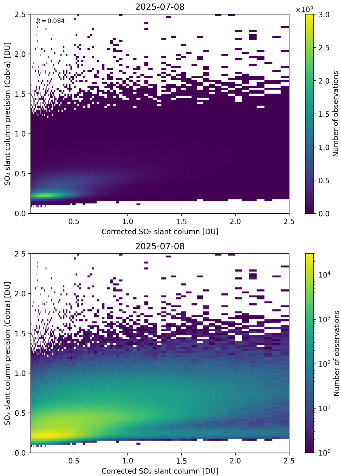
Figure 234: Scatter density plot of “Corrected SO 2 slant column” against “SO 2 slant column precision (Cobra)” for 2025-07-08 to 2025-07-09.
