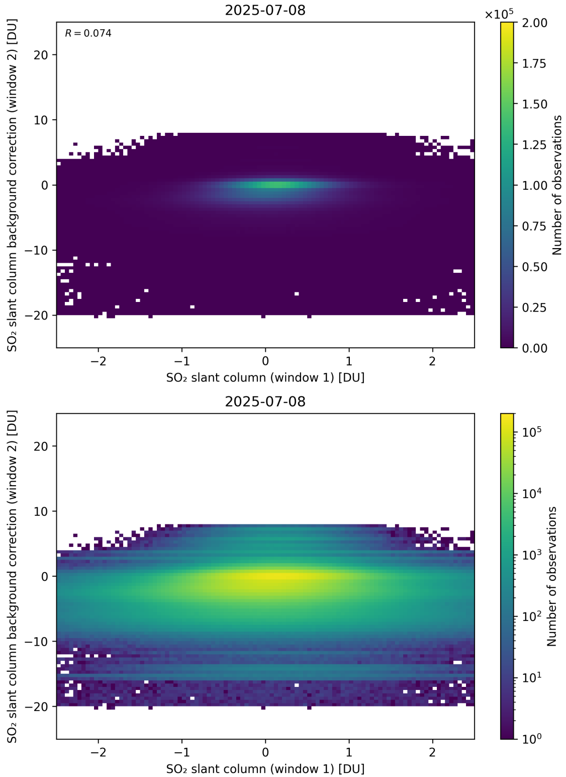
Figure 263: Scatter density plot of “SO 2 slant column (window 1)” against “SO 2 slant column background correction (window 2)” for 2025-07-08 to 2025-07-09.
