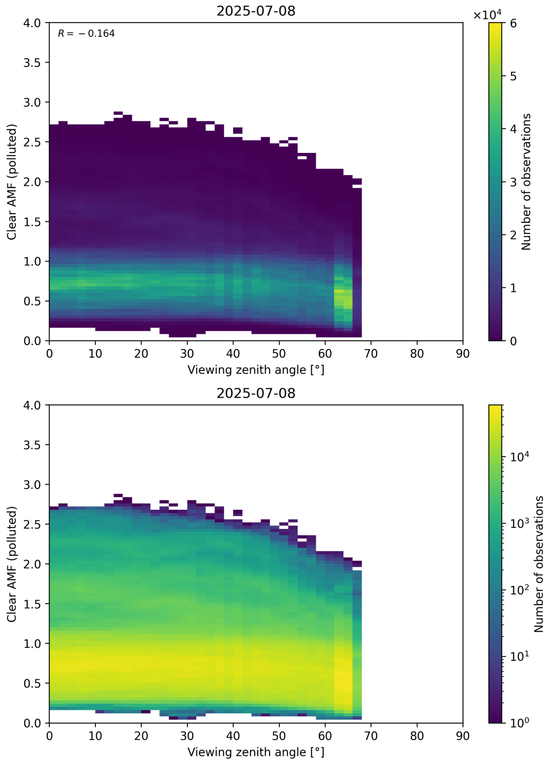
Figure 370: Scatter density plot of “Viewing zenith angle” against “Clear AMF (polluted)” for 2025-07-08 to 2025-07-09.
