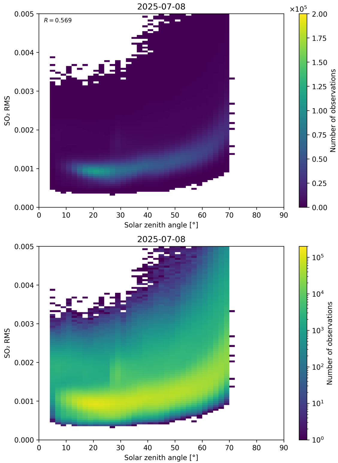
Figure 176: Scatter density plot of “Solar zenith angle” against “SO 2 RMS” for 2025-07-08 to 2025-07-09.
