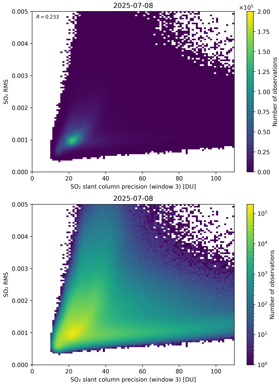
Figure 310: Scatter density plot of “SO 2 slant column precision (window 3)” against “SO 2 RMS” for 2025-07-08 to 2025-07-09.
