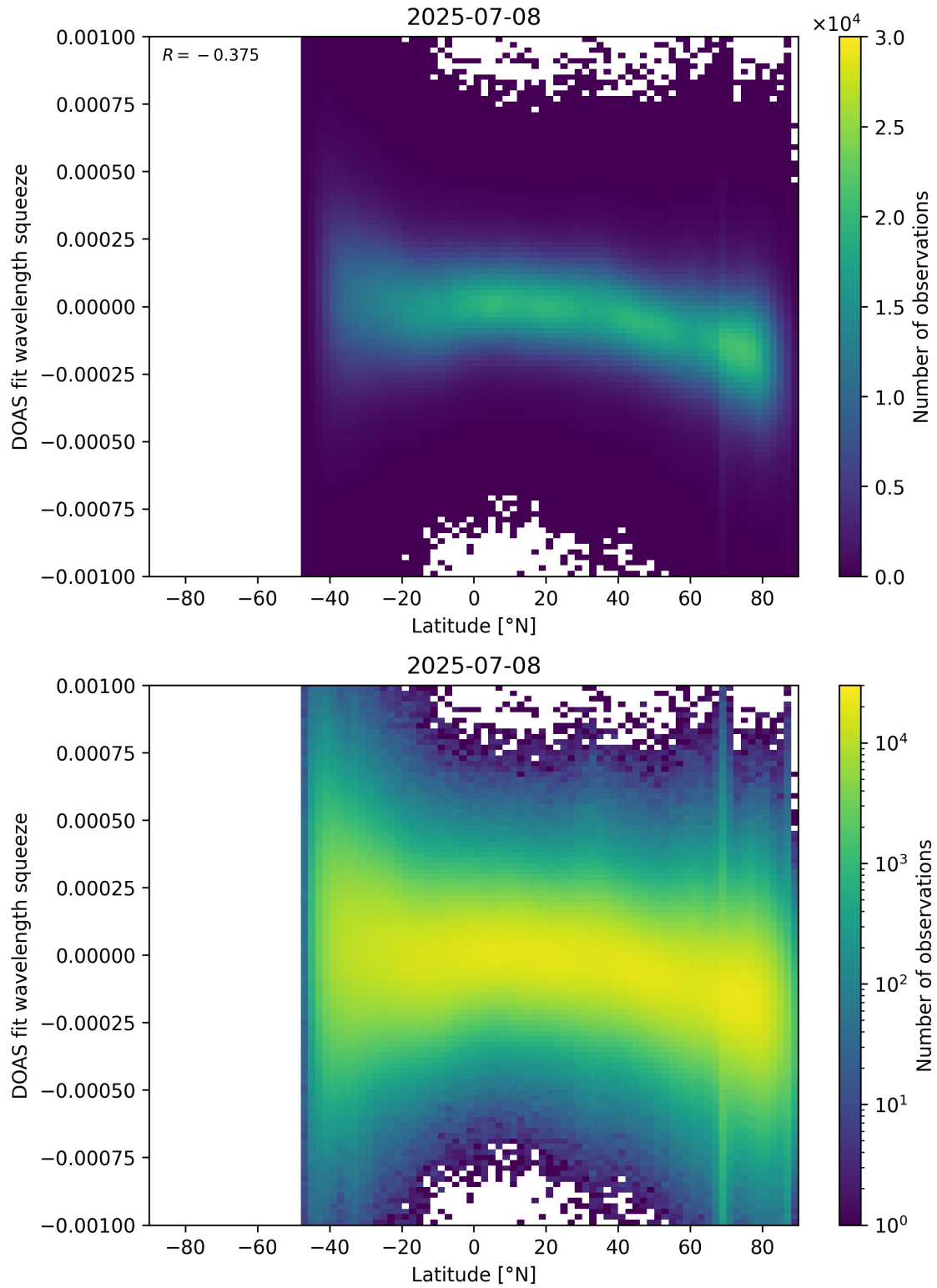
Figure 154: Scatter density plot of “Latitude” against “DOAS fit wavelength squeeze” for 2025-07-08 to 2025-07-09.
