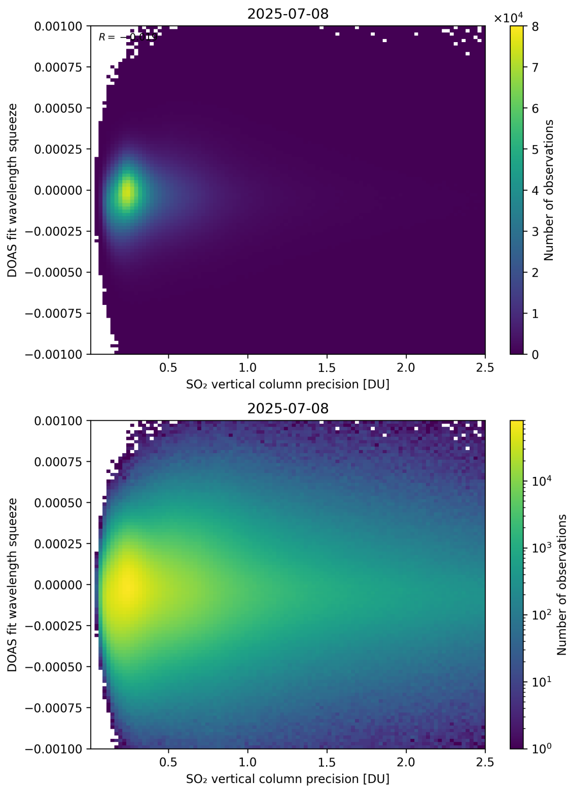
Figure 333: Scatter density plot of “SO 2 vertical column precision” against “DOAS fit wavelength squeeze” for 2025-07-08 to 2025-07-09.
