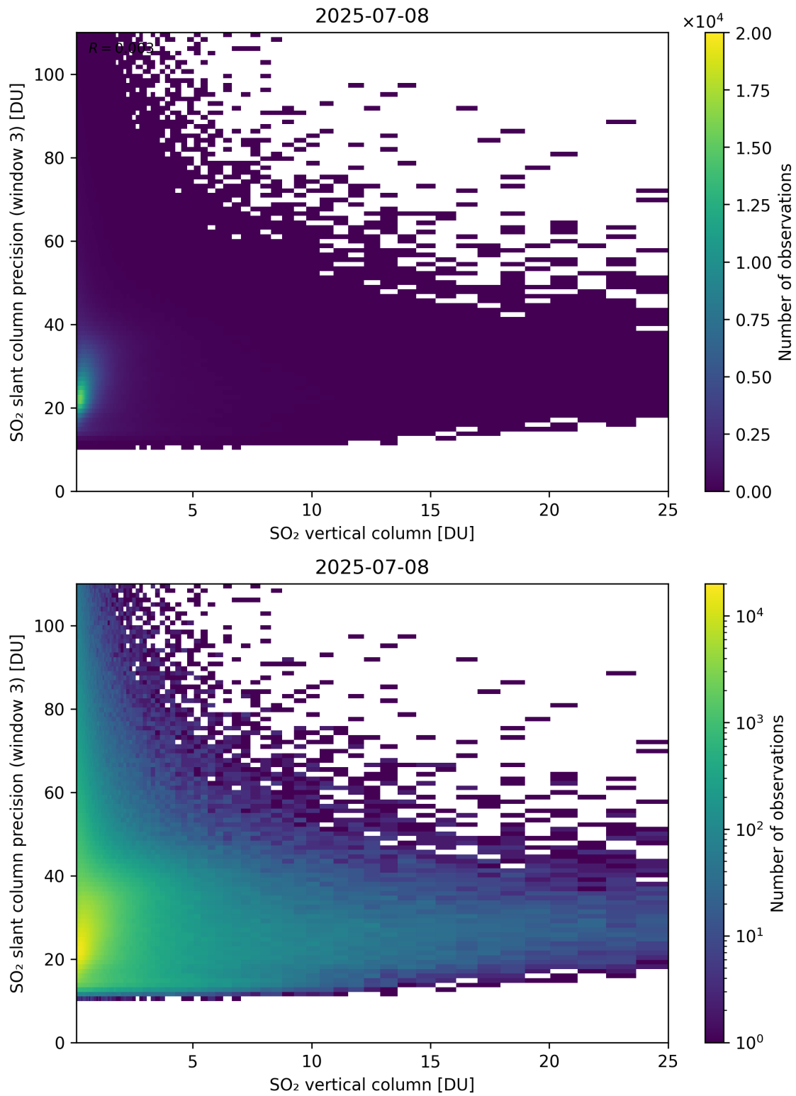
Figure 358: Scatter density plot of “SO 2 vertical column” against “SO 2 slant column precision (window 3)” for 2025-07-08 to 2025-07-09.
