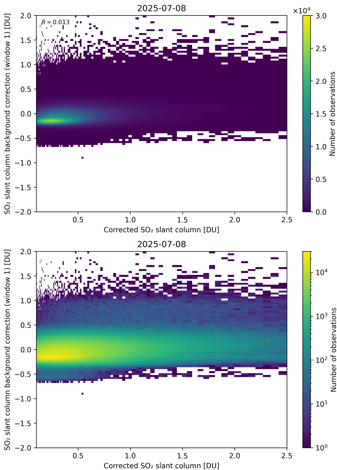
Figure 226: Scatter density plot of “Corrected SO 2 slant column” against “SO 2 slant column background correction (window 1)” for 2025-07-08 to 2025-07-09.
