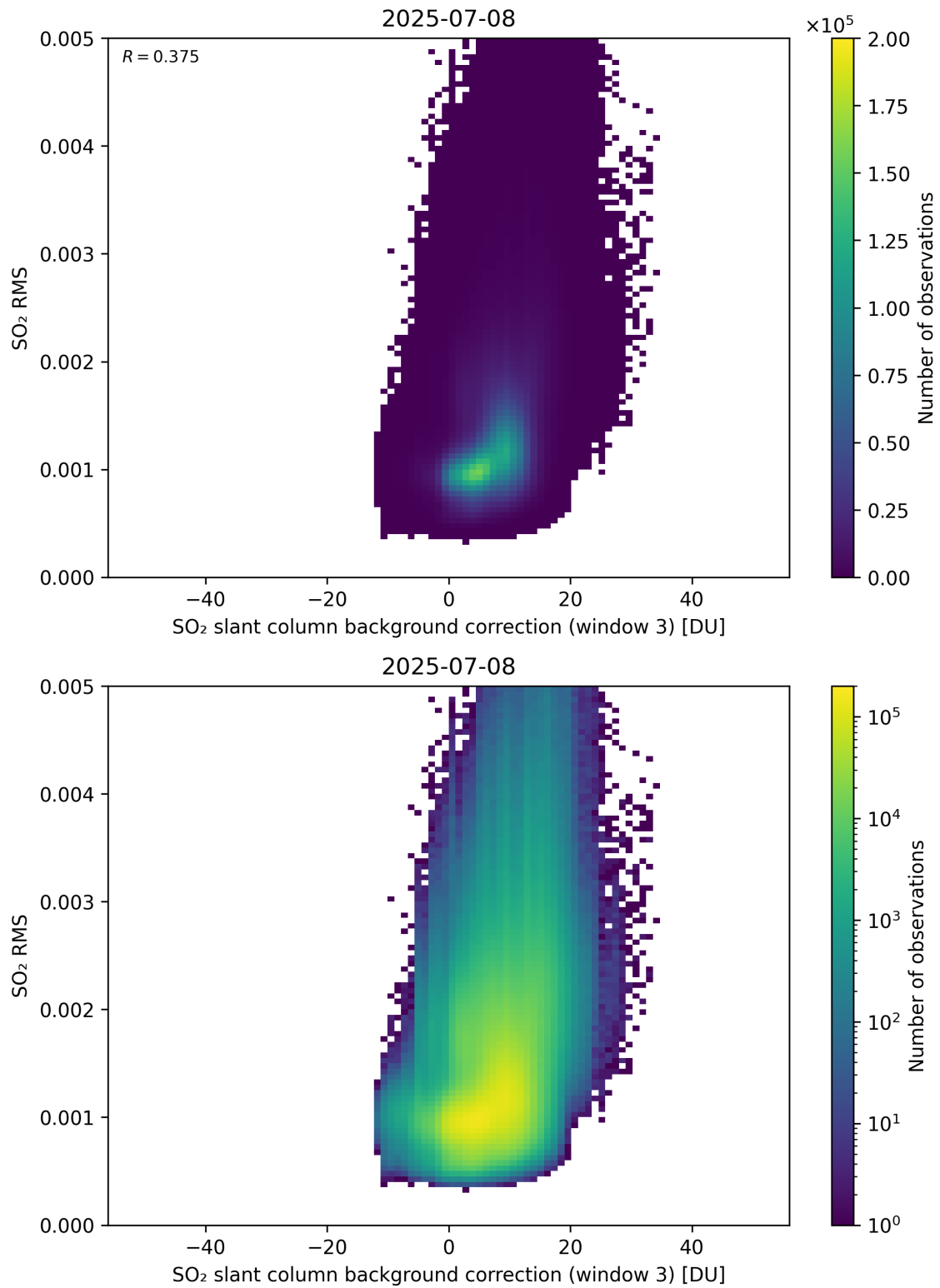
Figure 134: Scatter density plot of “SO 2 slant column background correction (window 3)” against “SO 2 RMS” for 2025-07-08 to 2025-07-09.
