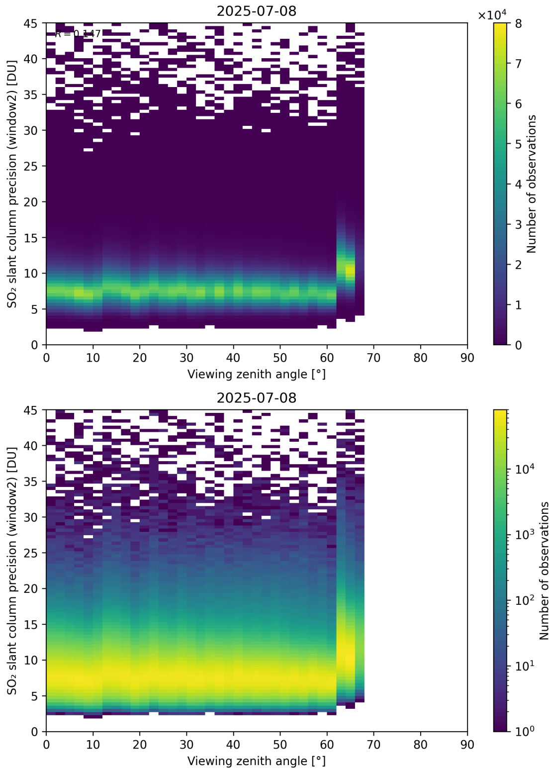
Figure 378: Scatter density plot of “Viewing zenith angle” against “SO 2 slant column precision (window2)” for 2025-07-08 to 2025-07-09.
