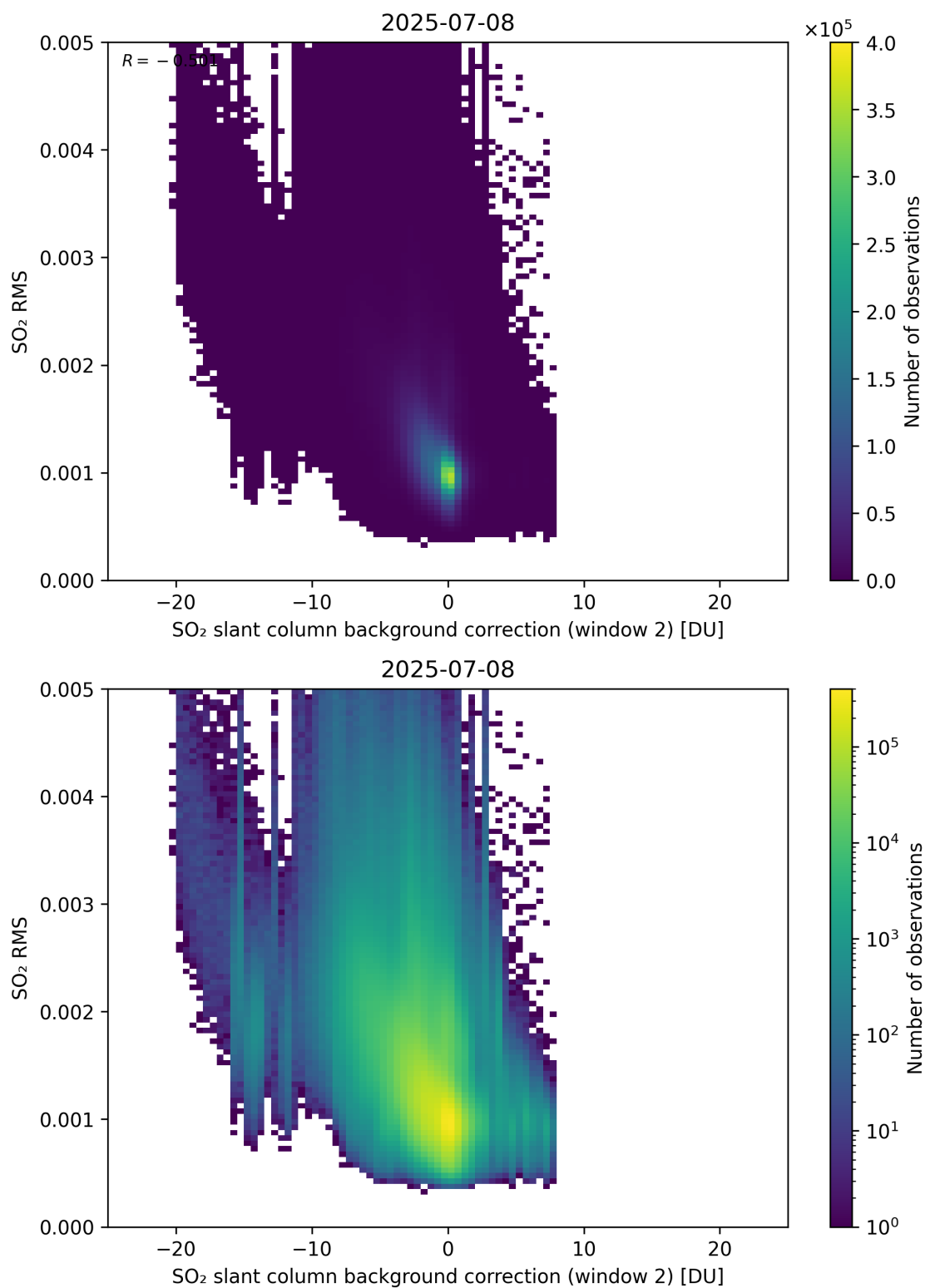
Figure 125: Scatter density plot of “SO 2 slant column background correction (window 2)” against “SO 2 RMS” for 2025-07-08 to 2025-07-09.
