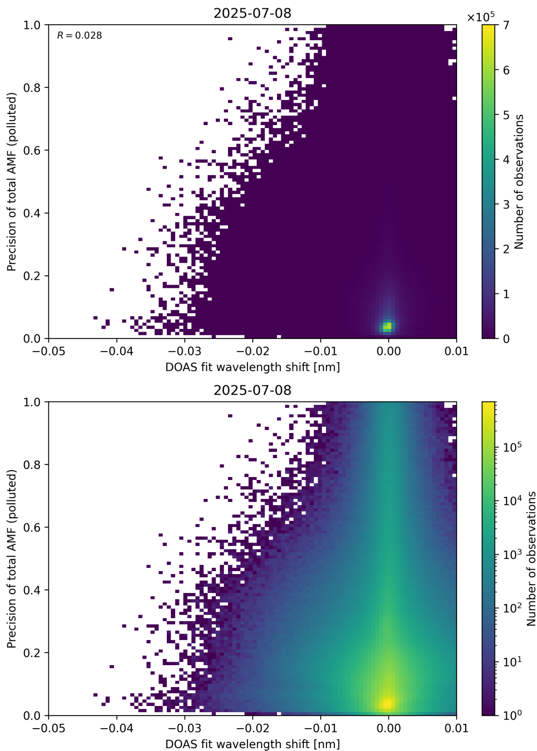
Figure 142: Scatter density plot of “DOAS fit wavelength shift” against “Precision of total AMF (polluted)” for 2025-07-08 to 2025-07-09.
