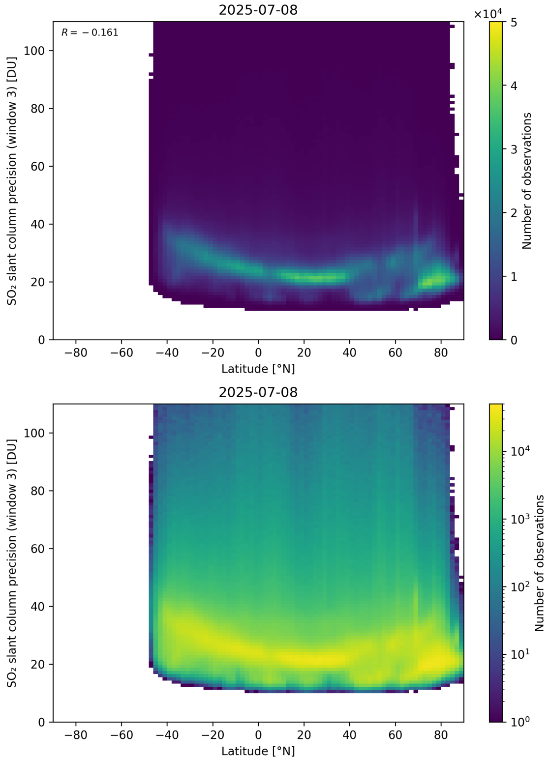
Figure 166: Scatter density plot of “Latitude” against “SO 2 slant column precision (window 3)” for 2025-07-08 to 2025-07-09.
