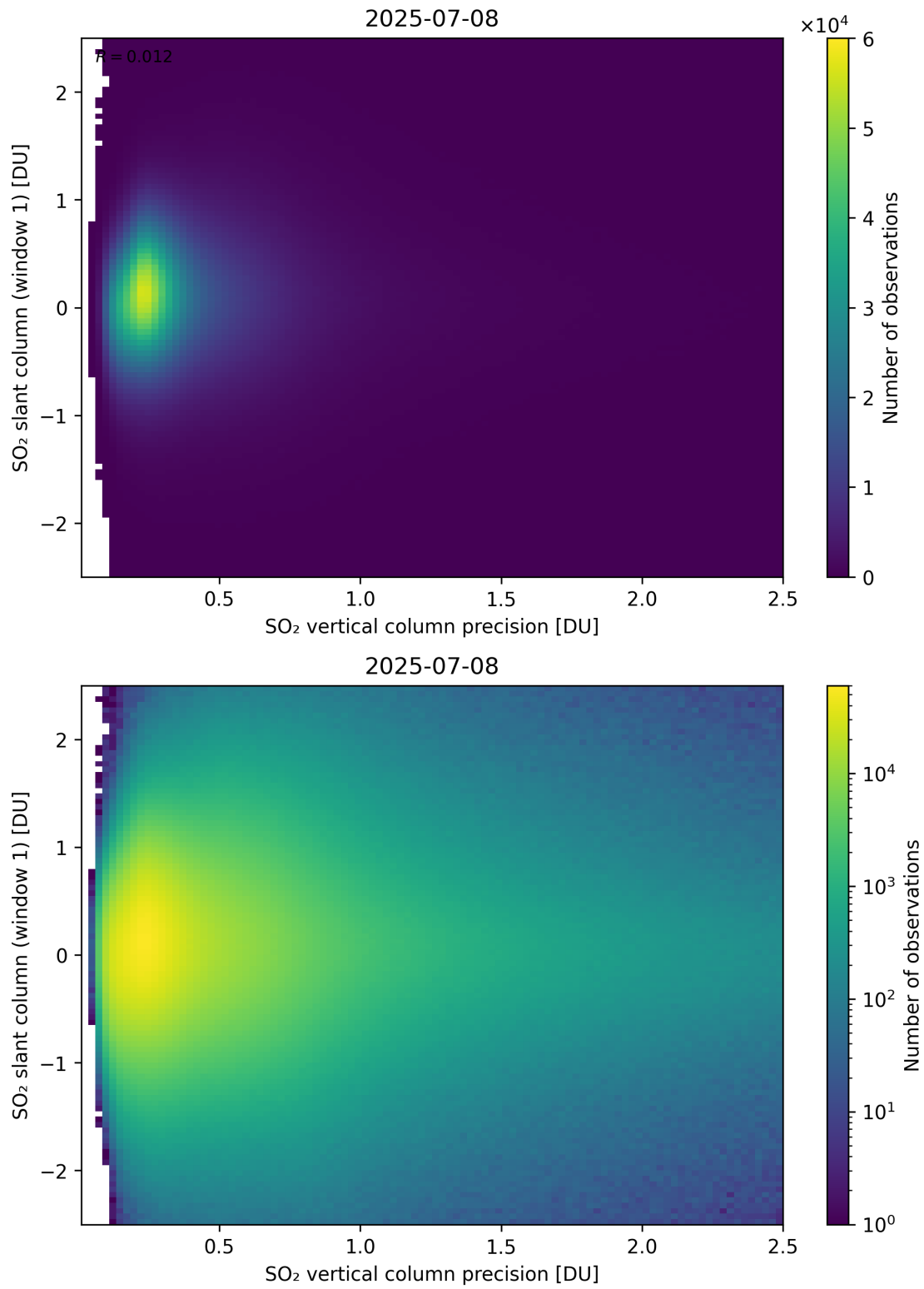
Figure 341: Scatter density plot of “SO 2 vertical column precision” against “SO 2 slant column (window 1)” for 2025-07-08 to 2025-07-09.
