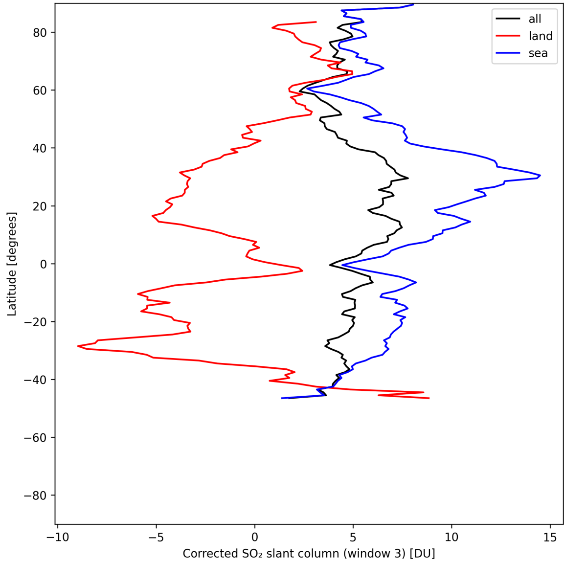
Figure 47: Zonal average of “Corrected SO 2 slant column (window 3)” for 2025-07-08 to 2025-07-09.
