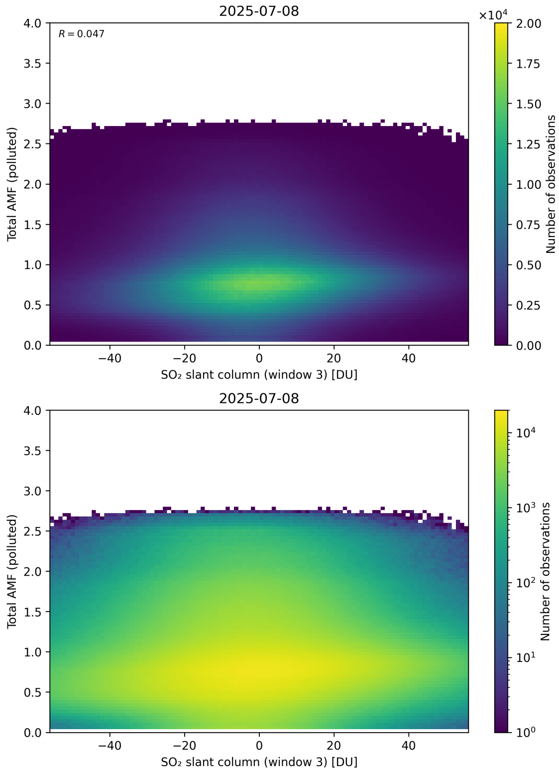
Figure 318: Scatter density plot of “SO 2 slant column (window 3)” against “Total AMF (polluted)” for 2025-07-08 to 2025-07-09.
