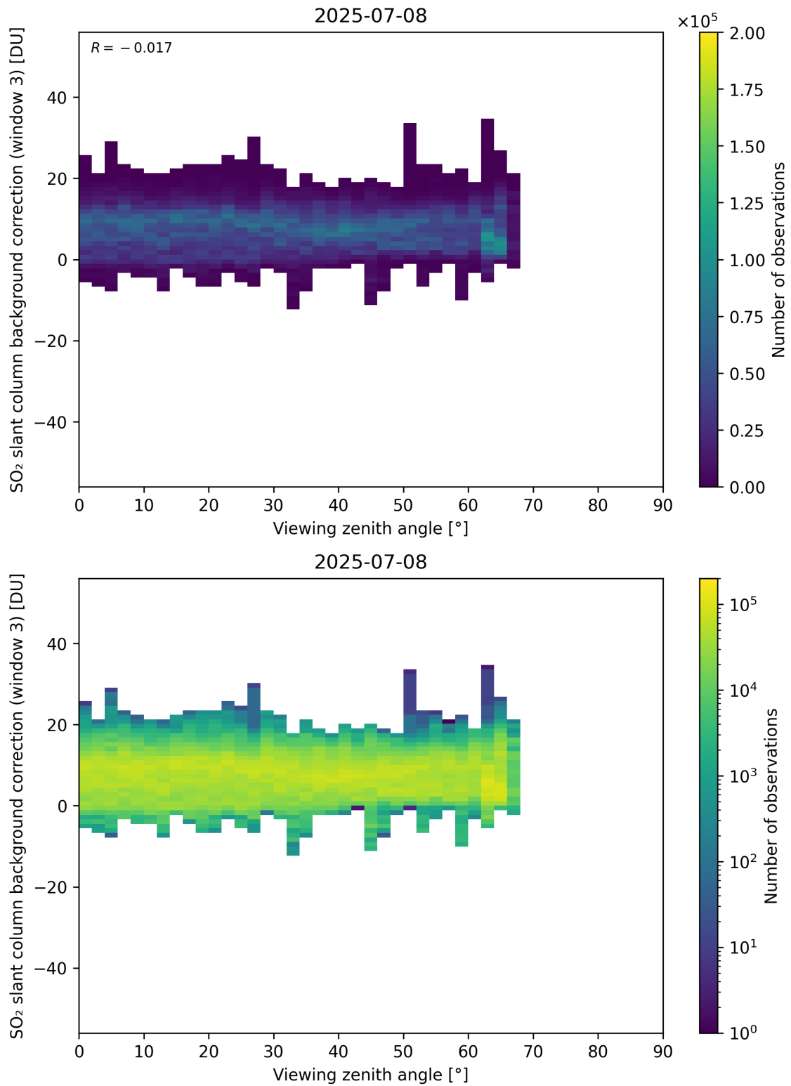
Figure 364: Scatter density plot of “Viewing zenith angle” against “SO 2 slant column background correction (window 3)” for 2025-07-08 to 2025-07-09.
