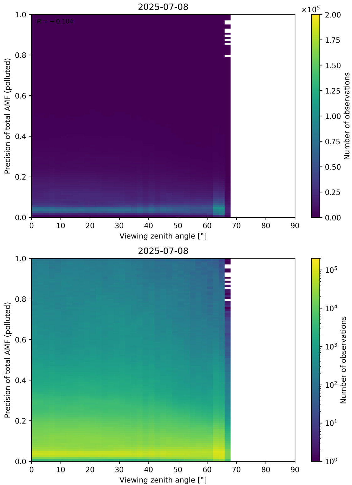
Figure 382: Scatter density plot of “Viewing zenith angle” against “Precision of total AMF (polluted)” for 2025-07-08 to 2025-07-09.
