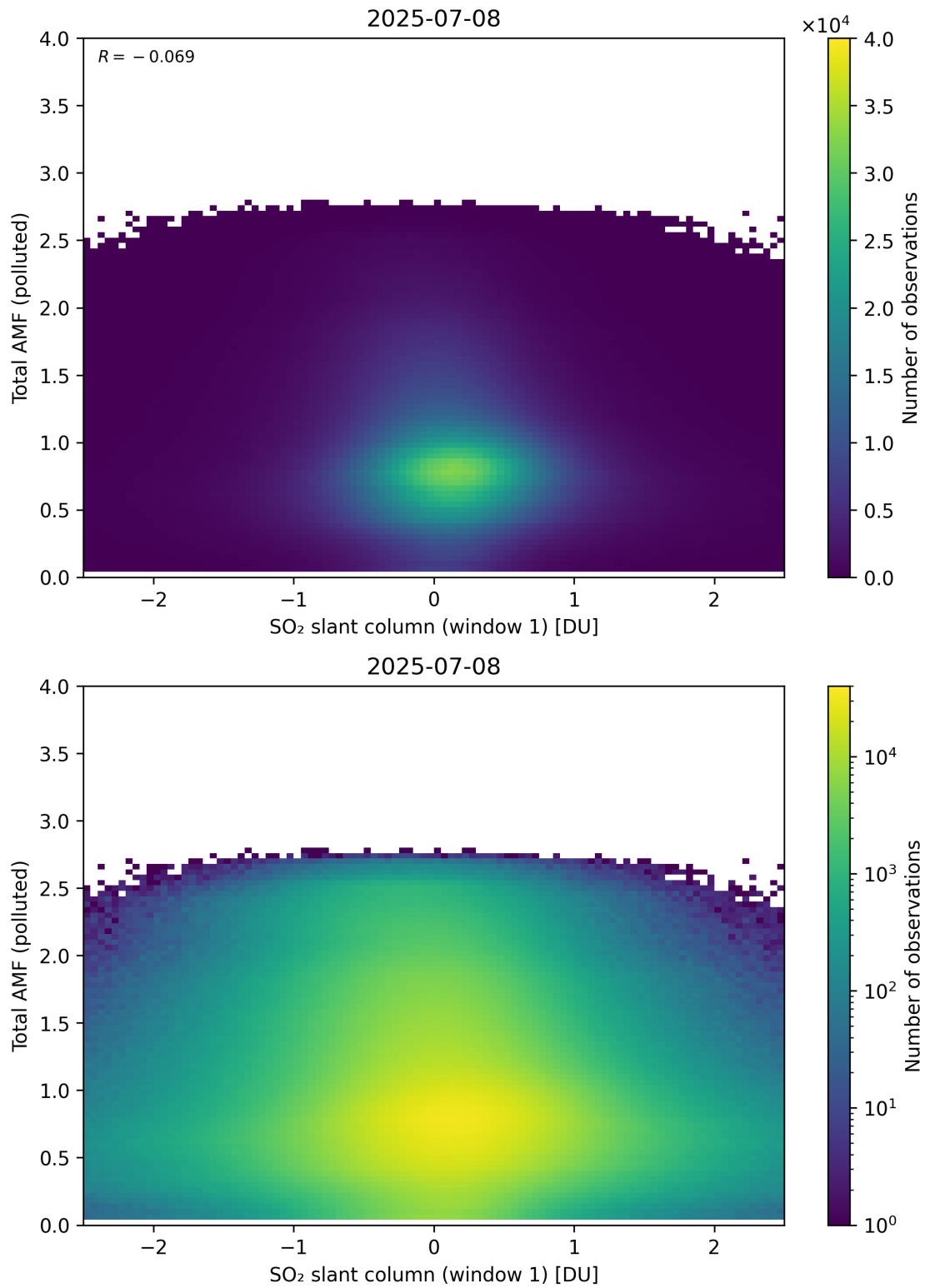
Figure 289: Scatter density plot of “SO 2 slant column (window 1)” against “Total AMF (polluted)” for 2025-07-08 to 2025-07-09.
