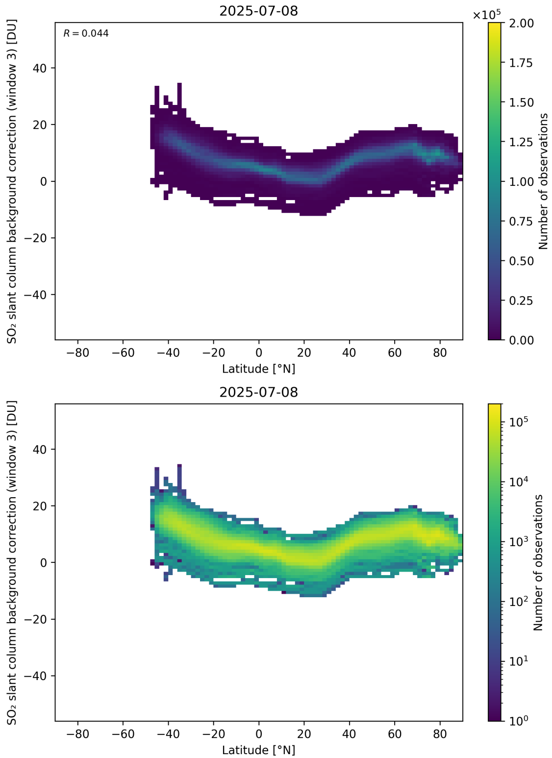
Figure 152: Scatter density plot of “Latitude” against “SO 2 slant column background correction (window 3)” for 2025-07-08 to 2025-07-09.
