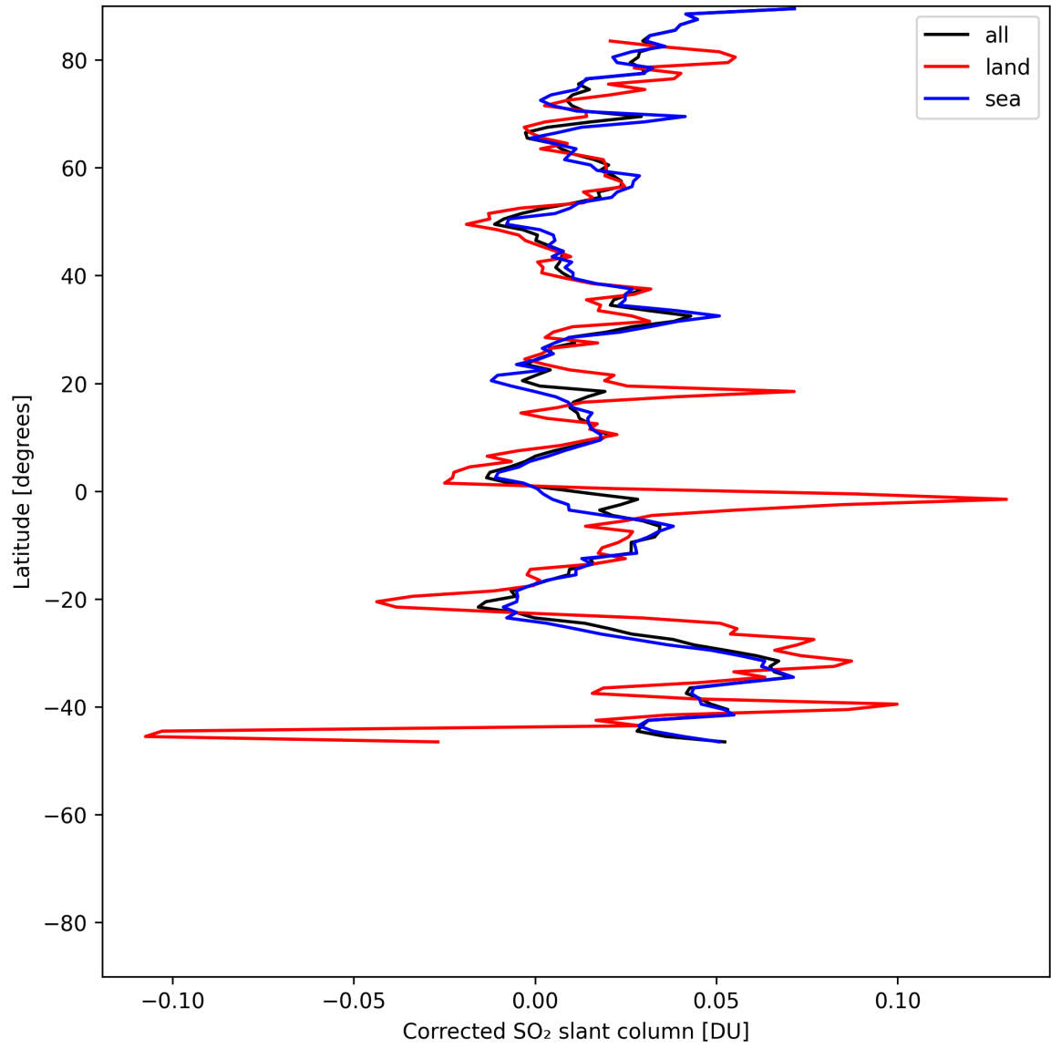
Figure 34: Zonal average of “Corrected SO 2 slant column” for 2025-07-08 to 2025-07-09.
