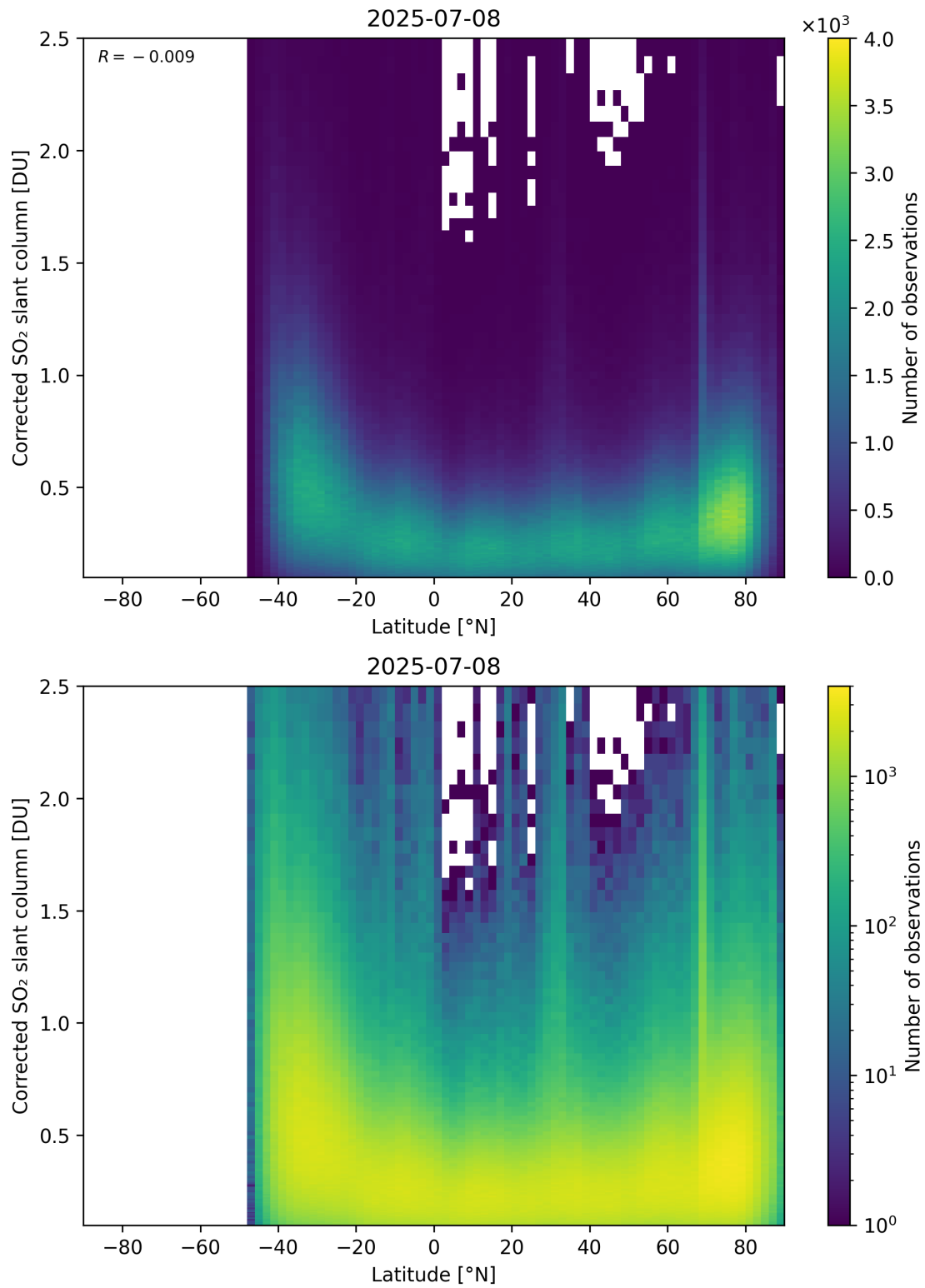
Figure 159: Scatter density plot of “Latitude” against “Corrected SO 2 slant column” for 2025-07-08 to 2025-07-09.
