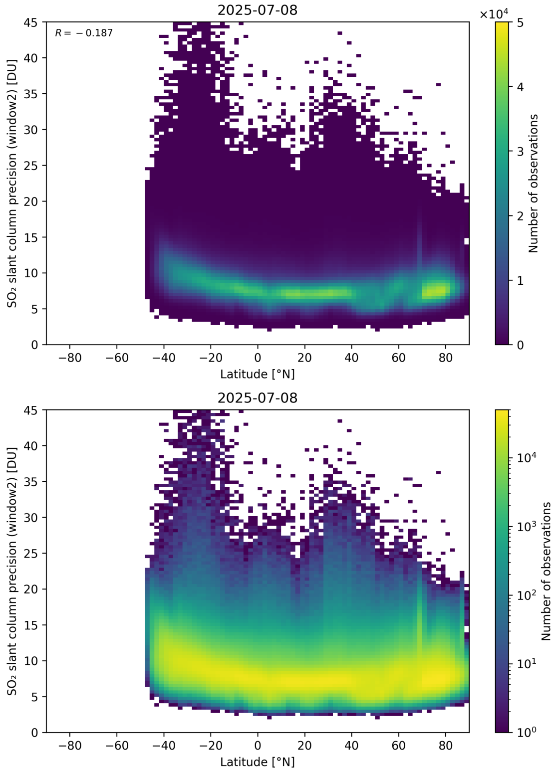
Figure 164: Scatter density plot of “Latitude” against “SO 2 slant column precision (window2)” for 2025-07-08 to 2025-07-09.
