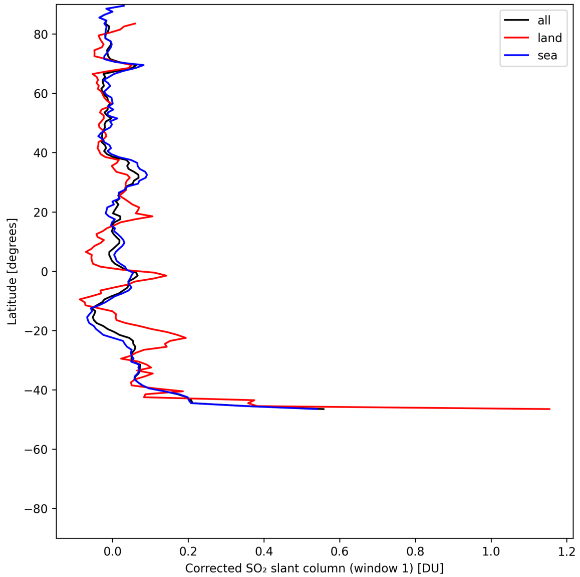
Figure 39: Zonal average of “Corrected SO 2 slant column (window 1)” for 2025-07-08 to 2025-07-09.
