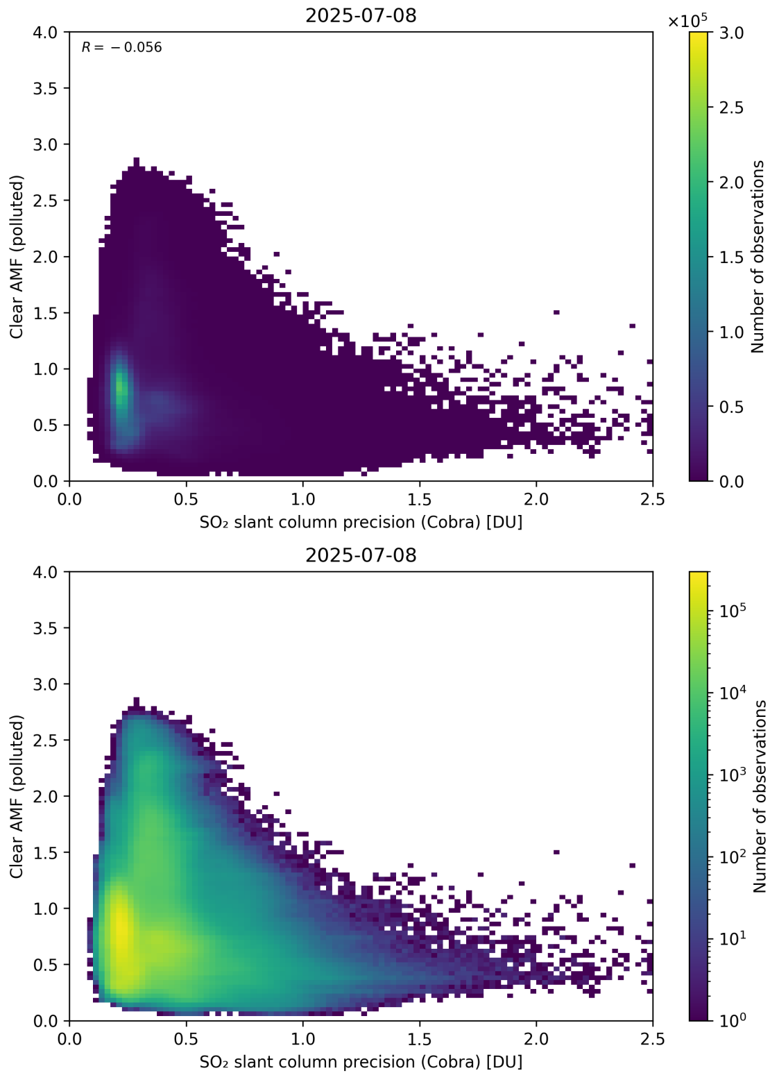
Figure 205: Scatter density plot of “SO 2 slant column precision (Cobra)” against “Clear AMF (polluted)” for 2025-07-08 to 2025-07-09.
