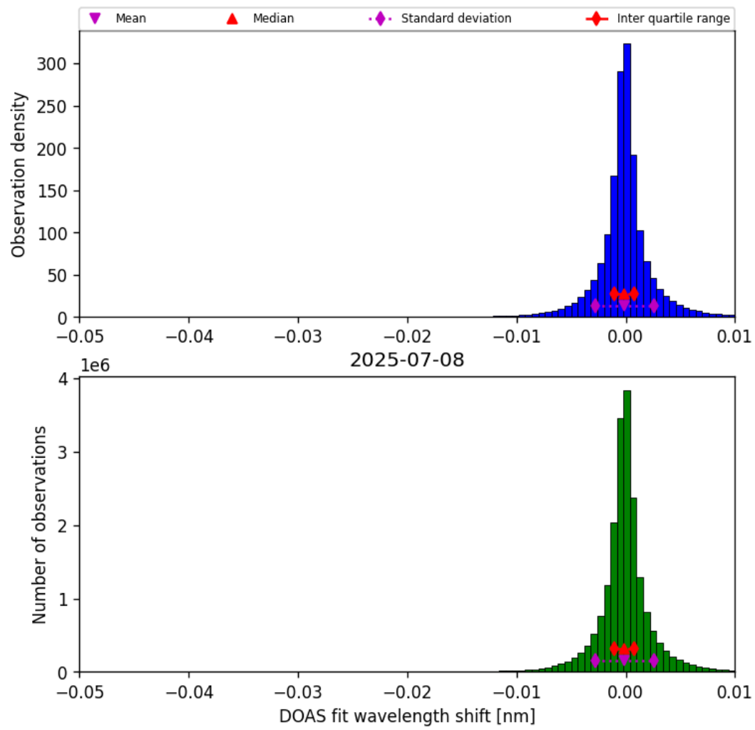
Figure 76: Histogram of “DOAS fit wavelength shift” for 2025-07-08 to 2025-07-09
