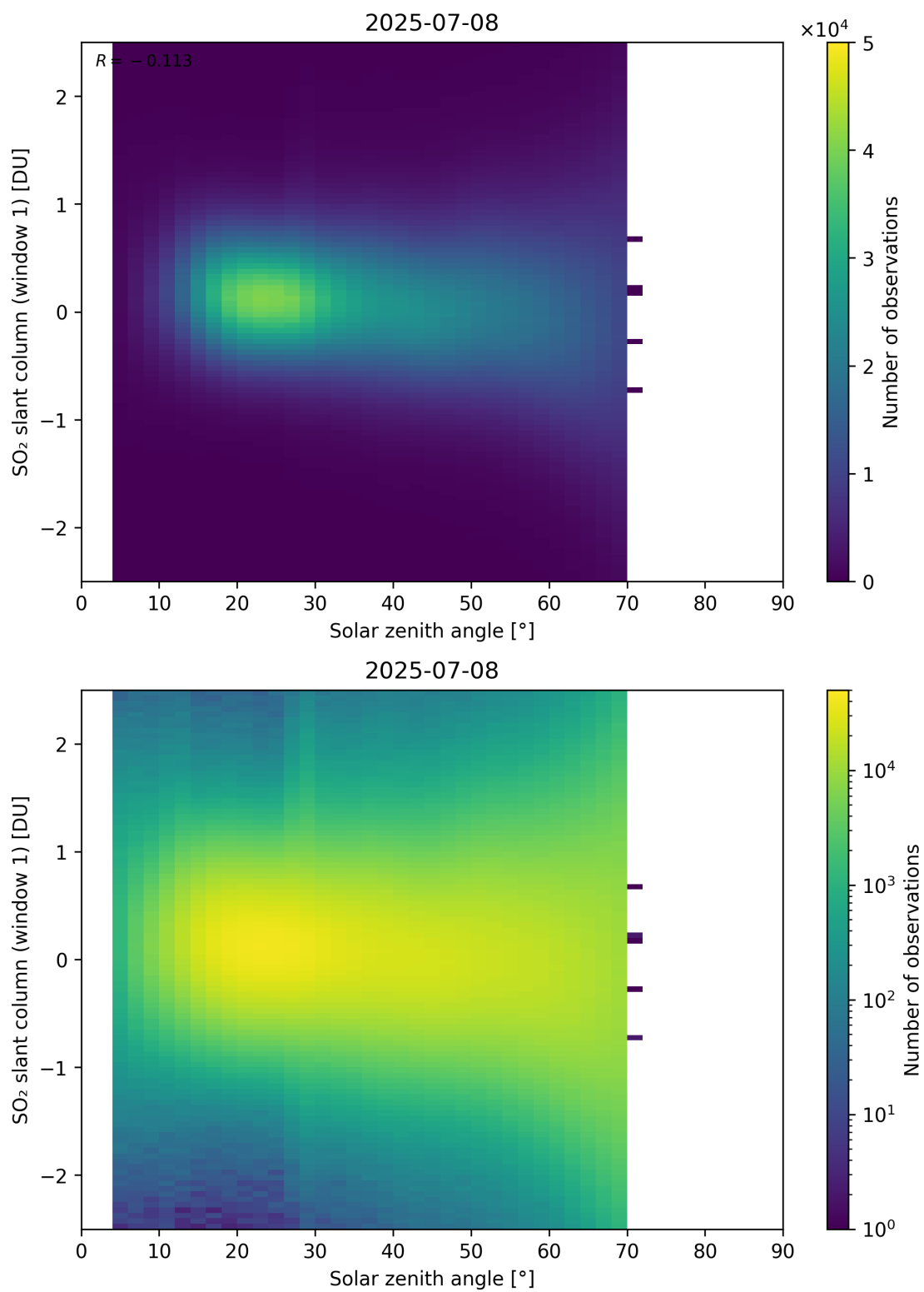
Figure 184: Scatter density plot of “Solar zenith angle” against “SO 2 slant column (window 1)” for 2025-07-08 to 2025-07-09.
