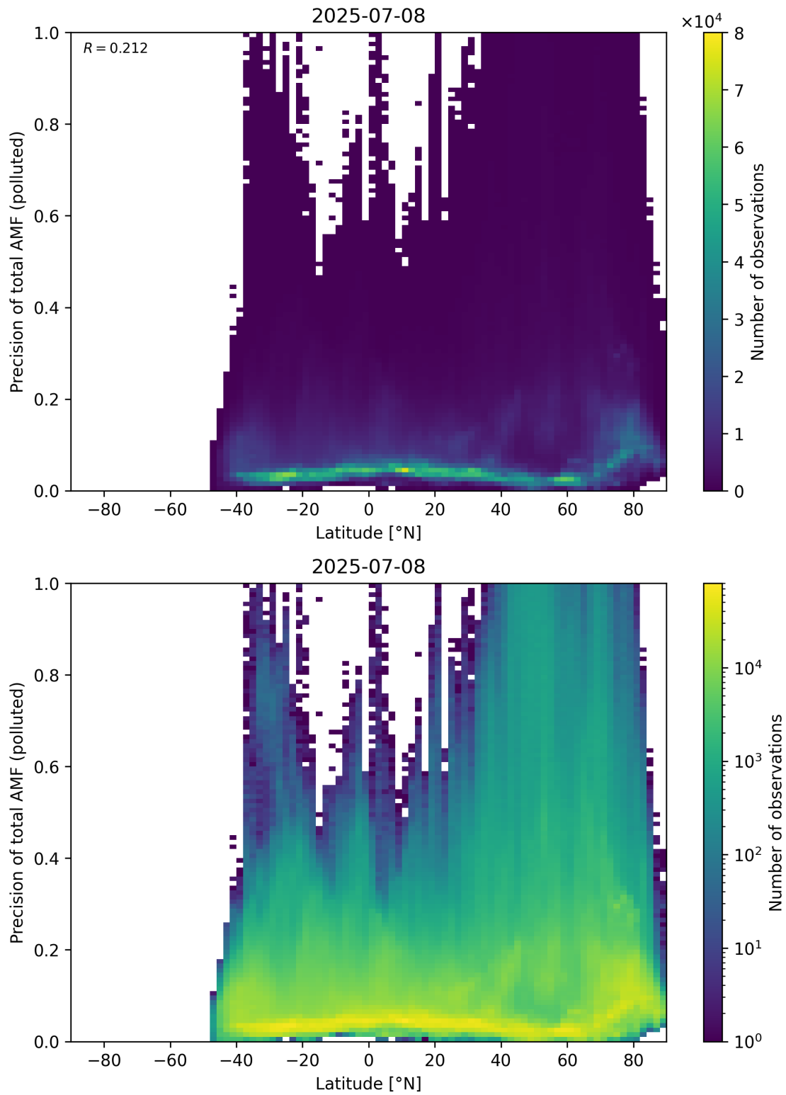
Figure 168: Scatter density plot of “Latitude” against “Precision of total AMF (polluted)” for 2025-07-08 to 2025-07-09.
