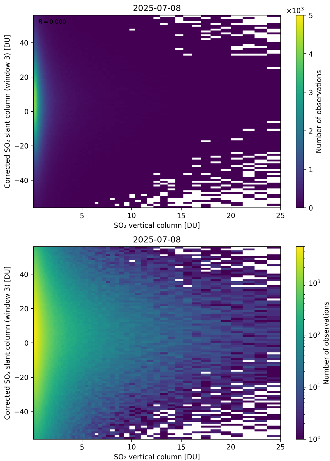
Figure 353: Scatter density plot of “SO 2 vertical column” against “Corrected SO 2 slant column (window 3)” for 2025-07-08 to 2025-07-09.
