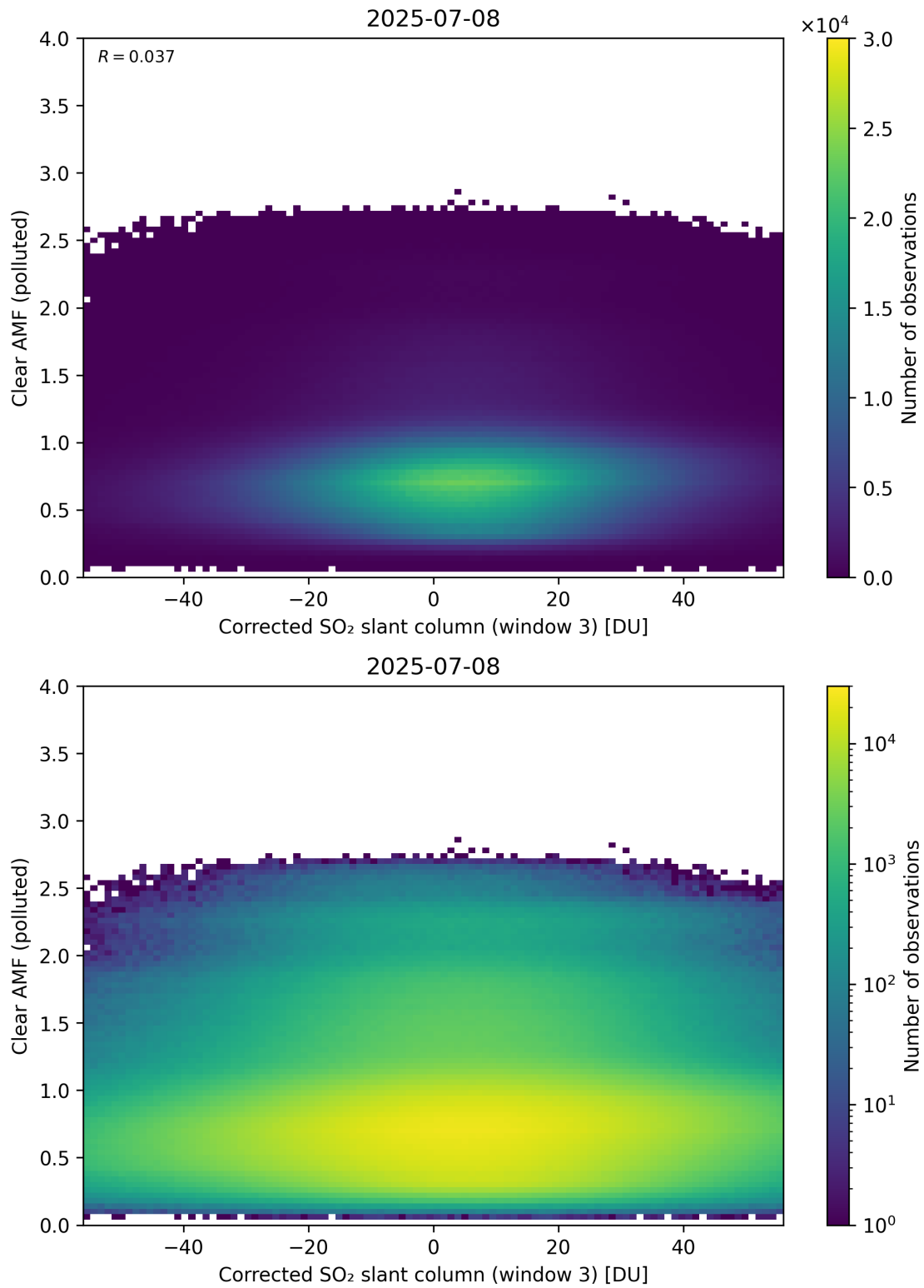
Figure 259: Scatter density plot of “Corrected SO 2 slant column (window 3)” against “Clear AMF (polluted)” for 2025-07-08 to 2025-07-09.
