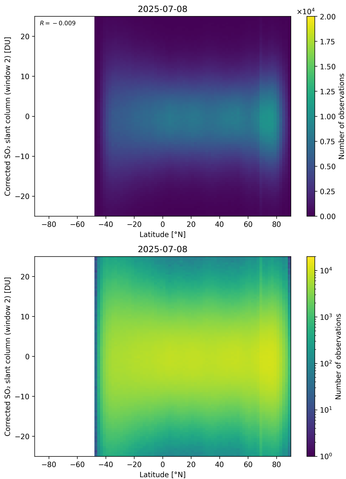
Figure 160: Scatter density plot of “Latitude” against “Corrected SO 2 slant column (window 2)” for 2025-07-08 to 2025-07-09.
