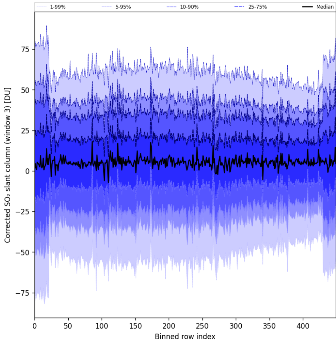
Figure 99: Along track statistics of “Corrected SO 2 slant column (window 3)” for 2025-07-08 to 2025-07-09
