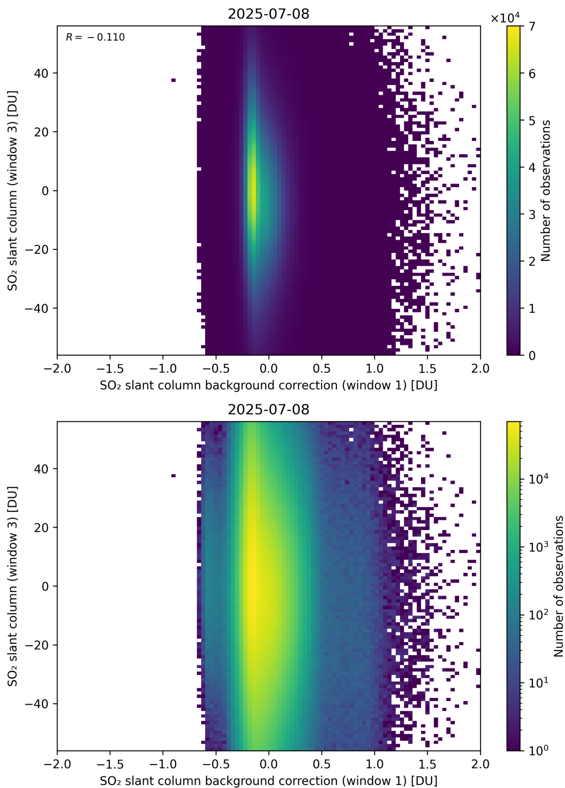
Figure 118: Scatter density plot of “SO 2 slant column background correction (window 1)” against “SO 2 slant column (window 3)” for 2025-07-08 to 2025-07-09.
