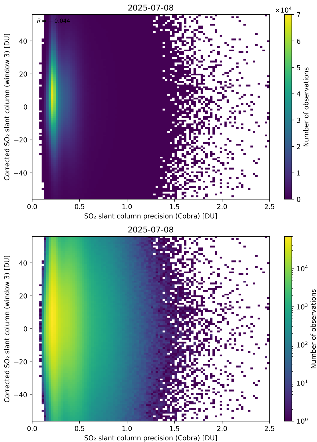
Figure 207: Scatter density plot of “SO 2 slant column precision (Cobra)” against “Corrected SO 2 slant column (window 3)” for 2025-07-08 to 2025-07-09.
