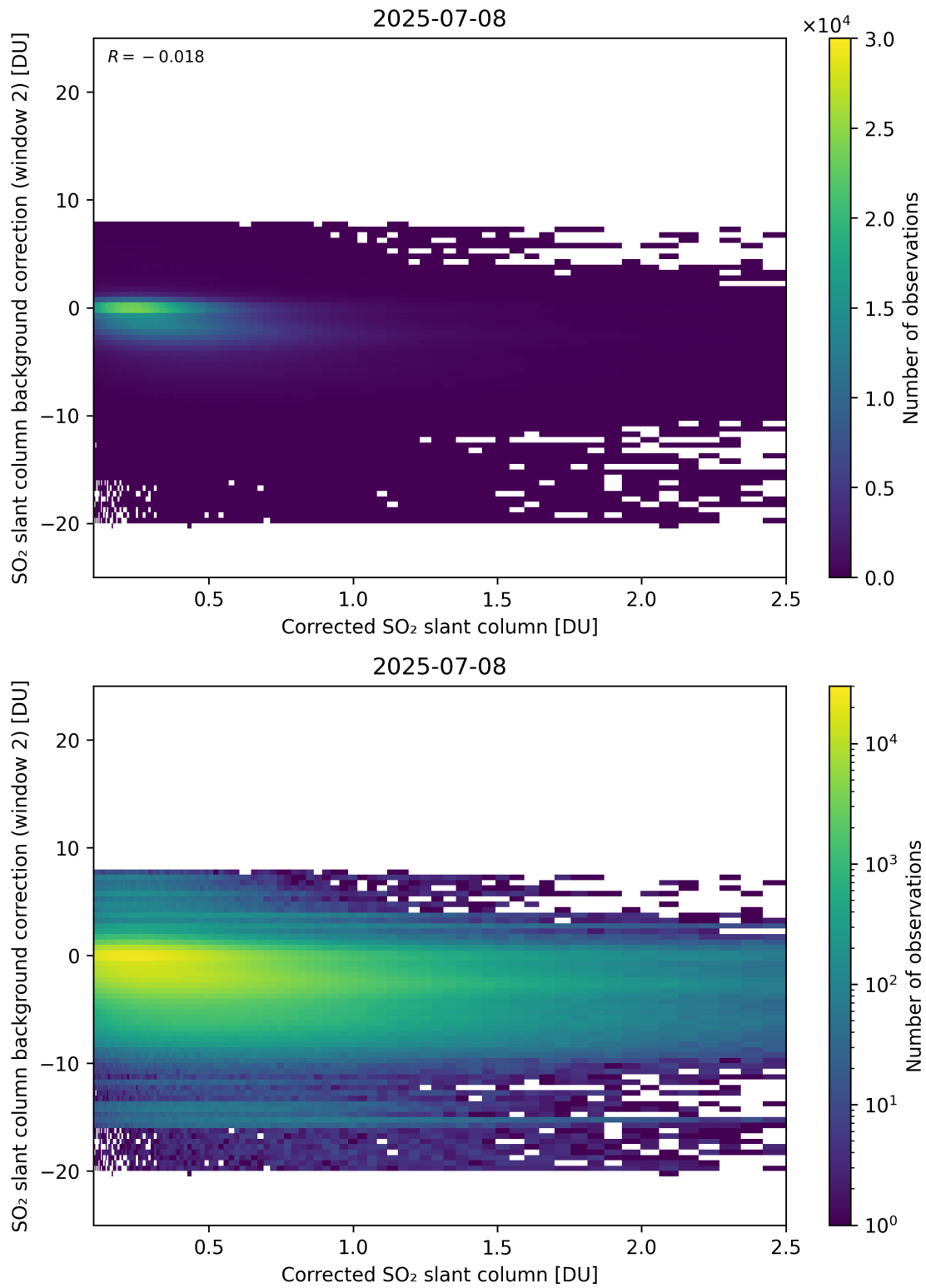
Figure 227: Scatter density plot of “Corrected SO 2 slant column” against “SO 2 slant column background correction (window 2)” for 2025-07-08 to 2025-07-09.
