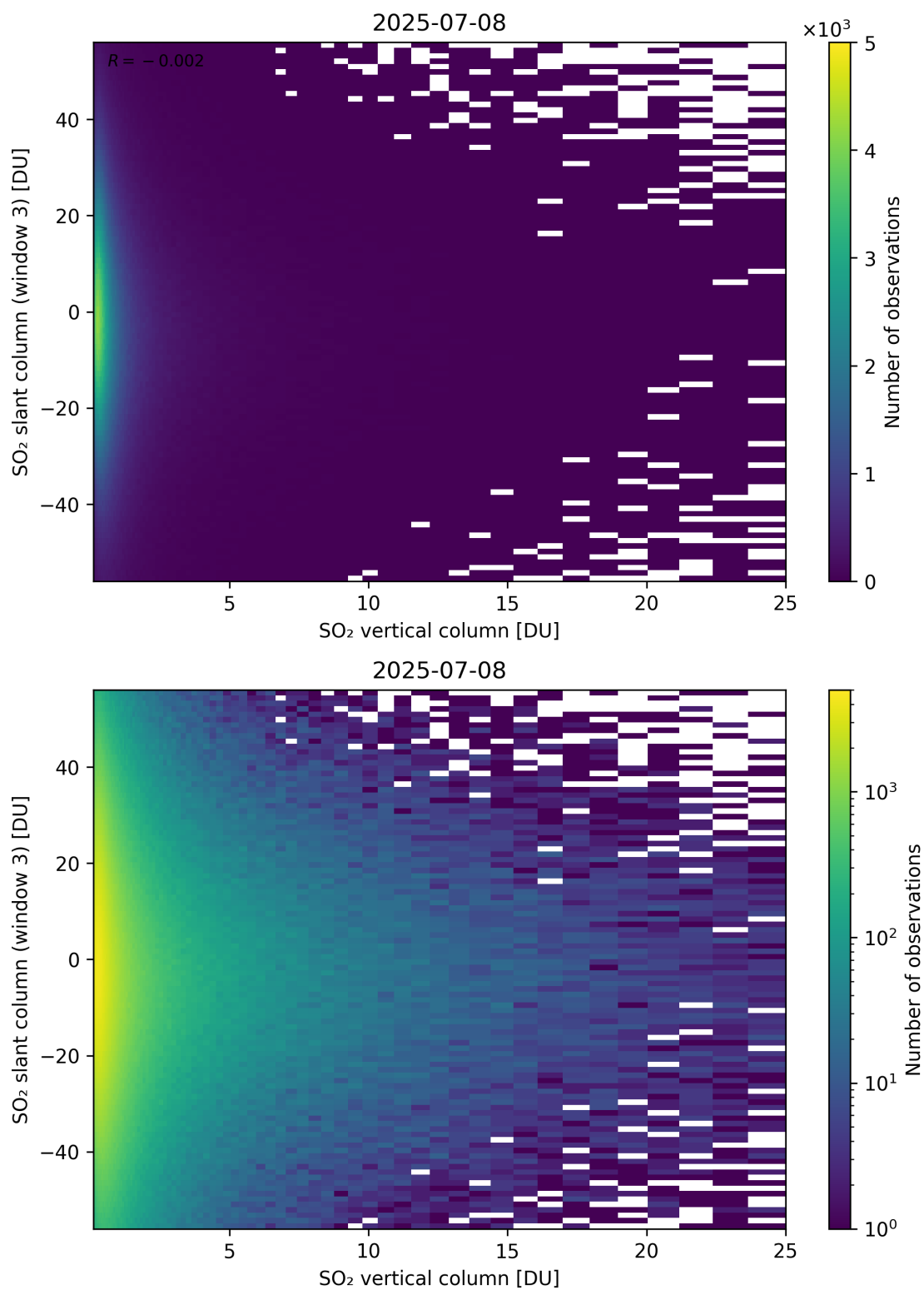
Figure 357: Scatter density plot of “SO 2 vertical column” against “SO 2 slant column (window 3)” for 2025-07-08 to 2025-07-09.
