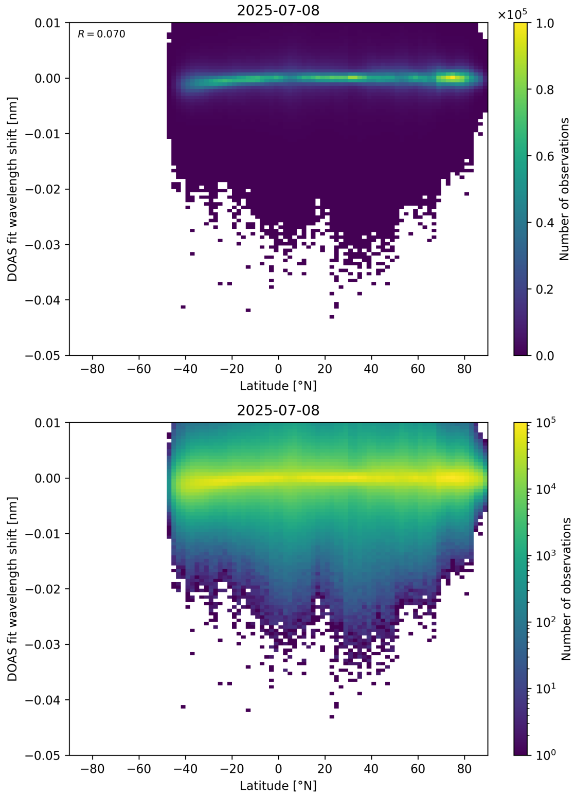
Figure 153: Scatter density plot of “Latitude” against “DOAS fit wavelength shift” for 2025-07-08 to 2025-07-09.
