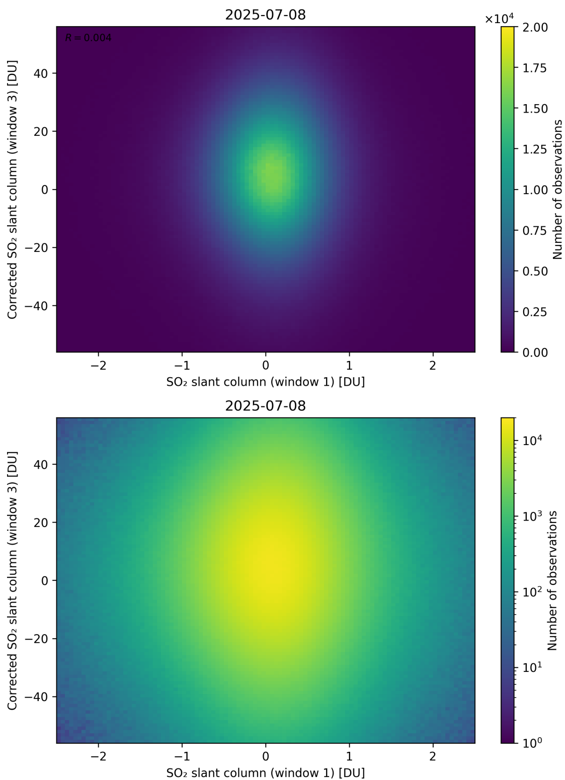
Figure 284: Scatter density plot of “SO 2 slant column (window 1)” against “Corrected SO 2 slant column (window 3)” for 2025-07-08 to 2025-07-09.
