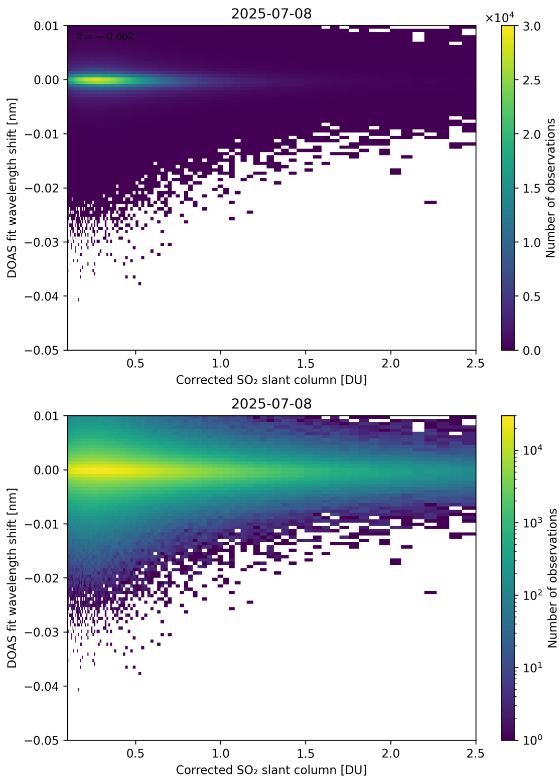
Figure 229: Scatter density plot of “Corrected SO 2 slant column” against “DOAS fit wavelength shift” for 2025-07-08 to 2025-07-09.
