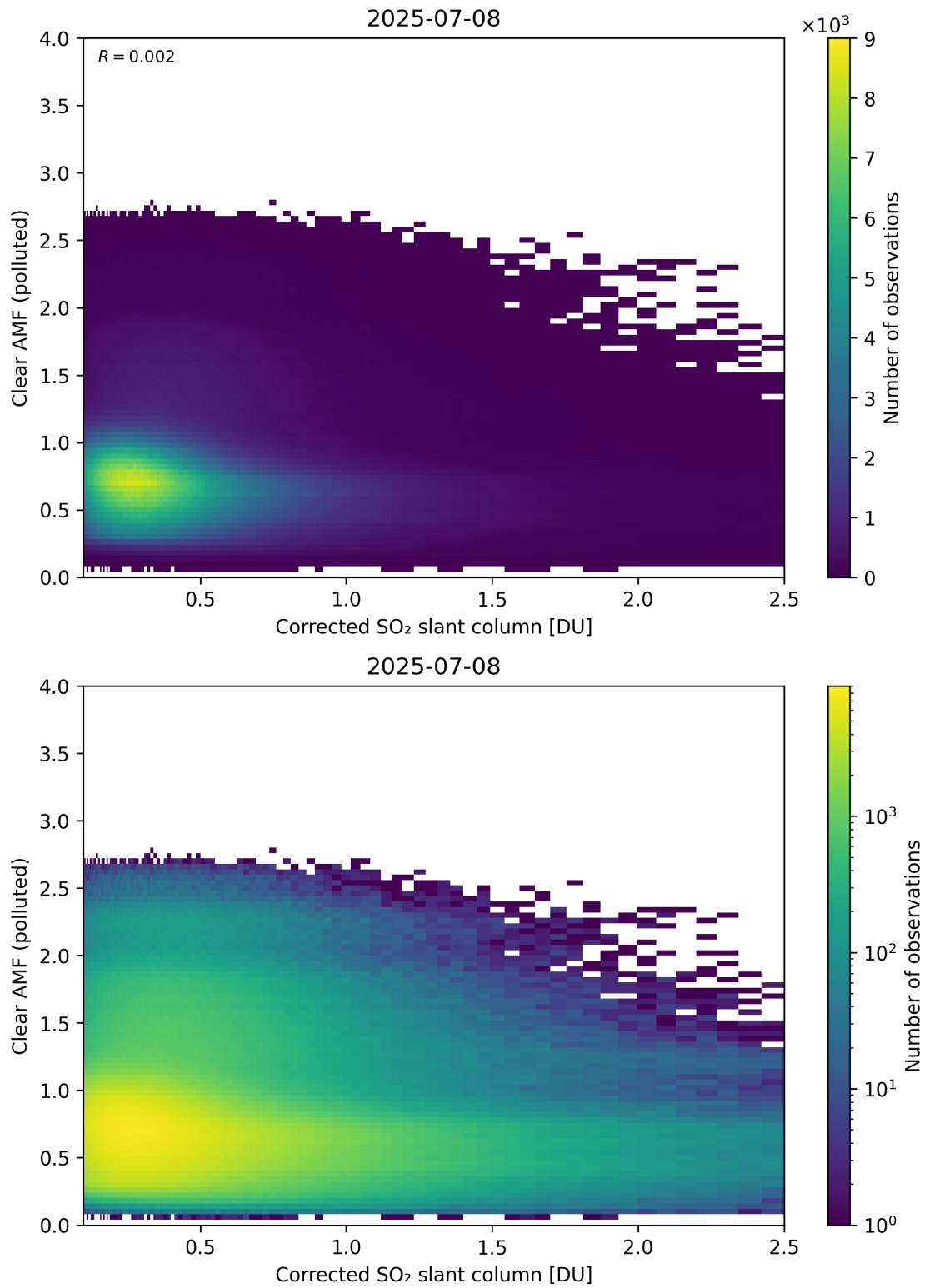
Figure 232: Scatter density plot of “Corrected SO 2 slant column” against “Clear AMF (polluted)” for 2025-07-08 to 2025-07-09.
