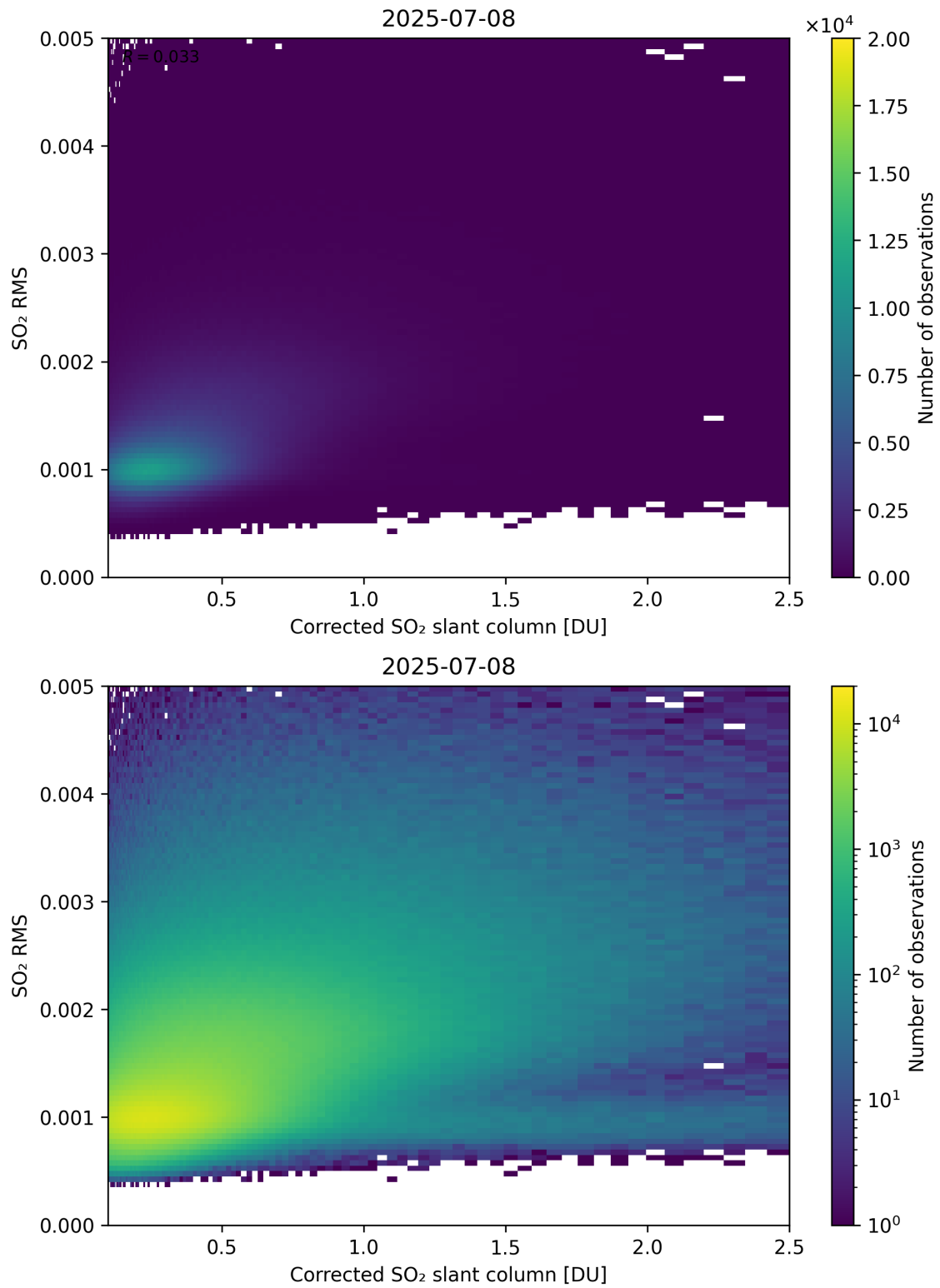
Figure 231: Scatter density plot of “Corrected SO 2 slant column” against “SO 2 RMS” for 2025-07-08 to 2025-07-09.
