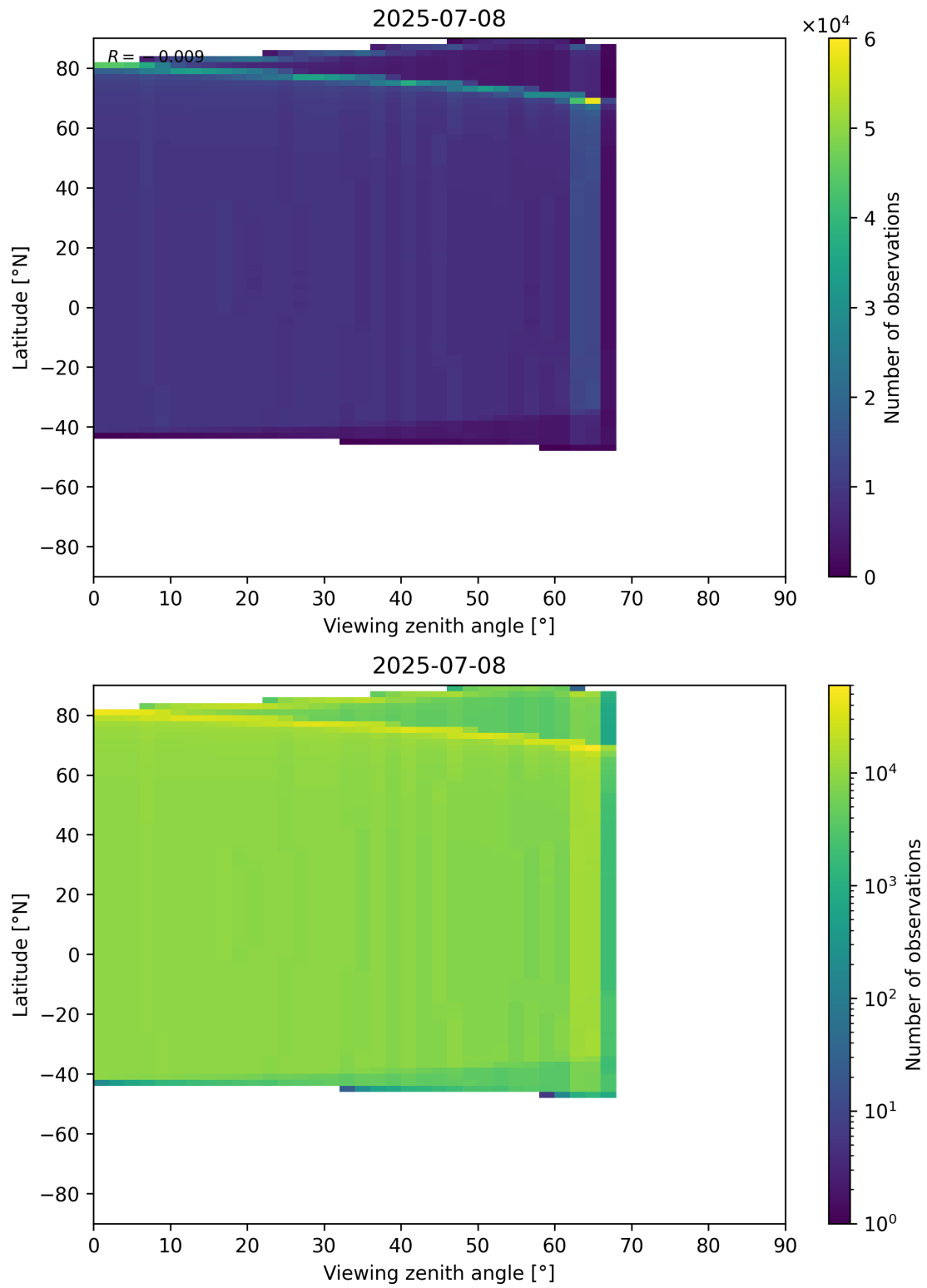
Figure 368: Scatter density plot of “Viewing zenith angle” against “Latitude” for 2025-07-08 to 2025-07-09.
