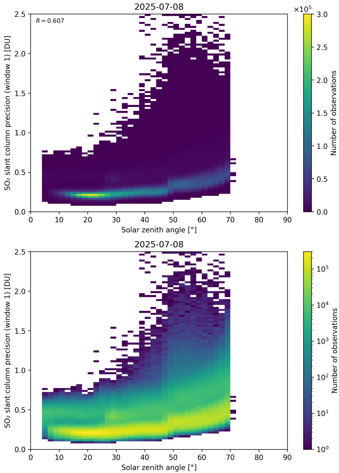
Figure 185: Scatter density plot of “Solar zenith angle” against “SO 2 slant column precision (window 1)” for 2025-07-08 to 2025-07-09.
