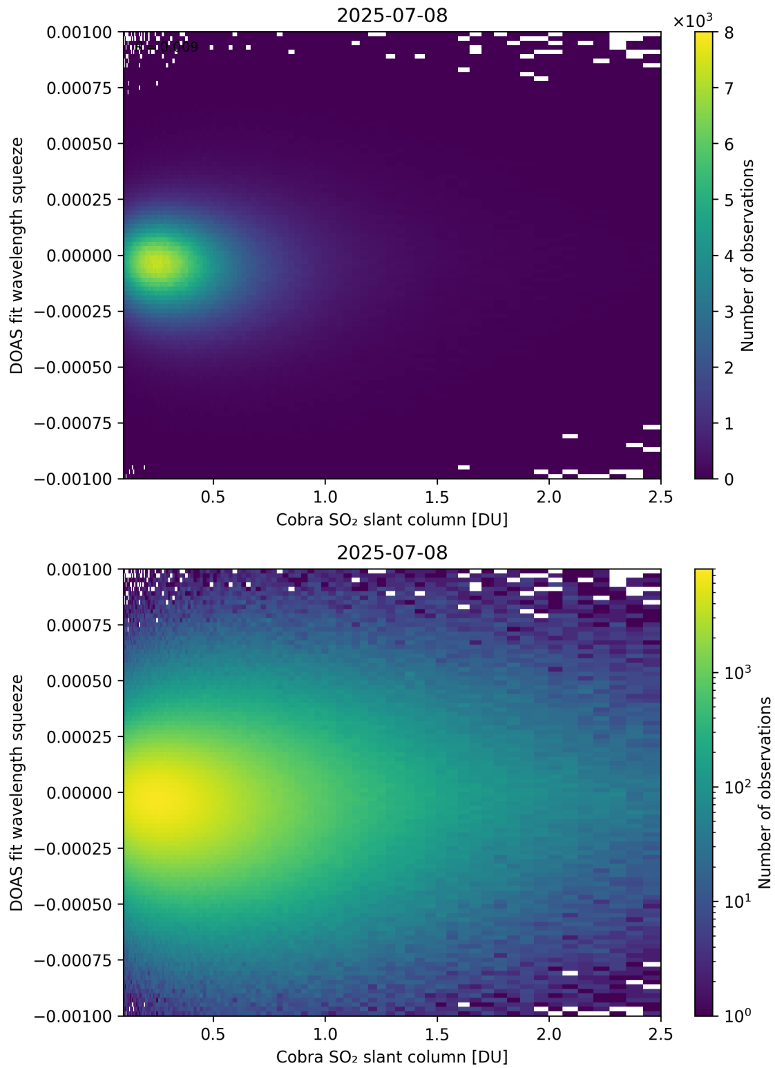
Figure 197: Scatter density plot of “Cobra SO 2 slant column” against “DOAS fit wavelength squeeze” for 2025-07-08 to 2025-07-09.
