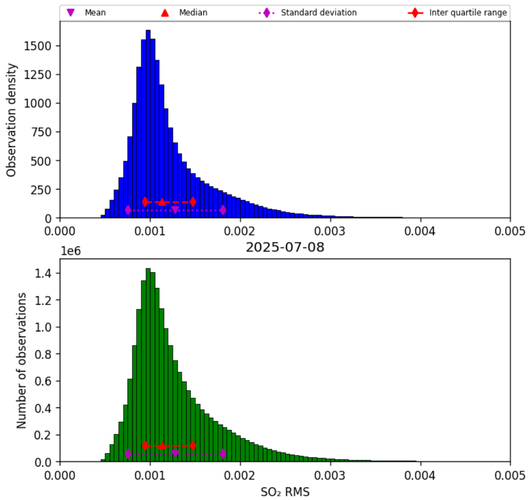
Figure 78: Histogram of “SO 2 RMS” for 2025-07-08 to 2025-07-09
