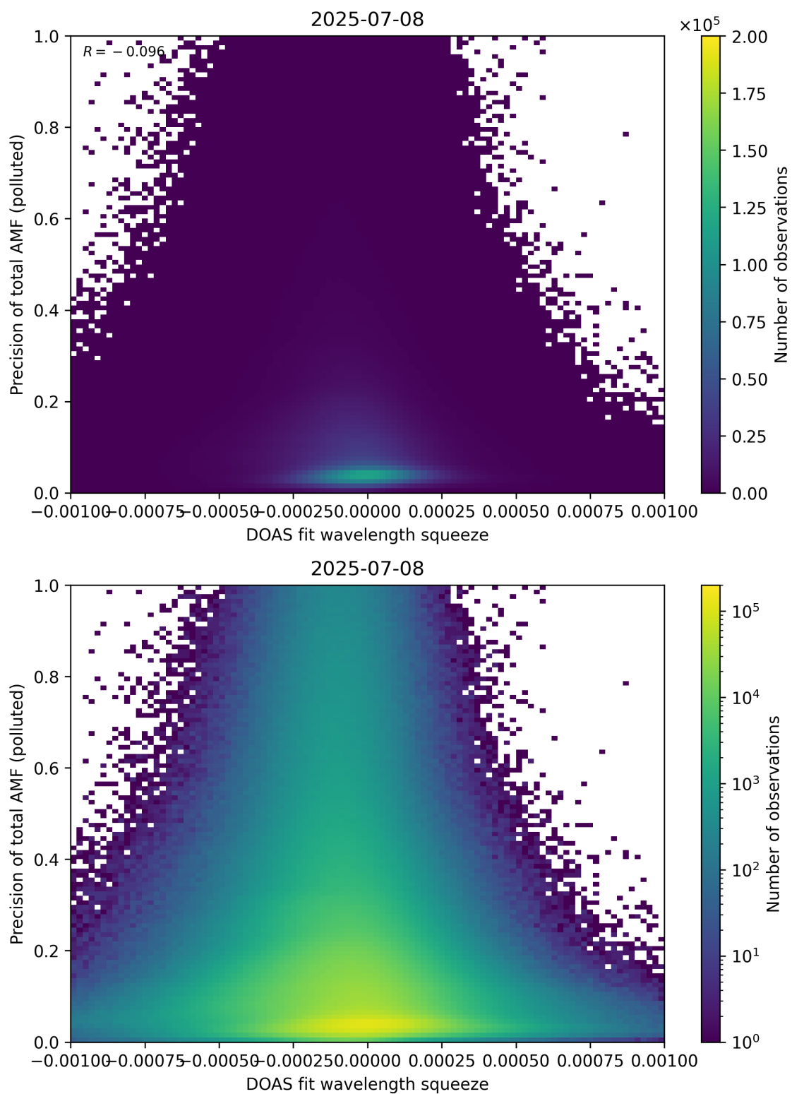
Figure 146: Scatter density plot of “DOAS fit wavelength squeeze” against “Precision of total AMF (polluted)” for 2025-07-08 to 2025-07-09.
