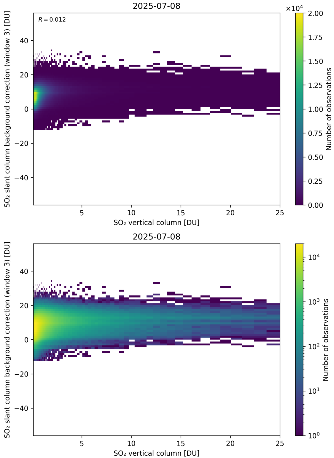
Figure 325: Scatter density plot of “SO 2 vertical column” against “SO 2 slant column background correction (window 3)” for 2025-07-08 to 2025-07-09.
