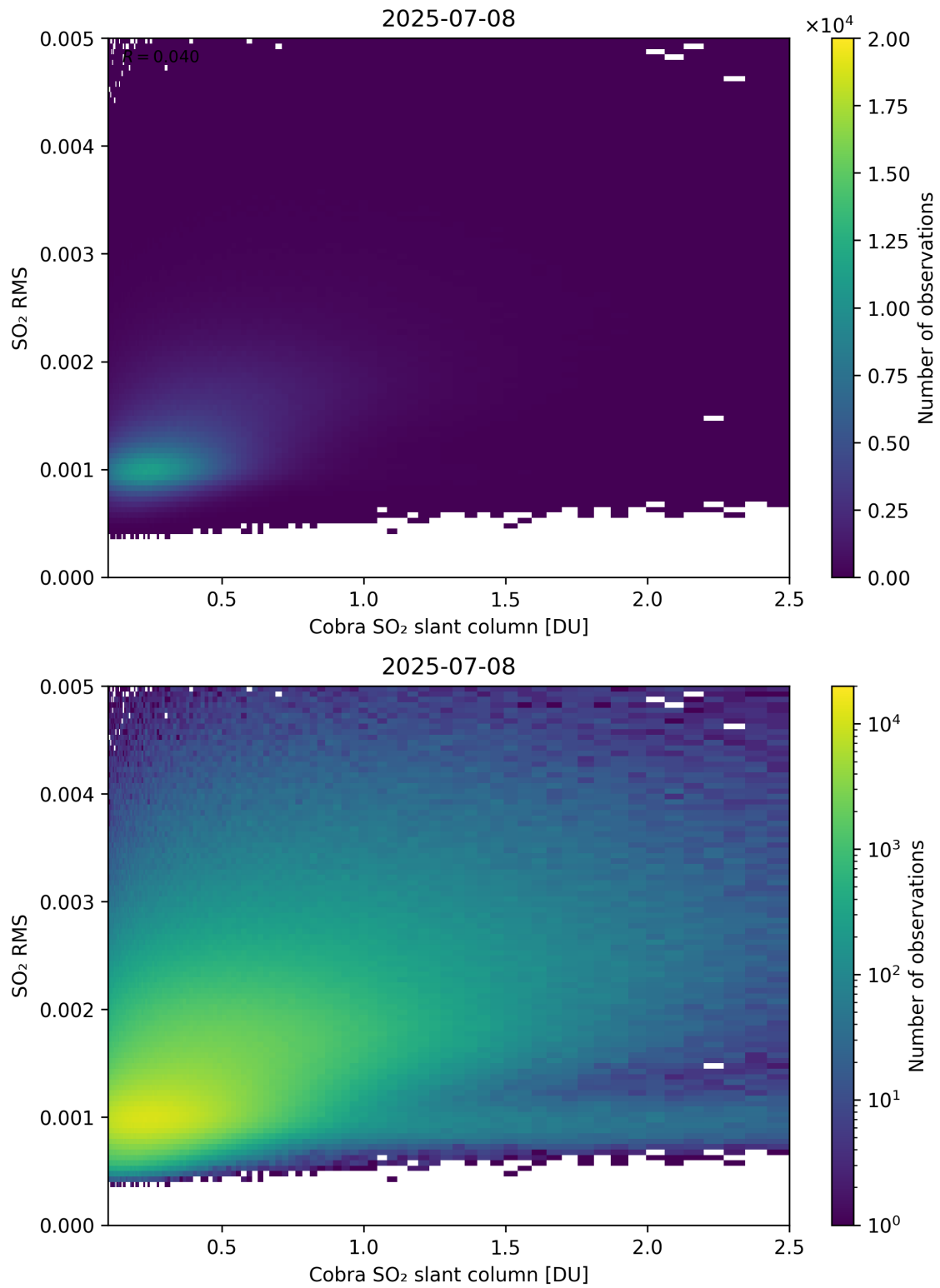
Figure 198: Scatter density plot of “Cobra SO 2 slant column” against “SO 2 RMS” for 2025-07-08 to 2025-07-09.
