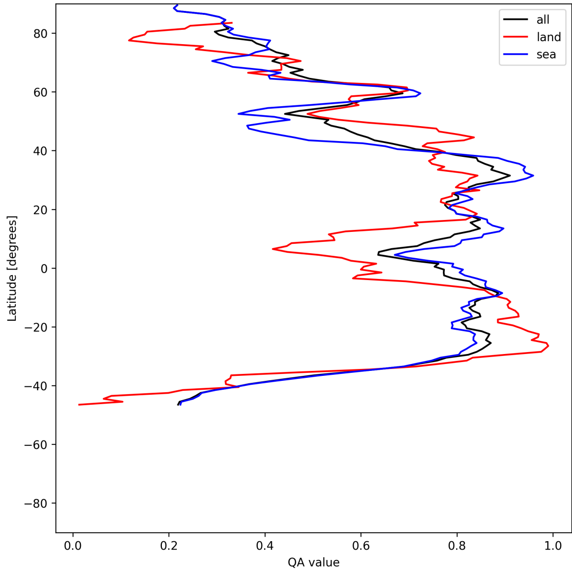
Figure 31: Zonal average of “QA value” for 2025-07-08 to 2025-07-09.
