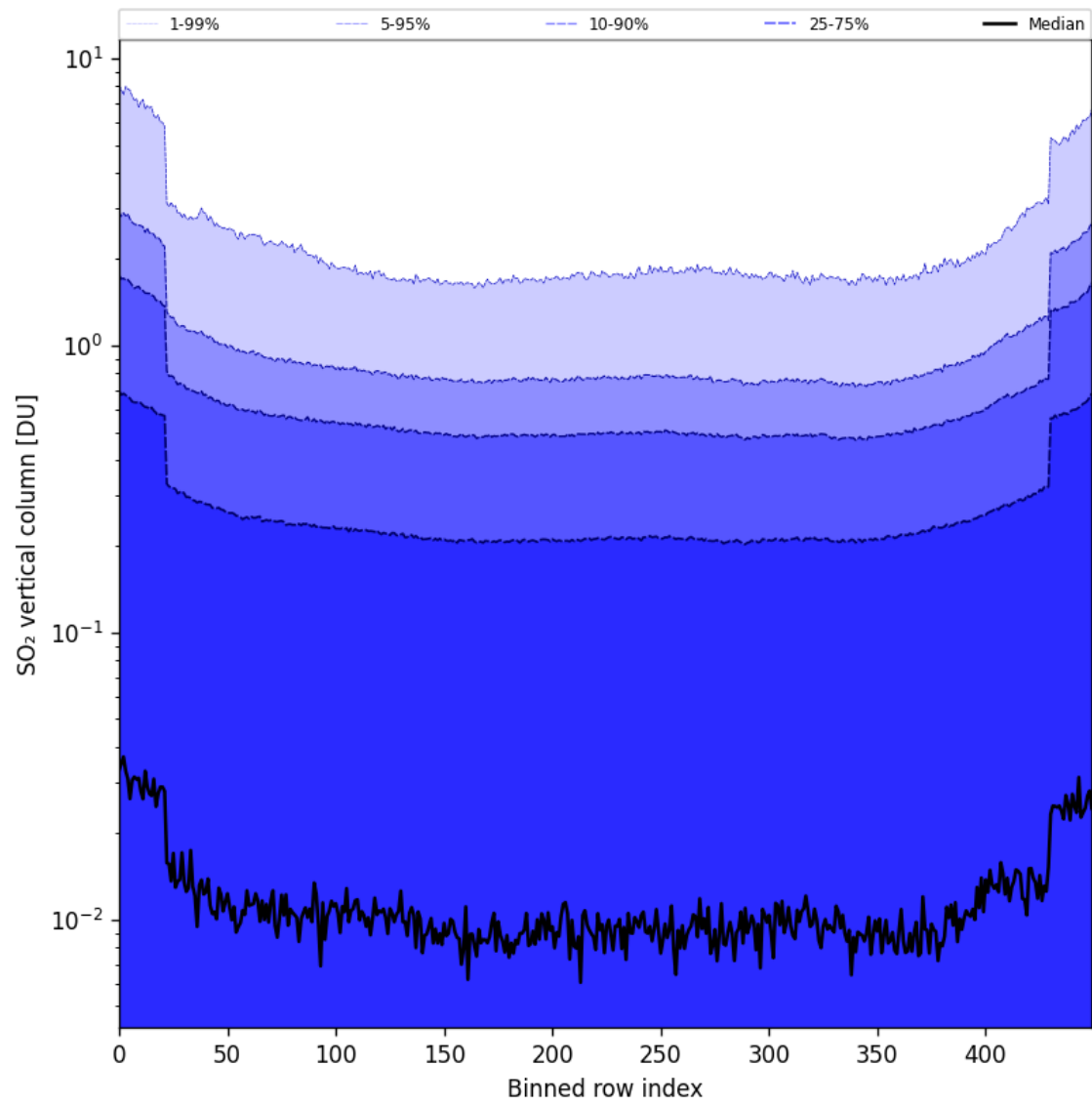
Figure 84: Along track statistics of “SO 2 vertical column” for 2025-07-08 to 2025-07-09
