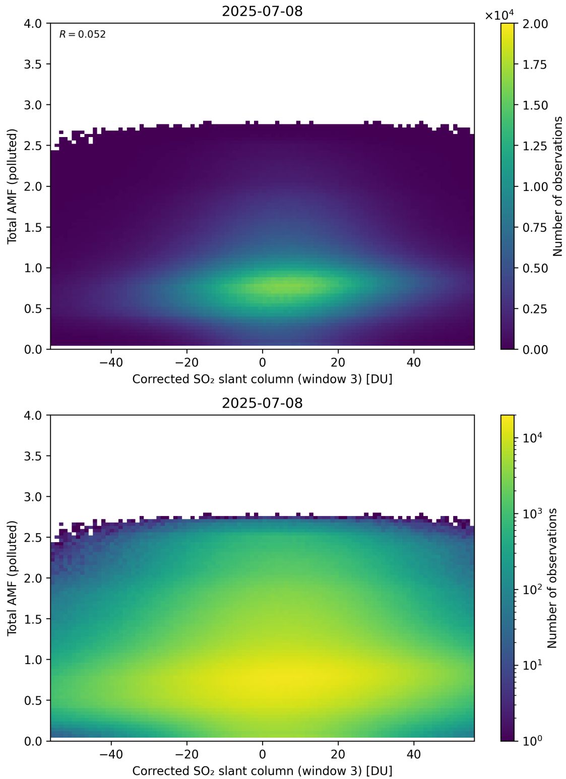
Figure 260: Scatter density plot of “Corrected SO 2 slant column (window 3)” against “Total AMF (polluted)” for 2025-07-08 to 2025-07-09.
