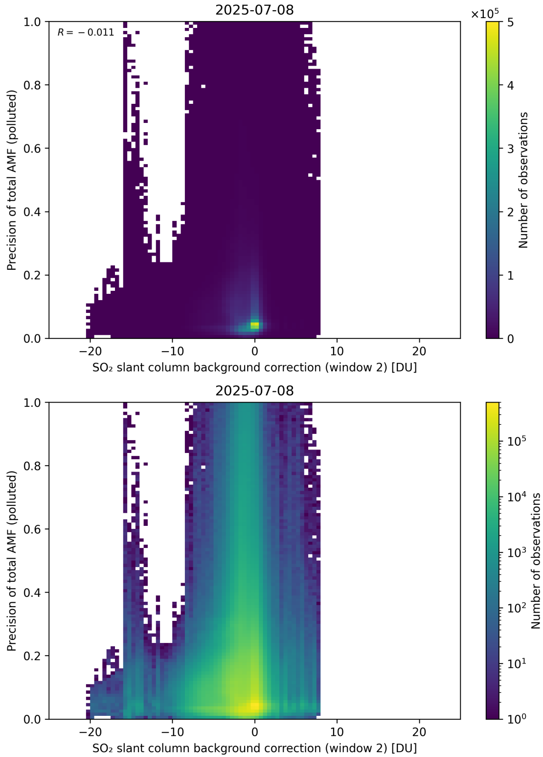
Figure 131: Scatter density plot of “SO 2 slant column background correction (window 2)” against “Precision of total AMF (polluted)” for 2025-07-08 to 2025-07-09.
