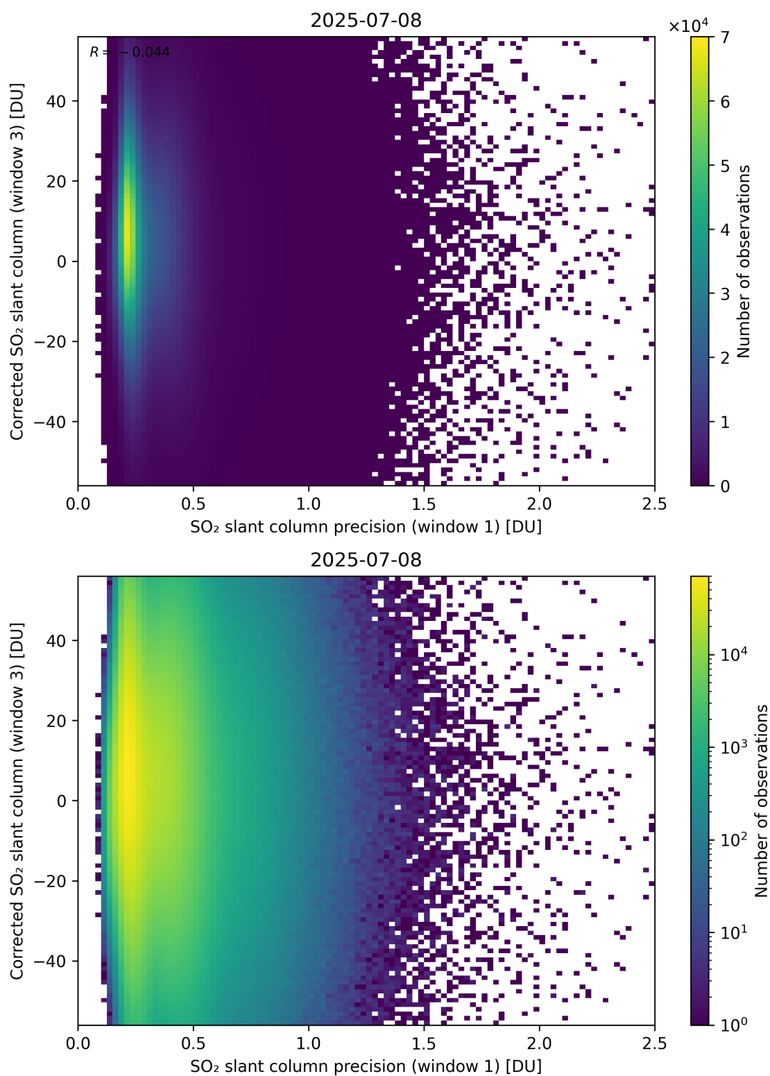
Figure 276: Scatter density plot of “SO 2 slant column precision (window 1)” against “Corrected SO 2 slant column (window 3)” for 2025-07-08 to 2025-07-09.
