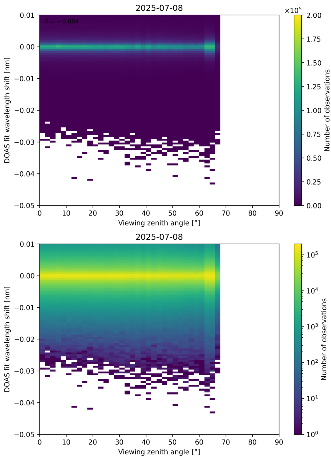
Figure 365: Scatter density plot of “Viewing zenith angle” against “DOAS fit wavelength shift” for 2025-07-08 to 2025-07-09.
