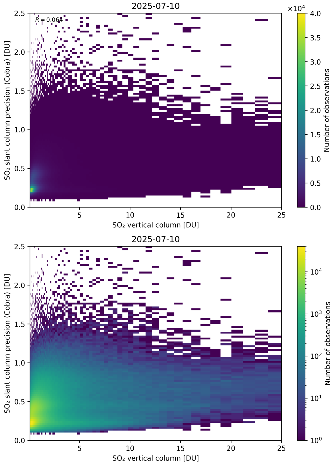
Figure 350: Scatter density plot of “SO 2 vertical column” against “SO 2 slant column precision (Cobra)” for 2025-07-09 to 2025-07-11.
