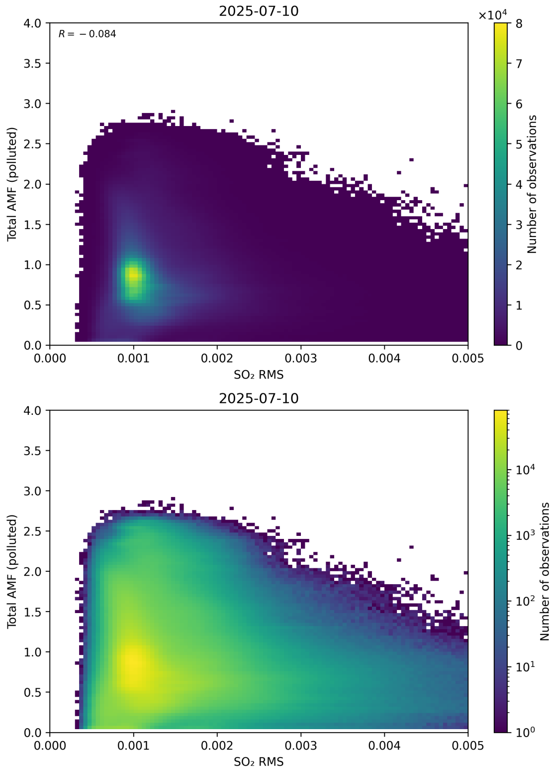
Figure 148: Scatter density plot of “SO 2 RMS” against “Total AMF (polluted)” for 2025-07-09 to 2025-07-11.
