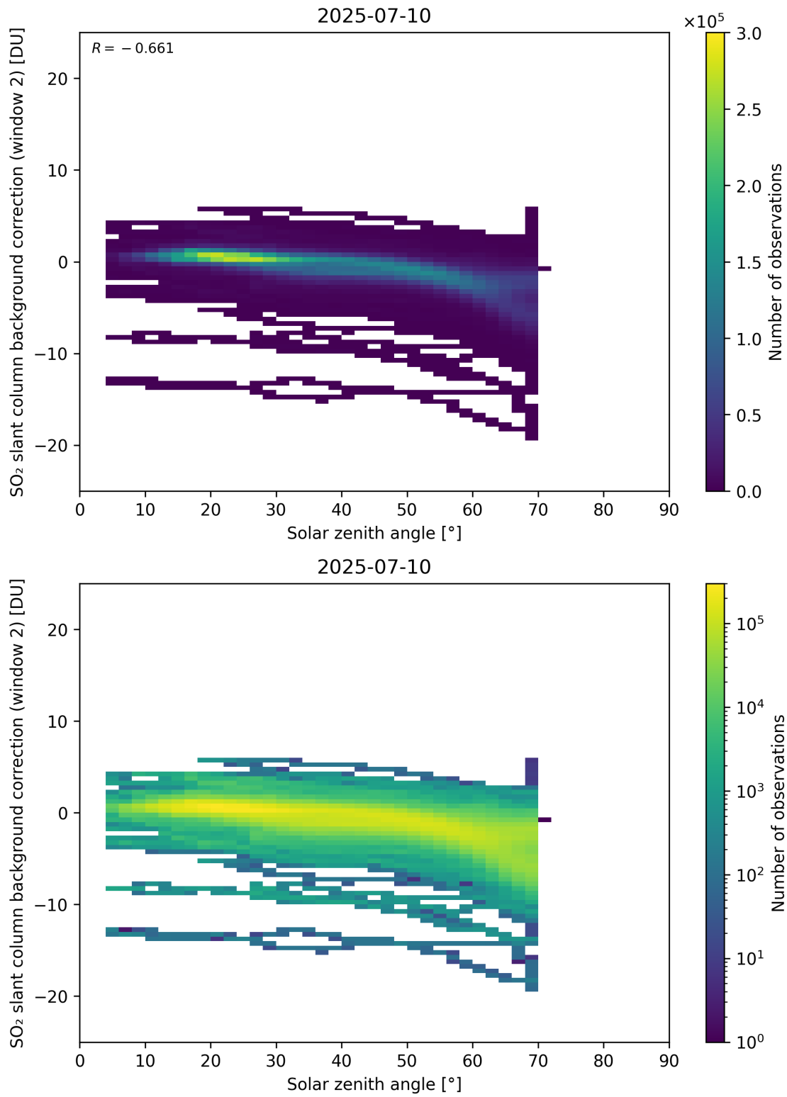
Figure 172: Scatter density plot of “Solar zenith angle” against “SO 2 slant column background correction (window 2)” for 2025-07-09 to 2025-07-11.
