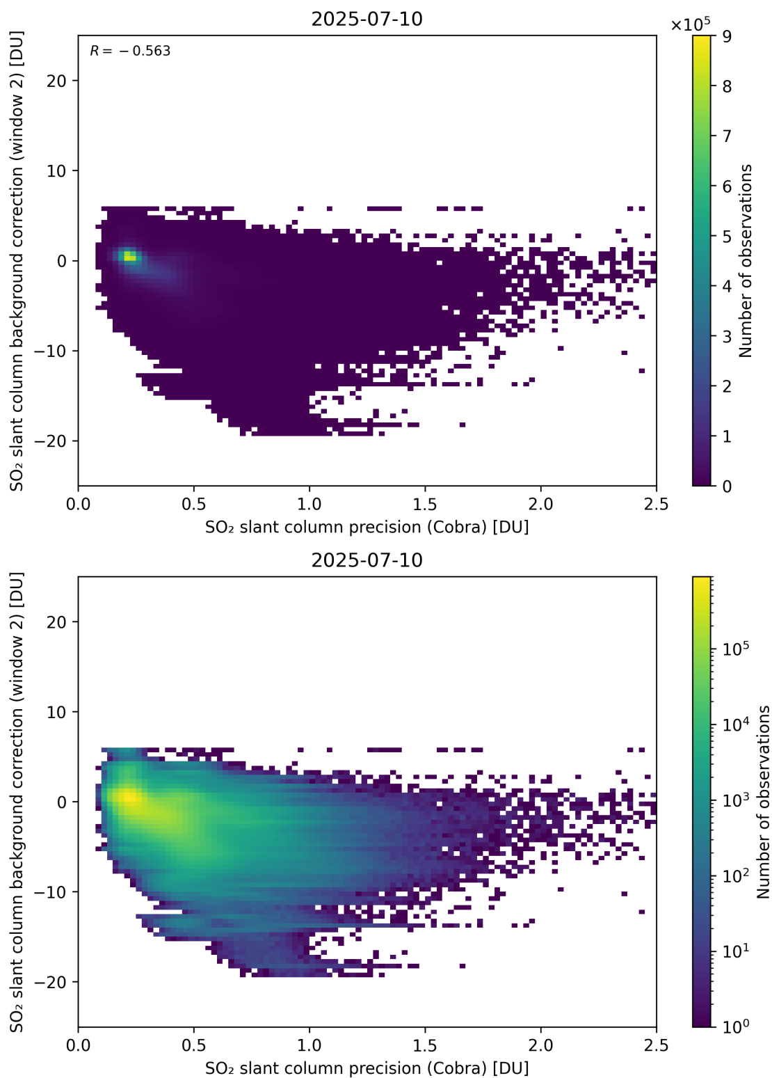
Figure 200: Scatter density plot of “SO 2 slant column precision (Cobra)” against “SO 2 slant column background correction (window 2)” for 2025-07-09 to 2025-07-11.
