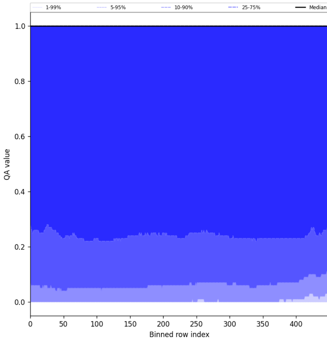
Figure 83: Along track statistics of “QA value” for 2025-07-09 to 2025-07-11
