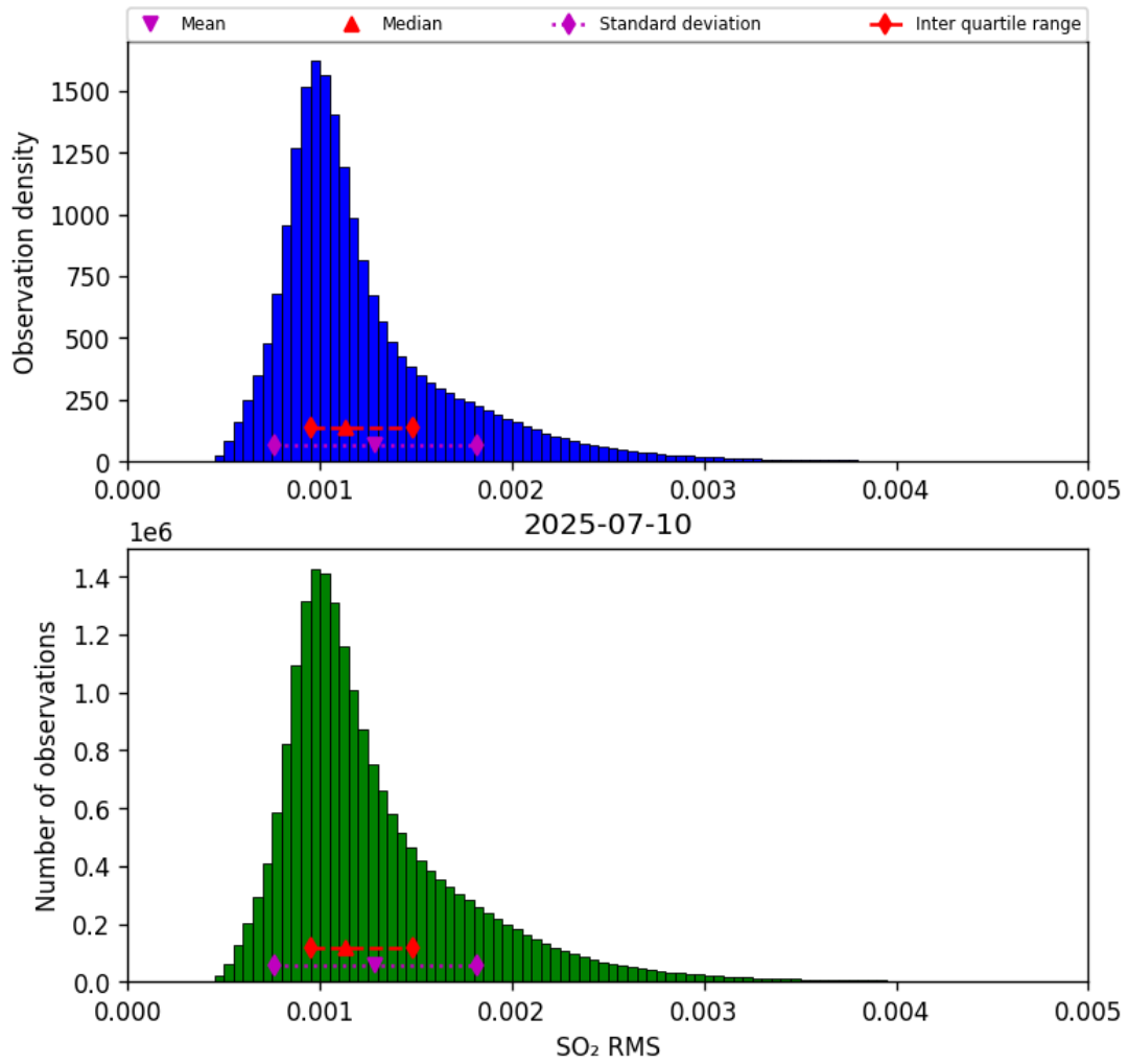
Figure 78: Histogram of “SO 2 RMS” for 2025-07-09 to 2025-07-11
