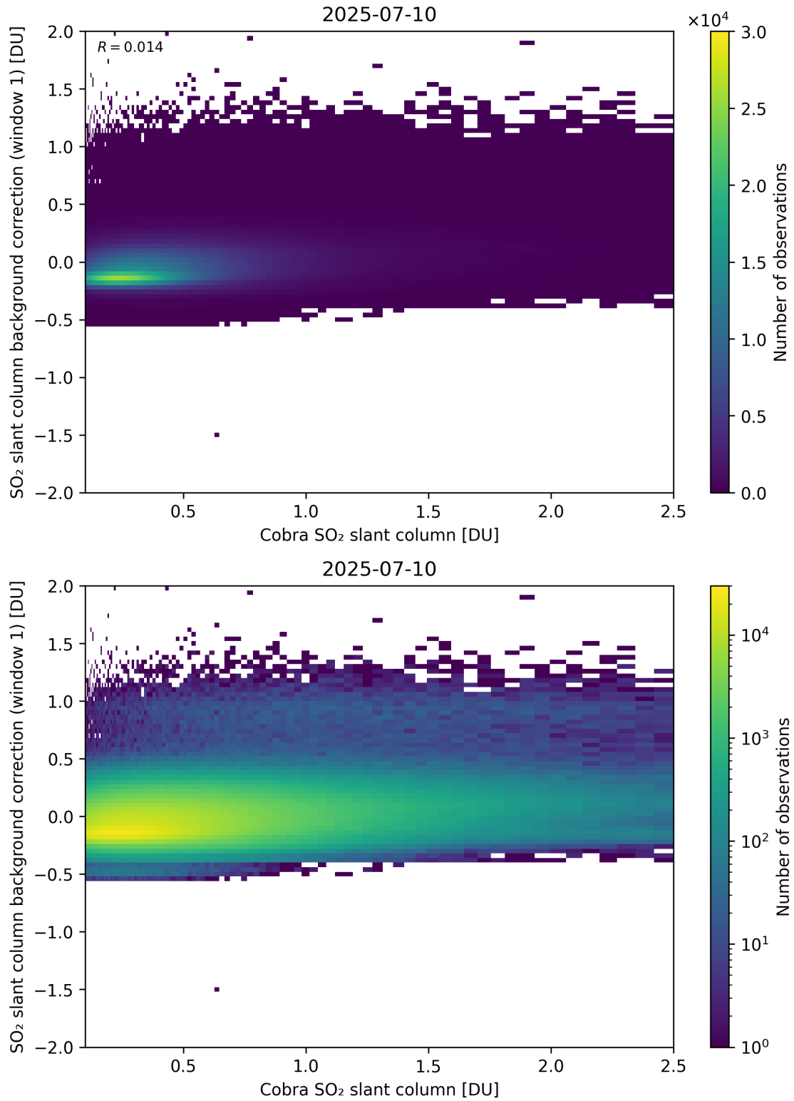
Figure 193: Scatter density plot of “Cobra SO 2 slant column” against “SO 2 slant column background correction (window 1)” for 2025-07-09 to 2025-07-11.
