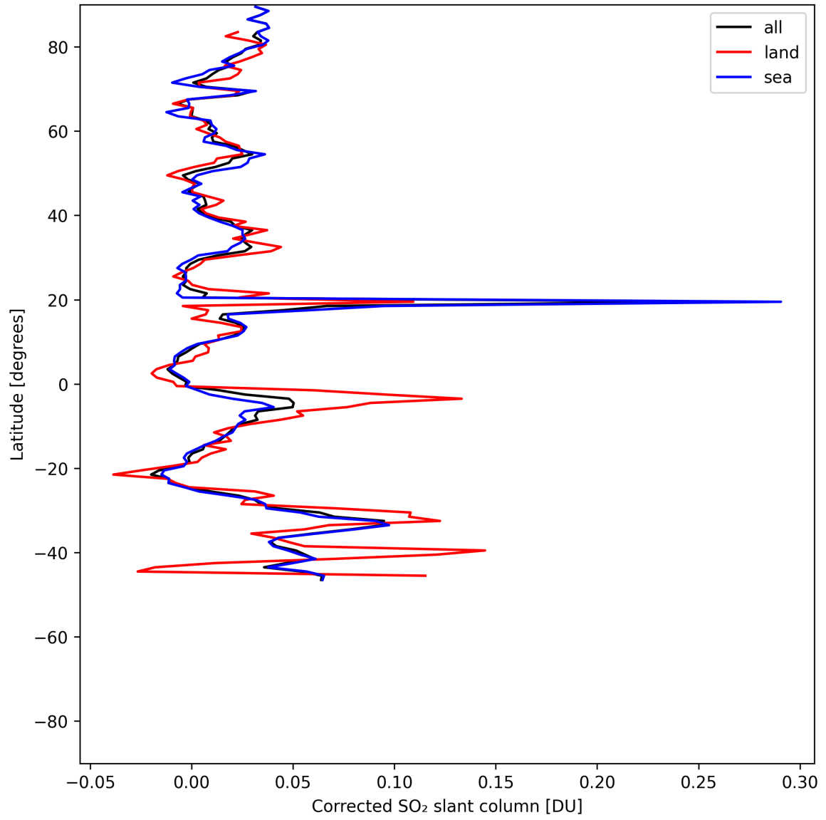
Figure 34: Zonal average of “Corrected SO 2 slant column” for 2025-07-09 to 2025-07-11.
