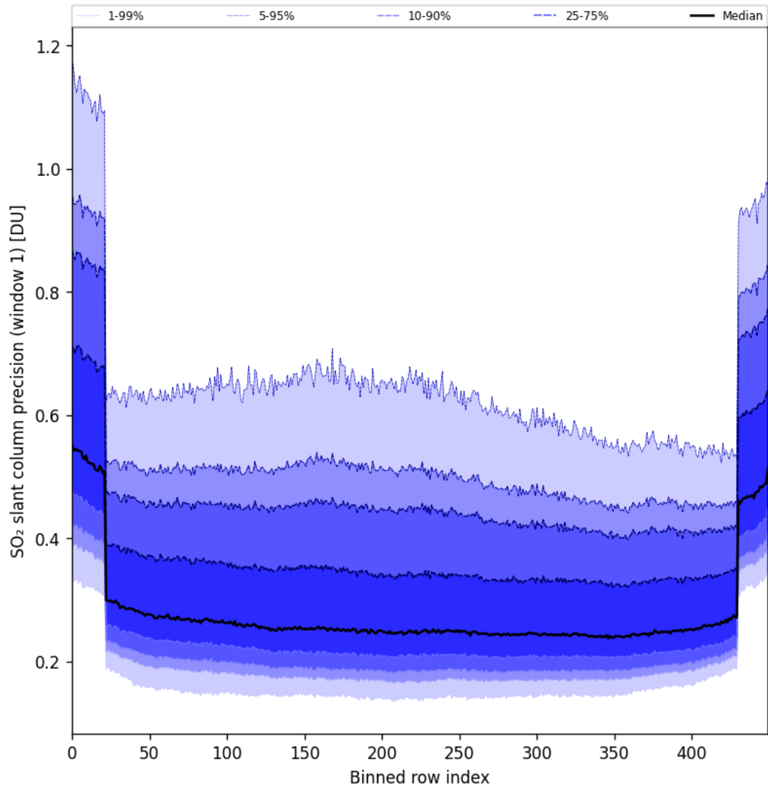
Figure 90: Along track statistics of “SO 2 slant column precision (window 1)” for 2025-07-09 to 2025-07-11
