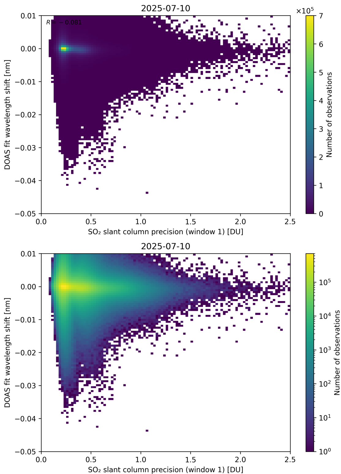
Figure 271: Scatter density plot of “SO 2 slant column precision (window 1)” against “DOAS fit wavelength shift” for 2025-07-09 to 2025-07-11.
