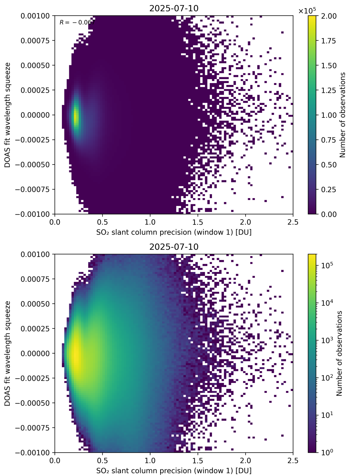
Figure 272: Scatter density plot of “SO 2 slant column precision (window 1)” against “DOAS fit wavelength squeeze” for 2025-07-09 to 2025-07-11.
