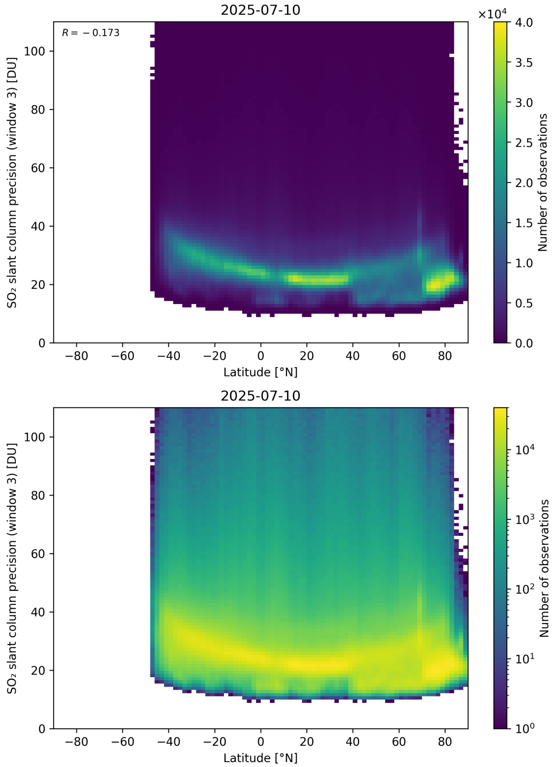
Figure 166: Scatter density plot of “Latitude” against “SO 2 slant column precision (window 3)” for 2025-07-09 to 2025-07-11.
