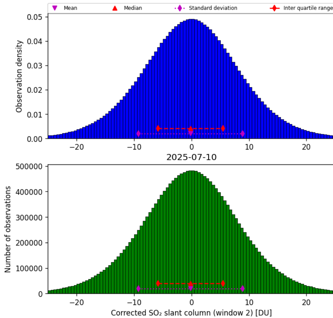
Figure 69: Histogram of “Corrected SO 2 slant column (window 2)” for 2025-07-09 to 2025-07-11
