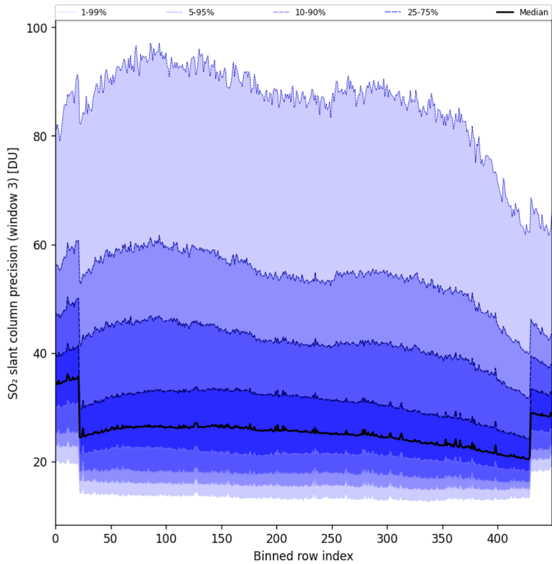
Figure 98: Along track statistics of “SO 2 slant column precision (window 3)” for 2025-07-09 to 2025-07-11
