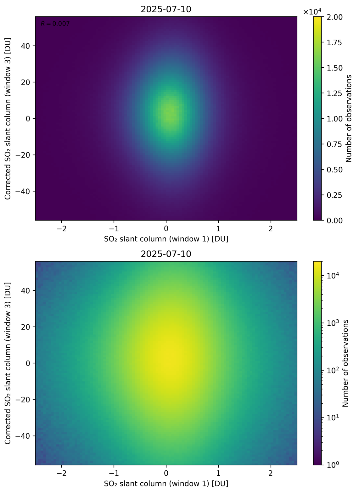
Figure 284: Scatter density plot of “SO 2 slant column (window 1)” against “Corrected SO 2 slant column (window 3)” for 2025-07-09 to 2025-07-11.
