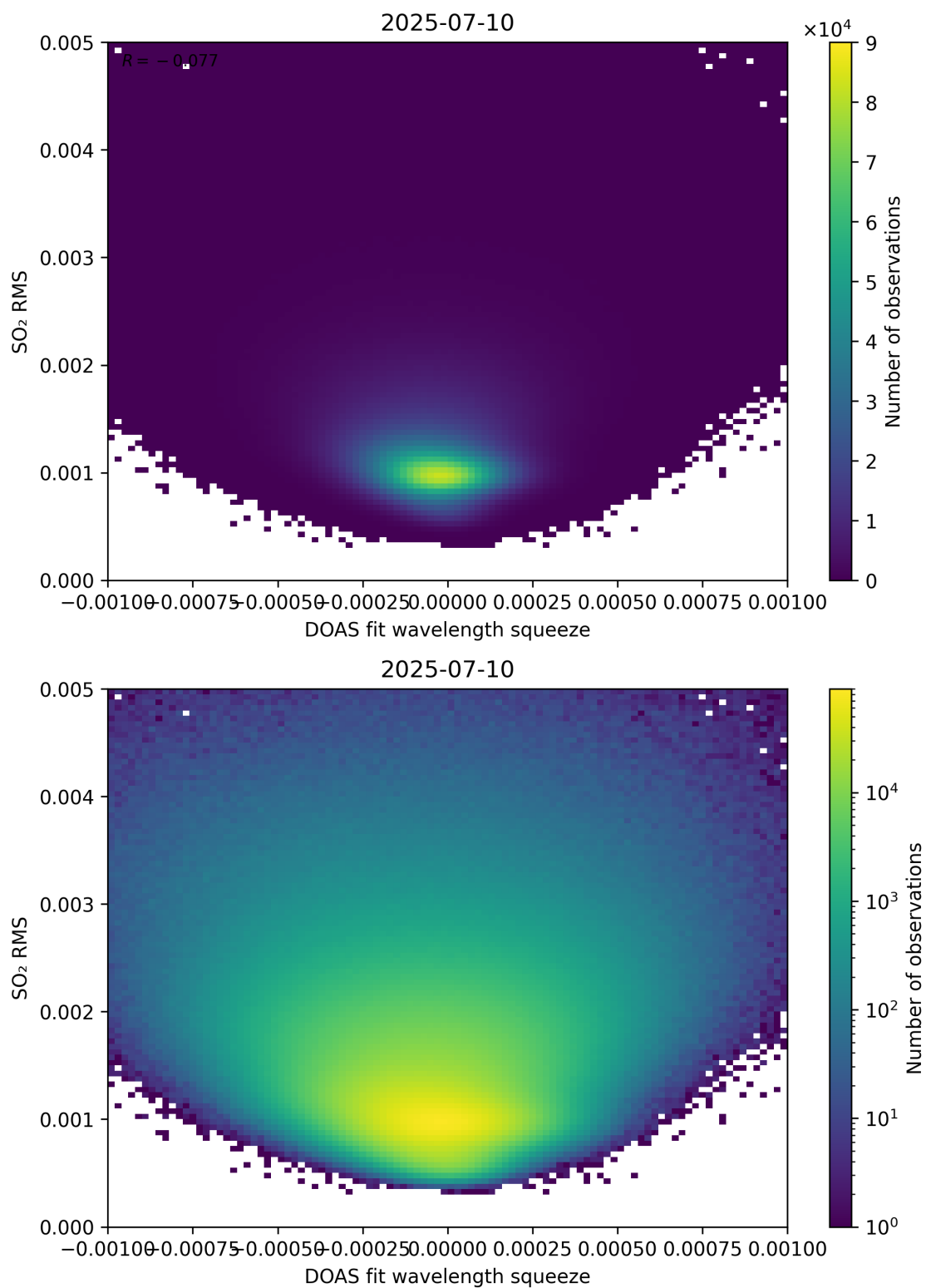
Figure 143: Scatter density plot of “DOAS fit wavelength squeeze” against “SO 2 RMS” for 2025-07-09 to 2025-07-11.
