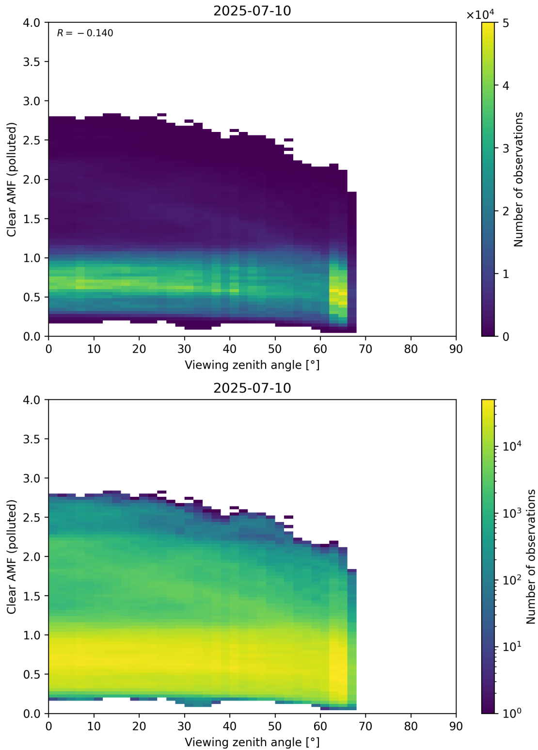
Figure 370: Scatter density plot of “Viewing zenith angle” against “Clear AMF (polluted)” for 2025-07-09 to 2025-07-11.
