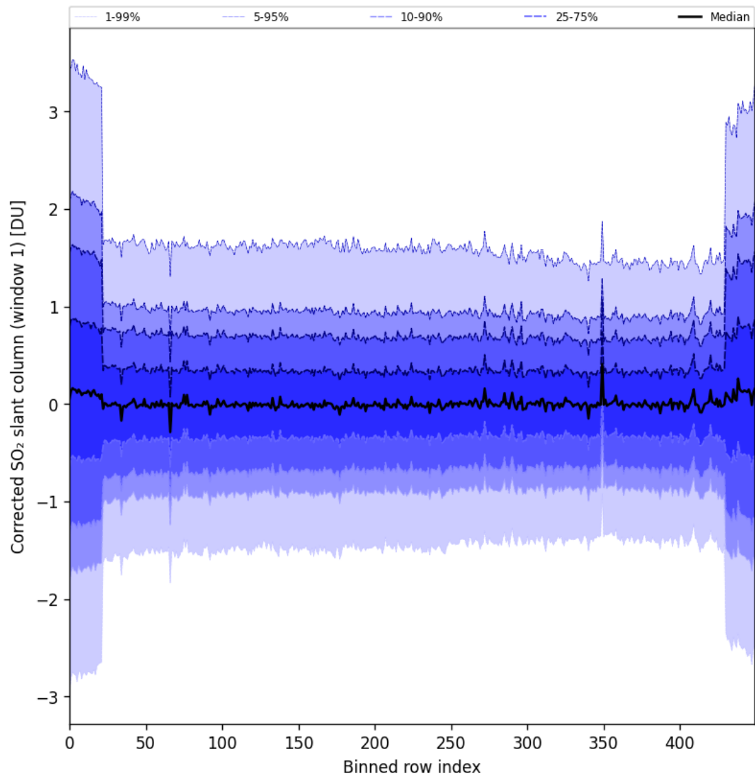
Figure 91: Along track statistics of “Corrected SO 2 slant column (window 1)” for 2025-07-09 to 2025-07-11
