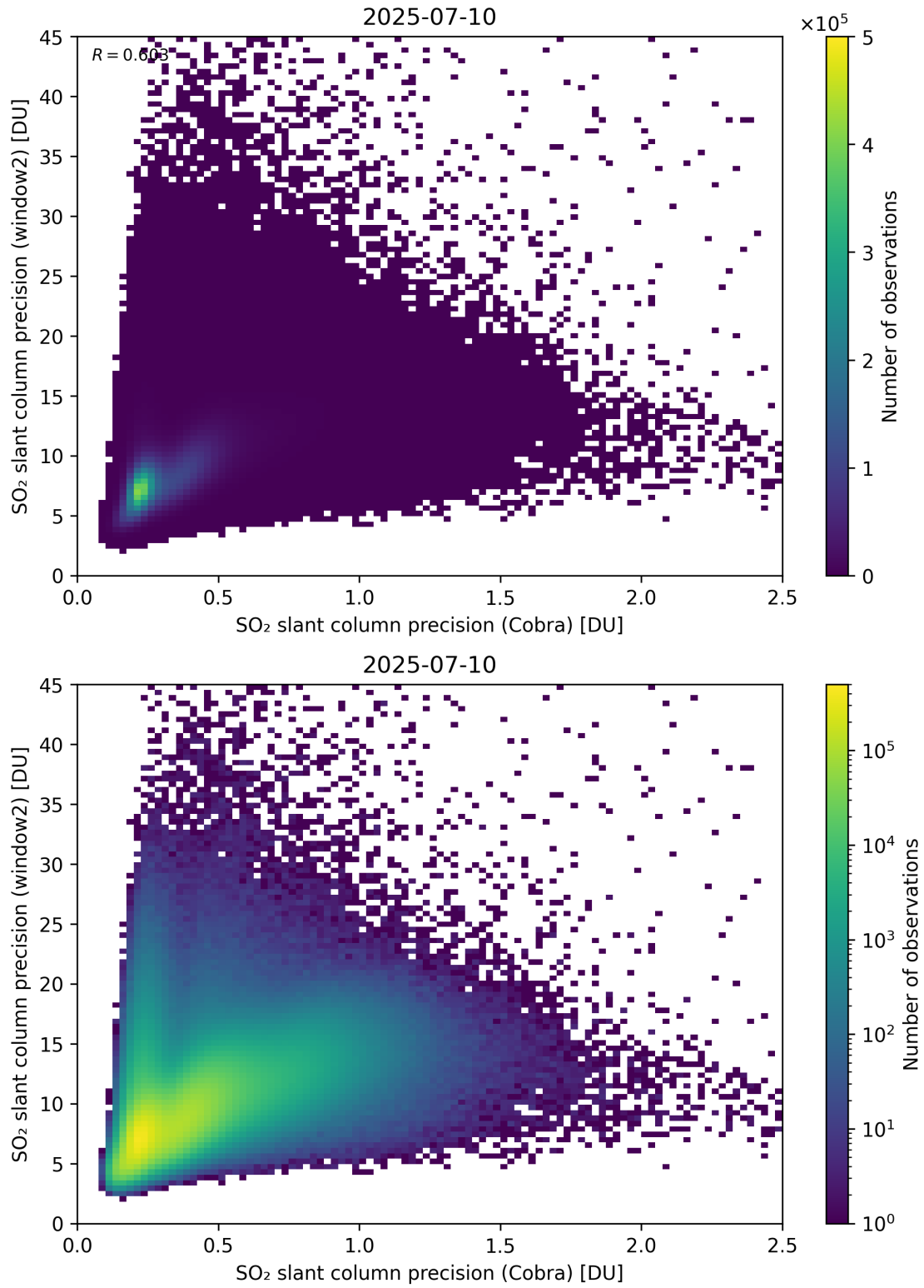
Figure 210: Scatter density plot of “SO 2 slant column precision (Cobra)” against “SO 2 slant column precision (window2)” for 2025-07-09 to 2025-07-11.
