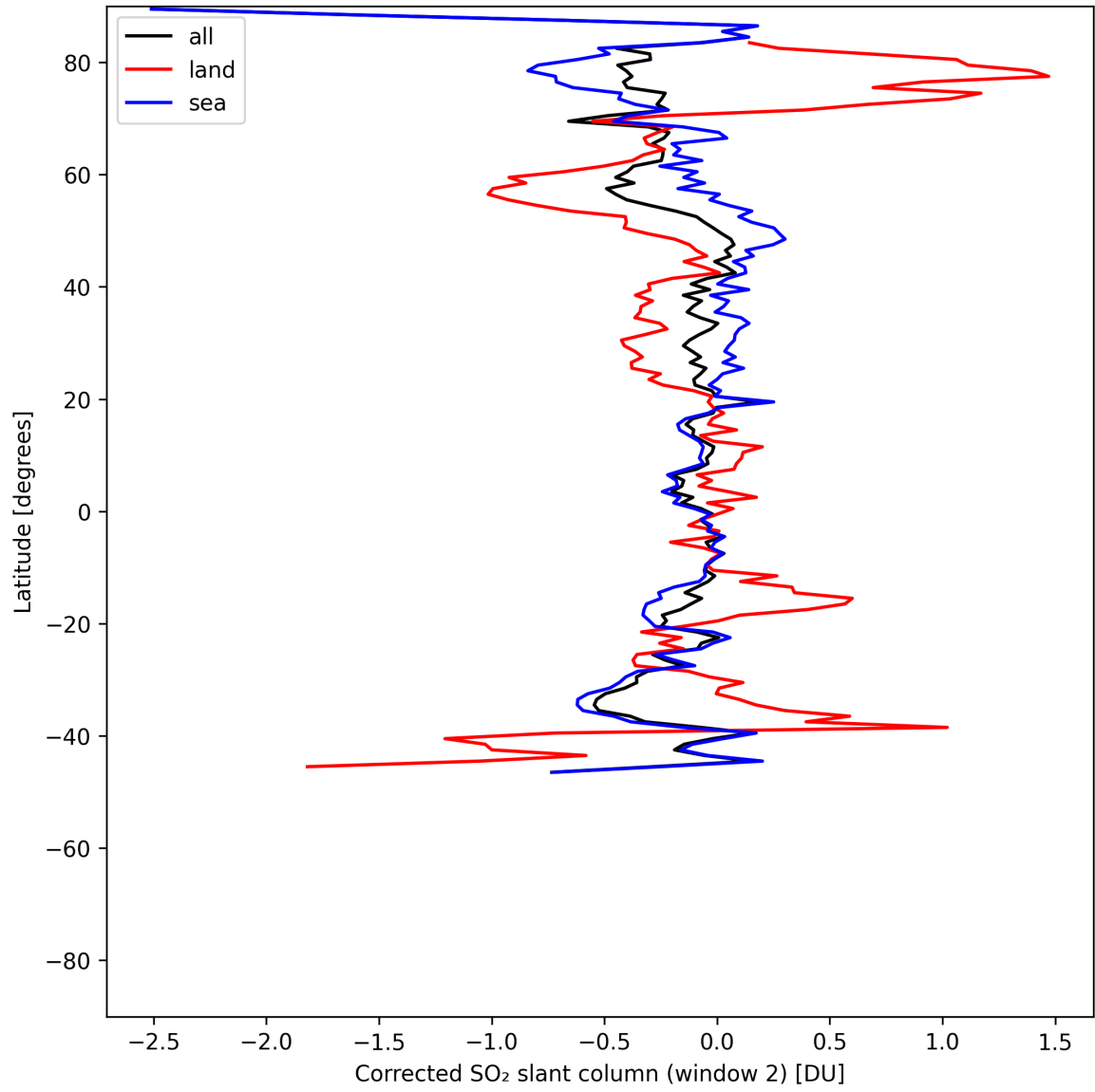
Figure 43: Zonal average of “Corrected SO 2 slant column (window 2)” for 2025-07-09 to 2025-07-11.
