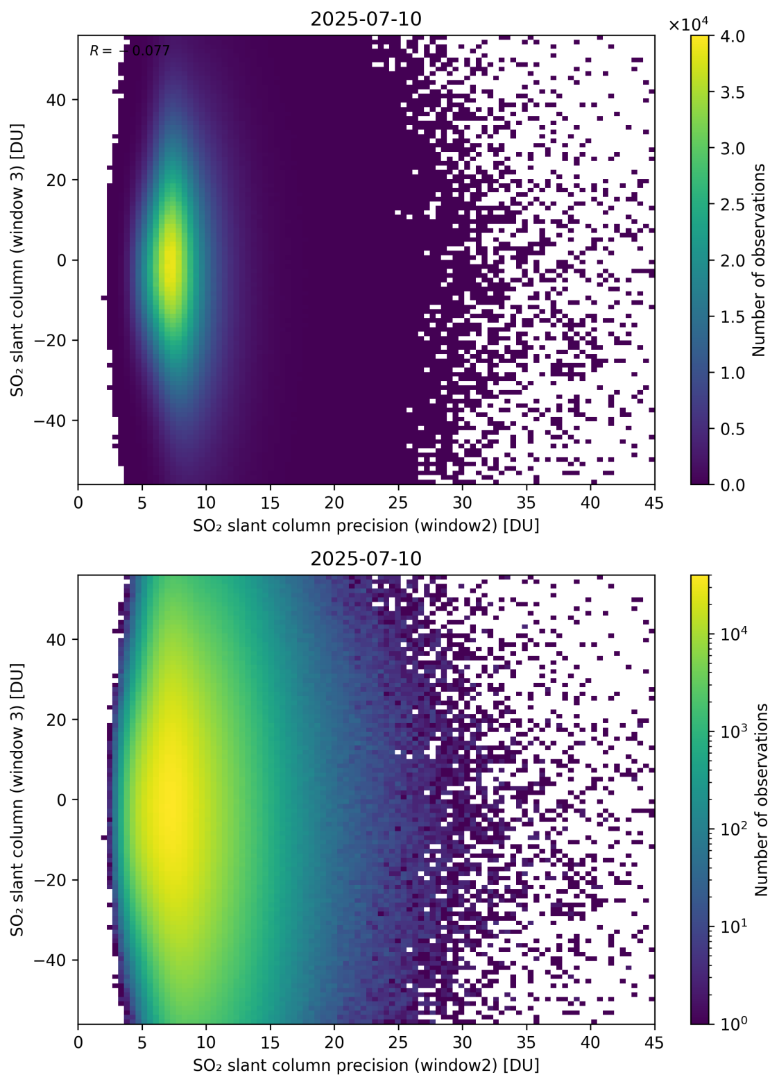
Figure 299: Scatter density plot of “SO 2 slant column precision (window2)” against “SO 2 slant column (window 3)” for 2025-07-09 to 2025-07-11.
