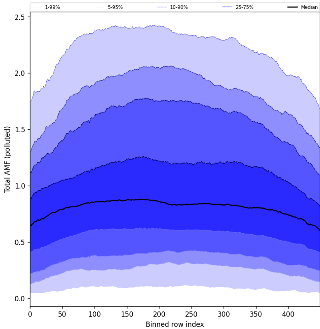
Figure 105: Along track statistics of “Total AMF (polluted)” for 2025-07-09 to 2025-07-11
