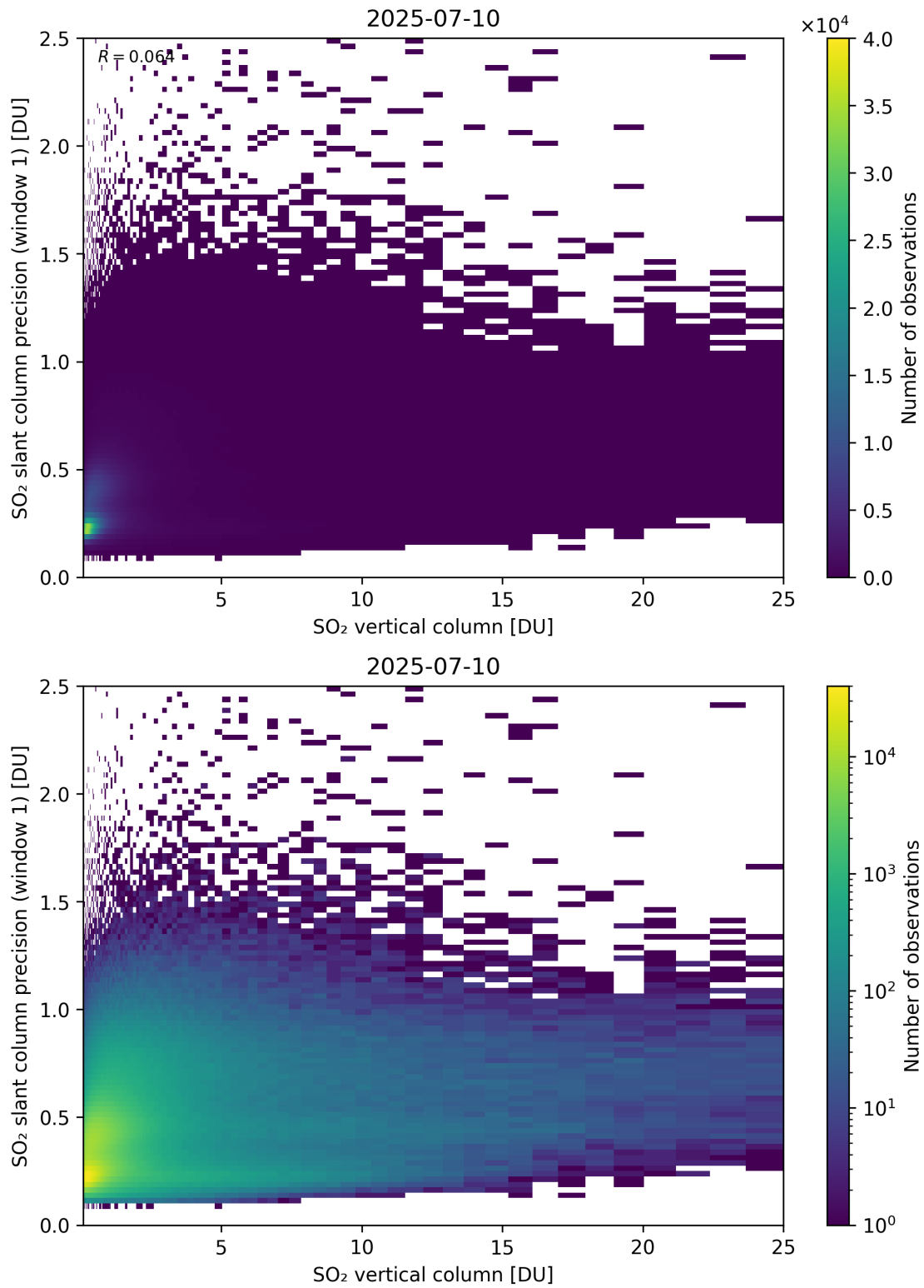
Figure 355: Scatter density plot of “SO 2 vertical column” against “SO 2 slant column precision (window 1)” for 2025-07-09 to 2025-07-11.
