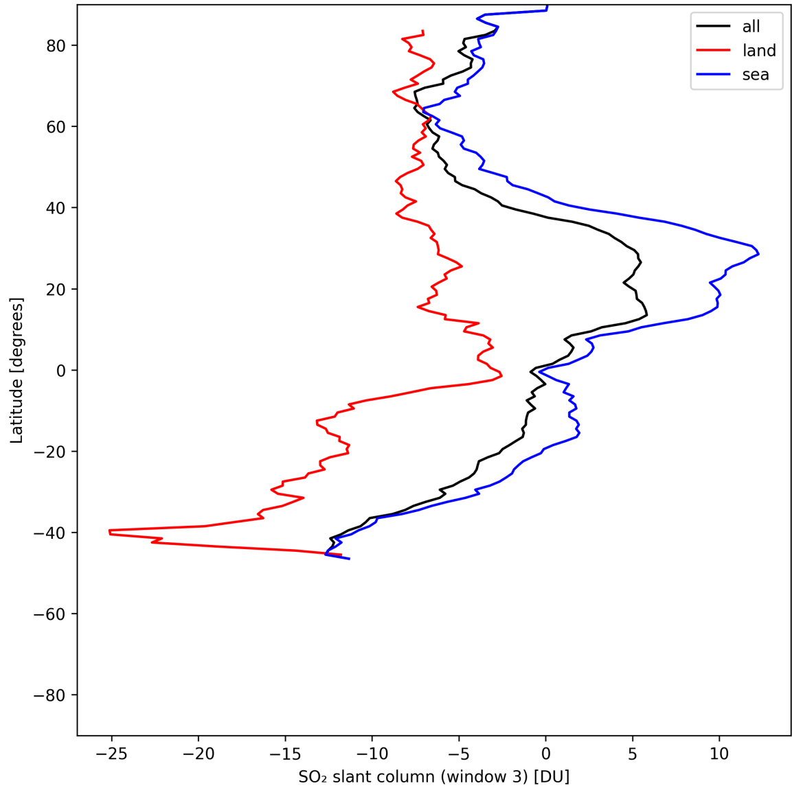
Figure 45: Zonal average of “SO 2 slant column (window 3)” for 2025-07-09 to 2025-07-11.
