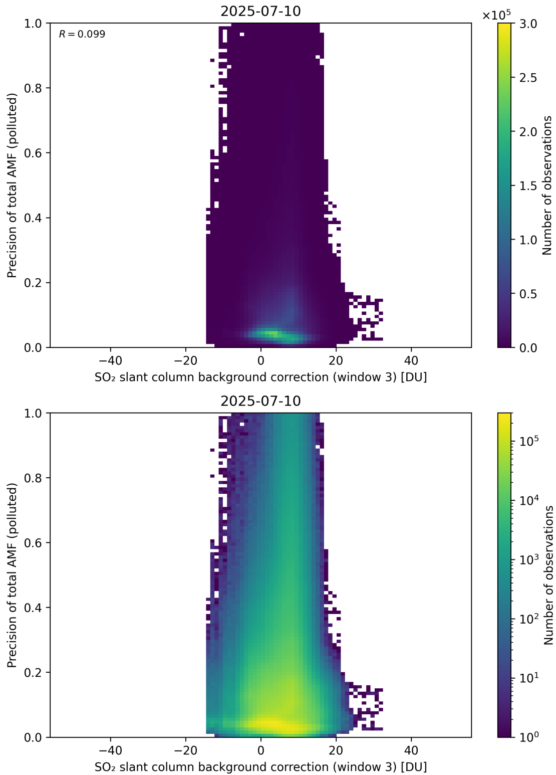
Figure 137: Scatter density plot of “SO 2 slant column background correction (window 3)” against “Precision of total AMF (polluted)” for 2025-07-09 to 2025-07-11.
