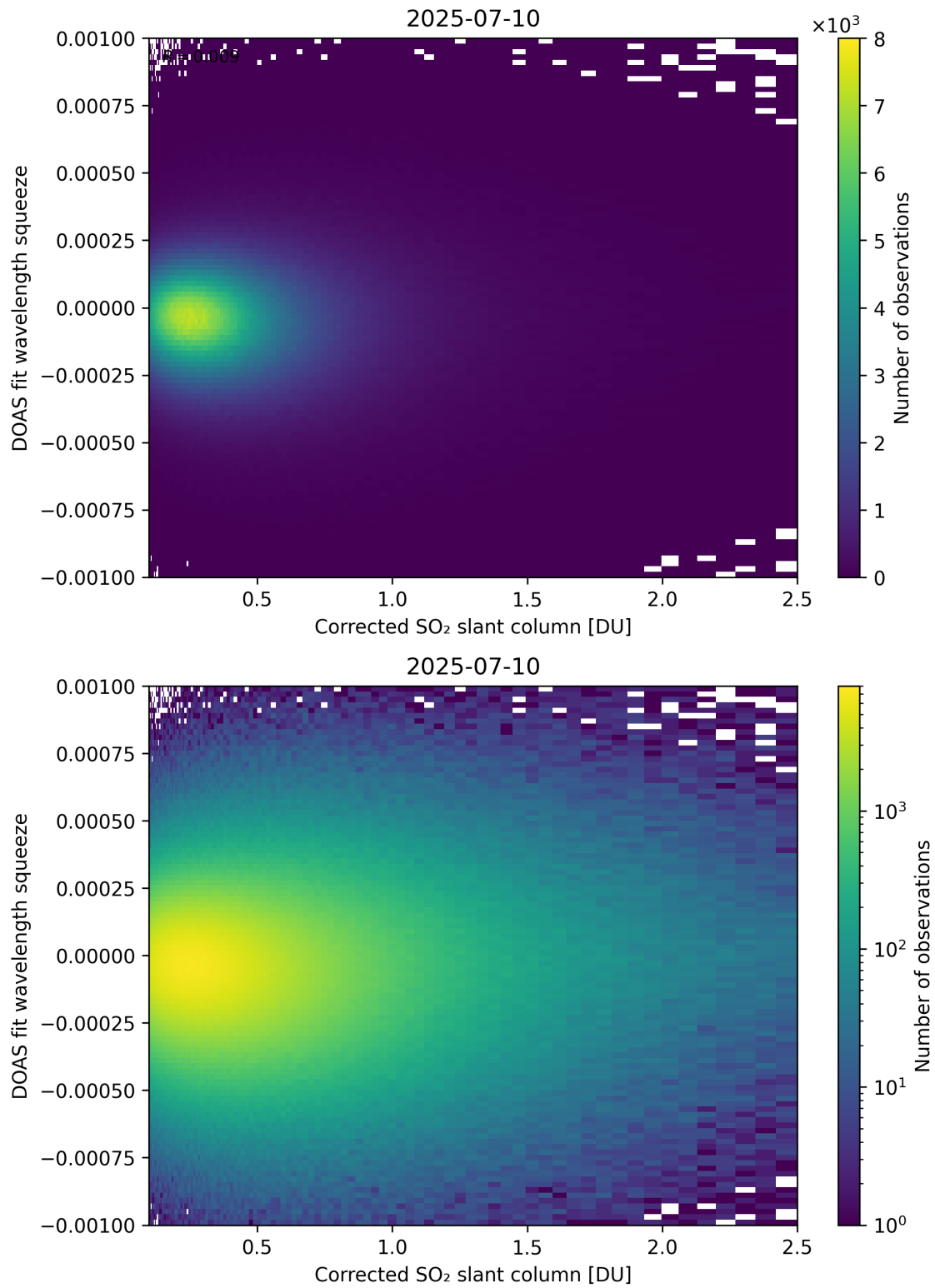
Figure 230: Scatter density plot of “Corrected SO 2 slant column” against “DOAS fit wavelength squeeze” for 2025-07-09 to 2025-07-11.
