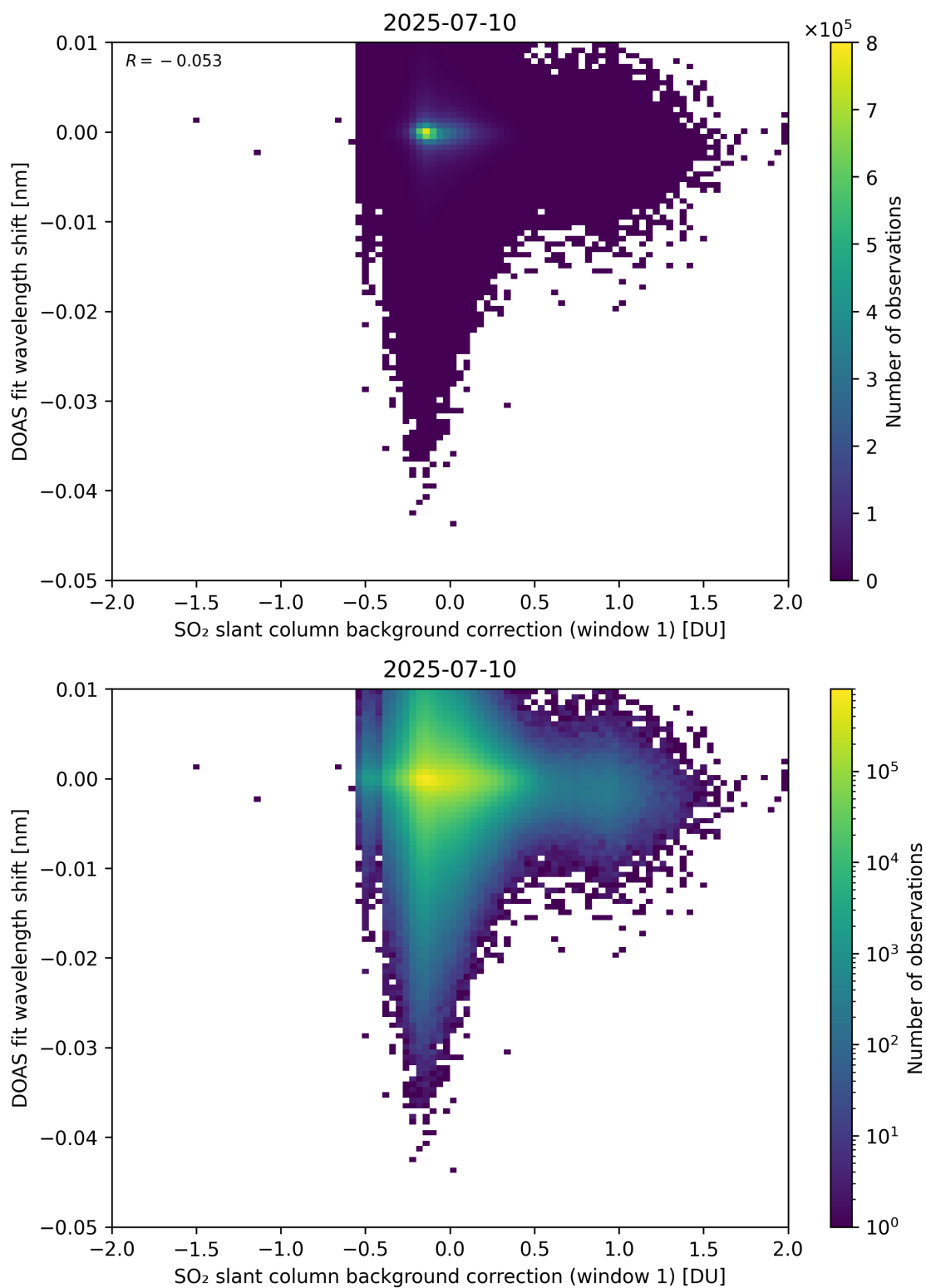
Figure 111: Scatter density plot of “SO 2 slant column background correction (window 1)” against “DOAS fit wavelength shift” for 2025-07-09 to 2025-07-11.
