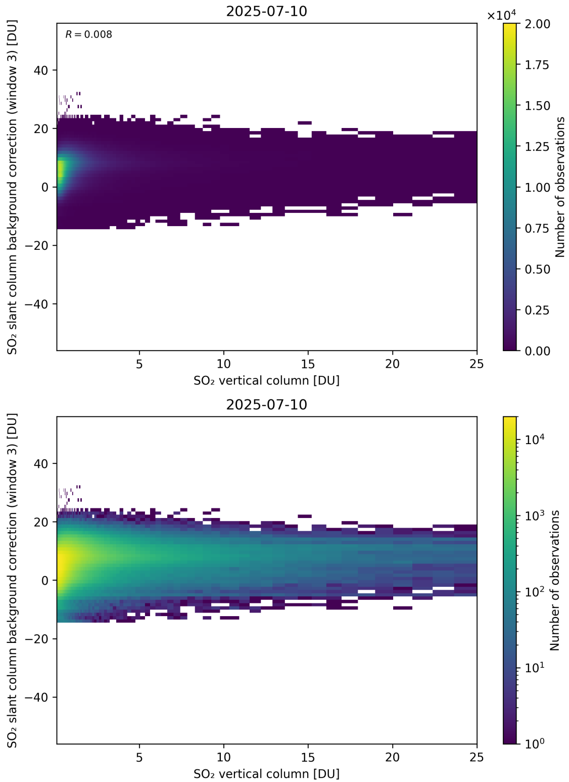
Figure 325: Scatter density plot of “SO 2 vertical column” against “SO 2 slant column background correction (window 3)” for 2025-07-09 to 2025-07-11.
