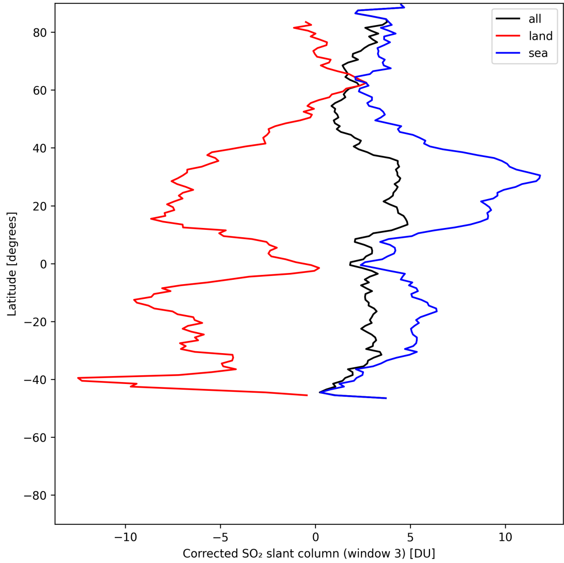
Figure 47: Zonal average of “Corrected SO 2 slant column (window 3)” for 2025-07-09 to 2025-07-11.
