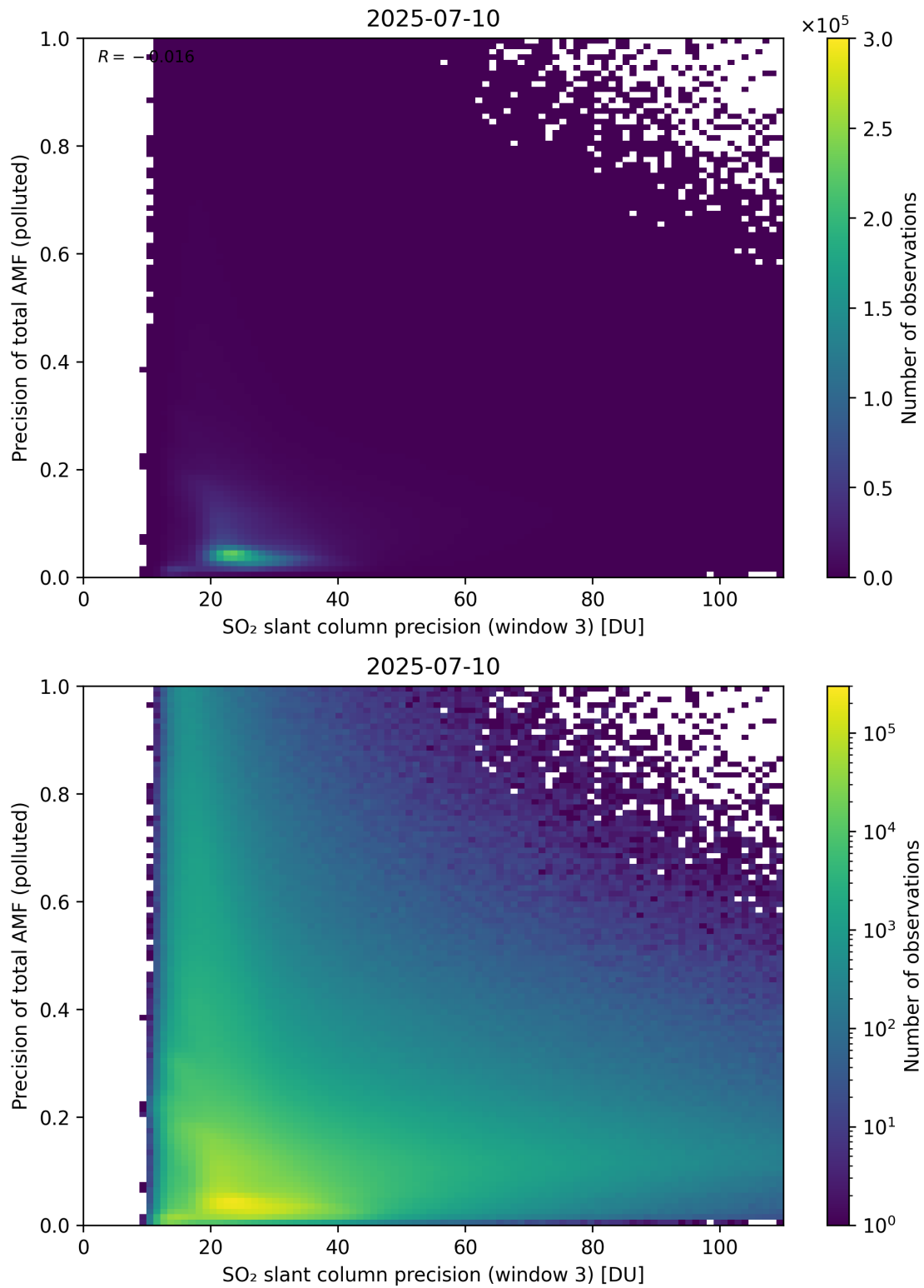
Figure 314: Scatter density plot of “SO 2 slant column precision (window 3)” against “Precision of total AMF (polluted)” for 2025-07-09 to 2025-07-11.
