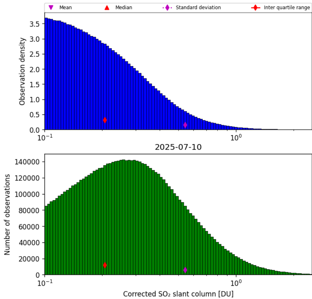
Figure 60: Histogram of “Corrected SO 2 slant column” for 2025-07-09 to 2025-07-11
