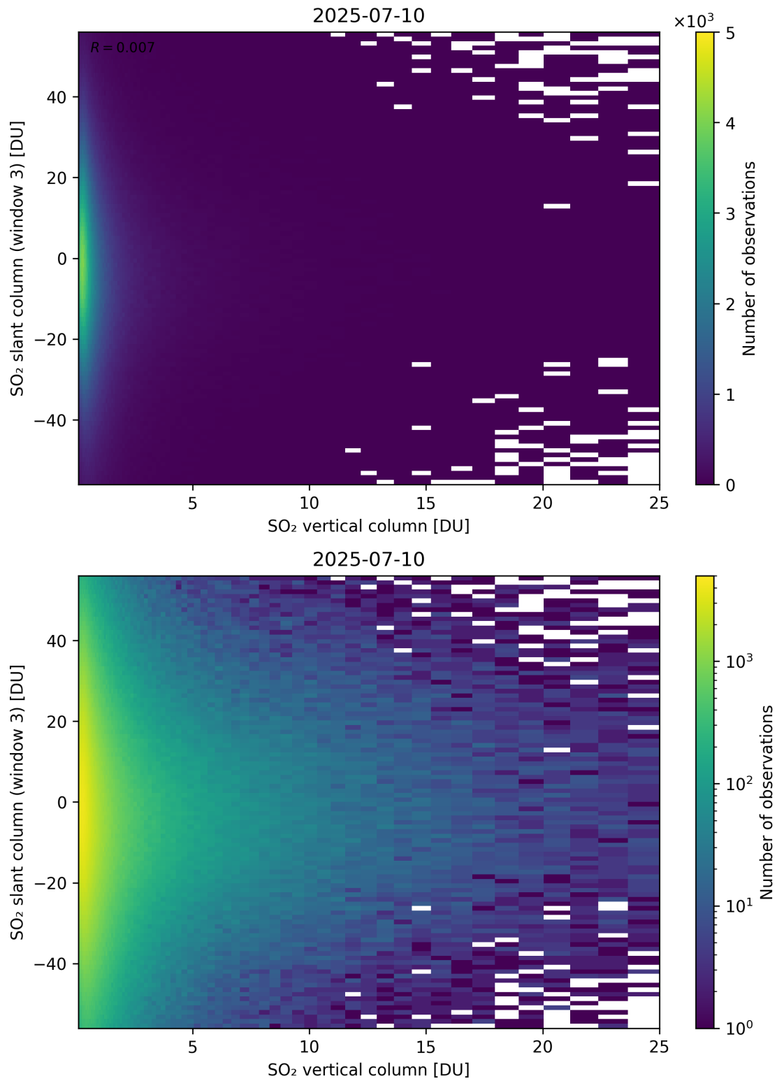
Figure 357: Scatter density plot of “SO 2 vertical column” against “SO 2 slant column (window 3)” for 2025-07-09 to 2025-07-11.
