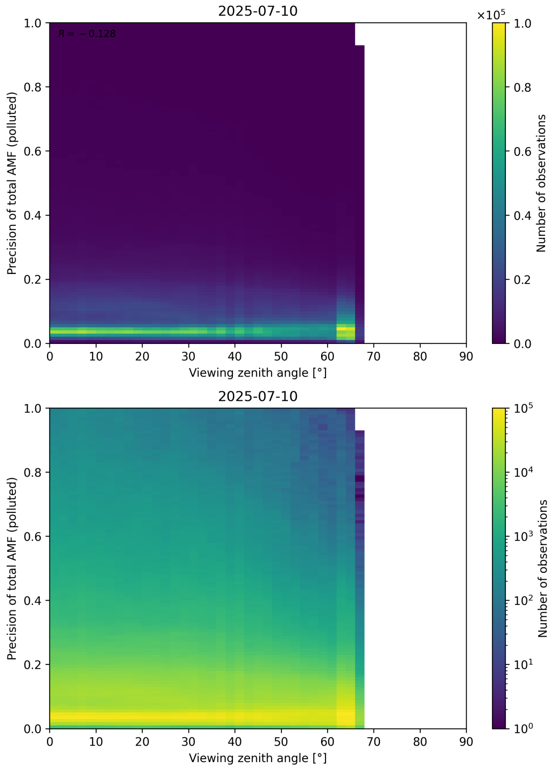
Figure 382: Scatter density plot of “Viewing zenith angle” against “Precision of total AMF (polluted)” for 2025-07-09 to 2025-07-11.
