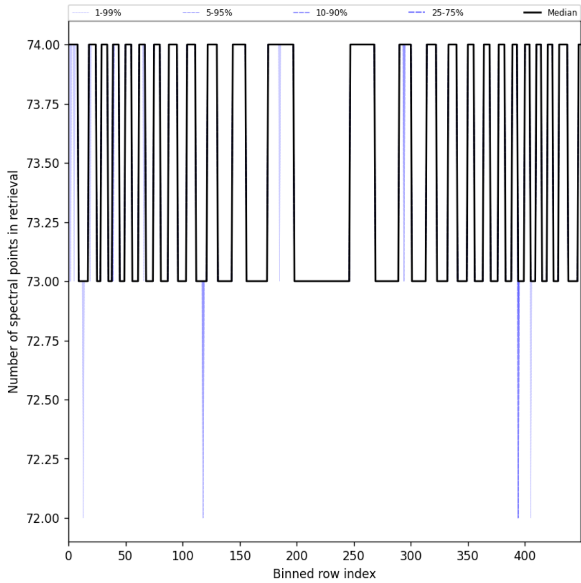
Figure 108: Along track statistics of “Number of spectral points in retrieval” for 2025-07-09 to 2025-07-11
