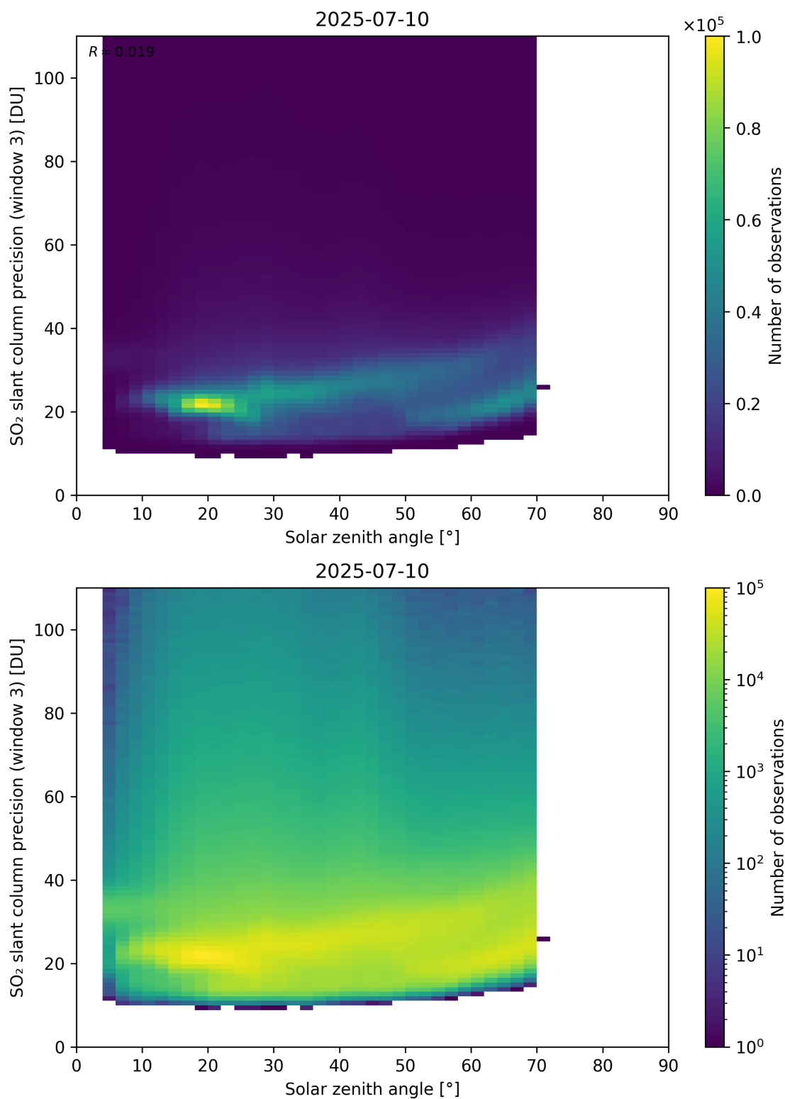
Figure 188: Scatter density plot of “Solar zenith angle” against “SO 2 slant column precision (window 3)” for 2025-07-09 to 2025-07-11.
