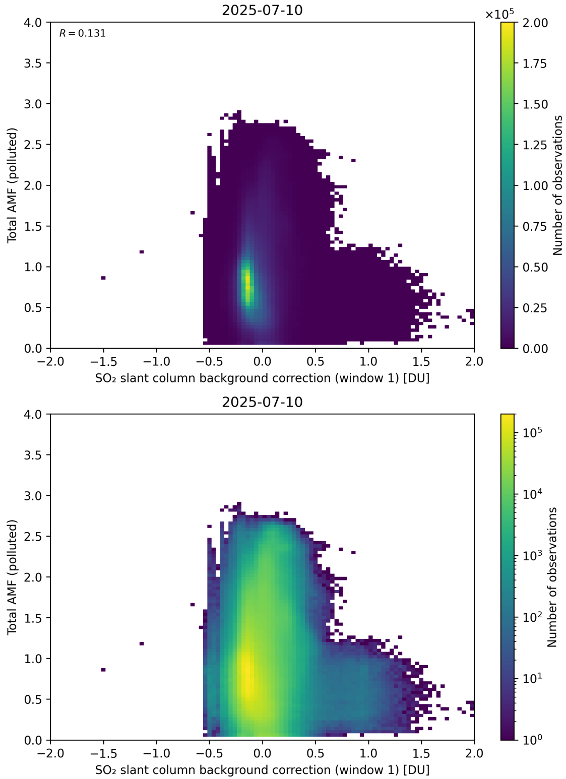
Figure 120: Scatter density plot of “SO 2 slant column background correction (window 1)” against “Total AMF (polluted)” for 2025-07-09 to 2025-07-11.
