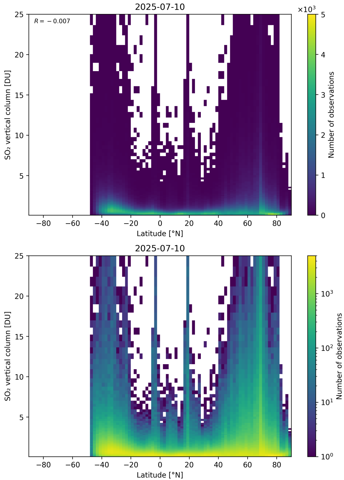
Figure 169: Scatter density plot of “Latitude” against “SO 2 vertical column” for 2025-07-09 to 2025-07-11.
