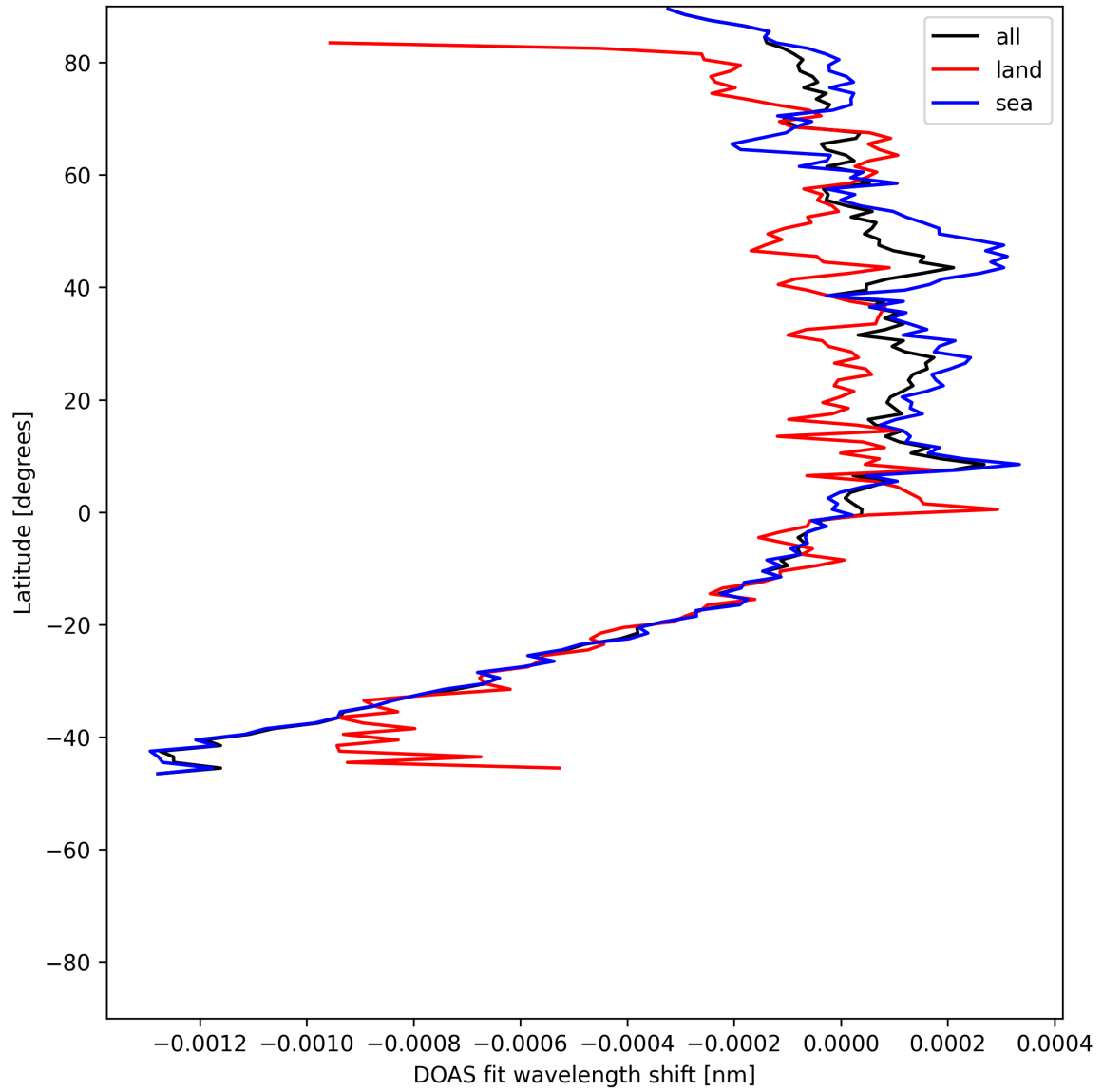
Figure 50: Zonal average of “DOAS fit wavelength shift” for 2025-07-09 to 2025-07-11.
