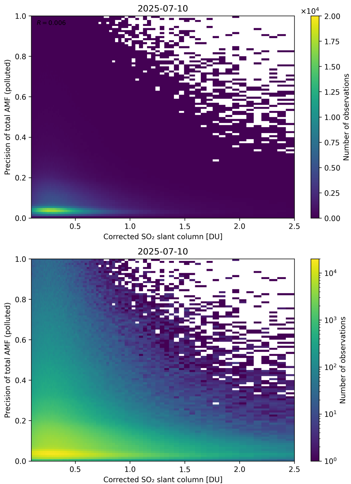
Figure 243: Scatter density plot of “Corrected SO 2 slant column” against “Precision of total AMF (polluted)” for 2025-07-09 to 2025-07-11.
