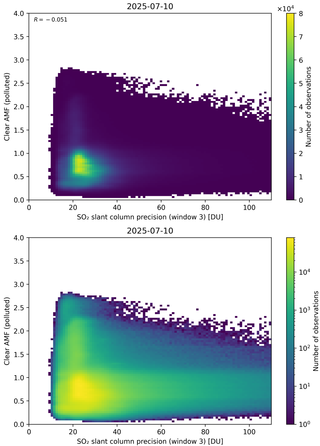
Figure 311: Scatter density plot of “SO 2 slant column precision (window 3)” against “Clear AMF (polluted)” for 2025-07-09 to 2025-07-11.
