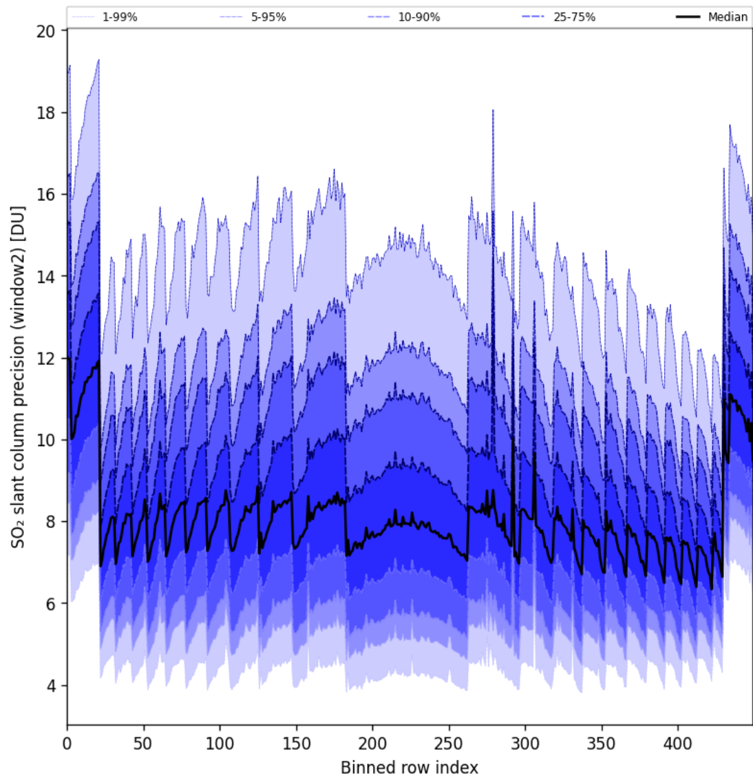
Figure 94: Along track statistics of “SO 2 slant column precision (window2)” for 2025-07-09 to 2025-07-11
