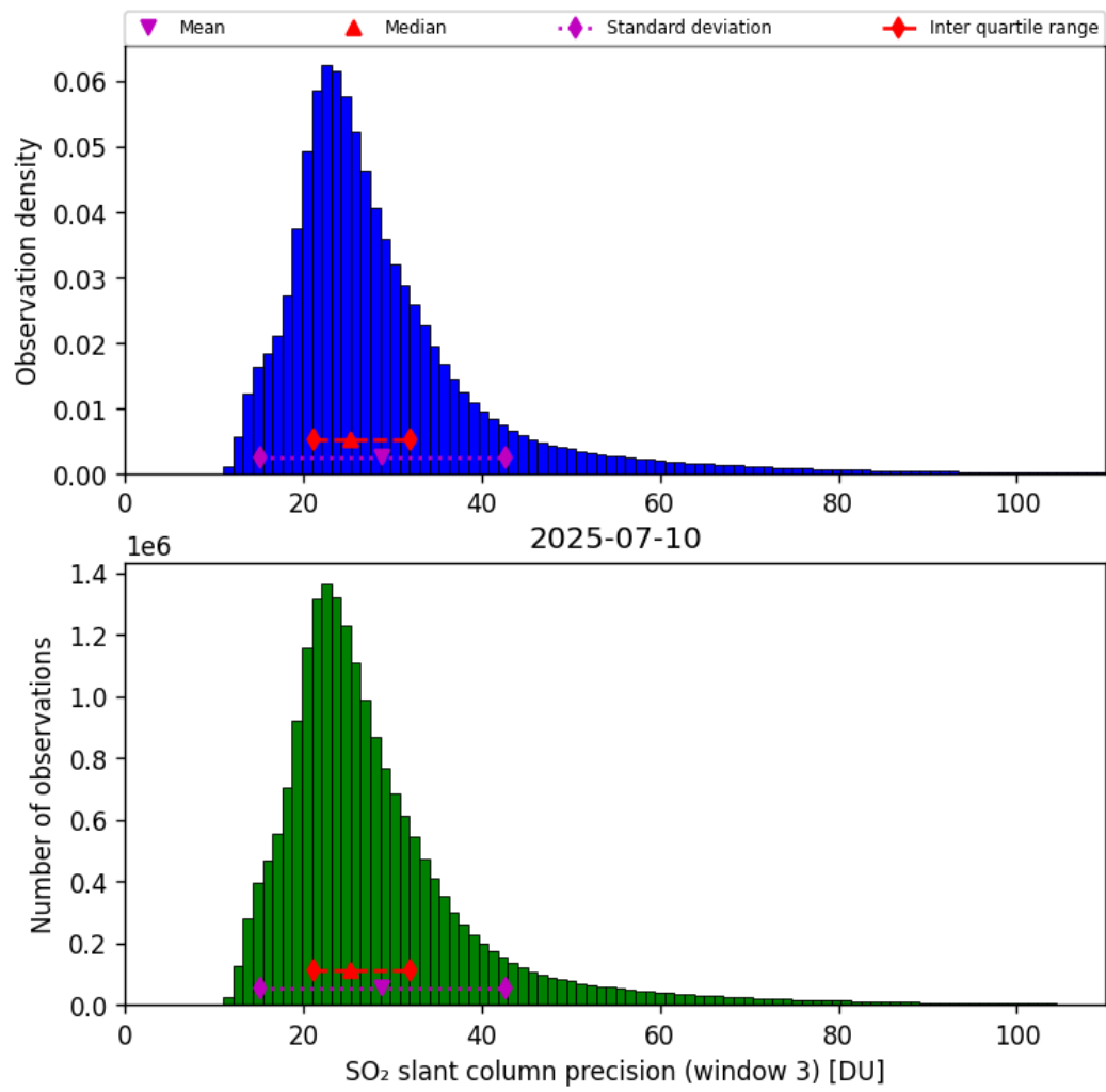
Figure 72: Histogram of “SO 2 slant column precision (window 3)” for 2025-07-09 to 2025-07-11
