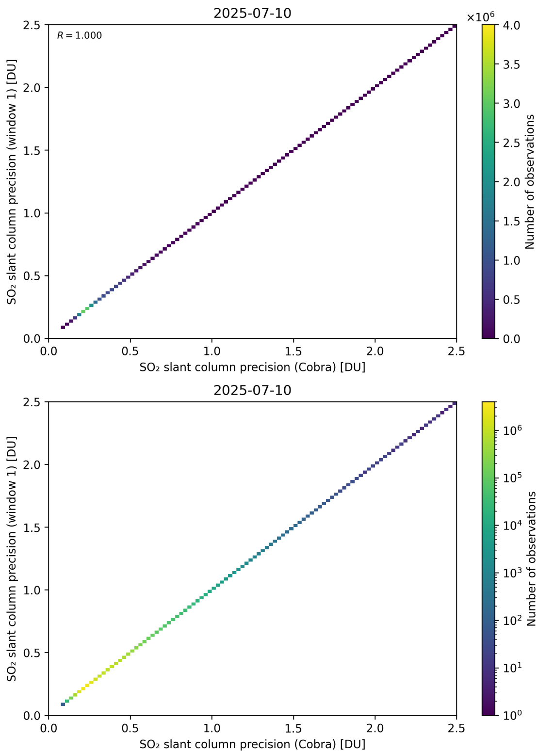
Figure 209: Scatter density plot of “SO 2 slant column precision (Cobra)” against “SO 2 slant column precision (window 1)” for 2025-07-09 to 2025-07-11.
