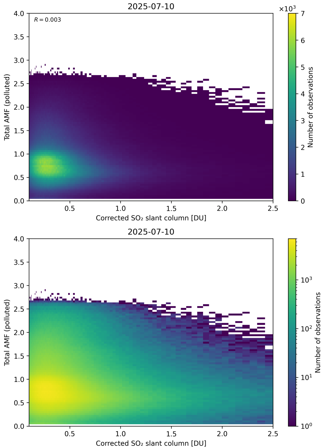
Figure 242: Scatter density plot of “Corrected SO 2 slant column” against “Total AMF (polluted)” for 2025-07-09 to 2025-07-11.
