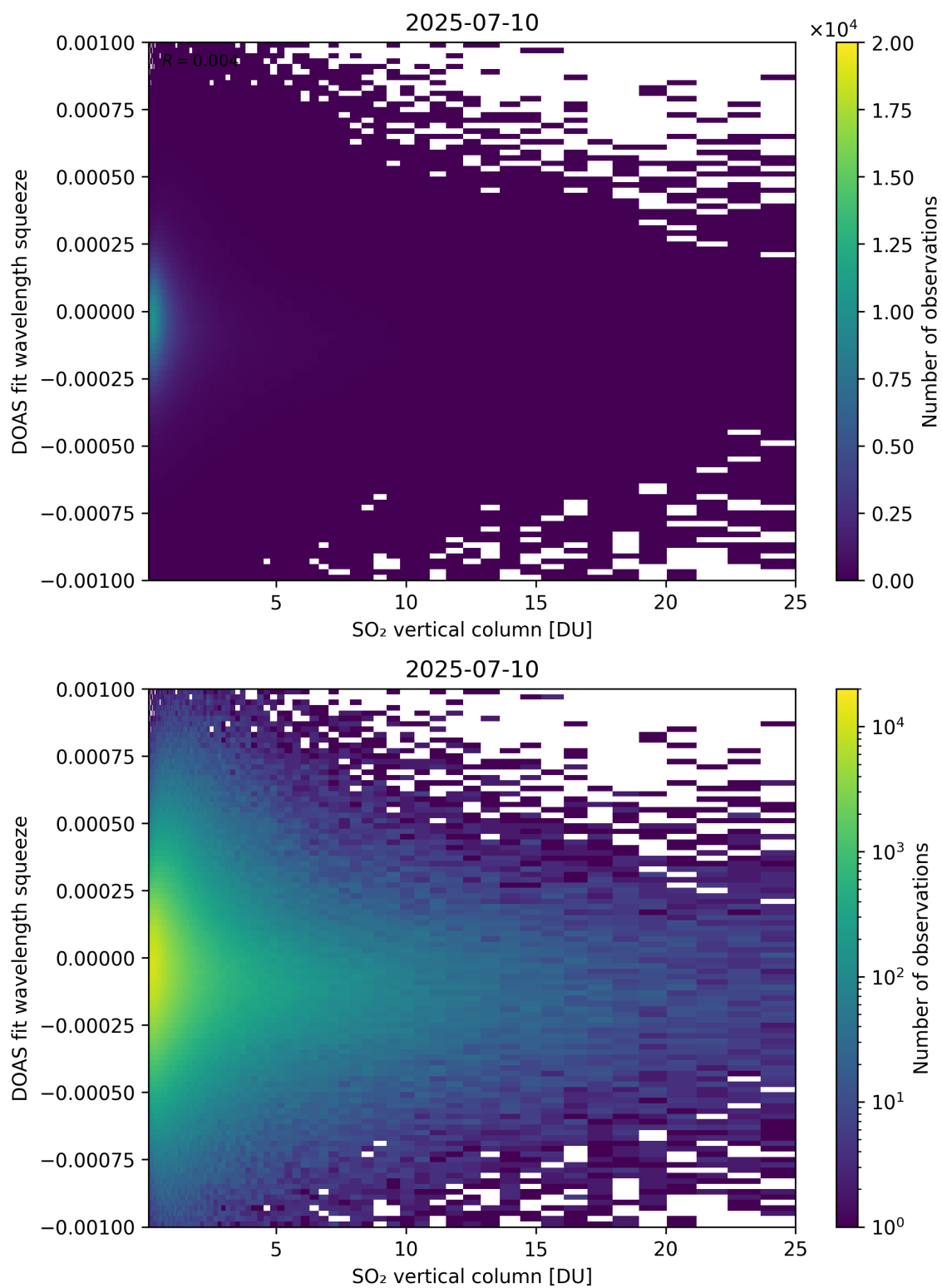
Figure 327: Scatter density plot of “SO 2 vertical column” against “DOAS fit wavelength squeeze” for 2025-07-09 to 2025-07-11.
