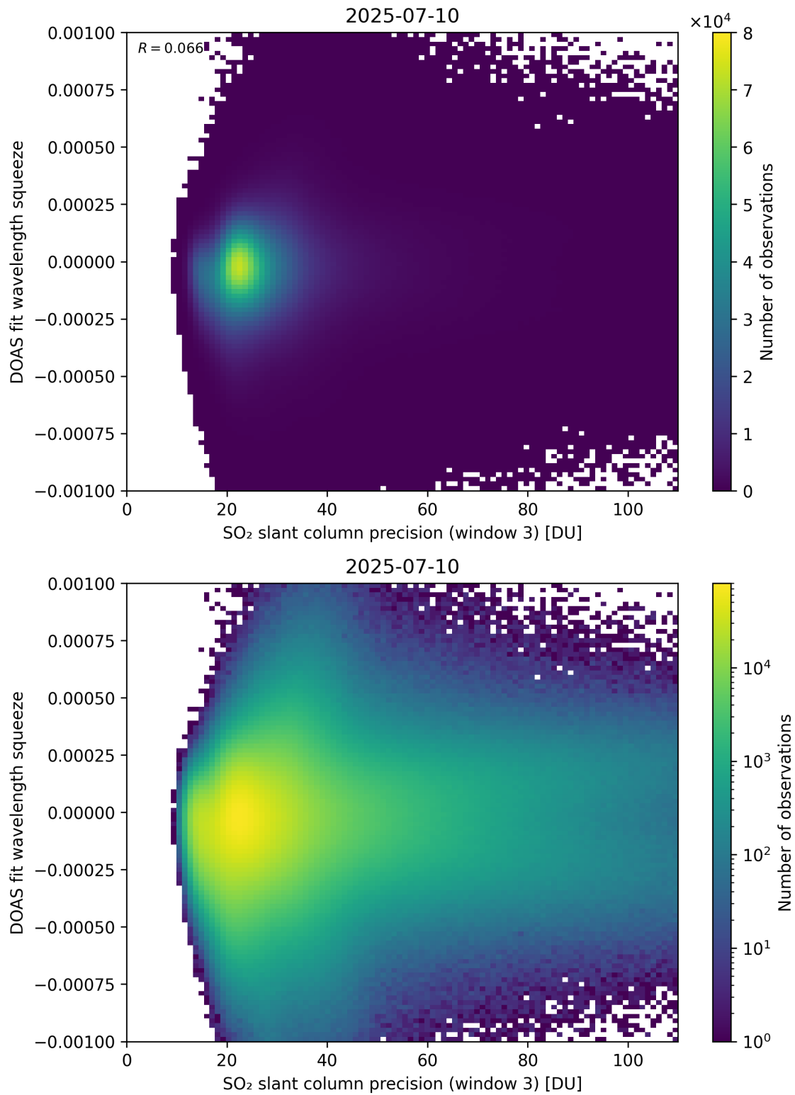
Figure 309: Scatter density plot of “SO 2 slant column precision (window 3)” against “DOAS fit wavelength squeeze” for 2025-07-09 to 2025-07-11.
