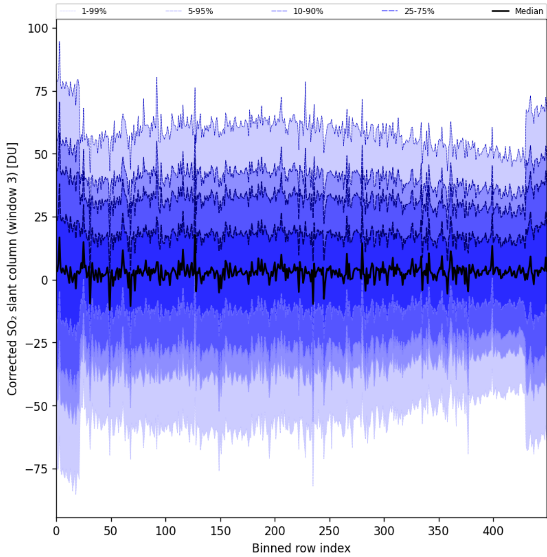
Figure 99: Along track statistics of “Corrected SO 2 slant column (window 3)” for 2025-07-09 to 2025-07-11
