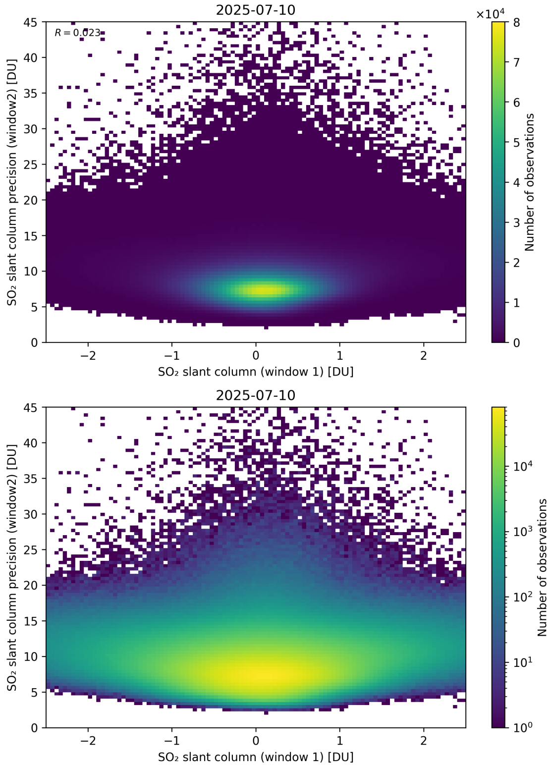
Figure 286: Scatter density plot of “SO 2 slant column (window 1)” against “SO 2 slant column precision (window2)” for 2025-07-09 to 2025-07-11.
