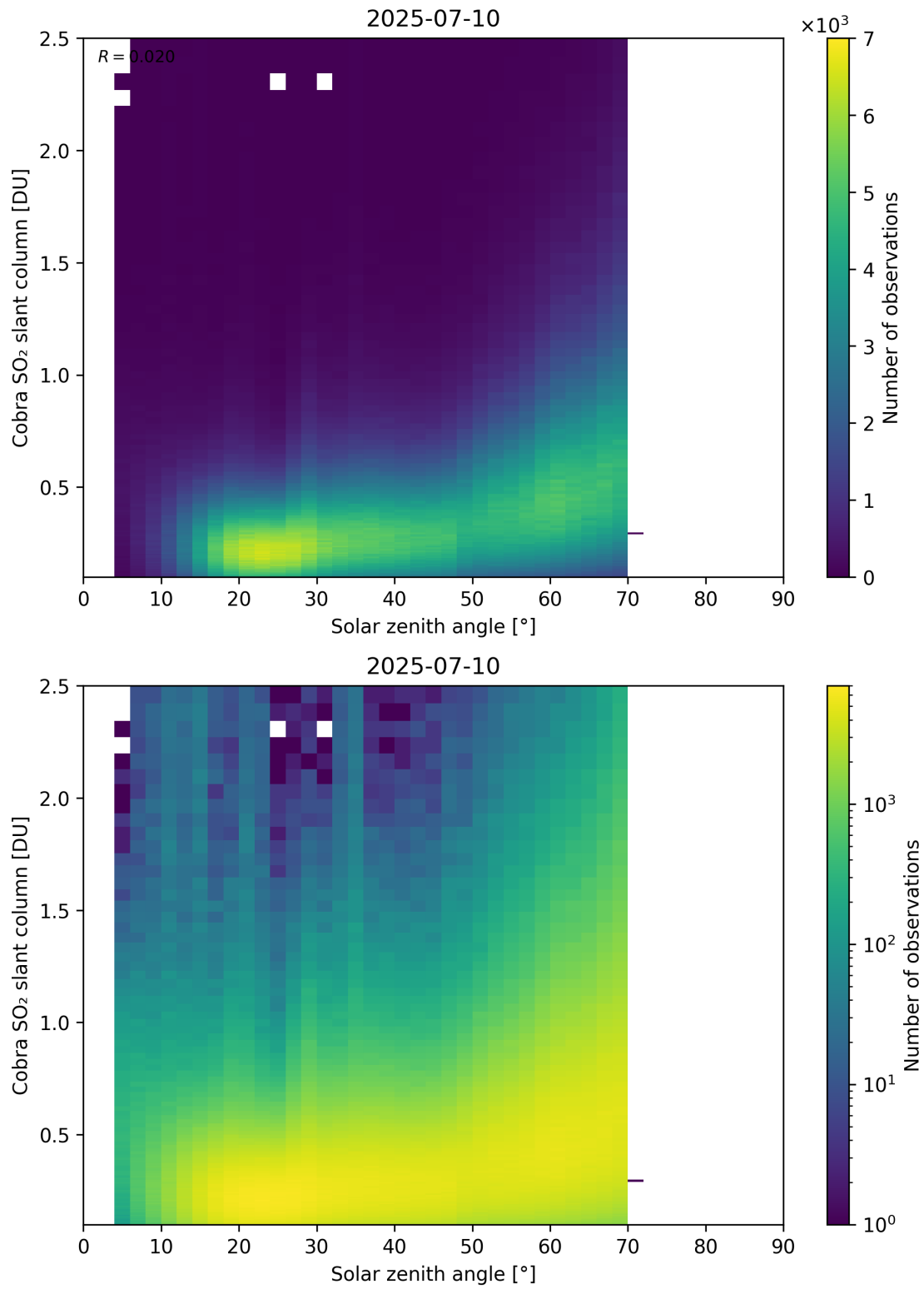
Figure 179: Scatter density plot of “Solar zenith angle” against “Cobra SO 2 slant column” for 2025-07-09 to 2025-07-11.
