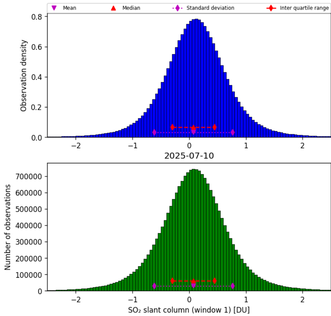
Figure 63: Histogram of “SO 2 slant column (window 1)” for 2025-07-09 to 2025-07-11
