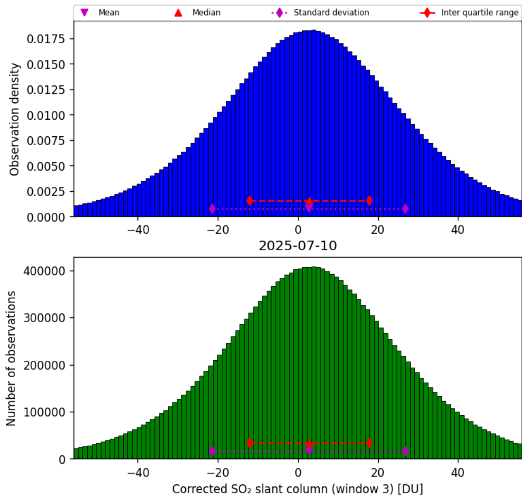
Figure 73: Histogram of “Corrected SO 2 slant column (window 3)” for 2025-07-09 to 2025-07-11
