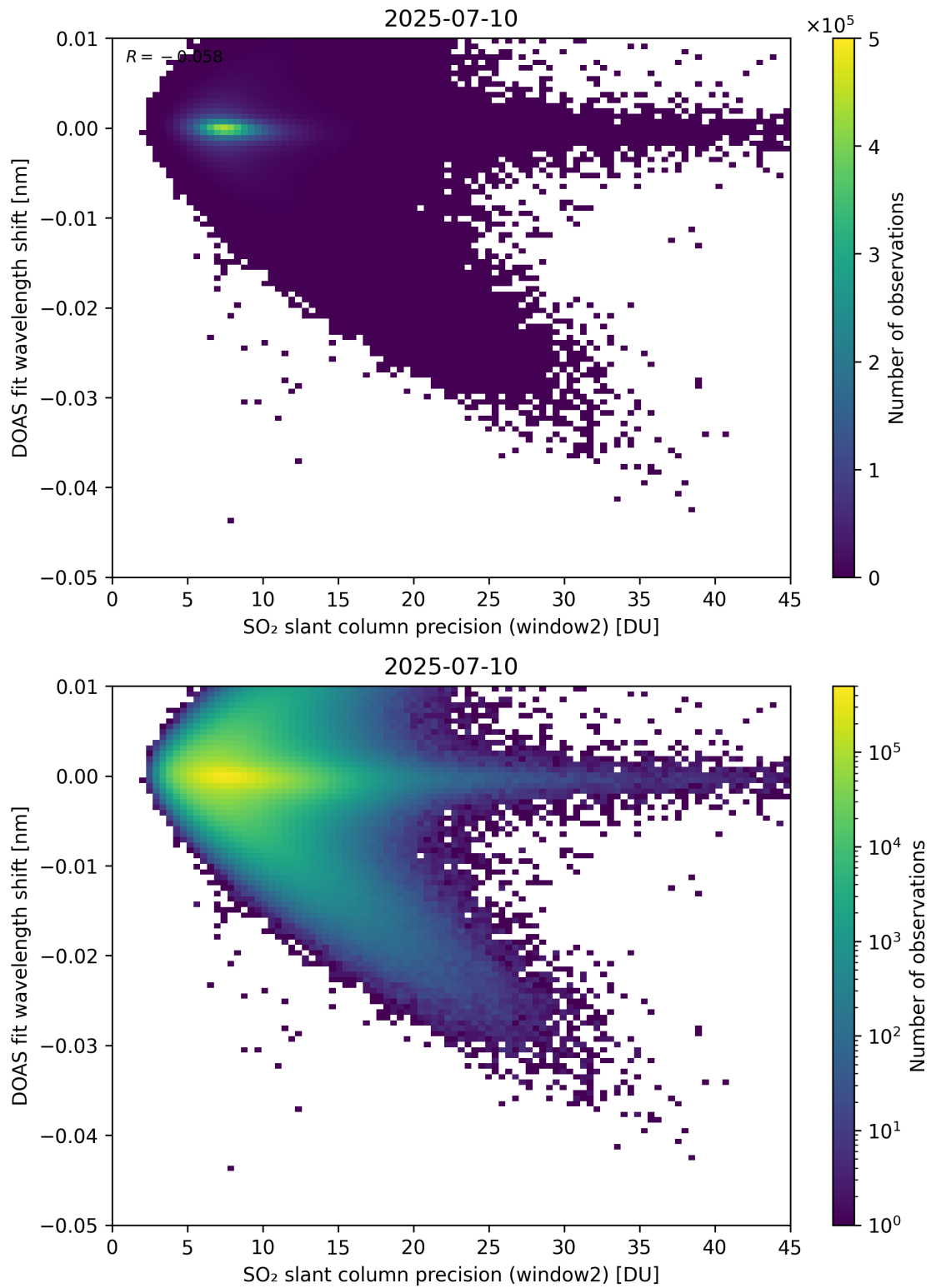
Figure 293: Scatter density plot of “SO 2 slant column precision (window2)” against “DOAS fit wavelength shift” for 2025-07-09 to 2025-07-11.
