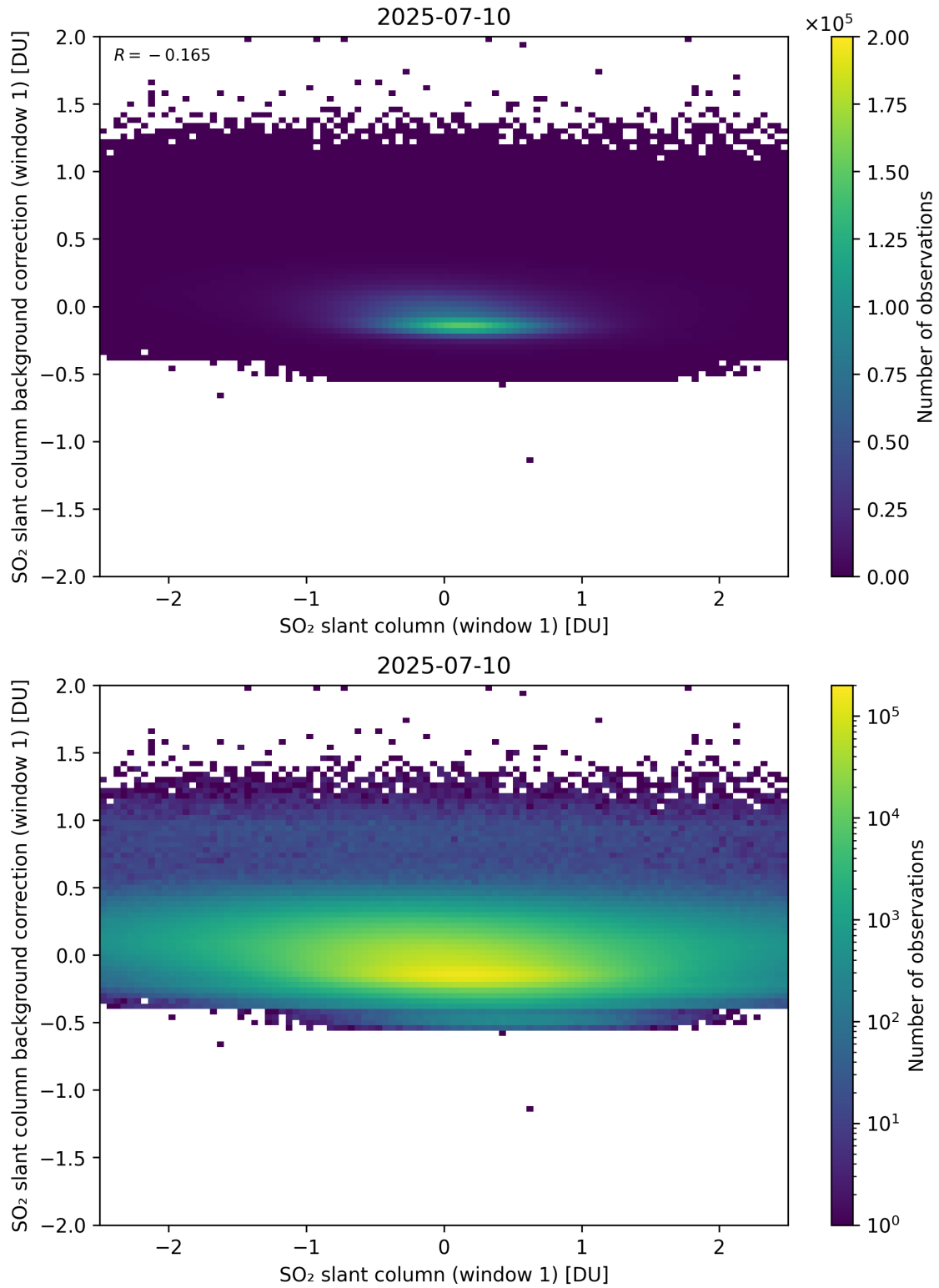
Figure 262: Scatter density plot of “SO 2 slant column (window 1)” against “SO 2 slant column background correction (window 1)” for 2025-07-09 to 2025-07-11.
