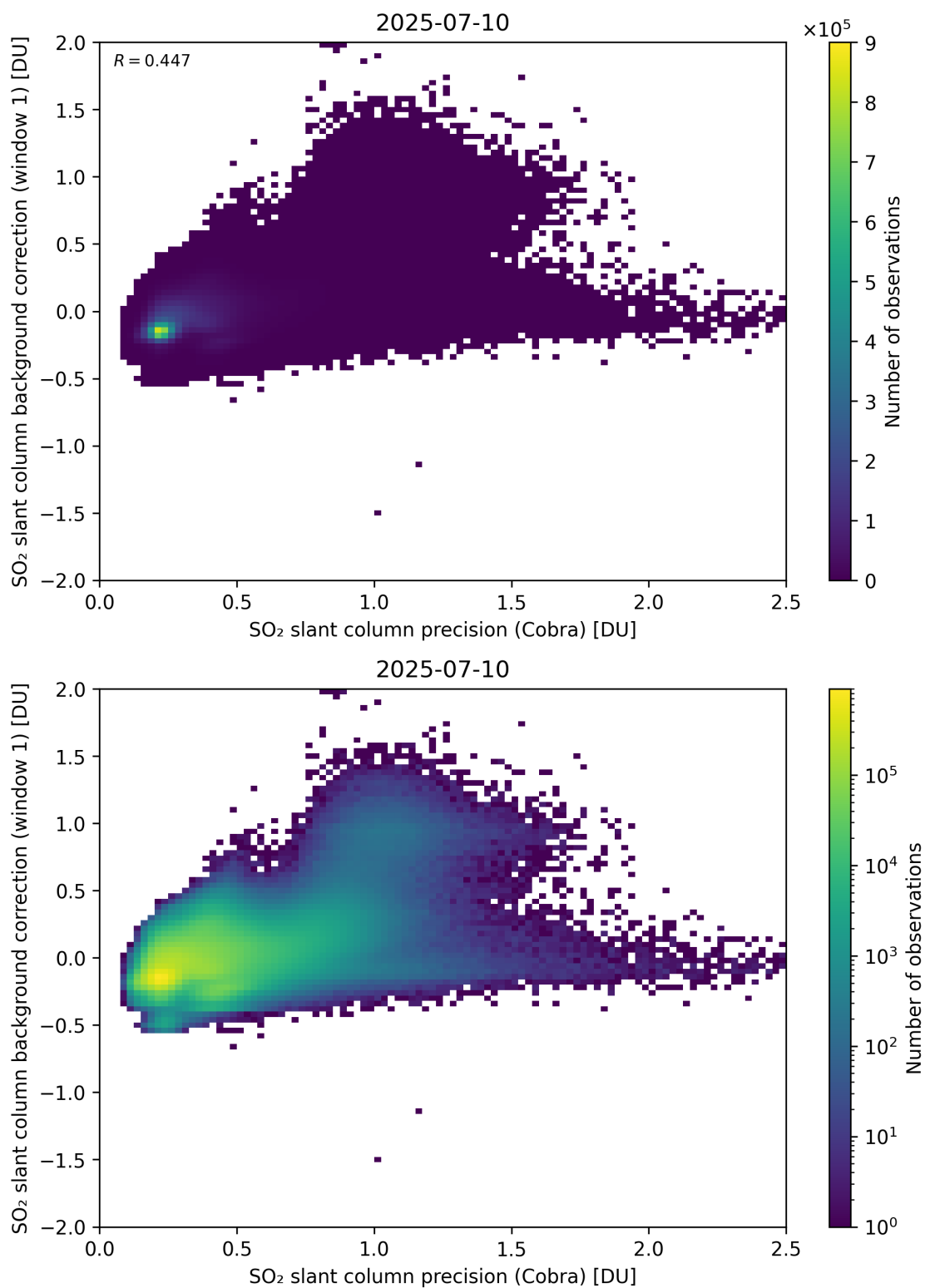
Figure 199: Scatter density plot of “SO 2 slant column precision (Cobra)” against “SO 2 slant column background correction (window 1)” for 2025-07-09 to 2025-07-11.
