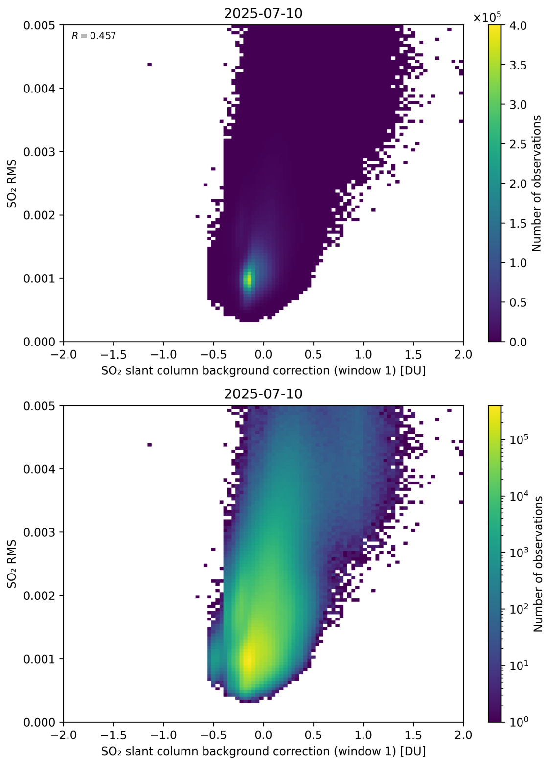
Figure 113: Scatter density plot of “SO 2 slant column background correction (window 1)” against “SO 2 RMS” for 2025-07-09 to 2025-07-11.
