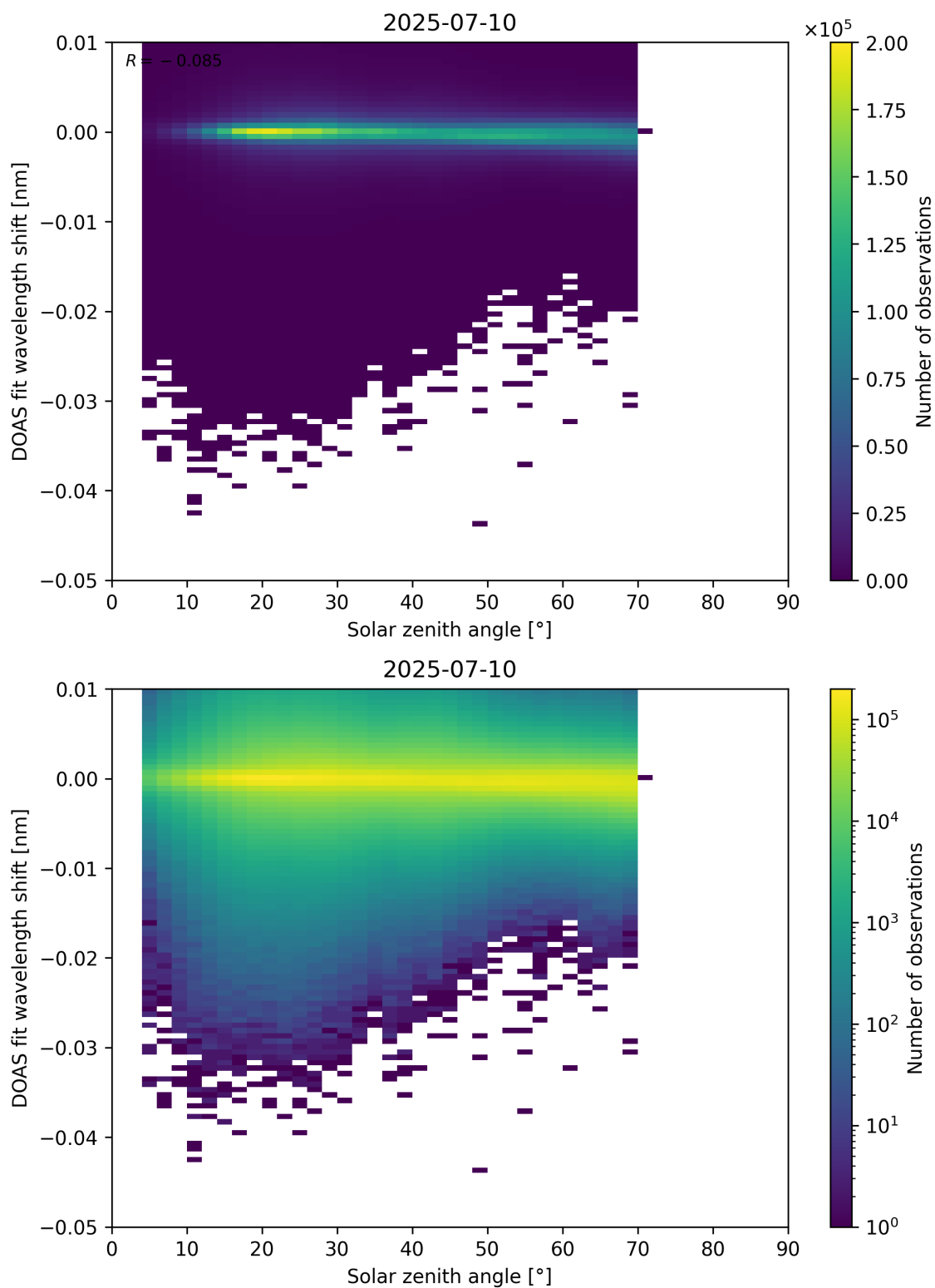
Figure 174: Scatter density plot of “Solar zenith angle” against “DOAS fit wavelength shift” for 2025-07-09 to 2025-07-11.
