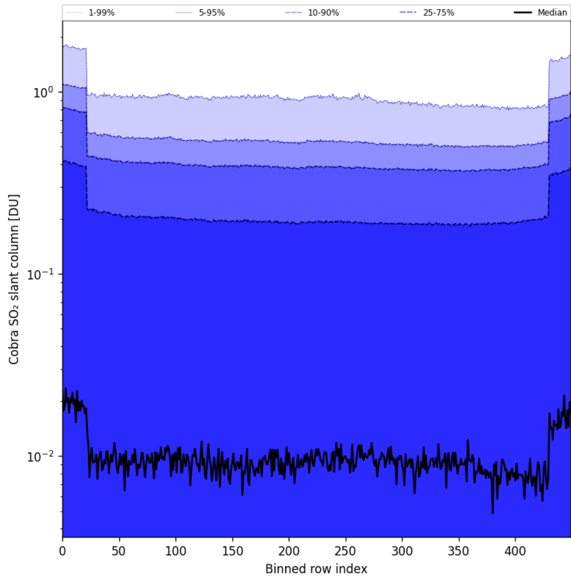
Figure 87: Along track statistics of “Cobra SO 2 slant column” for 2025-07-09 to 2025-07-11
