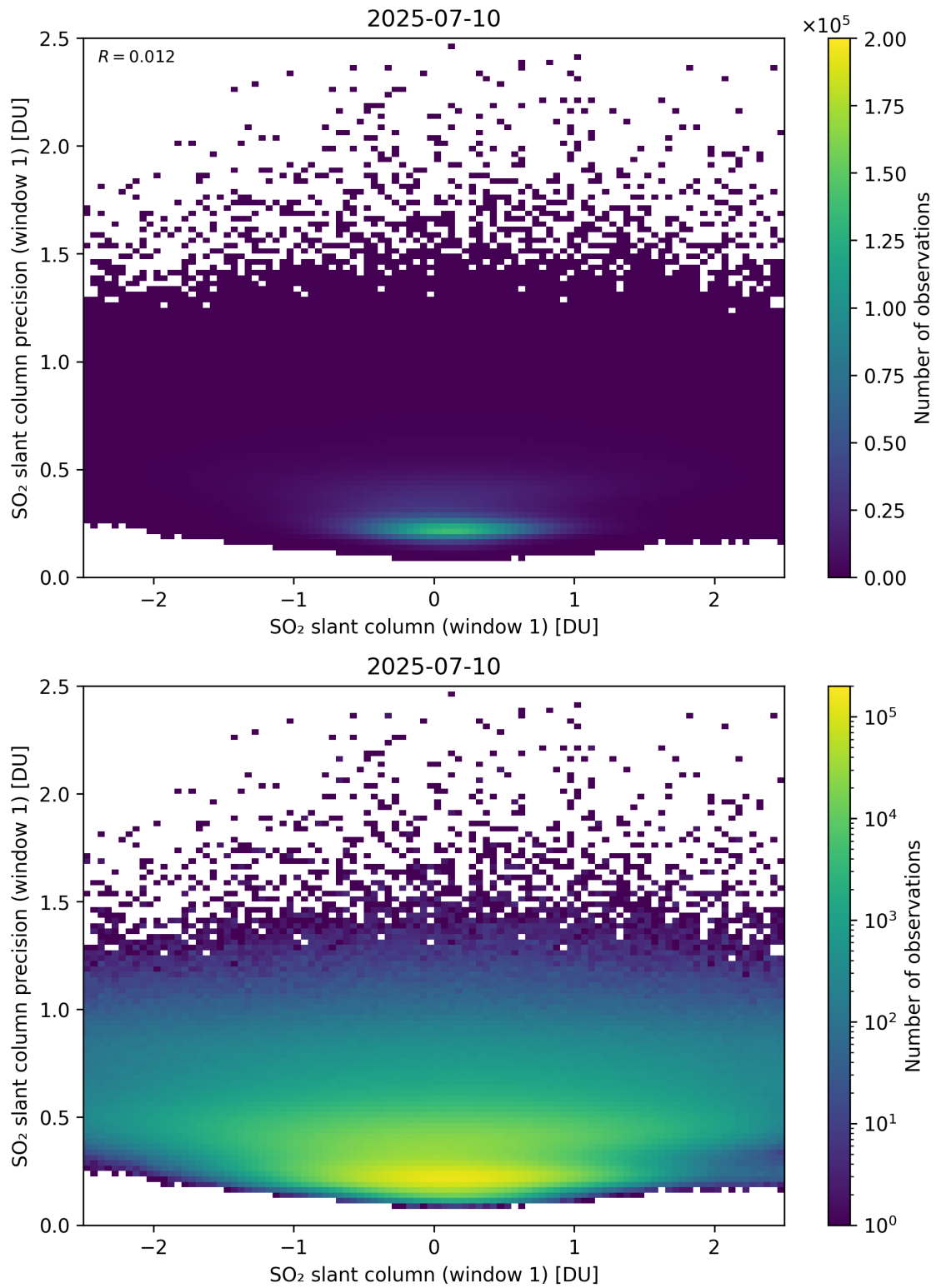
Figure 285: Scatter density plot of “SO 2 slant column (window 1)” against “SO 2 slant column precision (window 1)” for 2025-07-09 to 2025-07-11.
