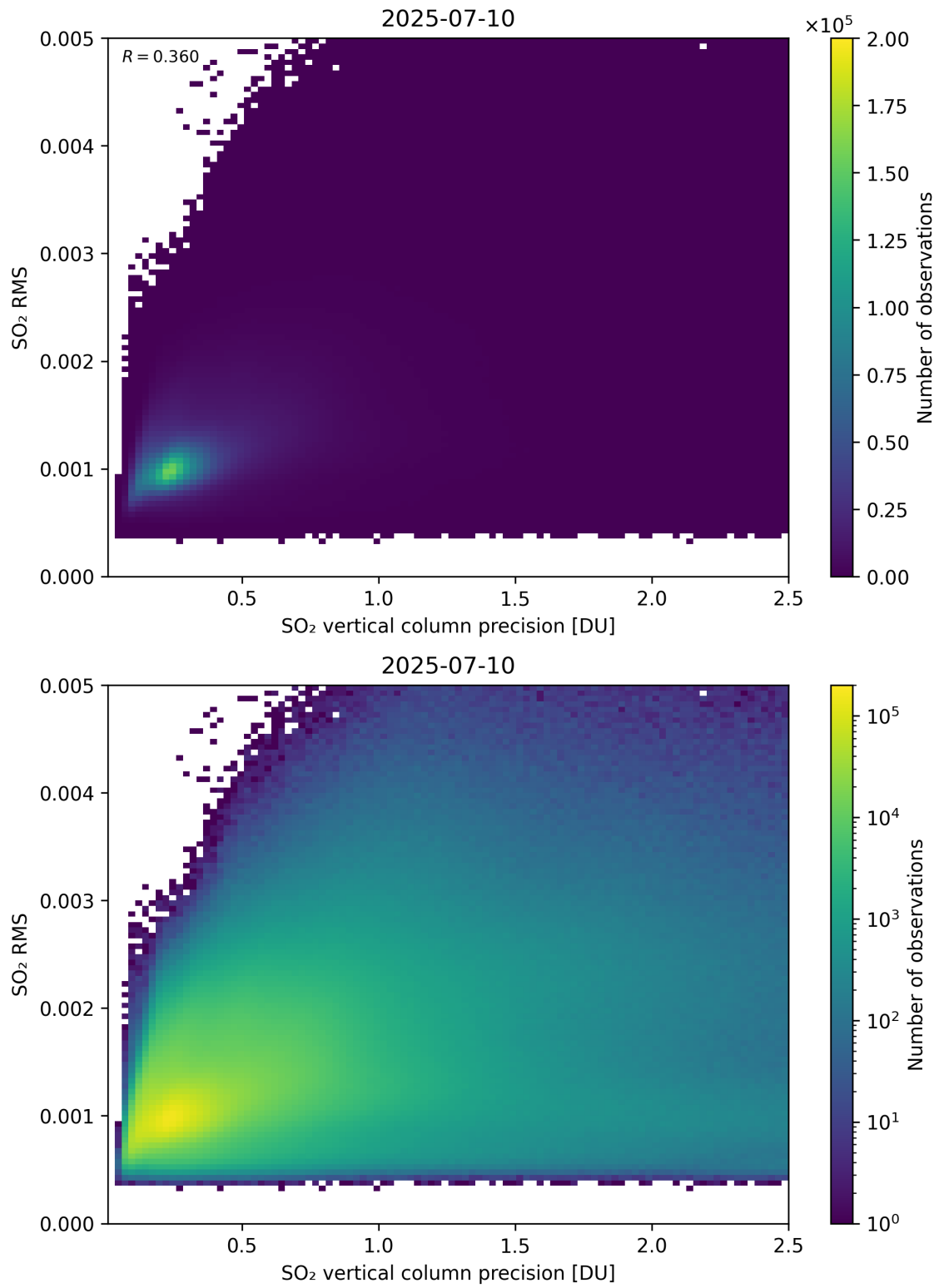
Figure 334: Scatter density plot of “SO 2 vertical column precision” against “SO 2 RMS” for 2025-07-09 to 2025-07-11.
