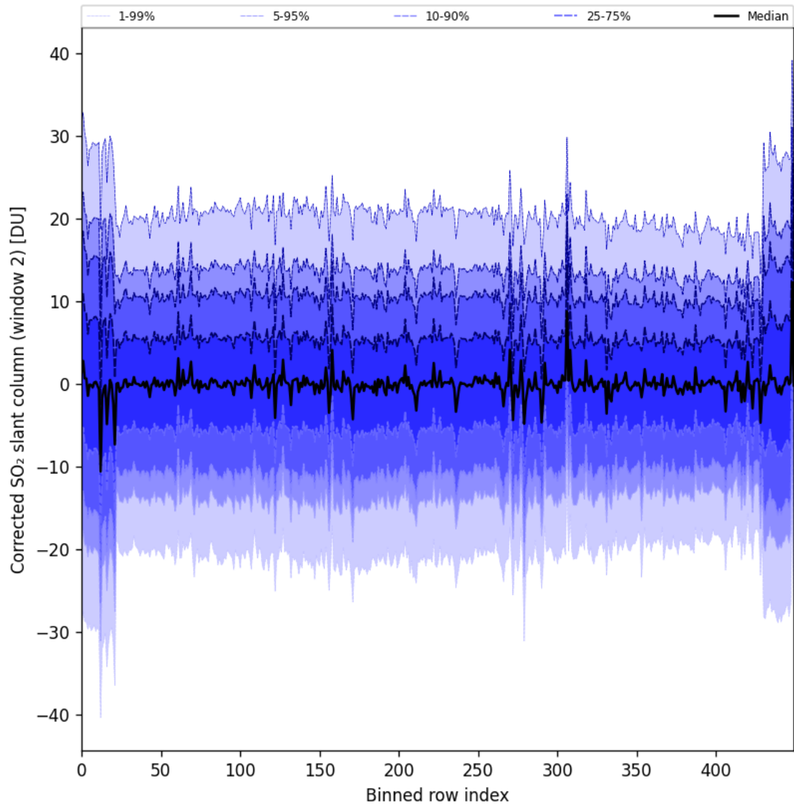
Figure 95: Along track statistics of “Corrected SO 2 slant column (window 2)” for 2025-07-09 to 2025-07-11
