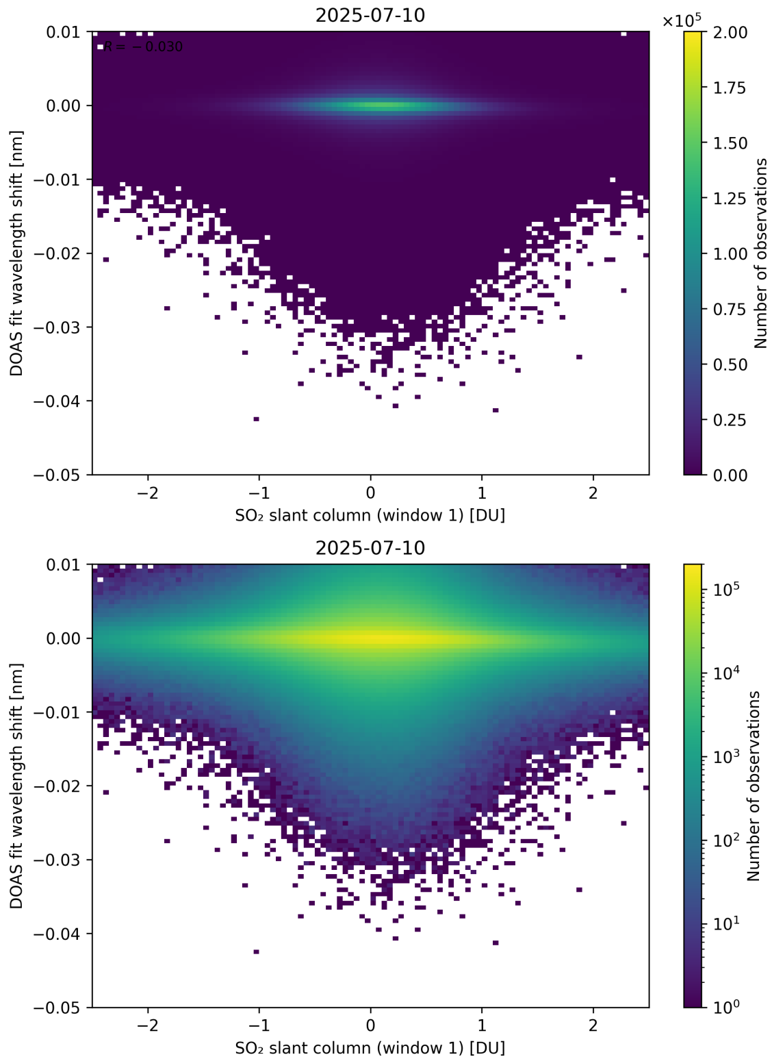
Figure 265: Scatter density plot of “SO 2 slant column (window 1)” against “DOAS fit wavelength shift” for 2025-07-09 to 2025-07-11.
