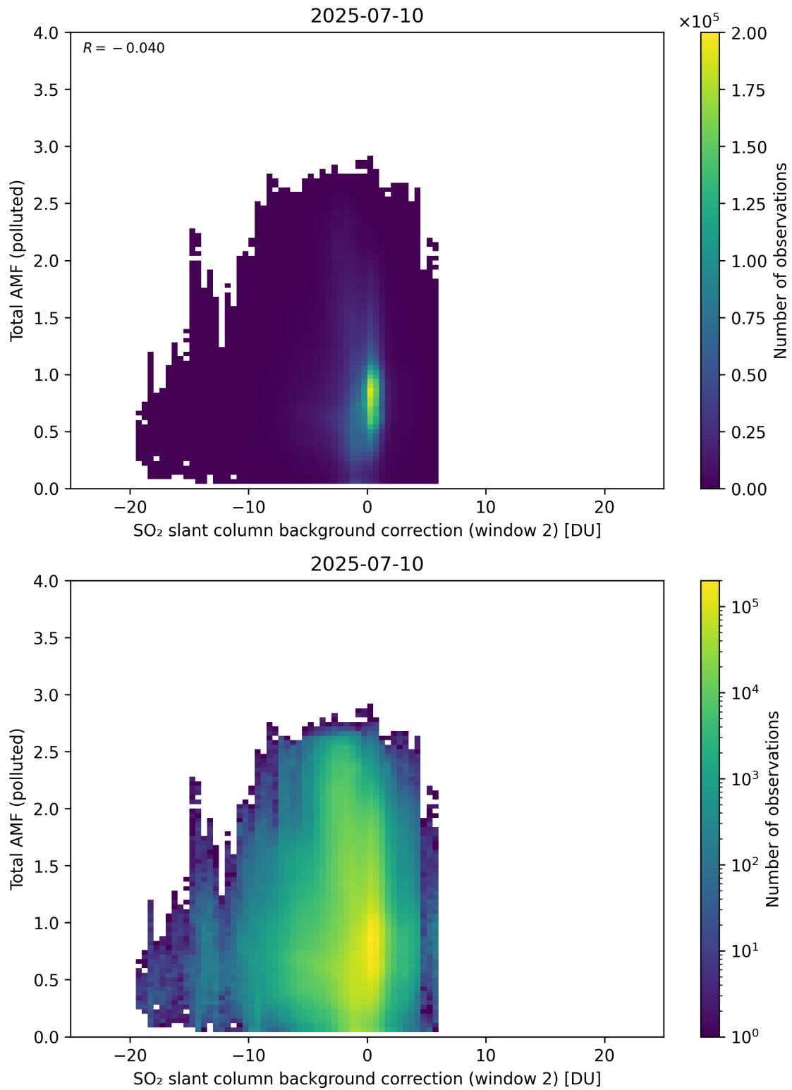
Figure 130: Scatter density plot of “SO 2 slant column background correction (window 2)” against “Total AMF (polluted)” for 2025-07-09 to 2025-07-11.
