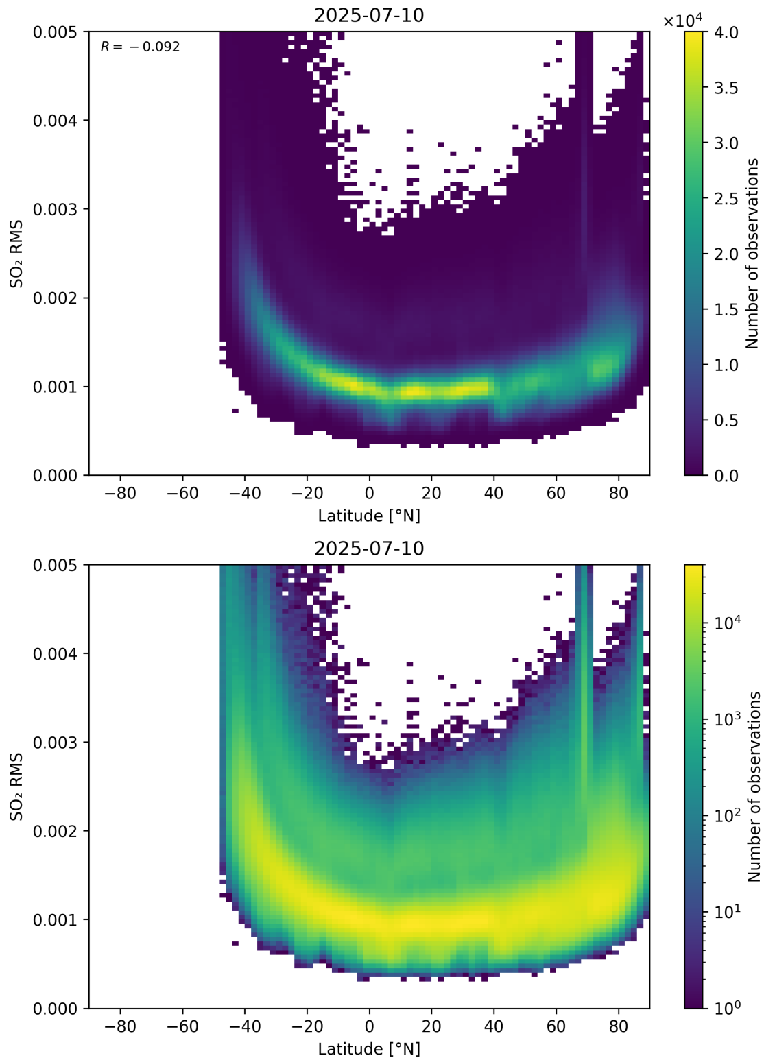
Figure 155: Scatter density plot of “Latitude” against “SO 2 RMS” for 2025-07-09 to 2025-07-11.
