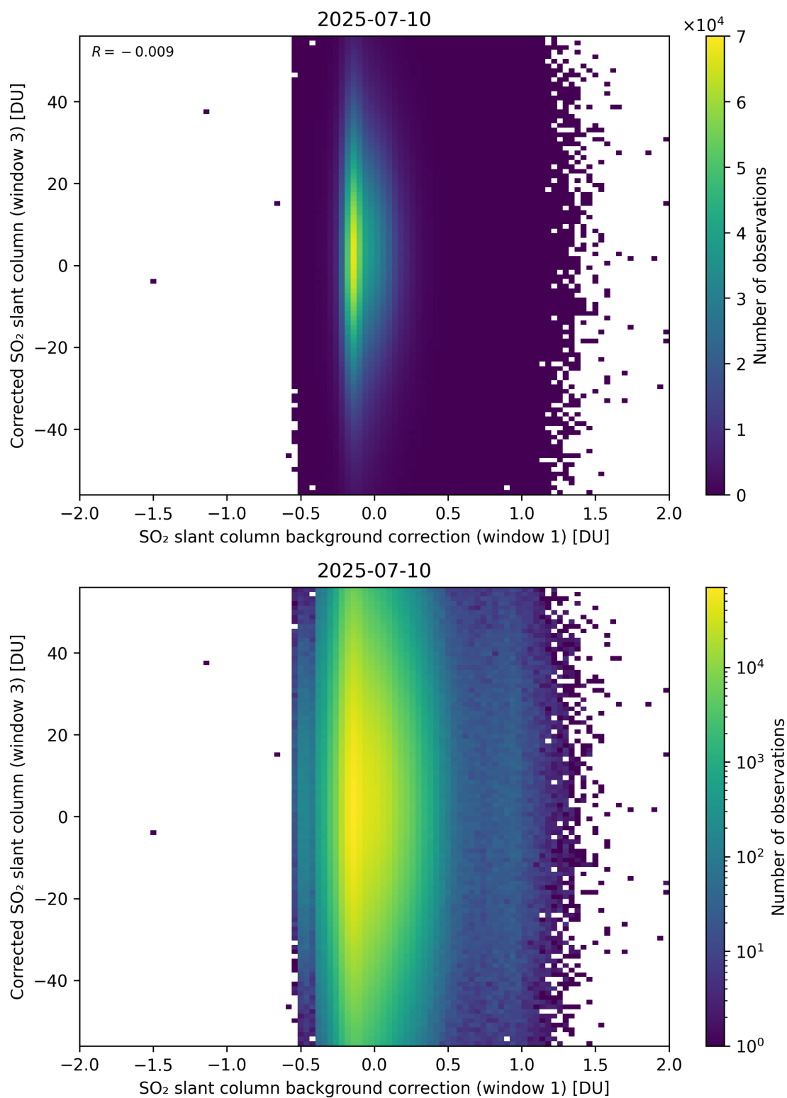
Figure 116: Scatter density plot of “SO 2 slant column background correction (window 1)” against “Corrected SO 2 slant column (window 3)” for 2025-07-09 to 2025-07-11.
