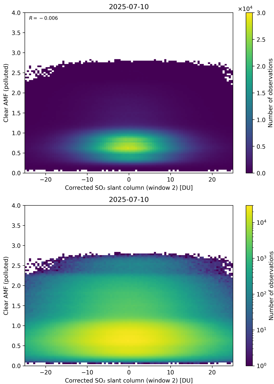
Figure 249: Scatter density plot of “Corrected SO 2 slant column (window 2)” against “Clear AMF (polluted)” for 2025-07-09 to 2025-07-11.
