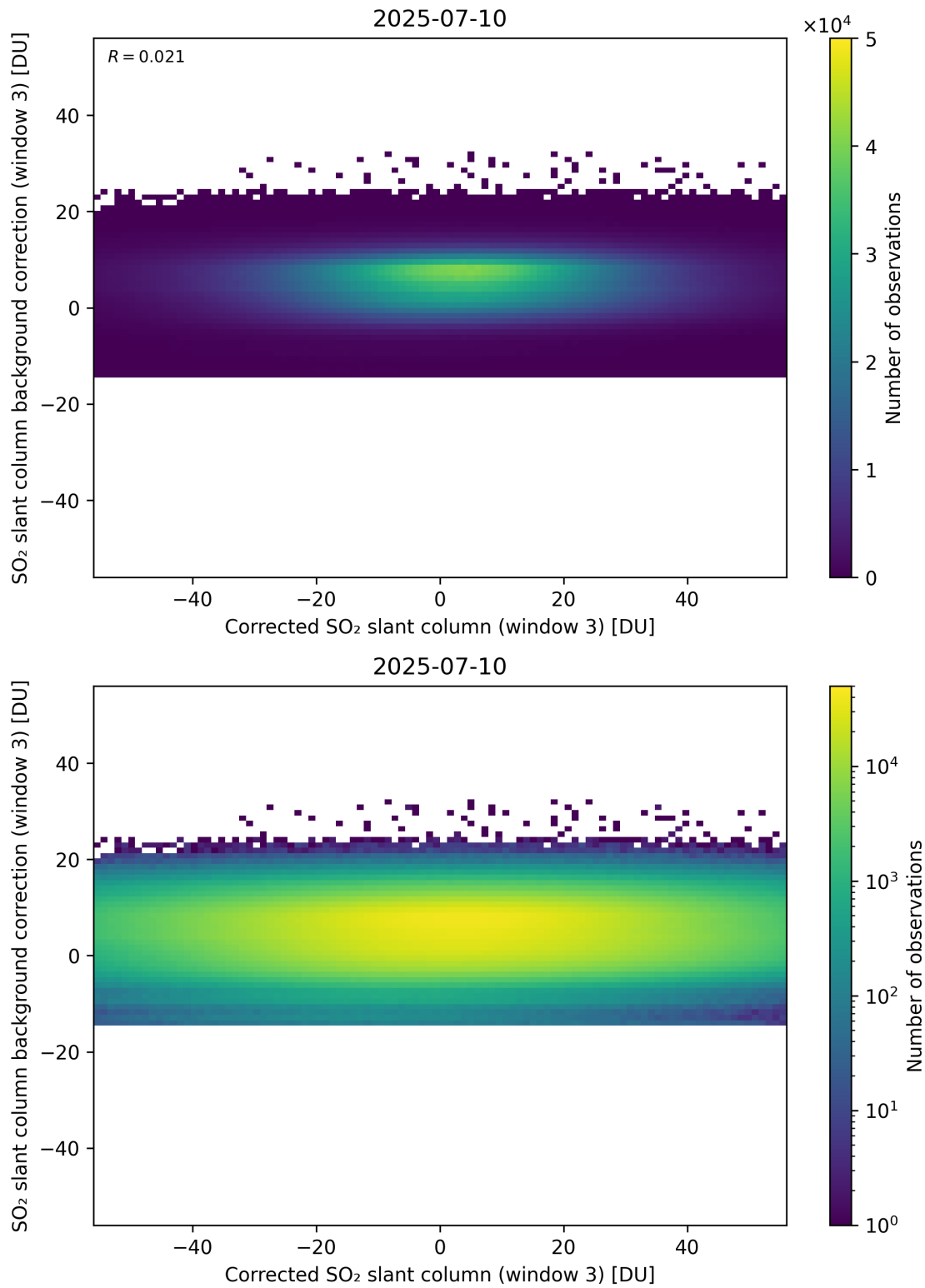
Figure 255: Scatter density plot of “Corrected SO 2 slant column (window 3)” against “SO 2 slant column background correction (window 3)” for 2025-07-09 to 2025-07-11.
