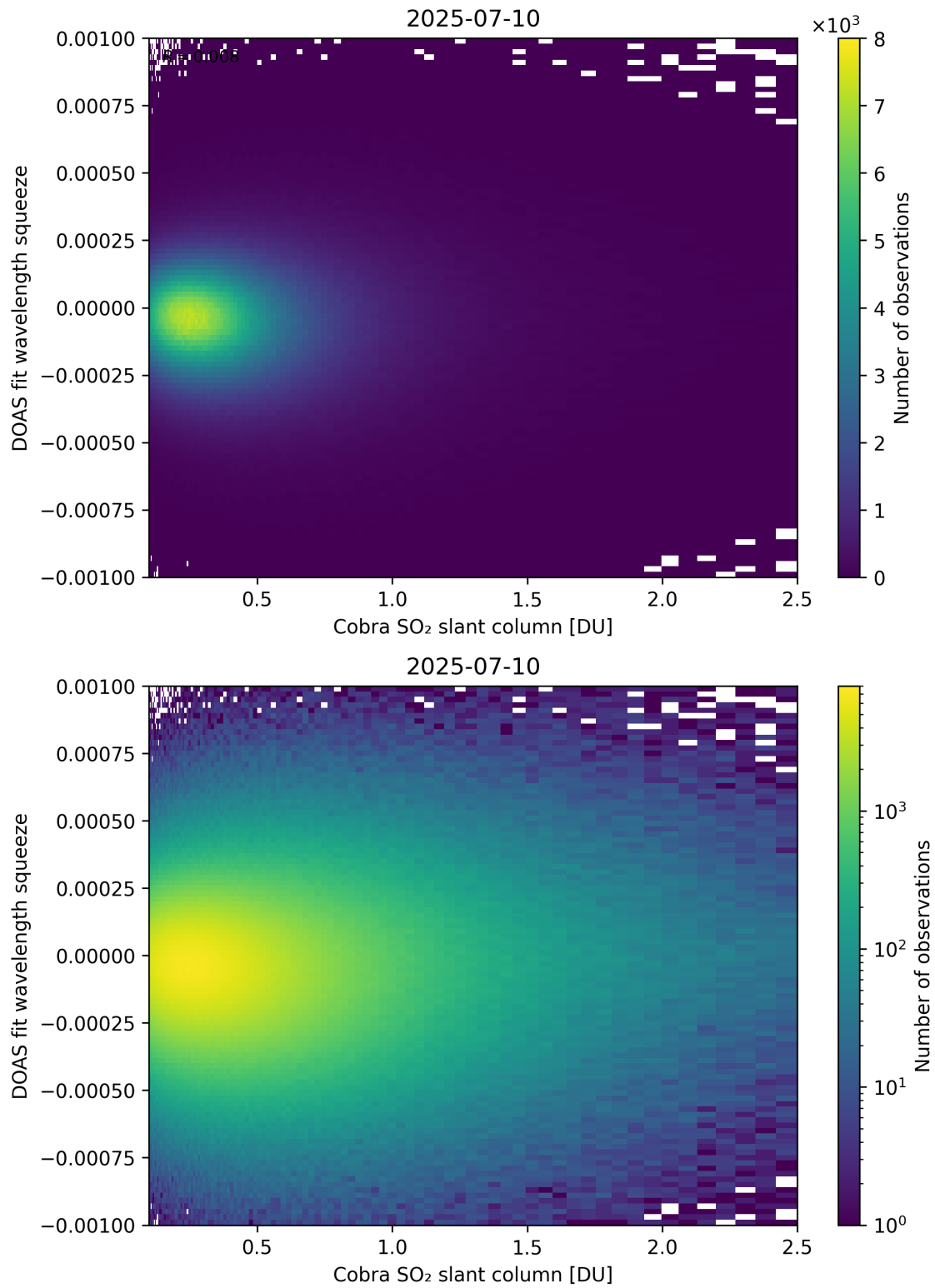
Figure 197: Scatter density plot of “Cobra SO 2 slant column” against “DOAS fit wavelength squeeze” for 2025-07-09 to 2025-07-11.
