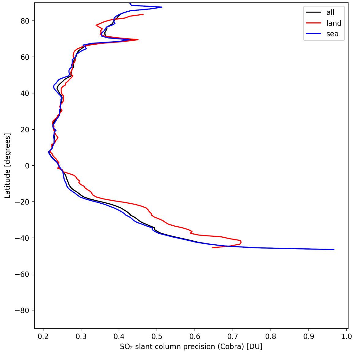
Figure 36: Zonal average of “SO 2 slant column precision (Cobra)” for 2025-07-09 to 2025-07-11.
