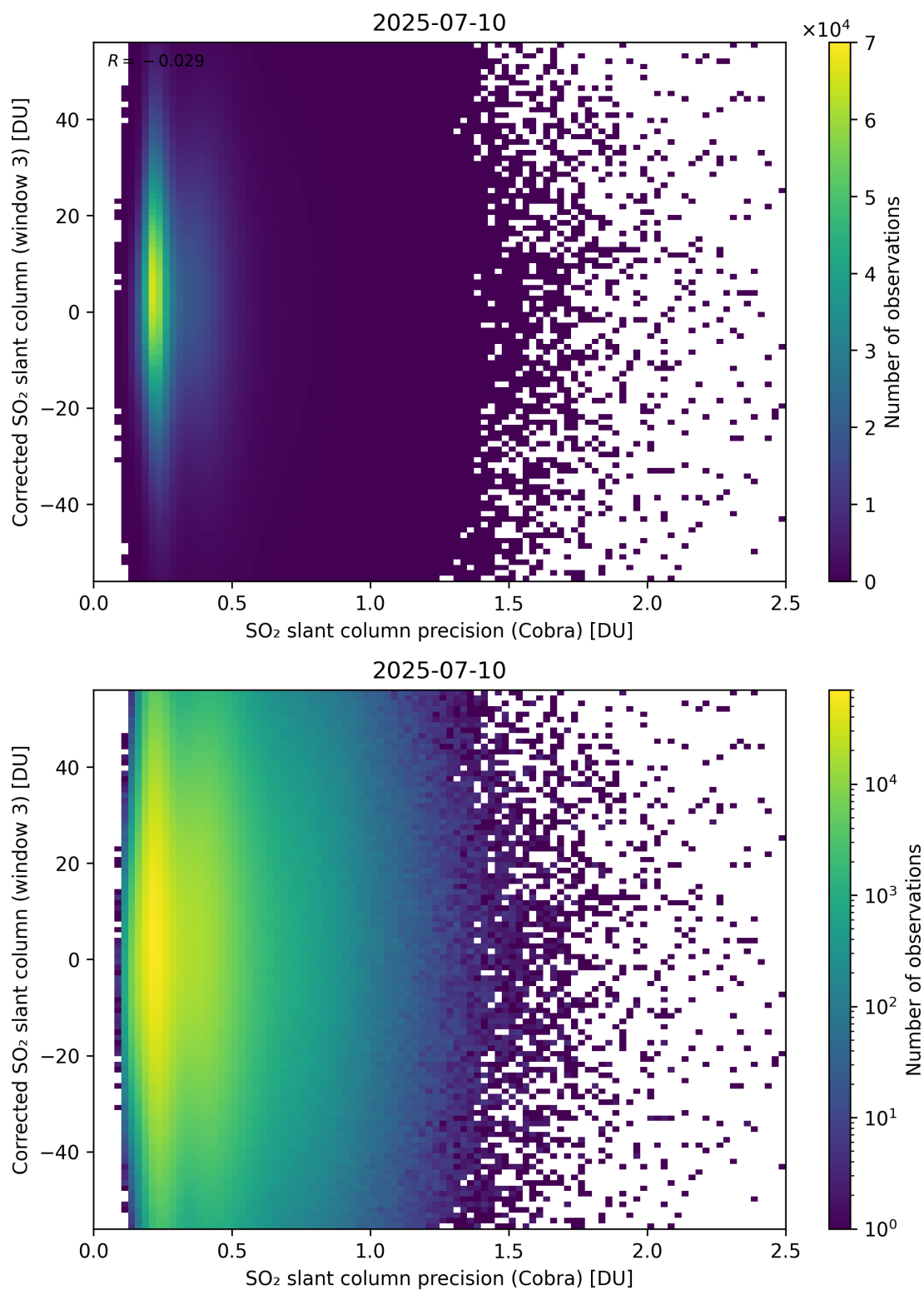
Figure 207: Scatter density plot of “SO 2 slant column precision (Cobra)” against “Corrected SO 2 slant column (window 3)” for 2025-07-09 to 2025-07-11.
