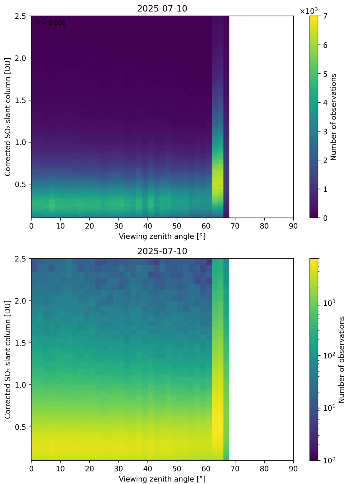
Figure 373: Scatter density plot of “Viewing zenith angle” against “Corrected SO 2 slant column” for 2025-07-09 to 2025-07-11.
