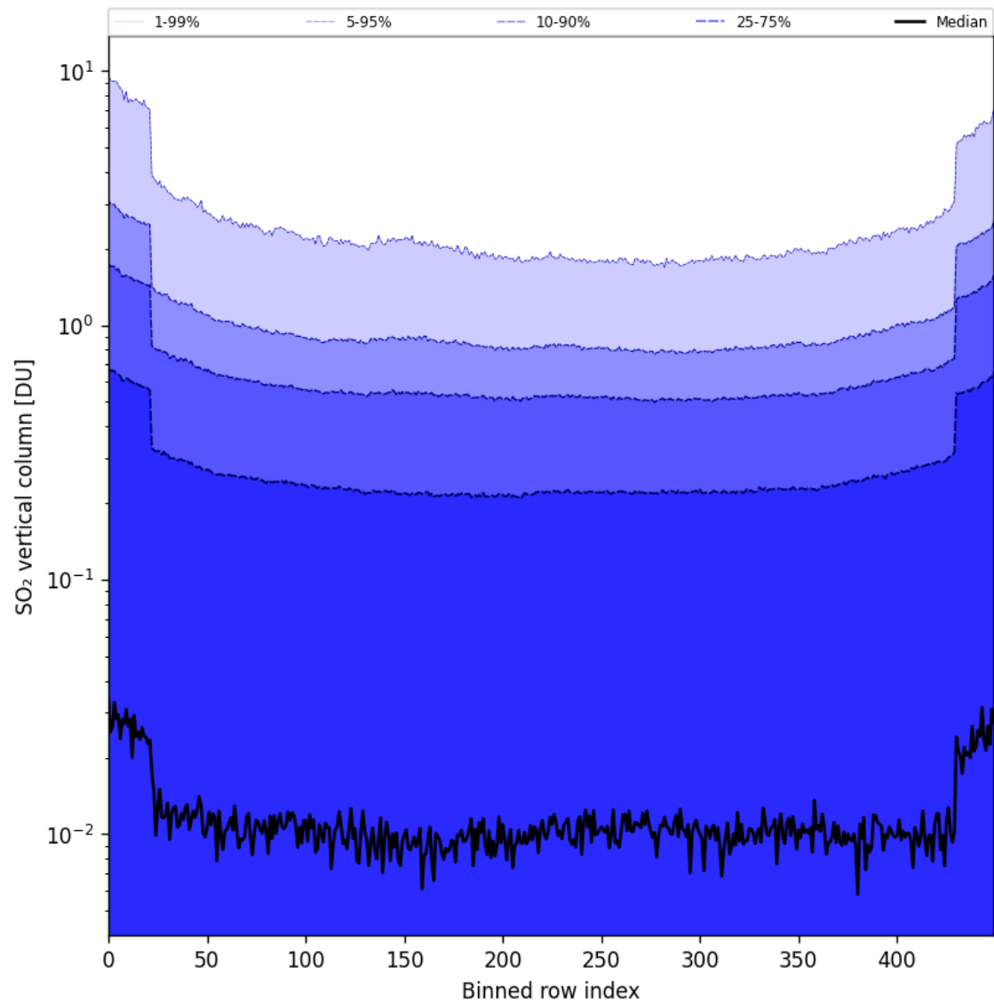
Figure 84: Along track statistics of “SO 2 vertical column” for 2025-07-09 to 2025-07-11
