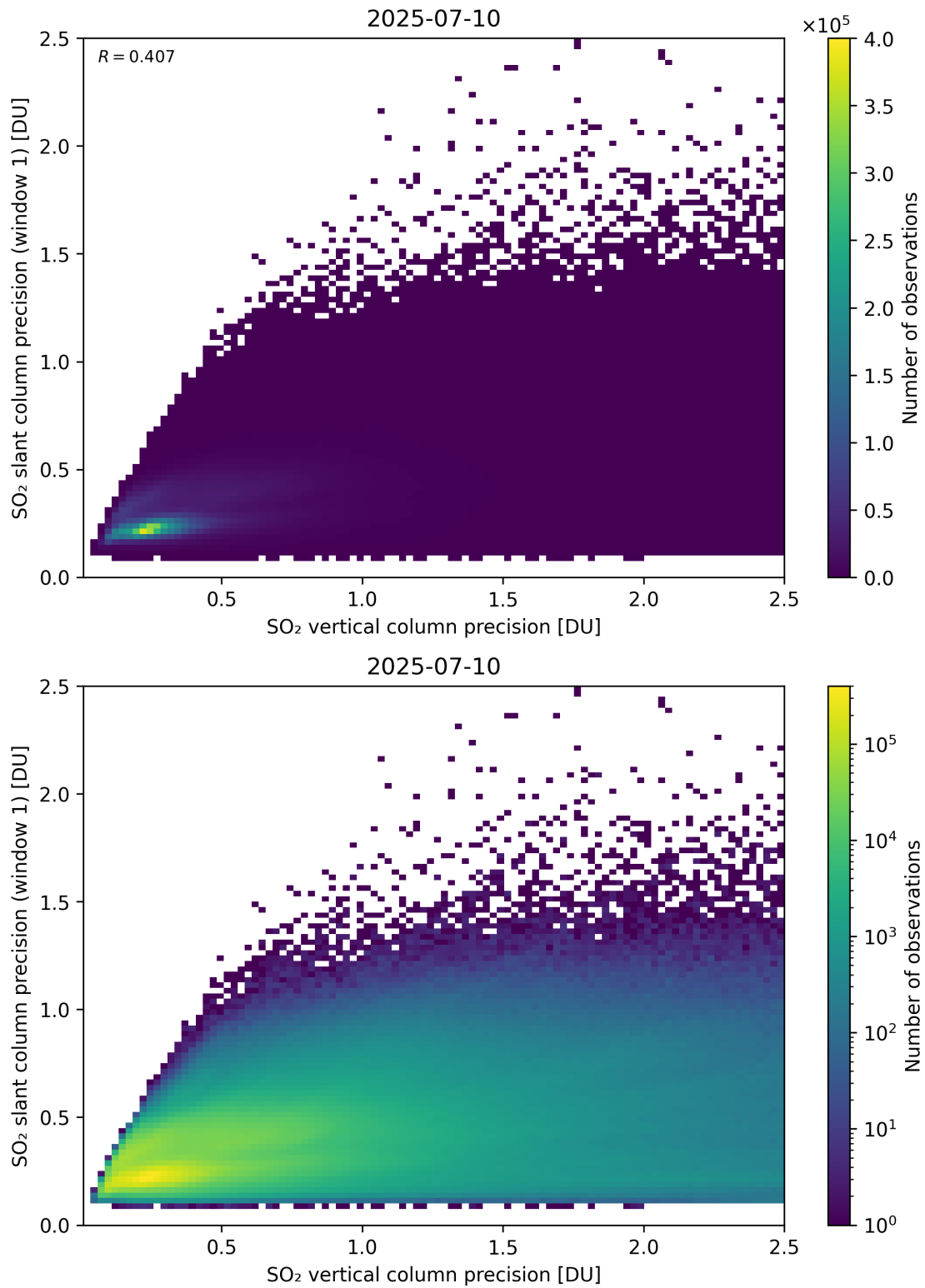
Figure 342: Scatter density plot of “SO 2 vertical column precision” against “SO 2 slant column precision (window 1)” for 2025-07-09 to 2025-07-11.
