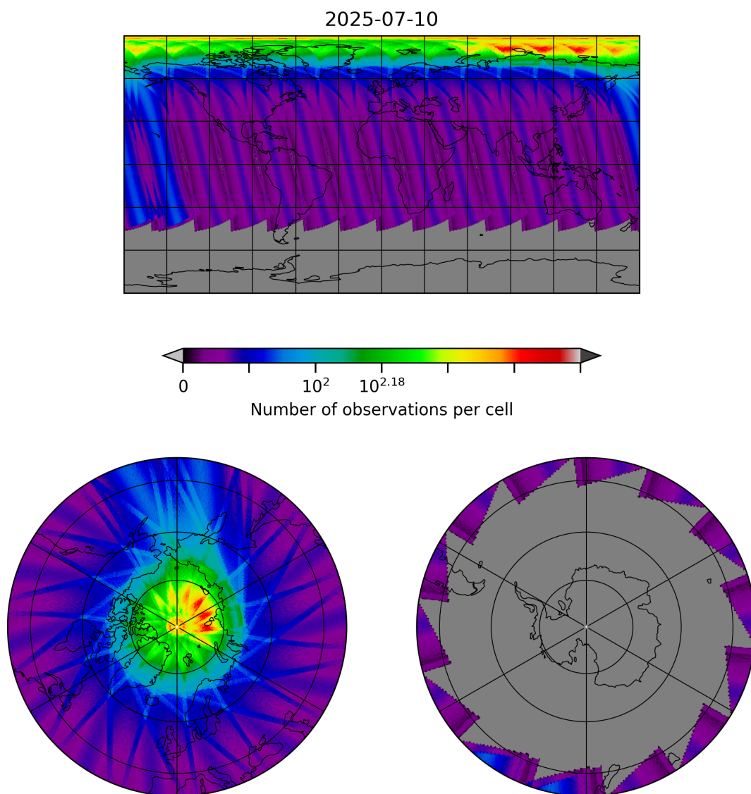
Figure 30: Map of the number of observations for 2025-07-09 to 2025-07-11
