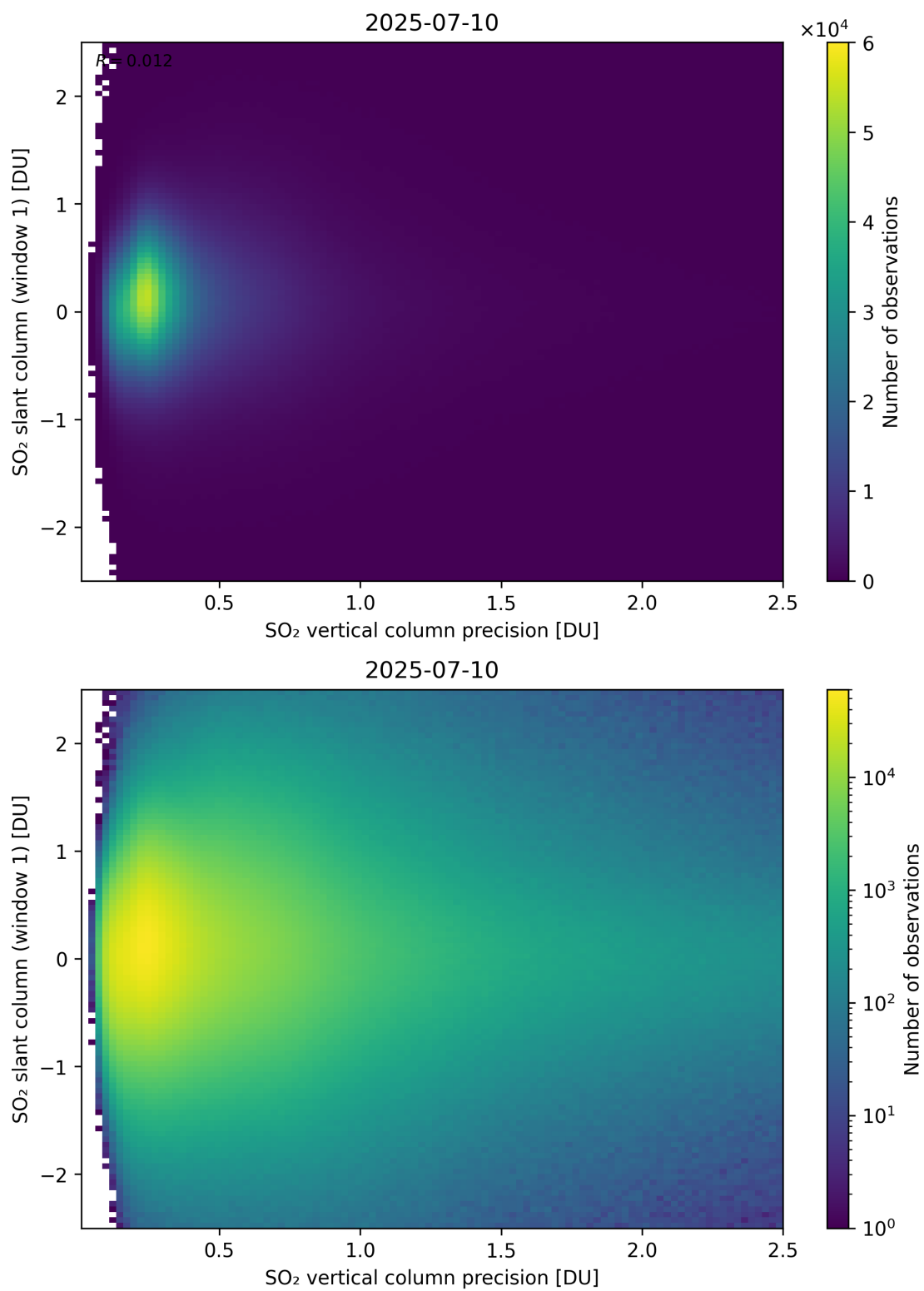
Figure 341: Scatter density plot of “SO 2 vertical column precision” against “SO 2 slant column (window 1)” for 2025-07-09 to 2025-07-11.
