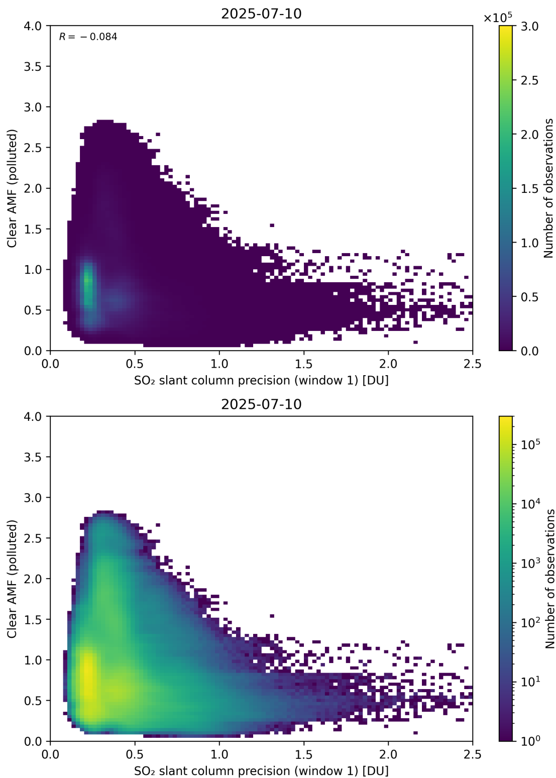
Figure 274: Scatter density plot of “SO 2 slant column precision (window 1)” against “Clear AMF (polluted)” for 2025-07-09 to 2025-07-11.
