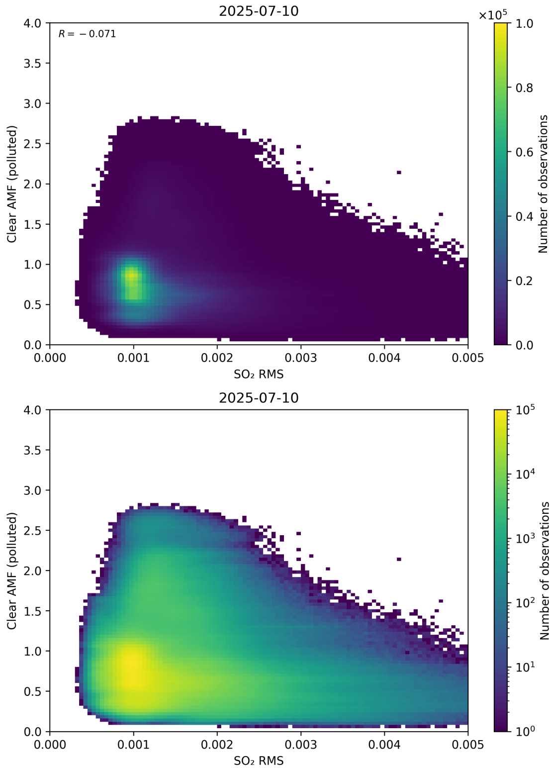
Figure 147: Scatter density plot of “SO 2 RMS” against “Clear AMF (polluted)” for 2025-07-09 to 2025-07-11.
