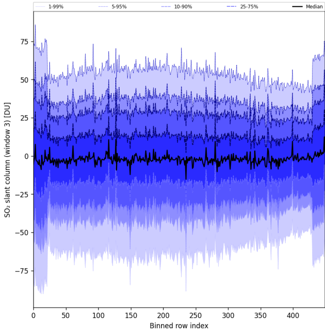
Figure 97: Along track statistics of “SO 2 slant column (window 3)” for 2025-07-09 to 2025-07-11
