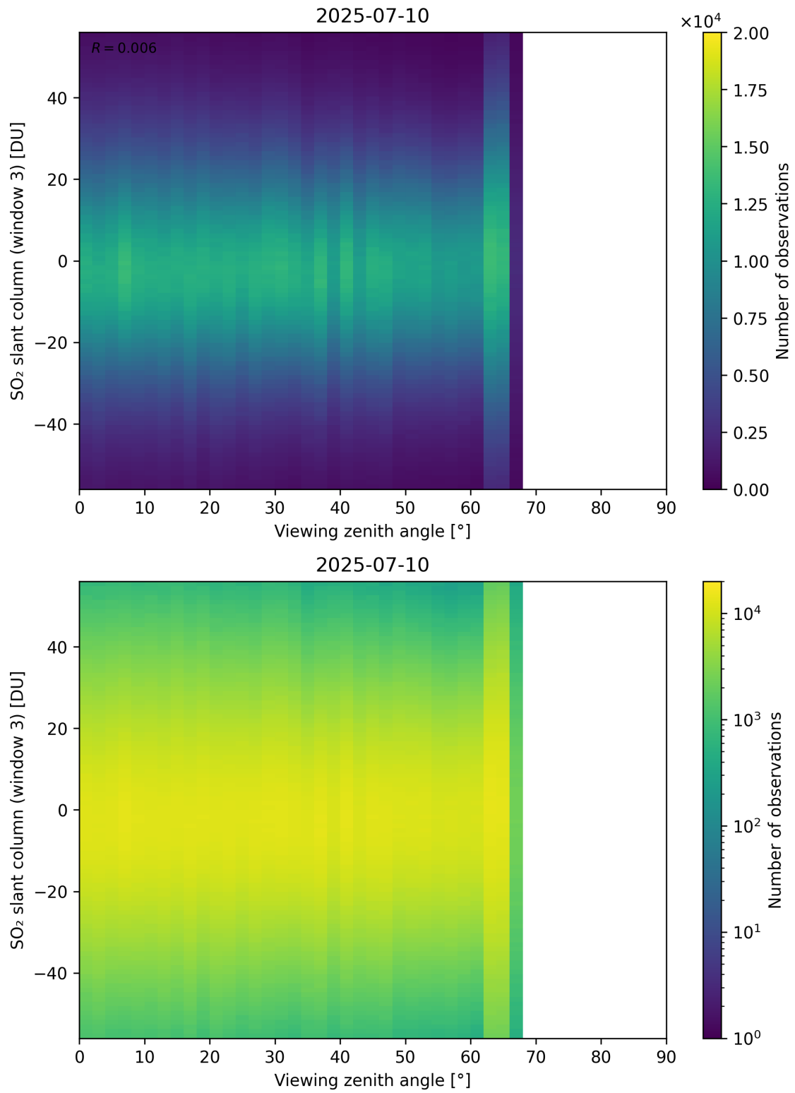
Figure 379: Scatter density plot of “Viewing zenith angle” against “SO 2 slant column (window 3)” for 2025-07-09 to 2025-07-11.
