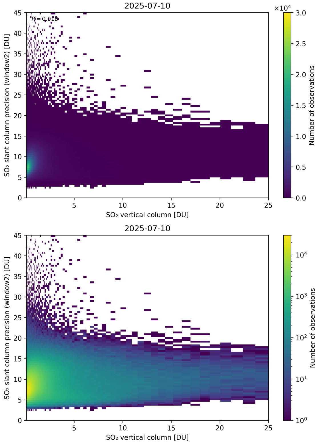
Figure 356: Scatter density plot of “SO 2 vertical column” against “SO 2 slant column precision (window2)” for 2025-07-09 to 2025-07-11.
