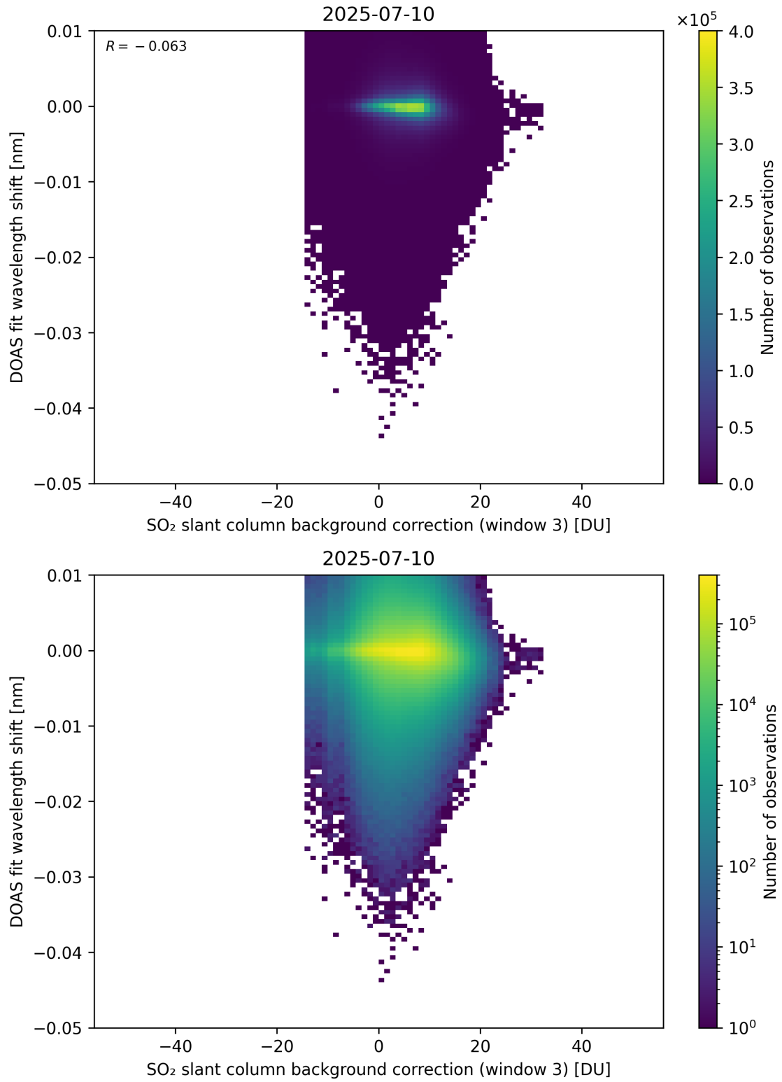
Figure 132: Scatter density plot of “SO 2 slant column background correction (window 3)” against “DOAS fit wavelength shift” for 2025-07-09 to 2025-07-11.
