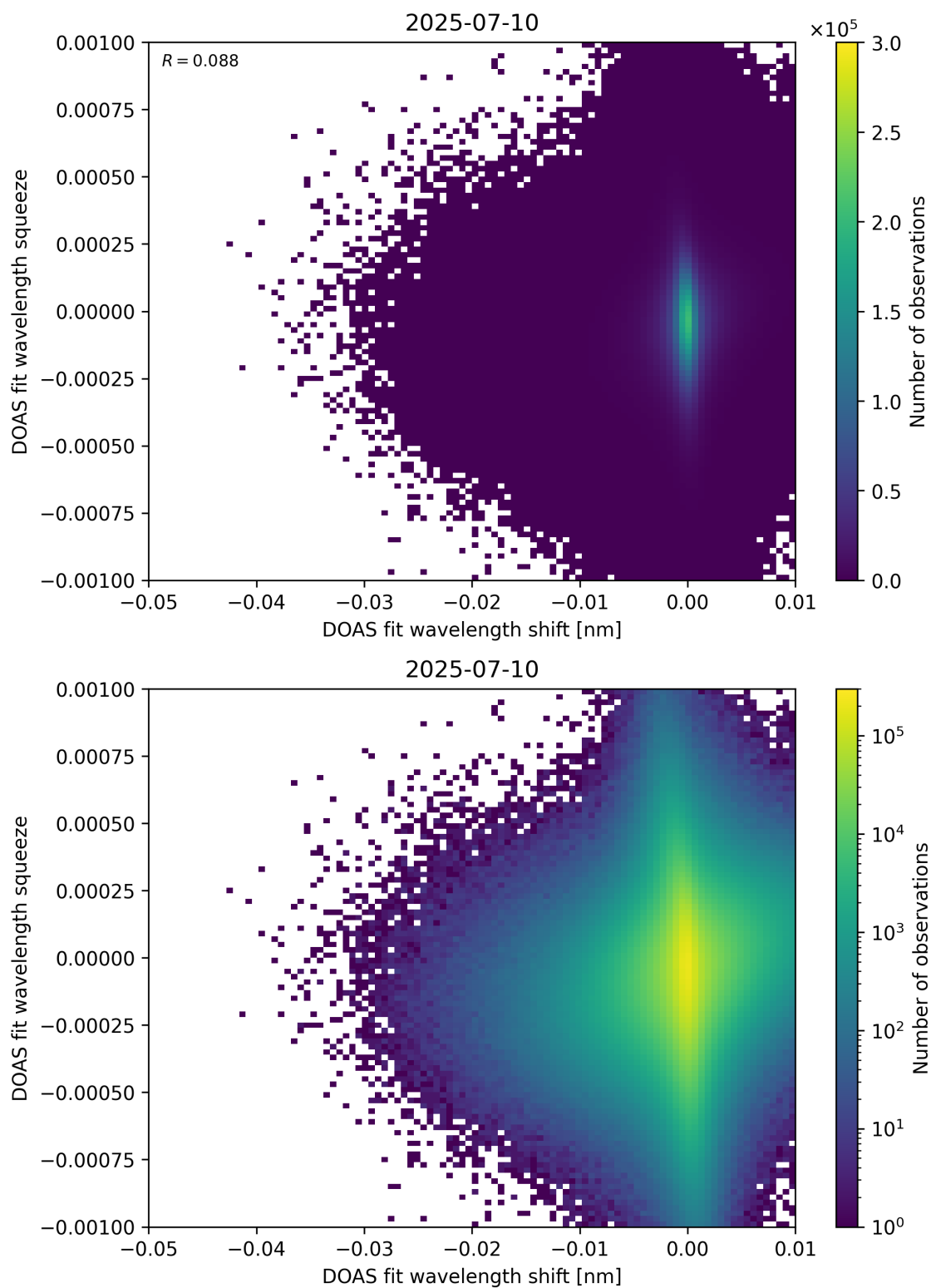
Figure 138: Scatter density plot of “DOAS fit wavelength shift” against “DOAS fit wavelength squeeze” for 2025-07-09 to 2025-07-11.
