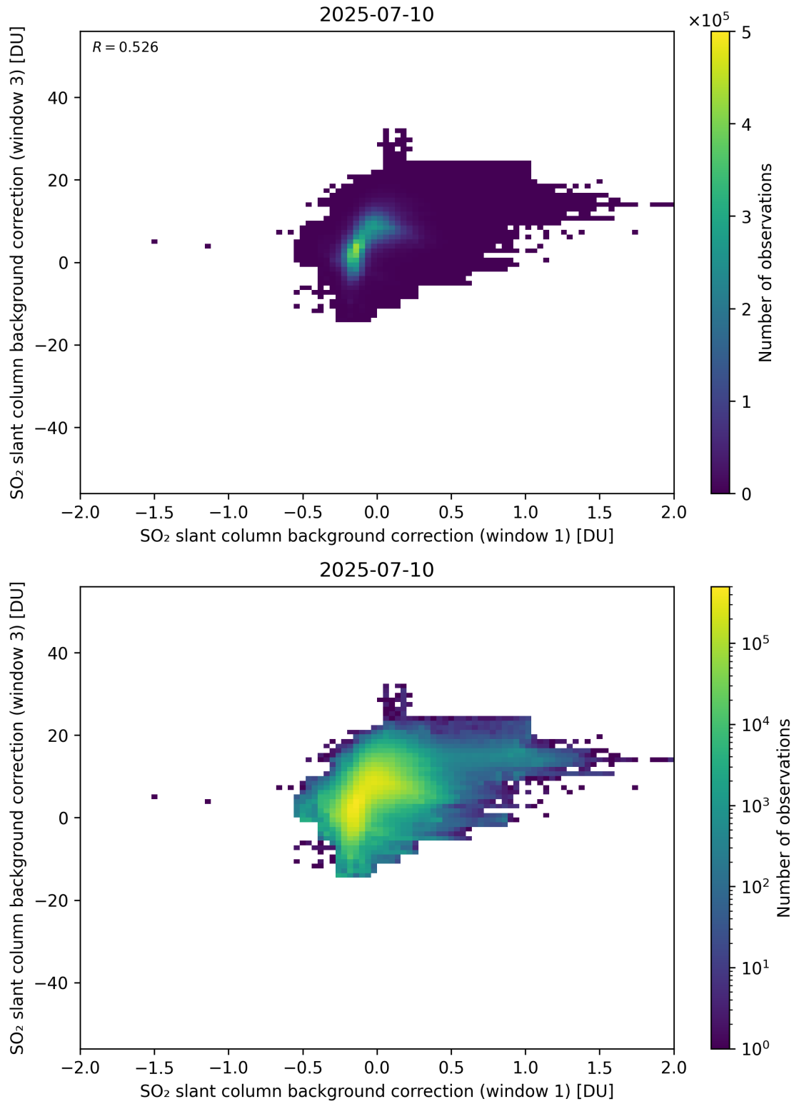
Figure 110: Scatter density plot of “SO 2 slant column background correction (window 1)” against “SO 2 slant column background correction (window 3)” for 2025-07-09 to 2025-07-11.
