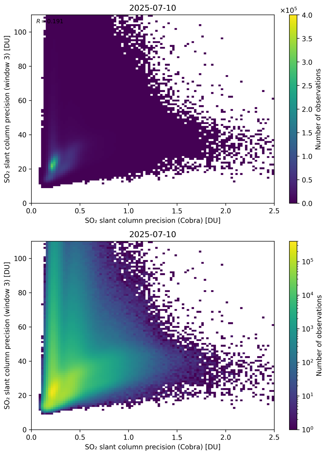
Figure 212: Scatter density plot of “SO 2 slant column precision (Cobra)” against “SO 2 slant column precision (window 3)” for 2025-07-09 to 2025-07-11.
