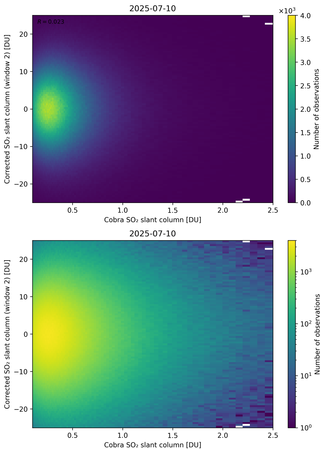
Figure 217: Scatter density plot of “Cobra SO 2 slant column” against “Corrected SO 2 slant column (window 2)” for 2025-07-09 to 2025-07-11.
