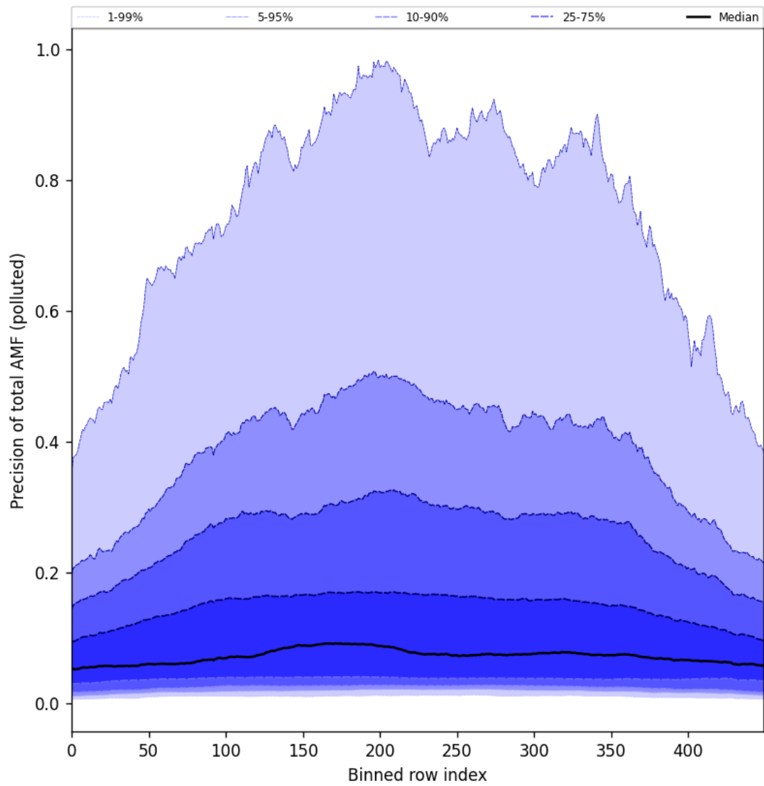
Figure 106: Along track statistics of “Precision of total AMF (polluted)” for 2025-07-09 to 2025-07-11
