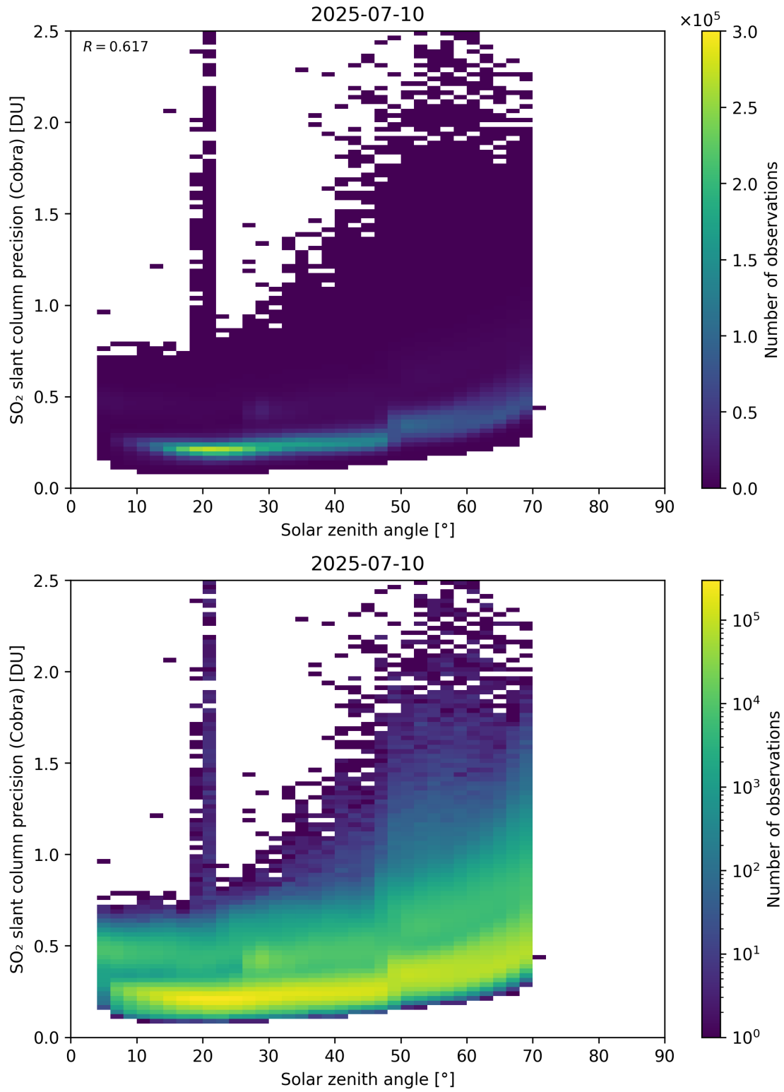
Figure 180: Scatter density plot of “Solar zenith angle” against “SO 2 slant column precision (Cobra)” for 2025-07-09 to 2025-07-11.
