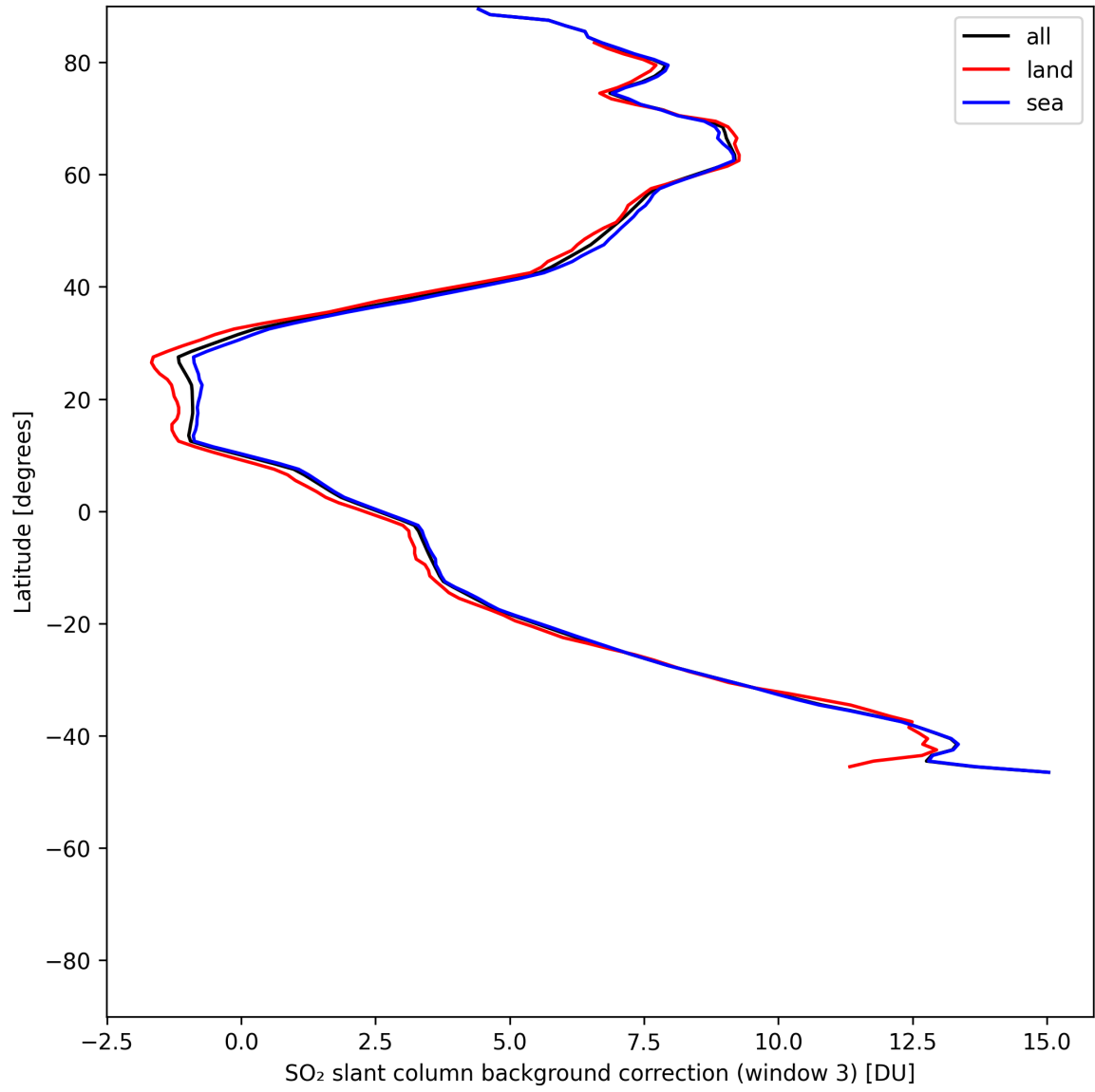
Figure 48: Zonal average of “SO 2 slant column background correction (window 3)” for 2025-07-09 to 2025-07-11.
