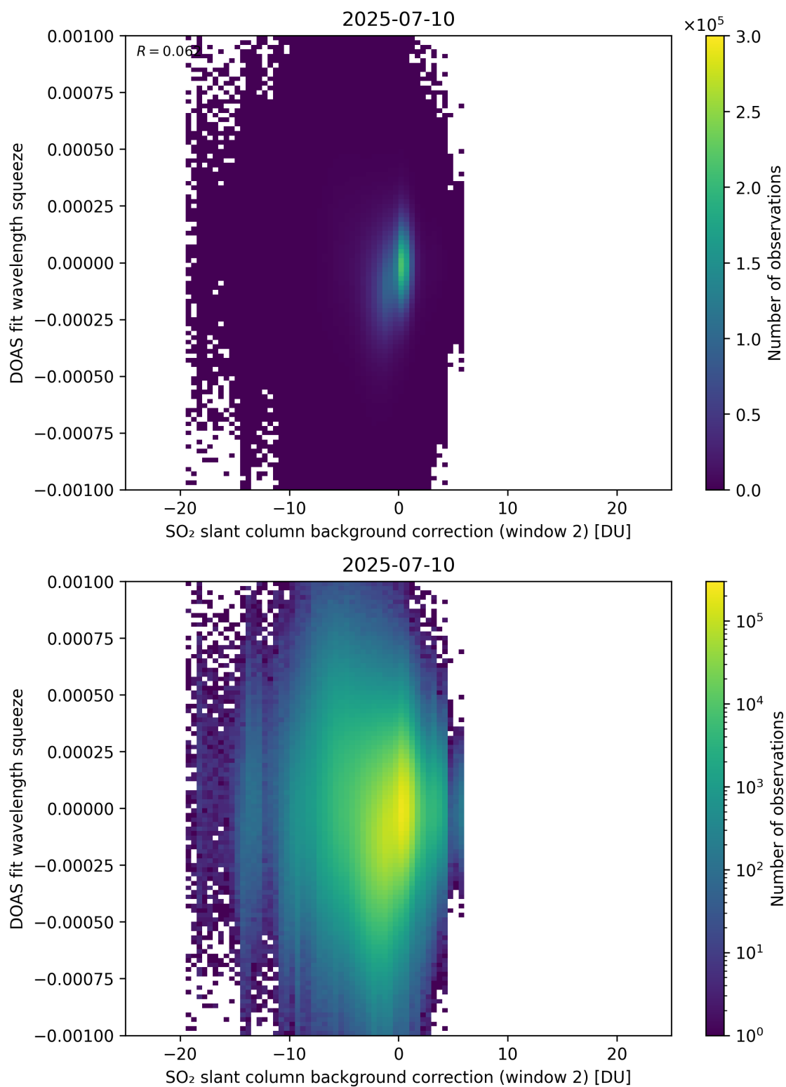
Figure 124: Scatter density plot of “SO 2 slant column background correction (window 2)” against “DOAS fit wavelength squeeze” for 2025-07-09 to 2025-07-11.
