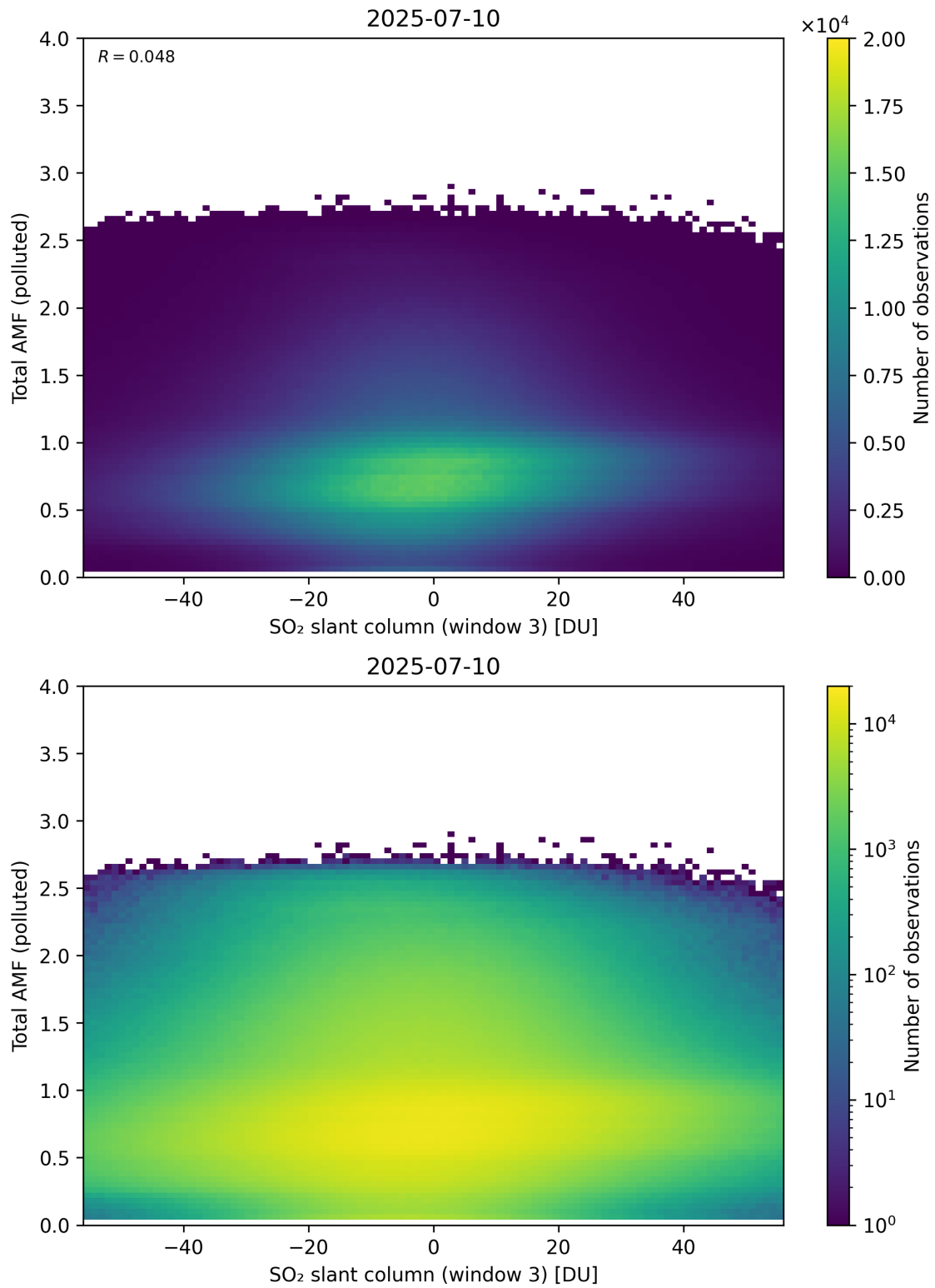
Figure 318: Scatter density plot of “SO 2 slant column (window 3)” against “Total AMF (polluted)” for 2025-07-09 to 2025-07-11.
