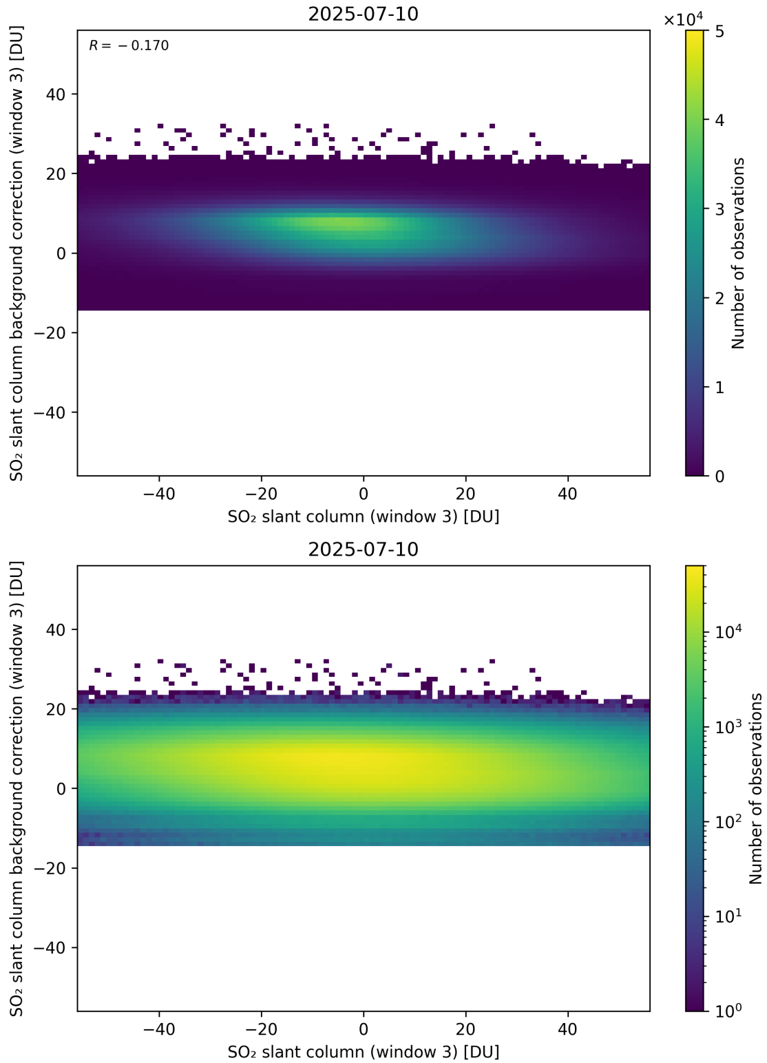
Figure 303: Scatter density plot of “SO 2 slant column (window 3)” against “SO 2 slant column background correction (window 3)” for 2025-07-09 to 2025-07-11.
