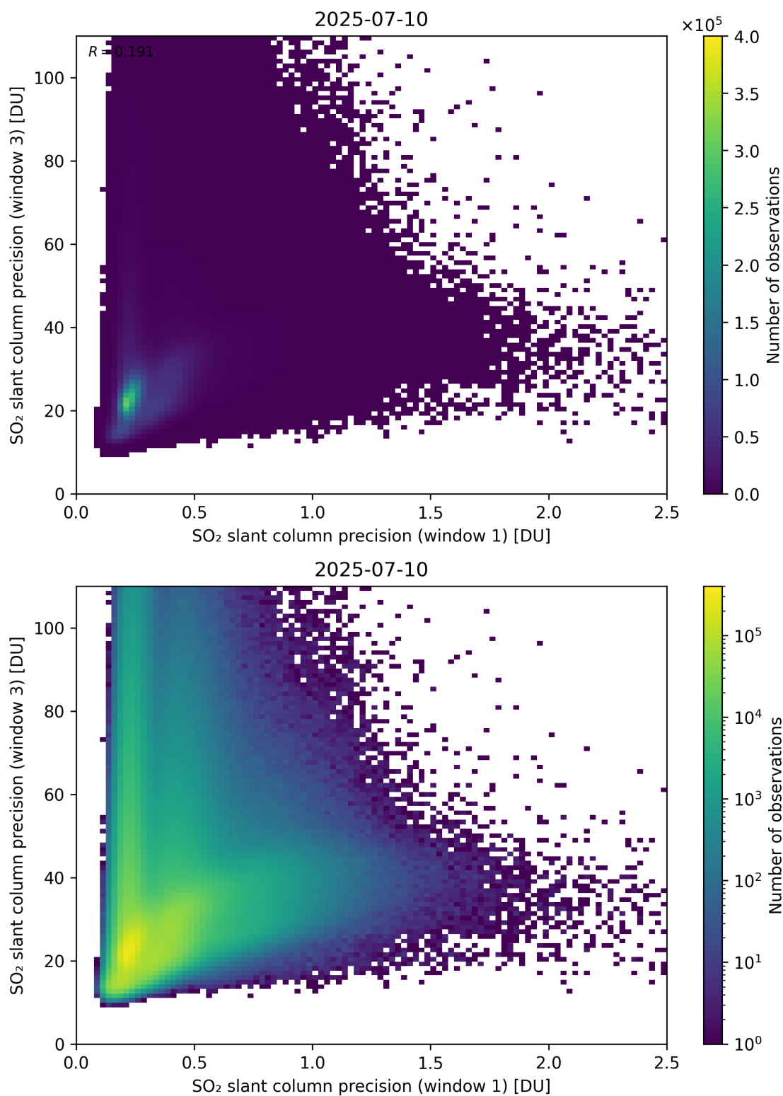
Figure 279: Scatter density plot of “SO 2 slant column precision (window 1)” against “SO 2 slant column precision (window 3)” for 2025-07-09 to 2025-07-11.
