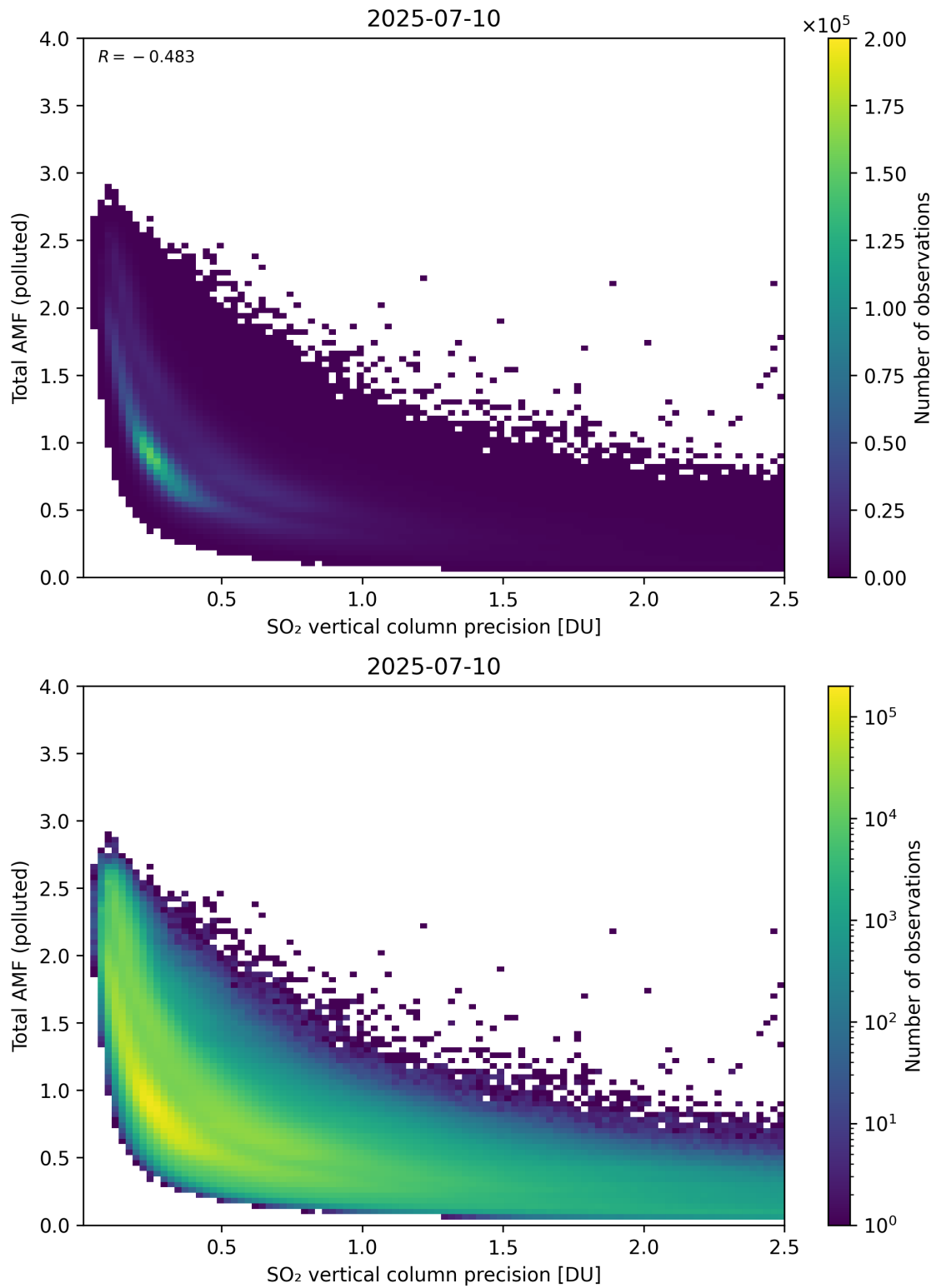
Figure 346: Scatter density plot of “SO 2 vertical column precision” against “Total AMF (polluted)” for 2025-07-09 to 2025-07-11.
