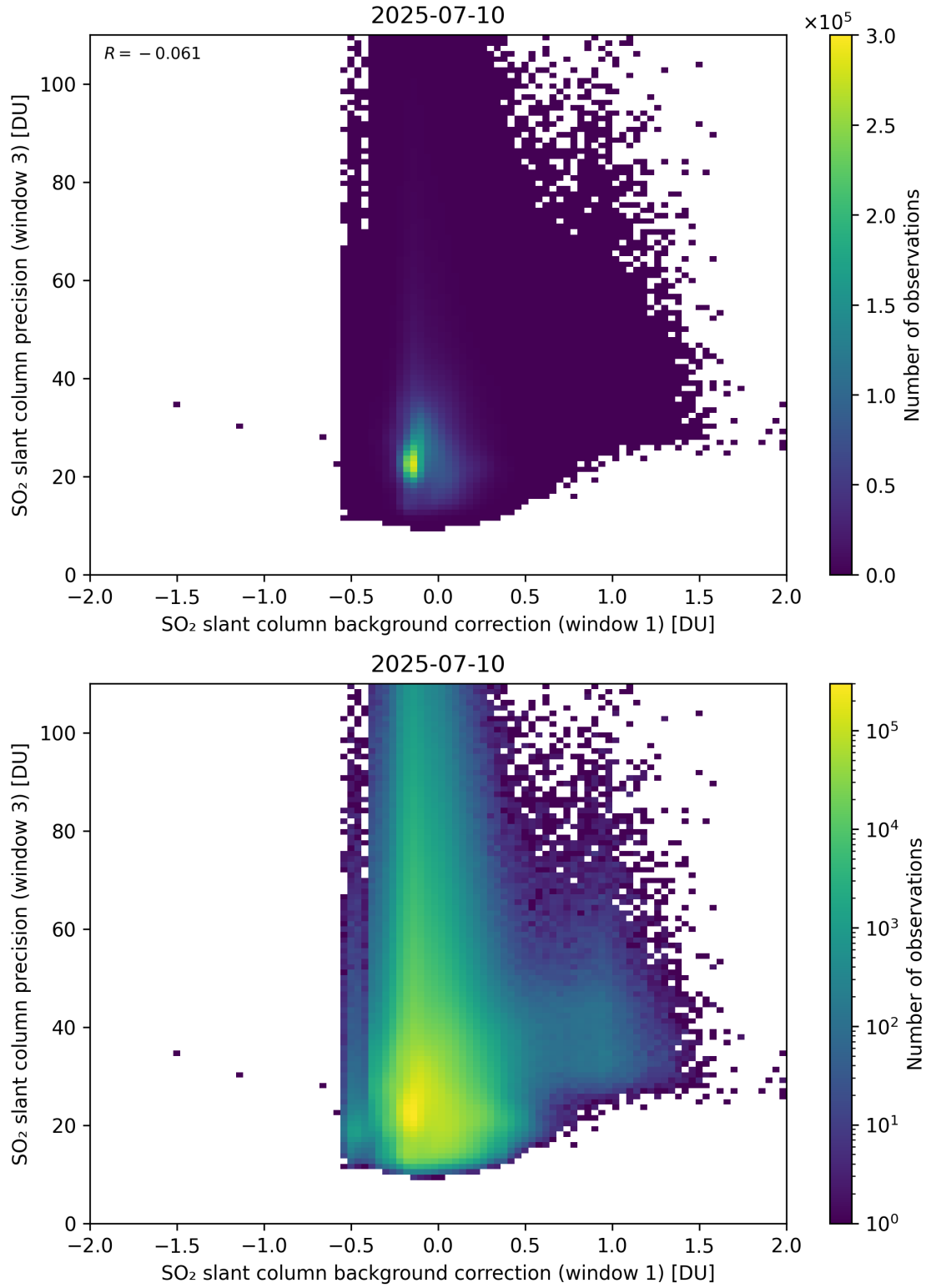
Figure 119: Scatter density plot of “SO 2 slant column background correction (window 1)” against “SO 2 slant column precision (window 3)” for 2025-07-09 to 2025-07-11.
