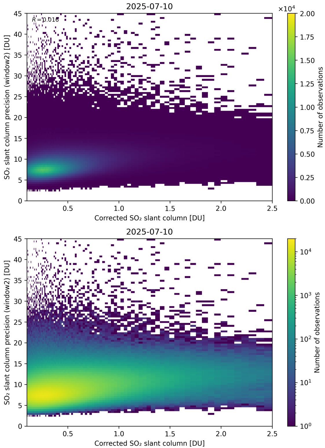
Figure 239: Scatter density plot of “Corrected SO 2 slant column” against “SO 2 slant column precision (window2)” for 2025-07-09 to 2025-07-11.
