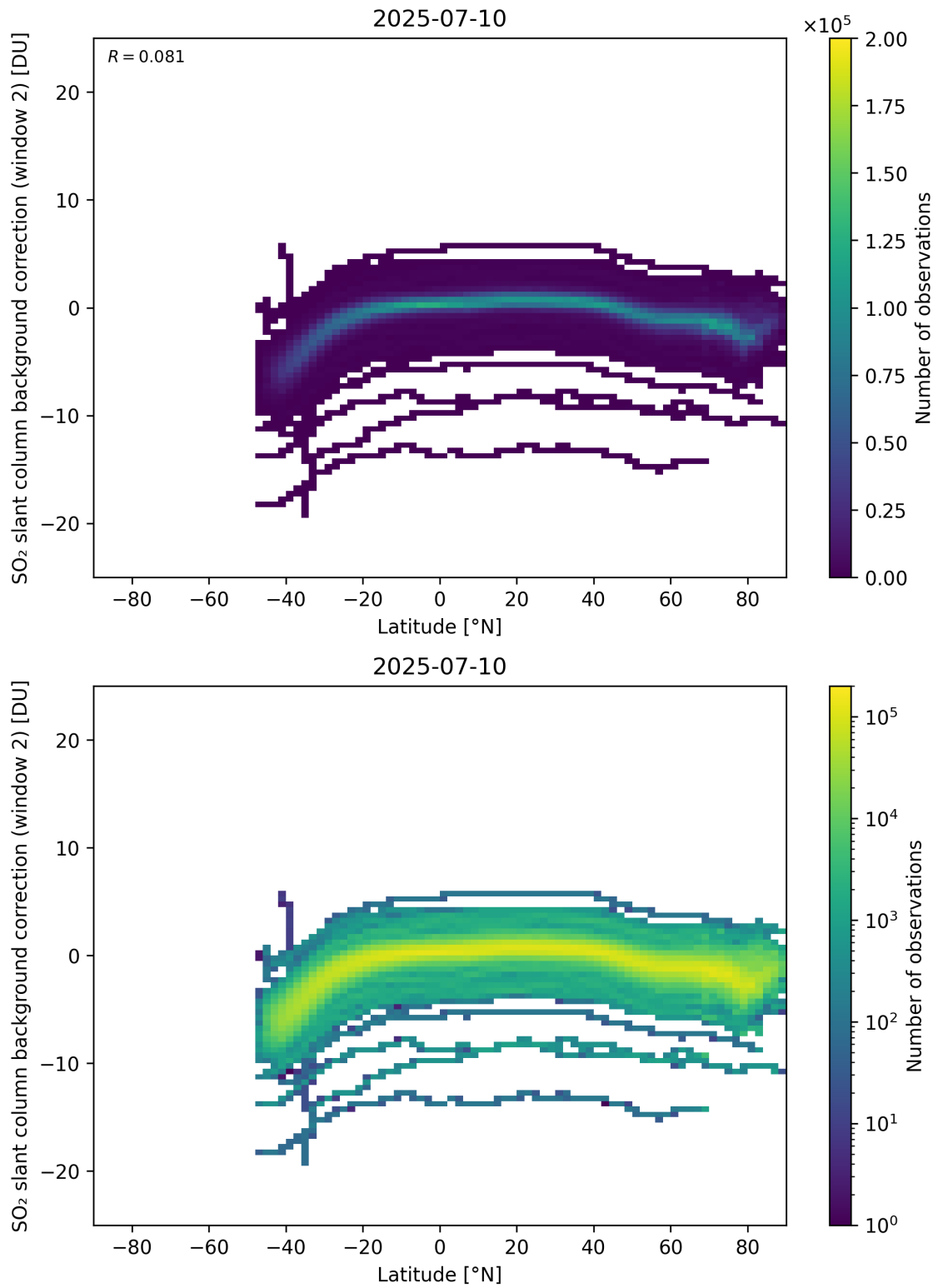
Figure 151: Scatter density plot of “Latitude” against “SO 2 slant column background correction (window 2)” for 2025-07-09 to 2025-07-11.
