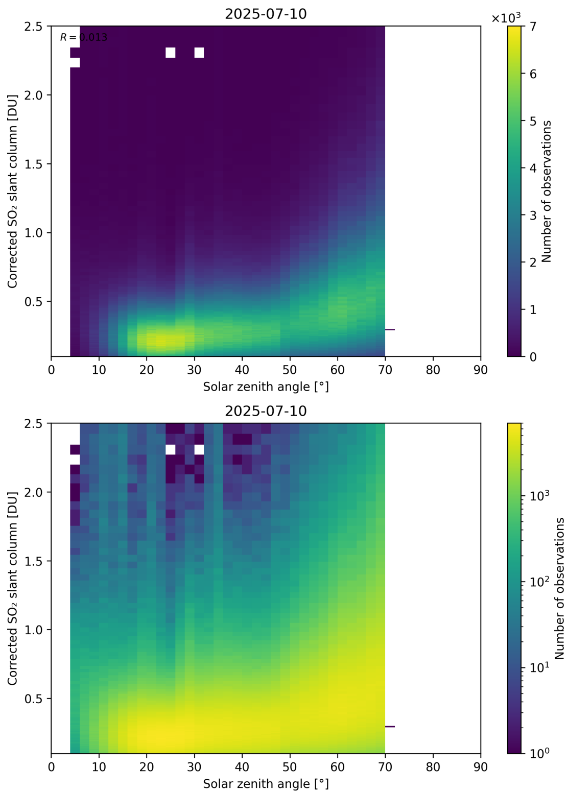
Figure 181: Scatter density plot of “Solar zenith angle” against “Corrected SO 2 slant column” for 2025-07-09 to 2025-07-11.
