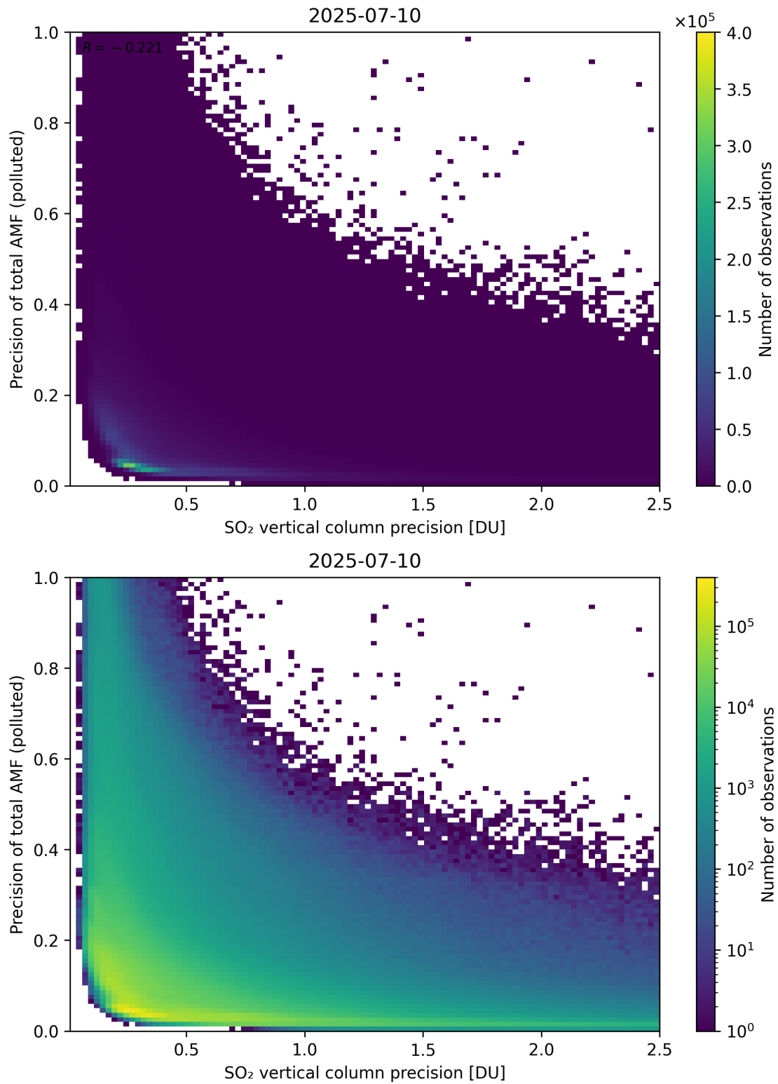
Figure 347: Scatter density plot of “SO 2 vertical column precision” against “Precision of total AMF (polluted)” for 2025-07-09 to 2025-07-11.
