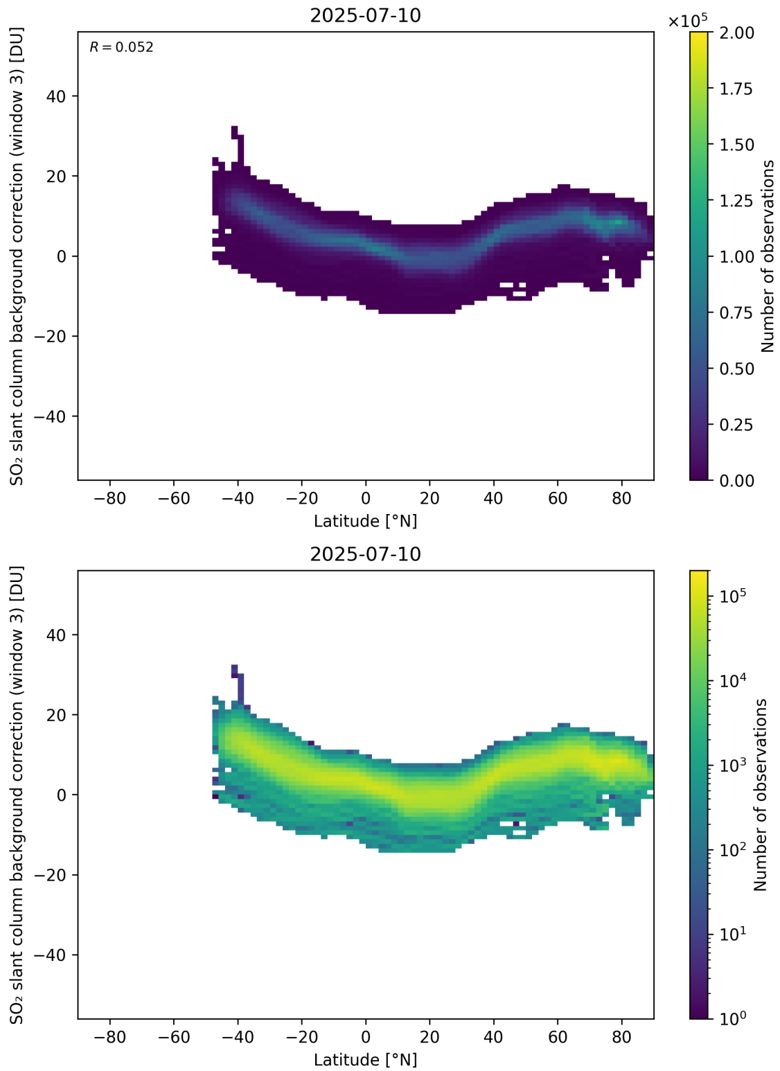
Figure 152: Scatter density plot of “Latitude” against “SO 2 slant column background correction (window 3)” for 2025-07-09 to 2025-07-11.
