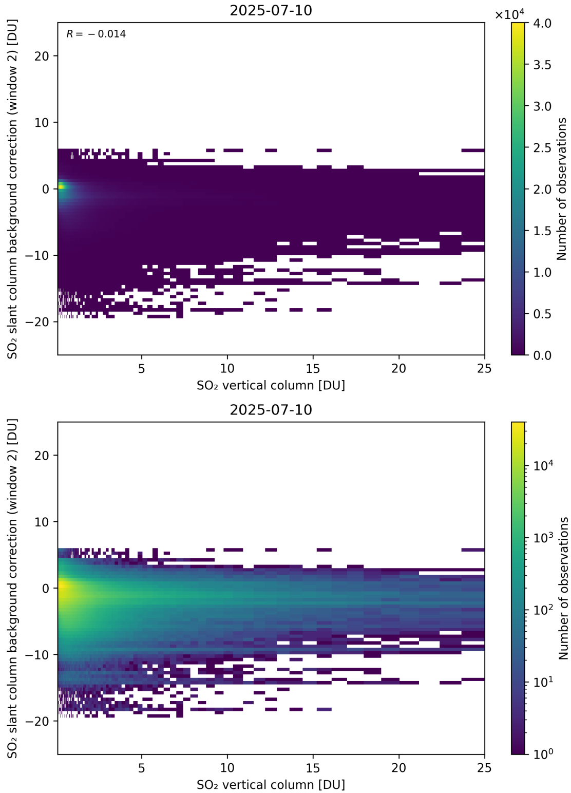
Figure 324: Scatter density plot of “SO 2 vertical column” against “SO 2 slant column background correction (window 2)” for 2025-07-09 to 2025-07-11.
