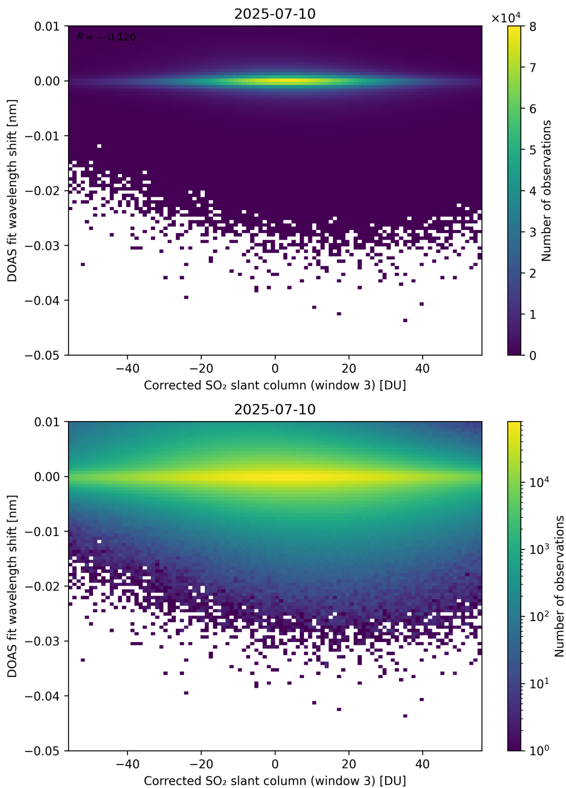
Figure 256: Scatter density plot of “Corrected SO 2 slant column (window 3)” against “DOAS fit wavelength shift” for 2025-07-09 to 2025-07-11.
