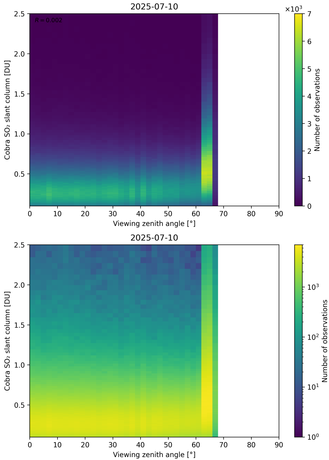
Figure 371: Scatter density plot of “Viewing zenith angle” against “Cobra SO 2 slant column” for 2025-07-09 to 2025-07-11.
