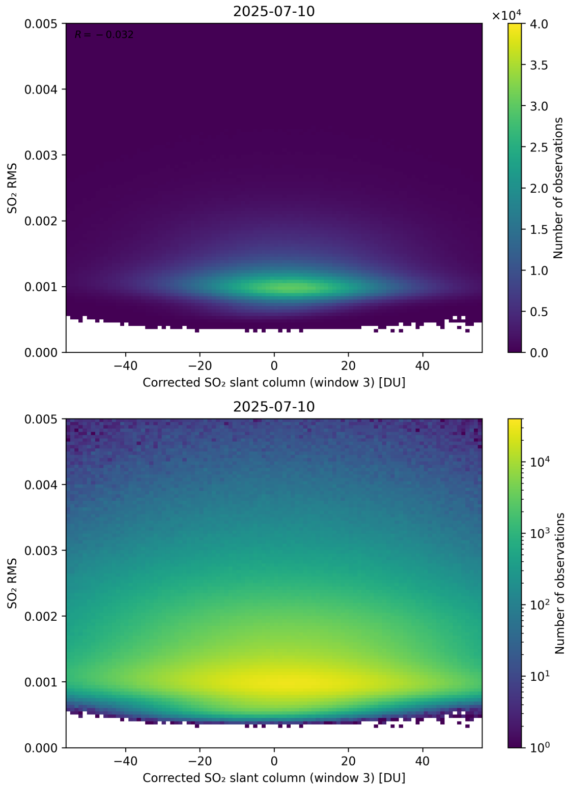
Figure 258: Scatter density plot of “Corrected SO 2 slant column (window 3)” against “SO 2 RMS” for 2025-07-09 to 2025-07-11.
