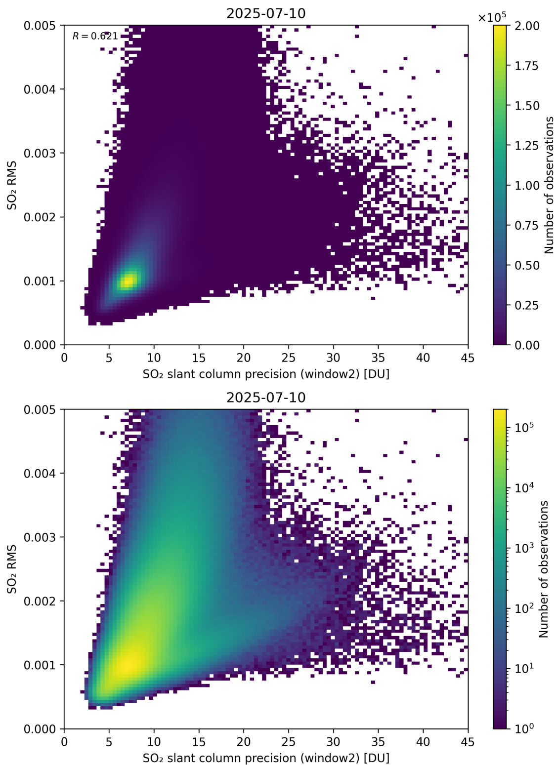
Figure 295: Scatter density plot of “SO 2 slant column precision (window2)” against “SO 2 RMS” for 2025-07-09 to 2025-07-11.
