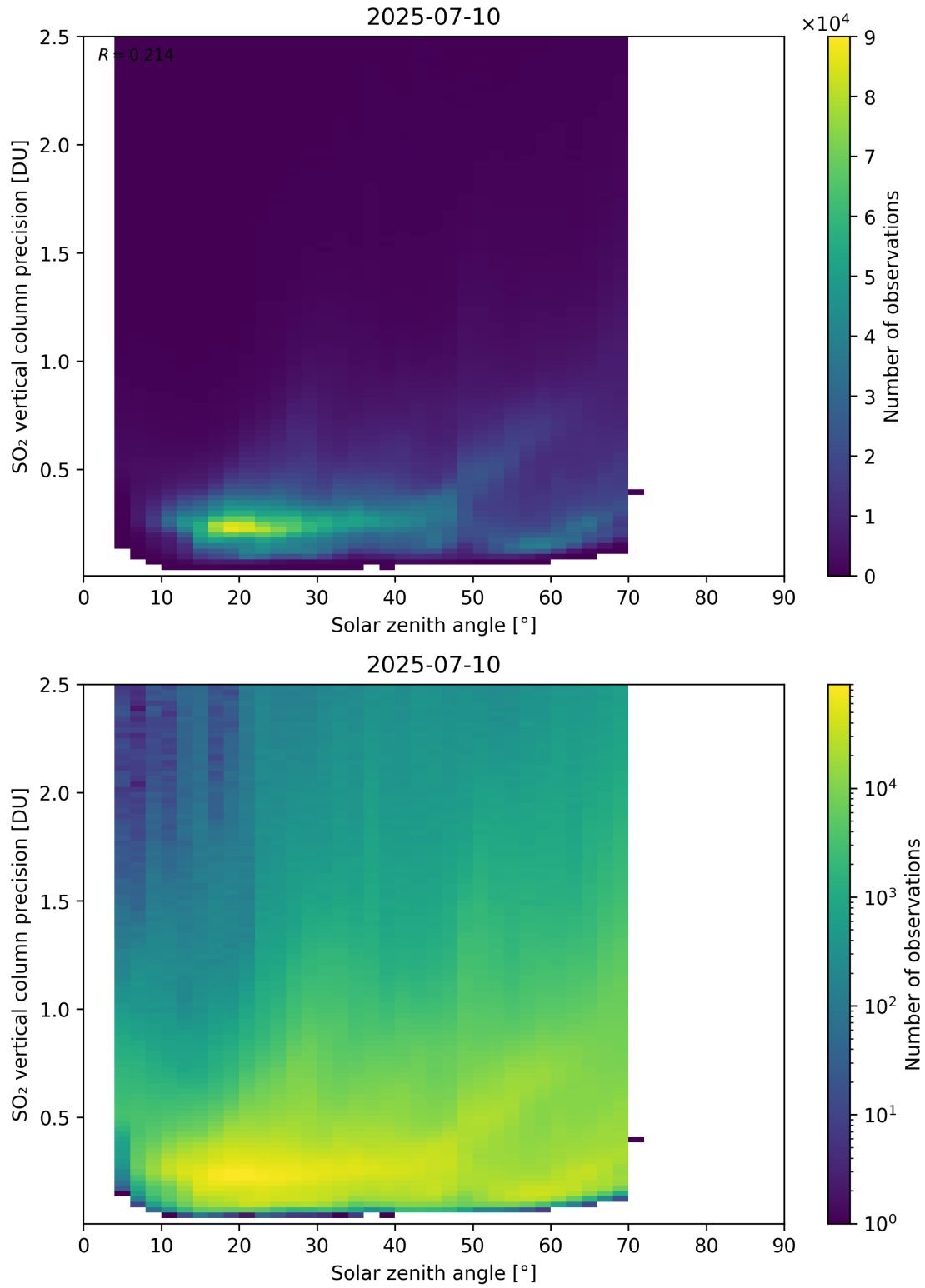
Figure 192: Scatter density plot of “Solar zenith angle” against “SO 2 vertical column precision” for 2025-07-09 to 2025-07-11.
