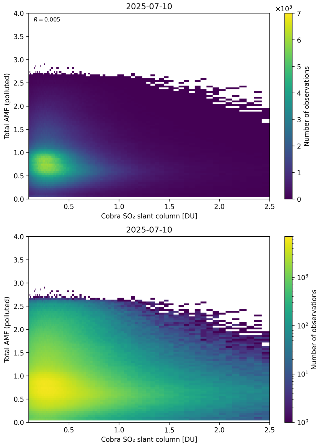
Figure 224: Scatter density plot of “Cobra SO 2 slant column” against “Total AMF (polluted)” for 2025-07-09 to 2025-07-11.
