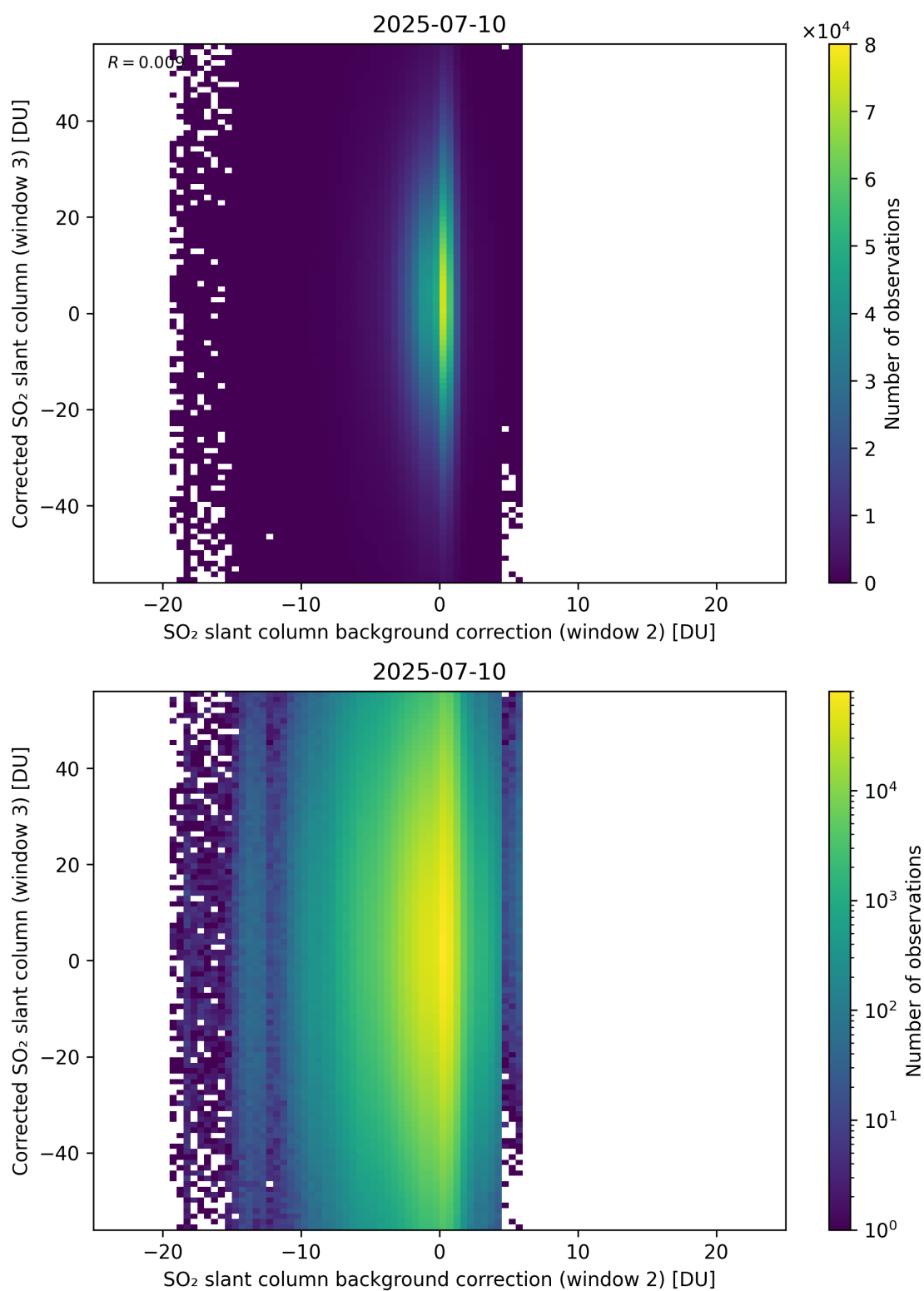
Figure 127: Scatter density plot of “SO 2 slant column background correction (window 2)” against “Corrected SO 2 slant column (window 3)” for 2025-07-09 to 2025-07-11.
