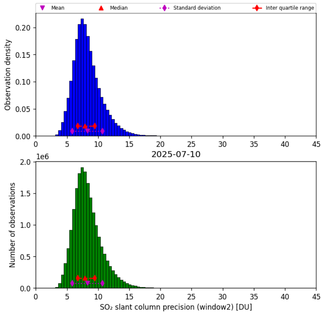
Figure 68: Histogram of “SO 2 slant column precision (window2)” for 2025-07-09 to 2025-07-11
