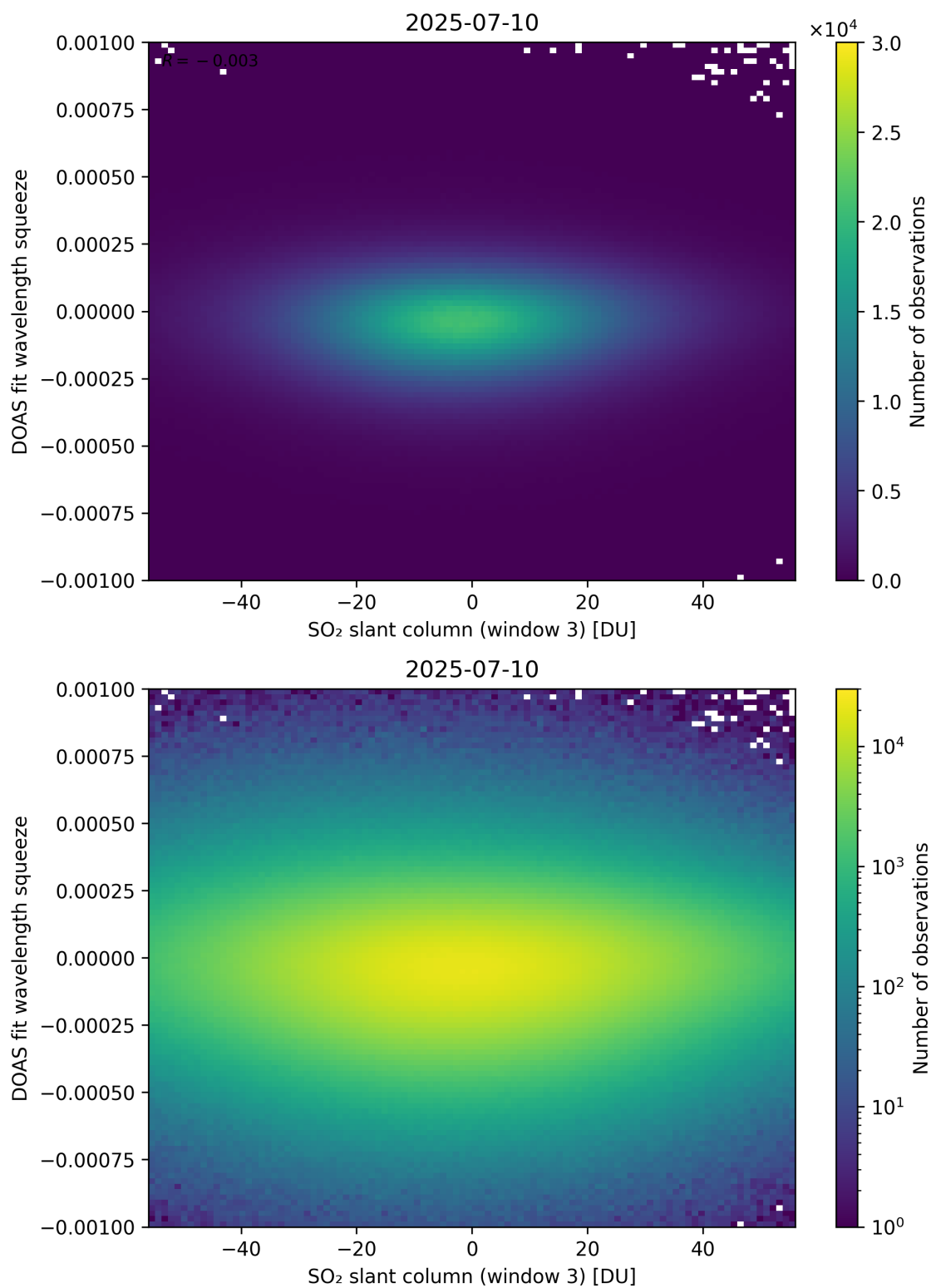
Figure 305: Scatter density plot of “SO 2 slant column (window 3)” against “DOAS fit wavelength squeeze” for 2025-07-09 to 2025-07-11.
