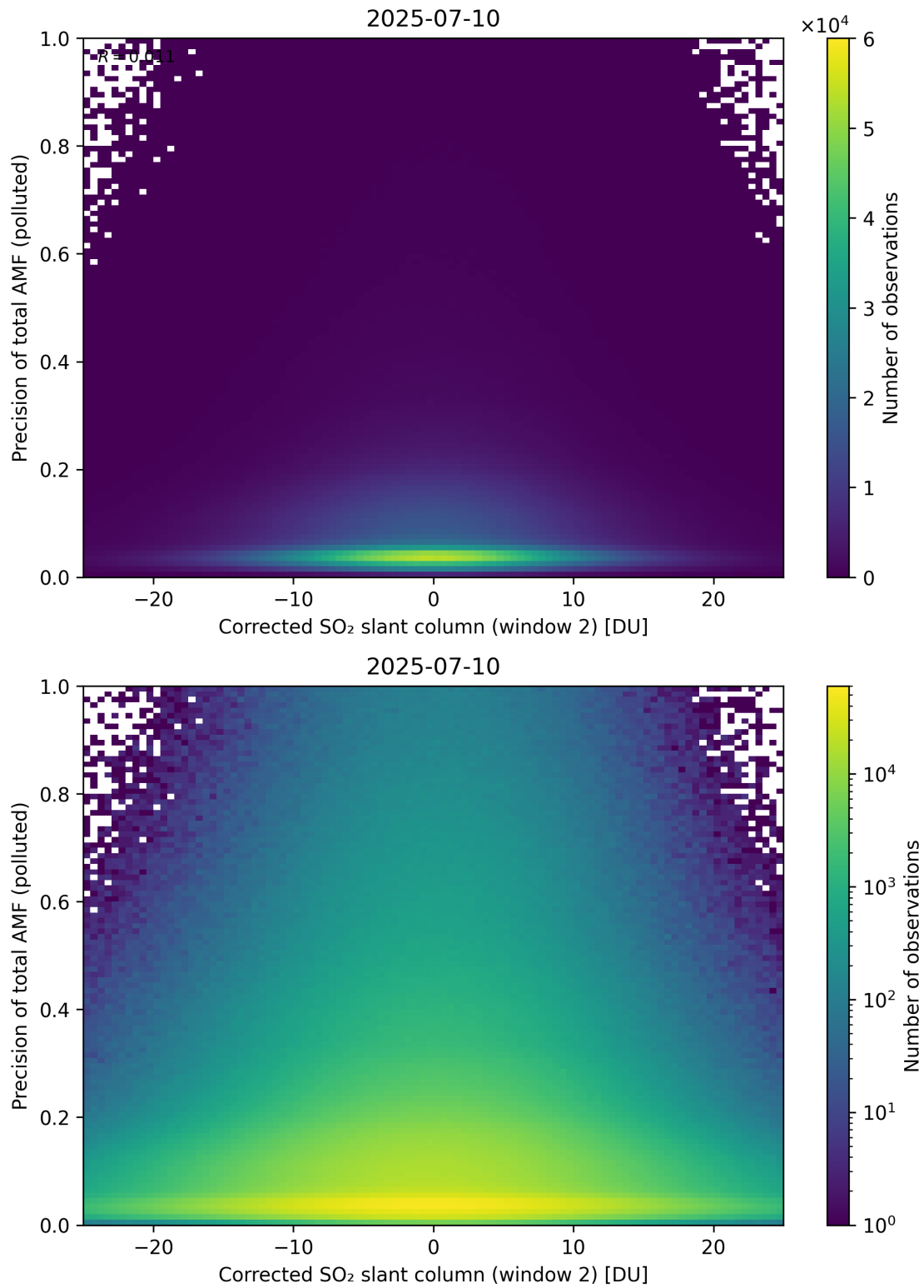
Figure 254: Scatter density plot of “Corrected SO 2 slant column (window 2)” against “Precision of total AMF (polluted)” for 2025-07-09 to 2025-07-11.
