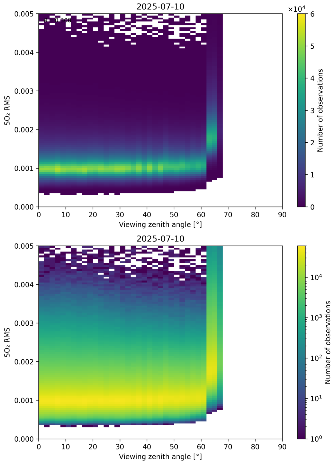
Figure 367: Scatter density plot of “Viewing zenith angle” against “SO 2 RMS” for 2025-07-09 to 2025-07-11.
