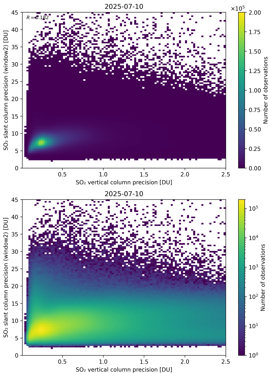
Figure 343: Scatter density plot of “SO 2 vertical column precision” against “SO 2 slant column precision (window2)” for 2025-07-09 to 2025-07-11.
