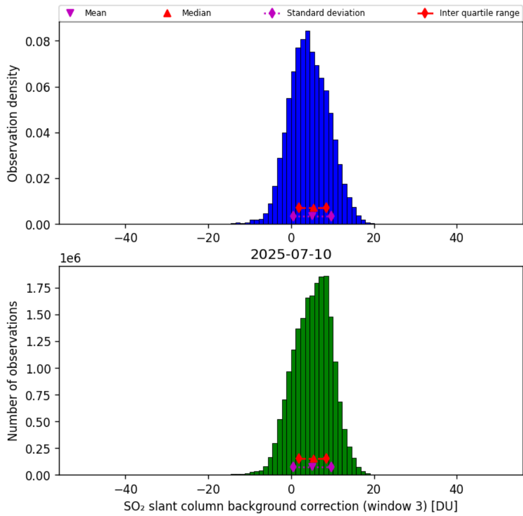
Figure 74: Histogram of “SO 2 slant column background correction (window 3)” for 2025-07-09 to 2025-07-11
