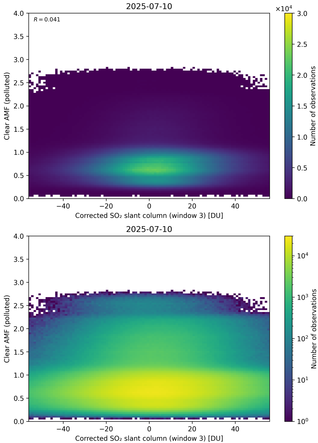
Figure 259: Scatter density plot of “Corrected SO 2 slant column (window 3)” against “Clear AMF (polluted)” for 2025-07-09 to 2025-07-11.
