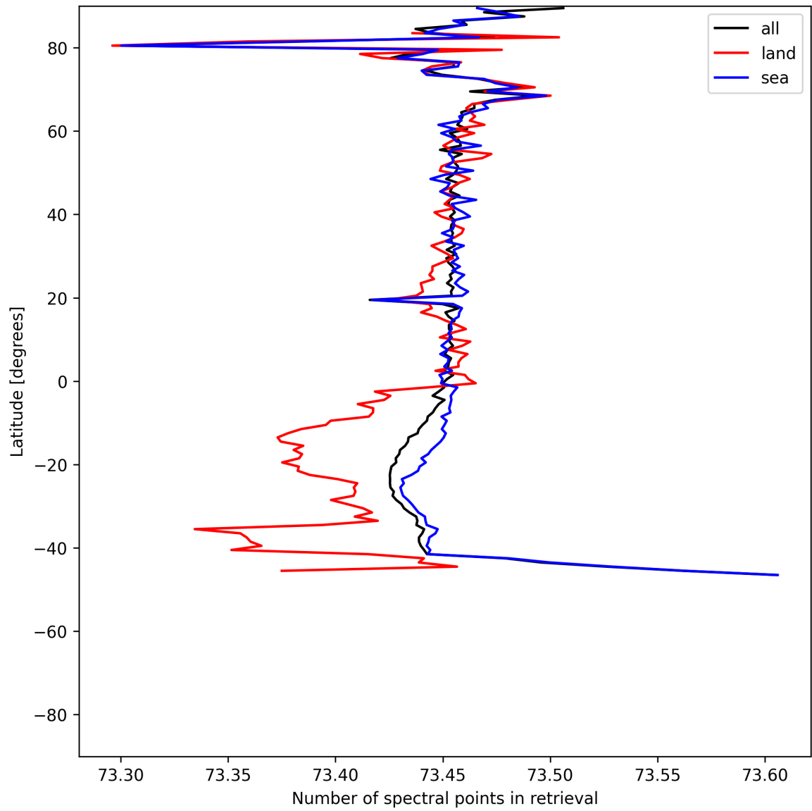
Figure 56: Zonal average of “Number of spectral points in retrieval” for 2025-07-09 to 2025-07-11.
