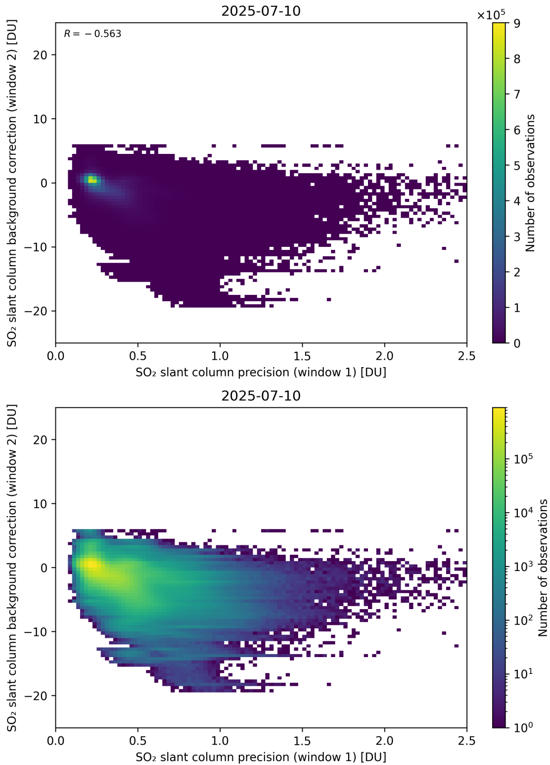
Figure 269: Scatter density plot of “SO 2 slant column precision (window 1)” against “SO 2 slant column background correction (window 2)” for 2025-07-09 to 2025-07-11.
