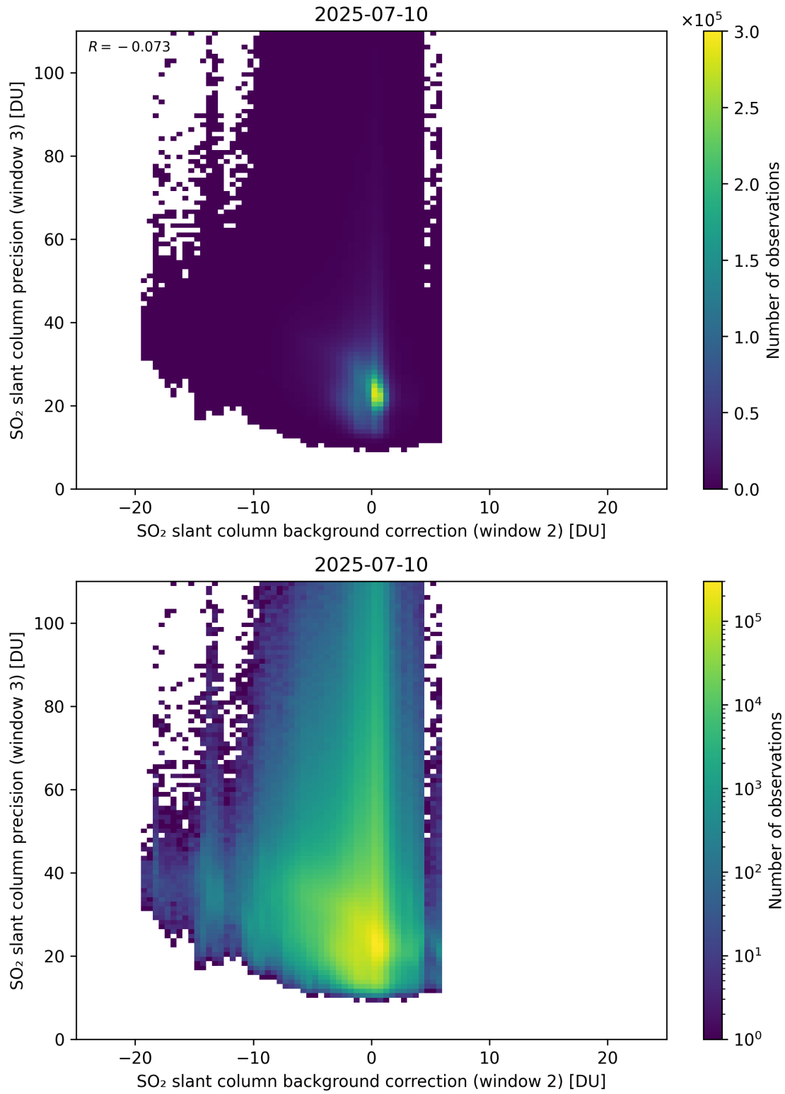
Figure 129: Scatter density plot of “SO 2 slant column background correction (window 2)” against “SO 2 slant column precision (window 3)” for 2025-07-09 to 2025-07-11.
