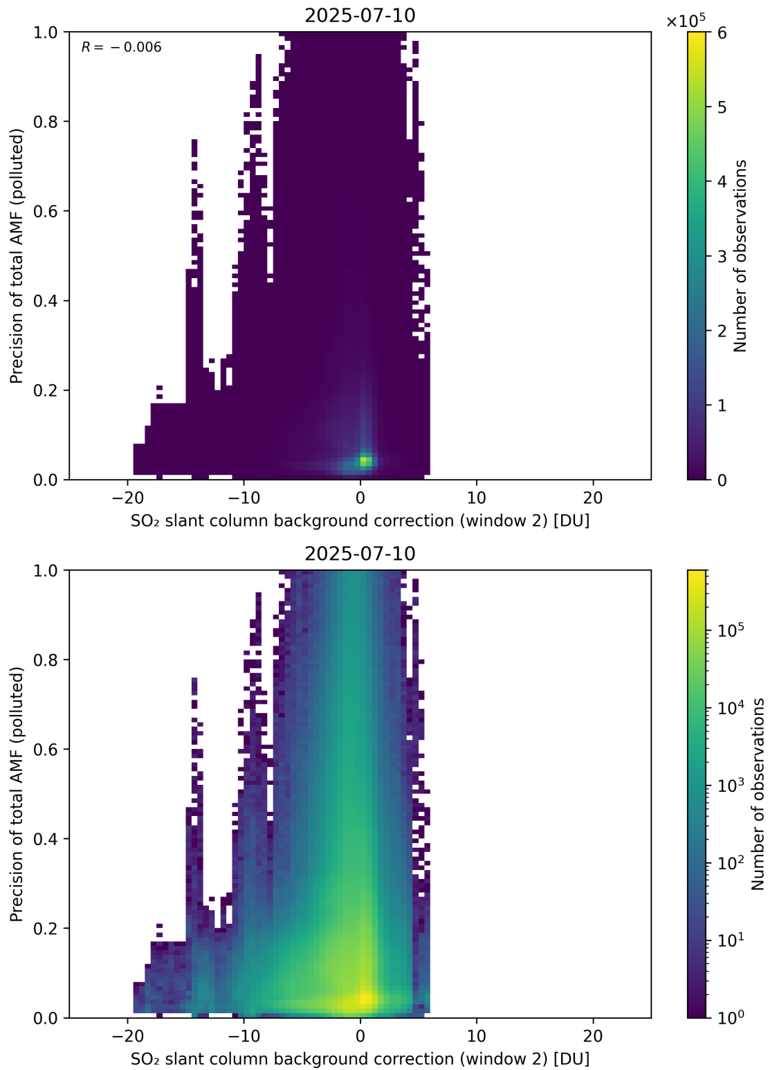
Figure 131: Scatter density plot of “SO 2 slant column background correction (window 2)” against “Precision of total AMF (polluted)” for 2025-07-09 to 2025-07-11.
