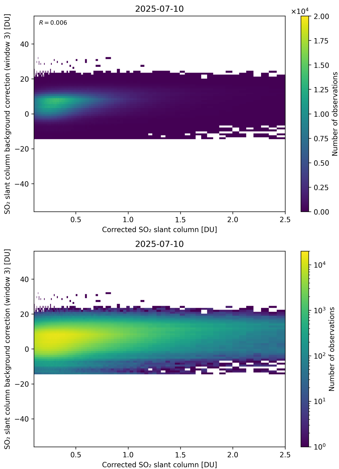
Figure 228: Scatter density plot of “Corrected SO 2 slant column” against “SO 2 slant column background correction (window 3)” for 2025-07-09 to 2025-07-11.
