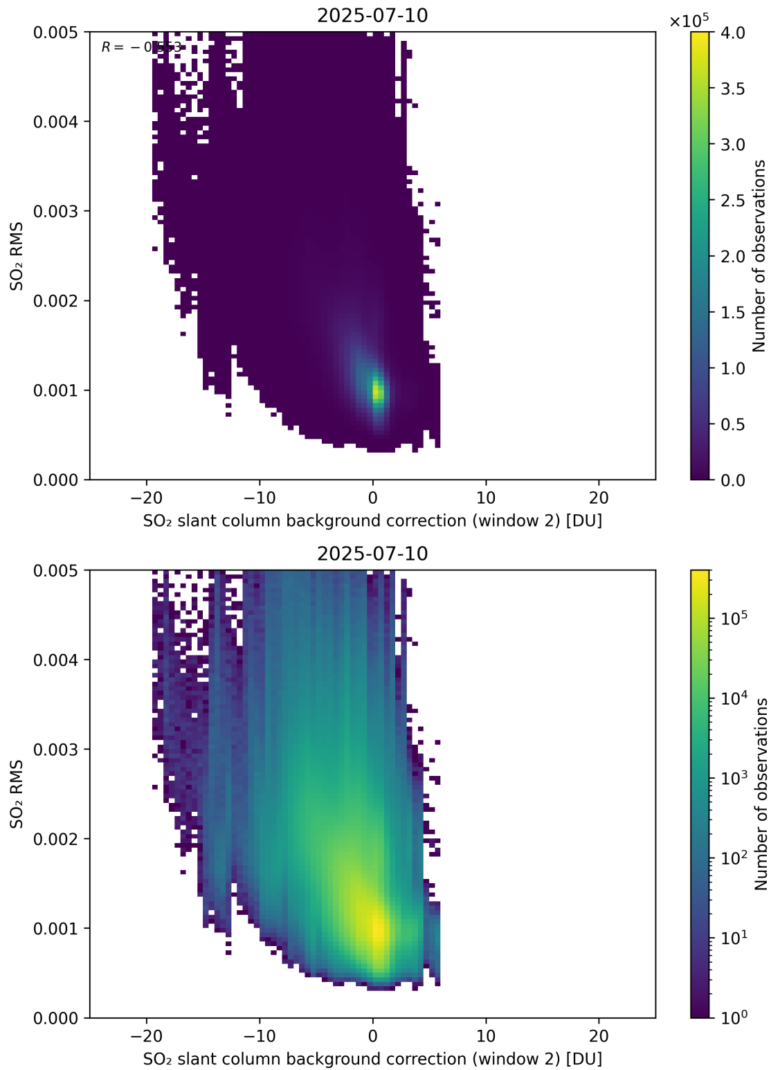
Figure 125: Scatter density plot of “SO 2 slant column background correction (window 2)” against “SO 2 RMS” for 2025-07-09 to 2025-07-11.
