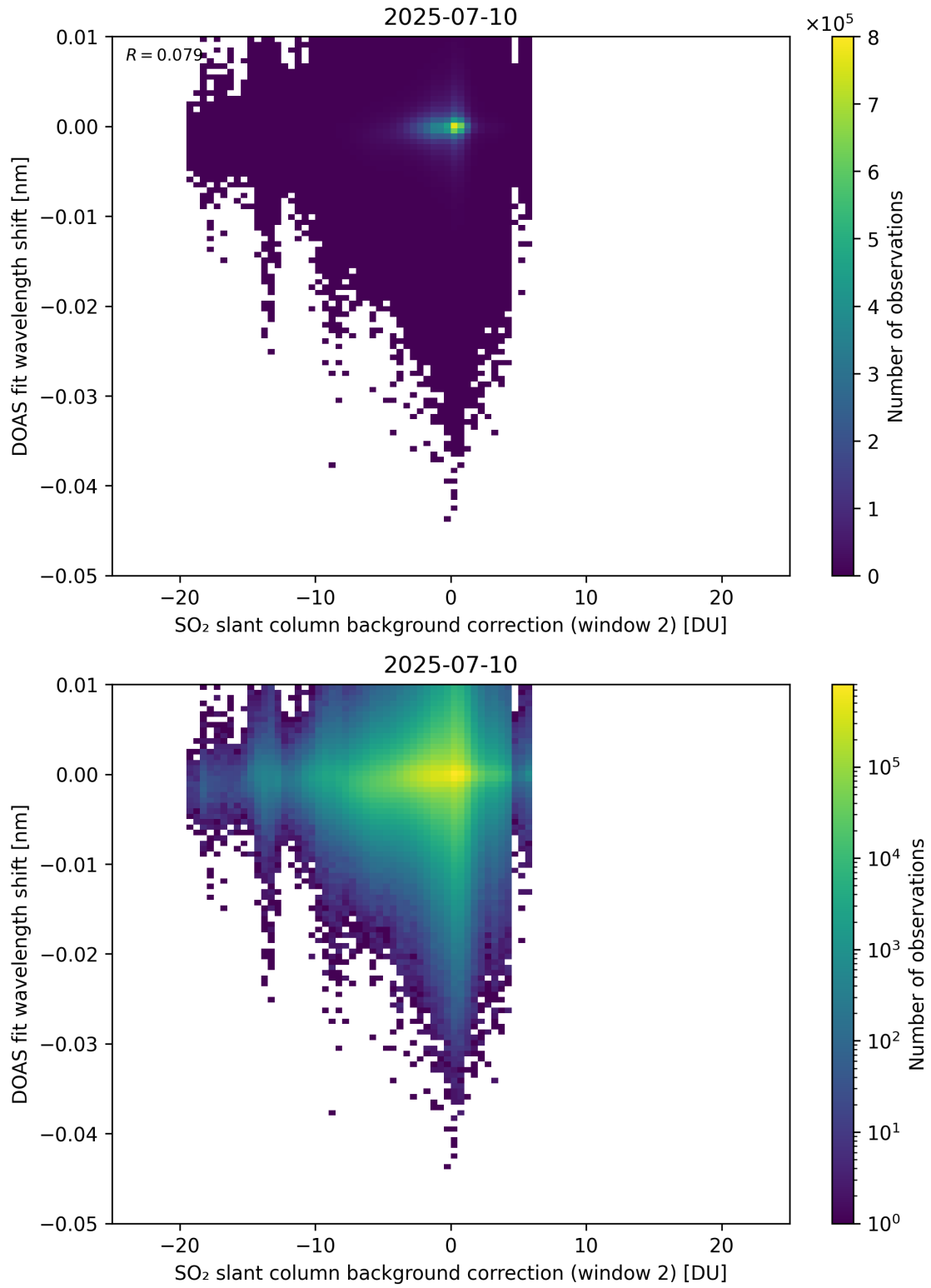
Figure 123: Scatter density plot of “SO 2 slant column background correction (window 2)” against “DOAS fit wavelength shift” for 2025-07-09 to 2025-07-11.
