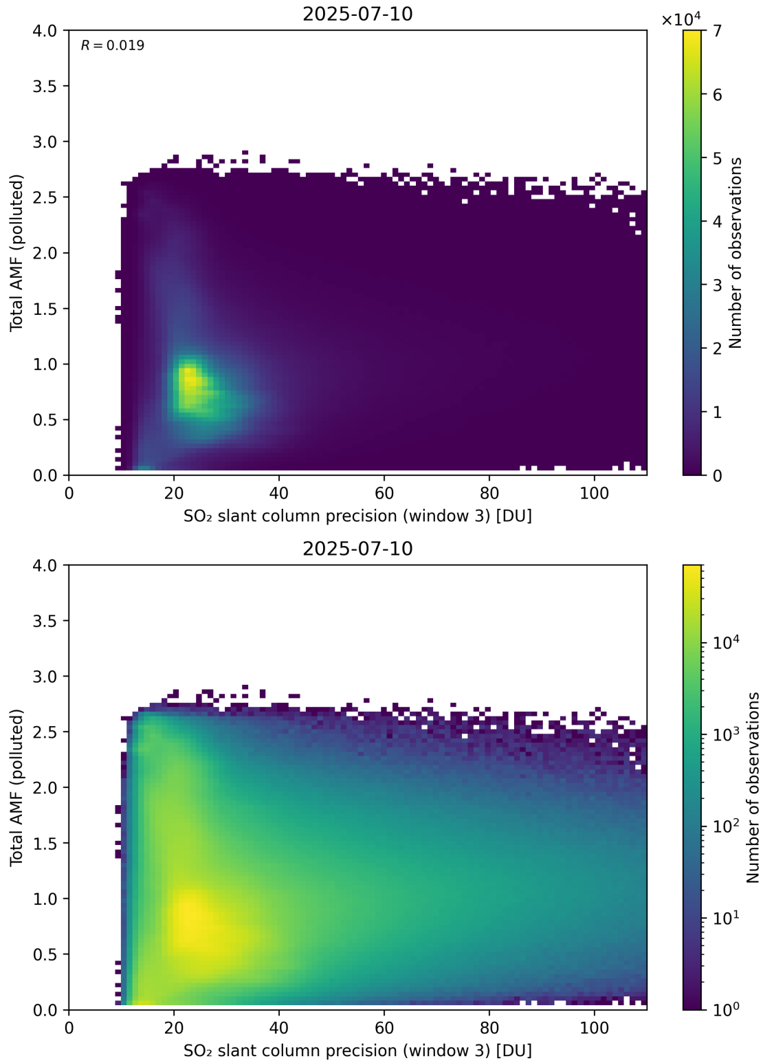
Figure 313: Scatter density plot of “SO 2 slant column precision (window 3)” against “Total AMF (polluted)” for 2025-07-09 to 2025-07-11.
