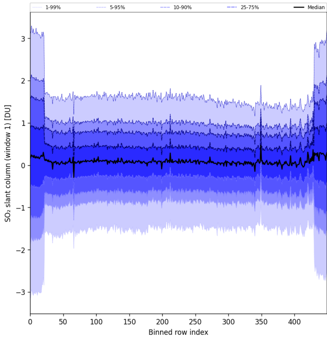
Figure 89: Along track statistics of “SO 2 slant column (window 1)” for 2025-07-09 to 2025-07-11
