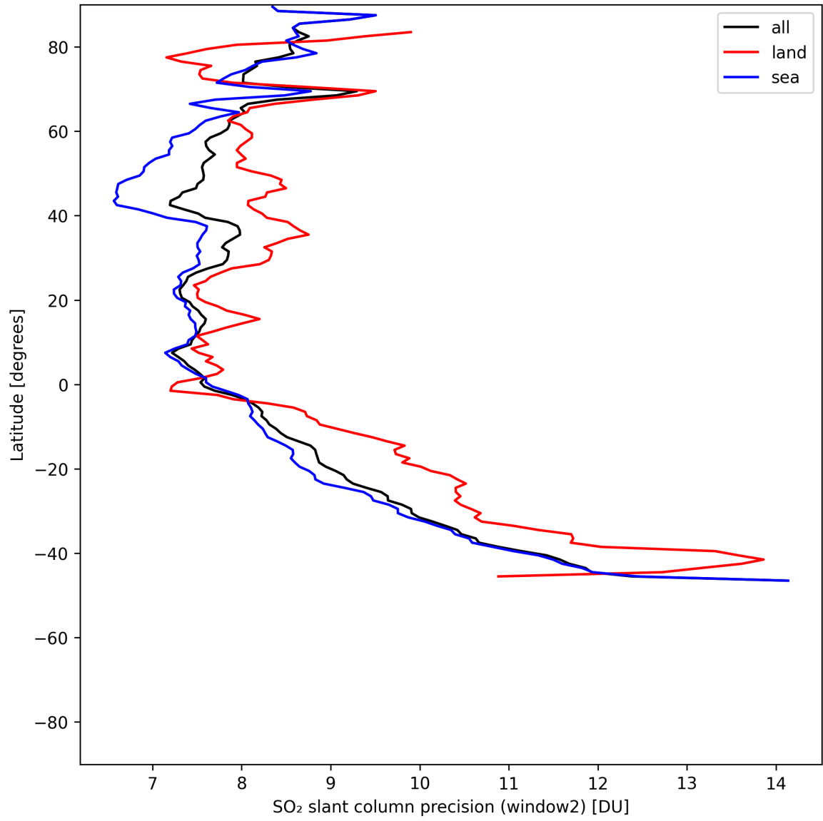
Figure 42: Zonal average of “SO 2 slant column precision (window2)” for 2025-07-09 to 2025-07-11.
