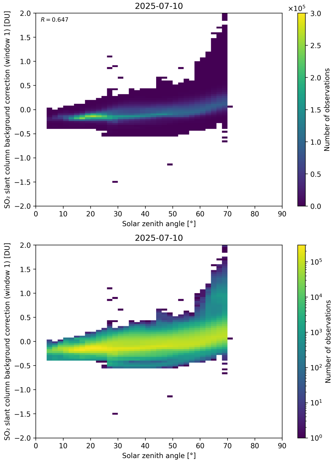
Figure 171: Scatter density plot of “Solar zenith angle” against “SO 2 slant column background correction (window 1)” for 2025-07-09 to 2025-07-11.
