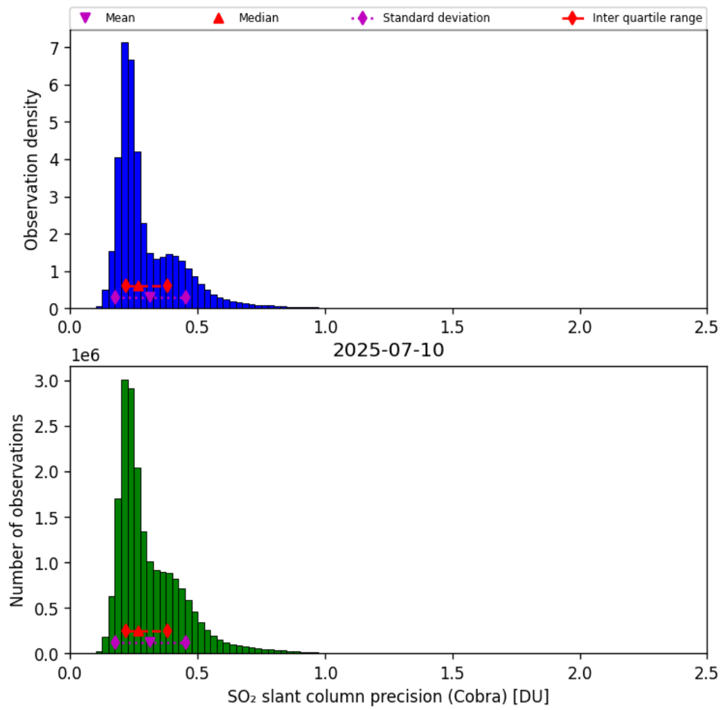
Figure 62: Histogram of “SO 2 slant column precision (Cobra)” for 2025-07-09 to 2025-07-11
