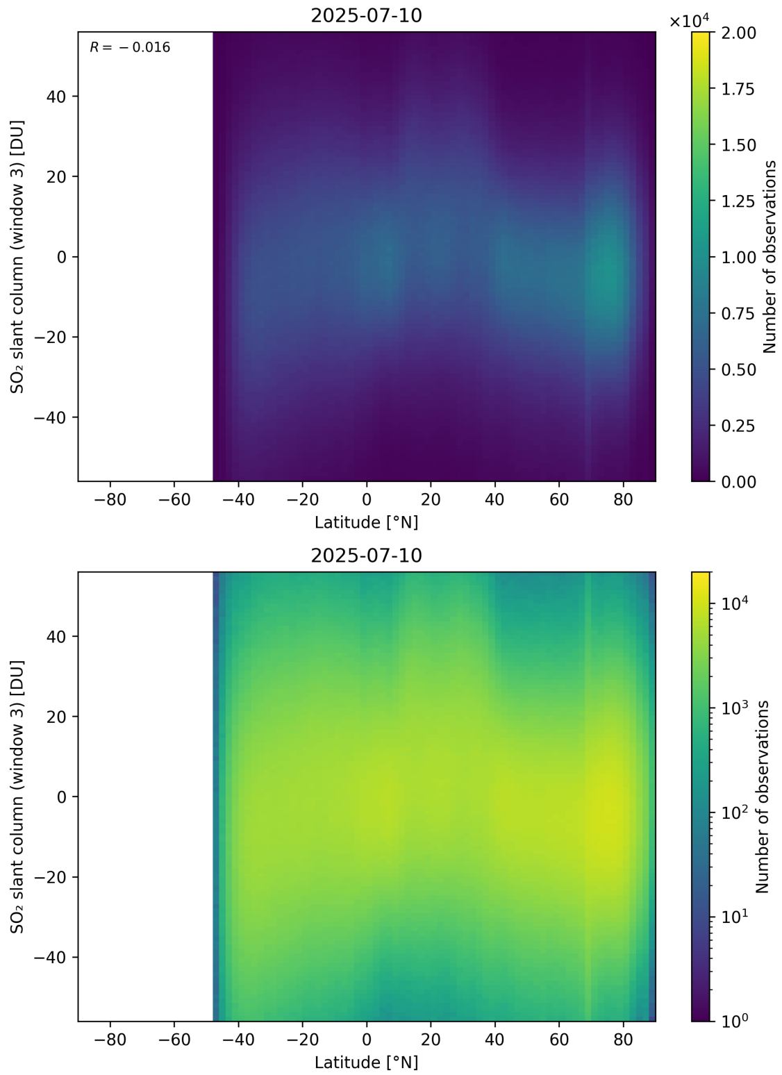
Figure 165: Scatter density plot of “Latitude” against “SO 2 slant column (window 3)” for 2025-07-09 to 2025-07-11.
