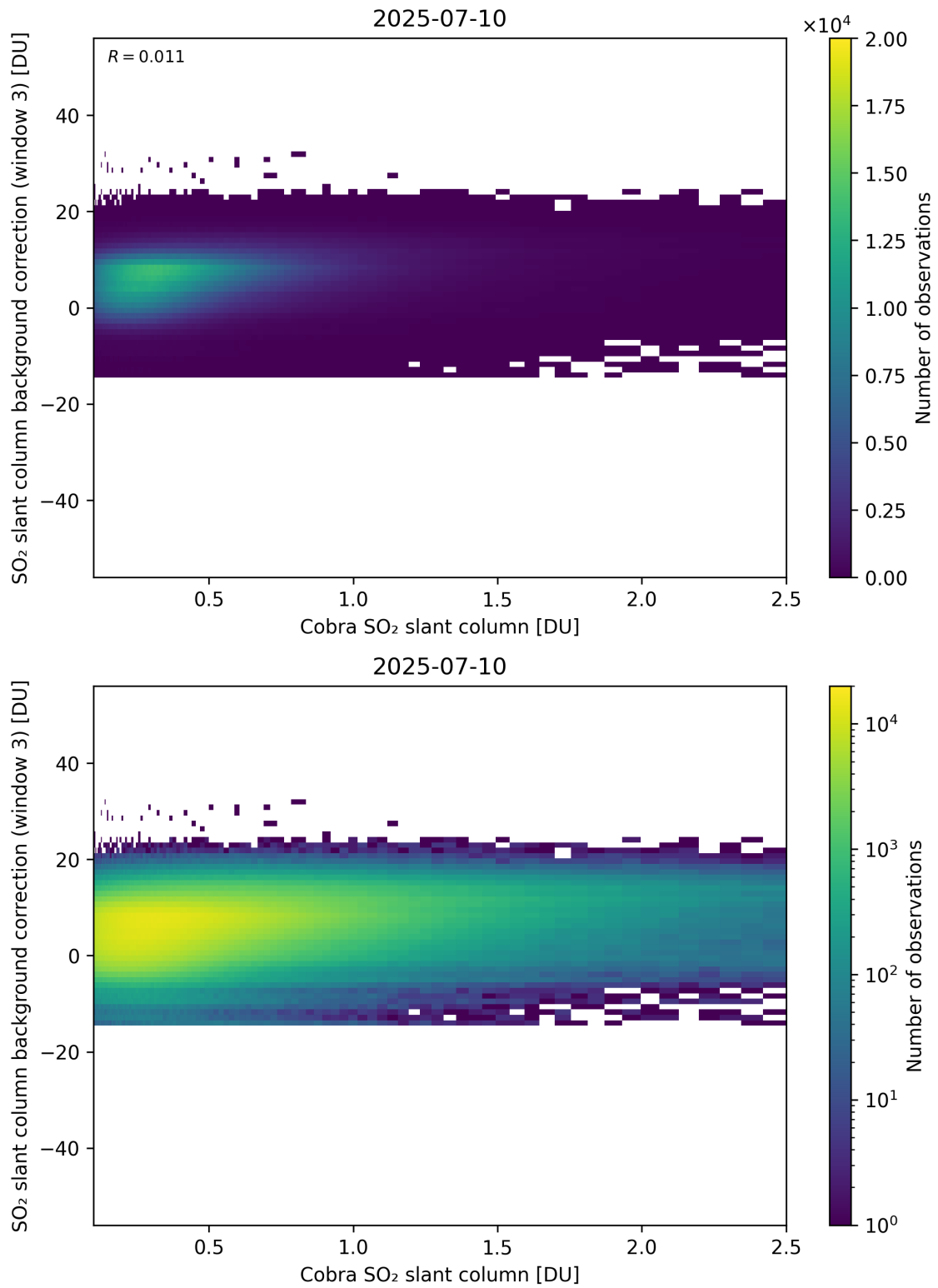
Figure 195: Scatter density plot of “Cobra SO 2 slant column” against “SO 2 slant column background correction (window 3)” for 2025-07-09 to 2025-07-11.
