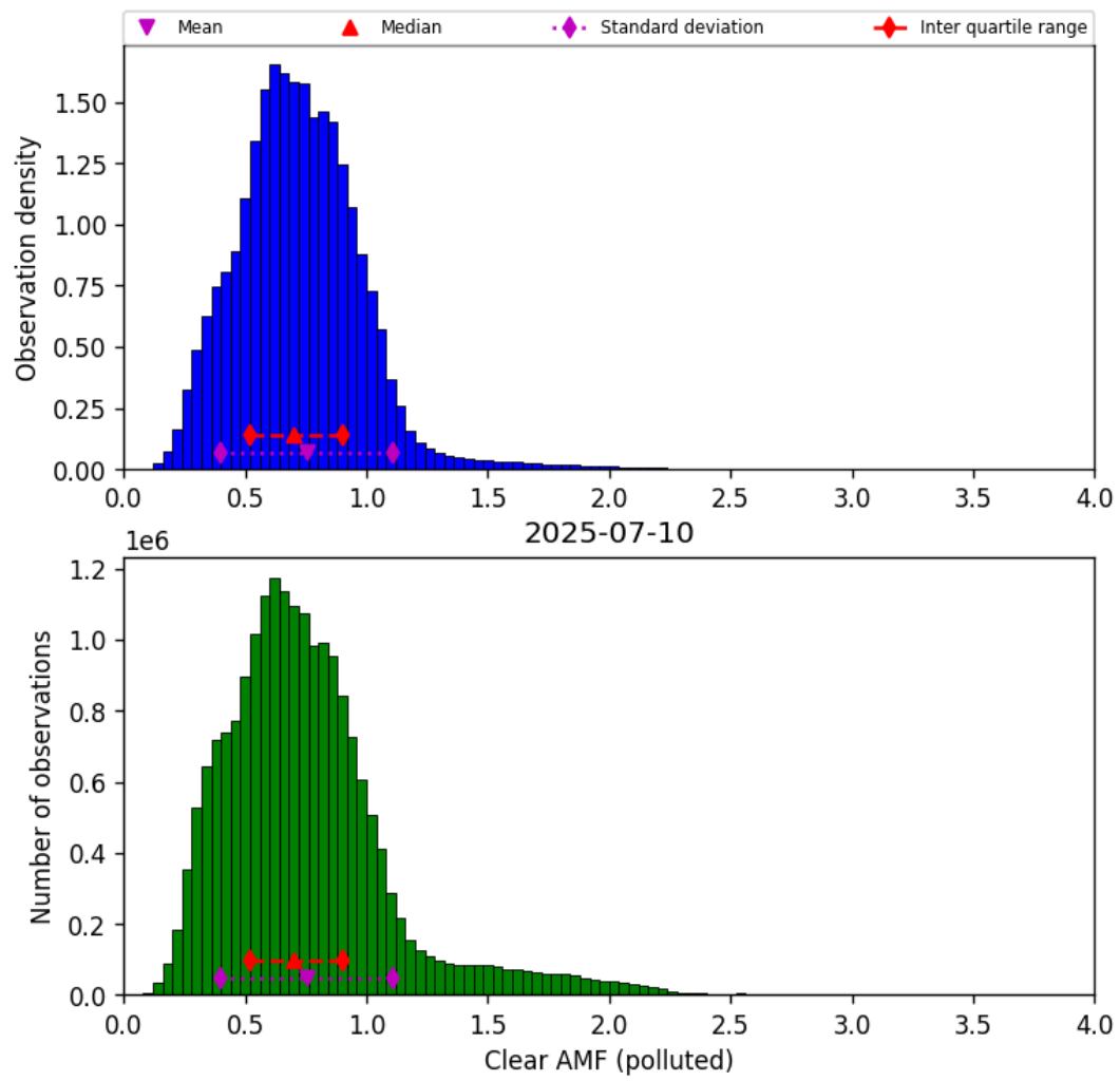
Figure 81: Histogram of “Clear AMF (polluted)” for 2025-07-09 to 2025-07-11
