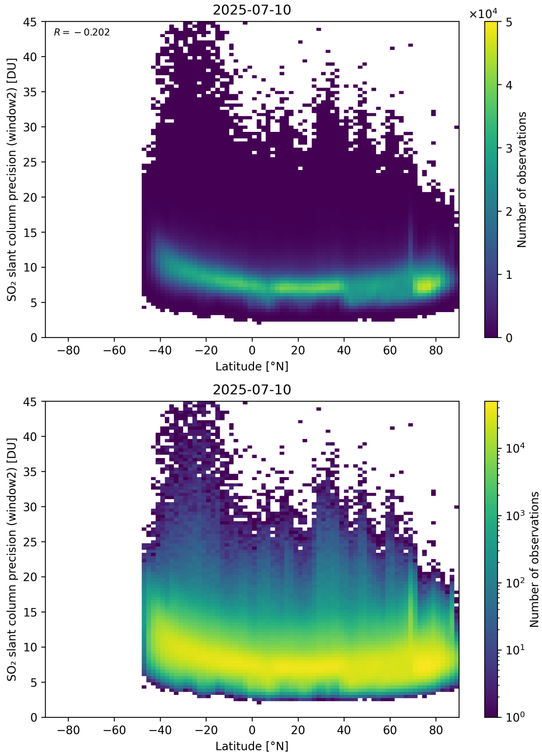
Figure 164: Scatter density plot of “Latitude” against “SO 2 slant column precision (window2)” for 2025-07-09 to 2025-07-11.
