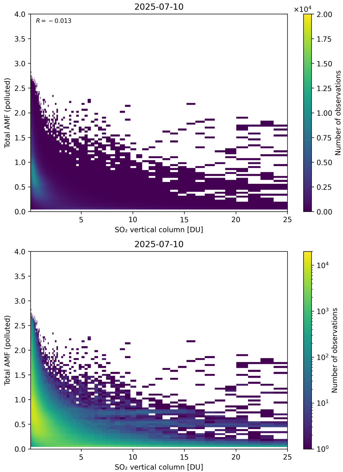
Figure 359: Scatter density plot of “SO 2 vertical column” against “Total AMF (polluted)” for 2025-07-09 to 2025-07-11.
