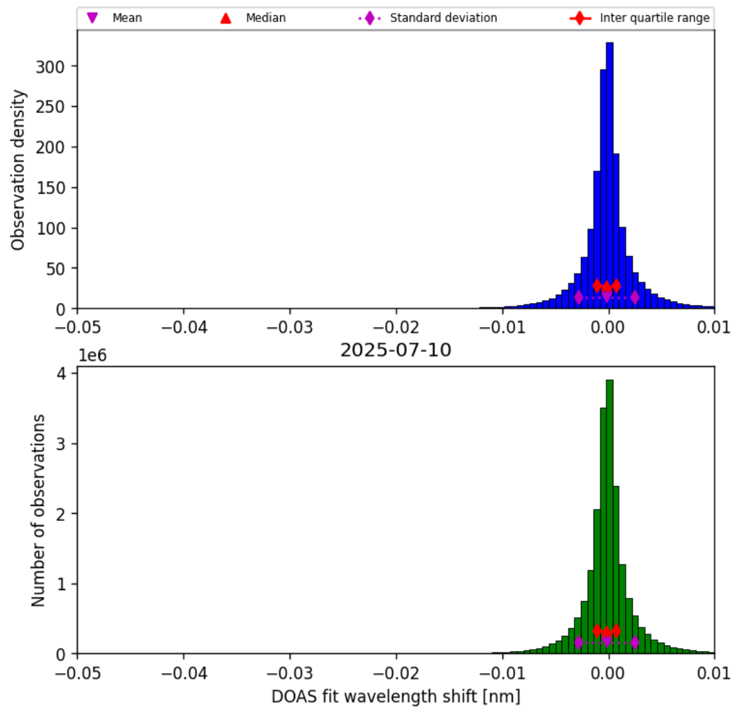
Figure 76: Histogram of “DOAS fit wavelength shift” for 2025-07-09 to 2025-07-11
