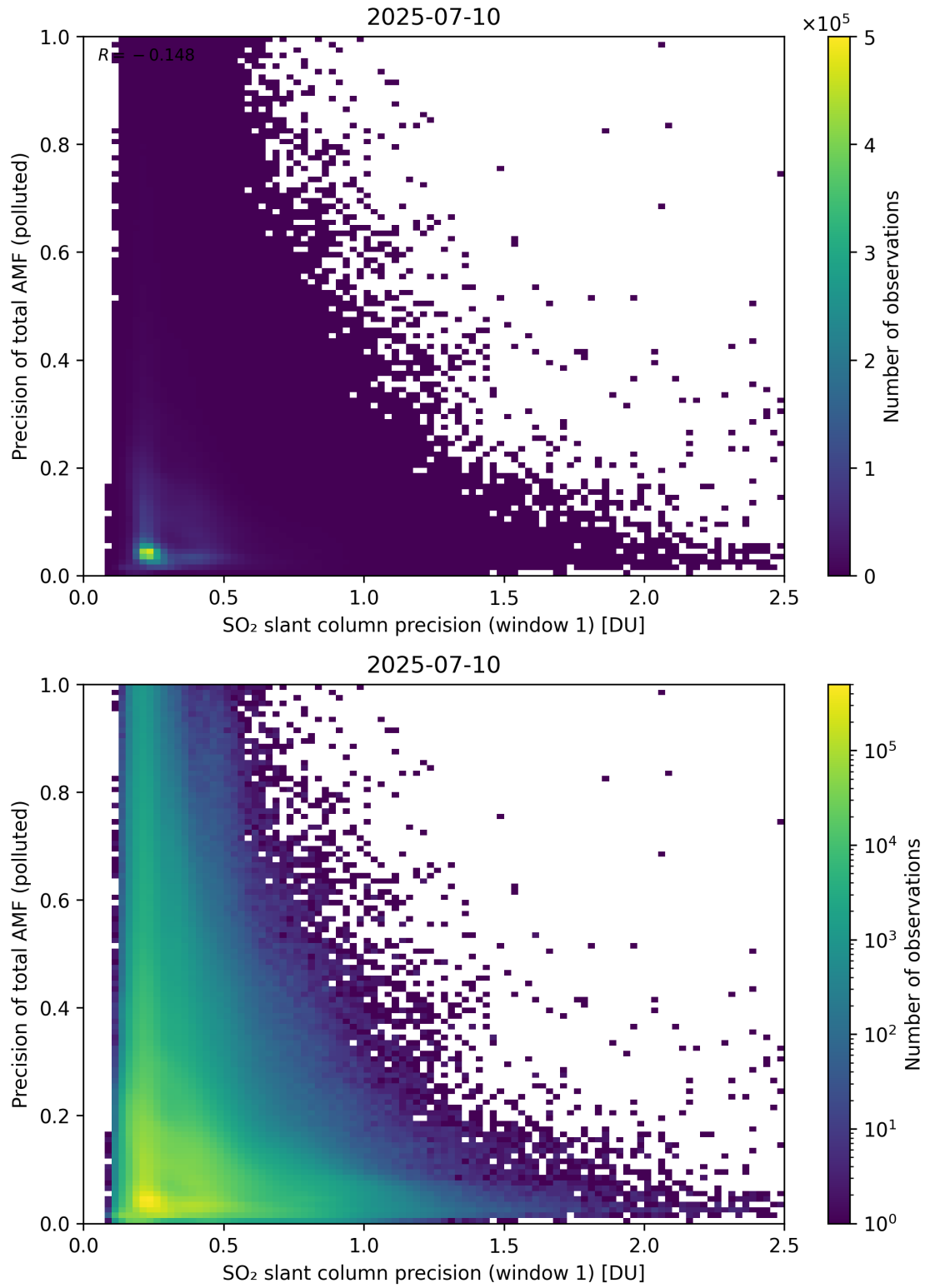
Figure 281: Scatter density plot of “SO 2 slant column precision (window 1)” against “Precision of total AMF (polluted)” for 2025-07-09 to 2025-07-11.
