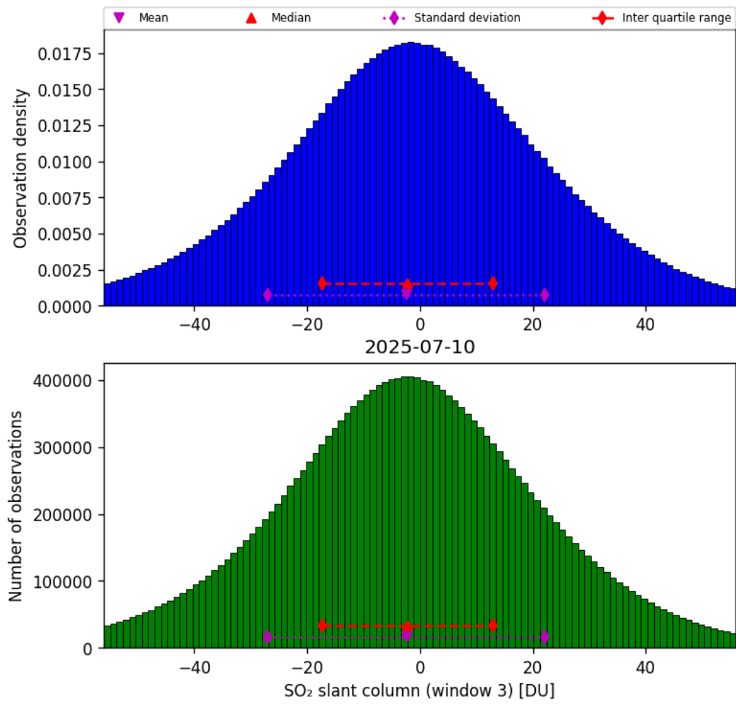
Figure 71: Histogram of “SO 2 slant column (window 3)” for 2025-07-09 to 2025-07-11
