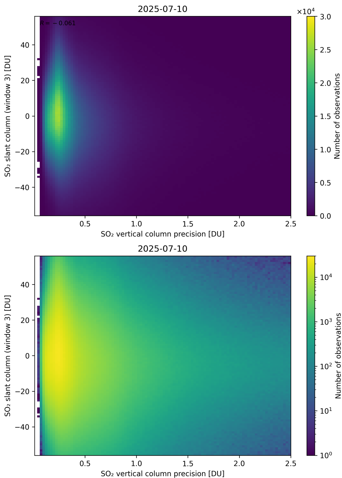
Figure 344: Scatter density plot of “SO 2 vertical column precision” against “SO 2 slant column (window 3)” for 2025-07-09 to 2025-07-11.
