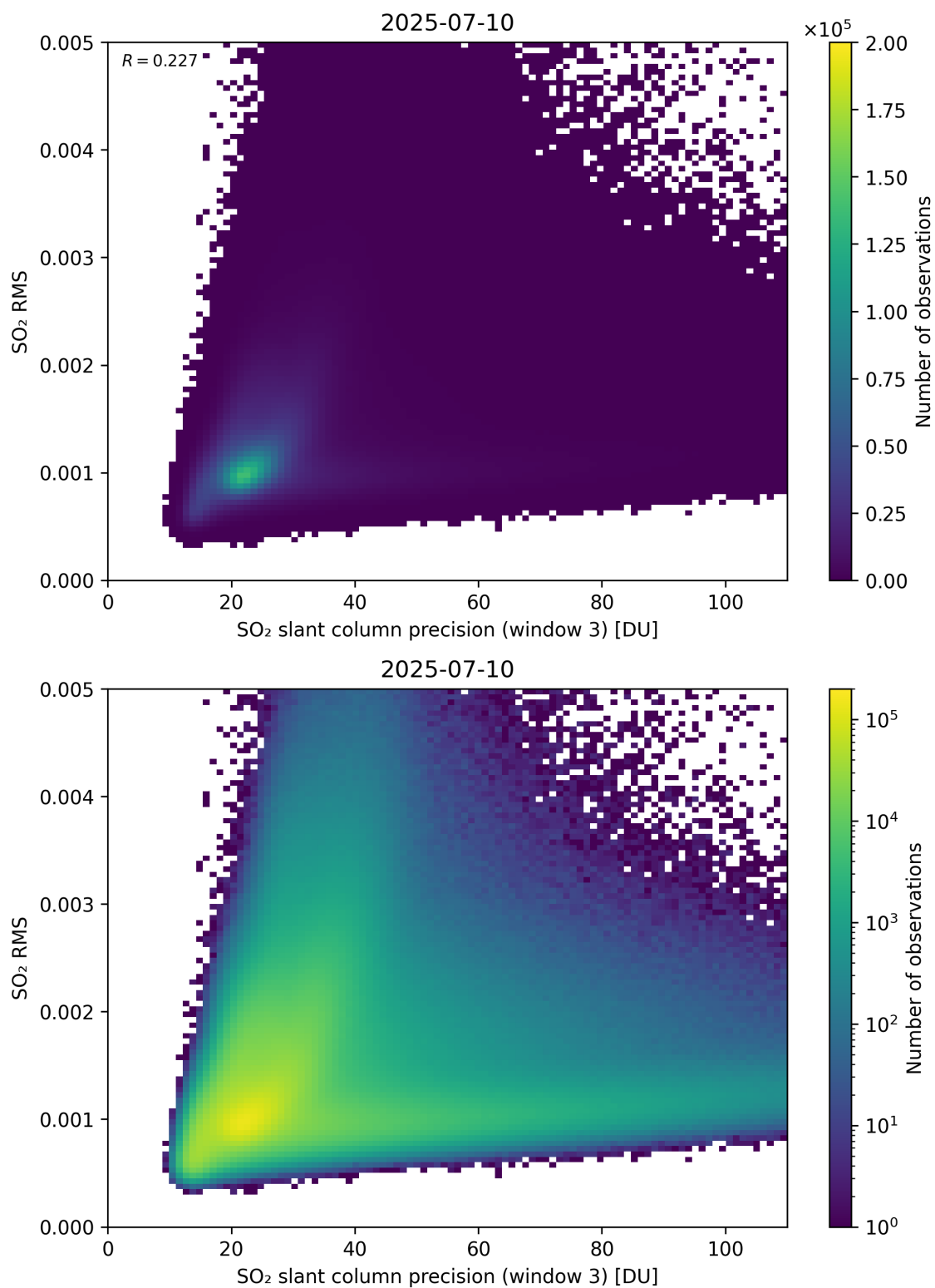
Figure 310: Scatter density plot of “SO 2 slant column precision (window 3)” against “SO 2 RMS” for 2025-07-09 to 2025-07-11.
