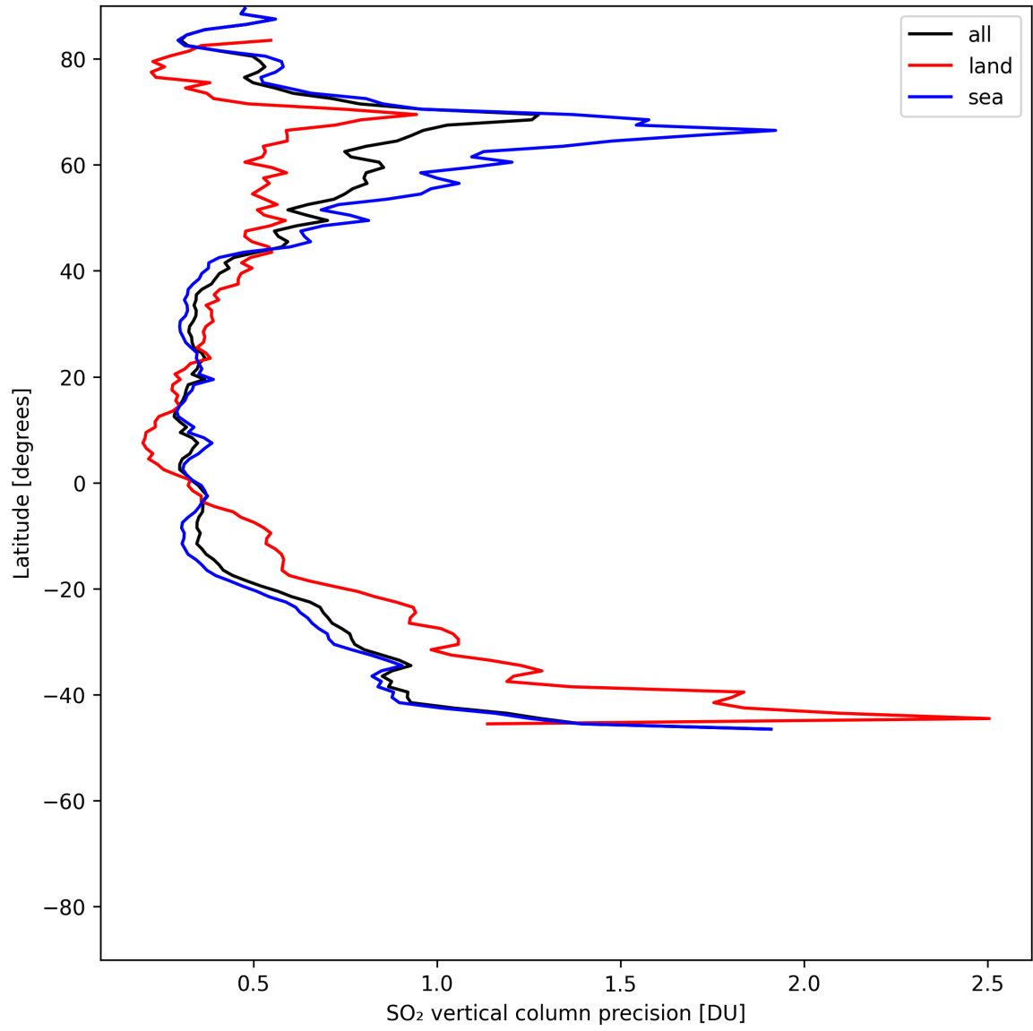
Figure 33: Zonal average of “SO 2 vertical column precision” for 2025-07-09 to 2025-07-11.
