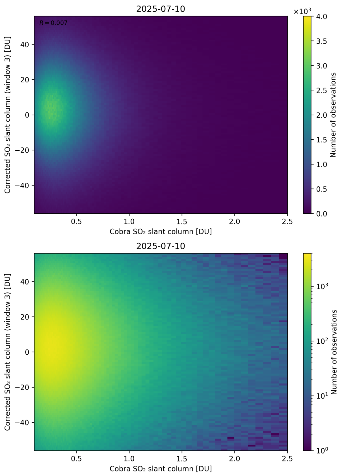
Figure 218: Scatter density plot of “Cobra SO 2 slant column” against “Corrected SO 2 slant column (window 3)” for 2025-07-09 to 2025-07-11.
