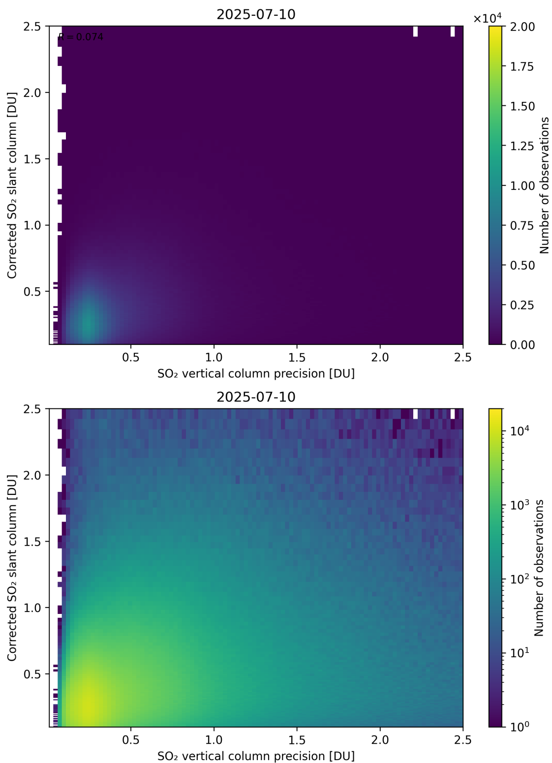
Figure 338: Scatter density plot of “SO 2 vertical column precision” against “Corrected SO 2 slant column” for 2025-07-09 to 2025-07-11.
