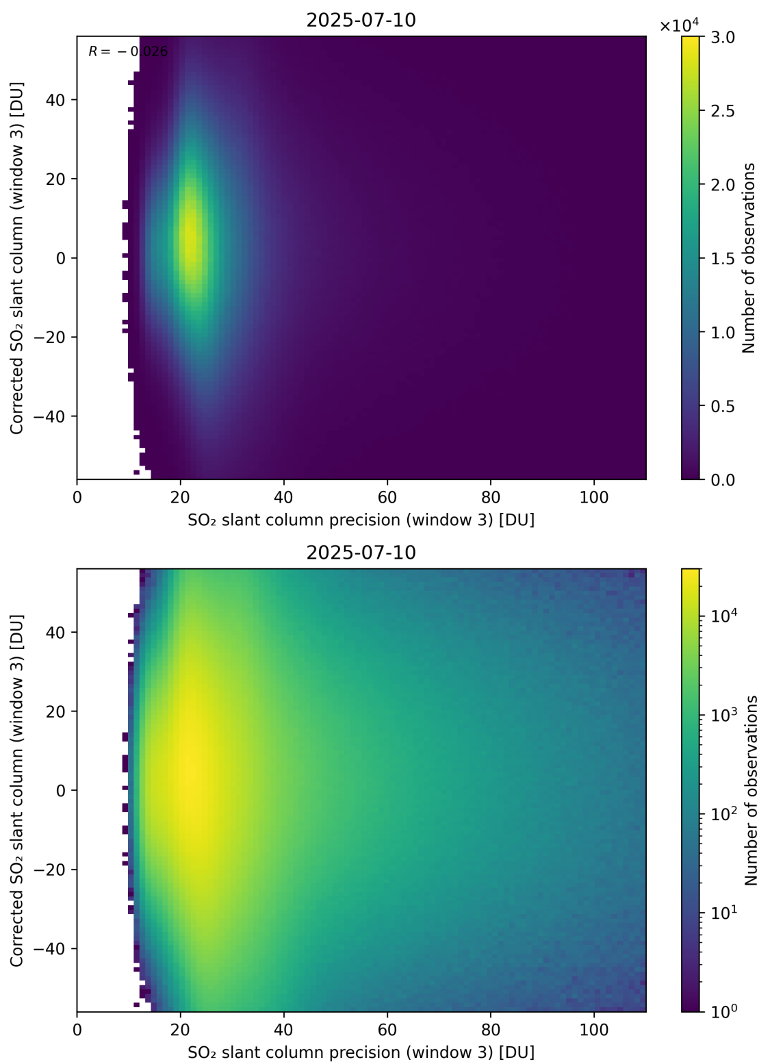
Figure 312: Scatter density plot of “SO 2 slant column precision (window 3)” against “Corrected SO 2 slant column (window 3)” for 2025-07-09 to 2025-07-11.
