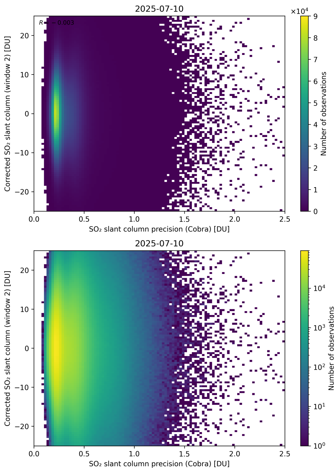
Figure 206: Scatter density plot of “SO 2 slant column precision (Cobra)” against “Corrected SO 2 slant column (window 2)” for 2025-07-09 to 2025-07-11.
