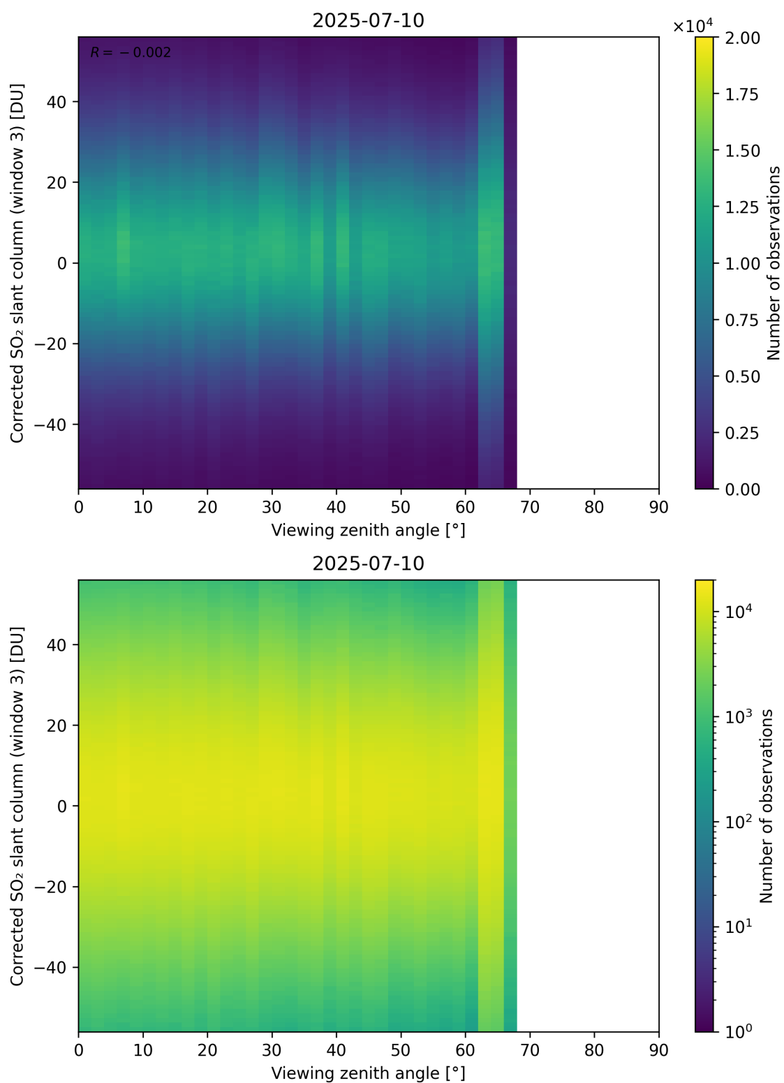
Figure 375: Scatter density plot of “Viewing zenith angle” against “Corrected SO 2 slant column (window 3)” for 2025-07-09 to 2025-07-11.
