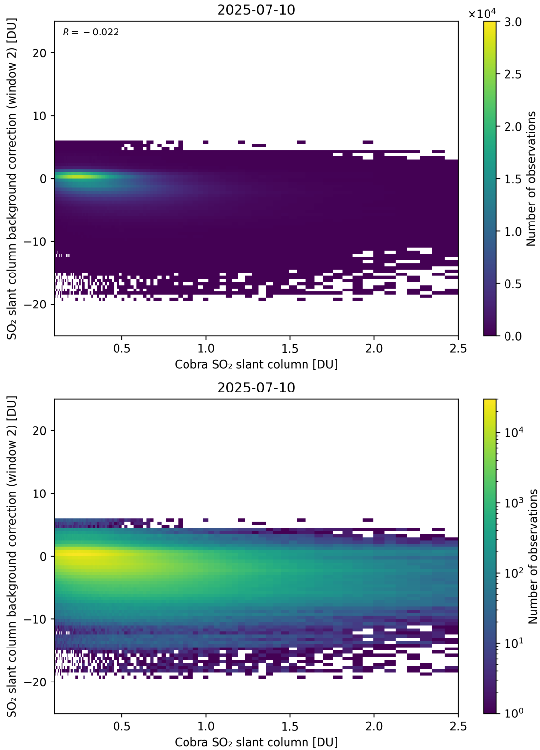
Figure 194: Scatter density plot of “Cobra SO 2 slant column” against “SO 2 slant column background correction (window 2)” for 2025-07-09 to 2025-07-11.
