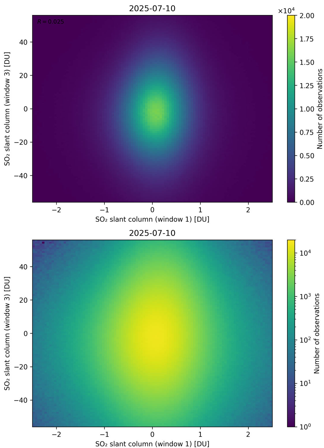
Figure 287: Scatter density plot of “SO 2 slant column (window 1)” against “SO 2 slant column (window 3)” for 2025-07-09 to 2025-07-11.
