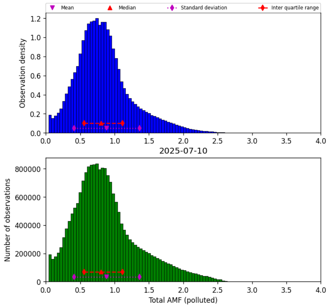
Figure 79: Histogram of “Total AMF (polluted)” for 2025-07-09 to 2025-07-11
