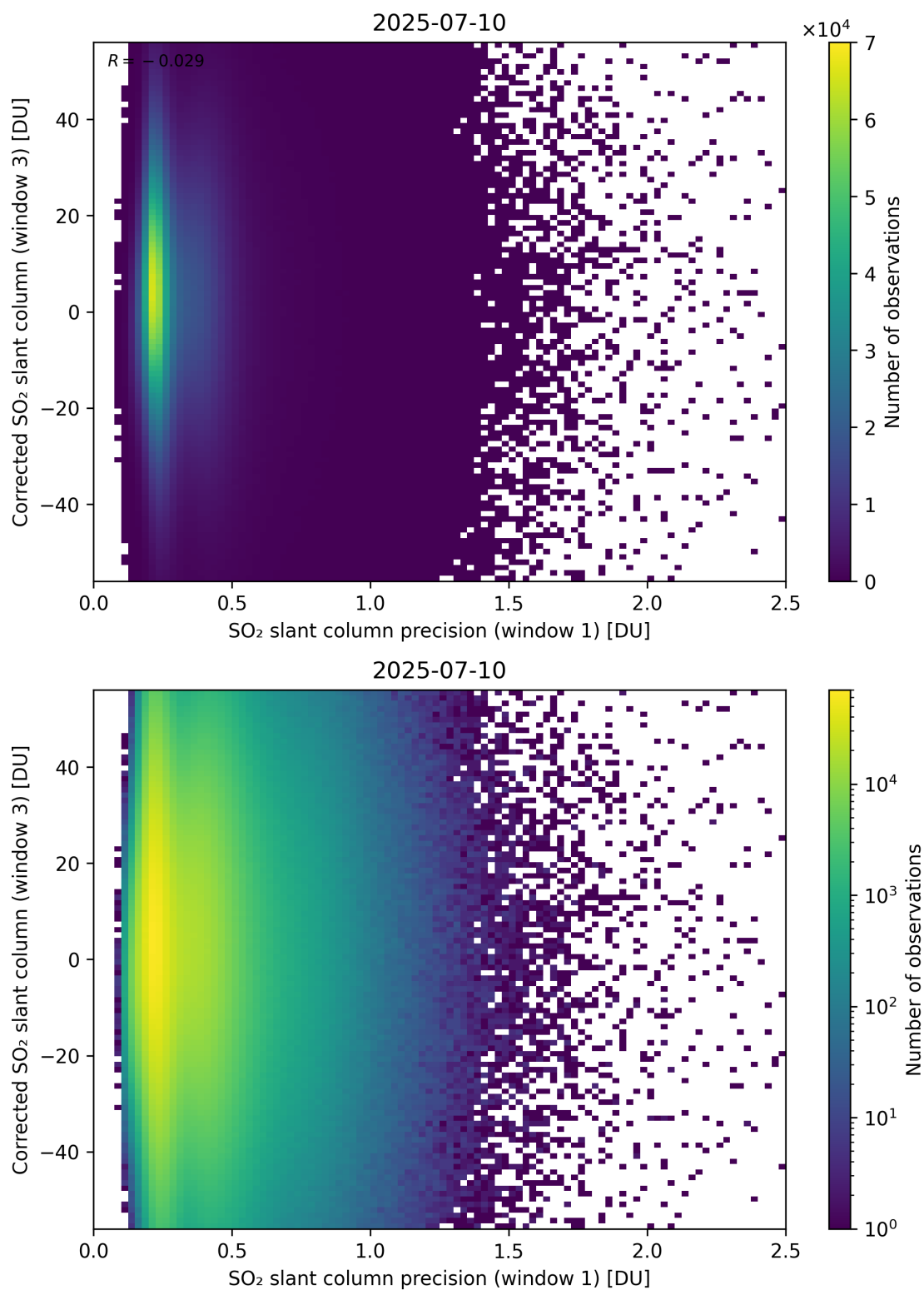
Figure 276: Scatter density plot of “SO 2 slant column precision (window 1)” against “Corrected SO 2 slant column (window 3)” for 2025-07-09 to 2025-07-11.
