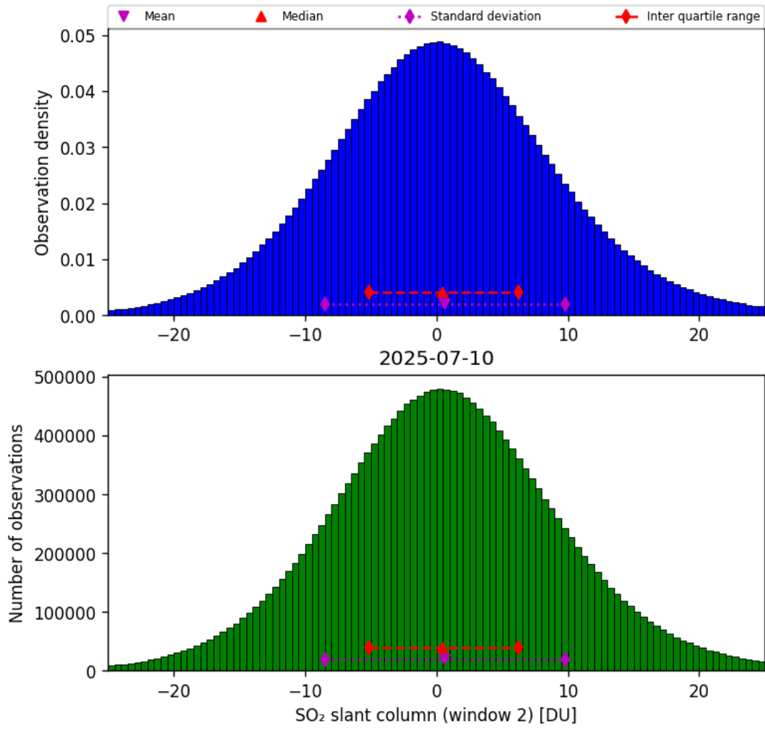
Figure 67: Histogram of “SO 2 slant column (window 2)” for 2025-07-09 to 2025-07-11
