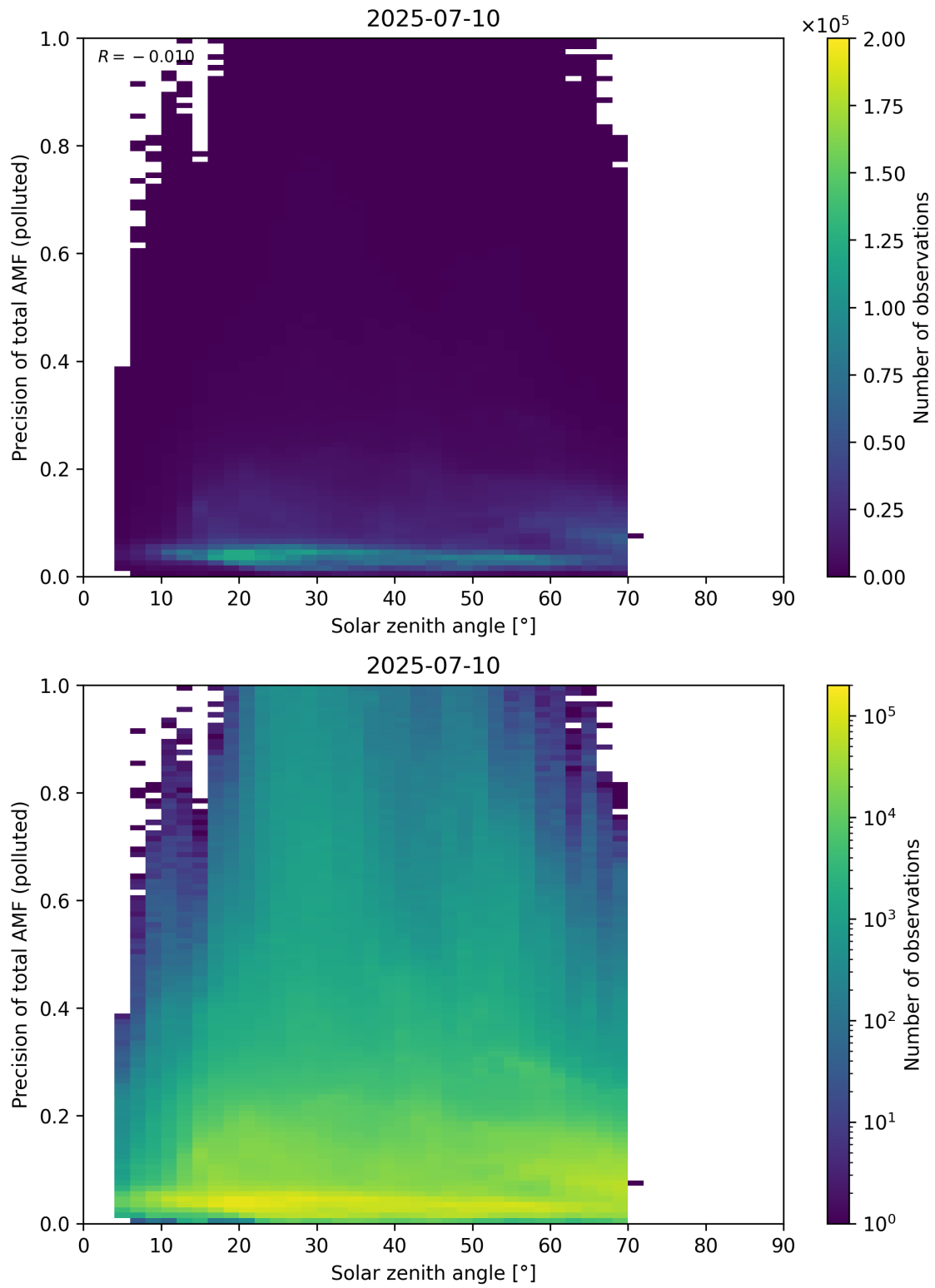
Figure 190: Scatter density plot of “Solar zenith angle” against “Precision of total AMF (polluted)” for 2025-07-09 to 2025-07-11.
