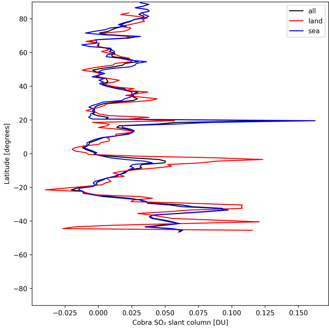
Figure 35: Zonal average of “Cobra SO 2 slant column” for 2025-07-09 to 2025-07-11.
