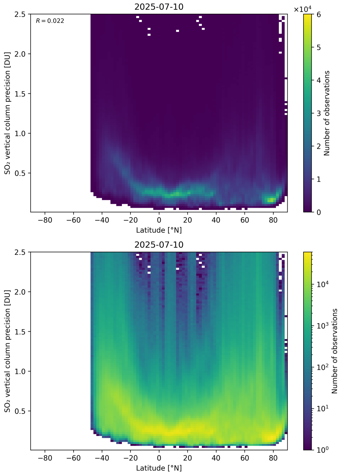
Figure 170: Scatter density plot of “Latitude” against “SO 2 vertical column precision” for 2025-07-09 to 2025-07-11.
