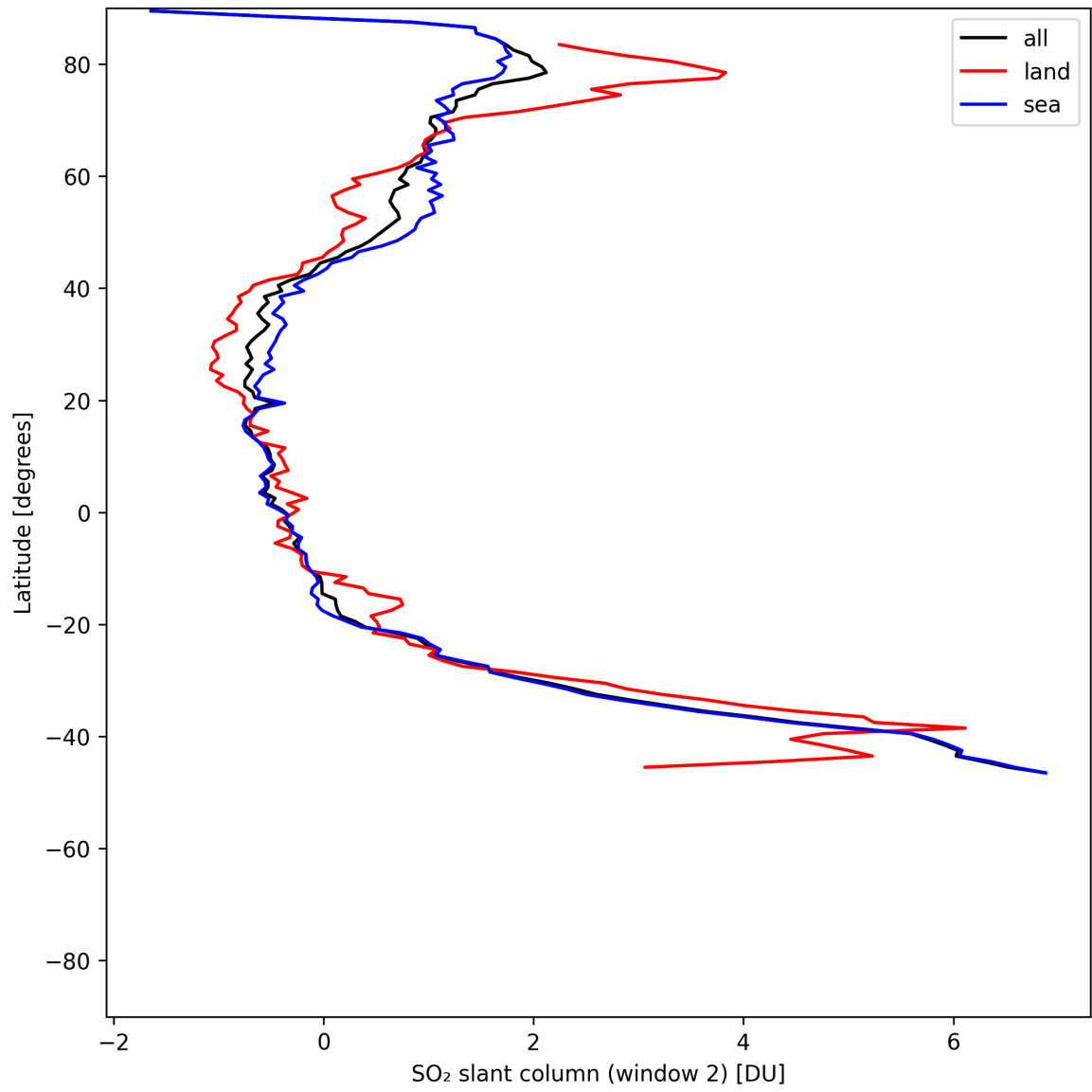
Figure 41: Zonal average of “SO 2 slant column (window 2)” for 2025-07-09 to 2025-07-11.
