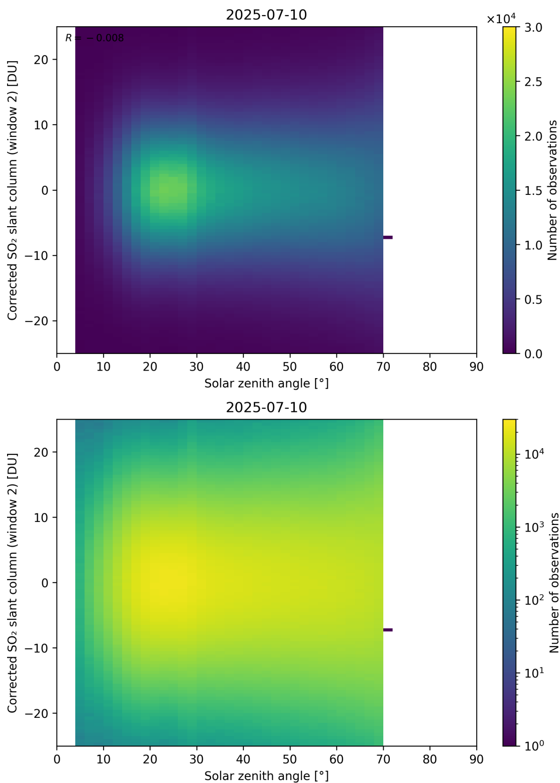
Figure 182: Scatter density plot of “Solar zenith angle” against “Corrected SO 2 slant column (window 2)” for 2025-07-09 to 2025-07-11.
