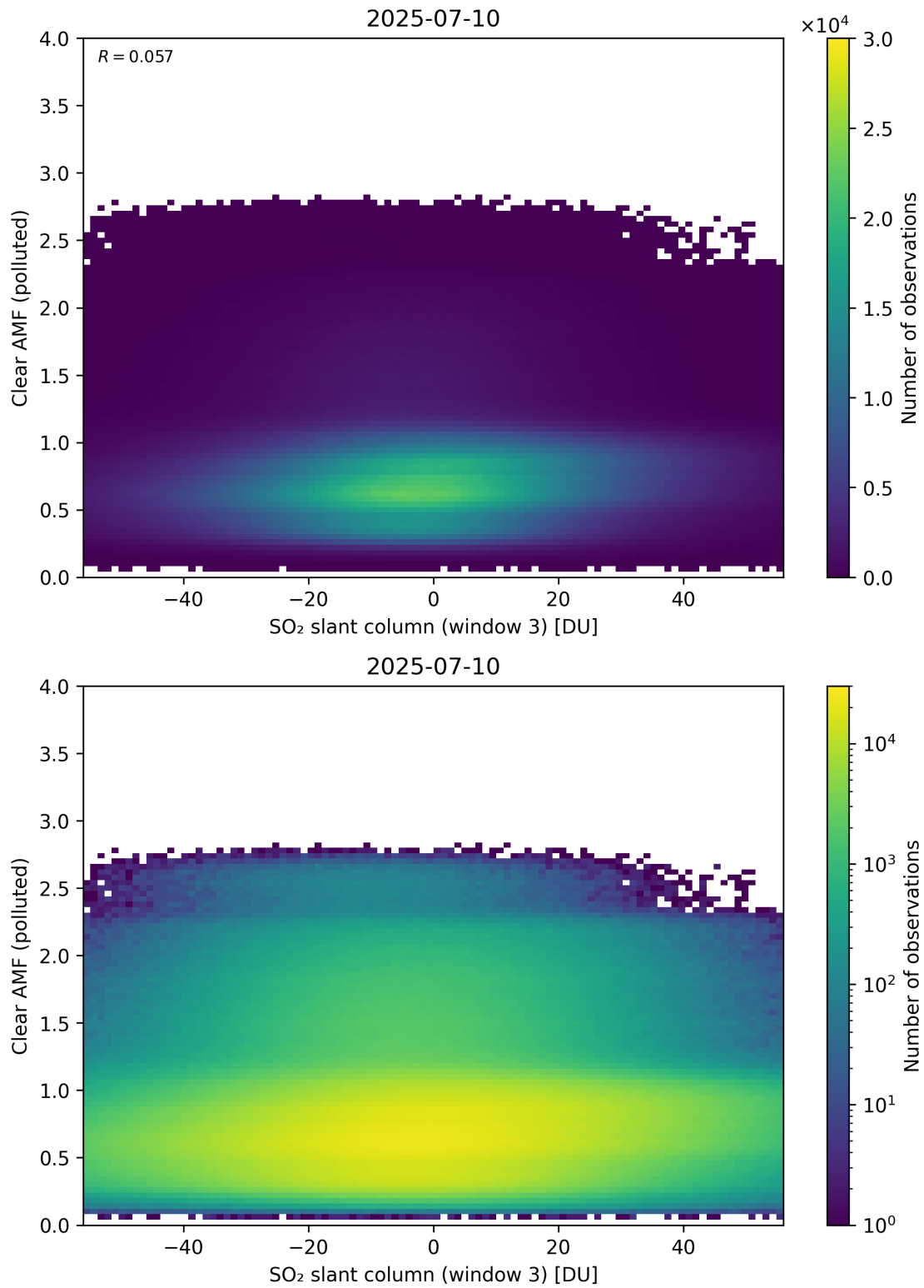
Figure 315: Scatter density plot of “SO 2 slant column (window 3)” against “Clear AMF (polluted)” for 2025-07-09 to 2025-07-11.
