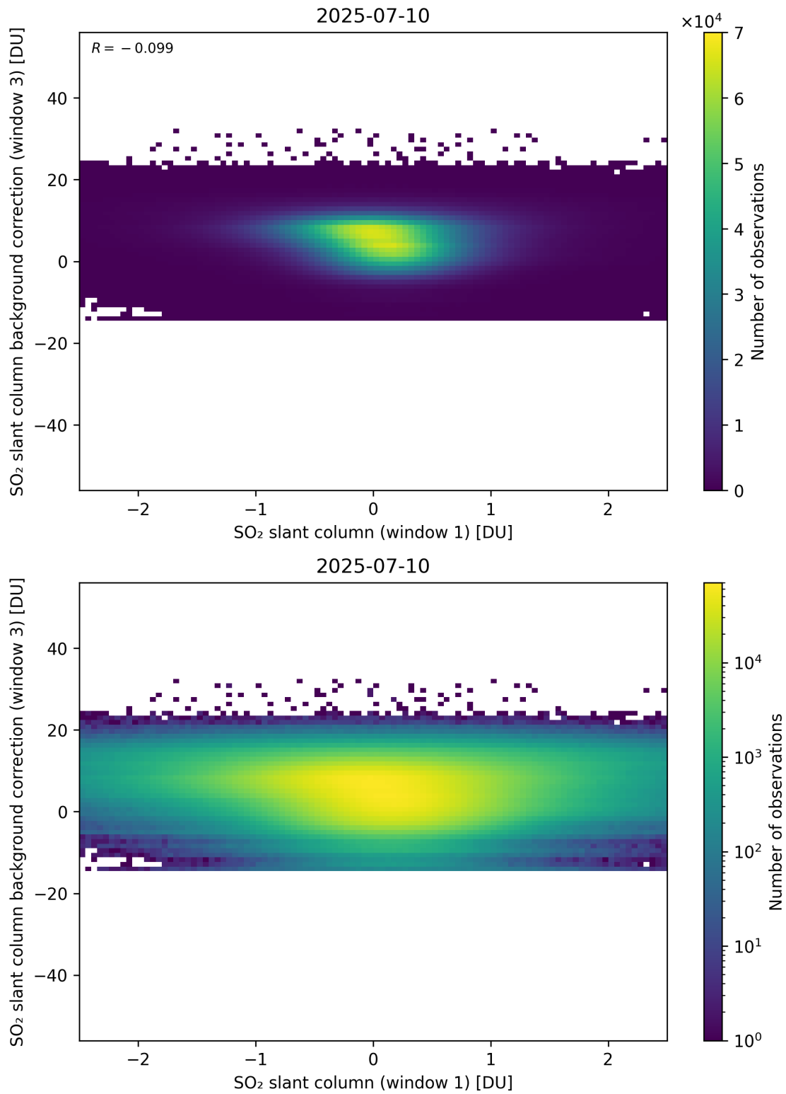
Figure 264: Scatter density plot of “SO 2 slant column (window 1)” against “SO 2 slant column background correction (window 3)” for 2025-07-09 to 2025-07-11.
