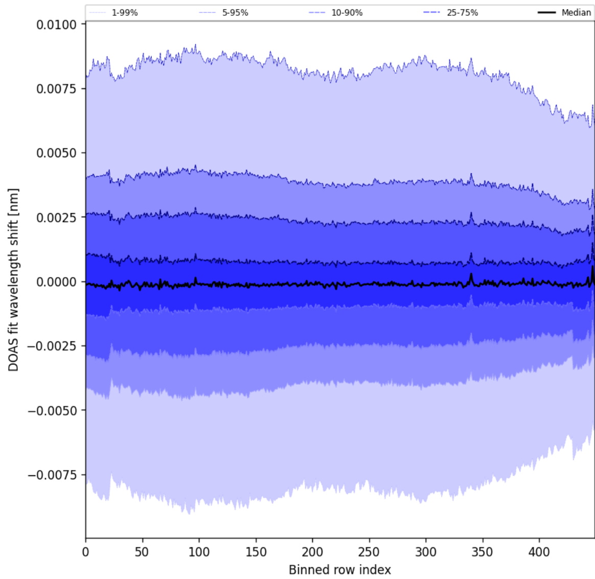
Figure 102: Along track statistics of “DOAS fit wavelength shift” for 2025-07-09 to 2025-07-11
