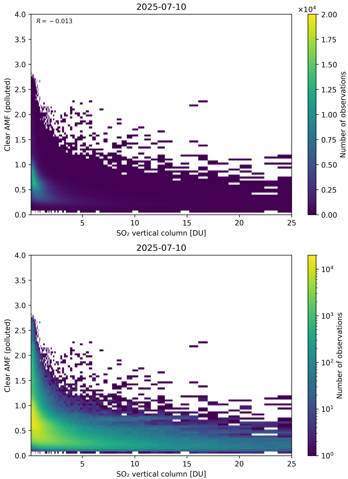
Figure 348: Scatter density plot of “SO 2 vertical column” against “Clear AMF (polluted)” for 2025-07-09 to 2025-07-11.
