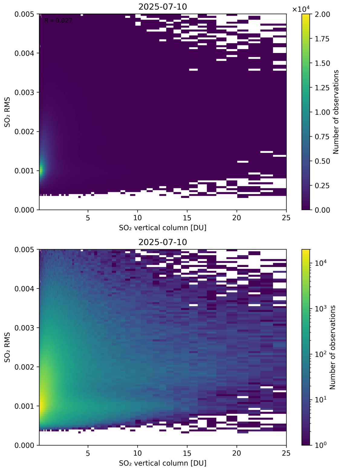
Figure 328: Scatter density plot of “SO 2 vertical column” against “SO 2 RMS” for 2025-07-09 to 2025-07-11.
