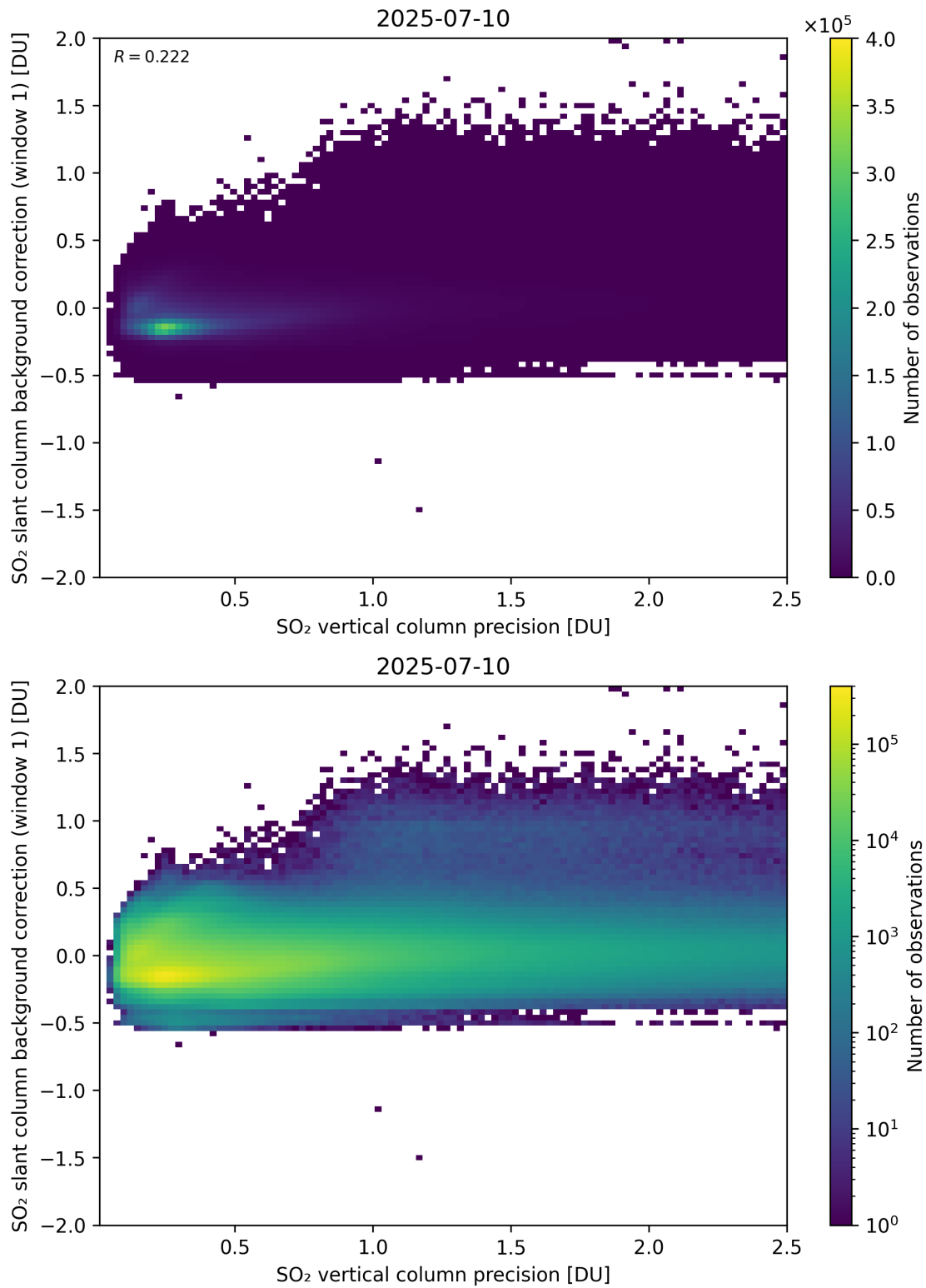
Figure 329: Scatter density plot of “SO 2 vertical column precision” against “SO 2 slant column background correction (window 1)” for 2025-07-09 to 2025-07-11.
