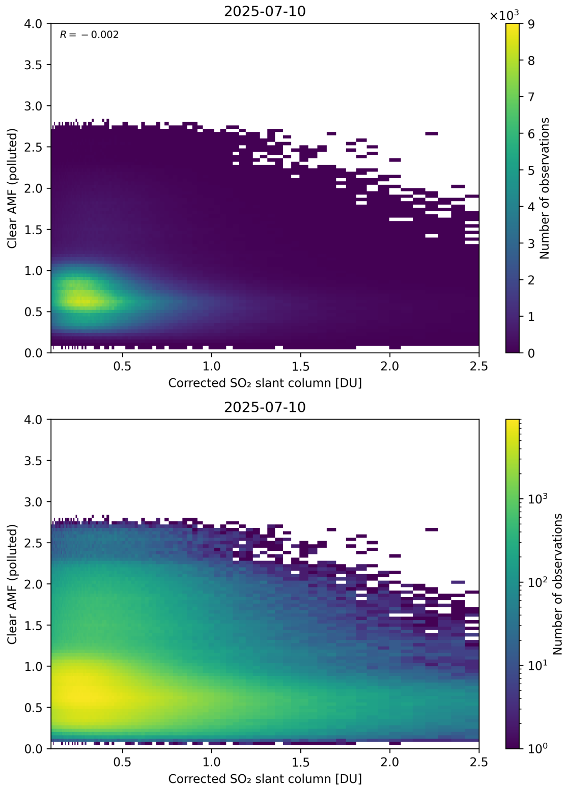
Figure 232: Scatter density plot of “Corrected SO 2 slant column” against “Clear AMF (polluted)” for 2025-07-09 to 2025-07-11.
