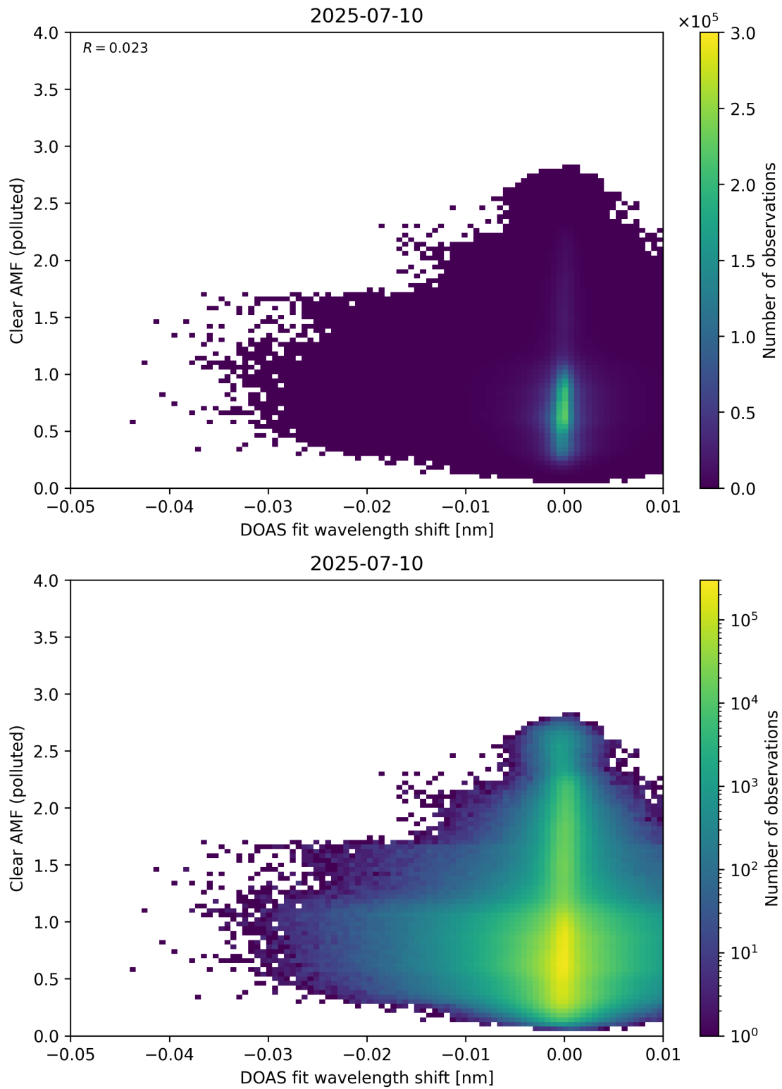
Figure 140: Scatter density plot of “DOAS fit wavelength shift” against “Clear AMF (polluted)” for 2025-07-09 to 2025-07-11.
