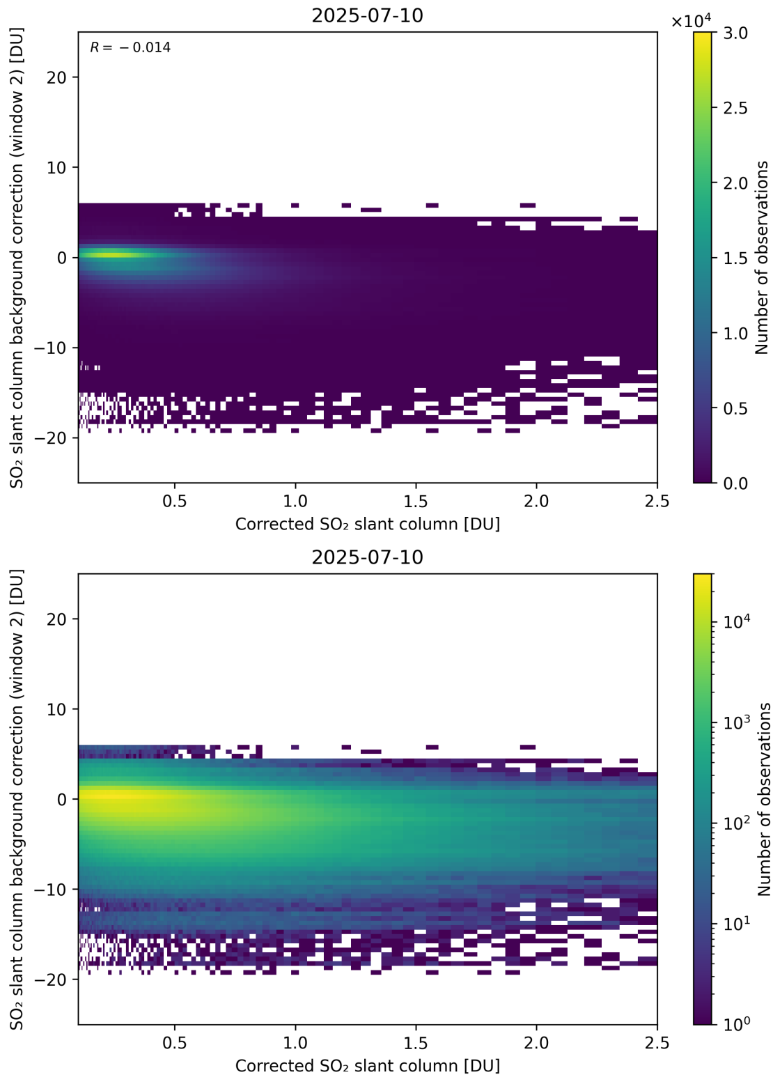
Figure 227: Scatter density plot of “Corrected SO 2 slant column” against “SO 2 slant column background correction (window 2)” for 2025-07-09 to 2025-07-11.
