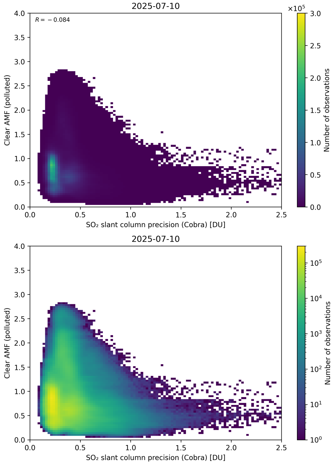
Figure 205: Scatter density plot of “SO 2 slant column precision (Cobra)” against “Clear AMF (polluted)” for 2025-07-09 to 2025-07-11.
