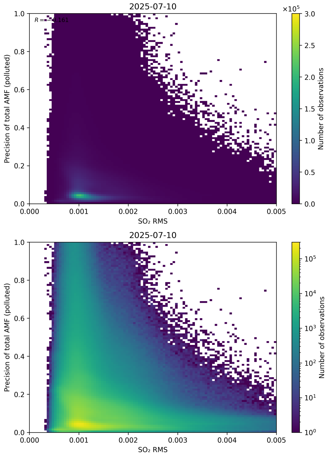
Figure 149: Scatter density plot of “SO 2 RMS” against “Precision of total AMF (polluted)” for 2025-07-09 to 2025-07-11.
