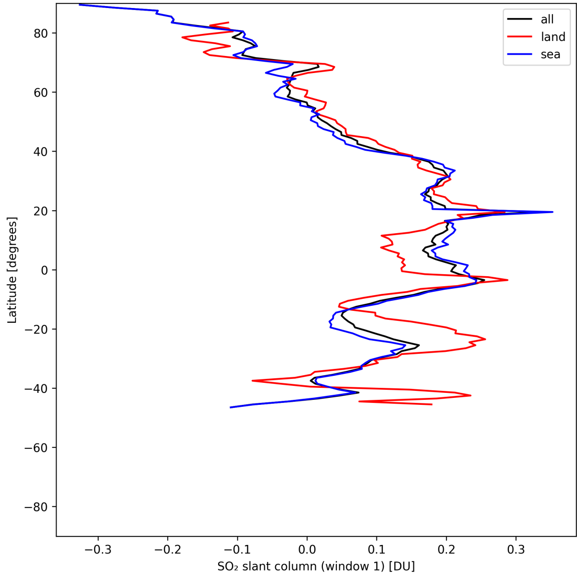
Figure 37: Zonal average of “SO 2 slant column (window 1)” for 2025-07-09 to 2025-07-11.
