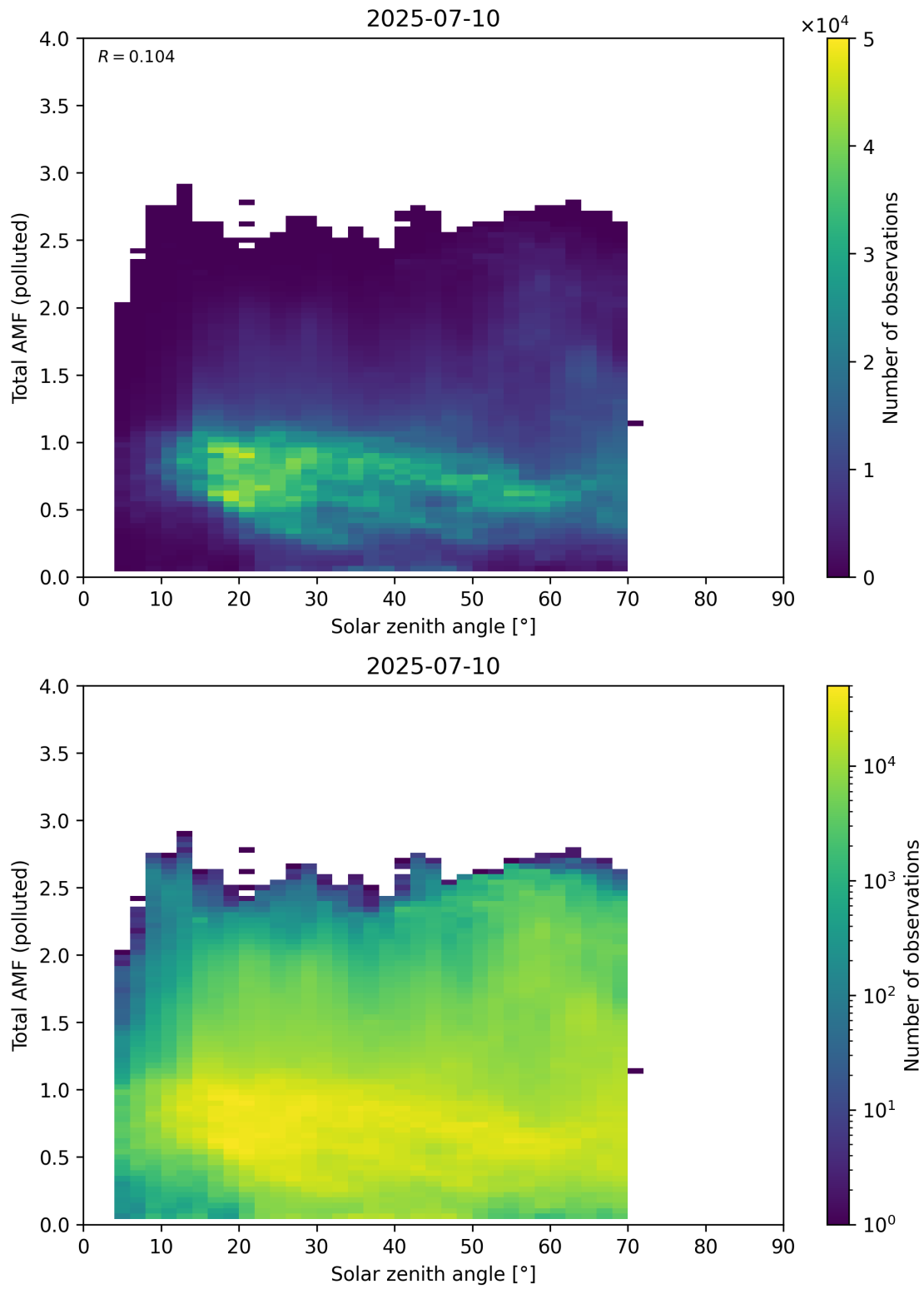
Figure 189: Scatter density plot of “Solar zenith angle” against “Total AMF (polluted)” for 2025-07-09 to 2025-07-11.
