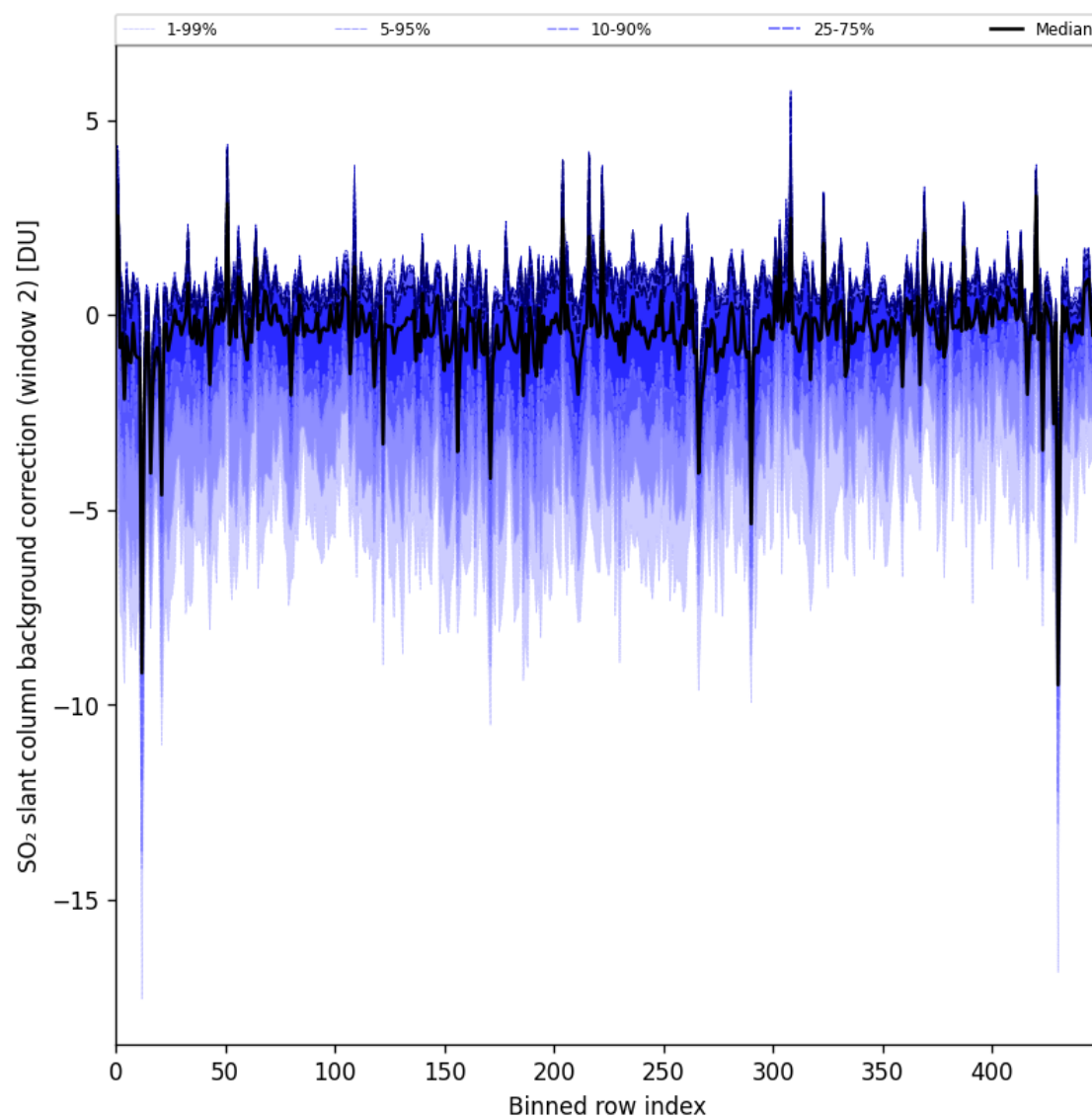
Figure 96: Along track statistics of “SO 2 slant column background correction (window 2)” for 2025-07-09 to 2025-07-11
