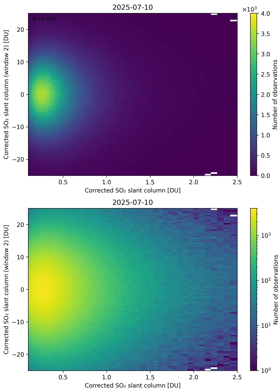
Figure 235: Scatter density plot of “Corrected SO 2 slant column” against “Corrected SO 2 slant column (window 2)” for 2025-07-09 to 2025-07-11.
