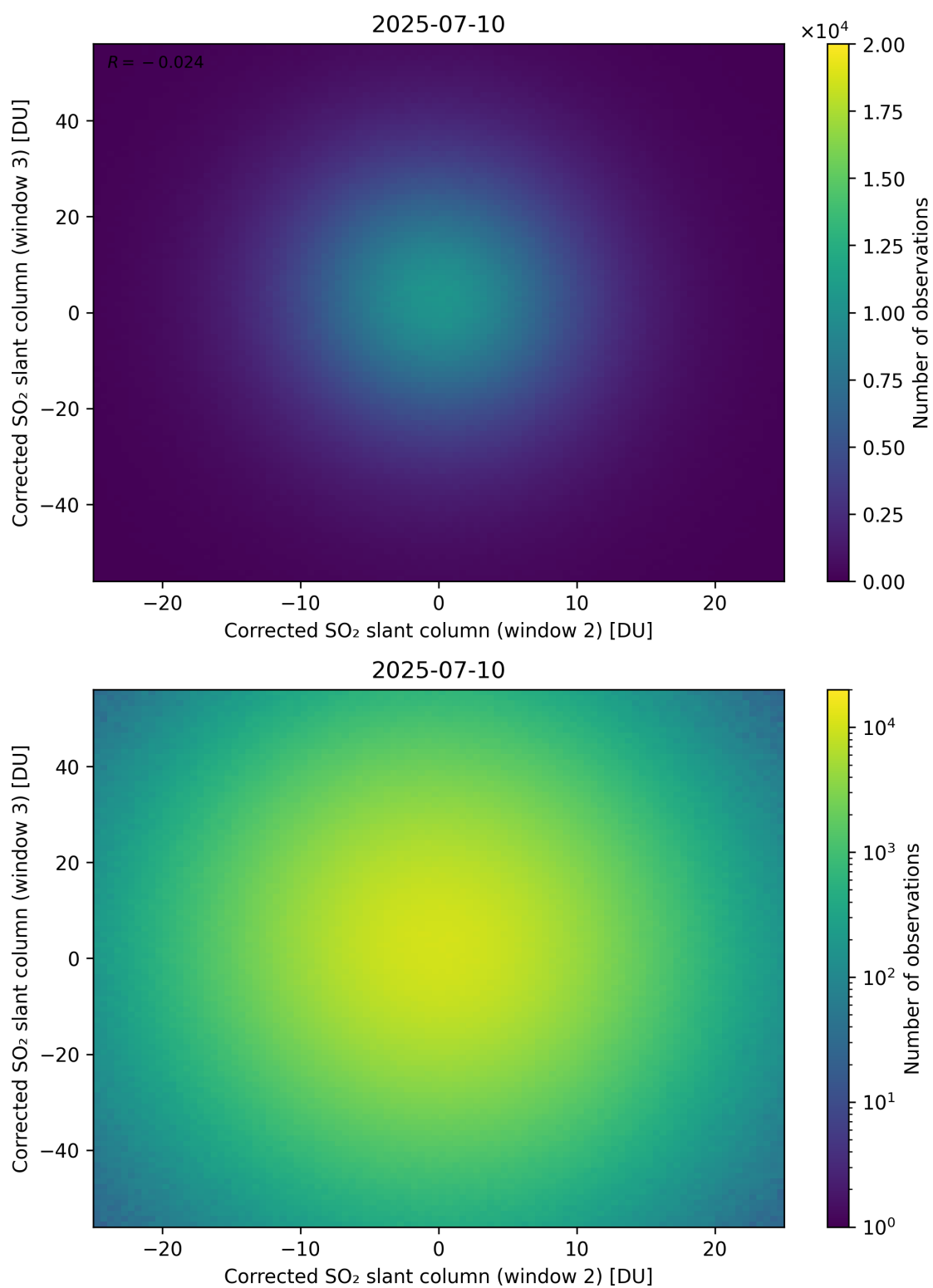
Figure 250: Scatter density plot of “Corrected SO 2 slant column (window 2)” against “Corrected SO 2 slant column (window 3)” for 2025-07-09 to 2025-07-11.
