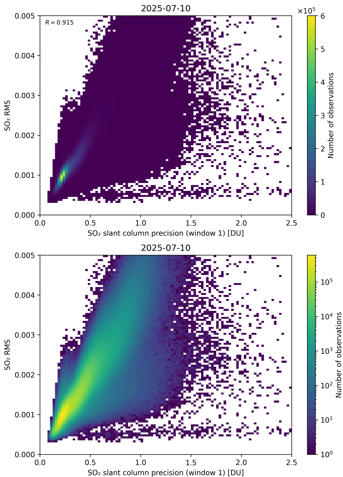
Figure 273: Scatter density plot of “SO 2 slant column precision (window 1)” against “SO 2 RMS” for 2025-07-09 to 2025-07-11.
