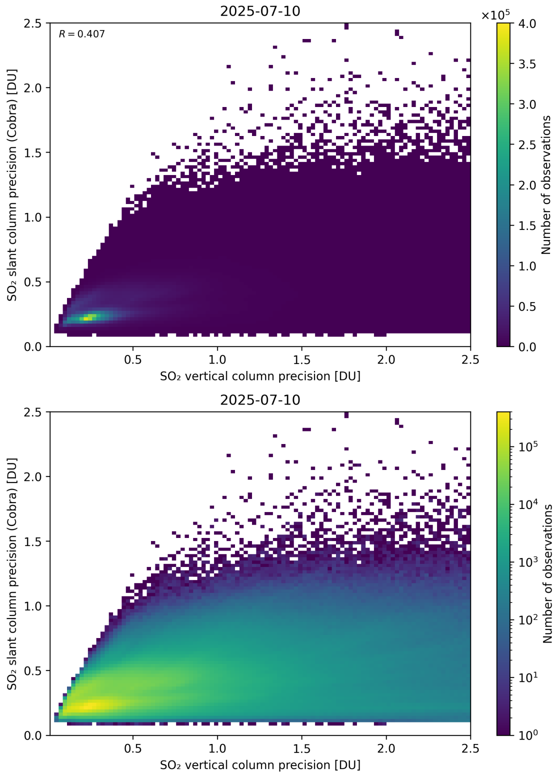
Figure 337: Scatter density plot of “SO 2 vertical column precision” against “SO 2 slant column precision (Cobra)” for 2025-07-09 to 2025-07-11.
