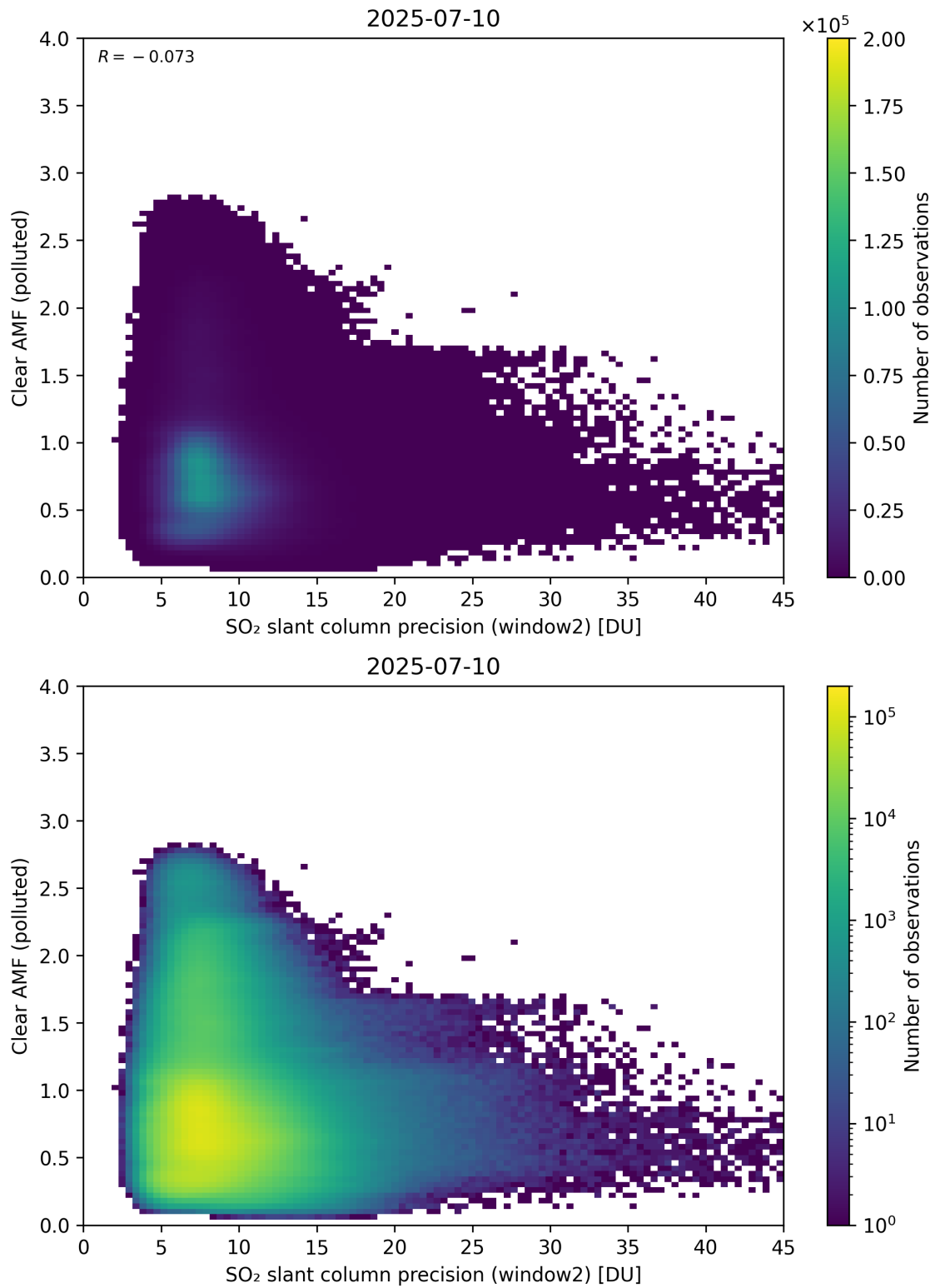
Figure 296: Scatter density plot of “SO 2 slant column precision (window2)” against “Clear AMF (polluted)” for 2025-07-09 to 2025-07-11.
