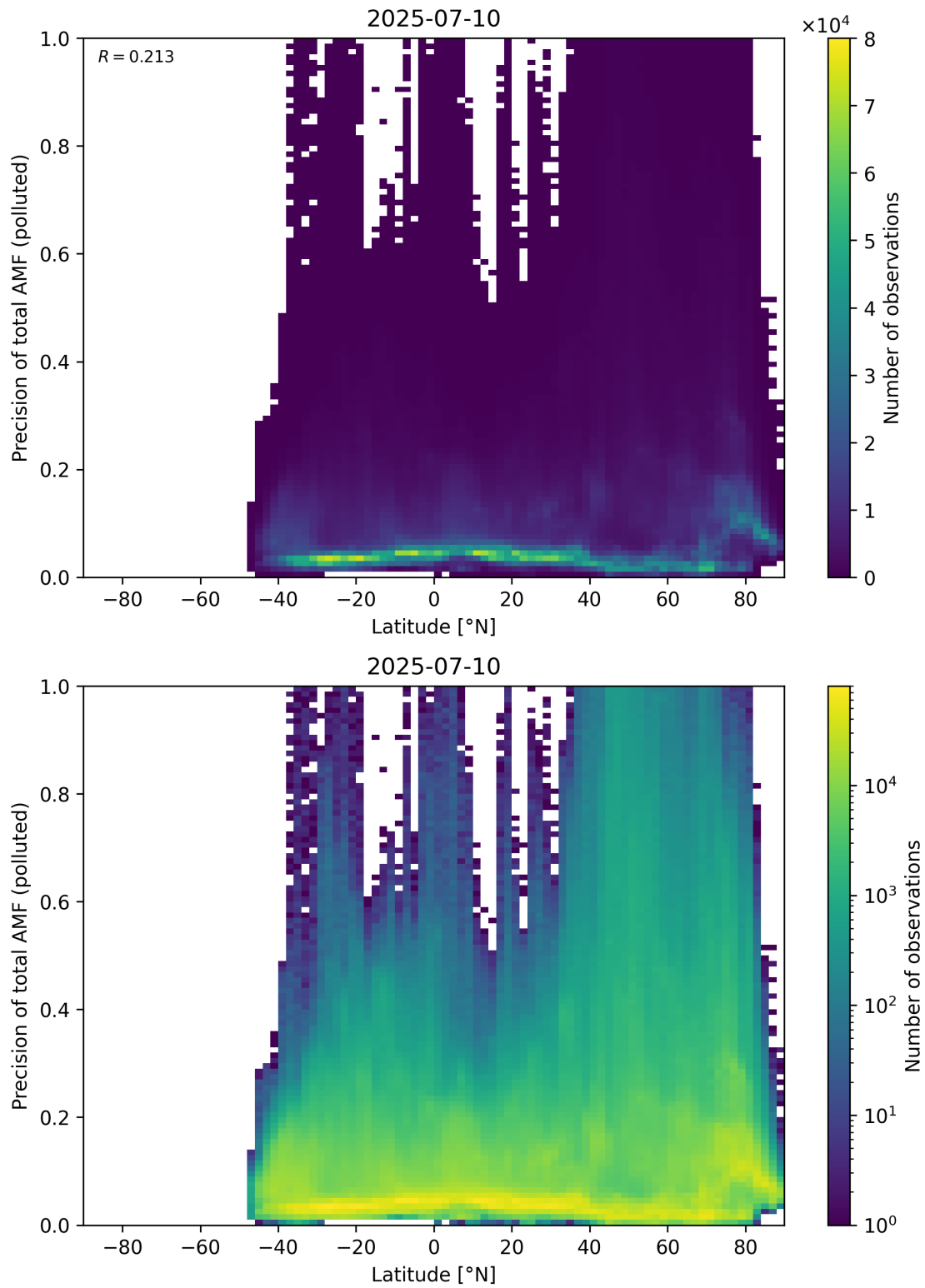
Figure 168: Scatter density plot of “Latitude” against “Precision of total AMF (polluted)” for 2025-07-09 to 2025-07-11.
