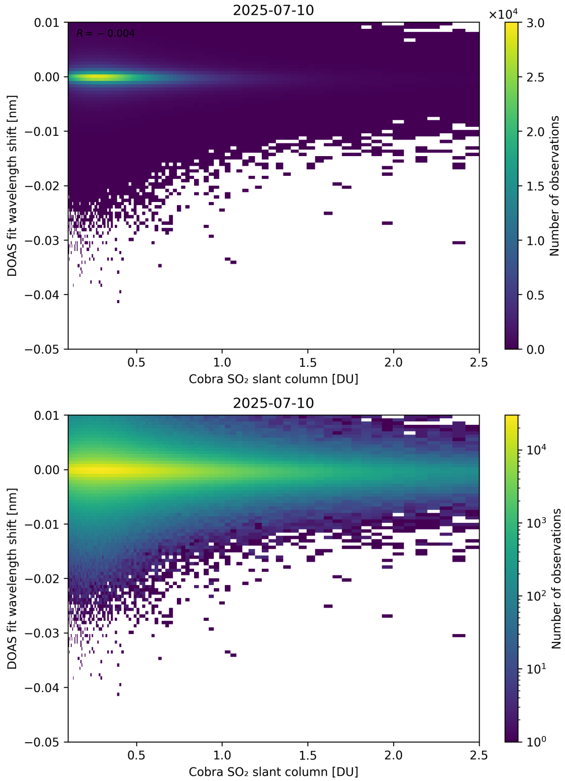
Figure 196: Scatter density plot of “Cobra SO 2 slant column” against “DOAS fit wavelength shift” for 2025-07-09 to 2025-07-11.
