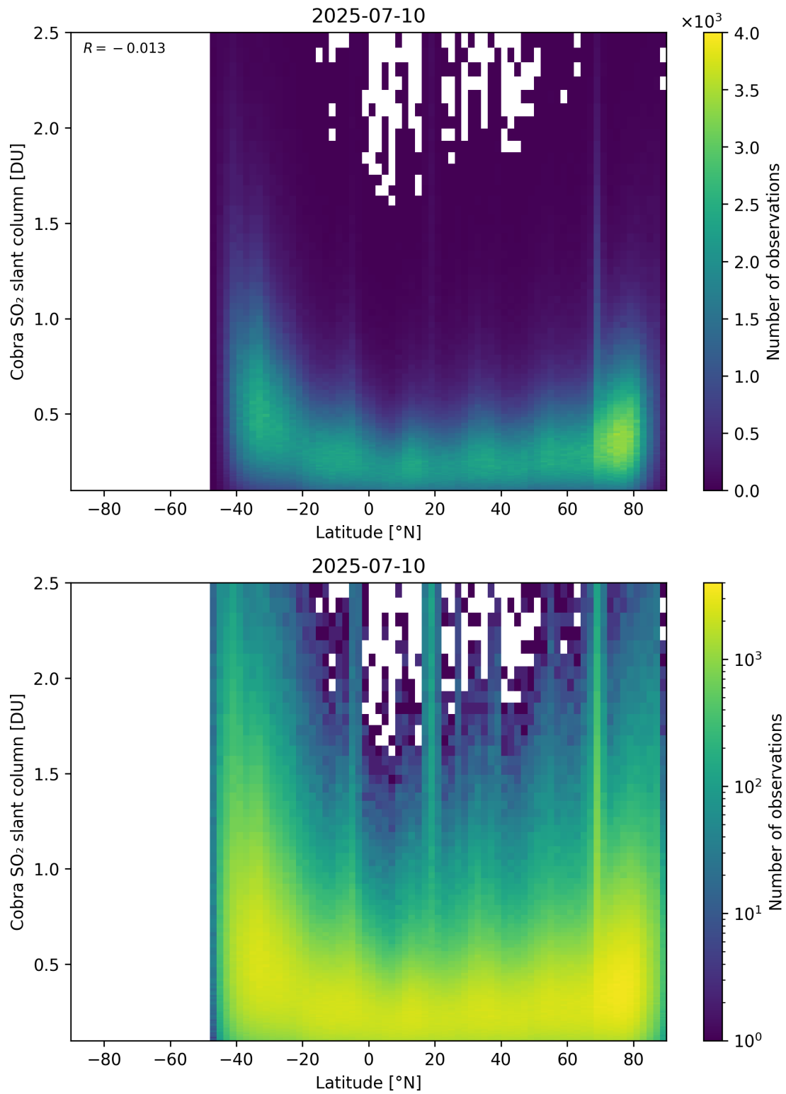
Figure 157: Scatter density plot of “Latitude” against “Cobra SO 2 slant column” for 2025-07-09 to 2025-07-11.
