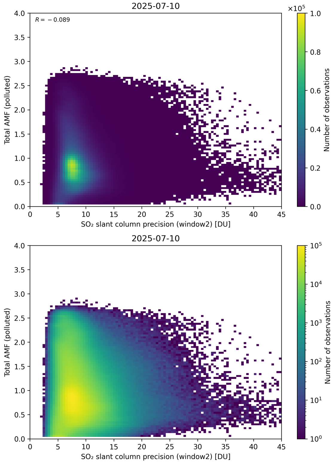
Figure 301: Scatter density plot of “SO 2 slant column precision (window2)” against “Total AMF (polluted)” for 2025-07-09 to 2025-07-11.
