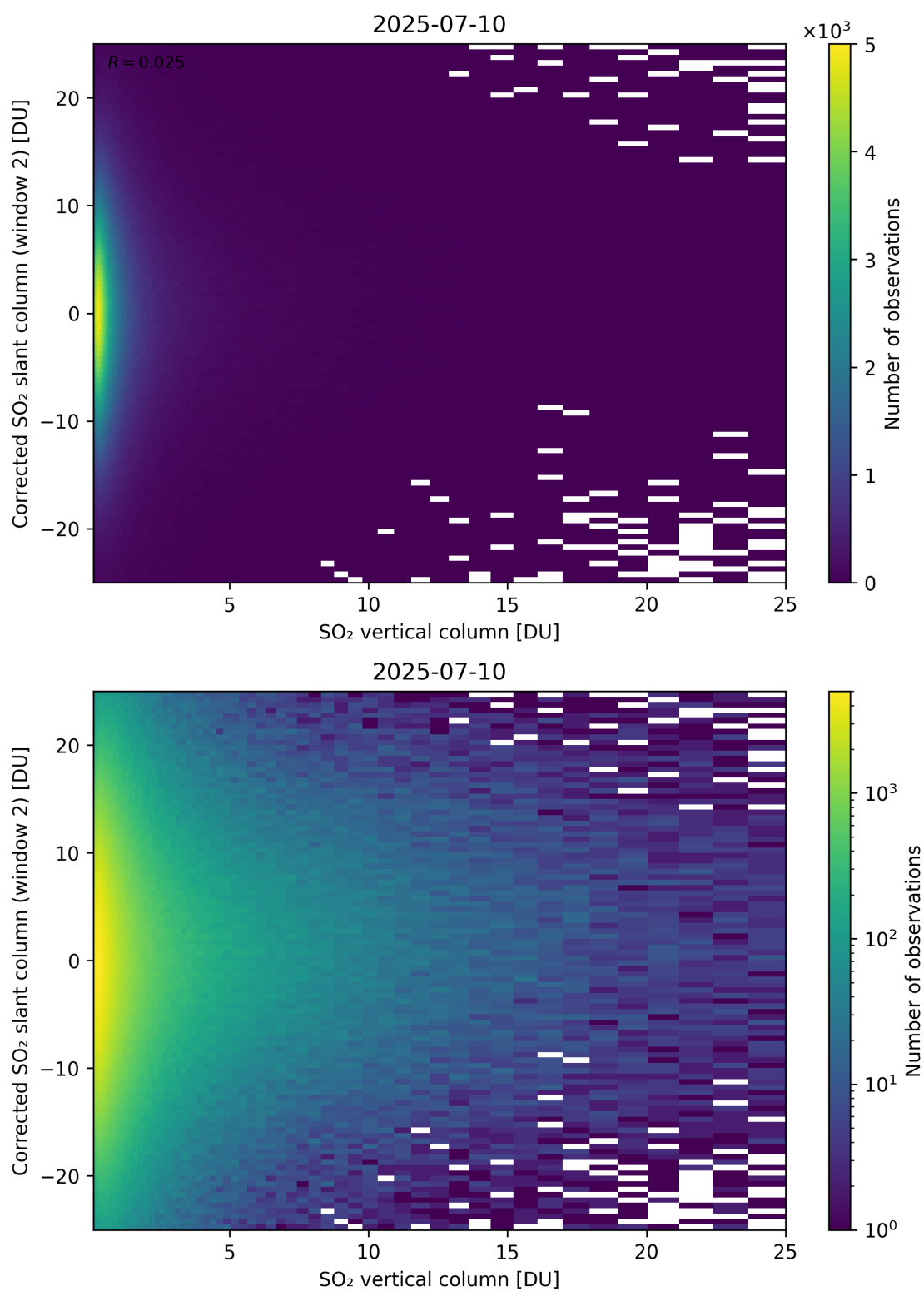
Figure 352: Scatter density plot of “SO 2 vertical column” against “Corrected SO 2 slant column (window 2)” for 2025-07-09 to 2025-07-11.
