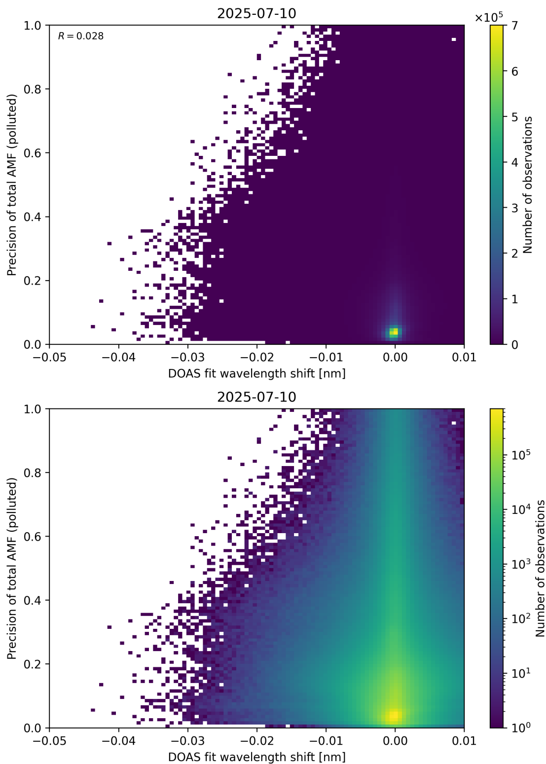
Figure 142: Scatter density plot of “DOAS fit wavelength shift” against “Precision of total AMF (polluted)” for 2025-07-09 to 2025-07-11.
