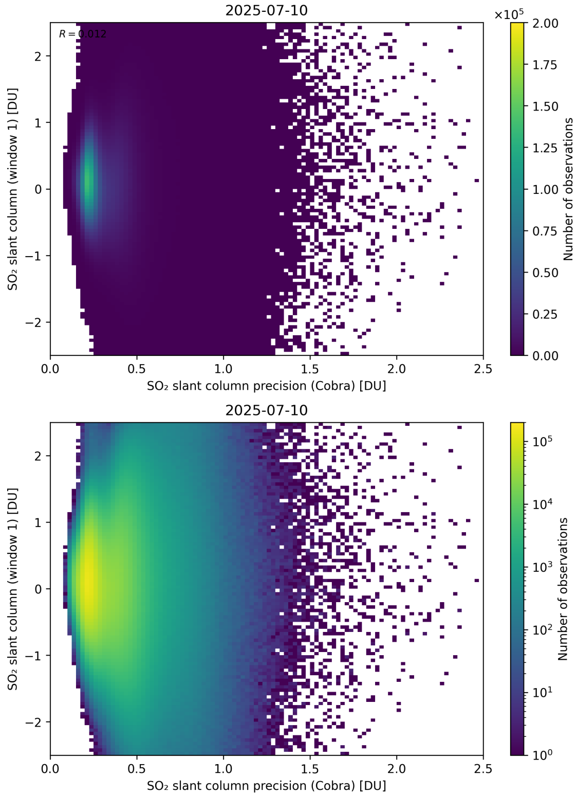
Figure 208: Scatter density plot of “SO 2 slant column precision (Cobra)” against “SO 2 slant column (window 1)” for 2025-07-09 to 2025-07-11.
