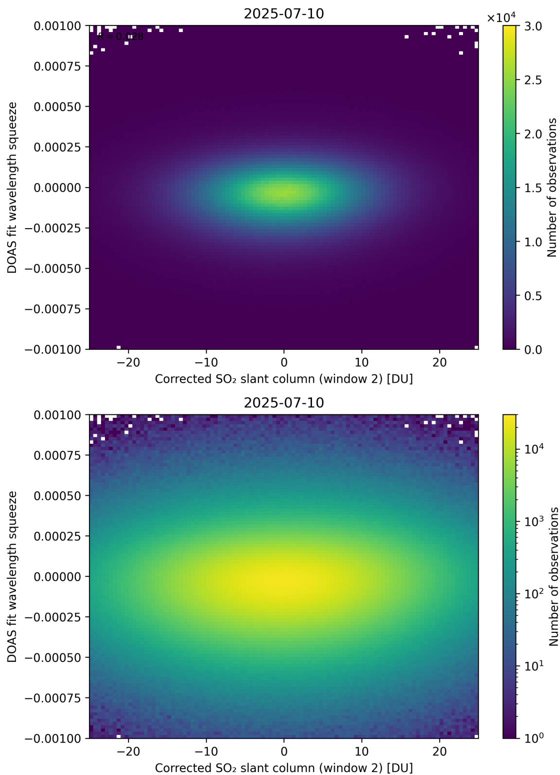
Figure 247: Scatter density plot of “Corrected SO 2 slant column (window 2)” against “DOAS fit wavelength squeeze” for 2025-07-09 to 2025-07-11.
