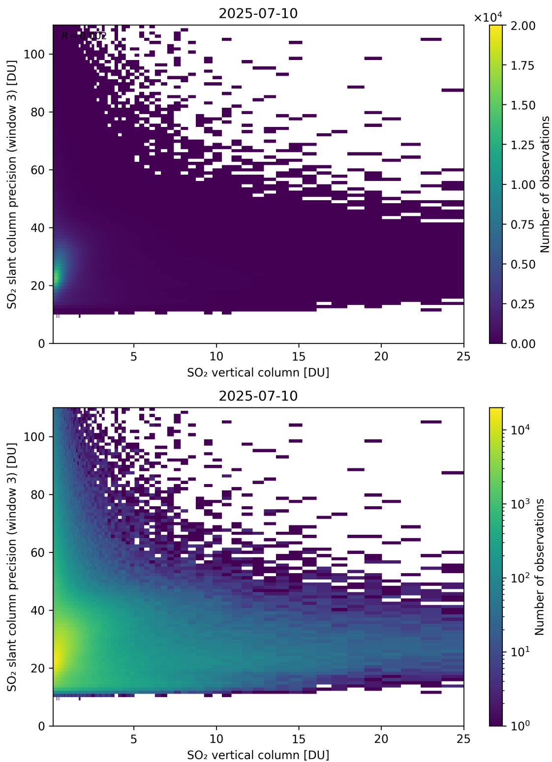
Figure 358: Scatter density plot of “SO 2 vertical column” against “SO 2 slant column precision (window 3)” for 2025-07-09 to 2025-07-11.
