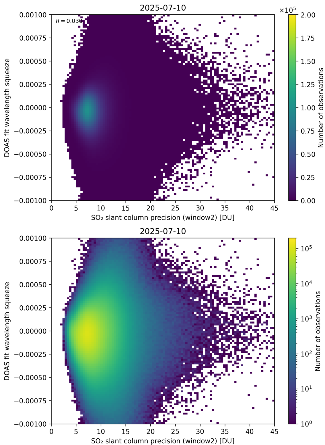
Figure 294: Scatter density plot of “SO 2 slant column precision (window2)” against “DOAS fit wavelength squeeze” for 2025-07-09 to 2025-07-11.
