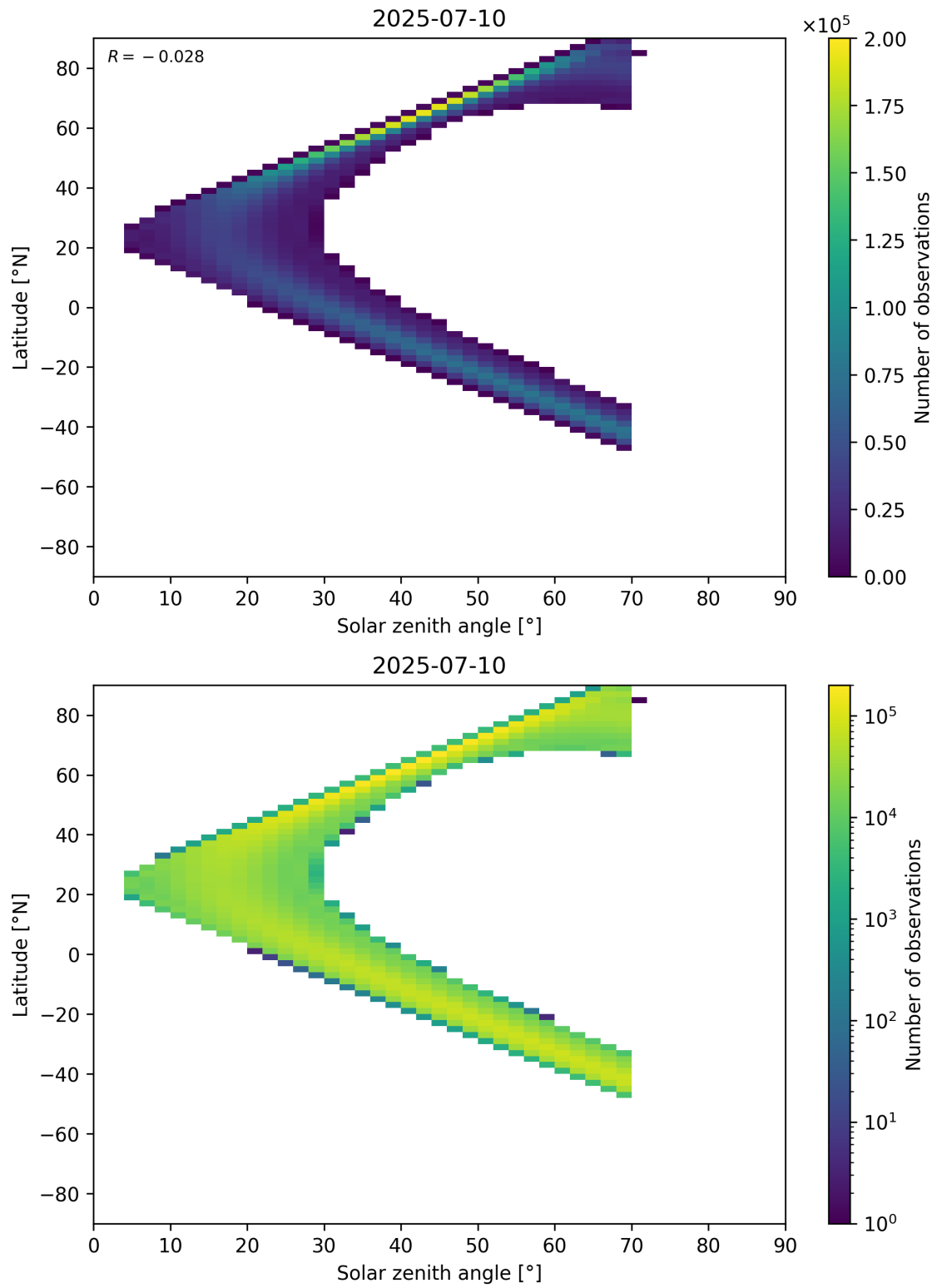
Figure 177: Scatter density plot of “Solar zenith angle” against “Latitude” for 2025-07-09 to 2025-07-11.
