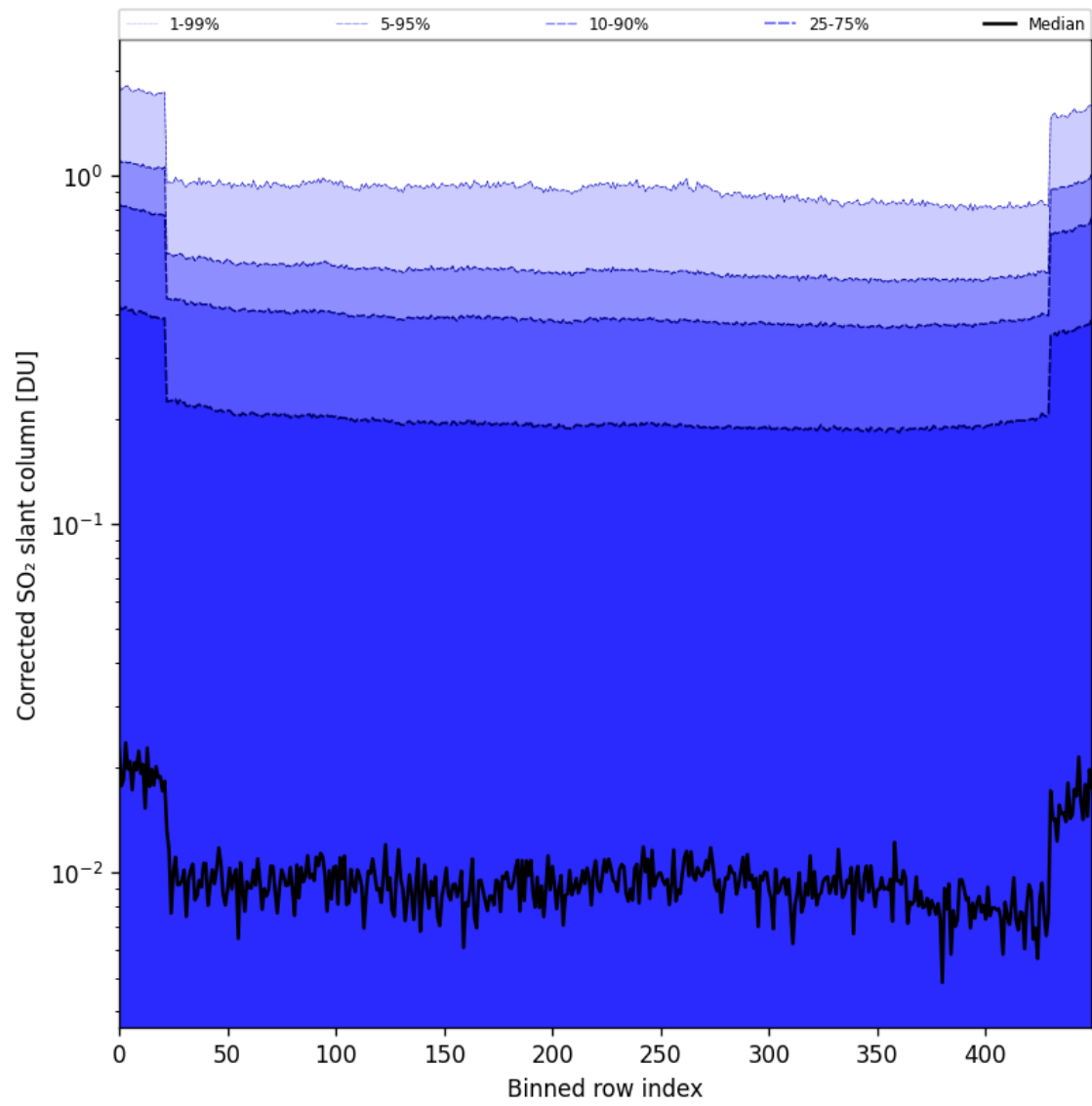
Figure 86: Along track statistics of “Corrected SO 2 slant column” for 2025-07-09 to 2025-07-11
