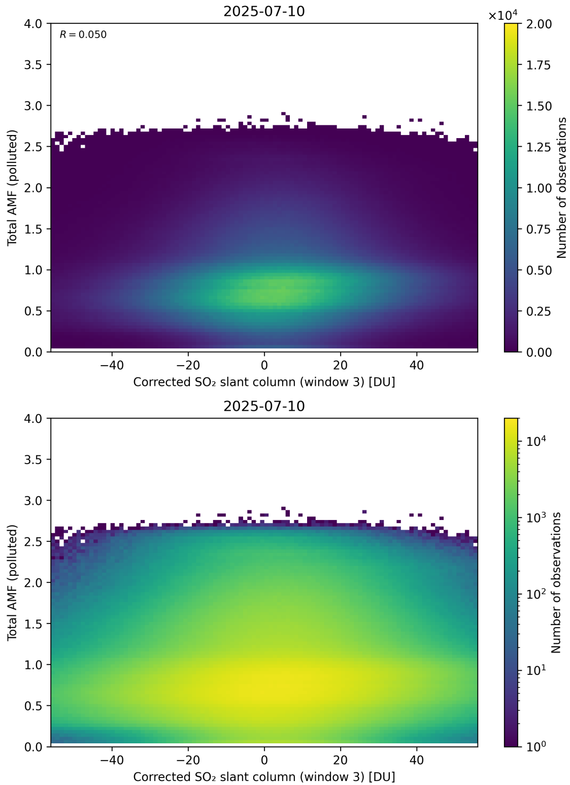
Figure 260: Scatter density plot of “Corrected SO 2 slant column (window 3)” against “Total AMF (polluted)” for 2025-07-09 to 2025-07-11.
