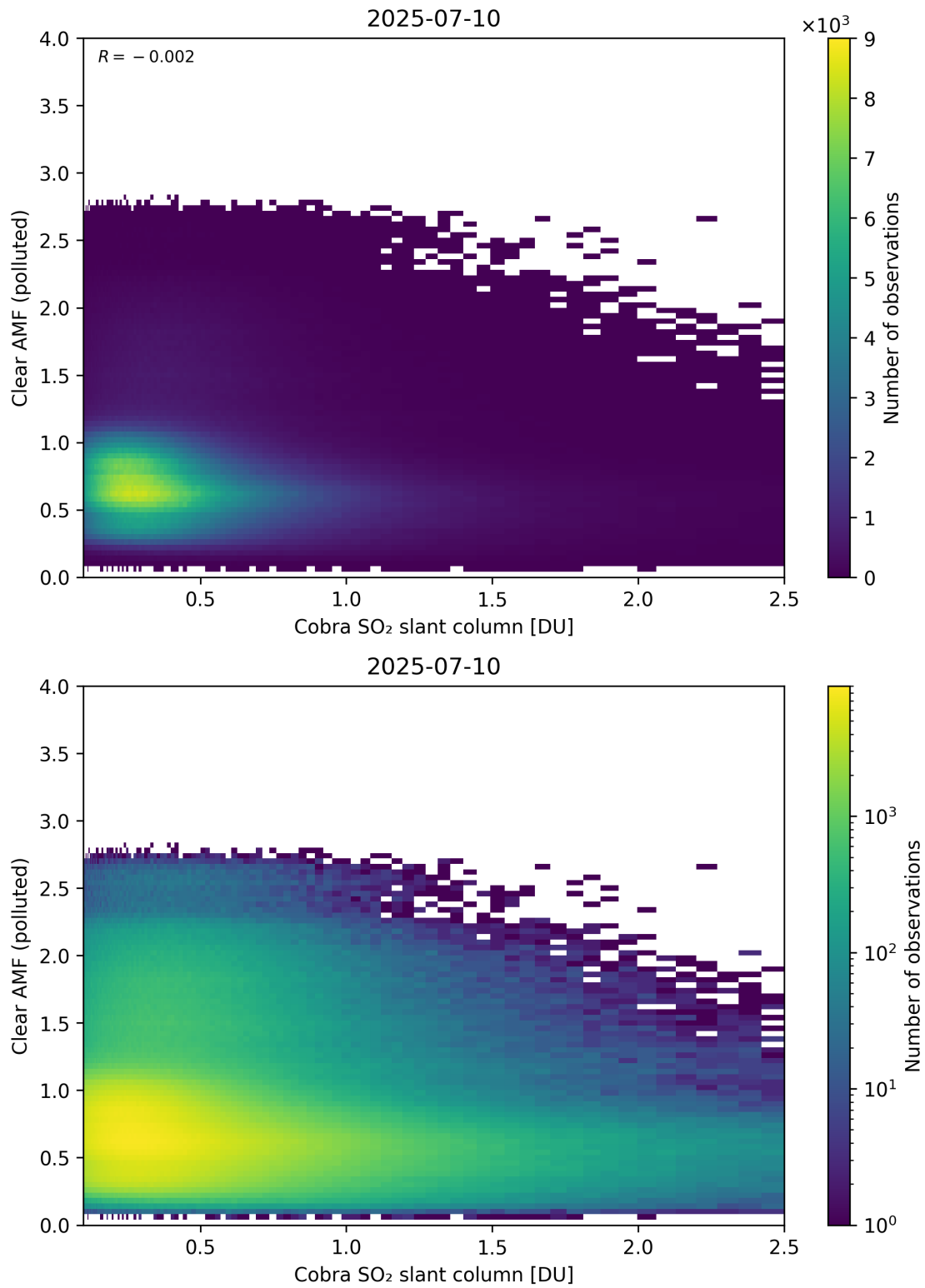
Figure 215: Scatter density plot of “Cobra SO 2 slant column” against “Clear AMF (polluted)” for 2025-07-09 to 2025-07-11.
