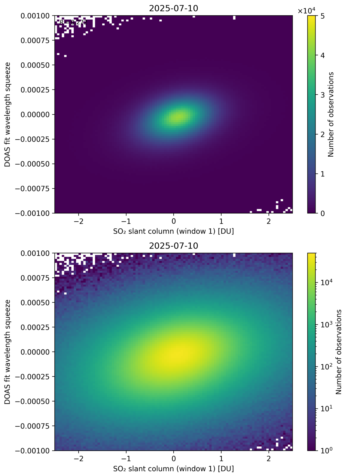
Figure 266: Scatter density plot of “SO 2 slant column (window 1)” against “DOAS fit wavelength squeeze” for 2025-07-09 to 2025-07-11.
