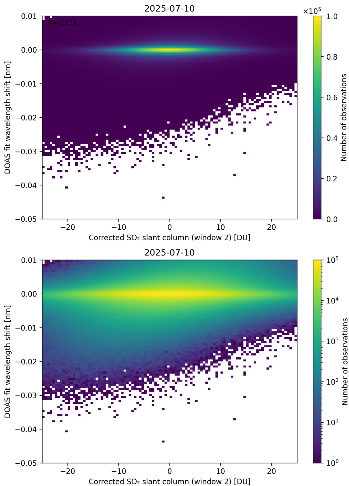
Figure 246: Scatter density plot of “Corrected SO 2 slant column (window 2)” against “DOAS fit wavelength shift” for 2025-07-09 to 2025-07-11.
