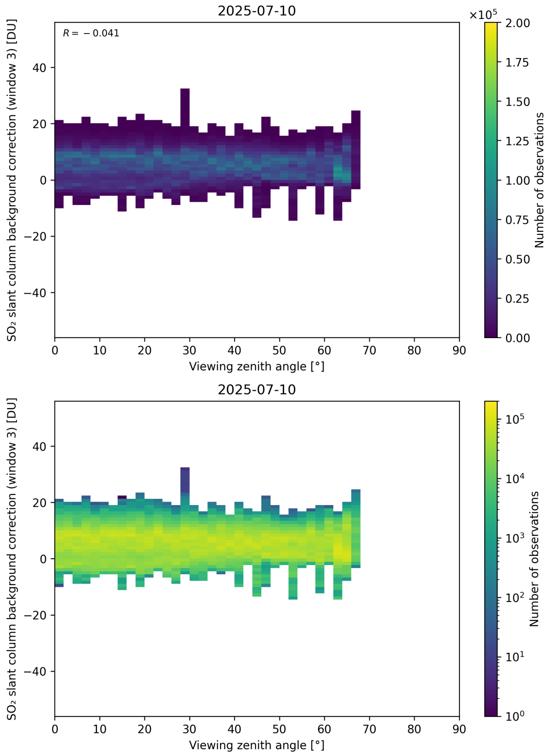
Figure 364: Scatter density plot of “Viewing zenith angle” against “SO 2 slant column background correction (window 3)” for 2025-07-09 to 2025-07-11.
