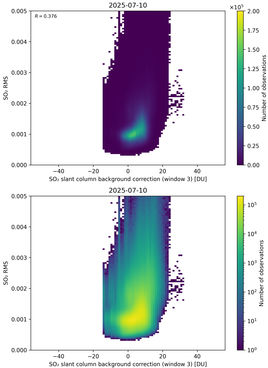
Figure 134: Scatter density plot of “SO 2 slant column background correction (window 3)” against “SO 2 RMS” for 2025-07-09 to 2025-07-11.
