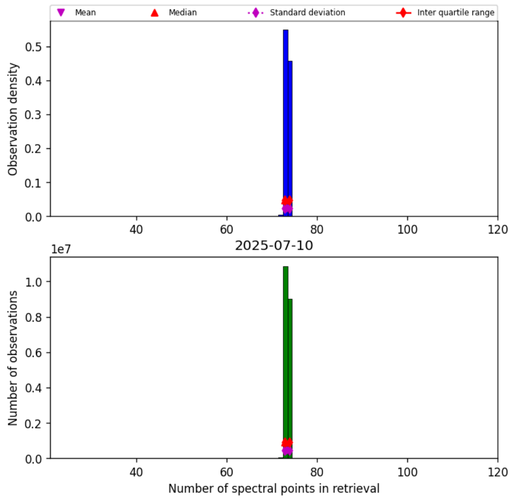
Figure 82: Histogram of “Number of spectral points in retrieval” for 2025-07-09 to 2025-07-11
