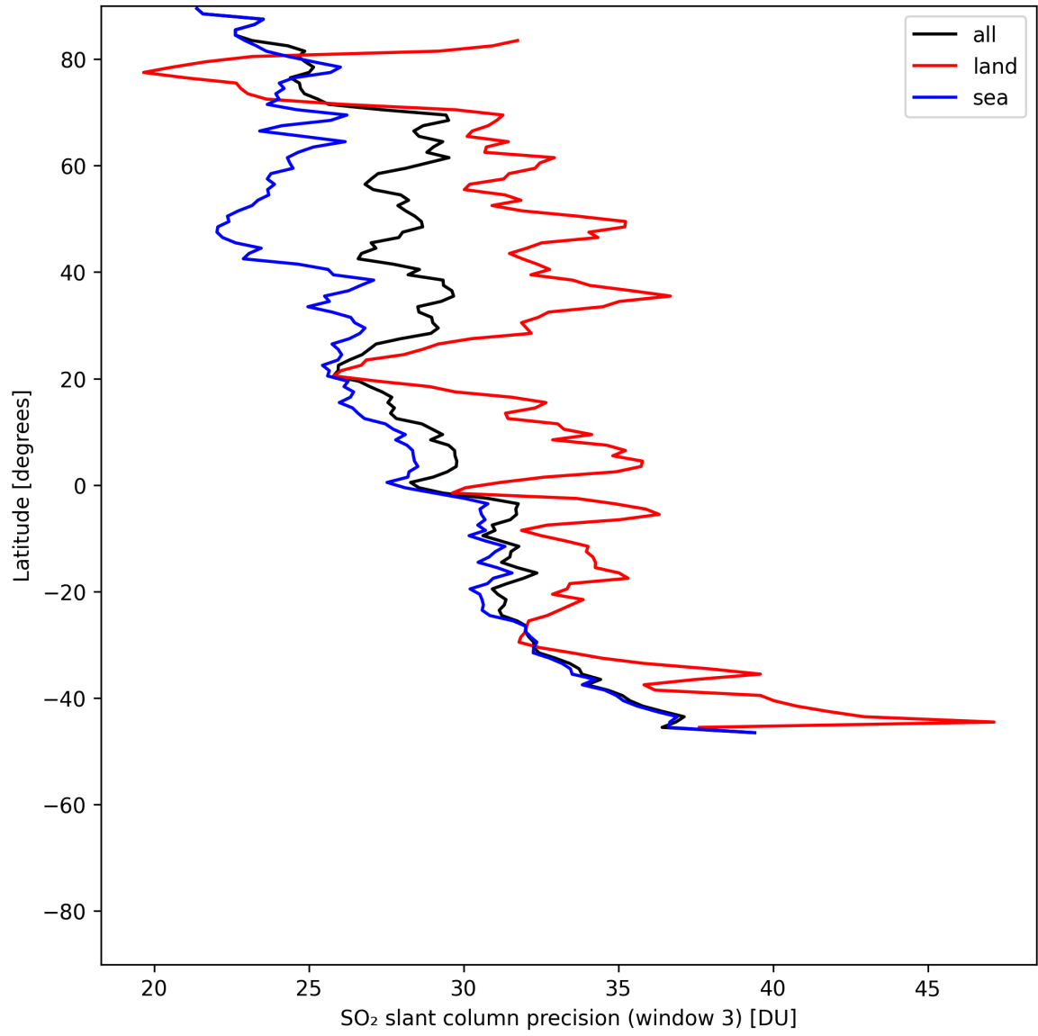
Figure 46: Zonal average of “SO 2 slant column precision (window 3)” for 2025-07-09 to 2025-07-11.
