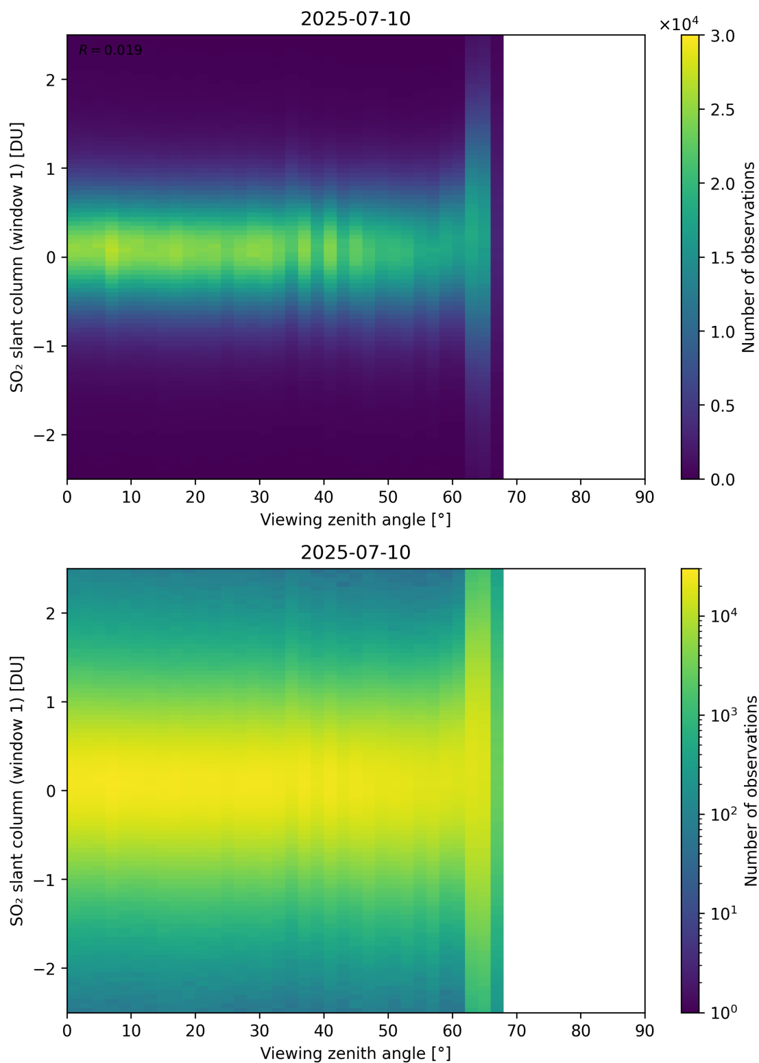
Figure 376: Scatter density plot of “Viewing zenith angle” against “SO 2 slant column (window 1)” for 2025-07-09 to 2025-07-11.
