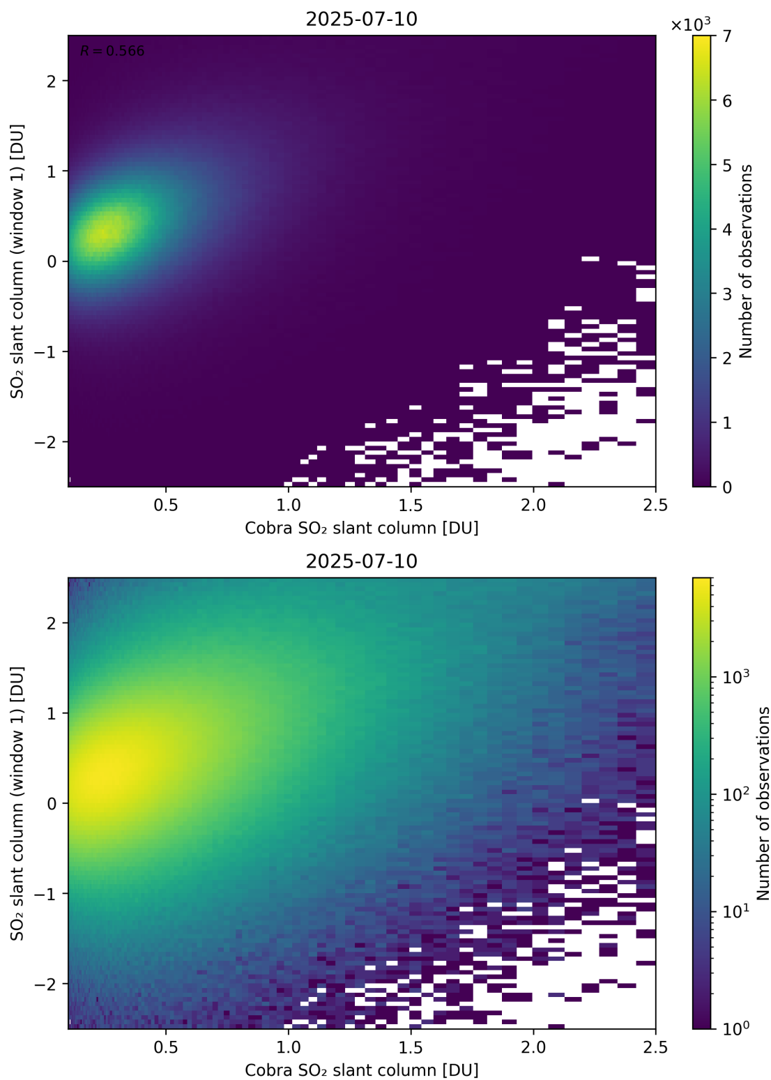
Figure 219: Scatter density plot of “Cobra SO 2 slant column” against “SO 2 slant column (window 1)” for 2025-07-09 to 2025-07-11.
