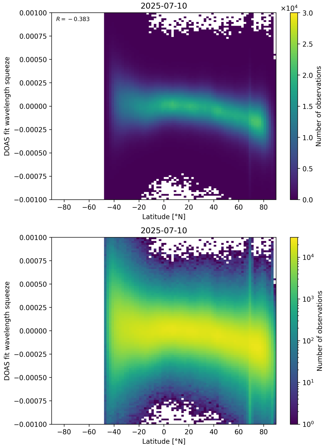
Figure 154: Scatter density plot of “Latitude” against “DOAS fit wavelength squeeze” for 2025-07-09 to 2025-07-11.
