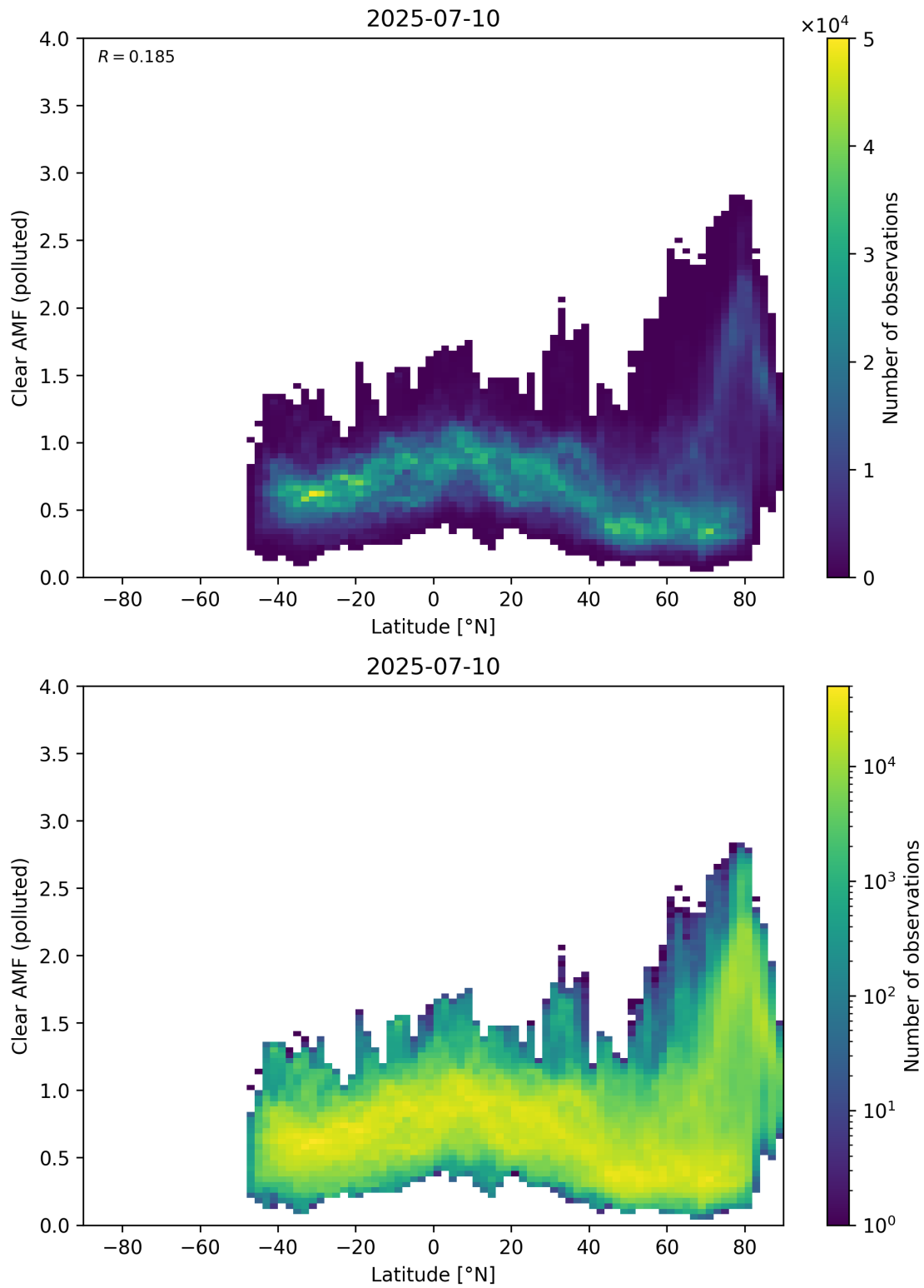
Figure 156: Scatter density plot of “Latitude” against “Clear AMF (polluted)” for 2025-07-09 to 2025-07-11.
