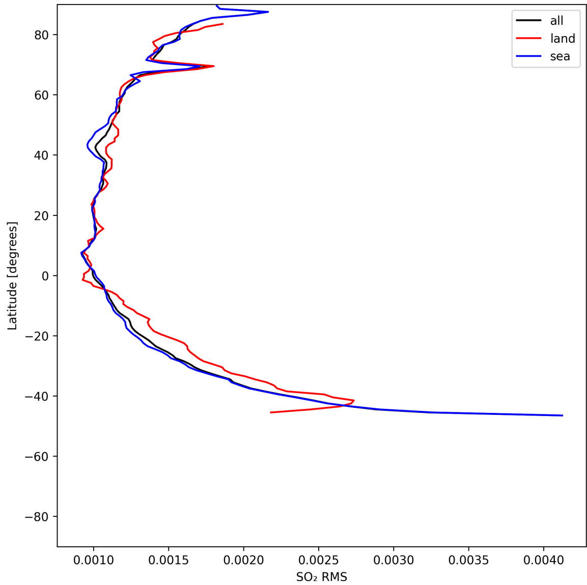
Figure 52: Zonal average of “SO 2 RMS” for 2025-07-09 to 2025-07-11.
