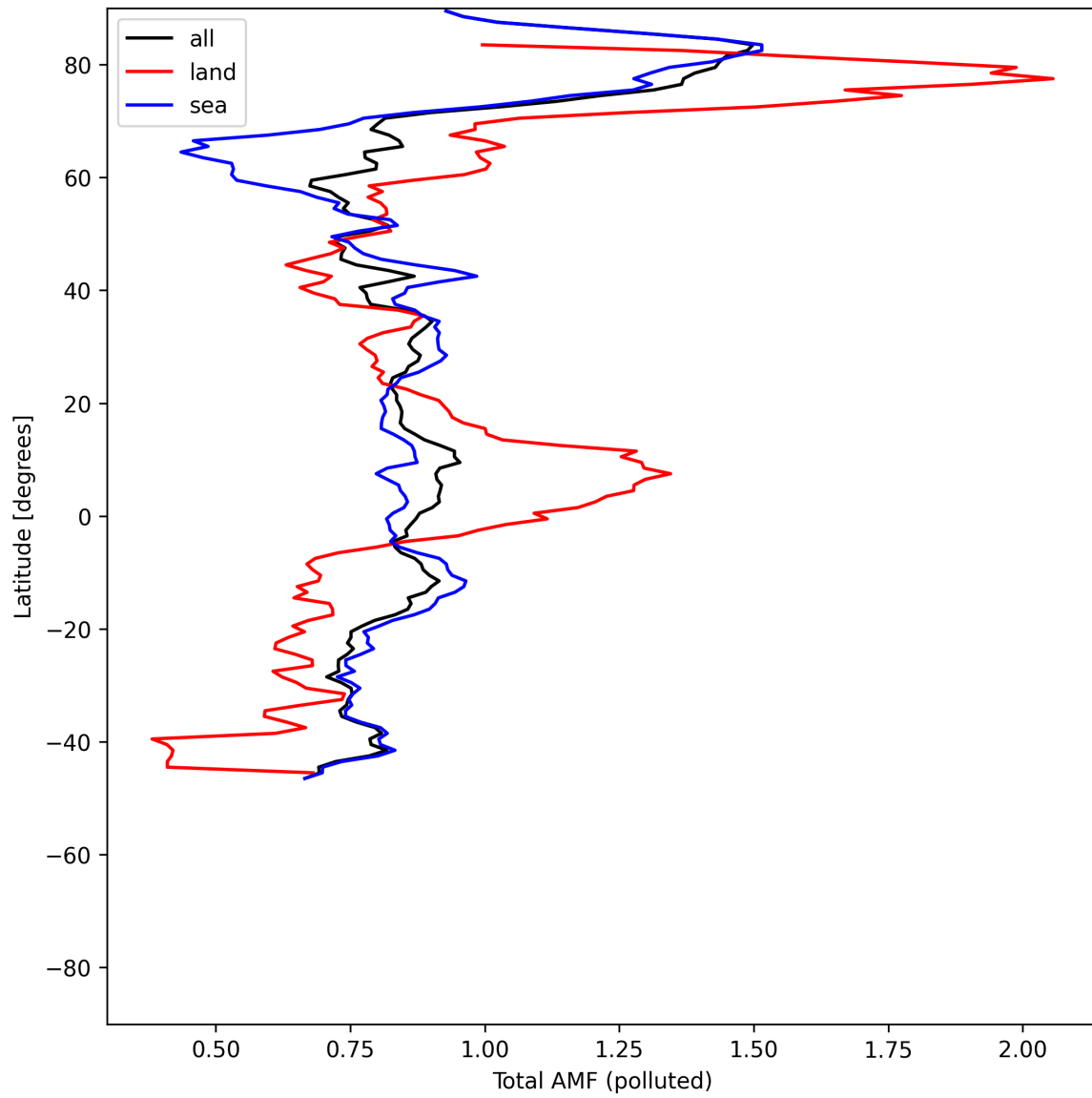
Figure 53: Zonal average of “Total AMF (polluted)” for 2025-07-09 to 2025-07-11.
