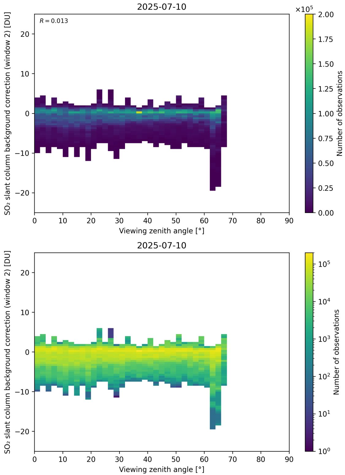
Figure 363: Scatter density plot of “Viewing zenith angle” against “SO 2 slant column background correction (window 2)” for 2025-07-09 to 2025-07-11.
