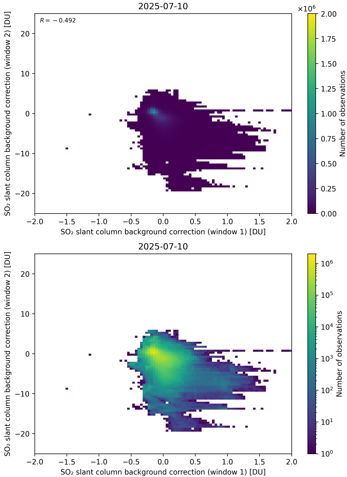
Figure 109: Scatter density plot of “SO 2 slant column background correction (window 1)” against “SO 2 slant column background correction (window 2)” for 2025-07-09 to 2025-07-11.
