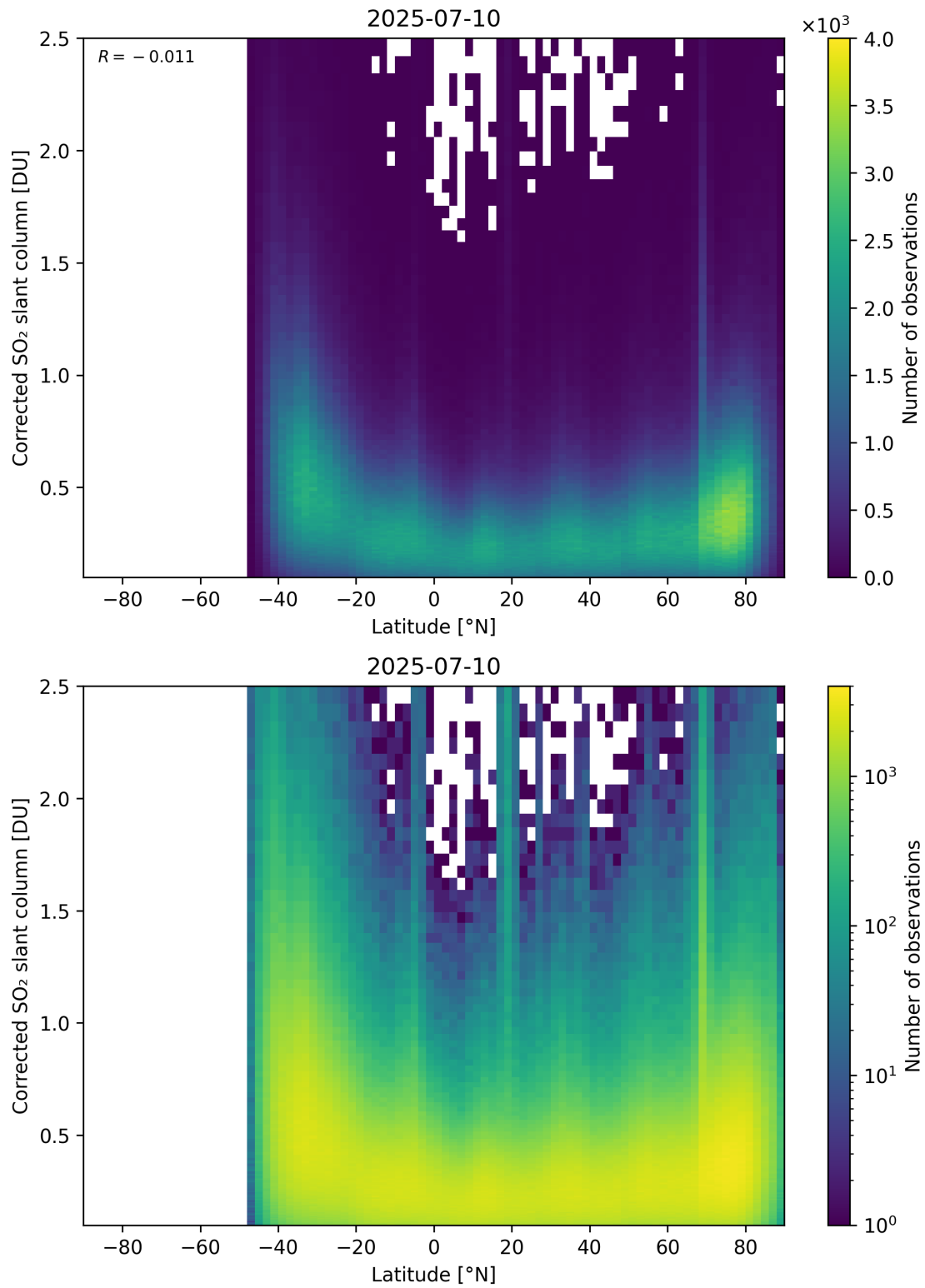
Figure 159: Scatter density plot of “Latitude” against “Corrected SO 2 slant column” for 2025-07-09 to 2025-07-11.
