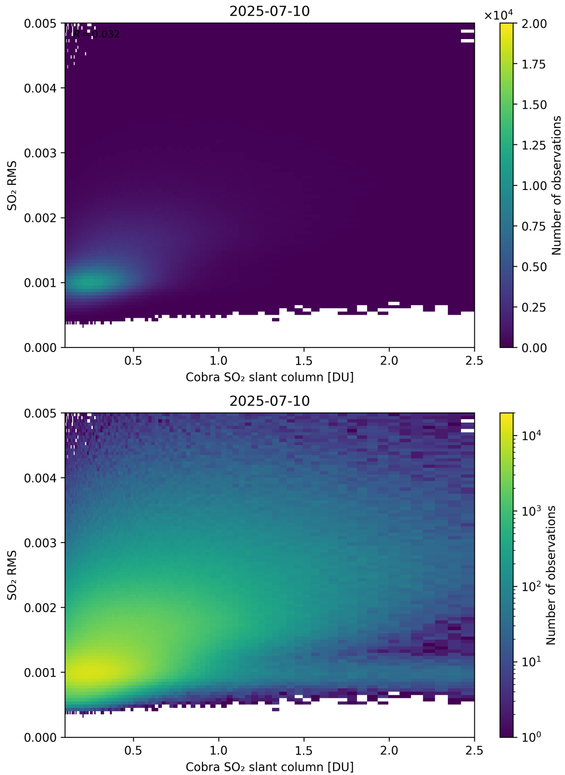
Figure 198: Scatter density plot of “Cobra SO 2 slant column” against “SO 2 RMS” for 2025-07-09 to 2025-07-11.
