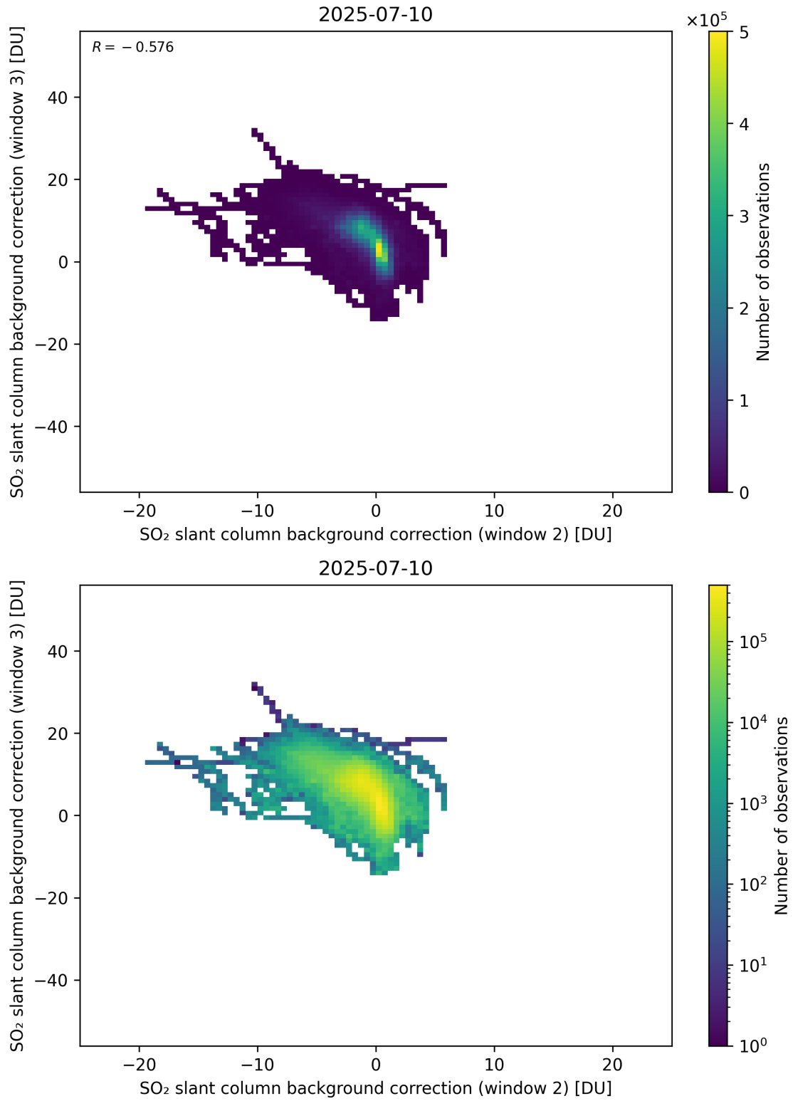
Figure 122: Scatter density plot of “SO 2 slant column background correction (window 2)” against “SO 2 slant column background correction (window 3)” for 2025-07-09 to 2025-07-11.
