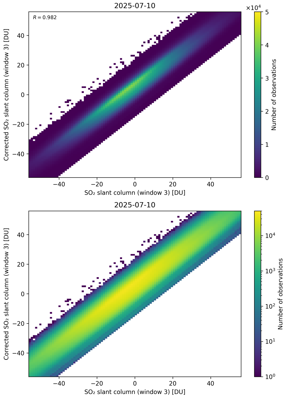
Figure 316: Scatter density plot of “SO 2 slant column (window 3)” against “Corrected SO 2 slant column (window 3)” for 2025-07-09 to 2025-07-11.
