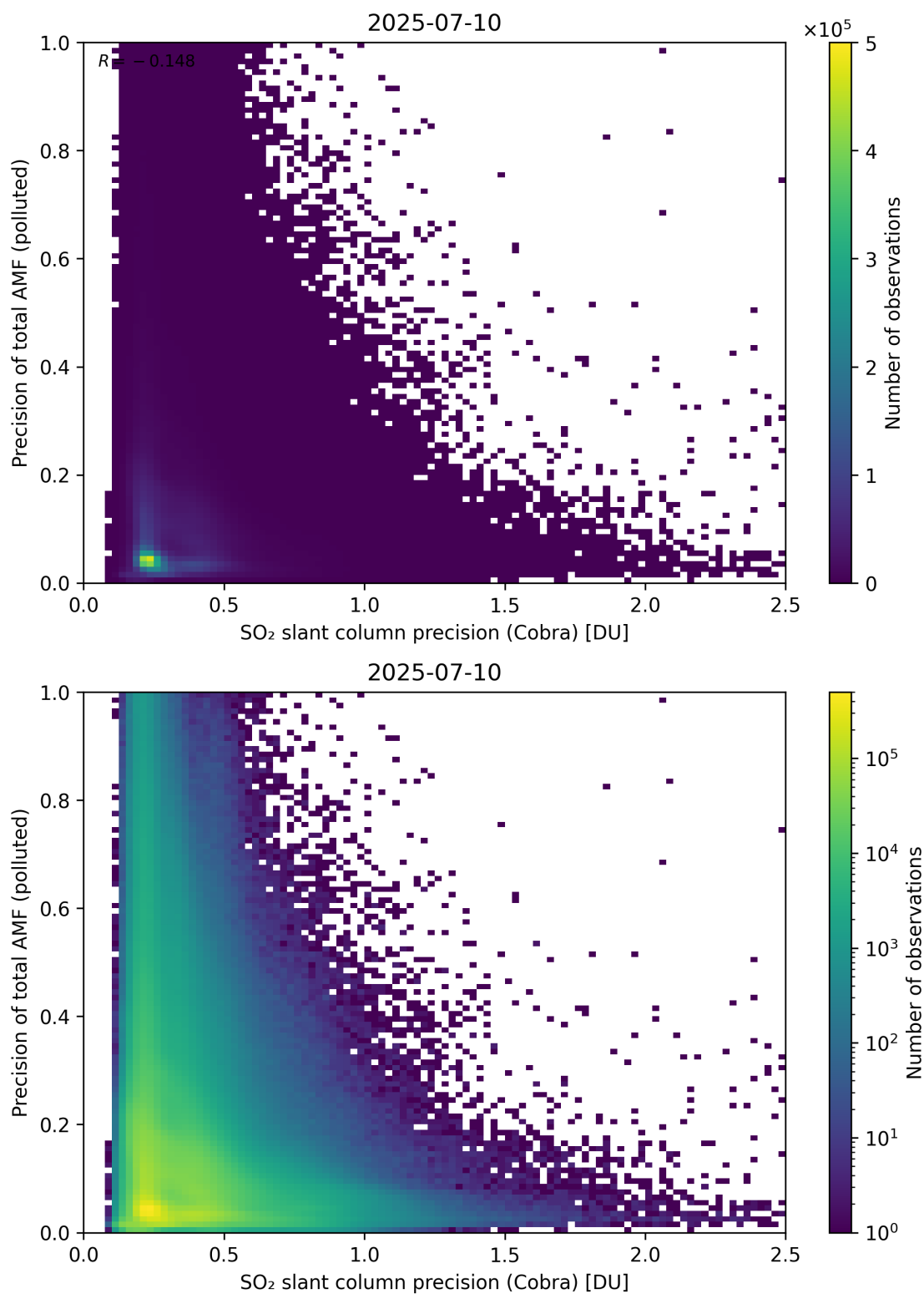
Figure 214: Scatter density plot of “SO 2 slant column precision (Cobra)” against “Precision of total AMF (polluted)” for 2025-07-09 to 2025-07-11.
