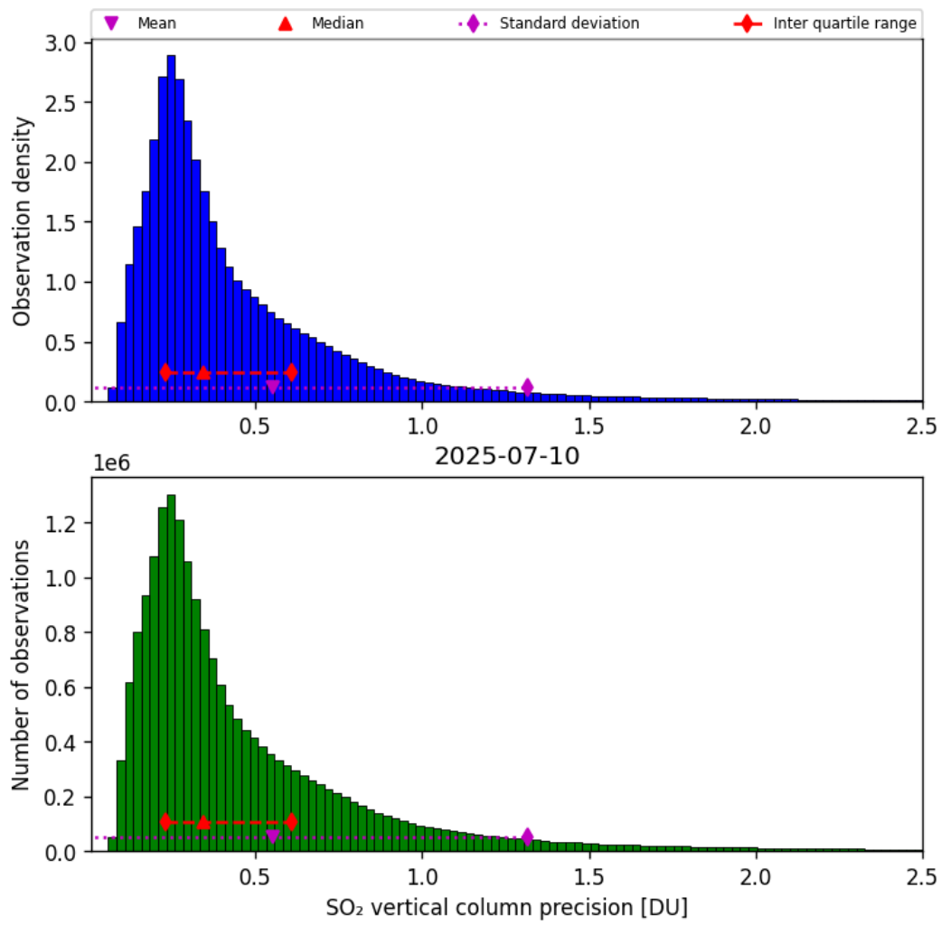
Figure 59: Histogram of “SO 2 vertical column precision” for 2025-07-09 to 2025-07-11
