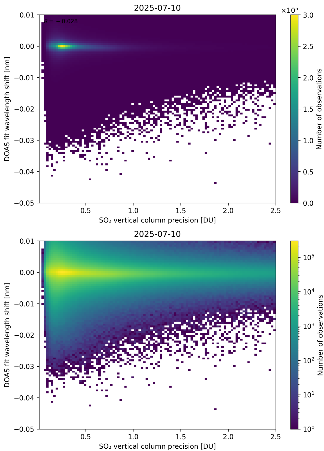
Figure 332: Scatter density plot of “SO 2 vertical column precision” against “DOAS fit wavelength shift” for 2025-07-09 to 2025-07-11.
