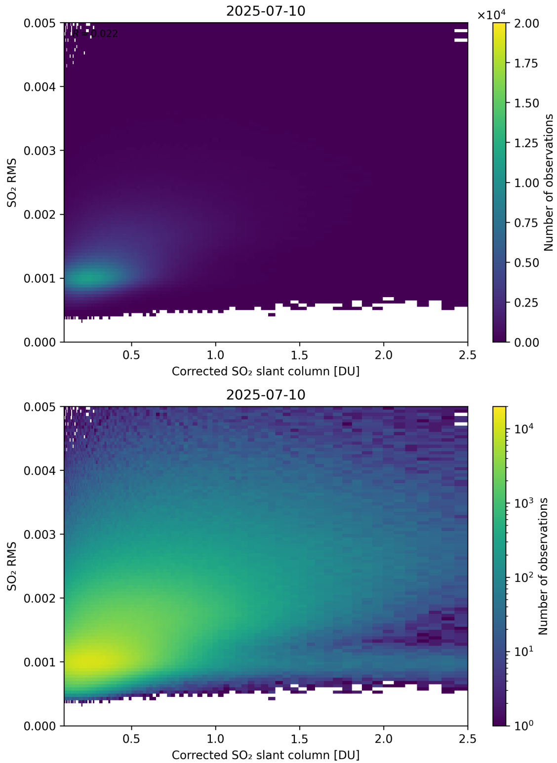
Figure 231: Scatter density plot of “Corrected SO 2 slant column” against “SO 2 RMS” for 2025-07-09 to 2025-07-11.
