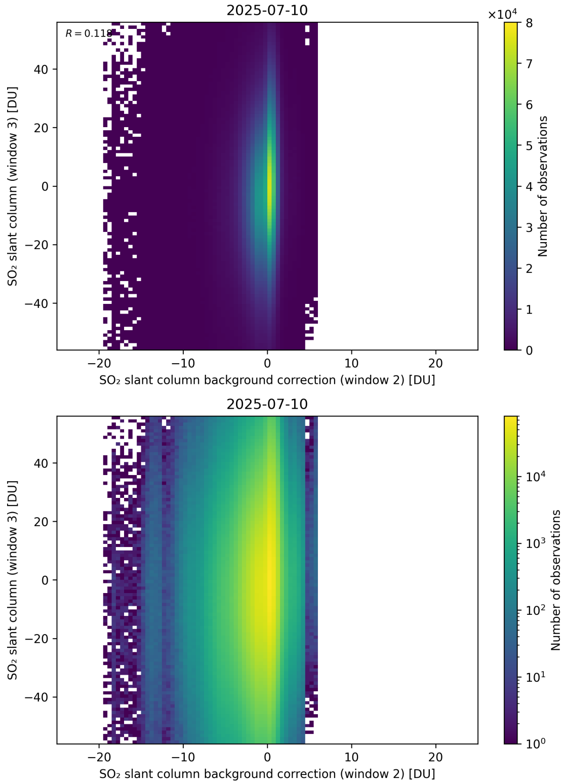
Figure 128: Scatter density plot of “SO 2 slant column background correction (window 2)” against “SO 2 slant column (window 3)” for 2025-07-09 to 2025-07-11.
