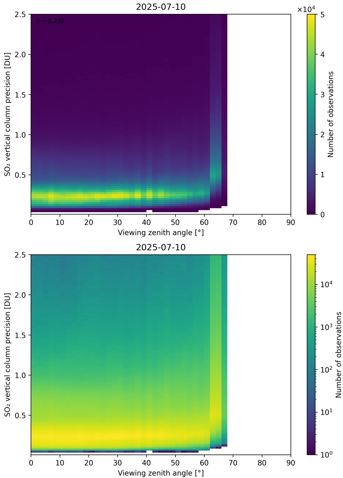
Figure 384: Scatter density plot of “Viewing zenith angle” against “SO 2 vertical column precision” for 2025-07-09 to 2025-07-11.
