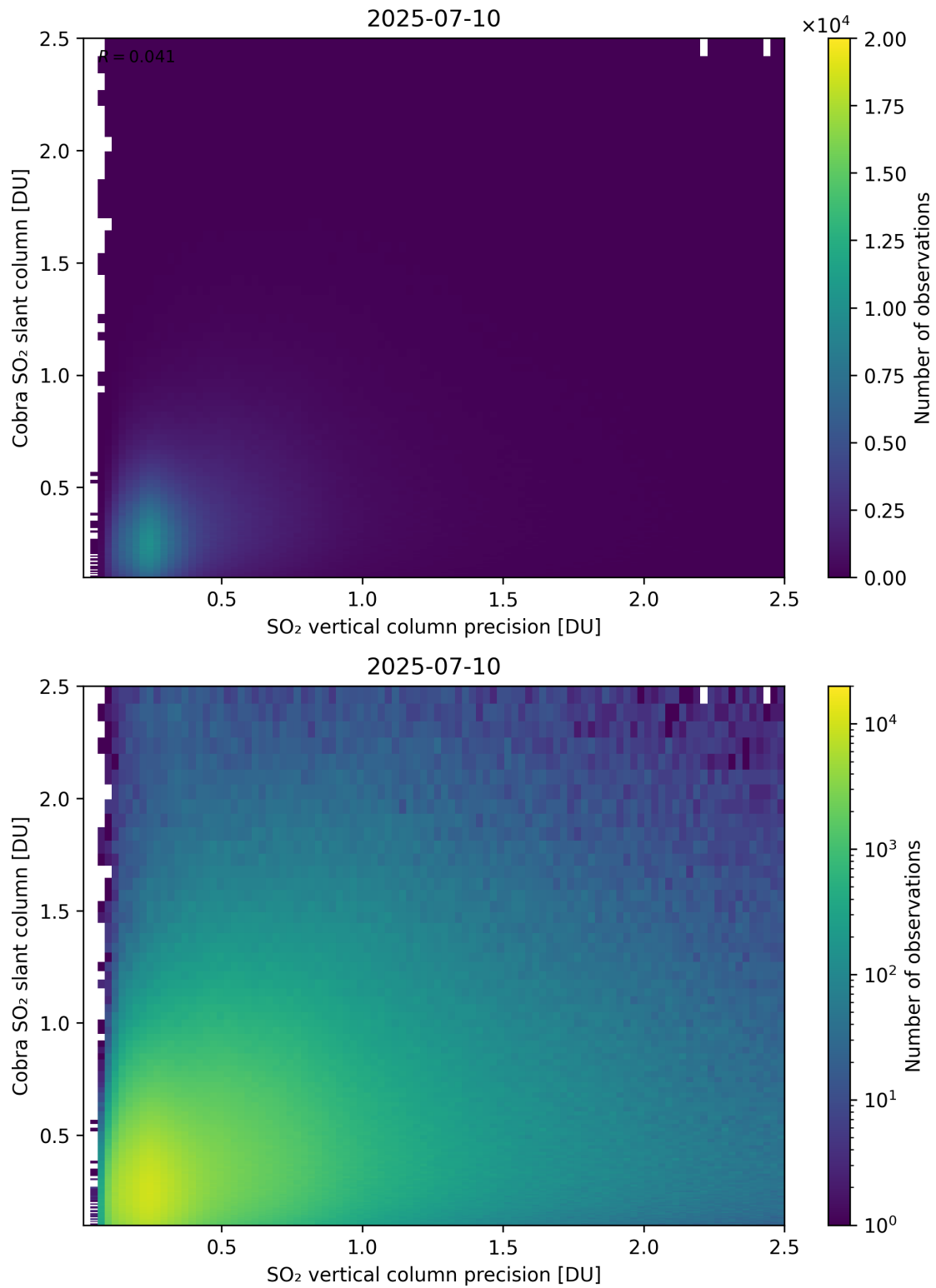
Figure 336: Scatter density plot of “SO 2 vertical column precision” against “Cobra SO 2 slant column” for 2025-07-09 to 2025-07-11.
