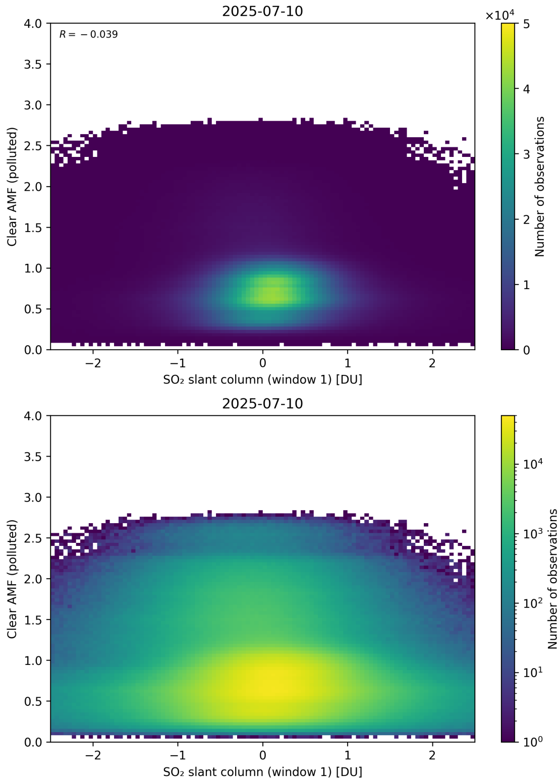
Figure 282: Scatter density plot of “SO 2 slant column (window 1)” against “Clear AMF (polluted)” for 2025-07-09 to 2025-07-11.
