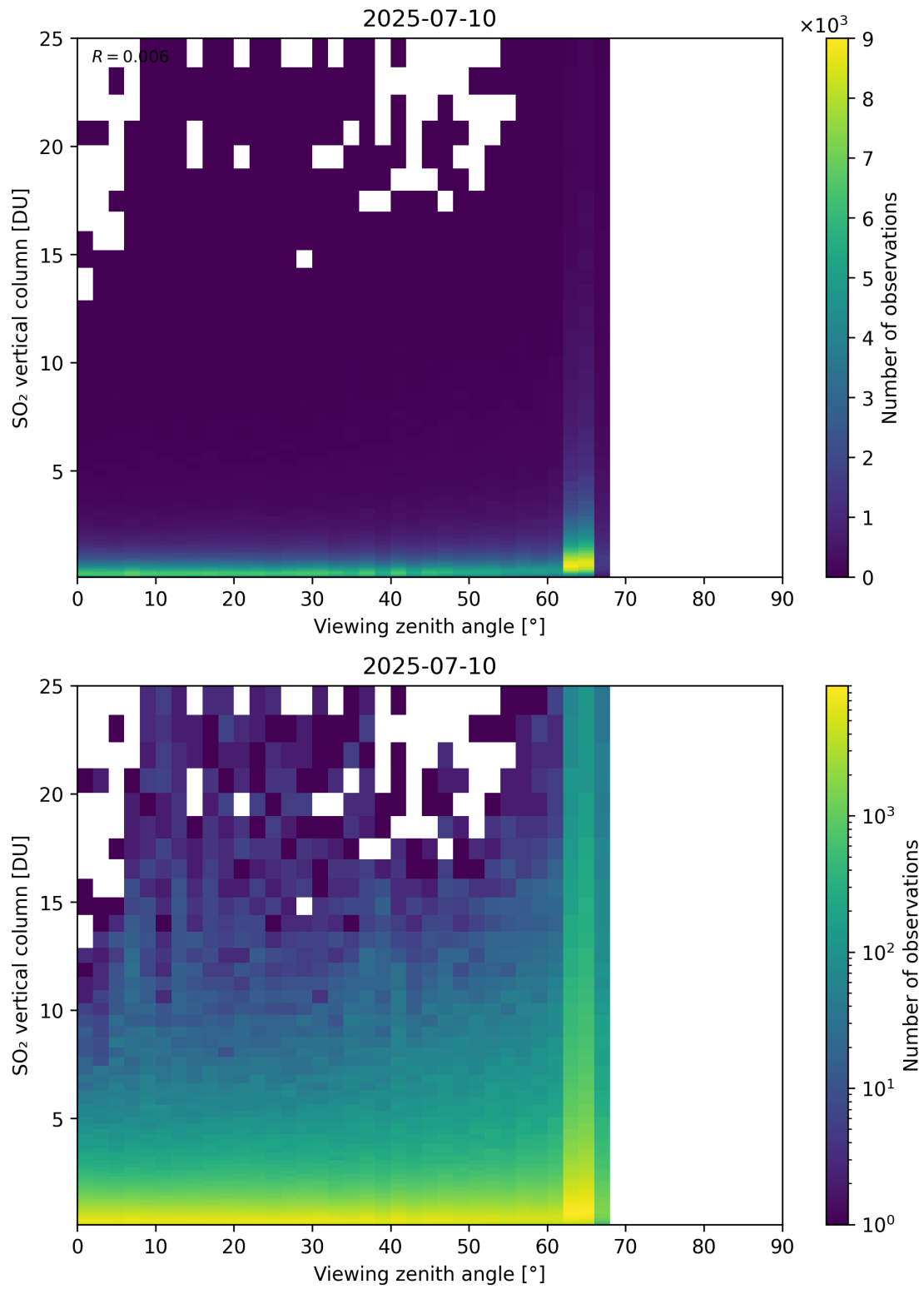
Figure 383: Scatter density plot of “Viewing zenith angle” against “SO 2 vertical column” for 2025-07-09 to 2025-07-11.
