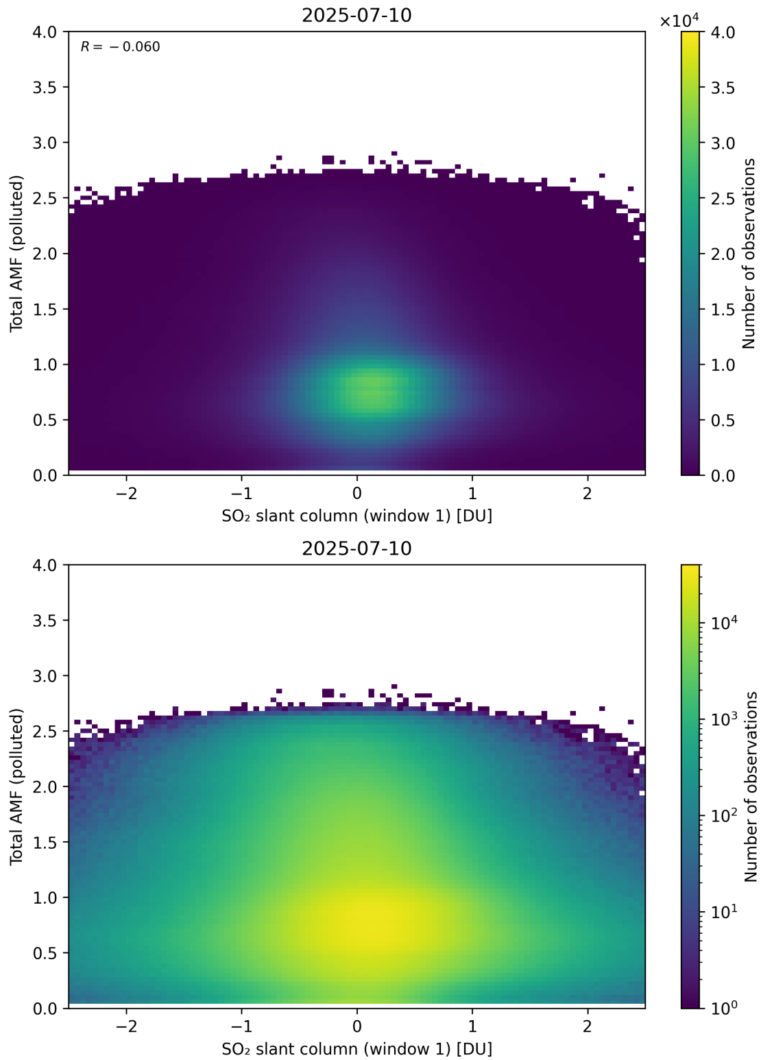
Figure 289: Scatter density plot of “SO 2 slant column (window 1)” against “Total AMF (polluted)” for 2025-07-09 to 2025-07-11.
