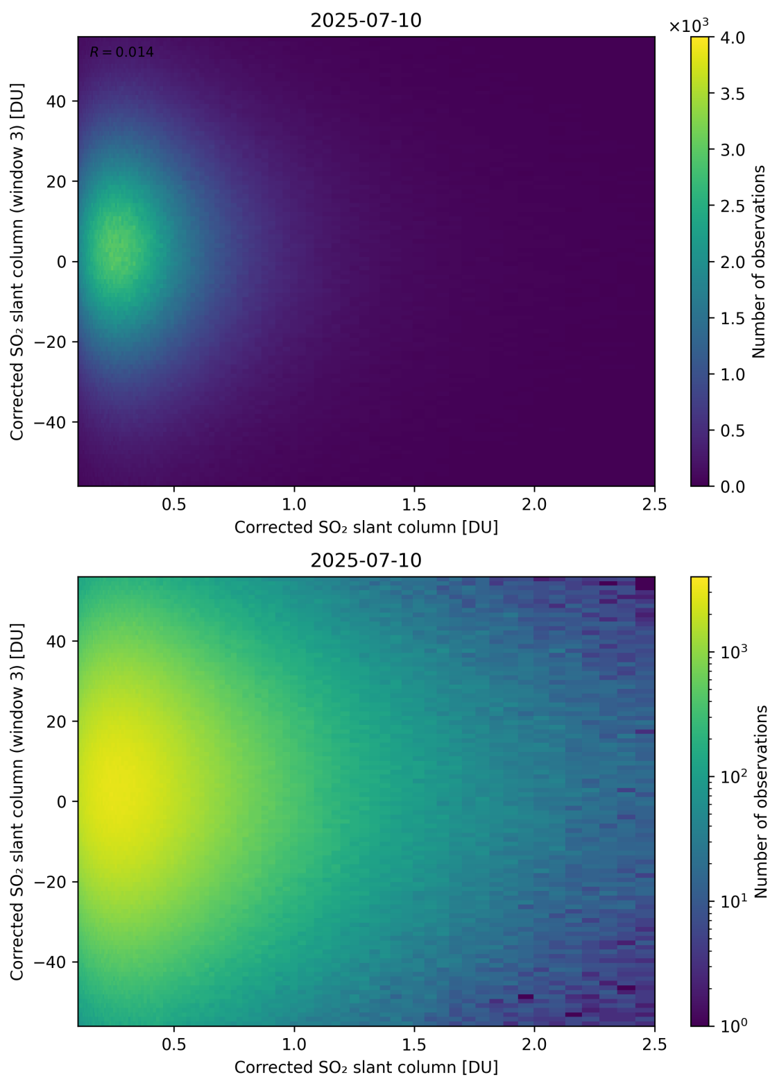
Figure 236: Scatter density plot of “Corrected SO 2 slant column” against “Corrected SO 2 slant column (window 3)” for 2025-07-09 to 2025-07-11.
