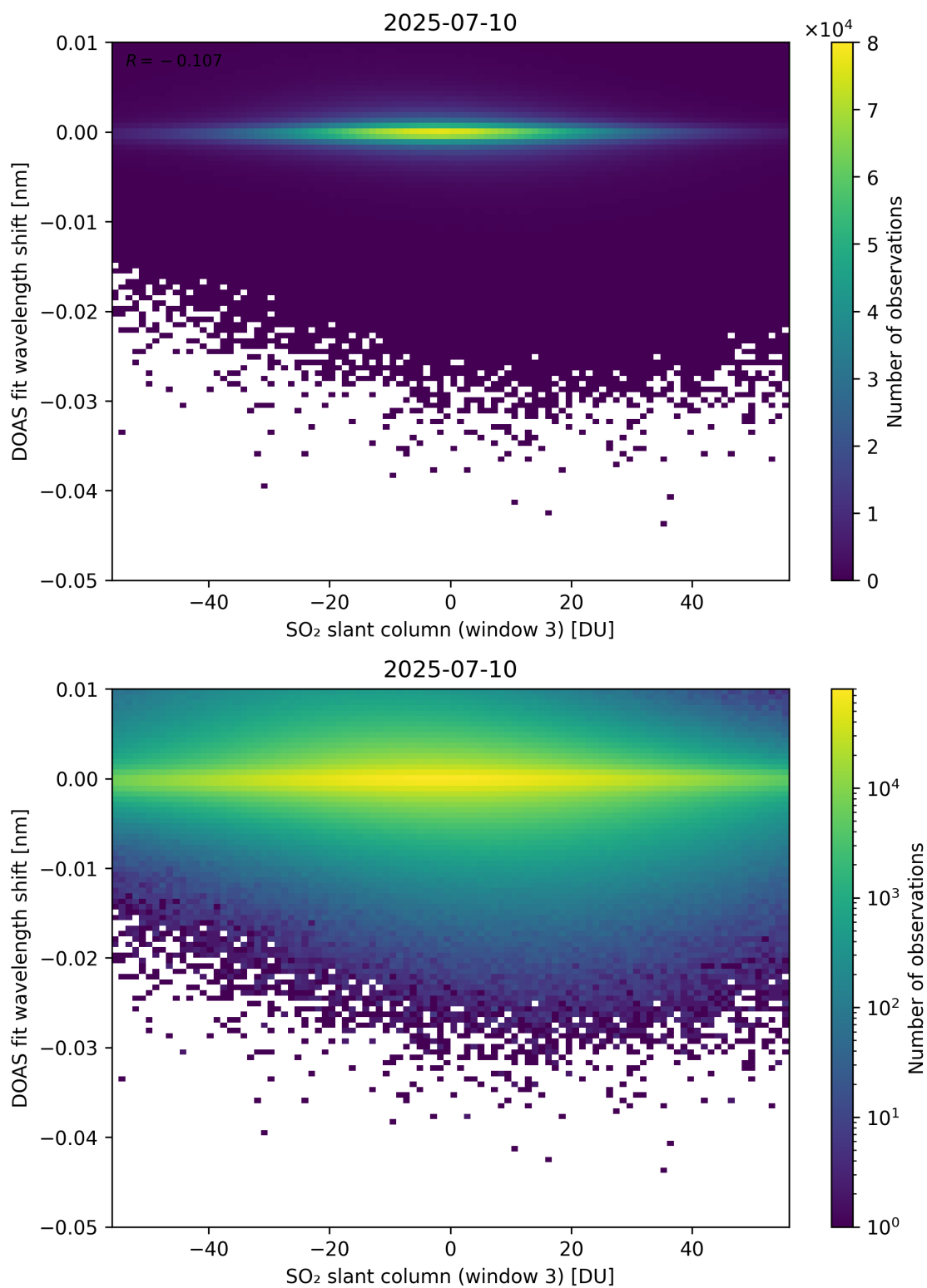
Figure 304: Scatter density plot of “SO 2 slant column (window 3)” against “DOAS fit wavelength shift” for 2025-07-09 to 2025-07-11.
