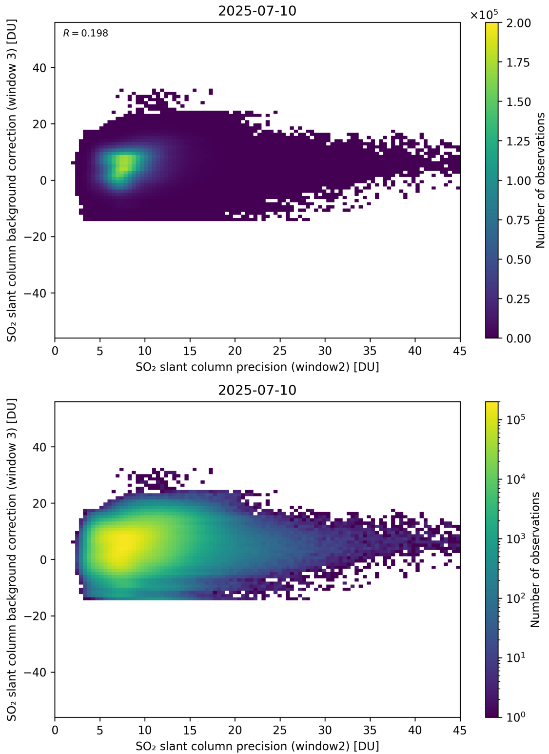
Figure 292: Scatter density plot of “SO 2 slant column precision (window2)” against “SO 2 slant column background correction (window 3)” for 2025-07-09 to 2025-07-11.
