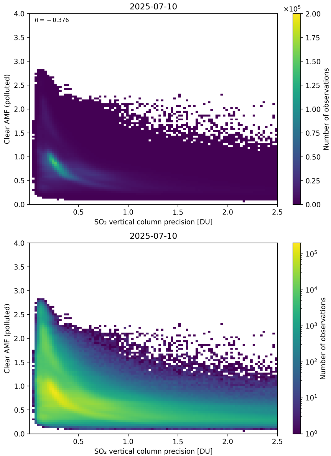
Figure 335: Scatter density plot of “SO 2 vertical column precision” against “Clear AMF (polluted)” for 2025-07-09 to 2025-07-11.
