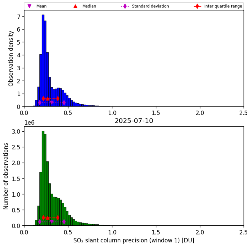
Figure 64: Histogram of “SO 2 slant column precision (window 1)” for 2025-07-09 to 2025-07-11
