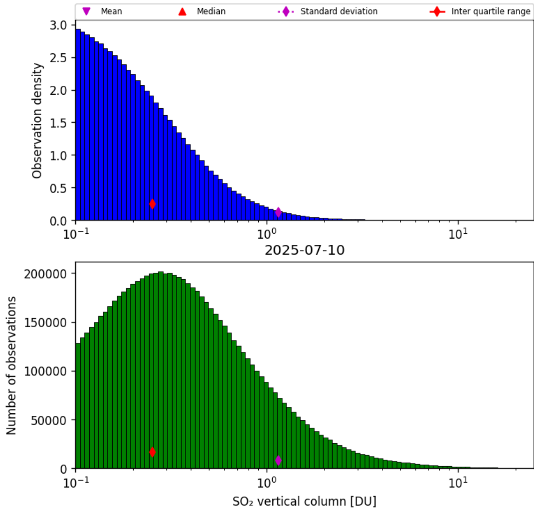
Figure 58: Histogram of “SO 2 vertical column” for 2025-07-09 to 2025-07-11
