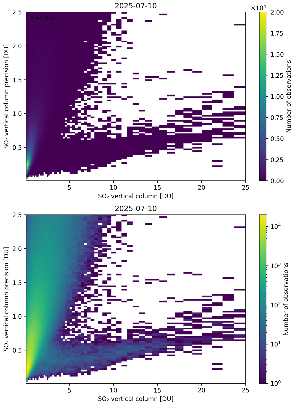
Figure 361: Scatter density plot of “SO 2 vertical column” against “SO 2 vertical column precision” for 2025-07-09 to 2025-07-11.
