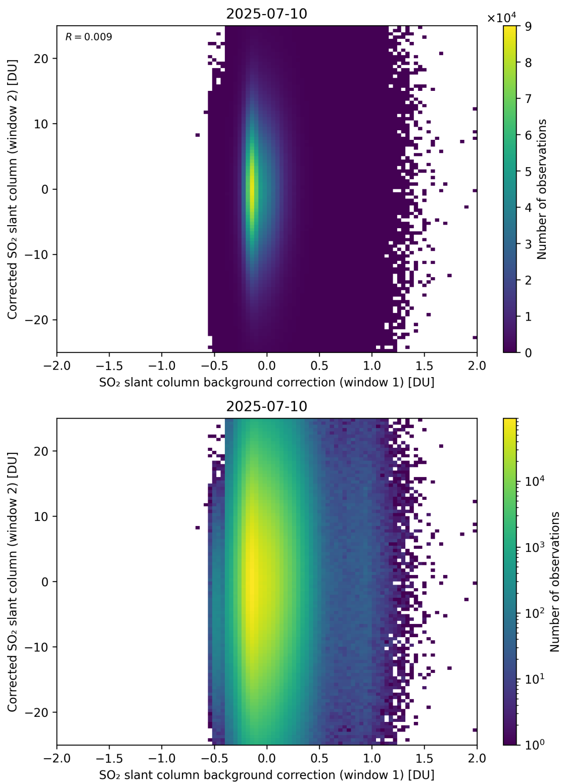
Figure 115: Scatter density plot of “SO 2 slant column background correction (window 1)” against “Corrected SO 2 slant column (window 2)” for 2025-07-09 to 2025-07-11.
