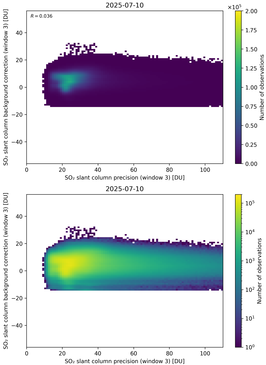
Figure 307: Scatter density plot of “SO 2 slant column precision (window 3)” against “SO 2 slant column background correction (window 3)” for 2025-07-09 to 2025-07-11.
