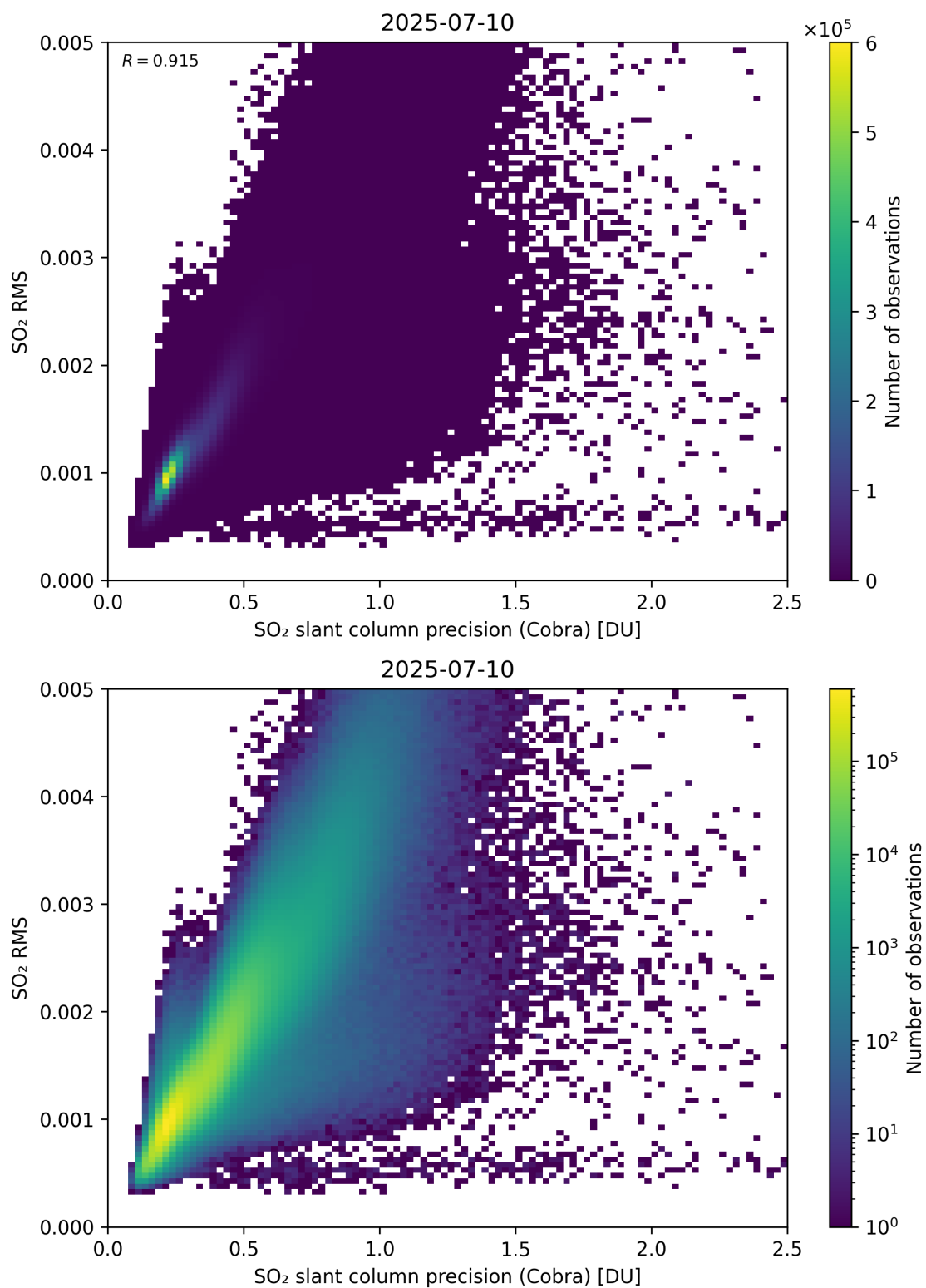
Figure 204: Scatter density plot of “SO 2 slant column precision (Cobra)” against “SO 2 RMS” for 2025-07-09 to 2025-07-11.
