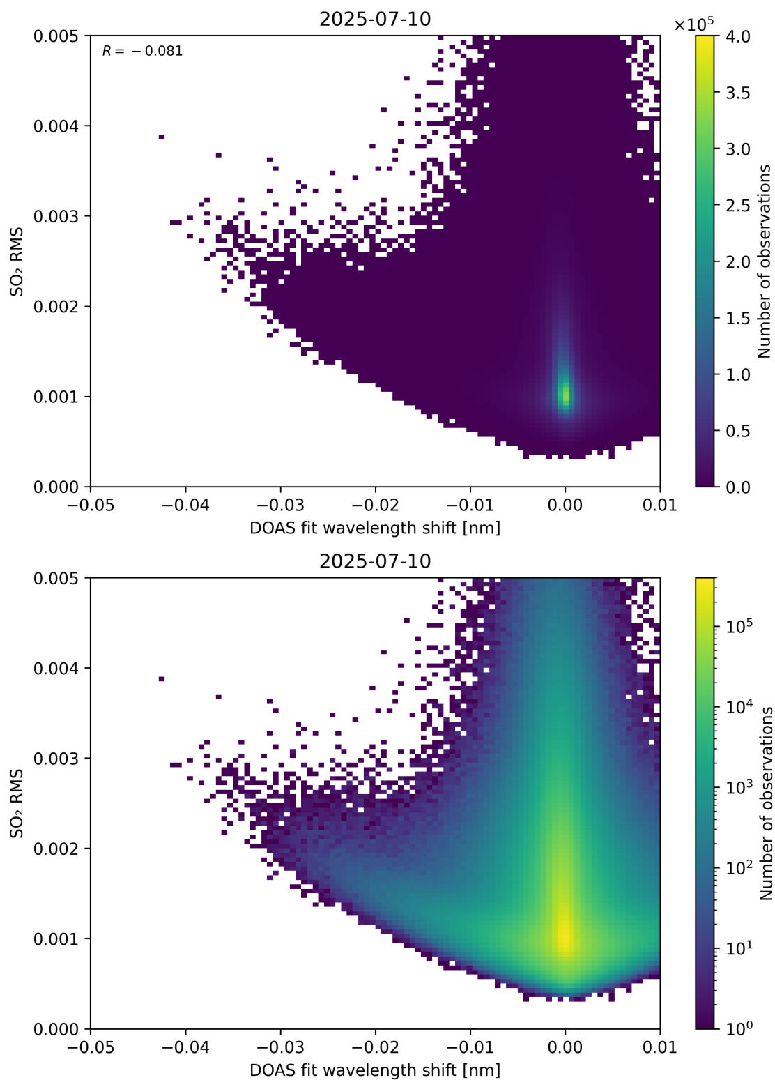
Figure 139: Scatter density plot of “DOAS fit wavelength shift” against “SO 2 RMS” for 2025-07-09 to 2025-07-11.
