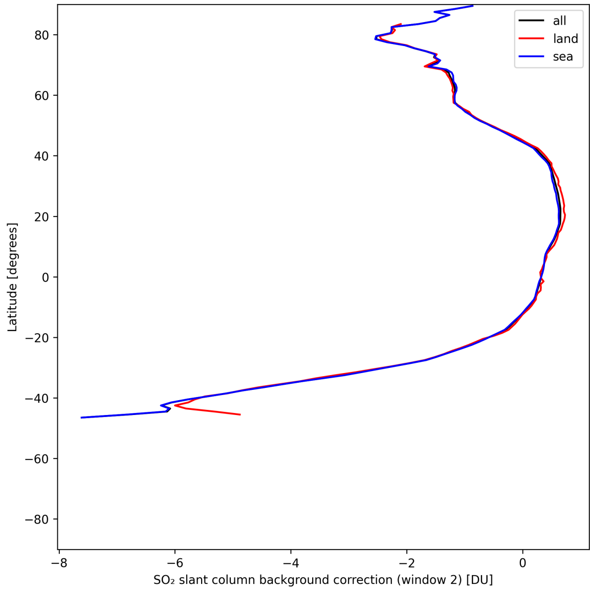
Figure 44: Zonal average of “SO 2 slant column background correction (window 2)” for 2025-07-09 to 2025-07-11.
