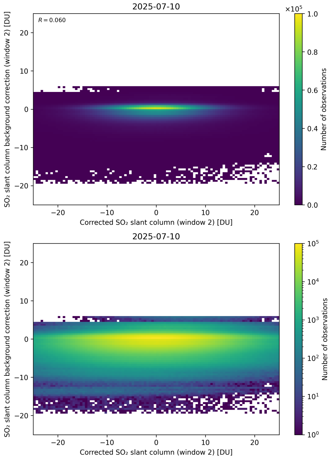
Figure 244: Scatter density plot of “Corrected SO 2 slant column (window 2)” against “SO 2 slant column background correction (window 2)” for 2025-07-09 to 2025-07-11.
