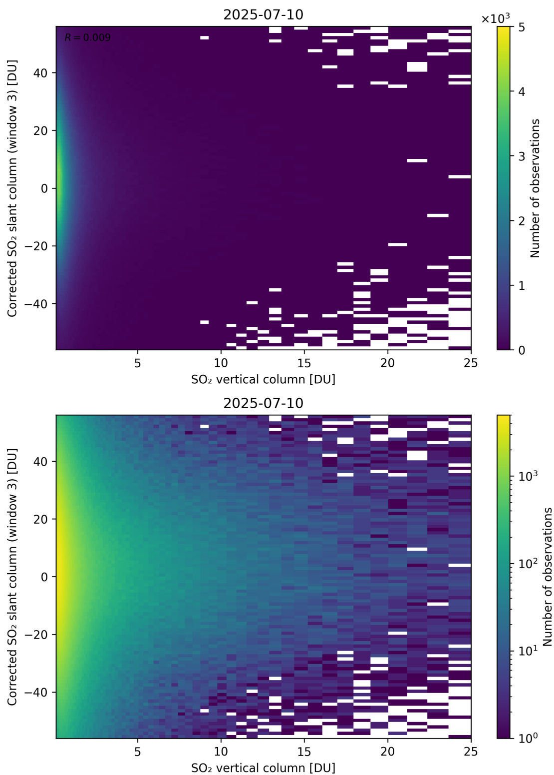
Figure 353: Scatter density plot of “SO 2 vertical column” against “Corrected SO 2 slant column (window 3)” for 2025-07-09 to 2025-07-11.
