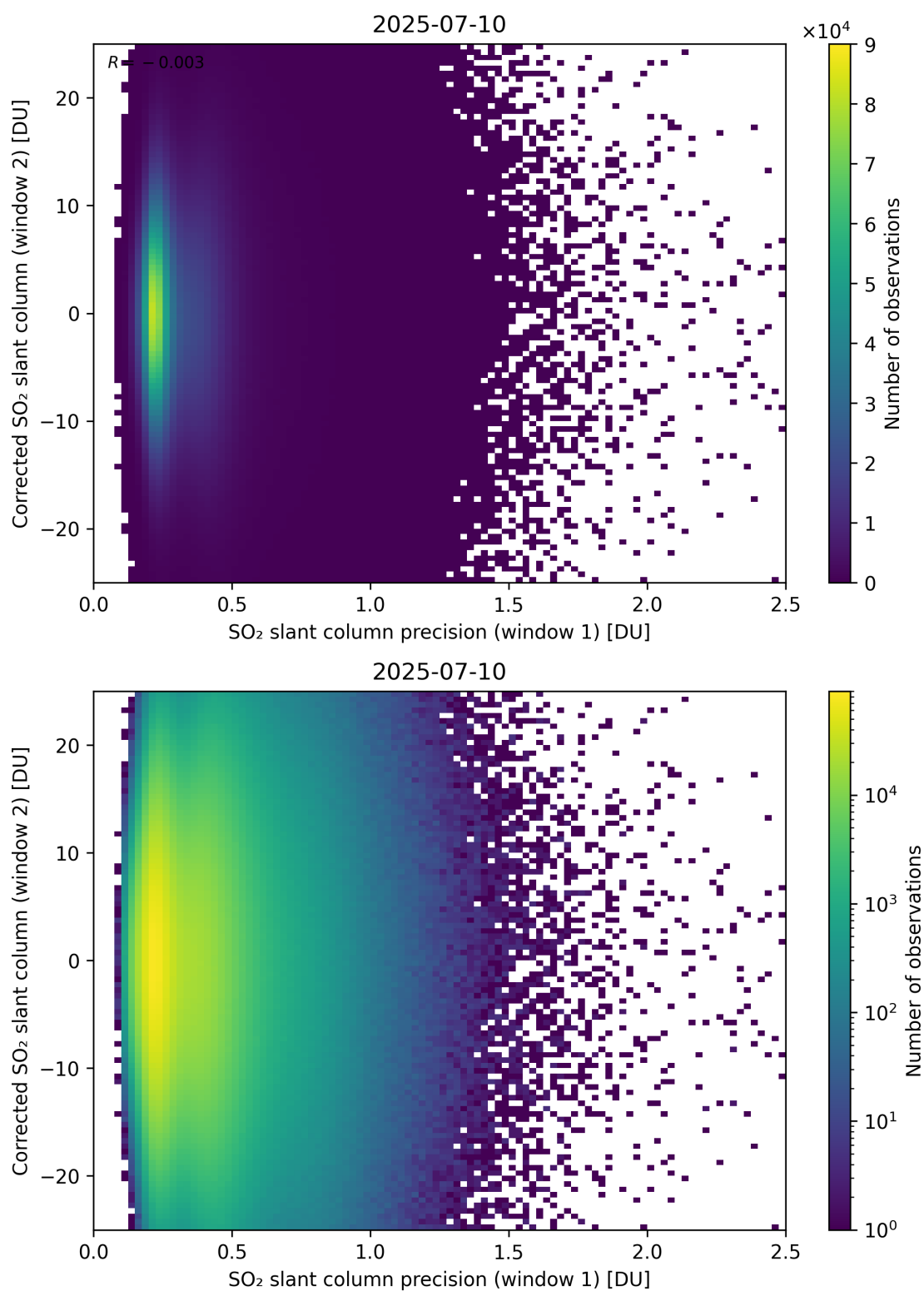
Figure 275: Scatter density plot of “SO 2 slant column precision (window 1)” against “Corrected SO 2 slant column (window 2)” for 2025-07-09 to 2025-07-11.
