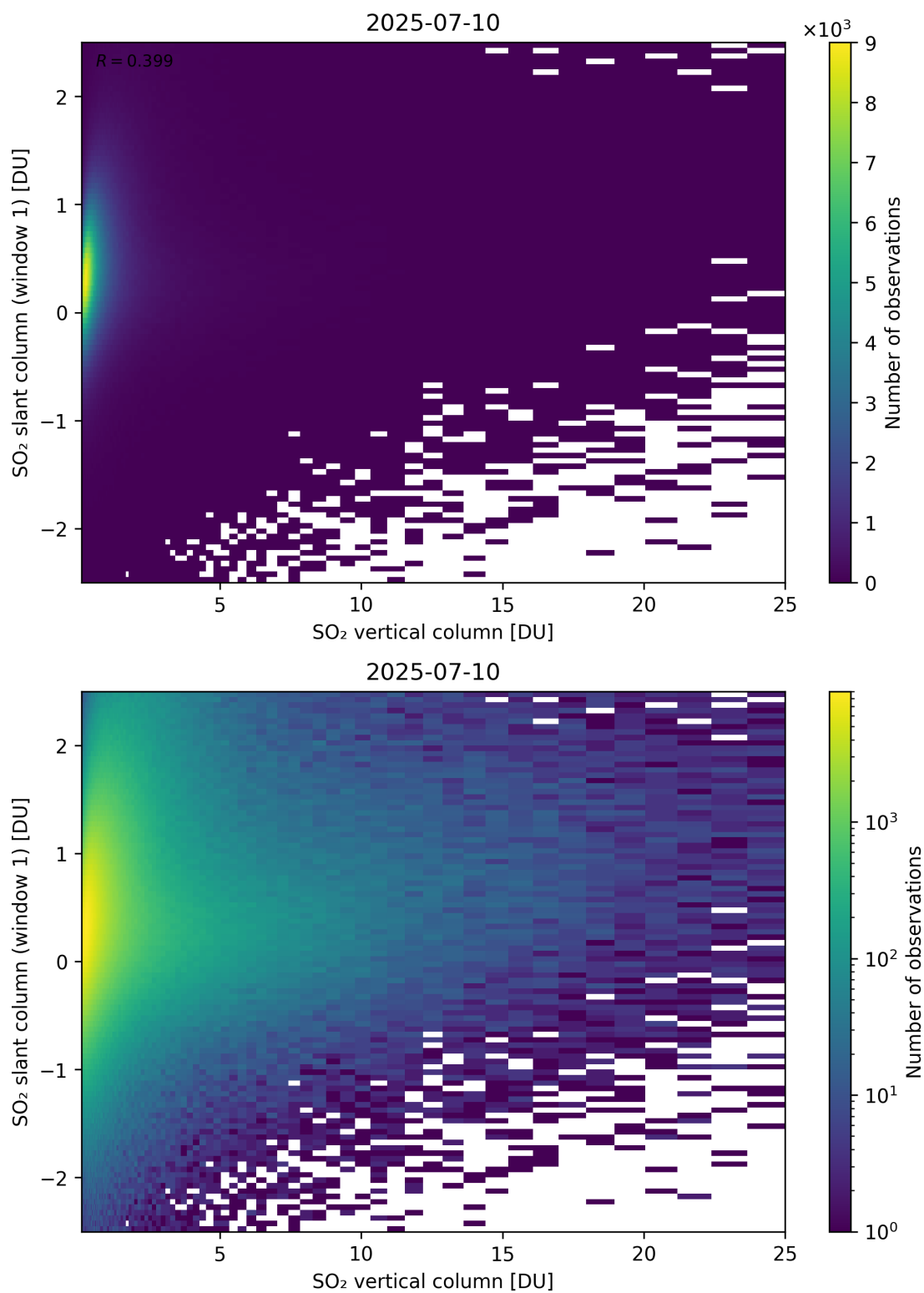
Figure 354: Scatter density plot of “SO 2 vertical column” against “SO 2 slant column (window 1)” for 2025-07-09 to 2025-07-11.
