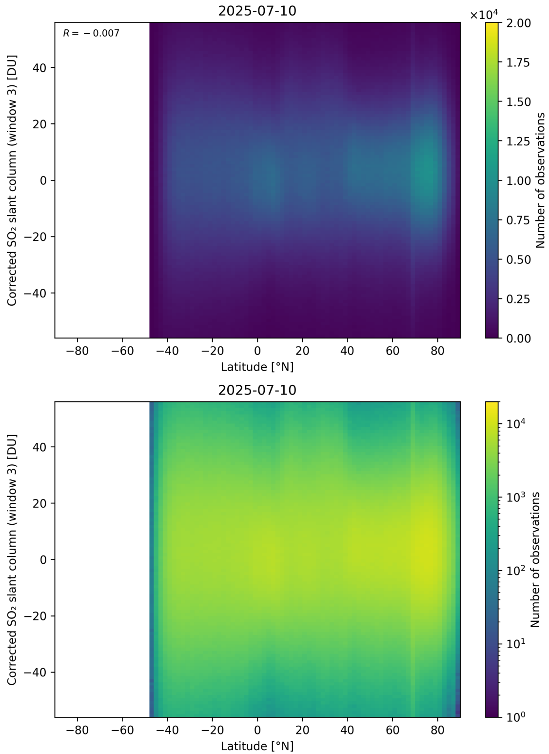
Figure 161: Scatter density plot of “Latitude” against “Corrected SO 2 slant column (window 3)” for 2025-07-09 to 2025-07-11.
