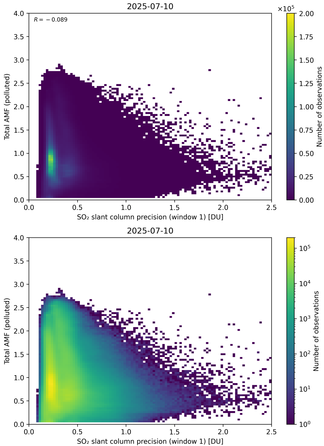
Figure 280: Scatter density plot of “SO 2 slant column precision (window 1)” against “Total AMF (polluted)” for 2025-07-09 to 2025-07-11.
