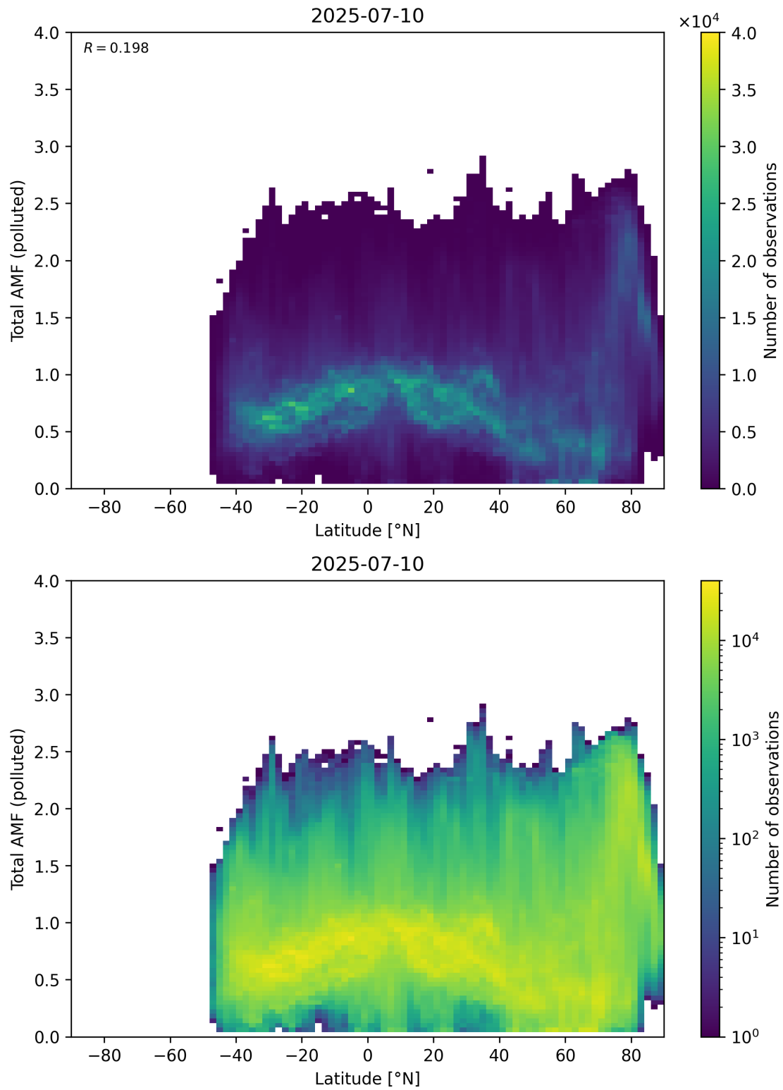
Figure 167: Scatter density plot of “Latitude” against “Total AMF (polluted)” for 2025-07-09 to 2025-07-11.
