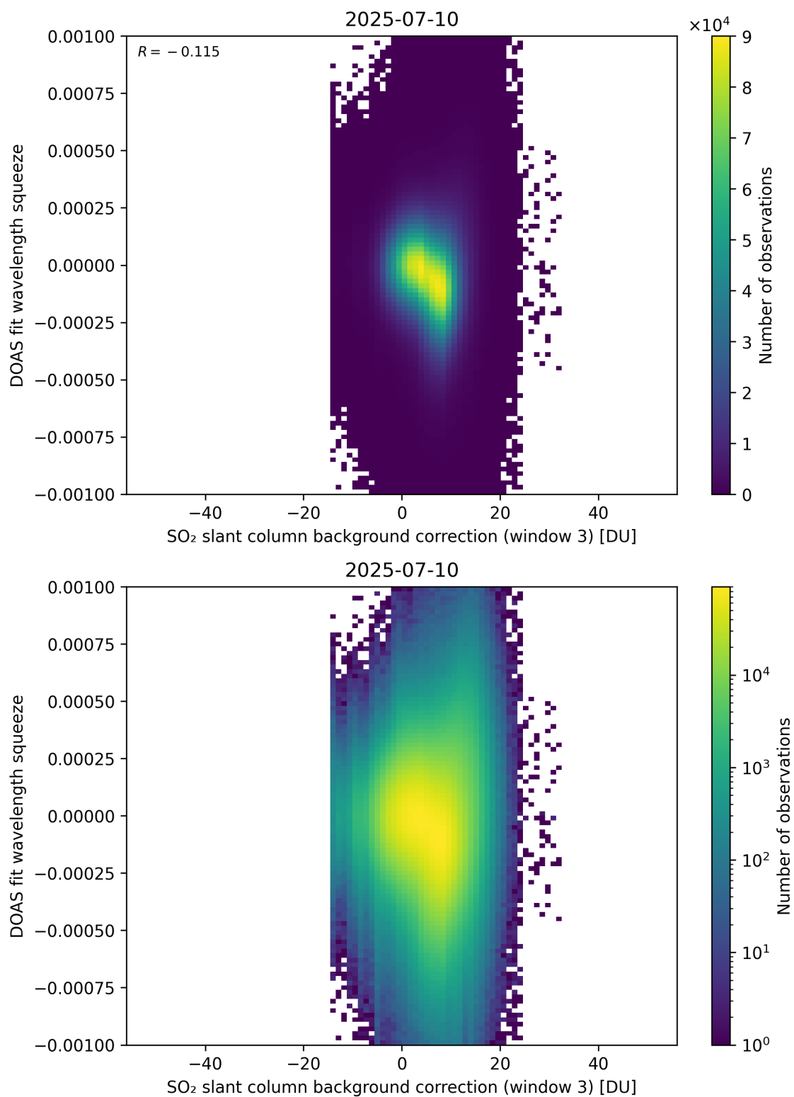
Figure 133: Scatter density plot of “SO 2 slant column background correction (window 3)” against “DOAS fit wavelength squeeze” for 2025-07-09 to 2025-07-11.
