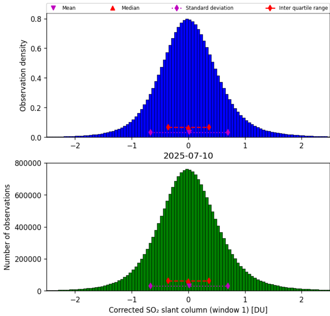
Figure 65: Histogram of “Corrected SO 2 slant column (window 1)” for 2025-07-09 to 2025-07-11
