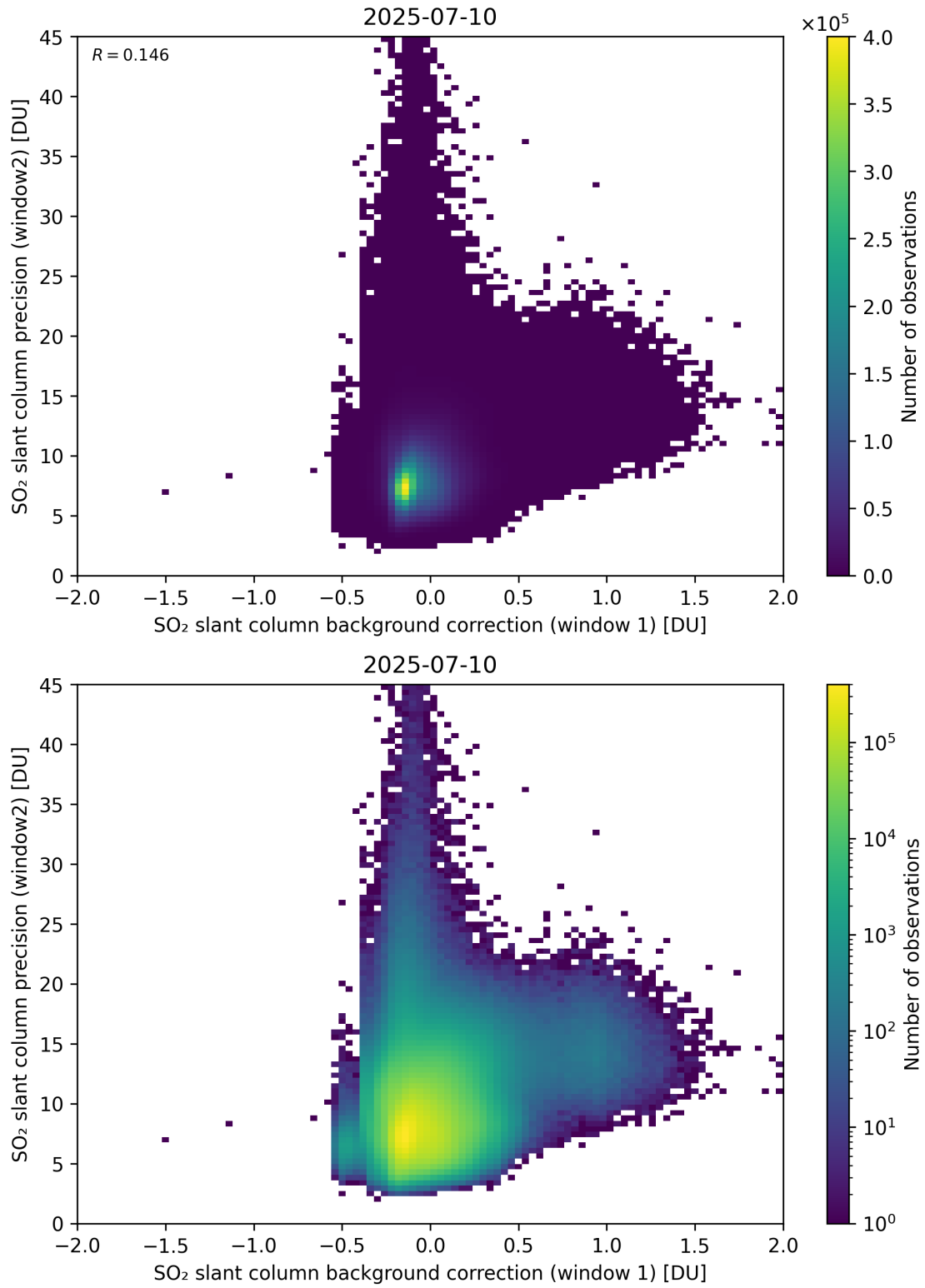
Figure 117: Scatter density plot of “SO 2 slant column background correction (window 1)” against “SO 2 slant column precision (window2)” for 2025-07-09 to 2025-07-11.
