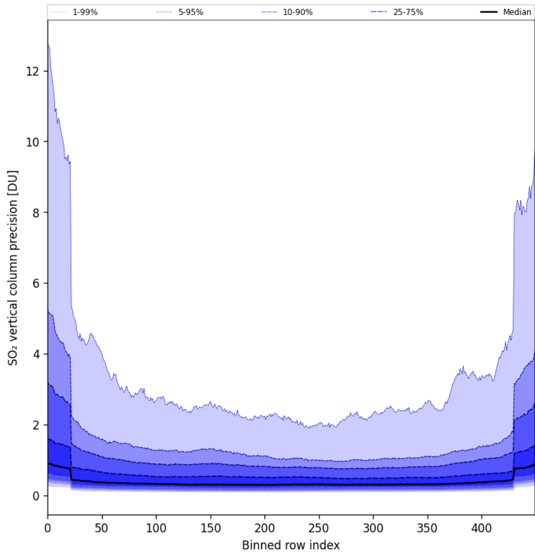
Figure 85: Along track statistics of “SO 2 vertical column precision” for 2025-07-09 to 2025-07-11
