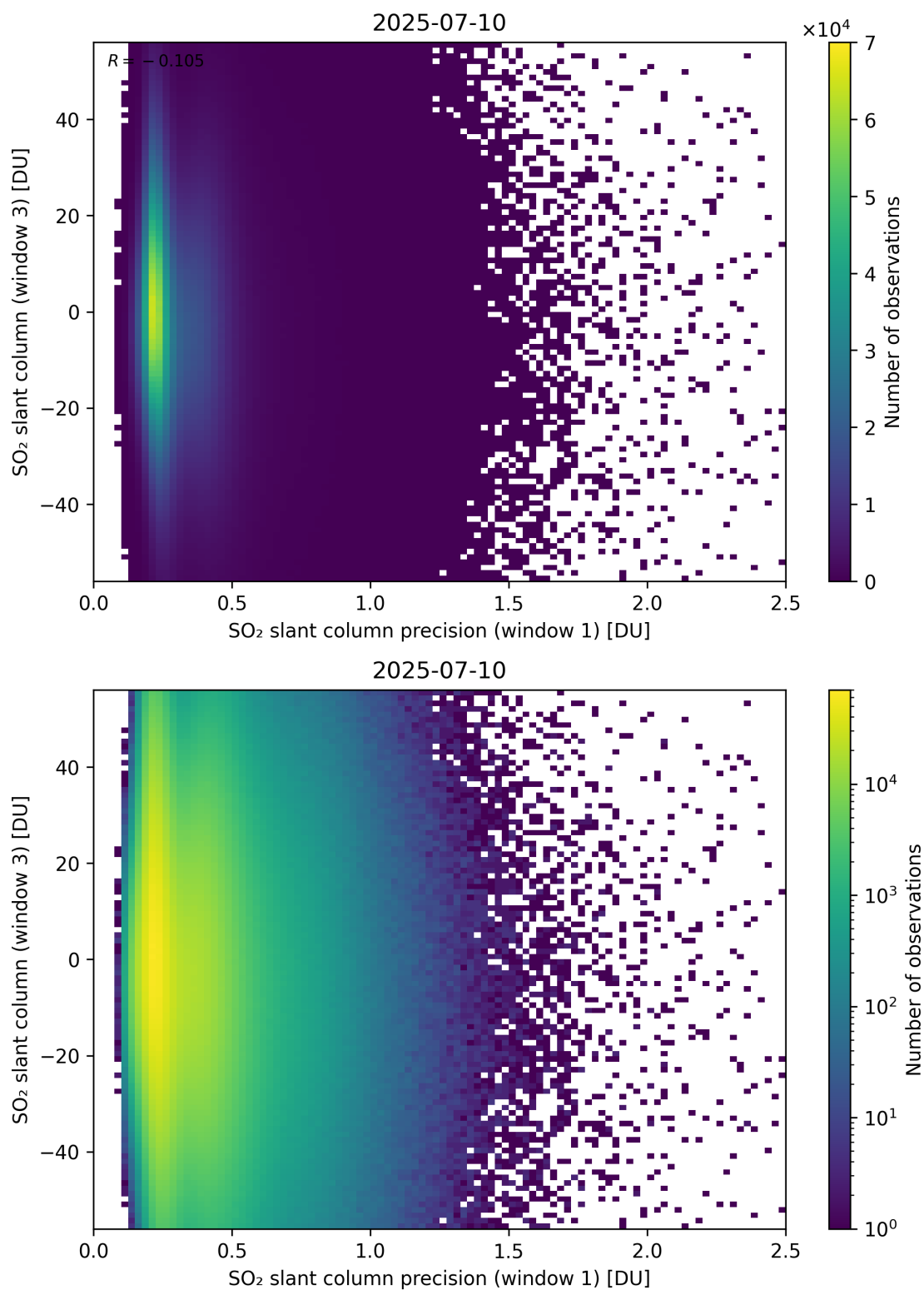
Figure 278: Scatter density plot of “SO 2 slant column precision (window 1)” against “SO 2 slant column (window 3)” for 2025-07-09 to 2025-07-11.
