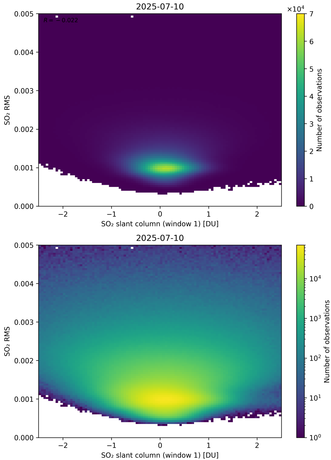
Figure 267: Scatter density plot of “SO 2 slant column (window 1)” against “SO 2 RMS” for 2025-07-09 to 2025-07-11.
