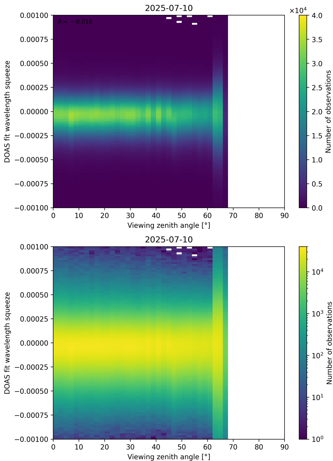
Figure 366: Scatter density plot of “Viewing zenith angle” against “DOAS fit wavelength squeeze” for 2025-07-09 to 2025-07-11.
