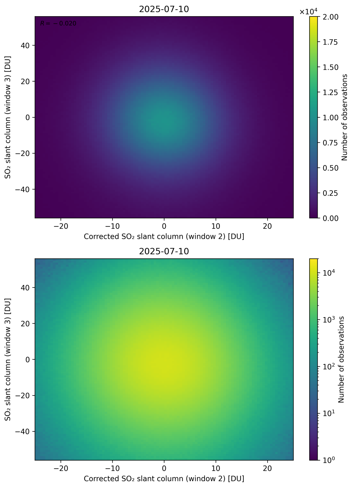
Figure 251: Scatter density plot of “Corrected SO 2 slant column (window 2)” against “SO 2 slant column (window 3)” for 2025-07-09 to 2025-07-11.
