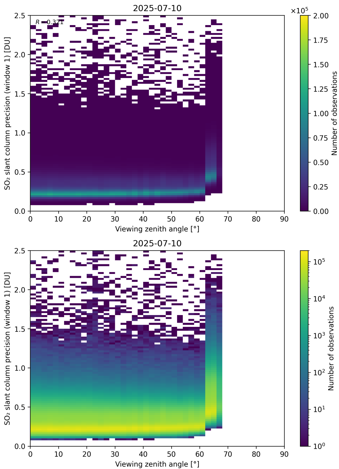
Figure 377: Scatter density plot of “Viewing zenith angle” against “SO 2 slant column precision (window 1)” for 2025-07-09 to 2025-07-11.
