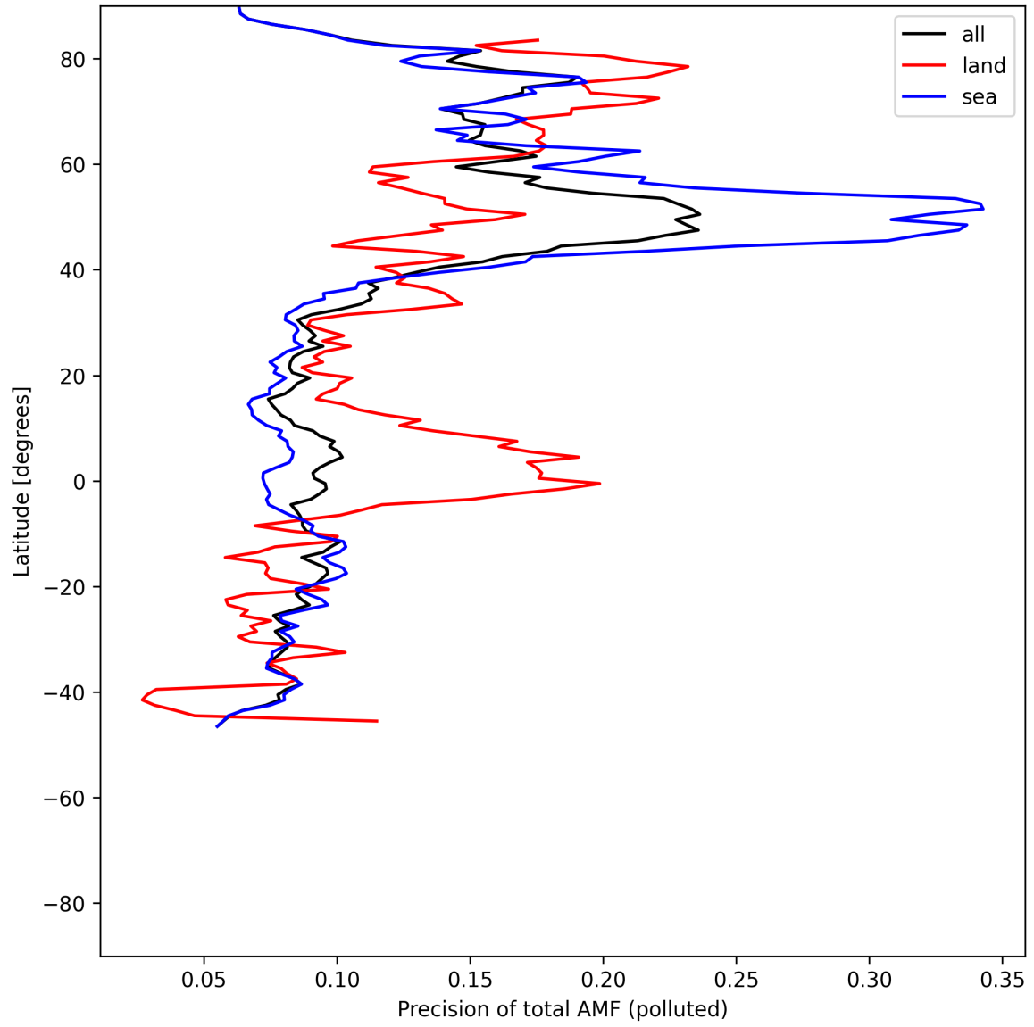
Figure 54: Zonal average of “Precision of total AMF (polluted)” for 2025-07-09 to 2025-07-11.
