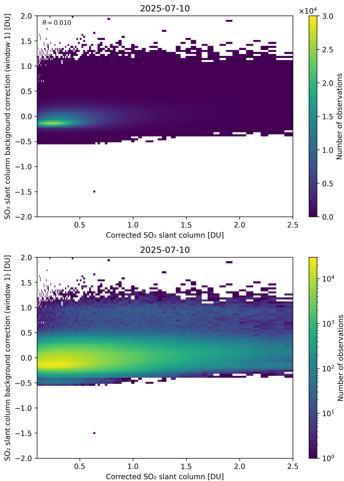
Figure 226: Scatter density plot of “Corrected SO 2 slant column” against “SO 2 slant column background correction (window 1)” for 2025-07-09 to 2025-07-11.
