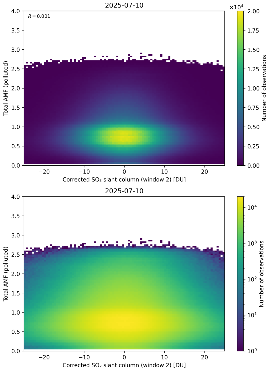
Figure 253: Scatter density plot of “Corrected SO 2 slant column (window 2)” against “Total AMF (polluted)” for 2025-07-09 to 2025-07-11.
