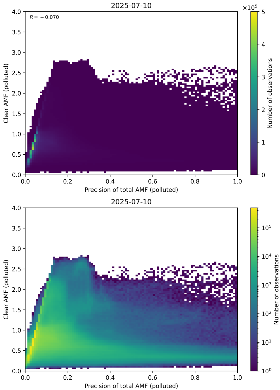
Figure 320: Scatter density plot of “Precision of total AMF (polluted)” against “Clear AMF (polluted)” for 2025-07-09 to 2025-07-11.
