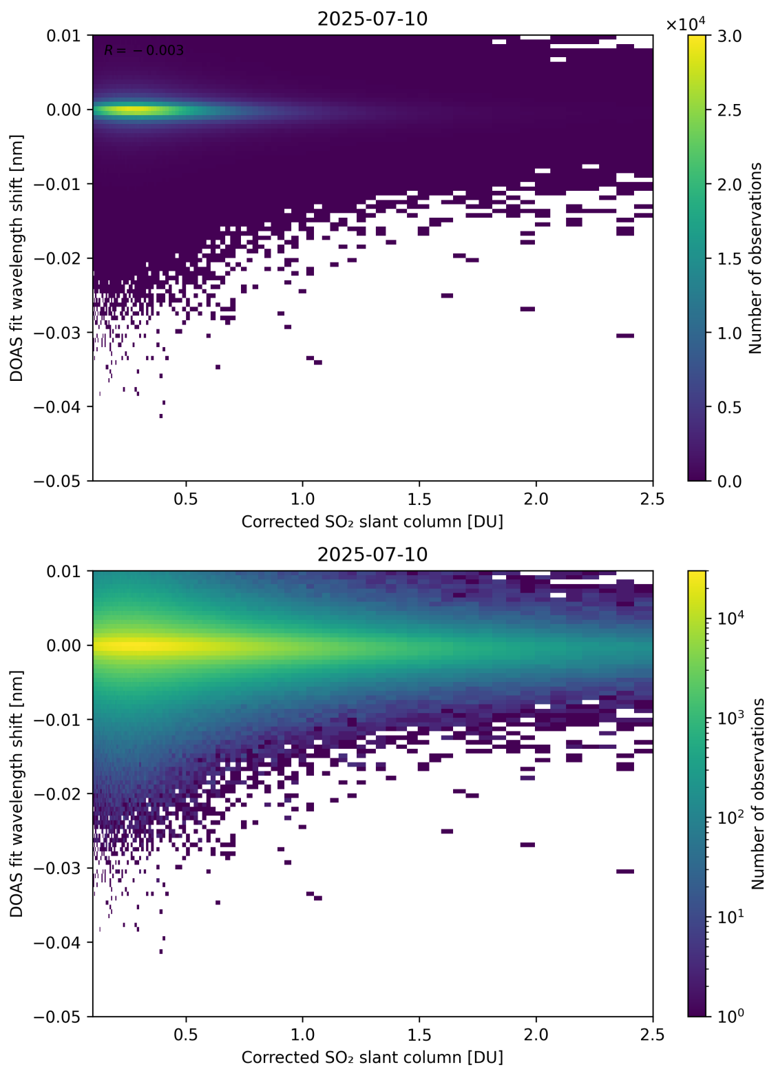
Figure 229: Scatter density plot of “Corrected SO 2 slant column” against “DOAS fit wavelength shift” for 2025-07-09 to 2025-07-11.
