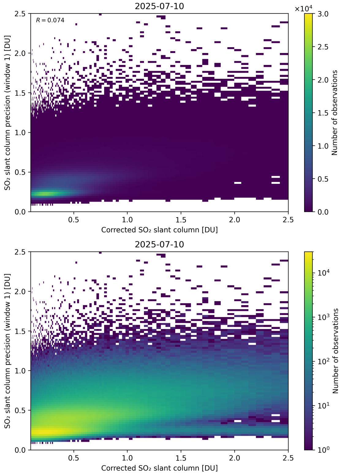
Figure 238: Scatter density plot of “Corrected SO 2 slant column” against “SO 2 slant column precision (window 1)” for 2025-07-09 to 2025-07-11.
