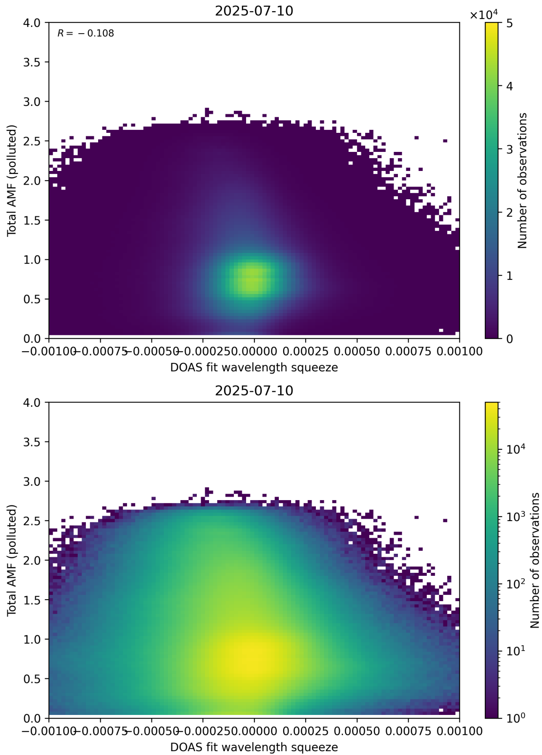
Figure 145: Scatter density plot of “DOAS fit wavelength squeeze” against “Total AMF (polluted)” for 2025-07-09 to 2025-07-11.
