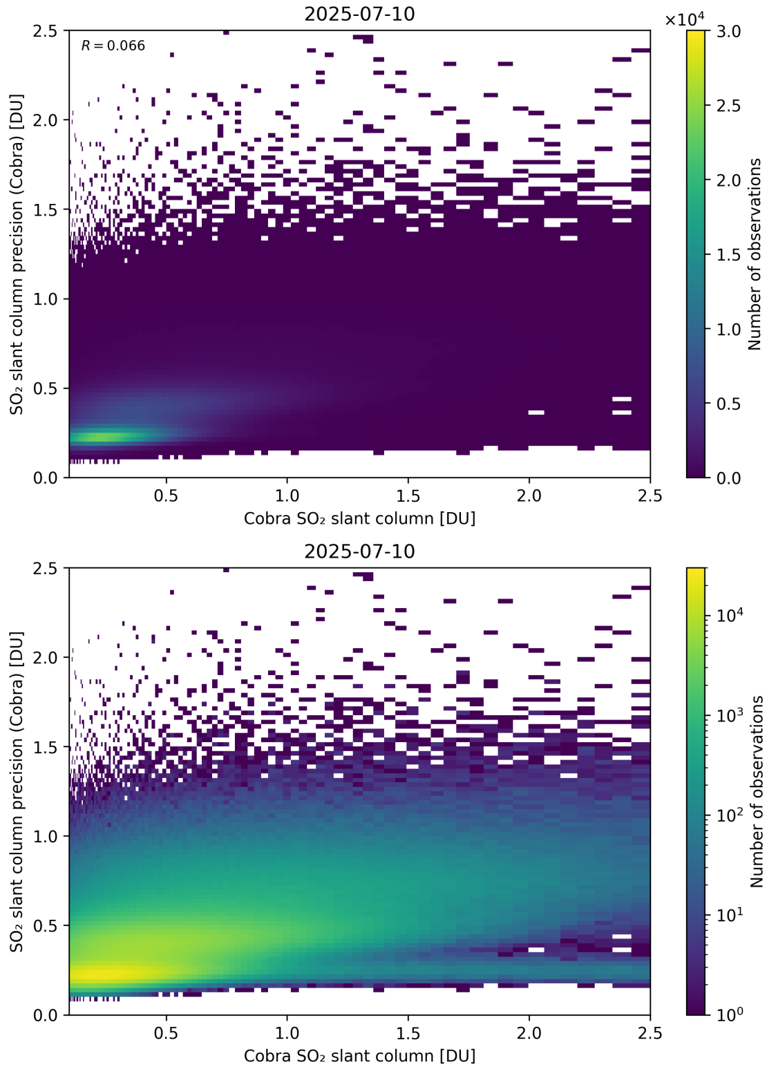
Figure 216: Scatter density plot of “Cobra SO 2 slant column” against “SO 2 slant column precision (Cobra)” for 2025-07-09 to 2025-07-11.
