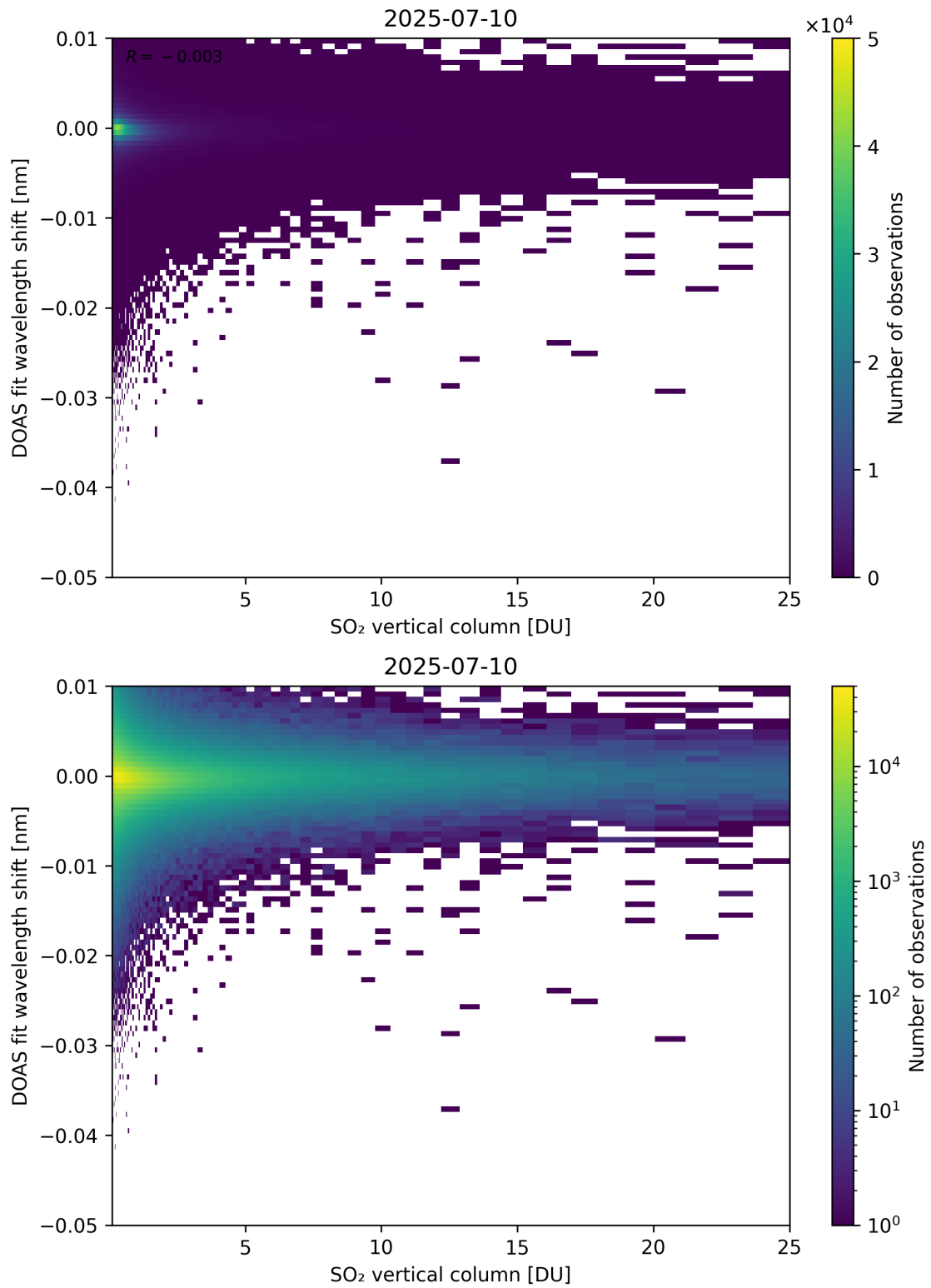
Figure 326: Scatter density plot of “SO 2 vertical column” against “DOAS fit wavelength shift” for 2025-07-09 to 2025-07-11.
