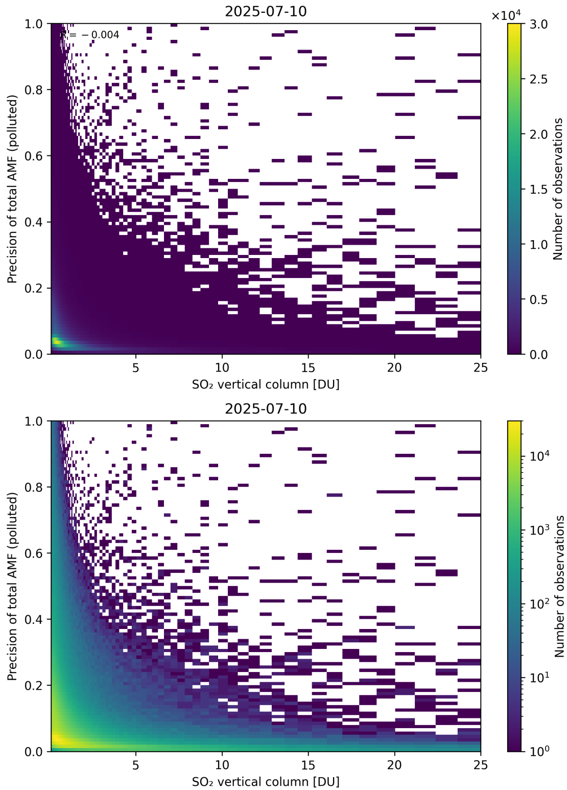
Figure 360: Scatter density plot of “SO 2 vertical column” against “Precision of total AMF (polluted)” for 2025-07-09 to 2025-07-11.
