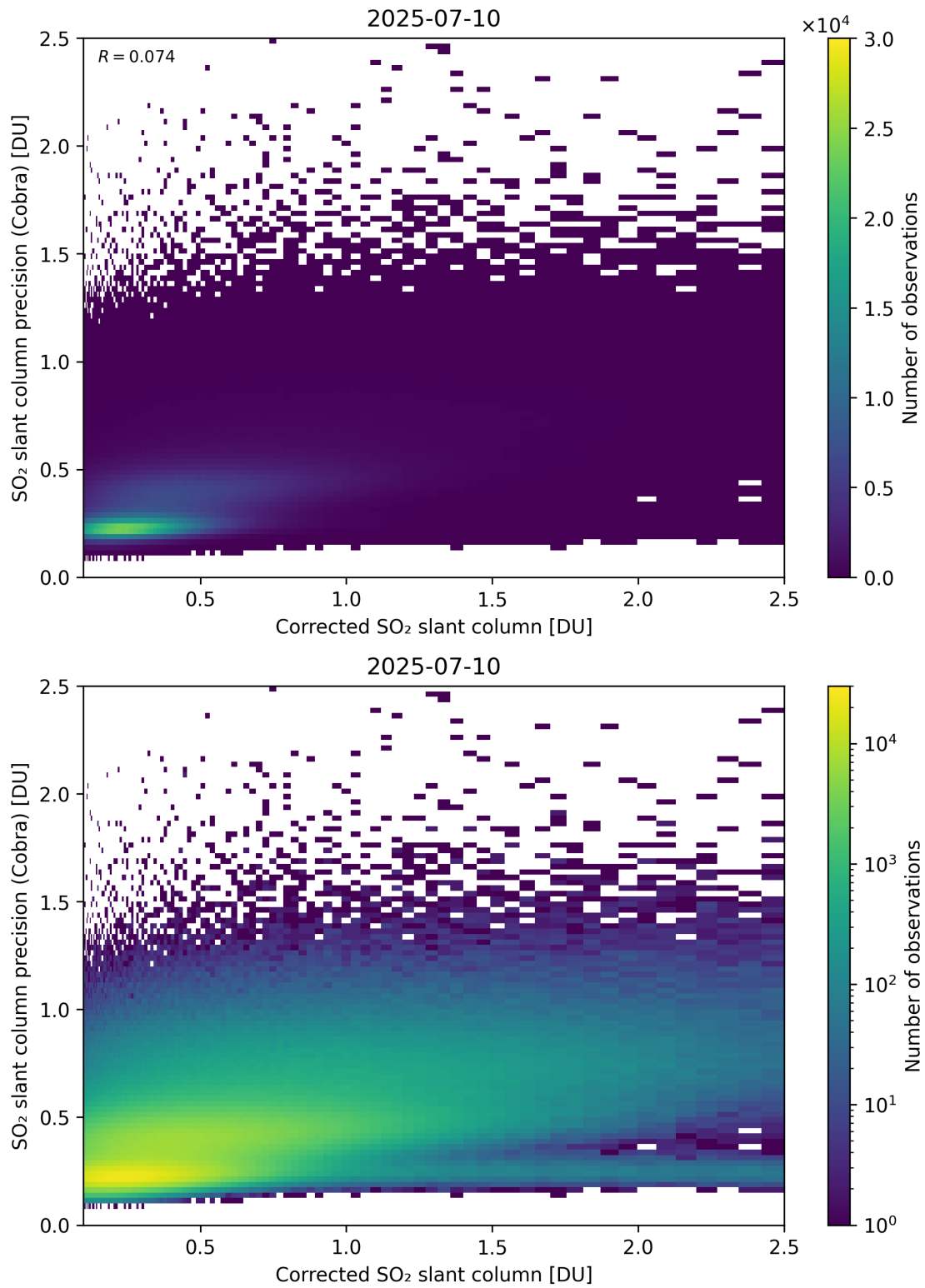
Figure 234: Scatter density plot of “Corrected SO 2 slant column” against “SO 2 slant column precision (Cobra)” for 2025-07-09 to 2025-07-11.
