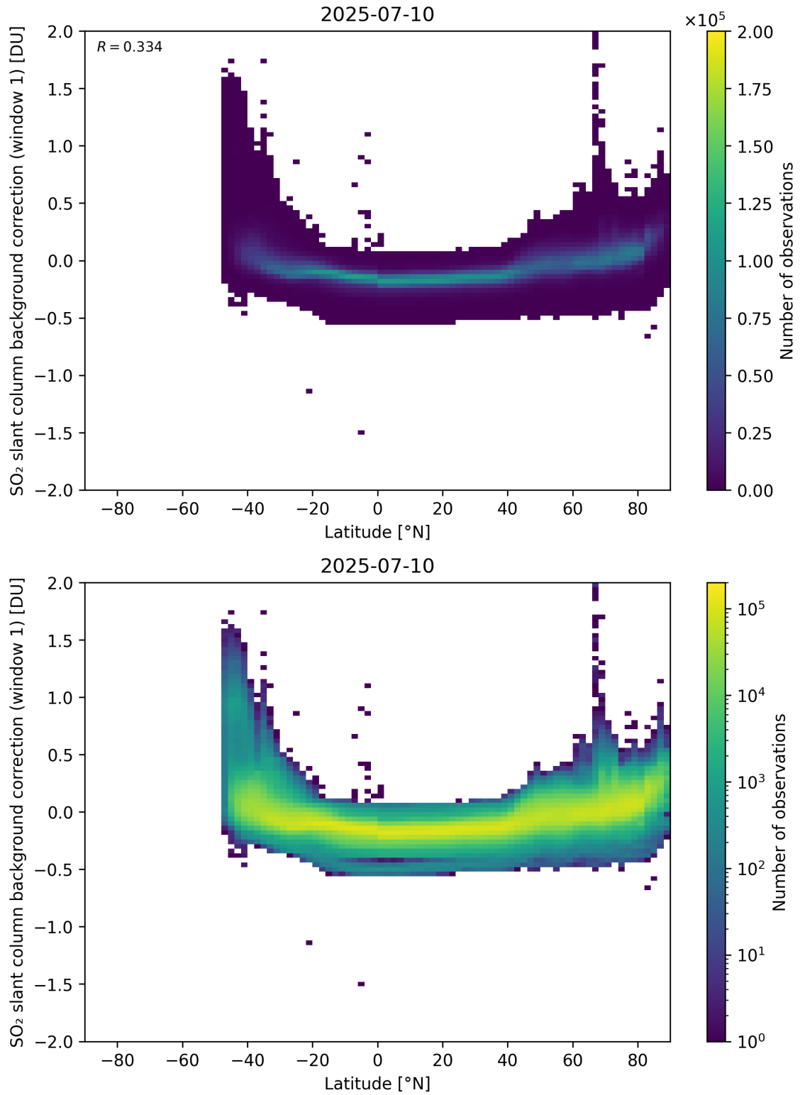
Figure 150: Scatter density plot of “Latitude” against “SO 2 slant column background correction (window 1)” for 2025-07-09 to 2025-07-11.
