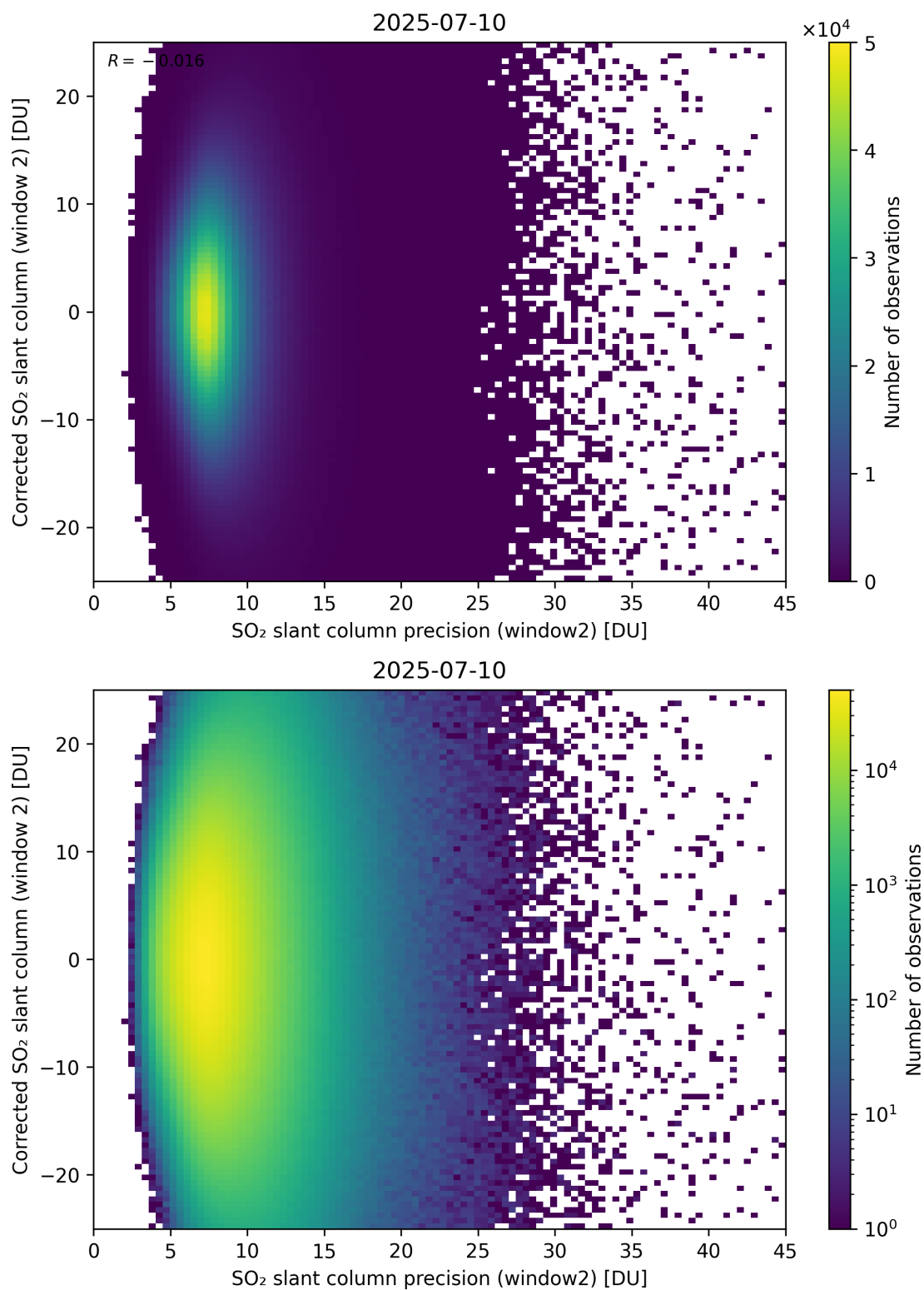
Figure 297: Scatter density plot of “SO 2 slant column precision (window2)” against “Corrected SO 2 slant column (window 2)” for 2025-07-09 to 2025-07-11.
