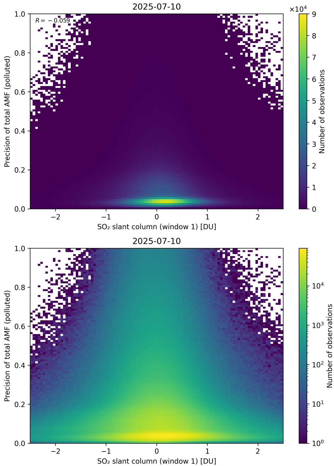
Figure 290: Scatter density plot of “SO 2 slant column (window 1)” against “Precision of total AMF (polluted)” for 2025-07-09 to 2025-07-11.
