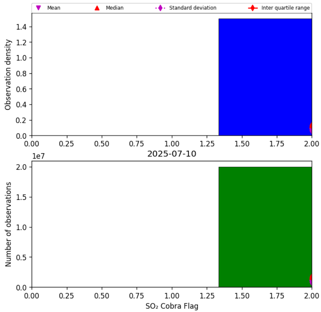
Figure 75: Histogram of “SO 2 Cobra Flag” for 2025-07-09 to 2025-07-11
