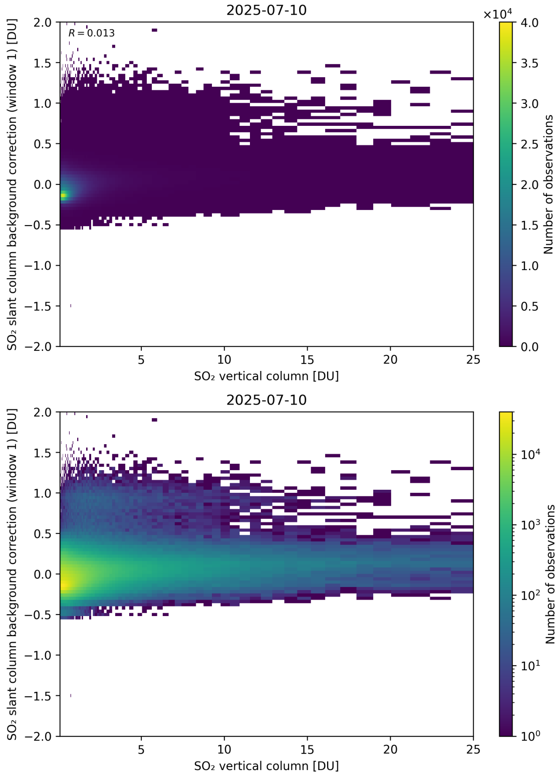
Figure 323: Scatter density plot of “SO 2 vertical column” against “SO 2 slant column background correction (window 1)” for 2025-07-09 to 2025-07-11.
