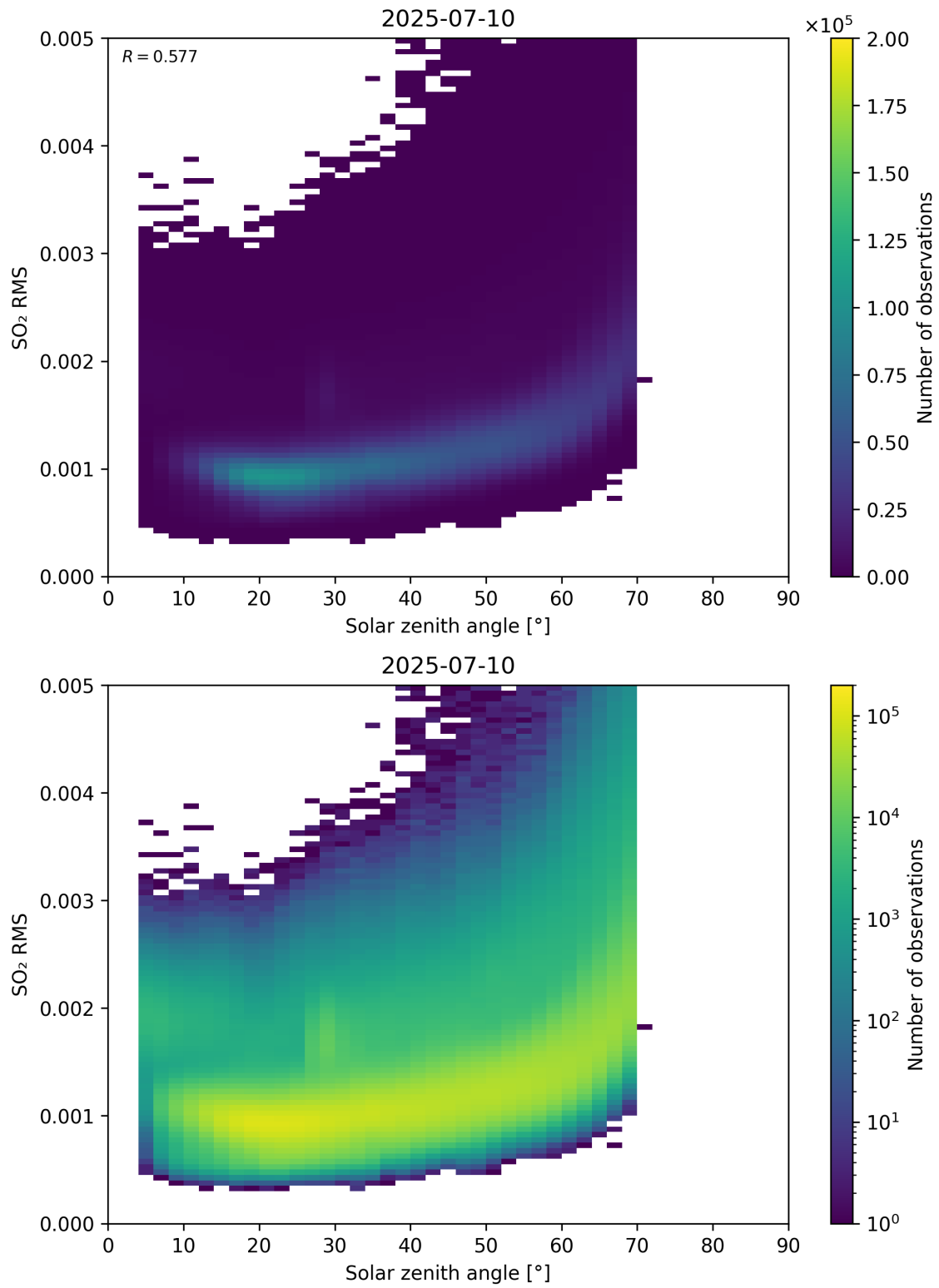
Figure 176: Scatter density plot of “Solar zenith angle” against “SO 2 RMS” for 2025-07-09 to 2025-07-11.
