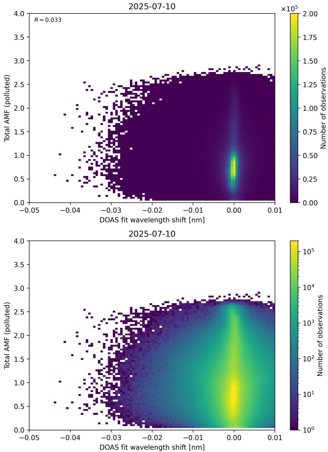
Figure 141: Scatter density plot of “DOAS fit wavelength shift” against “Total AMF (polluted)” for 2025-07-09 to 2025-07-11.
