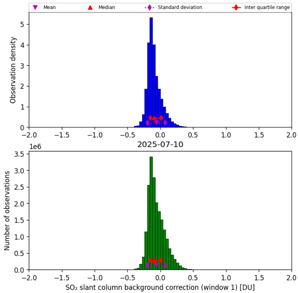
Figure 66: Histogram of “SO 2 slant column background correction (window 1)” for 2025-07-09 to 2025-07-11
