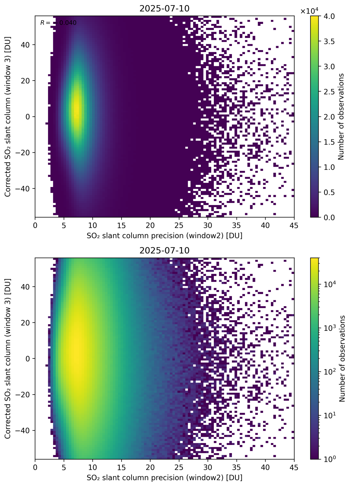
Figure 298: Scatter density plot of “SO 2 slant column precision (window2)” against “Corrected SO 2 slant column (window 3)” for 2025-07-09 to 2025-07-11.
