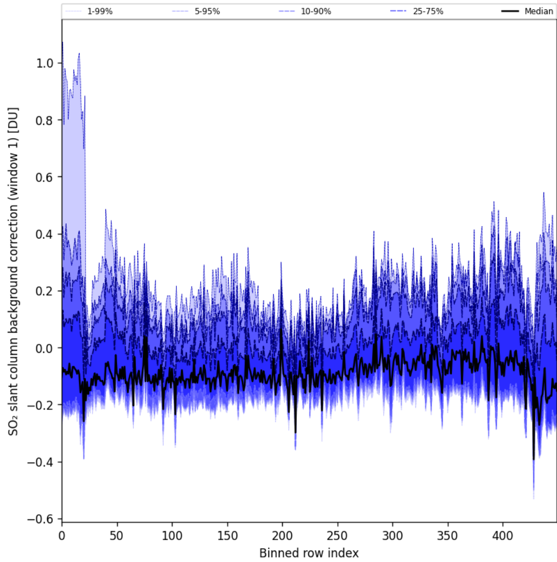
Figure 92: Along track statistics of “SO 2 slant column background correction (window 1)” for 2025-07-09 to 2025-07-11
