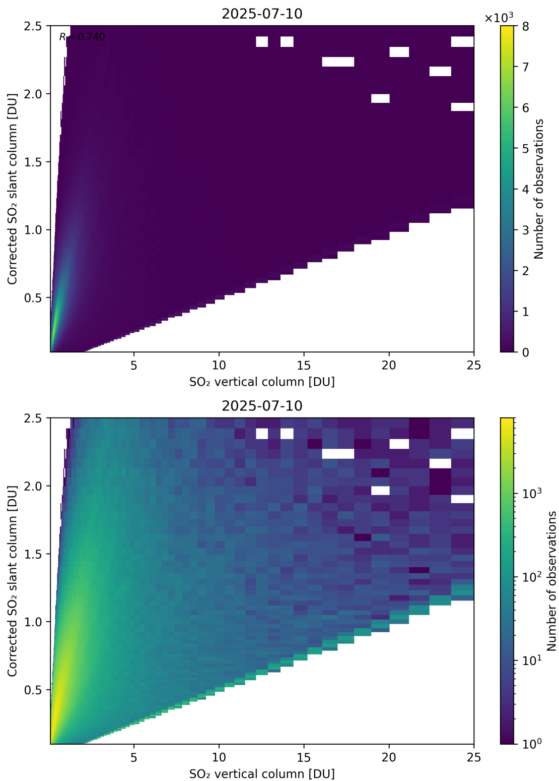
Figure 351: Scatter density plot of “SO 2 vertical column” against “Corrected SO 2 slant column” for 2025-07-09 to 2025-07-11.
