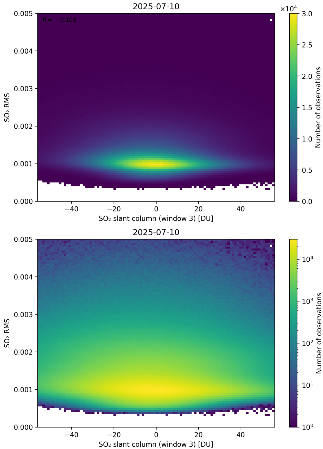
Figure 306: Scatter density plot of “SO 2 slant column (window 3)” against “SO 2 RMS” for 2025-07-09 to 2025-07-11.
