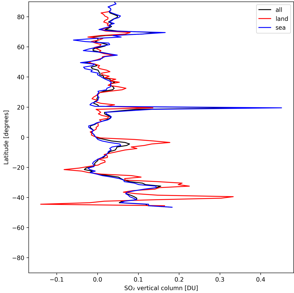
Figure 32: Zonal average of “SO 2 vertical column” for 2025-07-09 to 2025-07-11.
