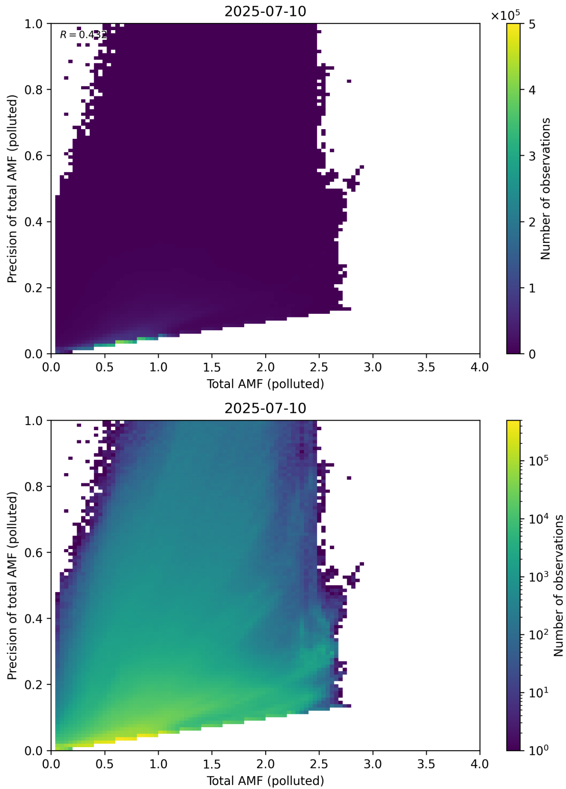
Figure 322: Scatter density plot of “Total AMF (polluted)” against “Precision of total AMF (polluted)” for 2025-07-09 to 2025-07-11.
