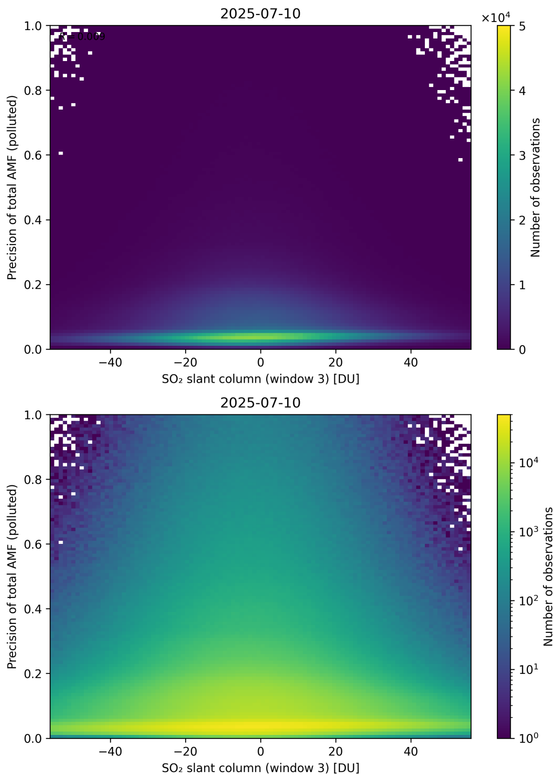
Figure 319: Scatter density plot of “SO 2 slant column (window 3)” against “Precision of total AMF (polluted)” for 2025-07-09 to 2025-07-11.
