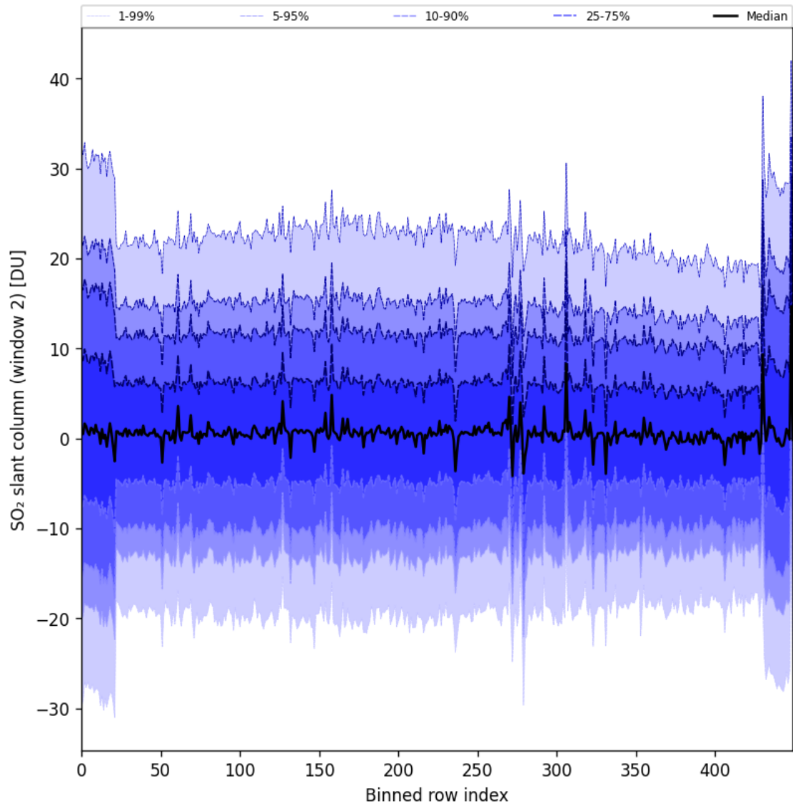
Figure 93: Along track statistics of “SO 2 slant column (window 2)” for 2025-07-09 to 2025-07-11
