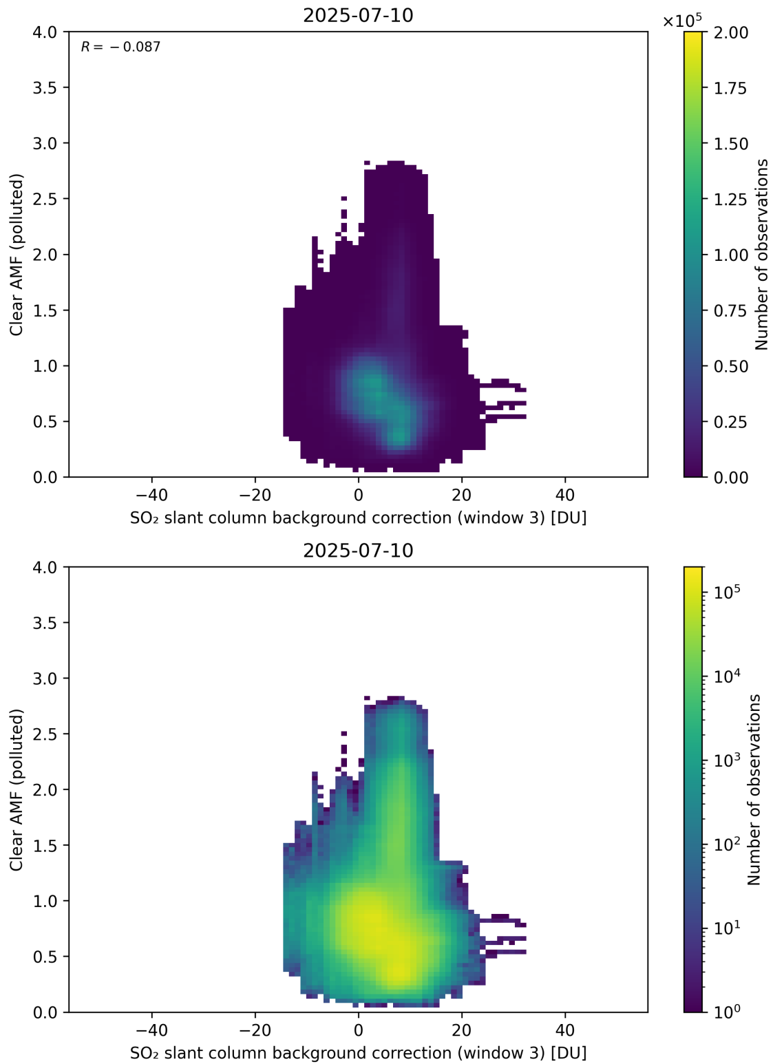
Figure 135: Scatter density plot of “SO 2 slant column background correction (window 3)” against “Clear AMF (polluted)” for 2025-07-09 to 2025-07-11.
