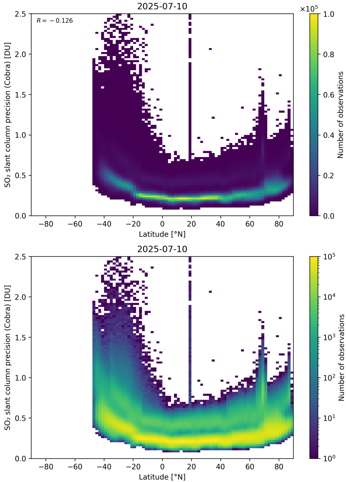
Figure 158: Scatter density plot of “Latitude” against “SO 2 slant column precision (Cobra)” for 2025-07-09 to 2025-07-11.
