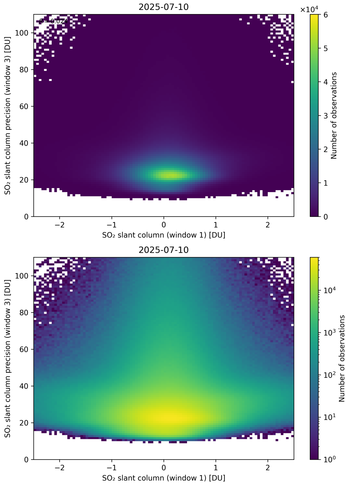
Figure 288: Scatter density plot of “SO 2 slant column (window 1)” against “SO 2 slant column precision (window 3)” for 2025-07-09 to 2025-07-11.
