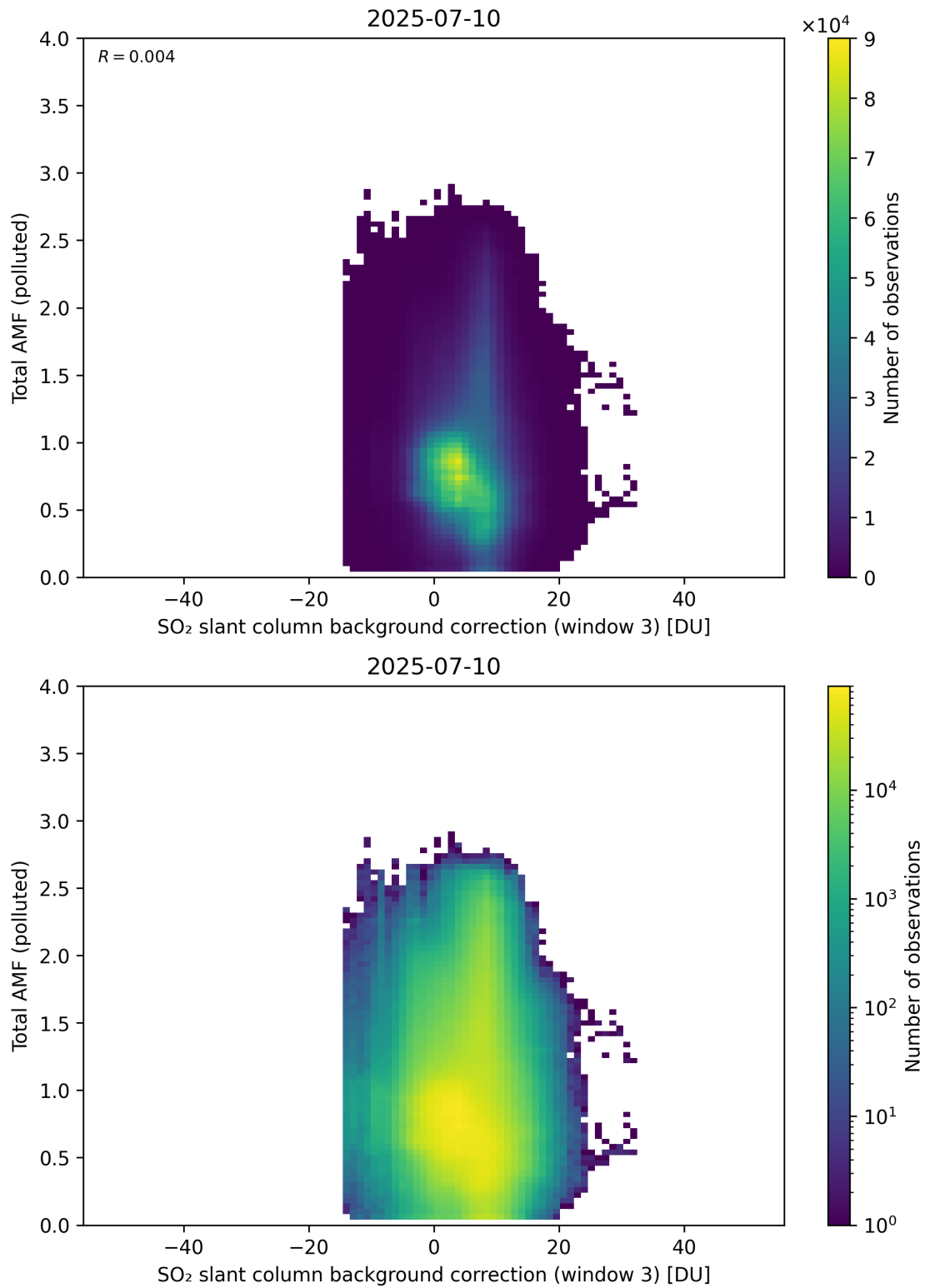
Figure 136: Scatter density plot of “SO 2 slant column background correction (window 3)” against “Total AMF (polluted)” for 2025-07-09 to 2025-07-11.
