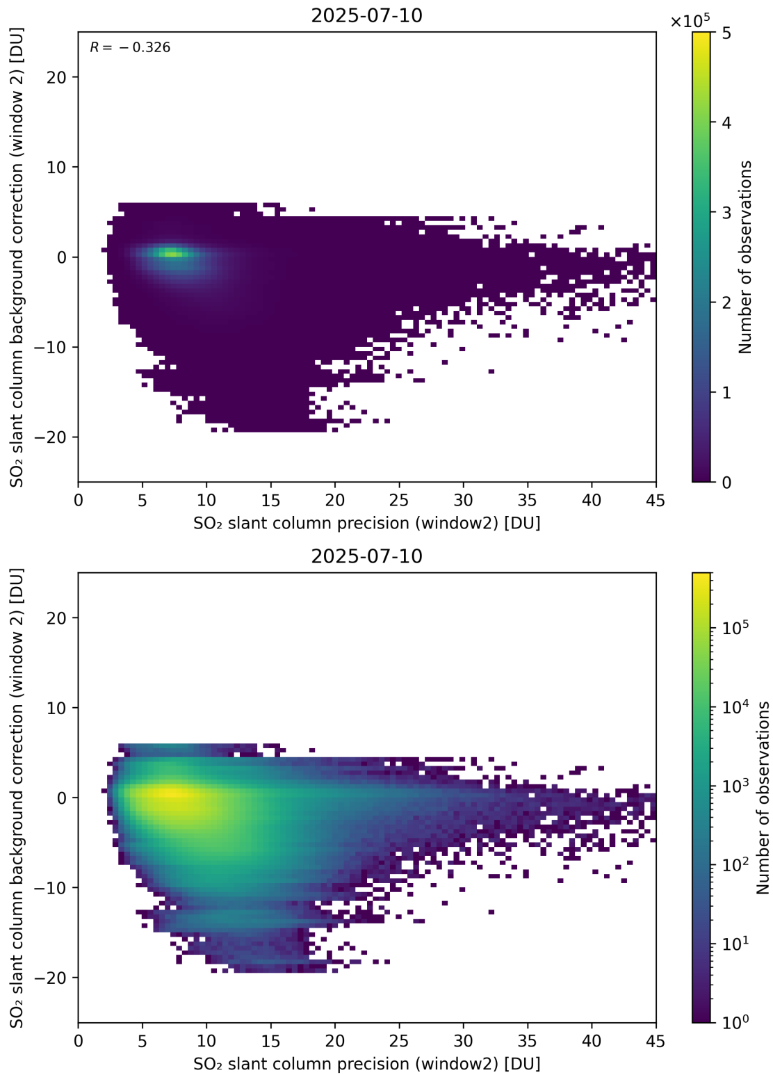
Figure 291: Scatter density plot of “SO 2 slant column precision (window2)” against “SO 2 slant column background correction (window 2)” for 2025-07-09 to 2025-07-11.
