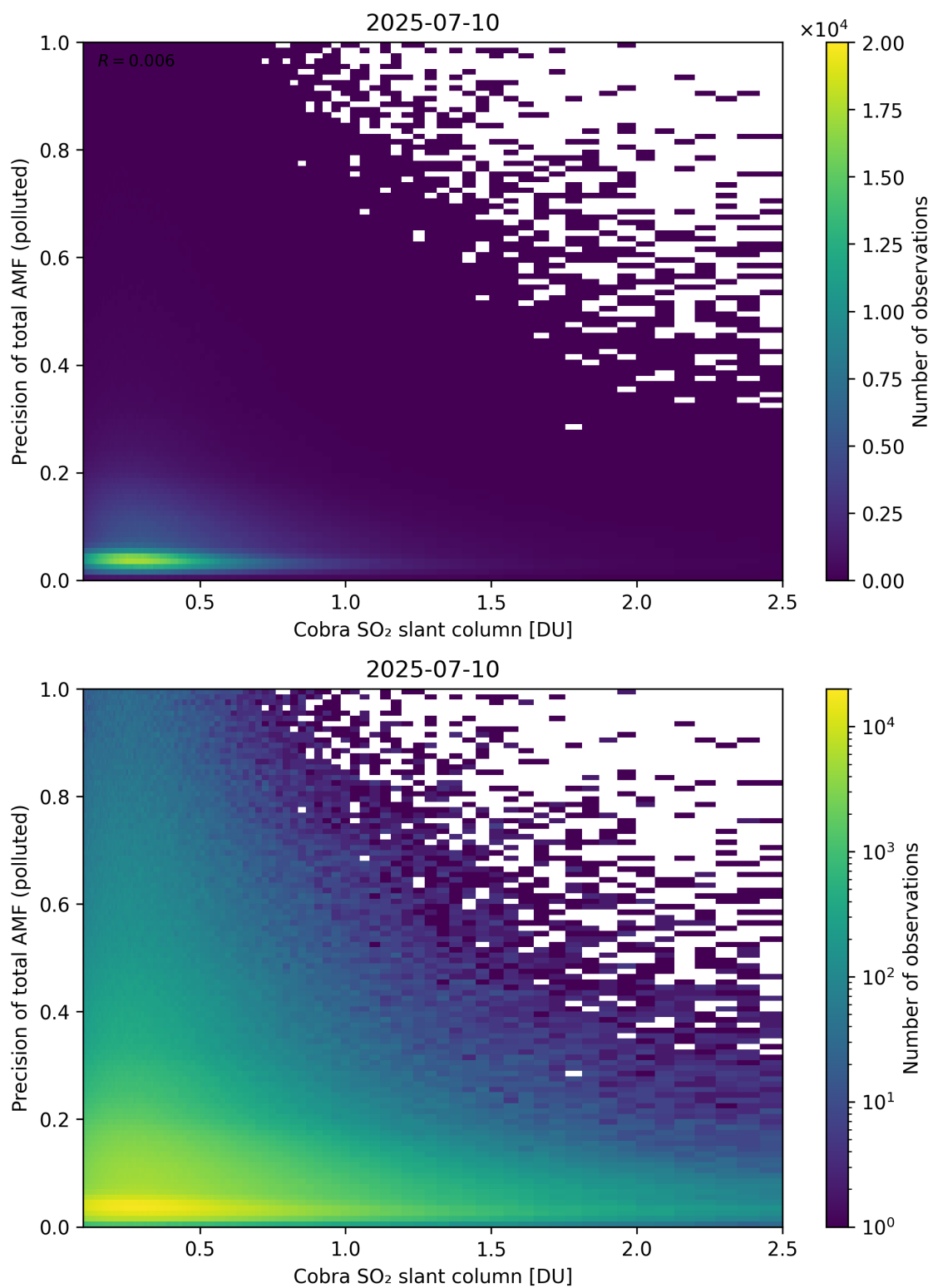
Figure 225: Scatter density plot of “Cobra SO 2 slant column” against “Precision of total AMF (polluted)” for 2025-07-09 to 2025-07-11.
