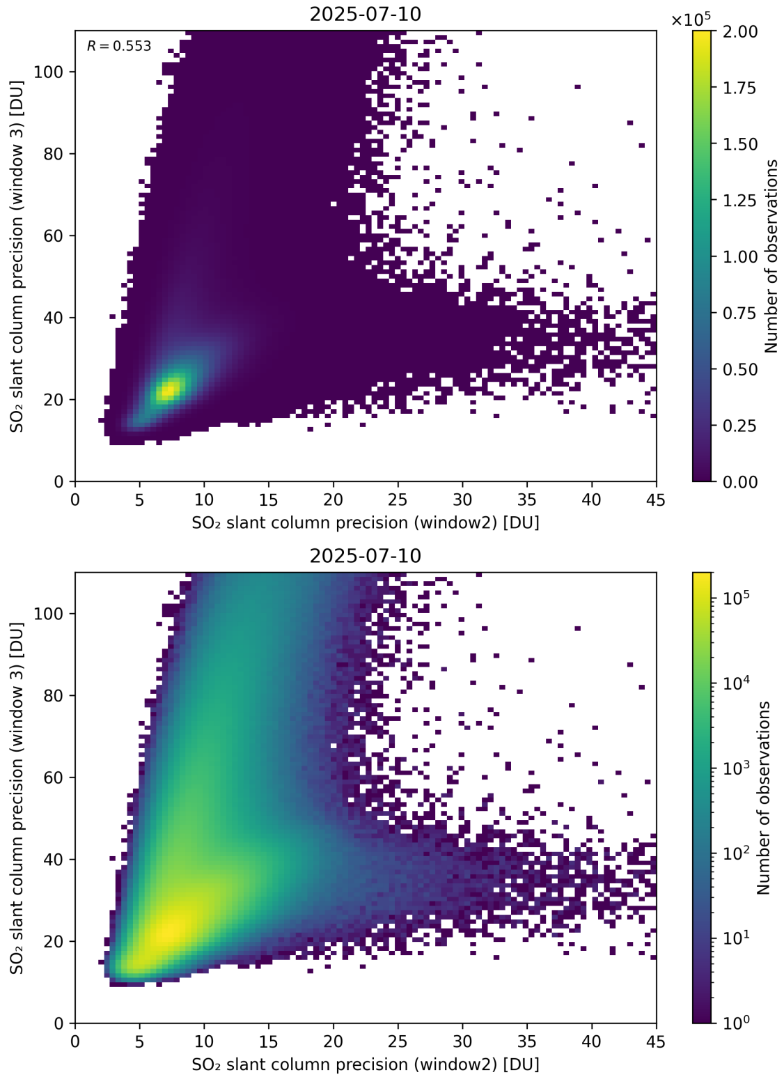
Figure 300: Scatter density plot of “SO 2 slant column precision (window2)” against “SO 2 slant column precision (window 3)” for 2025-07-09 to 2025-07-11.
