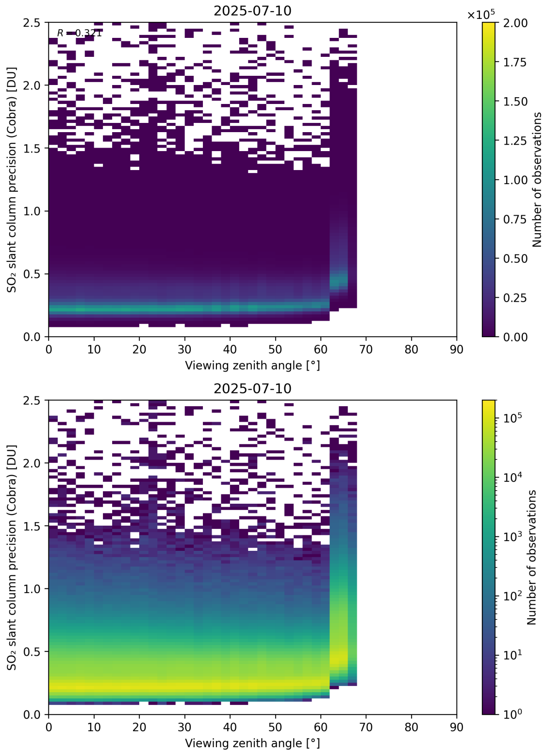
Figure 372: Scatter density plot of “Viewing zenith angle” against “SO 2 slant column precision (Cobra)” for 2025-07-09 to 2025-07-11.
