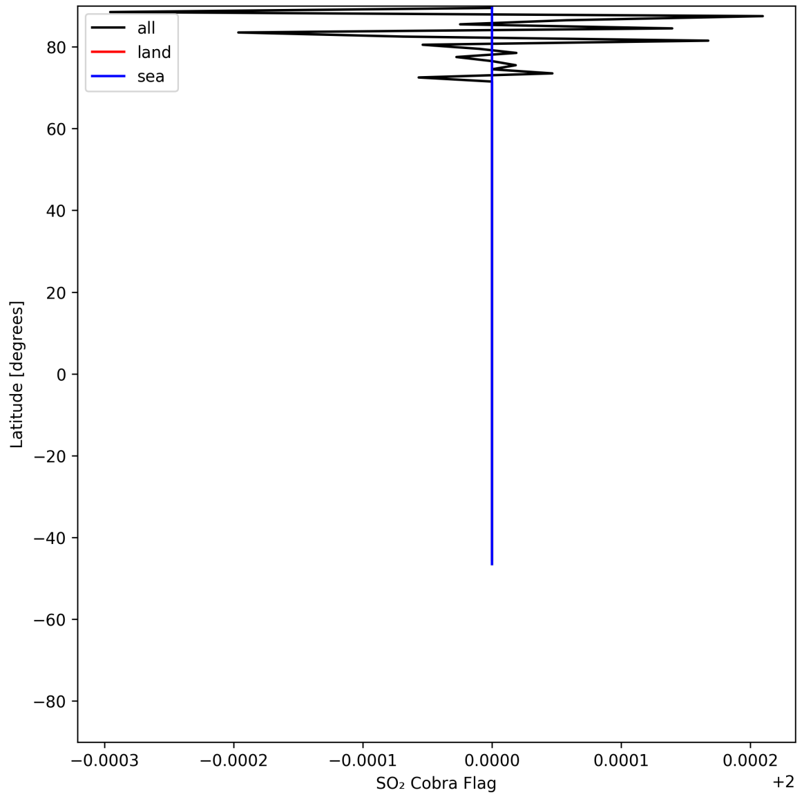
Figure 49: Zonal average of “SO 2 Cobra Flag” for 2025-07-09 to 2025-07-11.
