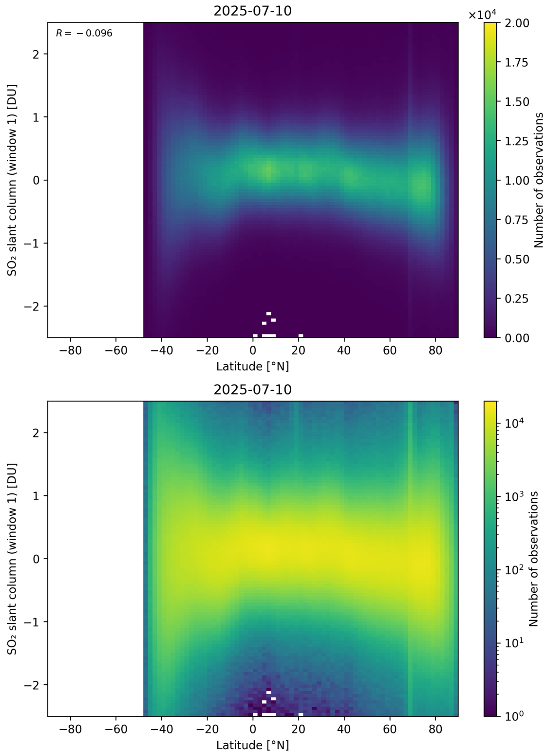
Figure 162: Scatter density plot of “Latitude” against “SO 2 slant column (window 1)” for 2025-07-09 to 2025-07-11.
