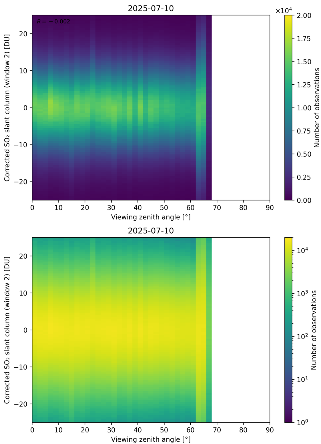
Figure 374: Scatter density plot of “Viewing zenith angle” against “Corrected SO 2 slant column (window 2)” for 2025-07-09 to 2025-07-11.
