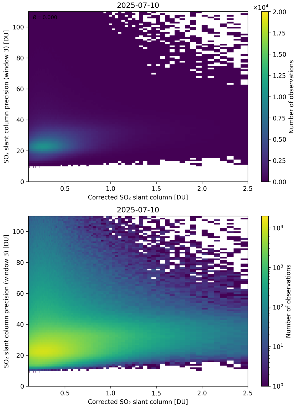
Figure 241: Scatter density plot of “Corrected SO 2 slant column” against “SO 2 slant column precision (window 3)” for 2025-07-09 to 2025-07-11.
