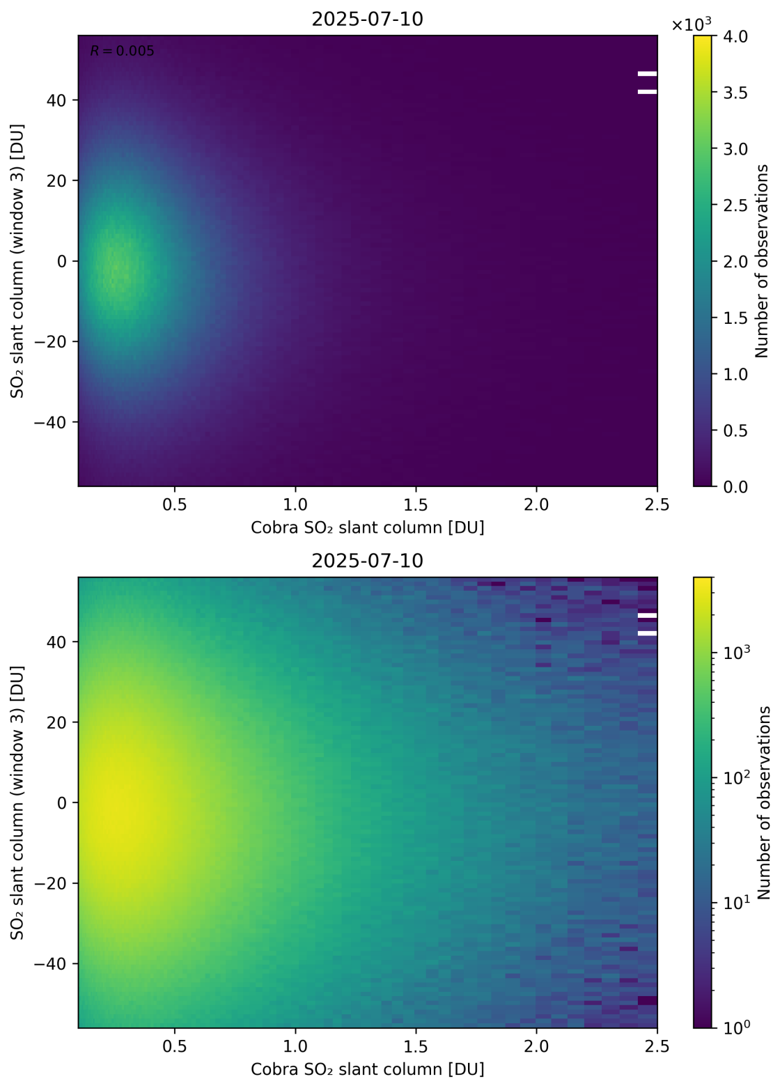
Figure 222: Scatter density plot of “Cobra SO 2 slant column” against “SO 2 slant column (window 3)” for 2025-07-09 to 2025-07-11.
