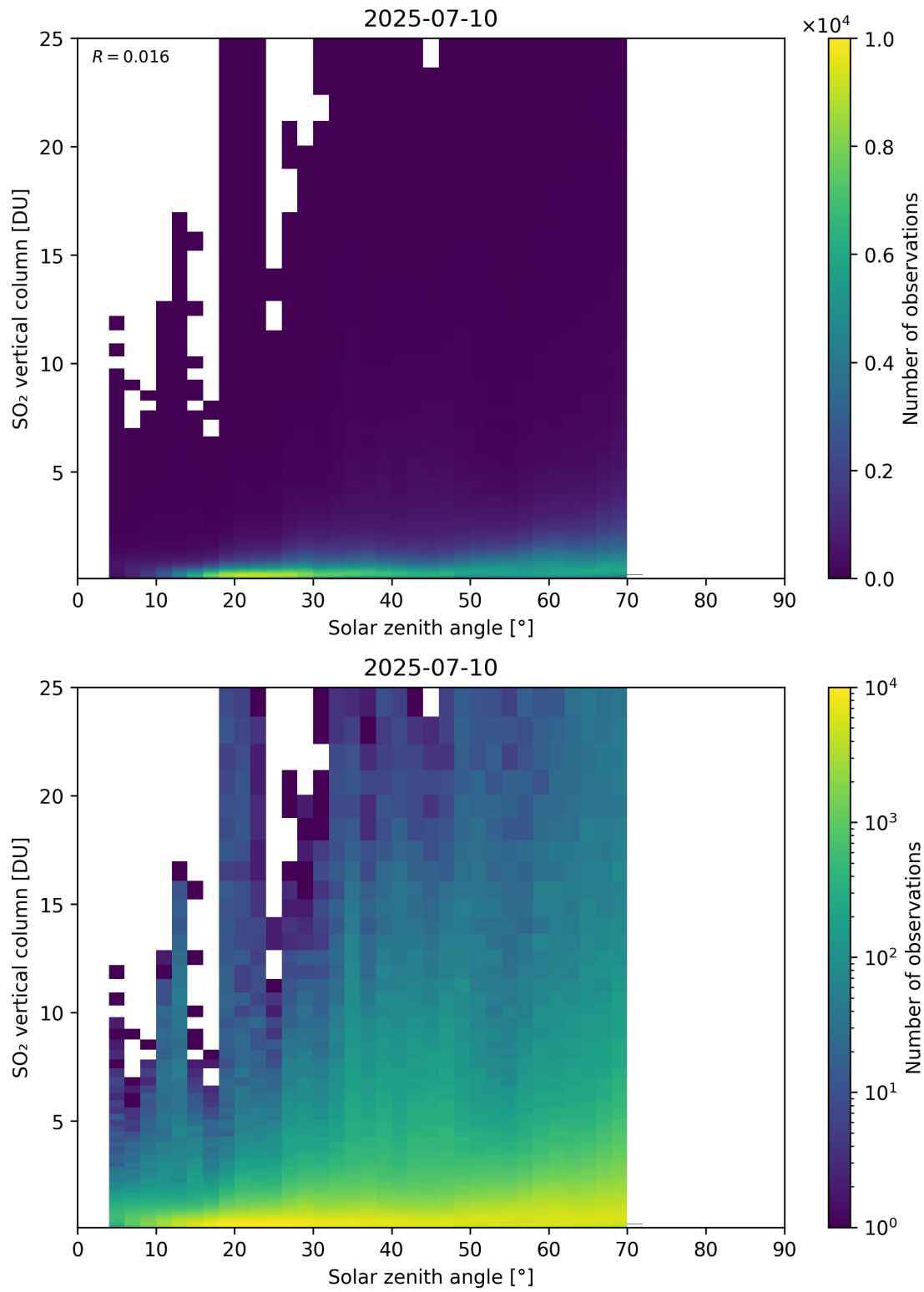
Figure 191: Scatter density plot of “Solar zenith angle” against “SO 2 vertical column” for 2025-07-09 to 2025-07-11.
