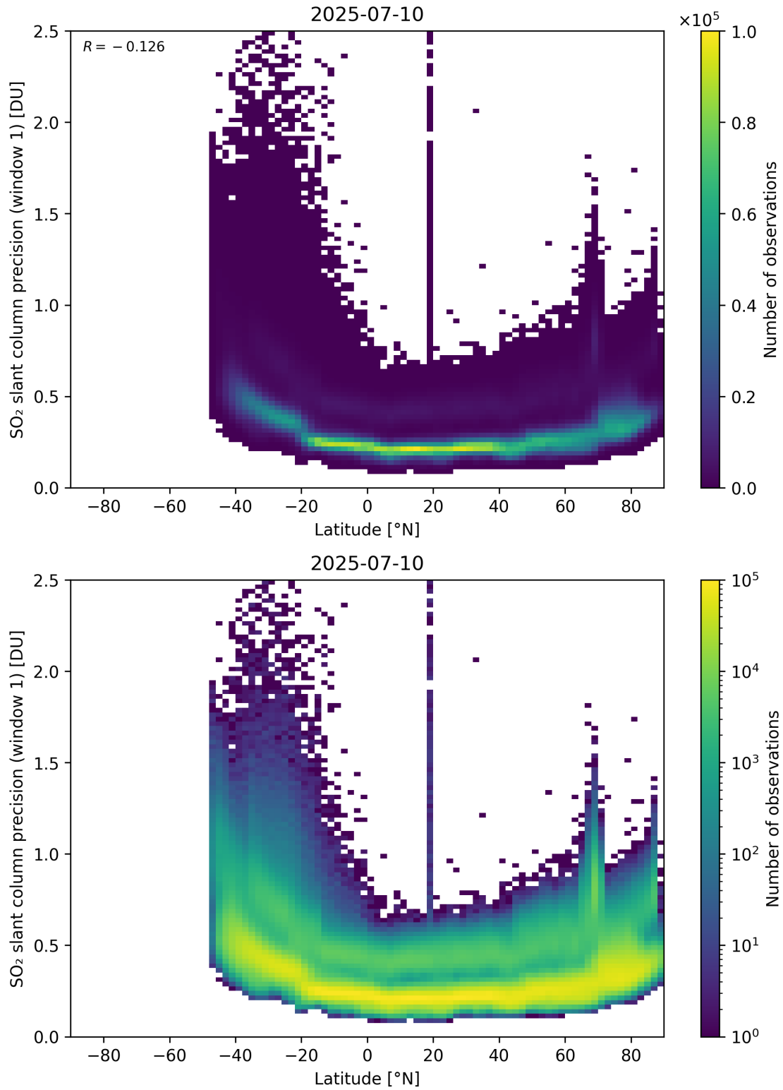
Figure 163: Scatter density plot of “Latitude” against “SO 2 slant column precision (window 1)” for 2025-07-09 to 2025-07-11.
