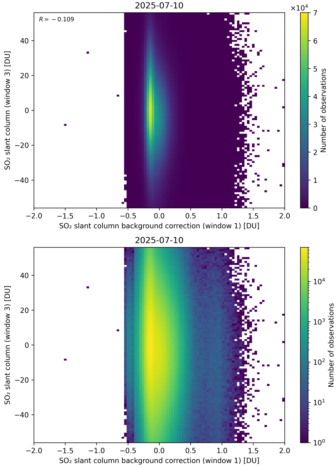
Figure 118: Scatter density plot of “SO 2 slant column background correction (window 1)” against “SO 2 slant column (window 3)” for 2025-07-09 to 2025-07-11.
