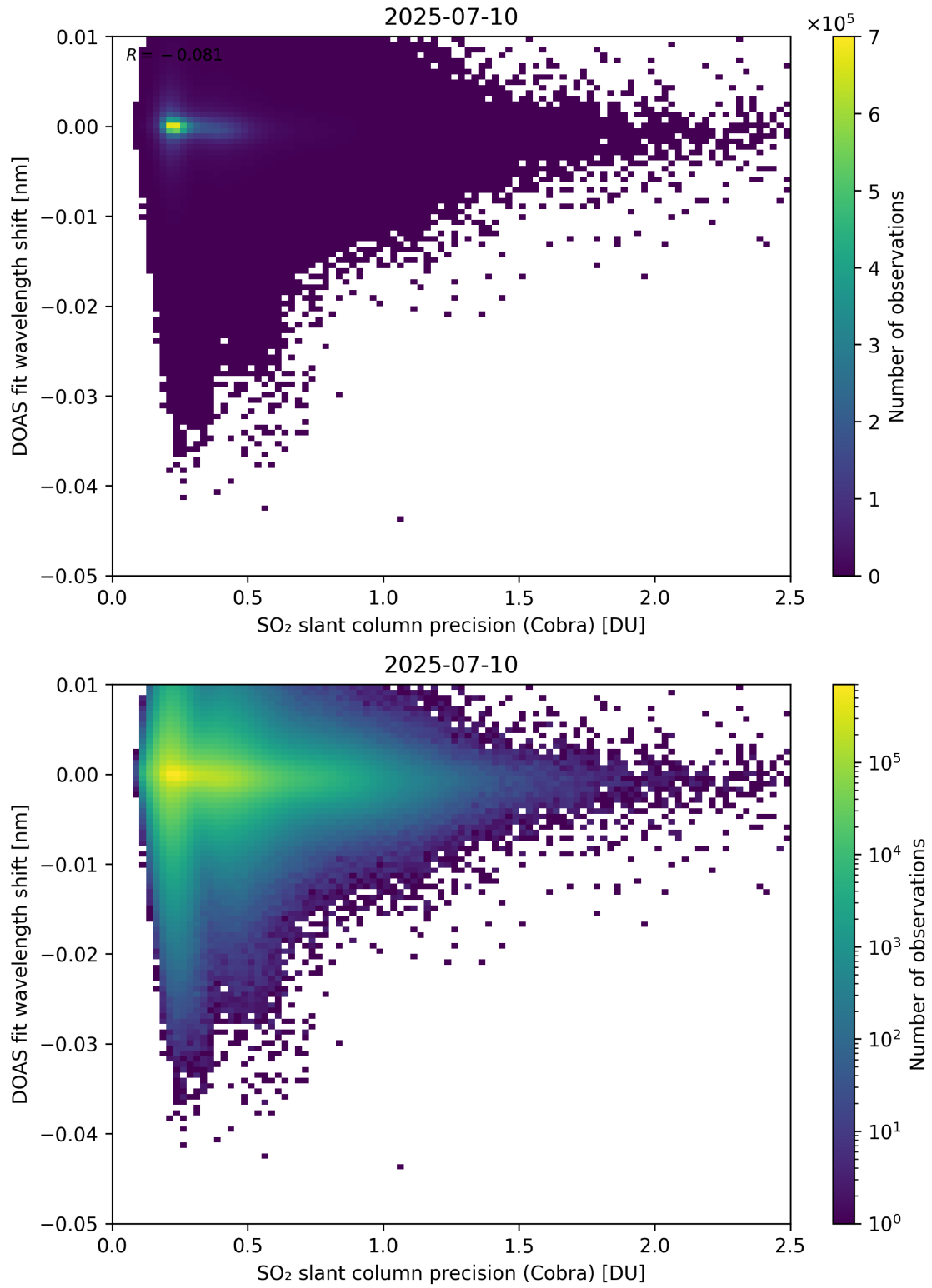
Figure 202: Scatter density plot of “SO 2 slant column precision (Cobra)” against “DOAS fit wavelength shift” for 2025-07-09 to 2025-07-11.
