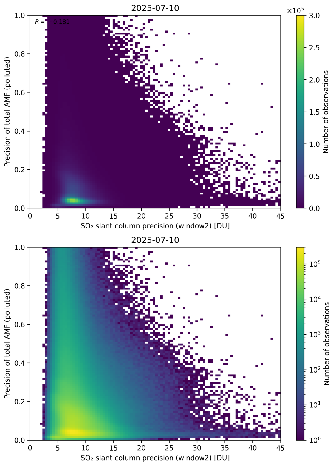
Figure 302: Scatter density plot of “SO 2 slant column precision (window2)” against “Precision of total AMF (polluted)” for 2025-07-09 to 2025-07-11.
