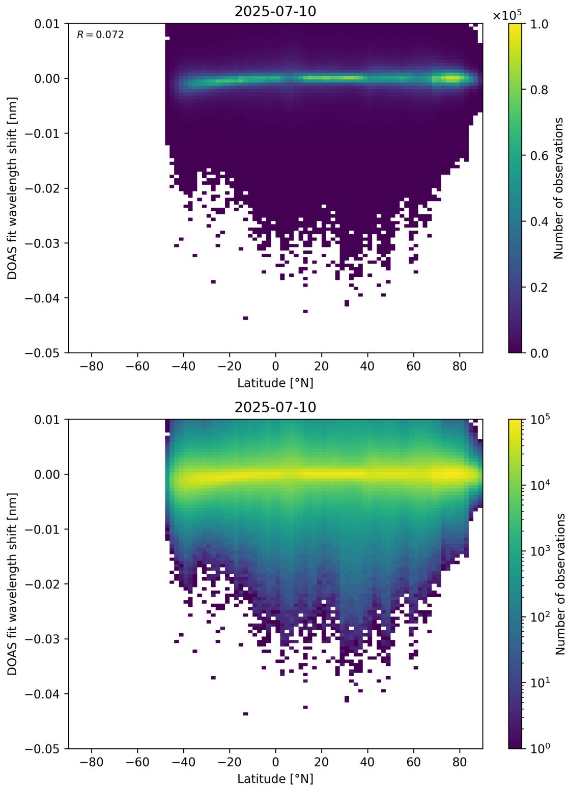
Figure 153: Scatter density plot of “Latitude” against “DOAS fit wavelength shift” for 2025-07-09 to 2025-07-11.
