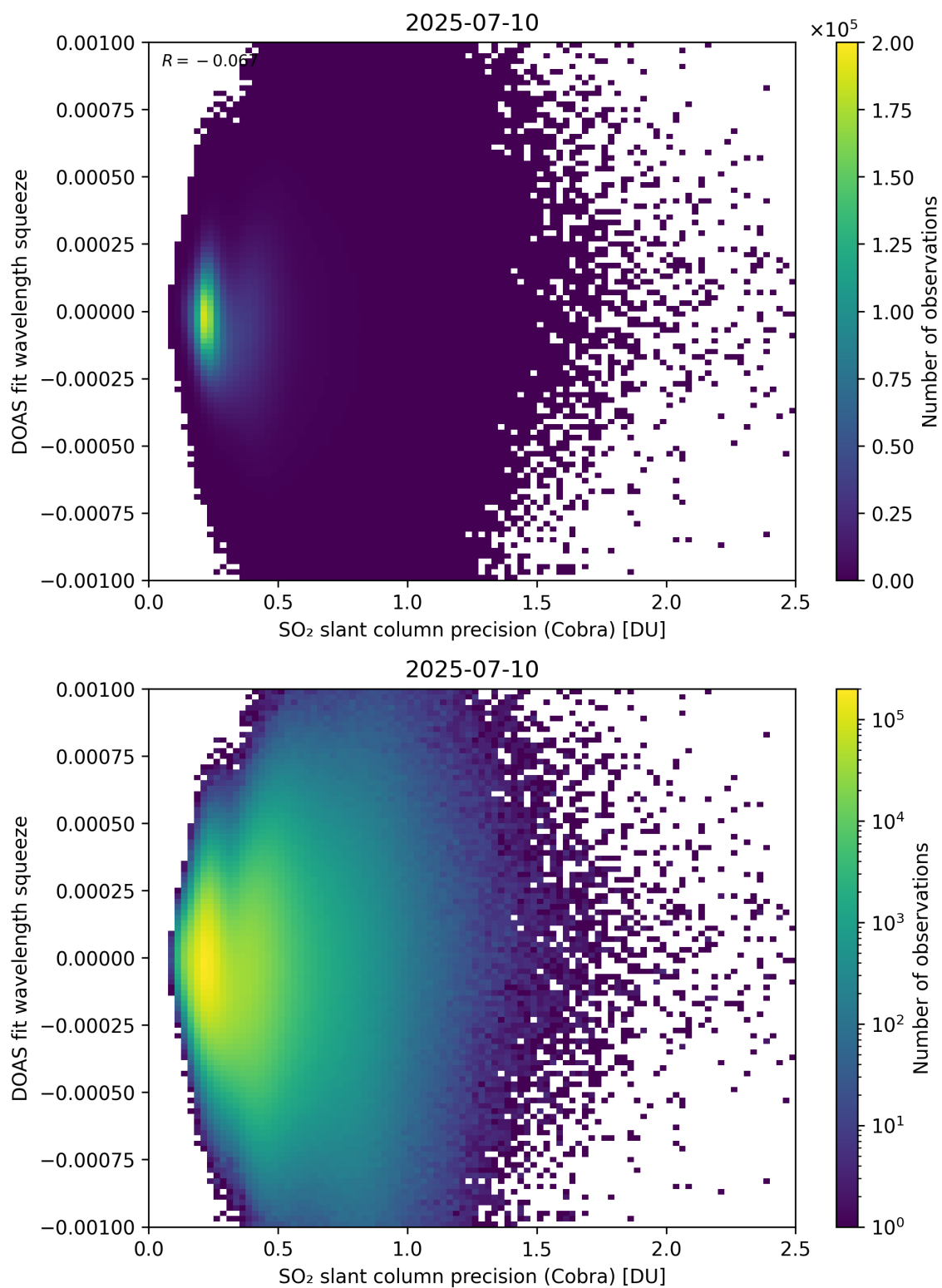
Figure 203: Scatter density plot of “SO 2 slant column precision (Cobra)” against “DOAS fit wavelength squeeze” for 2025-07-09 to 2025-07-11.
