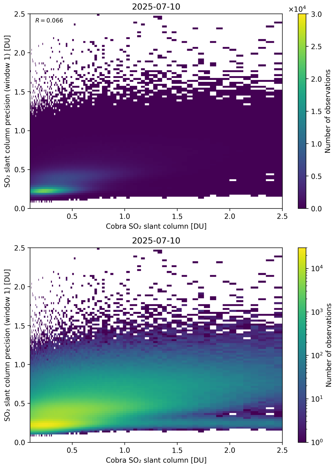
Figure 220: Scatter density plot of “Cobra SO 2 slant column” against “SO 2 slant column precision (window 1)” for 2025-07-09 to 2025-07-11.
