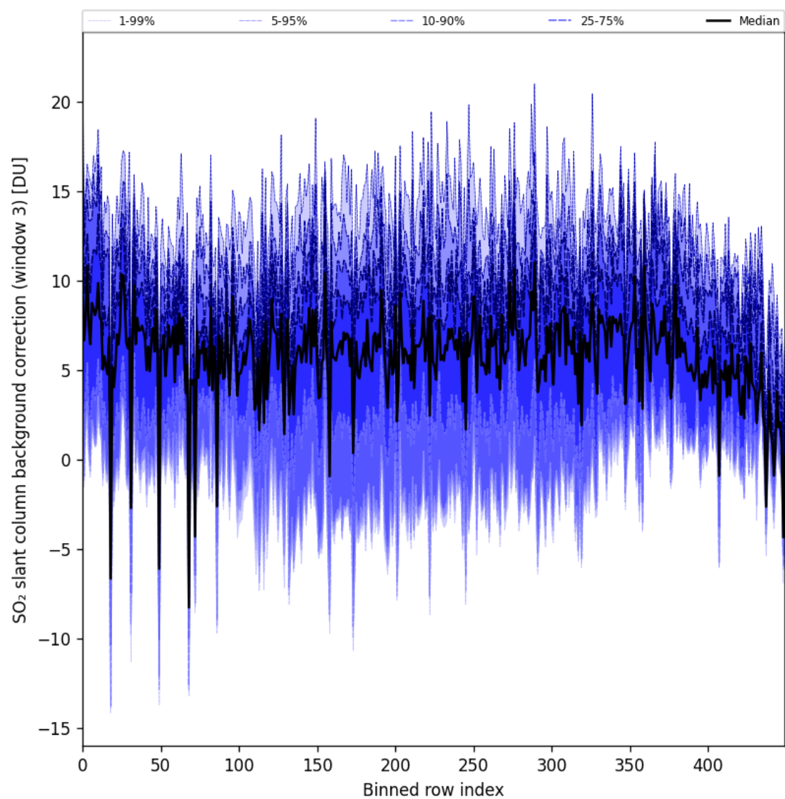
Figure 100: Along track statistics of “SO 2 slant column background correction (window 3)” for 2025-07-09 to 2025-07-11
