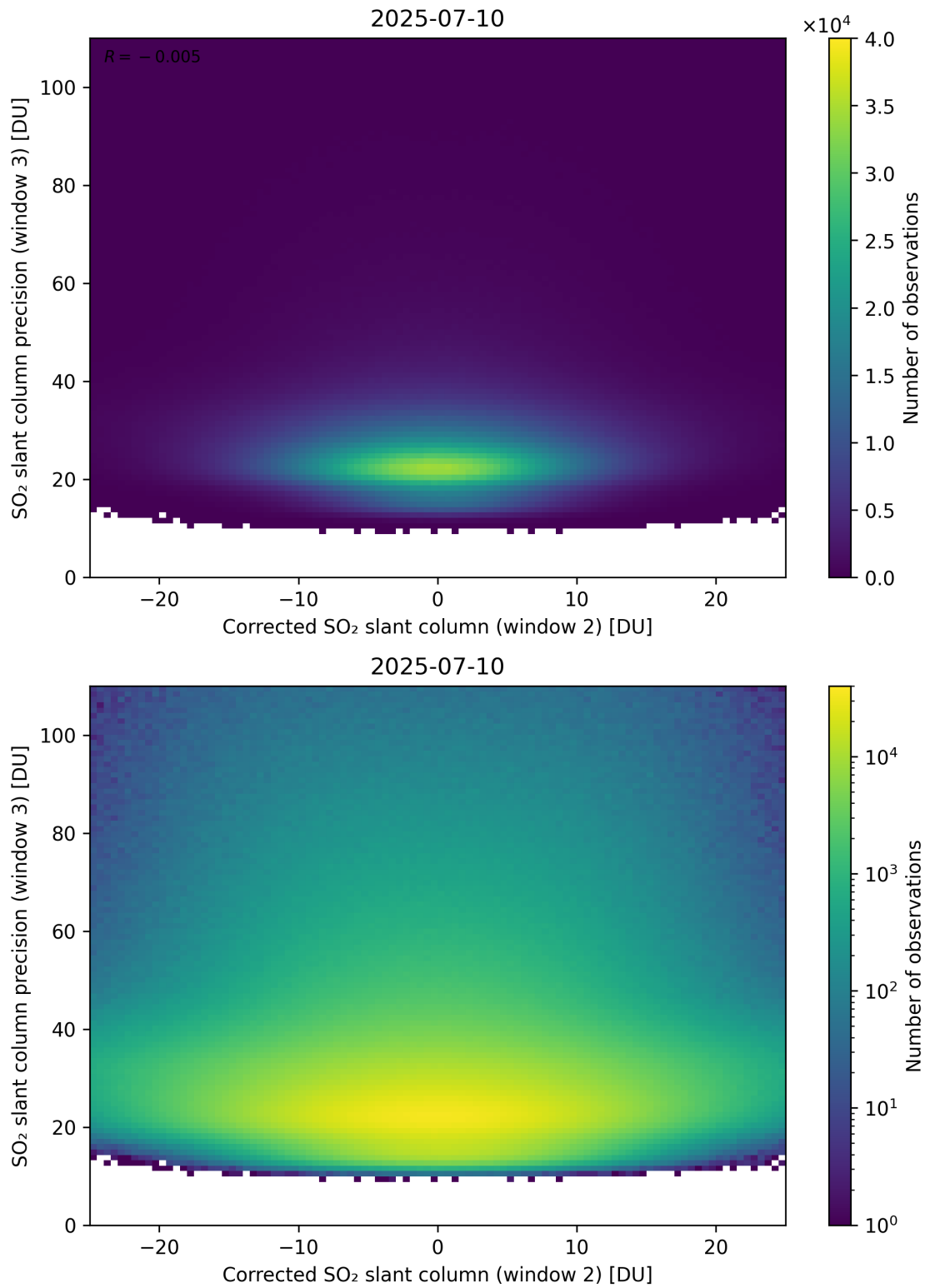
Figure 252: Scatter density plot of “Corrected SO 2 slant column (window 2)” against “SO 2 slant column precision (window 3)” for 2025-07-09 to 2025-07-11.
