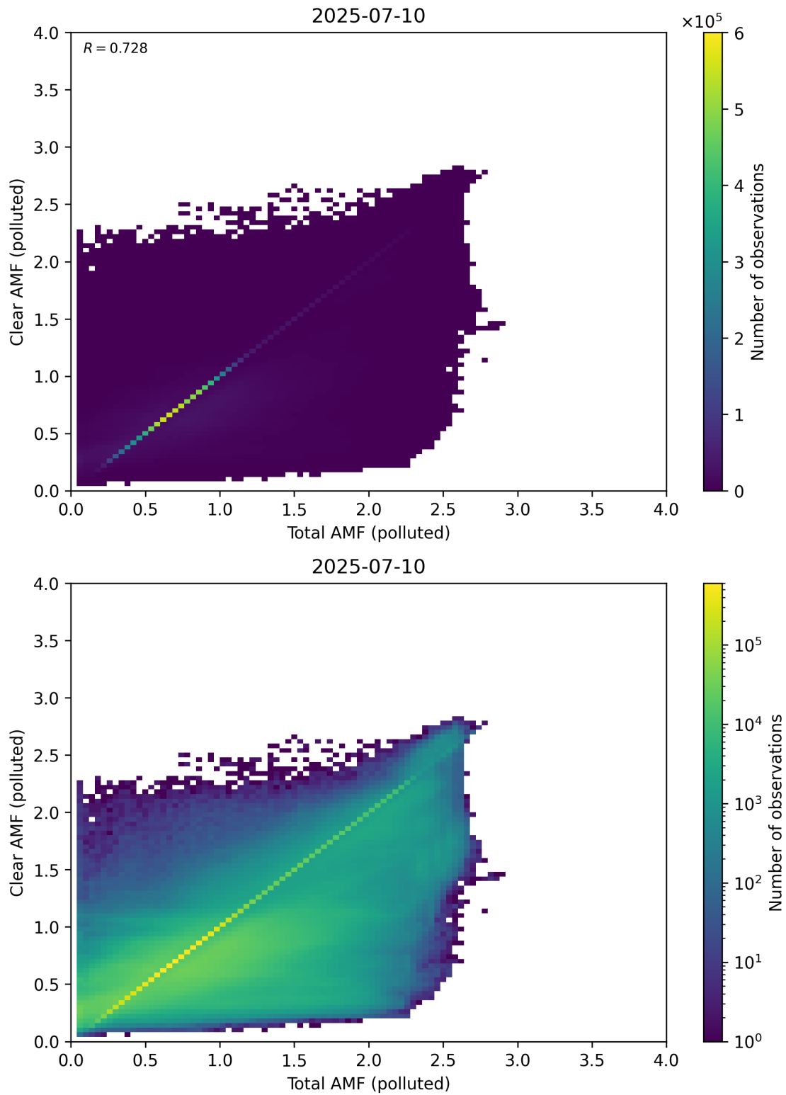
Figure 321: Scatter density plot of “Total AMF (polluted)” against “Clear AMF (polluted)” for 2025-07-09 to 2025-07-11.
