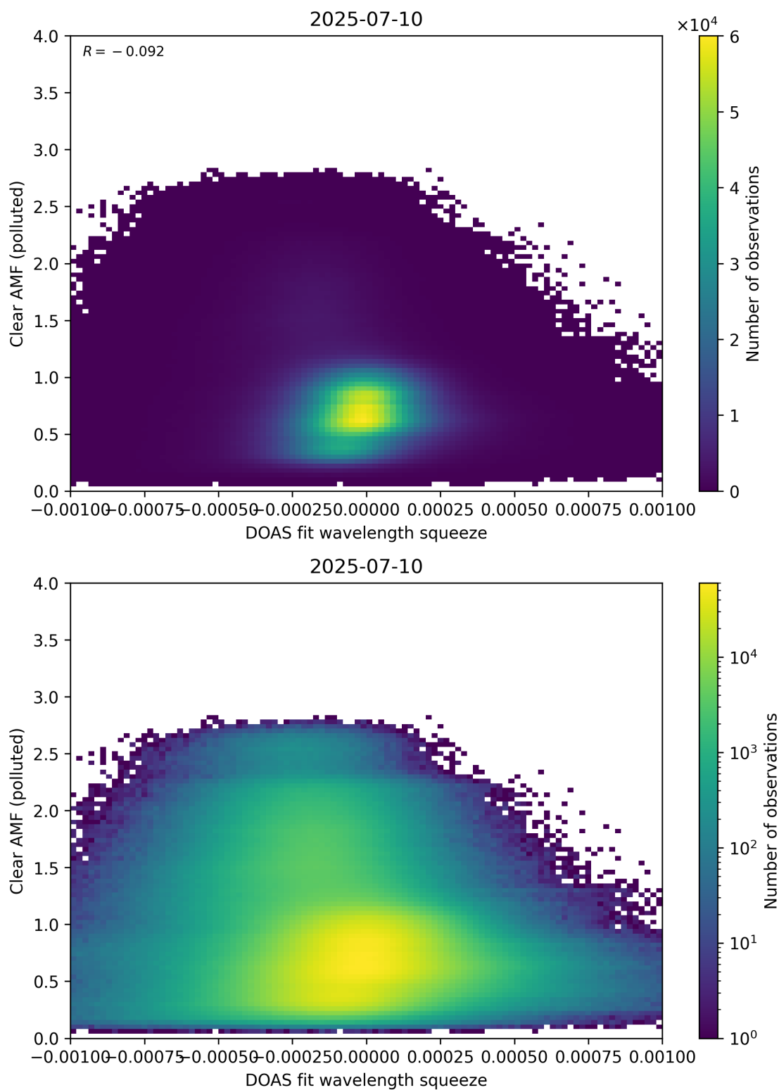
Figure 144: Scatter density plot of “DOAS fit wavelength squeeze” against “Clear AMF (polluted)” for 2025-07-09 to 2025-07-11.
