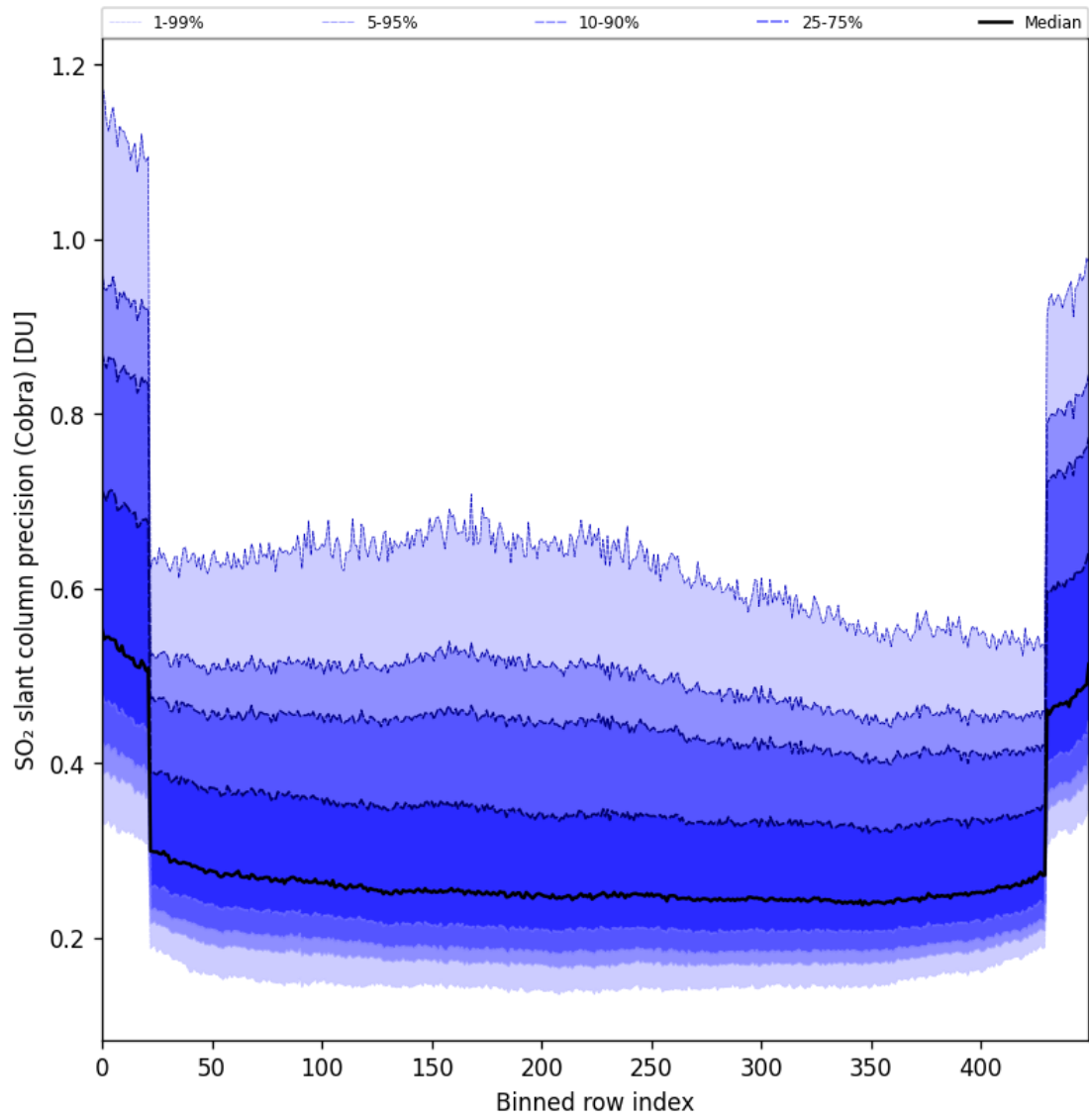
Figure 88: Along track statistics of “SO 2 slant column precision (Cobra)” for 2025-07-09 to 2025-07-11
