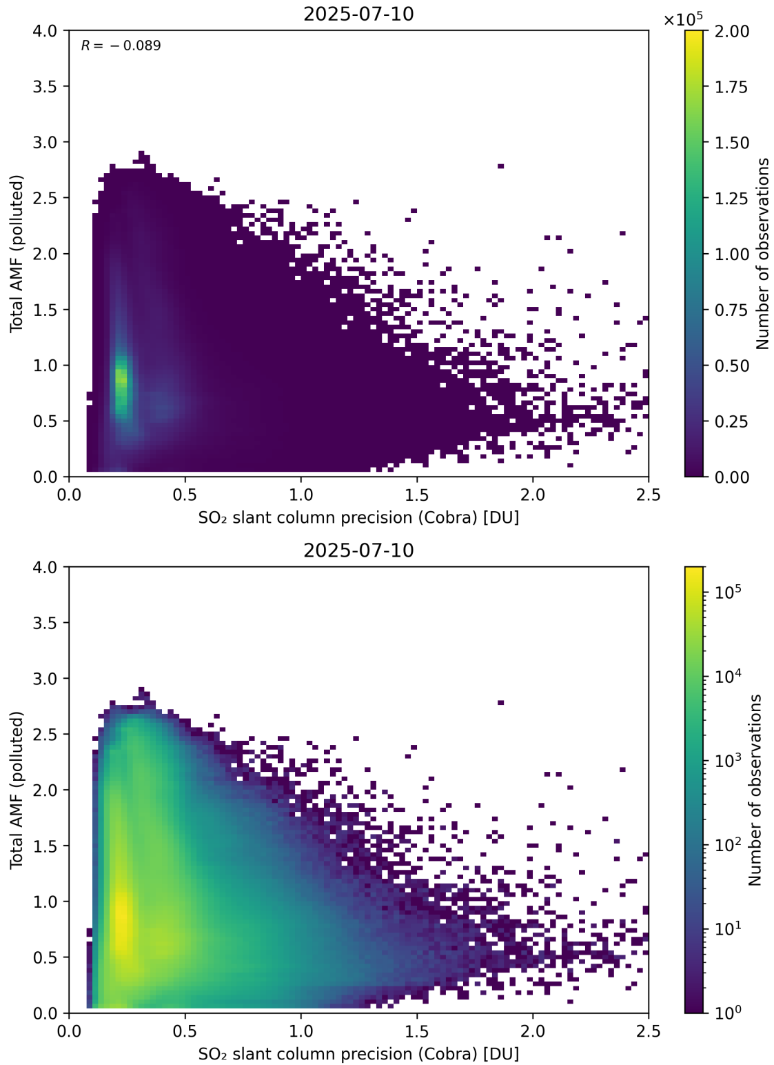
Figure 213: Scatter density plot of “SO 2 slant column precision (Cobra)” against “Total AMF (polluted)” for 2025-07-09 to 2025-07-11.
