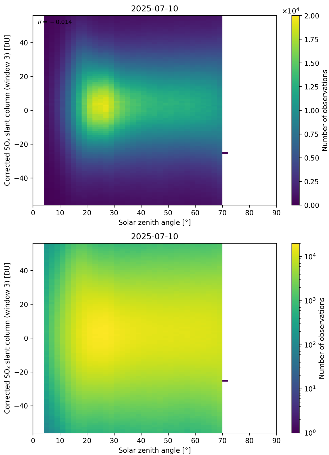
Figure 183: Scatter density plot of “Solar zenith angle” against “Corrected SO 2 slant column (window 3)” for 2025-07-09 to 2025-07-11.
