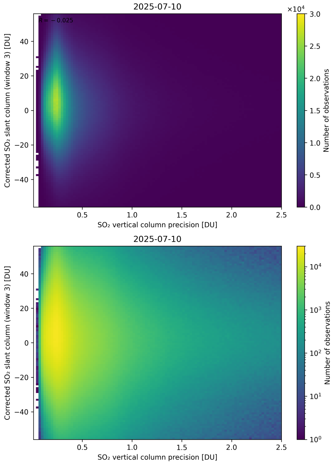
Figure 340: Scatter density plot of “SO 2 vertical column precision” against “Corrected SO 2 slant column (window 3)” for 2025-07-09 to 2025-07-11.
