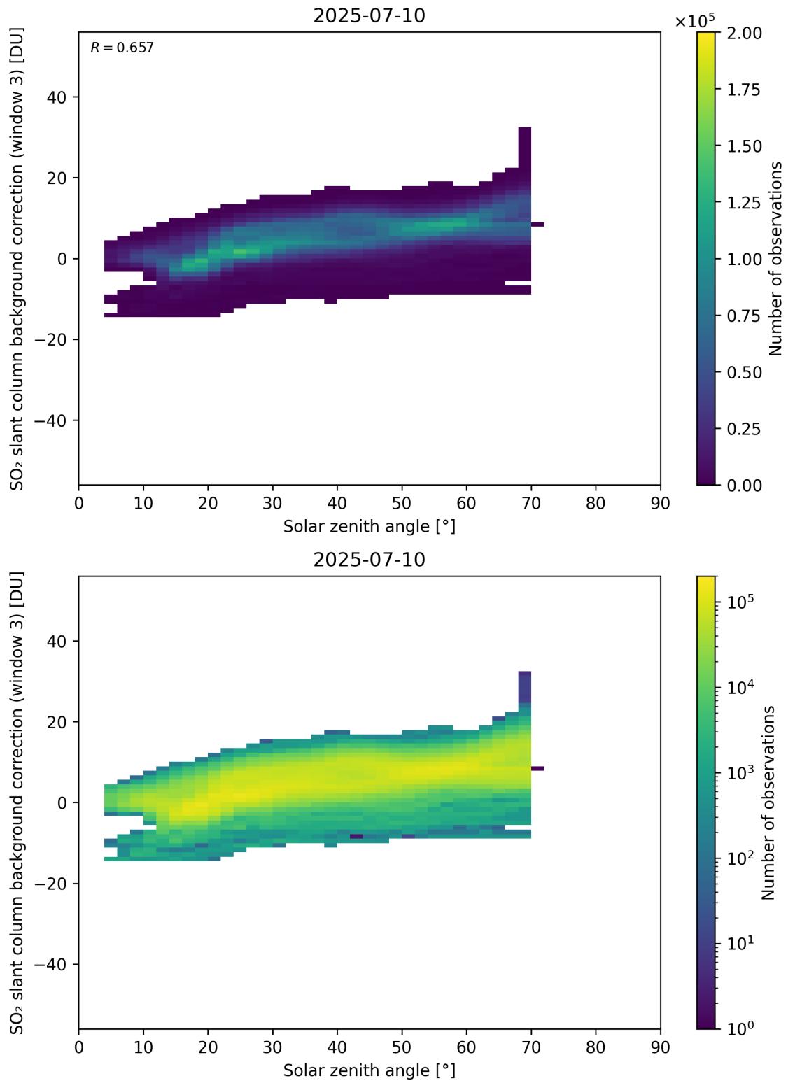
Figure 173: Scatter density plot of “Solar zenith angle” against “SO 2 slant column background correction (window 3)” for 2025-07-09 to 2025-07-11.
