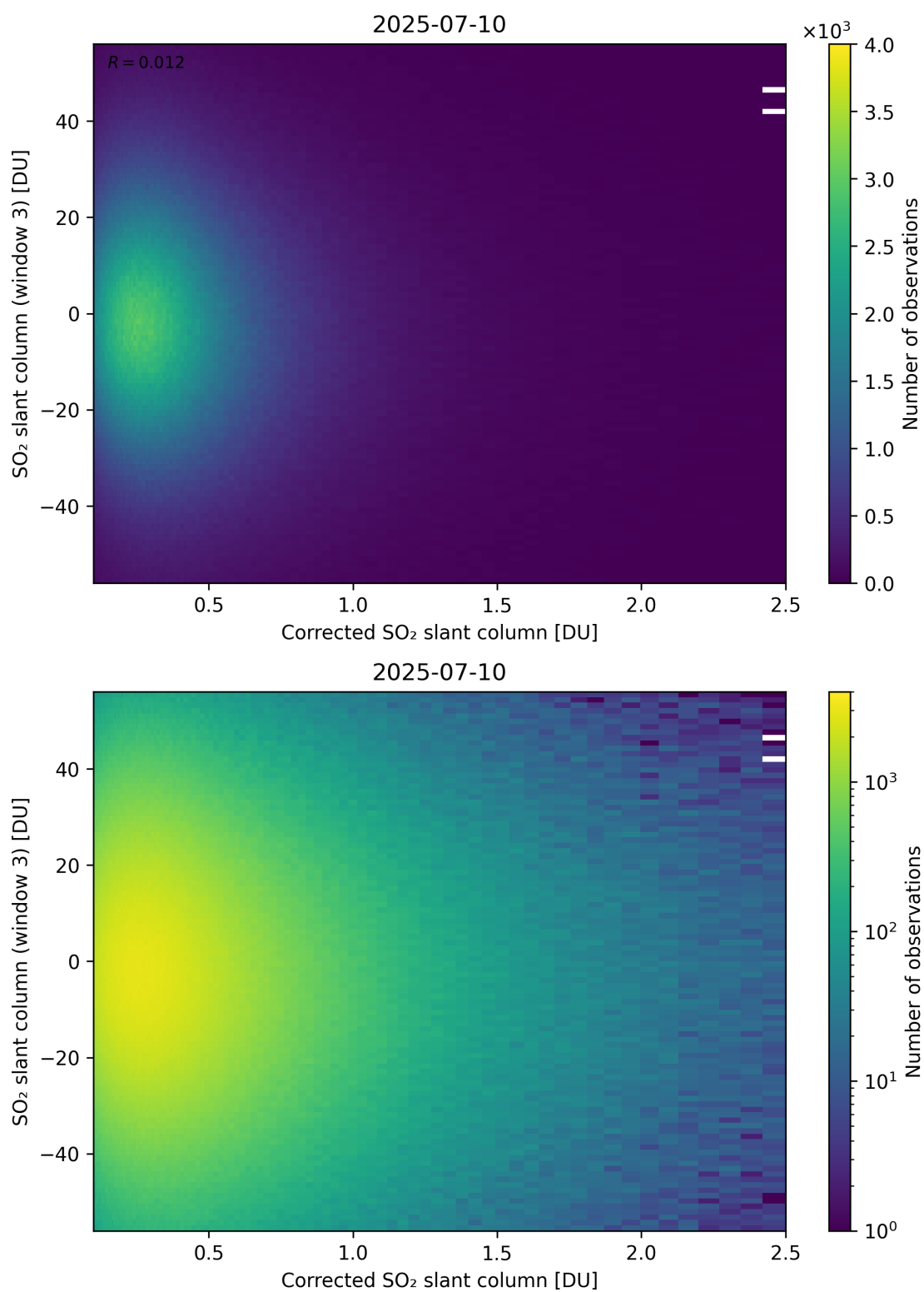
Figure 240: Scatter density plot of “Corrected SO 2 slant column” against “SO 2 slant column (window 3)” for 2025-07-09 to 2025-07-11.
