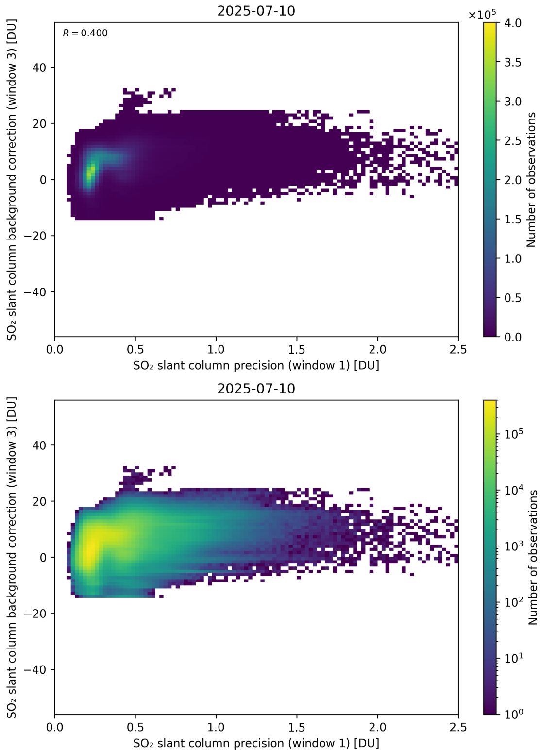
Figure 270: Scatter density plot of “SO 2 slant column precision (window 1)” against “SO 2 slant column background correction (window 3)” for 2025-07-09 to 2025-07-11.
