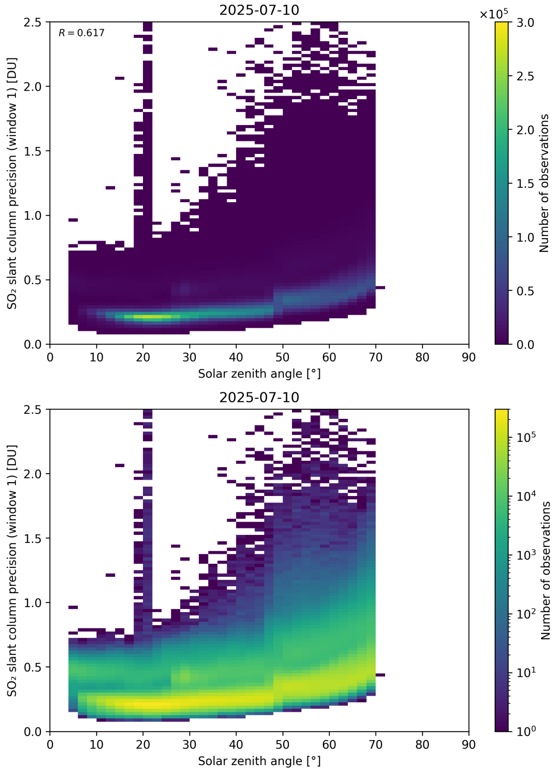
Figure 185: Scatter density plot of “Solar zenith angle” against “SO 2 slant column precision (window 1)” for 2025-07-09 to 2025-07-11.
