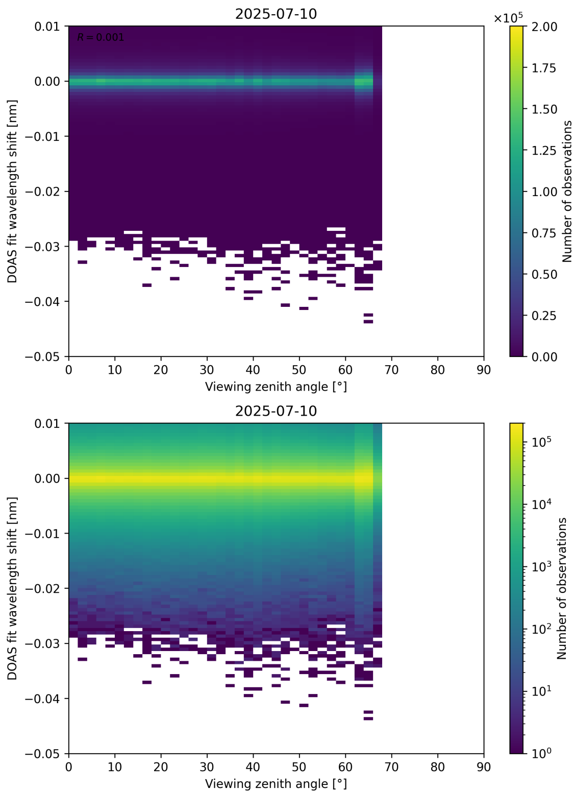
Figure 365: Scatter density plot of “Viewing zenith angle” against “DOAS fit wavelength shift” for 2025-07-09 to 2025-07-11.
