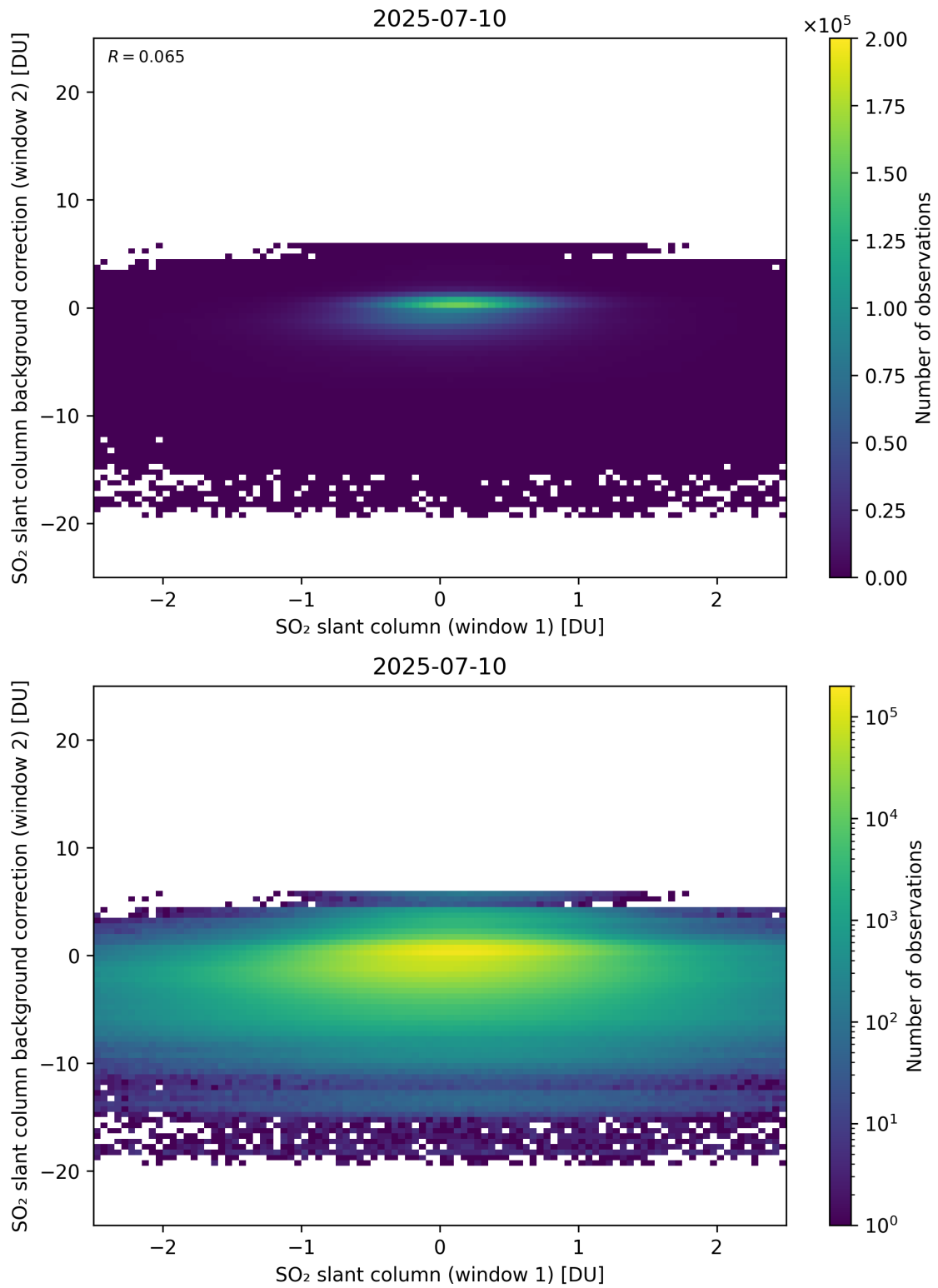
Figure 263: Scatter density plot of “SO 2 slant column (window 1)” against “SO 2 slant column background correction (window 2)” for 2025-07-09 to 2025-07-11.
