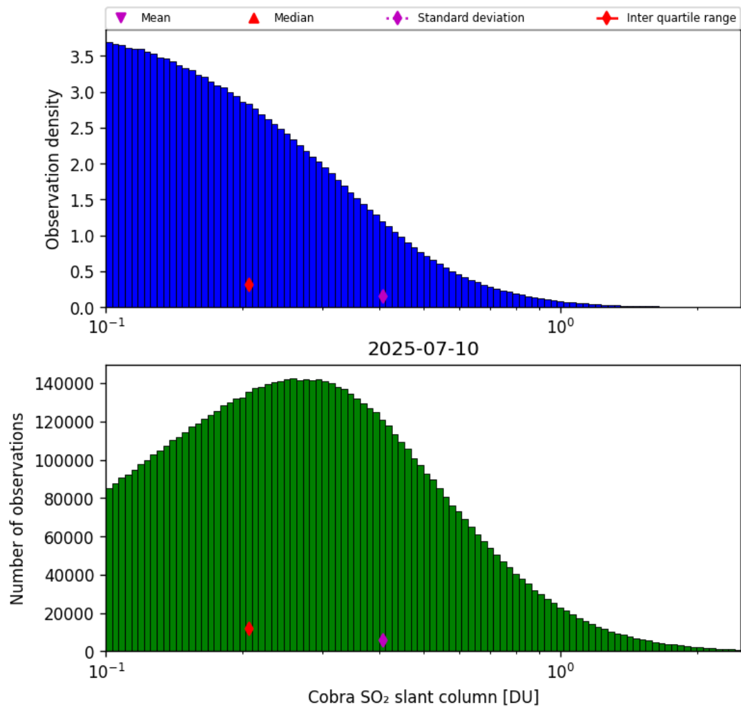
Figure 61: Histogram of “Cobra SO 2 slant column” for 2025-07-09 to 2025-07-11
