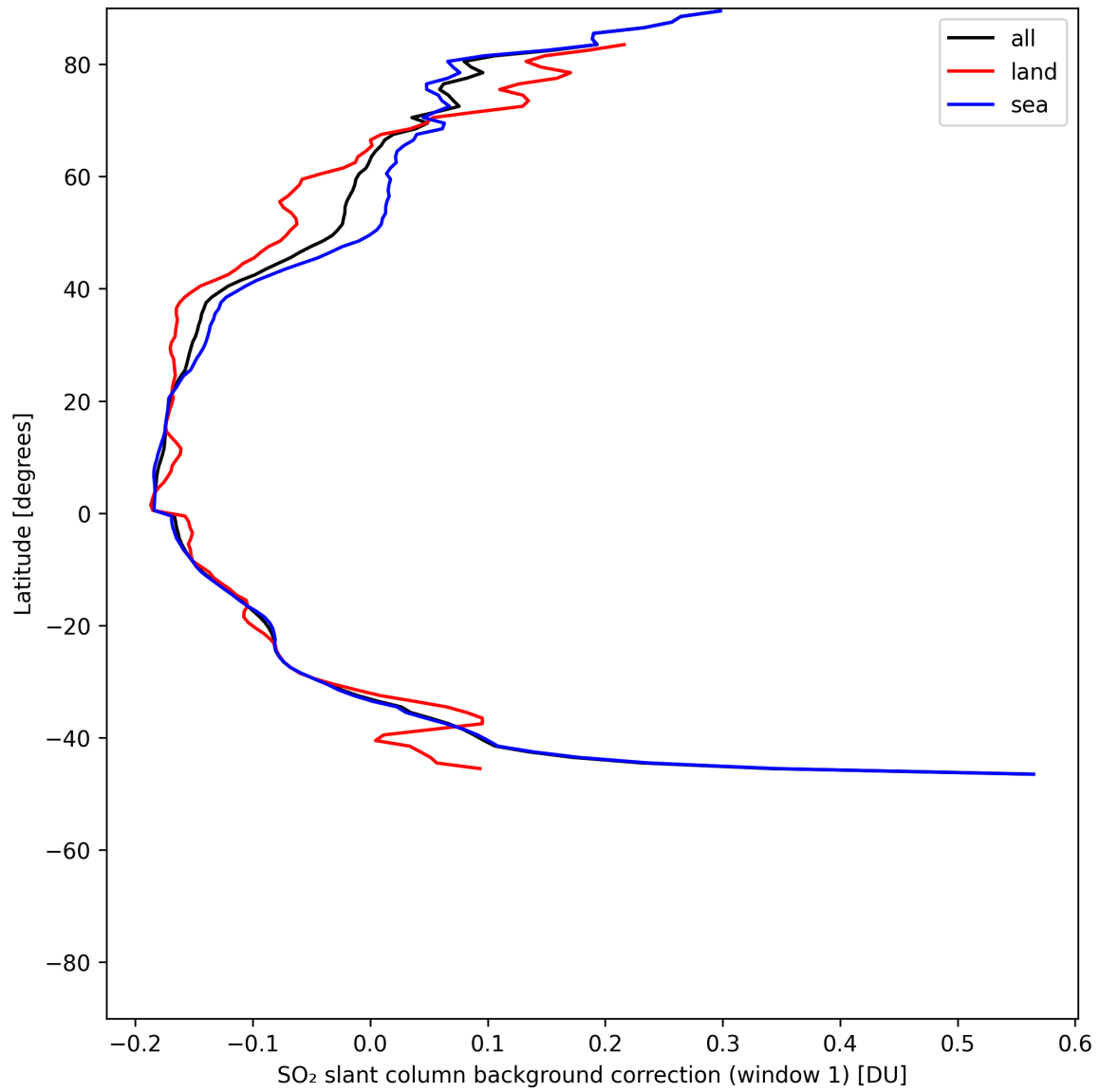
Figure 40: Zonal average of “SO 2 slant column background correction (window 1)” for 2025-07-09 to 2025-07-11.
