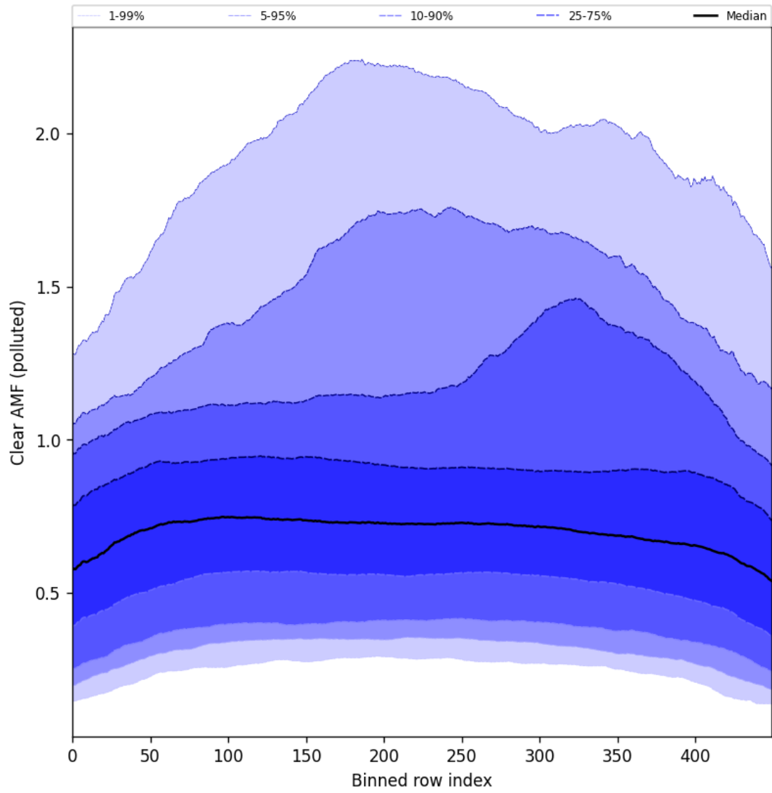
Figure 107: Along track statistics of “Clear AMF (polluted)” for 2025-07-09 to 2025-07-11
