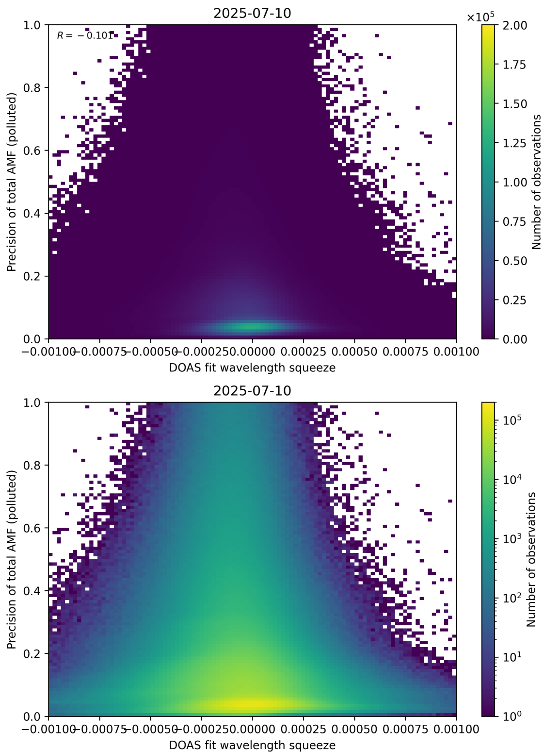
Figure 146: Scatter density plot of “DOAS fit wavelength squeeze” against “Precision of total AMF (polluted)” for 2025-07-09 to 2025-07-11.
