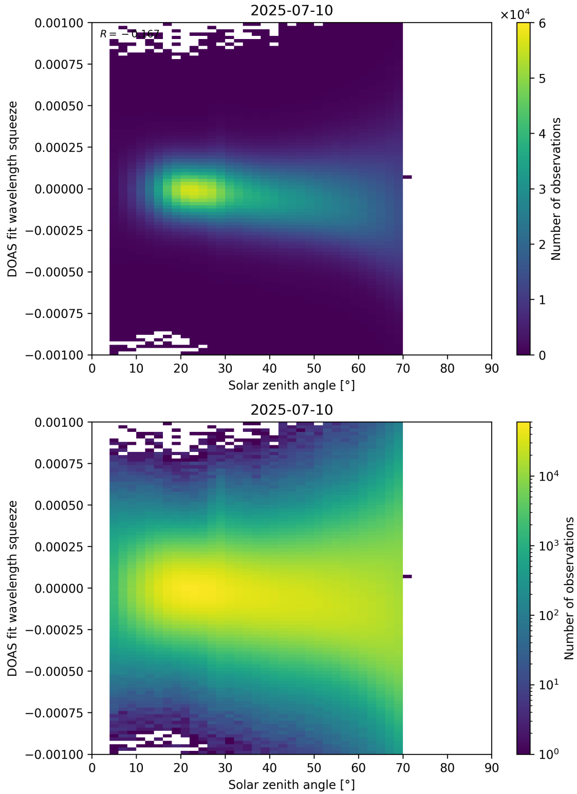
Figure 175: Scatter density plot of “Solar zenith angle” against “DOAS fit wavelength squeeze” for 2025-07-09 to 2025-07-11.
