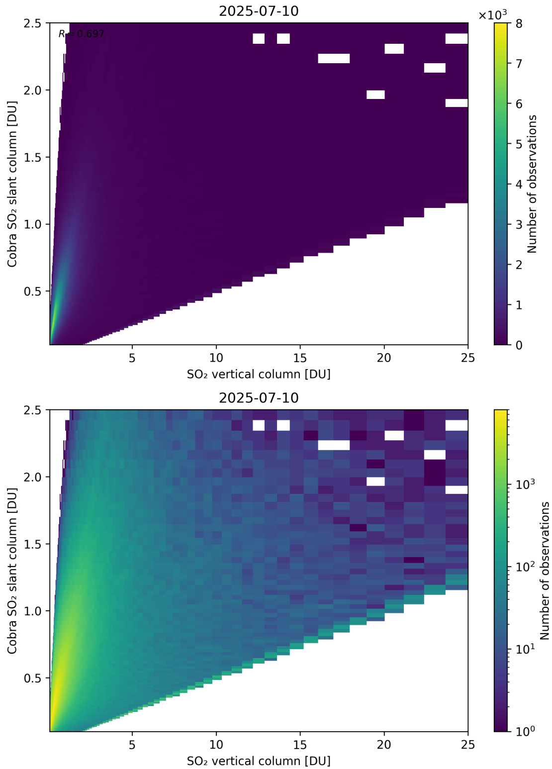
Figure 349: Scatter density plot of “SO 2 vertical column” against “Cobra SO 2 slant column” for 2025-07-09 to 2025-07-11.
