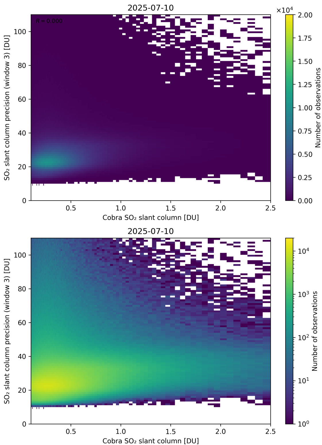
Figure 223: Scatter density plot of “Cobra SO 2 slant column” against “SO 2 slant column precision (window 3)” for 2025-07-09 to 2025-07-11.
