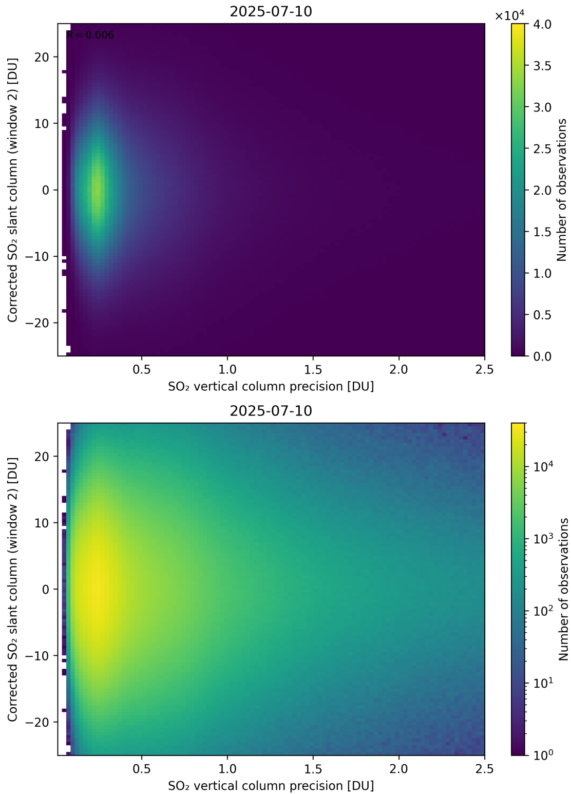
Figure 339: Scatter density plot of “SO 2 vertical column precision” against “Corrected SO 2 slant column (window 2)” for 2025-07-09 to 2025-07-11.
