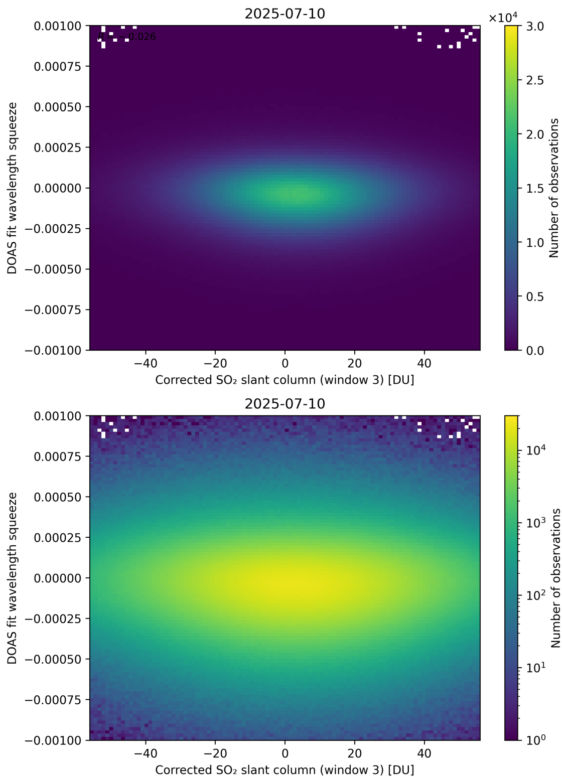
Figure 257: Scatter density plot of “Corrected SO 2 slant column (window 3)” against “DOAS fit wavelength squeeze” for 2025-07-09 to 2025-07-11.
