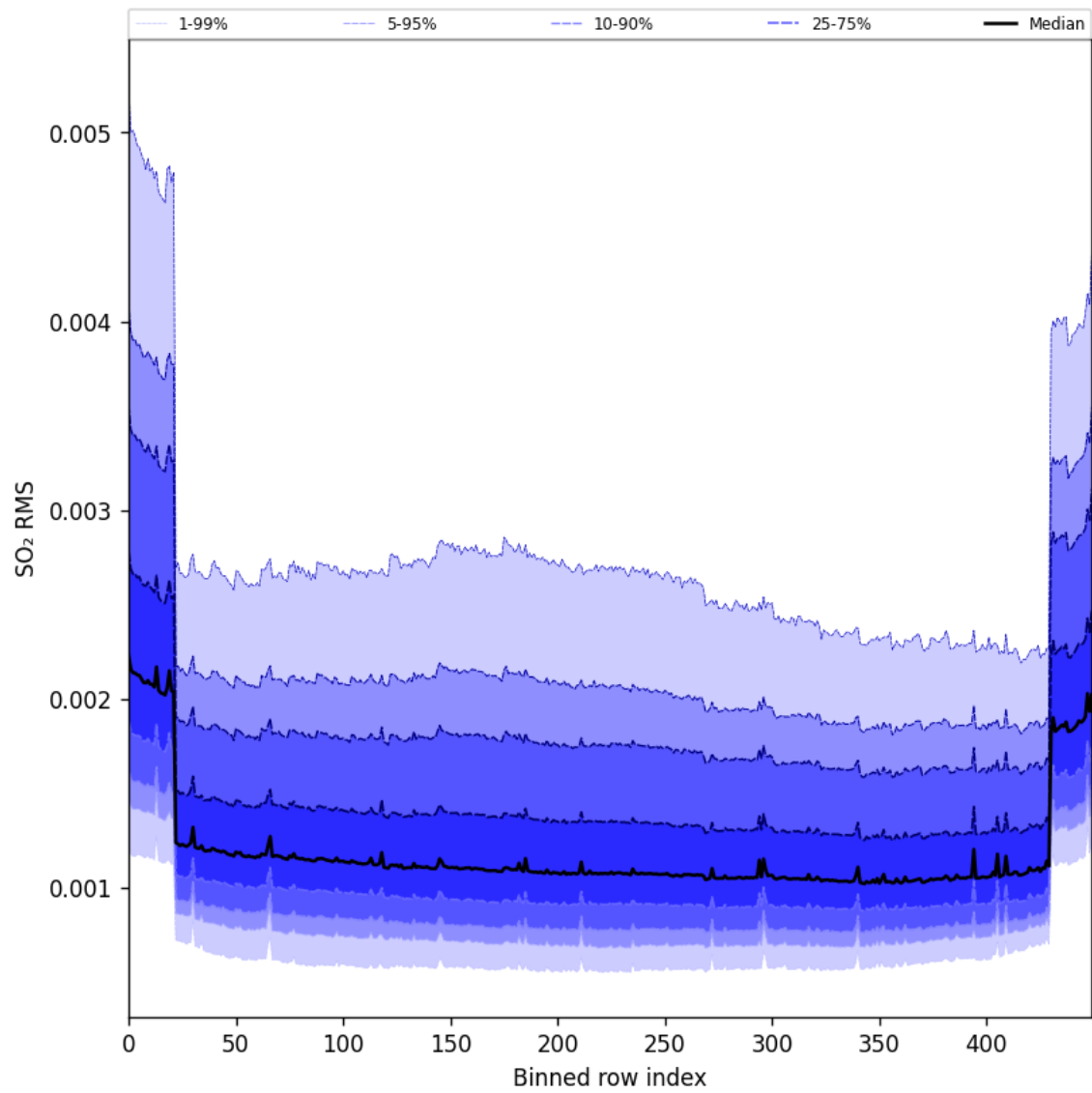
Figure 104: Along track statistics of “SO 2 RMS” for 2025-07-09 to 2025-07-11
