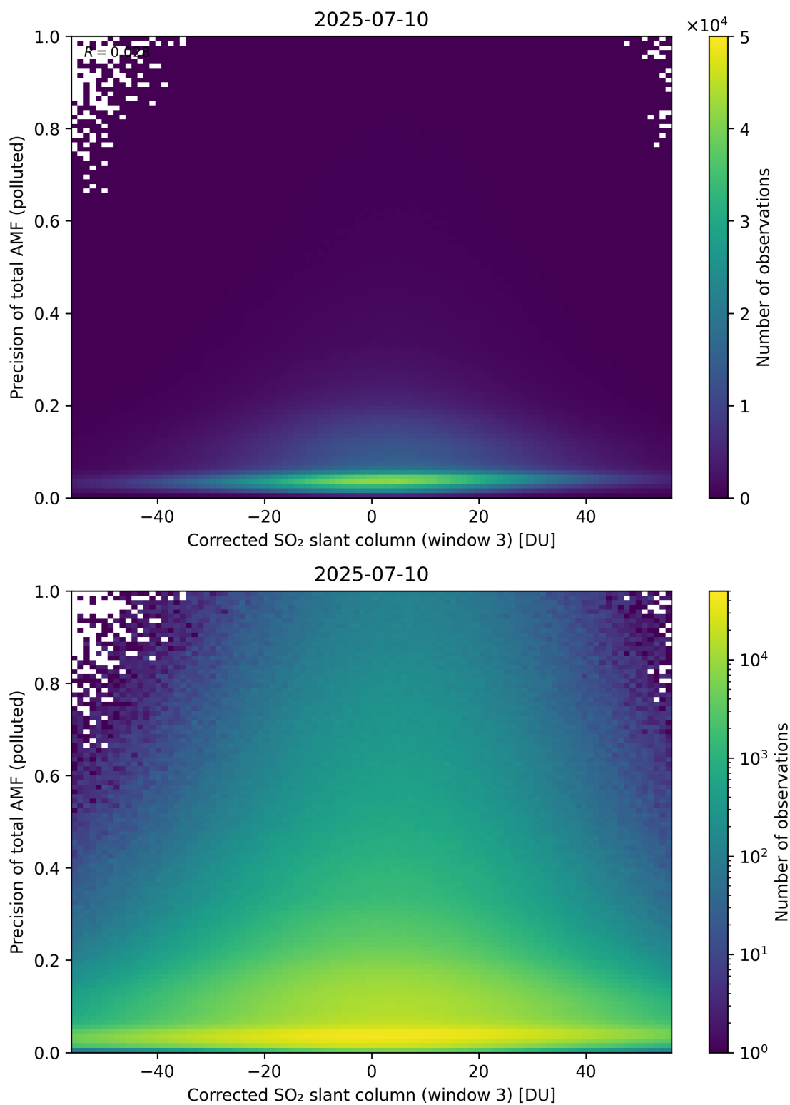
Figure 261: Scatter density plot of “Corrected SO 2 slant column (window 3)” against “Precision of total AMF (polluted)” for 2025-07-09 to 2025-07-11.
