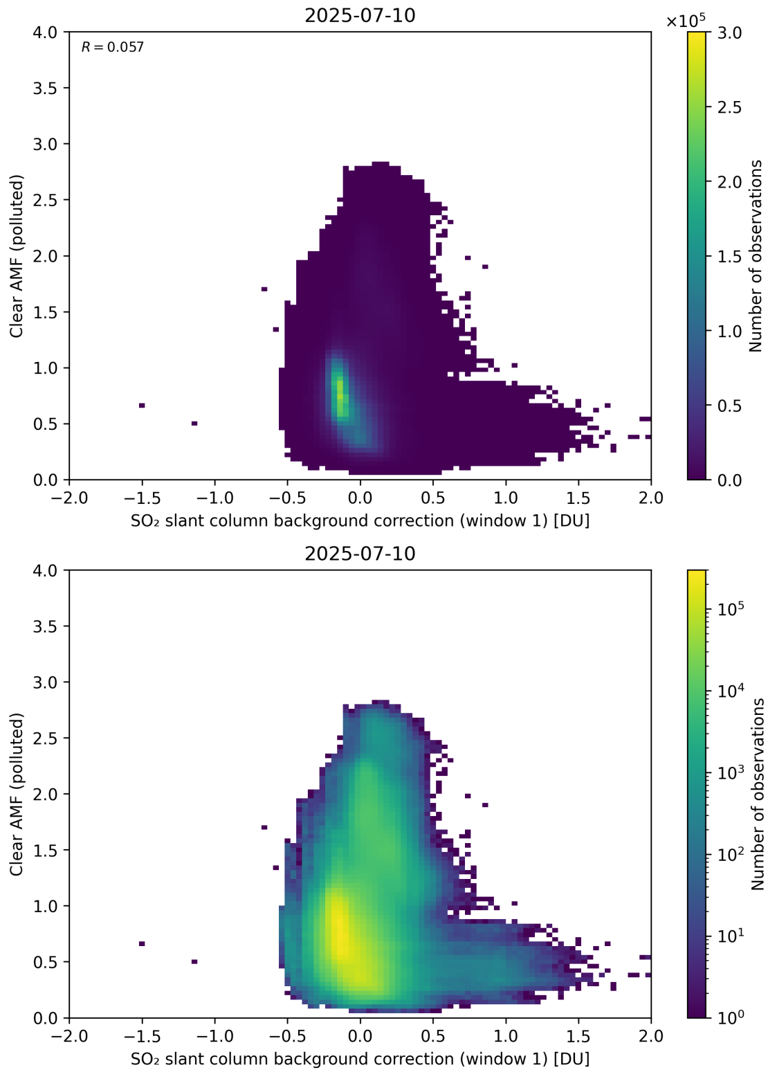
Figure 114: Scatter density plot of “SO 2 slant column background correction (window 1)” against “Clear AMF (polluted)” for 2025-07-09 to 2025-07-11.
