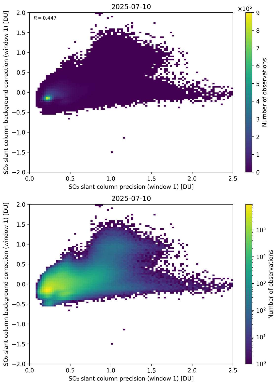
Figure 268: Scatter density plot of “SO 2 slant column precision (window 1)” against “SO 2 slant column background correction (window 1)” for 2025-07-09 to 2025-07-11.
