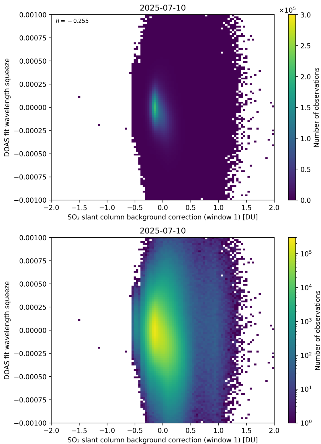
Figure 112: Scatter density plot of “SO 2 slant column background correction (window 1)” against “DOAS fit wavelength squeeze” for 2025-07-09 to 2025-07-11.
