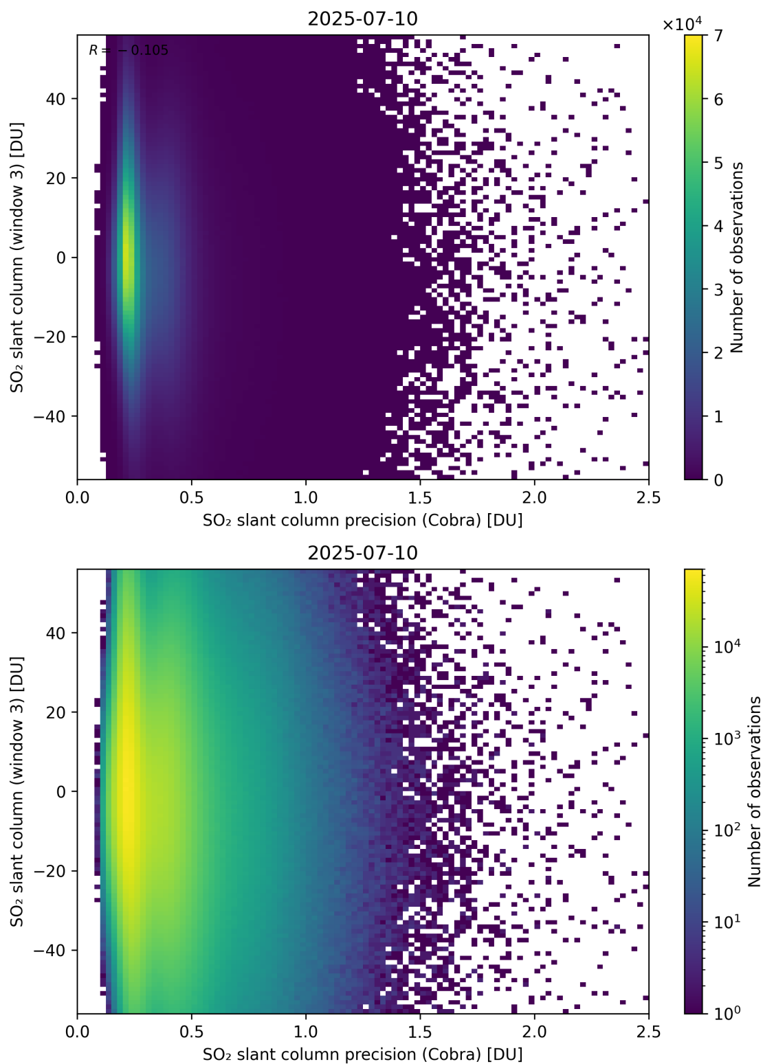
Figure 211: Scatter density plot of “SO 2 slant column precision (Cobra)” against “SO 2 slant column (window 3)” for 2025-07-09 to 2025-07-11.
