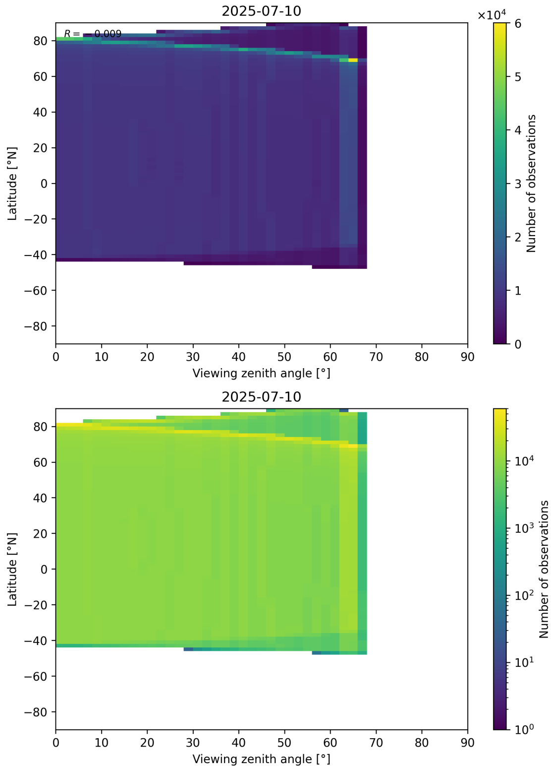
Figure 368: Scatter density plot of “Viewing zenith angle” against “Latitude” for 2025-07-09 to 2025-07-11.
