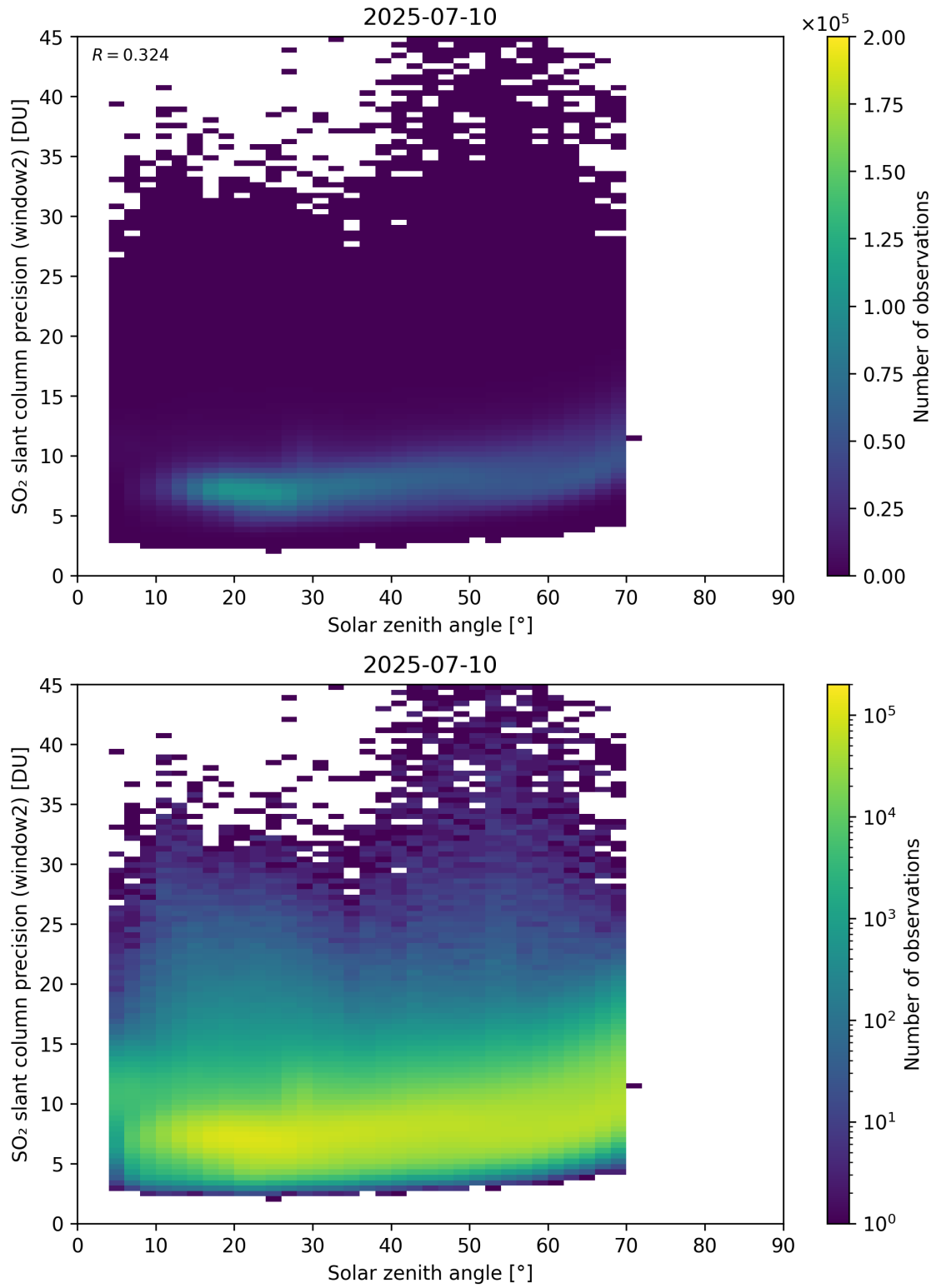
Figure 186: Scatter density plot of “Solar zenith angle” against “SO 2 slant column precision (window2)” for 2025-07-09 to 2025-07-11.
