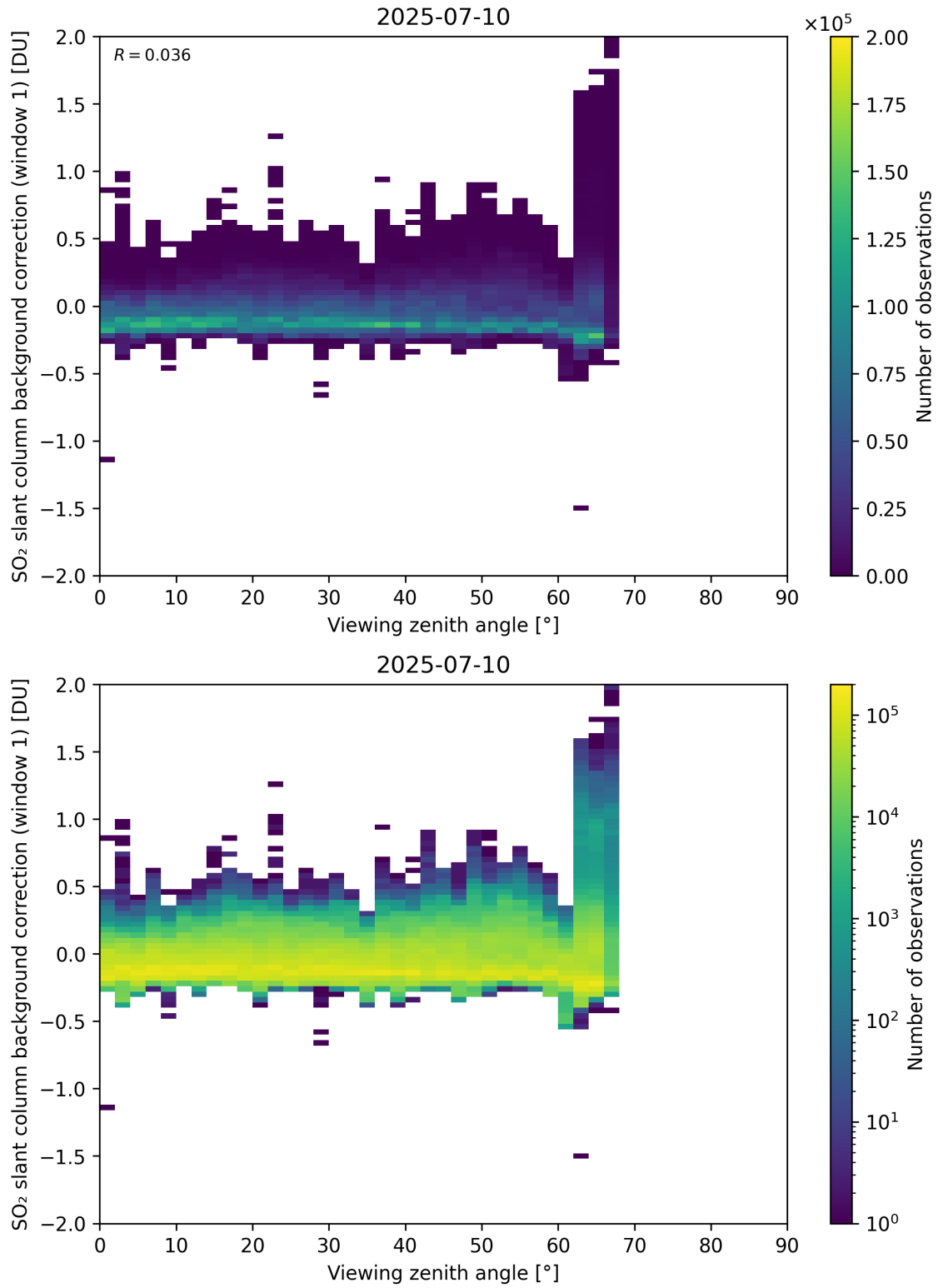
Figure 362: Scatter density plot of “Viewing zenith angle” against “SO 2 slant column background correction (window 1)” for 2025-07-09 to 2025-07-11.
