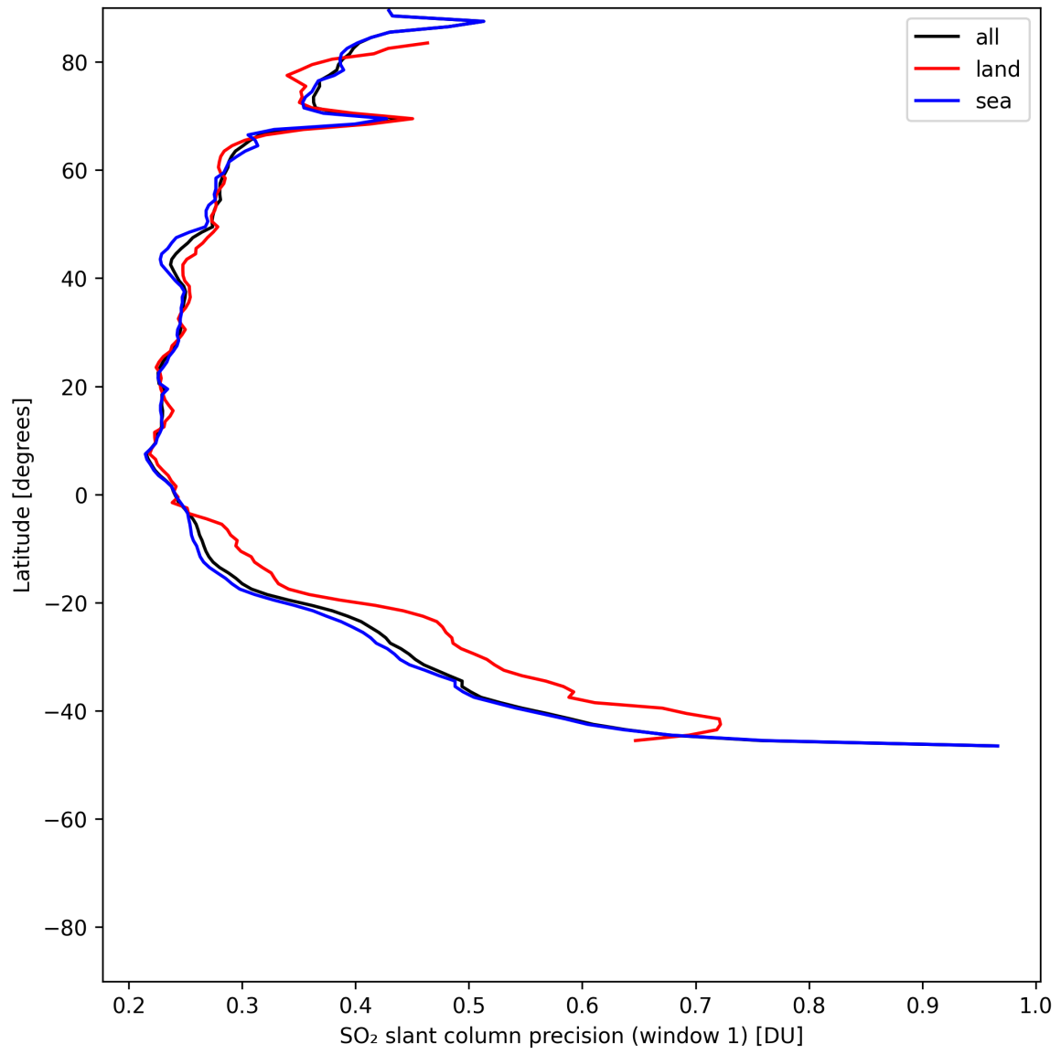
Figure 38: Zonal average of “SO 2 slant column precision (window 1)” for 2025-07-09 to 2025-07-11.
