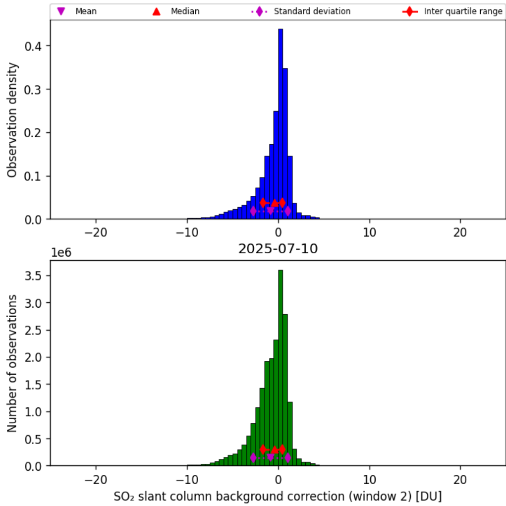
Figure 70: Histogram of “SO 2 slant column background correction (window 2)” for 2025-07-09 to 2025-07-11
