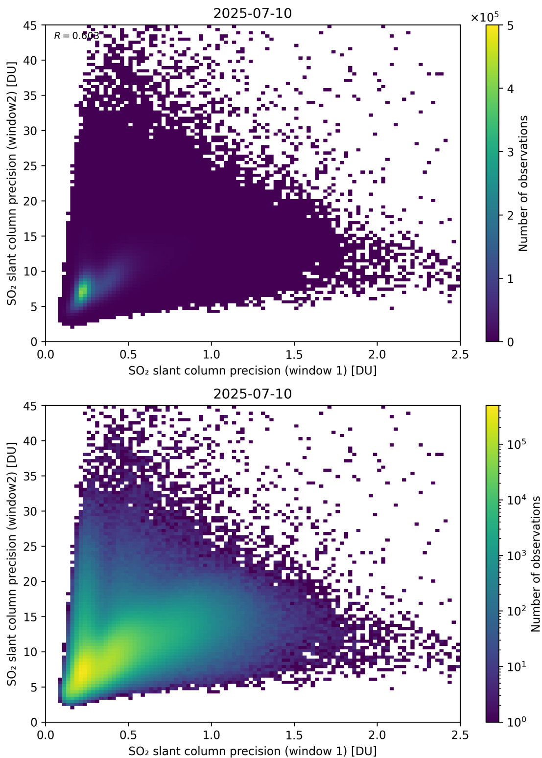
Figure 277: Scatter density plot of “SO 2 slant column precision (window 1)” against “SO 2 slant column precision (window2)” for 2025-07-09 to 2025-07-11.
