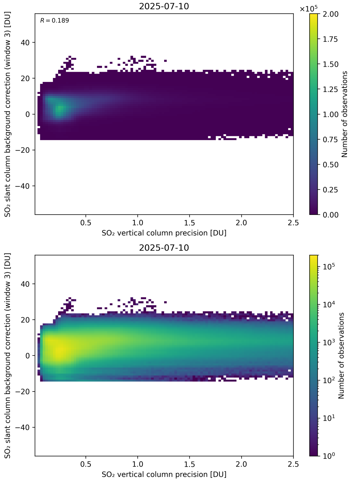
Figure 331: Scatter density plot of “SO 2 vertical column precision” against “SO 2 slant column background correction (window 3)” for 2025-07-09 to 2025-07-11.
