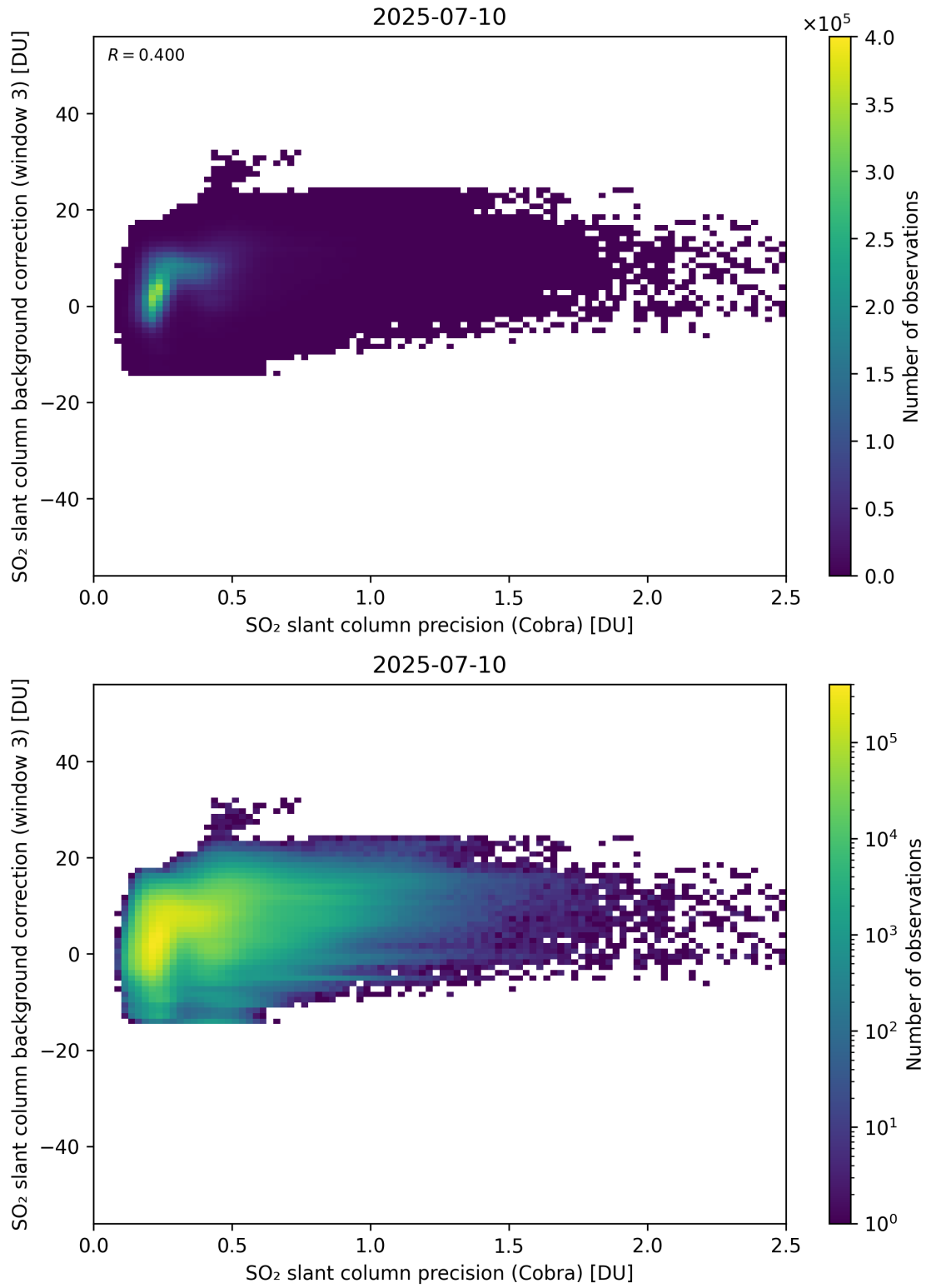
Figure 201: Scatter density plot of “SO 2 slant column precision (Cobra)” against “SO 2 slant column background correction (window 3)” for 2025-07-09 to 2025-07-11.
