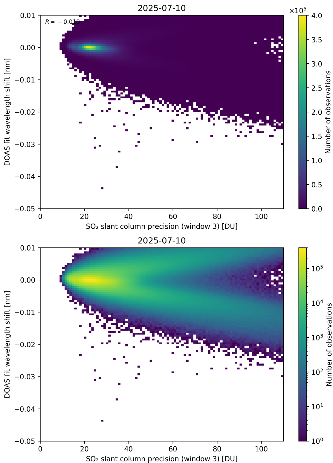
Figure 308: Scatter density plot of “SO 2 slant column precision (window 3)” against “DOAS fit wavelength shift” for 2025-07-09 to 2025-07-11.
