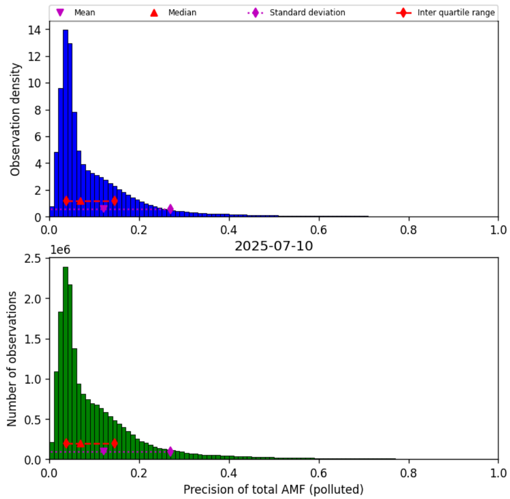
Figure 80: Histogram of “Precision of total AMF (polluted)” for 2025-07-09 to 2025-07-11
