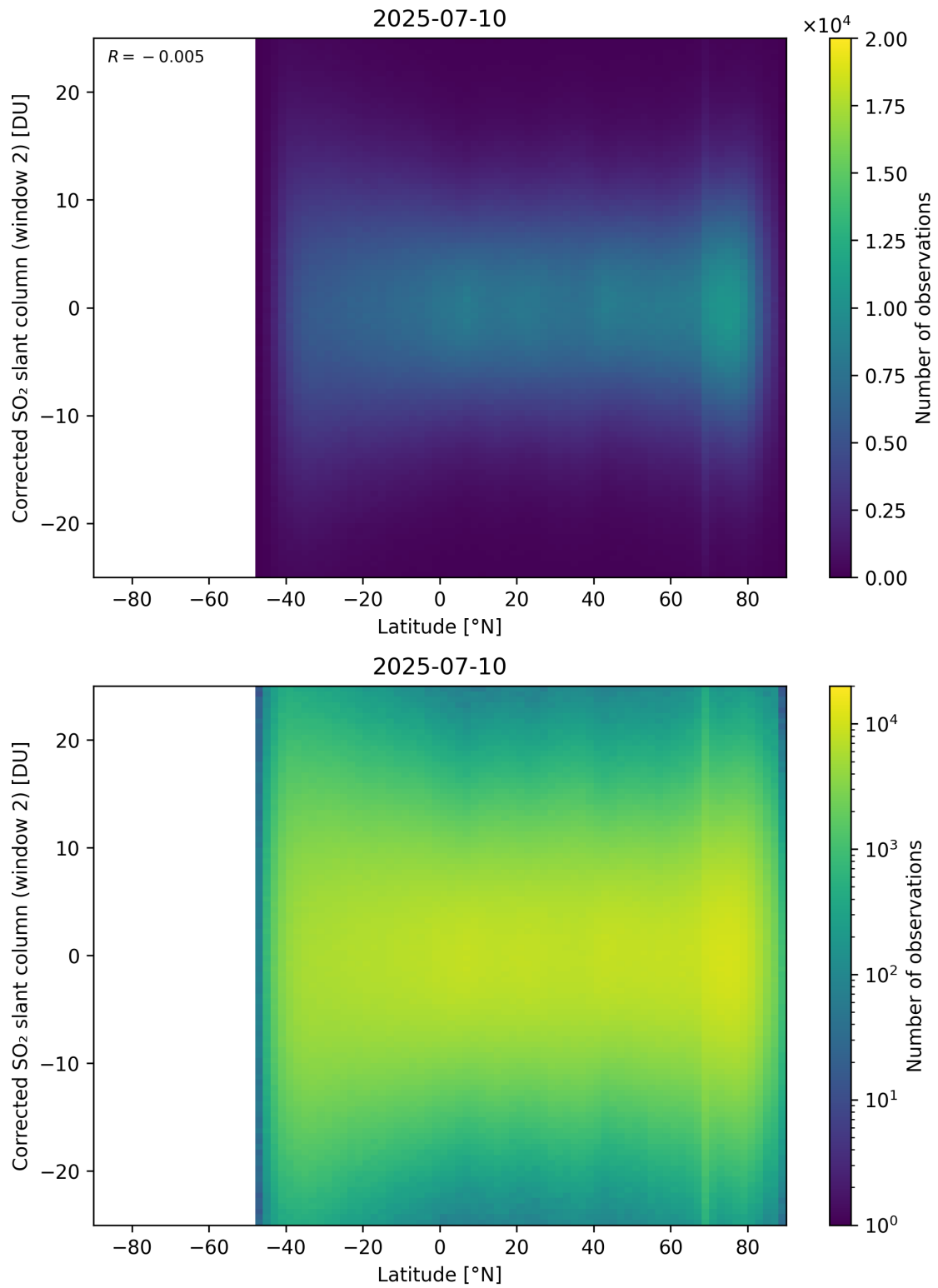
Figure 160: Scatter density plot of “Latitude” against “Corrected SO 2 slant column (window 2)” for 2025-07-09 to 2025-07-11.
