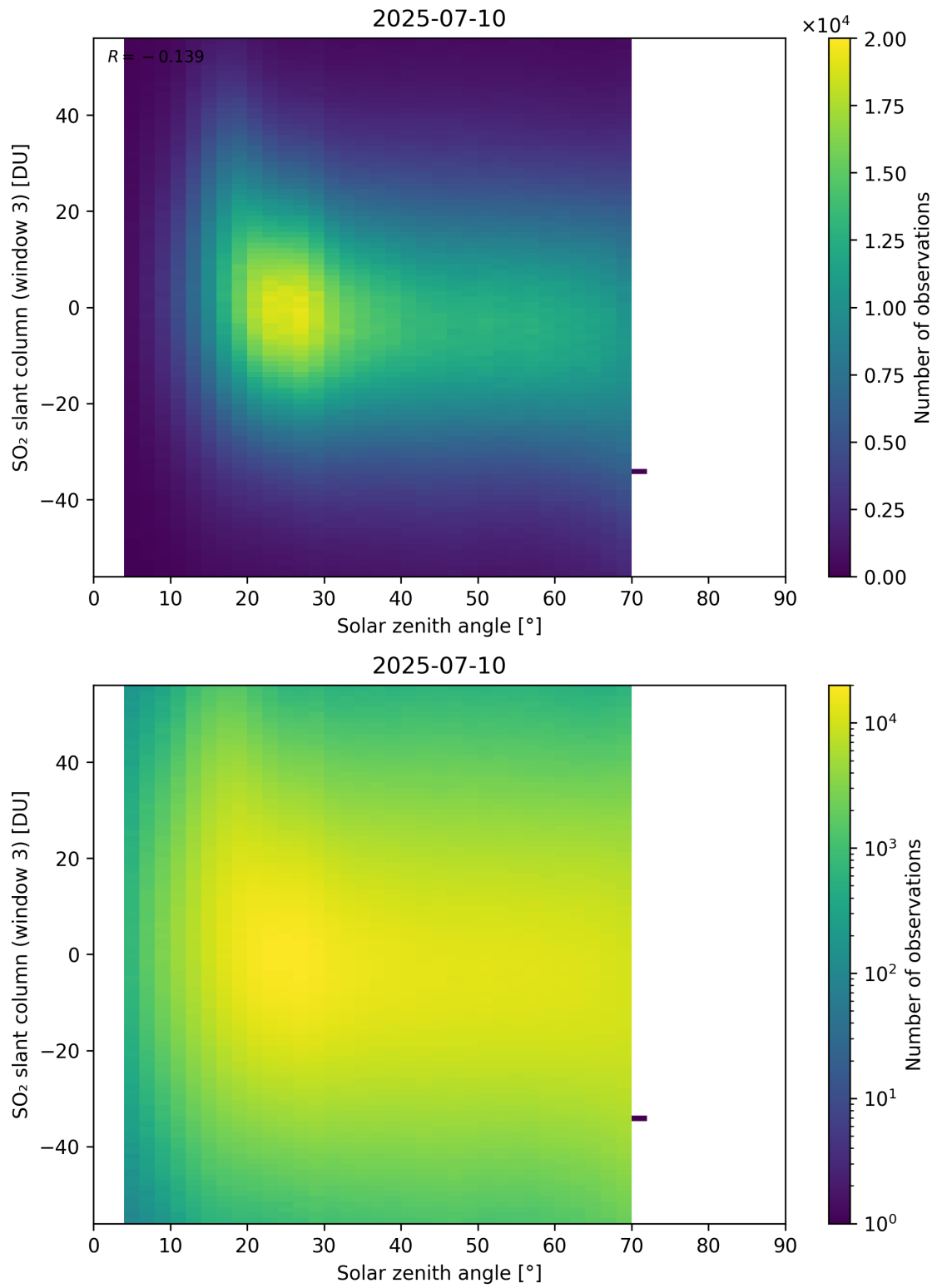
Figure 187: Scatter density plot of “Solar zenith angle” against “SO 2 slant column (window 3)” for 2025-07-09 to 2025-07-11.
