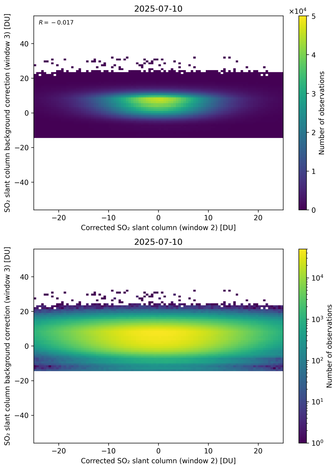
Figure 245: Scatter density plot of “Corrected SO 2 slant column (window 2)” against “SO 2 slant column background correction (window 3)” for 2025-07-09 to 2025-07-11.
