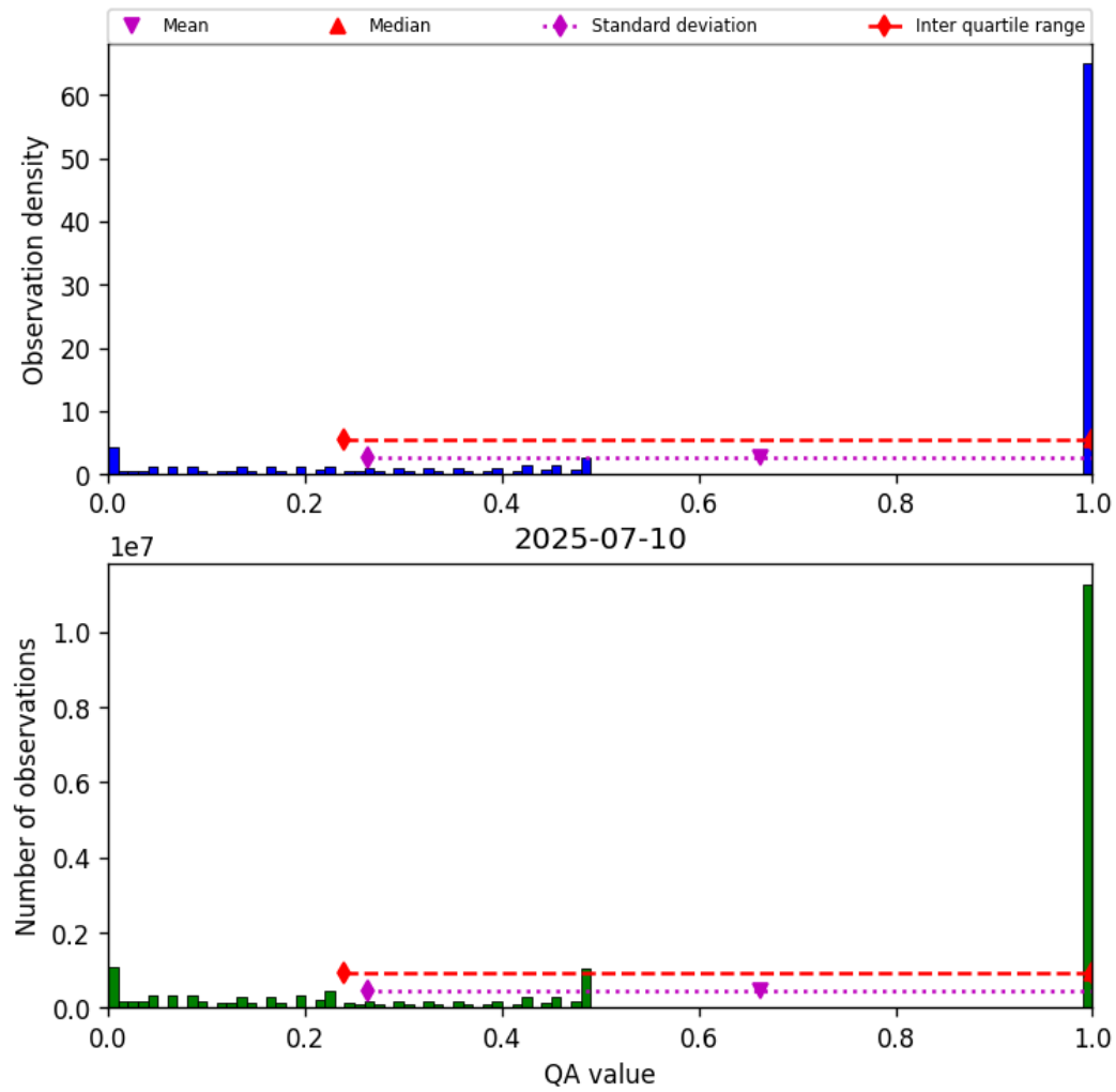
Figure 57: Histogram of “QA value” for 2025-07-09 to 2025-07-11
