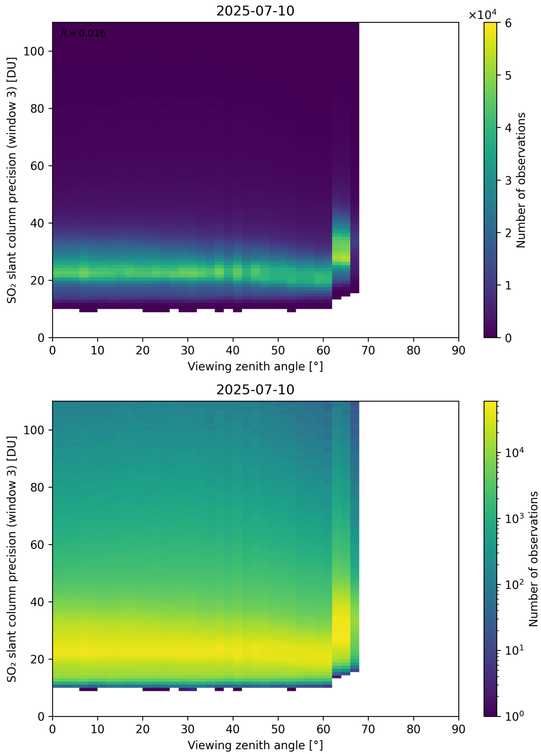
Figure 380: Scatter density plot of “Viewing zenith angle” against “SO 2 slant column precision (window 3)” for 2025-07-09 to 2025-07-11.
