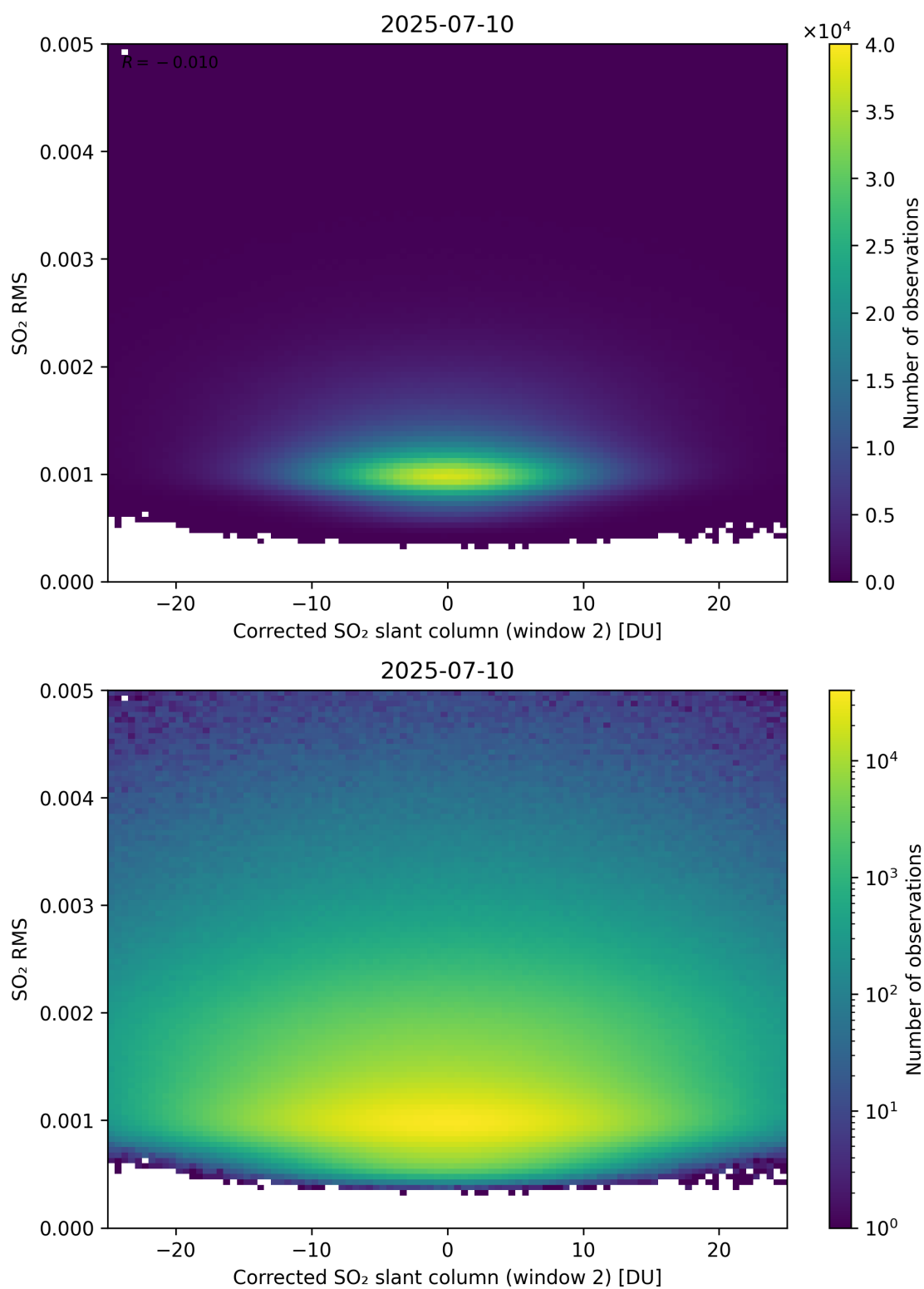
Figure 248: Scatter density plot of “Corrected SO 2 slant column (window 2)” against “SO 2 RMS” for 2025-07-09 to 2025-07-11.
