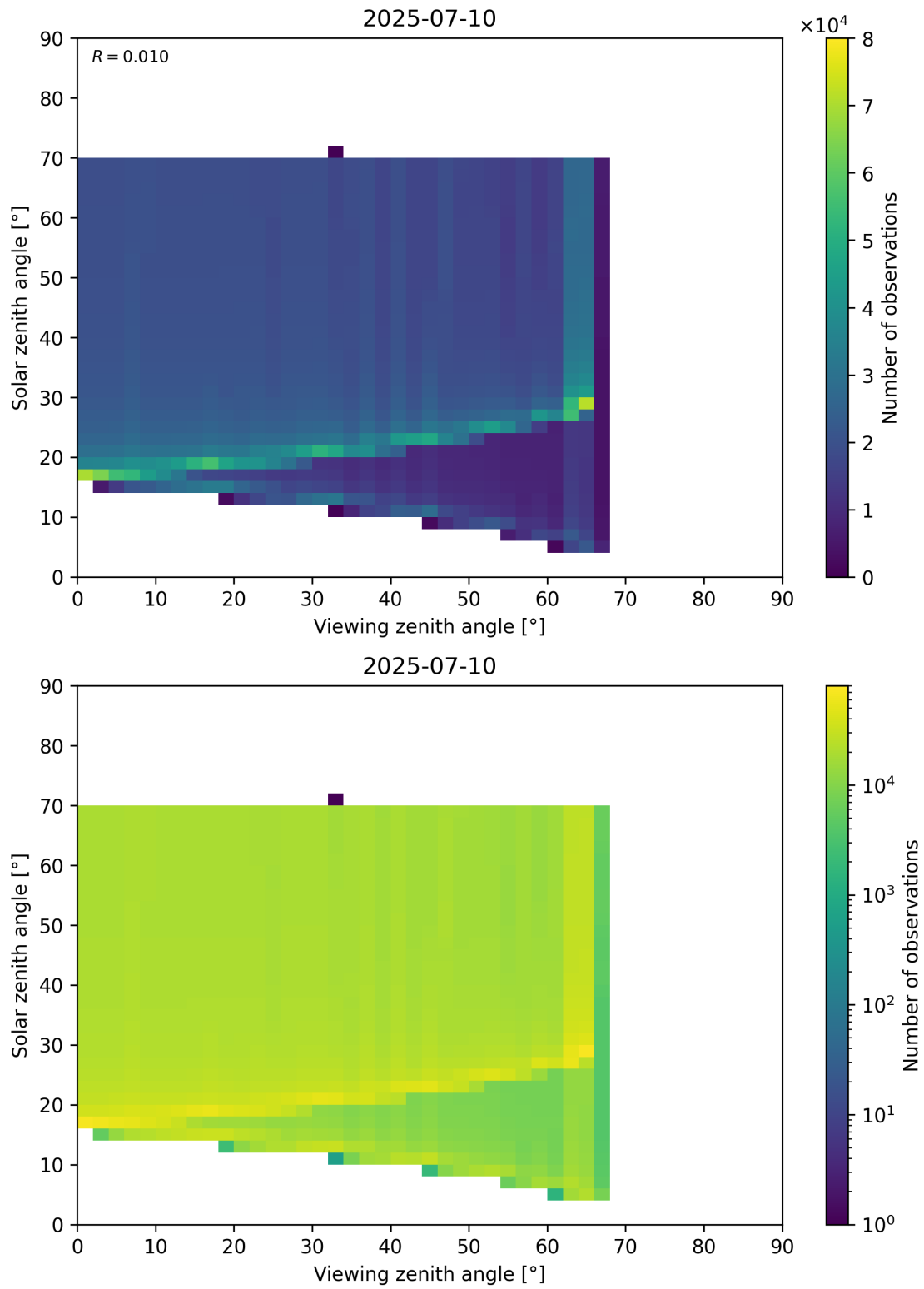
Figure 369: Scatter density plot of “Viewing zenith angle” against “Solar zenith angle” for 2025-07-09 to 2025-07-11.
