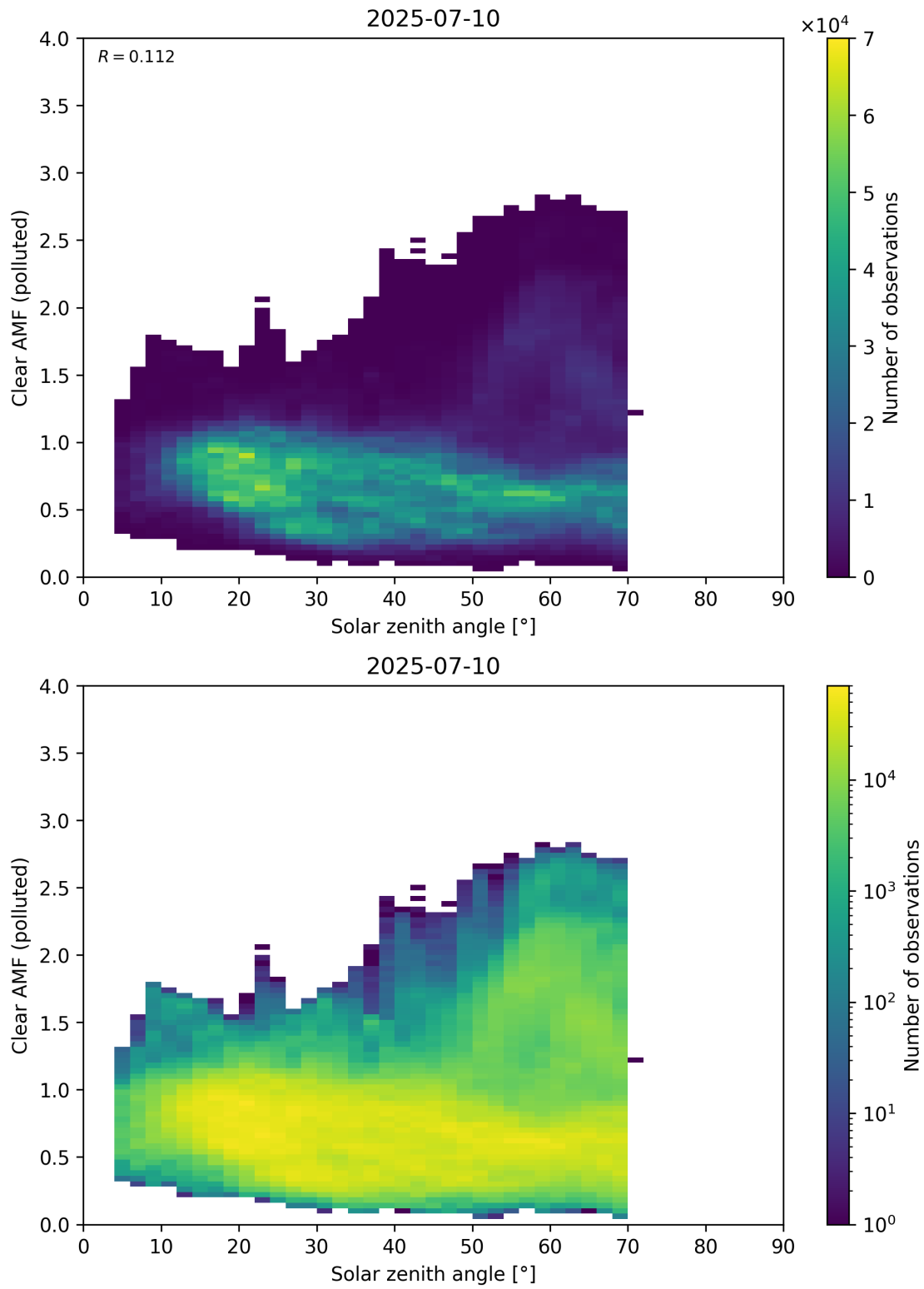
Figure 178: Scatter density plot of “Solar zenith angle” against “Clear AMF (polluted)” for 2025-07-09 to 2025-07-11.
