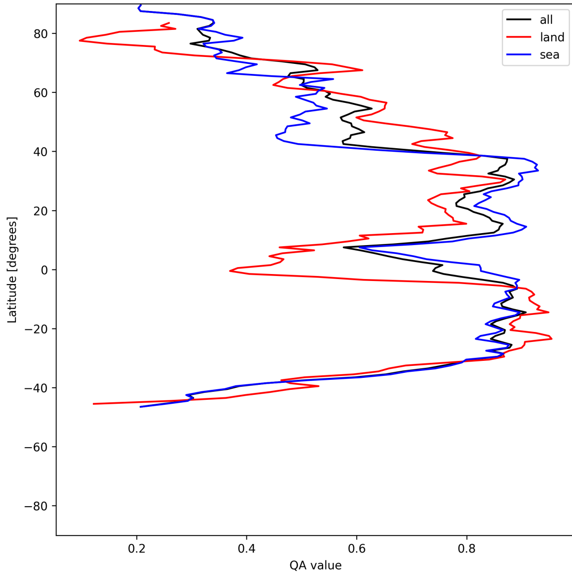
Figure 31: Zonal average of “QA value” for 2025-07-09 to 2025-07-11.
