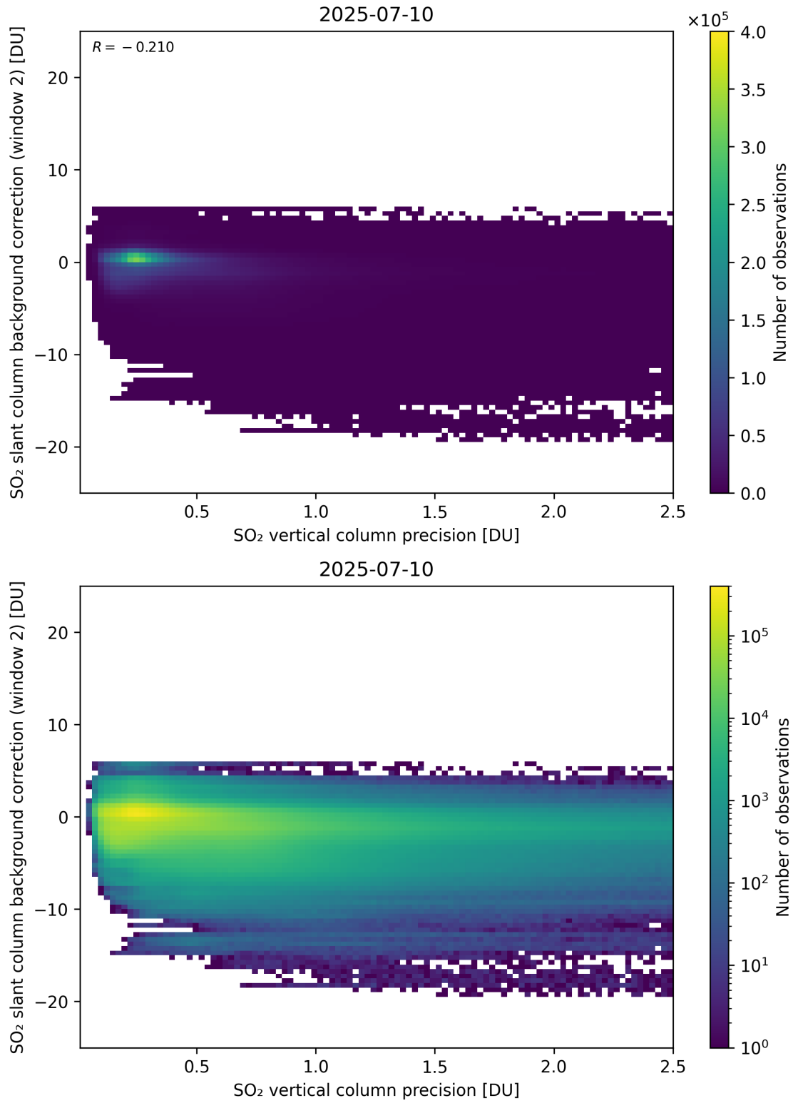
Figure 330: Scatter density plot of “SO 2 vertical column precision” against “SO 2 slant column background correction (window 2)” for 2025-07-09 to 2025-07-11.
