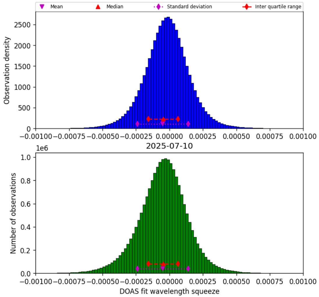
Figure 77: Histogram of “DOAS fit wavelength squeeze” for 2025-07-09 to 2025-07-11
