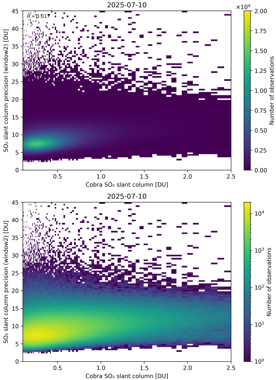
Figure 221: Scatter density plot of “Cobra SO 2 slant column” against “SO 2 slant column precision (window2)” for 2025-07-09 to 2025-07-11.
