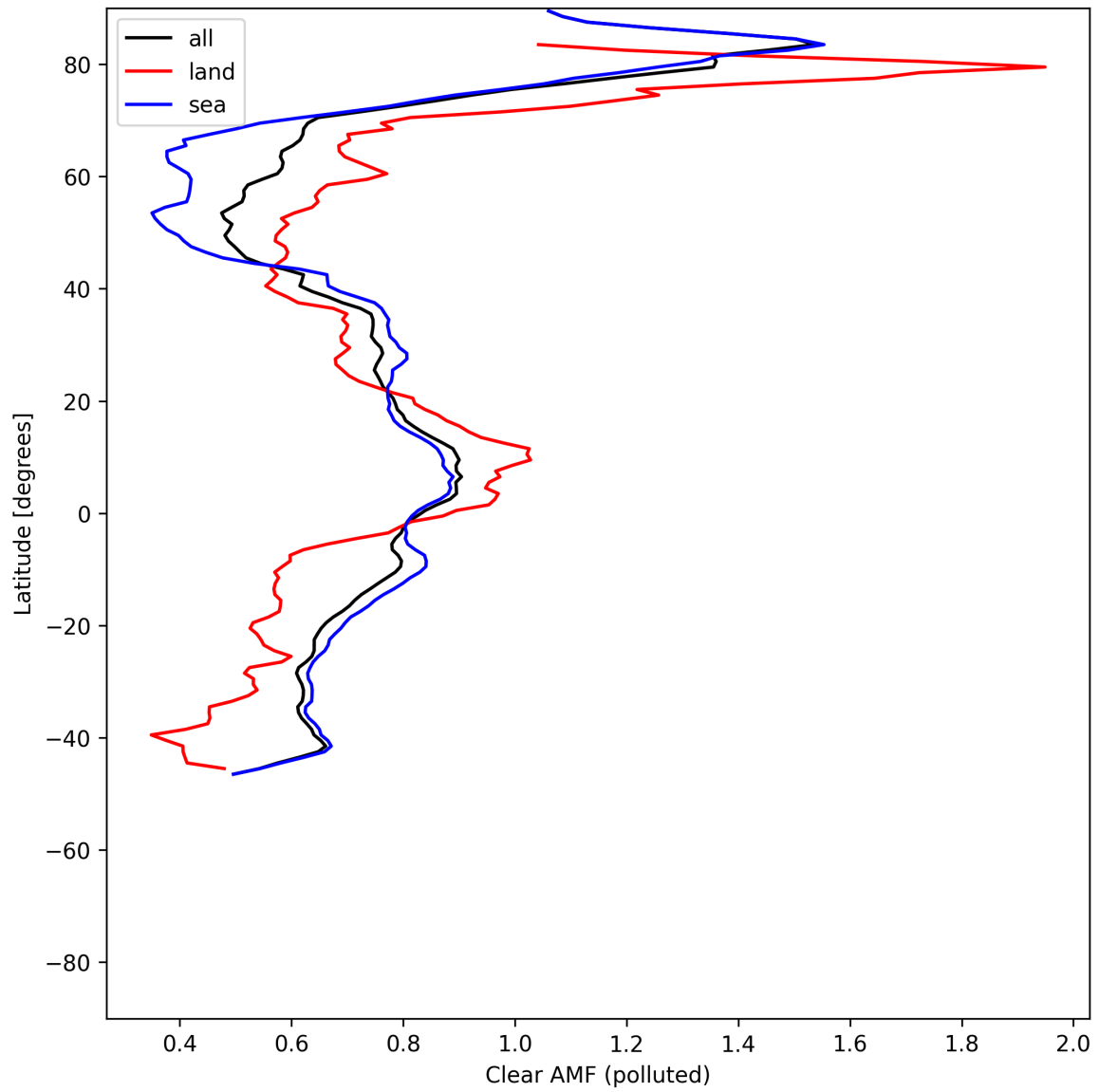
Figure 55: Zonal average of “Clear AMF (polluted)” for 2025-07-09 to 2025-07-11.
