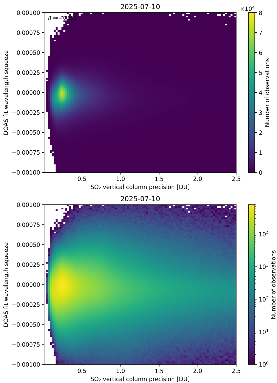
Figure 333: Scatter density plot of “SO 2 vertical column precision” against “DOAS fit wavelength squeeze” for 2025-07-09 to 2025-07-11.
