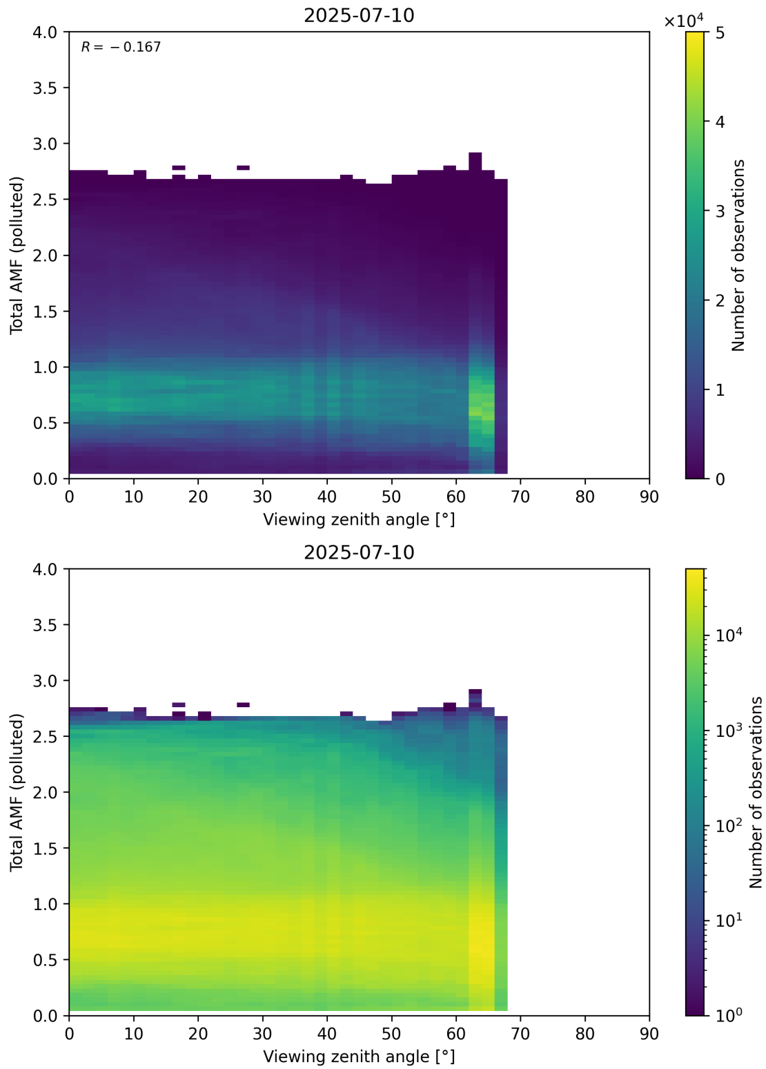
Figure 381: Scatter density plot of “Viewing zenith angle” against “Total AMF (polluted)” for 2025-07-09 to 2025-07-11.
