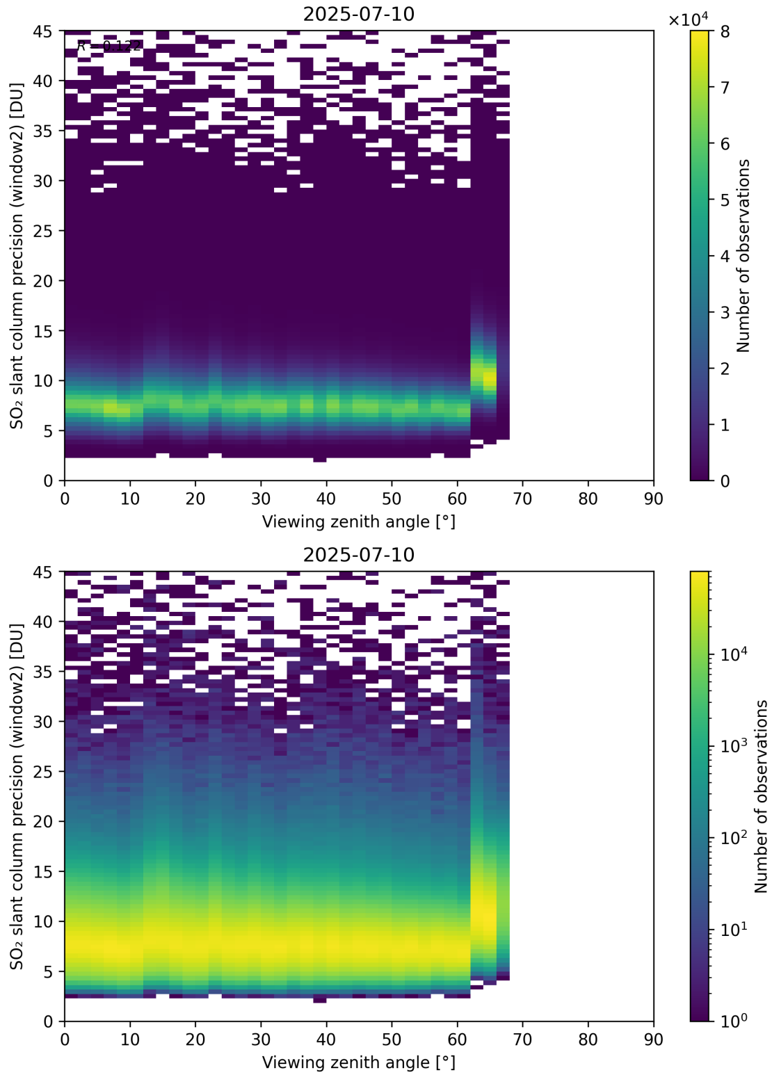
Figure 378: Scatter density plot of “Viewing zenith angle” against “SO 2 slant column precision (window2)” for 2025-07-09 to 2025-07-11.
