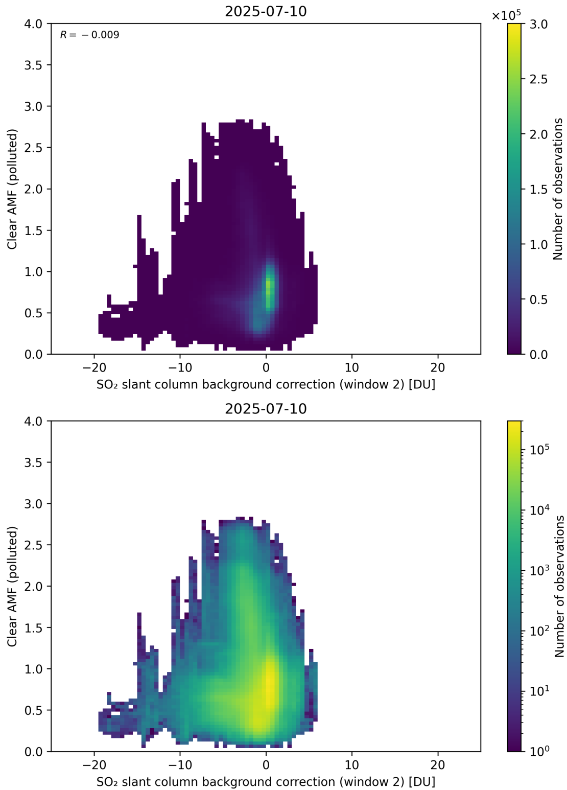
Figure 126: Scatter density plot of “SO 2 slant column background correction (window 2)” against “Clear AMF (polluted)” for 2025-07-09 to 2025-07-11.
