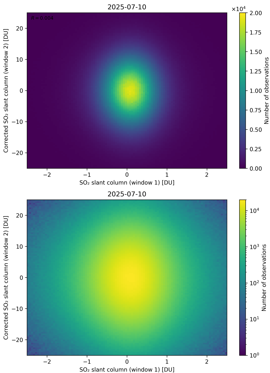
Figure 283: Scatter density plot of “SO 2 slant column (window 1)” against “Corrected SO 2 slant column (window 2)” for 2025-07-09 to 2025-07-11.
