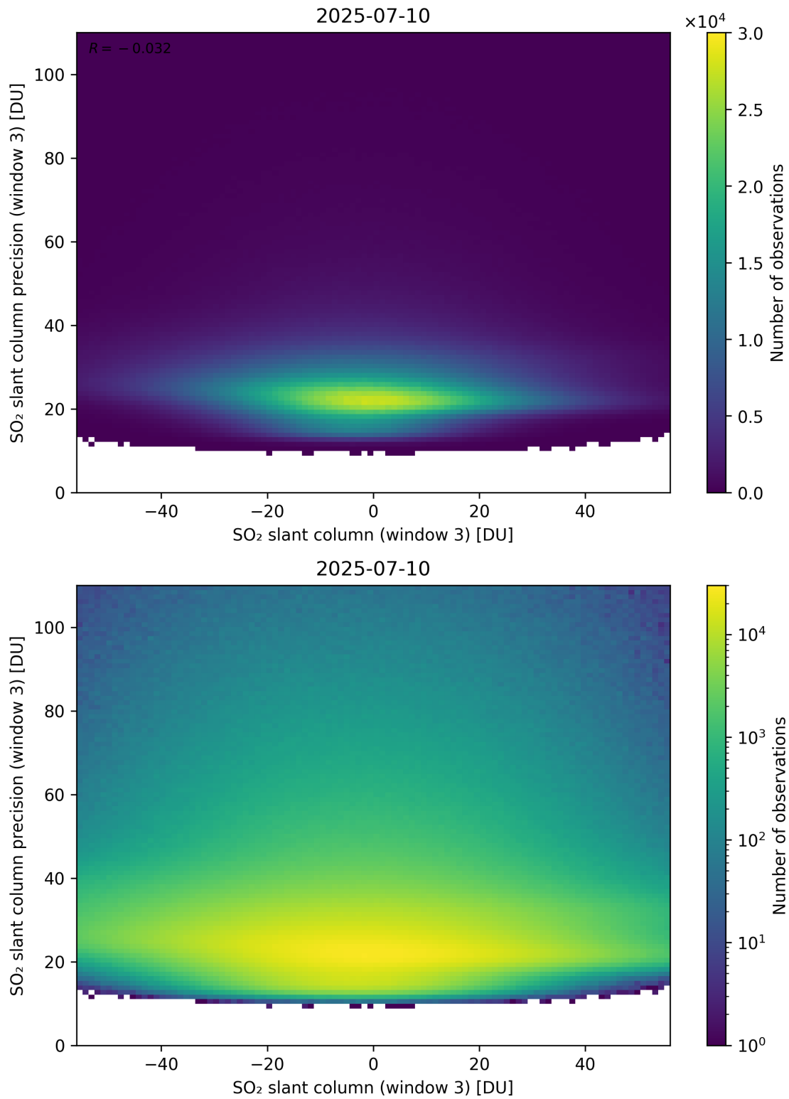
Figure 317: Scatter density plot of “SO 2 slant column (window 3)” against “SO 2 slant column precision (window 3)” for 2025-07-09 to 2025-07-11.
