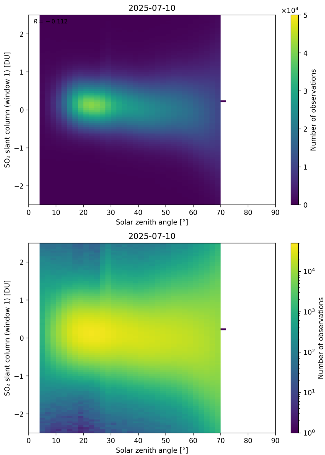
Figure 184: Scatter density plot of “Solar zenith angle” against “SO 2 slant column (window 1)” for 2025-07-09 to 2025-07-11.
