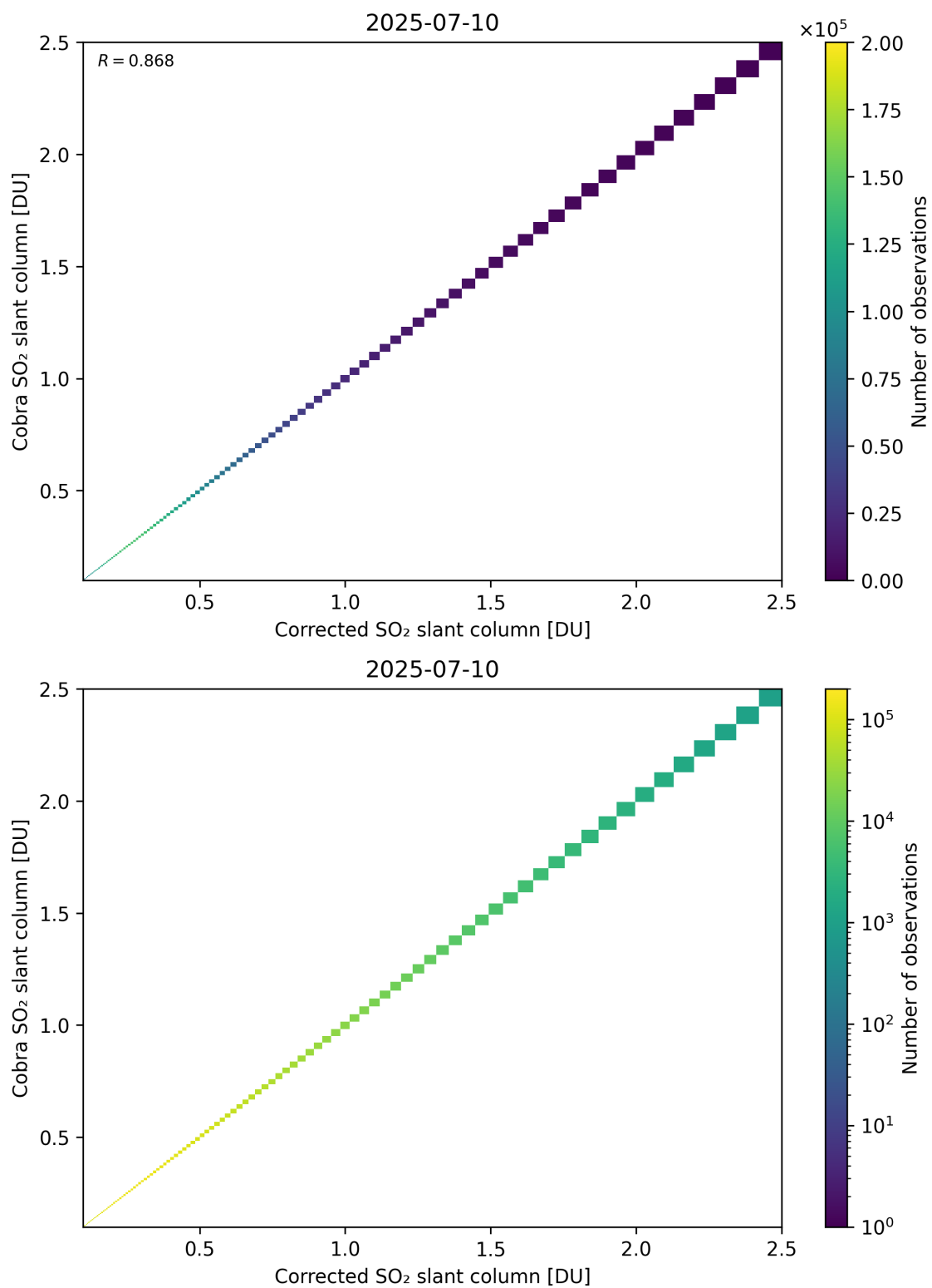
Figure 233: Scatter density plot of “Corrected SO 2 slant column” against “Cobra SO 2 slant column” for 2025-07-09 to 2025-07-11.
