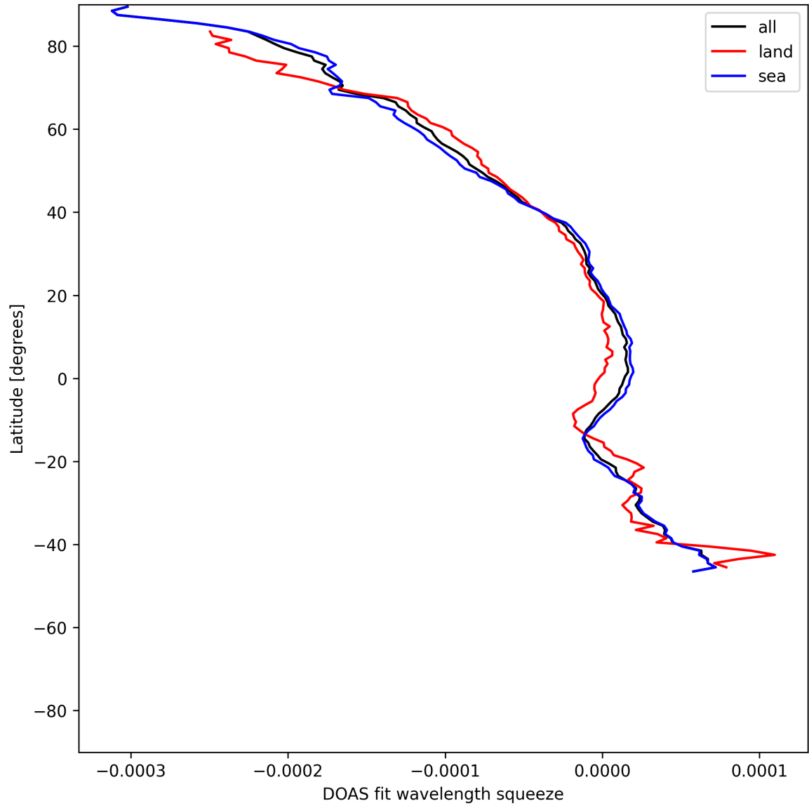
Figure 51: Zonal average of “DOAS fit wavelength squeeze” for 2025-07-09 to 2025-07-11.
