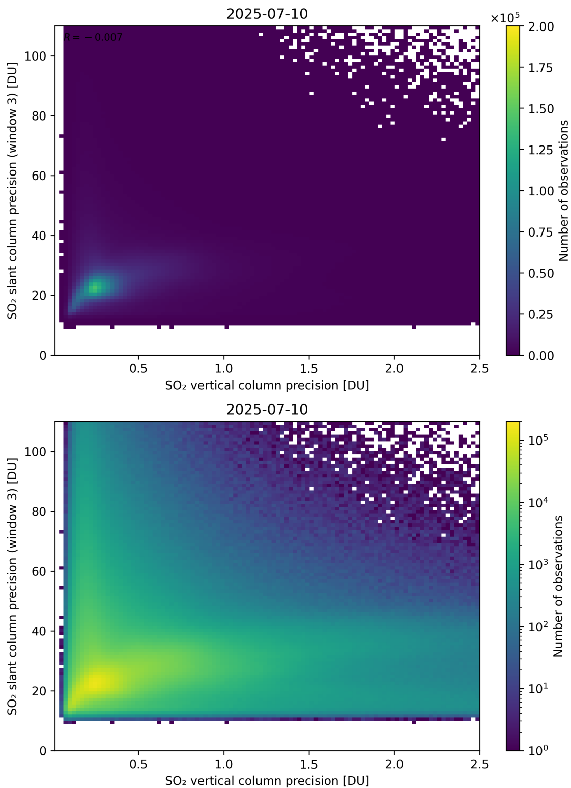
Figure 345: Scatter density plot of “SO 2 vertical column precision” against “SO 2 slant column precision (window 3)” for 2025-07-09 to 2025-07-11.
