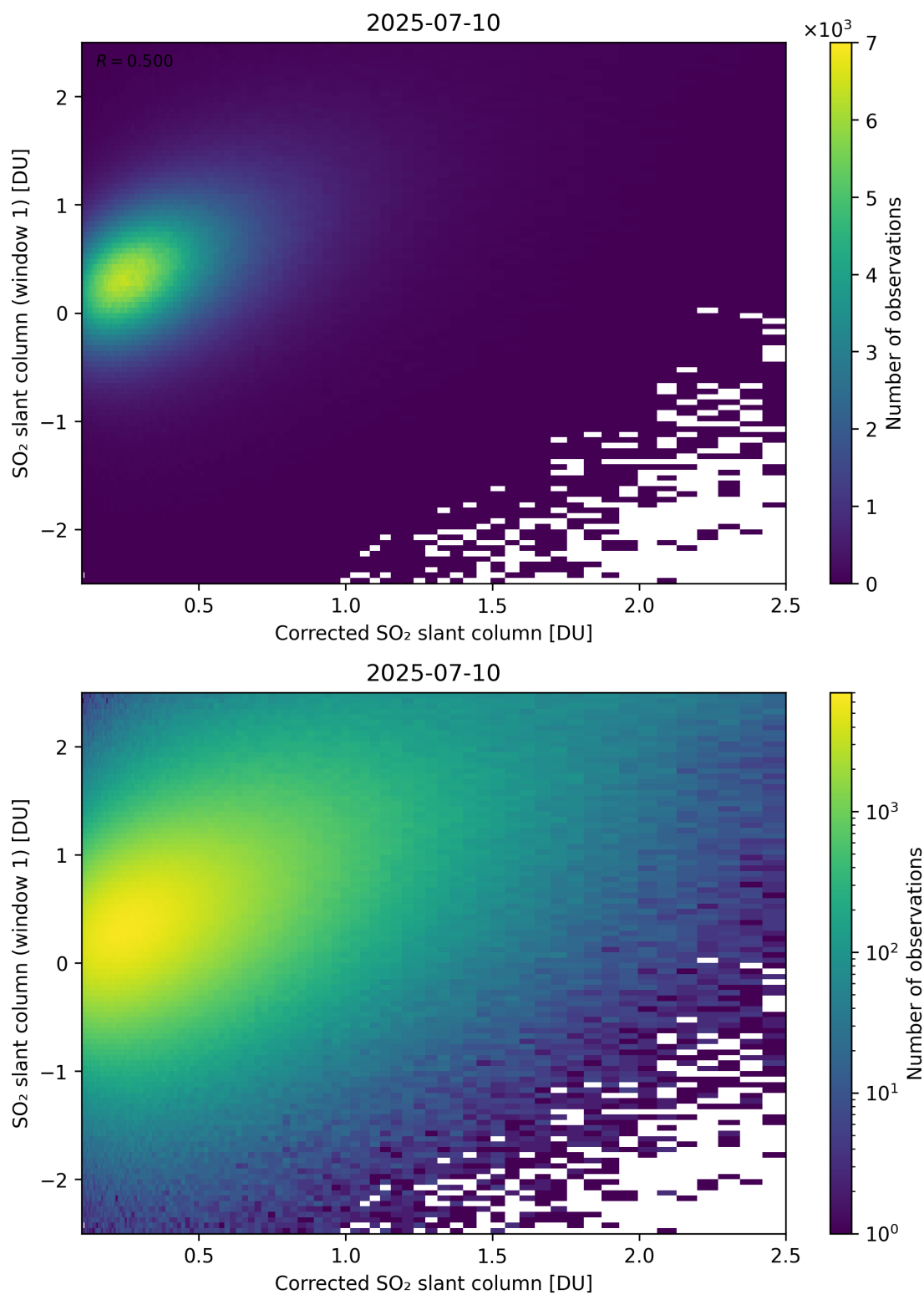
Figure 237: Scatter density plot of “Corrected SO 2 slant column” against “SO 2 slant column (window 1)” for 2025-07-09 to 2025-07-11.
