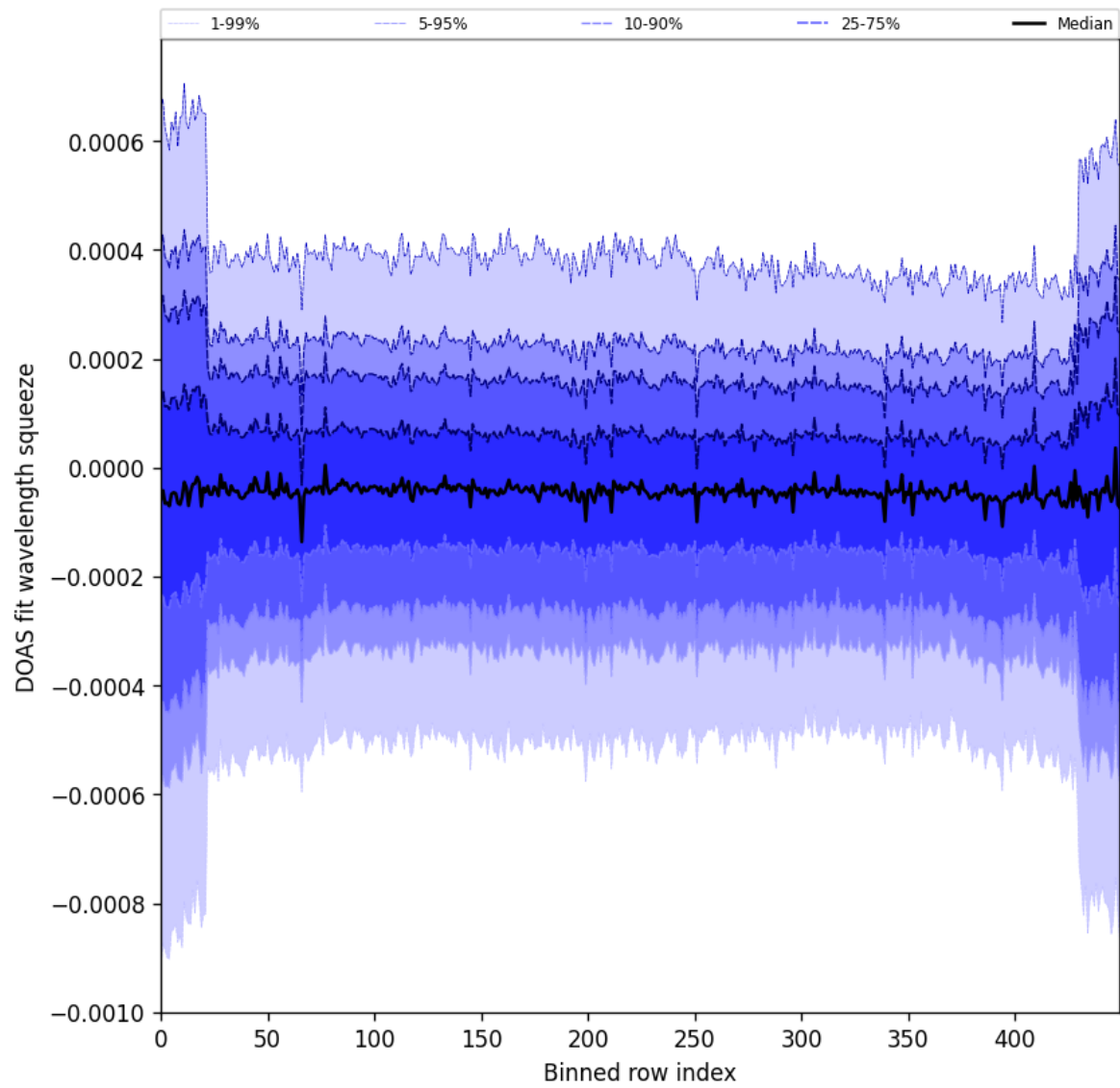
Figure 103: Along track statistics of “DOAS fit wavelength squeeze” for 2025-07-09 to 2025-07-11
