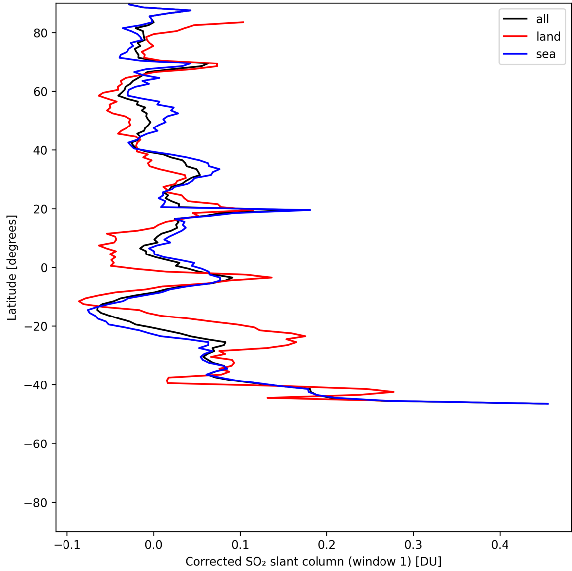
Figure 39: Zonal average of “Corrected SO 2 slant column (window 1)” for 2025-07-09 to 2025-07-11.
