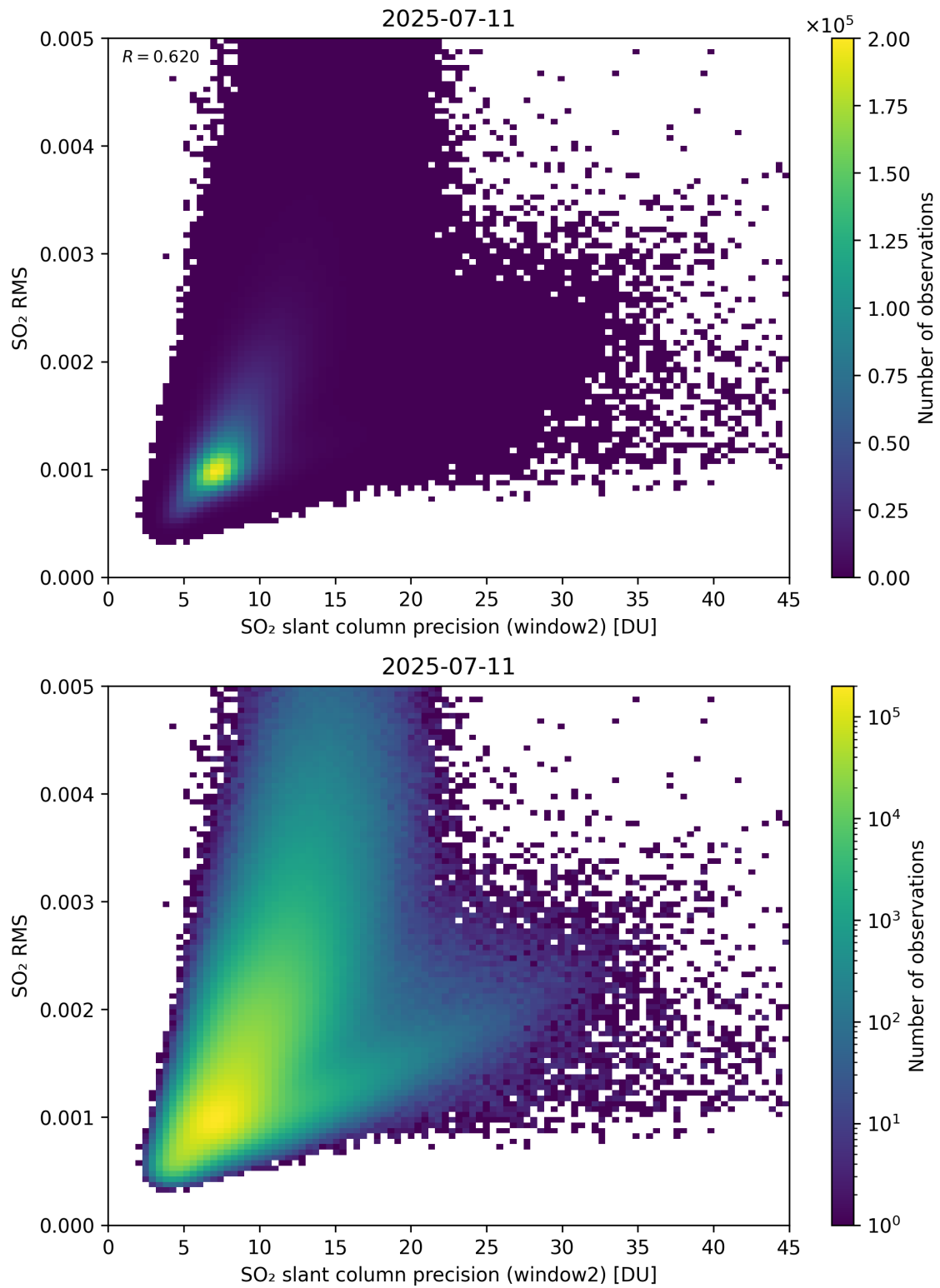
Figure 295: Scatter density plot of “SO 2 slant column precision (window2)” against “SO 2 RMS” for 2025-07-10 to 2025-07-12.
