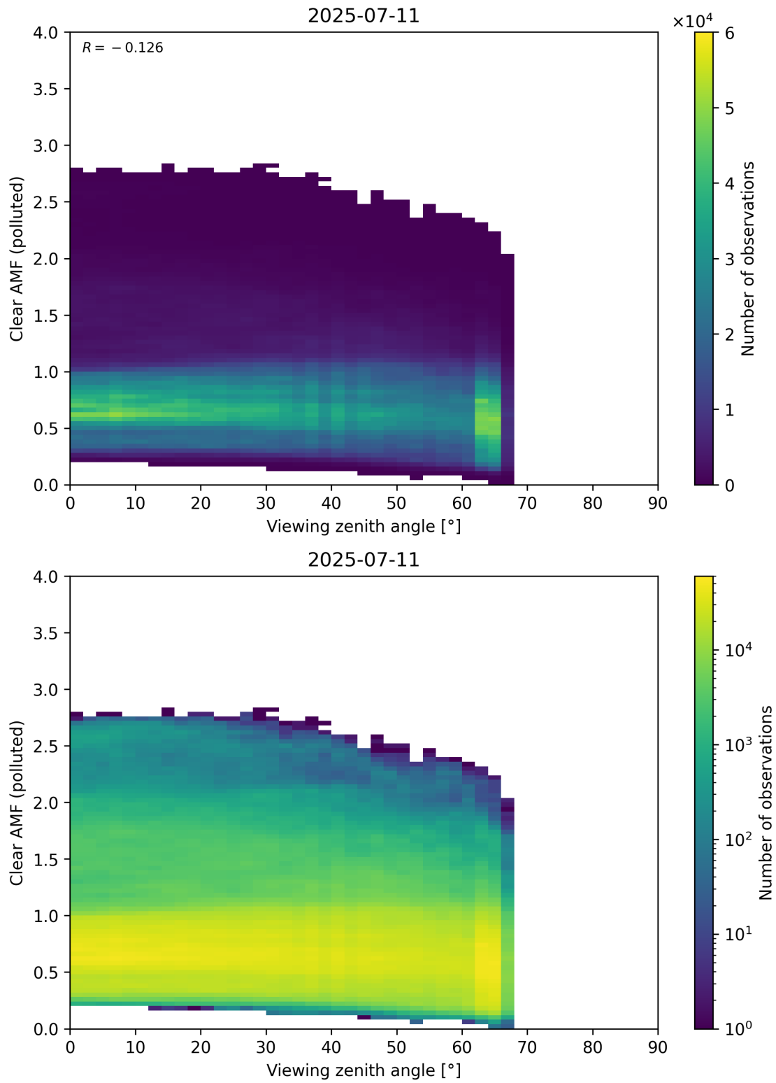
Figure 370: Scatter density plot of “Viewing zenith angle” against “Clear AMF (polluted)” for 2025-07-10 to 2025-07-12.
