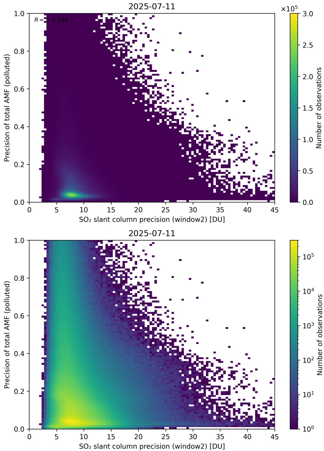
Figure 302: Scatter density plot of “SO 2 slant column precision (window2)” against “Precision of total AMF (polluted)” for 2025-07-10 to 2025-07-12.
