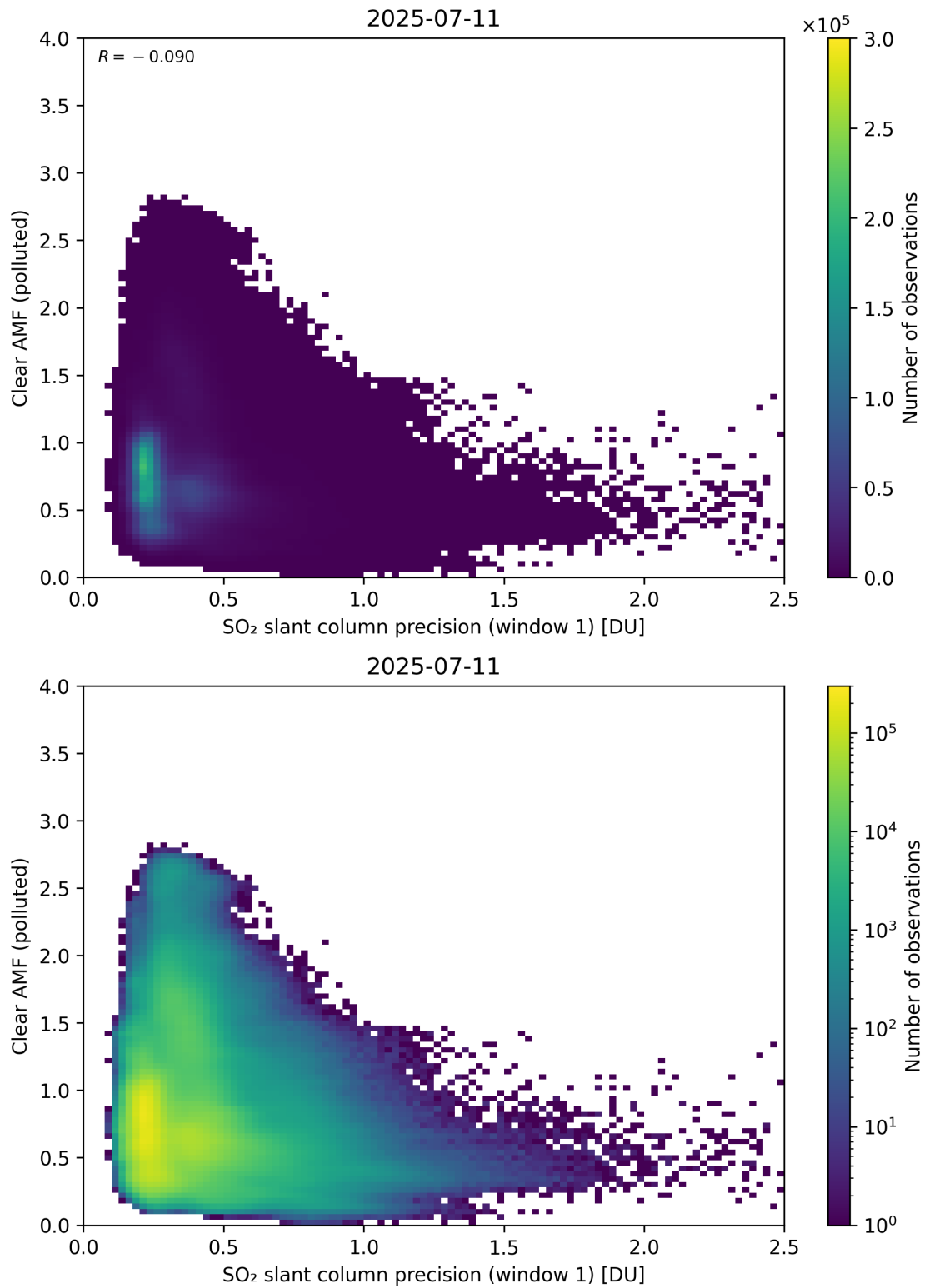
Figure 274: Scatter density plot of “SO 2 slant column precision (window 1)” against “Clear AMF (polluted)” for 2025-07-10 to 2025-07-12.
