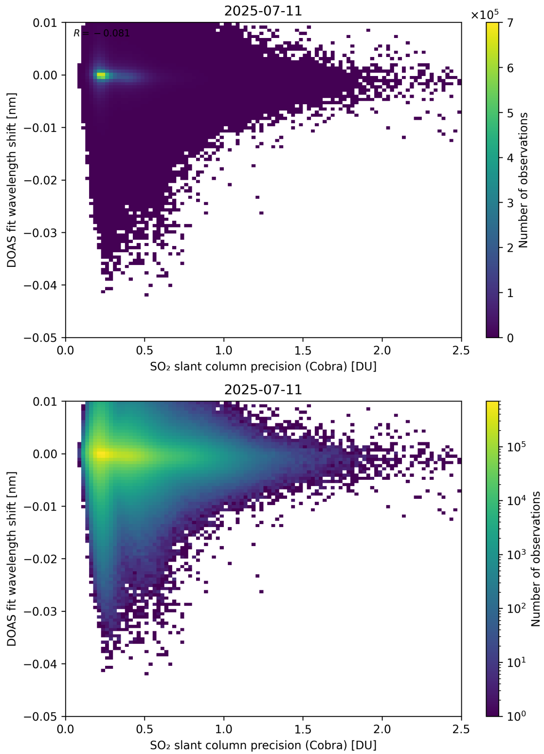
Figure 202: Scatter density plot of “SO 2 slant column precision (Cobra)” against “DOAS fit wavelength shift” for 2025-07-10 to 2025-07-12.
