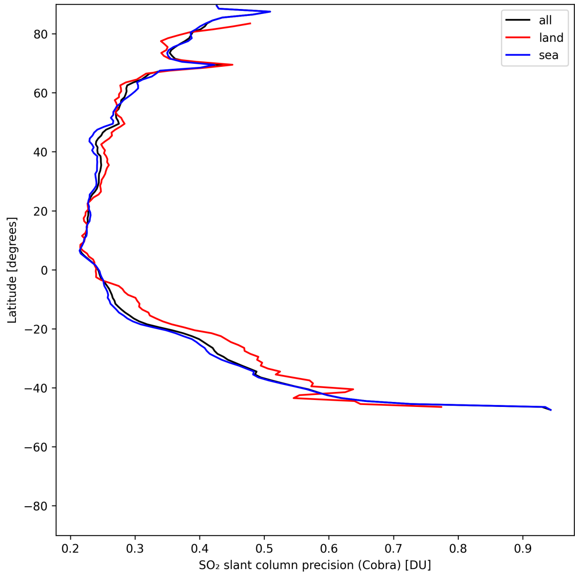
Figure 36: Zonal average of “SO 2 slant column precision (Cobra)” for 2025-07-10 to 2025-07-12.
