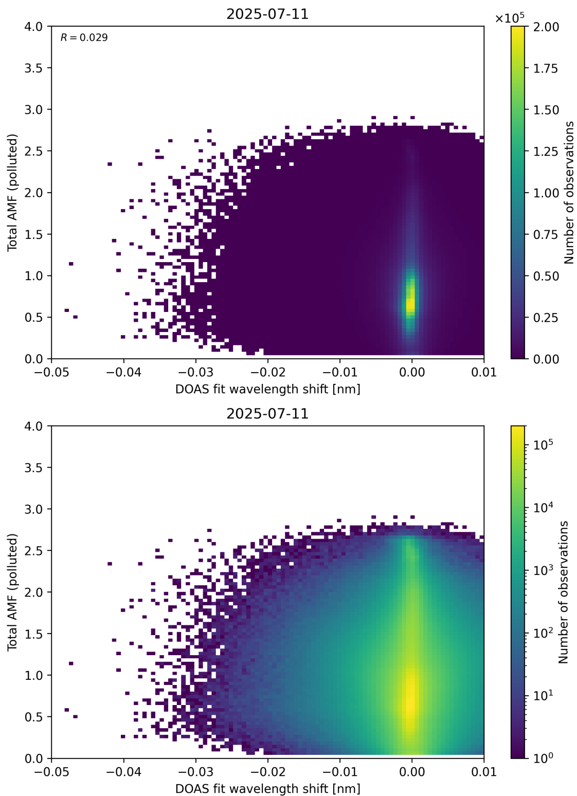
Figure 141: Scatter density plot of “DOAS fit wavelength shift” against “Total AMF (polluted)” for 2025-07-10 to 2025-07-12.
