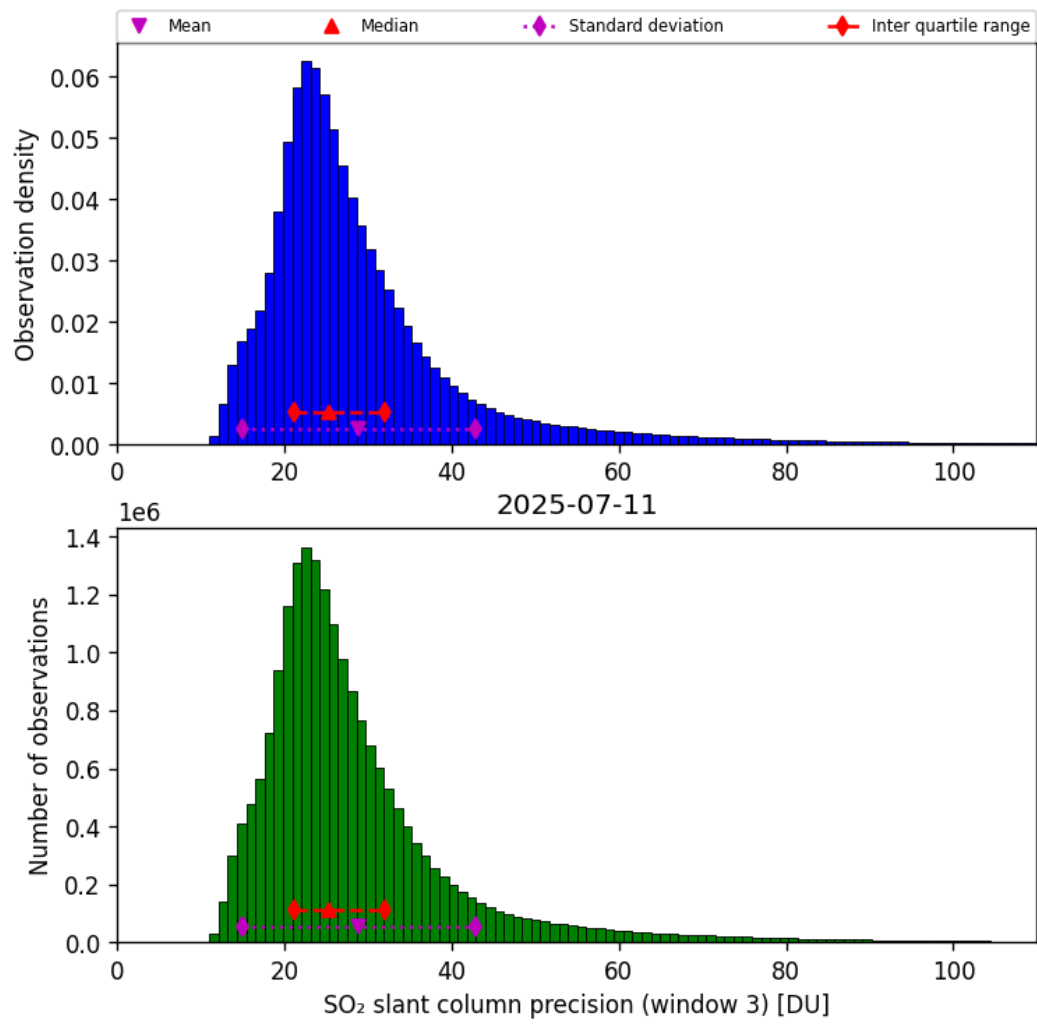
Figure 72: Histogram of “SO 2 slant column precision (window 3)” for 2025-07-10 to 2025-07-12
