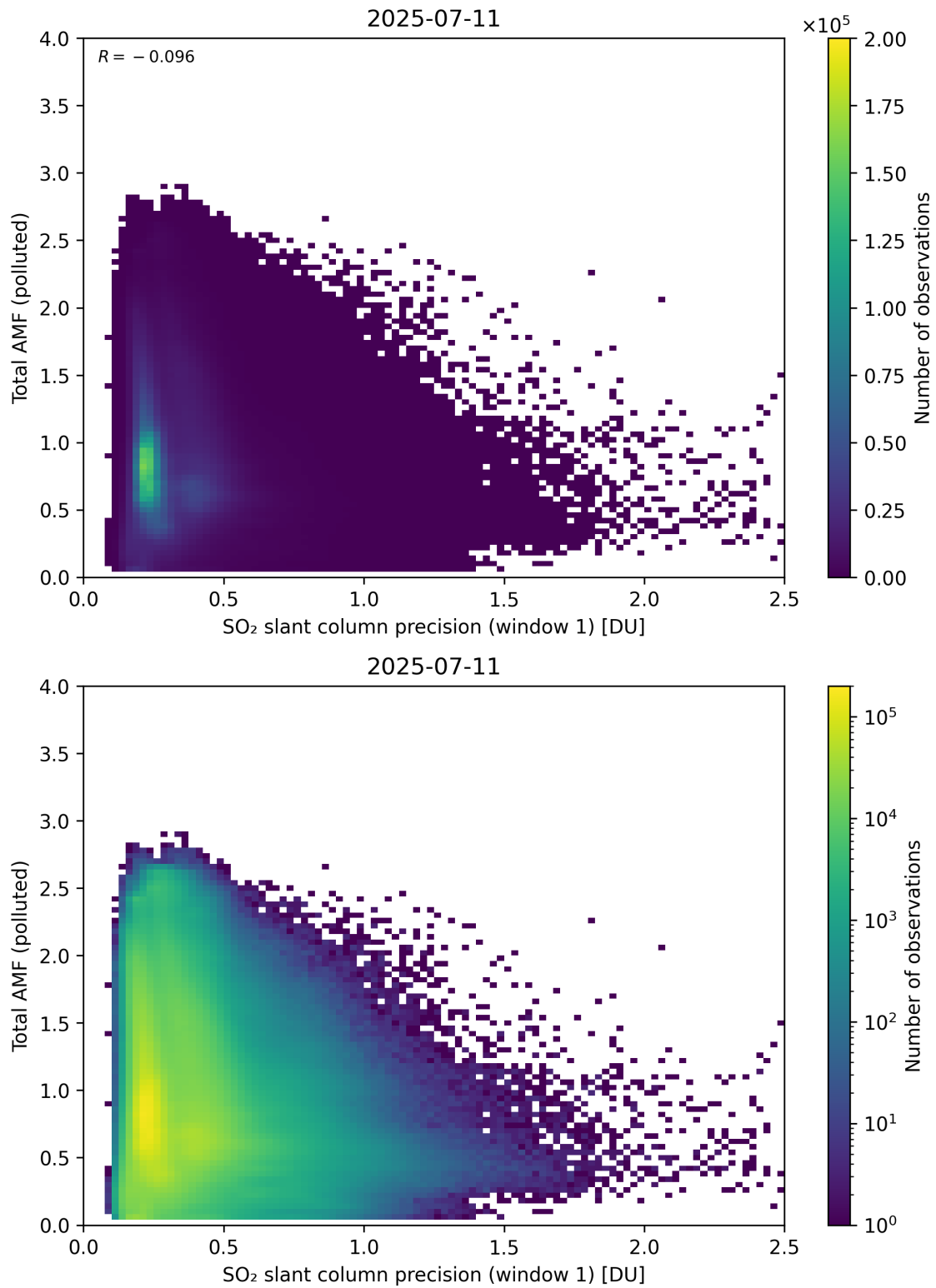
Figure 280: Scatter density plot of “SO 2 slant column precision (window 1)” against “Total AMF (polluted)” for 2025-07-10 to 2025-07-12.
