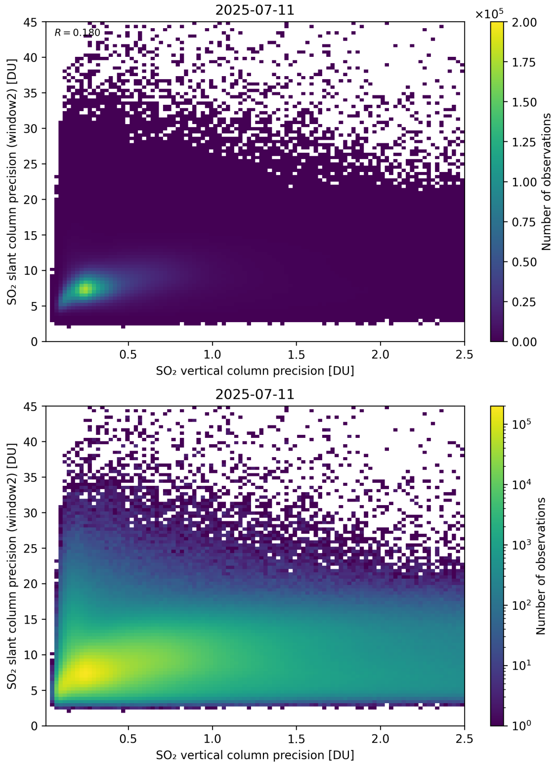
Figure 343: Scatter density plot of “SO 2 vertical column precision” against “SO 2 slant column precision (window2)” for 2025-07-10 to 2025-07-12.
