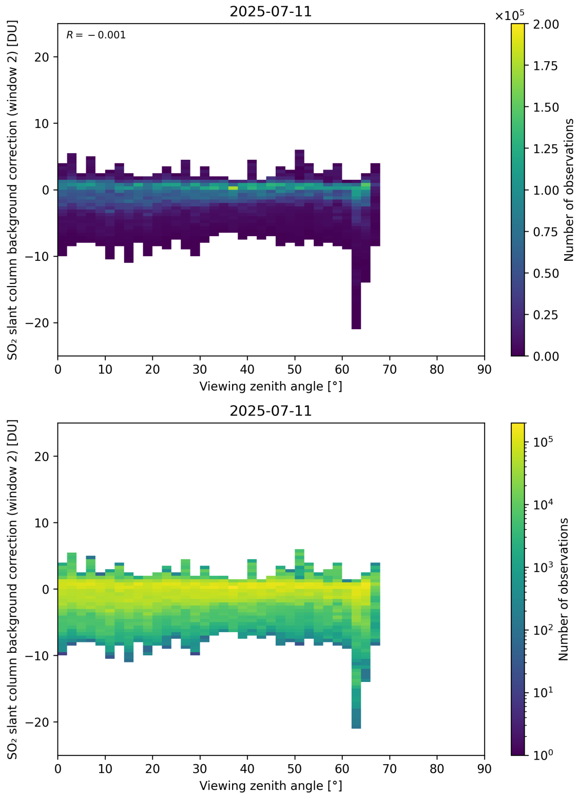
Figure 363: Scatter density plot of “Viewing zenith angle” against “SO 2 slant column background correction (window 2)” for 2025-07-10 to 2025-07-12.
