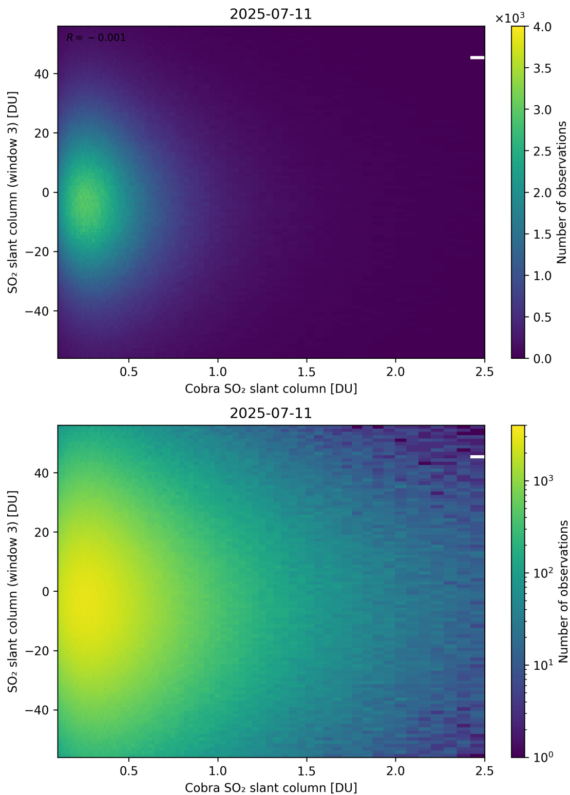
Figure 222: Scatter density plot of “Cobra SO 2 slant column” against “SO 2 slant column (window 3)” for 2025-07-10 to 2025-07-12.
