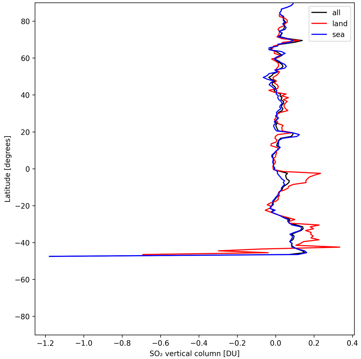
Figure 32: Zonal average of “SO 2 vertical column” for 2025-07-10 to 2025-07-12.
