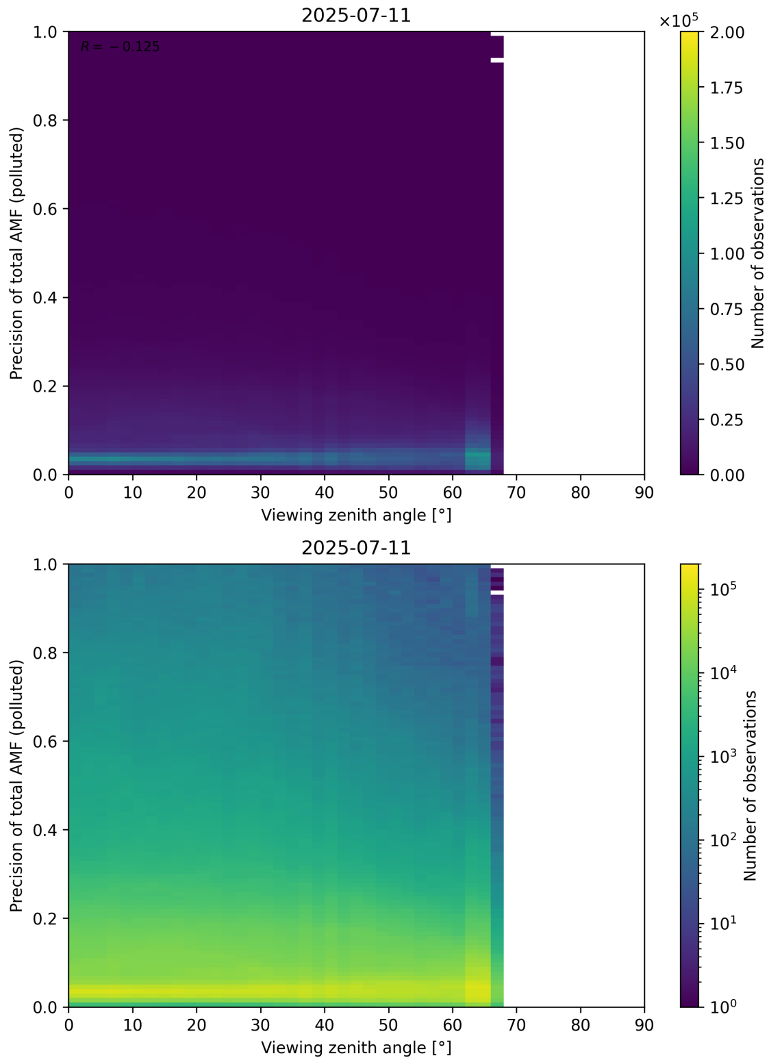
Figure 382: Scatter density plot of “Viewing zenith angle” against “Precision of total AMF (polluted)” for 2025-07-10 to 2025-07-12.
