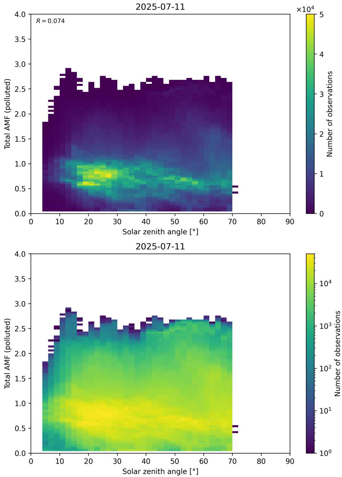
Figure 189: Scatter density plot of “Solar zenith angle” against “Total AMF (polluted)” for 2025-07-10 to 2025-07-12.
