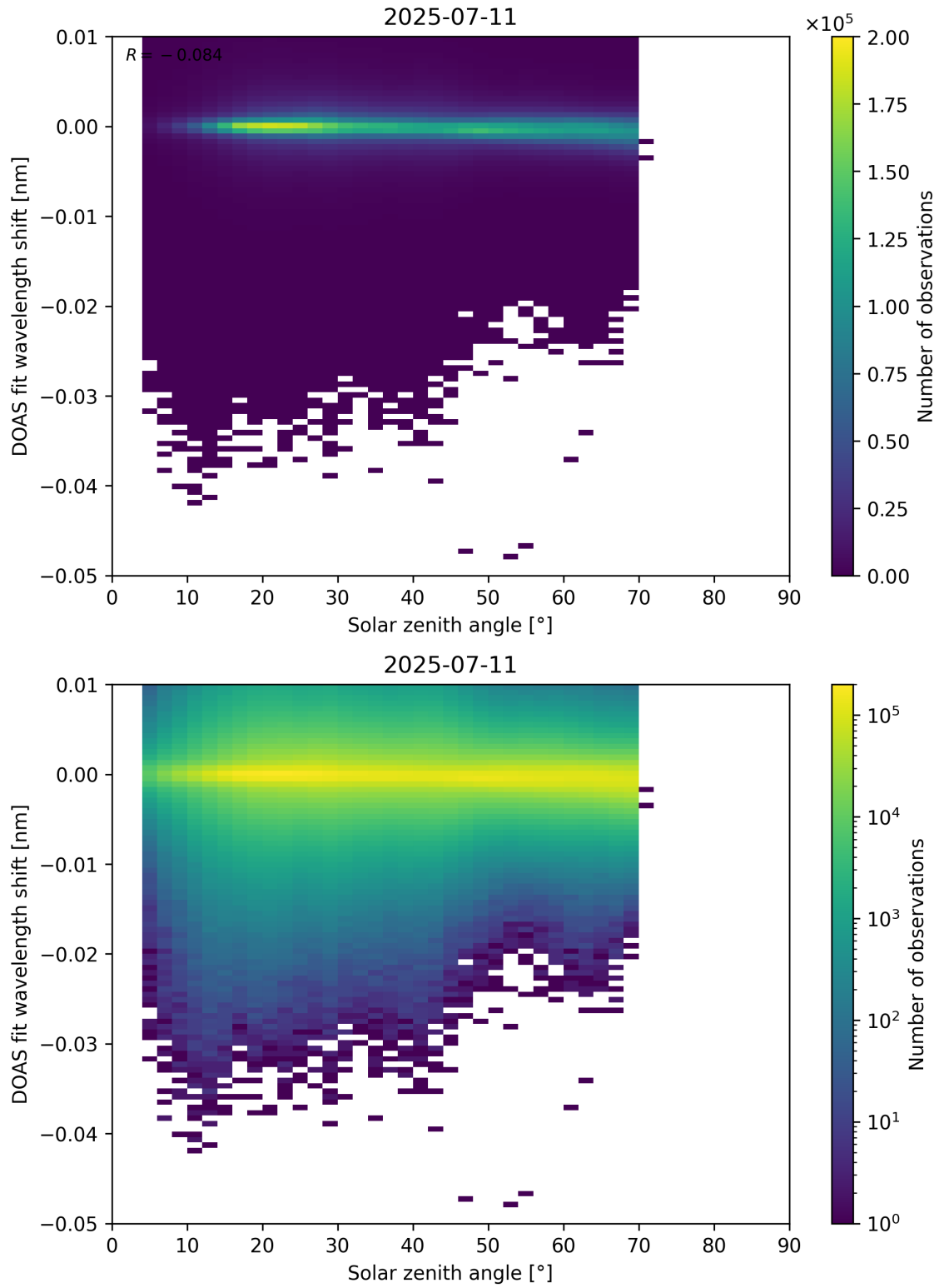
Figure 174: Scatter density plot of “Solar zenith angle” against “DOAS fit wavelength shift” for 2025-07-10 to 2025-07-12.
