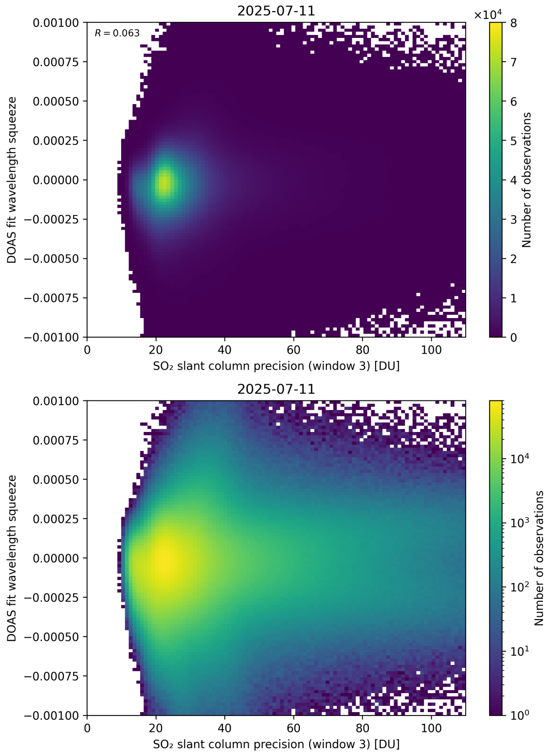
Figure 309: Scatter density plot of “SO 2 slant column precision (window 3)” against “DOAS fit wavelength squeeze” for 2025-07-10 to 2025-07-12.
