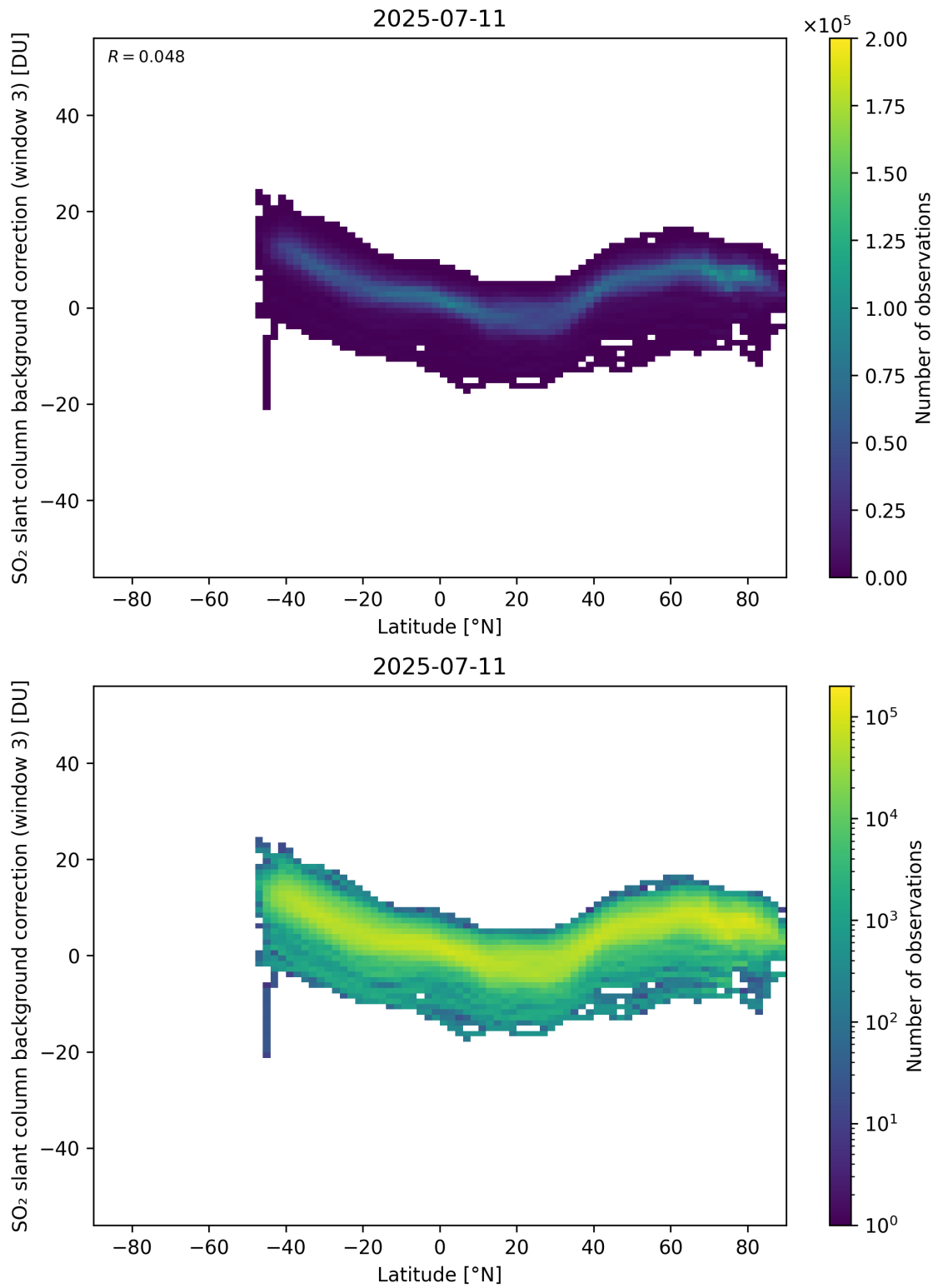
Figure 152: Scatter density plot of “Latitude” against “SO 2 slant column background correction (window 3)” for 2025-07-10 to 2025-07-12.
