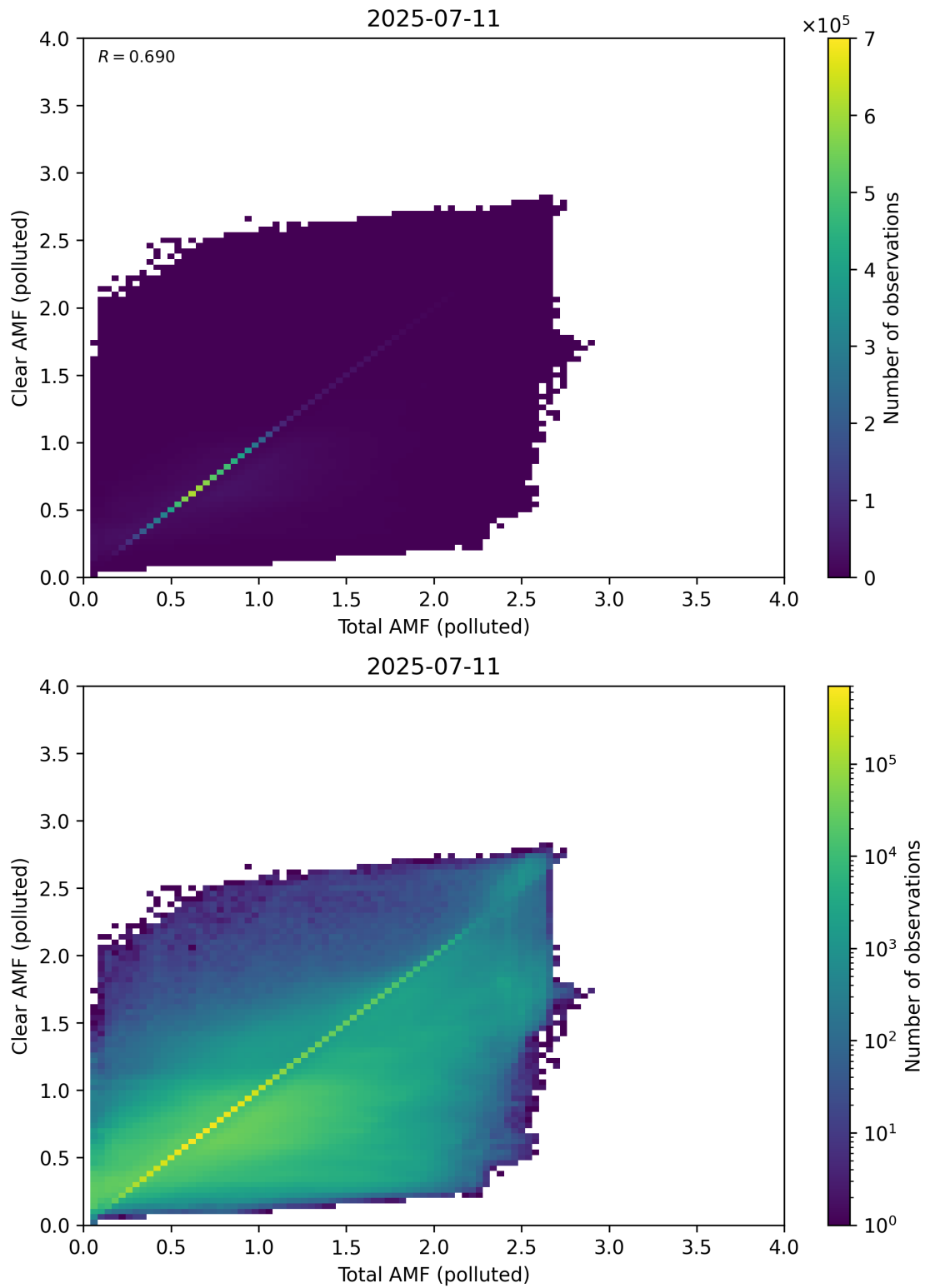
Figure 321: Scatter density plot of “Total AMF (polluted)” against “Clear AMF (polluted)” for 2025-07-10 to 2025-07-12.
