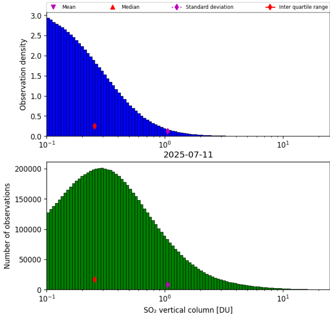
Figure 58: Histogram of “SO 2 vertical column” for 2025-07-10 to 2025-07-12
