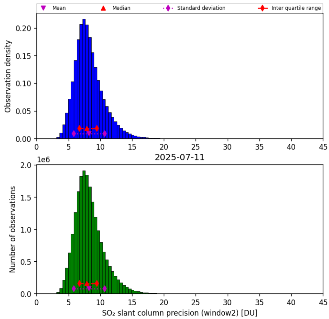
Figure 68: Histogram of “SO 2 slant column precision (window2)” for 2025-07-10 to 2025-07-12
