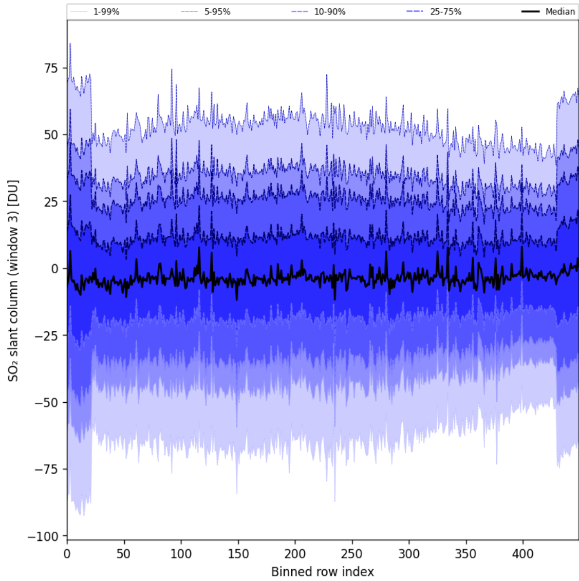
Figure 97: Along track statistics of “SO 2 slant column (window 3)” for 2025-07-10 to 2025-07-12
