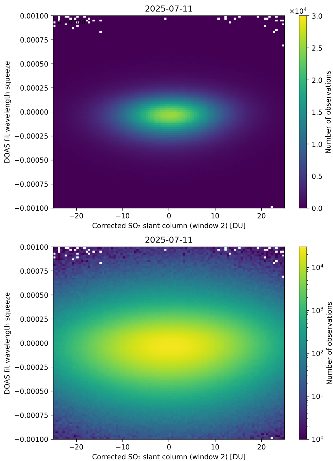
Figure 247: Scatter density plot of “Corrected SO 2 slant column (window 2)” against “DOAS fit wavelength squeeze” for 2025-07-10 to 2025-07-12.
