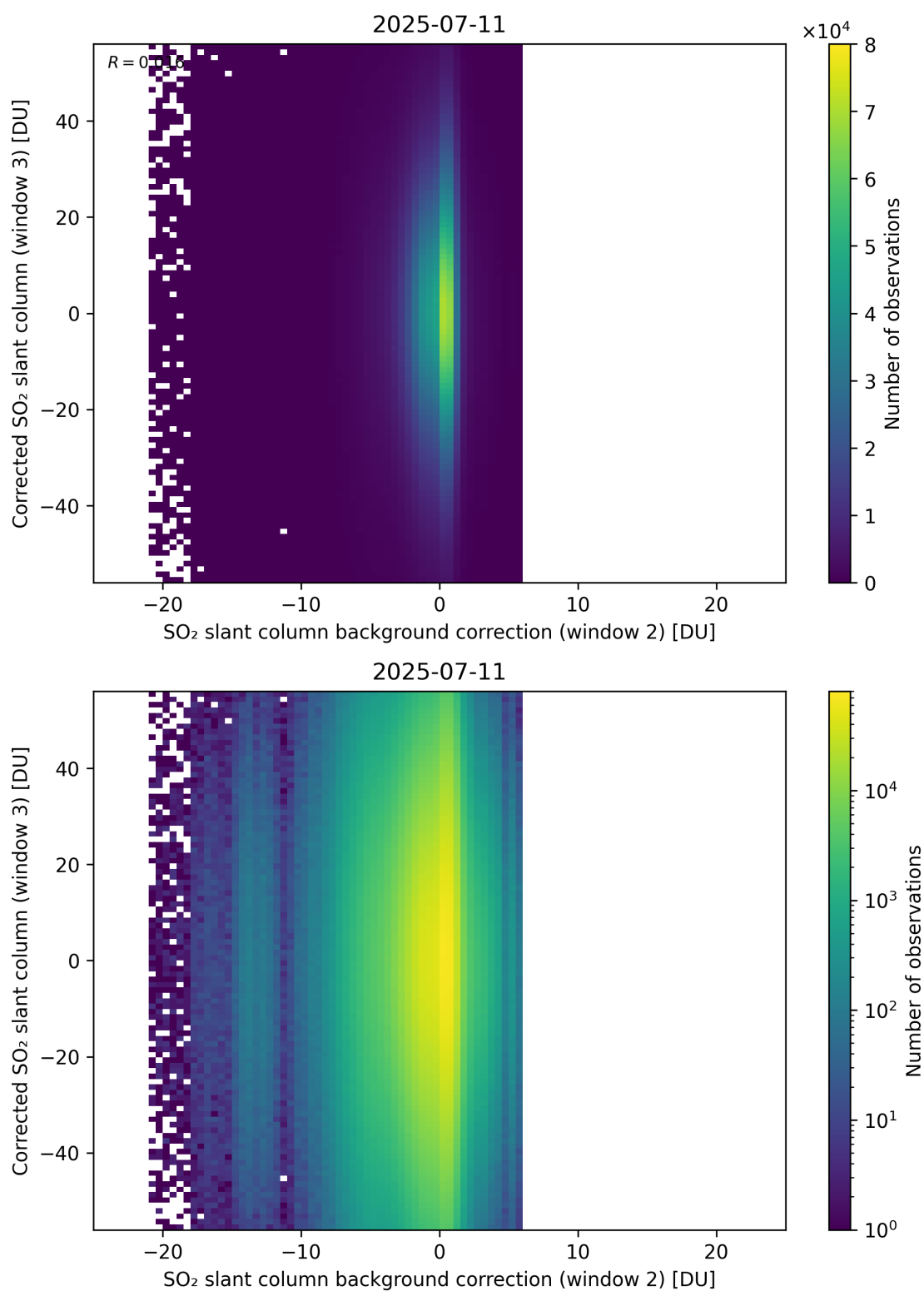
Figure 127: Scatter density plot of “SO 2 slant column background correction (window 2)” against “Corrected SO 2 slant column (window 3)” for 2025-07-10 to 2025-07-12.
