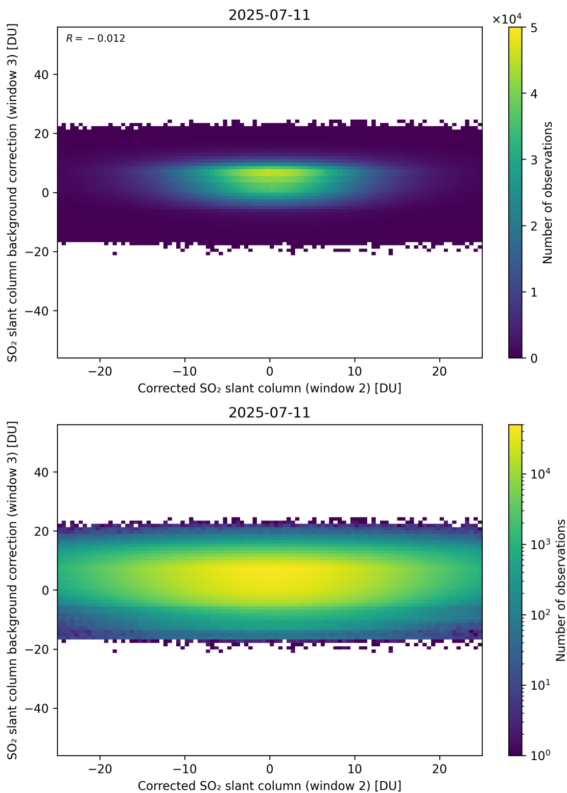
Figure 245: Scatter density plot of “Corrected SO 2 slant column (window 2)” against “SO 2 slant column background correction (window 3)” for 2025-07-10 to 2025-07-12.
