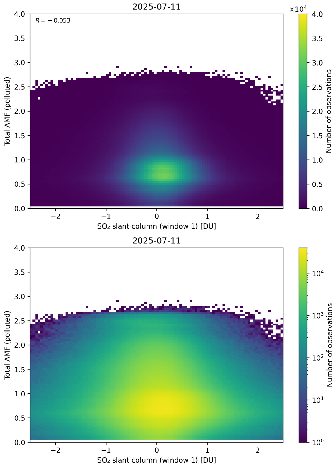
Figure 289: Scatter density plot of “SO 2 slant column (window 1)” against “Total AMF (polluted)” for 2025-07-10 to 2025-07-12.
