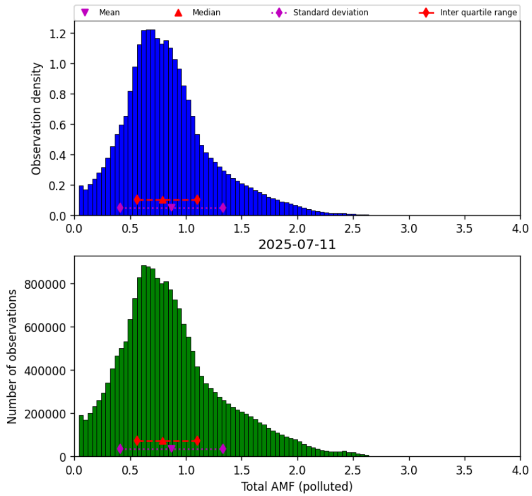
Figure 79: Histogram of “Total AMF (polluted)” for 2025-07-10 to 2025-07-12
