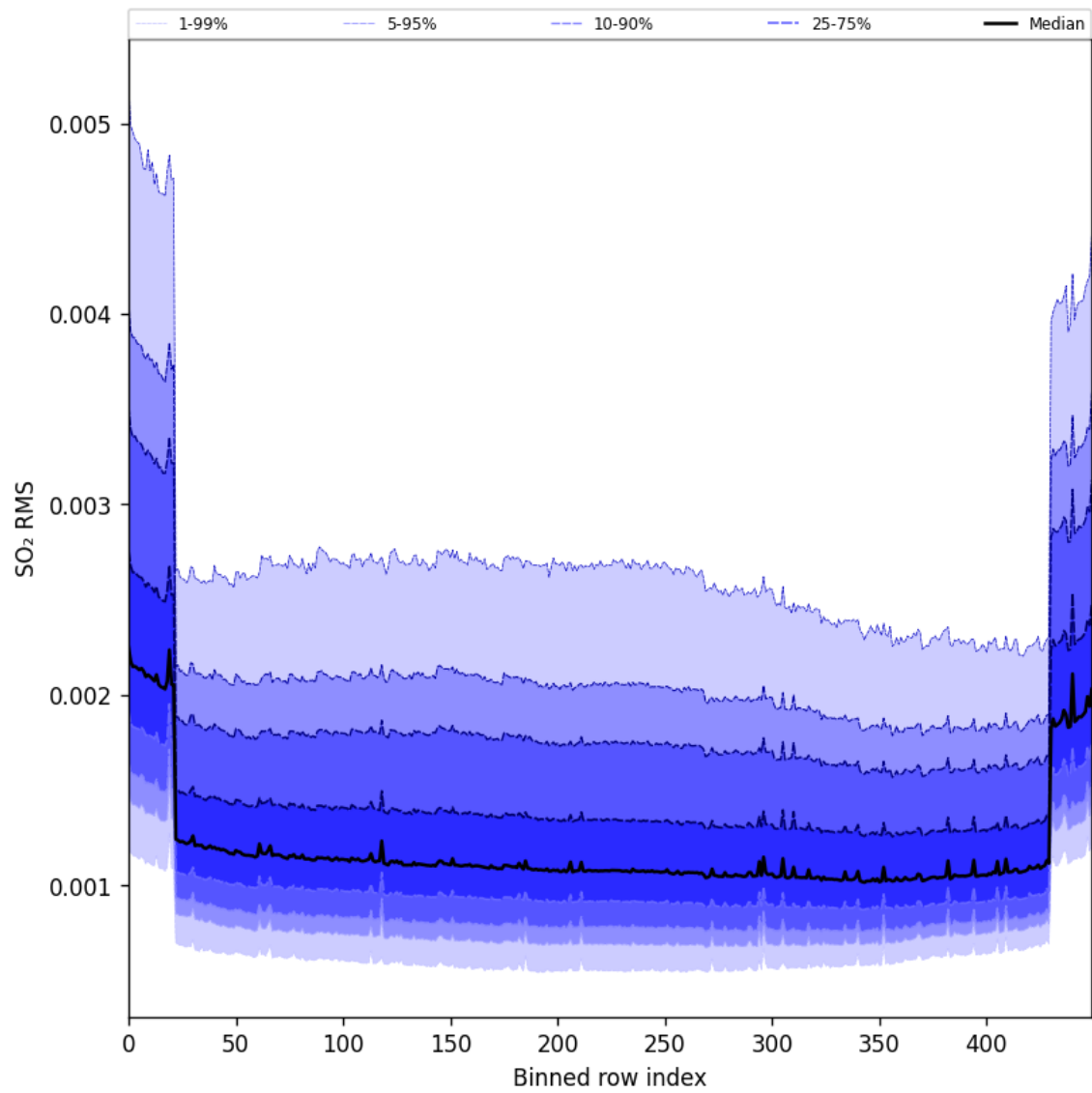
Figure 104: Along track statistics of “SO 2 RMS” for 2025-07-10 to 2025-07-12
