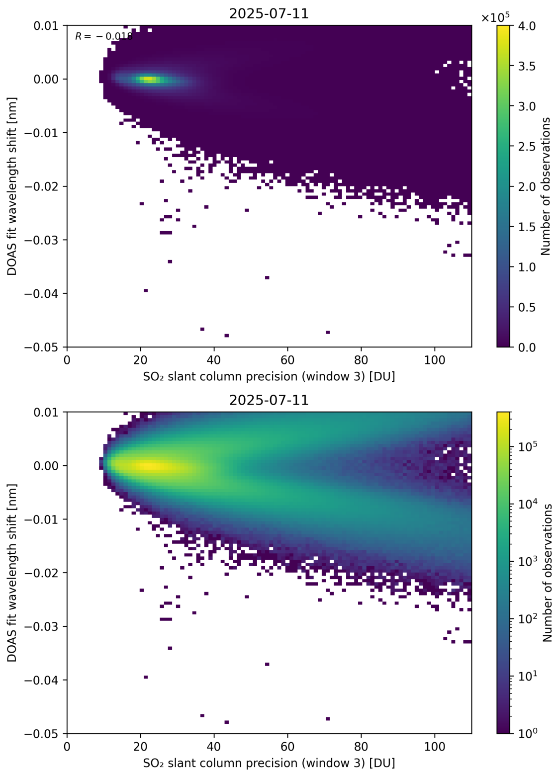
Figure 308: Scatter density plot of “SO 2 slant column precision (window 3)” against “DOAS fit wavelength shift” for 2025-07-10 to 2025-07-12.
