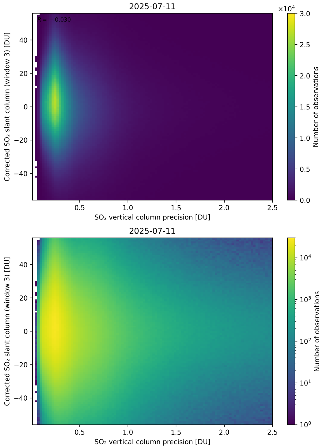
Figure 340: Scatter density plot of “SO 2 vertical column precision” against “Corrected SO 2 slant column (window 3)” for 2025-07-10 to 2025-07-12.
