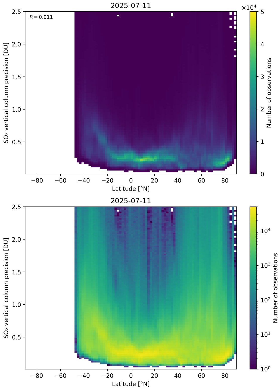
Figure 170: Scatter density plot of “Latitude” against “SO 2 vertical column precision” for 2025-07-10 to 2025-07-12.
