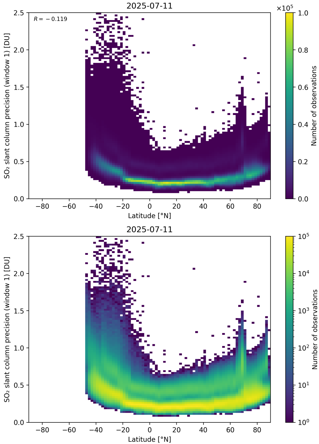
Figure 163: Scatter density plot of “Latitude” against “SO 2 slant column precision (window 1)” for 2025-07-10 to 2025-07-12.
