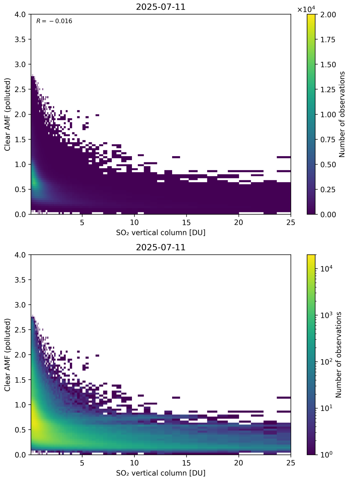
Figure 348: Scatter density plot of “SO 2 vertical column” against “Clear AMF (polluted)” for 2025-07-10 to 2025-07-12.
