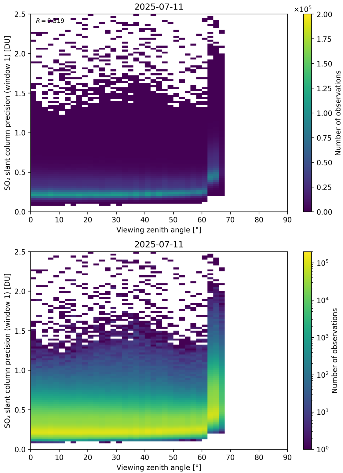
Figure 377: Scatter density plot of “Viewing zenith angle” against “SO 2 slant column precision (window 1)” for 2025-07-10 to 2025-07-12.
