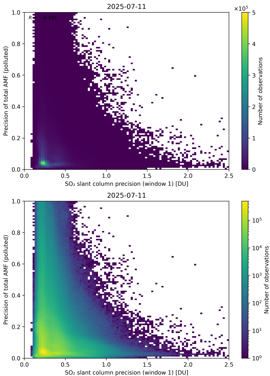
Figure 281: Scatter density plot of “SO 2 slant column precision (window 1)” against “Precision of total AMF (polluted)” for 2025-07-10 to 2025-07-12.
