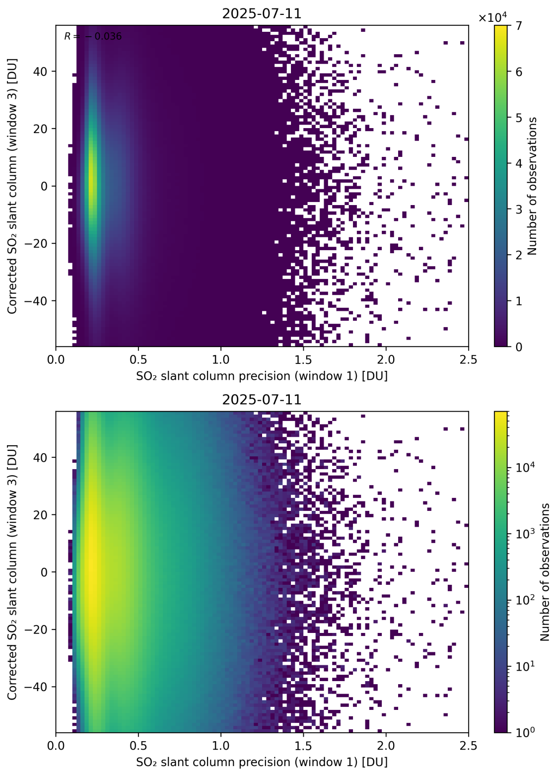
Figure 276: Scatter density plot of “SO 2 slant column precision (window 1)” against “Corrected SO 2 slant column (window 3)” for 2025-07-10 to 2025-07-12.
