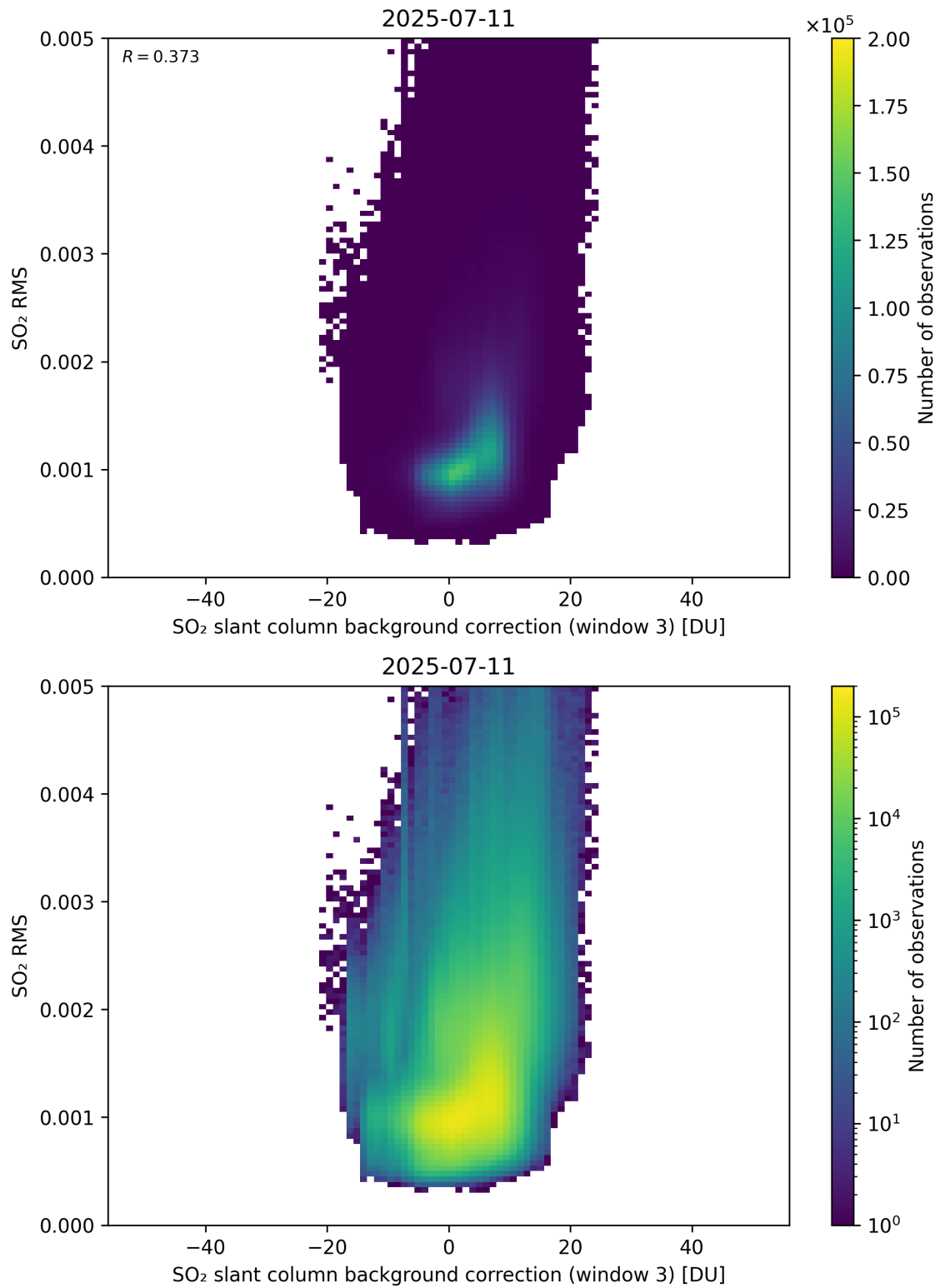
Figure 134: Scatter density plot of “SO 2 slant column background correction (window 3)” against “SO 2 RMS” for 2025-07-10 to 2025-07-12.
