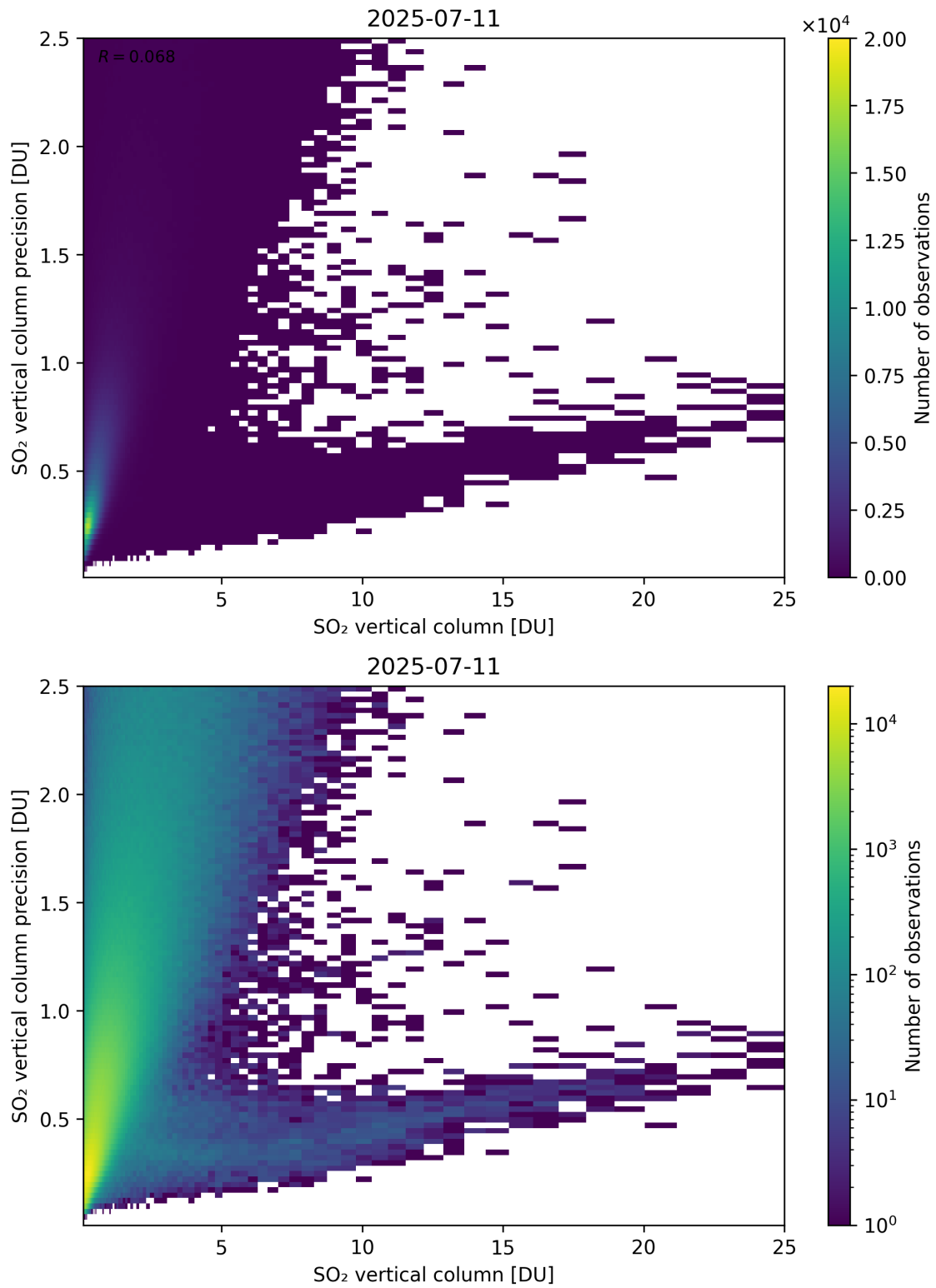
Figure 361: Scatter density plot of “SO 2 vertical column” against “SO 2 vertical column precision” for 2025-07-10 to 2025-07-12.
