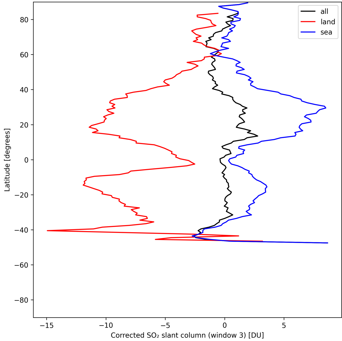
Figure 47: Zonal average of “Corrected SO 2 slant column (window 3)” for 2025-07-10 to 2025-07-12.
