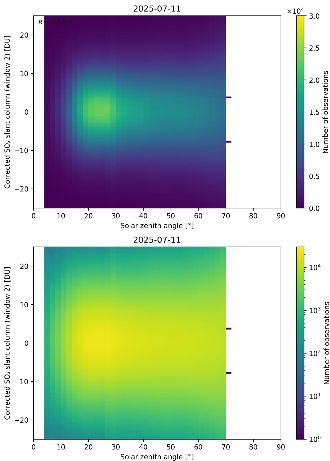
Figure 182: Scatter density plot of “Solar zenith angle” against “Corrected SO 2 slant column (window 2)” for 2025-07-10 to 2025-07-12.
