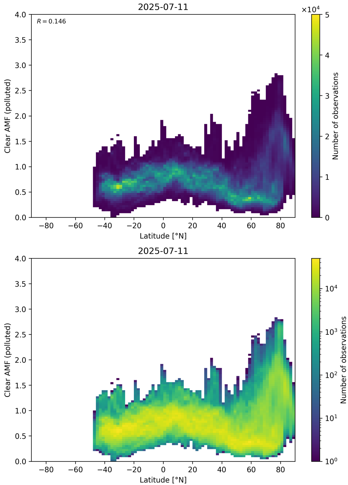
Figure 156: Scatter density plot of “Latitude” against “Clear AMF (polluted)” for 2025-07-10 to 2025-07-12.
