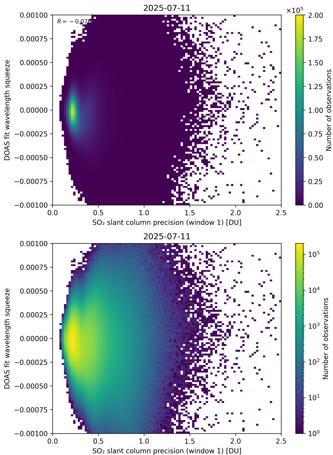
Figure 272: Scatter density plot of “SO 2 slant column precision (window 1)” against “DOAS fit wavelength squeeze” for 2025-07-10 to 2025-07-12.
