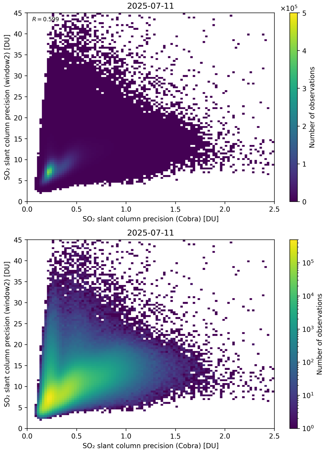
Figure 210: Scatter density plot of “SO 2 slant column precision (Cobra)” against “SO 2 slant column precision (window2)” for 2025-07-10 to 2025-07-12.
