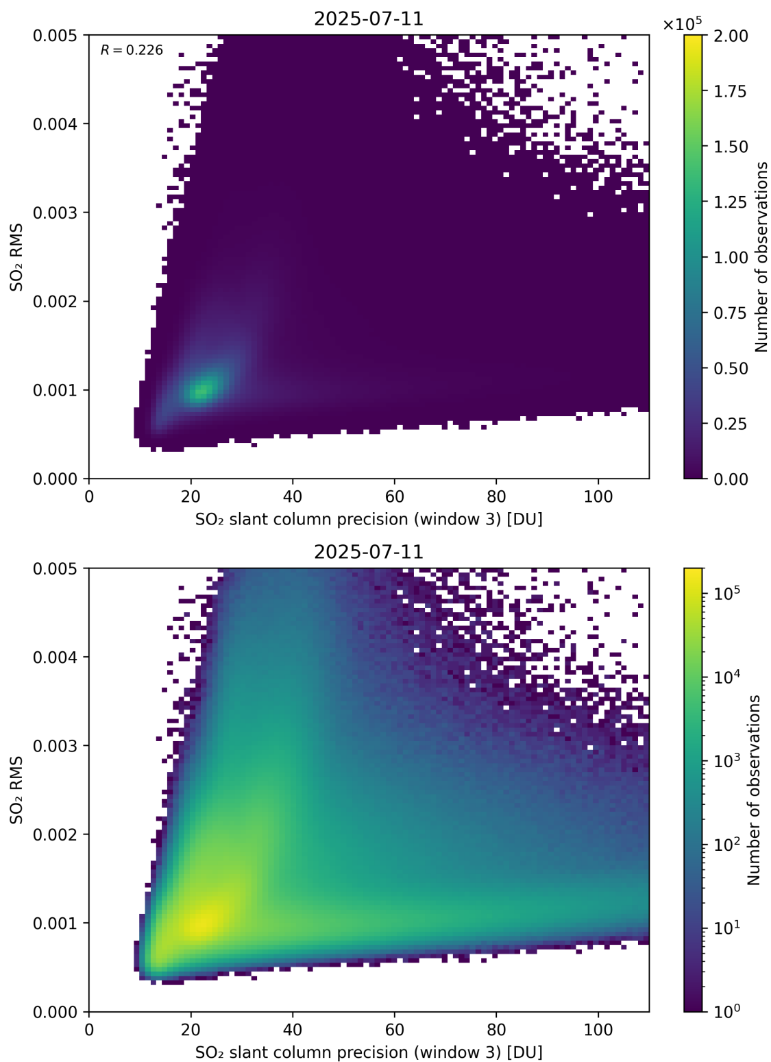
Figure 310: Scatter density plot of “SO 2 slant column precision (window 3)” against “SO 2 RMS” for 2025-07-10 to 2025-07-12.
