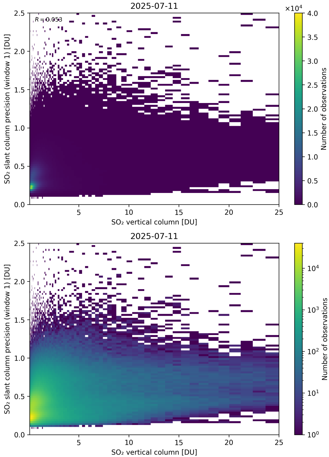
Figure 355: Scatter density plot of “SO 2 vertical column” against “SO 2 slant column precision (window 1)” for 2025-07-10 to 2025-07-12.
