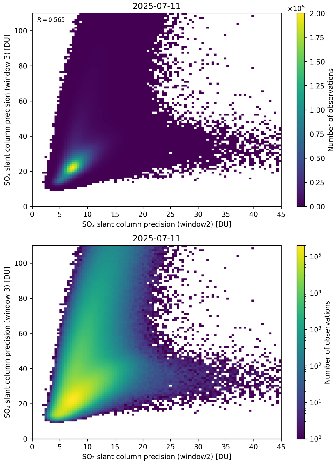
Figure 300: Scatter density plot of “SO 2 slant column precision (window2)” against “SO 2 slant column precision (window 3)” for 2025-07-10 to 2025-07-12.
