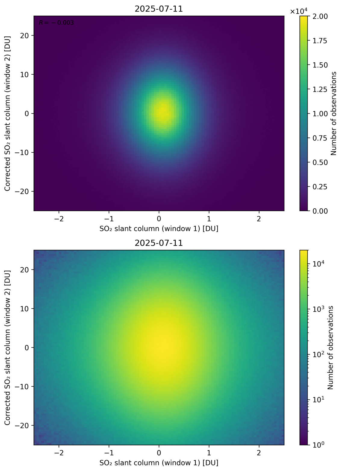
Figure 283: Scatter density plot of “SO 2 slant column (window 1)” against “Corrected SO 2 slant column (window 2)” for 2025-07-10 to 2025-07-12.
