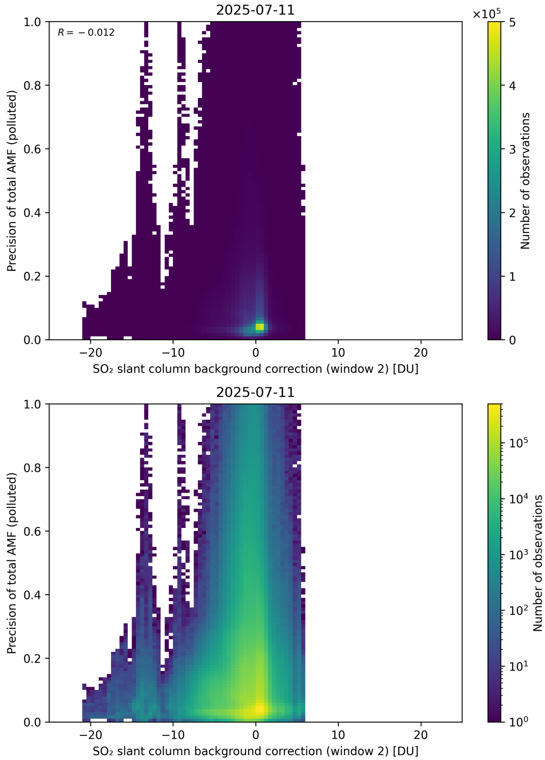
Figure 131: Scatter density plot of “SO 2 slant column background correction (window 2)” against “Precision of total AMF (polluted)” for 2025-07-10 to 2025-07-12.
