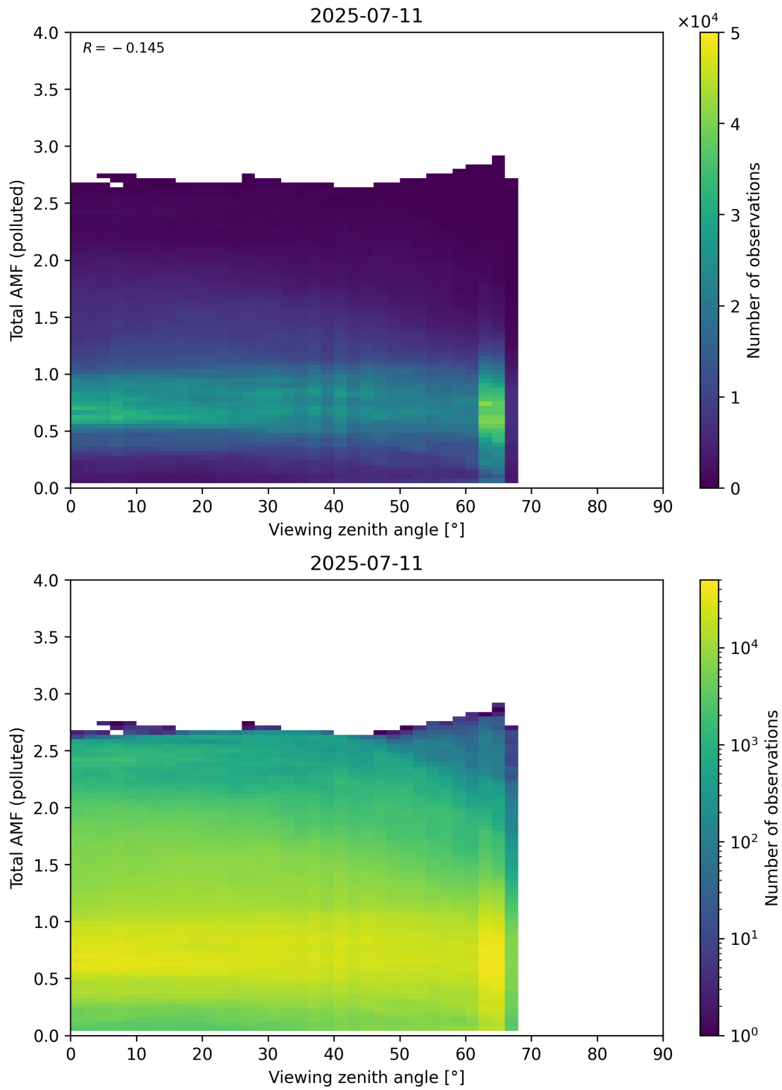
Figure 381: Scatter density plot of “Viewing zenith angle” against “Total AMF (polluted)” for 2025-07-10 to 2025-07-12.
