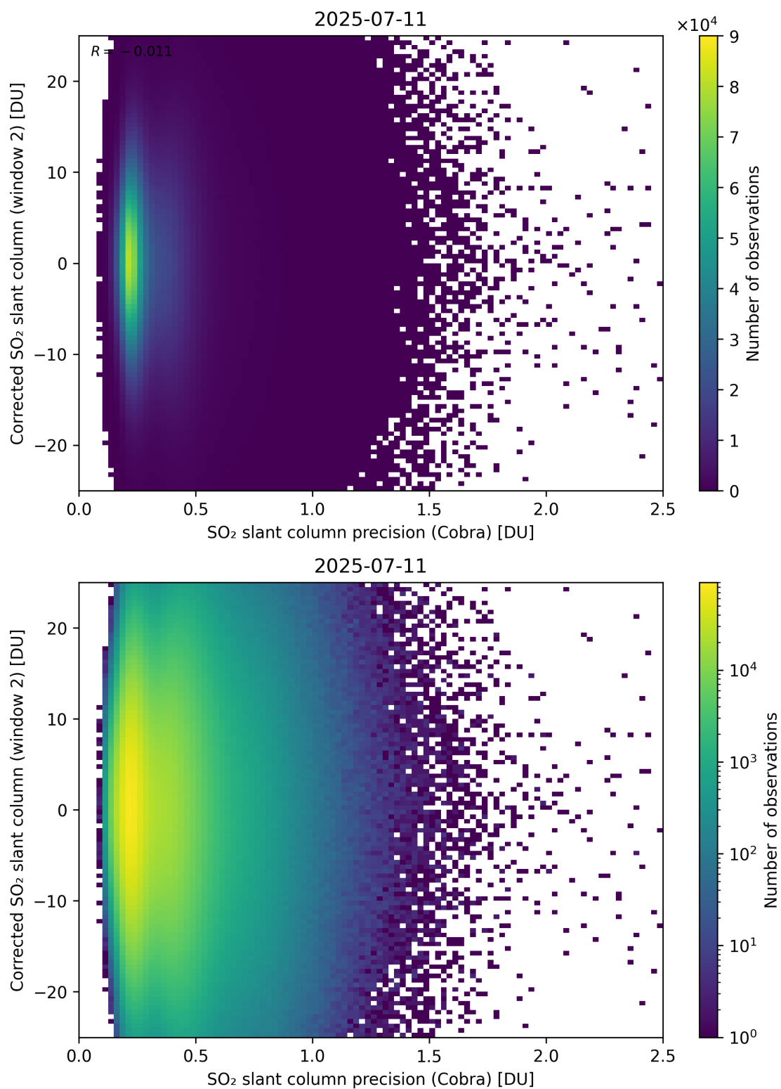
Figure 206: Scatter density plot of “SO 2 slant column precision (Cobra)” against “Corrected SO 2 slant column (window 2)” for 2025-07-10 to 2025-07-12.
