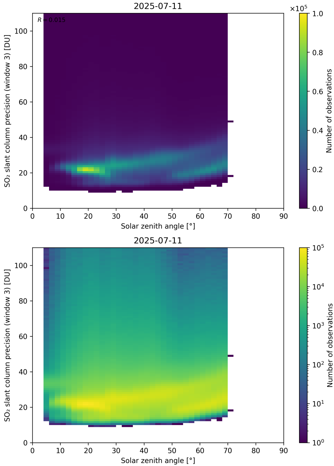
Figure 188: Scatter density plot of “Solar zenith angle” against “SO 2 slant column precision (window 3)” for 2025-07-10 to 2025-07-12.
