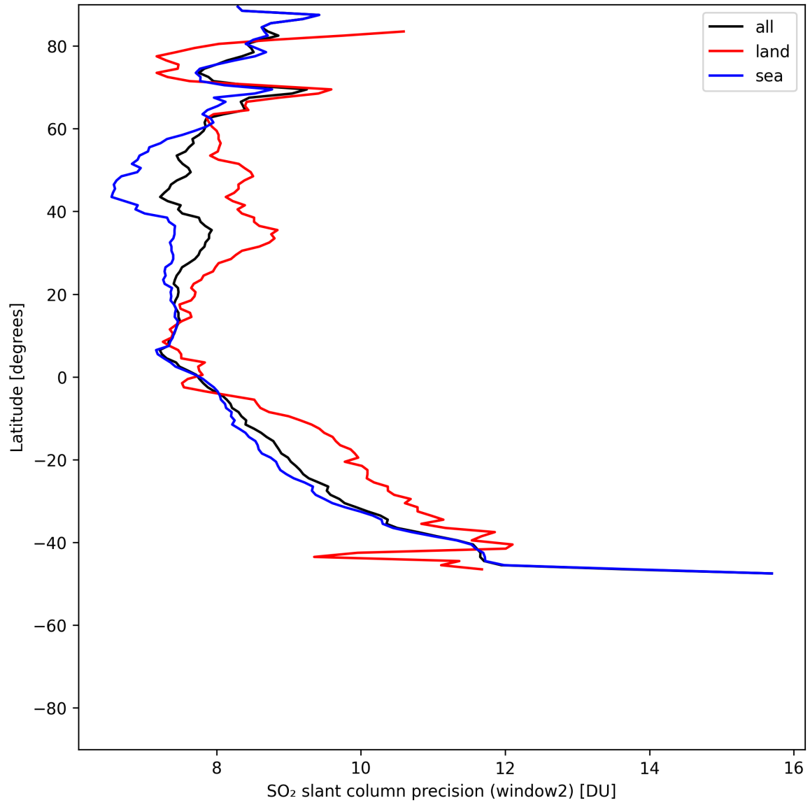
Figure 42: Zonal average of “SO 2 slant column precision (window2)” for 2025-07-10 to 2025-07-12.
