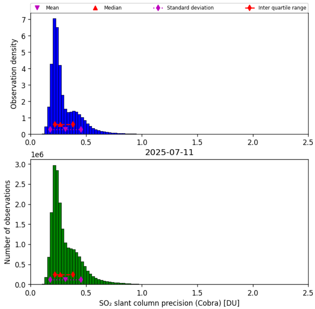
Figure 62: Histogram of “SO 2 slant column precision (Cobra)” for 2025-07-10 to 2025-07-12
