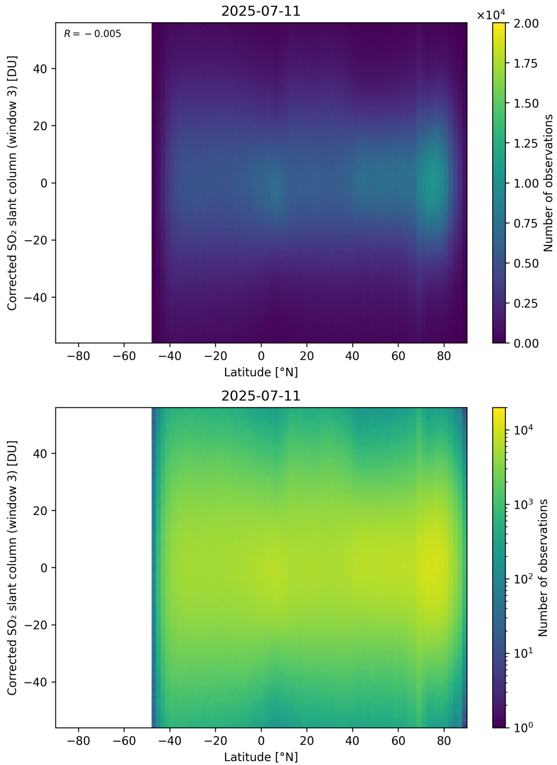
Figure 161: Scatter density plot of “Latitude” against “Corrected SO 2 slant column (window 3)” for 2025-07-10 to 2025-07-12.
