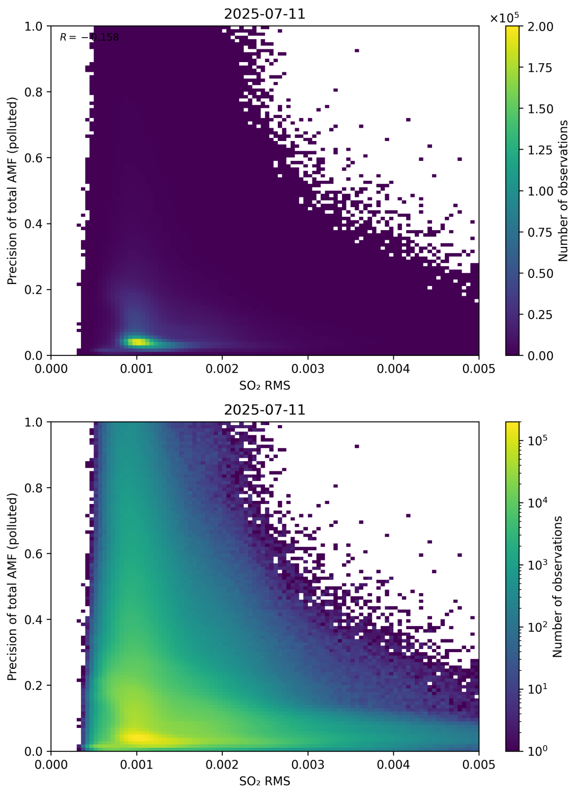
Figure 149: Scatter density plot of “SO 2 RMS” against “Precision of total AMF (polluted)” for 2025-07-10 to 2025-07-12.
