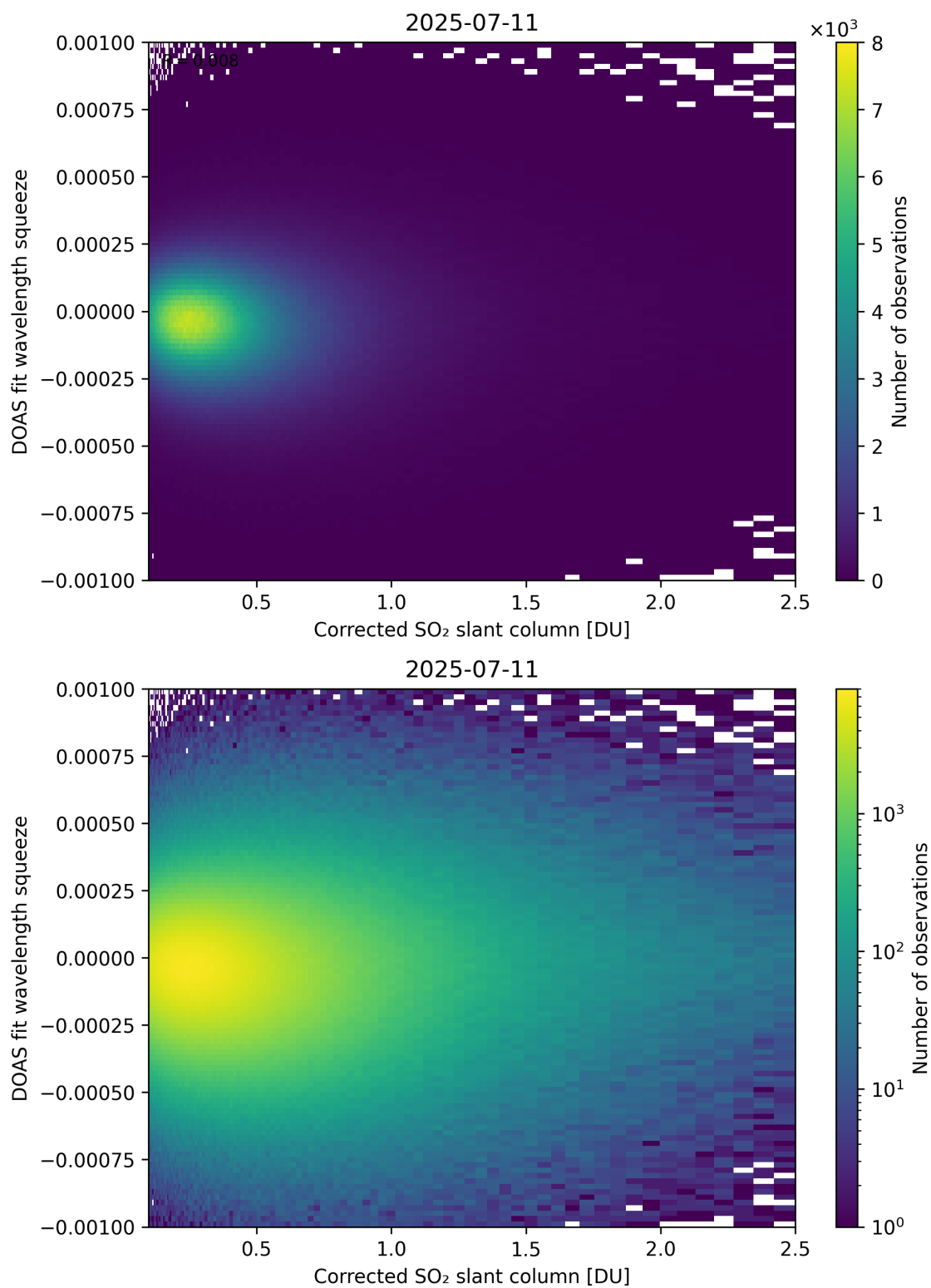
Figure 230: Scatter density plot of “Corrected SO 2 slant column” against “DOAS fit wavelength squeeze” for 2025-07-10 to 2025-07-12.
