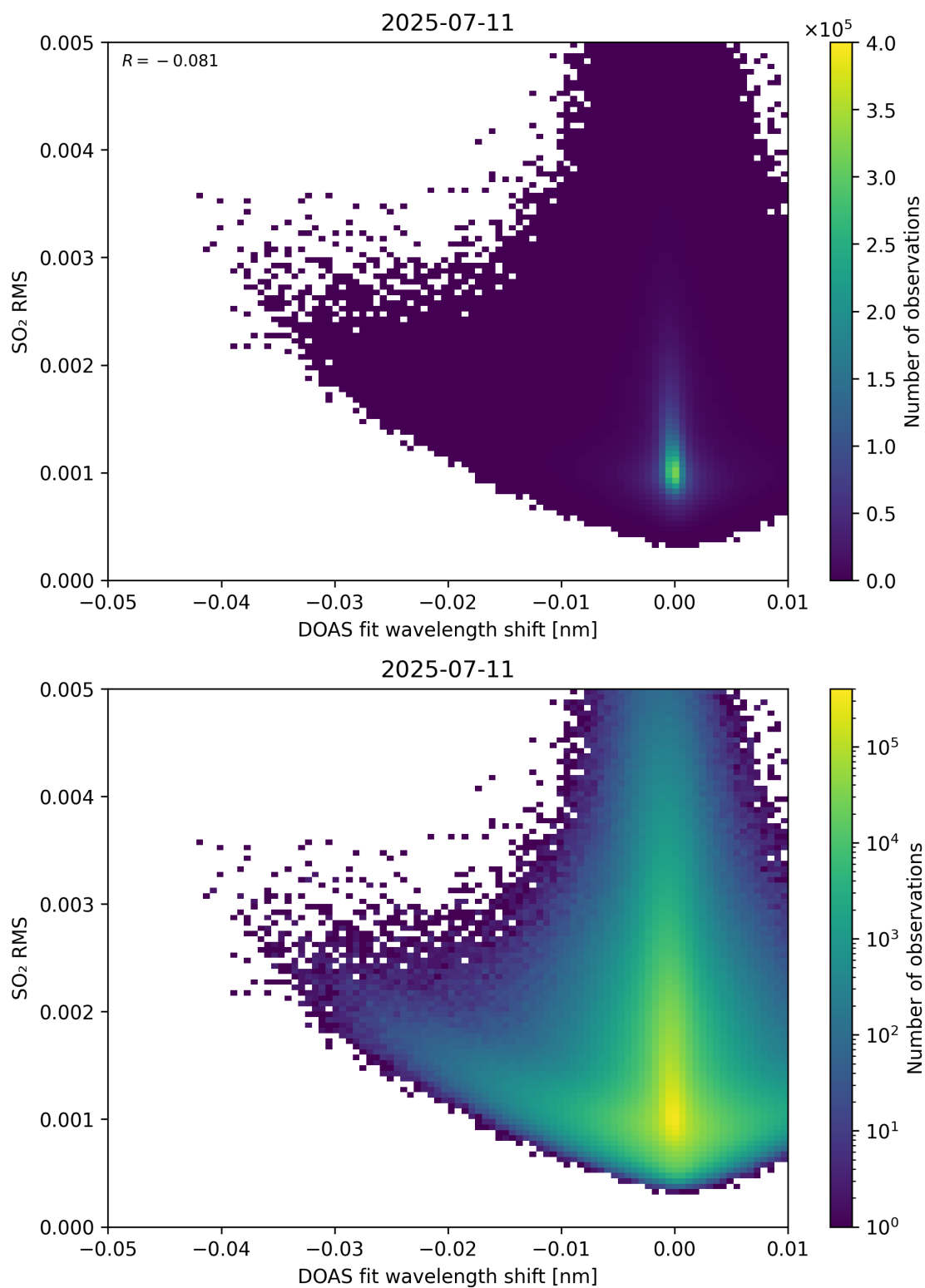
Figure 139: Scatter density plot of “DOAS fit wavelength shift” against “SO 2 RMS” for 2025-07-10 to 2025-07-12.
