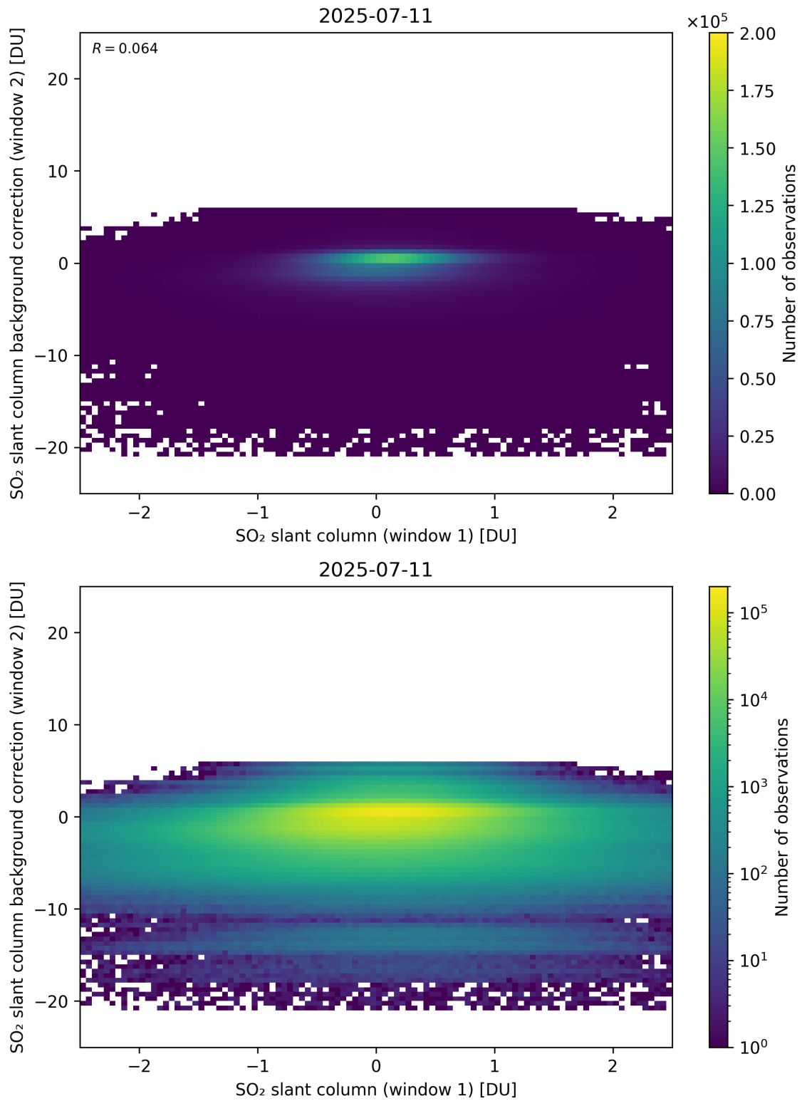
Figure 263: Scatter density plot of “SO 2 slant column (window 1)” against “SO 2 slant column background correction (window 2)” for 2025-07-10 to 2025-07-12.
