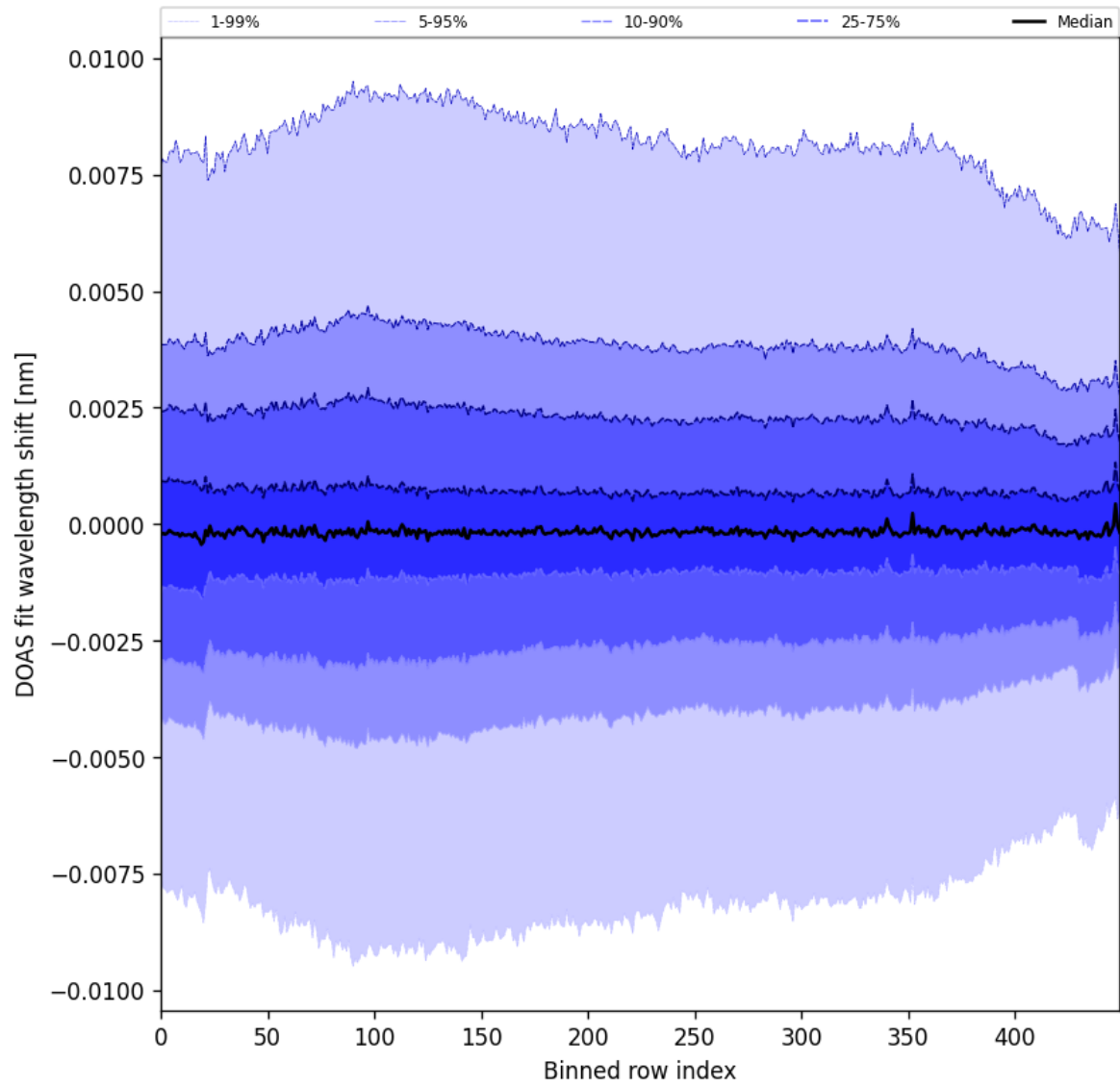
Figure 102: Along track statistics of “DOAS fit wavelength shift” for 2025-07-10 to 2025-07-12
