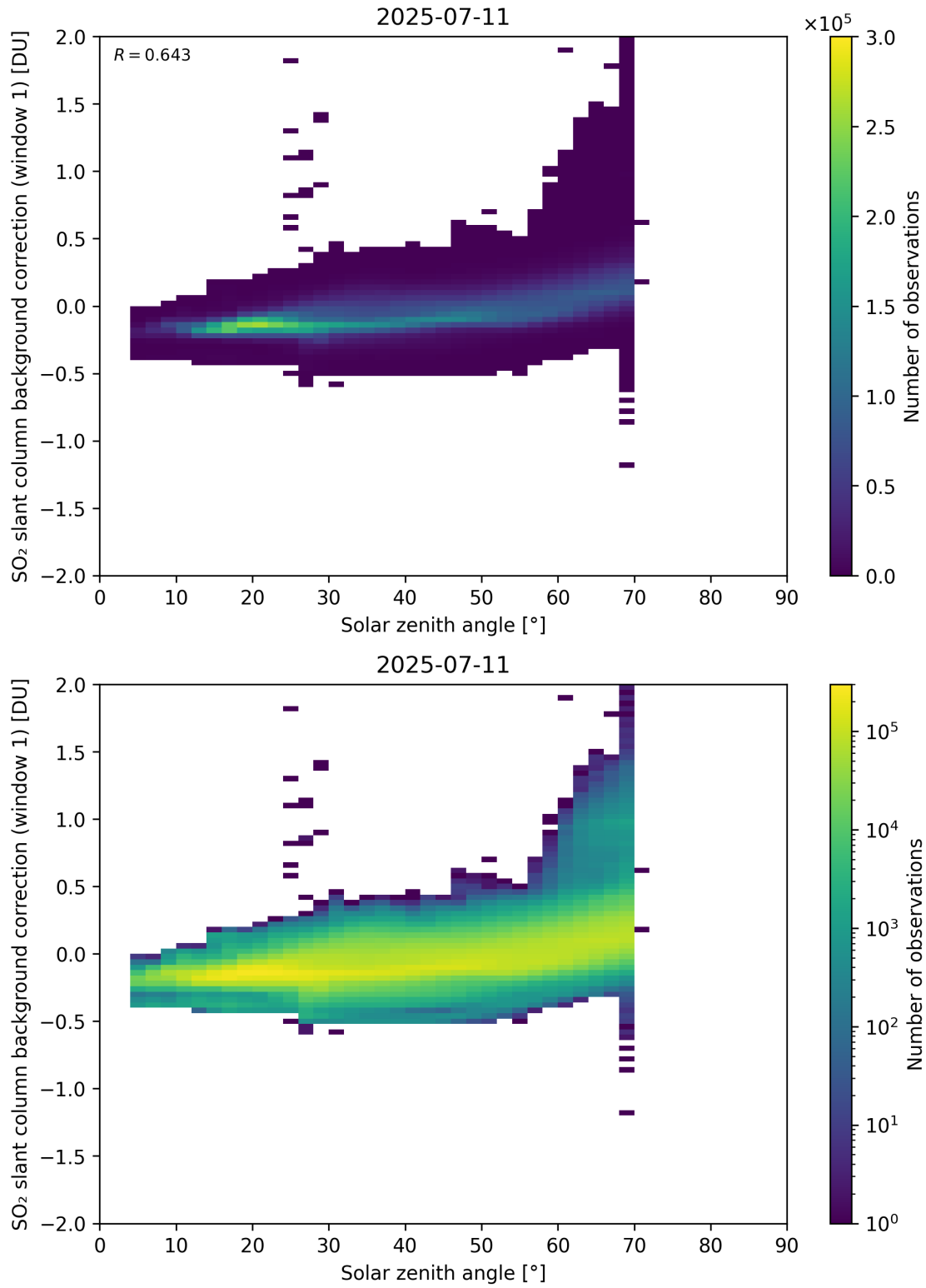
Figure 171: Scatter density plot of “Solar zenith angle” against “SO 2 slant column background correction (window 1)” for 2025-07-10 to 2025-07-12.
