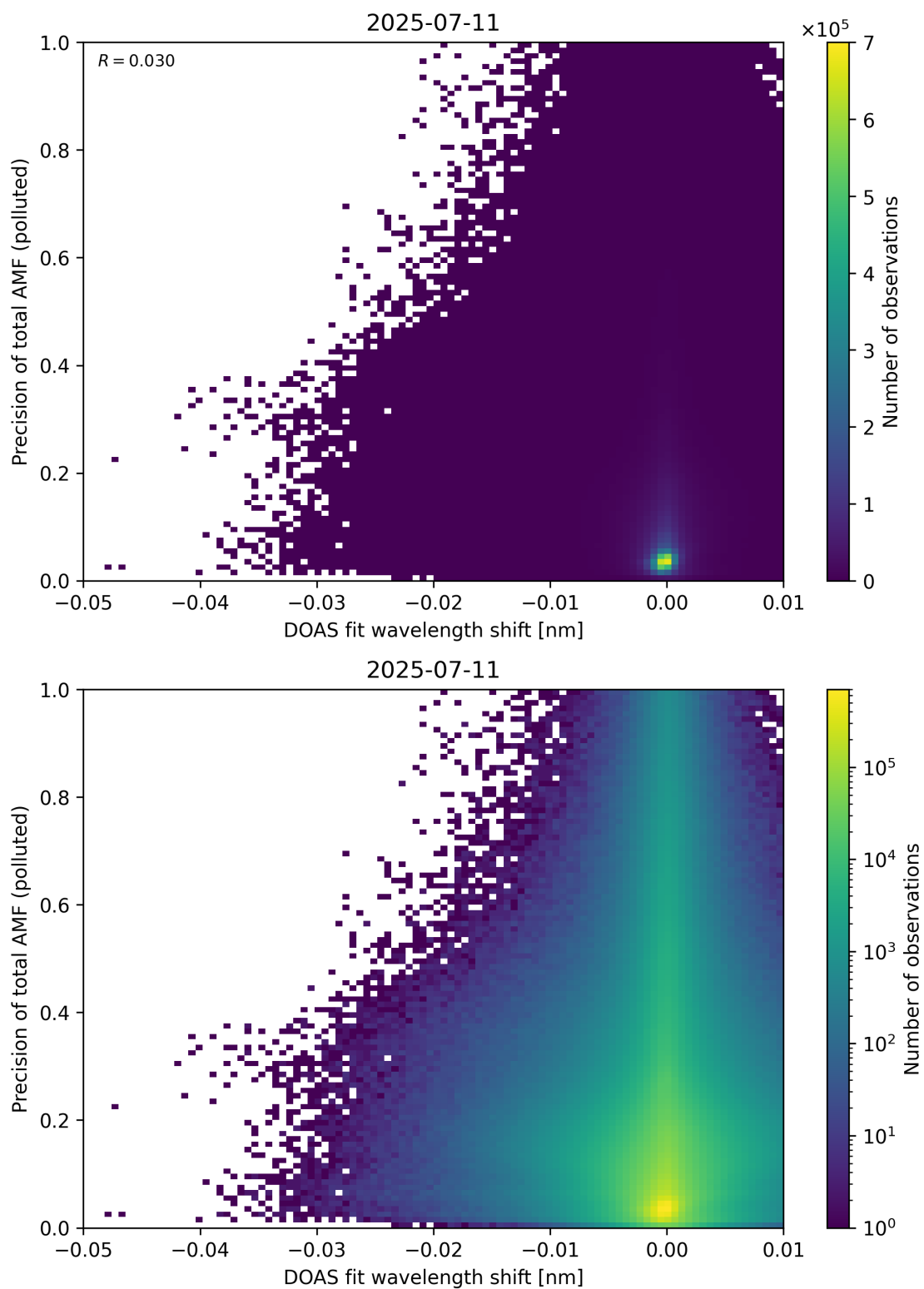
Figure 142: Scatter density plot of “DOAS fit wavelength shift” against “Precision of total AMF (polluted)” for 2025-07-10 to 2025-07-12.
