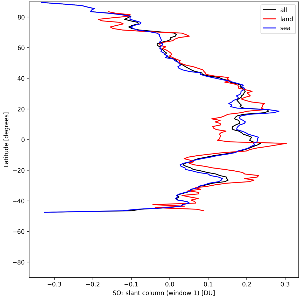
Figure 37: Zonal average of “SO 2 slant column (window 1)” for 2025-07-10 to 2025-07-12.
