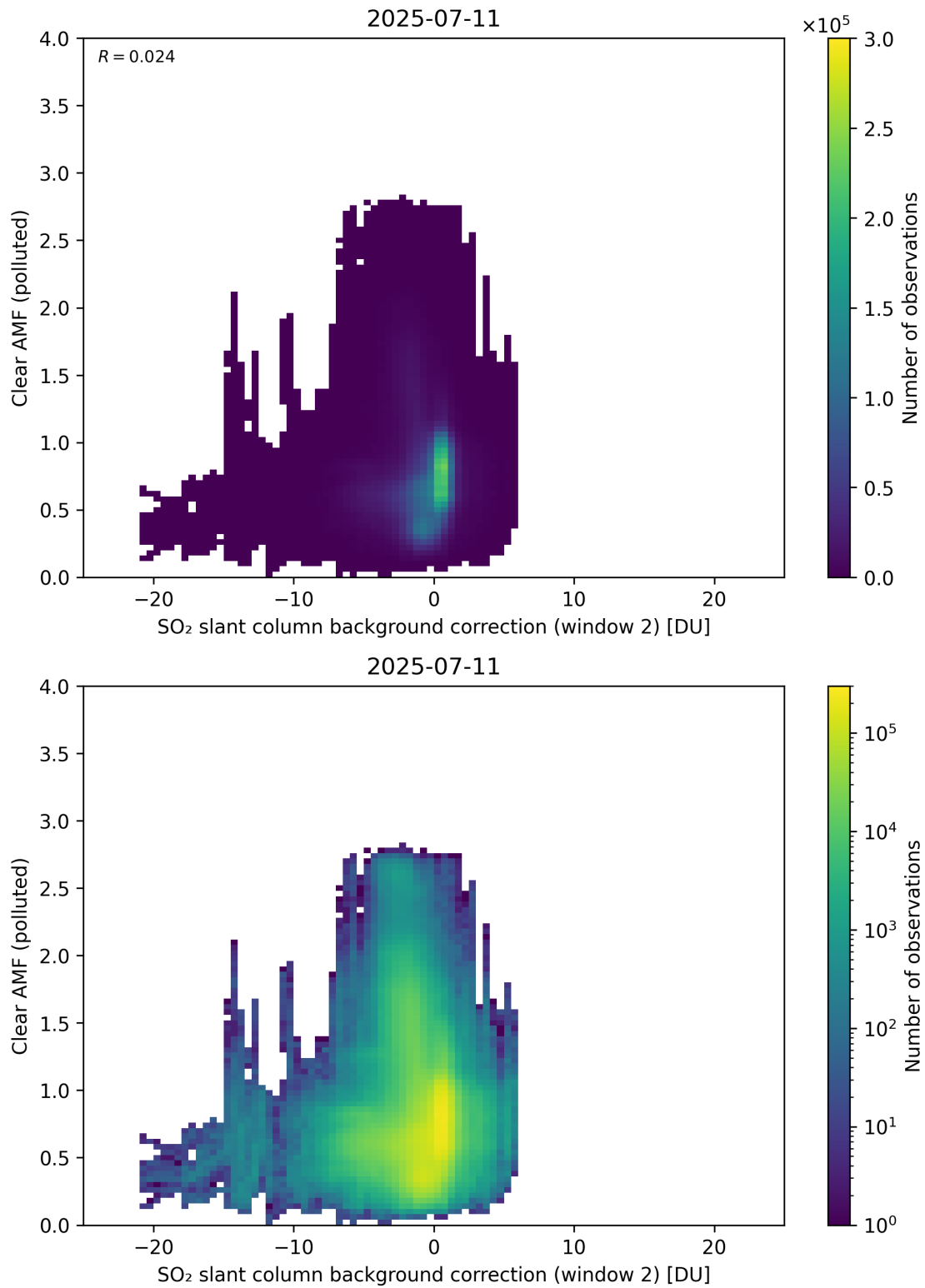
Figure 126: Scatter density plot of “SO 2 slant column background correction (window 2)” against “Clear AMF (polluted)” for 2025-07-10 to 2025-07-12.
