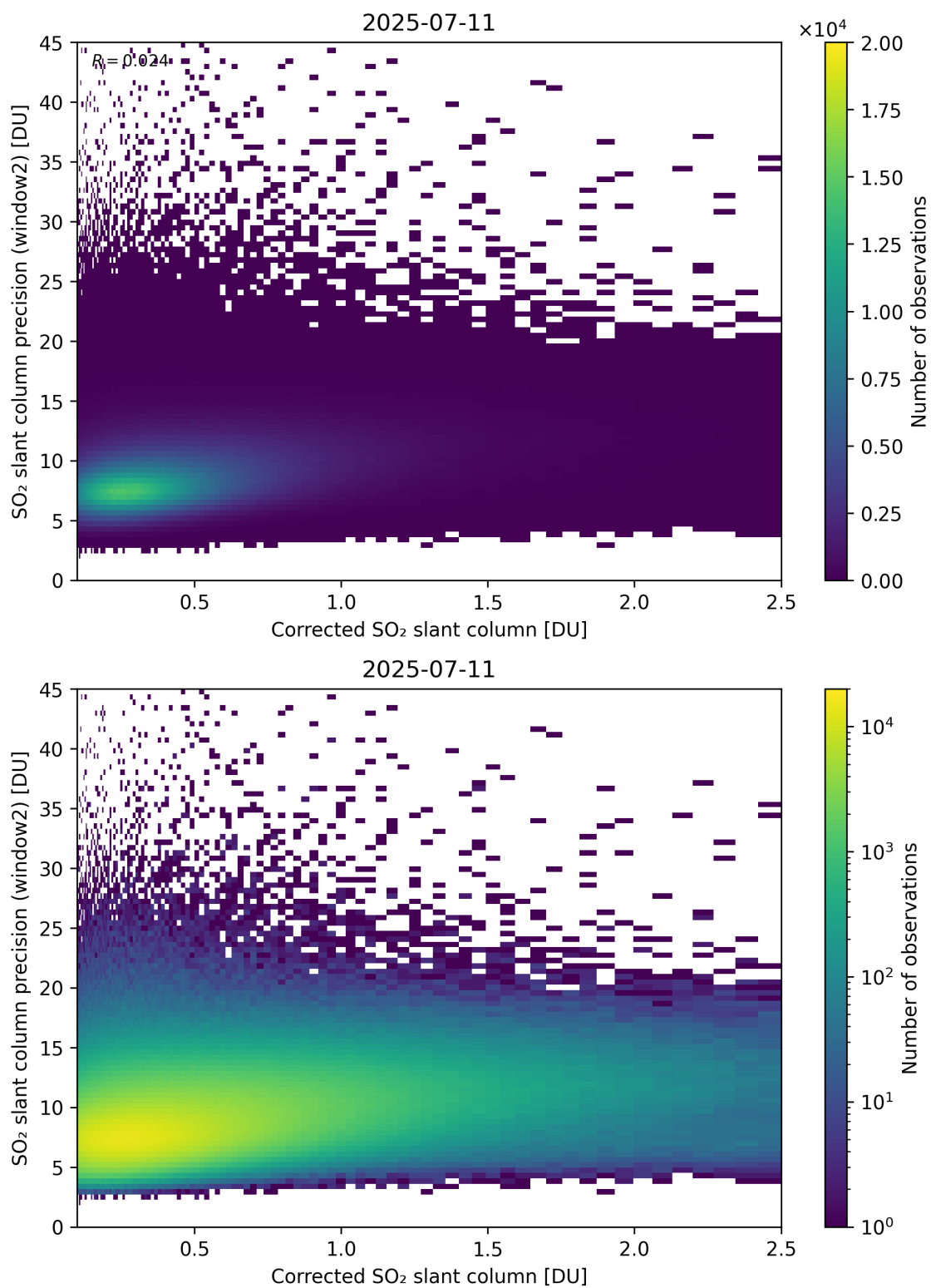
Figure 239: Scatter density plot of “Corrected SO 2 slant column” against “SO 2 slant column precision (window2)” for 2025-07-10 to 2025-07-12.
