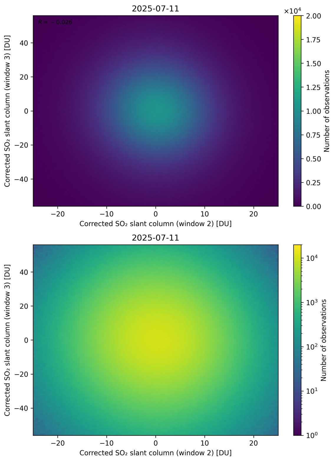
Figure 250: Scatter density plot of “Corrected SO 2 slant column (window 2)” against “Corrected SO 2 slant column (window 3)” for 2025-07-10 to 2025-07-12.
