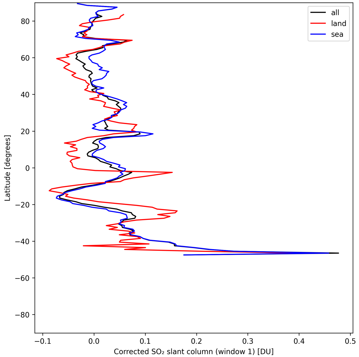
Figure 39: Zonal average of “Corrected SO 2 slant column (window 1)” for 2025-07-10 to 2025-07-12.
