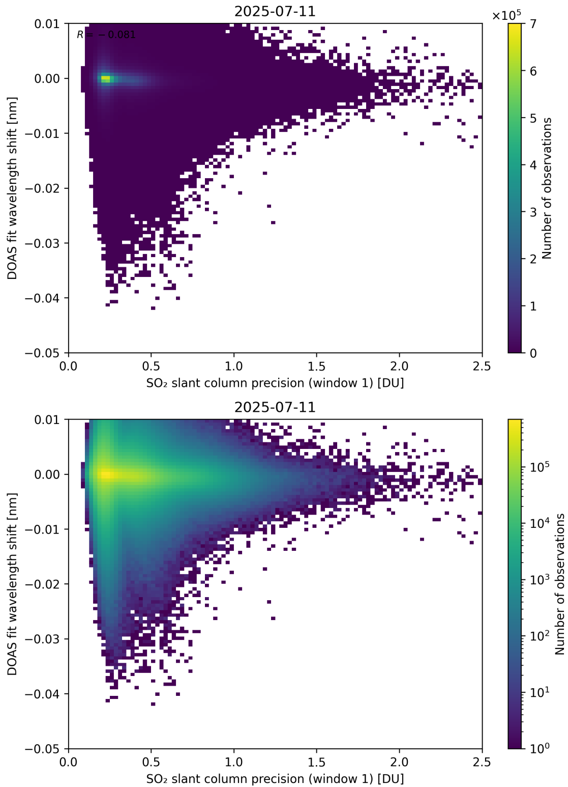
Figure 271: Scatter density plot of “SO 2 slant column precision (window 1)” against “DOAS fit wavelength shift” for 2025-07-10 to 2025-07-12.
