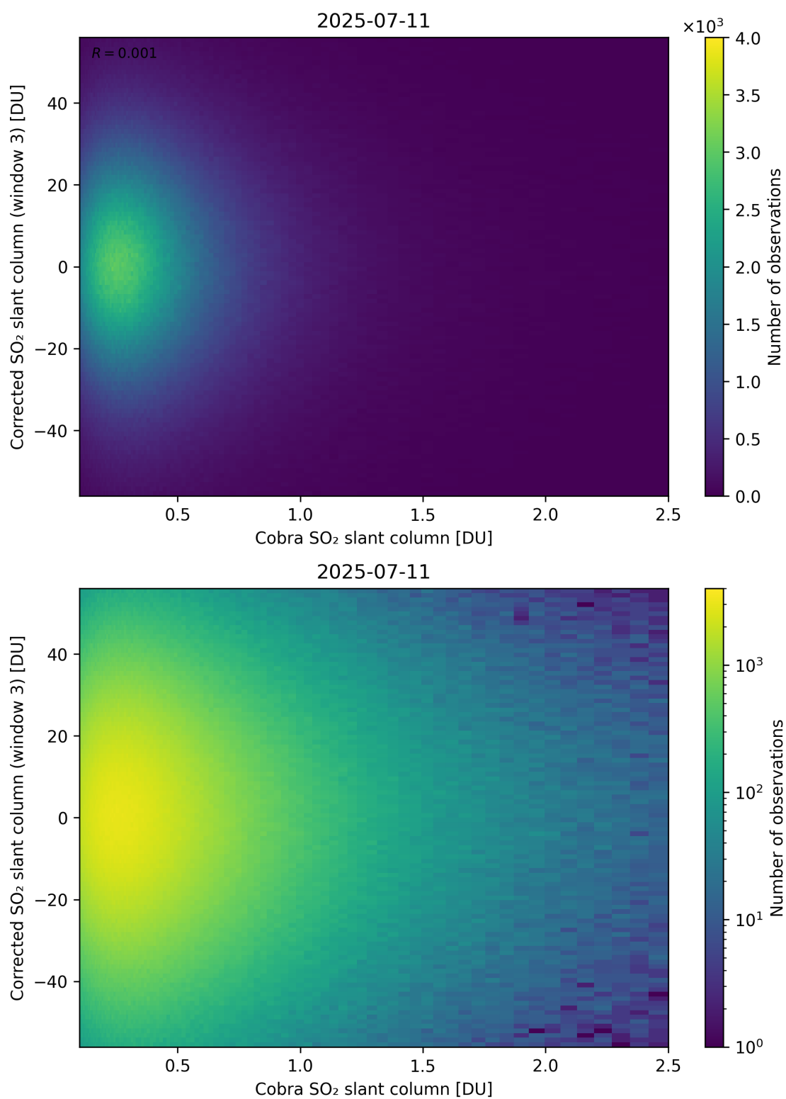
Figure 218: Scatter density plot of “Cobra SO 2 slant column” against “Corrected SO 2 slant column (window 3)” for 2025-07-10 to 2025-07-12.
