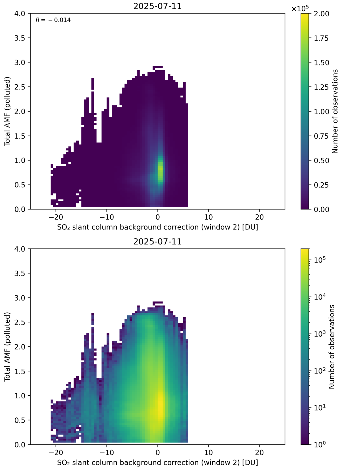
Figure 130: Scatter density plot of “SO 2 slant column background correction (window 2)” against “Total AMF (polluted)” for 2025-07-10 to 2025-07-12.
