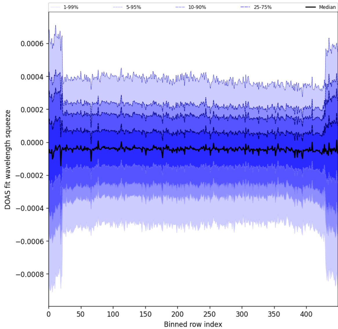
Figure 103: Along track statistics of “DOAS fit wavelength squeeze” for 2025-07-10 to 2025-07-12
