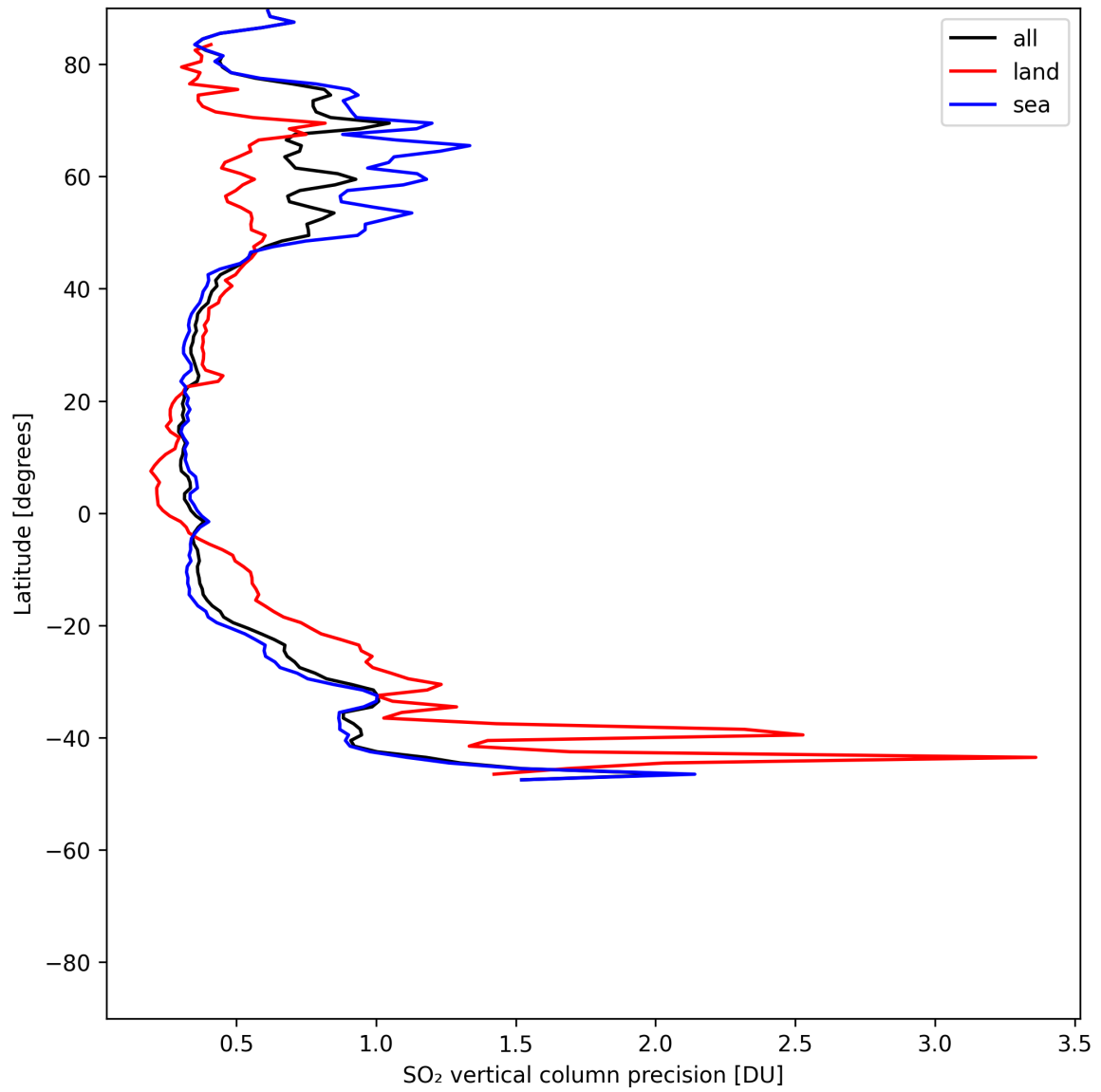
Figure 33: Zonal average of “SO 2 vertical column precision” for 2025-07-10 to 2025-07-12.
