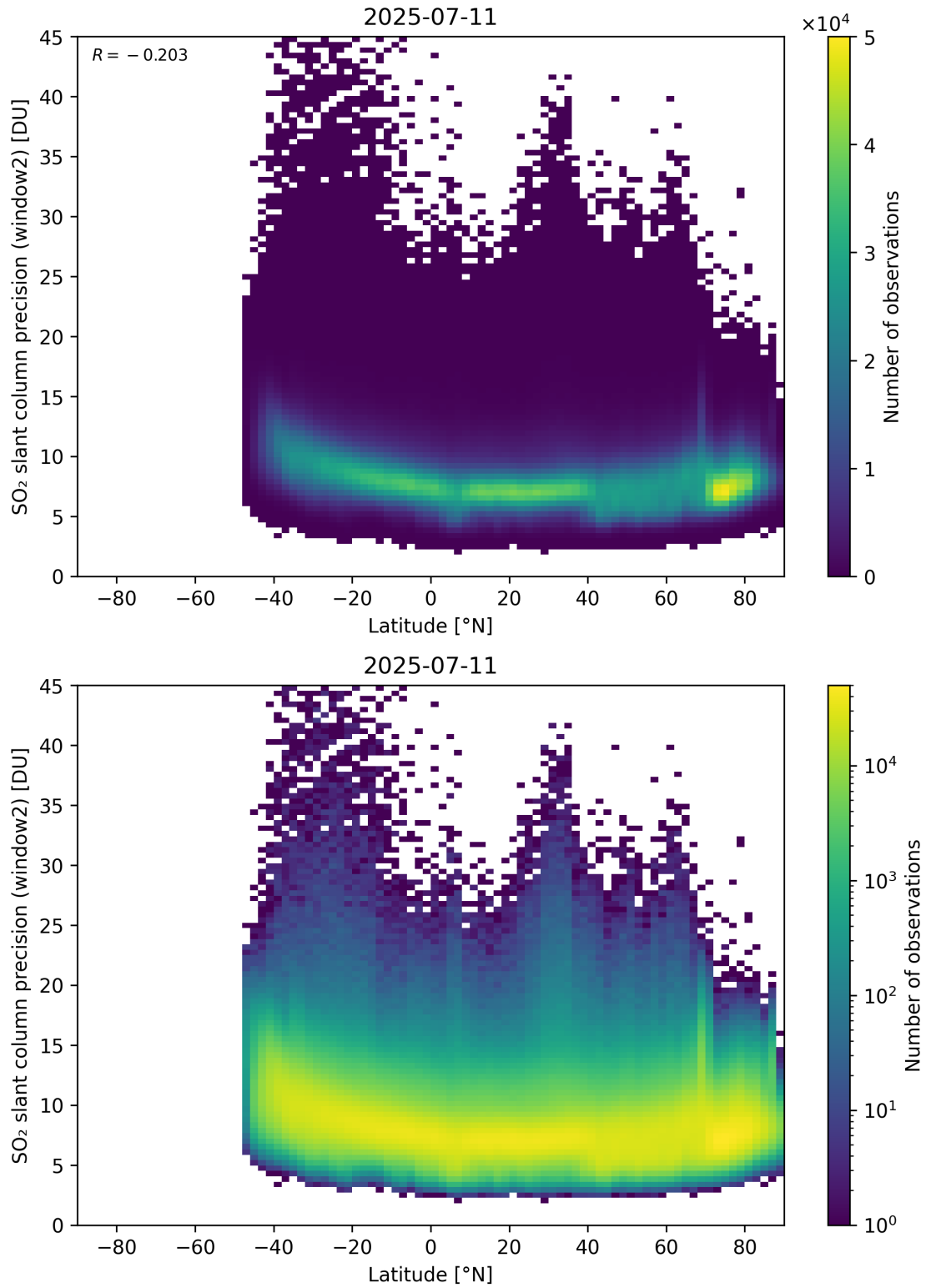
Figure 164: Scatter density plot of “Latitude” against “SO 2 slant column precision (window2)” for 2025-07-10 to 2025-07-12.
