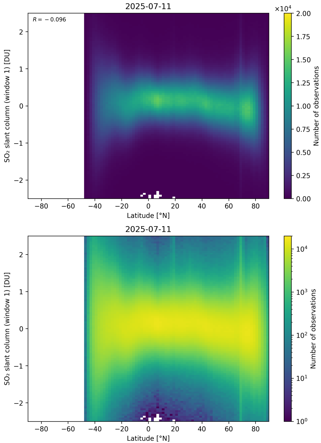
Figure 162: Scatter density plot of “Latitude” against “SO 2 slant column (window 1)” for 2025-07-10 to 2025-07-12.
