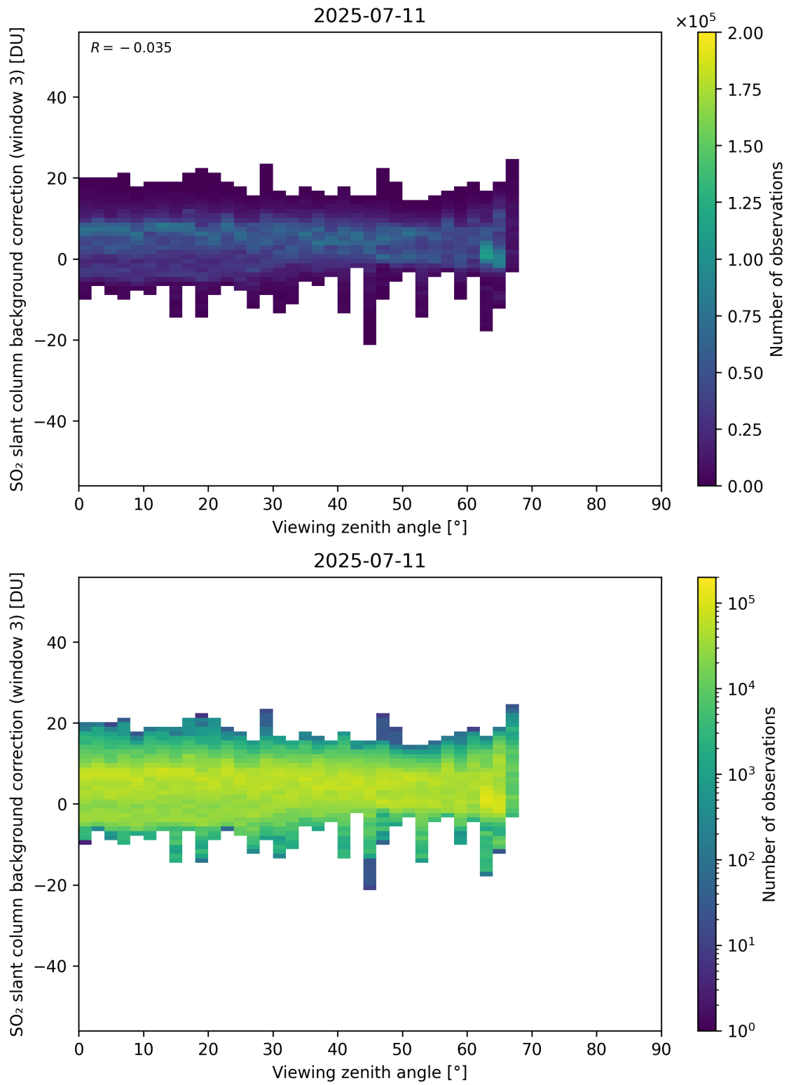
Figure 364: Scatter density plot of “Viewing zenith angle” against “SO 2 slant column background correction (window 3)” for 2025-07-10 to 2025-07-12.
