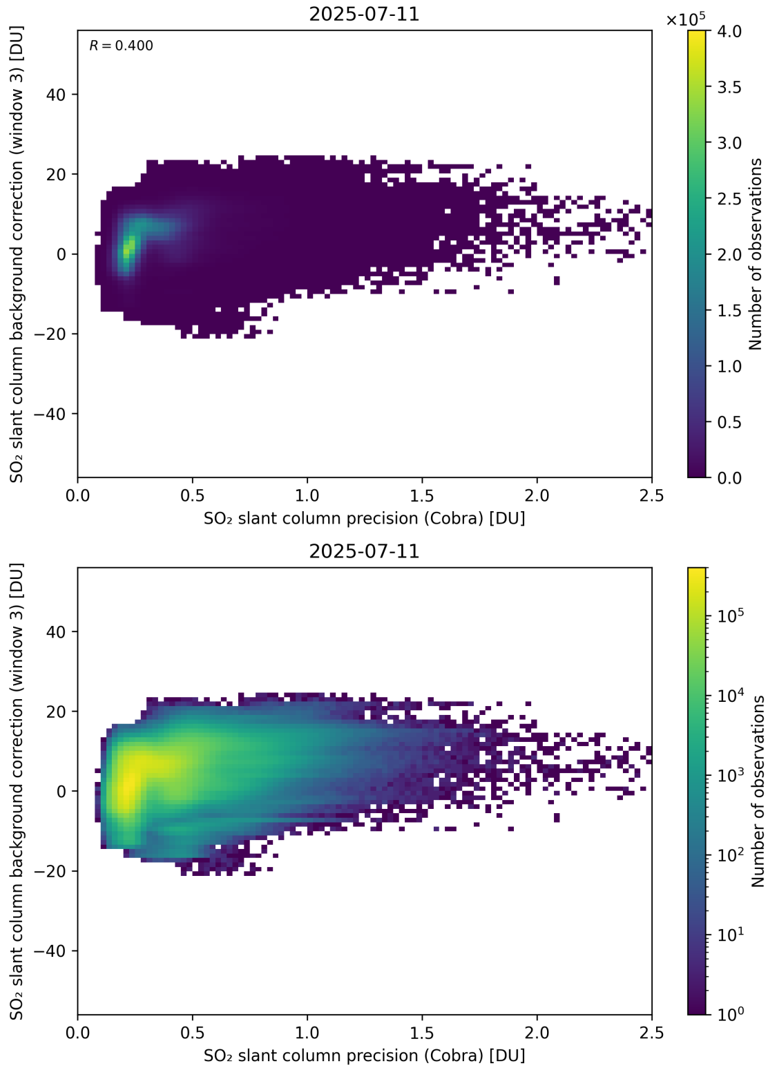
Figure 201: Scatter density plot of “SO 2 slant column precision (Cobra)” against “SO 2 slant column background correction (window 3)” for 2025-07-10 to 2025-07-12.
