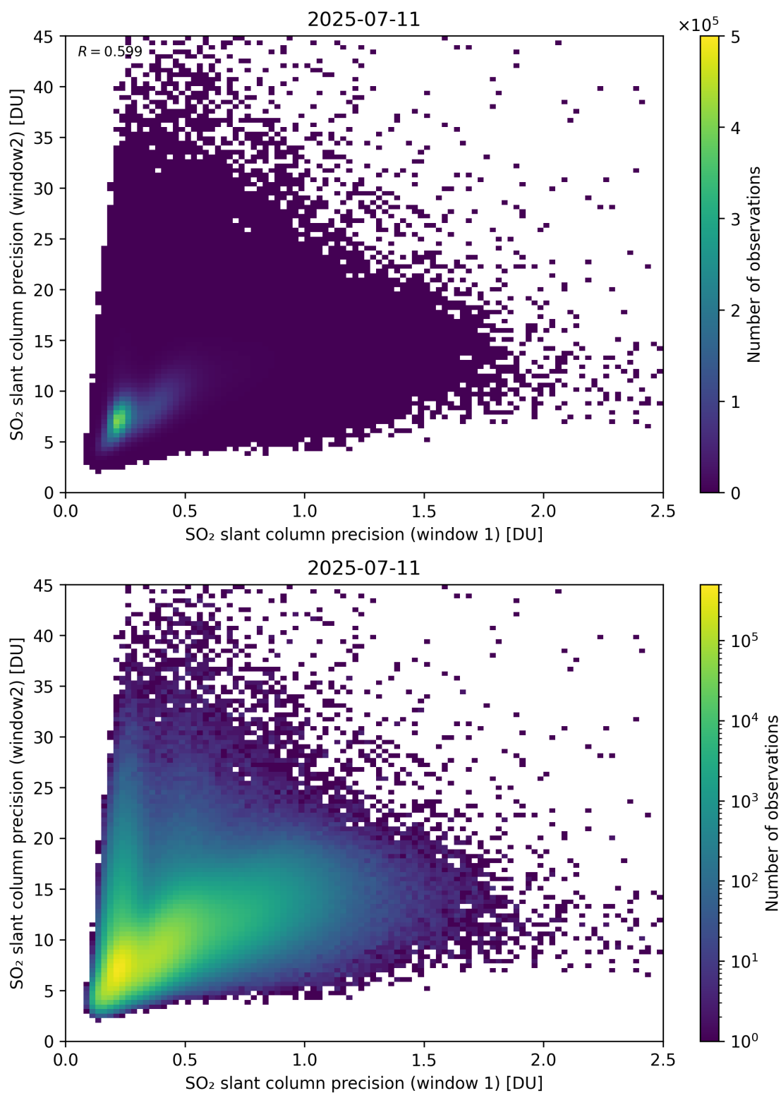
Figure 277: Scatter density plot of “SO 2 slant column precision (window 1)” against “SO 2 slant column precision (window 2)” for 2025-07-10 to 2025-07-12.
