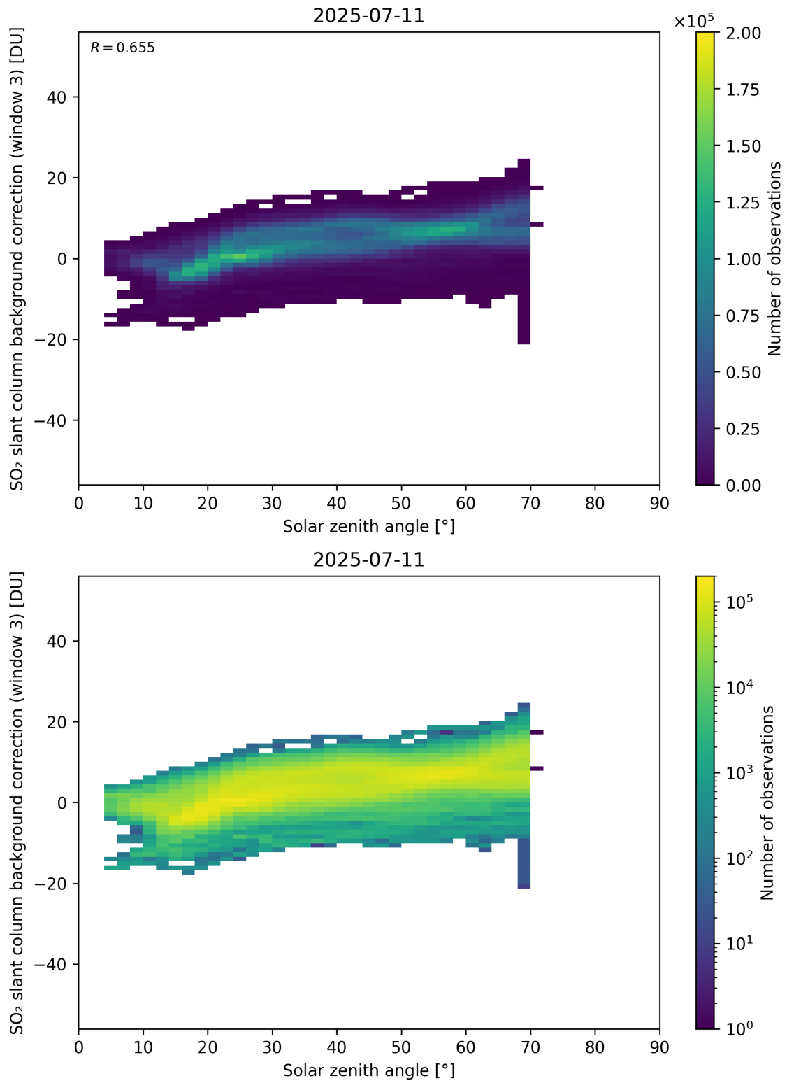
Figure 173: Scatter density plot of “Solar zenith angle” against “SO 2 slant column background correction (window 3)” for 2025-07-10 to 2025-07-12.
