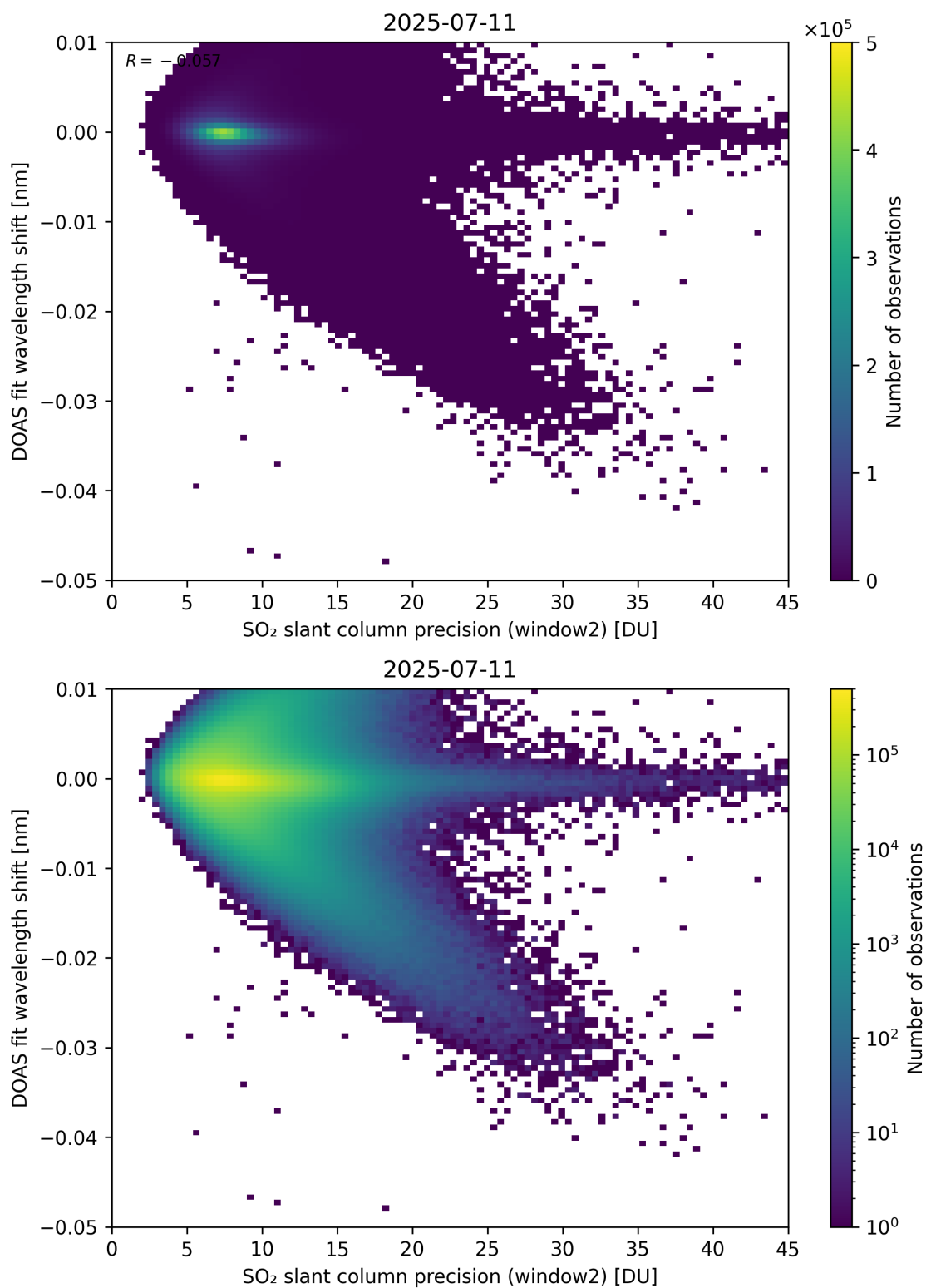
Figure 293: Scatter density plot of “SO 2 slant column precision (window2)” against “DOAS fit wavelength shift” for 2025-07-10 to 2025-07-12.
