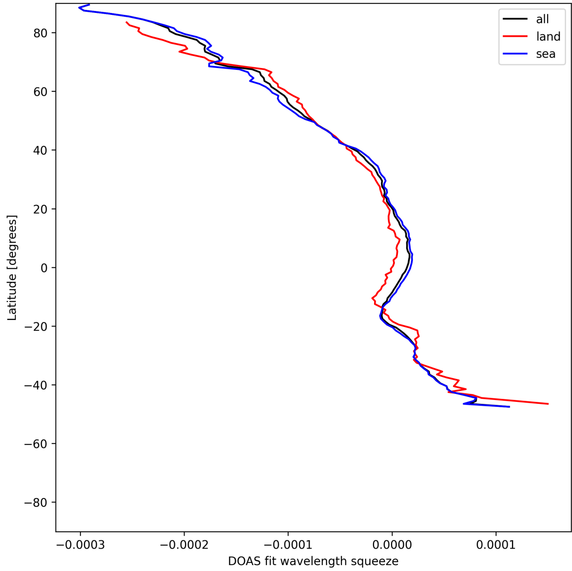
Figure 51: Zonal average of “DOAS fit wavelength squeeze” for 2025-07-10 to 2025-07-12.
