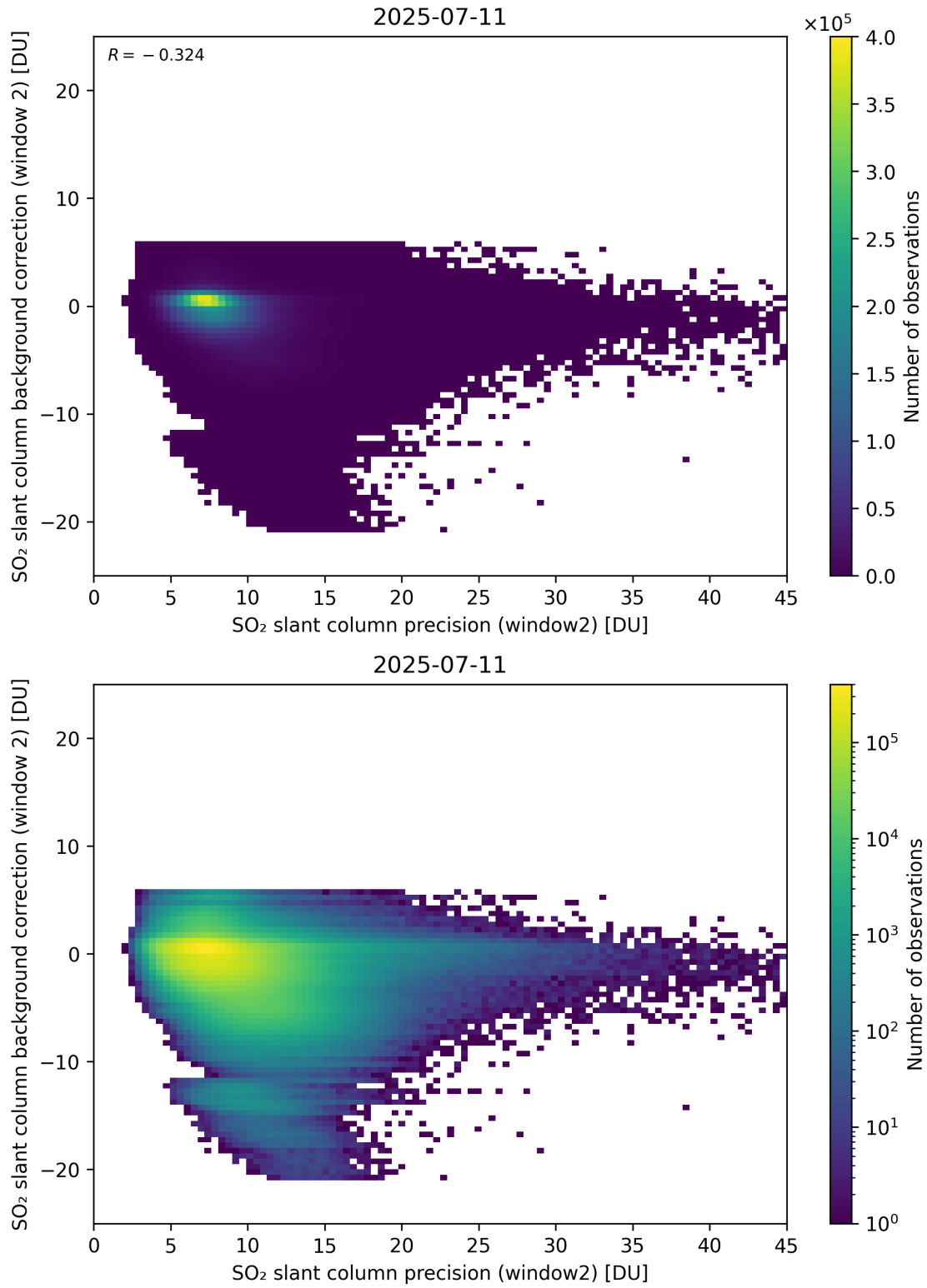
Figure 291: Scatter density plot of “SO 2 slant column precision (window2)” against “SO 2 slant column background correction (window 2)” for 2025-07-10 to 2025-07-12.
