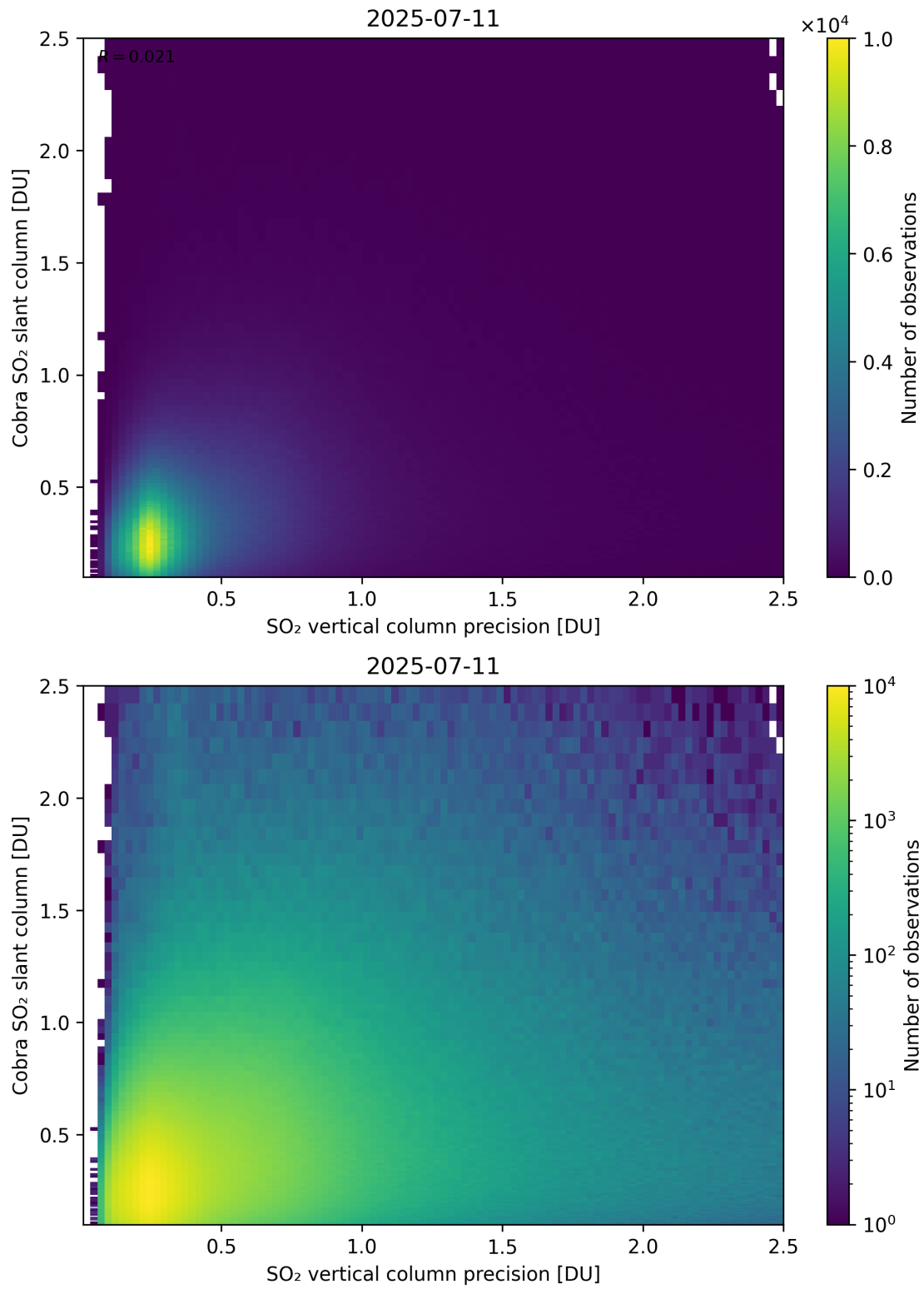
Figure 336: Scatter density plot of “SO 2 vertical column precision” against “Cobra SO 2 slant column” for 2025-07-10 to 2025-07-12.
