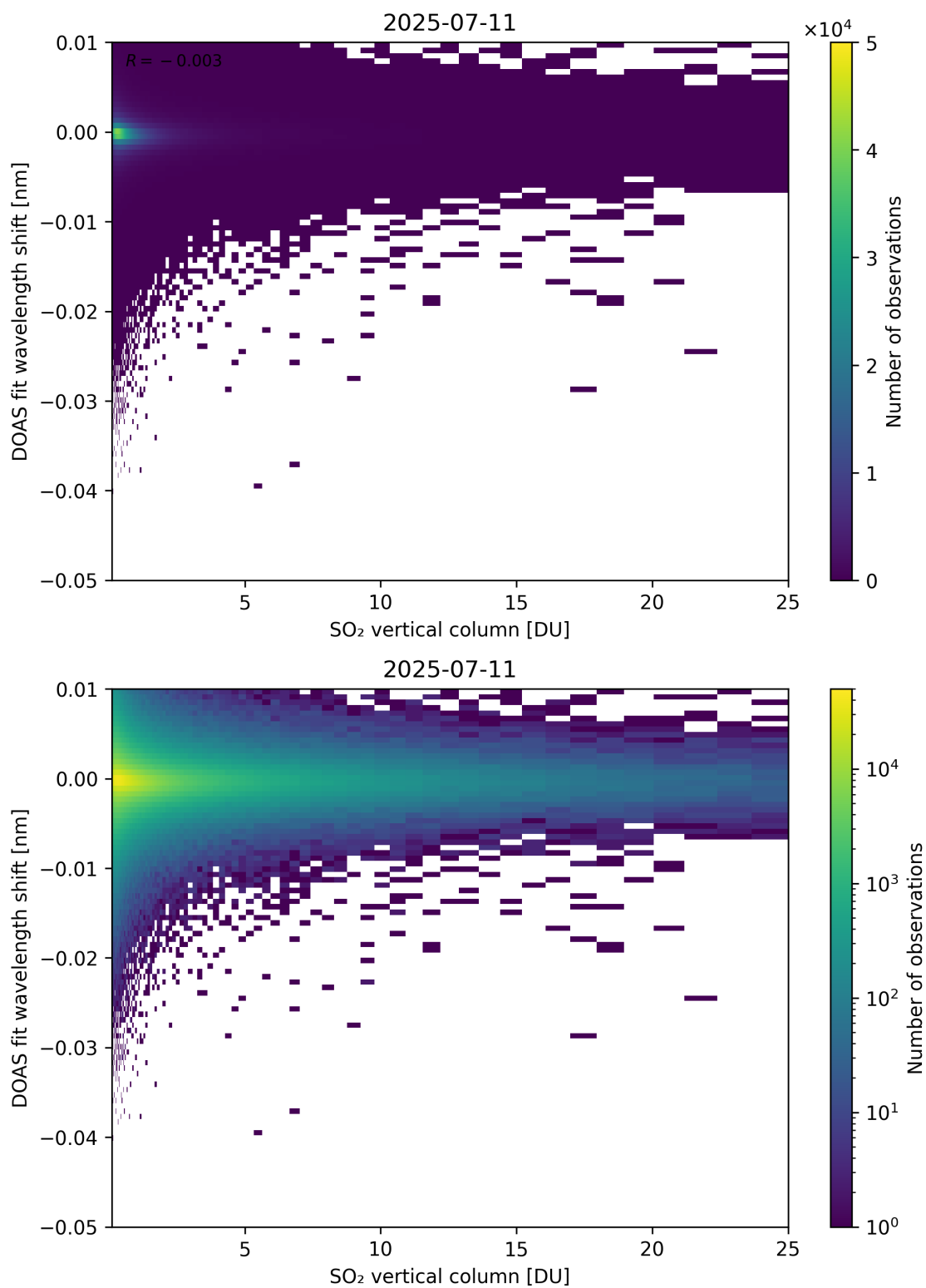
Figure 326: Scatter density plot of “SO 2 vertical column” against “DOAS fit wavelength shift” for 2025-07-10 to 2025-07-12.
