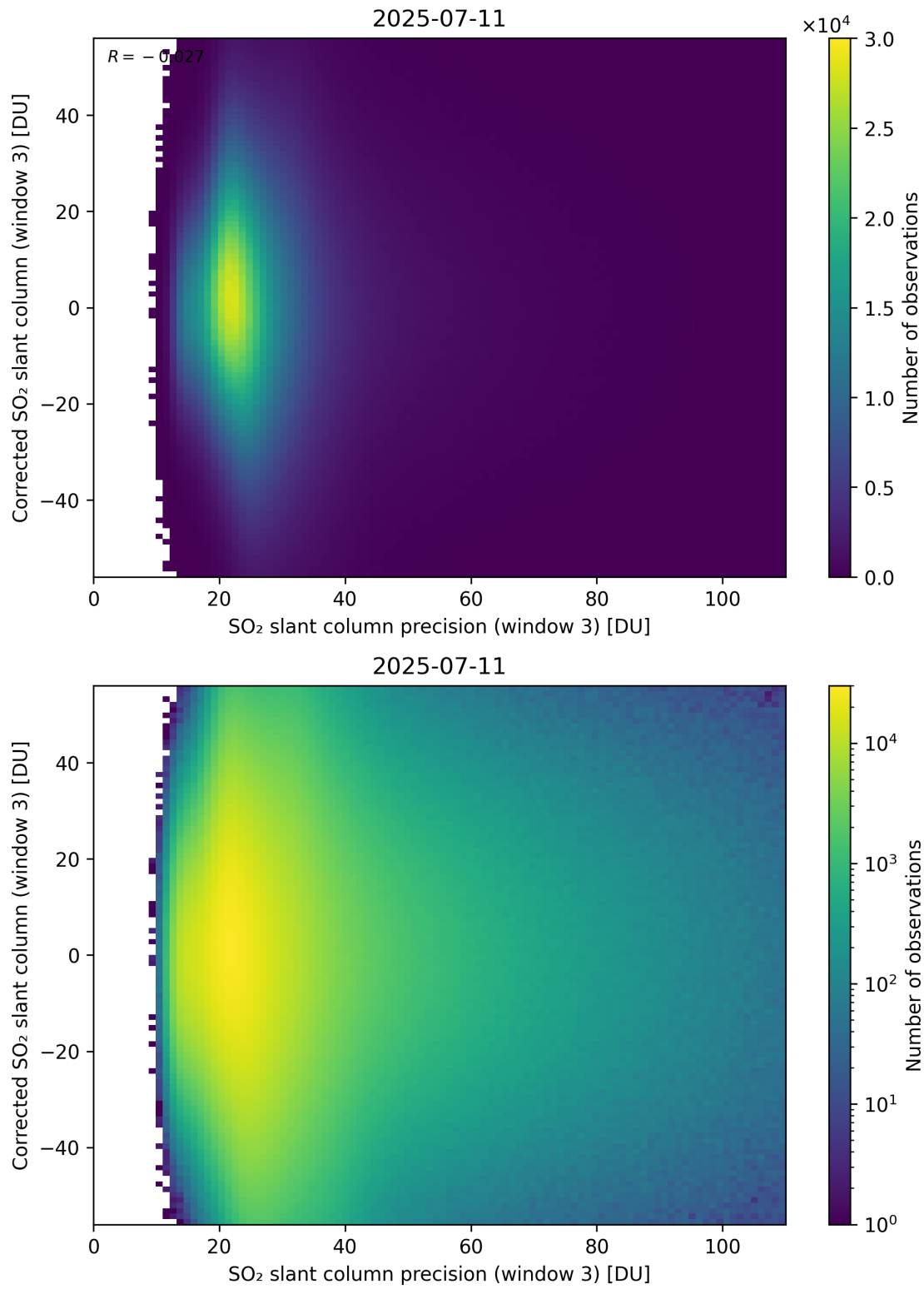
Figure 312: Scatter density plot of “SO 2 slant column precision (window 3)” against “Corrected SO 2 slant column (window 3)” for 2025-07-10 to 2025-07-12.
