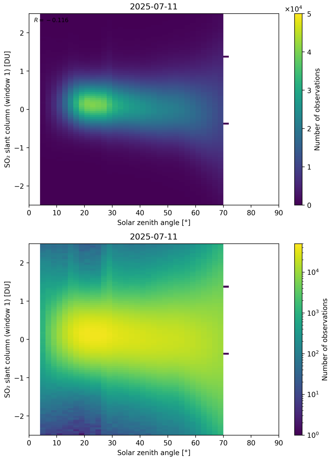
Figure 184: Scatter density plot of “Solar zenith angle” against “SO 2 slant column (window 1)” for 2025-07-10 to 2025-07-12.
