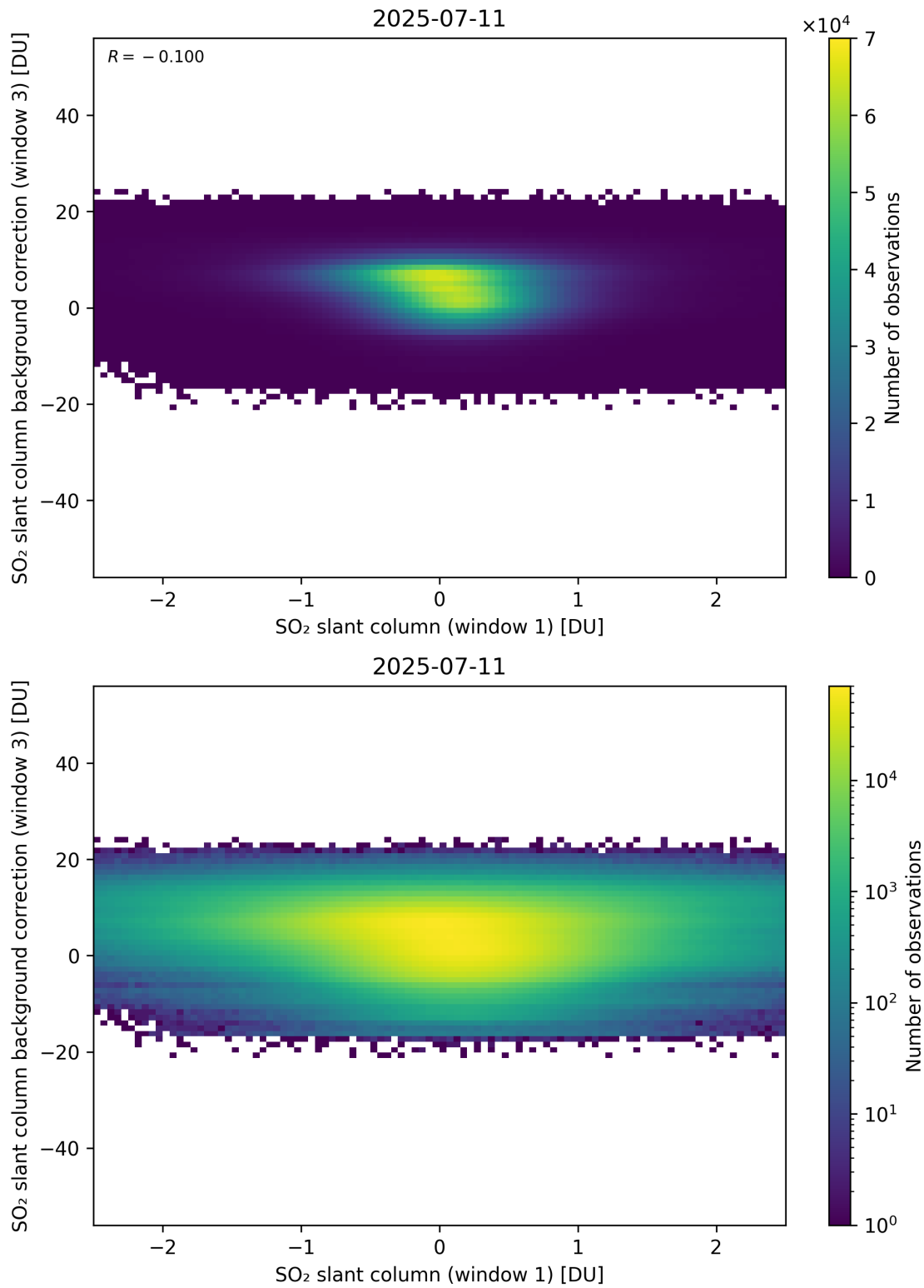
Figure 264: Scatter density plot of “SO 2 slant column (window 1)” against “SO 2 slant column background correction (window 3)” for 2025-07-10 to 2025-07-12.
