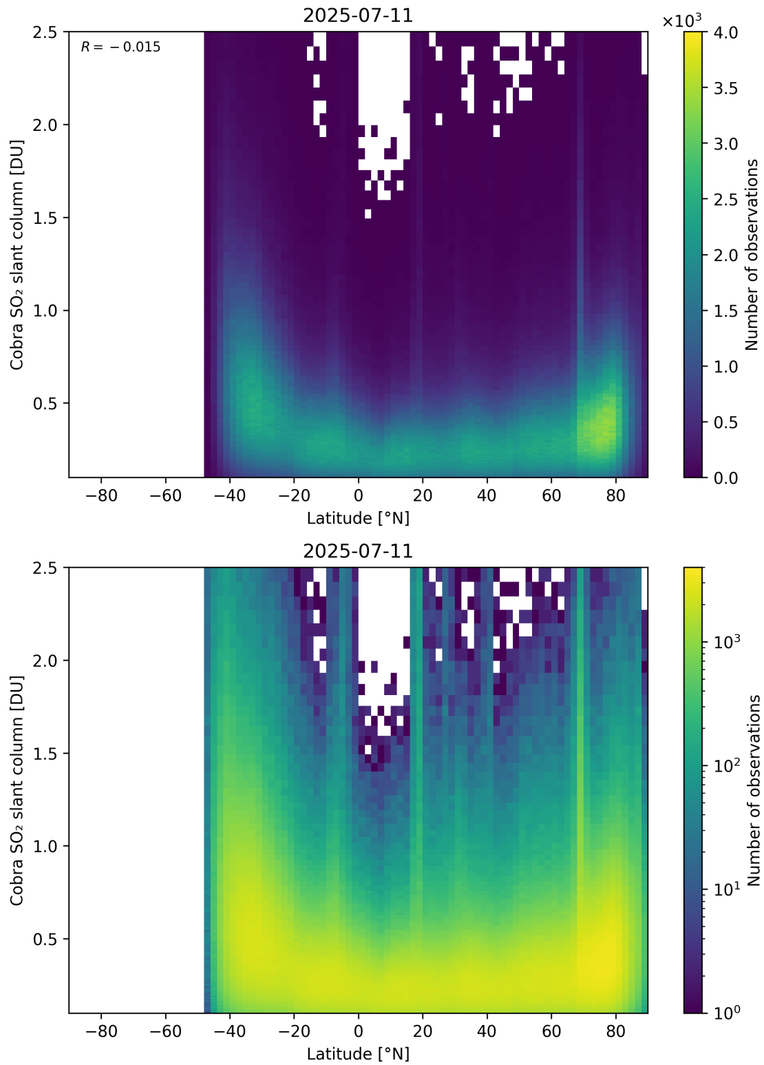
Figure 157: Scatter density plot of “Latitude” against “Cobra SO 2 slant column” for 2025-07-10 to 2025-07-12.
