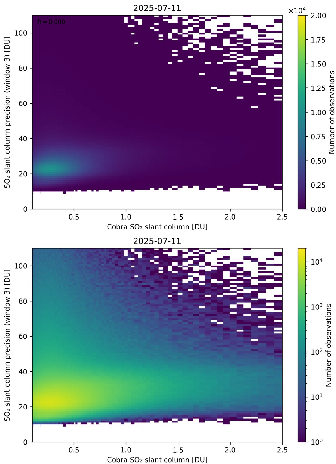
Figure 223: Scatter density plot of “Cobra SO 2 slant column” against “SO 2 slant column precision (window 3)” for 2025-07-10 to 2025-07-12.
