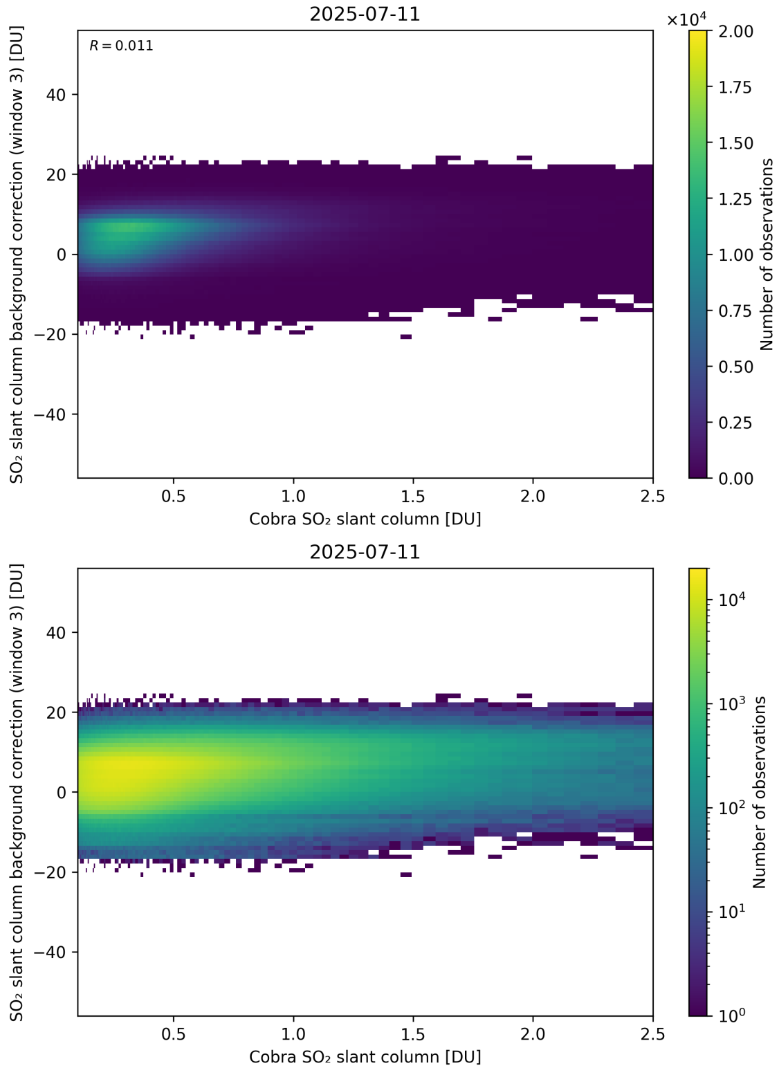
Figure 195: Scatter density plot of “Cobra SO 2 slant column” against “SO 2 slant column background correction (window 3)” for 2025-07-10 to 2025-07-12.
