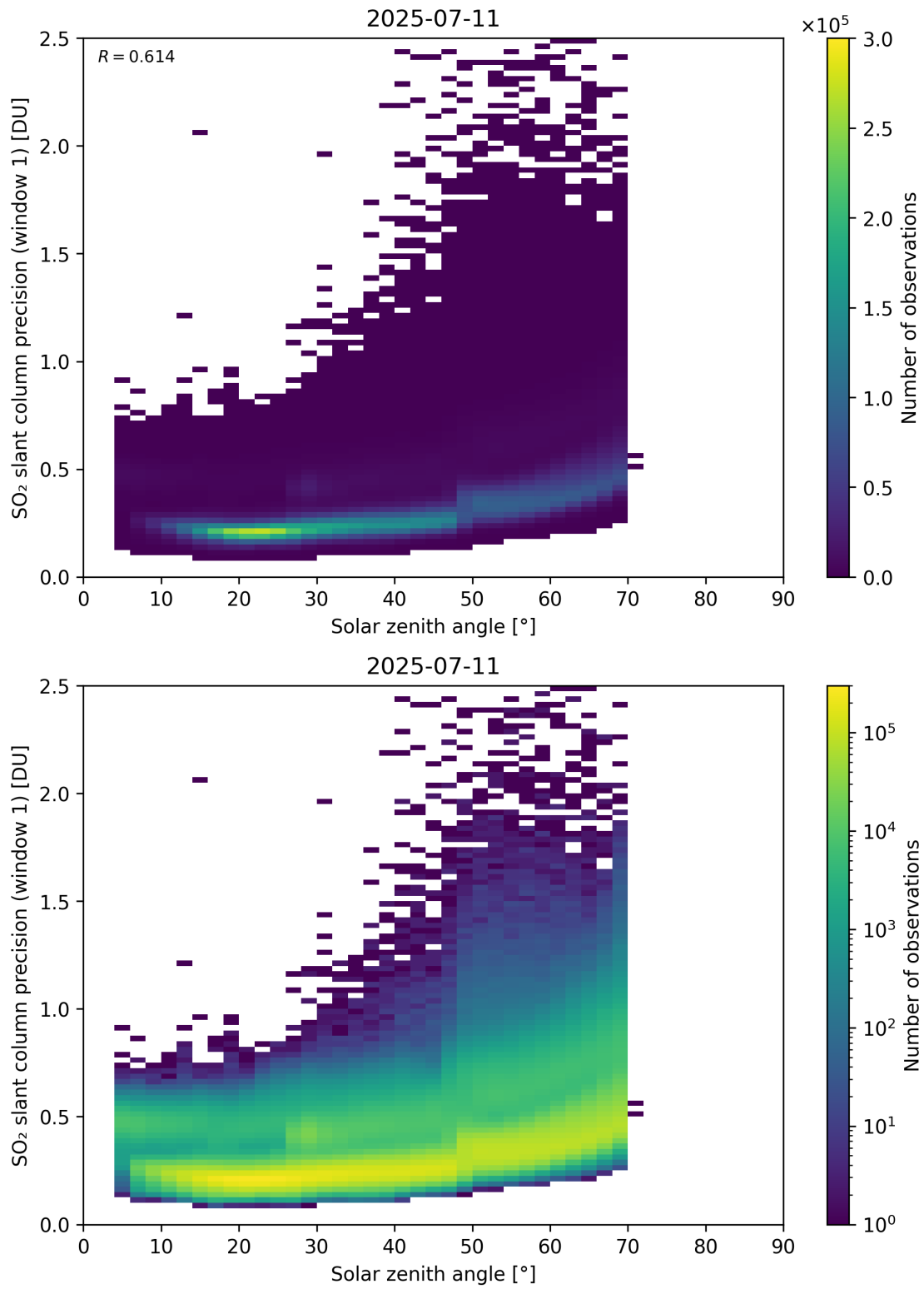
Figure 185: Scatter density plot of “Solar zenith angle” against “SO 2 slant column precision (window 1)” for 2025-07-10 to 2025-07-12.
