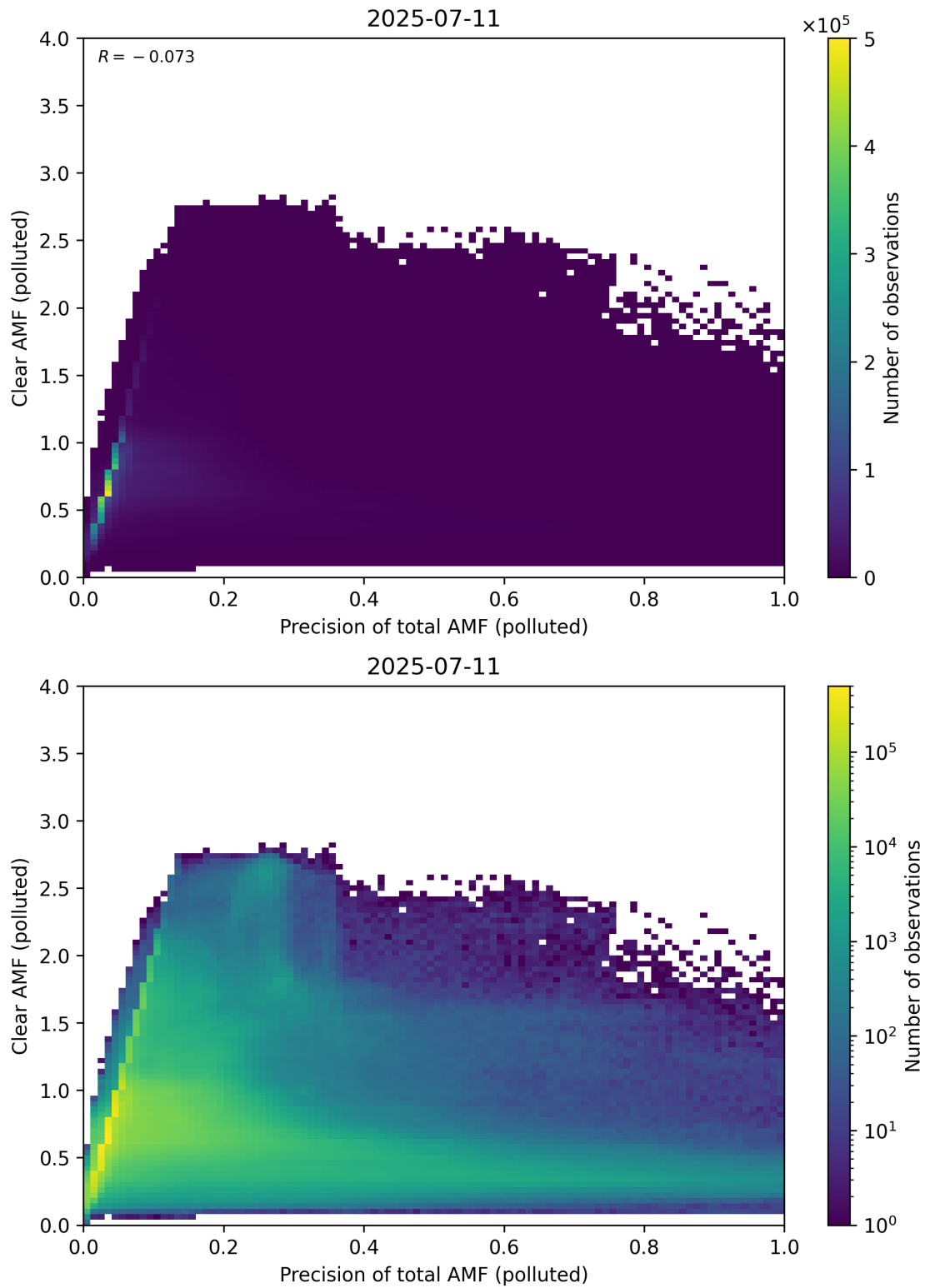
Figure 320: Scatter density plot of “Precision of total AMF (polluted)” against “Clear AMF (polluted)” for 2025-07-10 to 2025-07-12.
