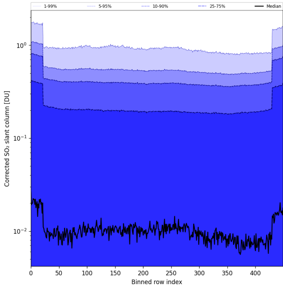
Figure 86: Along track statistics of “Corrected SO 2 slant column” for 2025-07-10 to 2025-07-12
