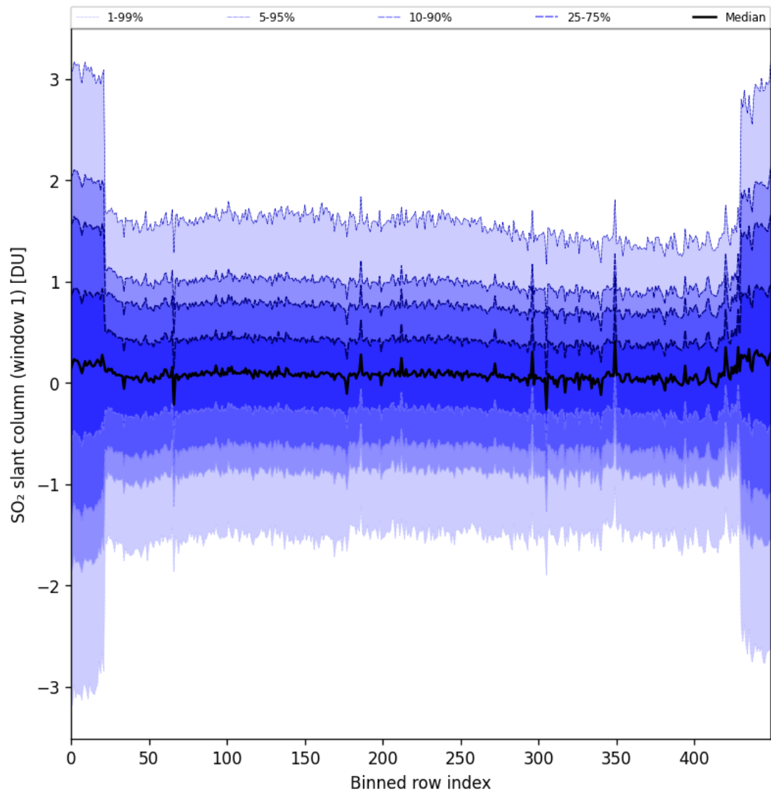
Figure 89: Along track statistics of “SO 2 slant column (window 1)” for 2025-07-10 to 2025-07-12
