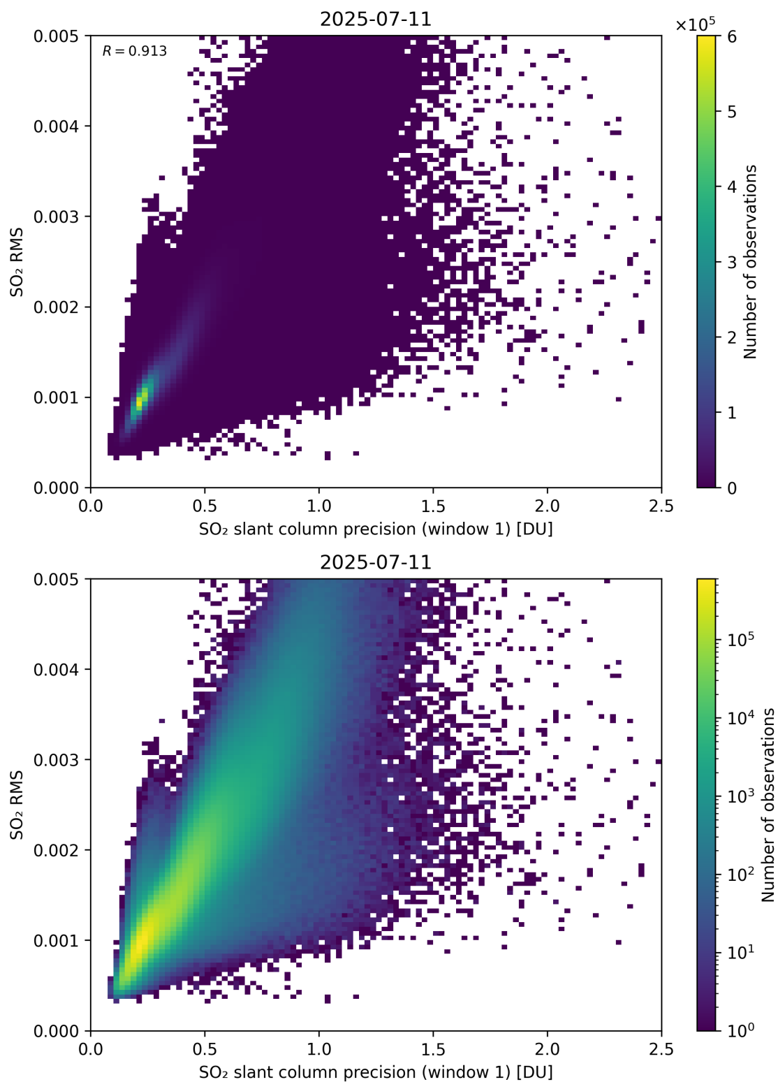
Figure 273: Scatter density plot of “SO 2 slant column precision (window 1)” against “SO 2 RMS” for 2025-07-10 to 2025-07-12.
