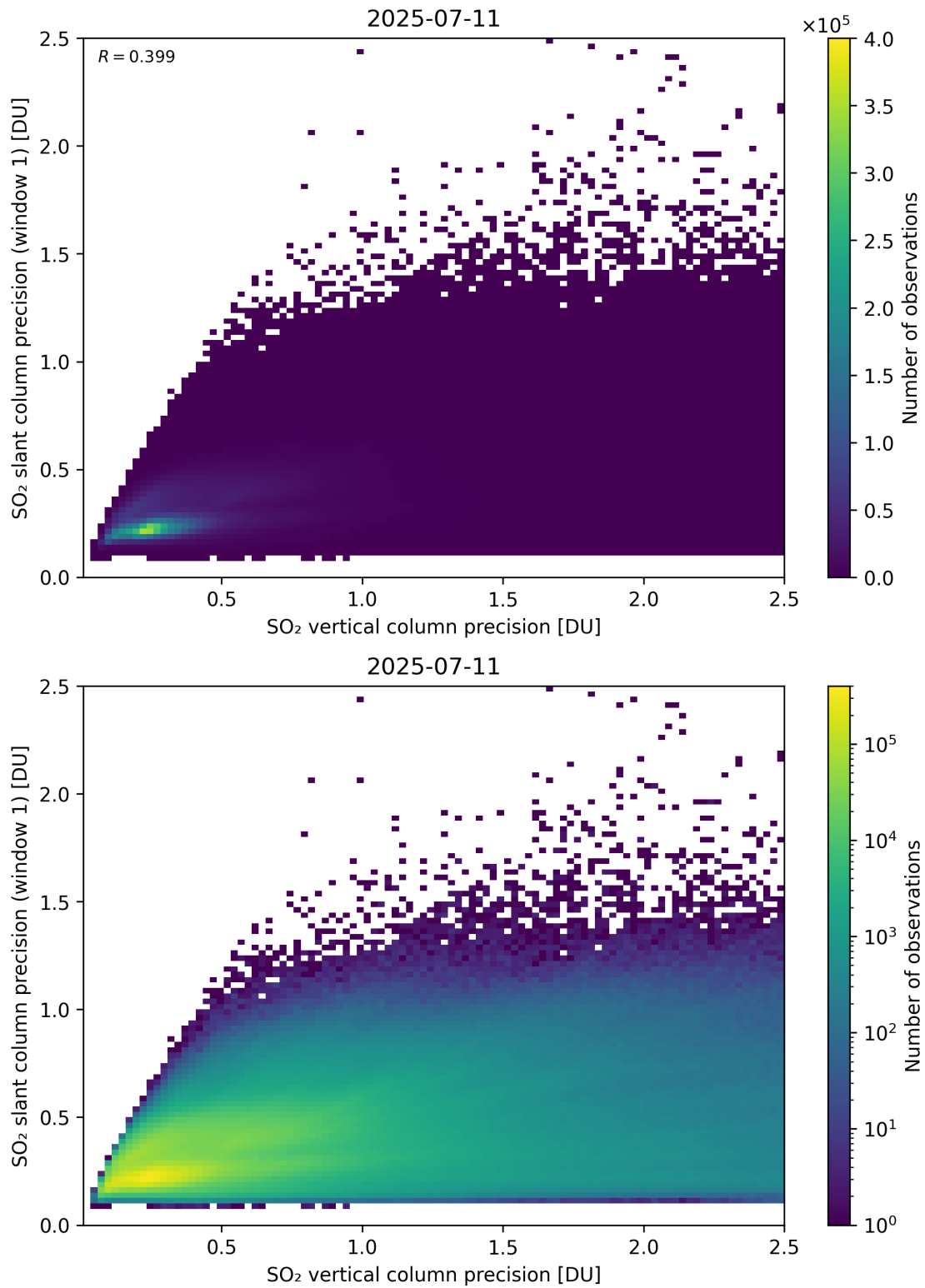
Figure 342: Scatter density plot of “SO 2 vertical column precision” against “SO 2 slant column precision (window 1)” for 2025-07-10 to 2025-07-12.
