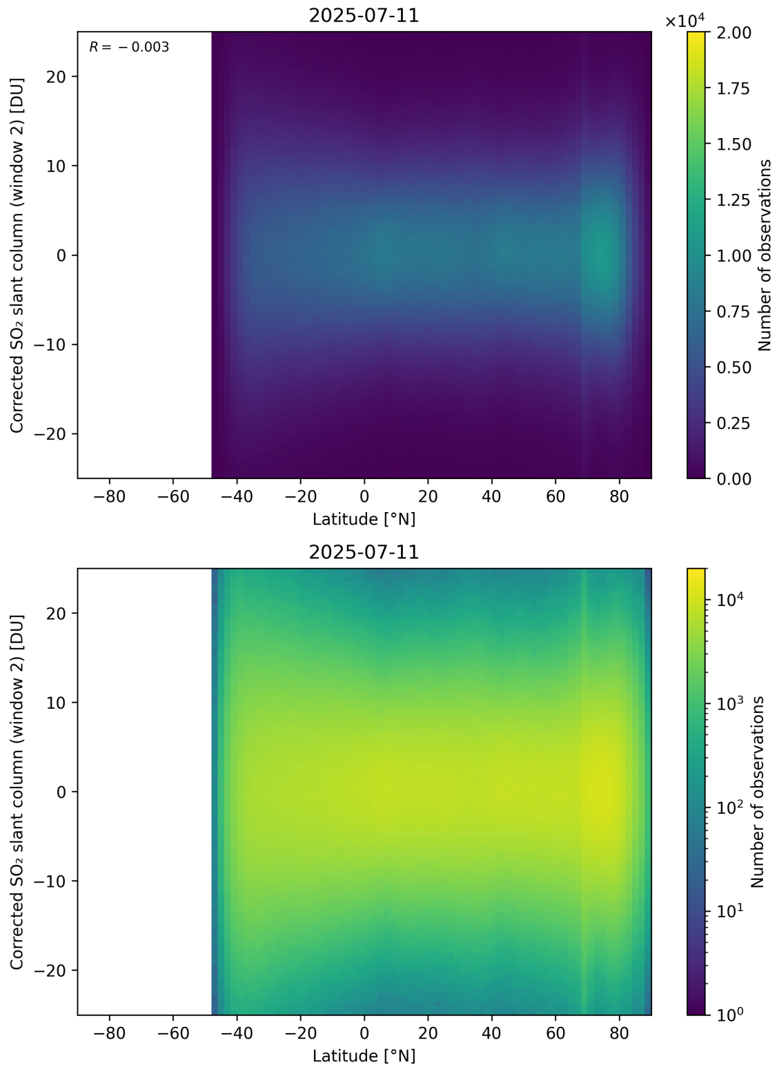
Figure 160: Scatter density plot of “Latitude” against “Corrected SO 2 slant column (window 2)” for 2025-07-10 to 2025-07-12.
