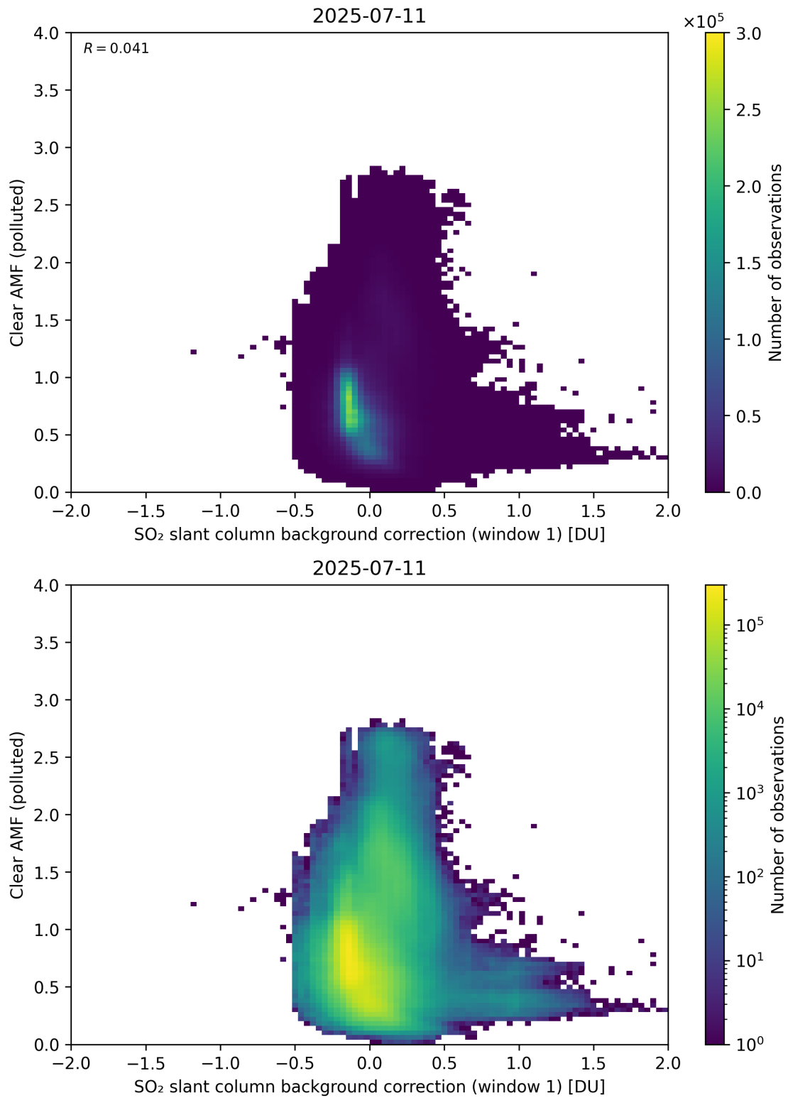
Figure 114: Scatter density plot of “SO 2 slant column background correction (window 1)” against “Clear AMF (polluted)” for 2025-07-10 to 2025-07-12.
