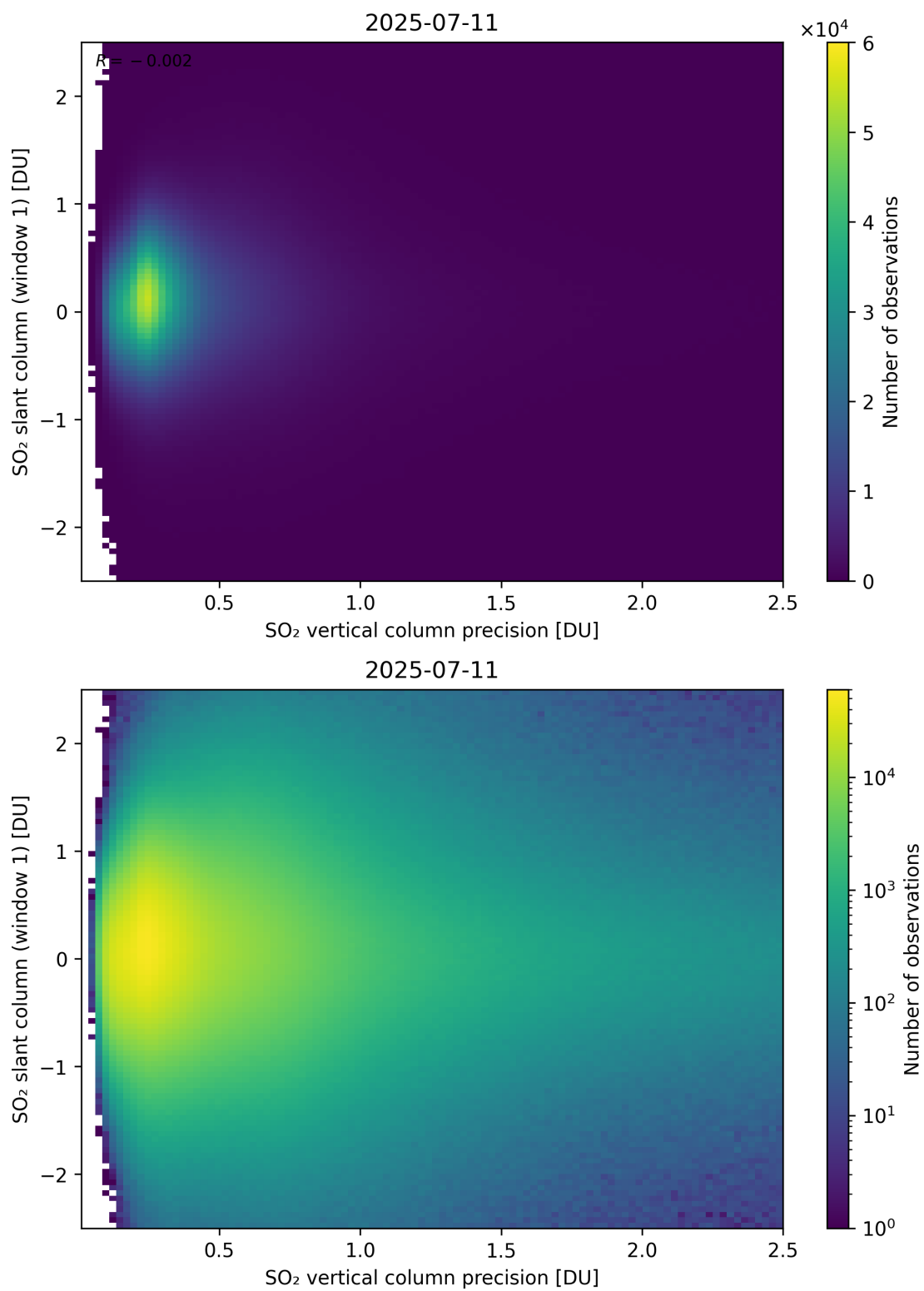
Figure 341: Scatter density plot of “SO 2 vertical column precision” against “SO 2 slant column (window 1)” for 2025-07-10 to 2025-07-12.
