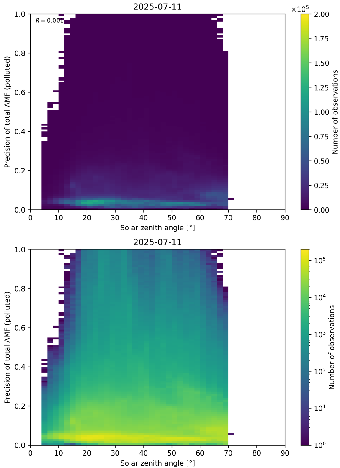
Figure 190: Scatter density plot of “Solar zenith angle” against “Precision of total AMF (polluted)” for 2025-07-10 to 2025-07-12.
