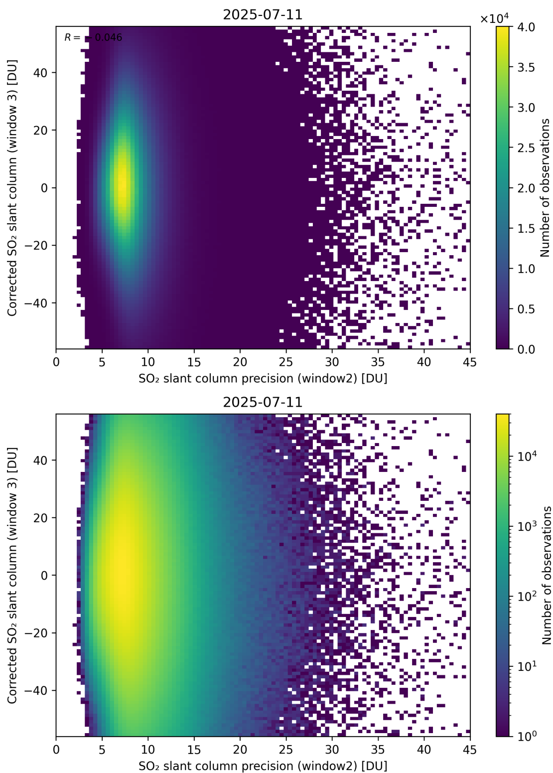
Figure 298: Scatter density plot of “SO 2 slant column precision (window2)” against “Corrected SO 2 slant column (window 3)” for 2025-07-10 to 2025-07-12.
