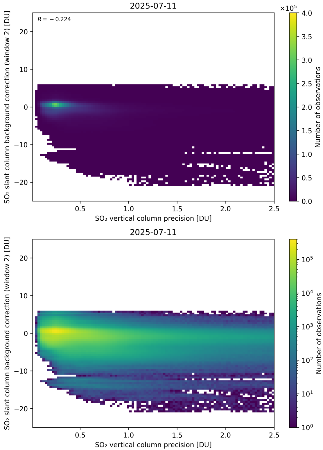
Figure 330: Scatter density plot of “SO 2 vertical column precision” against “SO 2 slant column background correction (window 2)” for 2025-07-10 to 2025-07-12.
