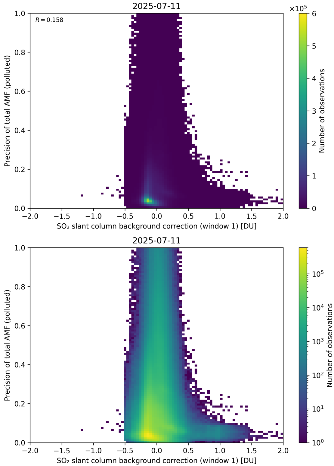
Figure 121: Scatter density plot of “SO 2 slant column background correction (window 1)” against “Precision of total AMF (polluted)” for 2025-07-10 to 2025-07-12.
