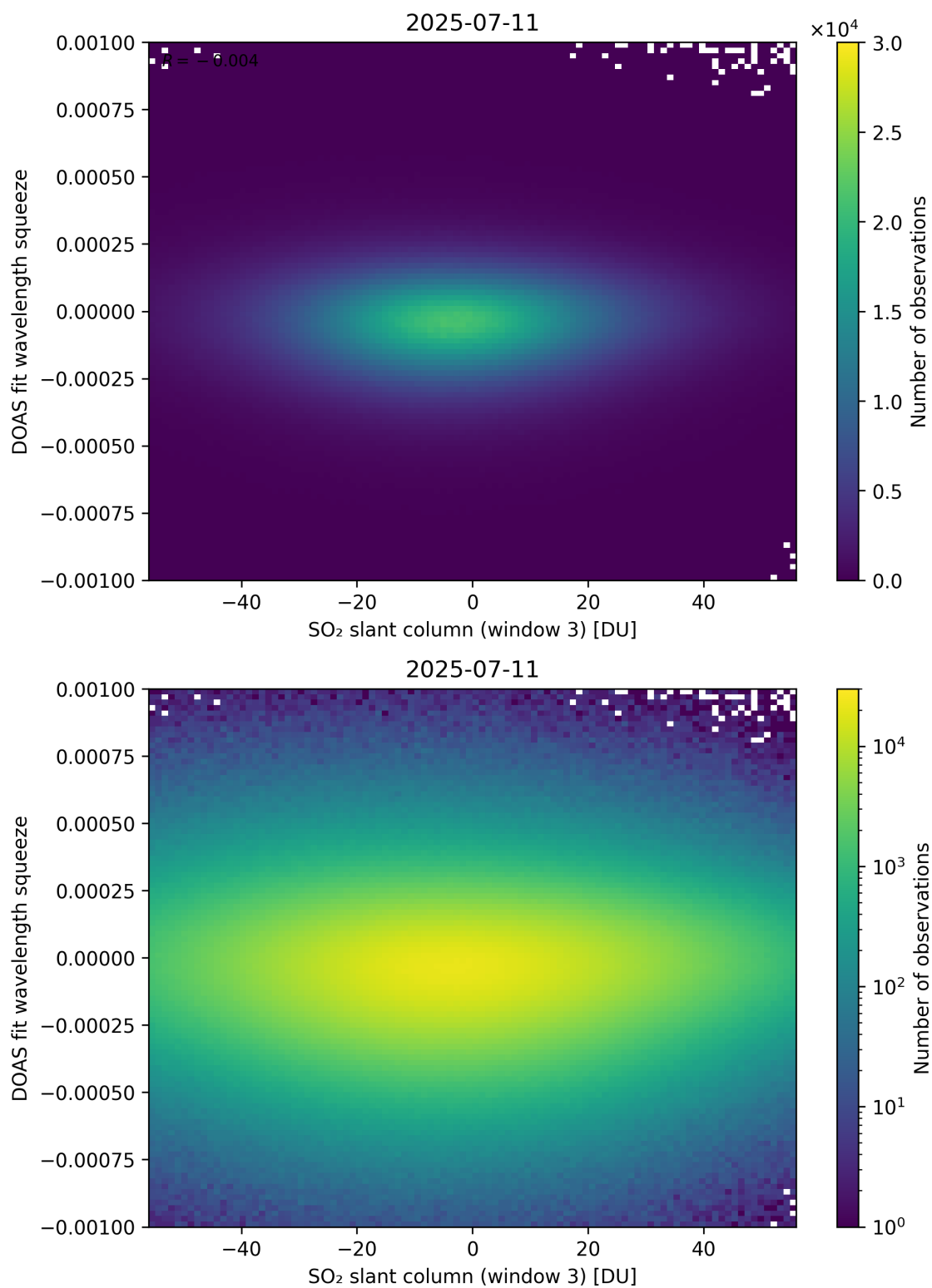
Figure 305: Scatter density plot of “SO 2 slant column (window 3)” against “DOAS fit wavelength squeeze” for 2025-07-10 to 2025-07-12.
