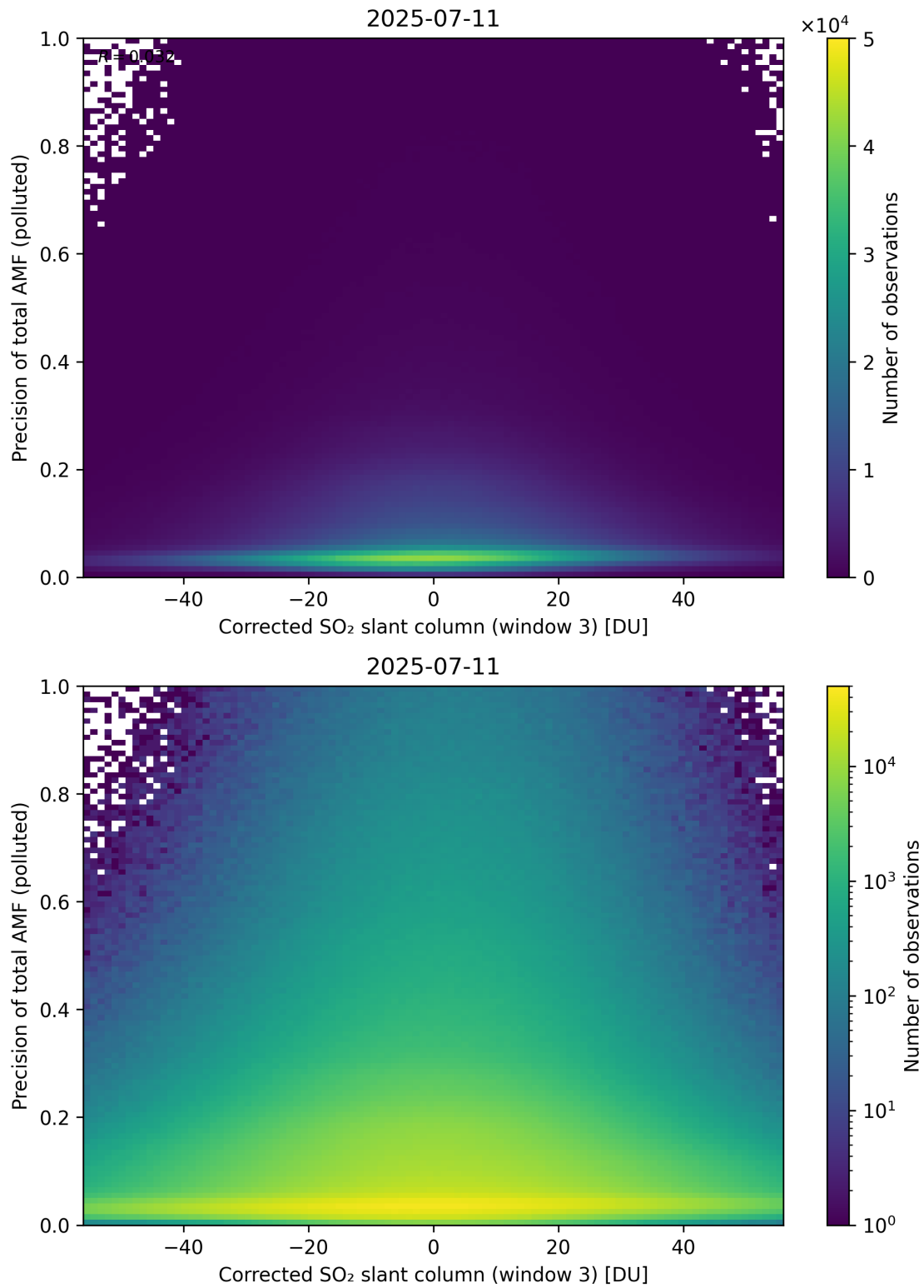
Figure 261: Scatter density plot of “Corrected SO 2 slant column (window 3)” against “Precision of total AMF (polluted)” for 2025-07-10 to 2025-07-12.
