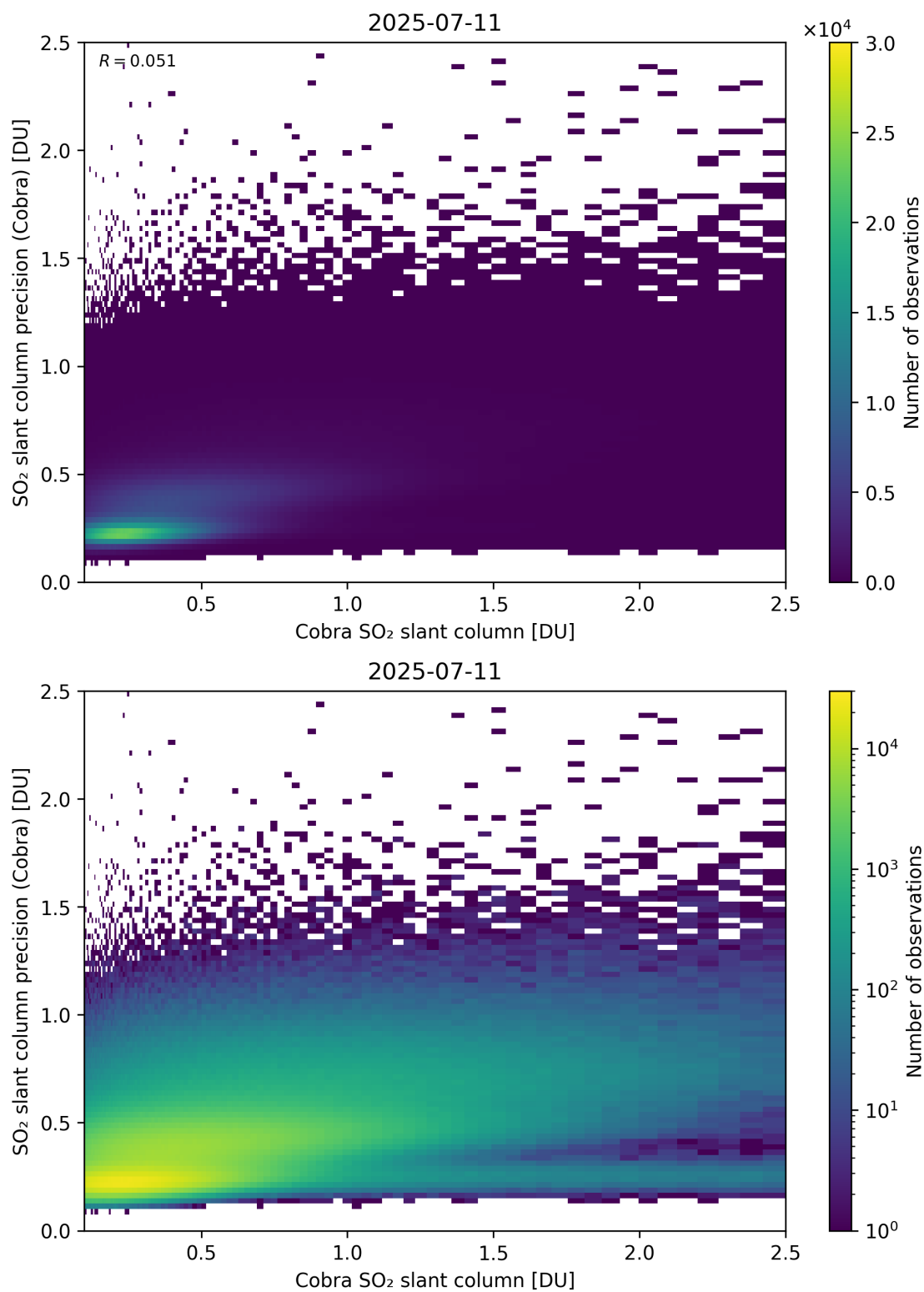
Figure 216: Scatter density plot of “Cobra SO 2 slant column” against “SO 2 slant column precision (Cobra)” for 2025-07-10 to 2025-07-12.
