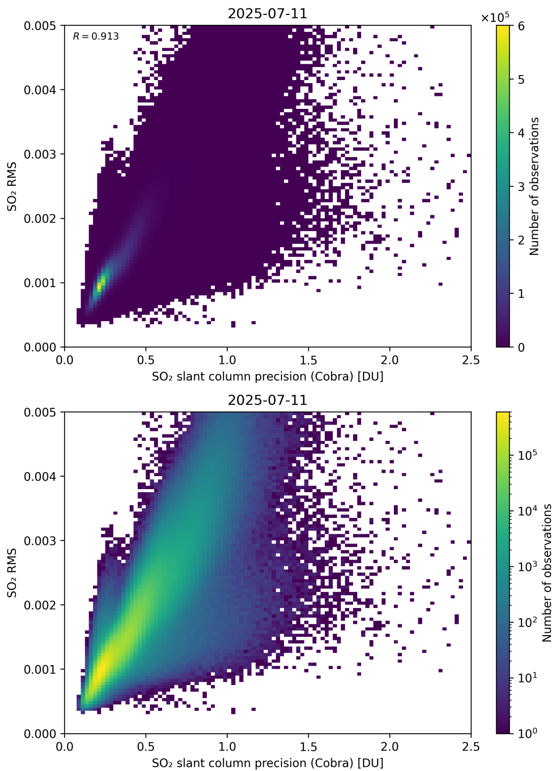
Figure 204: Scatter density plot of “SO 2 slant column precision (Cobra)” against “SO 2 RMS” for 2025-07-10 to 2025-07-12.
