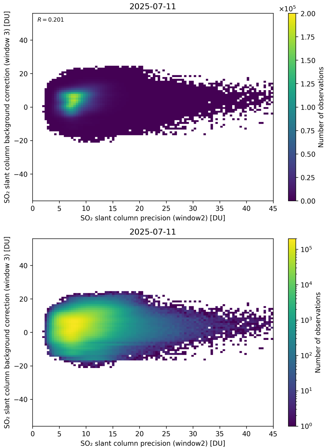
Figure 292: Scatter density plot of “SO 2 slant column precision (window2)” against “SO 2 slant column background correction (window 3)” for 2025-07-10 to 2025-07-12.
