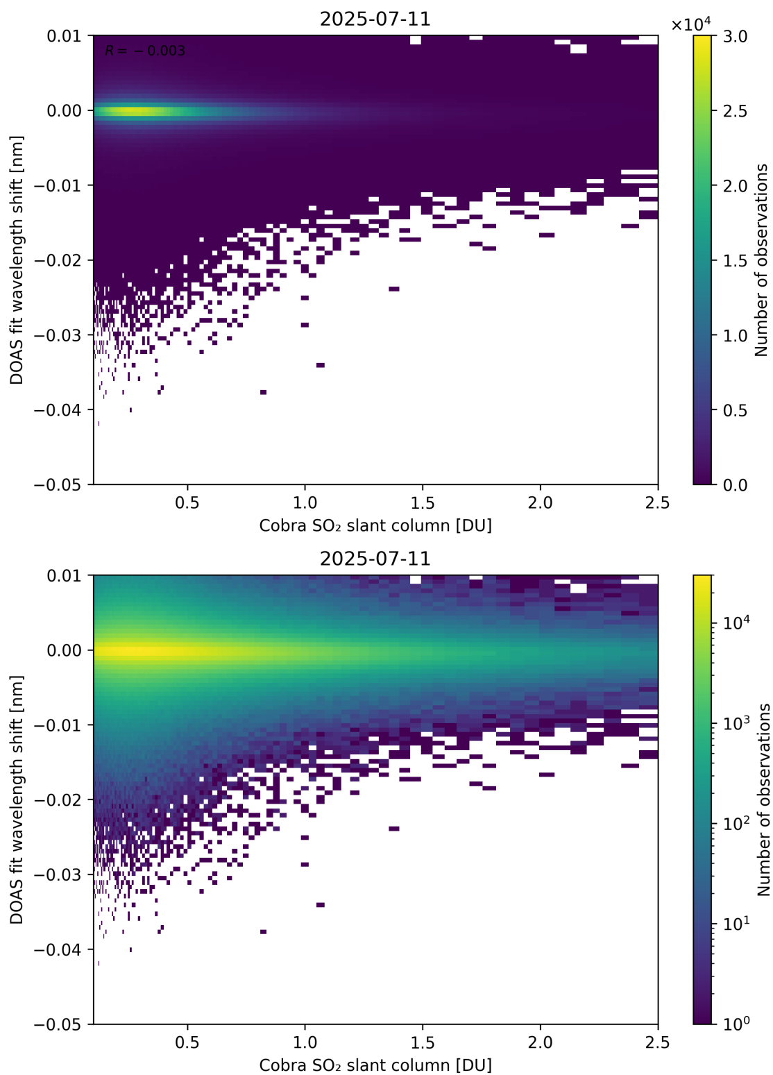
Figure 196: Scatter density plot of “Cobra SO 2 slant column” against “DOAS fit wavelength shift” for 2025-07-10 to 2025-07-12.
