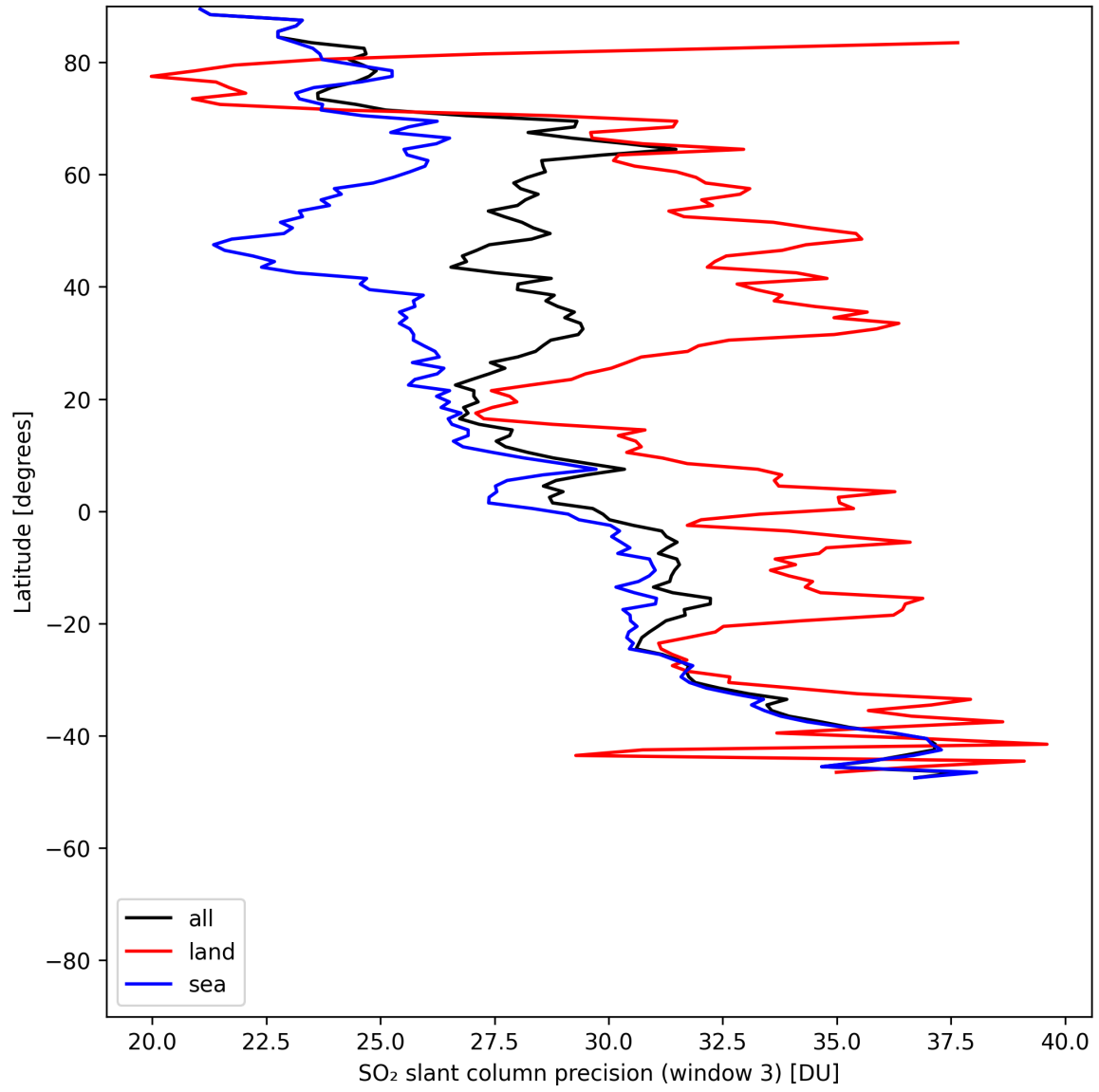
Figure 46: Zonal average of “SO 2 slant column precision (window 3)” for 2025-07-10 to 2025-07-12.
