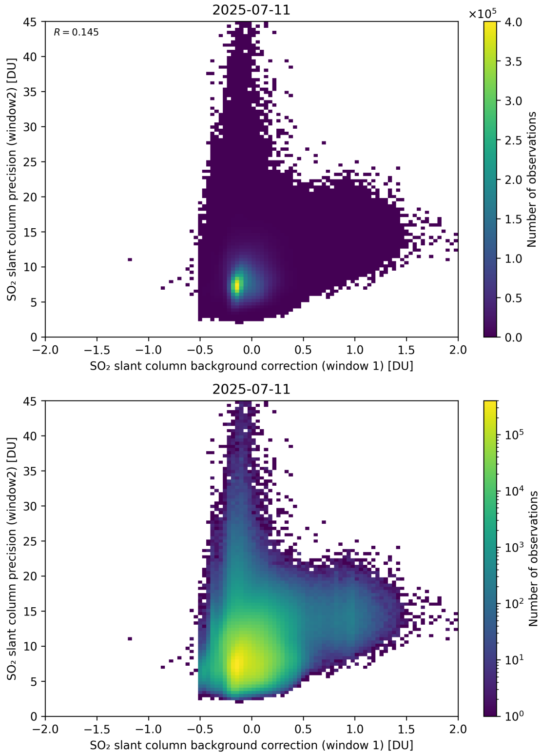
Figure 117: Scatter density plot of “SO 2 slant column background correction (window 1)” against “SO 2 slant column precision (window2)” for 2025-07-10 to 2025-07-12.
