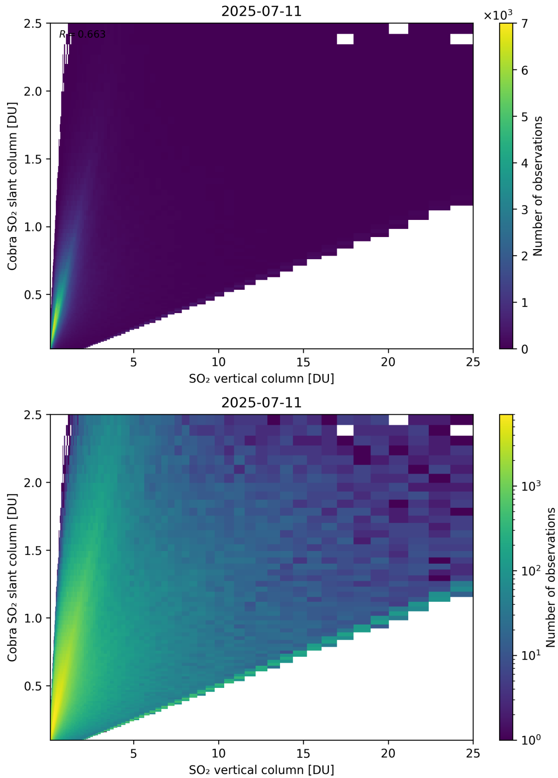
Figure 349: Scatter density plot of “SO 2 vertical column” against “Cobra SO 2 slant column” for 2025-07-10 to 2025-07-12.
