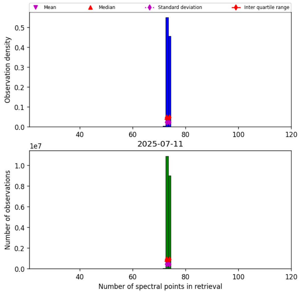
Figure 82: Histogram of “Number of spectral points in retrieval” for 2025-07-10 to 2025-07-12
