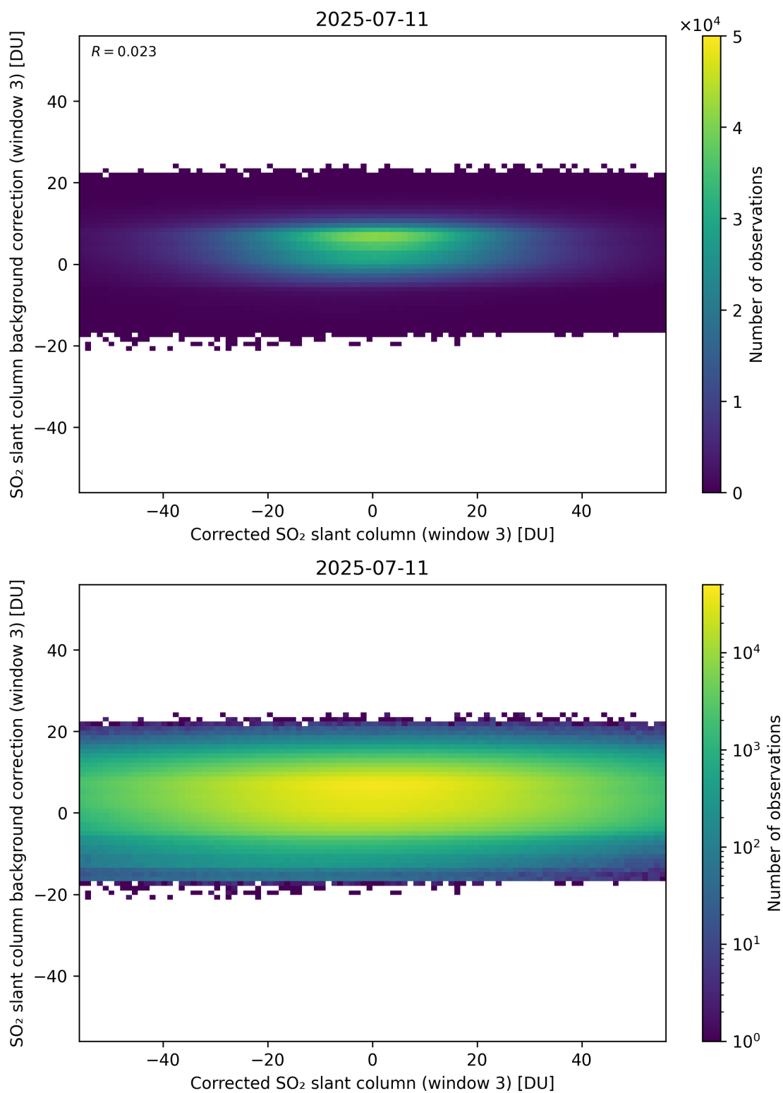
Figure 255: Scatter density plot of “Corrected SO 2 slant column (window 3)” against “SO 2 slant column background correction (window 3)” for 2025-07-10 to 2025-07-12.
