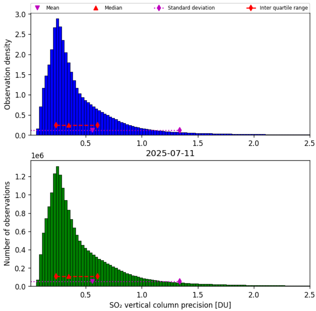
Figure 59: Histogram of “SO 2 vertical column precision” for 2025-07-10 to 2025-07-12
