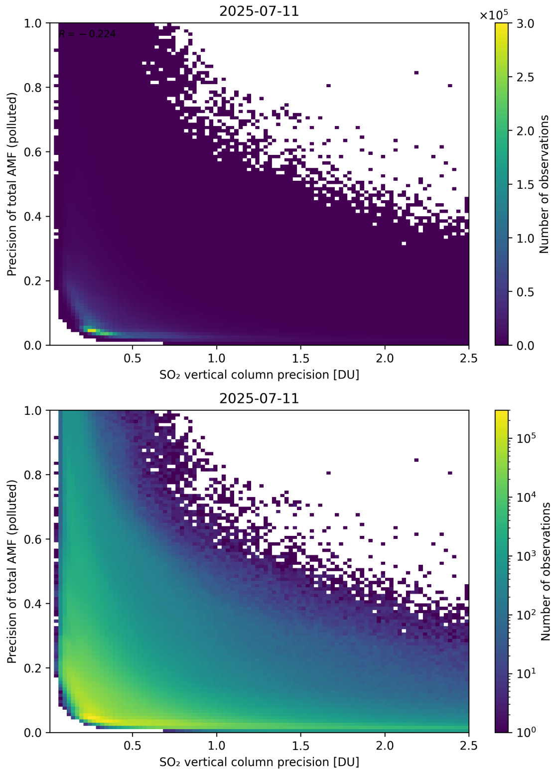
Figure 347: Scatter density plot of “SO 2 vertical column precision” against “Precision of total AMF (polluted)” for 2025-07-10 to 2025-07-12.
