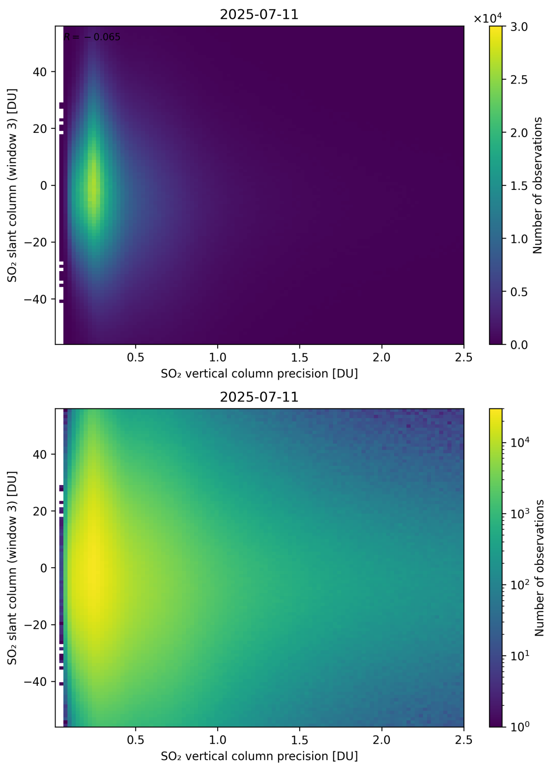
Figure 344: Scatter density plot of “SO 2 vertical column precision” against “SO 2 slant column (window 3)” for 2025-07-10 to 2025-07-12.
