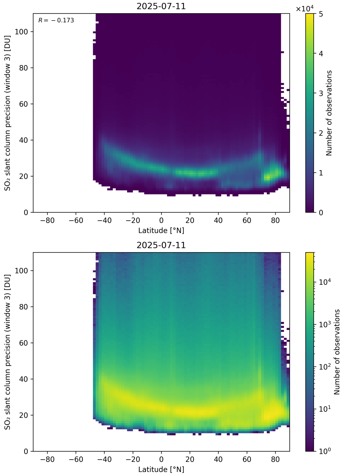
Figure 166: Scatter density plot of “Latitude” against “SO 2 slant column precision (window 3)” for 2025-07-10 to 2025-07-12.
