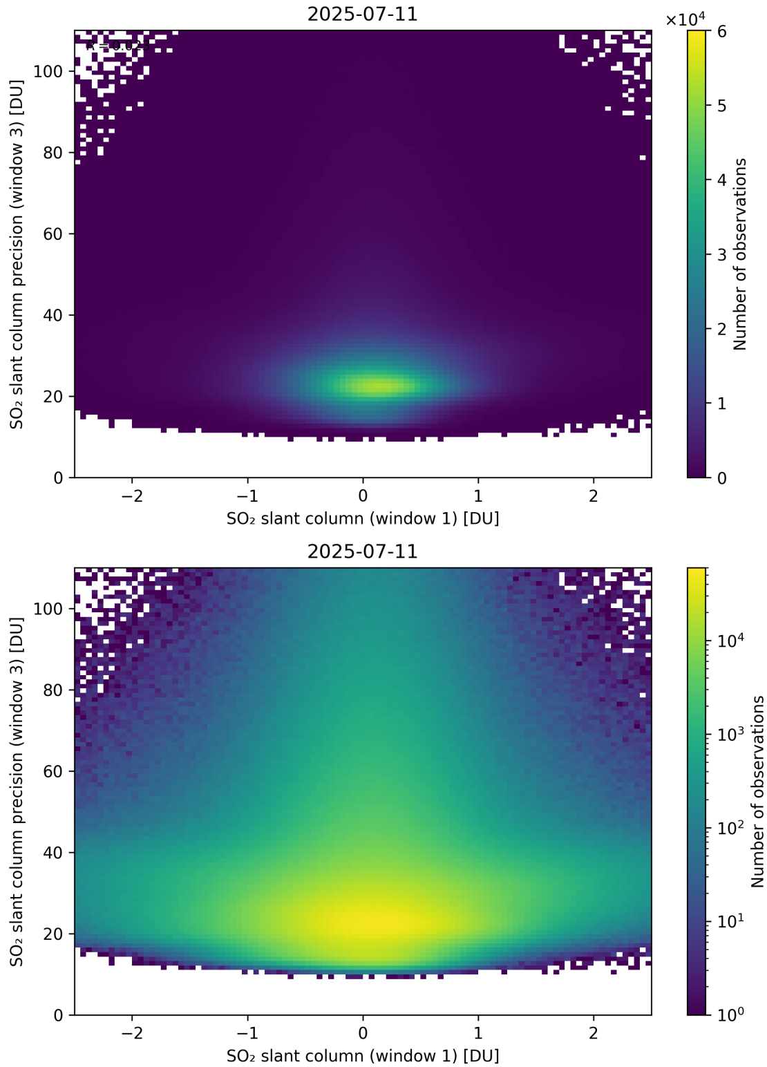
Figure 288: Scatter density plot of “SO 2 slant column (window 1)” against “SO 2 slant column precision (window 3)” for 2025-07-10 to 2025-07-12.
