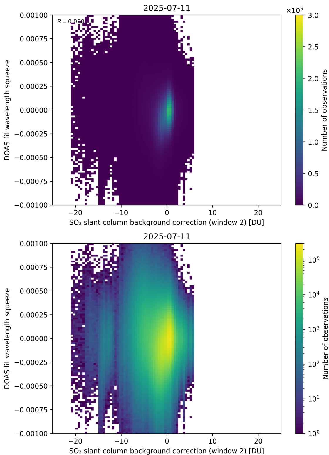
Figure 124: Scatter density plot of “SO 2 slant column background correction (window 2)” against “DOAS fit wavelength squeeze” for 2025-07-10 to 2025-07-12.
