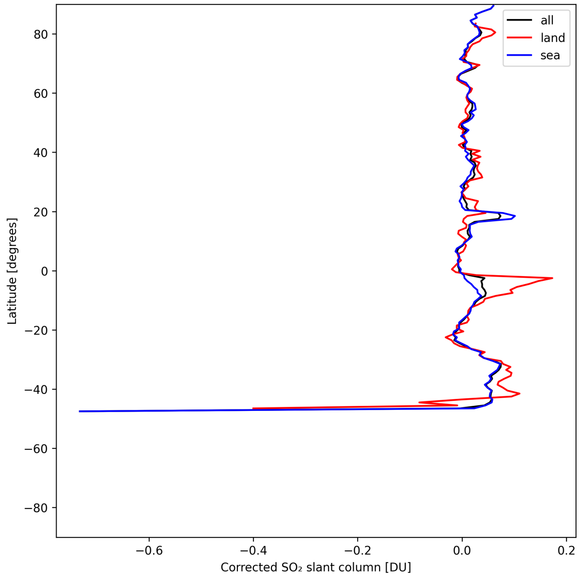
Figure 34: Zonal average of “Corrected SO 2 slant column” for 2025-07-10 to 2025-07-12.
