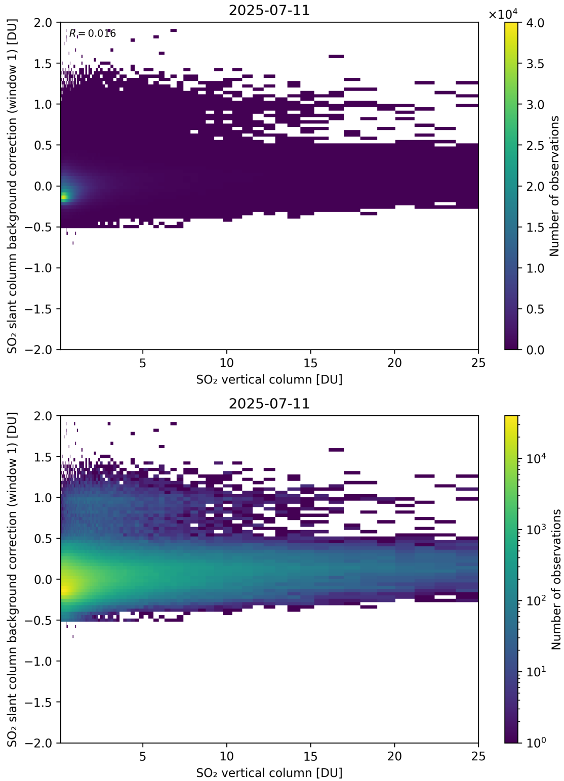
Figure 323: Scatter density plot of “SO 2 vertical column” against “SO 2 slant column background correction (window 1)” for 2025-07-10 to 2025-07-12.
