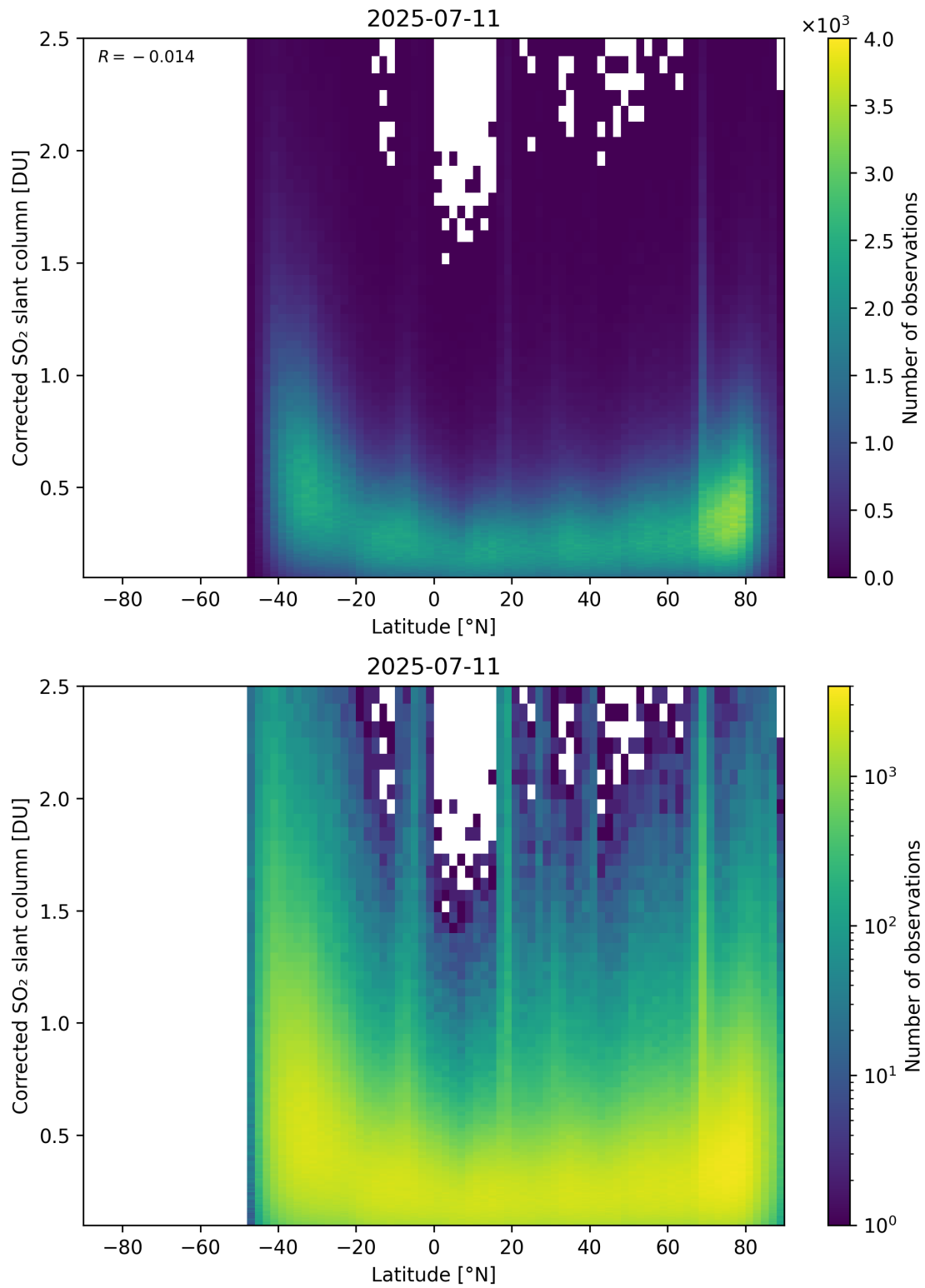
Figure 159: Scatter density plot of “Latitude” against “Corrected SO 2 slant column” for 2025-07-10 to 2025-07-12.
