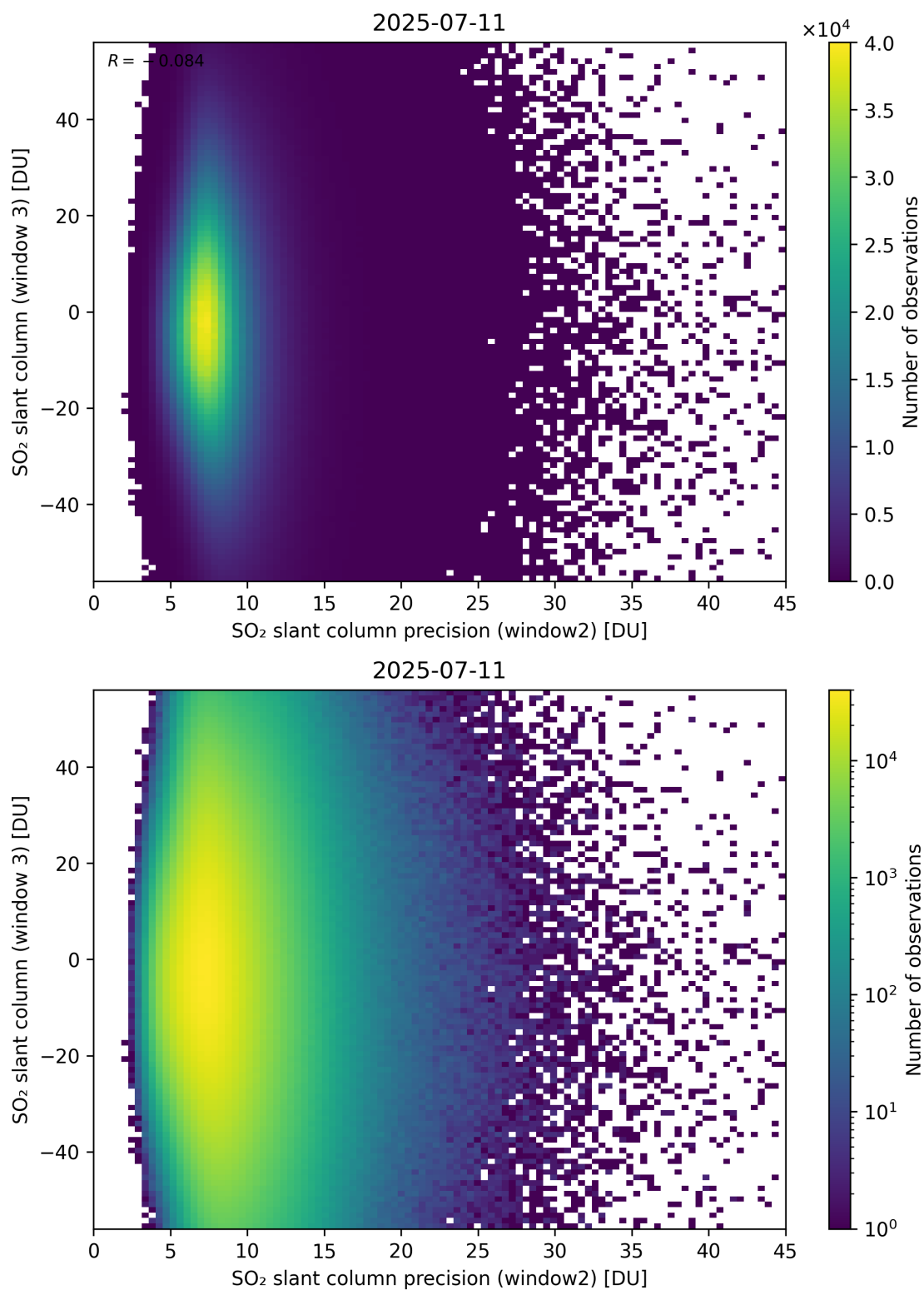
Figure 299: Scatter density plot of “SO 2 slant column precision (window2)” against “SO 2 slant column (window 3)” for 2025-07-10 to 2025-07-12.
