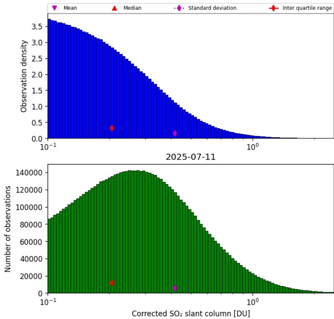
Figure 60: Histogram of "Corrected SO 2 slant column" for 2025-07-10 to 2025-07-12
