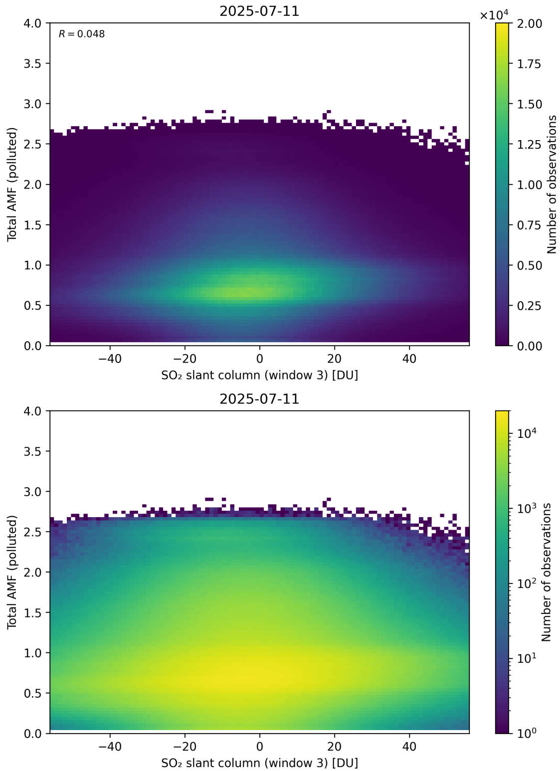
Figure 318: Scatter density plot of “SO 2 slant column (window 3)” against “Total AMF (polluted)” for 2025-07-10 to 2025-07-12.
