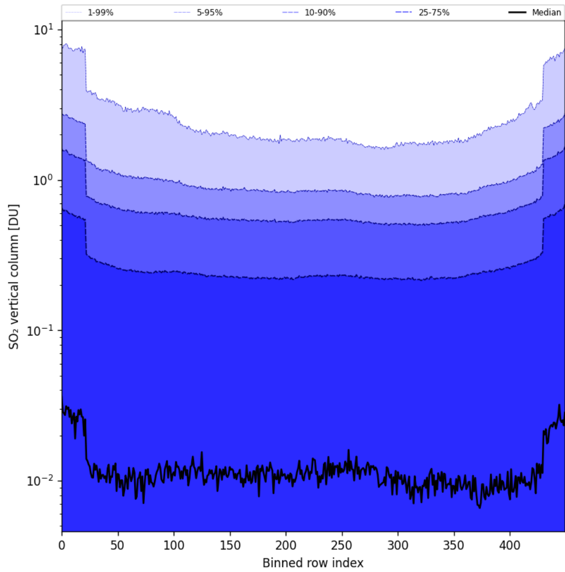
Figure 84: Along track statistics of “SO 2 vertical column” for 2025-07-10 to 2025-07-12
