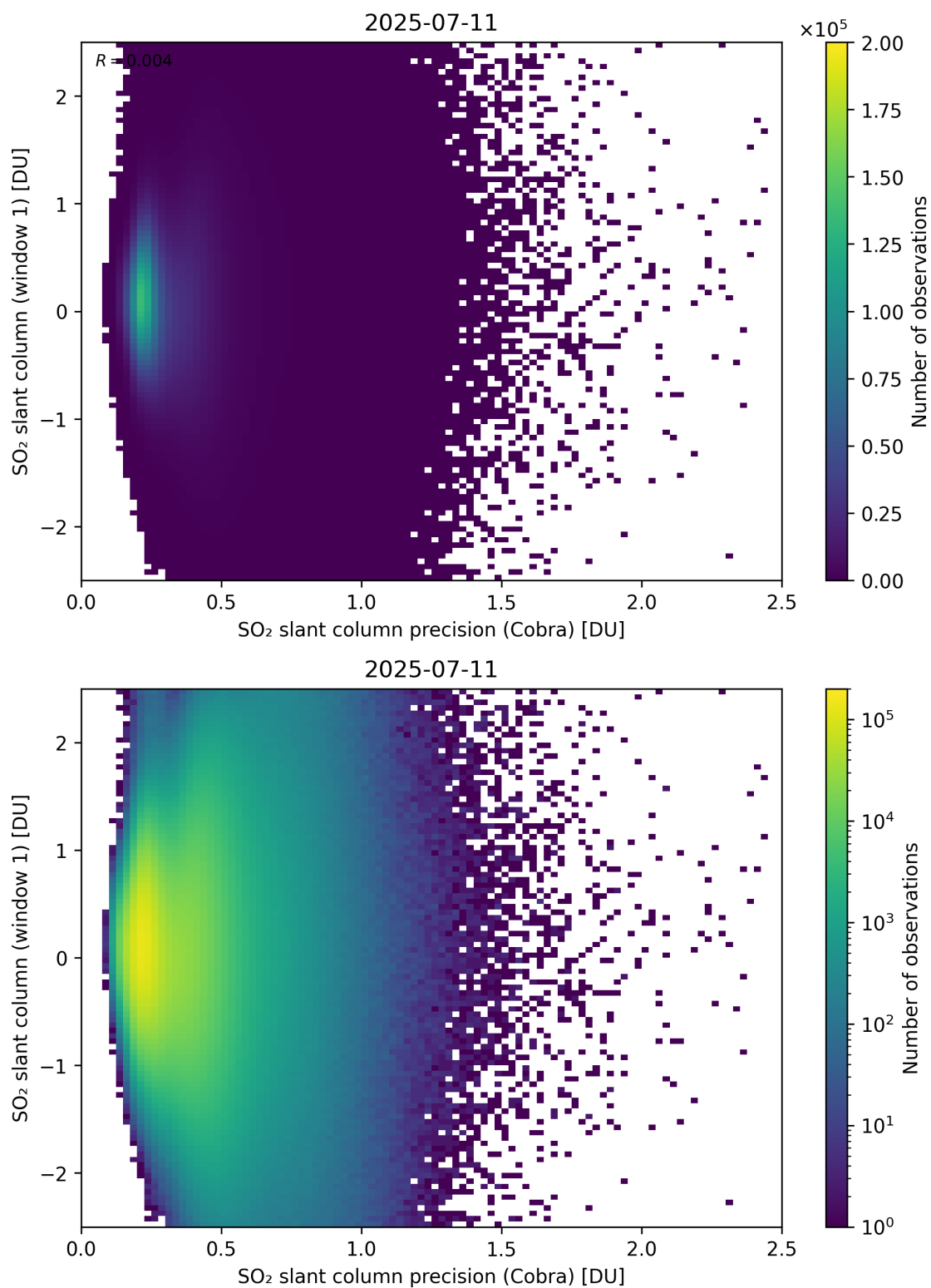
Figure 208: Scatter density plot of “SO 2 slant column precision (Cobra)” against “SO 2 slant column (window 1)” for 2025-07-10 to 2025-07-12.
