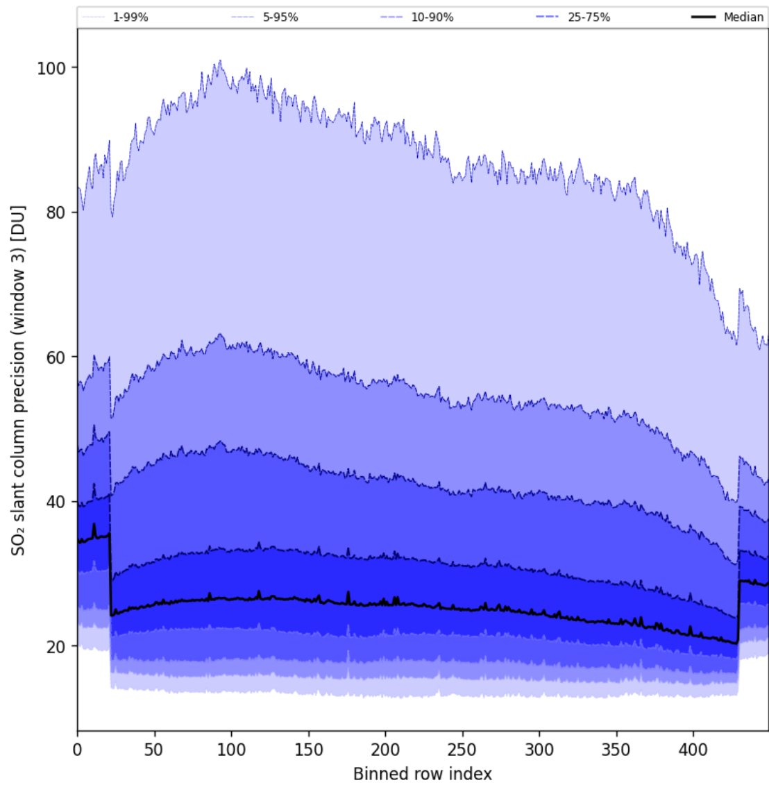
Figure 98: Along track statistics of “SO 2 slant column precision (window 3)” for 2025-07-10 to 2025-07-12
