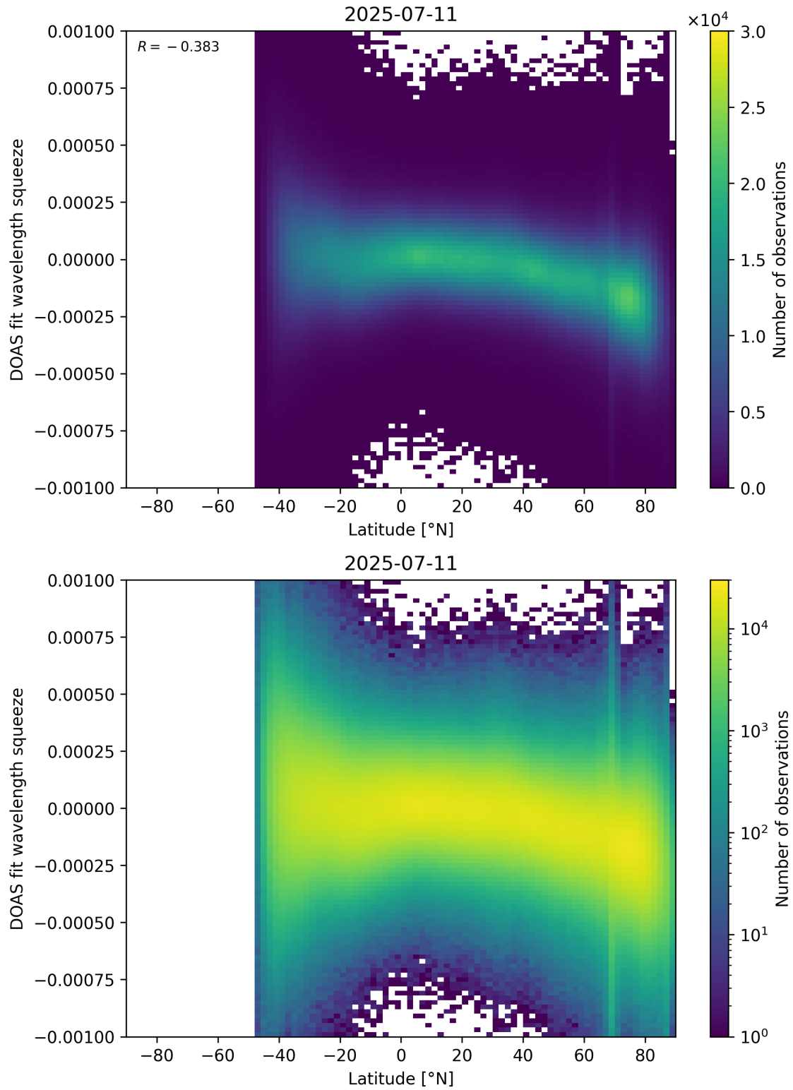
Figure 154: Scatter density plot of “Latitude” against “DOAS fit wavelength squeeze” for 2025-07-10 to 2025-07-12.
