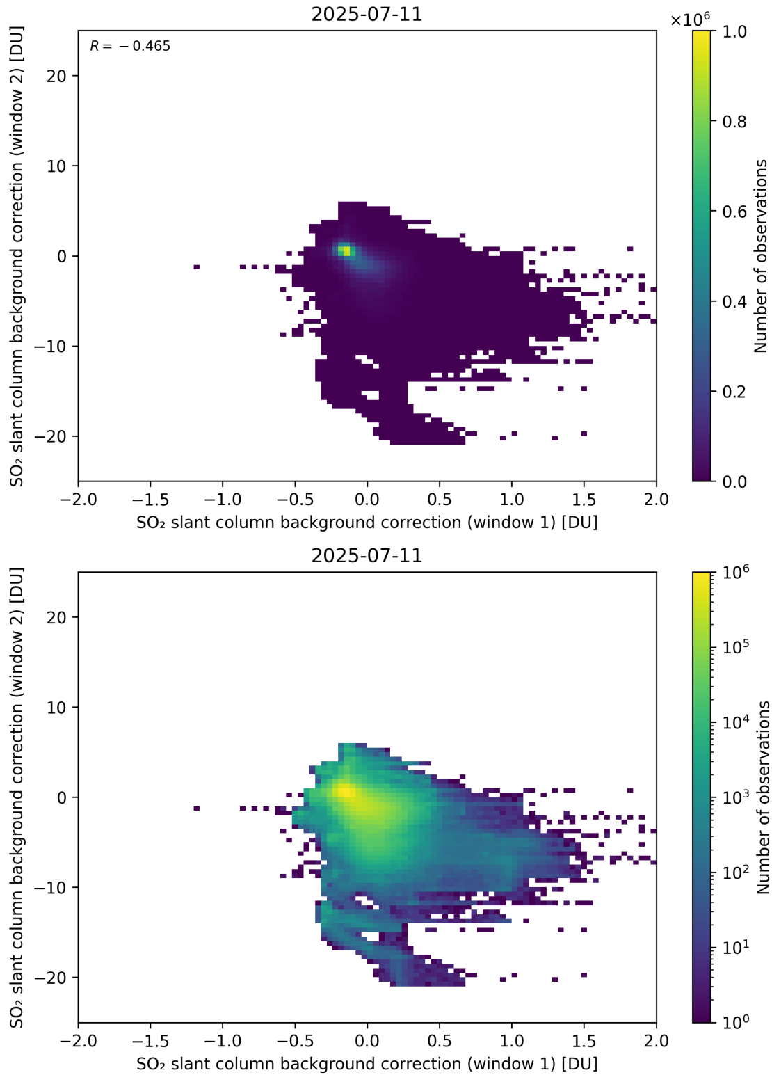
Figure 109: Scatter density plot of “SO 2 slant column background correction (window 1)” against “SO 2 slant column background correction (window 2)” for 2025-07-10 to 2025-07-12.
