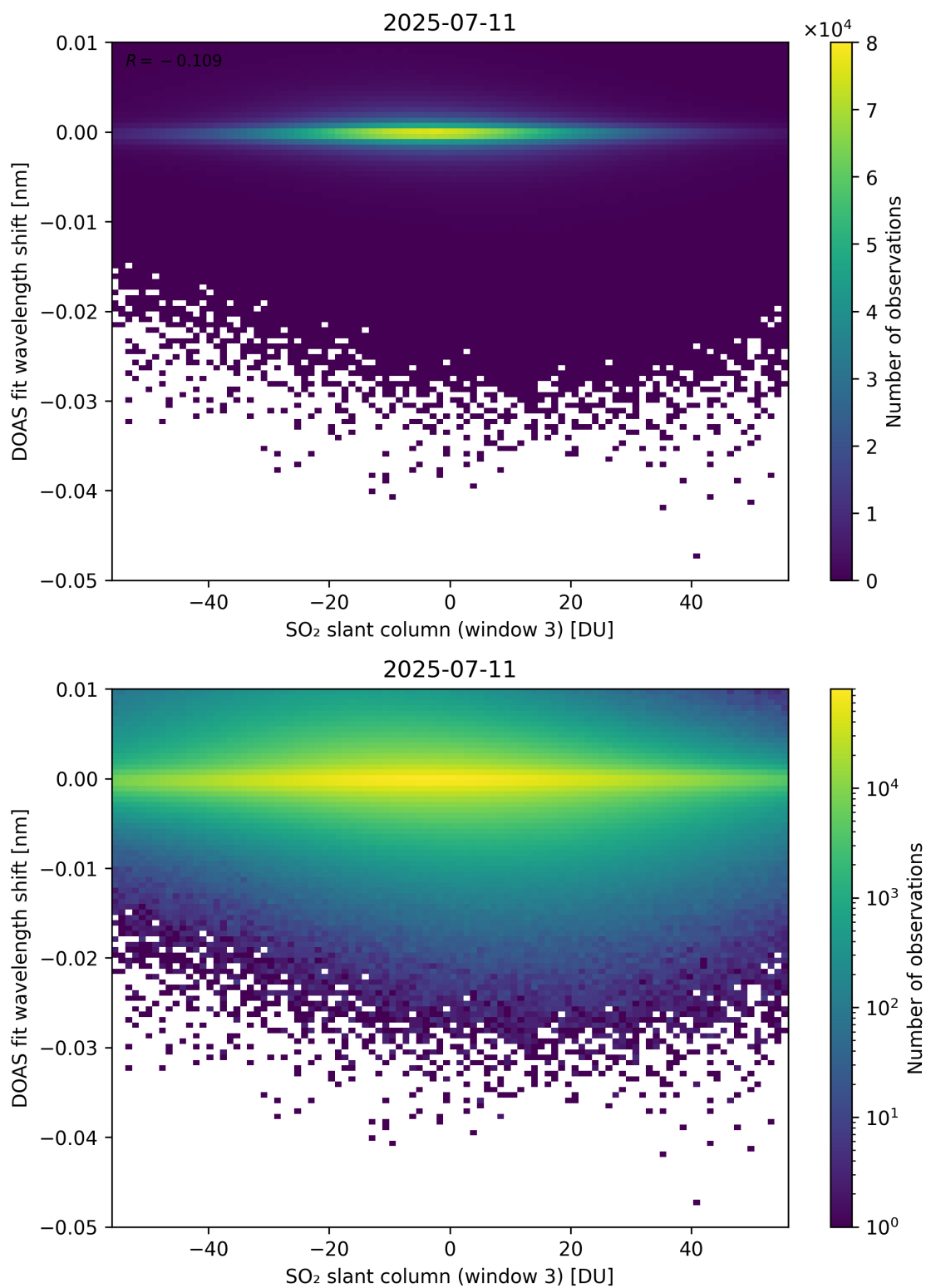
Figure 304: Scatter density plot of “SO 2 slant column (window 3)” against “DOAS fit wavelength shift” for 2025-07-10 to 2025-07-12.
