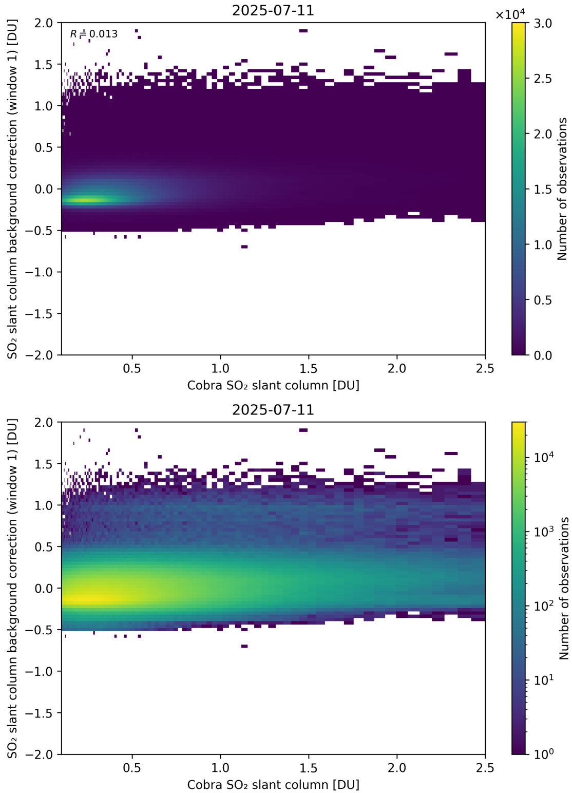
Figure 193: Scatter density plot of “Cobra SO 2 slant column” against “SO 2 slant column background correction (window 1)” for 2025-07-10 to 2025-07-12.
