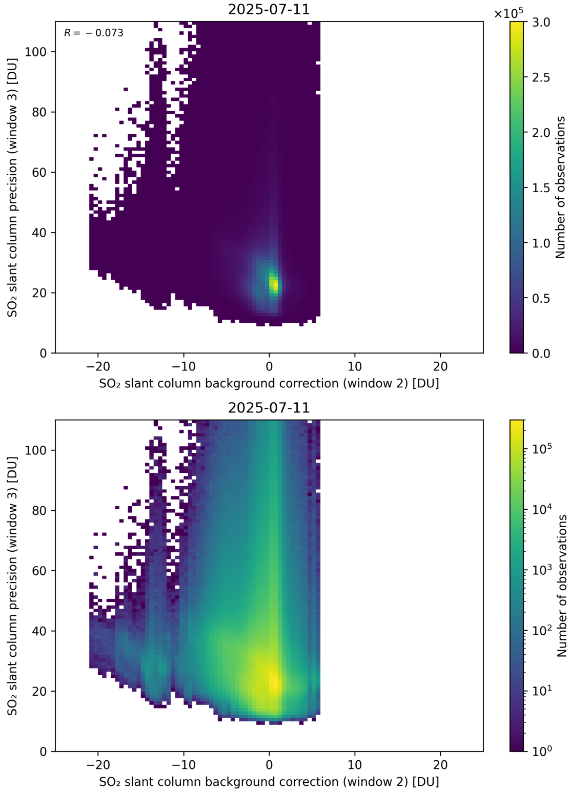
Figure 129: Scatter density plot of “SO 2 slant column background correction (window 2)” against “SO 2 slant column precision (window 3)” for 2025-07-10 to 2025-07-12.
