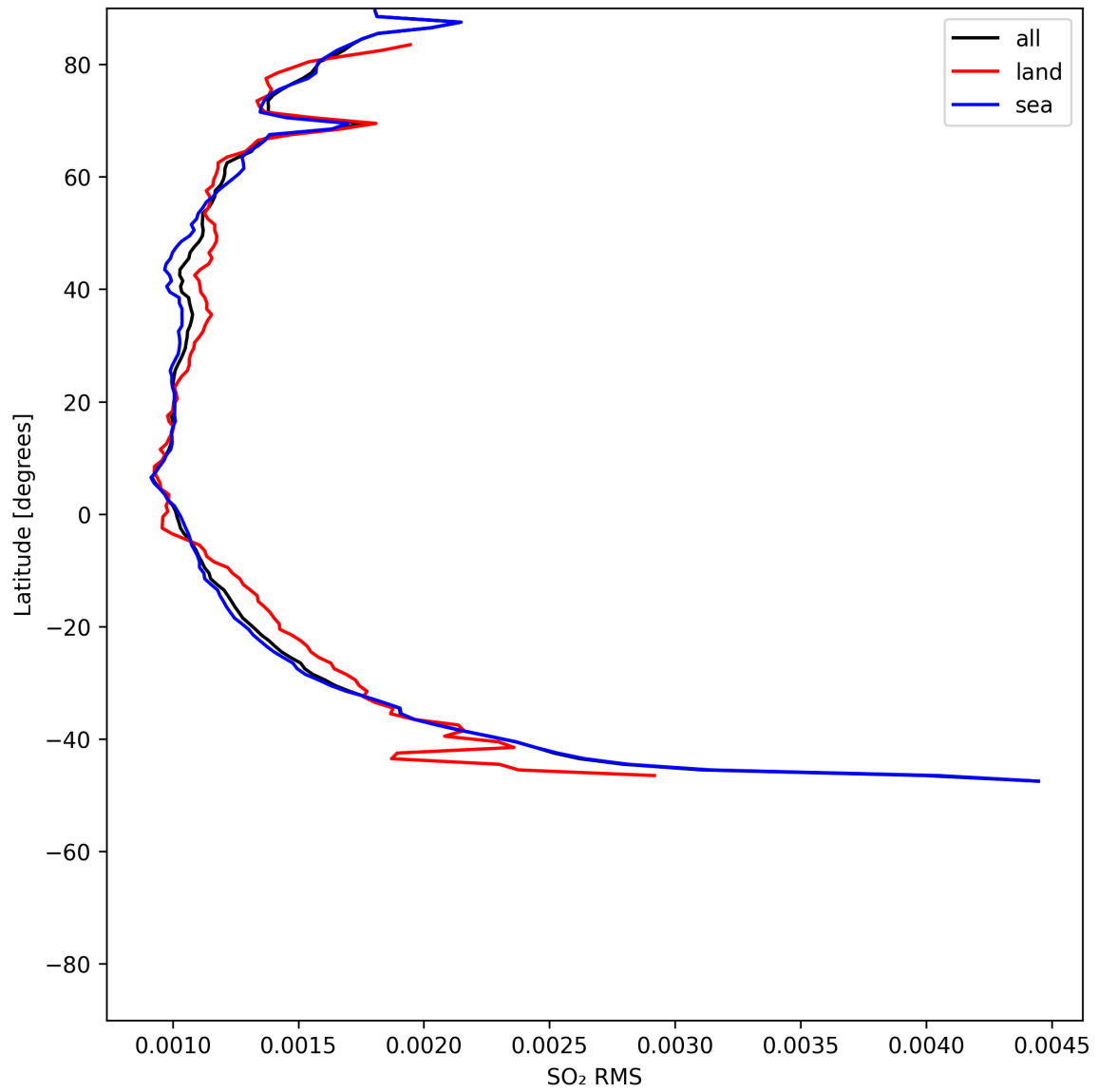
Figure 52: Zonal average of “SO 2 RMS” for 2025-07-10 to 2025-07-12.
