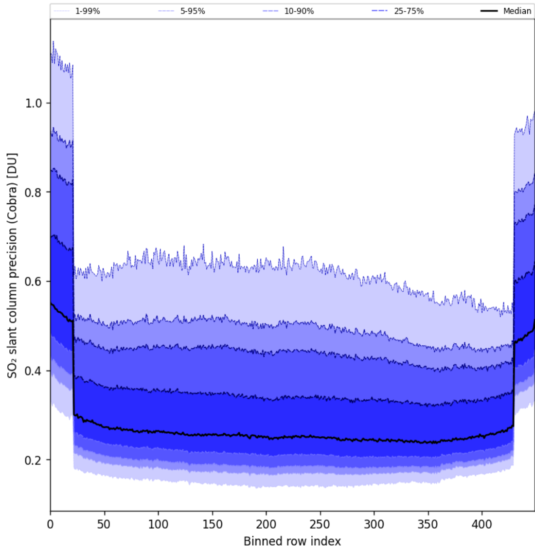
Figure 88: Along track statistics of “SO 2 slant column precision (Cobra)” for 2025-07-10 to 2025-07-12
