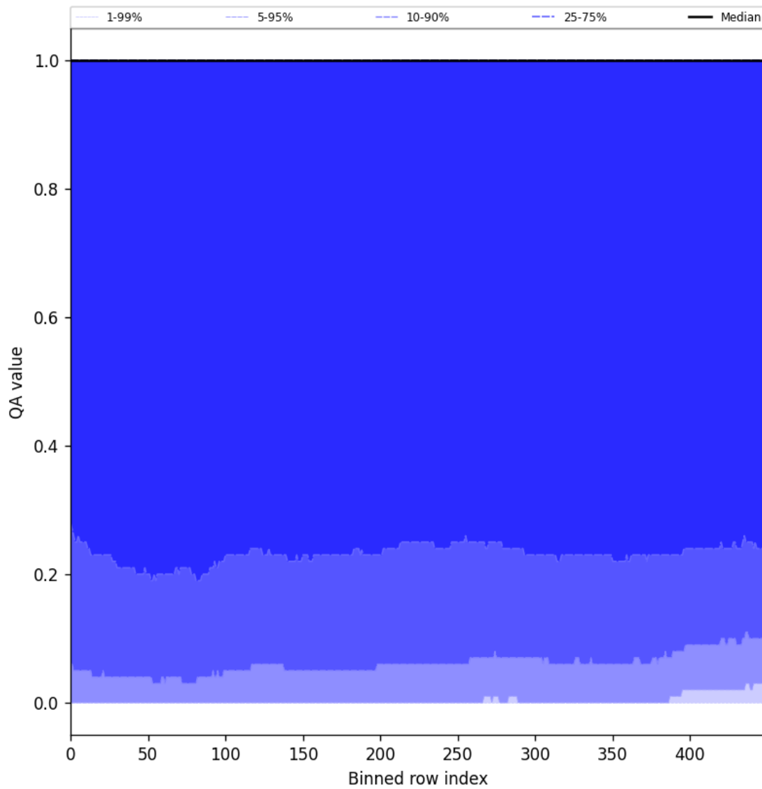
Figure 83: Along track statistics of “QA value” for 2025-07-10 to 2025-07-12
