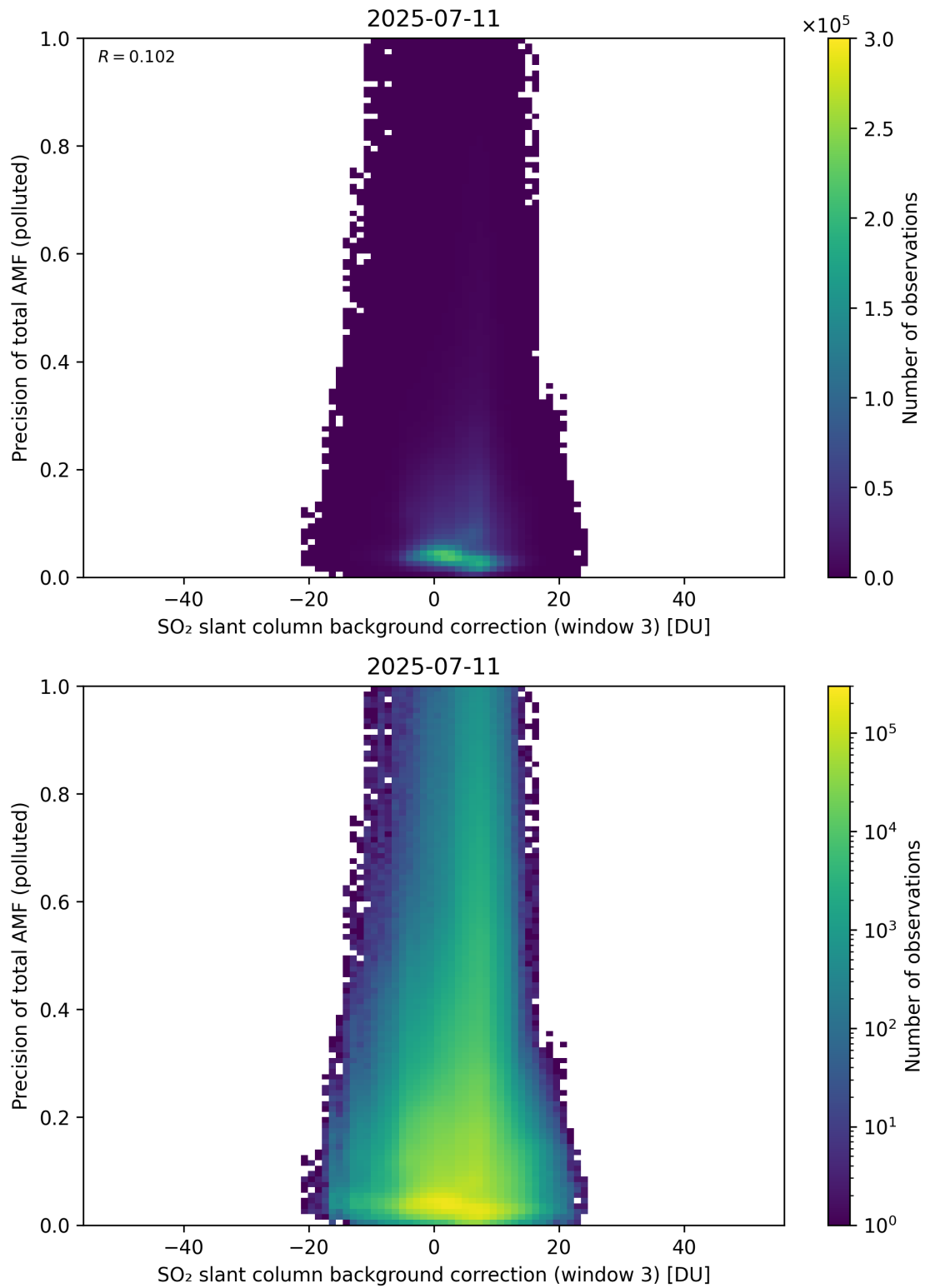
Figure 137: Scatter density plot of “SO 2 slant column background correction (window 3)” against “Precision of total AMF (polluted)” for 2025-07-10 to 2025-07-12.
