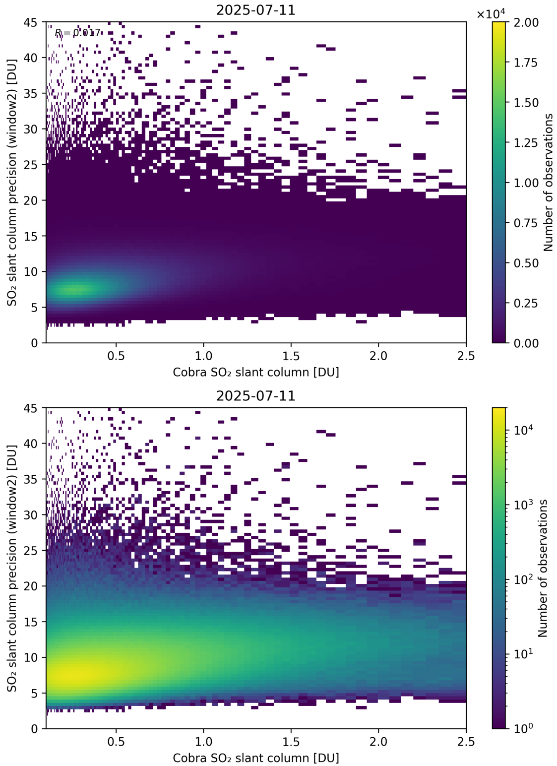
Figure 221: Scatter density plot of “Cobra SO 2 slant column” against “SO 2 slant column precision (window2)” for 2025-07-10 to 2025-07-12.
