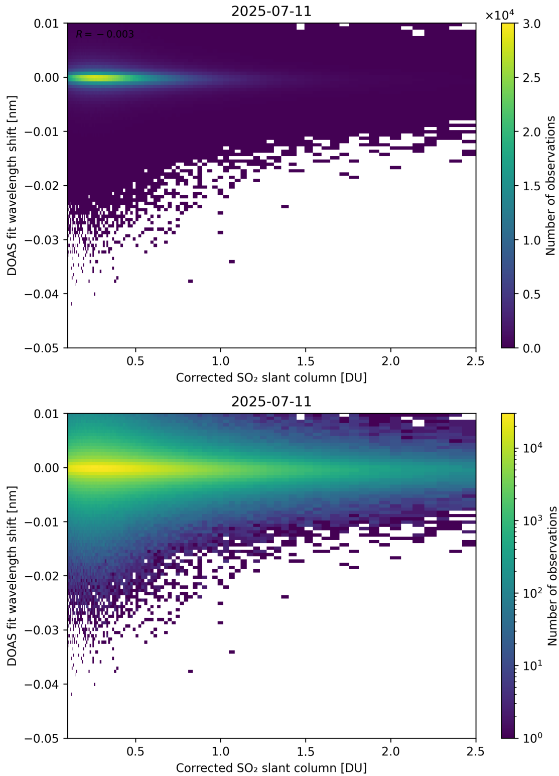
Figure 229: Scatter density plot of “Corrected SO 2 slant column” against “DOAS fit wavelength shift” for 2025-07-10 to 2025-07-12.
