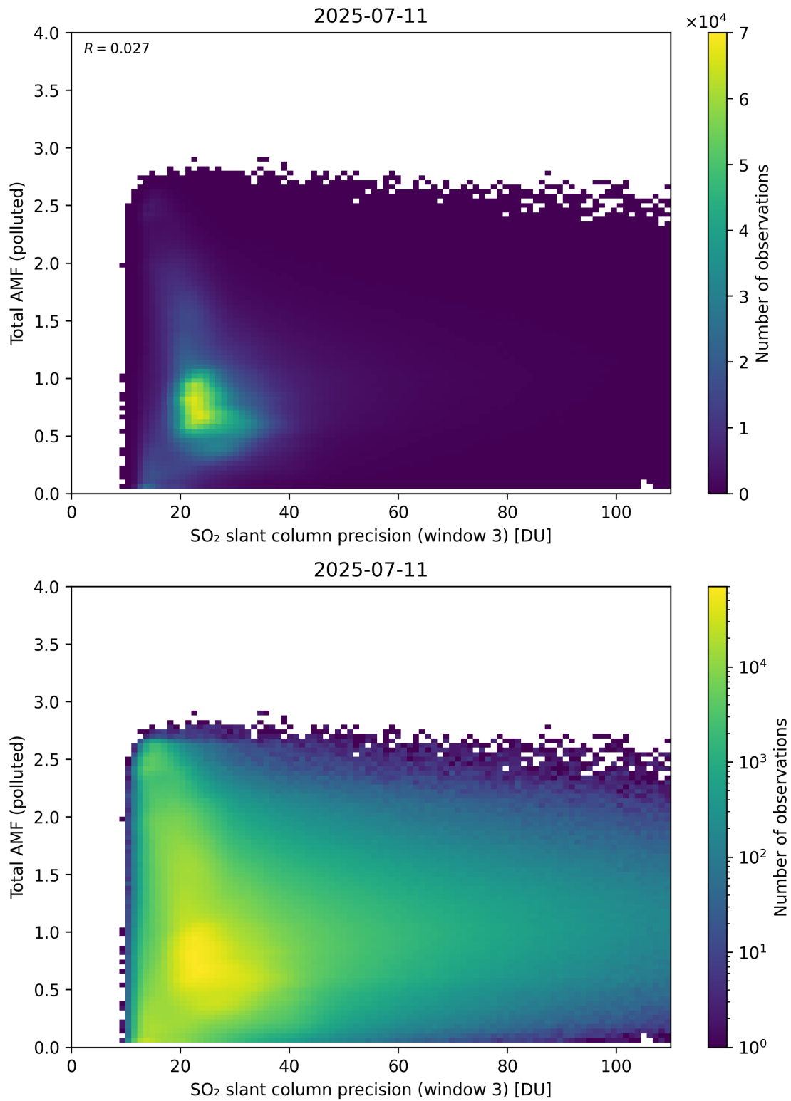
Figure 313: Scatter density plot of “SO 2 slant column precision (window 3)” against “Total AMF (polluted)” for 2025-07-10 to 2025-07-12.
