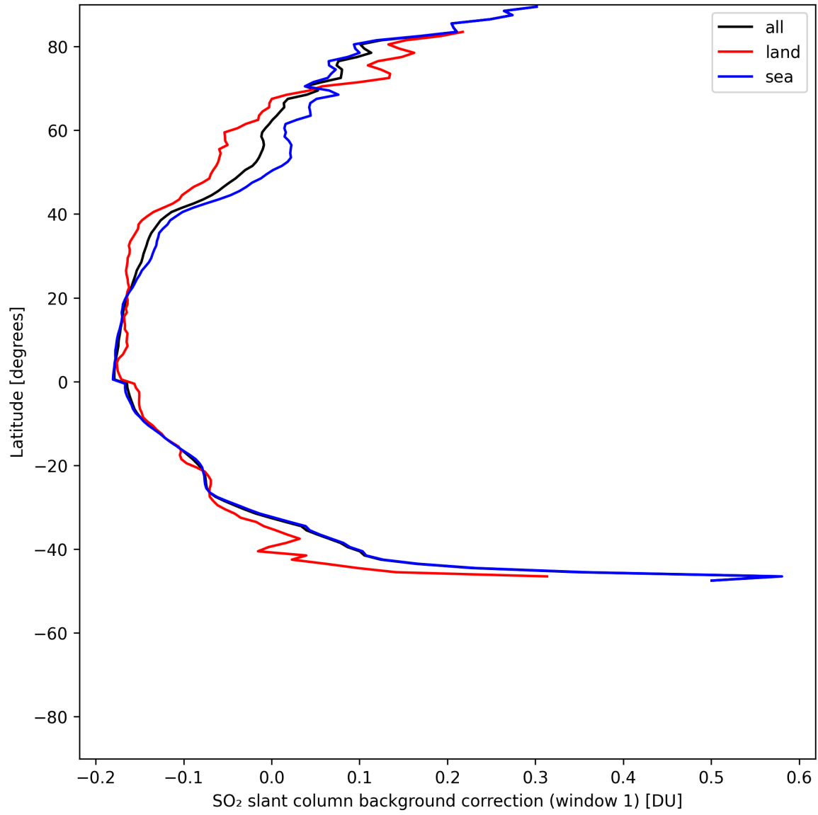
Figure 40: Zonal average of “SO 2 slant column background correction (window 1)” for 2025-07-10 to 2025-07-12.
