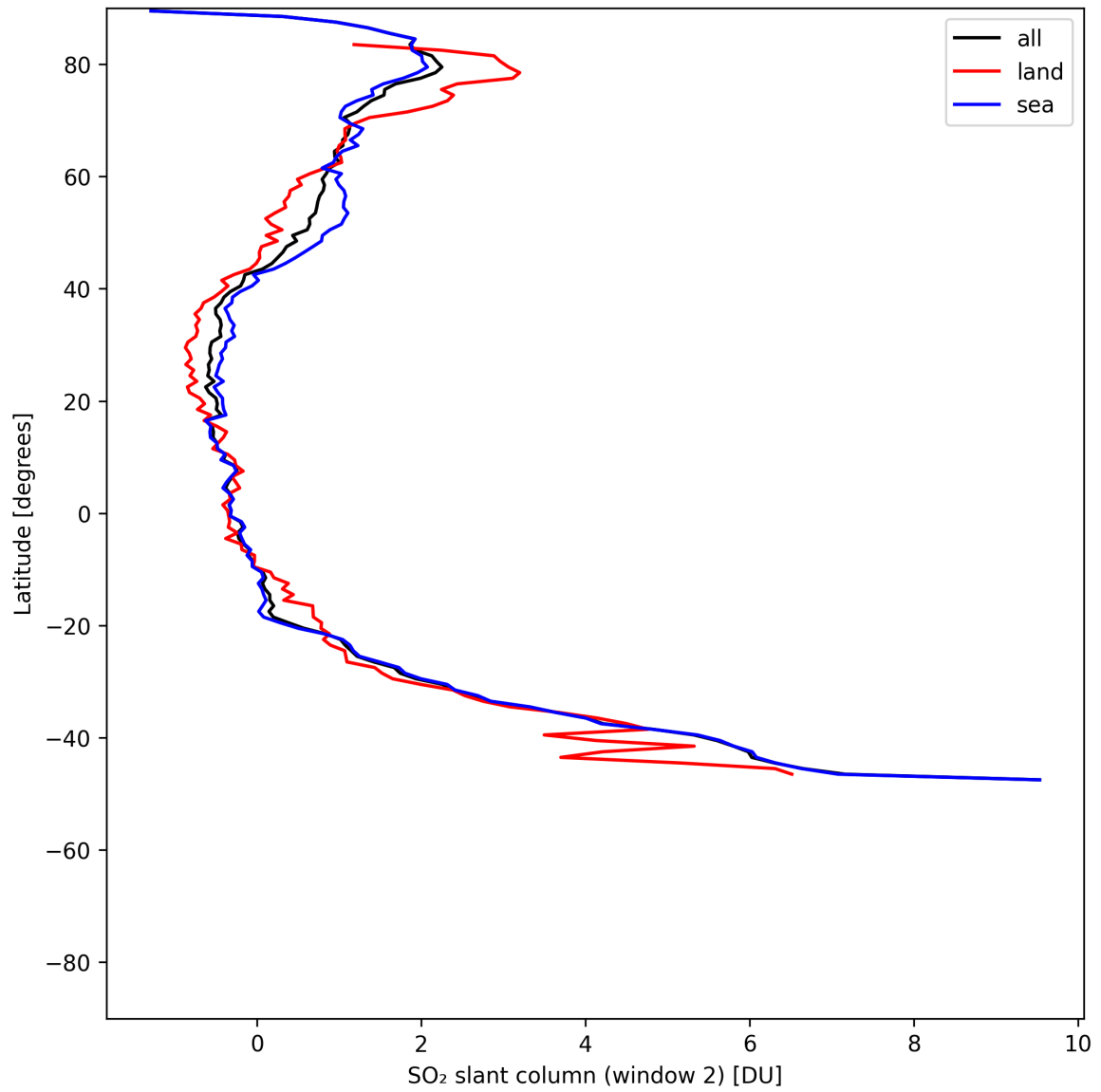
Figure 41: Zonal average of “SO 2 slant column (window 2)” for 2025-07-10 to 2025-07-12.
