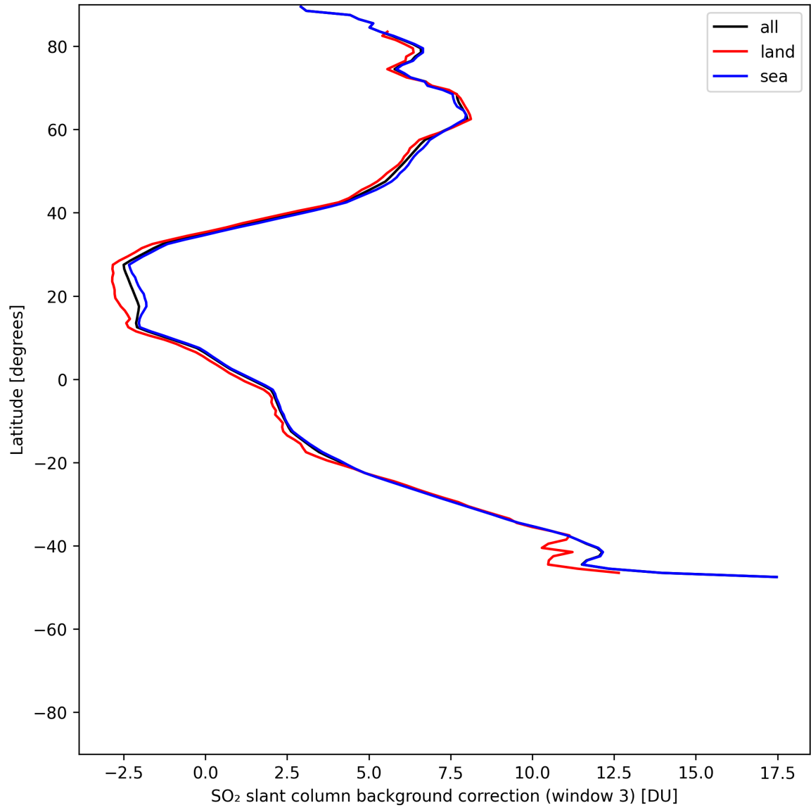
Figure 48: Zonal average of “SO 2 slant column background correction (window 3)” for 2025-07-10 to 2025-07-12.
