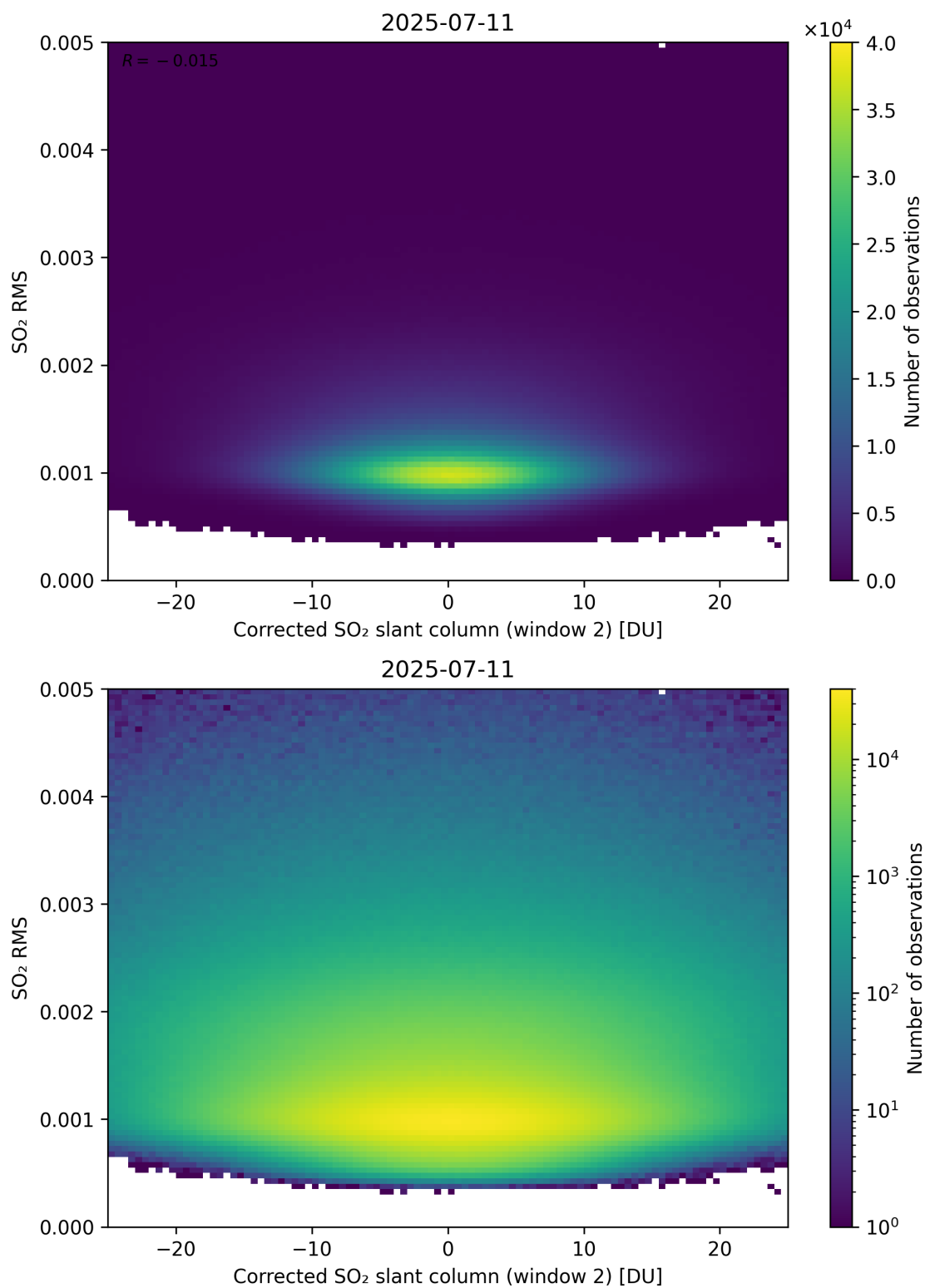
Figure 248: Scatter density plot of “Corrected SO 2 slant column (window 2)” against “SO 2 RMS” for 2025-07-10 to 2025-07-12.
