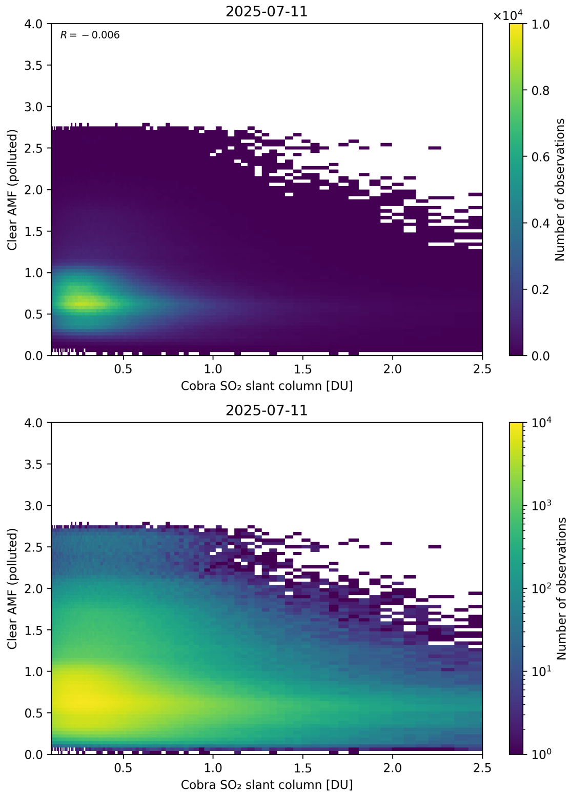
Figure 215: Scatter density plot of “Cobra SO 2 slant column” against “Clear AMF (polluted)” for 2025-07-10 to 2025-07-12.
