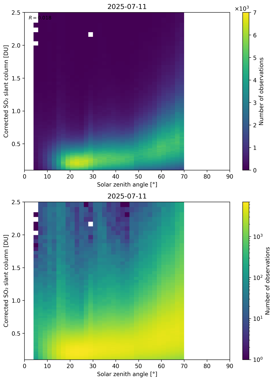
Figure 181: Scatter density plot of “Solar zenith angle” against “Corrected SO 2 slant column” for 2025-07-10 to 2025-07-12.
