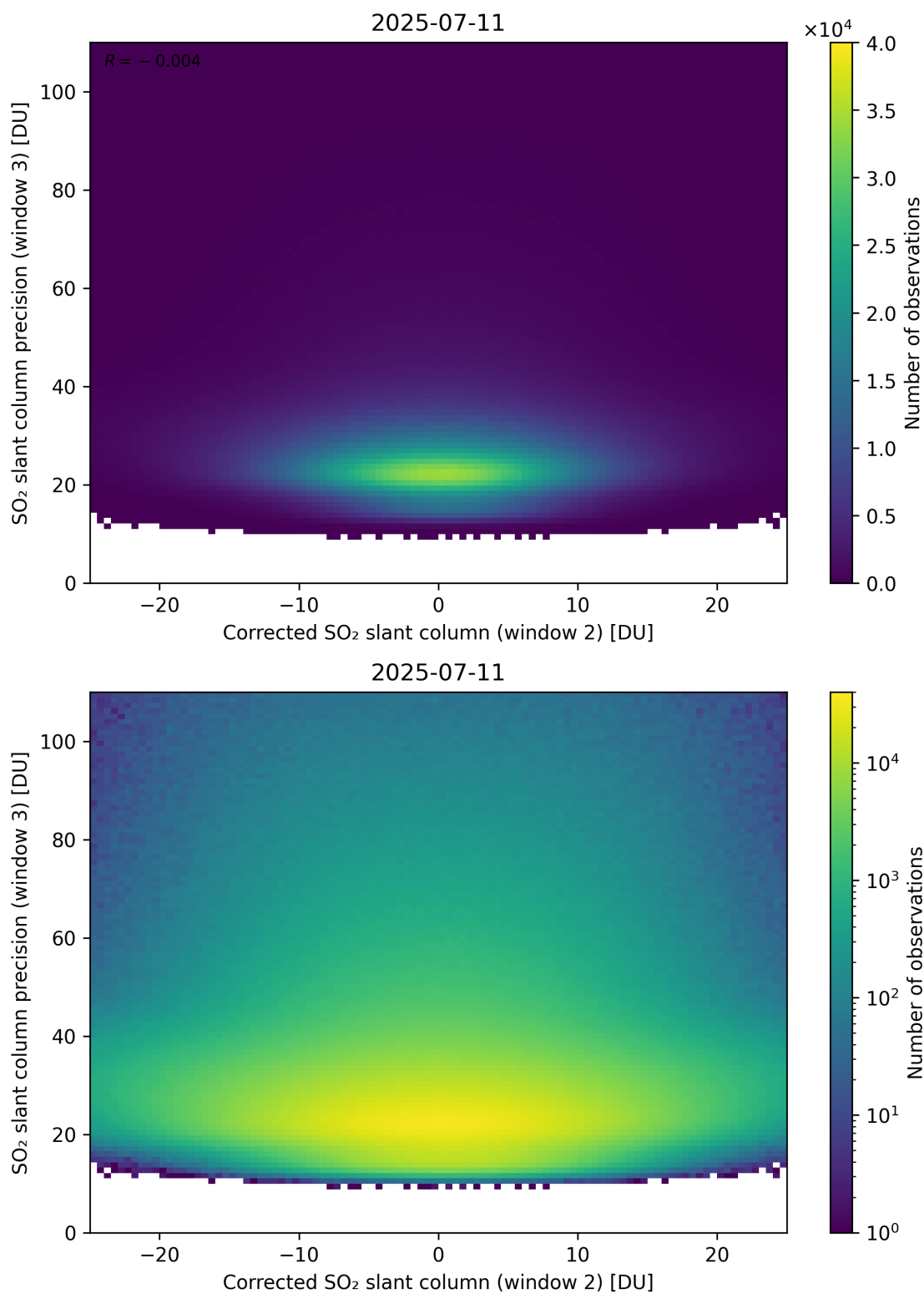
Figure 252: Scatter density plot of “Corrected SO 2 slant column (window 2)” against “SO 2 slant column precision (window 3)” for 2025-07-10 to 2025-07-12.
