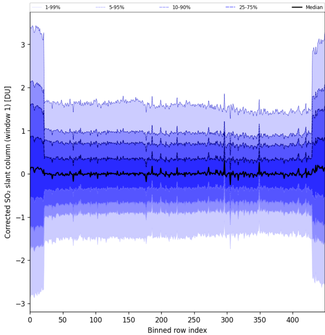
Figure 91: Along track statistics of “Corrected SO 2 slant column (window 1)” for 2025-07-10 to 2025-07-12
