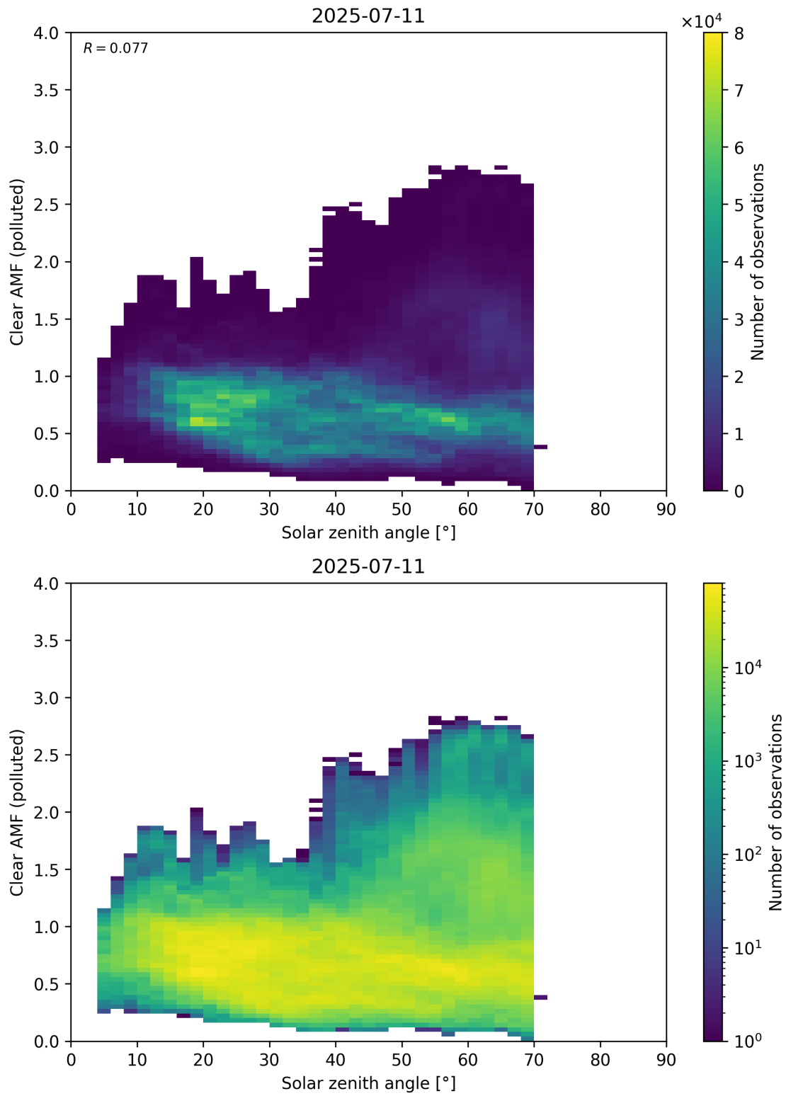
Figure 178: Scatter density plot of “Solar zenith angle” against “Clear AMF (polluted)” for 2025-07-10 to 2025-07-12.
