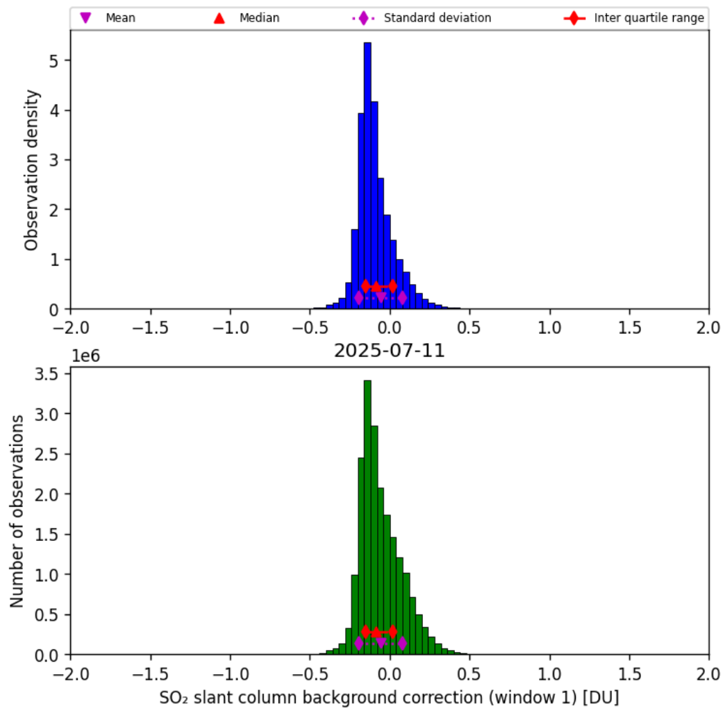
Figure 66: Histogram of “SO 2 slant column background correction (window 1)” for 2025-07-10 to 2025-07-12
