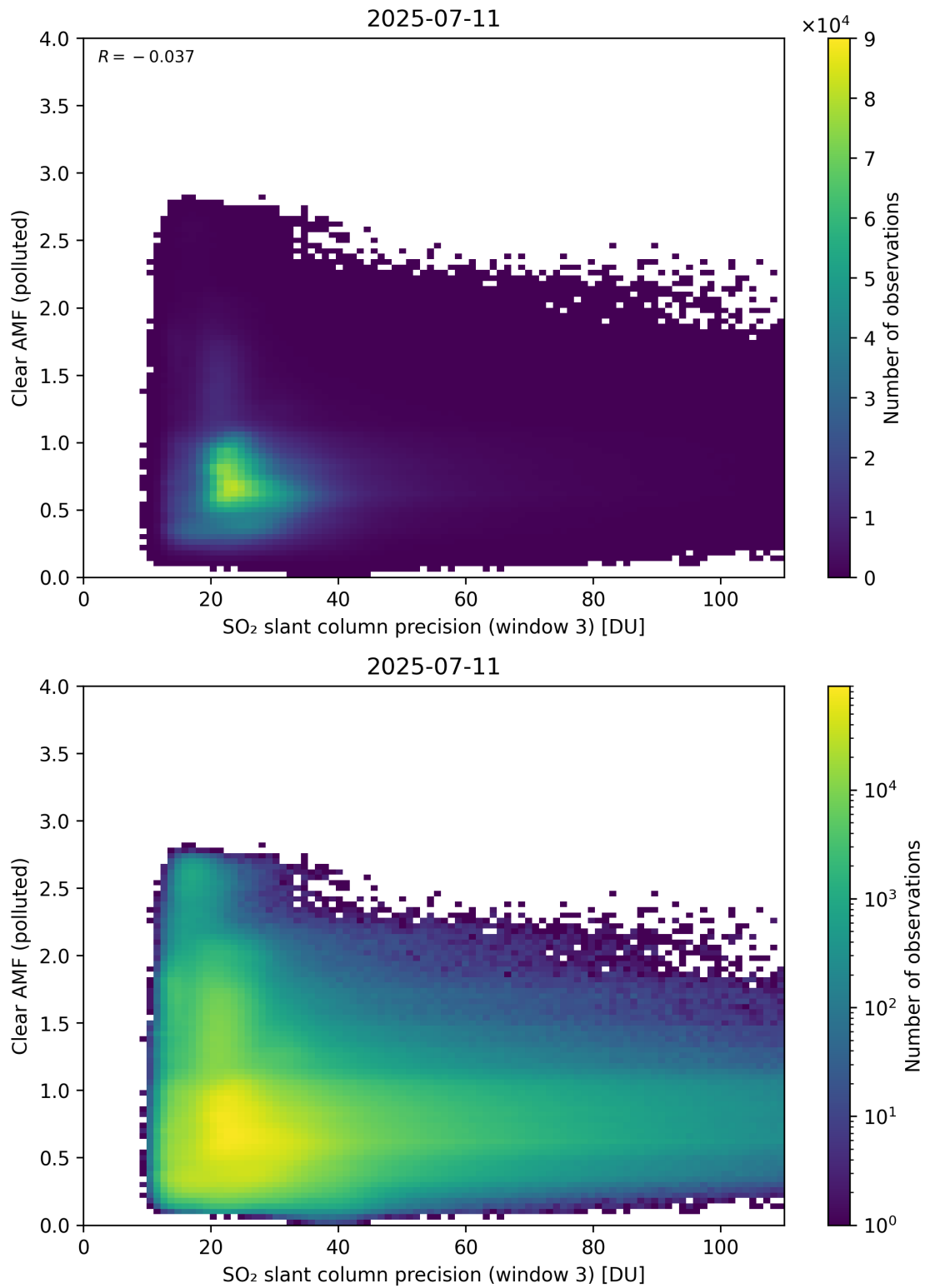
Figure 311: Scatter density plot of “SO 2 slant column precision (window 3)” against “Clear AMF (polluted)” for 2025-07-10 to 2025-07-12.
