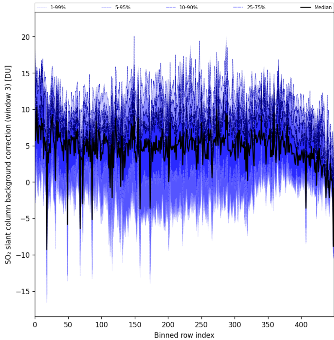
Figure 100: Along track statistics of “SO 2 slant column background correction (window 3)” for 2025-07-10 to 2025-07-12
