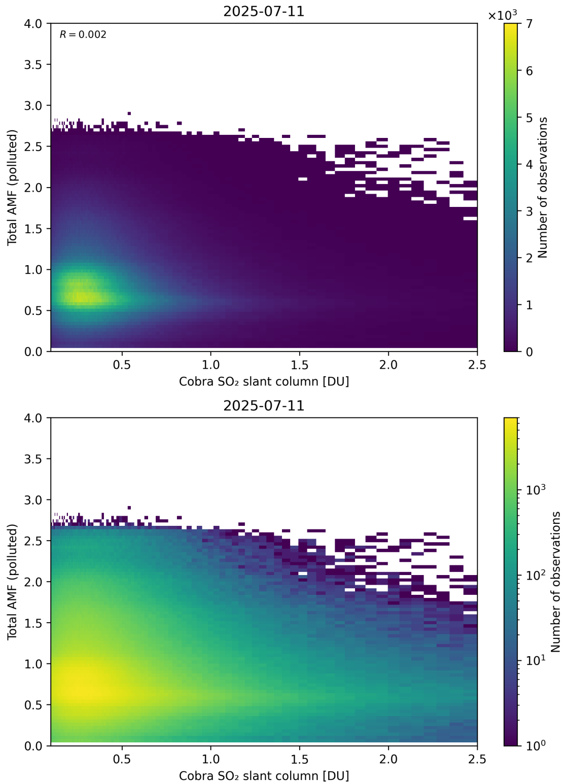
Figure 224: Scatter density plot of “Cobra SO 2 slant column” against “Total AMF (polluted)” for 2025-07-10 to 2025-07-12.
