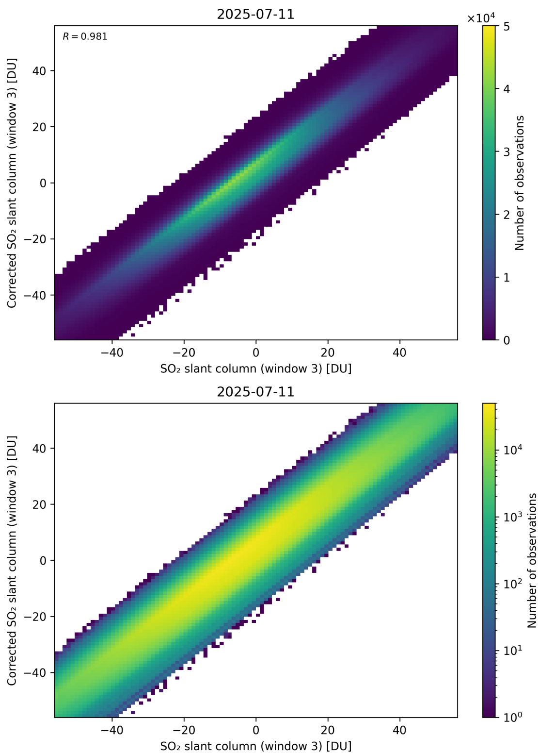
Figure 316: Scatter density plot of “SO 2 slant column (window 3)” against “Corrected SO 2 slant column (window 3)” for 2025-07-10 to 2025-07-12.
