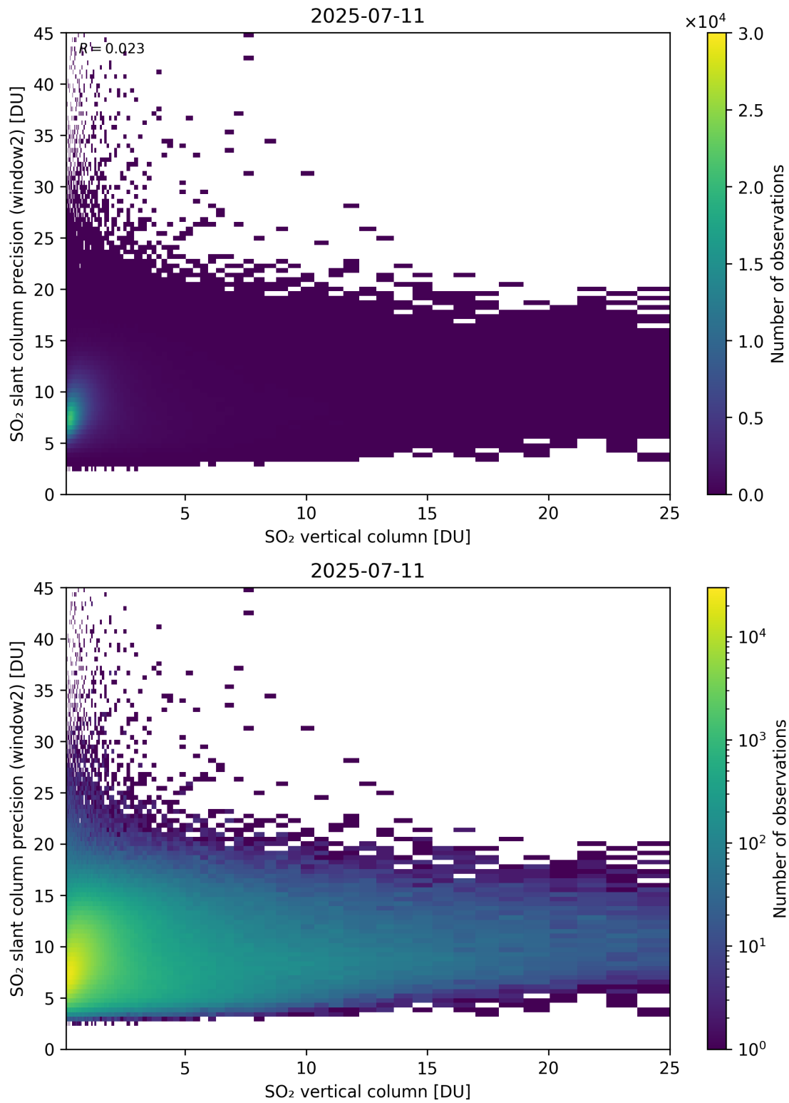
Figure 356: Scatter density plot of “SO 2 vertical column” against “SO 2 slant column precision (window2)” for 2025-07-10 to 2025-07-12.
