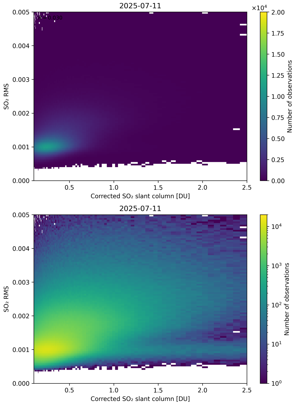
Figure 231: Scatter density plot of “Corrected SO 2 slant column” against “SO 2 RMS” for 2025-07-10 to 2025-07-12.
