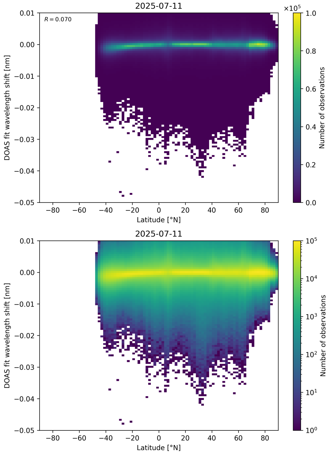
Figure 153: Scatter density plot of “Latitude” against “DOAS fit wavelength shift” for 2025-07-10 to 2025-07-12.
