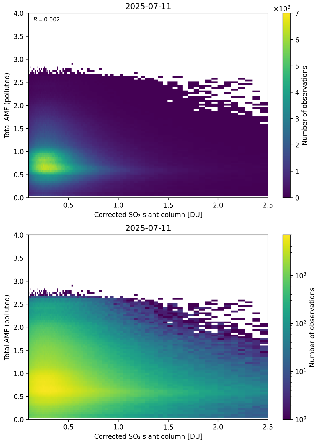
Figure 242: Scatter density plot of “Corrected SO 2 slant column” against “Total AMF (polluted)” for 2025-07-10 to 2025-07-12.
