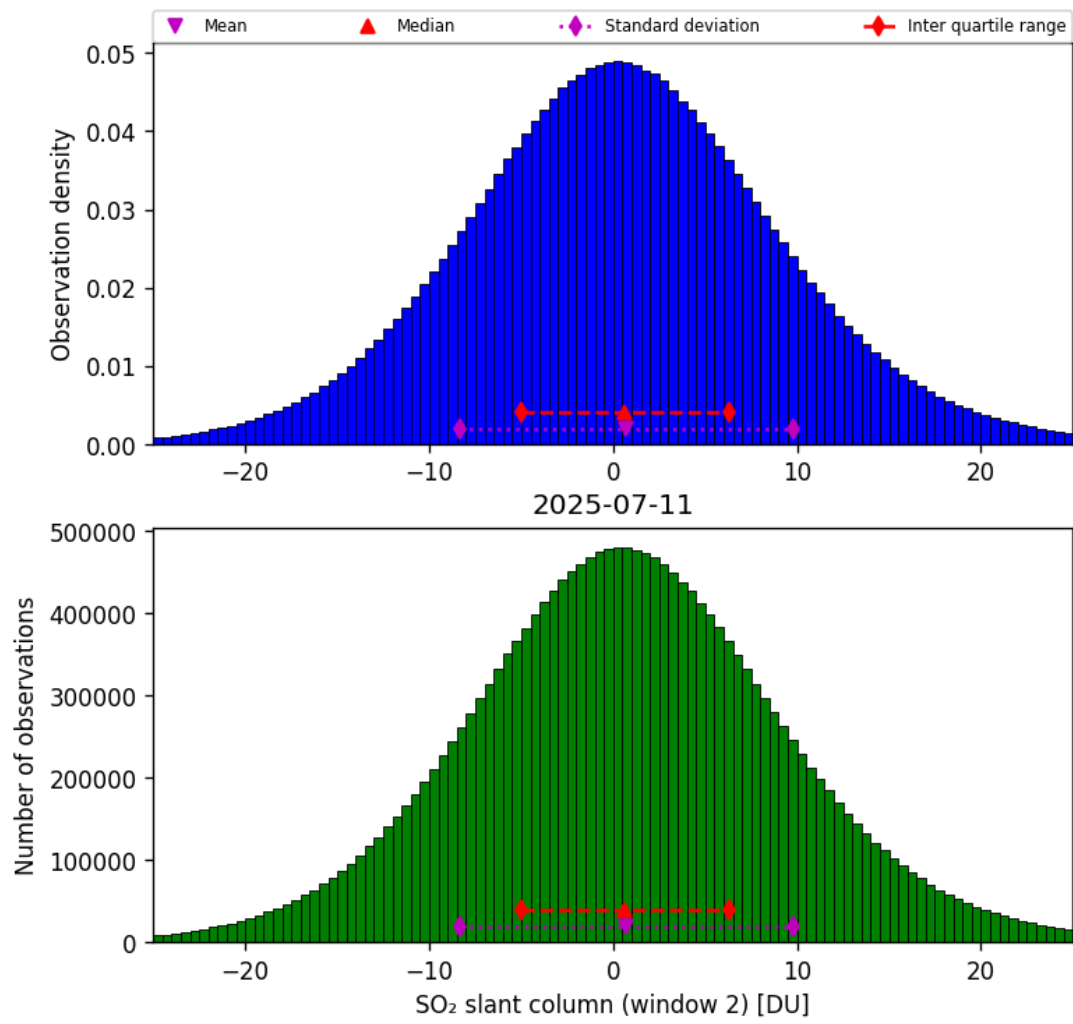
Figure 67: Histogram of “SO 2 slant column (window 2)” for 2025-07-10 to 2025-07-12
