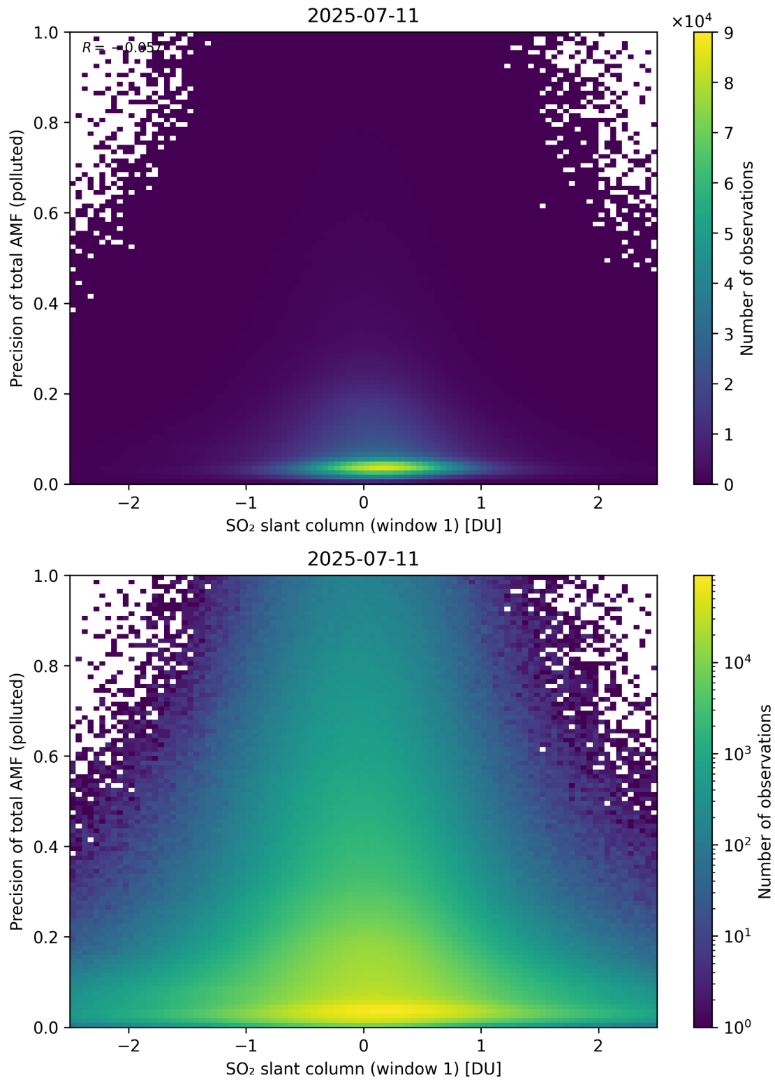
Figure 290: Scatter density plot of “SO 2 slant column (window 1)” against “Precision of total AMF (polluted)” for 2025-07-10 to 2025-07-12.
