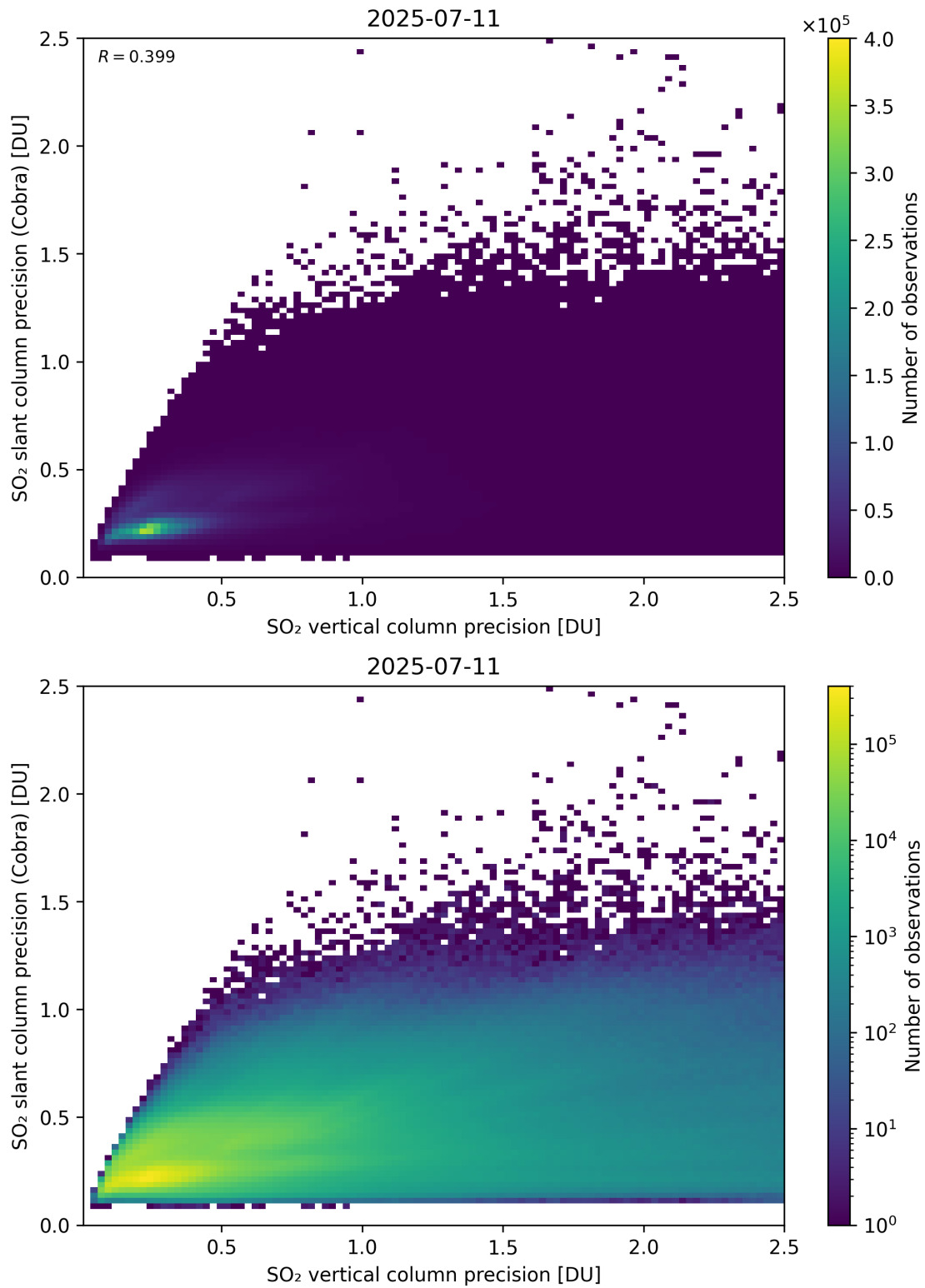
Figure 337: Scatter density plot of “SO 2 vertical column precision” against “SO 2 slant column precision (Cobra)” for 2025-07-10 to 2025-07-12.
