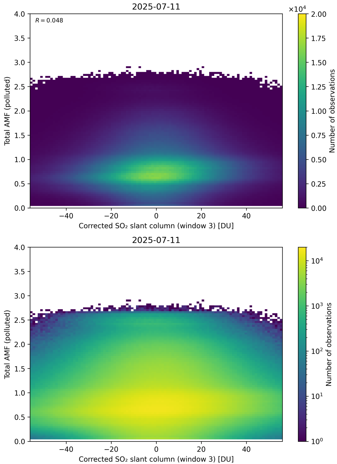
Figure 260: Scatter density plot of “Corrected SO 2 slant column (window 3)” against “Total AMF (polluted)” for 2025-07-10 to 2025-07-12.
