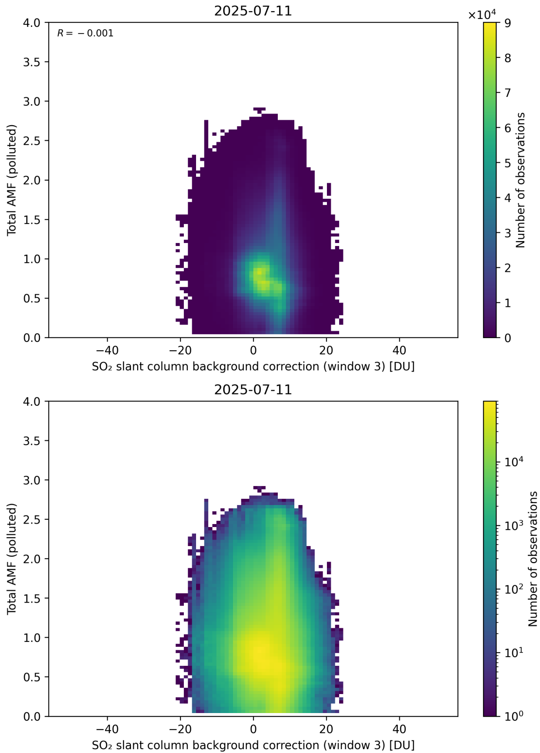
Figure 136: Scatter density plot of “SO 2 slant column background correction (window 3)” against “Total AMF (polluted)” for 2025-07-10 to 2025-07-12.
