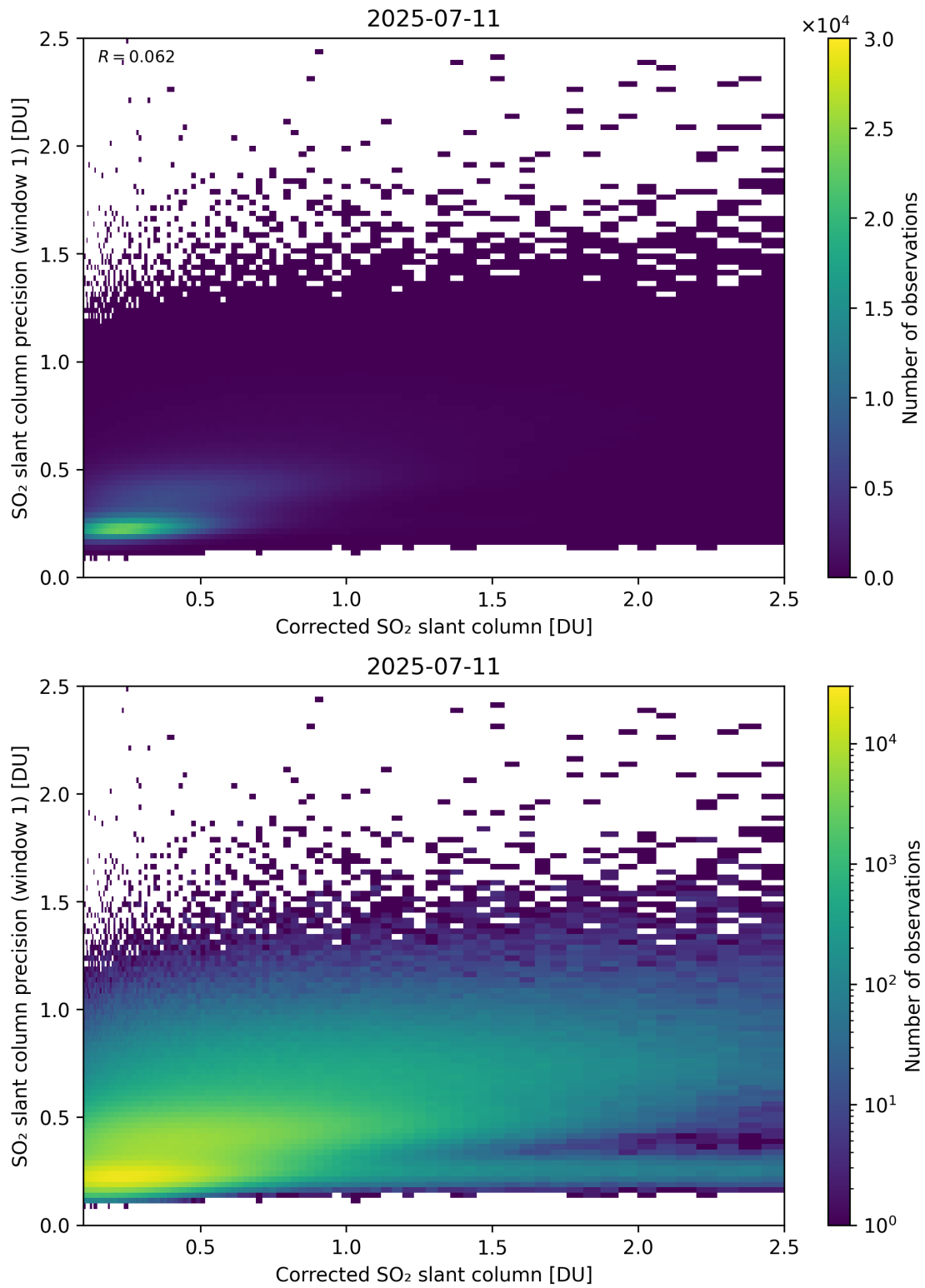
Figure 238: Scatter density plot of “Corrected SO 2 slant column” against “SO 2 slant column precision (window 1)” for 2025-07-10 to 2025-07-12.
