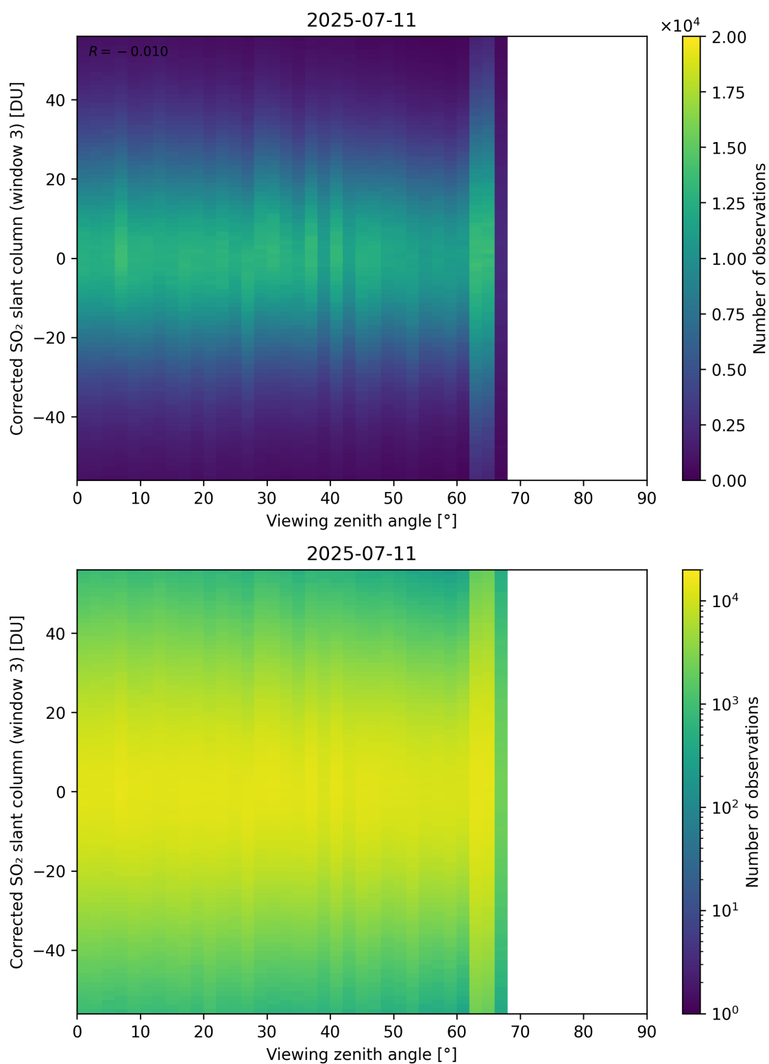
Figure 375: Scatter density plot of “Viewing zenith angle” against “Corrected SO 2 slant column (window 3)” for 2025-07-10 to 2025-07-12.
