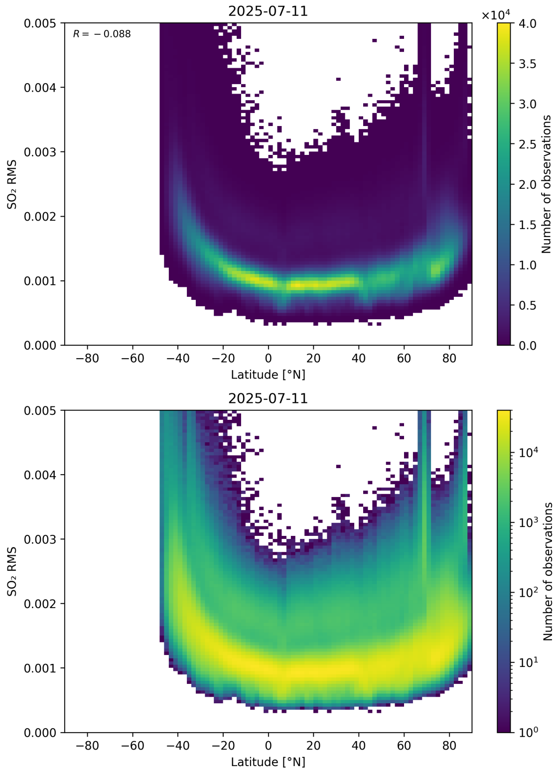
Figure 155: Scatter density plot of “Latitude” against “SO 2 RMS” for 2025-07-10 to 2025-07-12.
