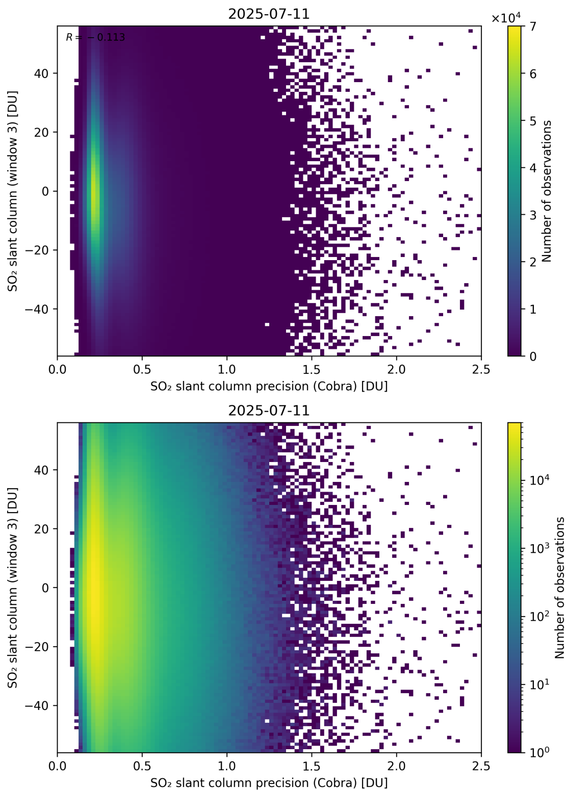
Figure 211: Scatter density plot of “SO 2 slant column precision (Cobra)” against “SO 2 slant column (window 3)” for 2025-07-10 to 2025-07-12.
