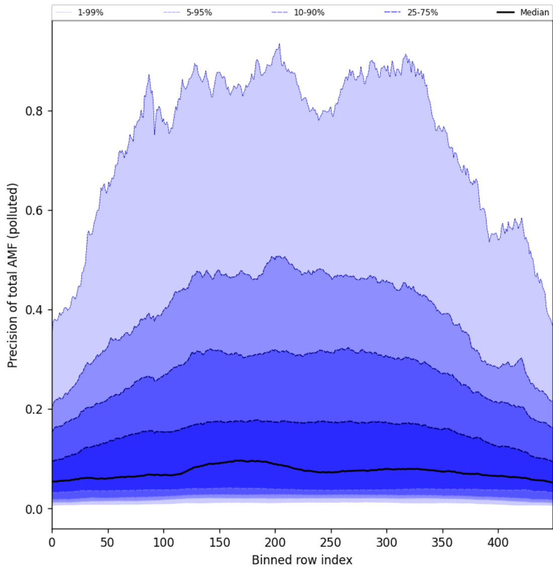
Figure 106: Along track statistics of “Precision of total AMF (polluted)” for 2025-07-10 to 2025-07-12
