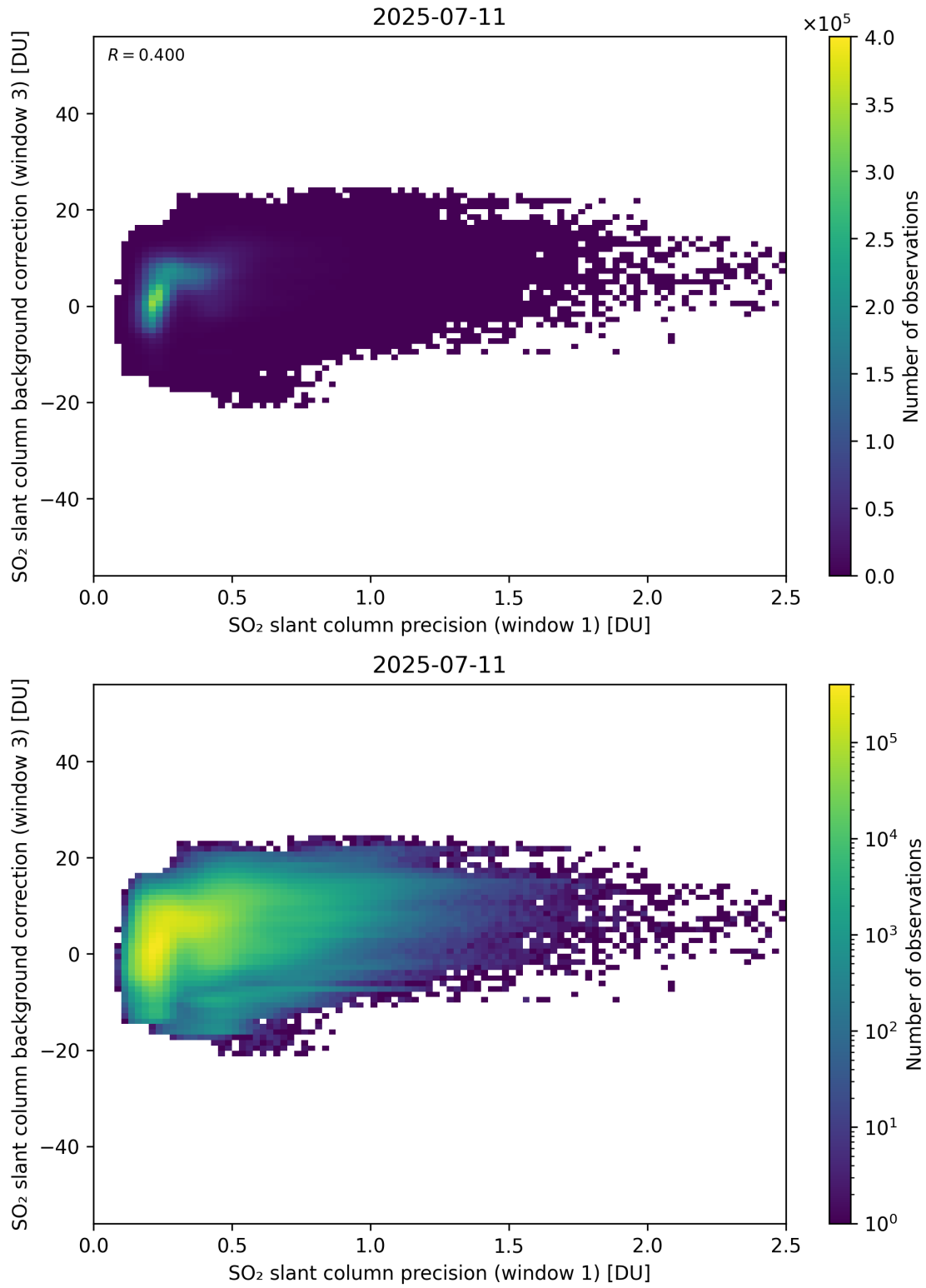
Figure 270: Scatter density plot of “SO 2 slant column precision (window 1)” against “SO 2 slant column background correction (window 3)” for 2025-07-10 to 2025-07-12.
