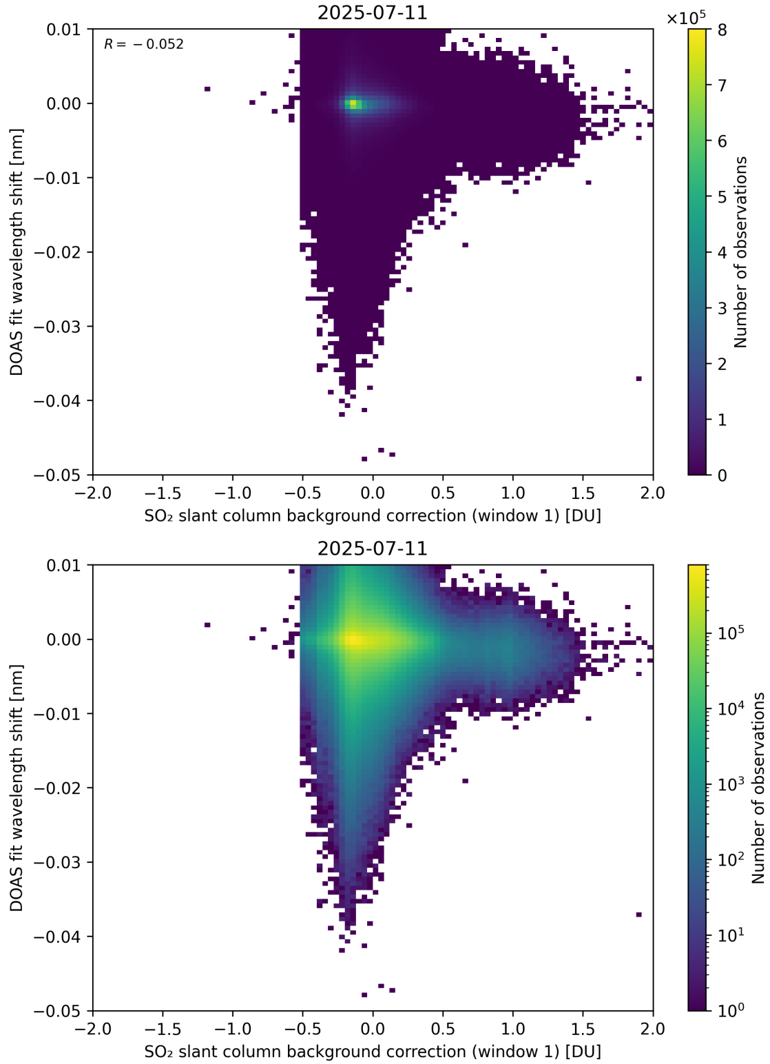
Figure 111: Scatter density plot of “SO 2 slant column background correction (window 1)” against “DOAS fit wavelength shift” for 2025-07-10 to 2025-07-12.
