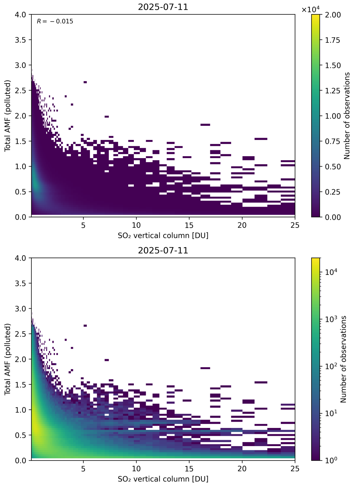
Figure 359: Scatter density plot of “SO 2 vertical column” against “Total AMF (polluted)” for 2025-07-10 to 2025-07-12.
