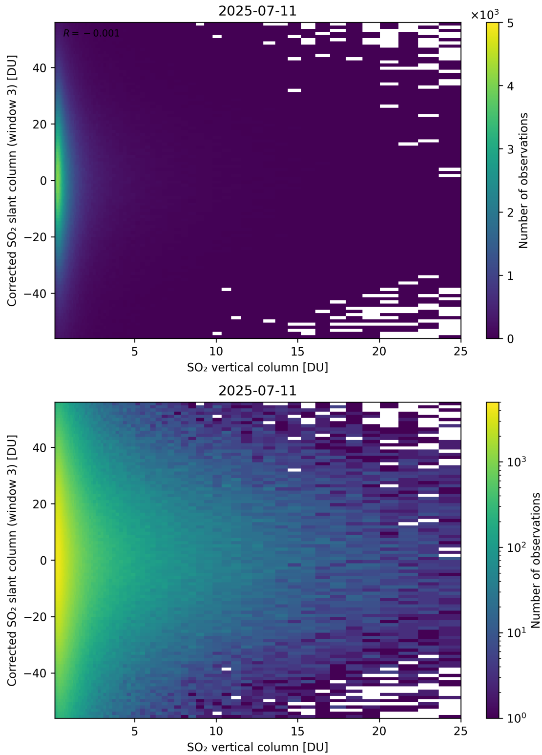
Figure 353: Scatter density plot of “SO 2 vertical column” against “Corrected SO 2 slant column (window 3)” for 2025-07-10 to 2025-07-12.
