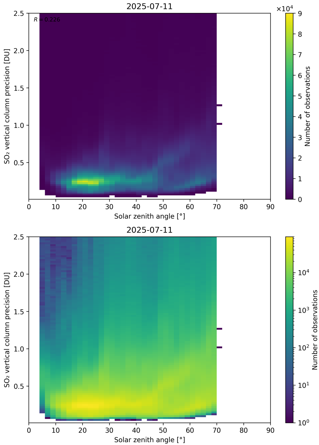
Figure 192: Scatter density plot of “Solar zenith angle” against “SO 2 vertical column precision” for 2025-07-10 to 2025-07-12.
