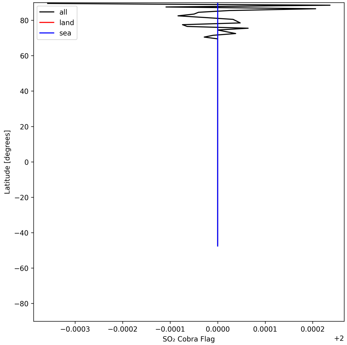
Figure 49: Zonal average of “SO 2 Cobra Flag” for 2025-07-10 to 2025-07-12.
