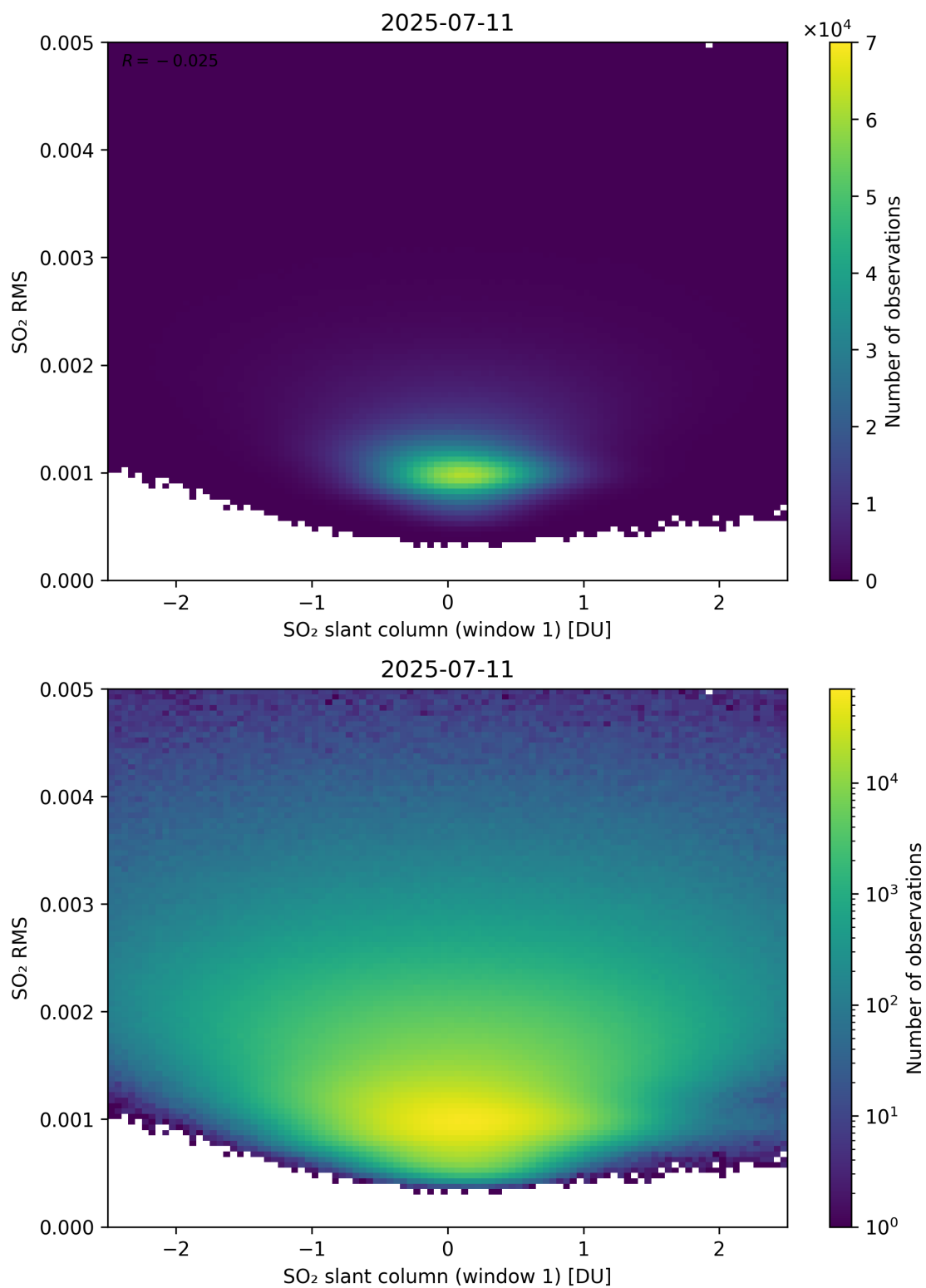
Figure 267: Scatter density plot of “SO 2 slant column (window 1)” against “SO 2 RMS” for 2025-07-10 to 2025-07-12.
