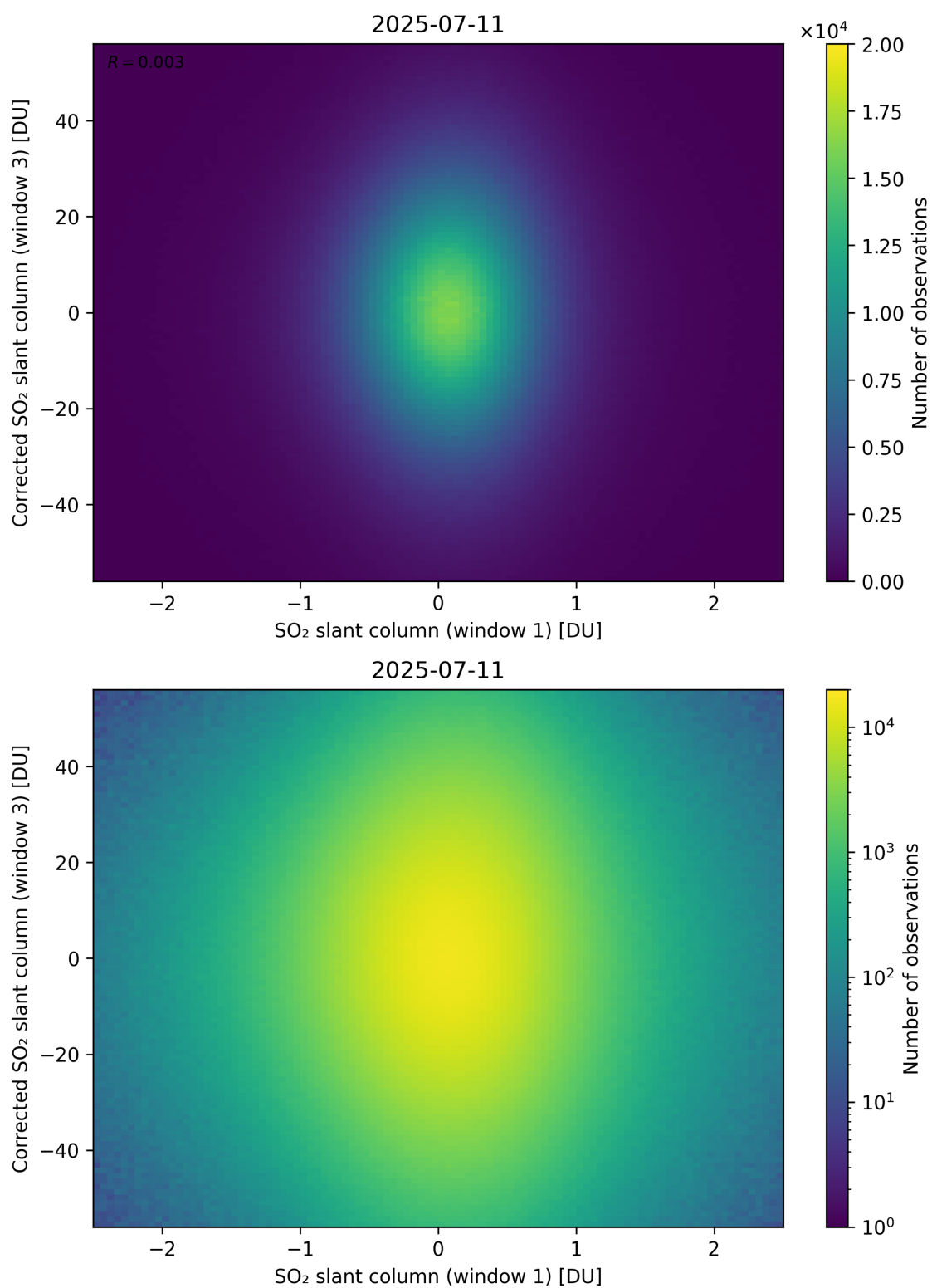
Figure 284: Scatter density plot of “SO 2 slant column (window 1)” against “Corrected SO 2 slant column (window 3)” for 2025-07-10 to 2025-07-12.
