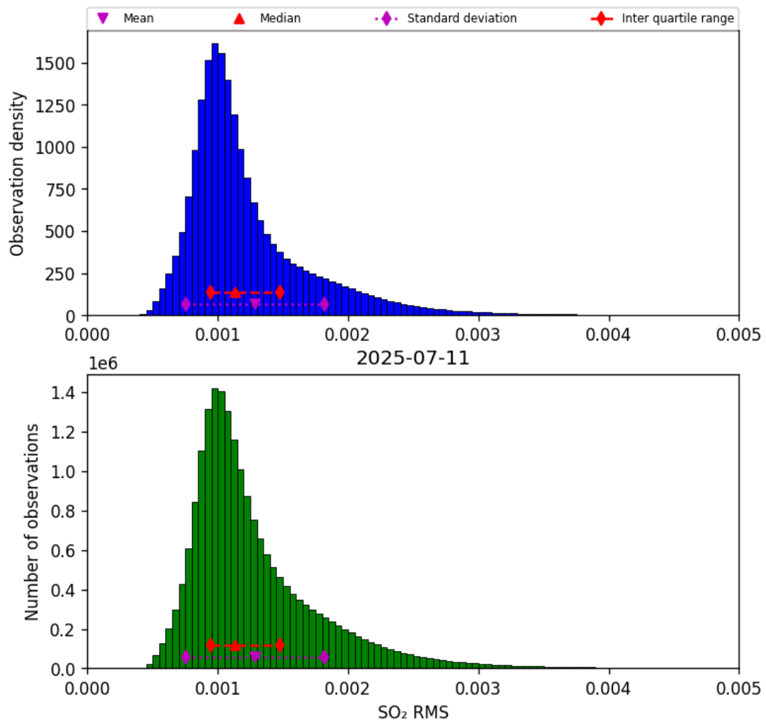
Figure 78: Histogram of “SO 2 RMS” for 2025-07-10 to 2025-07-12
