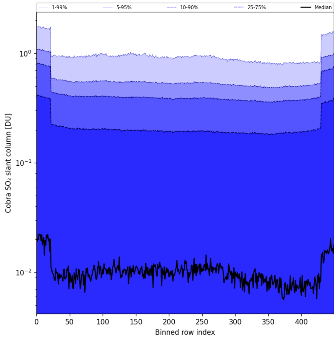
Figure 87: Along track statistics of “Cobra SO 2 slant column” for 2025-07-10 to 2025-07-12
