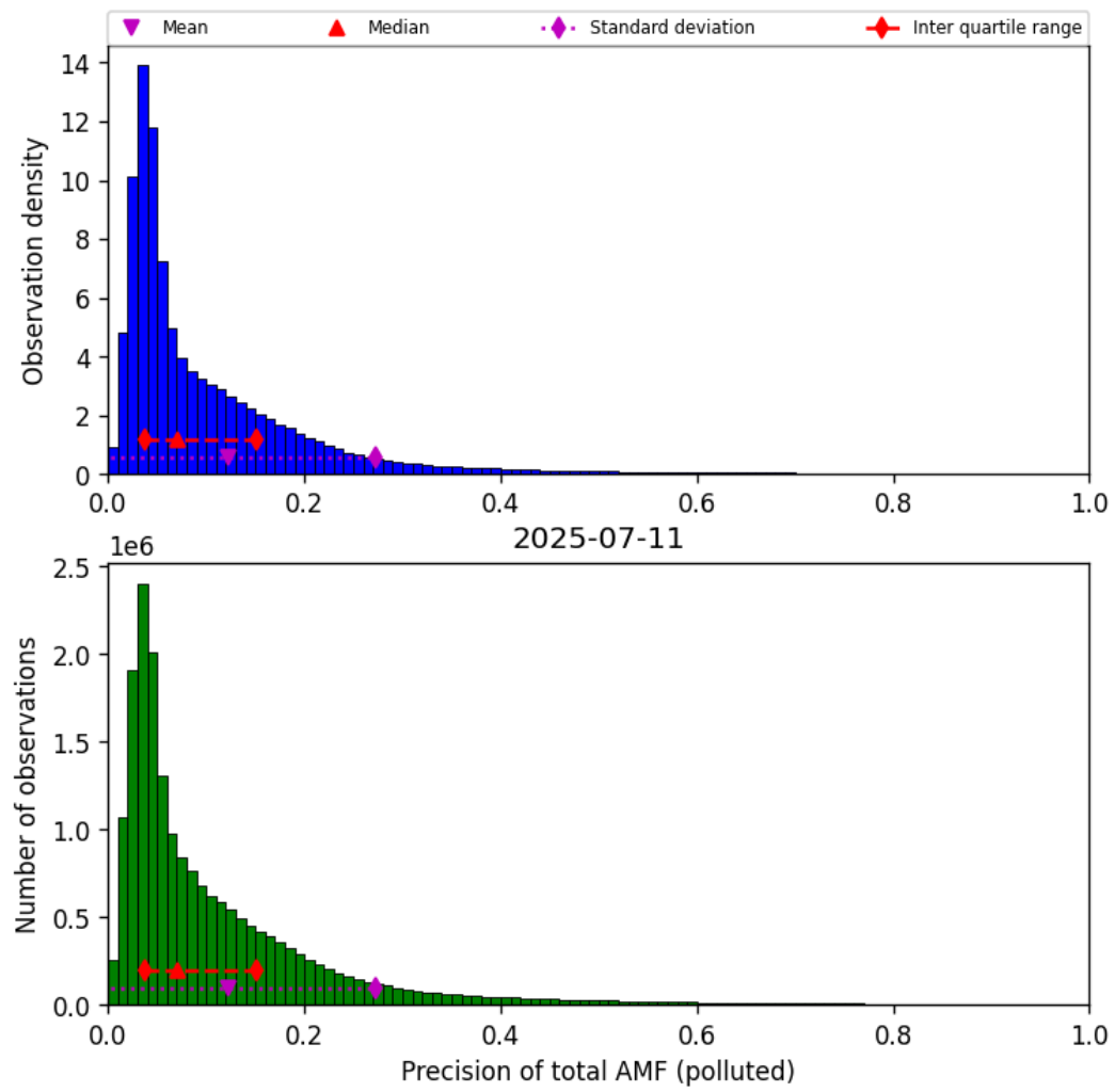
Figure 80: Histogram of “Precision of total AMF (polluted)” for 2025-07-10 to 2025-07-12
