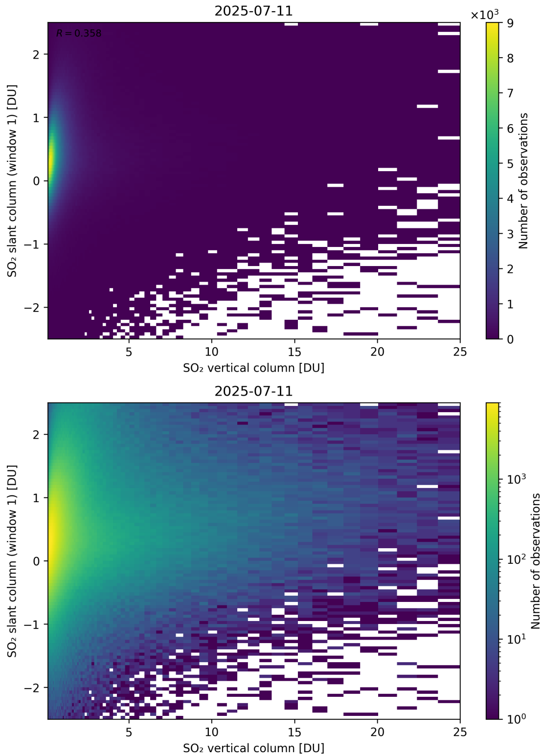
Figure 354: Scatter density plot of “SO 2 vertical column” against “SO 2 slant column (window 1)” for 2025-07-10 to 2025-07-12.
