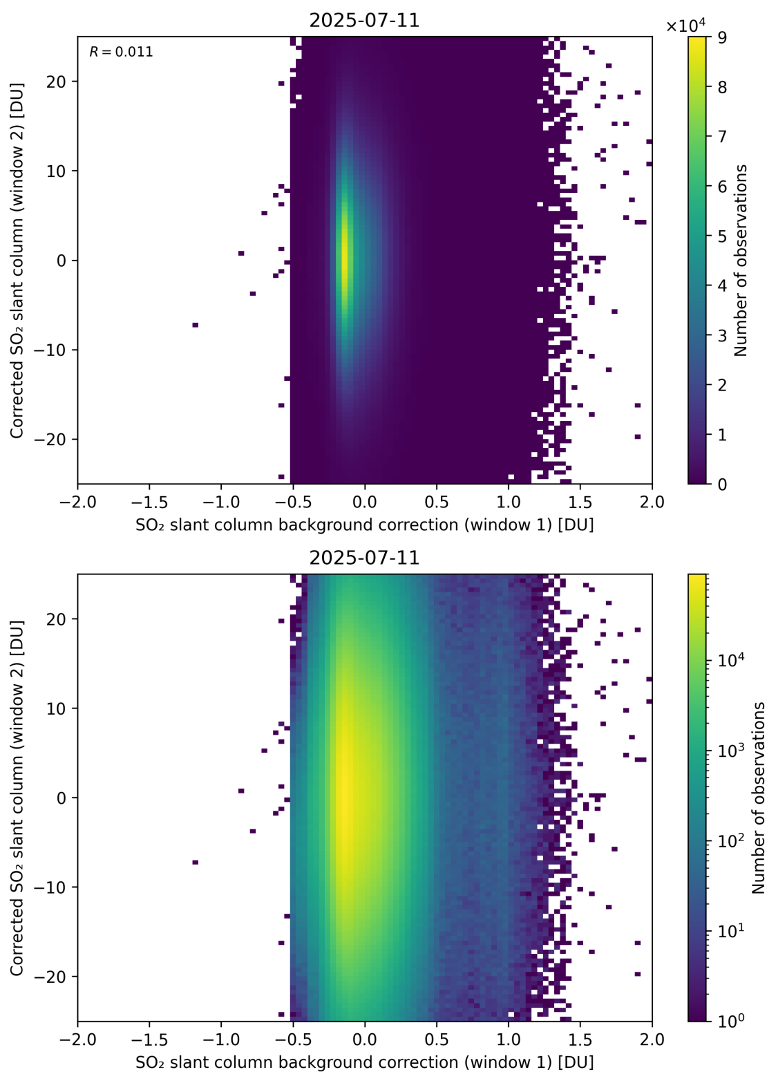
Figure 115: Scatter density plot of “SO 2 slant column background correction (window 1)” against “Corrected SO 2 slant column (window 2)” for 2025-07-10 to 2025-07-12.
