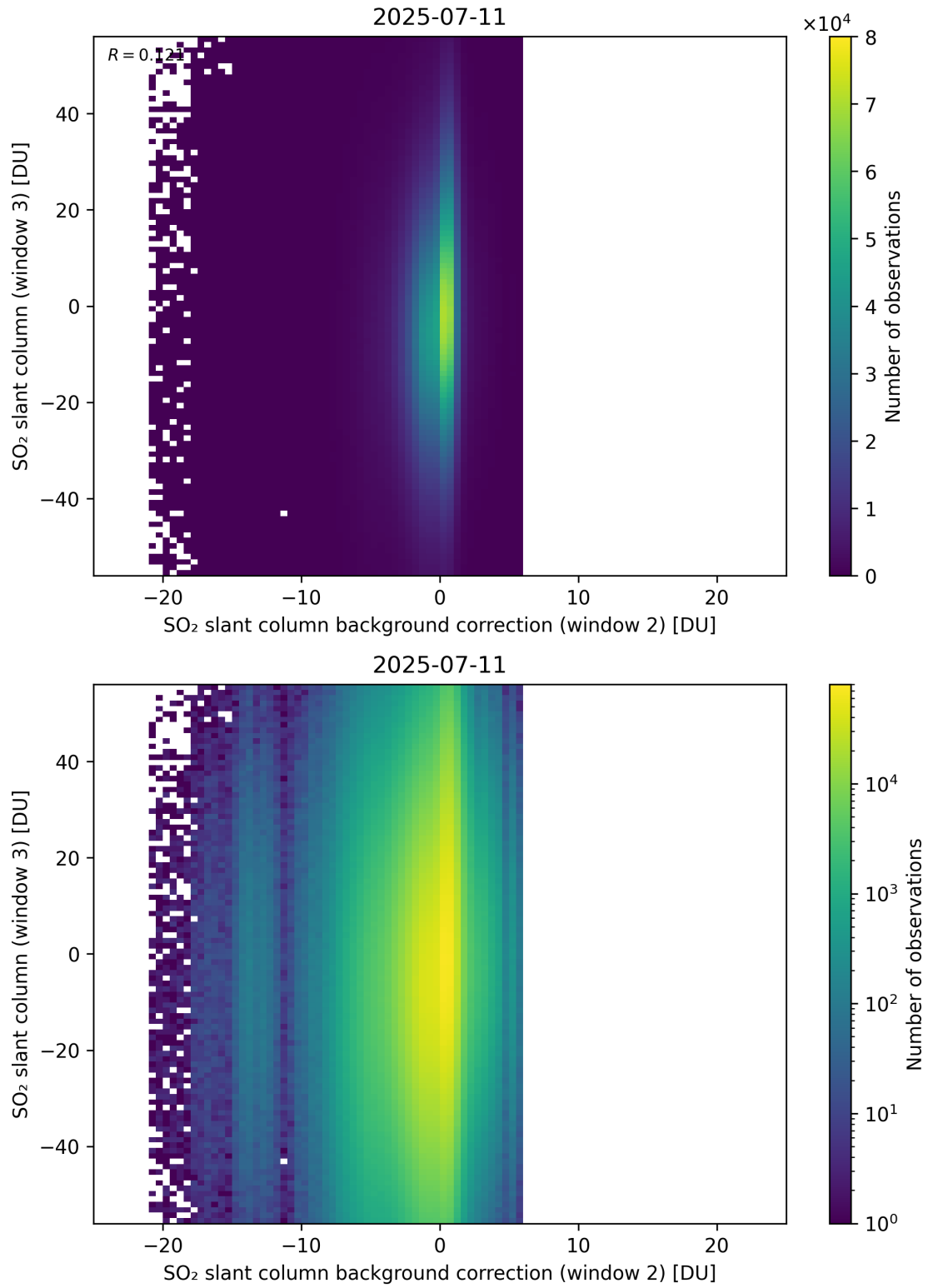
Figure 128: Scatter density plot of “SO 2 slant column background correction (window 2)” against “SO 2 slant column (window 3)” for 2025-07-10 to 2025-07-12.
