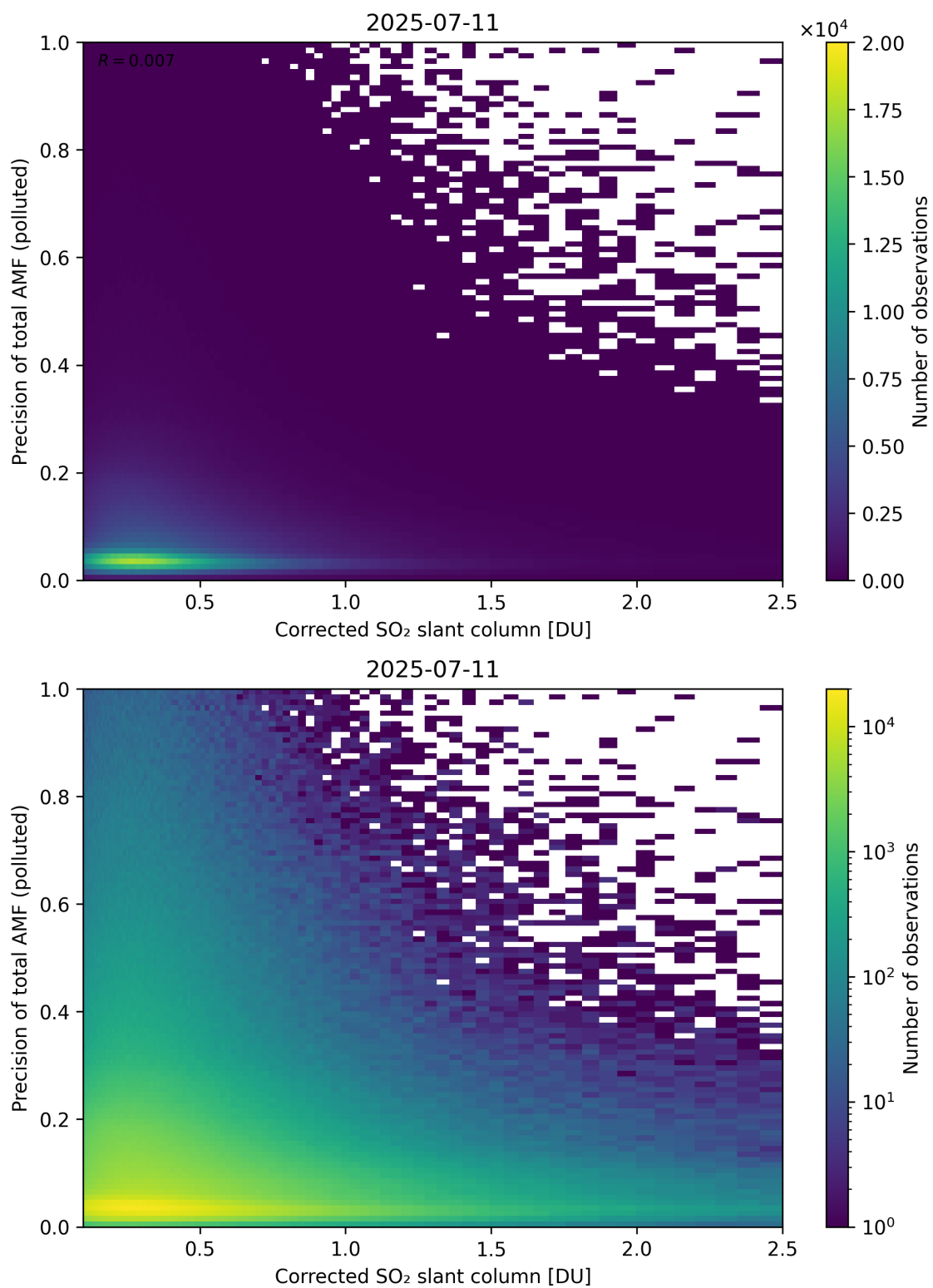
Figure 243: Scatter density plot of “Corrected SO 2 slant column” against “Precision of total AMF (polluted)” for 2025-07-10 to 2025-07-12.
