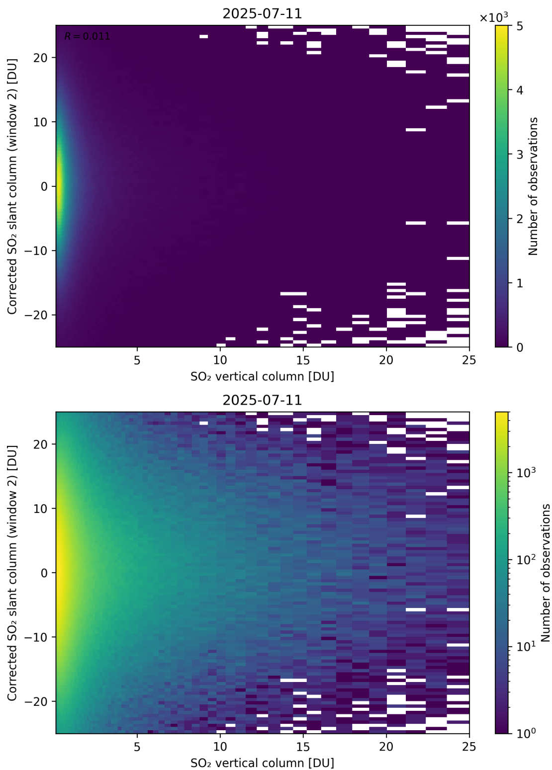
Figure 352: Scatter density plot of “SO 2 vertical column” against “Corrected SO 2 slant column (window 2)” for 2025-07-10 to 2025-07-12.
