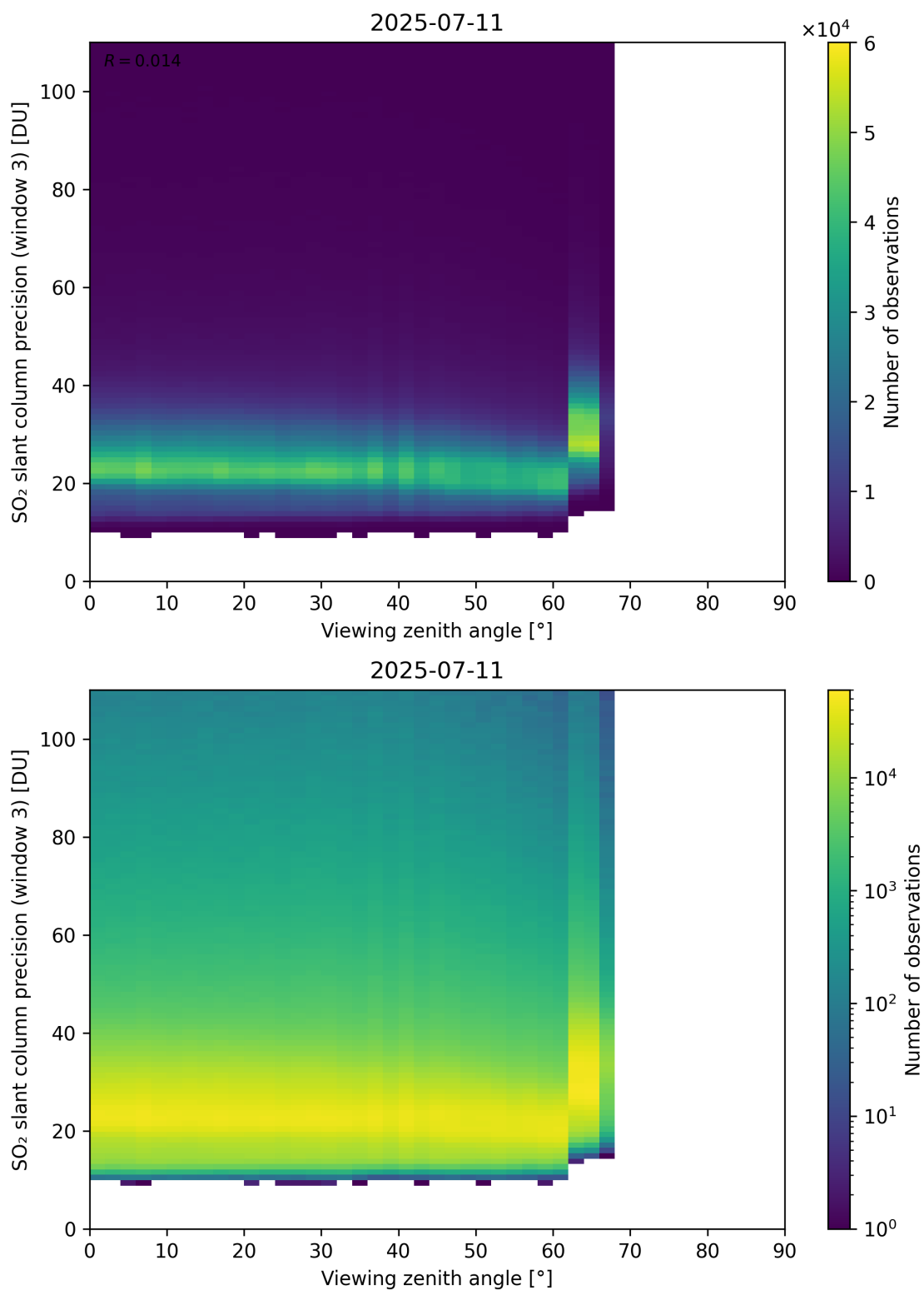
Figure 380: Scatter density plot of “Viewing zenith angle” against “SO 2 slant column precision (window 3)” for 2025-07-10 to 2025-07-12.
