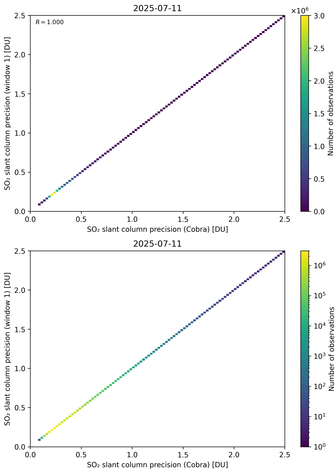
Figure 209: Scatter density plot of “SO 2 slant column precision (Cobra)” against “SO 2 slant column precision (window 1)” for 2025-07-10 to 2025-07-12.
