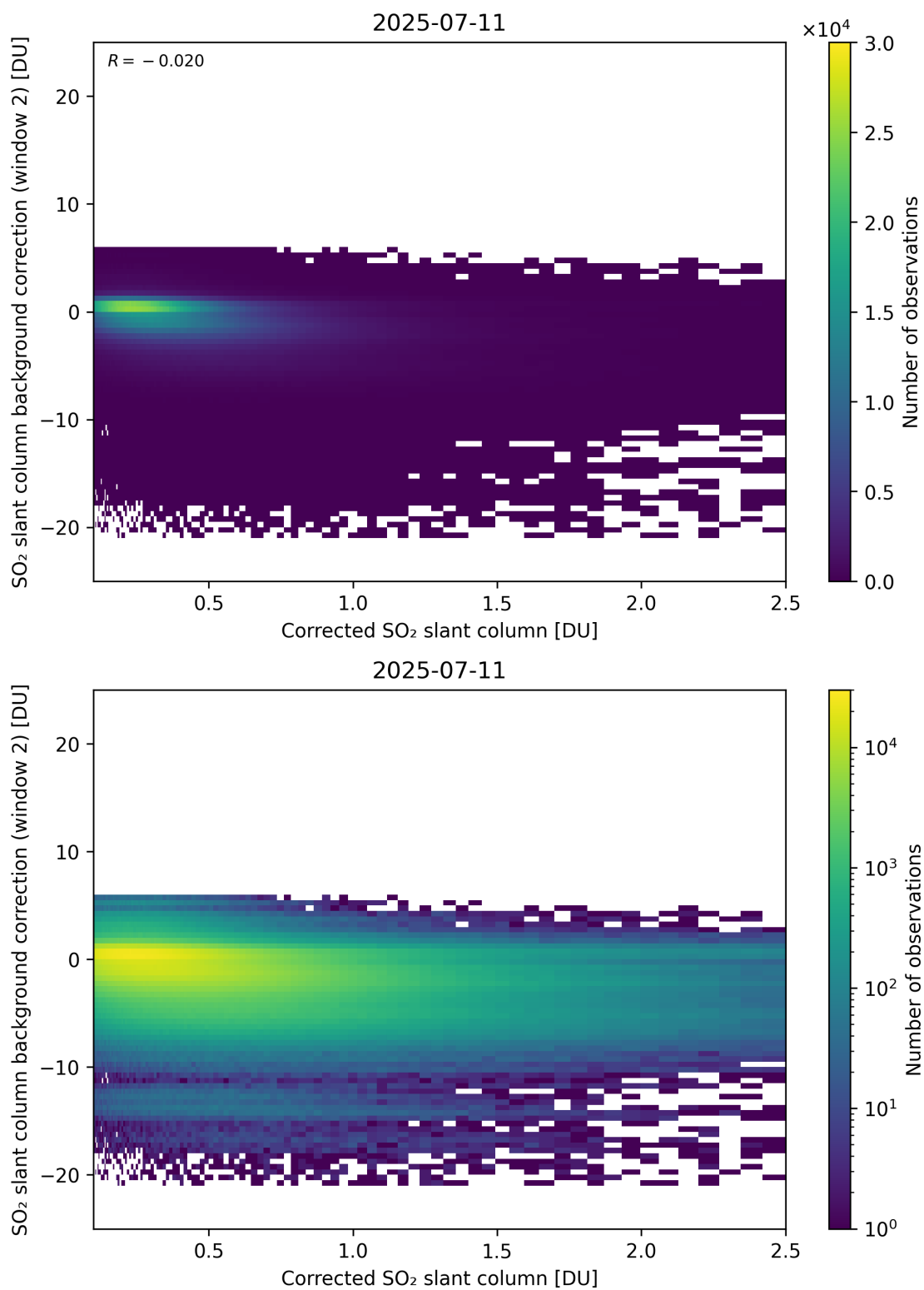
Figure 227: Scatter density plot of “Corrected SO 2 slant column” against “SO 2 slant column background correction (window 2)” for 2025-07-10 to 2025-07-12.
