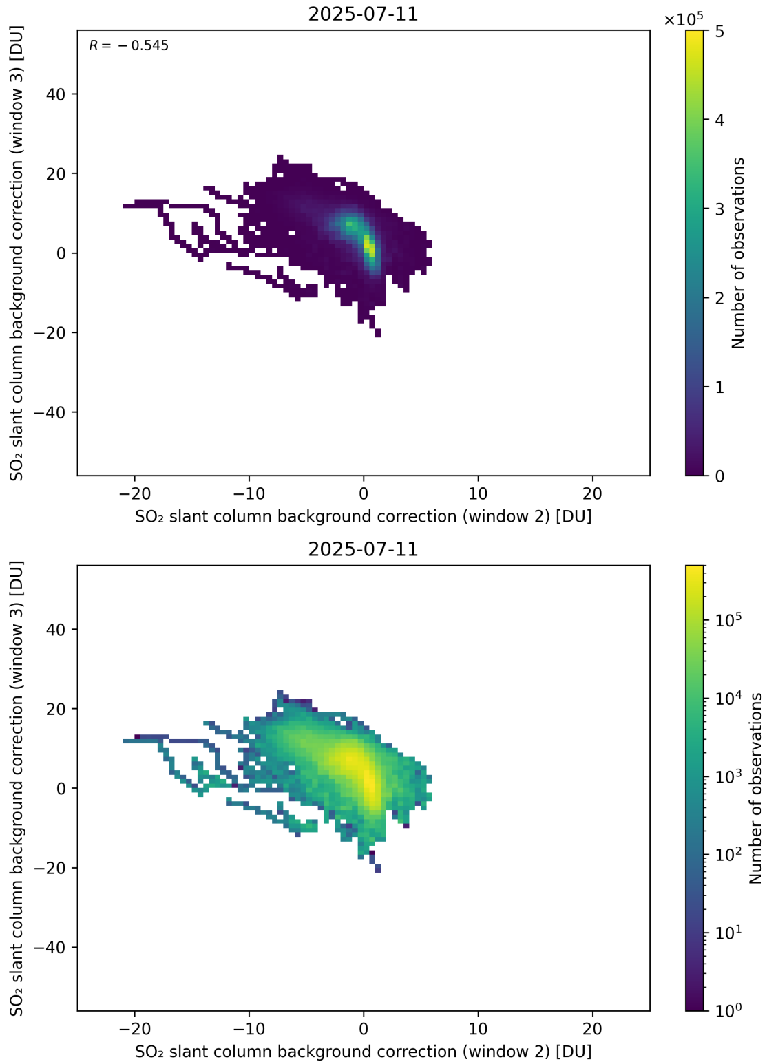
Figure 122: Scatter density plot of “SO 2 slant column background correction (window 2)” against “SO 2 slant column background correction (window 3)” for 2025-07-10 to 2025-07-12.
