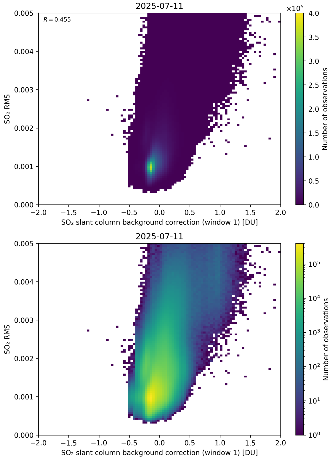
Figure 113: Scatter density plot of “SO 2 slant column background correction (window 1)” against “SO 2 RMS” for 2025-07-10 to 2025-07-12.
