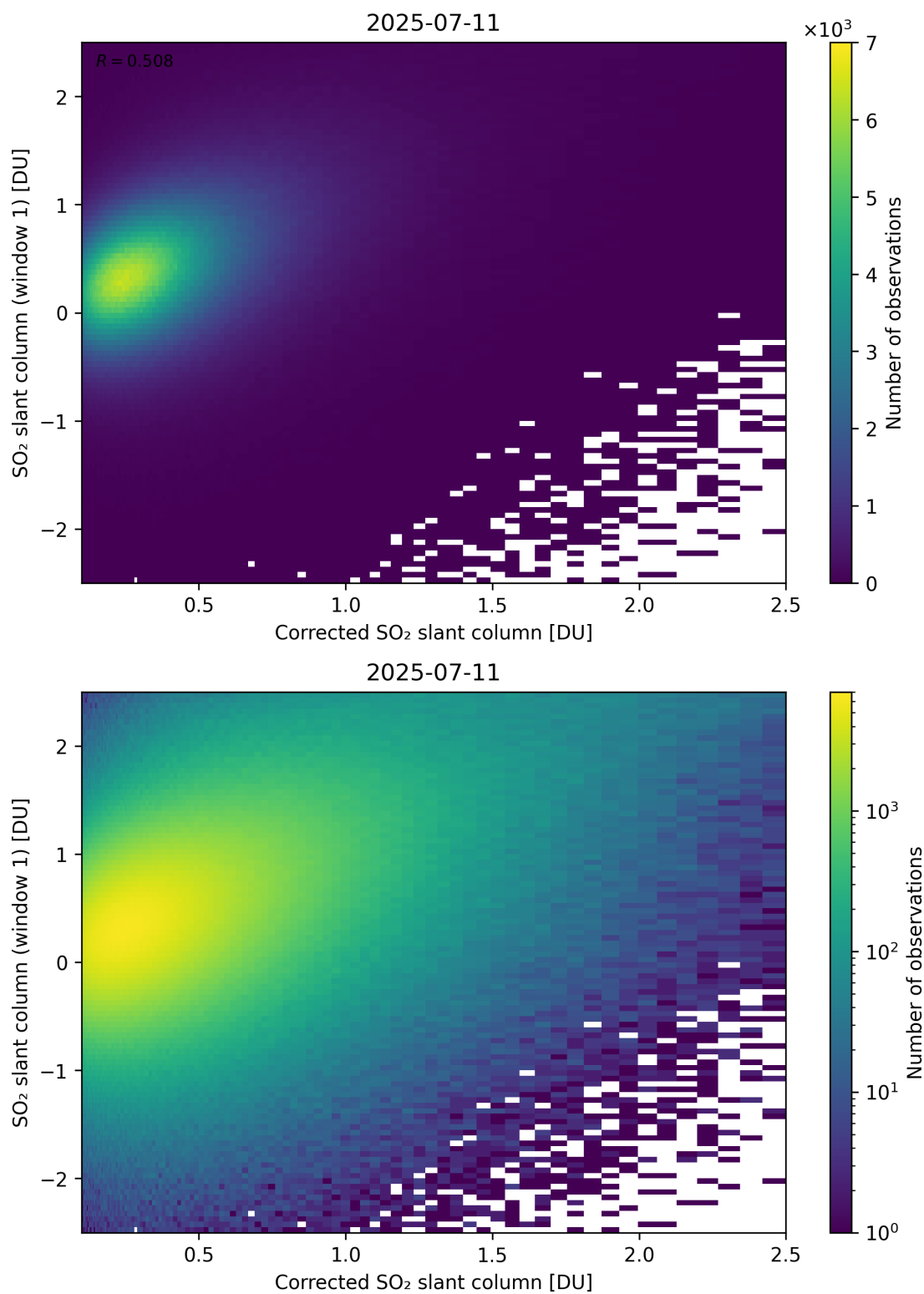
Figure 237: Scatter density plot of “Corrected SO 2 slant column” against “SO 2 slant column (window 1)” for 2025-07-10 to 2025-07-12.
