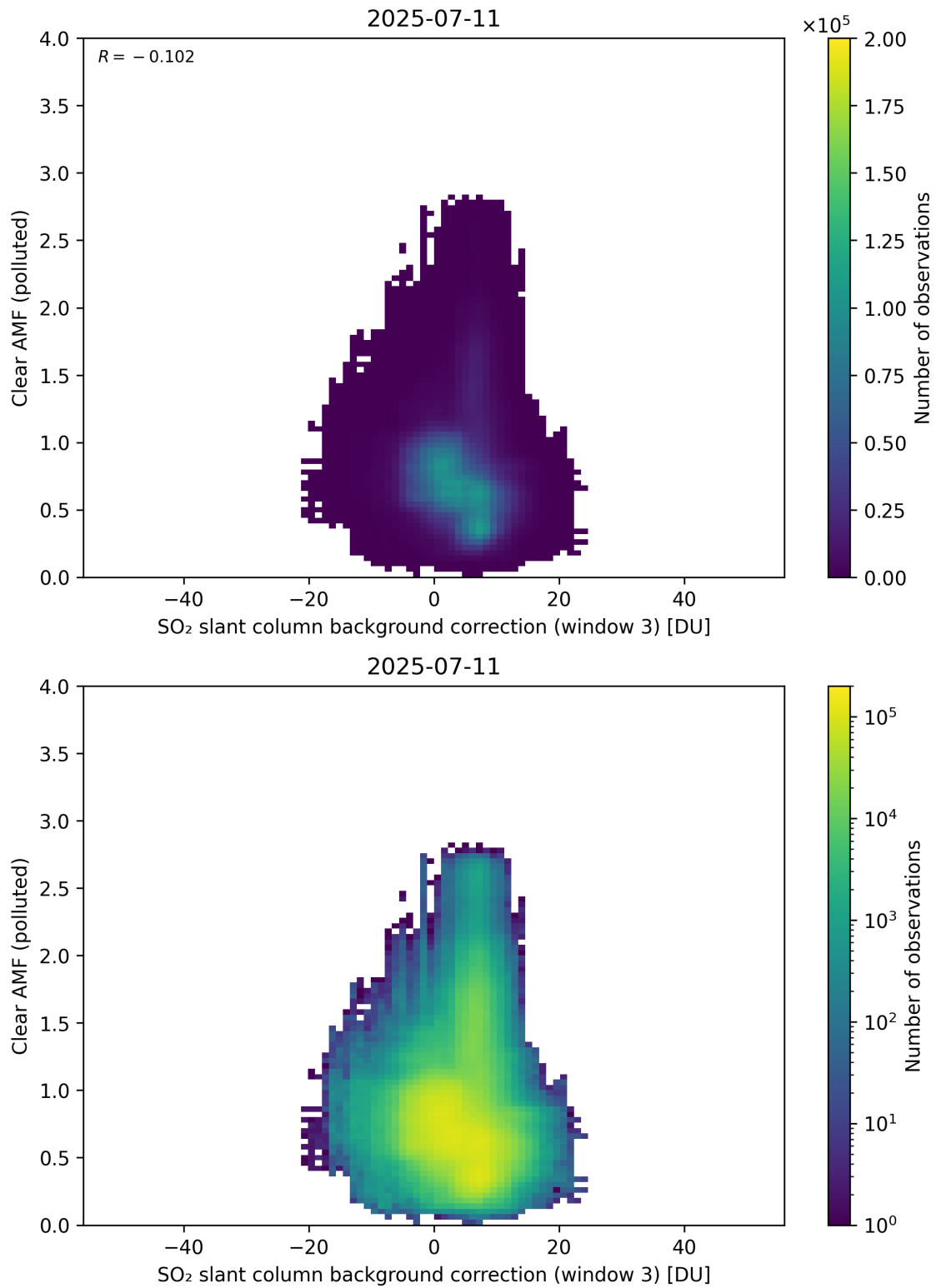
Figure 135: Scatter density plot of “SO 2 slant column background correction (window 3)” against “Clear AMF (polluted)” for 2025-07-10 to 2025-07-12.
