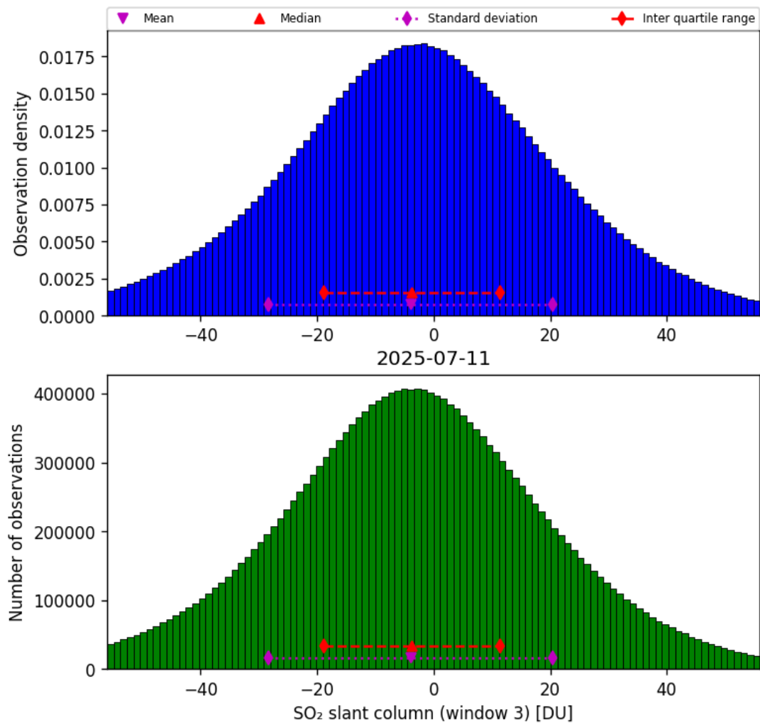
Figure 71: Histogram of “SO 2 slant column (window 3)” for 2025-07-10 to 2025-07-12
