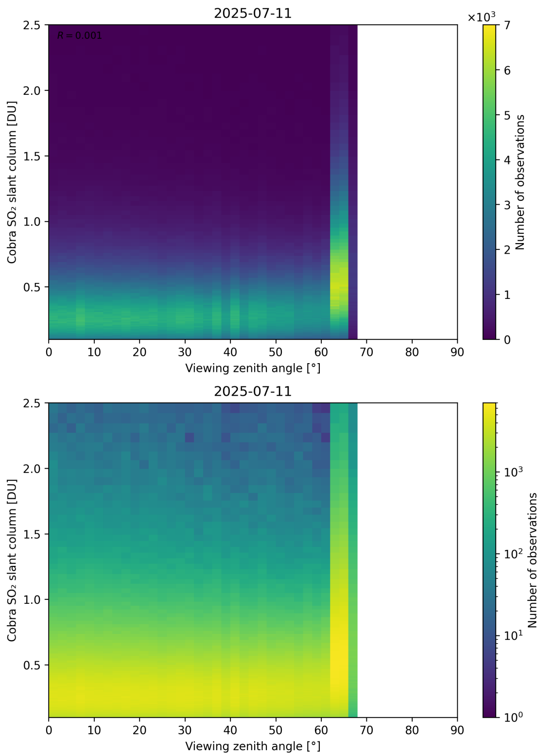
Figure 371: Scatter density plot of “Viewing zenith angle” against “Cobra SO 2 slant column” for 2025-07-10 to 2025-07-12.
