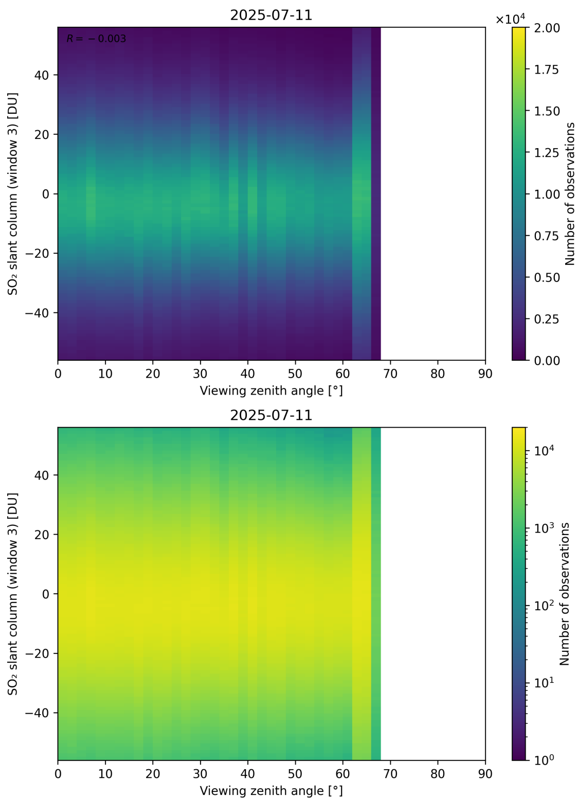
Figure 379: Scatter density plot of “Viewing zenith angle” against “SO 2 slant column (window 3)” for 2025-07-10 to 2025-07-12.
