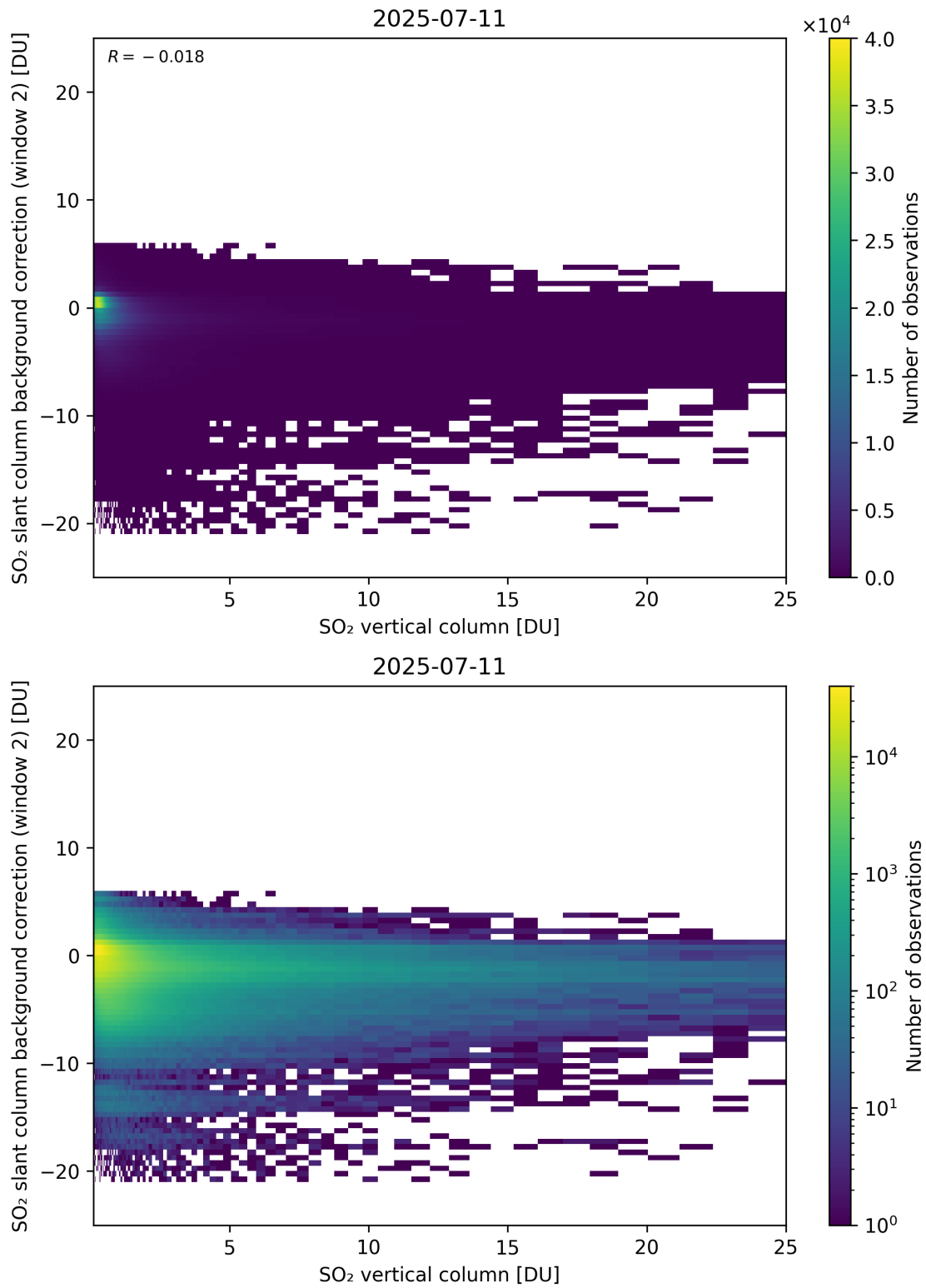
Figure 324: Scatter density plot of “SO 2 vertical column” against “SO 2 slant column background correction (window 2)” for 2025-07-10 to 2025-07-12.
