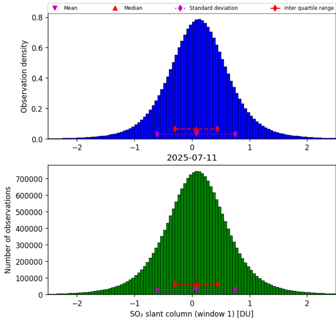
Figure 63: Histogram of “SO 2 slant column (window 1)” for 2025-07-10 to 2025-07-12
