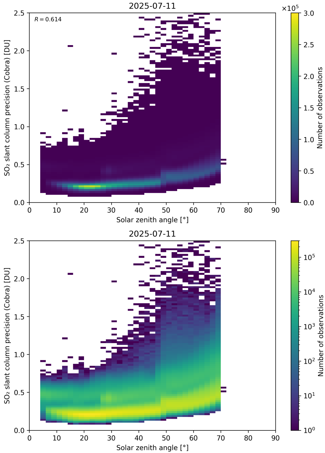
Figure 180: Scatter density plot of “Solar zenith angle” against “SO 2 slant column precision (Cobra)” for 2025-07-10 to 2025-07-12.
