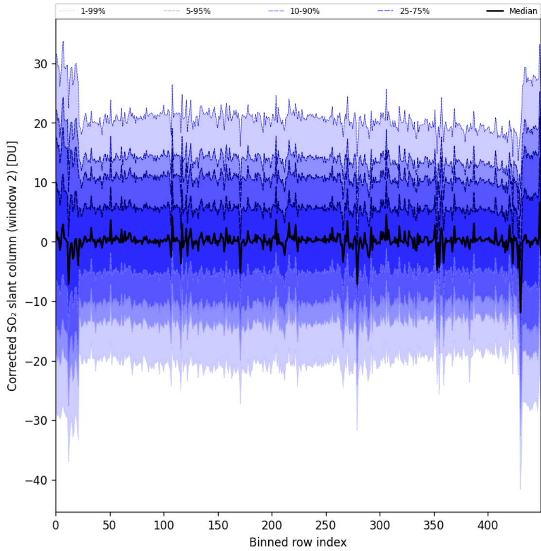
Figure 95: Along track statistics of “Corrected SO 2 slant column (window 2)” for 2025-07-10 to 2025-07-12
