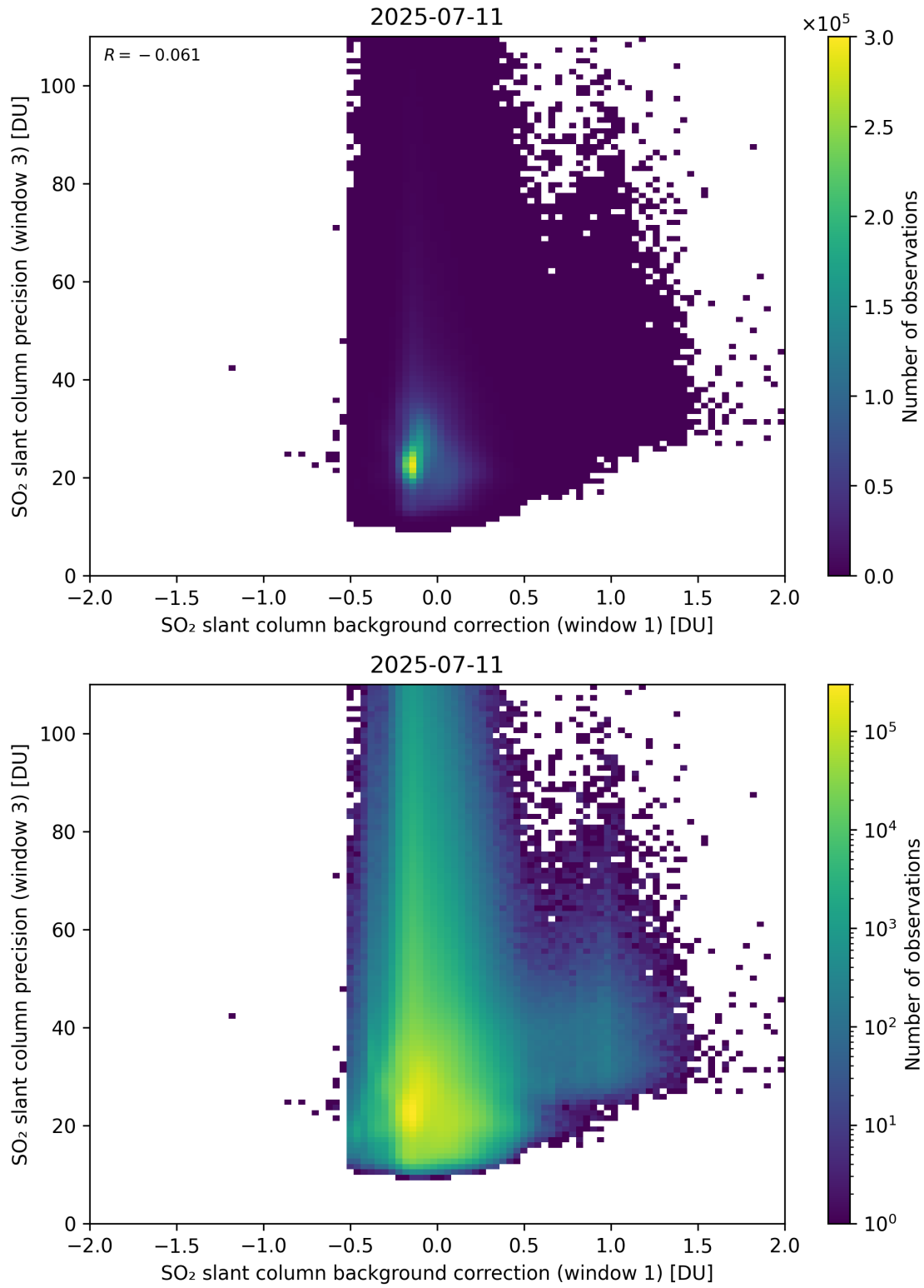
Figure 119: Scatter density plot of “SO 2 slant column background correction (window 1)” against “SO 2 slant column precision (window 3)” for 2025-07-10 to 2025-07-12.
