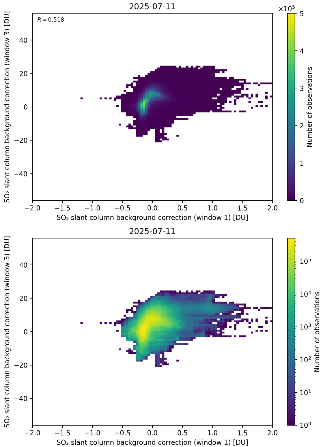
Figure 110: Scatter density plot of “SO 2 slant column background correction (window 1)” against “SO 2 slant column background correction (window 3)” for 2025-07-10 to 2025-07-12.
