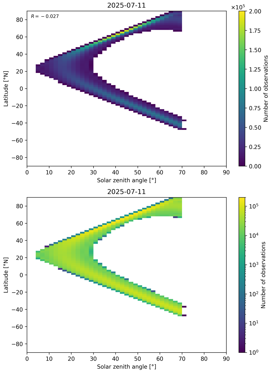
Figure 177: Scatter density plot of “Solar zenith angle” against “Latitude” for 2025-07-10 to 2025-07-12.
