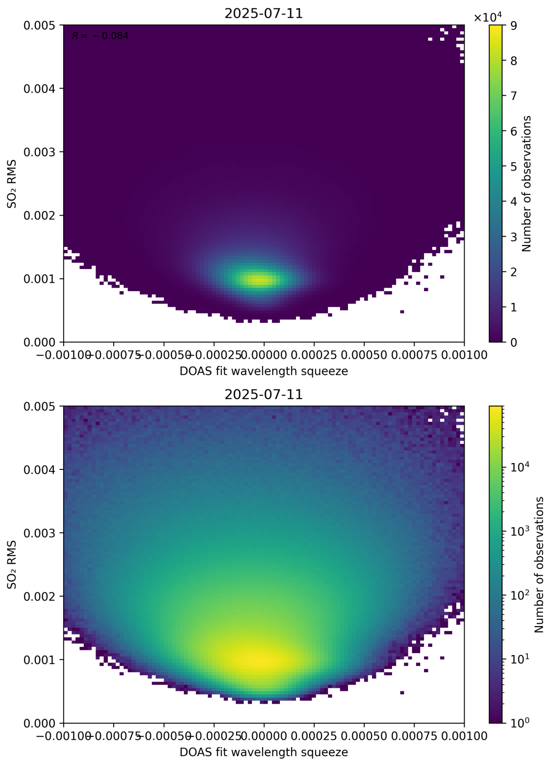
Figure 143: Scatter density plot of “DOAS fit wavelength squeeze” against “SO 2 RMS” for 2025-07-10 to 2025-07-12.
