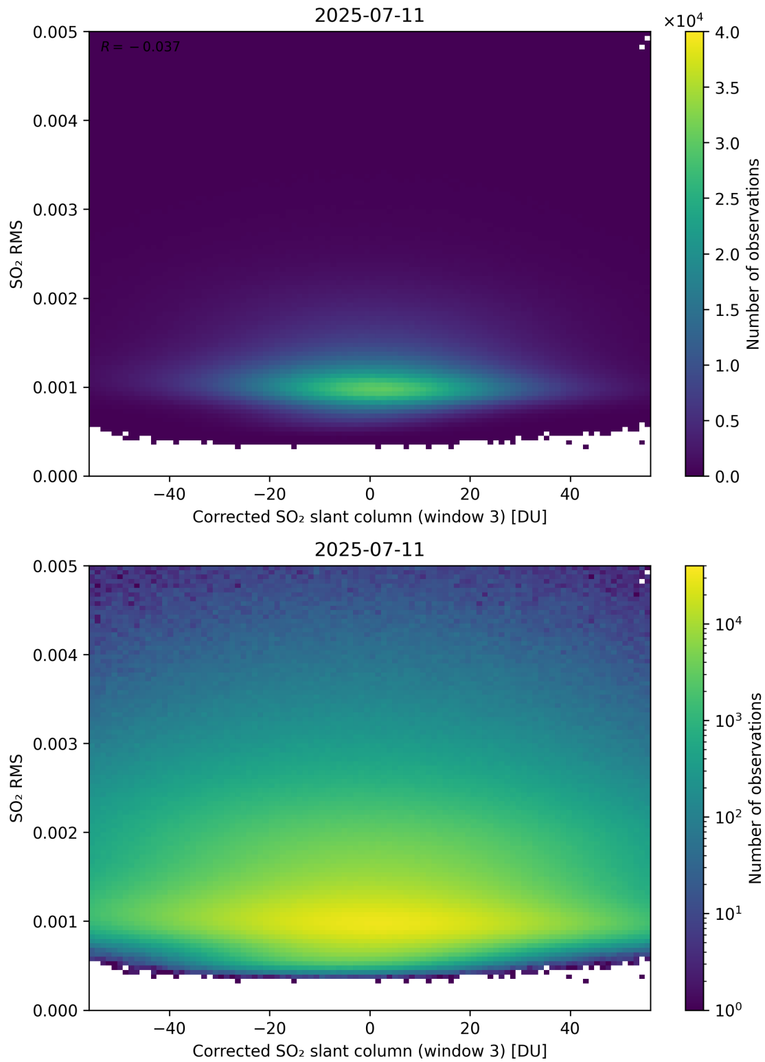
Figure 258: Scatter density plot of “Corrected SO 2 slant column (window 3)” against “SO 2 RMS” for 2025-07-10 to 2025-07-12.
