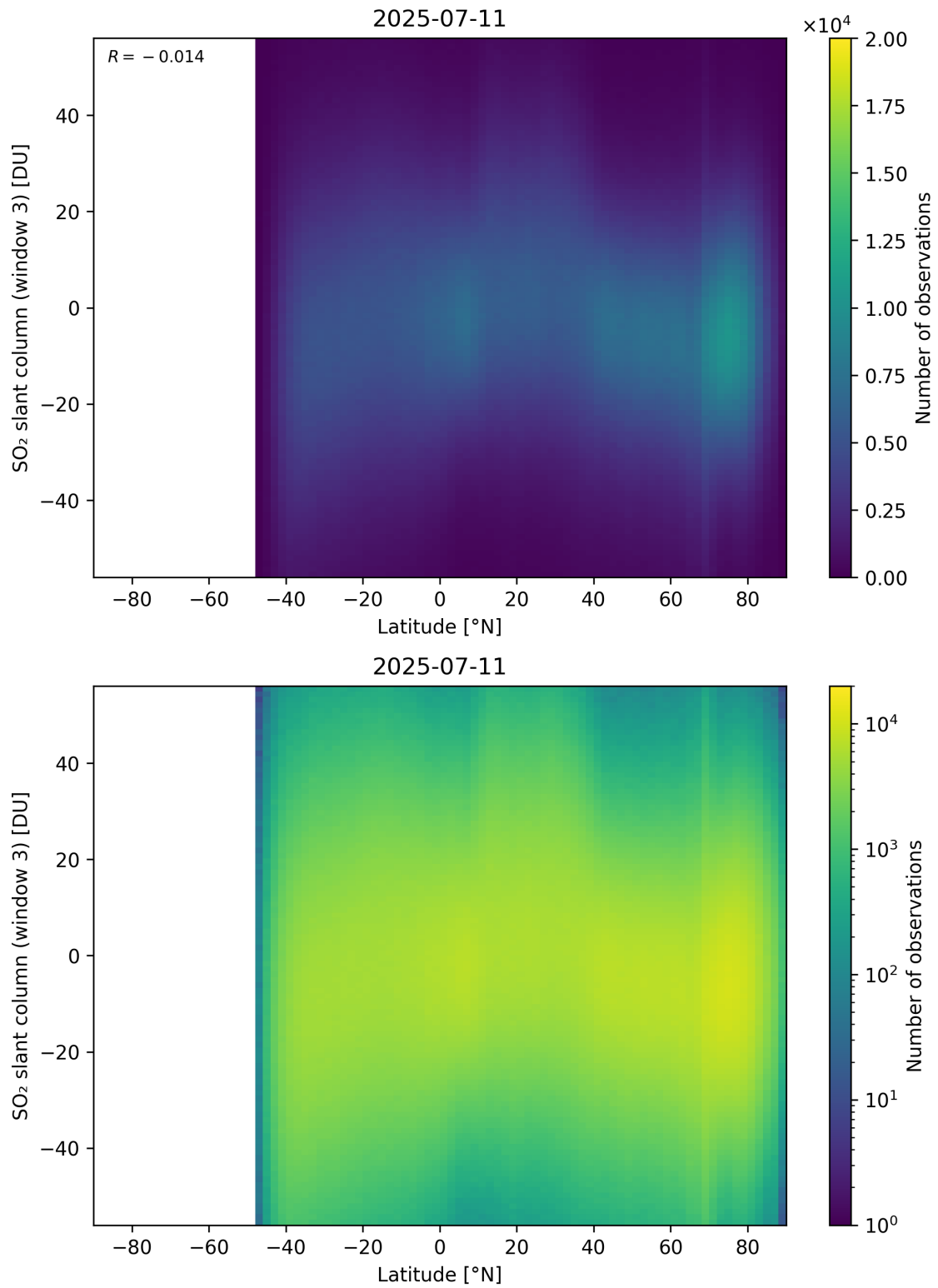
Figure 165: Scatter density plot of “Latitude” against “SO 2 slant column (window 3)” for 2025-07-10 to 2025-07-12.
