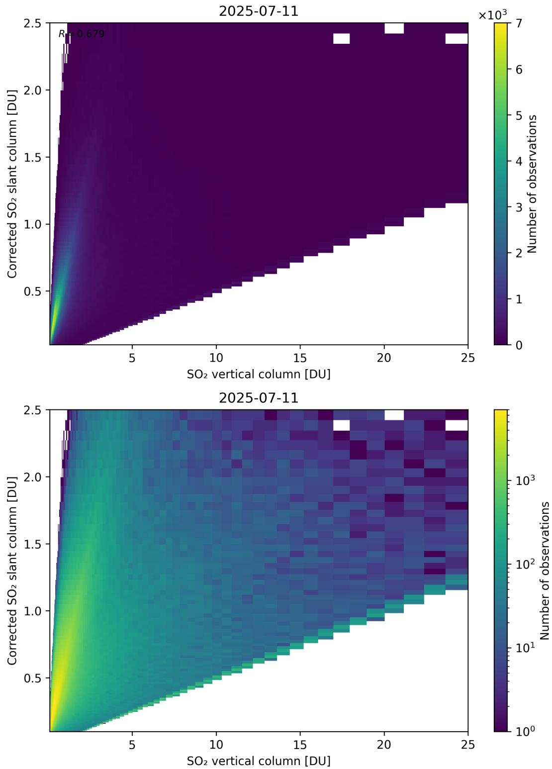
Figure 351: Scatter density plot of “SO 2 vertical column” against “Corrected SO 2 slant column” for 2025-07-10 to 2025-07-12.
