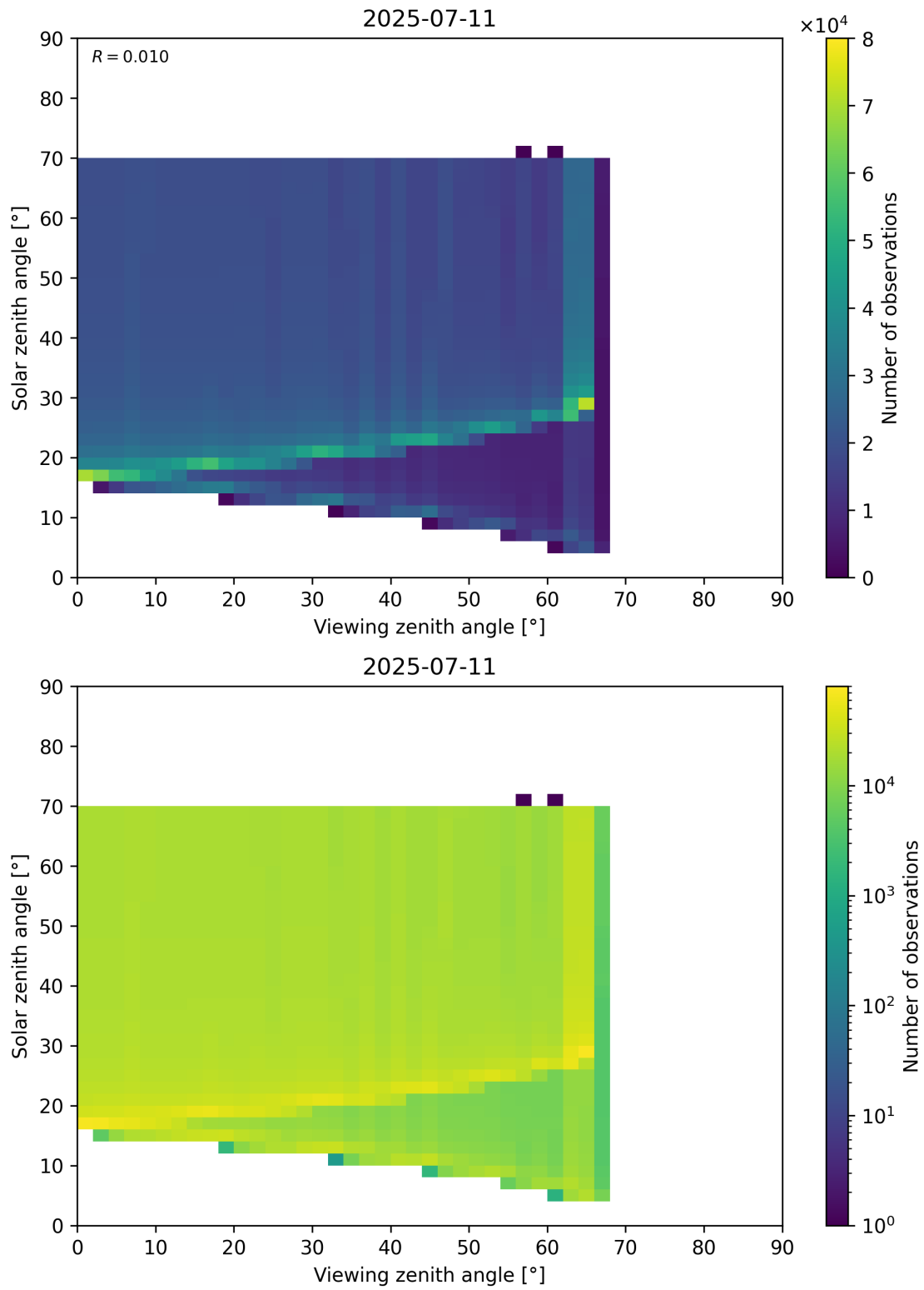
Figure 369: Scatter density plot of “Viewing zenith angle” against “Solar zenith angle” for 2025-07-10 to 2025-07-12.
