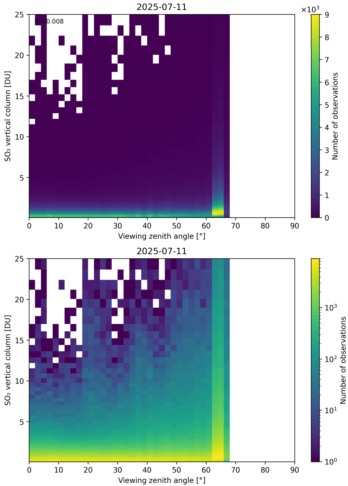
Figure 383: Scatter density plot of “Viewing zenith angle” against “SO 2 vertical column” for 2025-07-10 to 2025-07-12.
