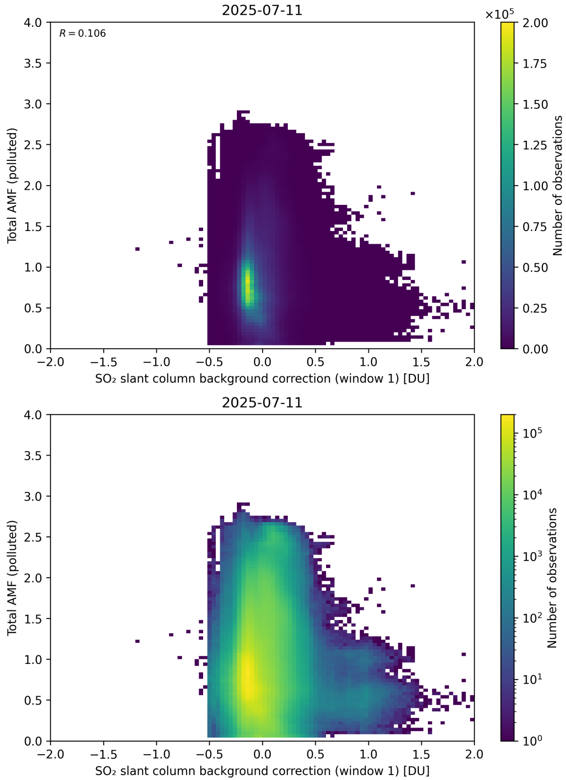
Figure 120: Scatter density plot of “SO 2 slant column background correction (window 1)” against “Total AMF (polluted)” for 2025-07-10 to 2025-07-12.
