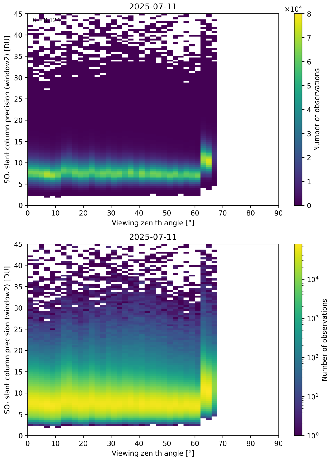
Figure 378: Scatter density plot of “Viewing zenith angle” against “SO 2 slant column precision (window2)” for 2025-07-10 to 2025-07-12.
