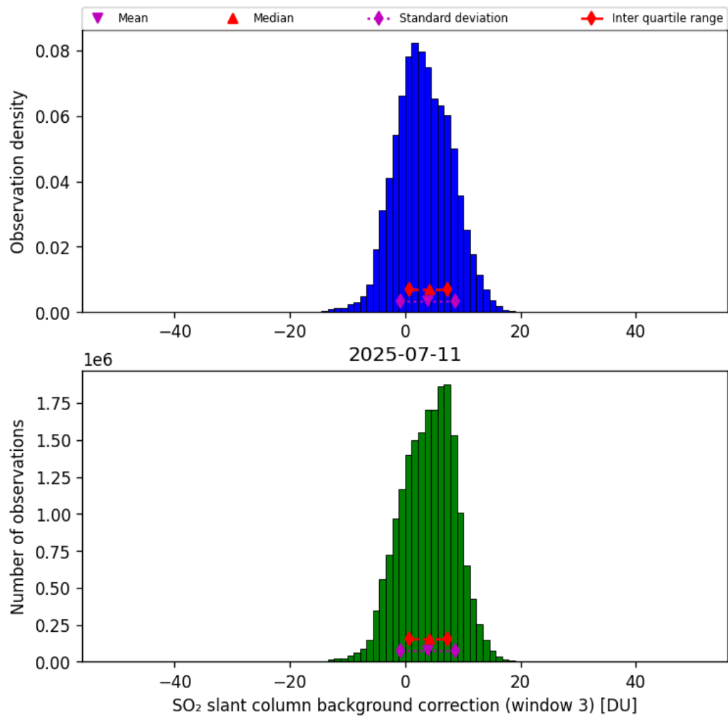
Figure 74: Histogram of “SO 2 slant column background correction (window 3)” for 2025-07-10 to 2025-07-12
