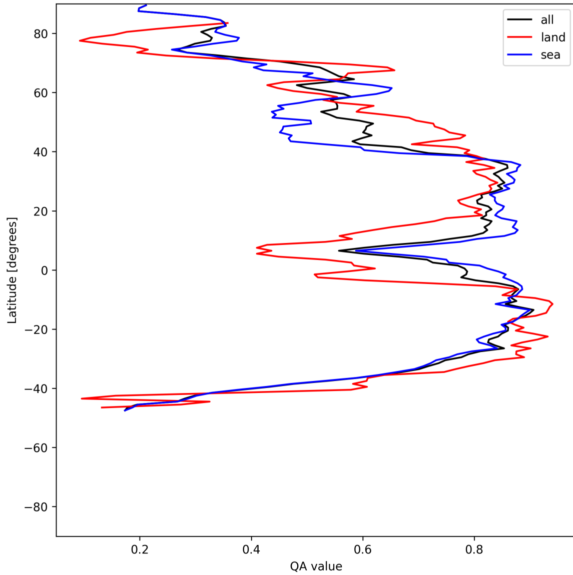
Figure 31: Zonal average of “QA value” for 2025-07-10 to 2025-07-12.
