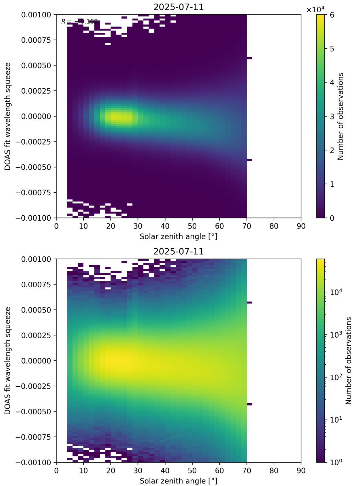
Figure 175: Scatter density plot of “Solar zenith angle” against “DOAS fit wavelength squeeze” for 2025-07-10 to 2025-07-12.
