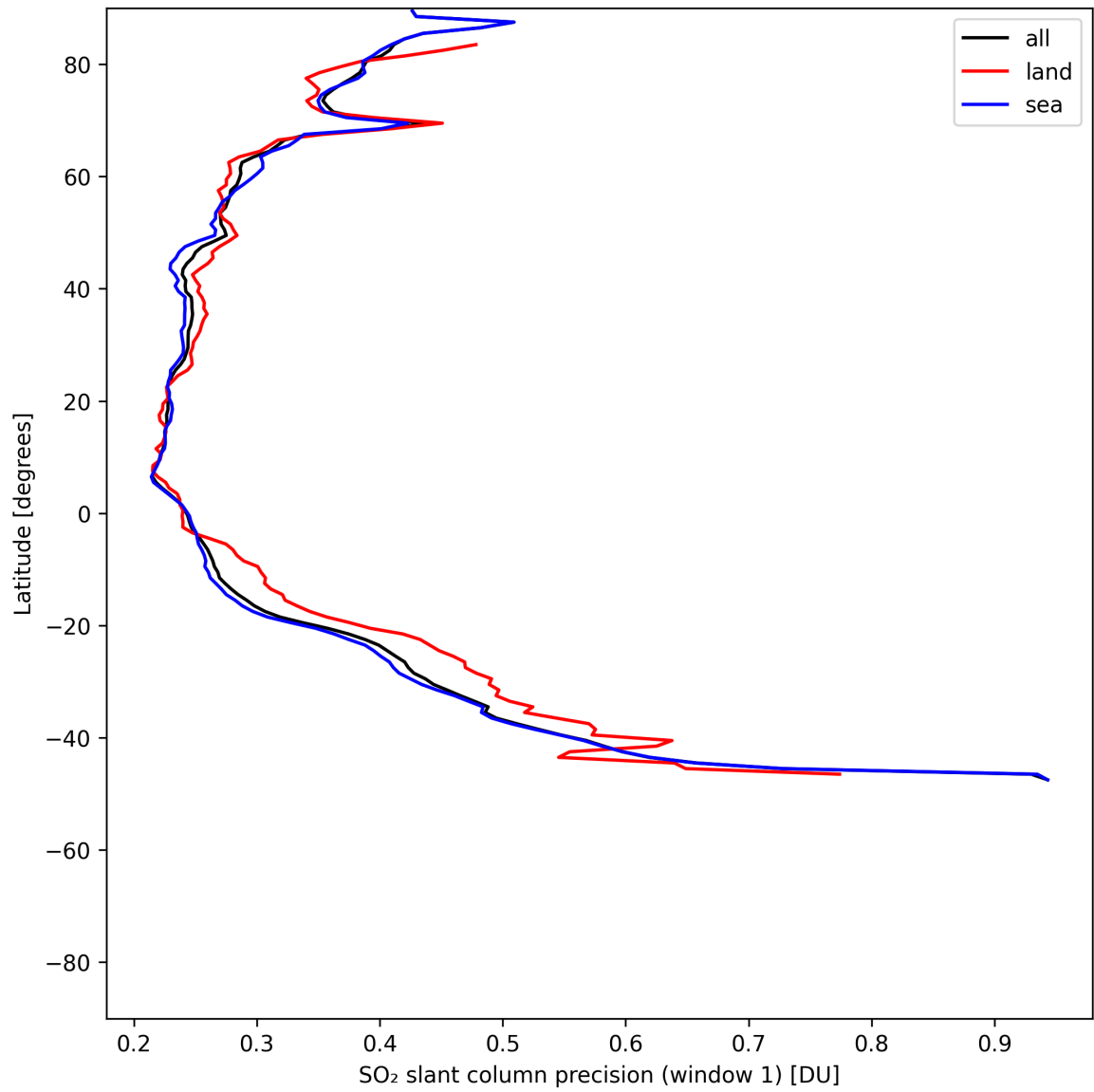
Figure 38: Zonal average of "SO 2 slant column precision (window 1)" for 2025-07-10 to 2025-07-12.
