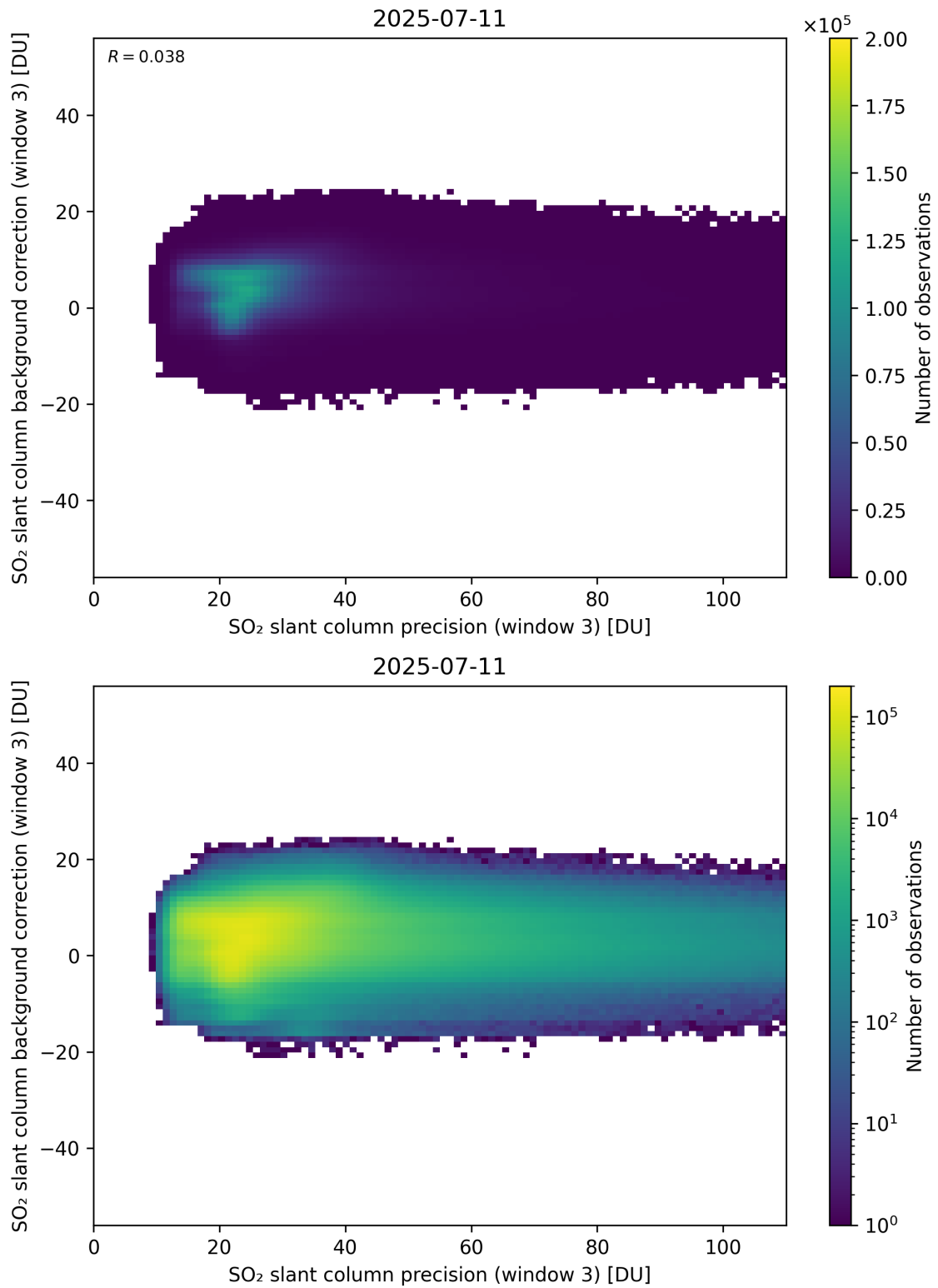
Figure 307: Scatter density plot of “SO 2 slant column precision (window 3)” against “SO 2 slant column background correction (window 3)” for 2025-07-10 to 2025-07-12.
