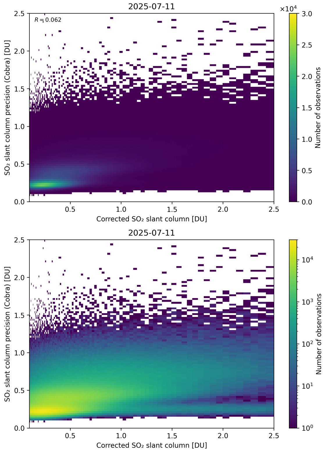
Figure 234: Scatter density plot of “Corrected SO 2 slant column” against “SO 2 slant column precision (Cobra)” for 2025-07-10 to 2025-07-12.
