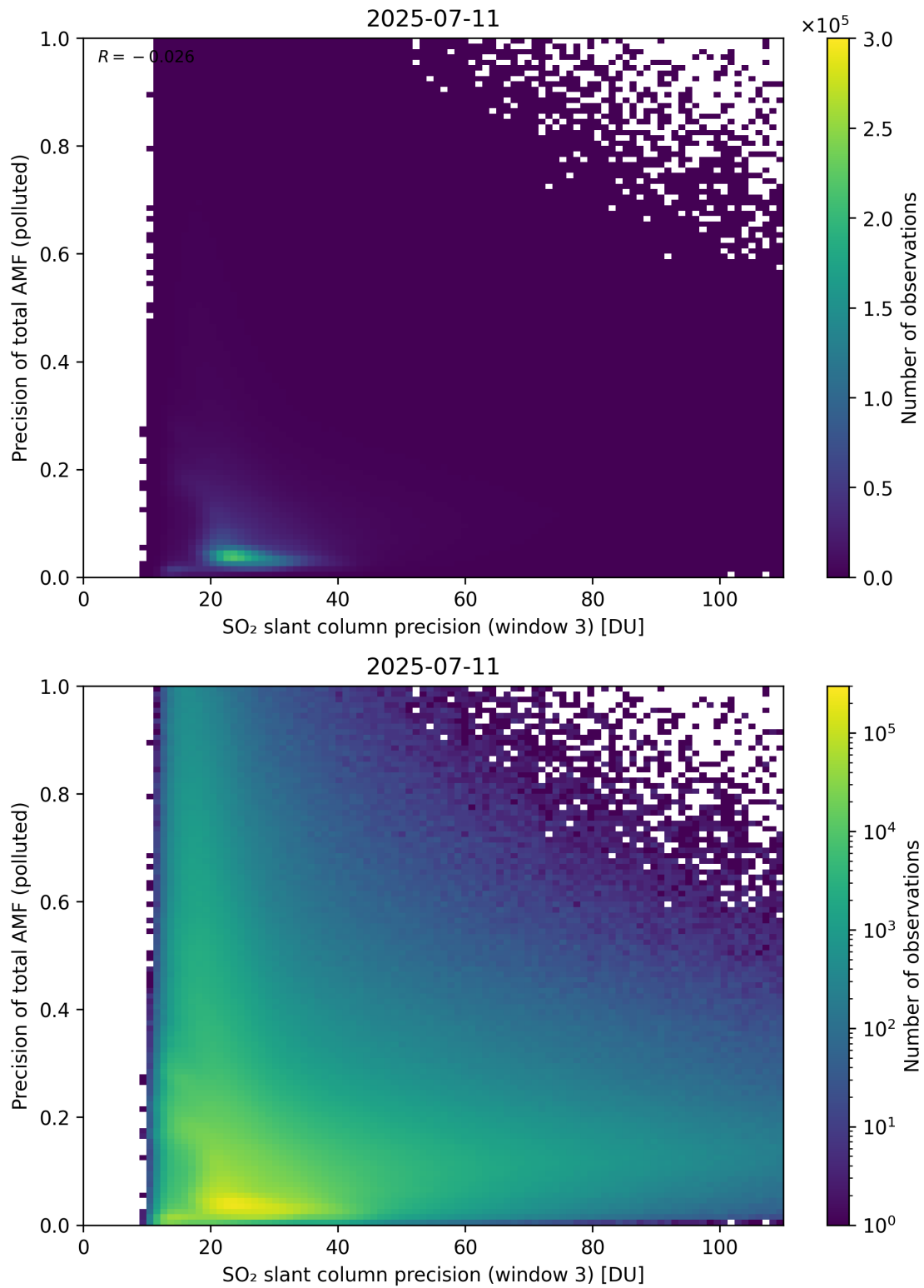
Figure 314: Scatter density plot of “SO 2 slant column precision (window 3)” against “Precision of total AMF (polluted)” for 2025-07-10 to 2025-07-12.
