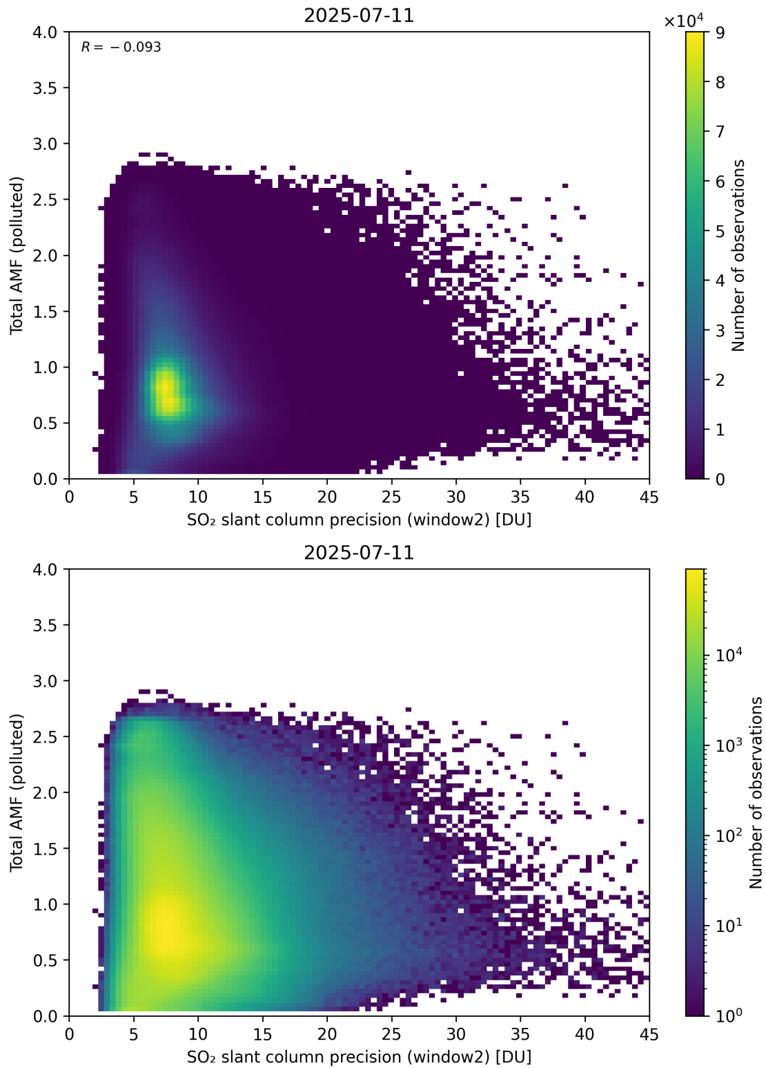
Figure 301: Scatter density plot of “SO 2 slant column precision (window2)” against “Total AMF (polluted)” for 2025-07-10 to 2025-07-12.
