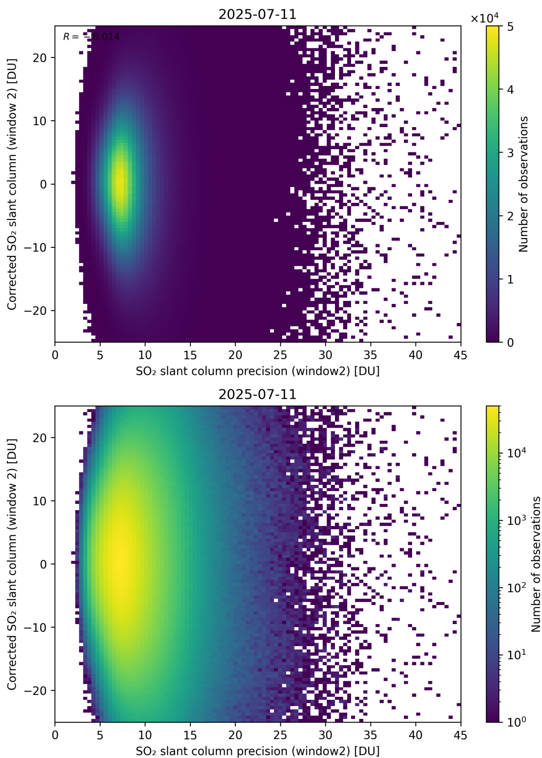
Figure 297: Scatter density plot of “SO 2 slant column precision (window2)” against “Corrected SO 2 slant column (window 2)” for 2025-07-10 to 2025-07-12.
