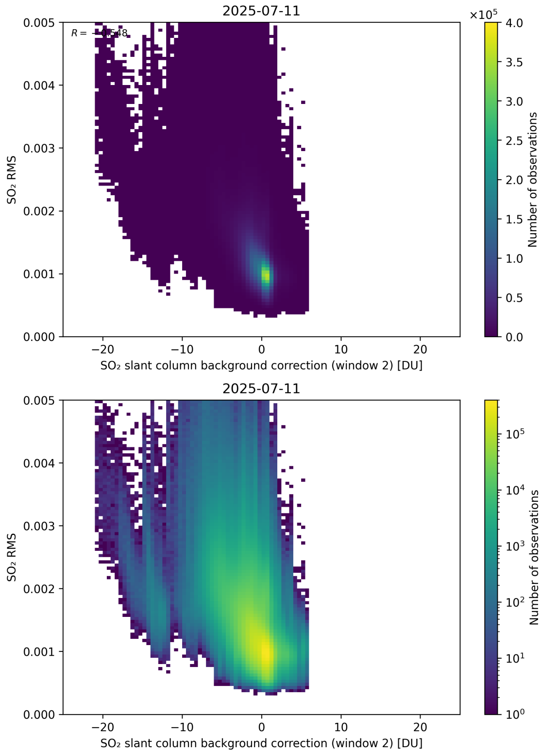
Figure 125: Scatter density plot of “SO 2 slant column background correction (window 2)” against “SO 2 RMS” for 2025-07-10 to 2025-07-12.
