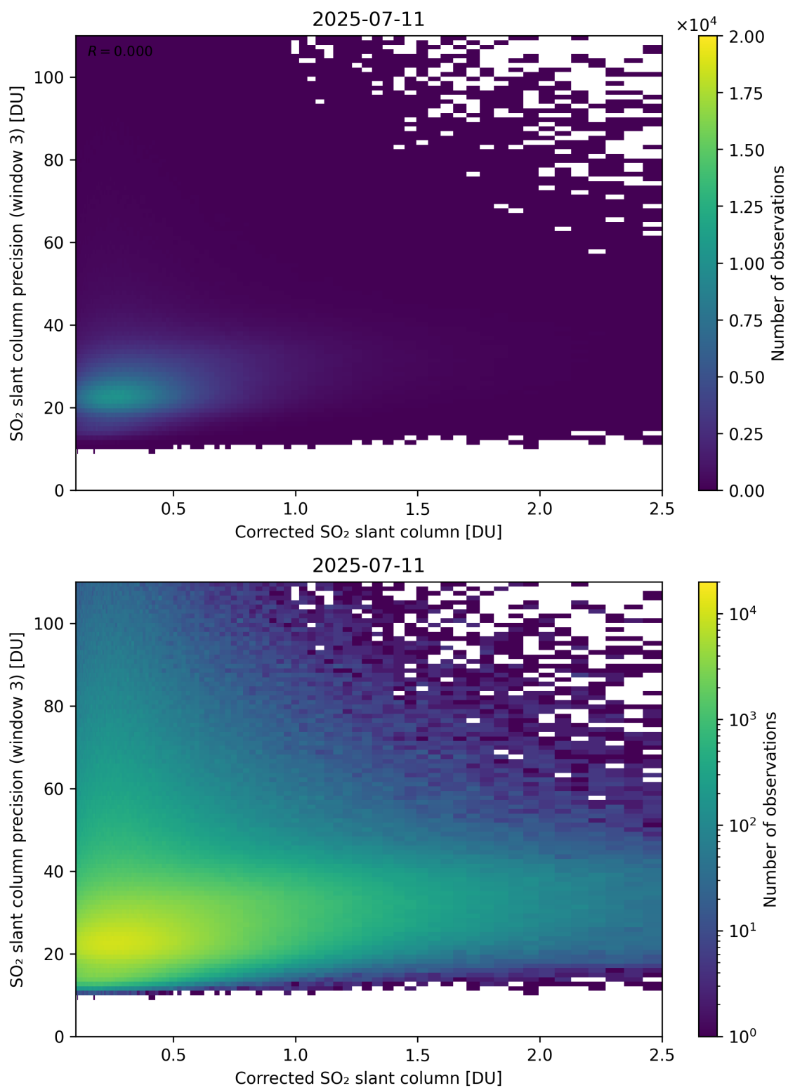
Figure 241: Scatter density plot of “Corrected SO 2 slant column” against “SO 2 slant column precision (window 3)” for 2025-07-10 to 2025-07-12.
