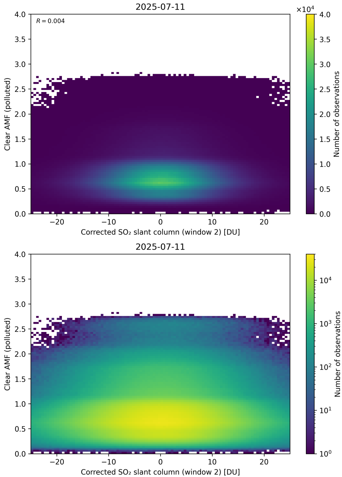
Figure 249: Scatter density plot of “Corrected SO 2 slant column (window 2)” against “Clear AMF (polluted)” for 2025-07-10 to 2025-07-12.
