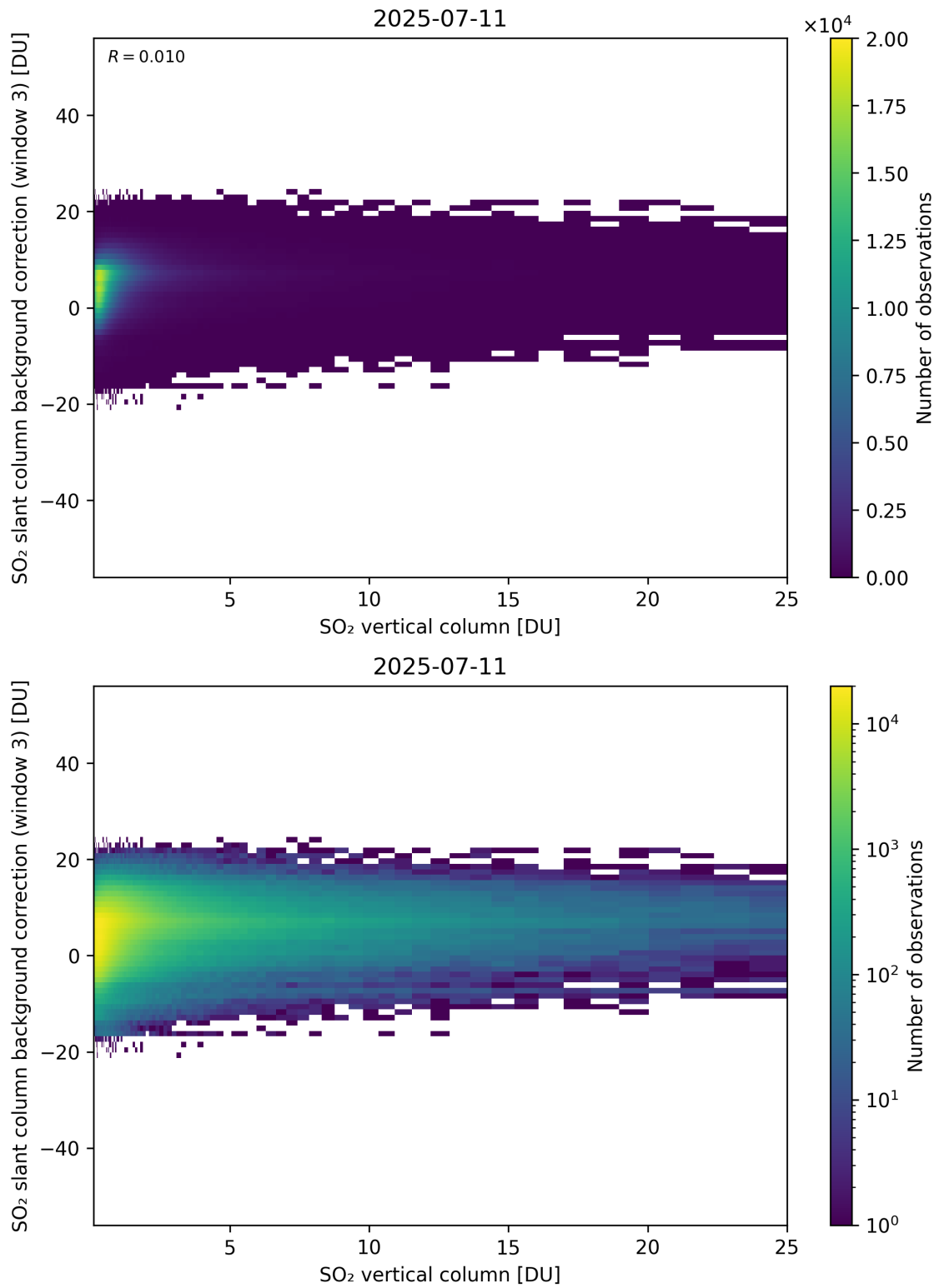
Figure 325: Scatter density plot of “SO 2 vertical column” against “SO 2 slant column background correction (window 3)” for 2025-07-10 to 2025-07-12.
