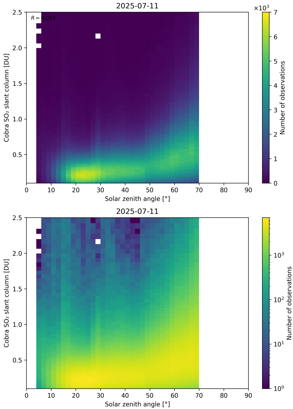
Figure 179: Scatter density plot of “Solar zenith angle” against “Cobra SO 2 slant column” for 2025-07-10 to 2025-07-12.
