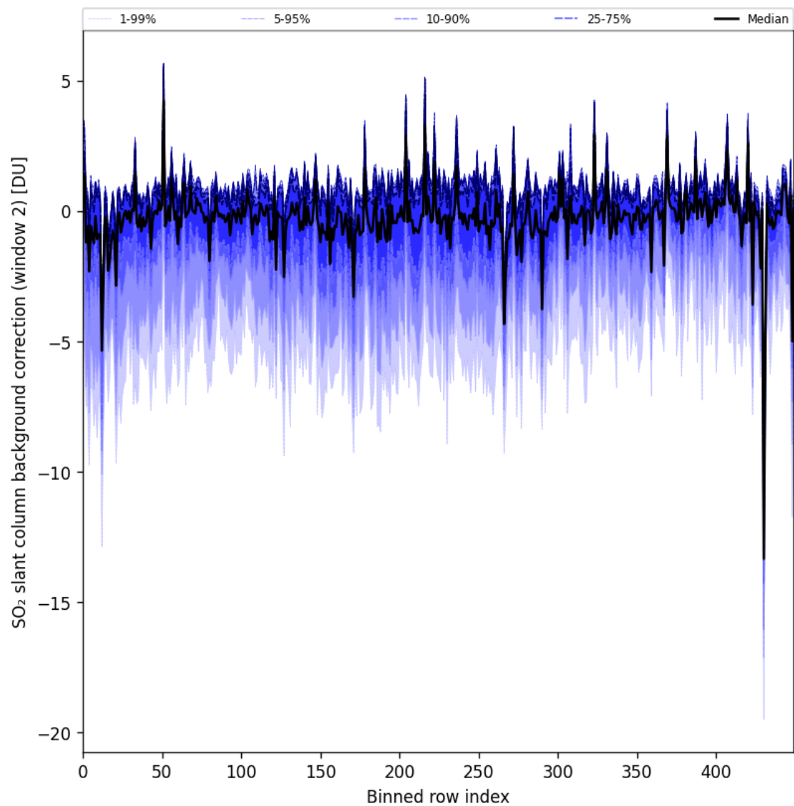
Figure 96: Along track statistics of “SO 2 slant column background correction (window 2)” for 2025-07-10 to 2025-07-12
