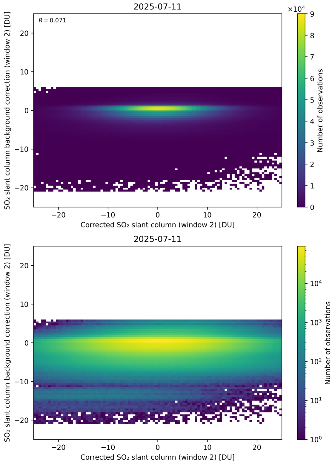
Figure 244: Scatter density plot of “Corrected SO 2 slant column (window 2)” against “SO 2 slant column background correction (window 2)” for 2025-07-10 to 2025-07-12.
