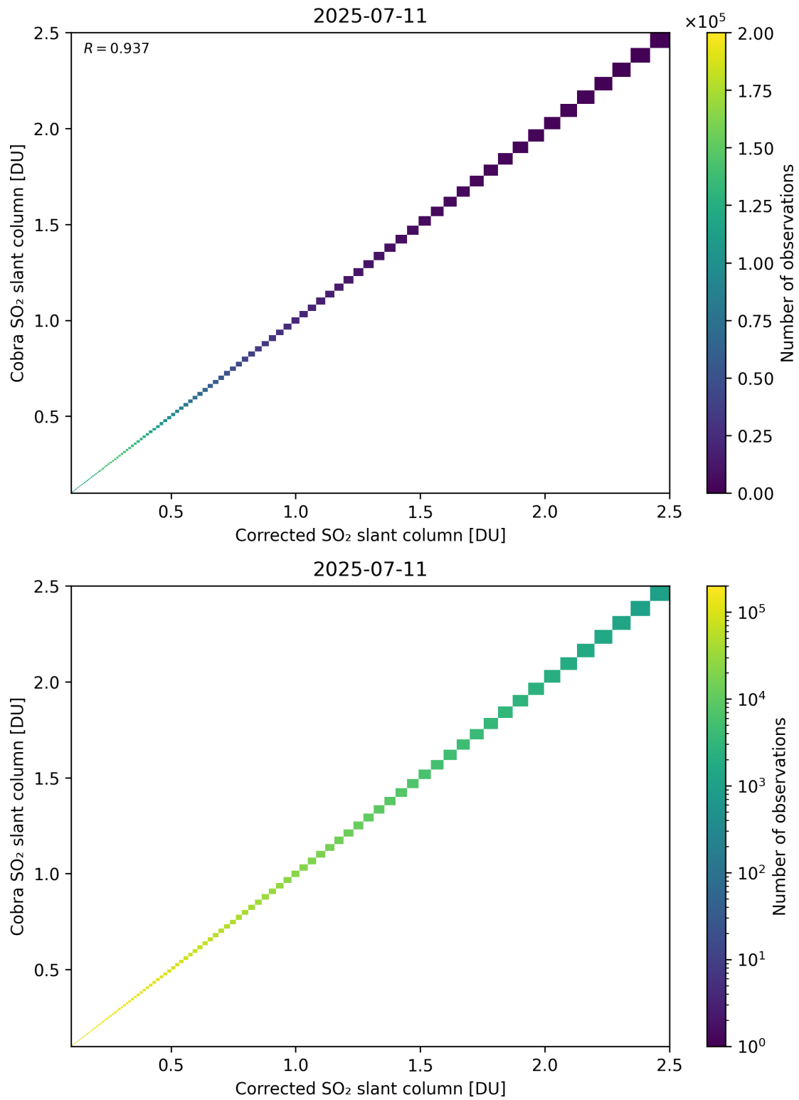
Figure 233: Scatter density plot of “Corrected SO 2 slant column” against “Cobra SO 2 slant column” for 2025-07-10 to 2025-07-12.
