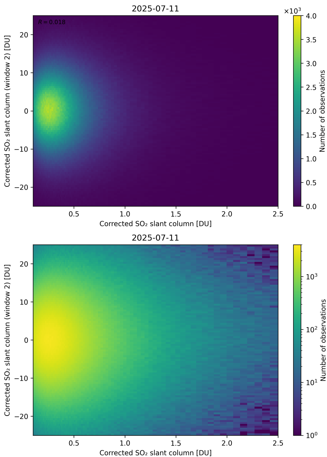
Figure 235: Scatter density plot of “Corrected SO 2 slant column” against “Corrected SO 2 slant column (window 2)” for 2025-07-10 to 2025-07-12.
