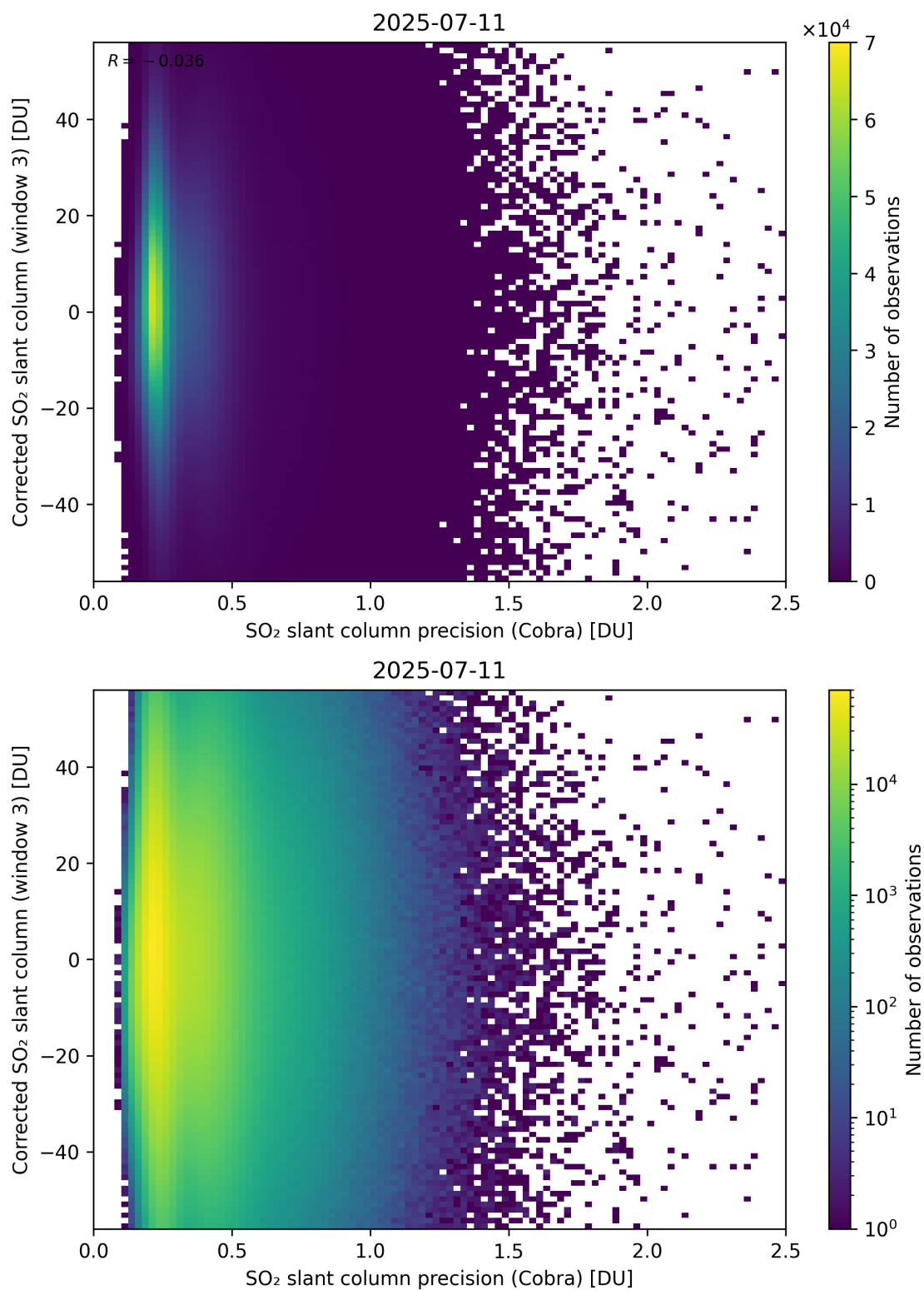
Figure 207: Scatter density plot of “SO 2 slant column precision (Cobra)” against “Corrected SO 2 slant column (window 3)” for 2025-07-10 to 2025-07-12.
