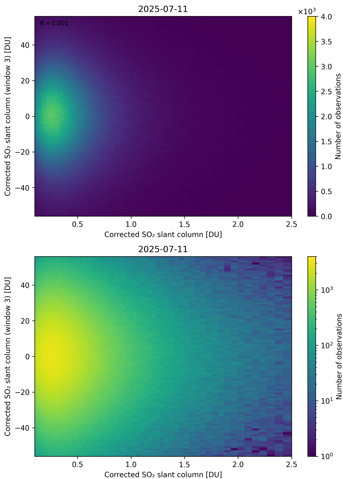
Figure 236: Scatter density plot of “Corrected SO 2 slant column” against “Corrected SO 2 slant column (window 3)” for 2025-07-10 to 2025-07-12.
