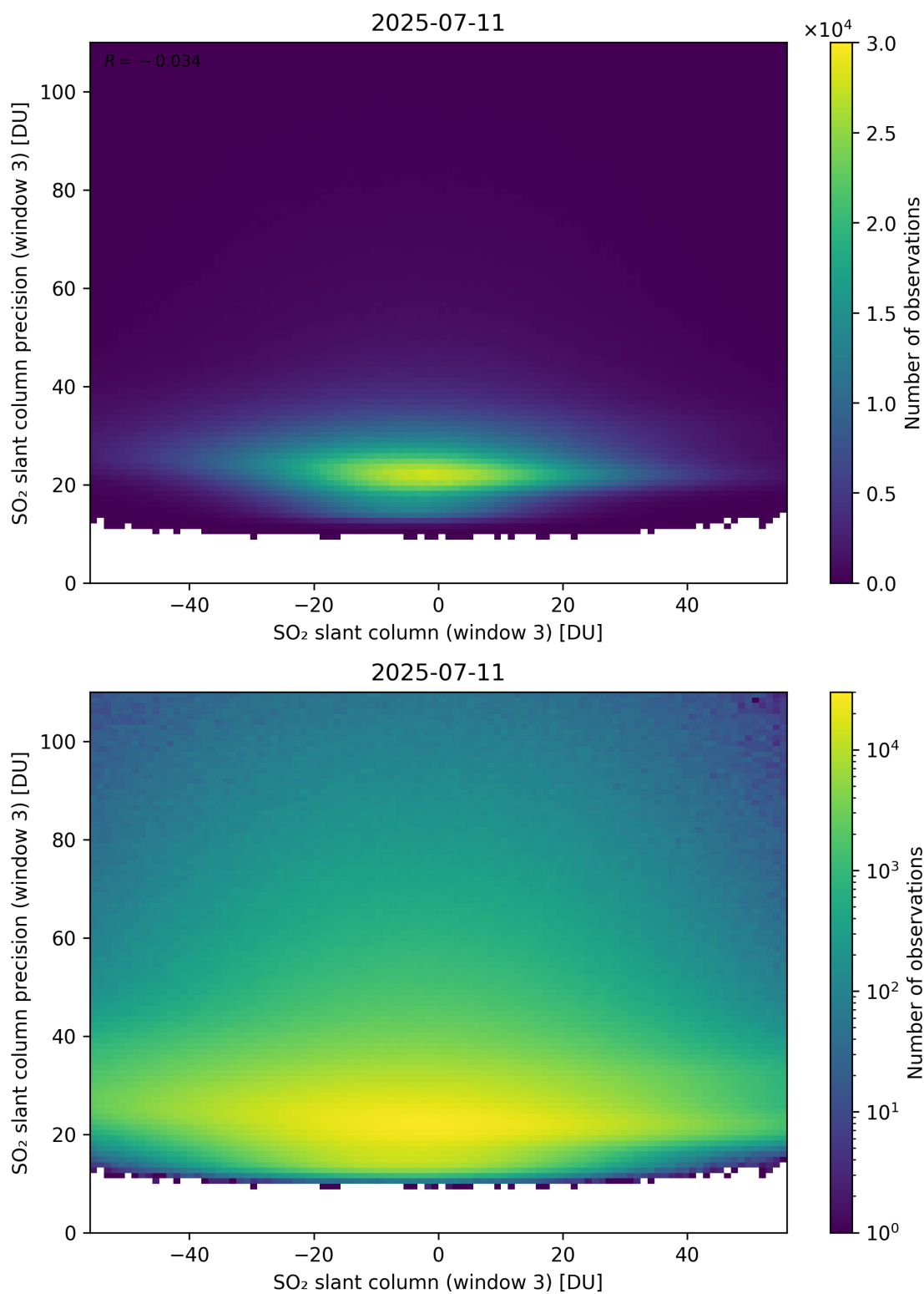
Figure 317: Scatter density plot of “SO 2 slant column (window 3)” against “SO 2 slant column precision (window 3)” for 2025-07-10 to 2025-07-12.
