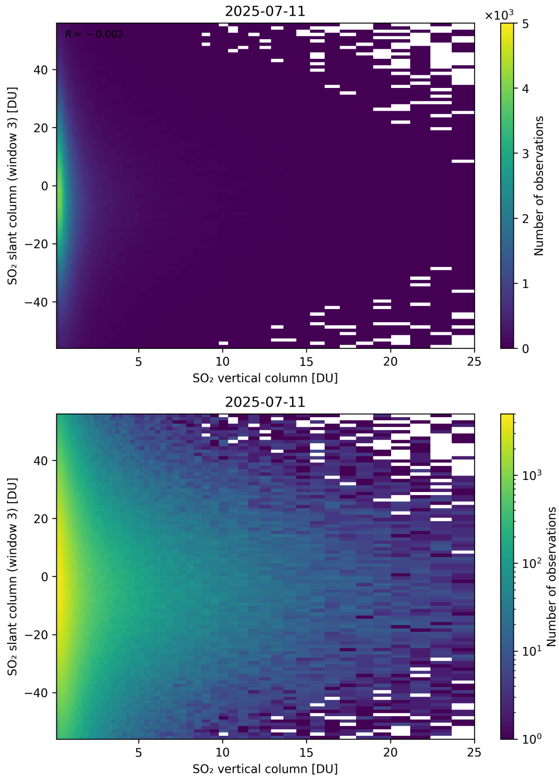
Figure 357: Scatter density plot of “SO 2 vertical column” against “SO 2 slant column (window 3)” for 2025-07-10 to 2025-07-12.
