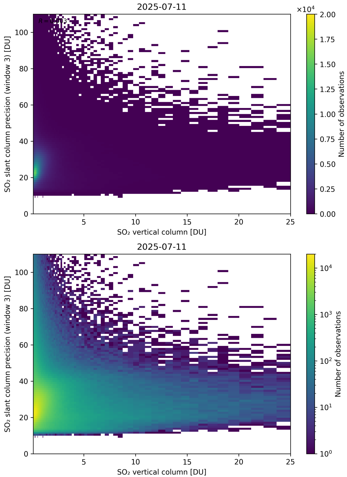
Figure 358: Scatter density plot of “SO 2 vertical column” against “SO 2 slant column precision (window 3)” for 2025-07-10 to 2025-07-12.
