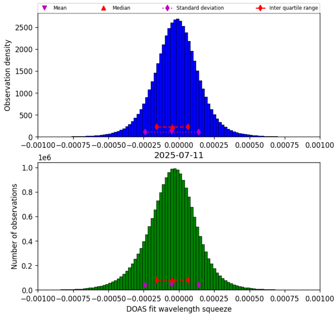
Figure 77: Histogram of “DOAS fit wavelength squeeze” for 2025-07-10 to 2025-07-12
