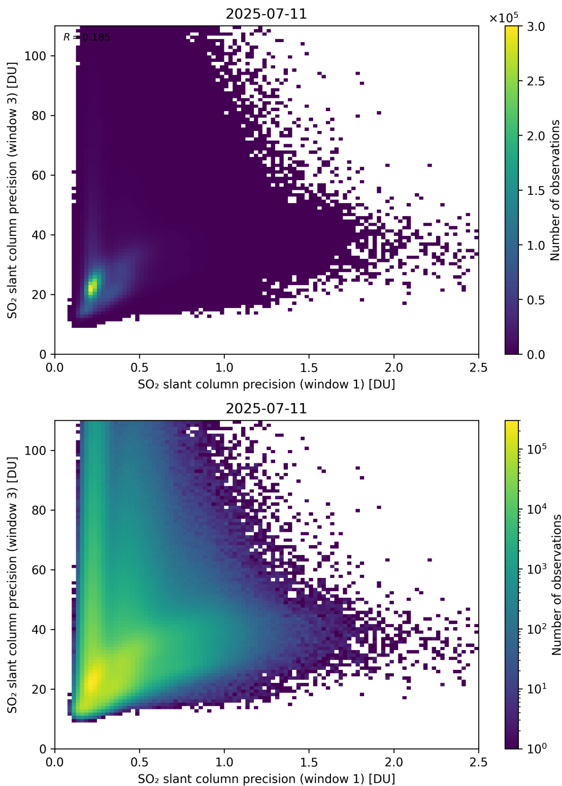
Figure 279: Scatter density plot of “SO 2 slant column precision (window 1)” against “SO 2 slant column precision (window 3)” for 2025-07-10 to 2025-07-12.
