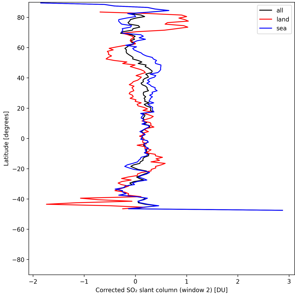
Figure 43: Zonal average of “Corrected SO 2 slant column (window 2)” for 2025-07-10 to 2025-07-12.
