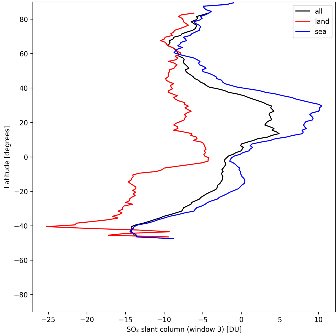
Figure 45: Zonal average of “SO 2 slant column (window 3)” for 2025-07-10 to 2025-07-12.
