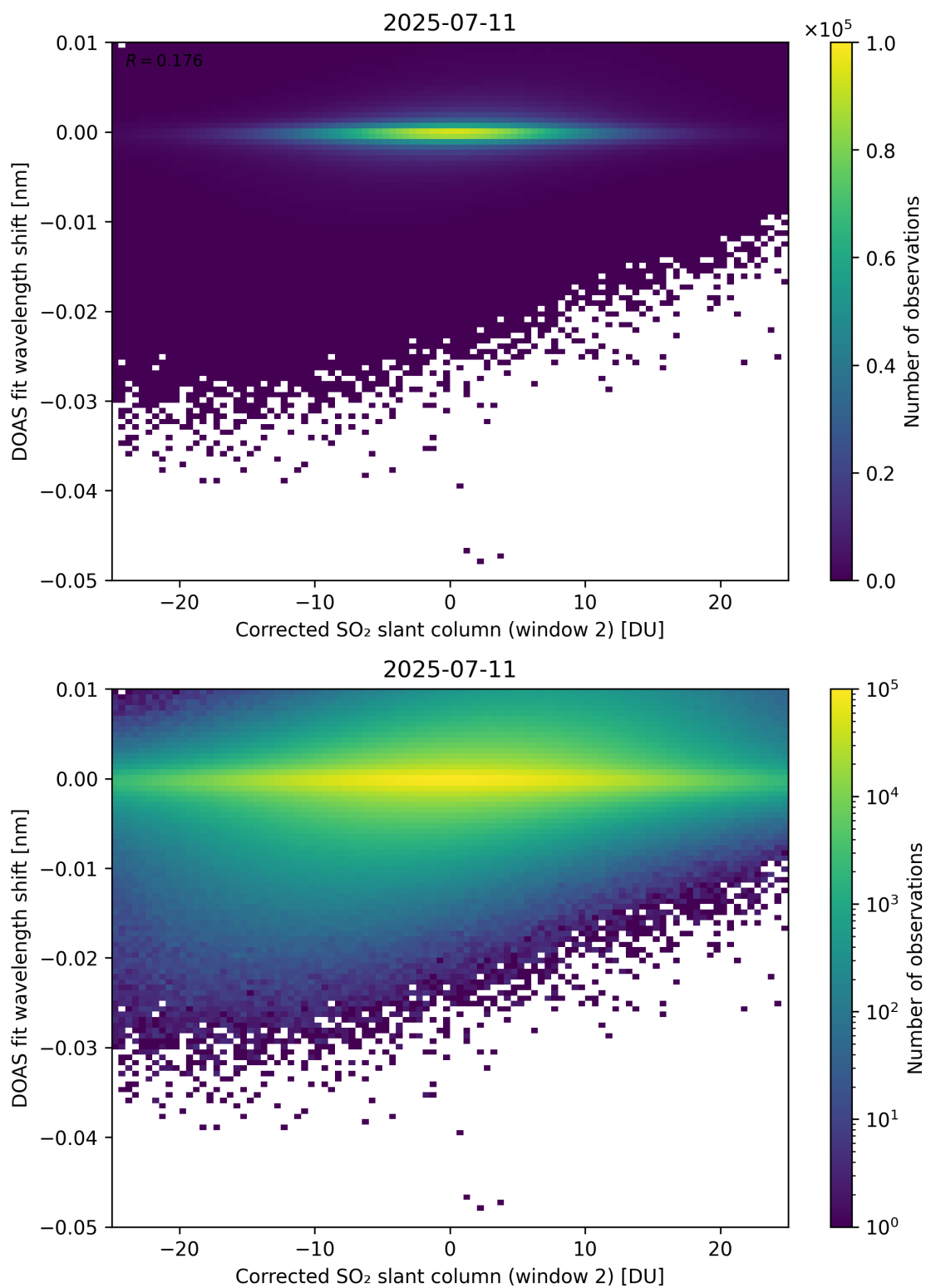
Figure 246: Scatter density plot of “Corrected SO 2 slant column (window 2)” against “DOAS fit wavelength shift” for 2025-07-10 to 2025-07-12.
