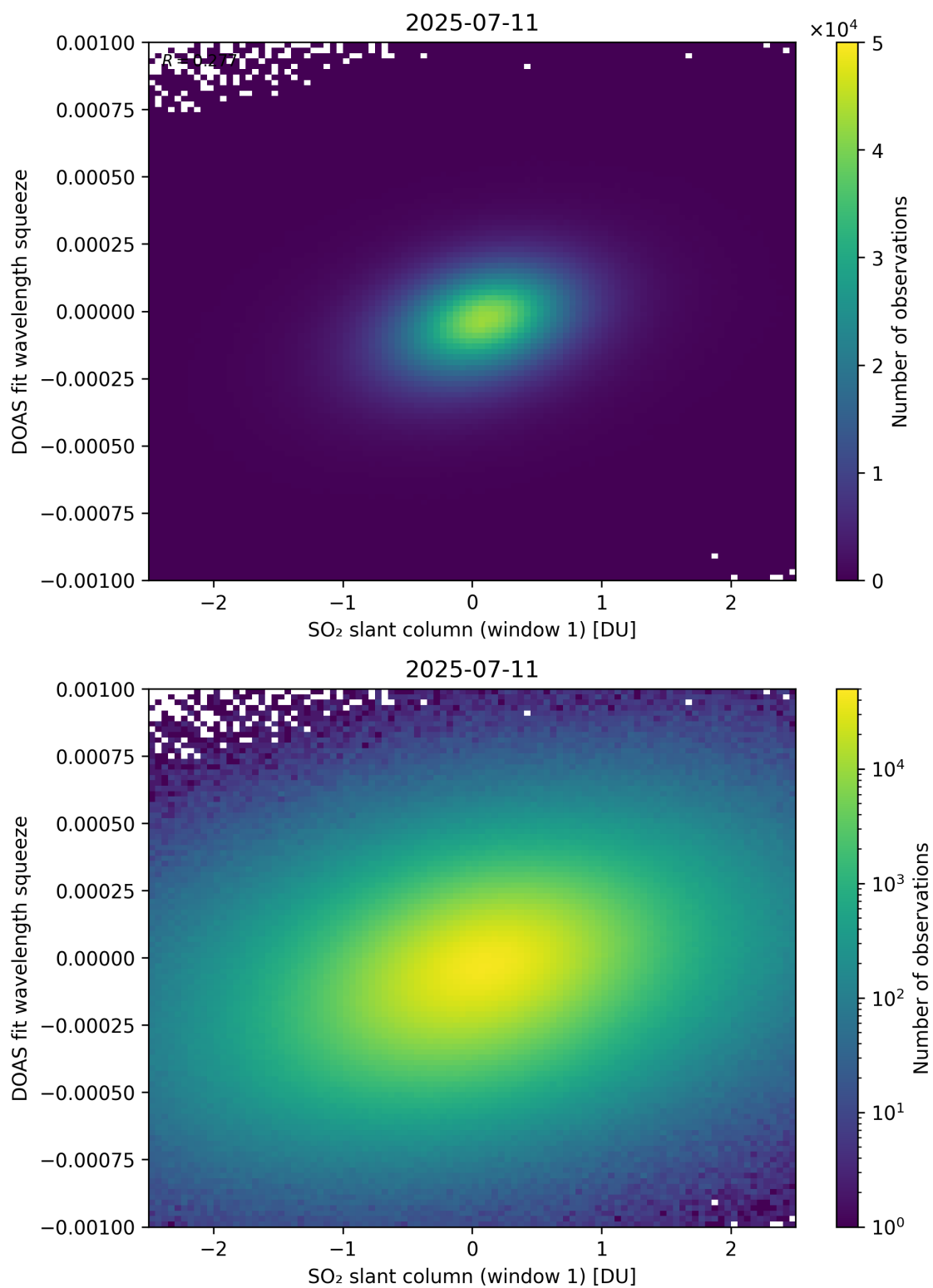
Figure 266: Scatter density plot of “SO 2 slant column (window 1)” against “DOAS fit wavelength squeeze” for 2025-07-10 to 2025-07-12.
