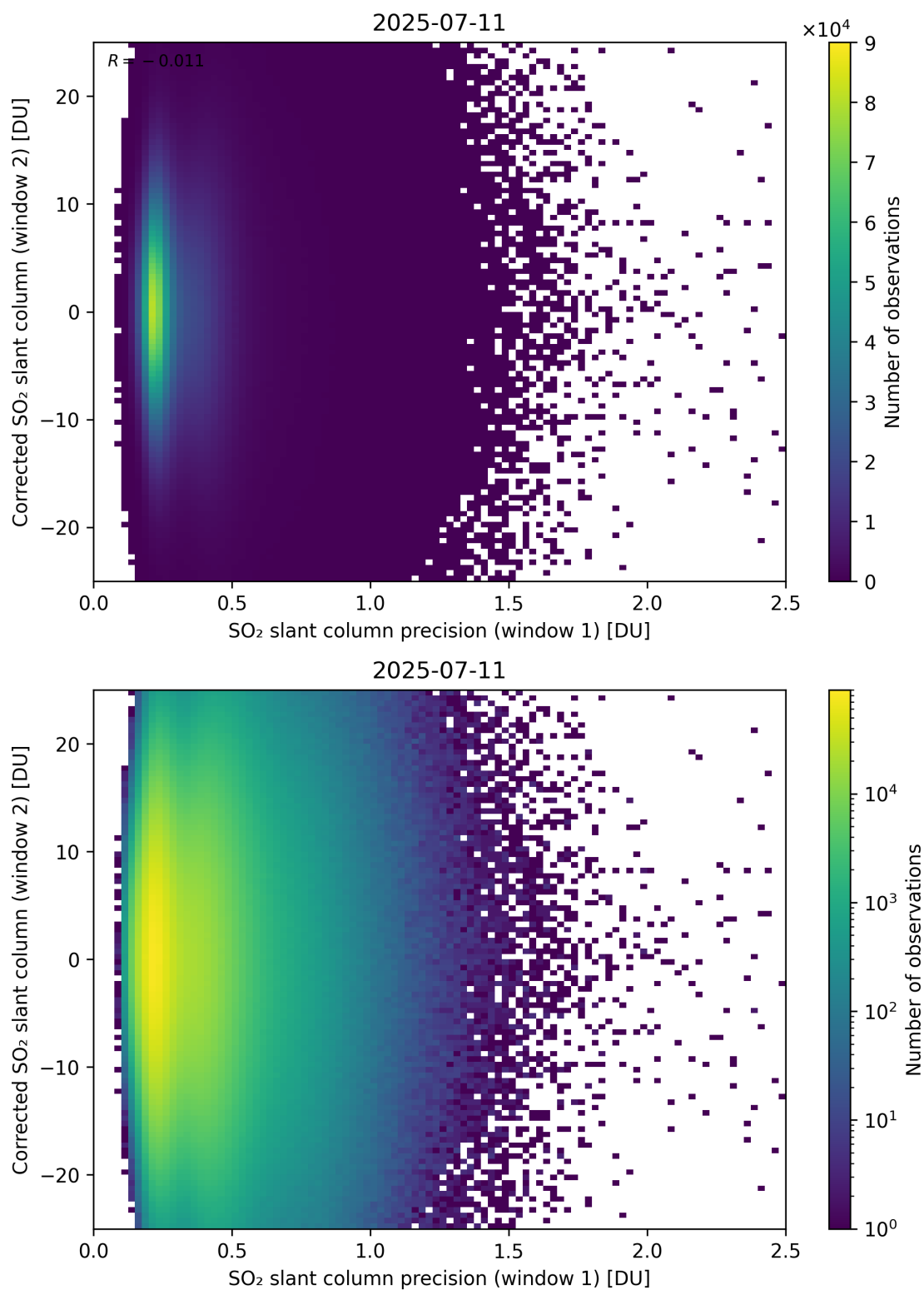
Figure 275: Scatter density plot of “SO 2 slant column precision (window 1)” against “Corrected SO 2 slant column (window 2)” for 2025-07-10 to 2025-07-12.
