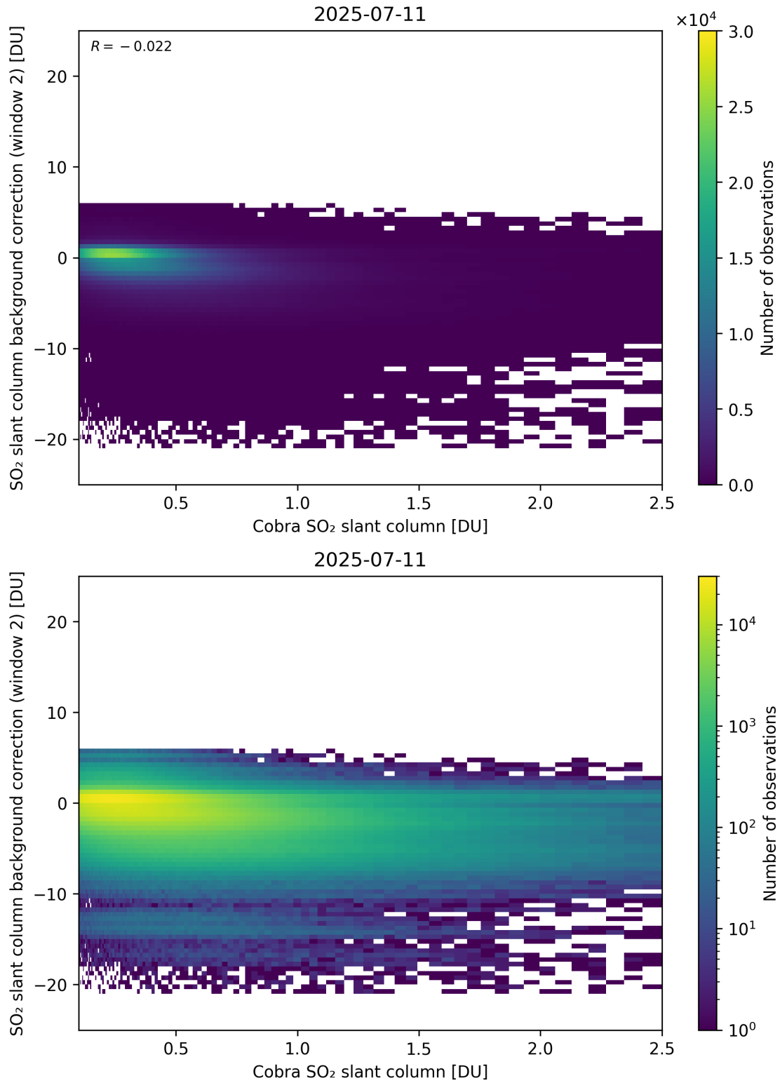
Figure 194: Scatter density plot of “Cobra SO 2 slant column” against “SO 2 slant column background correction (window 2)” for 2025-07-10 to 2025-07-12.
