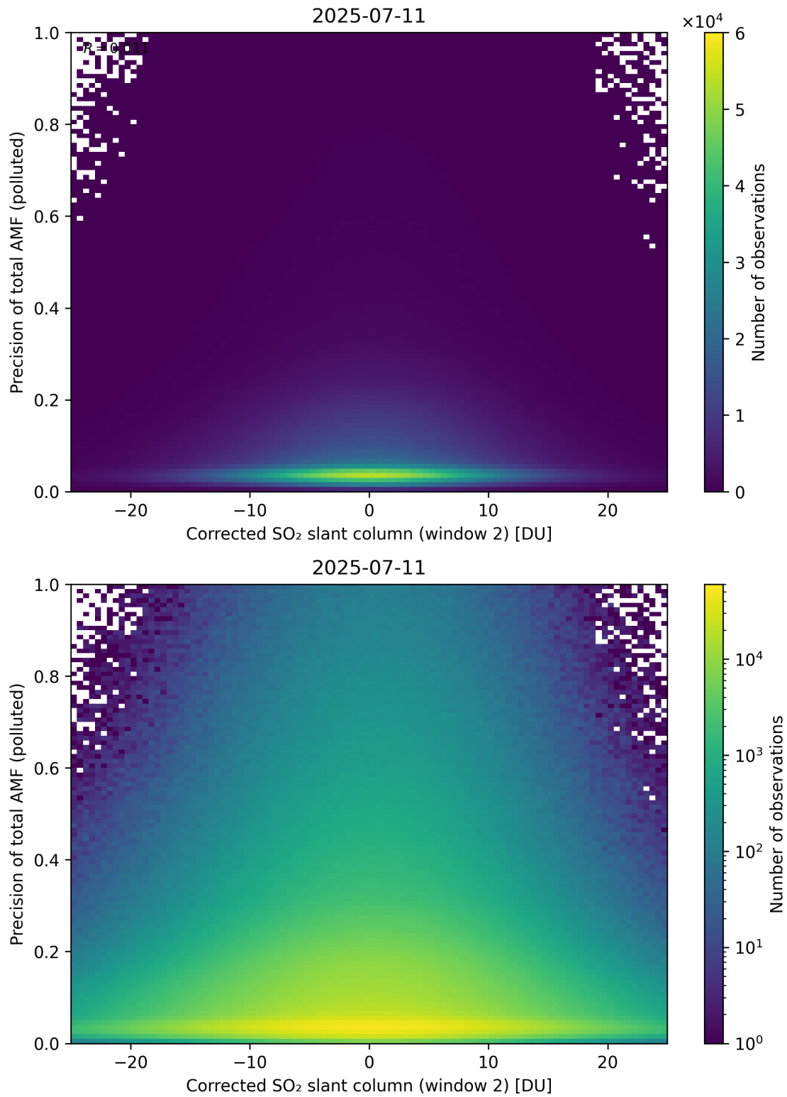
Figure 254: Scatter density plot of “Corrected SO 2 slant column (window 2)” against “Precision of total AMF (polluted)” for 2025-07-10 to 2025-07-12.
