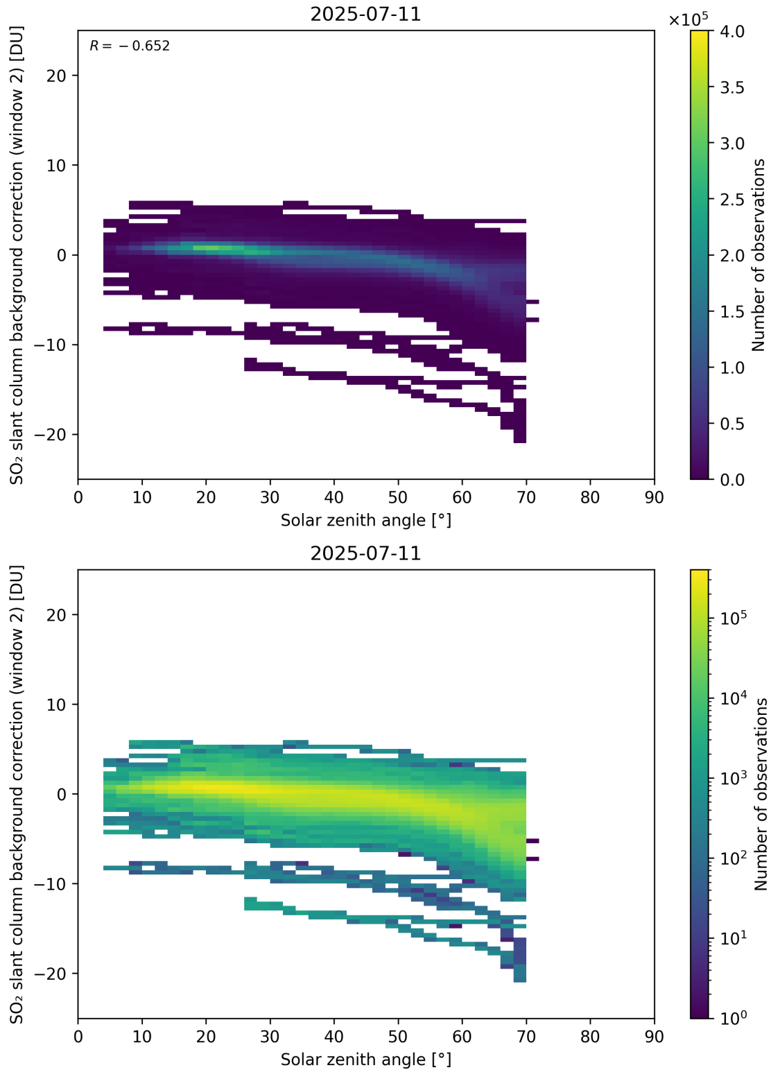
Figure 172: Scatter density plot of “Solar zenith angle” against “SO 2 slant column background correction (window 2)” for 2025-07-10 to 2025-07-12.
