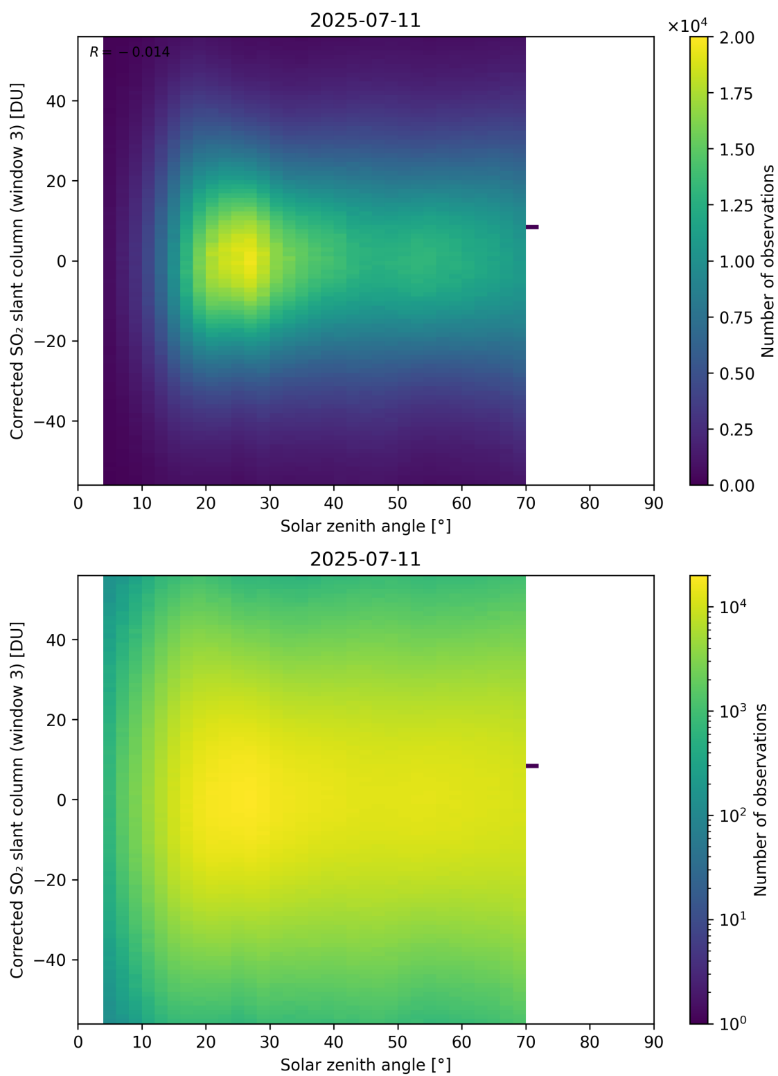
Figure 183: Scatter density plot of “Solar zenith angle” against “Corrected SO 2 slant column (window 3)” for 2025-07-10 to 2025-07-12.
