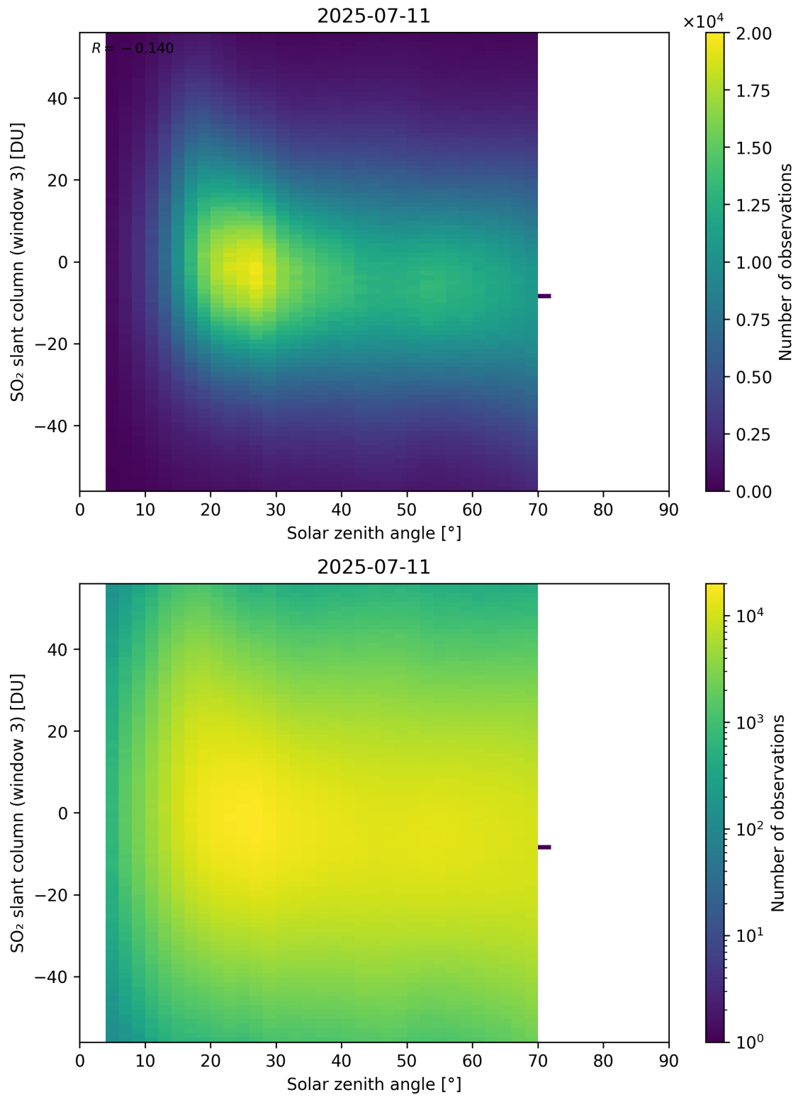
Figure 187: Scatter density plot of “Solar zenith angle” against “SO 2 slant column (window 3)” for 2025-07-10 to 2025-07-12.
