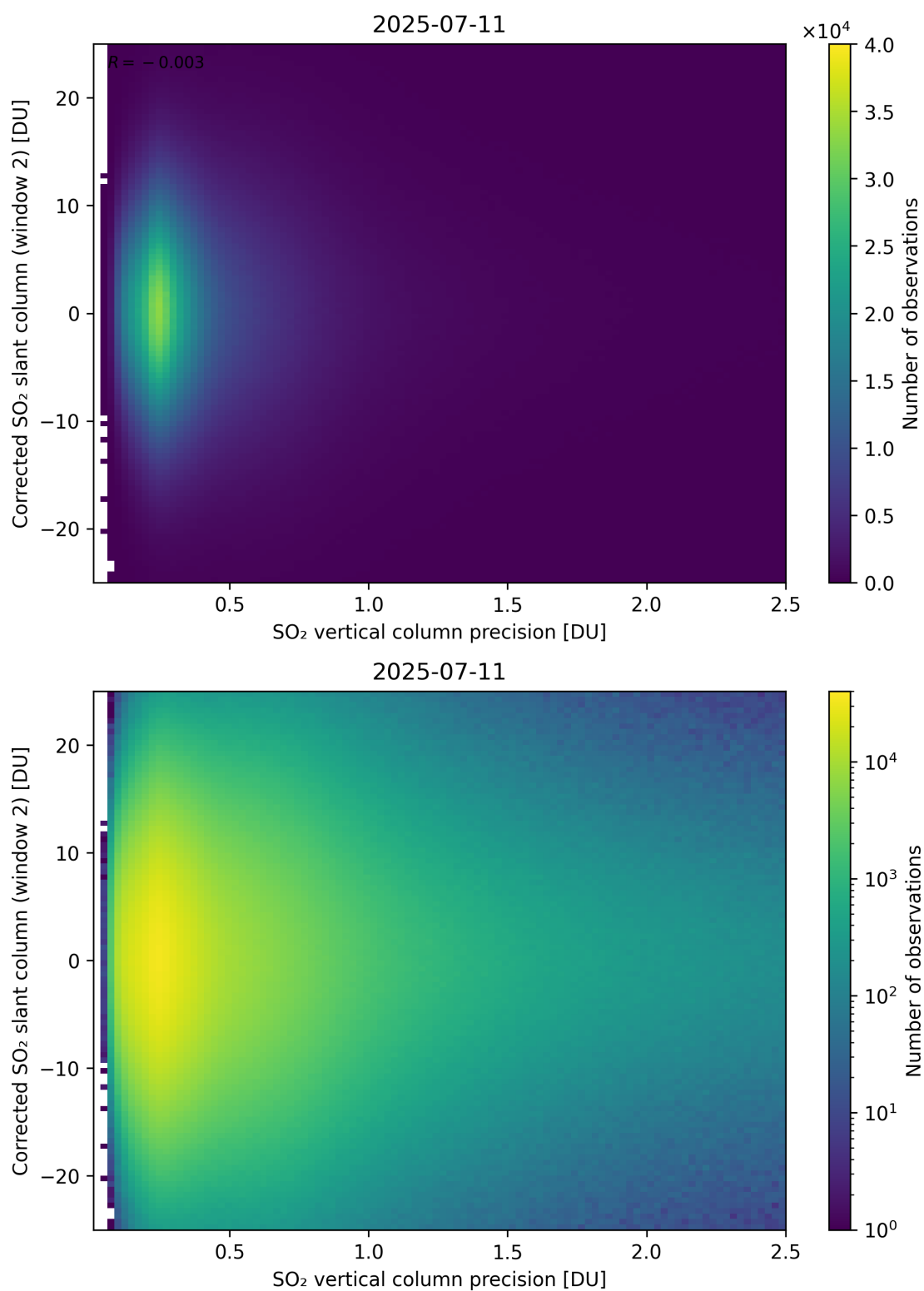
Figure 339: Scatter density plot of “SO 2 vertical column precision” against “Corrected SO 2 slant column (window 2)” for 2025-07-10 to 2025-07-12.
