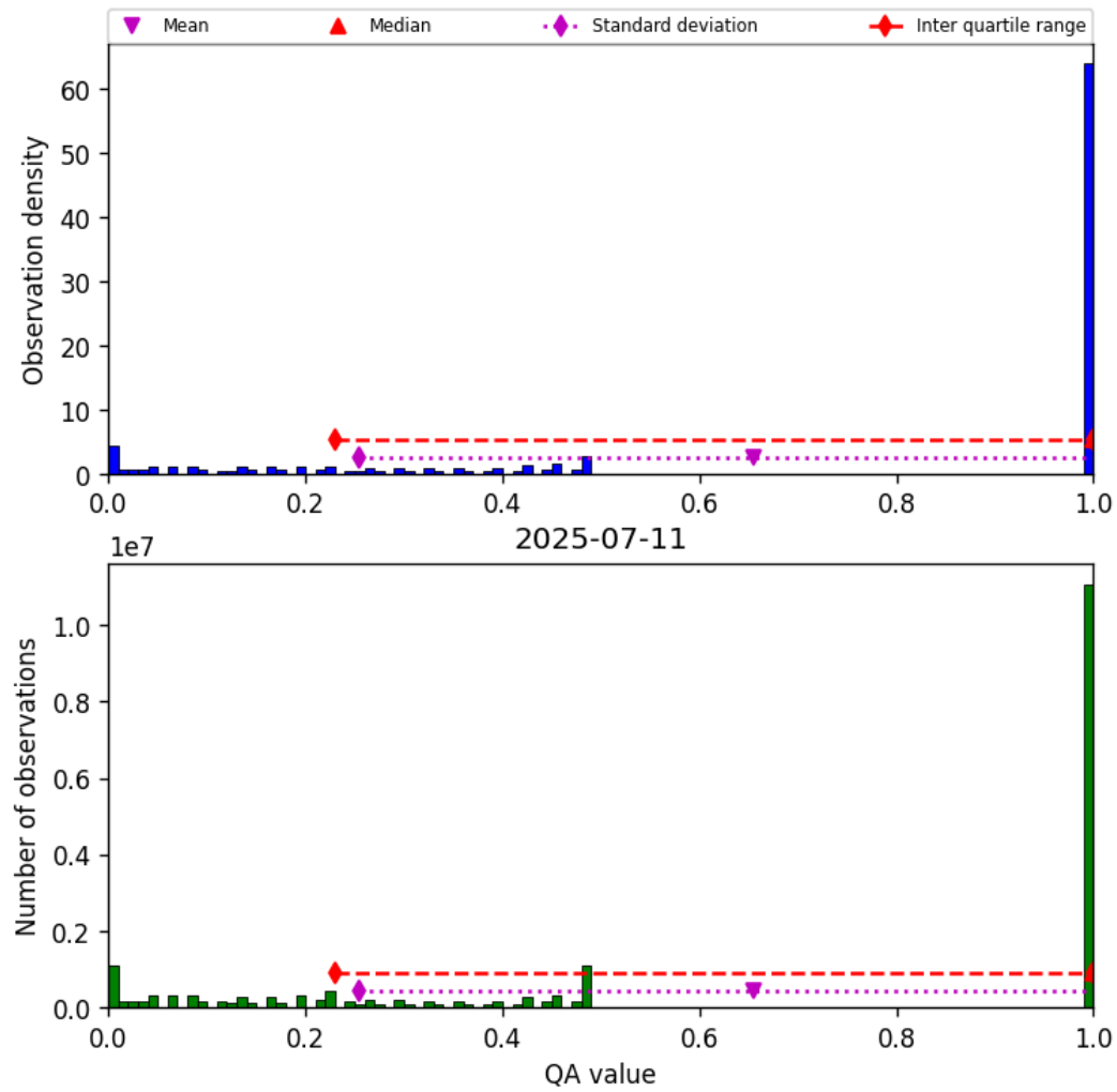
Figure 57: Histogram of “QA value” for 2025-07-10 to 2025-07-12
