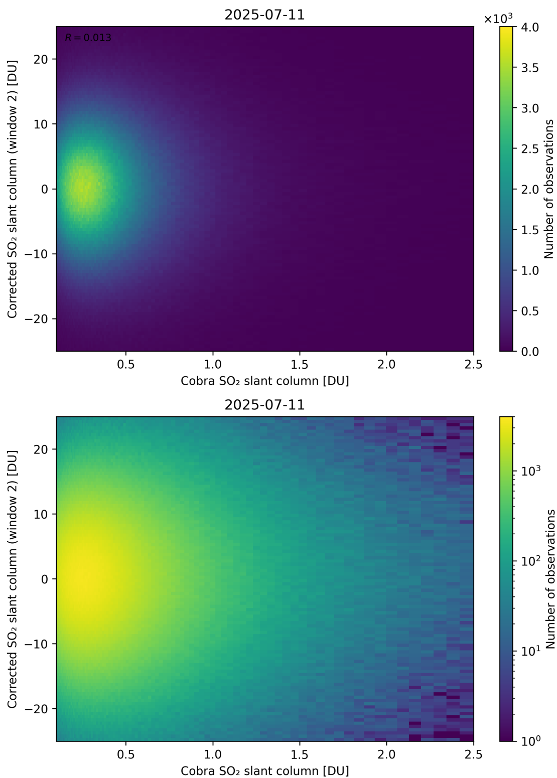
Figure 217: Scatter density plot of “Cobra SO 2 slant column” against “Corrected SO 2 slant column (window 2)” for 2025-07-10 to 2025-07-12.
