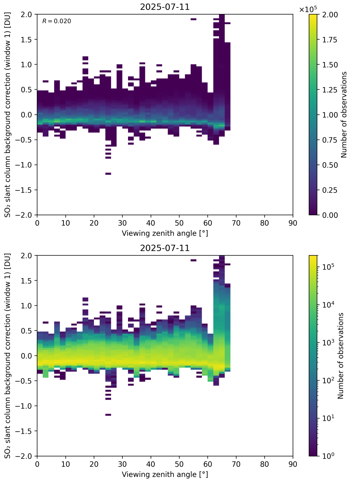
Figure 362: Scatter density plot of “Viewing zenith angle” against “SO 2 slant column background correction (window 1)” for 2025-07-10 to 2025-07-12.
