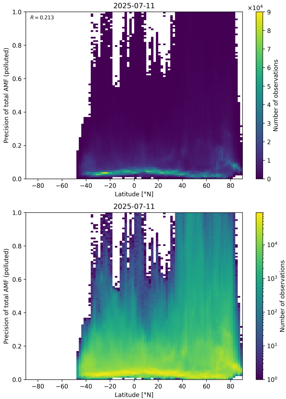
Figure 168: Scatter density plot of “Latitude” against “Precision of total AMF (polluted)” for 2025-07-10 to 2025-07-12.
