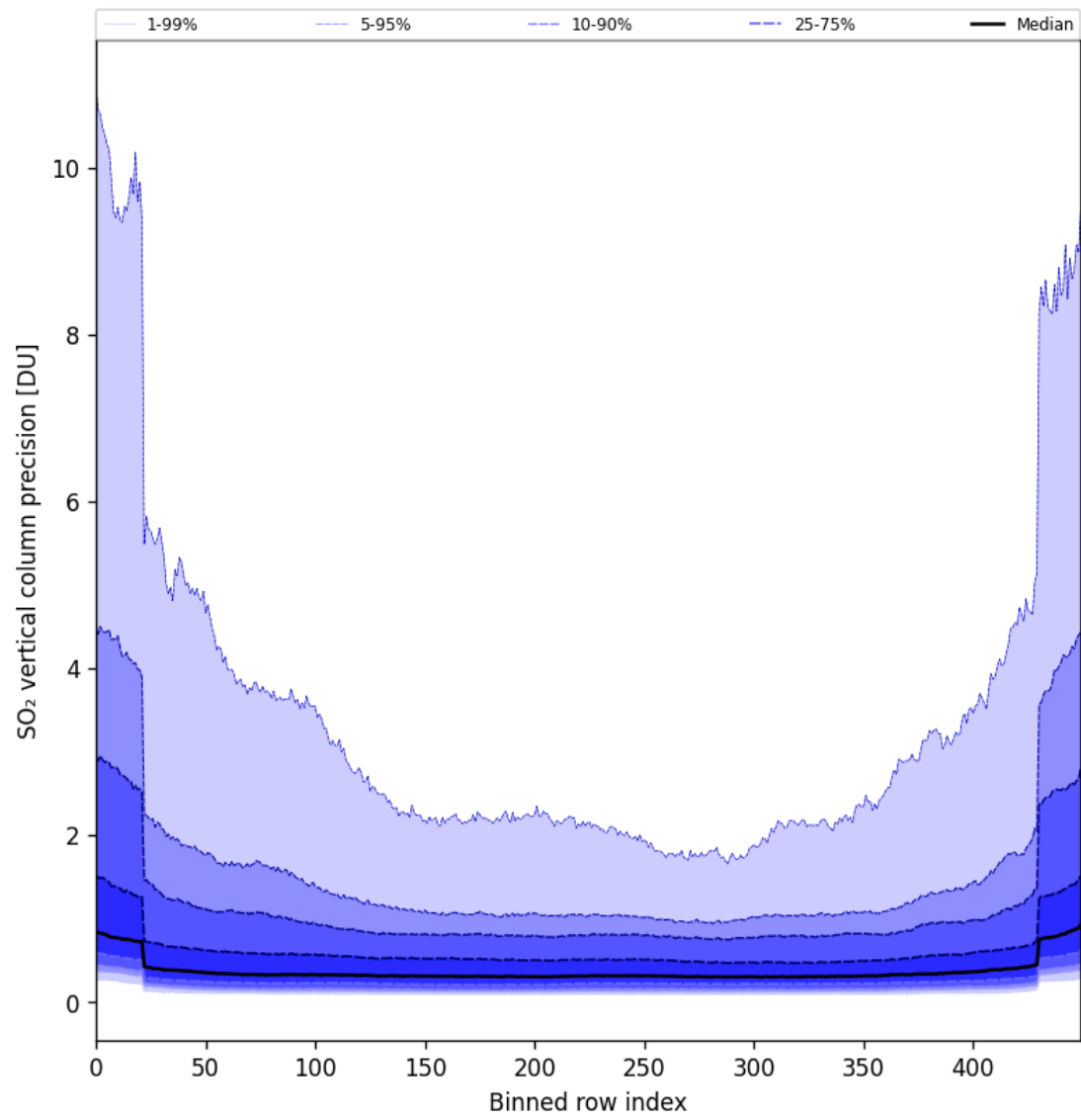
Figure 85: Along track statistics of “SO 2 vertical column precision” for 2025-07-10 to 2025-07-12
