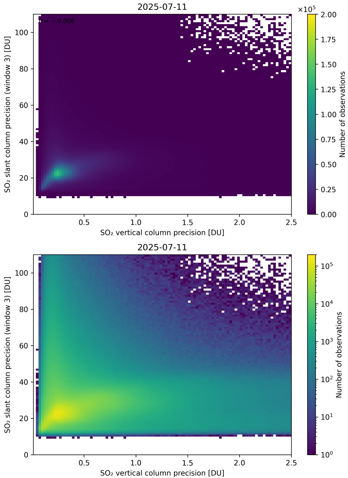
Figure 345: Scatter density plot of “SO 2 vertical column precision” against “SO 2 slant column precision (window 3)” for 2025-07-10 to 2025-07-12.
