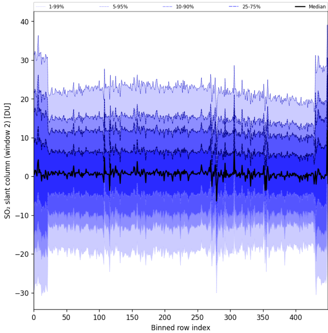
Figure 93: Along track statistics of “SO 2 slant column (window 2)” for 2025-07-10 to 2025-07-12
