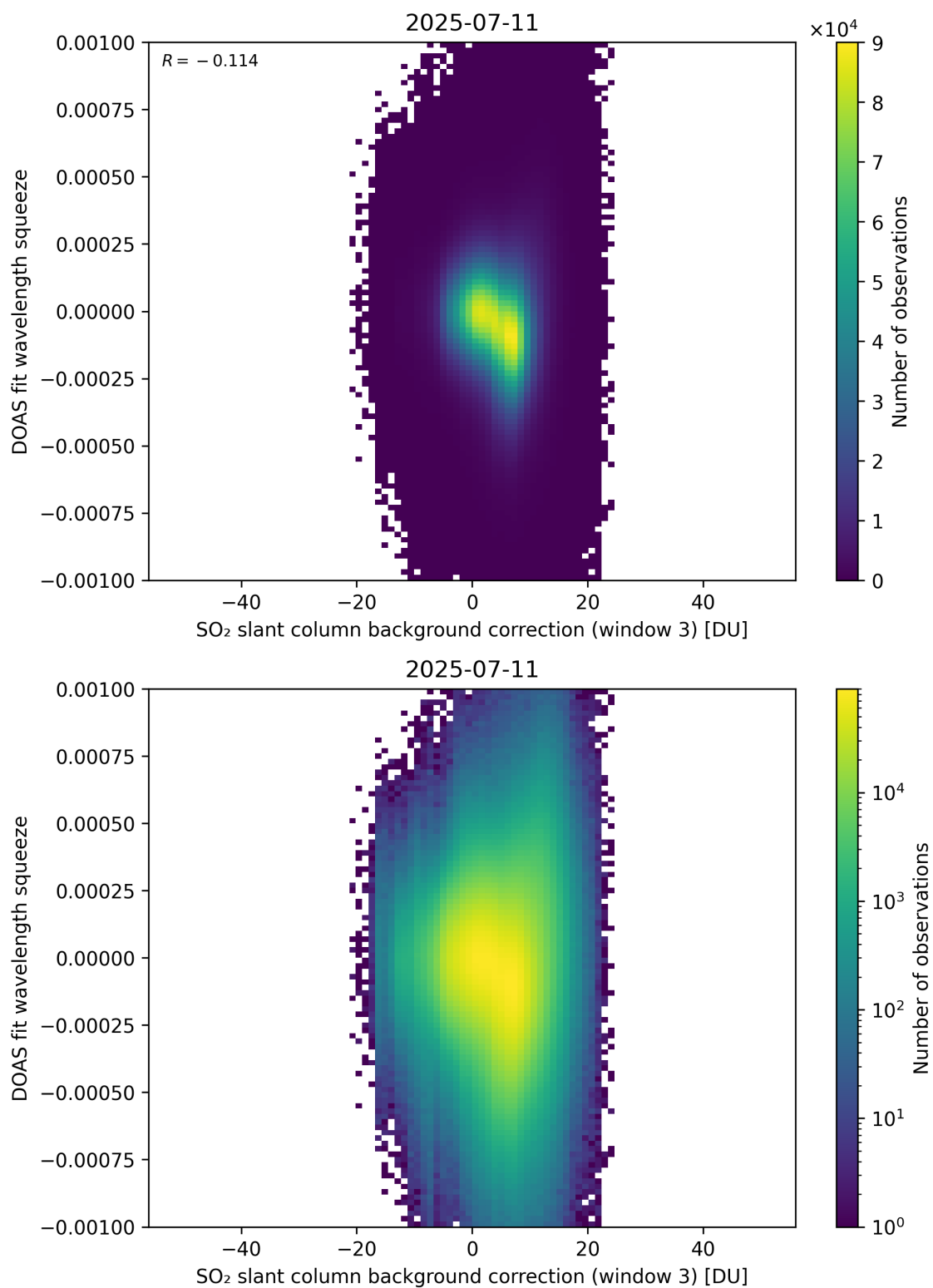
Figure 133: Scatter density plot of “SO 2 slant column background correction (window 3)” against “DOAS fit wavelength squeeze” for 2025-07-10 to 2025-07-12.
