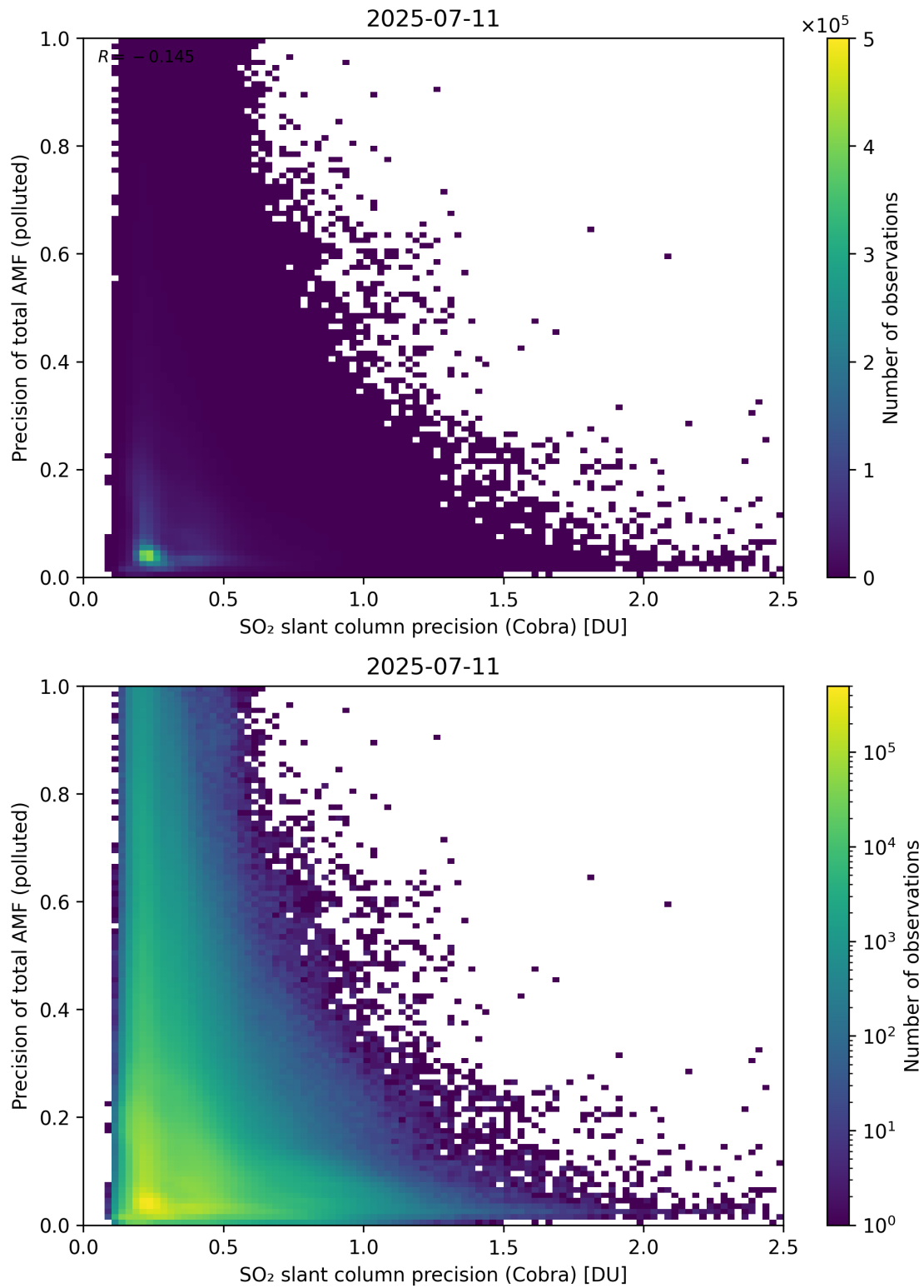
Figure 214: Scatter density plot of “SO 2 slant column precision (Cobra)” against “Precision of total AMF (polluted)” for 2025-07-10 to 2025-07-12.
