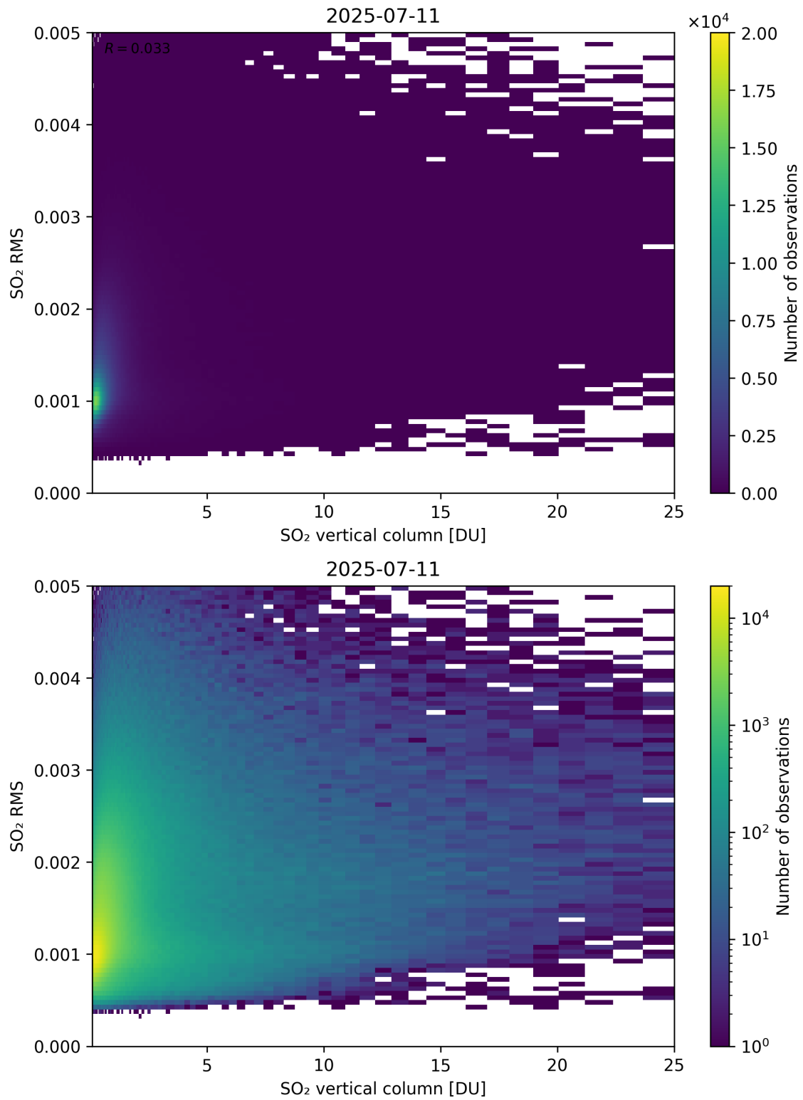
Figure 328: Scatter density plot of “SO 2 vertical column” against “SO 2 RMS” for 2025-07-10 to 2025-07-12.
