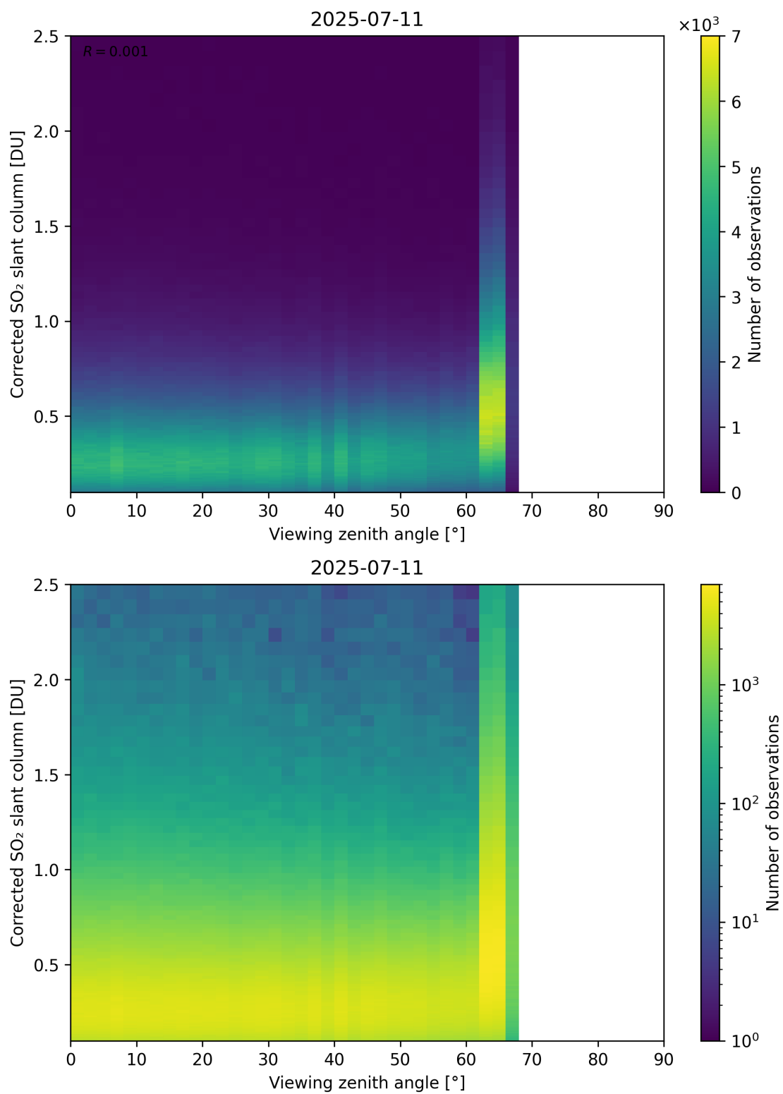
Figure 373: Scatter density plot of “Viewing zenith angle” against “Corrected SO 2 slant column” for 2025-07-10 to 2025-07-12.
