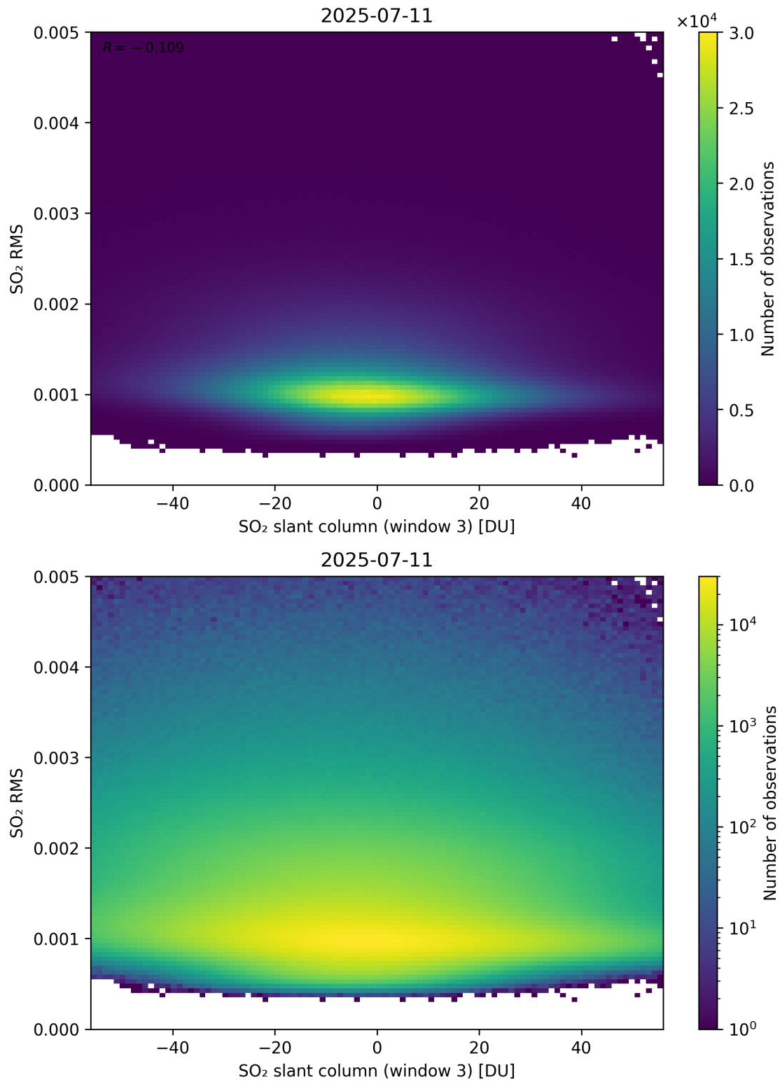
Figure 306: Scatter density plot of “SO 2 slant column (window 3)” against “SO 2 RMS” for 2025-07-10 to 2025-07-12.
