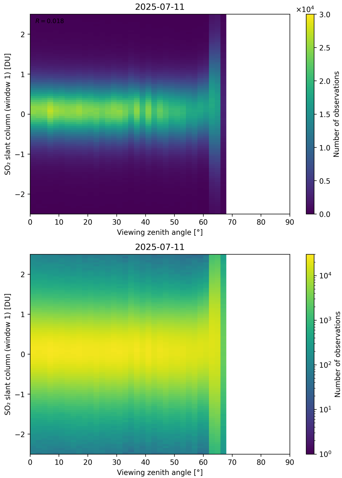
Figure 376: Scatter density plot of “Viewing zenith angle” against “SO 2 slant column (window 1)” for 2025-07-10 to 2025-07-12.
