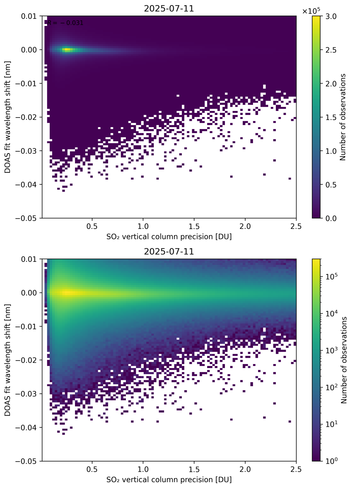
Figure 332: Scatter density plot of “SO 2 vertical column precision” against “DOAS fit wavelength shift” for 2025-07-10 to 2025-07-12.
