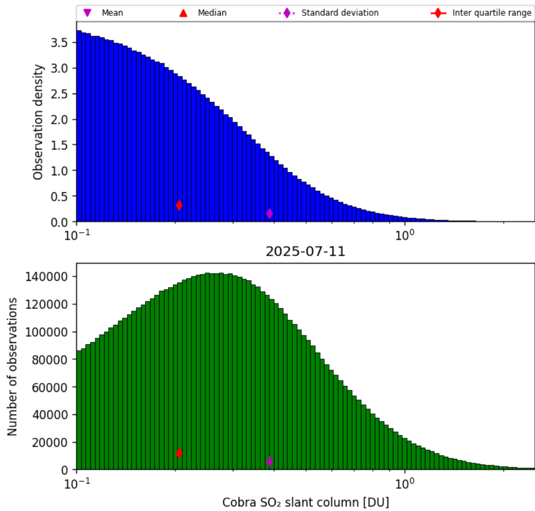
Figure 61: Histogram of “Cobra SO 2 slant column” for 2025-07-10 to 2025-07-12
