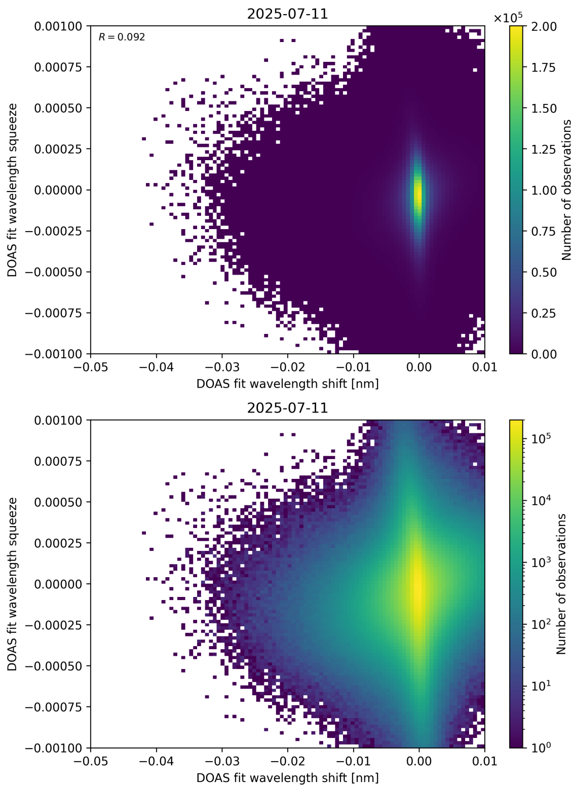
Figure 138: Scatter density plot of “DOAS fit wavelength shift” against “DOAS fit wavelength squeeze” for 2025-07-10 to 2025-07-12.
