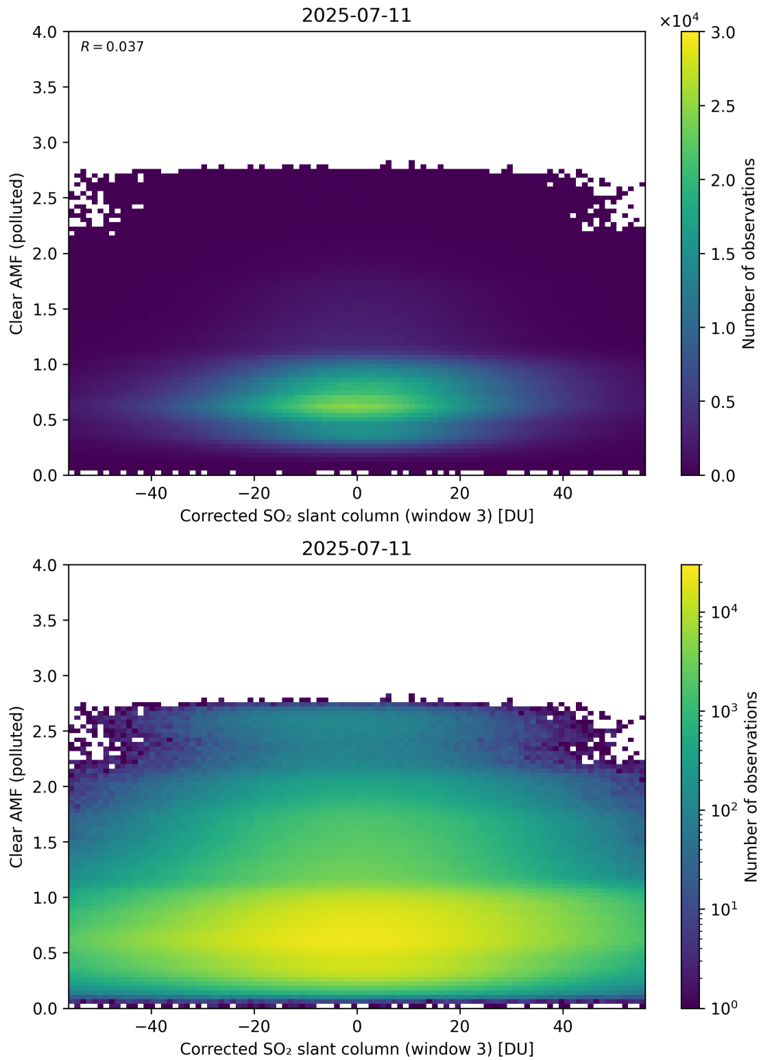
Figure 259: Scatter density plot of “Corrected SO 2 slant column (window 3)” against “Clear AMF (polluted)” for 2025-07-10 to 2025-07-12.
