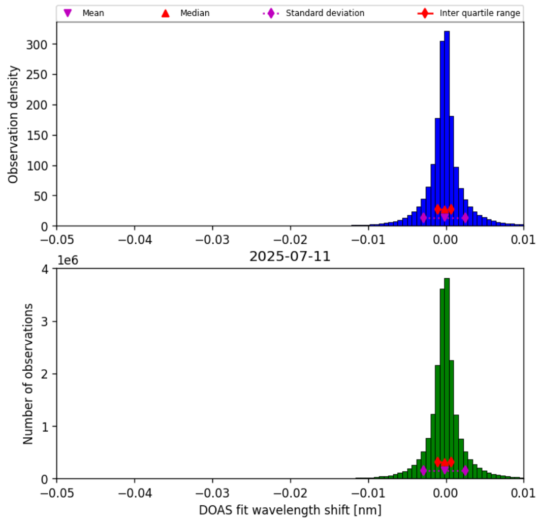
Figure 76: Histogram of “DOAS fit wavelength shift” for 2025-07-10 to 2025-07-12
