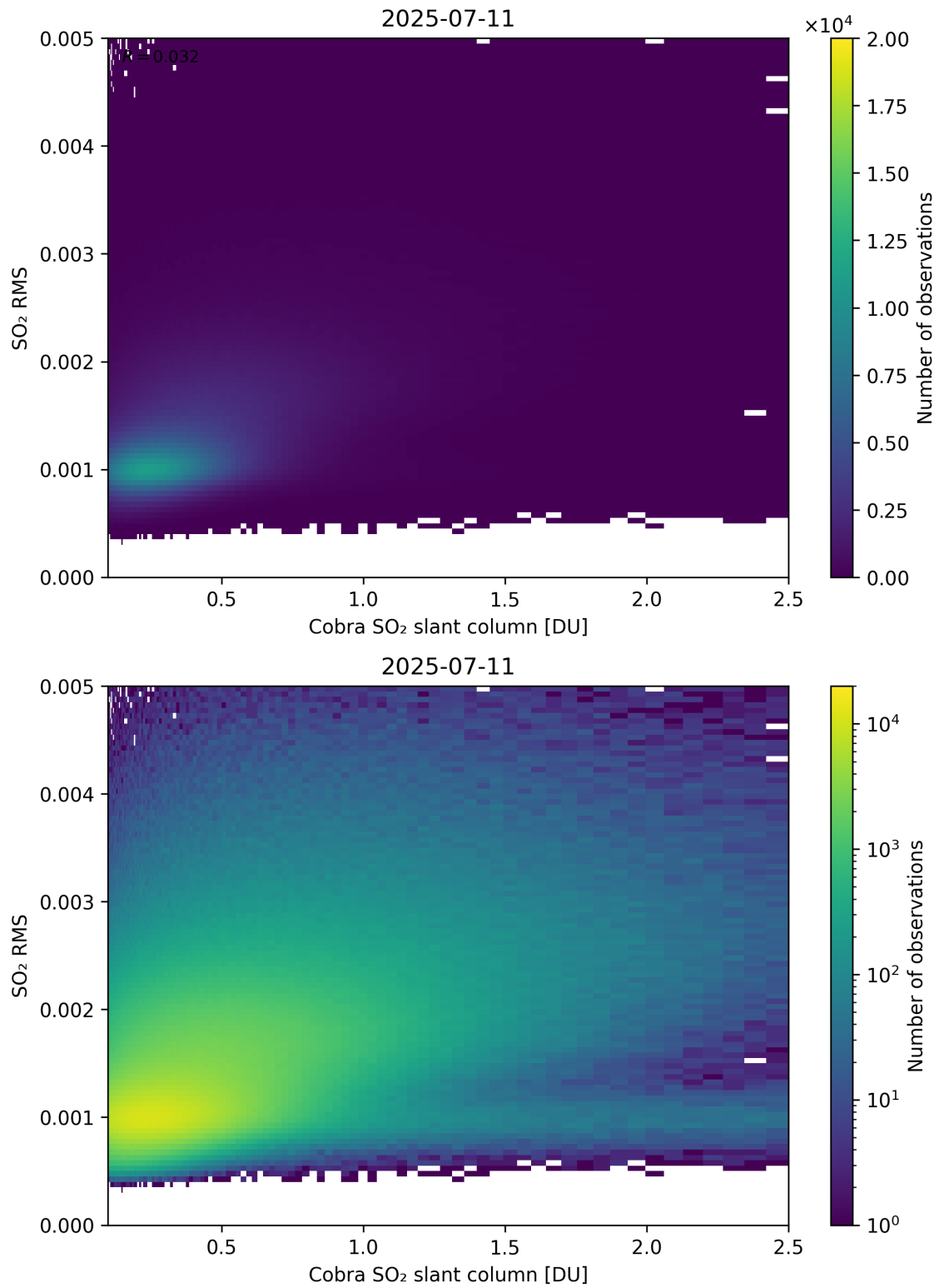
Figure 198: Scatter density plot of “Cobra SO 2 slant column” against “SO 2 RMS” for 2025-07-10 to 2025-07-12.
