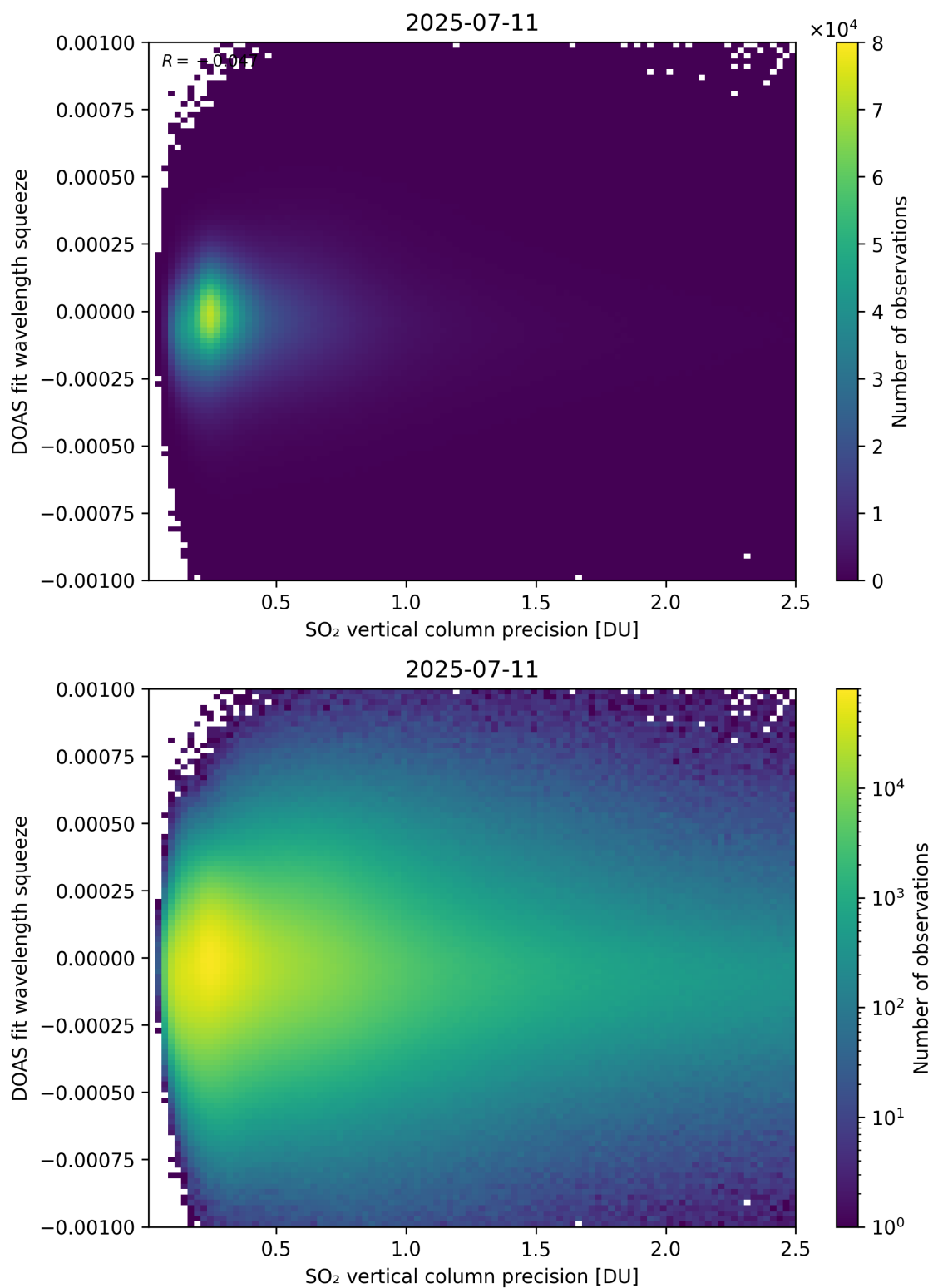
Figure 333: Scatter density plot of “SO 2 vertical column precision” against “DOAS fit wavelength squeeze” for 2025-07-10 to 2025-07-12.
