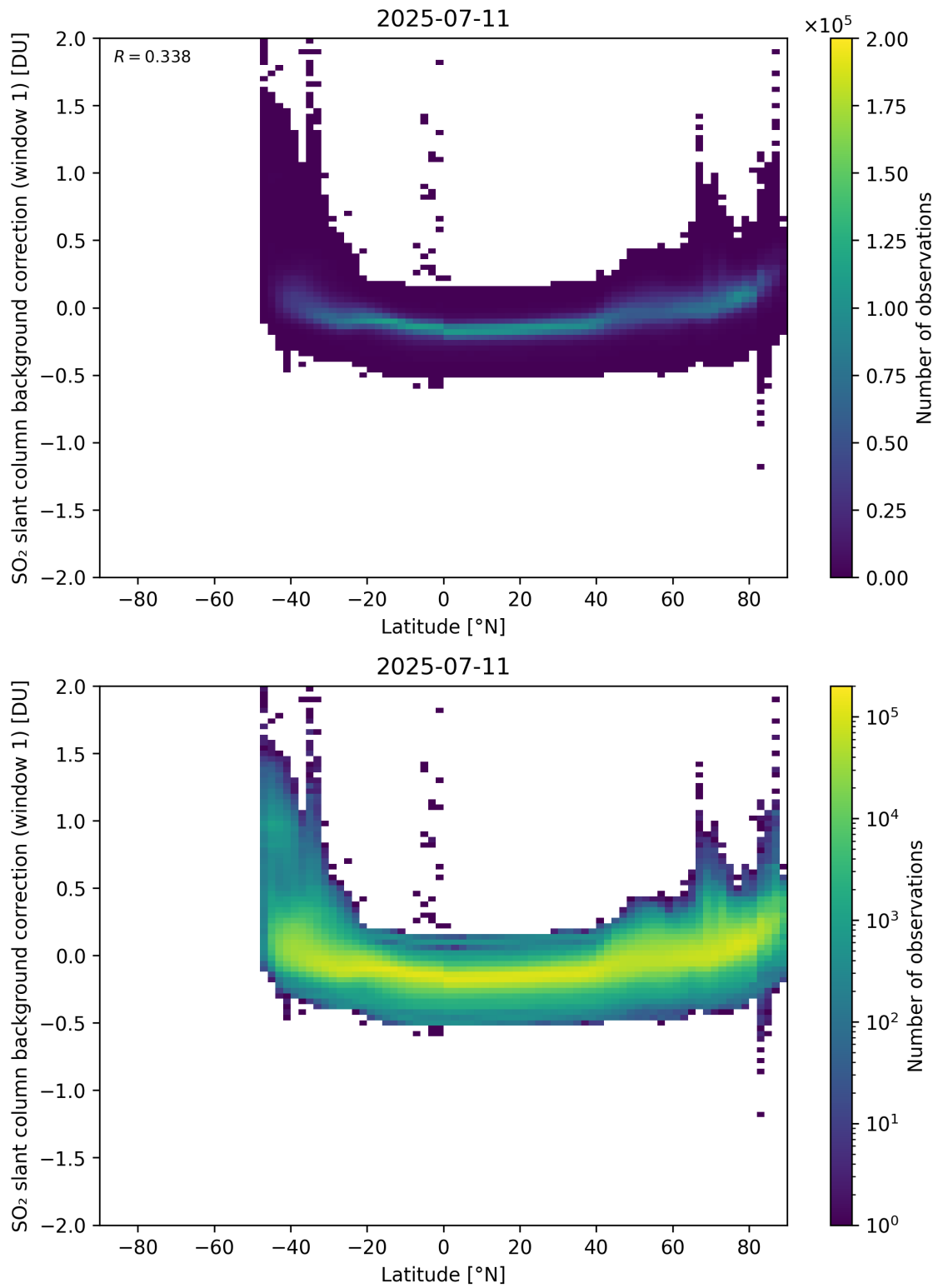
Figure 150: Scatter density plot of “Latitude” against “SO 2 slant column background correction (window 1)” for 2025-07-10 to 2025-07-12.
