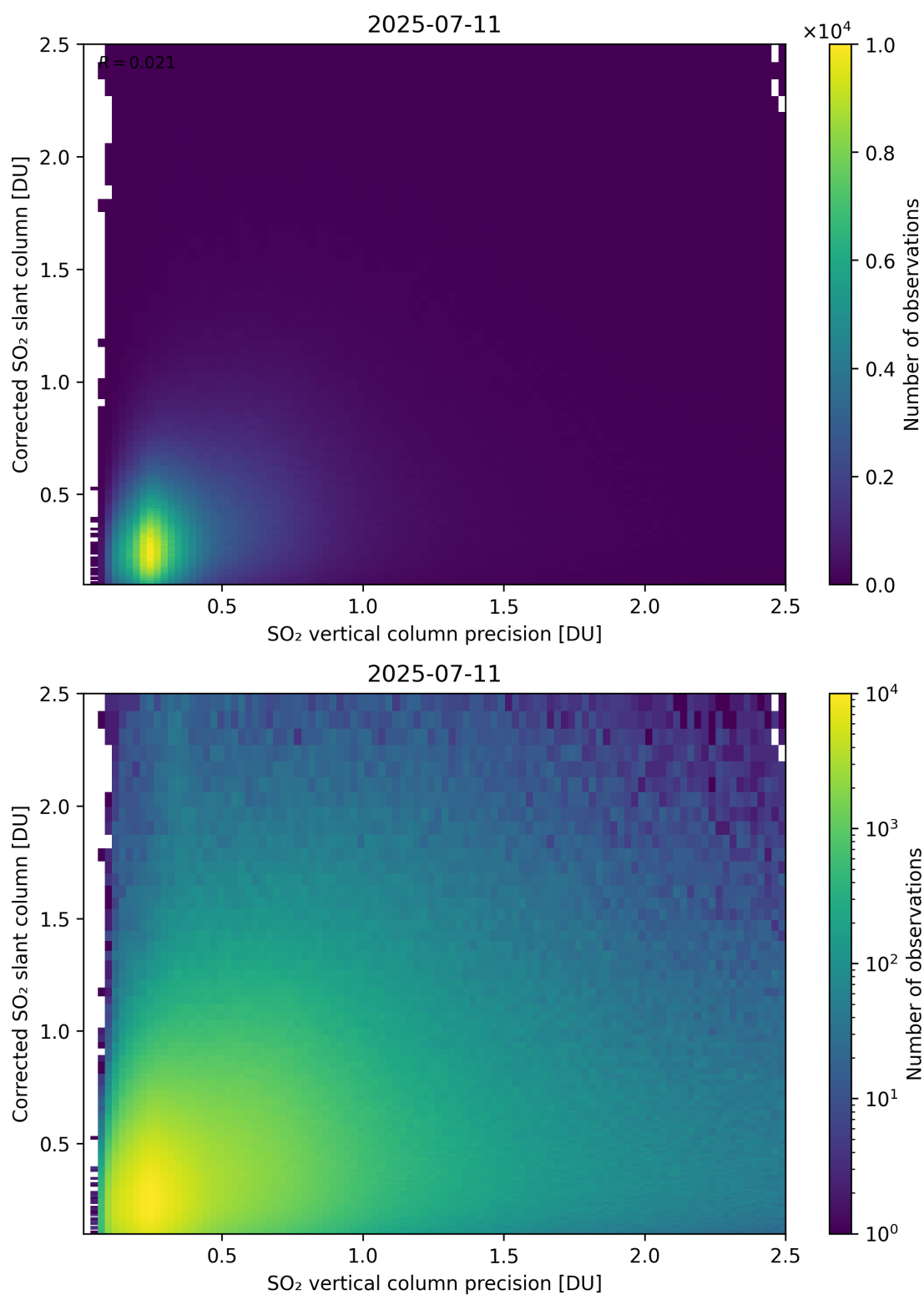
Figure 338: Scatter density plot of “SO 2 vertical column precision” against “Corrected SO 2 slant column” for 2025-07-10 to 2025-07-12.
