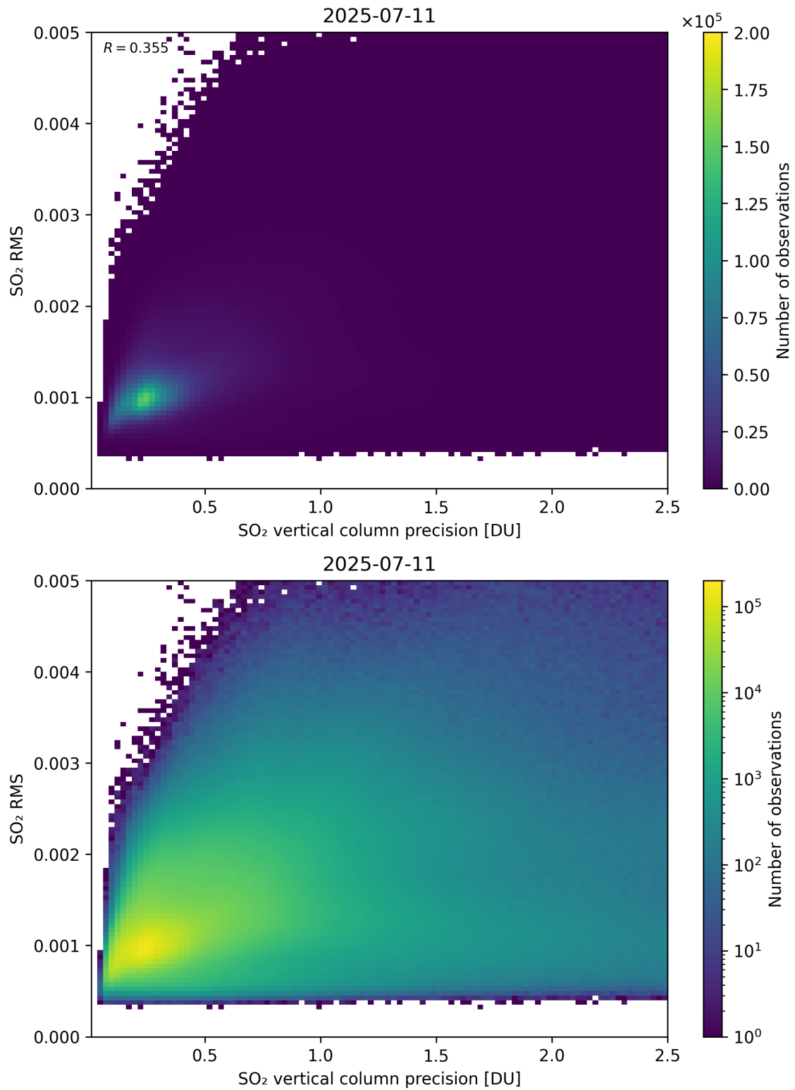
Figure 334: Scatter density plot of “SO 2 vertical column precision” against “SO 2 RMS” for 2025-07-10 to 2025-07-12.
