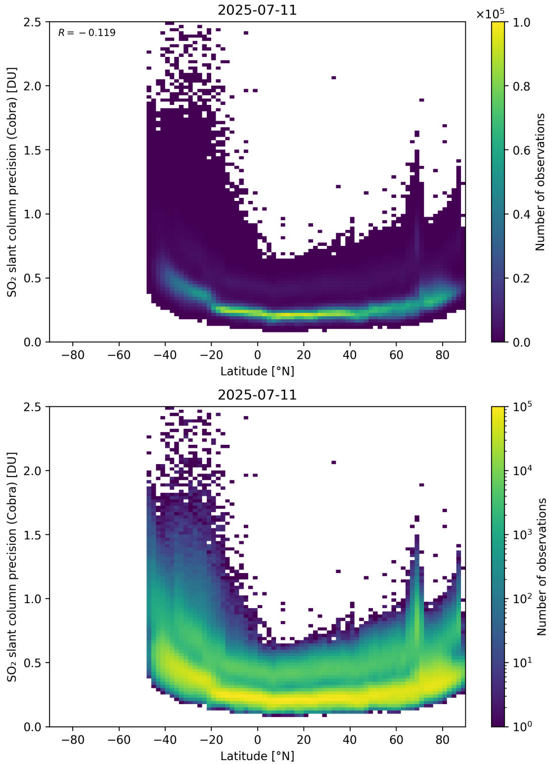
Figure 158: Scatter density plot of “Latitude” against “SO 2 slant column precision (Cobra)” for 2025-07-10 to 2025-07-12.
