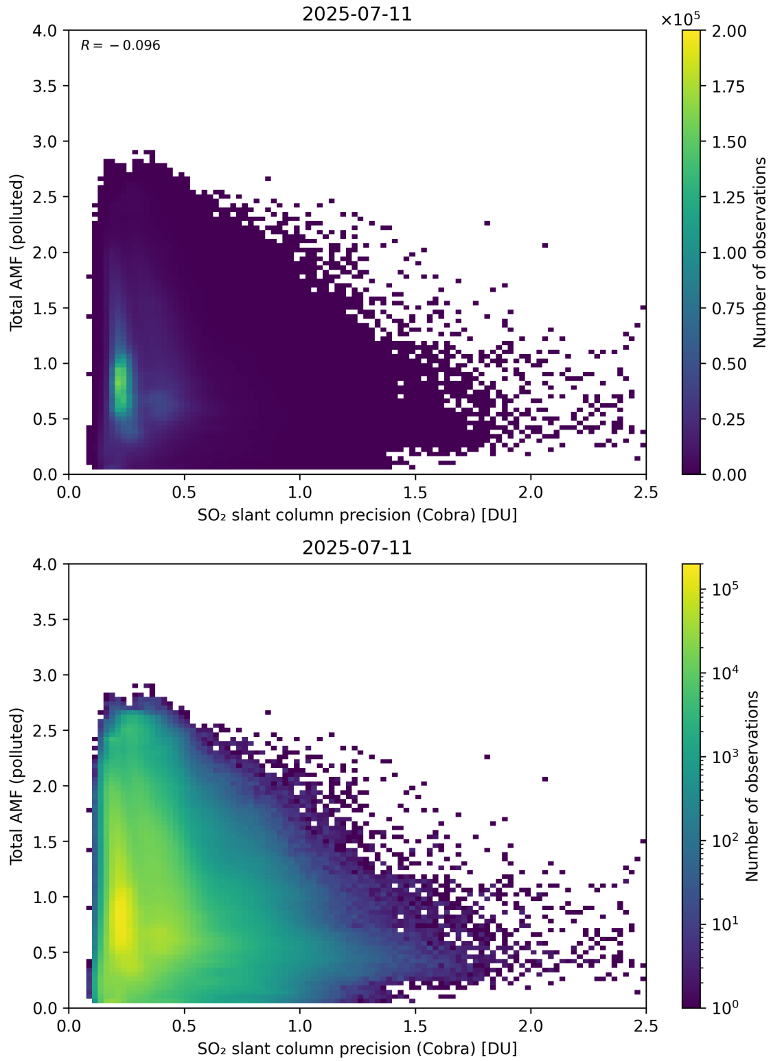
Figure 213: Scatter density plot of “SO 2 slant column precision (Cobra)” against “Total AMF (polluted)” for 2025-07-10 to 2025-07-12.
