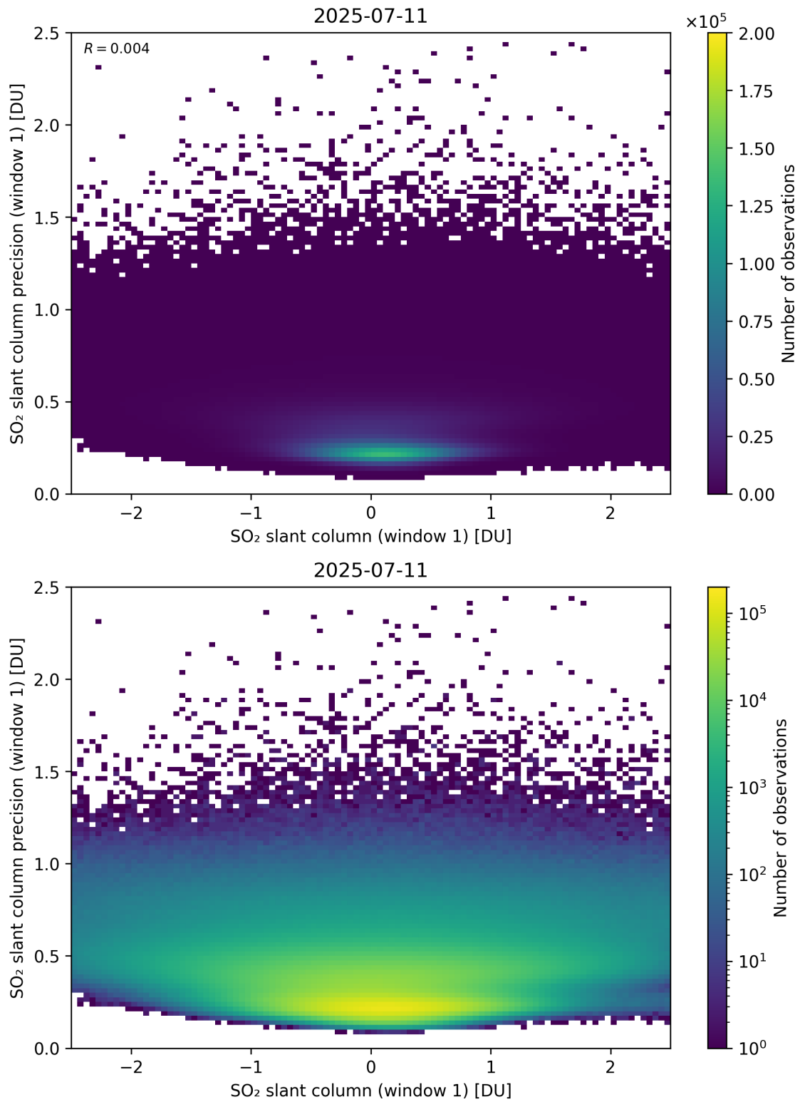
Figure 285: Scatter density plot of “SO 2 slant column (window 1)” against “SO 2 slant column precision (window 1)” for 2025-07-10 to 2025-07-12.
