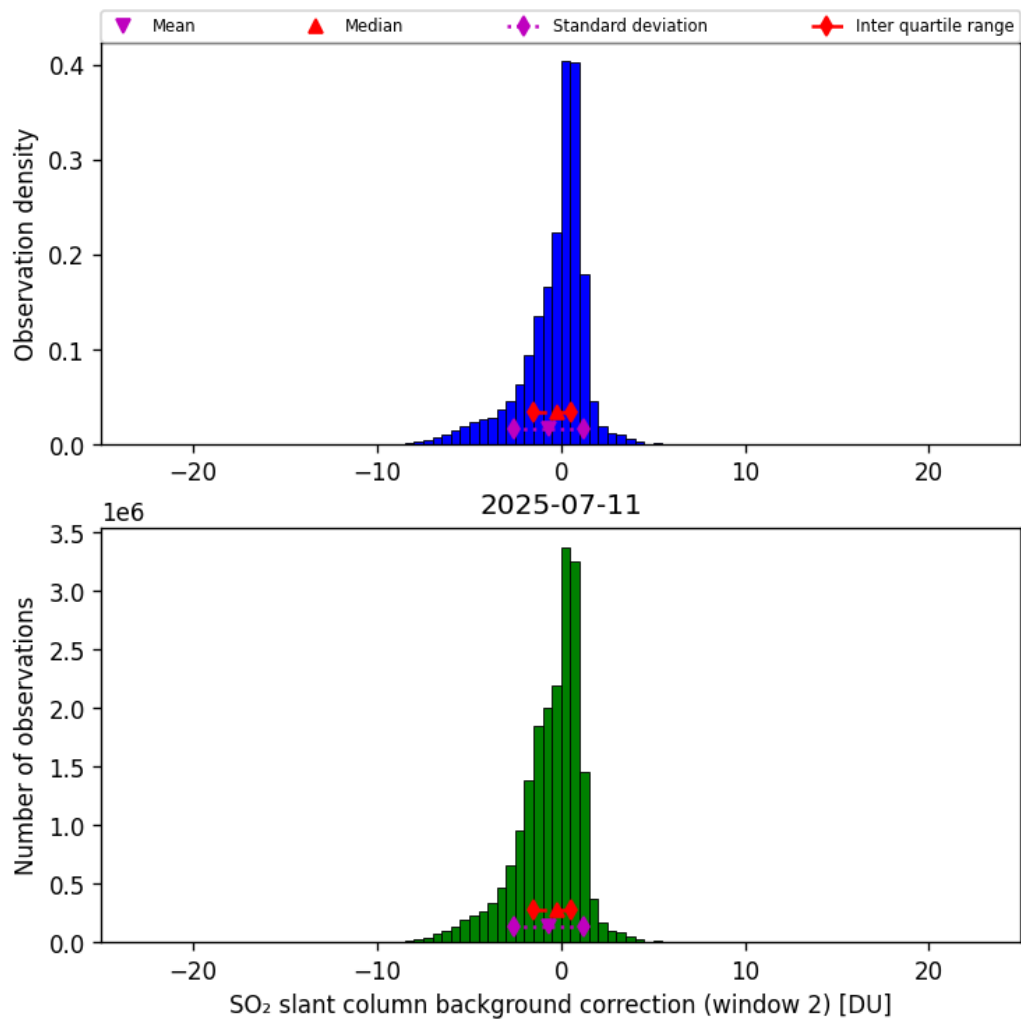
Figure 70: Histogram of “SO 2 slant column background correction (window 2)” for 2025-07-10 to 2025-07-12
