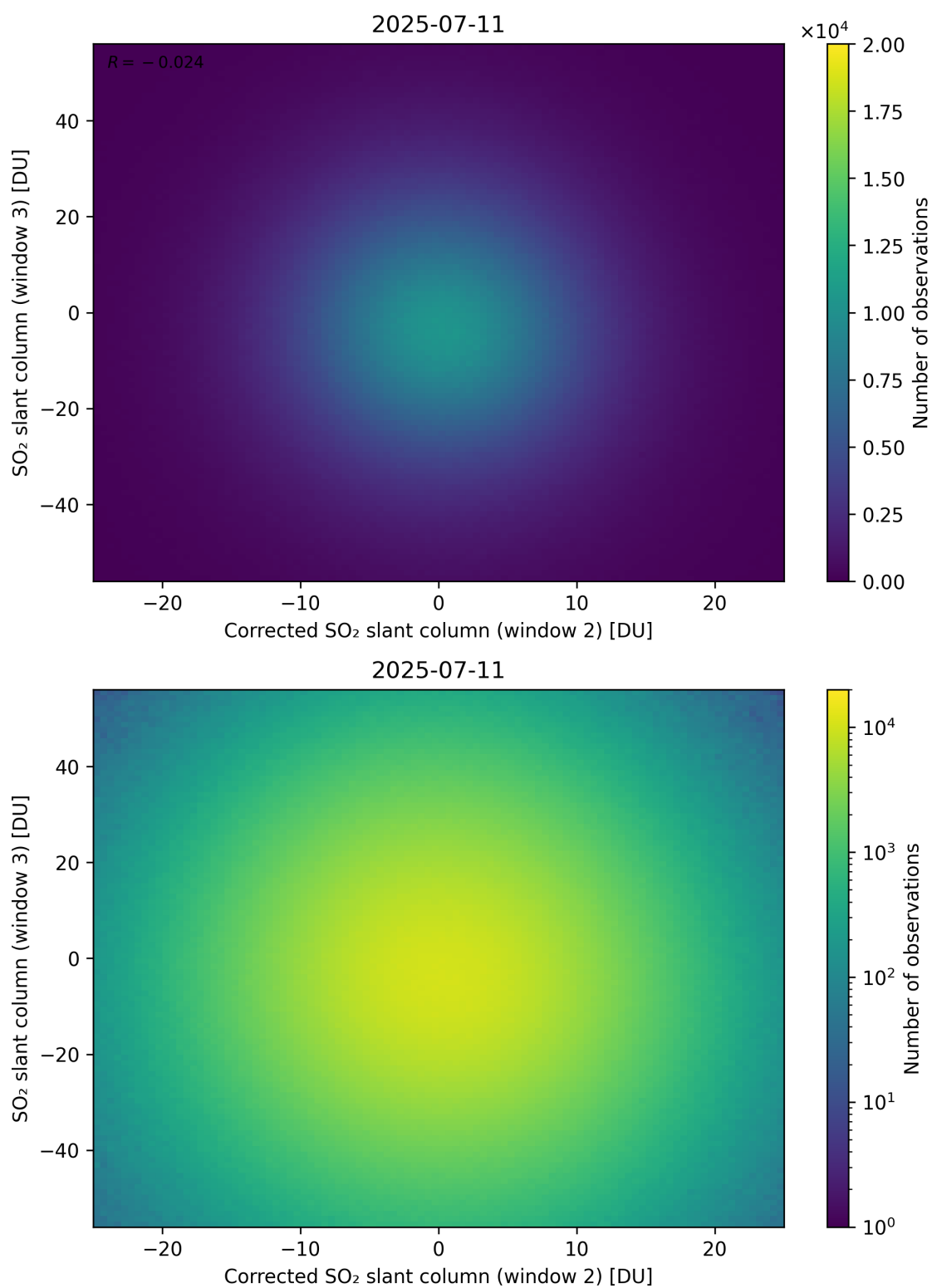
Figure 251: Scatter density plot of “Corrected SO 2 slant column (window 2)” against “SO 2 slant column (window 3)” for 2025-07-10 to 2025-07-12.
