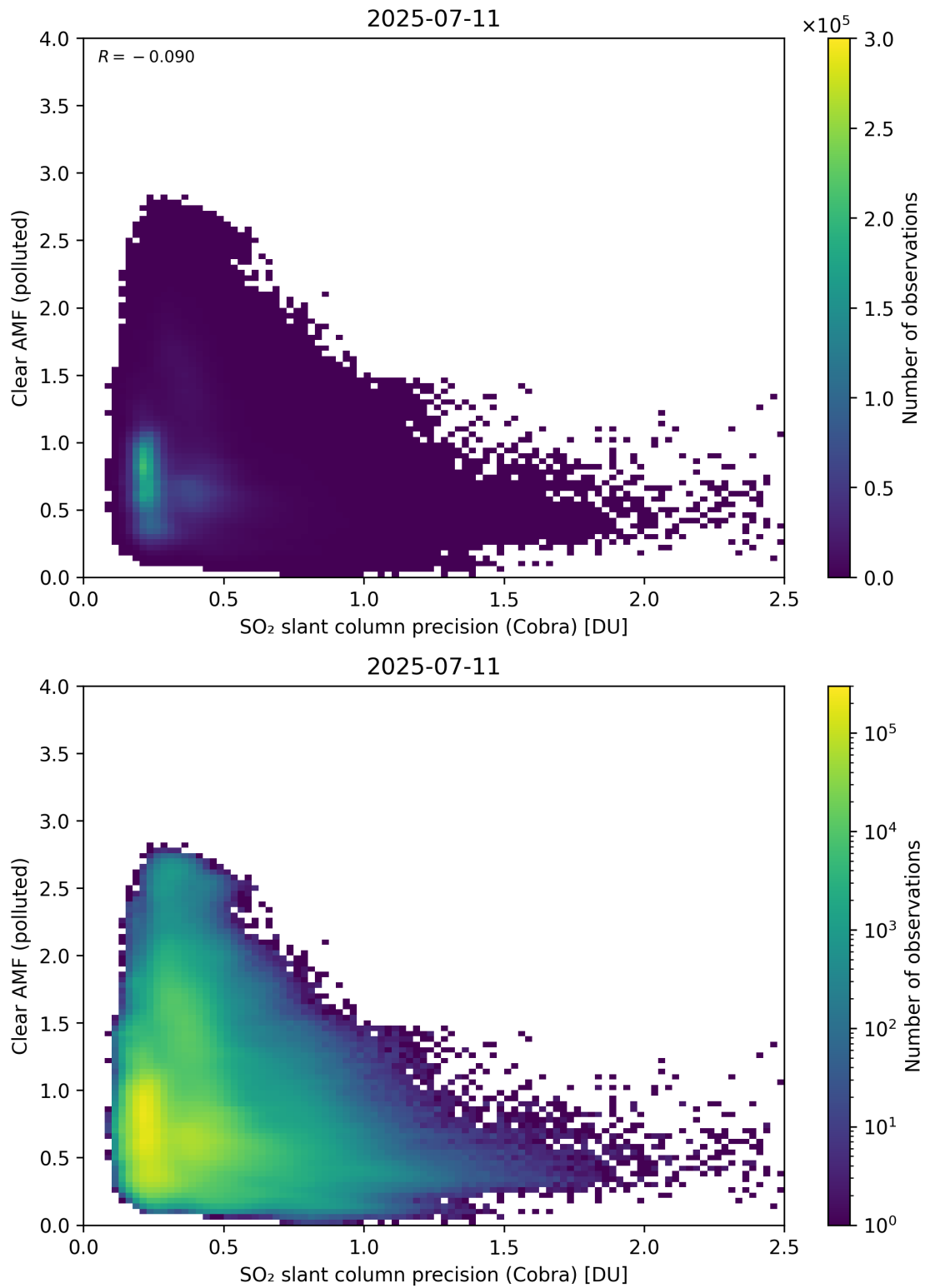
Figure 205: Scatter density plot of “SO 2 slant column precision (Cobra)” against “Clear AMF (polluted)” for 2025-07-10 to 2025-07-12.
