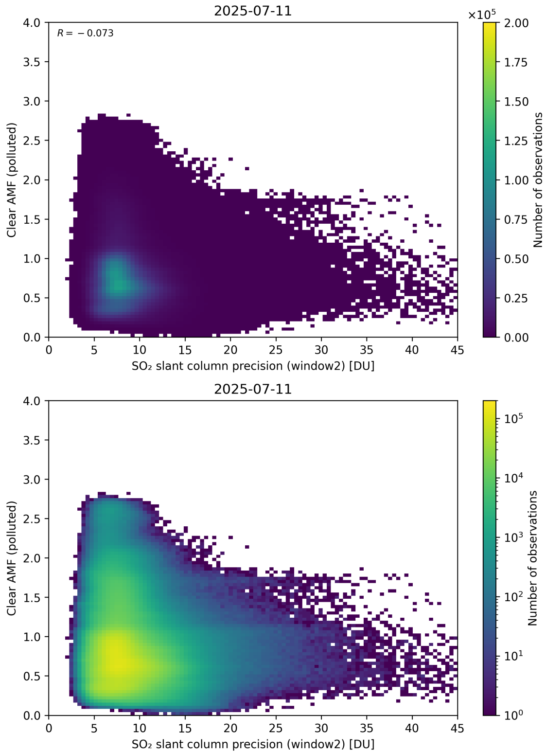
Figure 296: Scatter density plot of “SO 2 slant column precision (window2)” against “Clear AMF (polluted)” for 2025-07-10 to 2025-07-12.
