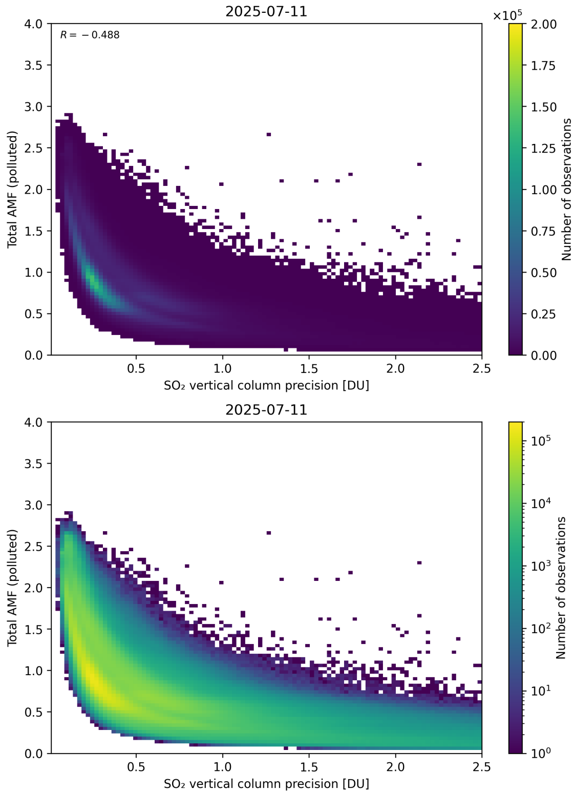
Figure 346: Scatter density plot of “SO 2 vertical column precision” against “Total AMF (polluted)” for 2025-07-10 to 2025-07-12.
