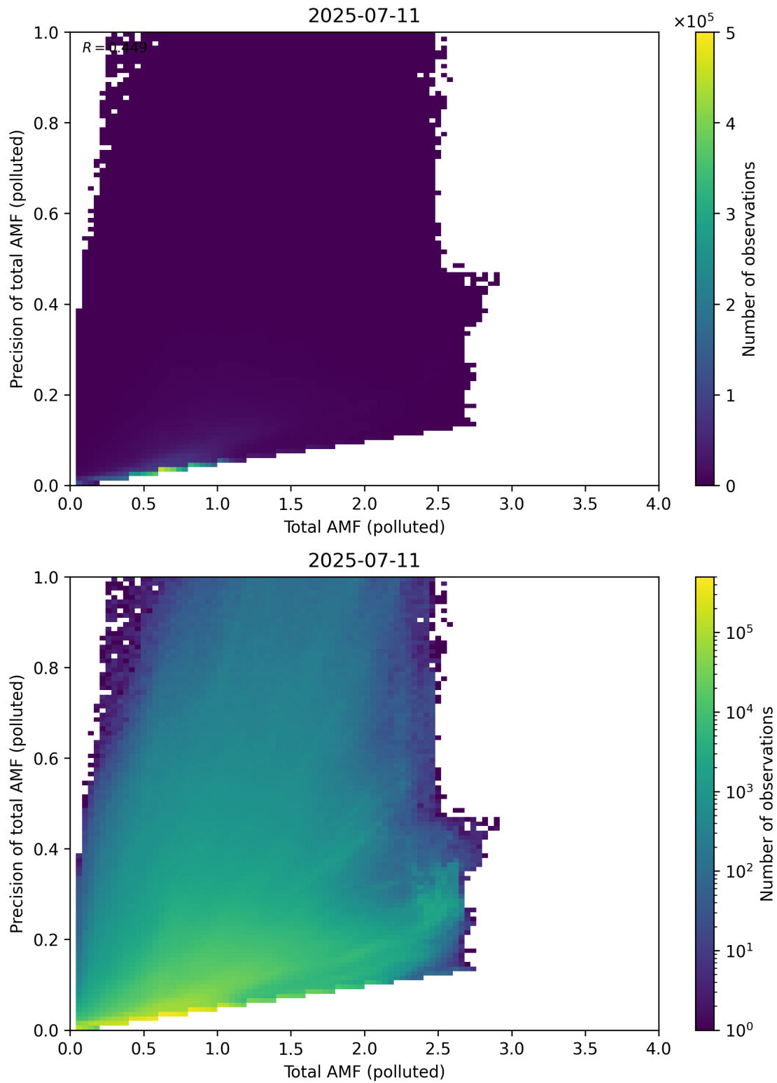
Figure 322: Scatter density plot of “Total AMF (polluted)” against “Precision of total AMF (polluted)” for 2025-07-10 to 2025-07-12.
