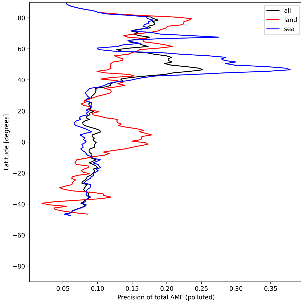
Figure 54: Zonal average of “Precision of total AMF (polluted)” for 2025-07-10 to 2025-07-12.
