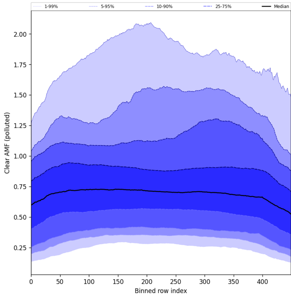
Figure 107: Along track statistics of “Clear AMF (polluted)” for 2025-07-10 to 2025-07-12
