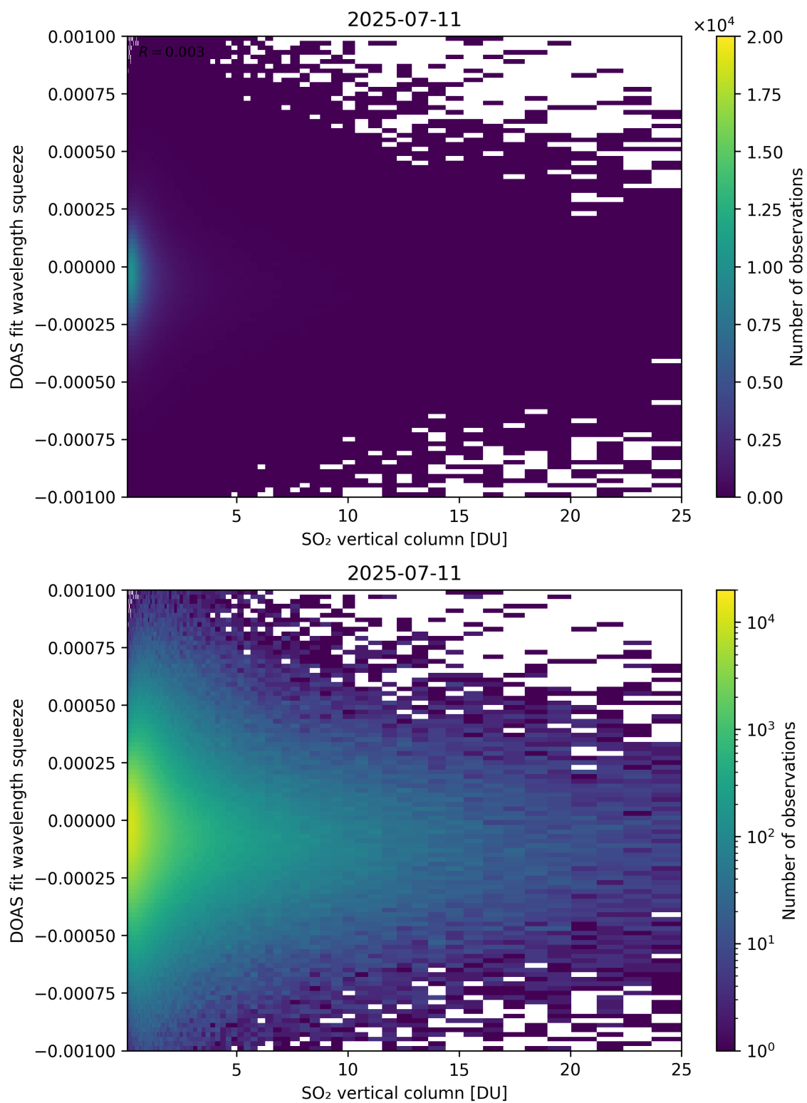
Figure 327: Scatter density plot of “SO 2 vertical column” against “DOAS fit wavelength squeeze” for 2025-07-10 to 2025-07-12.
