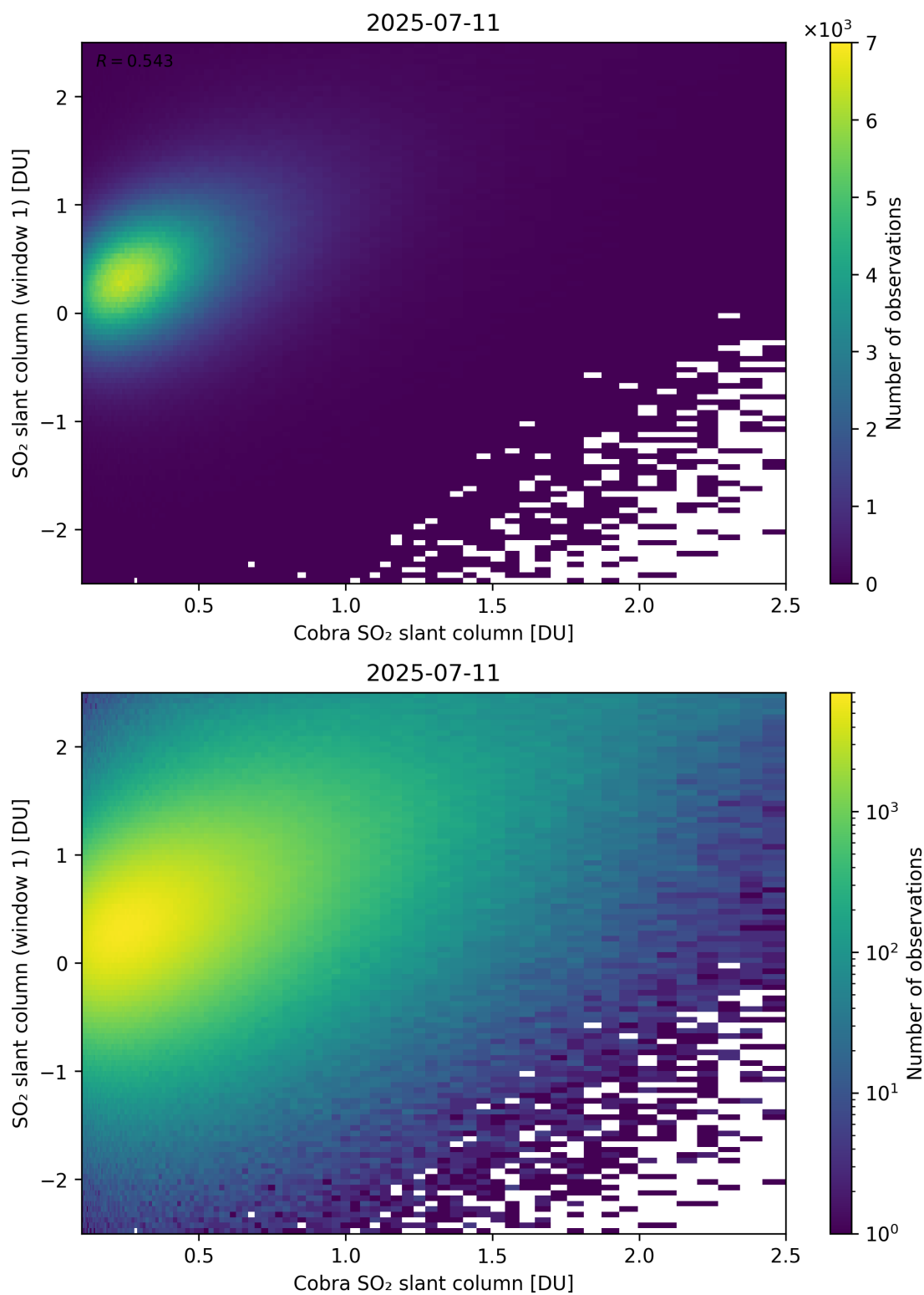
Figure 219: Scatter density plot of “Cobra SO 2 slant column” against “SO 2 slant column (window 1)” for 2025-07-10 to 2025-07-12.
