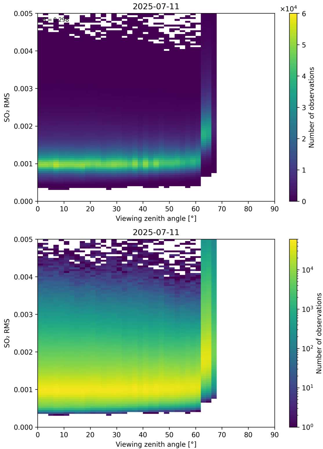
Figure 367: Scatter density plot of “Viewing zenith angle” against “SO 2 RMS” for 2025-07-10 to 2025-07-12.
