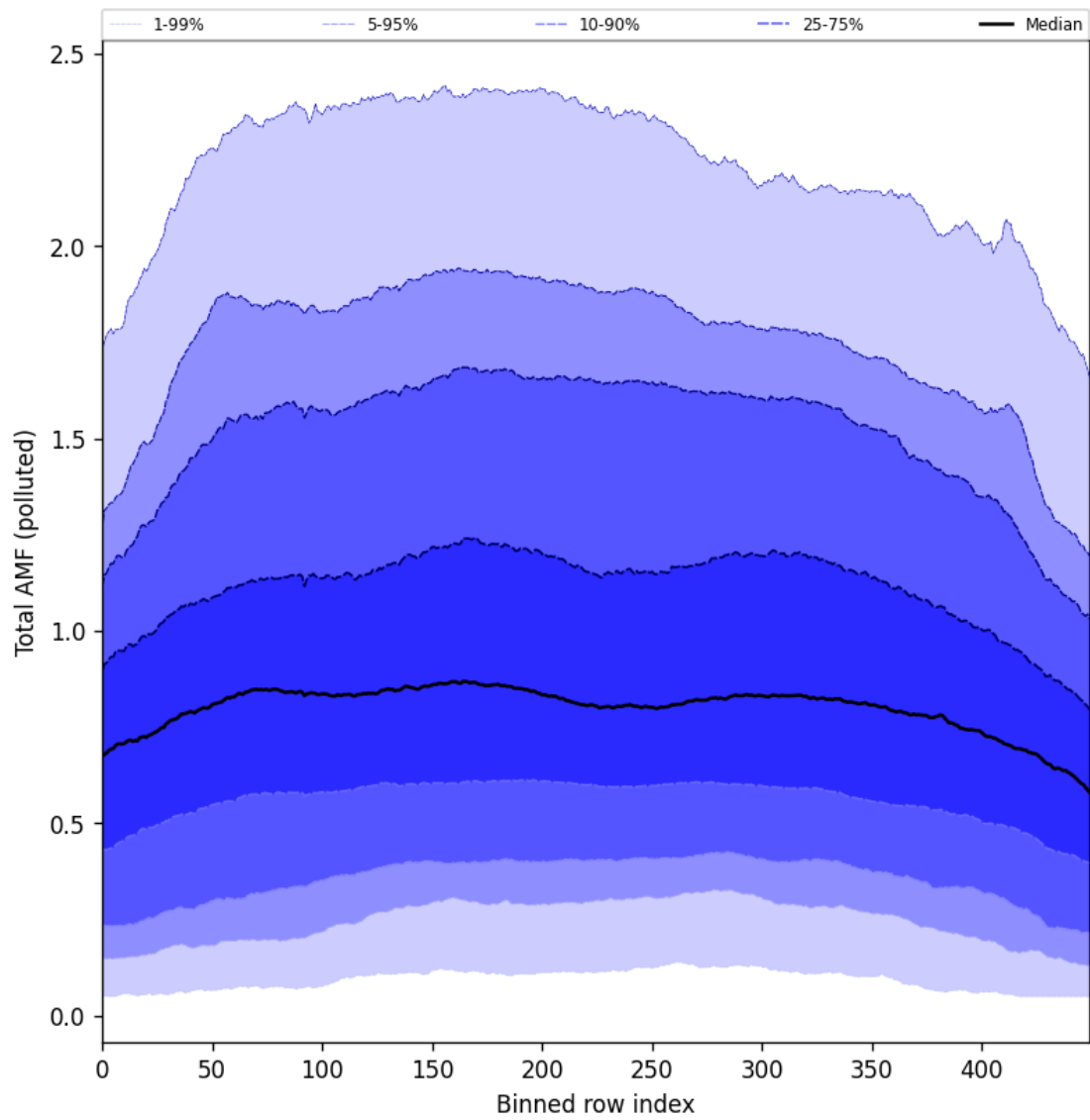
Figure 105: Along track statistics of “Total AMF (polluted)” for 2025-07-10 to 2025-07-12
