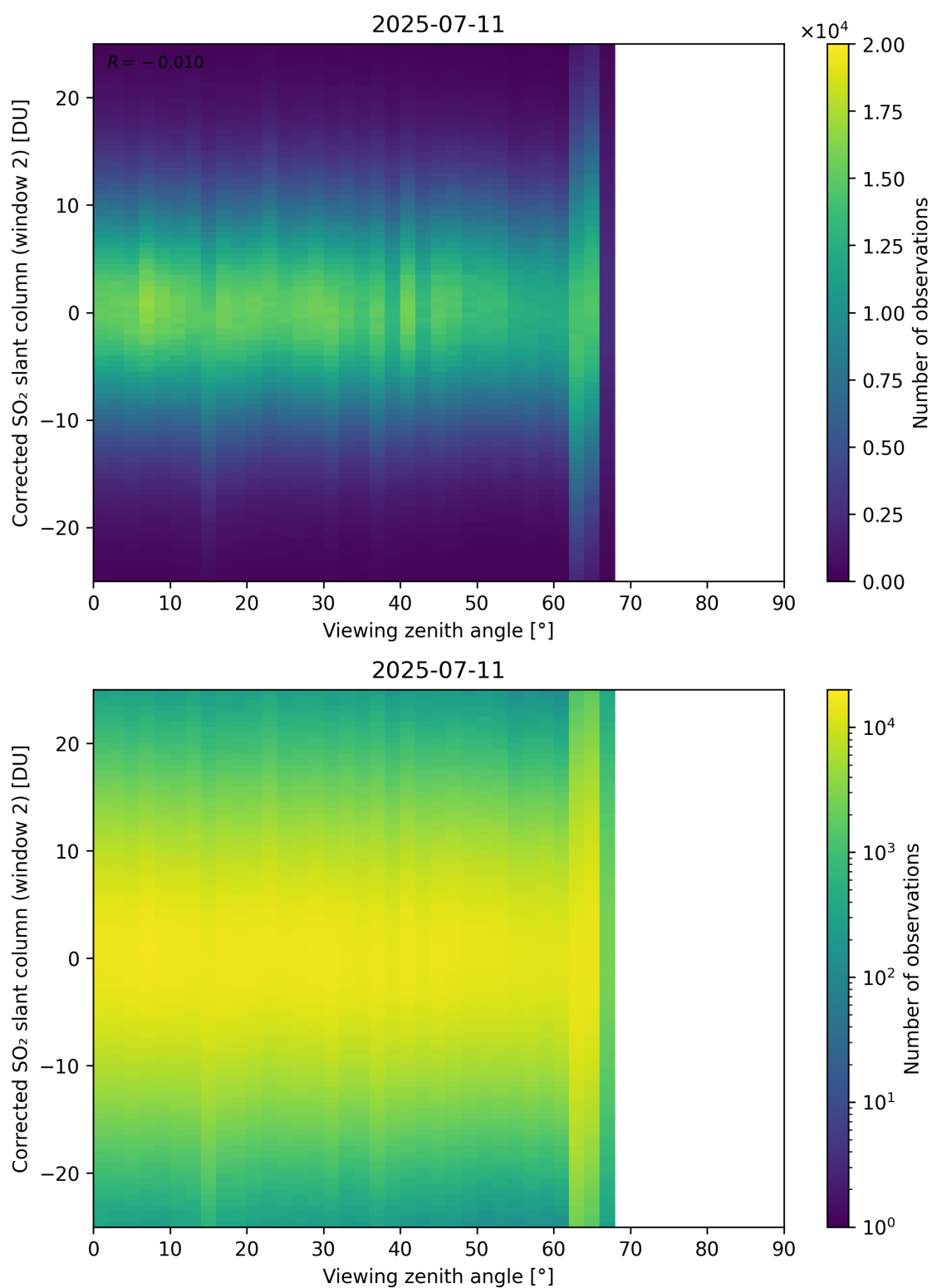
Figure 374: Scatter density plot of “Viewing zenith angle” against “Corrected SO 2 slant column (window 2)” for 2025-07-10 to 2025-07-12.
