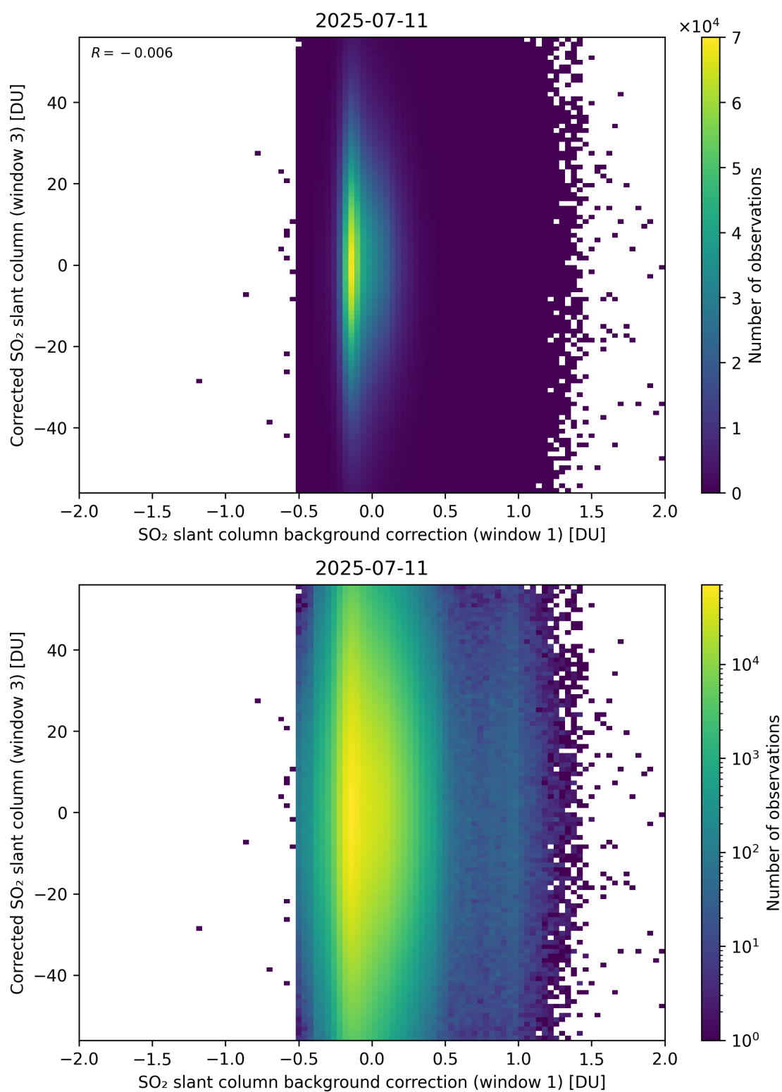
Figure 116: Scatter density plot of “SO 2 slant column background correction (window 1)” against “Corrected SO 2 slant column (window 3)” for 2025-07-10 to 2025-07-12.
