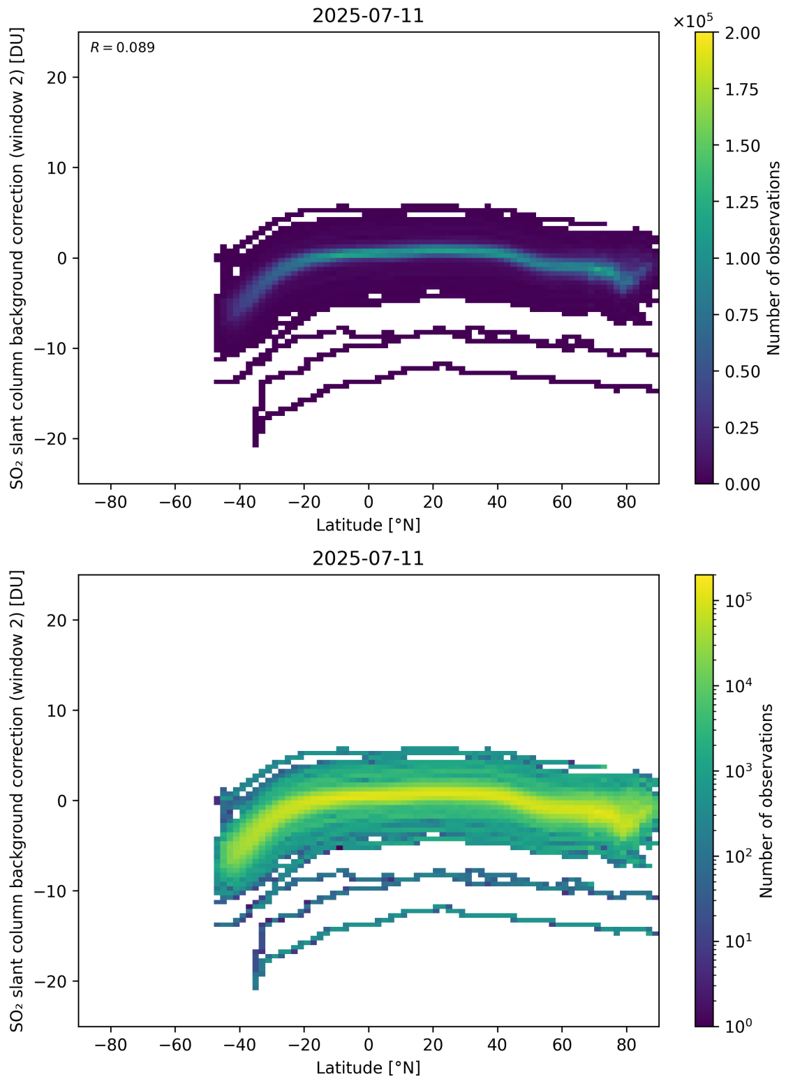
Figure 151: Scatter density plot of “Latitude” against “SO 2 slant column background correction (window 2)” for 2025-07-10 to 2025-07-12.
