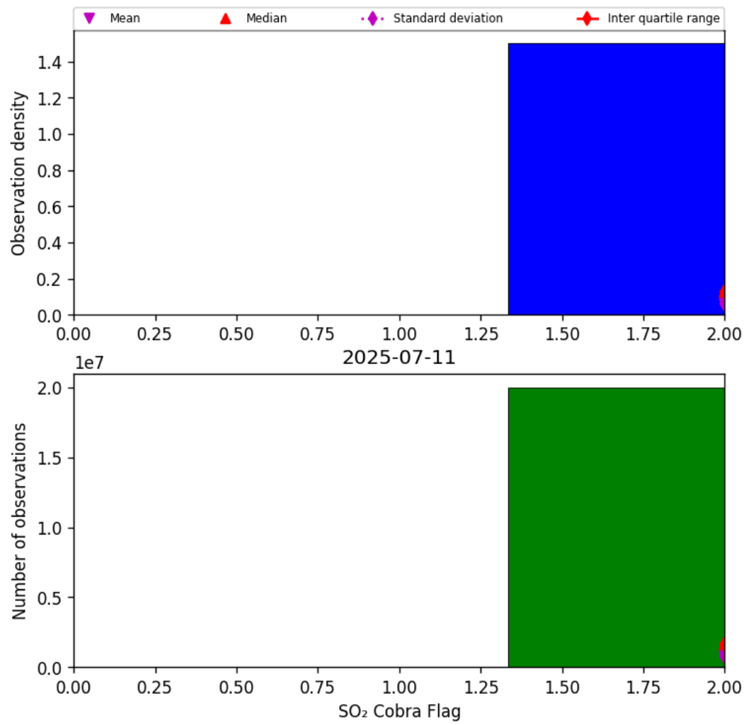
Figure 75: Histogram of “SO 2 Cobra Flag” for 2025-07-10 to 2025-07-12
