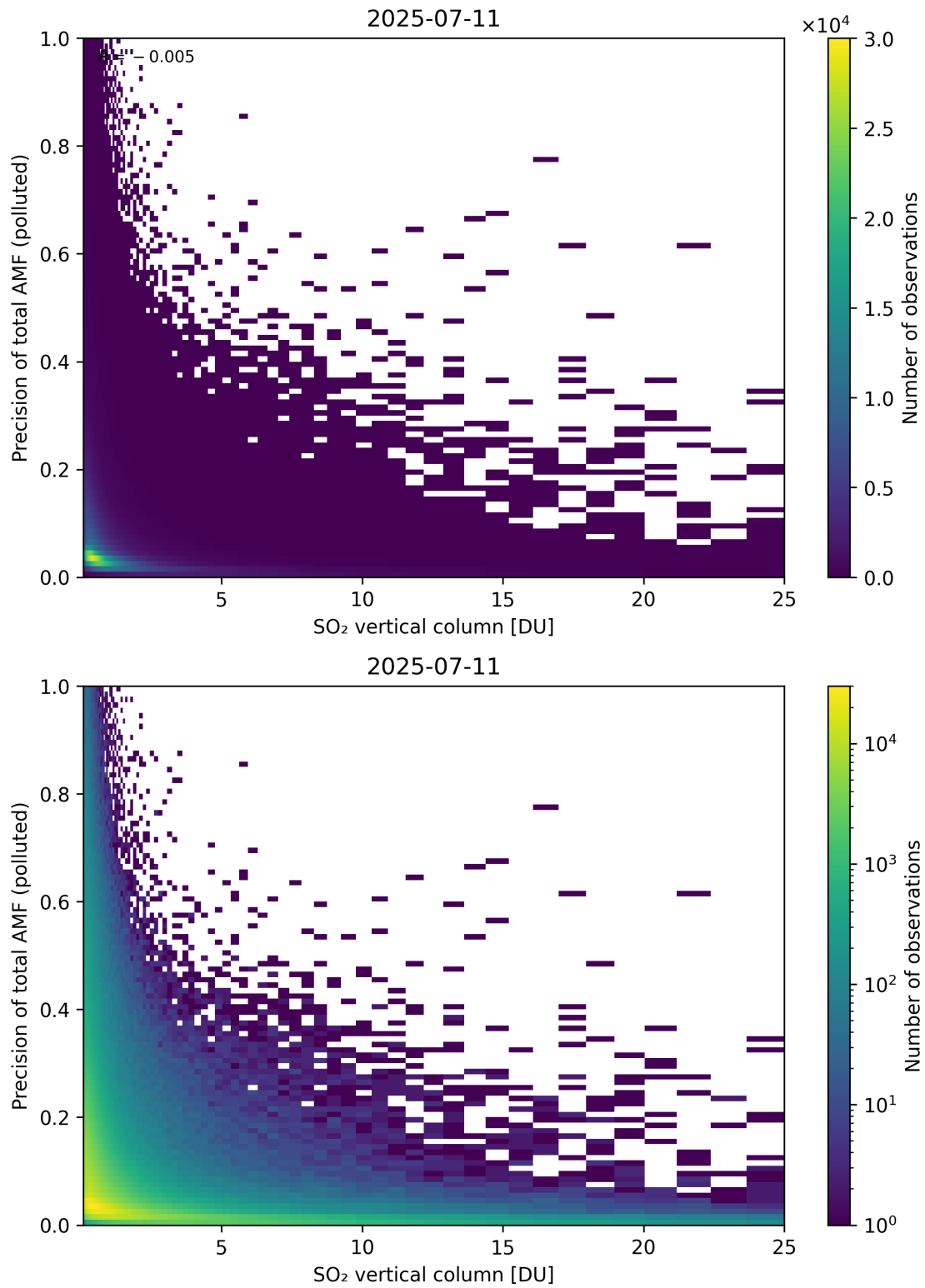
Figure 360: Scatter density plot of “SO 2 vertical column” against “Precision of total AMF (polluted)” for 2025-07-10 to 2025-07-12.
