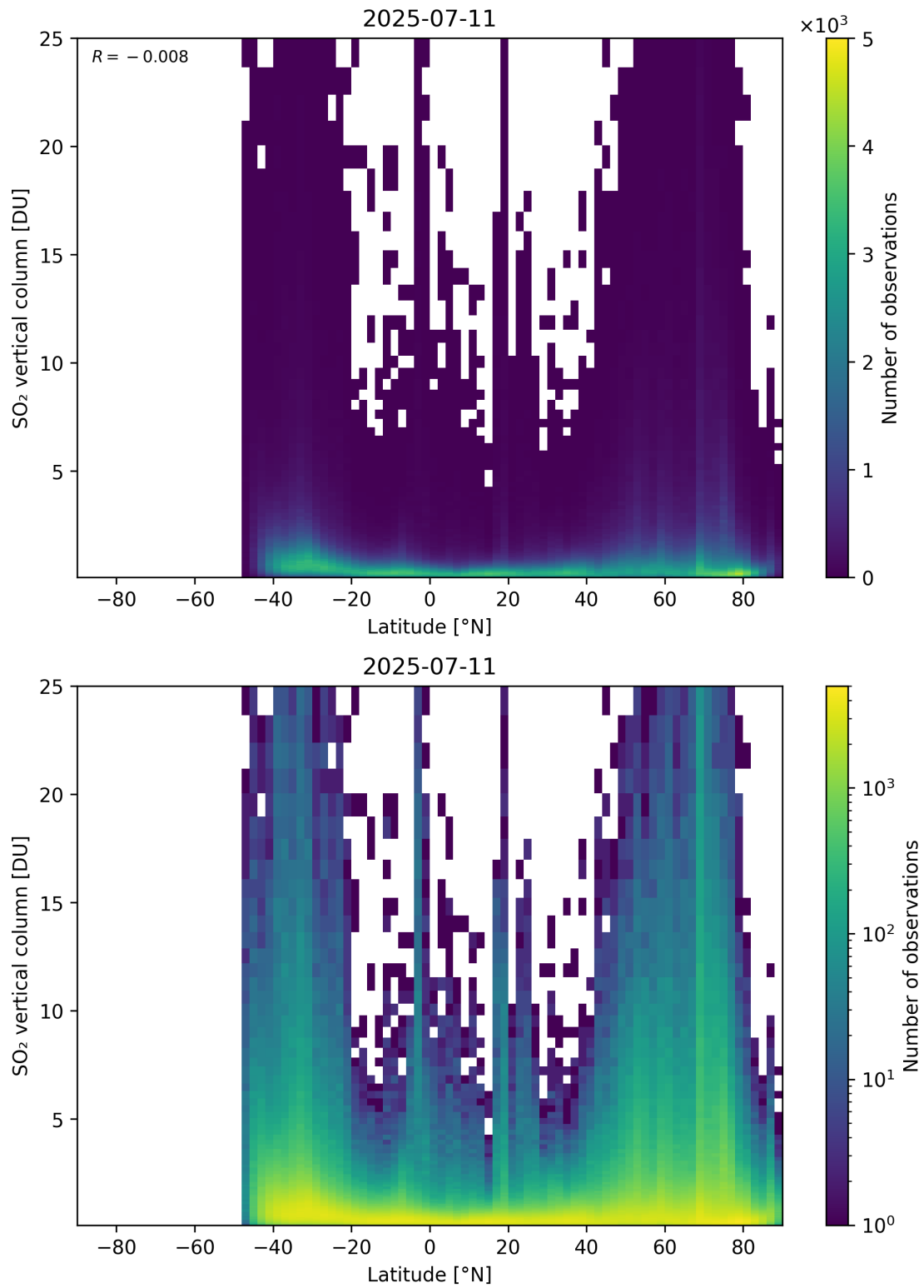
Figure 169: Scatter density plot of “Latitude” against “SO 2 vertical column” for 2025-07-10 to 2025-07-12.
