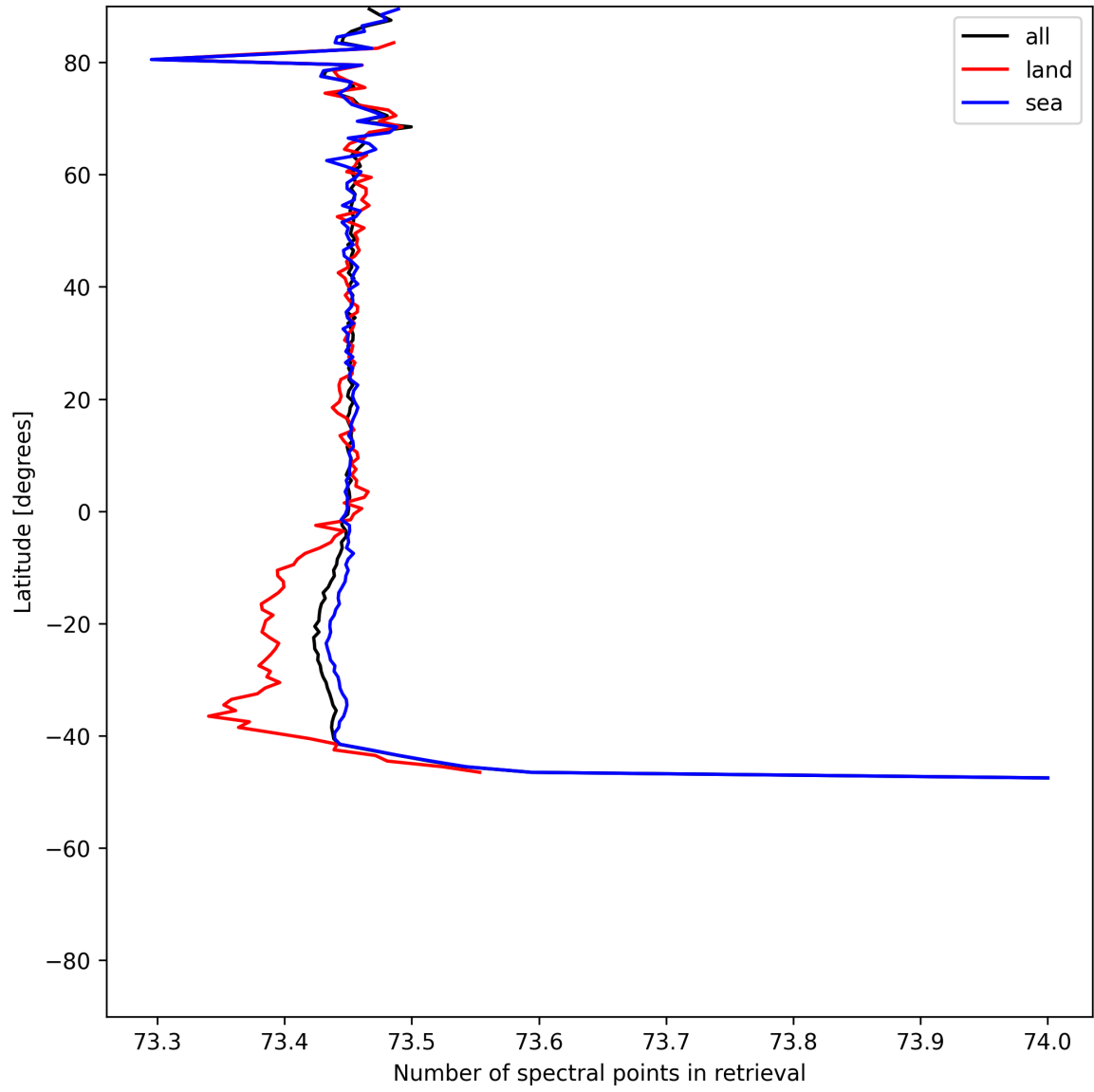
Figure 56: Zonal average of “Number of spectral points in retrieval” for 2025-07-10 to 2025-07-12.
