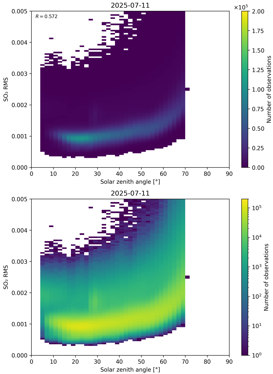
Figure 176: Scatter density plot of “Solar zenith angle” against “SO 2 RMS” for 2025-07-10 to 2025-07-12.
