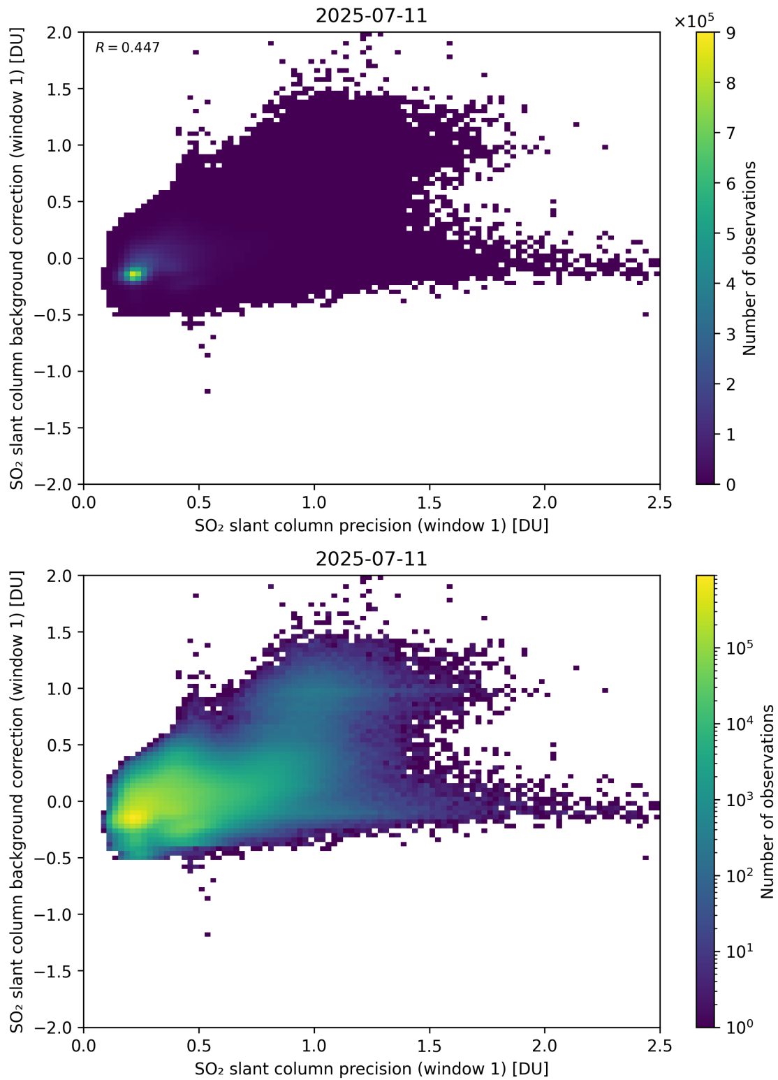
Figure 268: Scatter density plot of “SO 2 slant column precision (window 1)” against “SO 2 slant column background correction (window 1)” for 2025-07-10 to 2025-07-12.
