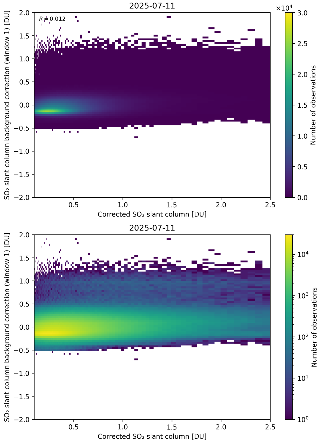
Figure 226: Scatter density plot of “Corrected SO 2 slant column” against “SO 2 slant column background correction (window 1)” for 2025-07-10 to 2025-07-12.
