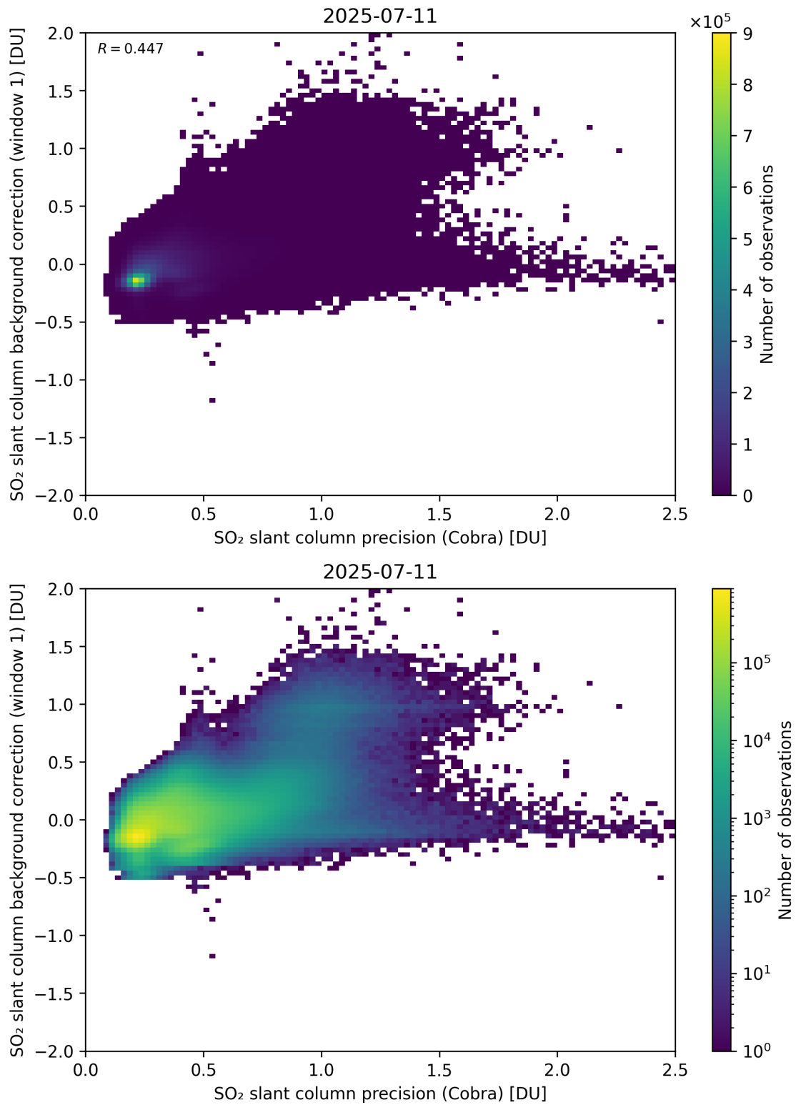
Figure 199: Scatter density plot of “SO 2 slant column precision (Cobra)” against “SO 2 slant column background correction (window 1)” for 2025-07-10 to 2025-07-12.
