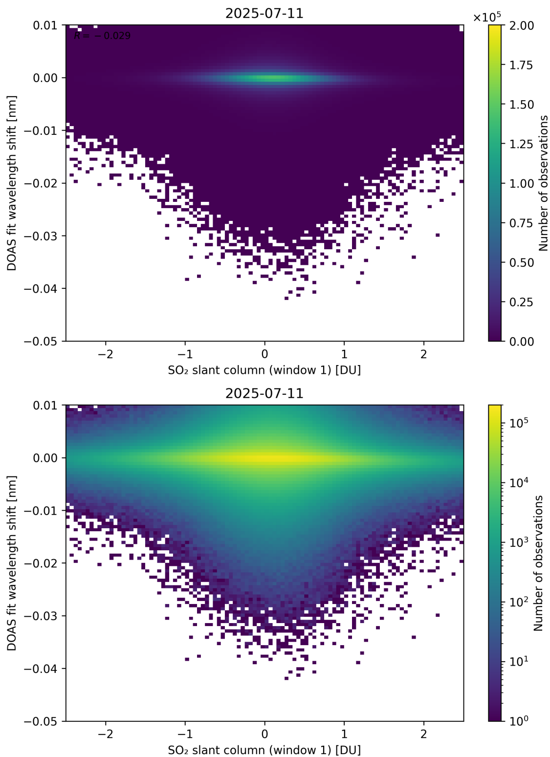
Figure 265: Scatter density plot of “SO 2 slant column (window 1)” against “DOAS fit wavelength shift” for 2025-07-10 to 2025-07-12.
