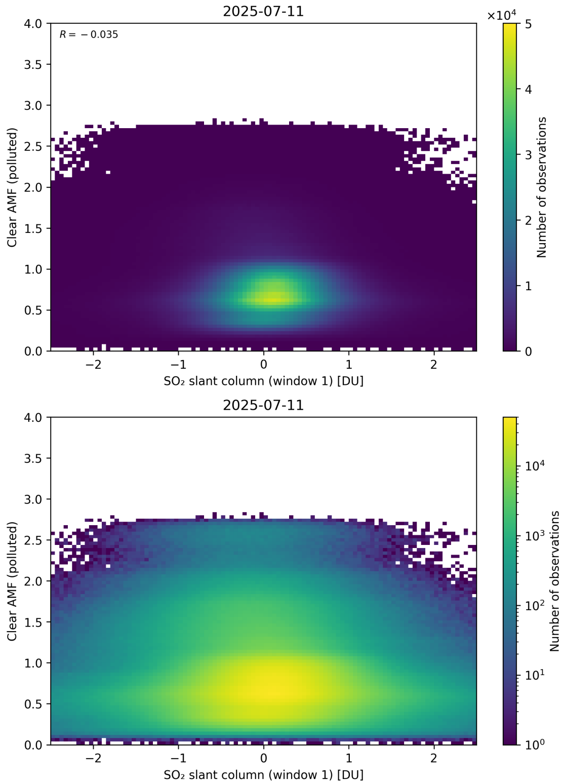
Figure 282: Scatter density plot of “SO 2 slant column (window 1)” against “Clear AMF (polluted)” for 2025-07-10 to 2025-07-12.
