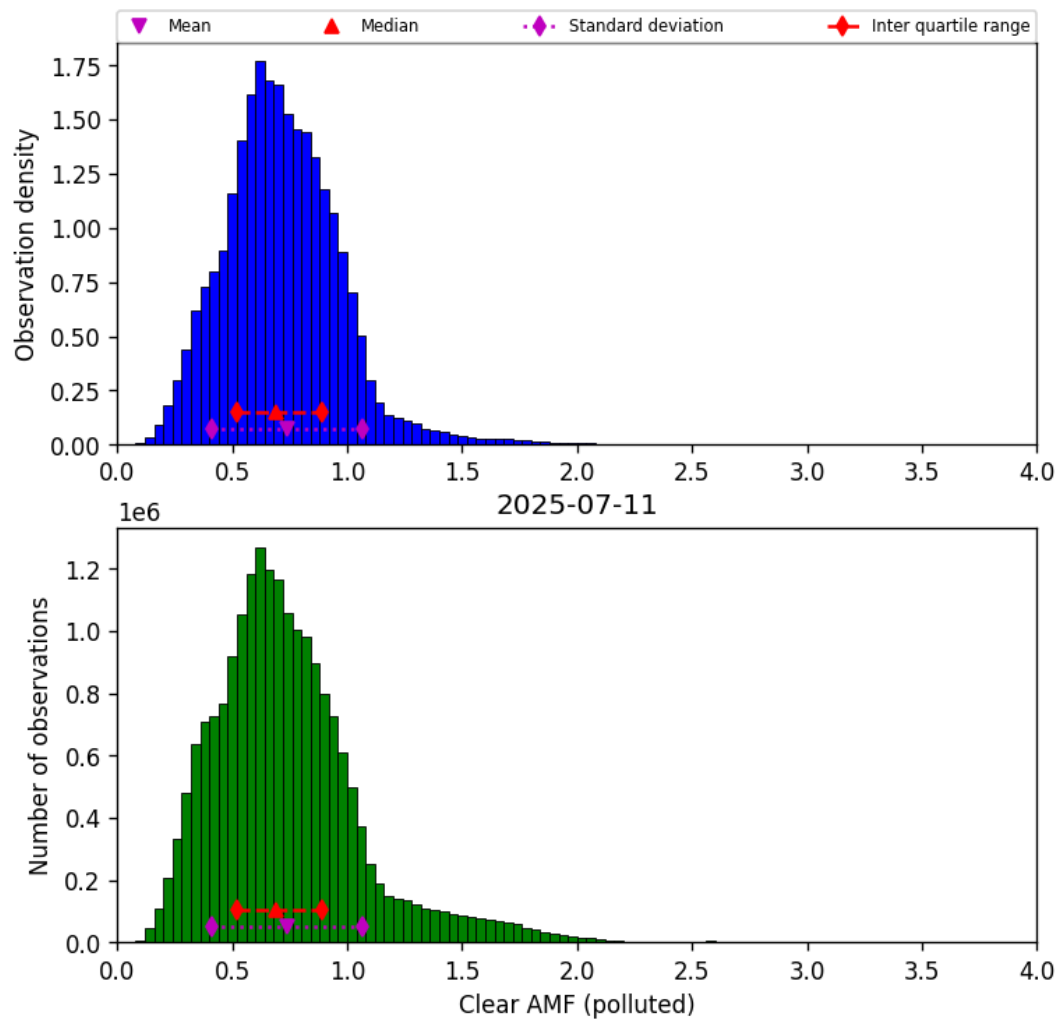
Figure 81: Histogram of “Clear AMF (polluted)” for 2025-07-10 to 2025-07-12
