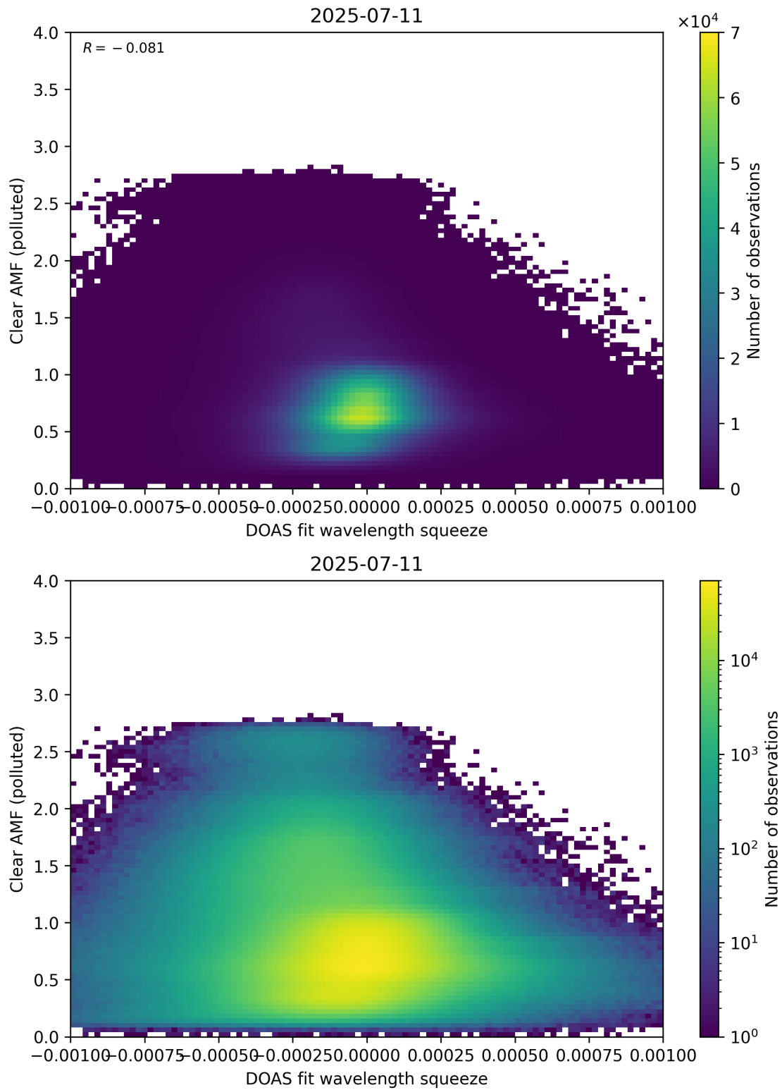
Figure 144: Scatter density plot of “DOAS fit wavelength squeeze” against “Clear AMF (polluted)” for 2025-07-10 to 2025-07-12.
