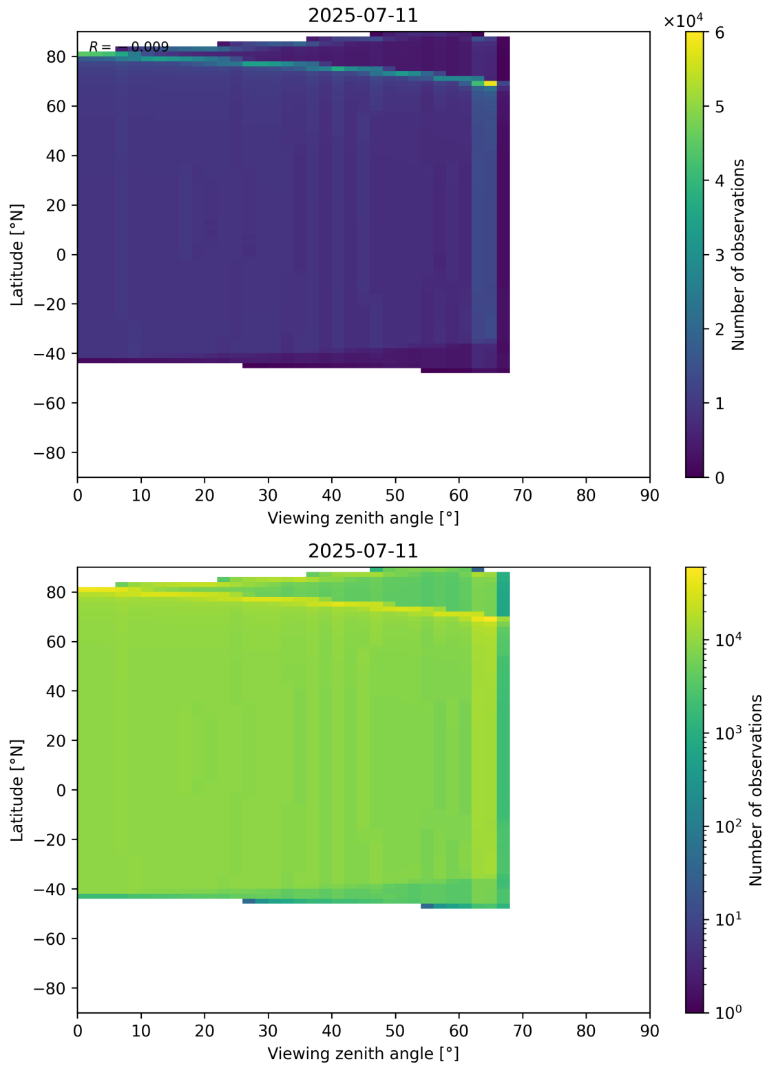
Figure 368: Scatter density plot of “Viewing zenith angle” against “Latitude” for 2025-07-10 to 2025-07-12.
