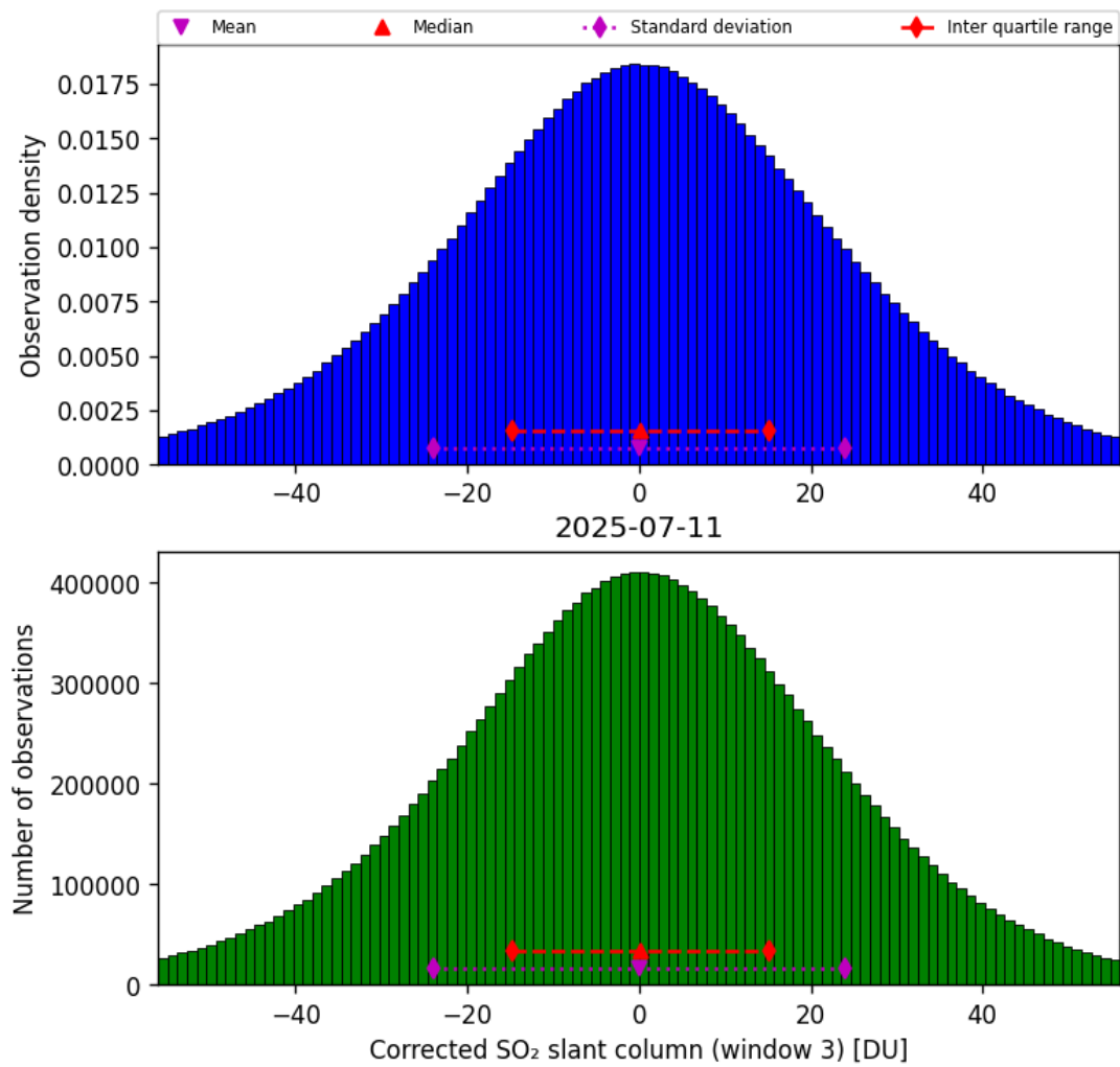
Figure 73: Histogram of “Corrected SO 2 slant column (window 3)” for 2025-07-10 to 2025-07-12
