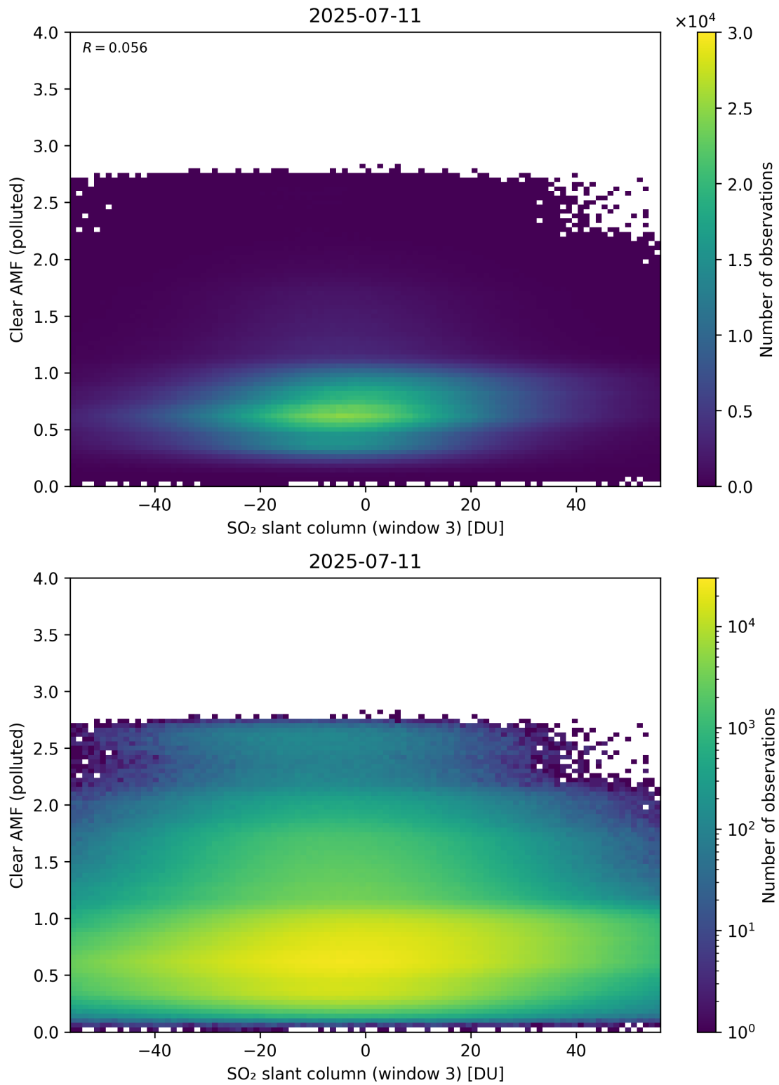
Figure 315: Scatter density plot of “SO 2 slant column (window 3)” against “Clear AMF (polluted)” for 2025-07-10 to 2025-07-12.
