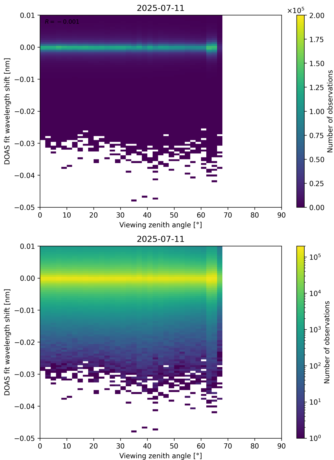
Figure 365: Scatter density plot of “Viewing zenith angle” against “DOAS fit wavelength shift” for 2025-07-10 to 2025-07-12.
