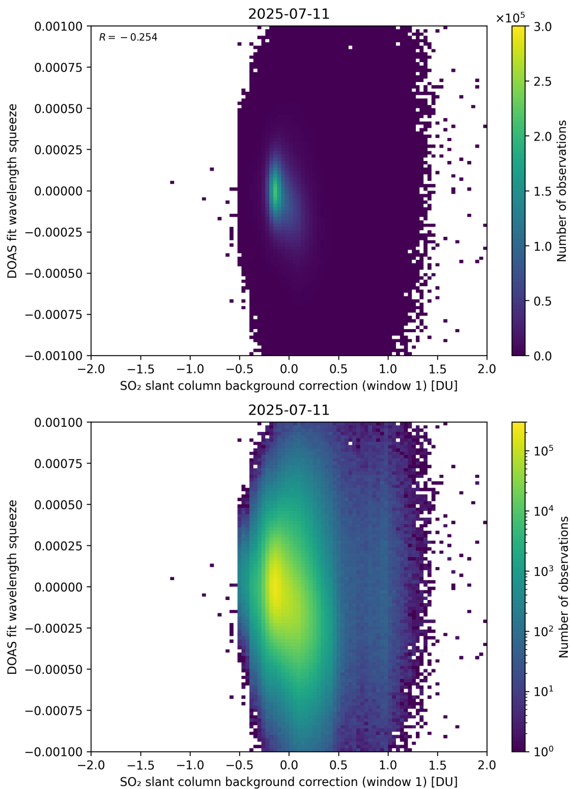
Figure 112: Scatter density plot of “SO 2 slant column background correction (window 1)” against “DOAS fit wavelength squeeze” for 2025-07-10 to 2025-07-12.
