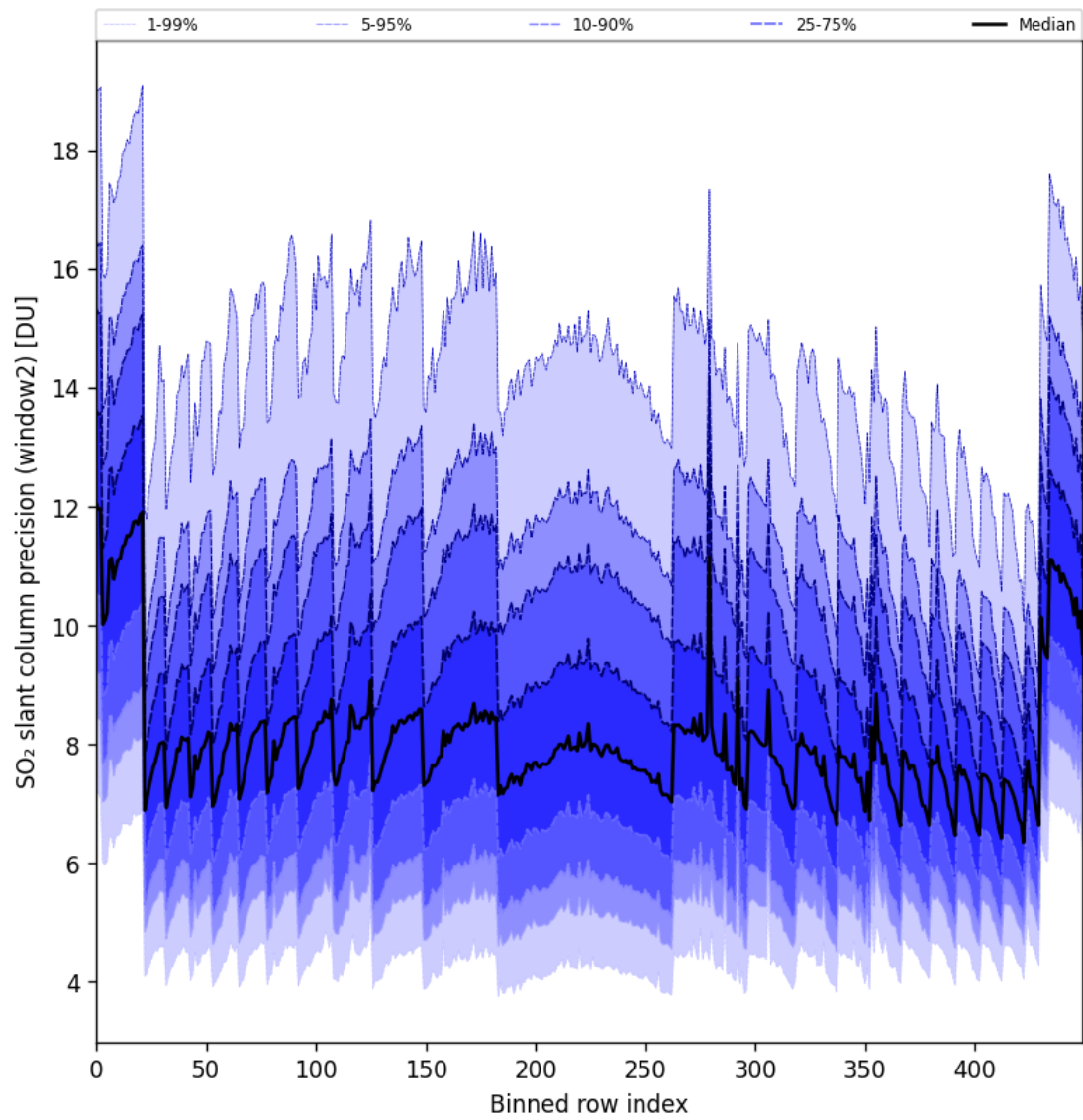
Figure 94: Along track statistics of “SO 2 slant column precision (window2)” for 2025-07-10 to 2025-07-12
