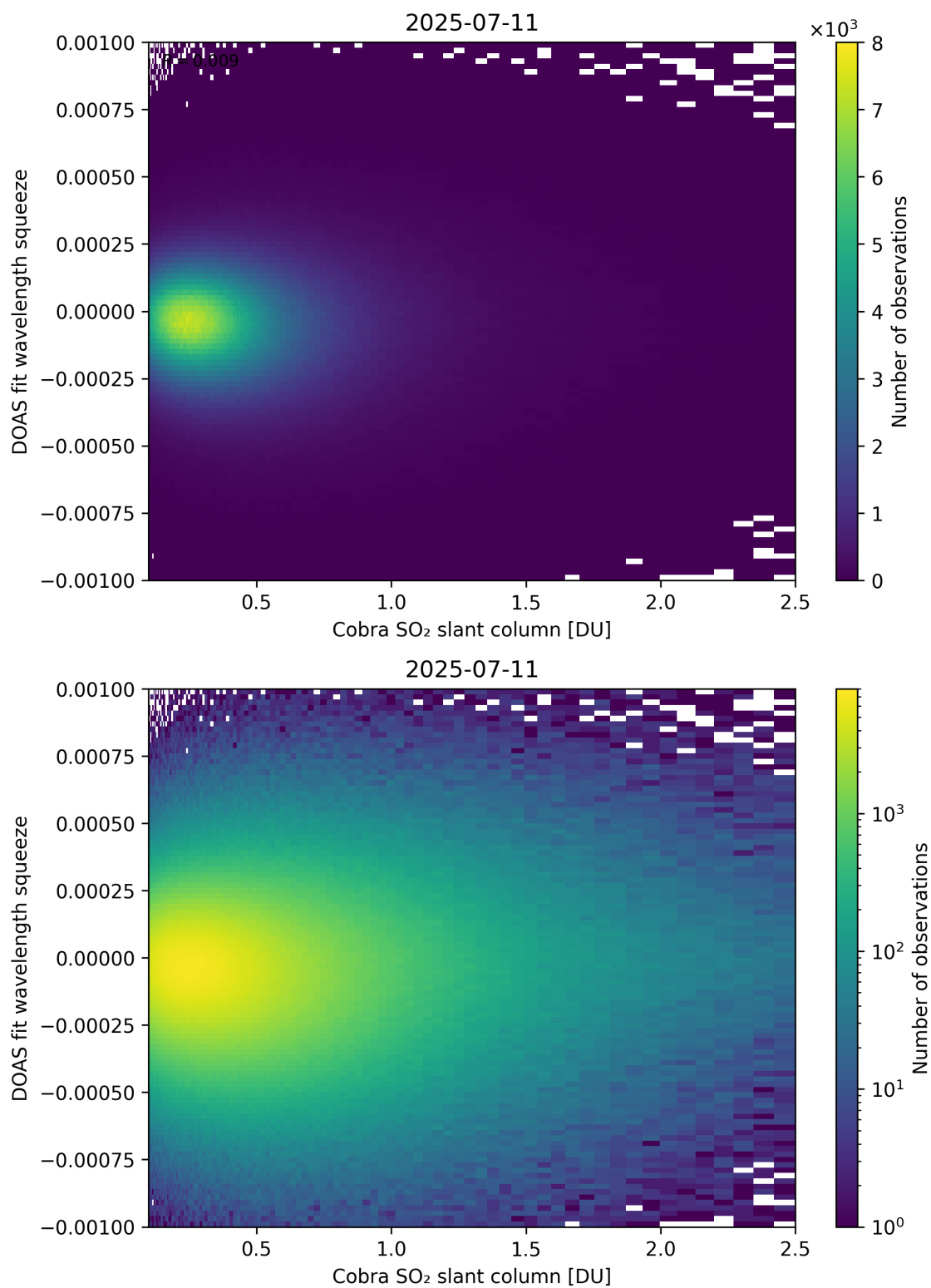
Figure 197: Scatter density plot of “Cobra SO 2 slant column” against “DOAS fit wavelength squeeze” for 2025-07-10 to 2025-07-12.
