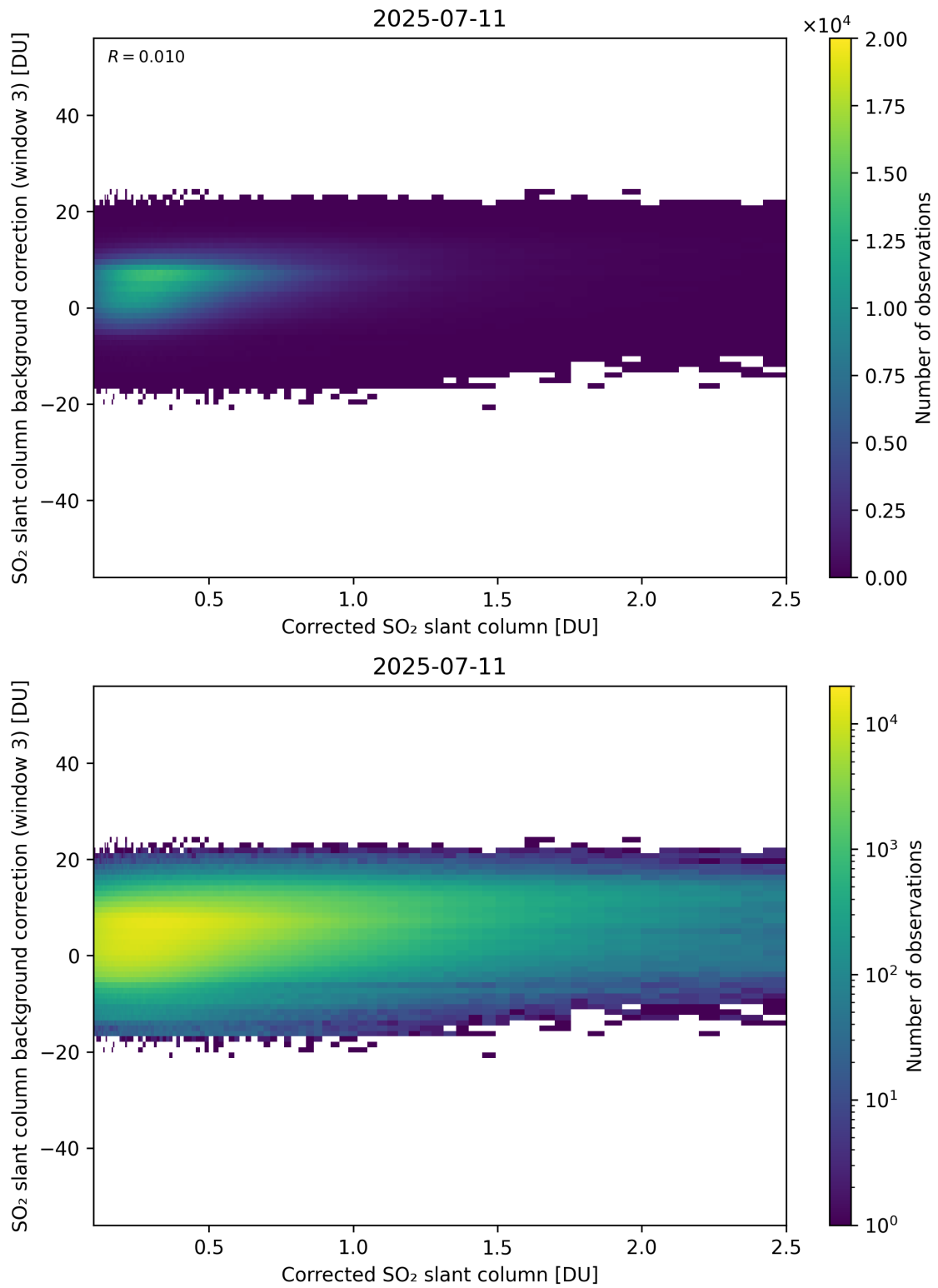
Figure 228: Scatter density plot of “Corrected SO 2 slant column” against “SO 2 slant column background correction (window 3)” for 2025-07-10 to 2025-07-12.
