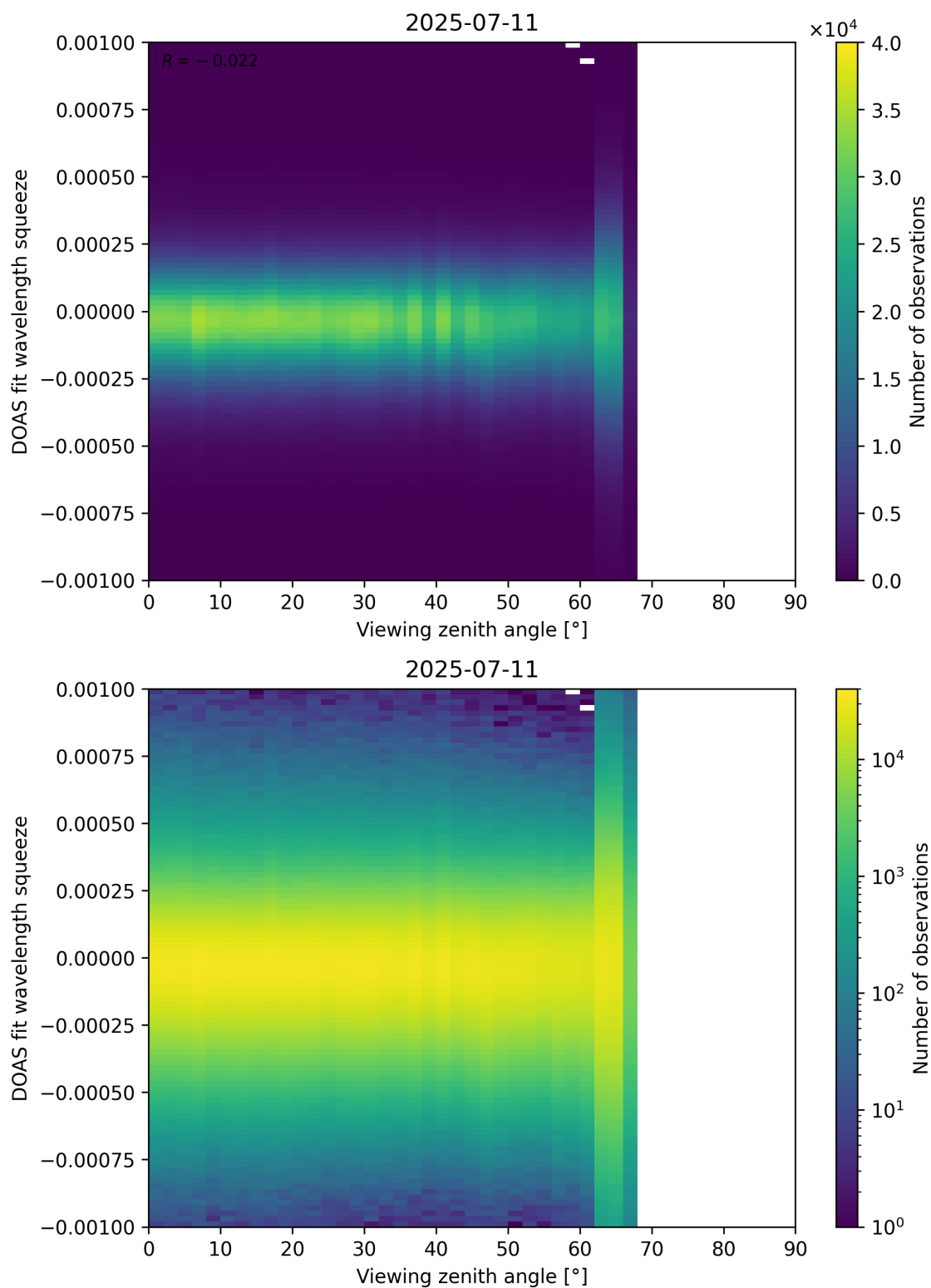
Figure 366: Scatter density plot of “Viewing zenith angle” against “DOAS fit wavelength squeeze” for 2025-07-10 to 2025-07-12.
