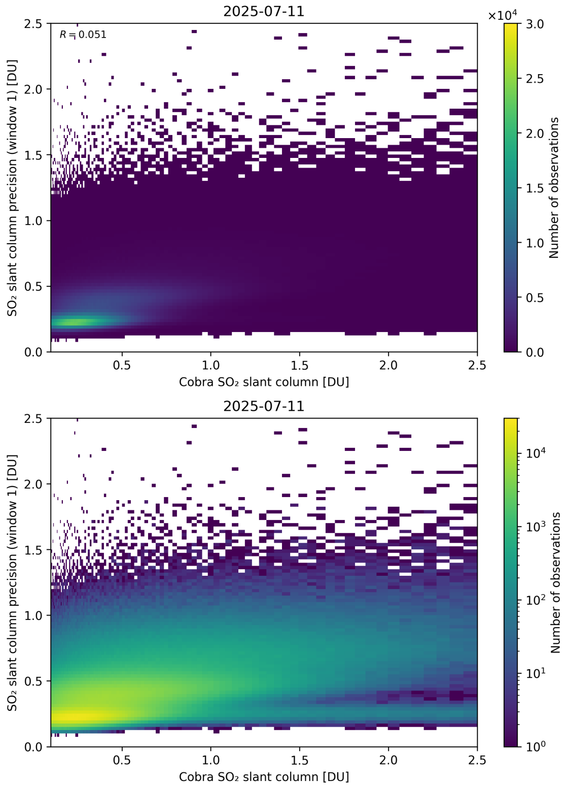
Figure 220: Scatter density plot of “Cobra SO 2 slant column” against “SO 2 slant column precision (window 1)” for 2025-07-10 to 2025-07-12.
