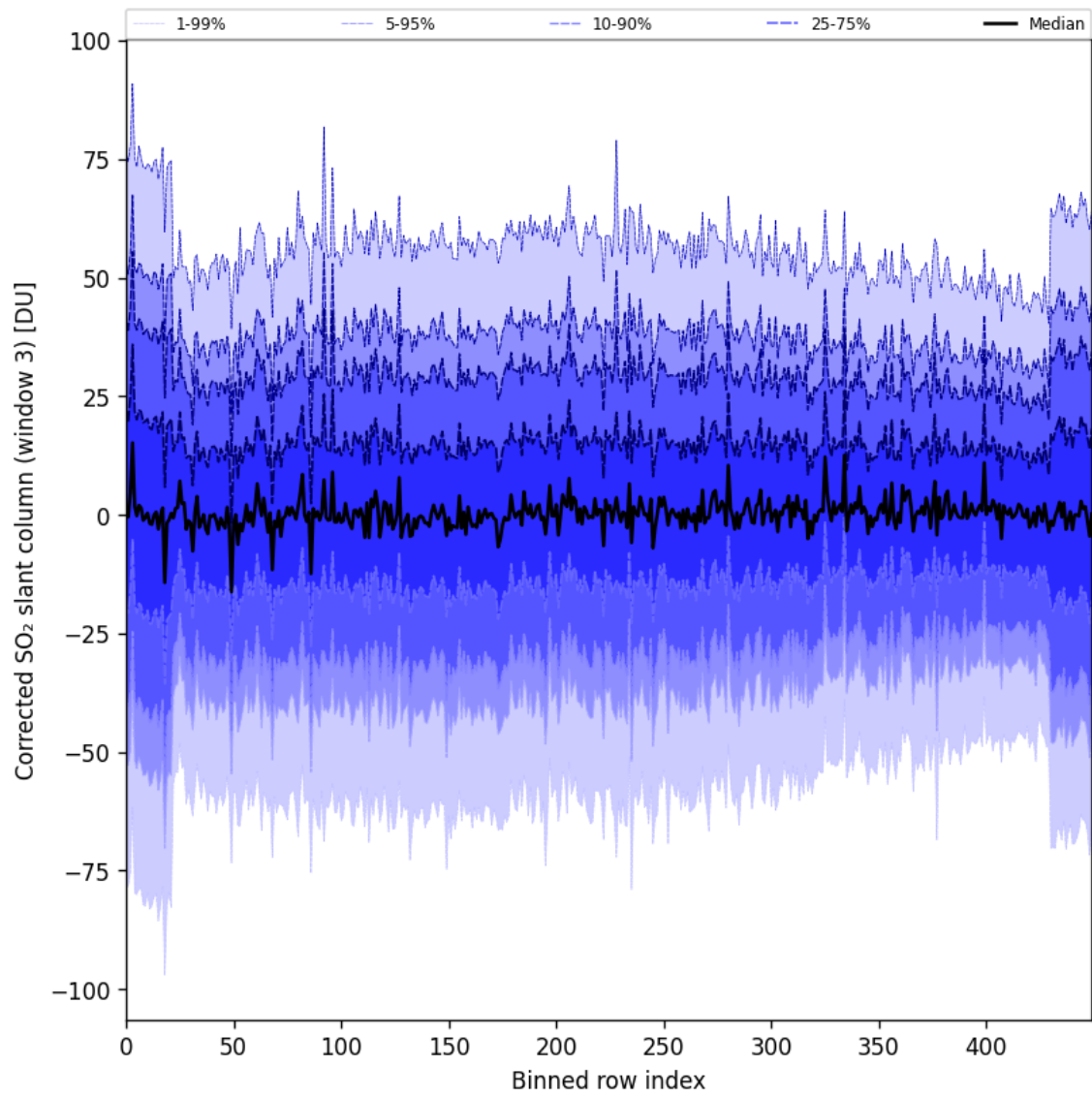
Figure 99: Along track statistics of “Corrected SO 2 slant column (window 3)” for 2025-07-10 to 2025-07-12
