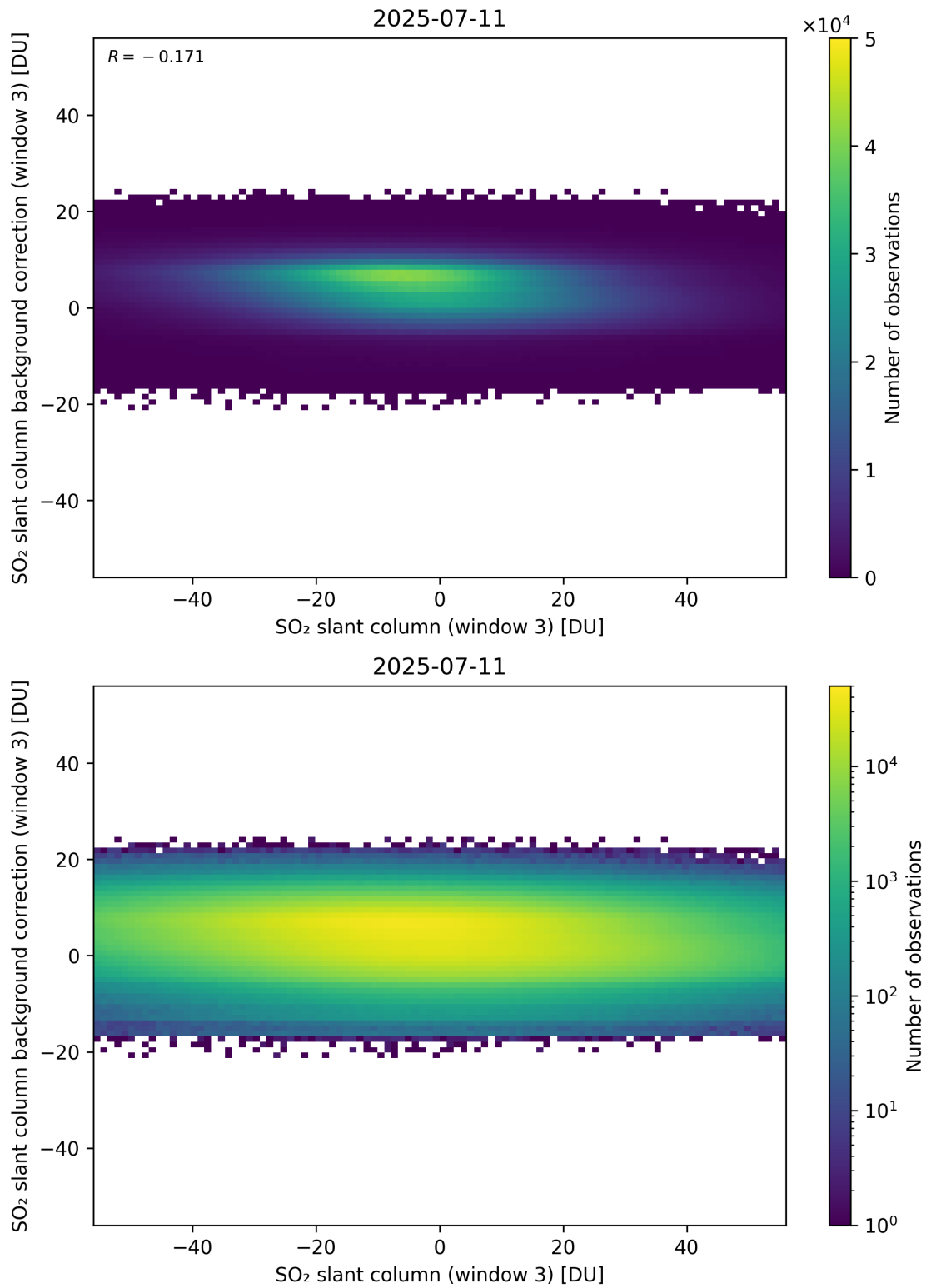
Figure 303: Scatter density plot of “SO 2 slant column (window 3)” against “SO 2 slant column background correction (window 3)” for 2025-07-10 to 2025-07-12.
