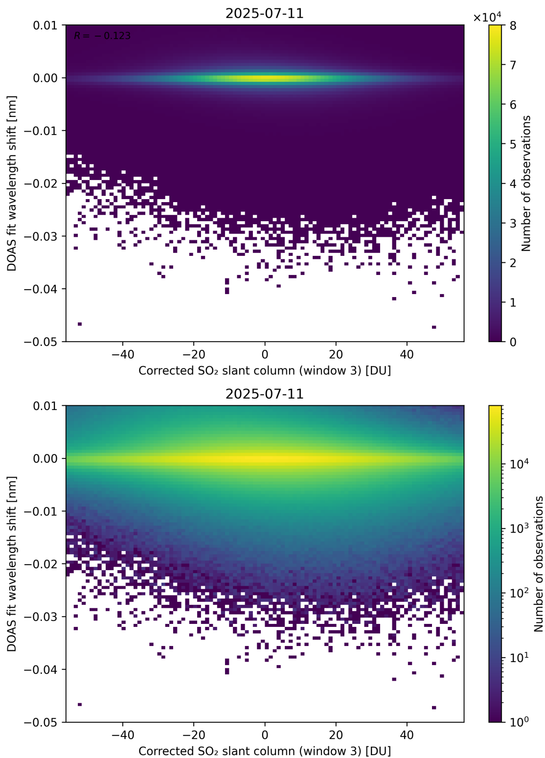
Figure 256: Scatter density plot of “Corrected SO 2 slant column (window 3)” against “DOAS fit wavelength shift” for 2025-07-10 to 2025-07-12.
