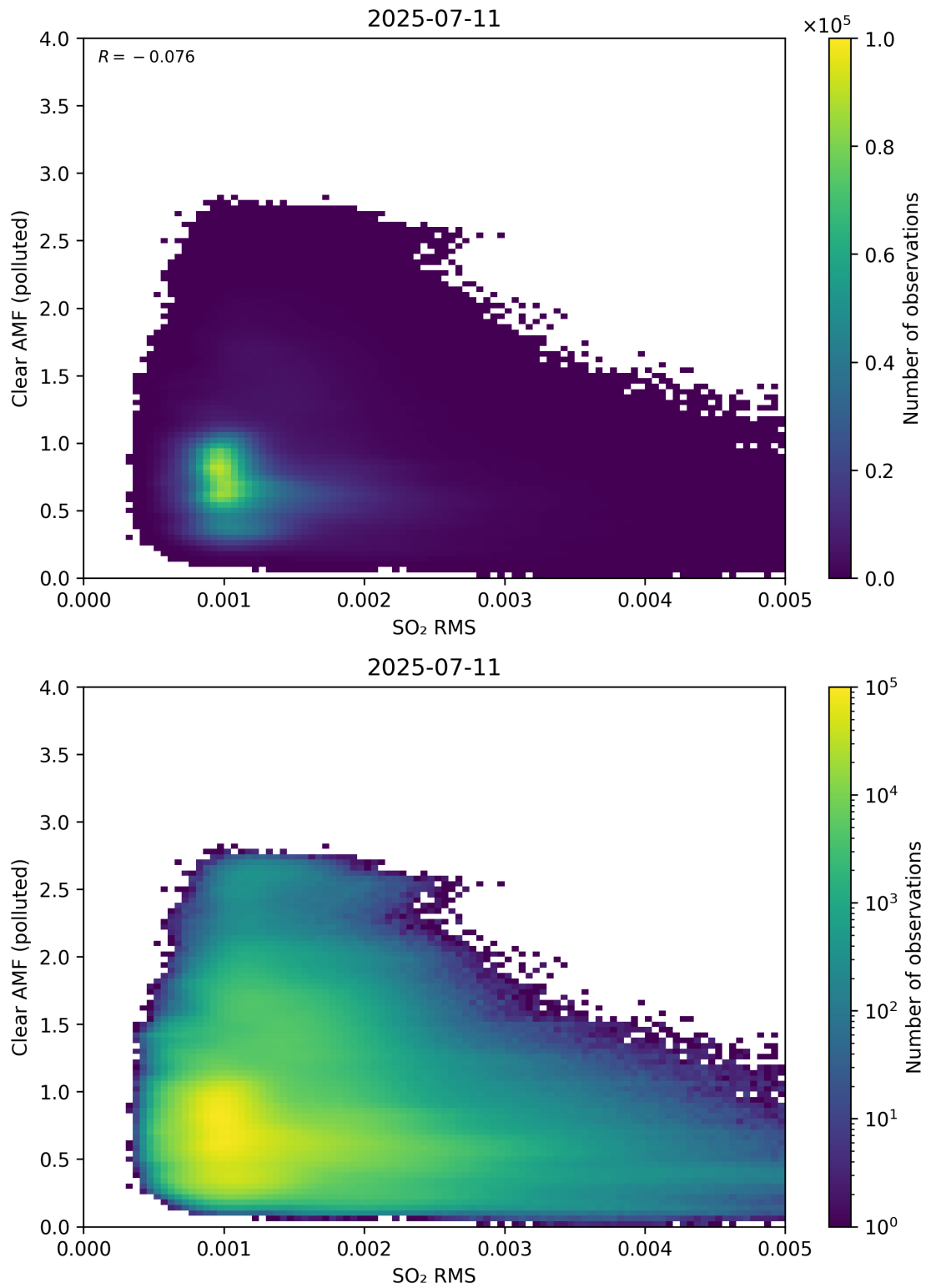
Figure 147: Scatter density plot of “SO 2 RMS” against “Clear AMF (polluted)” for 2025-07-10 to 2025-07-12.
