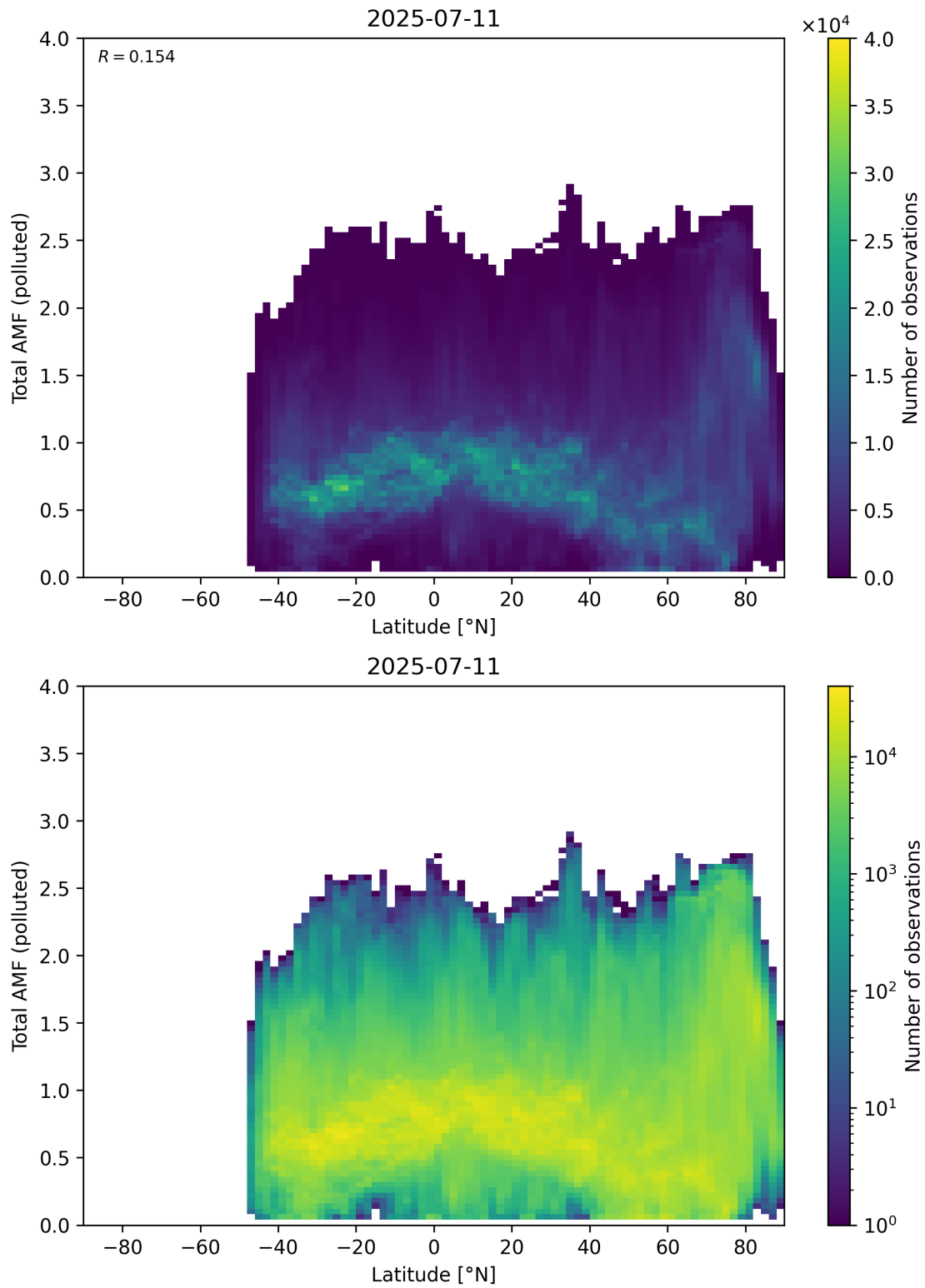
Figure 167: Scatter density plot of “Latitude” against “Total AMF (polluted)” for 2025-07-10 to 2025-07-12.
