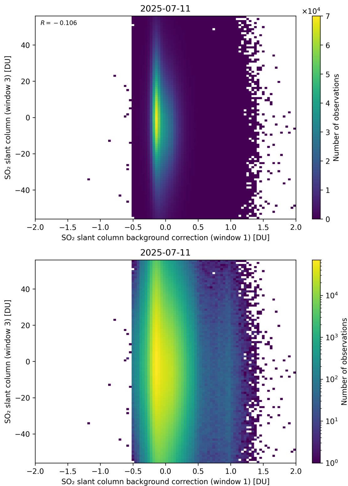
Figure 118: Scatter density plot of “SO 2 slant column background correction (window 1)” against “SO 2 slant column (window 3)” for 2025-07-10 to 2025-07-12.
