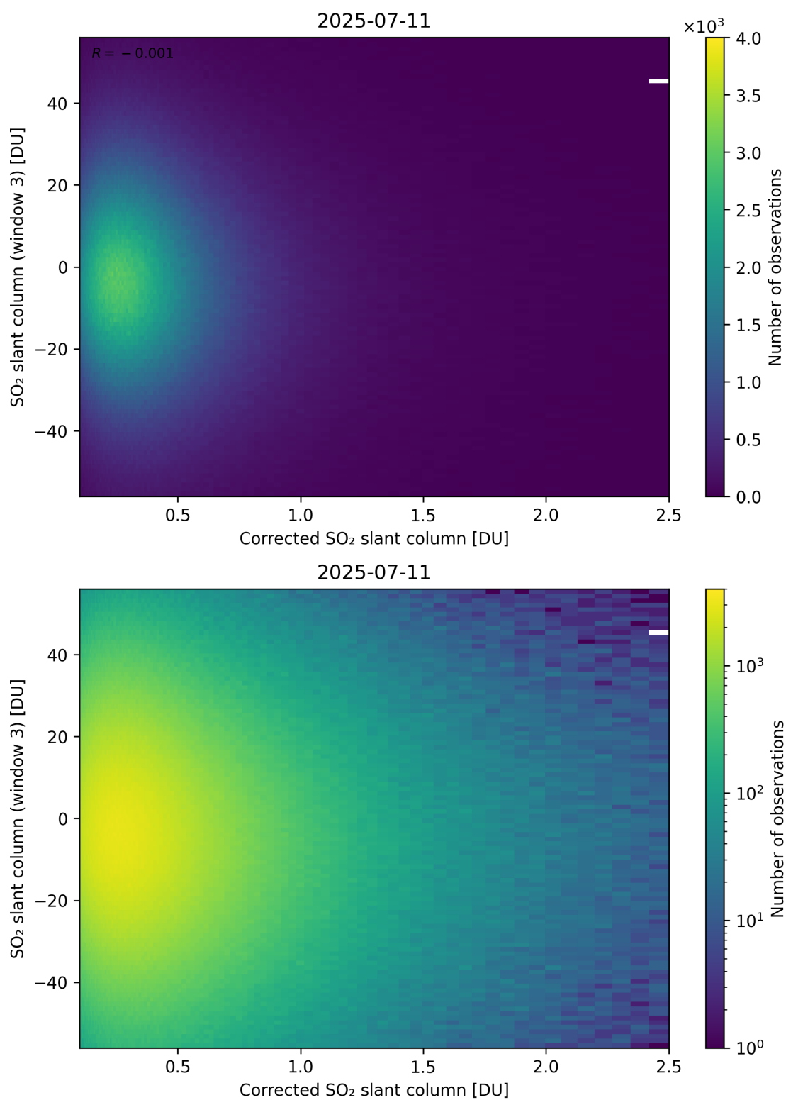
Figure 240: Scatter density plot of “Corrected SO 2 slant column” against “SO 2 slant column (window 3)” for 2025-07-10 to 2025-07-12.
