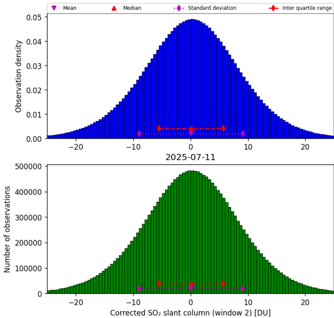
Figure 69: Histogram of “Corrected SO 2 slant column (window 2)” for 2025-07-10 to 2025-07-12
