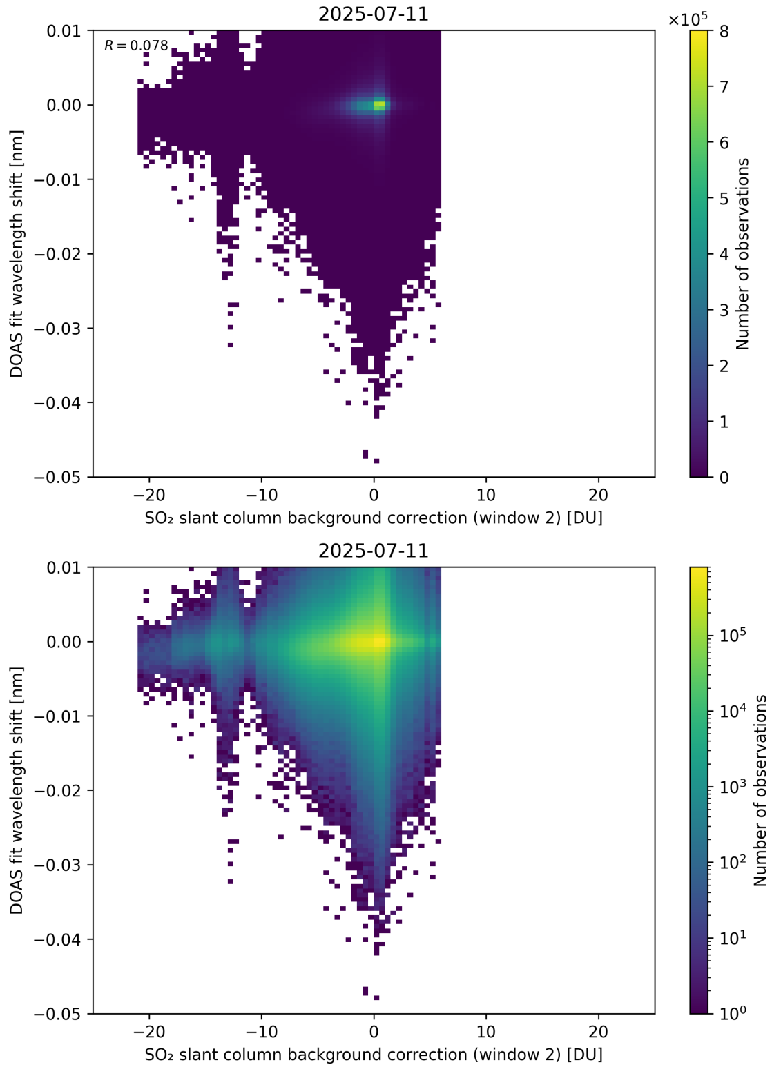
Figure 123: Scatter density plot of “SO 2 slant column background correction (window 2)” against “DOAS fit wavelength shift” for 2025-07-10 to 2025-07-12.
