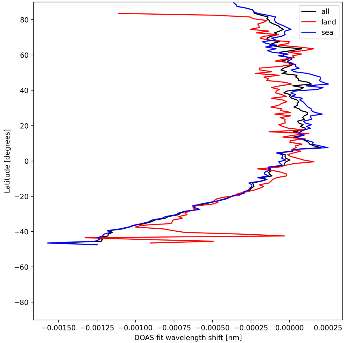
Figure 50: Zonal average of “DOAS fit wavelength shift” for 2025-07-10 to 2025-07-12.
