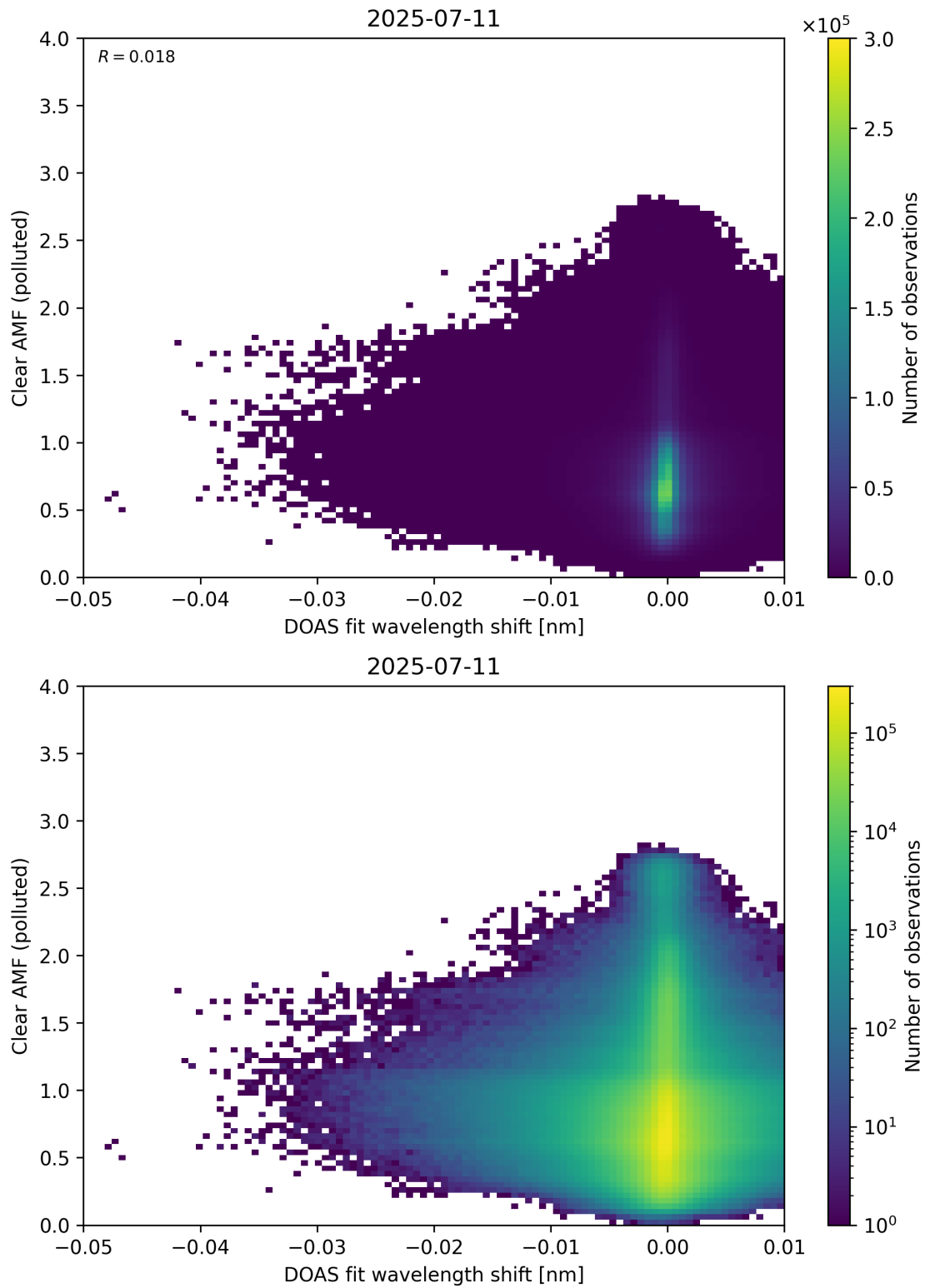
Figure 140: Scatter density plot of “DOAS fit wavelength shift” against “Clear AMF (polluted)” for 2025-07-10 to 2025-07-12.
