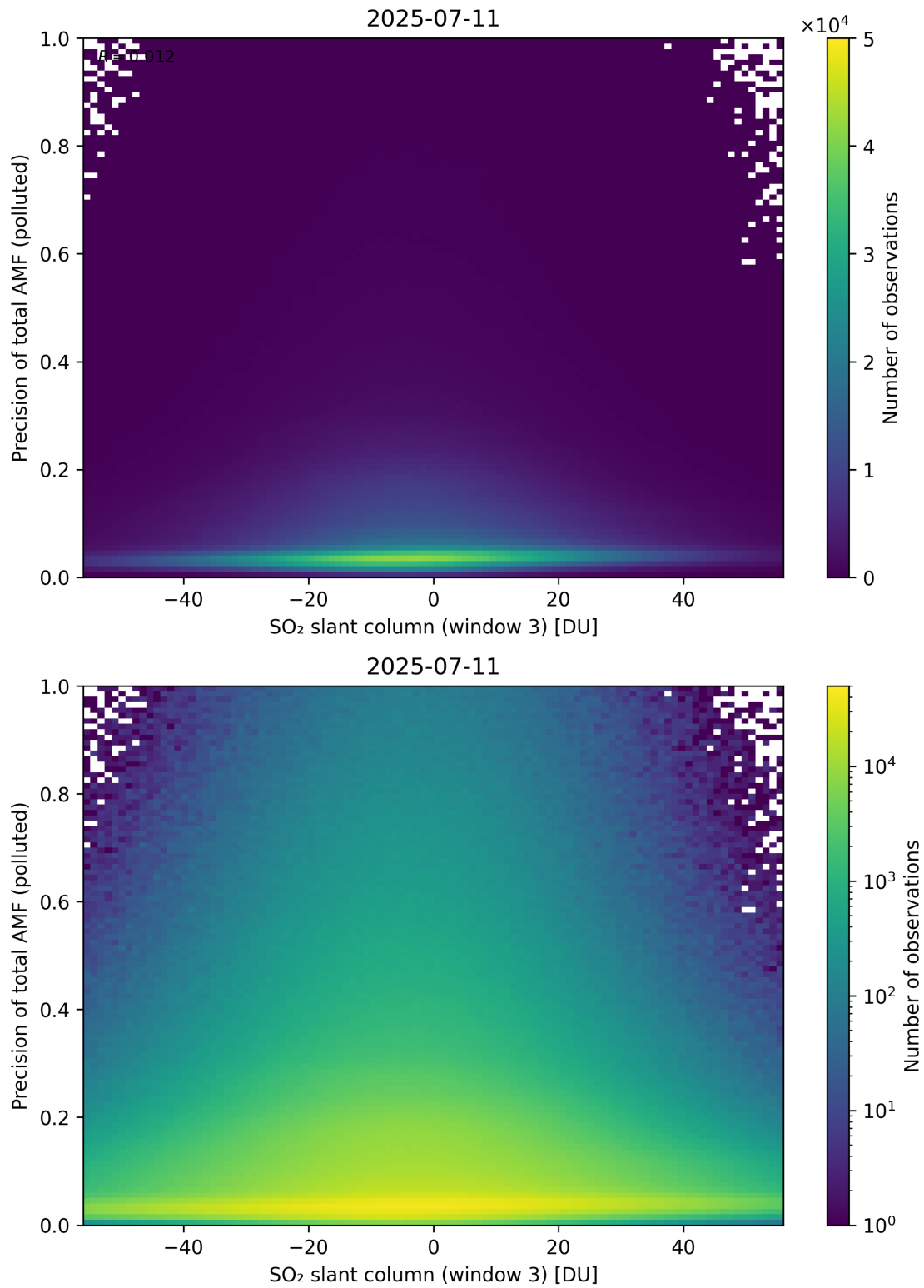
Figure 319: Scatter density plot of “SO 2 slant column (window 3)” against “Precision of total AMF (polluted)” for 2025-07-10 to 2025-07-12.
