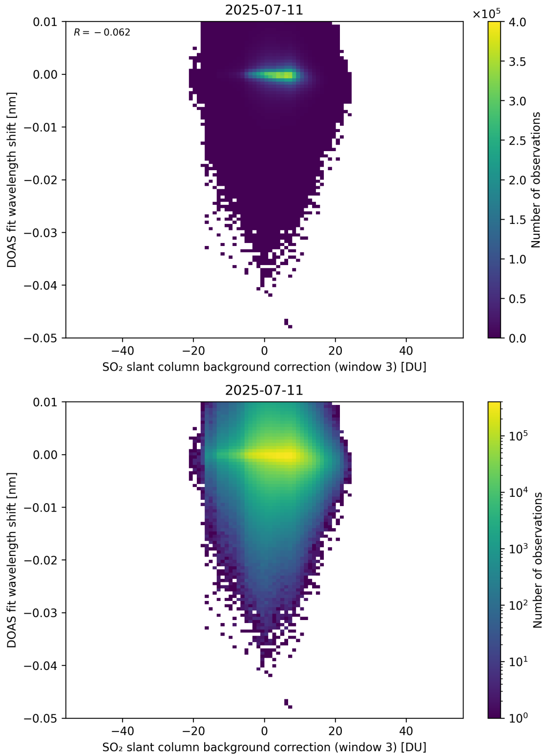
Figure 132: Scatter density plot of “SO 2 slant column background correction (window 3)” against “DOAS fit wavelength shift” for 2025-07-10 to 2025-07-12.
