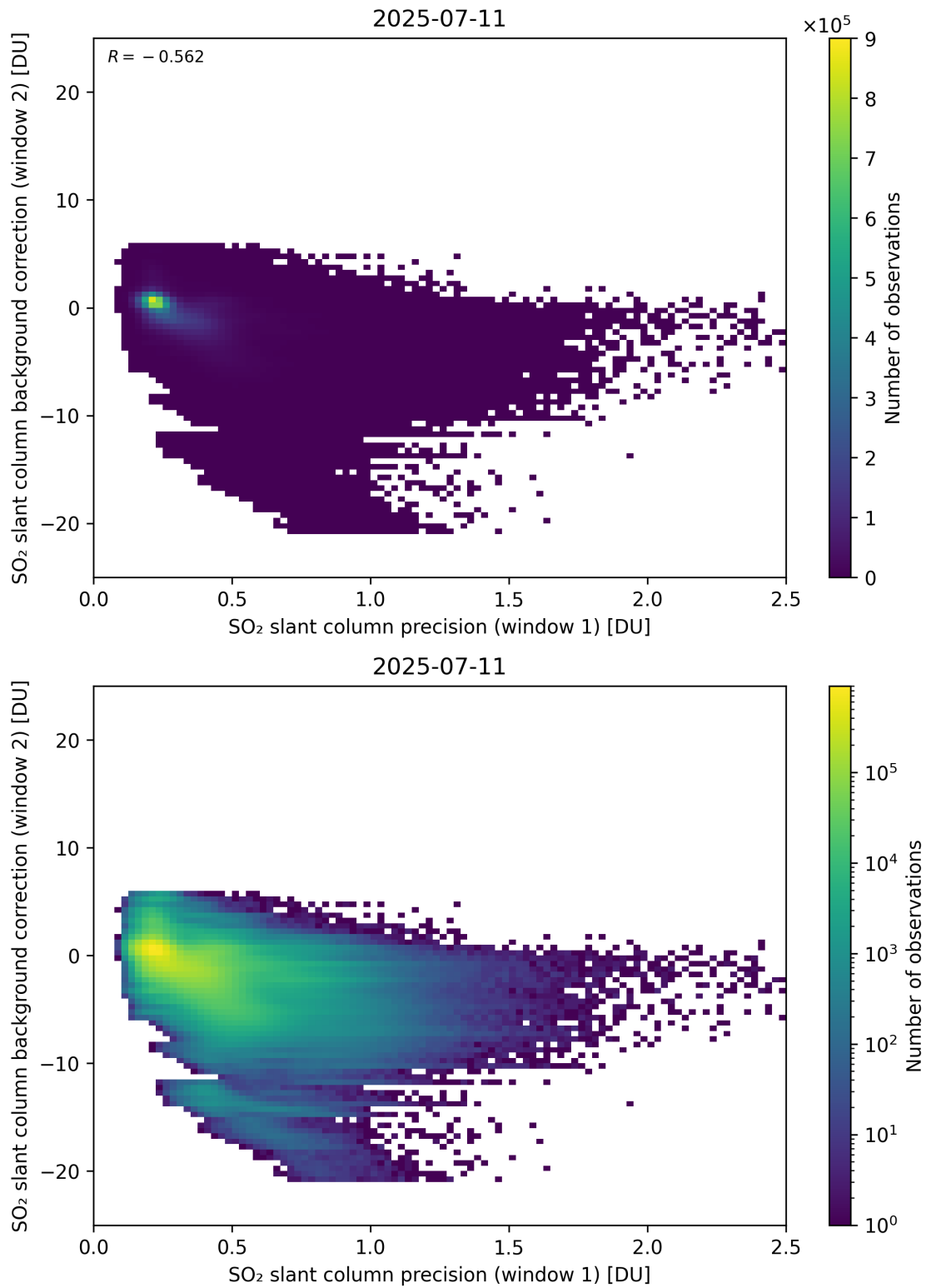
Figure 269: Scatter density plot of “SO 2 slant column precision (window 1)” against “SO 2 slant column background correction (window 2)” for 2025-07-10 to 2025-07-12.
