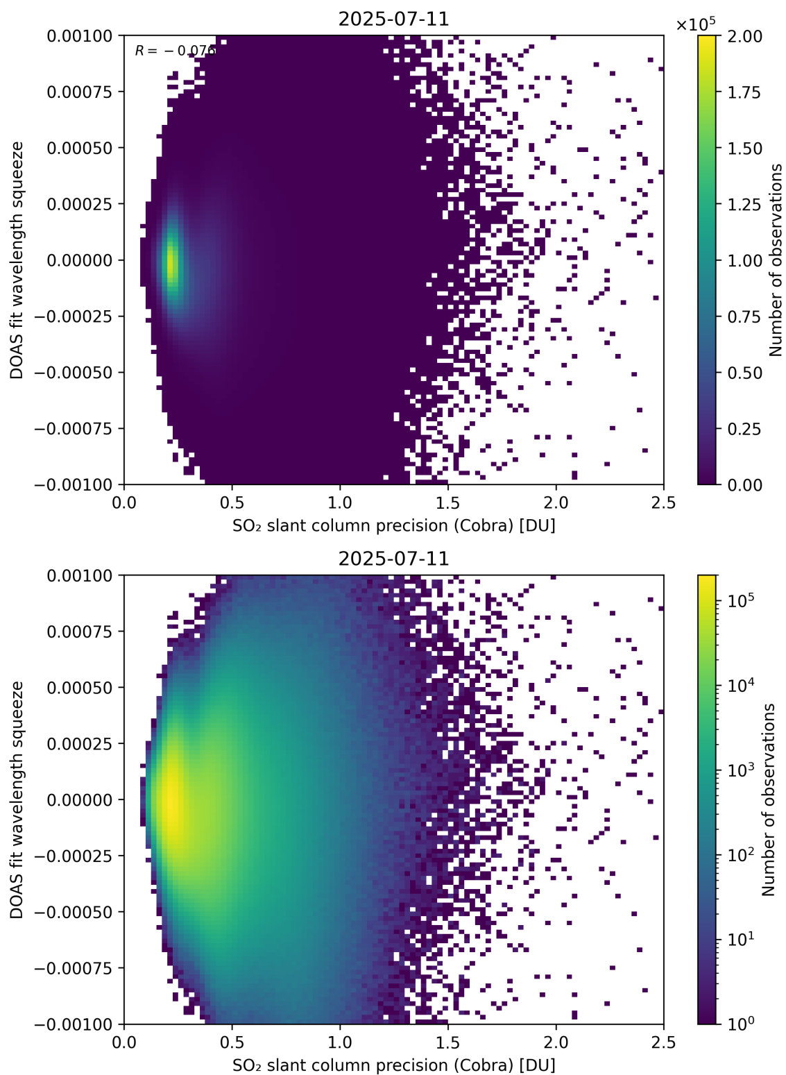
Figure 203: Scatter density plot of “SO 2 slant column precision (Cobra)” against “DOAS fit wavelength squeeze” for 2025-07-10 to 2025-07-12.
