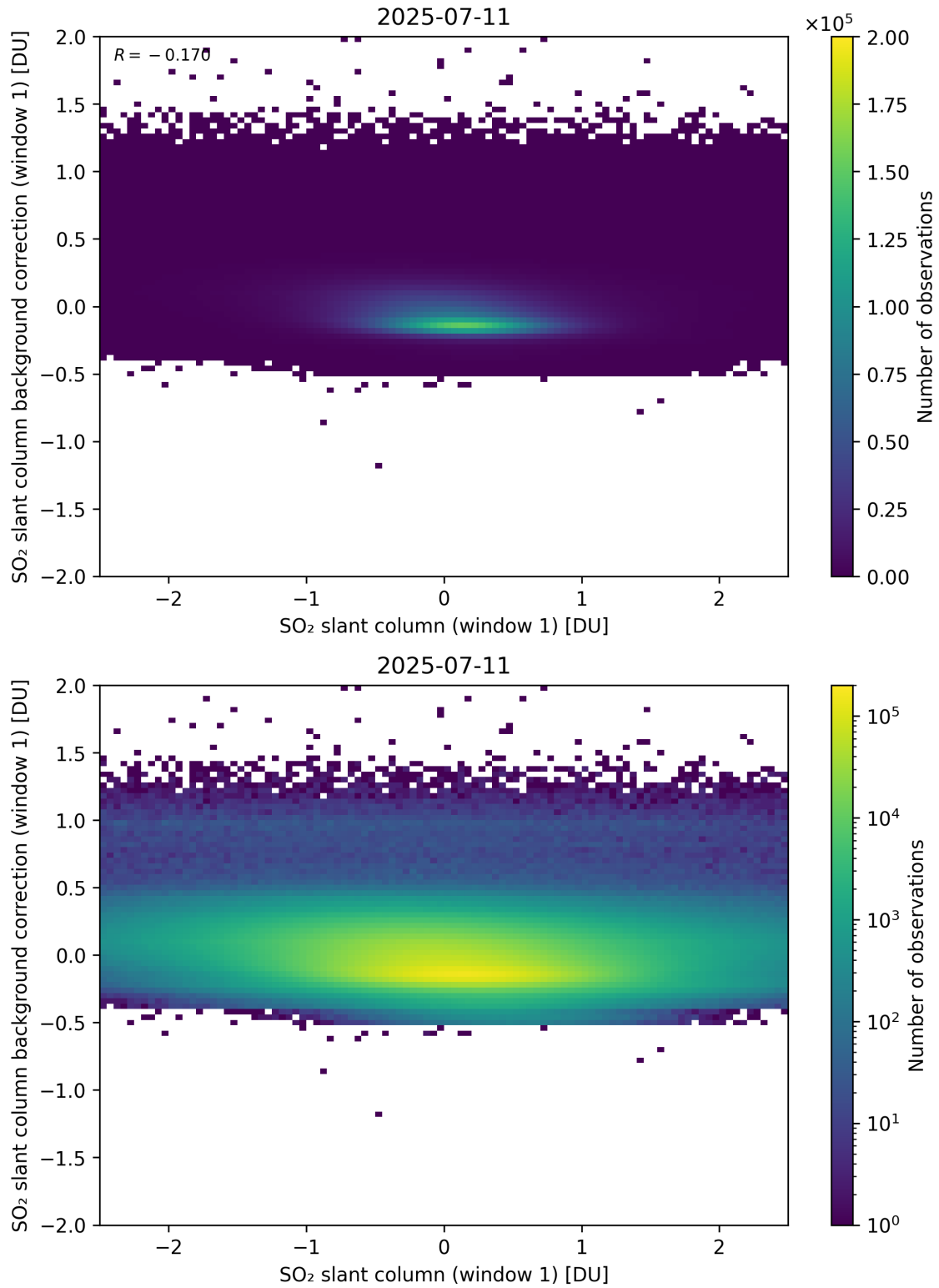
Figure 262: Scatter density plot of “SO 2 slant column (window 1)” against “SO 2 slant column background correction (window 1)” for 2025-07-10 to 2025-07-12.
