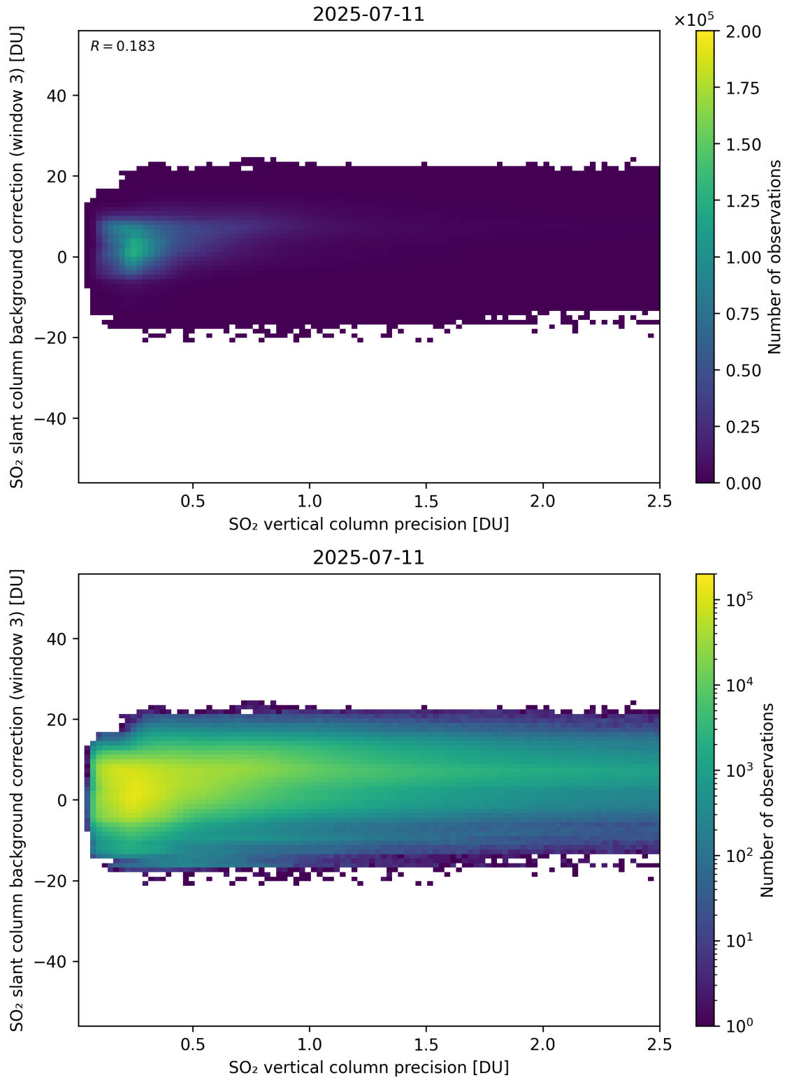
Figure 331: Scatter density plot of “SO 2 vertical column precision” against “SO 2 slant column background correction (window 3)” for 2025-07-10 to 2025-07-12.
