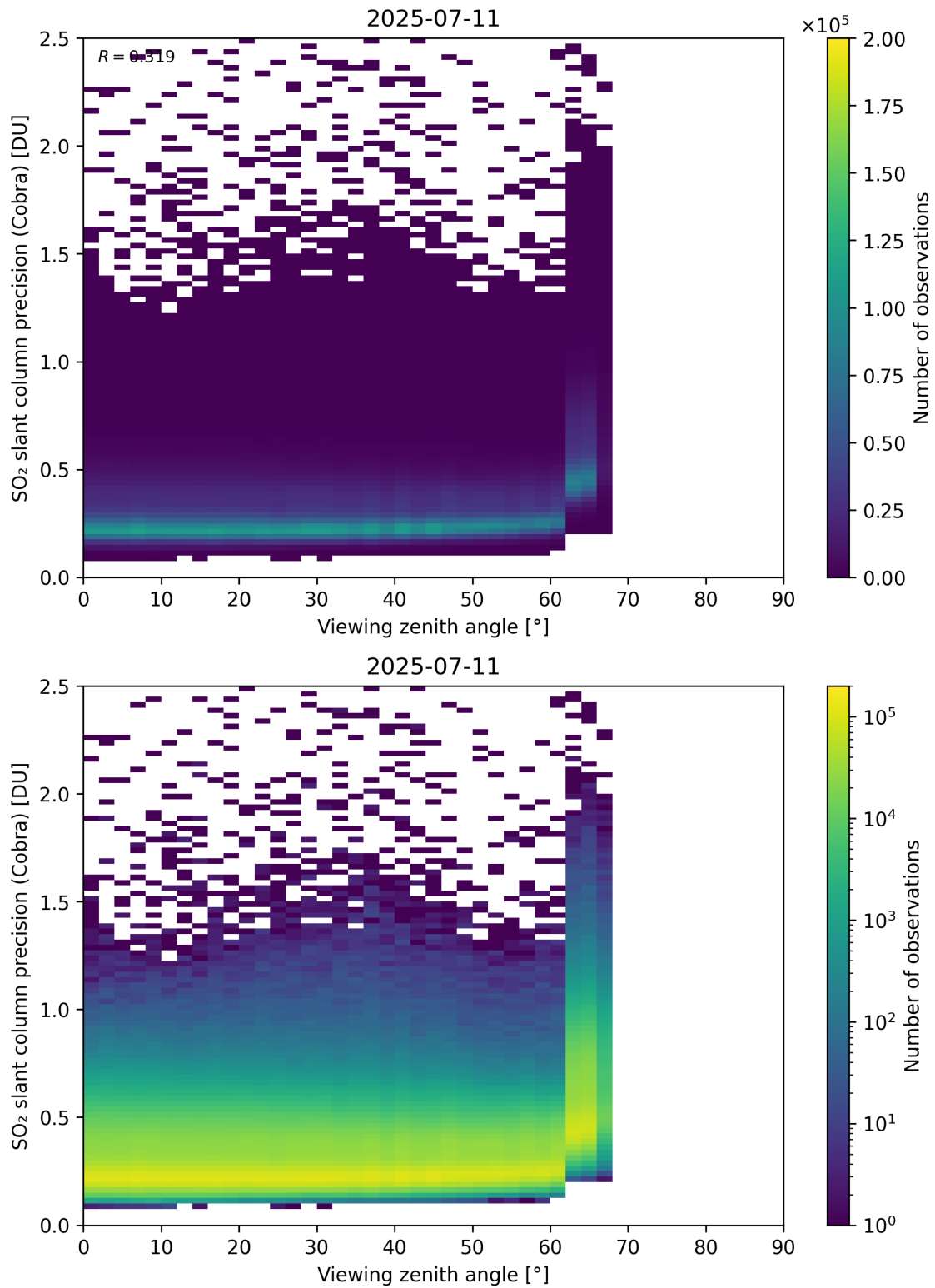
Figure 372: Scatter density plot of “Viewing zenith angle” against “SO 2 slant column precision (Cobra)” for 2025-07-10 to 2025-07-12.
