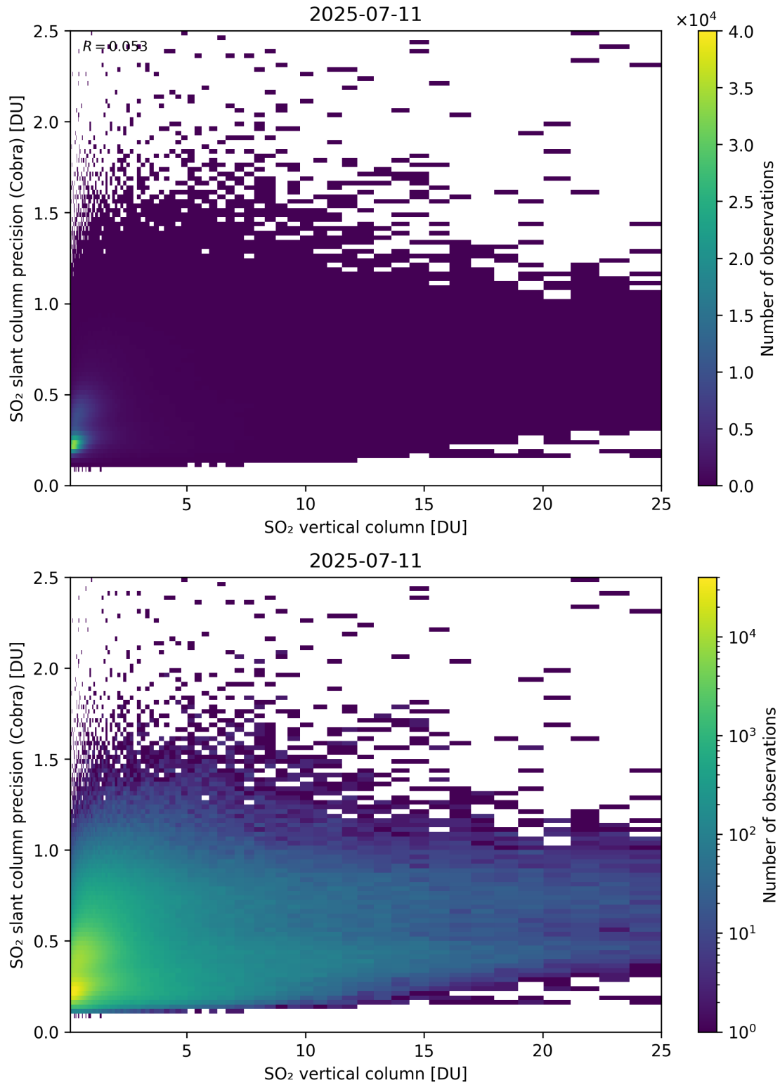
Figure 350: Scatter density plot of “SO 2 vertical column” against “SO 2 slant column precision (Cobra)” for 2025-07-10 to 2025-07-12.
