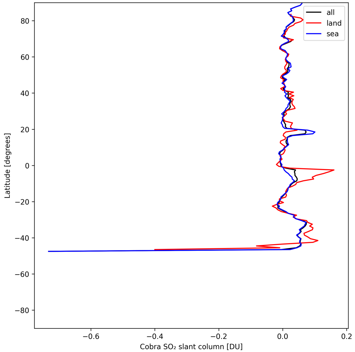
Figure 35: Zonal average of “Cobra SO 2 slant column” for 2025-07-10 to 2025-07-12.
