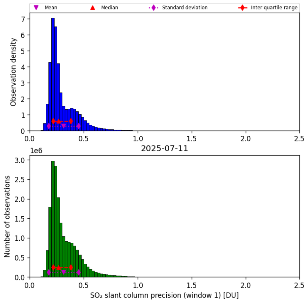
Figure 64: Histogram of “SO 2 slant column precision (window 1)” for 2025-07-10 to 2025-07-12
