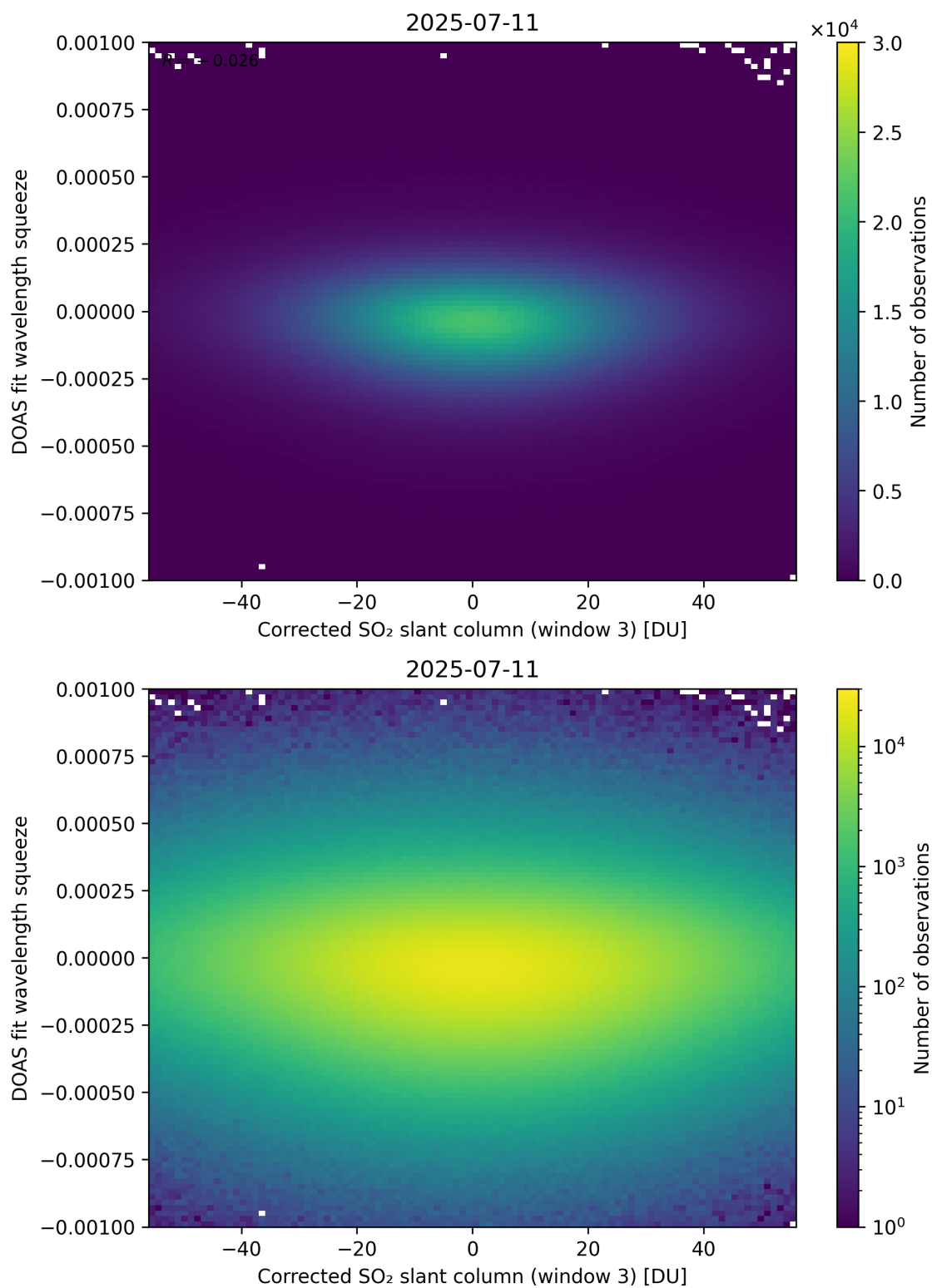
Figure 257: Scatter density plot of “Corrected SO 2 slant column (window 3)” against “DOAS fit wavelength squeeze” for 2025-07-10 to 2025-07-12.
