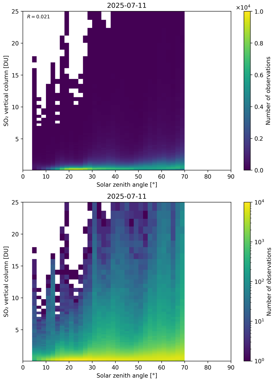
Figure 191: Scatter density plot of “Solar zenith angle” against “SO 2 vertical column” for 2025-07-10 to 2025-07-12.
