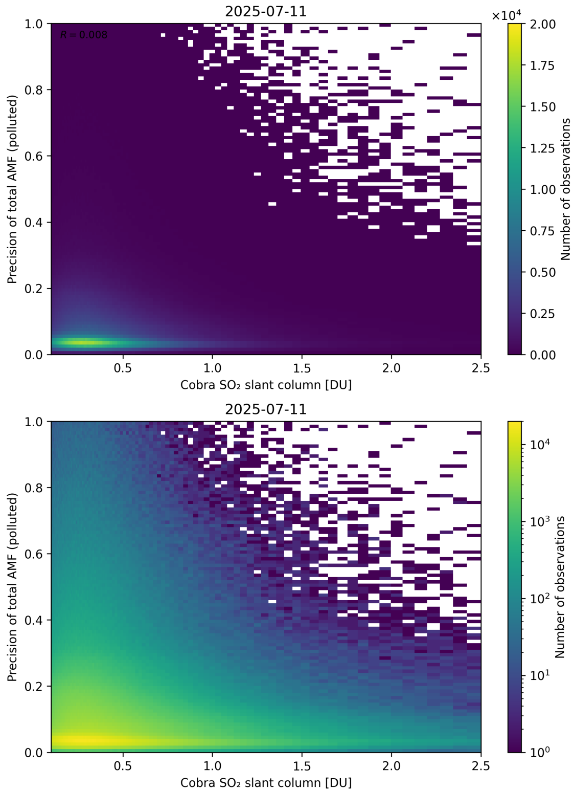
Figure 225: Scatter density plot of “Cobra SO 2 slant column” against “Precision of total AMF (polluted)” for 2025-07-10 to 2025-07-12.
