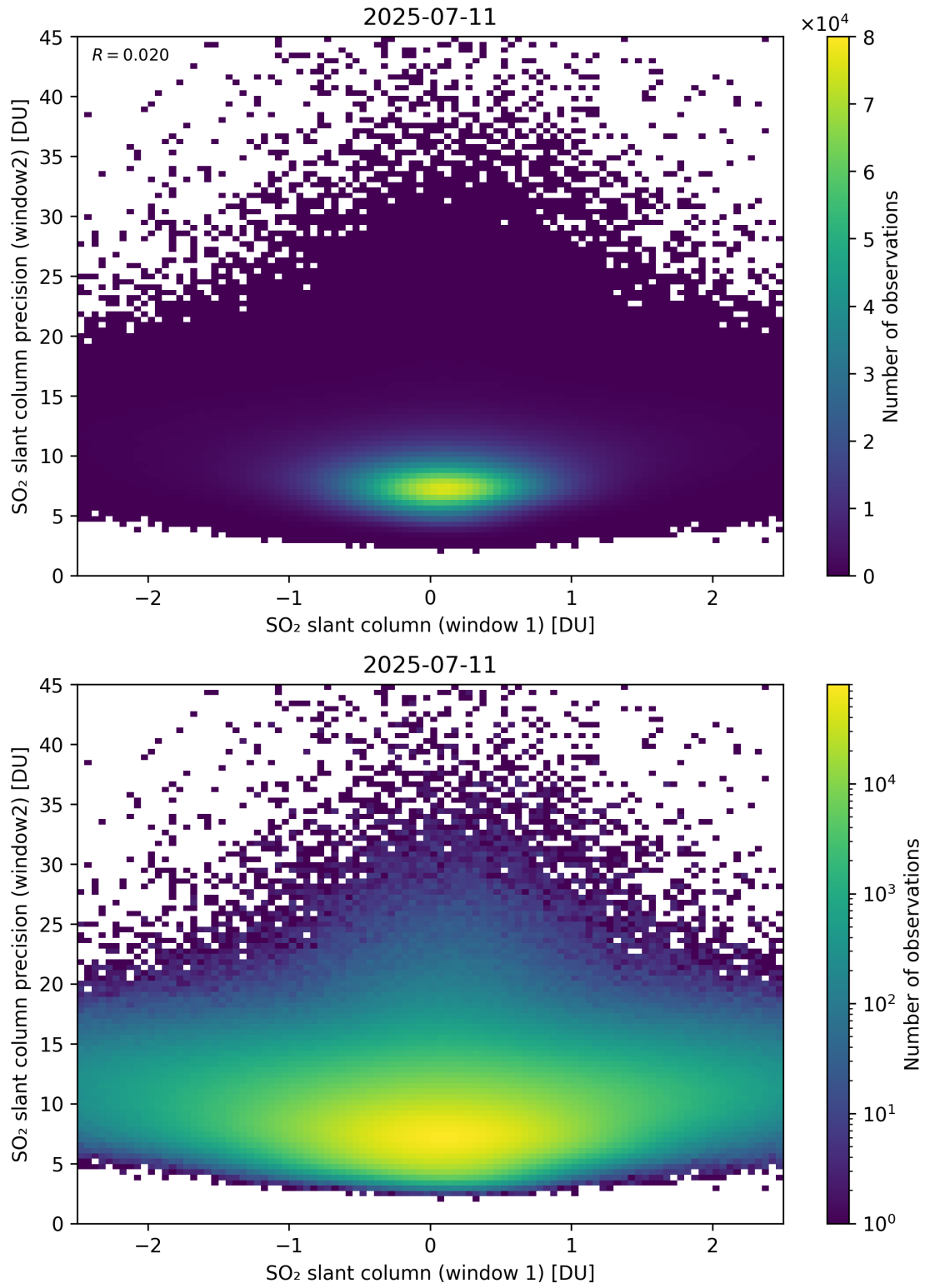
Figure 286: Scatter density plot of “SO 2 slant column (window 1)” against “SO 2 slant column precision (window2)” for 2025-07-10 to 2025-07-12.
