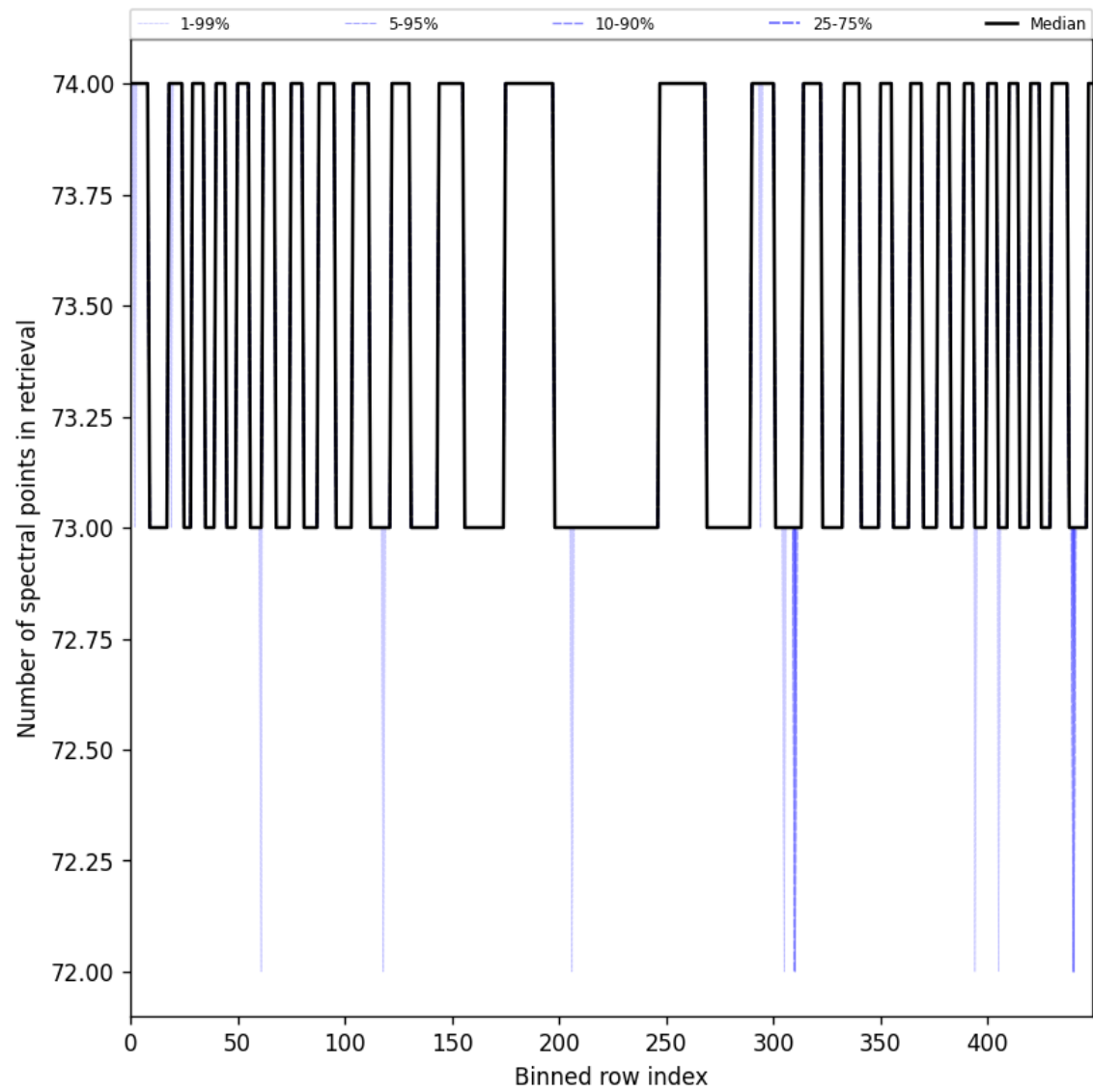
Figure 108: Along track statistics of “Number of spectral points in retrieval” for 2025-07-10 to 2025-07-12
