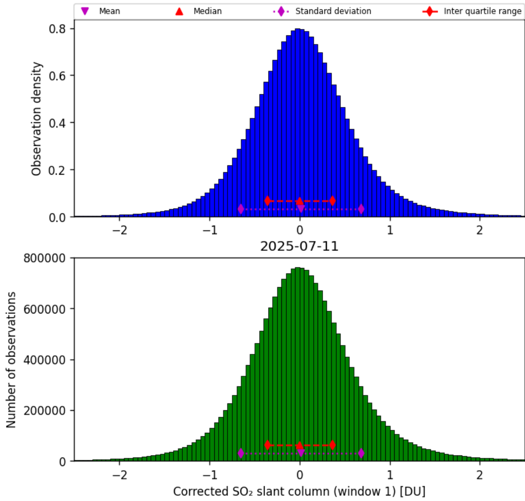
Figure 65: Histogram of “Corrected SO 2 slant column (window 1)” for 2025-07-10 to 2025-07-12
