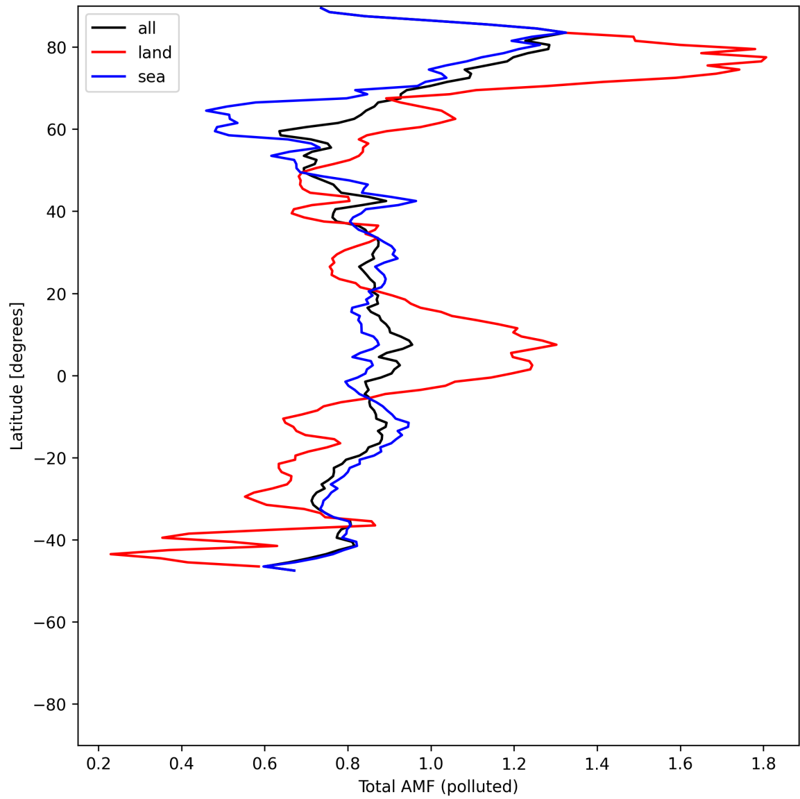
Figure 53: Zonal average of “Total AMF (polluted)” for 2025-07-10 to 2025-07-12.
