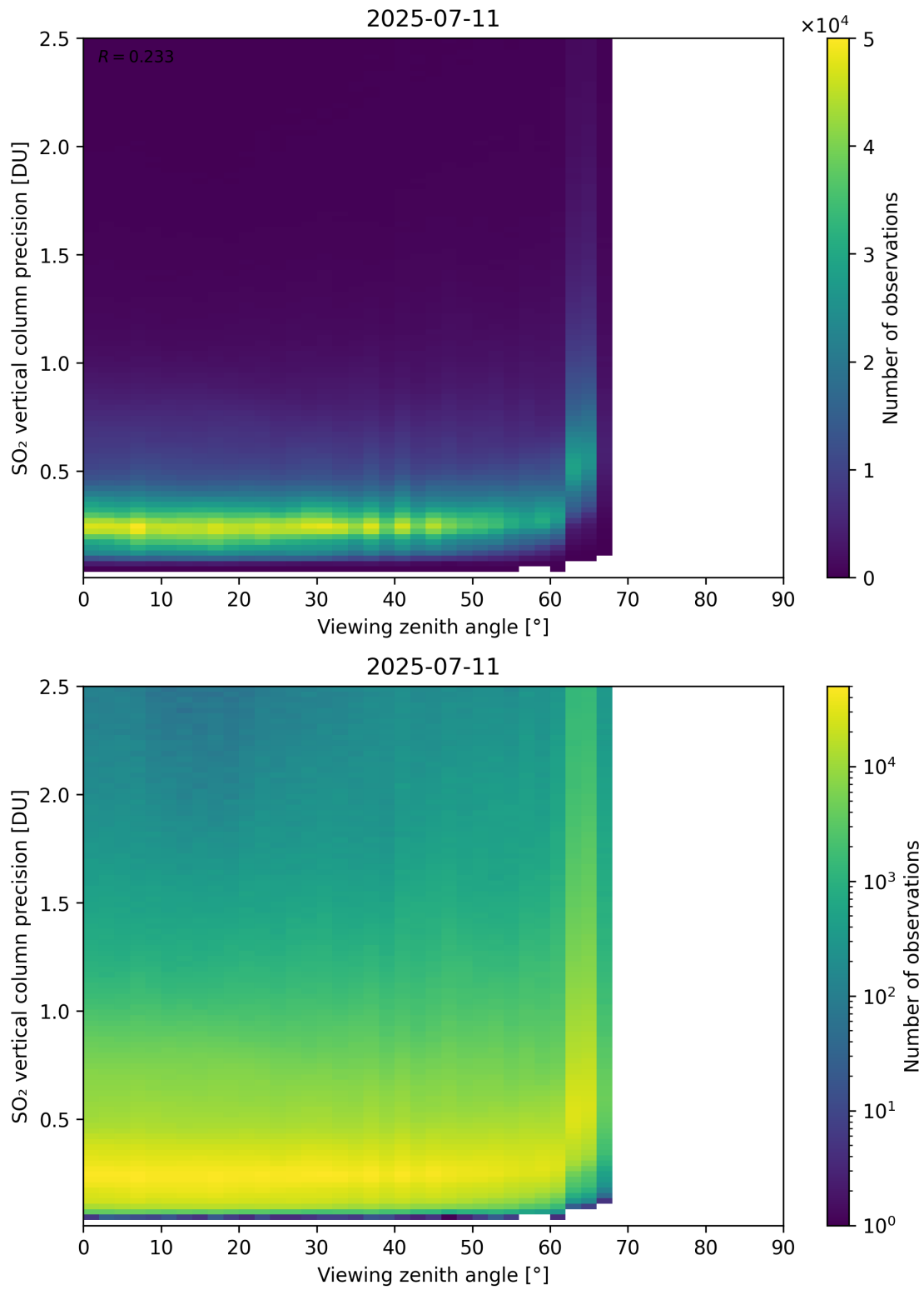
Figure 384: Scatter density plot of “Viewing zenith angle” against “SO 2 vertical column precision” for 2025-07-10 to 2025-07-12.
