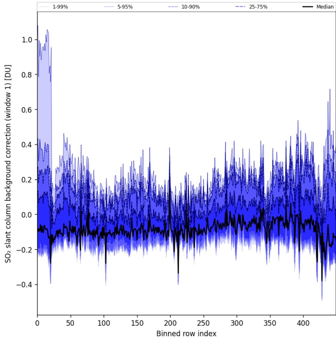
Figure 92: Along track statistics of “SO 2 slant column background correction (window 1)” for 2025-07-10 to 2025-07-12
