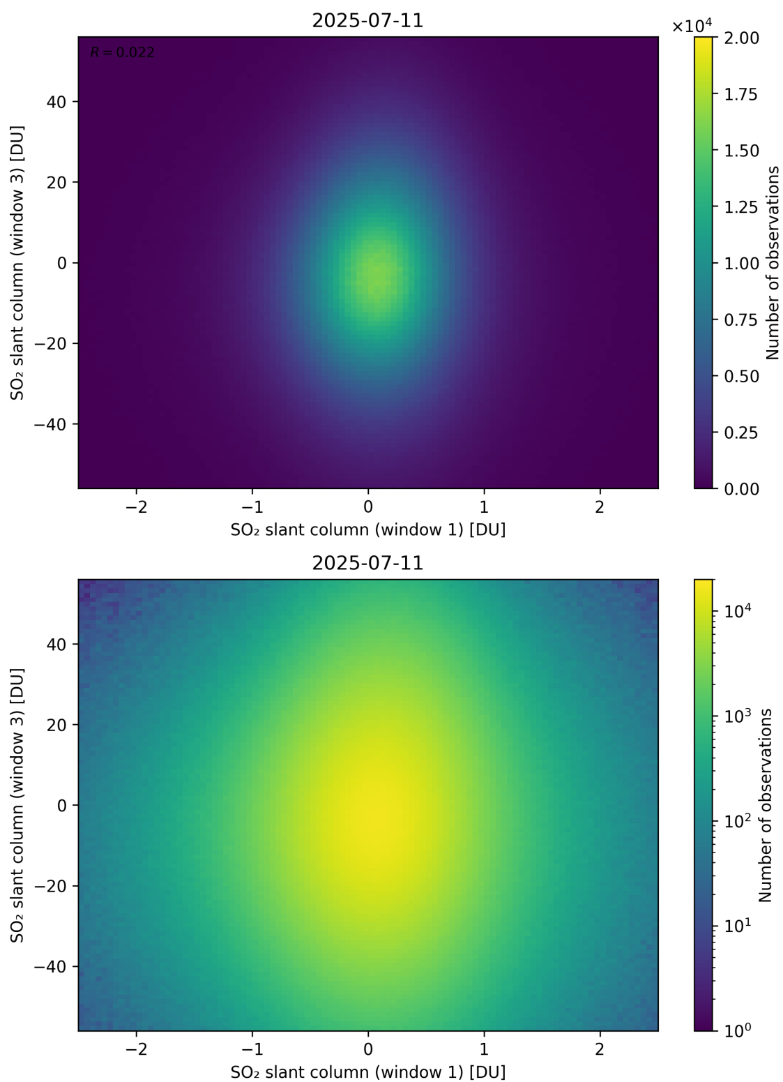
Figure 287: Scatter density plot of “SO 2 slant column (window 1)” against “SO 2 slant column (window 3)” for 2025-07-10 to 2025-07-12.
