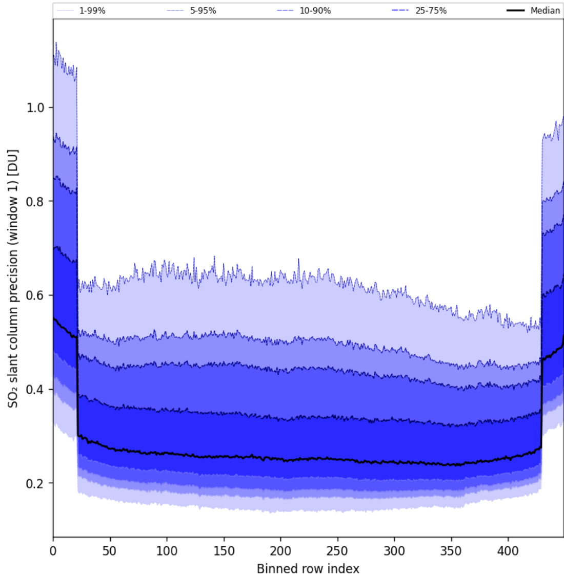
Figure 90: Along track statistics of “SO 2 slant column precision (window 1)” for 2025-07-10 to 2025-07-12
