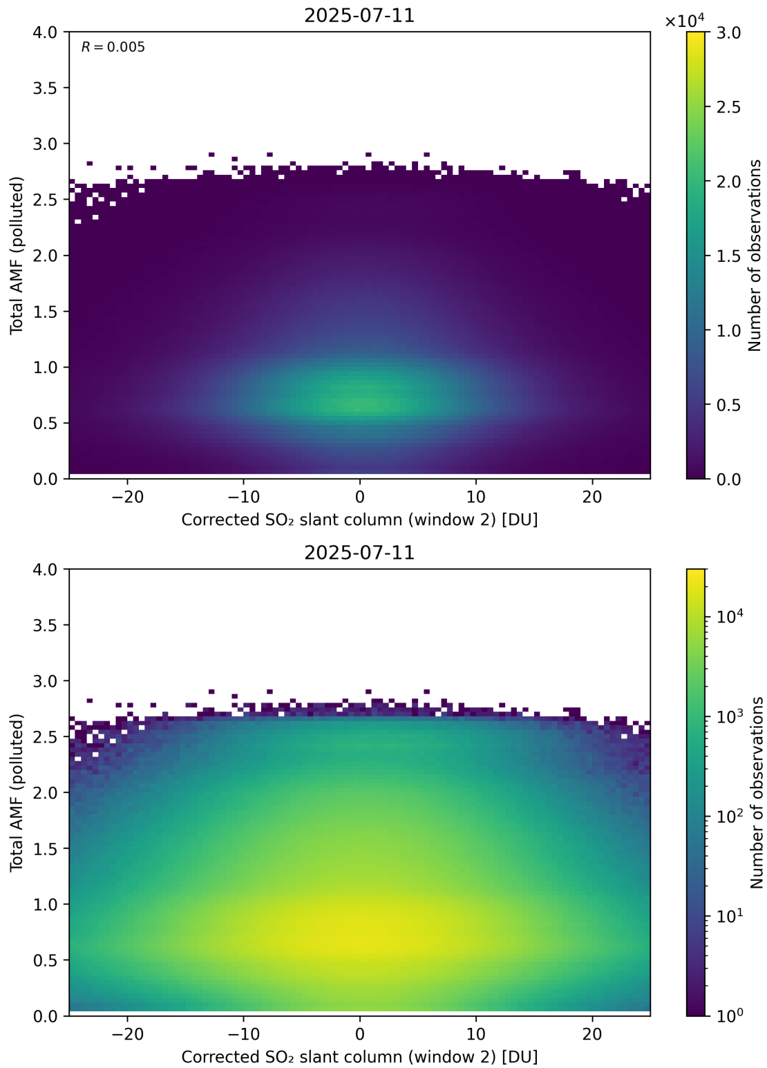
Figure 253: Scatter density plot of “Corrected SO 2 slant column (window 2)” against “Total AMF (polluted)” for 2025-07-10 to 2025-07-12.
