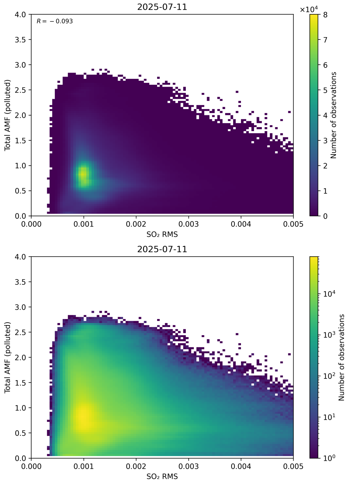
Figure 148: Scatter density plot of “SO 2 RMS” against “Total AMF (polluted)” for 2025-07-10 to 2025-07-12.
