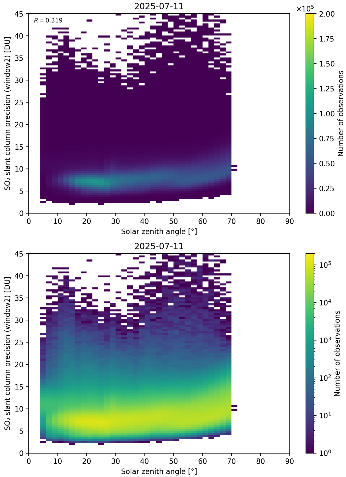
Figure 186: Scatter density plot of “Solar zenith angle” against “SO 2 slant column precision (window2)” for 2025-07-10 to 2025-07-12.
