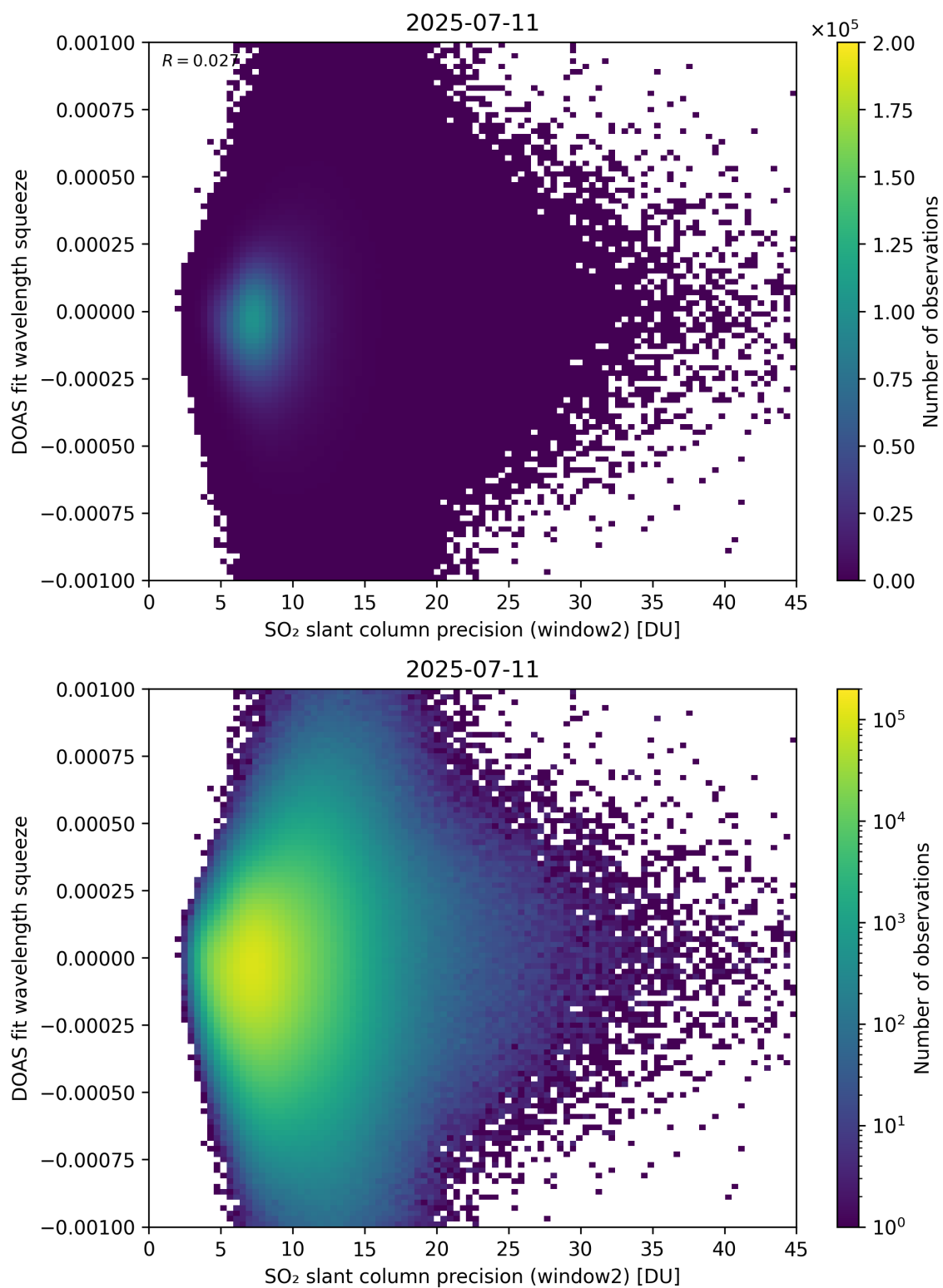
Figure 294: Scatter density plot of “SO 2 slant column precision (window2)” against “DOAS fit wavelength squeeze” for 2025-07-10 to 2025-07-12.
