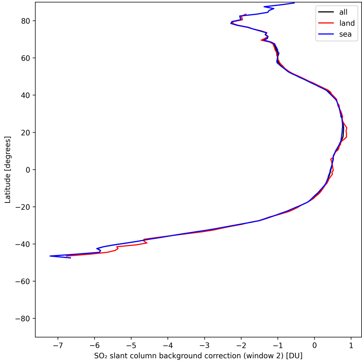
Figure 44: Zonal average of “SO 2 slant column background correction (window 2)” for 2025-07-10 to 2025-07-12.
