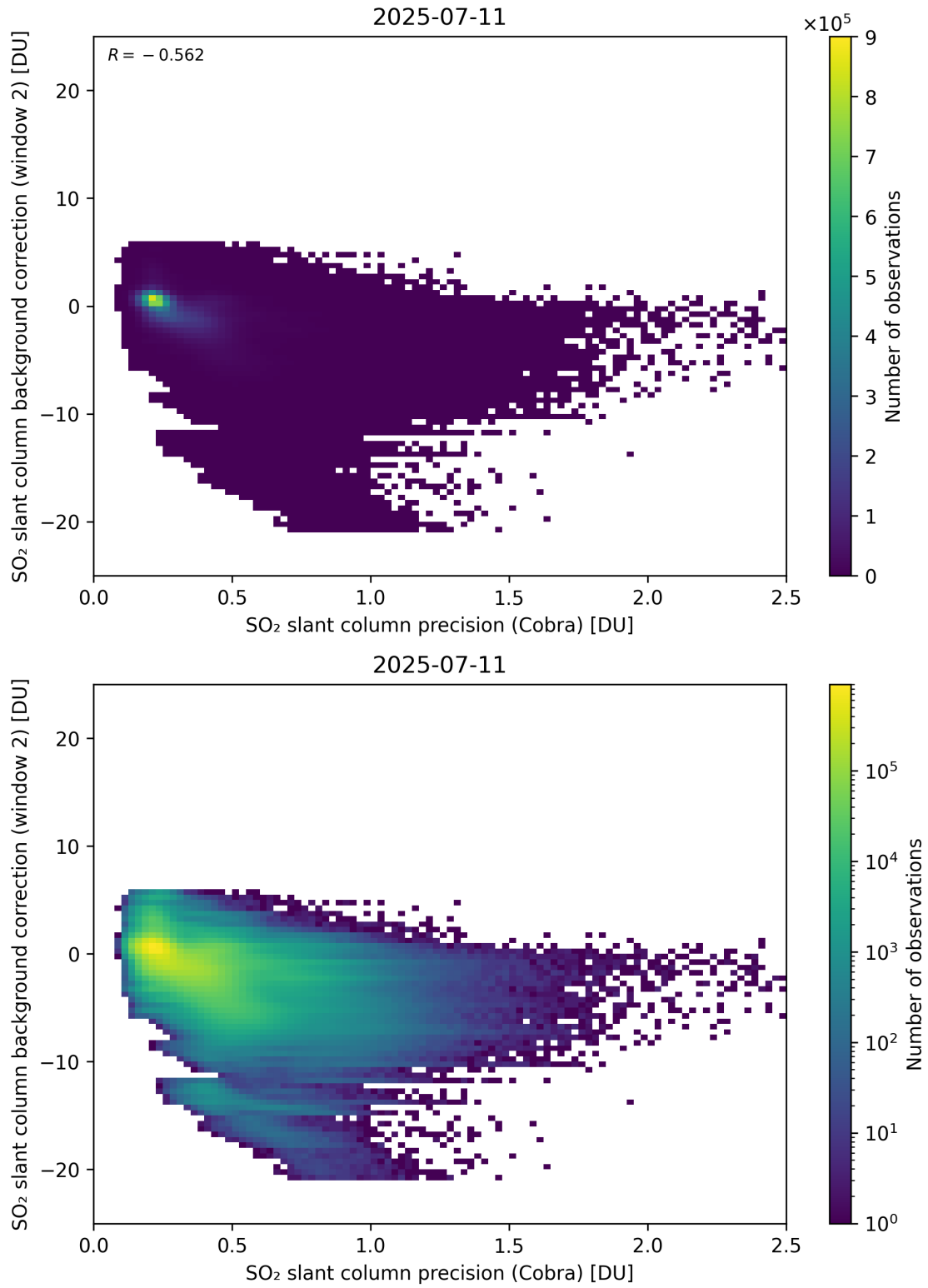
Figure 200: Scatter density plot of “SO 2 slant column precision (Cobra)” against “SO 2 slant column background correction (window 2)” for 2025-07-10 to 2025-07-12.
