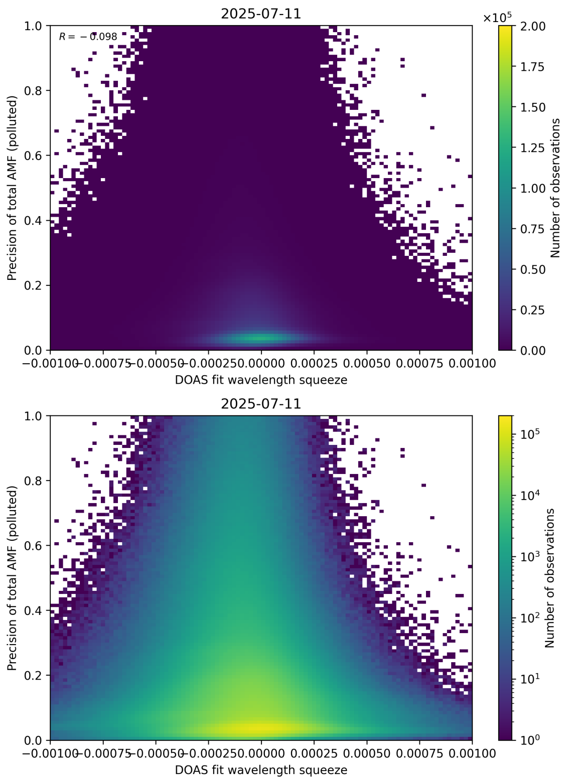
Figure 146: Scatter density plot of “DOAS fit wavelength squeeze” against “Precision of total AMF (polluted)” for 2025-07-10 to 2025-07-12.
