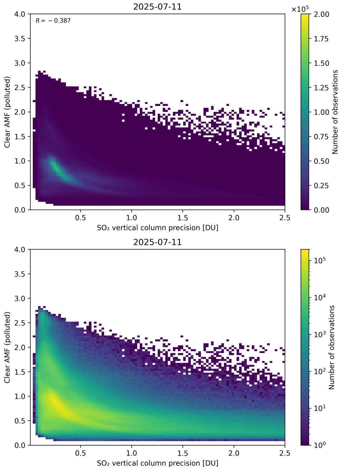
Figure 335: Scatter density plot of “SO 2 vertical column precision” against “Clear AMF (polluted)” for 2025-07-10 to 2025-07-12.
