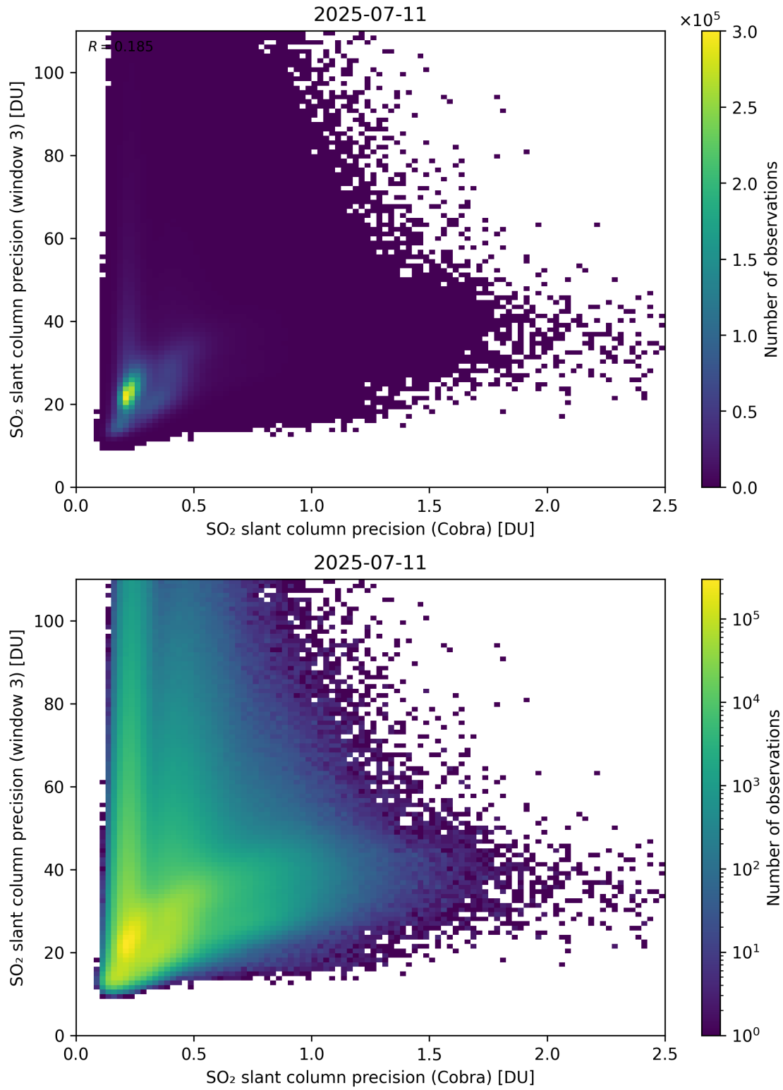
Figure 212: Scatter density plot of “SO 2 slant column precision (Cobra)” against “SO 2 slant column precision (window 3)” for 2025-07-10 to 2025-07-12.
