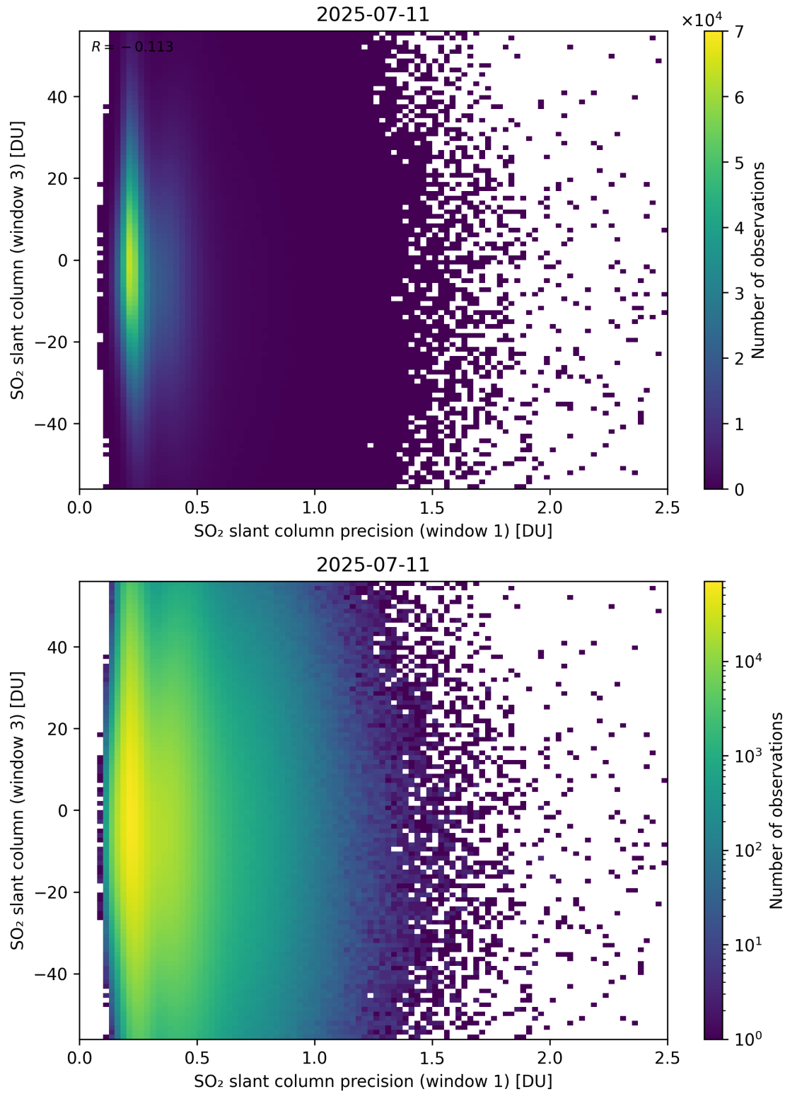
Figure 278: Scatter density plot of “SO 2 slant column precision (window 1)” against “SO 2 slant column (window 3)” for 2025-07-10 to 2025-07-12.
