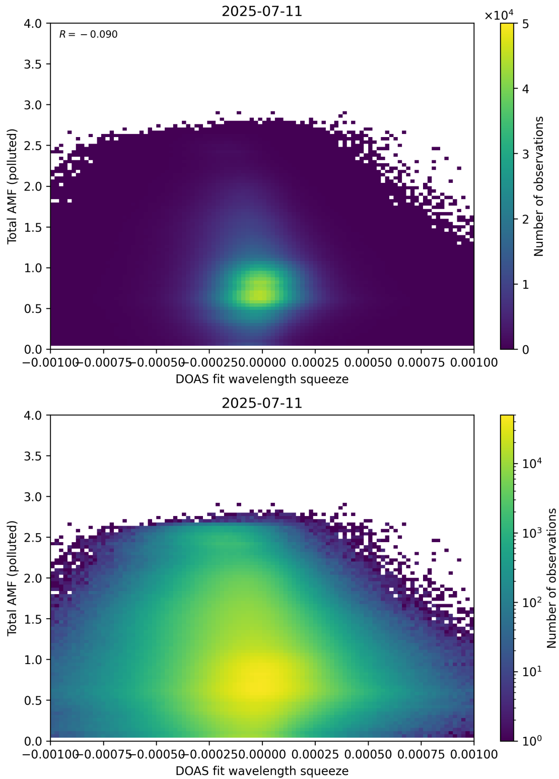
Figure 145: Scatter density plot of “DOAS fit wavelength squeeze” against “Total AMF (polluted)” for 2025-07-10 to 2025-07-12.
