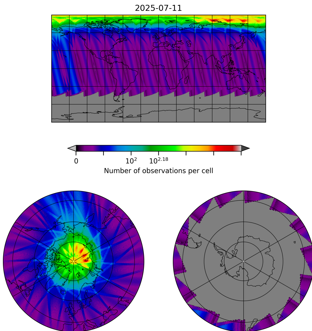
Figure 30: Map of the number of observations for 2025-07-10 to 2025-07-12
