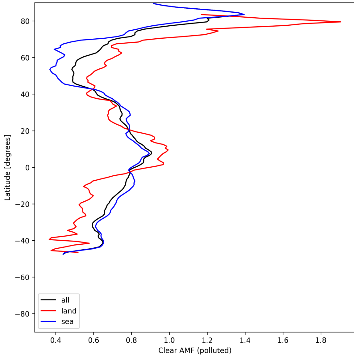
Figure 55: Zonal average of “Clear AMF (polluted)” for 2025-07-10 to 2025-07-12.
