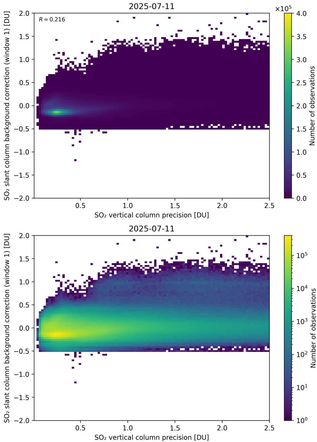
Figure 329: Scatter density plot of “SO 2 vertical column precision” against “SO 2 slant column background correction (window 1)” for 2025-07-10 to 2025-07-12.
