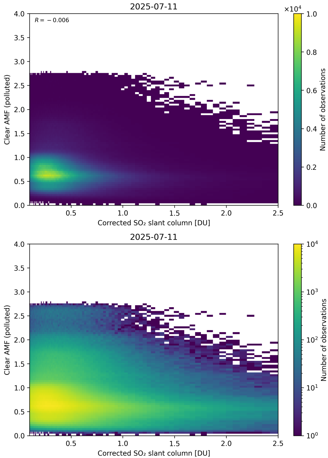
Figure 232: Scatter density plot of “Corrected SO 2 slant column” against “Clear AMF (polluted)” for 2025-07-10 to 2025-07-12.
