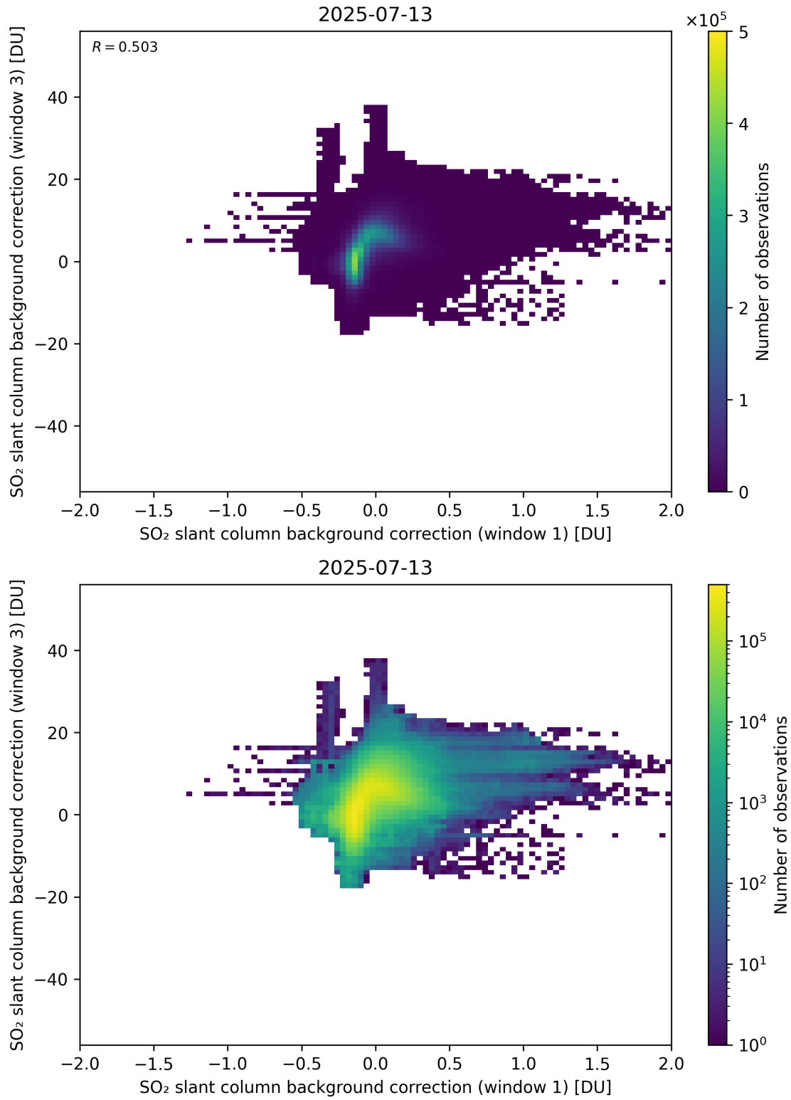
Figure 110: Scatter density plot of “SO 2 slant column background correction (window 1)” against “SO 2 slant column background correction (window 3)” for 2025-07-13 to 2025-07-14.
