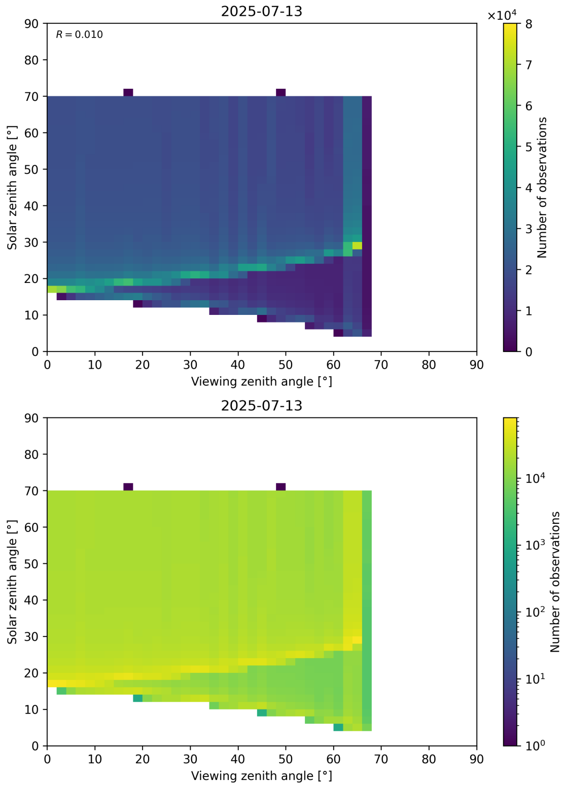
Figure 369: Scatter density plot of “Viewing zenith angle” against “Solar zenith angle” for 2025-07-13 to 2025-07-14.
