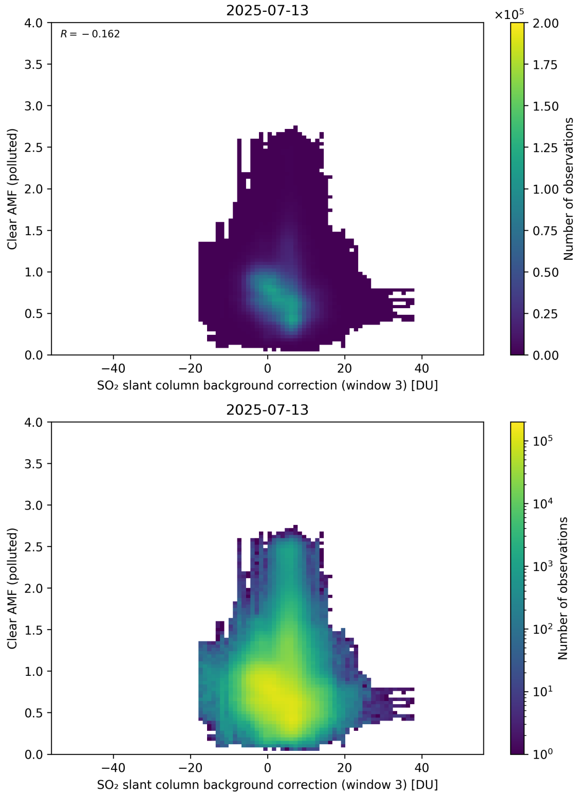
Figure 135: Scatter density plot of “SO 2 slant column background correction (window 3)” against “Clear AMF (polluted)” for 2025-07-13 to 2025-07-14.
