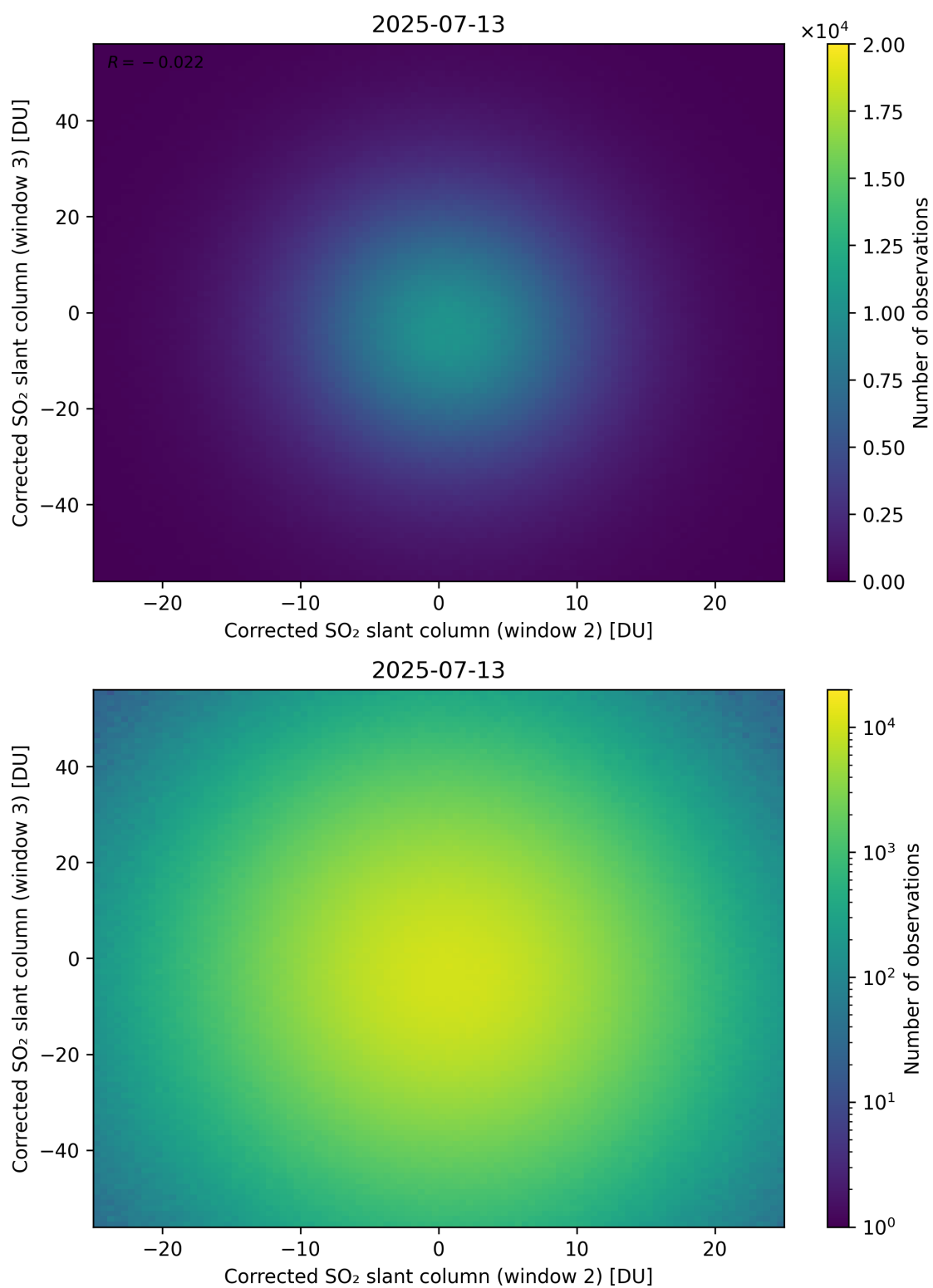
Figure 250: Scatter density plot of “Corrected SO 2 slant column (window 2)” against “Corrected SO 2 slant column (window 3)” for 2025-07-13 to 2025-07-14.
