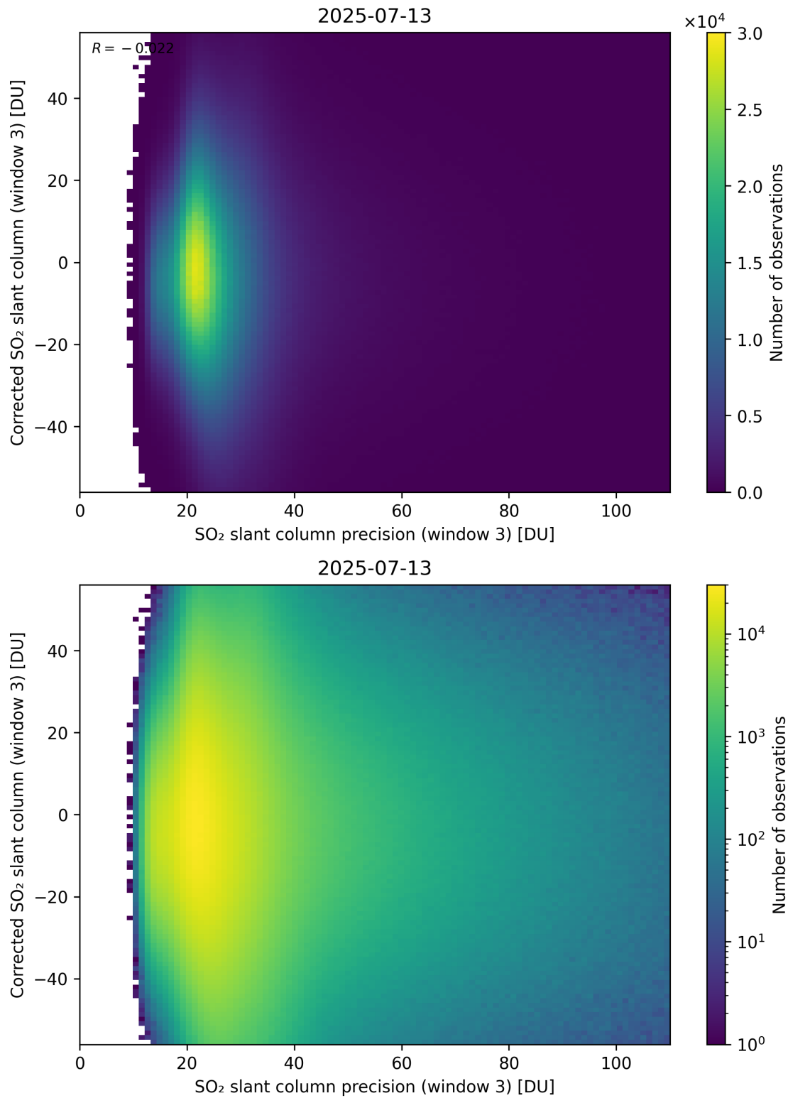
Figure 312: Scatter density plot of “SO 2 slant column precision (window 3)” against “Corrected SO 2 slant column (window 3)” for 2025-07-13 to 2025-07-14.
