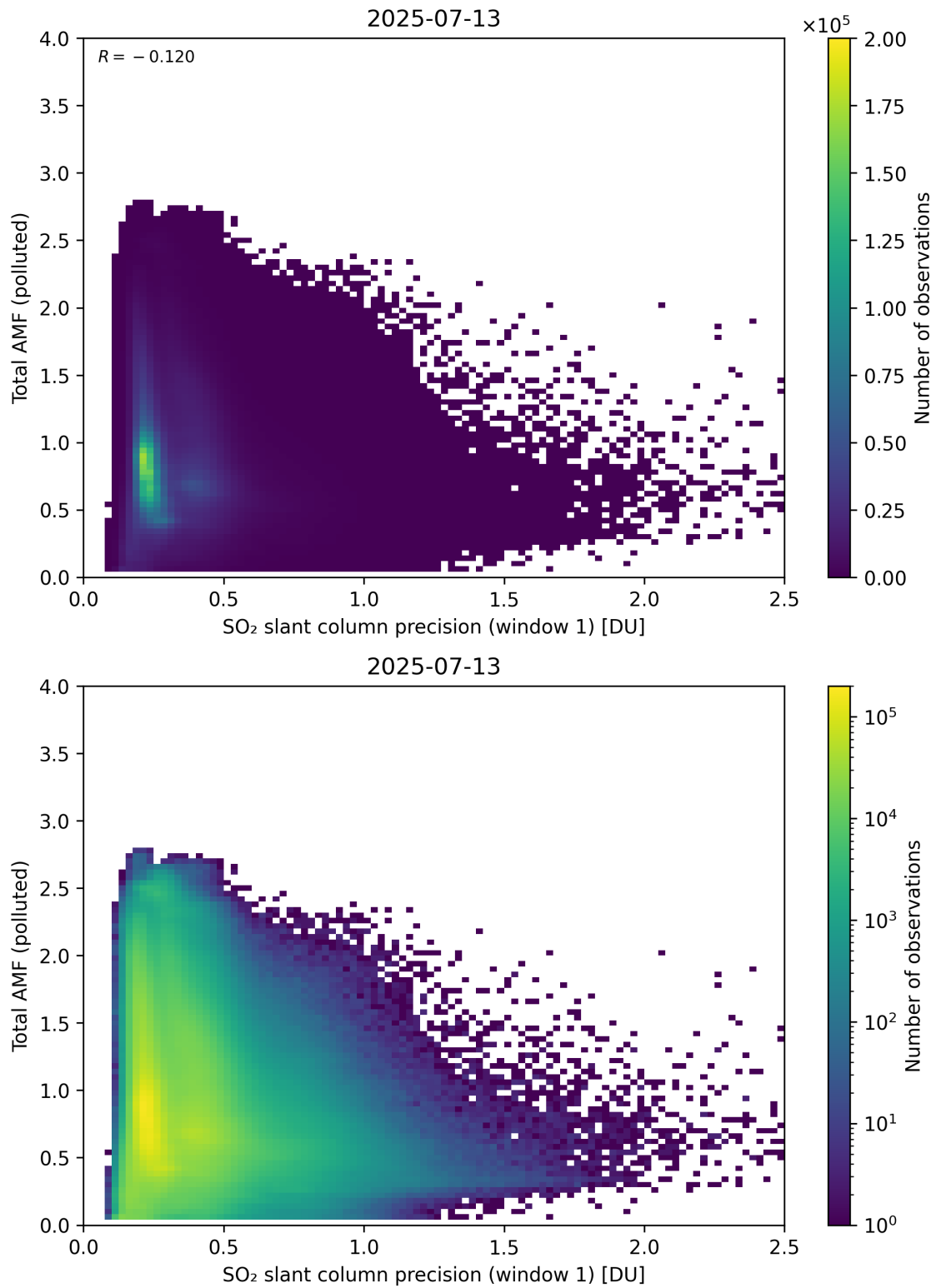
Figure 280: Scatter density plot of “SO 2 slant column precision (window 1)” against “Total AMF (polluted)” for 2025-07-13 to 2025-07-14.
