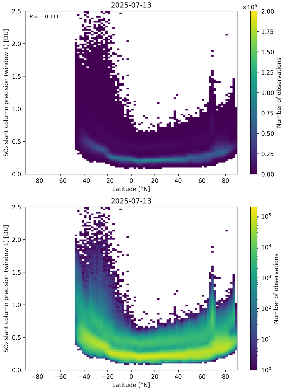
Figure 163: Scatter density plot of “Latitude” against “SO 2 slant column precision (window 1)” for 2025-07-13 to 2025-07-14.
