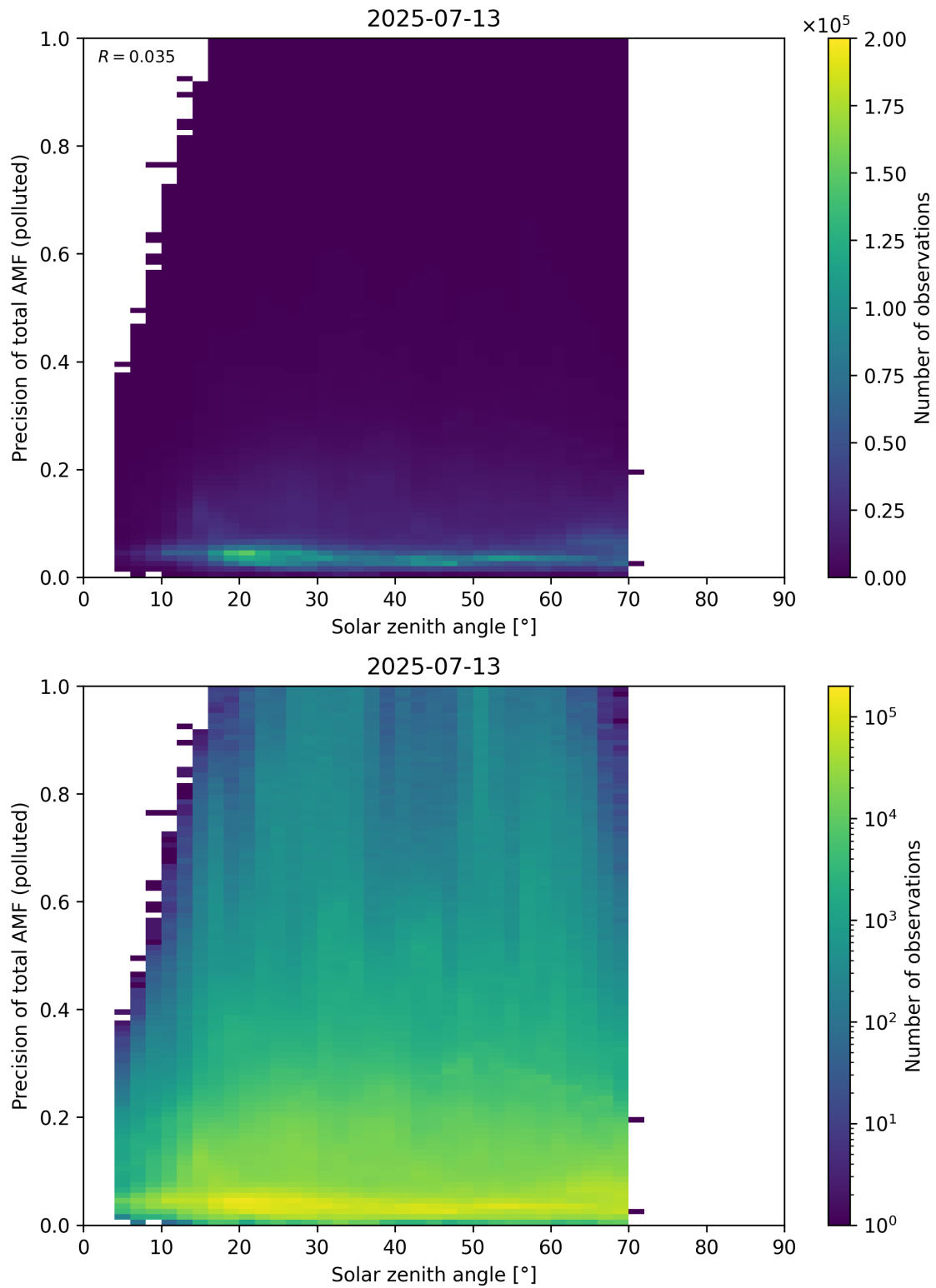
Figure 190: Scatter density plot of “Solar zenith angle” against “Precision of total AMF (polluted)” for 2025-07-13 to 2025-07-14.
