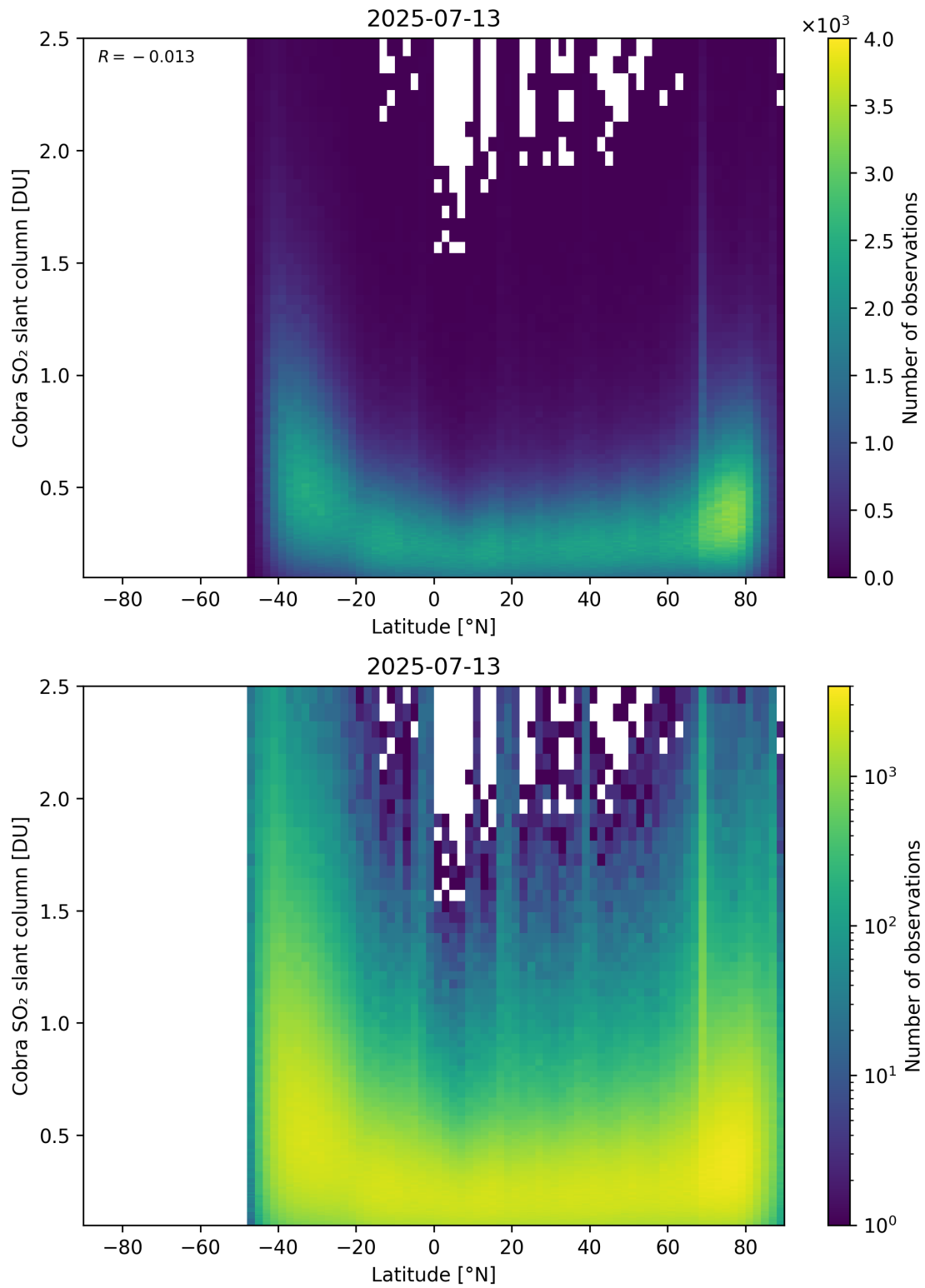
Figure 157: Scatter density plot of “Latitude” against “Cobra SO 2 slant column” for 2025-07-13 to 2025-07-14.
