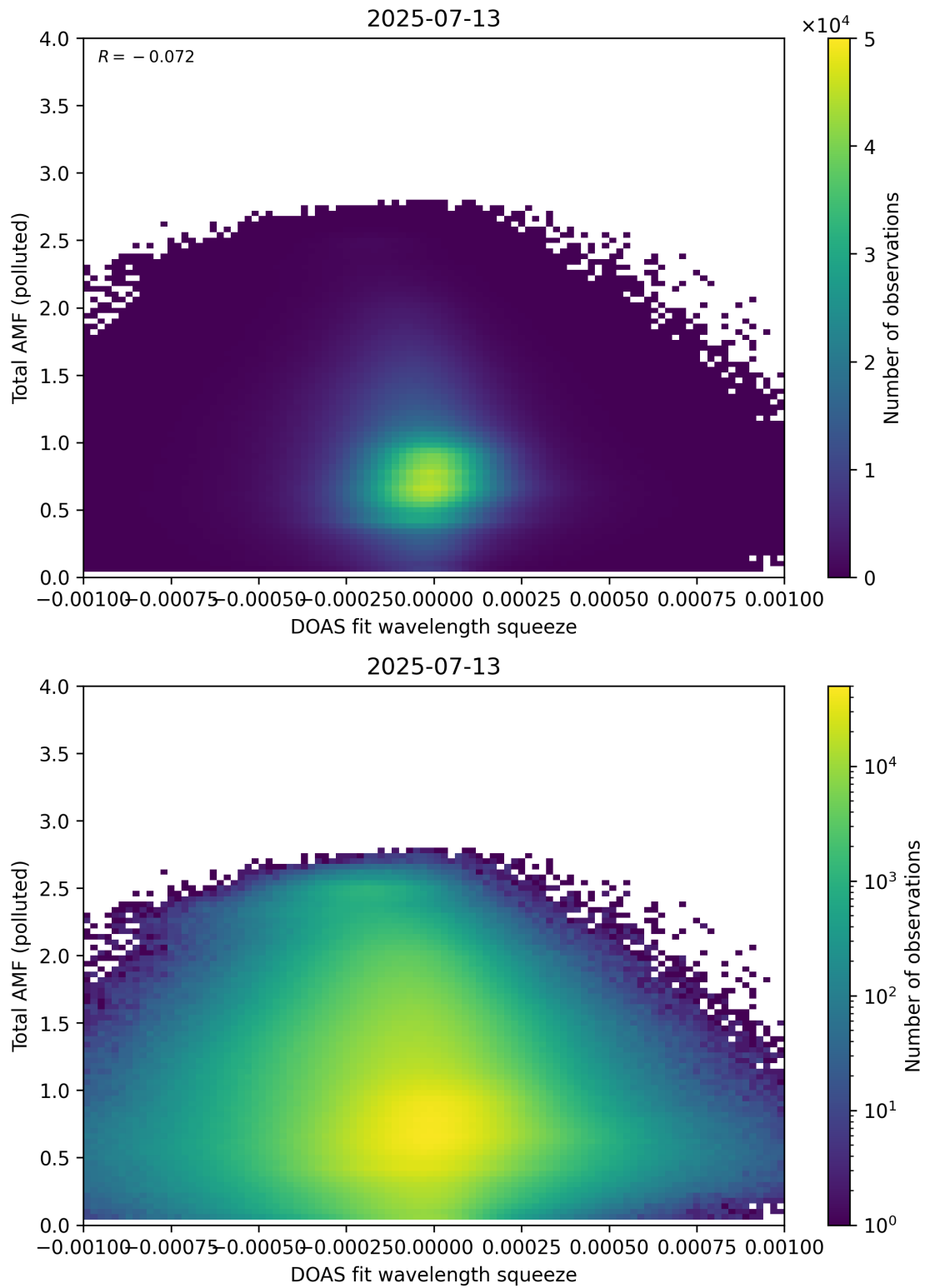
Figure 145: Scatter density plot of “DOAS fit wavelength squeeze” against “Total AMF (polluted)” for 2025-07-13 to 2025-07-14.
