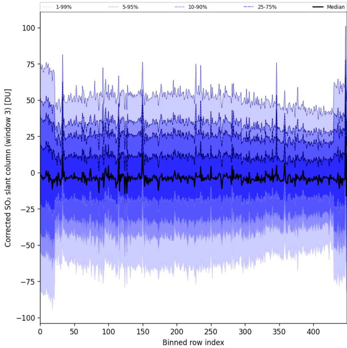
Figure 99: Along track statistics of “Corrected SO 2 slant column (window 3)” for 2025-07-13 to 2025-07-14
