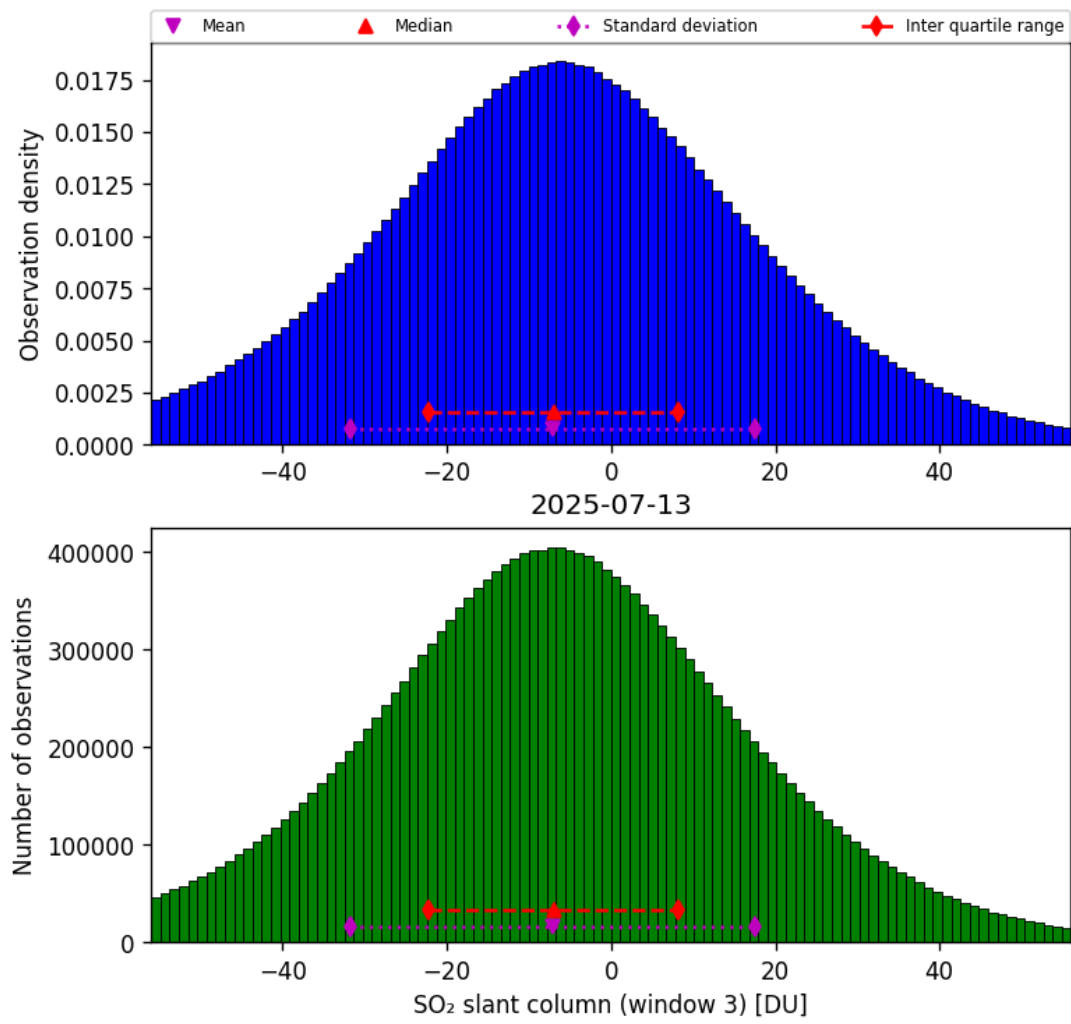
Figure 71: Histogram of “SO 2 slant column (window 3)” for 2025-07-13 to 2025-07-14
