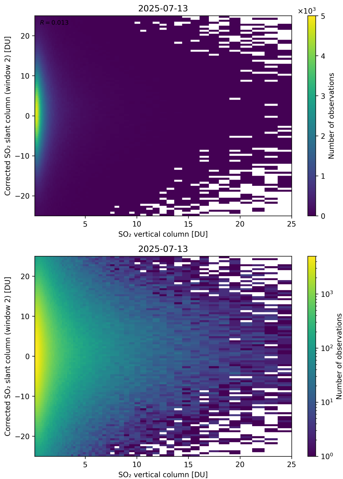
Figure 352: Scatter density plot of “SO 2 vertical column” against “Corrected SO 2 slant column (window 2)” for 2025-07-13 to 2025-07-14.
