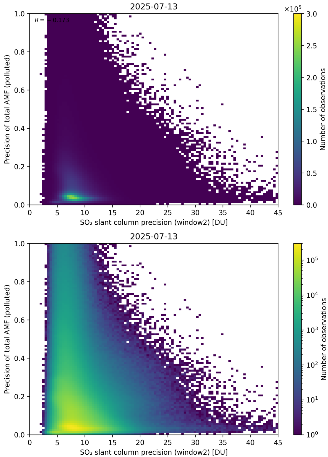
Figure 302: Scatter density plot of “SO 2 slant column precision (window2)” against “Precision of total AMF (polluted)” for 2025-07-13 to 2025-07-14.
