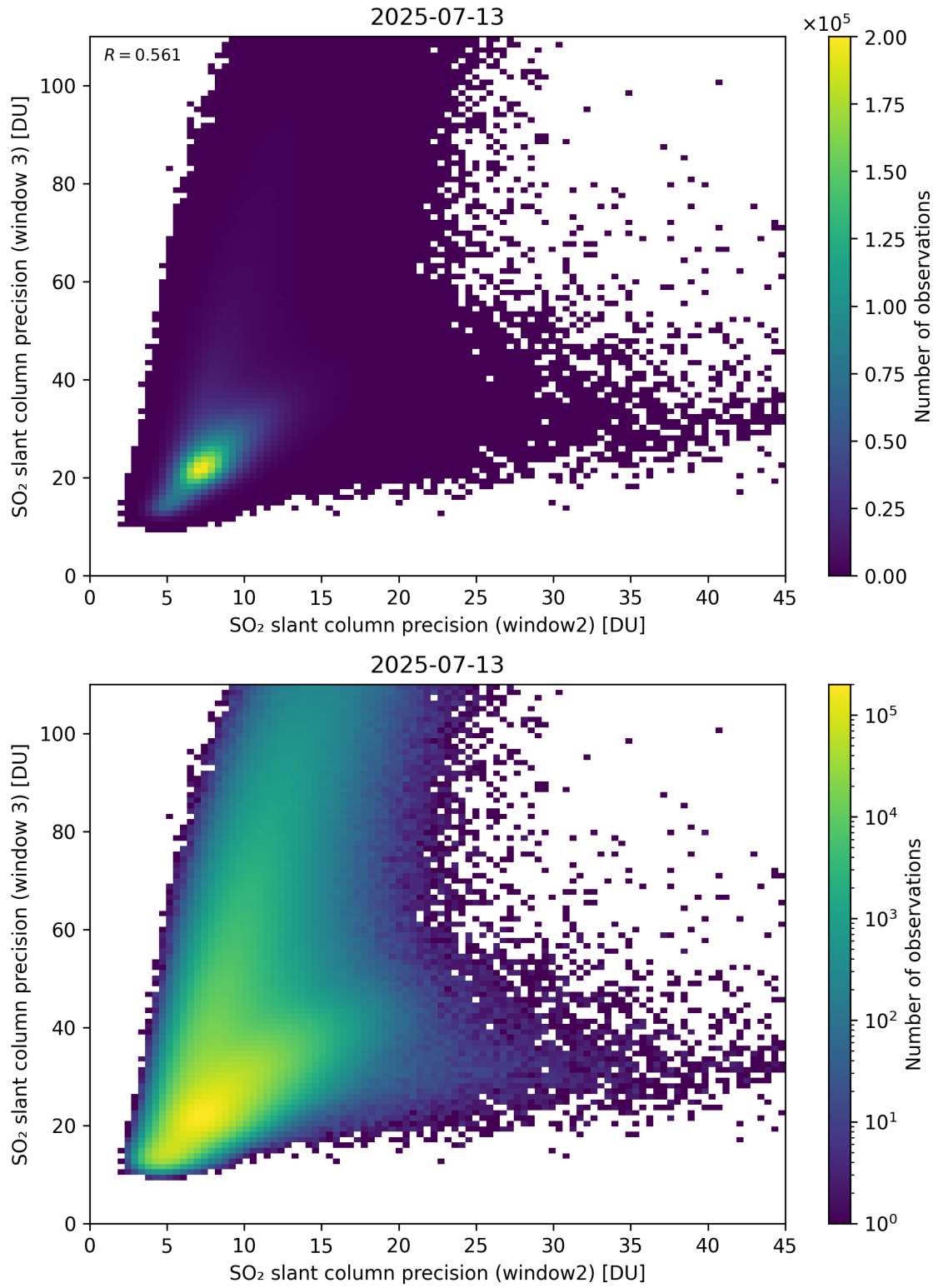
Figure 300: Scatter density plot of “SO 2 slant column precision (window2)” against “SO 2 slant column precision (window 3)” for 2025-07-13 to 2025-07-14.
