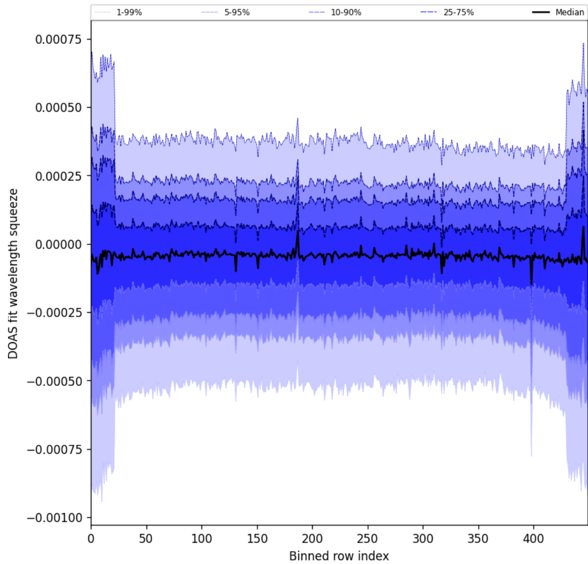
Figure 103: Along track statistics of “DOAS fit wavelength squeeze” for 2025-07-13 to 2025-07-14
