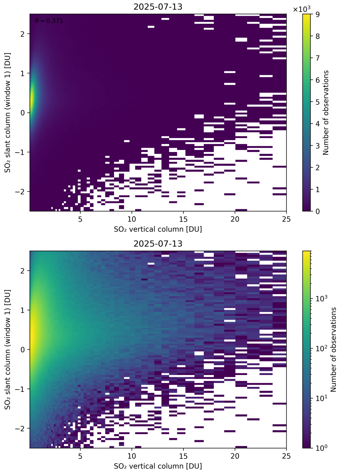
Figure 354: Scatter density plot of “SO 2 vertical column” against “SO 2 slant column (window 1)” for 2025-07-13 to 2025-07-14.
