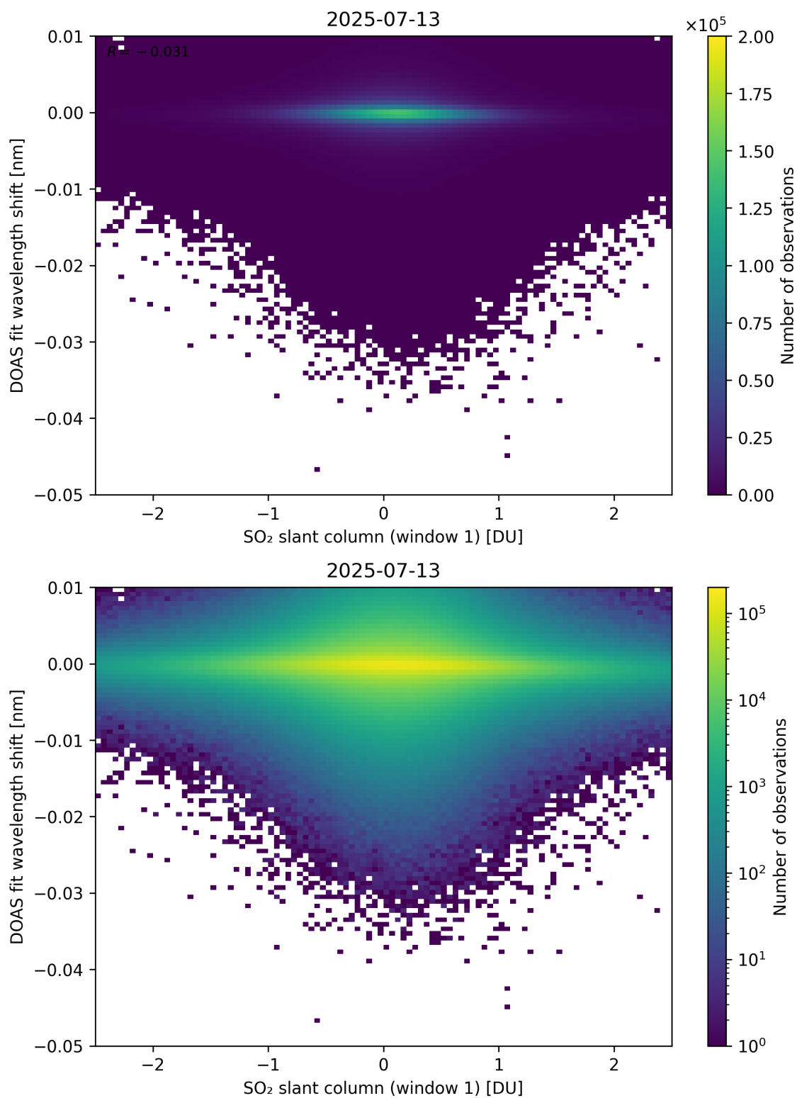
Figure 265: Scatter density plot of “SO 2 slant column (window 1)” against “DOAS fit wavelength shift” for 2025-07-13 to 2025-07-14.
