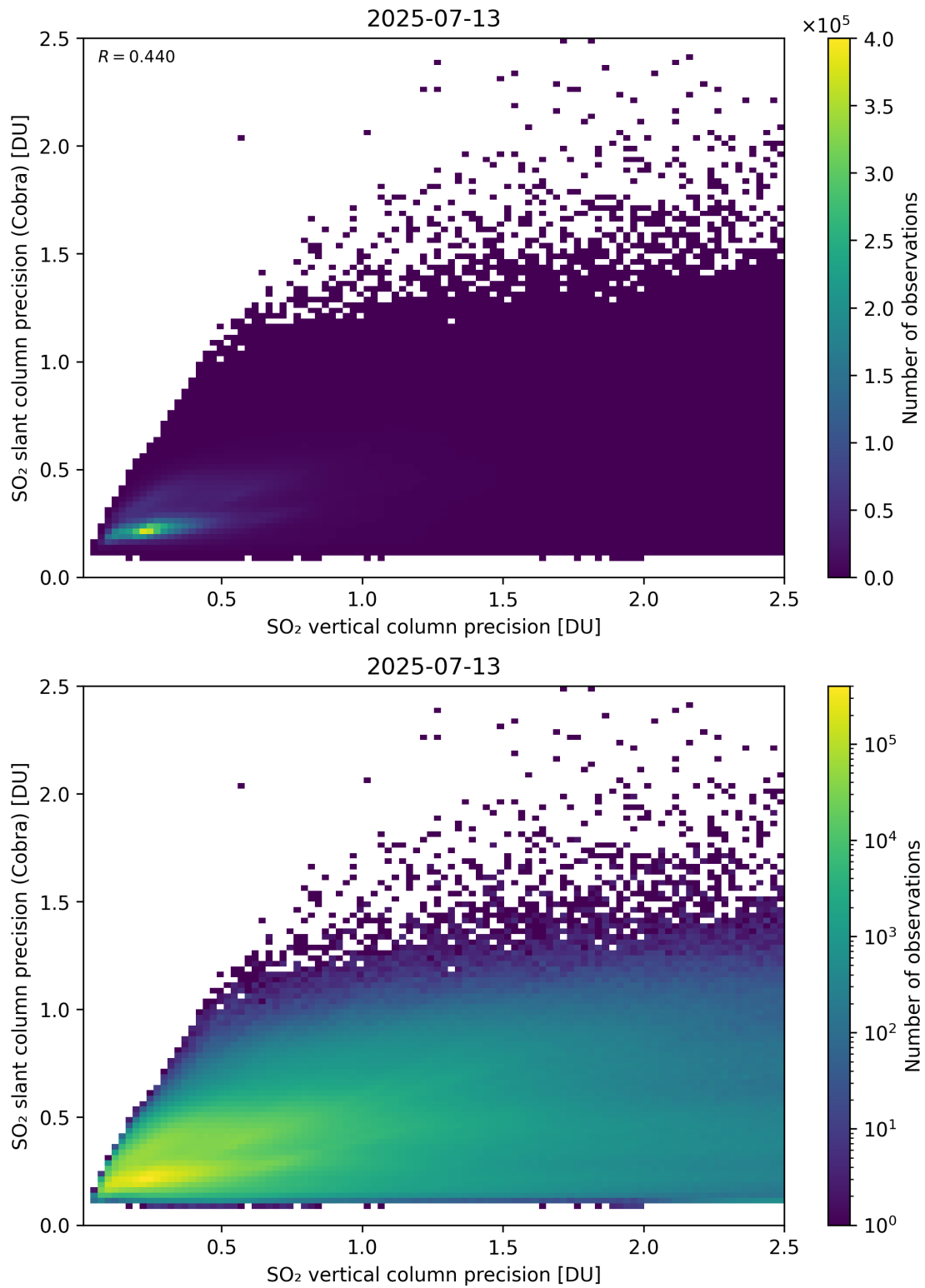
Figure 337: Scatter density plot of “SO 2 vertical column precision” against “SO 2 slant column precision (Cobra)” for 2025-07-13 to 2025-07-14.
