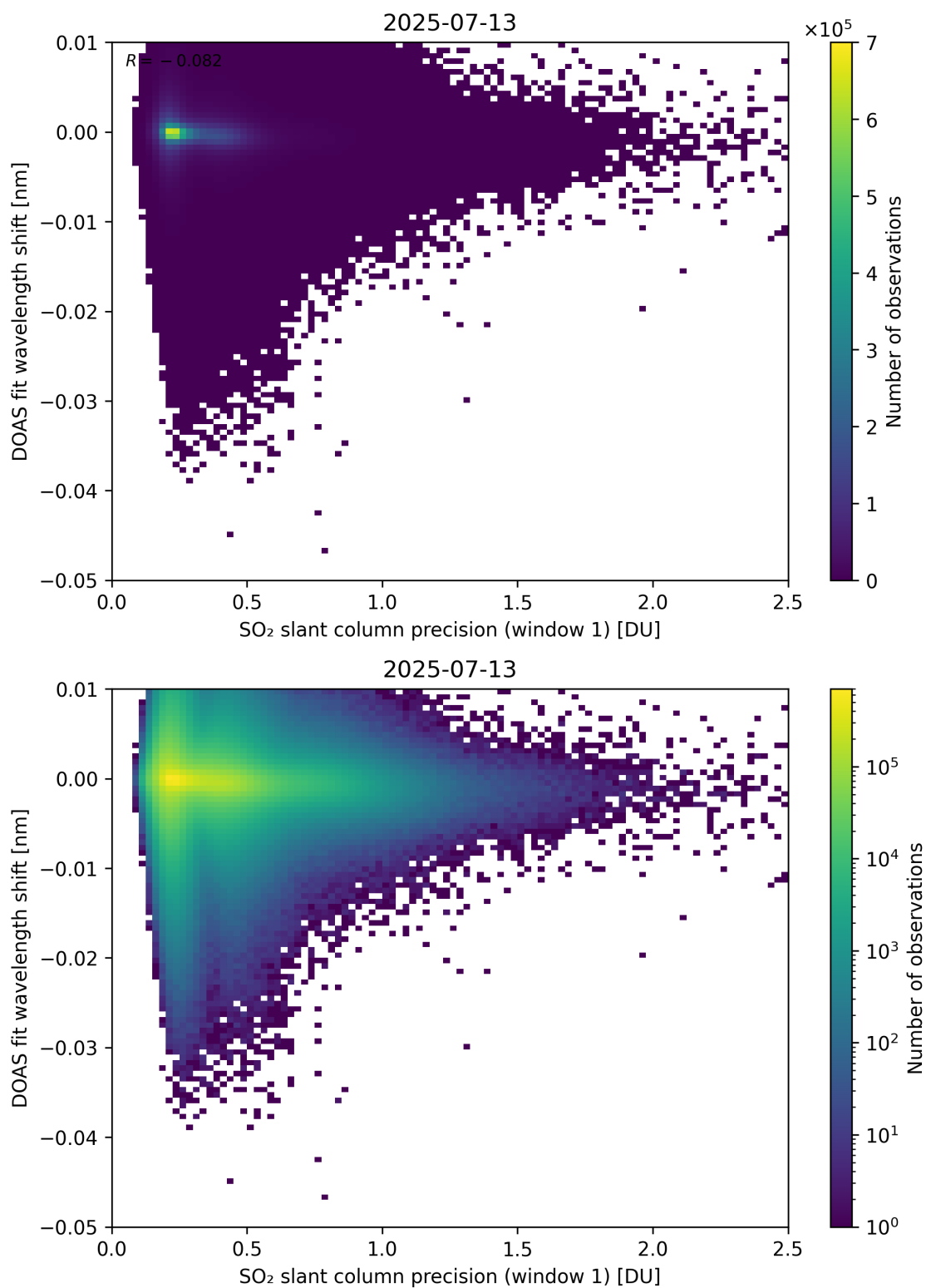
Figure 271: Scatter density plot of “SO 2 slant column precision (window 1)” against “DOAS fit wavelength shift” for 2025-07-13 to 2025-07-14.
