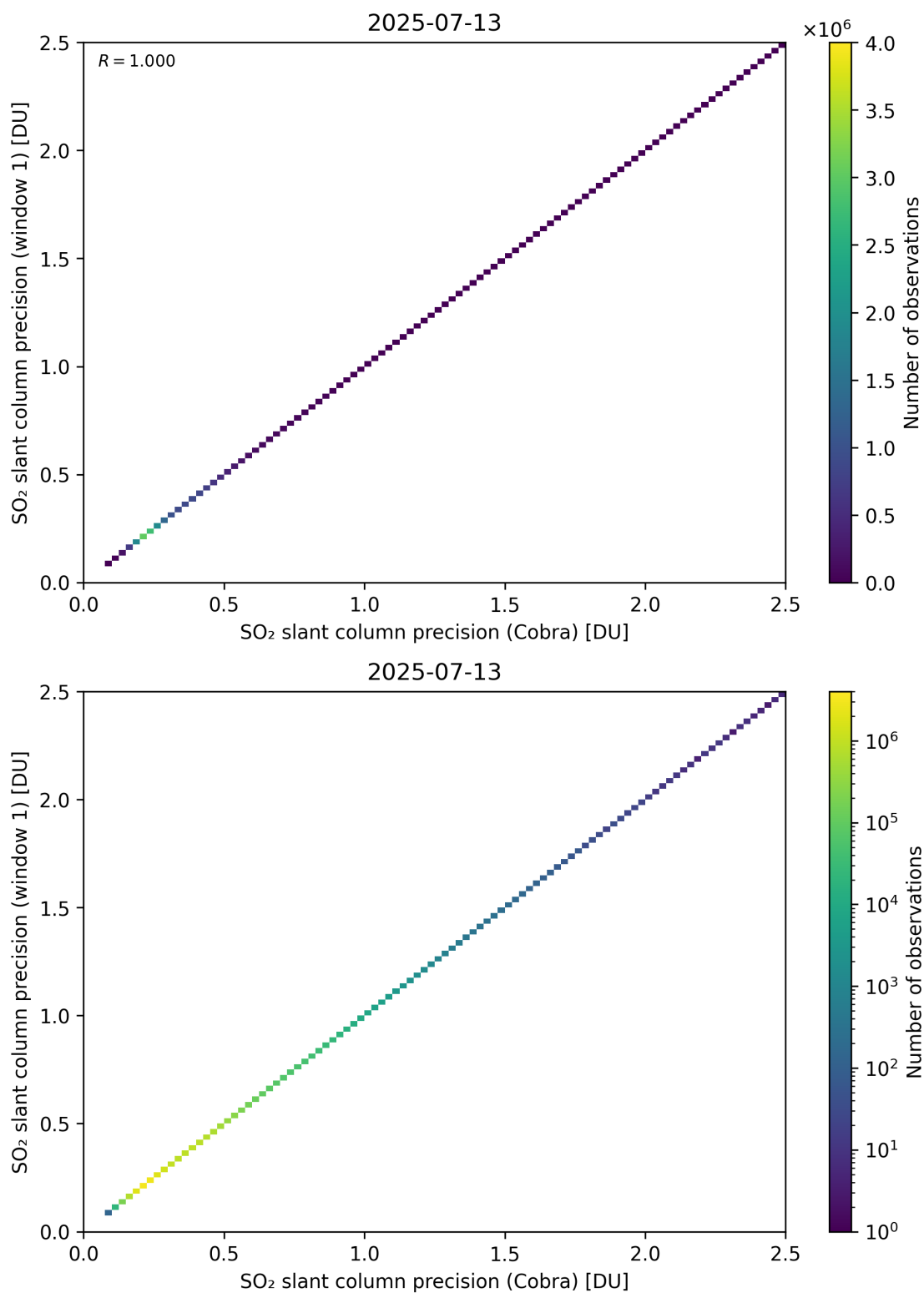
Figure 209: Scatter density plot of “SO 2 slant column precision (Cobra)” against “SO 2 slant column precision (window 1)” for 2025-07-13 to 2025-07-14.
