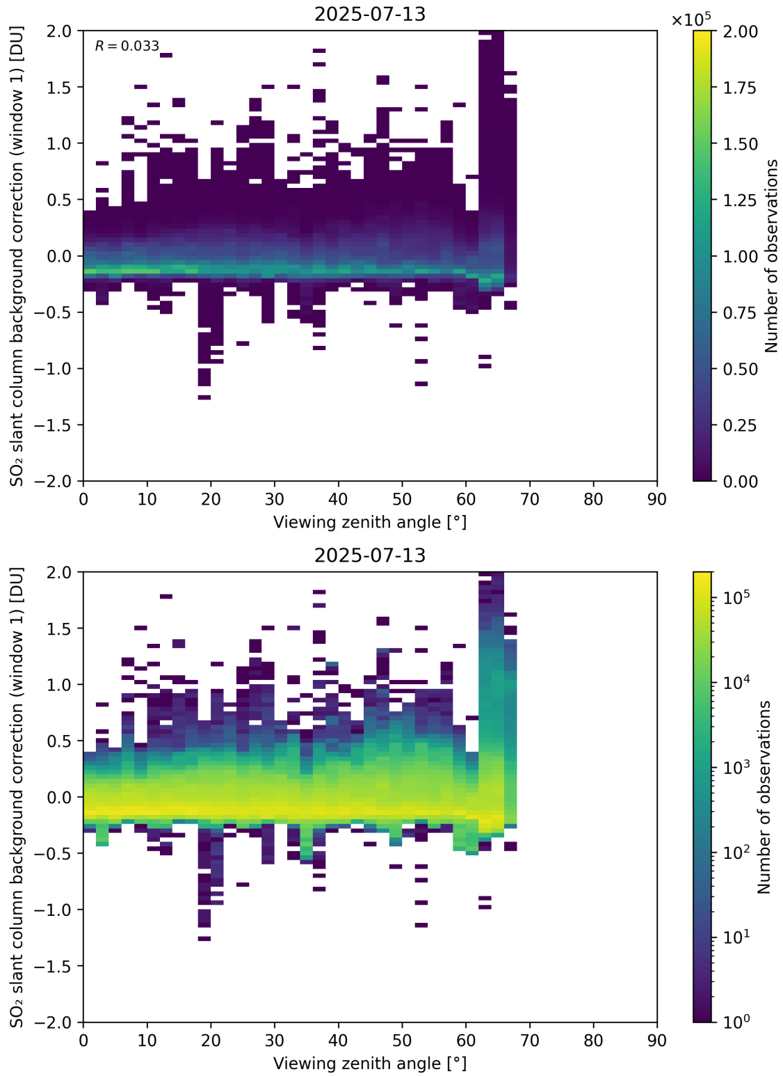
Figure 362: Scatter density plot of “Viewing zenith angle” against “SO 2 slant column background correction (window 1)” for 2025-07-13 to 2025-07-14.
