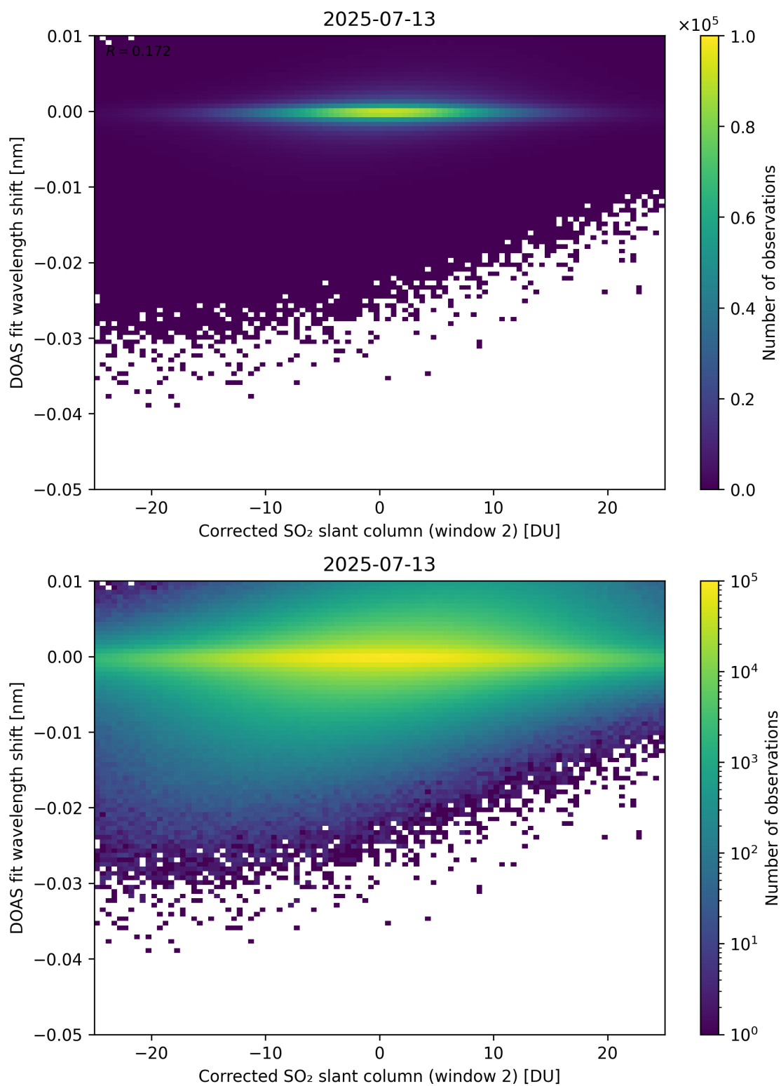
Figure 246: Scatter density plot of “Corrected SO 2 slant column (window 2)” against “DOAS fit wavelength shift” for 2025-07-13 to 2025-07-14.
