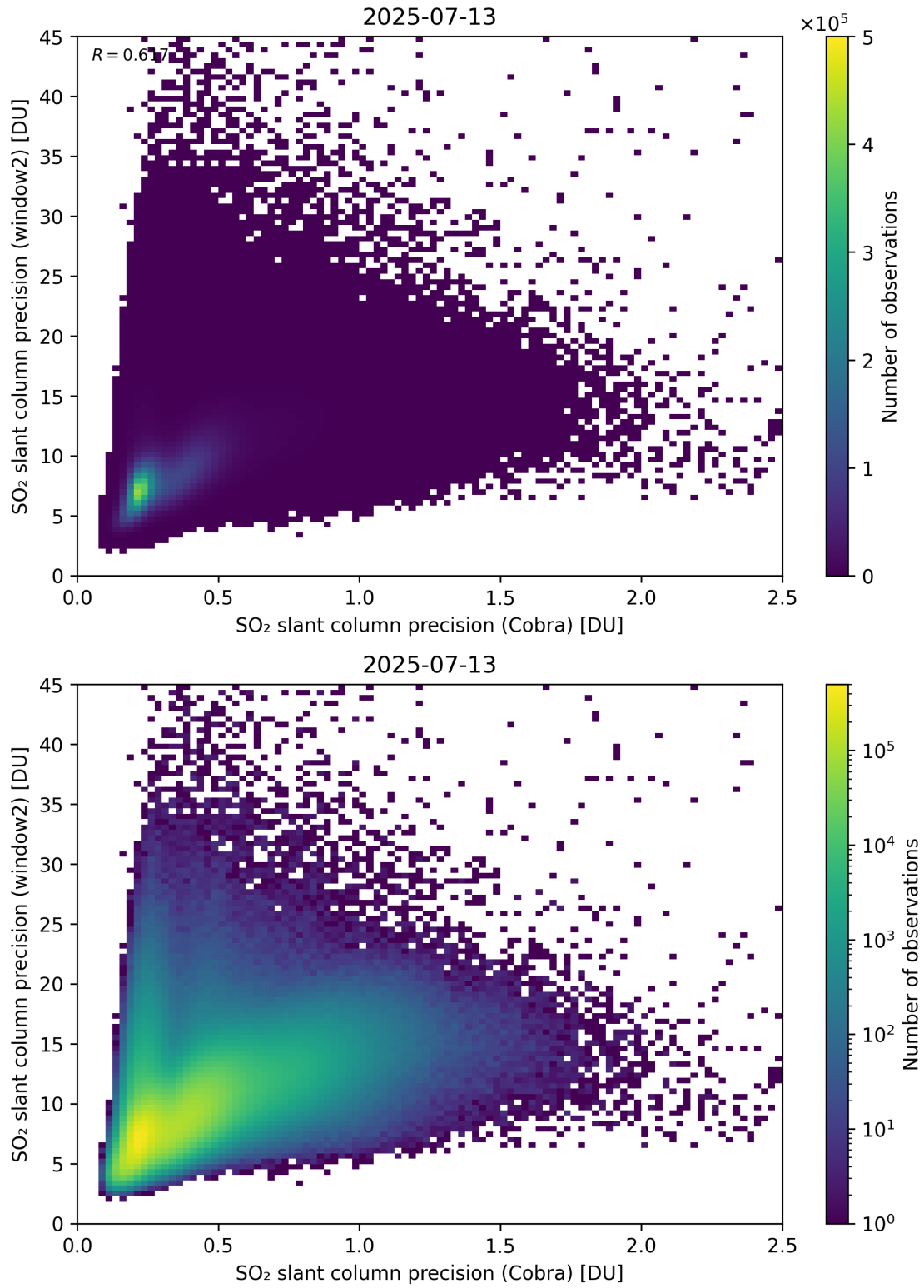
Figure 210: Scatter density plot of “SO 2 slant column precision (Cobra)” against “SO 2 slant column precision (window2)” for 2025-07-13 to 2025-07-14.
