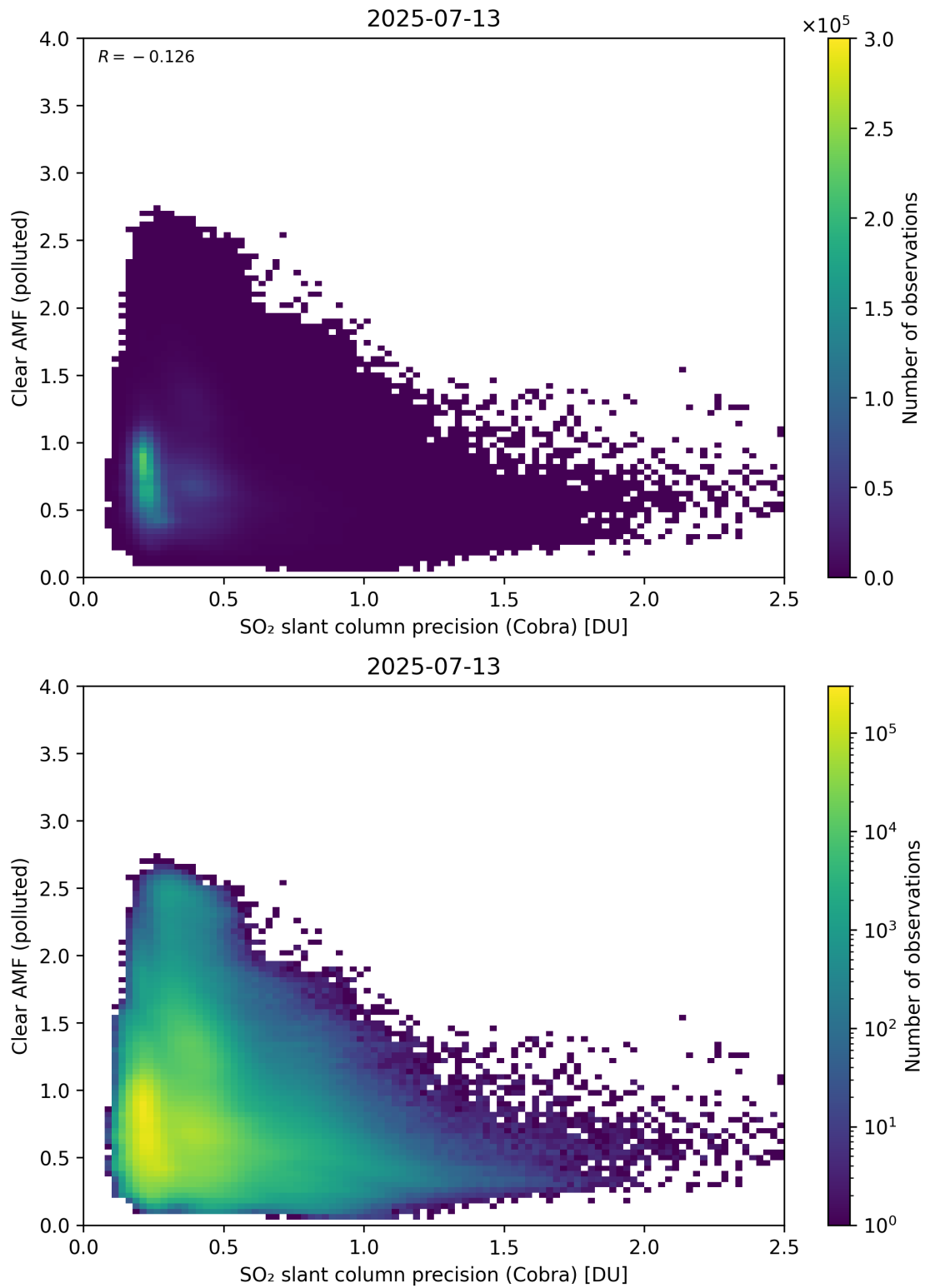
Figure 205: Scatter density plot of “SO 2 slant column precision (Cobra)” against “Clear AMF (polluted)” for 2025-07-13 to 2025-07-14.
