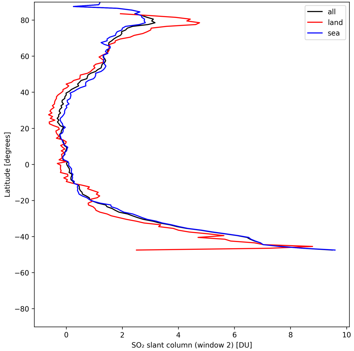
Figure 41: Zonal average of “SO 2 slant column (window 2)” for 2025-07-13 to 2025-07-14.
