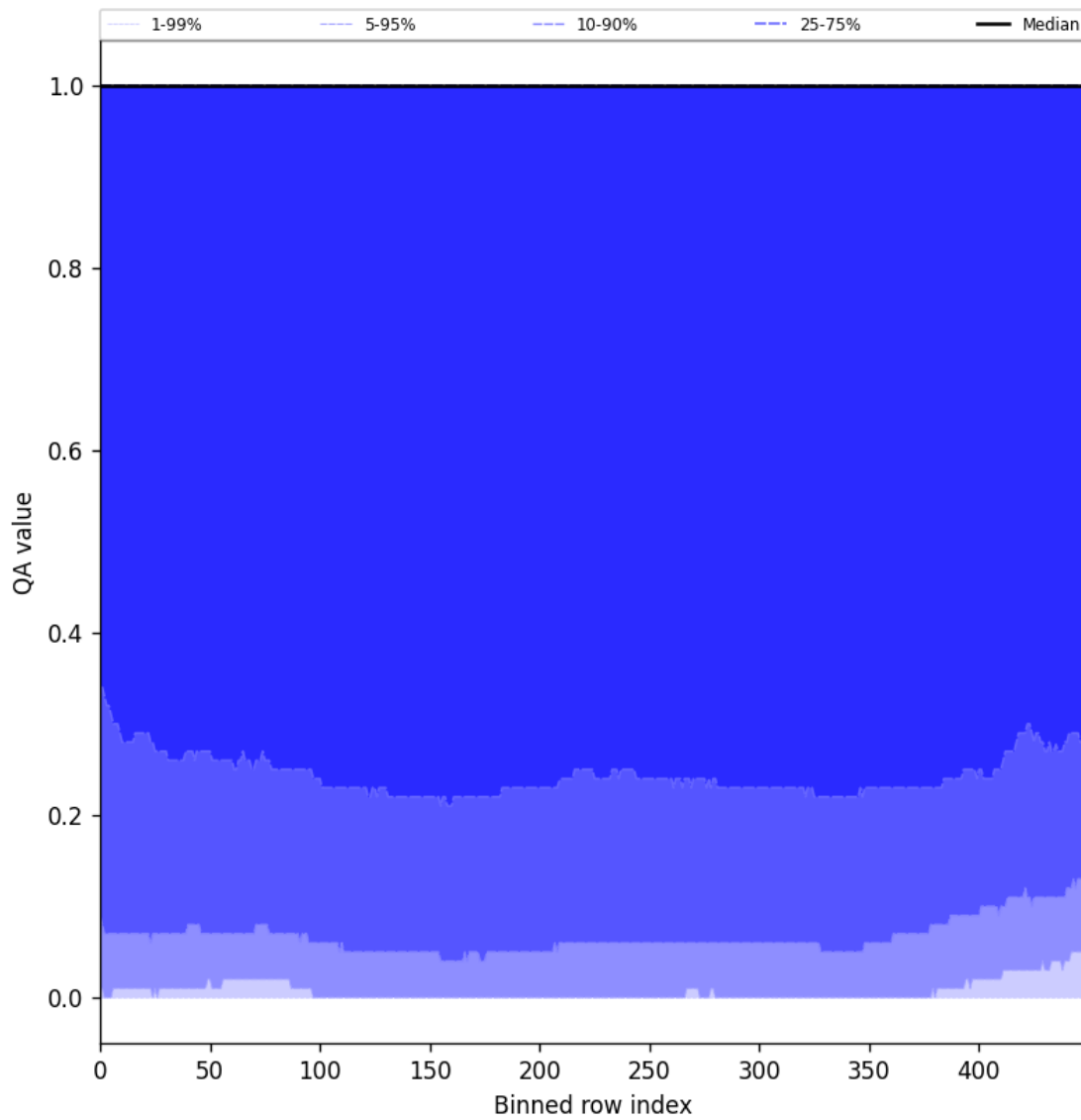
Figure 83: Along track statistics of “QA value” for 2025-07-13 to 2025-07-14
