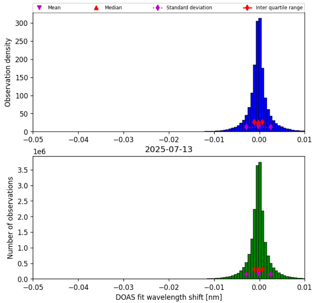
Figure 76: Histogram of “DOAS fit wavelength shift” for 2025-07-13 to 2025-07-14
