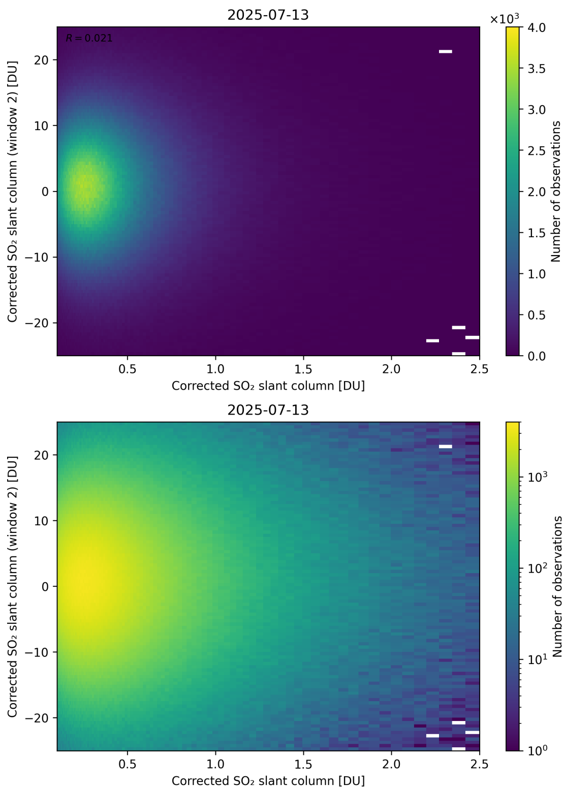
Figure 235: Scatter density plot of “Corrected SO 2 slant column” against “Corrected SO 2 slant column (window 2)” for 2025-07-13 to 2025-07-14.
