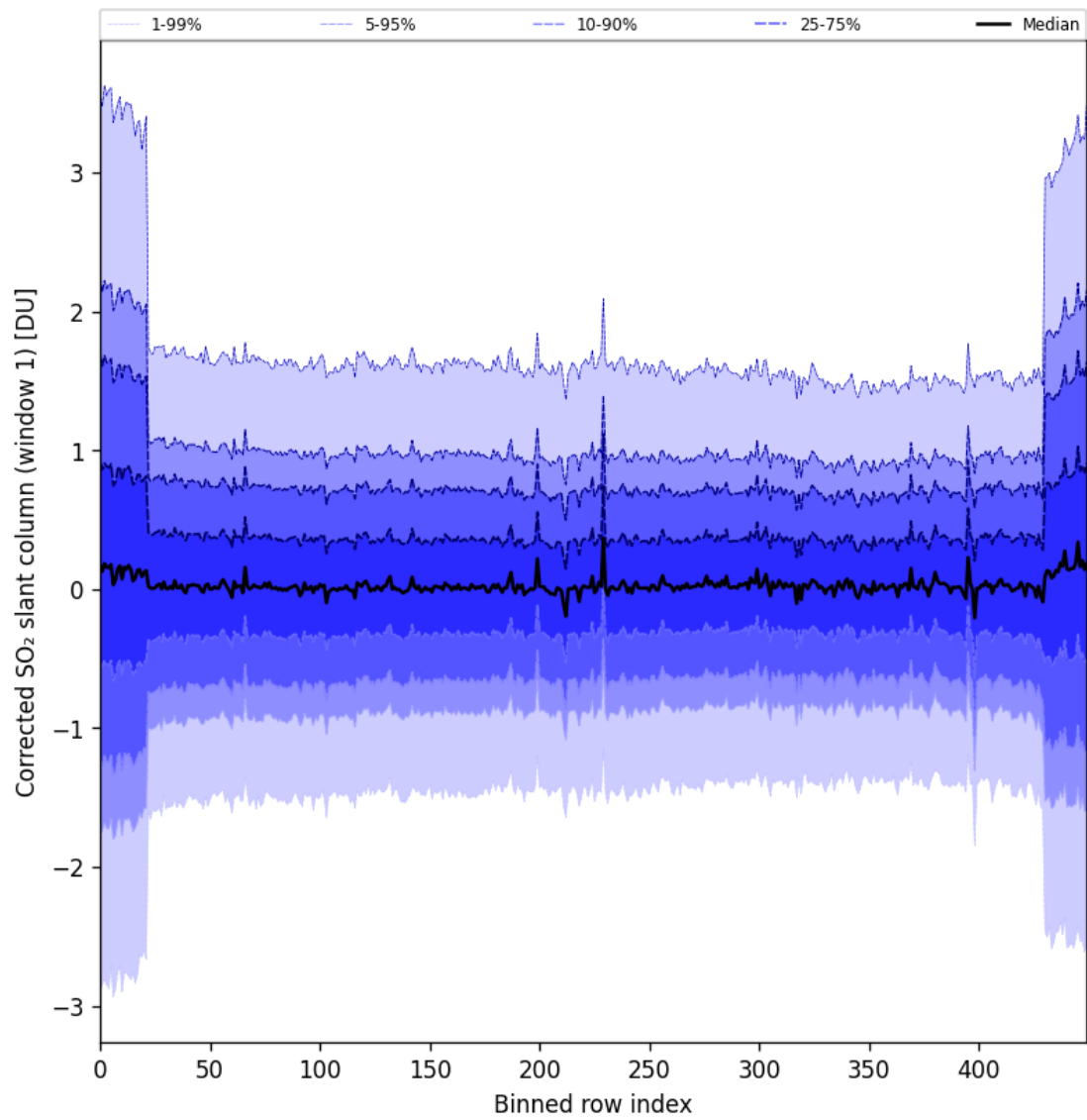
Figure 91: Along track statistics of “Corrected SO 2 slant column (window 1)” for 2025-07-13 to 2025-07-14
