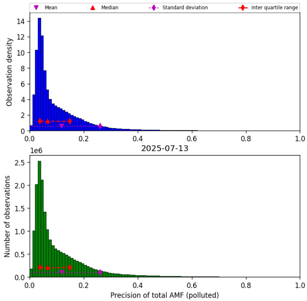
Figure 80: Histogram of “Precision of total AMF (polluted)” for 2025-07-13 to 2025-07-14
