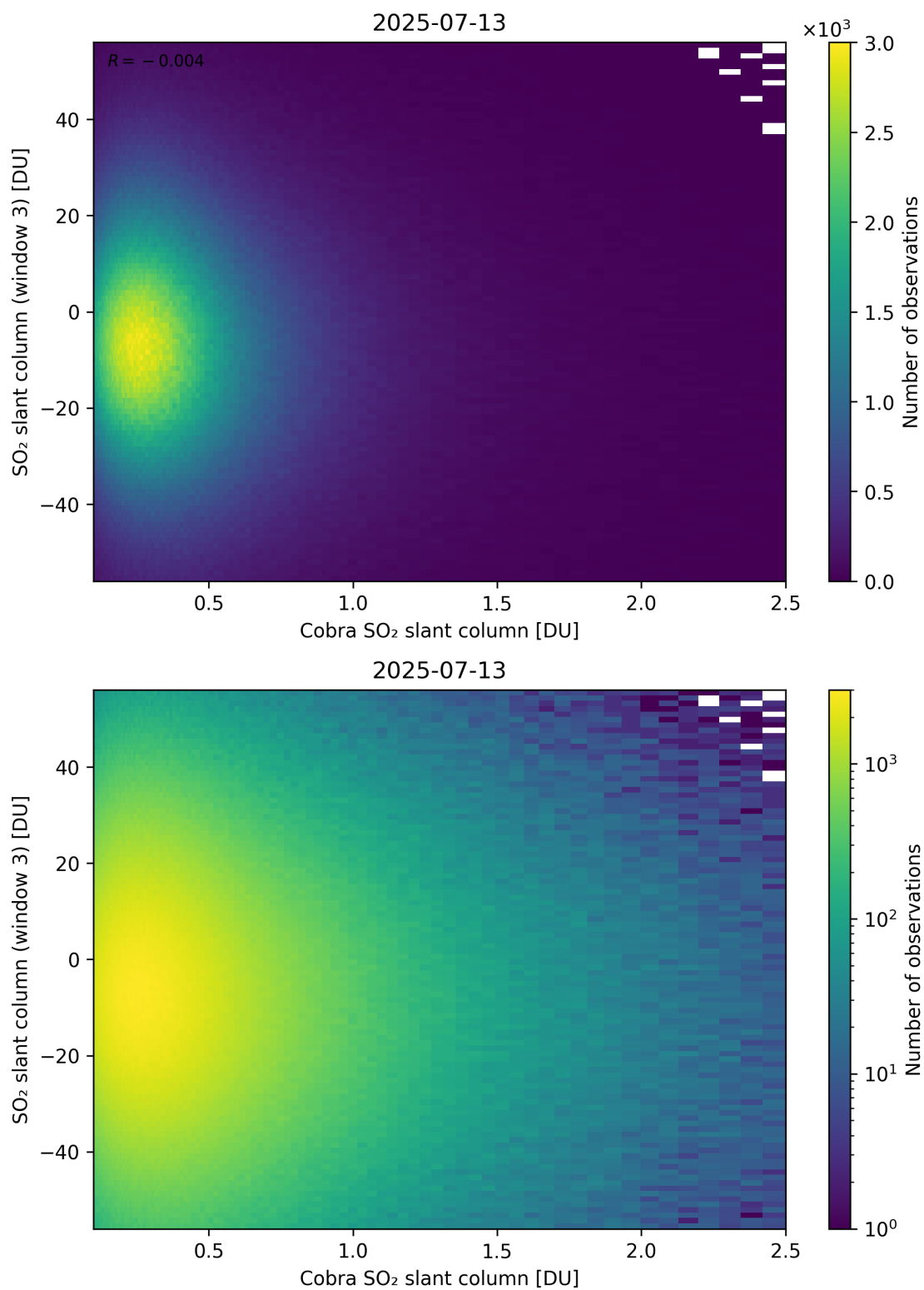
Figure 222: Scatter density plot of “Cobra SO 2 slant column” against “SO 2 slant column (window 3)” for 2025-07-13 to 2025-07-14.
