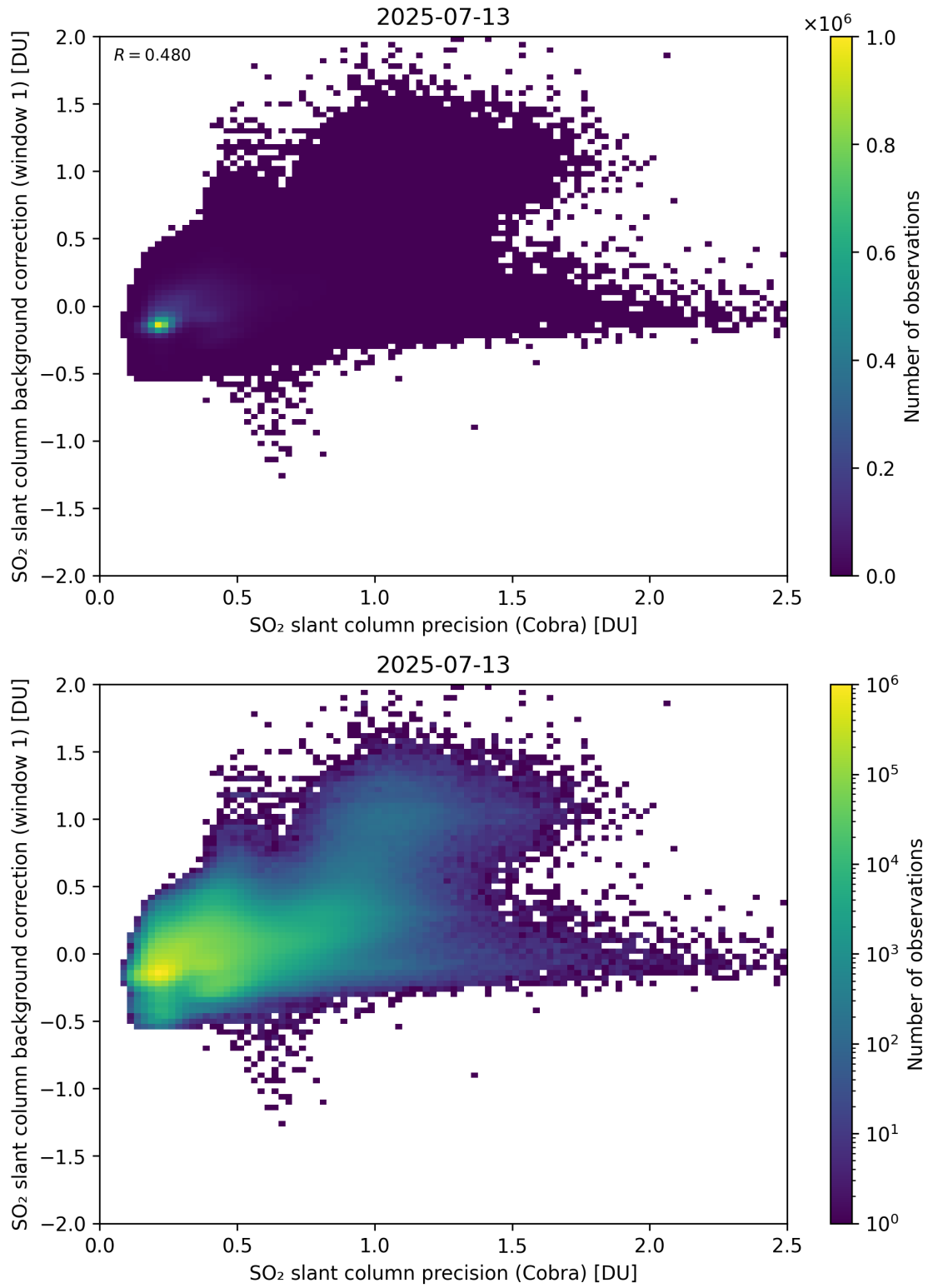
Figure 199: Scatter density plot of “SO 2 slant column precision (Cobra)” against “SO 2 slant column background correction (window 1)” for 2025-07-13 to 2025-07-14.
