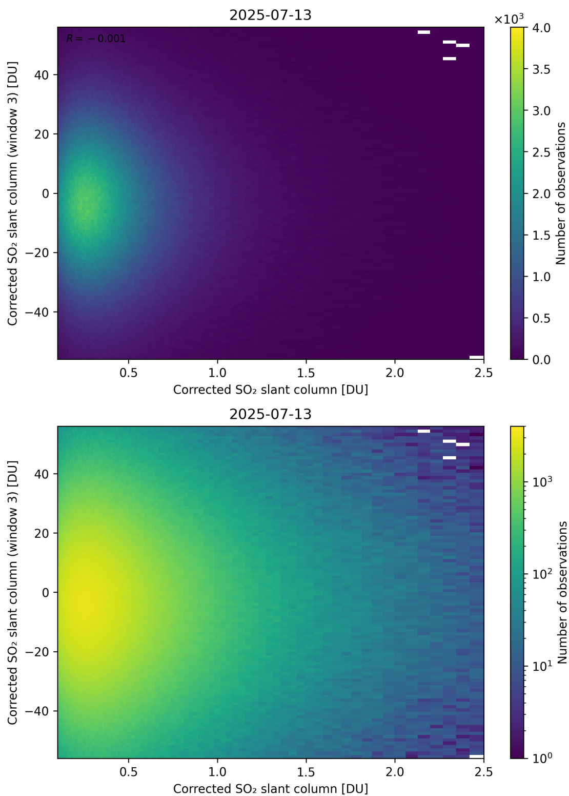
Figure 236: Scatter density plot of “Corrected SO 2 slant column” against “Corrected SO 2 slant column (window 3)” for 2025-07-13 to 2025-07-14.
