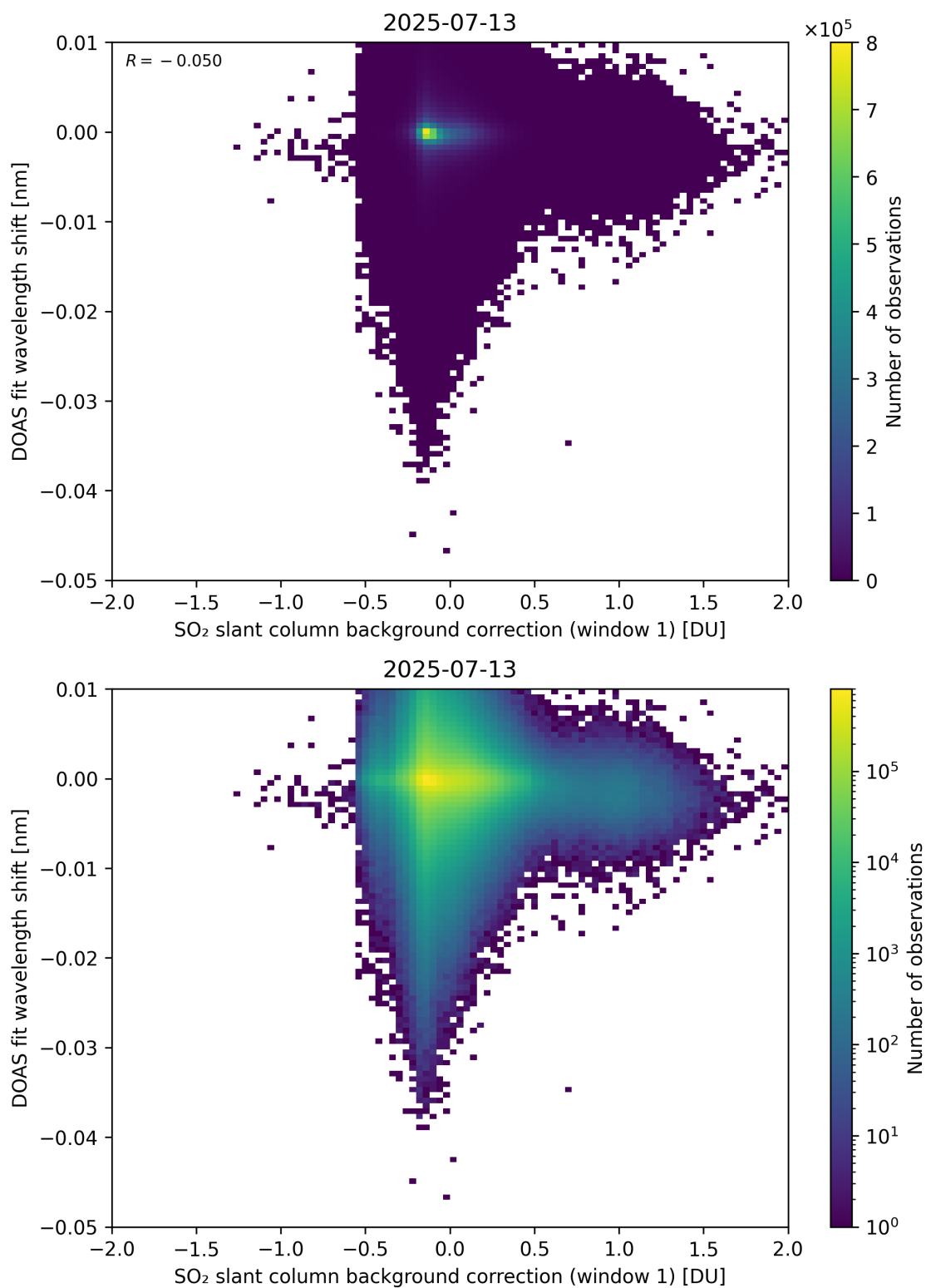
Figure 111: Scatter density plot of “SO 2 slant column background correction (window 1)” against “DOAS fit wavelength shift” for 2025-07-13 to 2025-07-14.
