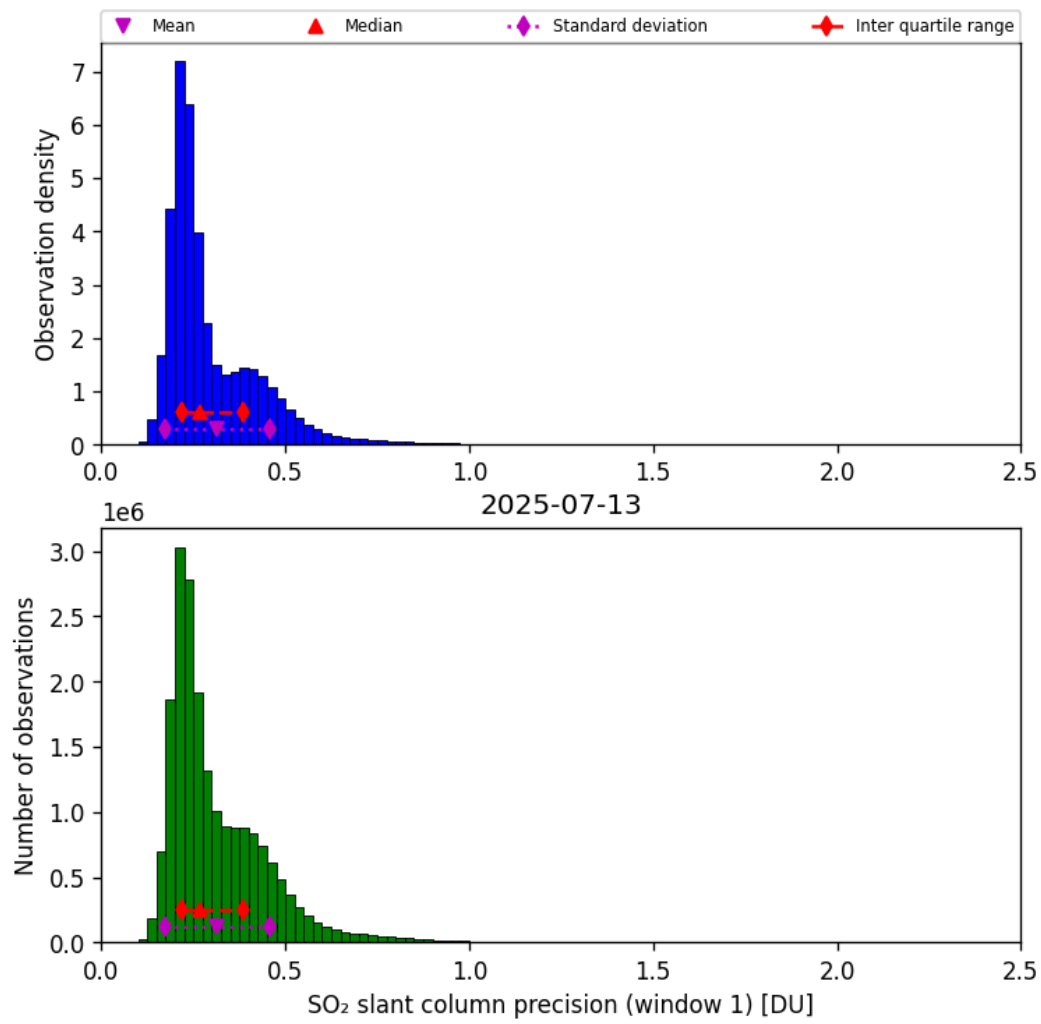
Figure 64: Histogram of “SO 2 slant column precision (window 1)” for 2025-07-13 to 2025-07-14
