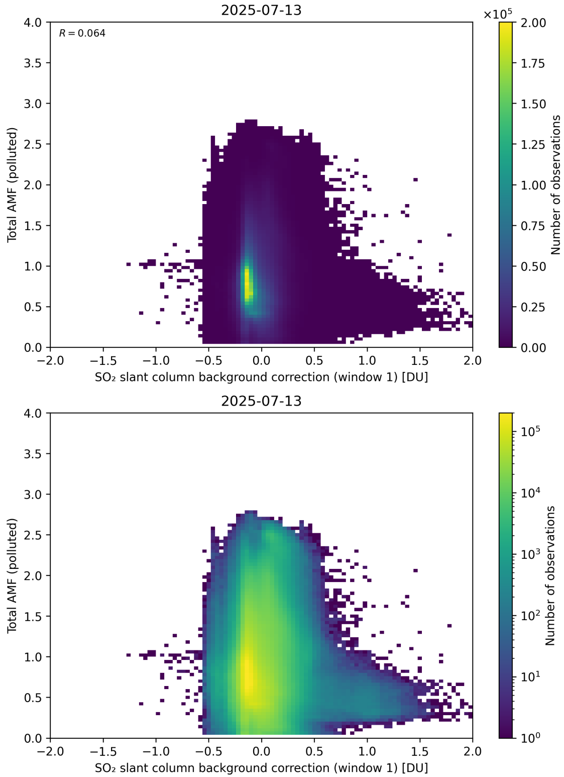
Figure 120: Scatter density plot of “SO 2 slant column background correction (window 1)” against “Total AMF (polluted)” for 2025-07-13 to 2025-07-14.
