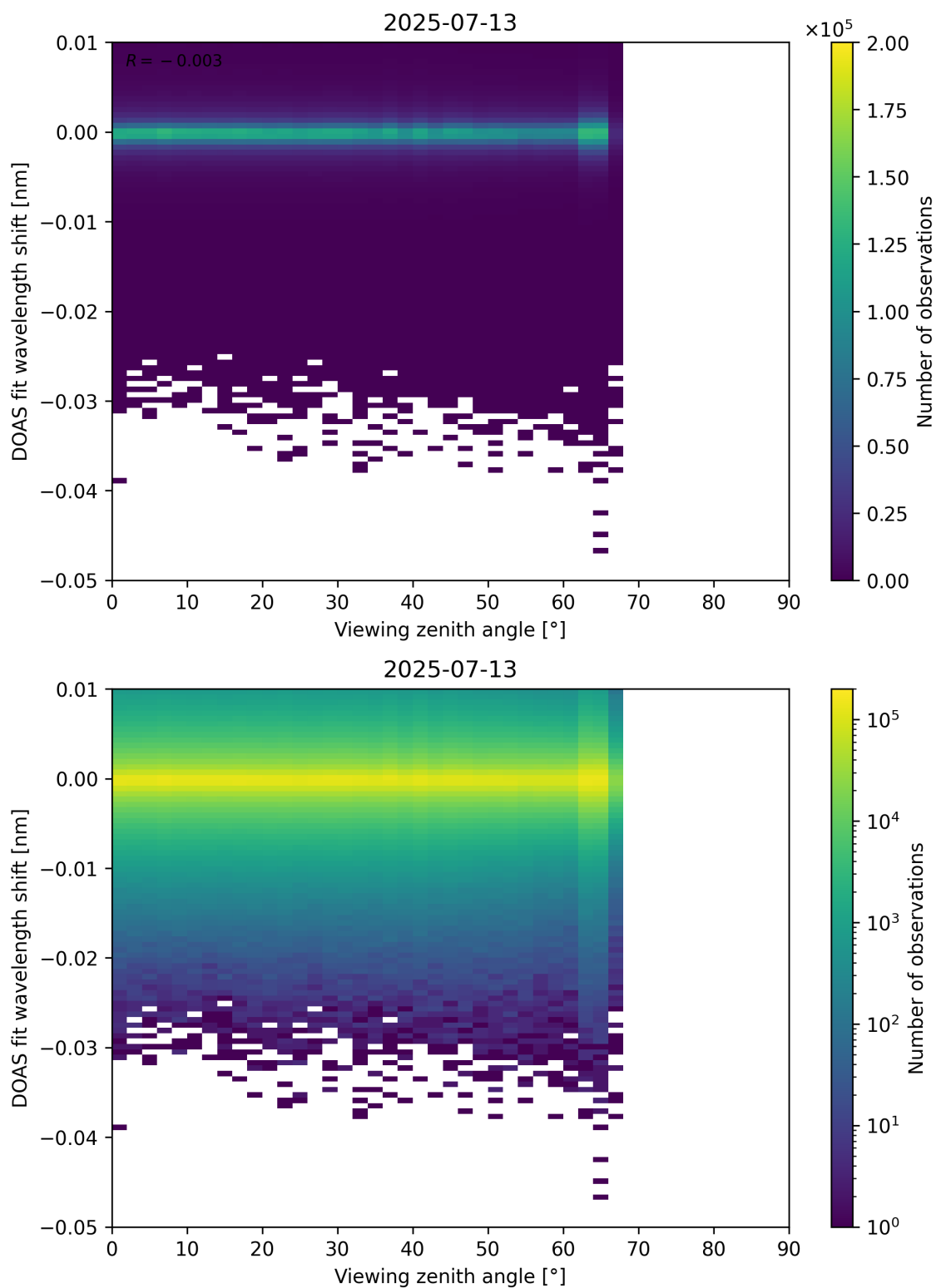
Figure 365: Scatter density plot of “Viewing zenith angle” against “DOAS fit wavelength shift” for 2025-07-13 to 2025-07-14.
