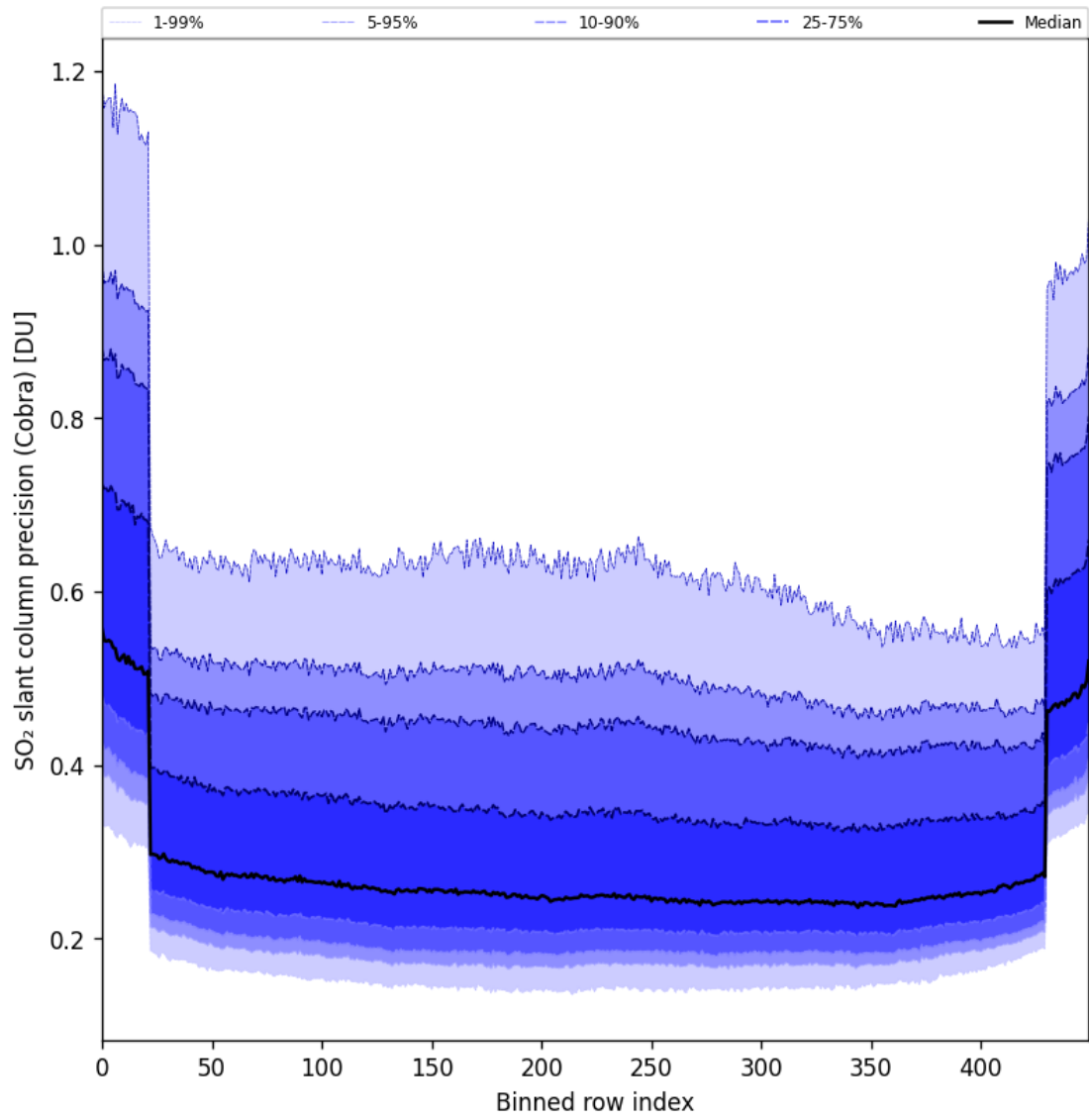
Figure 88: Along track statistics of “SO 2 slant column precision (Cobra)” for 2025-07-13 to 2025-07-14
