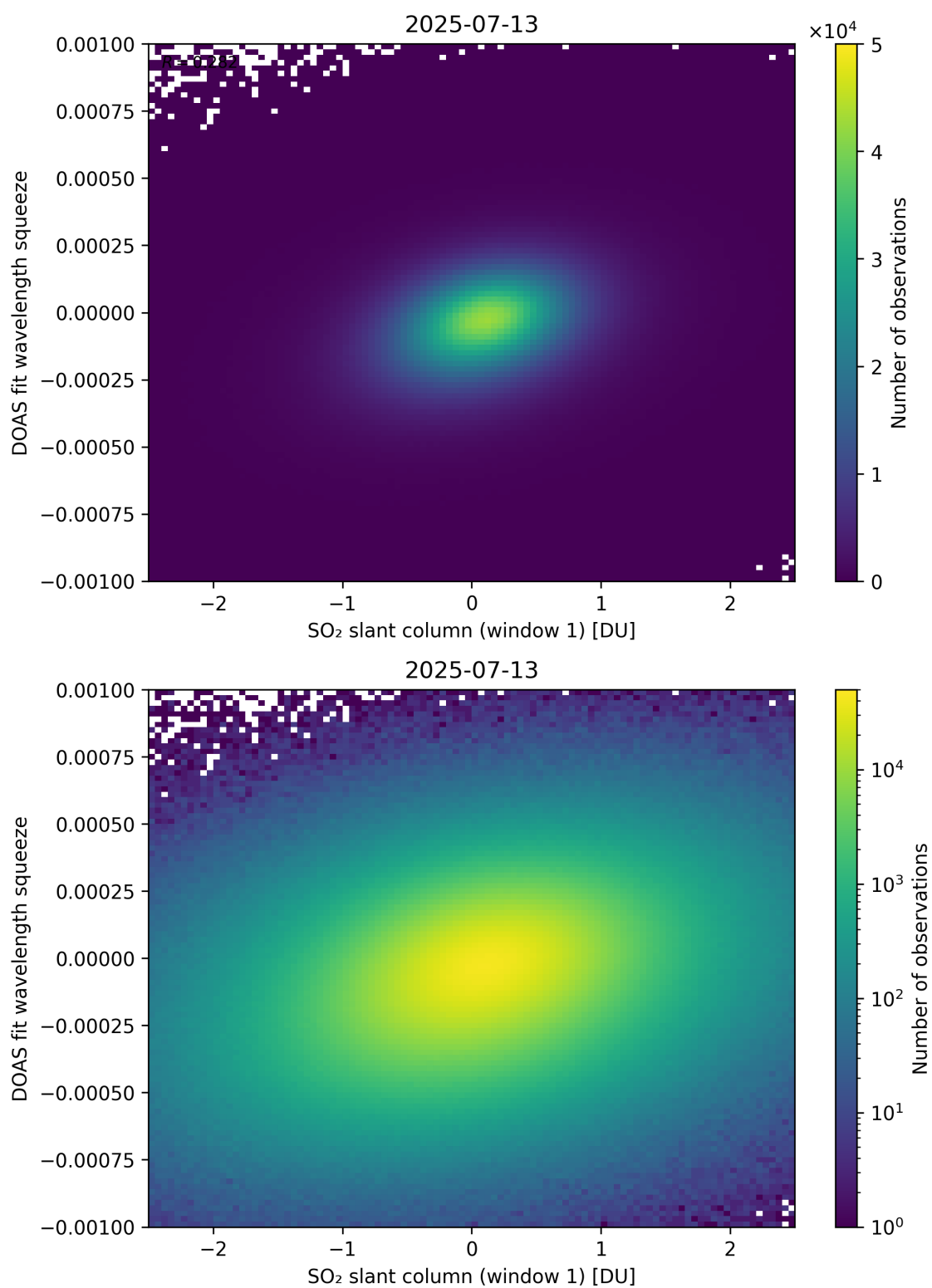
Figure 266: Scatter density plot of “SO 2 slant column (window 1)” against “DOAS fit wavelength squeeze” for 2025-07-13 to 2025-07-14.
