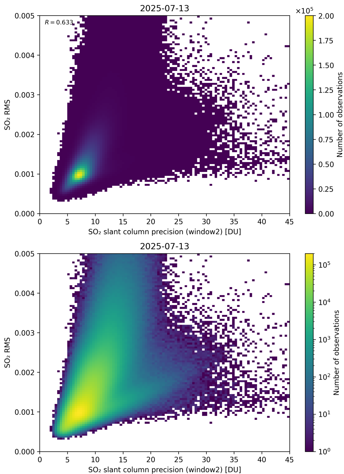
Figure 295: Scatter density plot of “SO 2 slant column precision (window2)” against “SO 2 RMS” for 2025-07-13 to 2025-07-14.
