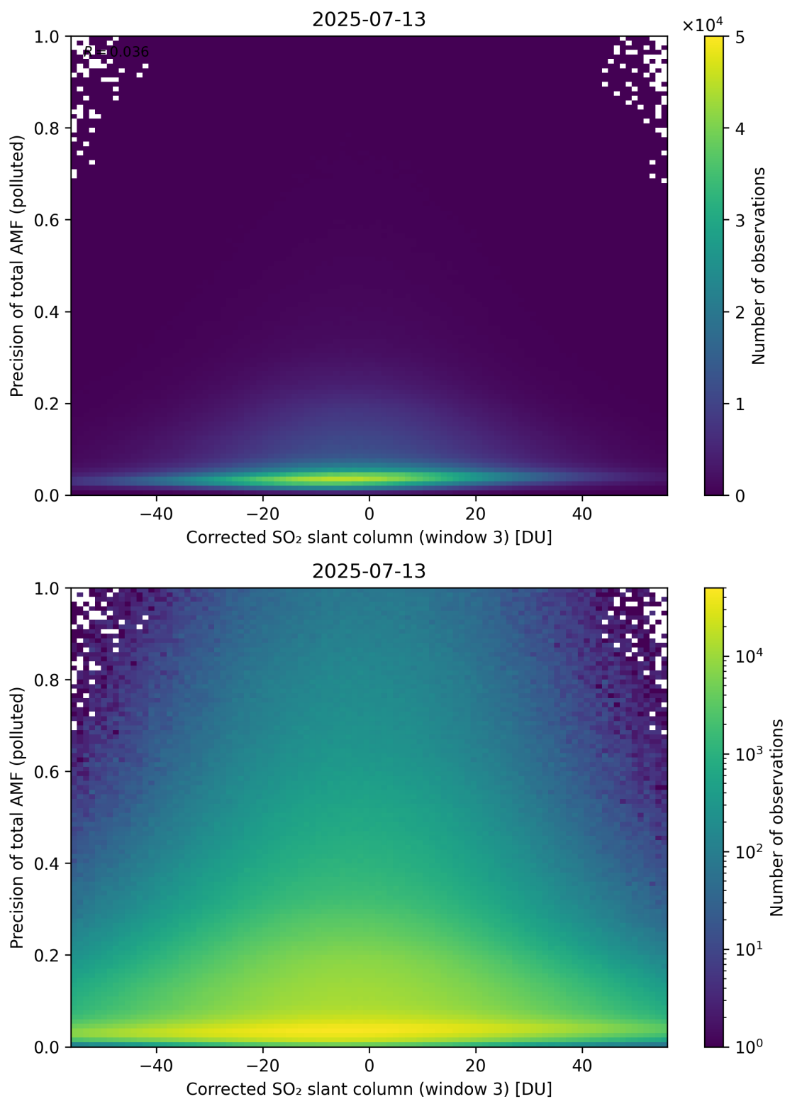
Figure 261: Scatter density plot of “Corrected SO 2 slant column (window 3)” against “Precision of total AMF (polluted)” for 2025-07-13 to 2025-07-14.
