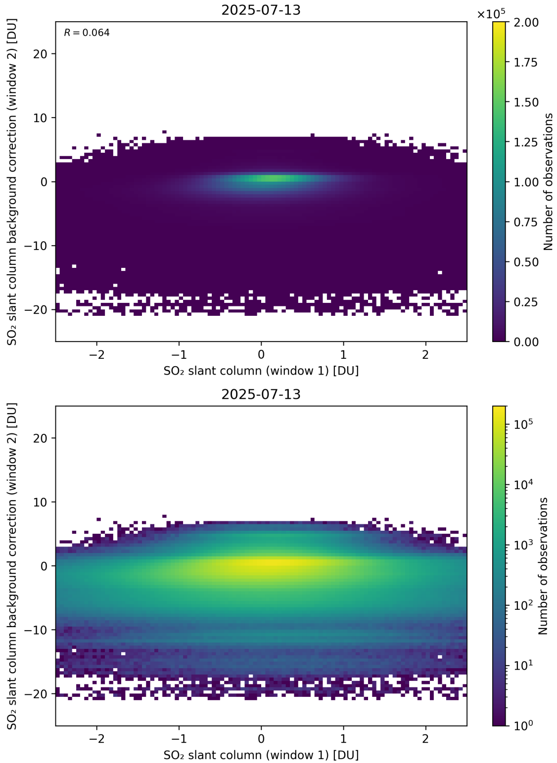
Figure 263: Scatter density plot of “SO 2 slant column (window 1)” against “SO 2 slant column background correction (window 2)” for 2025-07-13 to 2025-07-14.
