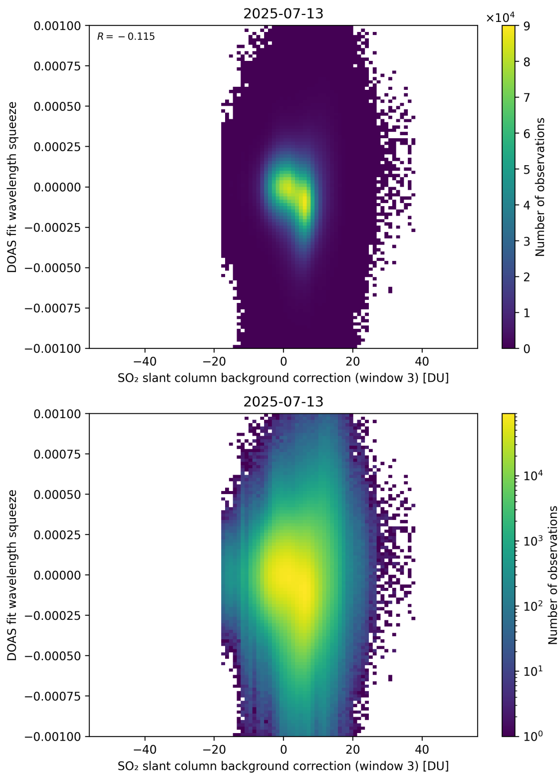
Figure 133: Scatter density plot of “SO 2 slant column background correction (window 3)” against “DOAS fit wavelength squeeze” for 2025-07-13 to 2025-07-14.
