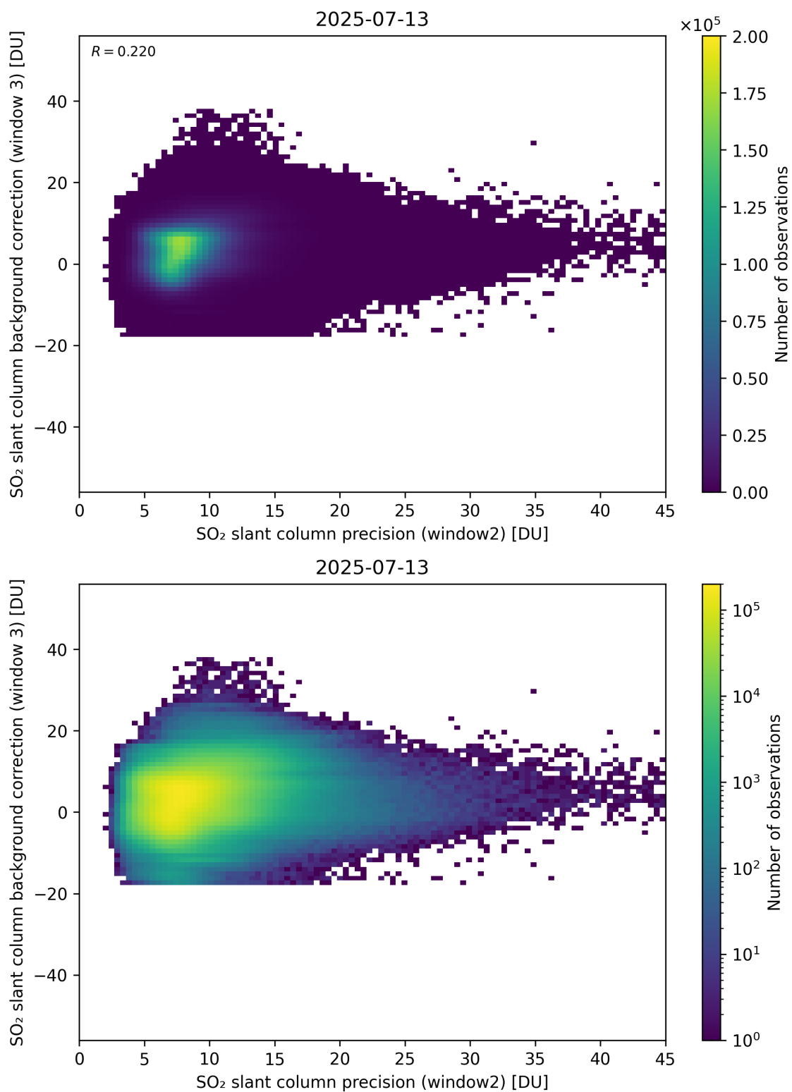
Figure 292: Scatter density plot of “SO 2 slant column precision (window2)” against “SO 2 slant column background correction (window 3)” for 2025-07-13 to 2025-07-14.
