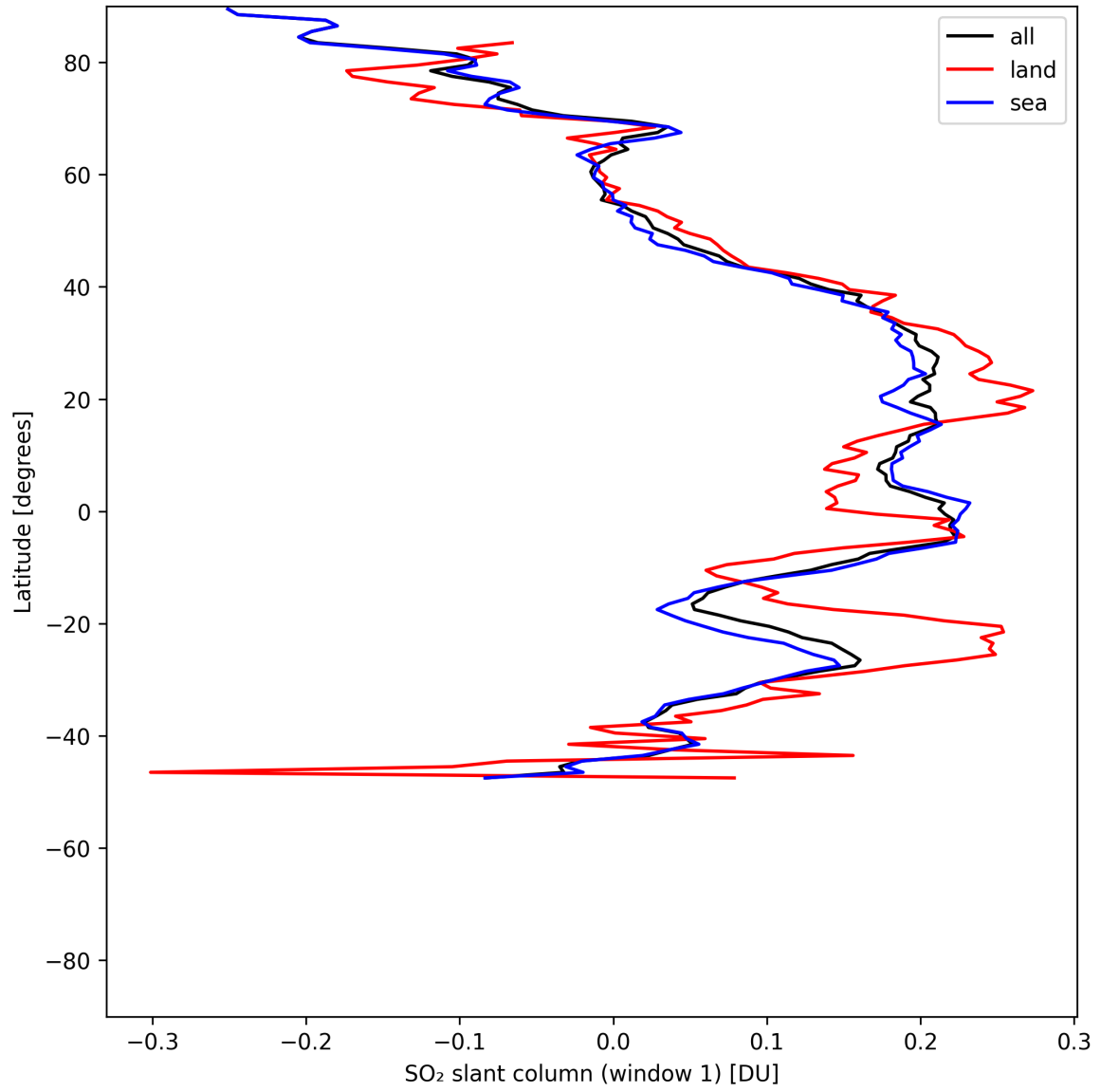
Figure 37: Zonal average of “SO 2 slant column (window 1)” for 2025-07-13 to 2025-07-14.
