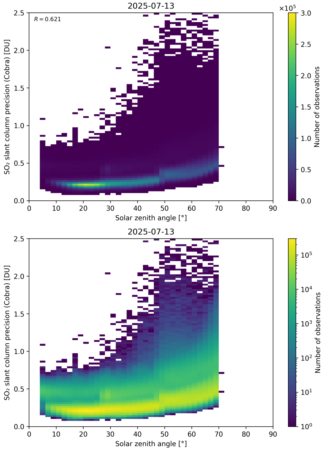
Figure 180: Scatter density plot of “Solar zenith angle” against “SO 2 slant column precision (Cobra)” for 2025-07-13 to 2025-07-14.
