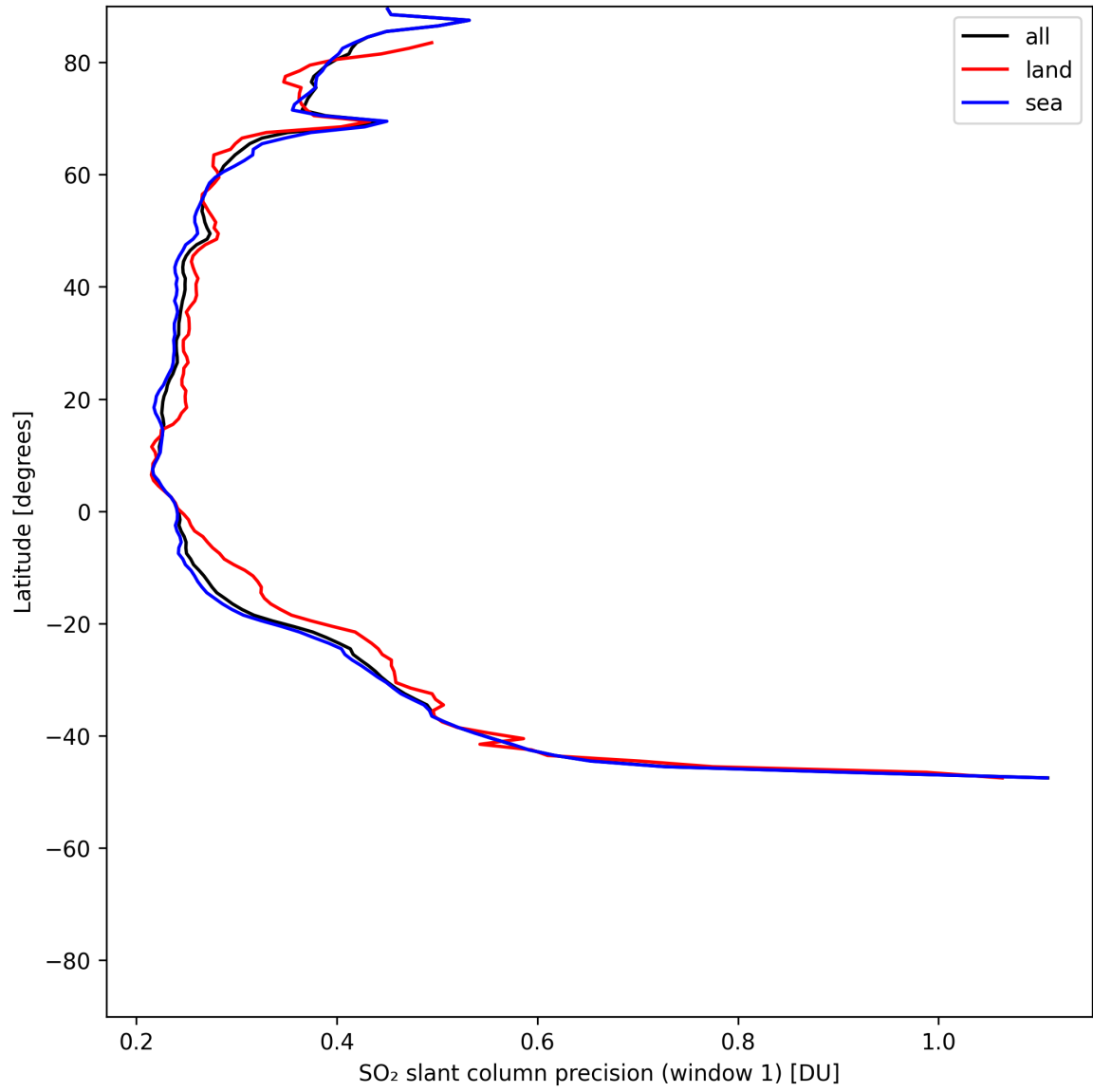
Figure 38: Zonal average of “SO 2 slant column precision (window 1)” for 2025-07-13 to 2025-07-14.
