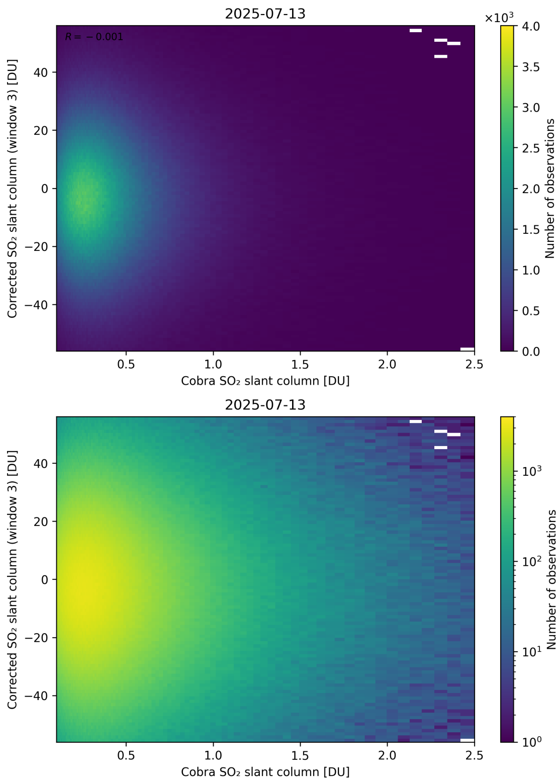
Figure 218: Scatter density plot of “Cobra SO 2 slant column” against “Corrected SO 2 slant column (window 3)” for 2025-07-13 to 2025-07-14.
