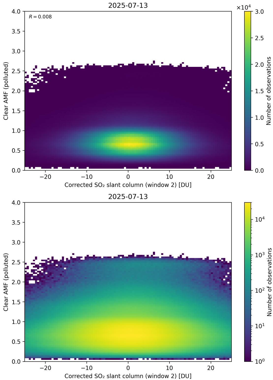
Figure 249: Scatter density plot of “Corrected SO 2 slant column (window 2)” against “Clear AMF (polluted)” for 2025-07-13 to 2025-07-14.
