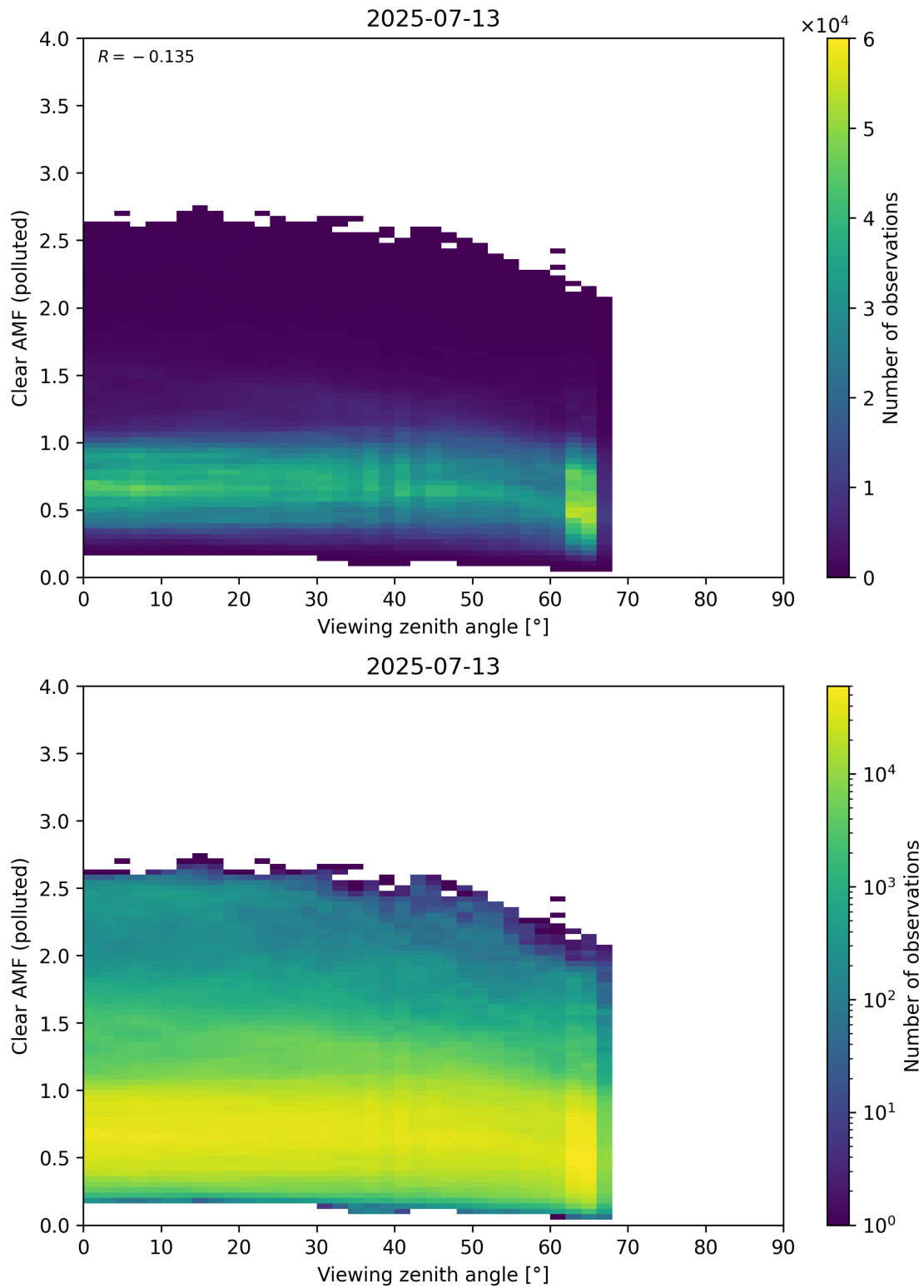
Figure 370: Scatter density plot of “Viewing zenith angle” against “Clear AMF (polluted)” for 2025-07-13 to 2025-07-14.
