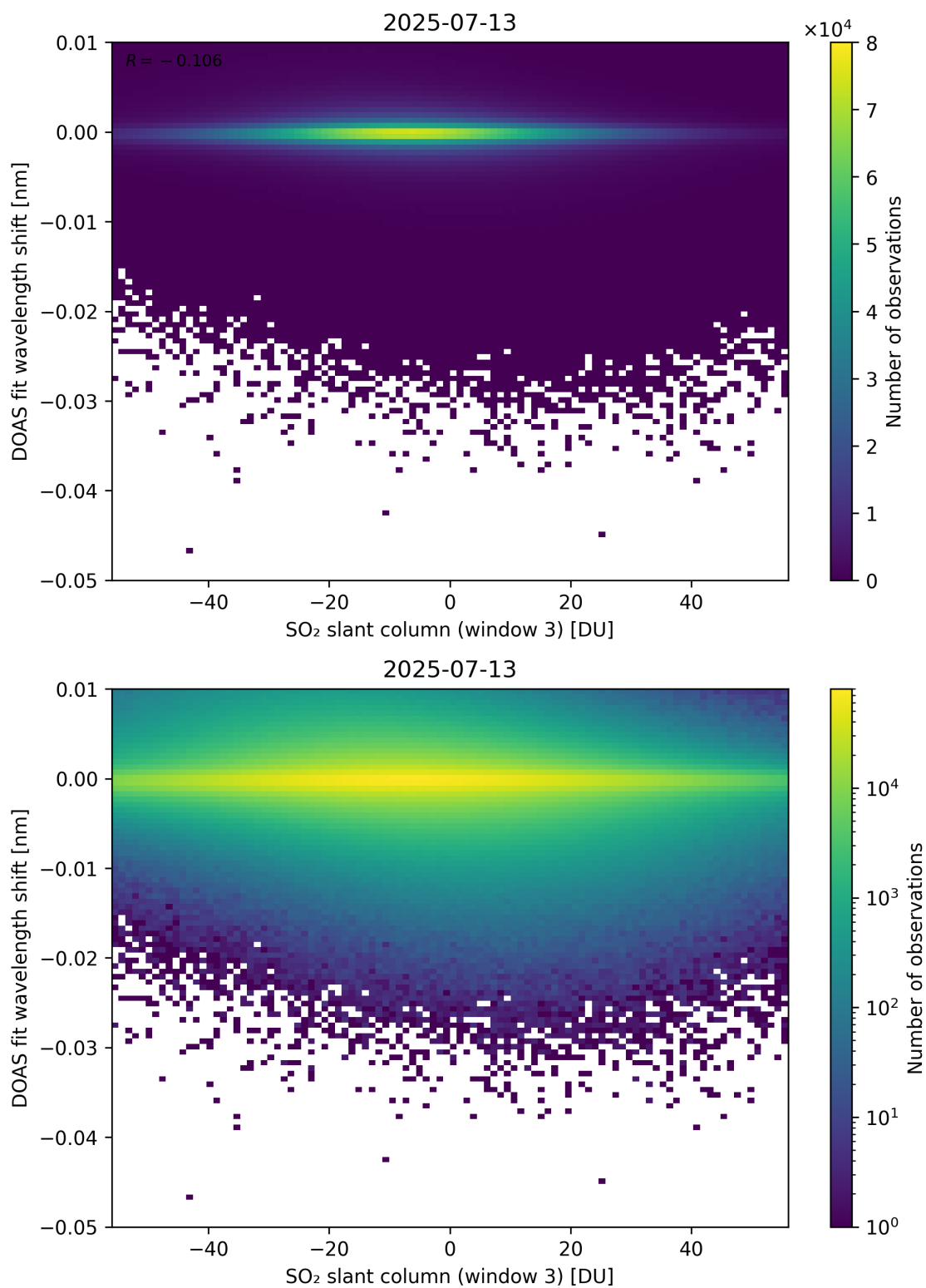
Figure 304: Scatter density plot of “SO 2 slant column (window 3)” against “DOAS fit wavelength shift” for 2025-07-13 to 2025-07-14.
