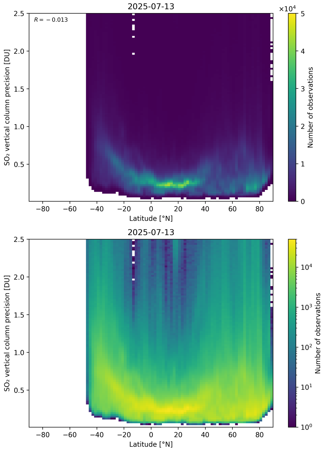
Figure 170: Scatter density plot of “Latitude” against “SO 2 vertical column precision” for 2025-07-13 to 2025-07-14.
