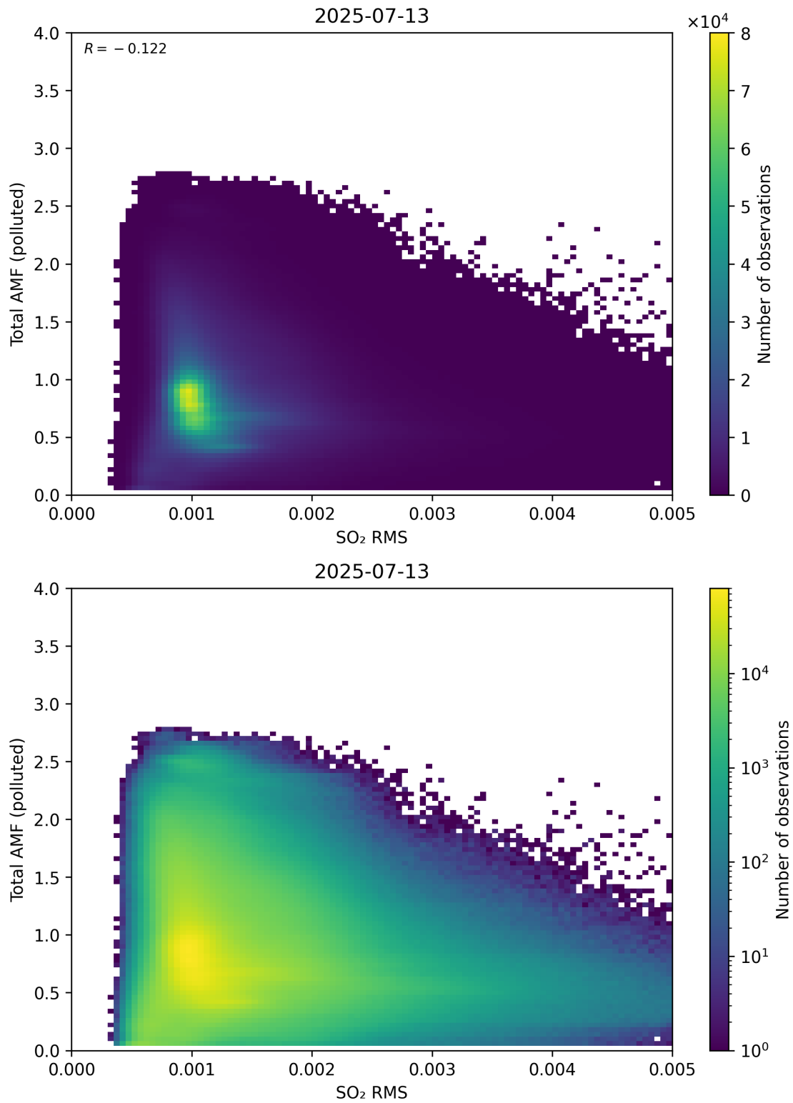
Figure 148: Scatter density plot of “SO 2 RMS” against “Total AMF (polluted)” for 2025-07-13 to 2025-07-14.
