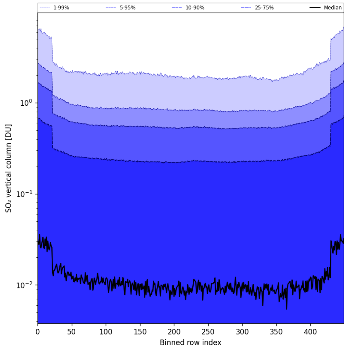
Figure 84: Along track statistics of “SO 2 vertical column” for 2025-07-13 to 2025-07-14
