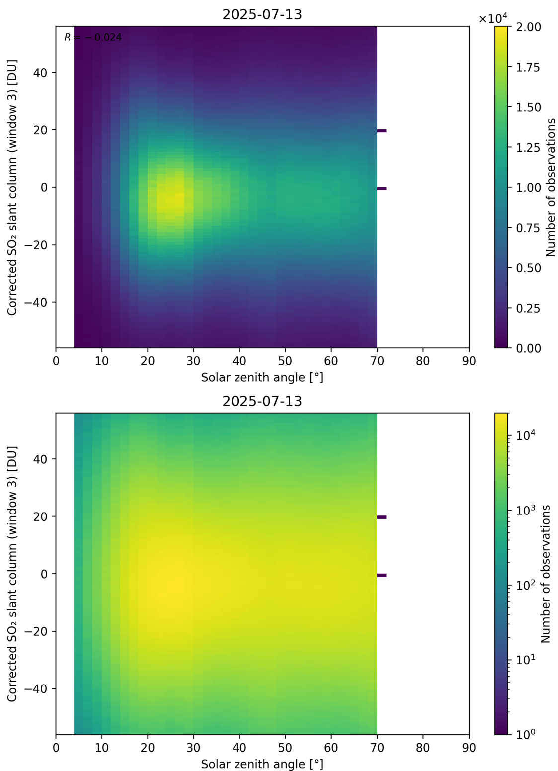
Figure 183: Scatter density plot of “Solar zenith angle” against “Corrected SO 2 slant column (window 3)” for 2025-07-13 to 2025-07-14.
