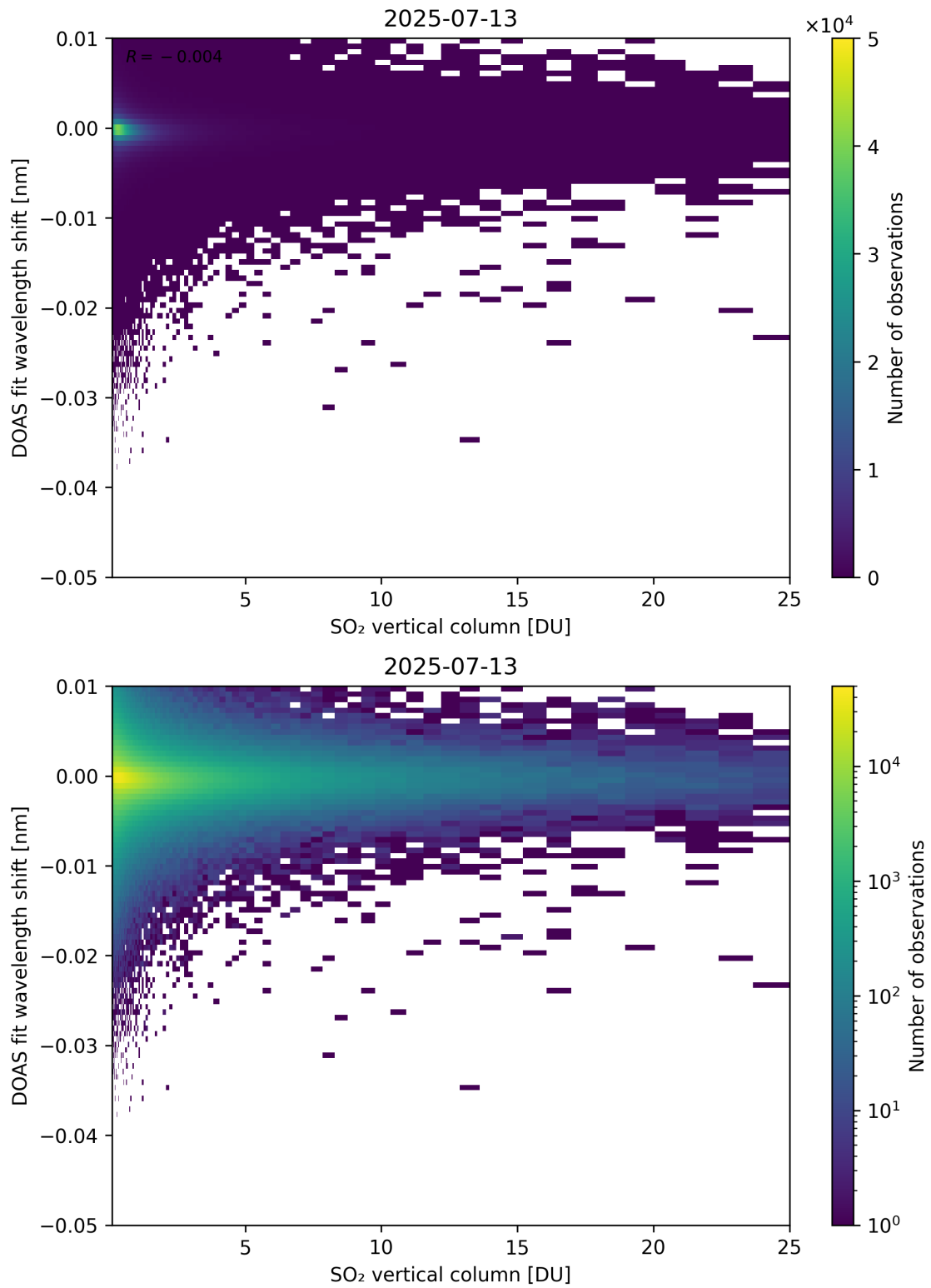
Figure 326: Scatter density plot of “SO 2 vertical column” against “DOAS fit wavelength shift” for 2025-07-13 to 2025-07-14.
