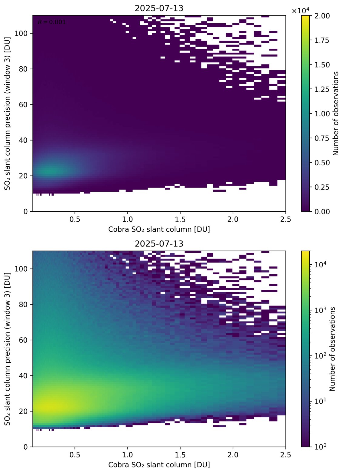
Figure 223: Scatter density plot of “Cobra SO 2 slant column” against “SO 2 slant column precision (window 3)” for 2025-07-13 to 2025-07-14.
