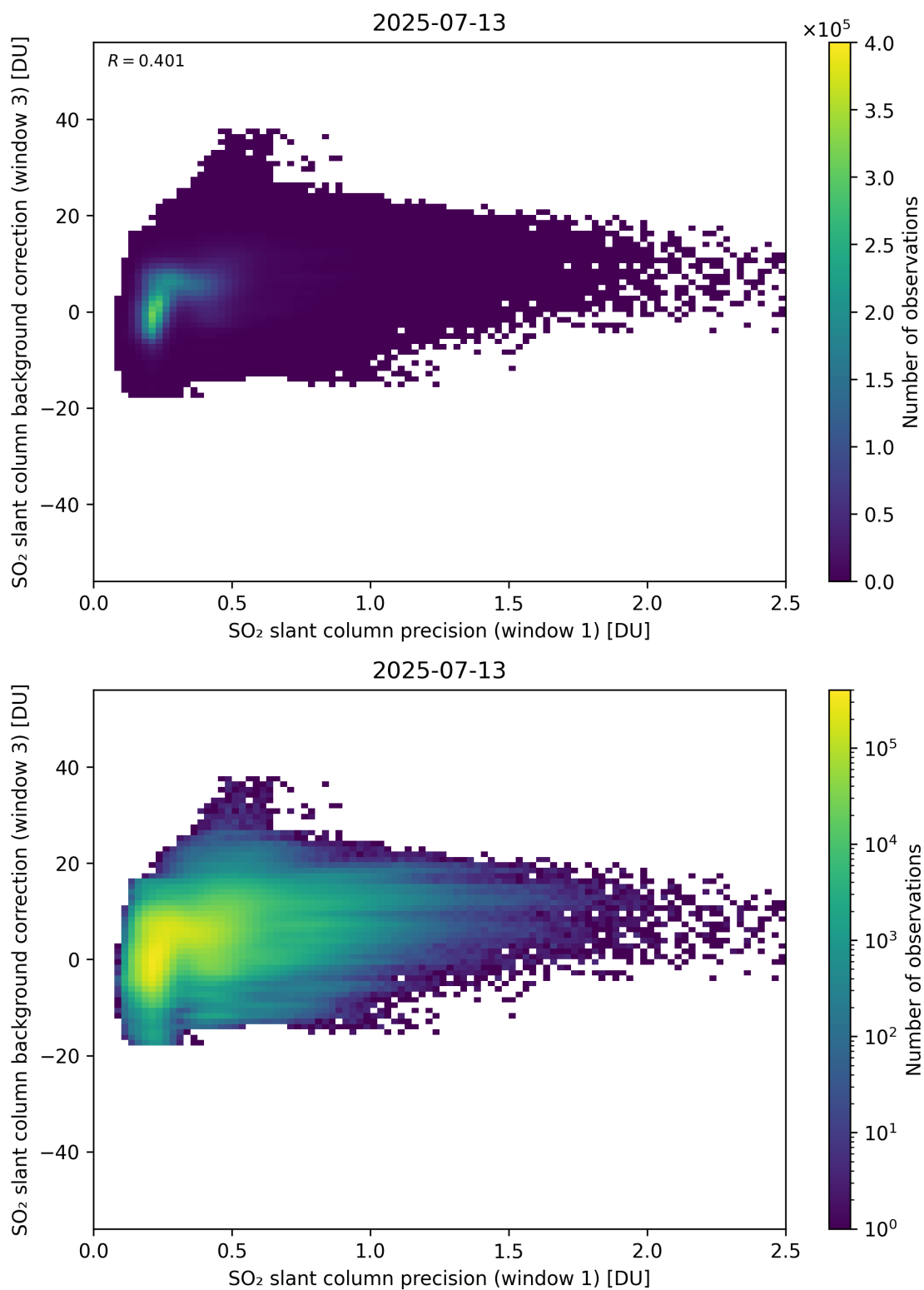
Figure 270: Scatter density plot of “SO 2 slant column precision (window 1)” against “SO 2 slant column background correction (window 3)” for 2025-07-13 to 2025-07-14.
