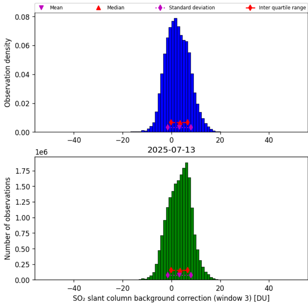
Figure 74: Histogram of “SO 2 slant column background correction (window 3)” for 2025-07-13 to 2025-07-14
