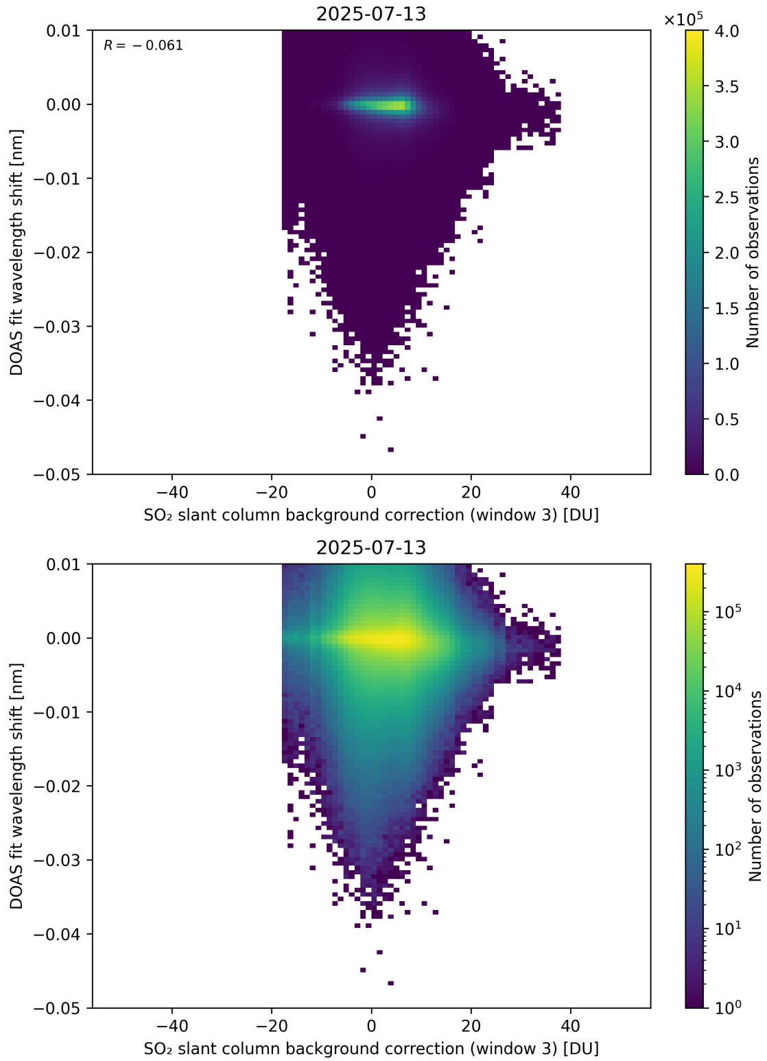
Figure 132: Scatter density plot of “SO 2 slant column background correction (window 3)” against “DOAS fit wavelength shift” for 2025-07-13 to 2025-07-14.
