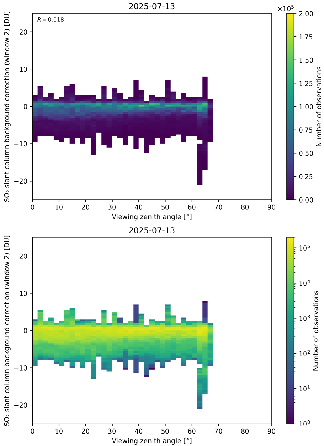
Figure 363: Scatter density plot of “Viewing zenith angle” against “SO 2 slant column background correction (window 2)” for 2025-07-13 to 2025-07-14.
