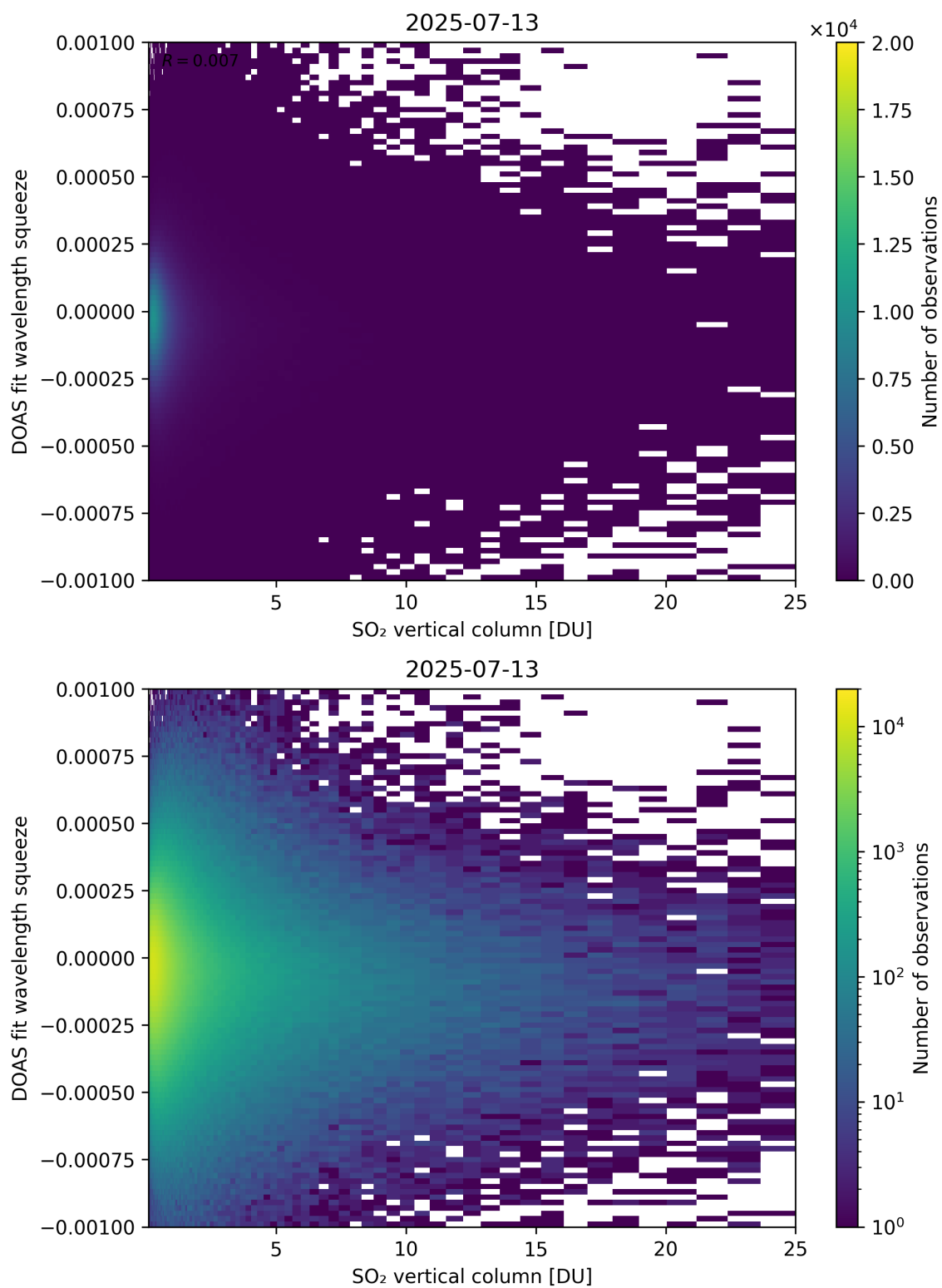
Figure 327: Scatter density plot of “SO 2 vertical column” against “DOAS fit wavelength squeeze” for 2025-07-13 to 2025-07-14.
