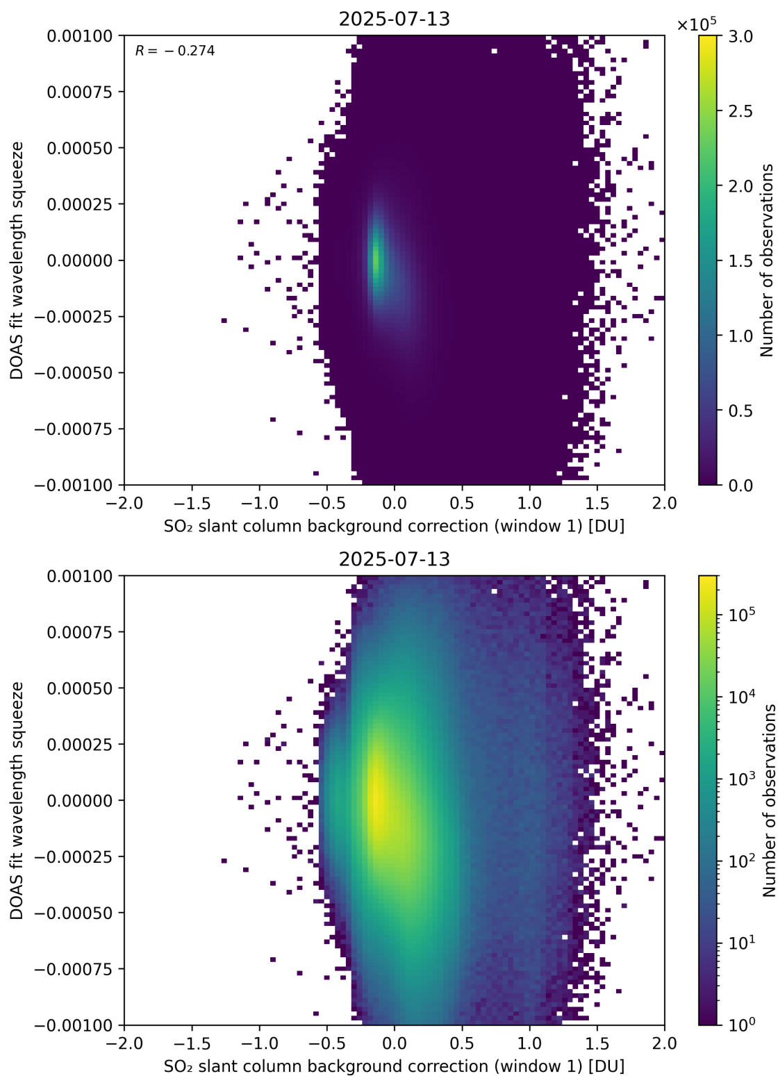
Figure 112: Scatter density plot of “SO 2 slant column background correction (window 1)” against “DOAS fit wavelength squeeze” for 2025-07-13 to 2025-07-14.
