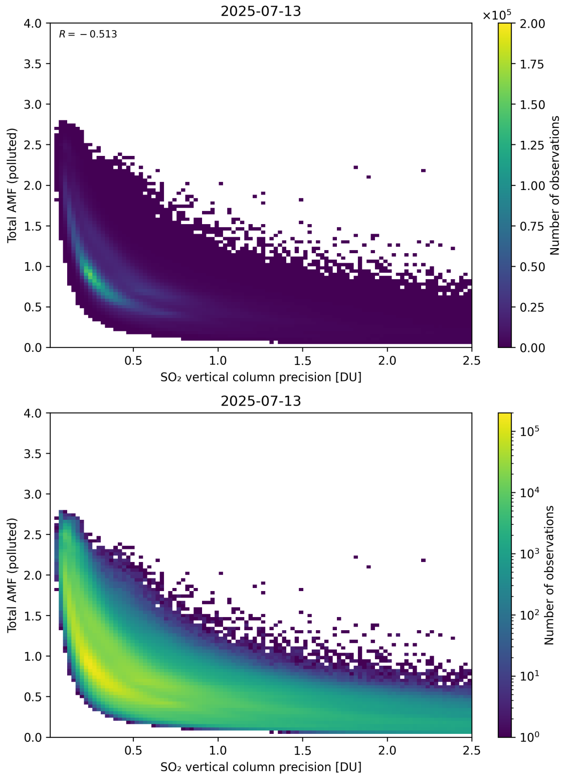
Figure 346: Scatter density plot of “SO 2 vertical column precision” against “Total AMF (polluted)” for 2025-07-13 to 2025-07-14.
