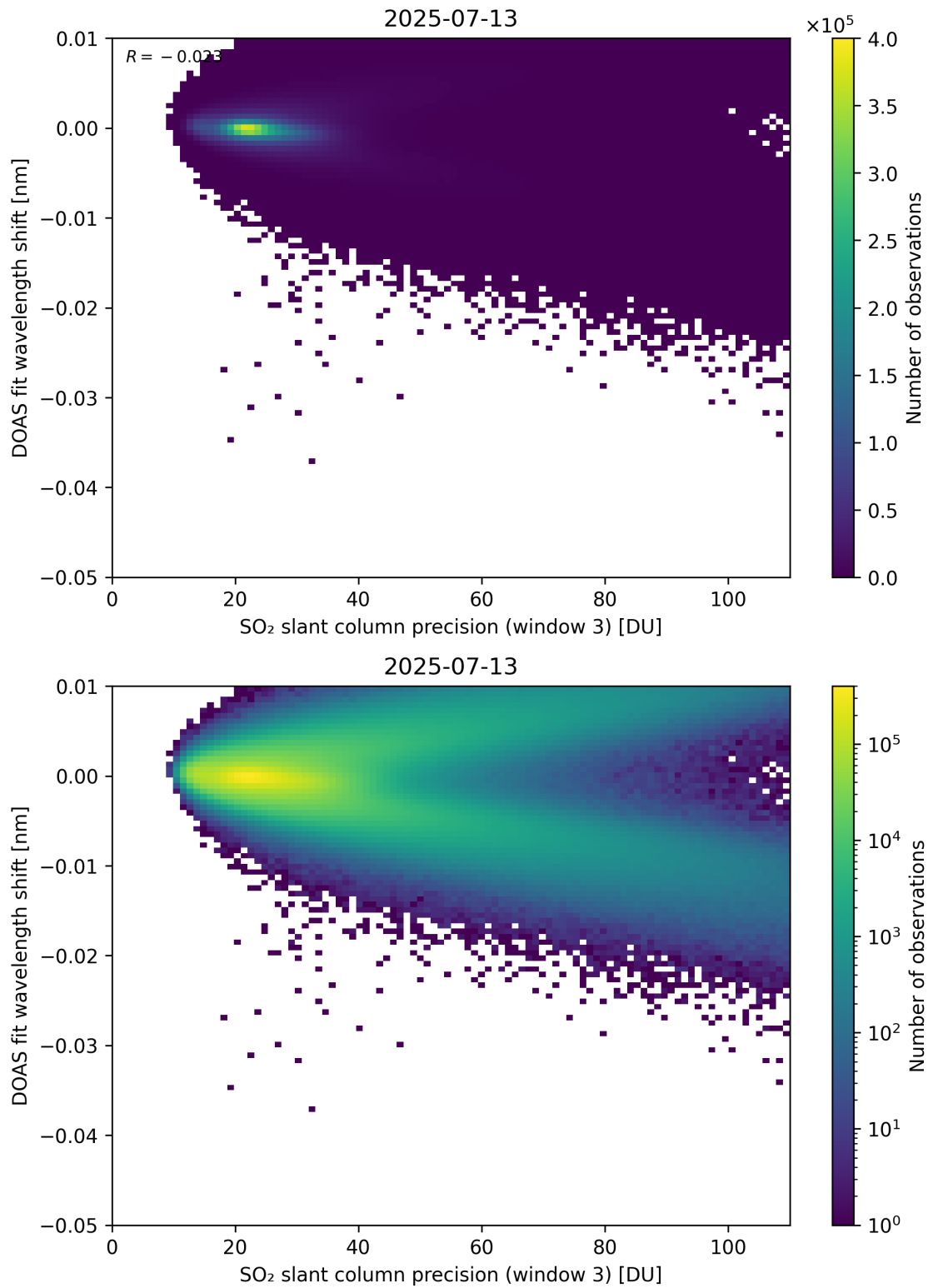
Figure 308: Scatter density plot of “SO 2 slant column precision (window 3)” against “DOAS fit wavelength shift” for 2025-07-13 to 2025-07-14.
