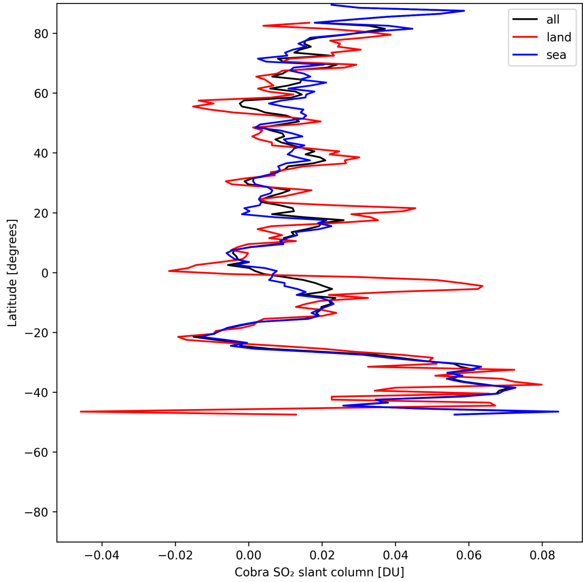
Figure 35: Zonal average of “Cobra SO 2 slant column” for 2025-07-13 to 2025-07-14.
