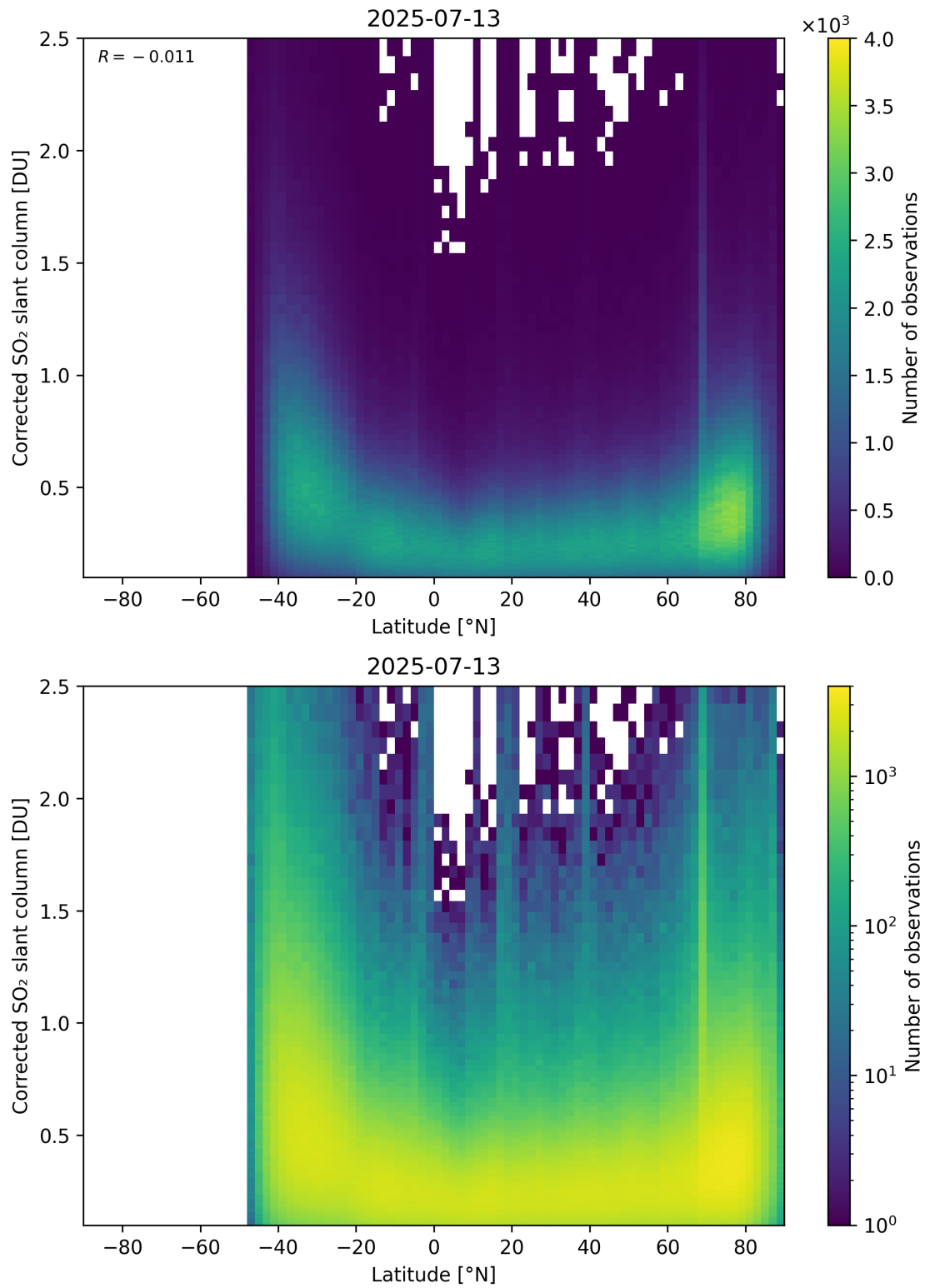
Figure 159: Scatter density plot of “Latitude” against “Corrected SO 2 slant column” for 2025-07-13 to 2025-07-14.
