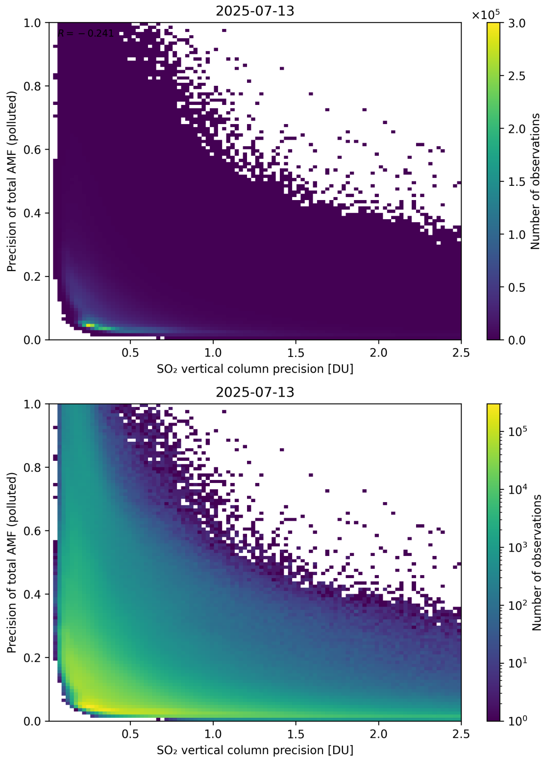
Figure 347: Scatter density plot of “SO 2 vertical column precision” against “Precision of total AMF (polluted)” for 2025-07-13 to 2025-07-14.
