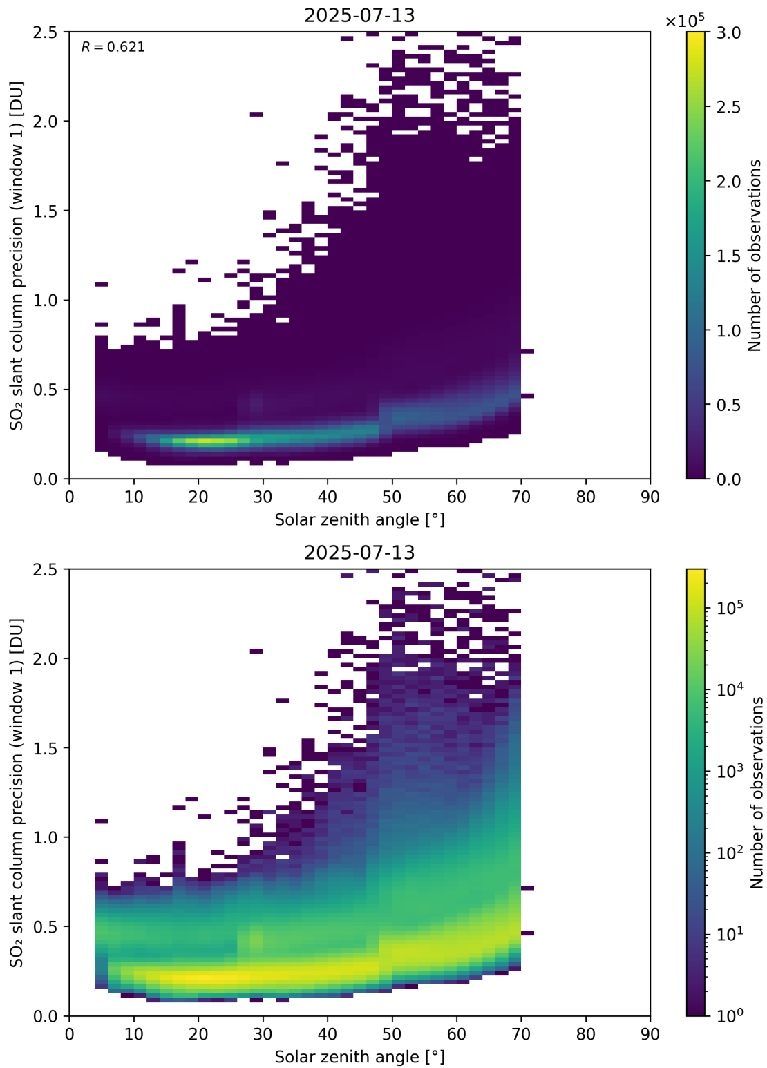
Figure 185: Scatter density plot of “Solar zenith angle” against “SO 2 slant column precision (window 1)” for 2025-07-13 to 2025-07-14.
