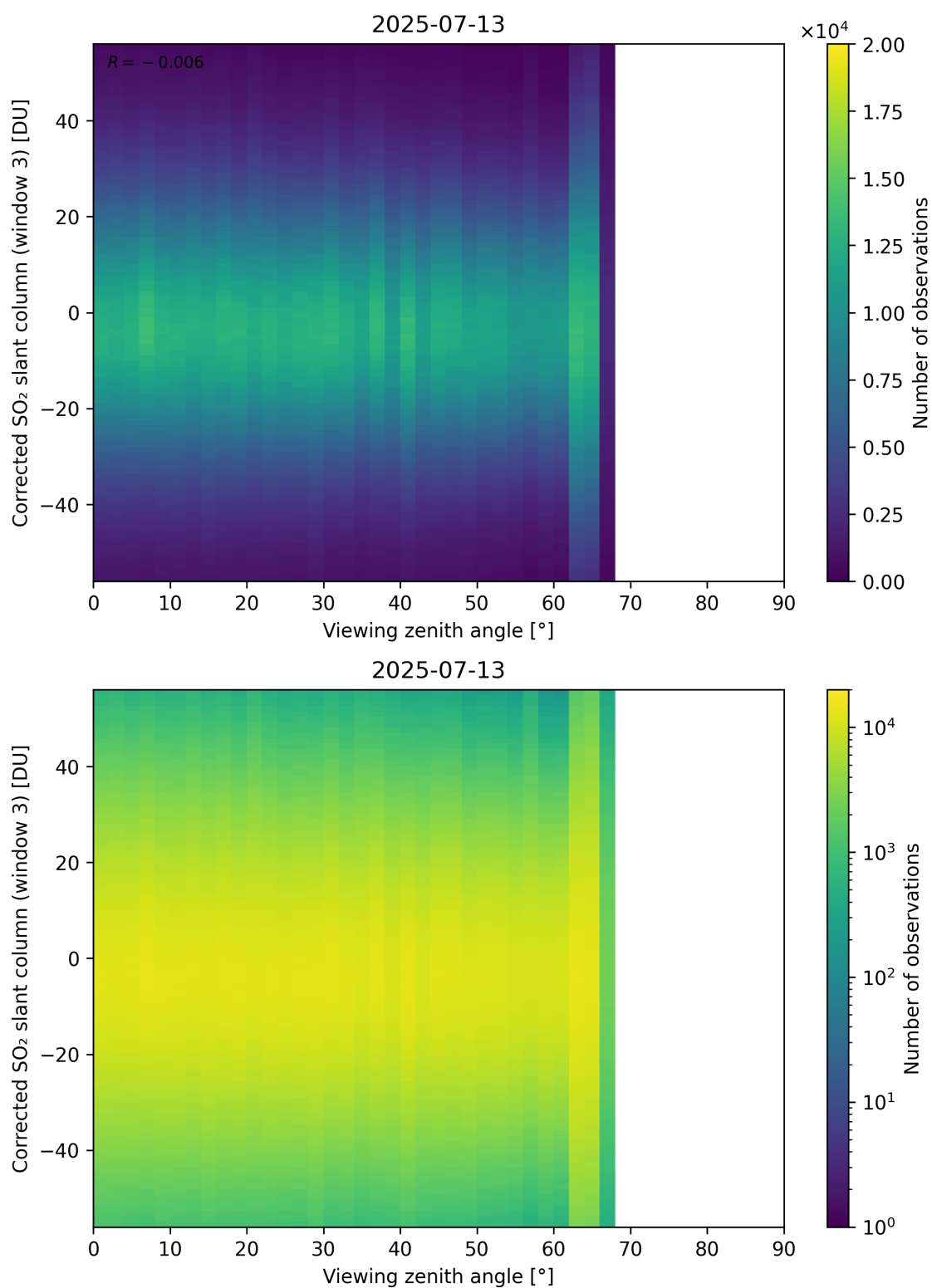
Figure 375: Scatter density plot of “Viewing zenith angle” against “Corrected SO 2 slant column (window 3)” for 2025-07-13 to 2025-07-14.
