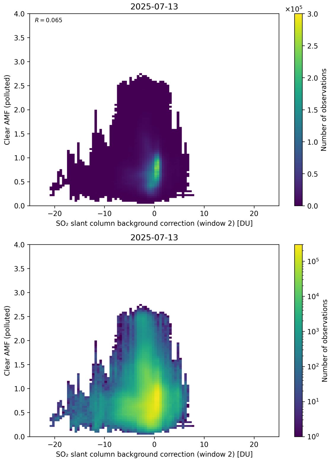
Figure 126: Scatter density plot of “SO 2 slant column background correction (window 2)” against “Clear AMF (polluted)” for 2025-07-13 to 2025-07-14.
