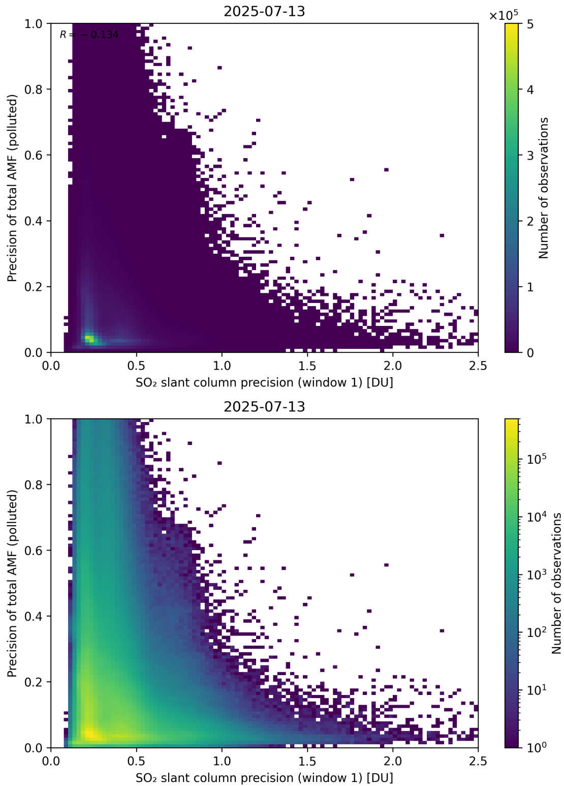
Figure 281: Scatter density plot of “SO 2 slant column precision (window 1)” against “Precision of total AMF (polluted)” for 2025-07-13 to 2025-07-14.
