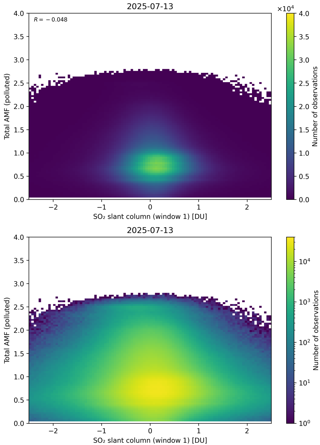
Figure 289: Scatter density plot of “SO 2 slant column (window 1)” against “Total AMF (polluted)” for 2025-07-13 to 2025-07-14.
