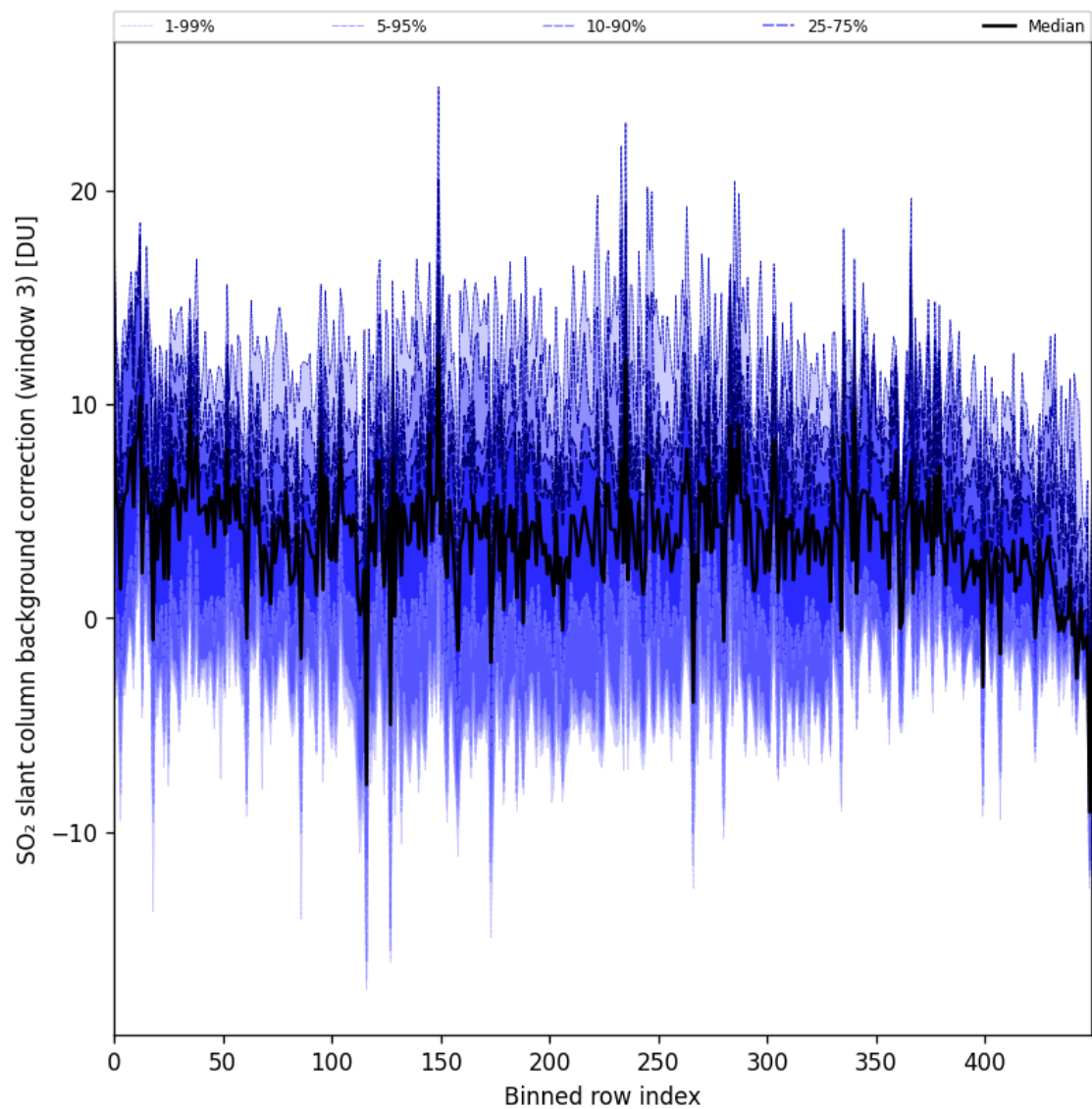
Figure 100: Along track statistics of “SO 2 slant column background correction (window 3)” for 2025-07-13 to 2025-07-14
