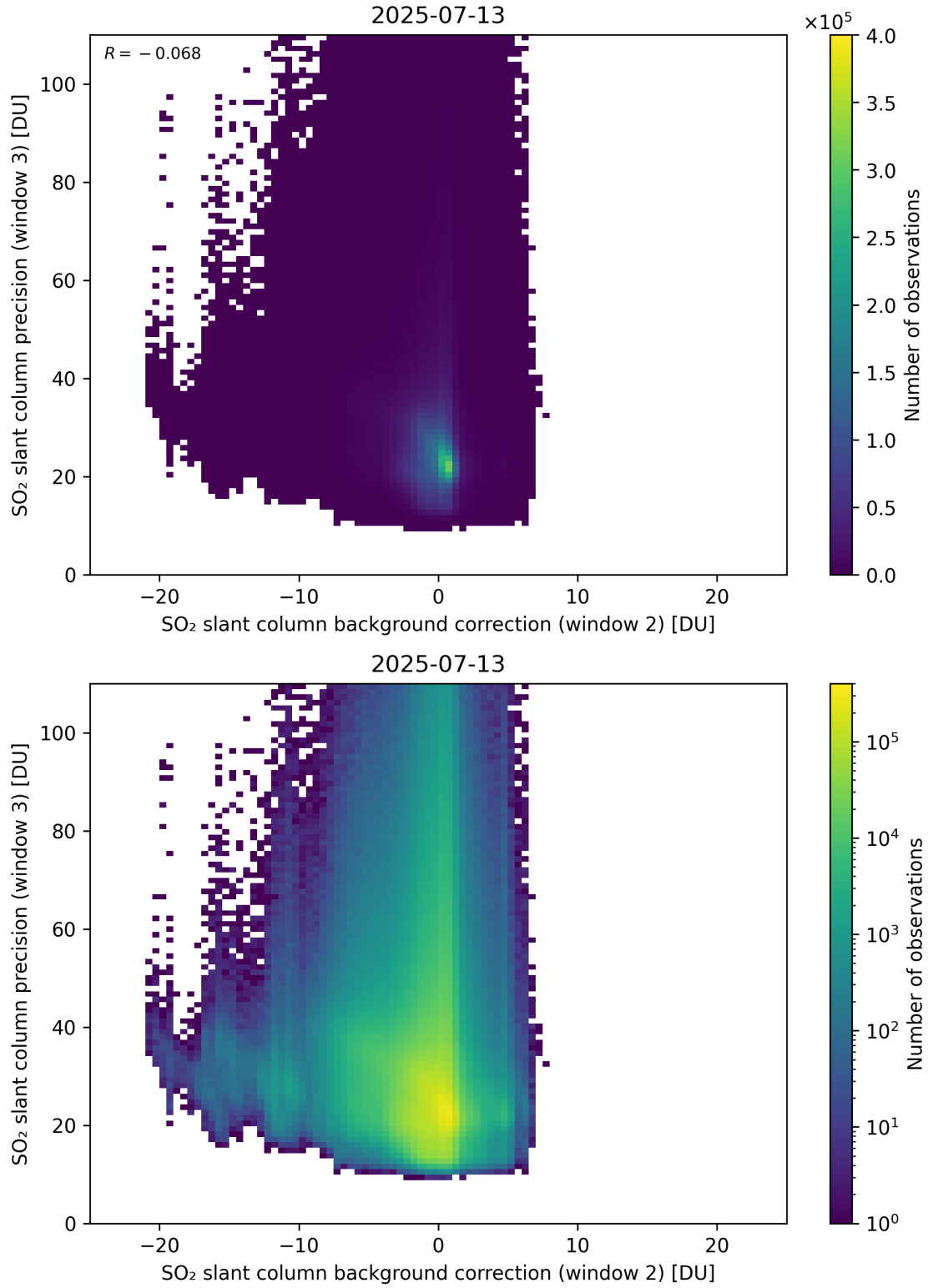
Figure 129: Scatter density plot of “SO 2 slant column background correction (window 2)” against “SO 2 slant column precision (window 3)” for 2025-07-13 to 2025-07-14.
