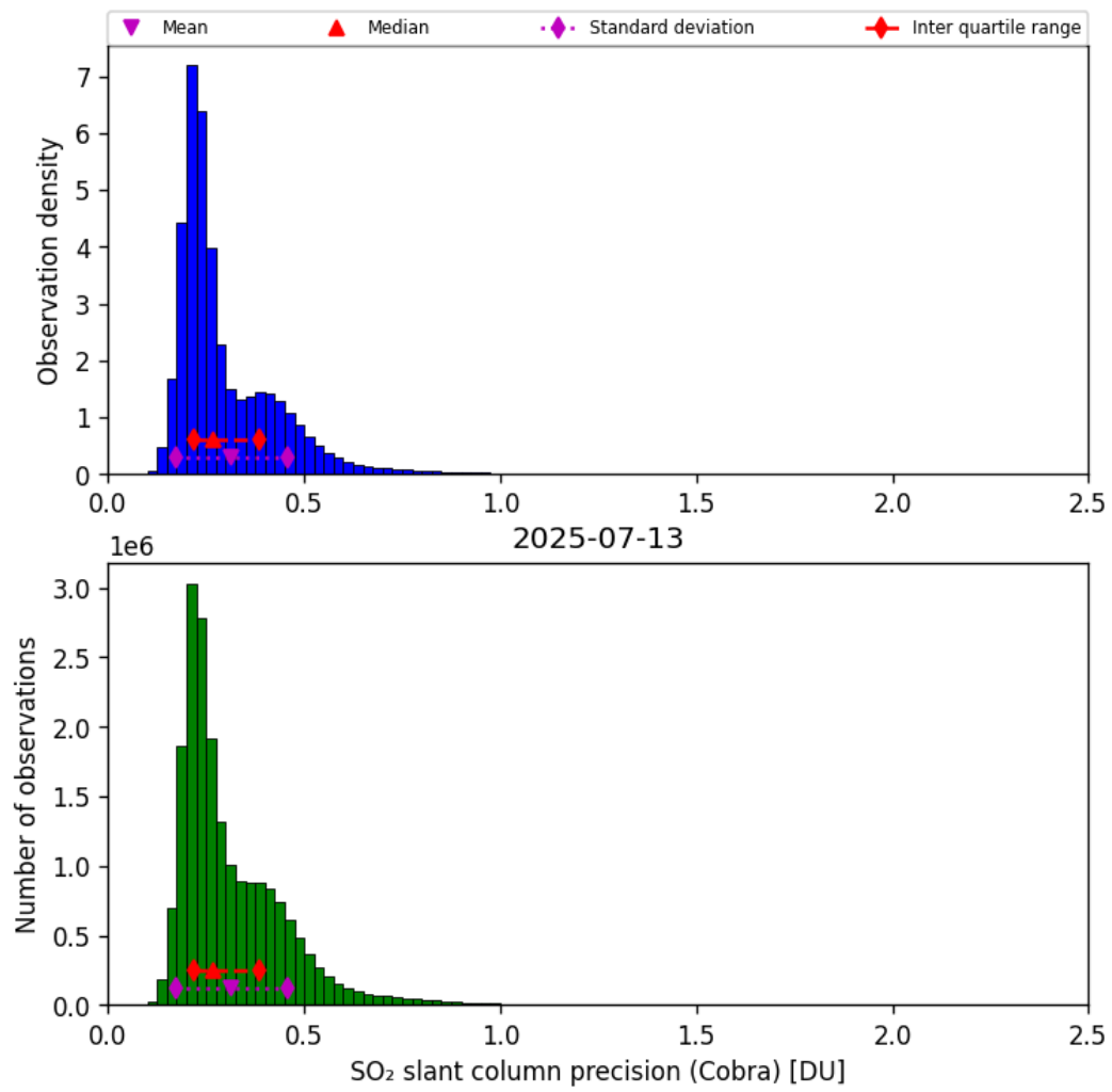
Figure 62: Histogram of “SO 2 slant column precision (Cobra)” for 2025-07-13 to 2025-07-14
