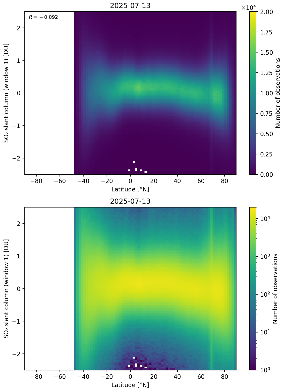
Figure 162: Scatter density plot of “Latitude” against “SO 2 slant column (window 1)” for 2025-07-13 to 2025-07-14.
