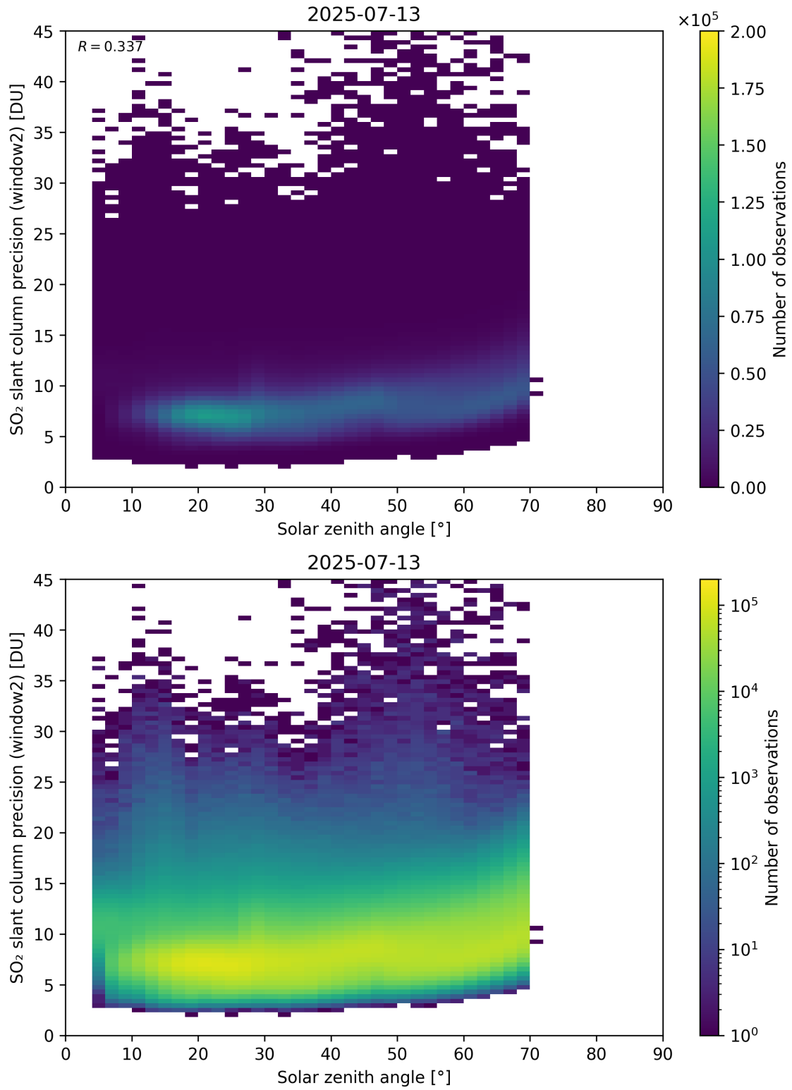
Figure 186: Scatter density plot of “Solar zenith angle” against “SO 2 slant column precision (window2)” for 2025-07-13 to 2025-07-14.
