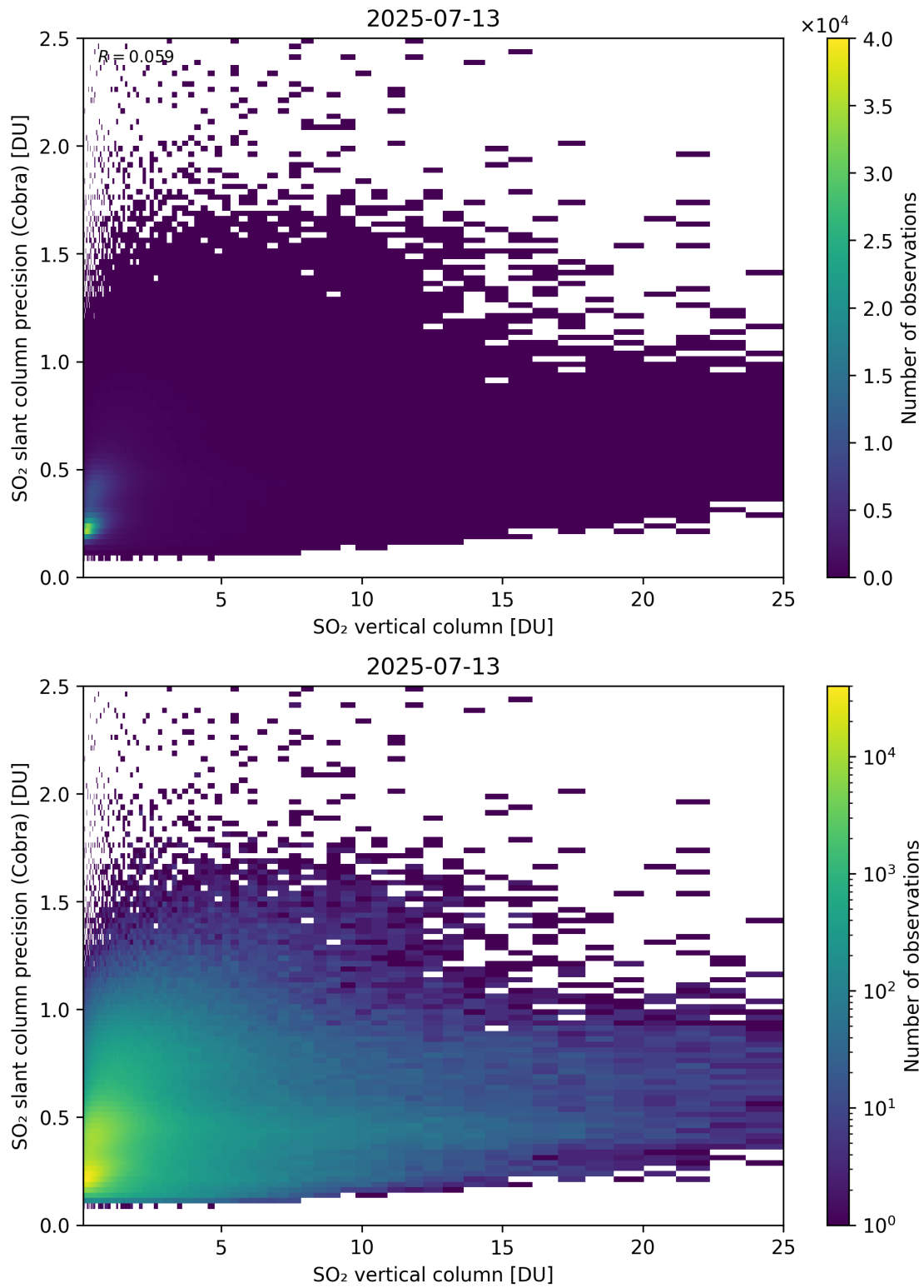
Figure 350: Scatter density plot of “SO 2 vertical column” against “SO 2 slant column precision (Cobra)” for 2025-07-13 to 2025-07-14.
