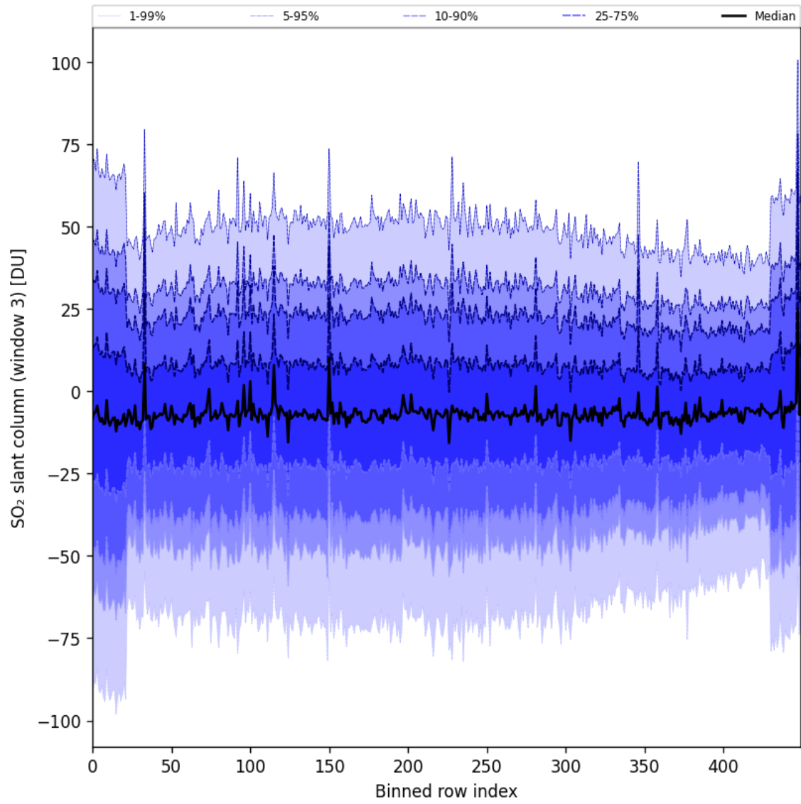
Figure 97: Along track statistics of “SO 2 slant column (window 3)” for 2025-07-13 to 2025-07-14
