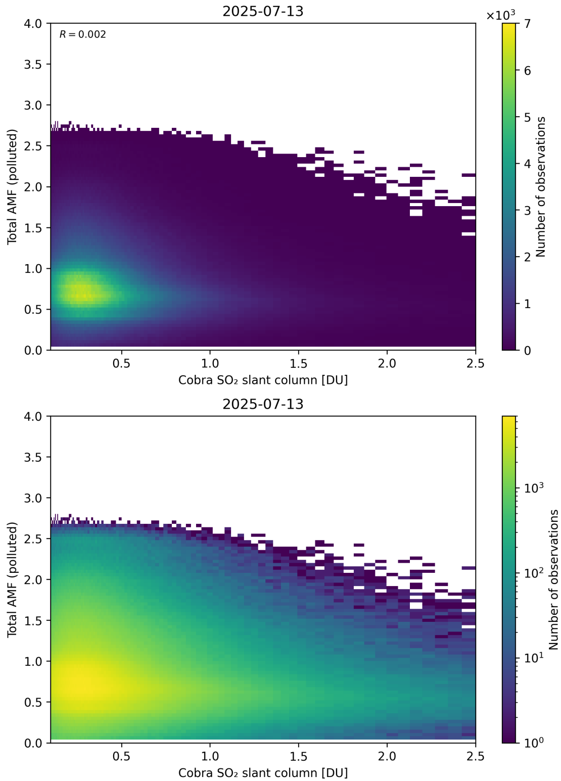
Figure 224: Scatter density plot of “Cobra SO 2 slant column” against “Total AMF (polluted)” for 2025-07-13 to 2025-07-14.
