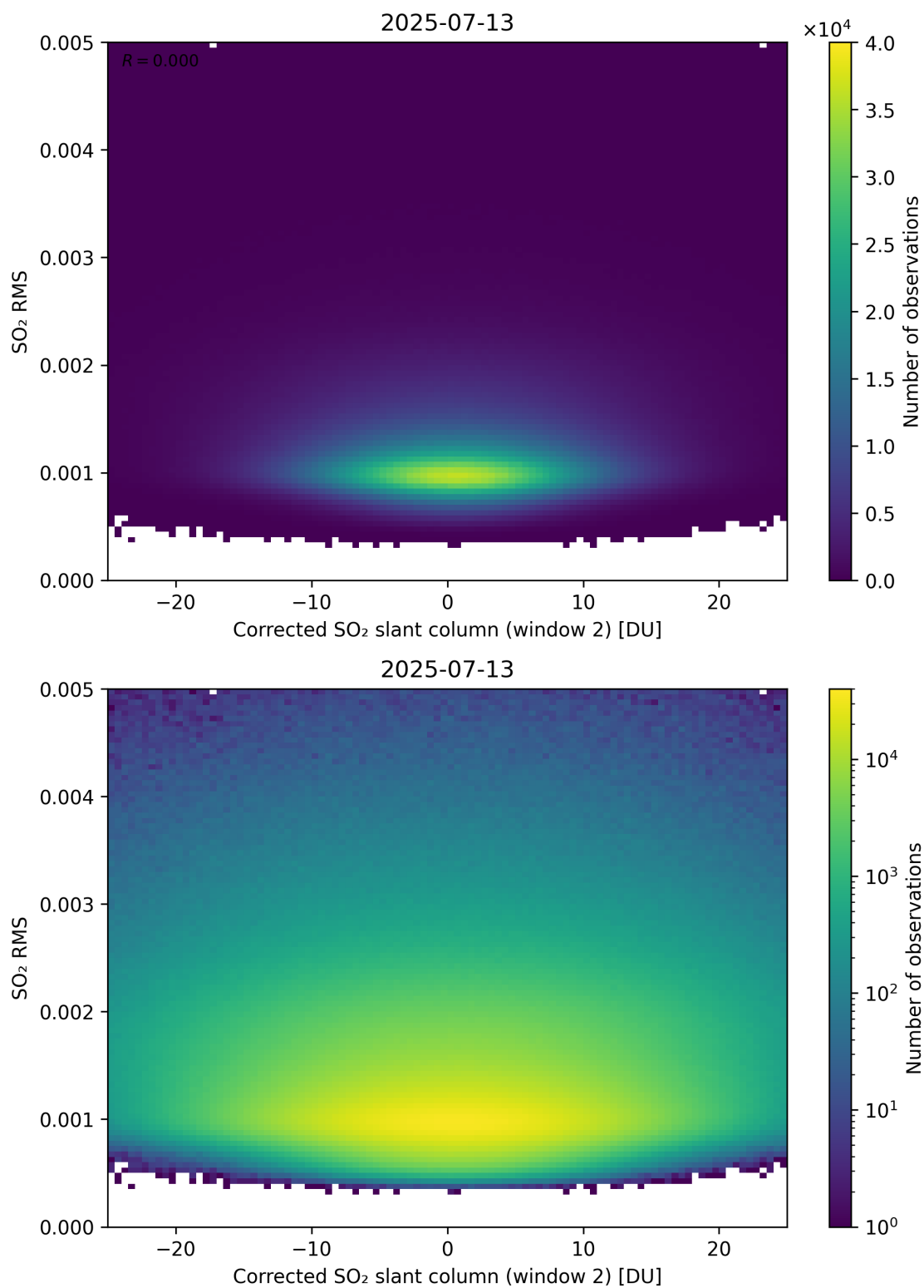
Figure 248: Scatter density plot of “Corrected SO 2 slant column (window 2)” against “SO 2 RMS” for 2025-07-13 to 2025-07-14.
