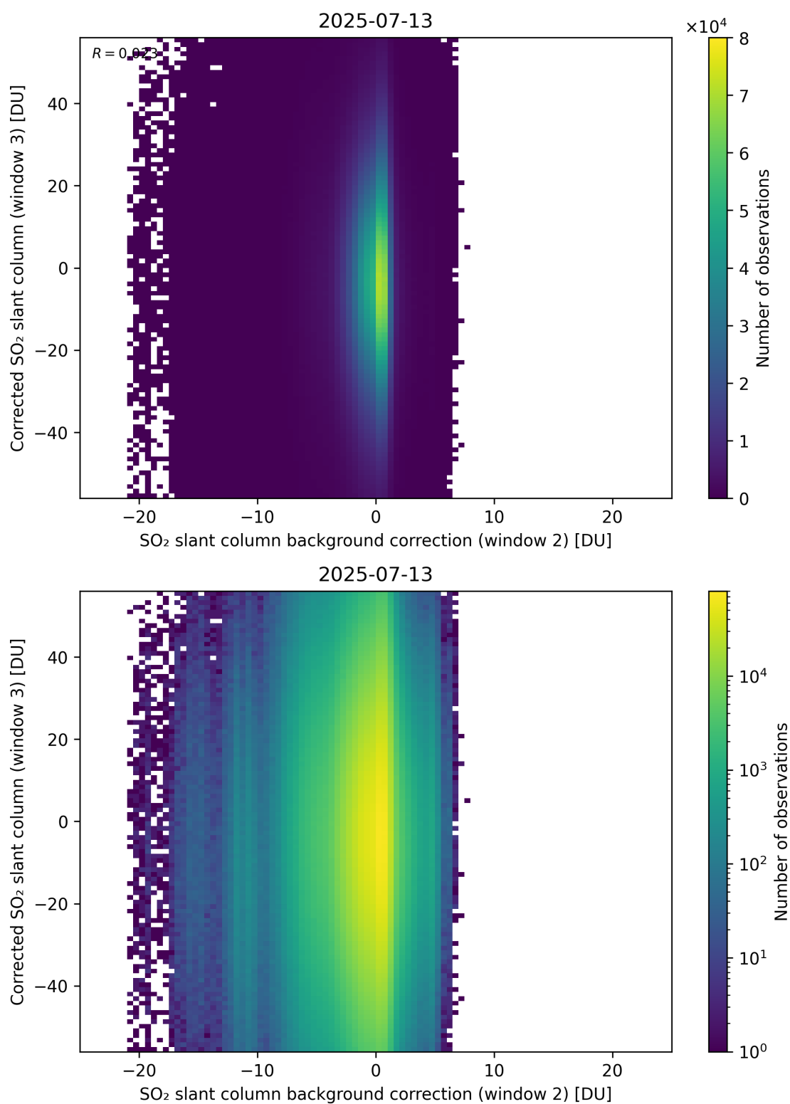
Figure 127: Scatter density plot of “SO 2 slant column background correction (window 2)” against “Corrected SO 2 slant column (window 3)” for 2025-07-13 to 2025-07-14.
