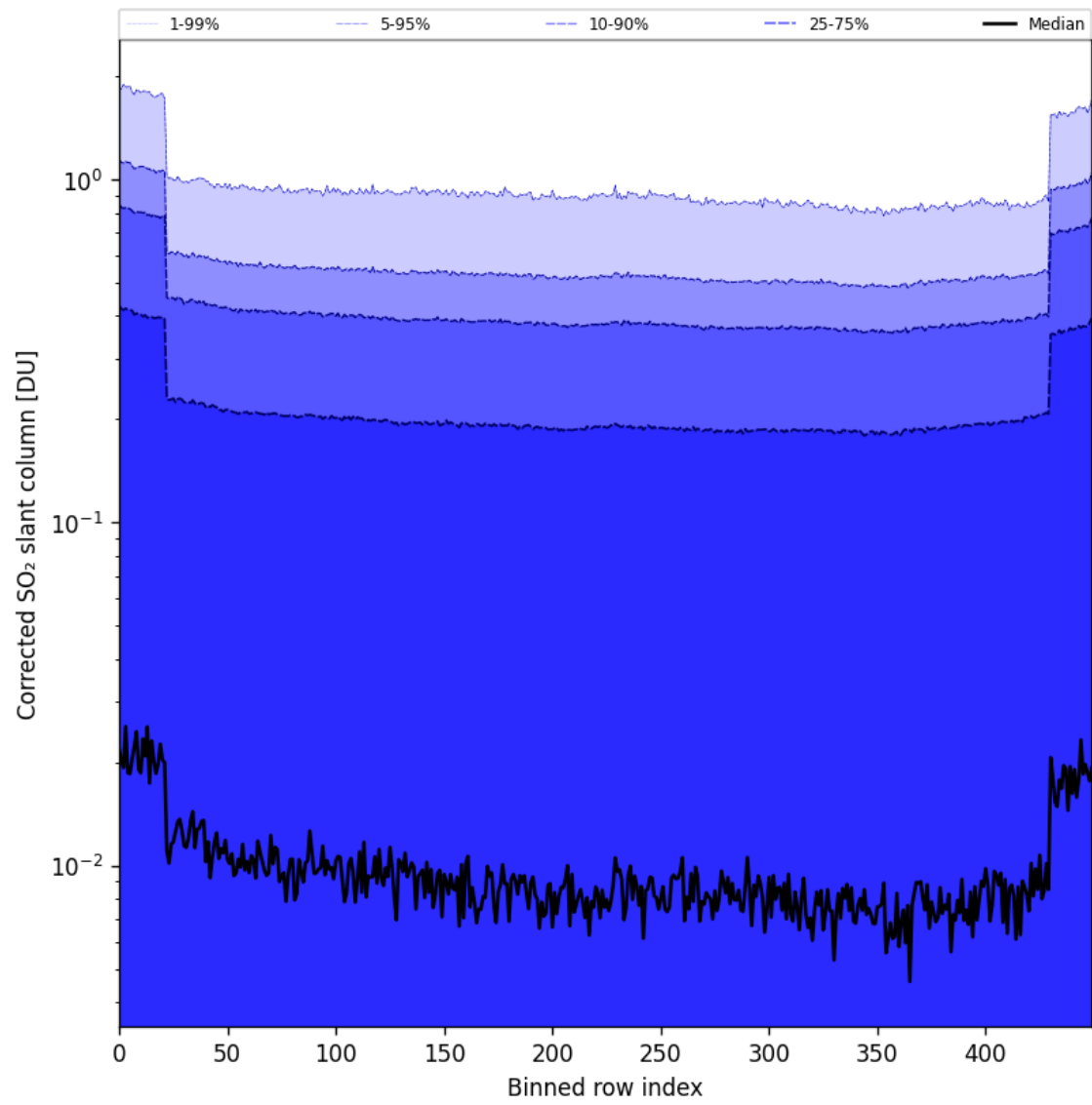
Figure 86: Along track statistics of "Corrected SO 2 slant column" for 2025-07-13 to 2025-07-14
