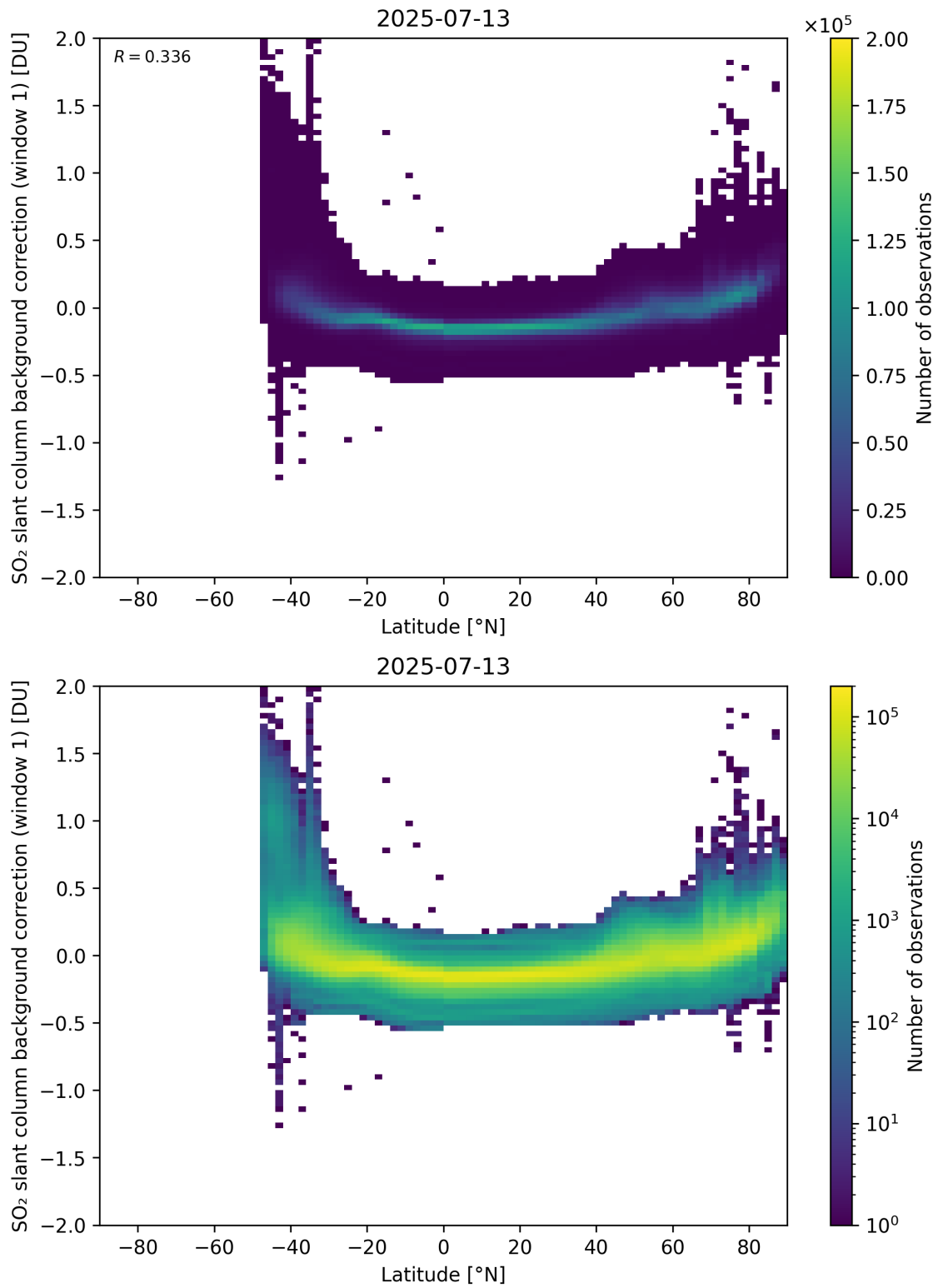
Figure 150: Scatter density plot of “Latitude” against “SO 2 slant column background correction (window 1)” for 2025-07-13 to 2025-07-14.
