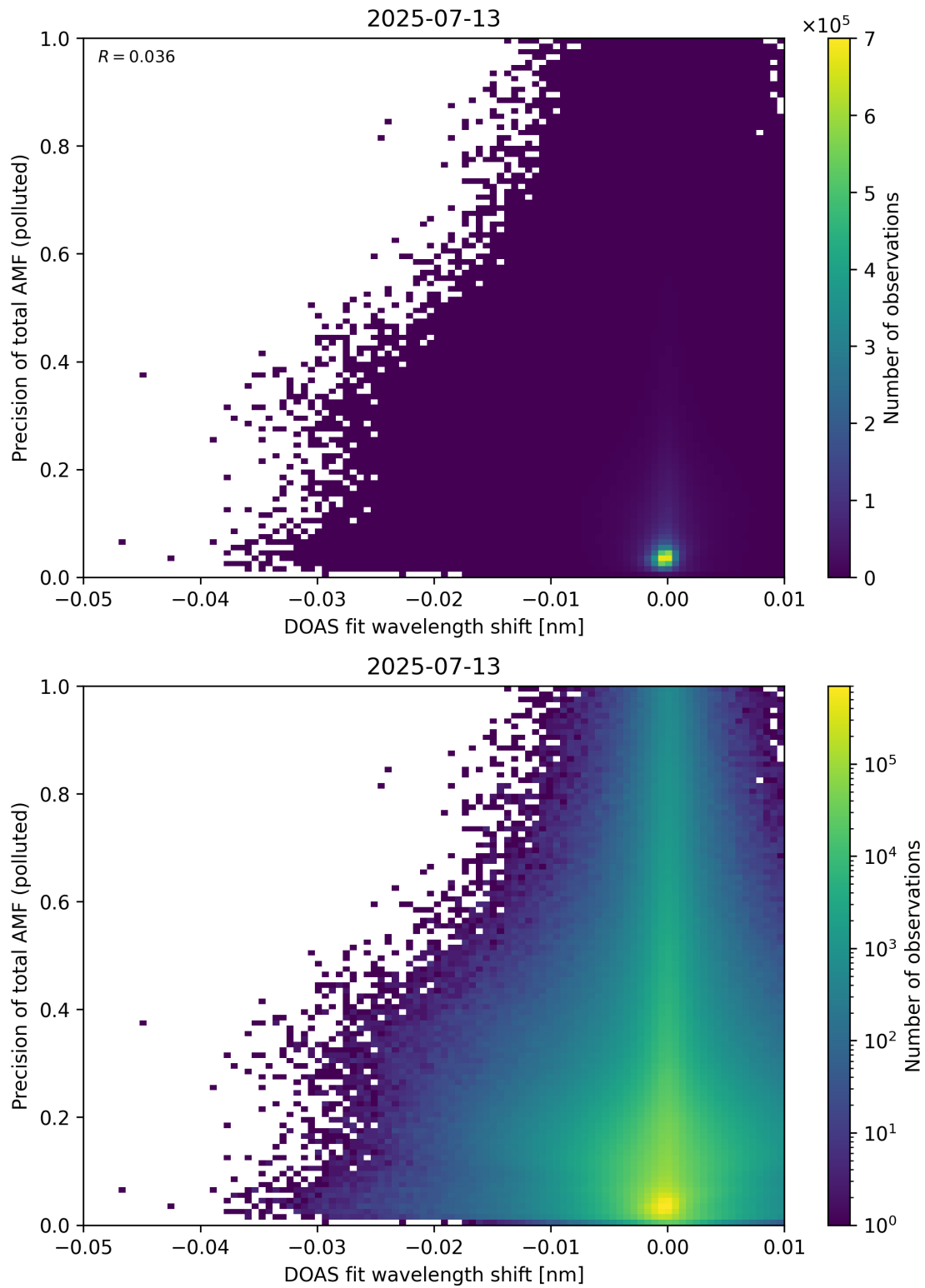
Figure 142: Scatter density plot of “DOAS fit wavelength shift” against “Precision of total AMF (polluted)” for 2025-07-13 to 2025-07-14.
