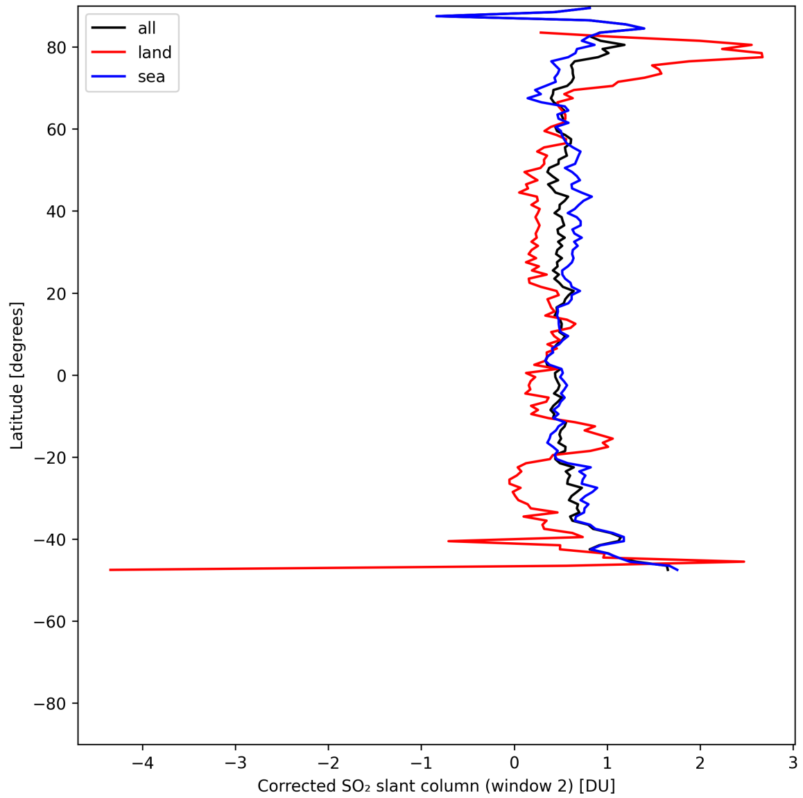
Figure 43: Zonal average of “Corrected SO 2 slant column (window 2)” for 2025-07-13 to 2025-07-14.
