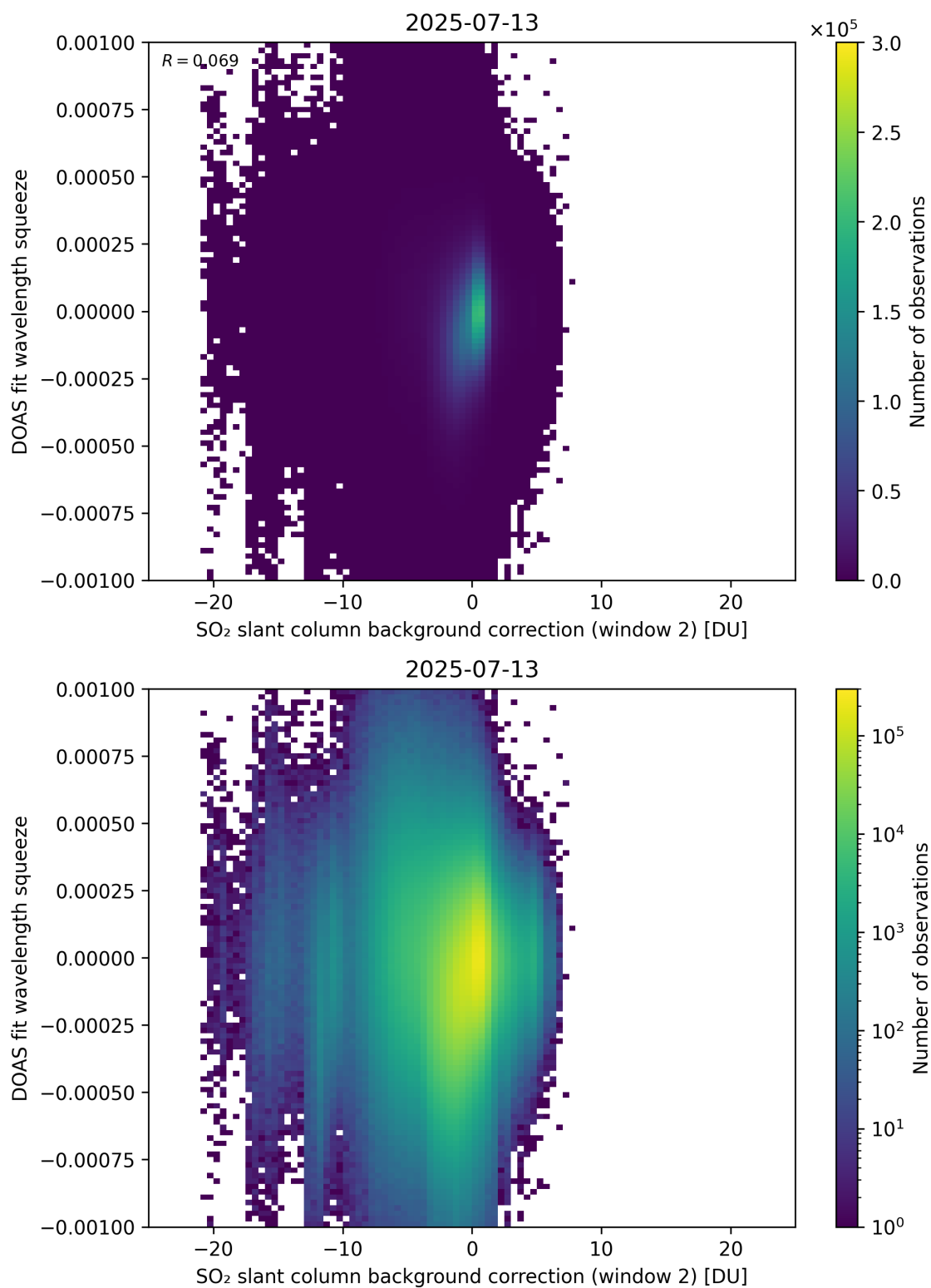
Figure 124: Scatter density plot of “SO 2 slant column background correction (window 2)” against “DOAS fit wavelength squeeze” for 2025-07-13 to 2025-07-14.
