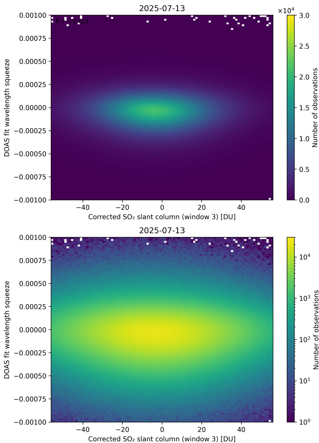
Figure 257: Scatter density plot of “Corrected SO 2 slant column (window 3)” against “DOAS fit wavelength squeeze” for 2025-07-13 to 2025-07-14.
