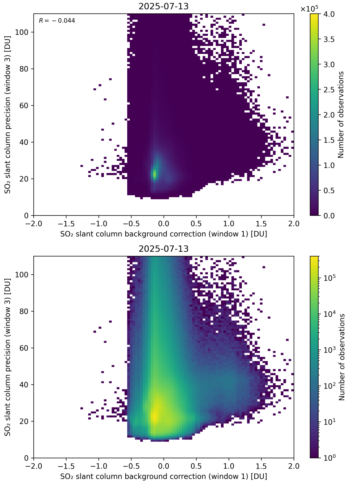
Figure 119: Scatter density plot of “SO 2 slant column background correction (window 1)” against “SO 2 slant column precision (window 3)” for 2025-07-13 to 2025-07-14.
