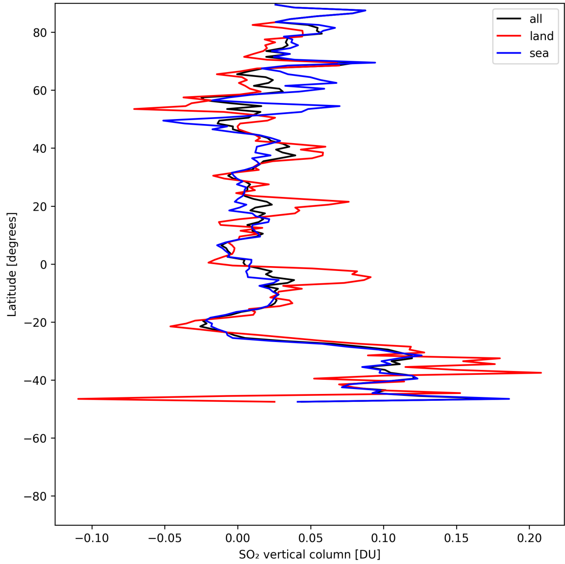
Figure 32: Zonal average of “SO 2 vertical column” for 2025-07-13 to 2025-07-14.
