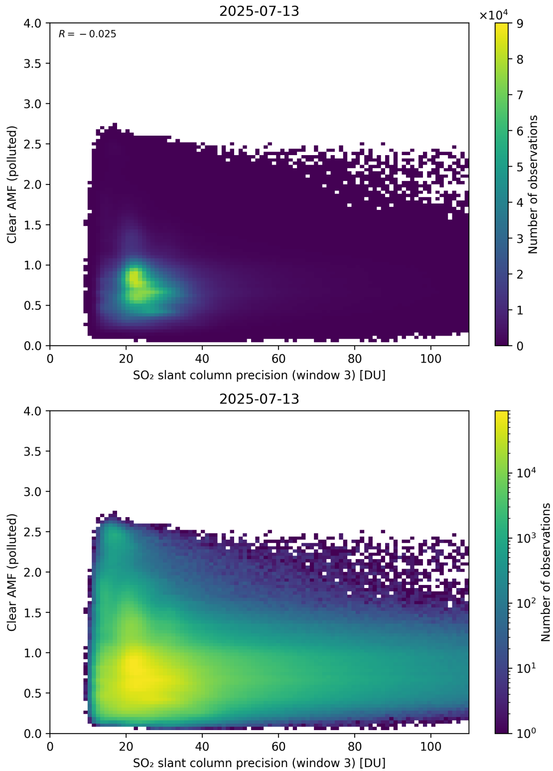
Figure 311: Scatter density plot of “SO 2 slant column precision (window 3)” against “Clear AMF (polluted)” for 2025-07-13 to 2025-07-14.
