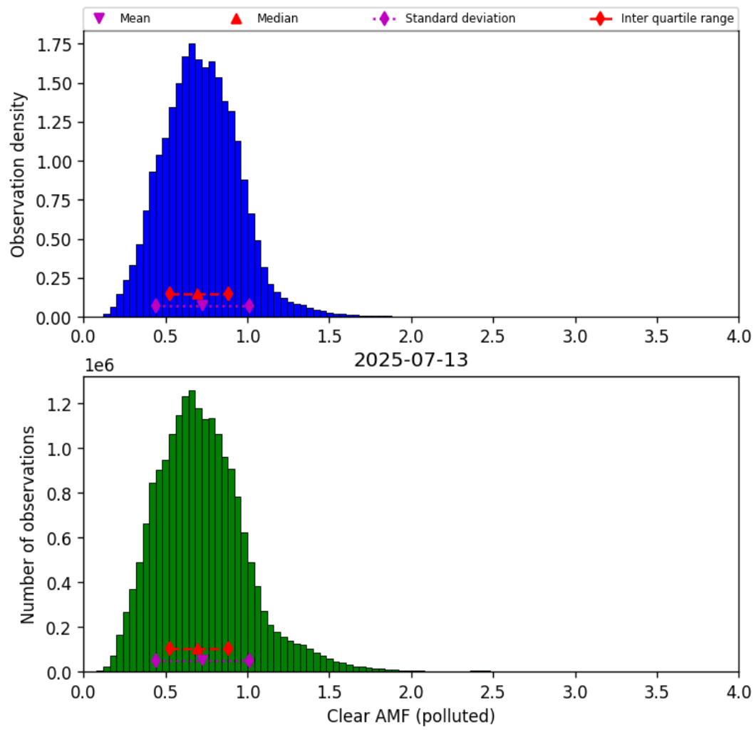
Figure 81: Histogram of “Clear AMF (polluted)” for 2025-07-13 to 2025-07-14
