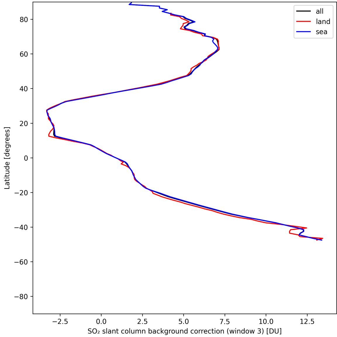
Figure 48: Zonal average of “SO 2 slant column background correction (window 3)” for 2025-07-13 to 2025-07-14.
