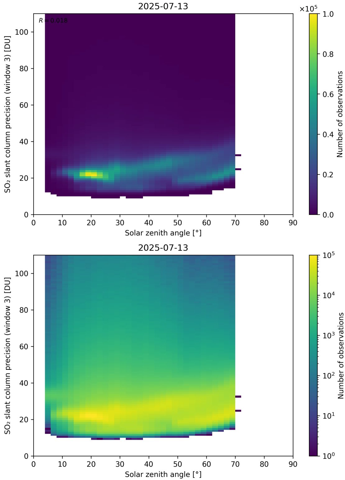
Figure 188: Scatter density plot of “Solar zenith angle” against “SO 2 slant column precision (window 3)” for 2025-07-13 to 2025-07-14.
