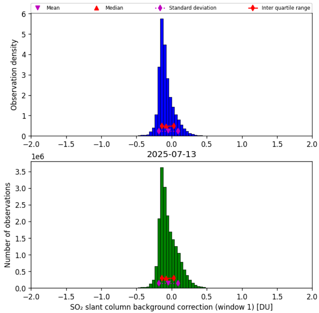
Figure 66: Histogram of “SO 2 slant column background correction (window 1)” for 2025-07-13 to 2025-07-14
