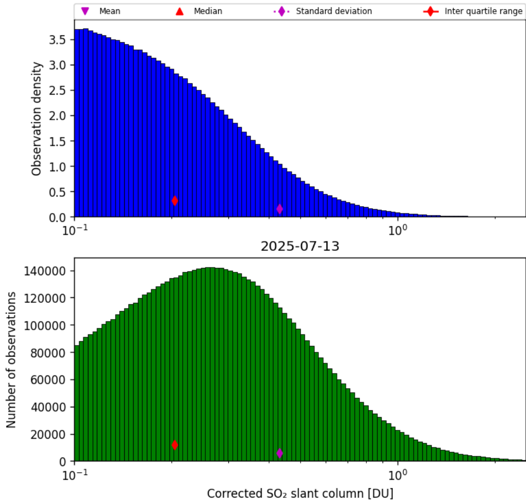
Figure 60: Histogram of “Corrected SO 2 slant column” for 2025-07-13 to 2025-07-14
