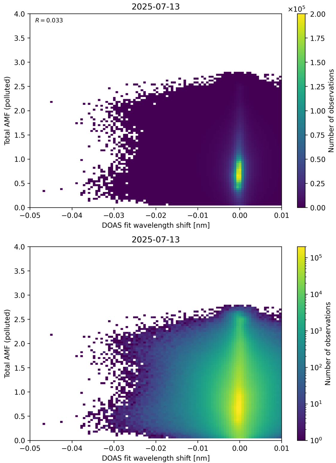
Figure 141: Scatter density plot of “DOAS fit wavelength shift” against “Total AMF (polluted)” for 2025-07-13 to 2025-07-14.
