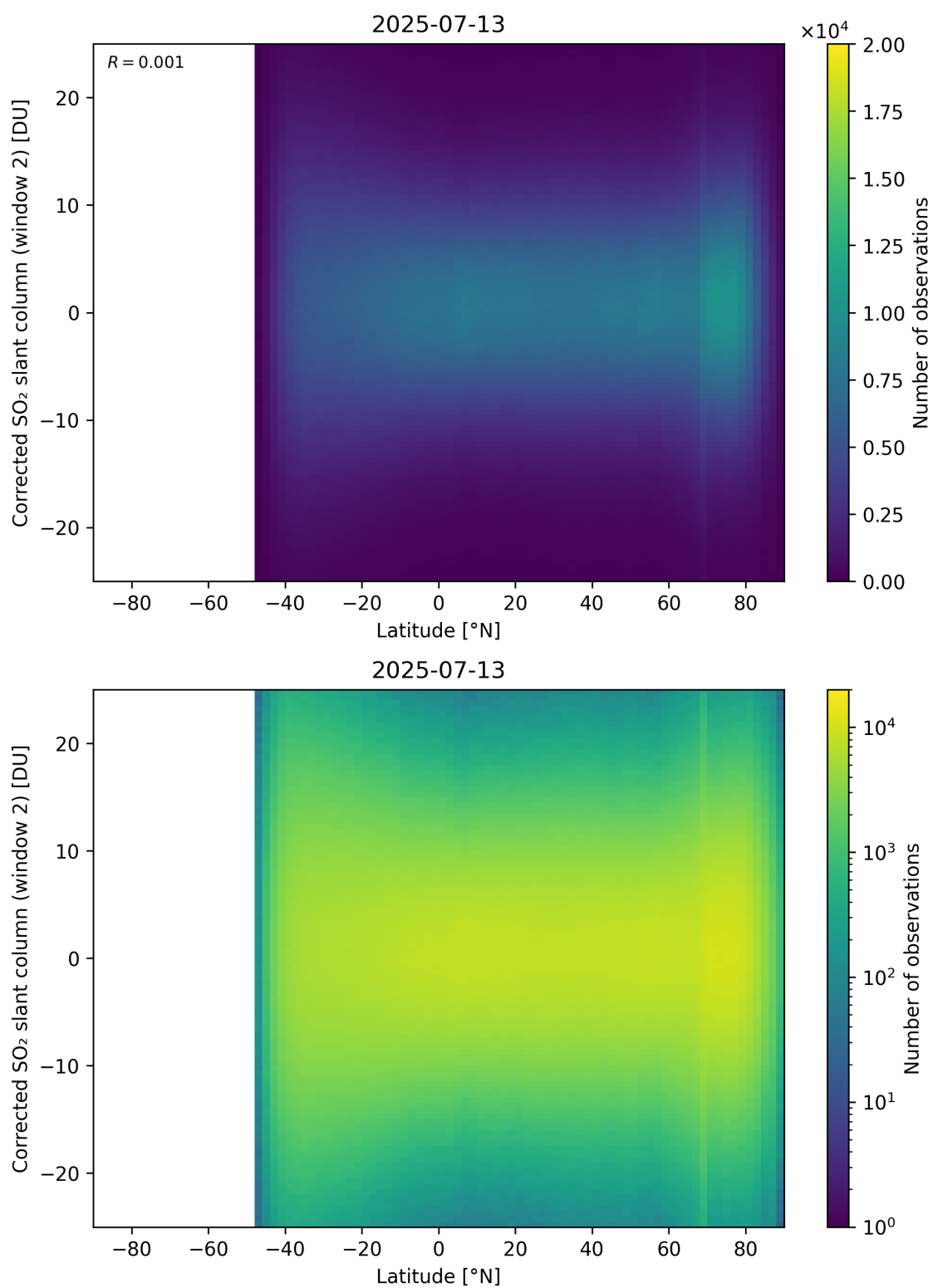
Figure 160: Scatter density plot of “Latitude” against “Corrected SO 2 slant column (window 2)” for 2025-07-13 to 2025-07-14.
