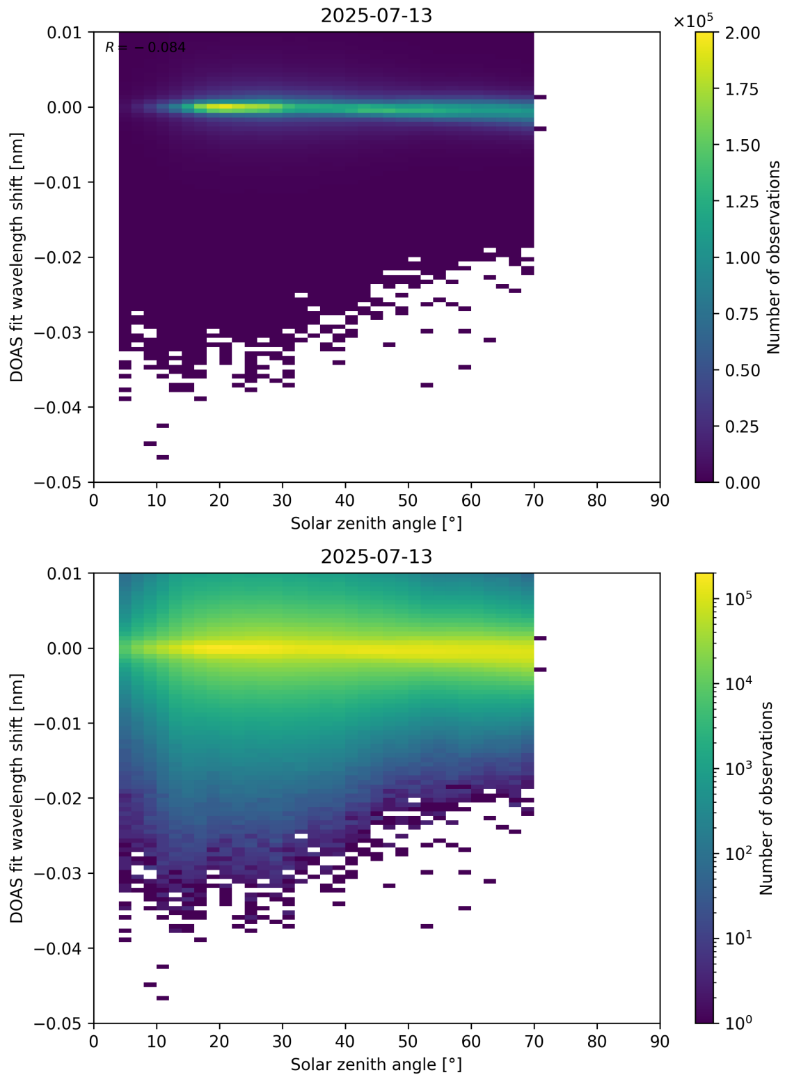
Figure 174: Scatter density plot of “Solar zenith angle” against “DOAS fit wavelength shift” for 2025-07-13 to 2025-07-14.
