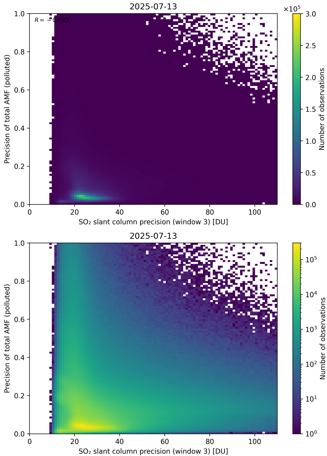
Figure 314: Scatter density plot of “SO 2 slant column precision (window 3)” against “Precision of total AMF (polluted)” for 2025-07-13 to 2025-07-14.
