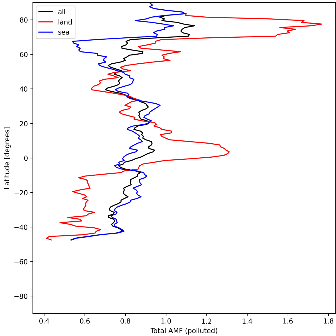
Figure 53: Zonal average of “Total AMF (polluted)” for 2025-07-13 to 2025-07-14.
