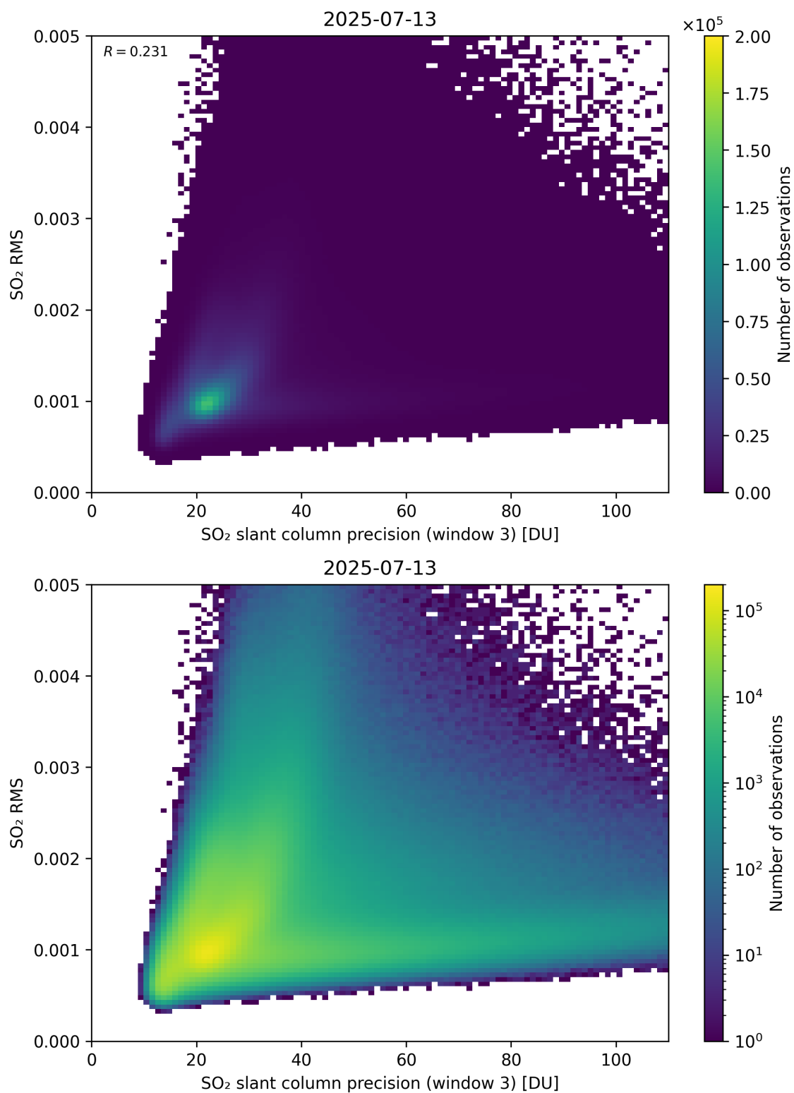
Figure 310: Scatter density plot of “SO 2 slant column precision (window 3)” against “SO 2 RMS” for 2025-07-13 to 2025-07-14.
