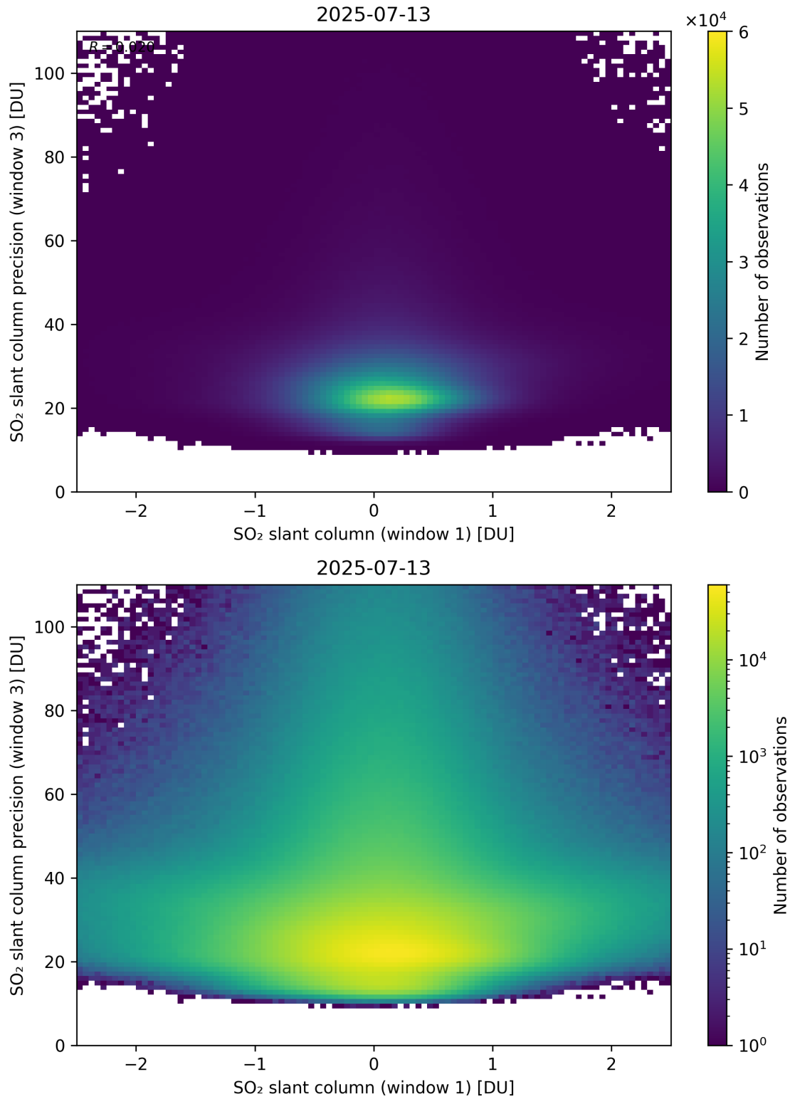
Figure 288: Scatter density plot of “SO 2 slant column (window 1)” against “SO 2 slant column precision (window 3)” for 2025-07-13 to 2025-07-14.
