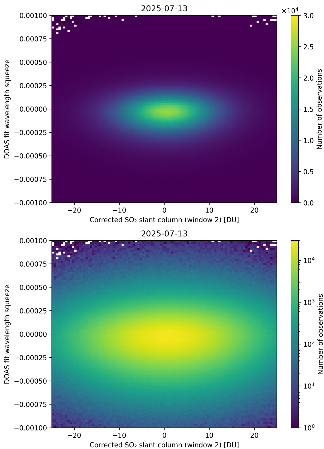
Figure 247: Scatter density plot of “Corrected SO 2 slant column (window 2)” against “DOAS fit wavelength squeeze” for 2025-07-13 to 2025-07-14.
