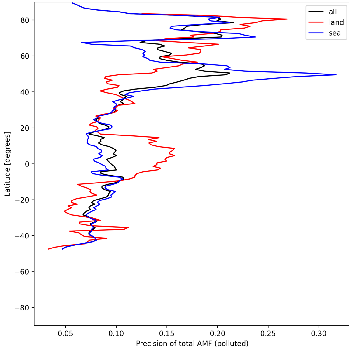
Figure 54: Zonal average of “Precision of total AMF (polluted)” for 2025-07-13 to 2025-07-14.
