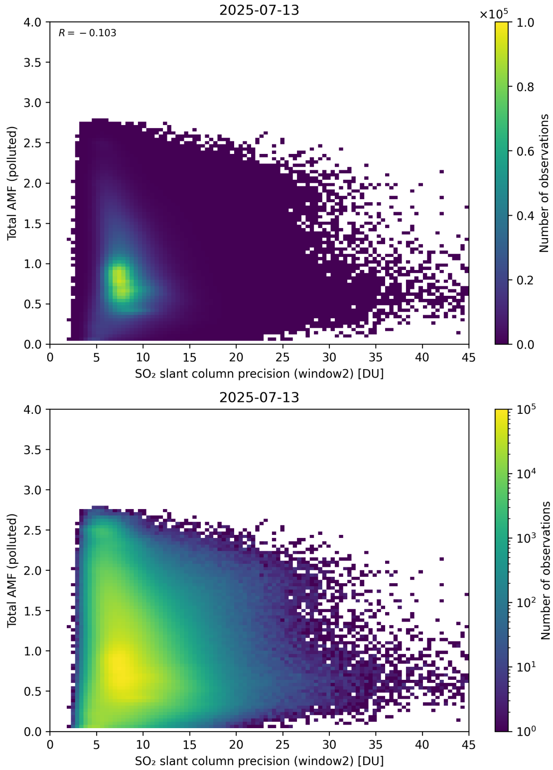
Figure 301: Scatter density plot of “SO 2 slant column precision (window2)” against “Total AMF (polluted)” for 2025-07-13 to 2025-07-14.
