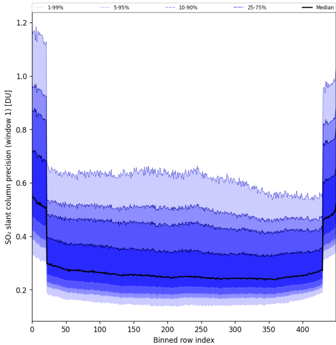
Figure 90: Along track statistics of “SO 2 slant column precision (window 1)” for 2025-07-13 to 2025-07-14
