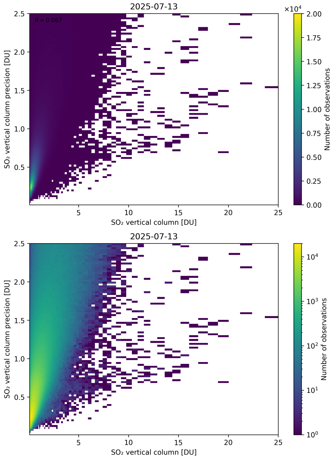
Figure 361: Scatter density plot of “SO 2 vertical column” against “SO 2 vertical column precision” for 2025-07-13 to 2025-07-14.
