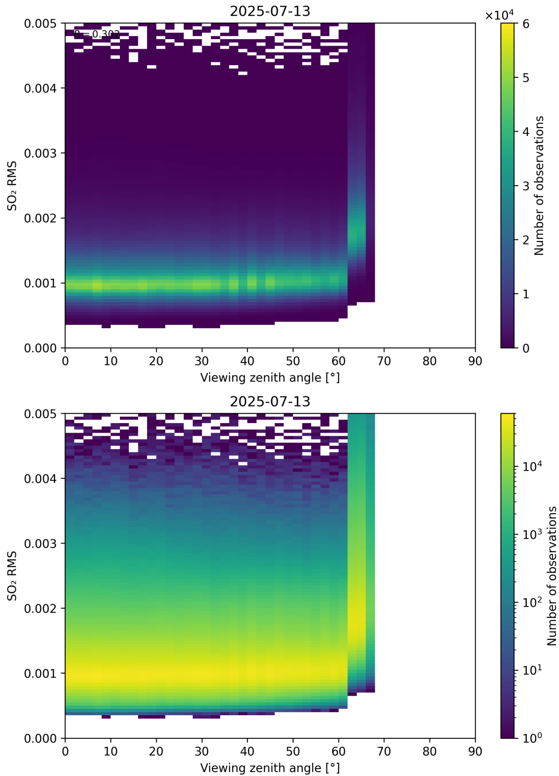
Figure 367: Scatter density plot of “Viewing zenith angle” against “SO 2 RMS” for 2025-07-13 to 2025-07-14.
