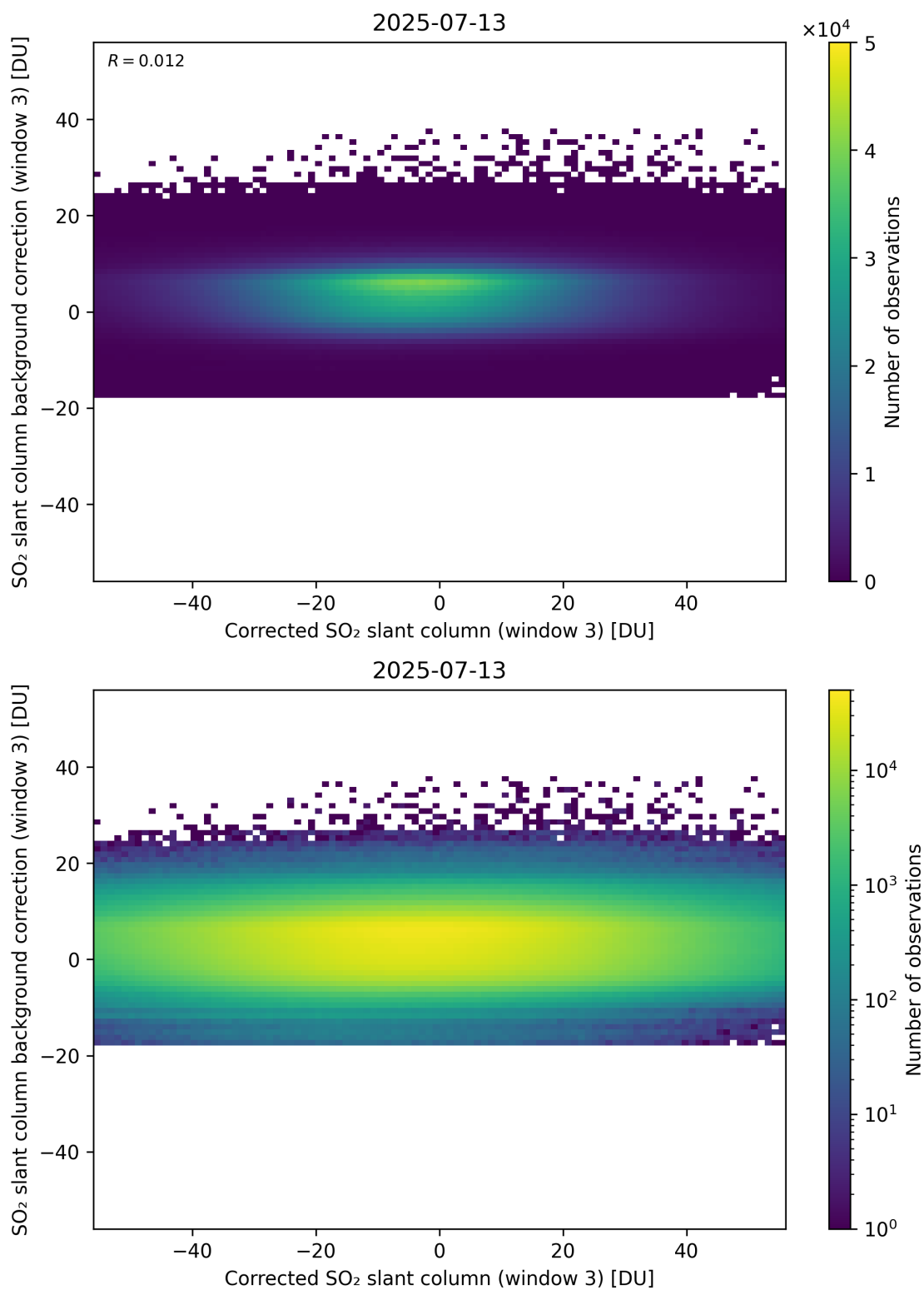
Figure 255: Scatter density plot of “Corrected SO 2 slant column (window 3)” against “SO 2 slant column background correction (window 3)” for 2025-07-13 to 2025-07-14.
