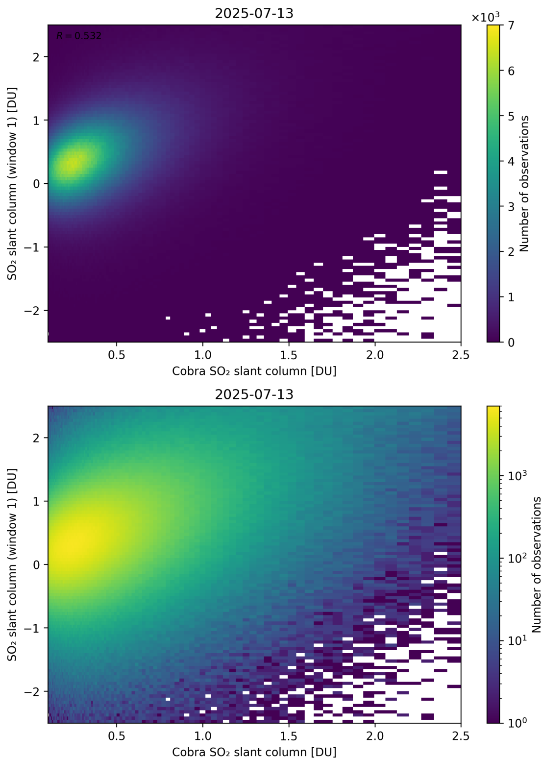
Figure 219: Scatter density plot of “Cobra SO 2 slant column” against “SO 2 slant column (window 1)” for 2025-07-13 to 2025-07-14.
