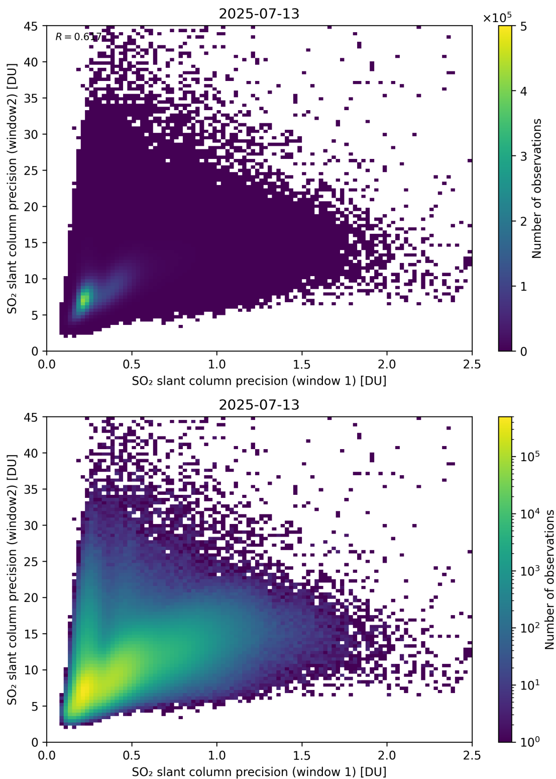
Figure 277: Scatter density plot of “SO 2 slant column precision (window 1)” against “SO 2 slant column precision (window2)” for 2025-07-13 to 2025-07-14.
