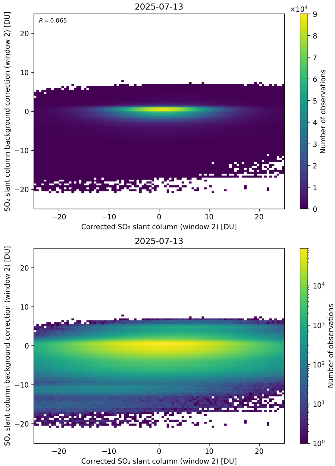
Figure 244: Scatter density plot of “Corrected SO 2 slant column (window 2)” against “SO 2 slant column background correction (window 2)” for 2025-07-13 to 2025-07-14.
