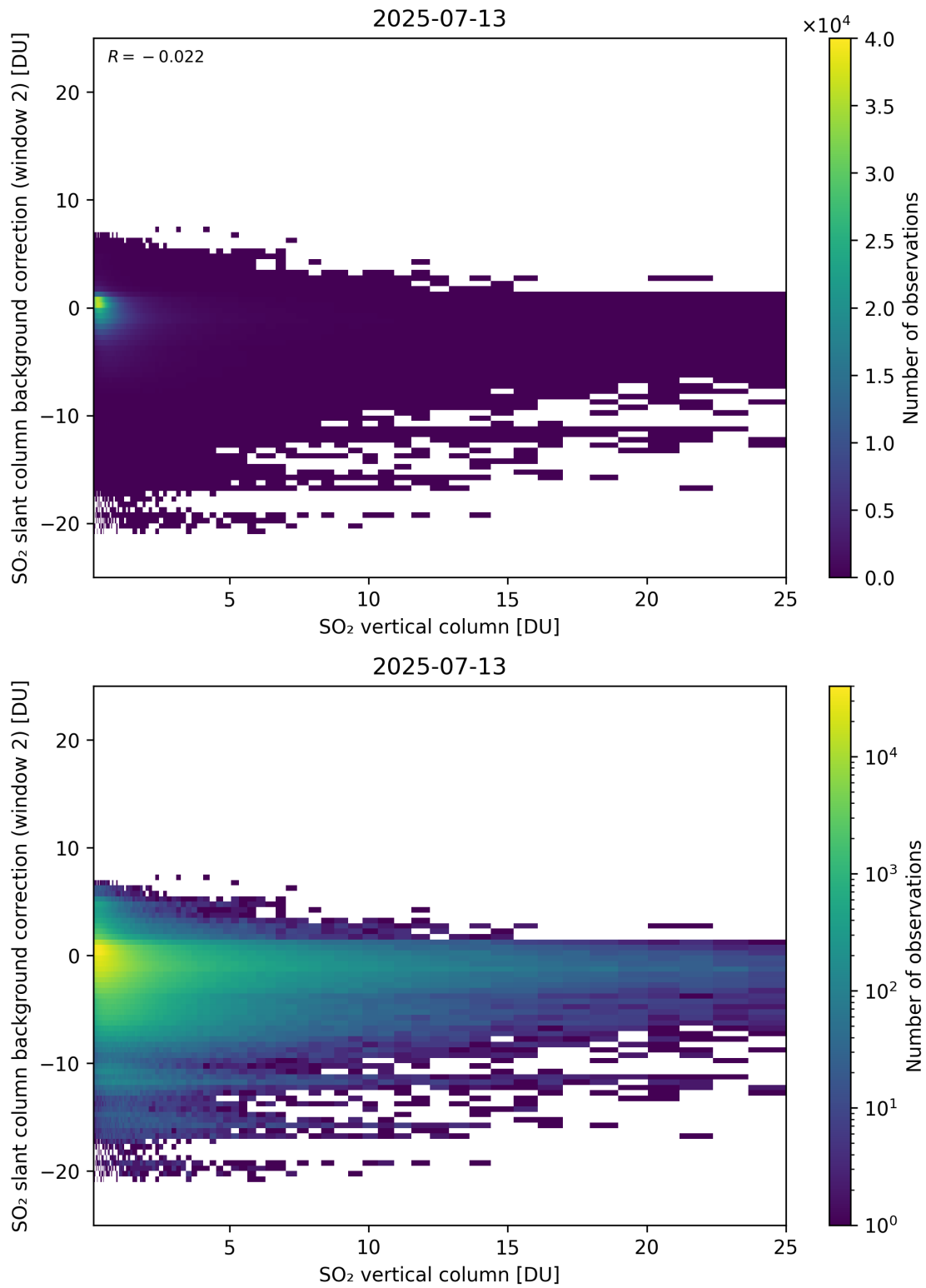
Figure 324: Scatter density plot of “SO 2 vertical column” against “SO 2 slant column background correction (window 2)” for 2025-07-13 to 2025-07-14.
