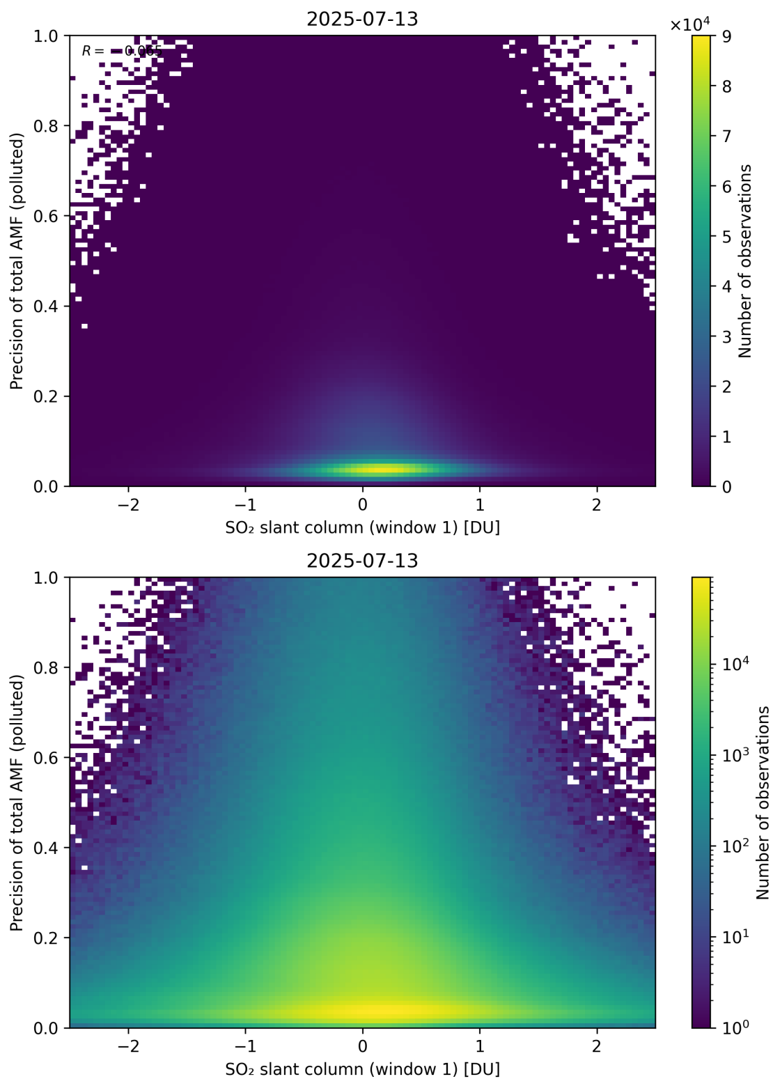
Figure 290: Scatter density plot of “SO 2 slant column (window 1)” against “Precision of total AMF (polluted)” for 2025-07-13 to 2025-07-14.
