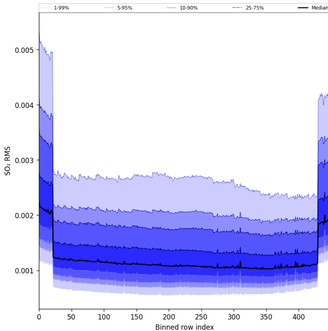
Figure 104: Along track statistics of “SO 2 RMS” for 2025-07-13 to 2025-07-14
