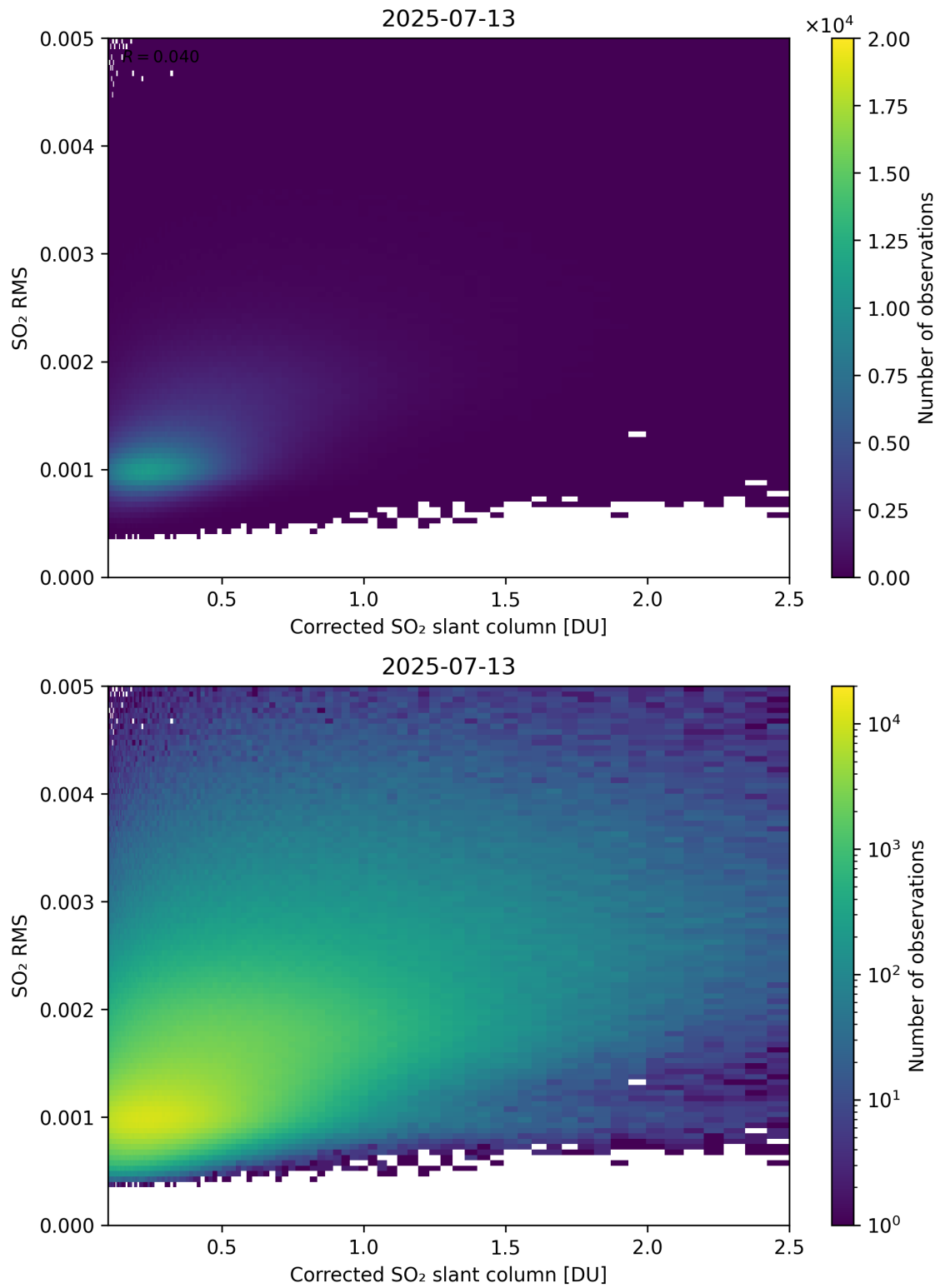
Figure 231: Scatter density plot of “Corrected SO 2 slant column” against “SO 2 RMS” for 2025-07-13 to 2025-07-14.
