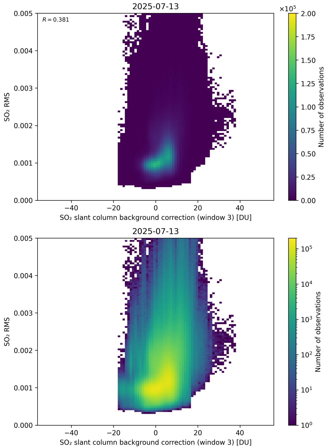
Figure 134: Scatter density plot of “SO 2 slant column background correction (window 3)” against “SO 2 RMS” for 2025-07-13 to 2025-07-14.
