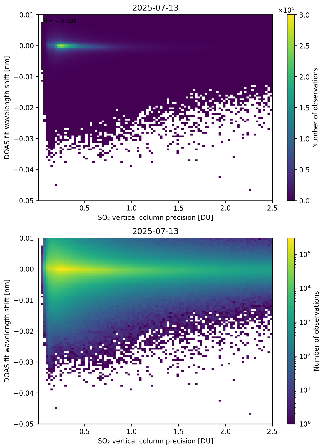
Figure 332: Scatter density plot of “SO 2 vertical column precision” against “DOAS fit wavelength shift” for 2025-07-13 to 2025-07-14.
