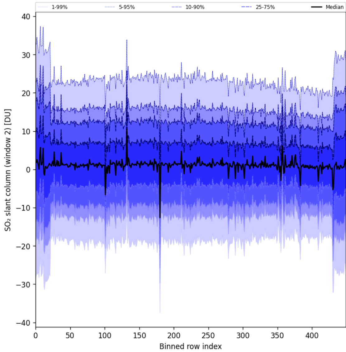
Figure 93: Along track statistics of “SO 2 slant column (window 2)” for 2025-07-13 to 2025-07-14
