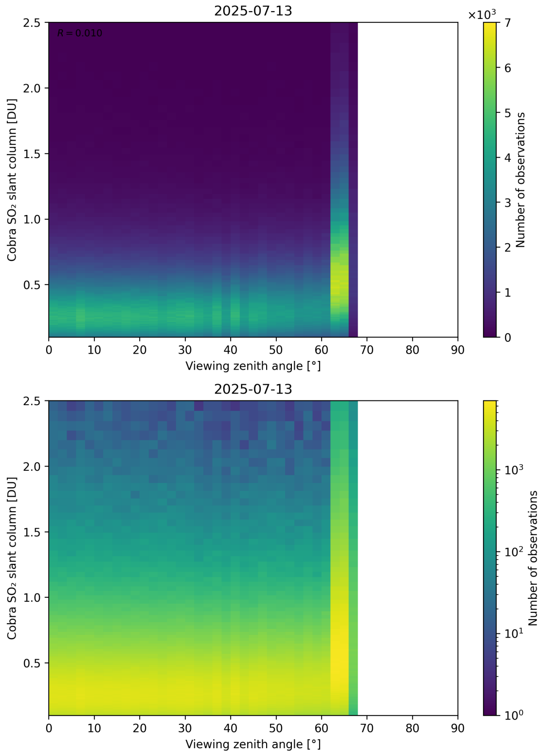
Figure 371: Scatter density plot of “Viewing zenith angle” against “Cobra SO 2 slant column” for 2025-07-13 to 2025-07-14.
