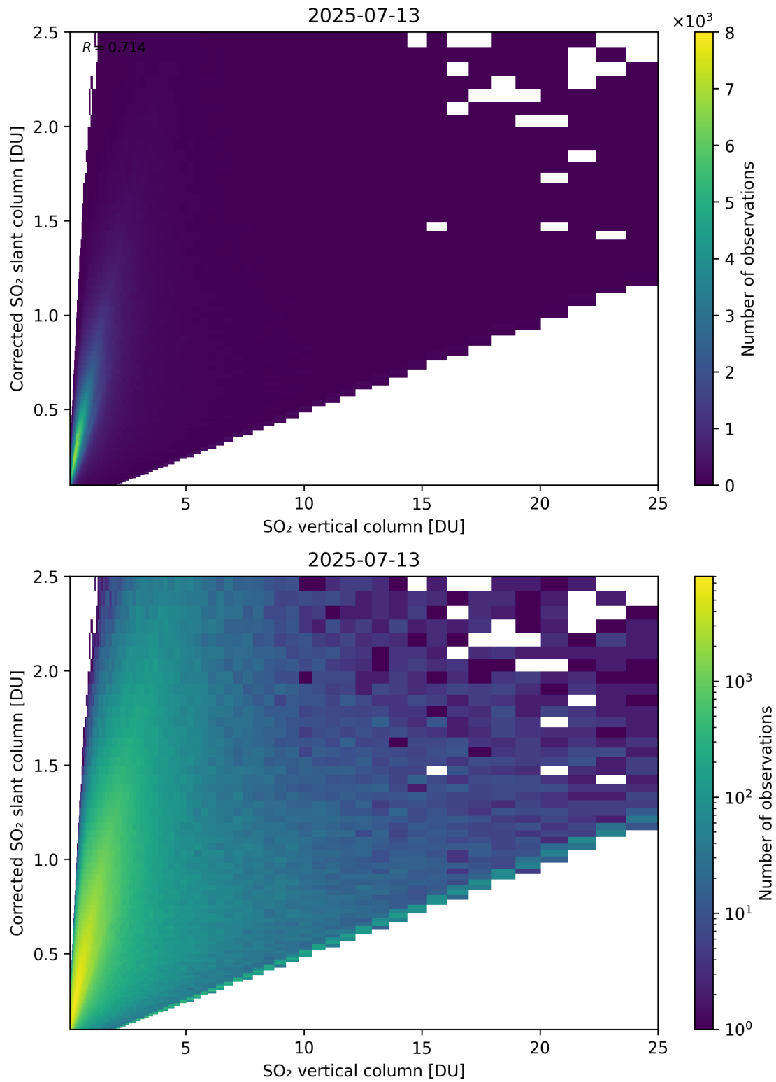
Figure 351: Scatter density plot of “SO 2 vertical column” against “Corrected SO 2 slant column” for 2025-07-13 to 2025-07-14.
