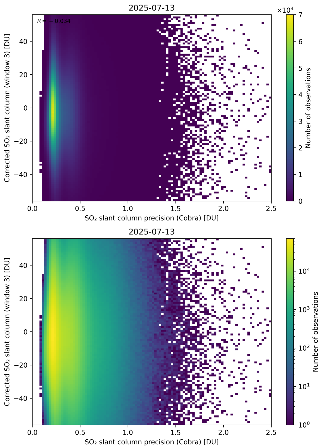
Figure 207: Scatter density plot of “SO 2 slant column precision (Cobra)” against “Corrected SO 2 slant column (window 3)” for 2025-07-13 to 2025-07-14.
