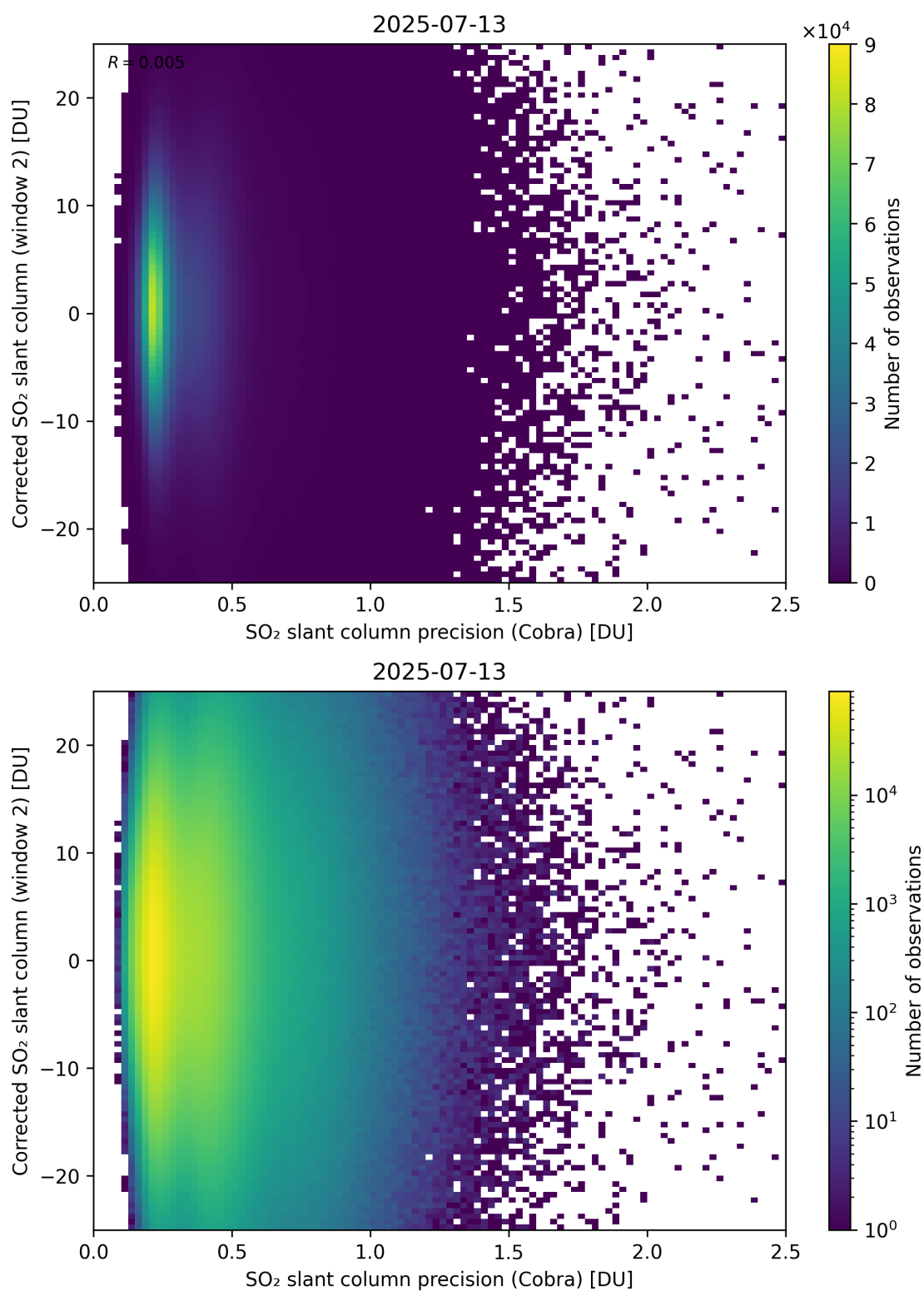
Figure 206: Scatter density plot of “SO 2 slant column precision (Cobra)” against “Corrected SO 2 slant column (window 2)” for 2025-07-13 to 2025-07-14.
