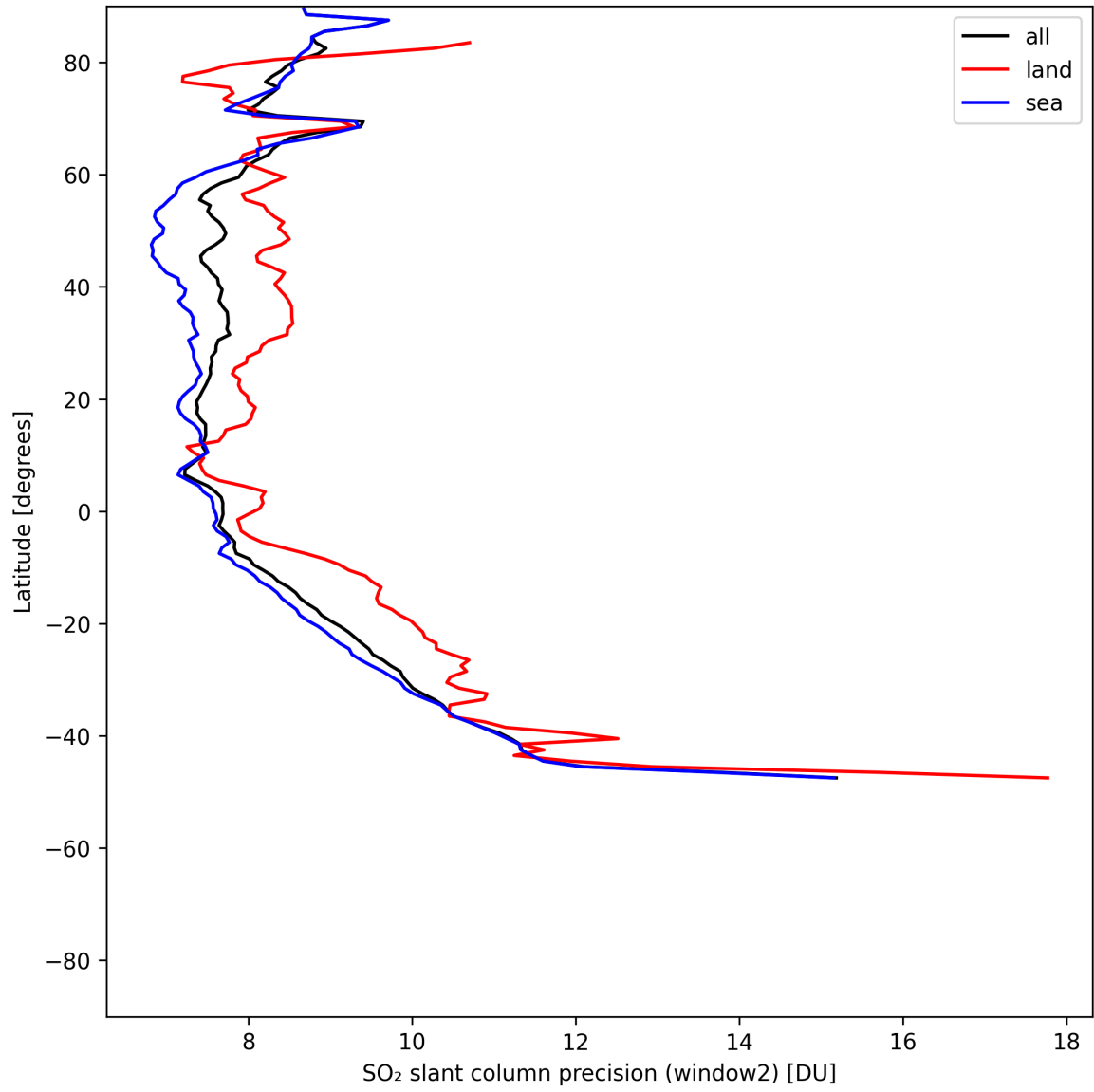
Figure 42: Zonal average of “SO 2 slant column precision (window2)” for 2025-07-13 to 2025-07-14.
