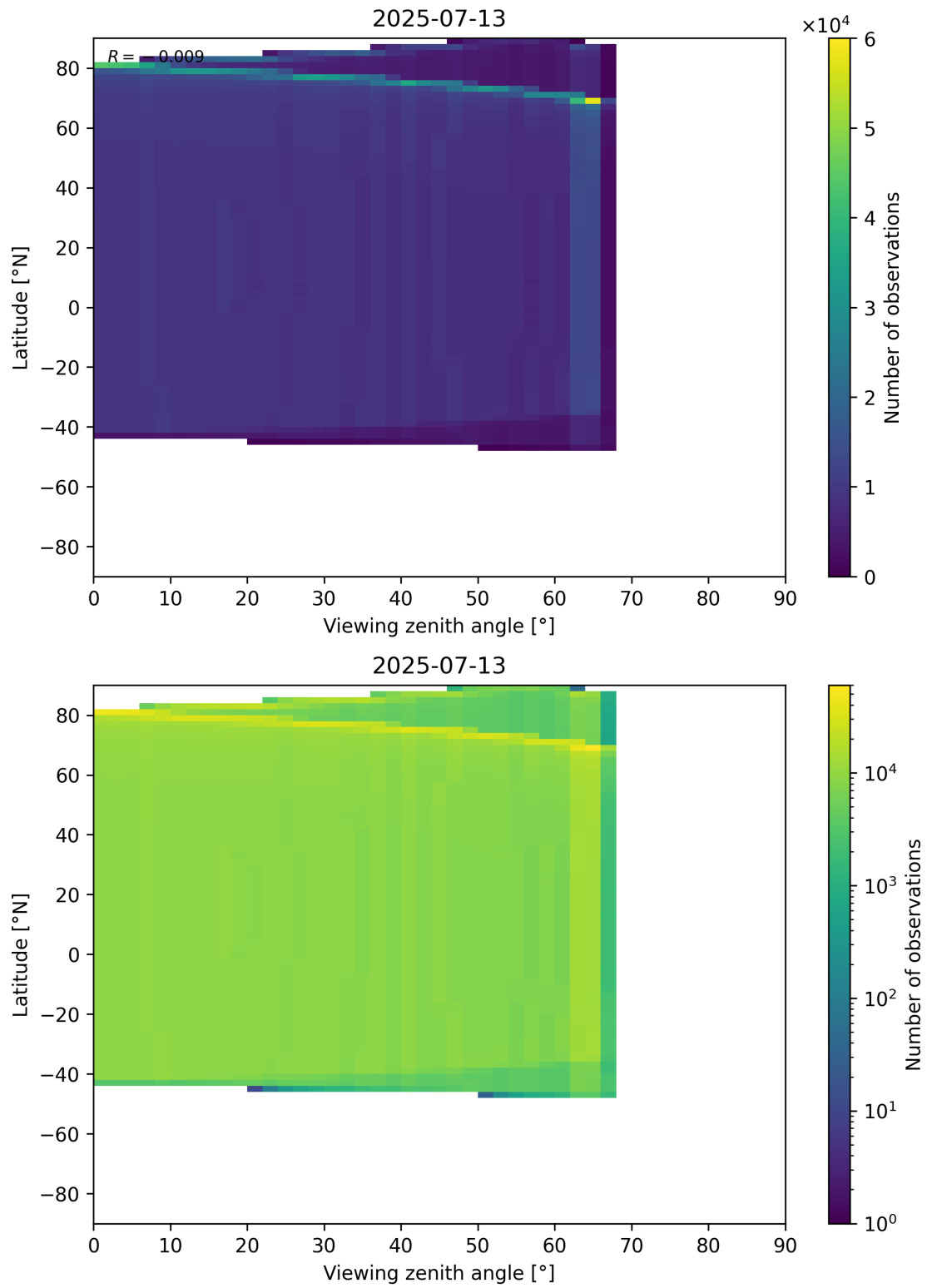
Figure 368: Scatter density plot of “Viewing zenith angle” against “Latitude” for 2025-07-13 to 2025-07-14.
