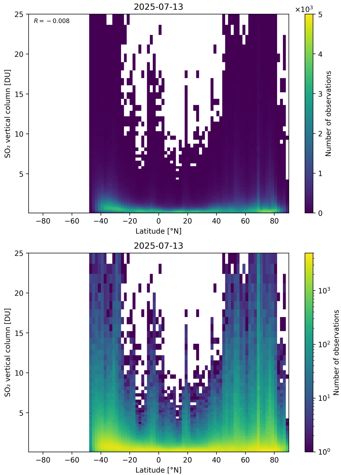
Figure 169: Scatter density plot of “Latitude” against “SO 2 vertical column” for 2025-07-13 to 2025-07-14.
