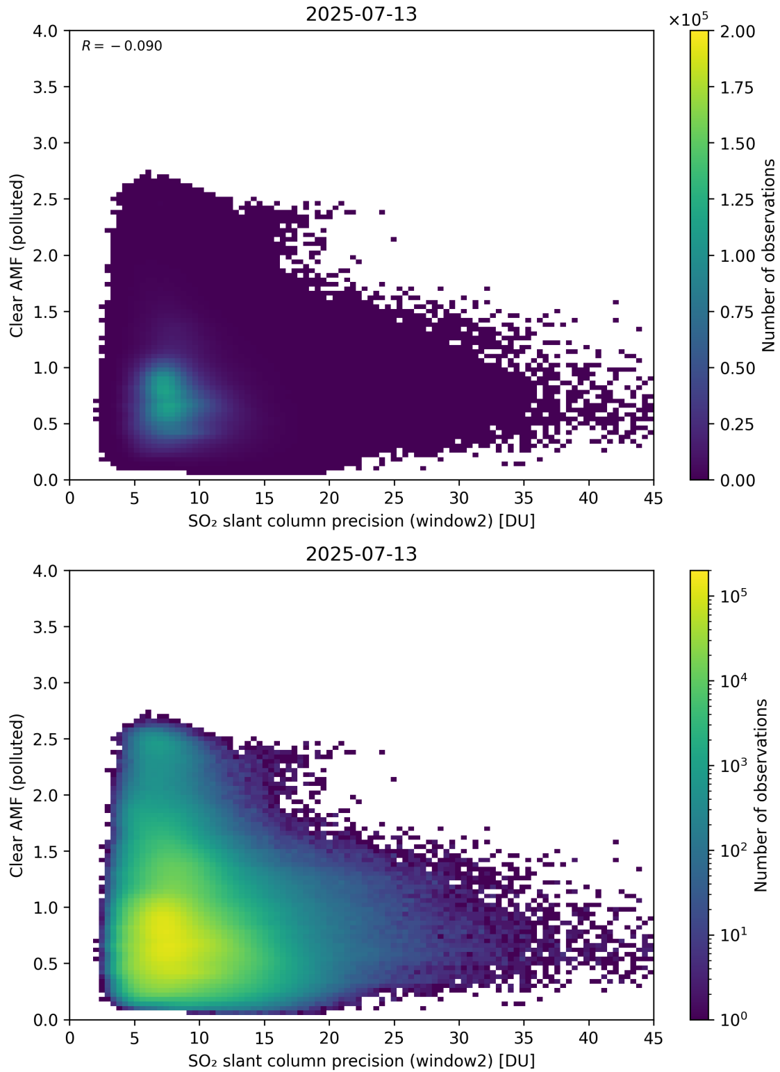
Figure 296: Scatter density plot of “SO 2 slant column precision (window2)” against “Clear AMF (polluted)” for 2025-07-13 to 2025-07-14.
