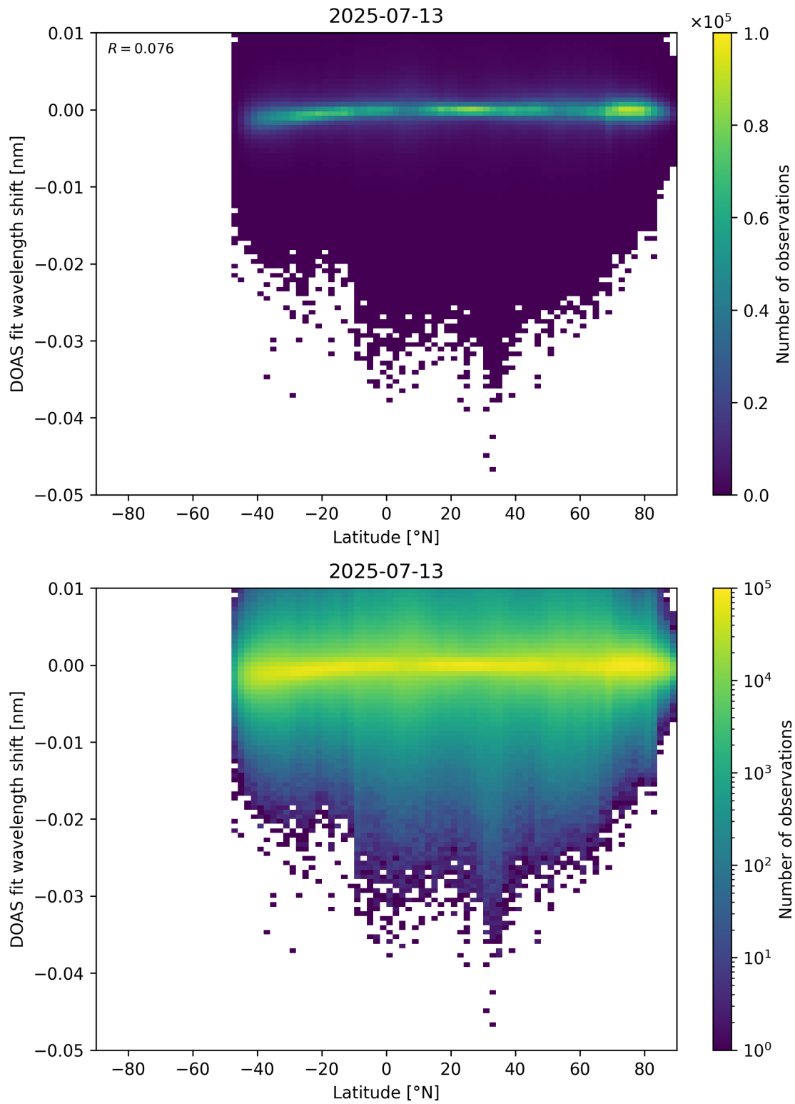
Figure 153: Scatter density plot of “Latitude” against “DOAS fit wavelength shift” for 2025-07-13 to 2025-07-14.
