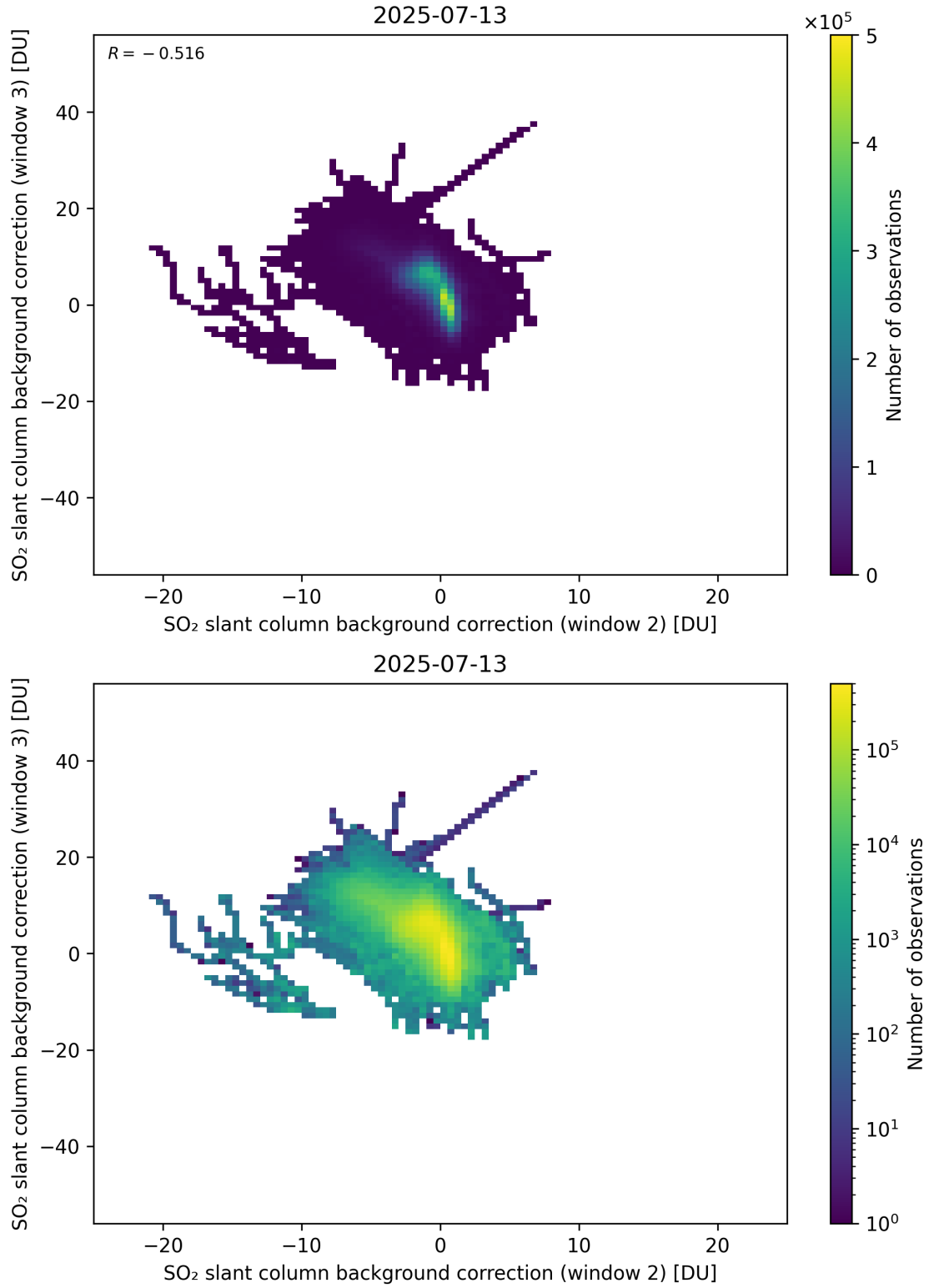
Figure 122: Scatter density plot of “SO 2 slant column background correction (window 2)” against “SO 2 slant column background correction (window 3)” for 2025-07-13 to 2025-07-14.
