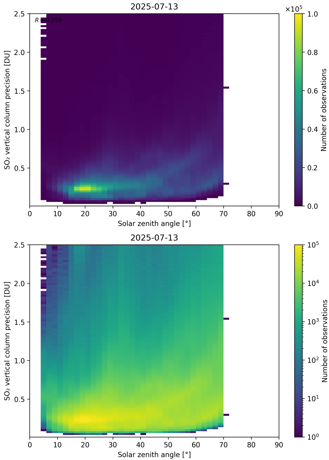
Figure 192: Scatter density plot of “Solar zenith angle” against “SO 2 vertical column precision” for 2025-07-13 to 2025-07-14.
