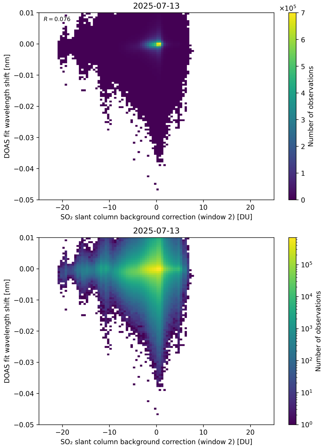
Figure 123: Scatter density plot of “SO 2 slant column background correction (window 2)” against “DOAS fit wavelength shift” for 2025-07-13 to 2025-07-14.
