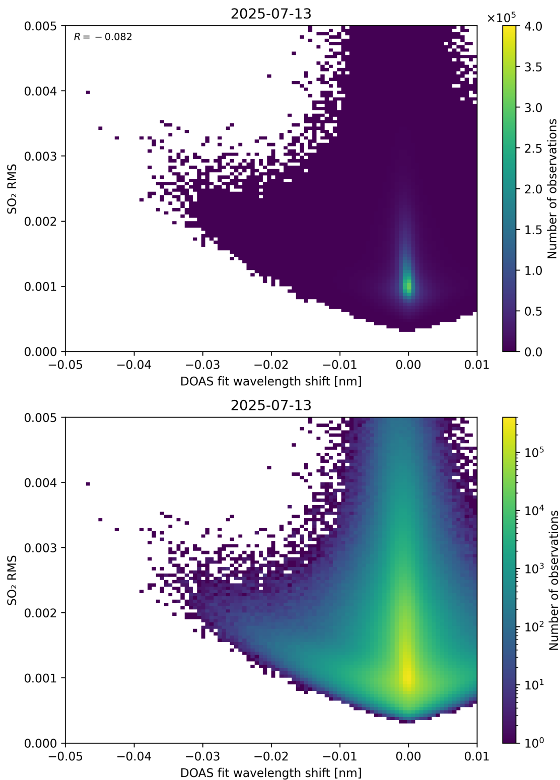
Figure 139: Scatter density plot of “DOAS fit wavelength shift” against “SO 2 RMS” for 2025-07-13 to 2025-07-14.
