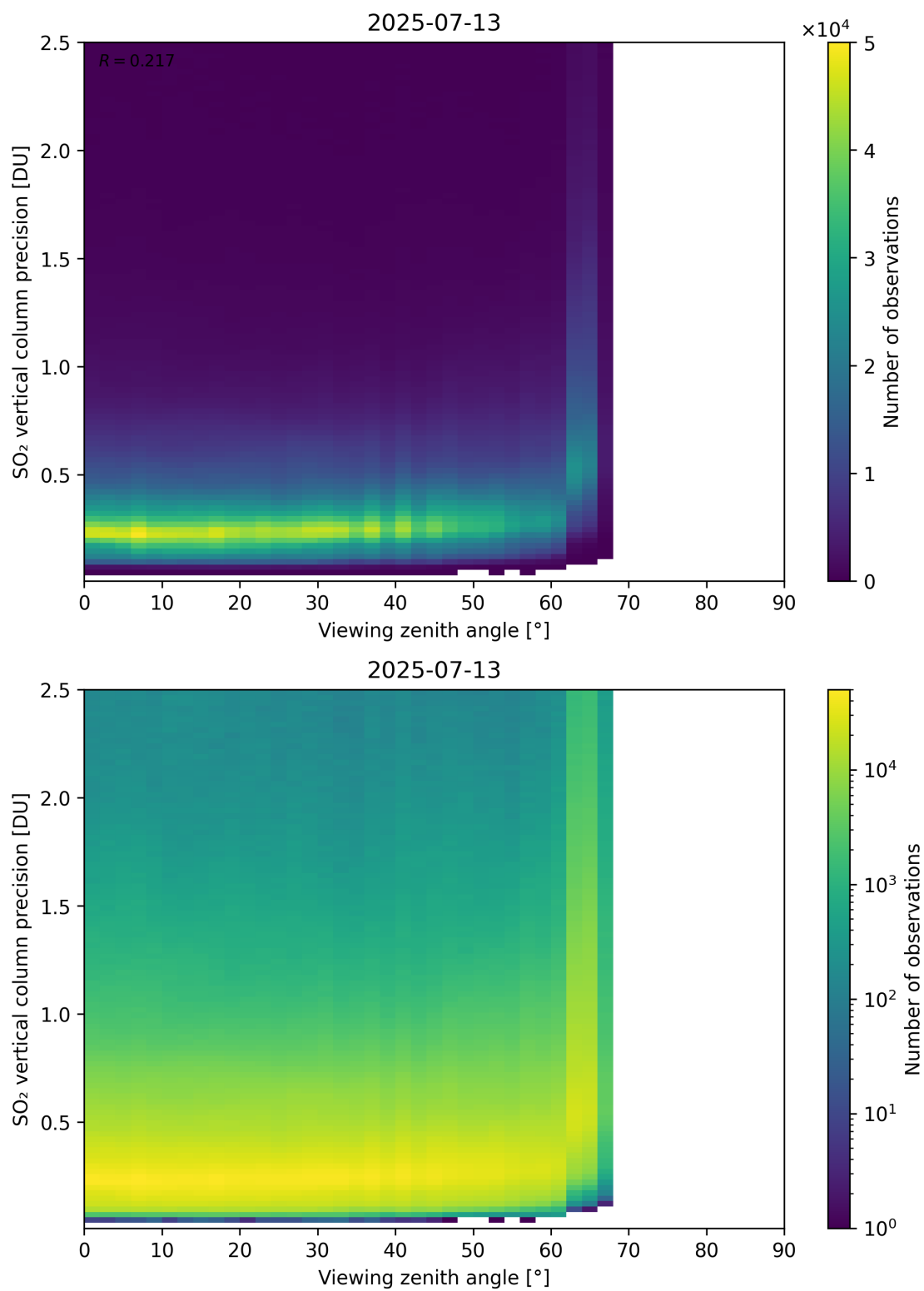
Figure 384: Scatter density plot of “Viewing zenith angle” against “SO 2 vertical column precision” for 2025-07-13 to 2025-07-14.
