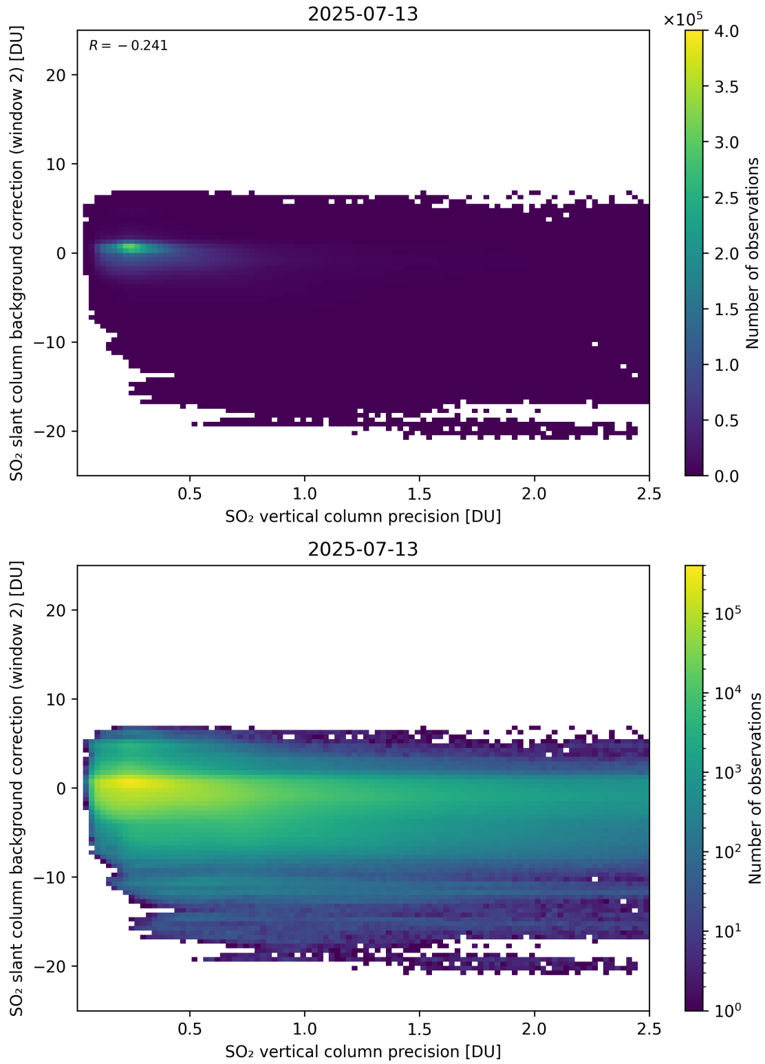
Figure 330: Scatter density plot of “SO 2 vertical column precision” against “SO 2 slant column background correction (window 2)” for 2025-07-13 to 2025-07-14.
