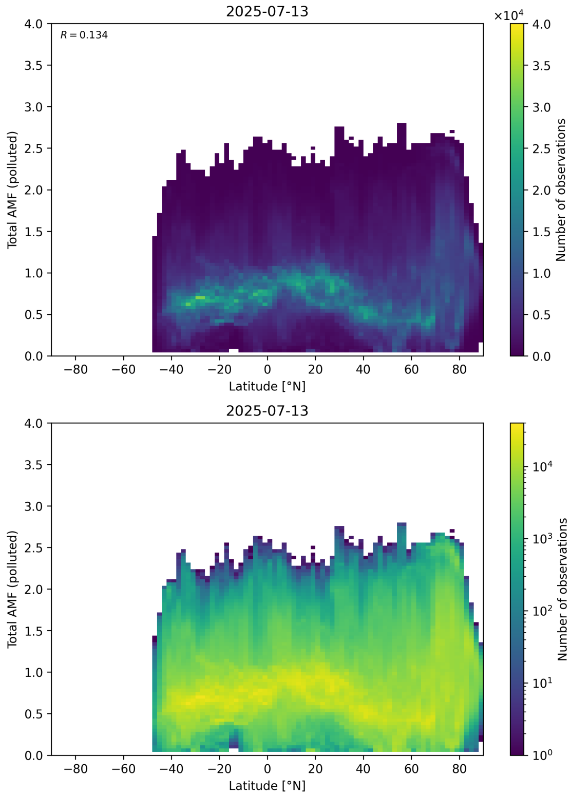
Figure 167: Scatter density plot of “Latitude” against “Total AMF (polluted)” for 2025-07-13 to 2025-07-14.
