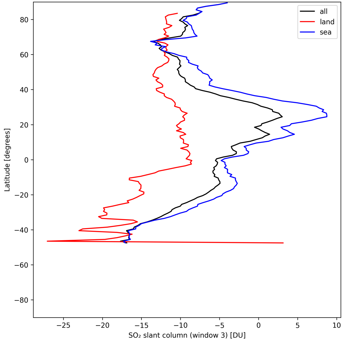
Figure 45: Zonal average of “SO 2 slant column (window 3)” for 2025-07-13 to 2025-07-14.
