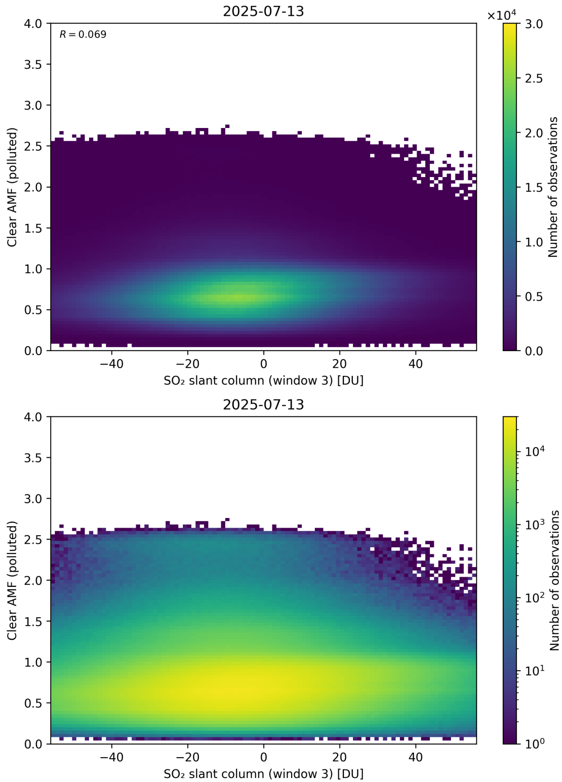
Figure 315: Scatter density plot of “SO 2 slant column (window 3)” against “Clear AMF (polluted)” for 2025-07-13 to 2025-07-14.
