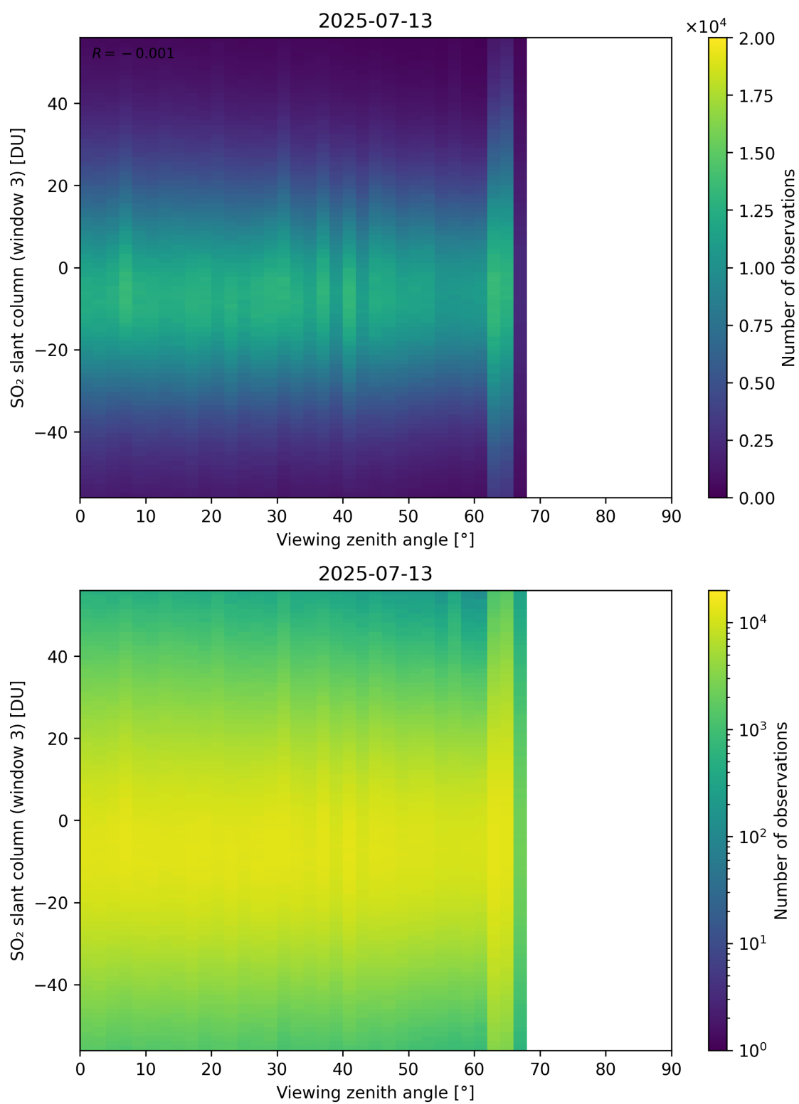
Figure 379: Scatter density plot of “Viewing zenith angle” against “SO 2 slant column (window 3)” for 2025-07-13 to 2025-07-14.
