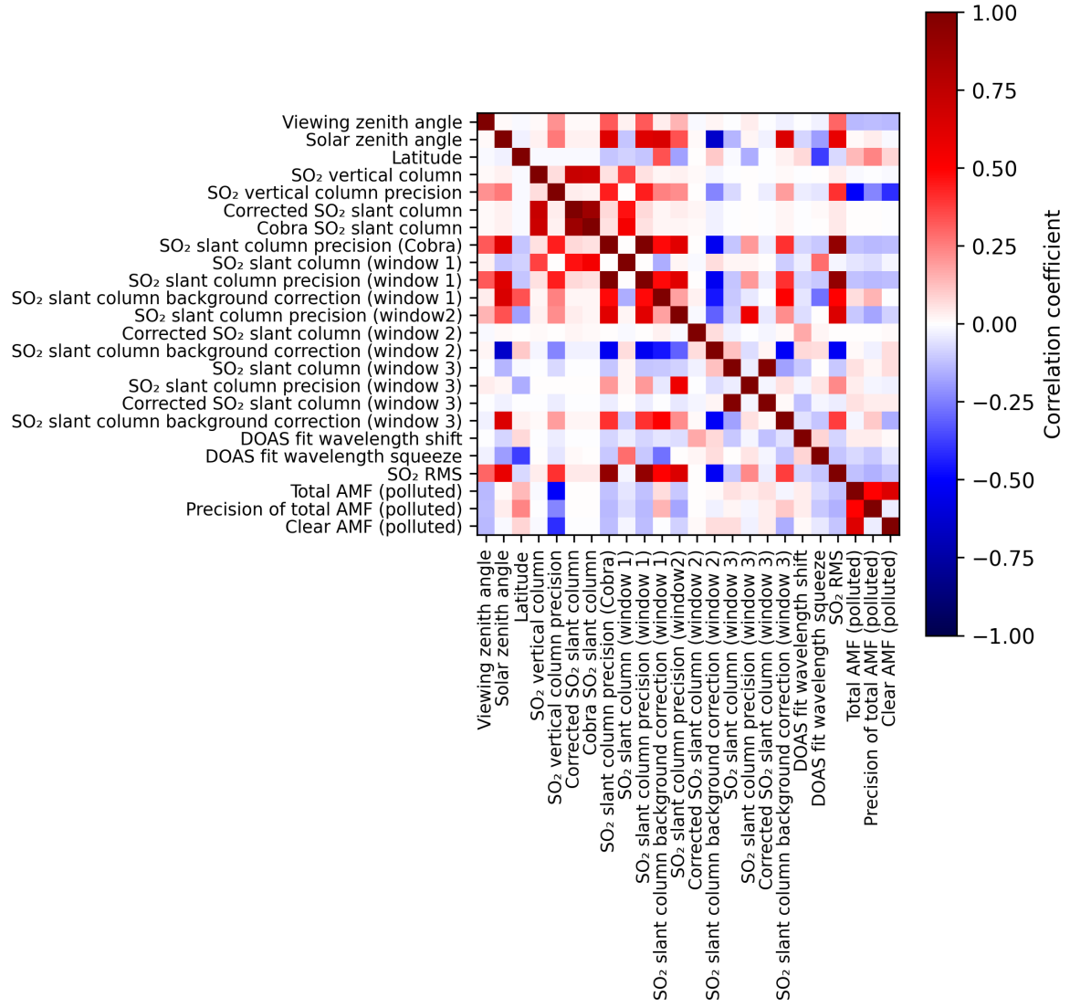
Figure 2: Map of correlation matrix for 2025-07-13 to 2025-07-14.
