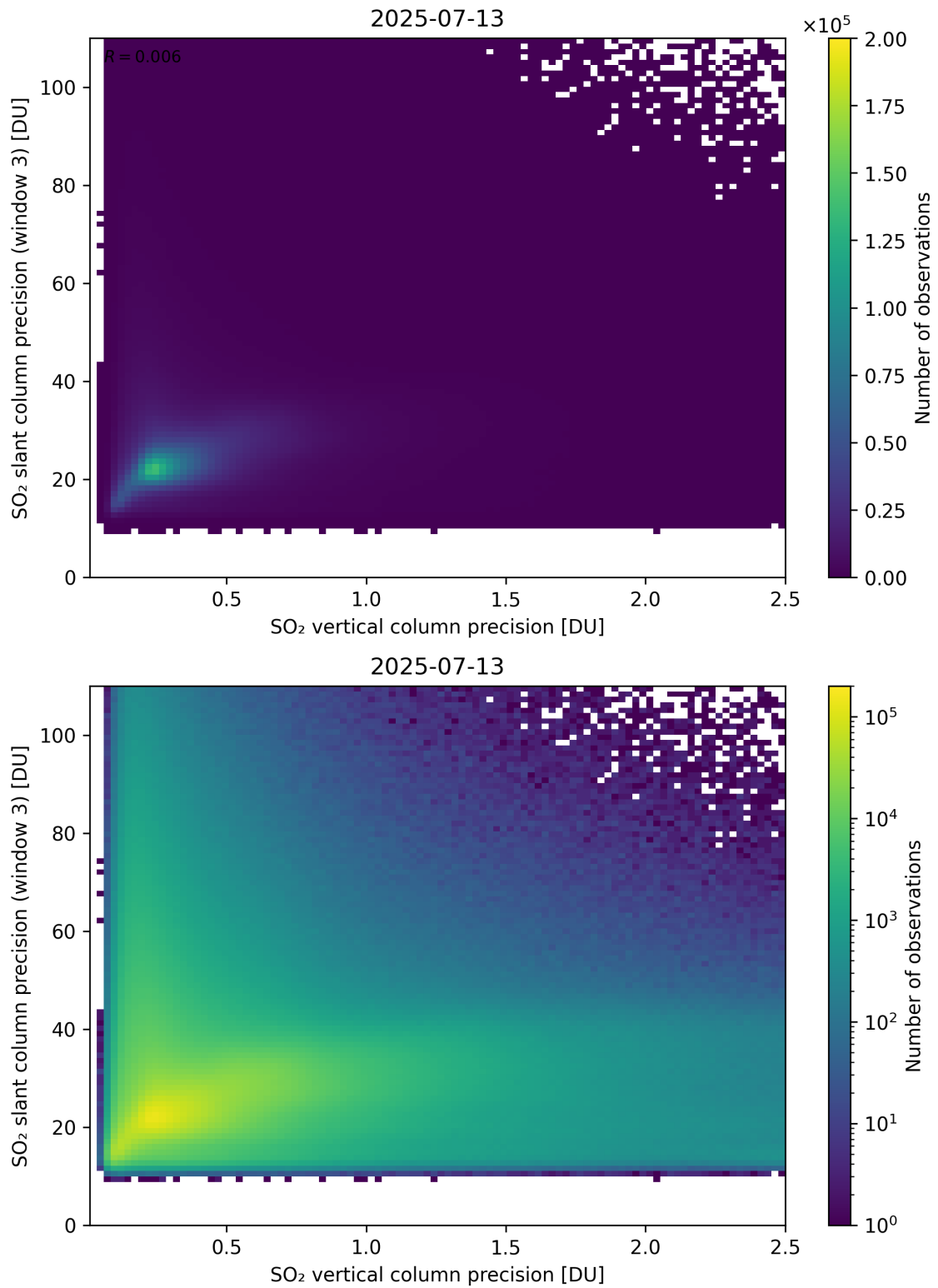
Figure 345: Scatter density plot of “SO 2 vertical column precision” against “SO 2 slant column precision (window 3)” for 2025-07-13 to 2025-07-14.
