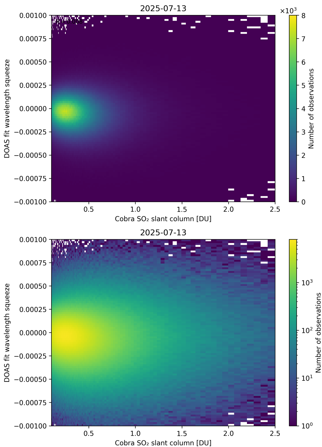
Figure 197: Scatter density plot of “Cobra SO 2 slant column” against “DOAS fit wavelength squeeze” for 2025-07-13 to 2025-07-14.
