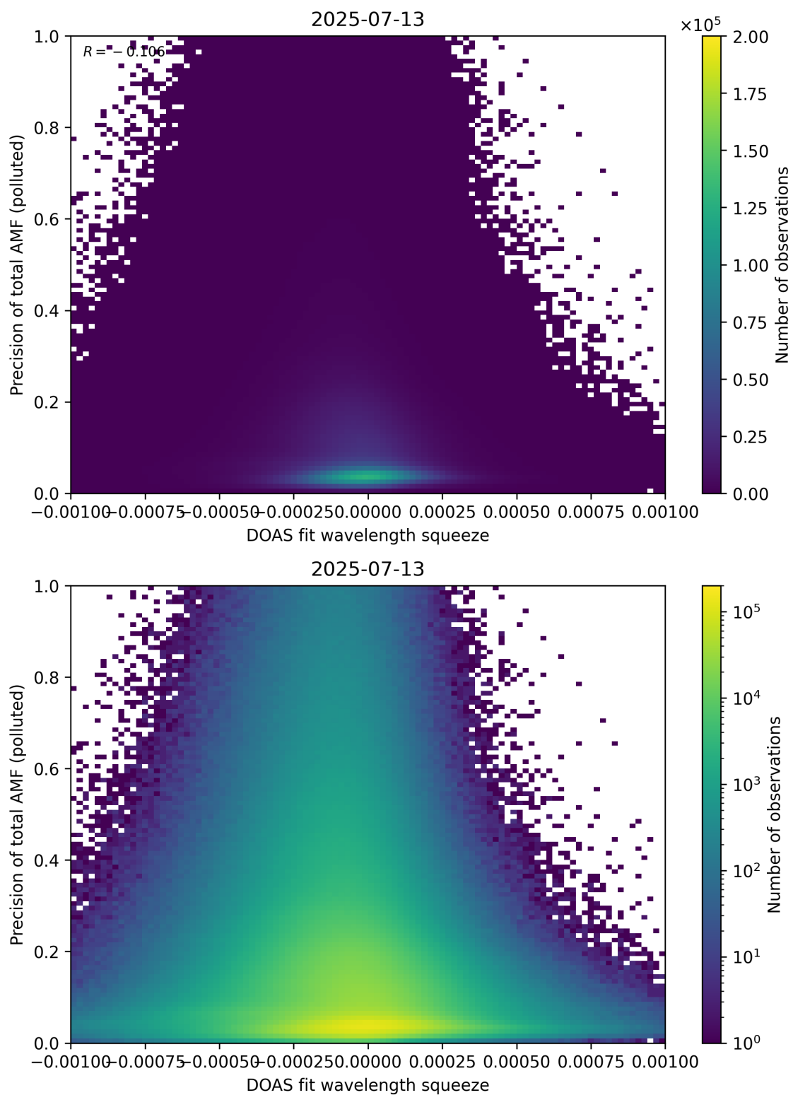
Figure 146: Scatter density plot of “DOAS fit wavelength squeeze” against “Precision of total AMF (polluted)” for 2025-07-13 to 2025-07-14.
