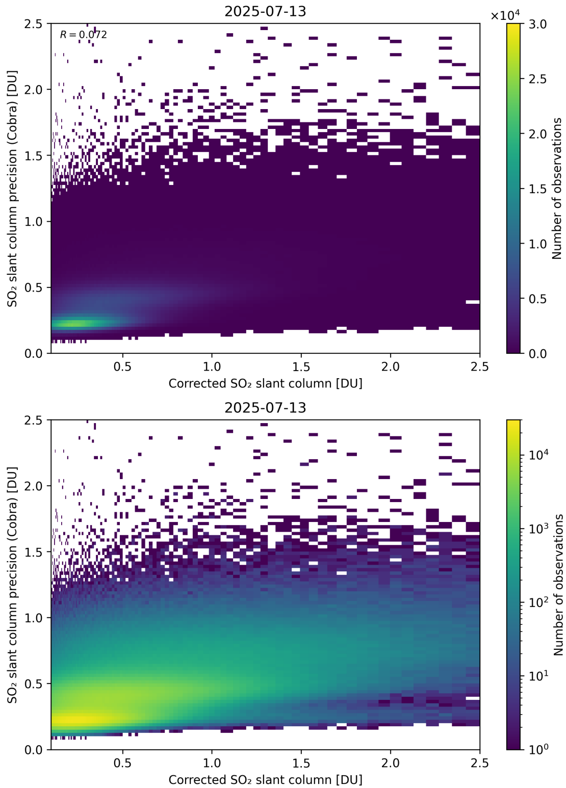
Figure 234: Scatter density plot of “Corrected SO 2 slant column” against “SO 2 slant column precision (Cobra)” for 2025-07-13 to 2025-07-14.
