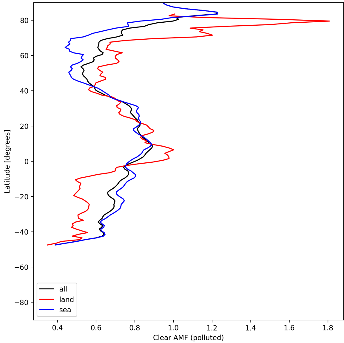
Figure 55: Zonal average of “Clear AMF (polluted)” for 2025-07-13 to 2025-07-14.
