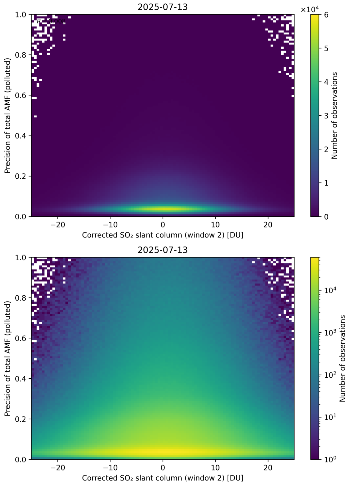
Figure 254: Scatter density plot of “Corrected SO 2 slant column (window 2)” against “Precision of total AMF (polluted)” for 2025-07-13 to 2025-07-14.
