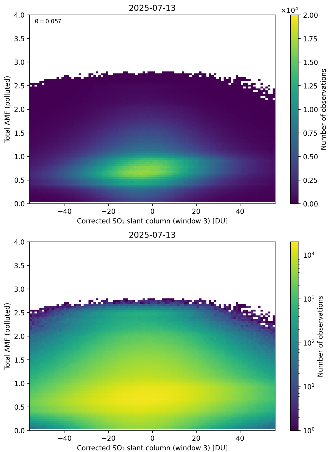
Figure 260: Scatter density plot of “Corrected SO 2 slant column (window 3)” against “Total AMF (polluted)” for 2025-07-13 to 2025-07-14.
