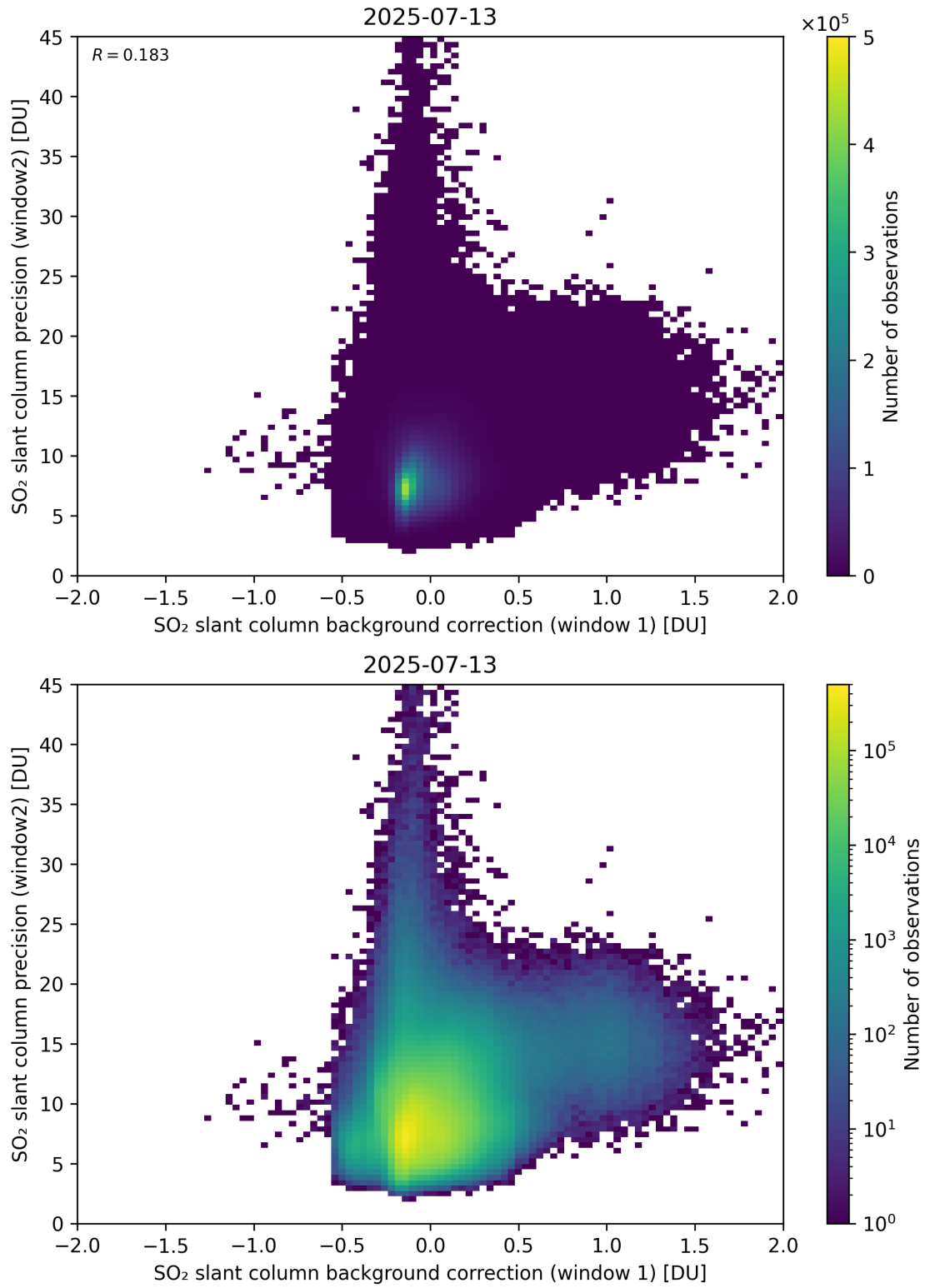
Figure 117: Scatter density plot of “SO 2 slant column background correction (window 1)” against “SO 2 slant column precision (window2)” for 2025-07-13 to 2025-07-14.
