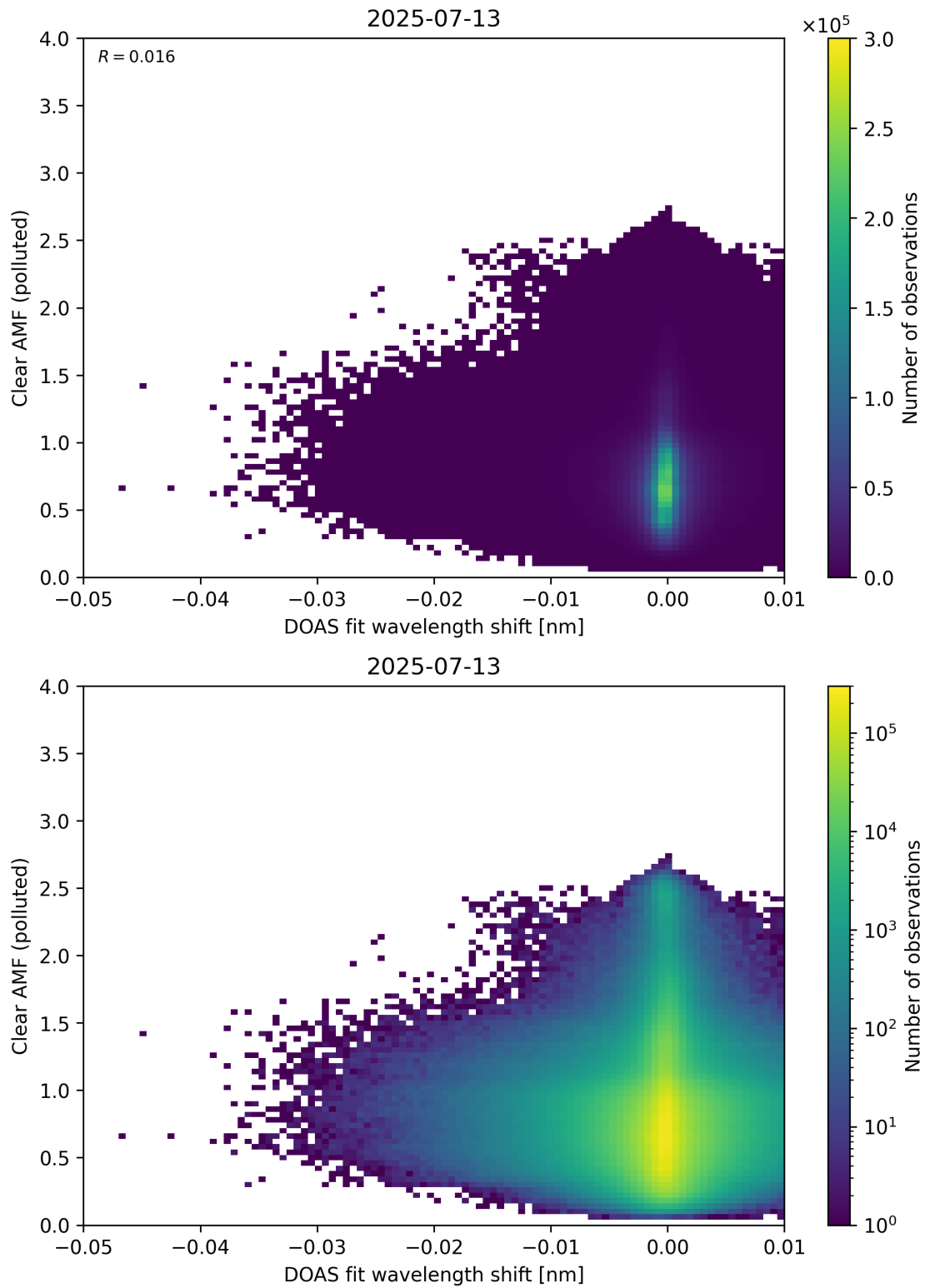
Figure 140: Scatter density plot of “DOAS fit wavelength shift” against “Clear AMF (polluted)” for 2025-07-13 to 2025-07-14.
