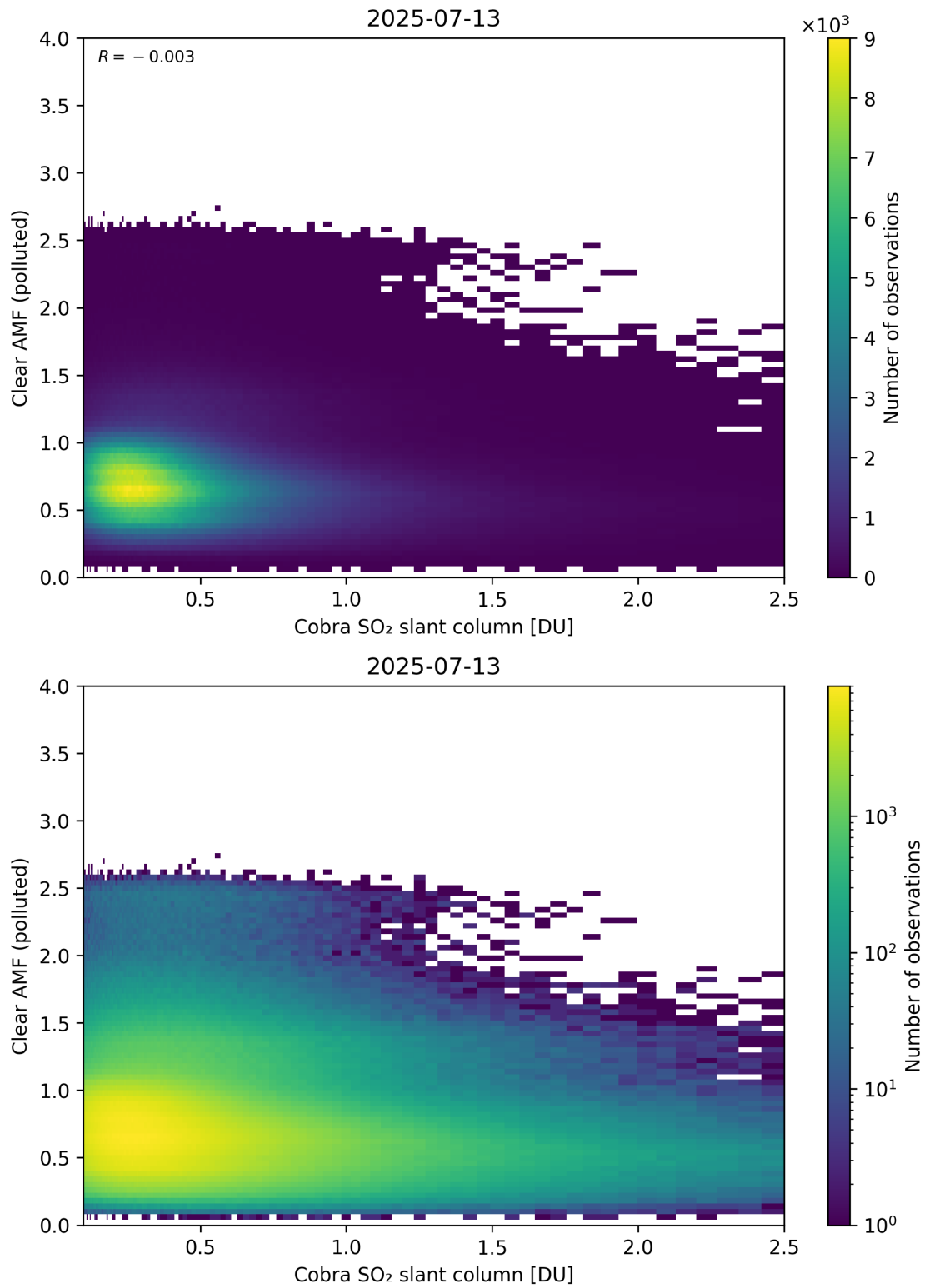
Figure 215: Scatter density plot of “Cobra SO 2 slant column” against “Clear AMF (polluted)” for 2025-07-13 to 2025-07-14.
