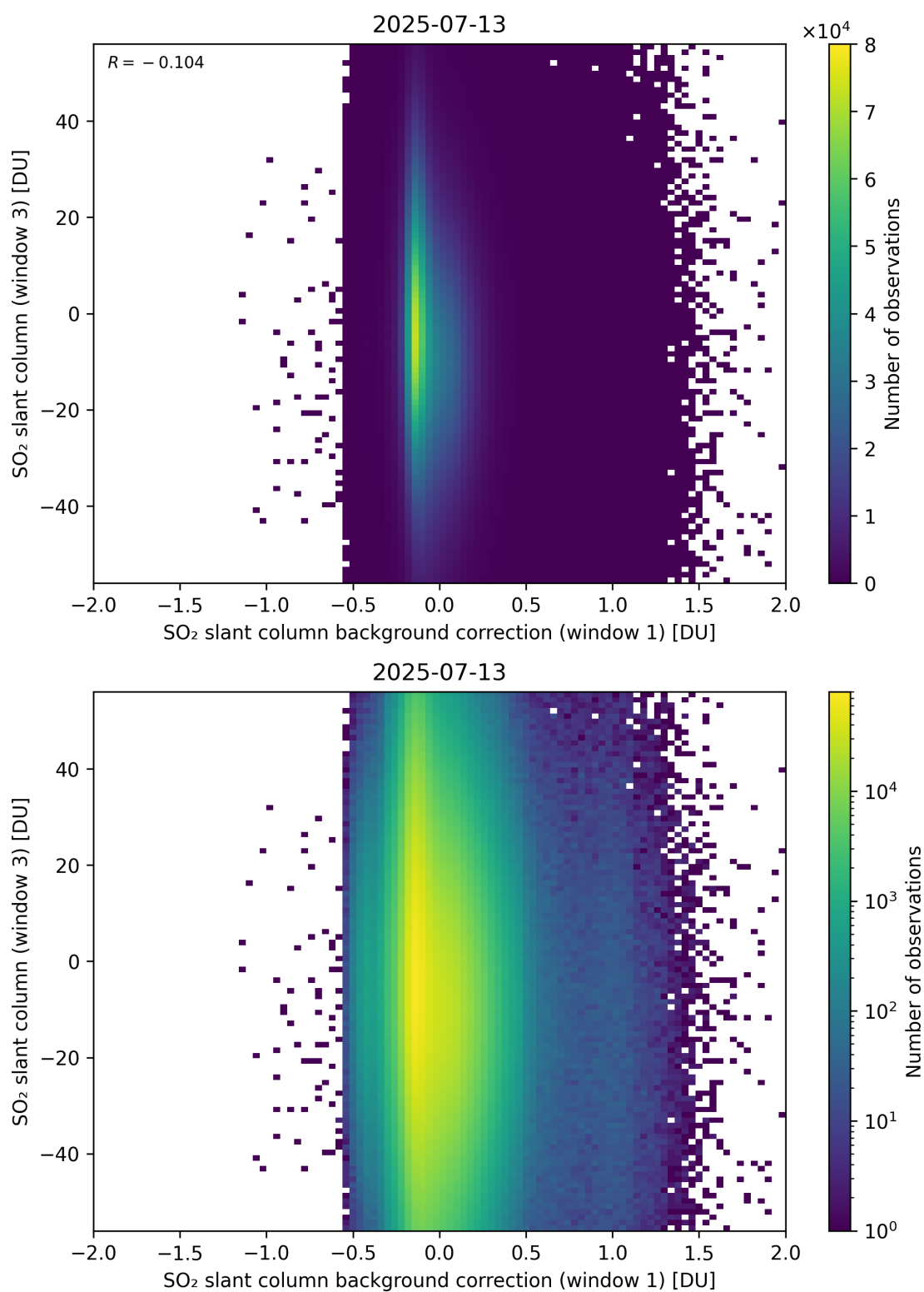
Figure 118: Scatter density plot of “SO 2 slant column background correction (window 1)” against “SO 2 slant column (window 3)” for 2025-07-13 to 2025-07-14.
