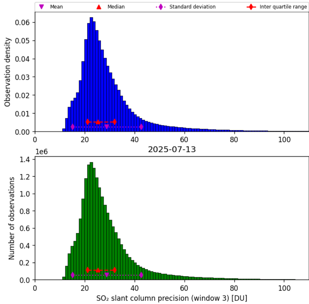
Figure 72: Histogram of “SO 2 slant column precision (window 3)” for 2025-07-13 to 2025-07-14
