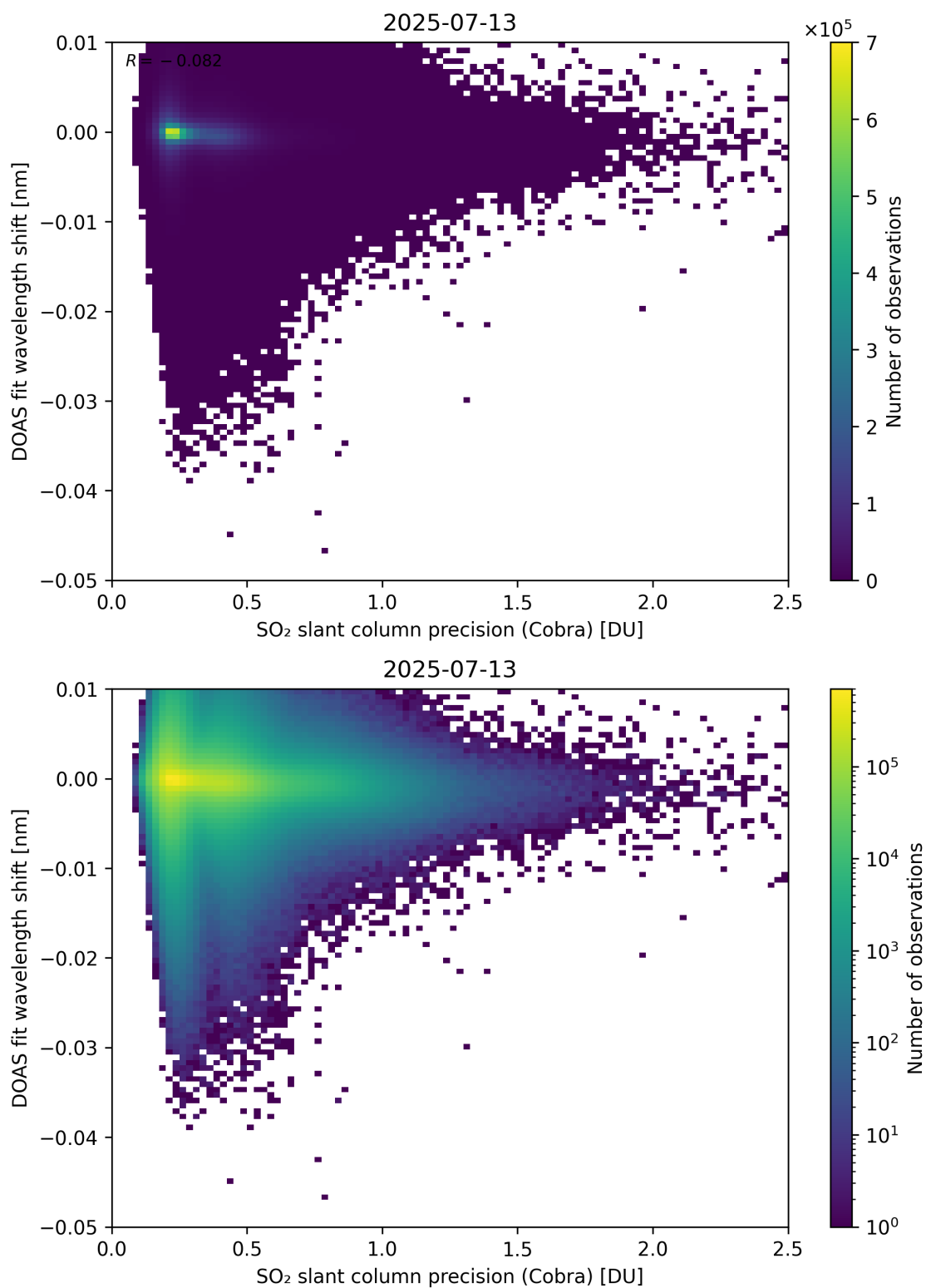
Figure 202: Scatter density plot of “SO 2 slant column precision (Cobra)” against “DOAS fit wavelength shift” for 2025-07-13 to 2025-07-14.
