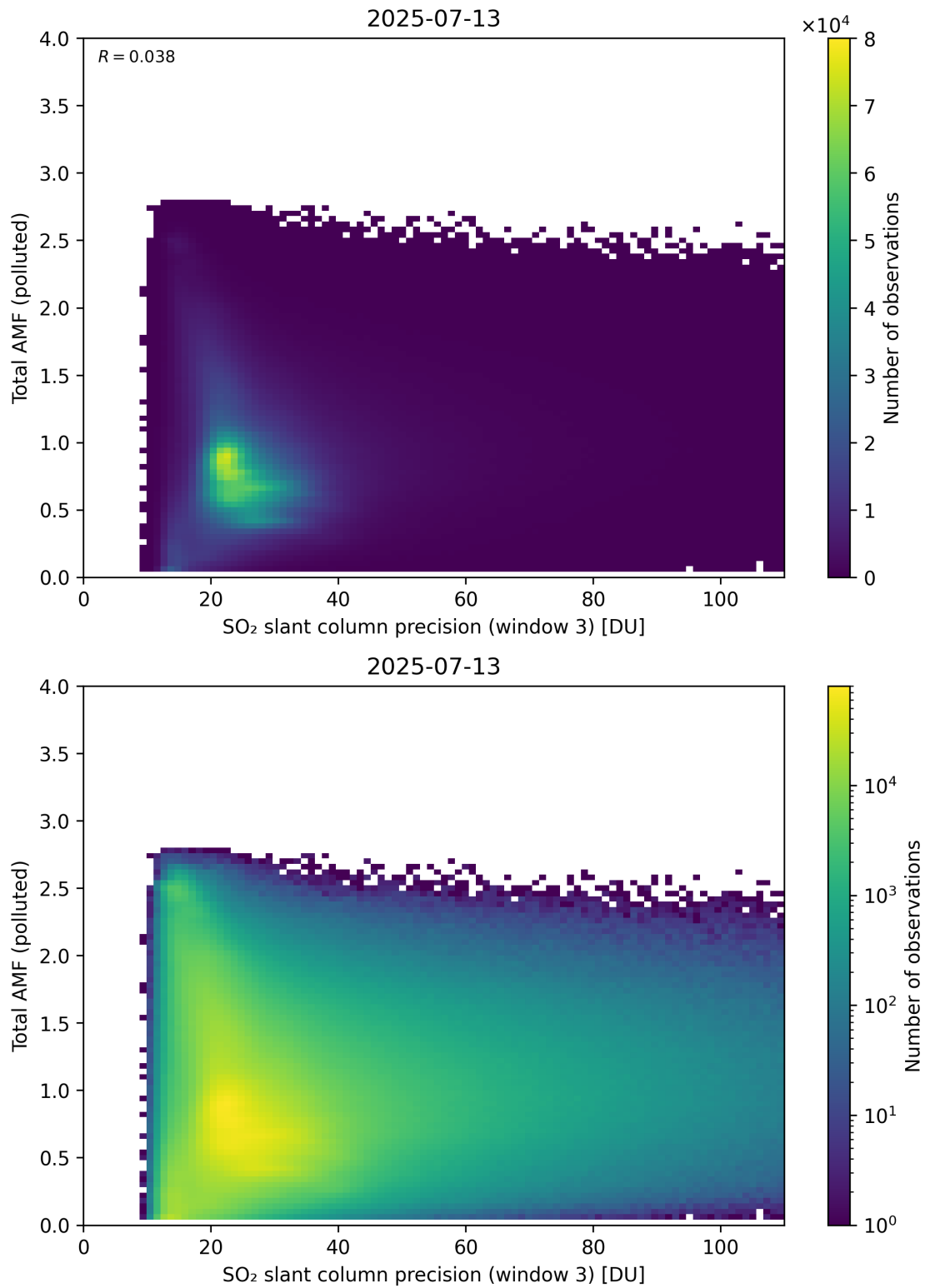
Figure 313: Scatter density plot of “SO 2 slant column precision (window 3)” against “Total AMF (polluted)” for 2025-07-13 to 2025-07-14.
