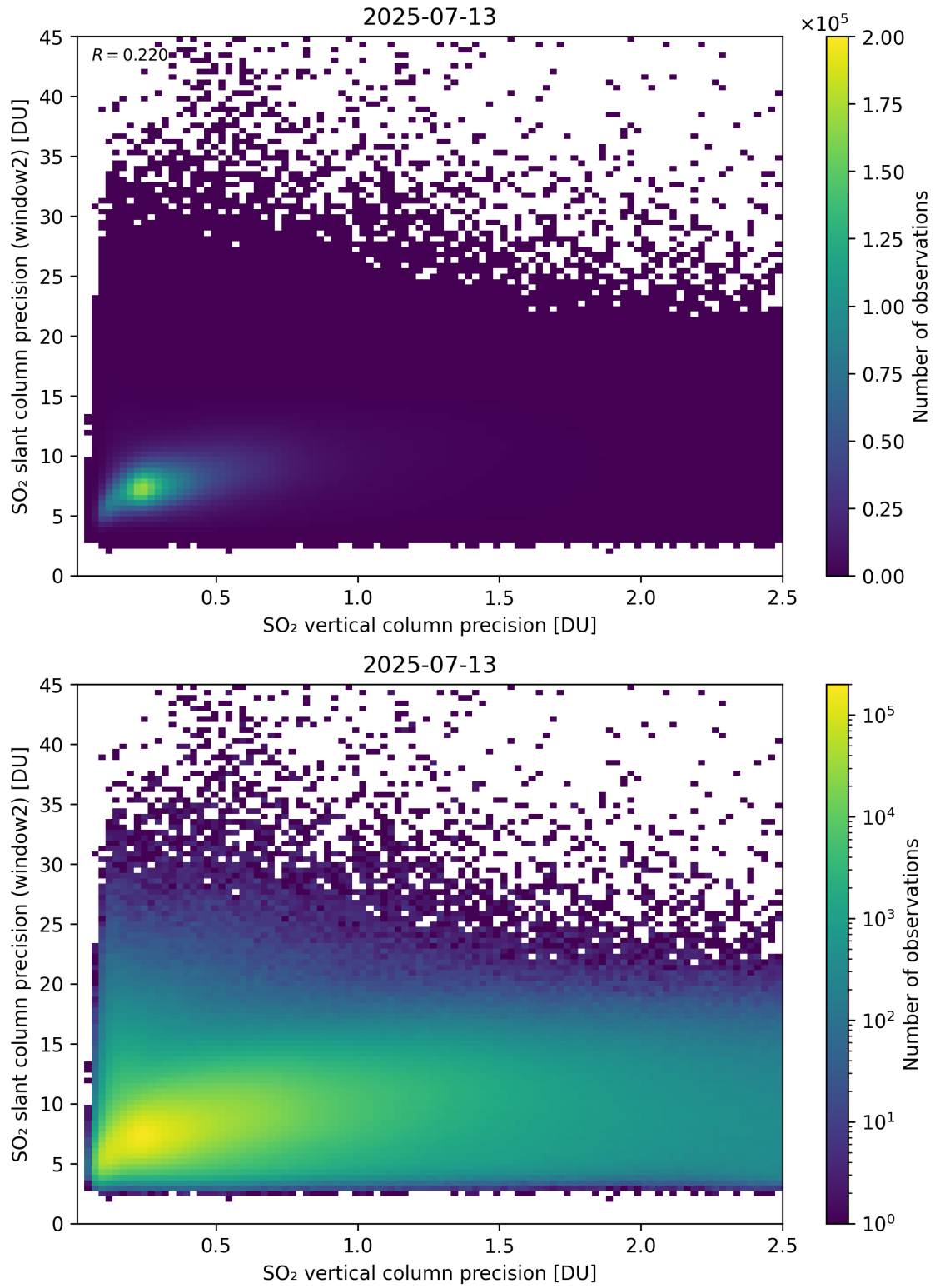
Figure 343: Scatter density plot of “SO 2 vertical column precision” against “SO 2 slant column precision (window2)” for 2025-07-13 to 2025-07-14.
