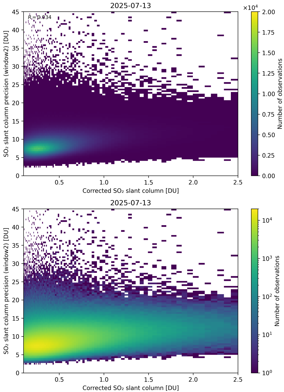
Figure 239: Scatter density plot of “Corrected SO 2 slant column” against “SO 2 slant column precision (window2)” for 2025-07-13 to 2025-07-14.
