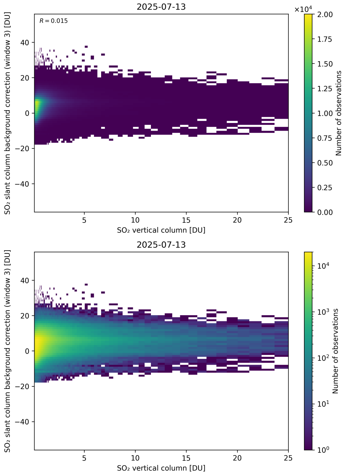
Figure 325: Scatter density plot of “SO 2 vertical column” against “SO 2 slant column background correction (window 3)” for 2025-07-13 to 2025-07-14.
