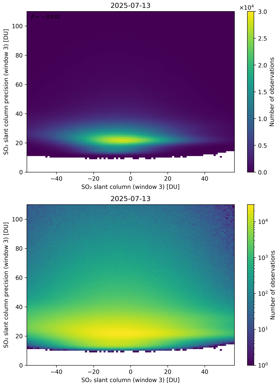
Figure 317: Scatter density plot of “SO 2 slant column (window 3)” against “SO 2 slant column precision (window 3)” for 2025-07-13 to 2025-07-14.
