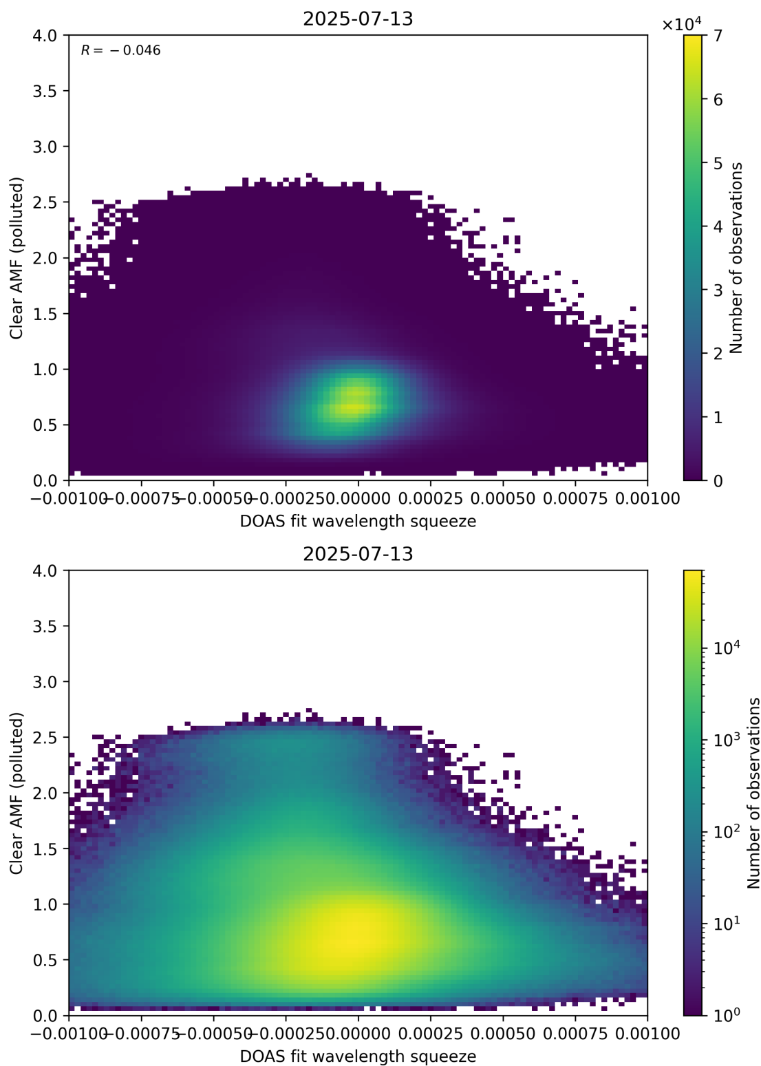
Figure 144: Scatter density plot of “DOAS fit wavelength squeeze” against “Clear AMF (polluted)” for 2025-07-13 to 2025-07-14.
