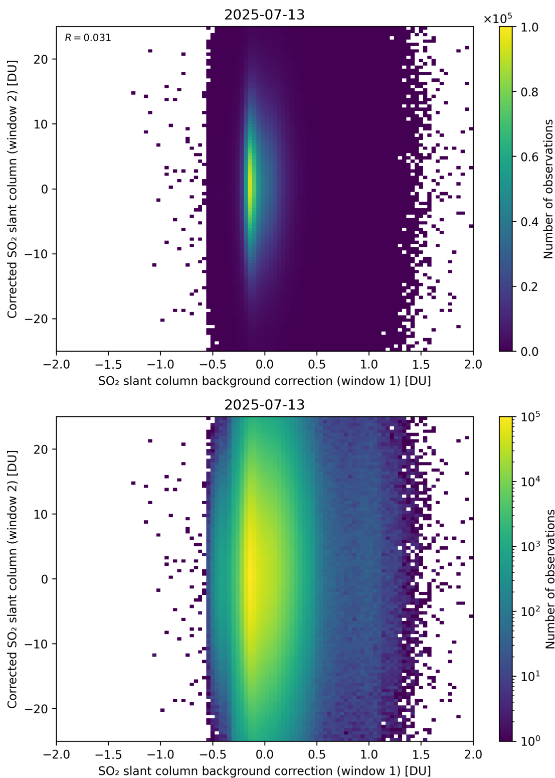
Figure 115: Scatter density plot of “SO 2 slant column background correction (window 1)” against “Corrected SO 2 slant column (window 2)” for 2025-07-13 to 2025-07-14.
