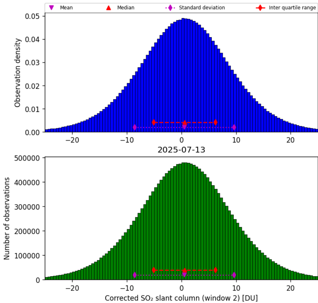
Figure 69: Histogram of “Corrected SO 2 slant column (window 2)” for 2025-07-13 to 2025-07-14
