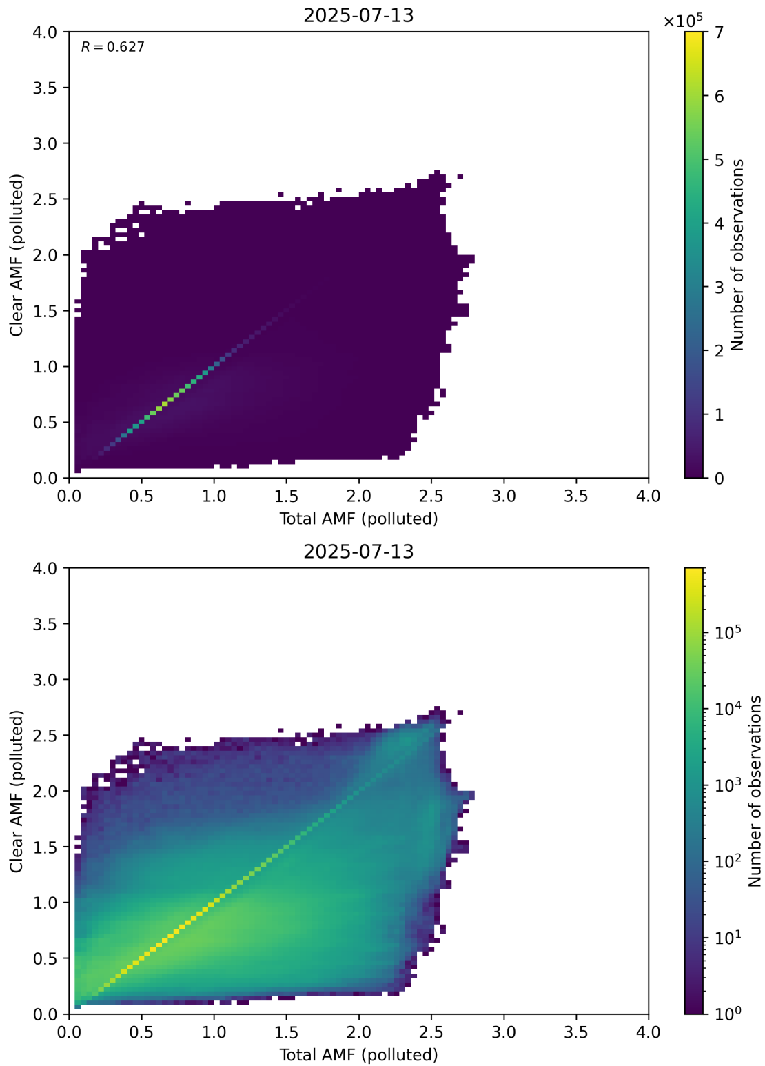
Figure 321: Scatter density plot of “Total AMF (polluted)” against “Clear AMF (polluted)” for 2025-07-13 to 2025-07-14.
