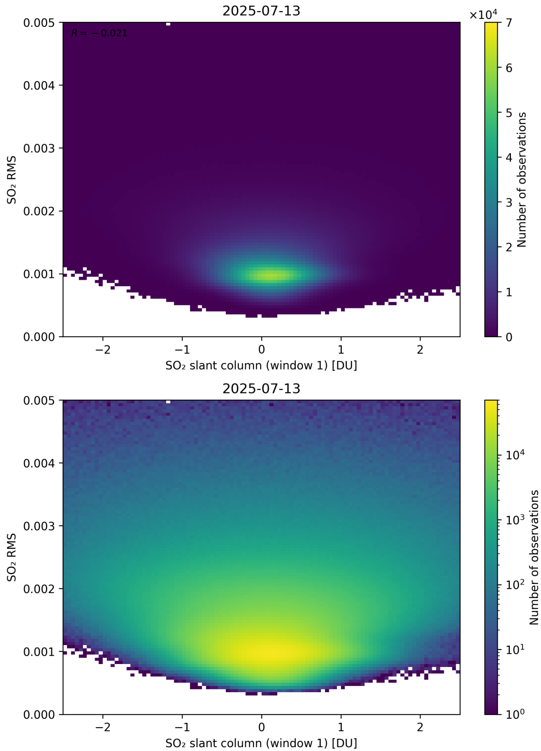
Figure 267: Scatter density plot of “SO 2 slant column (window 1)” against “SO 2 RMS” for 2025-07-13 to 2025-07-14.
