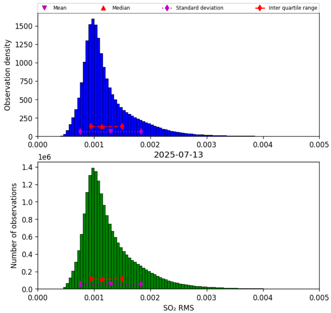
Figure 78: Histogram of “SO 2 RMS” for 2025-07-13 to 2025-07-14
