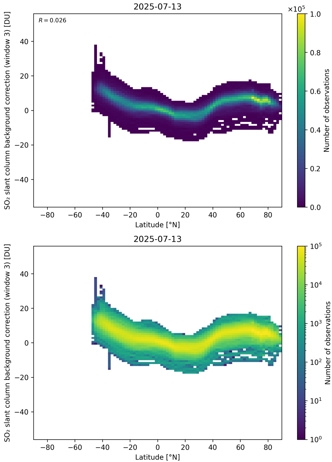
Figure 152: Scatter density plot of “Latitude” against “SO 2 slant column background correction (window 3)” for 2025-07-13 to 2025-07-14.
