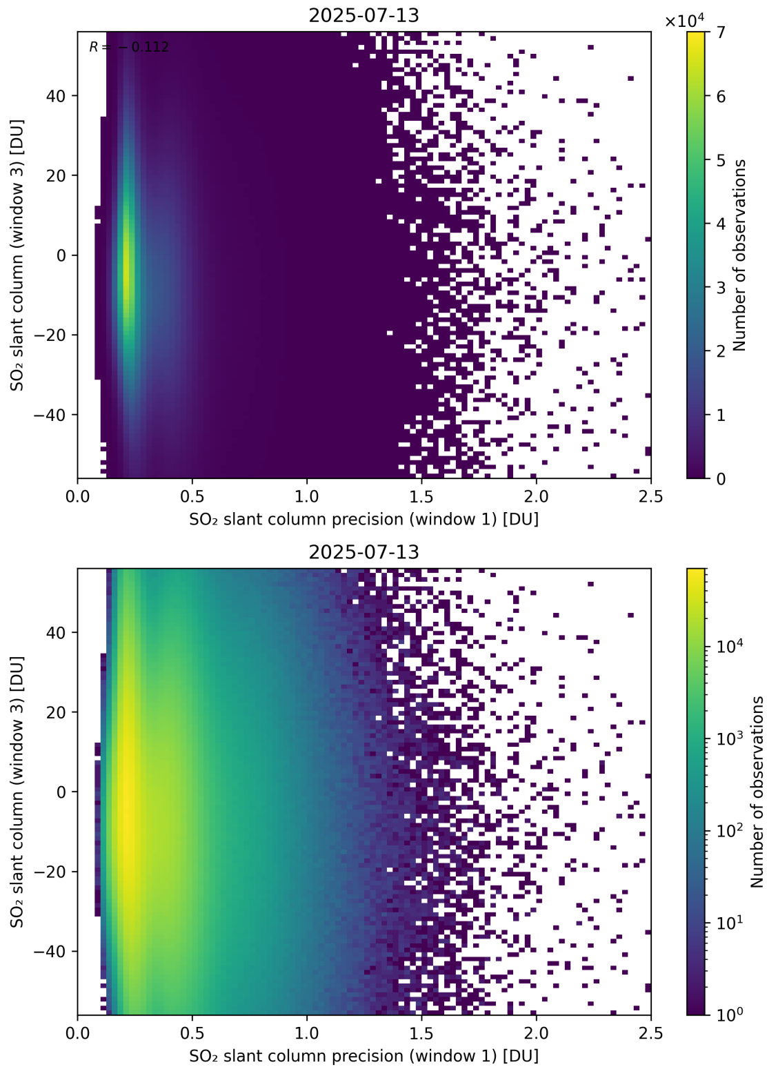
Figure 278: Scatter density plot of “SO 2 slant column precision (window 1)” against “SO 2 slant column (window 3)” for 2025-07-13 to 2025-07-14.
