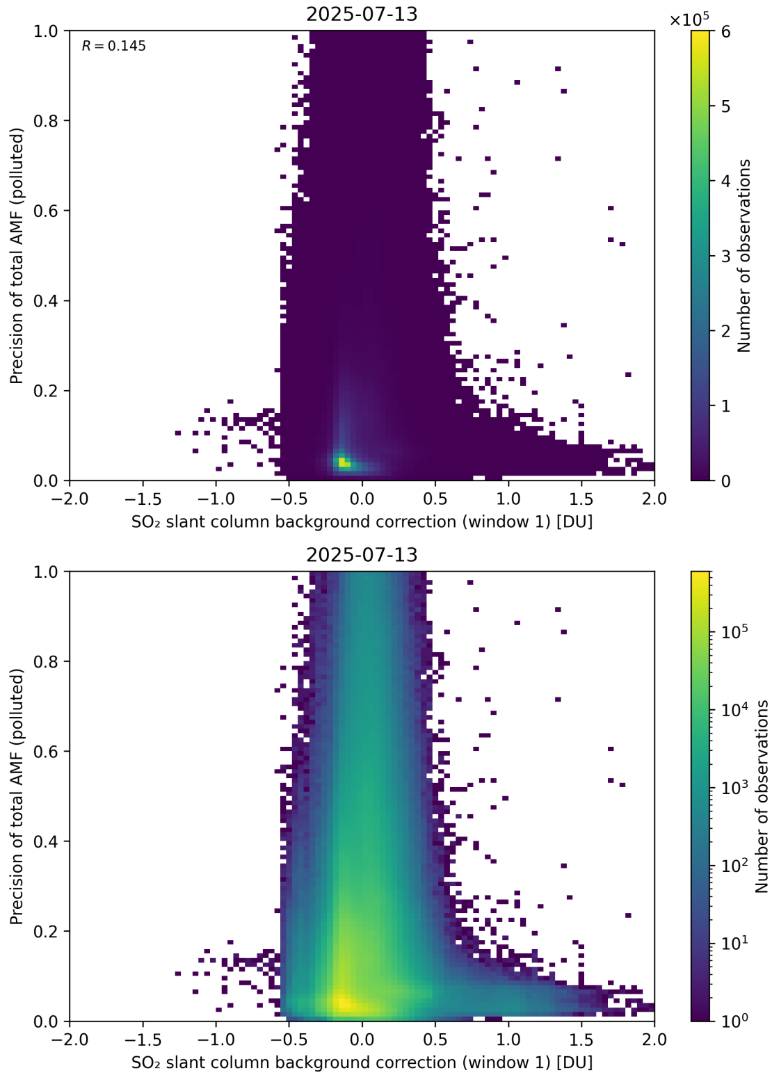
Figure 121: Scatter density plot of “SO 2 slant column background correction (window 1)” against “Precision of total AMF (polluted)” for 2025-07-13 to 2025-07-14.
