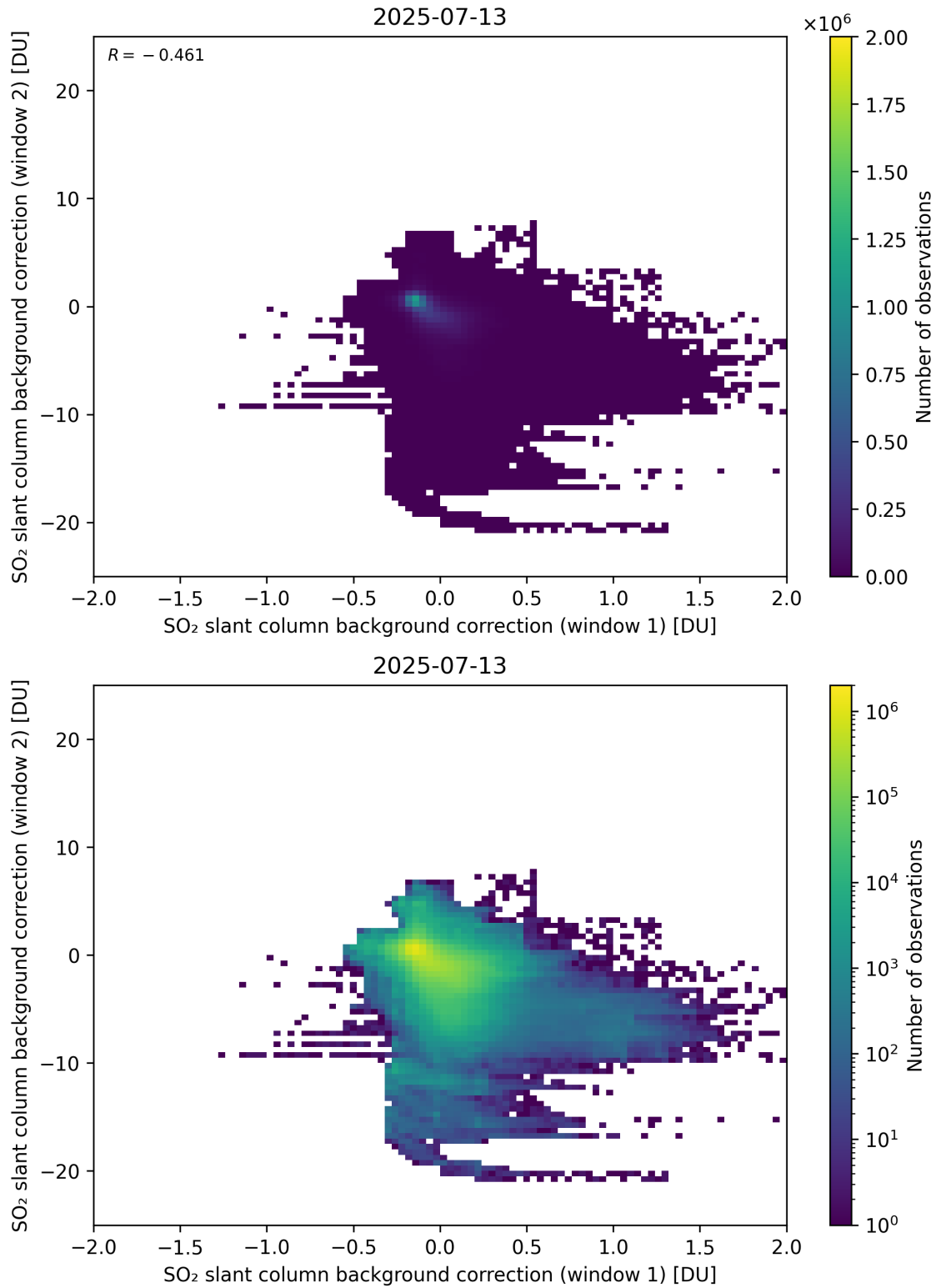
Figure 109: Scatter density plot of “SO 2 slant column background correction (window 1)” against “SO 2 slant column background correction (window 2)” for 2025-07-13 to 2025-07-14.
