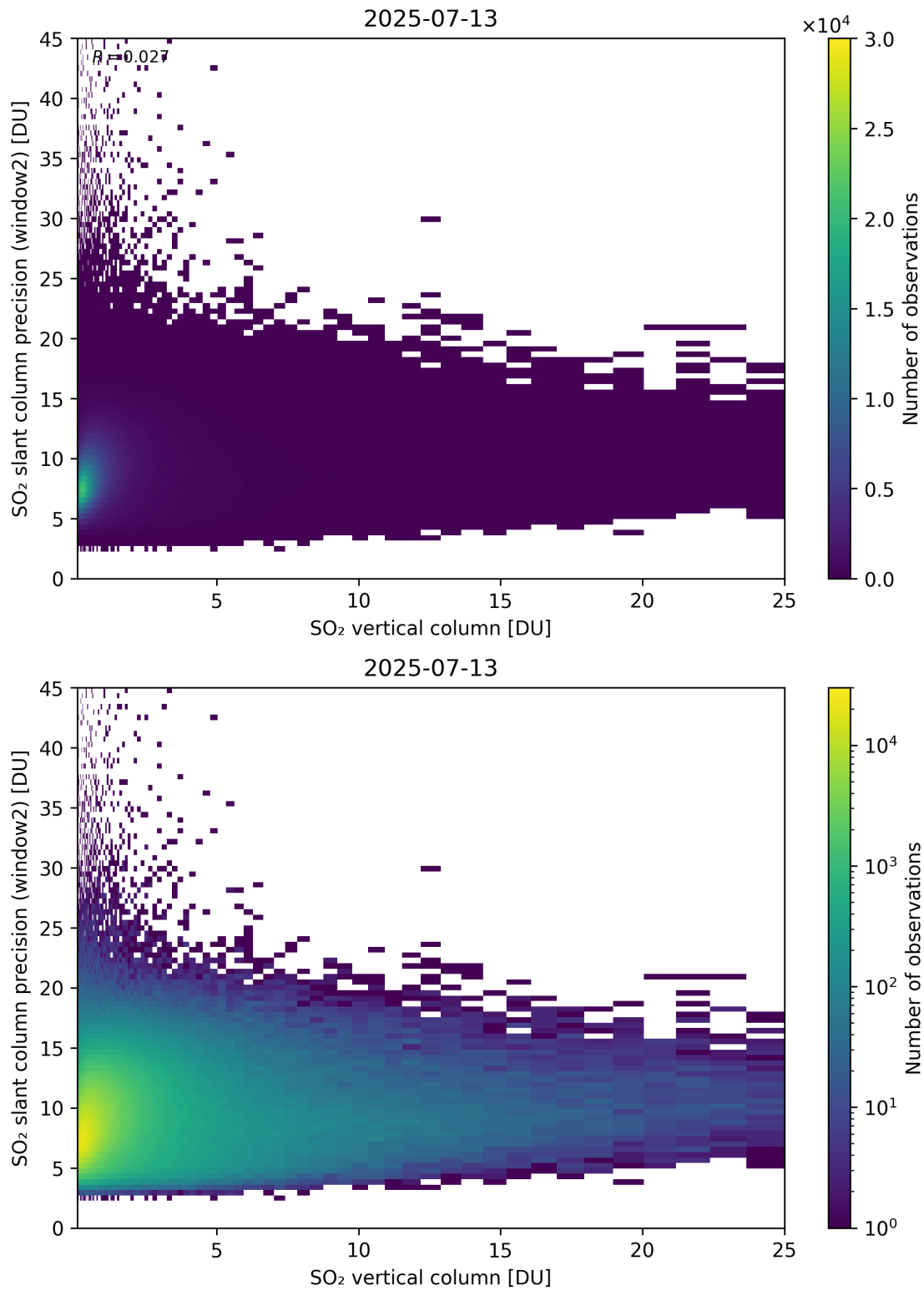
Figure 356: Scatter density plot of “SO 2 vertical column” against “SO 2 slant column precision (window2)” for 2025-07-13 to 2025-07-14.
