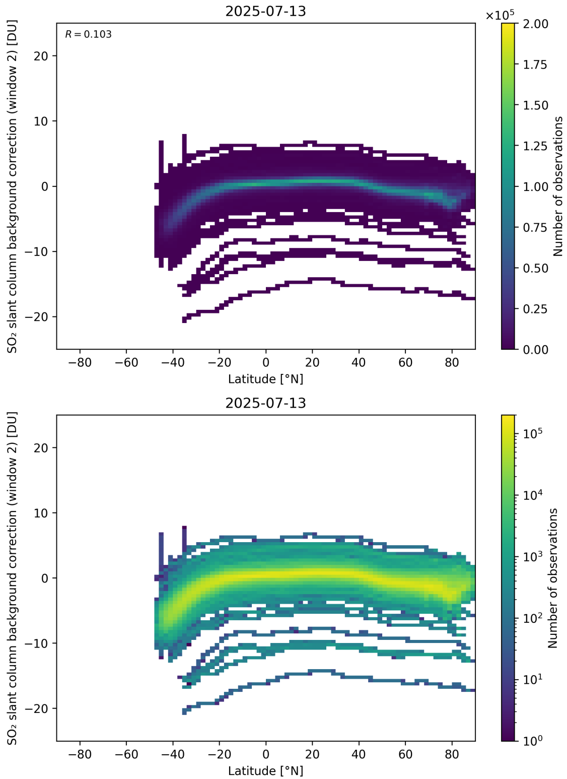
Figure 151: Scatter density plot of “Latitude” against “SO 2 slant column background correction (window 2)” for 2025-07-13 to 2025-07-14.
