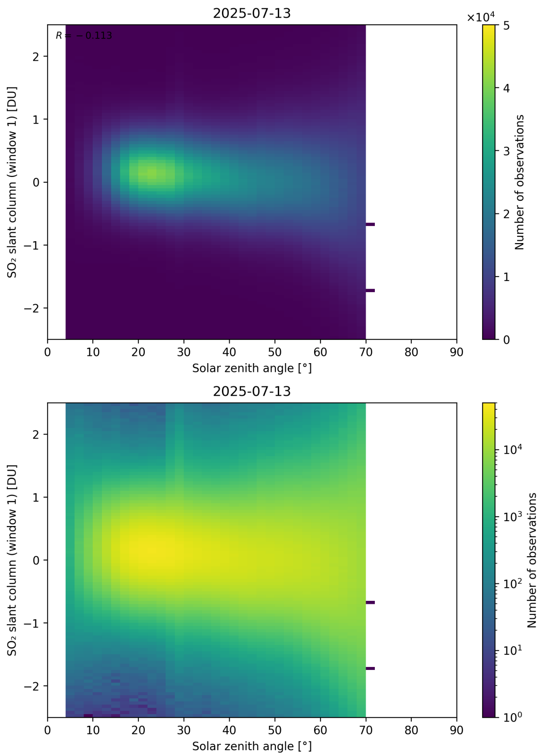
Figure 184: Scatter density plot of “Solar zenith angle” against “SO 2 slant column (window 1)” for 2025-07-13 to 2025-07-14.
