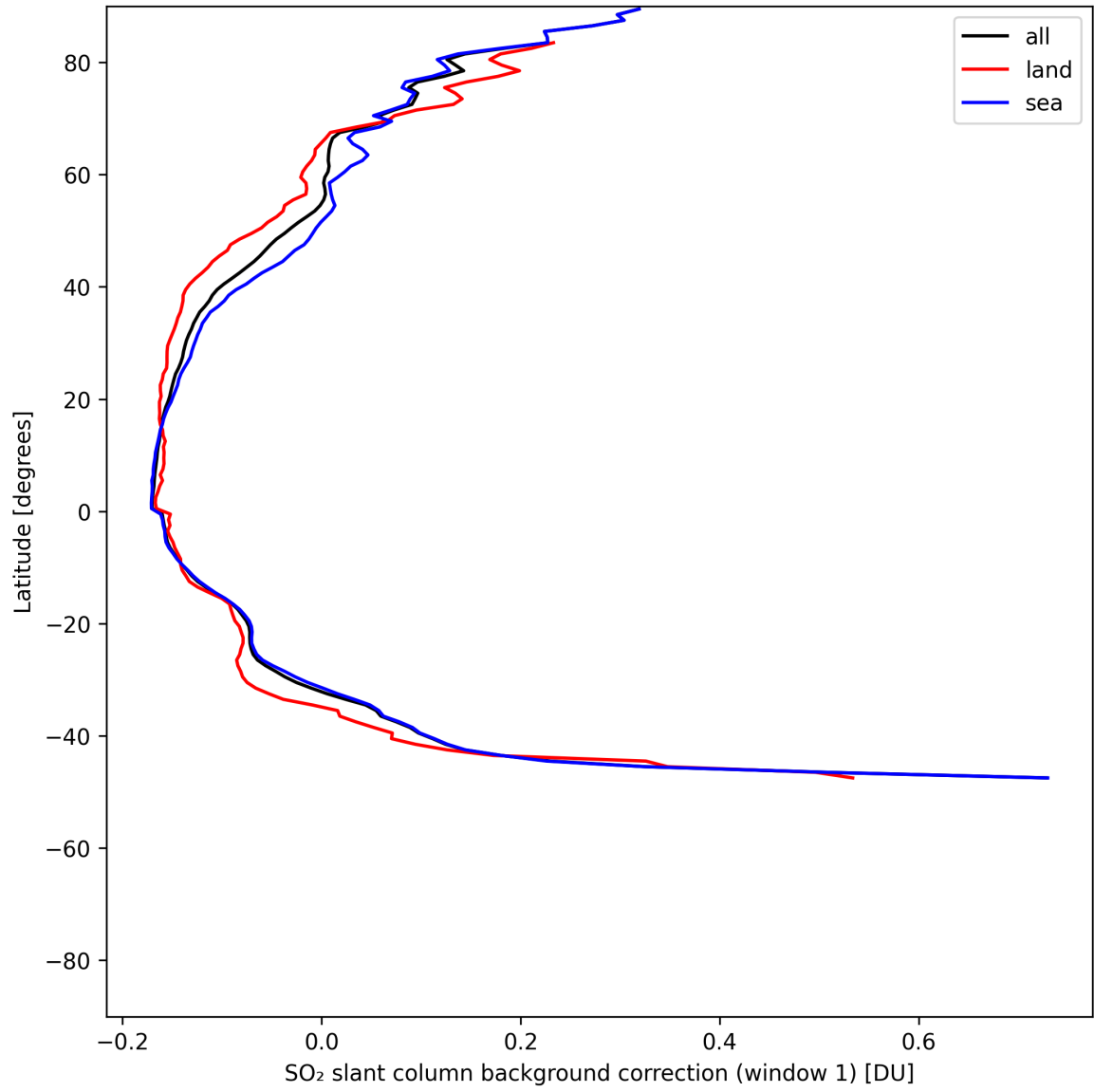
Figure 40: Zonal average of “SO 2 slant column background correction (window 1)” for 2025-07-13 to 2025-07-14.
