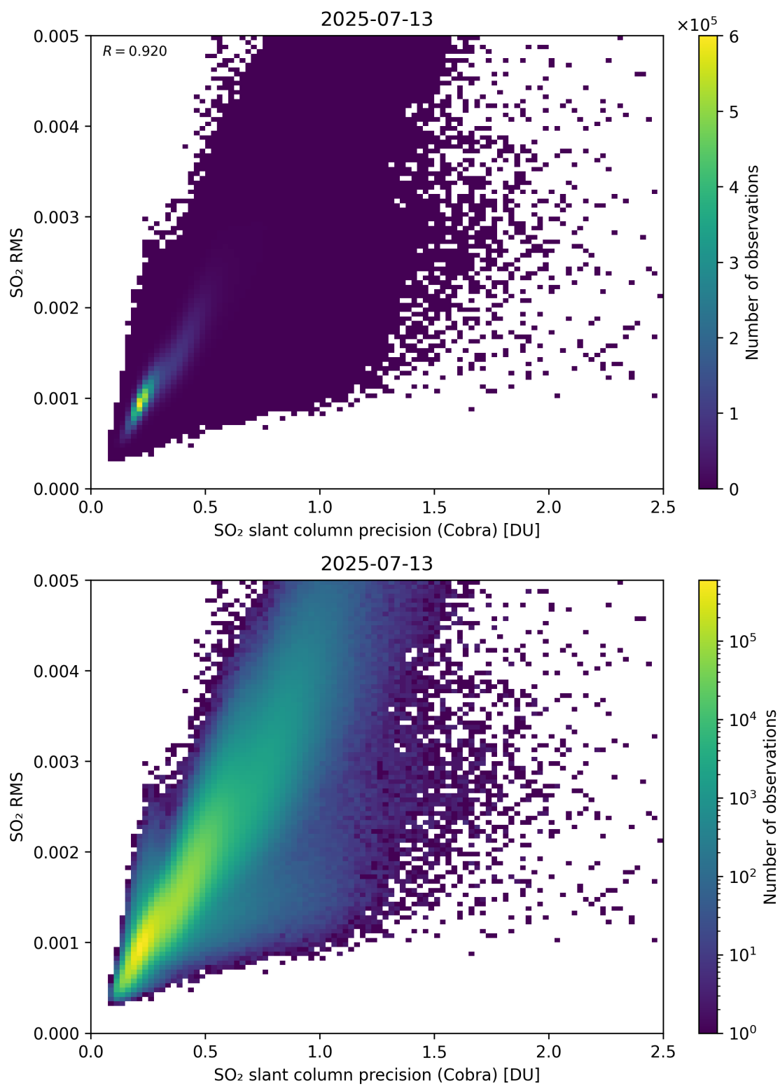
Figure 204: Scatter density plot of “SO 2 slant column precision (Cobra)” against “SO 2 RMS” for 2025-07-13 to 2025-07-14.
