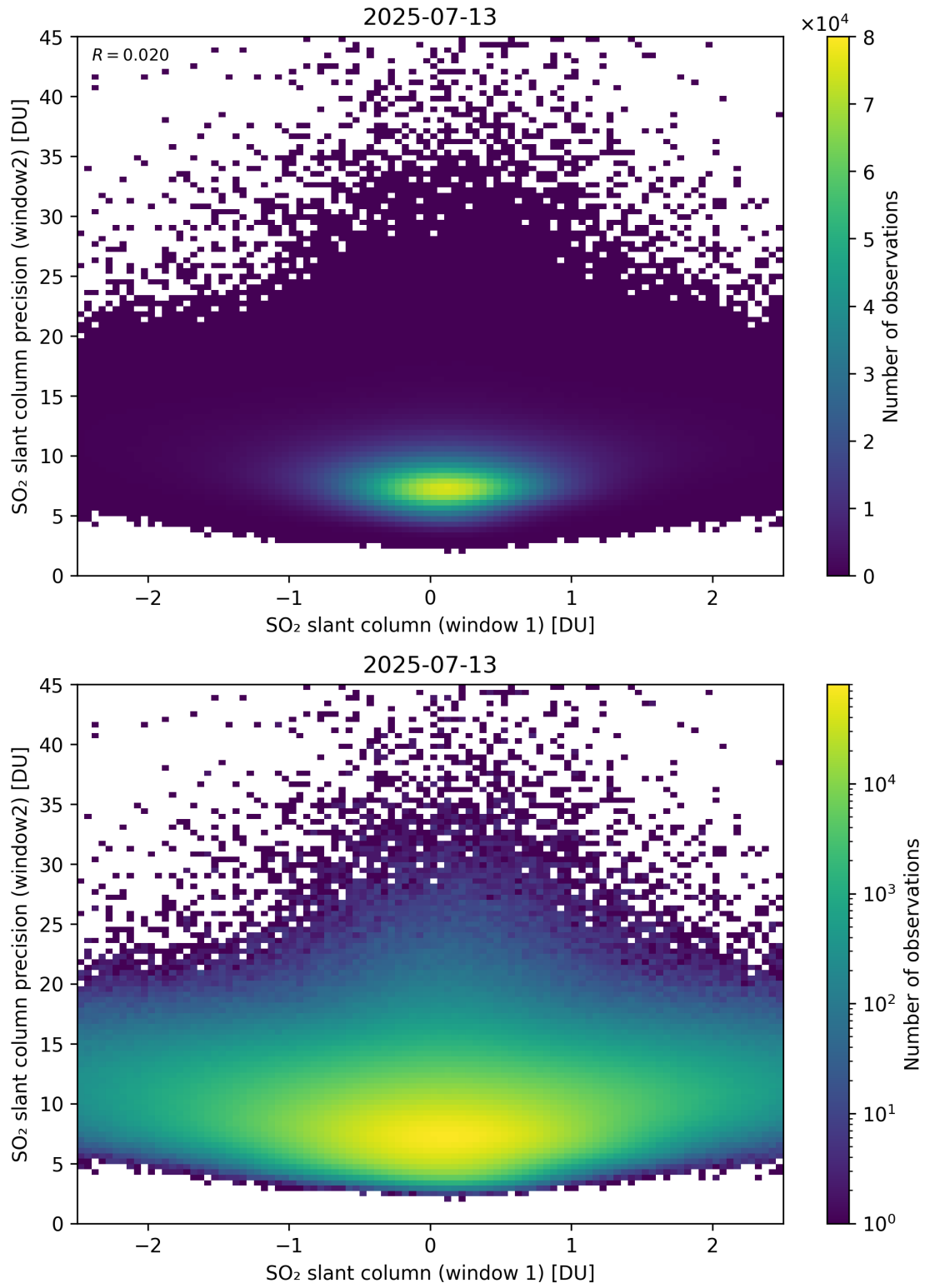
Figure 286: Scatter density plot of “SO 2 slant column (window 1)” against “SO 2 slant column precision (window2)” for 2025-07-13 to 2025-07-14.
