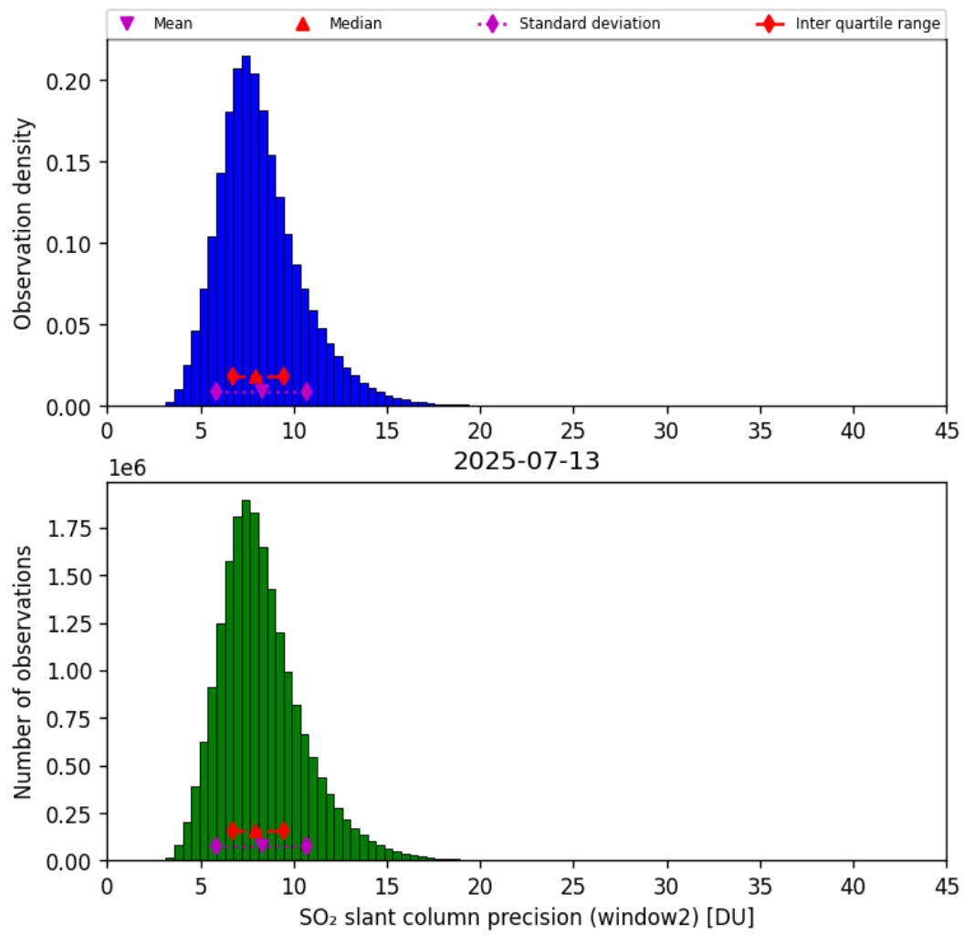
Figure 68: Histogram of “SO 2 slant column precision (window2)” for 2025-07-13 to 2025-07-14
