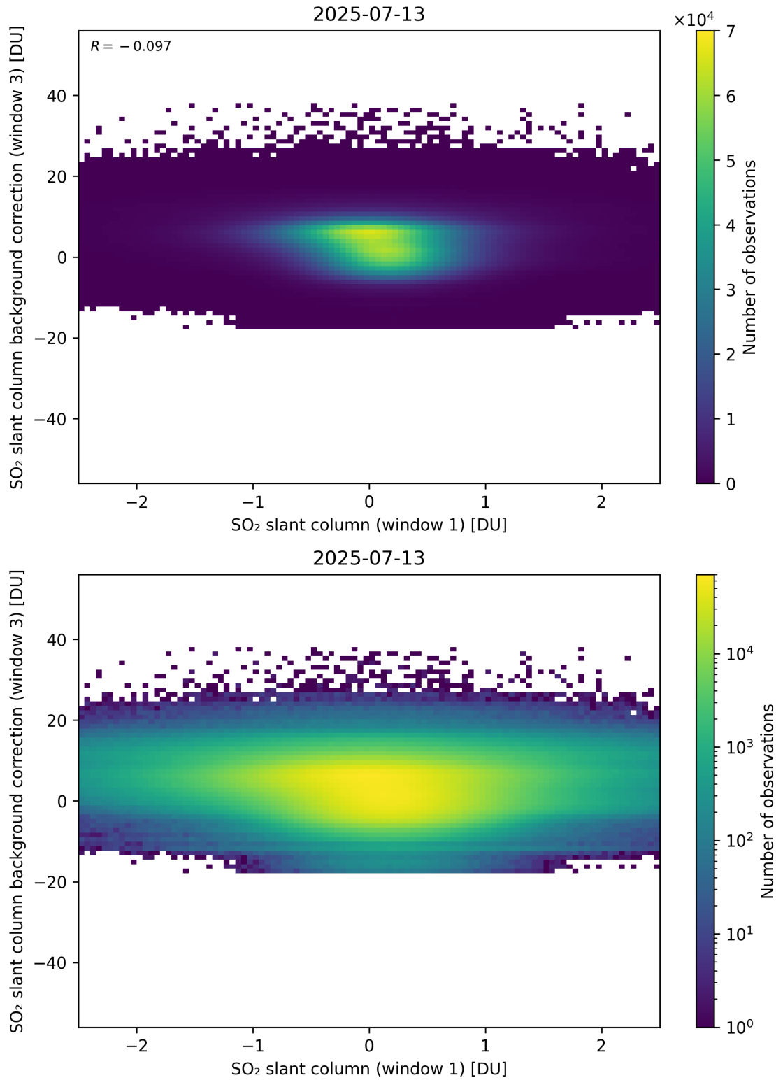
Figure 264: Scatter density plot of “SO 2 slant column (window 1)” against “SO 2 slant column background correction (window 3)” for 2025-07-13 to 2025-07-14.
