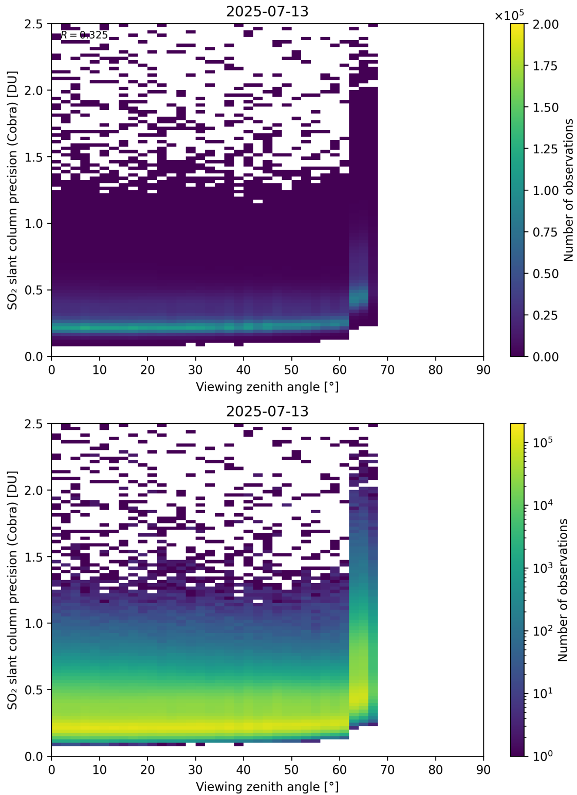
Figure 372: Scatter density plot of “Viewing zenith angle” against “SO 2 slant column precision (Cobra)” for 2025-07-13 to 2025-07-14.
