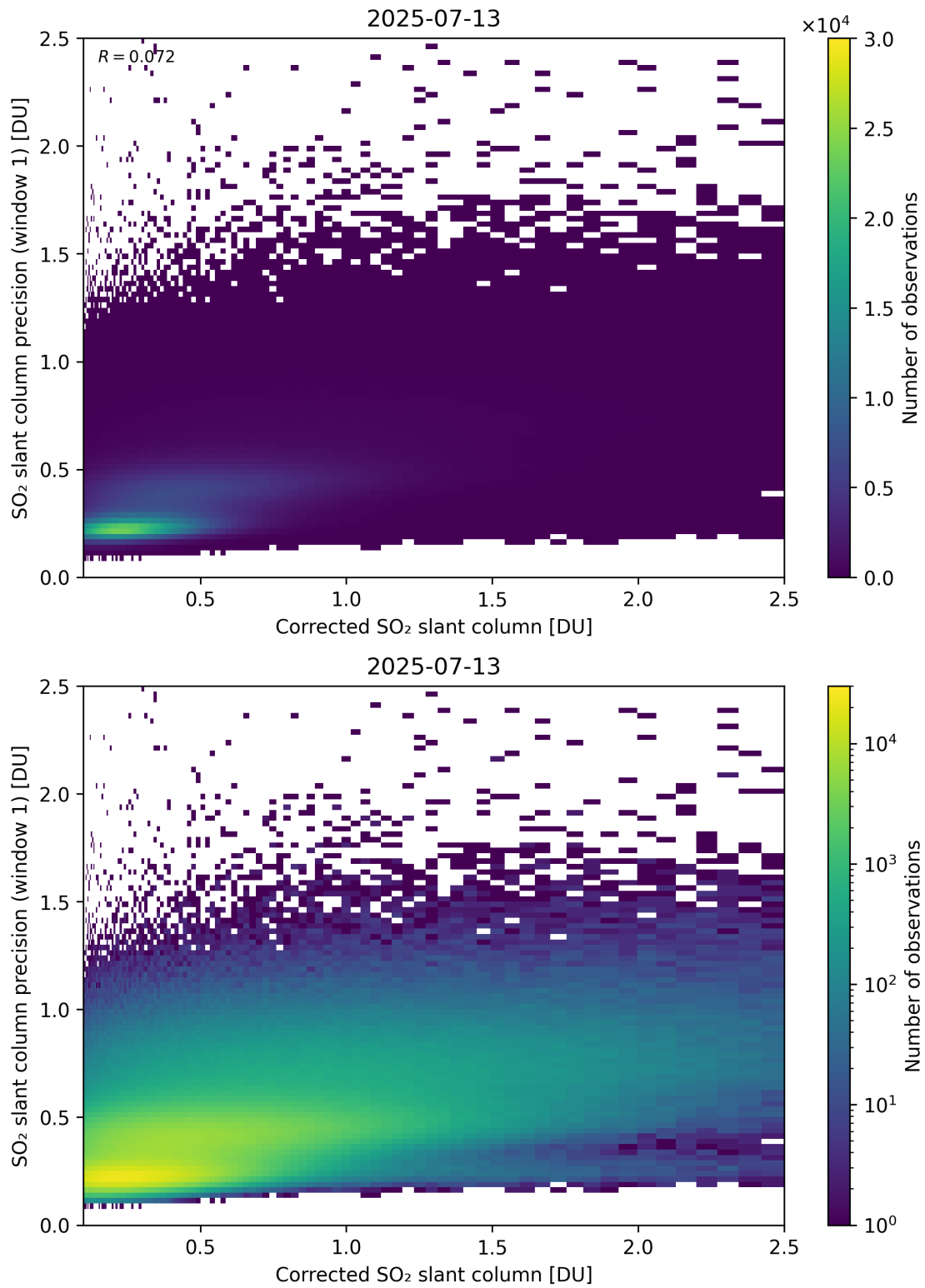
Figure 238: Scatter density plot of “Corrected SO 2 slant column” against “SO 2 slant column precision (window 1)” for 2025-07-13 to 2025-07-14.
