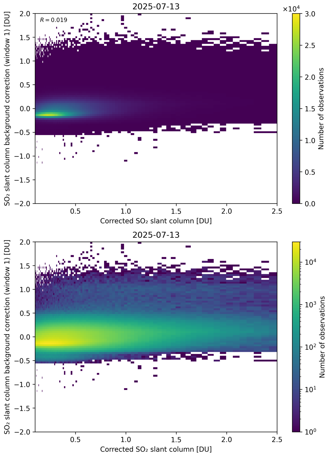
Figure 226: Scatter density plot of “Corrected SO 2 slant column” against “SO 2 slant column background correction (window 1)” for 2025-07-13 to 2025-07-14.
