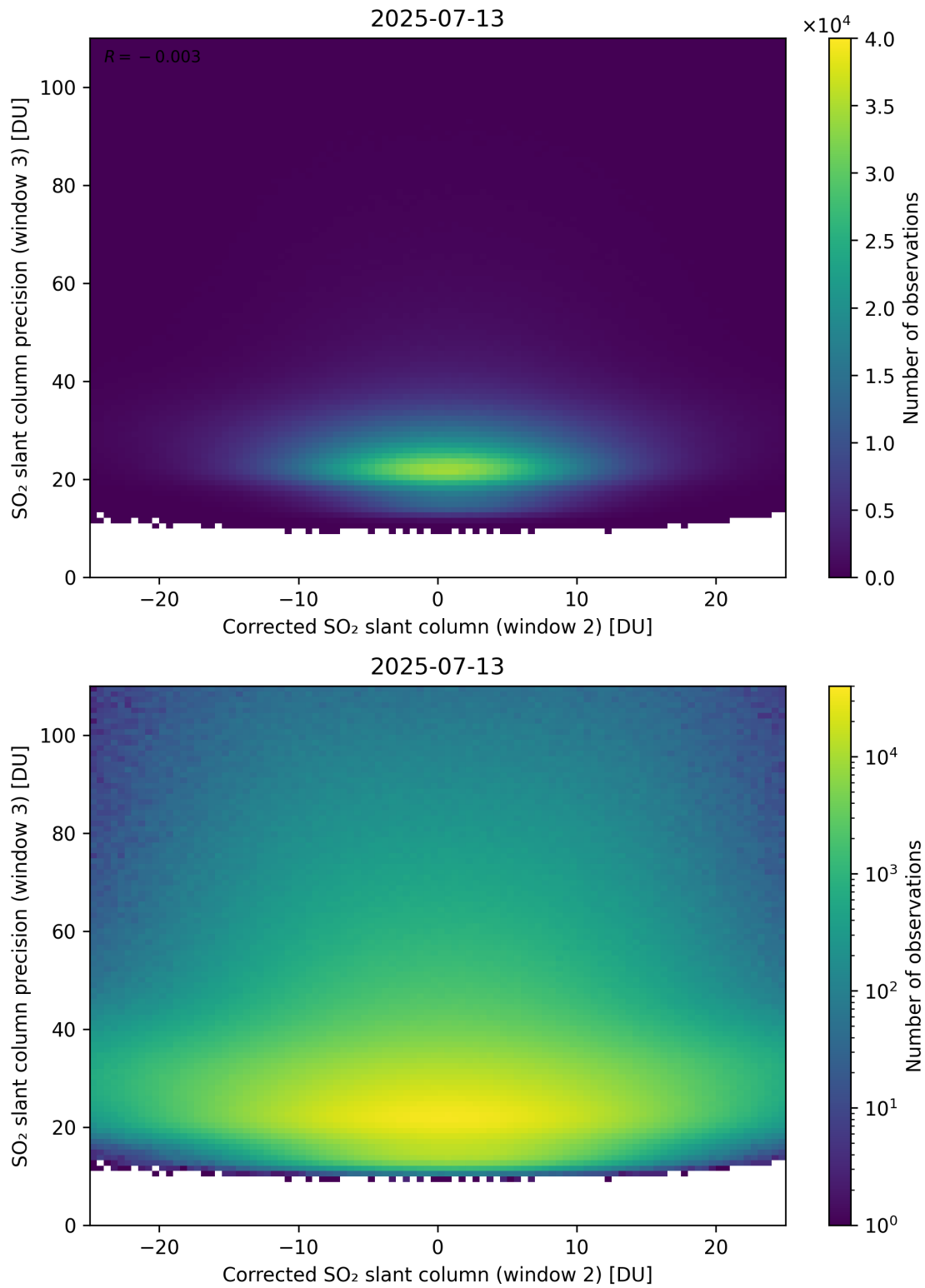
Figure 252: Scatter density plot of “Corrected SO 2 slant column (window 2)” against “SO 2 slant column precision (window 3)” for 2025-07-13 to 2025-07-14.
