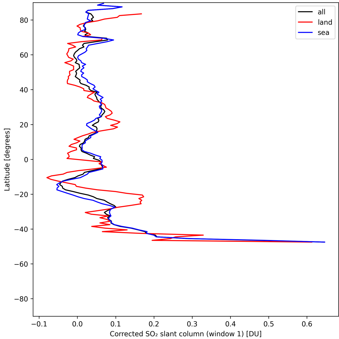
Figure 39: Zonal average of “Corrected SO 2 slant column (window 1)” for 2025-07-13 to 2025-07-14.
