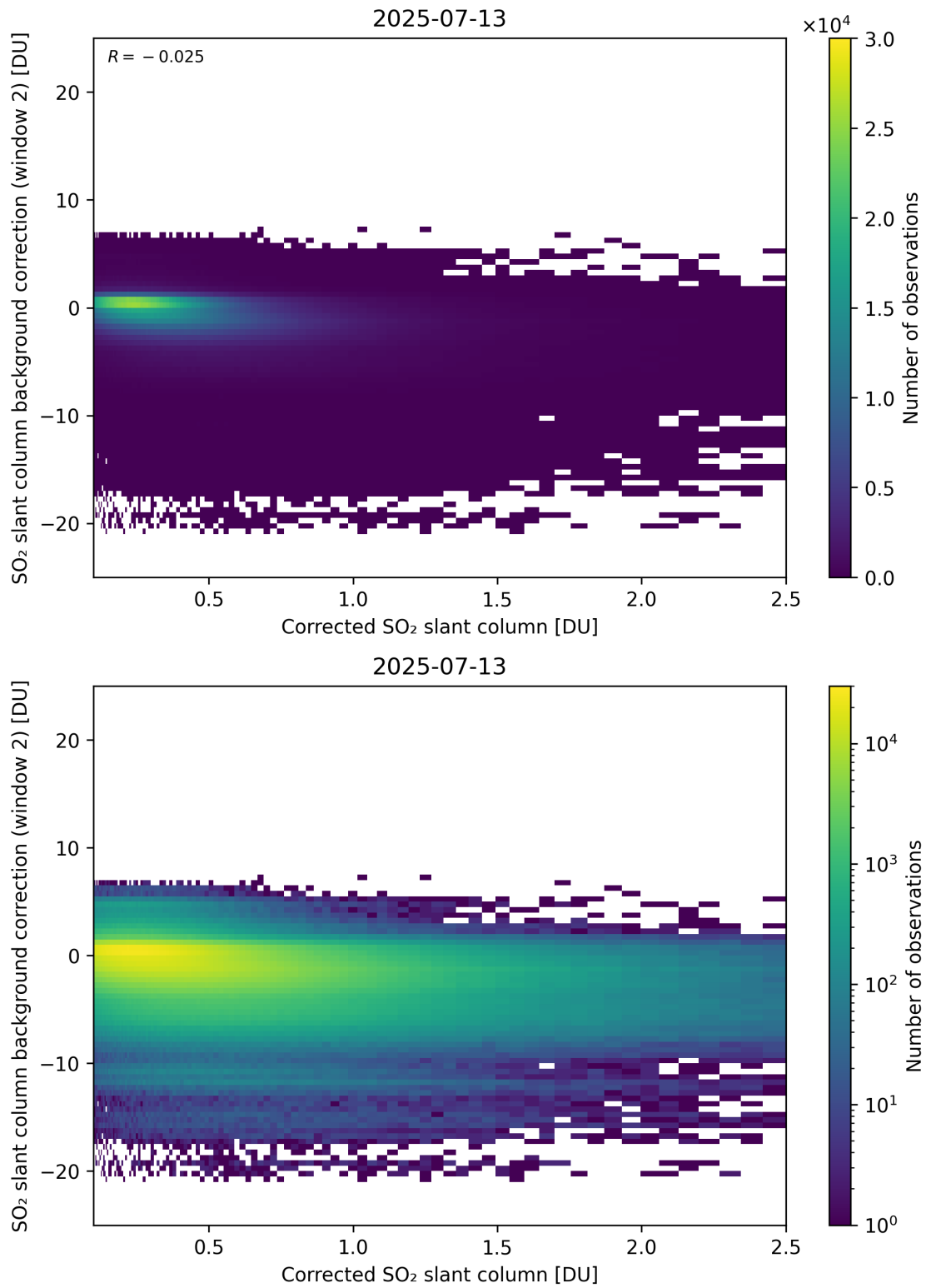
Figure 227: Scatter density plot of “Corrected SO 2 slant column” against “SO 2 slant column background correction (window 2)” for 2025-07-13 to 2025-07-14.
