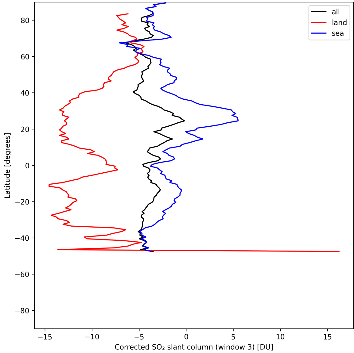
Figure 47: Zonal average of “Corrected SO 2 slant column (window 3)” for 2025-07-13 to 2025-07-14.
