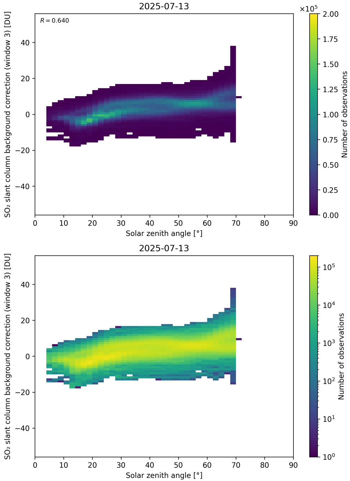
Figure 173: Scatter density plot of “Solar zenith angle” against “SO 2 slant column background correction (window 3)” for 2025-07-13 to 2025-07-14.
