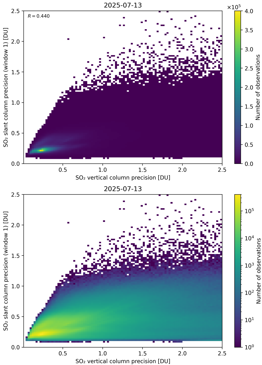
Figure 342: Scatter density plot of “SO 2 vertical column precision” against “SO 2 slant column precision (window 1)” for 2025-07-13 to 2025-07-14.
