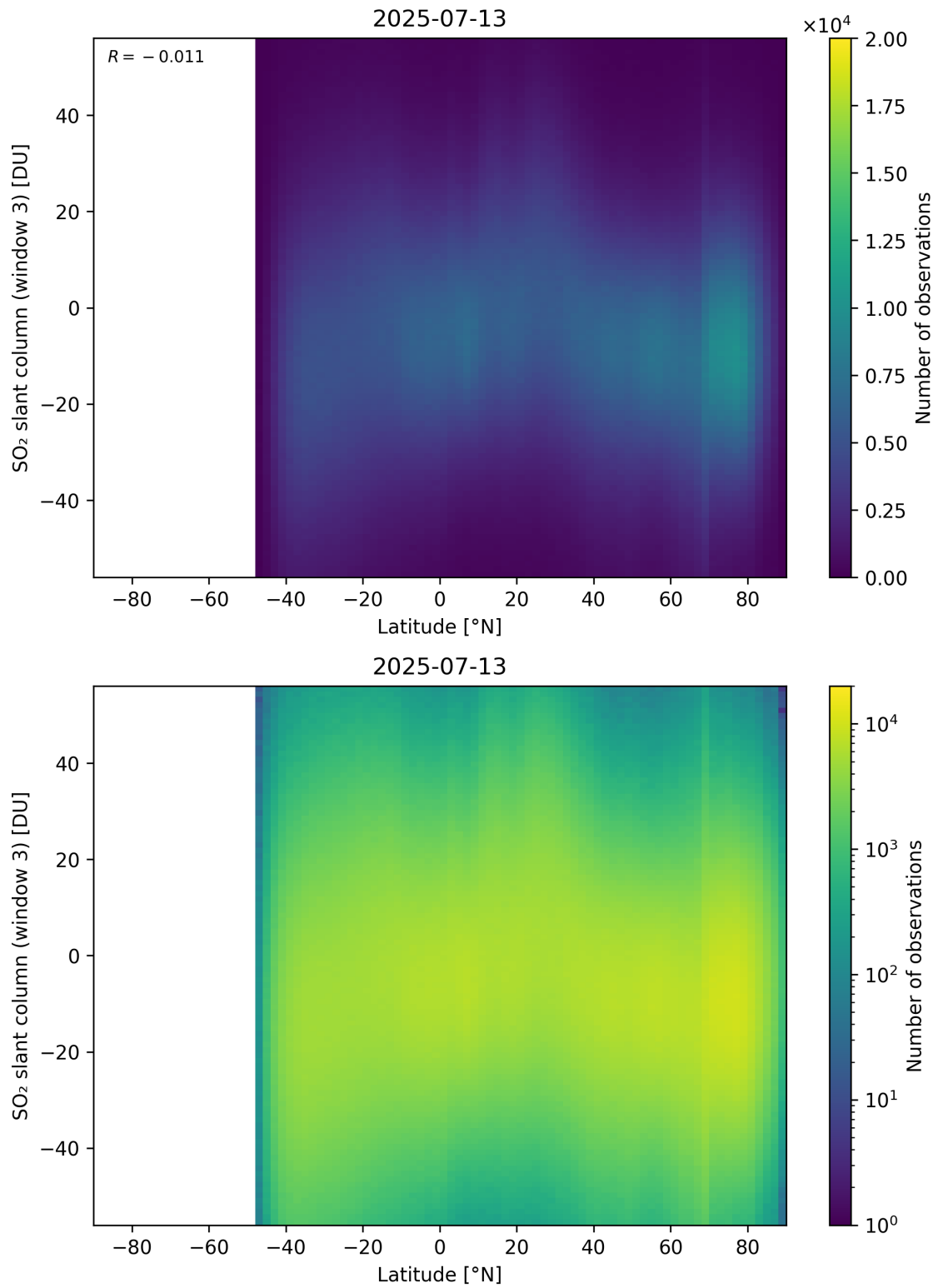
Figure 165: Scatter density plot of “Latitude” against “SO 2 slant column (window 3)” for 2025-07-13 to 2025-07-14.
