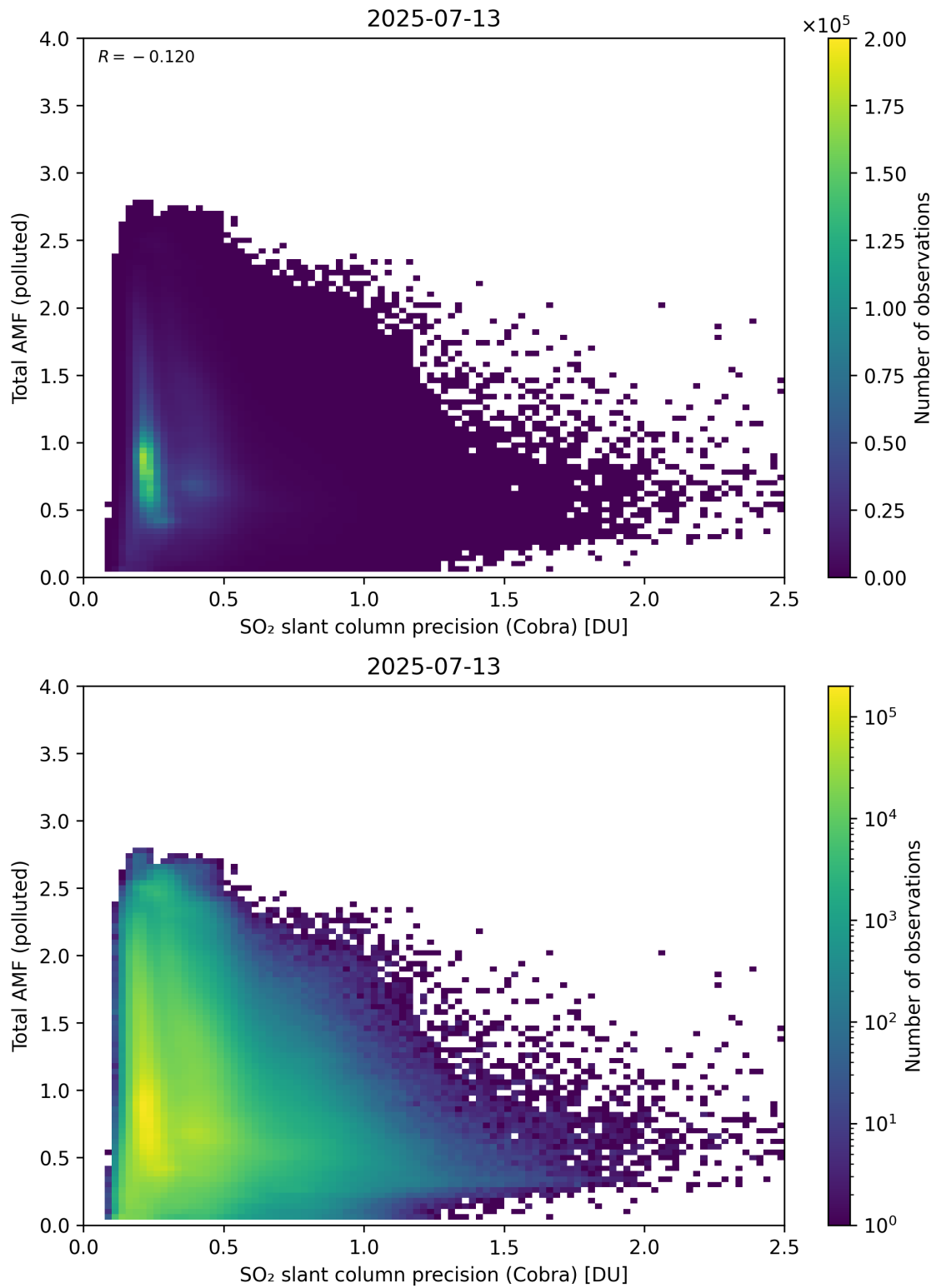
Figure 213: Scatter density plot of “SO 2 slant column precision (Cobra)” against “Total AMF (polluted)” for 2025-07-13 to 2025-07-14.
