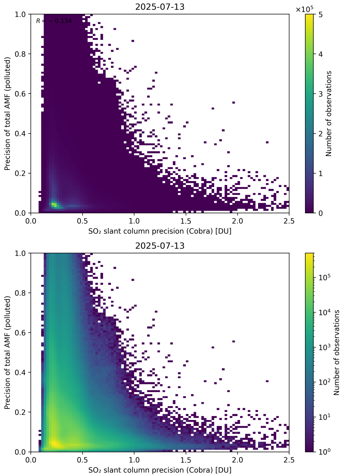
Figure 214: Scatter density plot of “SO 2 slant column precision (Cobra)” against “Precision of total AMF (polluted)” for 2025-07-13 to 2025-07-14.
