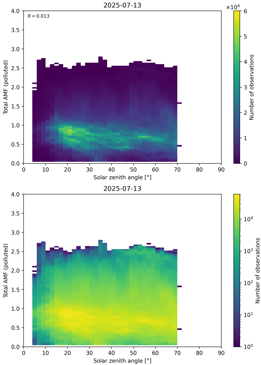
Figure 189: Scatter density plot of “Solar zenith angle” against “Total AMF (polluted)” for 2025-07-13 to 2025-07-14.
