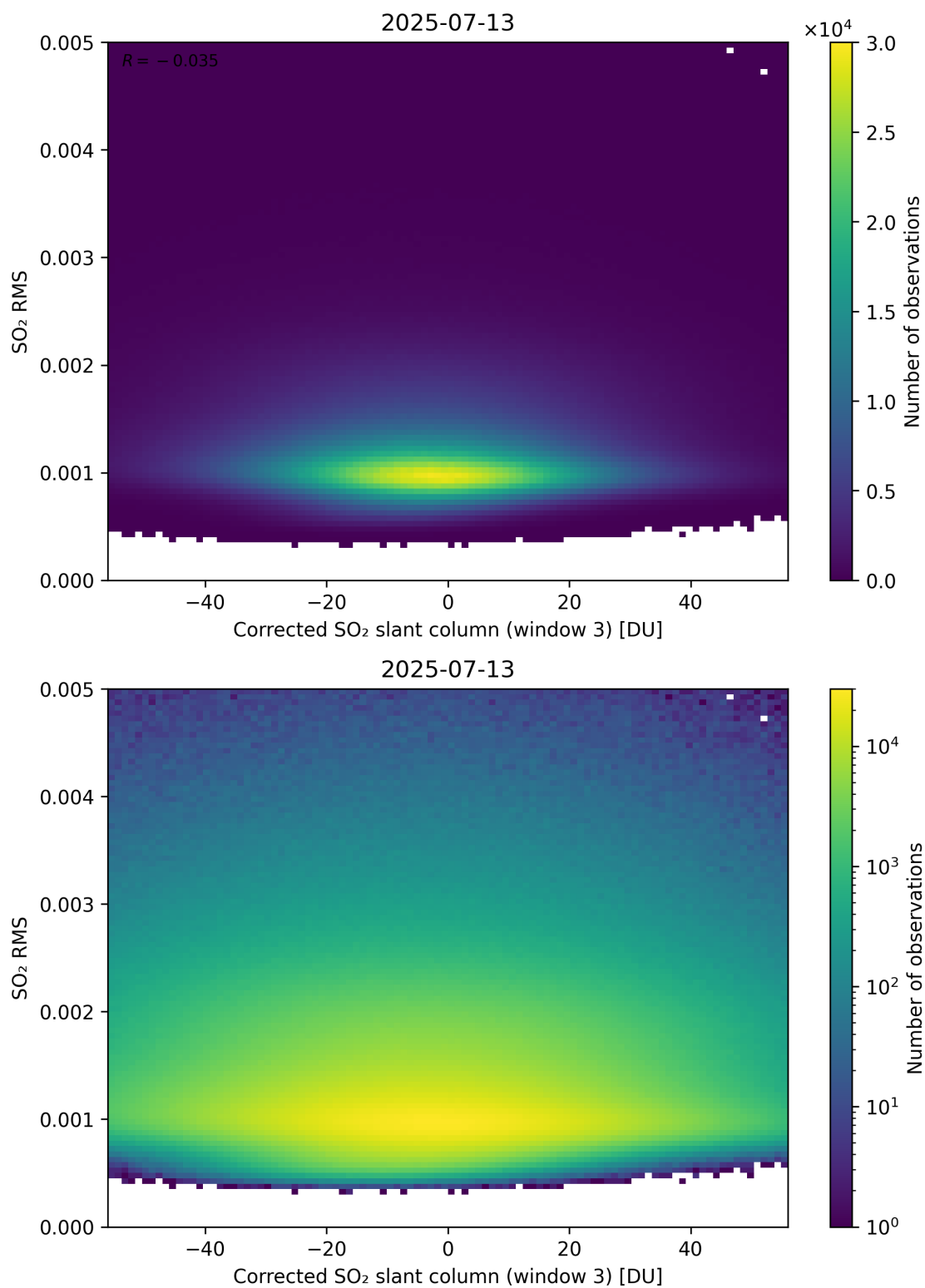
Figure 258: Scatter density plot of “Corrected SO 2 slant column (window 3)” against “SO 2 RMS” for 2025-07-13 to 2025-07-14.
