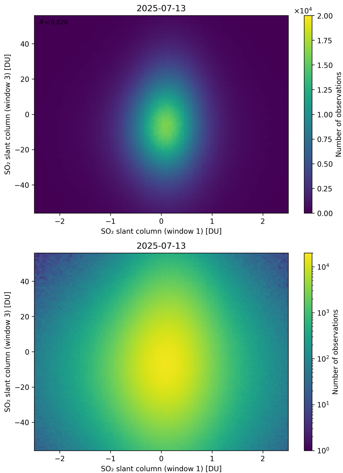
Figure 287: Scatter density plot of “SO 2 slant column (window 1)” against “SO 2 slant column (window 3)” for 2025-07-13 to 2025-07-14.
