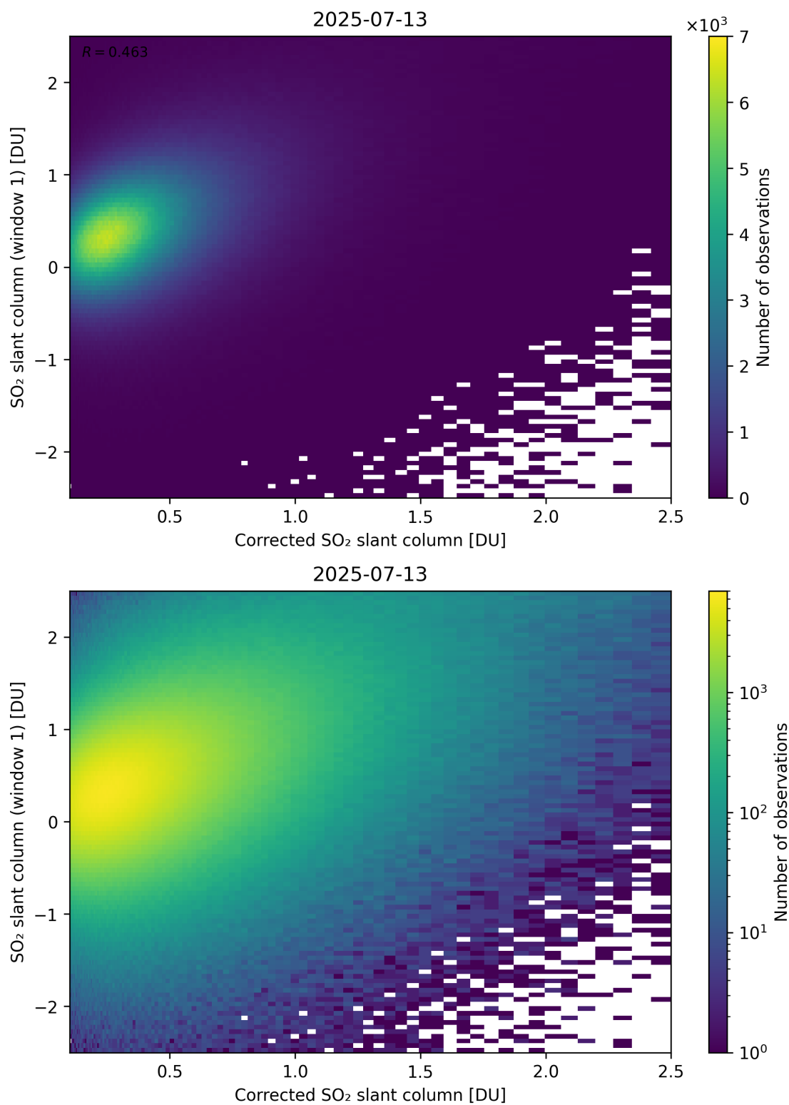
Figure 237: Scatter density plot of “Corrected SO 2 slant column” against “SO 2 slant column (window 1)” for 2025-07-13 to 2025-07-14.
