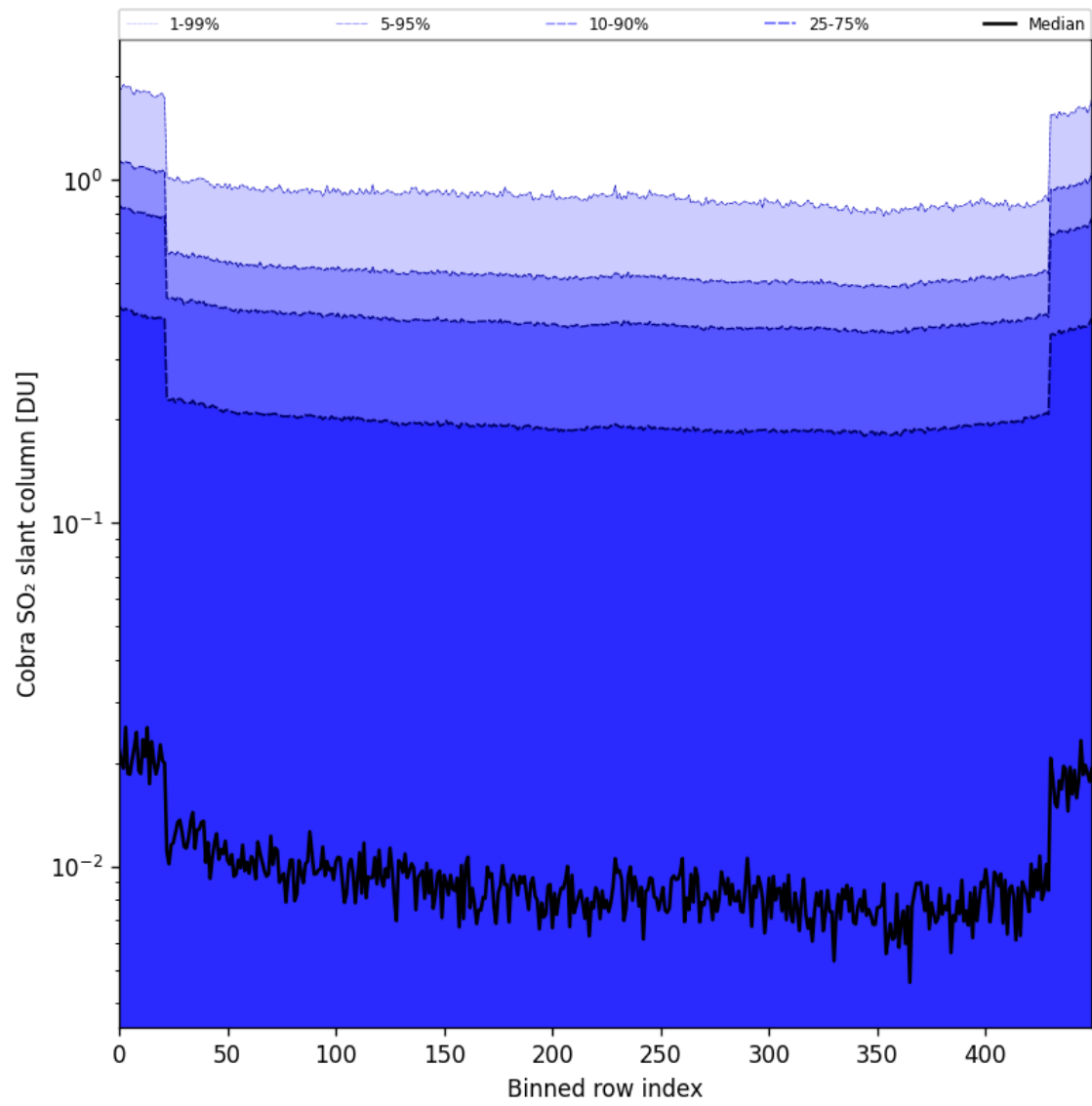
Figure 87: Along track statistics of "Cobra SO 2 slant column" for 2025-07-13 to 2025-07-14
