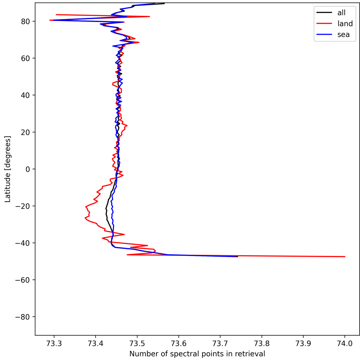
Figure 56: Zonal average of “Number of spectral points in retrieval” for 2025-07-13 to 2025-07-14.
