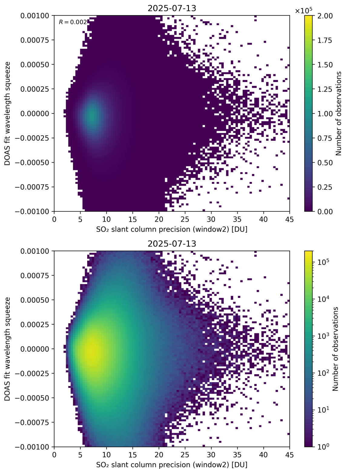
Figure 294: Scatter density plot of “SO 2 slant column precision (window2)” against “DOAS fit wavelength squeeze” for 2025-07-13 to 2025-07-14.
