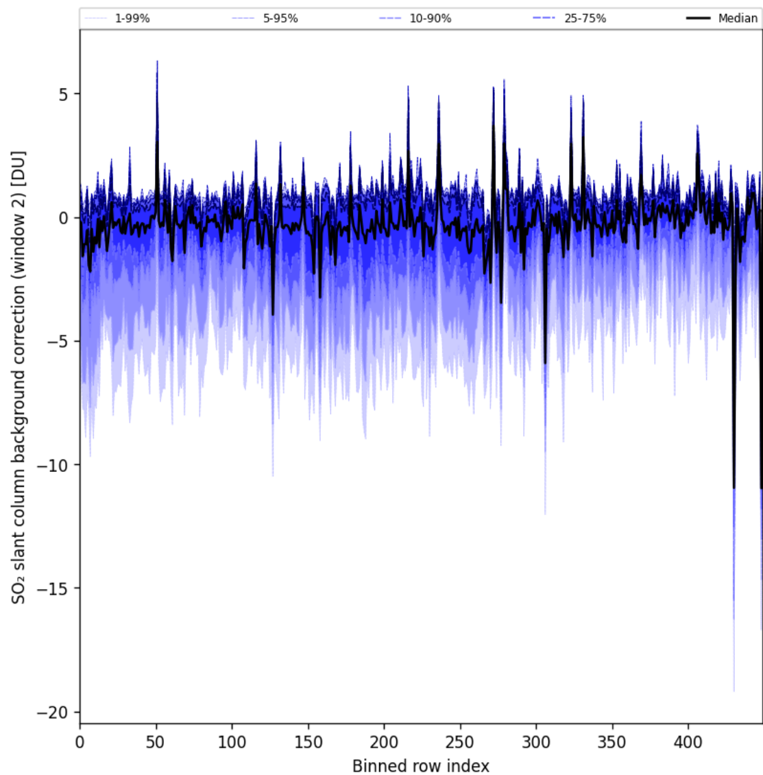
Figure 96: Along track statistics of “SO 2 slant column background correction (window 2)” for 2025-07-13 to 2025-07-14
