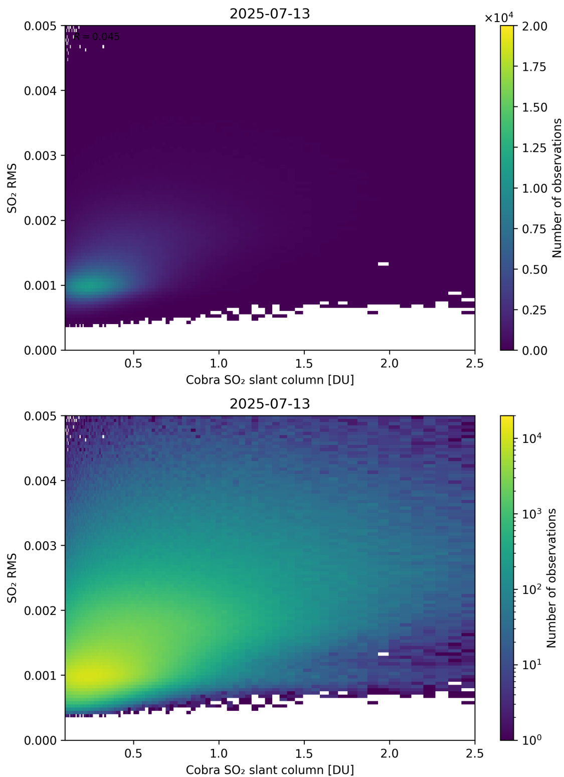
Figure 198: Scatter density plot of “Cobra SO 2 slant column” against “SO 2 RMS” for 2025-07-13 to 2025-07-14.
