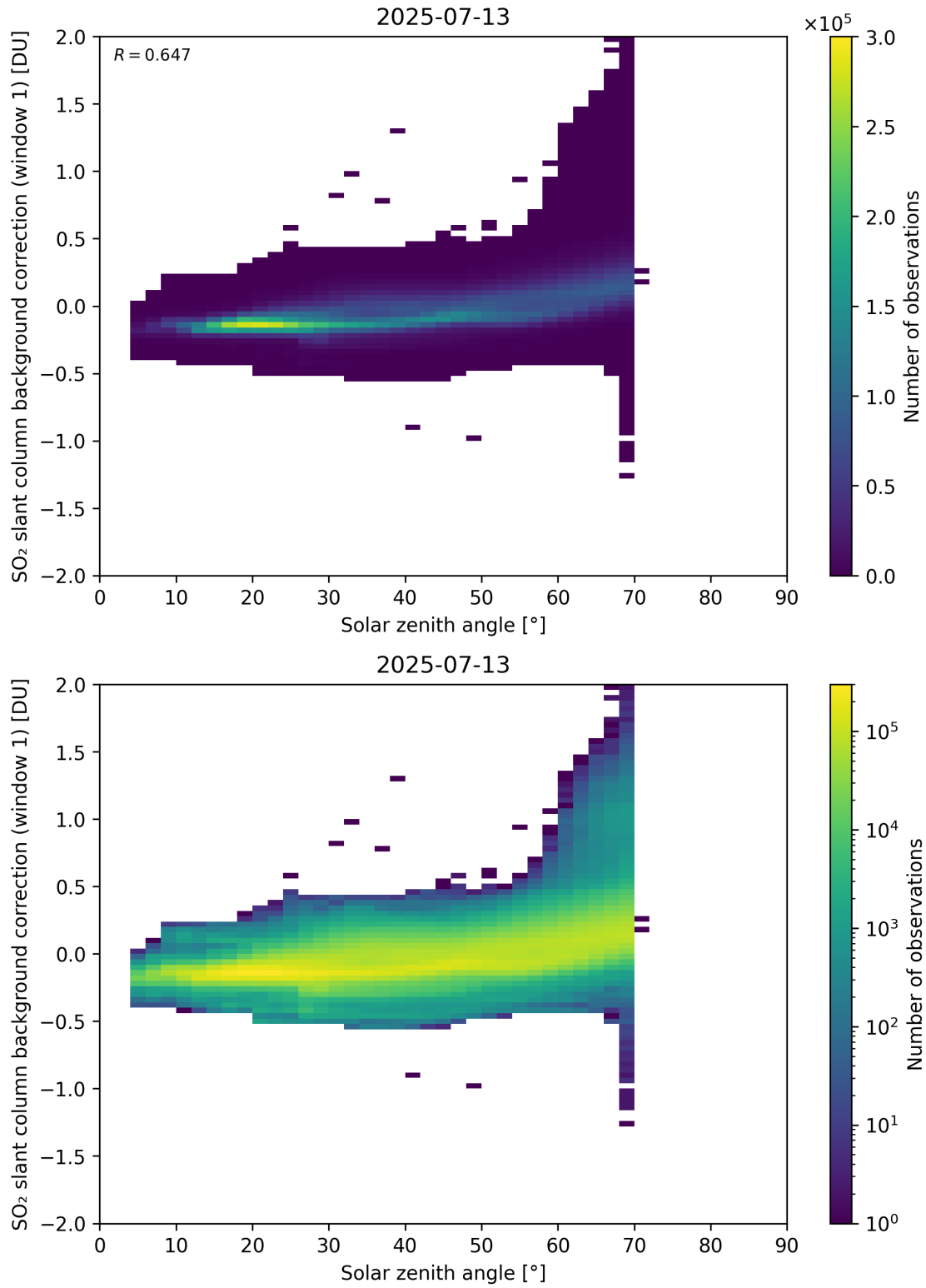
Figure 171: Scatter density plot of “Solar zenith angle” against “SO 2 slant column background correction (window 1)” for 2025-07-13 to 2025-07-14.
