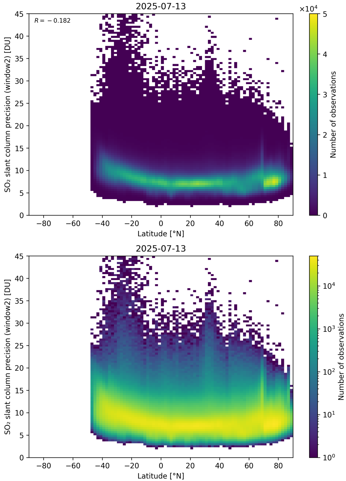
Figure 164: Scatter density plot of “Latitude” against “SO 2 slant column precision (window2)” for 2025-07-13 to 2025-07-14.
