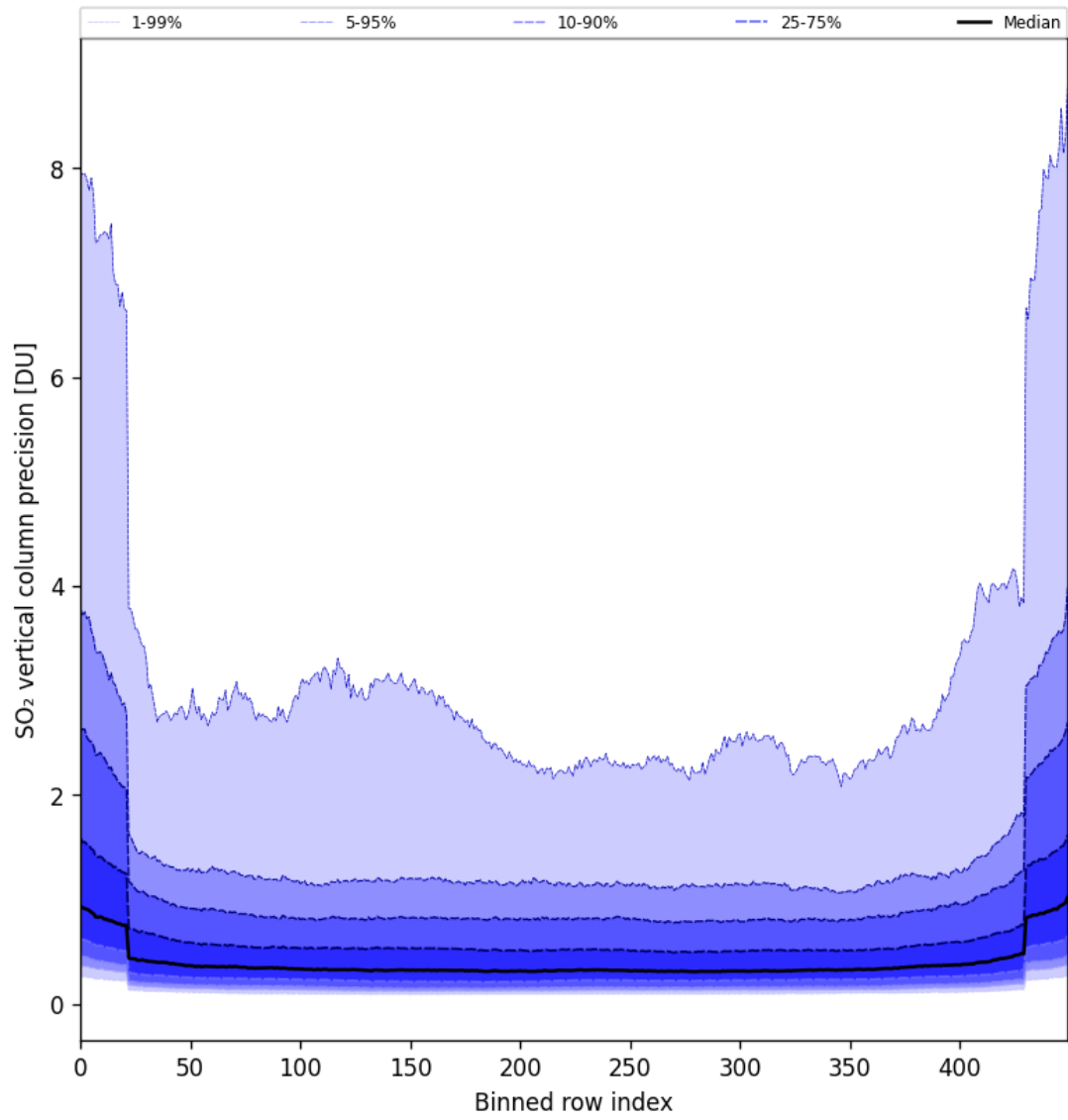
Figure 85: Along track statistics of “SO 2 vertical column precision” for 2025-07-13 to 2025-07-14
