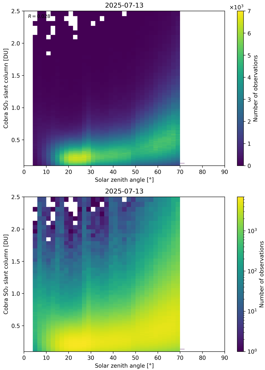
Figure 179: Scatter density plot of “Solar zenith angle” against “Cobra SO 2 slant column” for 2025-07-13 to 2025-07-14.
