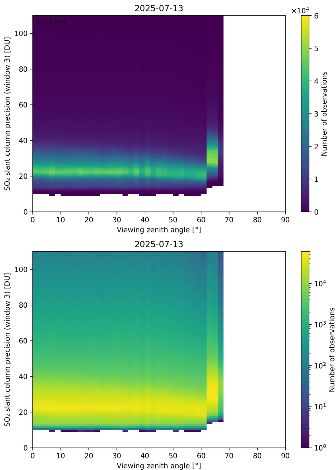
Figure 380: Scatter density plot of “Viewing zenith angle” against “SO 2 slant column precision (window 3)” for 2025-07-13 to 2025-07-14.
