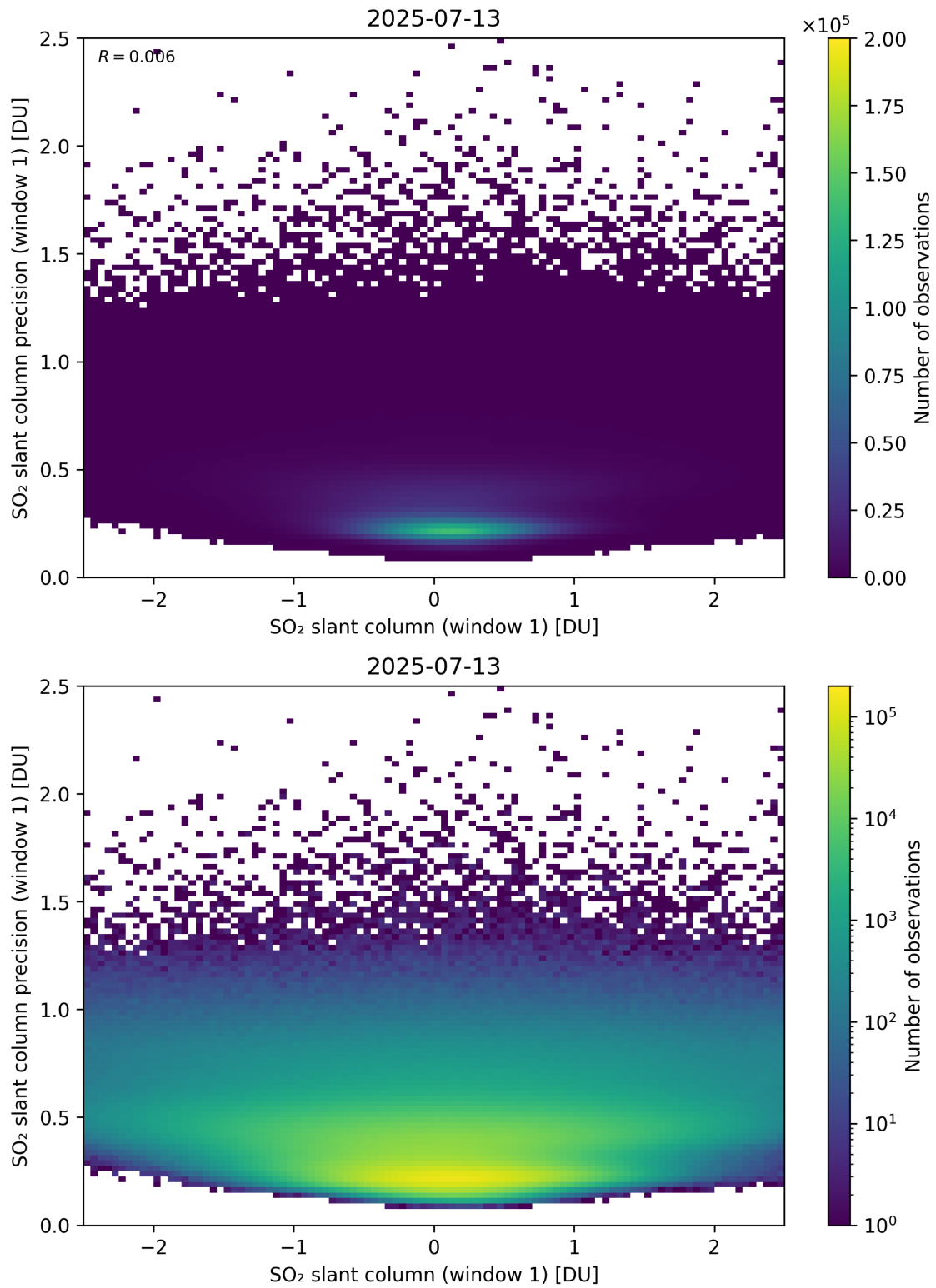
Figure 285: Scatter density plot of “SO 2 slant column (window 1)” against “SO 2 slant column precision (window 1)” for 2025-07-13 to 2025-07-14.
