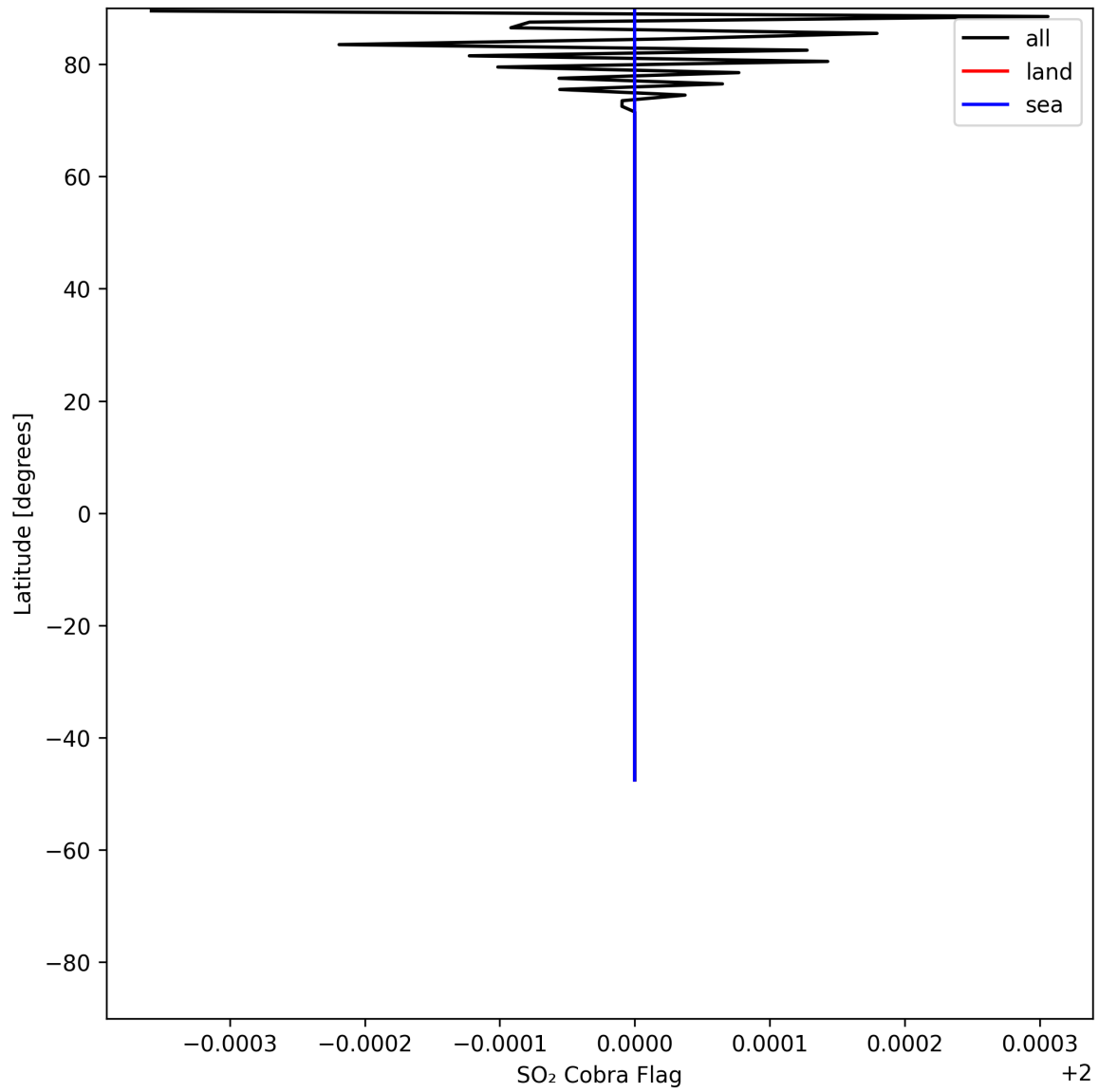
Figure 49: Zonal average of "SO 2 Cobra Flag" for 2025-07-13 to 2025-07-14.
