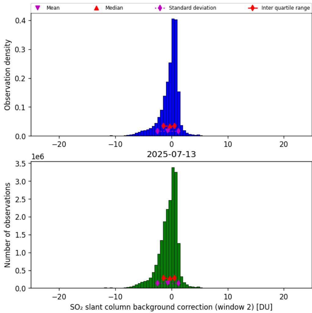
Figure 70: Histogram of “SO 2 slant column background correction (window 2)” for 2025-07-13 to 2025-07-14
