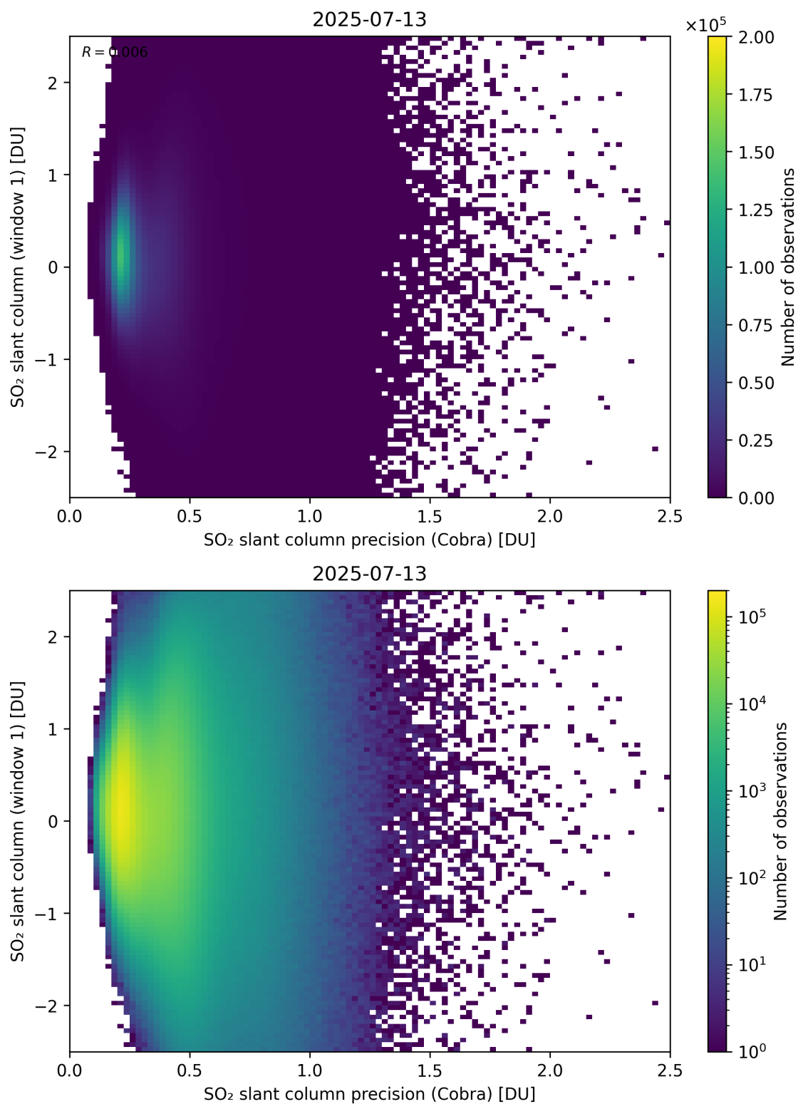
Figure 208: Scatter density plot of “SO 2 slant column precision (Cobra)” against “SO 2 slant column (window 1)” for 2025-07-13 to 2025-07-14.
