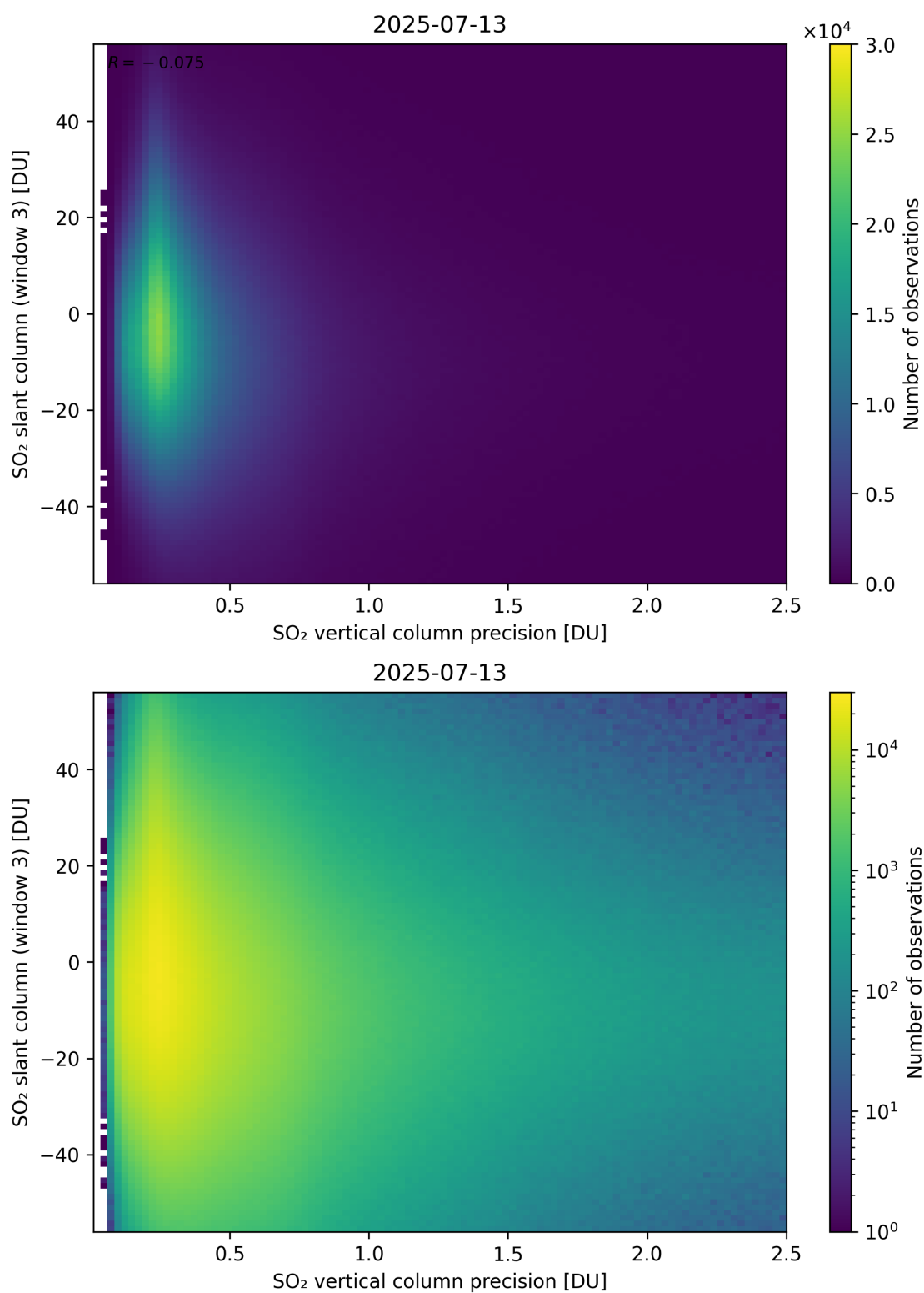
Figure 344: Scatter density plot of “SO 2 vertical column precision” against “SO 2 slant column (window 3)” for 2025-07-13 to 2025-07-14.
