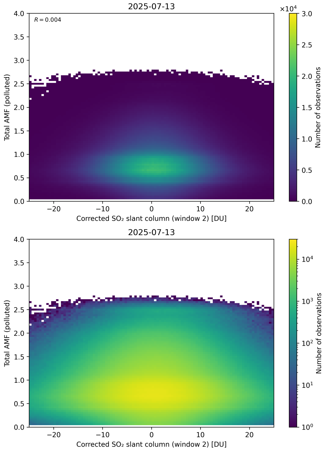
Figure 253: Scatter density plot of “Corrected SO 2 slant column (window 2)” against “Total AMF (polluted)” for 2025-07-13 to 2025-07-14.
