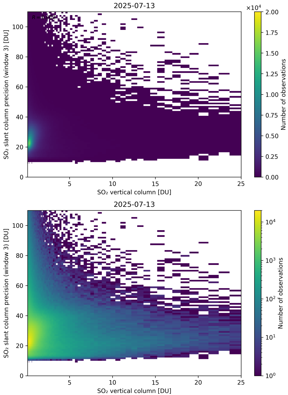
Figure 358: Scatter density plot of “SO 2 vertical column” against “SO 2 slant column precision (window 3)” for 2025-07-13 to 2025-07-14.
