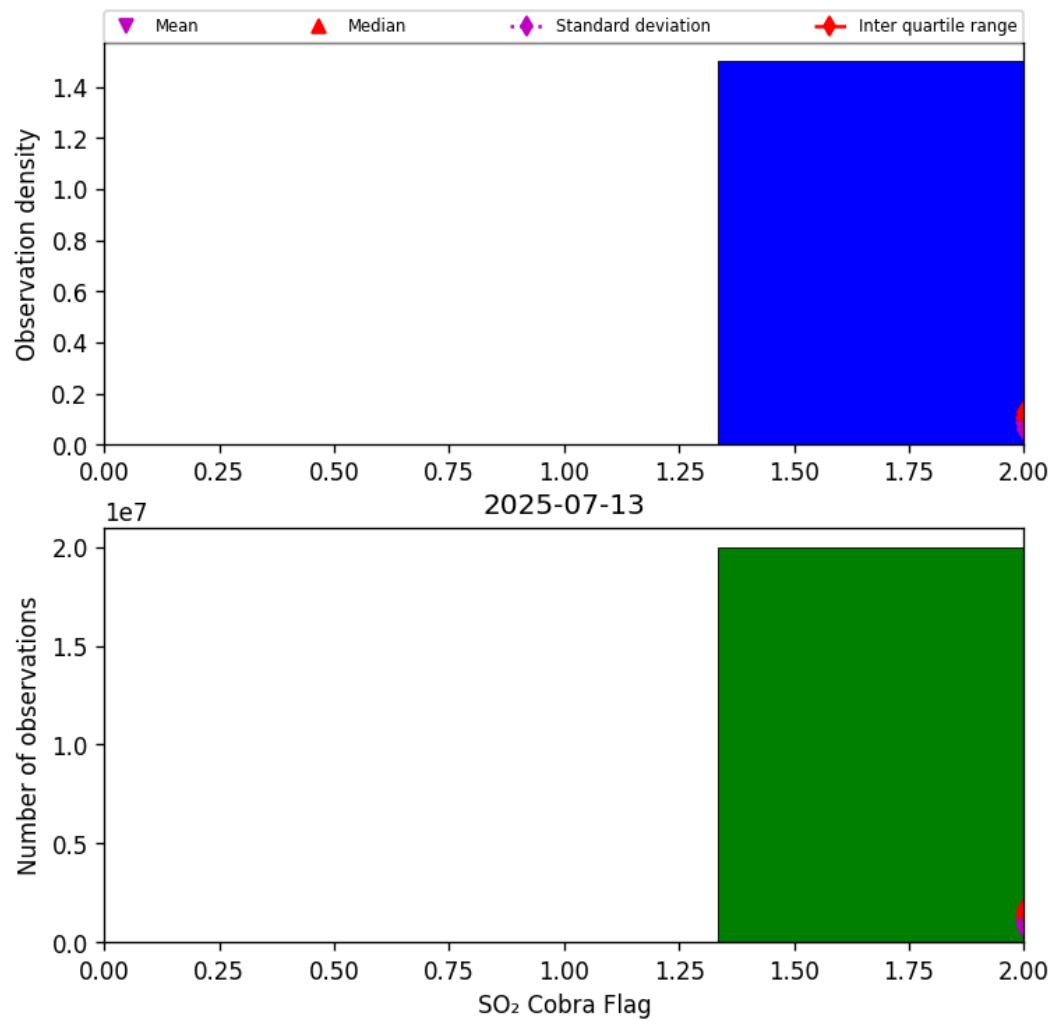
Figure 75: Histogram of “SO 2 Cobra Flag” for 2025-07-13 to 2025-07-14
