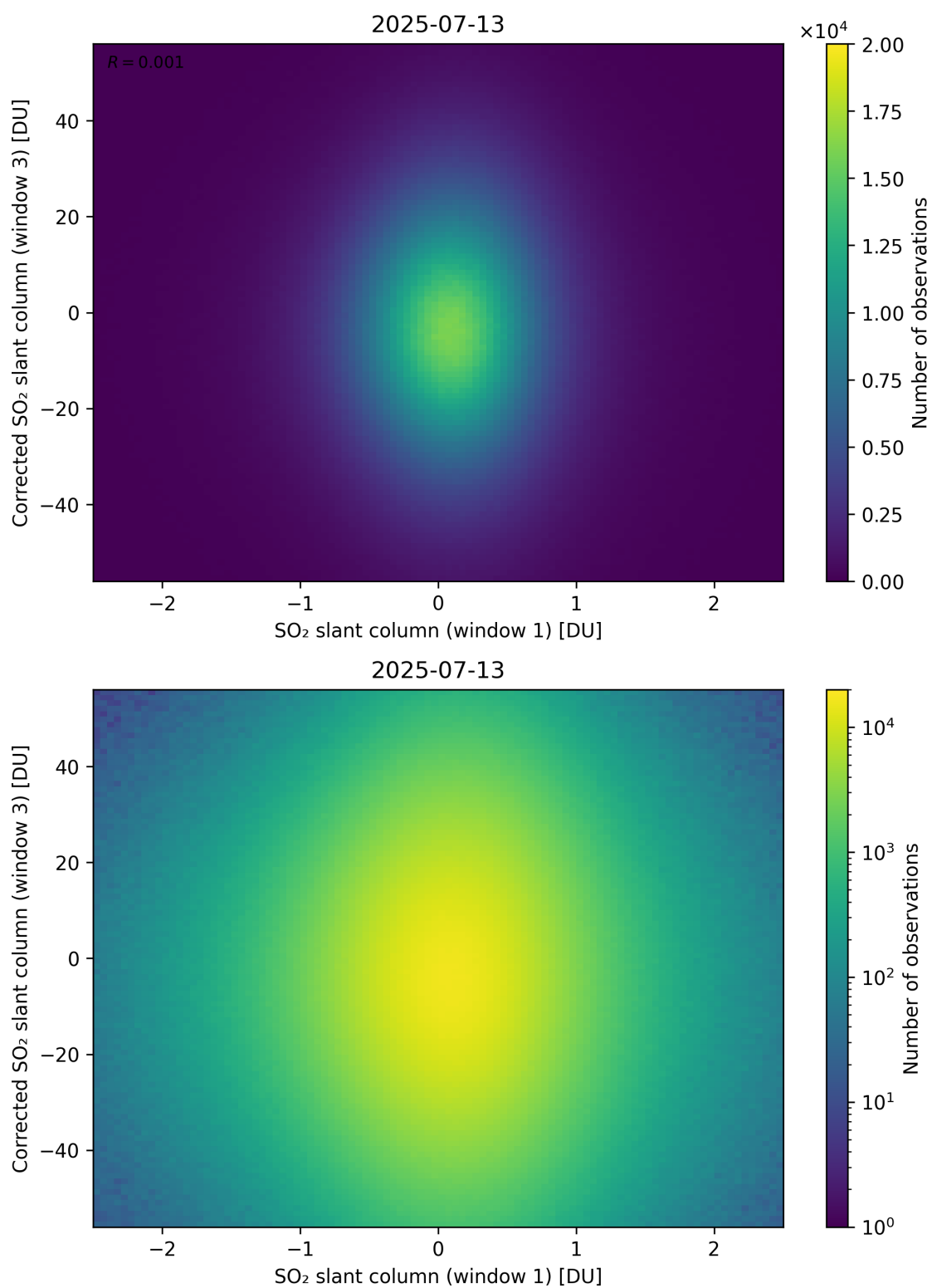
Figure 284: Scatter density plot of “SO 2 slant column (window 1)” against “Corrected SO 2 slant column (window 3)” for 2025-07-13 to 2025-07-14.
