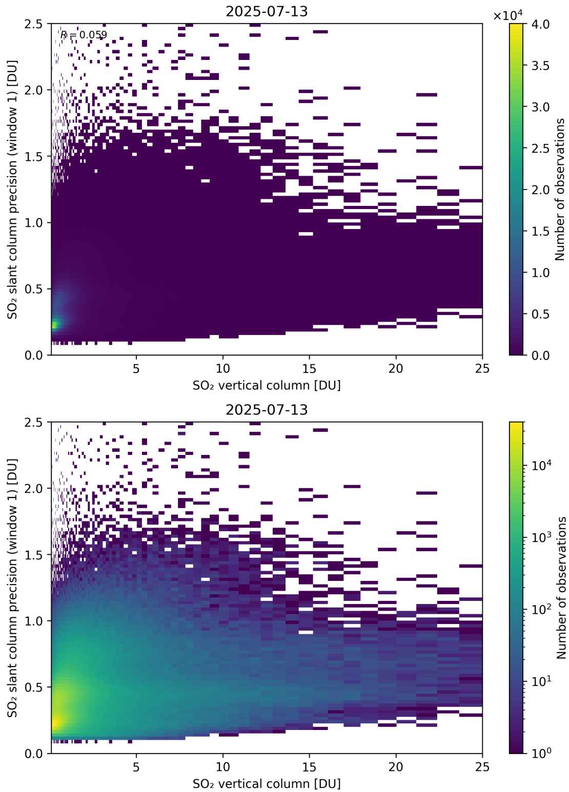
Figure 355: Scatter density plot of “SO 2 vertical column” against “SO 2 slant column precision (window 1)” for 2025-07-13 to 2025-07-14.
