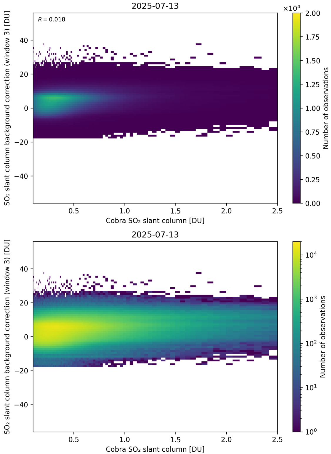
Figure 195: Scatter density plot of “Cobra SO 2 slant column” against “SO 2 slant column background correction (window 3)” for 2025-07-13 to 2025-07-14.
