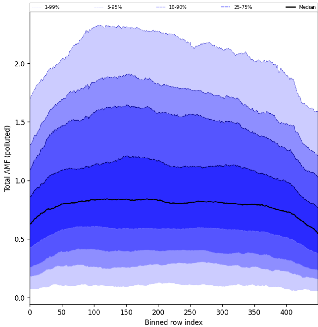
Figure 105: Along track statistics of “Total AMF (polluted)” for 2025-07-13 to 2025-07-14
