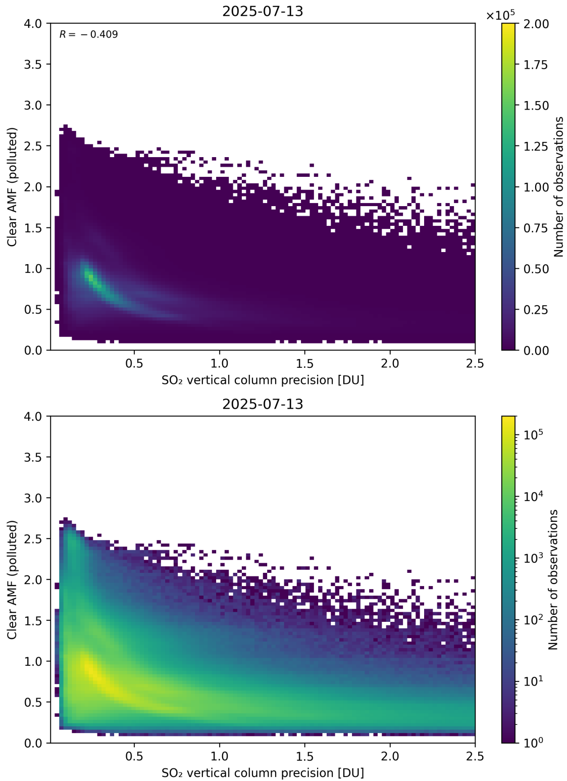
Figure 335: Scatter density plot of “SO 2 vertical column precision” against “Clear AMF (polluted)” for 2025-07-13 to 2025-07-14.
