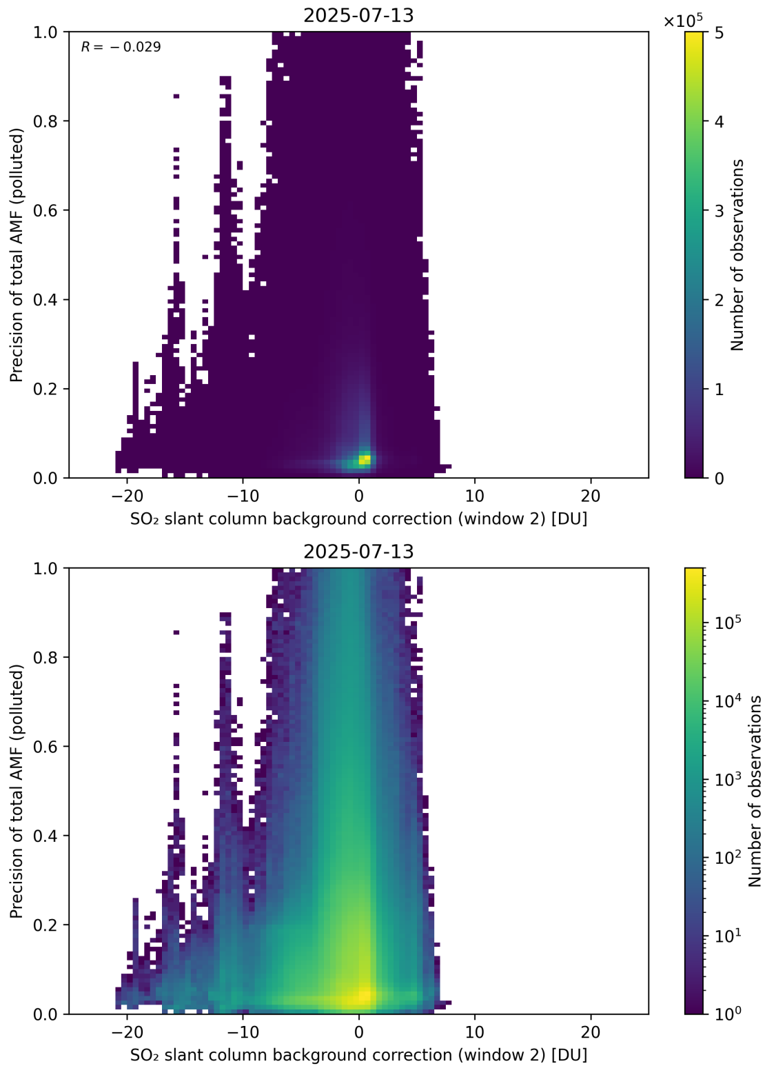
Figure 131: Scatter density plot of “SO 2 slant column background correction (window 2)” against “Precision of total AMF (polluted)” for 2025-07-13 to 2025-07-14.
