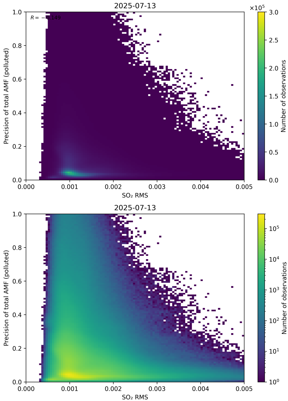
Figure 149: Scatter density plot of “SO 2 RMS” against “Precision of total AMF (polluted)” for 2025-07-13 to 2025-07-14.
