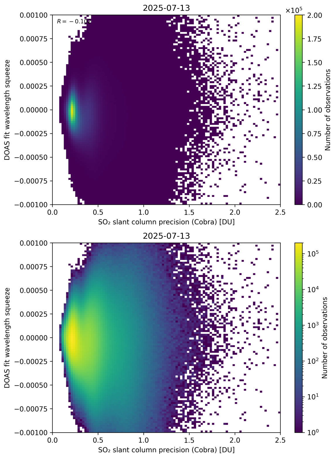
Figure 203: Scatter density plot of “SO 2 slant column precision (Cobra)” against “DOAS fit wavelength squeeze” for 2025-07-13 to 2025-07-14.
