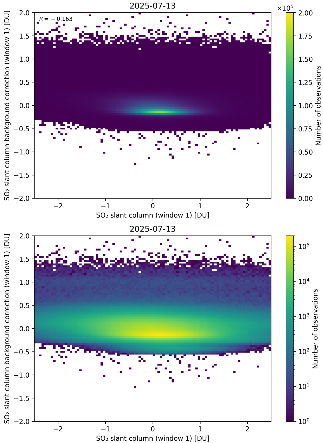
Figure 262: Scatter density plot of “SO 2 slant column (window 1)” against “SO 2 slant column background correction (window 1)” for 2025-07-13 to 2025-07-14.
