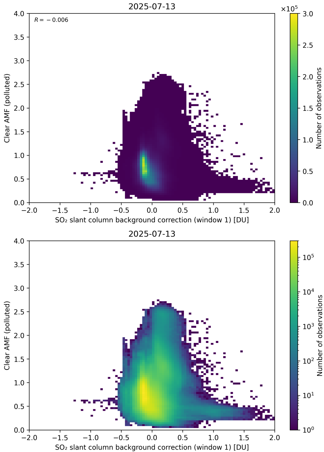
Figure 114: Scatter density plot of “SO 2 slant column background correction (window 1)” against “Clear AMF (polluted)” for 2025-07-13 to 2025-07-14.
