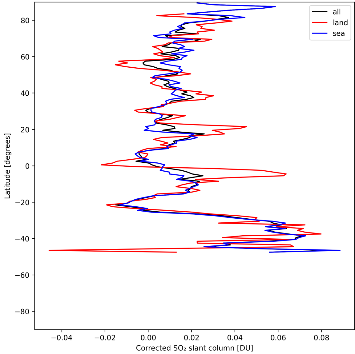
Figure 34: Zonal average of “Corrected SO 2 slant column” for 2025-07-13 to 2025-07-14.
