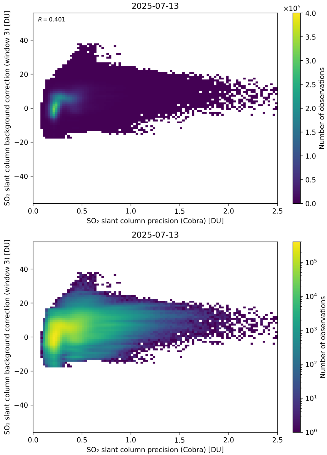
Figure 201: Scatter density plot of “SO 2 slant column precision (Cobra)” against “SO 2 slant column background correction (window 3)” for 2025-07-13 to 2025-07-14.
