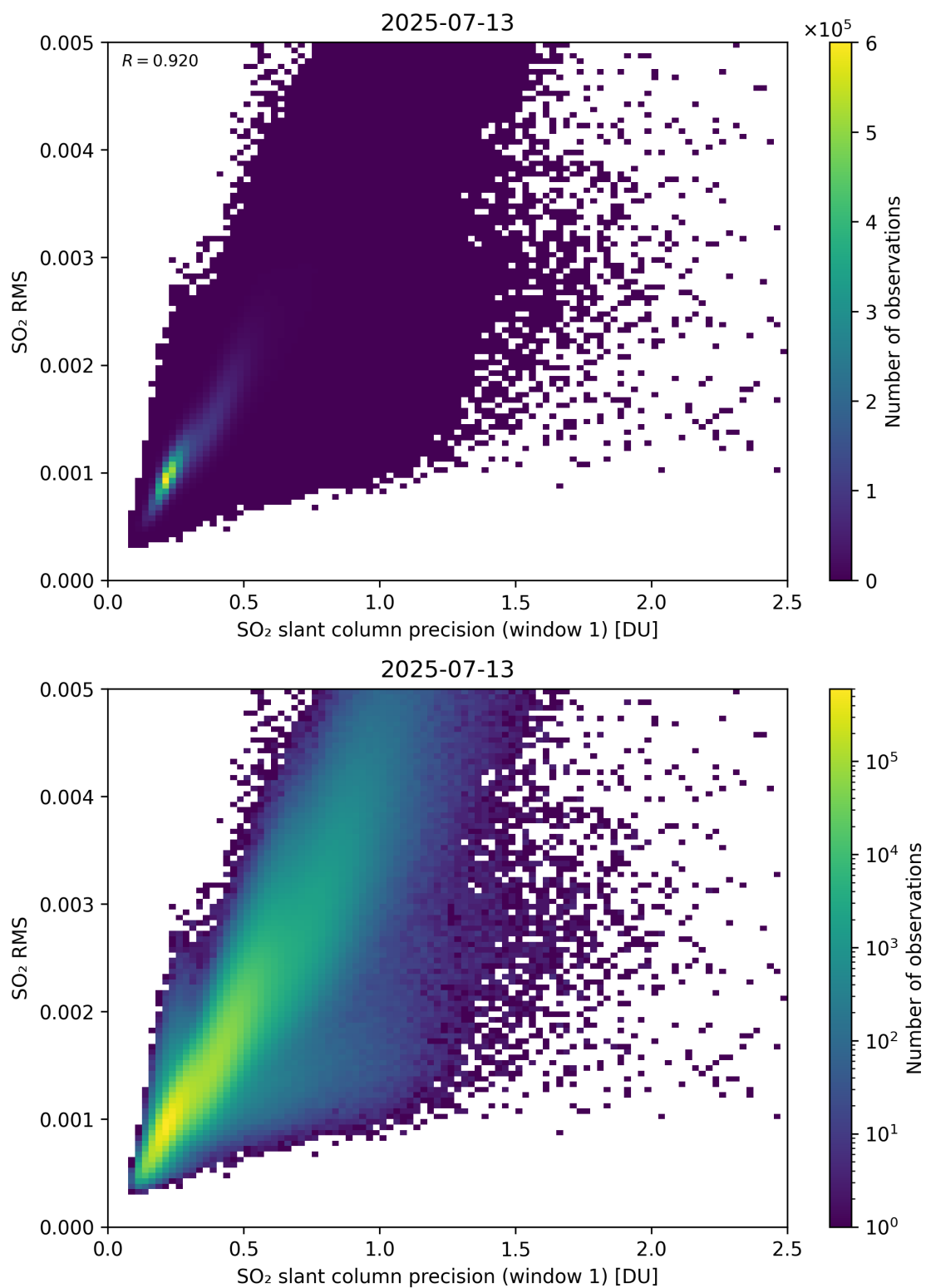
Figure 273: Scatter density plot of “SO 2 slant column precision (window 1)” against “SO 2 RMS” for 2025-07-13 to 2025-07-14.
