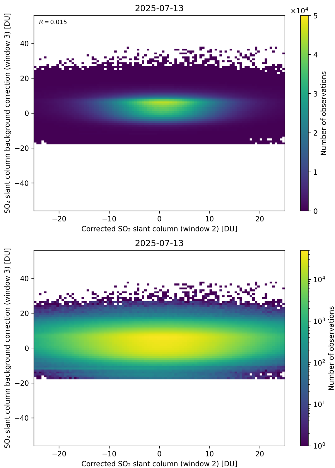
Figure 245: Scatter density plot of “Corrected SO 2 slant column (window 2)” against “SO 2 slant column background correction (window 3)” for 2025-07-13 to 2025-07-14.
