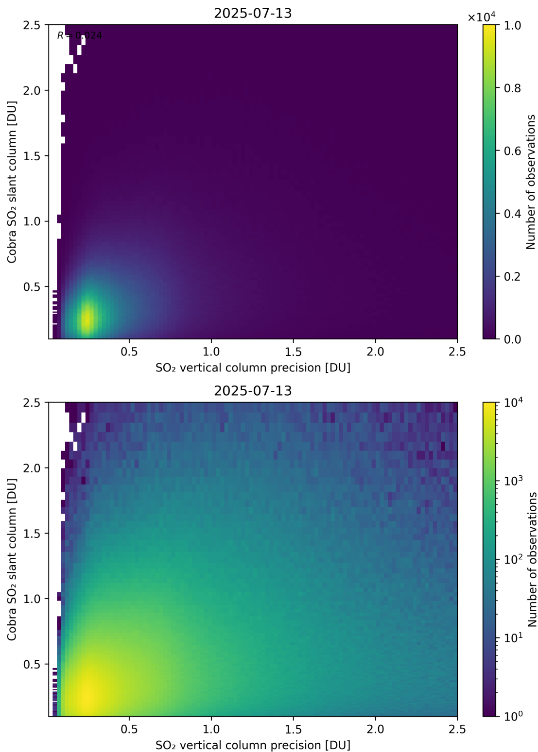
Figure 336: Scatter density plot of “SO 2 vertical column precision” against “Cobra SO 2 slant column” for 2025-07-13 to 2025-07-14.
