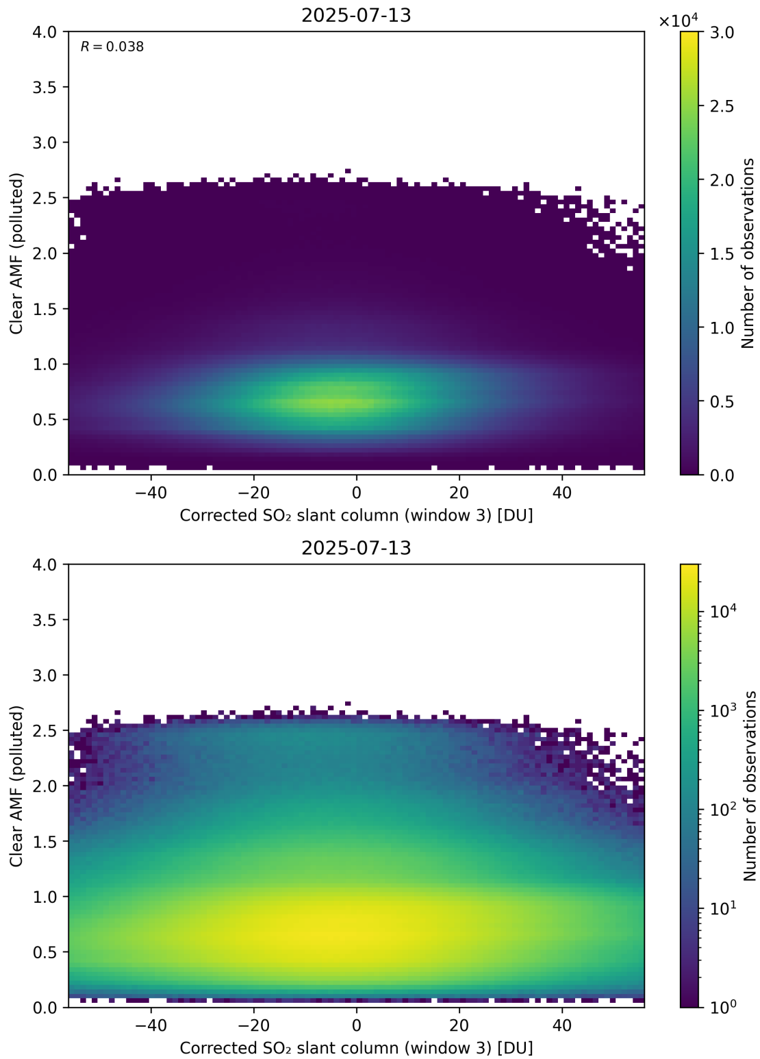
Figure 259: Scatter density plot of “Corrected SO 2 slant column (window 3)” against “Clear AMF (polluted)” for 2025-07-13 to 2025-07-14.
