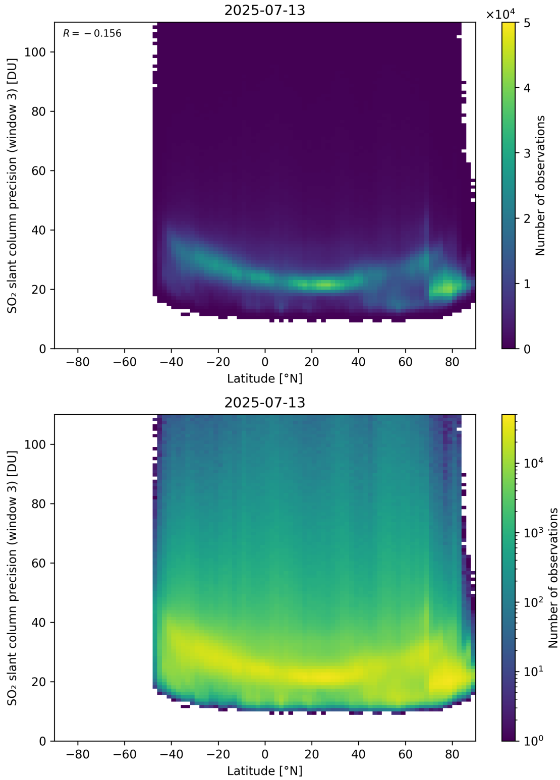
Figure 166: Scatter density plot of “Latitude” against “SO 2 slant column precision (window 3)” for 2025-07-13 to 2025-07-14.
