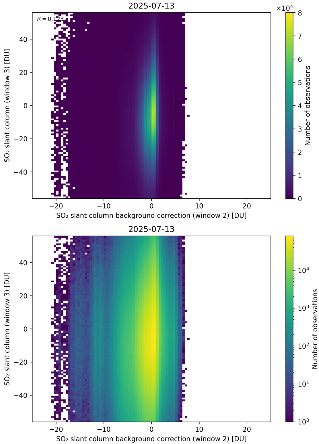
Figure 128: Scatter density plot of “SO 2 slant column background correction (window 2)” against “SO 2 slant column (window 3)” for 2025-07-13 to 2025-07-14.
