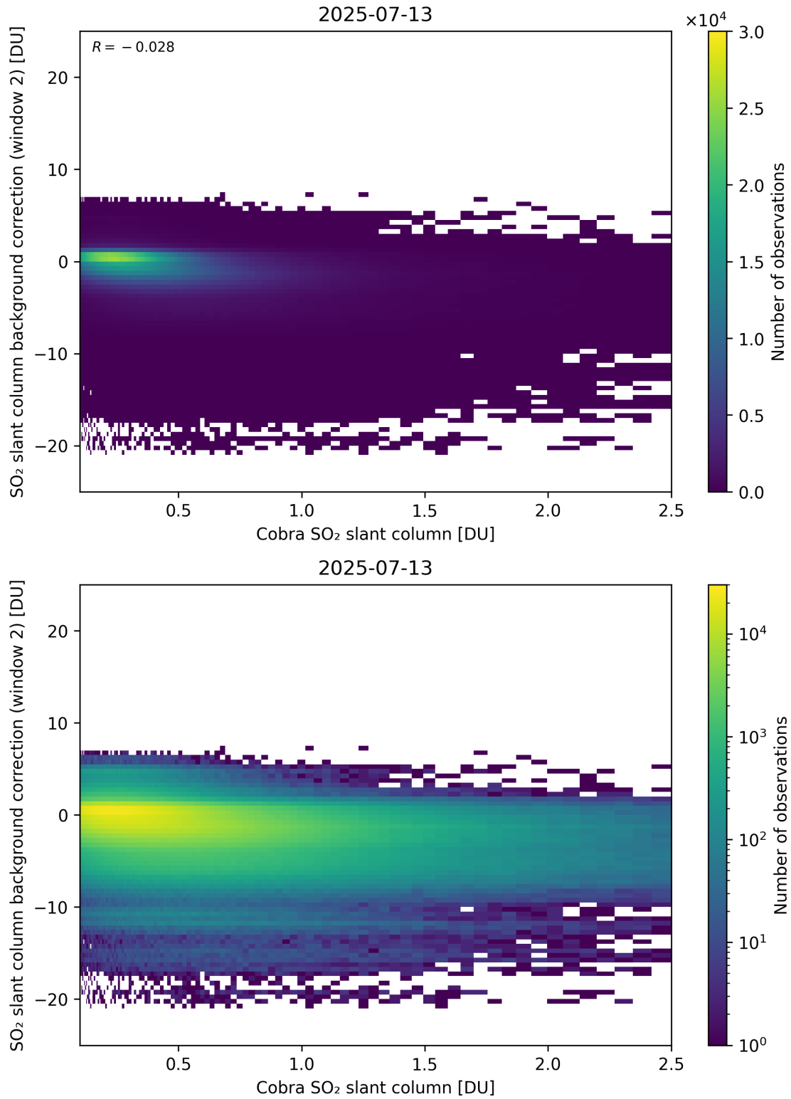
Figure 194: Scatter density plot of “Cobra SO 2 slant column” against “SO 2 slant column background correction (window 2)” for 2025-07-13 to 2025-07-14.
