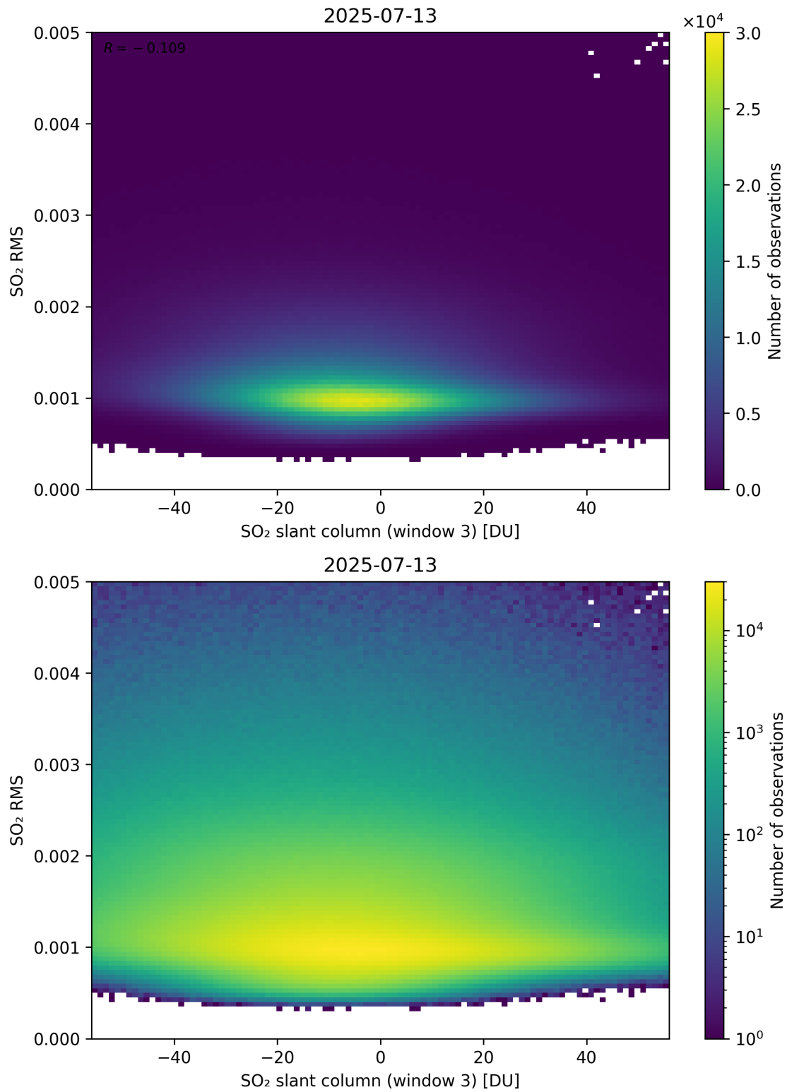
Figure 306: Scatter density plot of “SO 2 slant column (window 3)” against “SO 2 RMS” for 2025-07-13 to 2025-07-14.
