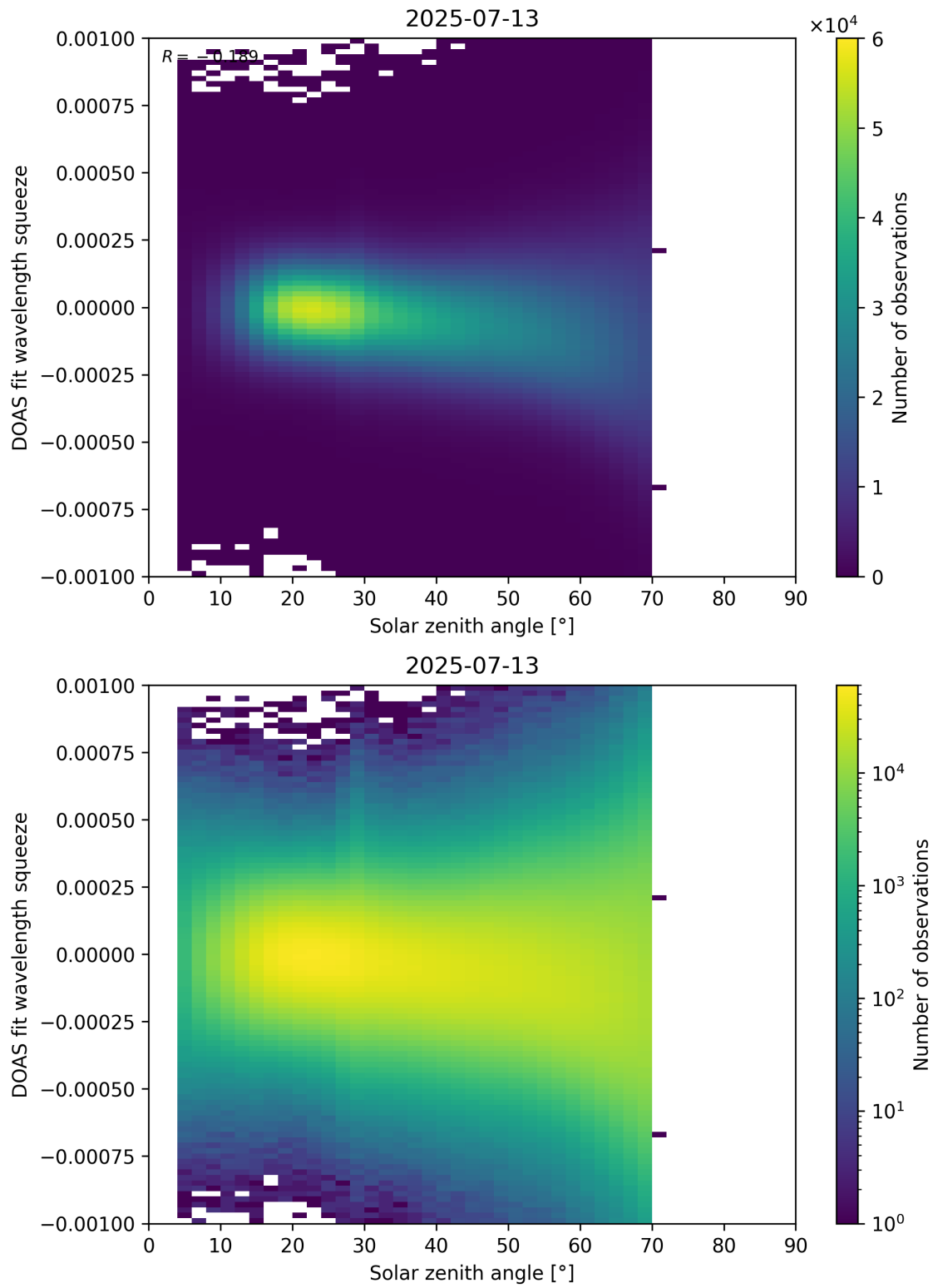
Figure 175: Scatter density plot of “Solar zenith angle” against “DOAS fit wavelength squeeze” for 2025-07-13 to 2025-07-14.
