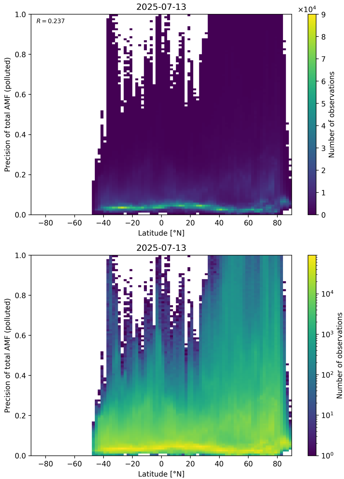
Figure 168: Scatter density plot of “Latitude” against “Precision of total AMF (polluted)” for 2025-07-13 to 2025-07-14.
