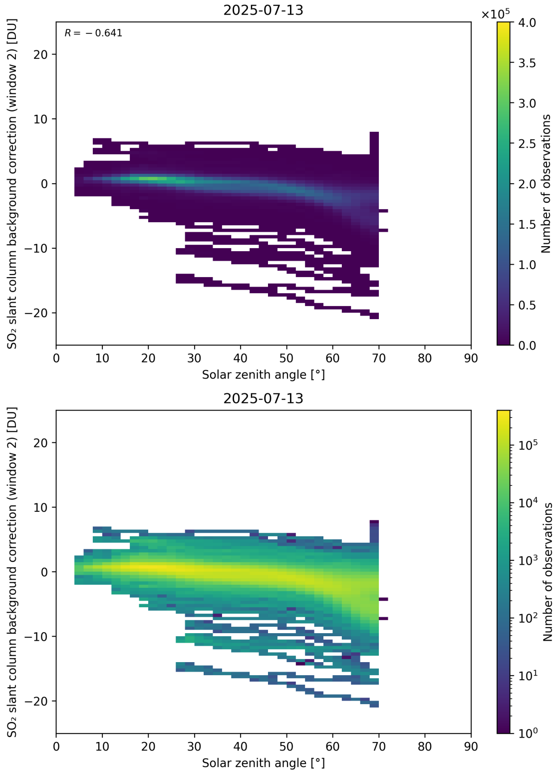
Figure 172: Scatter density plot of “Solar zenith angle” against “SO 2 slant column background correction (window 2)” for 2025-07-13 to 2025-07-14.
