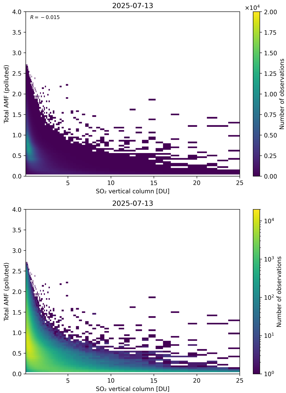
Figure 359: Scatter density plot of “SO 2 vertical column” against “Total AMF (polluted)” for 2025-07-13 to 2025-07-14.
