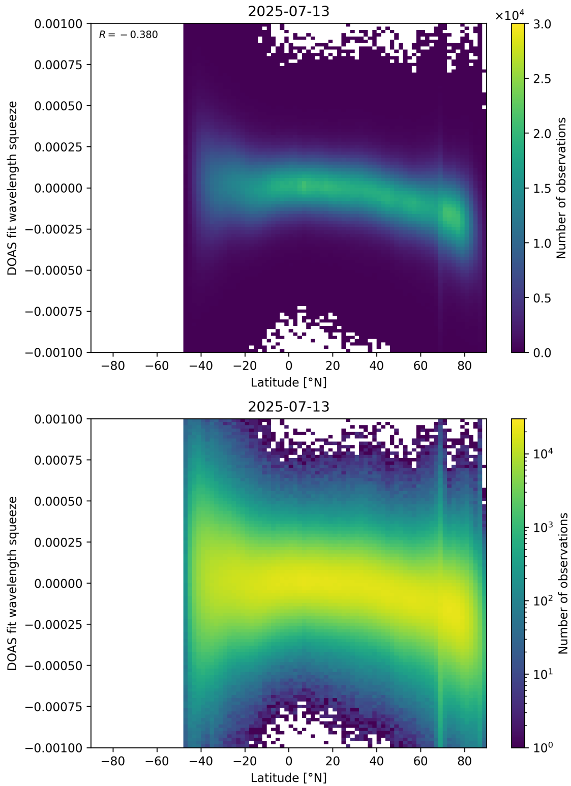
Figure 154: Scatter density plot of “Latitude” against “DOAS fit wavelength squeeze” for 2025-07-13 to 2025-07-14.
