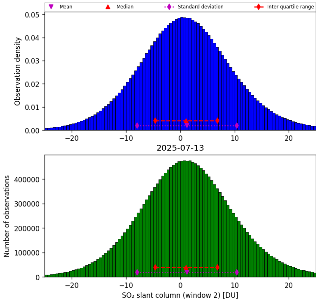
Figure 67: Histogram of “SO 2 slant column (window 2)” for 2025-07-13 to 2025-07-14
