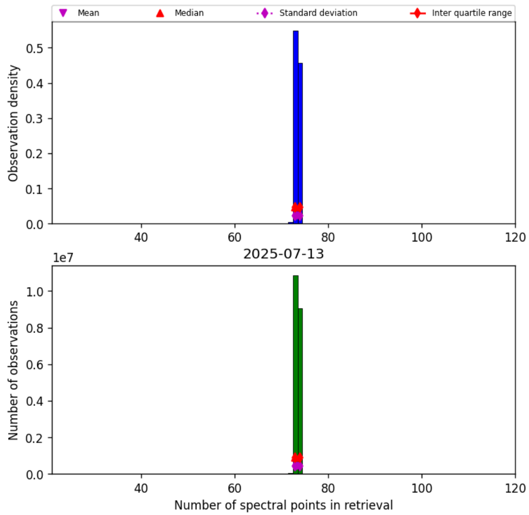
Figure 82: Histogram of “Number of spectral points in retrieval” for 2025-07-13 to 2025-07-14
