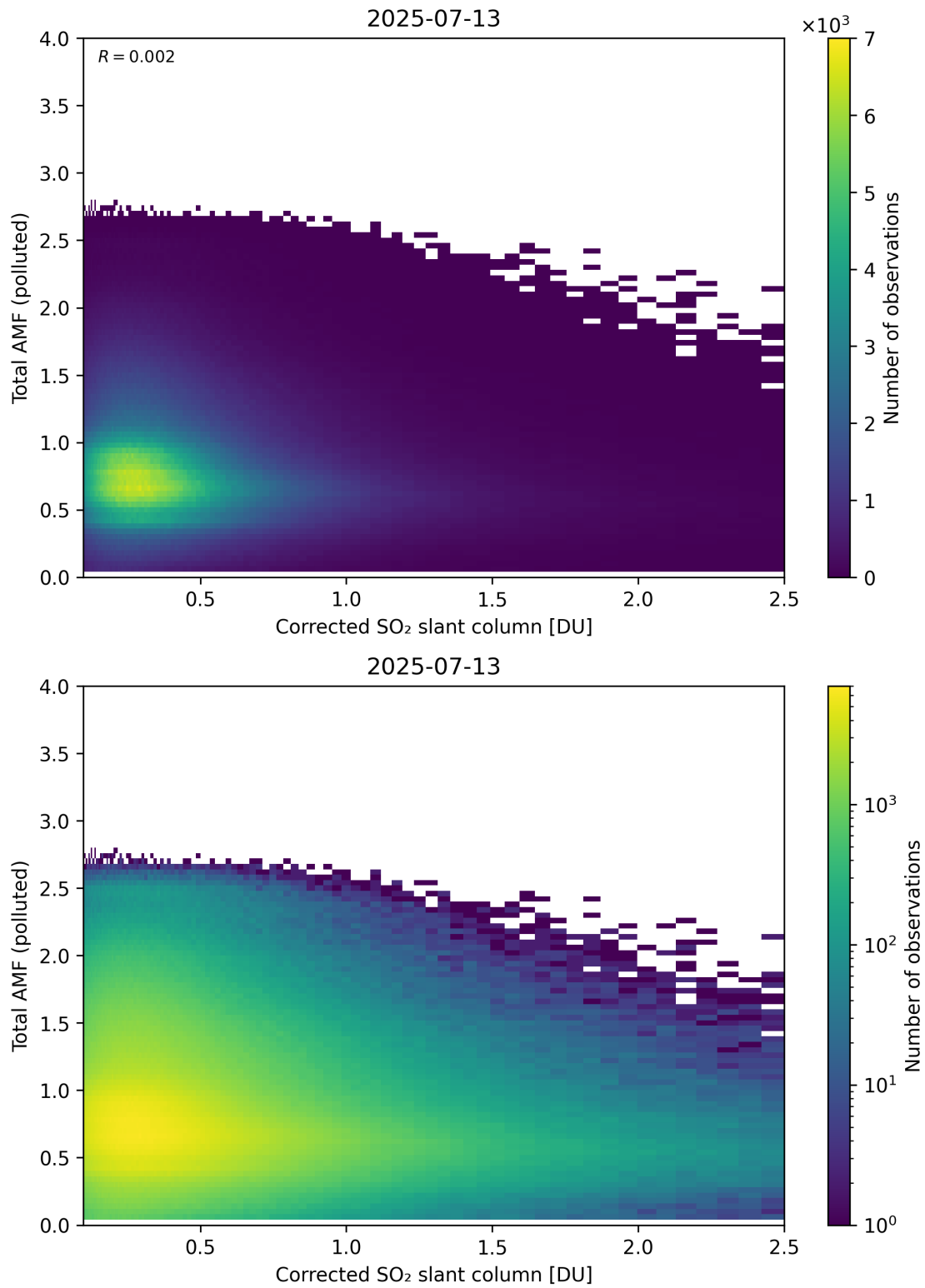
Figure 242: Scatter density plot of “Corrected SO 2 slant column” against “Total AMF (polluted)” for 2025-07-13 to 2025-07-14.
