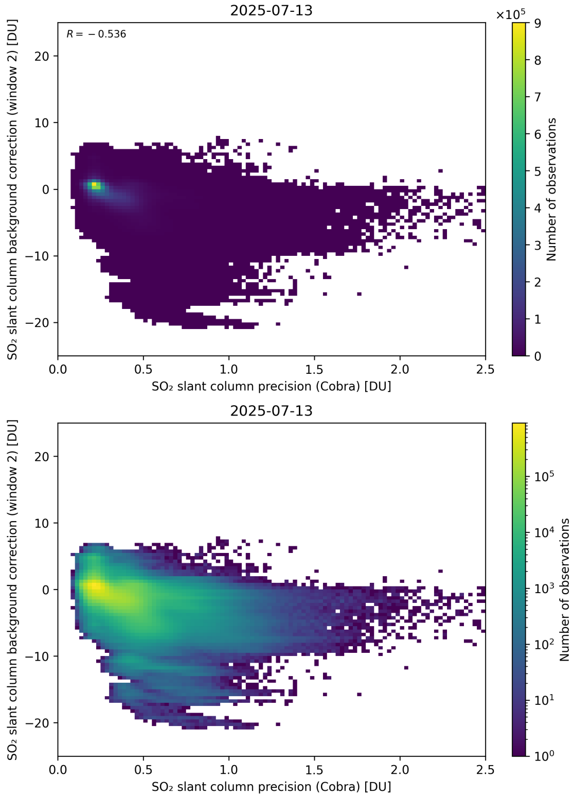
Figure 200: Scatter density plot of “SO 2 slant column precision (Cobra)” against “SO 2 slant column background correction (window 2)” for 2025-07-13 to 2025-07-14.
