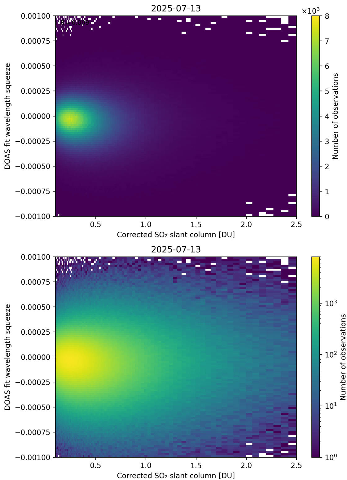
Figure 230: Scatter density plot of “Corrected SO 2 slant column” against “DOAS fit wavelength squeeze” for 2025-07-13 to 2025-07-14.
