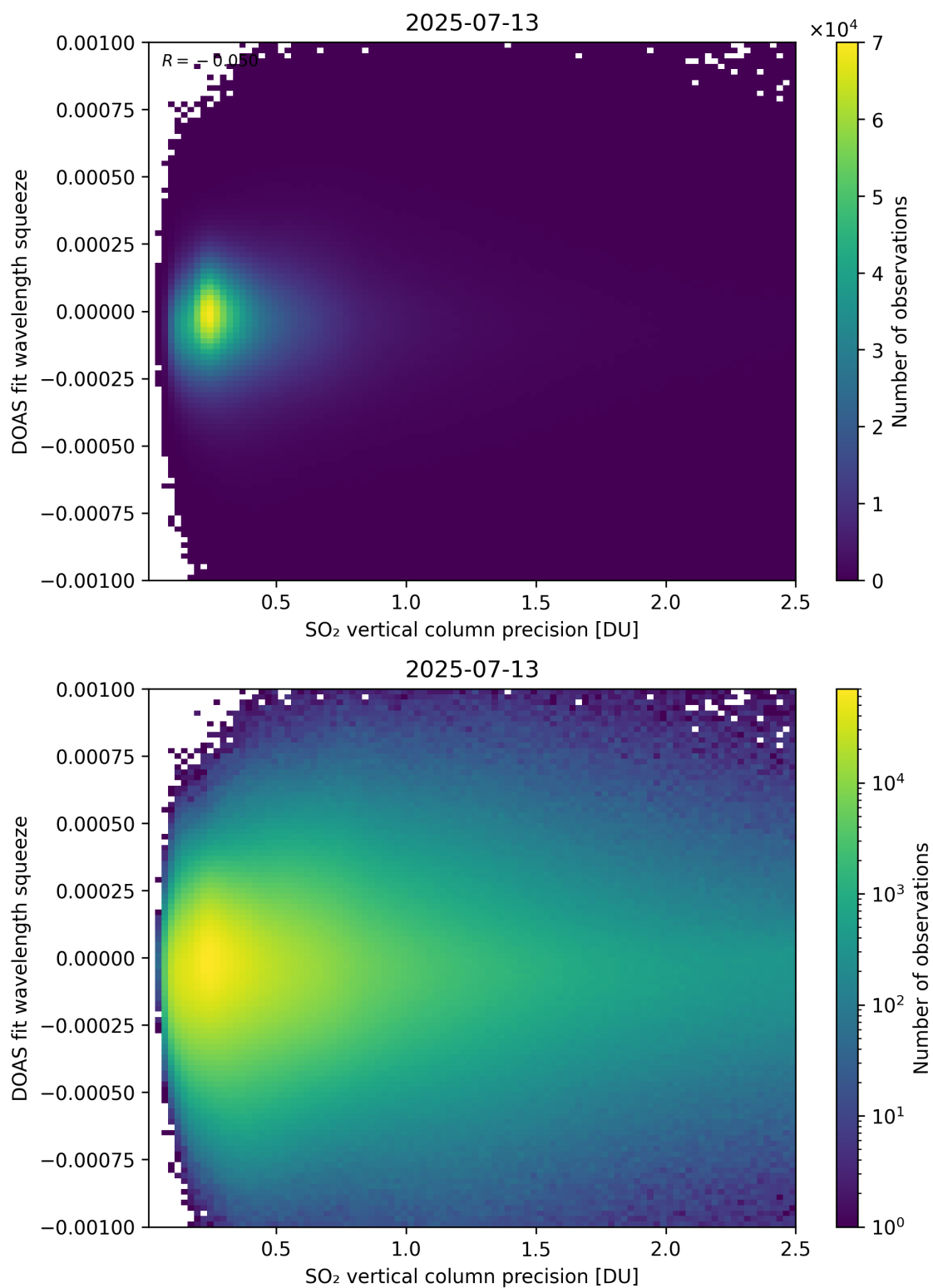
Figure 333: Scatter density plot of “SO 2 vertical column precision” against “DOAS fit wavelength squeeze” for 2025-07-13 to 2025-07-14.
