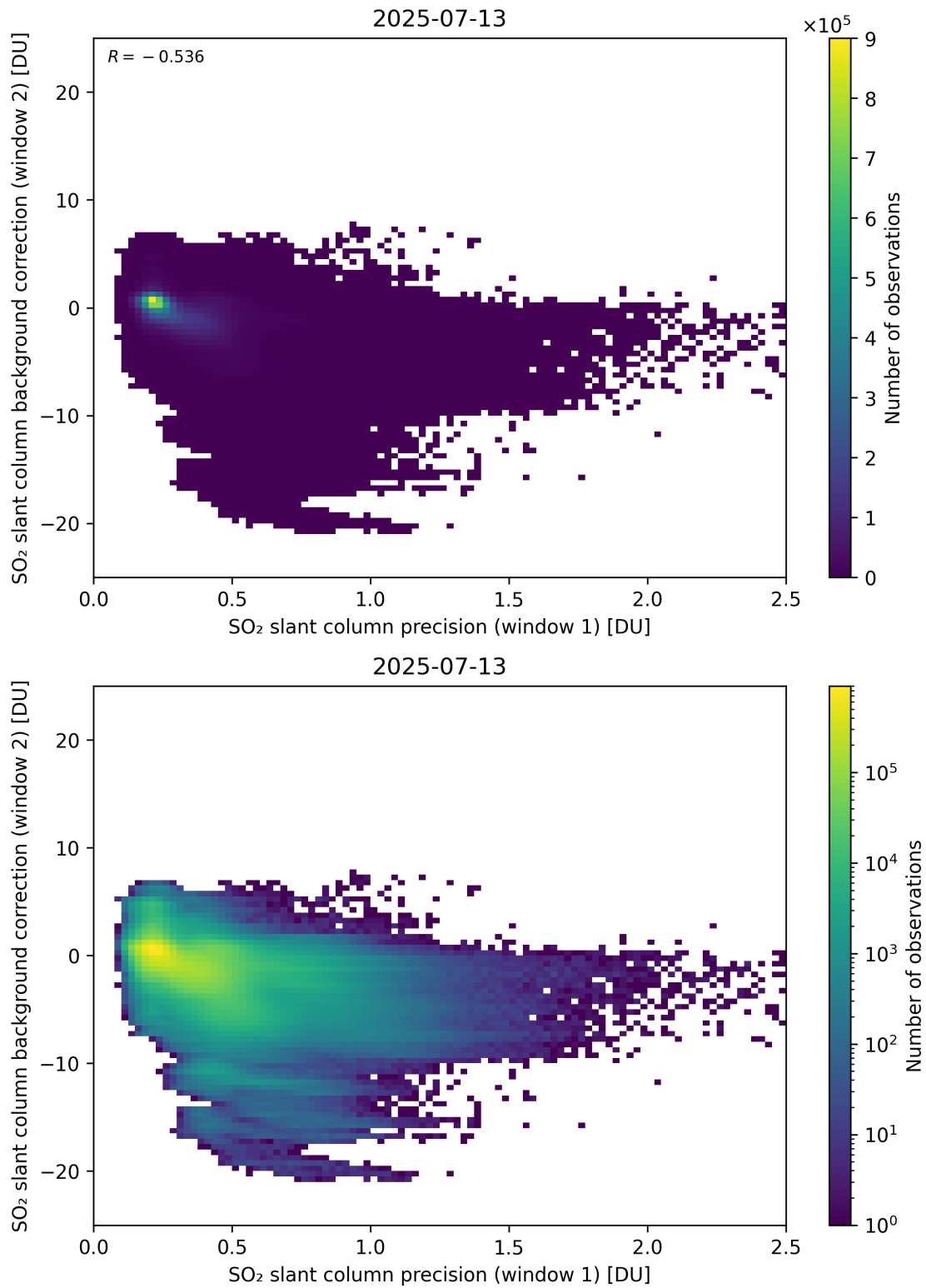
Figure 269: Scatter density plot of “SO 2 slant column precision (window 1)” against “SO 2 slant column background correction (window 2)” for 2025-07-13 to 2025-07-14.
