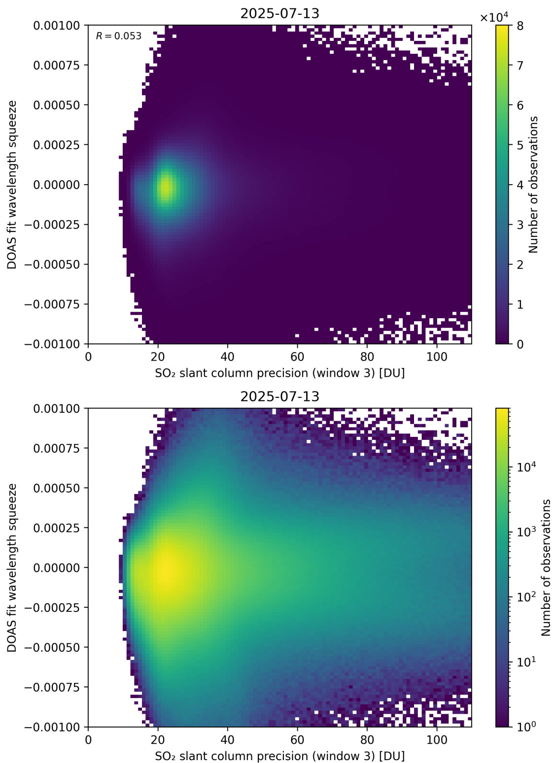
Figure 309: Scatter density plot of “SO 2 slant column precision (window 3)” against “DOAS fit wavelength squeeze” for 2025-07-13 to 2025-07-14.
