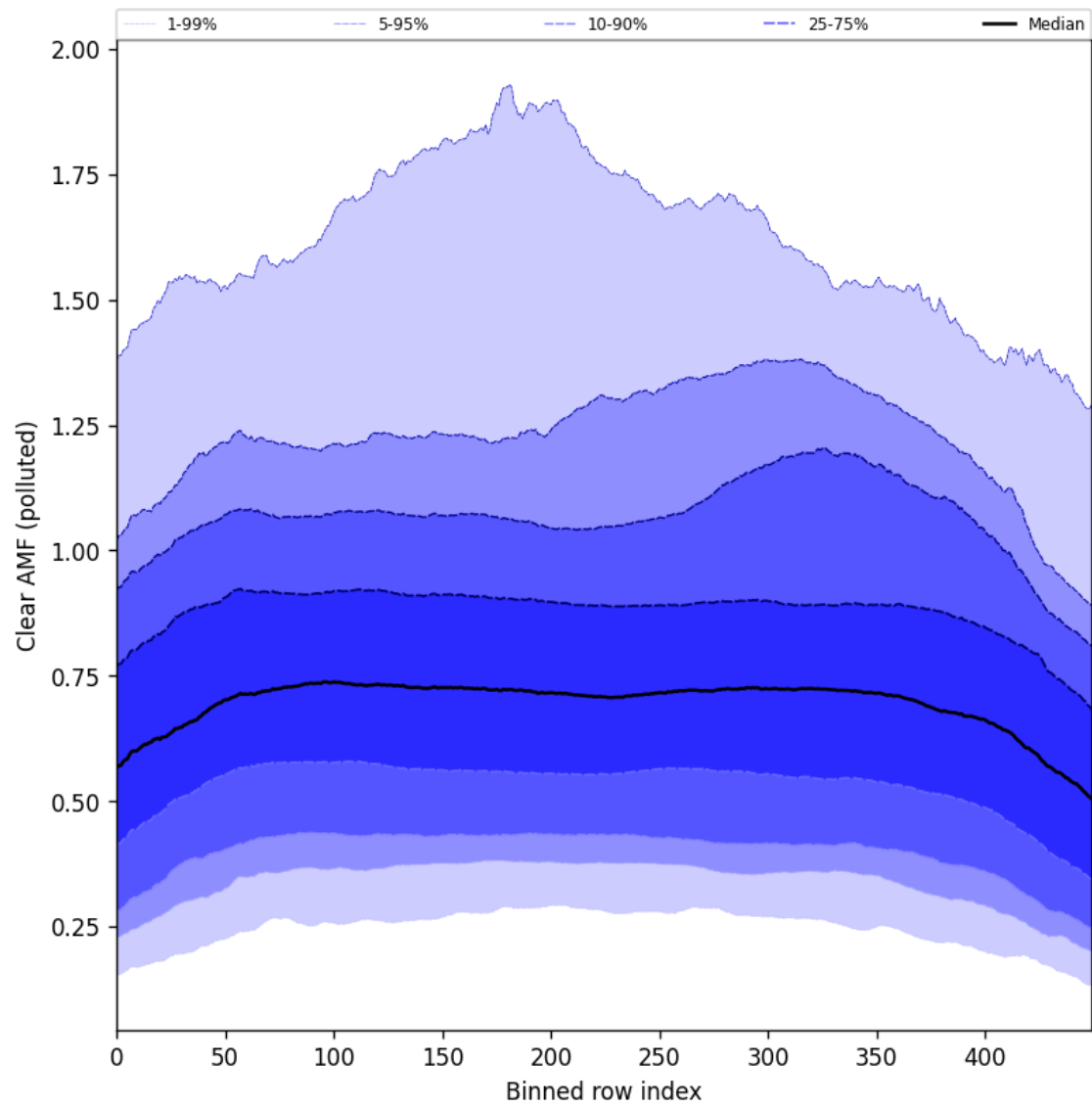
Figure 107: Along track statistics of “Clear AMF (polluted)” for 2025-07-13 to 2025-07-14
