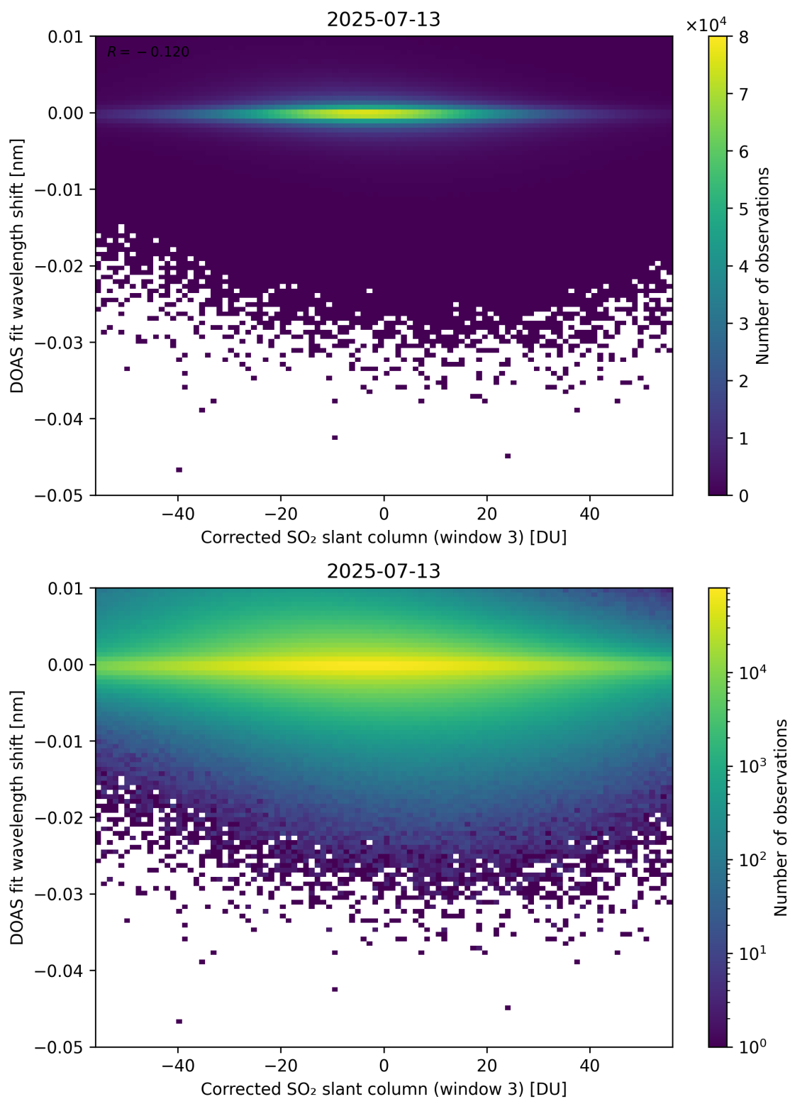
Figure 256: Scatter density plot of “Corrected SO 2 slant column (window 3)” against “DOAS fit wavelength shift” for 2025-07-13 to 2025-07-14.
