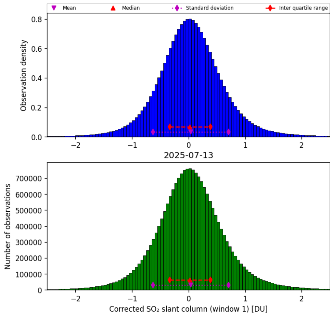
Figure 65: Histogram of “Corrected SO 2 slant column (window 1)” for 2025-07-13 to 2025-07-14
