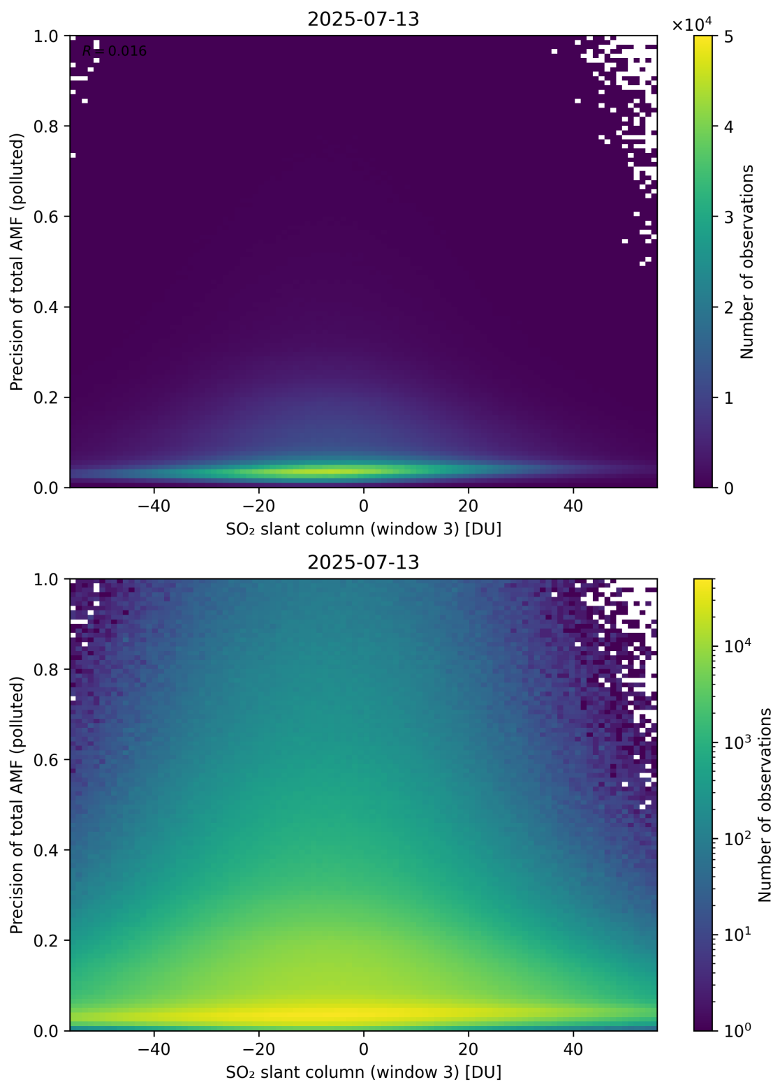
Figure 319: Scatter density plot of “SO 2 slant column (window 3)” against “Precision of total AMF (polluted)” for 2025-07-13 to 2025-07-14.
