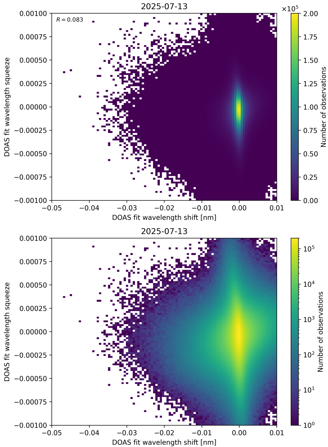
Figure 138: Scatter density plot of “DOAS fit wavelength shift” against “DOAS fit wavelength squeeze” for 2025-07-13 to 2025-07-14.
