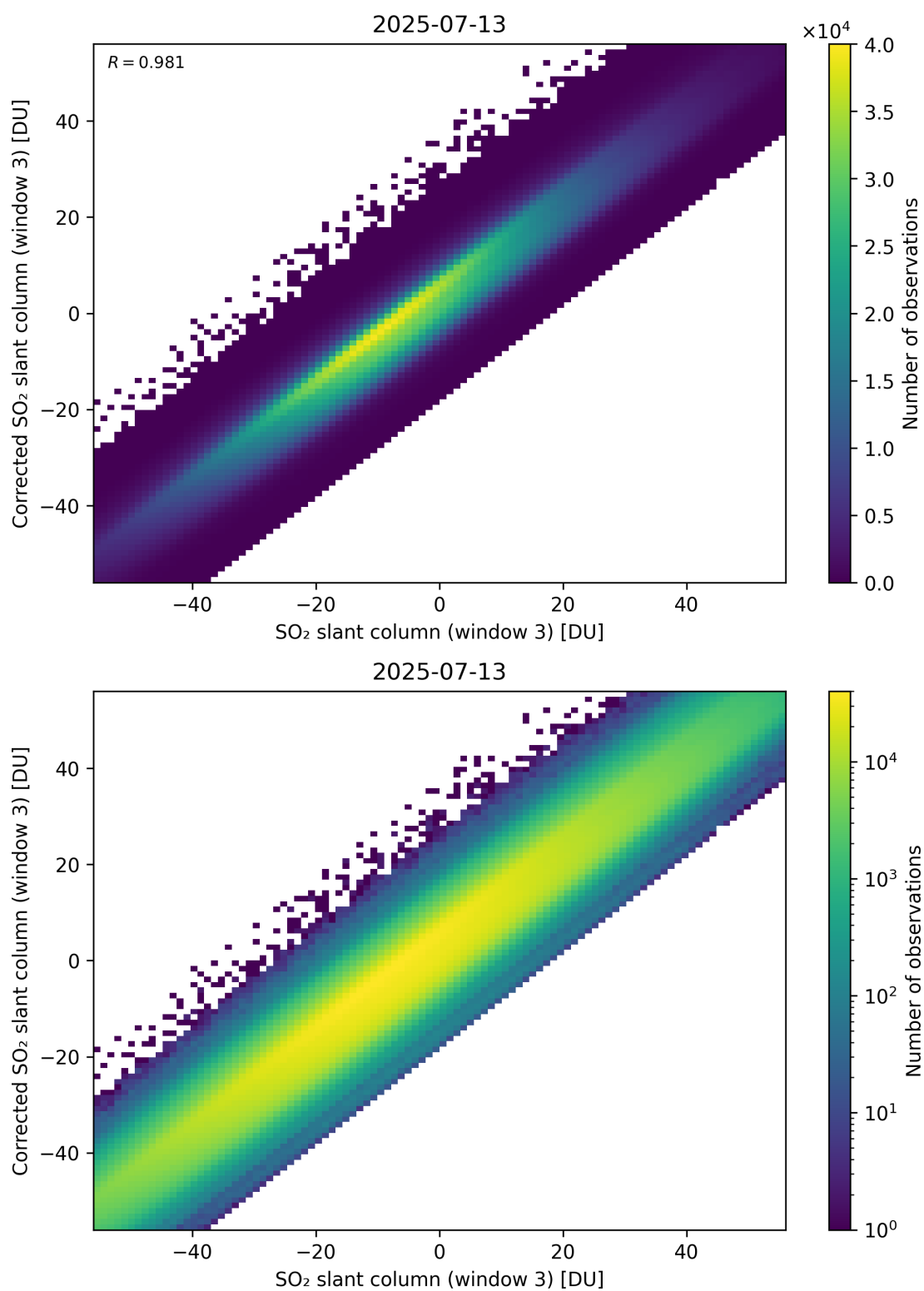
Figure 316: Scatter density plot of “SO 2 slant column (window 3)” against “Corrected SO 2 slant column (window 3)” for 2025-07-13 to 2025-07-14.
