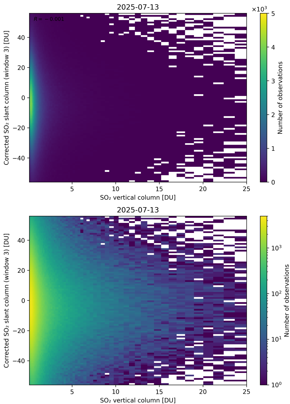
Figure 353: Scatter density plot of “SO 2 vertical column” against “Corrected SO 2 slant column (window 3)” for 2025-07-13 to 2025-07-14.
