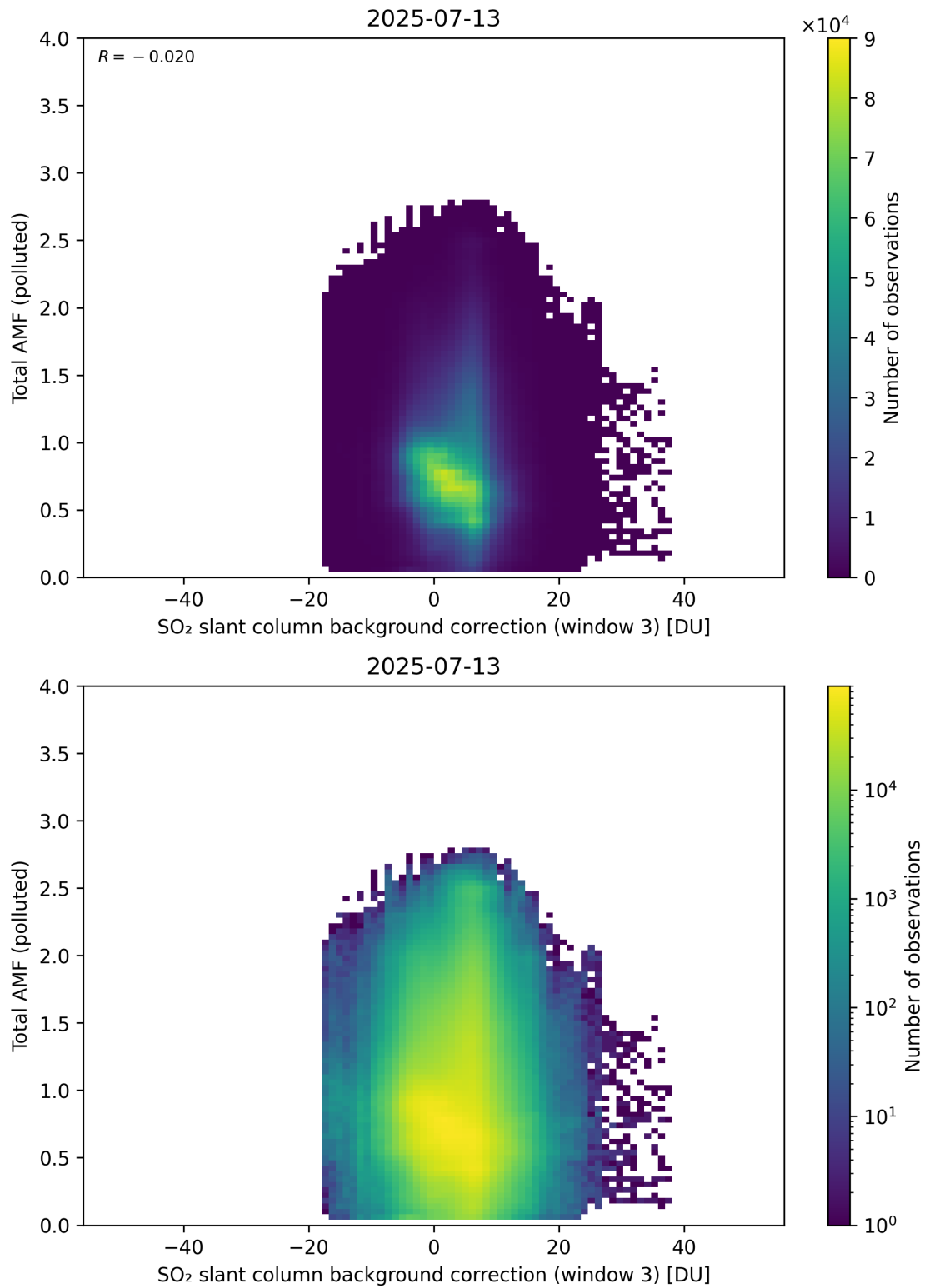
Figure 136: Scatter density plot of “SO 2 slant column background correction (window 3)” against “Total AMF (polluted)” for 2025-07-13 to 2025-07-14.
