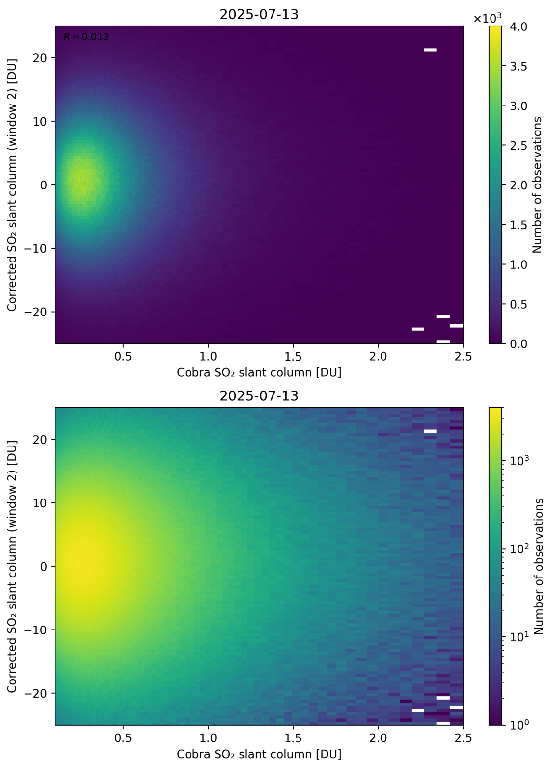
Figure 217: Scatter density plot of “Cobra SO 2 slant column” against “Corrected SO 2 slant column (window 2)” for 2025-07-13 to 2025-07-14.
