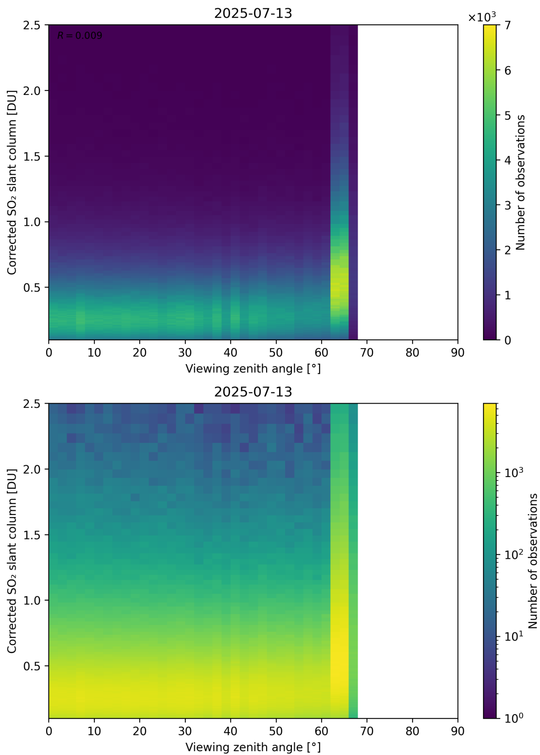
Figure 373: Scatter density plot of “Viewing zenith angle” against “Corrected SO 2 slant column” for 2025-07-13 to 2025-07-14.
