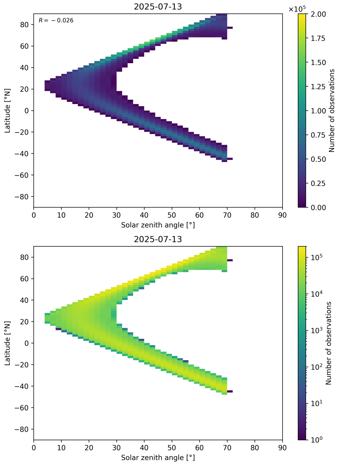
Figure 177: Scatter density plot of “Solar zenith angle” against “Latitude” for 2025-07-13 to 2025-07-14.
