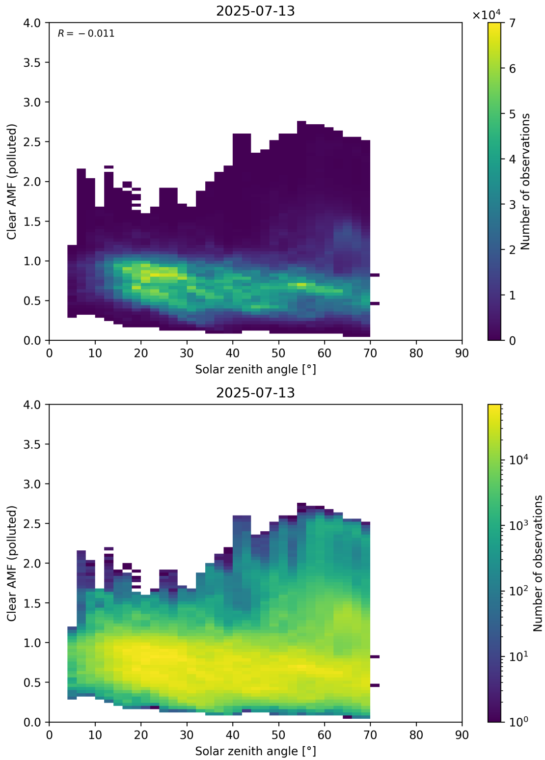
Figure 178: Scatter density plot of “Solar zenith angle” against “Clear AMF (polluted)” for 2025-07-13 to 2025-07-14.
