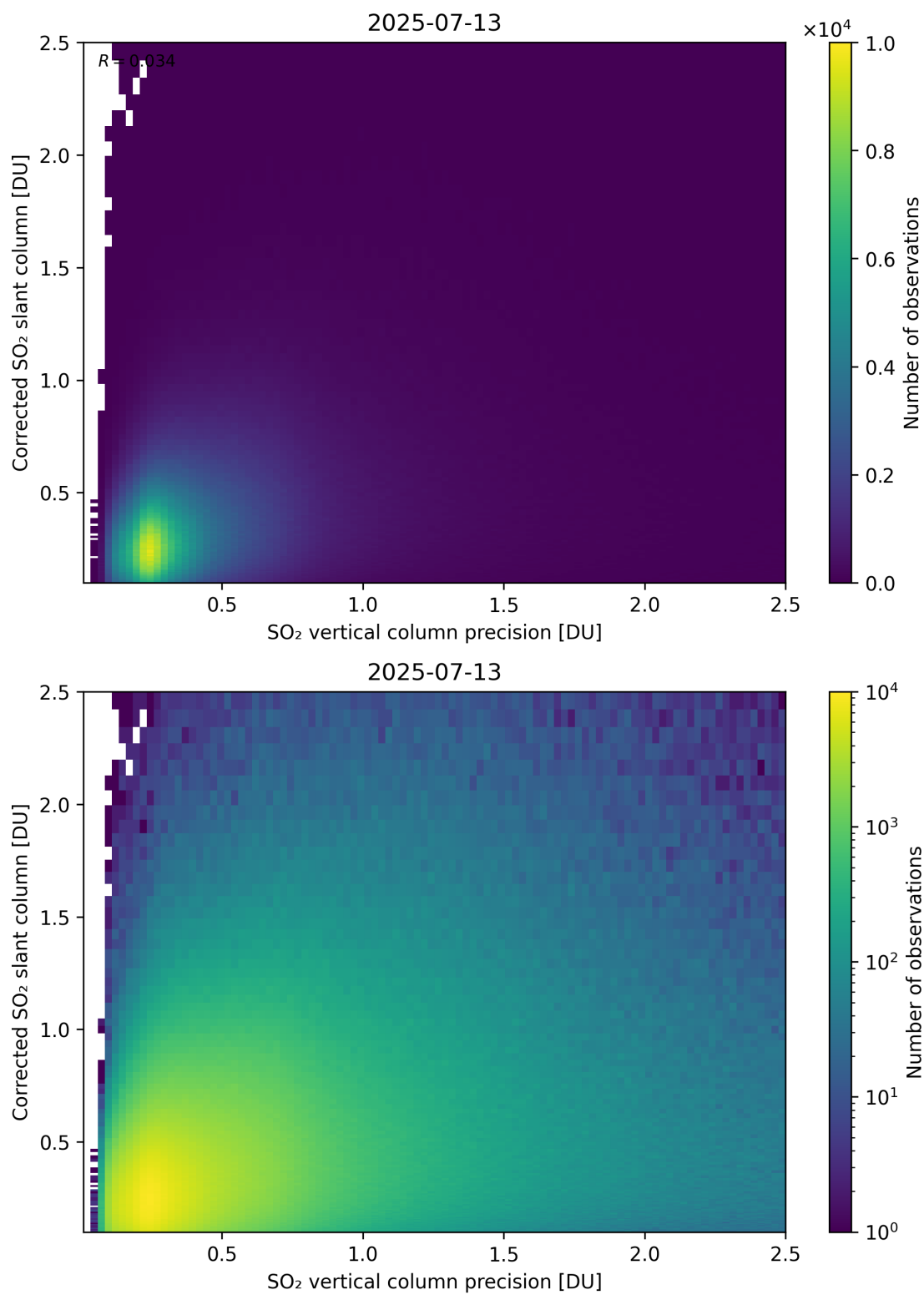
Figure 338: Scatter density plot of “SO 2 vertical column precision” against “Corrected SO 2 slant column” for 2025-07-13 to 2025-07-14.
