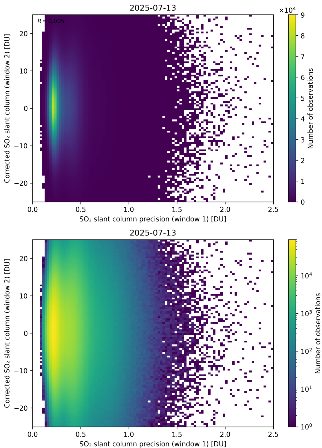
Figure 275: Scatter density plot of “SO 2 slant column precision (window 1)” against “Corrected SO 2 slant column (window 2)” for 2025-07-13 to 2025-07-14.
