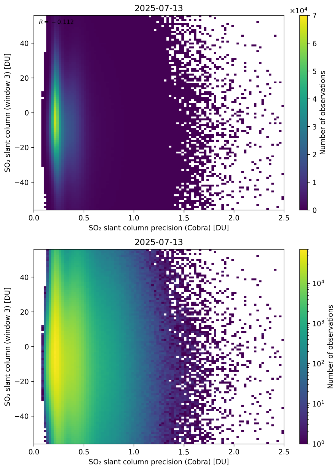
Figure 211: Scatter density plot of “SO 2 slant column precision (Cobra)” against “SO 2 slant column (window 3)” for 2025-07-13 to 2025-07-14.
