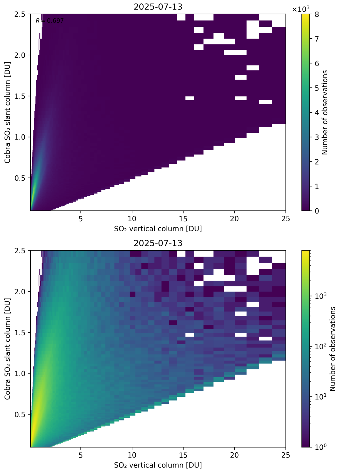
Figure 349: Scatter density plot of “SO 2 vertical column” against “Cobra SO 2 slant column” for 2025-07-13 to 2025-07-14.
