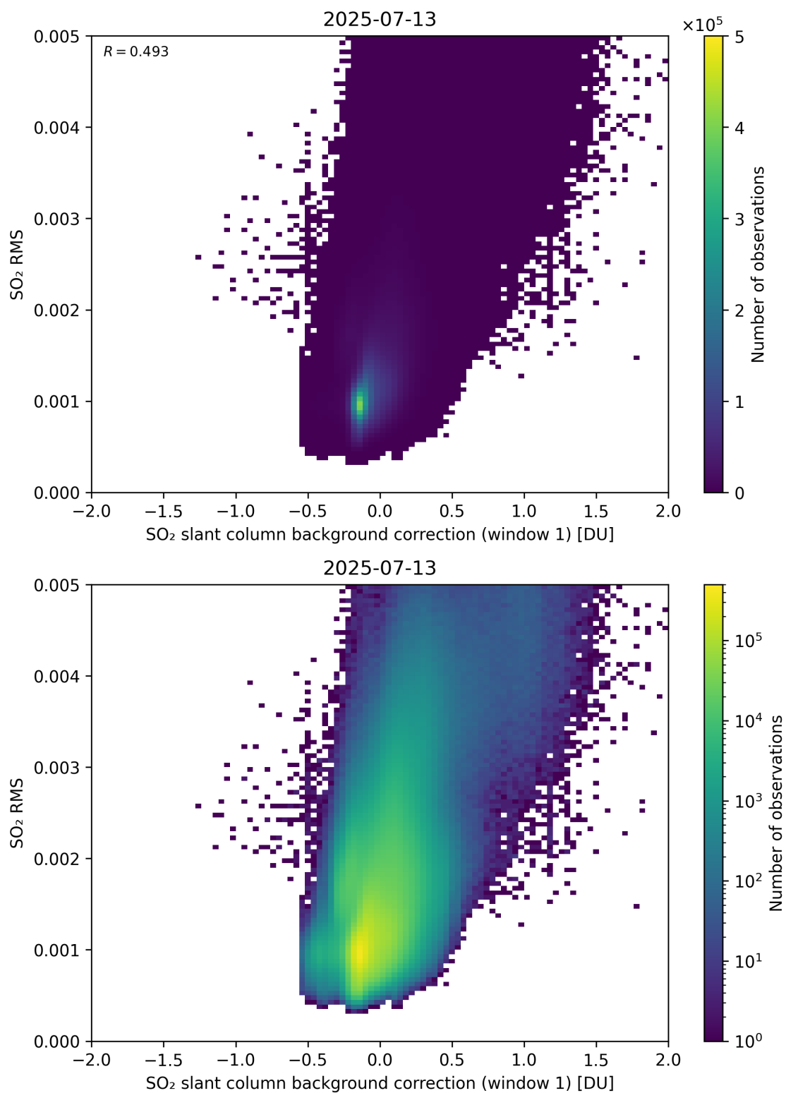
Figure 113: Scatter density plot of “SO 2 slant column background correction (window 1)” against “SO 2 RMS” for 2025-07-13 to 2025-07-14.
