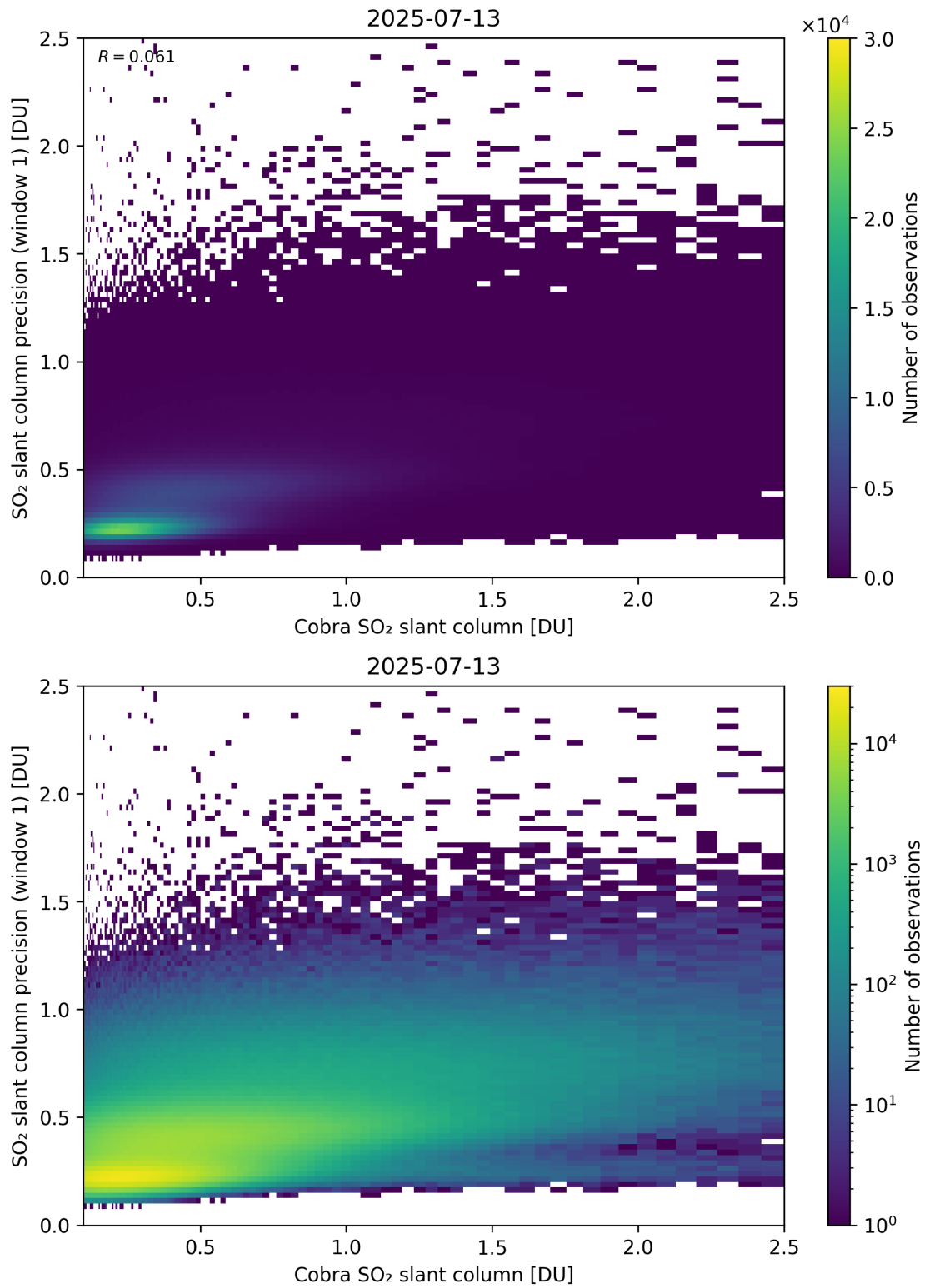
Figure 220: Scatter density plot of “Cobra SO 2 slant column” against “SO 2 slant column precision (window 1)” for 2025-07-13 to 2025-07-14.
