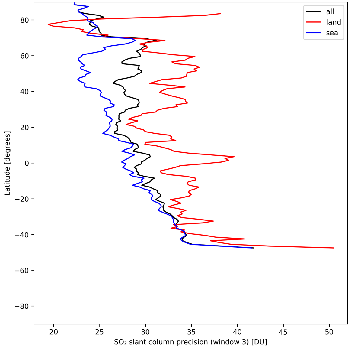
Figure 46: Zonal average of “SO 2 slant column precision (window 3)” for 2025-07-13 to 2025-07-14.
