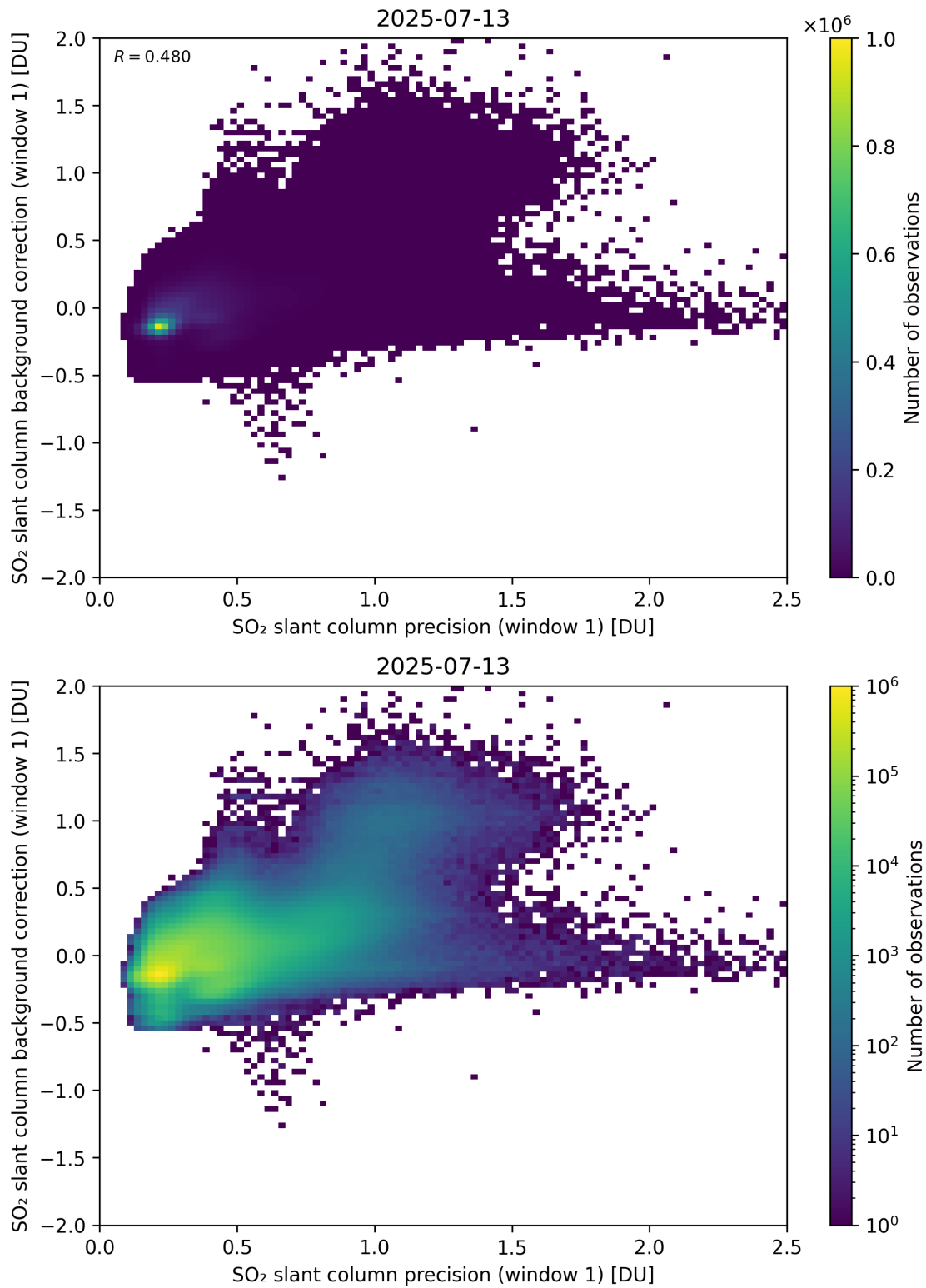
Figure 268: Scatter density plot of “SO 2 slant column precision (window 1)” against “SO 2 slant column background correction (window 1)” for 2025-07-13 to 2025-07-14.
