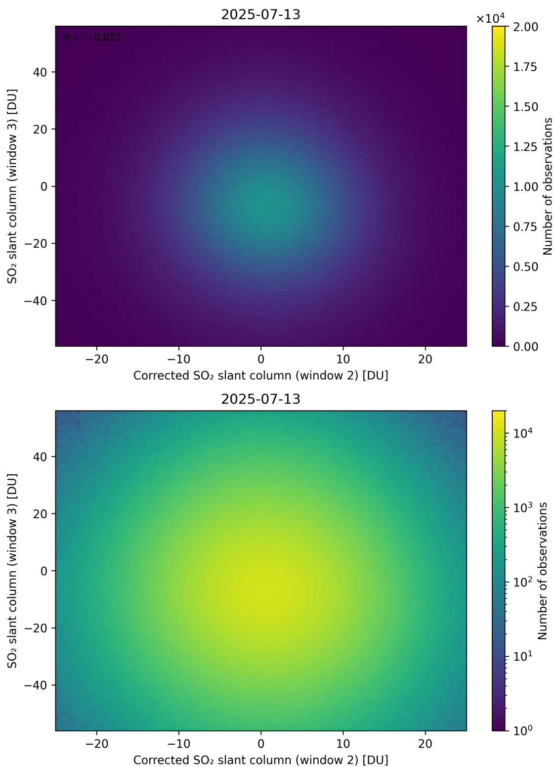
Figure 251: Scatter density plot of “Corrected SO 2 slant column (window 2)” against “SO 2 slant column (window 3)” for 2025-07-13 to 2025-07-14.
