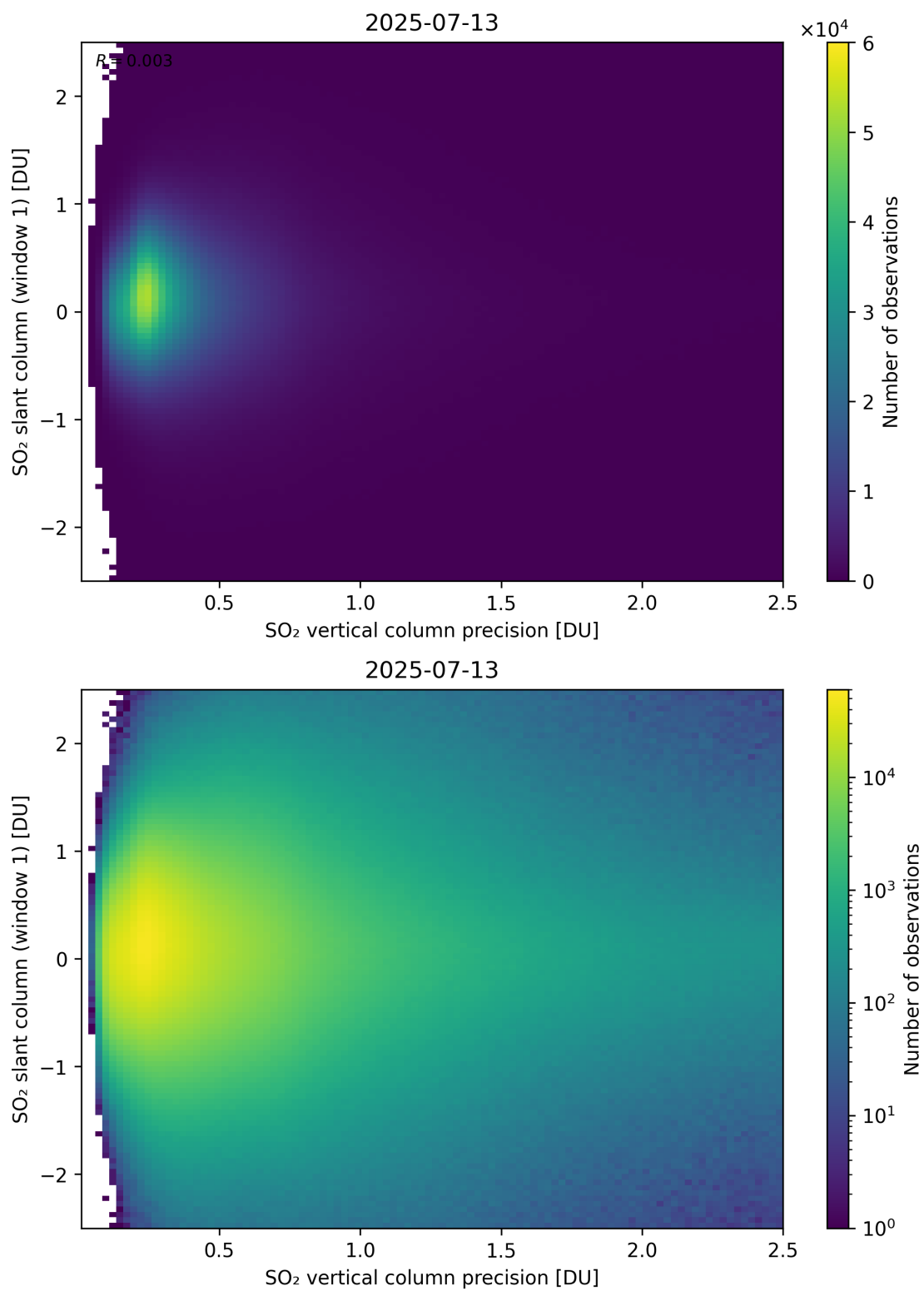
Figure 341: Scatter density plot of “SO 2 vertical column precision” against “SO 2 slant column (window 1)” for 2025-07-13 to 2025-07-14.
