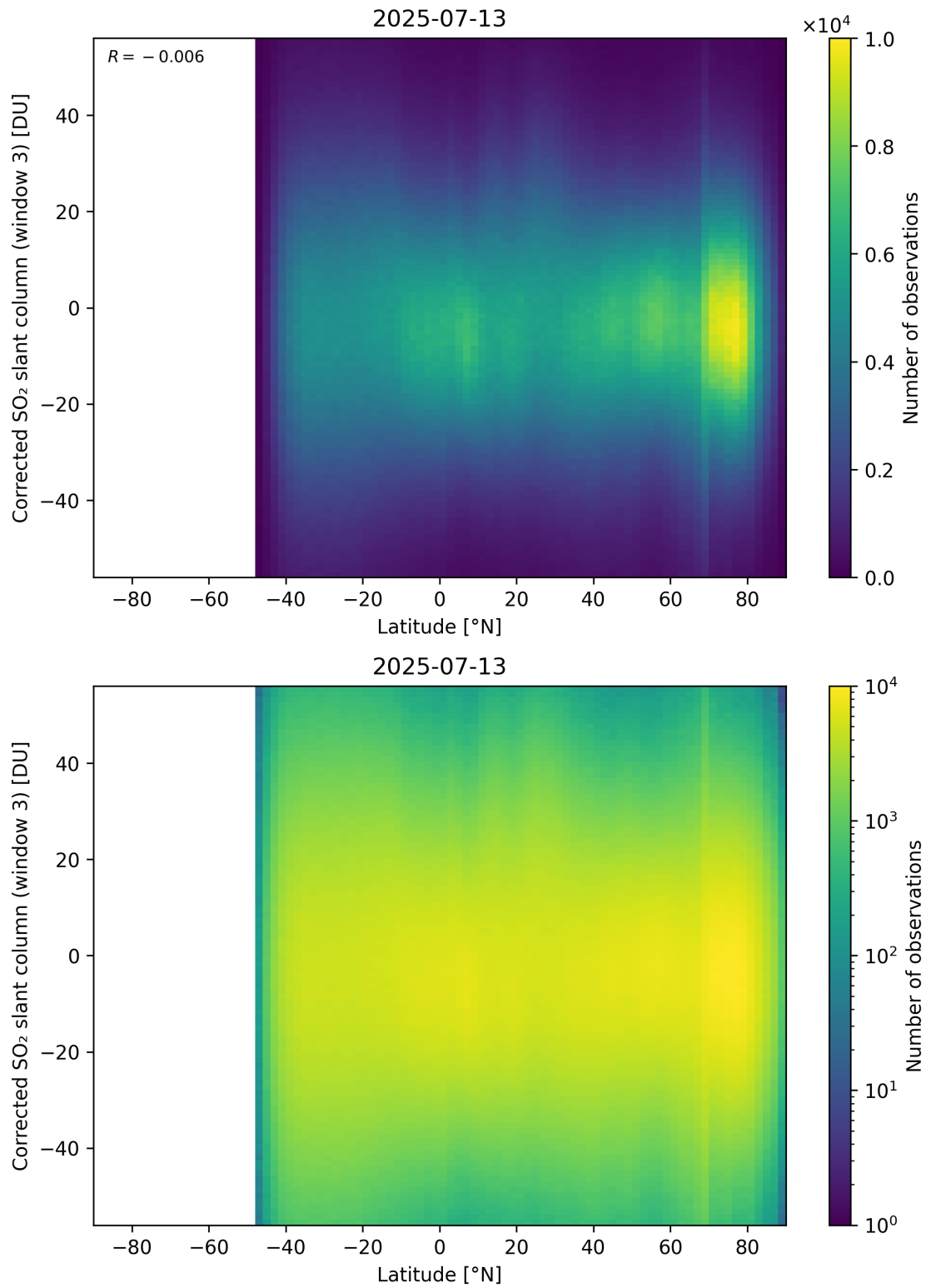
Figure 161: Scatter density plot of “Latitude” against “Corrected SO 2 slant column (window 3)” for 2025-07-13 to 2025-07-14.
