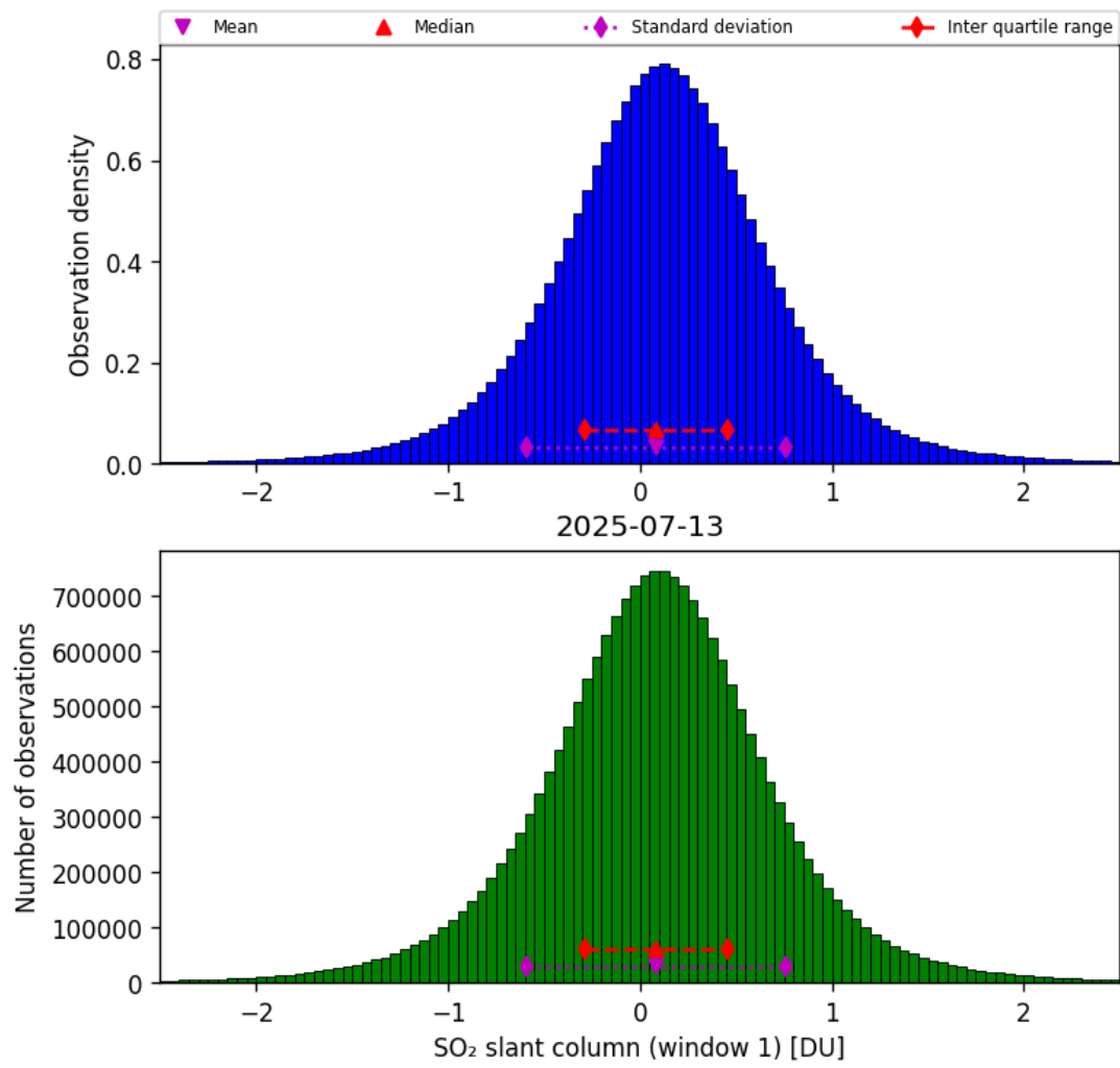
Figure 63: Histogram of “SO 2 slant column (window 1)” for 2025-07-13 to 2025-07-14
