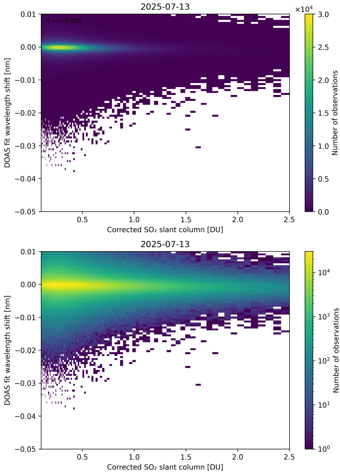
Figure 229: Scatter density plot of “Corrected SO 2 slant column” against “DOAS fit wavelength shift” for 2025-07-13 to 2025-07-14.
