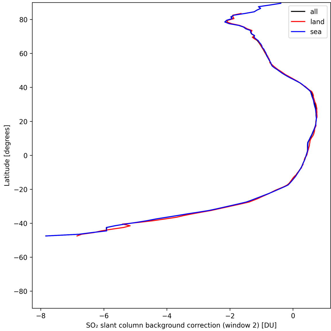
Figure 44: Zonal average of “SO 2 slant column background correction (window 2)” for 2025-07-13 to 2025-07-14.
