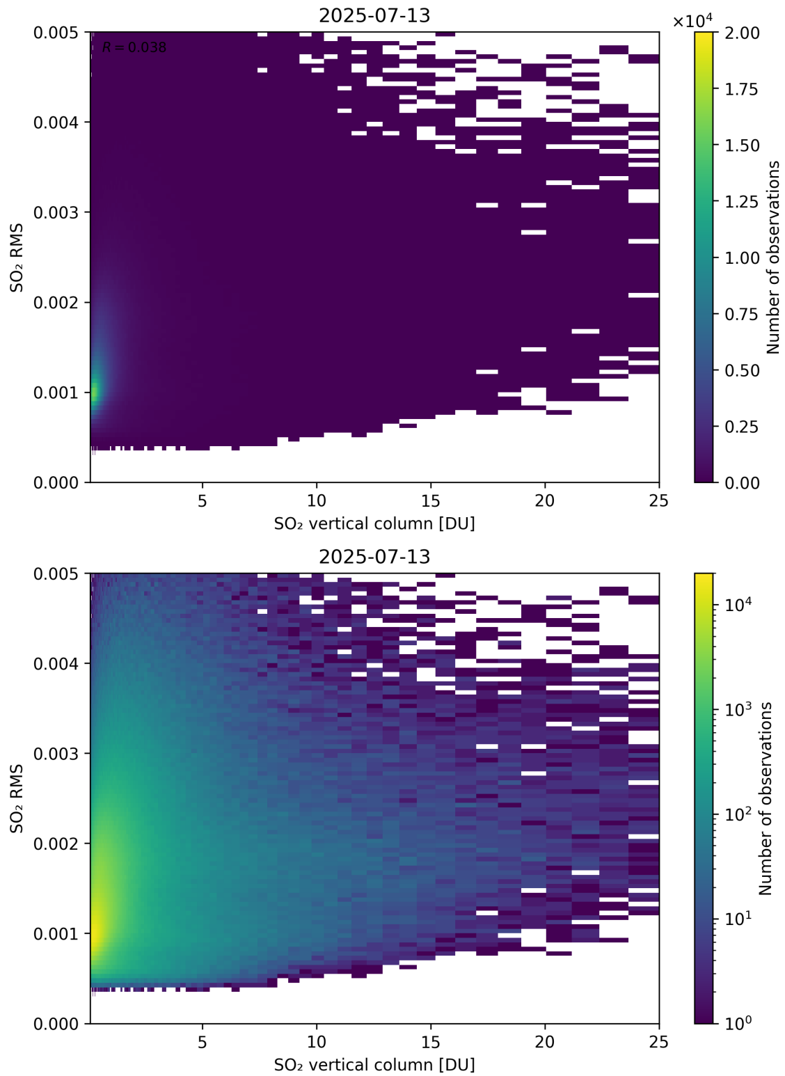
Figure 328: Scatter density plot of “SO 2 vertical column” against “SO 2 RMS” for 2025-07-13 to 2025-07-14.
