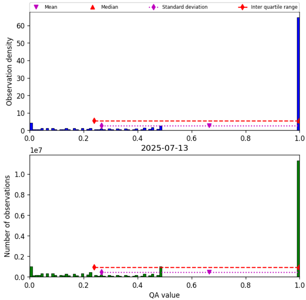
Figure 57: Histogram of “QA value” for 2025-07-13 to 2025-07-14
