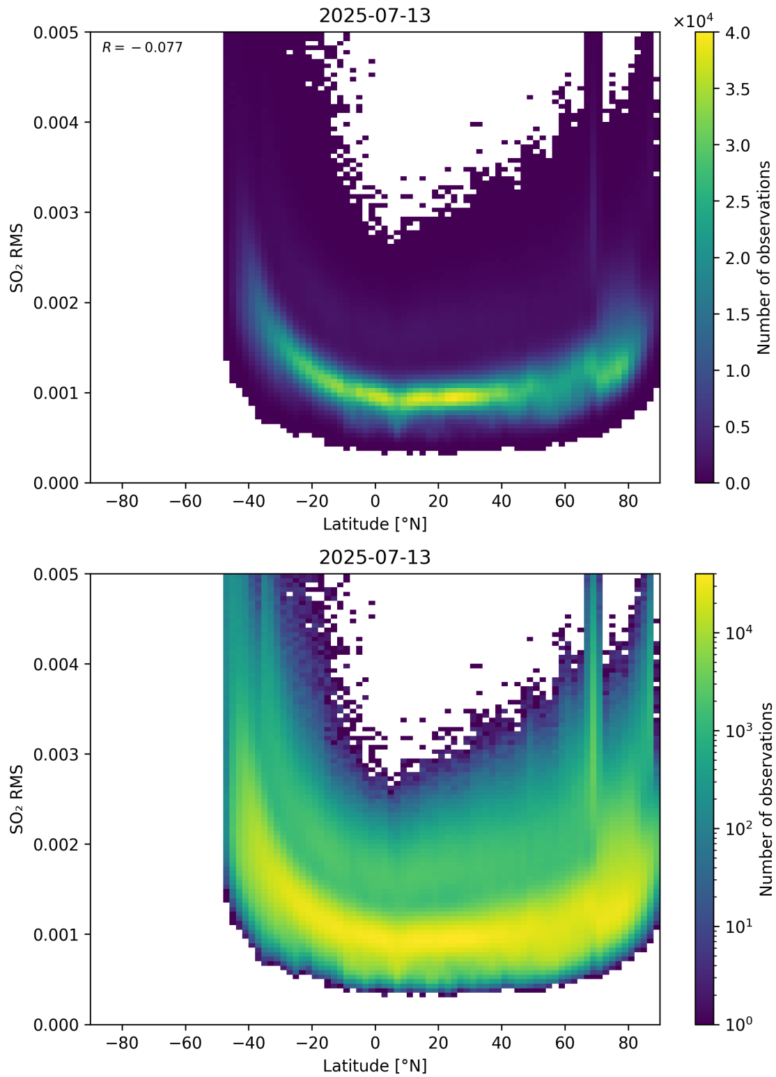
Figure 155: Scatter density plot of “Latitude” against “SO 2 RMS” for 2025-07-13 to 2025-07-14.
