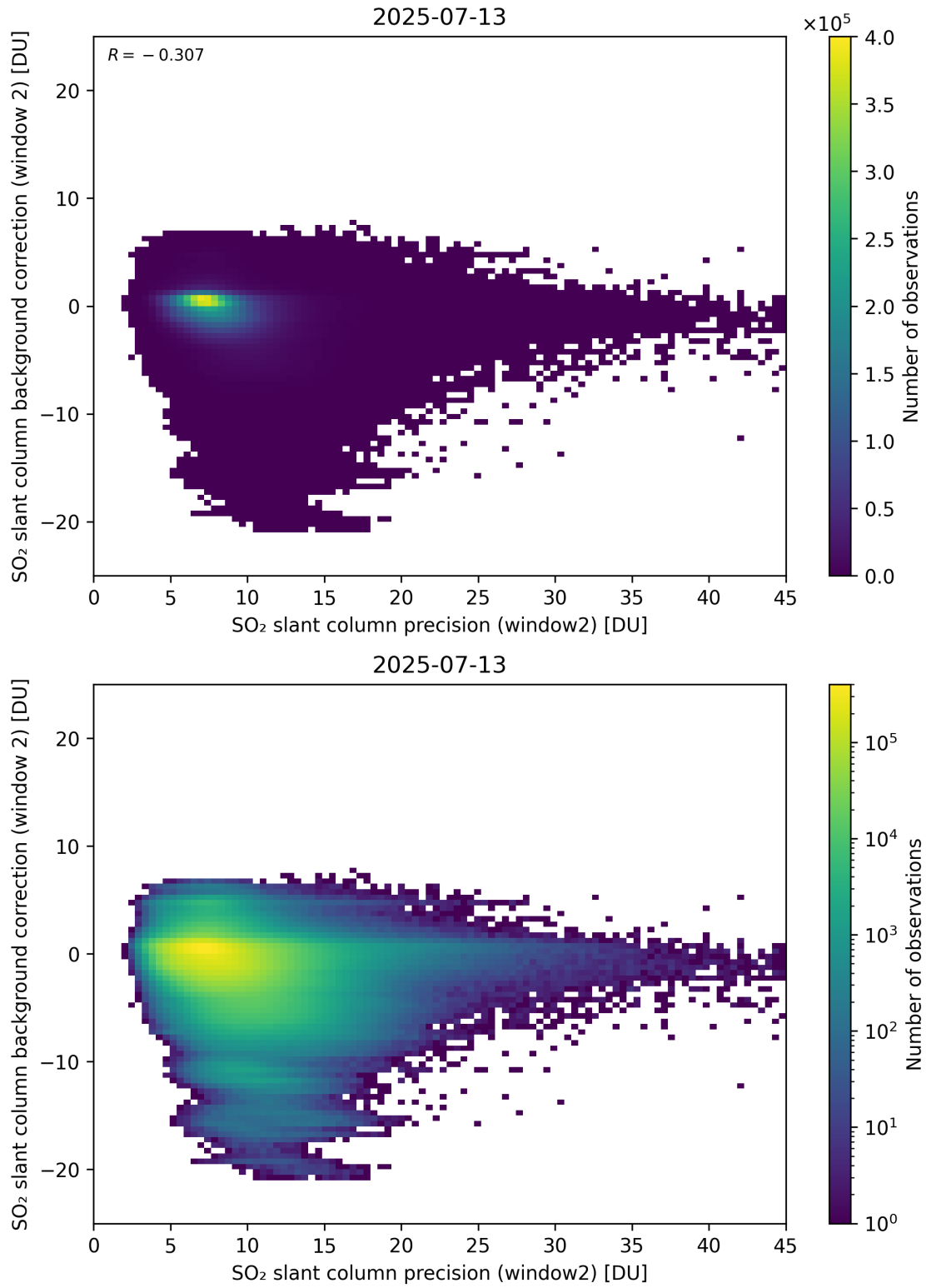
Figure 291: Scatter density plot of “SO 2 slant column precision (window2)” against “SO 2 slant column background correction (window 2)” for 2025-07-13 to 2025-07-14.
