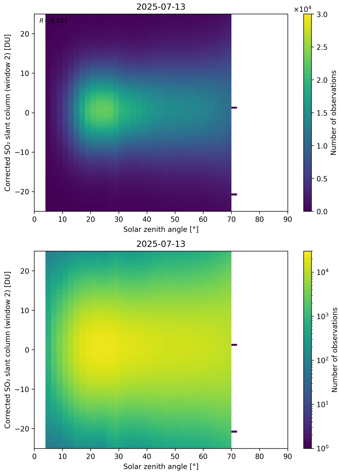
Figure 182: Scatter density plot of “Solar zenith angle” against “Corrected SO 2 slant column (window 2)” for 2025-07-13 to 2025-07-14.
