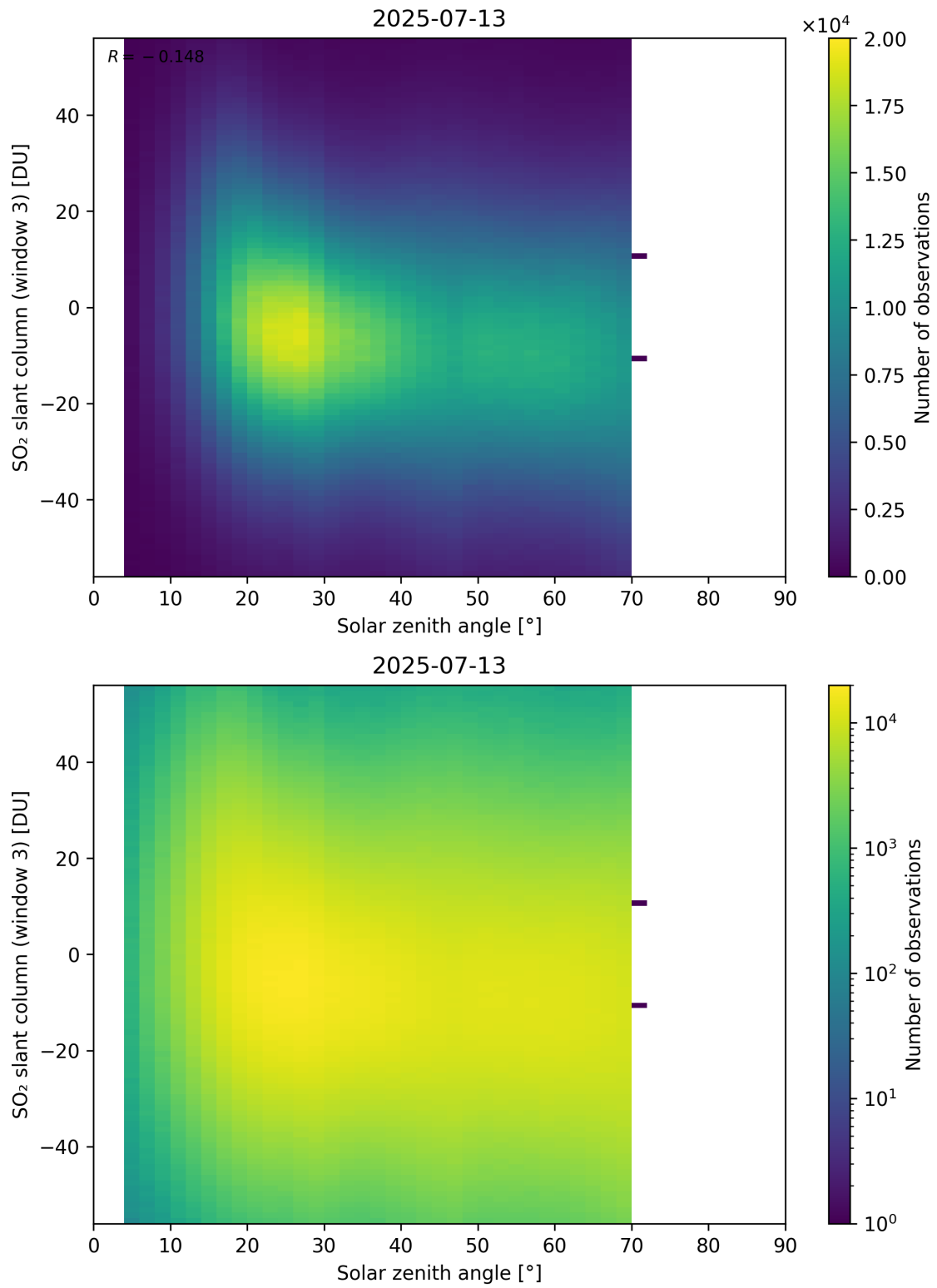
Figure 187: Scatter density plot of “Solar zenith angle” against “SO 2 slant column (window 3)” for 2025-07-13 to 2025-07-14.
