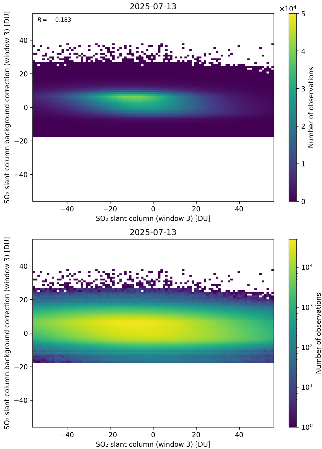
Figure 303: Scatter density plot of “SO 2 slant column (window 3)” against “SO 2 slant column background correction (window 3)” for 2025-07-13 to 2025-07-14.
