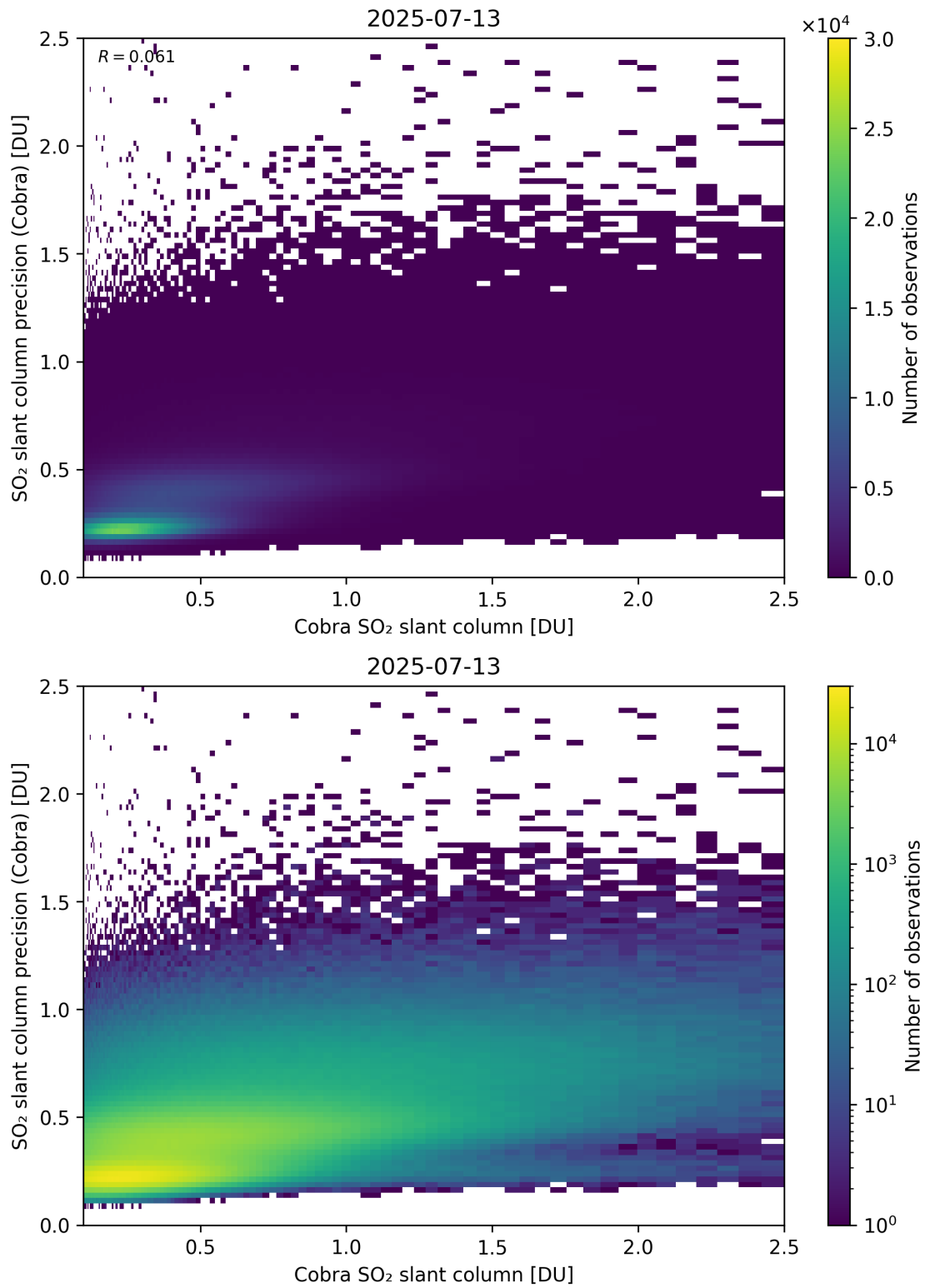
Figure 216: Scatter density plot of “Cobra SO 2 slant column” against “SO 2 slant column precision (Cobra)” for 2025-07-13 to 2025-07-14.
