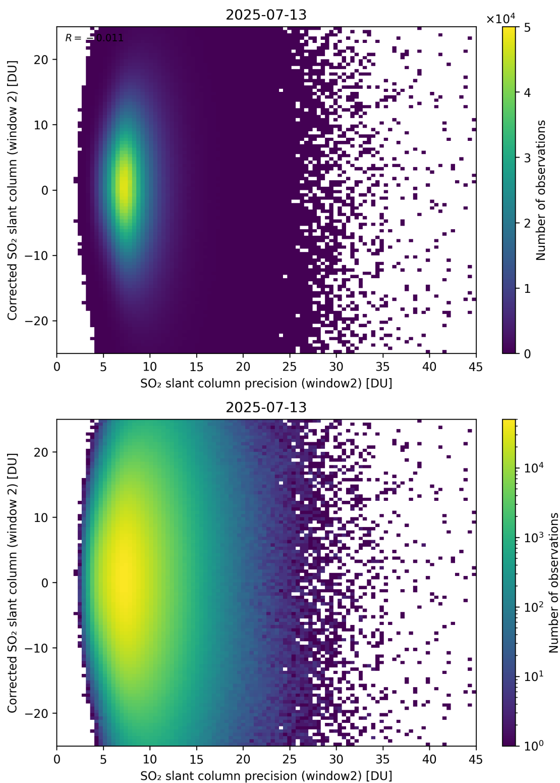
Figure 297: Scatter density plot of “SO 2 slant column precision (window2)” against “Corrected SO 2 slant column (window 2)” for 2025-07-13 to 2025-07-14.
