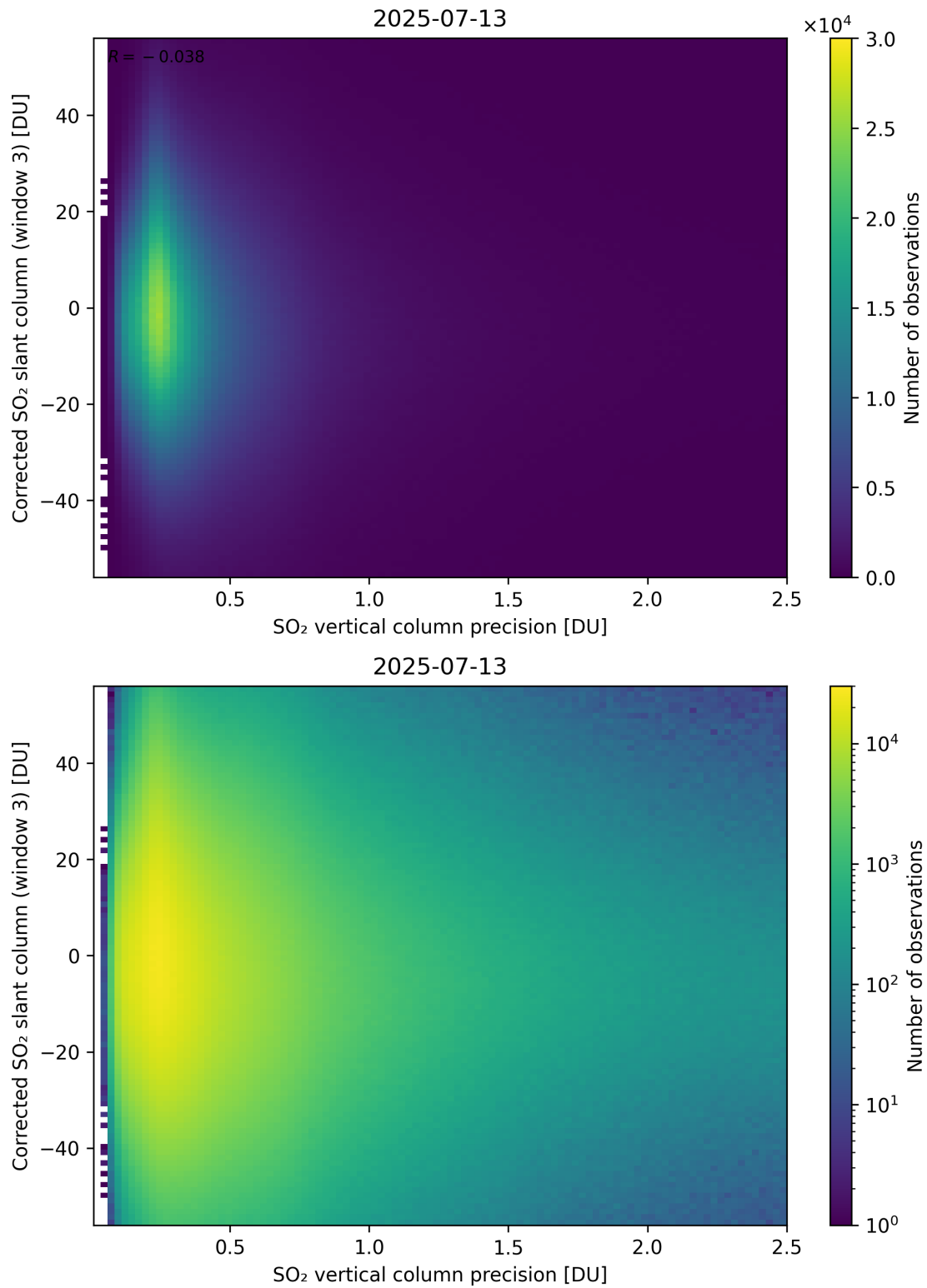
Figure 340: Scatter density plot of “SO 2 vertical column precision” against “Corrected SO 2 slant column (window 3)” for 2025-07-13 to 2025-07-14.
