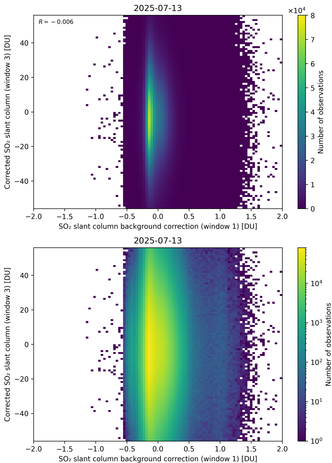
Figure 116: Scatter density plot of “SO 2 slant column background correction (window 1)” against “Corrected SO 2 slant column (window 3)” for 2025-07-13 to 2025-07-14.
