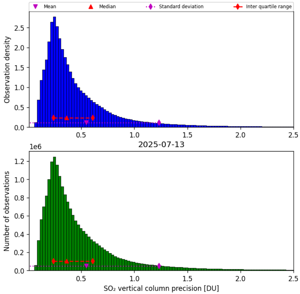
Figure 59: Histogram of “SO 2 vertical column precision” for 2025-07-13 to 2025-07-14
