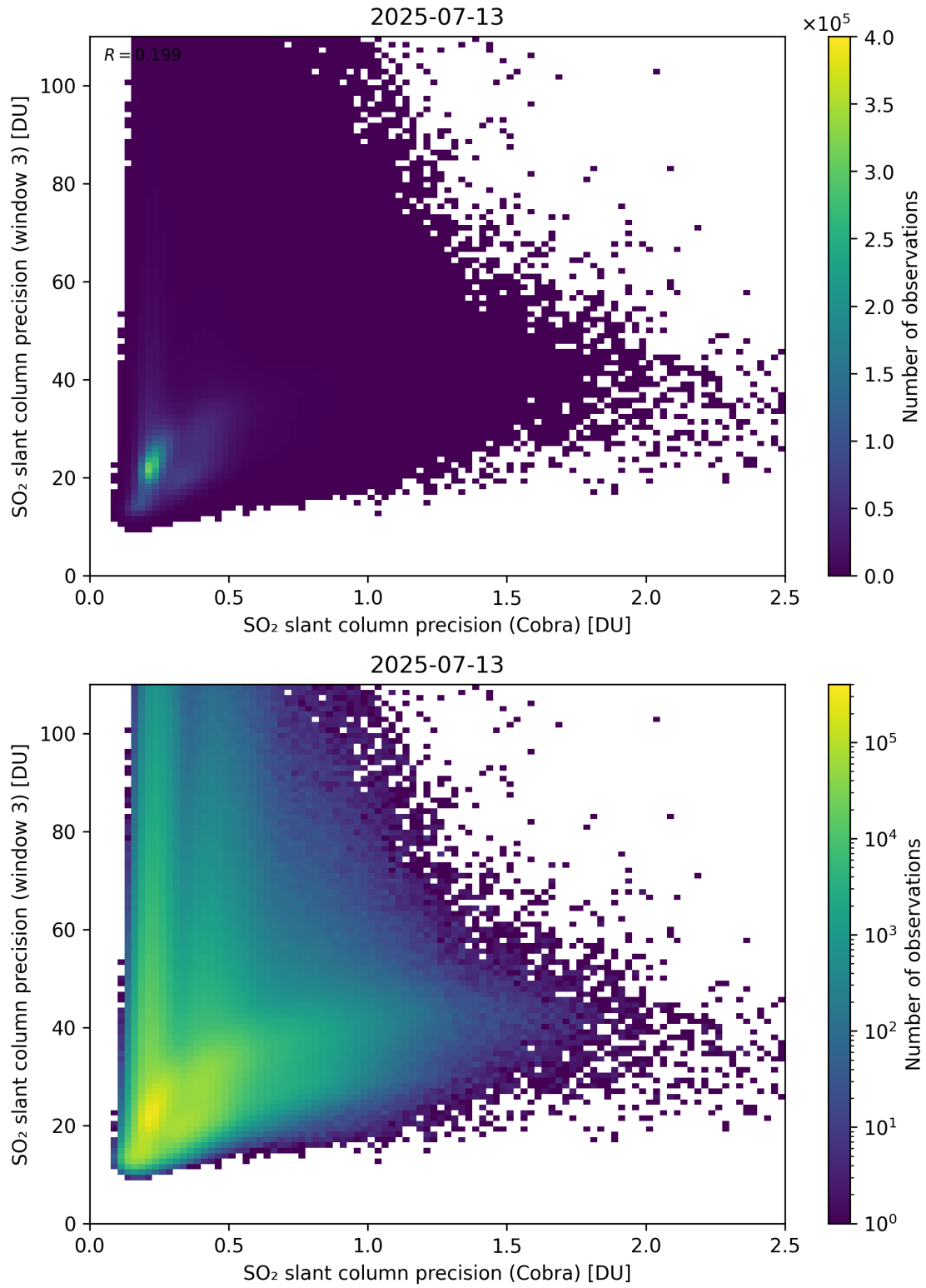
Figure 212: Scatter density plot of “SO 2 slant column precision (Cobra)” against “SO 2 slant column precision (window 3)” for 2025-07-13 to 2025-07-14.
