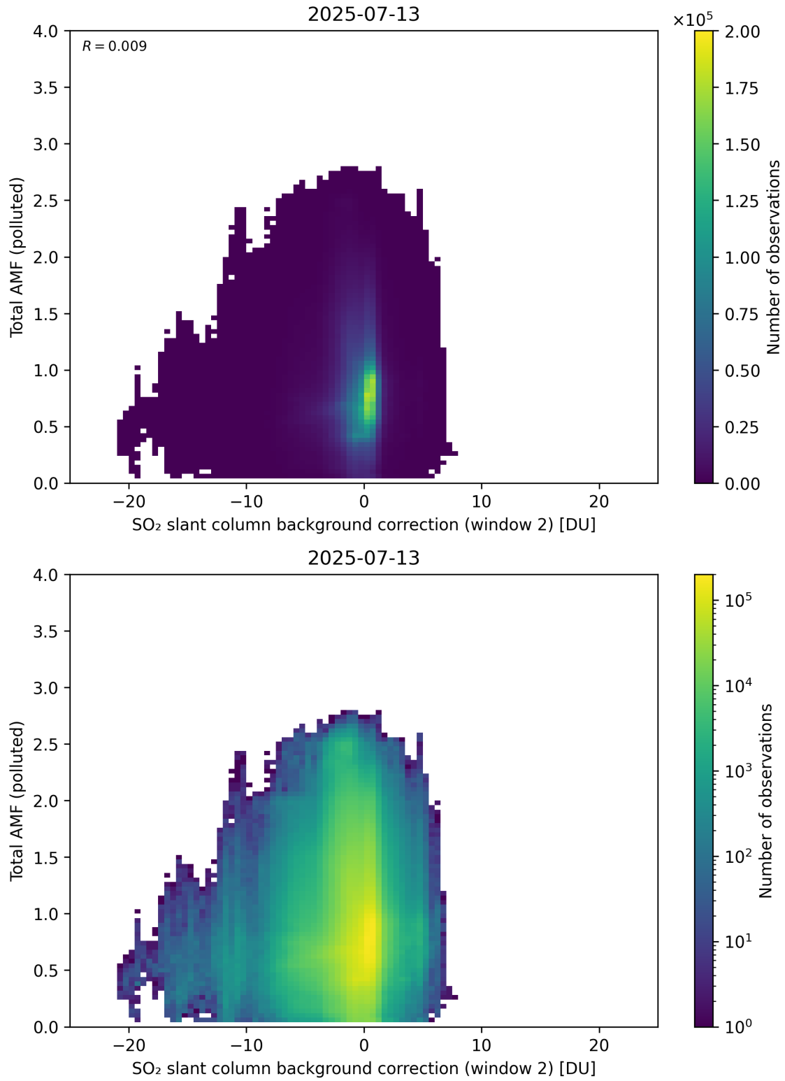
Figure 130: Scatter density plot of “SO 2 slant column background correction (window 2)” against “Total AMF (polluted)” for 2025-07-13 to 2025-07-14.
