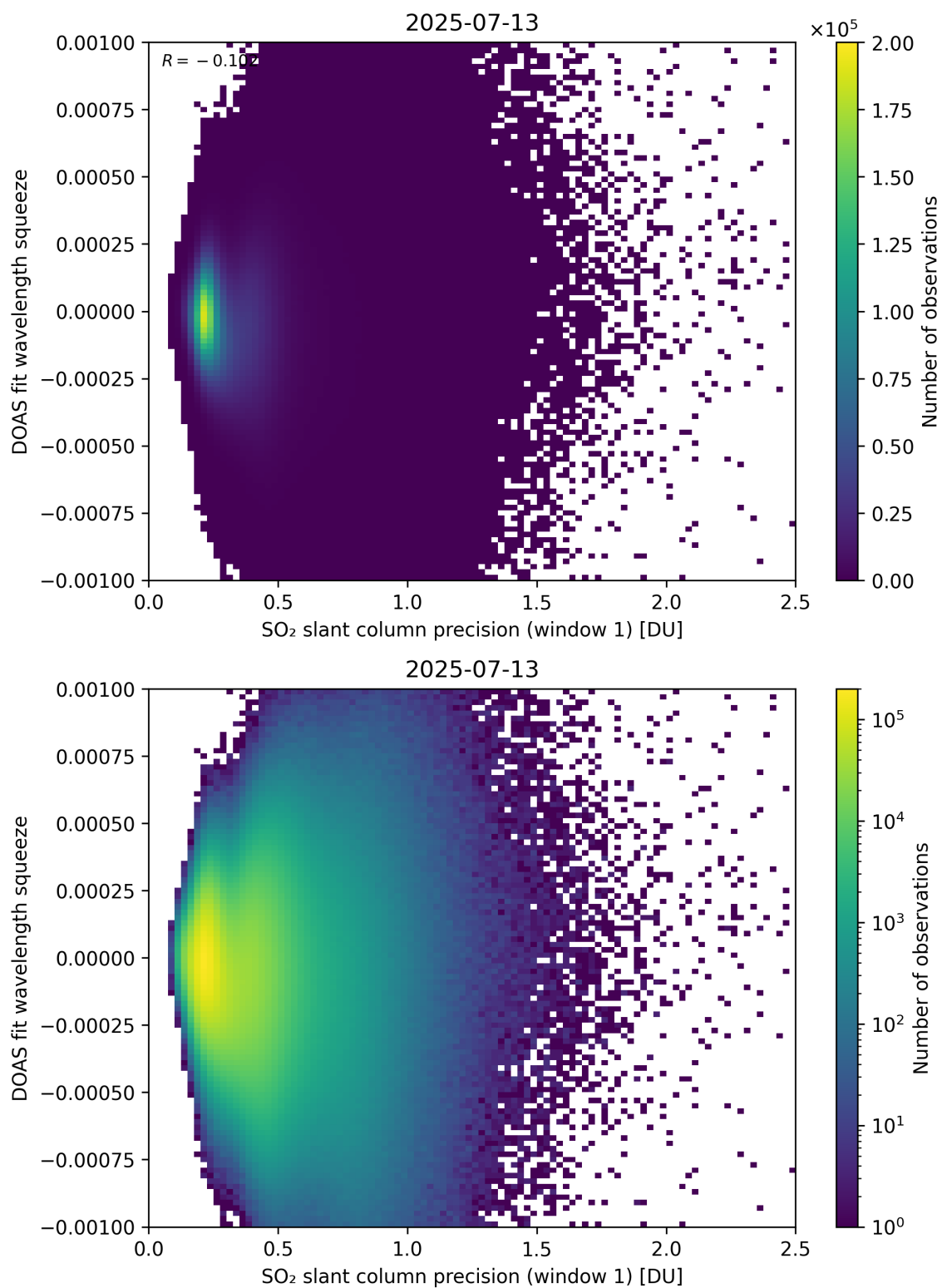
Figure 272: Scatter density plot of “SO 2 slant column precision (window 1)” against “DOAS fit wavelength squeeze” for 2025-07-13 to 2025-07-14.
