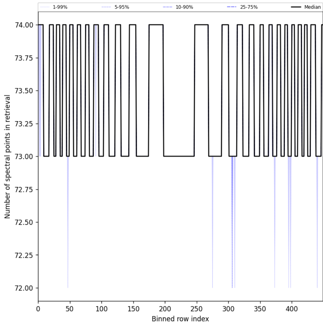
Figure 108: Along track statistics of “Number of spectral points in retrieval” for 2025-07-13 to 2025-07-14
