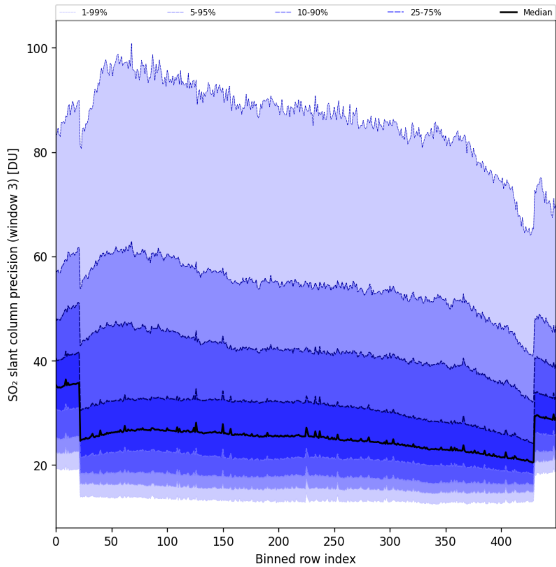
Figure 98: Along track statistics of “SO 2 slant column precision (window 3)” for 2025-07-13 to 2025-07-14
