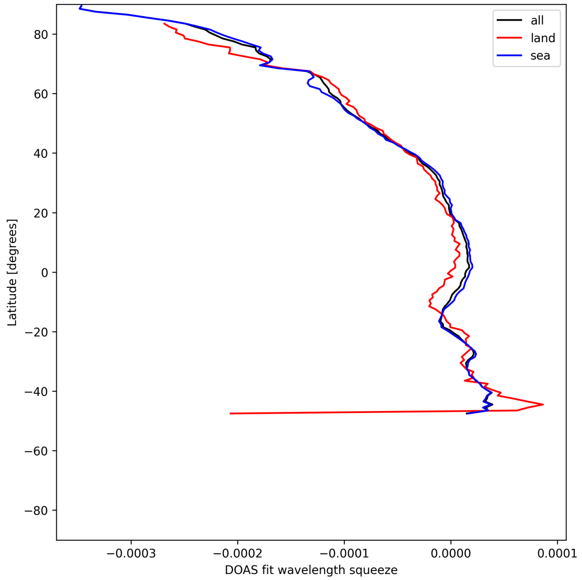
Figure 51: Zonal average of “DOAS fit wavelength squeeze” for 2025-07-13 to 2025-07-14.
