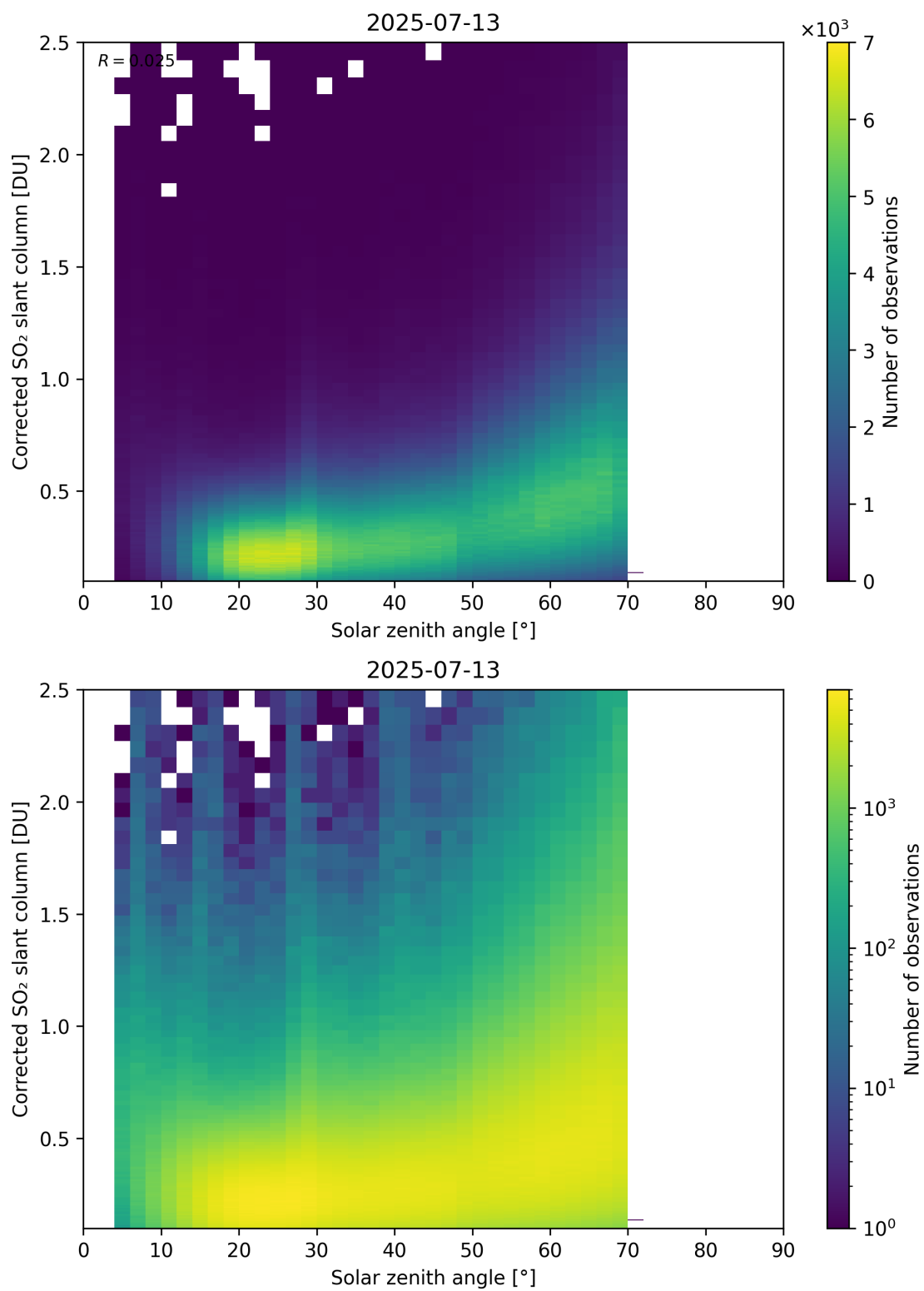
Figure 181: Scatter density plot of “Solar zenith angle” against “Corrected SO 2 slant column” for 2025-07-13 to 2025-07-14.
