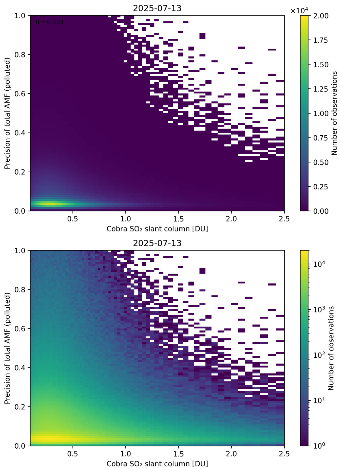
Figure 225: Scatter density plot of “Cobra SO 2 slant column” against “Precision of total AMF (polluted)” for 2025-07-13 to 2025-07-14.
