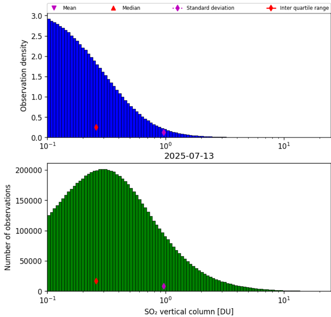
Figure 58: Histogram of “SO 2 vertical column” for 2025-07-13 to 2025-07-14
