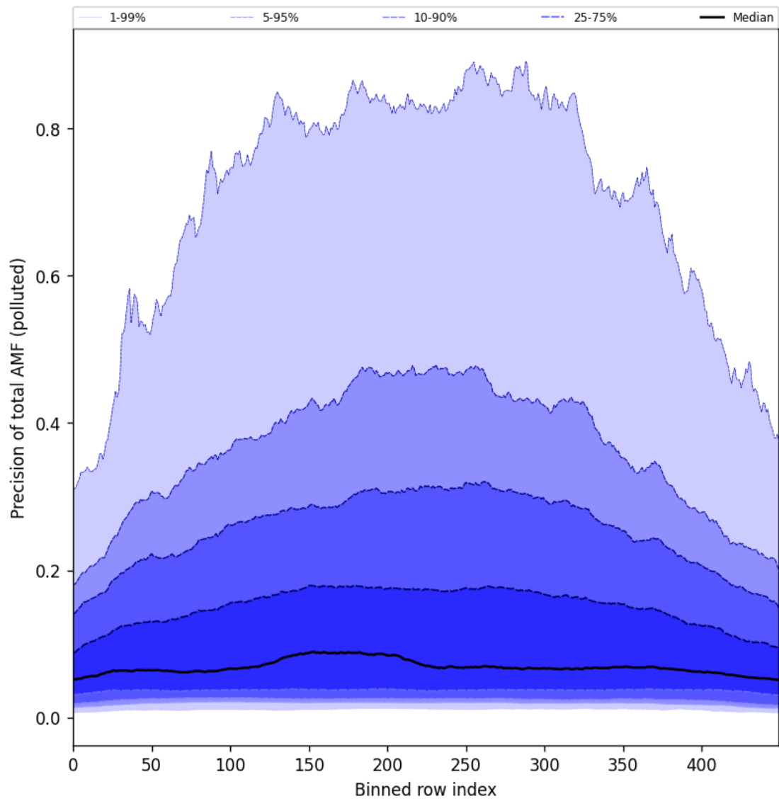
Figure 106: Along track statistics of “Precision of total AMF (polluted)” for 2025-07-13 to 2025-07-14
