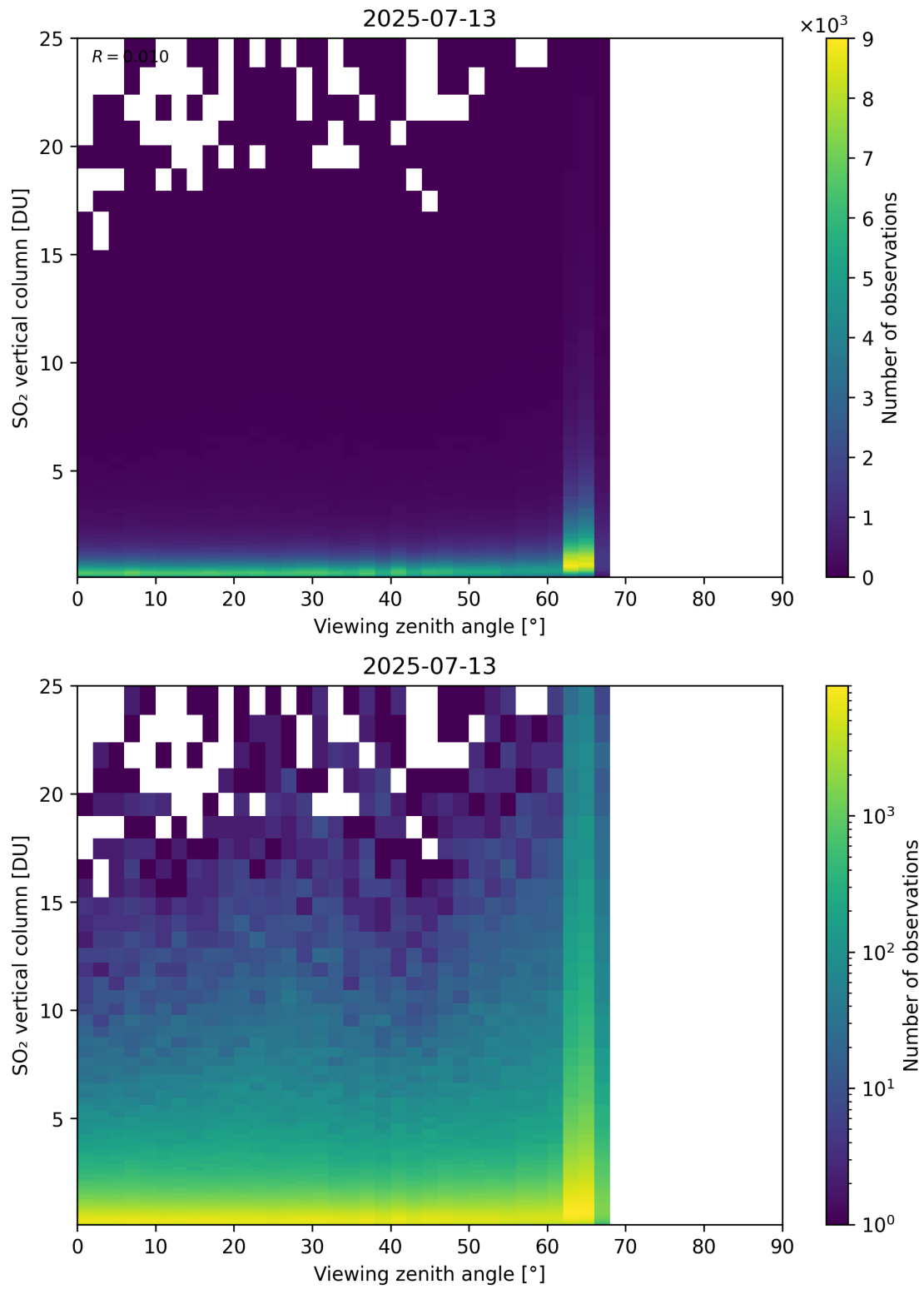
Figure 383: Scatter density plot of “Viewing zenith angle” against “SO 2 vertical column” for 2025-07-13 to 2025-07-14.
