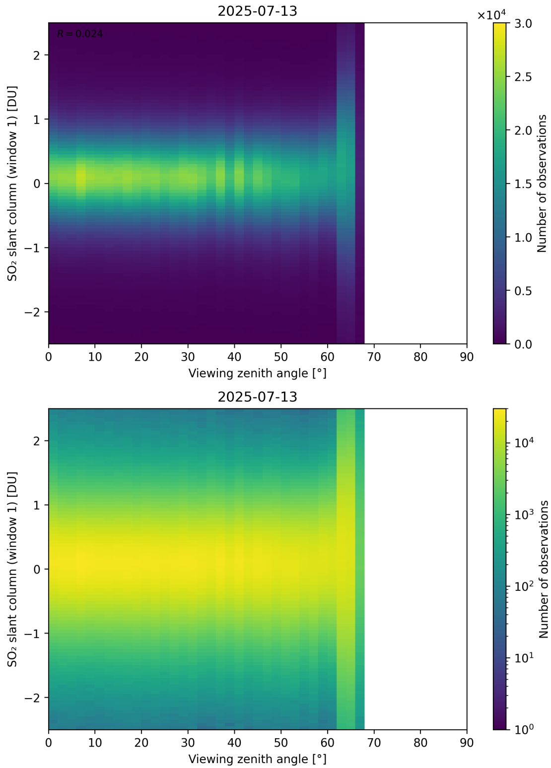
Figure 376: Scatter density plot of “Viewing zenith angle” against “SO 2 slant column (window 1)” for 2025-07-13 to 2025-07-14.
