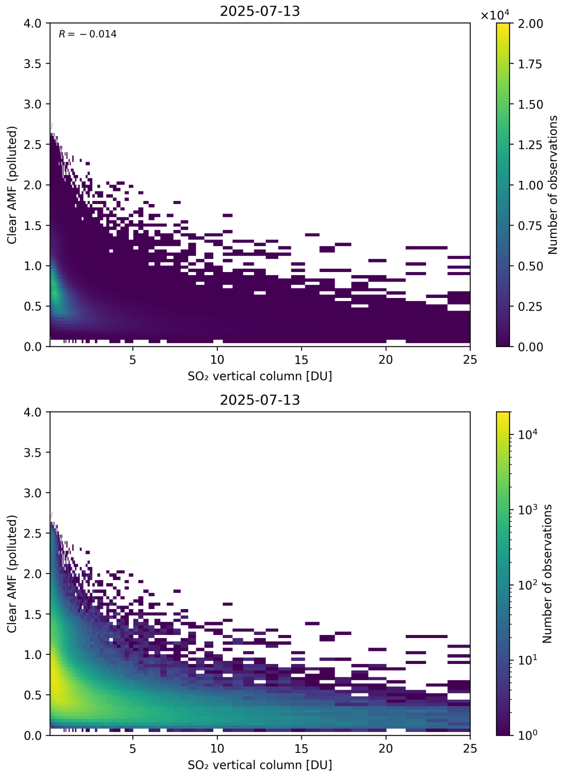
Figure 348: Scatter density plot of “SO 2 vertical column” against “Clear AMF (polluted)” for 2025-07-13 to 2025-07-14.
