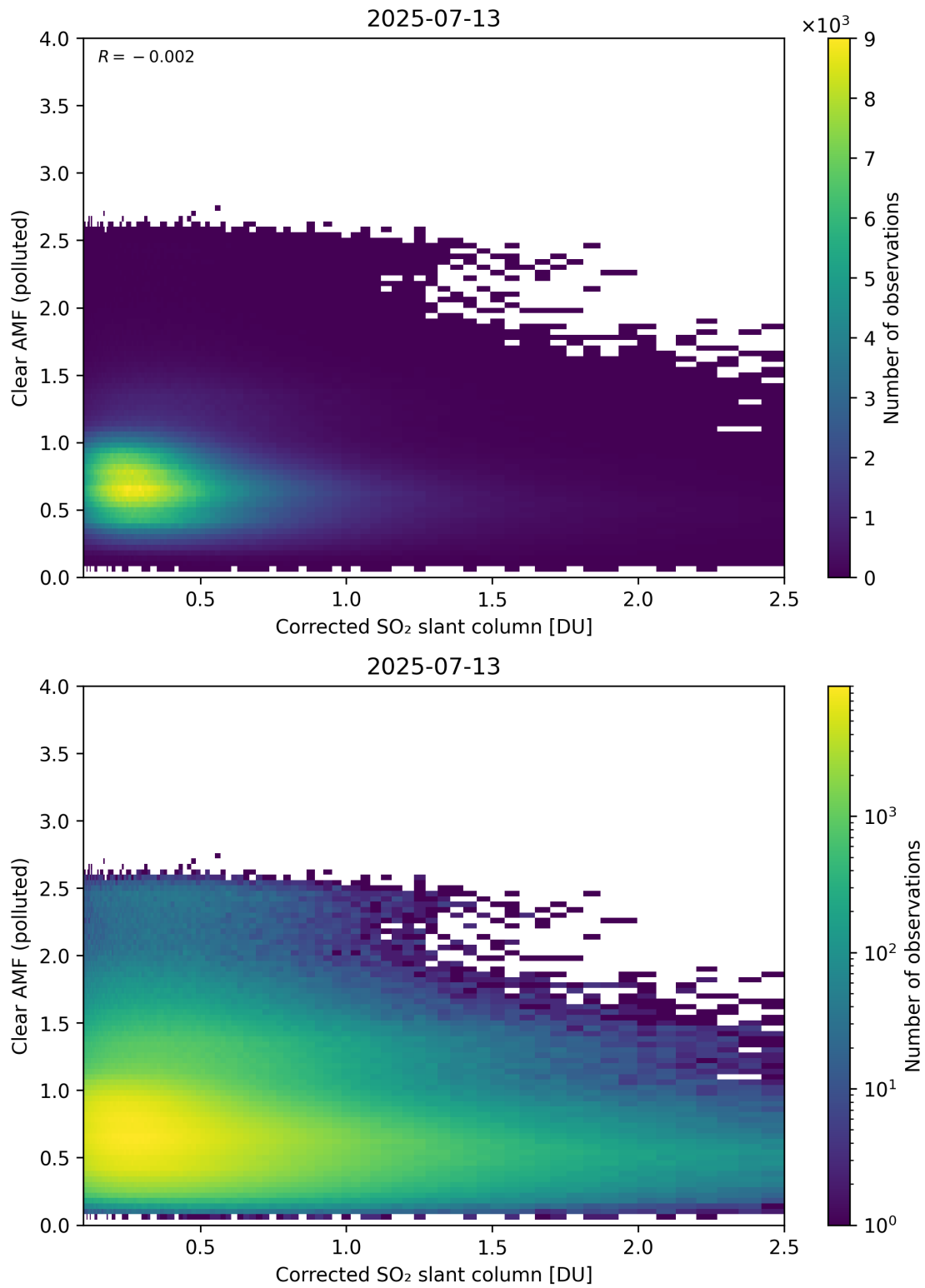
Figure 232: Scatter density plot of “Corrected SO 2 slant column” against “Clear AMF (polluted)” for 2025-07-13 to 2025-07-14.
