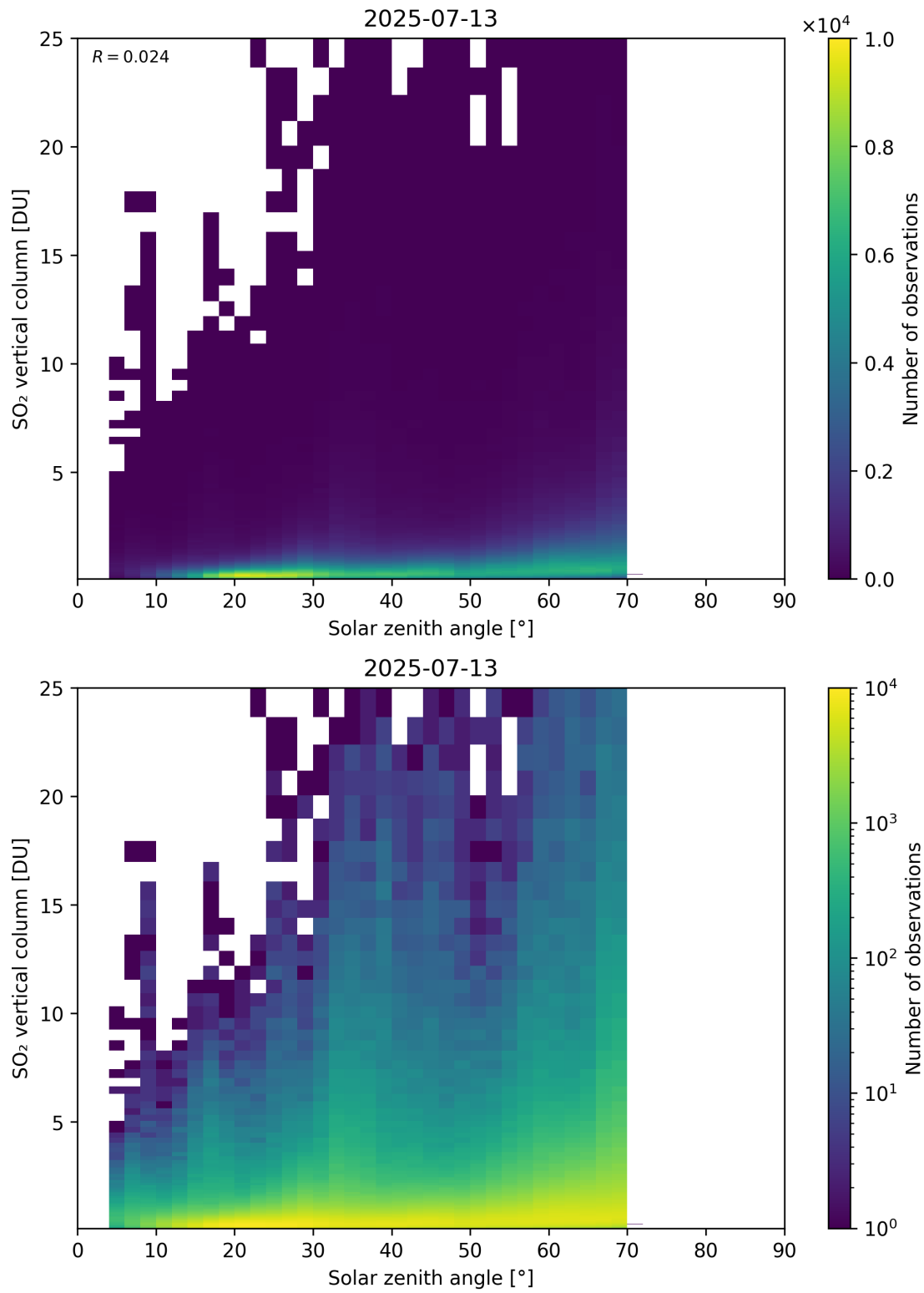
Figure 191: Scatter density plot of “Solar zenith angle” against “SO 2 vertical column” for 2025-07-13 to 2025-07-14.
