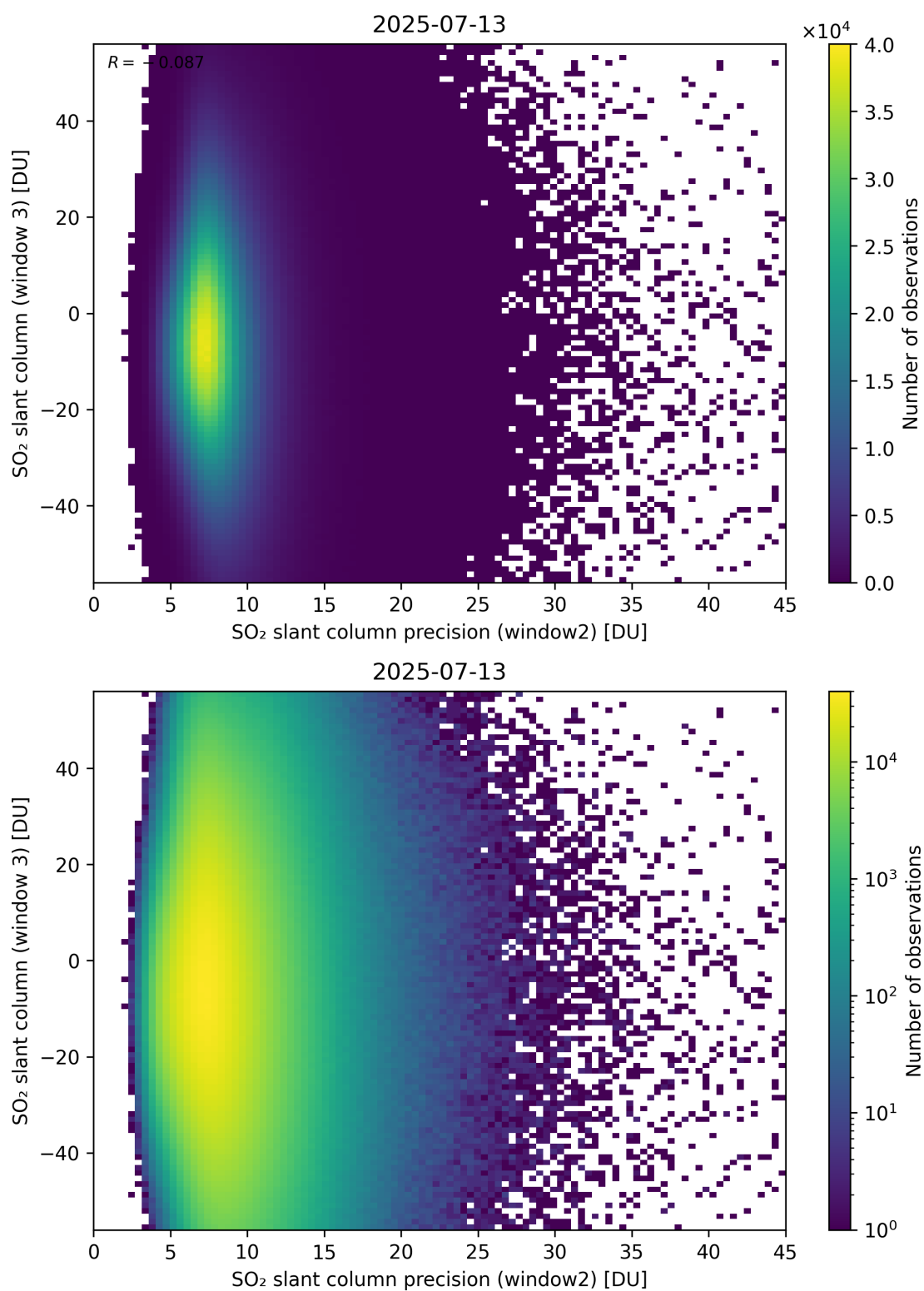
Figure 299: Scatter density plot of “SO 2 slant column precision (window2)” against “SO 2 slant column (window 3)” for 2025-07-13 to 2025-07-14.
