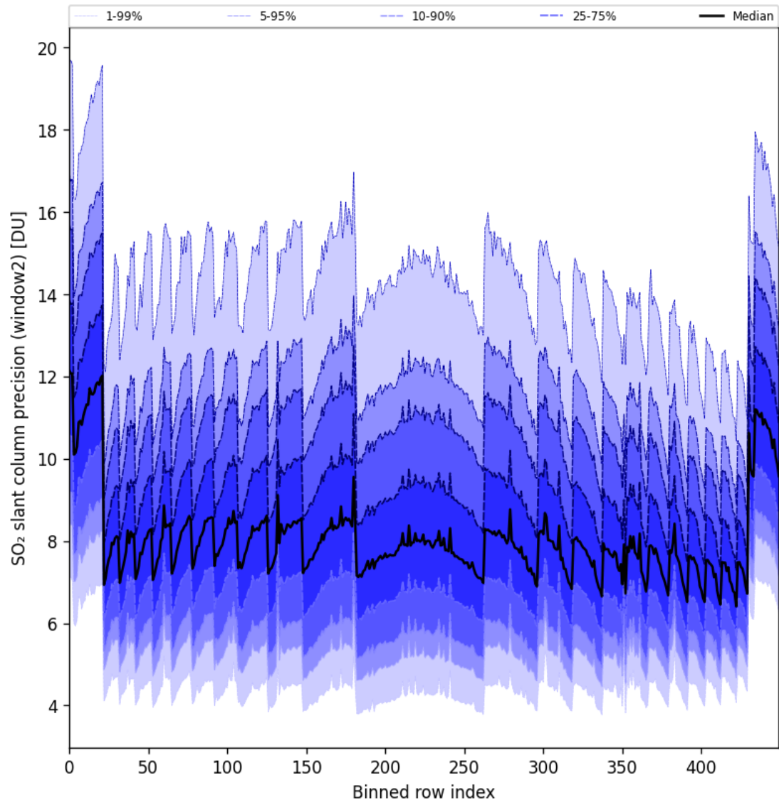
Figure 94: Along track statistics of “SO 2 slant column precision (window2)” for 2025-07-13 to 2025-07-14
