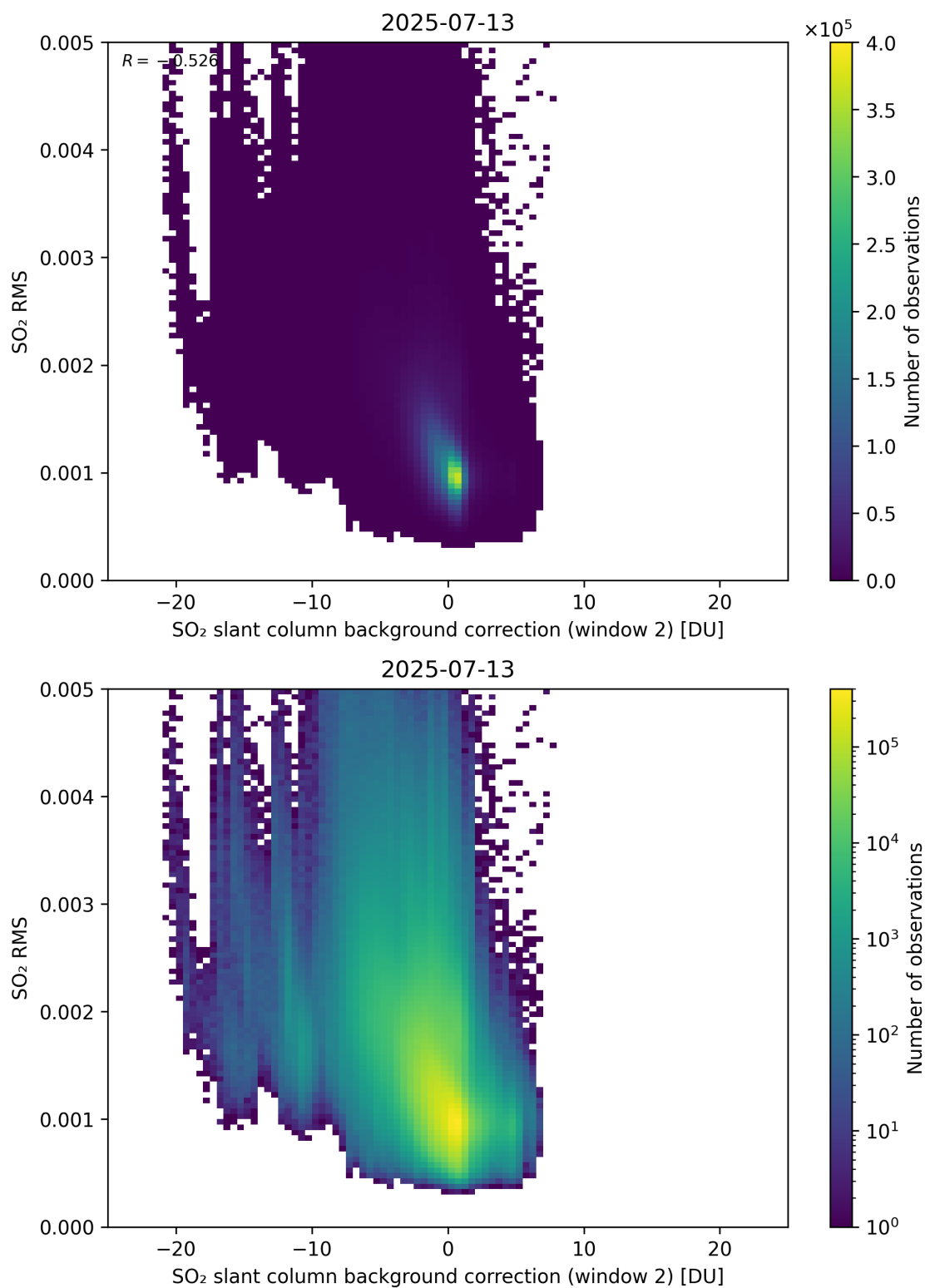
Figure 125: Scatter density plot of “SO 2 slant column background correction (window 2)” against “SO 2 RMS” for 2025-07-13 to 2025-07-14.
