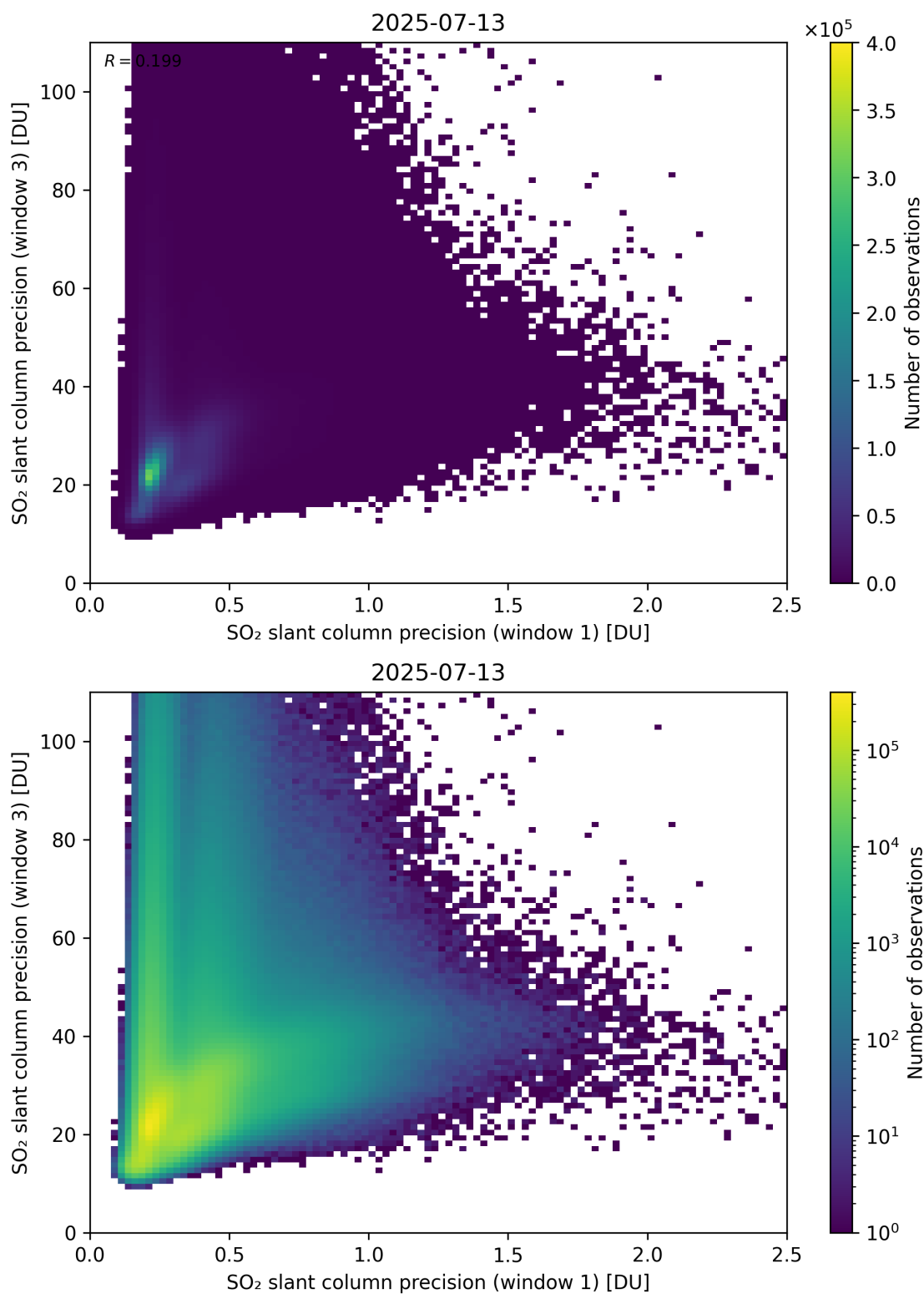
Figure 279: Scatter density plot of “SO 2 slant column precision (window 1)” against “SO 2 slant column precision (window 3)” for 2025-07-13 to 2025-07-14.
