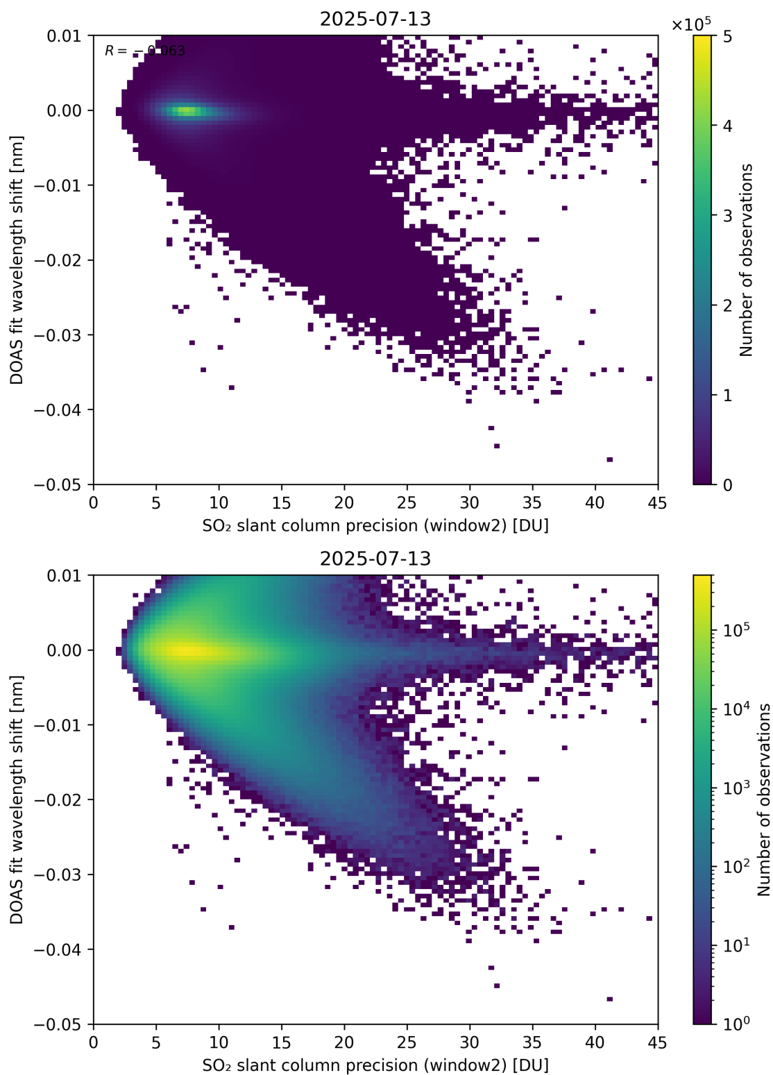
Figure 293: Scatter density plot of “SO 2 slant column precision (window2)” against “DOAS fit wavelength shift” for 2025-07-13 to 2025-07-14.
