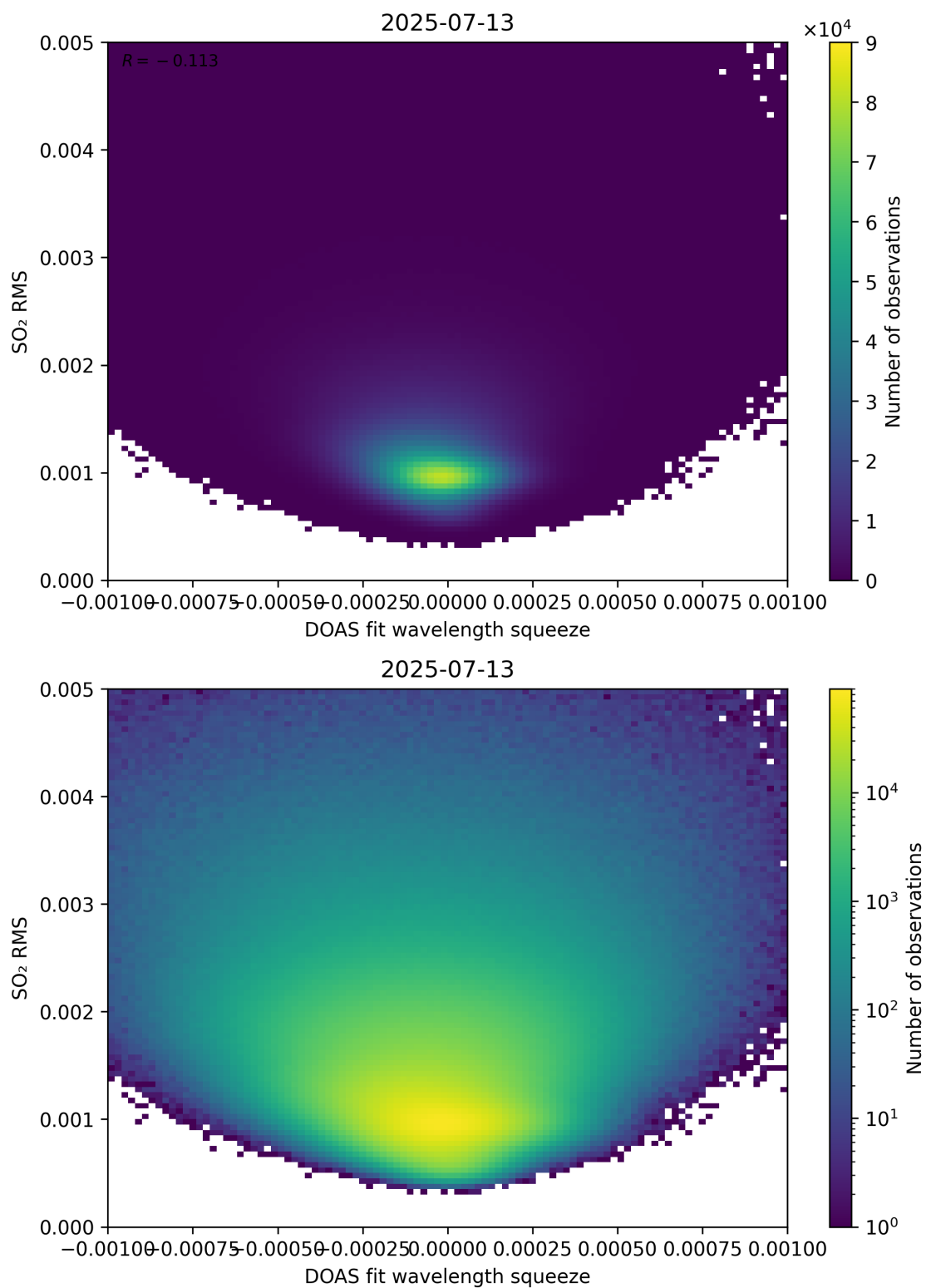
Figure 143: Scatter density plot of “DOAS fit wavelength squeeze” against “SO 2 RMS” for 2025-07-13 to 2025-07-14.
