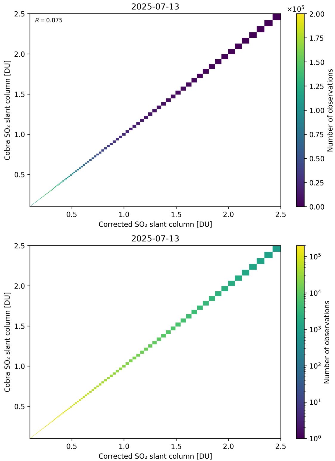
Figure 233: Scatter density plot of “Corrected SO 2 slant column” against “Cobra SO 2 slant column” for 2025-07-13 to 2025-07-14.
