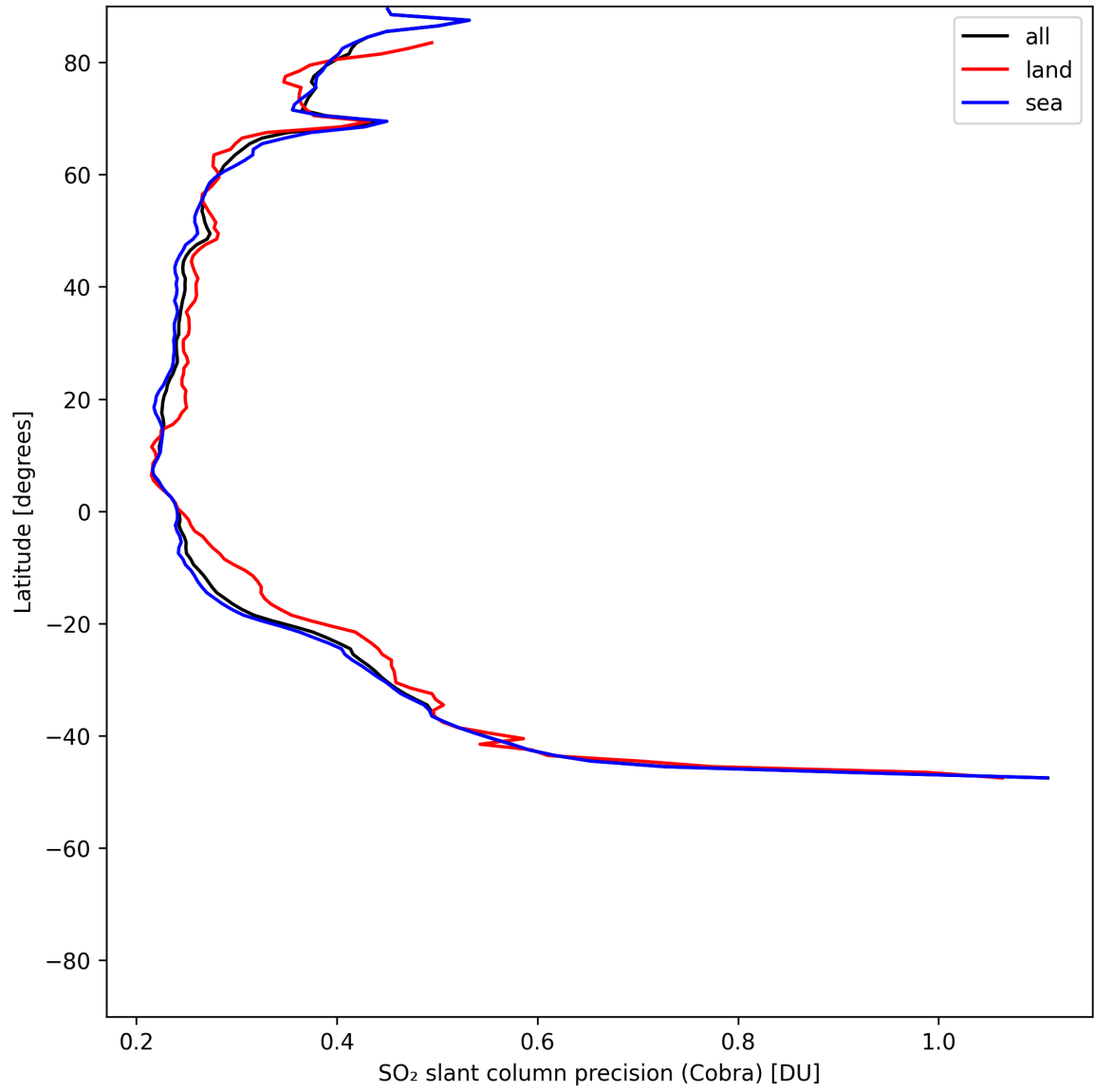
Figure 36: Zonal average of "SO 2 slant column precision (Cobra)" for 2025-07-13 to 2025-07-14.
