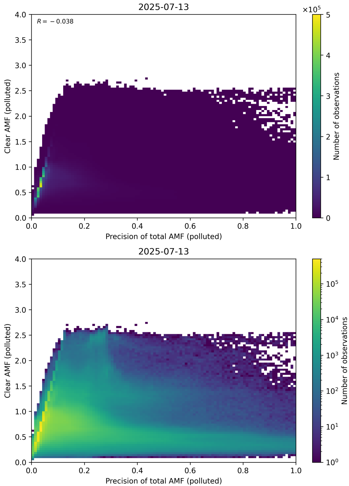
Figure 320: Scatter density plot of “Precision of total AMF (polluted)” against “Clear AMF (polluted)” for 2025-07-13 to 2025-07-14.
