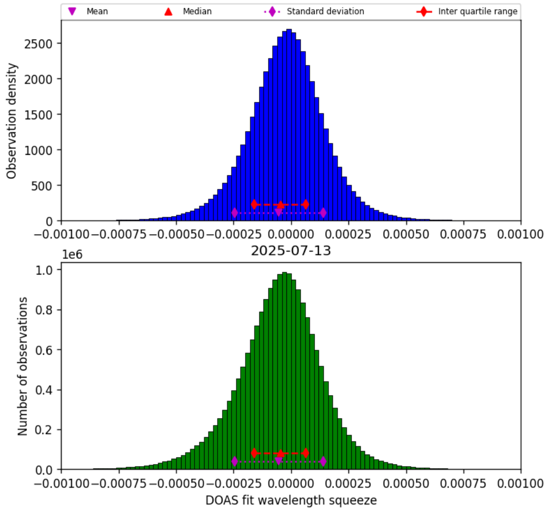
Figure 77: Histogram of “DOAS fit wavelength squeeze” for 2025-07-13 to 2025-07-14
