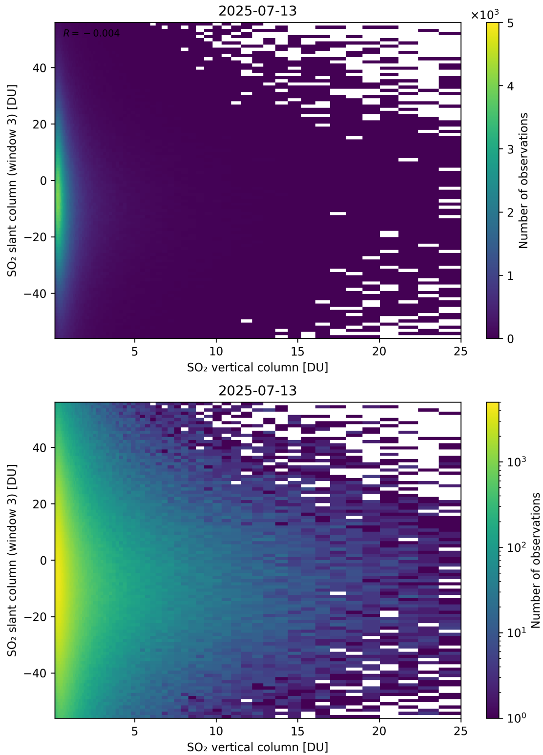
Figure 357: Scatter density plot of “SO 2 vertical column” against “SO 2 slant column (window 3)” for 2025-07-13 to 2025-07-14.
