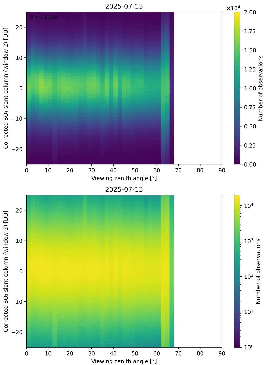
Figure 374: Scatter density plot of “Viewing zenith angle” against “Corrected SO 2 slant column (window 2)” for 2025-07-13 to 2025-07-14.
