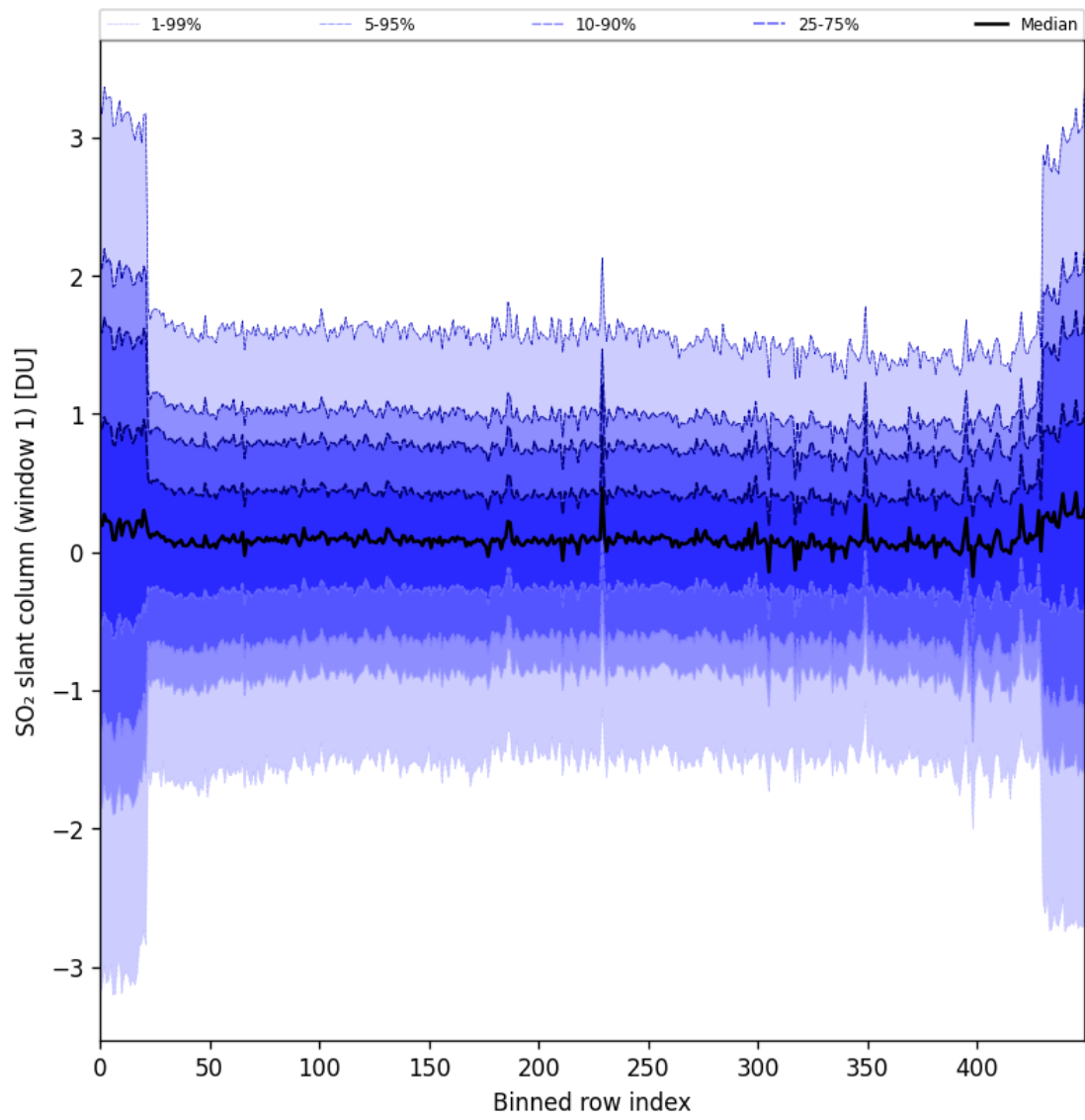
Figure 89: Along track statistics of “SO 2 slant column (window 1)” for 2025-07-13 to 2025-07-14
