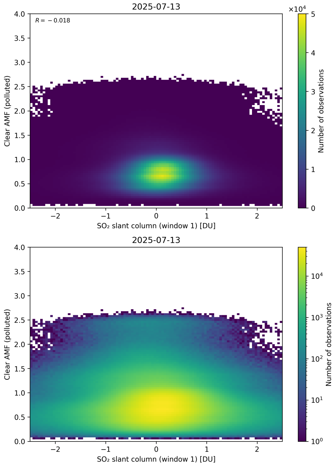
Figure 282: Scatter density plot of “SO 2 slant column (window 1)” against “Clear AMF (polluted)” for 2025-07-13 to 2025-07-14.
