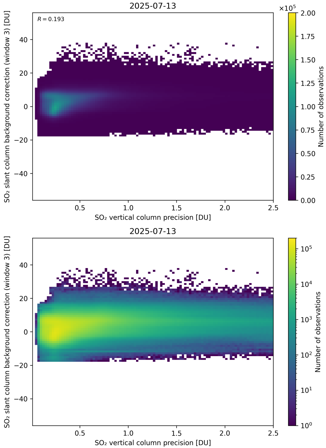
Figure 331: Scatter density plot of “SO 2 vertical column precision” against “SO 2 slant column background correction (window 3)” for 2025-07-13 to 2025-07-14.
