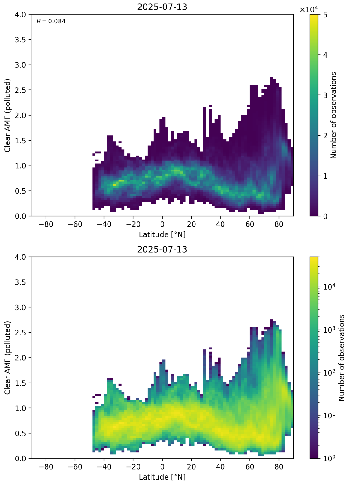
Figure 156: Scatter density plot of “Latitude” against “Clear AMF (polluted)” for 2025-07-13 to 2025-07-14.
