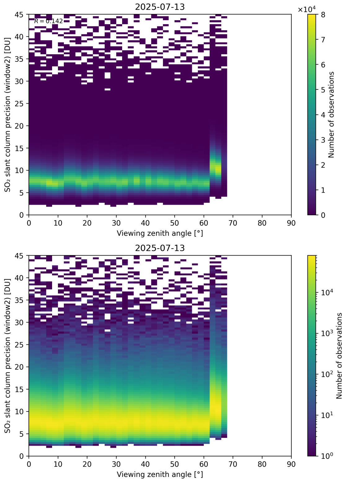
Figure 378: Scatter density plot of “Viewing zenith angle” against “SO 2 slant column precision (window2)” for 2025-07-13 to 2025-07-14.
