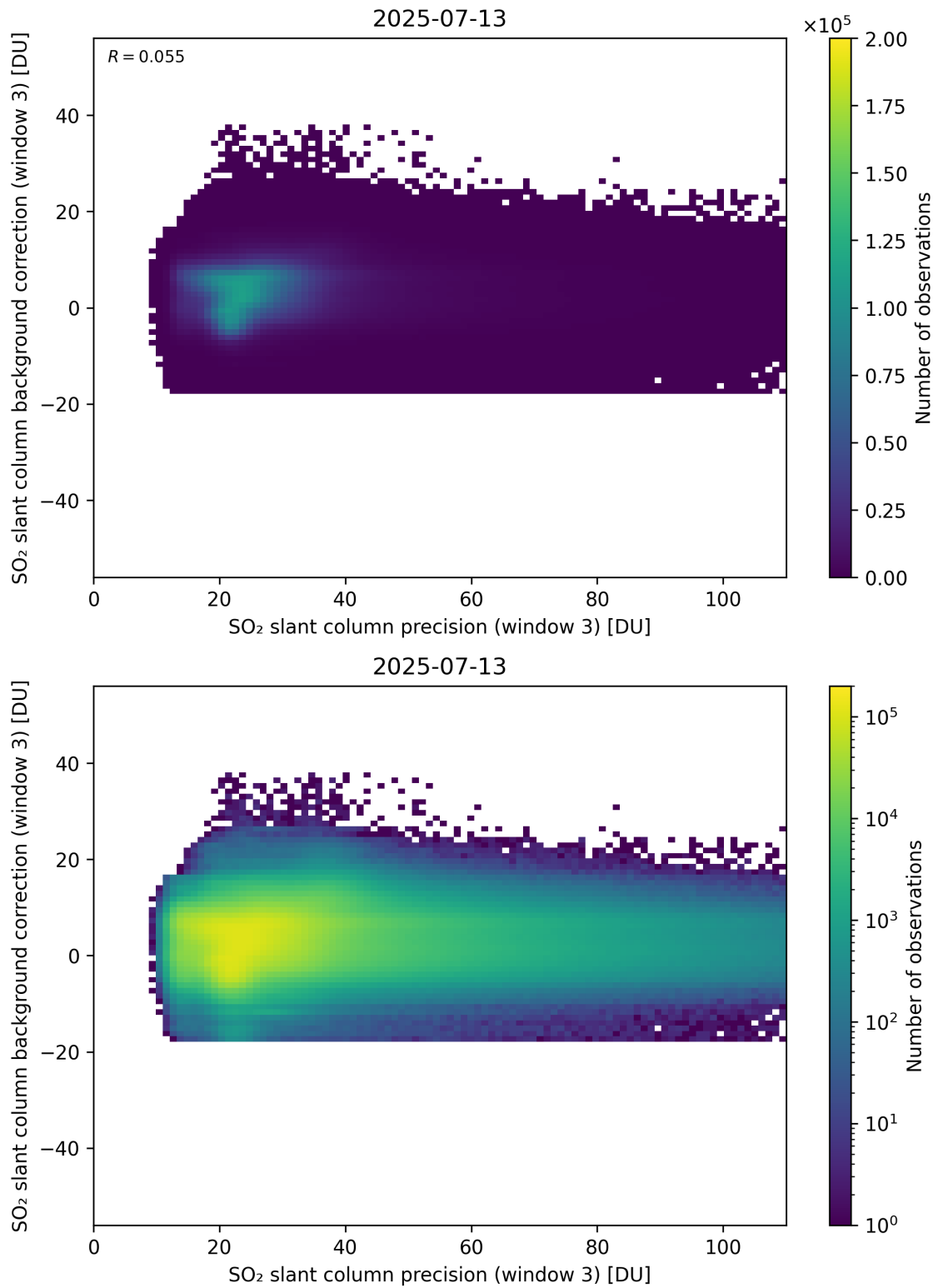
Figure 307: Scatter density plot of “SO 2 slant column precision (window 3)” against “SO 2 slant column background correction (window 3)” for 2025-07-13 to 2025-07-14.
