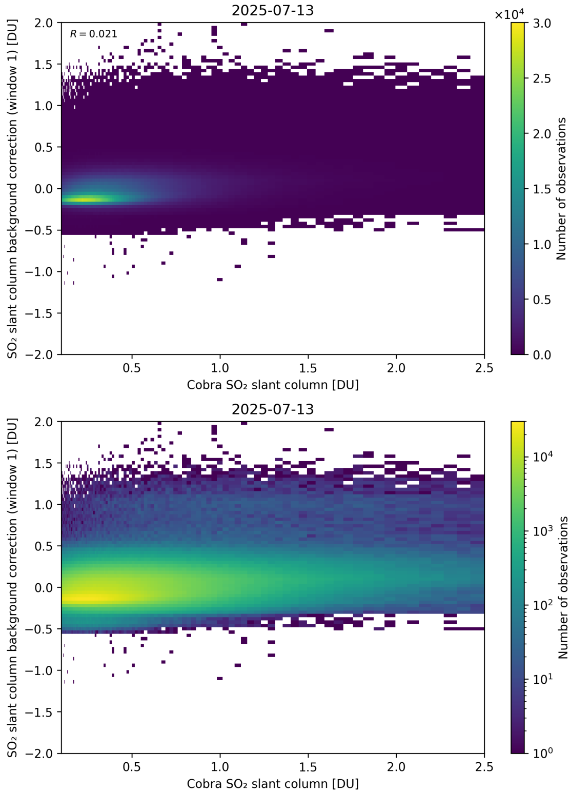
Figure 193: Scatter density plot of “Cobra SO 2 slant column” against “SO 2 slant column background correction (window 1)” for 2025-07-13 to 2025-07-14.
