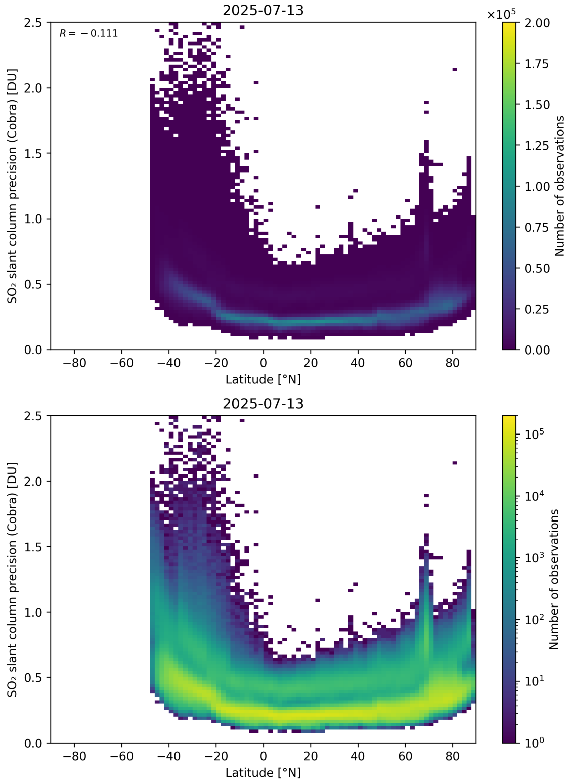
Figure 158: Scatter density plot of “Latitude” against “SO 2 slant column precision (Cobra)” for 2025-07-13 to 2025-07-14.
