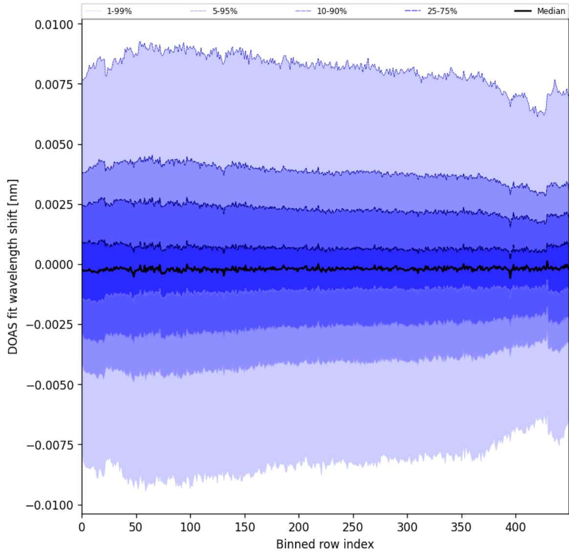
Figure 102: Along track statistics of “DOAS fit wavelength shift” for 2025-07-13 to 2025-07-14
