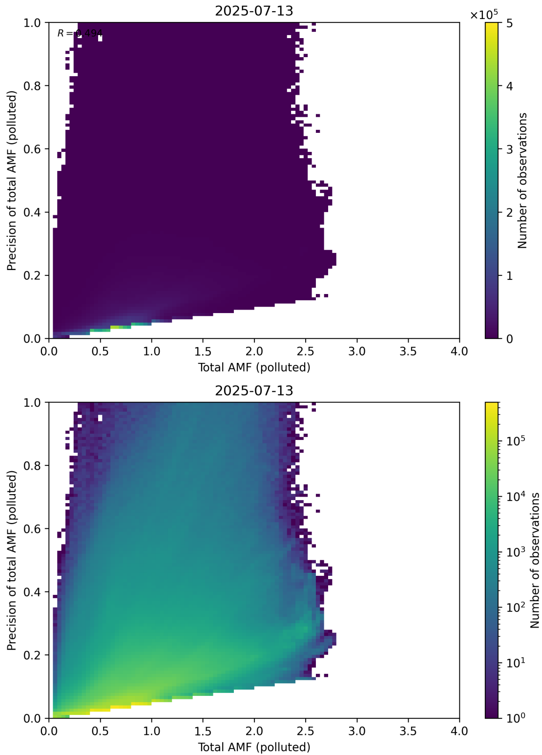
Figure 322: Scatter density plot of “Total AMF (polluted)” against “Precision of total AMF (polluted)” for 2025-07-13 to 2025-07-14.
