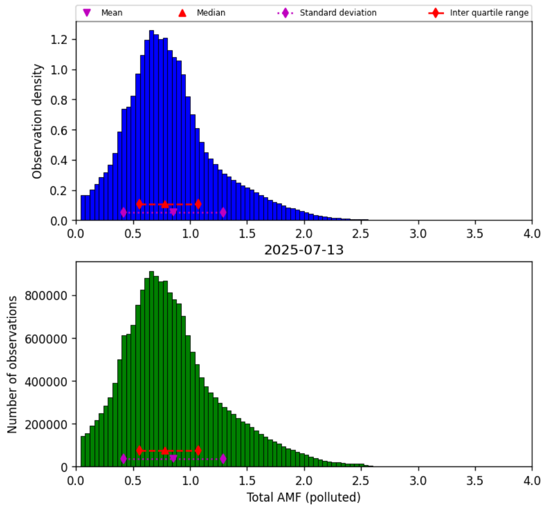
Figure 79: Histogram of “Total AMF (polluted)” for 2025-07-13 to 2025-07-14
