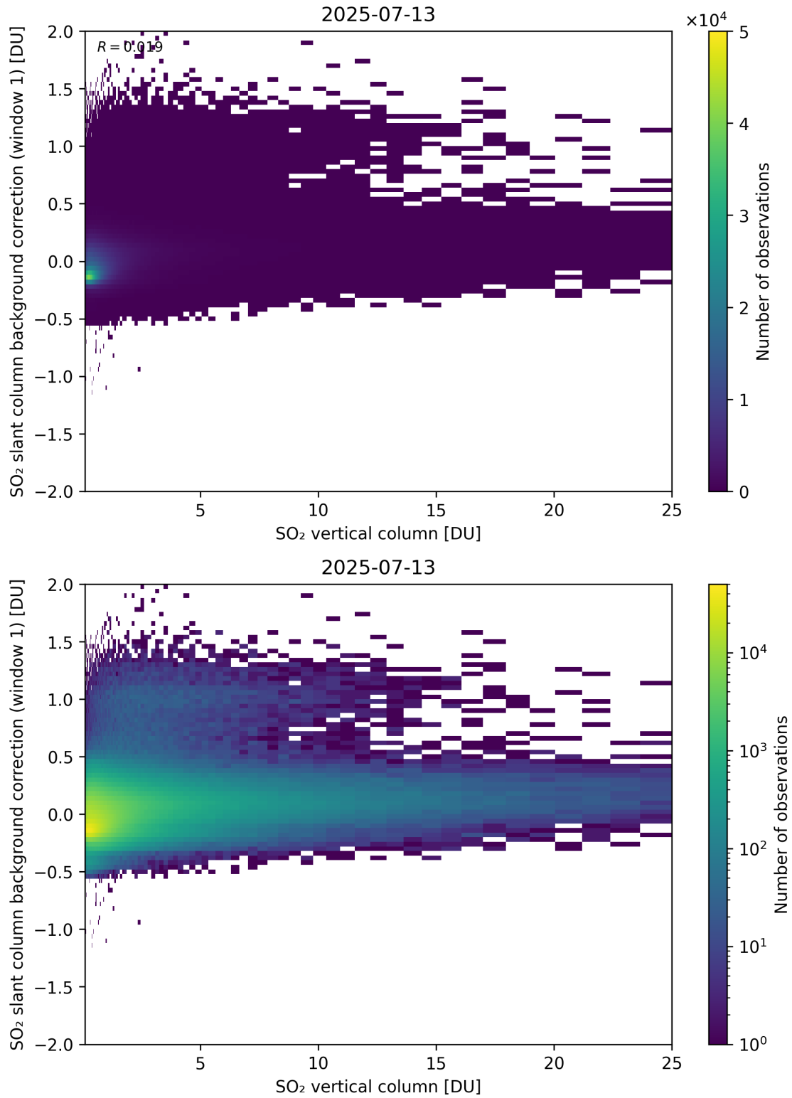
Figure 323: Scatter density plot of “SO 2 vertical column” against “SO 2 slant column background correction (window 1)” for 2025-07-13 to 2025-07-14.
