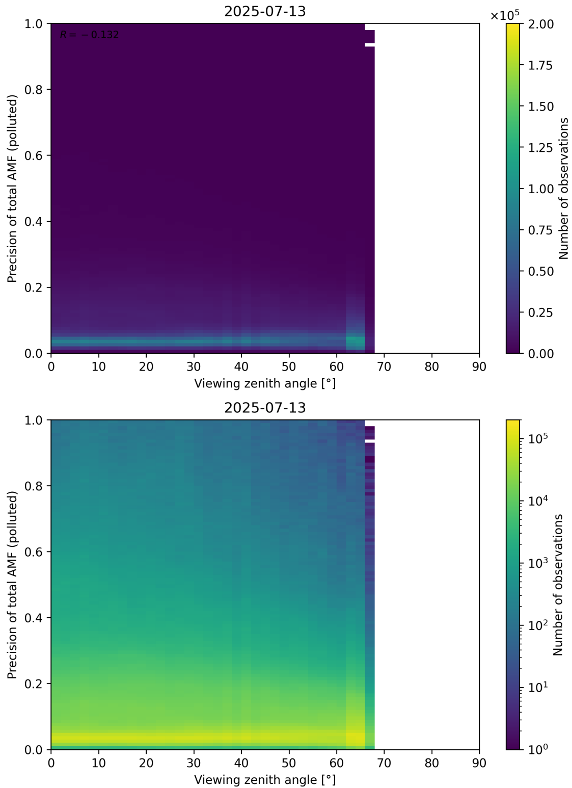
Figure 382: Scatter density plot of “Viewing zenith angle” against “Precision of total AMF (polluted)” for 2025-07-13 to 2025-07-14.
