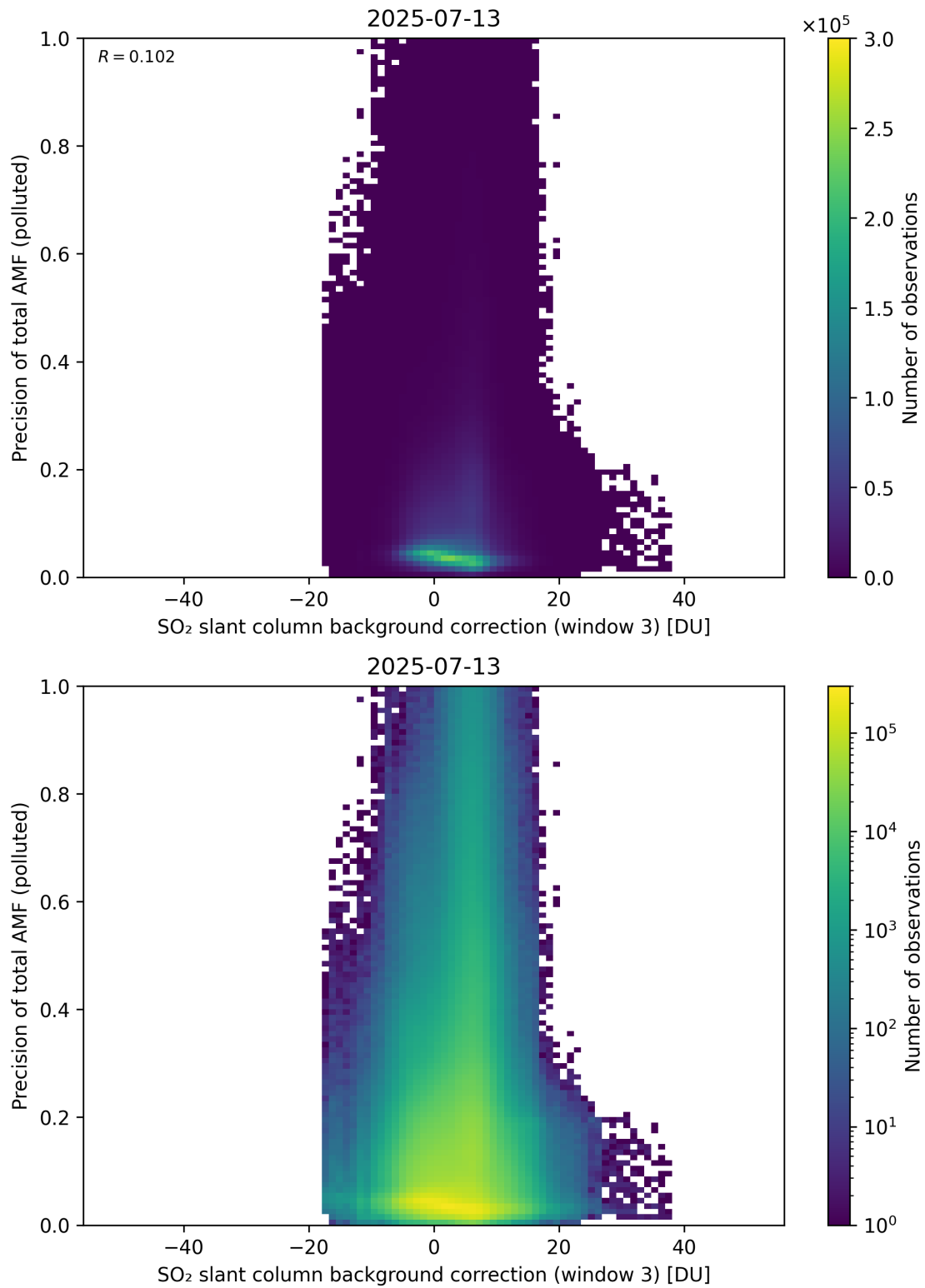
Figure 137: Scatter density plot of “SO 2 slant column background correction (window 3)” against “Precision of total AMF (polluted)” for 2025-07-13 to 2025-07-14.
