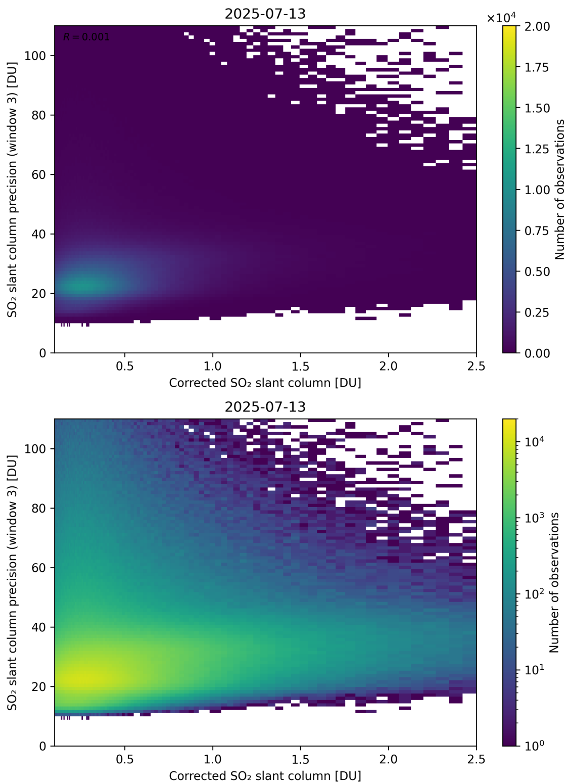
Figure 241: Scatter density plot of “Corrected SO 2 slant column” against “SO 2 slant column precision (window 3)” for 2025-07-13 to 2025-07-14.
