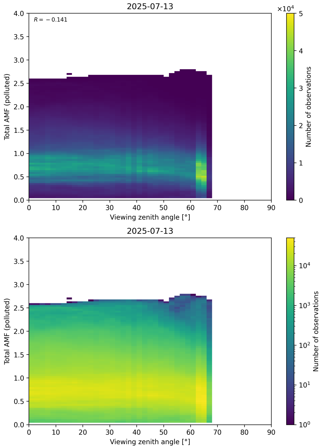
Figure 381: Scatter density plot of “Viewing zenith angle” against “Total AMF (polluted)” for 2025-07-13 to 2025-07-14.
