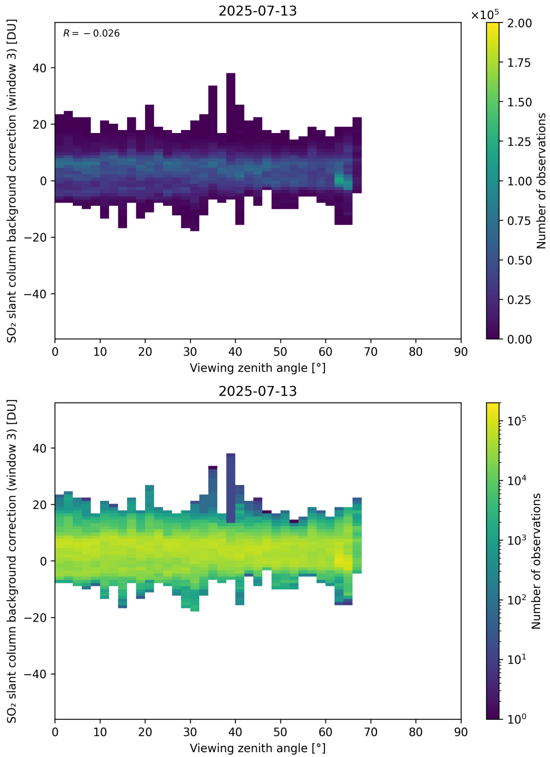
Figure 364: Scatter density plot of “Viewing zenith angle” against “SO 2 slant column background correction (window 3)” for 2025-07-13 to 2025-07-14.
