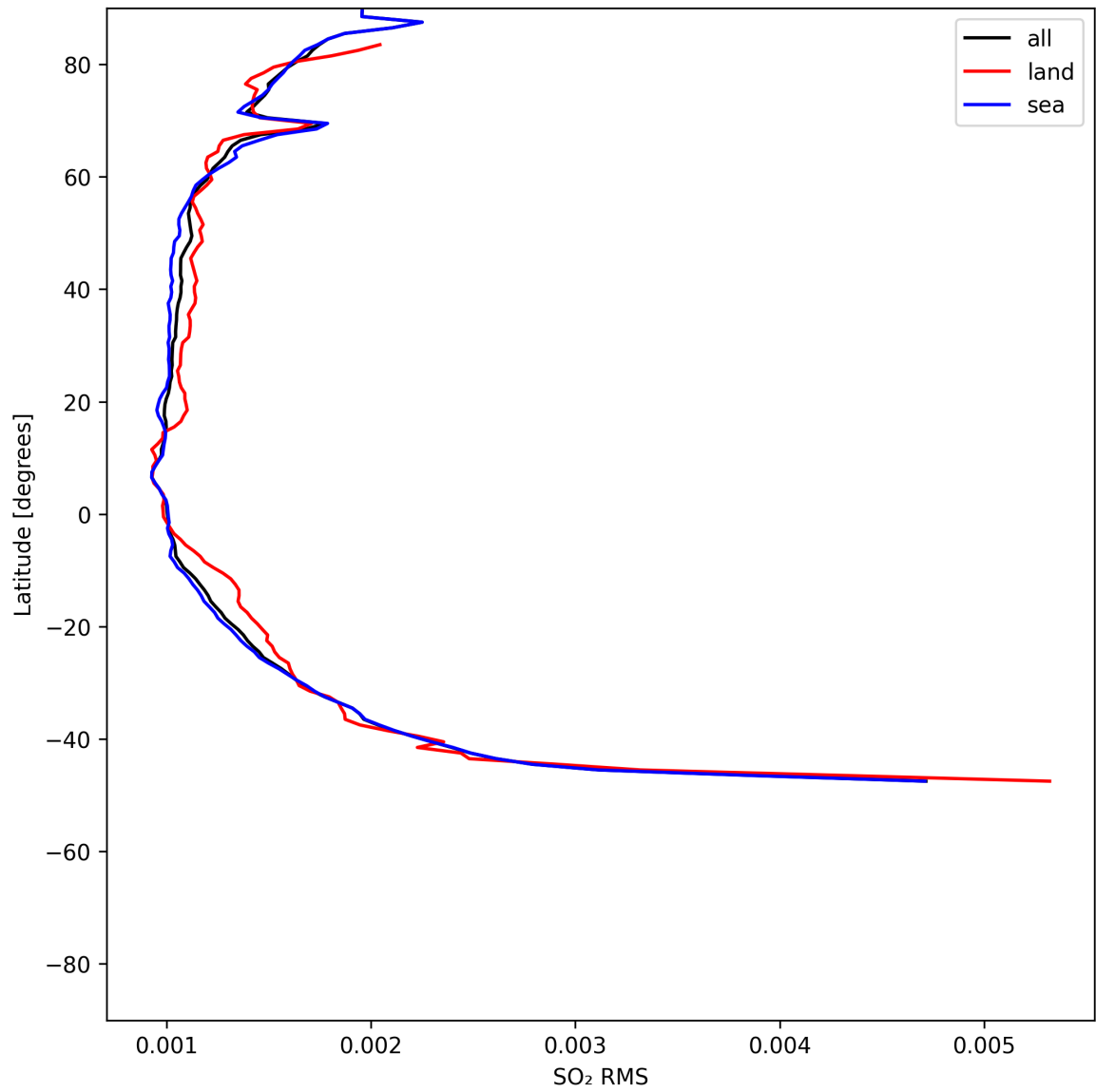
Figure 52: Zonal average of “SO 2 RMS” for 2025-07-13 to 2025-07-14.
