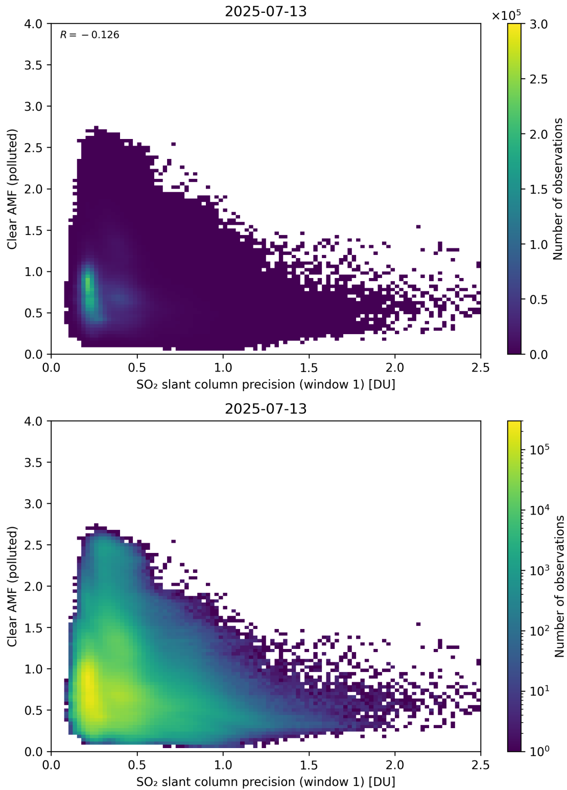
Figure 274: Scatter density plot of “SO 2 slant column precision (window 1)” against “Clear AMF (polluted)” for 2025-07-13 to 2025-07-14.
