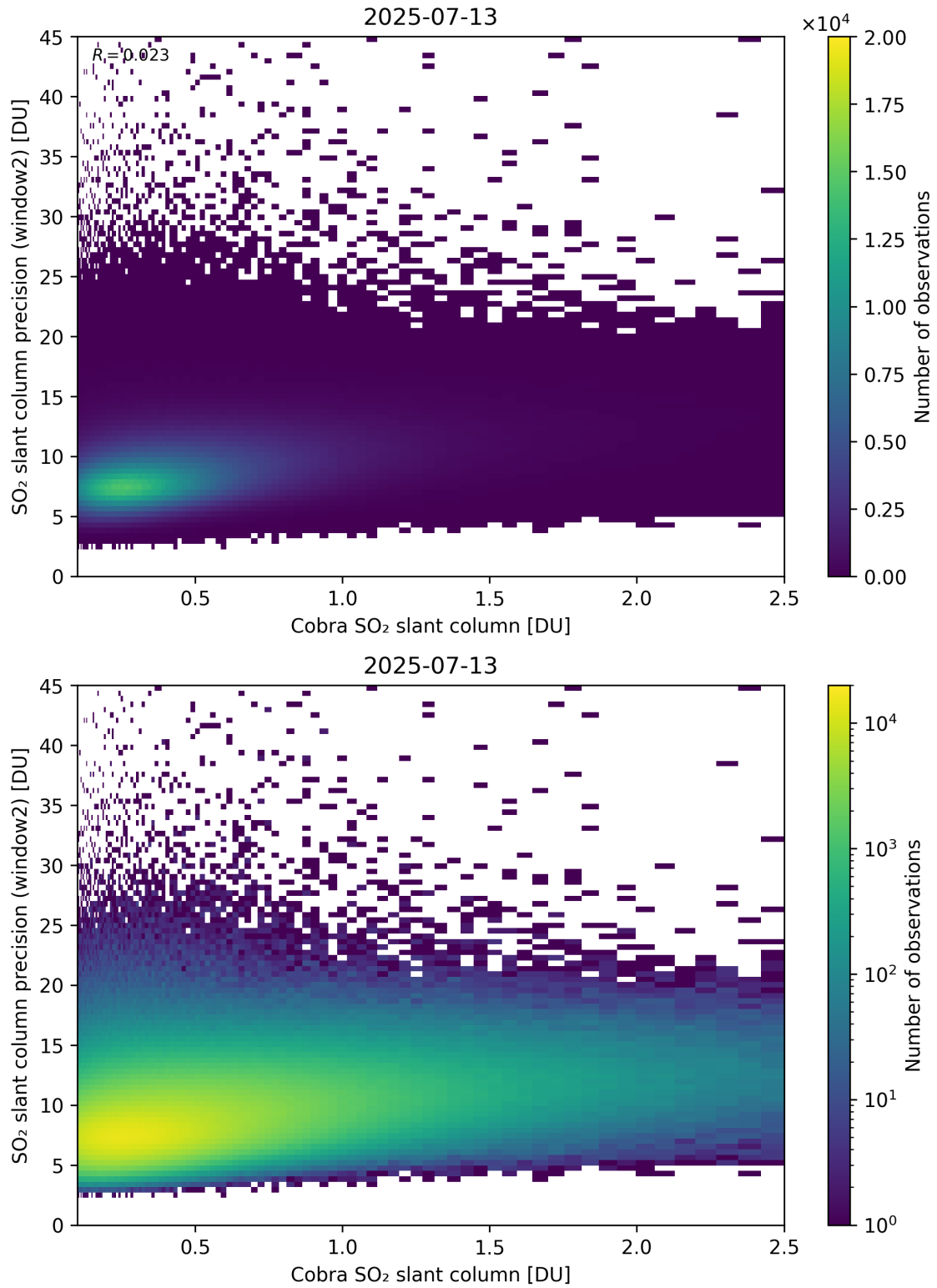
Figure 221: Scatter density plot of “Cobra SO 2 slant column” against “SO 2 slant column precision (window2)” for 2025-07-13 to 2025-07-14.
