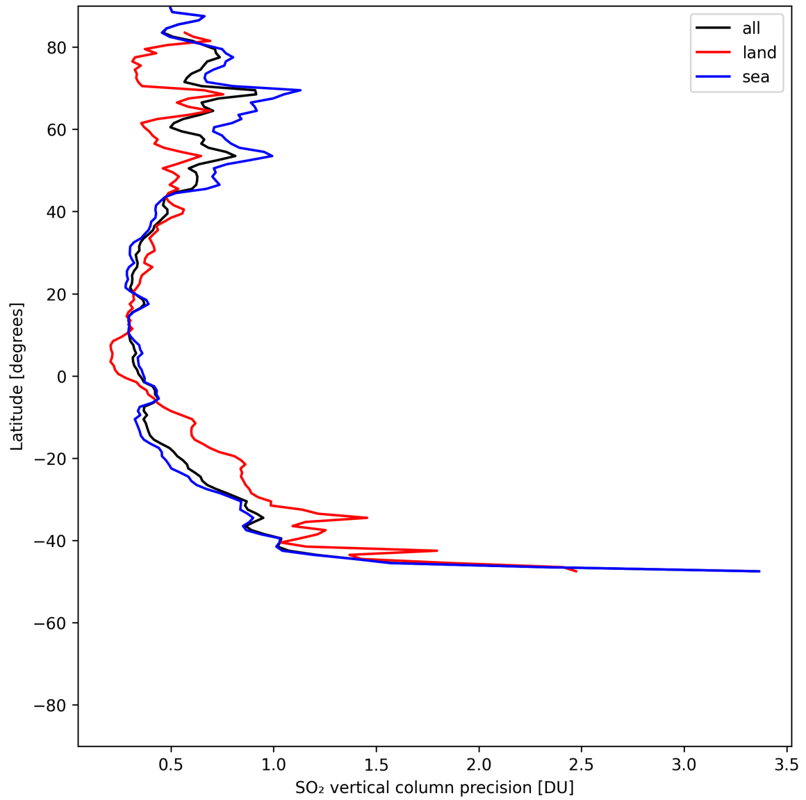
Figure 33: Zonal average of “SO 2 vertical column precision” for 2025-07-13 to 2025-07-14.
