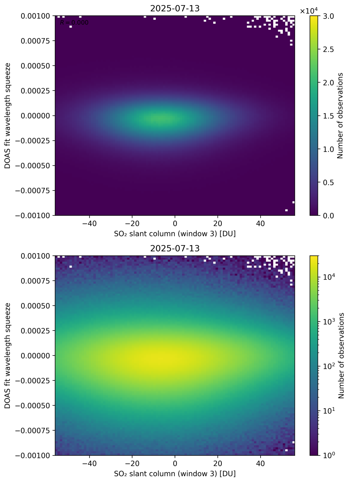
Figure 305: Scatter density plot of “SO 2 slant column (window 3)” against “DOAS fit wavelength squeeze” for 2025-07-13 to 2025-07-14.
