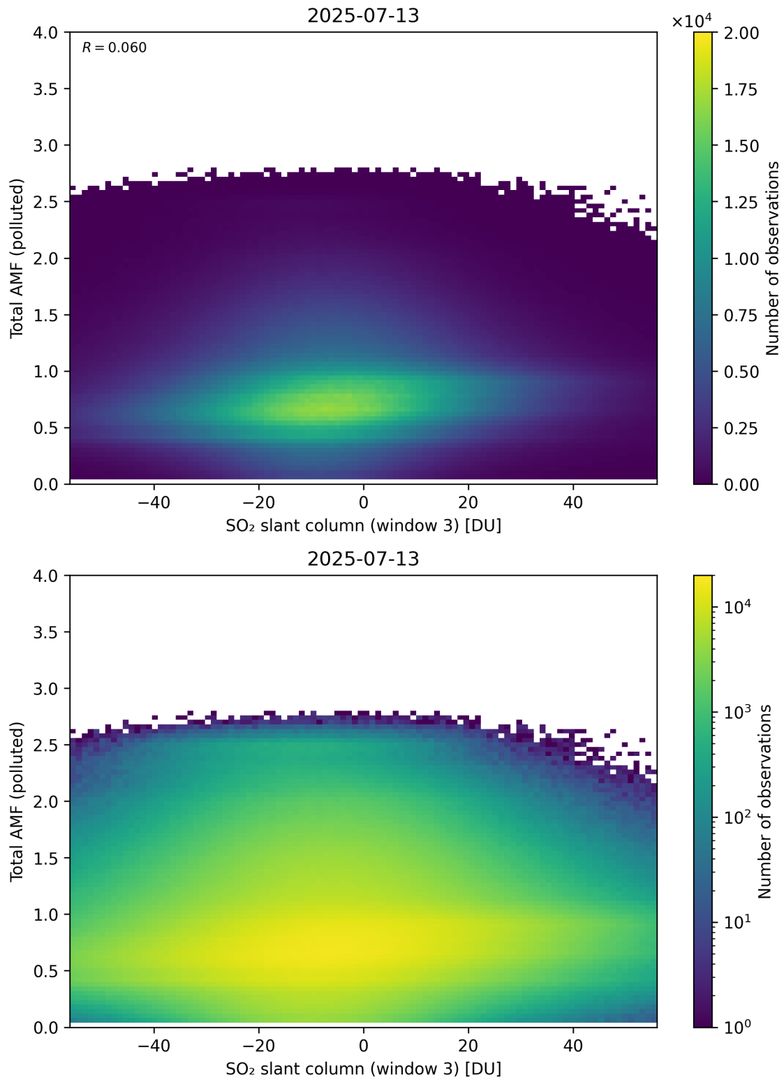
Figure 318: Scatter density plot of “SO 2 slant column (window 3)” against “Total AMF (polluted)” for 2025-07-13 to 2025-07-14.
