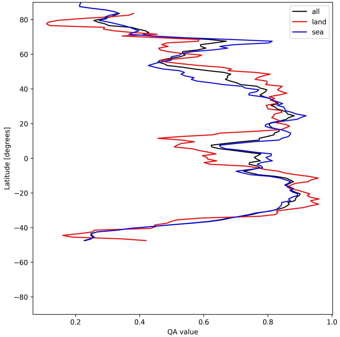
Figure 31: Zonal average of “QA value” for 2025-07-13 to 2025-07-14.
