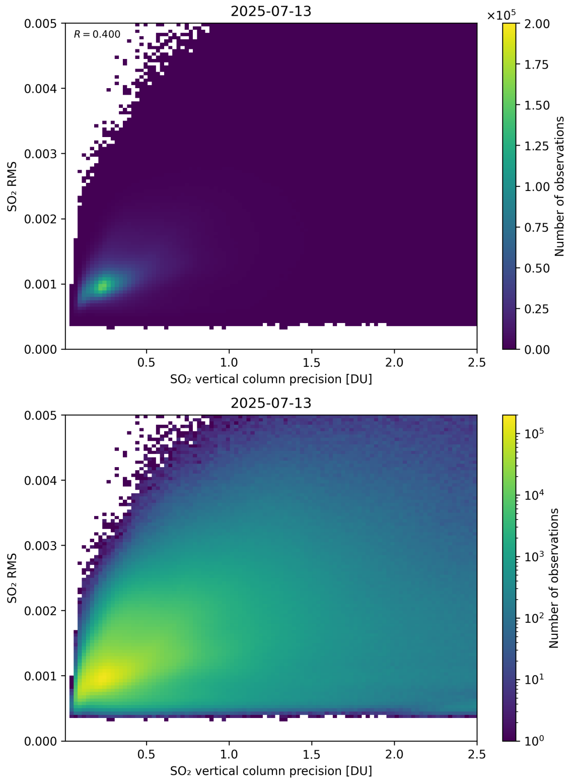
Figure 334: Scatter density plot of “SO 2 vertical column precision” against “SO 2 RMS” for 2025-07-13 to 2025-07-14.
