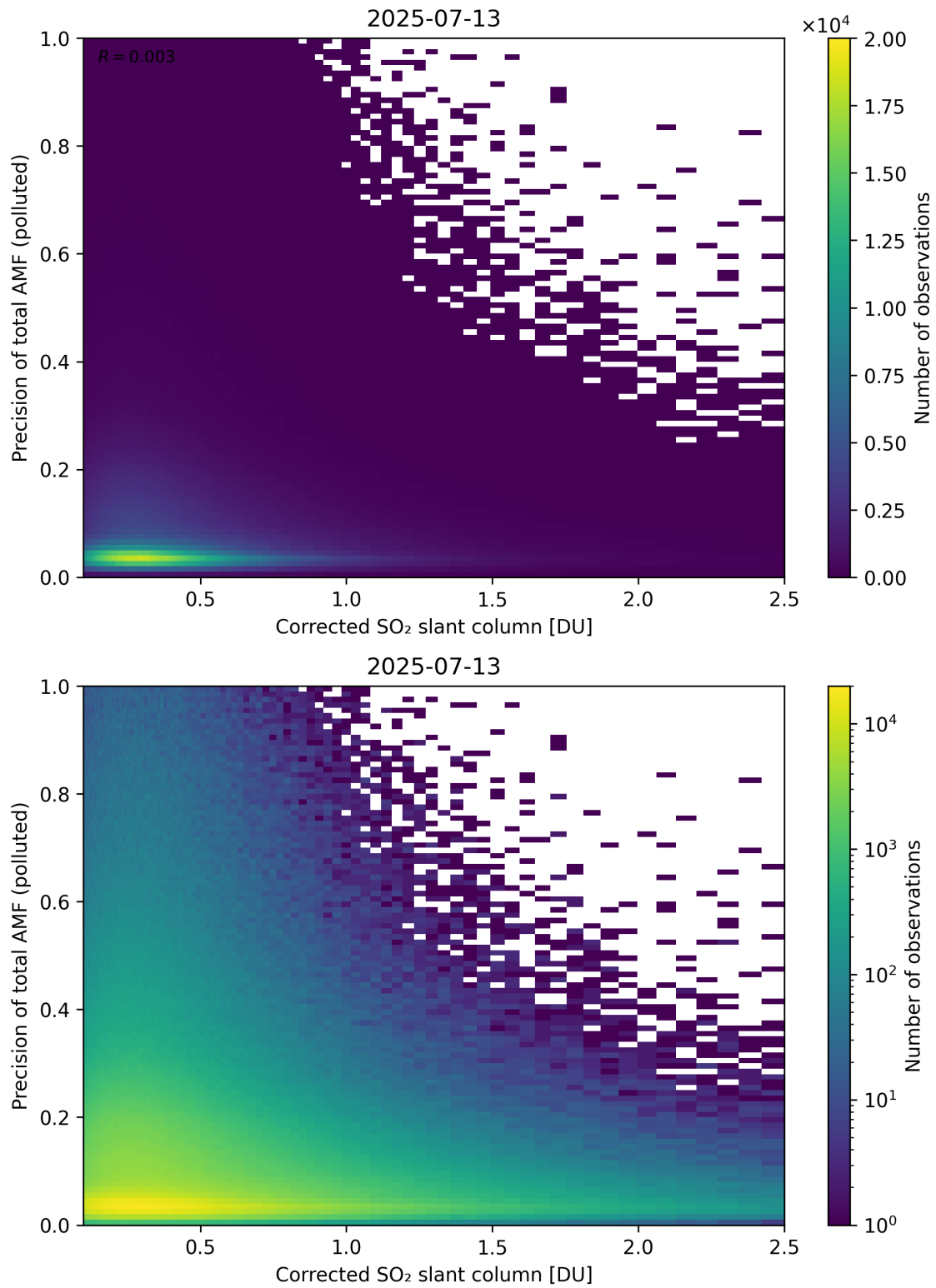
Figure 243: Scatter density plot of “Corrected SO 2 slant column” against “Precision of total AMF (polluted)” for 2025-07-13 to 2025-07-14.
