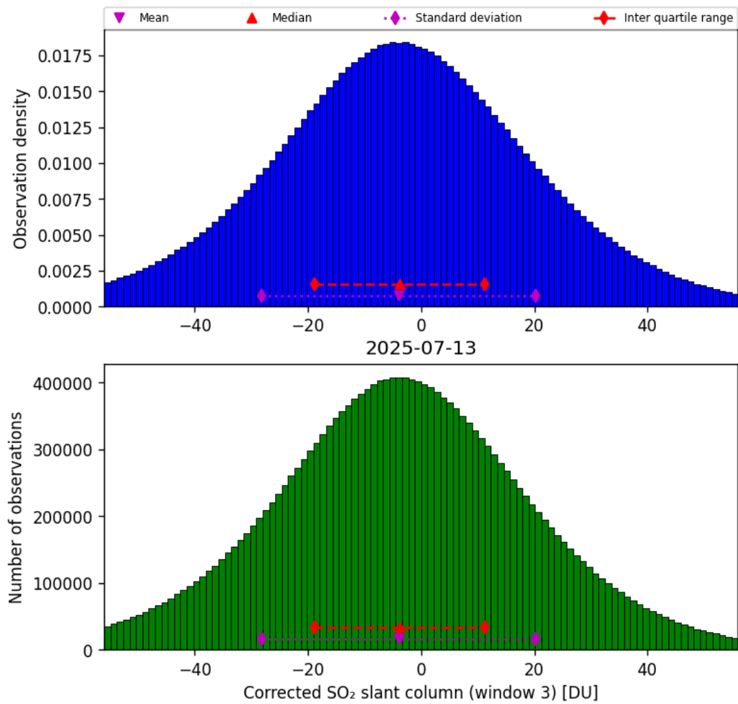
Figure 73: Histogram of “Corrected SO 2 slant column (window 3)” for 2025-07-13 to 2025-07-14
