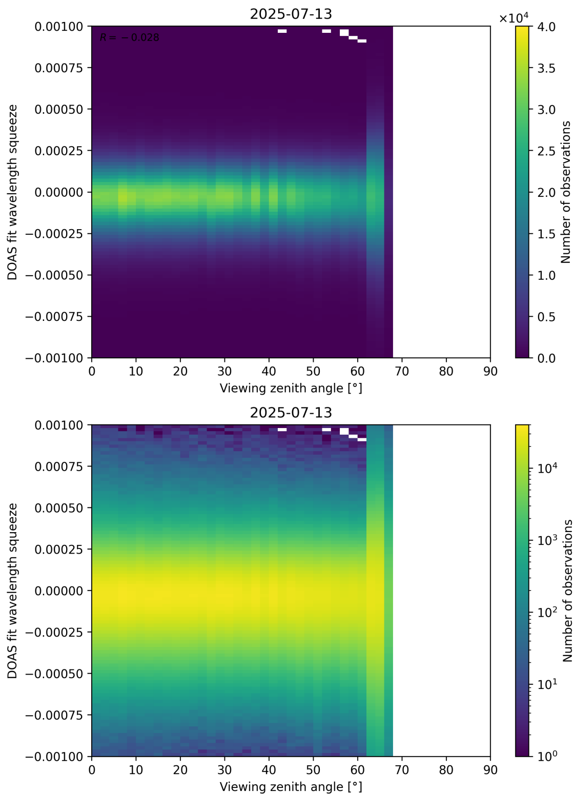
Figure 366: Scatter density plot of “Viewing zenith angle” against “DOAS fit wavelength squeeze” for 2025-07-13 to 2025-07-14.
