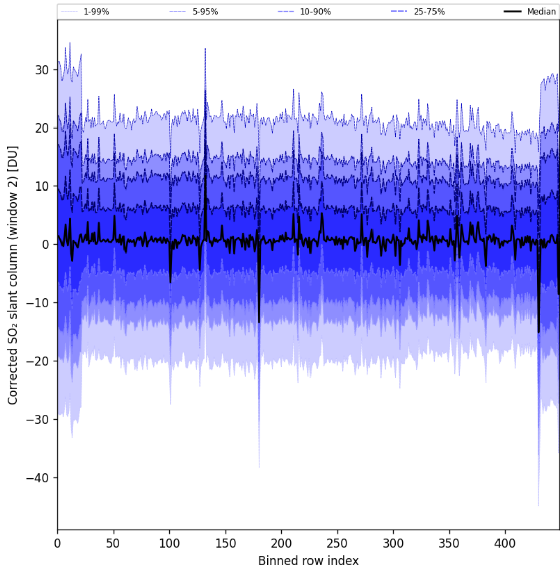
Figure 95: Along track statistics of “Corrected SO 2 slant column (window 2)” for 2025-07-13 to 2025-07-14
