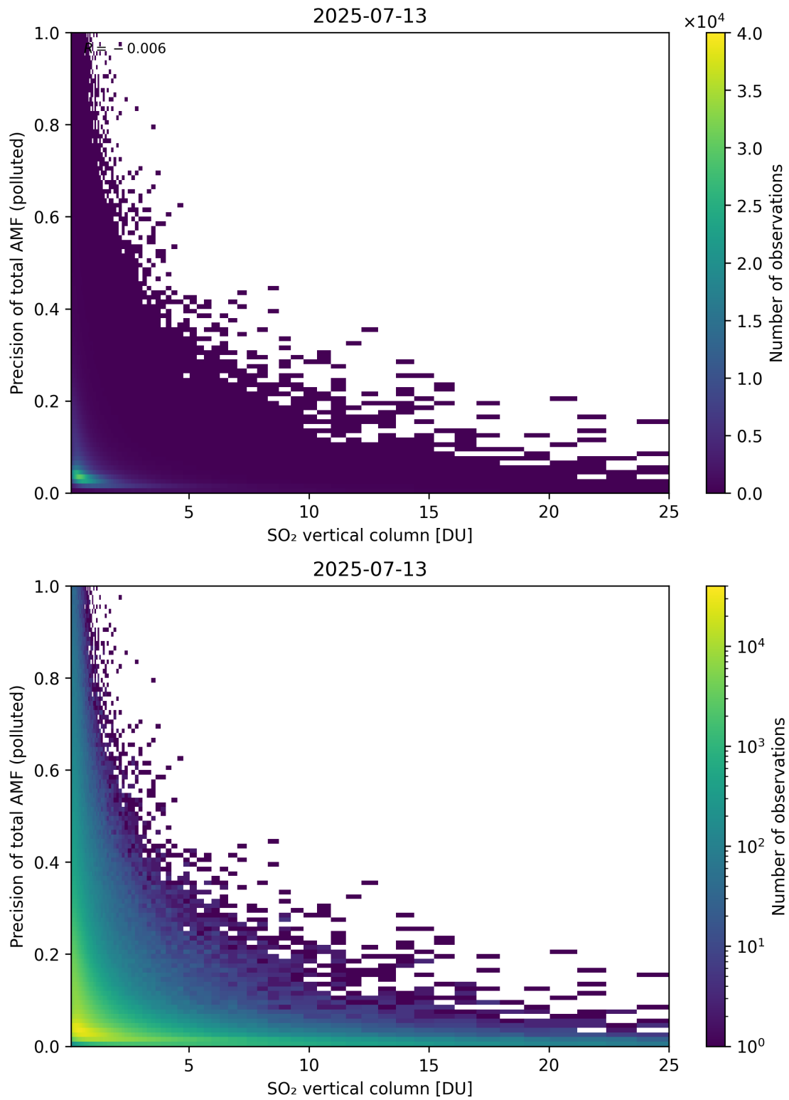
Figure 360: Scatter density plot of “SO 2 vertical column” against “Precision of total AMF (polluted)” for 2025-07-13 to 2025-07-14.
