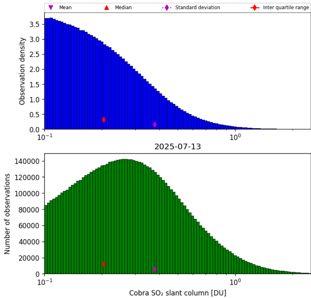
Figure 61: Histogram of “Cobra SO 2 slant column” for 2025-07-13 to 2025-07-14
