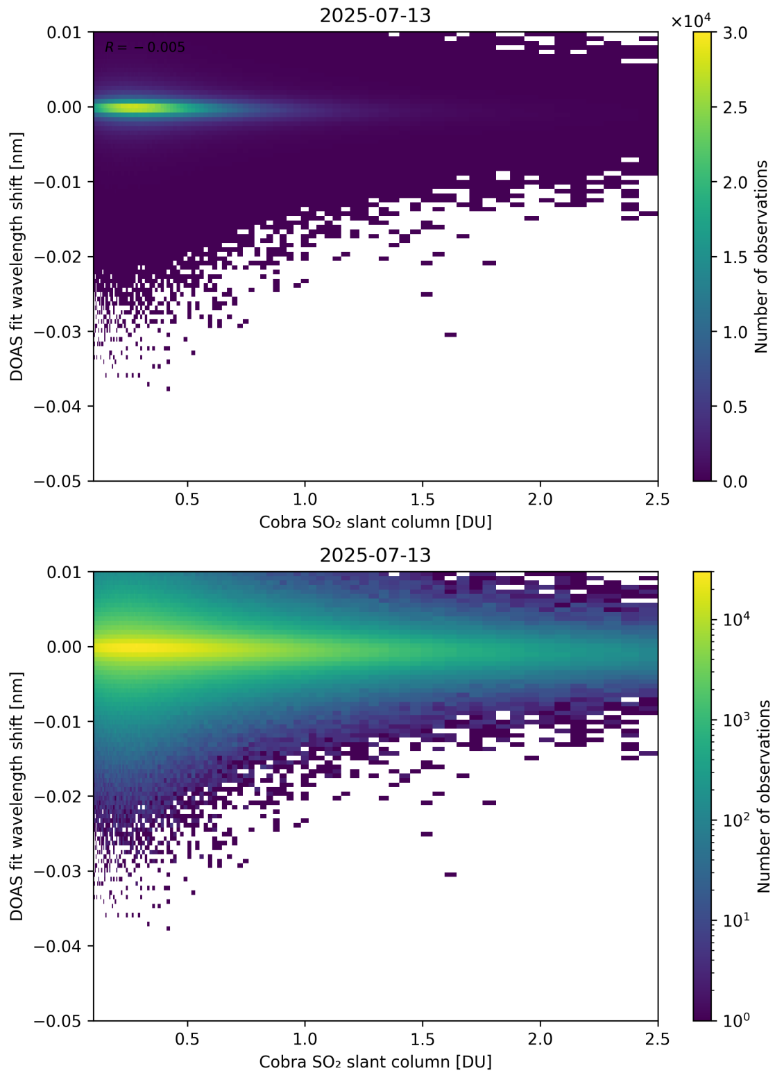
Figure 196: Scatter density plot of “Cobra SO 2 slant column” against “DOAS fit wavelength shift” for 2025-07-13 to 2025-07-14.
