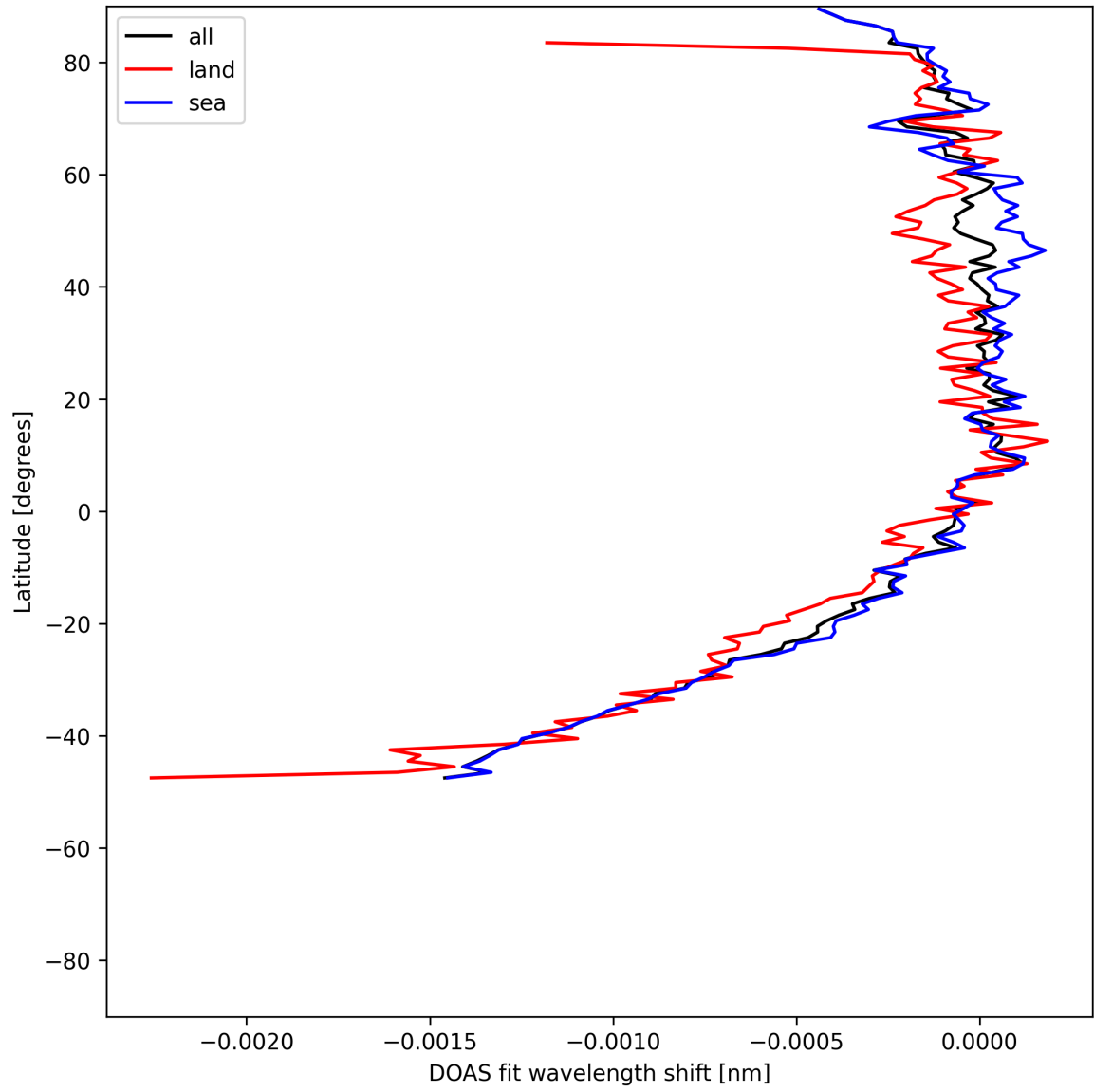
Figure 50: Zonal average of “DOAS fit wavelength shift” for 2025-07-13 to 2025-07-14.
