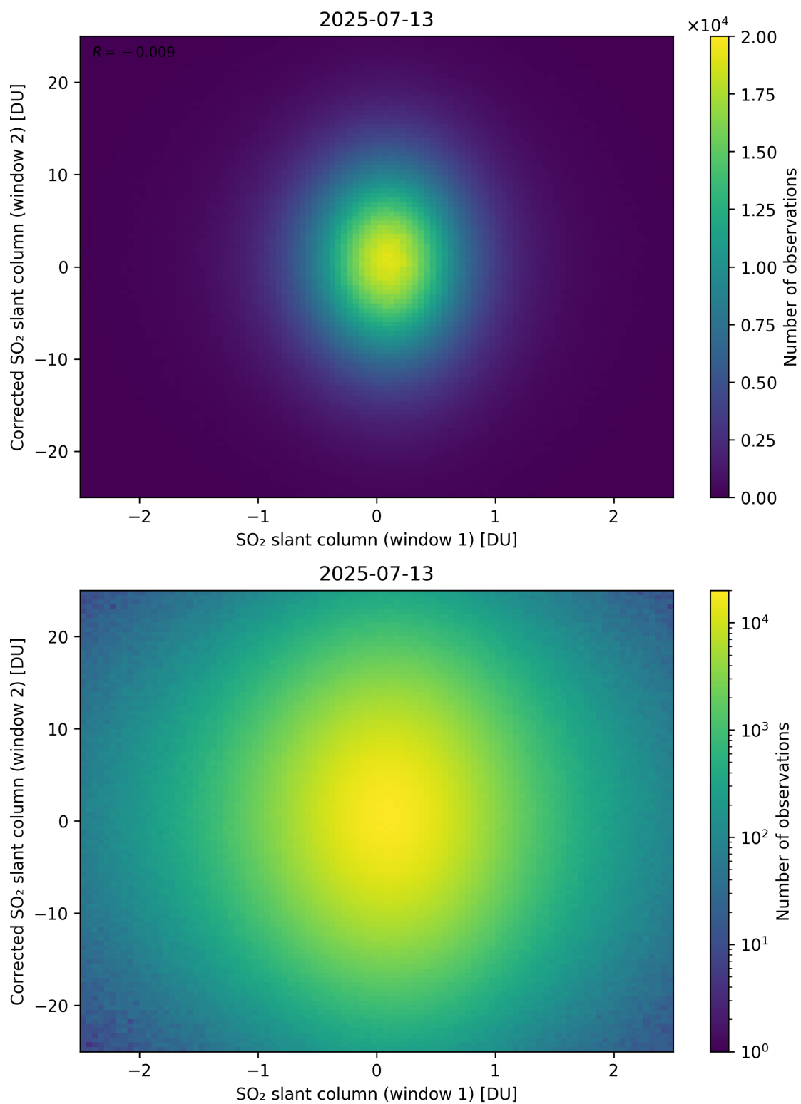
Figure 283: Scatter density plot of “SO 2 slant column (window 1)” against “Corrected SO 2 slant column (window 2)” for 2025-07-13 to 2025-07-14.
