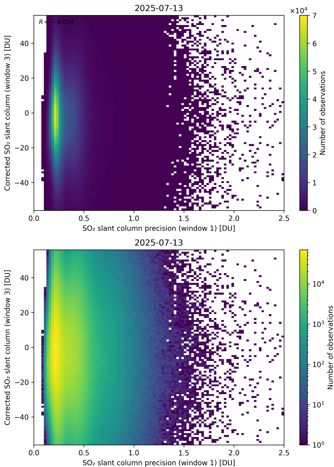
Figure 276: Scatter density plot of “SO 2 slant column precision (window 1)” against “Corrected SO 2 slant column (window 3)” for 2025-07-13 to 2025-07-14.
