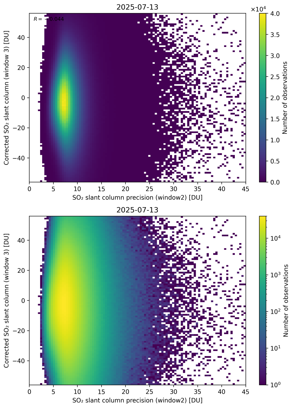
Figure 298: Scatter density plot of “SO 2 slant column precision (window2)” against “Corrected SO 2 slant column (window 3)” for 2025-07-13 to 2025-07-14.
