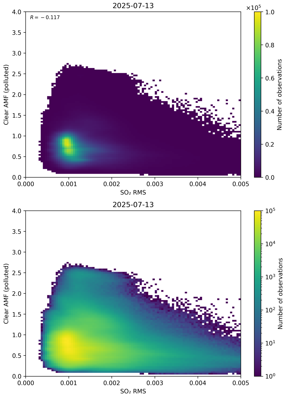
Figure 147: Scatter density plot of “SO 2 RMS” against “Clear AMF (polluted)” for 2025-07-13 to 2025-07-14.
