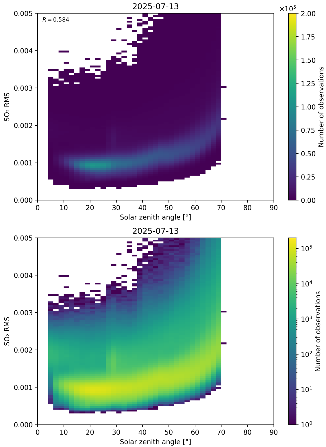
Figure 176: Scatter density plot of “Solar zenith angle” against “SO 2 RMS” for 2025-07-13 to 2025-07-14.
