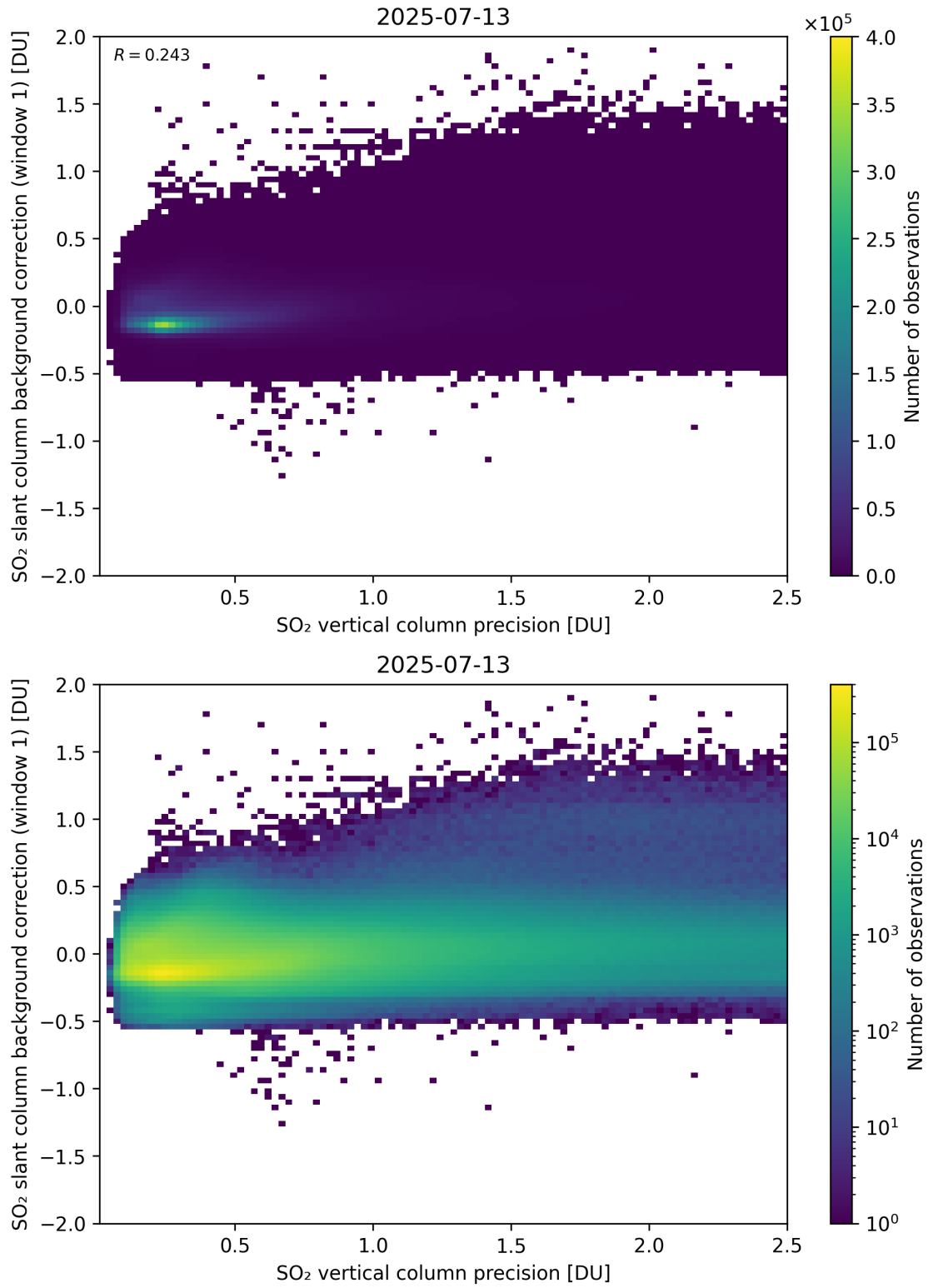
Figure 329: Scatter density plot of “SO 2 vertical column precision” against “SO 2 slant column background correction (window 1)” for 2025-07-13 to 2025-07-14.
