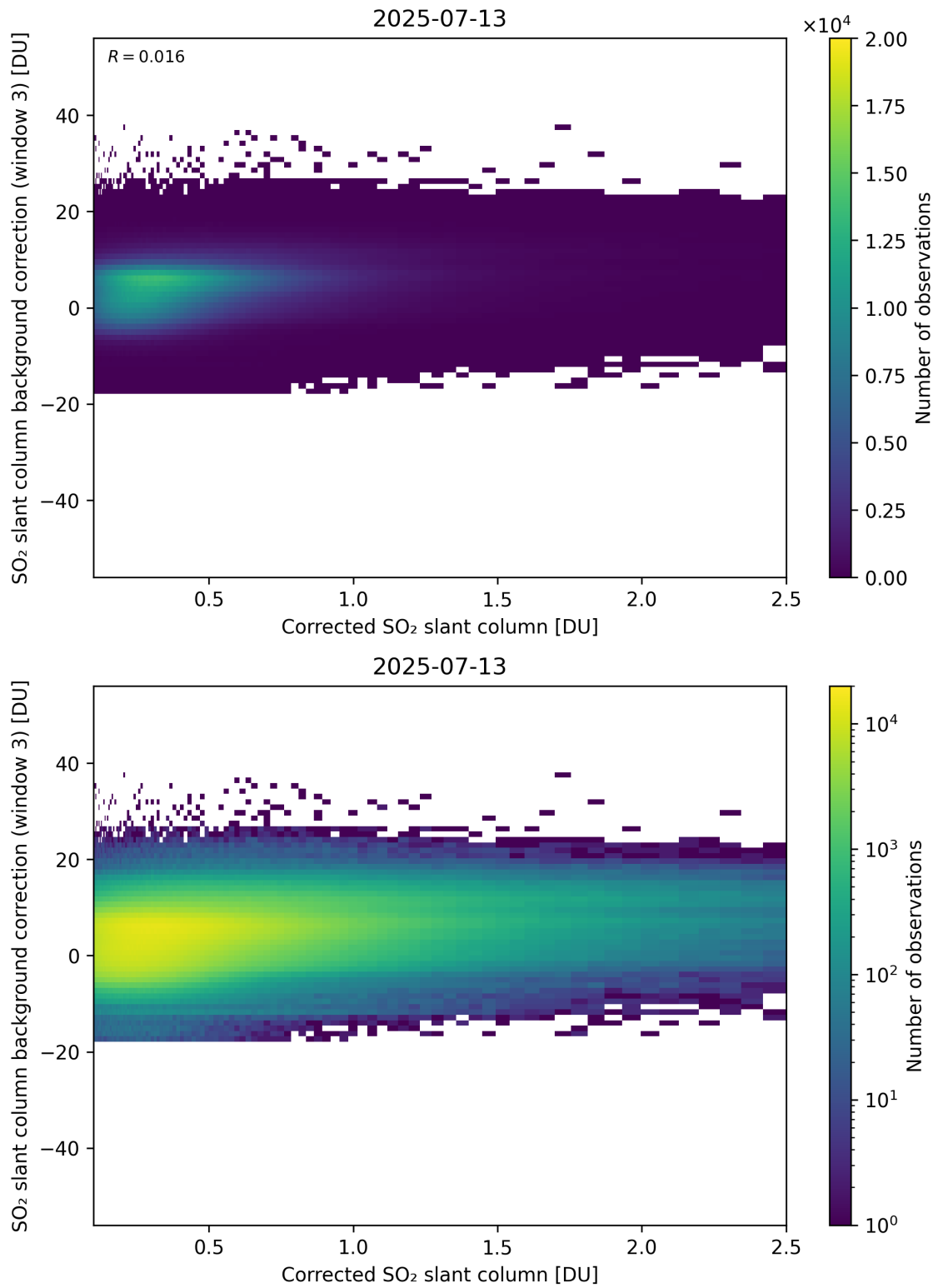
Figure 228: Scatter density plot of “Corrected SO 2 slant column” against “SO 2 slant column background correction (window 3)” for 2025-07-13 to 2025-07-14.
