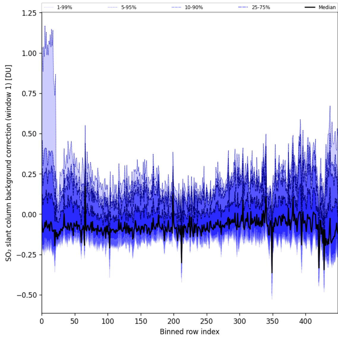
Figure 92: Along track statistics of “SO 2 slant column background correction (window 1)” for 2025-07-13 to 2025-07-14
