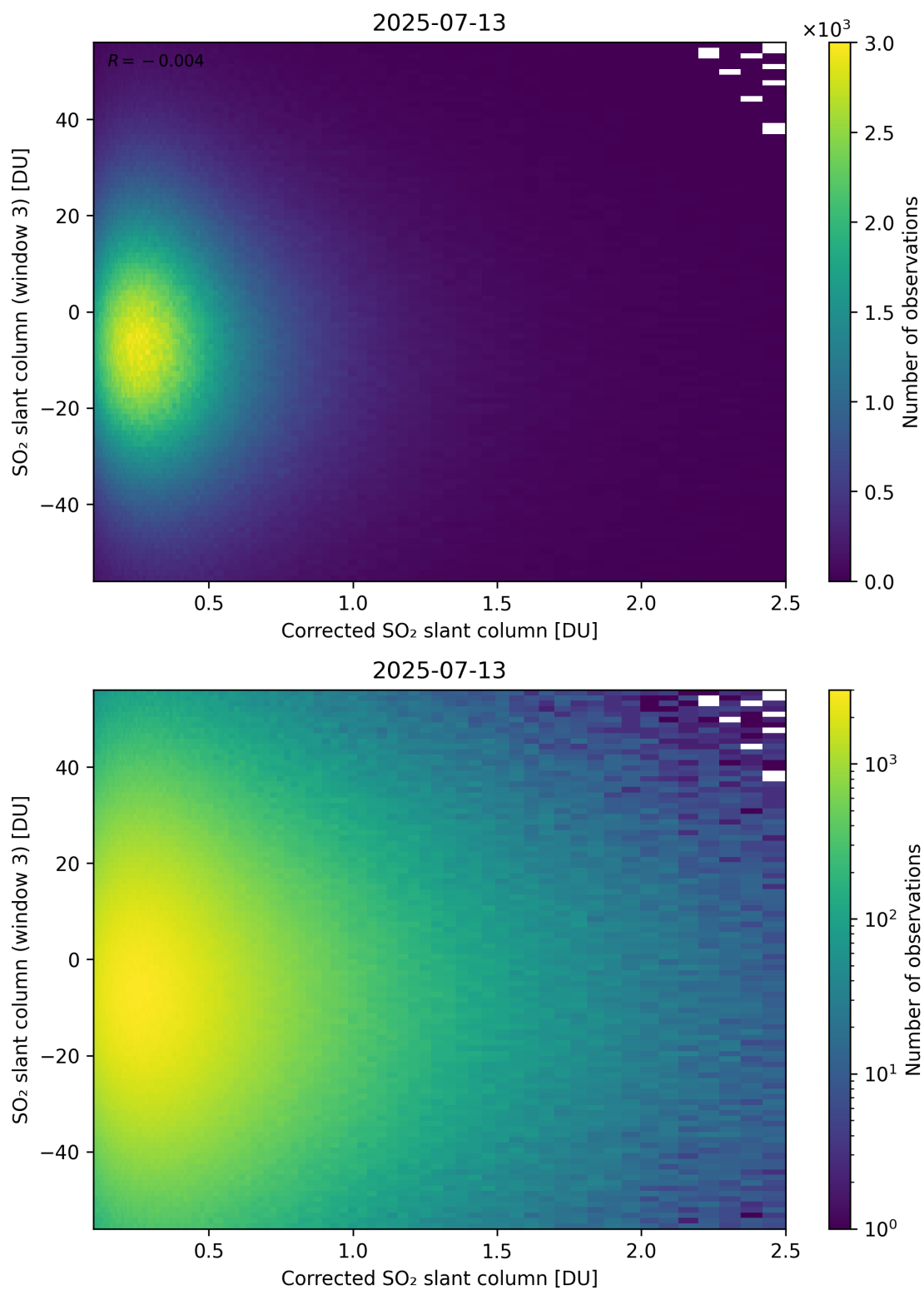
Figure 240: Scatter density plot of “Corrected SO 2 slant column” against “SO 2 slant column (window 3)” for 2025-07-13 to 2025-07-14.
