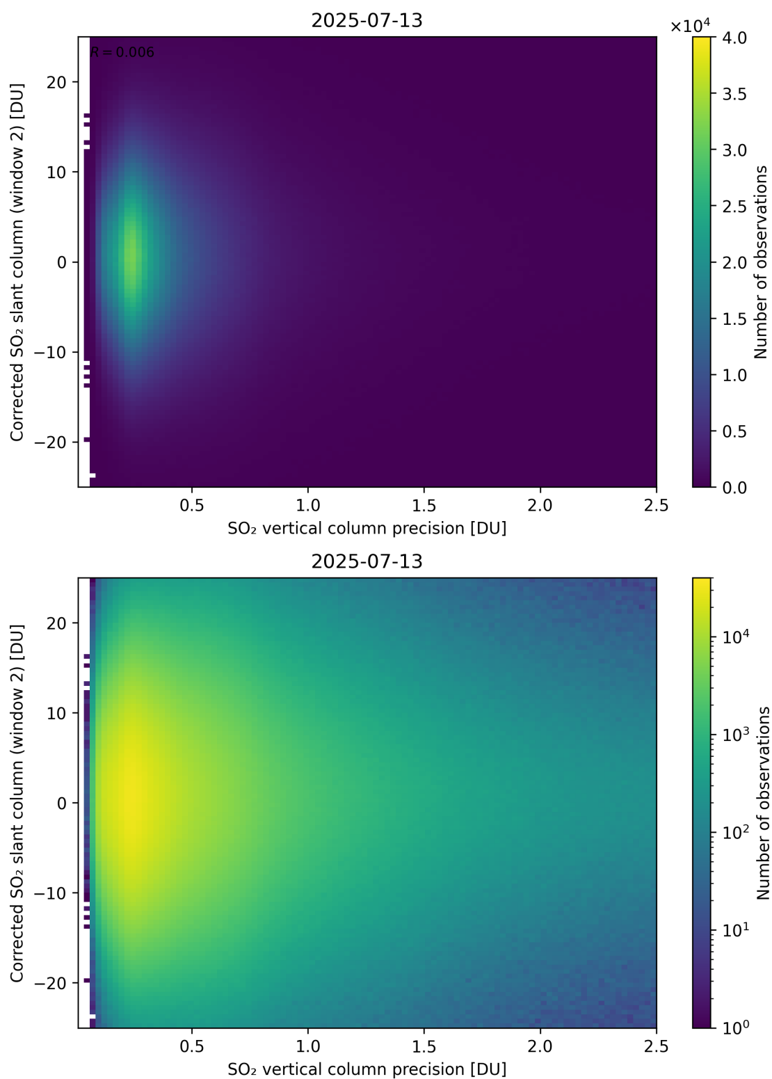
Figure 339: Scatter density plot of “SO 2 vertical column precision” against “Corrected SO 2 slant column (window 2)” for 2025-07-13 to 2025-07-14.
