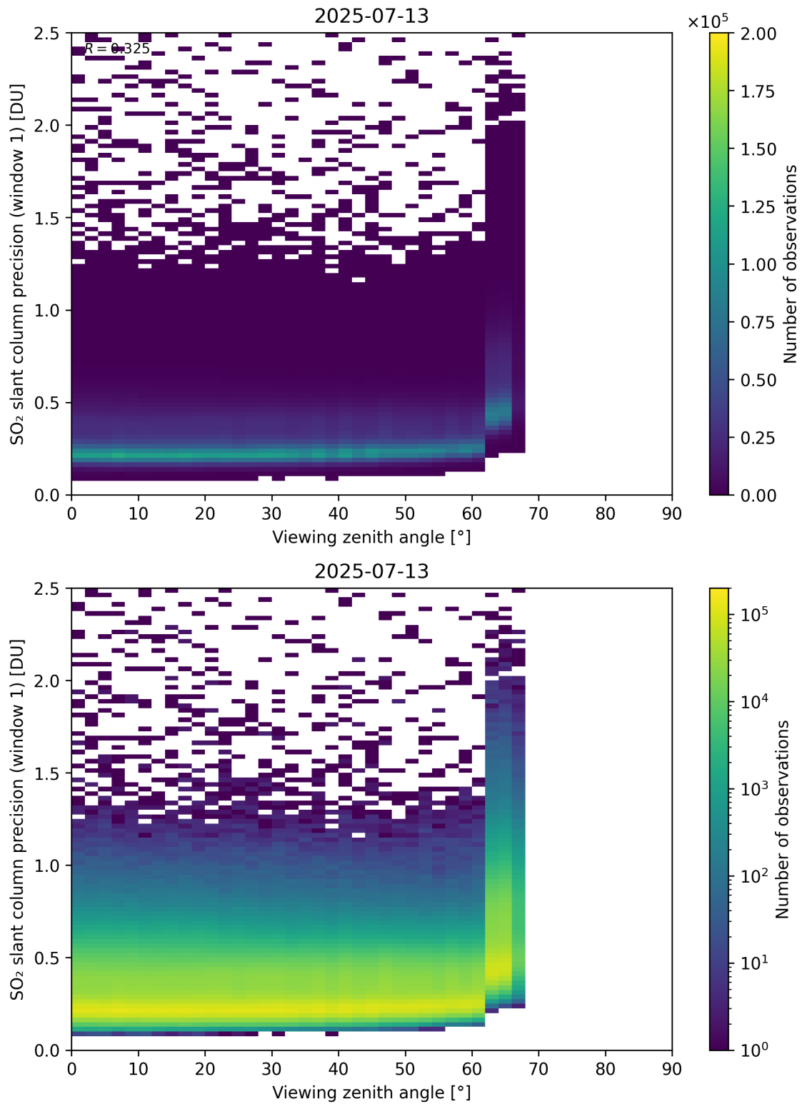
Figure 377: Scatter density plot of “Viewing zenith angle” against “SO 2 slant column precision (window 1)” for 2025-07-13 to 2025-07-14.
