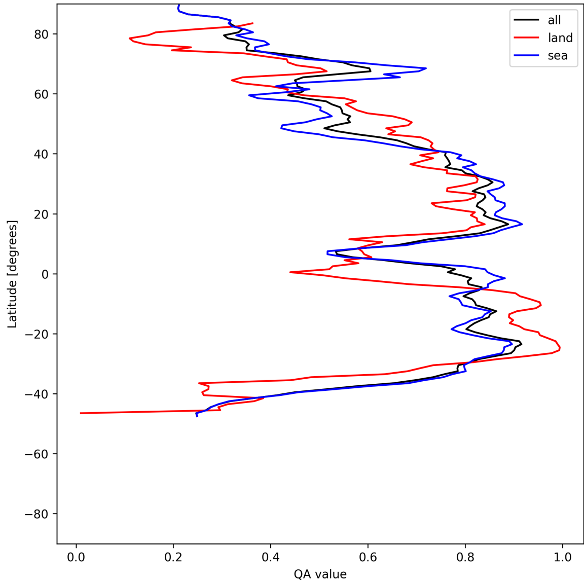
Figure 31: Zonal average of “QA value” for 2025-07-14 to 2025-07-16.
