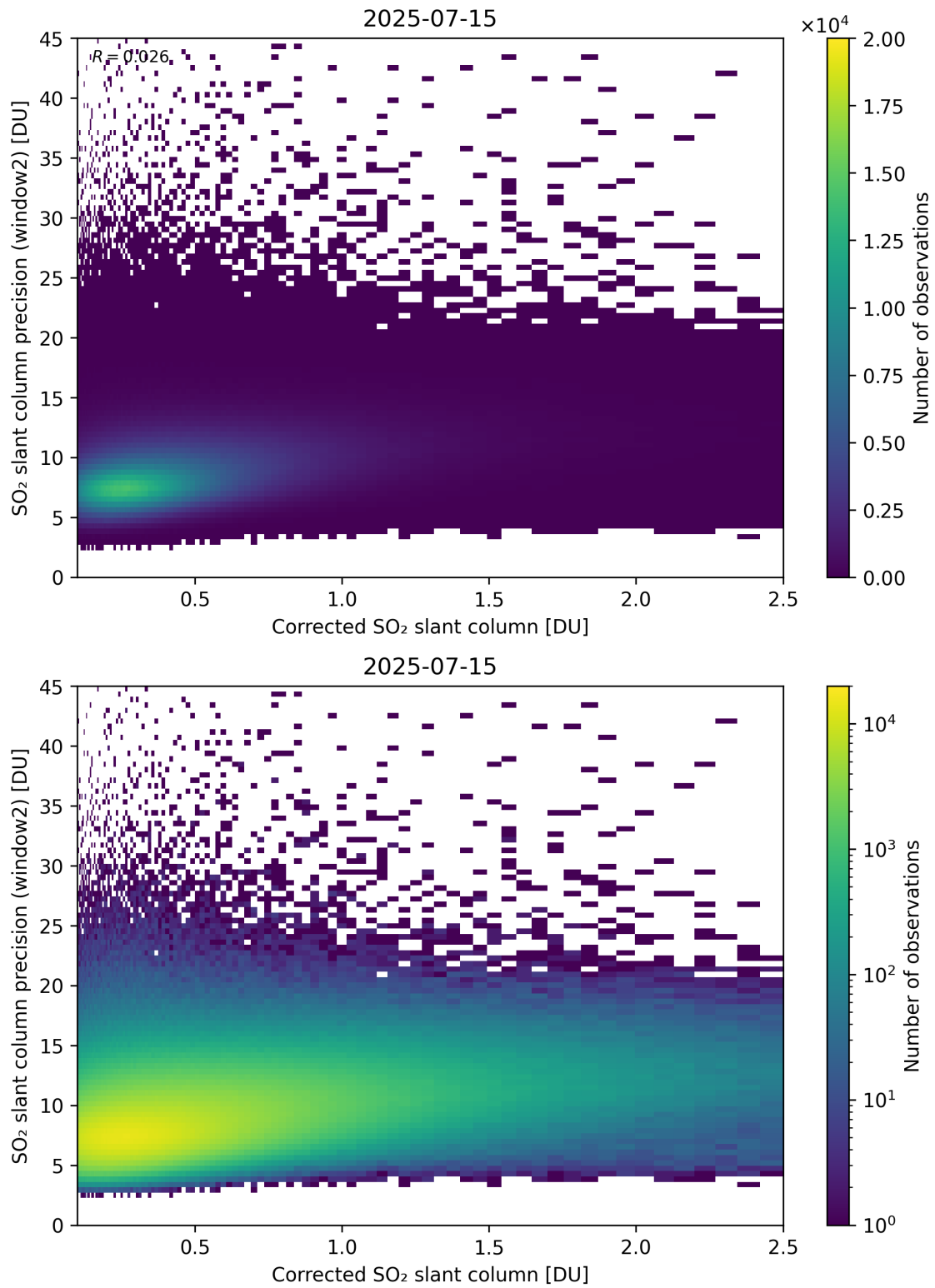
Figure 239: Scatter density plot of “Corrected SO 2 slant column” against “SO 2 slant column precision (window2)” for 2025-07-14 to 2025-07-16.
