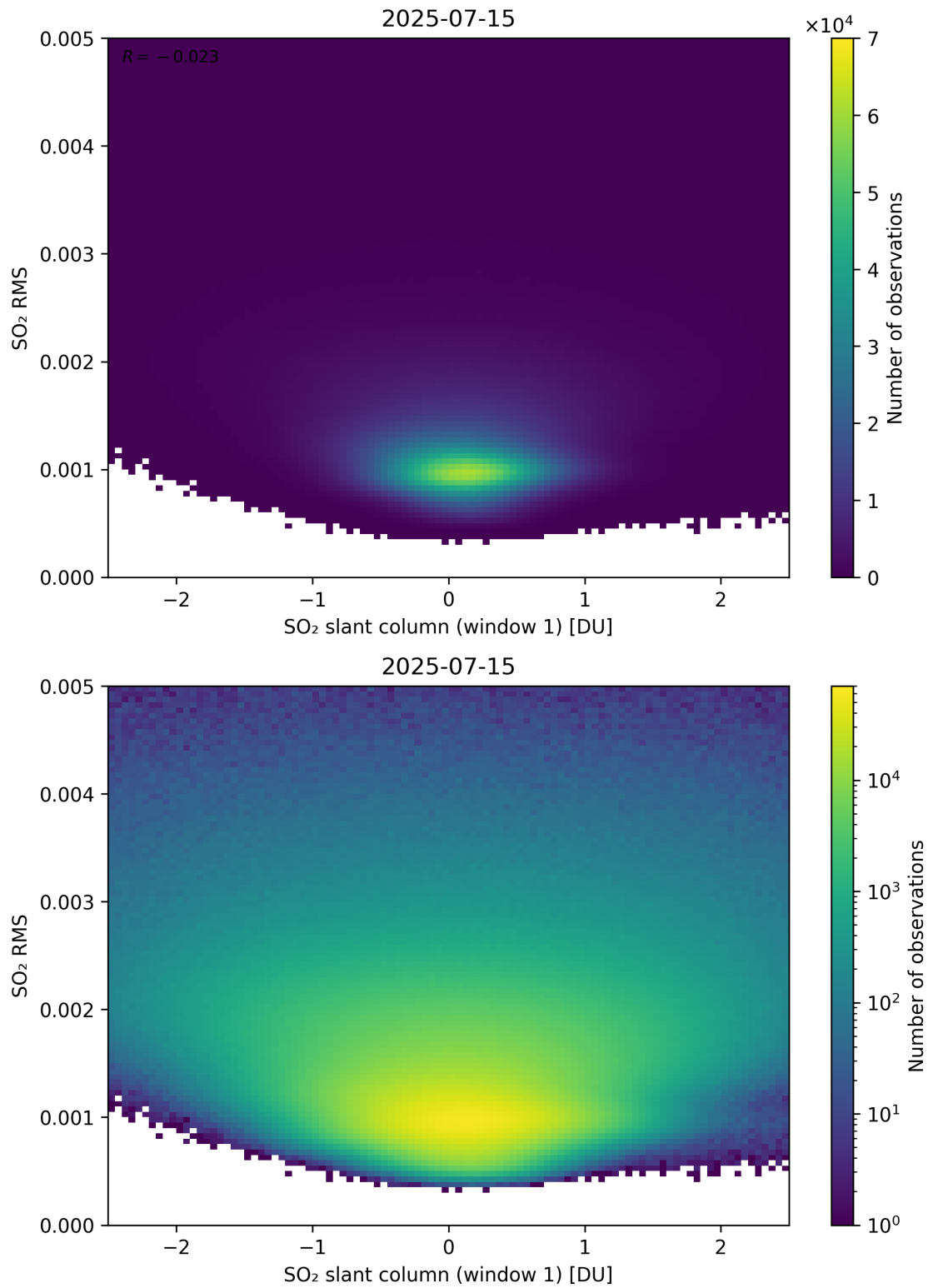
Figure 267: Scatter density plot of “SO 2 slant column (window 1)” against “SO 2 RMS” for 2025-07-14 to 2025-07-16.
