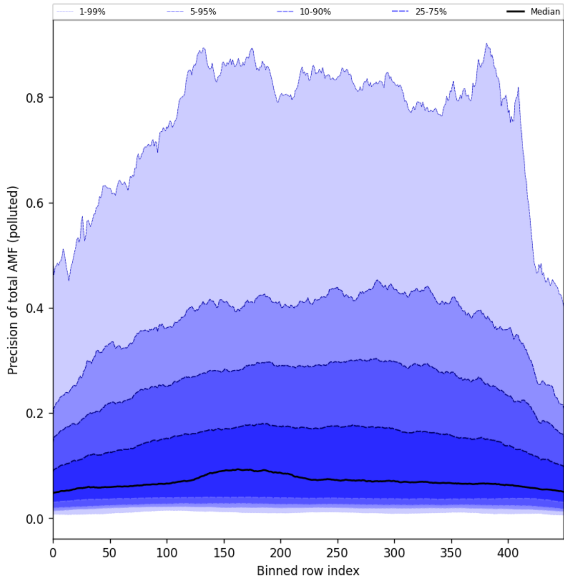
Figure 106: Along track statistics of “Precision of total AMF (polluted)” for 2025-07-14 to 2025-07-16
