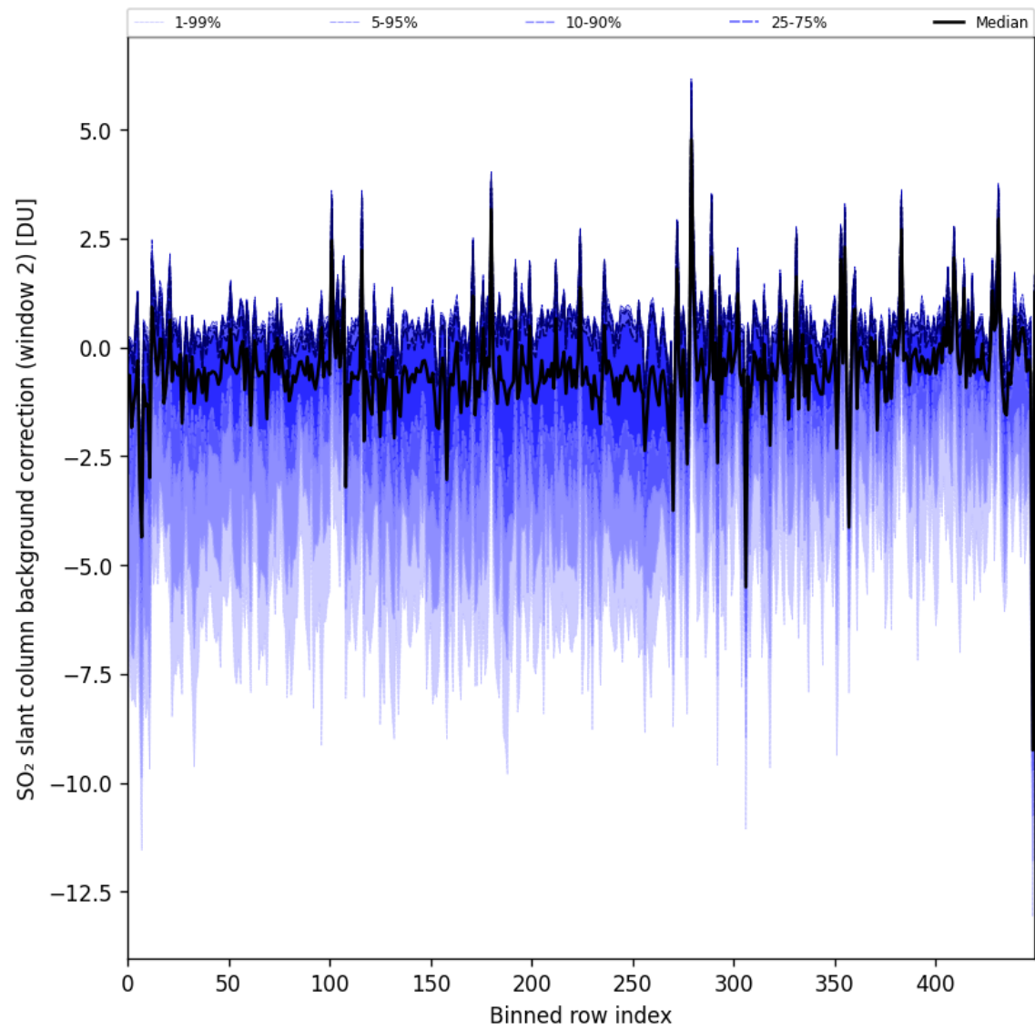
Figure 96: Along track statistics of “SO 2 slant column background correction (window 2)” for 2025-07-14 to 2025-07-16
