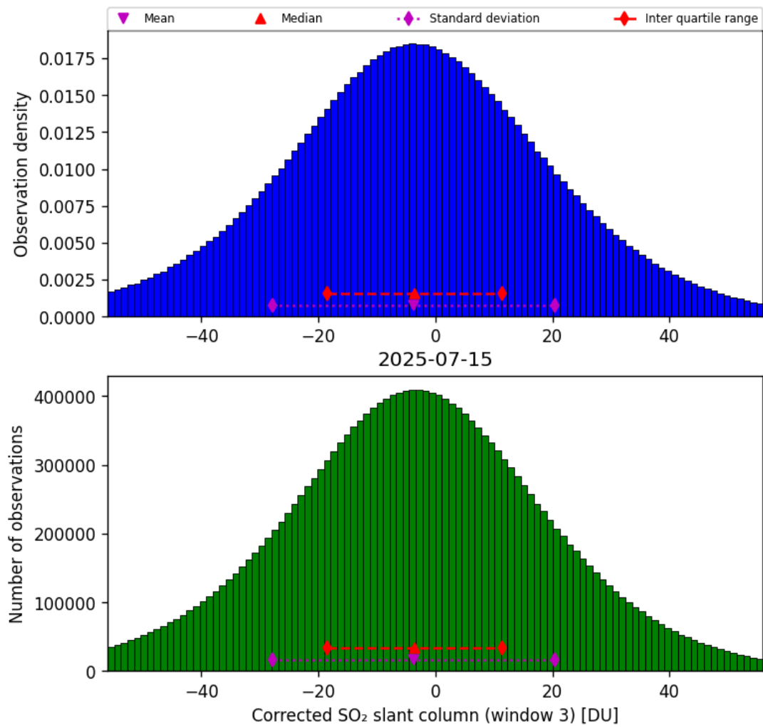
Figure 73: Histogram of “Corrected SO 2 slant column (window 3)” for 2025-07-14 to 2025-07-16
