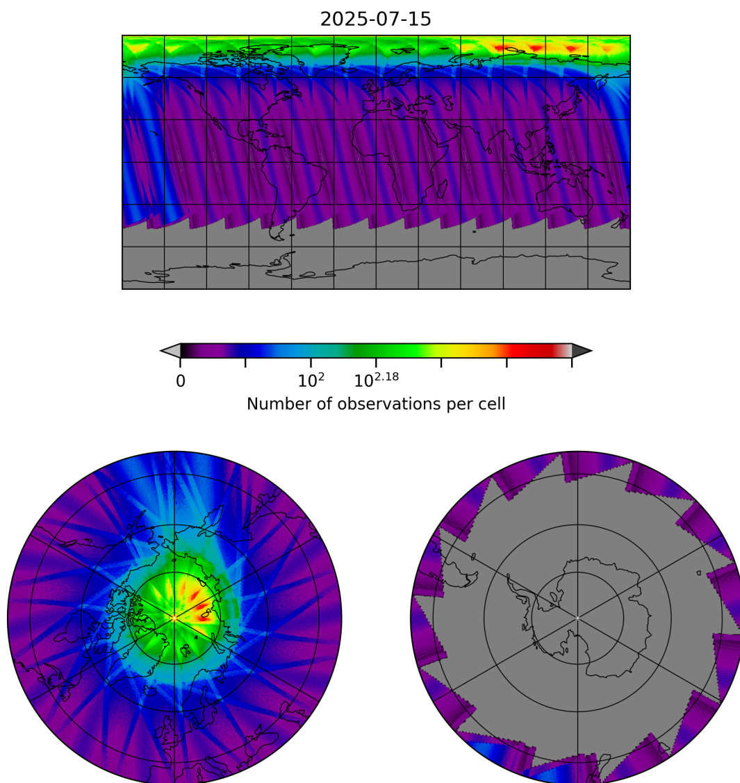
Figure 30: Map of the number of observations for 2025-07-14 to 2025-07-16
