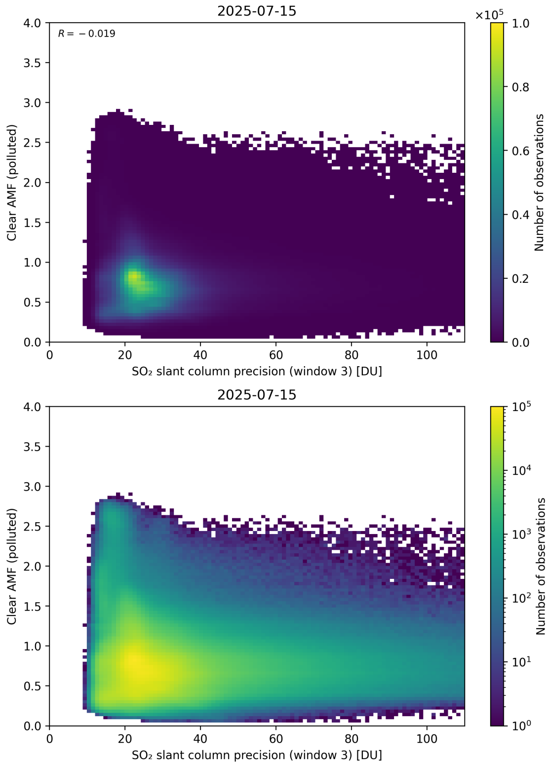
Figure 311: Scatter density plot of “SO 2 slant column precision (window 3)” against “Clear AMF (polluted)” for 2025-07-14 to 2025-07-16.
