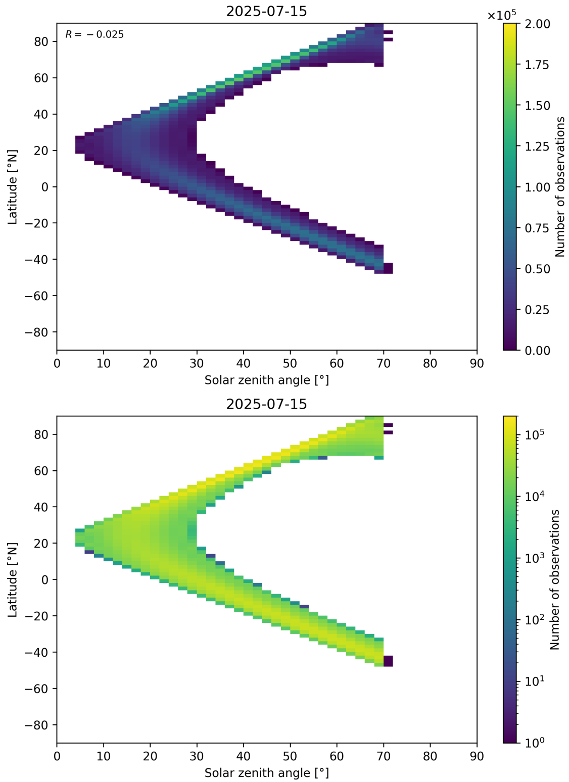
Figure 177: Scatter density plot of “Solar zenith angle” against “Latitude” for 2025-07-14 to 2025-07-16.
