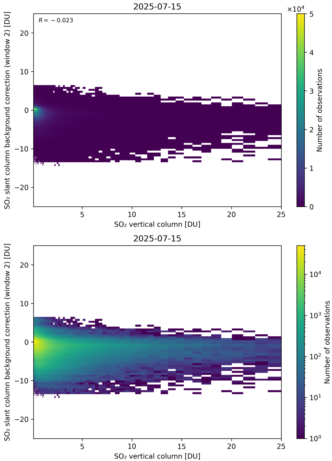
Figure 324: Scatter density plot of “SO 2 vertical column” against “SO 2 slant column background correction (window 2)” for 2025-07-14 to 2025-07-16.
