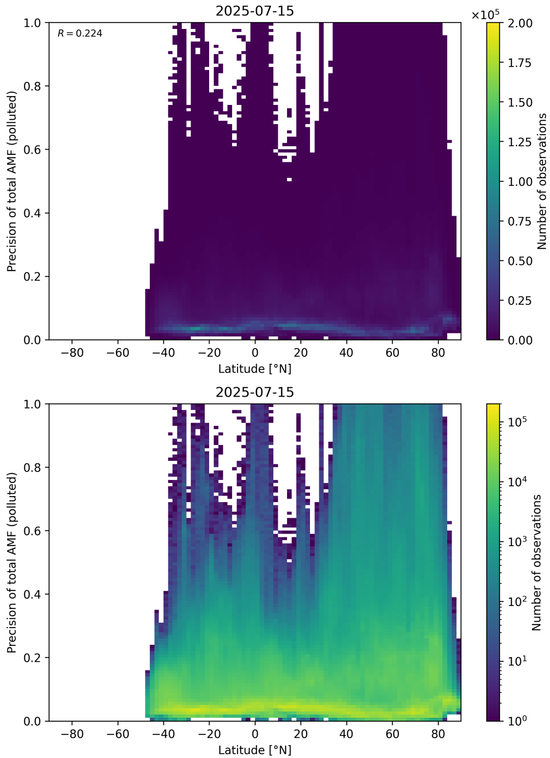
Figure 168: Scatter density plot of “Latitude” against “Precision of total AMF (polluted)” for 2025-07-14 to 2025-07-16.
