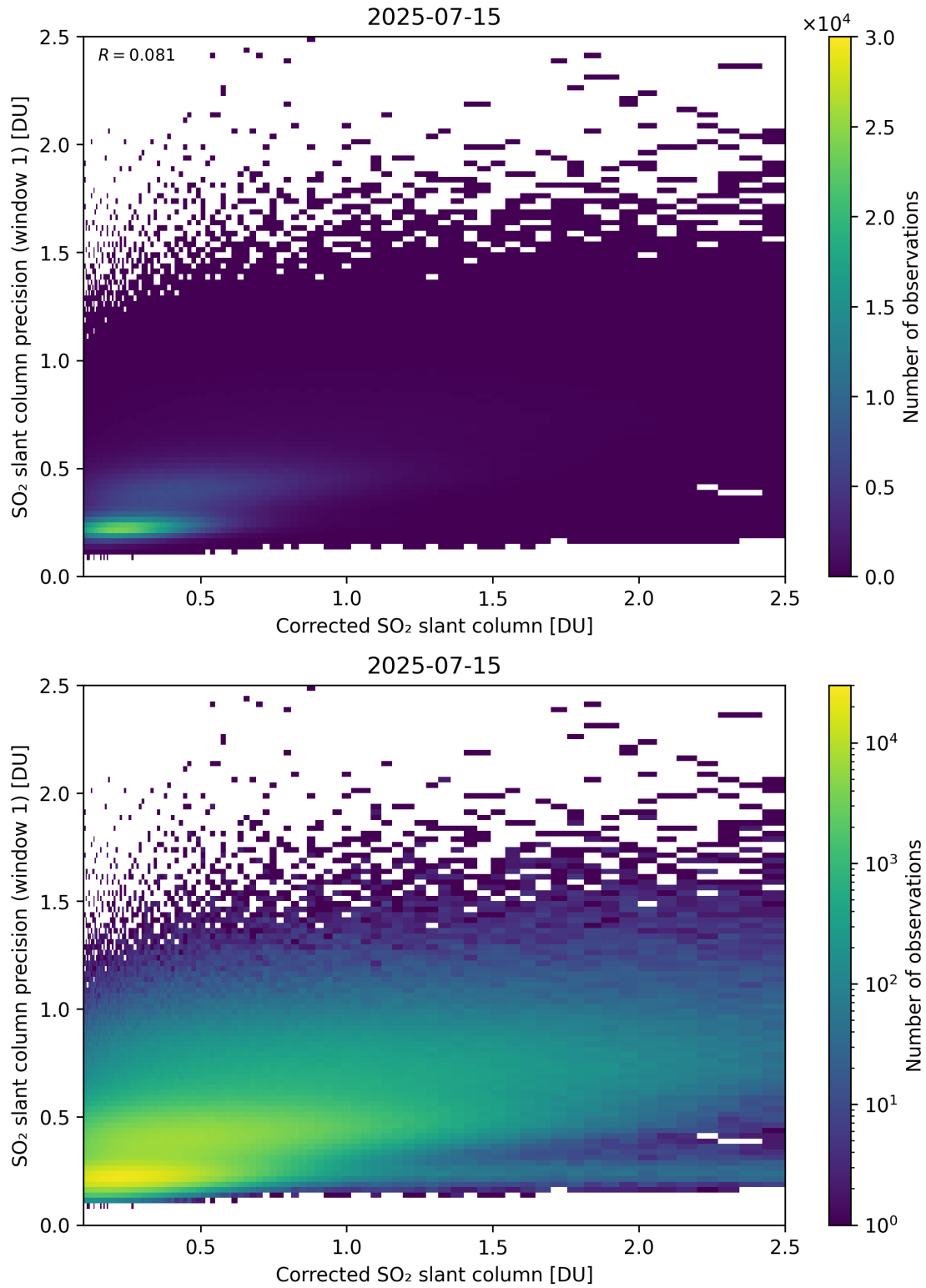
Figure 238: Scatter density plot of “Corrected SO 2 slant column” against “SO 2 slant column precision (window 1)” for 2025-07-14 to 2025-07-16.
