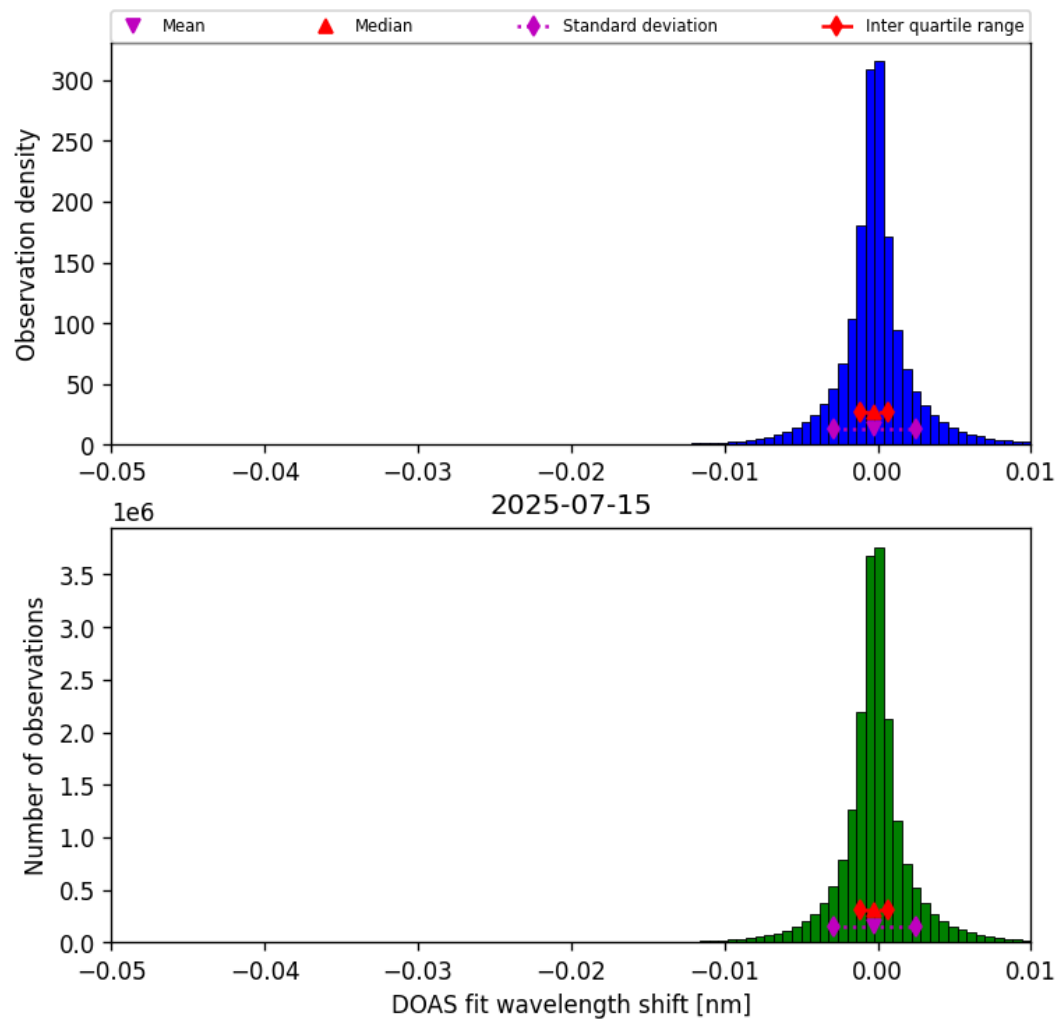
Figure 76: Histogram of “DOAS fit wavelength shift” for 2025-07-14 to 2025-07-16
