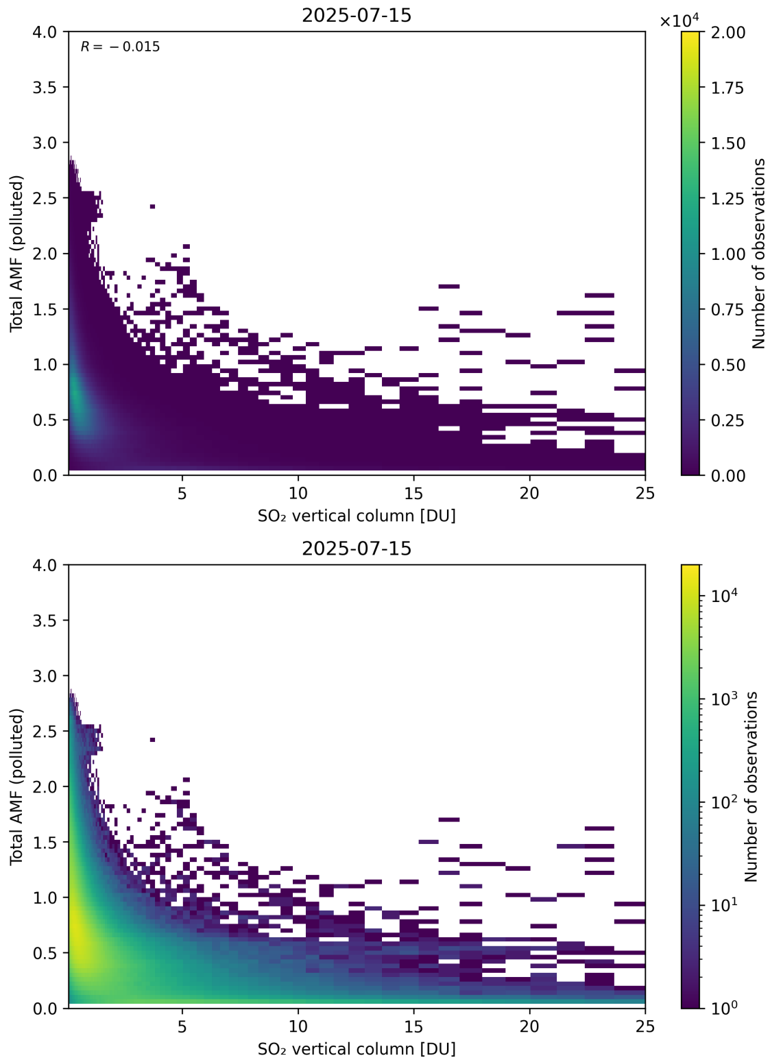
Figure 359: Scatter density plot of “SO 2 vertical column” against “Total AMF (polluted)” for 2025-07-14 to 2025-07-16.
