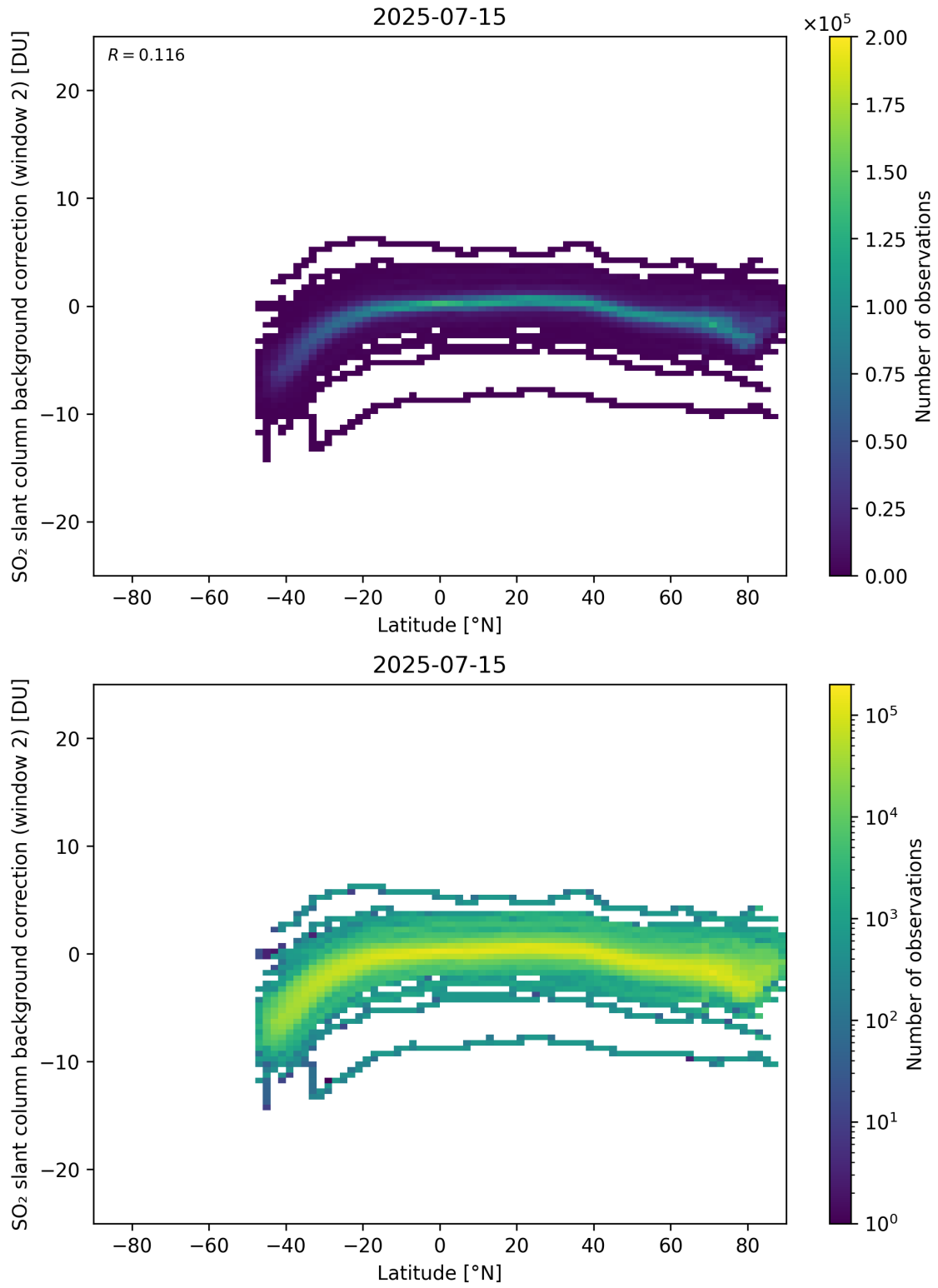
Figure 151: Scatter density plot of “Latitude” against “SO 2 slant column background correction (window 2)” for 2025-07-14 to 2025-07-16.
