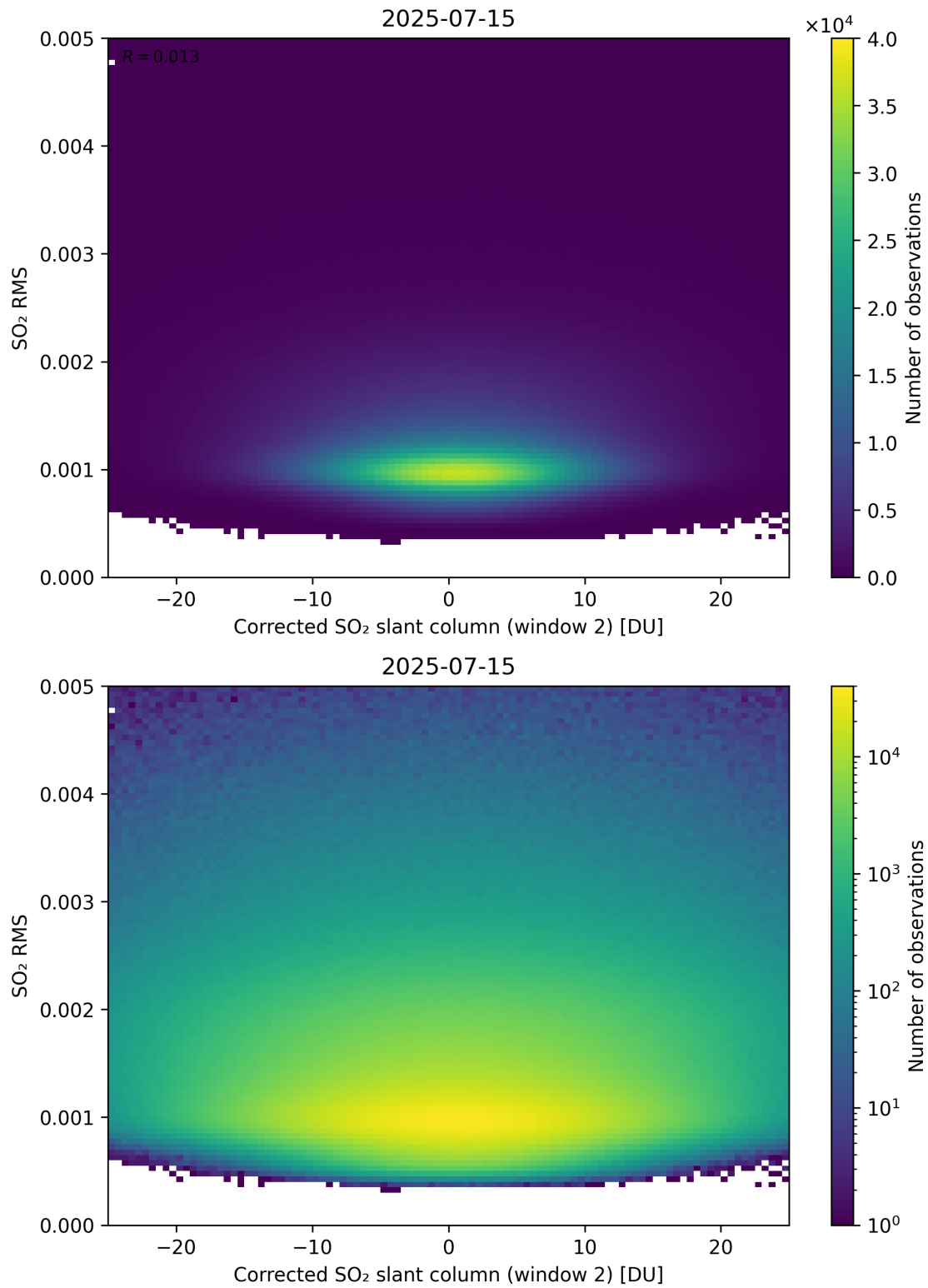
Figure 248: Scatter density plot of “Corrected SO 2 slant column (window 2)” against “SO 2 RMS” for 2025-07-14 to 2025-07-16.
