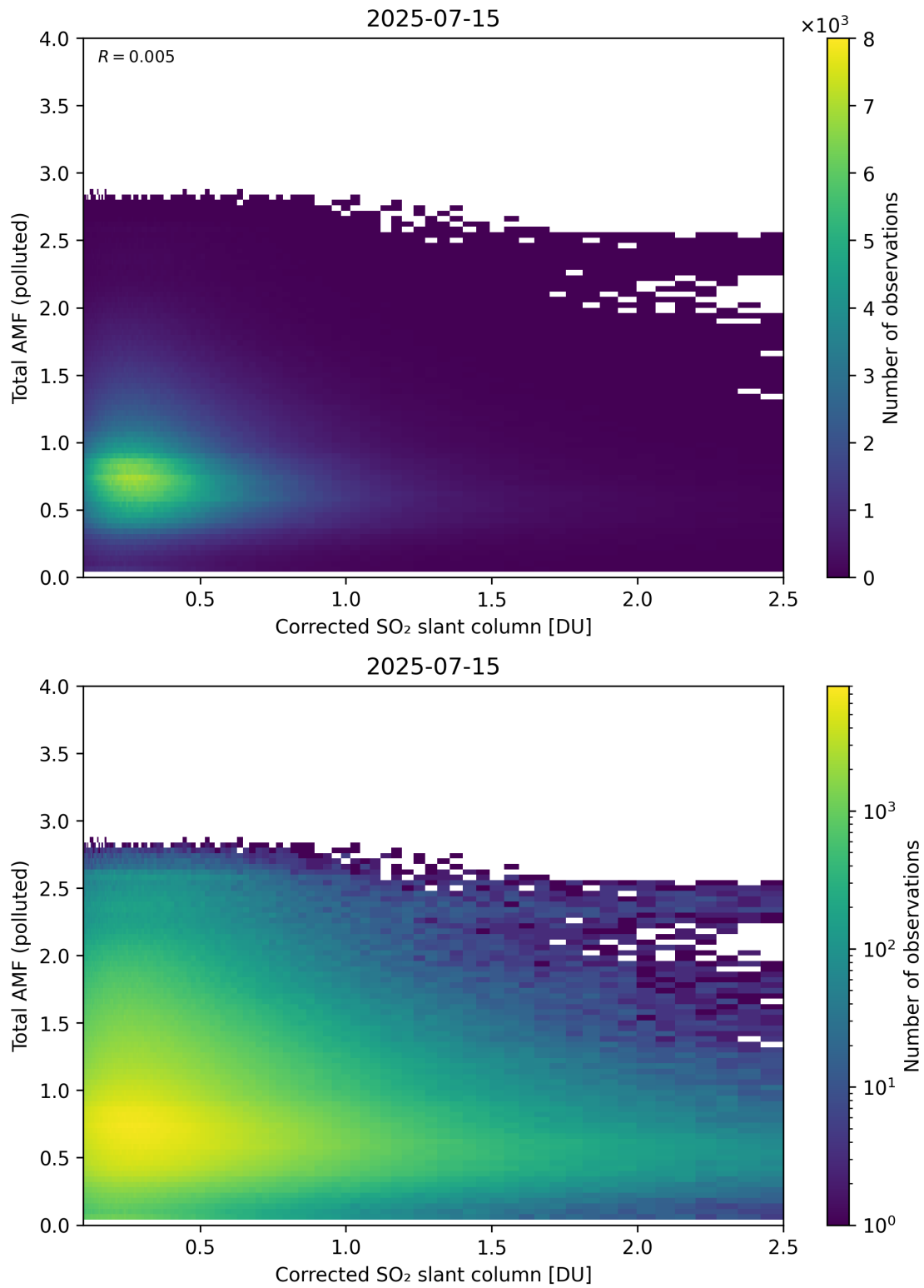
Figure 242: Scatter density plot of “Corrected SO 2 slant column” against “Total AMF (polluted)” for 2025-07-14 to 2025-07-16.
