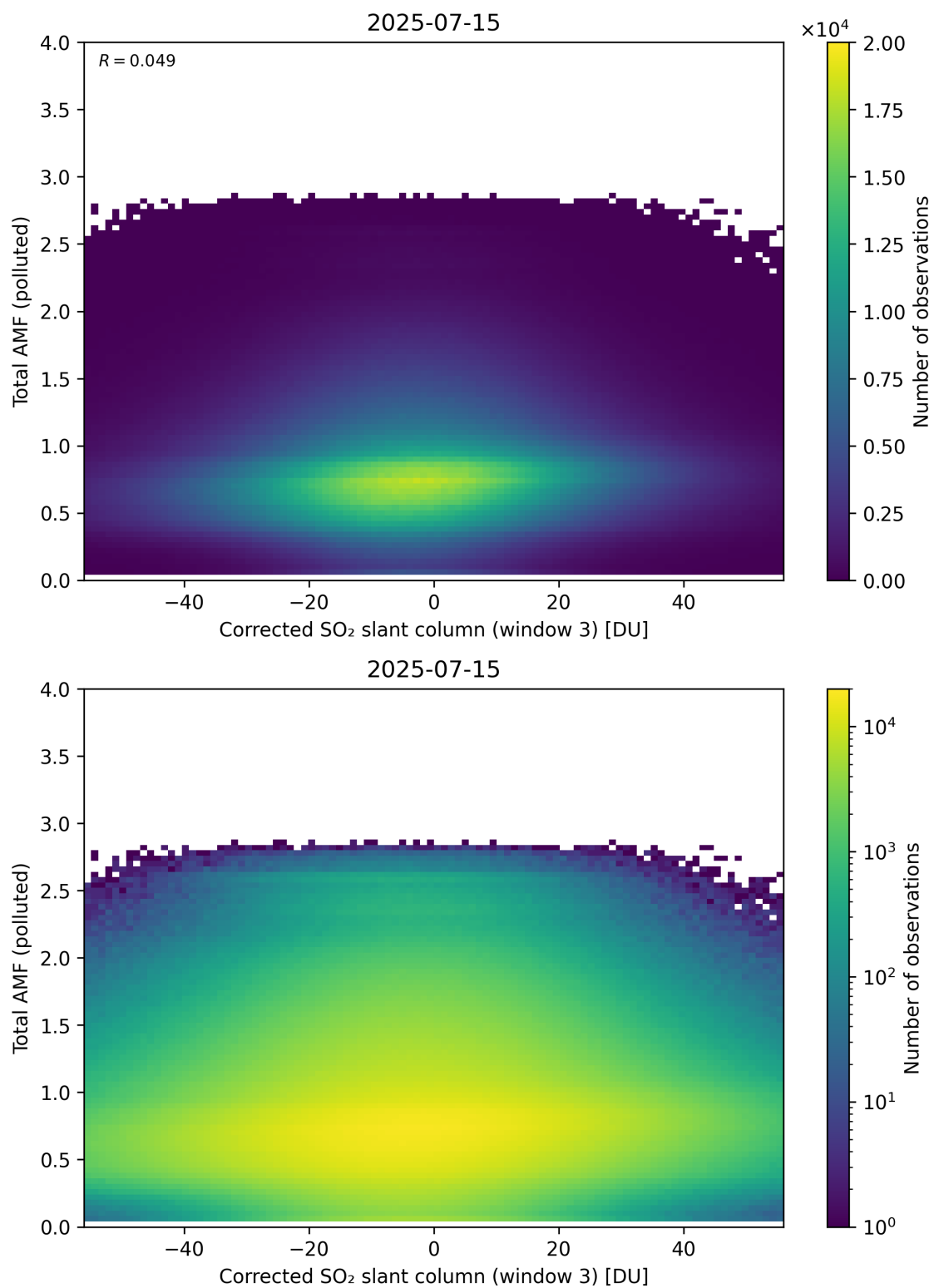
Figure 260: Scatter density plot of “Corrected SO 2 slant column (window 3)” against “Total AMF (polluted)” for 2025-07-14 to 2025-07-16.
