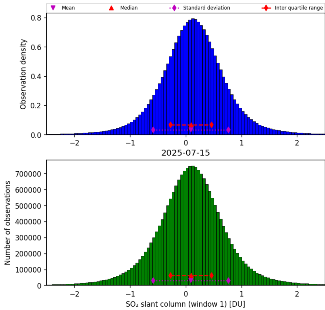
Figure 63: Histogram of “SO 2 slant column (window 1)” for 2025-07-14 to 2025-07-16
