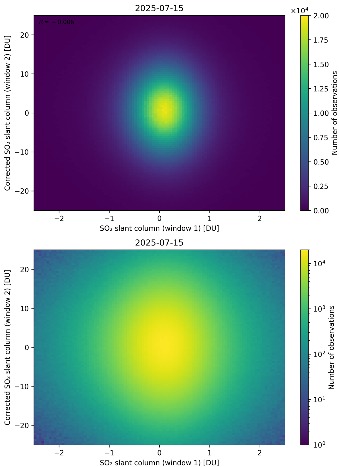
Figure 283: Scatter density plot of “SO 2 slant column (window 1)” against “Corrected SO 2 slant column (window 2)” for 2025-07-14 to 2025-07-16.
