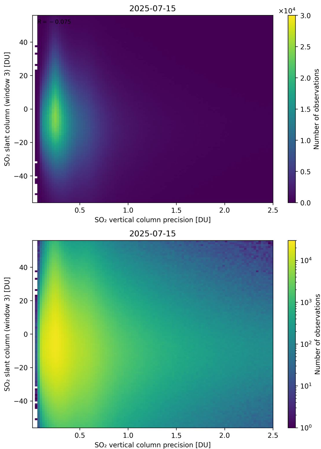
Figure 344: Scatter density plot of “SO 2 vertical column precision” against “SO 2 slant column (window 3)” for 2025-07-14 to 2025-07-16.
