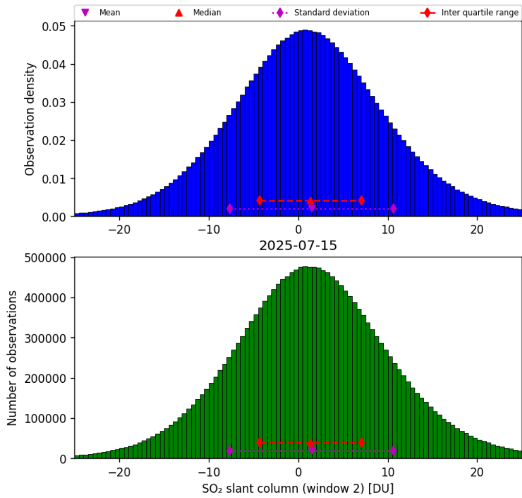
Figure 67: Histogram of “SO 2 slant column (window 2)” for 2025-07-14 to 2025-07-16
