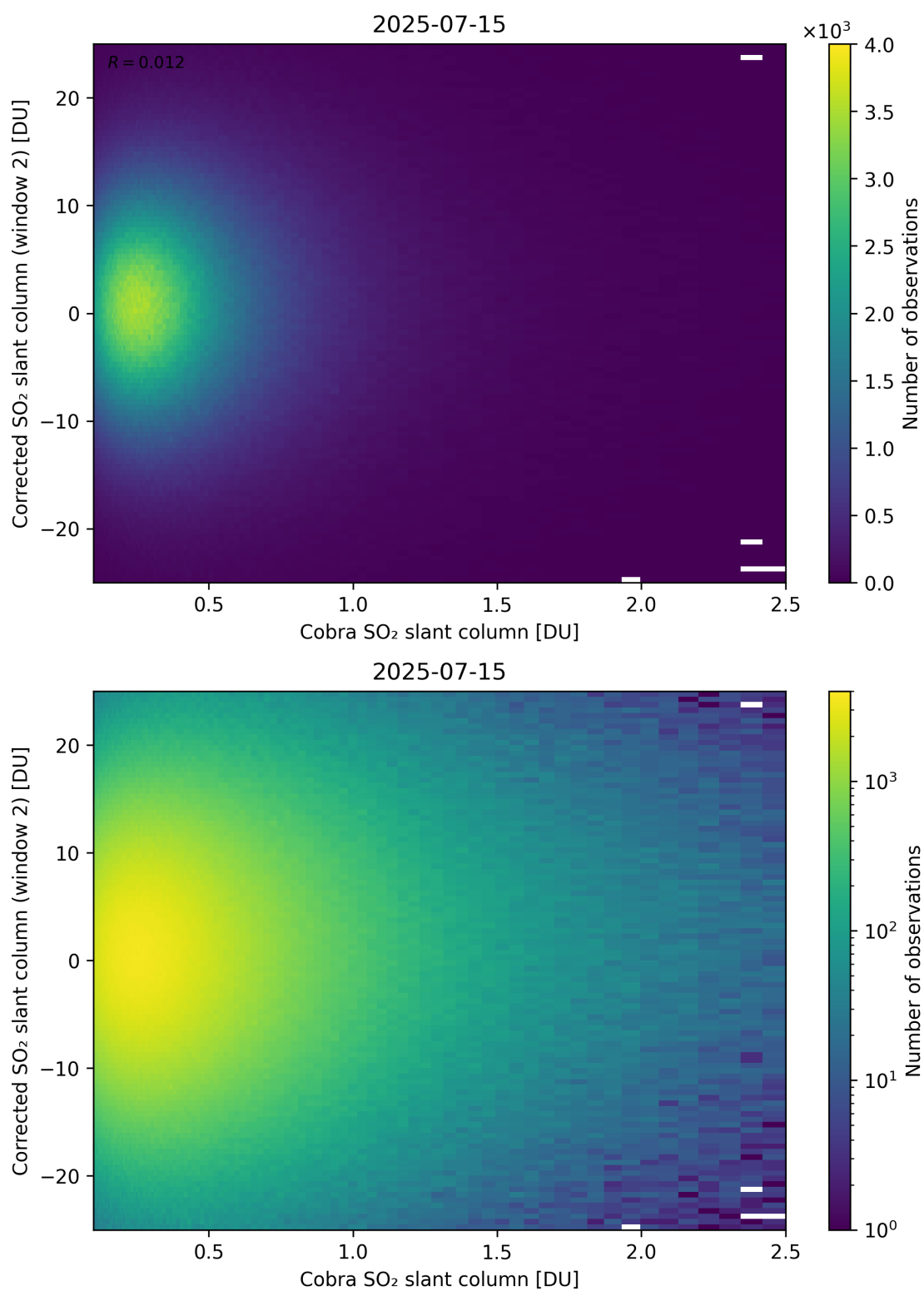
Figure 217: Scatter density plot of “Cobra SO 2 slant column” against “Corrected SO 2 slant column (window 2)” for 2025-07-14 to 2025-07-16.
