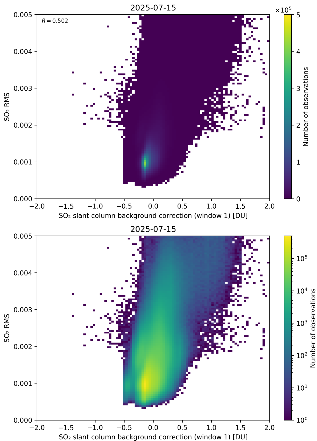
Figure 113: Scatter density plot of “SO 2 slant column background correction (window 1)” against “SO 2 RMS” for 2025-07-14 to 2025-07-16.
