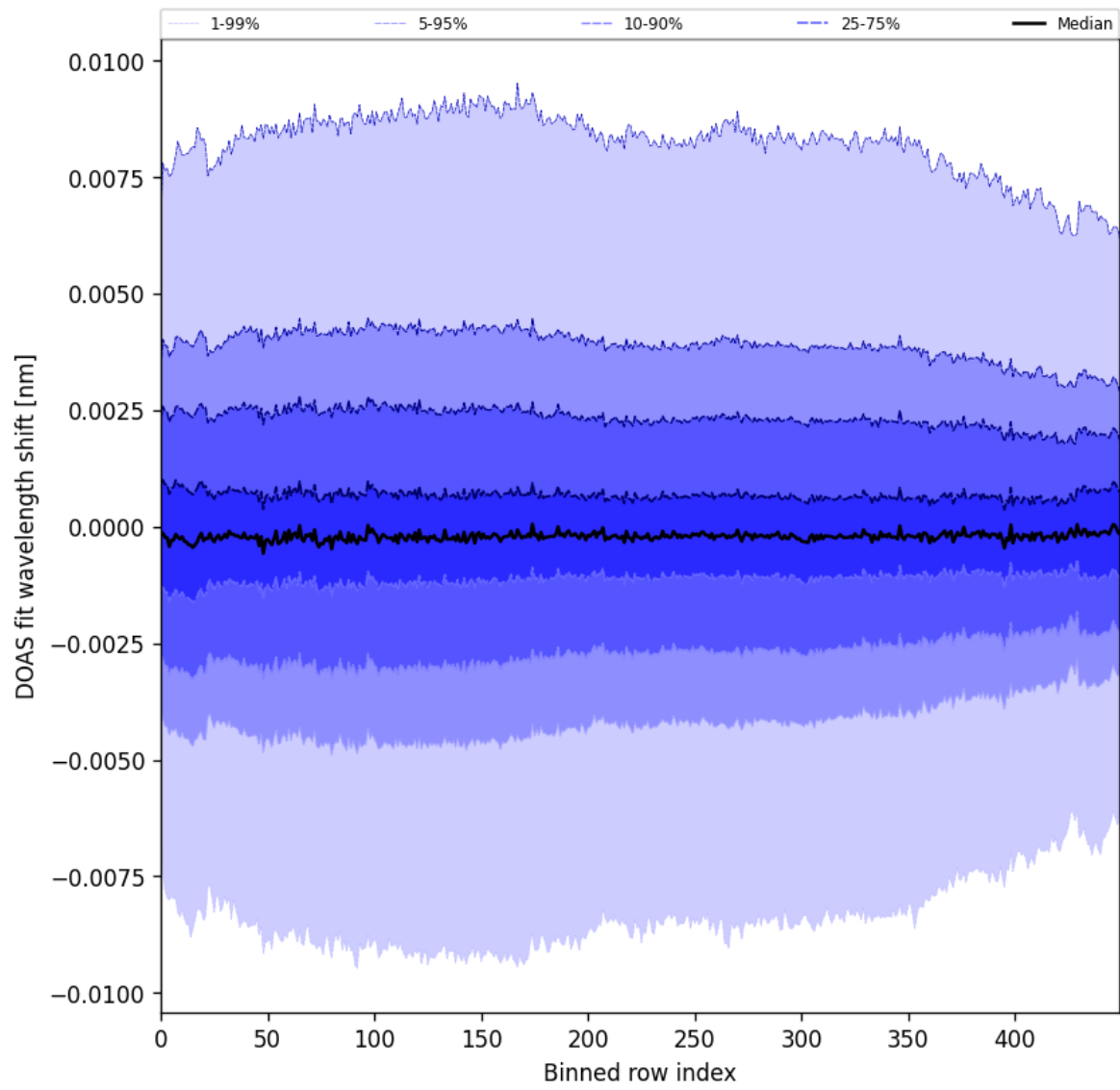
Figure 102: Along track statistics of “DOAS fit wavelength shift” for 2025-07-14 to 2025-07-16
