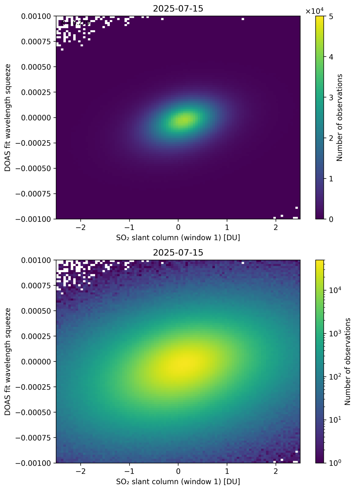
Figure 266: Scatter density plot of “SO 2 slant column (window 1)” against “DOAS fit wavelength squeeze” for 2025-07-14 to 2025-07-16.
