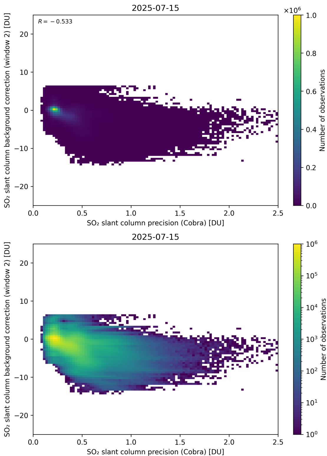
Figure 200: Scatter density plot of “SO 2 slant column precision (Cobra)” against “SO 2 slant column background correction (window 2)” for 2025-07-14 to 2025-07-16.
