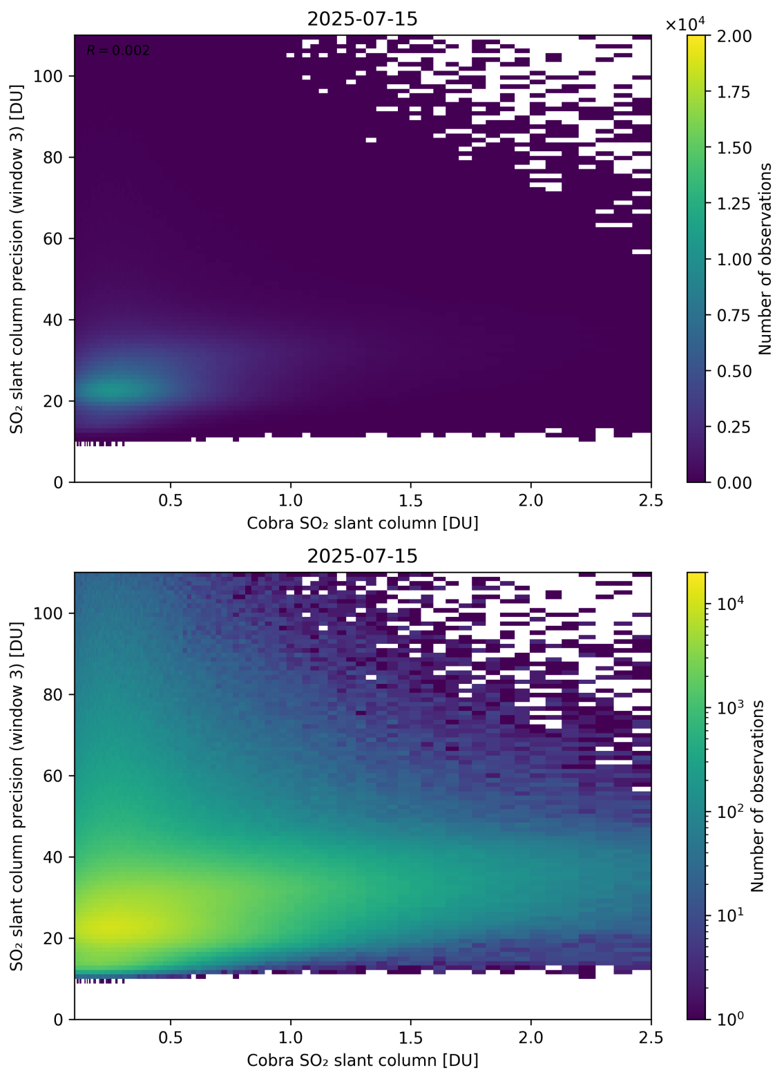
Figure 223: Scatter density plot of “Cobra SO 2 slant column” against “SO 2 slant column precision (window 3)” for 2025-07-14 to 2025-07-16.
