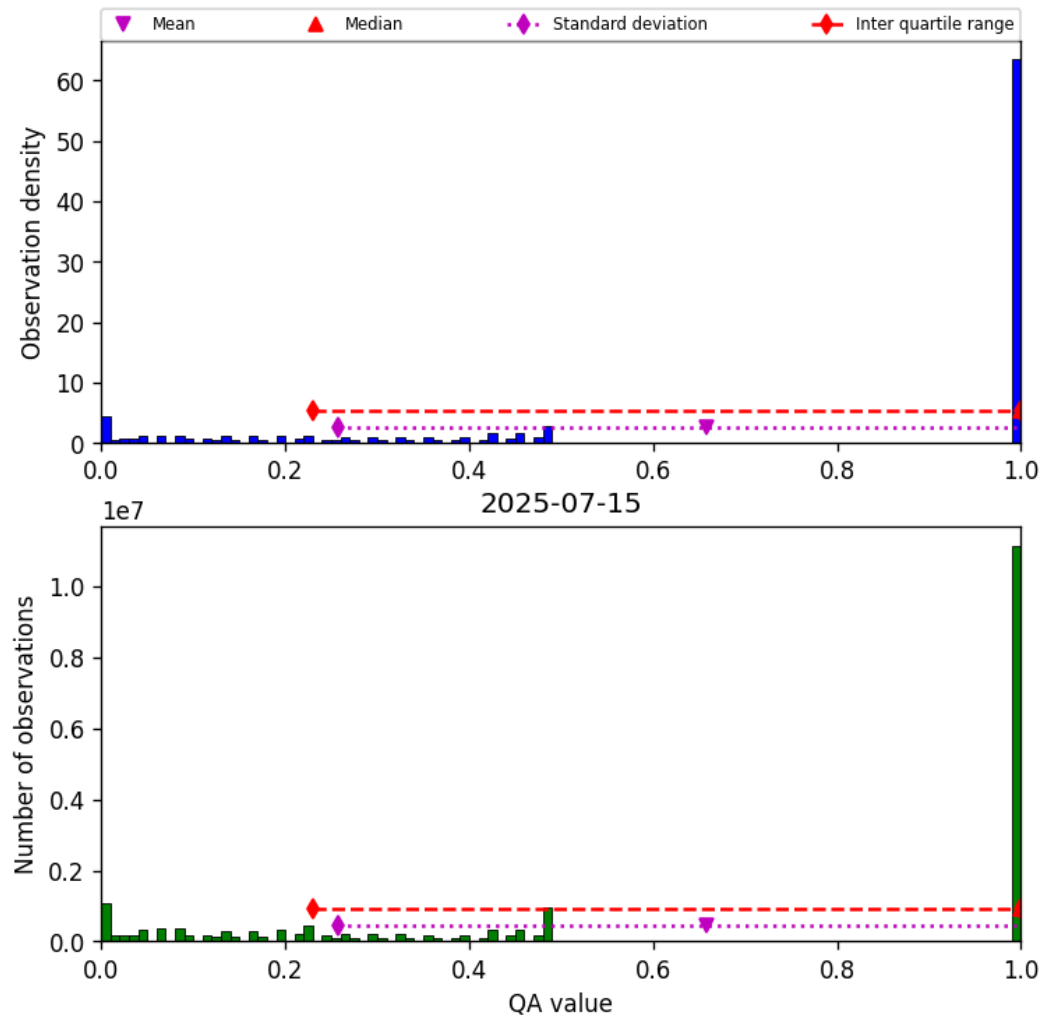
Figure 57: Histogram of “QA value” for 2025-07-14 to 2025-07-16
