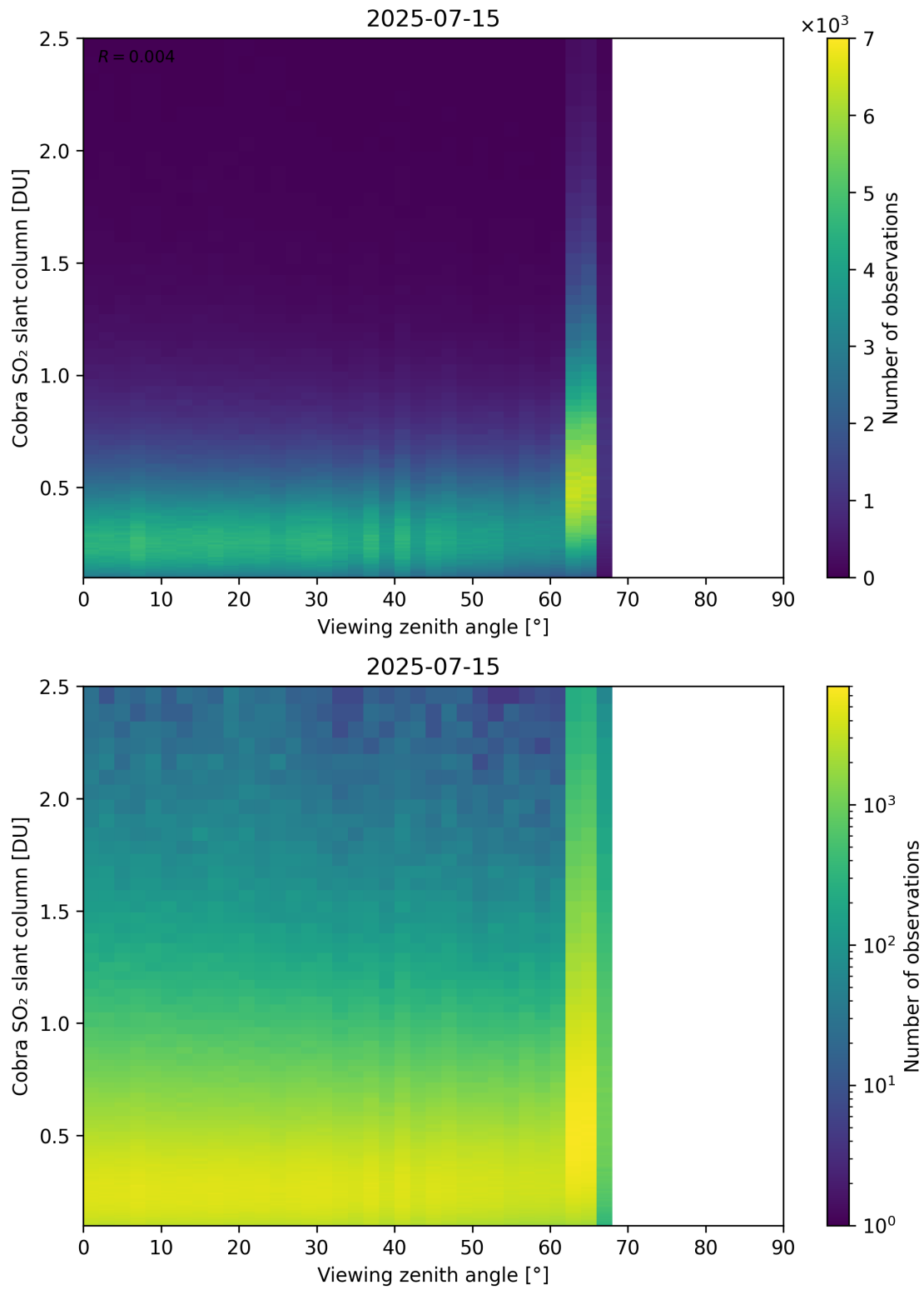
Figure 371: Scatter density plot of “Viewing zenith angle” against “Cobra SO 2 slant column” for 2025-07-14 to 2025-07-16.
