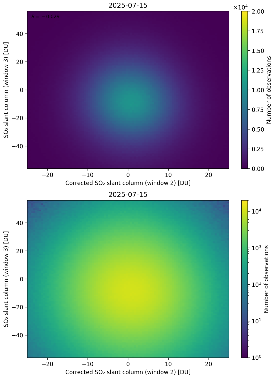
Figure 251: Scatter density plot of “Corrected SO 2 slant column (window 2)” against “SO 2 slant column (window 3)” for 2025-07-14 to 2025-07-16.
