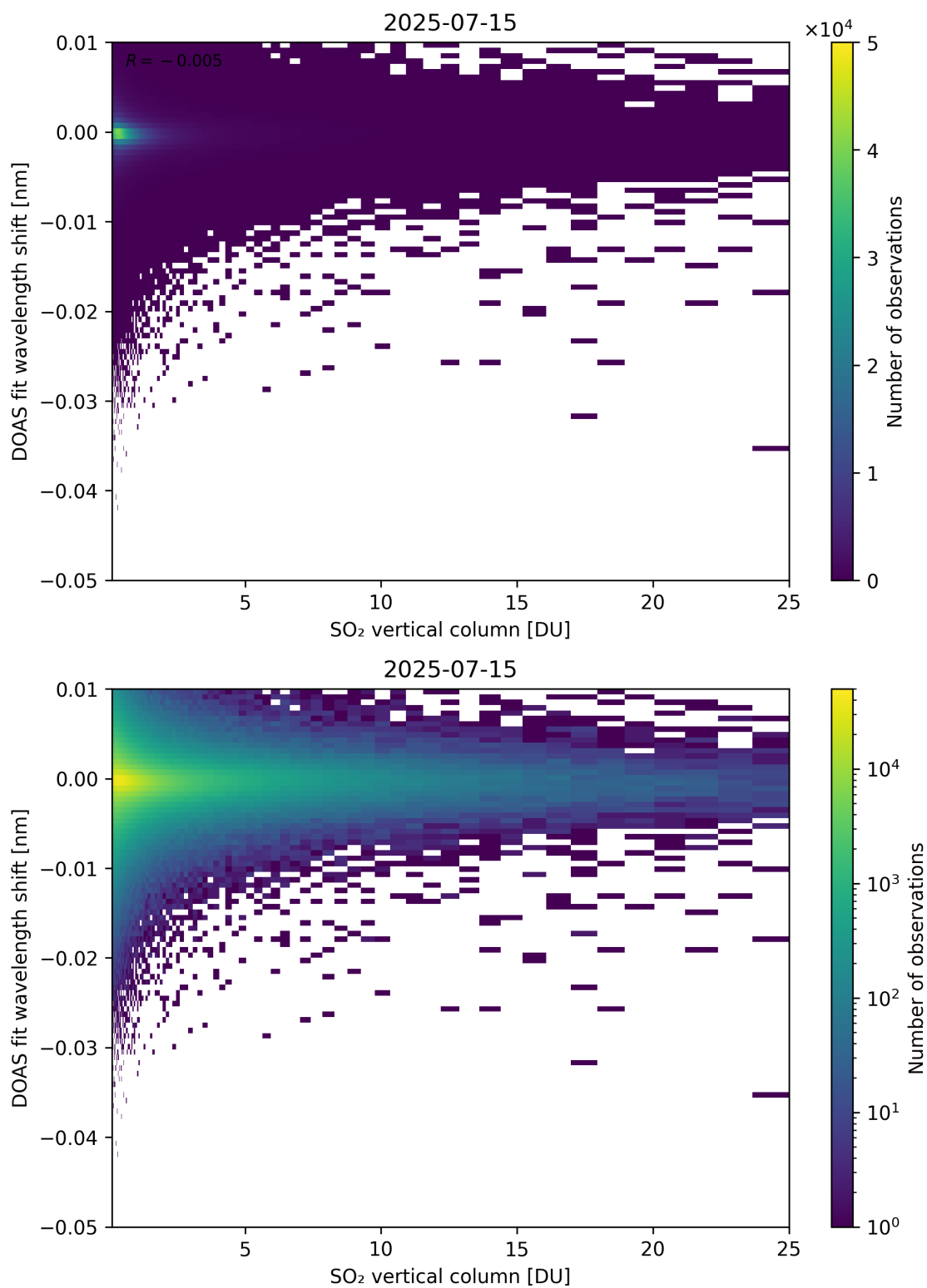
Figure 326: Scatter density plot of “SO 2 vertical column” against “DOAS fit wavelength shift” for 2025-07-14 to 2025-07-16.
