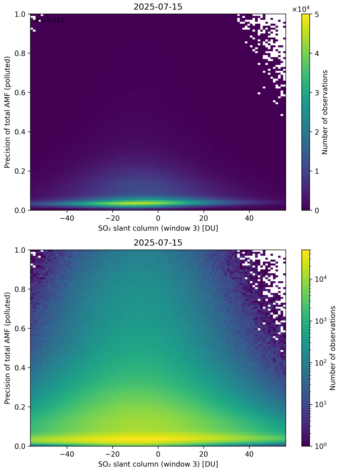
Figure 319: Scatter density plot of “SO 2 slant column (window 3)” against “Precision of total AMF (polluted)” for 2025-07-14 to 2025-07-16.
