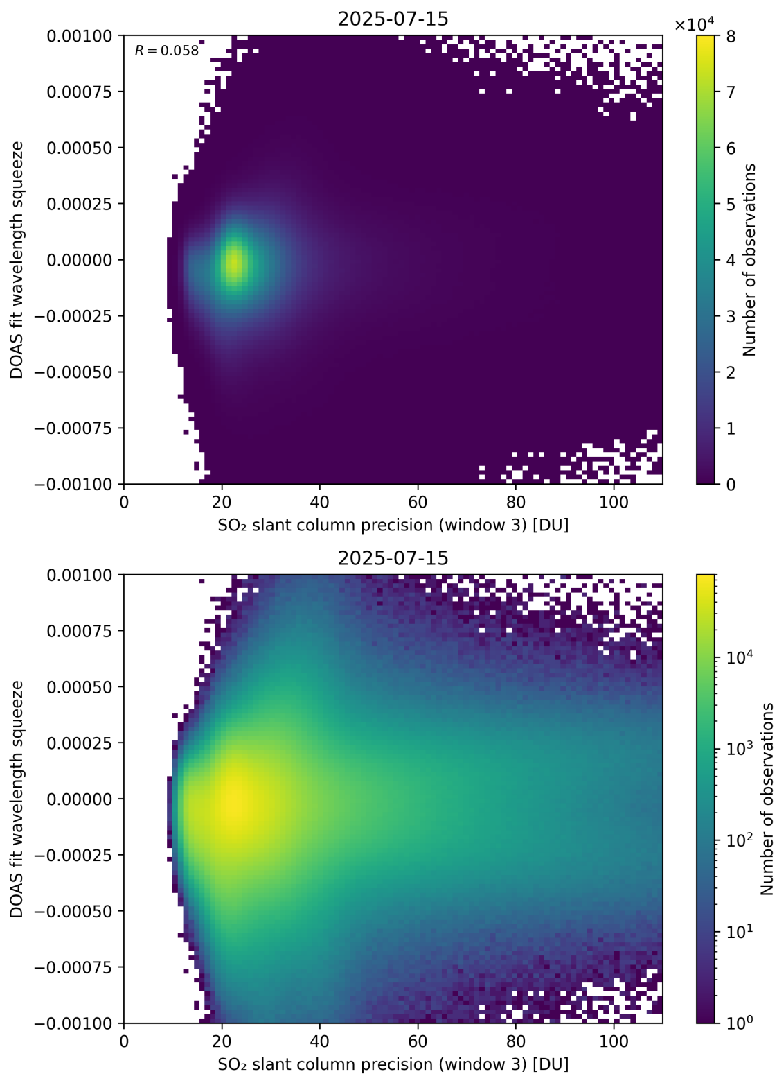
Figure 309: Scatter density plot of “SO 2 slant column precision (window 3)” against “DOAS fit wavelength squeeze” for 2025-07-14 to 2025-07-16.
