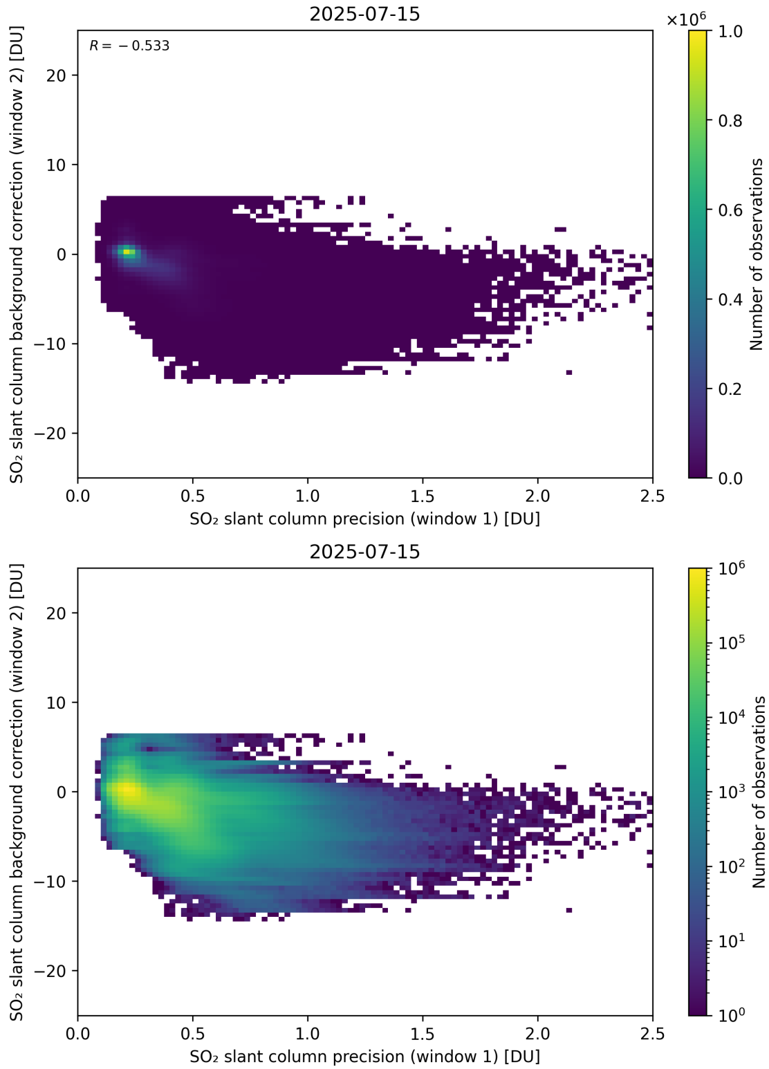
Figure 269: Scatter density plot of “SO 2 slant column precision (window 1)” against “SO 2 slant column background correction (window 2)” for 2025-07-14 to 2025-07-16.
