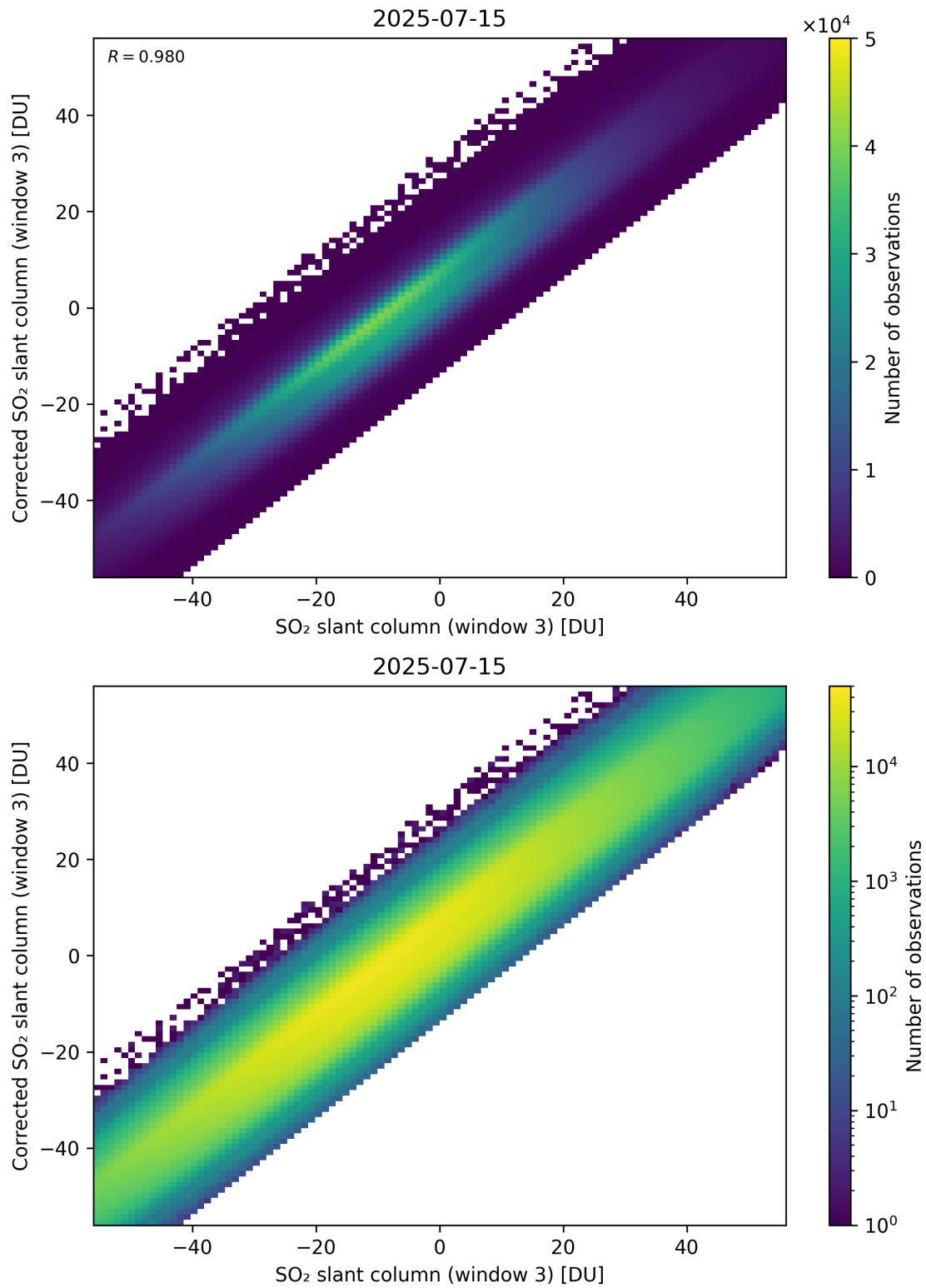
Figure 316: Scatter density plot of “SO 2 slant column (window 3)” against “Corrected SO 2 slant column (window 3)” for 2025-07-14 to 2025-07-16.
