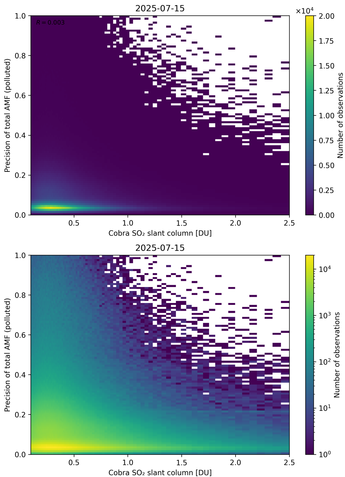
Figure 225: Scatter density plot of “Cobra SO 2 slant column” against “Precision of total AMF (polluted)” for 2025-07-14 to 2025-07-16.
