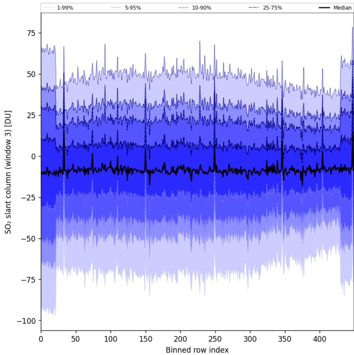
Figure 97: Along track statistics of “SO 2 slant column (window 3)” for 2025-07-14 to 2025-07-16
