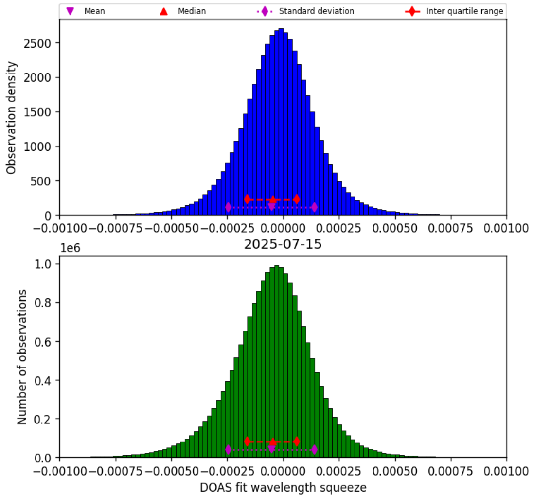
Figure 77: Histogram of “DOAS fit wavelength squeeze” for 2025-07-14 to 2025-07-16
