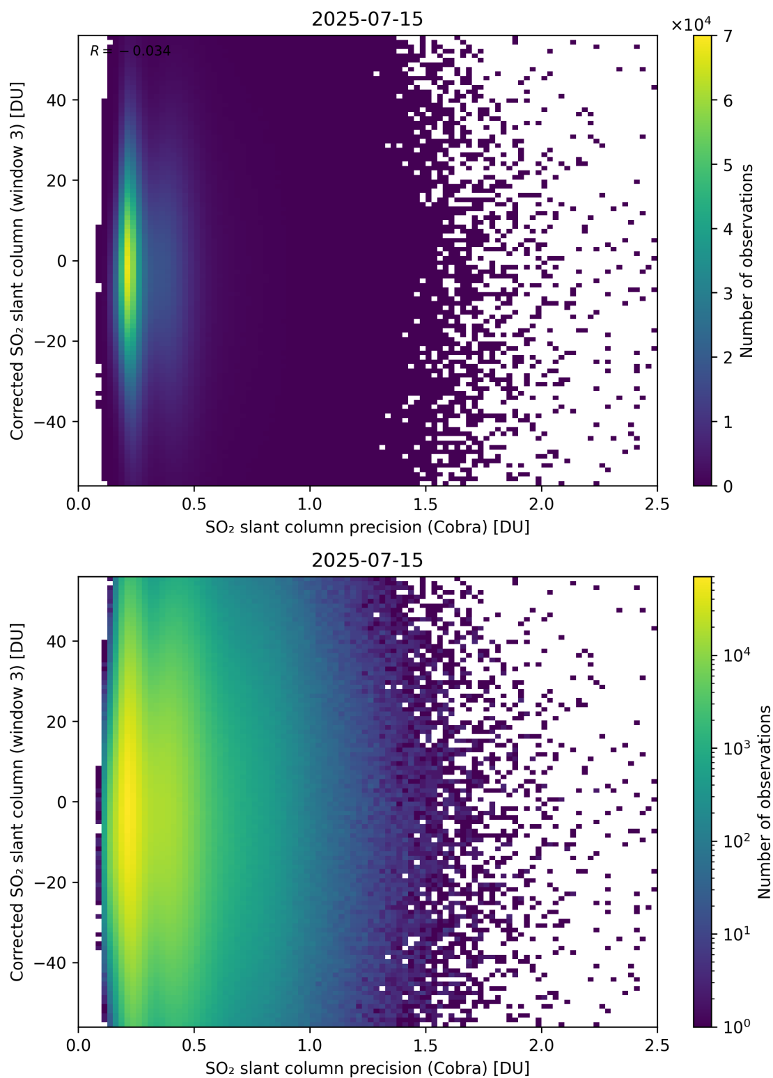
Figure 207: Scatter density plot of “SO 2 slant column precision (Cobra)” against “Corrected SO 2 slant column (window 3)” for 2025-07-14 to 2025-07-16.
