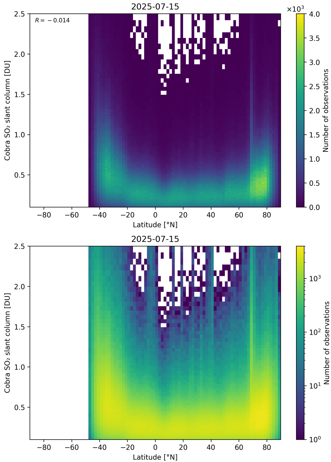
Figure 157: Scatter density plot of “Latitude” against “Cobra SO 2 slant column” for 2025-07-14 to 2025-07-16.
