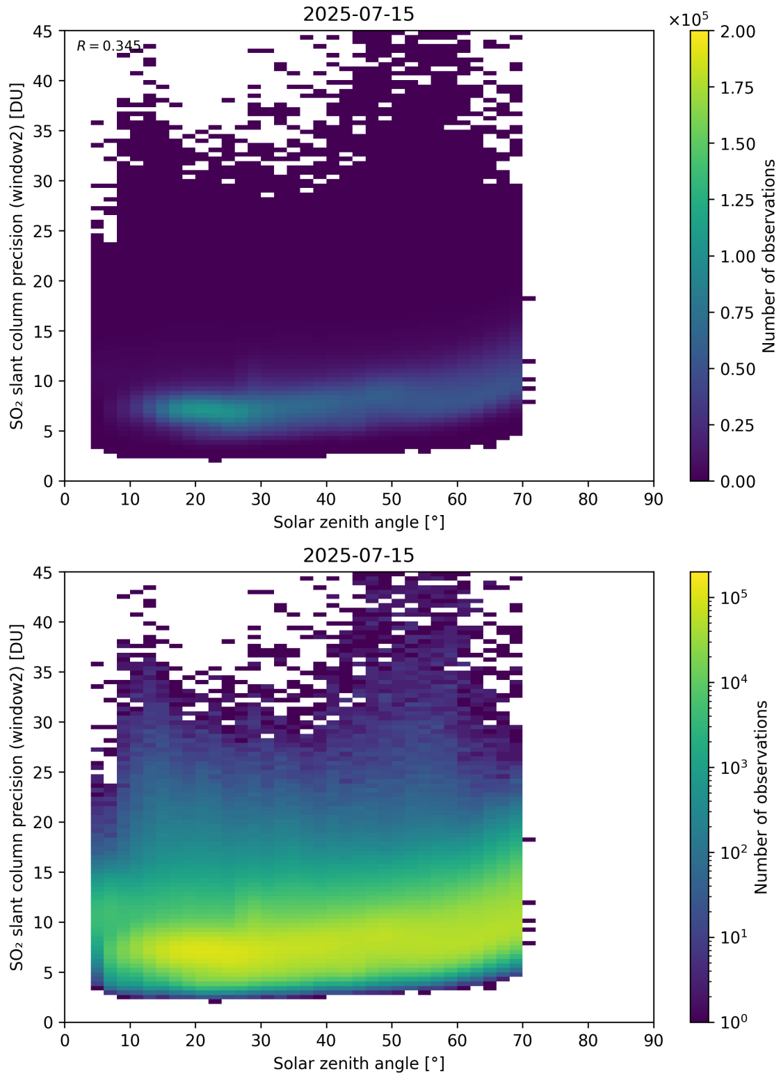
Figure 186: Scatter density plot of “Solar zenith angle” against “SO 2 slant column precision (window2)” for 2025-07-14 to 2025-07-16.
