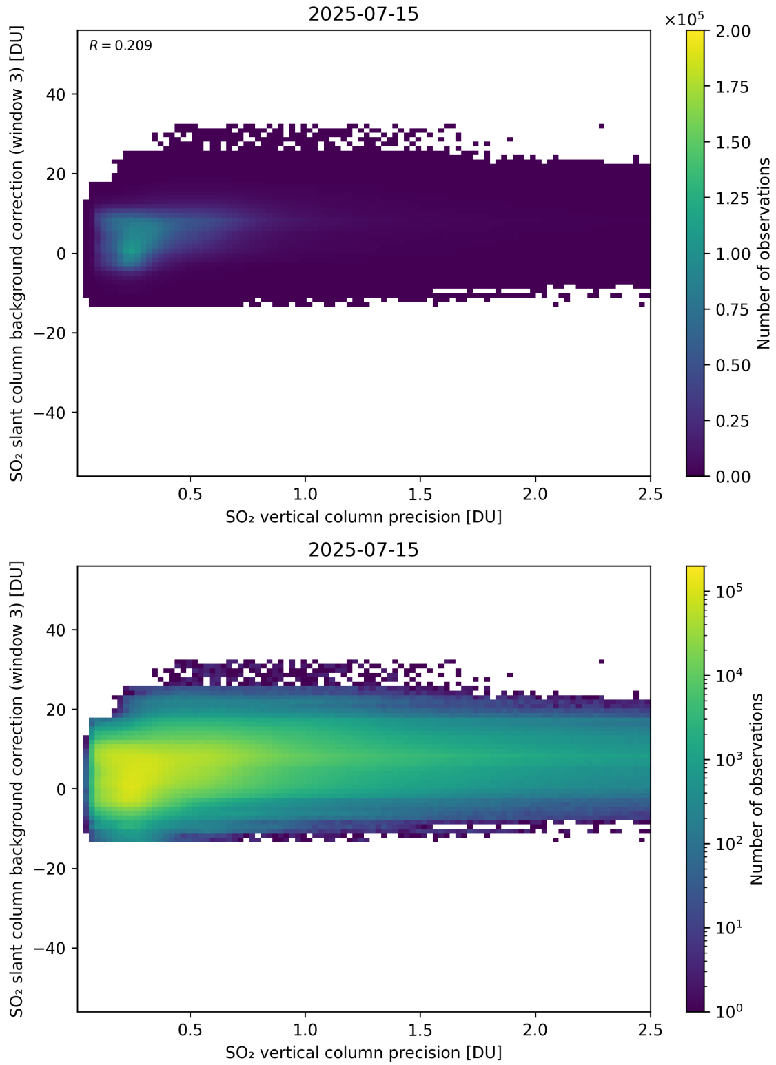
Figure 331: Scatter density plot of “SO 2 vertical column precision” against “SO 2 slant column background correction (window 3)” for 2025-07-14 to 2025-07-16.
