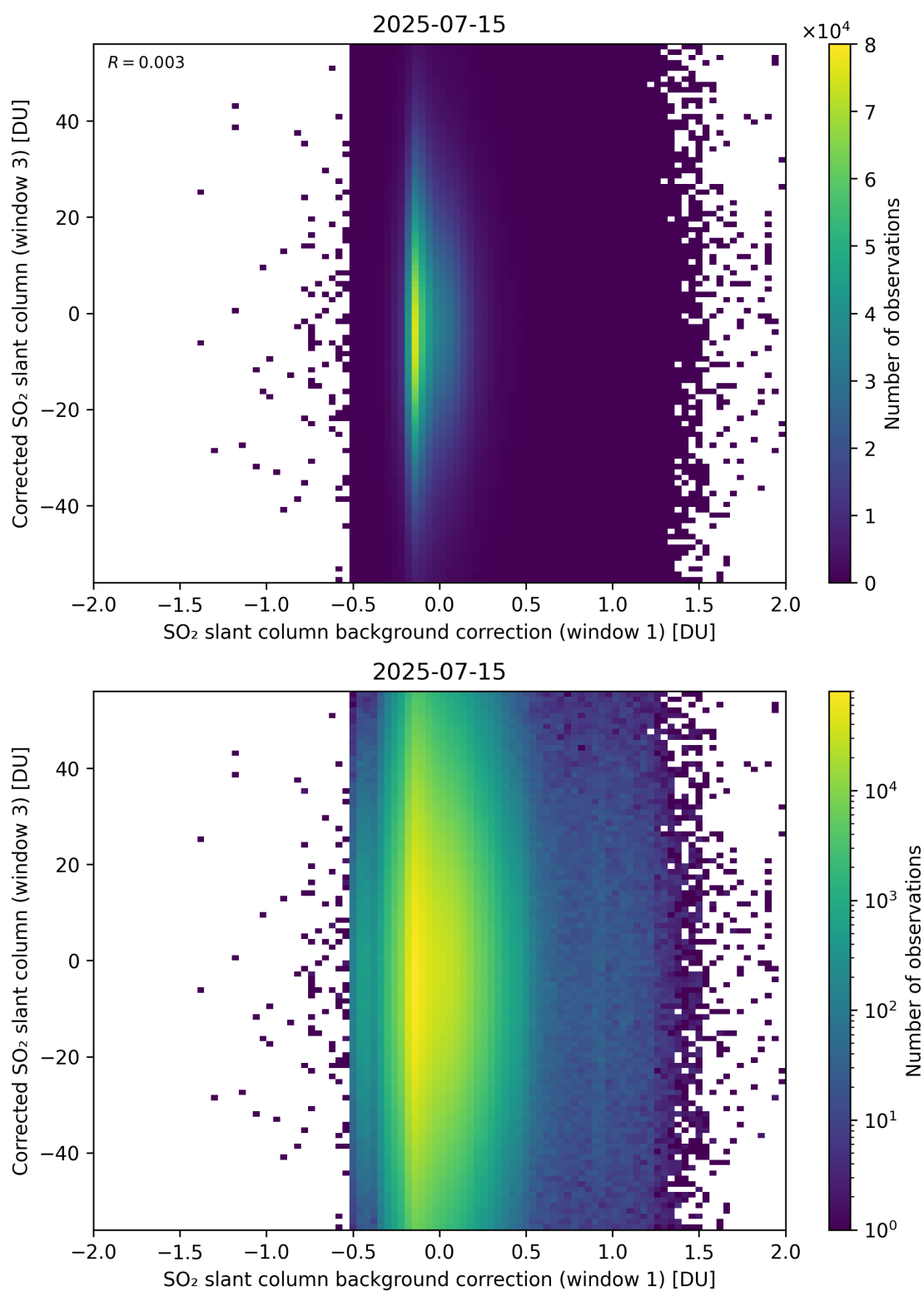
Figure 116: Scatter density plot of “SO 2 slant column background correction (window 1)” against “Corrected SO 2 slant column (window 3)” for 2025-07-14 to 2025-07-16.
