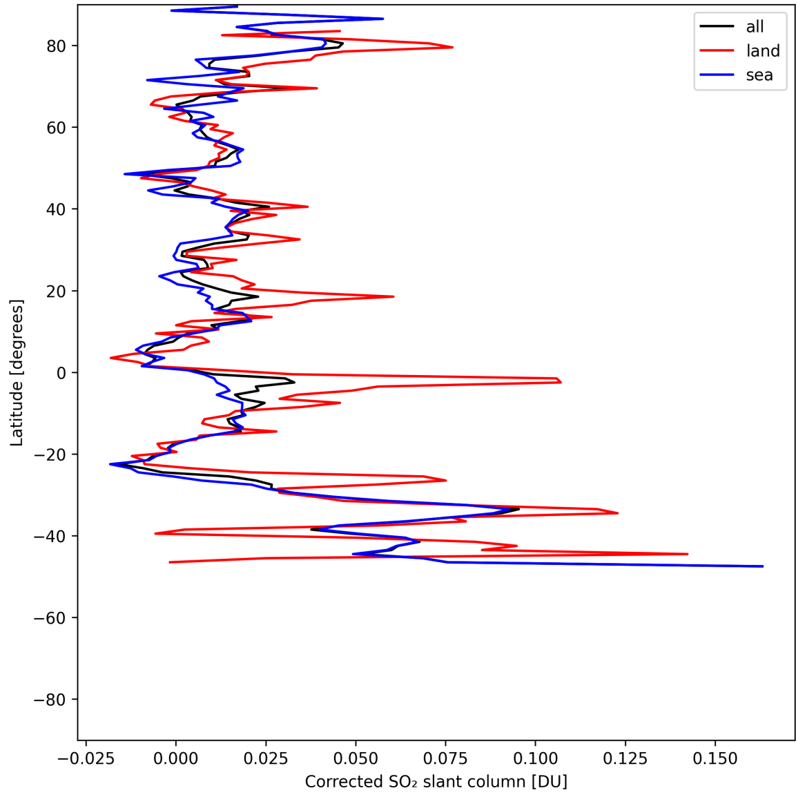
Figure 34: Zonal average of “Corrected SO 2 slant column” for 2025-07-14 to 2025-07-16.
