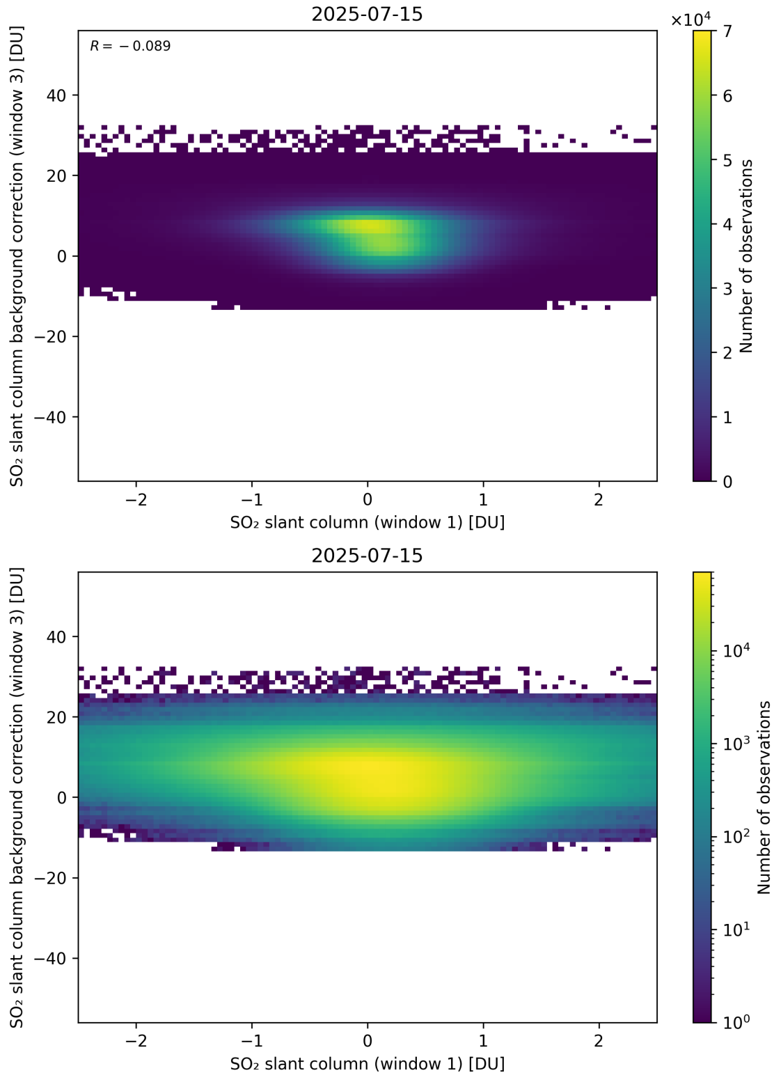
Figure 264: Scatter density plot of “SO 2 slant column (window 1)” against “SO 2 slant column background correction (window 3)” for 2025-07-14 to 2025-07-16.
