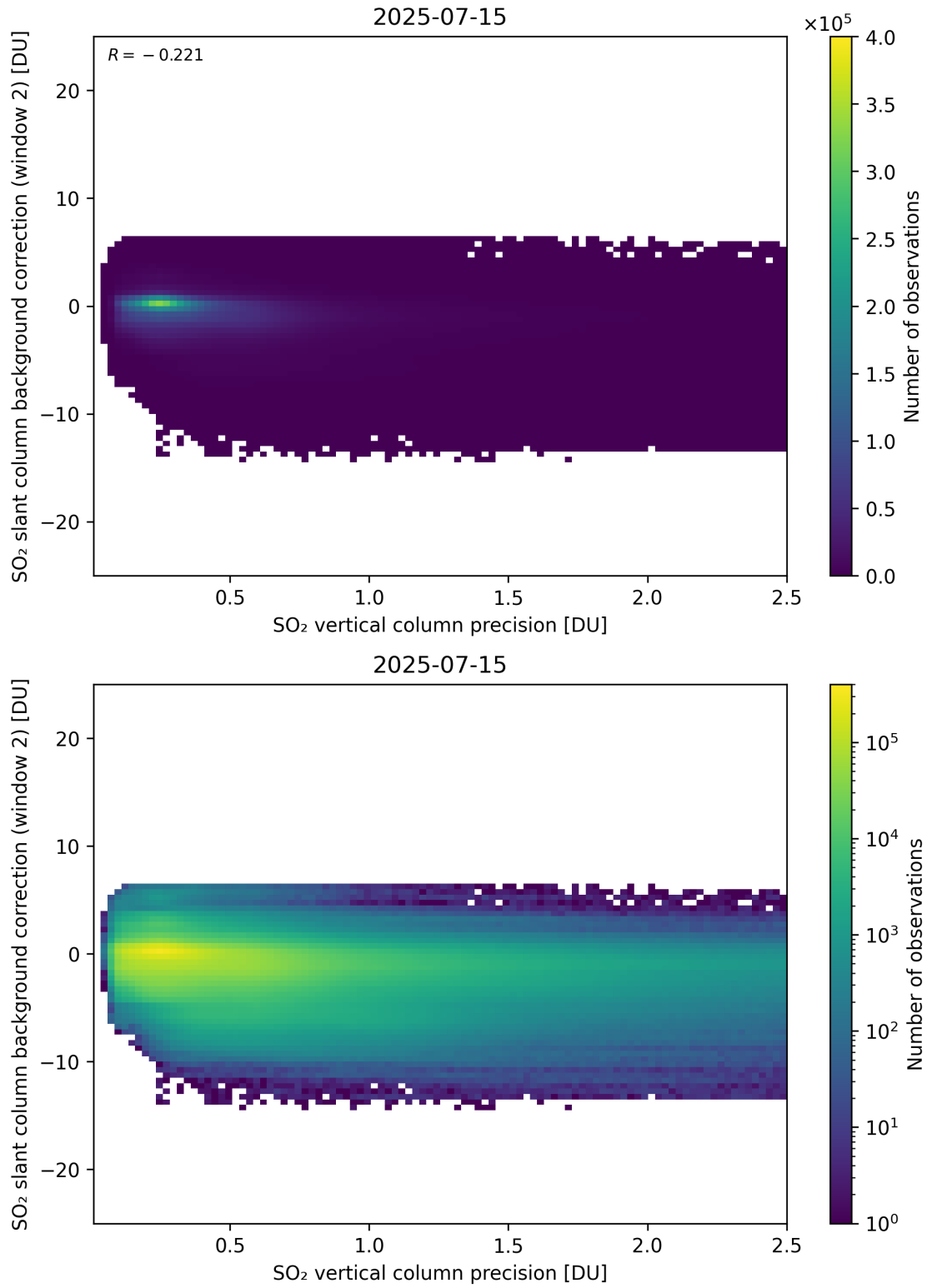
Figure 330: Scatter density plot of “SO 2 vertical column precision” against “SO 2 slant column background correction (window 2)” for 2025-07-14 to 2025-07-16.
