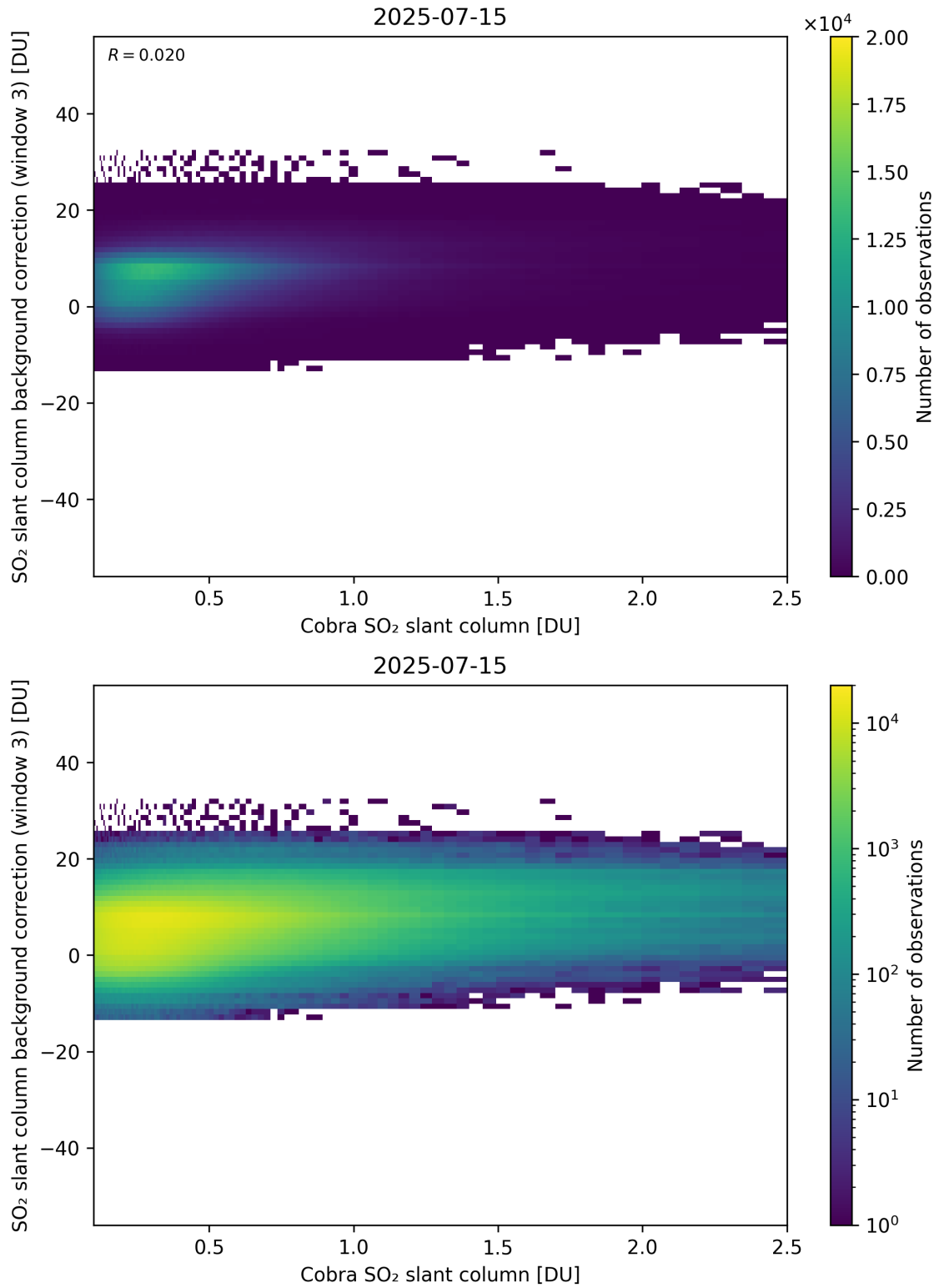
Figure 195: Scatter density plot of “Cobra SO 2 slant column” against “SO 2 slant column background correction (window 3)” for 2025-07-14 to 2025-07-16.
