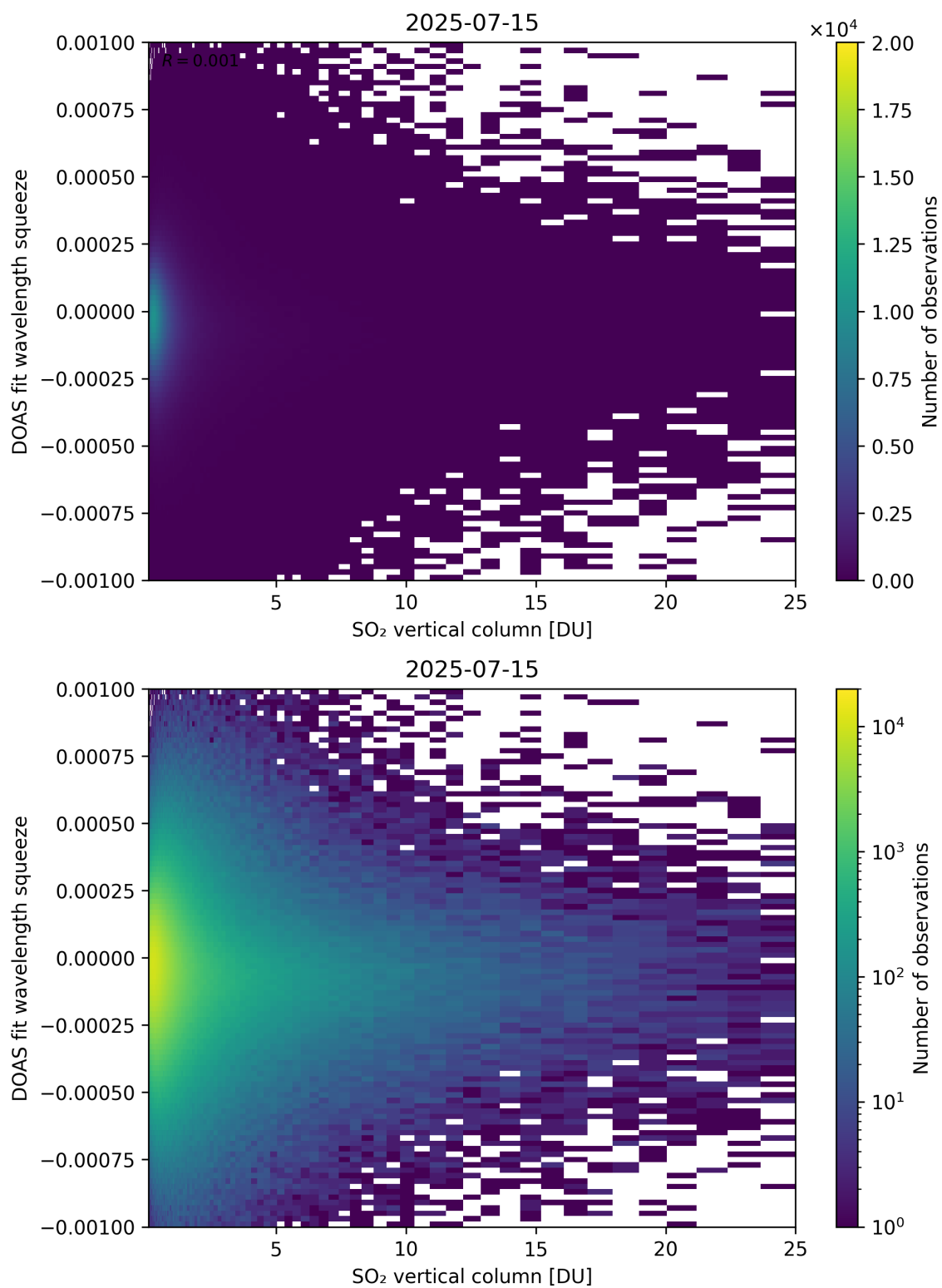
Figure 327: Scatter density plot of “SO 2 vertical column” against “DOAS fit wavelength squeeze” for 2025-07-14 to 2025-07-16.
