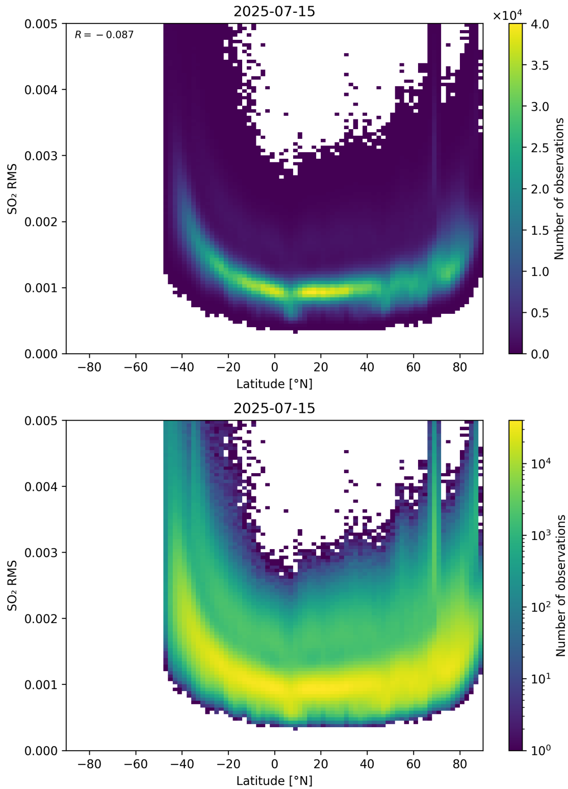
Figure 155: Scatter density plot of “Latitude” against “SO 2 RMS” for 2025-07-14 to 2025-07-16.
