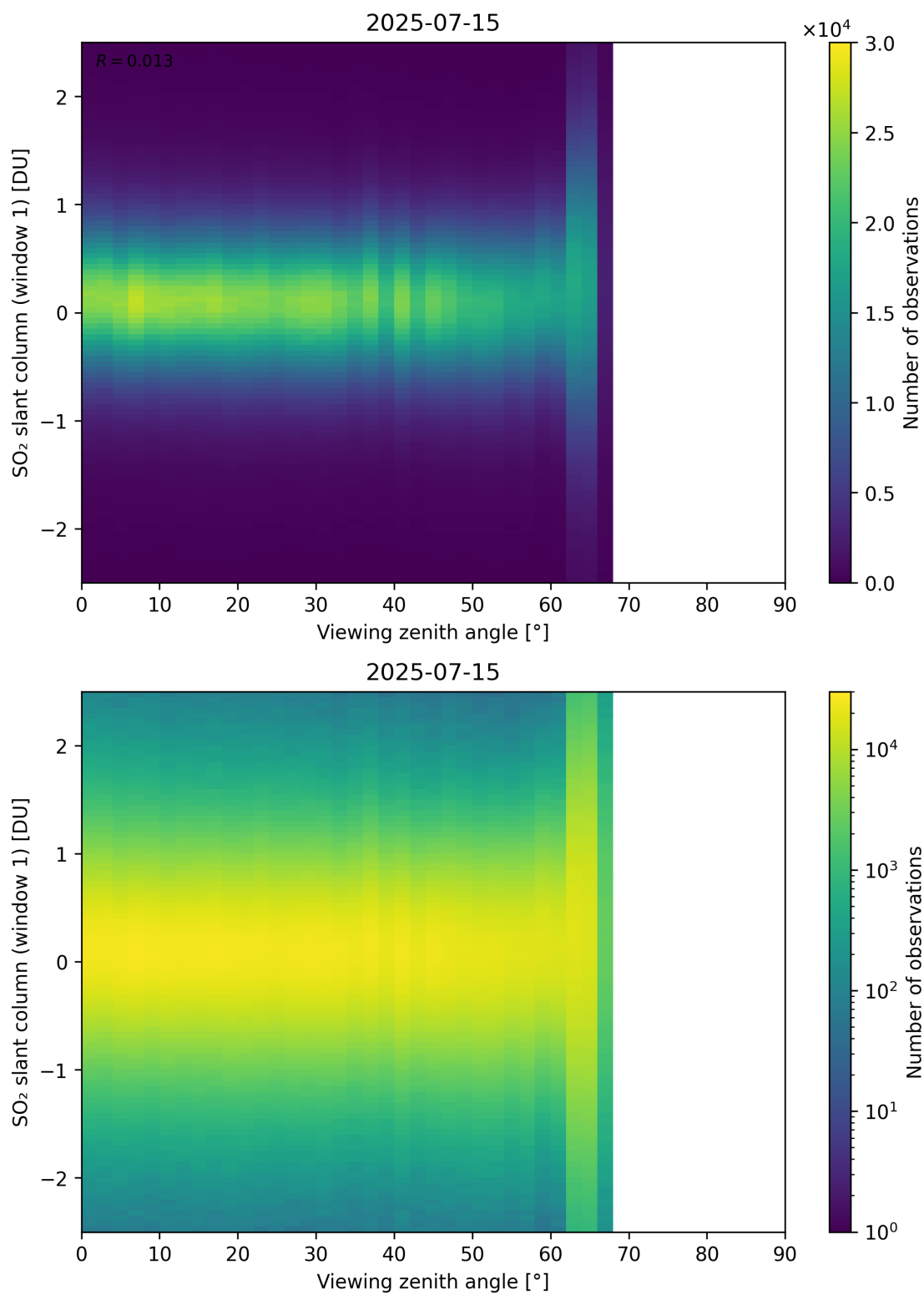
Figure 376: Scatter density plot of “Viewing zenith angle” against “SO 2 slant column (window 1)” for 2025-07-14 to 2025-07-16.
