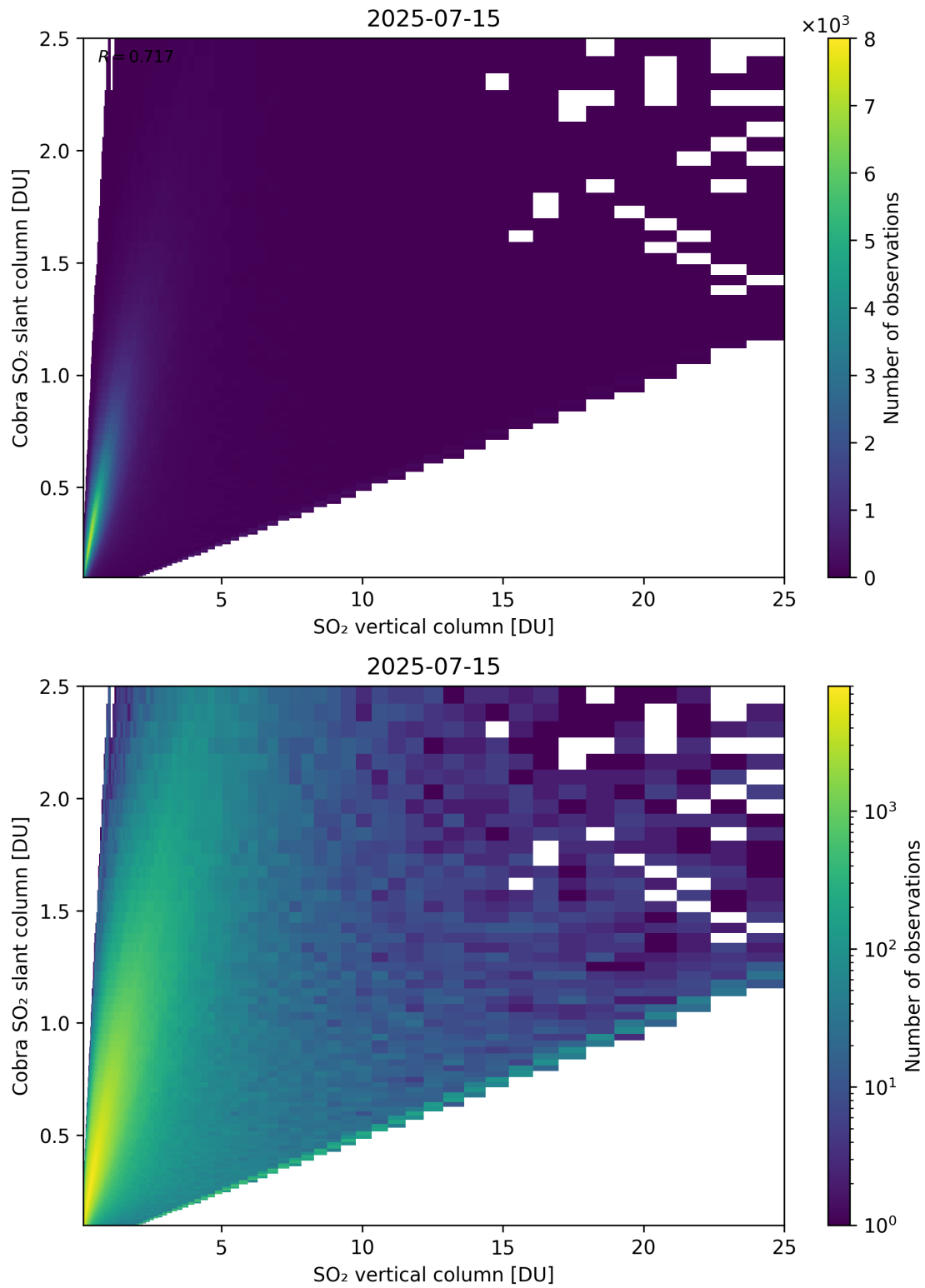
Figure 349: Scatter density plot of “SO 2 vertical column” against “Cobra SO 2 slant column” for 2025-07-14 to 2025-07-16.
