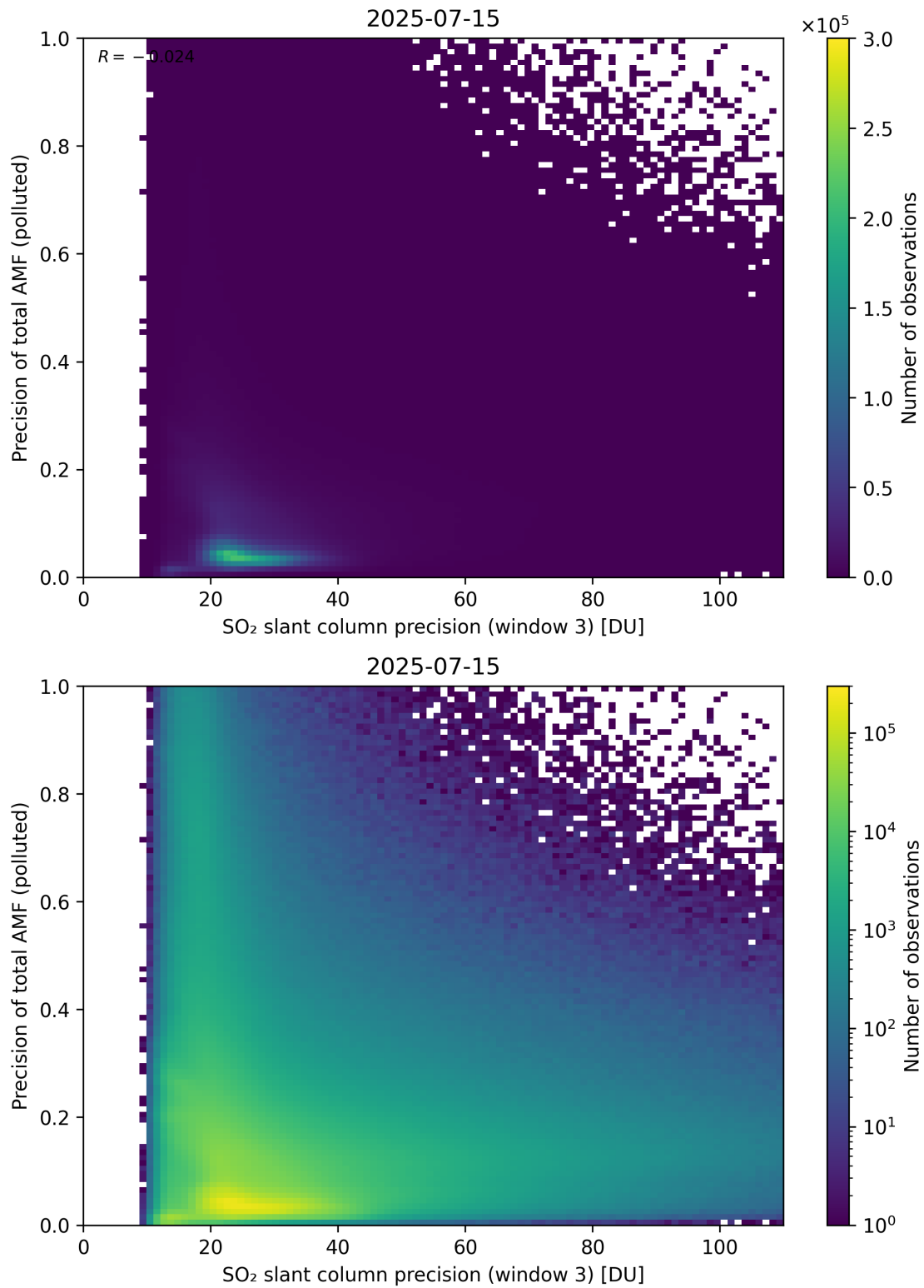
Figure 314: Scatter density plot of “SO 2 slant column precision (window 3)” against “Precision of total AMF (polluted)” for 2025-07-14 to 2025-07-16.
