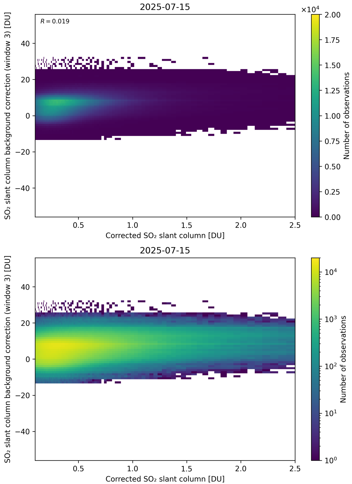
Figure 228: Scatter density plot of “Corrected SO 2 slant column” against “SO 2 slant column background correction (window 3)” for 2025-07-14 to 2025-07-16.
