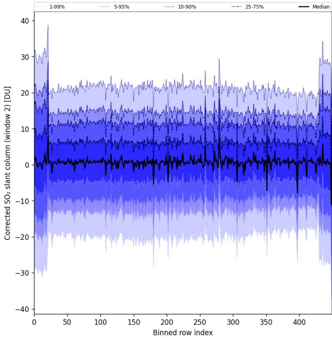
Figure 95: Along track statistics of "Corrected SO 2 slant column (window 2)" for 2025-07-14 to 2025-07-16
