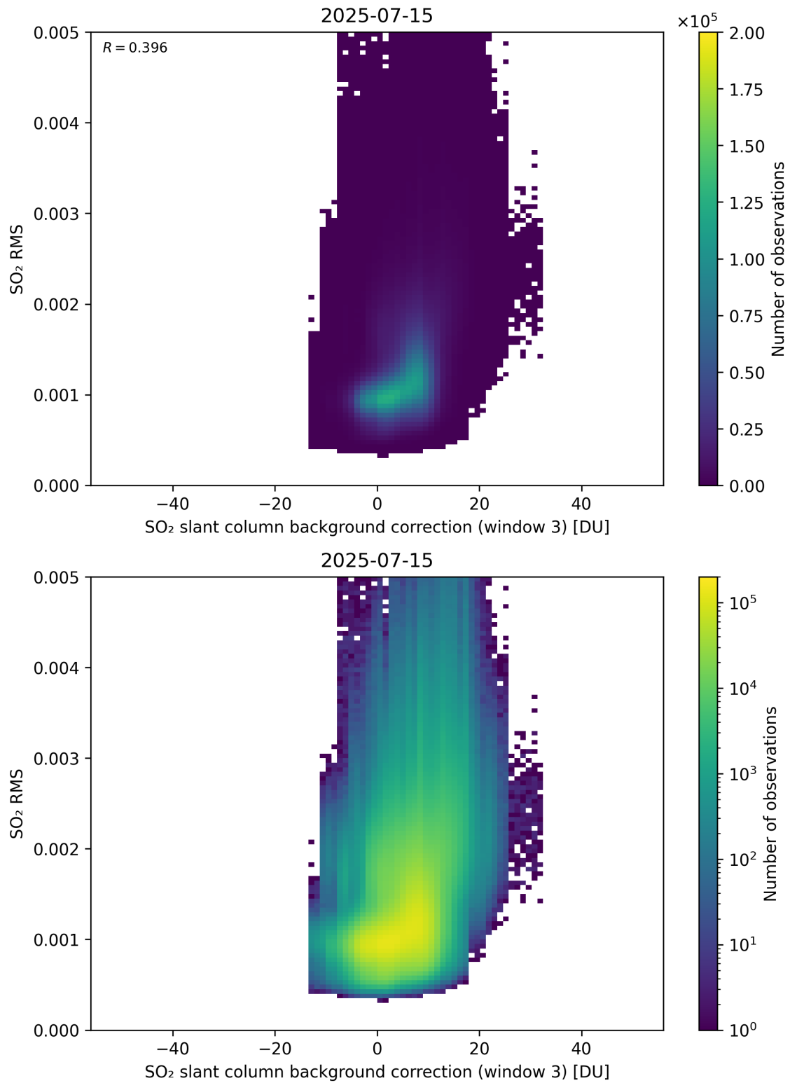
Figure 134: Scatter density plot of “SO 2 slant column background correction (window 3)” against “SO 2 RMS” for 2025-07-14 to 2025-07-16.
