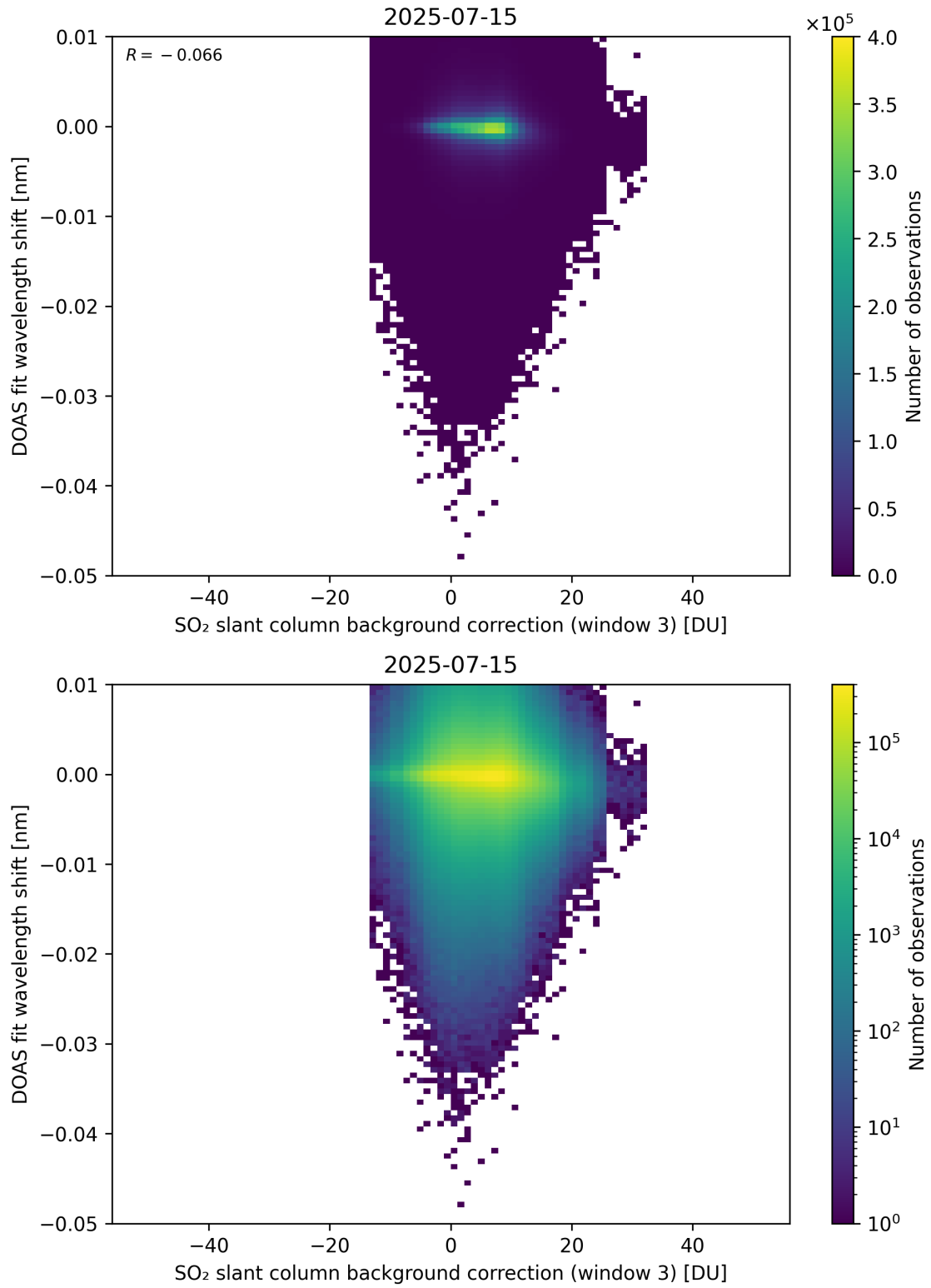
Figure 132: Scatter density plot of “SO 2 slant column background correction (window 3)” against “DOAS fit wavelength shift” for 2025-07-14 to 2025-07-16.
