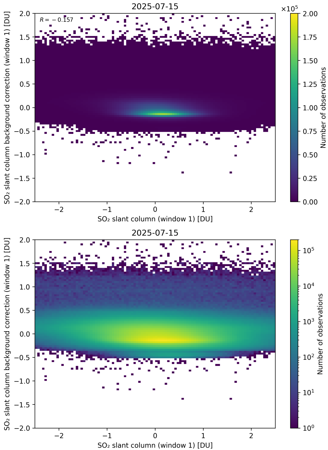
Figure 262: Scatter density plot of “SO 2 slant column (window 1)” against “SO 2 slant column background correction (window 1)” for 2025-07-14 to 2025-07-16.
