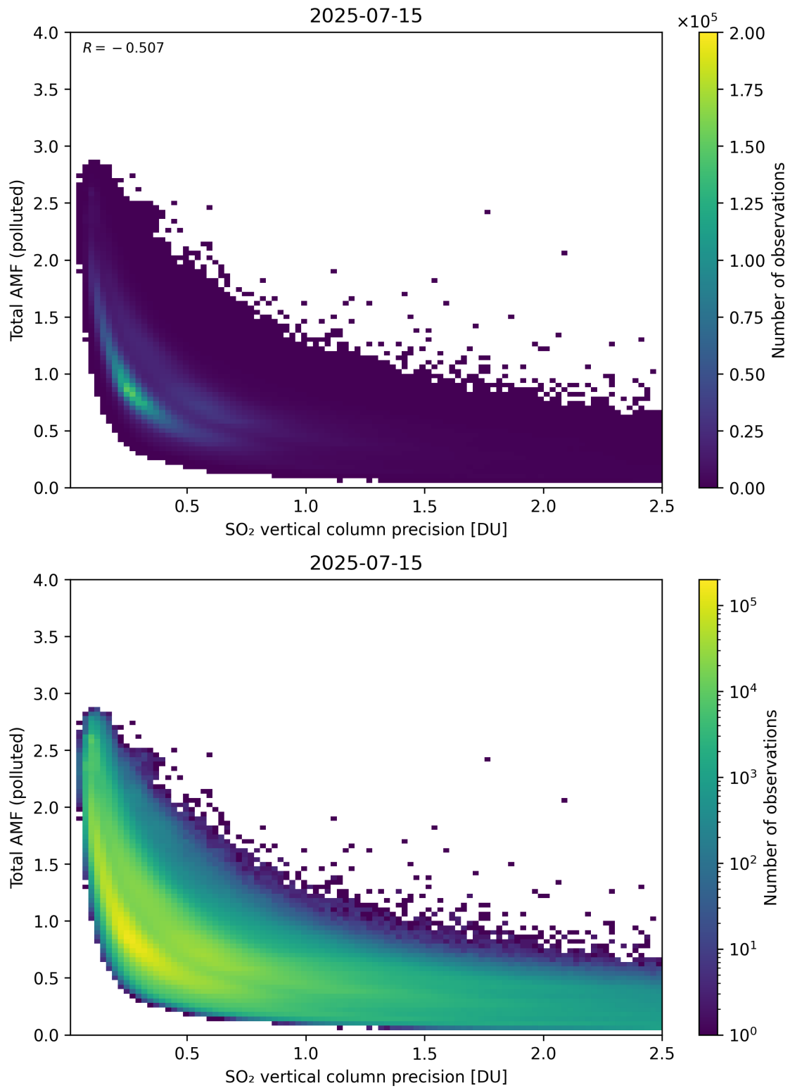
Figure 346: Scatter density plot of “SO 2 vertical column precision” against “Total AMF (polluted)” for 2025-07-14 to 2025-07-16.
