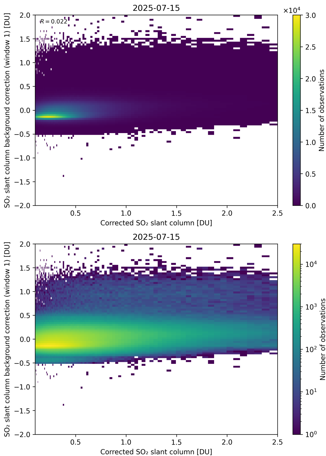
Figure 226: Scatter density plot of “Corrected SO 2 slant column” against “SO 2 slant column background correction (window 1)” for 2025-07-14 to 2025-07-16.
