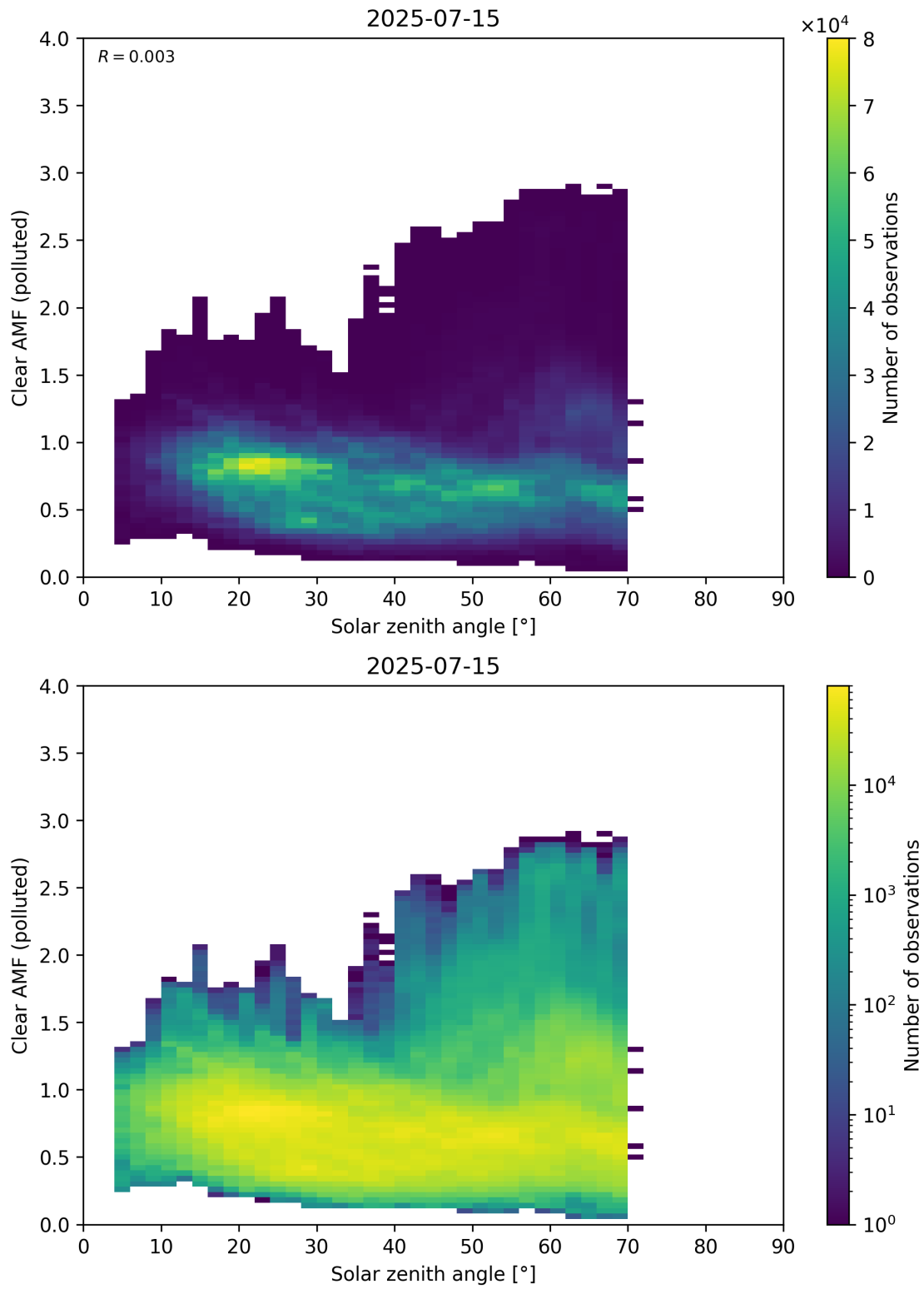
Figure 178: Scatter density plot of “Solar zenith angle” against “Clear AMF (polluted)” for 2025-07-14 to 2025-07-16.
