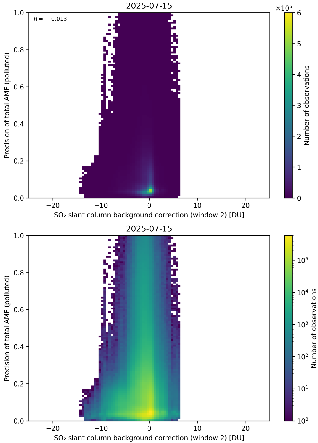
Figure 131: Scatter density plot of “SO 2 slant column background correction (window 2)” against “Precision of total AMF (polluted)” for 2025-07-14 to 2025-07-16.
