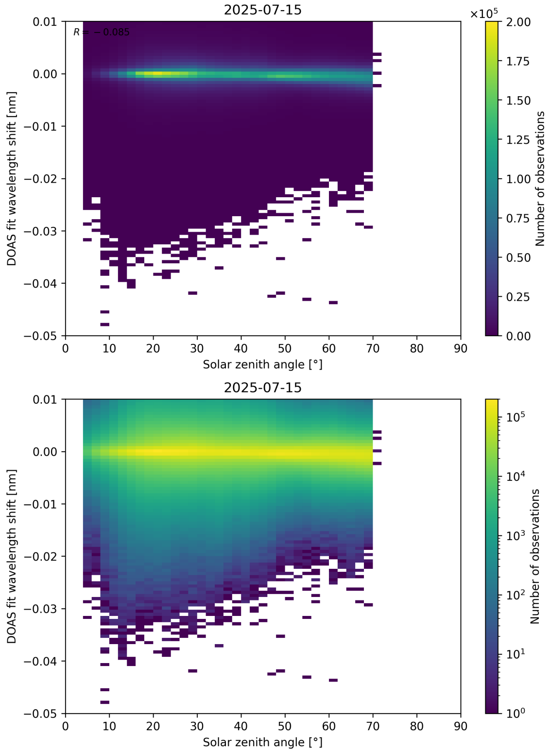
Figure 174: Scatter density plot of “Solar zenith angle” against “DOAS fit wavelength shift” for 2025-07-14 to 2025-07-16.
