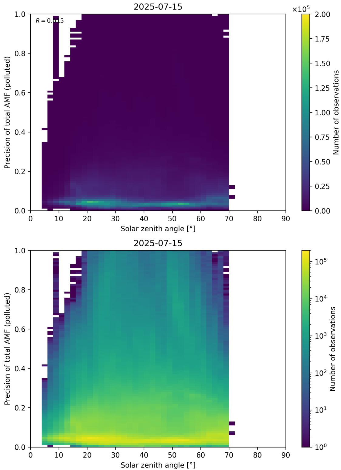
Figure 190: Scatter density plot of “Solar zenith angle” against “Precision of total AMF (polluted)” for 2025-07-14 to 2025-07-16.
