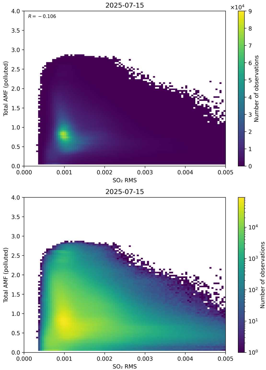
Figure 148: Scatter density plot of “SO 2 RMS” against “Total AMF (polluted)” for 2025-07-14 to 2025-07-16.
