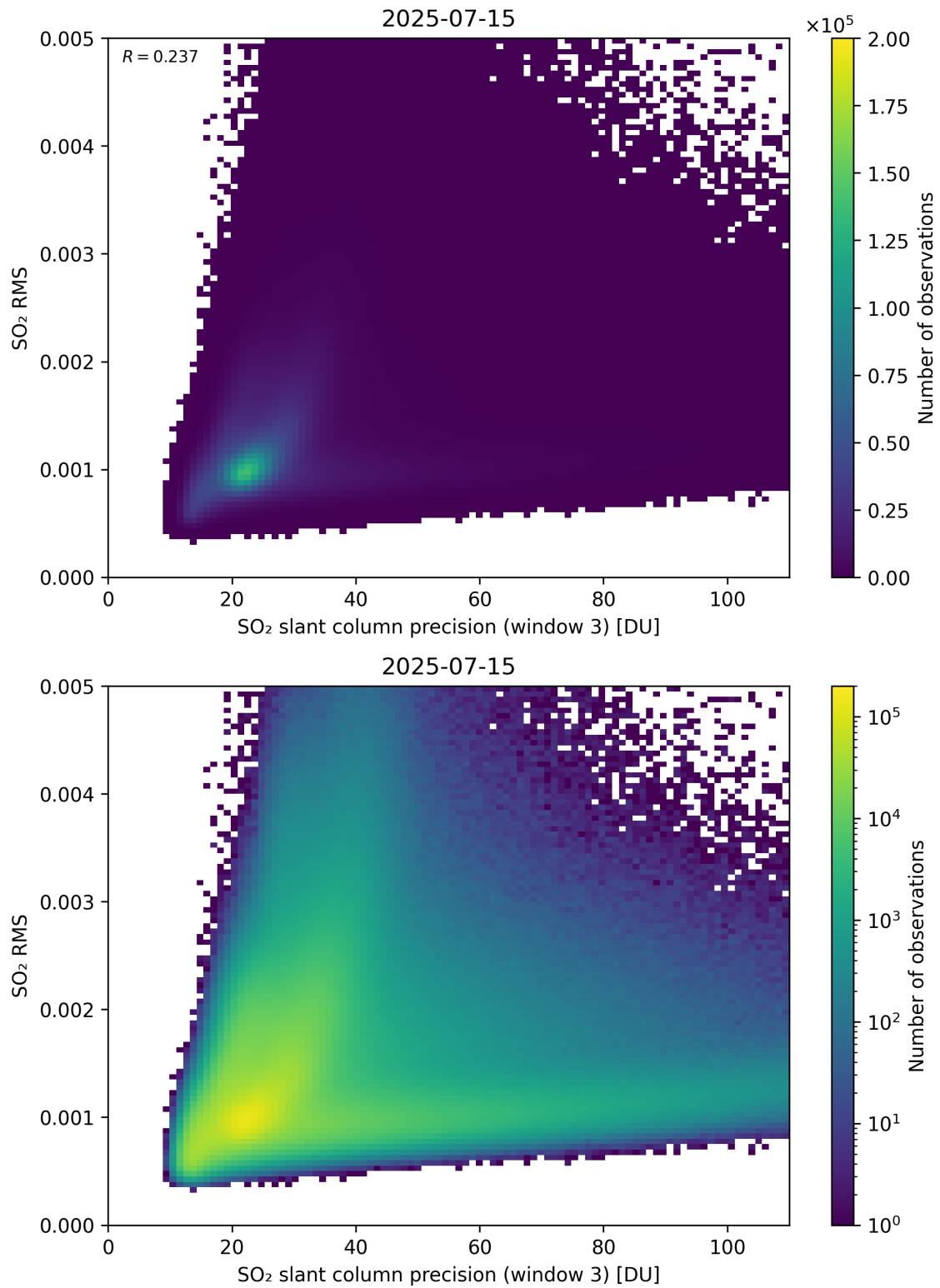
Figure 310: Scatter density plot of “SO 2 slant column precision (window 3)” against “SO 2 RMS” for 2025-07-14 to 2025-07-16.
