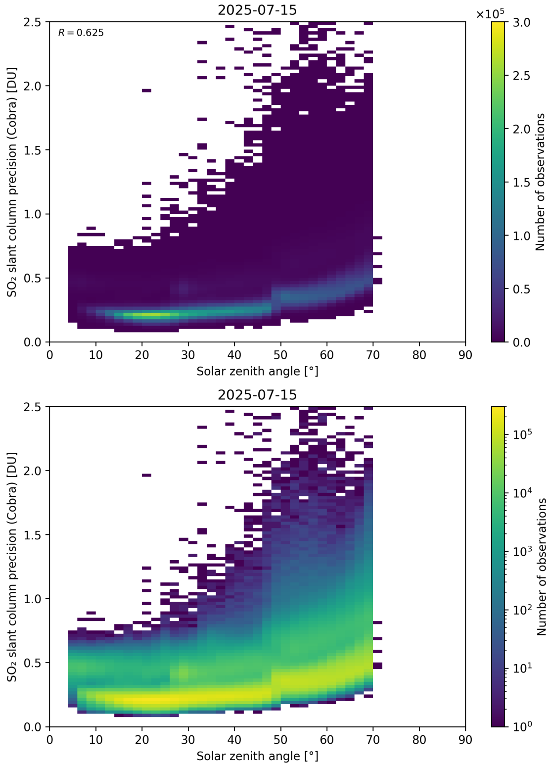
Figure 180: Scatter density plot of “Solar zenith angle” against “SO 2 slant column precision (Cobra)” for 2025-07-14 to 2025-07-16.
