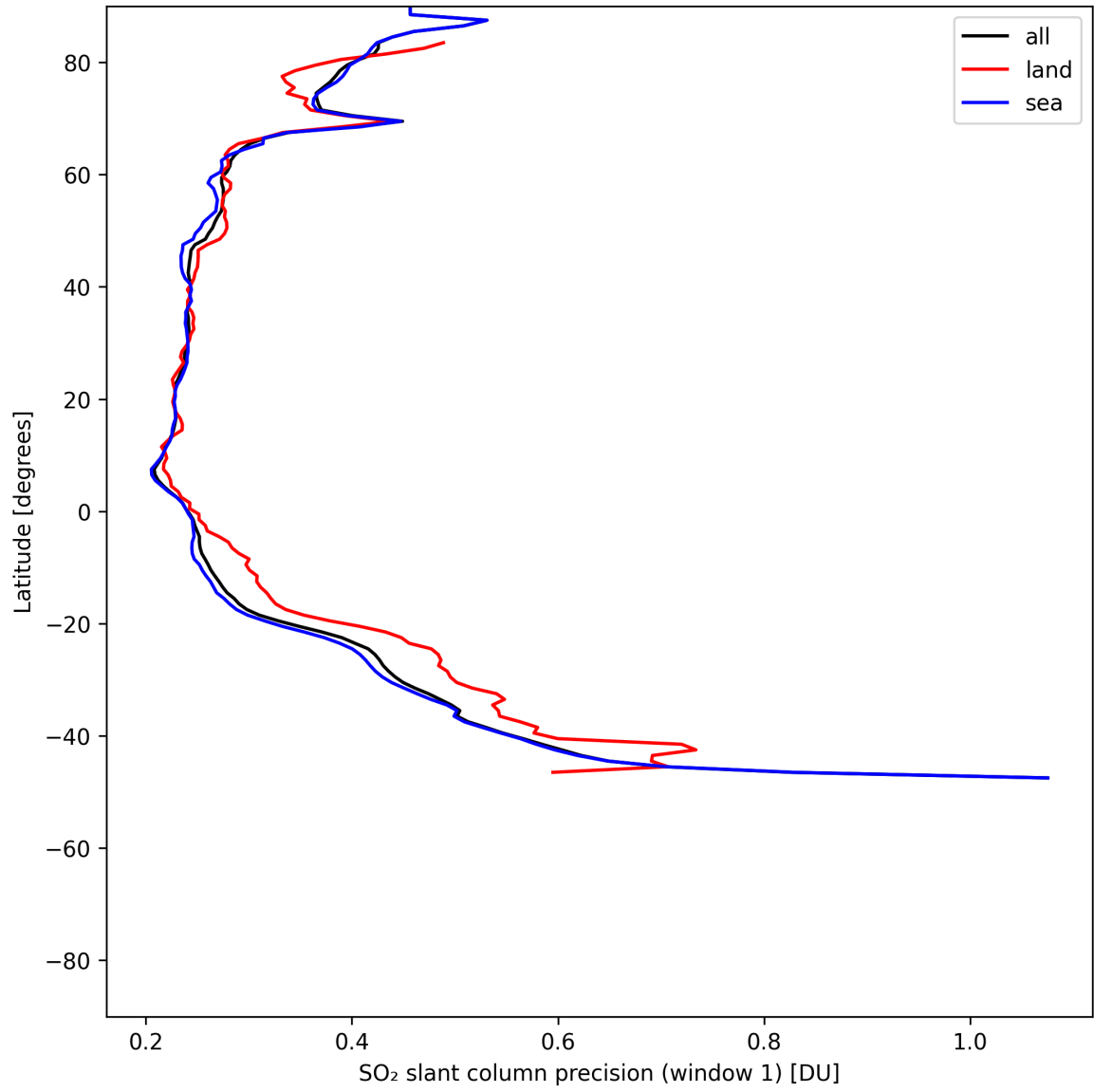
Figure 38: Zonal average of “SO 2 slant column precision (window 1)” for 2025-07-14 to 2025-07-16.
