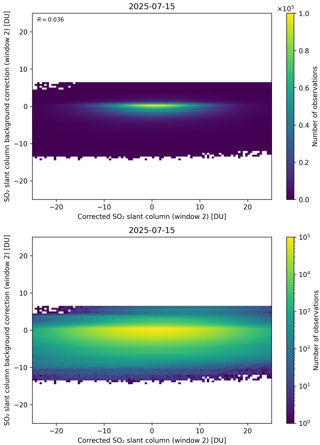
Figure 244: Scatter density plot of “Corrected SO 2 slant column (window 2)” against “SO 2 slant column background correction (window 2)” for 2025-07-14 to 2025-07-16.
