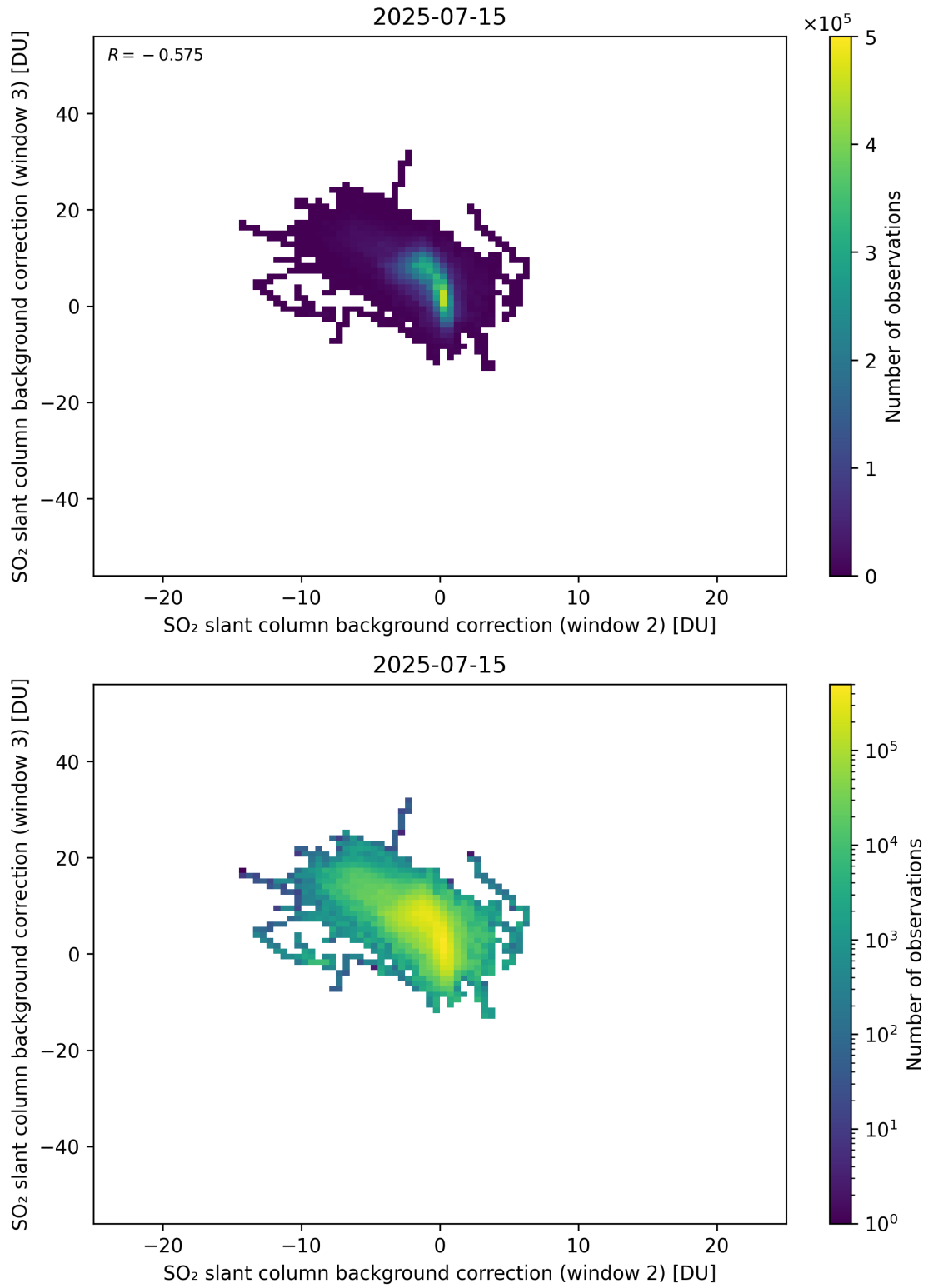
Figure 122: Scatter density plot of “SO 2 slant column background correction (window 2)” against “SO 2 slant column background correction (window 3)” for 2025-07-14 to 2025-07-16.
