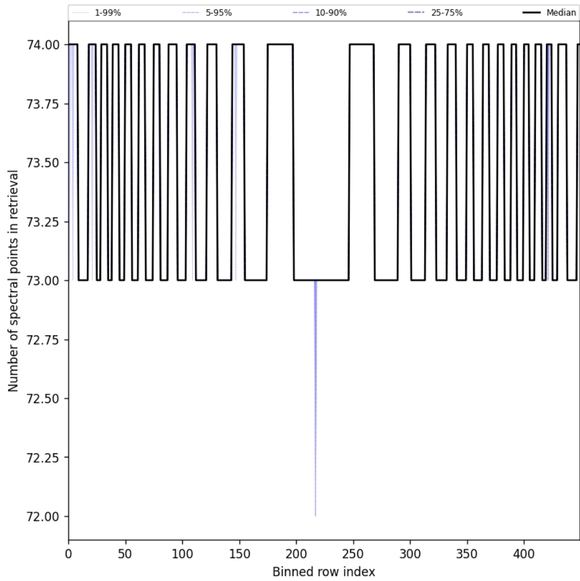
Figure 108: Along track statistics of “Number of spectral points in retrieval” for 2025-07-14 to 2025-07-16
