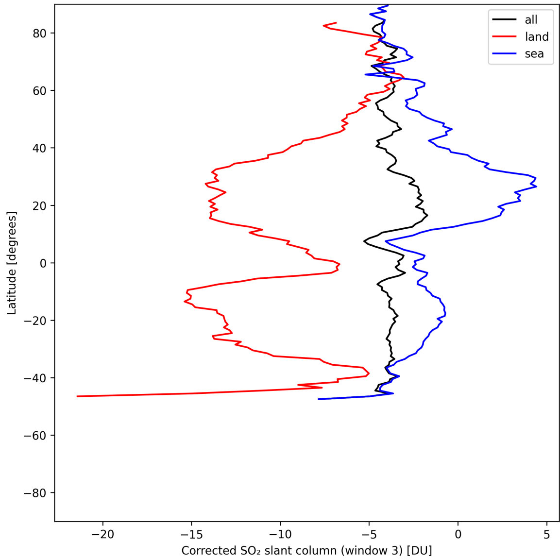
Figure 47: Zonal average of “Corrected SO 2 slant column (window 3)” for 2025-07-14 to 2025-07-16.
