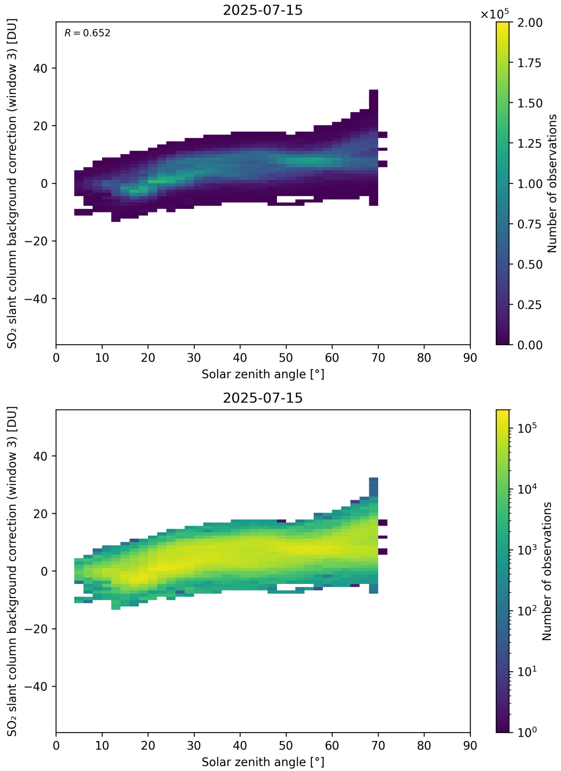
Figure 173: Scatter density plot of “Solar zenith angle” against “SO 2 slant column background correction (window 3)” for 2025-07-14 to 2025-07-16.
