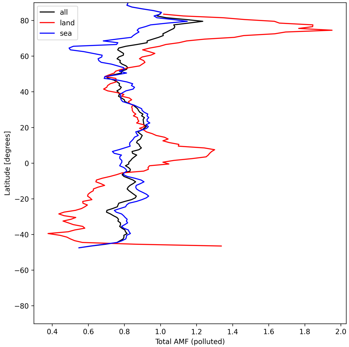
Figure 53: Zonal average of “Total AMF (polluted)” for 2025-07-14 to 2025-07-16.
