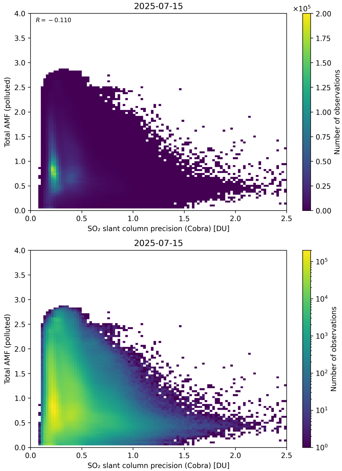
Figure 213: Scatter density plot of “SO 2 slant column precision (Cobra)” against “Total AMF (polluted)” for 2025-07-14 to 2025-07-16.
