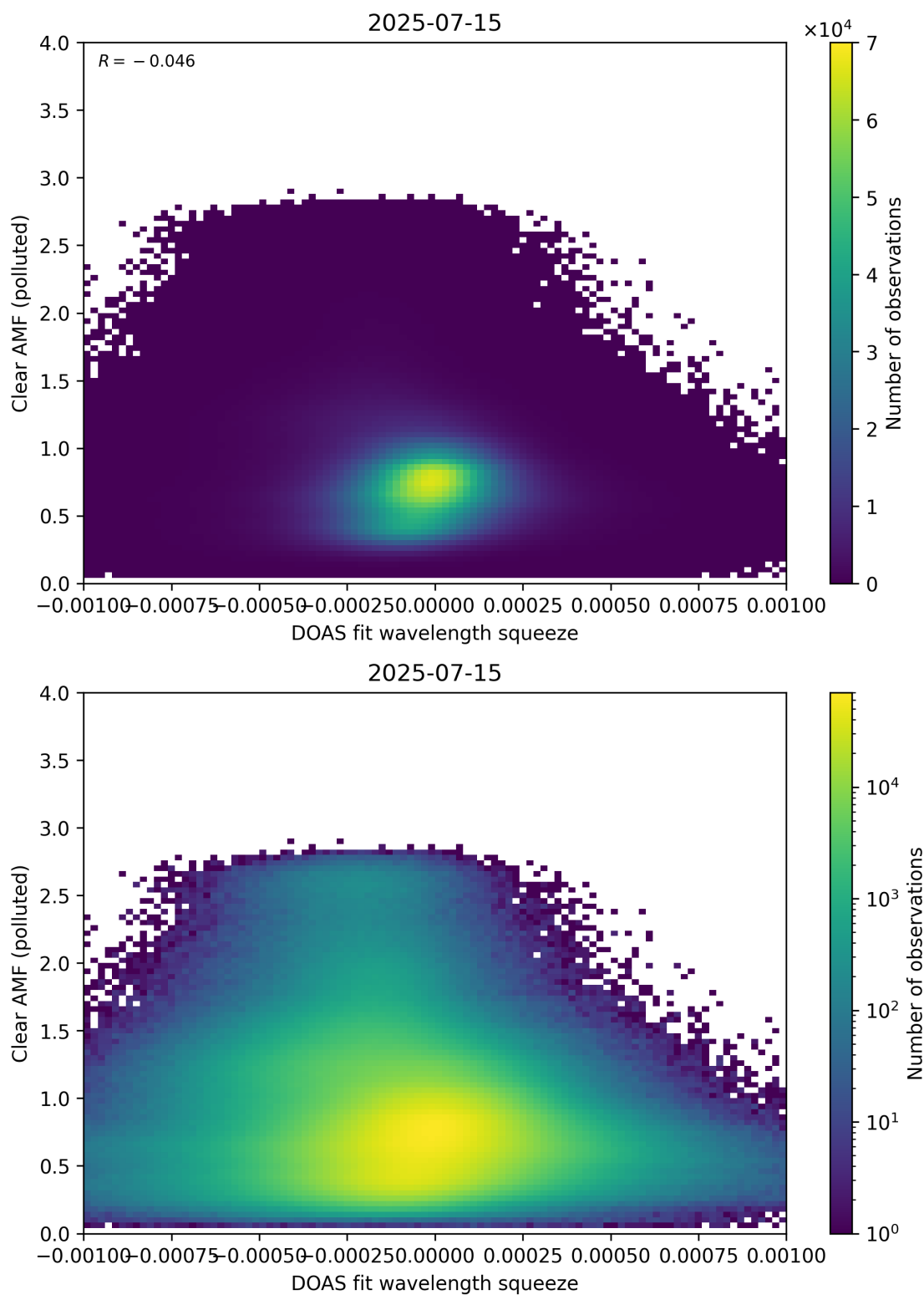
Figure 144: Scatter density plot of “DOAS fit wavelength squeeze” against “Clear AMF (polluted)” for 2025-07-14 to 2025-07-16.
