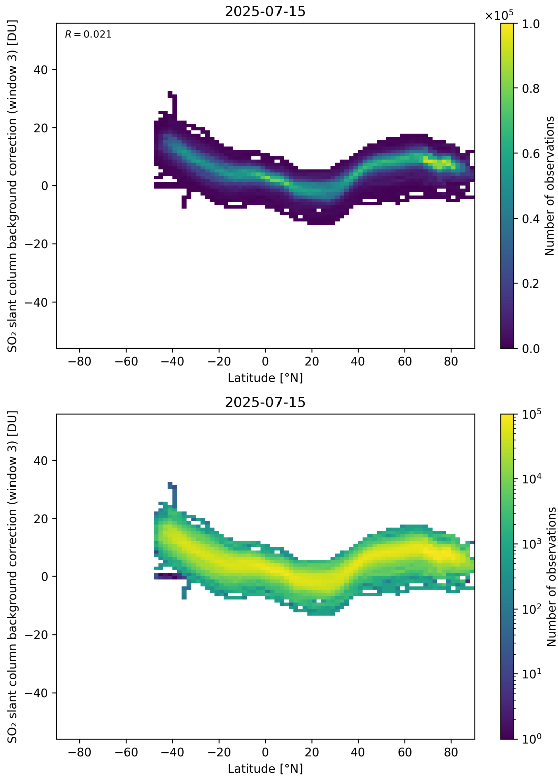
Figure 152: Scatter density plot of “Latitude” against “SO 2 slant column background correction (window 3)” for 2025-07-14 to 2025-07-16.
