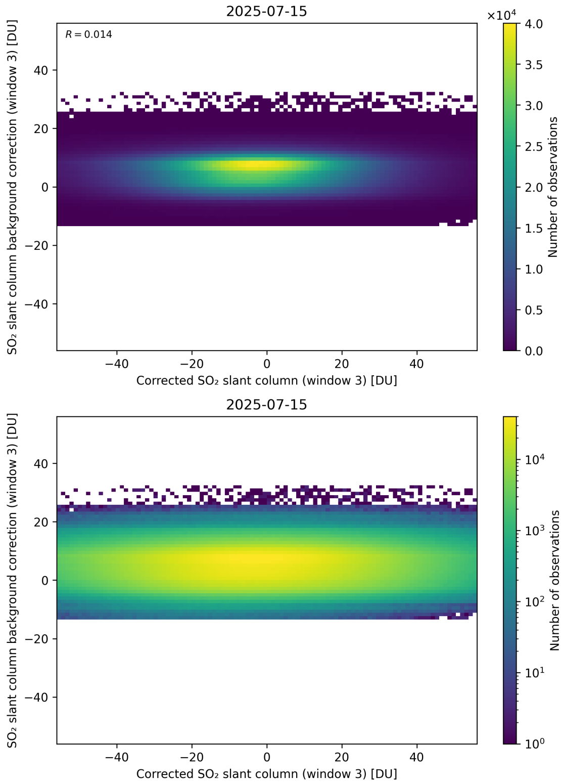
Figure 255: Scatter density plot of “Corrected SO 2 slant column (window 3)” against “SO 2 slant column background correction (window 3)” for 2025-07-14 to 2025-07-16.
