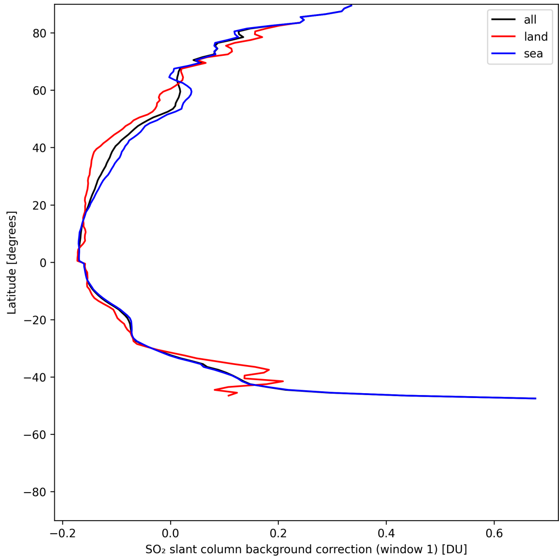
Figure 40: Zonal average of “SO 2 slant column background correction (window 1)” for 2025-07-14 to 2025-07-16.
