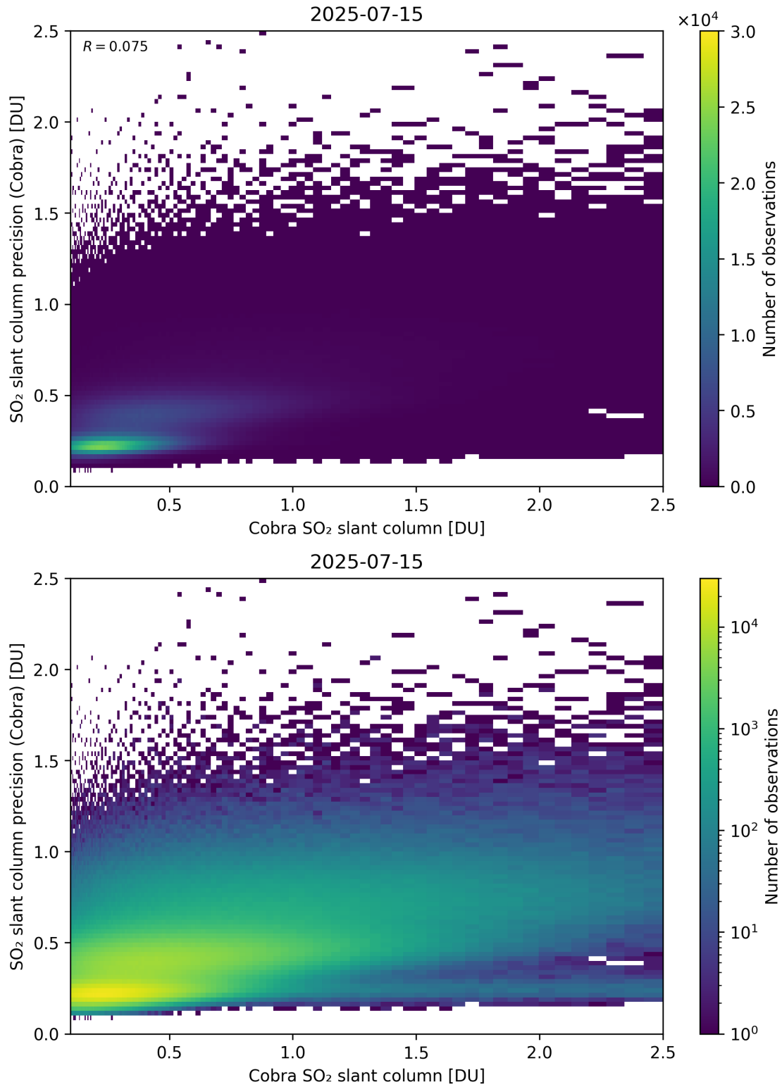
Figure 216: Scatter density plot of “Cobra SO 2 slant column” against “SO 2 slant column precision (Cobra)” for 2025-07-14 to 2025-07-16.
