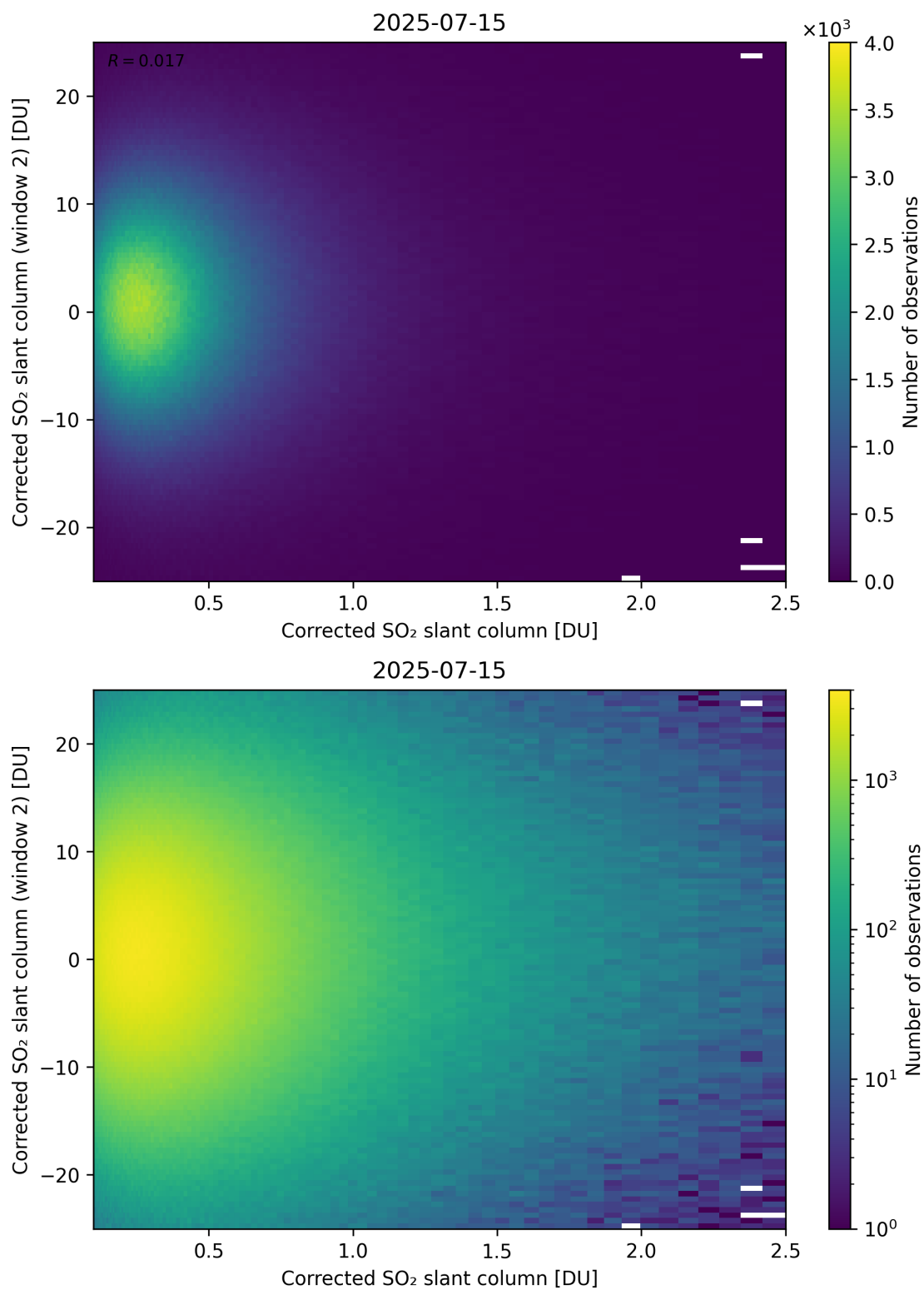
Figure 235: Scatter density plot of “Corrected SO 2 slant column” against “Corrected SO 2 slant column (window 2)” for 2025-07-14 to 2025-07-16.
