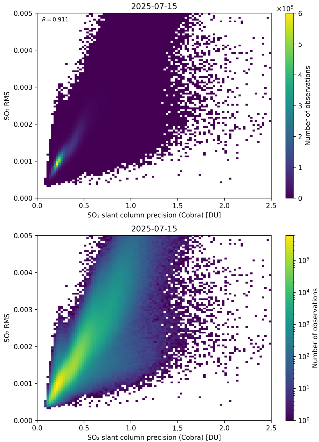
Figure 204: Scatter density plot of “SO 2 slant column precision (Cobra)” against “SO 2 RMS” for 2025-07-14 to 2025-07-16.
