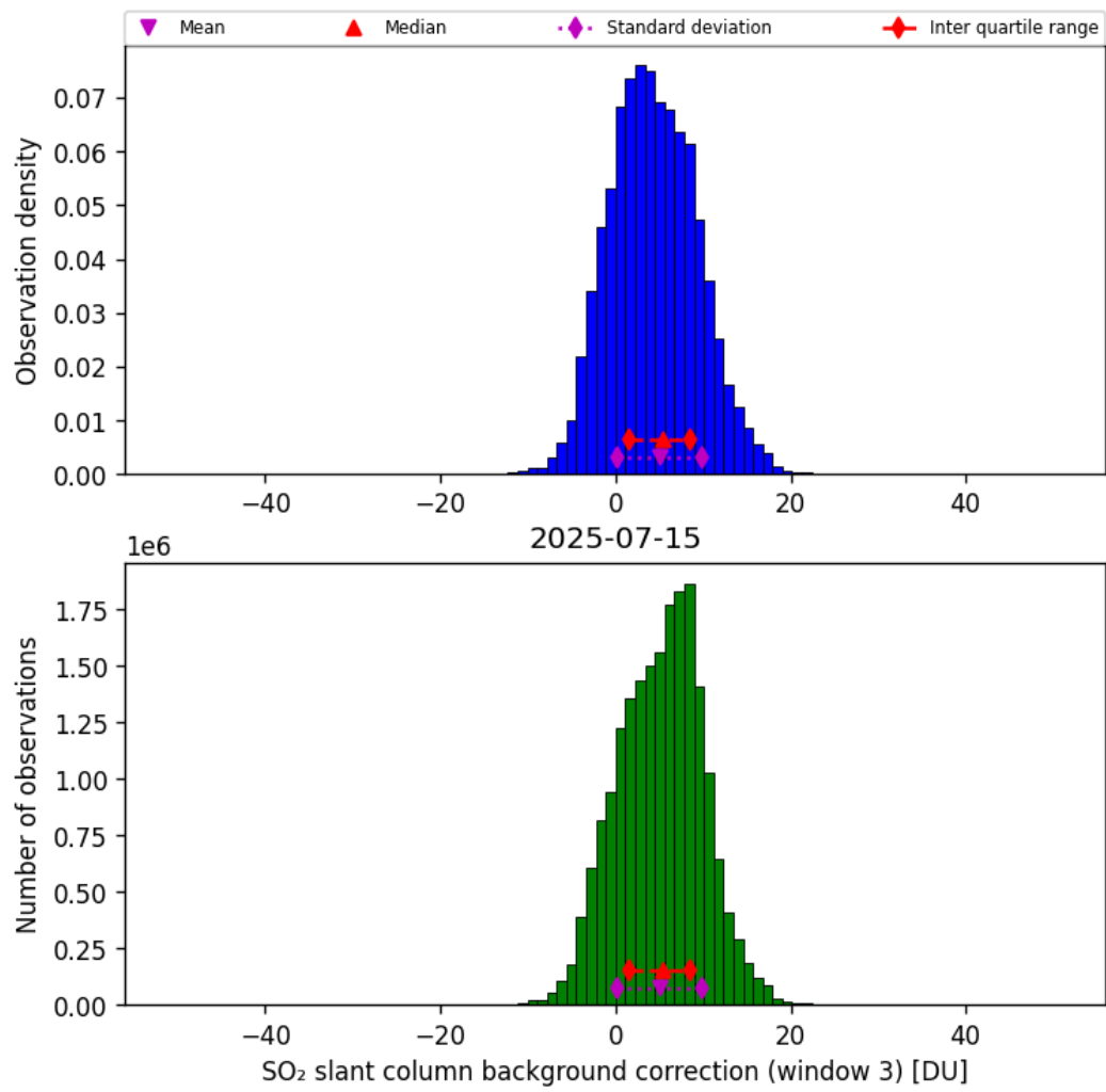
Figure 74: Histogram of “SO 2 slant column background correction (window 3)” for 2025-07-14 to 2025-07-16
