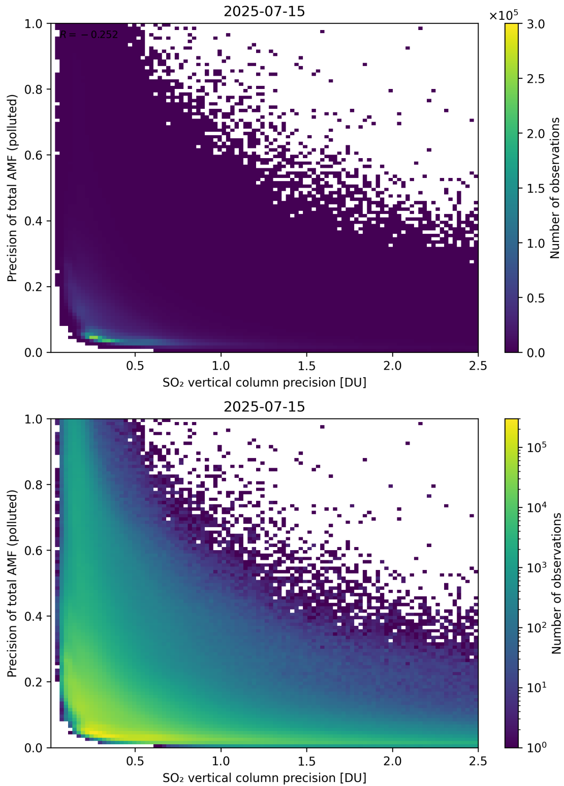
Figure 347: Scatter density plot of “SO 2 vertical column precision” against “Precision of total AMF (polluted)” for 2025-07-14 to 2025-07-16.
