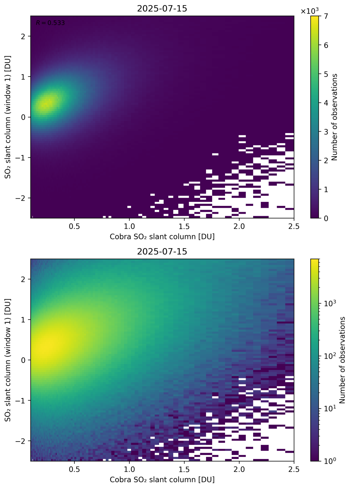
Figure 219: Scatter density plot of “Cobra SO 2 slant column” against “SO 2 slant column (window 1)” for 2025-07-14 to 2025-07-16.
