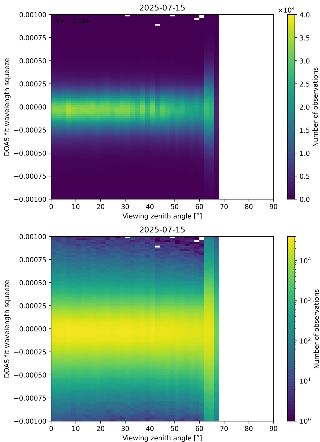
Figure 366: Scatter density plot of “Viewing zenith angle” against “DOAS fit wavelength squeeze” for 2025-07-14 to 2025-07-16.
