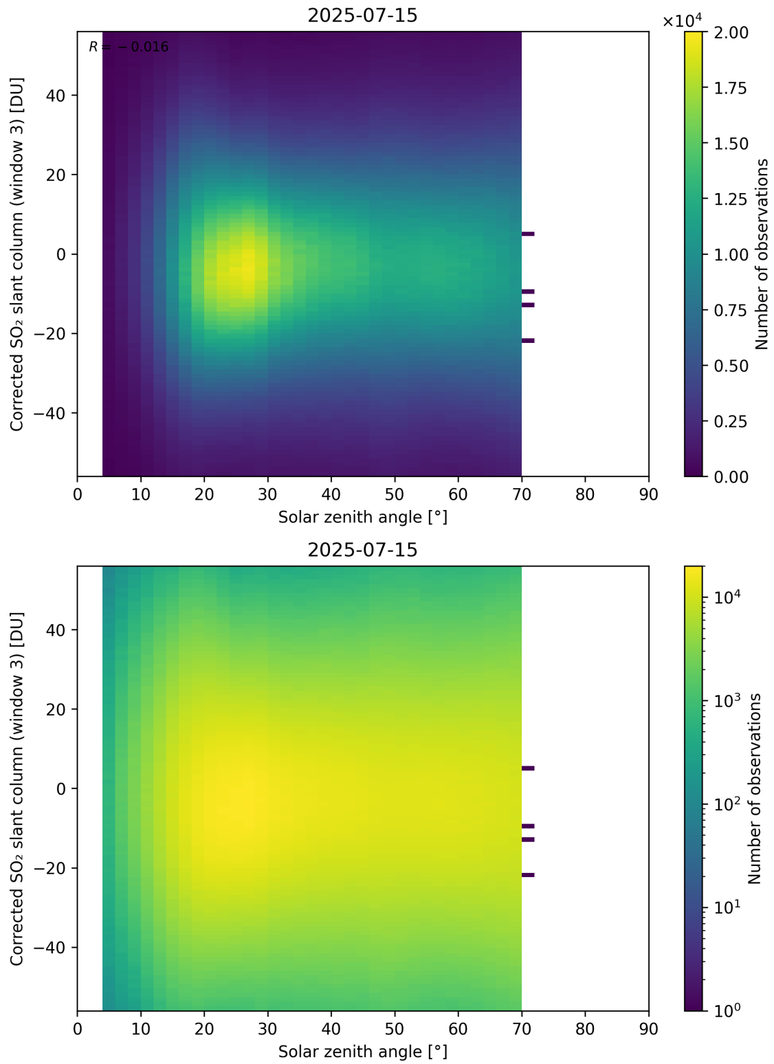
Figure 183: Scatter density plot of “Solar zenith angle” against “Corrected SO 2 slant column (window 3)” for 2025-07-14 to 2025-07-16.
