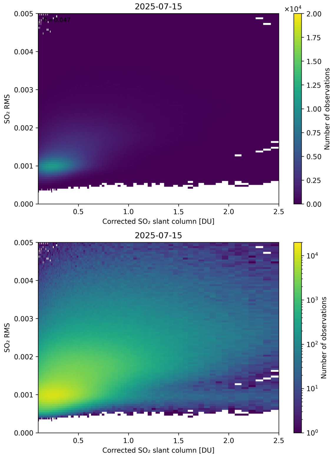
Figure 231: Scatter density plot of “Corrected SO 2 slant column” against “SO 2 RMS” for 2025-07-14 to 2025-07-16.
