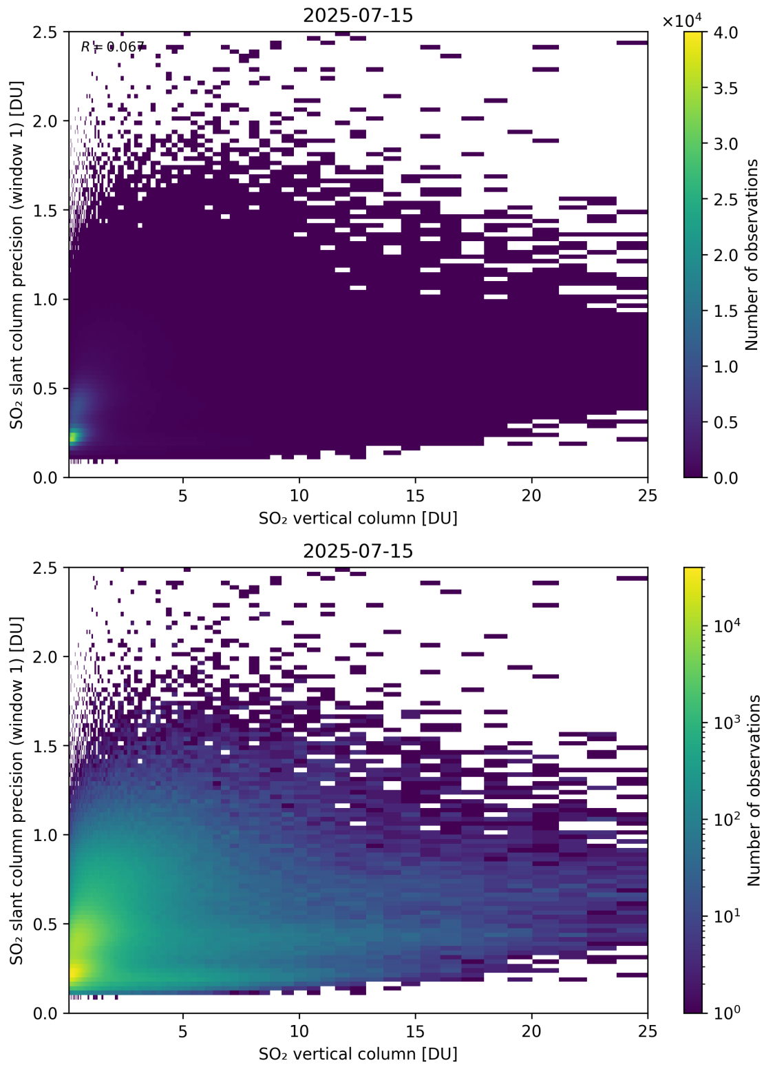
Figure 355: Scatter density plot of “SO 2 vertical column” against “SO 2 slant column precision (window 1)” for 2025-07-14 to 2025-07-16.
