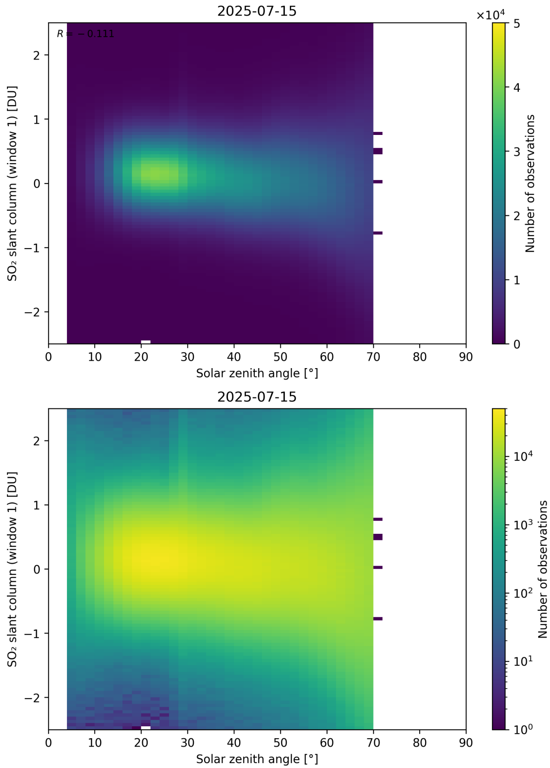
Figure 184: Scatter density plot of “Solar zenith angle” against “SO 2 slant column (window 1)” for 2025-07-14 to 2025-07-16.
