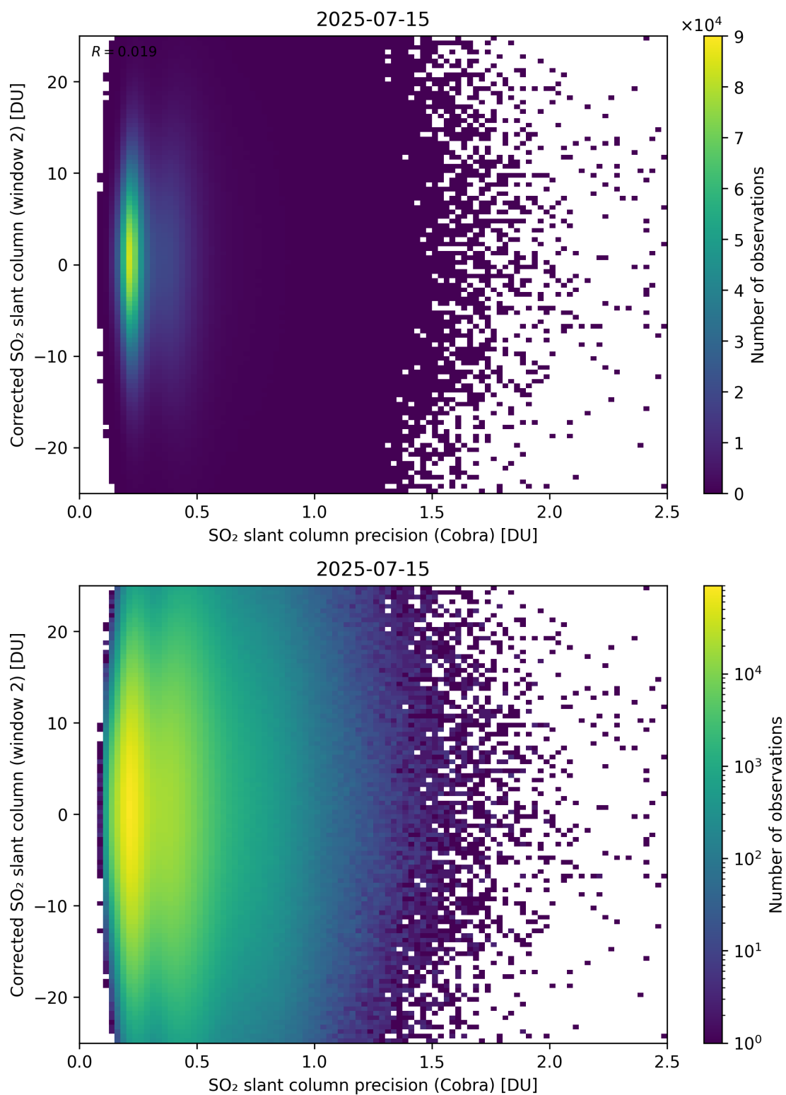
Figure 206: Scatter density plot of “SO 2 slant column precision (Cobra)” against “Corrected SO 2 slant column (window 2)” for 2025-07-14 to 2025-07-16.
