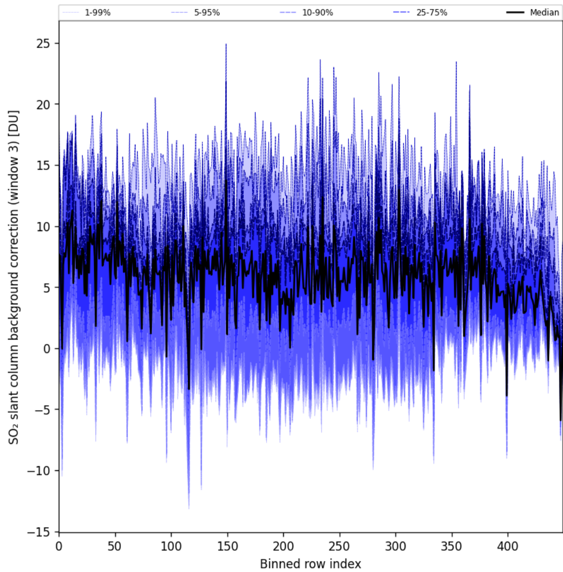
Figure 100: Along track statistics of “SO 2 slant column background correction (window 3)” for 2025-07-14 to 2025-07-16
