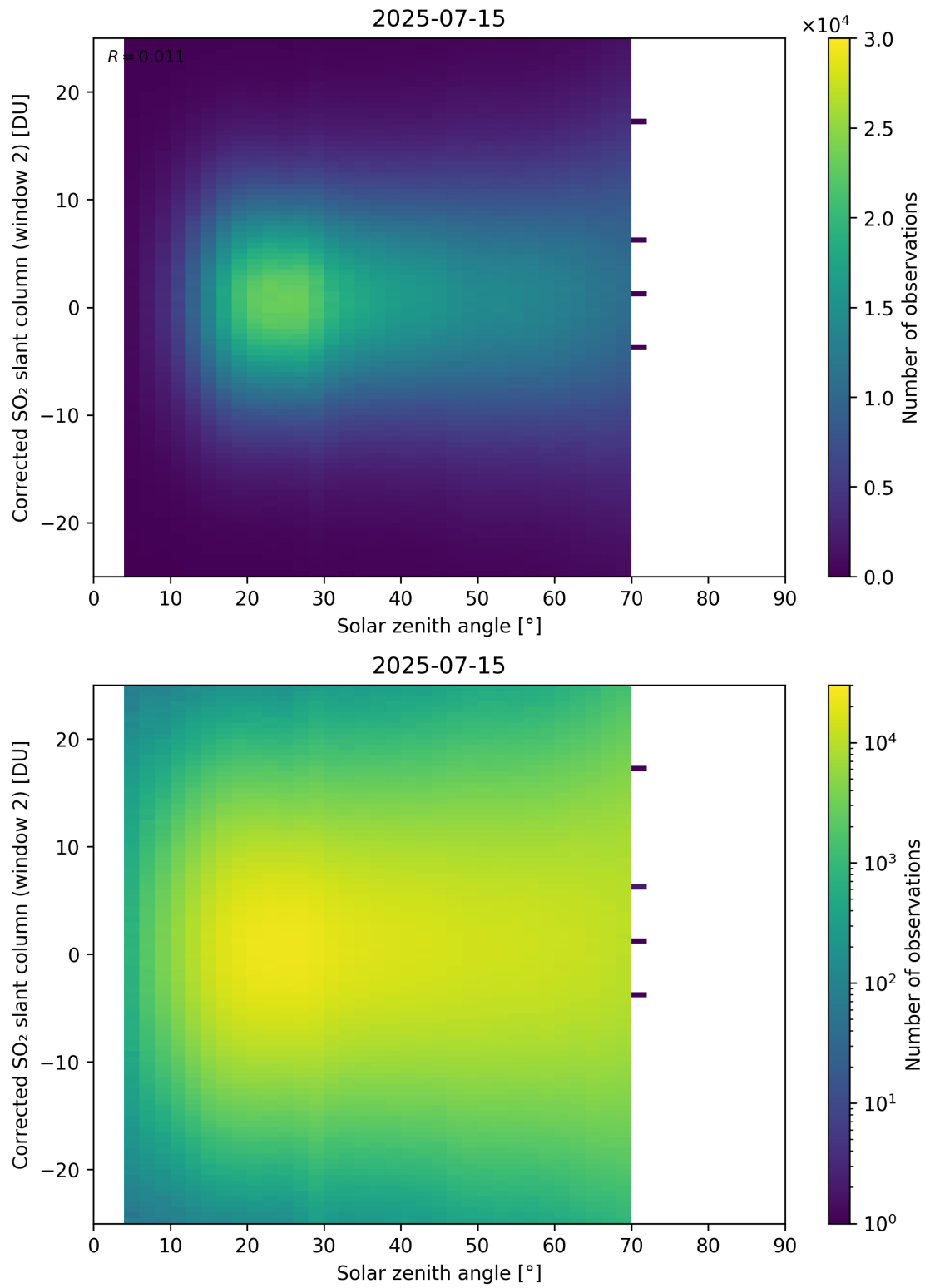
Figure 182: Scatter density plot of “Solar zenith angle” against “Corrected SO 2 slant column (window 2)” for 2025-07-14 to 2025-07-16.
