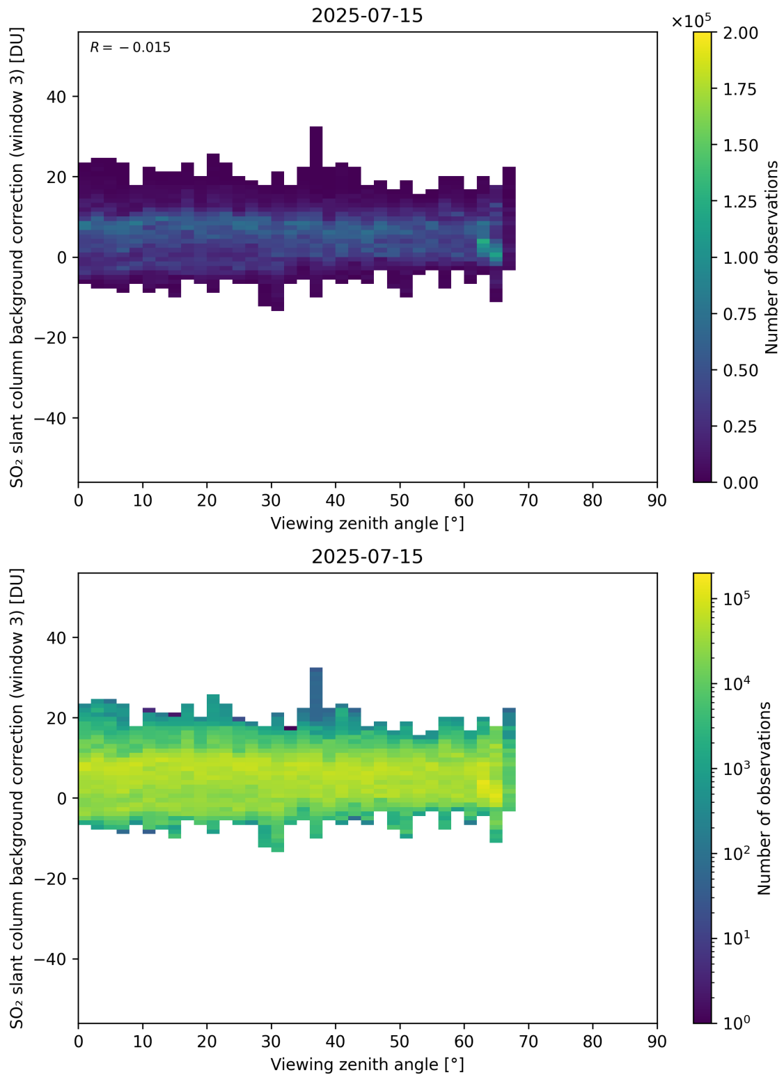
Figure 364: Scatter density plot of “Viewing zenith angle” against “SO 2 slant column background correction (window 3)” for 2025-07-14 to 2025-07-16.
