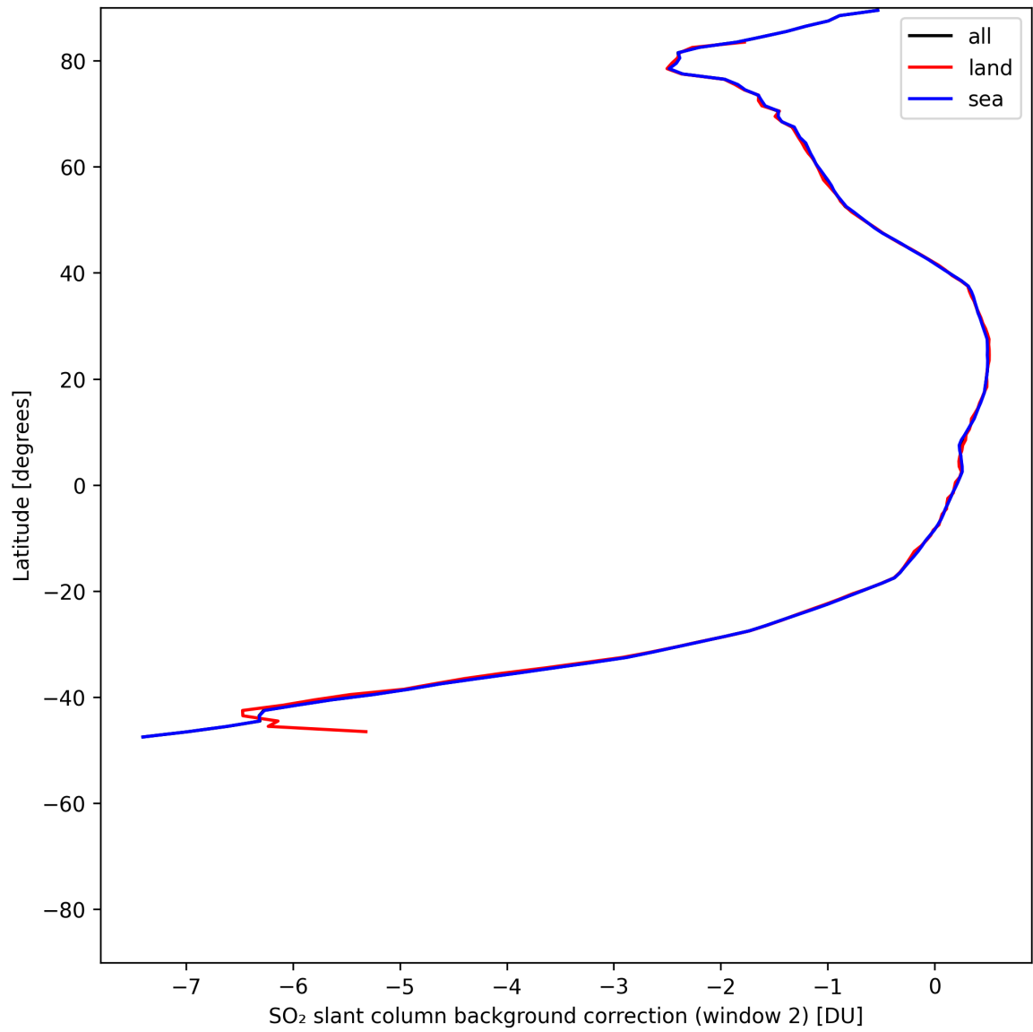
Figure 44: Zonal average of “SO 2 slant column background correction (window 2)” for 2025-07-14 to 2025-07-16.
