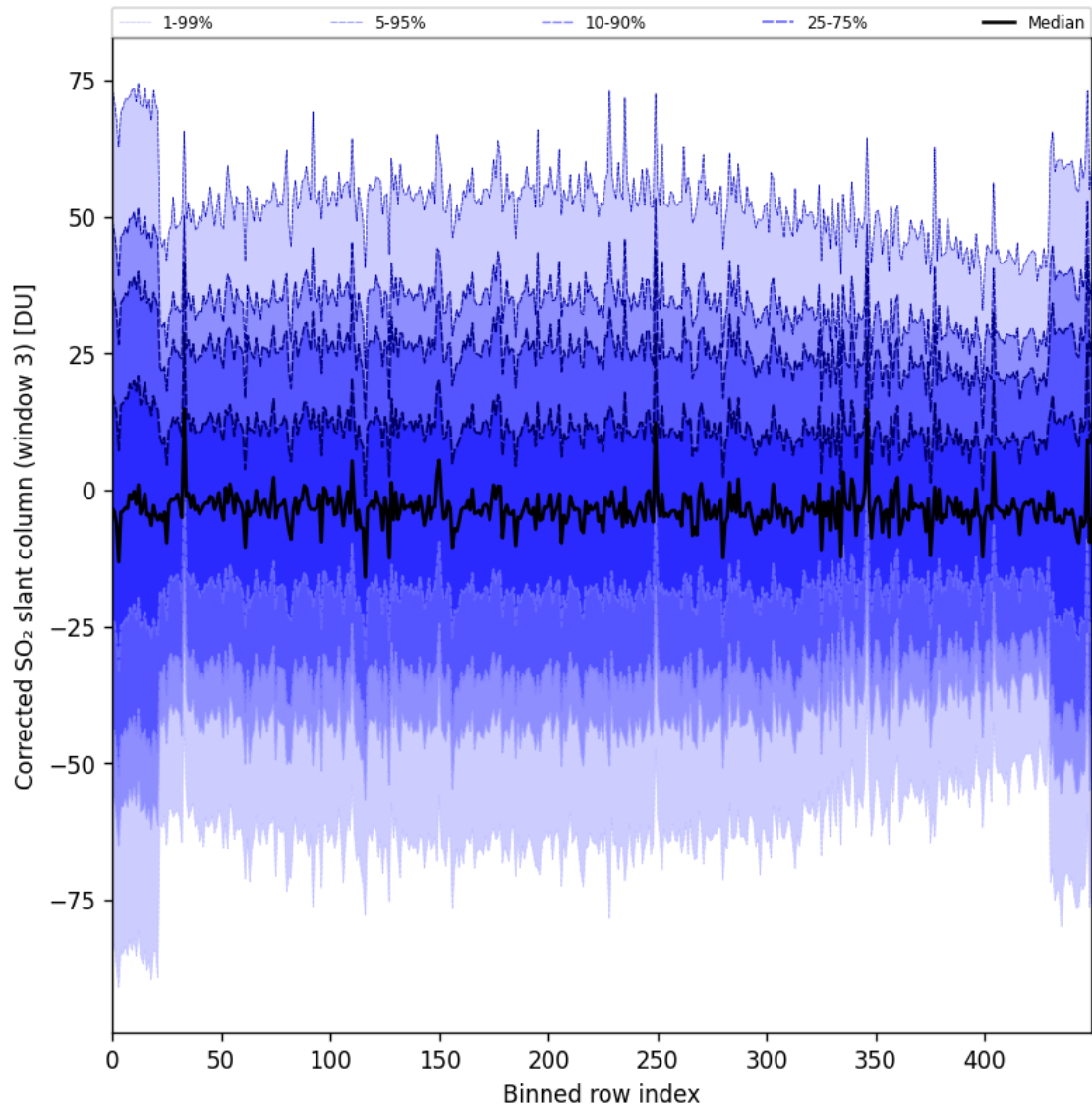
Figure 99: Along track statistics of “Corrected SO 2 slant column (window 3)” for 2025-07-14 to 2025-07-16
