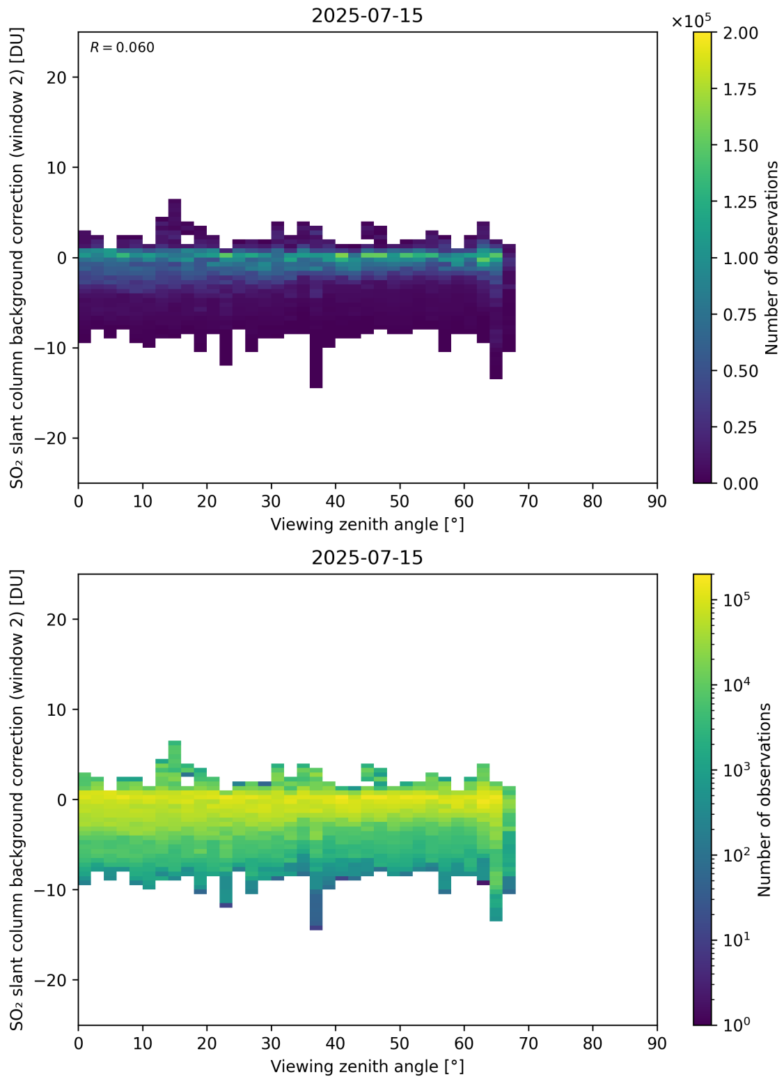
Figure 363: Scatter density plot of “Viewing zenith angle” against “SO 2 slant column background correction (window 2)” for 2025-07-14 to 2025-07-16.
