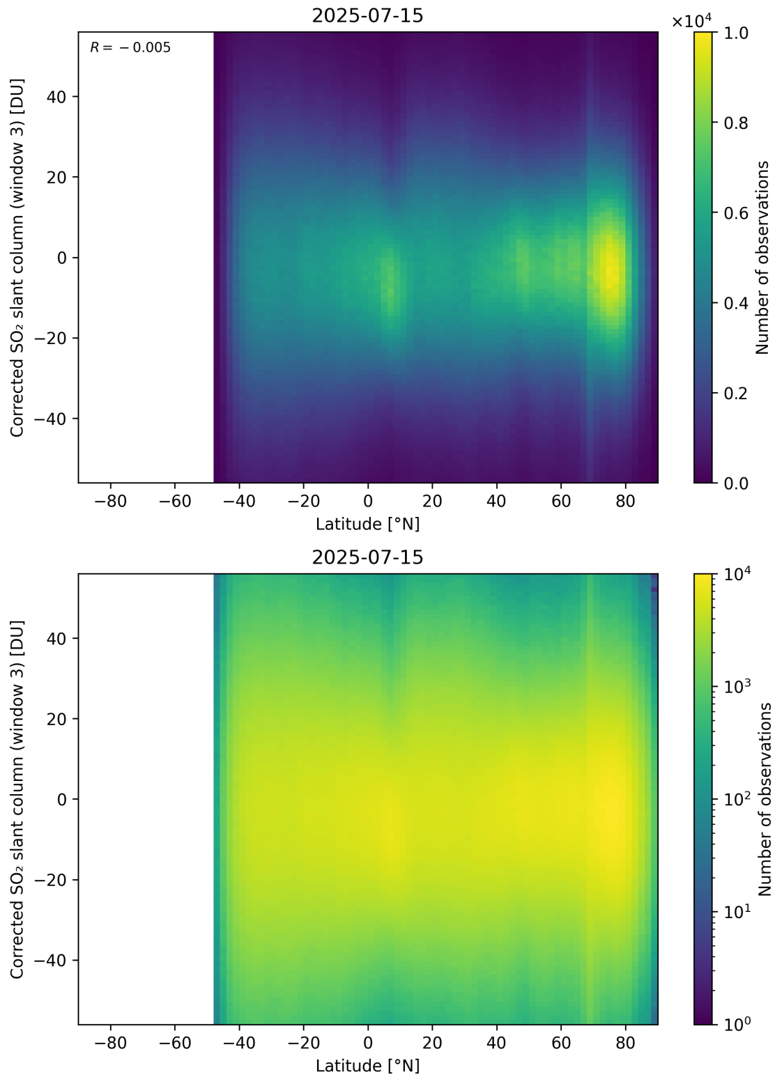
Figure 161: Scatter density plot of “Latitude” against “Corrected SO 2 slant column (window 3)” for 2025-07-14 to 2025-07-16.
