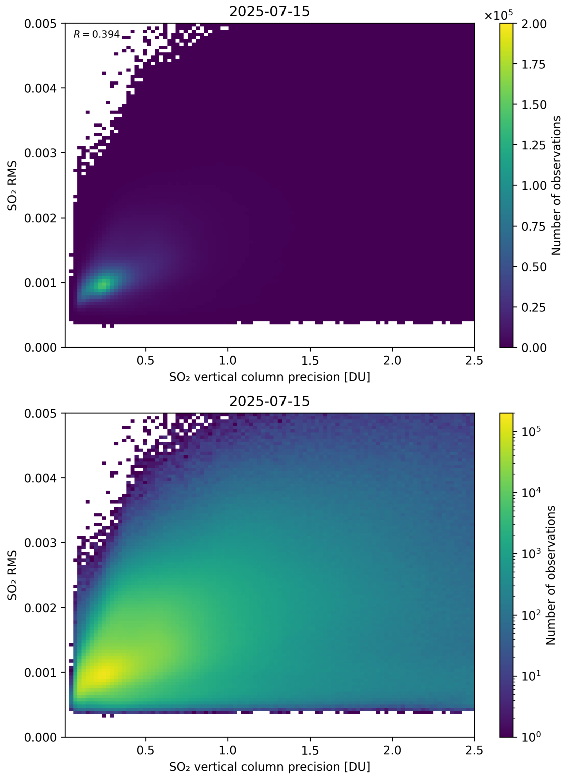
Figure 334: Scatter density plot of “SO 2 vertical column precision” against “SO 2 RMS” for 2025-07-14 to 2025-07-16.
