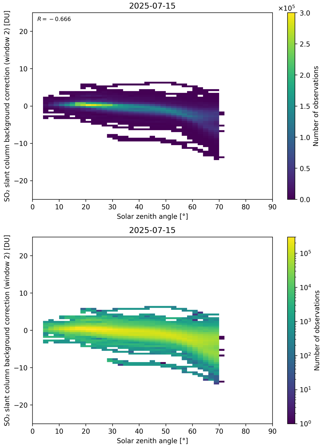
Figure 172: Scatter density plot of “Solar zenith angle” against “SO 2 slant column background correction (window 2)” for 2025-07-14 to 2025-07-16.
