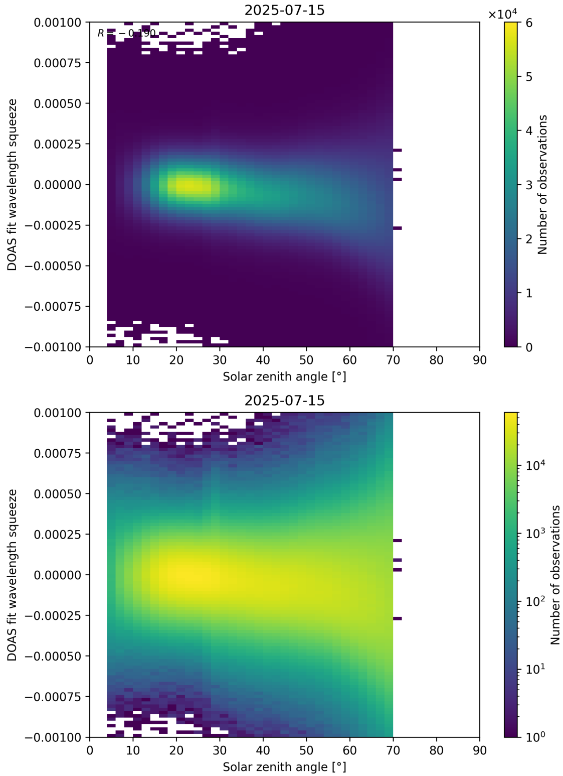
Figure 175: Scatter density plot of “Solar zenith angle” against “DOAS fit wavelength squeeze” for 2025-07-14 to 2025-07-16.
