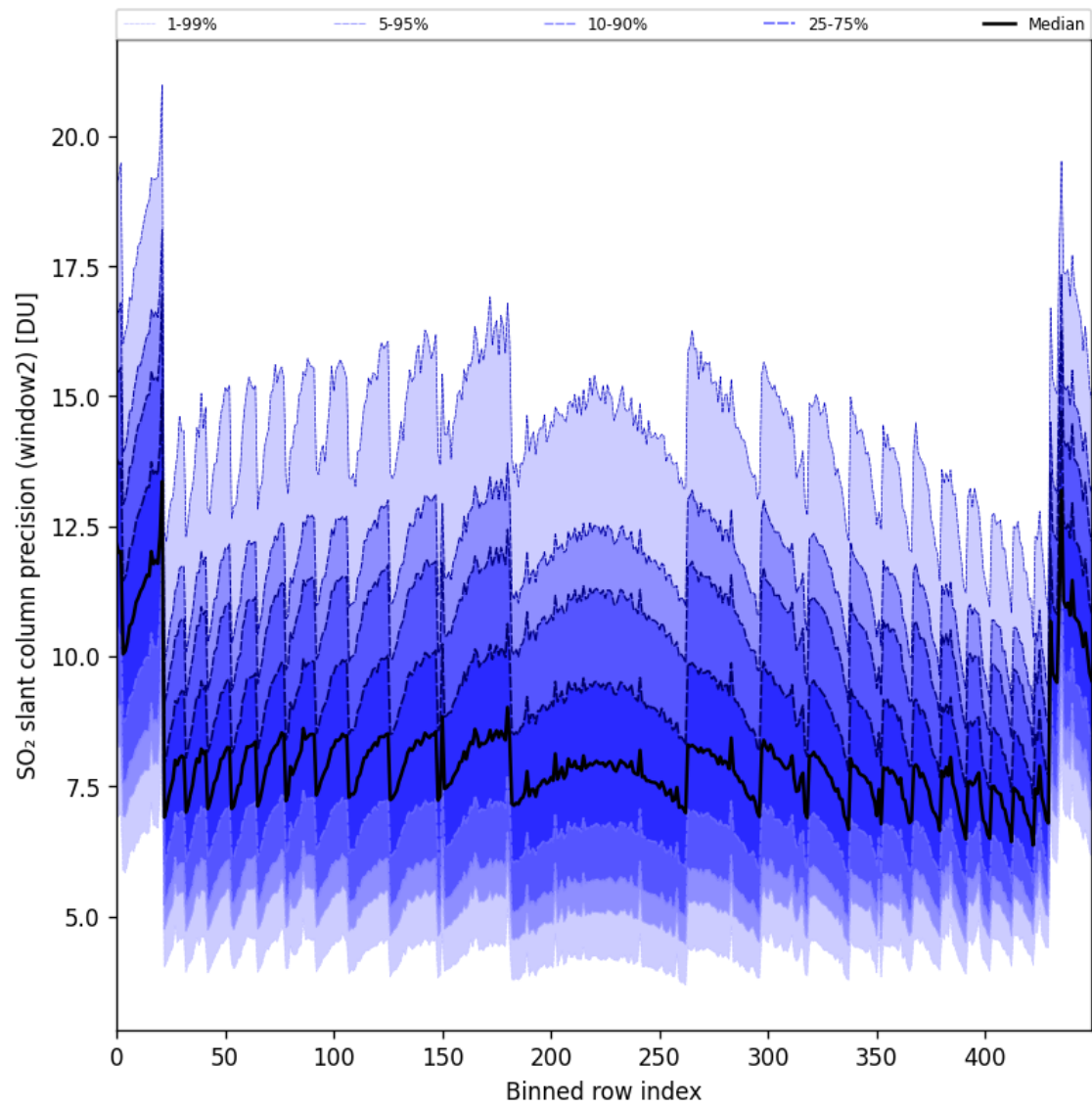
Figure 94: Along track statistics of “SO 2 slant column precision (window2)” for 2025-07-14 to 2025-07-16
