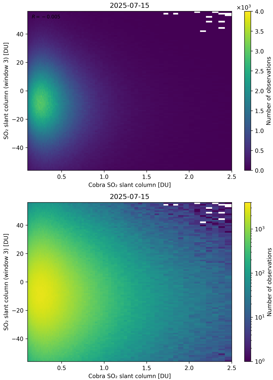
Figure 222: Scatter density plot of “Cobra SO 2 slant column” against “SO 2 slant column (window 3)” for 2025-07-14 to 2025-07-16.
