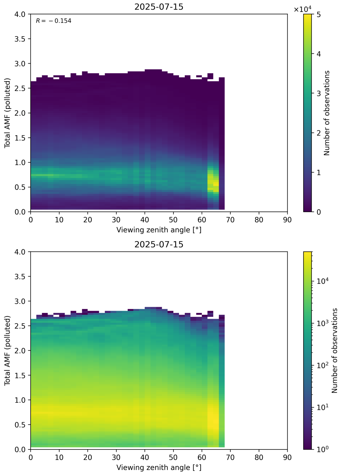
Figure 381: Scatter density plot of “Viewing zenith angle” against “Total AMF (polluted)” for 2025-07-14 to 2025-07-16.
