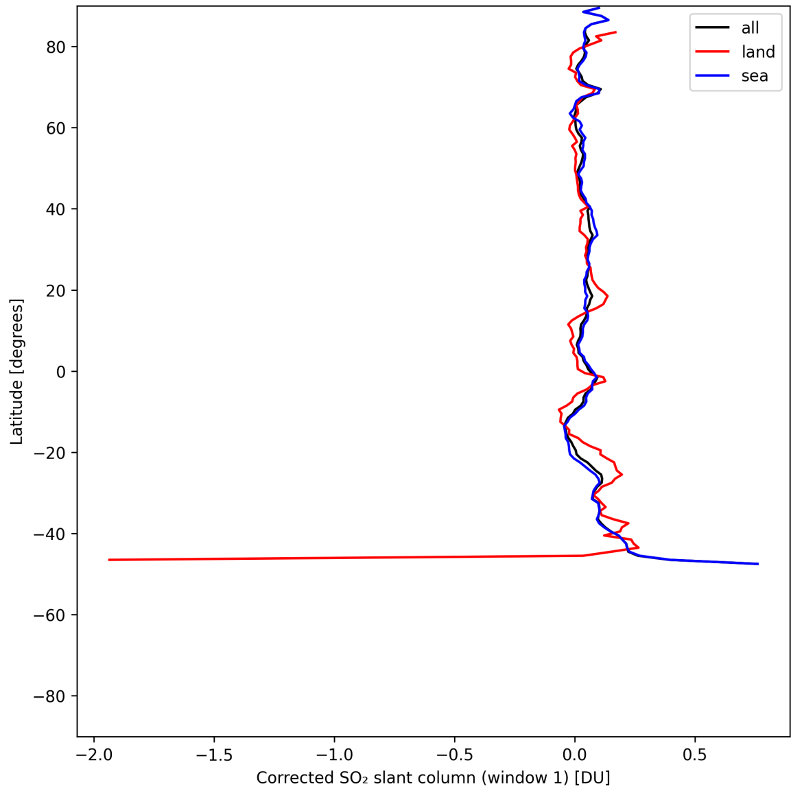
Figure 39: Zonal average of “Corrected SO 2 slant column (window 1)” for 2025-07-14 to 2025-07-16.
