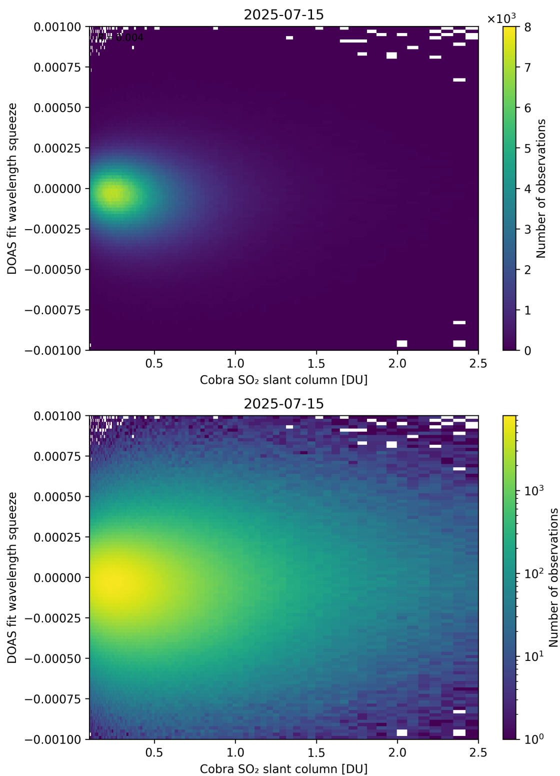
Figure 197: Scatter density plot of “Cobra SO 2 slant column” against “DOAS fit wavelength squeeze” for 2025-07-14 to 2025-07-16.
