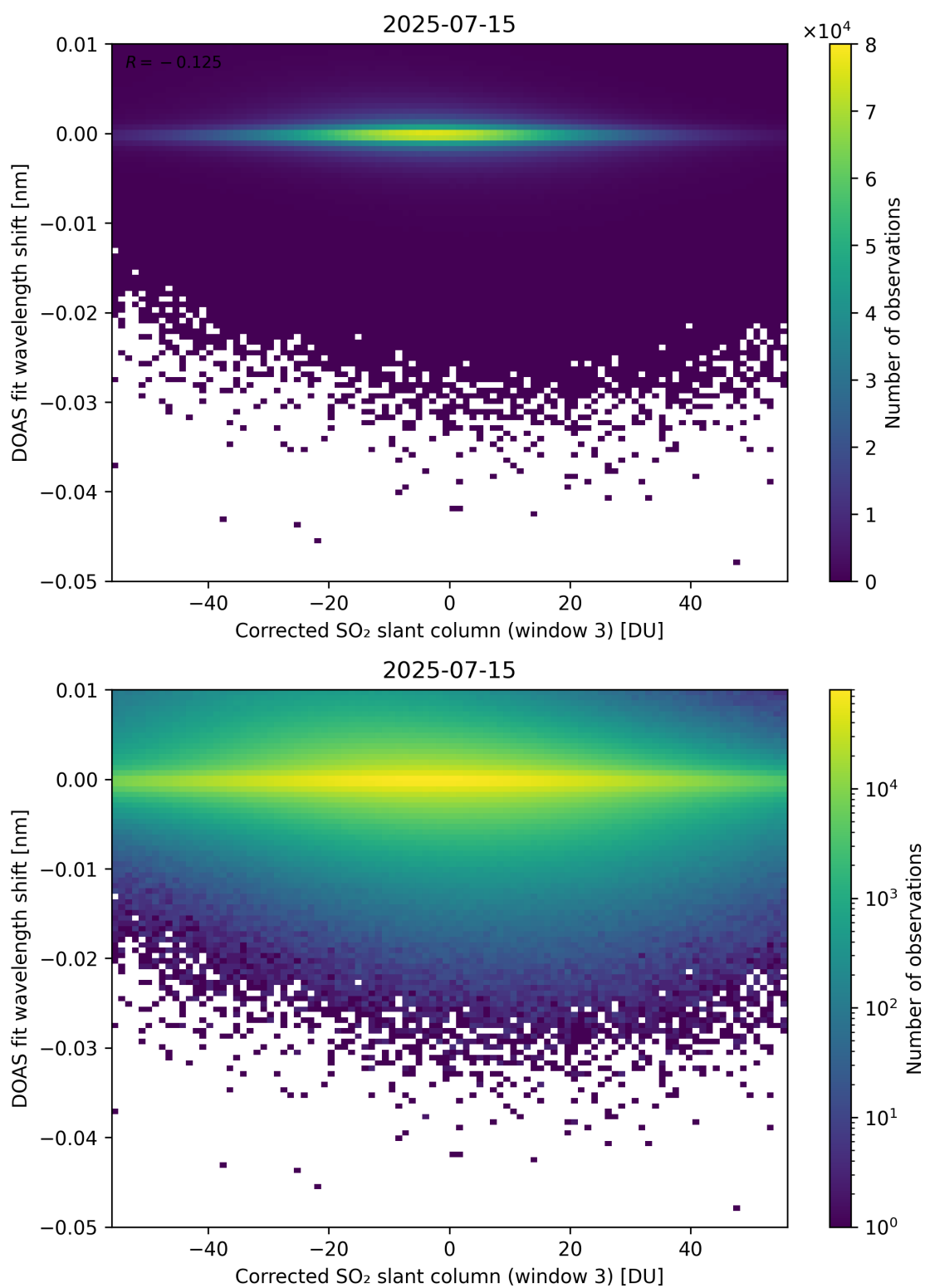
Figure 256: Scatter density plot of “Corrected SO 2 slant column (window 3)” against “DOAS fit wavelength shift” for 2025-07-14 to 2025-07-16.
