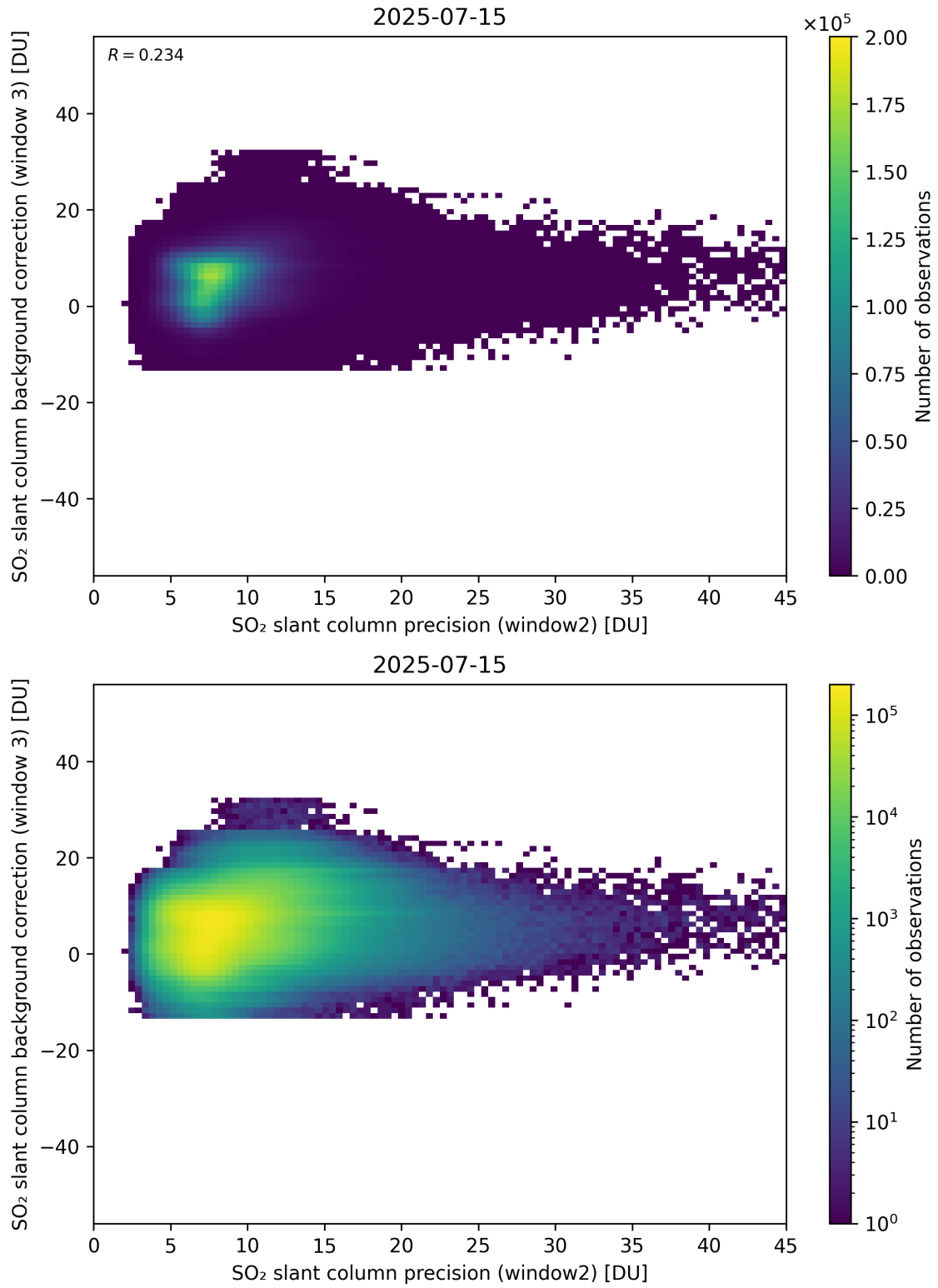
Figure 292: Scatter density plot of “SO 2 slant column precision (window2)” against “SO 2 slant column background correction (window 3)” for 2025-07-14 to 2025-07-16.
