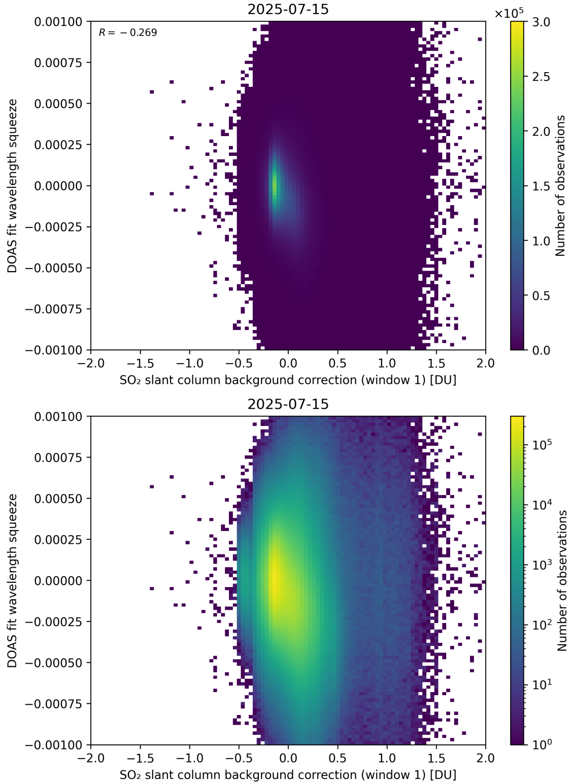
Figure 112: Scatter density plot of “SO 2 slant column background correction (window 1)” against “DOAS fit wavelength squeeze” for 2025-07-14 to 2025-07-16.
