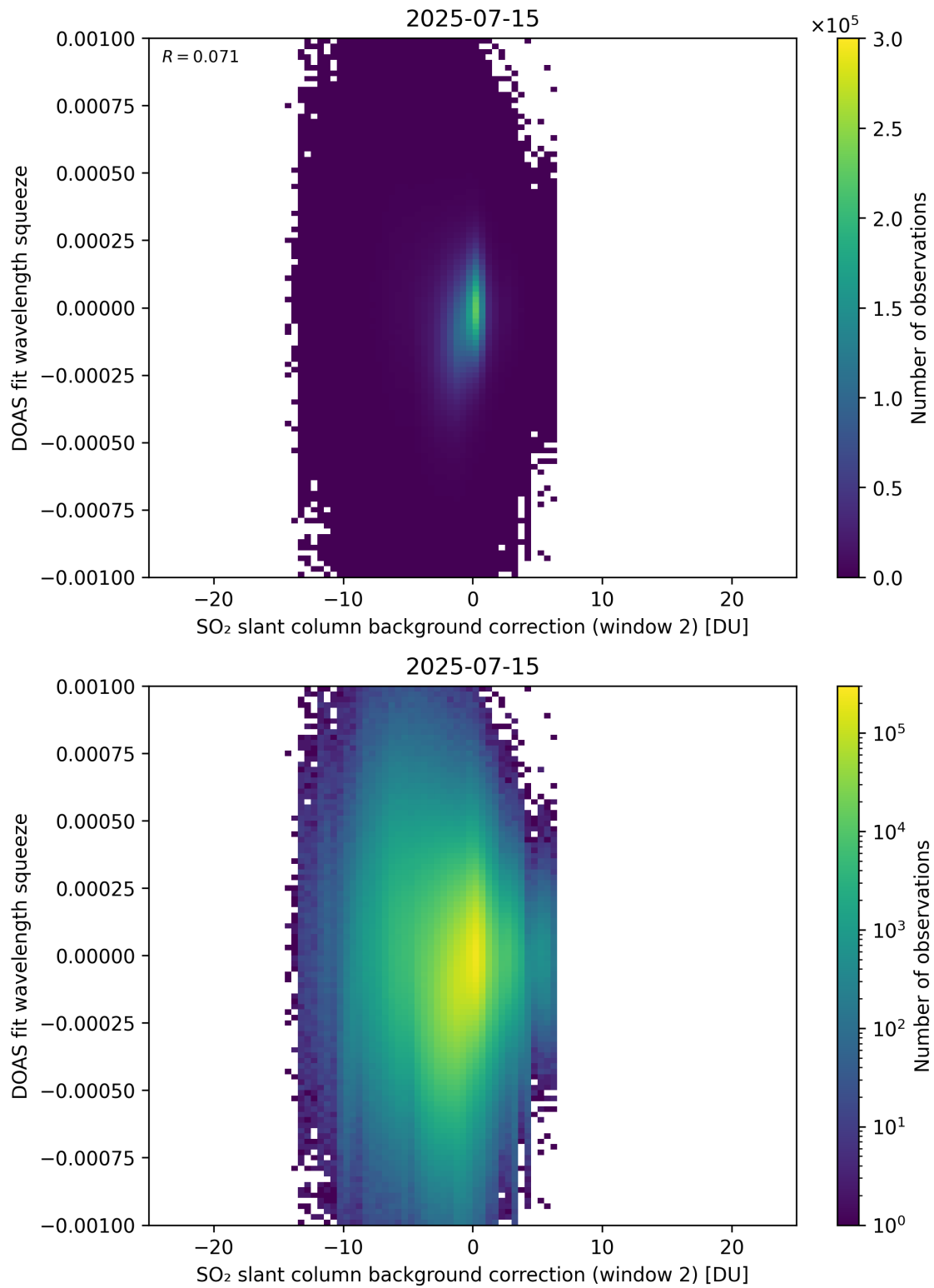
Figure 124: Scatter density plot of “SO 2 slant column background correction (window 2)” against “DOAS fit wavelength squeeze” for 2025-07-14 to 2025-07-16.
