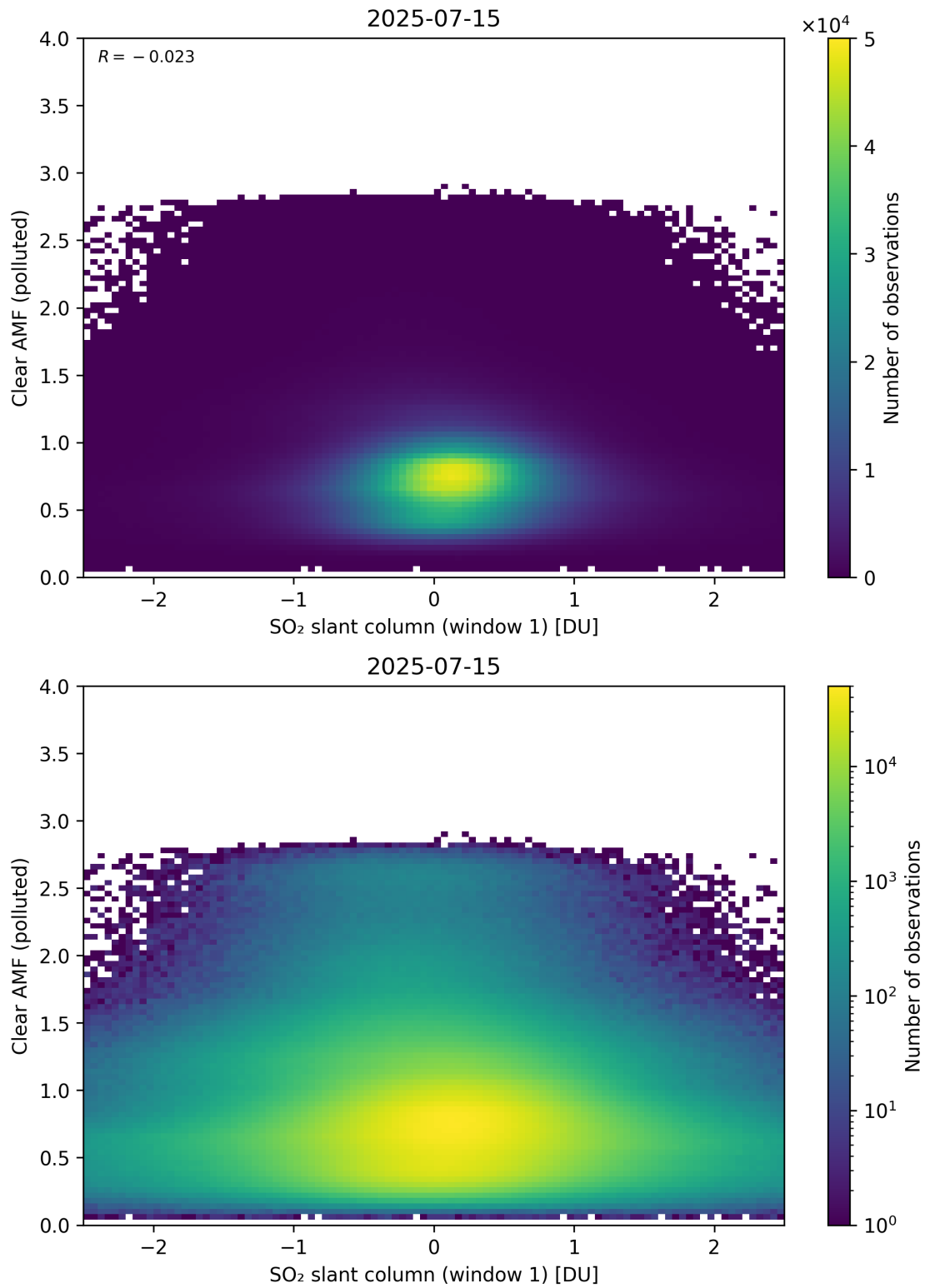
Figure 282: Scatter density plot of “SO 2 slant column (window 1)” against “Clear AMF (polluted)” for 2025-07-14 to 2025-07-16.
