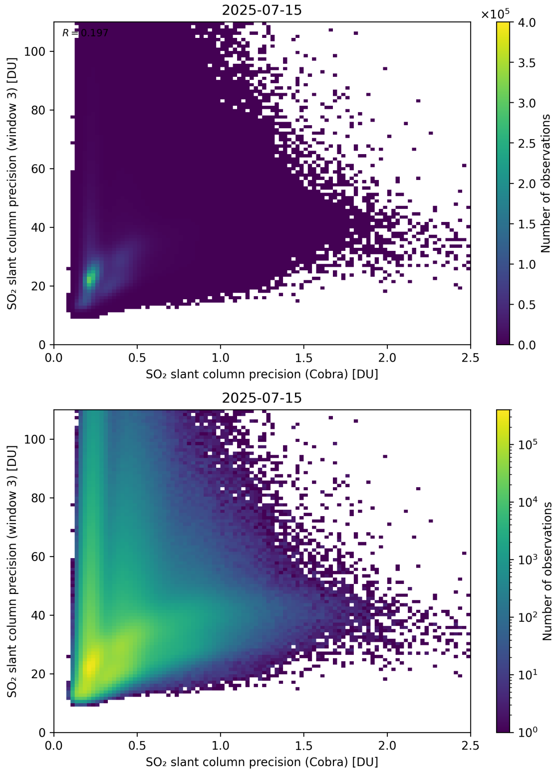
Figure 212: Scatter density plot of “SO 2 slant column precision (Cobra)” against “SO 2 slant column precision (window 3)” for 2025-07-14 to 2025-07-16.
