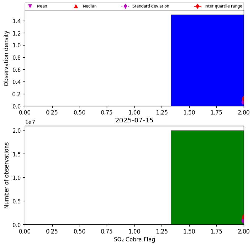
Figure 75: Histogram of “SO 2 Cobra Flag” for 2025-07-14 to 2025-07-16
