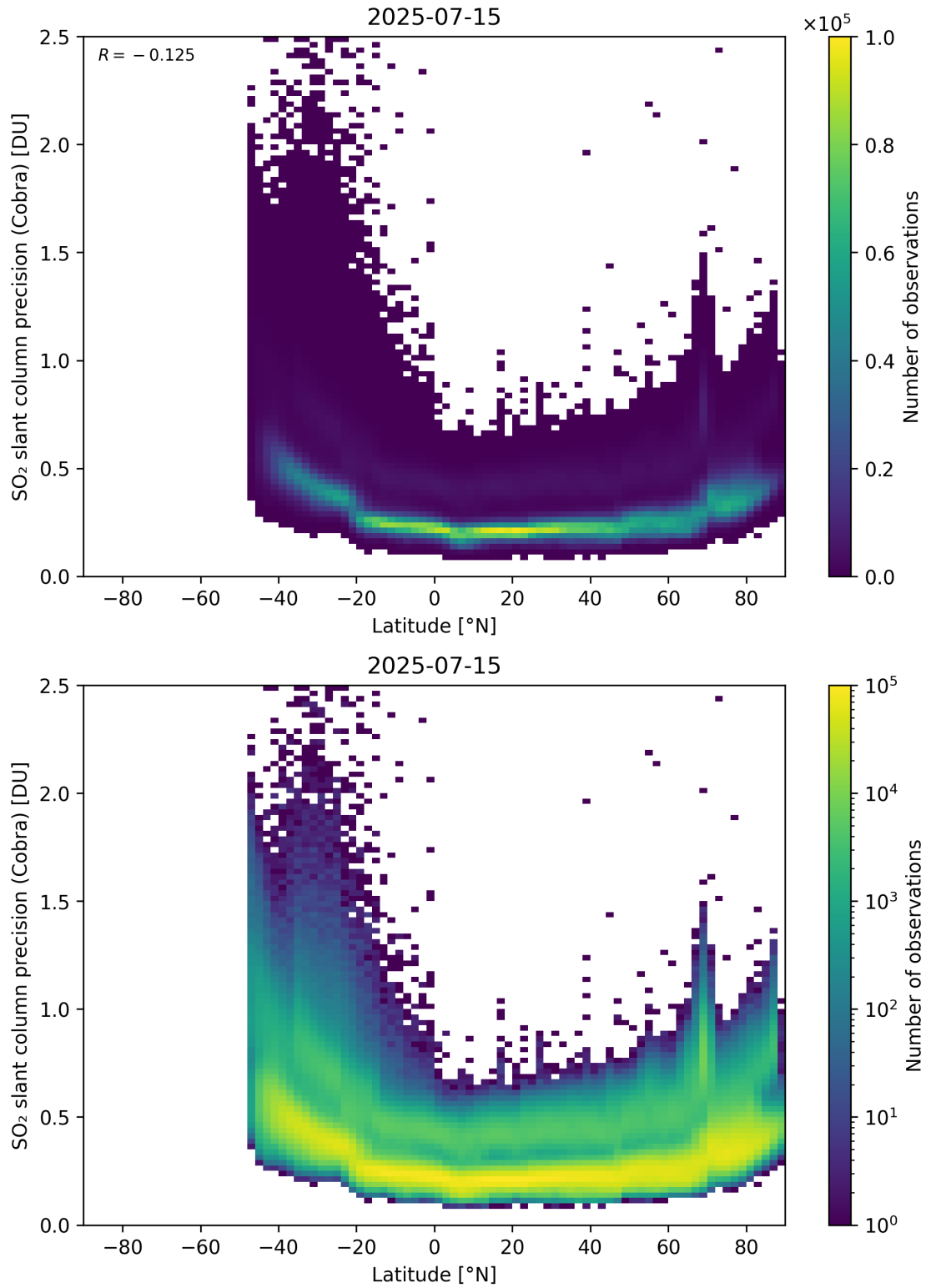
Figure 158: Scatter density plot of “Latitude” against “SO 2 slant column precision (Cobra)” for 2025-07-14 to 2025-07-16.
