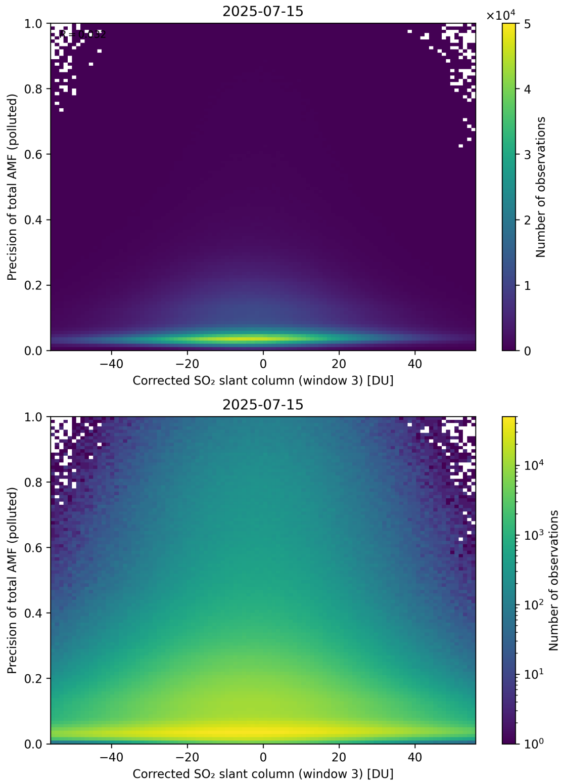
Figure 261: Scatter density plot of “Corrected SO 2 slant column (window 3)” against “Precision of total AMF (polluted)” for 2025-07-14 to 2025-07-16.
