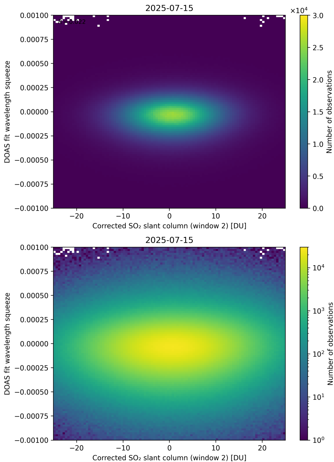
Figure 247: Scatter density plot of “Corrected SO 2 slant column (window 2)” against “DOAS fit wavelength squeeze” for 2025-07-14 to 2025-07-16.
