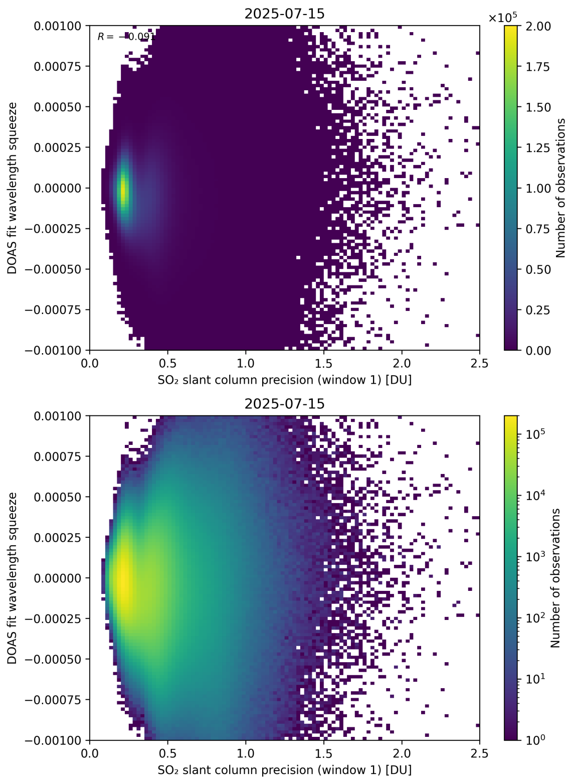
Figure 272: Scatter density plot of “SO 2 slant column precision (window 1)” against “DOAS fit wavelength squeeze” for 2025-07-14 to 2025-07-16.
