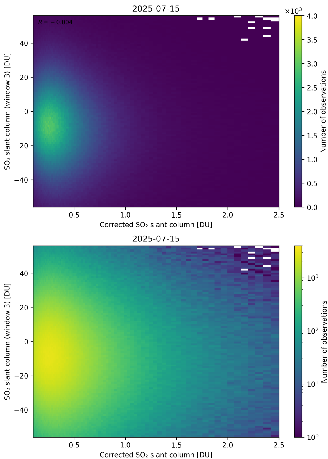
Figure 240: Scatter density plot of “Corrected SO 2 slant column” against “SO 2 slant column (window 3)” for 2025-07-14 to 2025-07-16.
