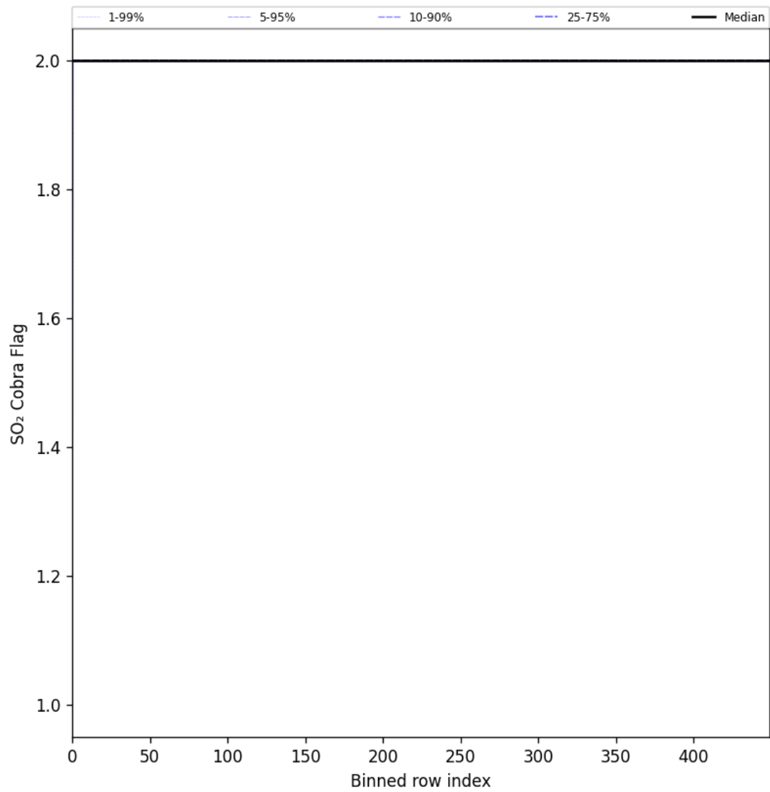
Figure 101: Along track statistics of “SO 2 Cobra Flag” for 2025-07-14 to 2025-07-16
