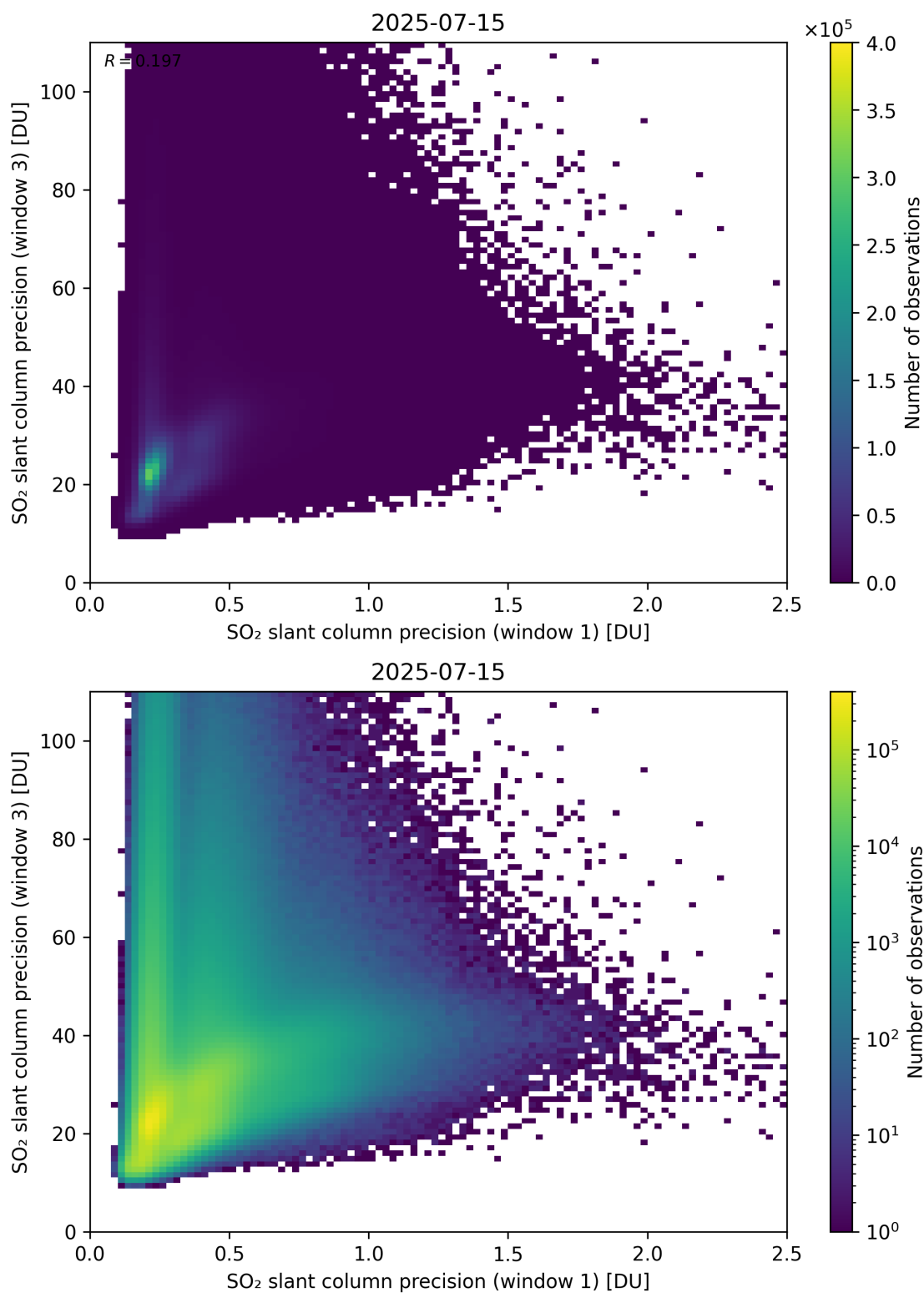
Figure 279: Scatter density plot of “SO 2 slant column precision (window 1)” against “SO 2 slant column precision (window 3)” for 2025-07-14 to 2025-07-16.
