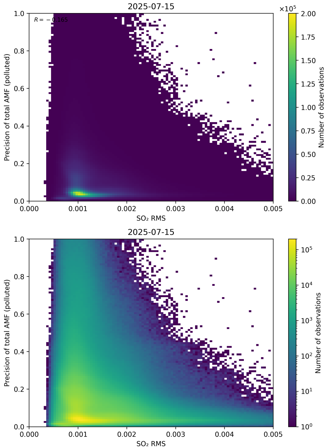
Figure 149: Scatter density plot of “SO 2 RMS” against “Precision of total AMF (polluted)” for 2025-07-14 to 2025-07-16.
