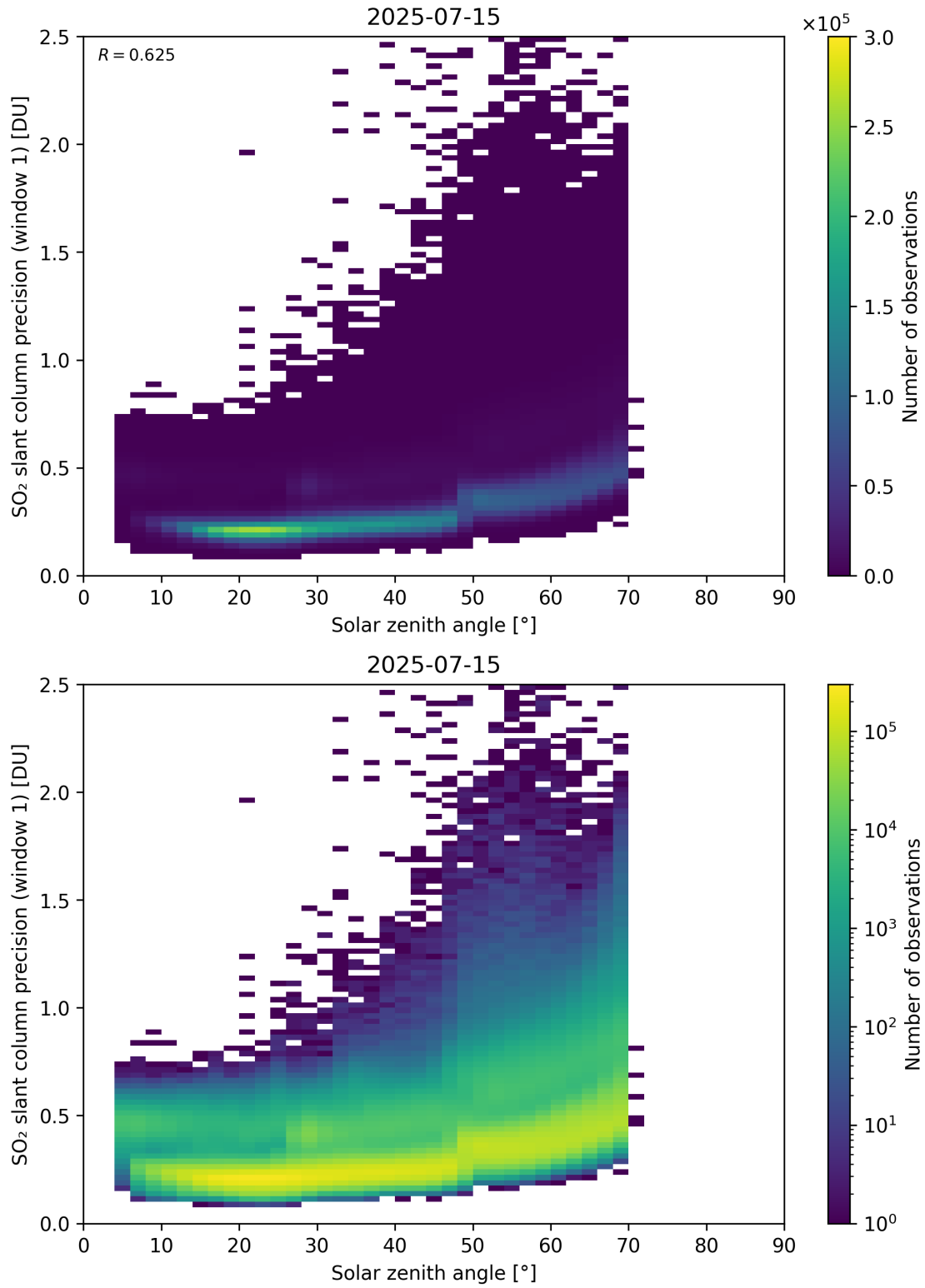
Figure 185: Scatter density plot of “Solar zenith angle” against “SO 2 slant column precision (window 1)” for 2025-07-14 to 2025-07-16.
