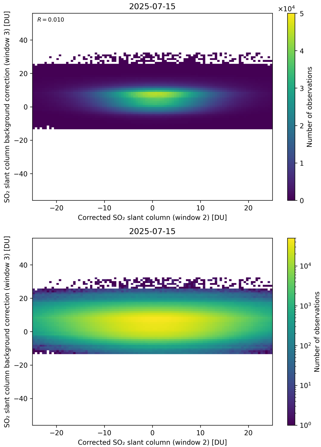
Figure 245: Scatter density plot of “Corrected SO 2 slant column (window 2)” against “SO 2 slant column background correction (window 3)” for 2025-07-14 to 2025-07-16.
