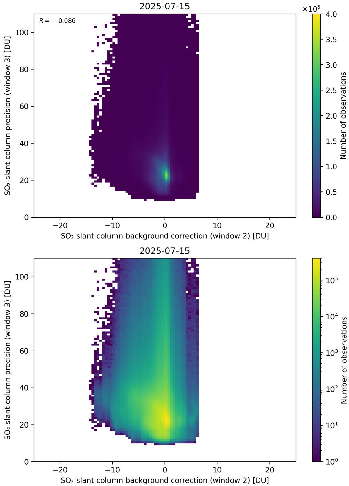
Figure 129: Scatter density plot of “SO 2 slant column background correction (window 2)” against “SO 2 slant column precision (window 3)” for 2025-07-14 to 2025-07-16.
