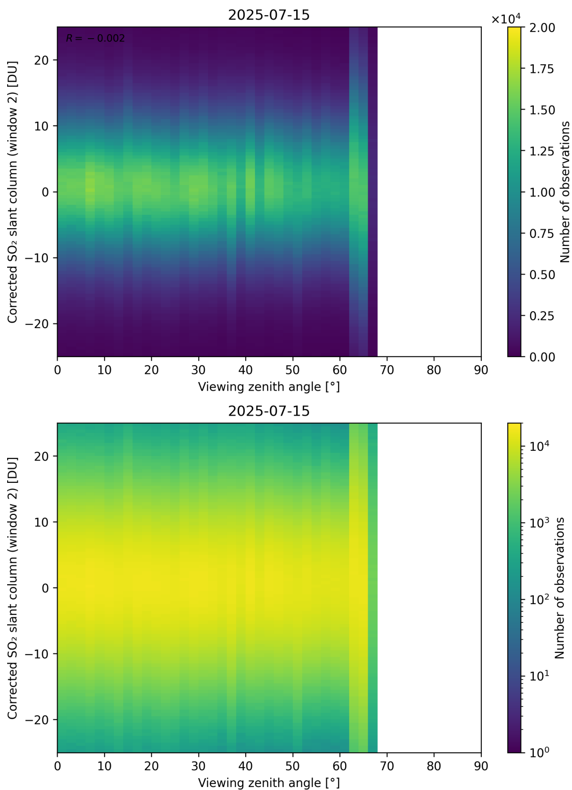
Figure 374: Scatter density plot of “Viewing zenith angle” against “Corrected SO 2 slant column (window 2)” for 2025-07-14 to 2025-07-16.
