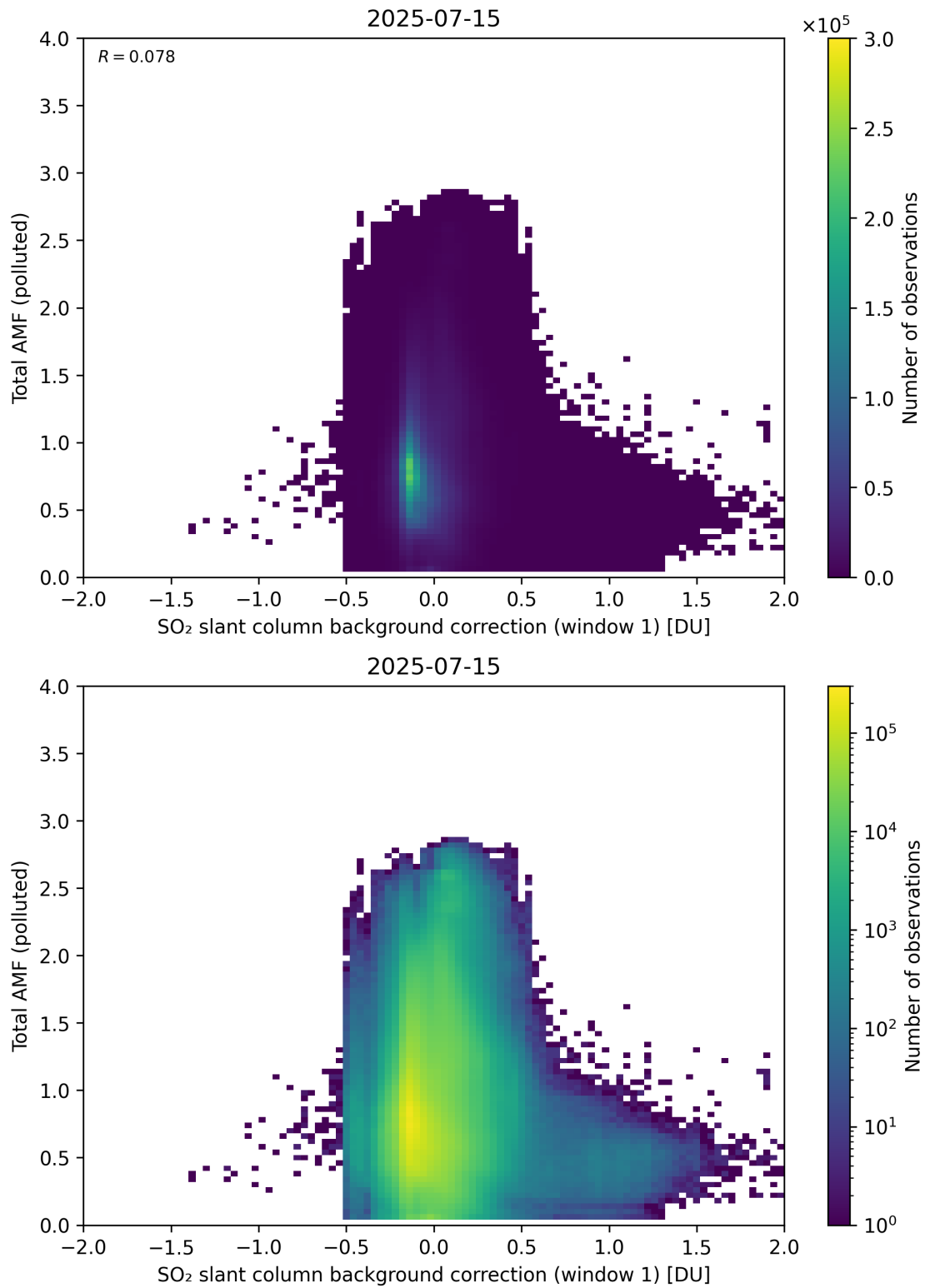
Figure 120: Scatter density plot of “SO 2 slant column background correction (window 1)” against “Total AMF (polluted)” for 2025-07-14 to 2025-07-16.
