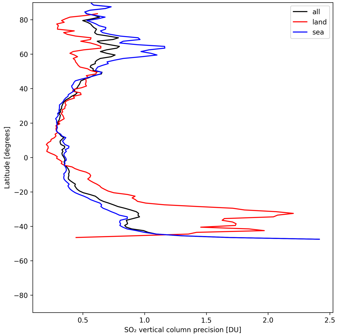
Figure 33: Zonal average of “SO 2 vertical column precision” for 2025-07-14 to 2025-07-16.
