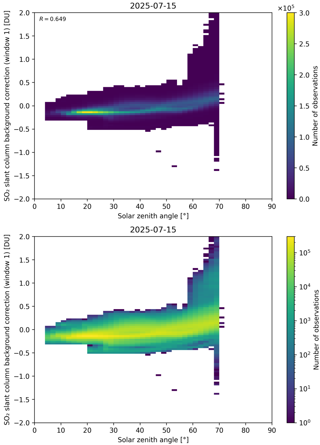
Figure 171: Scatter density plot of “Solar zenith angle” against “SO 2 slant column background correction (window 1)” for 2025-07-14 to 2025-07-16.
