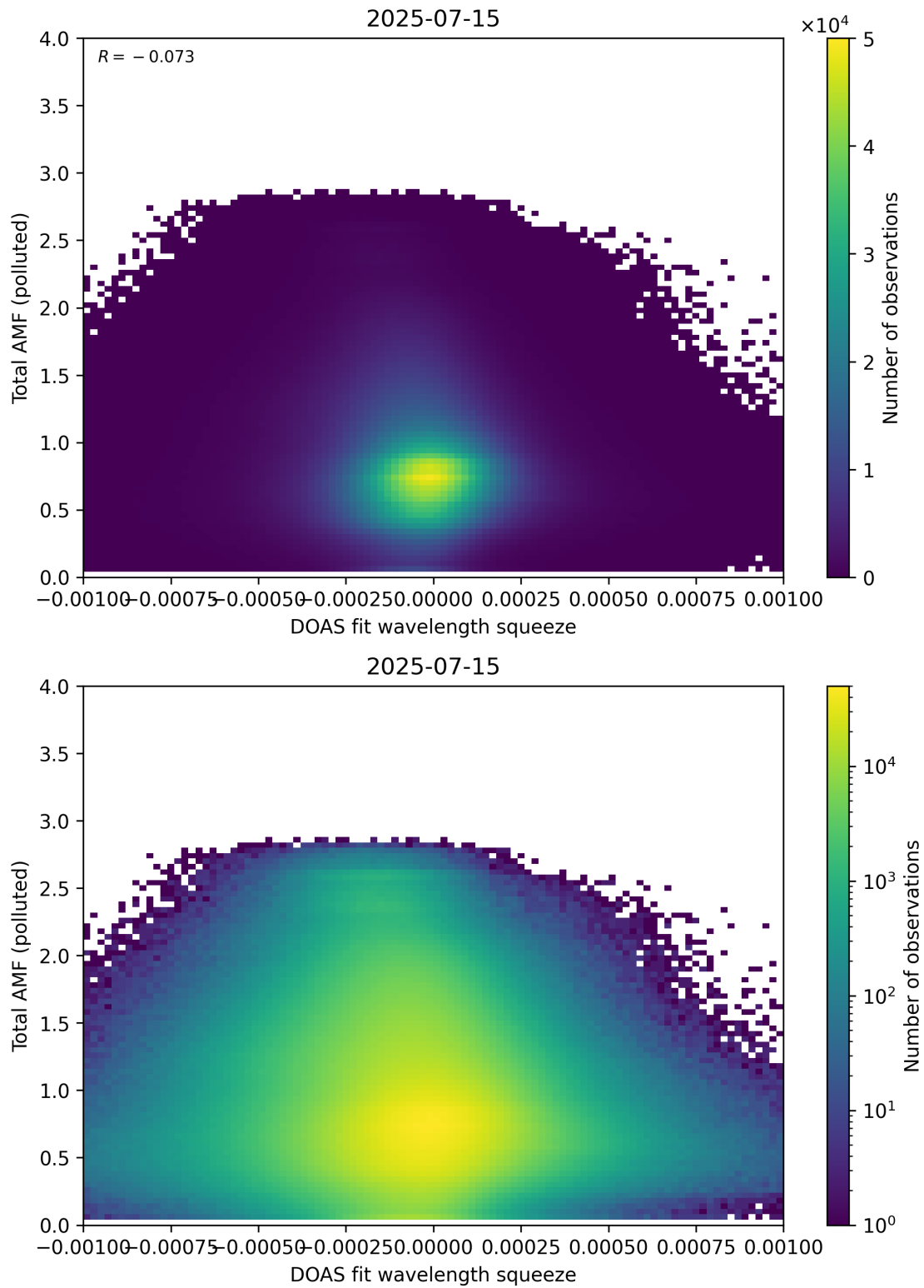
Figure 145: Scatter density plot of “DOAS fit wavelength squeeze” against “Total AMF (polluted)” for 2025-07-14 to 2025-07-16.
