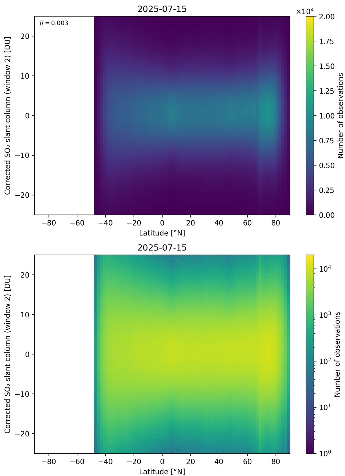
Figure 160: Scatter density plot of “Latitude” against “Corrected SO 2 slant column (window 2)” for 2025-07-14 to 2025-07-16.
