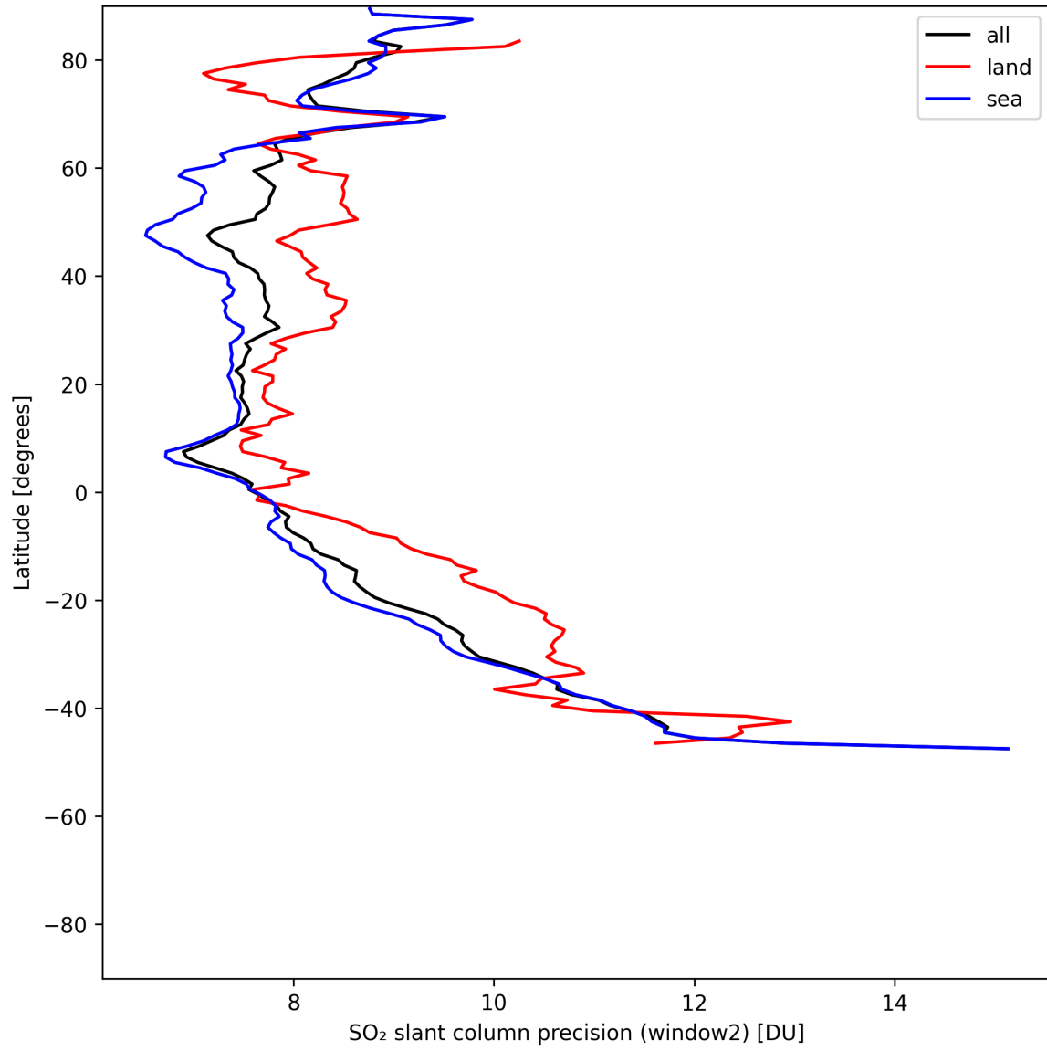
Figure 42: Zonal average of “SO 2 slant column precision (window2)” for 2025-07-14 to 2025-07-16.
