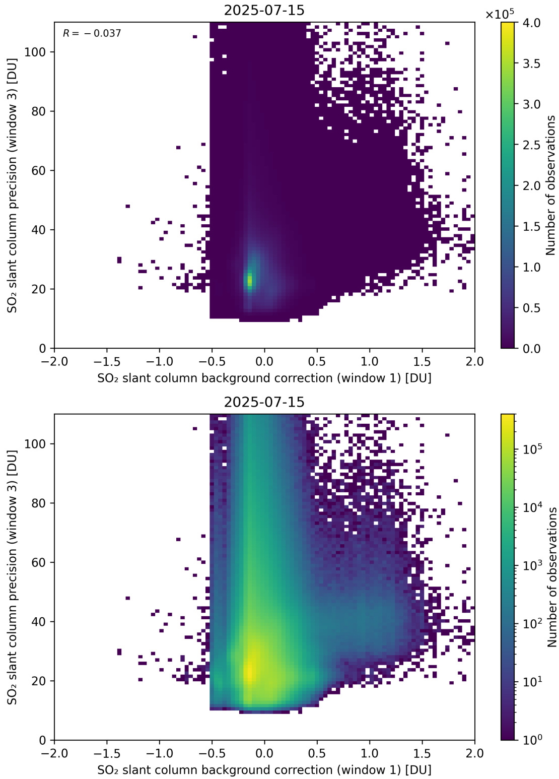
Figure 119: Scatter density plot of “SO 2 slant column background correction (window 1)” against “SO 2 slant column precision (window 3)” for 2025-07-14 to 2025-07-16.
