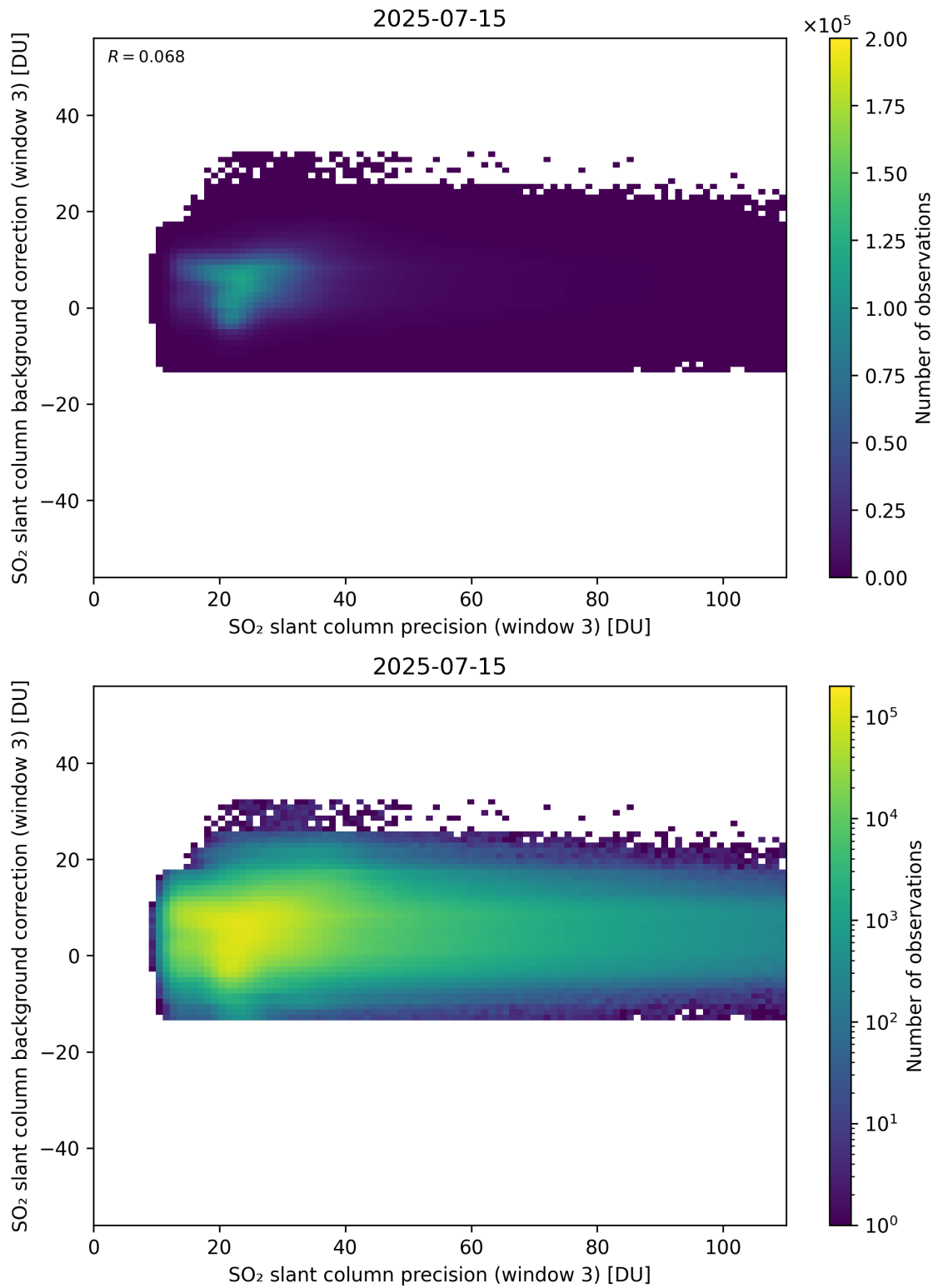
Figure 307: Scatter density plot of “SO 2 slant column precision (window 3)” against “SO 2 slant column background correction (window 3)” for 2025-07-14 to 2025-07-16.
