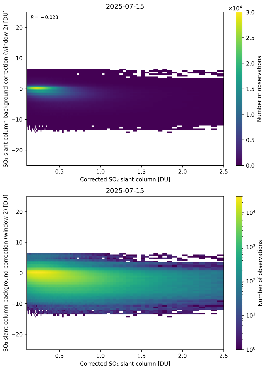
Figure 227: Scatter density plot of “Corrected SO 2 slant column” against “SO 2 slant column background correction (window 2)” for 2025-07-14 to 2025-07-16.
