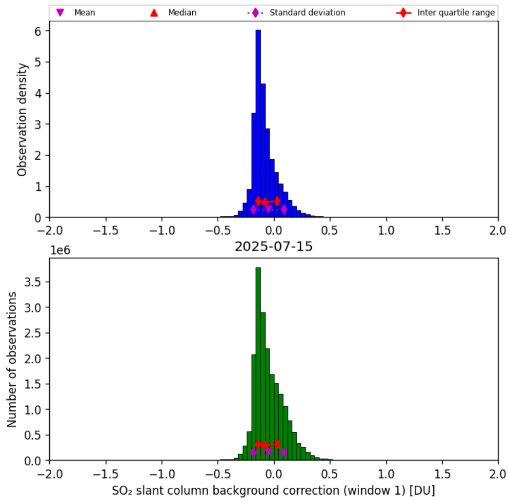
Figure 66: Histogram of “SO 2 slant column background correction (window 1)” for 2025-07-14 to 2025-07-16
