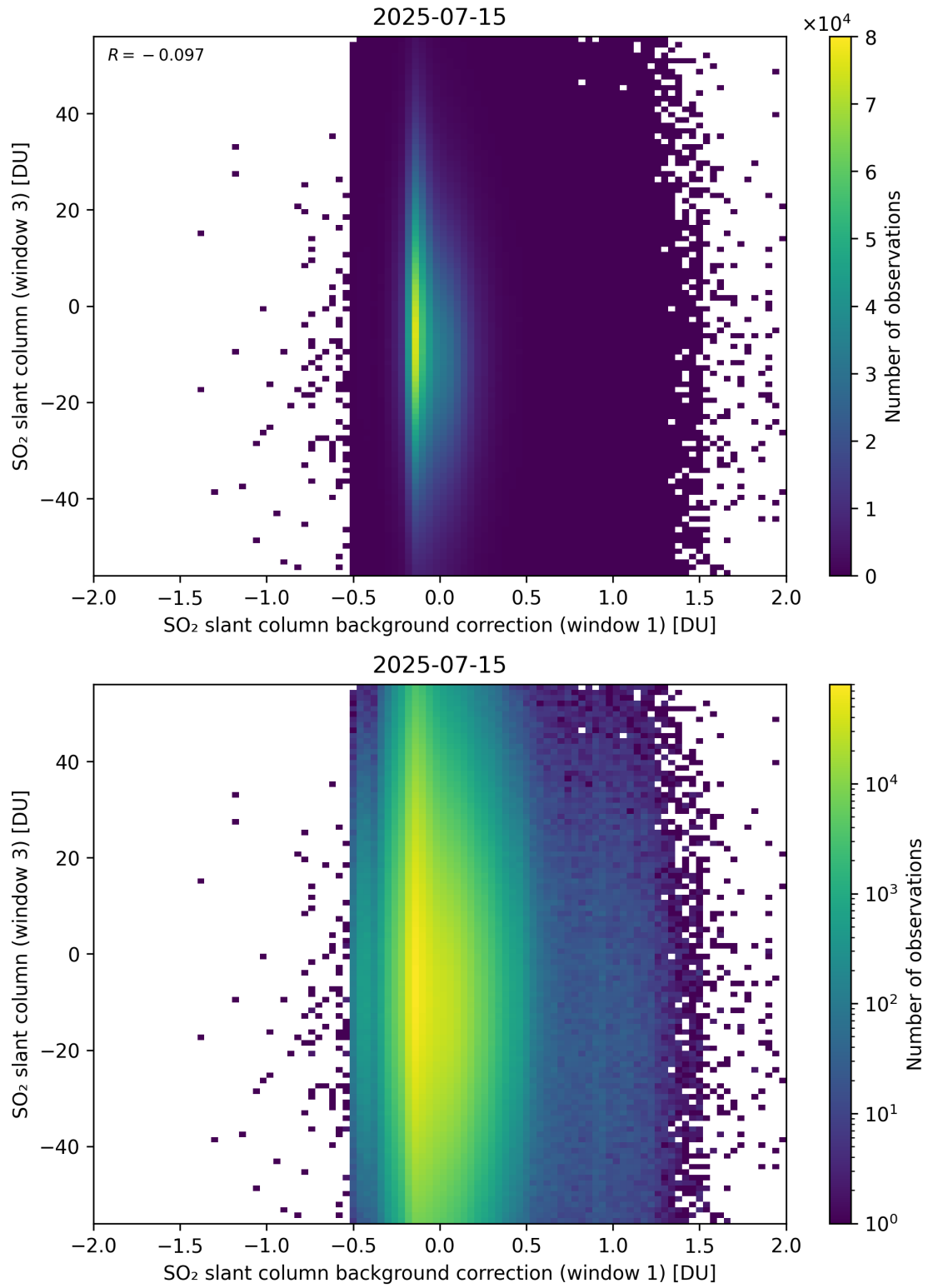
Figure 118: Scatter density plot of “SO 2 slant column background correction (window 1)” against “SO 2 slant column (window 3)” for 2025-07-14 to 2025-07-16.
