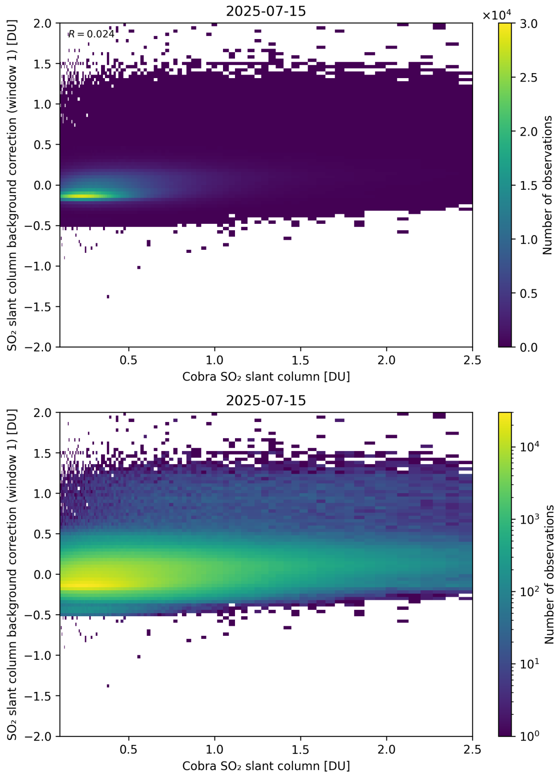
Figure 193: Scatter density plot of “Cobra SO 2 slant column” against “SO 2 slant column background correction (window 1)” for 2025-07-14 to 2025-07-16.
