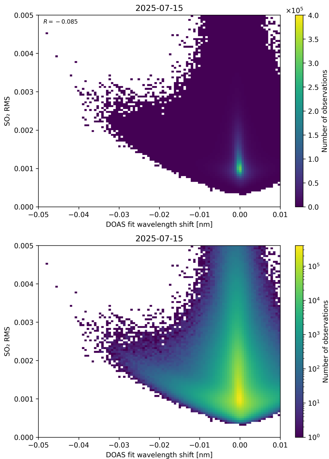
Figure 139: Scatter density plot of “DOAS fit wavelength shift” against “SO 2 RMS” for 2025-07-14 to 2025-07-16.
