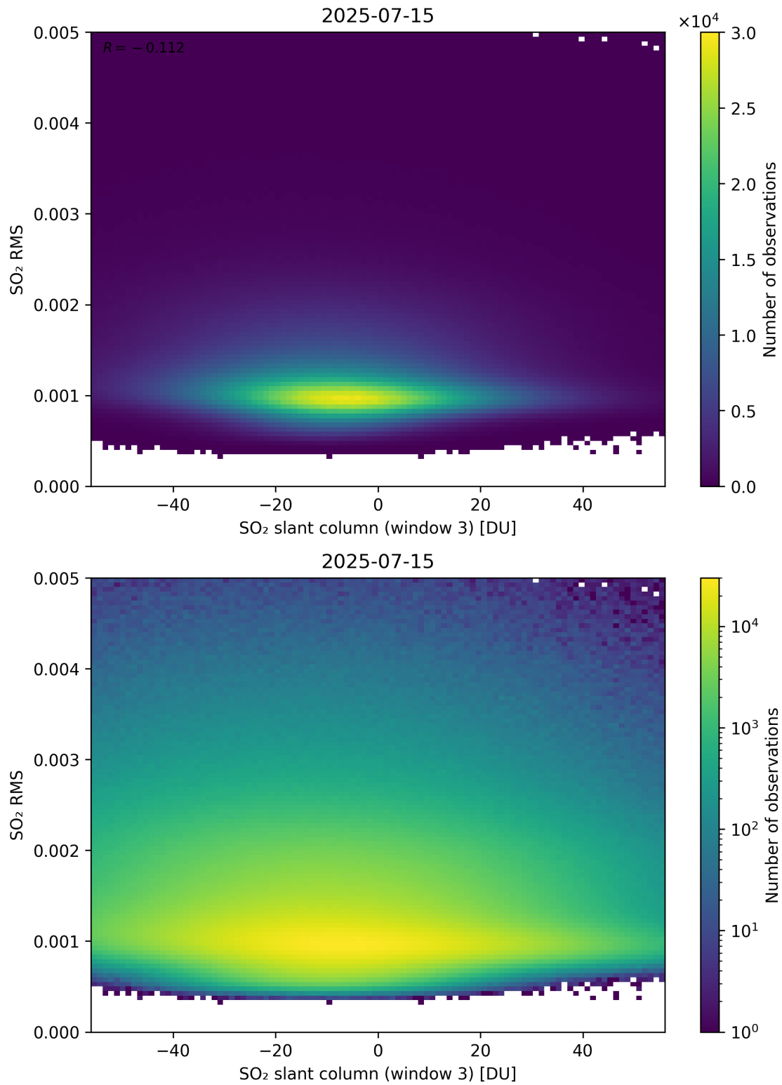
Figure 306: Scatter density plot of “SO 2 slant column (window 3)” against “SO 2 RMS” for 2025-07-14 to 2025-07-16.
