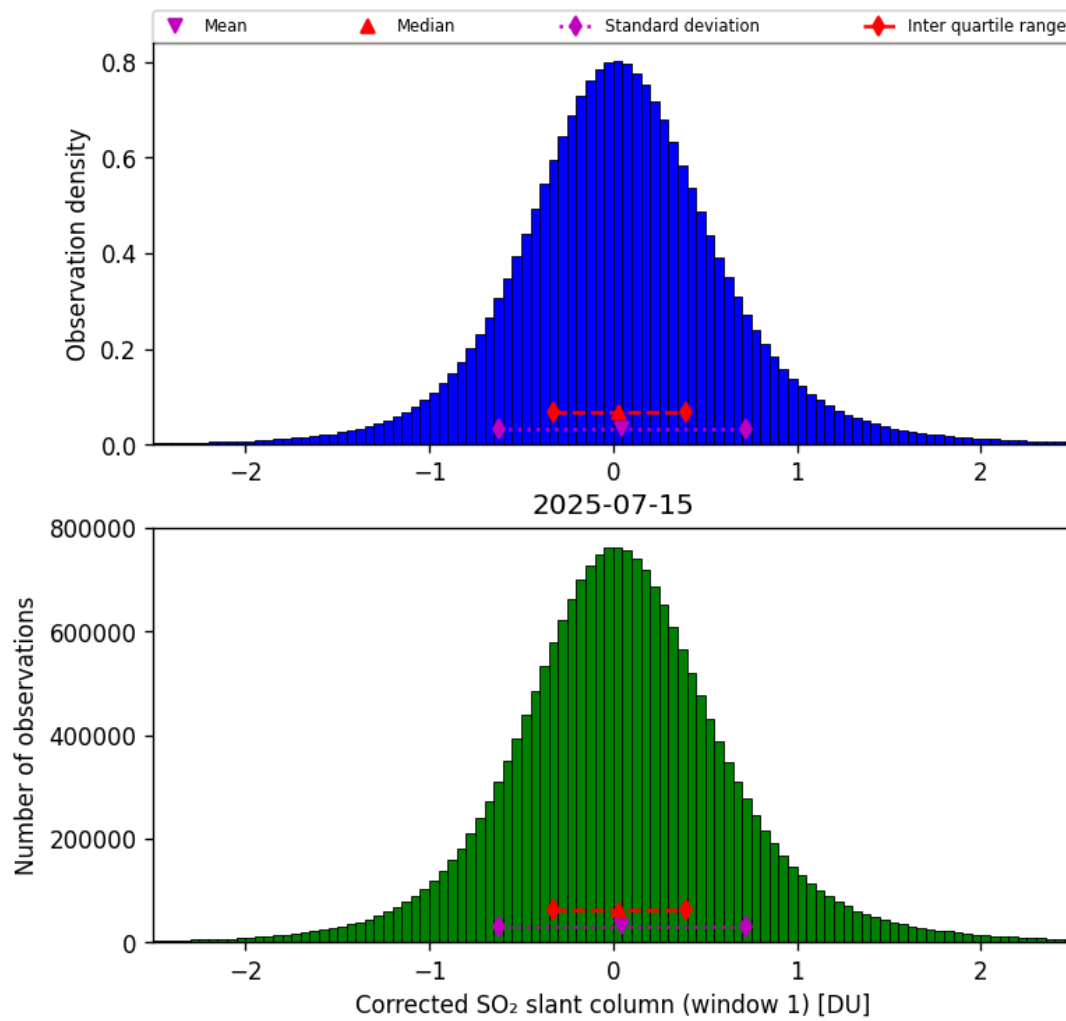
Figure 65: Histogram of “Corrected SO 2 slant column (window 1)” for 2025-07-14 to 2025-07-16
