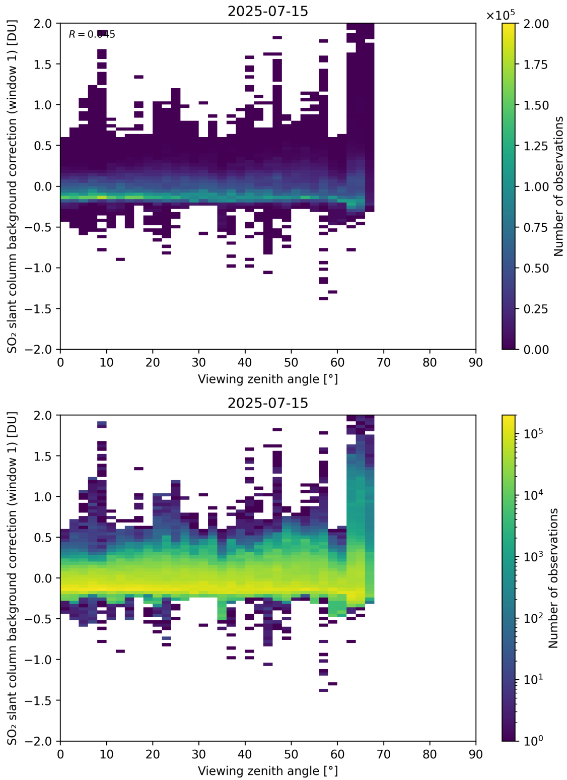
Figure 362: Scatter density plot of “Viewing zenith angle” against “SO 2 slant column background correction (window 1)” for 2025-07-14 to 2025-07-16.
