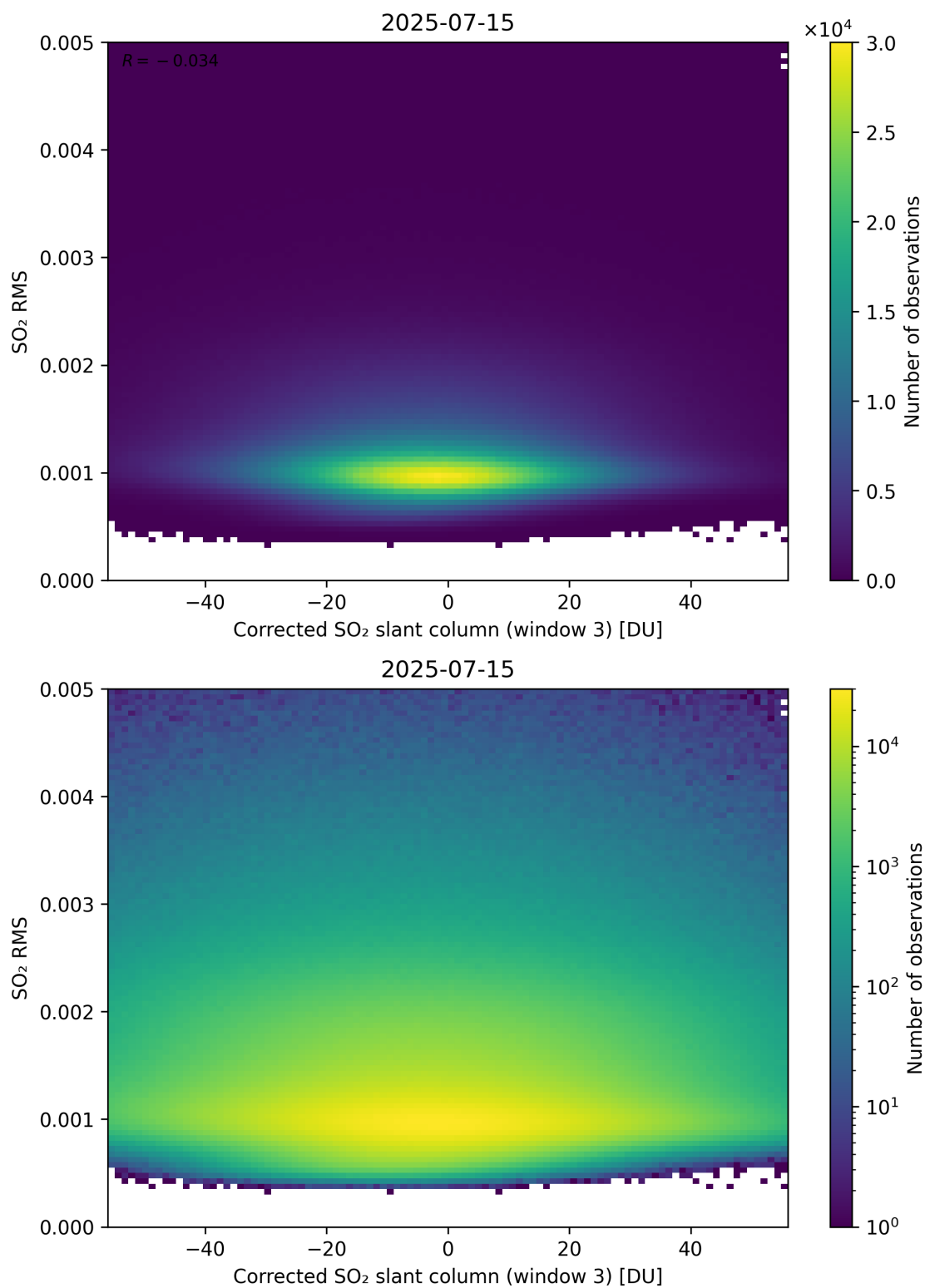
Figure 258: Scatter density plot of “Corrected SO 2 slant column (window 3)” against “SO 2 RMS” for 2025-07-14 to 2025-07-16.
