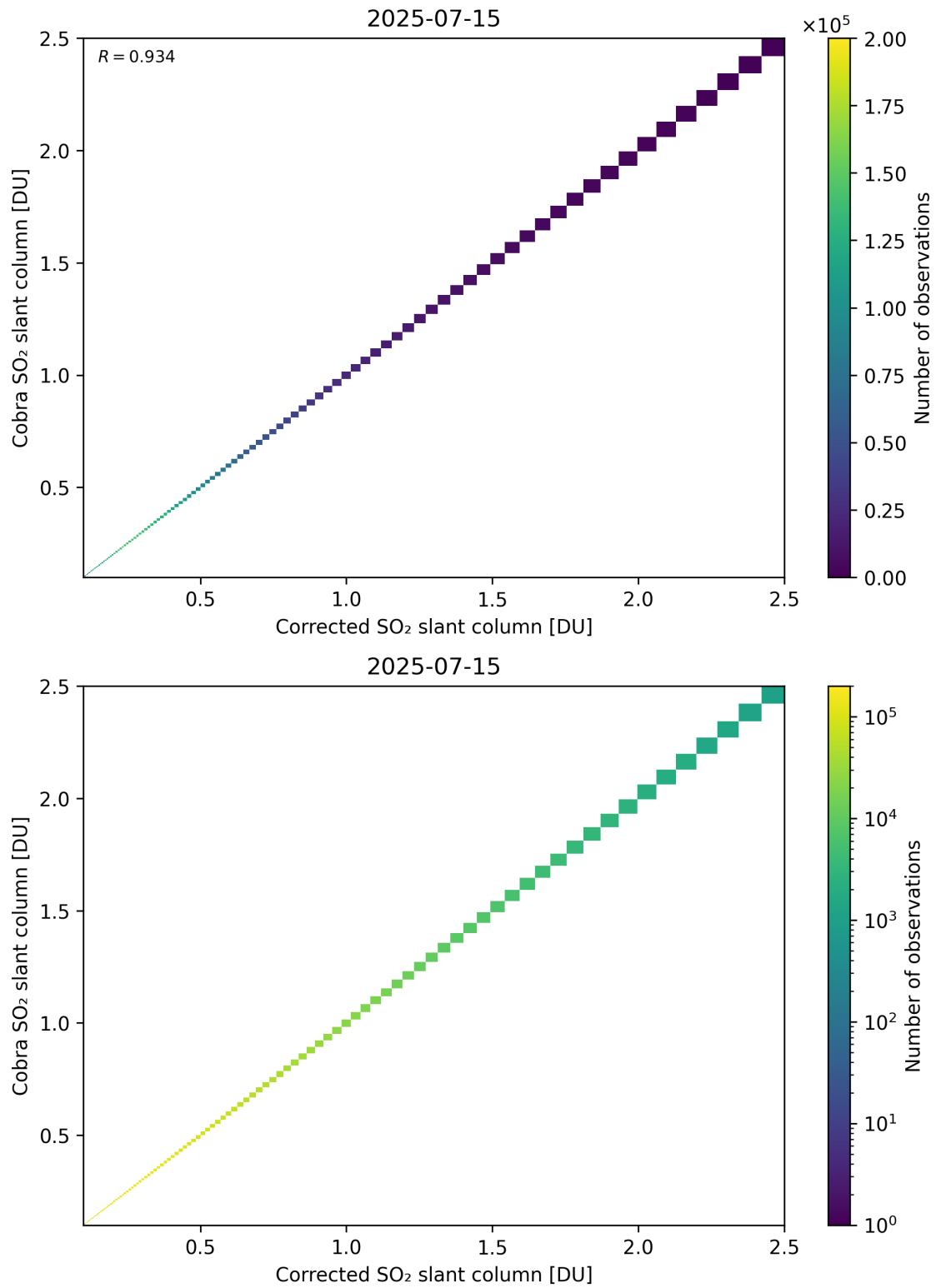
Figure 233: Scatter density plot of “Corrected SO 2 slant column” against “Cobra SO 2 slant column” for 2025-07-14 to 2025-07-16.
