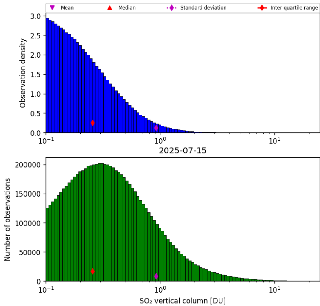
Figure 58: Histogram of “SO 2 vertical column” for 2025-07-14 to 2025-07-16
