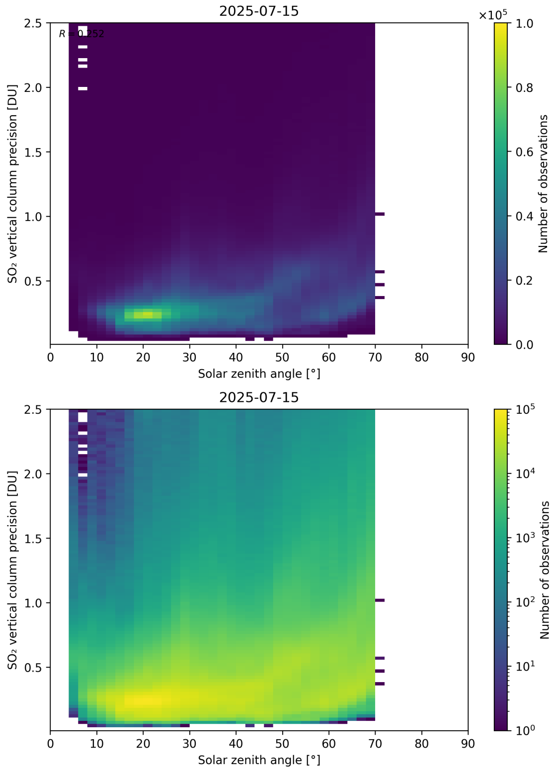
Figure 192: Scatter density plot of “Solar zenith angle” against “SO 2 vertical column precision” for 2025-07-14 to 2025-07-16.
