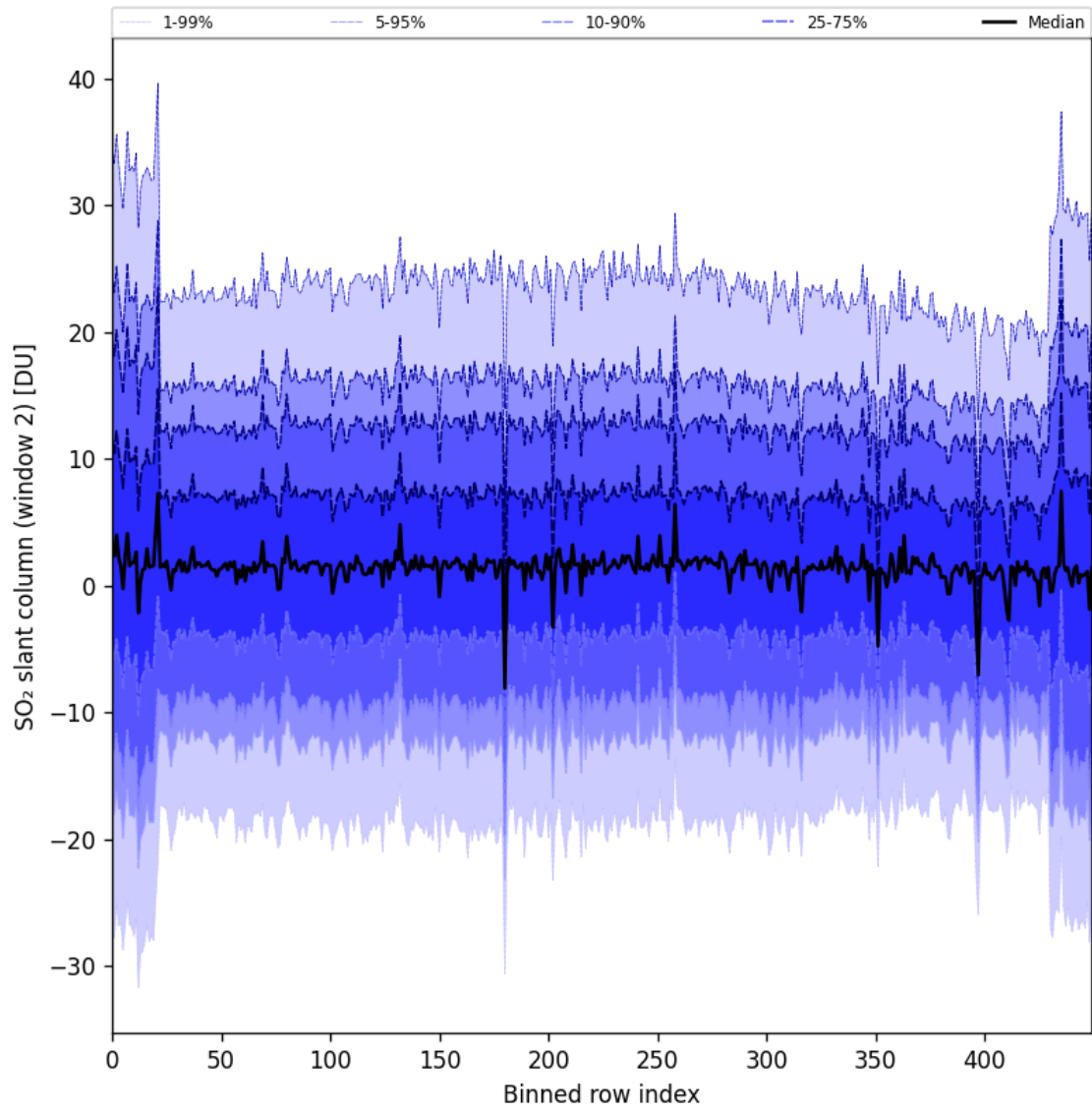
Figure 93: Along track statistics of “SO 2 slant column (window 2)” for 2025-07-14 to 2025-07-16
