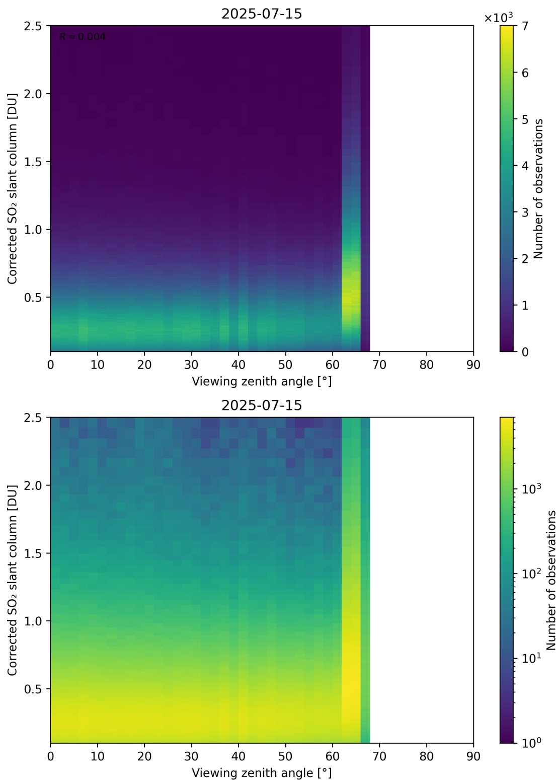
Figure 373: Scatter density plot of “Viewing zenith angle” against “Corrected SO 2 slant column” for 2025-07-14 to 2025-07-16.
