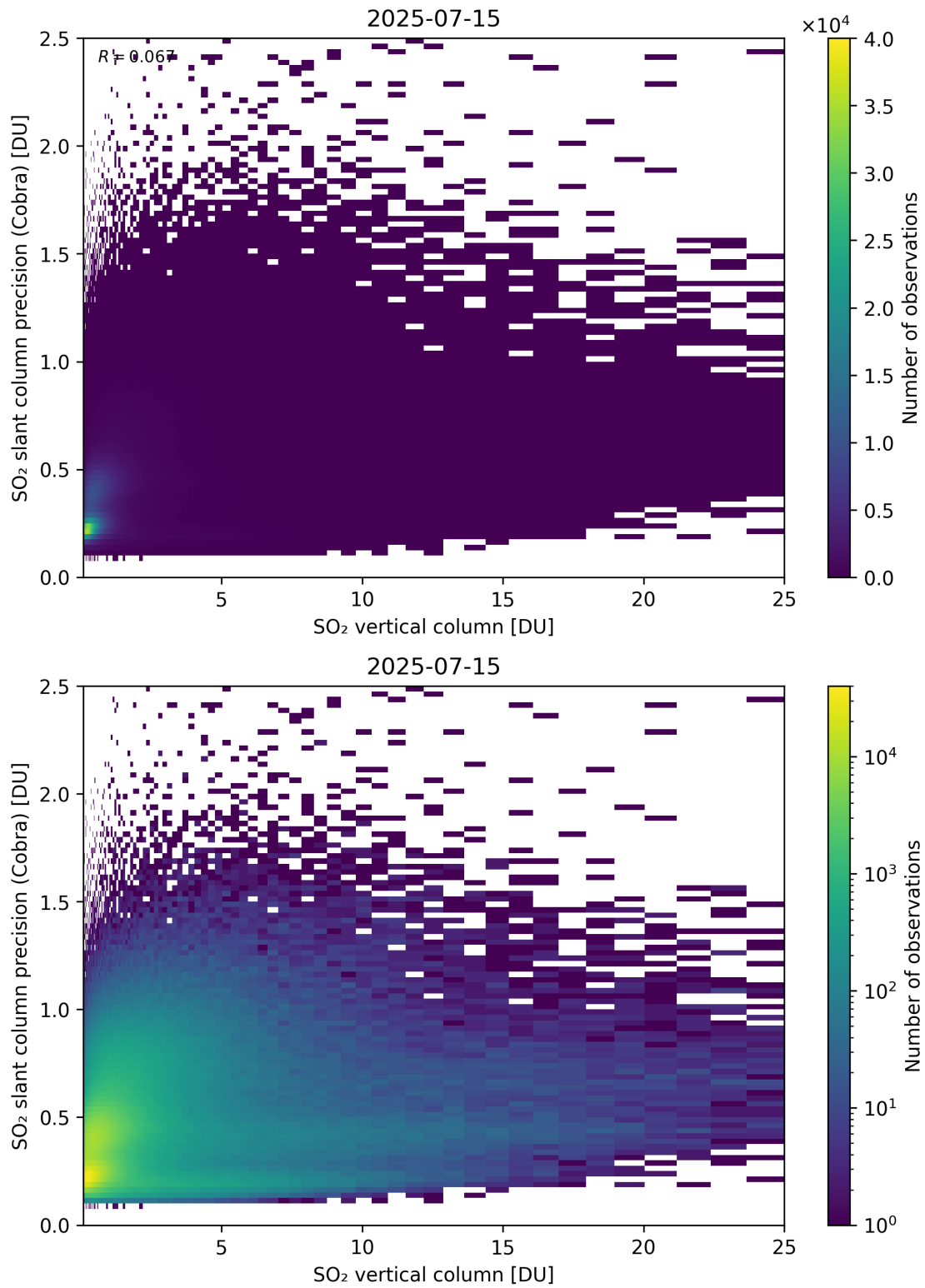
Figure 350: Scatter density plot of “SO 2 vertical column” against “SO 2 slant column precision (Cobra)” for 2025-07-14 to 2025-07-16.
