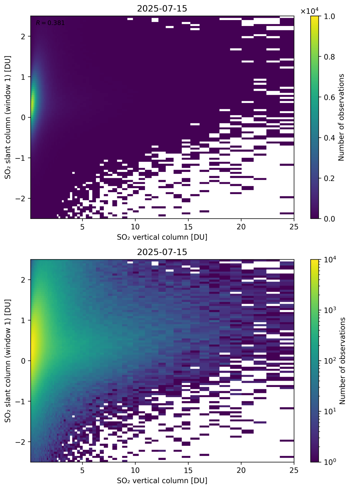
Figure 354: Scatter density plot of “SO 2 vertical column” against “SO 2 slant column (window 1)” for 2025-07-14 to 2025-07-16.
