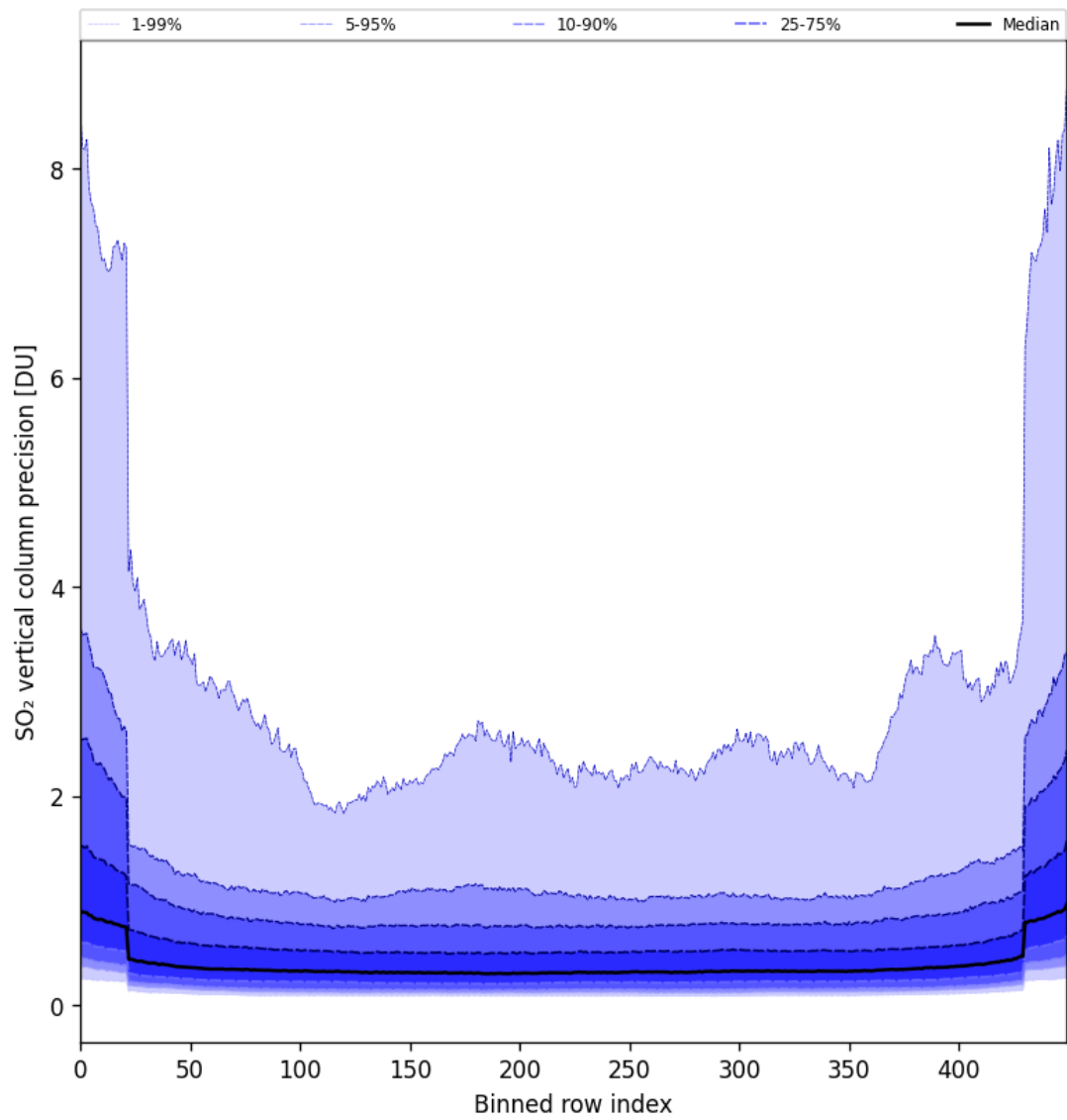
Figure 85: Along track statistics of “SO 2 vertical column precision” for 2025-07-14 to 2025-07-16
