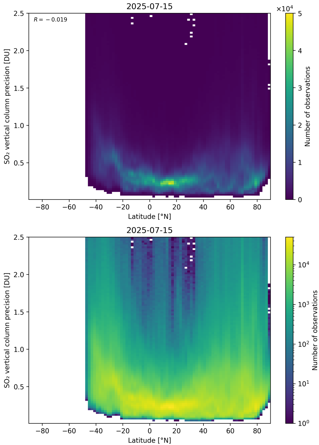
Figure 170: Scatter density plot of “Latitude” against “SO 2 vertical column precision” for 2025-07-14 to 2025-07-16.
