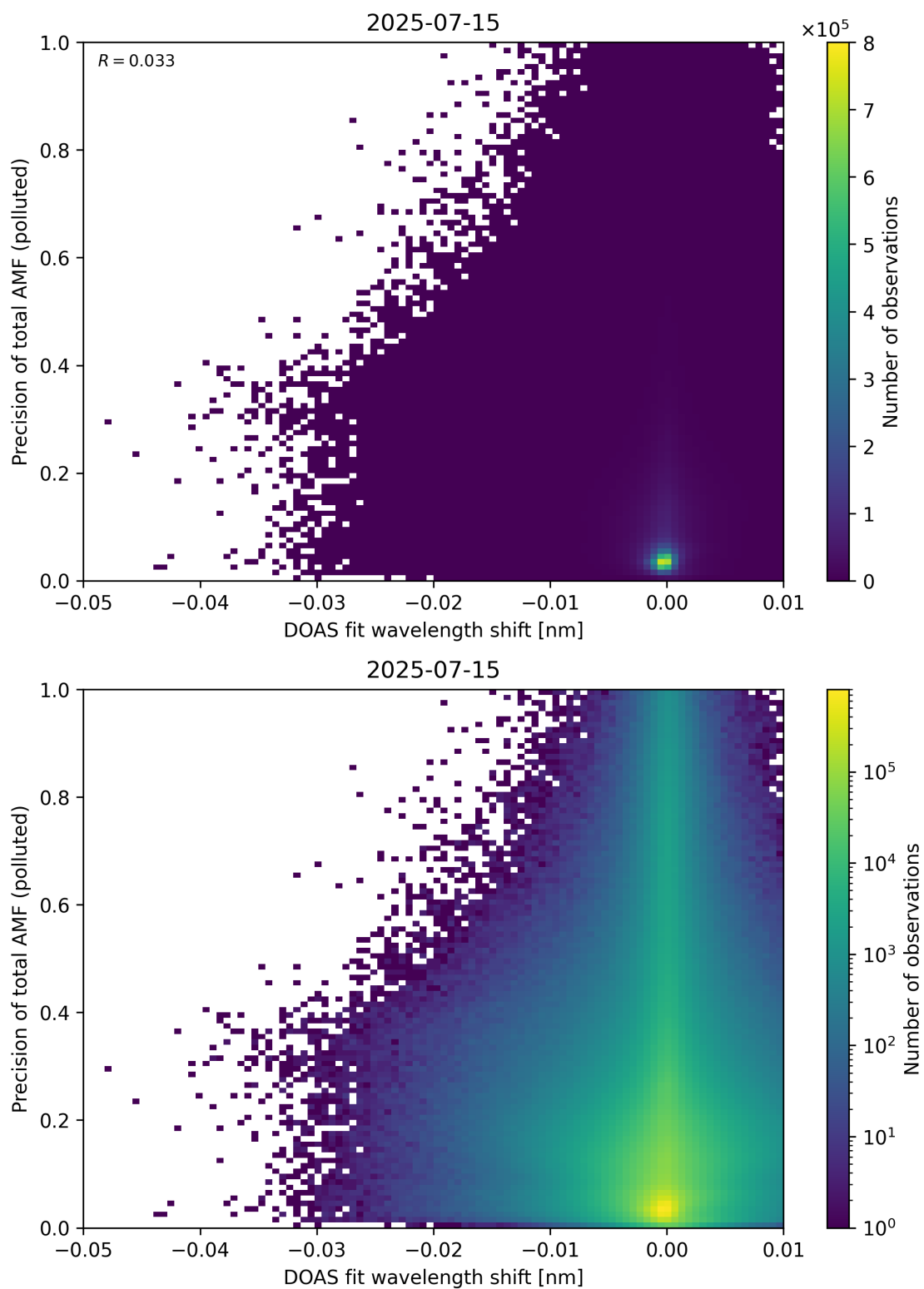
Figure 142: Scatter density plot of “DOAS fit wavelength shift” against “Precision of total AMF (polluted)” for 2025-07-14 to 2025-07-16.
