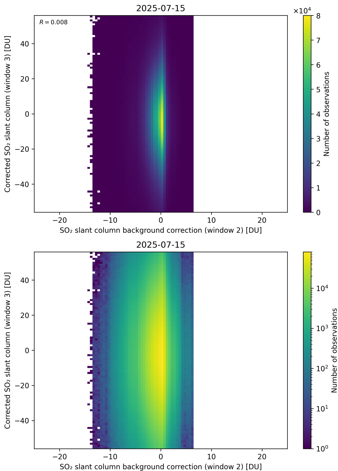
Figure 127: Scatter density plot of “SO 2 slant column background correction (window 2)” against “Corrected SO 2 slant column (window 3)” for 2025-07-14 to 2025-07-16.
