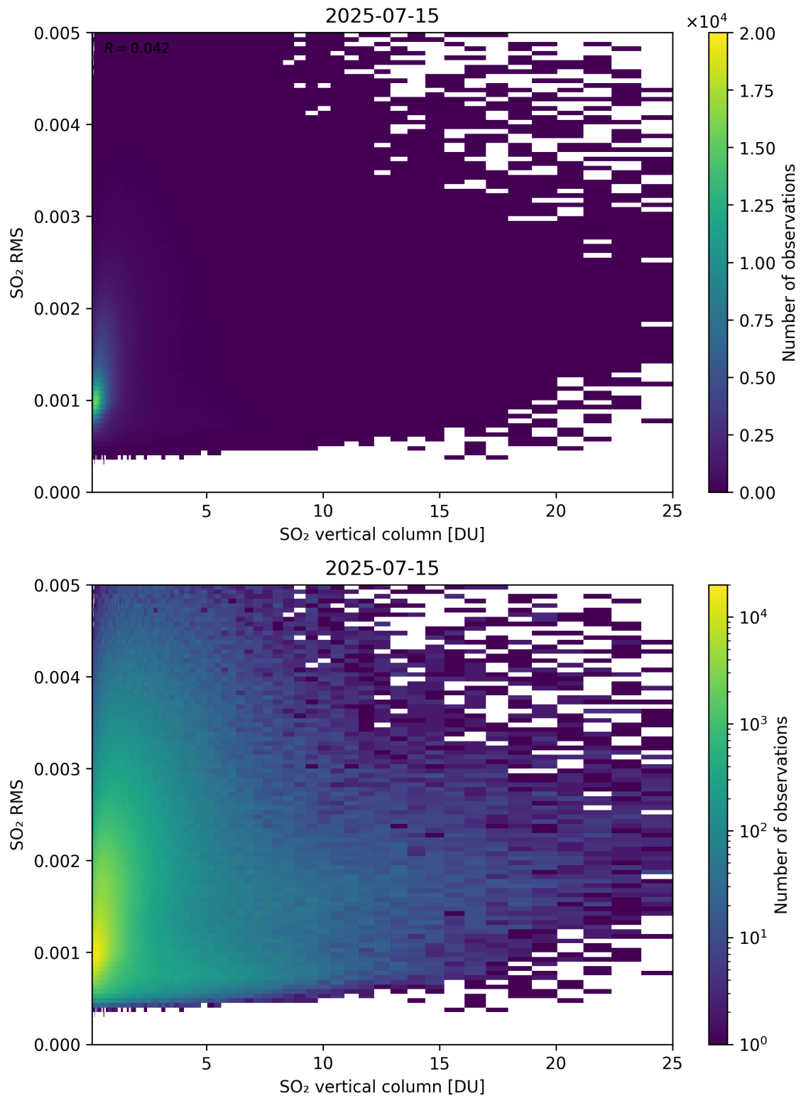
Figure 328: Scatter density plot of “SO 2 vertical column” against “SO 2 RMS” for 2025-07-14 to 2025-07-16.
