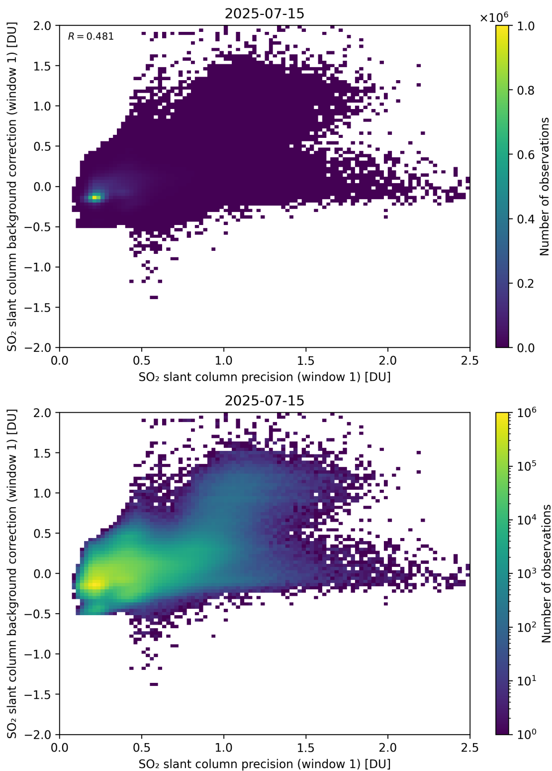
Figure 268: Scatter density plot of “SO 2 slant column precision (window 1)” against “SO 2 slant column background correction (window 1)” for 2025-07-14 to 2025-07-16.
