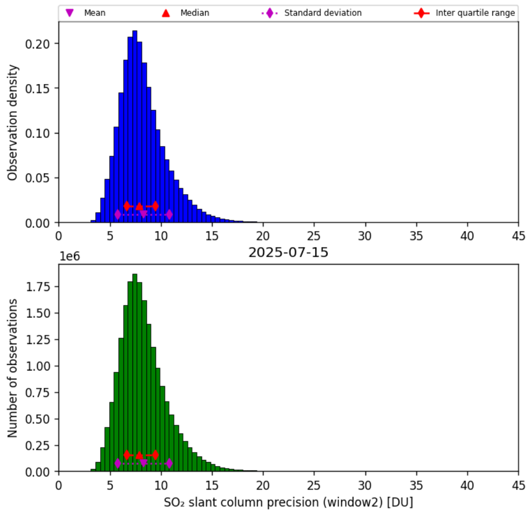
Figure 68: Histogram of “SO 2 slant column precision (window2)” for 2025-07-14 to 2025-07-16
