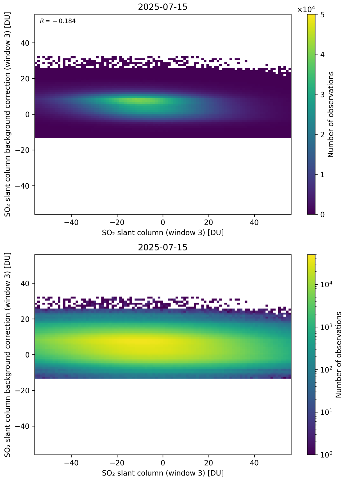
Figure 303: Scatter density plot of “SO 2 slant column (window 3)” against “SO 2 slant column background correction (window 3)” for 2025-07-14 to 2025-07-16.
