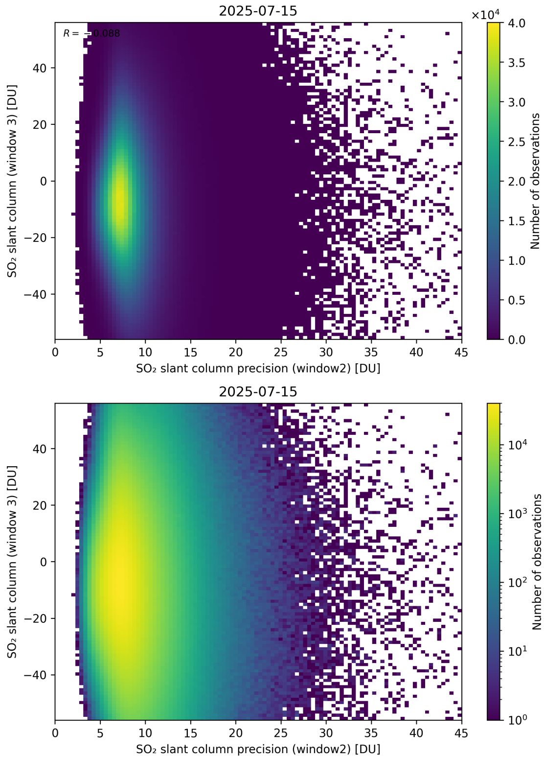
Figure 299: Scatter density plot of “SO 2 slant column precision (window2)” against “SO 2 slant column (window 3)” for 2025-07-14 to 2025-07-16.
