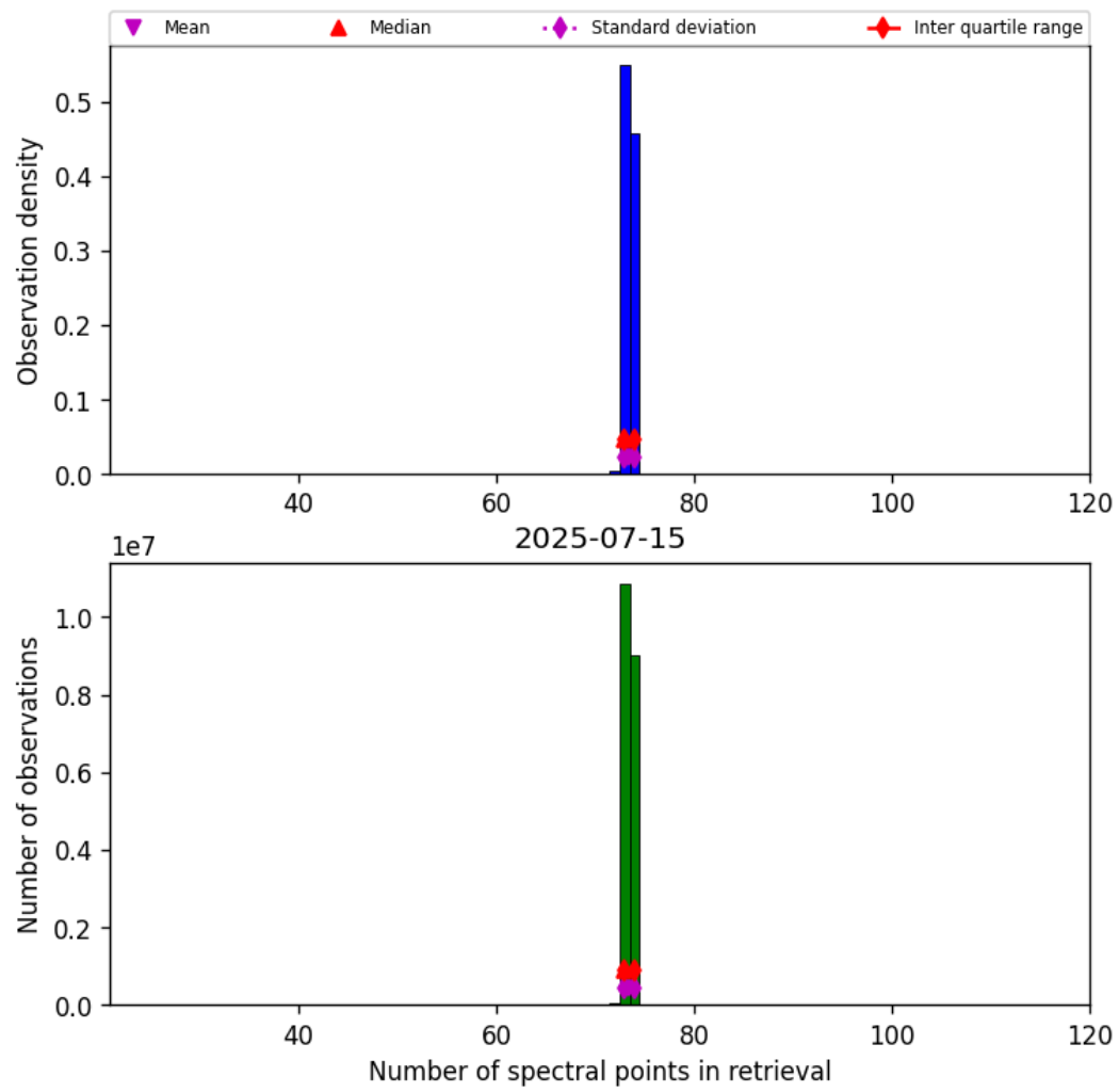
Figure 82: Histogram of “Number of spectral points in retrieval” for 2025-07-14 to 2025-07-16
