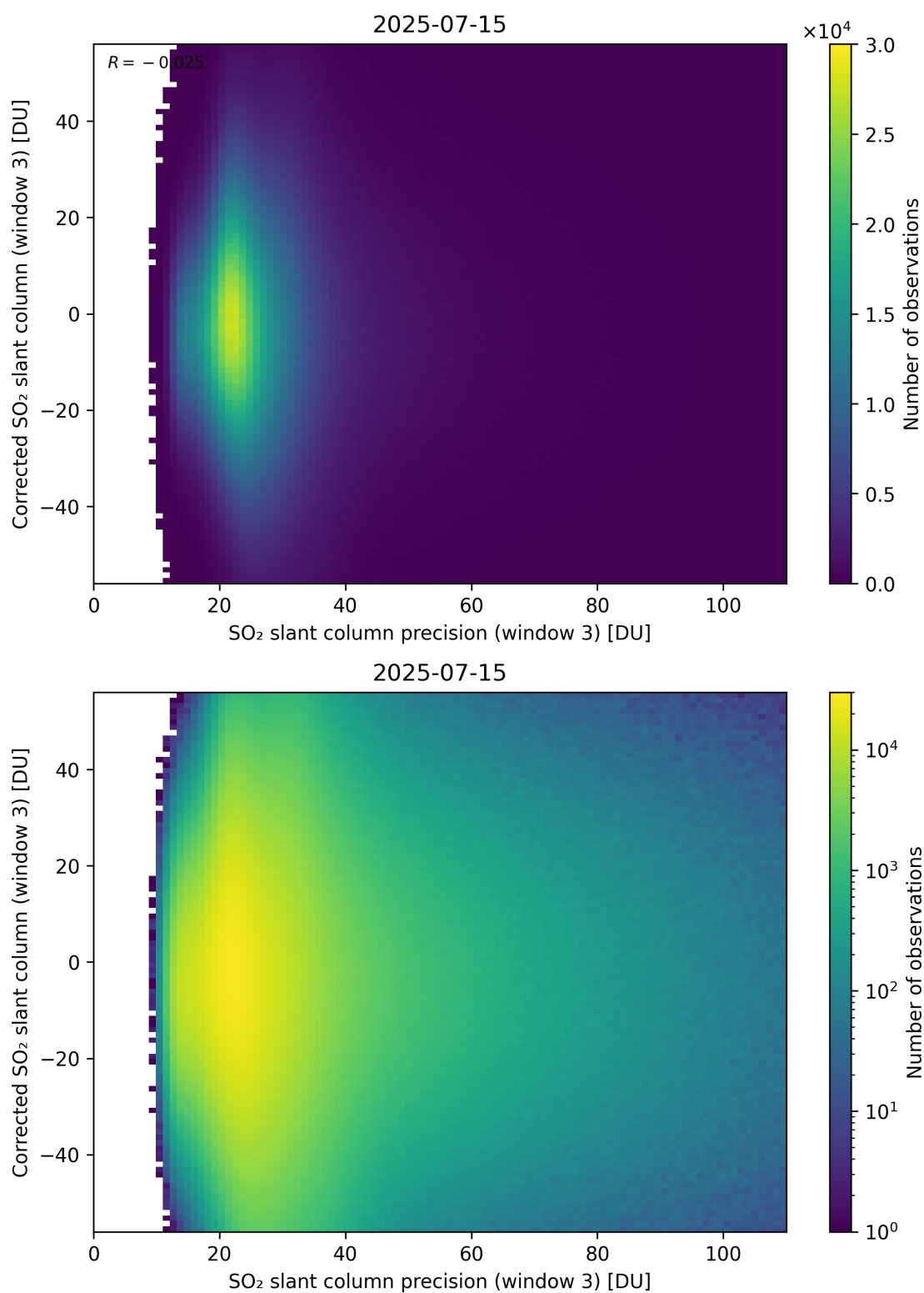
Figure 312: Scatter density plot of “SO 2 slant column precision (window 3)” against “Corrected SO 2 slant column (window 3)” for 2025-07-14 to 2025-07-16.
