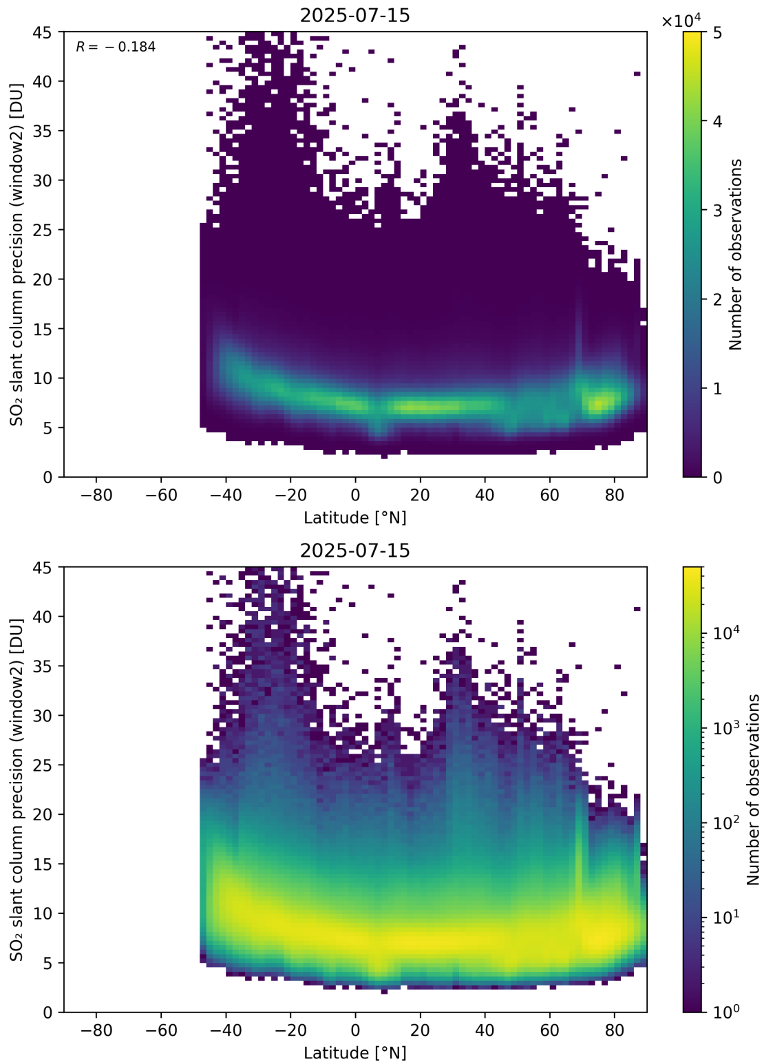
Figure 164: Scatter density plot of “Latitude” against “SO 2 slant column precision (window2)” for 2025-07-14 to 2025-07-16.
