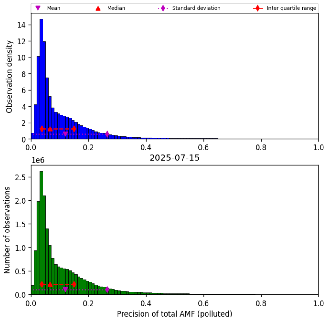
Figure 80: Histogram of “Precision of total AMF (polluted)” for 2025-07-14 to 2025-07-16
