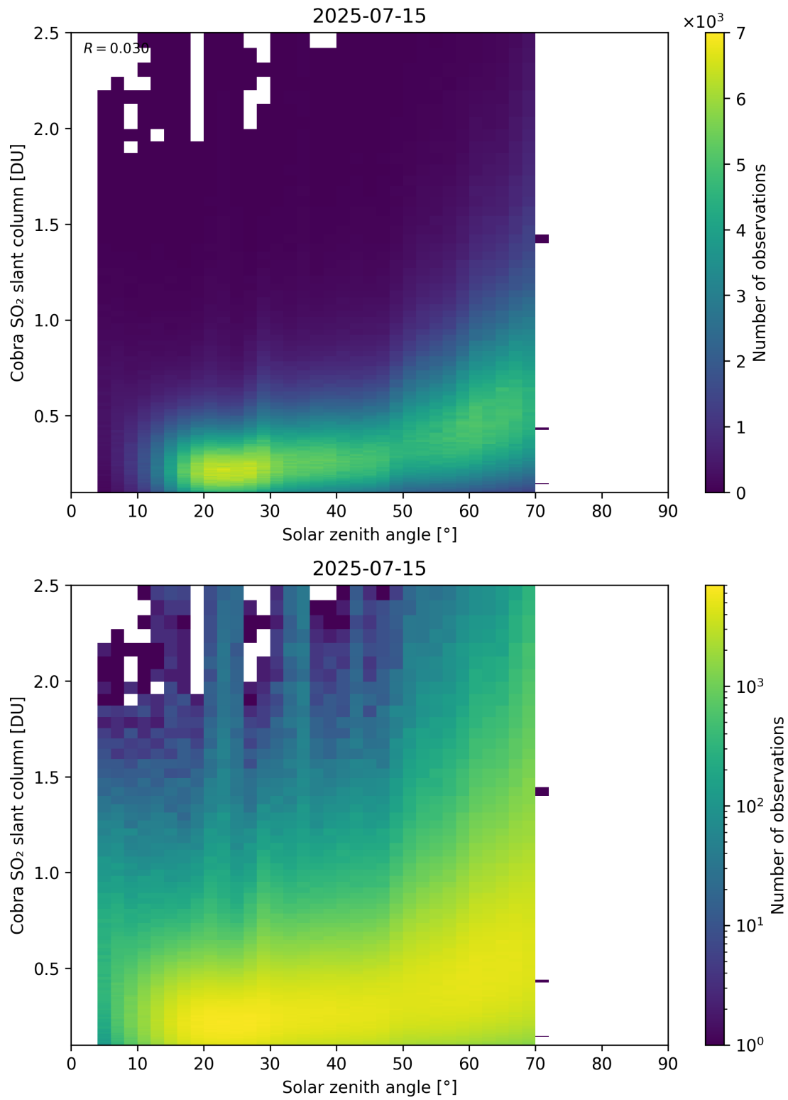
Figure 179: Scatter density plot of “Solar zenith angle” against “Cobra SO 2 slant column” for 2025-07-14 to 2025-07-16.
