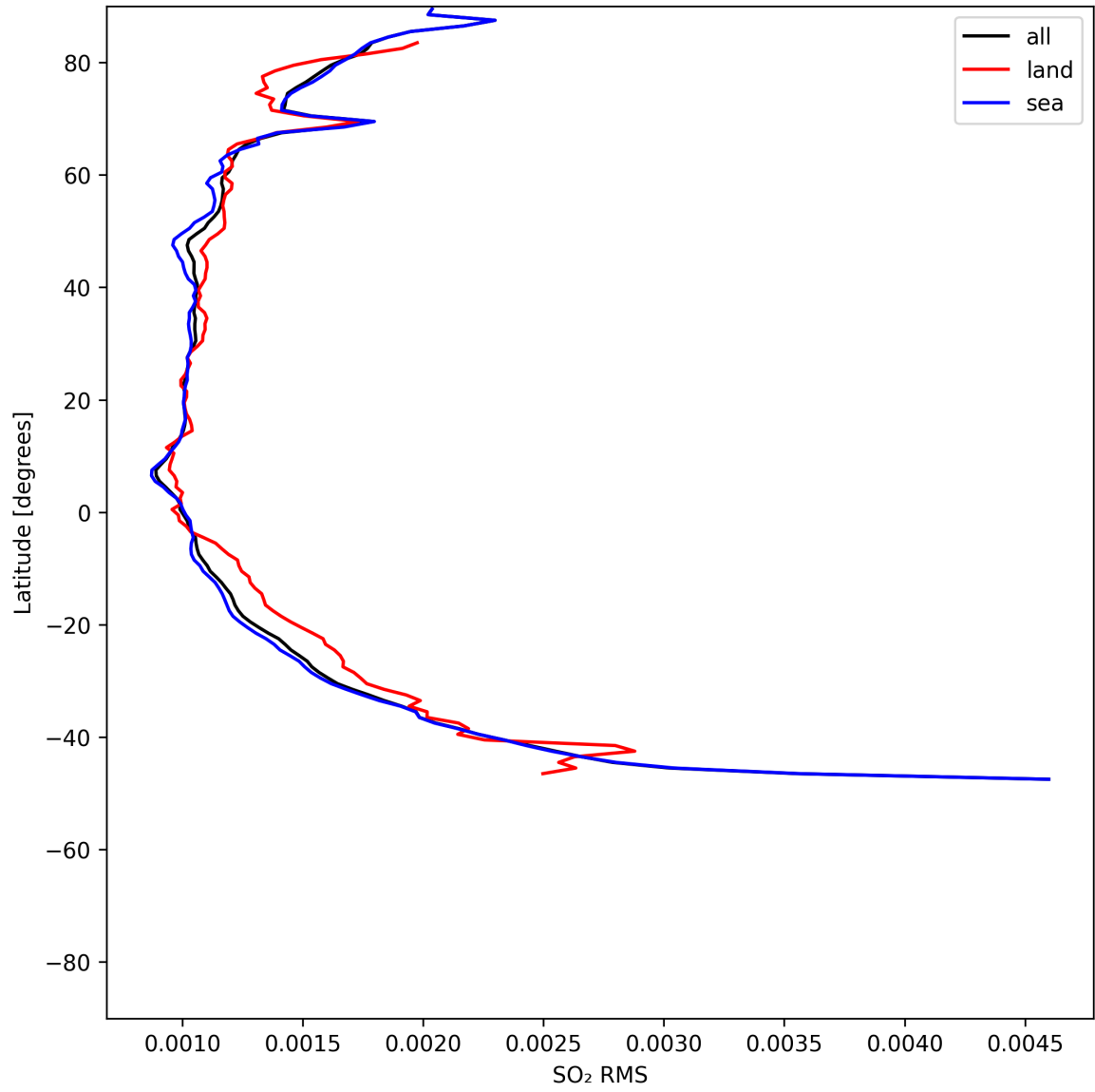
Figure 52: Zonal average of “SO 2 RMS” for 2025-07-14 to 2025-07-16.
