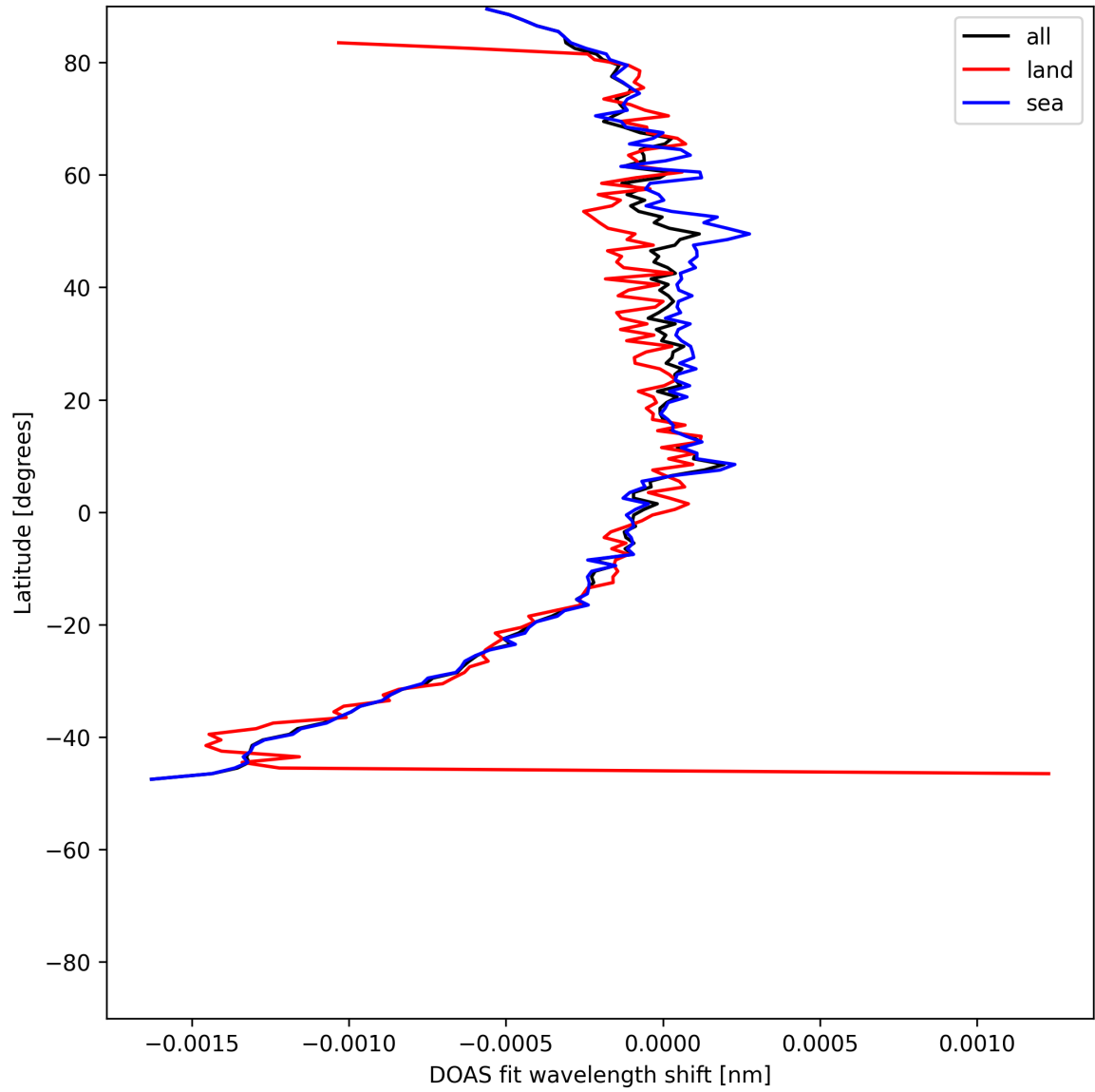
Figure 50: Zonal average of “DOAS fit wavelength shift” for 2025-07-14 to 2025-07-16.
