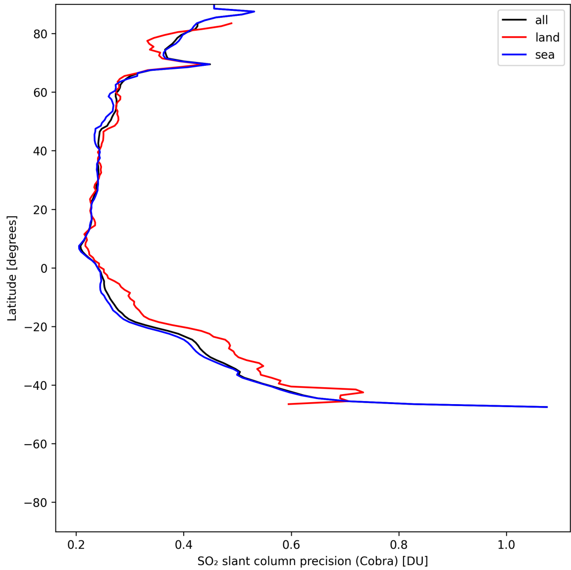
Figure 36: Zonal average of "SO 2 slant column precision (Cobra)" for 2025-07-14 to 2025-07-16.
