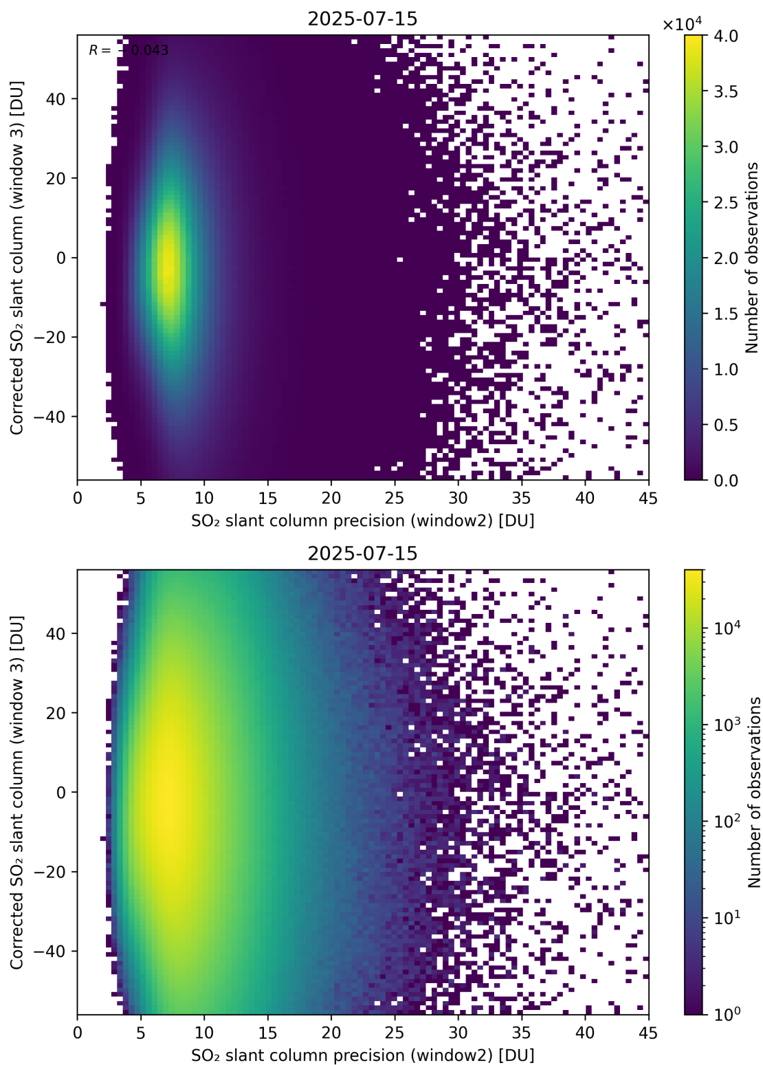
Figure 298: Scatter density plot of “SO 2 slant column precision (window2)” against “Corrected SO 2 slant column (window 3)” for 2025-07-14 to 2025-07-16.
