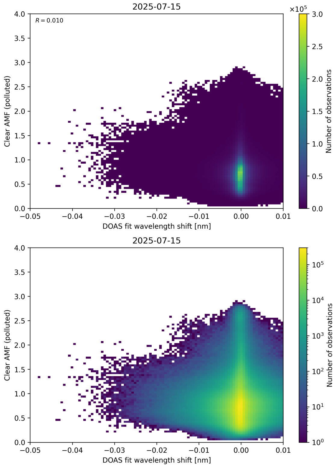
Figure 140: Scatter density plot of “DOAS fit wavelength shift” against “Clear AMF (polluted)” for 2025-07-14 to 2025-07-16.
