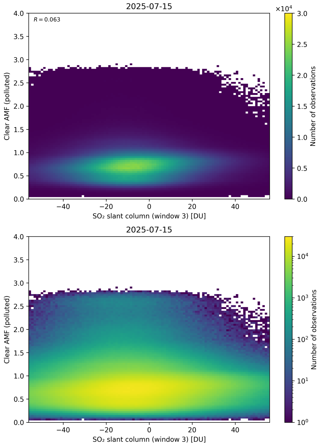
Figure 315: Scatter density plot of “SO 2 slant column (window 3)” against “Clear AMF (polluted)” for 2025-07-14 to 2025-07-16.
