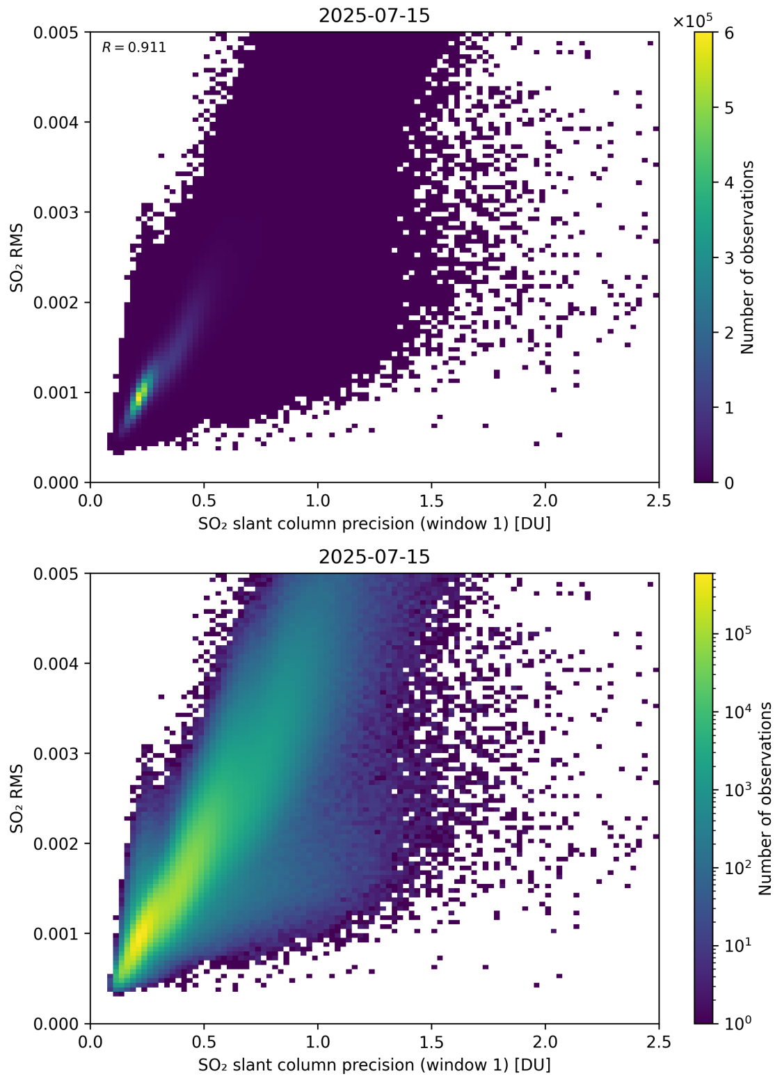
Figure 273: Scatter density plot of “SO 2 slant column precision (window 1)” against “SO 2 RMS” for 2025-07-14 to 2025-07-16.
