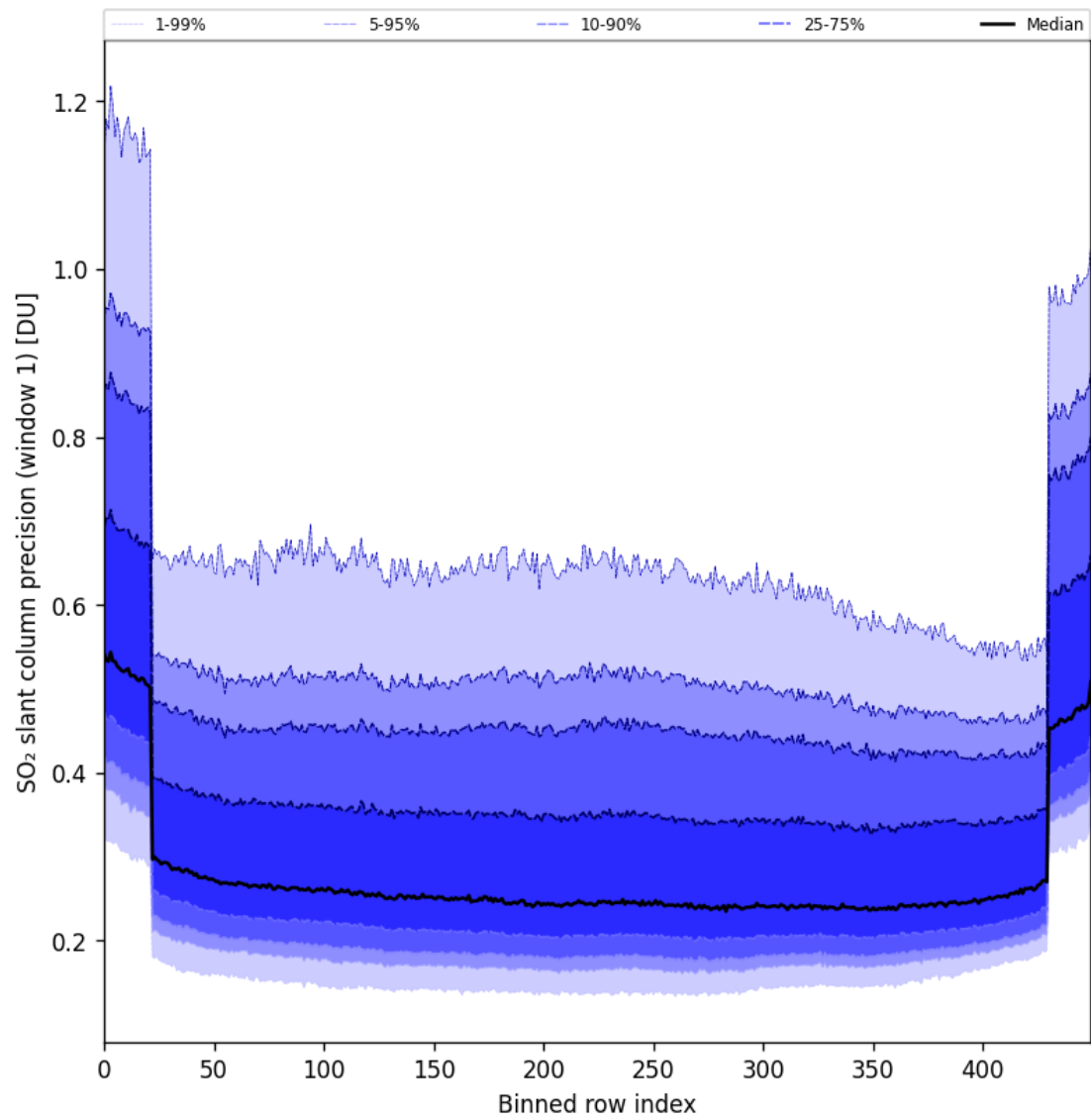
Figure 90: Along track statistics of "SO 2 slant column precision (window 1)" for 2025-07-14 to 2025-07-16
