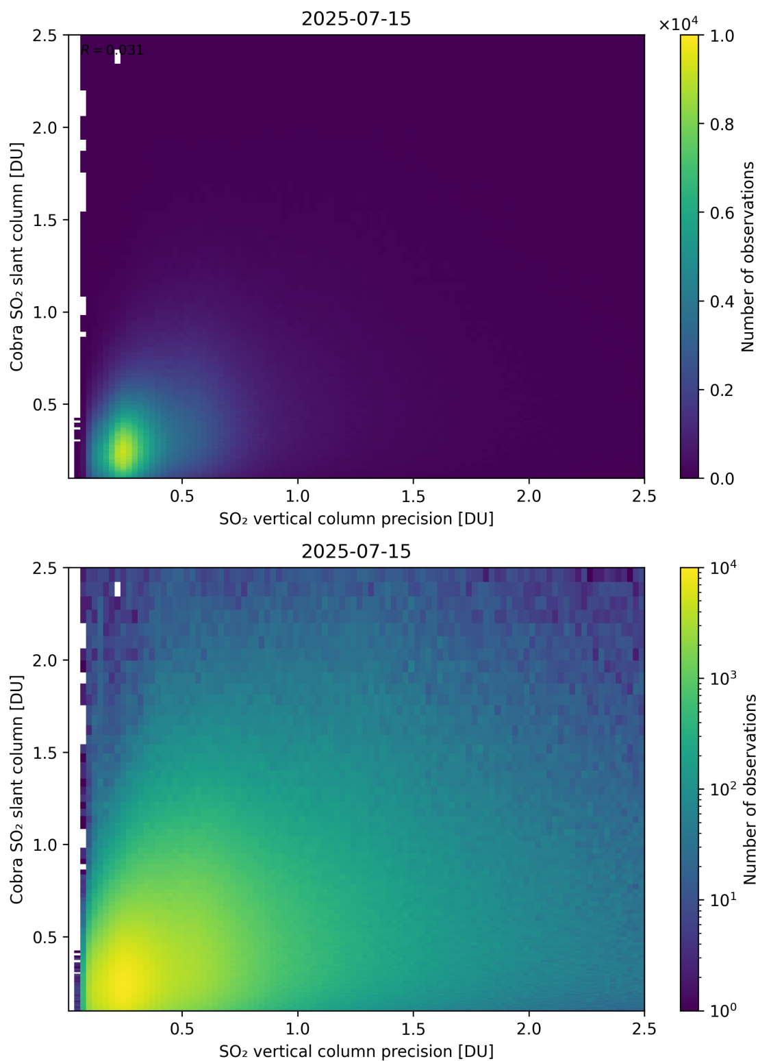
Figure 336: Scatter density plot of “SO 2 vertical column precision” against “Cobra SO 2 slant column” for 2025-07-14 to 2025-07-16.
