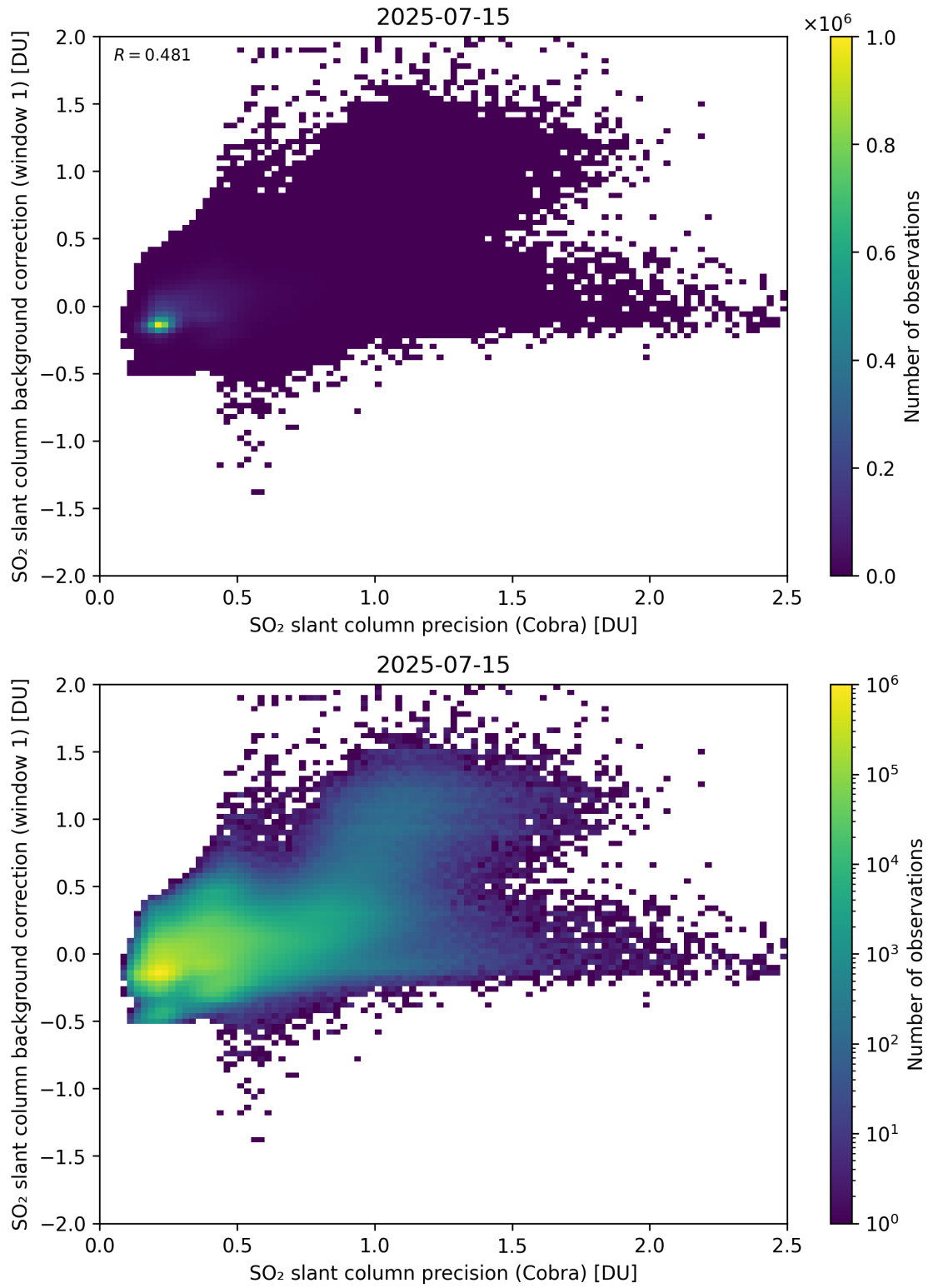
Figure 199: Scatter density plot of “SO 2 slant column precision (Cobra)” against “SO 2 slant column background correction (window 1)” for 2025-07-14 to 2025-07-16.
