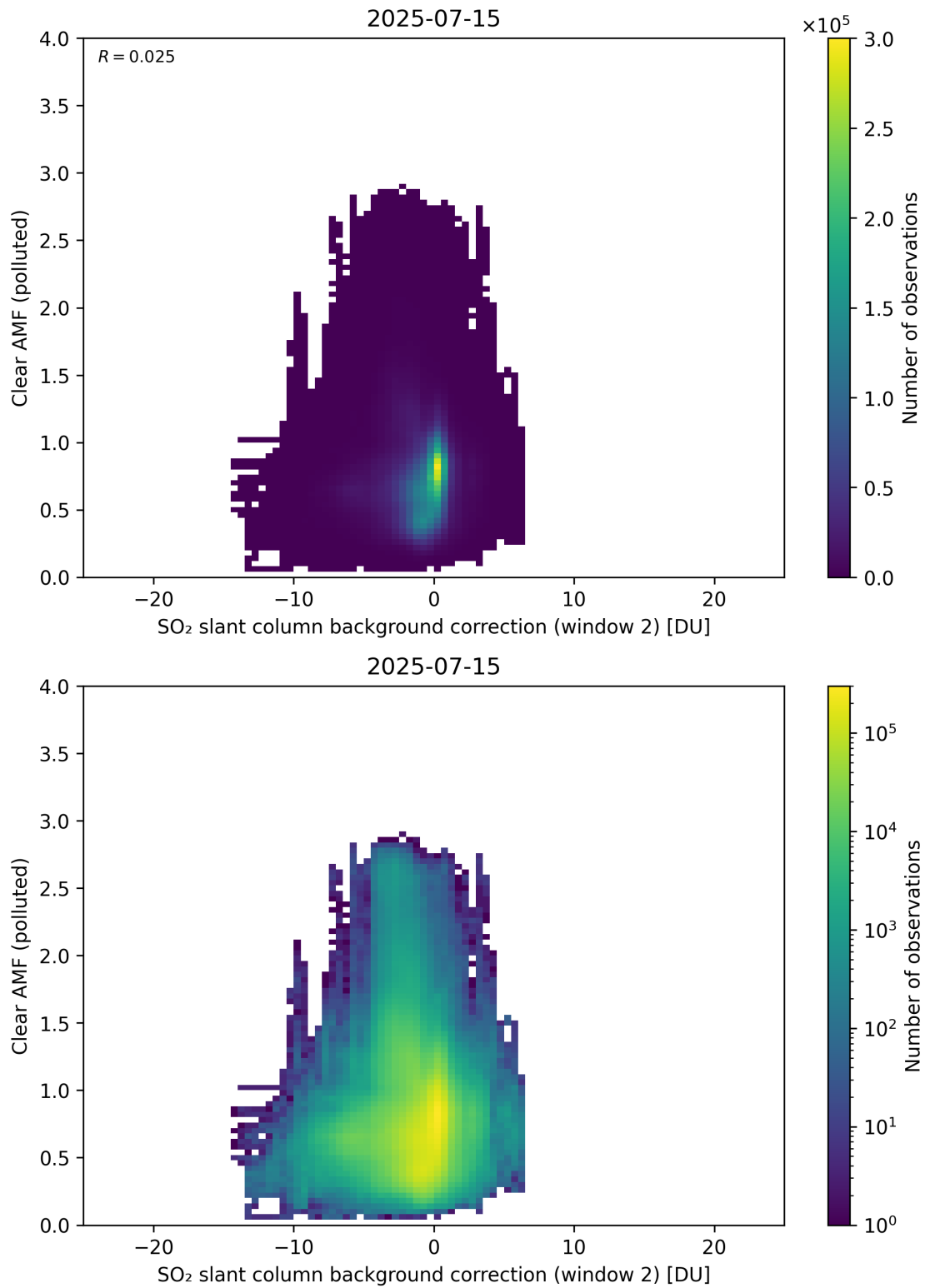
Figure 126: Scatter density plot of “SO 2 slant column background correction (window 2)” against “Clear AMF (polluted)” for 2025-07-14 to 2025-07-16.
