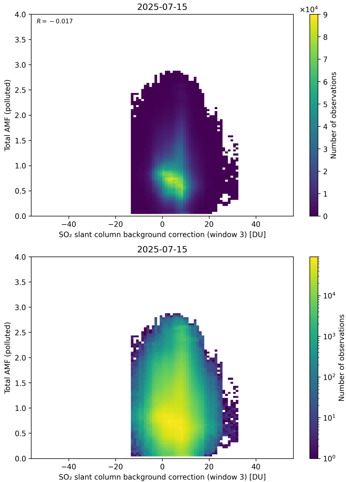
Figure 136: Scatter density plot of “SO 2 slant column background correction (window 3)” against “Total AMF (polluted)” for 2025-07-14 to 2025-07-16.
