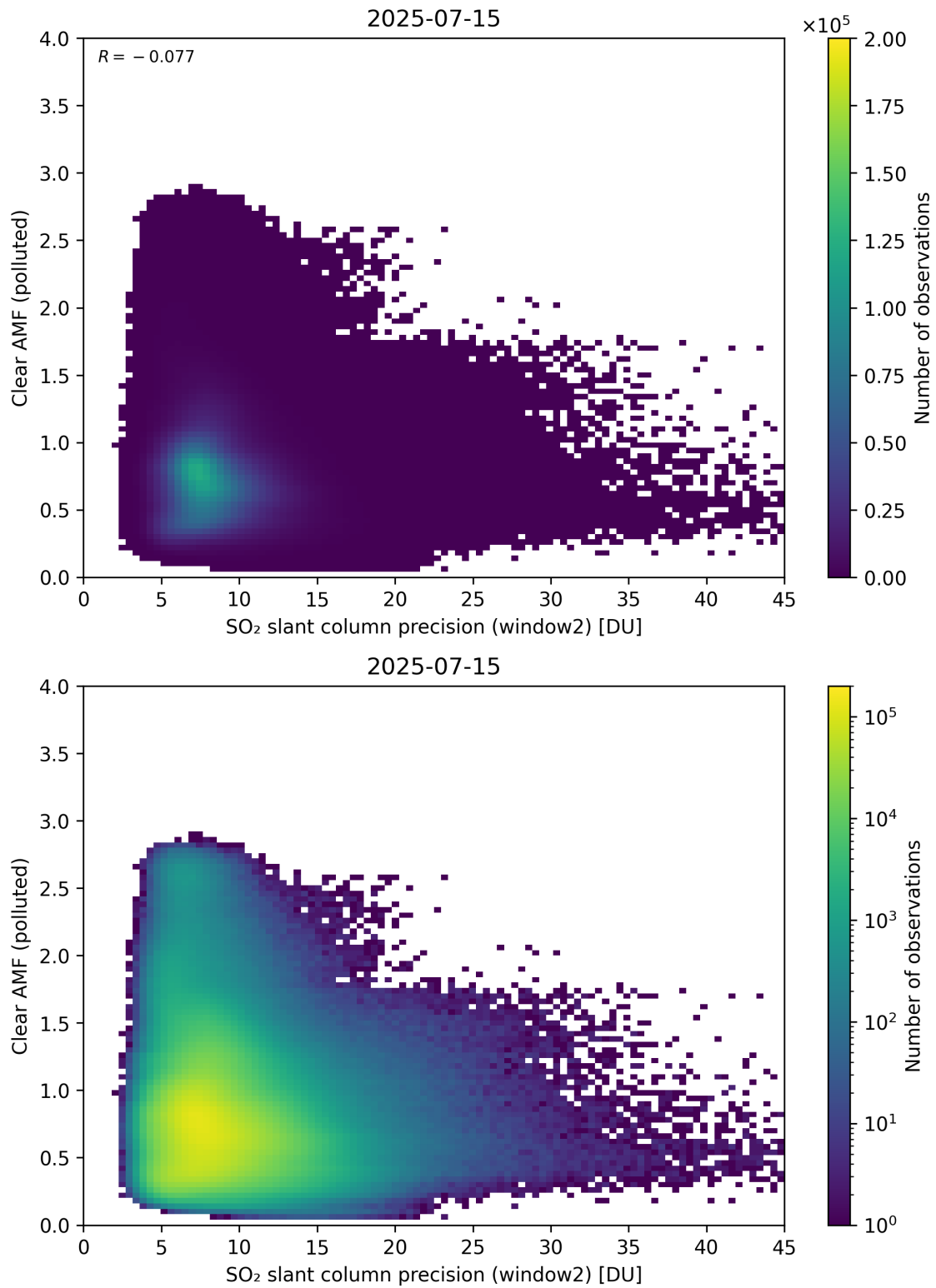
Figure 296: Scatter density plot of “SO 2 slant column precision (window2)” against “Clear AMF (polluted)” for 2025-07-14 to 2025-07-16.
