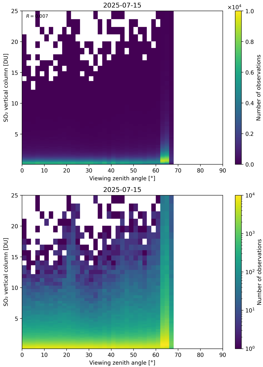
Figure 383: Scatter density plot of “Viewing zenith angle” against “SO 2 vertical column” for 2025-07-14 to 2025-07-16.
