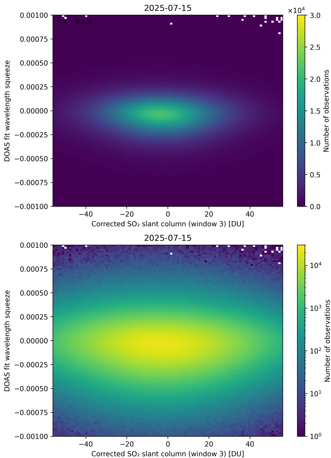
Figure 257: Scatter density plot of “Corrected SO 2 slant column (window 3)” against “DOAS fit wavelength squeeze” for 2025-07-14 to 2025-07-16.
