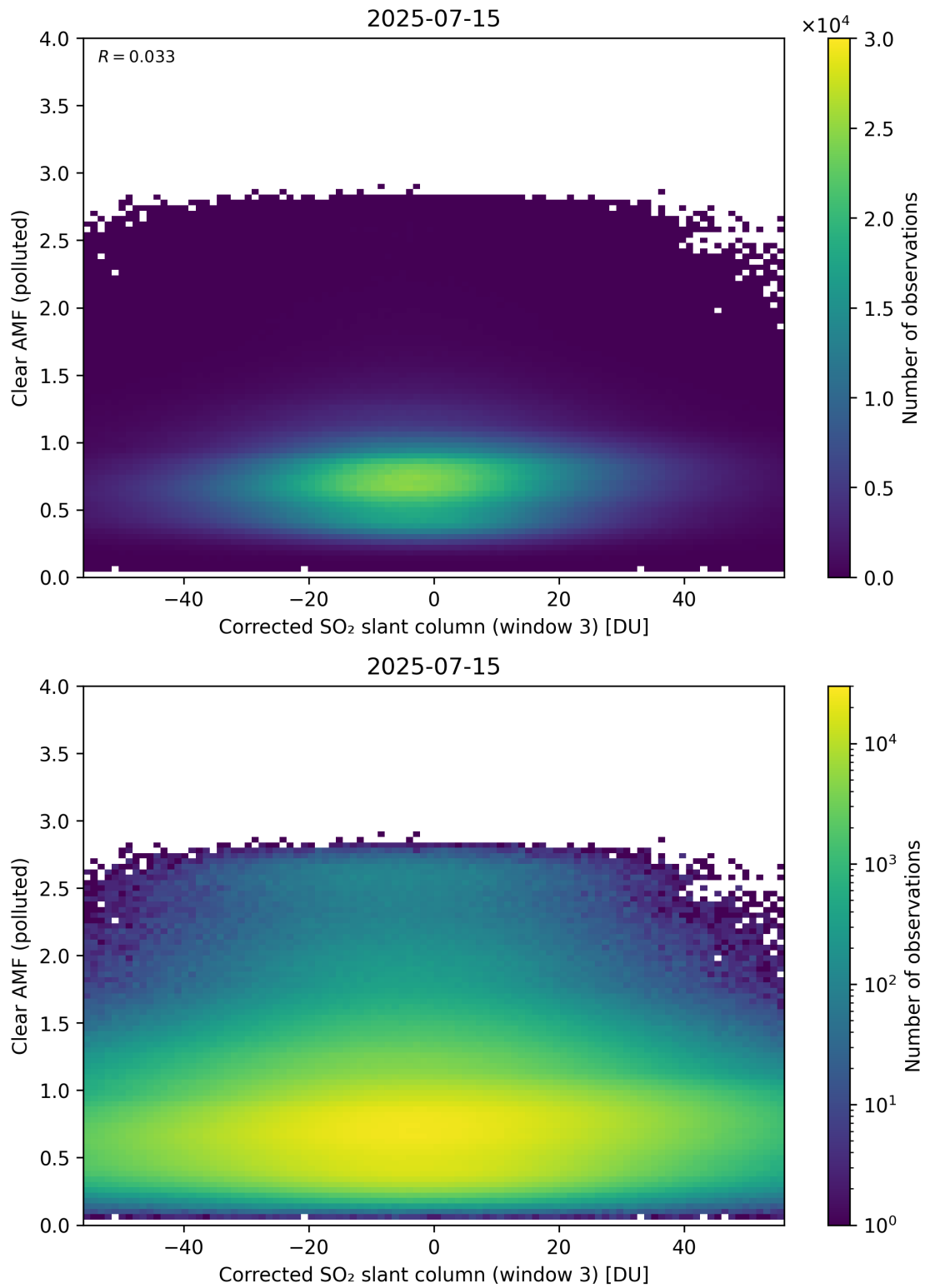
Figure 259: Scatter density plot of “Corrected SO 2 slant column (window 3)” against “Clear AMF (polluted)” for 2025-07-14 to 2025-07-16.
