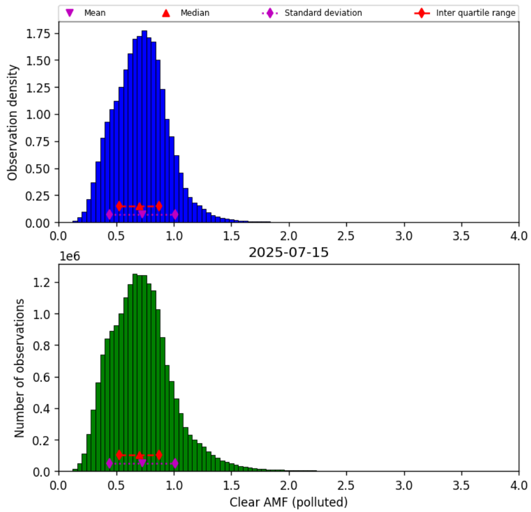
Figure 81: Histogram of “Clear AMF (polluted)” for 2025-07-14 to 2025-07-16
