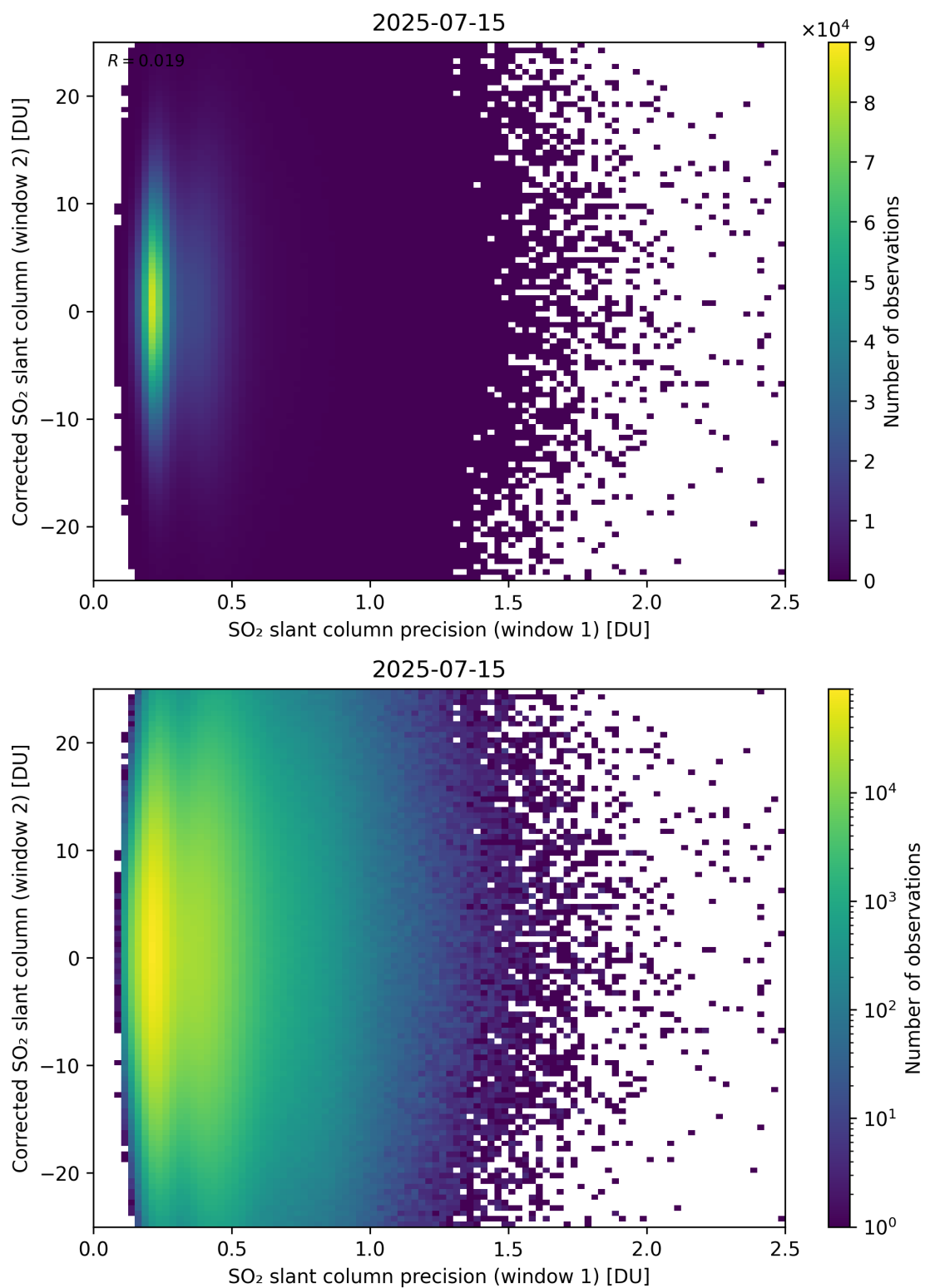
Figure 275: Scatter density plot of “SO 2 slant column precision (window 1)” against “Corrected SO 2 slant column (window 2)” for 2025-07-14 to 2025-07-16.
