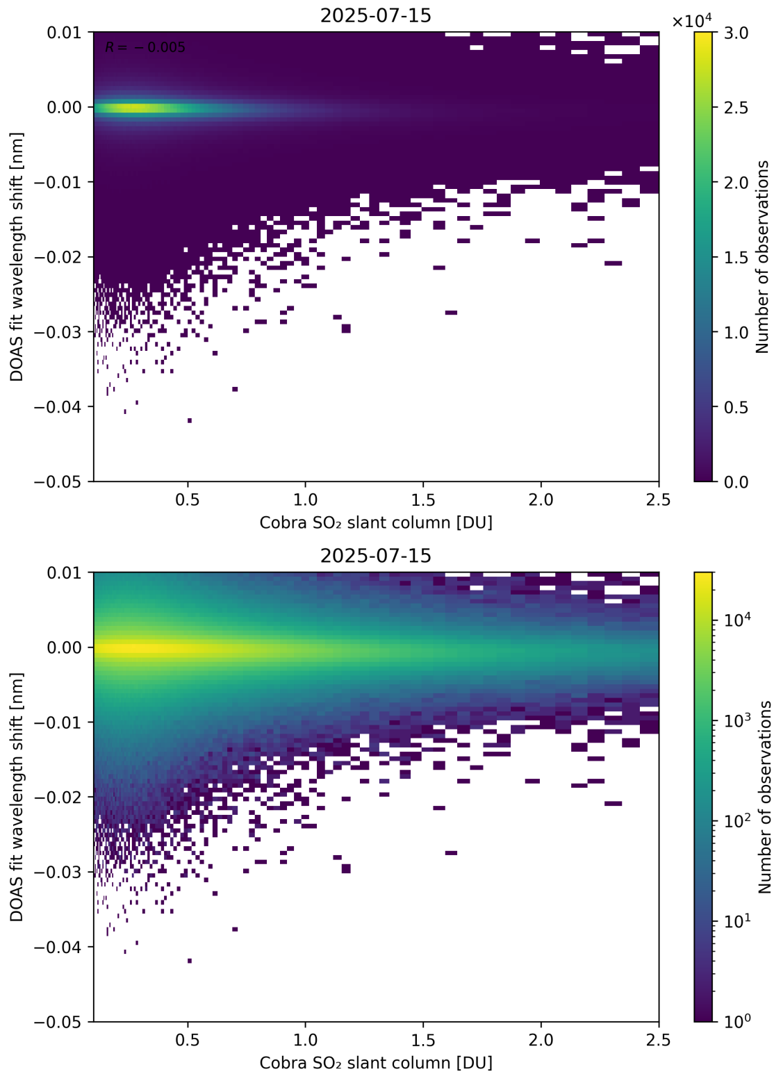
Figure 196: Scatter density plot of “Cobra SO 2 slant column” against “DOAS fit wavelength shift” for 2025-07-14 to 2025-07-16.
