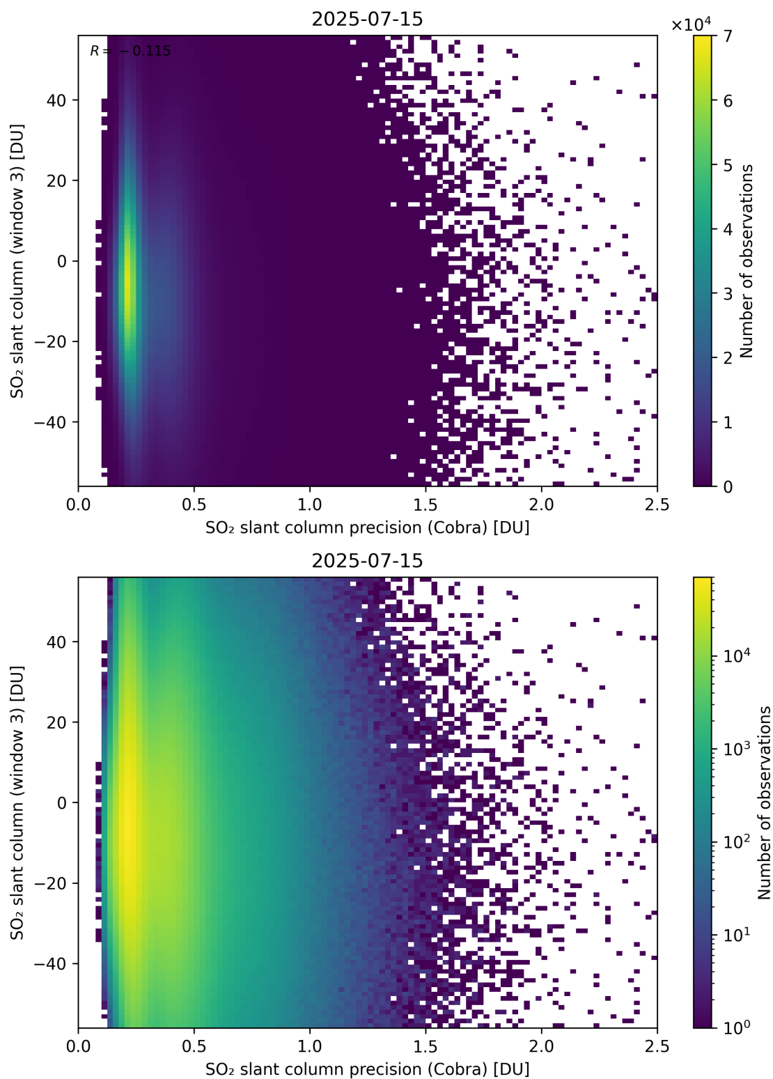
Figure 211: Scatter density plot of “SO 2 slant column precision (Cobra)” against “SO 2 slant column (window 3)” for 2025-07-14 to 2025-07-16.
