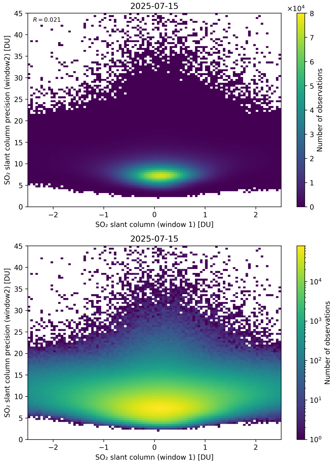
Figure 286: Scatter density plot of “SO 2 slant column (window 1)” against “SO 2 slant column precision (window2)” for 2025-07-14 to 2025-07-16.
