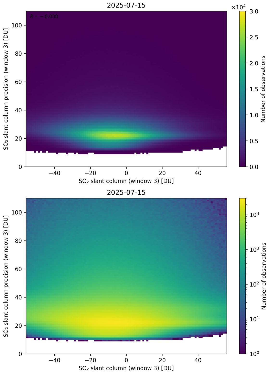
Figure 317: Scatter density plot of “SO 2 slant column (window 3)” against “SO 2 slant column precision (window 3)” for 2025-07-14 to 2025-07-16.
