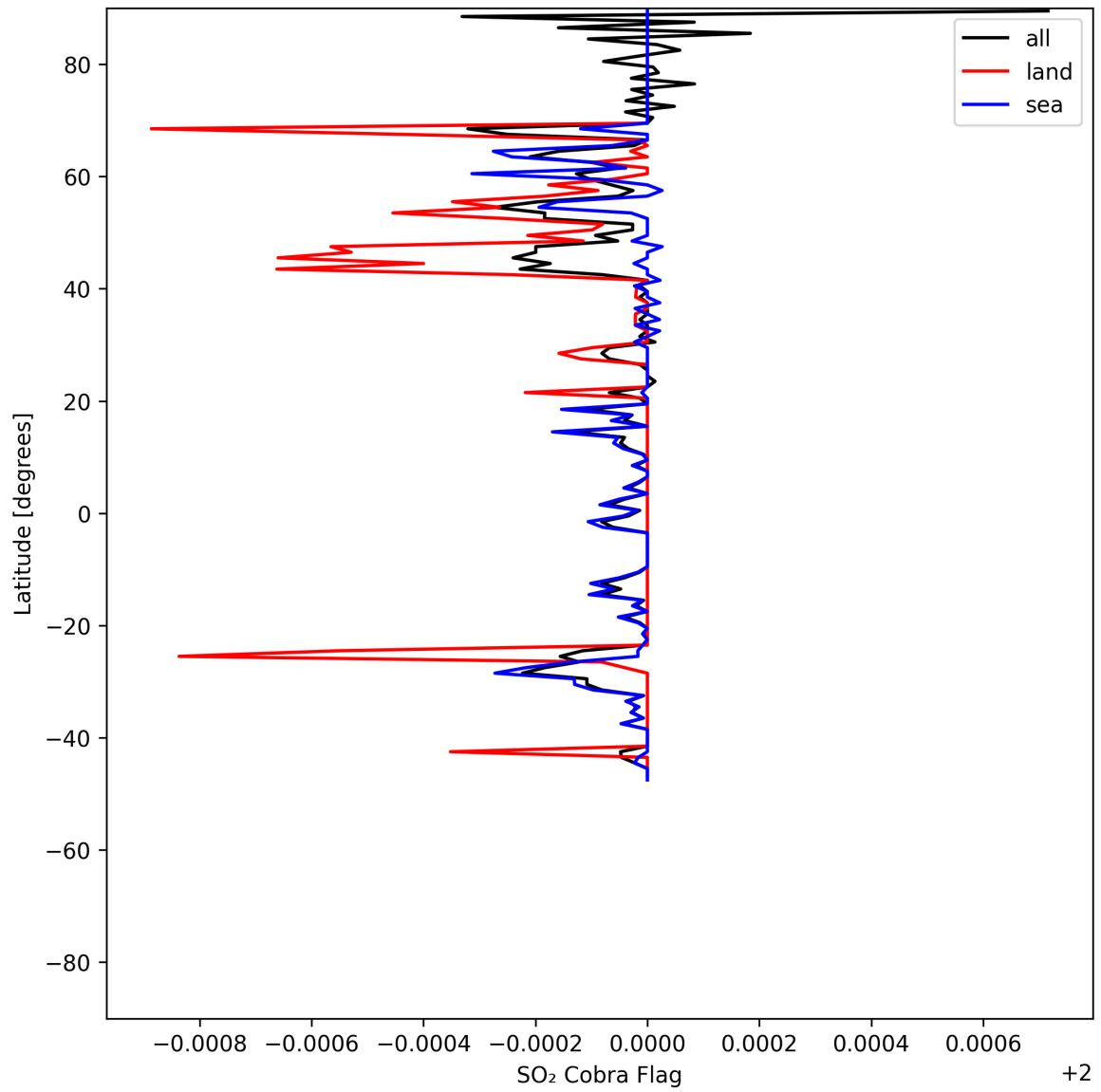
Figure 49: Zonal average of “SO 2 Cobra Flag” for 2025-07-14 to 2025-07-16.
