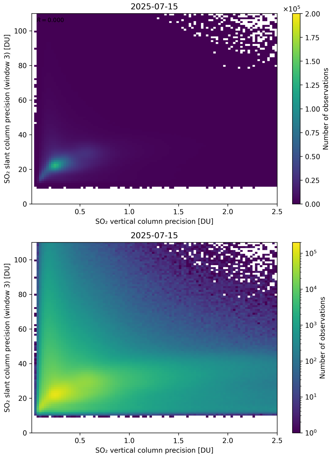
Figure 345: Scatter density plot of “SO 2 vertical column precision” against “SO 2 slant column precision (window 3)” for 2025-07-14 to 2025-07-16.
