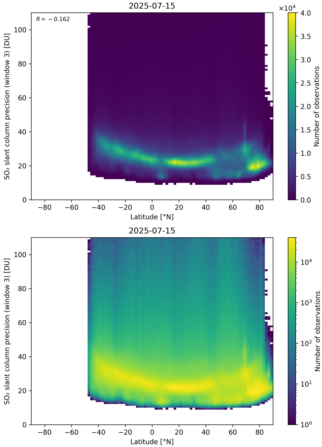
Figure 166: Scatter density plot of “Latitude” against “SO 2 slant column precision (window 3)” for 2025-07-14 to 2025-07-16.
