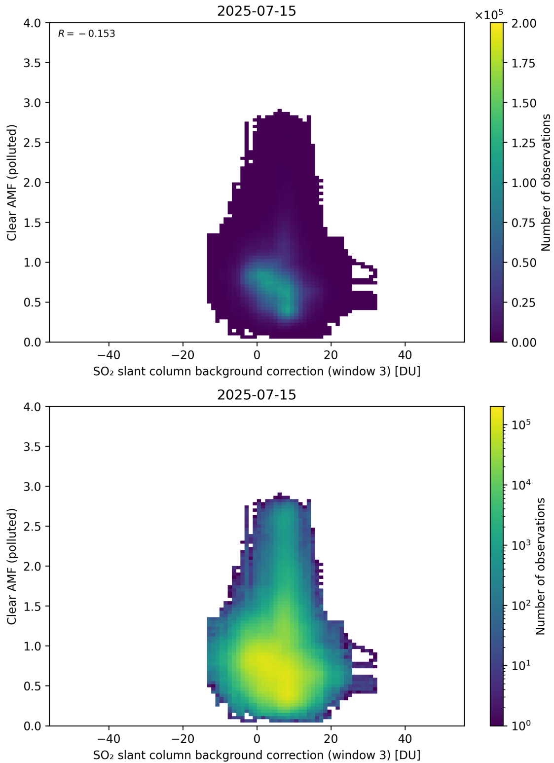
Figure 135: Scatter density plot of “SO 2 slant column background correction (window 3)” against “Clear AMF (polluted)” for 2025-07-14 to 2025-07-16.
