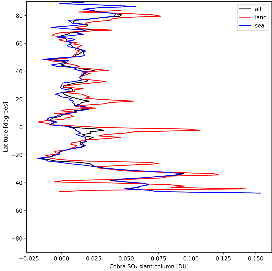
Figure 35: Zonal average of “Cobra SO 2 slant column” for 2025-07-14 to 2025-07-16.
