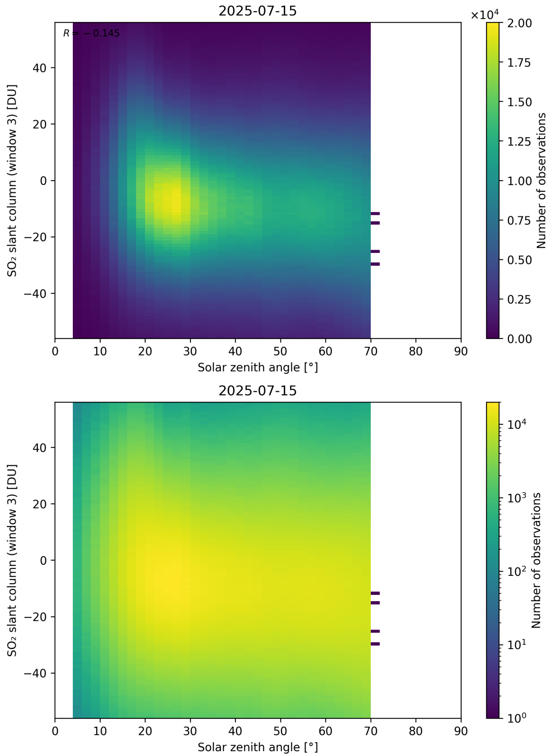
Figure 187: Scatter density plot of “Solar zenith angle” against “SO 2 slant column (window 3)” for 2025-07-14 to 2025-07-16.
