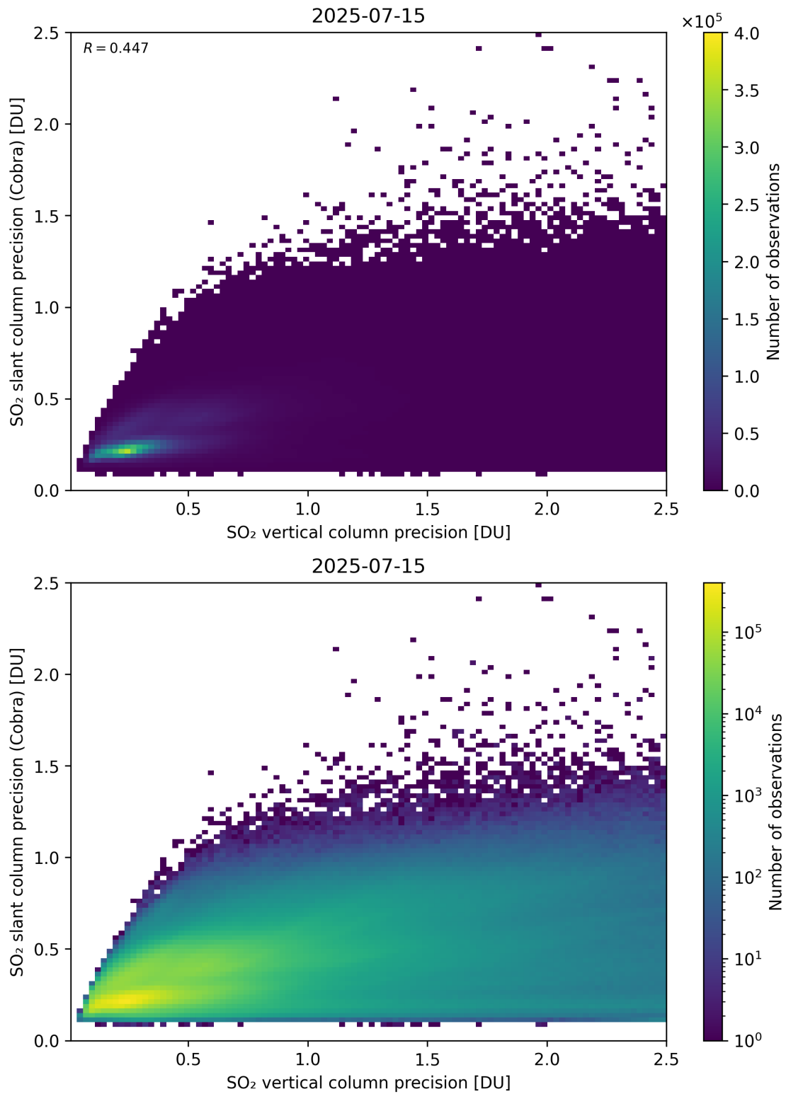
Figure 337: Scatter density plot of “SO 2 vertical column precision” against “SO 2 slant column precision (Cobra)” for 2025-07-14 to 2025-07-16.
