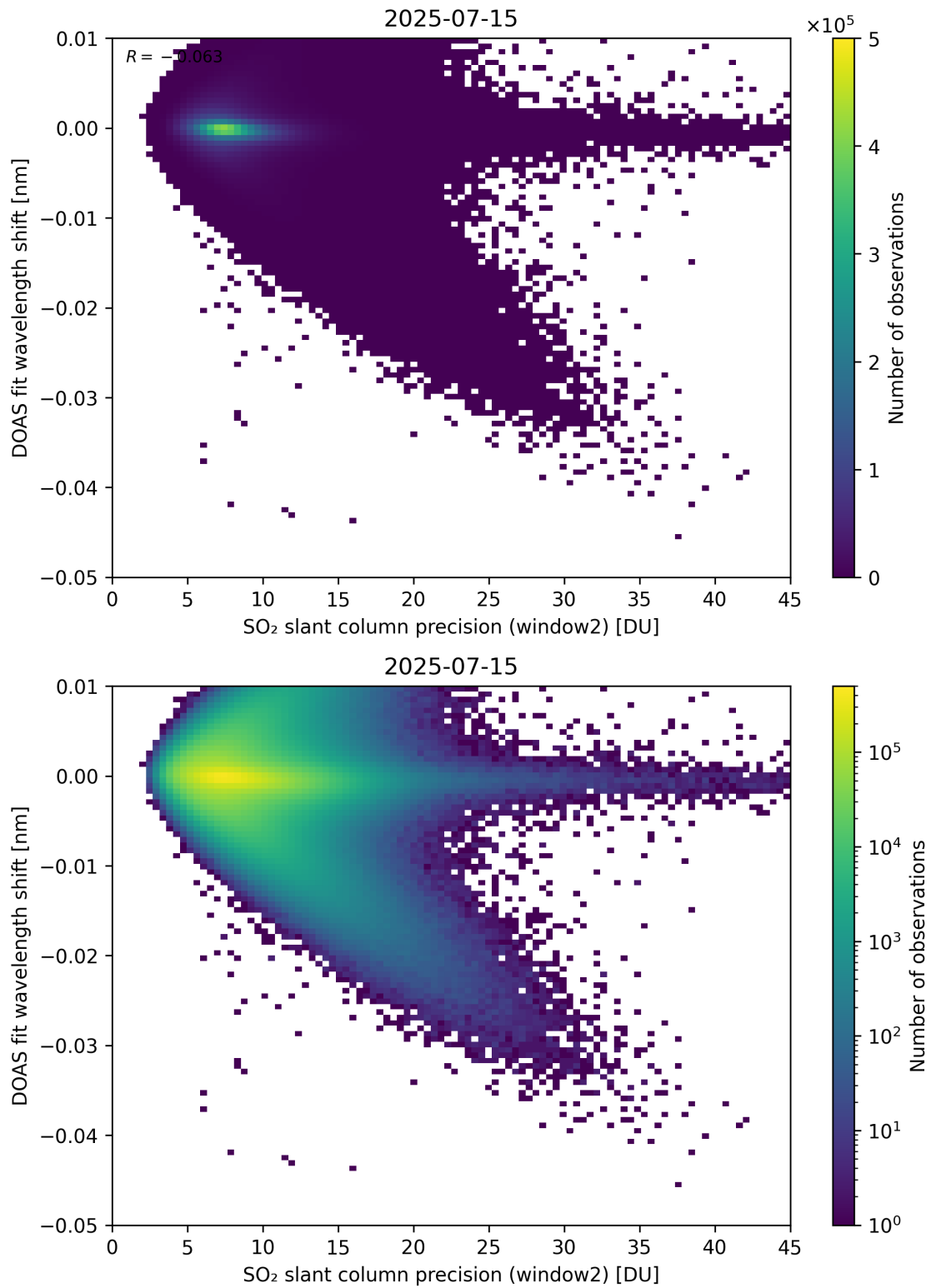
Figure 293: Scatter density plot of “SO 2 slant column precision (window2)” against “DOAS fit wavelength shift” for 2025-07-14 to 2025-07-16.
