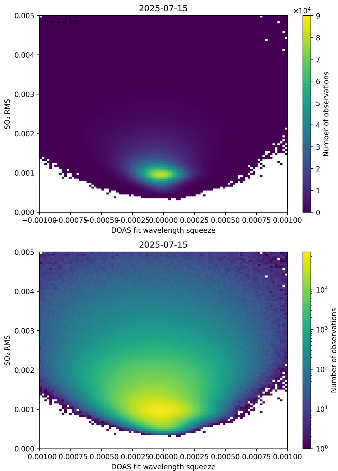
Figure 143: Scatter density plot of “DOAS fit wavelength squeeze” against “SO 2 RMS” for 2025-07-14 to 2025-07-16.
