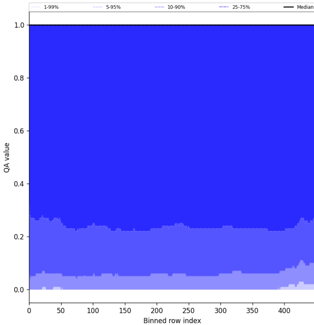
Figure 83: Along track statistics of “QA value” for 2025-07-14 to 2025-07-16
