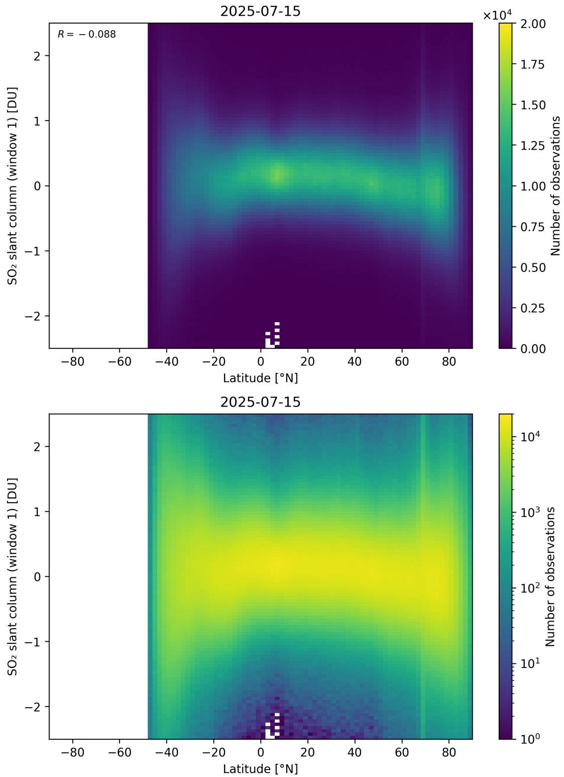
Figure 162: Scatter density plot of “Latitude” against “SO 2 slant column (window 1)” for 2025-07-14 to 2025-07-16.
