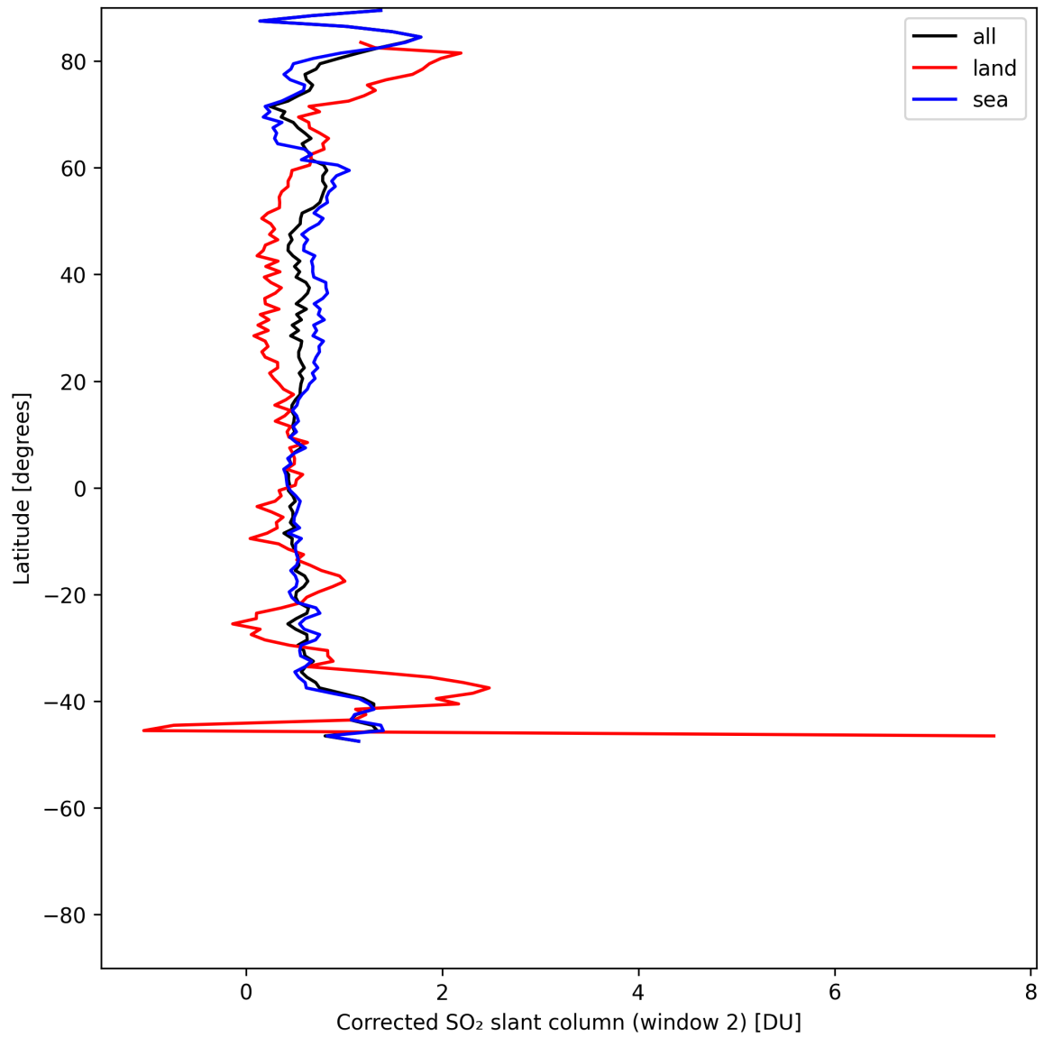
Figure 43: Zonal average of “Corrected SO 2 slant column (window 2)” for 2025-07-14 to 2025-07-16.
