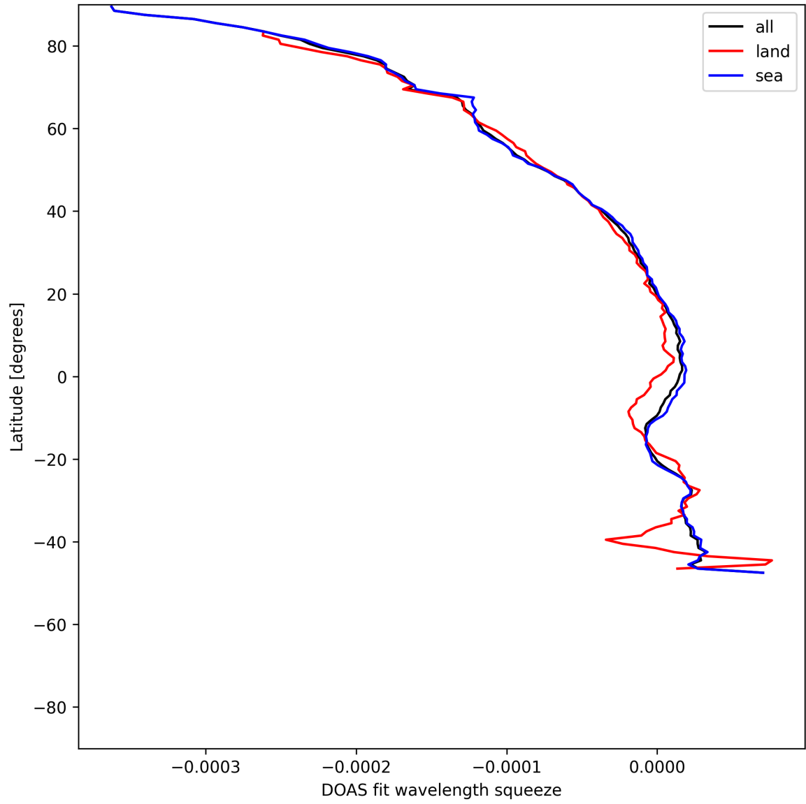
Figure 51: Zonal average of “DOAS fit wavelength squeeze” for 2025-07-14 to 2025-07-16.
