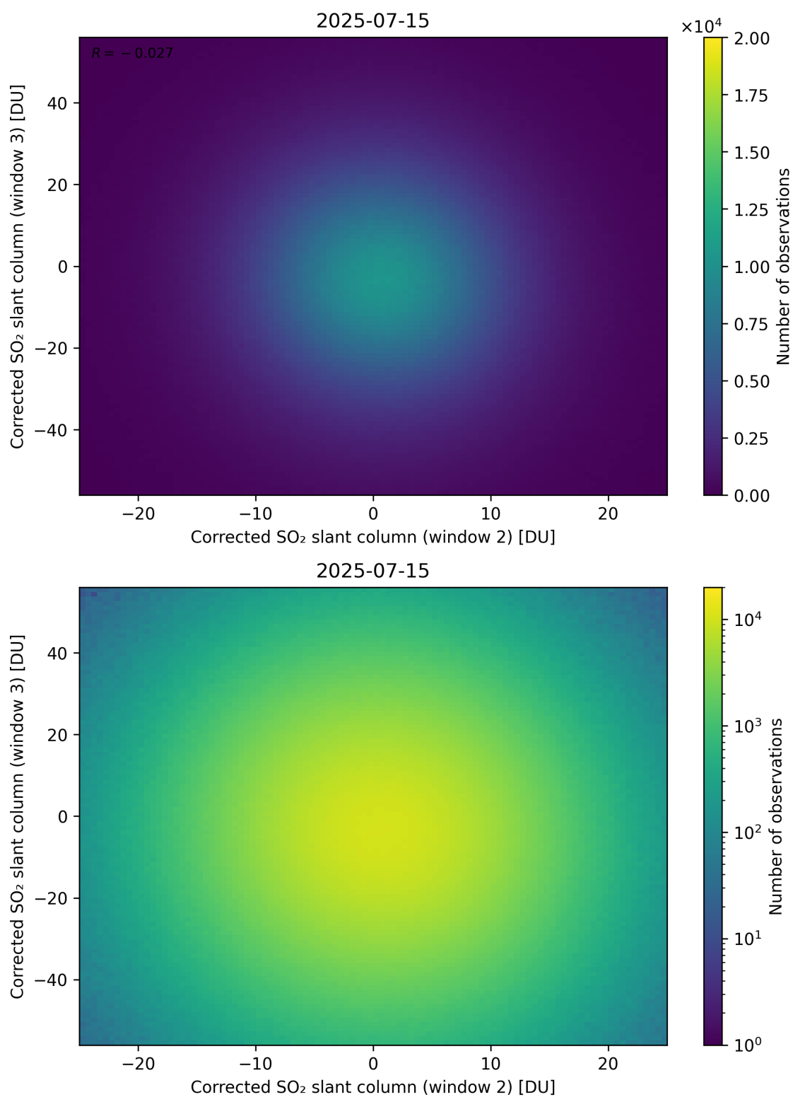
Figure 250: Scatter density plot of “Corrected SO 2 slant column (window 2)” against “Corrected SO 2 slant column (window 3)” for 2025-07-14 to 2025-07-16.
