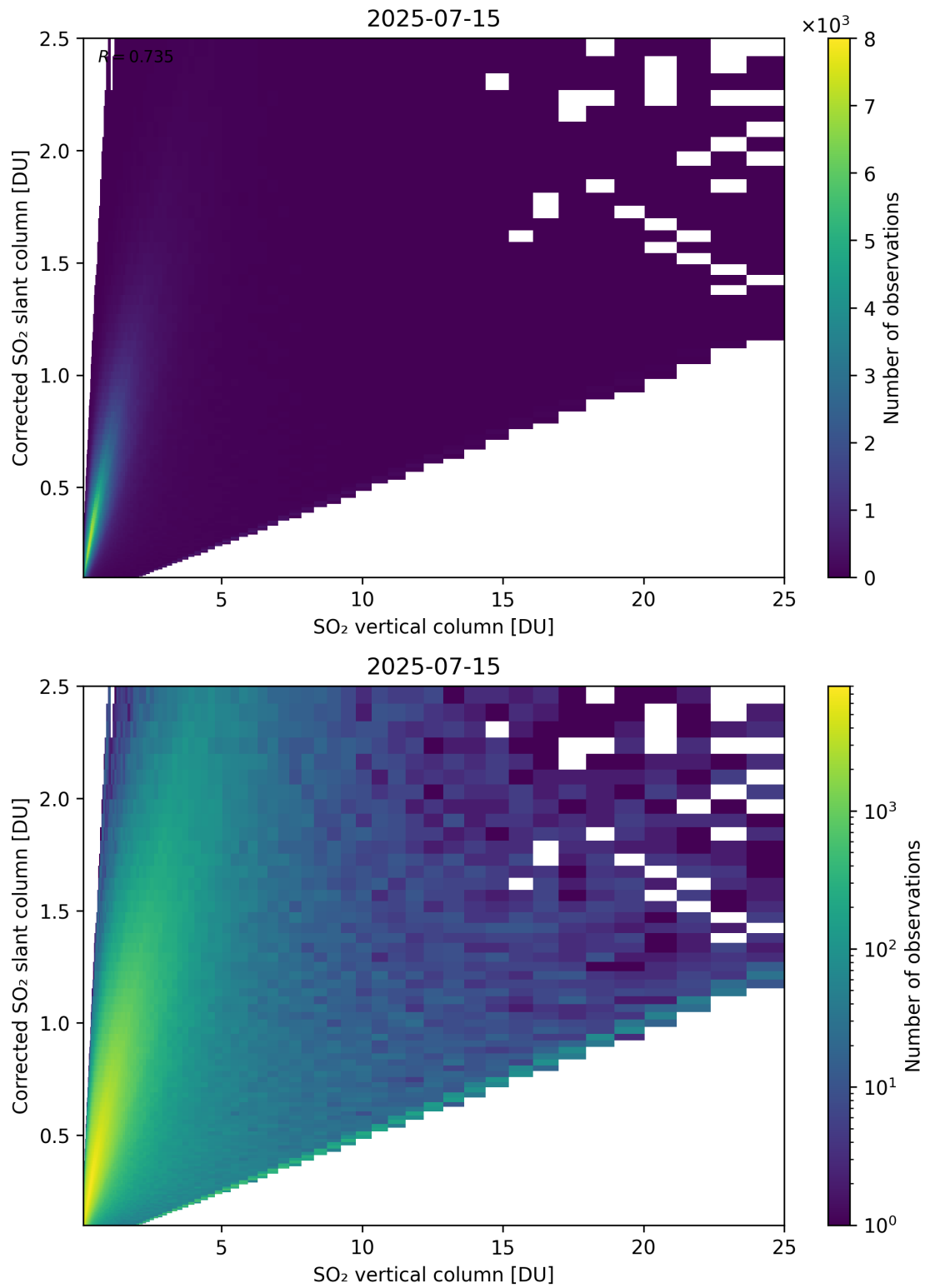
Figure 351: Scatter density plot of “SO 2 vertical column” against “Corrected SO 2 slant column” for 2025-07-14 to 2025-07-16.
