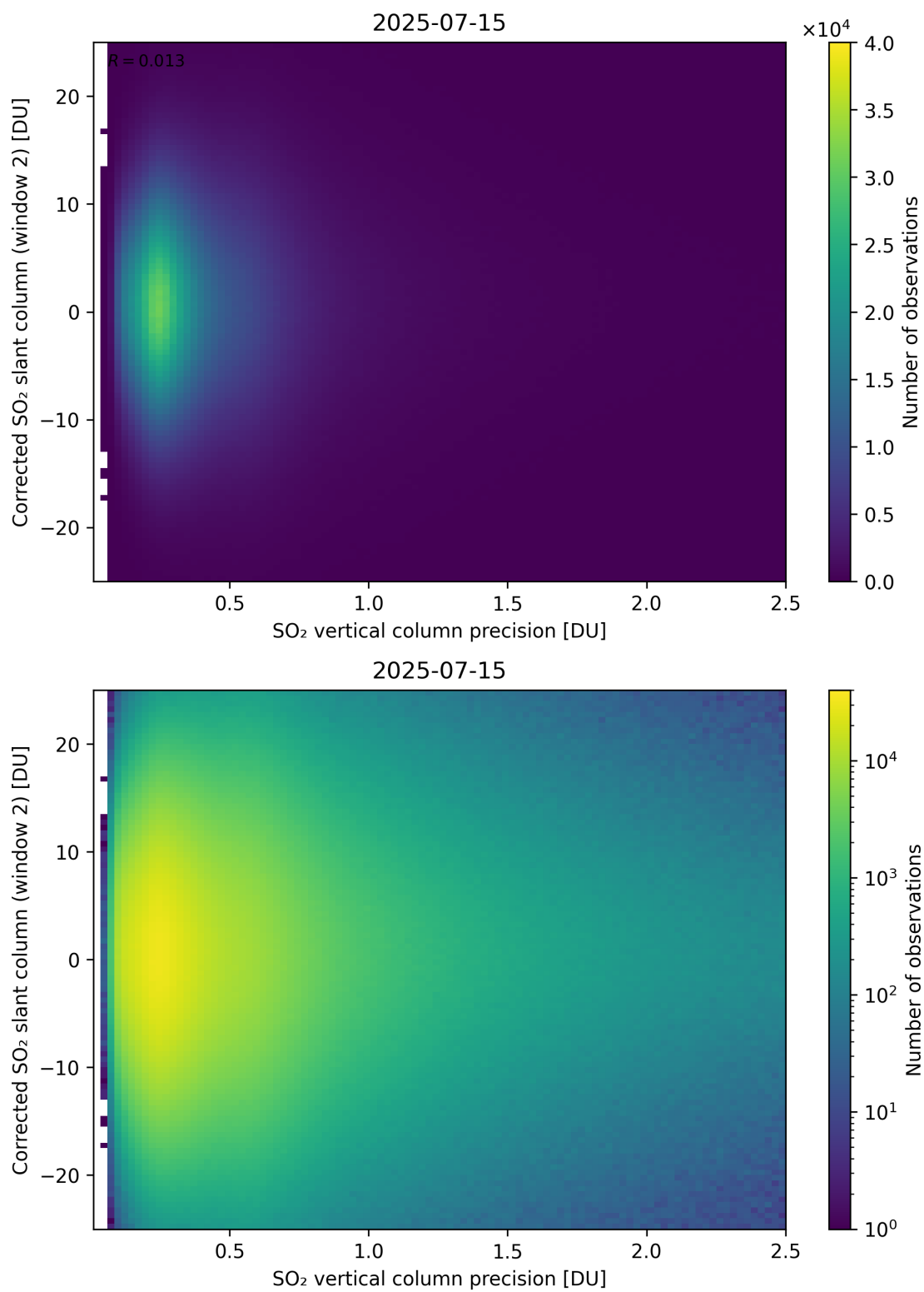
Figure 339: Scatter density plot of “SO 2 vertical column precision” against “Corrected SO 2 slant column (window 2)” for 2025-07-14 to 2025-07-16.
