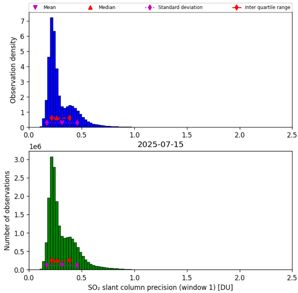
Figure 64: Histogram of “SO 2 slant column precision (window 1)” for 2025-07-14 to 2025-07-16
