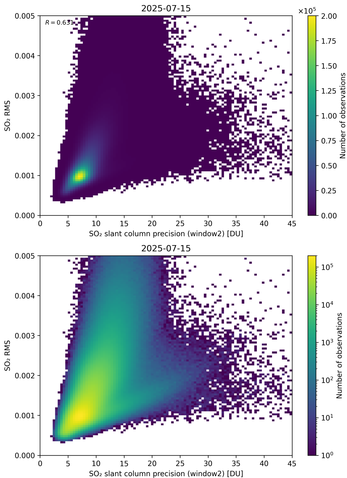
Figure 295: Scatter density plot of “SO 2 slant column precision (window2)” against “SO 2 RMS” for 2025-07-14 to 2025-07-16.
