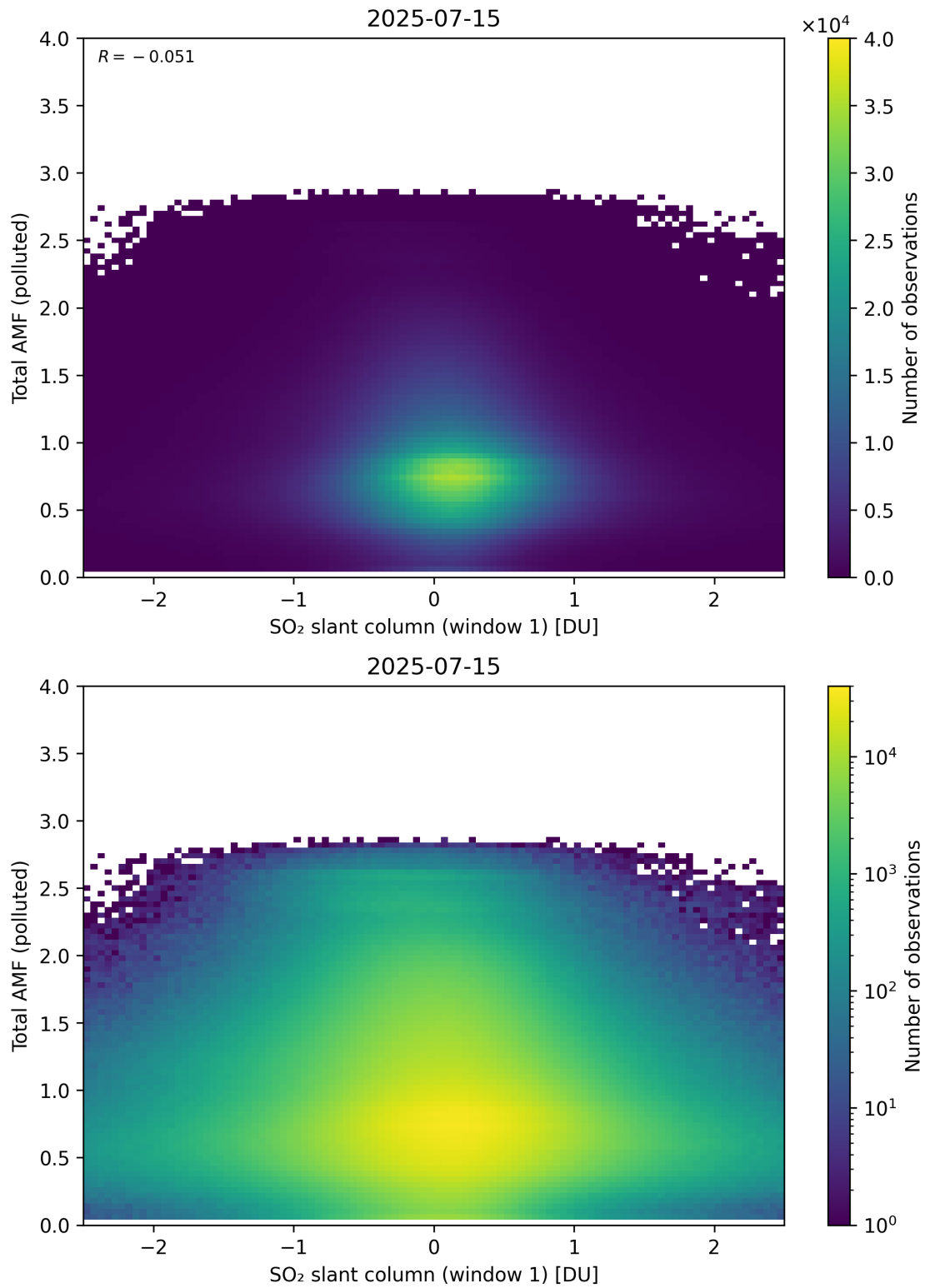
Figure 289: Scatter density plot of “SO 2 slant column (window 1)” against “Total AMF (polluted)” for 2025-07-14 to 2025-07-16.
