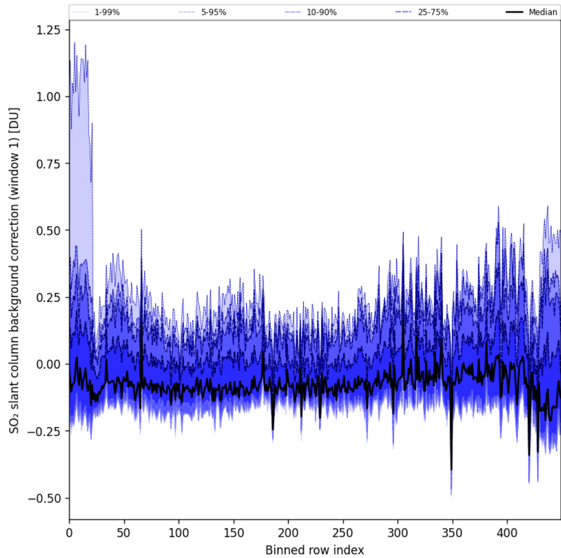
Figure 92: Along track statistics of “SO 2 slant column background correction (window 1)” for 2025-07-14 to 2025-07-16
