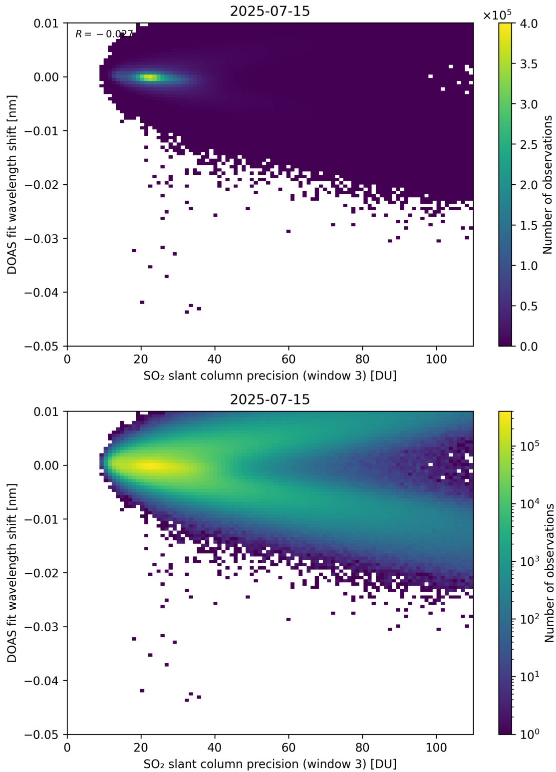
Figure 308: Scatter density plot of “SO 2 slant column precision (window 3)” against “DOAS fit wavelength shift” for 2025-07-14 to 2025-07-16.
