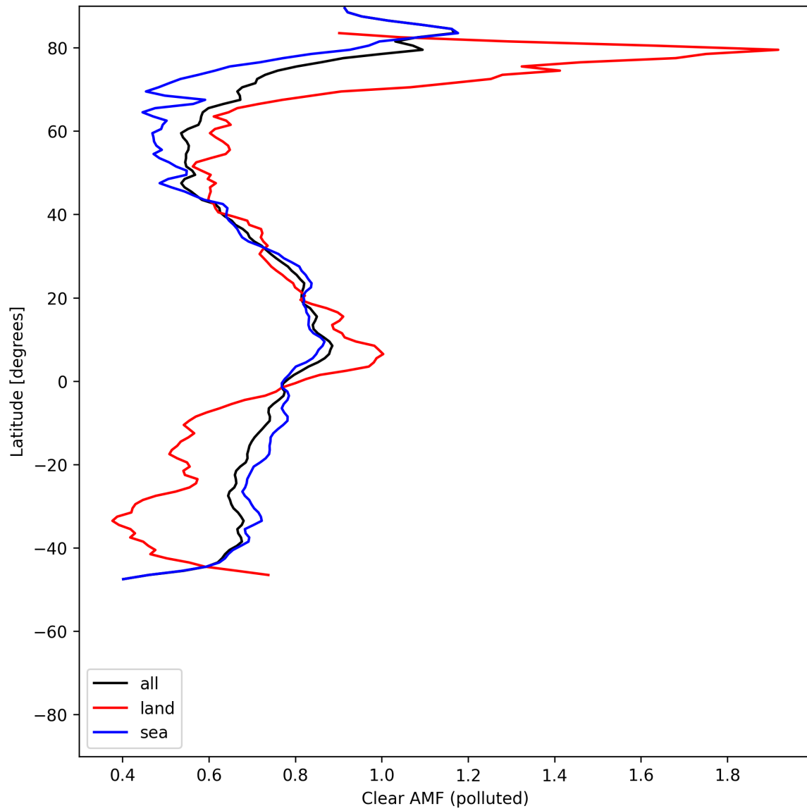
Figure 55: Zonal average of “Clear AMF (polluted)” for 2025-07-14 to 2025-07-16.
