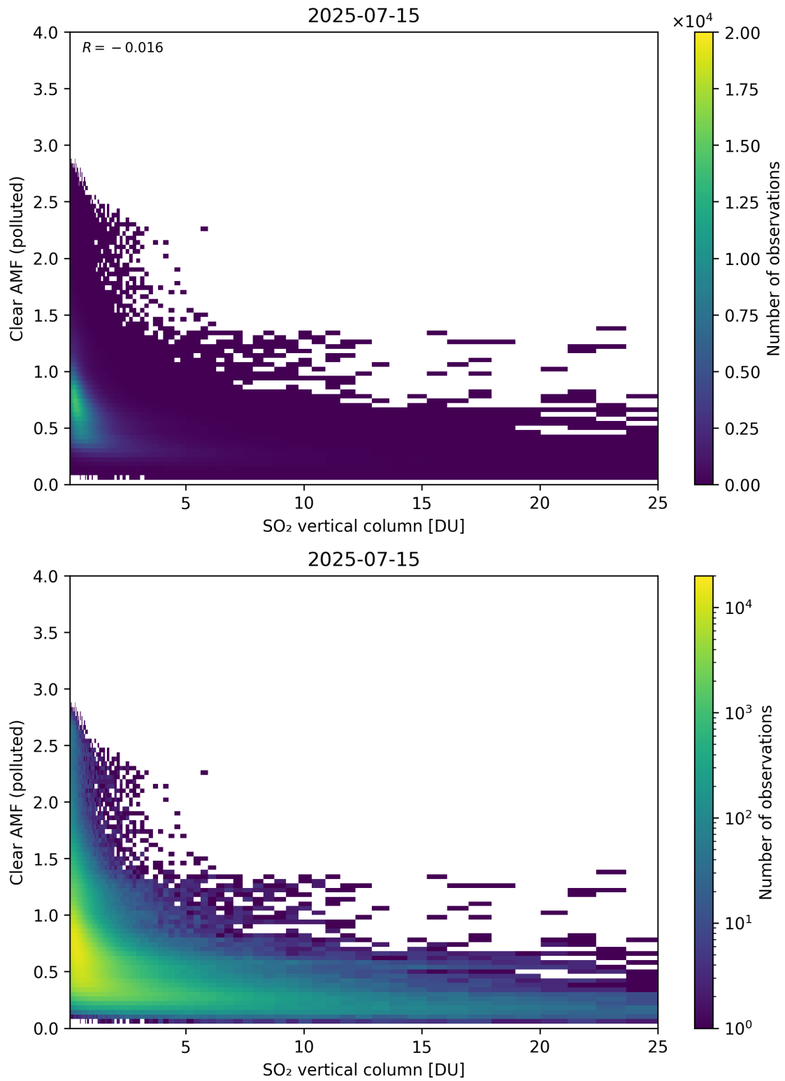
Figure 348: Scatter density plot of “SO 2 vertical column” against “Clear AMF (polluted)” for 2025-07-14 to 2025-07-16.
