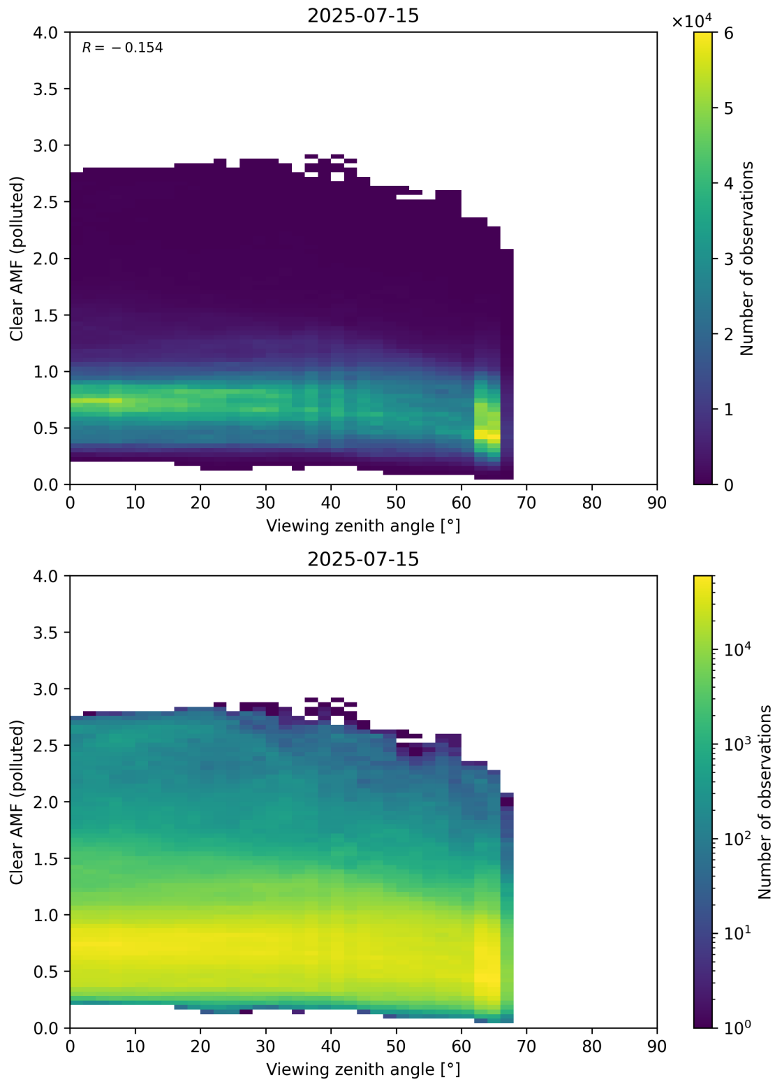
Figure 370: Scatter density plot of “Viewing zenith angle” against “Clear AMF (polluted)” for 2025-07-14 to 2025-07-16.
