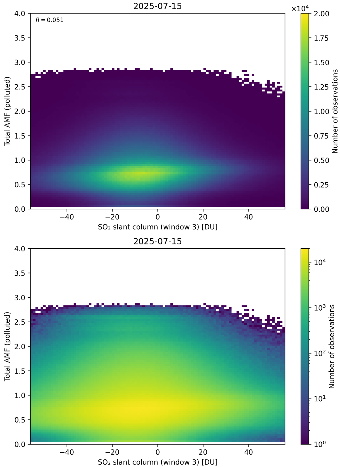
Figure 318: Scatter density plot of “SO 2 slant column (window 3)” against “Total AMF (polluted)” for 2025-07-14 to 2025-07-16.
