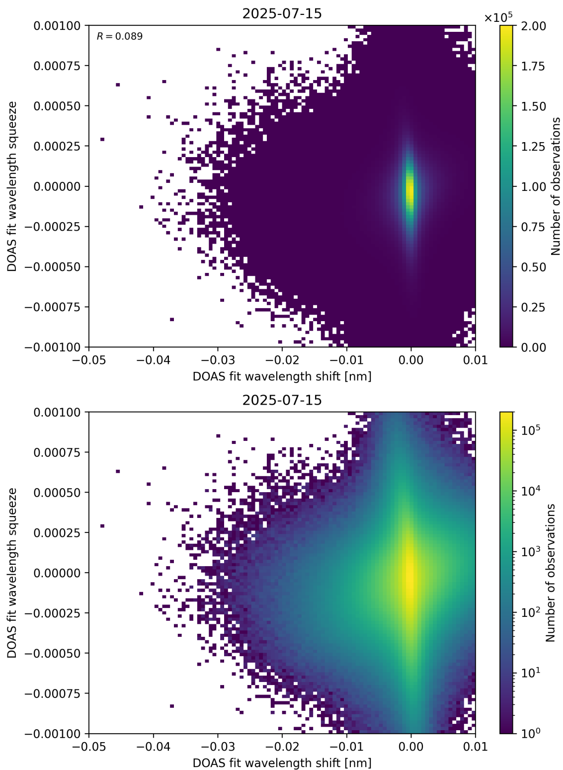
Figure 138: Scatter density plot of “DOAS fit wavelength shift” against “DOAS fit wavelength squeeze” for 2025-07-14 to 2025-07-16.
