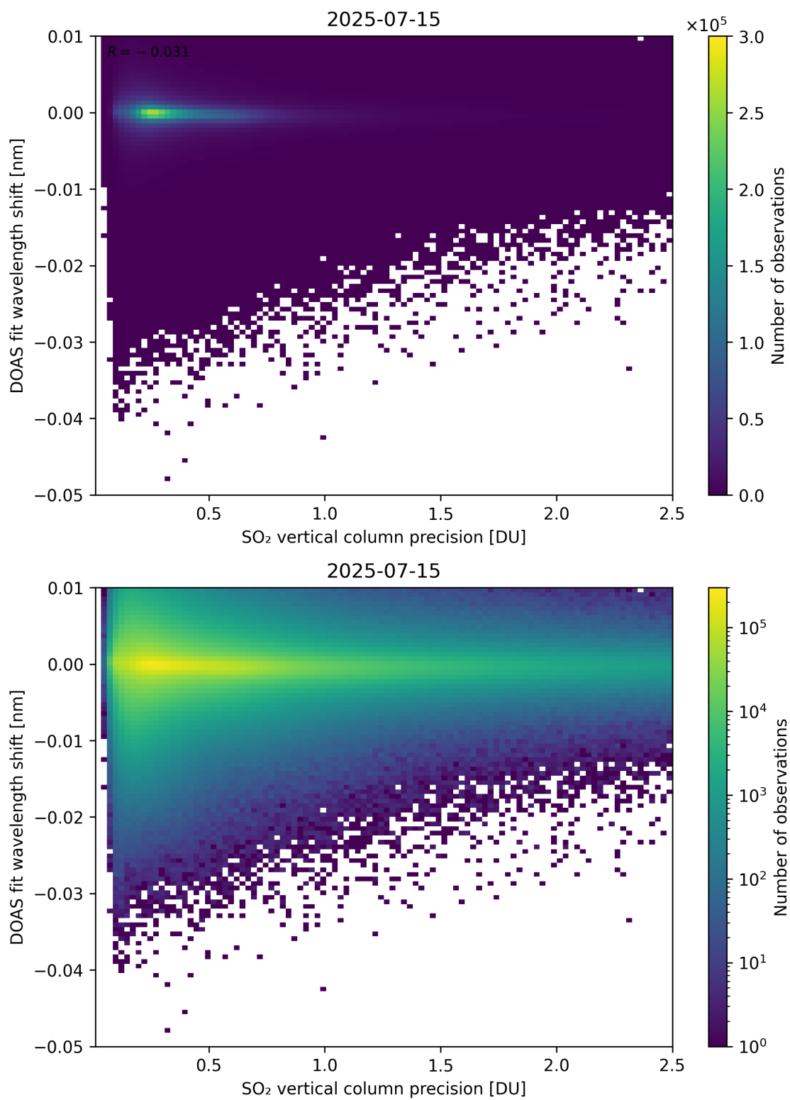
Figure 332: Scatter density plot of “SO 2 vertical column precision” against “DOAS fit wavelength shift” for 2025-07-14 to 2025-07-16.
