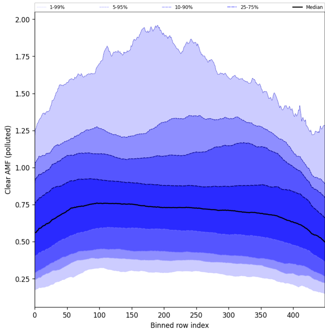
Figure 107: Along track statistics of “Clear AMF (polluted)” for 2025-07-14 to 2025-07-16
