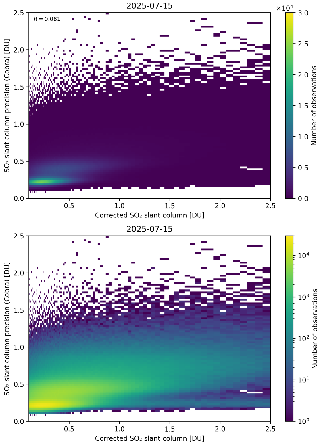
Figure 234: Scatter density plot of “Corrected SO 2 slant column” against “SO 2 slant column precision (Cobra)” for 2025-07-14 to 2025-07-16.
