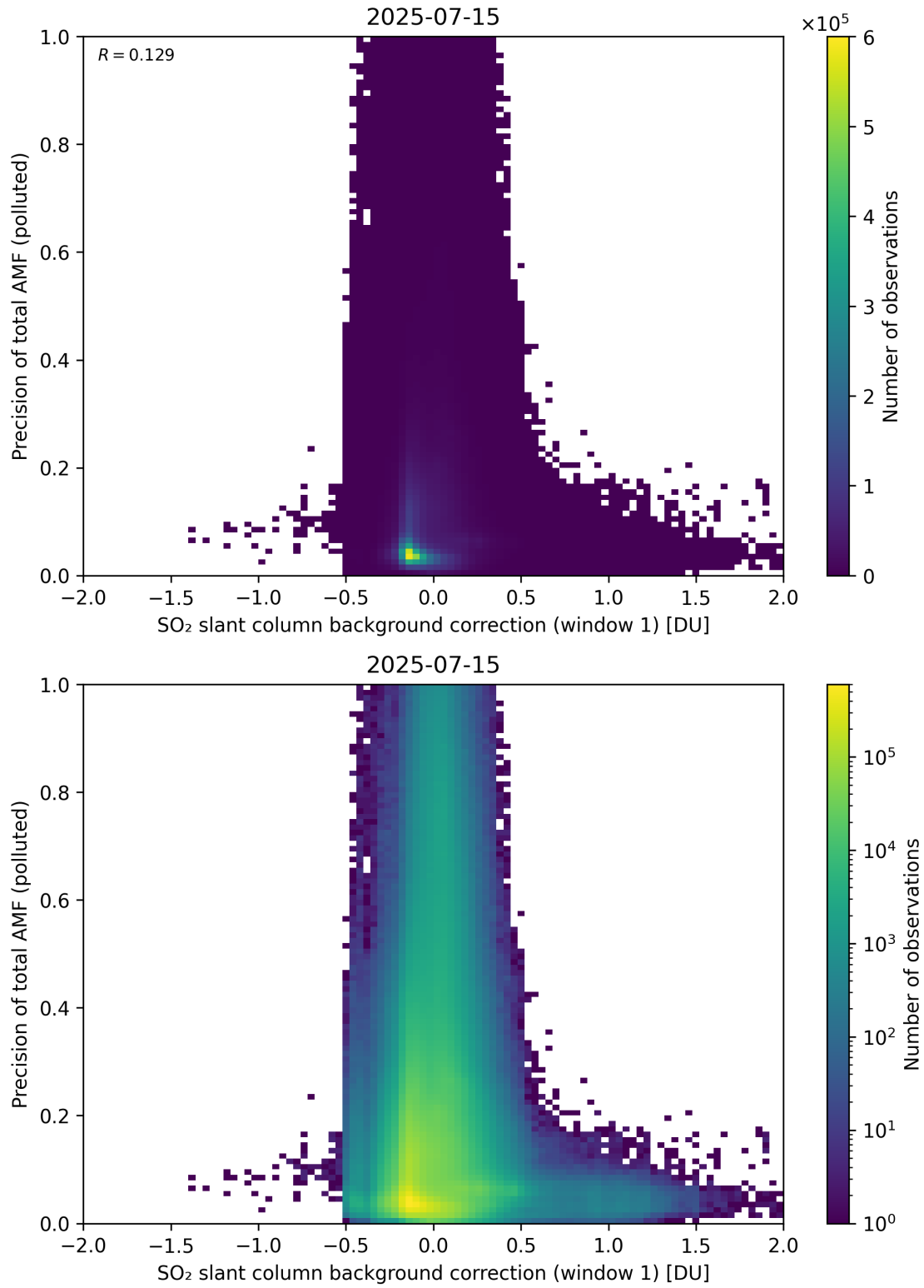
Figure 121: Scatter density plot of “SO 2 slant column background correction (window 1)” against “Precision of total AMF (polluted)” for 2025-07-14 to 2025-07-16.
