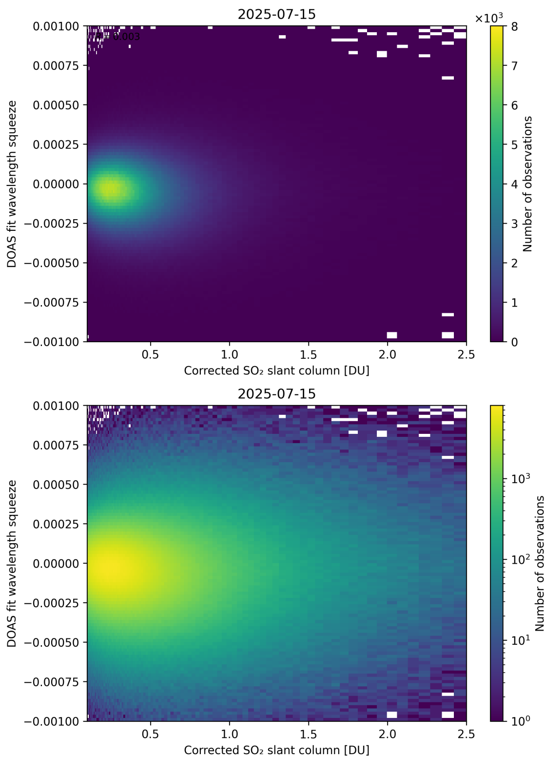
Figure 230: Scatter density plot of “Corrected SO 2 slant column” against “DOAS fit wavelength squeeze” for 2025-07-14 to 2025-07-16.
