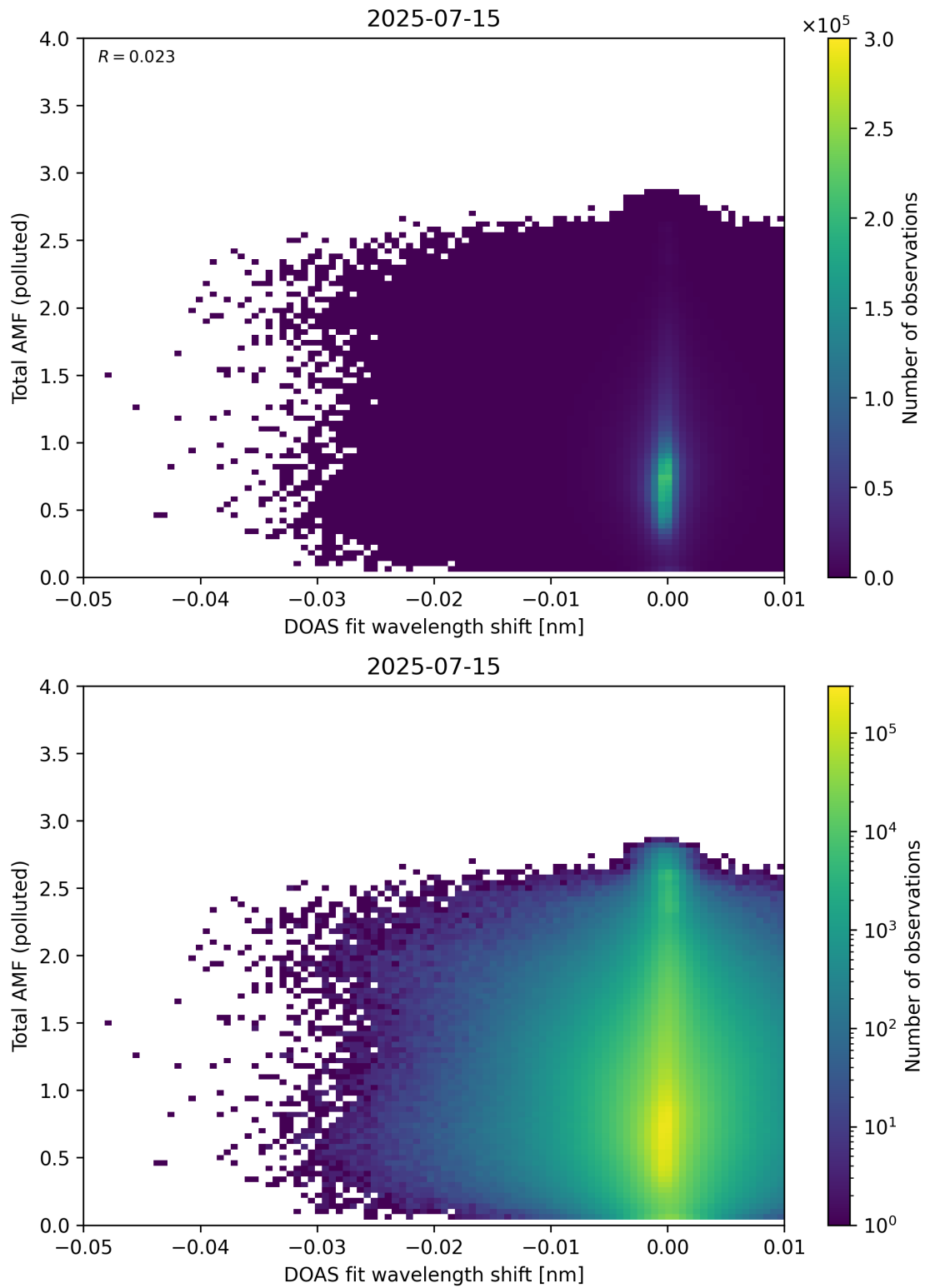
Figure 141: Scatter density plot of “DOAS fit wavelength shift” against “Total AMF (polluted)” for 2025-07-14 to 2025-07-16.
