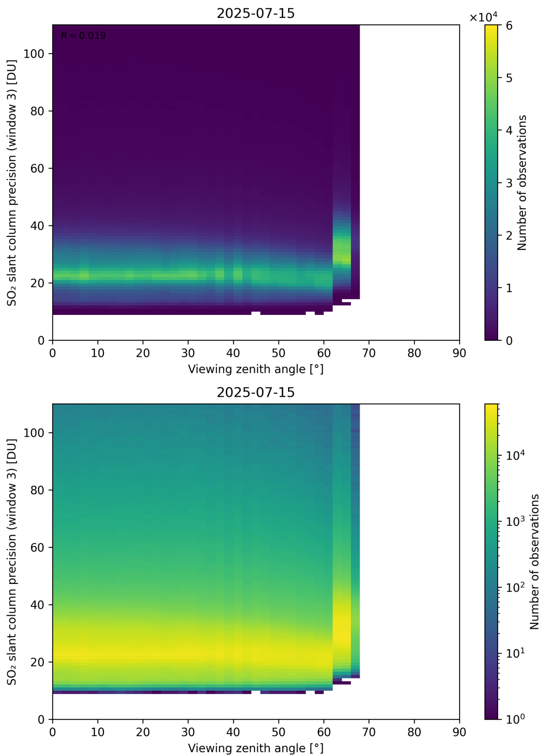
Figure 380: Scatter density plot of “Viewing zenith angle” against “SO 2 slant column precision (window 3)” for 2025-07-14 to 2025-07-16.
