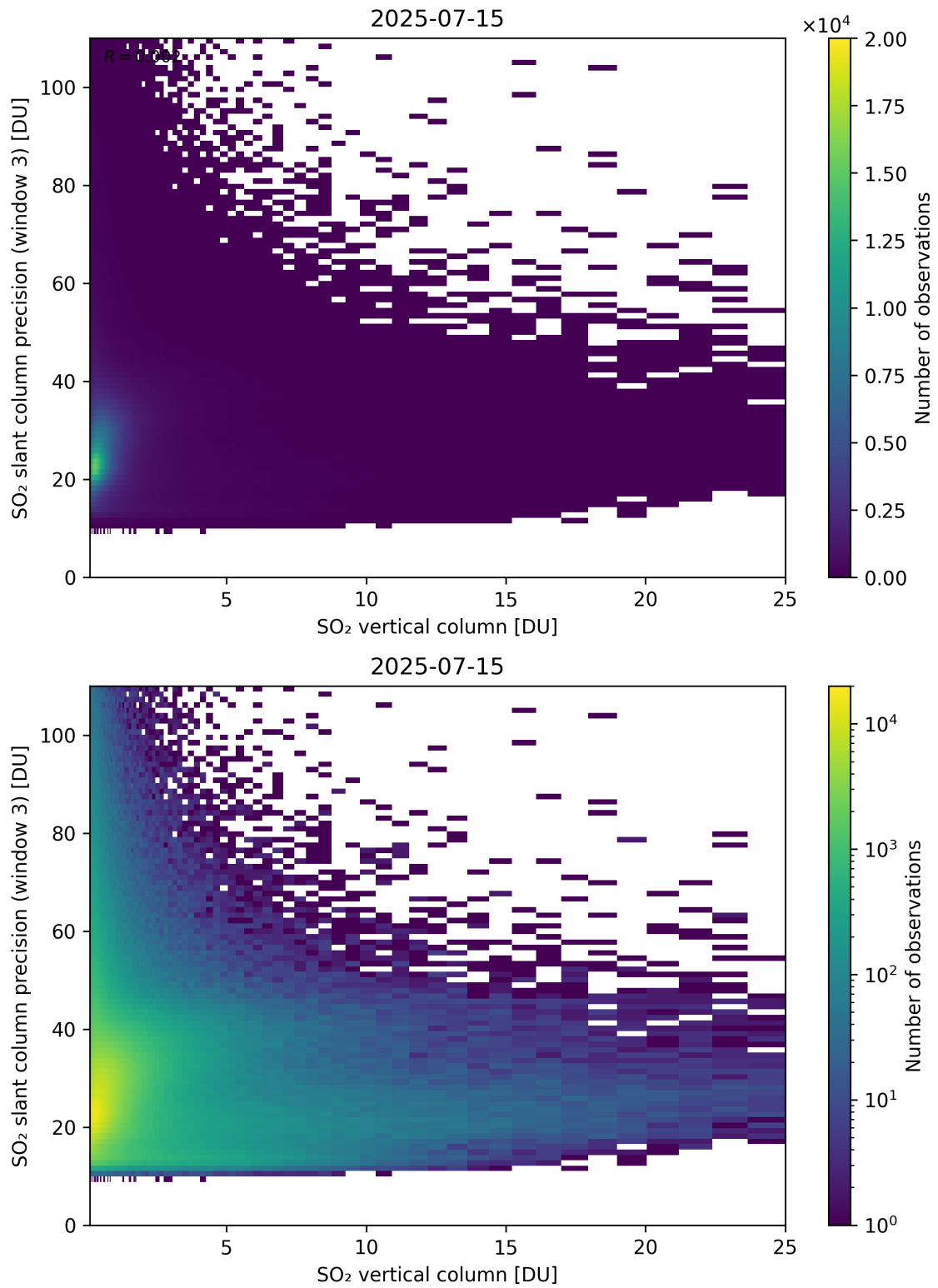
Figure 358: Scatter density plot of “SO 2 vertical column” against “SO 2 slant column precision (window 3)” for 2025-07-14 to 2025-07-16.
