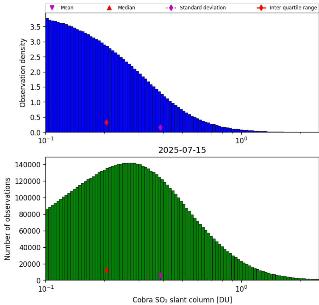
Figure 61: Histogram of “Cobra SO 2 slant column” for 2025-07-14 to 2025-07-16
