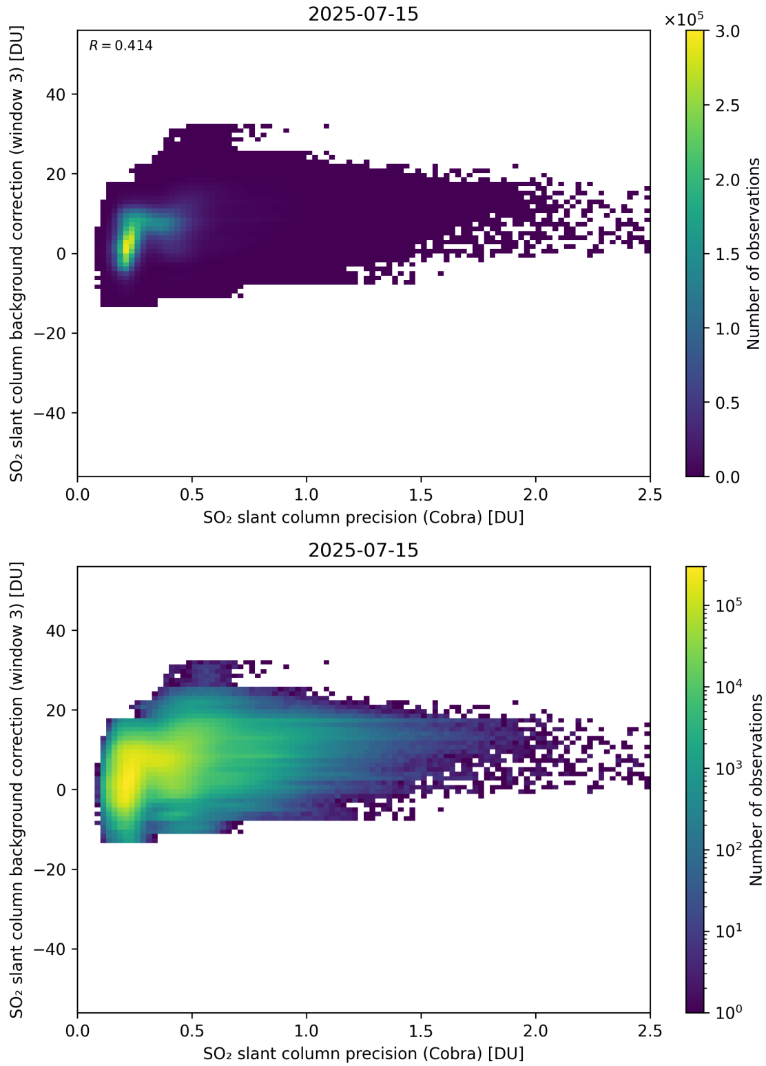
Figure 201: Scatter density plot of “SO 2 slant column precision (Cobra)” against “SO 2 slant column background correction (window 3)” for 2025-07-14 to 2025-07-16.
