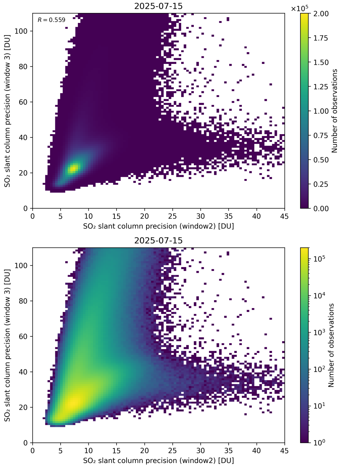
Figure 300: Scatter density plot of “SO 2 slant column precision (window2)” against “SO 2 slant column precision (window 3)” for 2025-07-14 to 2025-07-16.
