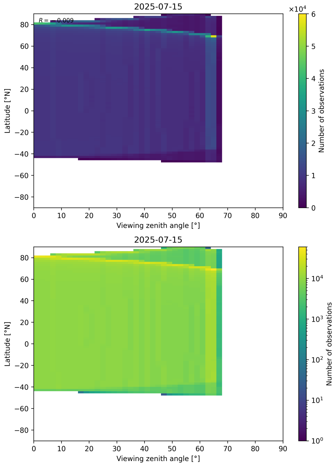
Figure 368: Scatter density plot of “Viewing zenith angle” against “Latitude” for 2025-07-14 to 2025-07-16.
