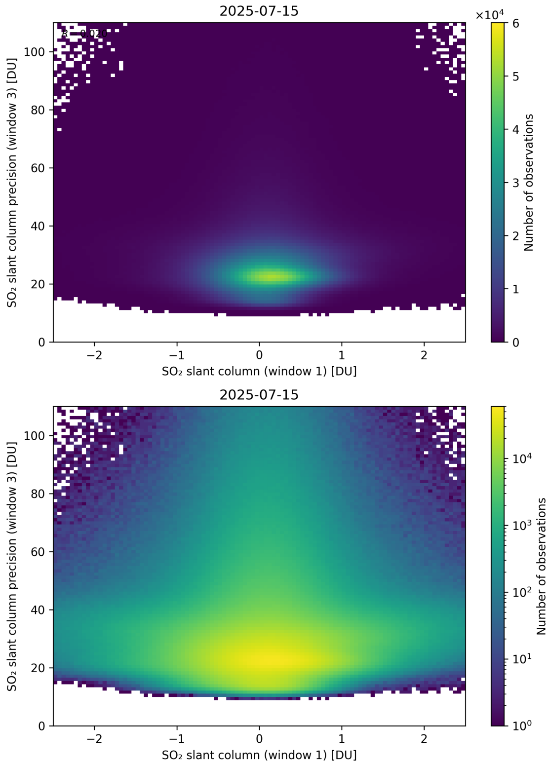
Figure 288: Scatter density plot of “SO 2 slant column (window 1)” against “SO 2 slant column precision (window 3)” for 2025-07-14 to 2025-07-16.
