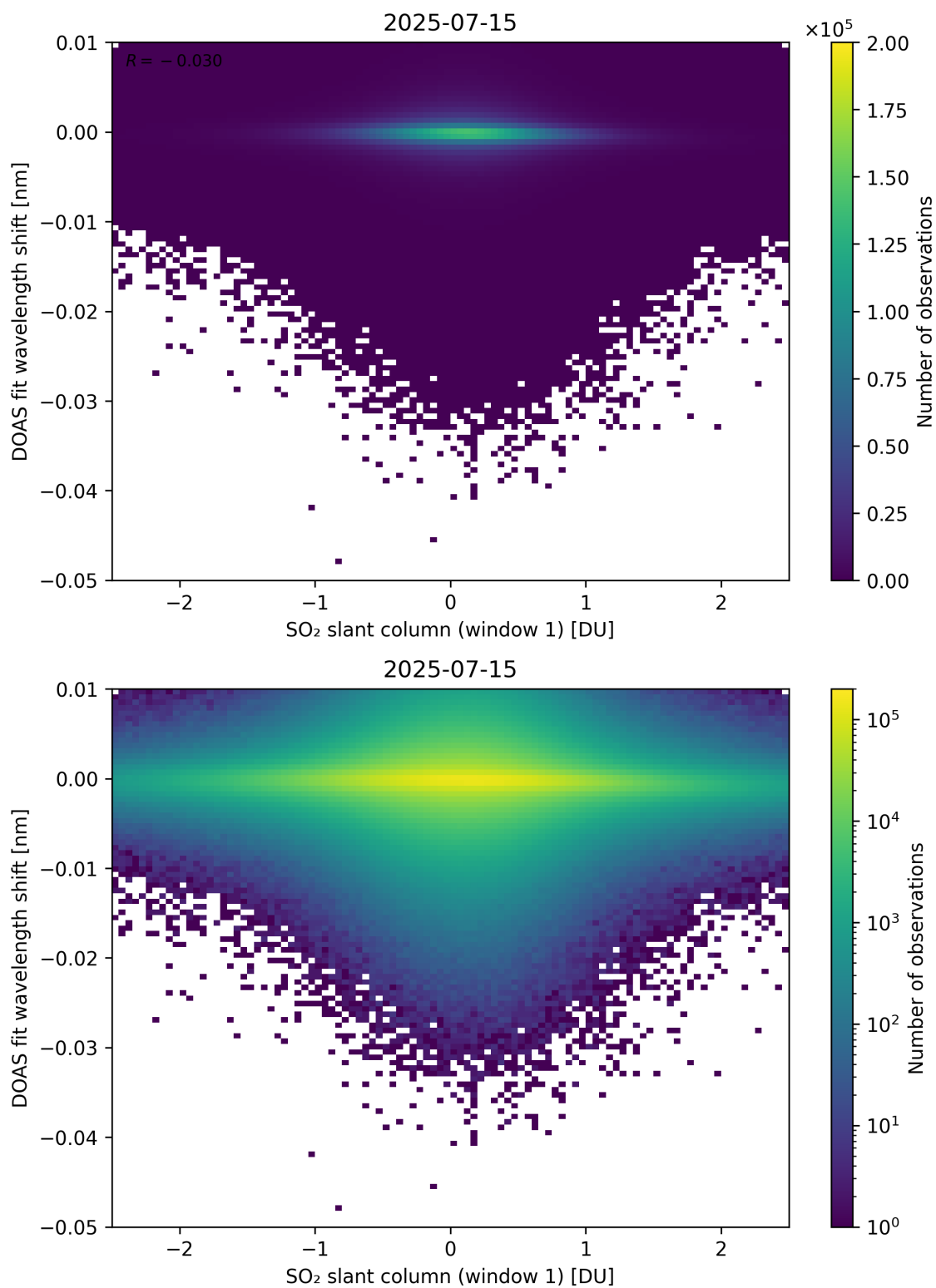
Figure 265: Scatter density plot of “SO 2 slant column (window 1)” against “DOAS fit wavelength shift” for 2025-07-14 to 2025-07-16.
