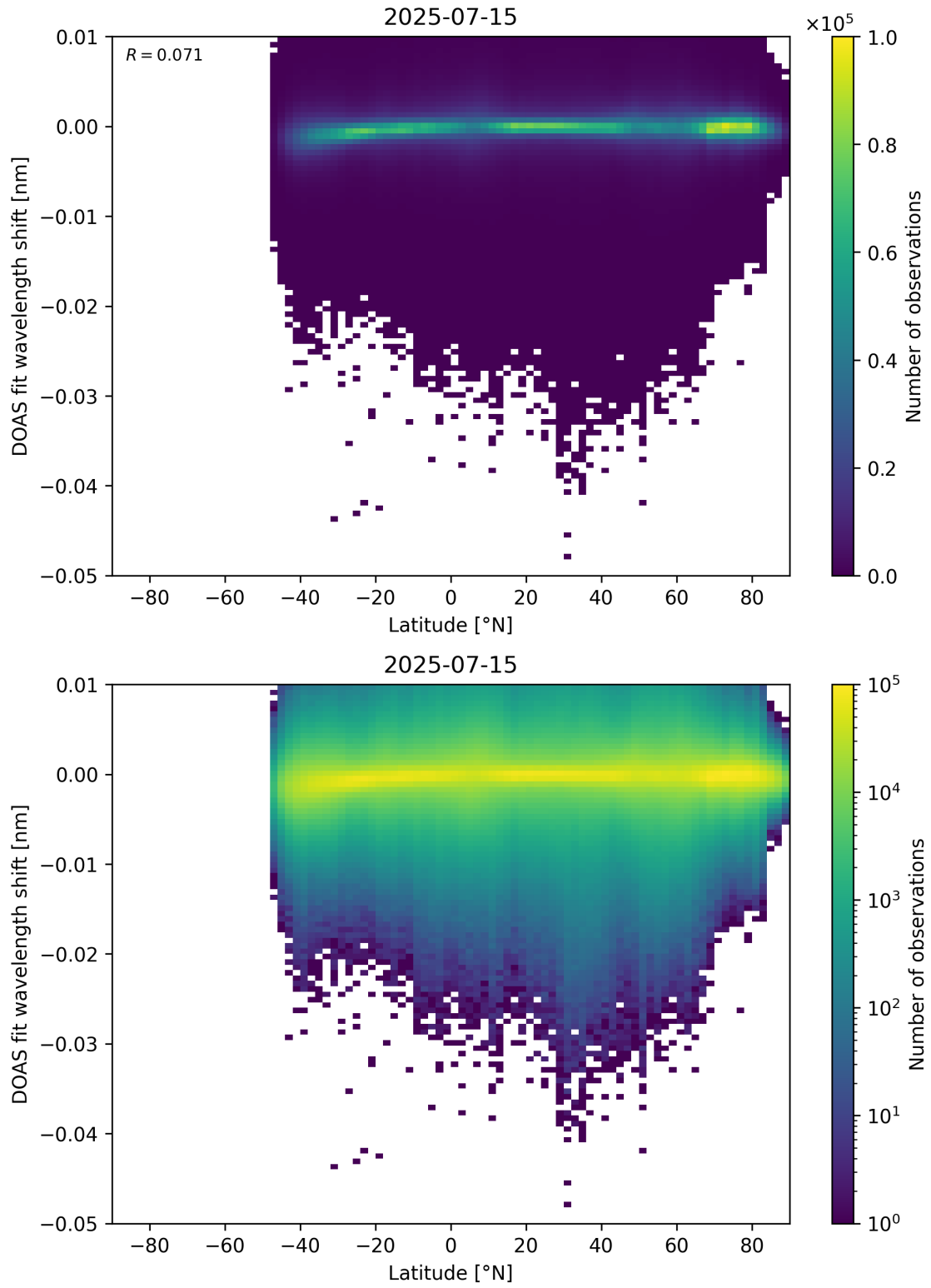
Figure 153: Scatter density plot of “Latitude” against “DOAS fit wavelength shift” for 2025-07-14 to 2025-07-16.
