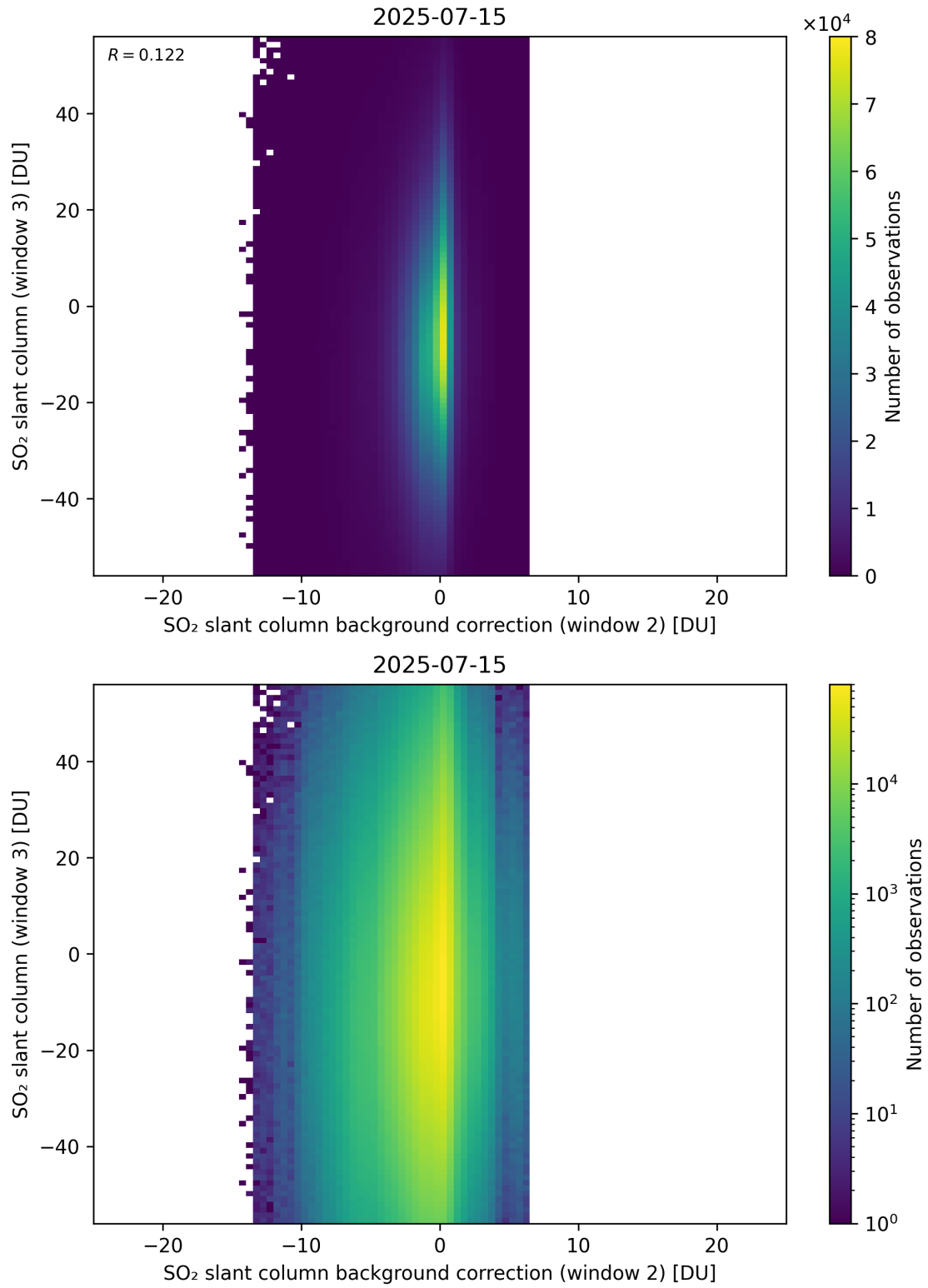
Figure 128: Scatter density plot of “SO 2 slant column background correction (window 2)” against “SO 2 slant column (window 3)” for 2025-07-14 to 2025-07-16.
