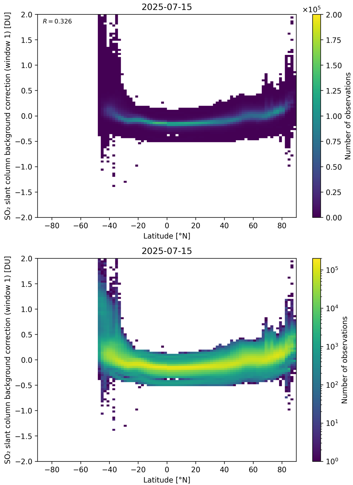
Figure 150: Scatter density plot of “Latitude” against “SO 2 slant column background correction (window 1)” for 2025-07-14 to 2025-07-16.
