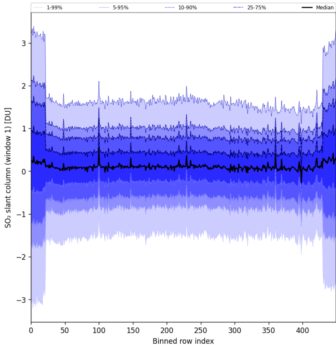
Figure 89: Along track statistics of “SO 2 slant column (window 1)” for 2025-07-14 to 2025-07-16
