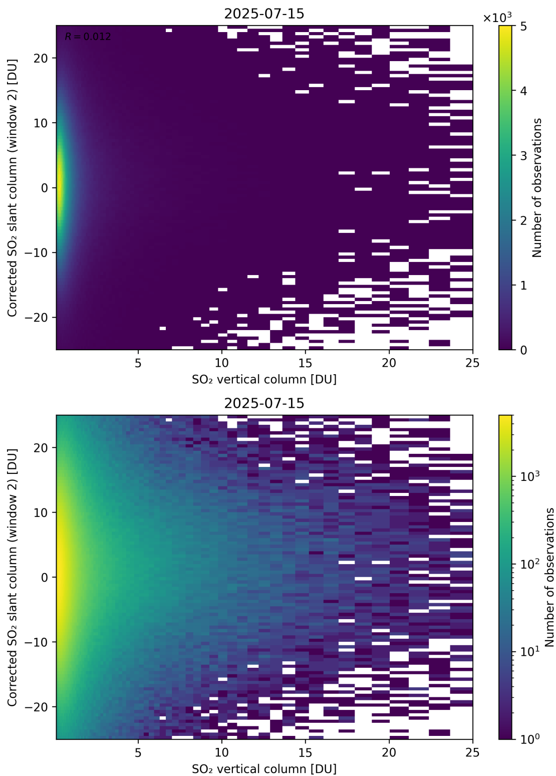
Figure 352: Scatter density plot of “SO 2 vertical column” against “Corrected SO 2 slant column (window 2)” for 2025-07-14 to 2025-07-16.
