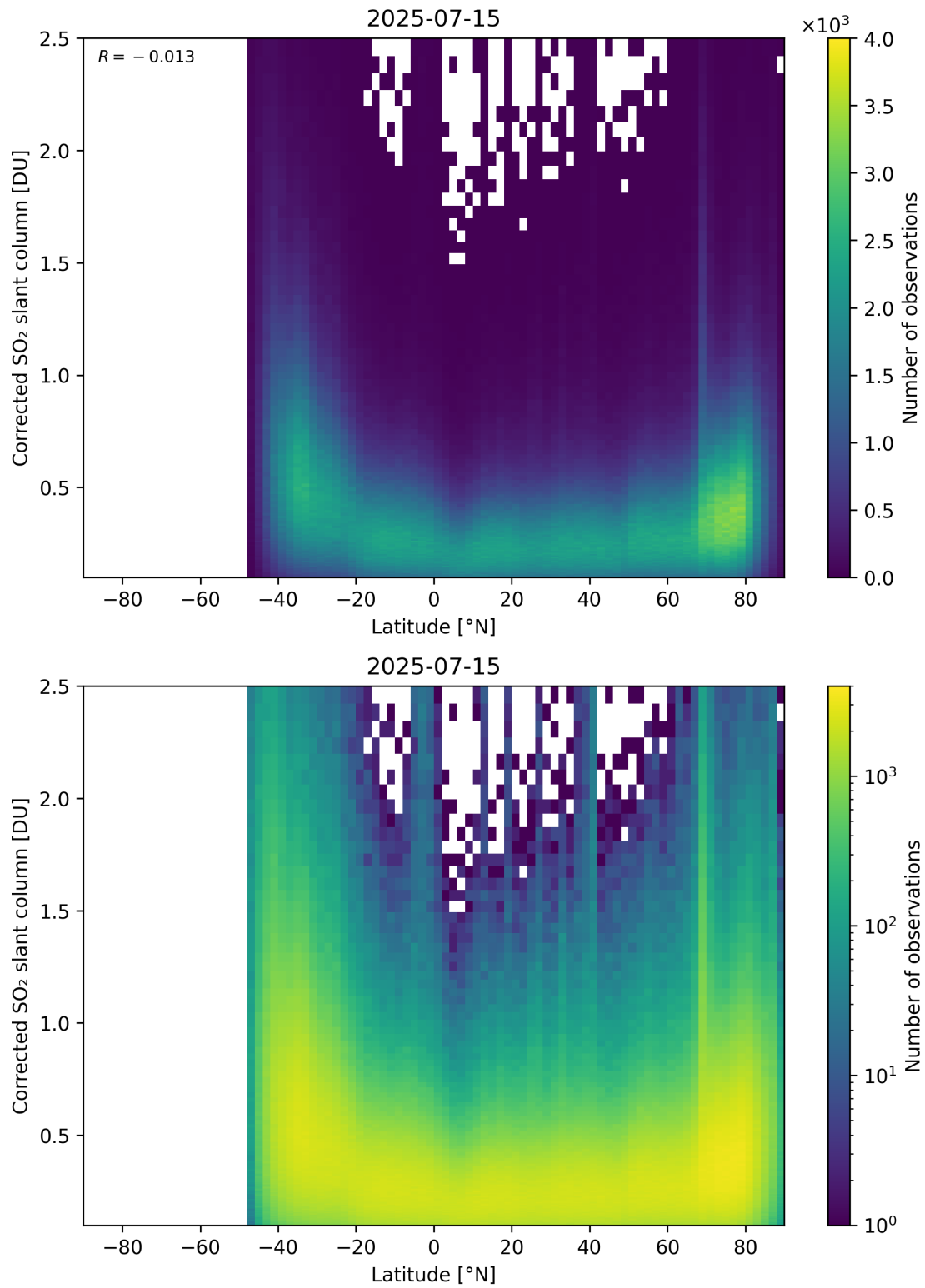
Figure 159: Scatter density plot of “Latitude” against “Corrected SO 2 slant column” for 2025-07-14 to 2025-07-16.
