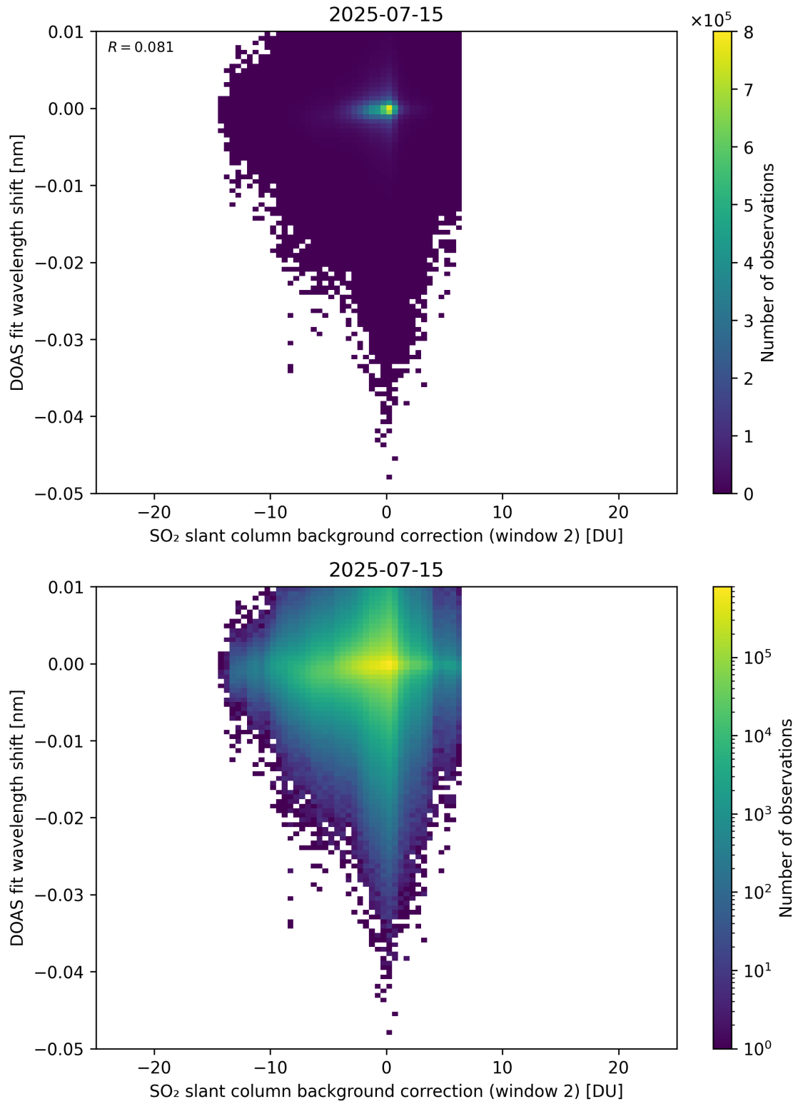
Figure 123: Scatter density plot of “SO 2 slant column background correction (window 2)” against “DOAS fit wavelength shift” for 2025-07-14 to 2025-07-16.
