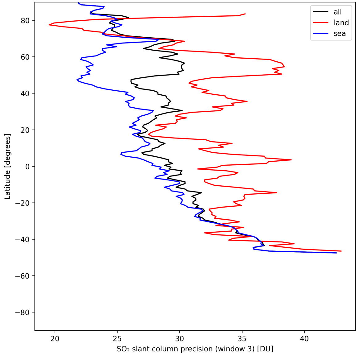
Figure 46: Zonal average of “SO 2 slant column precision (window 3)” for 2025-07-14 to 2025-07-16.
