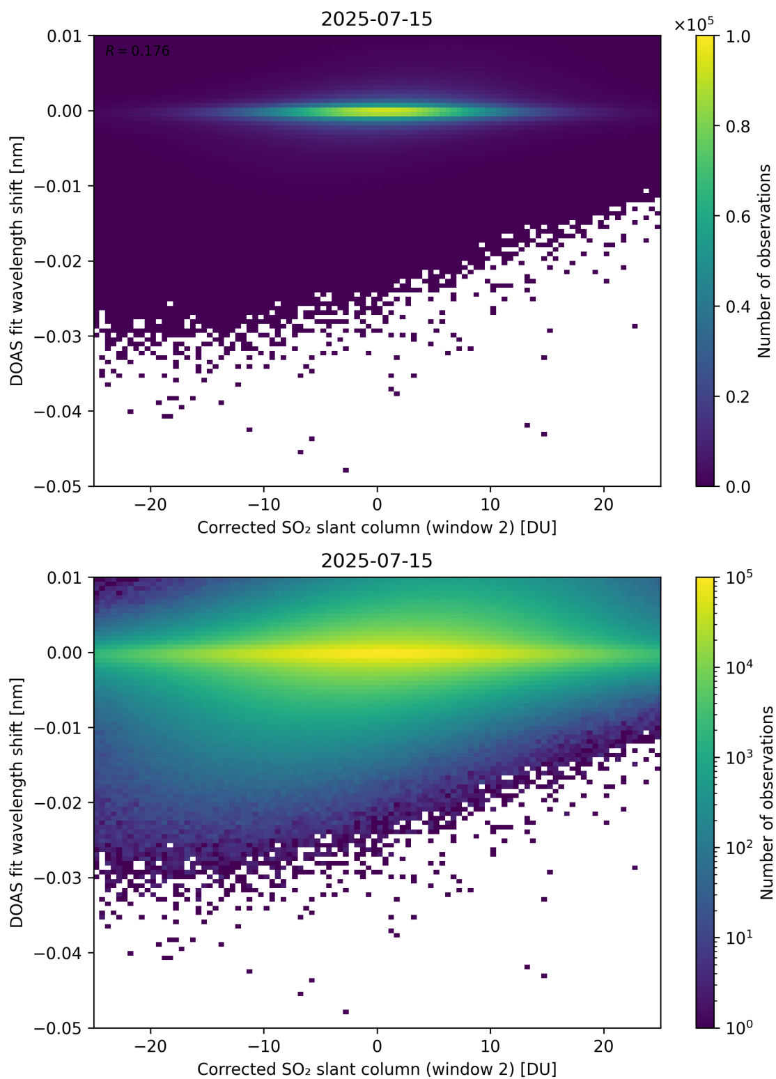
Figure 246: Scatter density plot of “Corrected SO 2 slant column (window 2)” against “DOAS fit wavelength shift” for 2025-07-14 to 2025-07-16.
