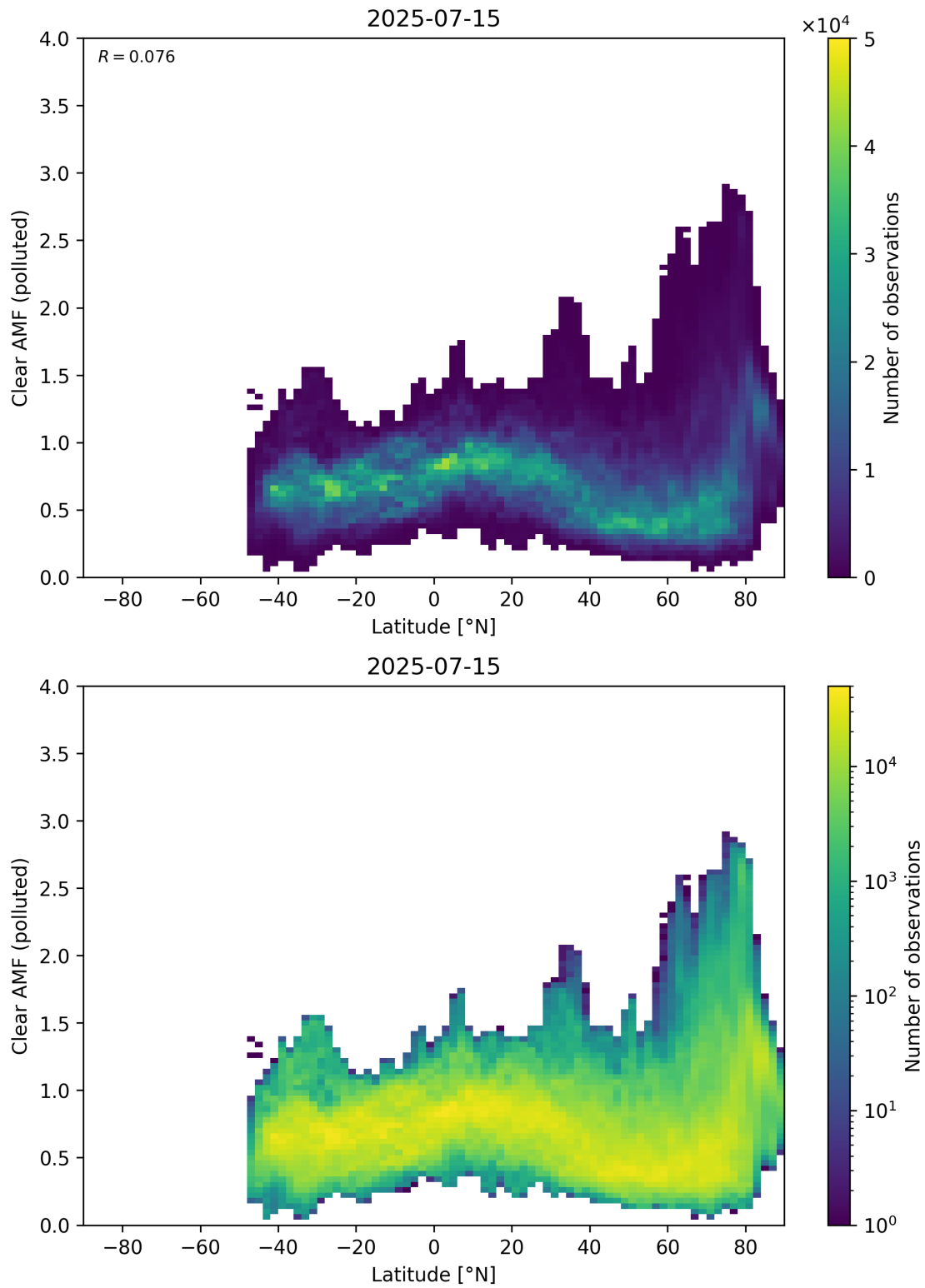
Figure 156: Scatter density plot of “Latitude” against “Clear AMF (polluted)” for 2025-07-14 to 2025-07-16.
