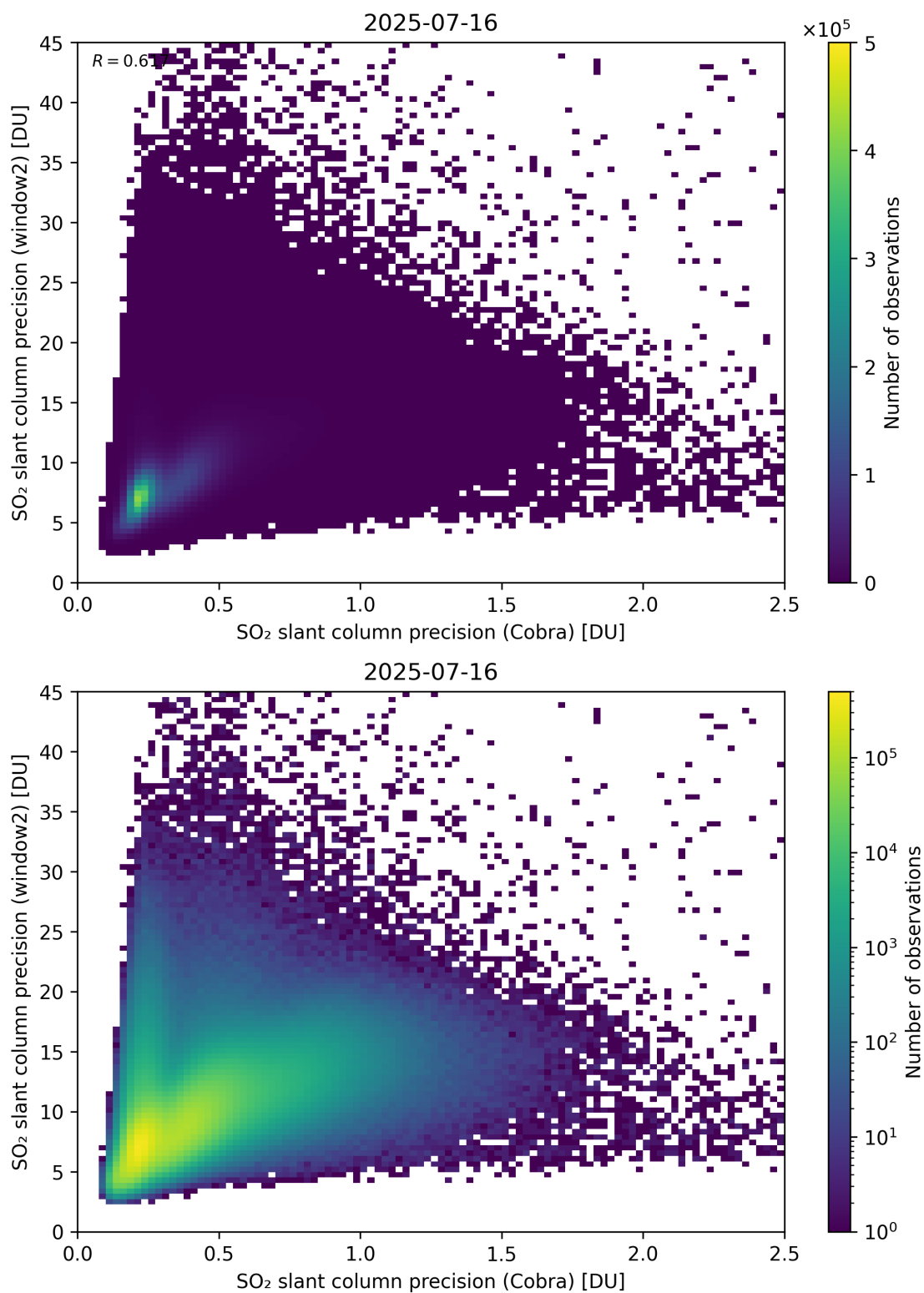
Figure 210: Scatter density plot of “SO 2 slant column precision (Cobra)” against “SO 2 slant column precision (window2)” for 2025-07-15 to 2025-07-17.
