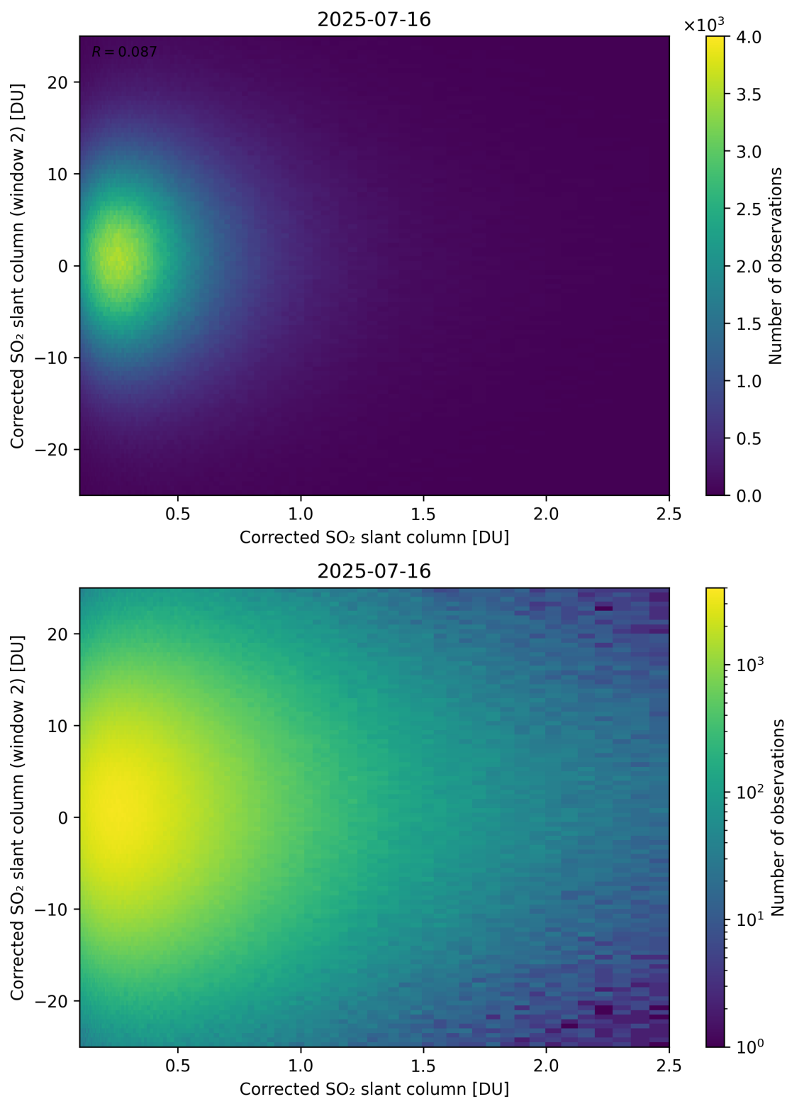
Figure 235: Scatter density plot of “Corrected SO 2 slant column” against “Corrected SO 2 slant column (window 2)” for 2025-07-15 to 2025-07-17.
