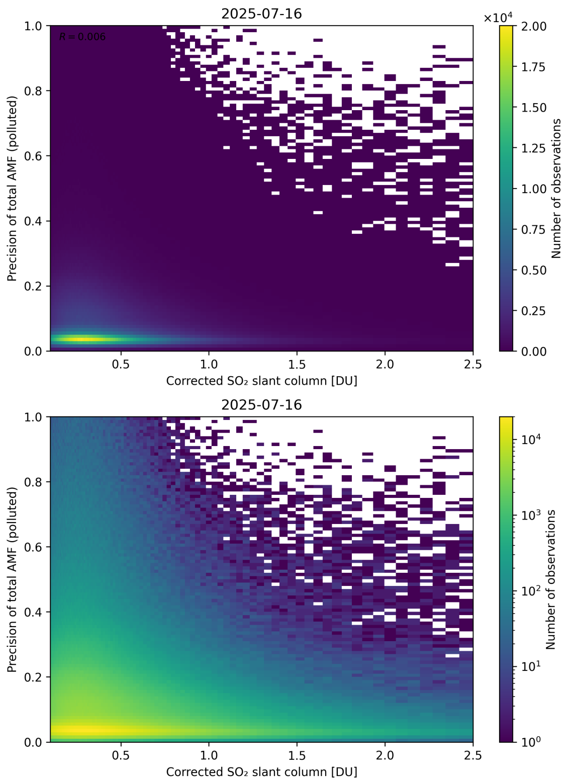
Figure 243: Scatter density plot of “Corrected SO 2 slant column” against “Precision of total AMF (polluted)” for 2025-07-15 to 2025-07-17.
