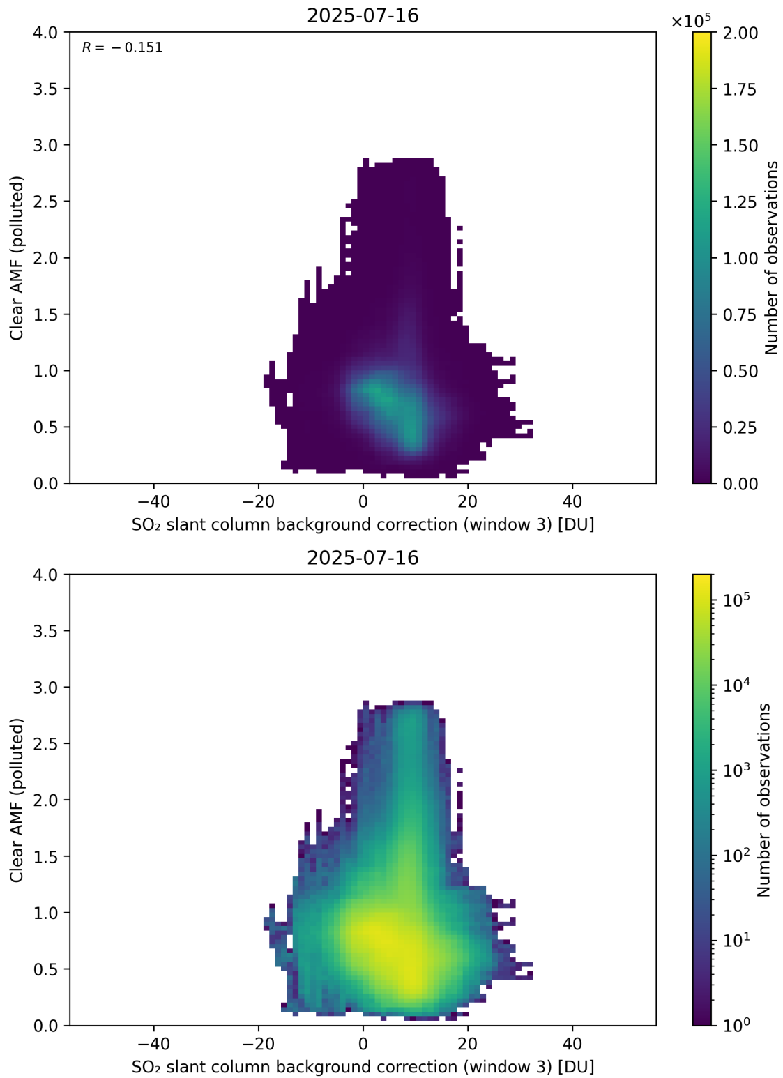
Figure 135: Scatter density plot of “SO 2 slant column background correction (window 3)” against “Clear AMF (polluted)” for 2025-07-15 to 2025-07-17.
