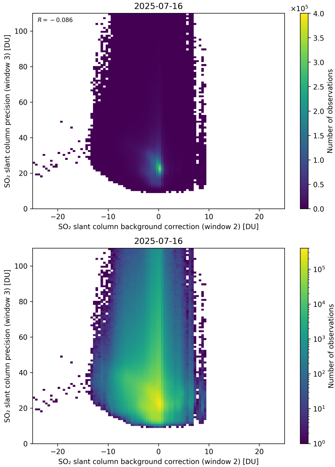
Figure 129: Scatter density plot of “SO 2 slant column background correction (window 2)” against “SO 2 slant column precision (window 3)” for 2025-07-15 to 2025-07-17.
