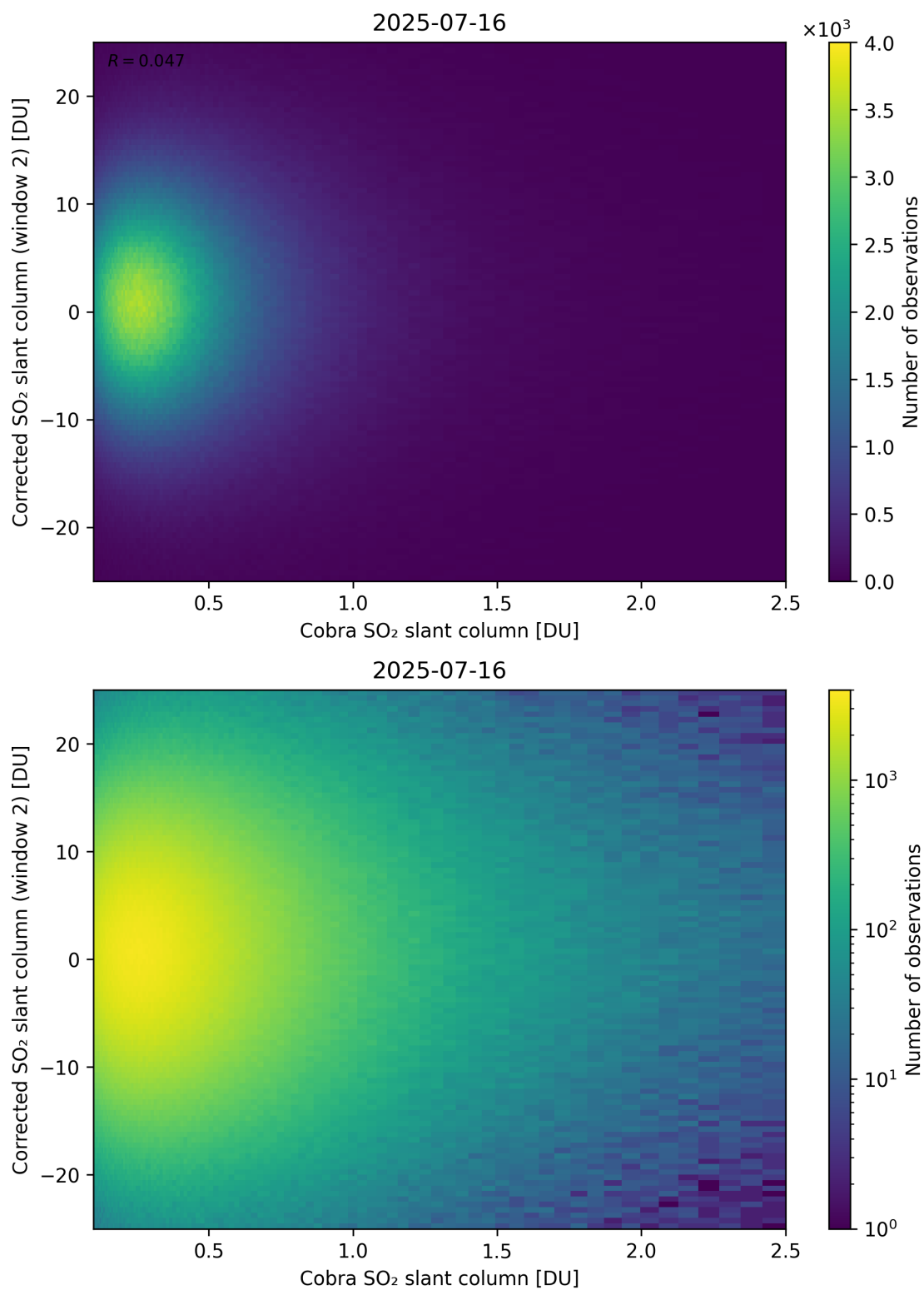
Figure 217: Scatter density plot of “Cobra SO 2 slant column” against “Corrected SO 2 slant column (window 2)” for 2025-07-15 to 2025-07-17.
