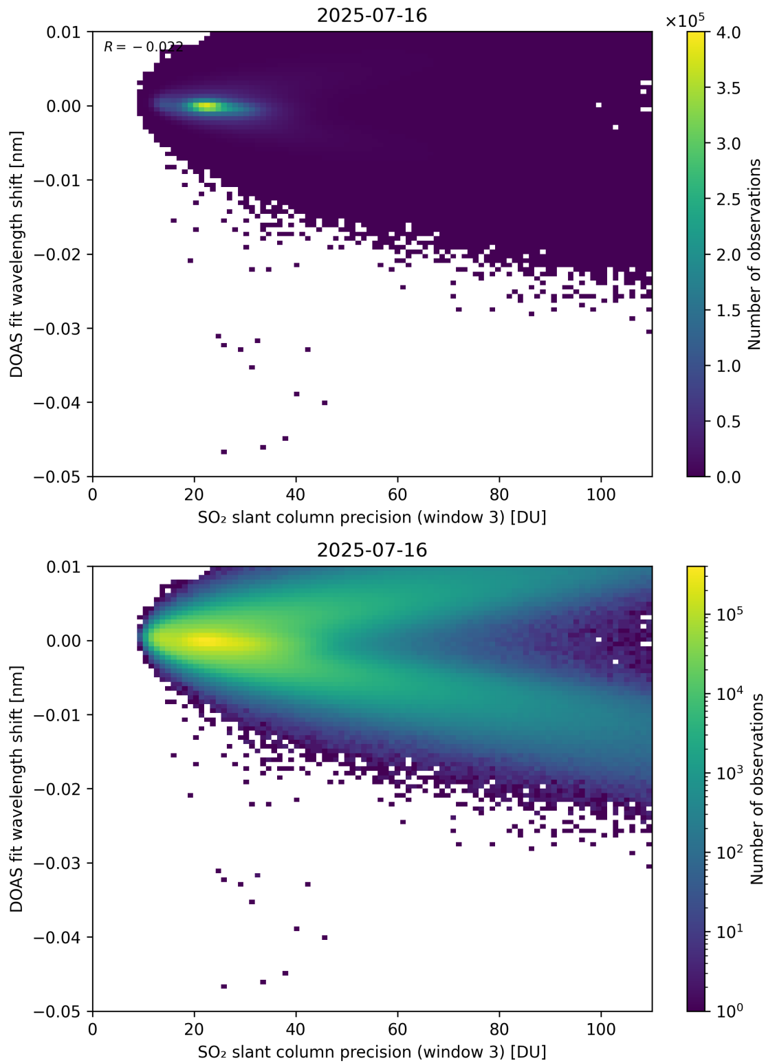
Figure 308: Scatter density plot of “SO 2 slant column precision (window 3)” against “DOAS fit wavelength shift” for 2025-07-15 to 2025-07-17.
