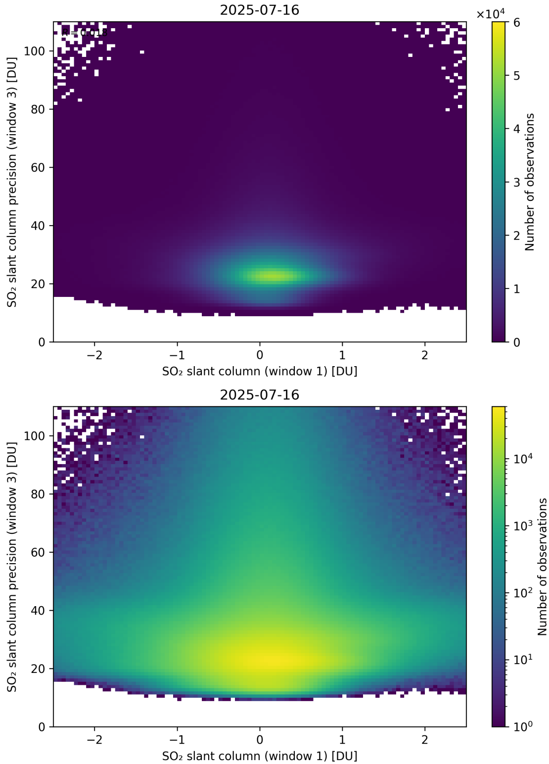
Figure 288: Scatter density plot of “SO 2 slant column (window 1)” against “SO 2 slant column precision (window 3)” for 2025-07-15 to 2025-07-17.
