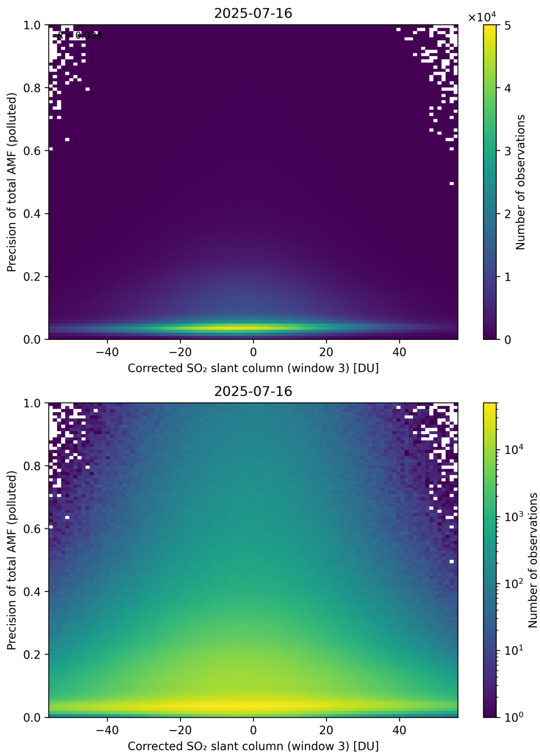
Figure 261: Scatter density plot of “Corrected SO 2 slant column (window 3)” against “Precision of total AMF (polluted)” for 2025-07-15 to 2025-07-17.
