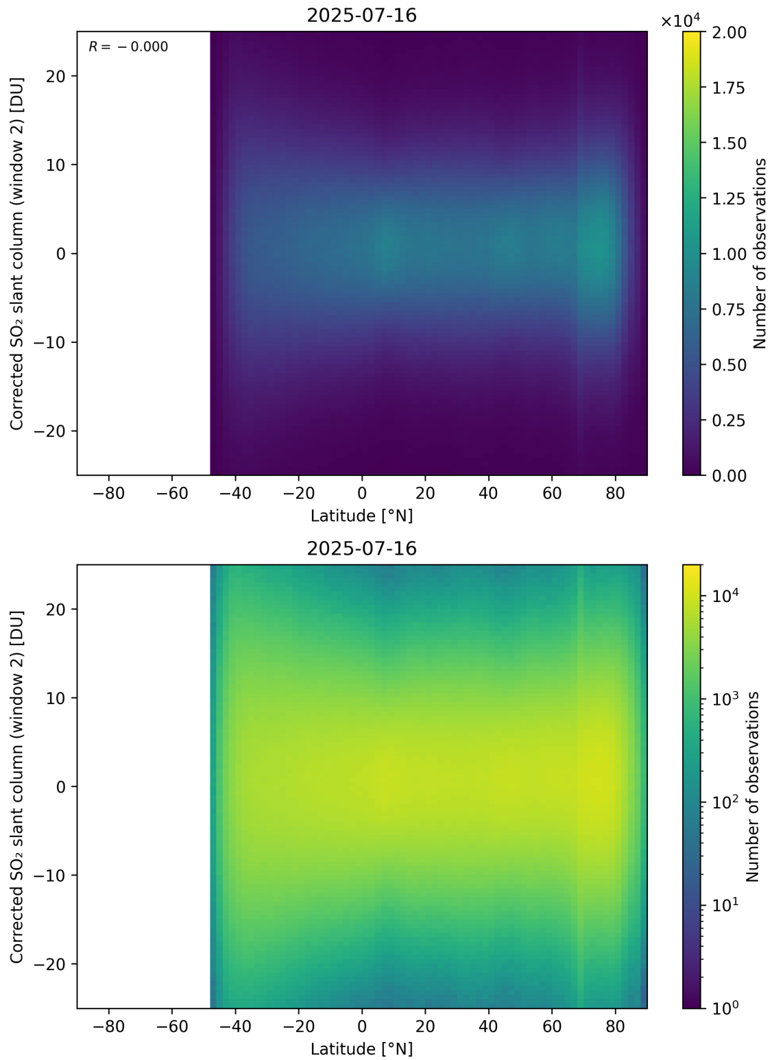
Figure 160: Scatter density plot of “Latitude” against “Corrected SO 2 slant column (window 2)” for 2025-07-15 to 2025-07-17.
