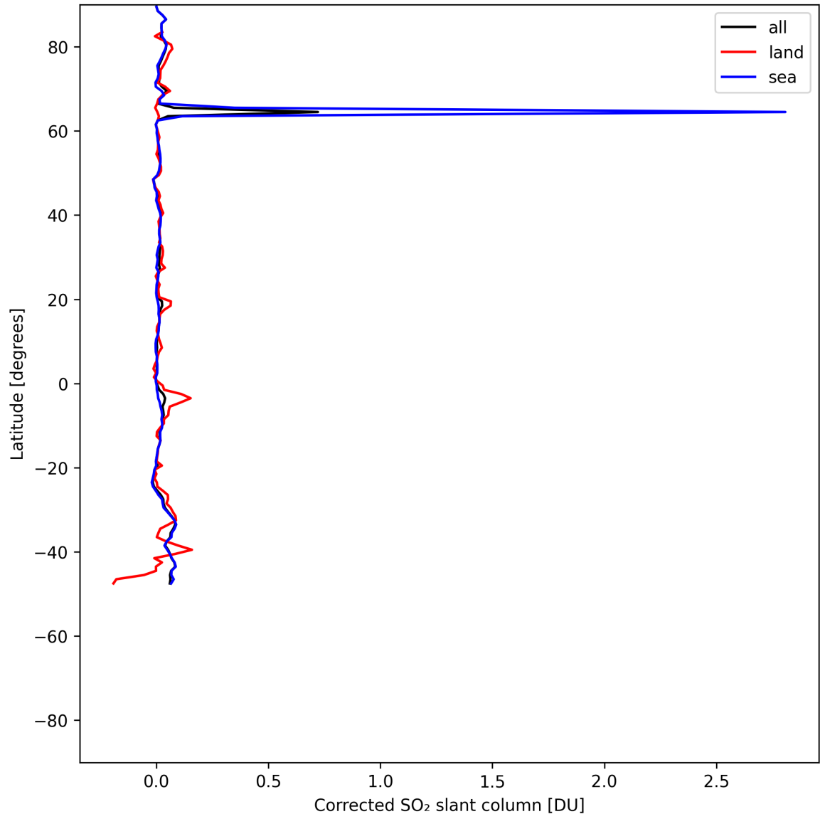
Figure 34: Zonal average of “Corrected SO 2 slant column” for 2025-07-15 to 2025-07-17.
