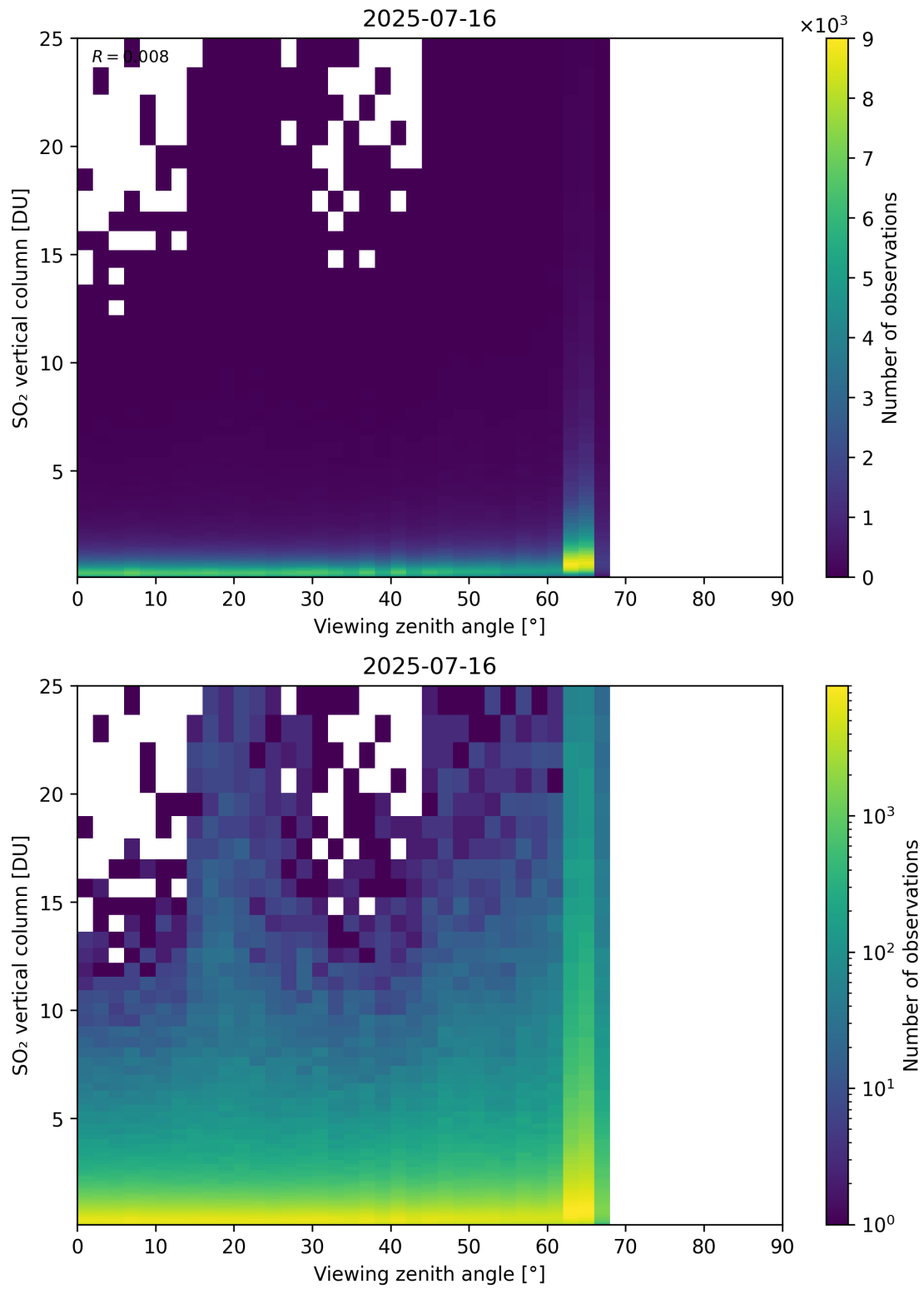
Figure 383: Scatter density plot of “Viewing zenith angle” against “SO 2 vertical column” for 2025-07-15 to 2025-07-17.
