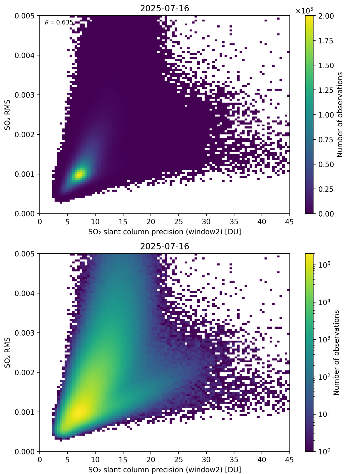
Figure 295: Scatter density plot of “SO 2 slant column precision (window2)” against “SO 2 RMS” for 2025-07-15 to 2025-07-17.
