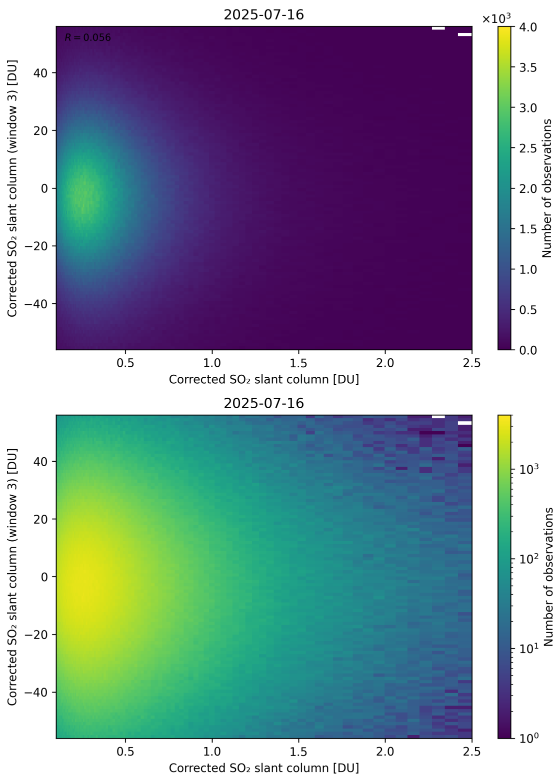
Figure 236: Scatter density plot of “Corrected SO 2 slant column” against “Corrected SO 2 slant column (window 3)” for 2025-07-15 to 2025-07-17.
