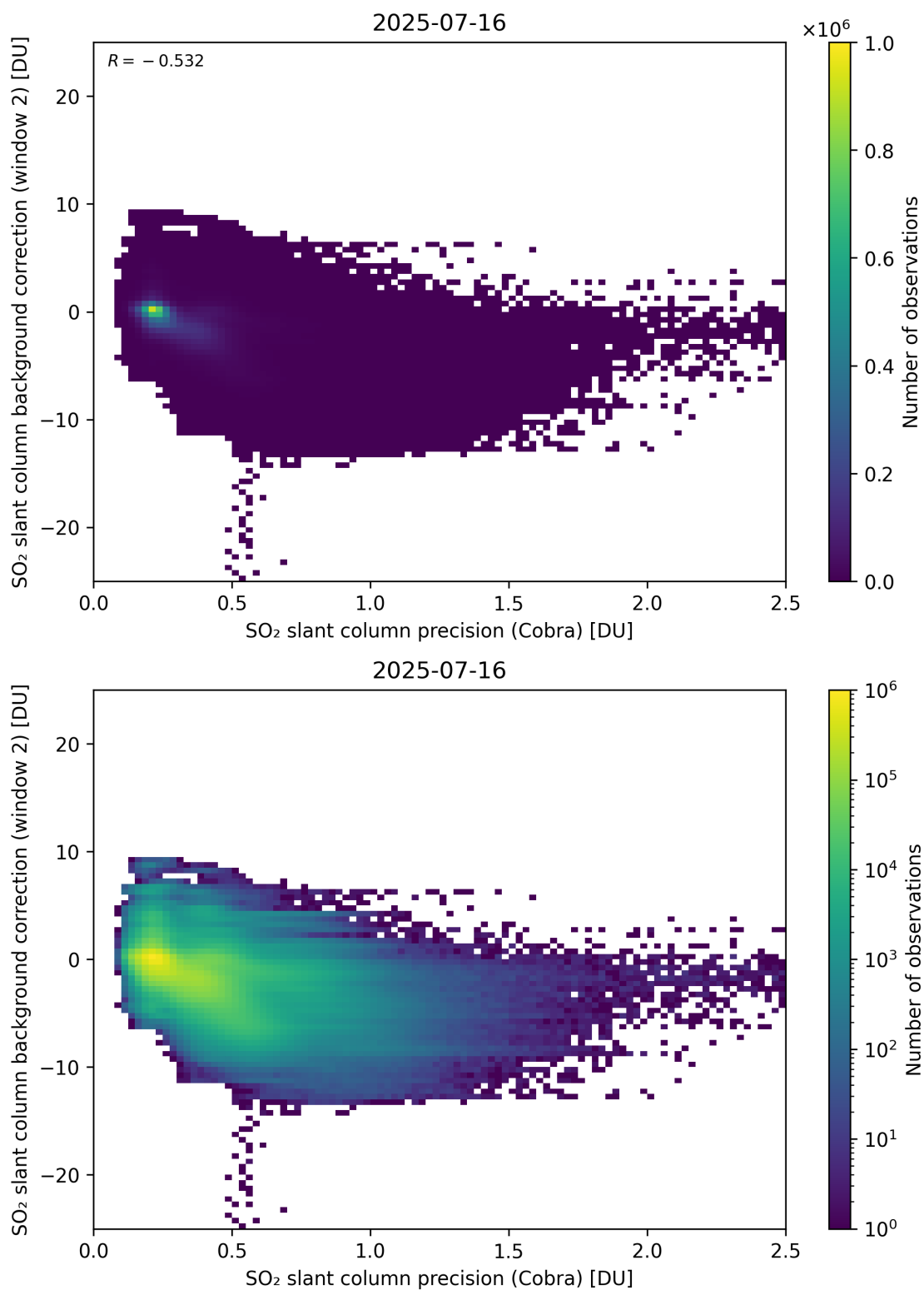
Figure 200: Scatter density plot of “SO 2 slant column precision (Cobra)” against “SO 2 slant column background correction (window 2)” for 2025-07-15 to 2025-07-17.
