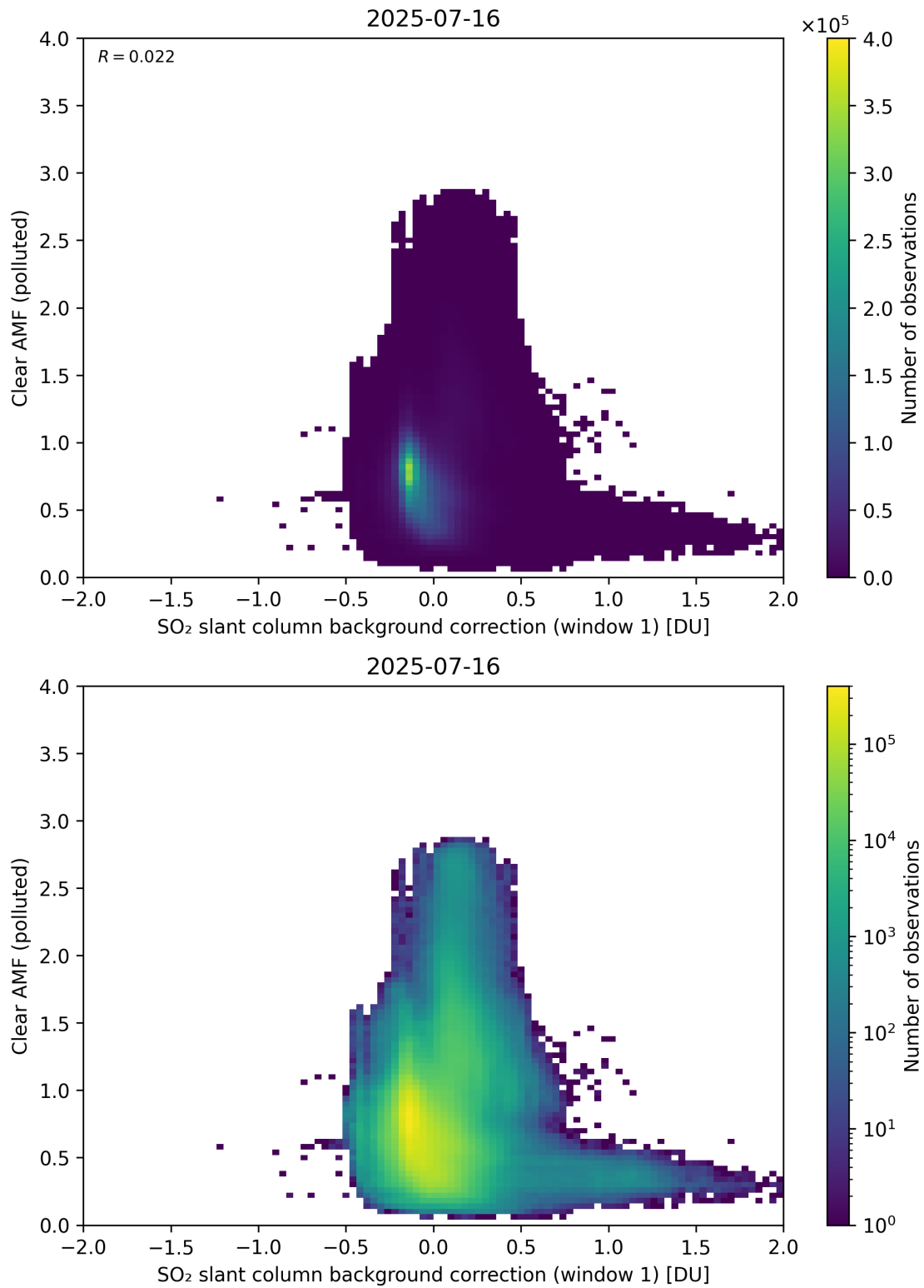
Figure 114: Scatter density plot of “SO 2 slant column background correction (window 1)” against “Clear AMF (polluted)” for 2025-07-15 to 2025-07-17.
