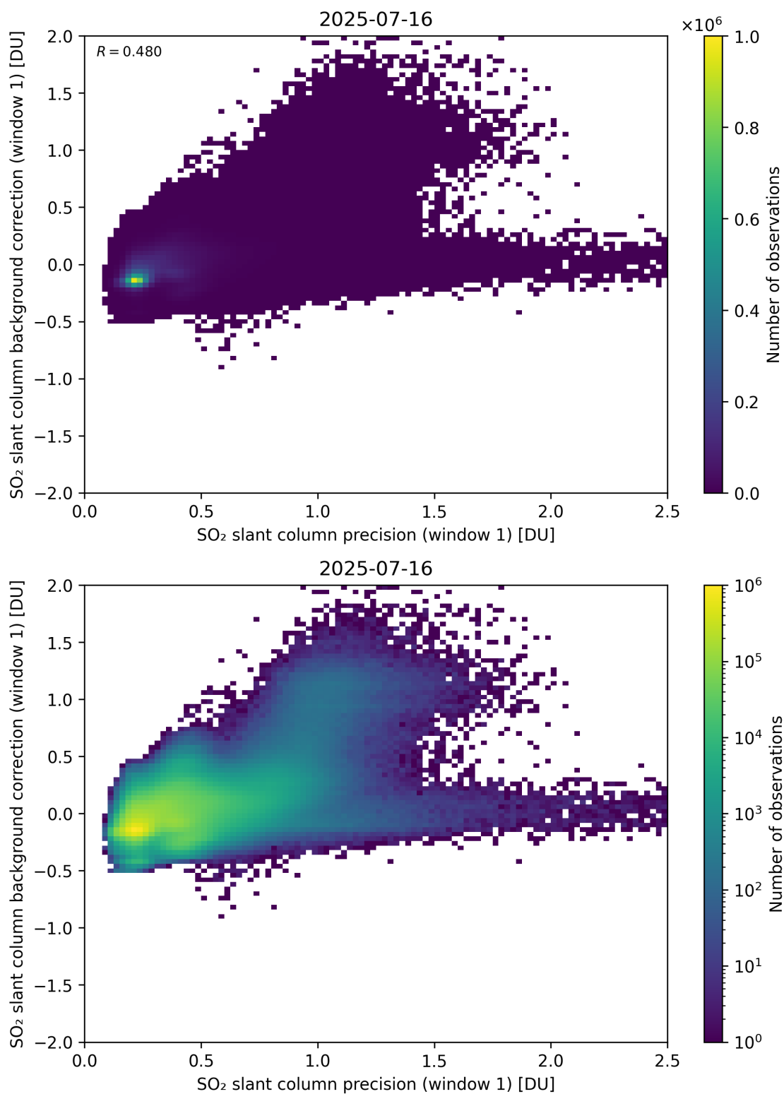
Figure 268: Scatter density plot of “SO 2 slant column precision (window 1)” against “SO 2 slant column background correction (window 1)” for 2025-07-15 to 2025-07-17.
