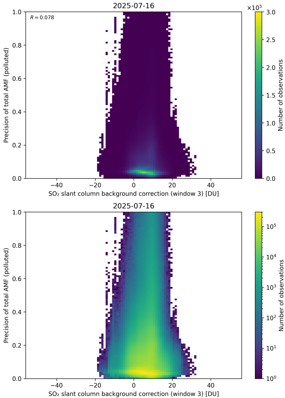
Figure 137: Scatter density plot of “SO 2 slant column background correction (window 3)” against “Precision of total AMF (polluted)” for 2025-07-15 to 2025-07-17.
