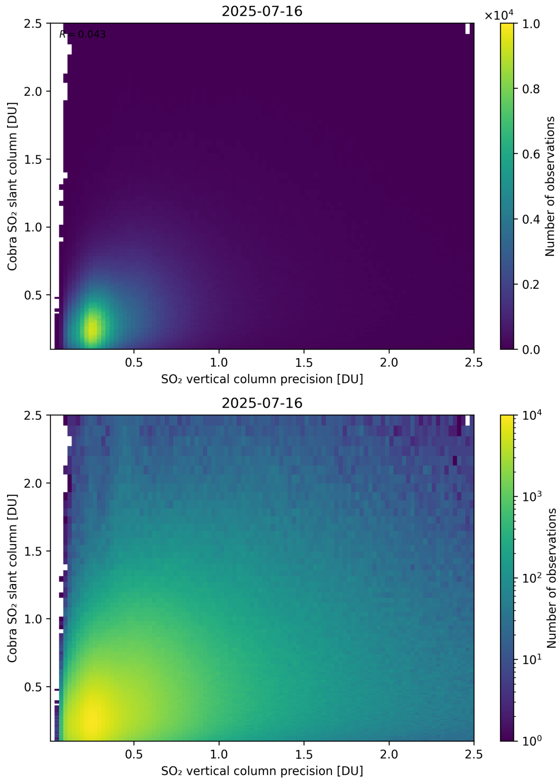
Figure 336: Scatter density plot of “SO 2 vertical column precision” against “Cobra SO 2 slant column” for 2025-07-15 to 2025-07-17.
