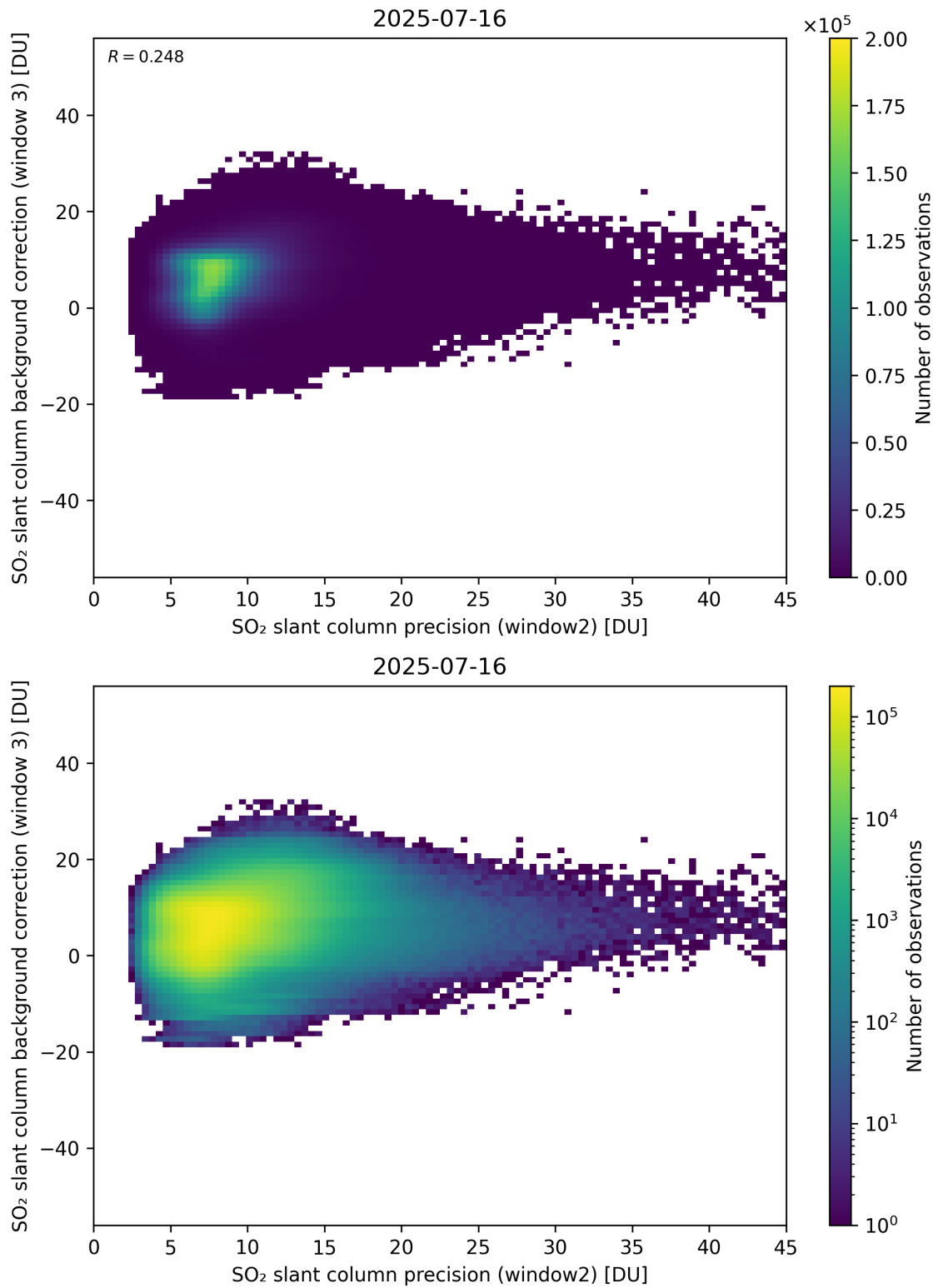
Figure 292: Scatter density plot of “SO 2 slant column precision (window2)” against “SO 2 slant column background correction (window 3)” for 2025-07-15 to 2025-07-17.
