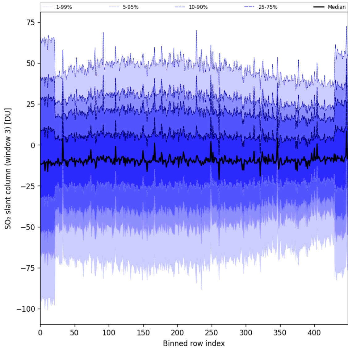
Figure 97: Along track statistics of “SO 2 slant column (window 3)” for 2025-07-15 to 2025-07-17
