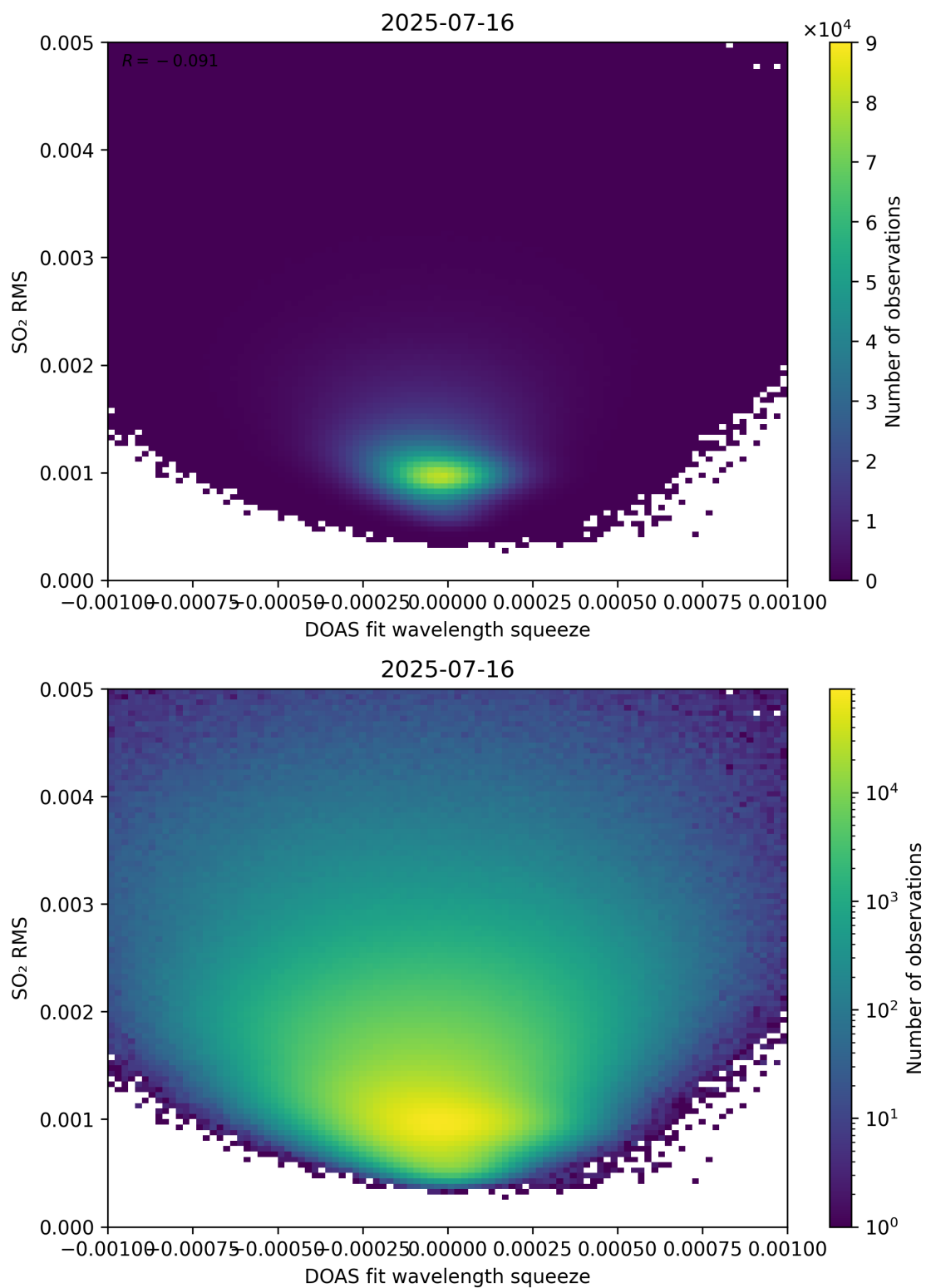
Figure 143: Scatter density plot of “DOAS fit wavelength squeeze” against “SO 2 RMS” for 2025-07-15 to 2025-07-17.
