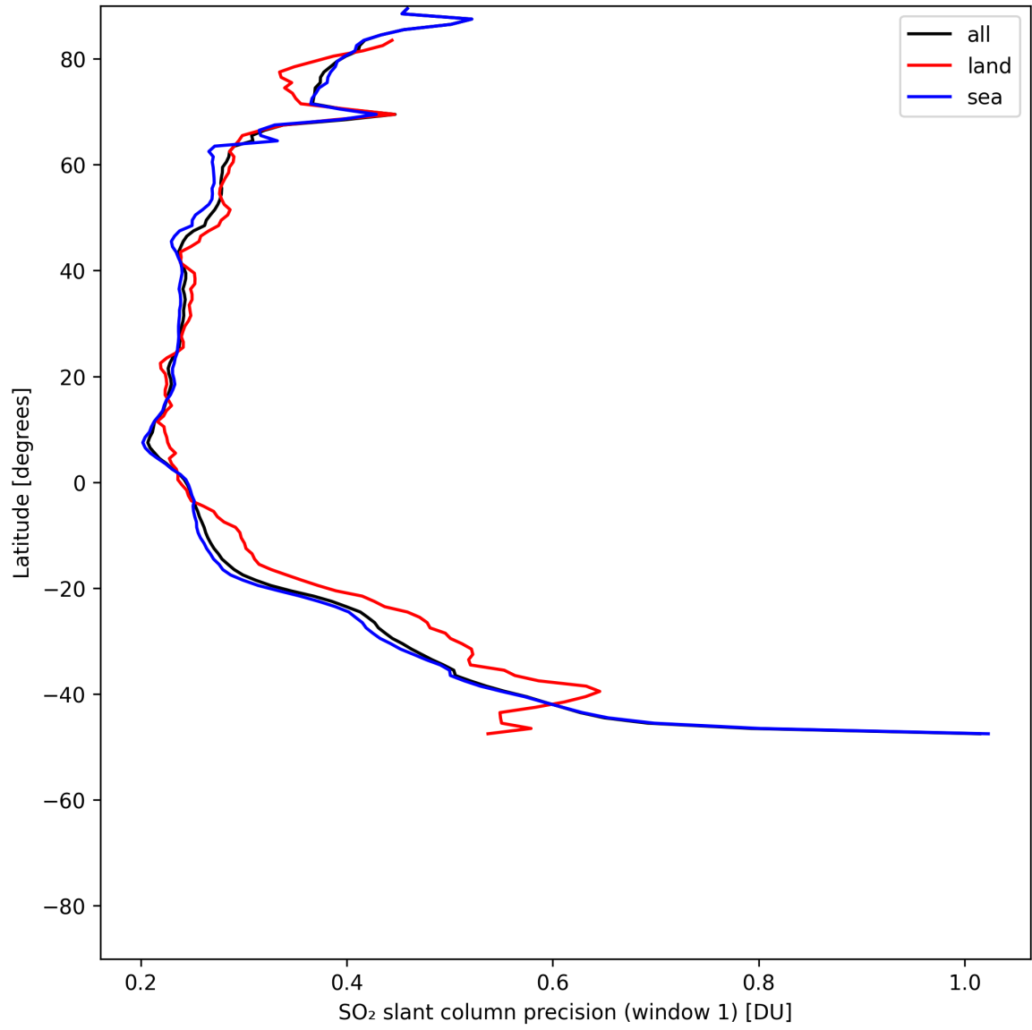
Figure 38: Zonal average of “SO 2 slant column precision (window 1)” for 2025-07-15 to 2025-07-17.
