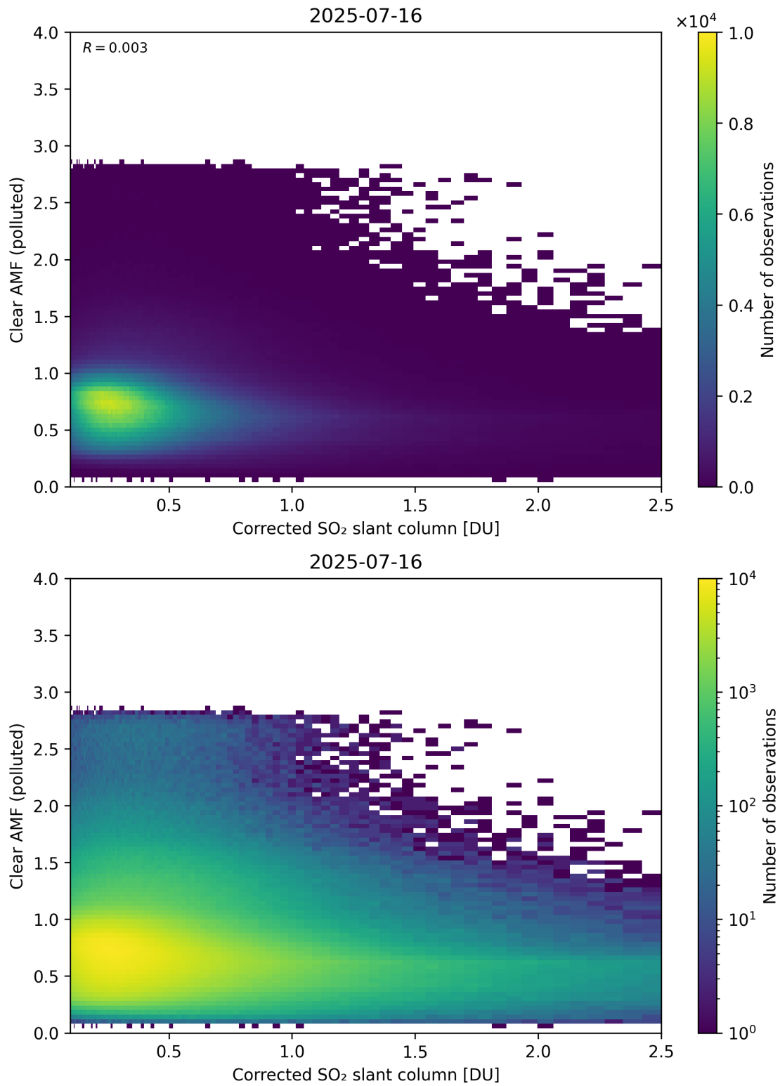
Figure 232: Scatter density plot of “Corrected SO 2 slant column” against “Clear AMF (polluted)” for 2025-07-15 to 2025-07-17.
