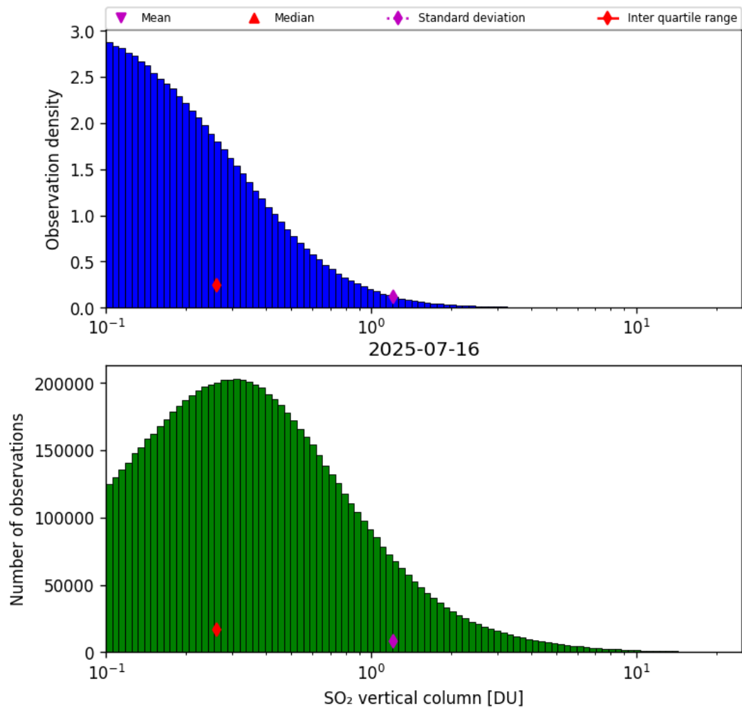
Figure 58: Histogram of “SO 2 vertical column” for 2025-07-15 to 2025-07-17
