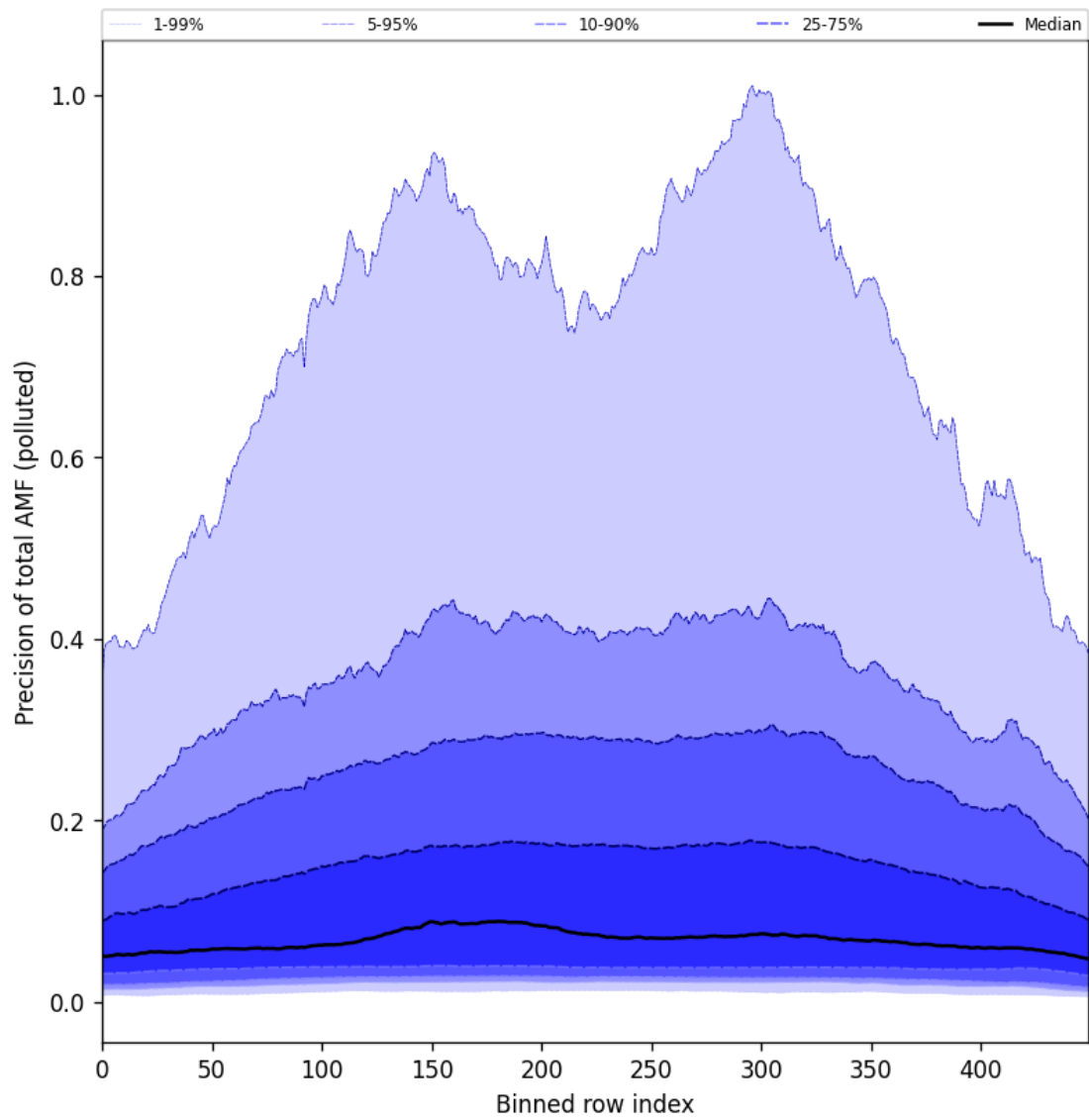
Figure 106: Along track statistics of “Precision of total AMF (polluted)” for 2025-07-15 to 2025-07-17
