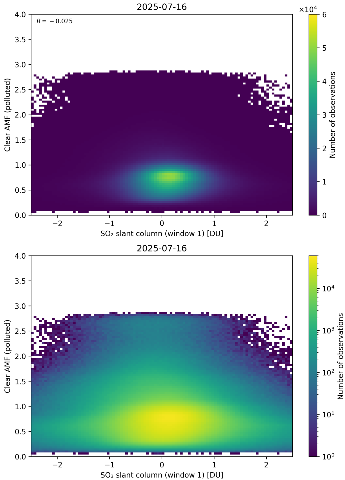
Figure 282: Scatter density plot of “SO 2 slant column (window 1)” against “Clear AMF (polluted)” for 2025-07-15 to 2025-07-17.
