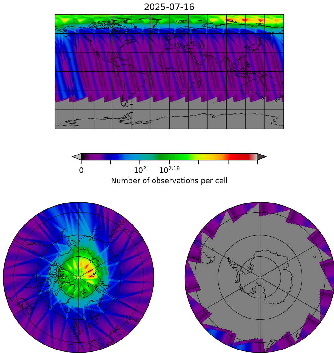
Figure 30: Map of the number of observations for 2025-07-15 to 2025-07-17
