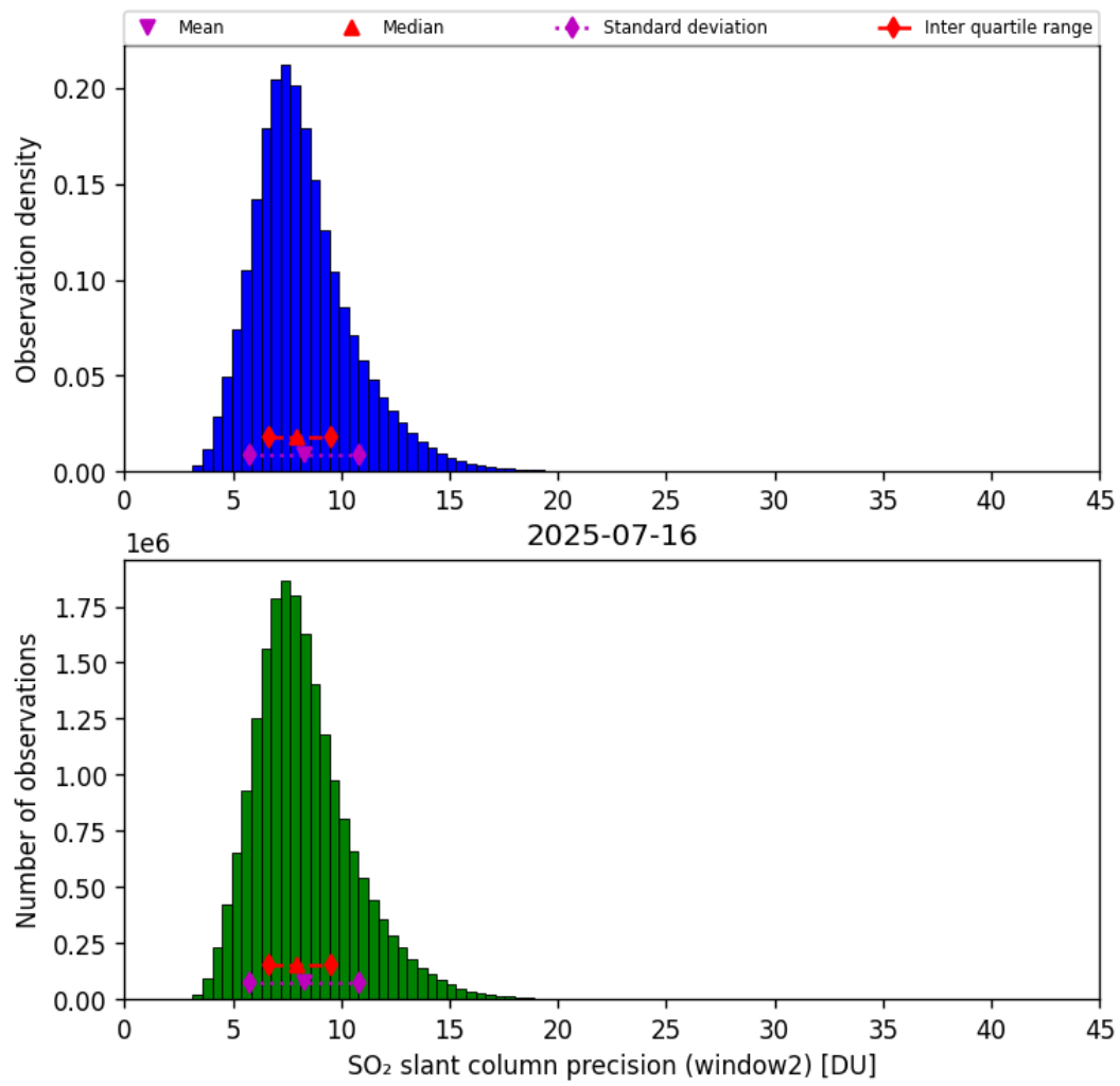
Figure 68: Histogram of “SO 2 slant column precision (window2)” for 2025-07-15 to 2025-07-17
