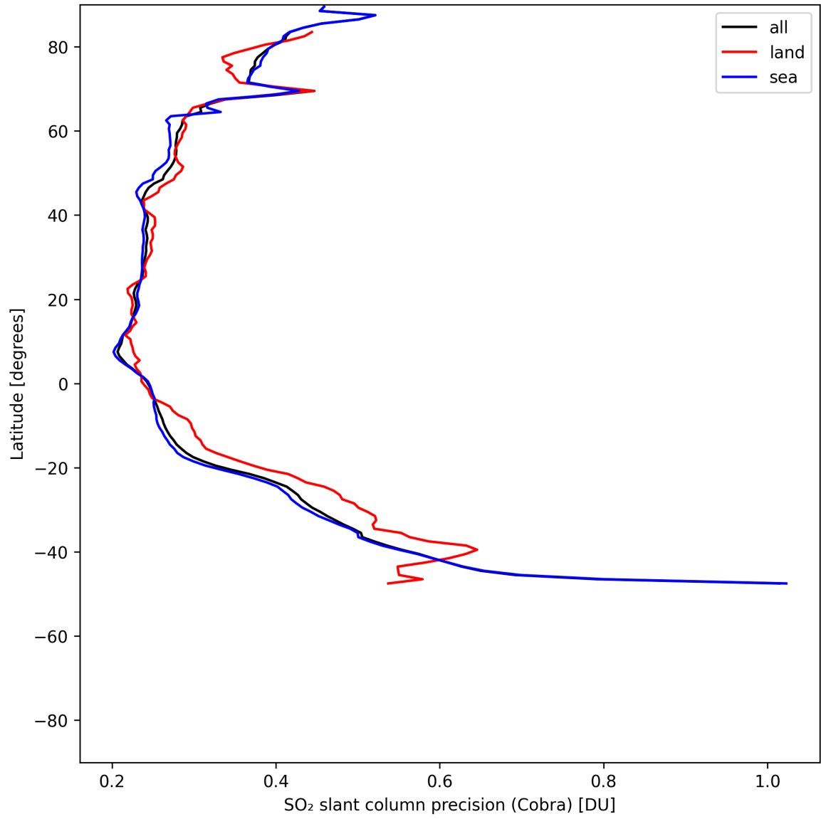
Figure 36: Zonal average of “SO 2 slant column precision (Cobra)” for 2025-07-15 to 2025-07-17.
