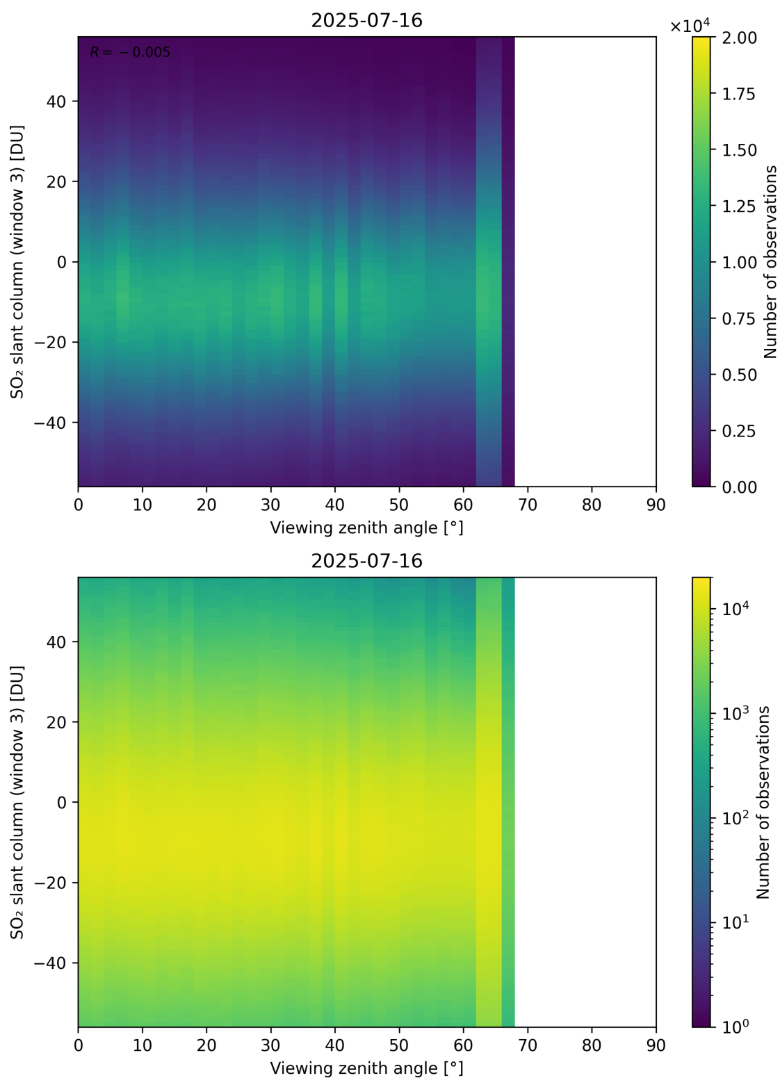
Figure 379: Scatter density plot of “Viewing zenith angle” against “SO 2 slant column (window 3)” for 2025-07-15 to 2025-07-17.
