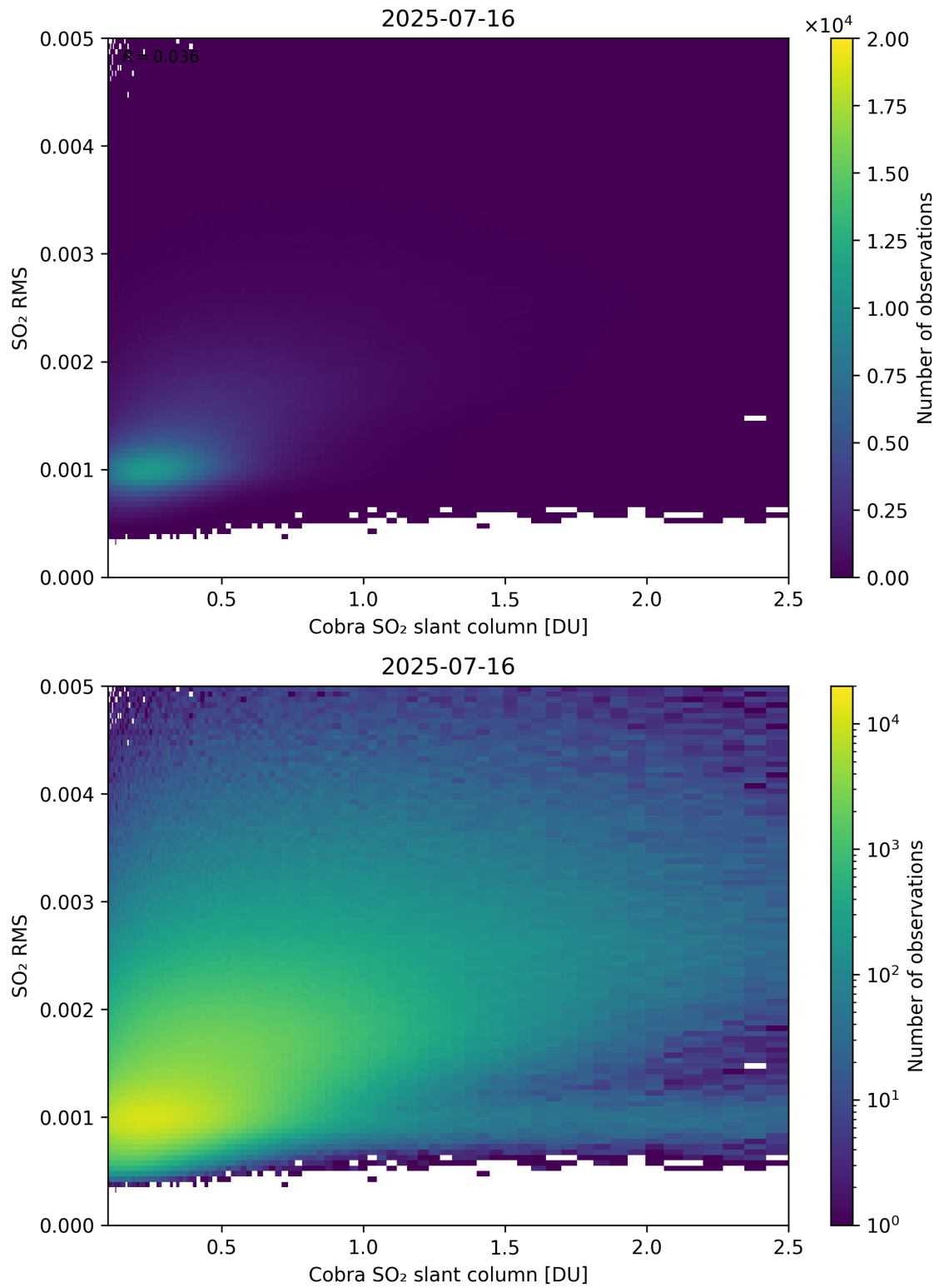
Figure 198: Scatter density plot of “Cobra SO 2 slant column” against “SO 2 RMS” for 2025-07-15 to 2025-07-17.
