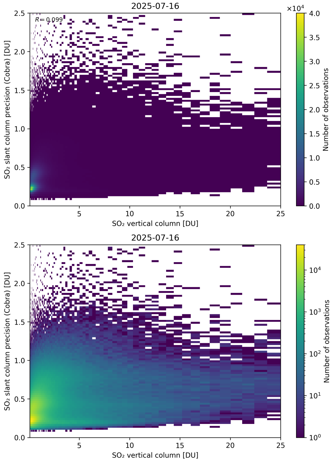
Figure 350: Scatter density plot of “SO 2 vertical column” against “SO 2 slant column precision (Cobra)” for 2025-07-15 to 2025-07-17.
