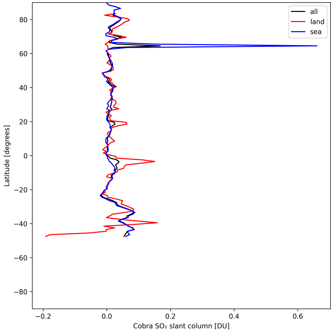
Figure 35: Zonal average of “Cobra SO 2 slant column” for 2025-07-15 to 2025-07-17.
