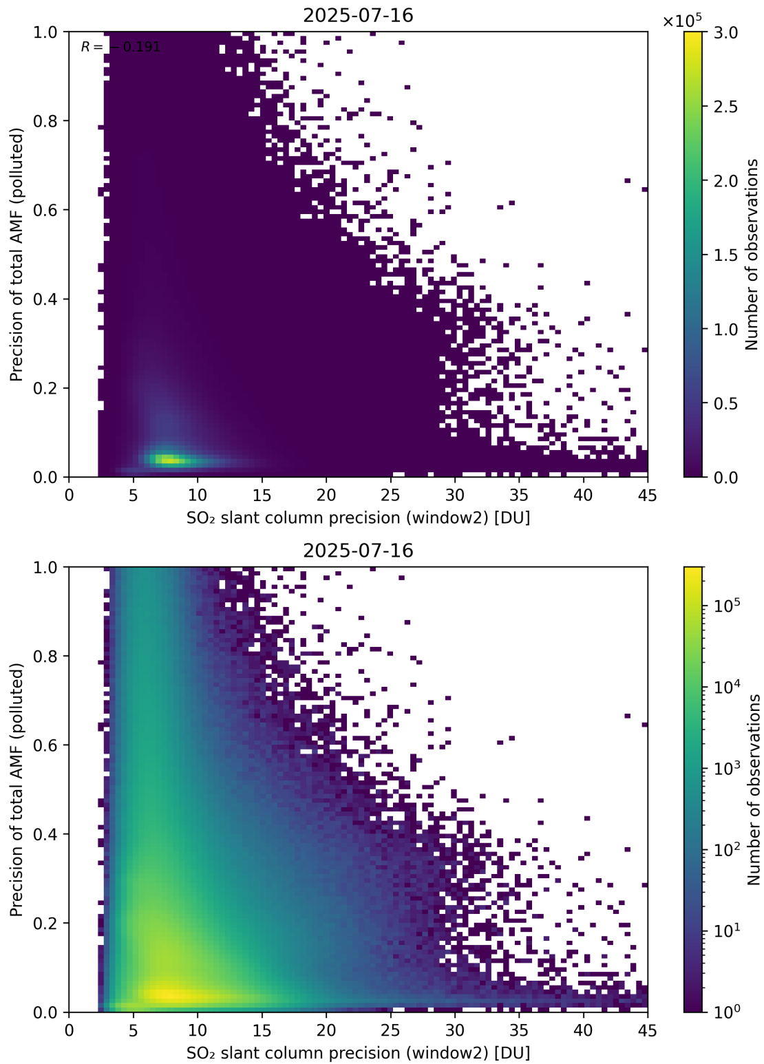
Figure 302: Scatter density plot of “SO 2 slant column precision (window2)” against “Precision of total AMF (polluted)” for 2025-07-15 to 2025-07-17.
