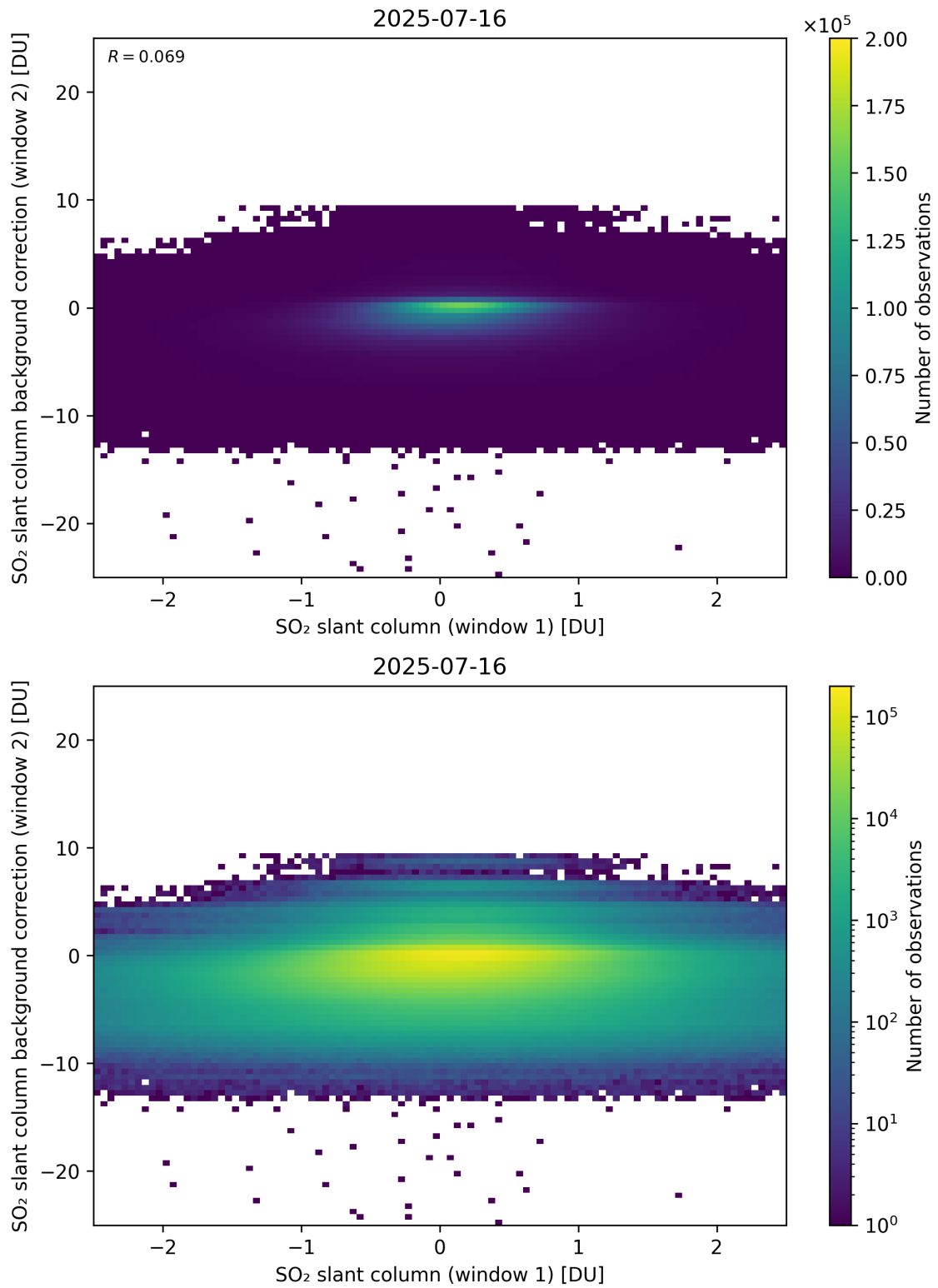
Figure 263: Scatter density plot of “SO 2 slant column (window 1)” against “SO 2 slant column background correction (window 2)” for 2025-07-15 to 2025-07-17.
