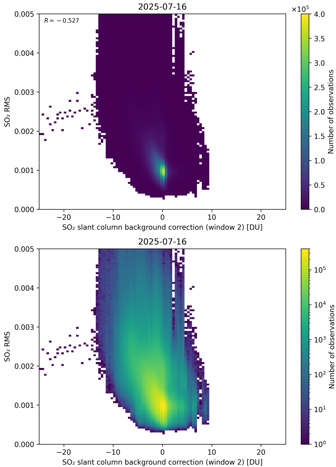
Figure 125: Scatter density plot of “SO 2 slant column background correction (window 2)” against “SO 2 RMS” for 2025-07-15 to 2025-07-17.
