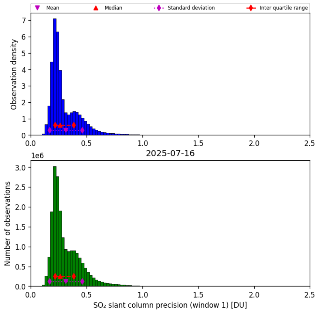
Figure 64: Histogram of “SO 2 slant column precision (window 1)” for 2025-07-15 to 2025-07-17
