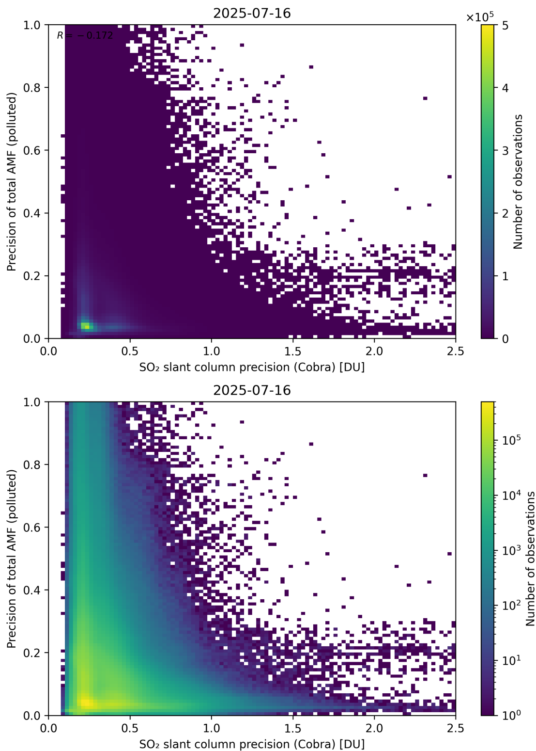
Figure 214: Scatter density plot of “SO 2 slant column precision (Cobra)” against “Precision of total AMF (polluted)” for 2025-07-15 to 2025-07-17.
