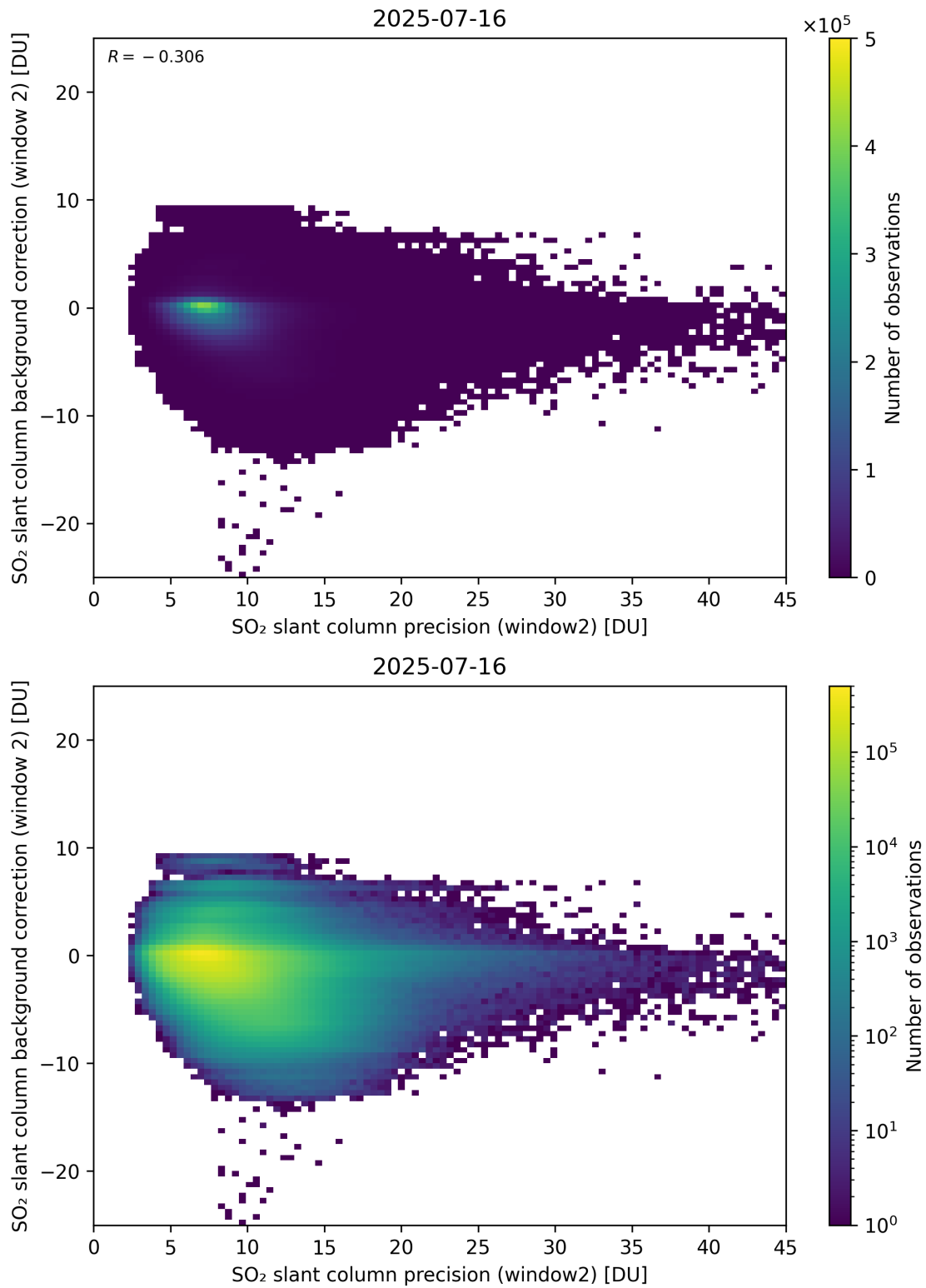
Figure 291: Scatter density plot of “SO 2 slant column precision (window2)” against “SO 2 slant column background correction (window 2)” for 2025-07-15 to 2025-07-17.
