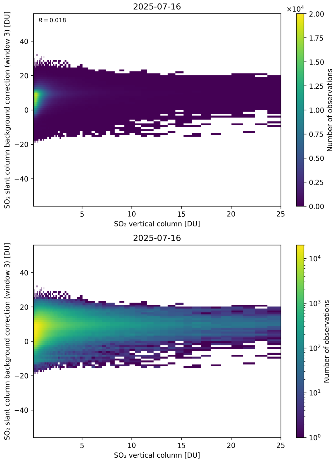
Figure 325: Scatter density plot of “SO 2 vertical column” against “SO 2 slant column background correction (window 3)” for 2025-07-15 to 2025-07-17.
