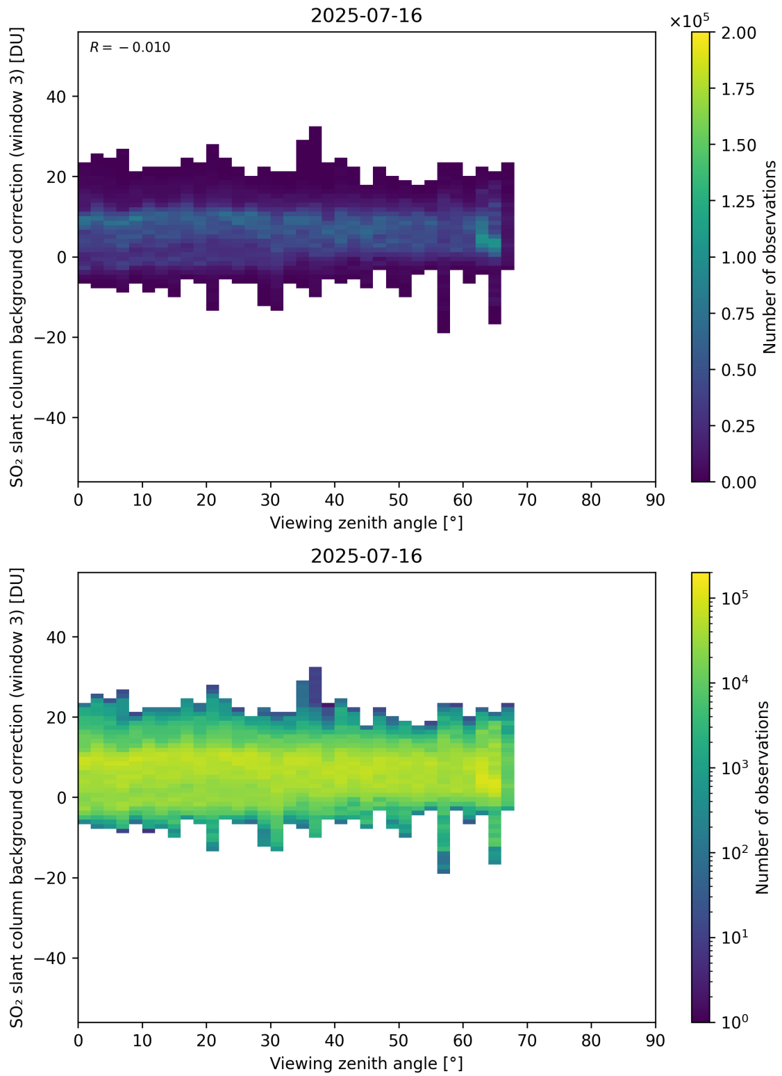
Figure 364: Scatter density plot of “Viewing zenith angle” against “SO 2 slant column background correction (window 3)” for 2025-07-15 to 2025-07-17.
