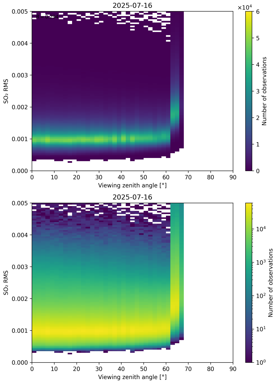
Figure 367: Scatter density plot of “Viewing zenith angle” against “SO 2 RMS” for 2025-07-15 to 2025-07-17.
