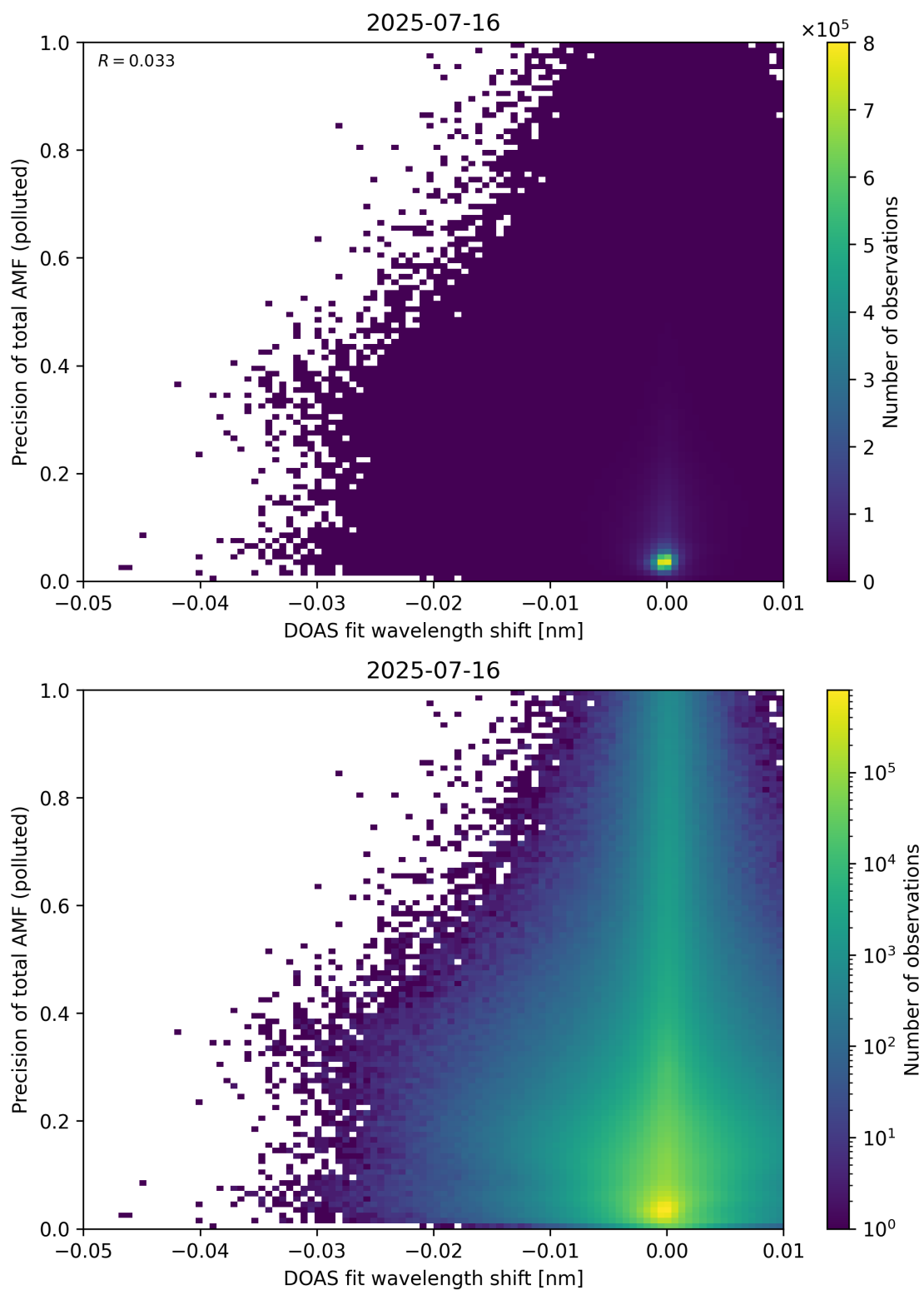
Figure 142: Scatter density plot of “DOAS fit wavelength shift” against “Precision of total AMF (polluted)” for 2025-07-15 to 2025-07-17.
