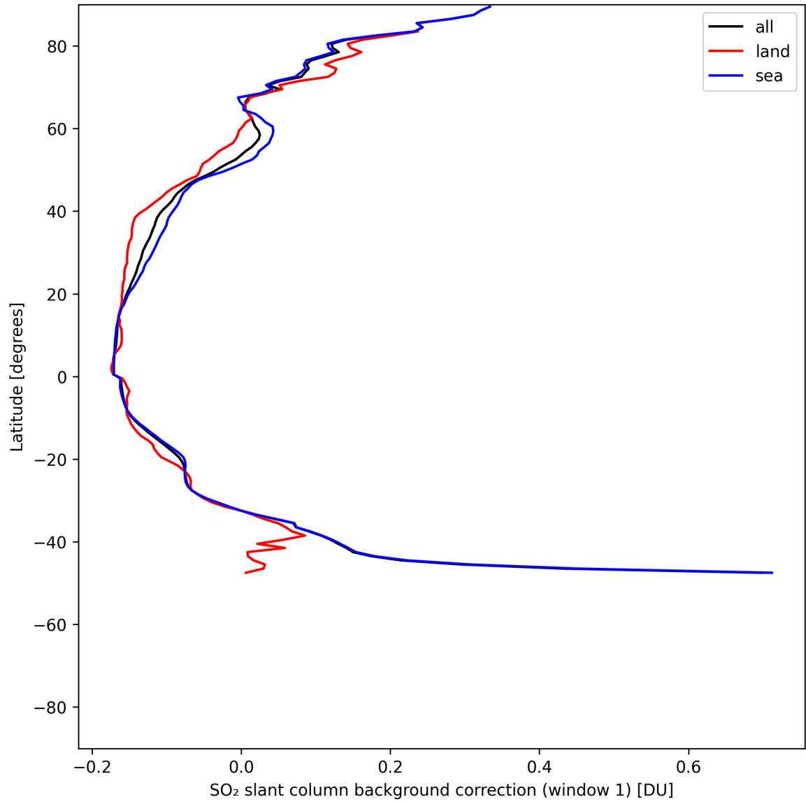
Figure 40: Zonal average of “SO 2 slant column background correction (window 1)” for 2025-07-15 to 2025-07-17.
