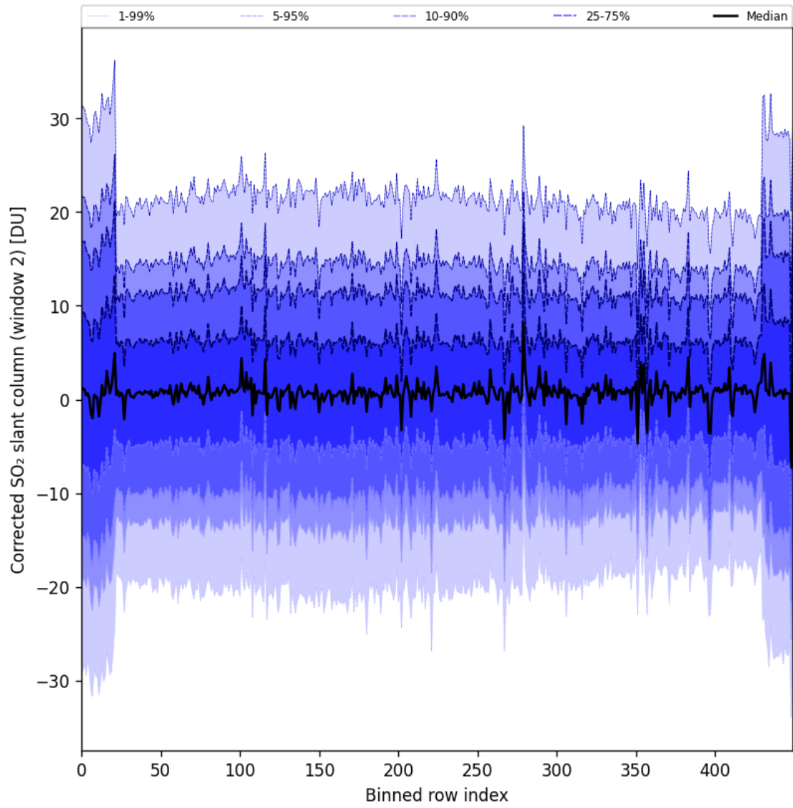
Figure 95: Along track statistics of “Corrected SO 2 slant column (window 2)” for 2025-07-15 to 2025-07-17
