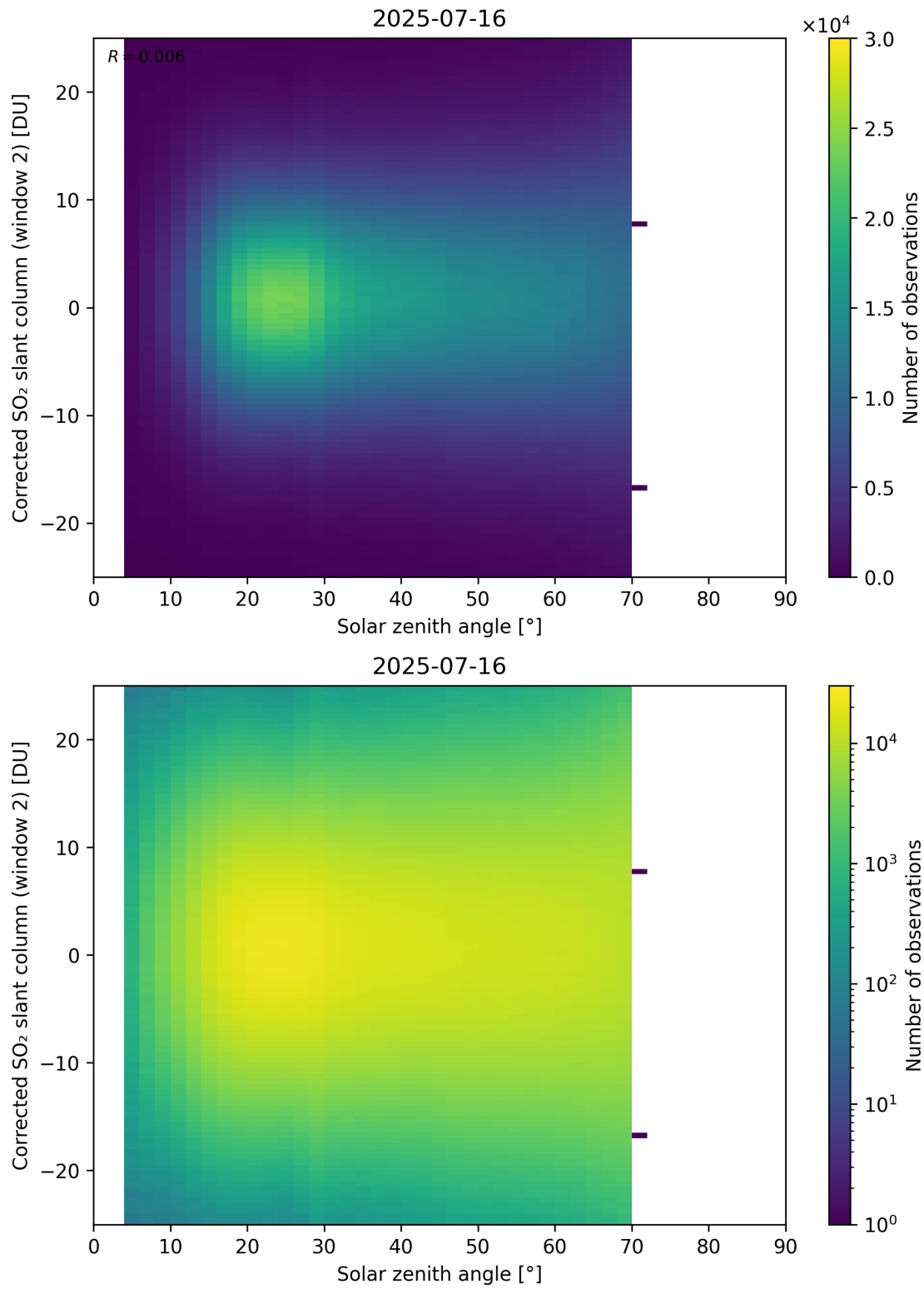
Figure 182: Scatter density plot of “Solar zenith angle” against “Corrected SO 2 slant column (window 2)” for 2025-07-15 to 2025-07-17.
