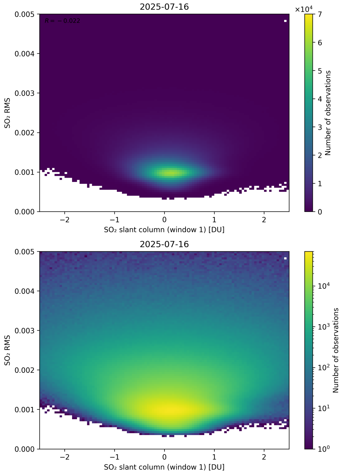
Figure 267: Scatter density plot of “SO 2 slant column (window 1)” against “SO 2 RMS” for 2025-07-15 to 2025-07-17.
