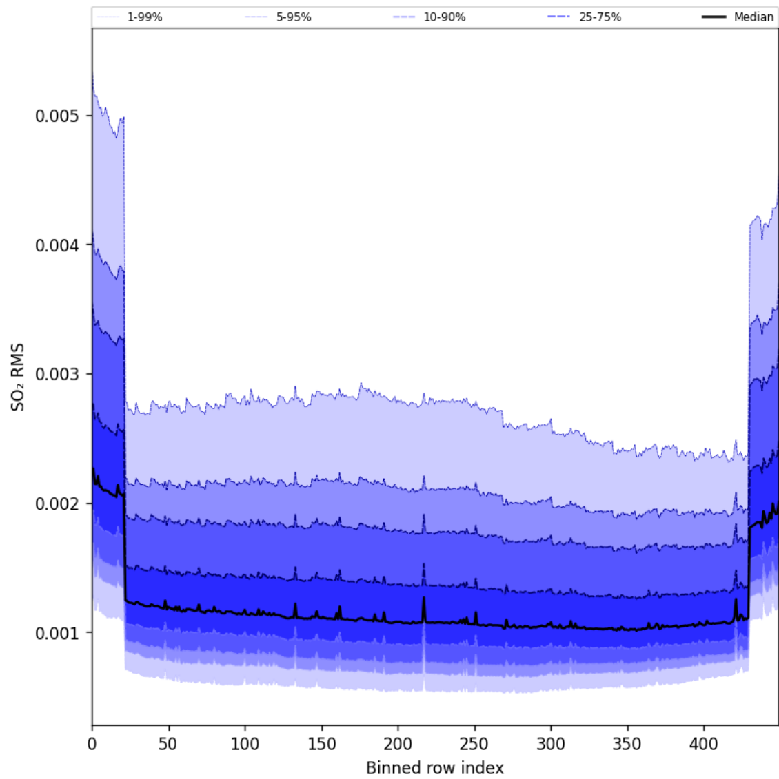
Figure 104: Along track statistics of “SO 2 RMS” for 2025-07-15 to 2025-07-17
