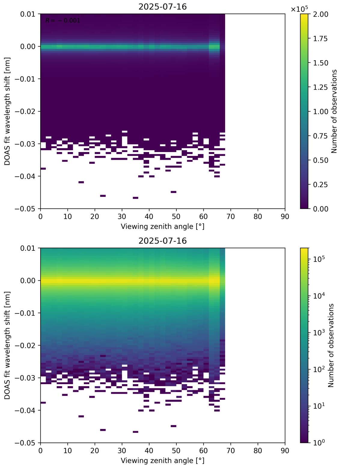
Figure 365: Scatter density plot of “Viewing zenith angle” against “DOAS fit wavelength shift” for 2025-07-15 to 2025-07-17.
