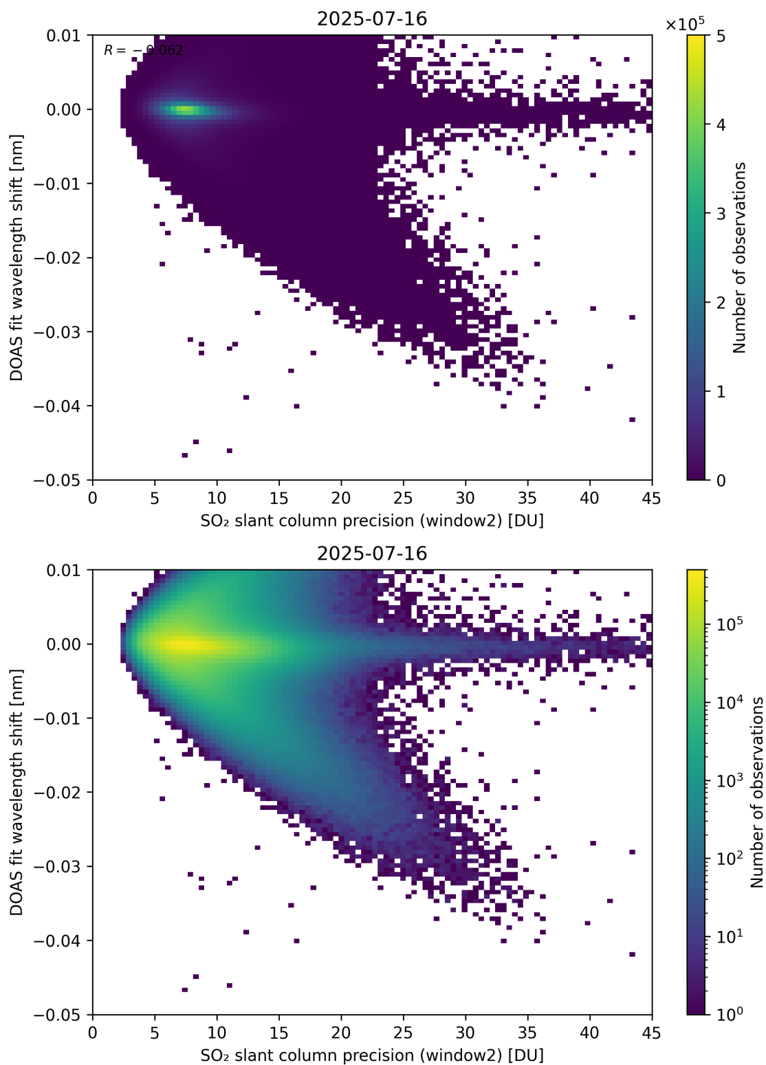
Figure 293: Scatter density plot of “SO 2 slant column precision (window2)” against “DOAS fit wavelength shift” for 2025-07-15 to 2025-07-17.
