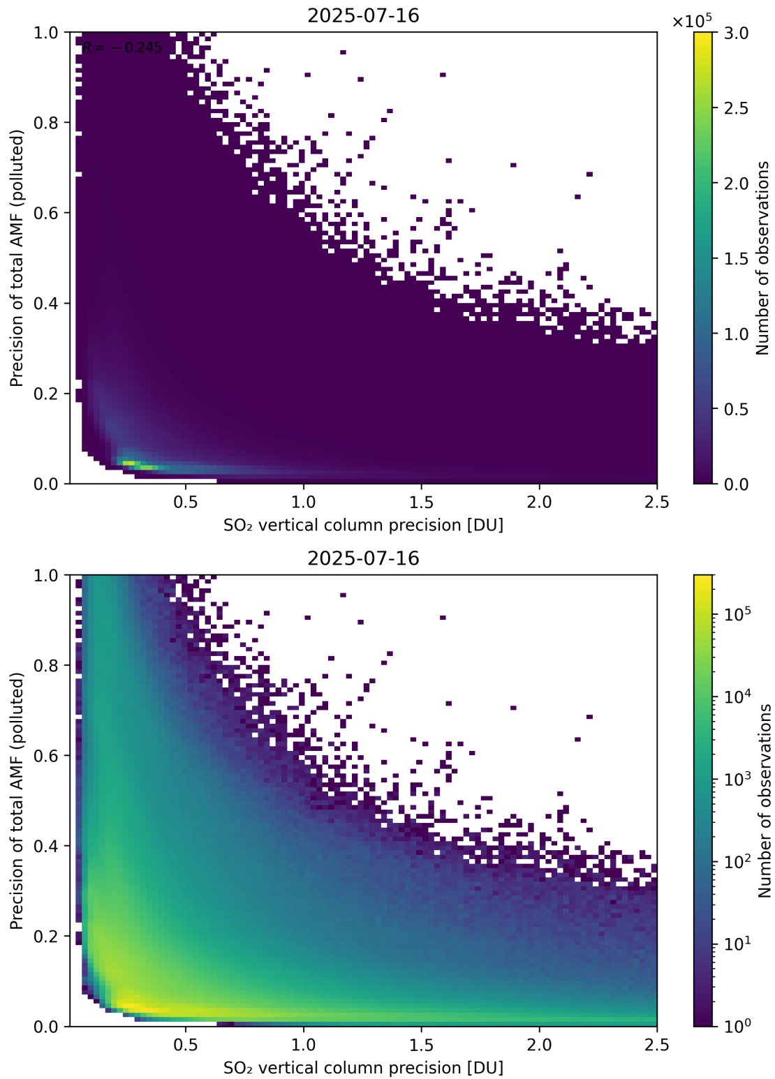
Figure 347: Scatter density plot of “SO 2 vertical column precision” against “Precision of total AMF (polluted)” for 2025-07-15 to 2025-07-17.
