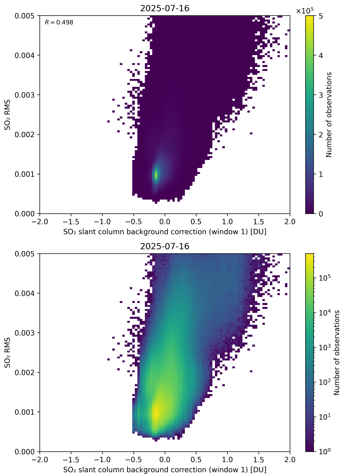
Figure 113: Scatter density plot of “SO 2 slant column background correction (window 1)” against “SO 2 RMS” for 2025-07-15 to 2025-07-17.
