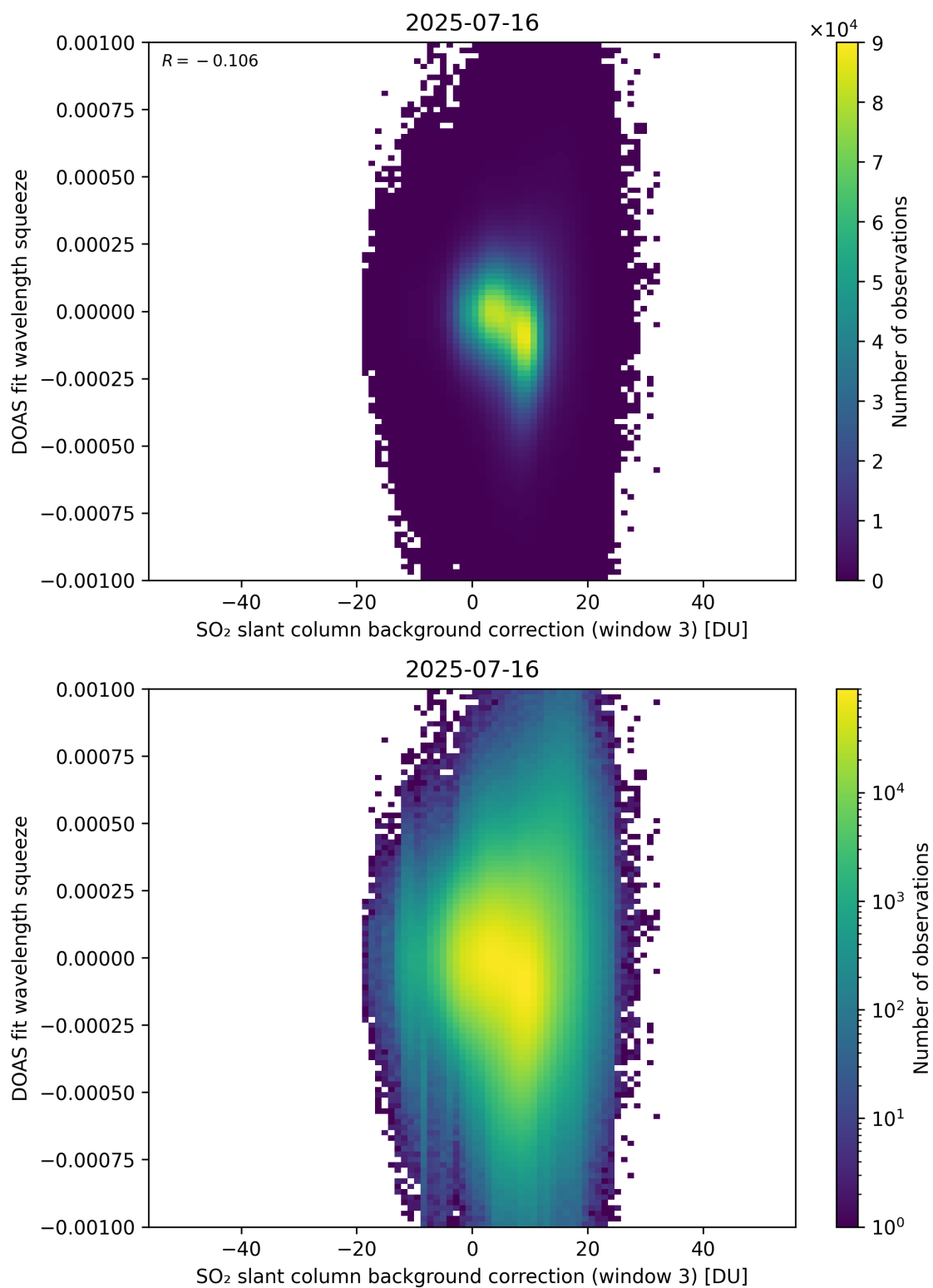
Figure 133: Scatter density plot of “SO 2 slant column background correction (window 3)” against “DOAS fit wavelength squeeze” for 2025-07-15 to 2025-07-17.
