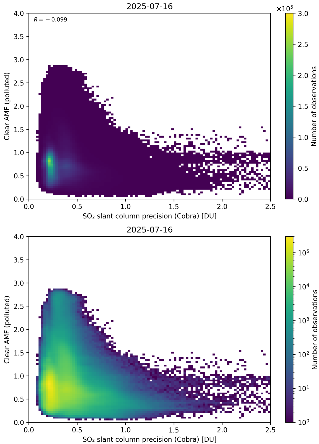
Figure 205: Scatter density plot of “SO 2 slant column precision (Cobra)” against “Clear AMF (polluted)” for 2025-07-15 to 2025-07-17.
