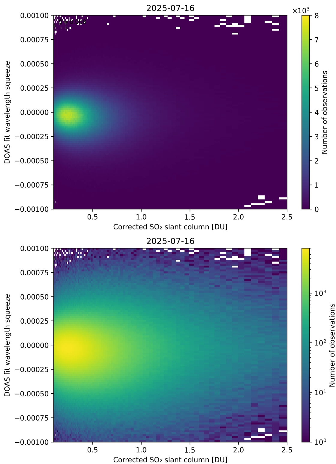
Figure 230: Scatter density plot of “Corrected SO 2 slant column” against “DOAS fit wavelength squeeze” for 2025-07-15 to 2025-07-17.
