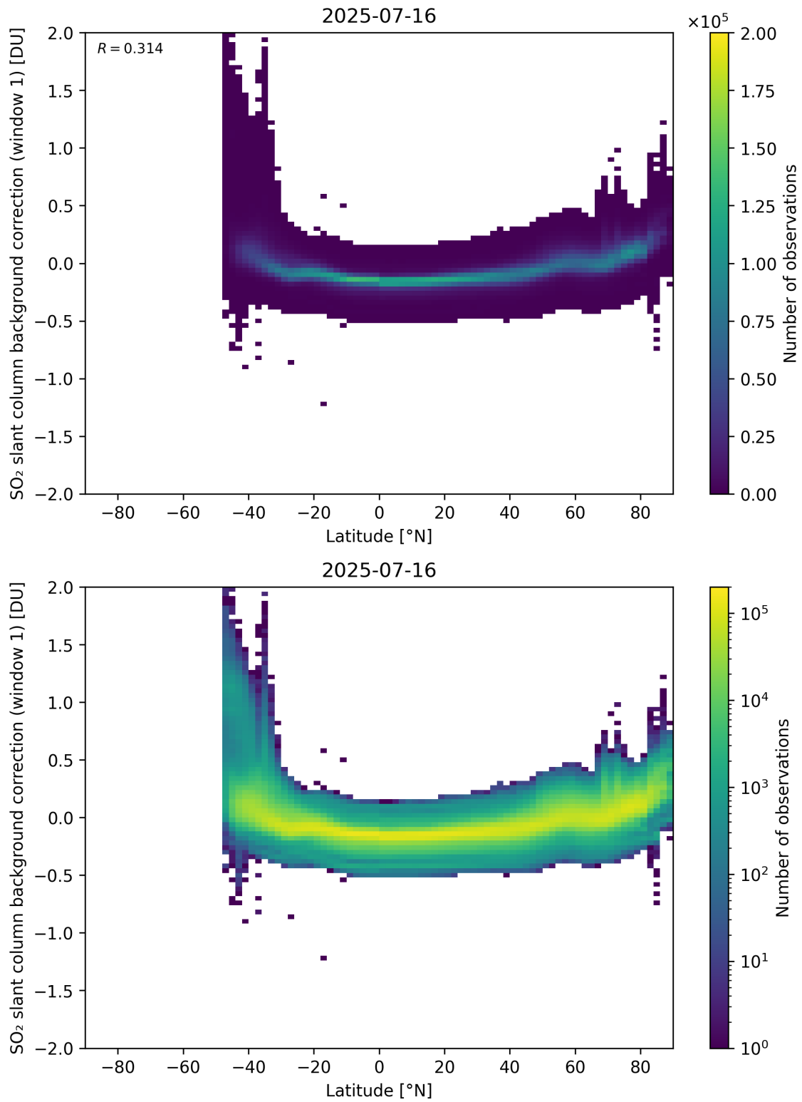
Figure 150: Scatter density plot of “Latitude” against “SO 2 slant column background correction (window 1)” for 2025-07-15 to 2025-07-17.
