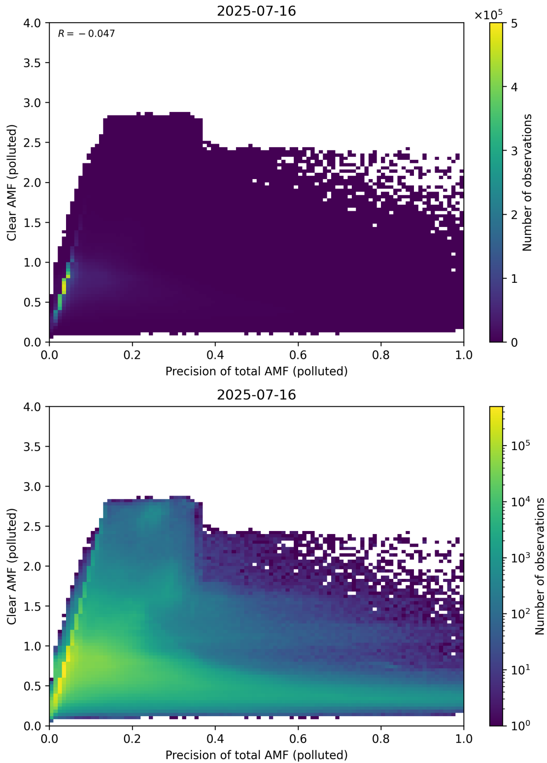
Figure 320: Scatter density plot of “Precision of total AMF (polluted)” against “Clear AMF (polluted)” for 2025-07-15 to 2025-07-17.
