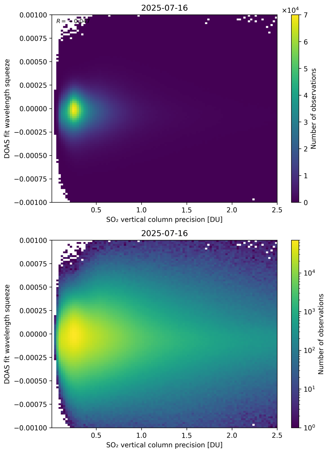
Figure 333: Scatter density plot of “SO 2 vertical column precision” against “DOAS fit wavelength squeeze” for 2025-07-15 to 2025-07-17.
