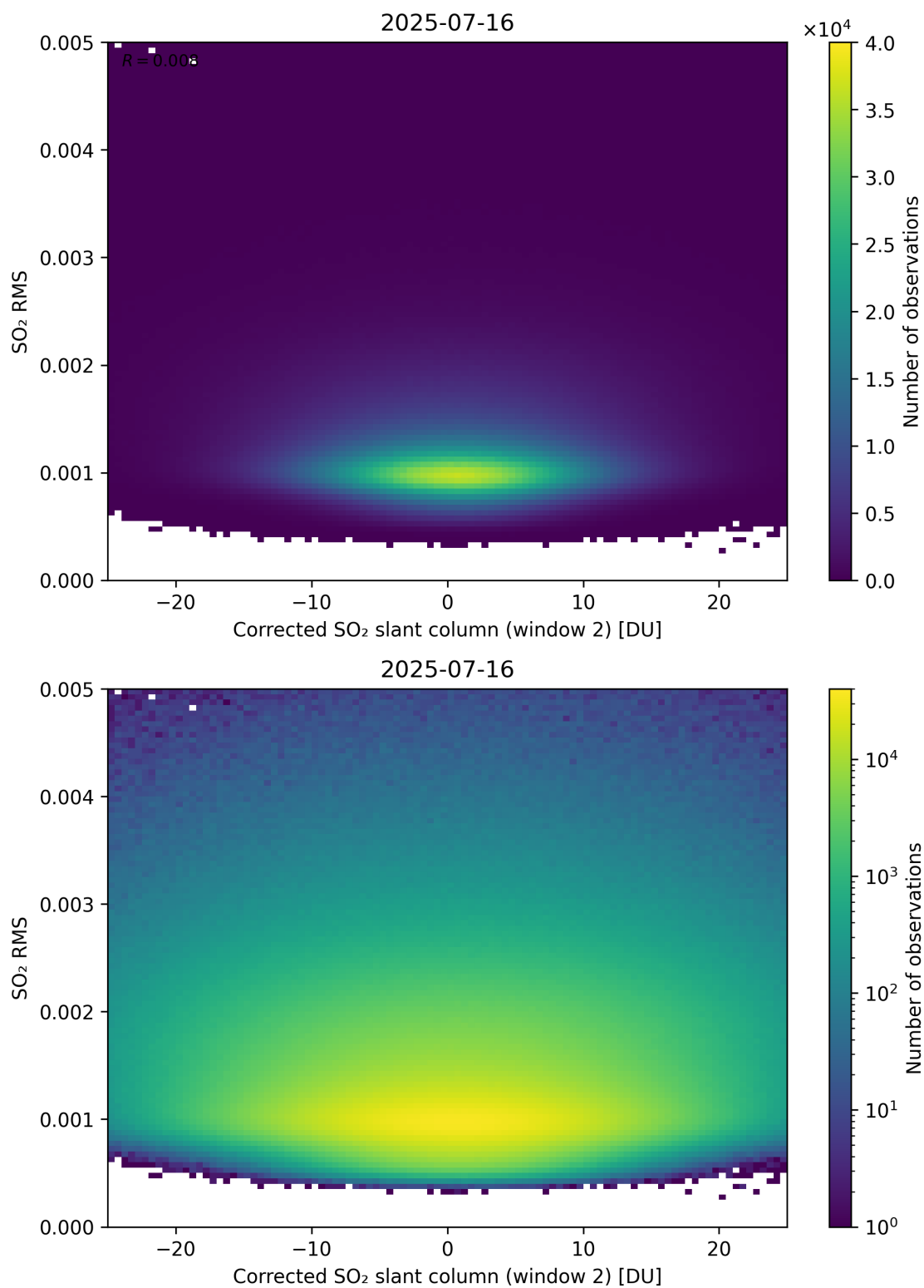
Figure 248: Scatter density plot of “Corrected SO 2 slant column (window 2)” against “SO 2 RMS” for 2025-07-15 to 2025-07-17.
