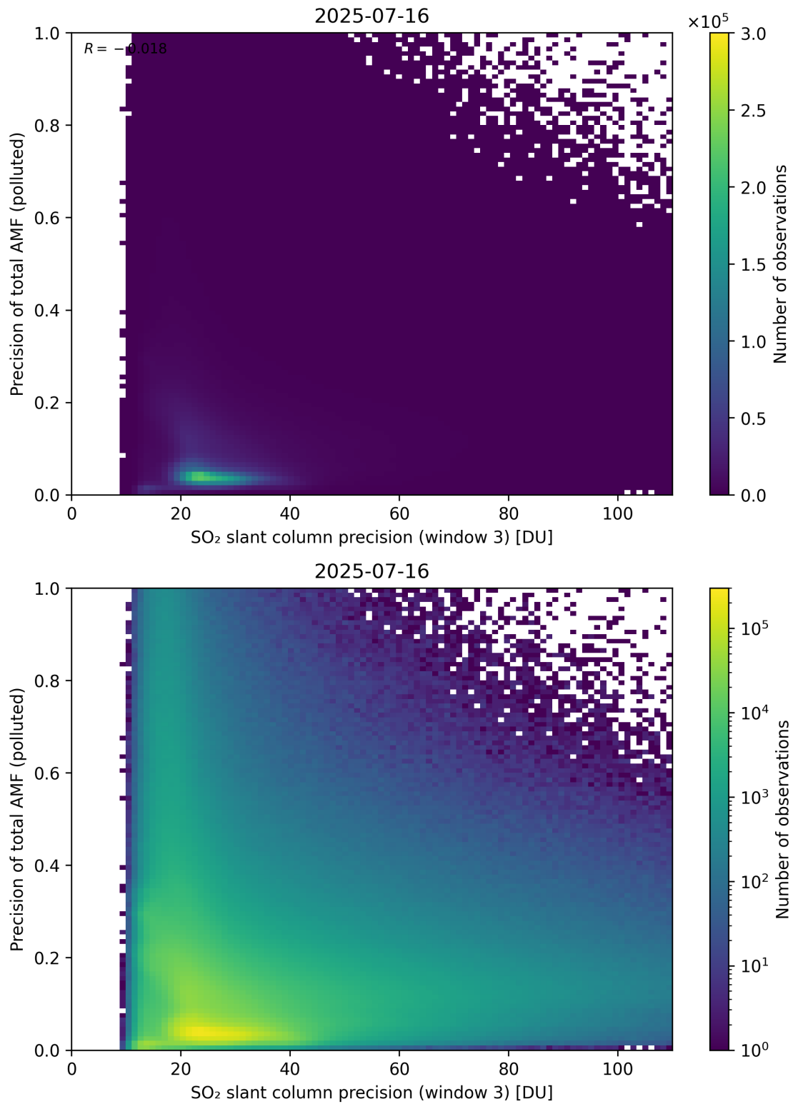
Figure 314: Scatter density plot of “SO 2 slant column precision (window 3)” against “Precision of total AMF (polluted)” for 2025-07-15 to 2025-07-17.
