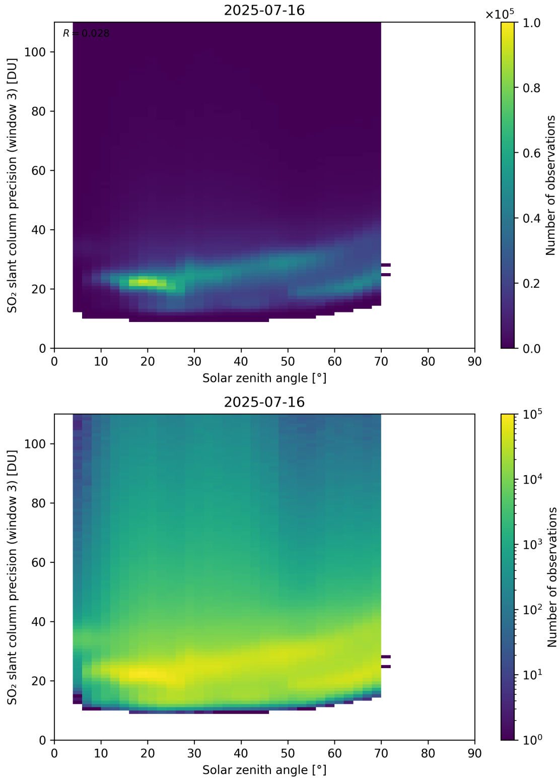
Figure 188: Scatter density plot of “Solar zenith angle” against “SO 2 slant column precision (window 3)” for 2025-07-15 to 2025-07-17.
