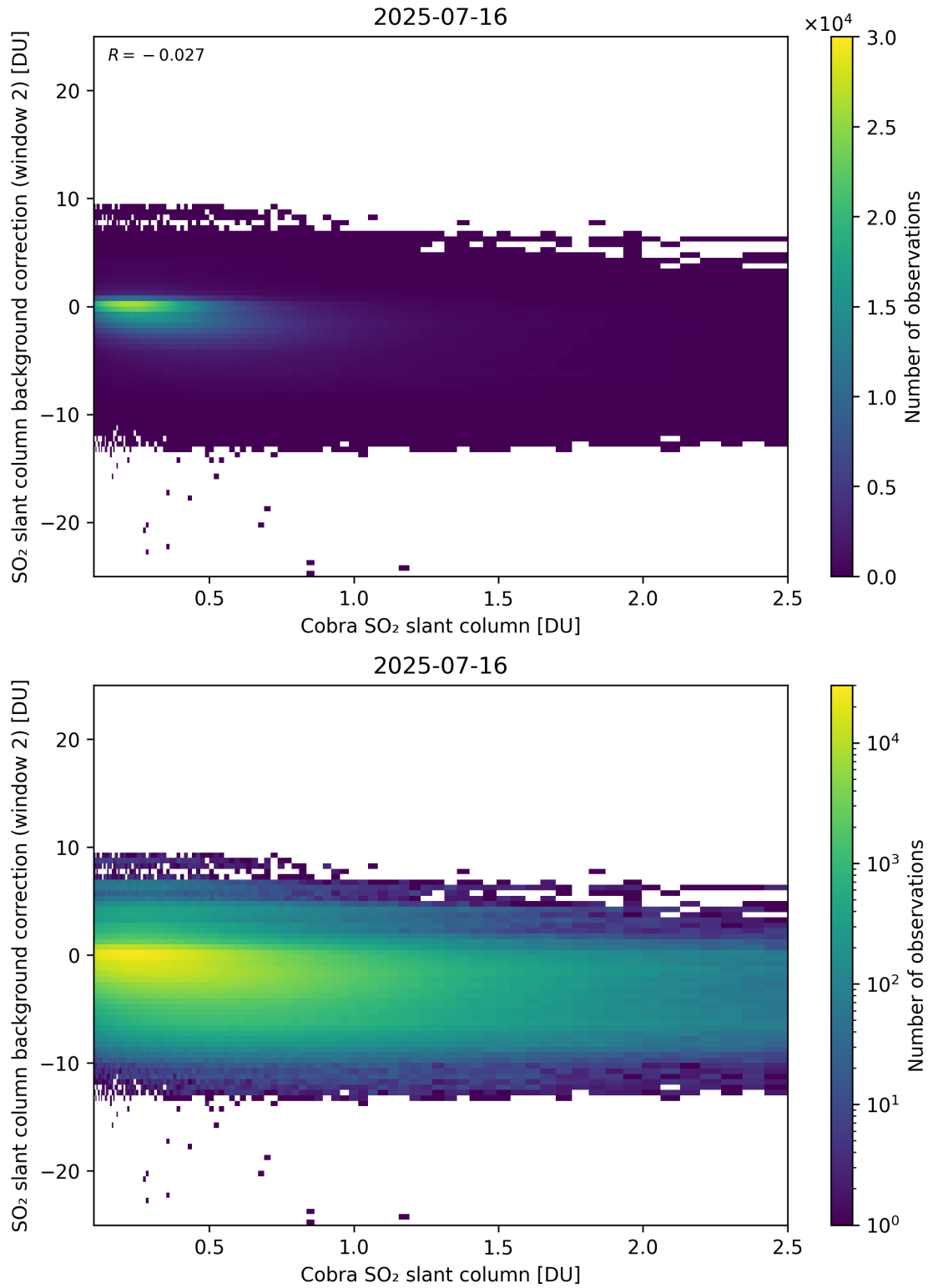
Figure 194: Scatter density plot of “Cobra SO 2 slant column” against “SO 2 slant column background correction (window 2)” for 2025-07-15 to 2025-07-17.
