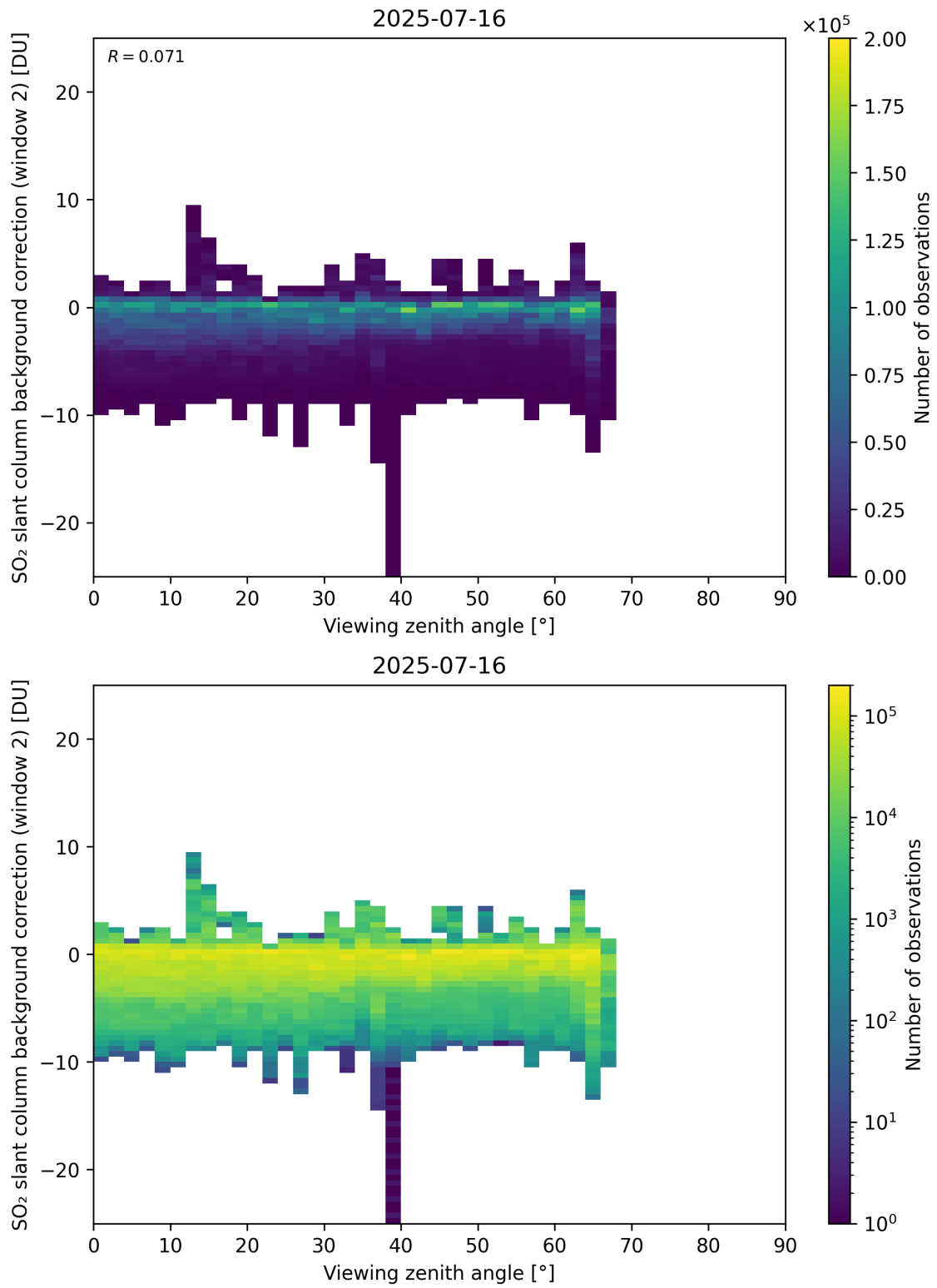
Figure 363: Scatter density plot of “Viewing zenith angle” against “SO 2 slant column background correction (window 2)” for 2025-07-15 to 2025-07-17.
