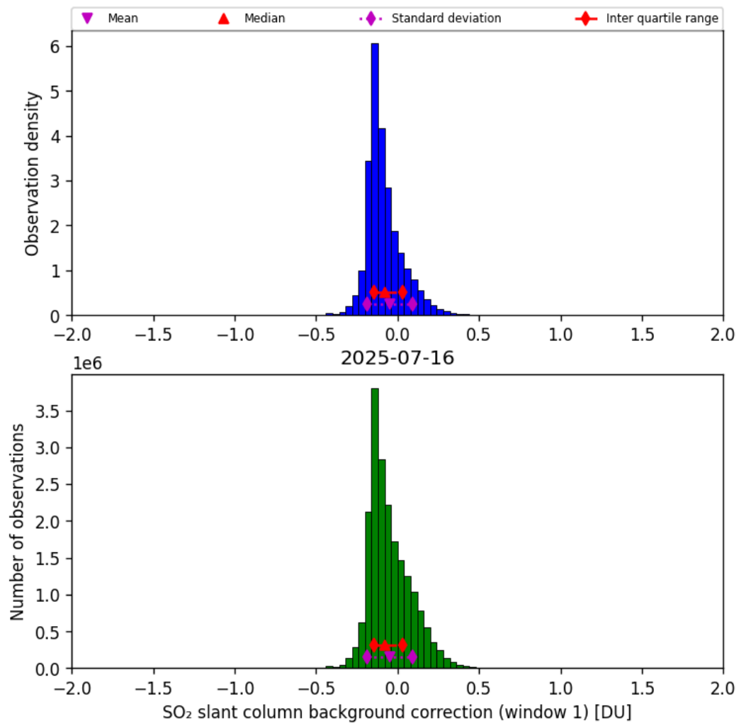
Figure 66: Histogram of “SO 2 slant column background correction (window 1)” for 2025-07-15 to 2025-07-17
