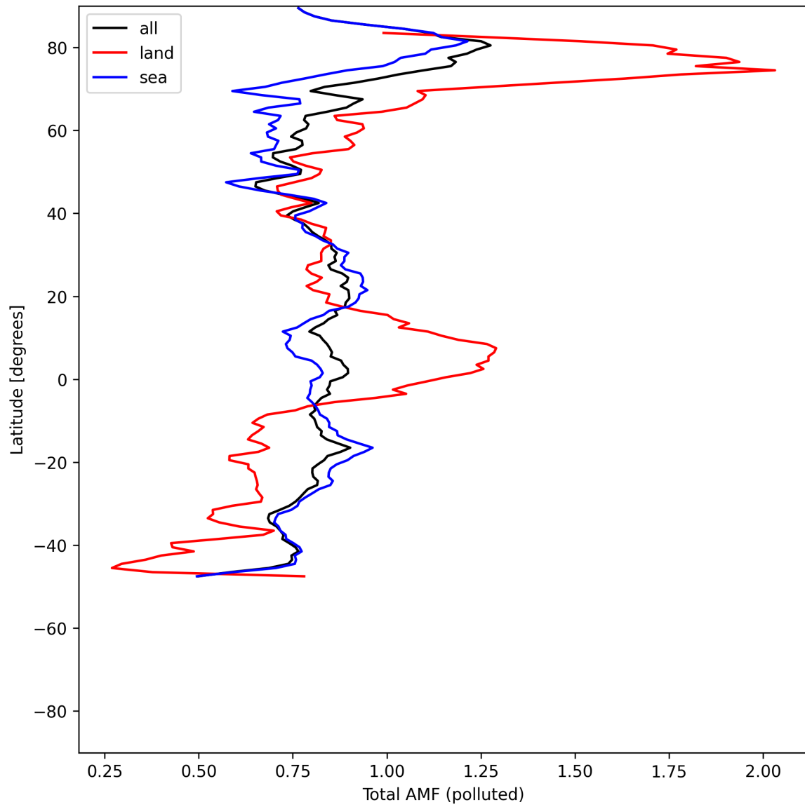
Figure 53: Zonal average of “Total AMF (polluted)” for 2025-07-15 to 2025-07-17.
