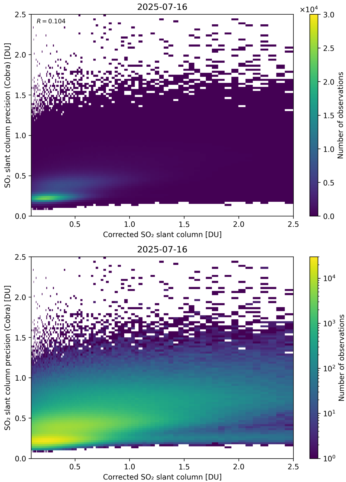
Figure 234: Scatter density plot of “Corrected SO 2 slant column” against “SO 2 slant column precision (Cobra)” for 2025-07-15 to 2025-07-17.
