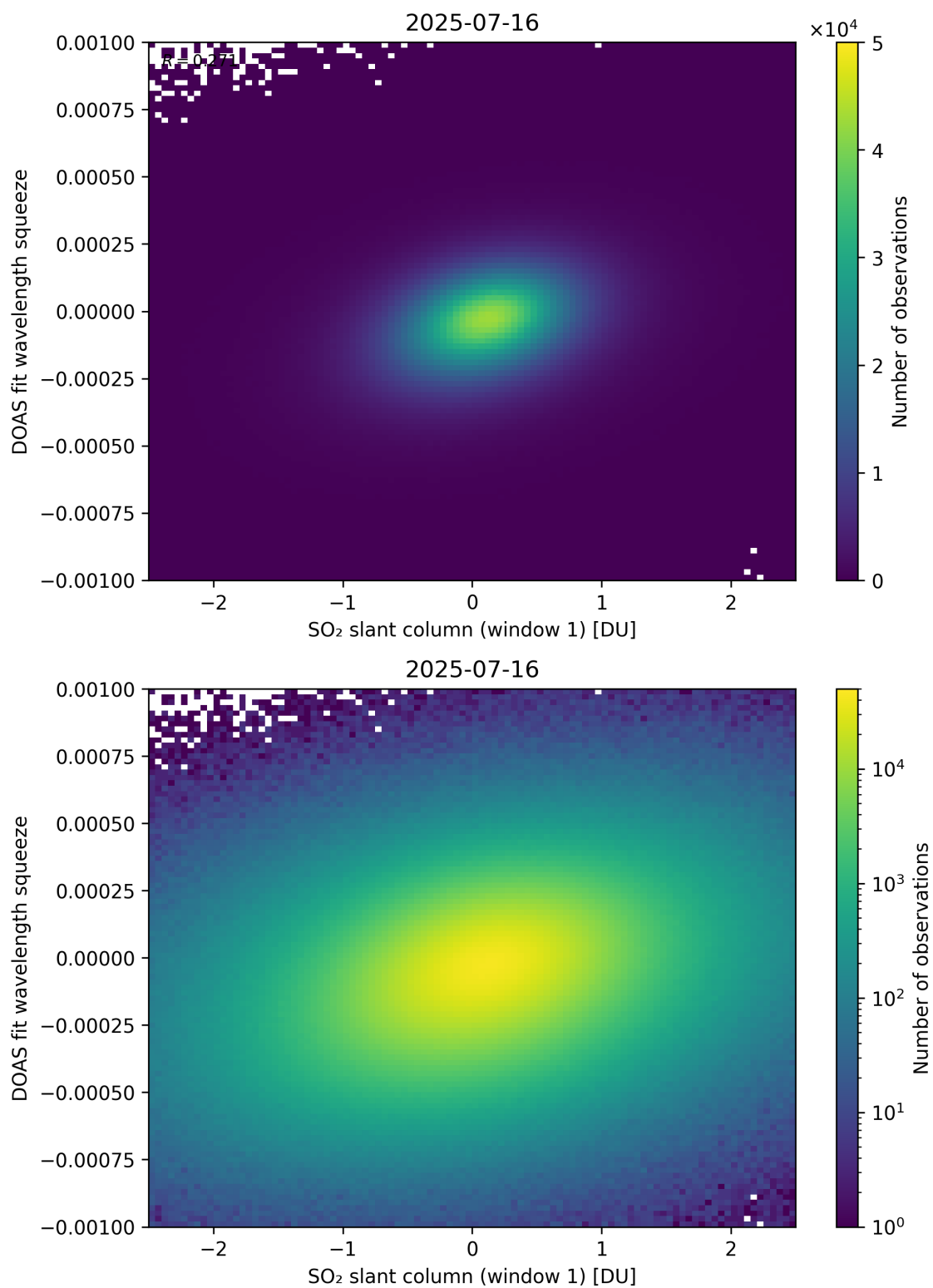
Figure 266: Scatter density plot of “SO 2 slant column (window 1)” against “DOAS fit wavelength squeeze” for 2025-07-15 to 2025-07-17.
