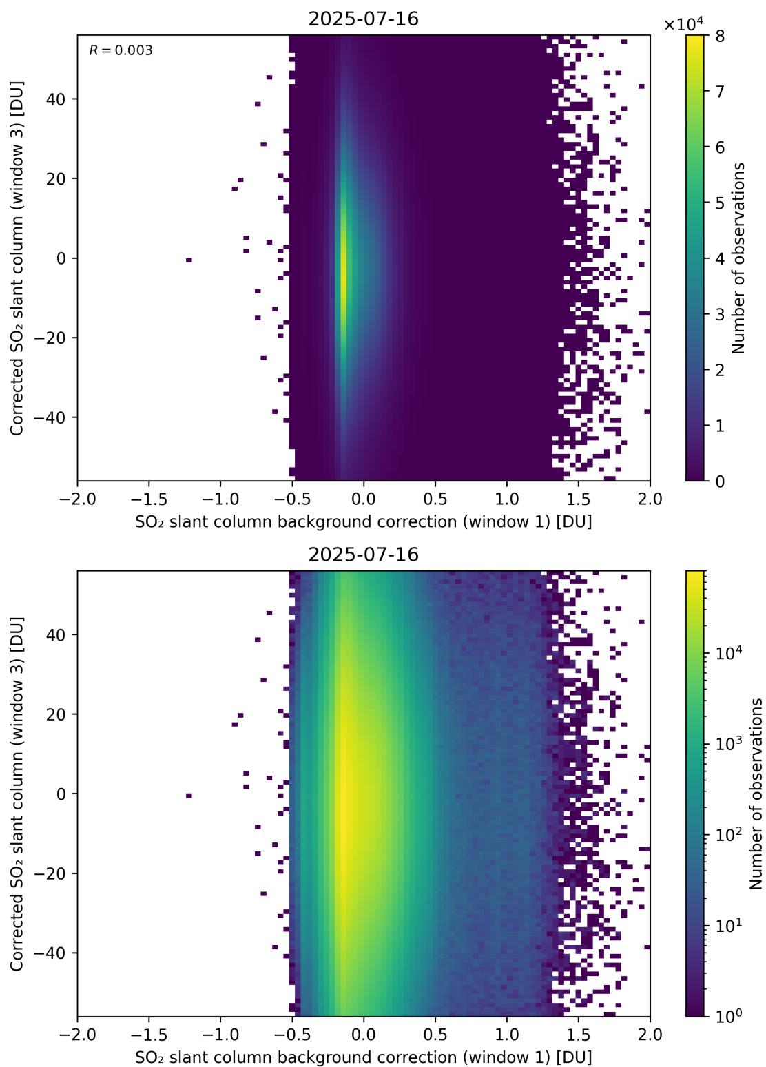
Figure 116: Scatter density plot of “SO 2 slant column background correction (window 1)” against “Corrected SO 2 slant column (window 3)” for 2025-07-15 to 2025-07-17.
