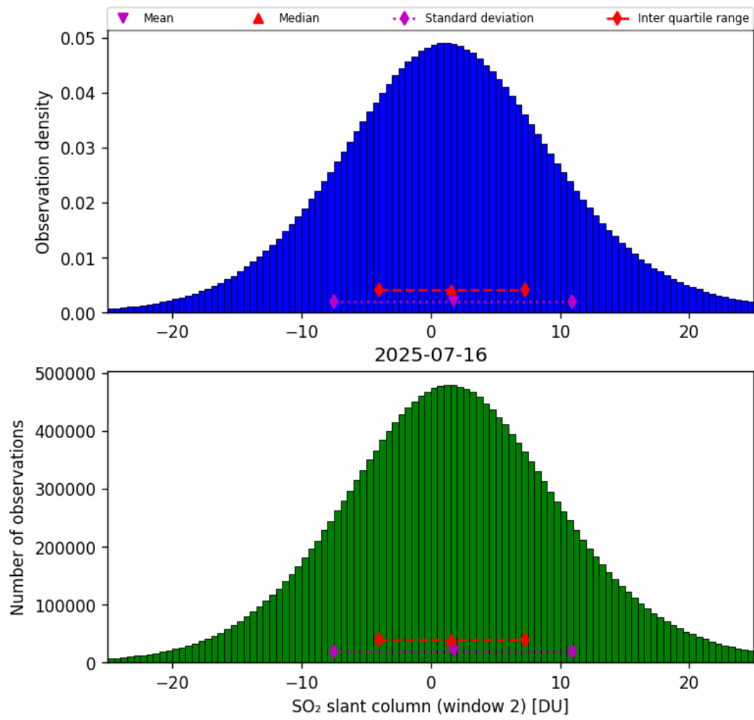
Figure 67: Histogram of “SO 2 slant column (window 2)” for 2025-07-15 to 2025-07-17
