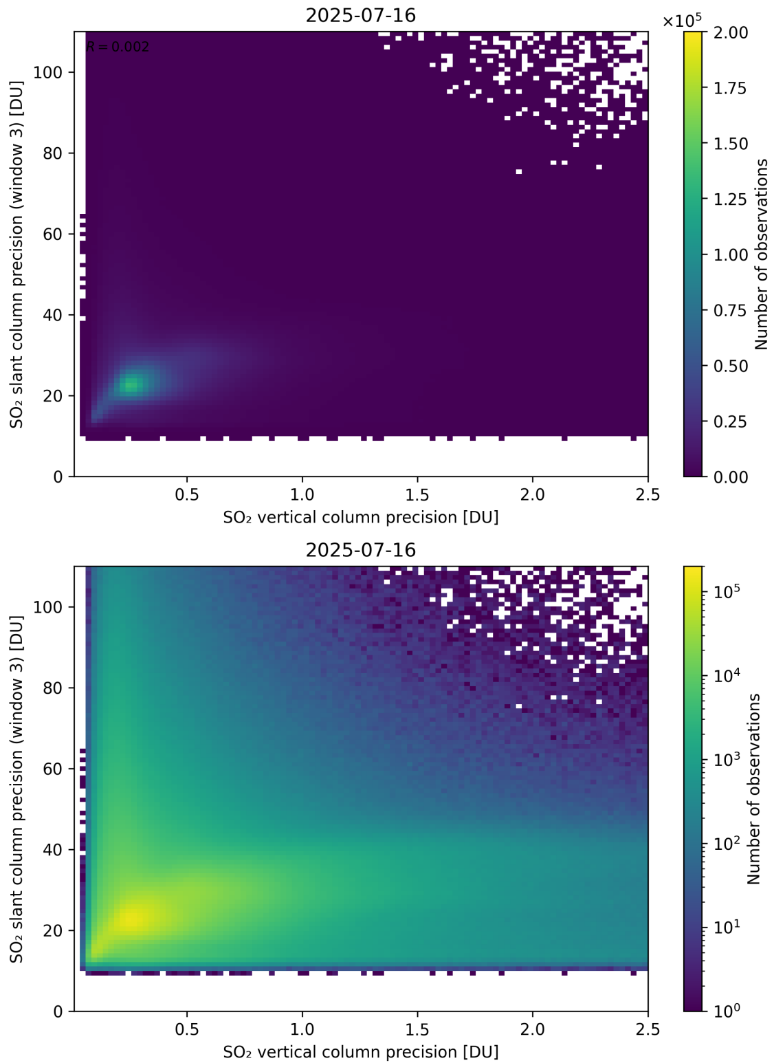
Figure 345: Scatter density plot of “SO 2 vertical column precision” against “SO 2 slant column precision (window 3)” for 2025-07-15 to 2025-07-17.
