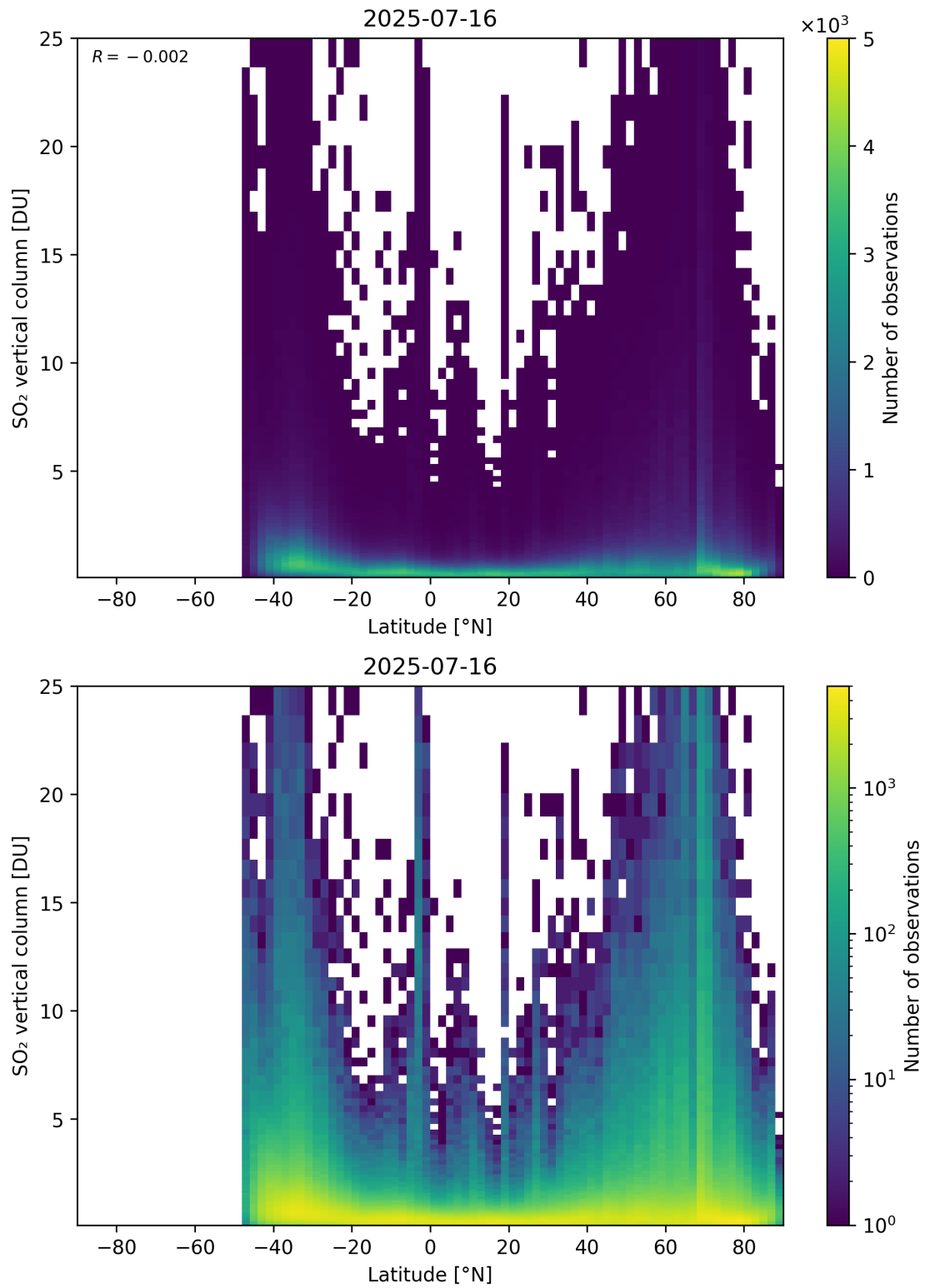
Figure 169: Scatter density plot of “Latitude” against “SO 2 vertical column” for 2025-07-15 to 2025-07-17.
