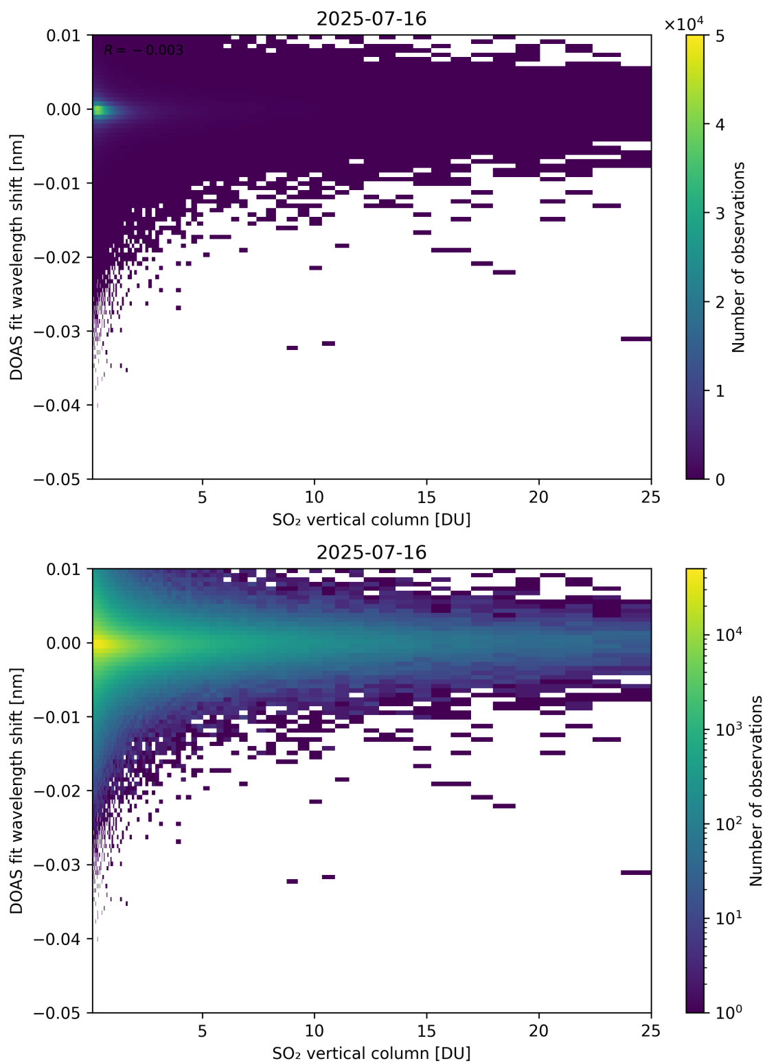
Figure 326: Scatter density plot of “SO 2 vertical column” against “DOAS fit wavelength shift” for 2025-07-15 to 2025-07-17.
