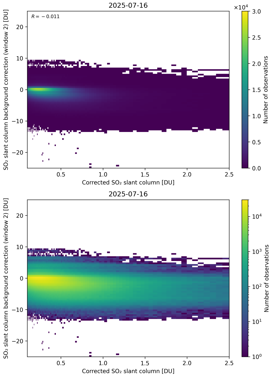
Figure 227: Scatter density plot of “Corrected SO 2 slant column” against “SO 2 slant column background correction (window 2)” for 2025-07-15 to 2025-07-17.
