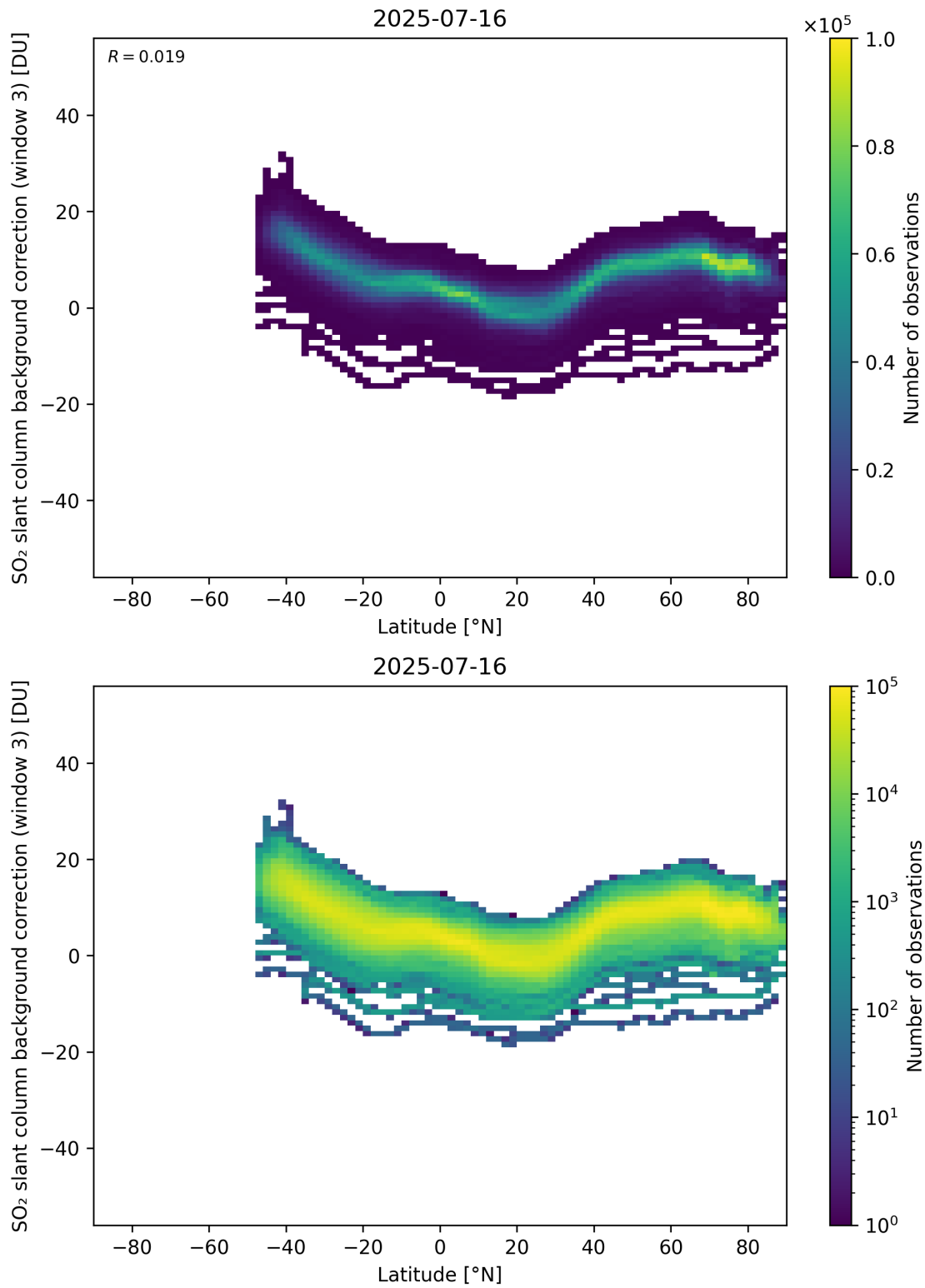
Figure 152: Scatter density plot of “Latitude” against “SO 2 slant column background correction (window 3)” for 2025-07-15 to 2025-07-17.
