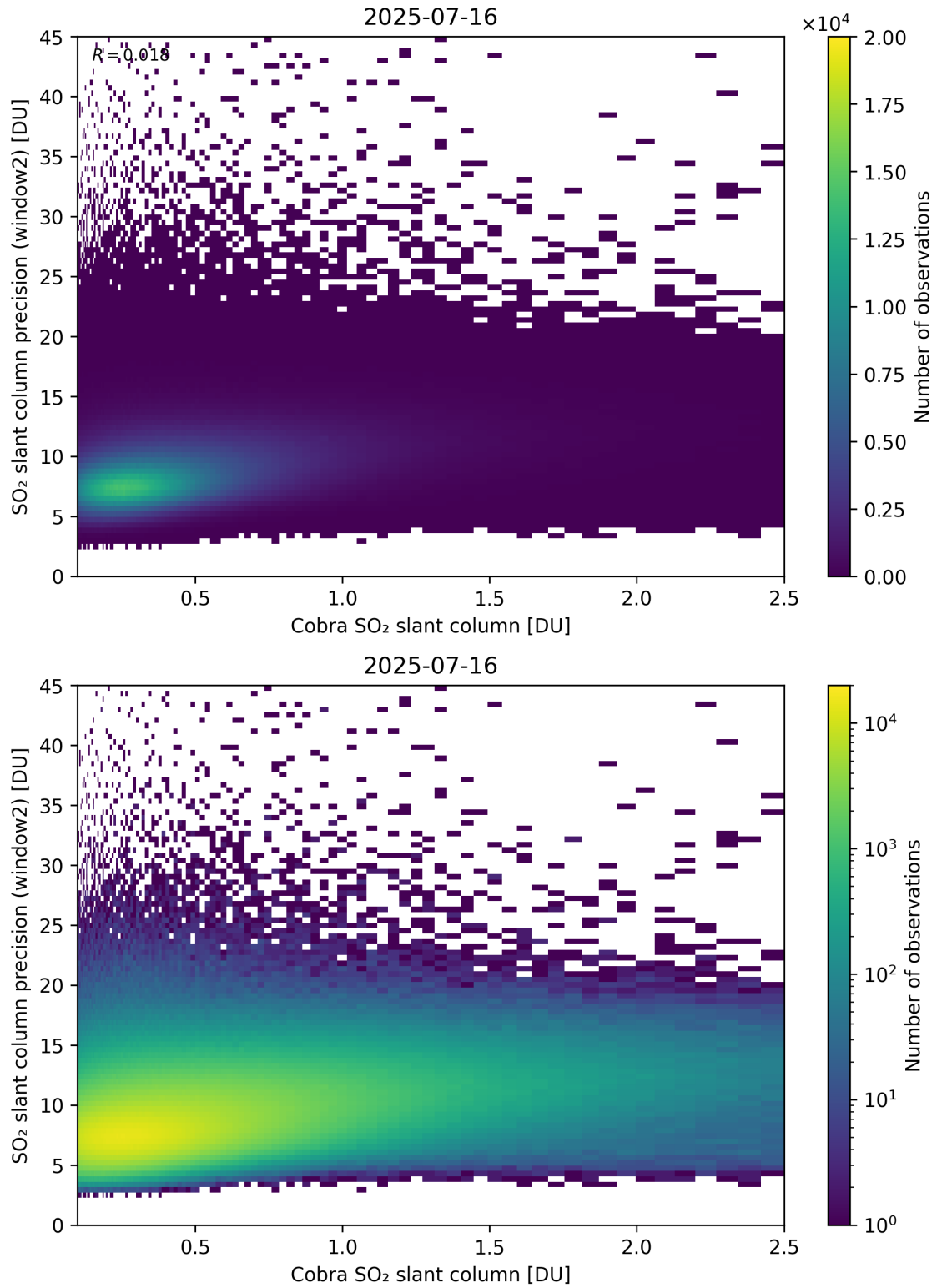
Figure 221: Scatter density plot of “Cobra SO 2 slant column” against “SO 2 slant column precision (window2)” for 2025-07-15 to 2025-07-17.
