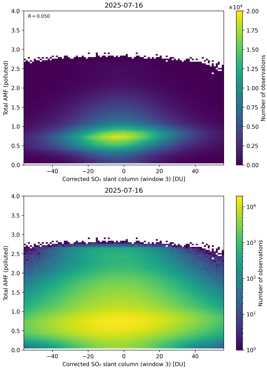
Figure 260: Scatter density plot of “Corrected SO 2 slant column (window 3)” against “Total AMF (polluted)” for 2025-07-15 to 2025-07-17.
