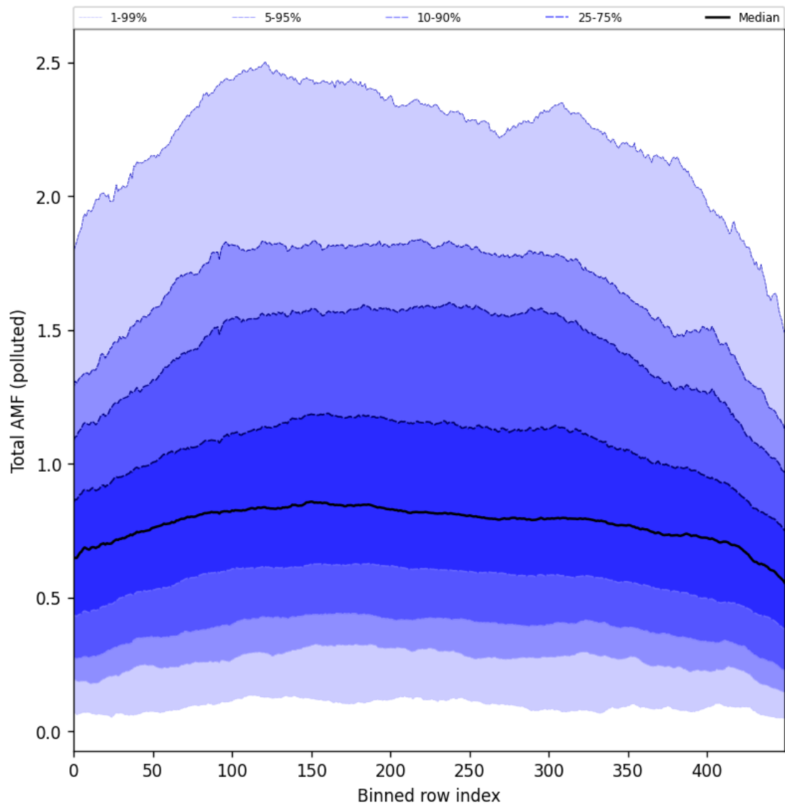
Figure 105: Along track statistics of “Total AMF (polluted)” for 2025-07-15 to 2025-07-17
