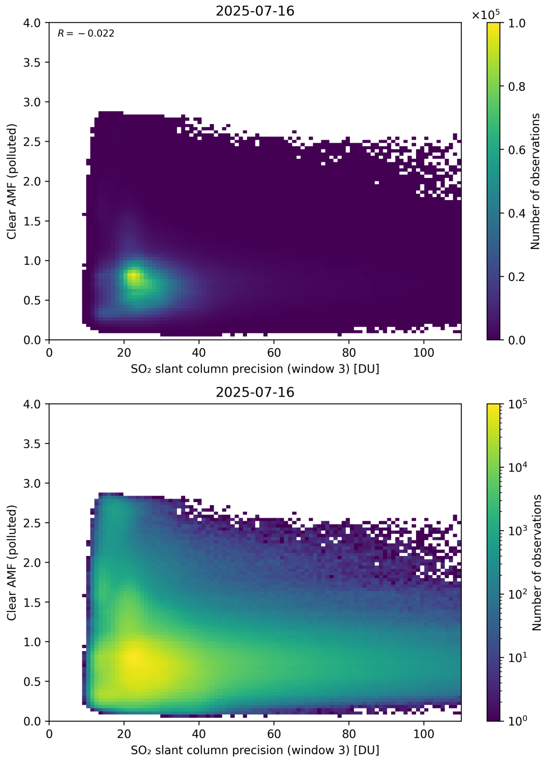
Figure 311: Scatter density plot of “SO 2 slant column precision (window 3)” against “Clear AMF (polluted)” for 2025-07-15 to 2025-07-17.
