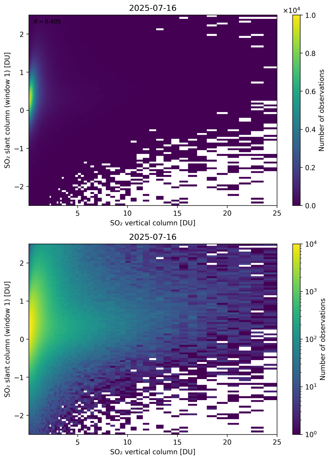
Figure 354: Scatter density plot of “SO 2 vertical column” against “SO 2 slant column (window 1)” for 2025-07-15 to 2025-07-17.
