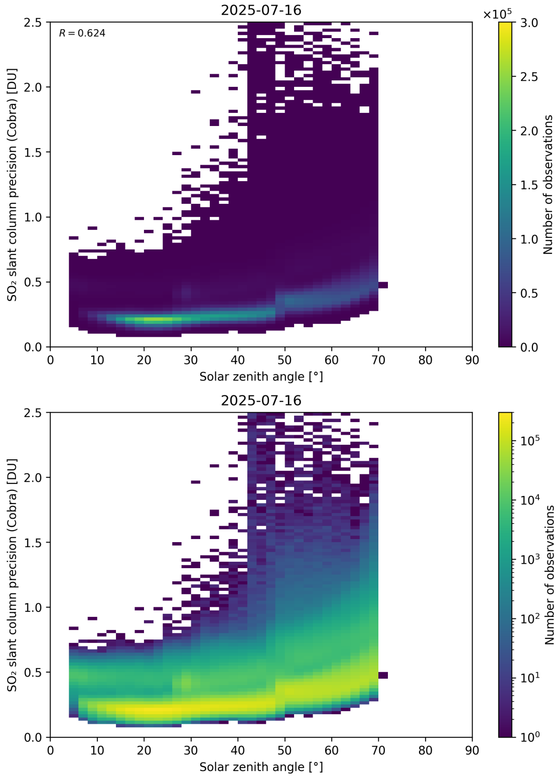
Figure 180: Scatter density plot of “Solar zenith angle” against “SO 2 slant column precision (Cobra)” for 2025-07-15 to 2025-07-17.
