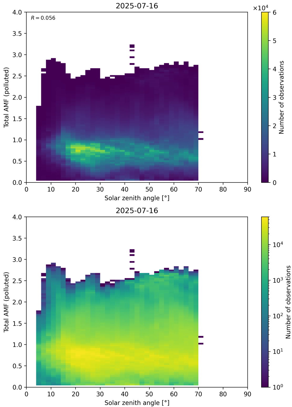
Figure 189: Scatter density plot of “Solar zenith angle” against “Total AMF (polluted)” for 2025-07-15 to 2025-07-17.
