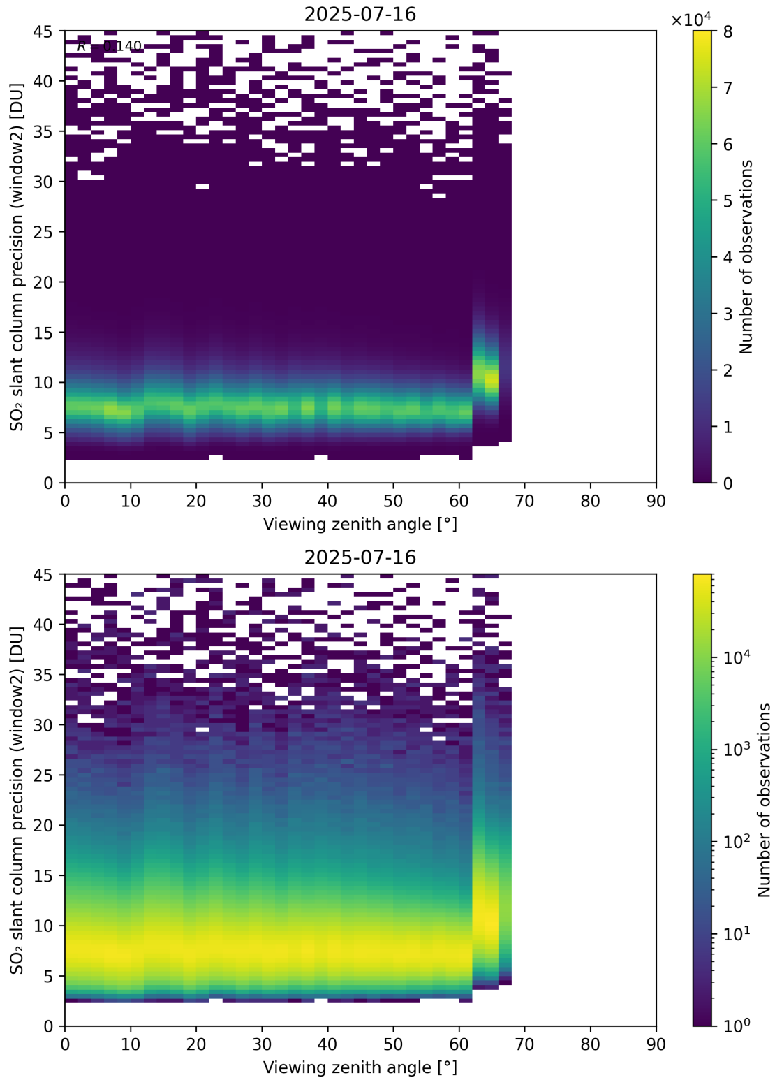
Figure 378: Scatter density plot of “Viewing zenith angle” against “SO 2 slant column precision (window2)” for 2025-07-15 to 2025-07-17.
