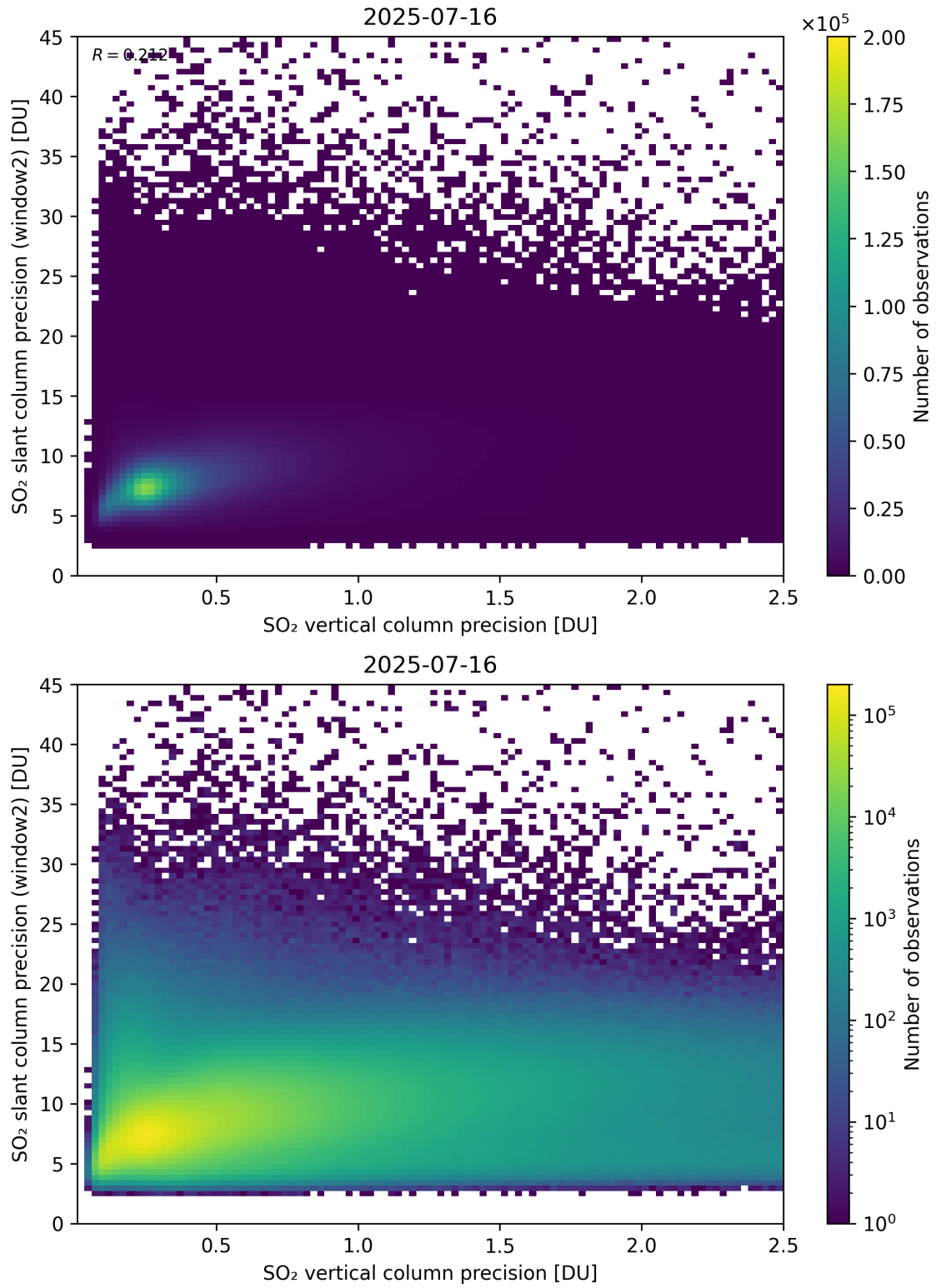
Figure 343: Scatter density plot of “SO 2 vertical column precision” against “SO 2 slant column precision (window2)” for 2025-07-15 to 2025-07-17.
