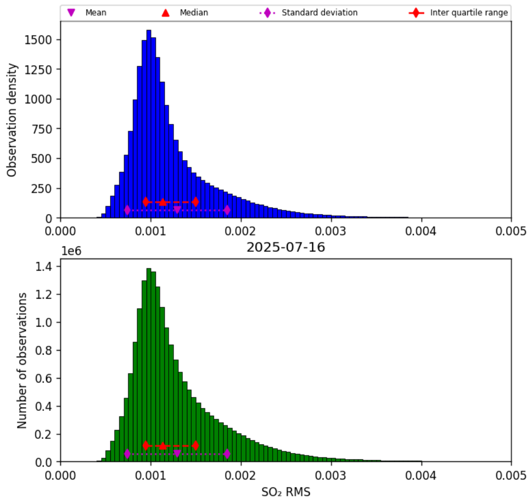
Figure 78: Histogram of “SO 2 RMS” for 2025-07-15 to 2025-07-17
