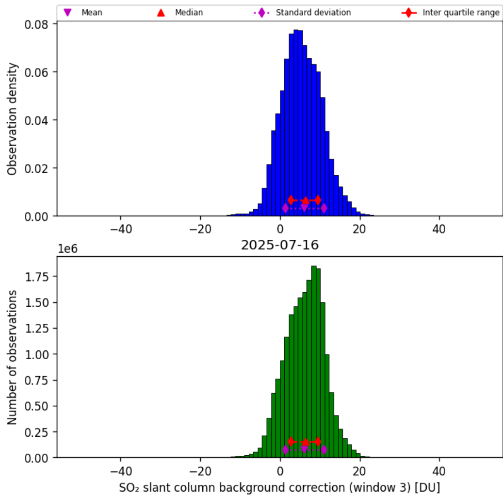
Figure 74: Histogram of “SO 2 slant column background correction (window 3)” for 2025-07-15 to 2025-07-17
