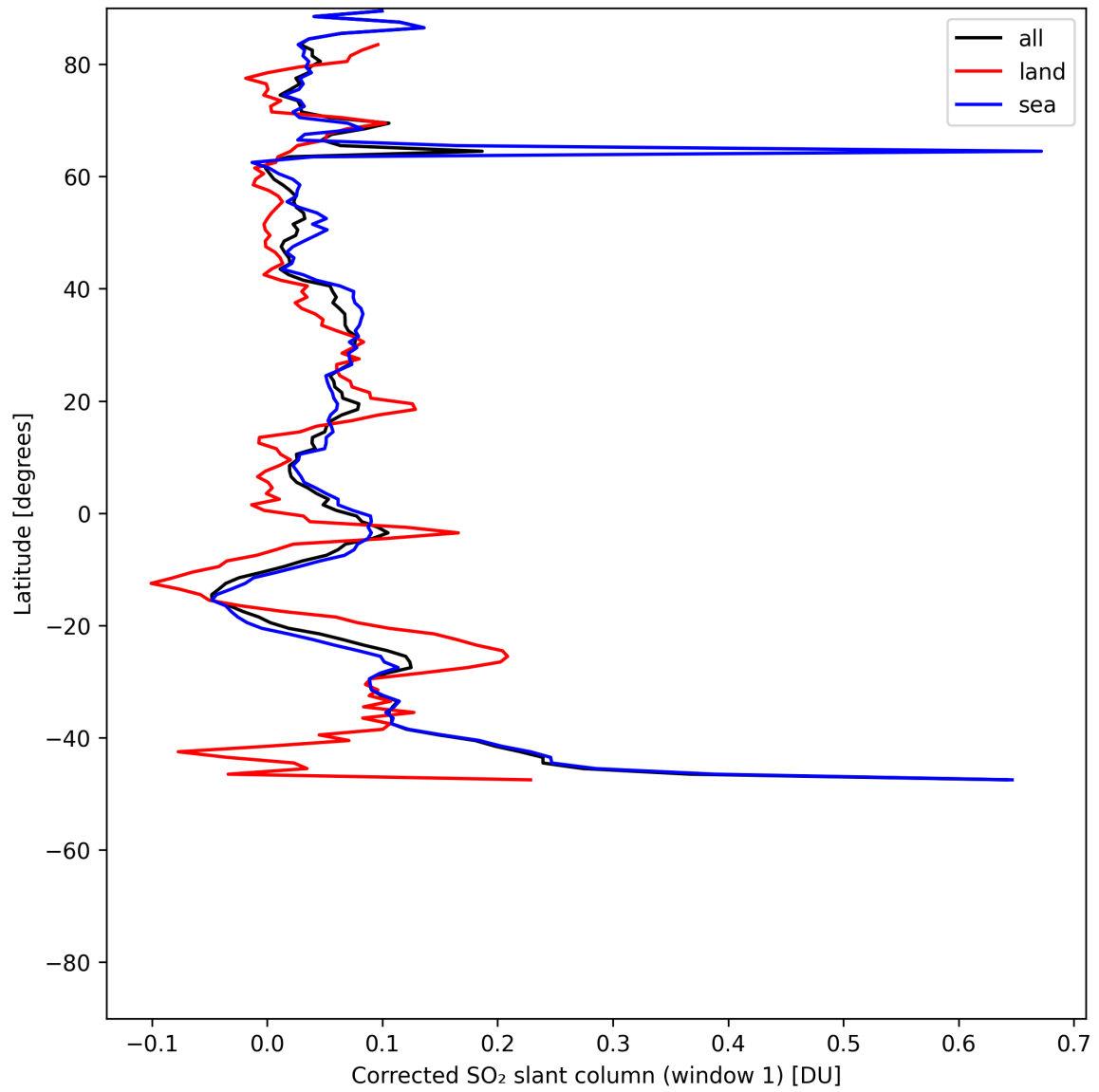
Figure 39: Zonal average of “Corrected SO 2 slant column (window 1)” for 2025-07-15 to 2025-07-17.
