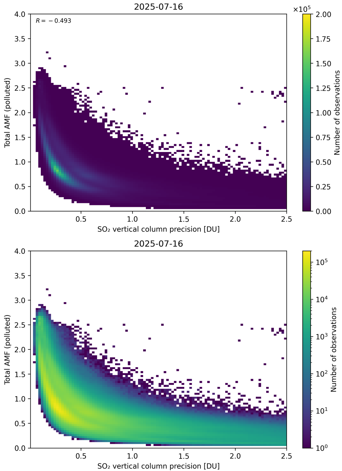
Figure 346: Scatter density plot of “SO 2 vertical column precision” against “Total AMF (polluted)” for 2025-07-15 to 2025-07-17.
