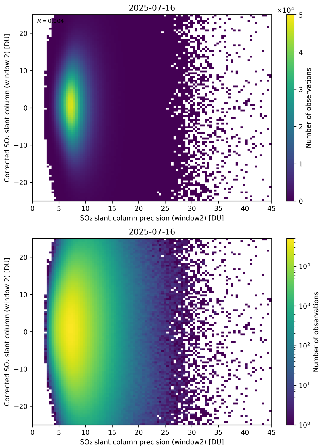
Figure 297: Scatter density plot of “SO 2 slant column precision (window2)” against “Corrected SO 2 slant column (window 2)” for 2025-07-15 to 2025-07-17.
