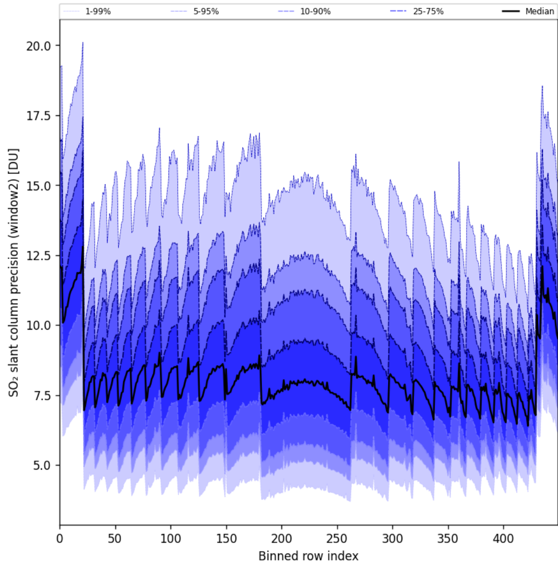
Figure 94: Along track statistics of “SO 2 slant column precision (window2)” for 2025-07-15 to 2025-07-17
