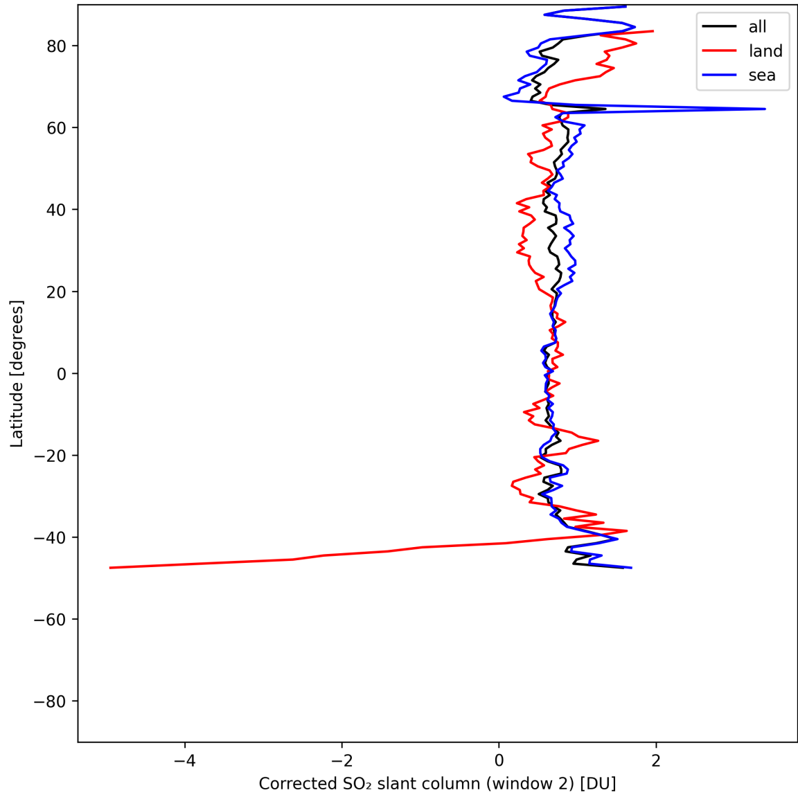
Figure 43: Zonal average of “Corrected SO 2 slant column (window 2)” for 2025-07-15 to 2025-07-17.
