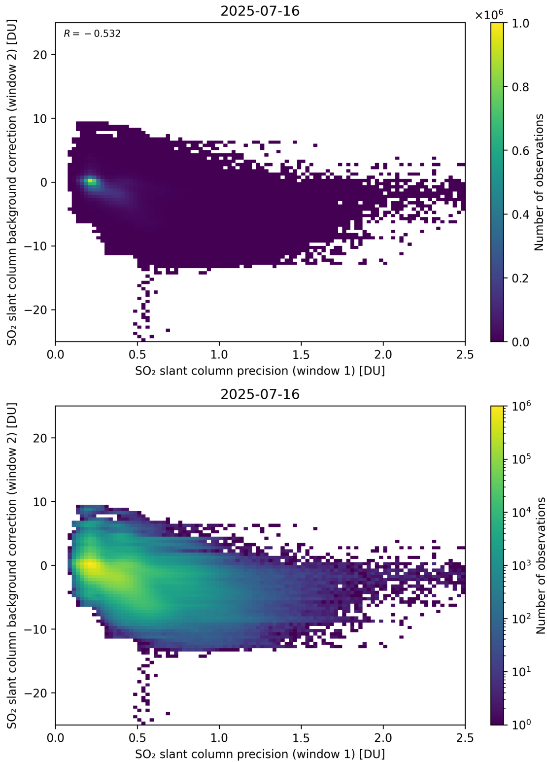
Figure 269: Scatter density plot of “SO 2 slant column precision (window 1)” against “SO 2 slant column background correction (window 2)” for 2025-07-15 to 2025-07-17.
