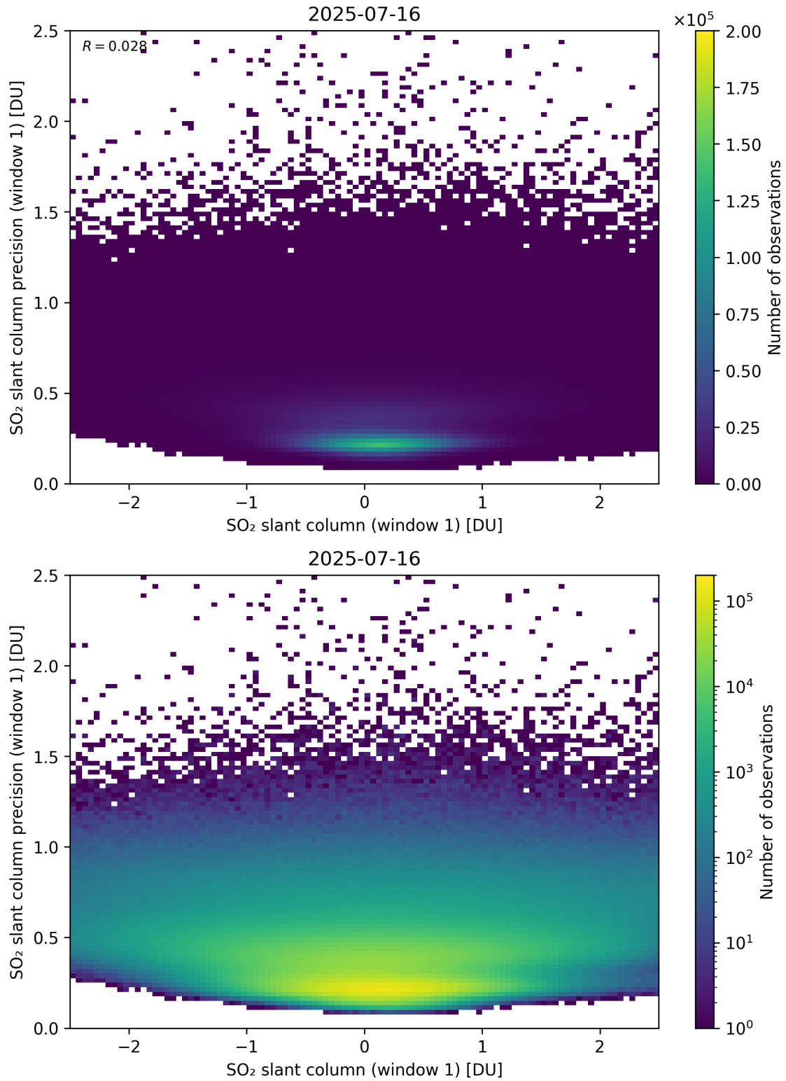
Figure 285: Scatter density plot of “SO 2 slant column (window 1)” against “SO 2 slant column precision (window 1)” for 2025-07-15 to 2025-07-17.
