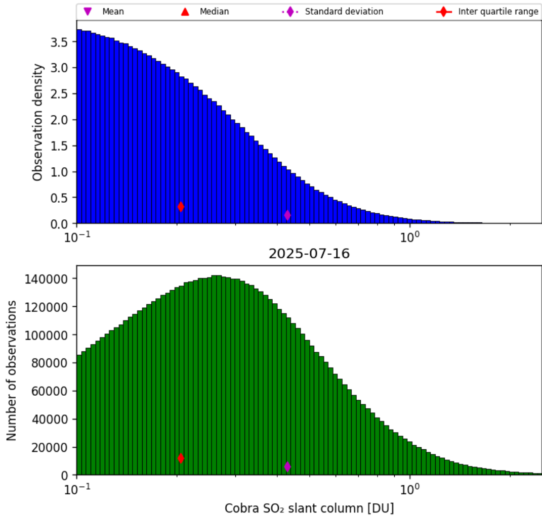
Figure 61: Histogram of “Cobra SO 2 slant column” for 2025-07-15 to 2025-07-17
