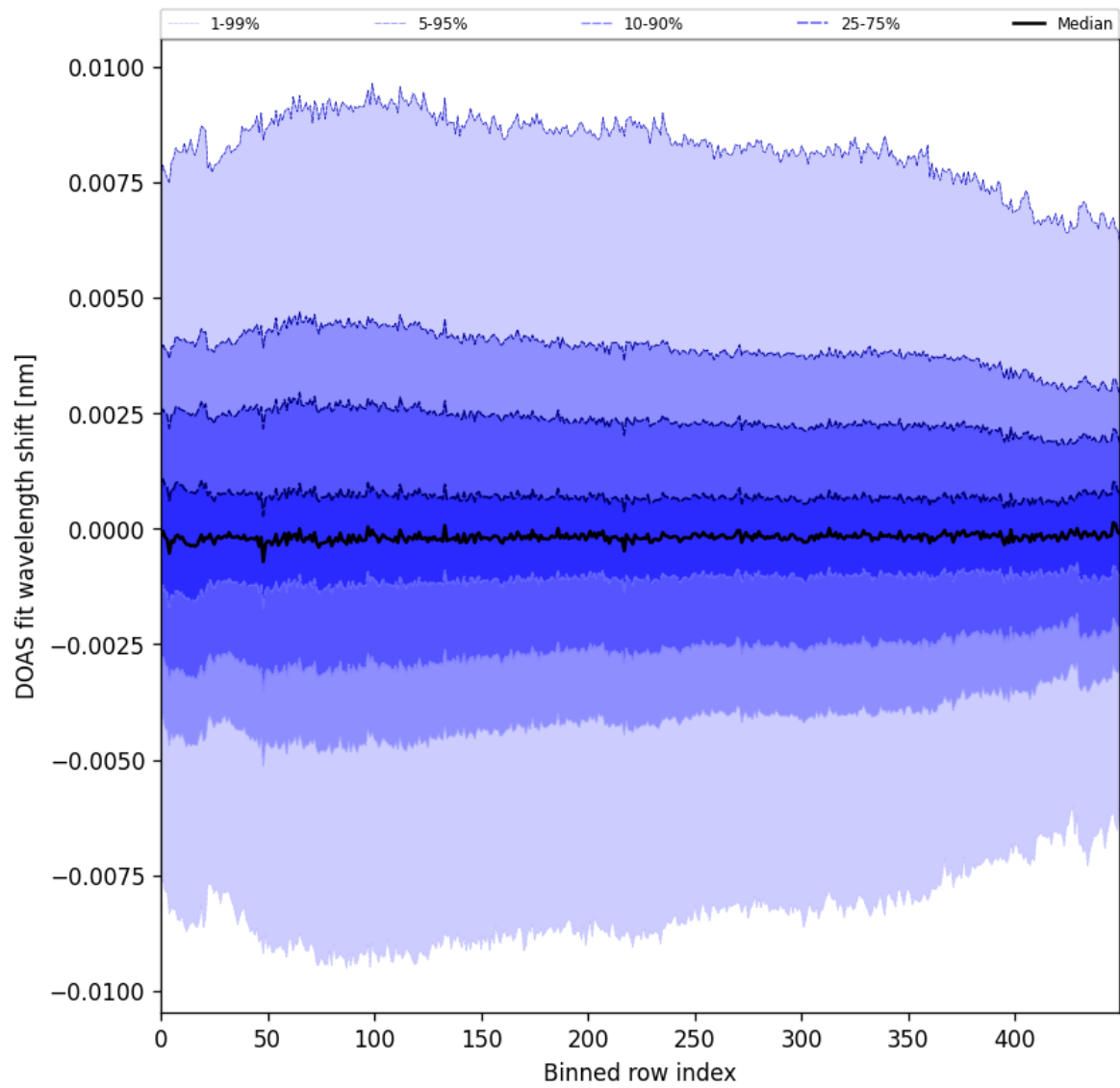
Figure 102: Along track statistics of “DOAS fit wavelength shift” for 2025-07-15 to 2025-07-17
