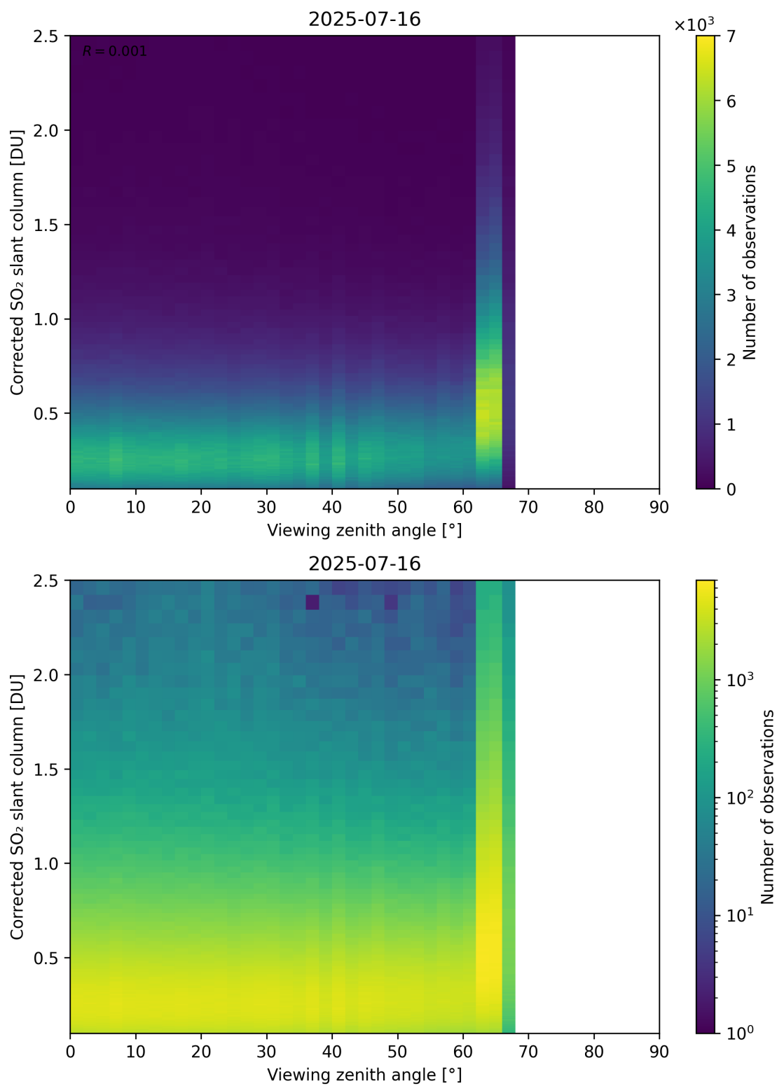
Figure 373: Scatter density plot of “Viewing zenith angle” against “Corrected SO 2 slant column” for 2025-07-15 to 2025-07-17.
