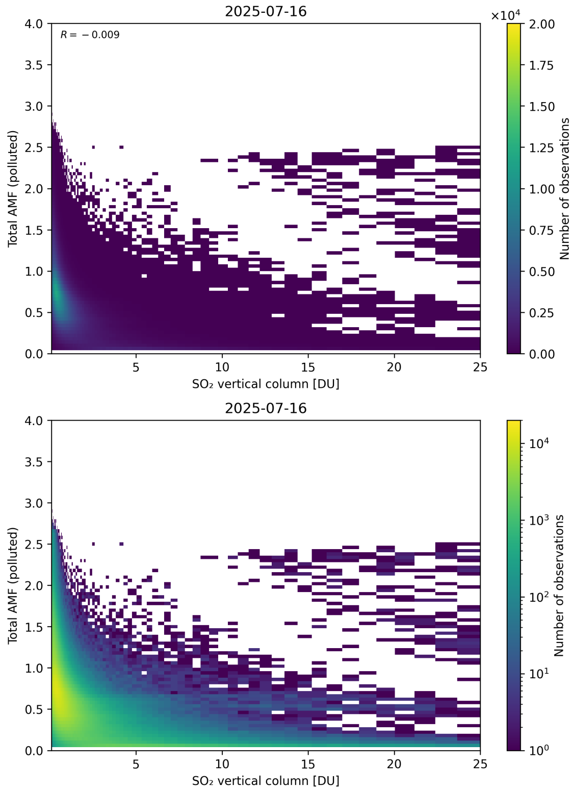
Figure 359: Scatter density plot of “SO 2 vertical column” against “Total AMF (polluted)” for 2025-07-15 to 2025-07-17.
