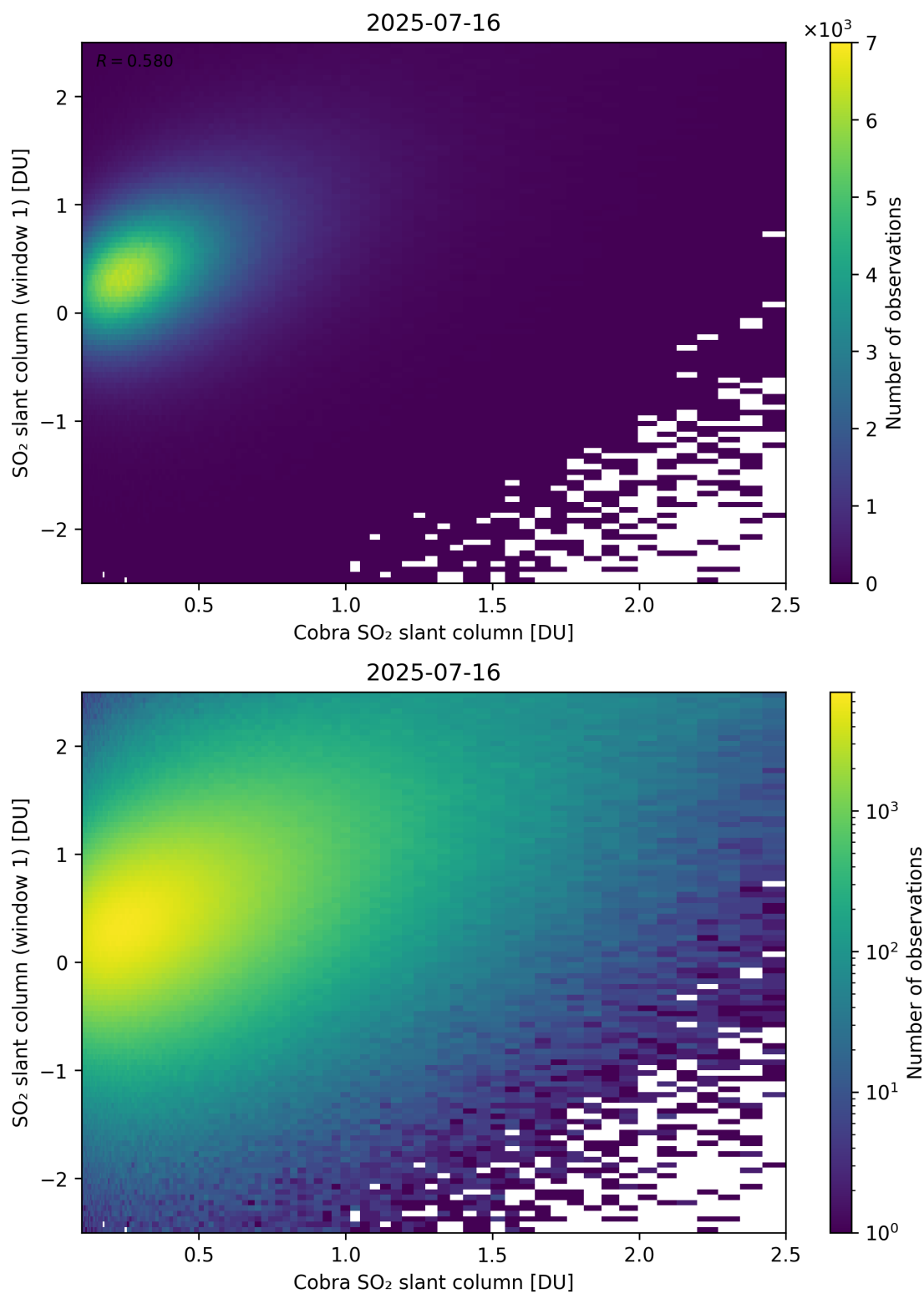
Figure 219: Scatter density plot of “Cobra SO 2 slant column” against “SO 2 slant column (window 1)” for 2025-07-15 to 2025-07-17.
