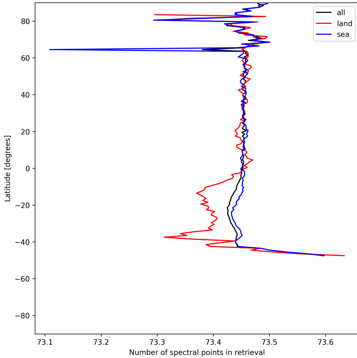
Figure 56: Zonal average of “Number of spectral points in retrieval” for 2025-07-15 to 2025-07-17.
