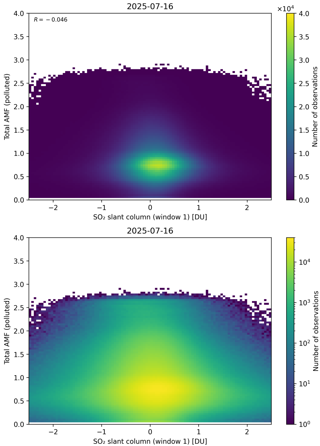
Figure 289: Scatter density plot of “SO 2 slant column (window 1)” against “Total AMF (polluted)” for 2025-07-15 to 2025-07-17.
