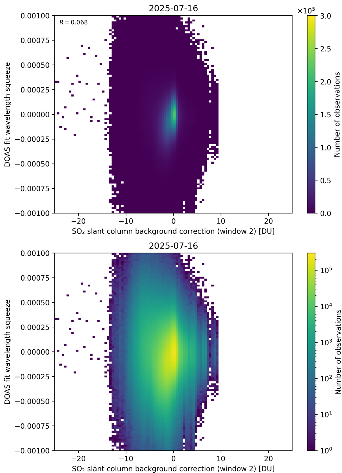
Figure 124: Scatter density plot of “SO 2 slant column background correction (window 2)” against “DOAS fit wavelength squeeze” for 2025-07-15 to 2025-07-17.
