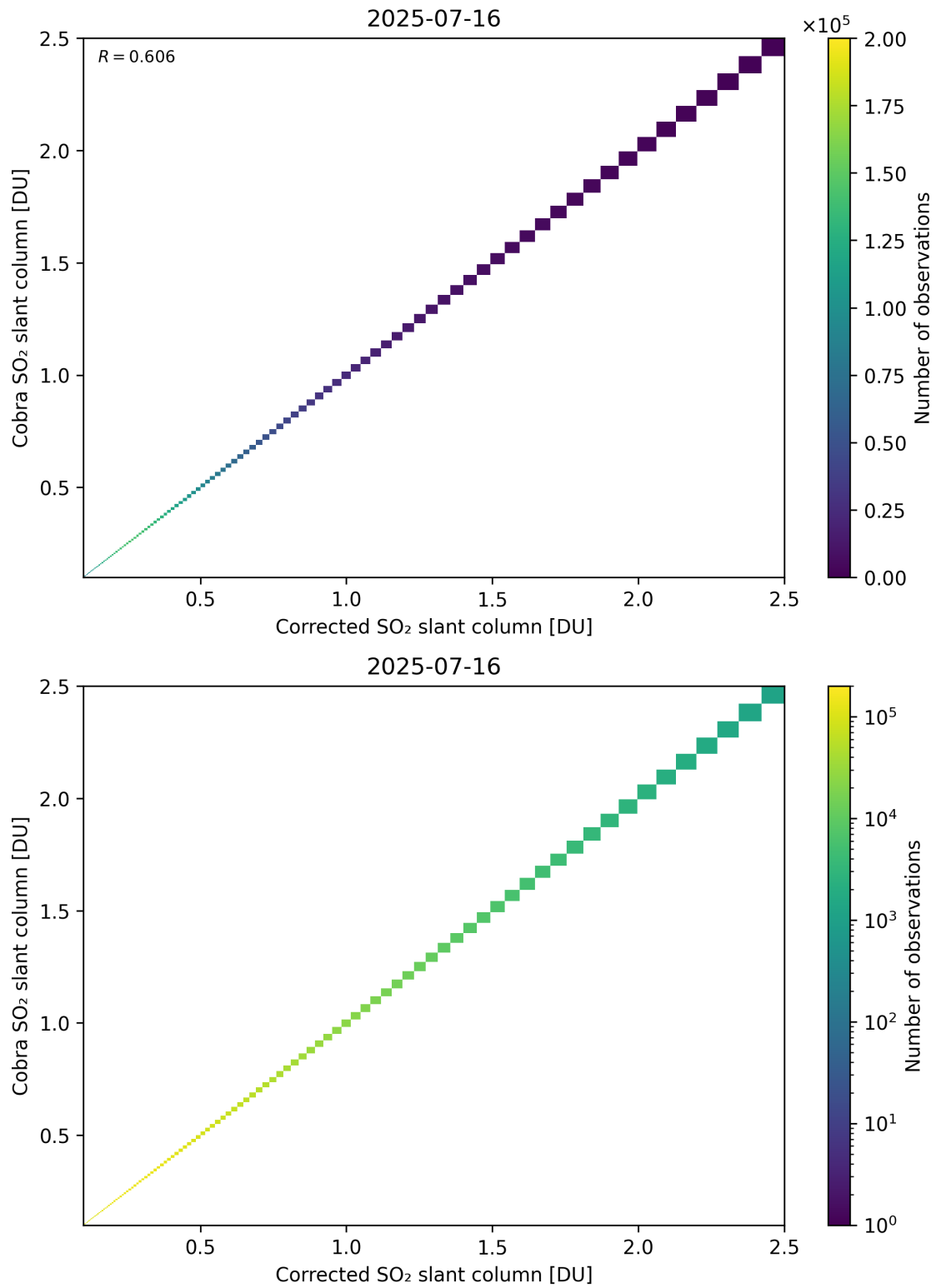
Figure 233: Scatter density plot of “Corrected SO 2 slant column” against “Cobra SO 2 slant column” for 2025-07-15 to 2025-07-17.
