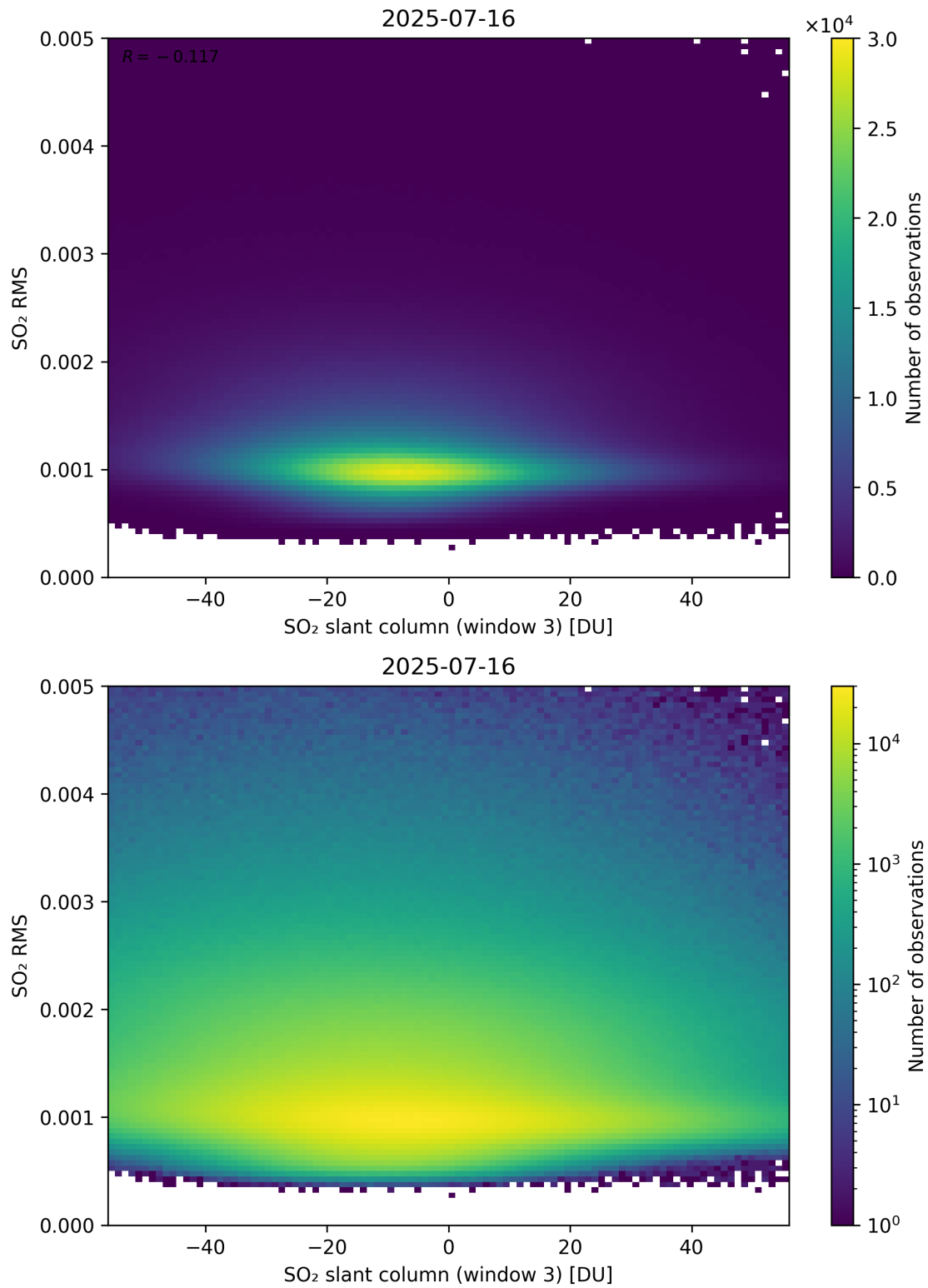
Figure 306: Scatter density plot of “SO 2 slant column (window 3)” against “SO 2 RMS” for 2025-07-15 to 2025-07-17.
