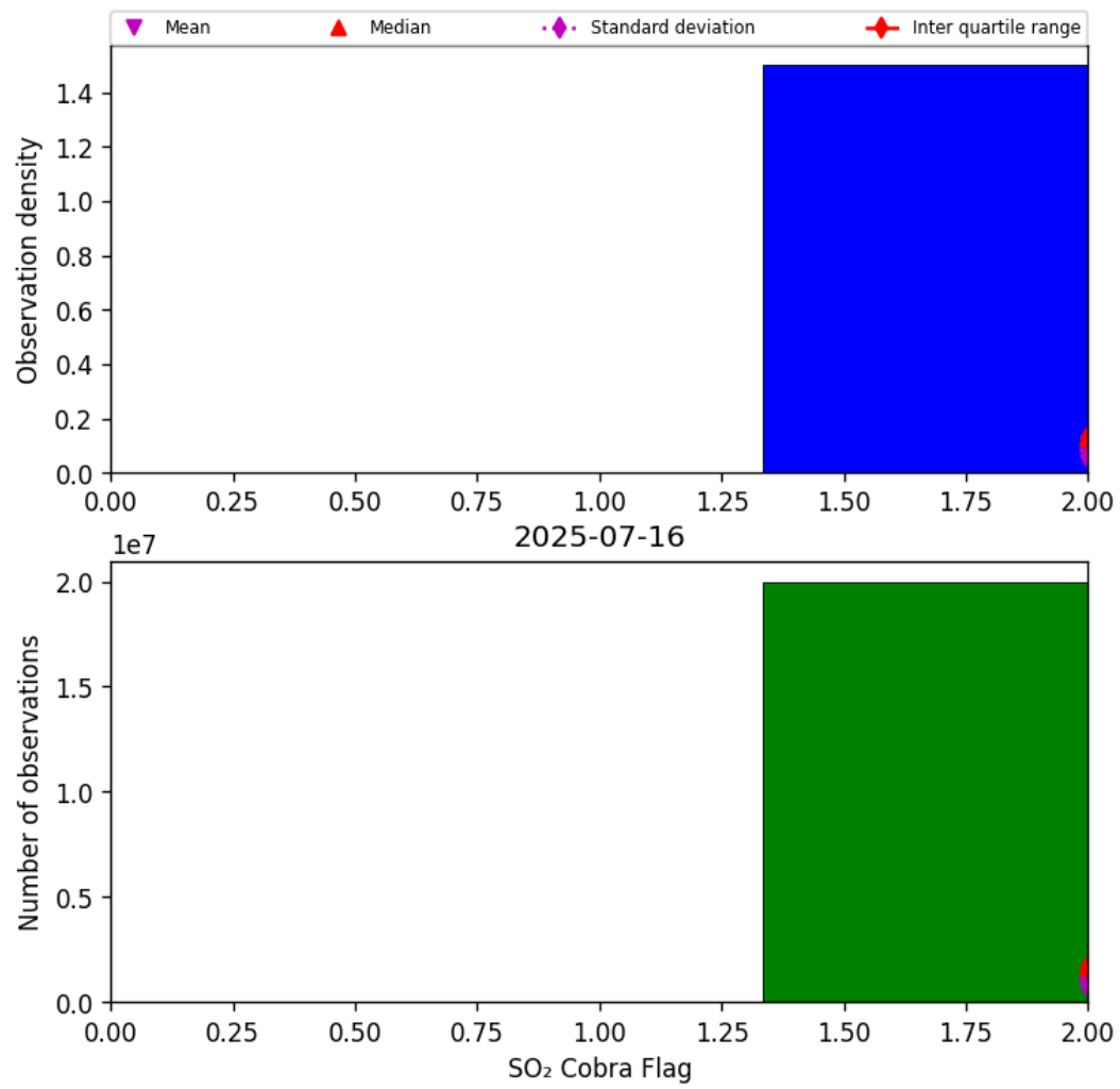
Figure 75: Histogram of “SO 2 Cobra Flag” for 2025-07-15 to 2025-07-17
