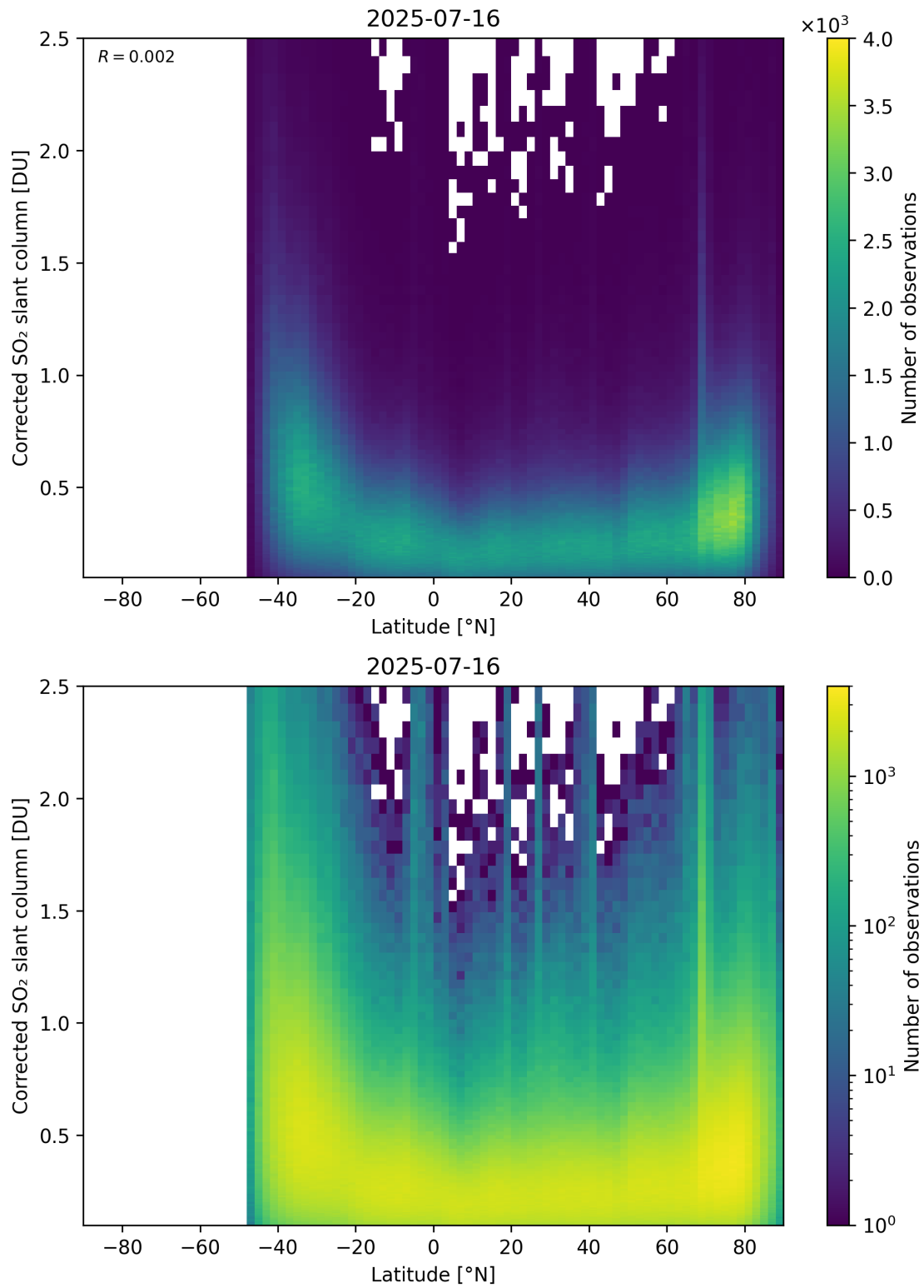
Figure 159: Scatter density plot of “Latitude” against “Corrected SO 2 slant column” for 2025-07-15 to 2025-07-17.
