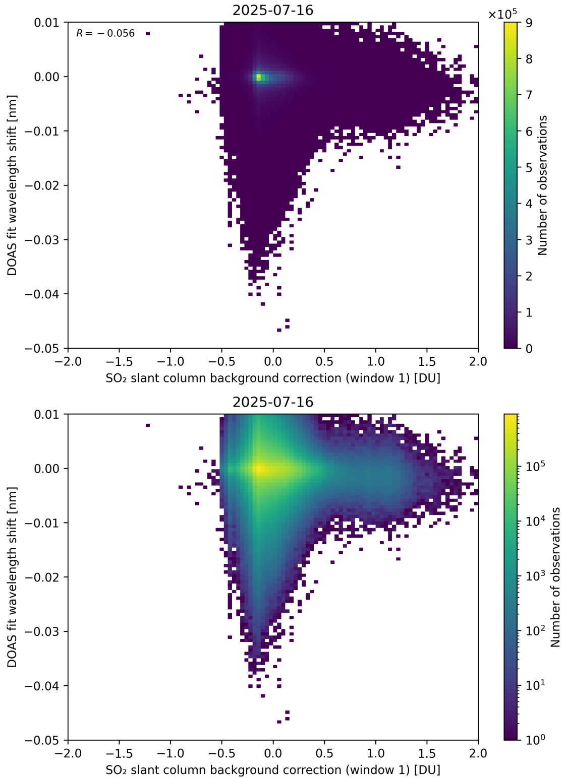
Figure 111: Scatter density plot of “SO 2 slant column background correction (window 1)” against “DOAS fit wavelength shift” for 2025-07-15 to 2025-07-17.
