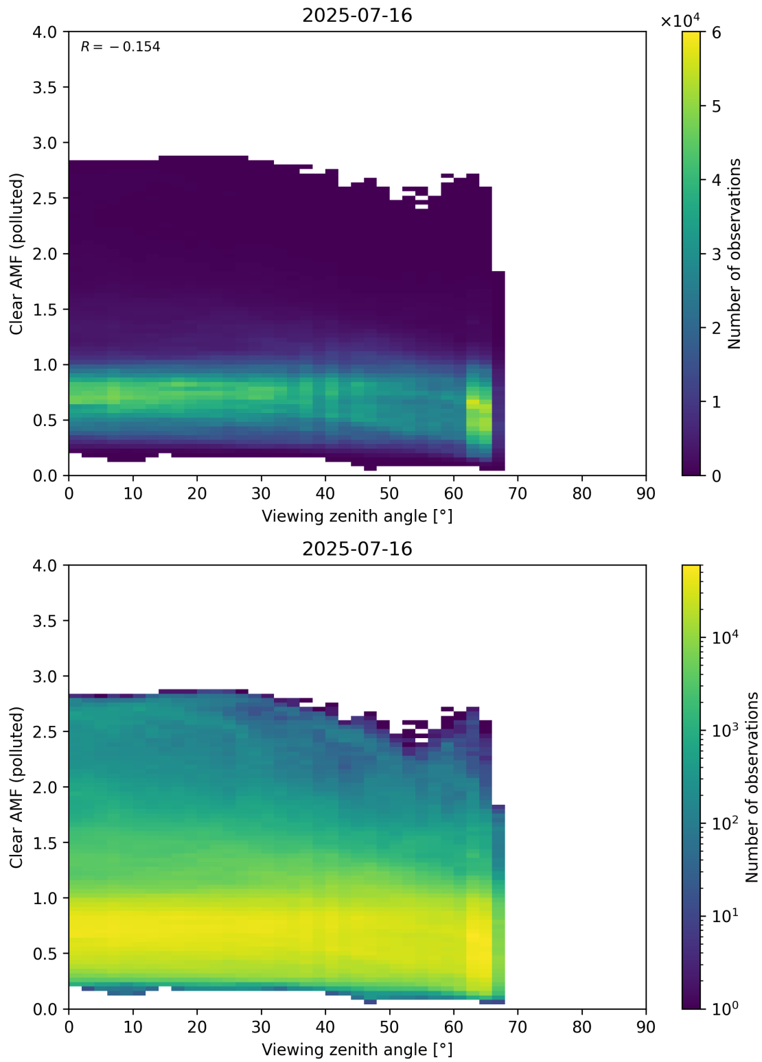
Figure 370: Scatter density plot of “Viewing zenith angle” against “Clear AMF (polluted)” for 2025-07-15 to 2025-07-17.
