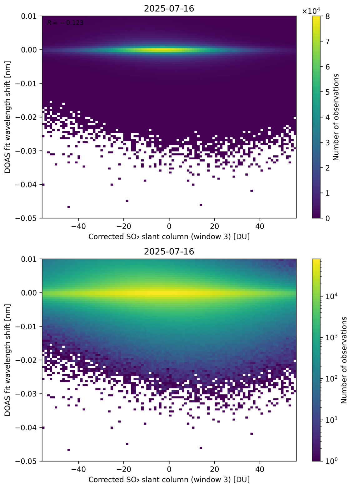
Figure 256: Scatter density plot of “Corrected SO 2 slant column (window 3)” against “DOAS fit wavelength shift” for 2025-07-15 to 2025-07-17.
