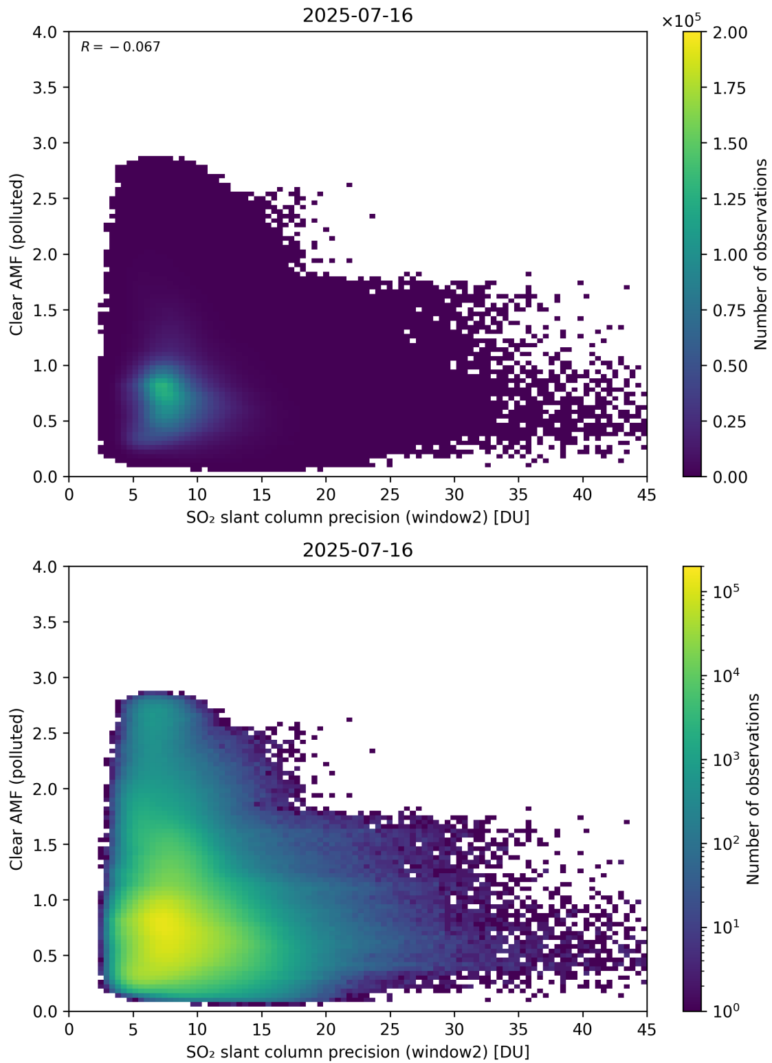
Figure 296: Scatter density plot of “SO 2 slant column precision (window2)” against “Clear AMF (polluted)” for 2025-07-15 to 2025-07-17.
