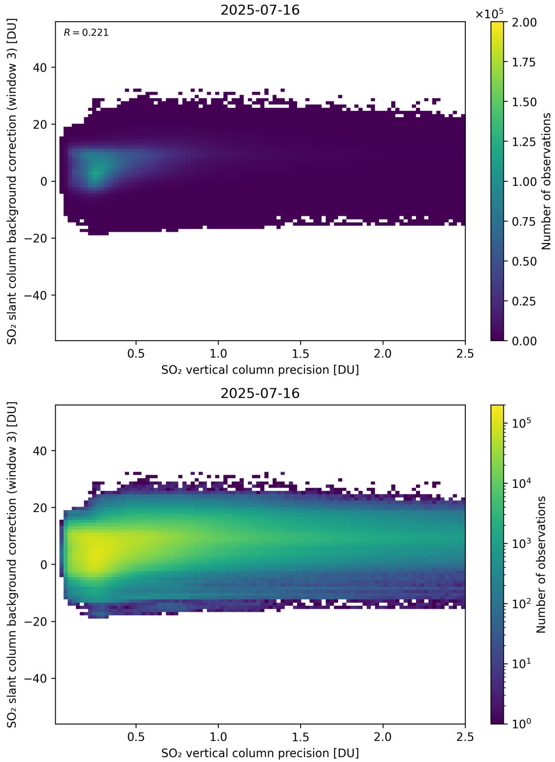
Figure 331: Scatter density plot of “SO 2 vertical column precision” against “SO 2 slant column background correction (window 3)” for 2025-07-15 to 2025-07-17.
