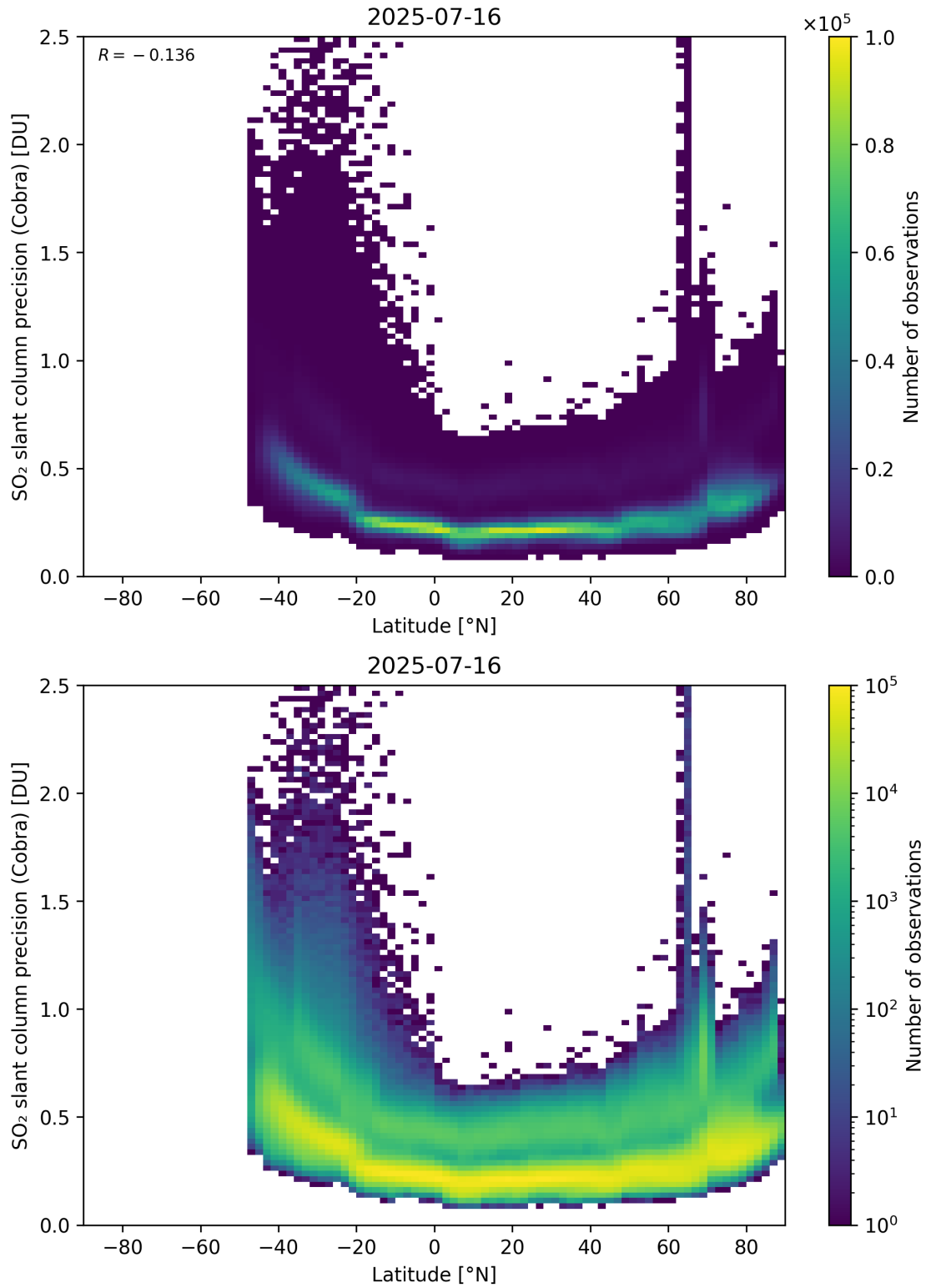
Figure 158: Scatter density plot of “Latitude” against “SO 2 slant column precision (Cobra)” for 2025-07-15 to 2025-07-17.
