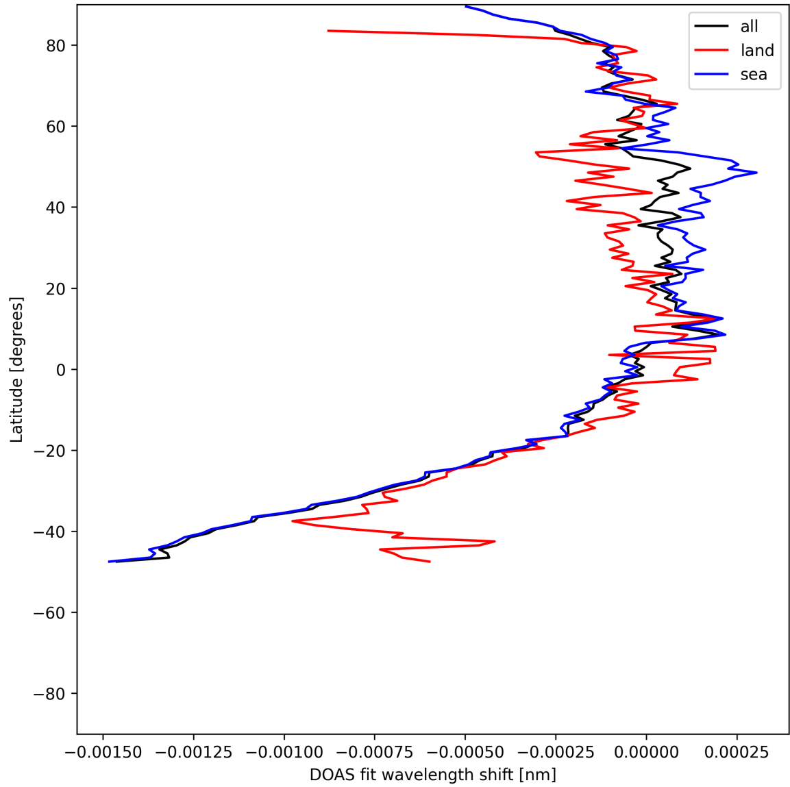
Figure 50: Zonal average of “DOAS fit wavelength shift” for 2025-07-15 to 2025-07-17.
