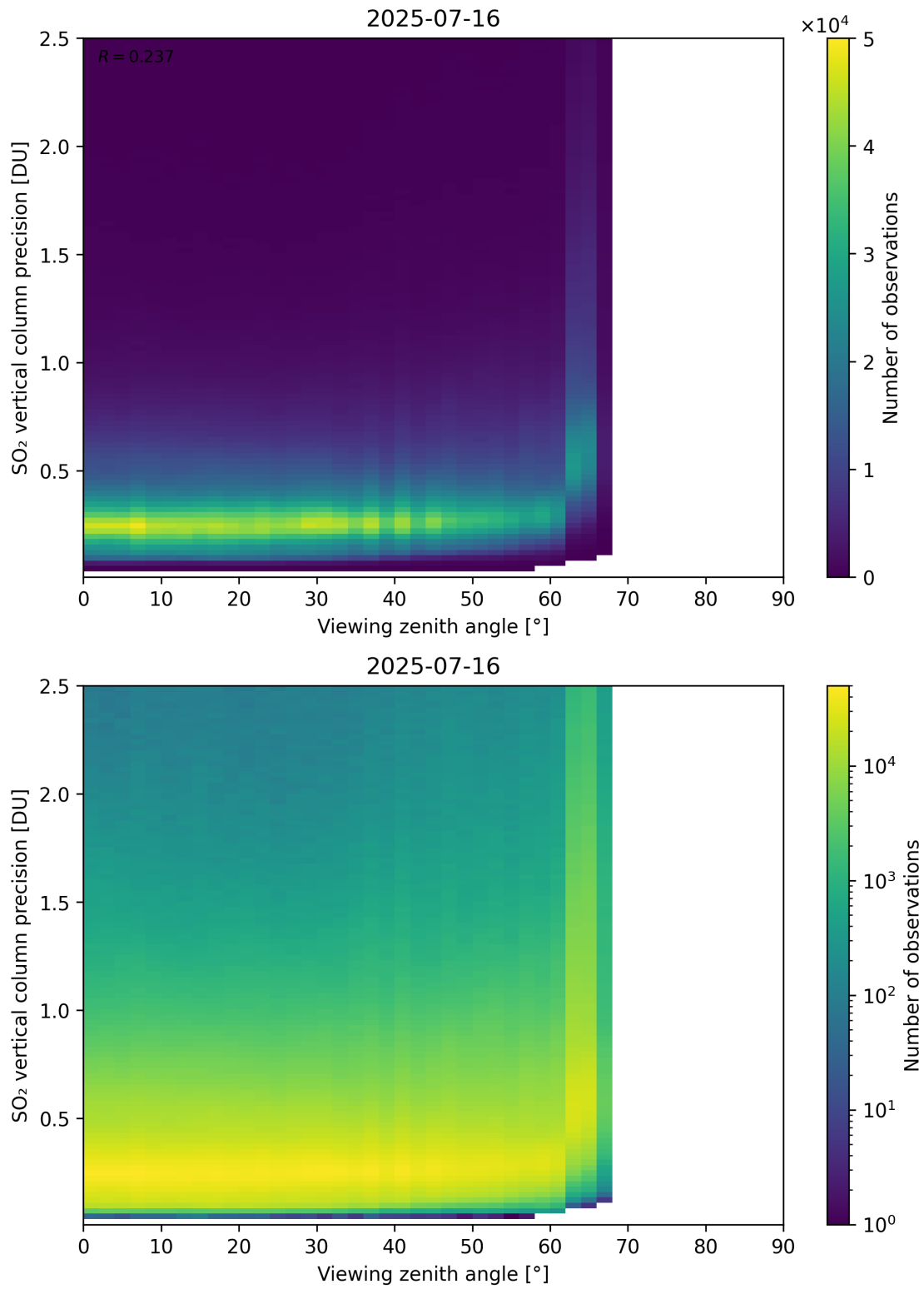
Figure 384: Scatter density plot of “Viewing zenith angle” against “SO 2 vertical column precision” for 2025-07-15 to 2025-07-17.
