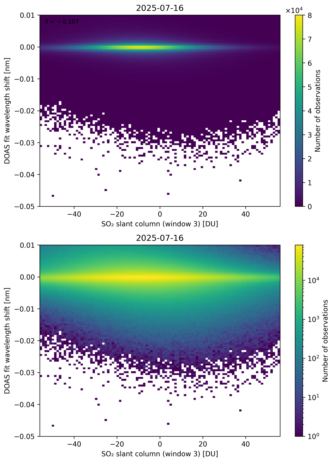
Figure 304: Scatter density plot of “SO 2 slant column (window 3)” against “DOAS fit wavelength shift” for 2025-07-15 to 2025-07-17.
