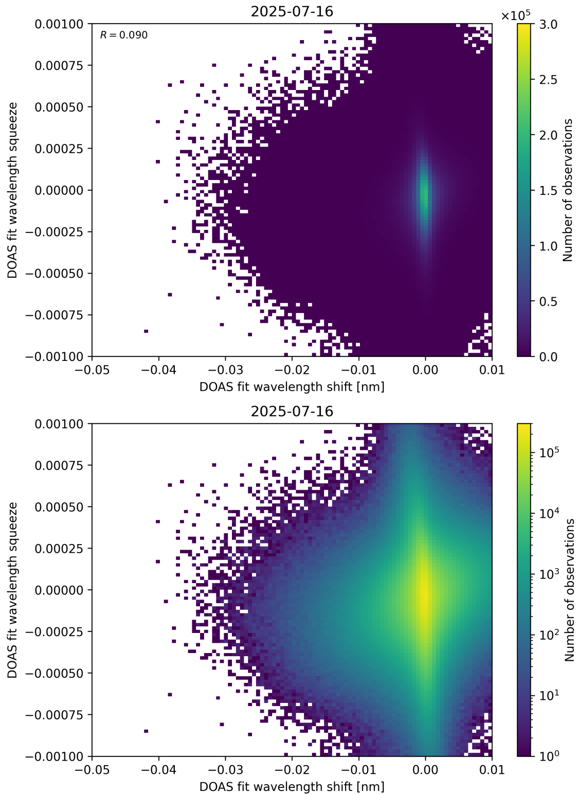
Figure 138: Scatter density plot of “DOAS fit wavelength shift” against “DOAS fit wavelength squeeze” for 2025-07-15 to 2025-07-17.
