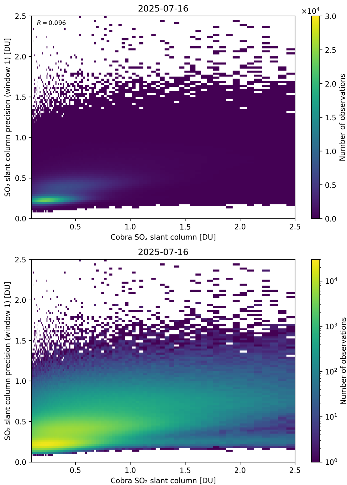
Figure 220: Scatter density plot of “Cobra SO 2 slant column” against “SO 2 slant column precision (window 1)” for 2025-07-15 to 2025-07-17.
