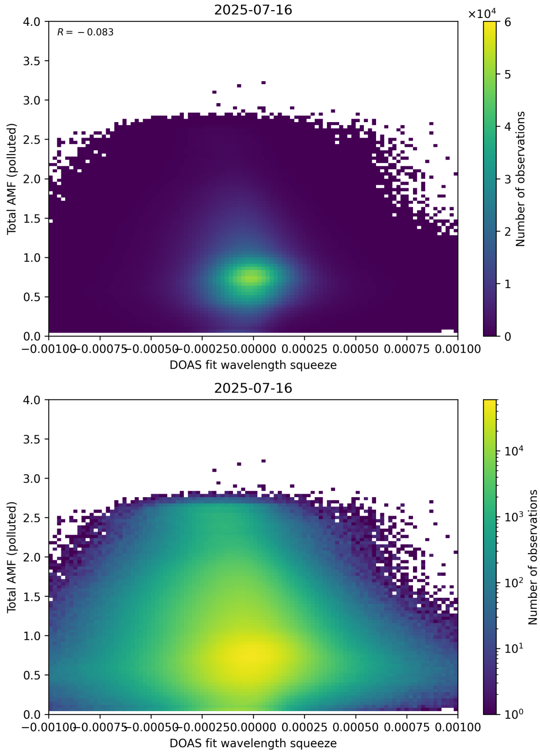
Figure 145: Scatter density plot of “DOAS fit wavelength squeeze” against “Total AMF (polluted)” for 2025-07-15 to 2025-07-17.
