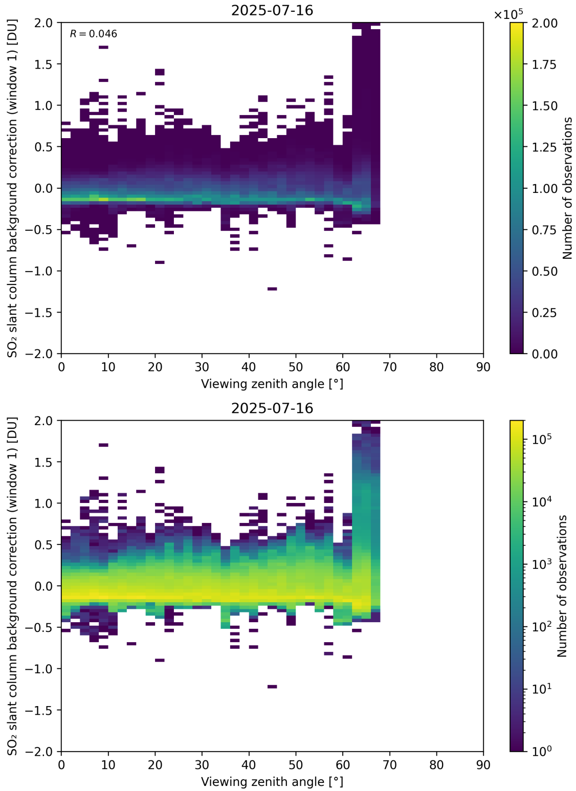
Figure 362: Scatter density plot of “Viewing zenith angle” against “SO 2 slant column background correction (window 1)” for 2025-07-15 to 2025-07-17.
