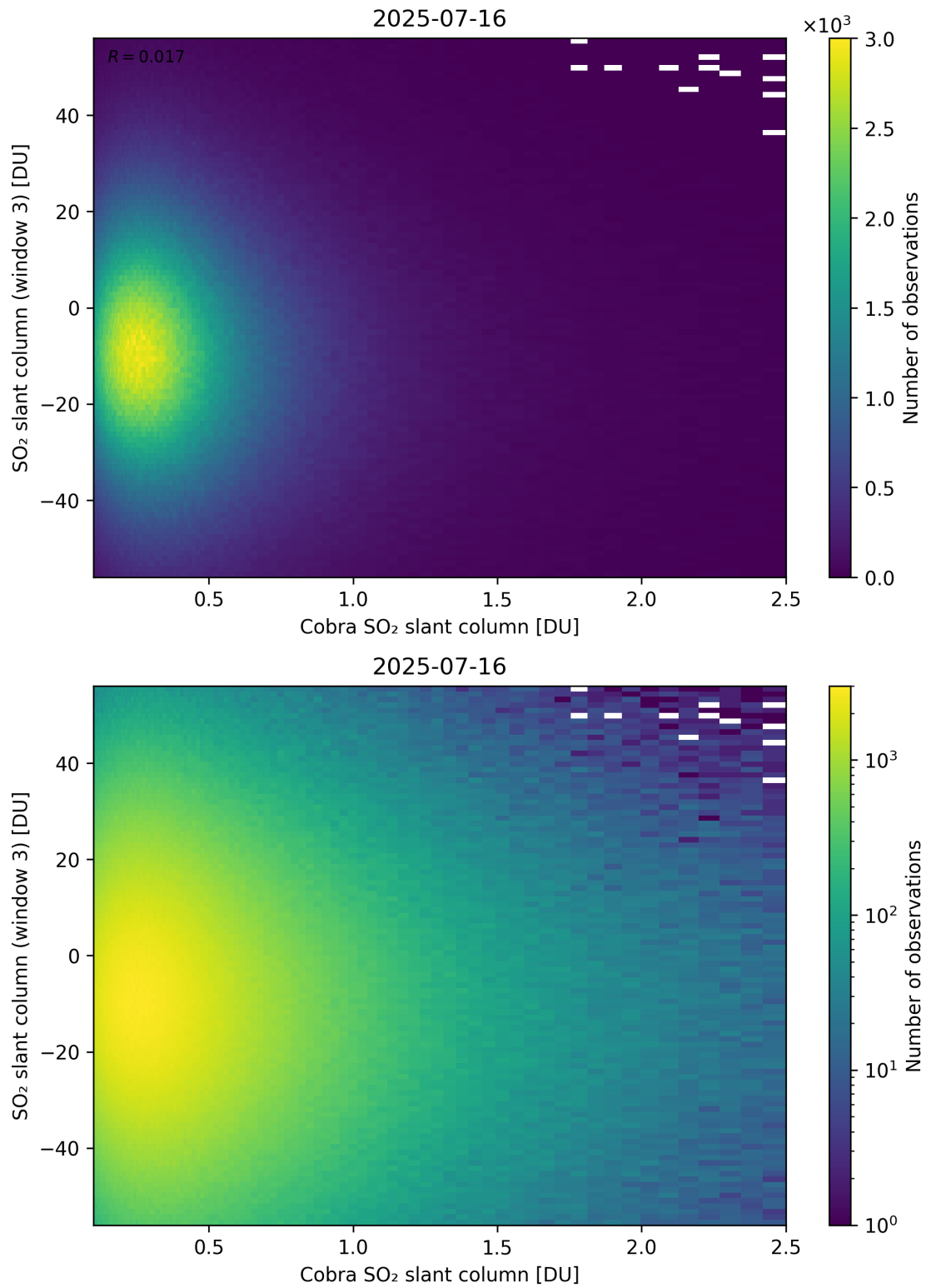
Figure 222: Scatter density plot of “Cobra SO 2 slant column” against “SO 2 slant column (window 3)” for 2025-07-15 to 2025-07-17.
