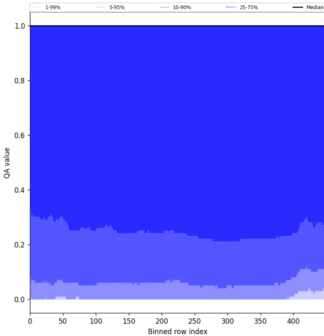
Figure 83: Along track statistics of “QA value” for 2025-07-15 to 2025-07-17
