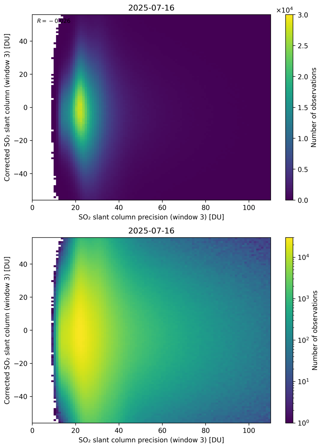
Figure 312: Scatter density plot of “SO 2 slant column precision (window 3)” against “Corrected SO 2 slant column (window 3)” for 2025-07-15 to 2025-07-17.
