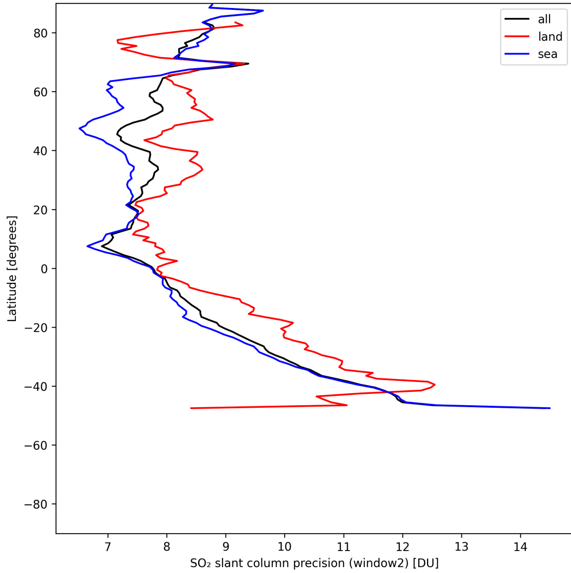
Figure 42: Zonal average of “SO 2 slant column precision (window2)” for 2025-07-15 to 2025-07-17.
