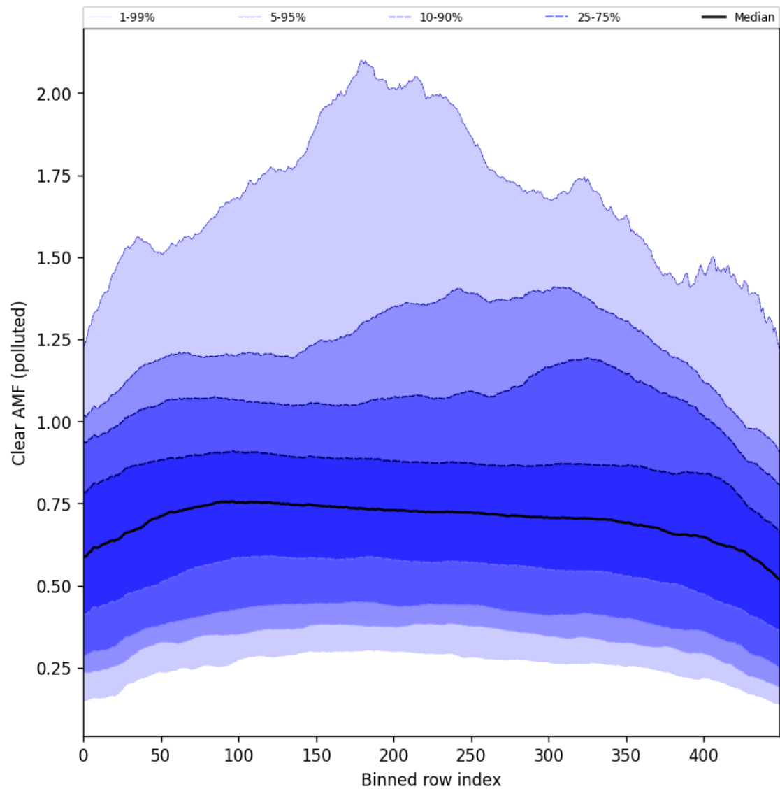
Figure 107: Along track statistics of “Clear AMF (polluted)” for 2025-07-15 to 2025-07-17
