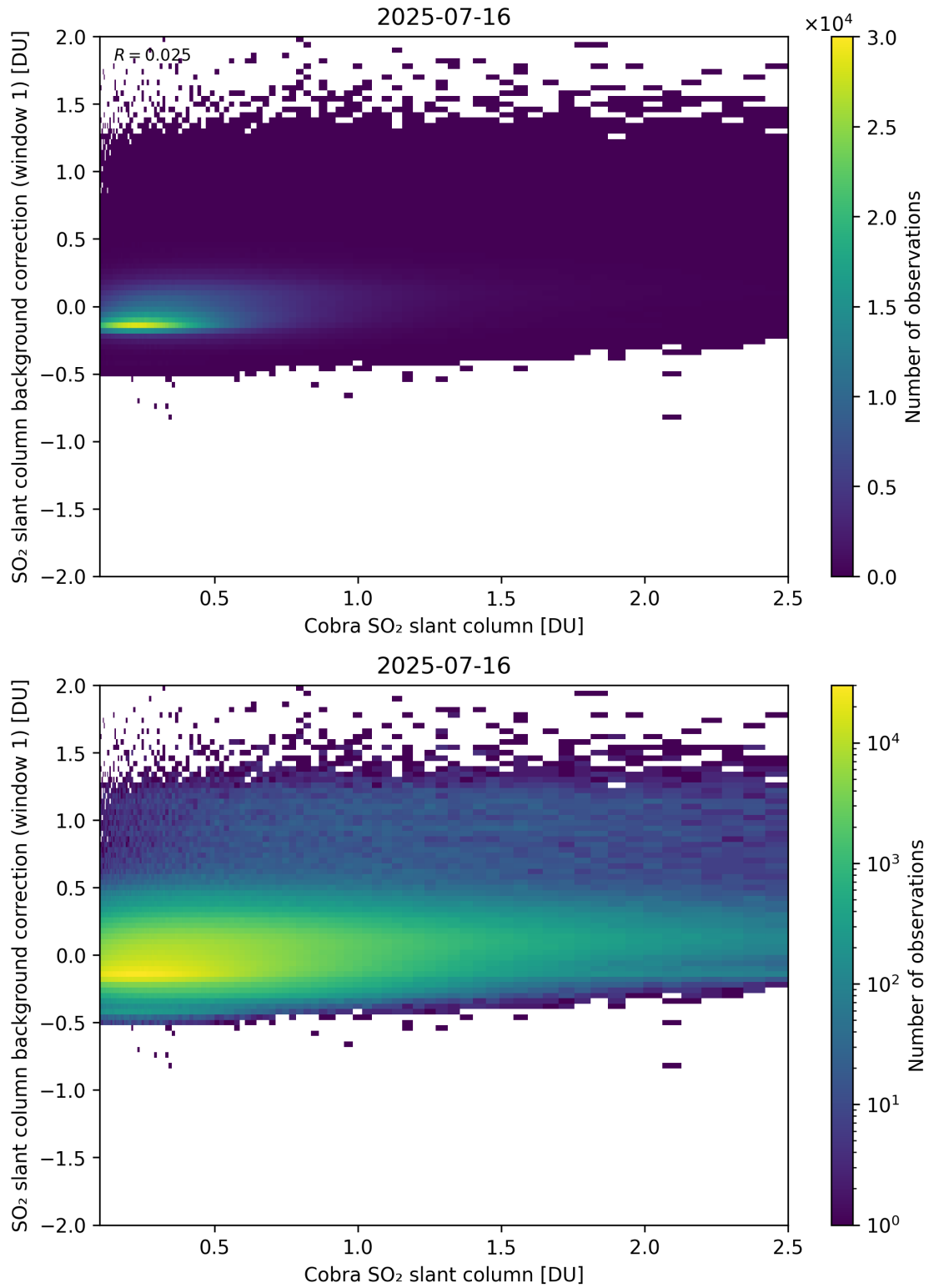
Figure 193: Scatter density plot of “Cobra SO 2 slant column” against “SO 2 slant column background correction (window 1)” for 2025-07-15 to 2025-07-17.
