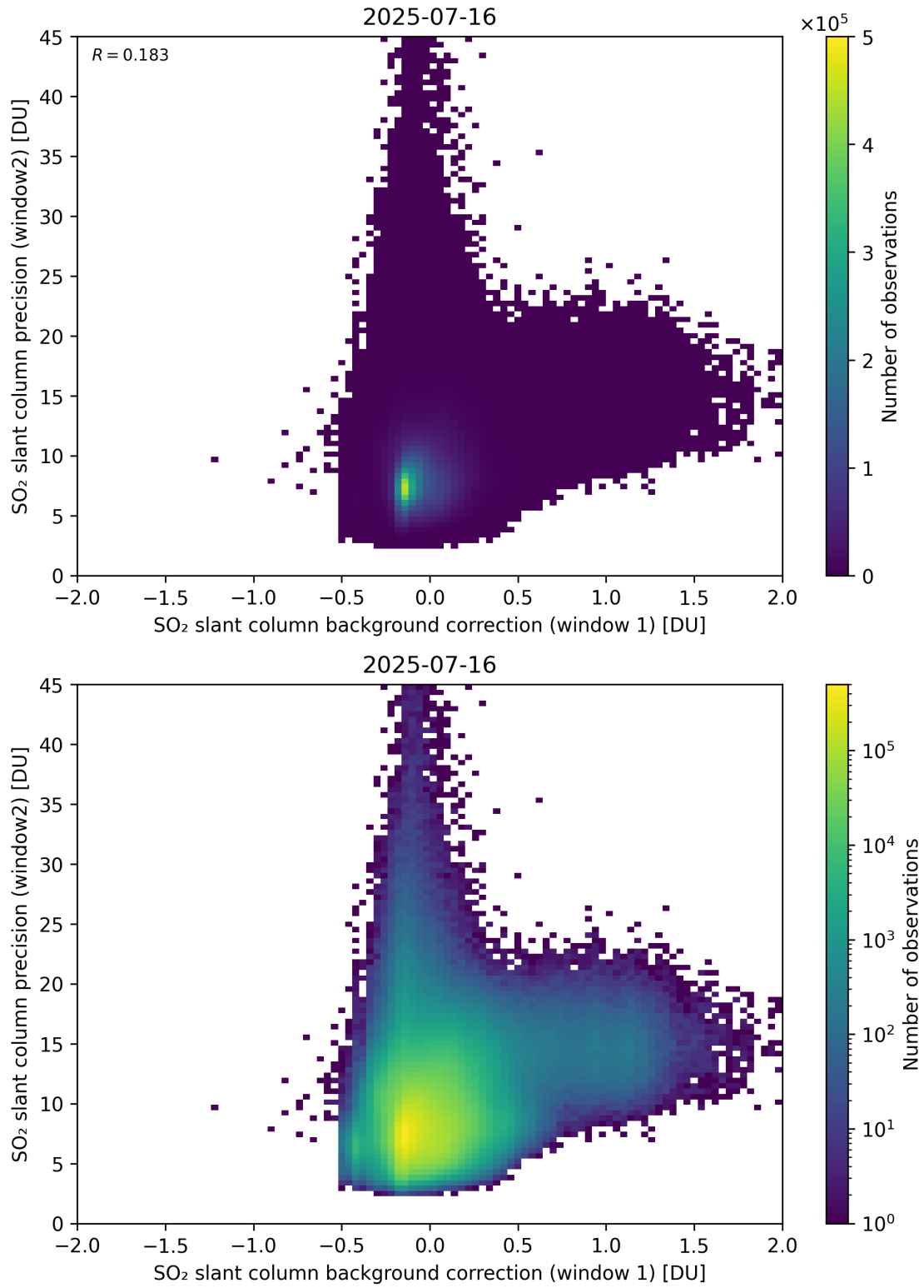
Figure 117: Scatter density plot of “SO 2 slant column background correction (window 1)” against “SO 2 slant column precision (window2)” for 2025-07-15 to 2025-07-17.
