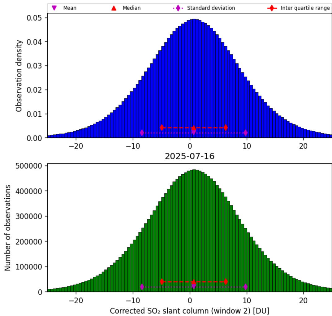
Figure 69: Histogram of “Corrected SO 2 slant column (window 2)” for 2025-07-15 to 2025-07-17
