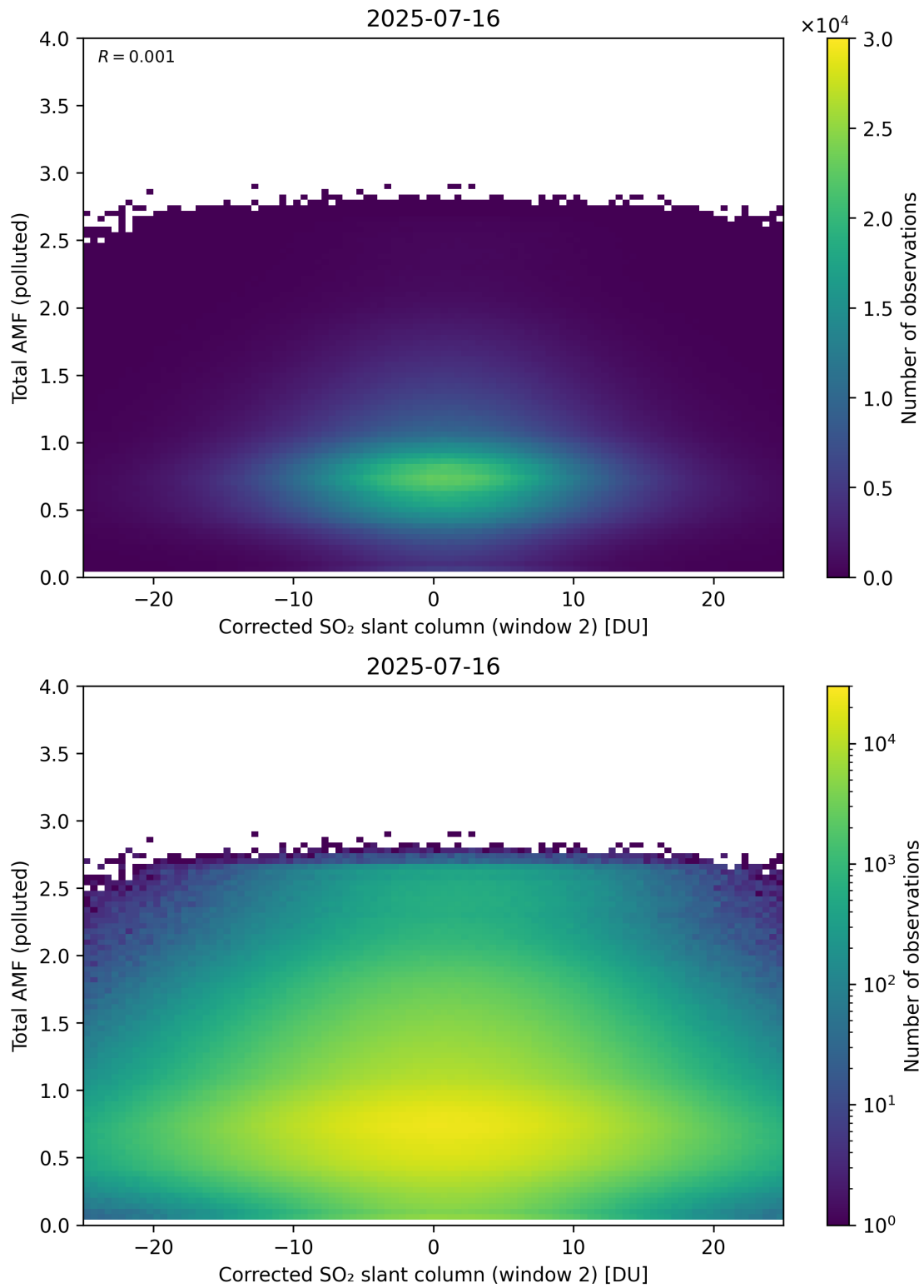
Figure 253: Scatter density plot of “Corrected SO 2 slant column (window 2)” against “Total AMF (polluted)” for 2025-07-15 to 2025-07-17.
