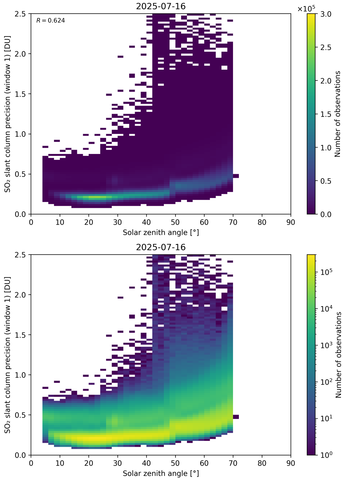
Figure 185: Scatter density plot of “Solar zenith angle” against “SO 2 slant column precision (window 1)” for 2025-07-15 to 2025-07-17.
