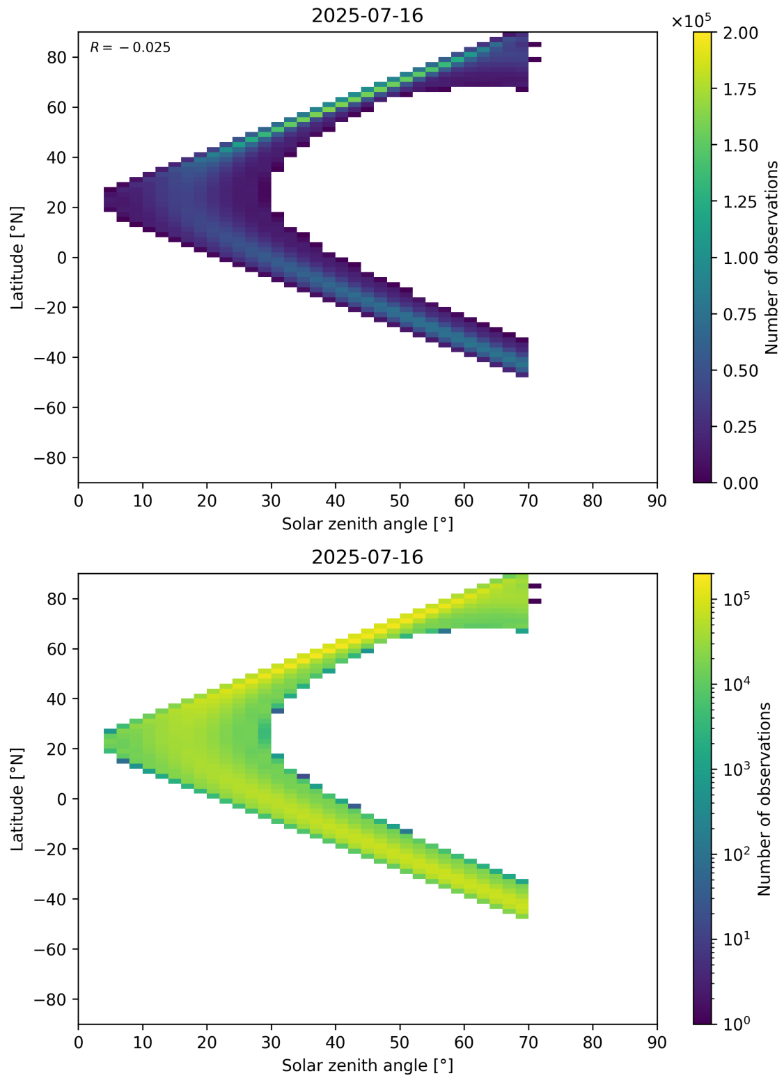
Figure 177: Scatter density plot of “Solar zenith angle” against “Latitude” for 2025-07-15 to 2025-07-17.
