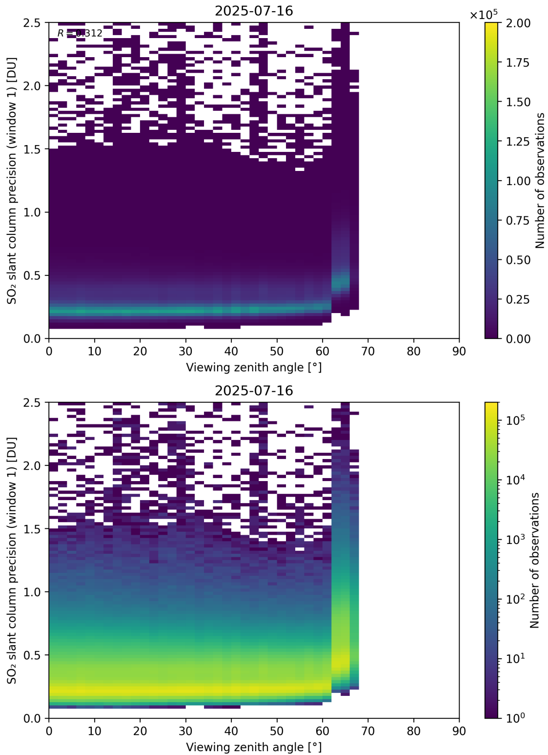
Figure 377: Scatter density plot of “Viewing zenith angle” against “SO 2 slant column precision (window 1)” for 2025-07-15 to 2025-07-17.
