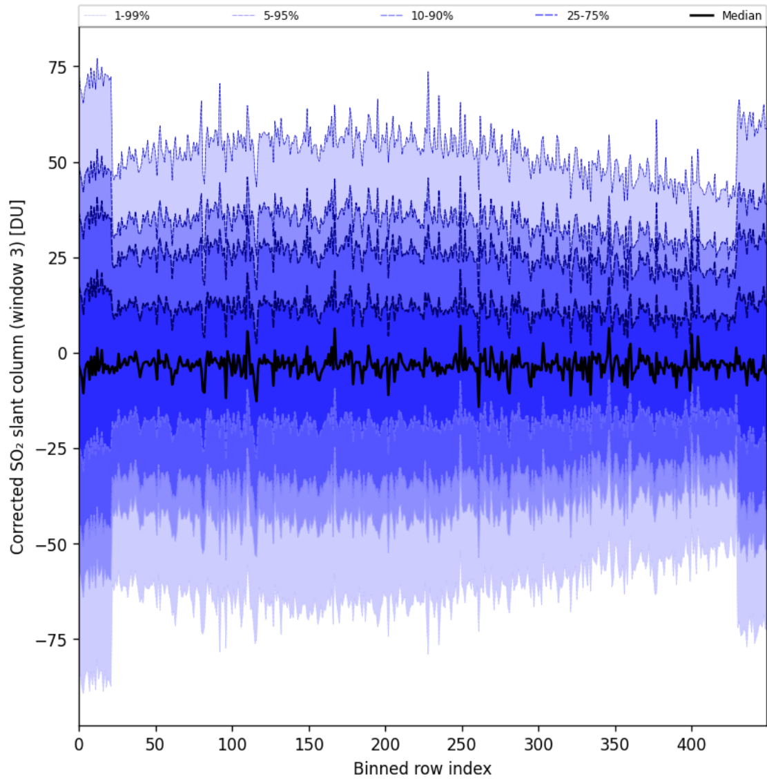
Figure 99: Along track statistics of “Corrected SO 2 slant column (window 3)” for 2025-07-15 to 2025-07-17
