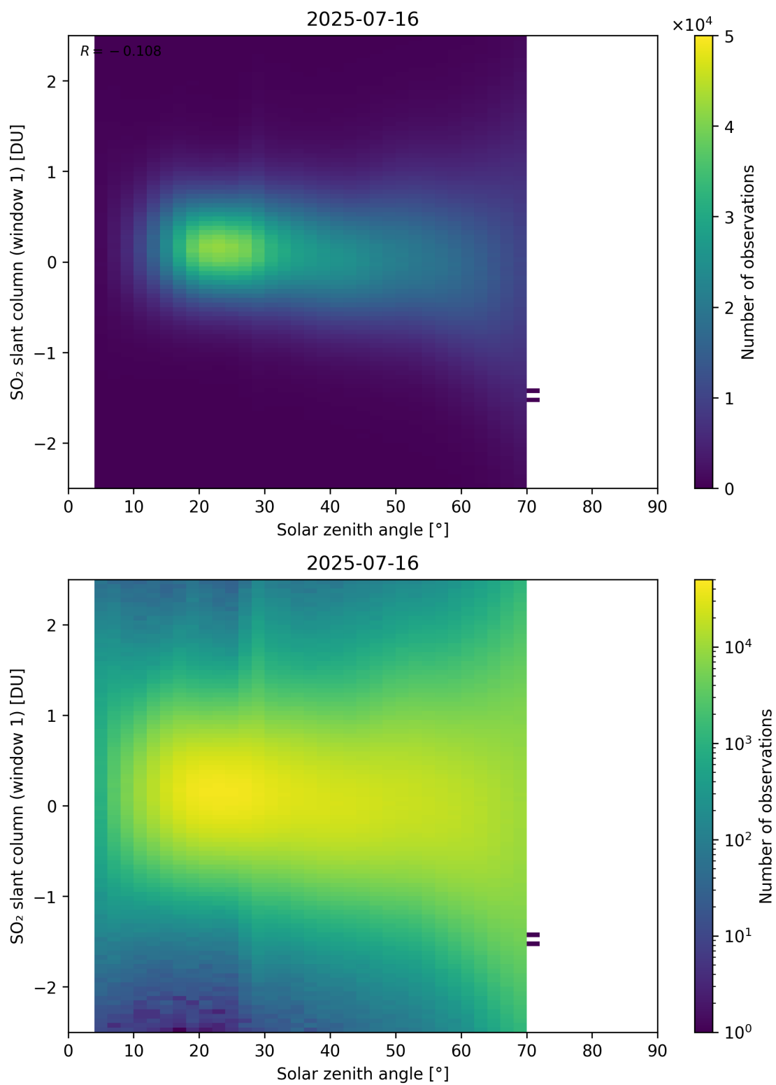
Figure 184: Scatter density plot of “Solar zenith angle” against “SO 2 slant column (window 1)” for 2025-07-15 to 2025-07-17.
