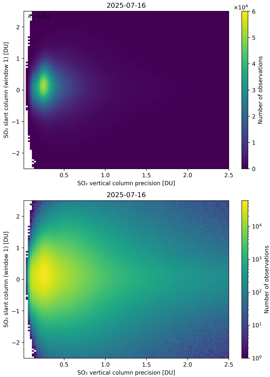
Figure 341: Scatter density plot of “SO 2 vertical column precision” against “SO 2 slant column (window 1)” for 2025-07-15 to 2025-07-17.
