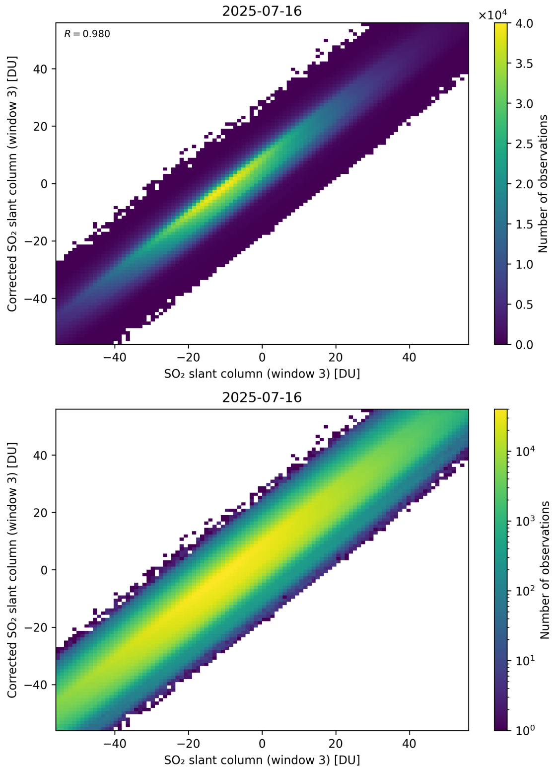
Figure 316: Scatter density plot of “SO 2 slant column (window 3)” against “Corrected SO 2 slant column (window 3)” for 2025-07-15 to 2025-07-17.
