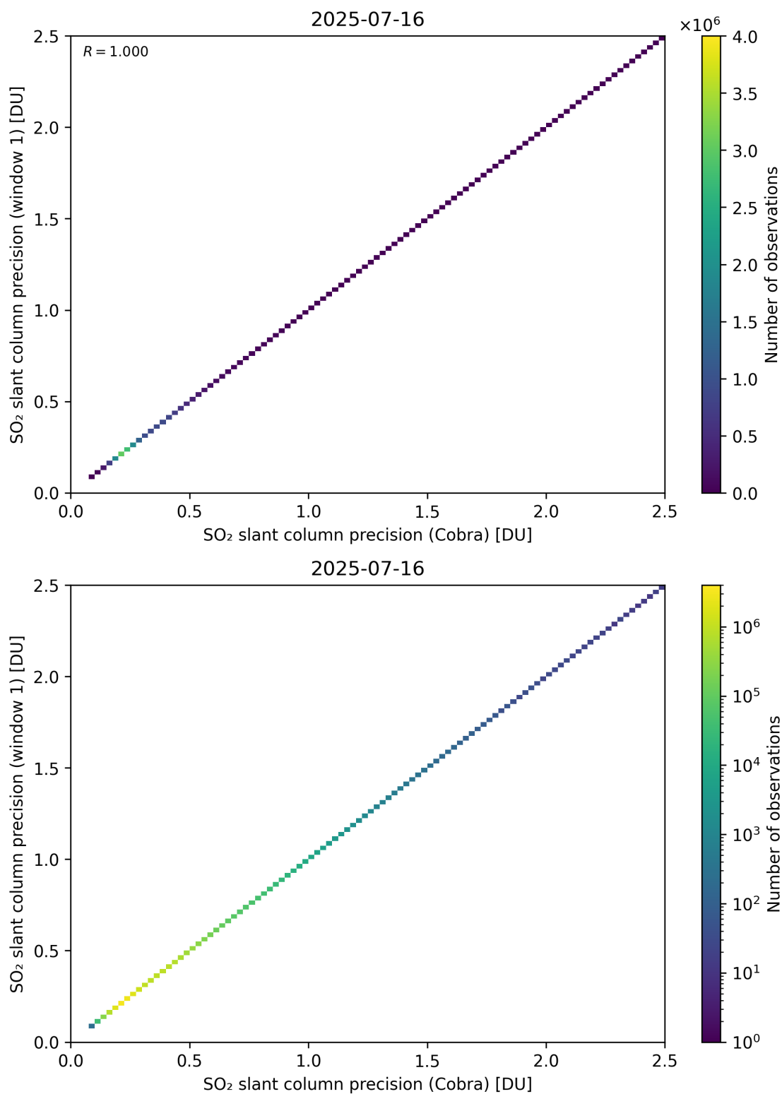
Figure 209: Scatter density plot of “SO 2 slant column precision (Cobra)” against “SO 2 slant column precision (window 1)” for 2025-07-15 to 2025-07-17.
