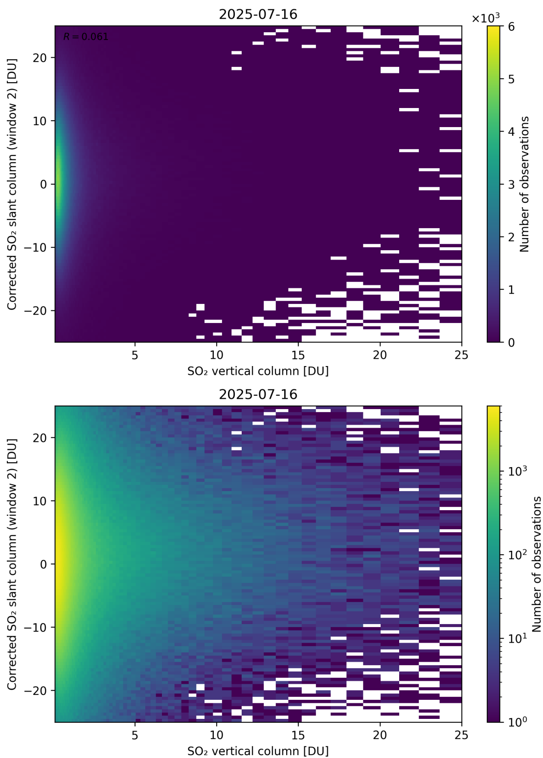
Figure 352: Scatter density plot of “SO 2 vertical column” against “Corrected SO 2 slant column (window 2)” for 2025-07-15 to 2025-07-17.
