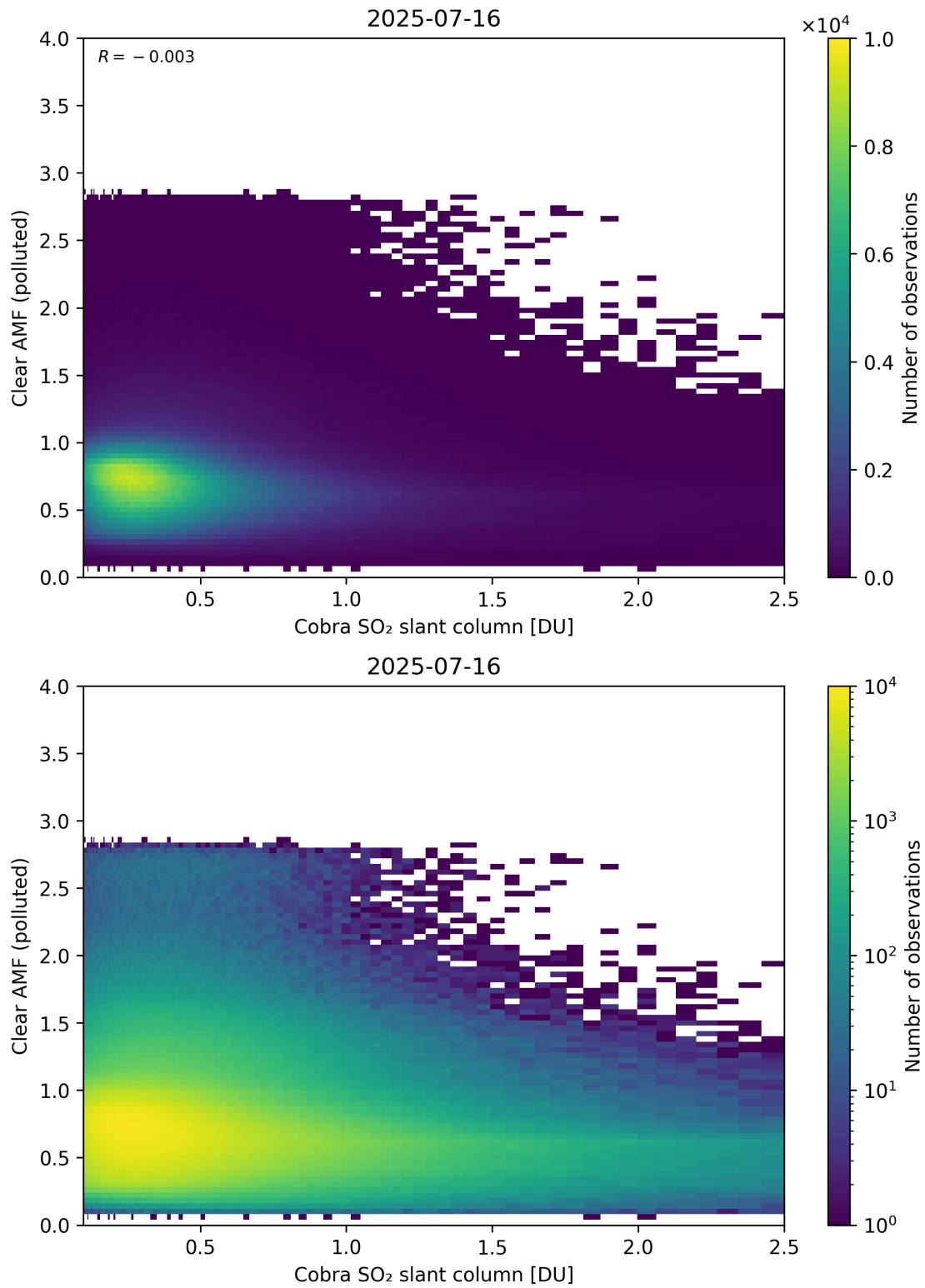
Figure 215: Scatter density plot of “Cobra SO 2 slant column” against “Clear AMF (polluted)” for 2025-07-15 to 2025-07-17.
