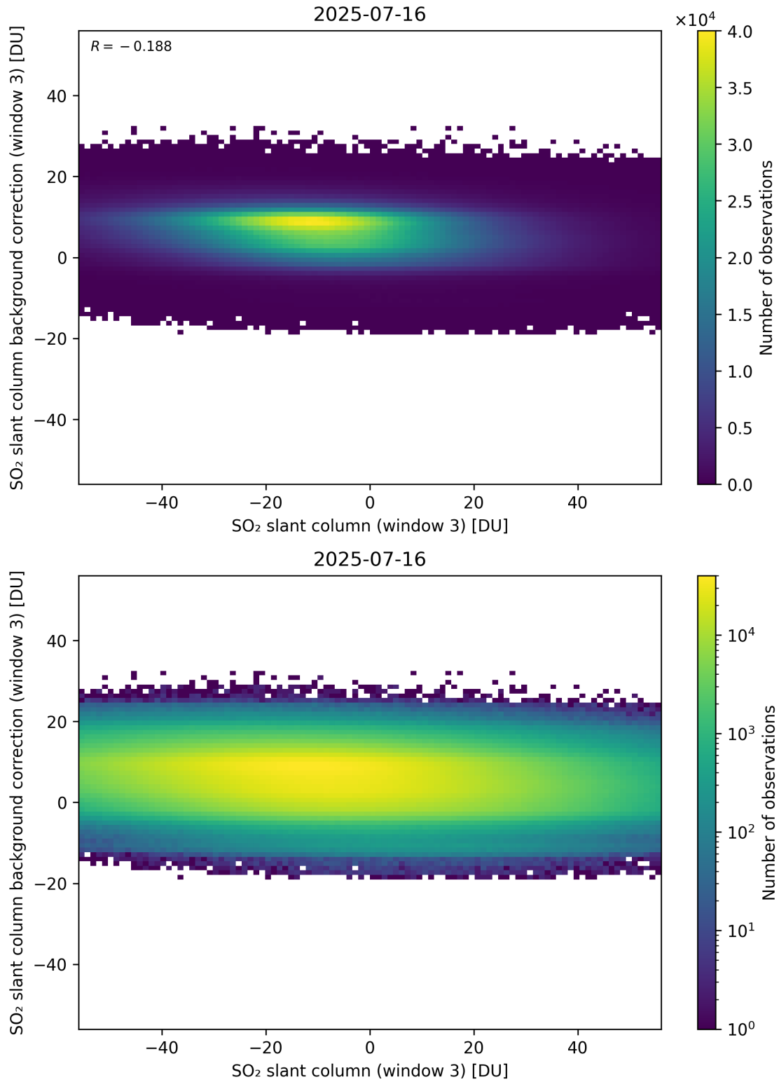
Figure 303: Scatter density plot of “SO 2 slant column (window 3)” against “SO 2 slant column background correction (window 3)” for 2025-07-15 to 2025-07-17.
