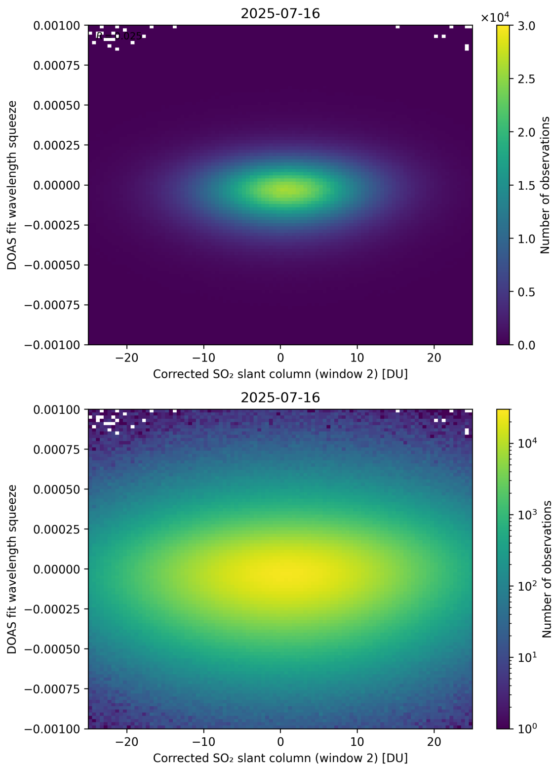
Figure 247: Scatter density plot of “Corrected SO 2 slant column (window 2)” against “DOAS fit wavelength squeeze” for 2025-07-15 to 2025-07-17.
