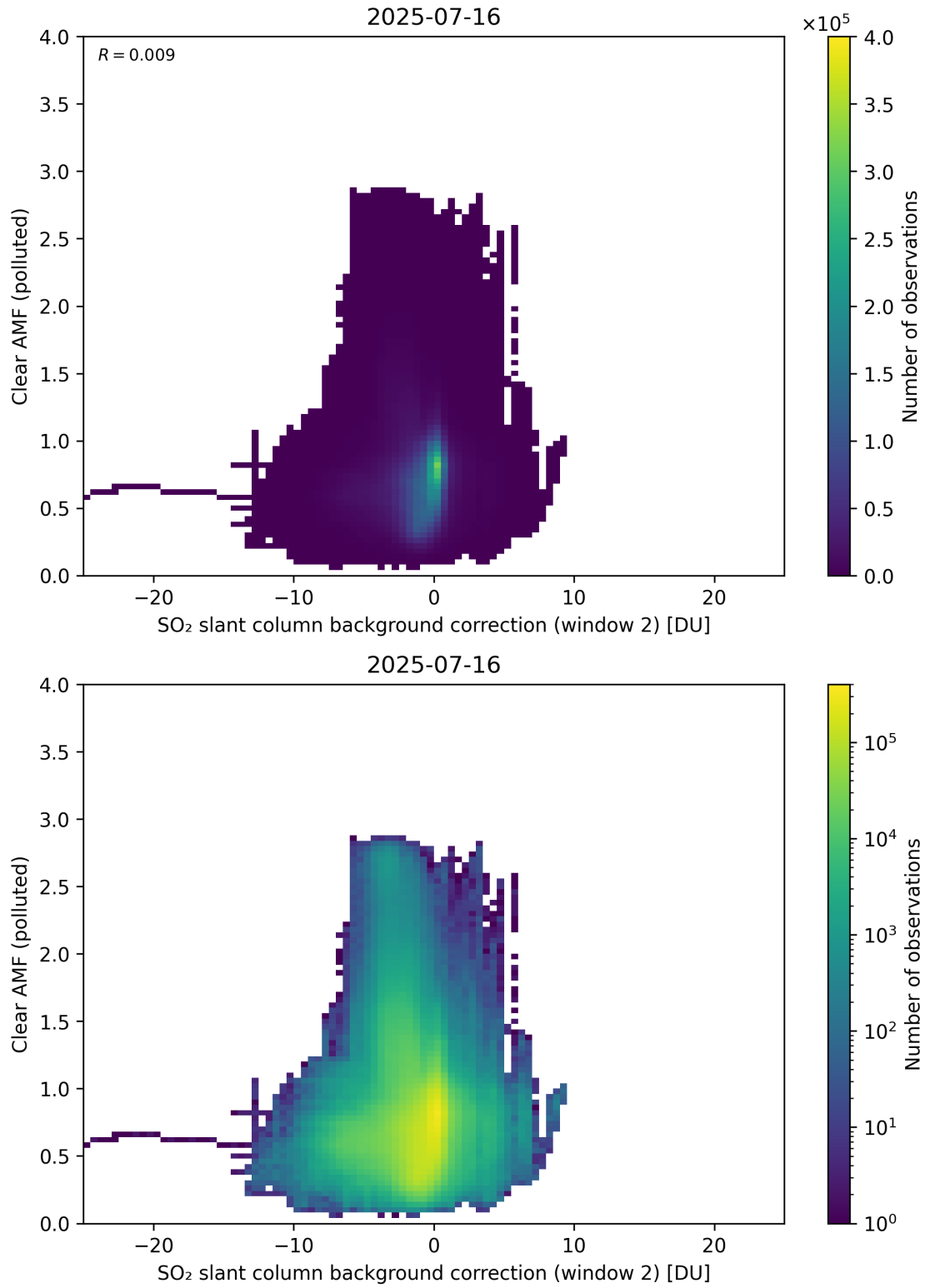
Figure 126: Scatter density plot of “SO 2 slant column background correction (window 2)” against “Clear AMF (polluted)” for 2025-07-15 to 2025-07-17.
