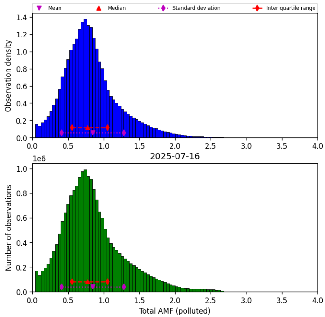
Figure 79: Histogram of “Total AMF (polluted)” for 2025-07-15 to 2025-07-17
