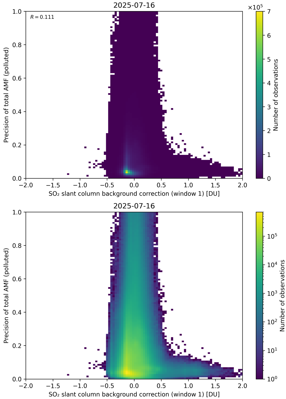
Figure 121: Scatter density plot of “SO 2 slant column background correction (window 1)” against “Precision of total AMF (polluted)” for 2025-07-15 to 2025-07-17.
