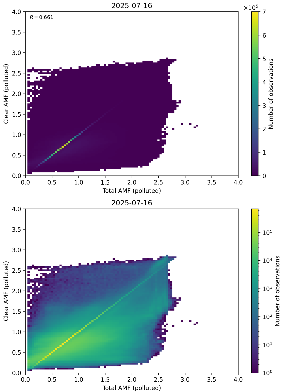
Figure 321: Scatter density plot of “Total AMF (polluted)” against “Clear AMF (polluted)” for 2025-07-15 to 2025-07-17.
