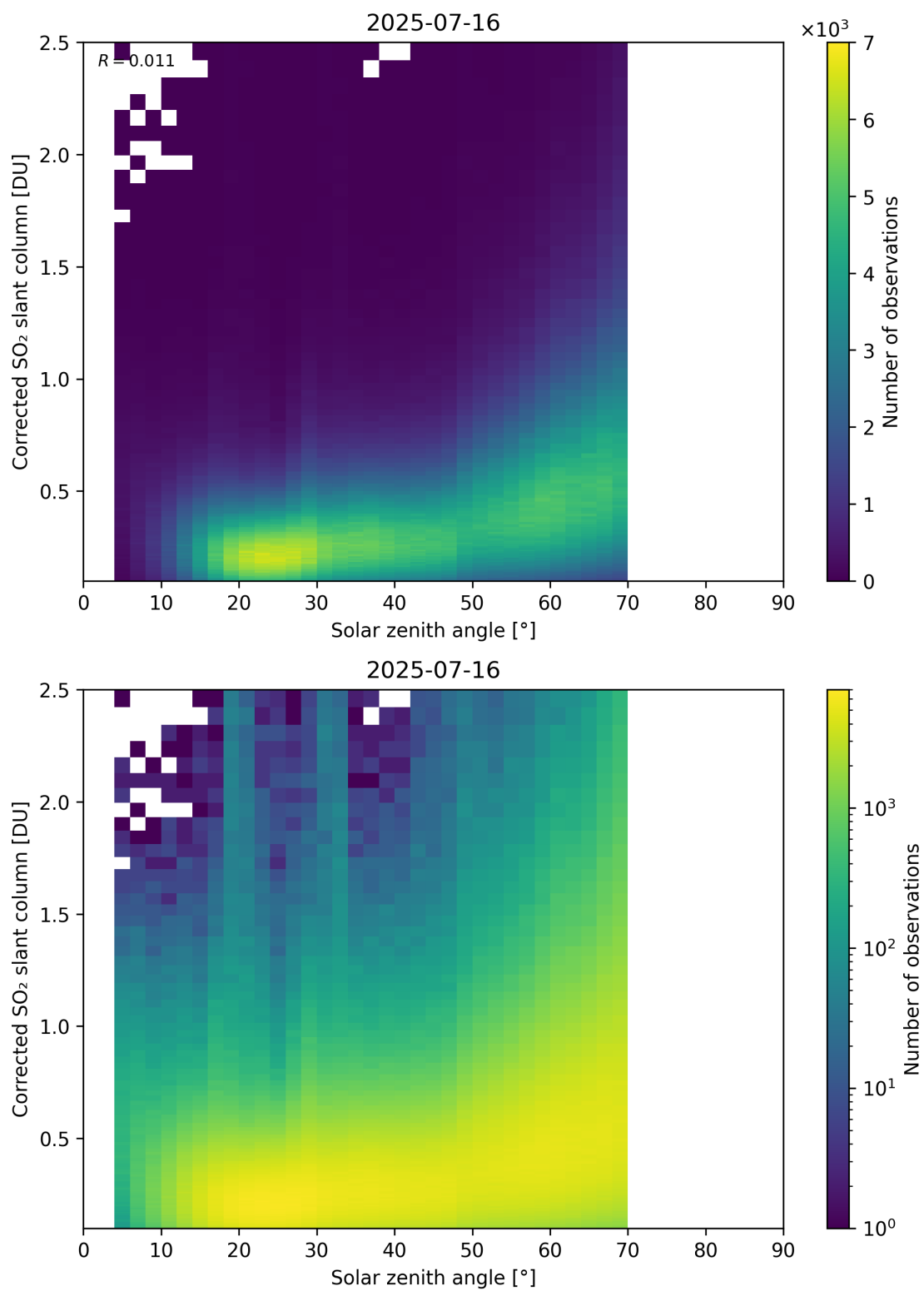
Figure 181: Scatter density plot of “Solar zenith angle” against “Corrected SO 2 slant column” for 2025-07-15 to 2025-07-17.
