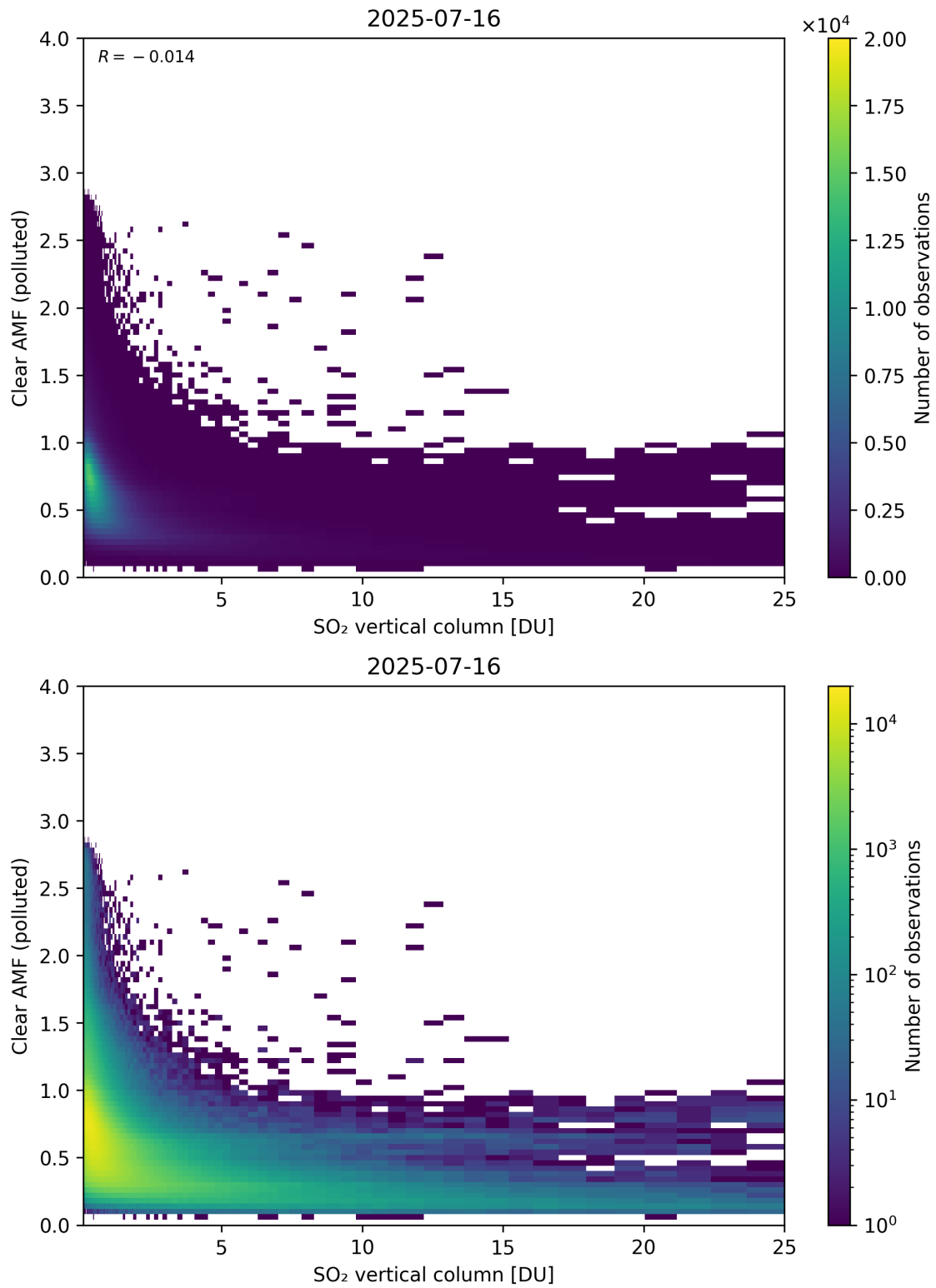
Figure 348: Scatter density plot of “SO 2 vertical column” against “Clear AMF (polluted)” for 2025-07-15 to 2025-07-17.
