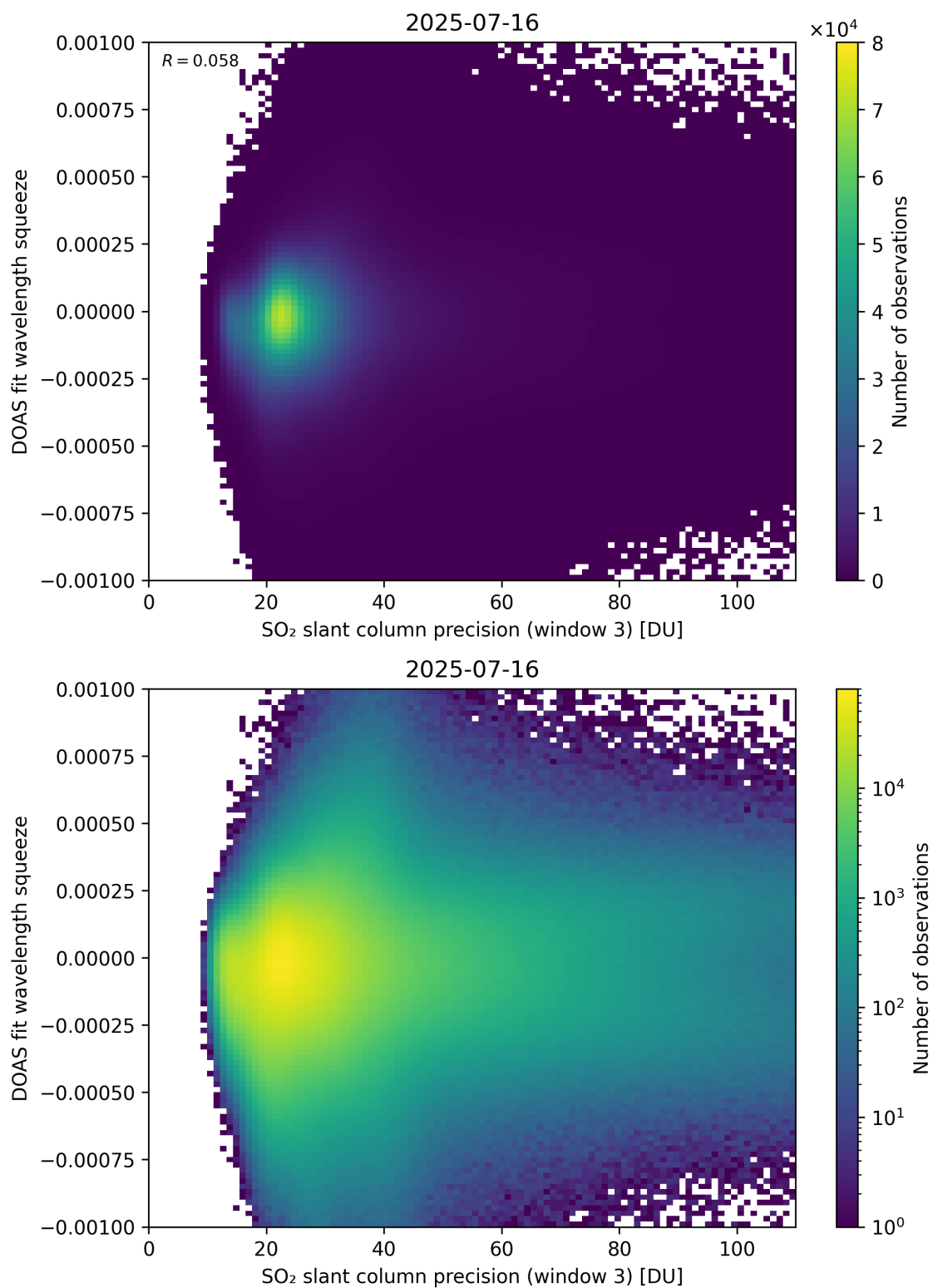
Figure 309: Scatter density plot of “SO 2 slant column precision (window 3)” against “DOAS fit wavelength squeeze” for 2025-07-15 to 2025-07-17.
