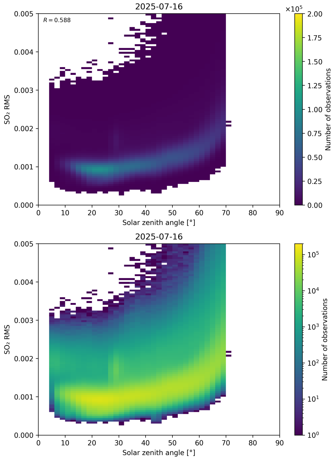
Figure 176: Scatter density plot of “Solar zenith angle” against “SO 2 RMS” for 2025-07-15 to 2025-07-17.
