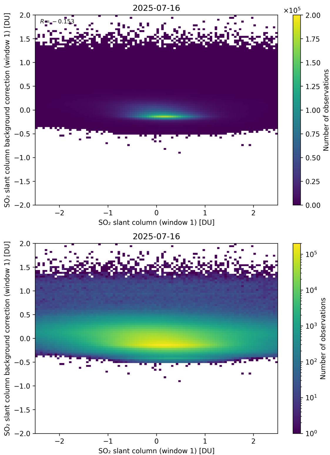
Figure 262: Scatter density plot of “SO 2 slant column (window 1)” against “SO 2 slant column background correction (window 1)” for 2025-07-15 to 2025-07-17.
