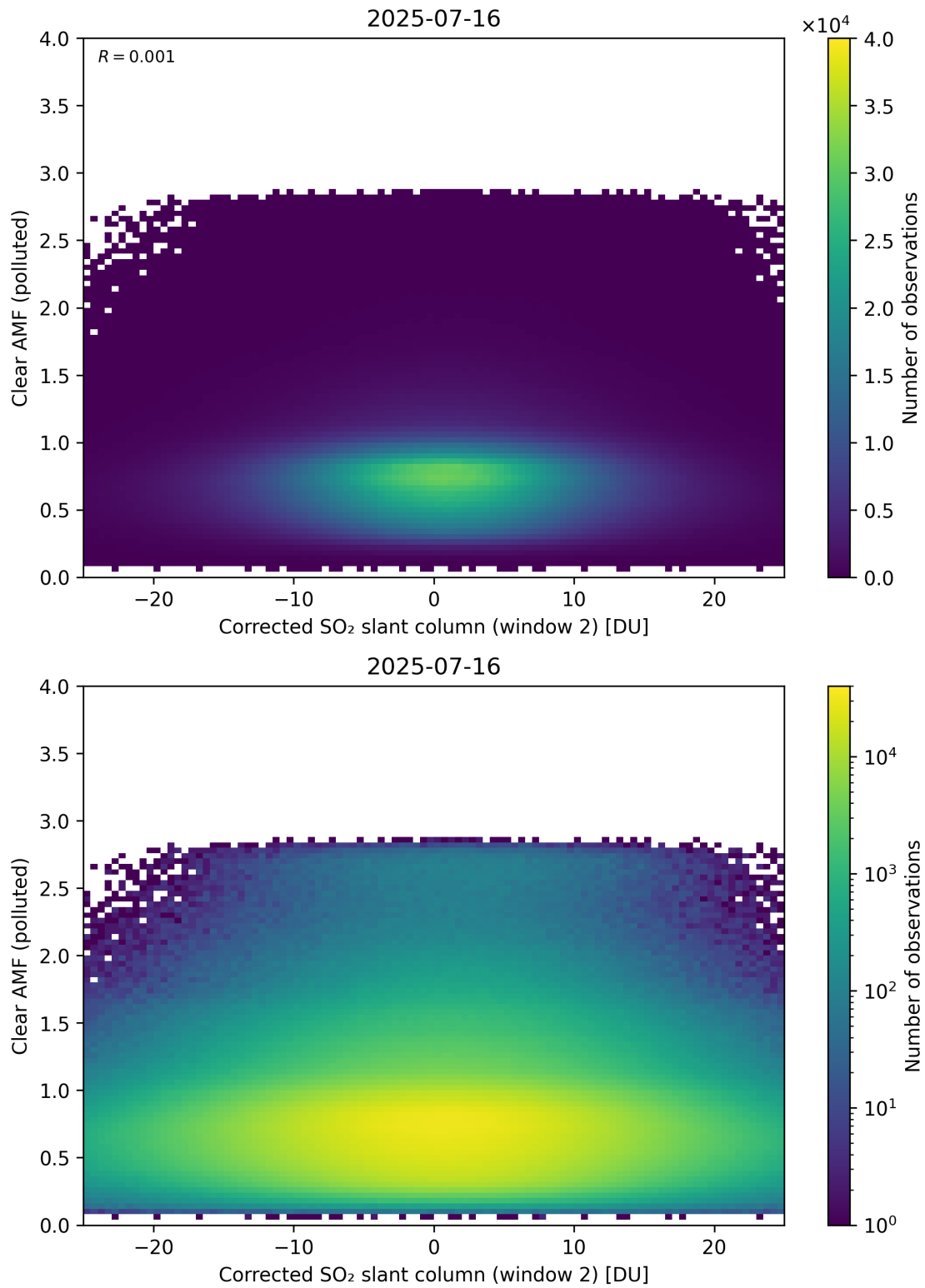
Figure 249: Scatter density plot of “Corrected SO 2 slant column (window 2)” against “Clear AMF (polluted)” for 2025-07-15 to 2025-07-17.
