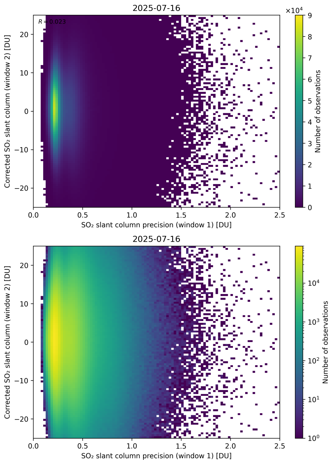
Figure 275: Scatter density plot of “SO 2 slant column precision (window 1)” against “Corrected SO 2 slant column (window 2)” for 2025-07-15 to 2025-07-17.
