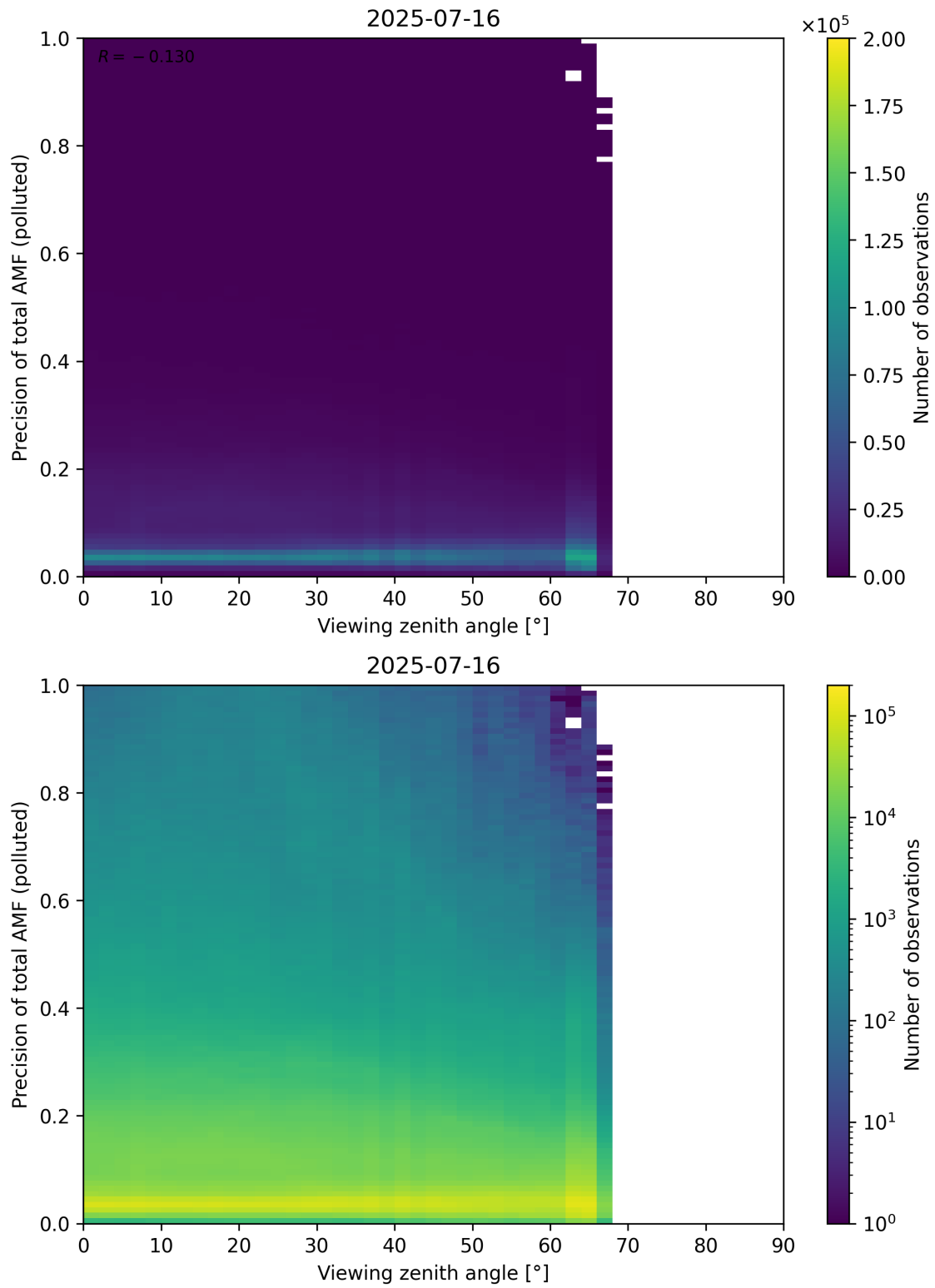
Figure 382: Scatter density plot of “Viewing zenith angle” against “Precision of total AMF (polluted)” for 2025-07-15 to 2025-07-17.
