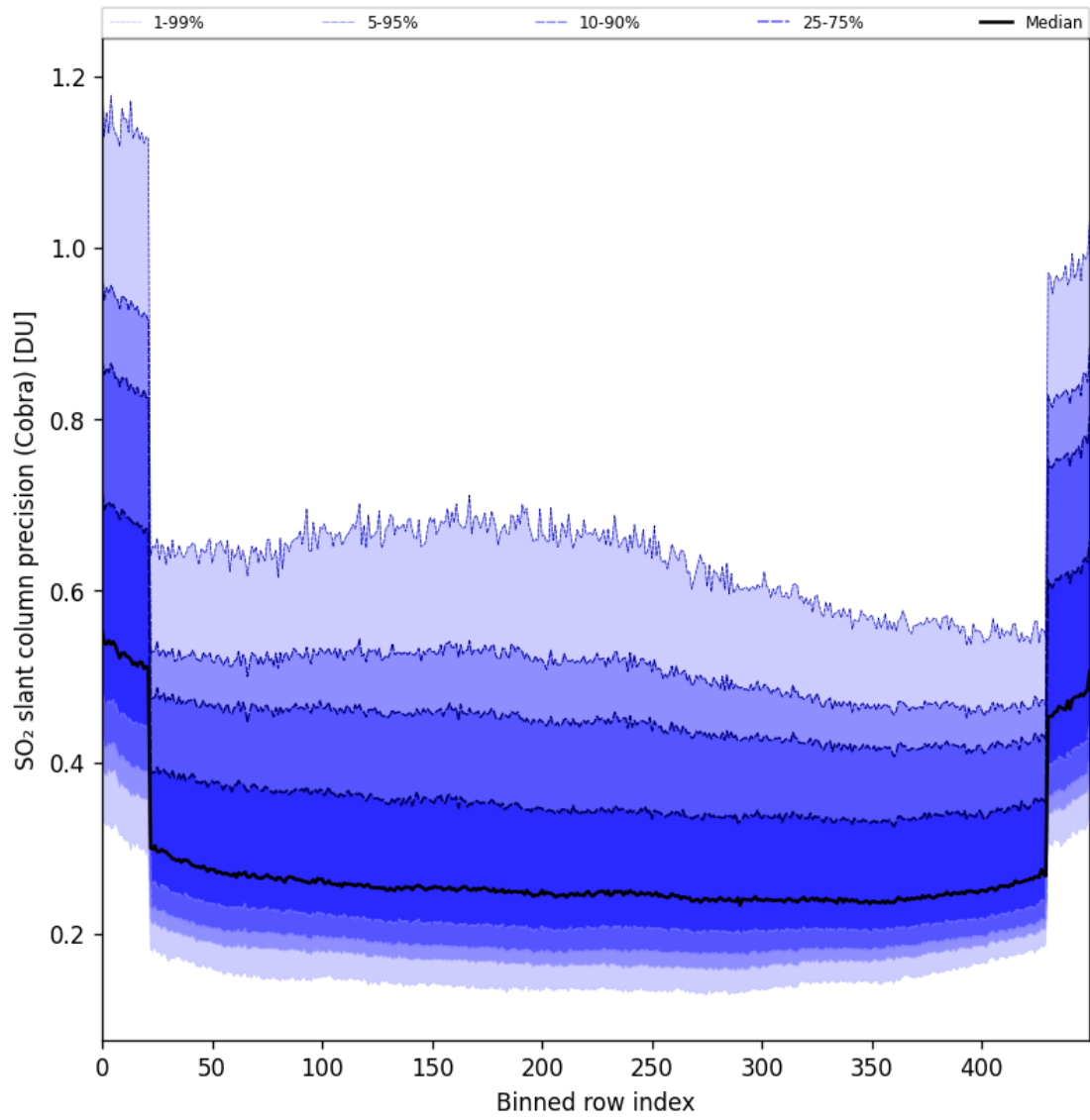
Figure 88: Along track statistics of “SO 2 slant column precision (Cobra)” for 2025-07-15 to 2025-07-17
