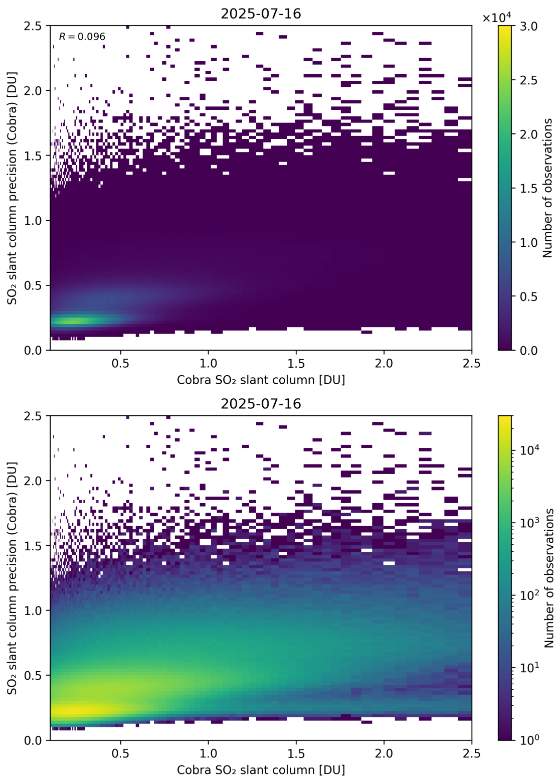
Figure 216: Scatter density plot of “Cobra SO 2 slant column” against “SO 2 slant column precision (Cobra)” for 2025-07-15 to 2025-07-17.
