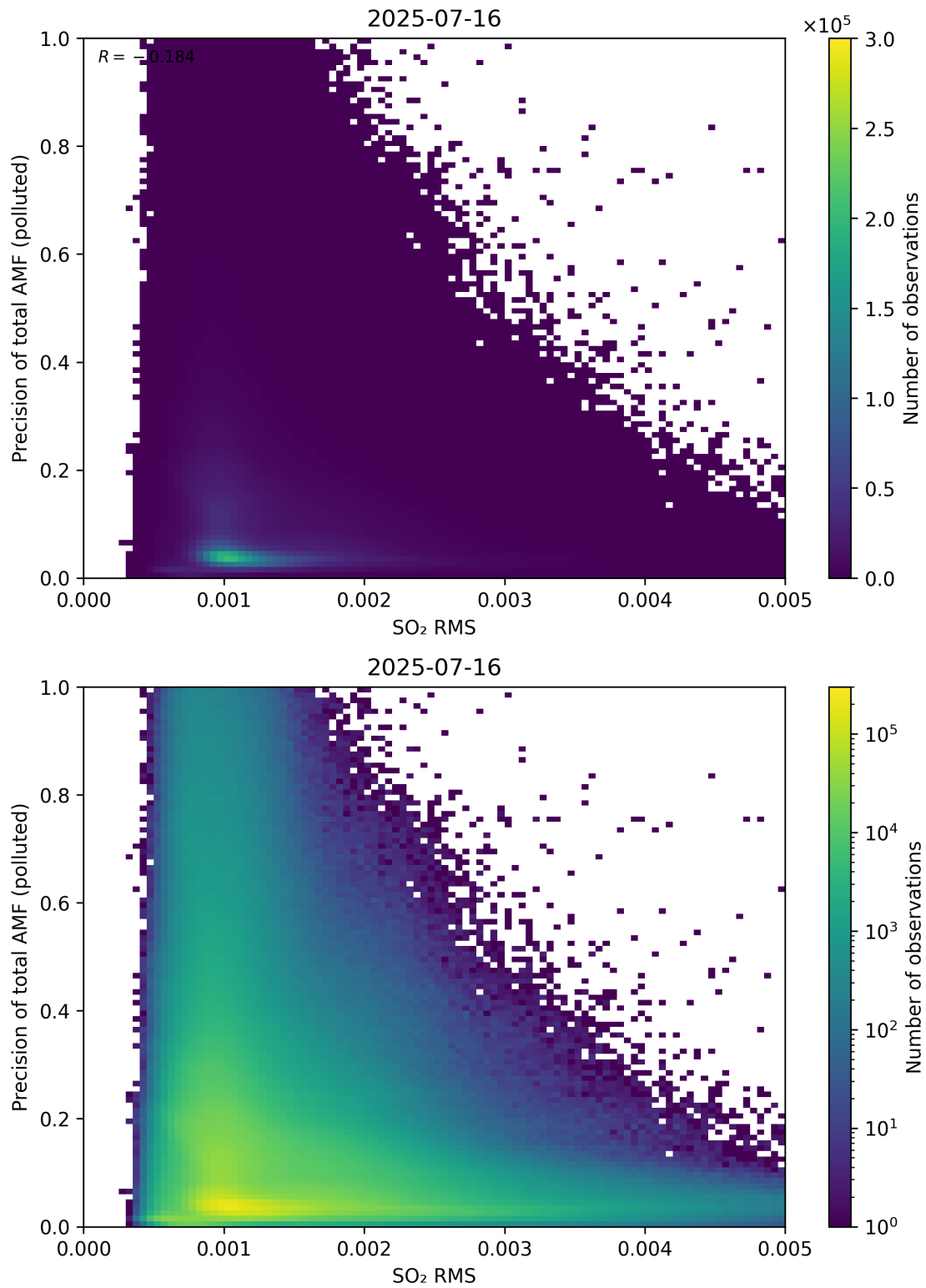
Figure 149: Scatter density plot of “SO 2 RMS” against “Precision of total AMF (polluted)” for 2025-07-15 to 2025-07-17.
