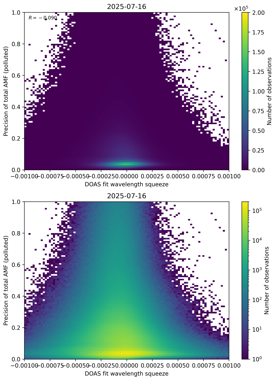
Figure 146: Scatter density plot of “DOAS fit wavelength squeeze” against “Precision of total AMF (polluted)” for 2025-07-15 to 2025-07-17.
