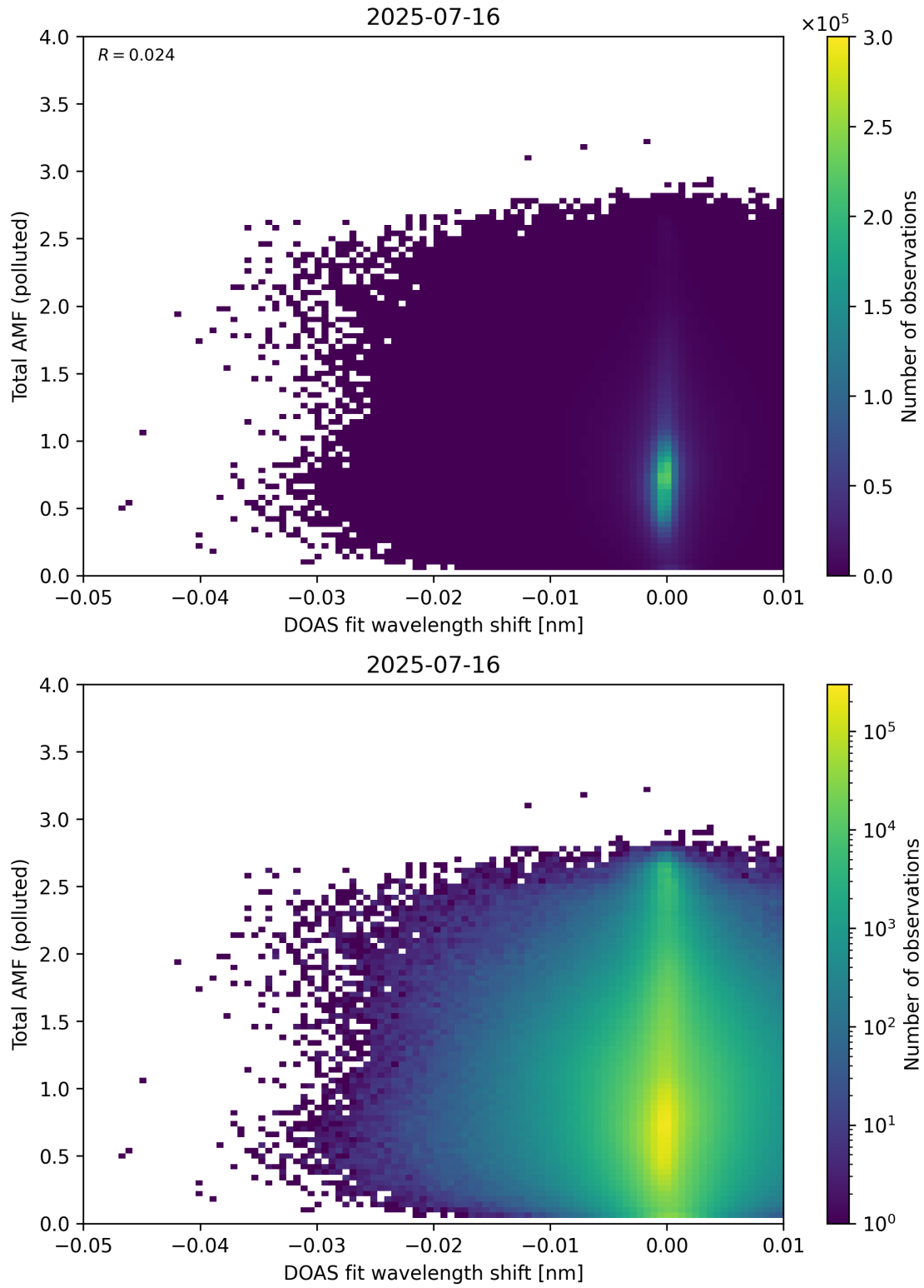
Figure 141: Scatter density plot of “DOAS fit wavelength shift” against “Total AMF (polluted)” for 2025-07-15 to 2025-07-17.
