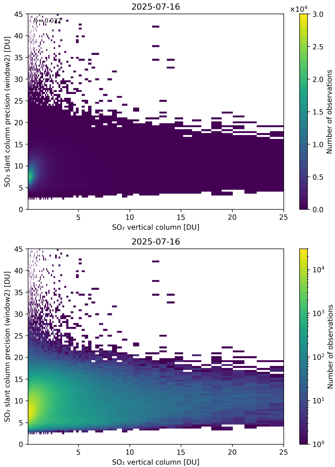
Figure 356: Scatter density plot of “SO 2 vertical column” against “SO 2 slant column precision (window2)” for 2025-07-15 to 2025-07-17.
