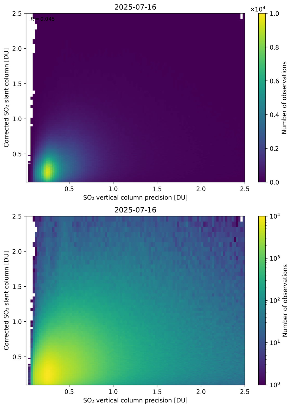
Figure 338: Scatter density plot of “SO 2 vertical column precision” against “Corrected SO 2 slant column” for 2025-07-15 to 2025-07-17.
