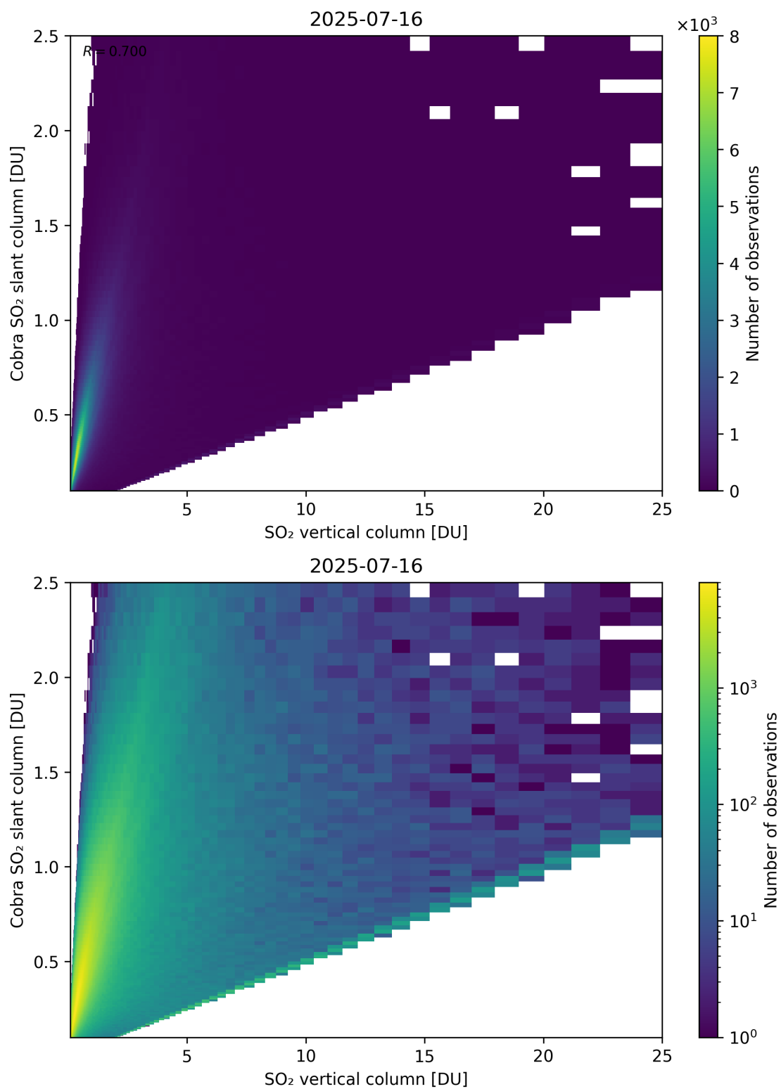
Figure 349: Scatter density plot of “SO 2 vertical column” against “Cobra SO 2 slant column” for 2025-07-15 to 2025-07-17.
