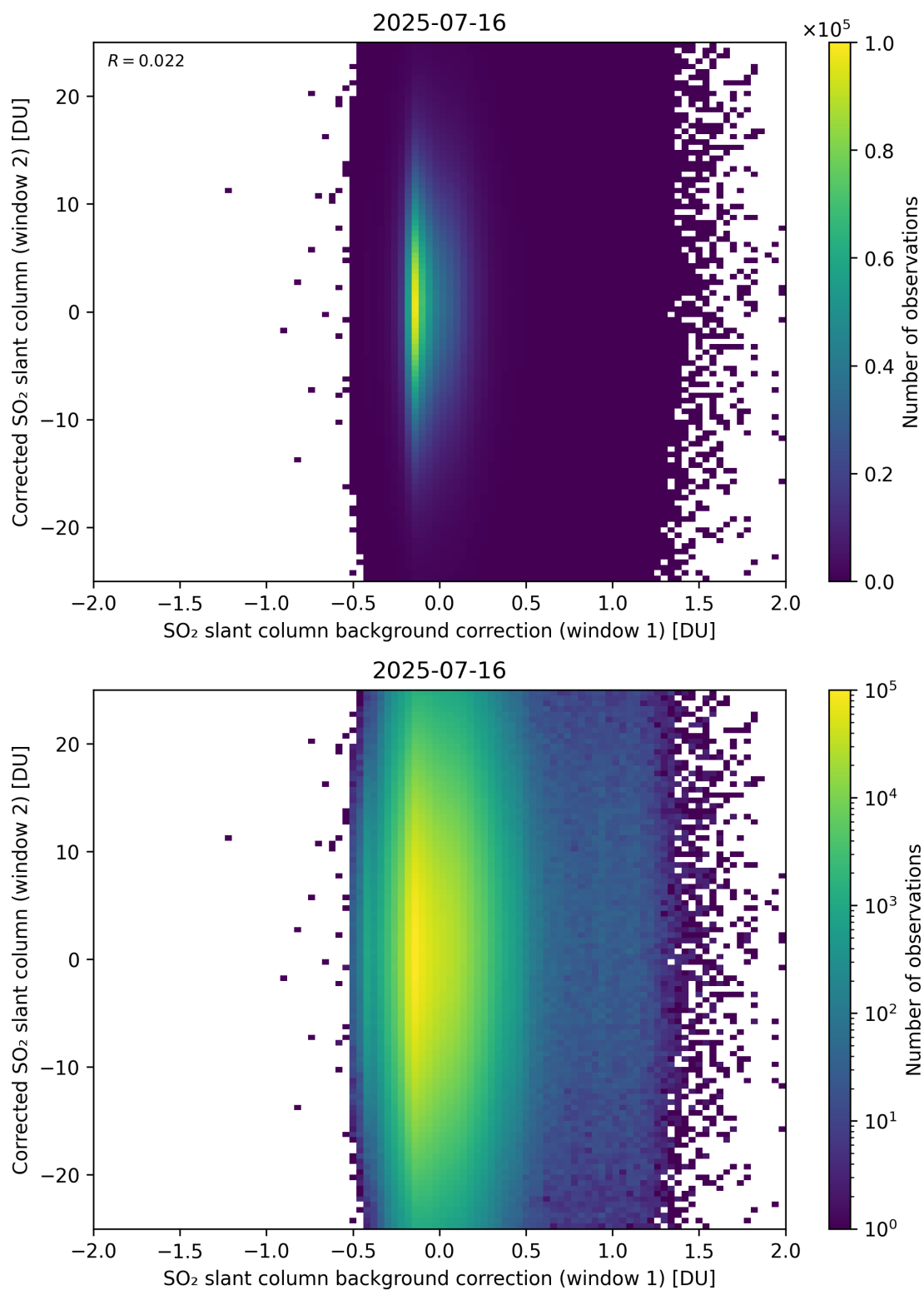
Figure 115: Scatter density plot of “SO 2 slant column background correction (window 1)” against “Corrected SO 2 slant column (window 2)” for 2025-07-15 to 2025-07-17.
