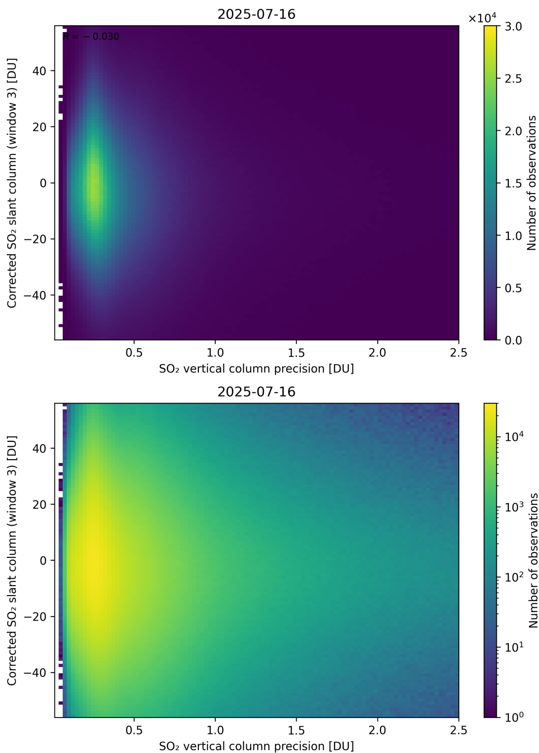
Figure 340: Scatter density plot of “SO 2 vertical column precision” against “Corrected SO 2 slant column (window 3)” for 2025-07-15 to 2025-07-17.
