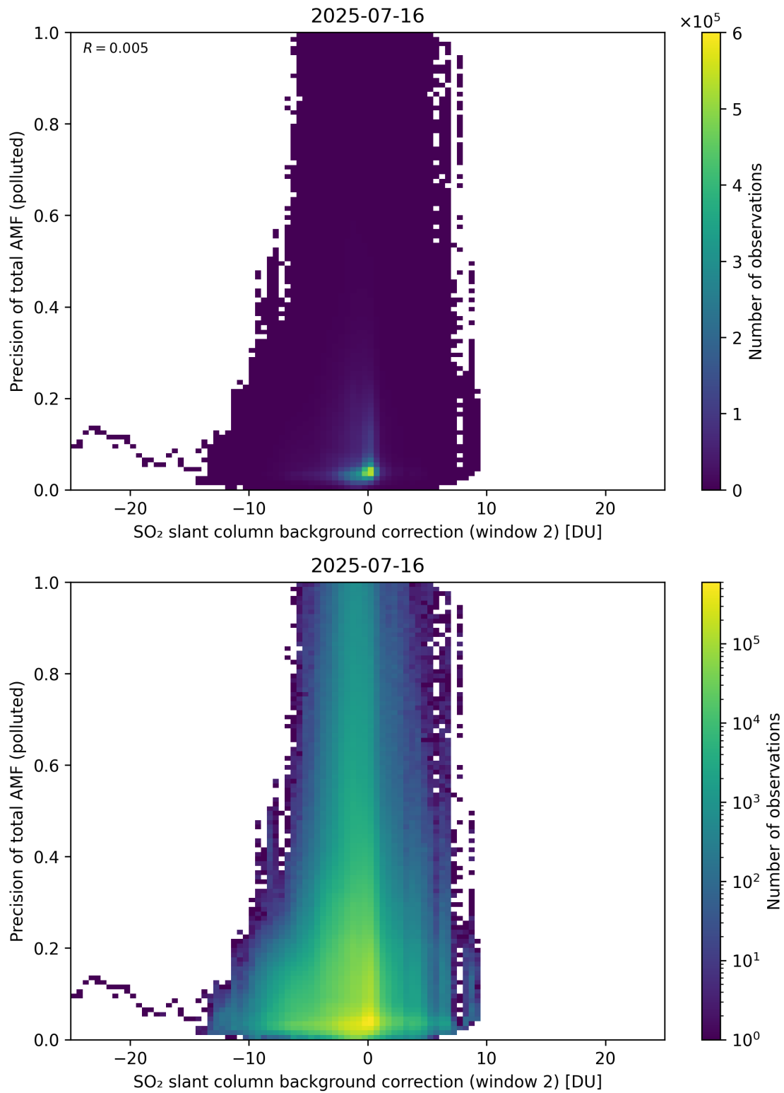
Figure 131: Scatter density plot of “SO 2 slant column background correction (window 2)” against “Precision of total AMF (polluted)” for 2025-07-15 to 2025-07-17.
