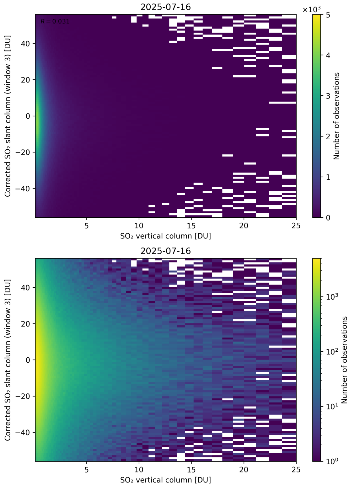
Figure 353: Scatter density plot of “SO 2 vertical column” against “Corrected SO 2 slant column (window 3)” for 2025-07-15 to 2025-07-17.
