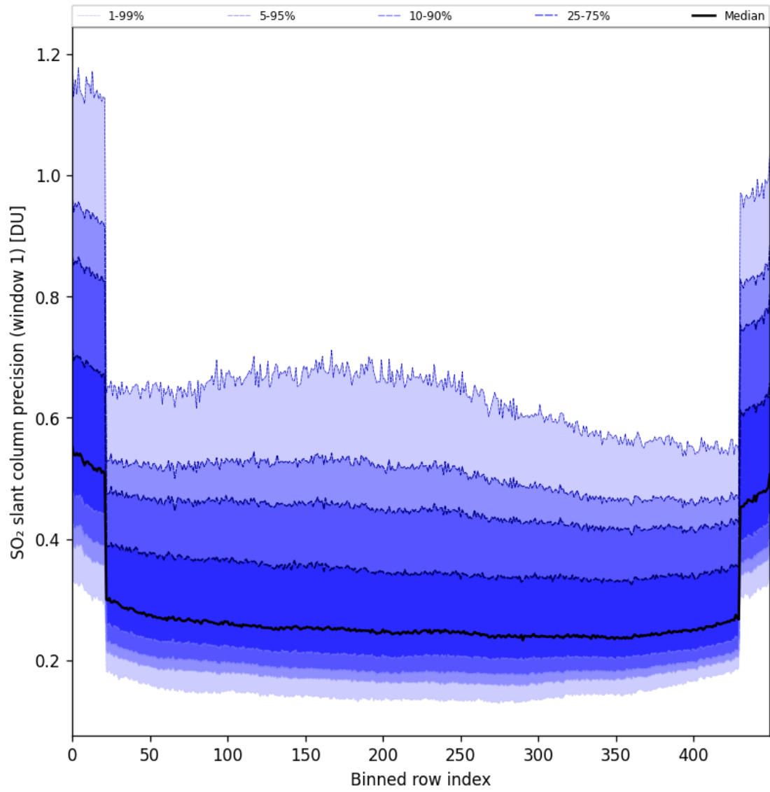
Figure 90: Along track statistics of “SO 2 slant column precision (window 1)” for 2025-07-15 to 2025-07-17
