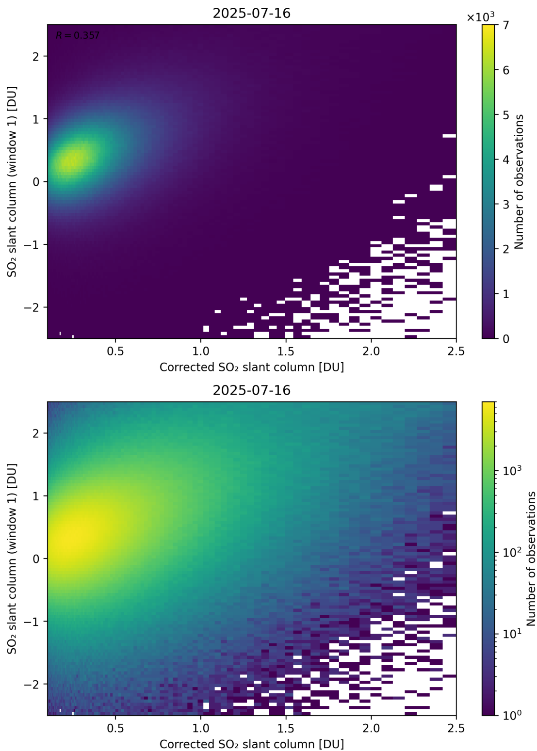
Figure 237: Scatter density plot of “Corrected SO 2 slant column” against “SO 2 slant column (window 1)” for 2025-07-15 to 2025-07-17.
