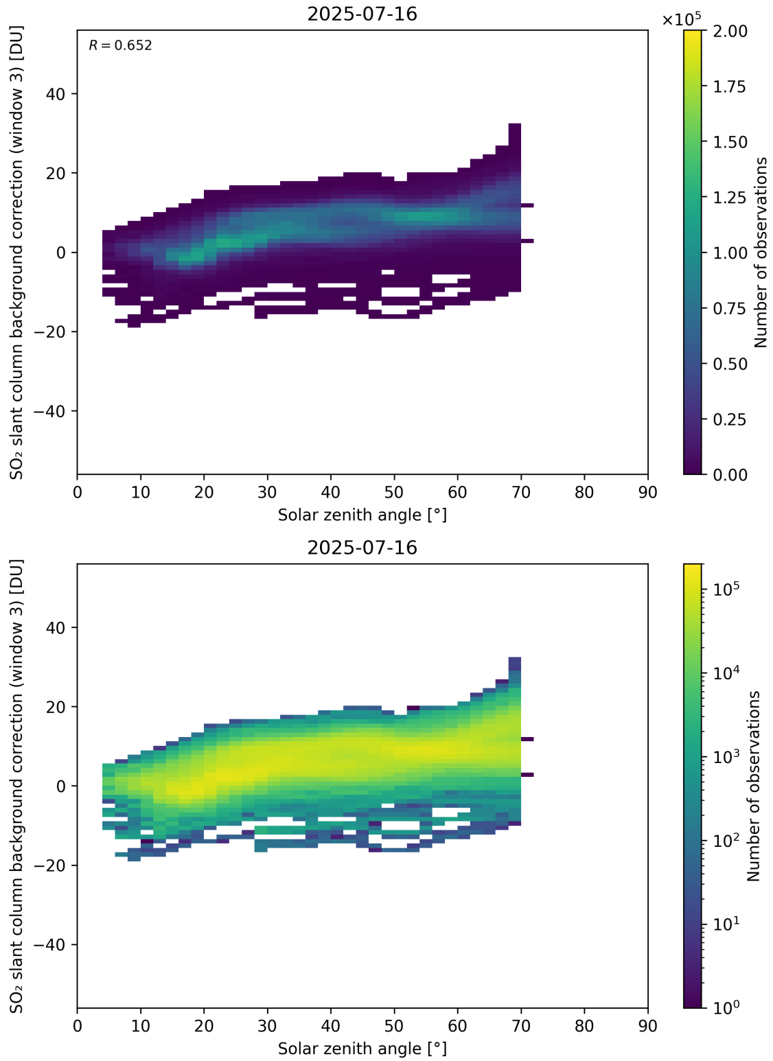
Figure 173: Scatter density plot of “Solar zenith angle” against “SO 2 slant column background correction (window 3)” for 2025-07-15 to 2025-07-17.
