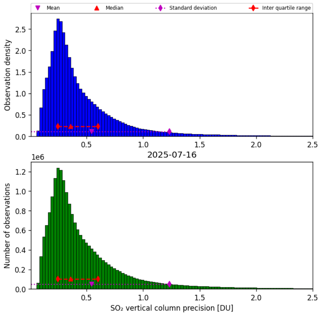
Figure 59: Histogram of “SO 2 vertical column precision” for 2025-07-15 to 2025-07-17
