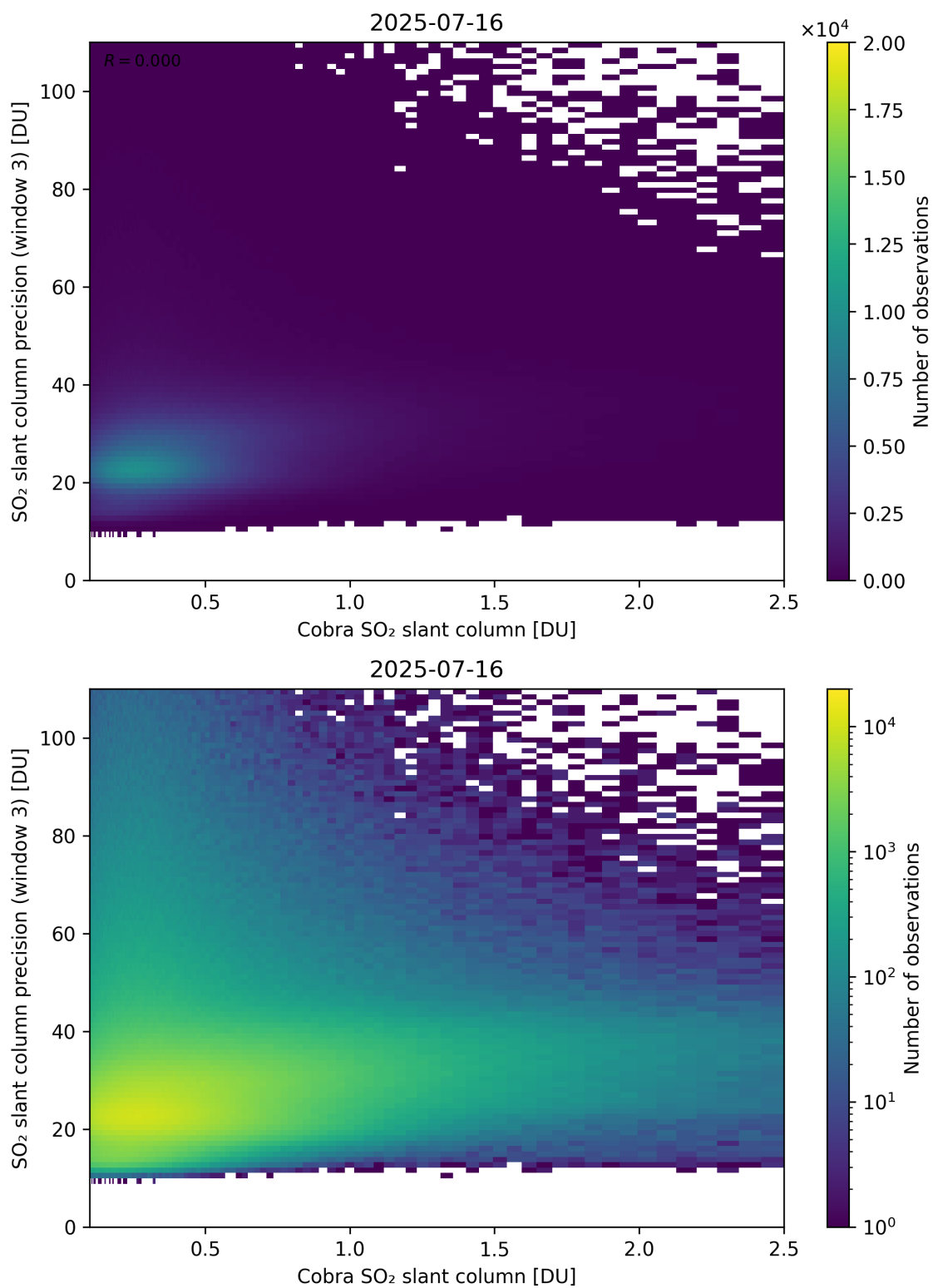
Figure 223: Scatter density plot of “Cobra SO 2 slant column” against “SO 2 slant column precision (window 3)” for 2025-07-15 to 2025-07-17.
