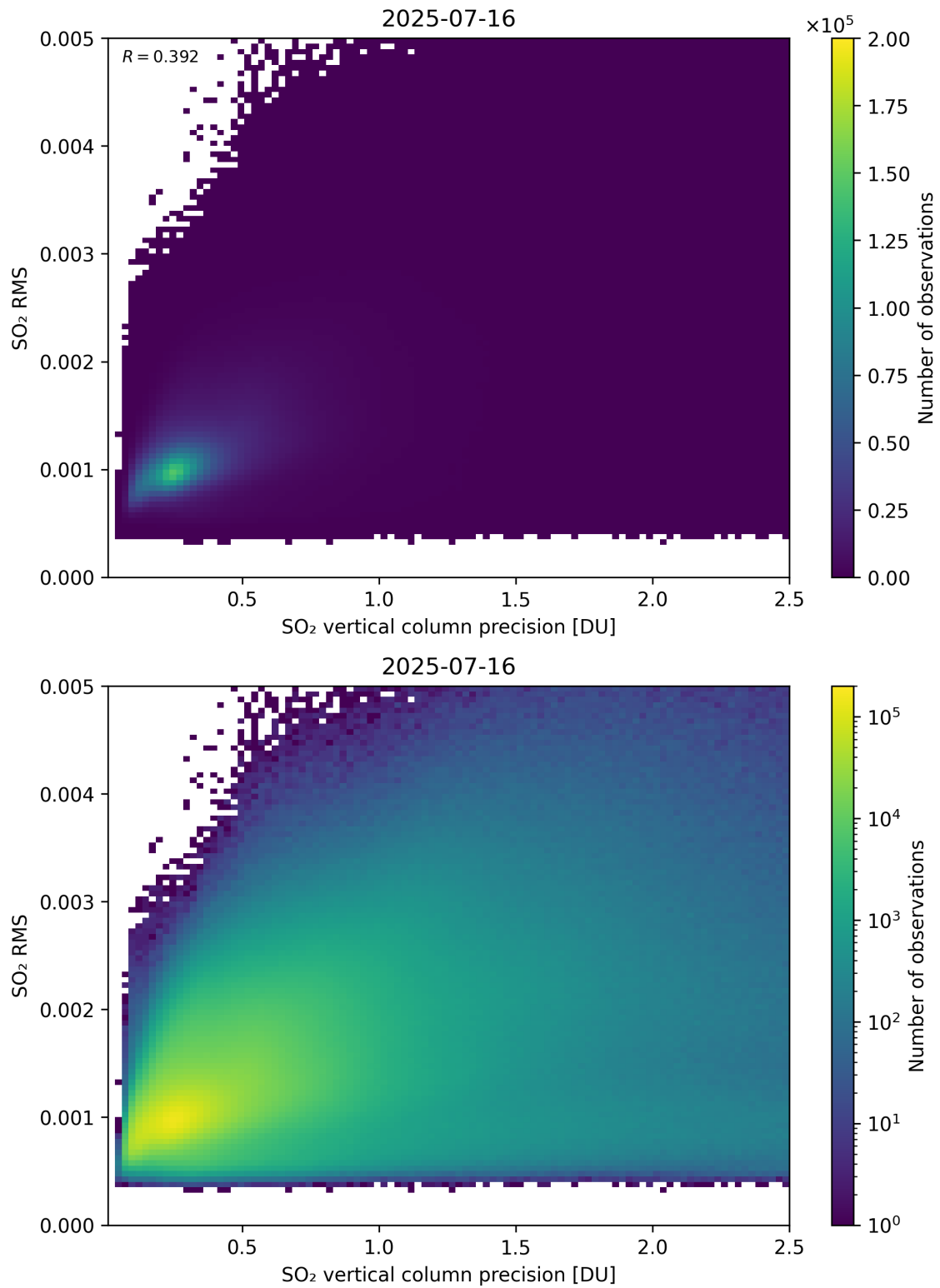
Figure 334: Scatter density plot of “SO 2 vertical column precision” against “SO 2 RMS” for 2025-07-15 to 2025-07-17.
