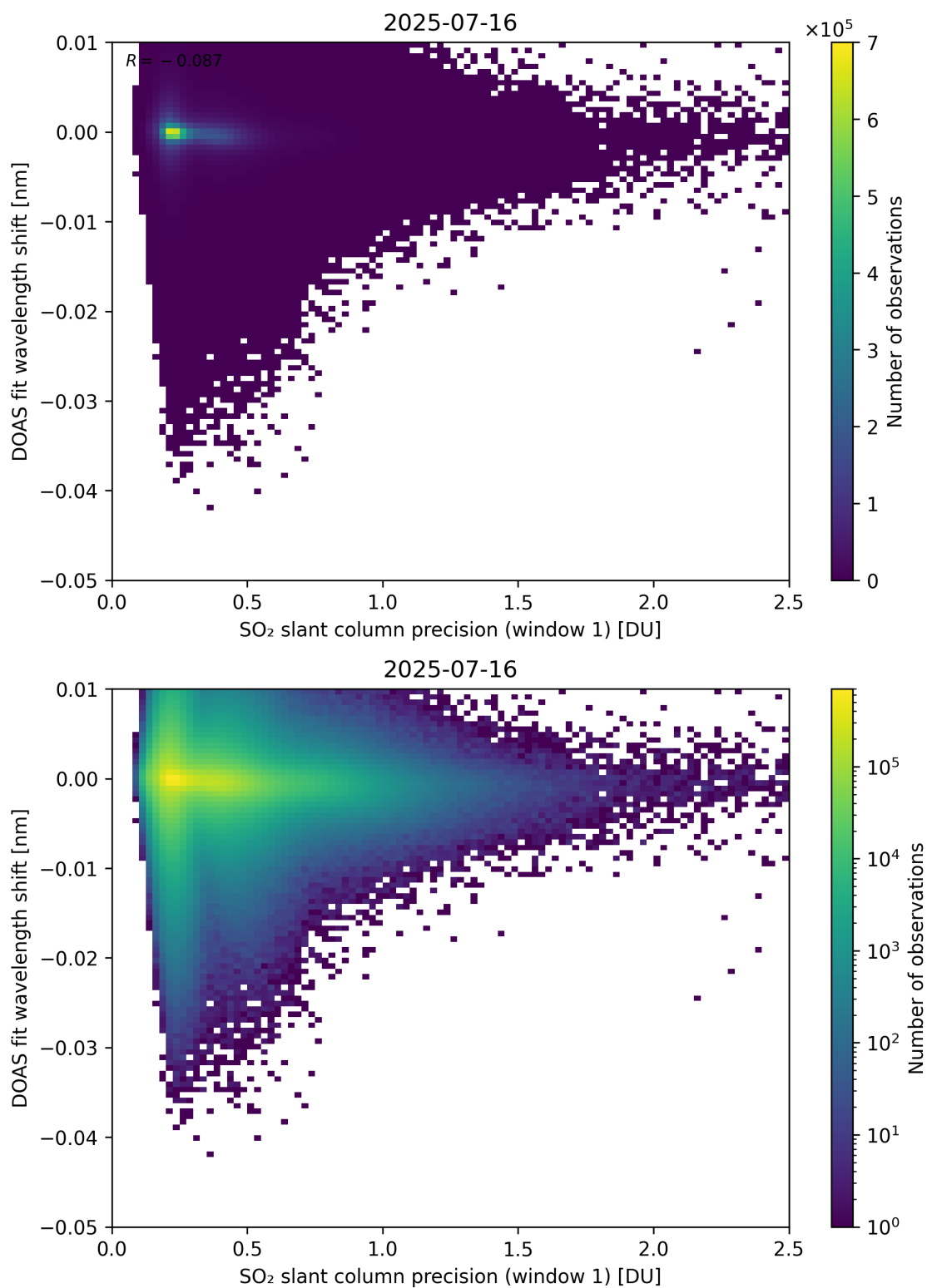
Figure 271: Scatter density plot of “SO 2 slant column precision (window 1)” against “DOAS fit wavelength shift” for 2025-07-15 to 2025-07-17.
