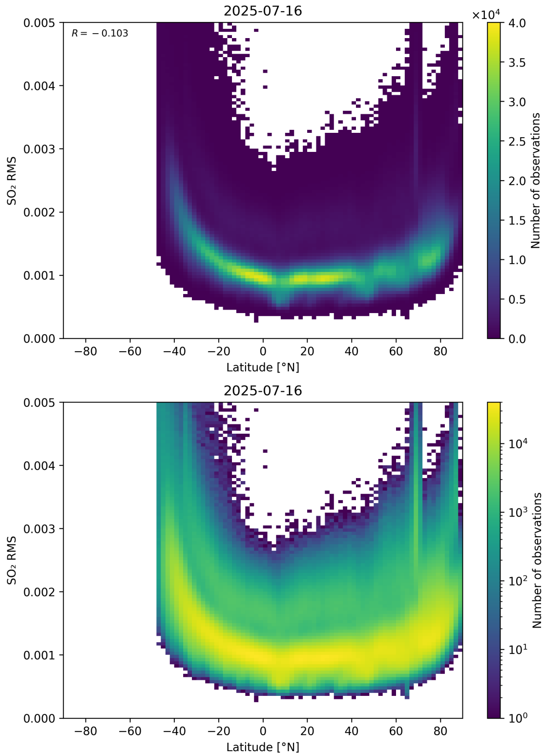
Figure 155: Scatter density plot of “Latitude” against “SO 2 RMS” for 2025-07-15 to 2025-07-17.
