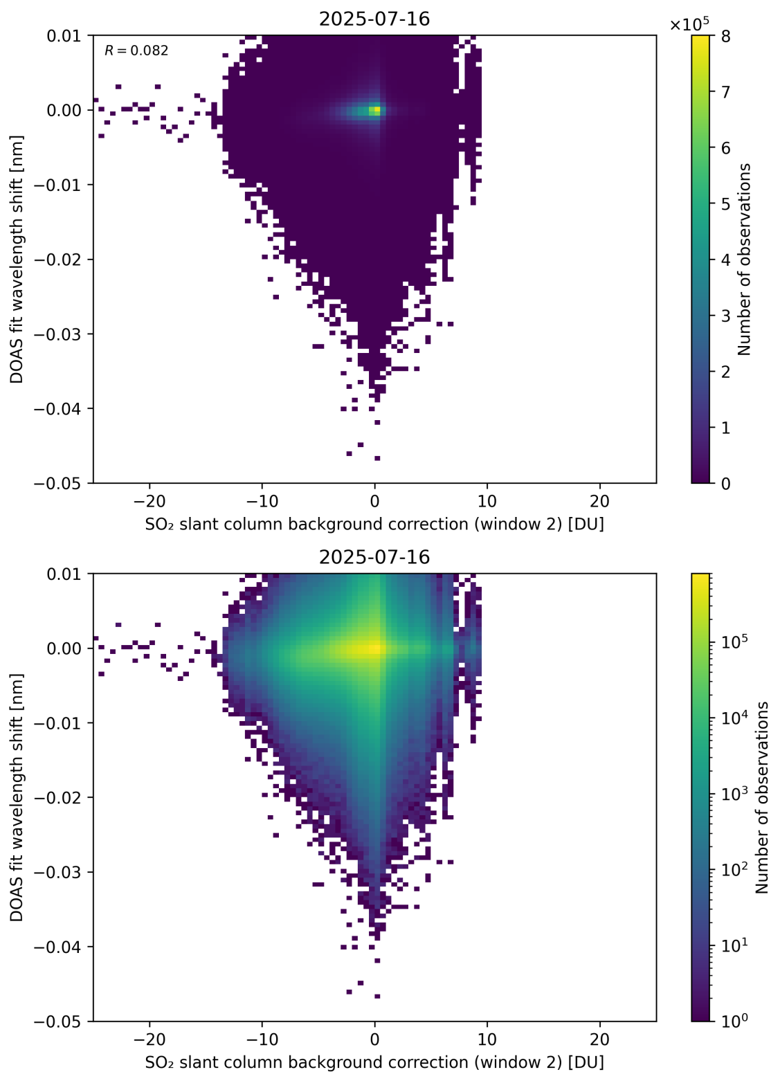
Figure 123: Scatter density plot of “SO 2 slant column background correction (window 2)” against “DOAS fit wavelength shift” for 2025-07-15 to 2025-07-17.
