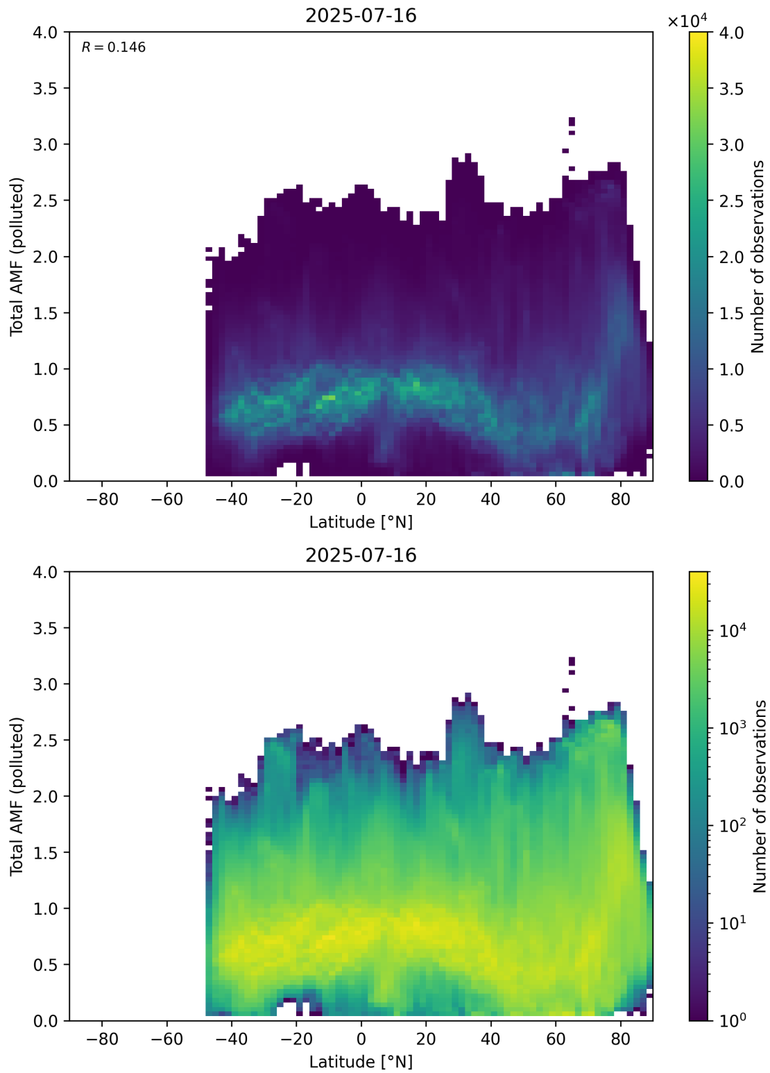
Figure 167: Scatter density plot of “Latitude” against “Total AMF (polluted)” for 2025-07-15 to 2025-07-17.
