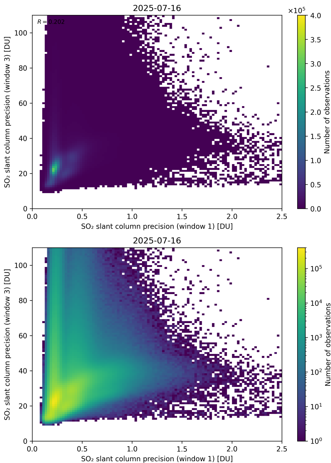
Figure 279: Scatter density plot of “SO 2 slant column precision (window 1)” against “SO 2 slant column precision (window 3)” for 2025-07-15 to 2025-07-17.
