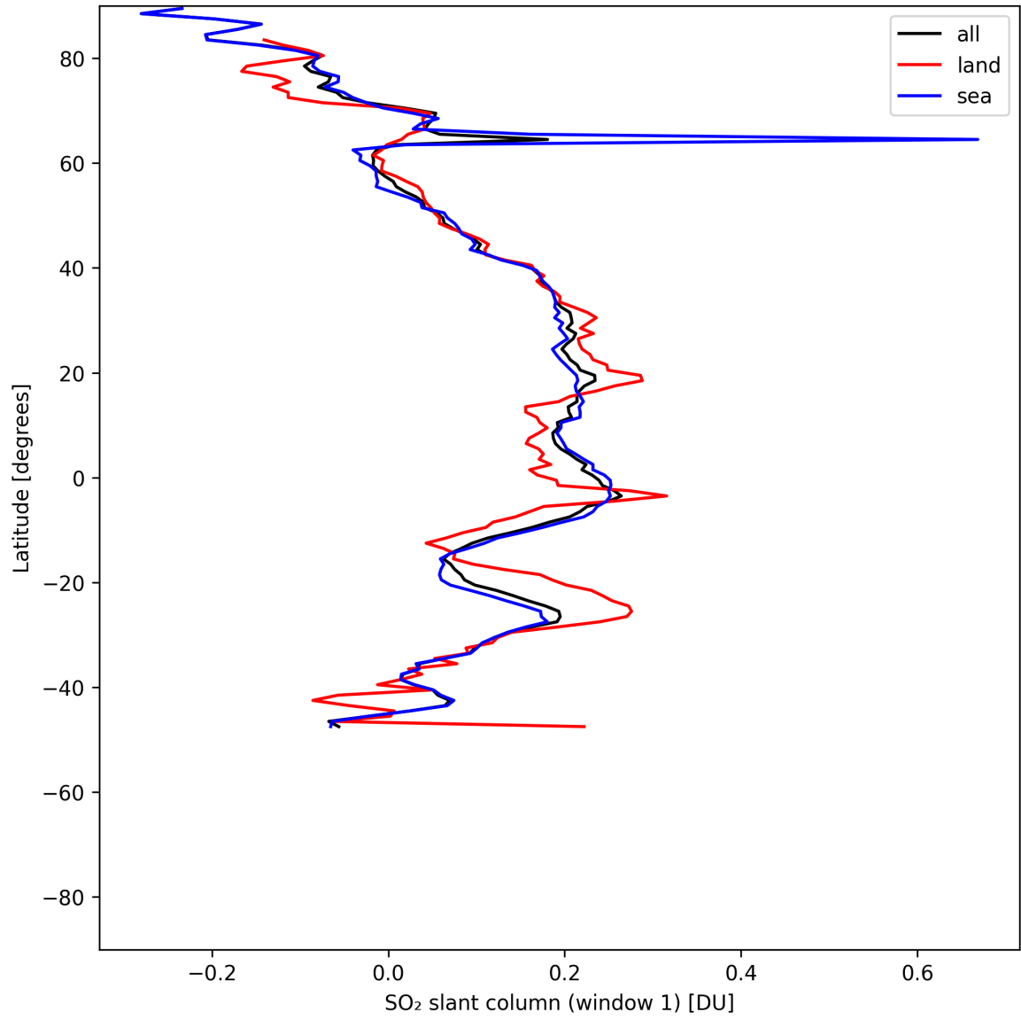
Figure 37: Zonal average of “SO 2 slant column (window 1)” for 2025-07-15 to 2025-07-17.
