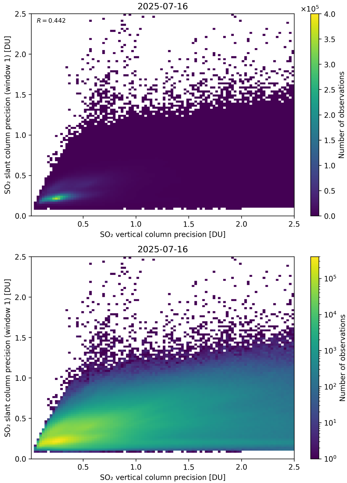
Figure 342: Scatter density plot of “SO 2 vertical column precision” against “SO 2 slant column precision (window 1)” for 2025-07-15 to 2025-07-17.
