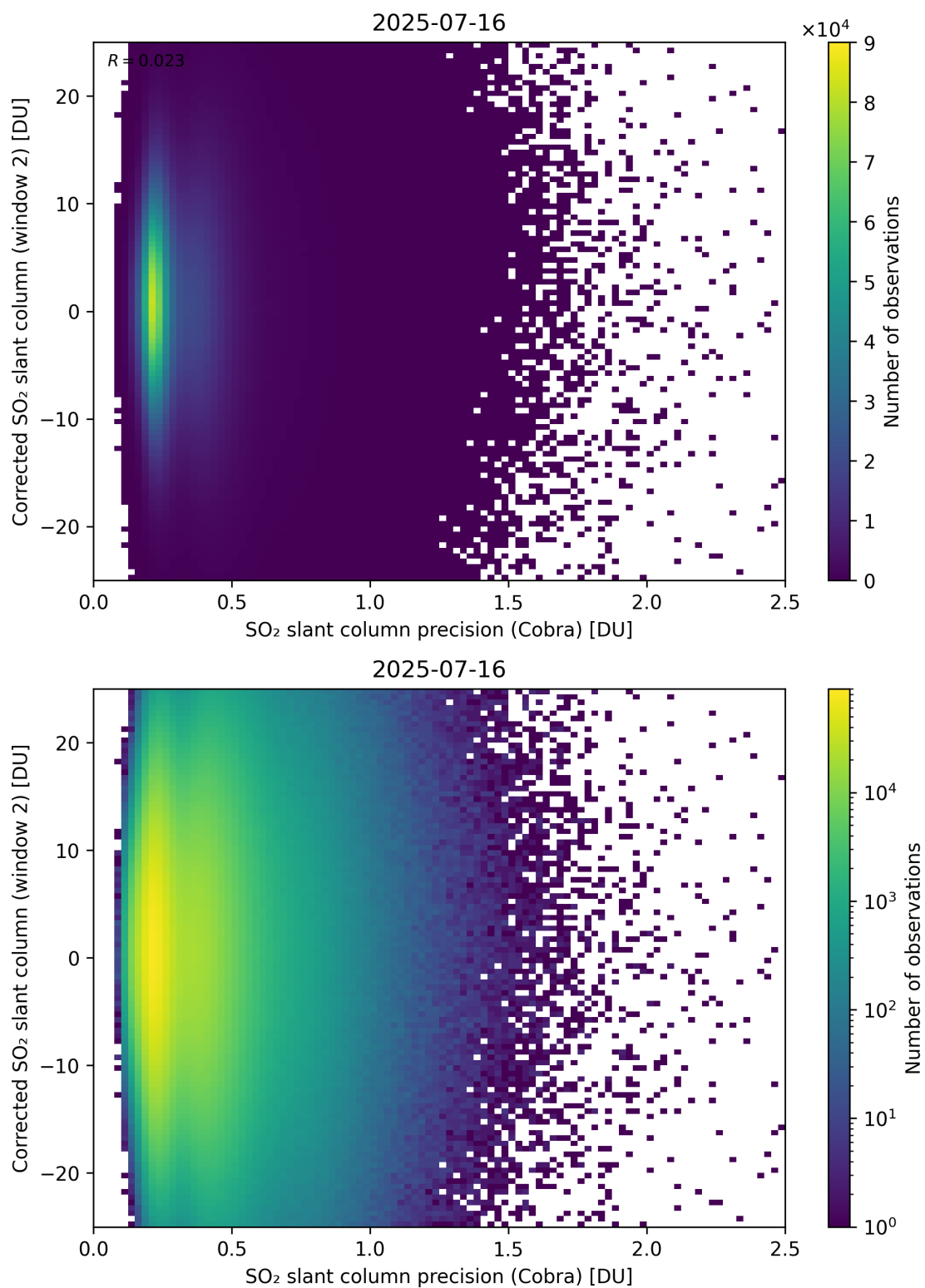
Figure 206: Scatter density plot of “SO 2 slant column precision (Cobra)” against “Corrected SO 2 slant column (window 2)” for 2025-07-15 to 2025-07-17.
