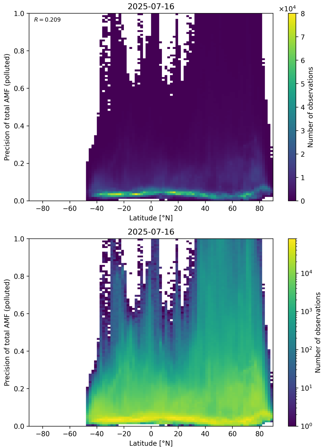
Figure 168: Scatter density plot of “Latitude” against “Precision of total AMF (polluted)” for 2025-07-15 to 2025-07-17.
