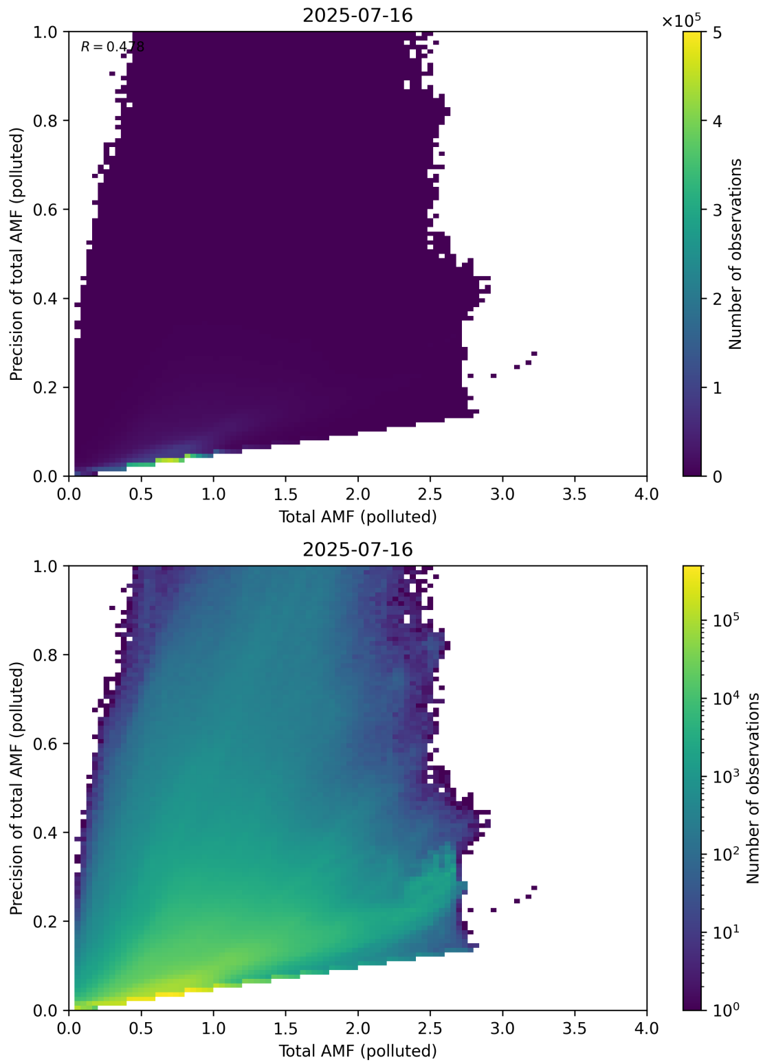
Figure 322: Scatter density plot of “Total AMF (polluted)” against “Precision of total AMF (polluted)” for 2025-07-15 to 2025-07-17.
