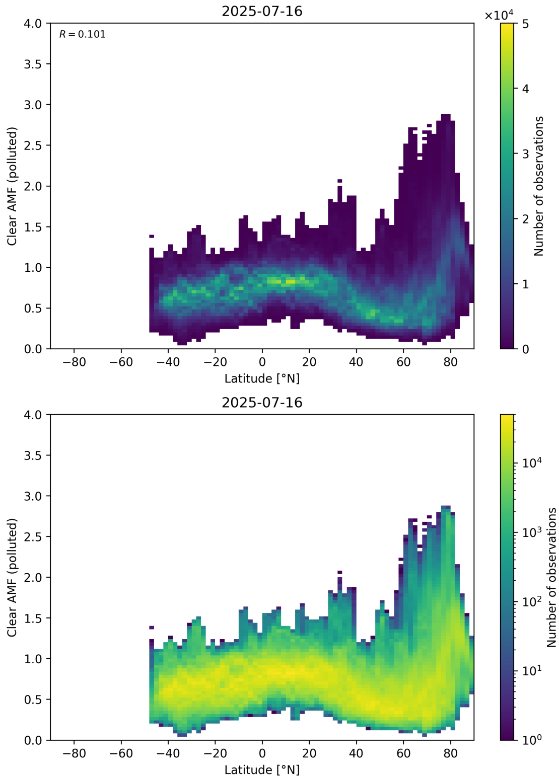
Figure 156: Scatter density plot of “Latitude” against “Clear AMF (polluted)” for 2025-07-15 to 2025-07-17.
