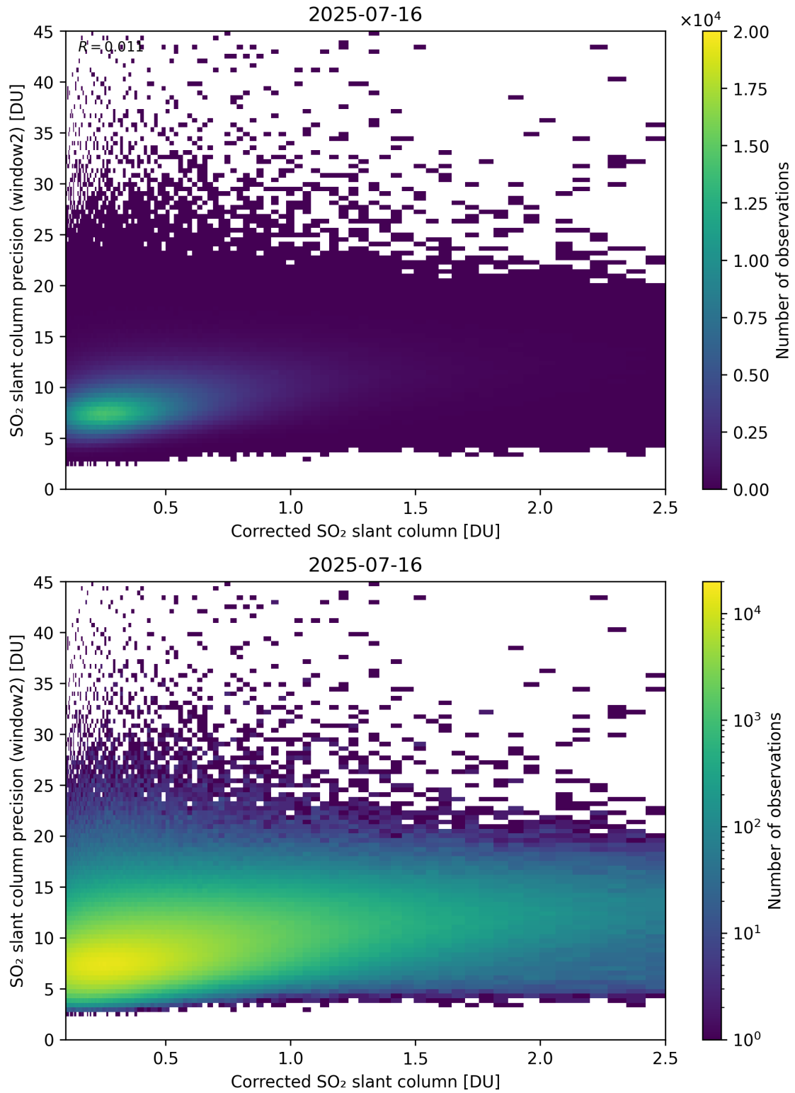
Figure 239: Scatter density plot of “Corrected SO 2 slant column” against “SO 2 slant column precision (window2)” for 2025-07-15 to 2025-07-17.
