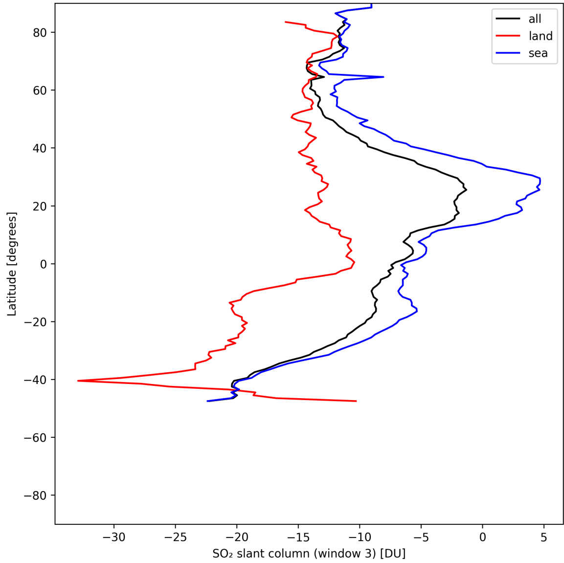
Figure 45: Zonal average of “SO 2 slant column (window 3)” for 2025-07-15 to 2025-07-17.
