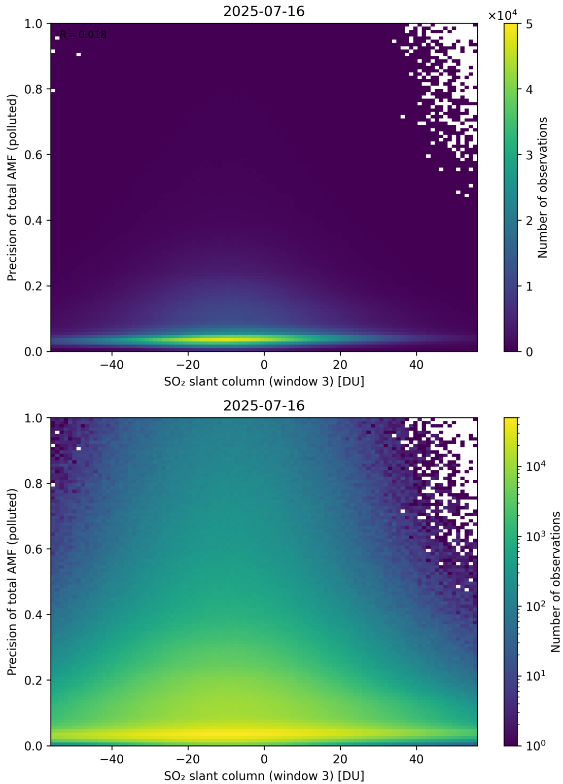
Figure 319: Scatter density plot of “SO 2 slant column (window 3)” against “Precision of total AMF (polluted)” for 2025-07-15 to 2025-07-17.
