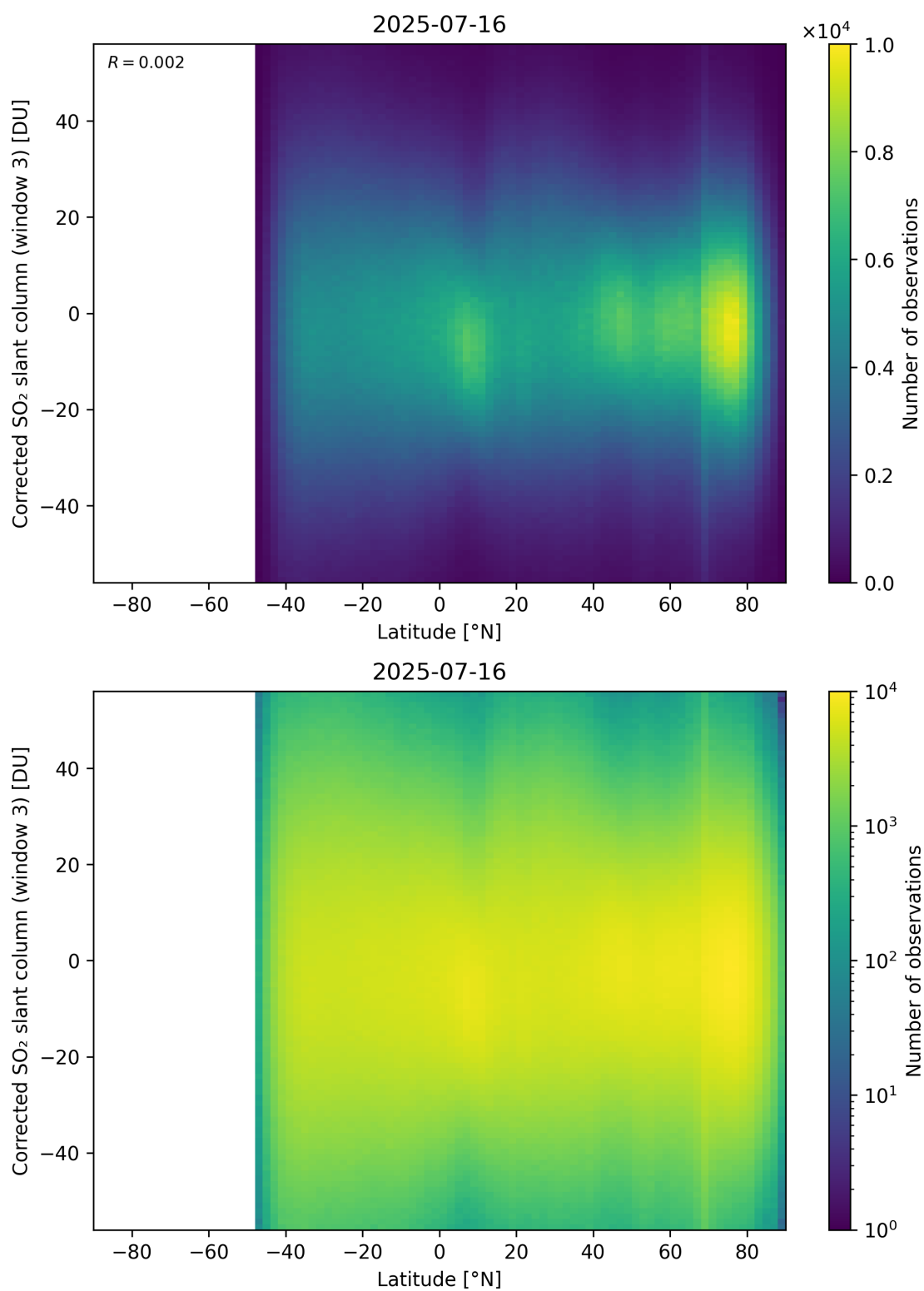
Figure 161: Scatter density plot of “Latitude” against “Corrected SO 2 slant column (window 3)” for 2025-07-15 to 2025-07-17.
