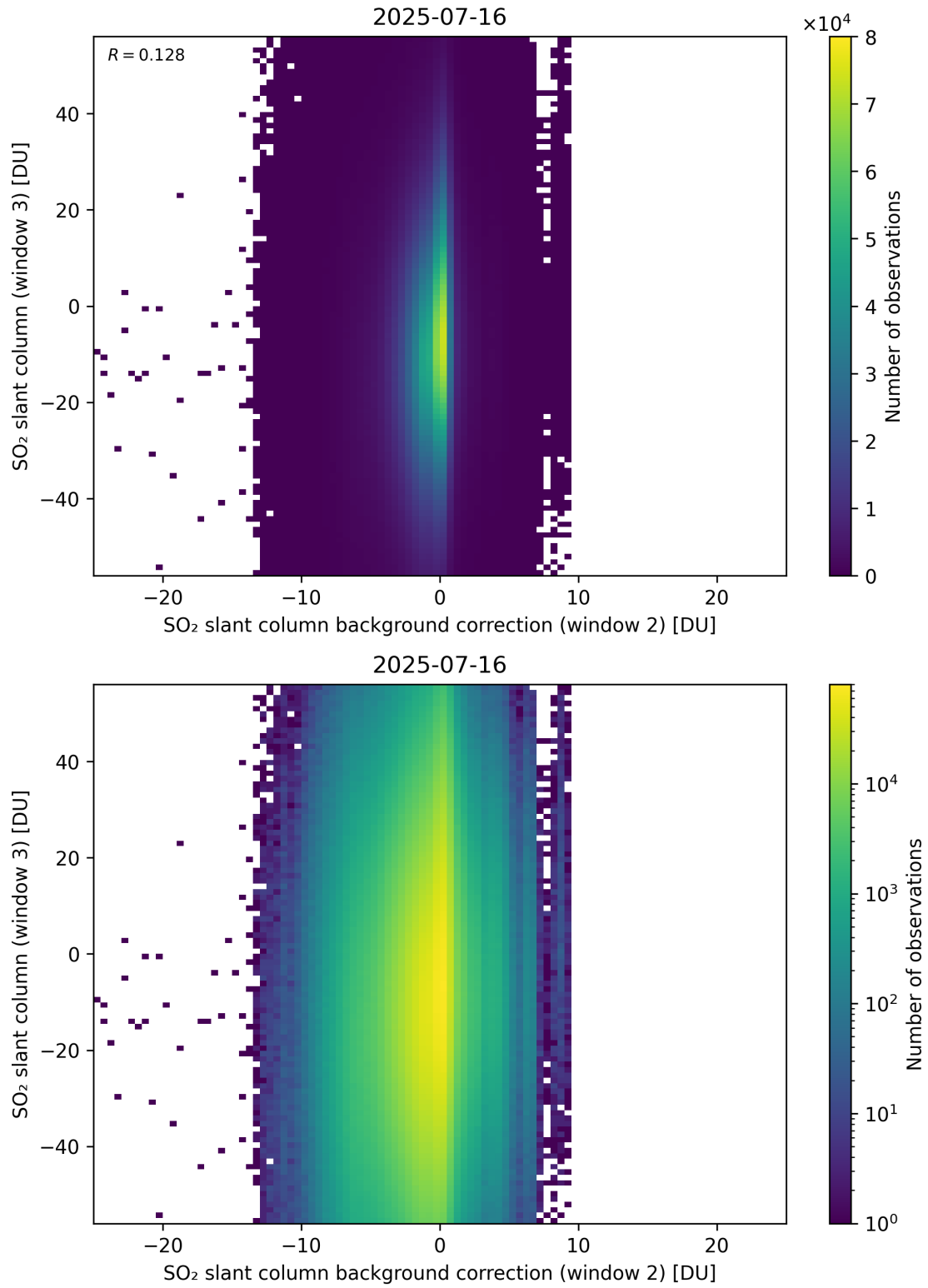
Figure 128: Scatter density plot of “SO 2 slant column background correction (window 2)” against “SO 2 slant column (window 3)” for 2025-07-15 to 2025-07-17.
