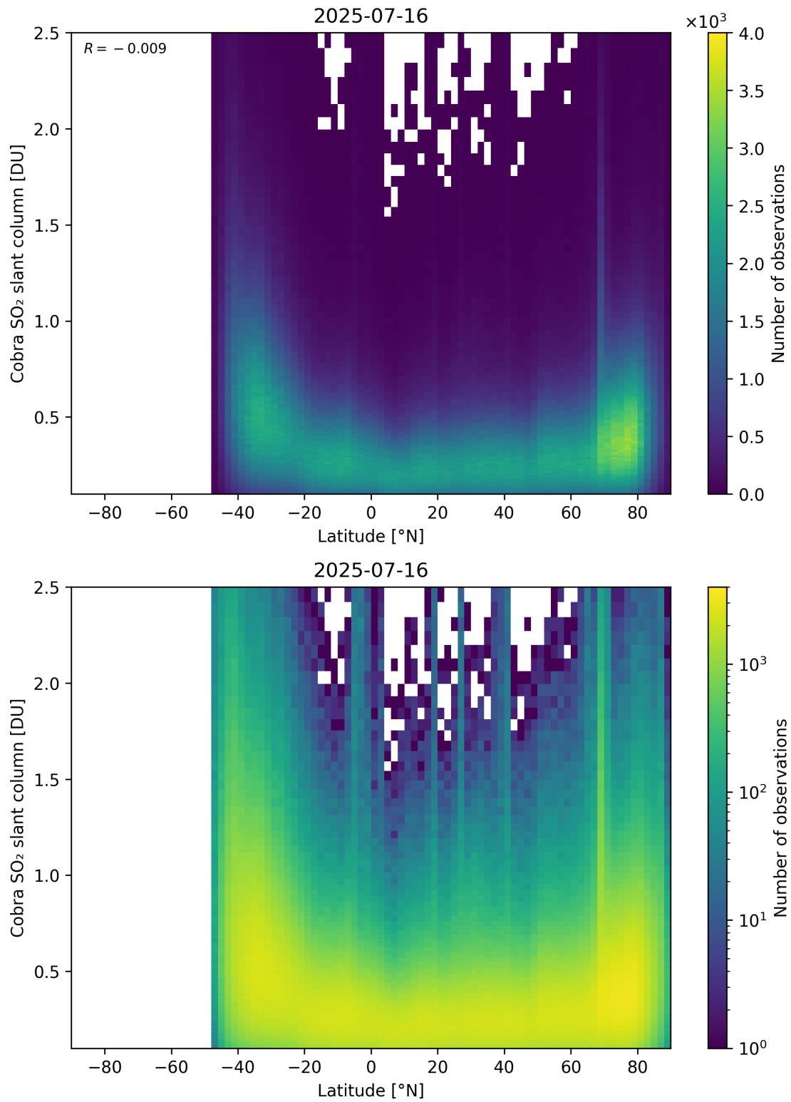
Figure 157: Scatter density plot of “Latitude” against “Cobra SO 2 slant column” for 2025-07-15 to 2025-07-17.
