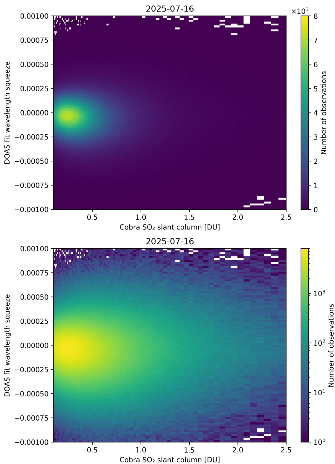
Figure 197: Scatter density plot of “Cobra SO 2 slant column” against “DOAS fit wavelength squeeze” for 2025-07-15 to 2025-07-17.
