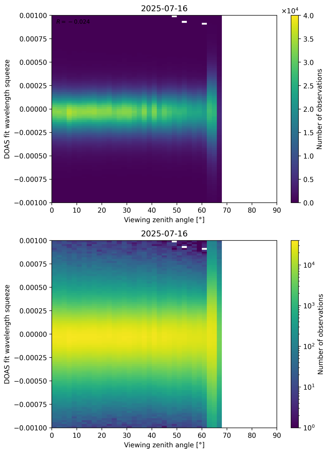
Figure 366: Scatter density plot of “Viewing zenith angle” against “DOAS fit wavelength squeeze” for 2025-07-15 to 2025-07-17.
