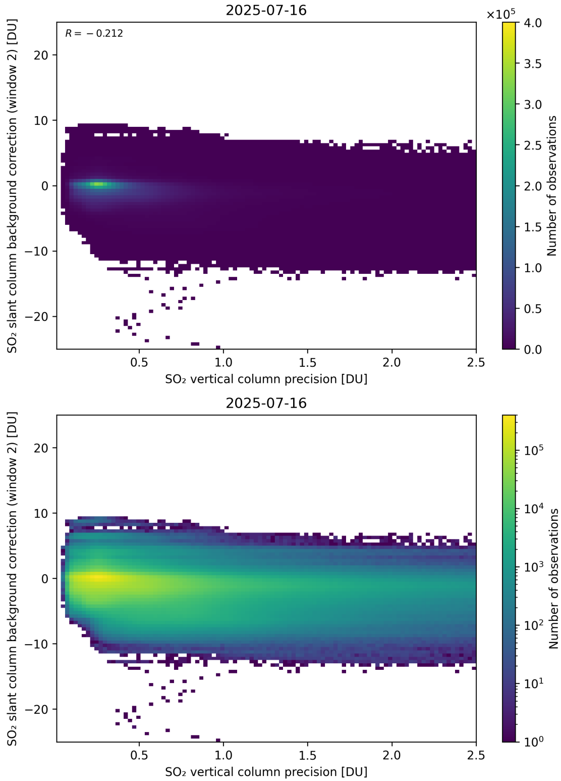
Figure 330: Scatter density plot of “SO 2 vertical column precision” against “SO 2 slant column background correction (window 2)” for 2025-07-15 to 2025-07-17.
