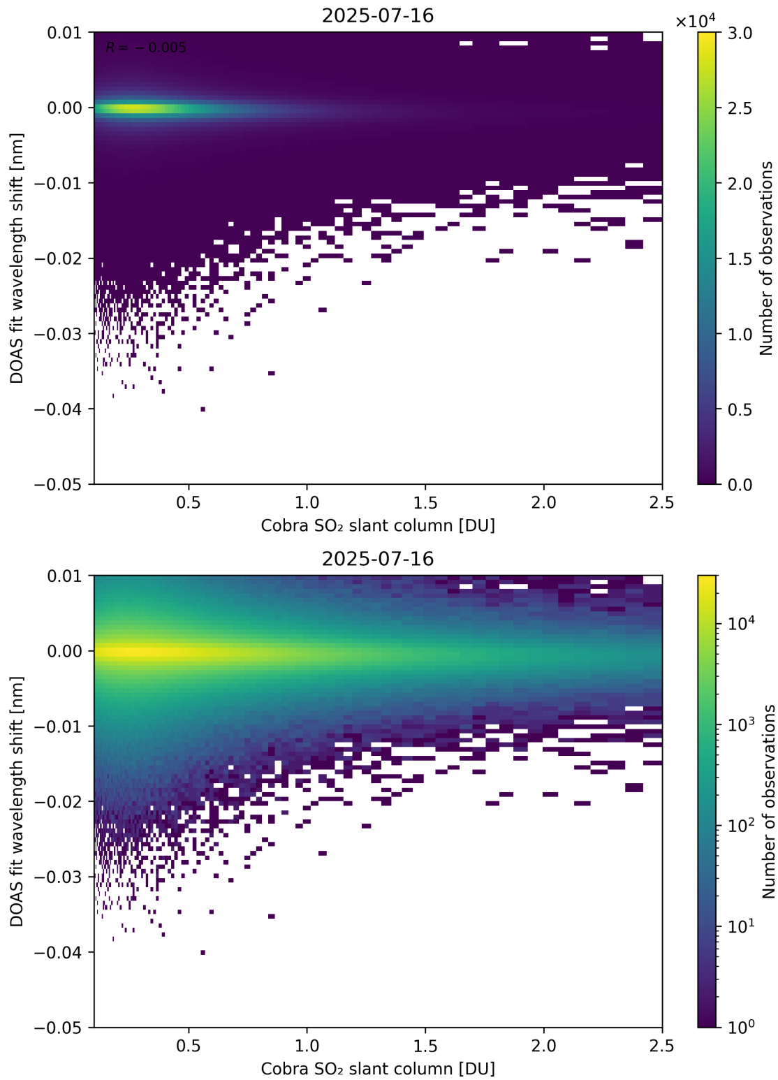
Figure 196: Scatter density plot of “Cobra SO 2 slant column” against “DOAS fit wavelength shift” for 2025-07-15 to 2025-07-17.
