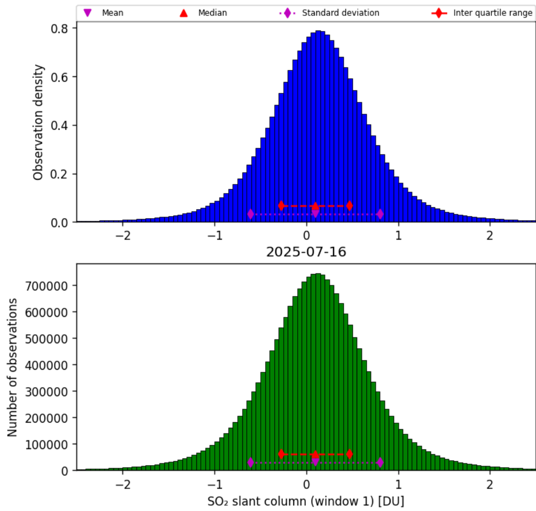
Figure 63: Histogram of “SO 2 slant column (window 1)” for 2025-07-15 to 2025-07-17
