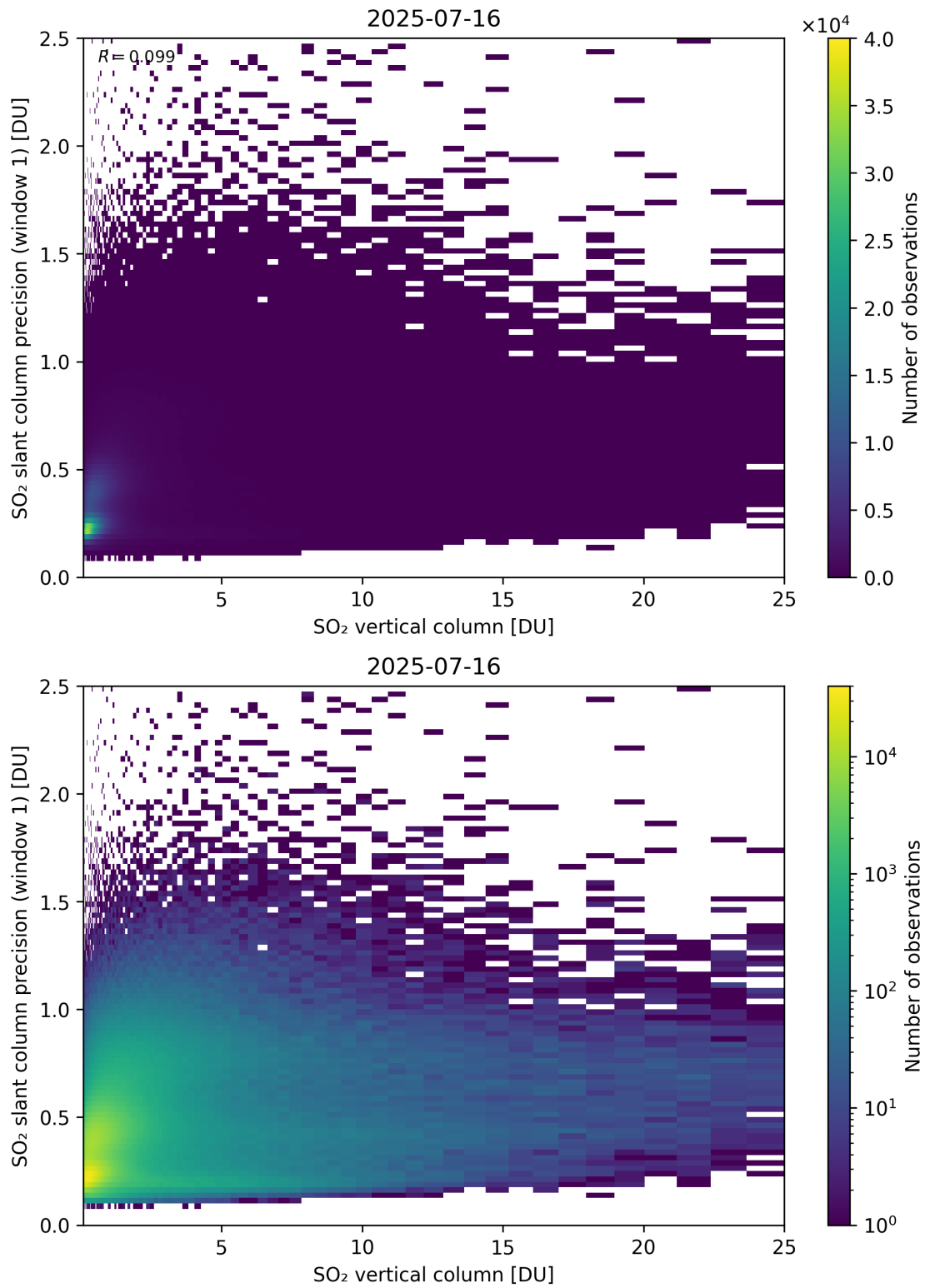
Figure 355: Scatter density plot of “SO 2 vertical column” against “SO 2 slant column precision (window 1)” for 2025-07-15 to 2025-07-17.
