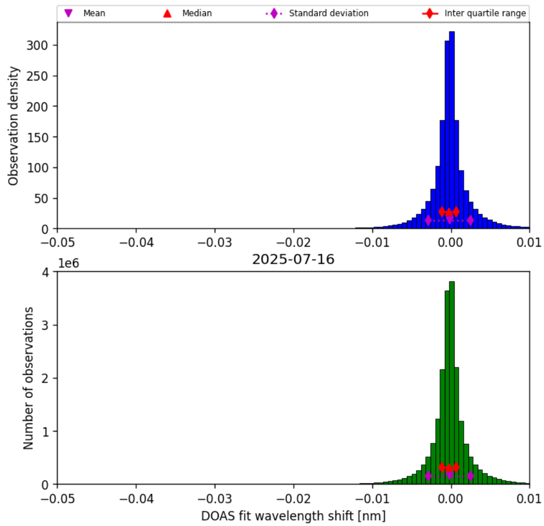
Figure 76: Histogram of “DOAS fit wavelength shift” for 2025-07-15 to 2025-07-17
