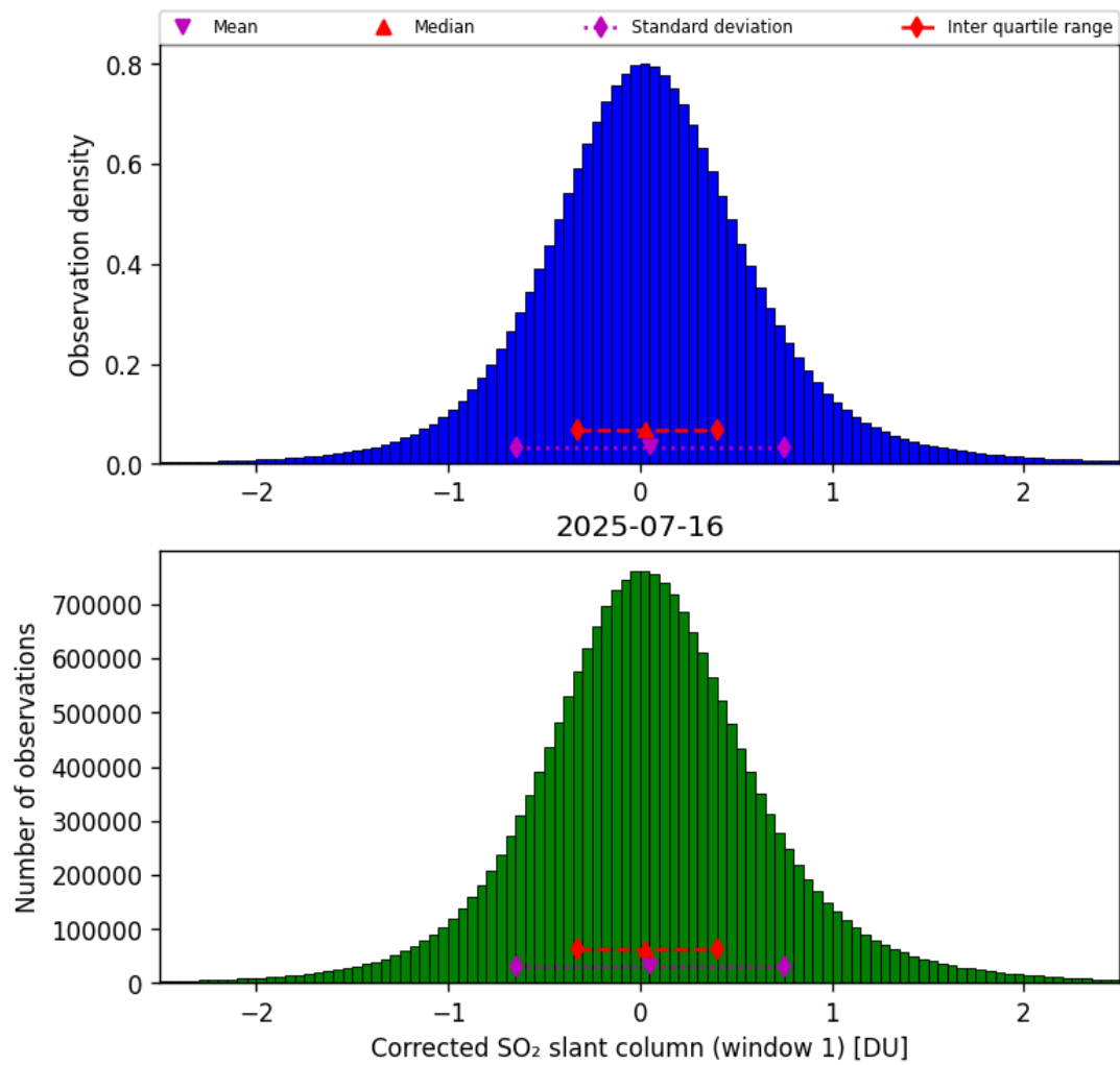
Figure 65: Histogram of “Corrected SO 2 slant column (window 1)” for 2025-07-15 to 2025-07-17
