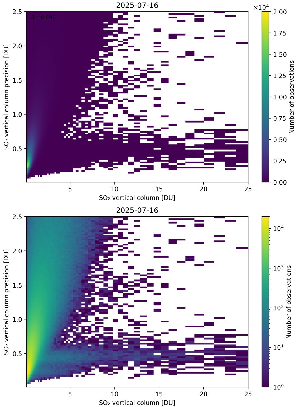
Figure 361: Scatter density plot of “SO 2 vertical column” against “SO 2 vertical column precision” for 2025-07-15 to 2025-07-17.
