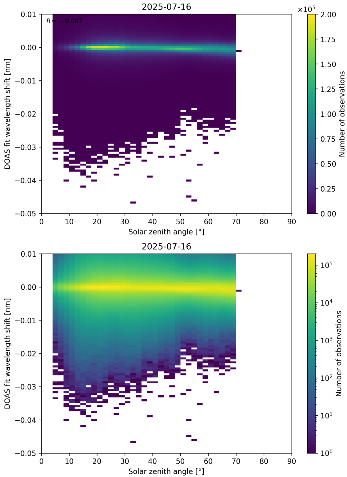
Figure 174: Scatter density plot of “Solar zenith angle” against “DOAS fit wavelength shift” for 2025-07-15 to 2025-07-17.
