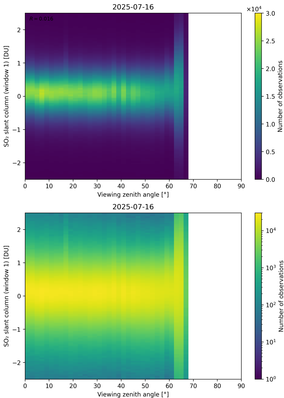
Figure 376: Scatter density plot of “Viewing zenith angle” against “SO 2 slant column (window 1)” for 2025-07-15 to 2025-07-17.
