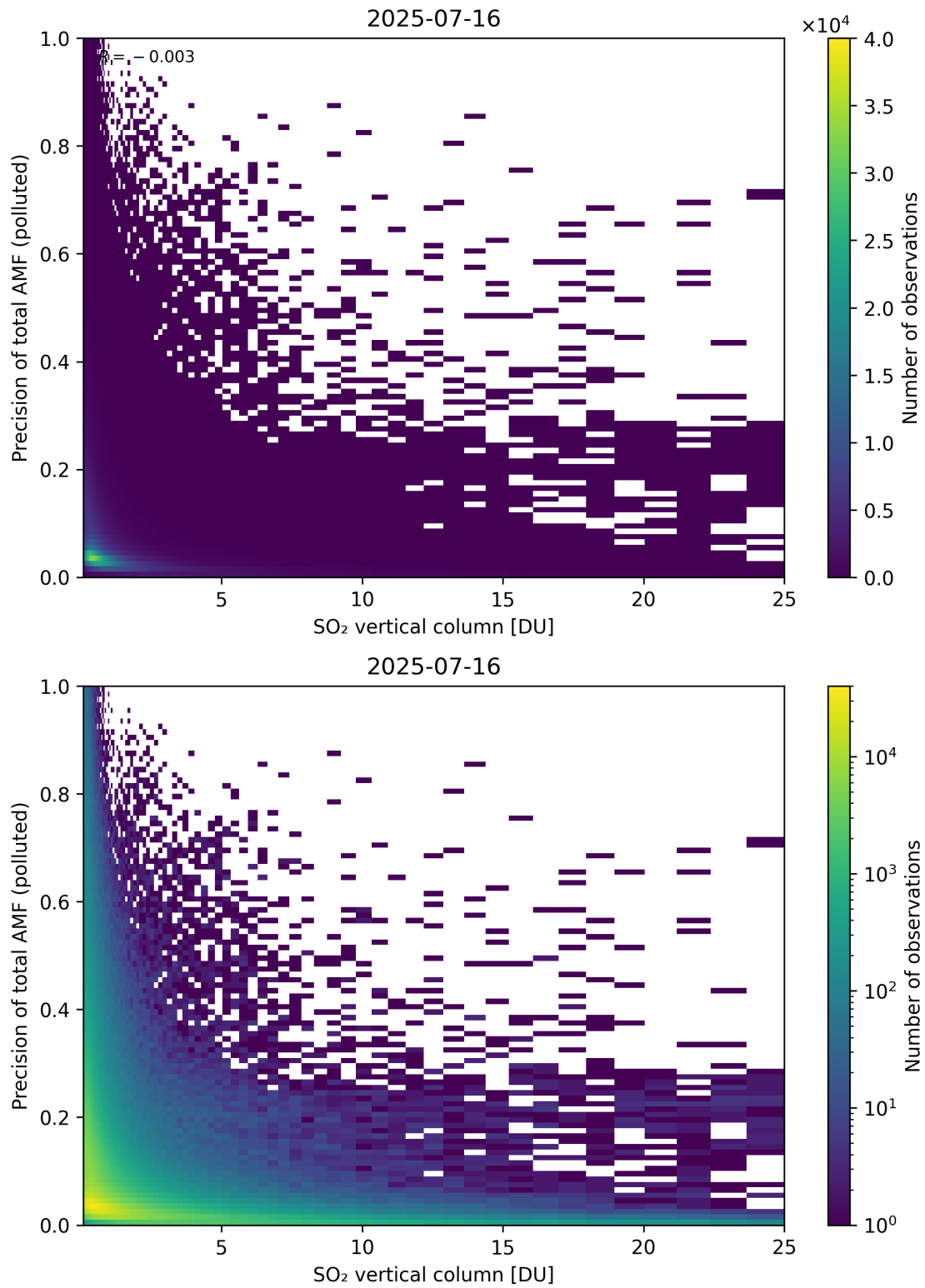
Figure 360: Scatter density plot of “SO 2 vertical column” against “Precision of total AMF (polluted)” for 2025-07-15 to 2025-07-17.
