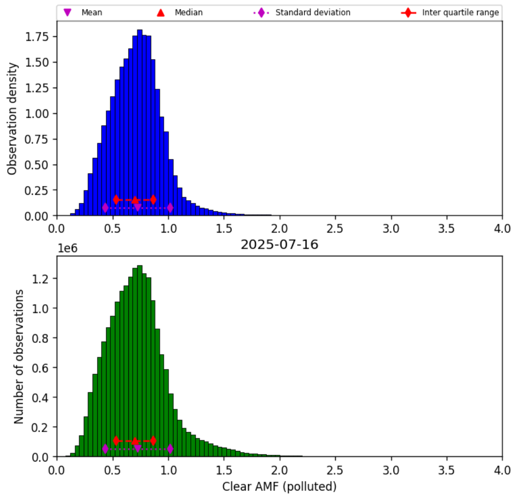
Figure 81: Histogram of “Clear AMF (polluted)” for 2025-07-15 to 2025-07-17
