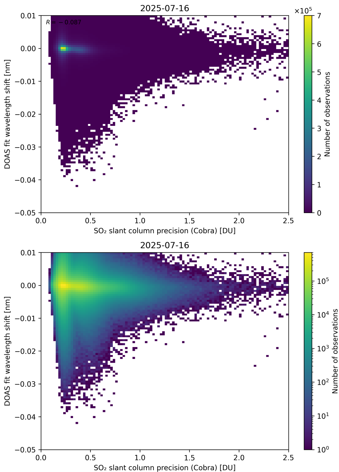
Figure 202: Scatter density plot of “SO 2 slant column precision (Cobra)” against “DOAS fit wavelength shift” for 2025-07-15 to 2025-07-17.
