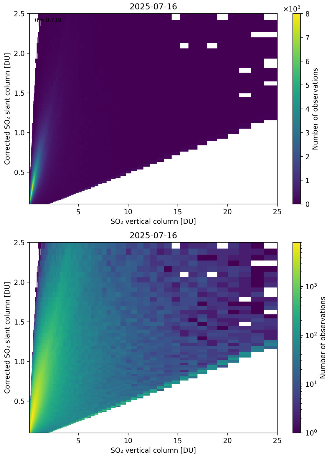
Figure 351: Scatter density plot of “SO 2 vertical column” against “Corrected SO 2 slant column” for 2025-07-15 to 2025-07-17.
