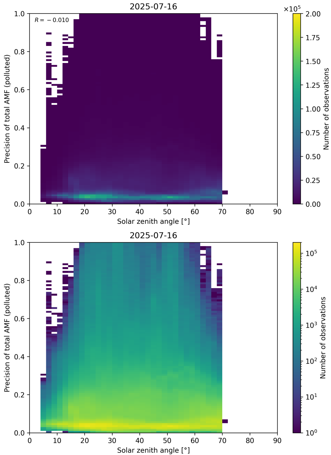
Figure 190: Scatter density plot of “Solar zenith angle” against “Precision of total AMF (polluted)” for 2025-07-15 to 2025-07-17.
