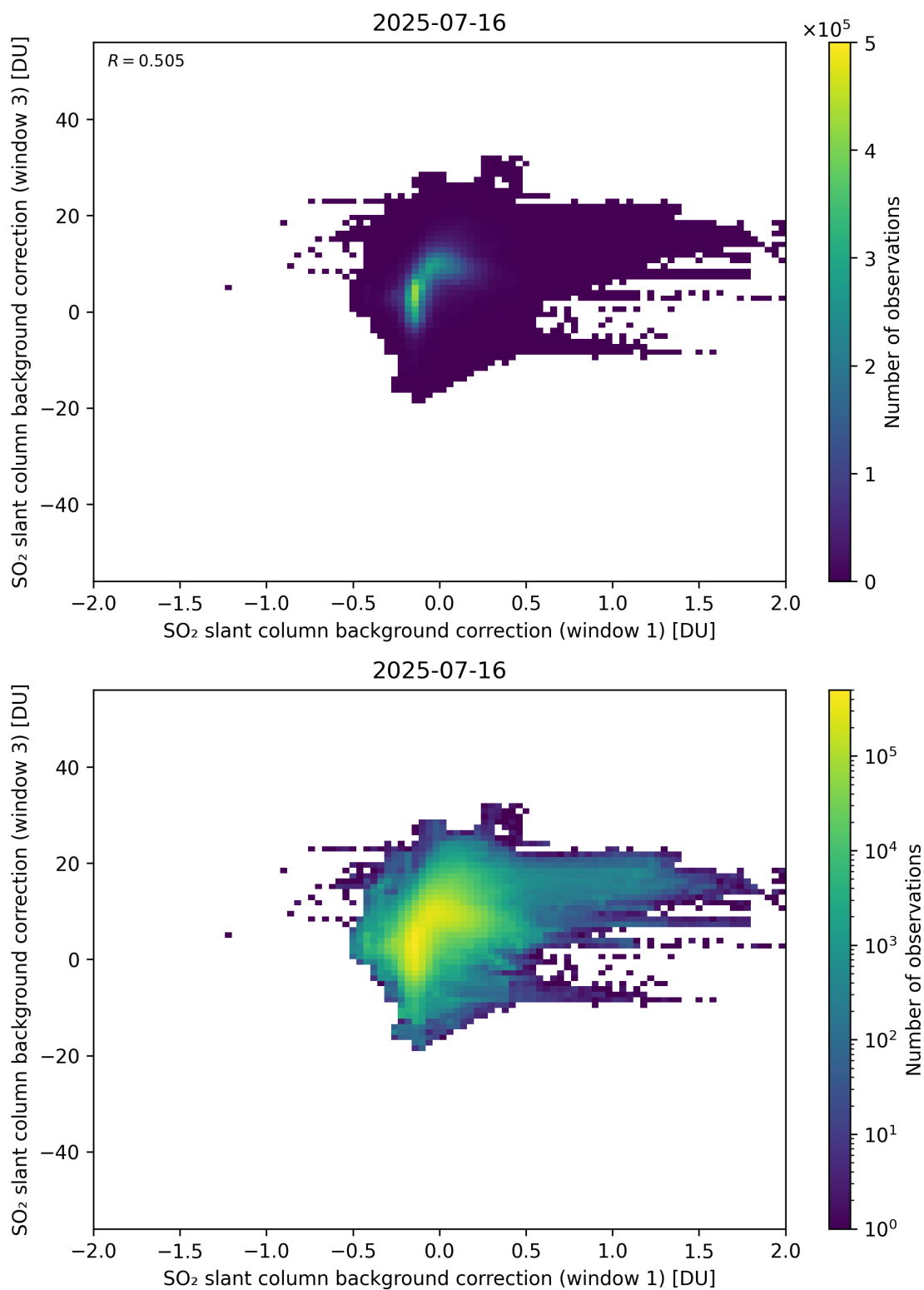
Figure 110: Scatter density plot of “SO 2 slant column background correction (window 1)” against “SO 2 slant column background correction (window 3)” for 2025-07-15 to 2025-07-17.
