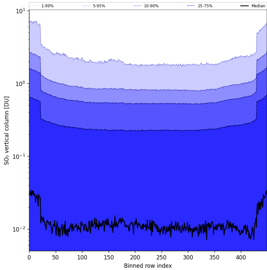
Figure 84: Along track statistics of “SO 2 vertical column” for 2025-07-15 to 2025-07-17
