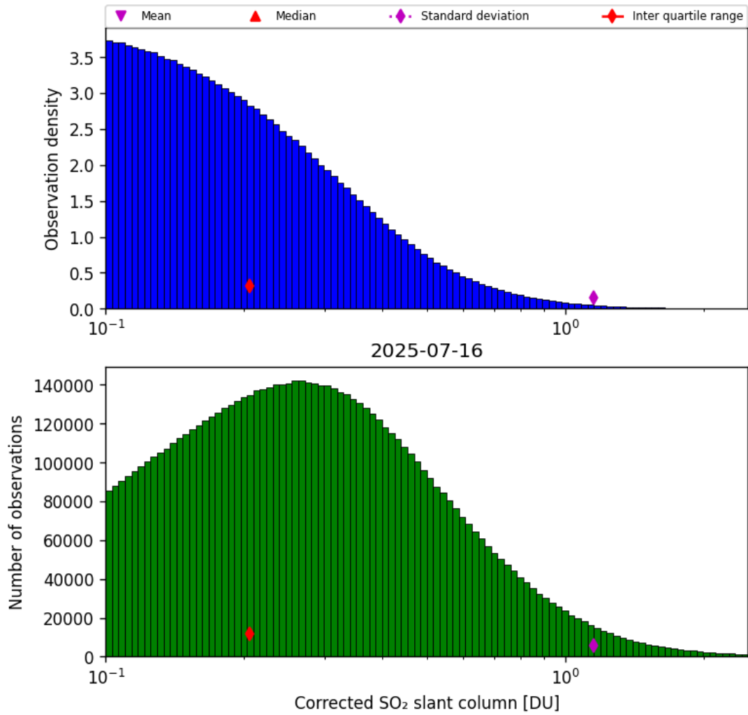
Figure 60: Histogram of “Corrected SO 2 slant column” for 2025-07-15 to 2025-07-17
