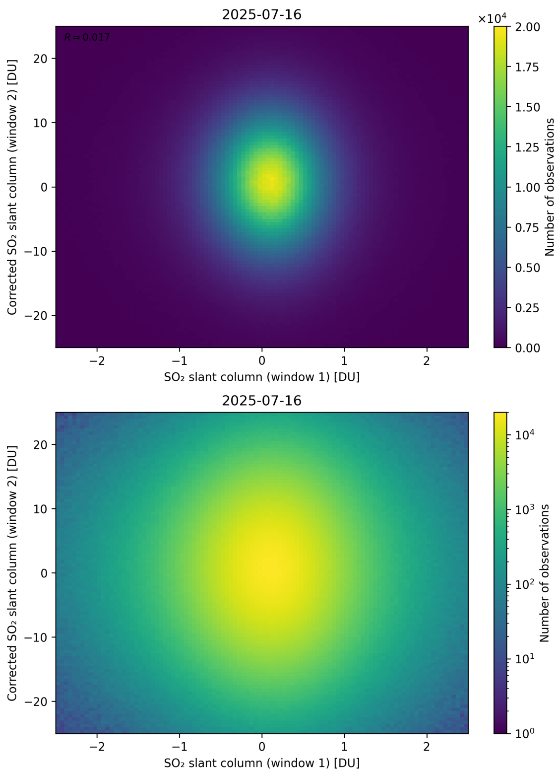
Figure 283: Scatter density plot of “SO 2 slant column (window 1)” against “Corrected SO 2 slant column (window 2)” for 2025-07-15 to 2025-07-17.
