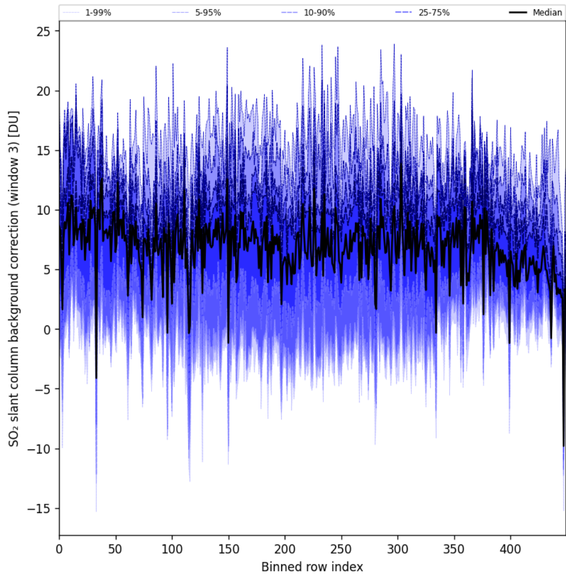
Figure 100: Along track statistics of “SO 2 slant column background correction (window 3)” for 2025-07-15 to 2025-07-17
