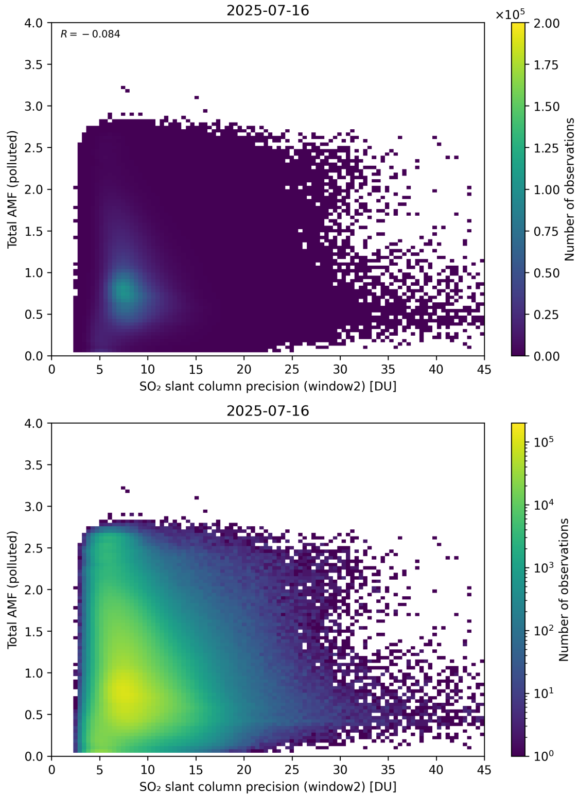
Figure 301: Scatter density plot of “SO 2 slant column precision (window2)” against “Total AMF (polluted)” for 2025-07-15 to 2025-07-17.
