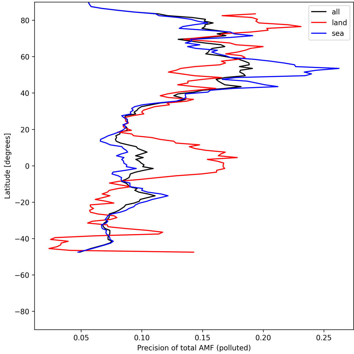
Figure 54: Zonal average of “Precision of total AMF (polluted)” for 2025-07-15 to 2025-07-17.
