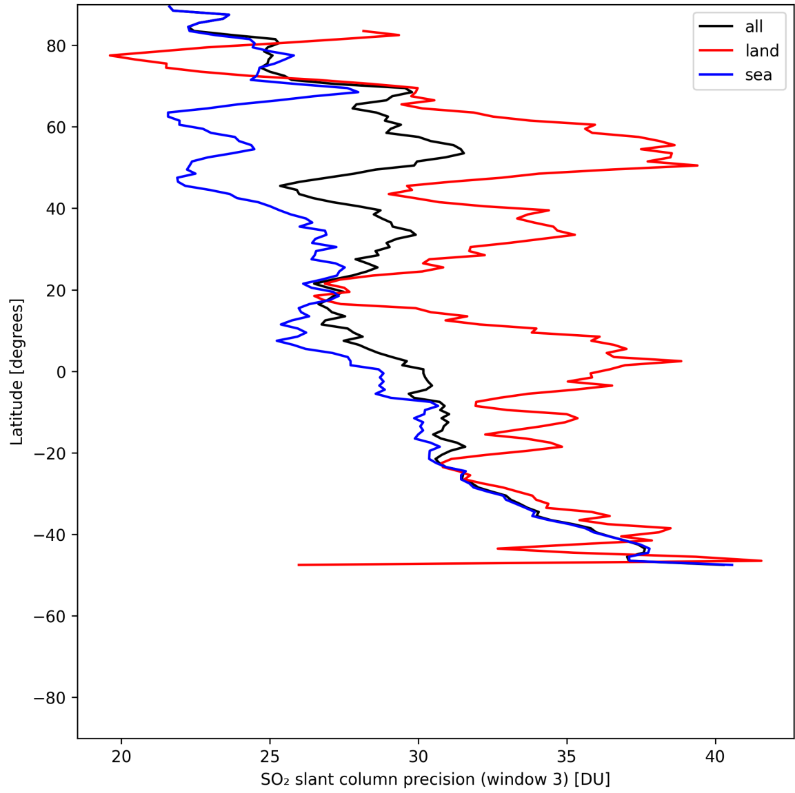
Figure 46: Zonal average of “SO 2 slant column precision (window 3)” for 2025-07-15 to 2025-07-17.
