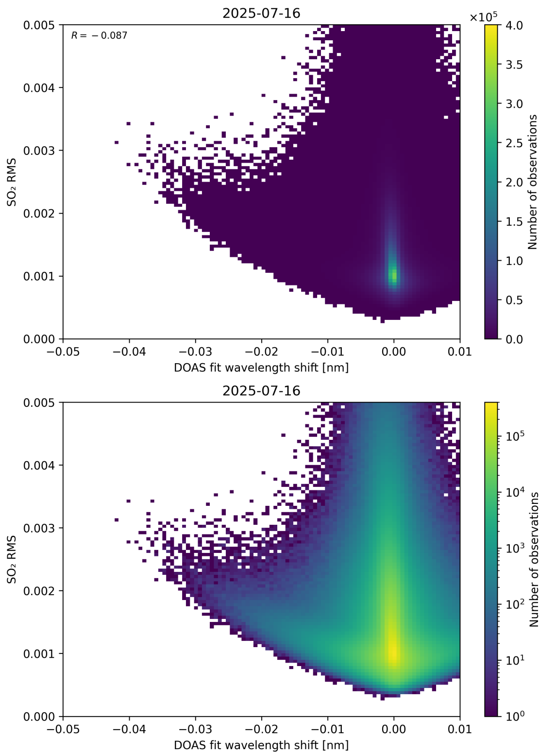
Figure 139: Scatter density plot of “DOAS fit wavelength shift” against “SO 2 RMS” for 2025-07-15 to 2025-07-17.
