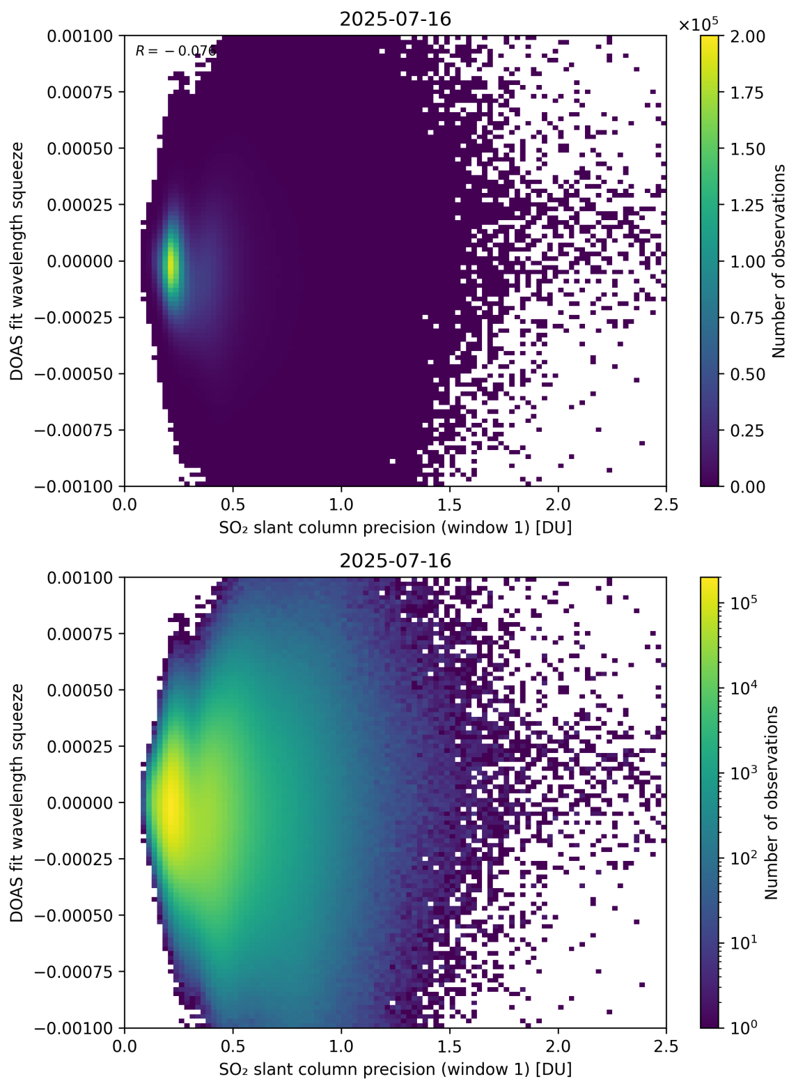
Figure 272: Scatter density plot of “SO 2 slant column precision (window 1)” against “DOAS fit wavelength squeeze” for 2025-07-15 to 2025-07-17.
