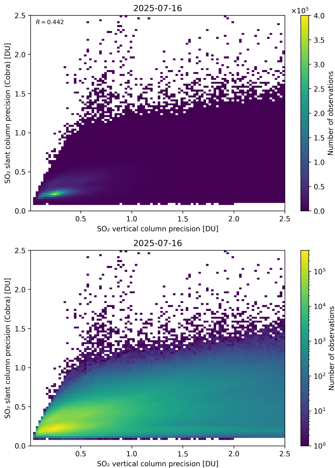
Figure 337: Scatter density plot of “SO 2 vertical column precision” against “SO 2 slant column precision (Cobra)” for 2025-07-15 to 2025-07-17.
