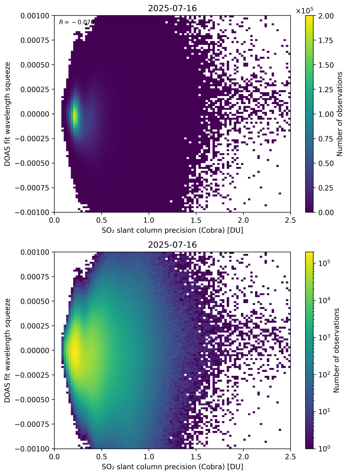
Figure 203: Scatter density plot of “SO 2 slant column precision (Cobra)” against “DOAS fit wavelength squeeze” for 2025-07-15 to 2025-07-17.
