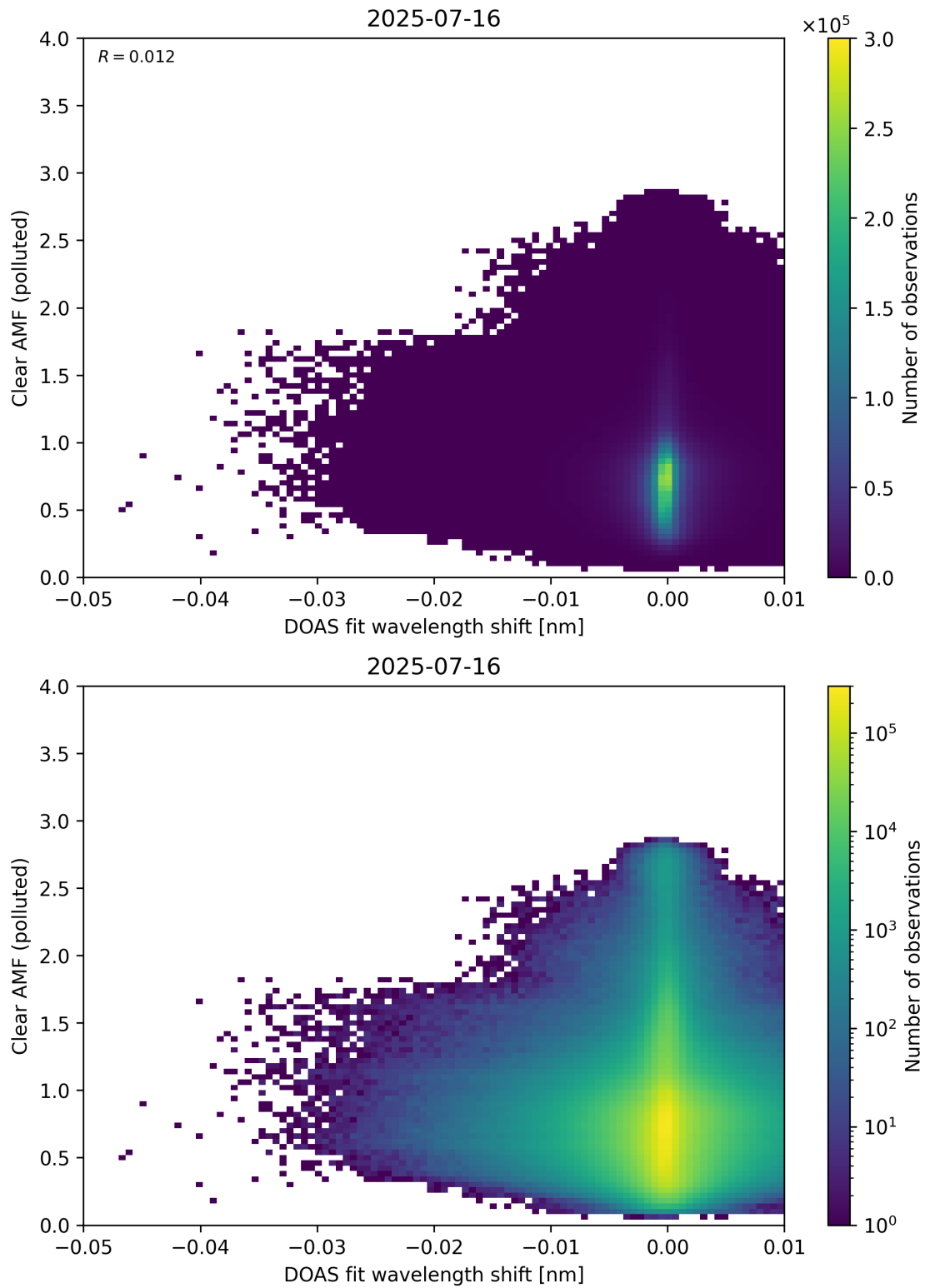
Figure 140: Scatter density plot of “DOAS fit wavelength shift” against “Clear AMF (polluted)” for 2025-07-15 to 2025-07-17.
