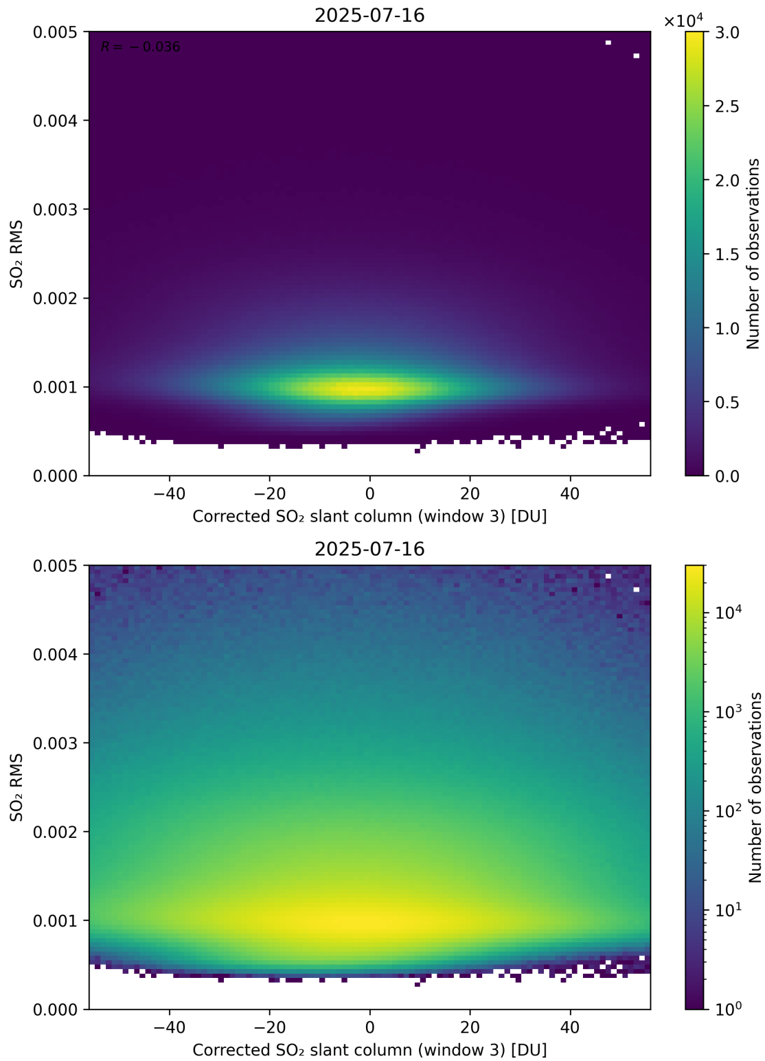
Figure 258: Scatter density plot of “Corrected SO 2 slant column (window 3)” against “SO 2 RMS” for 2025-07-15 to 2025-07-17.
