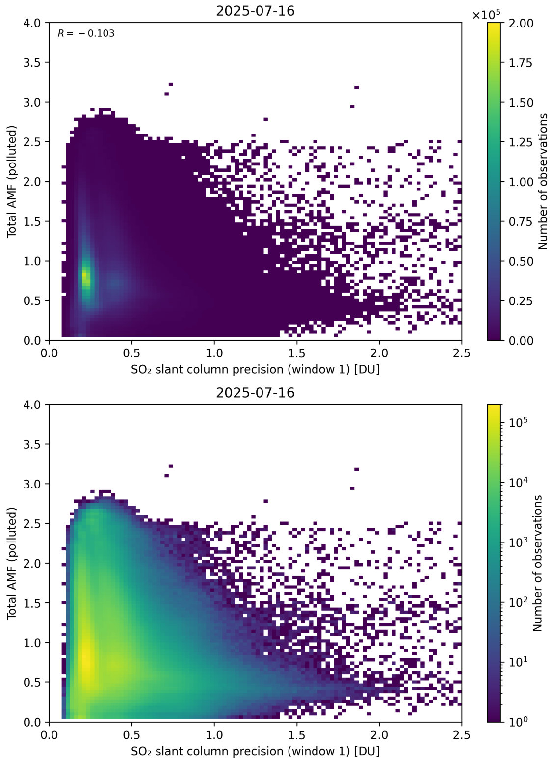
Figure 280: Scatter density plot of “SO 2 slant column precision (window 1)” against “Total AMF (polluted)” for 2025-07-15 to 2025-07-17.
