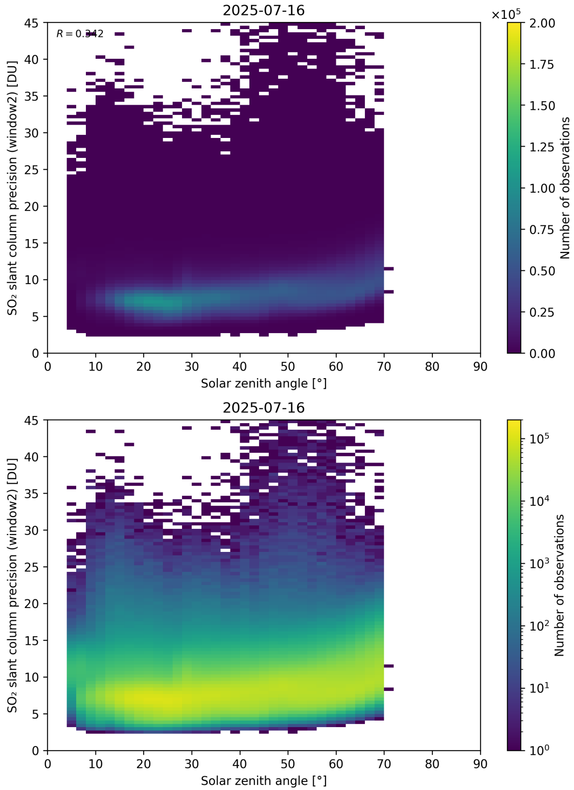
Figure 186: Scatter density plot of “Solar zenith angle” against “SO 2 slant column precision (window2)” for 2025-07-15 to 2025-07-17.
