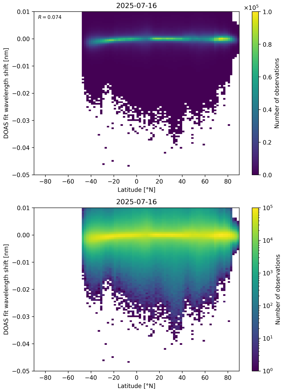
Figure 153: Scatter density plot of “Latitude” against “DOAS fit wavelength shift” for 2025-07-15 to 2025-07-17.
