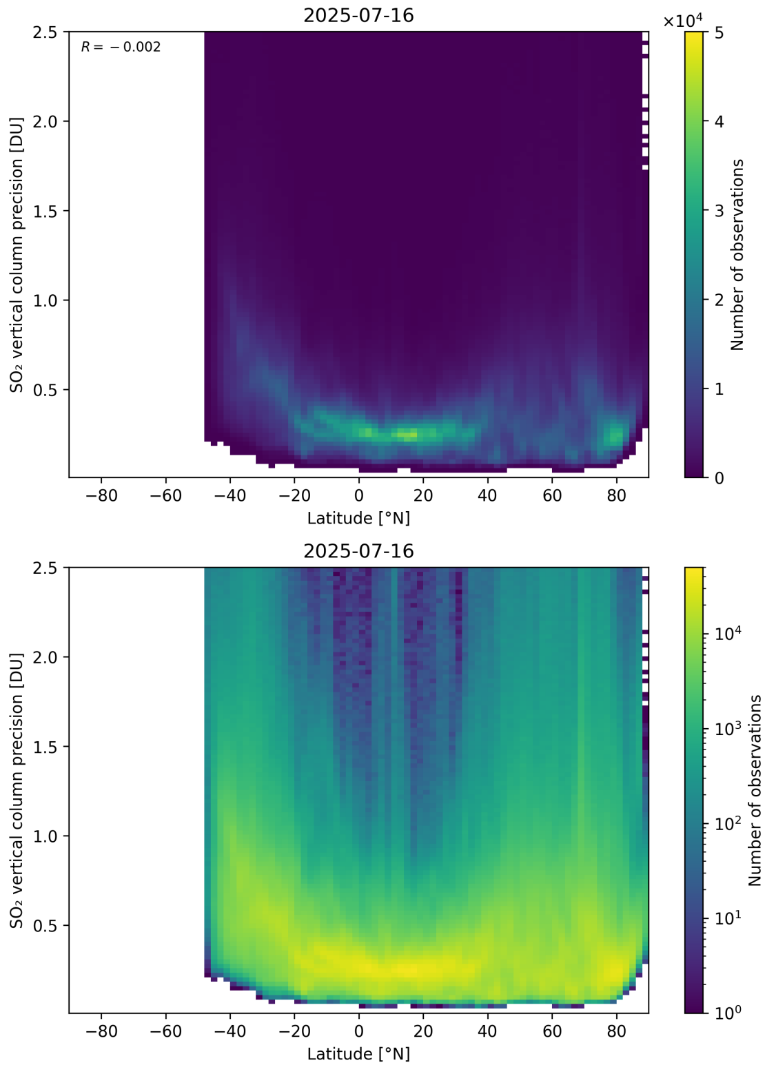
Figure 170: Scatter density plot of “Latitude” against “SO 2 vertical column precision” for 2025-07-15 to 2025-07-17.
