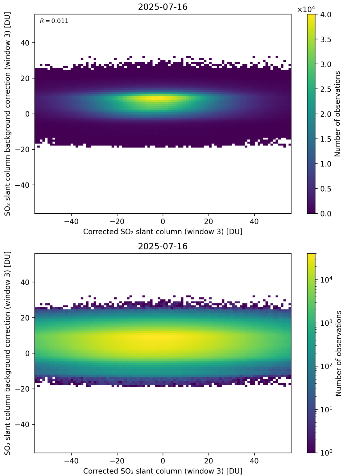
Figure 255: Scatter density plot of “Corrected SO 2 slant column (window 3)” against “SO 2 slant column background correction (window 3)” for 2025-07-15 to 2025-07-17.
