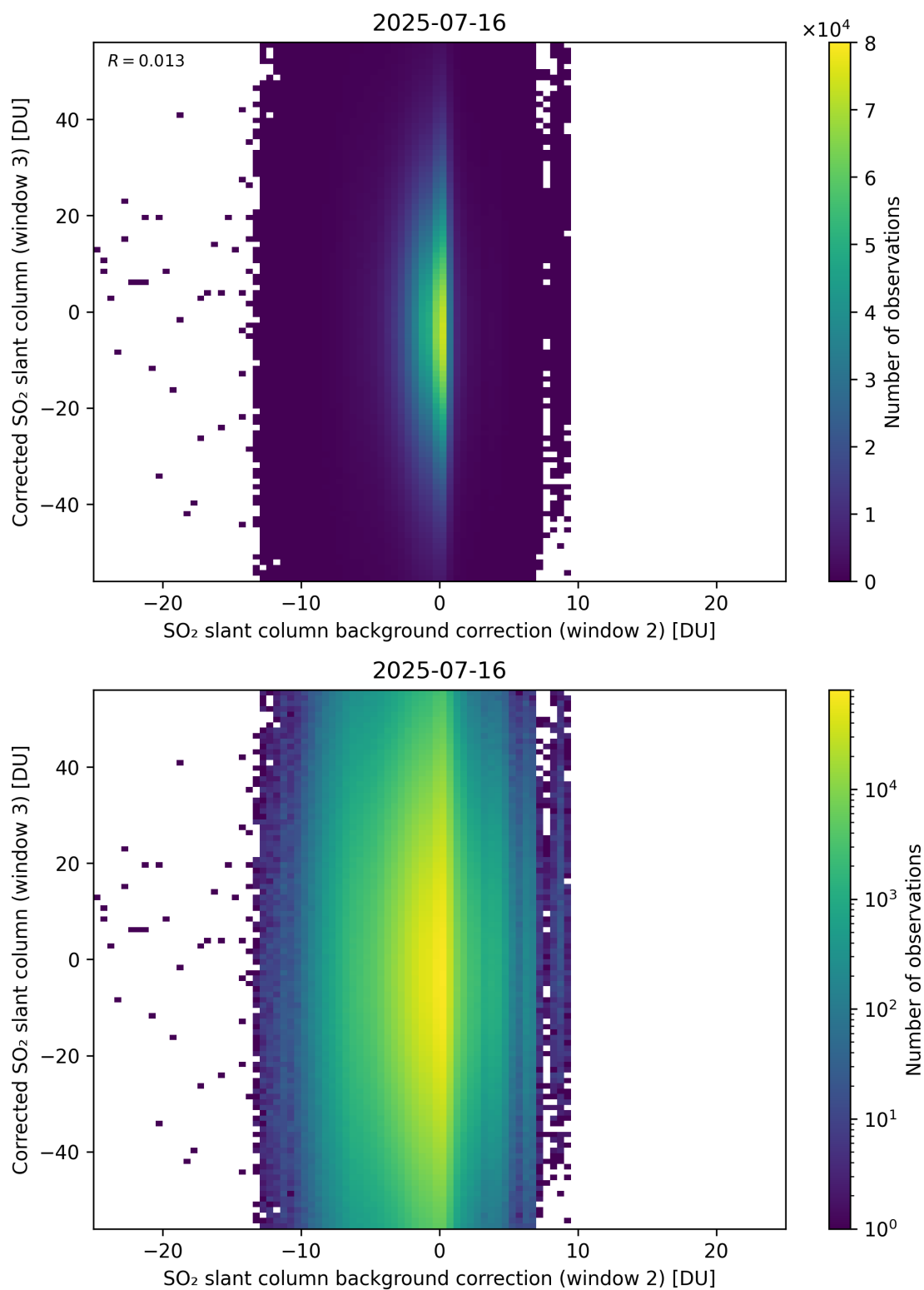
Figure 127: Scatter density plot of “SO 2 slant column background correction (window 2)” against “Corrected SO 2 slant column (window 3)” for 2025-07-15 to 2025-07-17.
