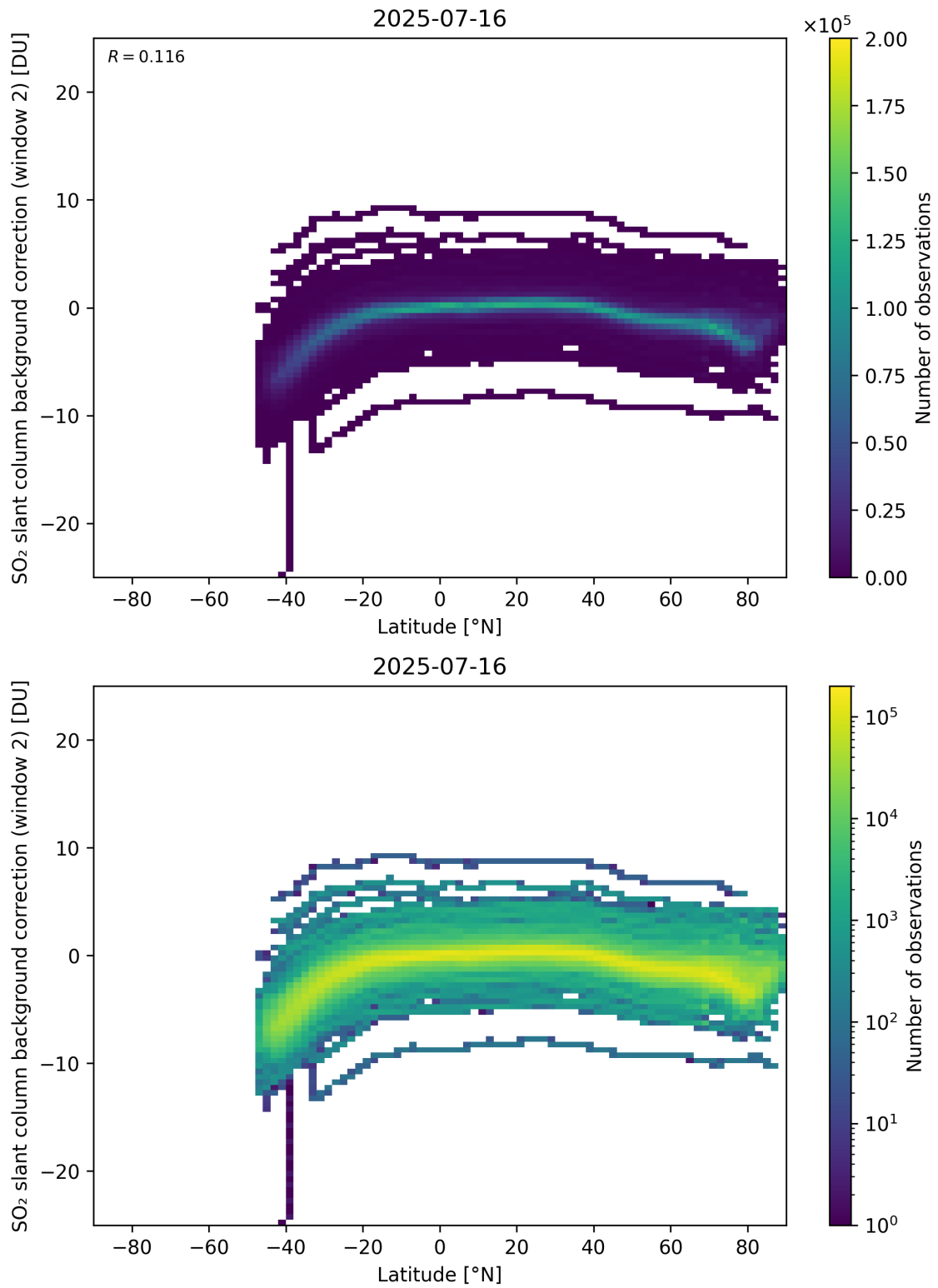
Figure 151: Scatter density plot of “Latitude” against “SO 2 slant column background correction (window 2)” for 2025-07-15 to 2025-07-17.
