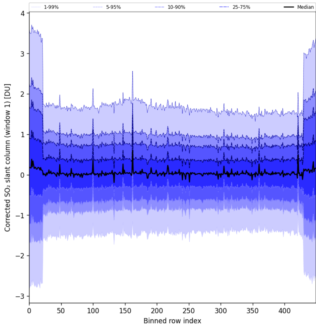
Figure 91: Along track statistics of “Corrected SO 2 slant column (window 1)” for 2025-07-15 to 2025-07-17
