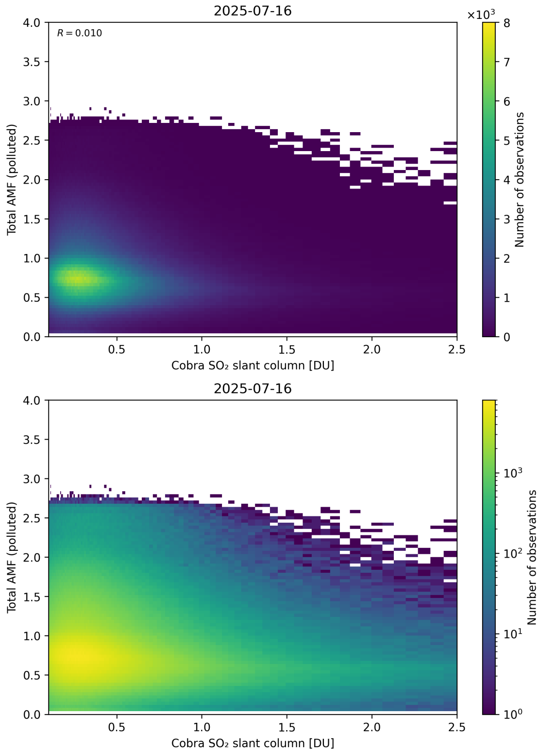
Figure 224: Scatter density plot of “Cobra SO 2 slant column” against “Total AMF (polluted)” for 2025-07-15 to 2025-07-17.
