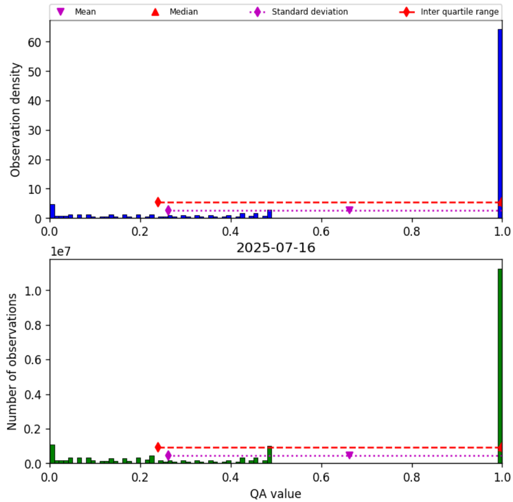
Figure 57: Histogram of “QA value” for 2025-07-15 to 2025-07-17
