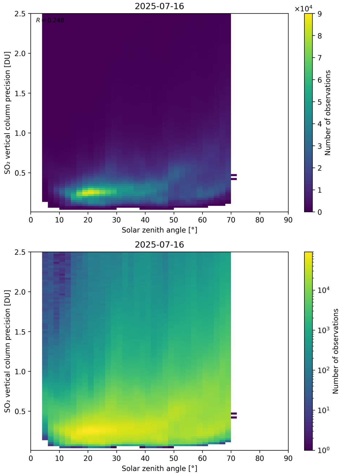
Figure 192: Scatter density plot of “Solar zenith angle” against “SO 2 vertical column precision” for 2025-07-15 to 2025-07-17.
