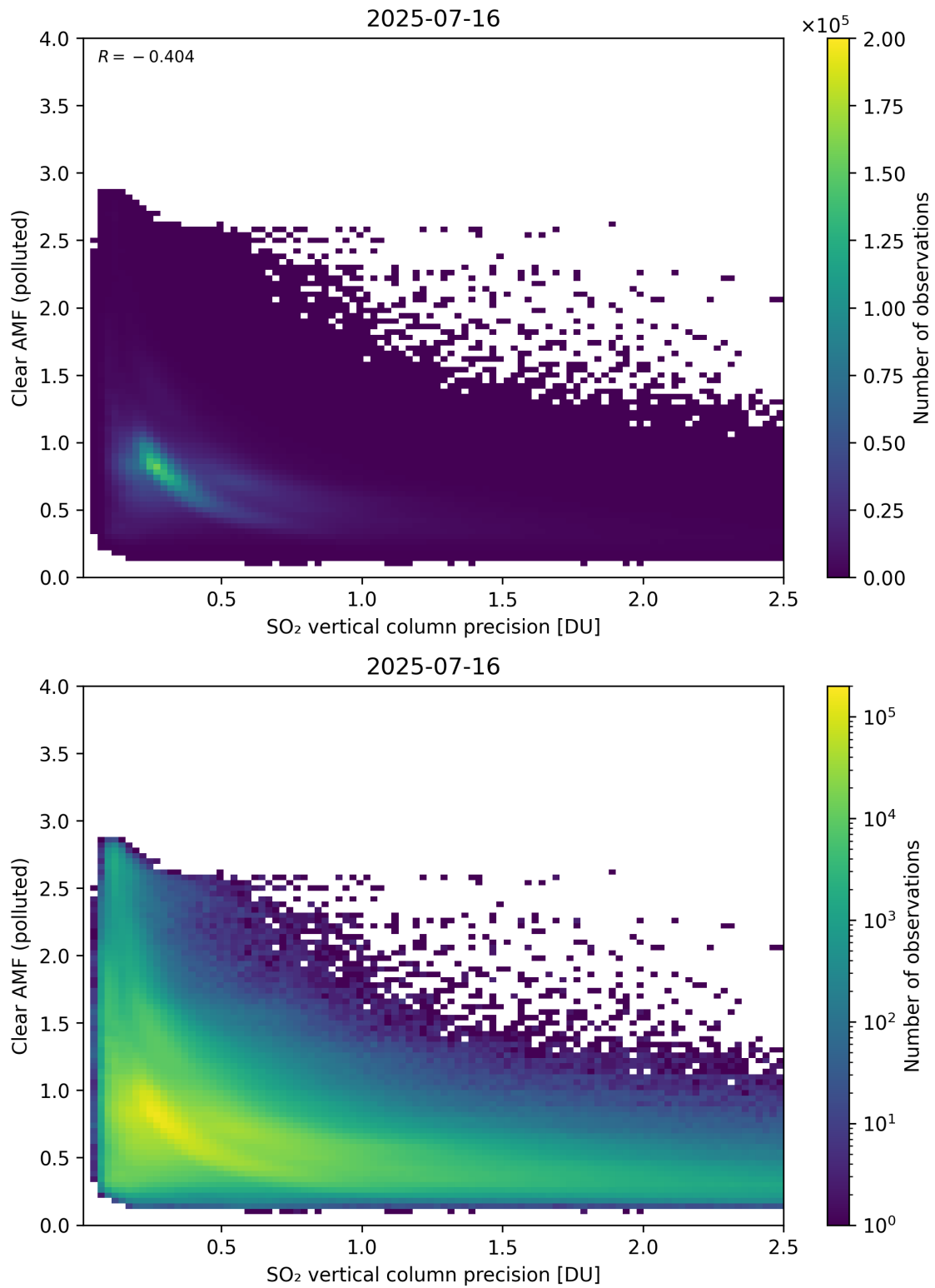
Figure 335: Scatter density plot of “SO 2 vertical column precision” against “Clear AMF (polluted)” for 2025-07-15 to 2025-07-17.
