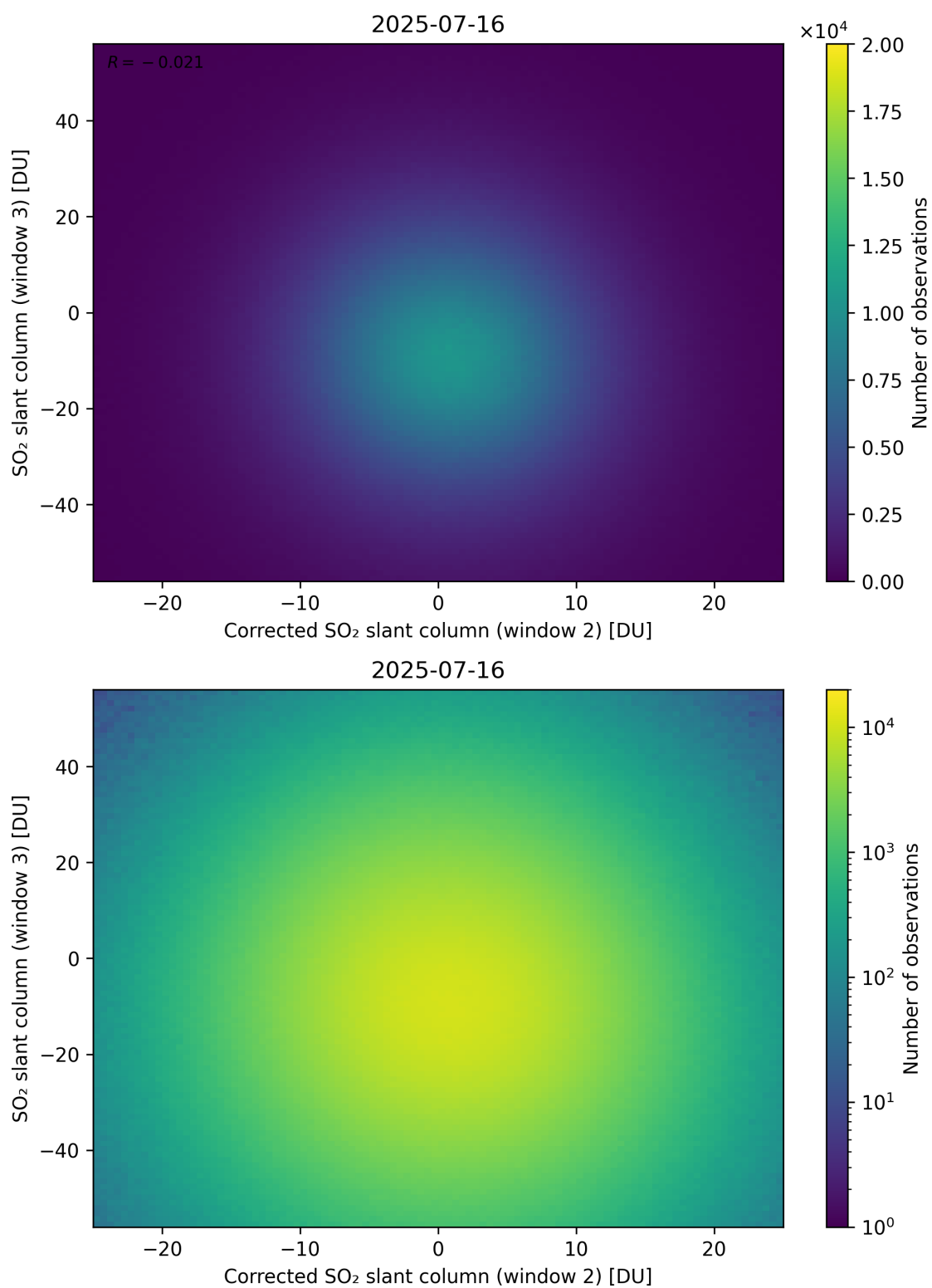
Figure 251: Scatter density plot of “Corrected SO 2 slant column (window 2)” against “SO 2 slant column (window 3)” for 2025-07-15 to 2025-07-17.
