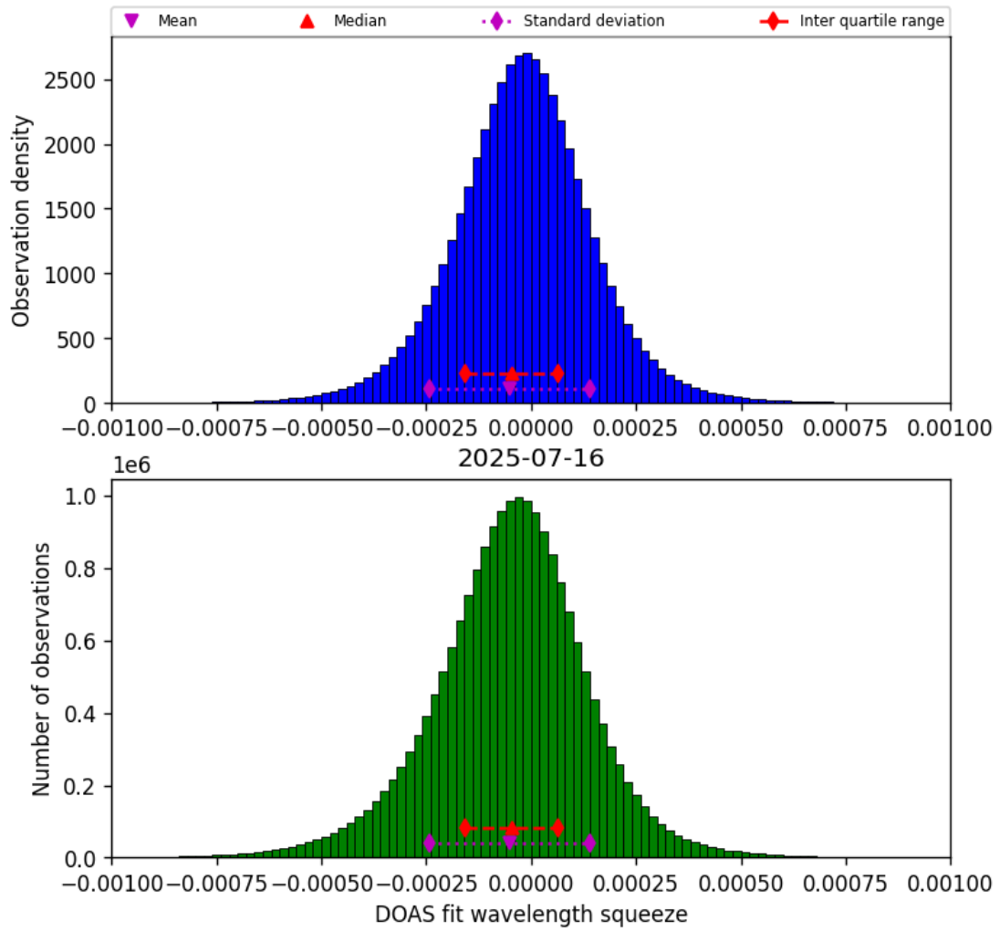
Figure 77: Histogram of “DOAS fit wavelength squeeze” for 2025-07-15 to 2025-07-17
