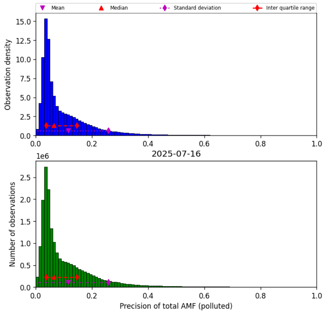
Figure 80: Histogram of “Precision of total AMF (polluted)” for 2025-07-15 to 2025-07-17
