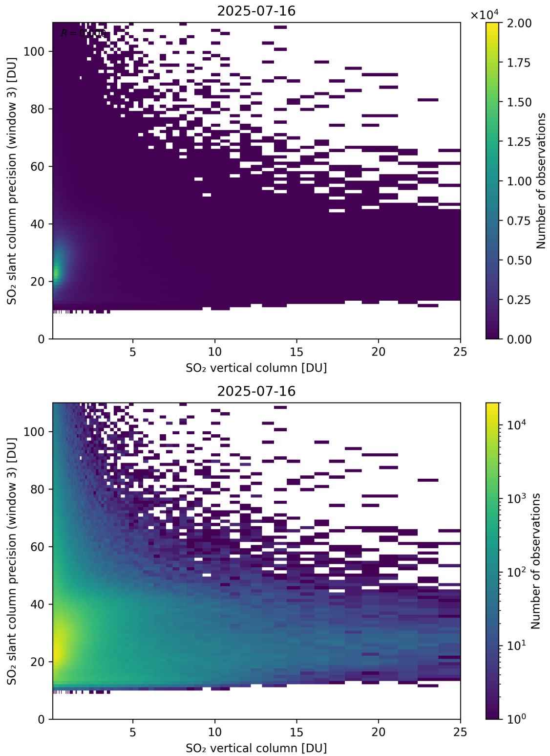
Figure 358: Scatter density plot of “SO 2 vertical column” against “SO 2 slant column precision (window 3)” for 2025-07-15 to 2025-07-17.
