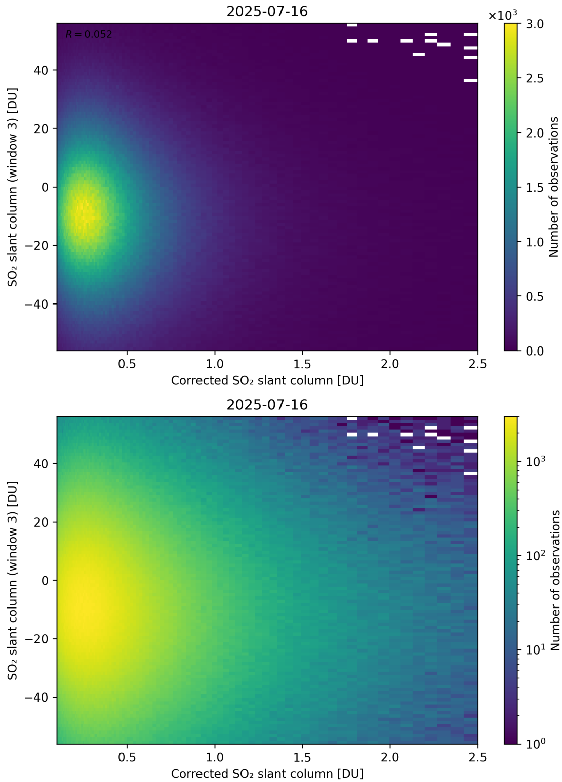
Figure 240: Scatter density plot of “Corrected SO 2 slant column” against “SO 2 slant column (window 3)” for 2025-07-15 to 2025-07-17.
