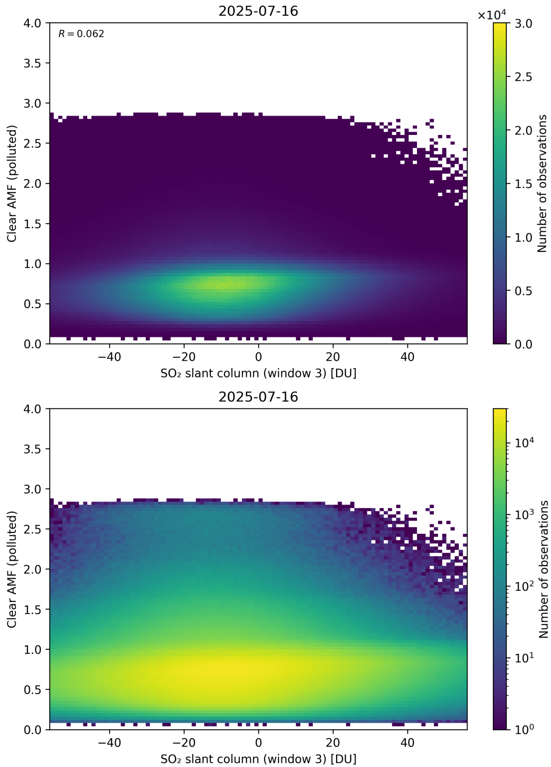
Figure 315: Scatter density plot of “SO 2 slant column (window 3)” against “Clear AMF (polluted)” for 2025-07-15 to 2025-07-17.
