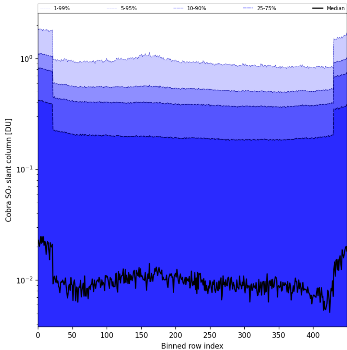
Figure 87: Along track statistics of “Cobra SO 2 slant column” for 2025-07-15 to 2025-07-17
