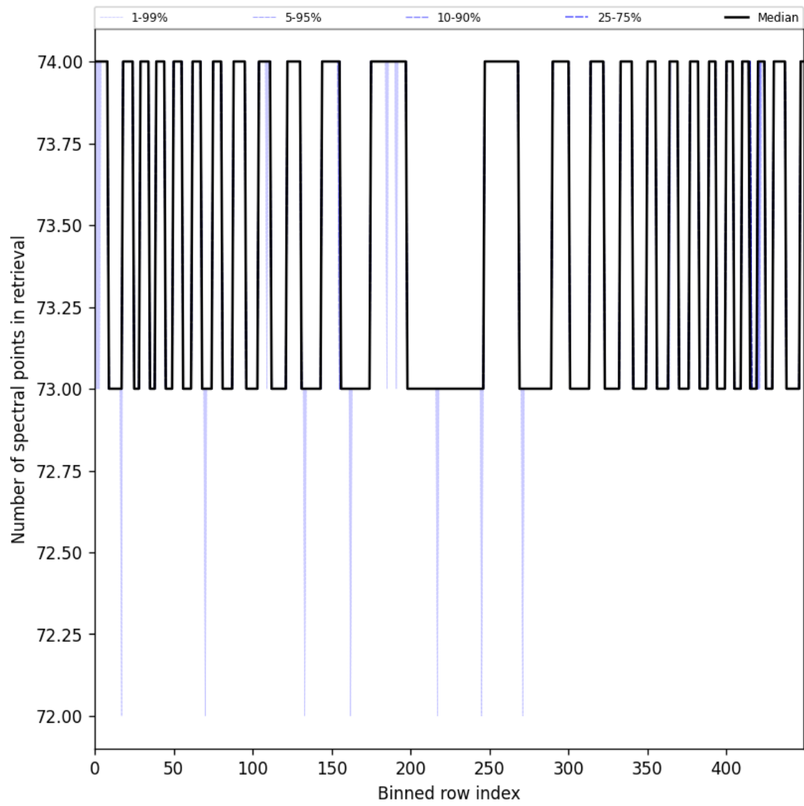
Figure 108: Along track statistics of “Number of spectral points in retrieval” for 2025-07-15 to 2025-07-17
