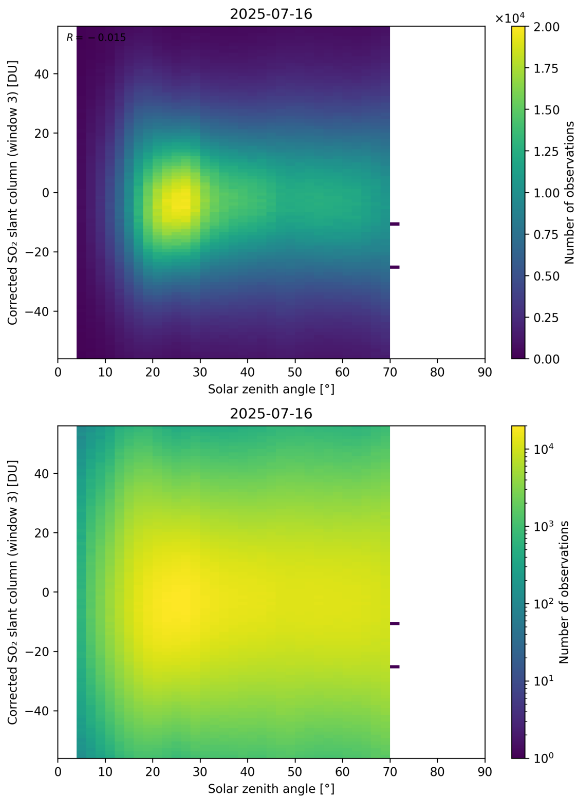
Figure 183: Scatter density plot of “Solar zenith angle” against “Corrected SO 2 slant column (window 3)” for 2025-07-15 to 2025-07-17.
