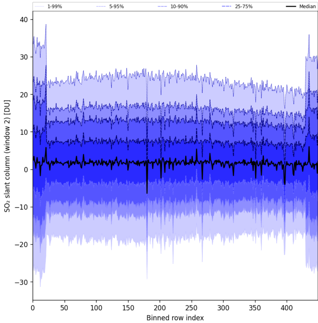
Figure 93: Along track statistics of “SO 2 slant column (window 2)” for 2025-07-15 to 2025-07-17
