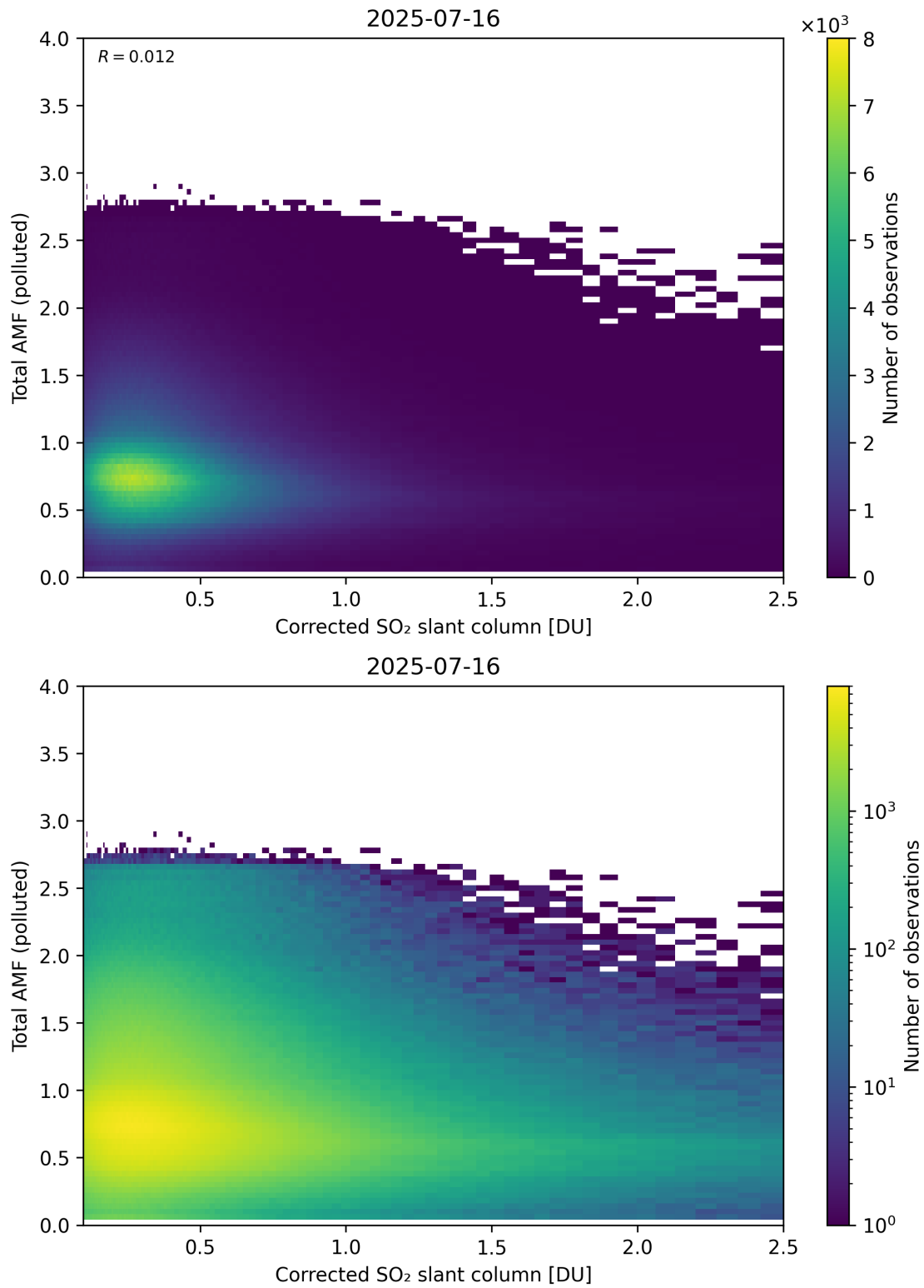
Figure 242: Scatter density plot of “Corrected SO 2 slant column” against “Total AMF (polluted)” for 2025-07-15 to 2025-07-17.
