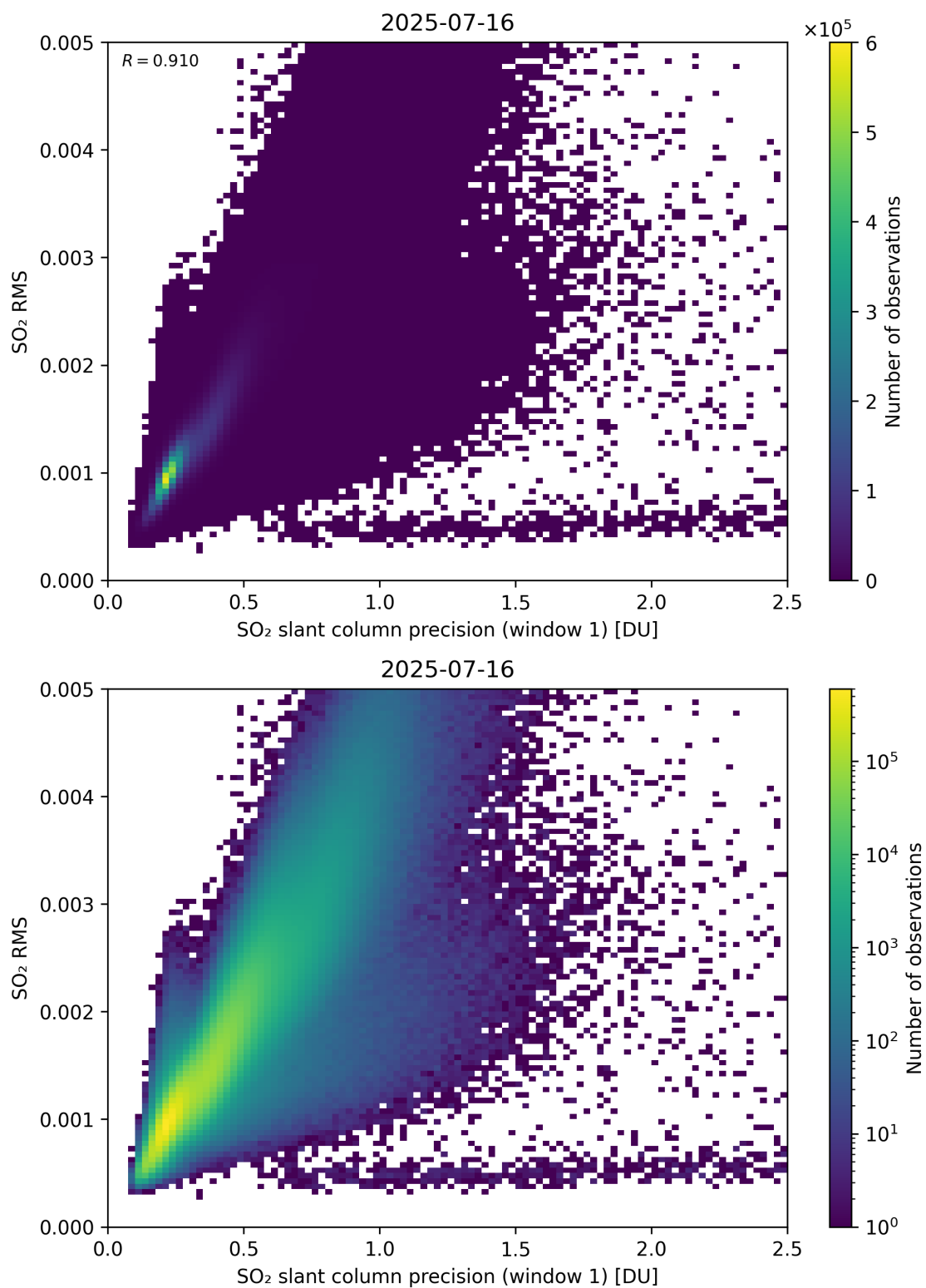
Figure 273: Scatter density plot of “SO 2 slant column precision (window 1)” against “SO 2 RMS” for 2025-07-15 to 2025-07-17.
