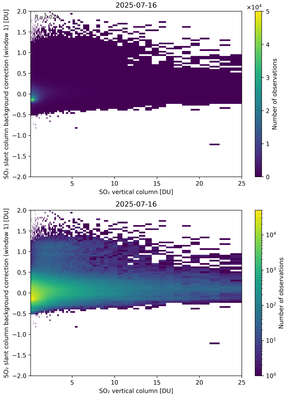
Figure 323: Scatter density plot of “SO 2 vertical column” against “SO 2 slant column background correction (window 1)” for 2025-07-15 to 2025-07-17.
