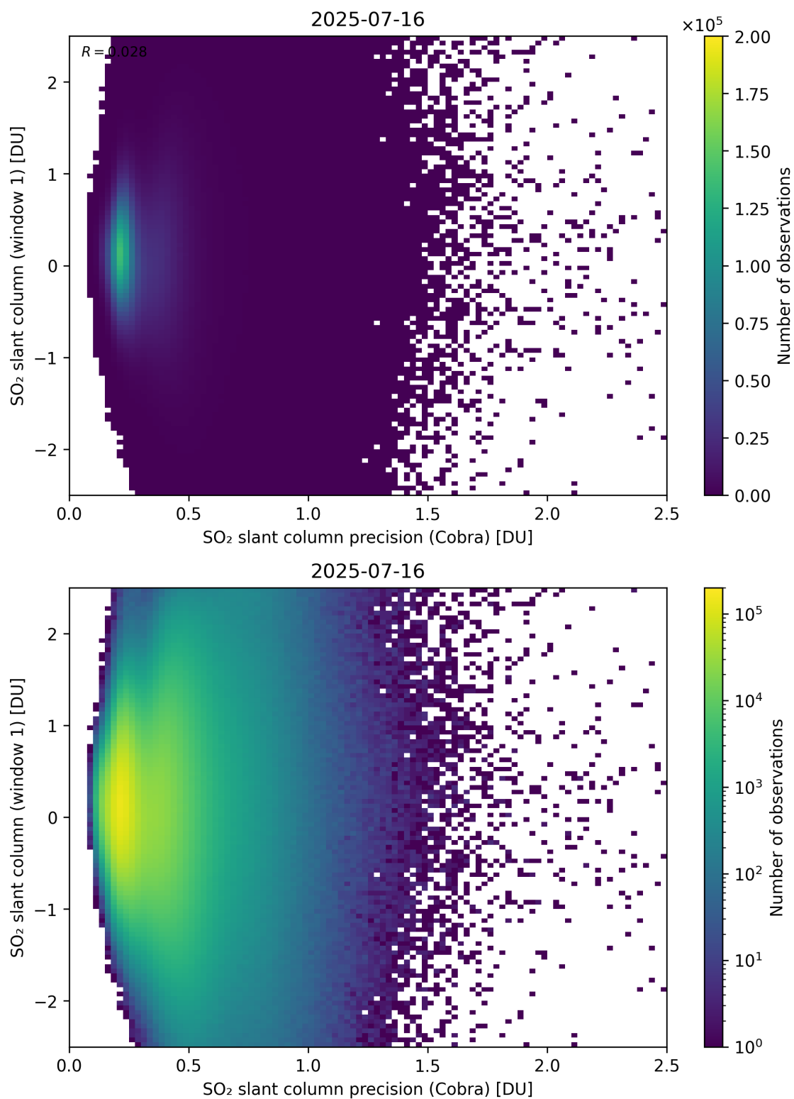
Figure 208: Scatter density plot of “SO 2 slant column precision (Cobra)” against “SO 2 slant column (window 1)” for 2025-07-15 to 2025-07-17.
