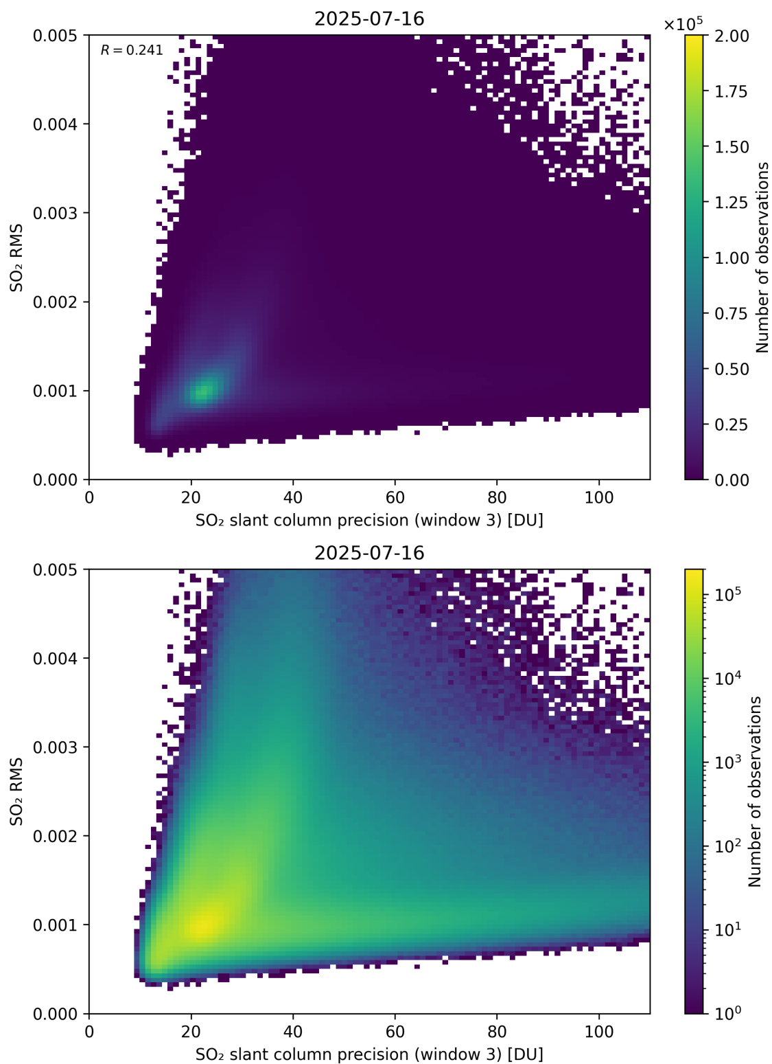
Figure 310: Scatter density plot of “SO 2 slant column precision (window 3)” against “SO 2 RMS” for 2025-07-15 to 2025-07-17.
