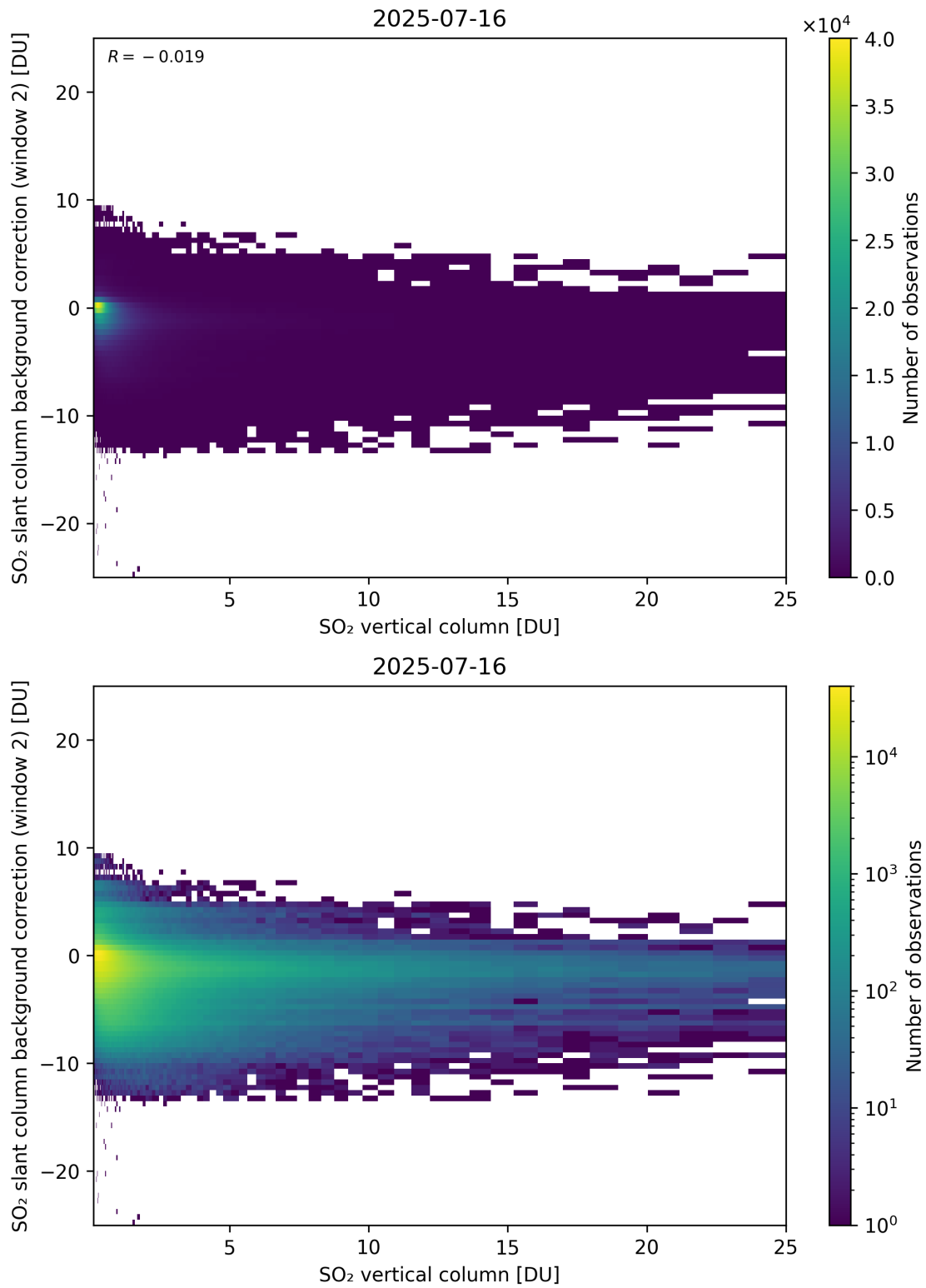
Figure 324: Scatter density plot of “SO 2 vertical column” against “SO 2 slant column background correction (window 2)” for 2025-07-15 to 2025-07-17.
