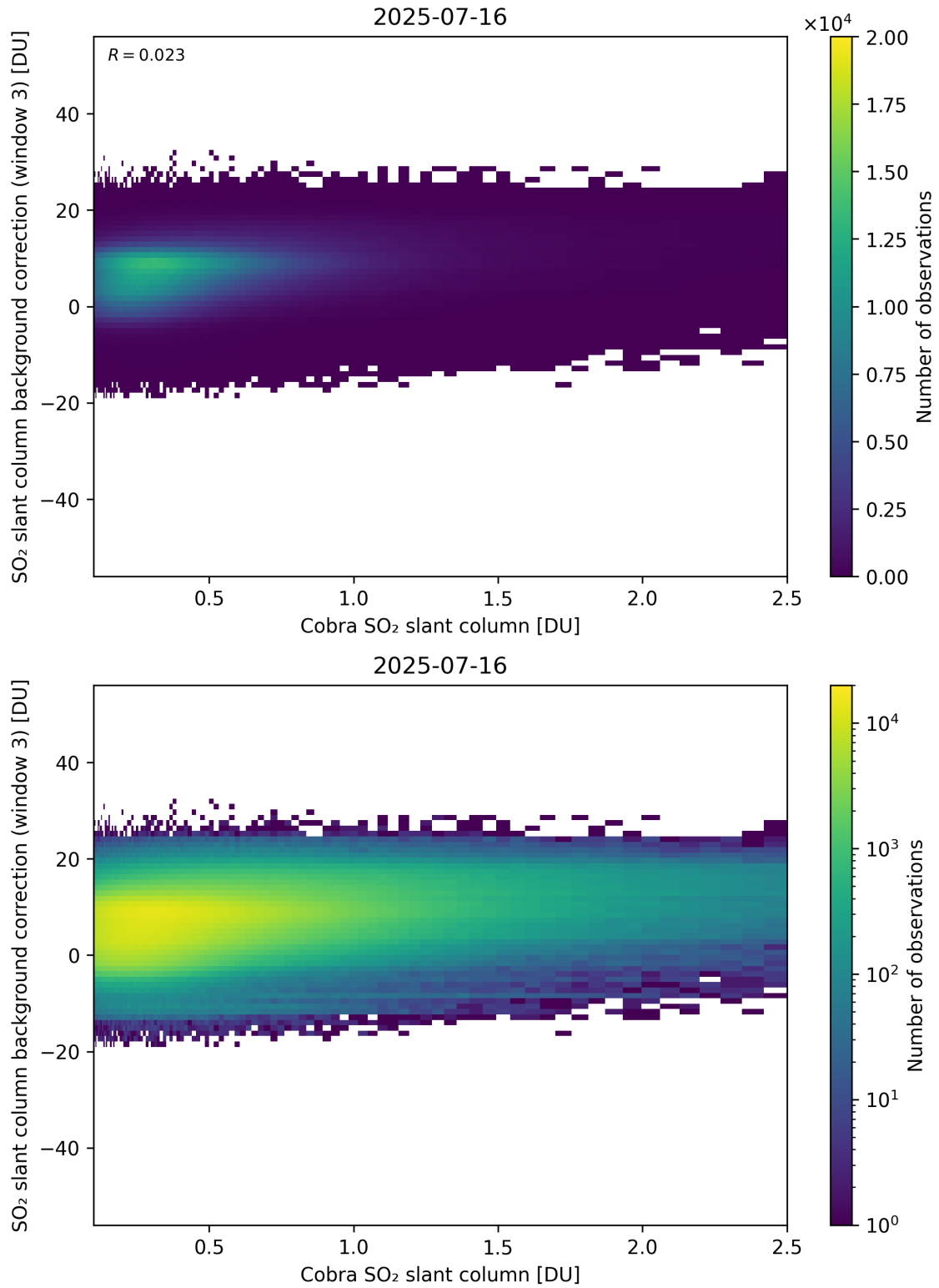
Figure 195: Scatter density plot of “Cobra SO 2 slant column” against “SO 2 slant column background correction (window 3)” for 2025-07-15 to 2025-07-17.
