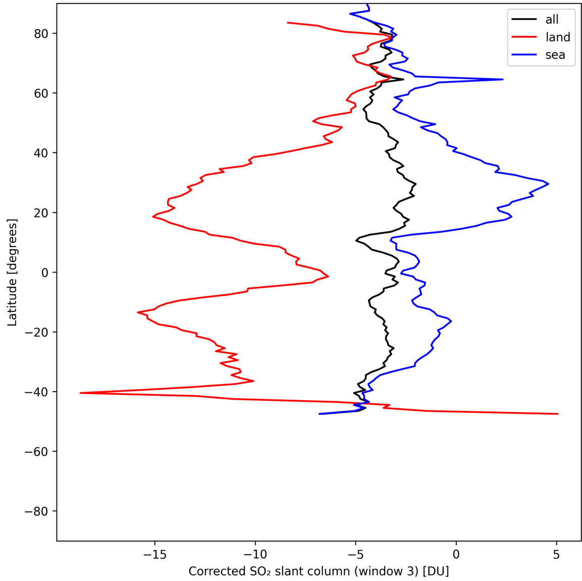
Figure 47: Zonal average of “Corrected SO 2 slant column (window 3)” for 2025-07-15 to 2025-07-17.
