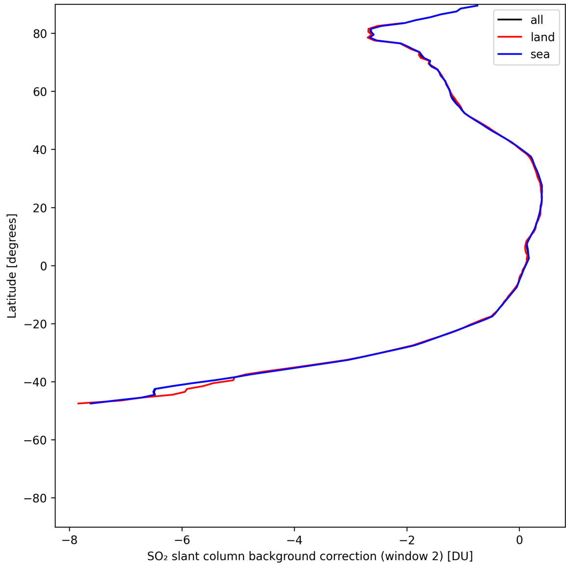
Figure 44: Zonal average of “SO 2 slant column background correction (window 2)” for 2025-07-15 to 2025-07-17.
