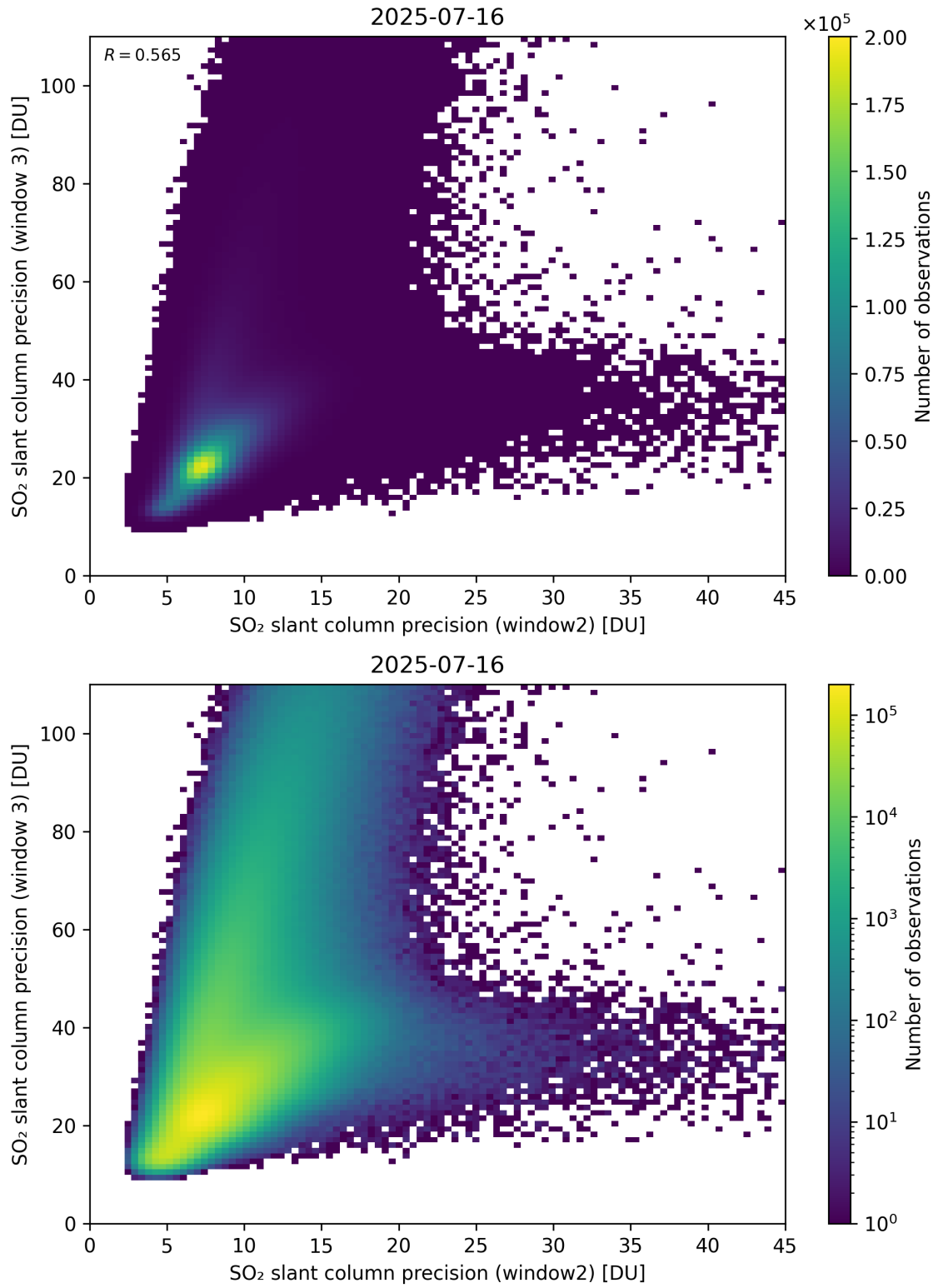
Figure 300: Scatter density plot of “SO 2 slant column precision (window2)” against “SO 2 slant column precision (window 3)” for 2025-07-15 to 2025-07-17.
