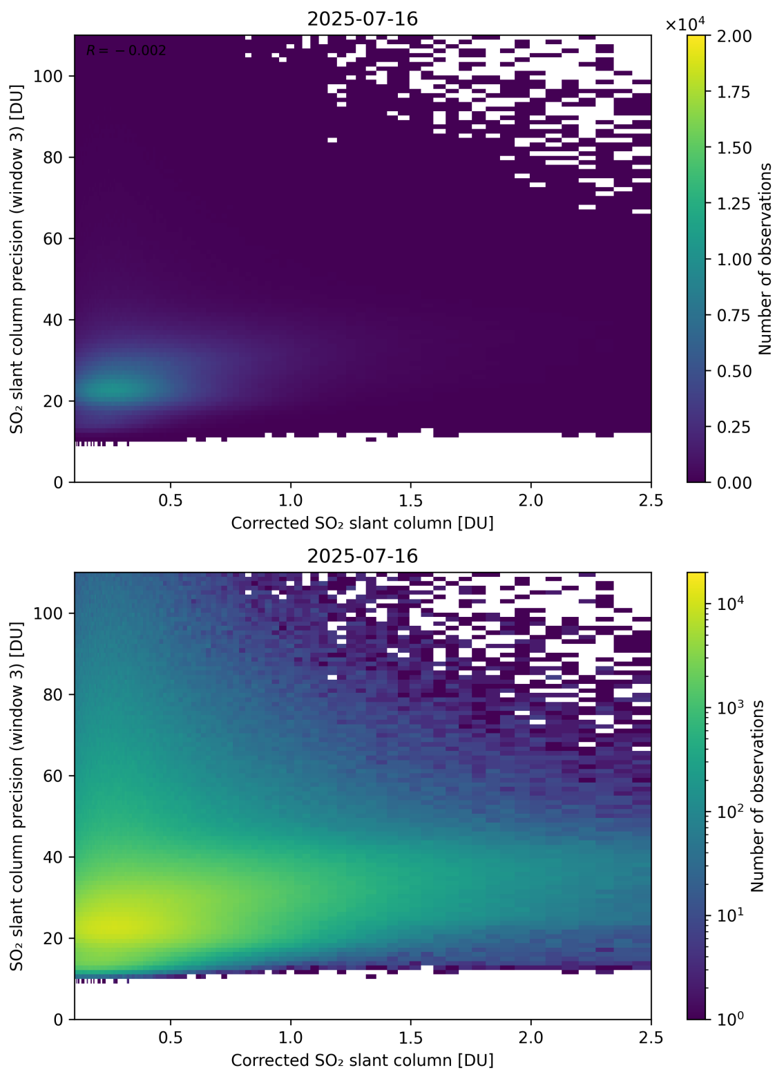
Figure 241: Scatter density plot of “Corrected SO 2 slant column” against “SO 2 slant column precision (window 3)” for 2025-07-15 to 2025-07-17.
