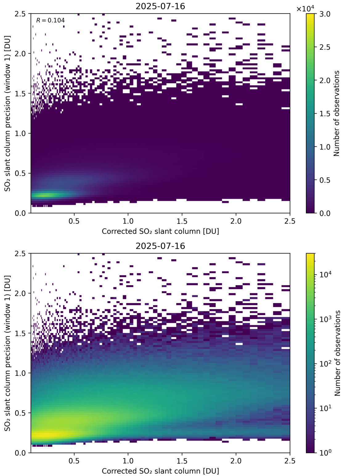
Figure 238: Scatter density plot of “Corrected SO 2 slant column” against “SO 2 slant column precision (window 1)” for 2025-07-15 to 2025-07-17.
