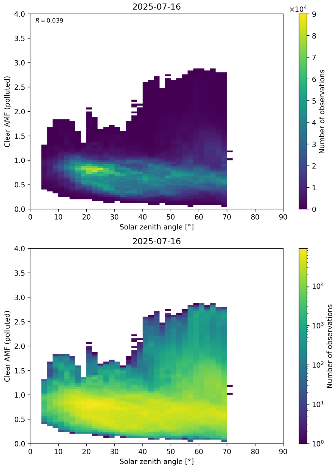
Figure 178: Scatter density plot of “Solar zenith angle” against “Clear AMF (polluted)” for 2025-07-15 to 2025-07-17.
