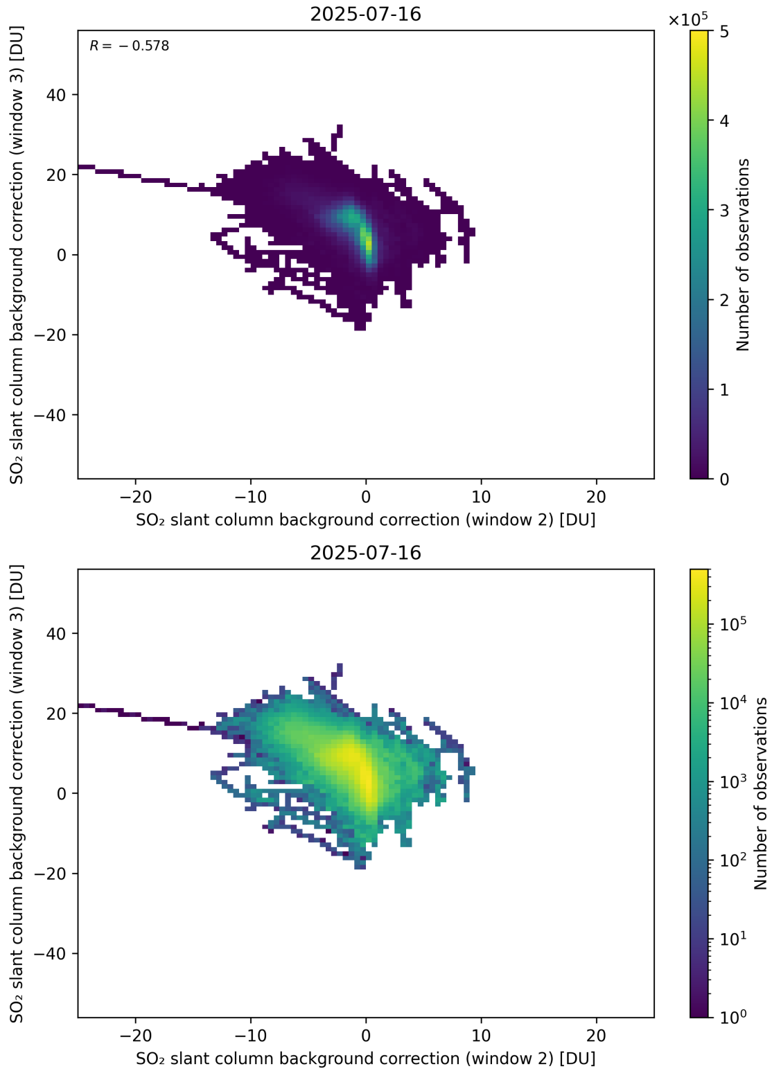
Figure 122: Scatter density plot of “SO 2 slant column background correction (window 2)” against “SO 2 slant column background correction (window 3)” for 2025-07-15 to 2025-07-17.
