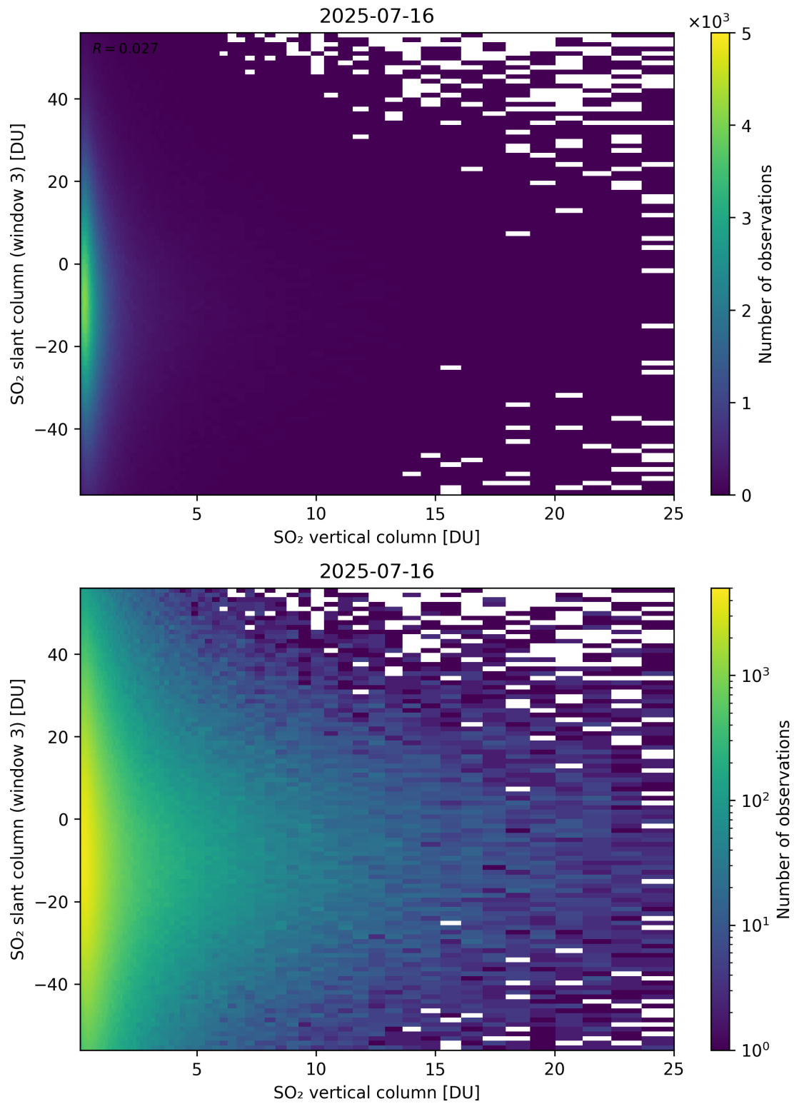
Figure 357: Scatter density plot of “SO 2 vertical column” against “SO 2 slant column (window 3)” for 2025-07-15 to 2025-07-17.
