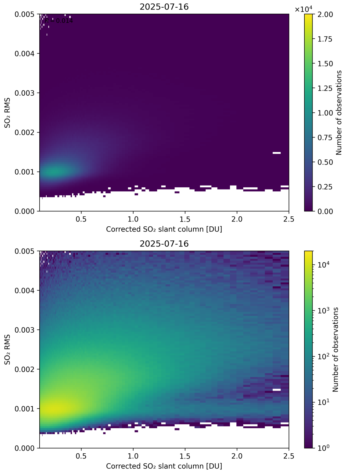
Figure 231: Scatter density plot of “Corrected SO 2 slant column” against “SO 2 RMS” for 2025-07-15 to 2025-07-17.
