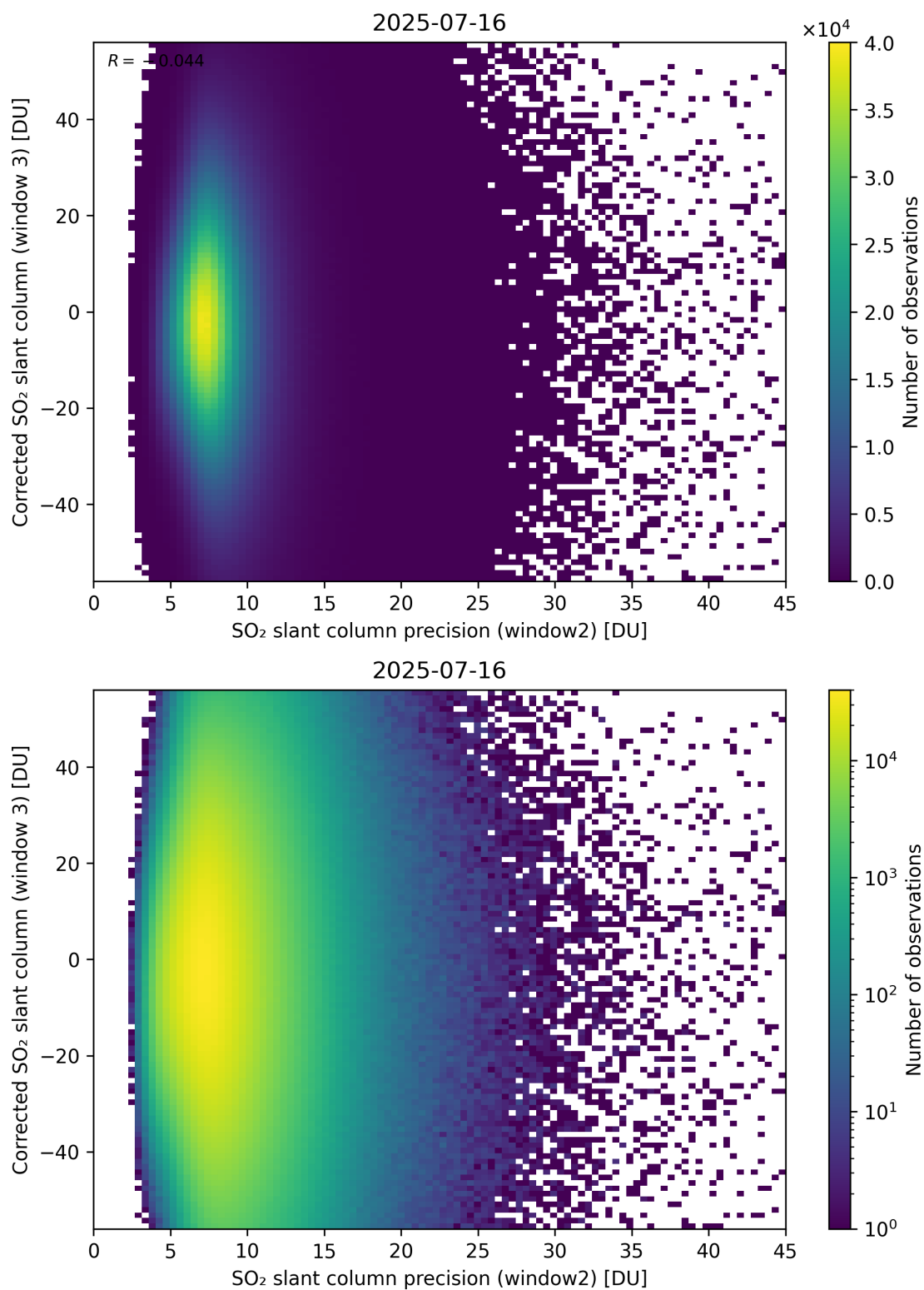
Figure 298: Scatter density plot of “SO 2 slant column precision (window2)” against “Corrected SO 2 slant column (window 3)” for 2025-07-15 to 2025-07-17.
