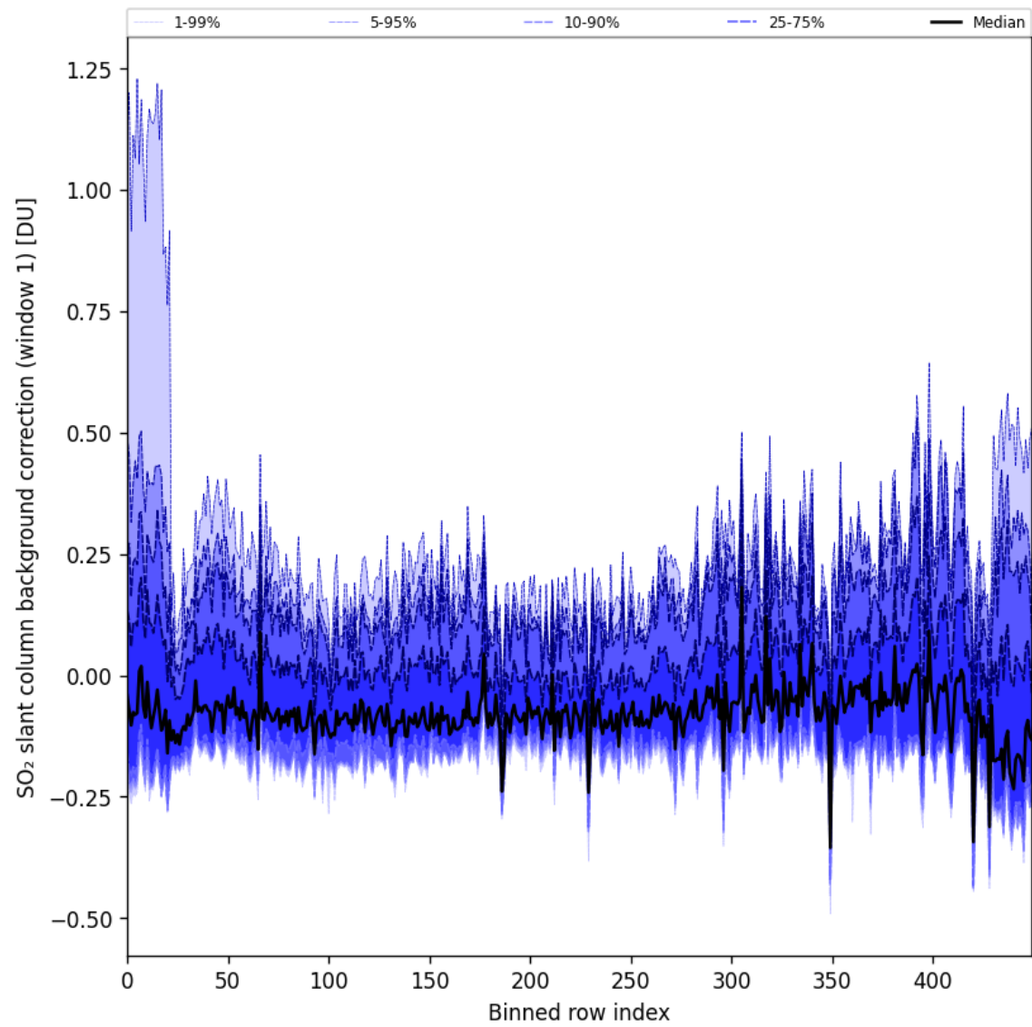
Figure 92: Along track statistics of “SO 2 slant column background correction (window 1)” for 2025-07-15 to 2025-07-17
