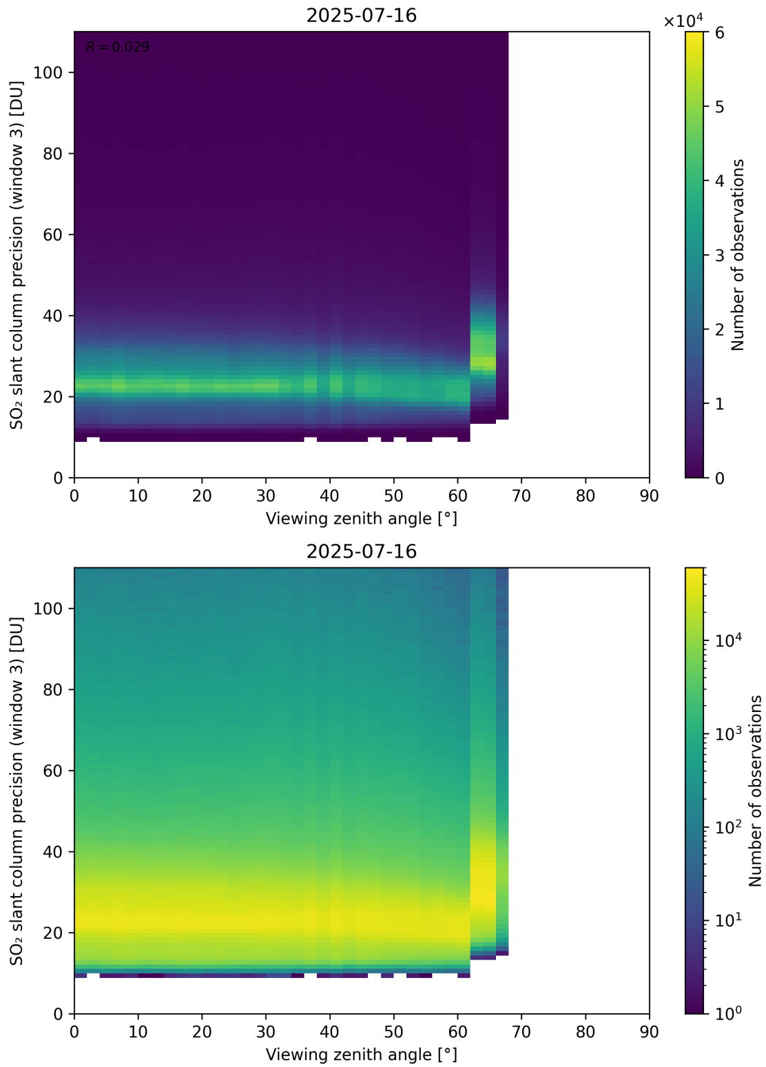
Figure 380: Scatter density plot of “Viewing zenith angle” against “SO 2 slant column precision (window 3)” for 2025-07-15 to 2025-07-17.
