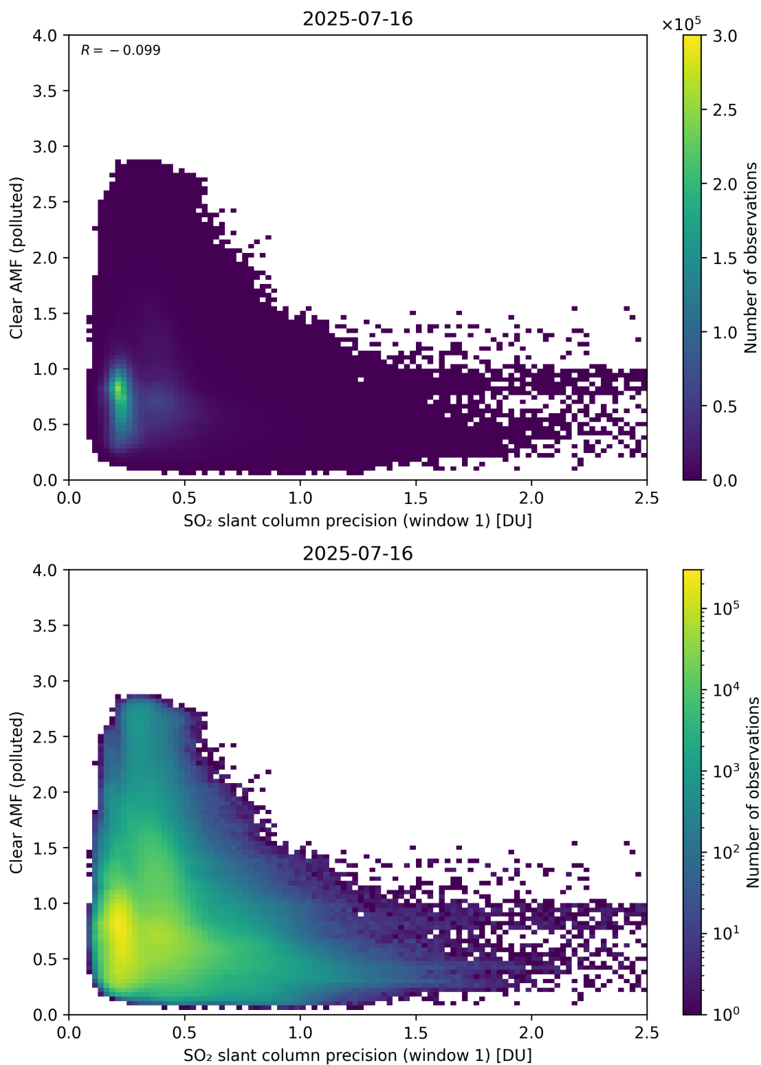
Figure 274: Scatter density plot of “SO 2 slant column precision (window 1)” against “Clear AMF (polluted)” for 2025-07-15 to 2025-07-17.
