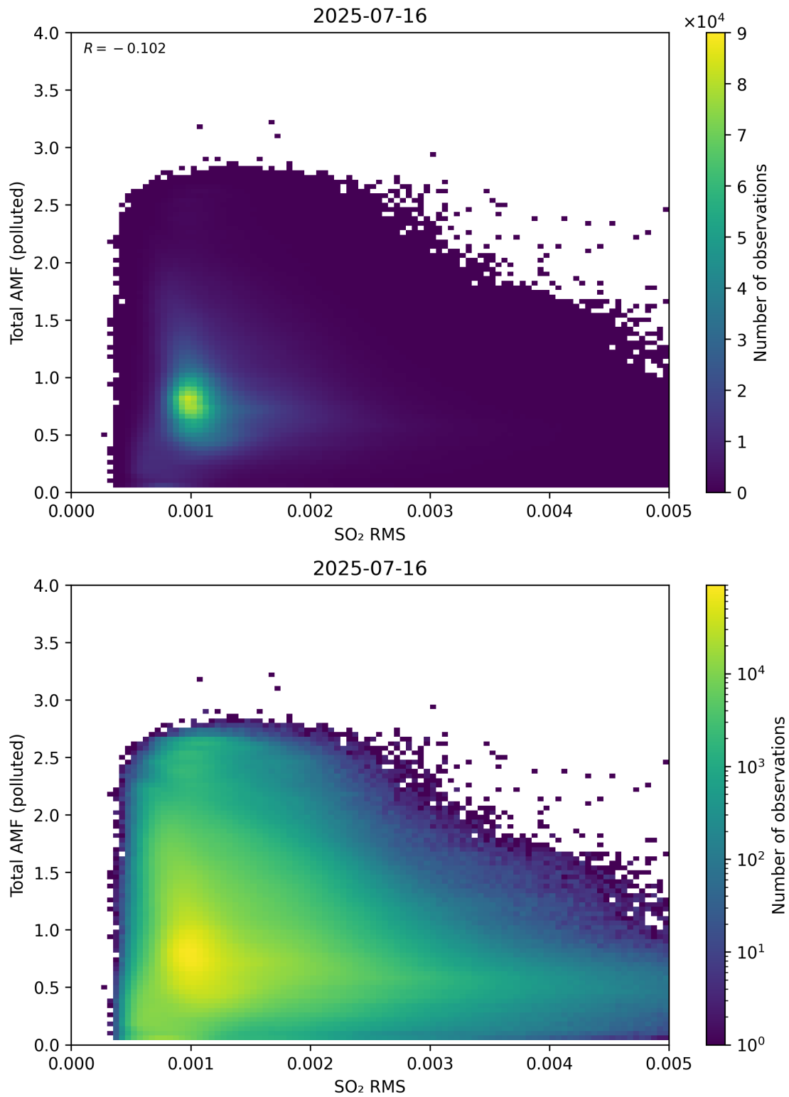
Figure 148: Scatter density plot of “SO 2 RMS” against “Total AMF (polluted)” for 2025-07-15 to 2025-07-17.
