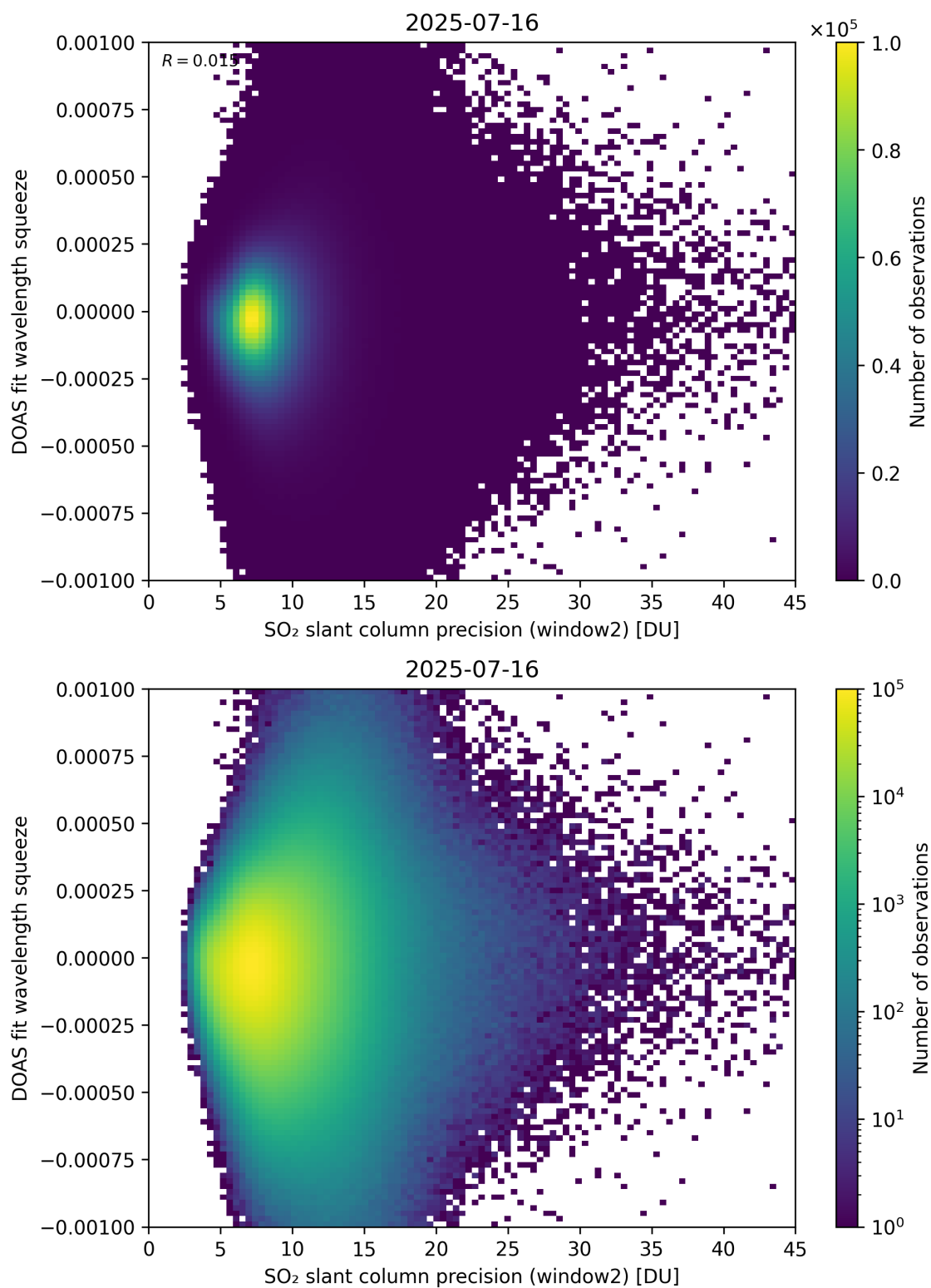
Figure 294: Scatter density plot of “SO 2 slant column precision (window2)” against “DOAS fit wavelength squeeze” for 2025-07-15 to 2025-07-17.
