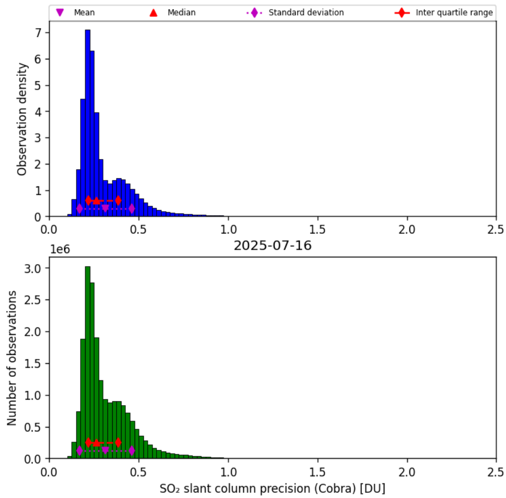
Figure 62: Histogram of “SO 2 slant column precision (Cobra)” for 2025-07-15 to 2025-07-17
