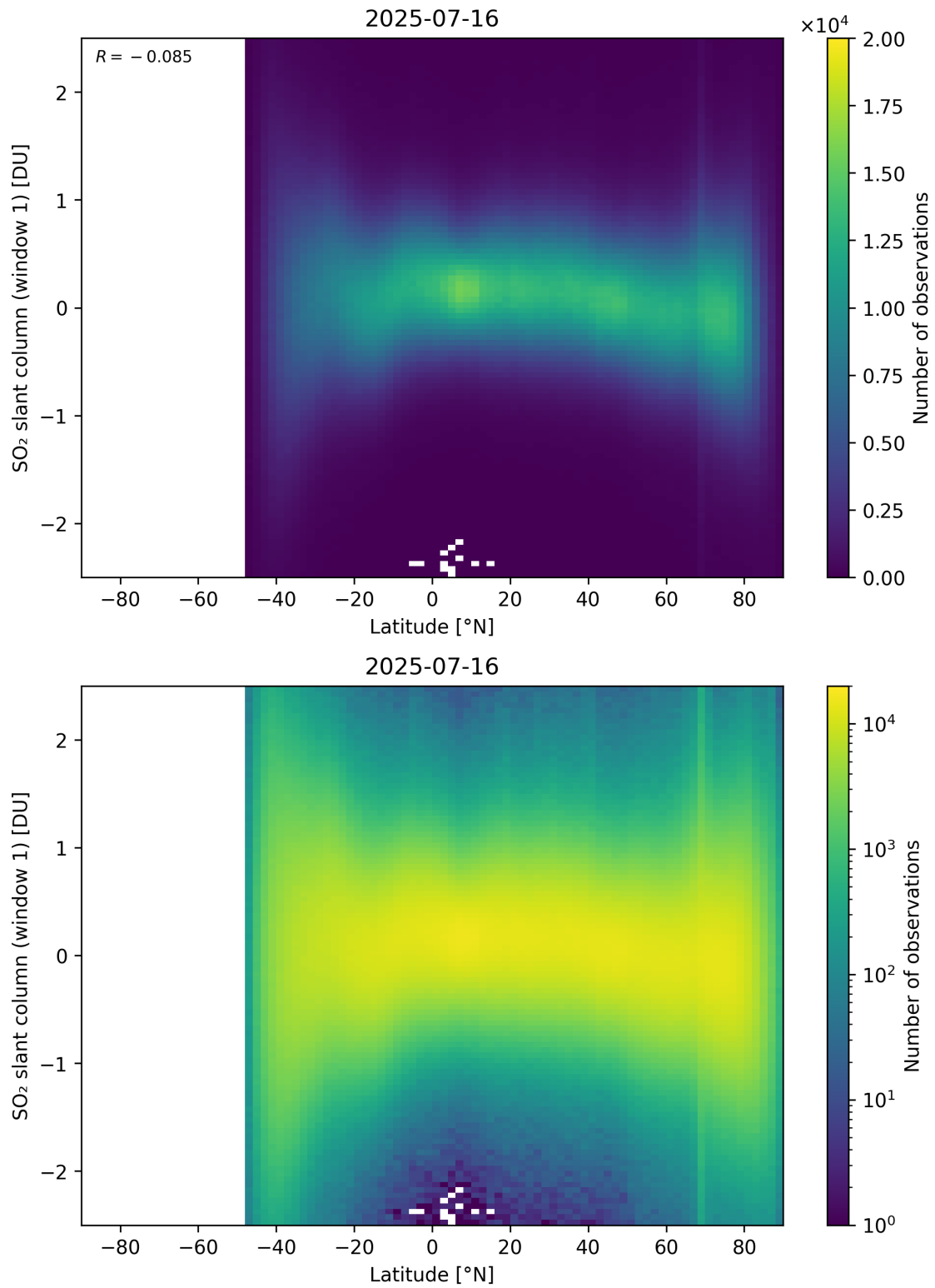
Figure 162: Scatter density plot of “Latitude” against “SO 2 slant column (window 1)” for 2025-07-15 to 2025-07-17.
