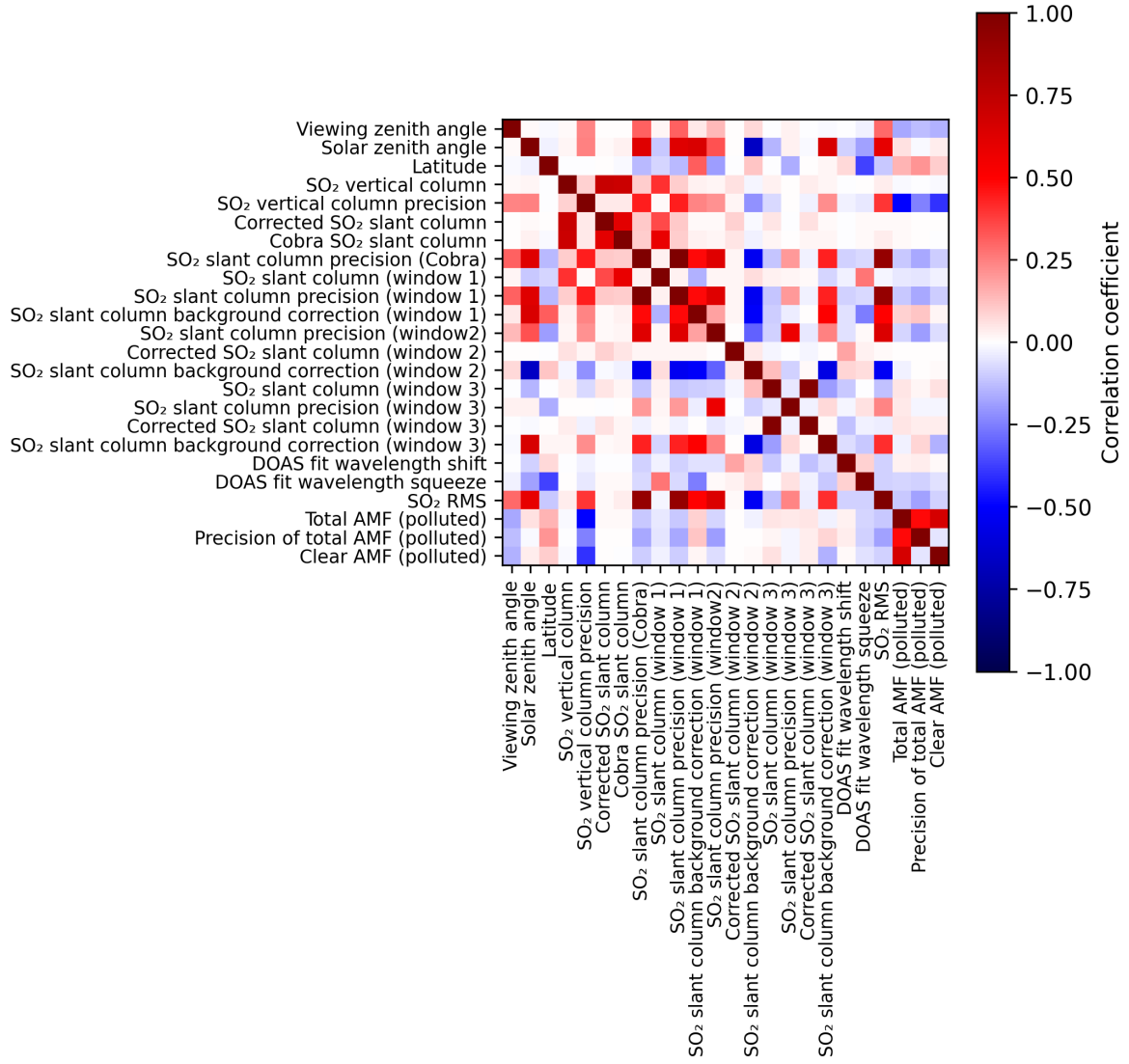
Figure 2: Map of correlation matrix for 2025-07-15 to 2025-07-17.
