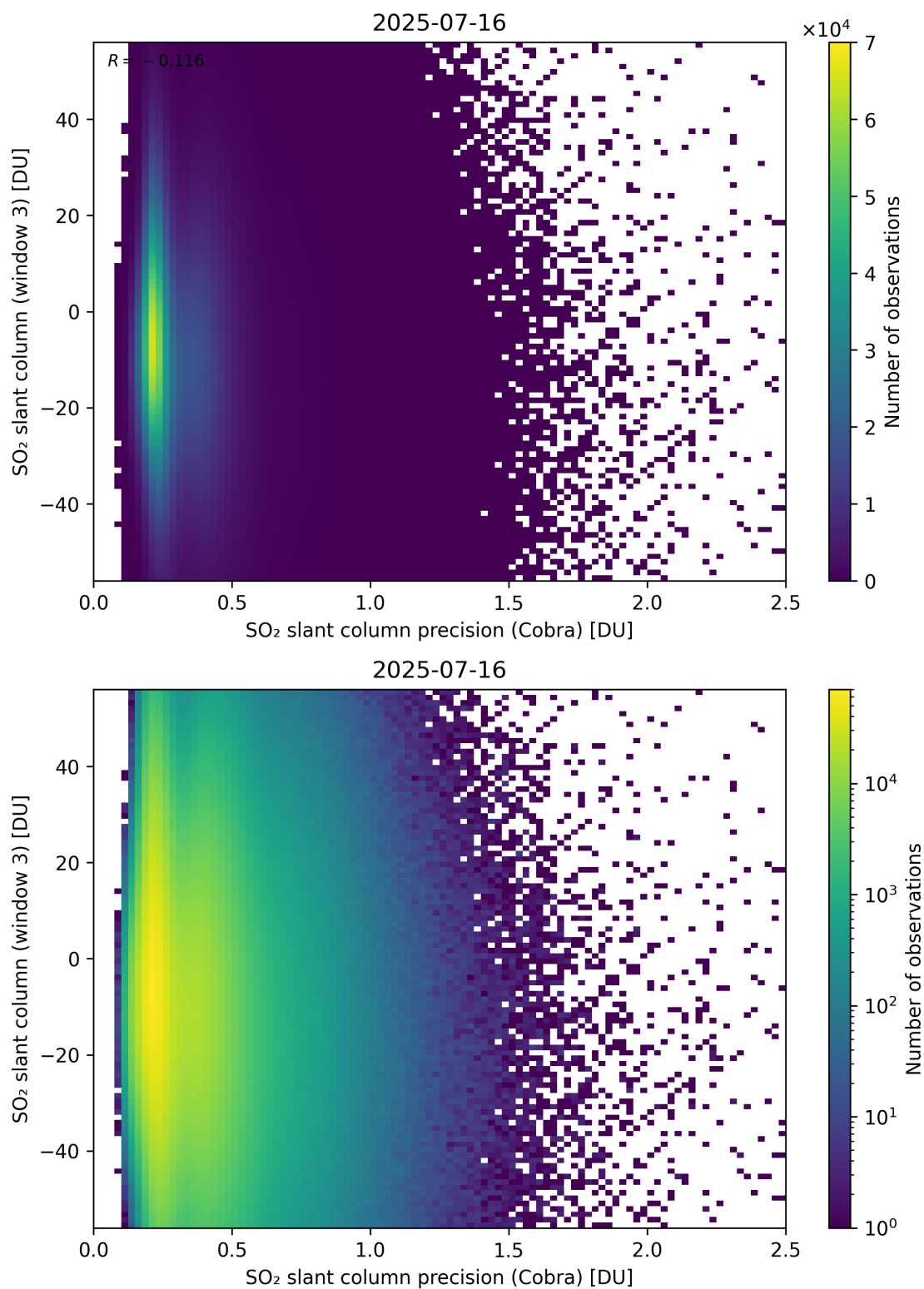
Figure 211: Scatter density plot of “SO 2 slant column precision (Cobra)” against “SO 2 slant column (window 3)” for 2025-07-15 to 2025-07-17.
