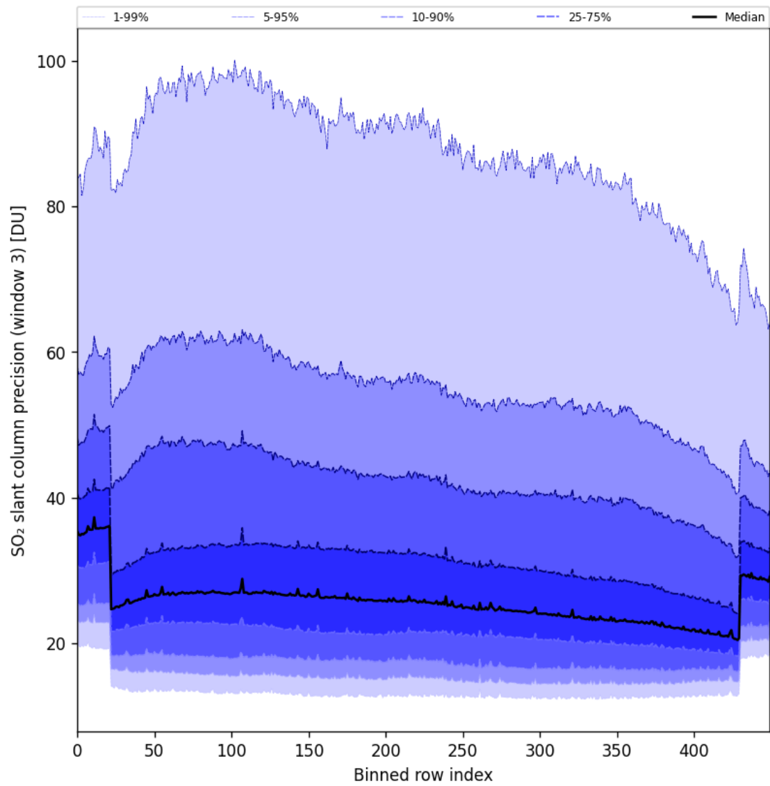
Figure 98: Along track statistics of “SO 2 slant column precision (window 3)” for 2025-07-15 to 2025-07-17
