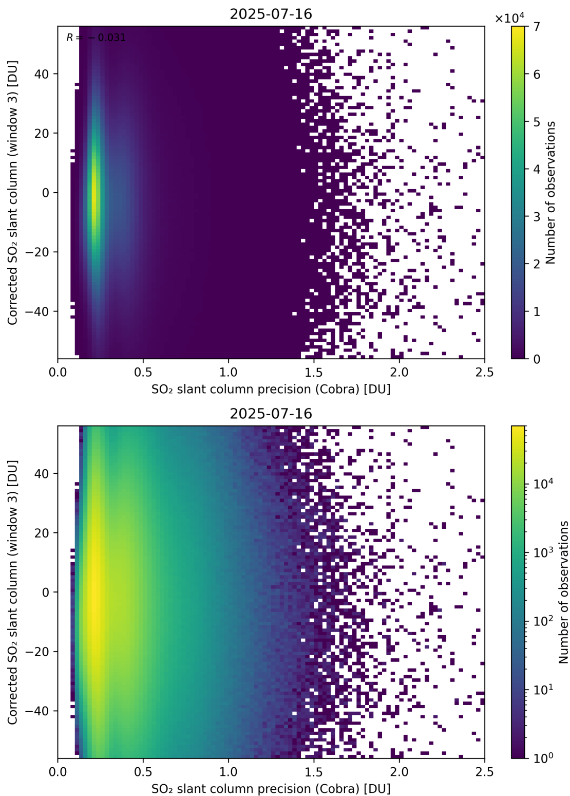
Figure 207: Scatter density plot of “SO 2 slant column precision (Cobra)” against “Corrected SO 2 slant column (window 3)” for 2025-07-15 to 2025-07-17.
