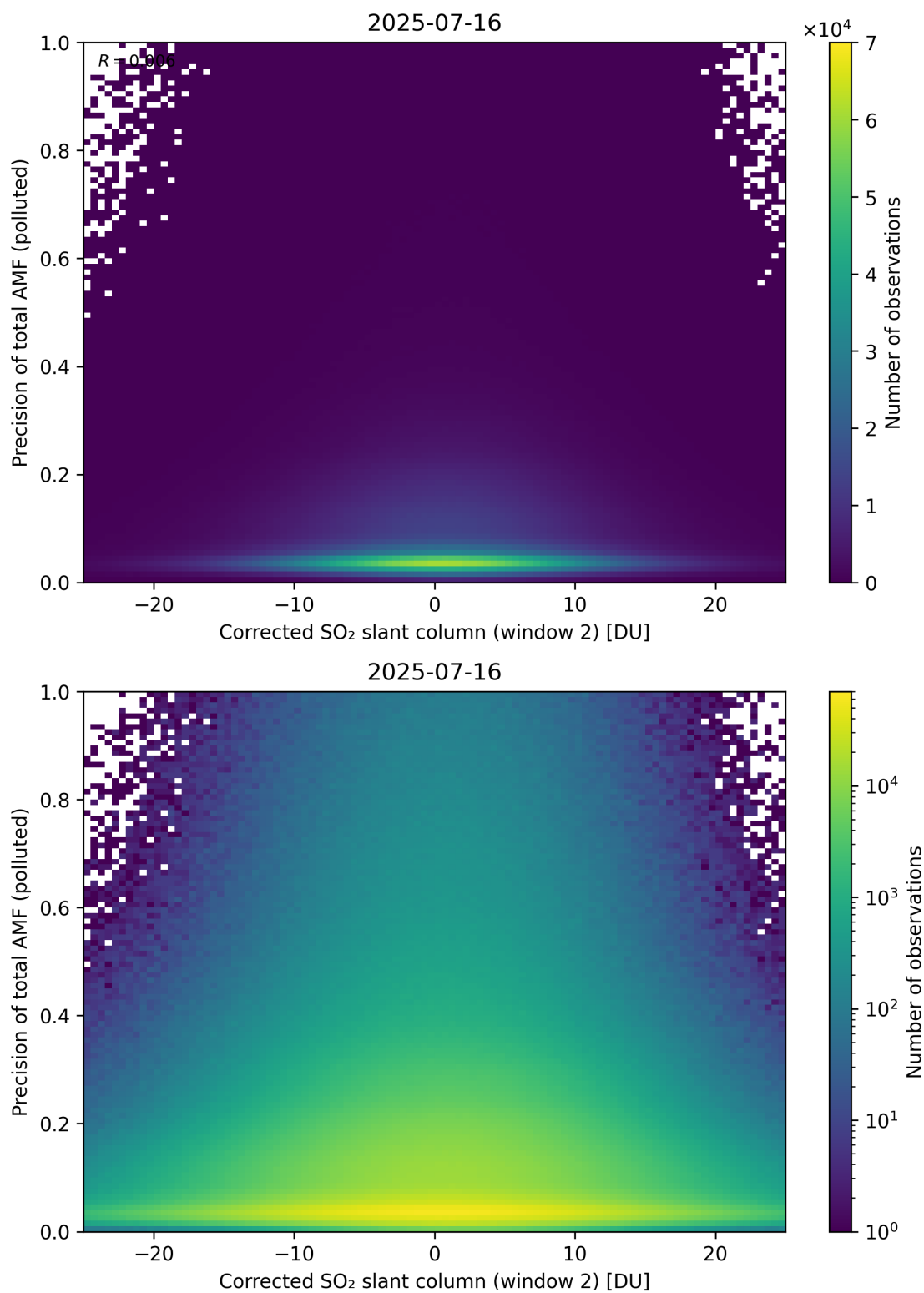
Figure 254: Scatter density plot of “Corrected SO 2 slant column (window 2)” against “Precision of total AMF (polluted)” for 2025-07-15 to 2025-07-17.
