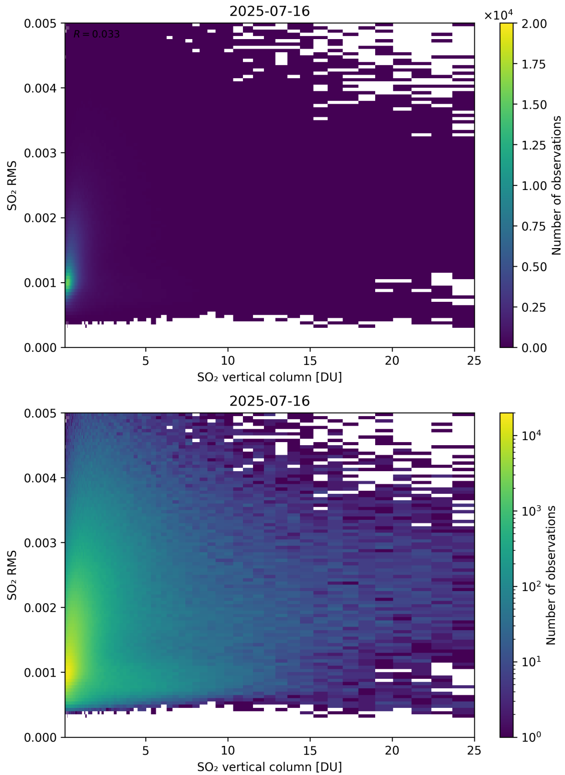
Figure 328: Scatter density plot of “SO 2 vertical column” against “SO 2 RMS” for 2025-07-15 to 2025-07-17.
