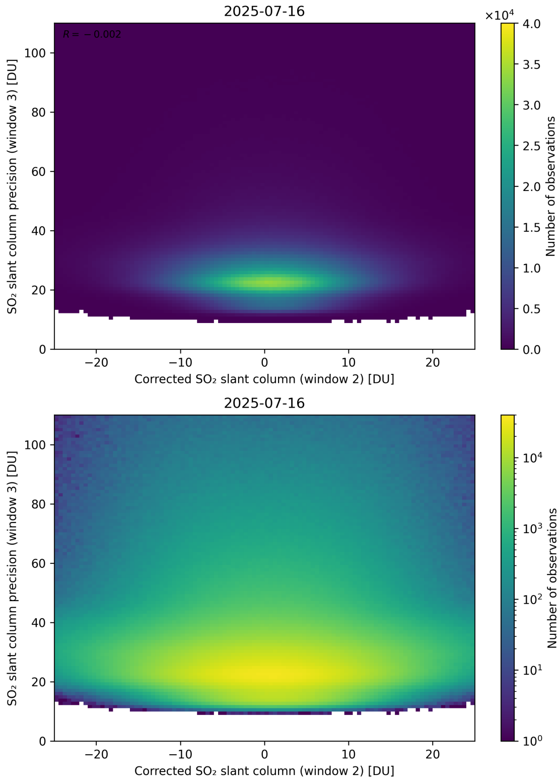
Figure 252: Scatter density plot of “Corrected SO 2 slant column (window 2)” against “SO 2 slant column precision (window 3)” for 2025-07-15 to 2025-07-17.
