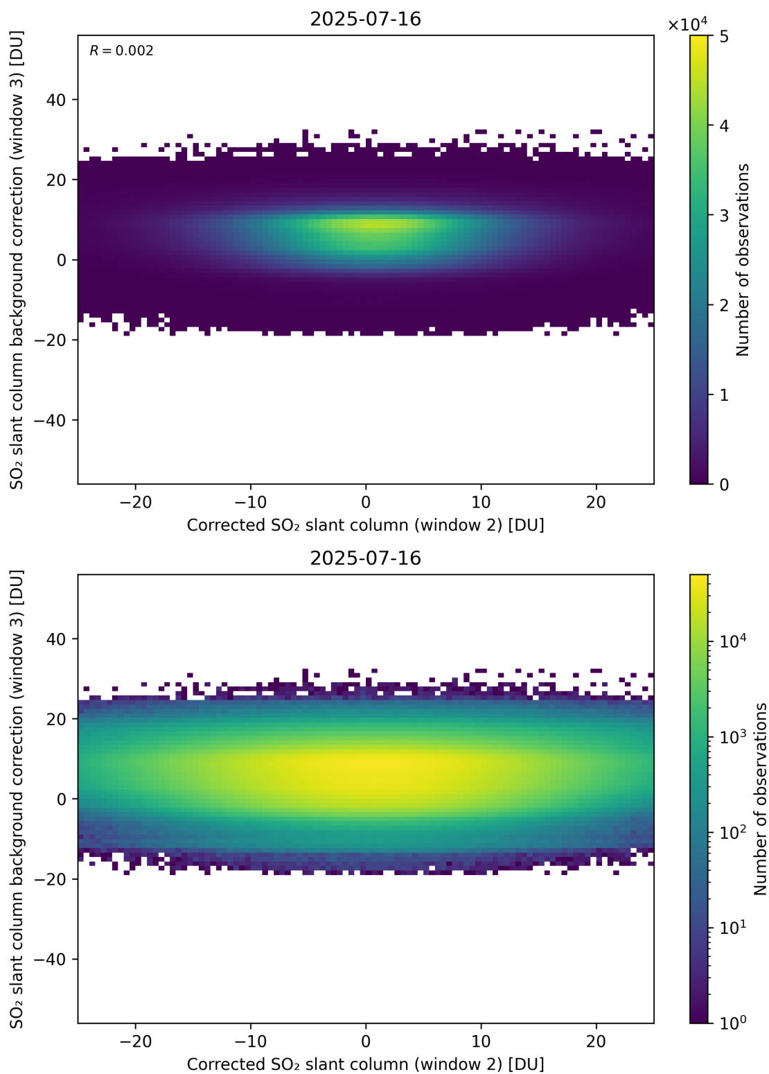
Figure 245: Scatter density plot of “Corrected SO 2 slant column (window 2)” against “SO 2 slant column background correction (window 3)” for 2025-07-15 to 2025-07-17.
