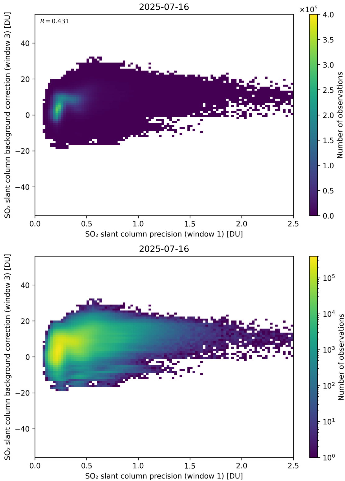
Figure 270: Scatter density plot of “SO 2 slant column precision (window 1)” against “SO 2 slant column background correction (window 3)” for 2025-07-15 to 2025-07-17.
