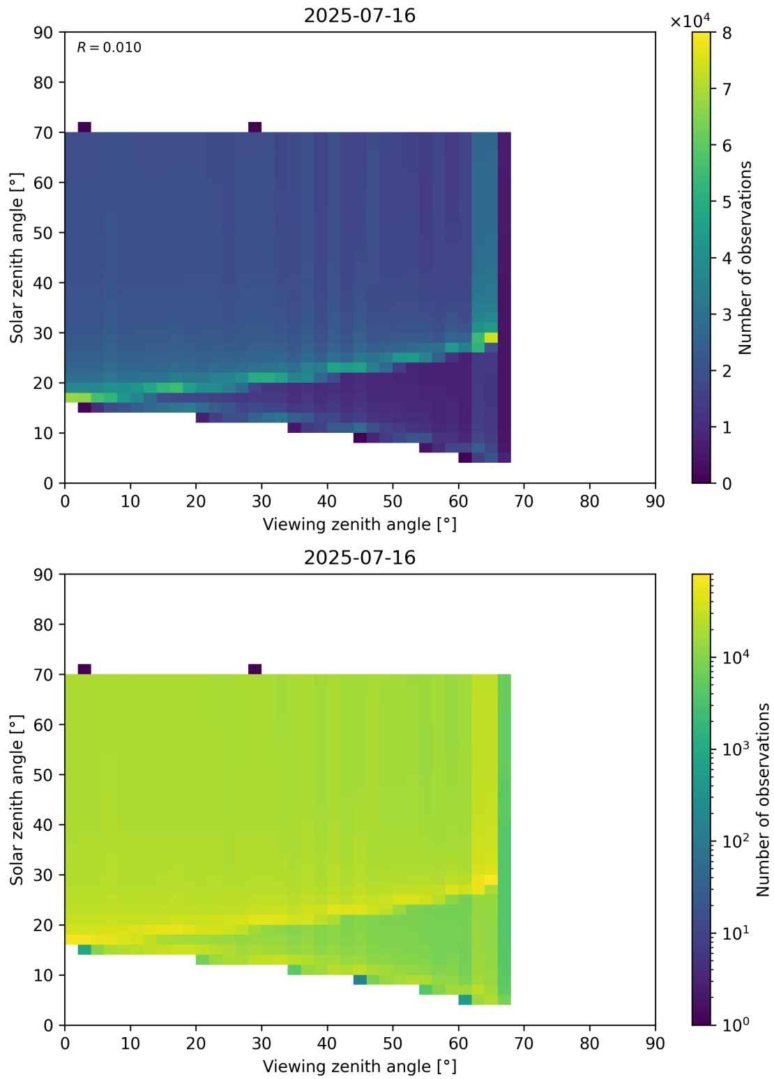
Figure 369: Scatter density plot of “Viewing zenith angle” against “Solar zenith angle” for 2025-07-15 to 2025-07-17.
