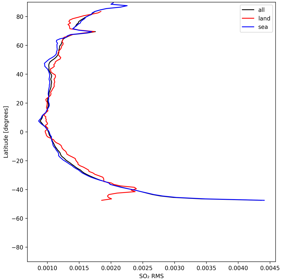
Figure 52: Zonal average of “SO 2 RMS” for 2025-07-15 to 2025-07-17.
