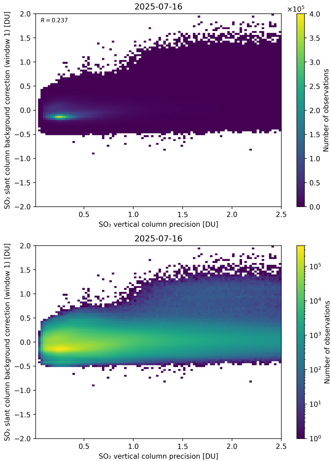
Figure 329: Scatter density plot of “SO 2 vertical column precision” against “SO 2 slant column background correction (window 1)” for 2025-07-15 to 2025-07-17.
