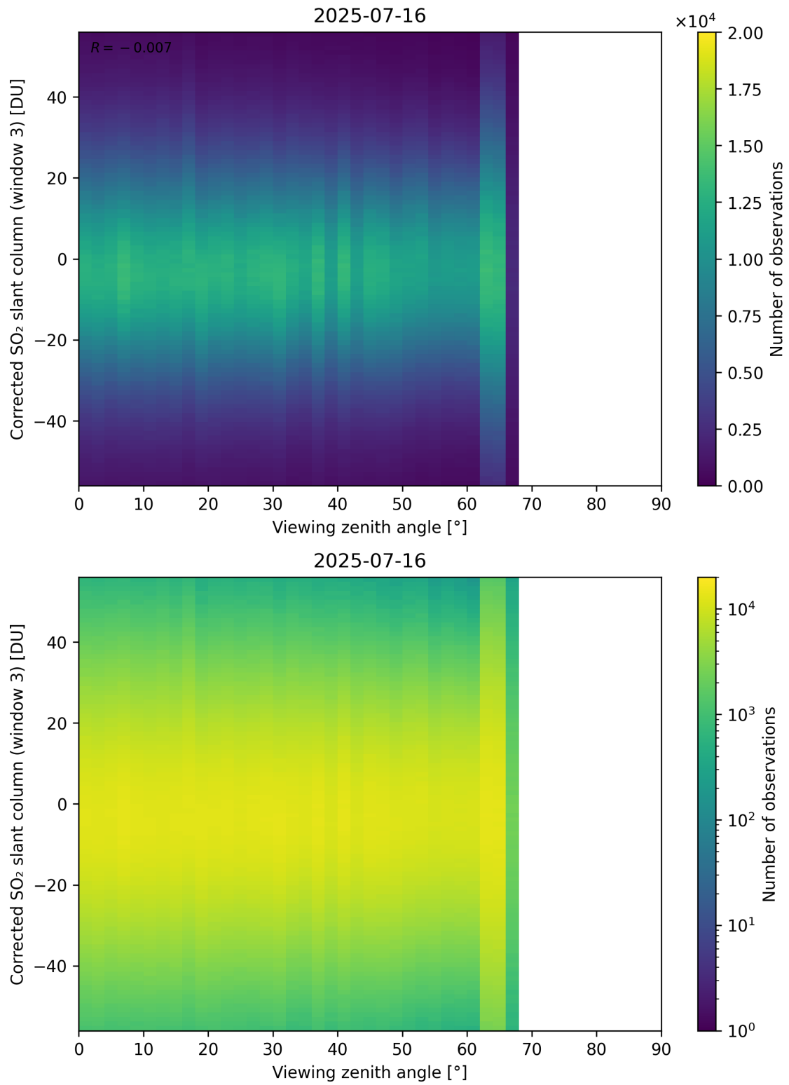
Figure 375: Scatter density plot of “Viewing zenith angle” against “Corrected SO 2 slant column (window 3)” for 2025-07-15 to 2025-07-17.
