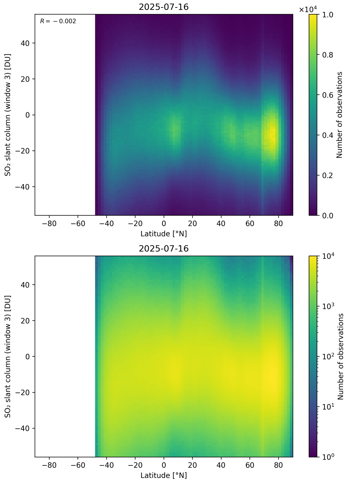
Figure 165: Scatter density plot of “Latitude” against “SO 2 slant column (window 3)” for 2025-07-15 to 2025-07-17.
