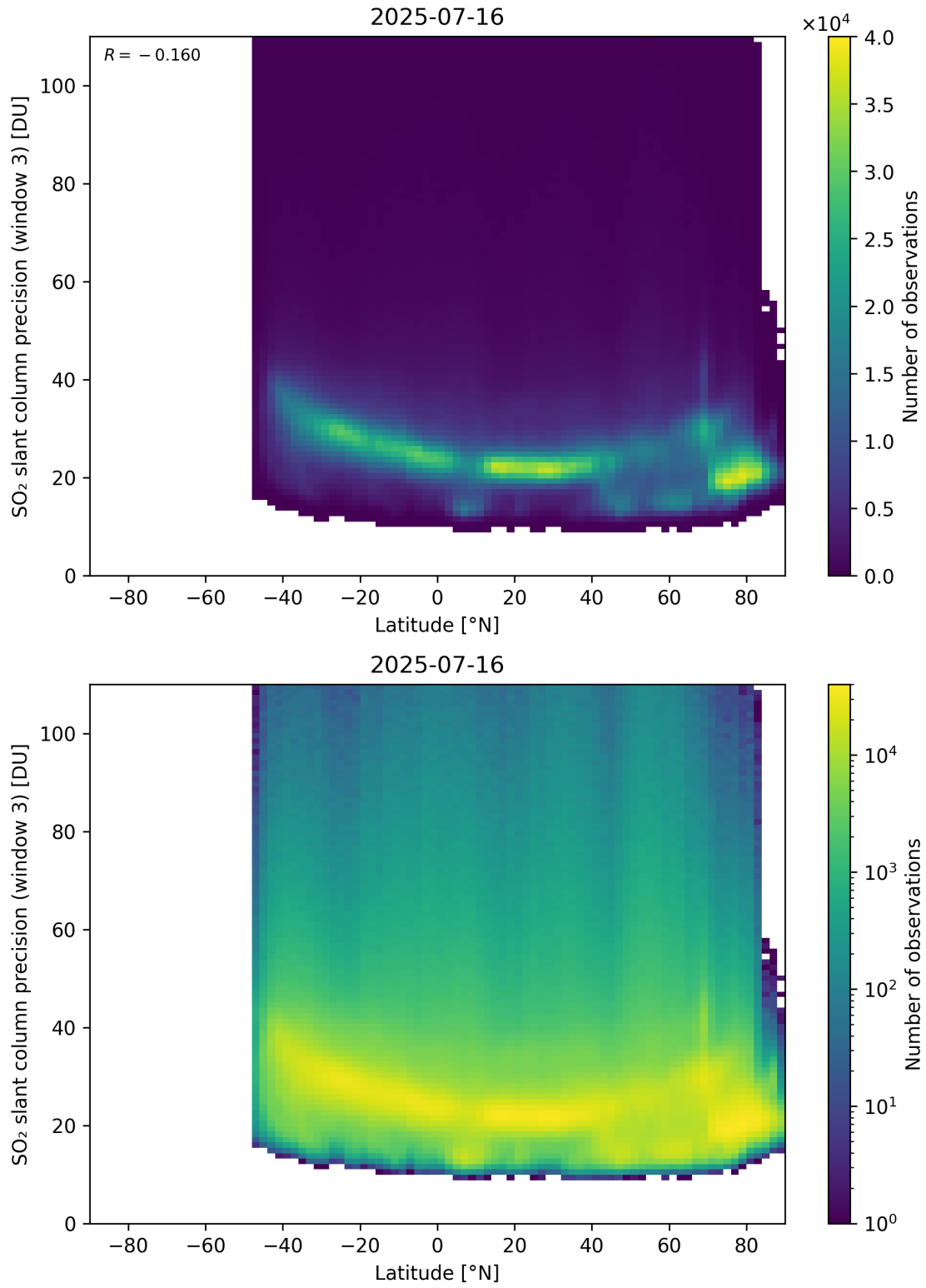
Figure 166: Scatter density plot of “Latitude” against “SO 2 slant column precision (window 3)” for 2025-07-15 to 2025-07-17.
