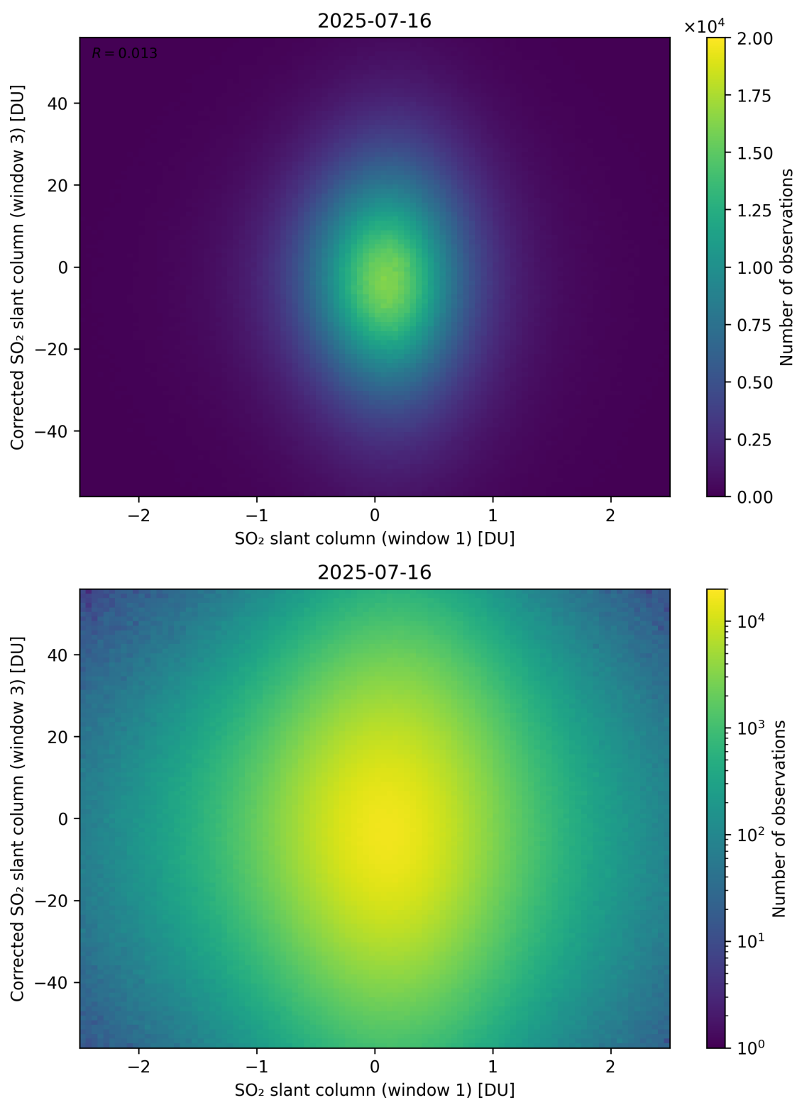
Figure 284: Scatter density plot of “SO 2 slant column (window 1)” against “Corrected SO 2 slant column (window 3)” for 2025-07-15 to 2025-07-17.
