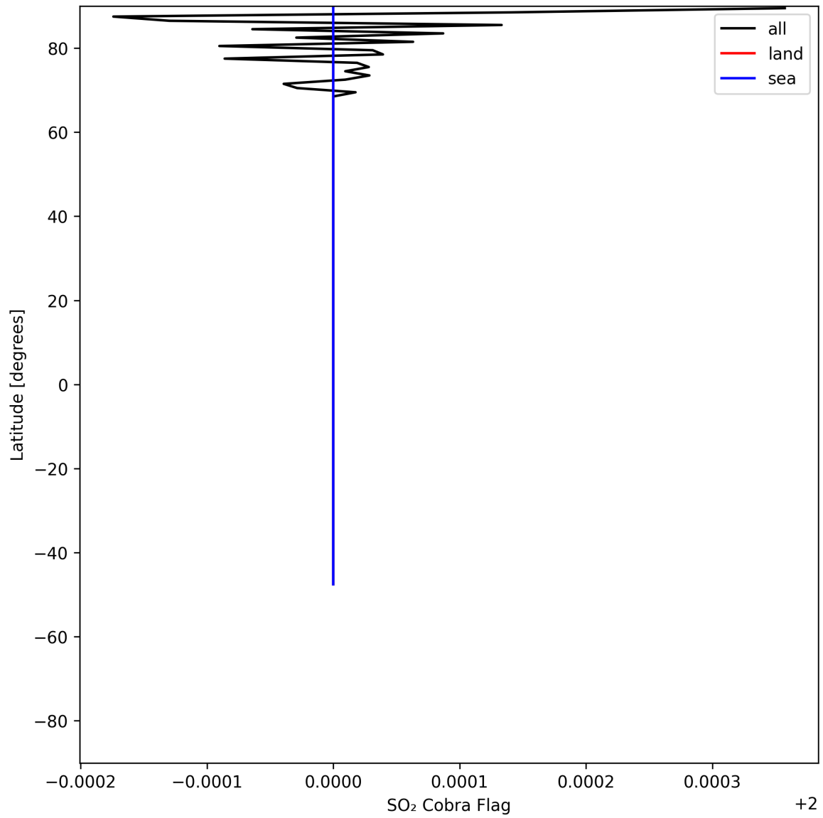
Figure 49: Zonal average of “SO 2 Cobra Flag” for 2025-07-15 to 2025-07-17.
