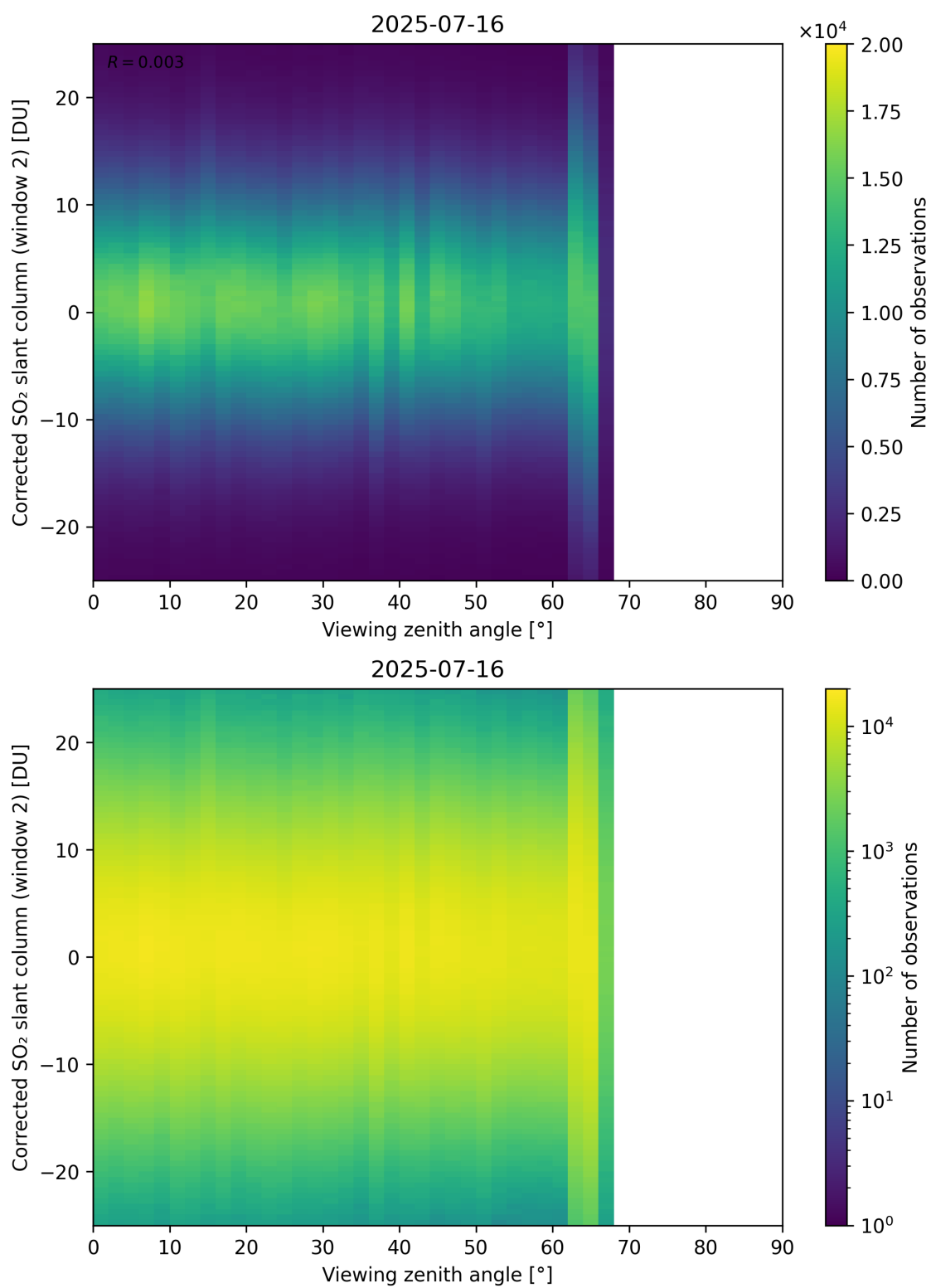
Figure 374: Scatter density plot of “Viewing zenith angle” against “Corrected SO 2 slant column (window 2)” for 2025-07-15 to 2025-07-17.
