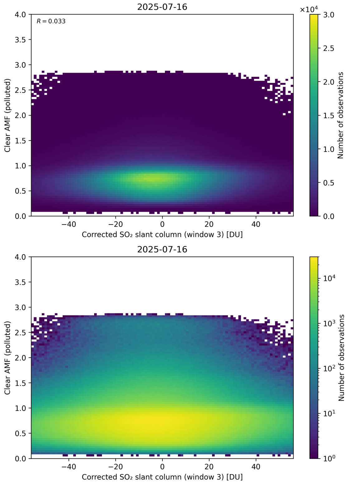
Figure 259: Scatter density plot of “Corrected SO 2 slant column (window 3)” against “Clear AMF (polluted)” for 2025-07-15 to 2025-07-17.
