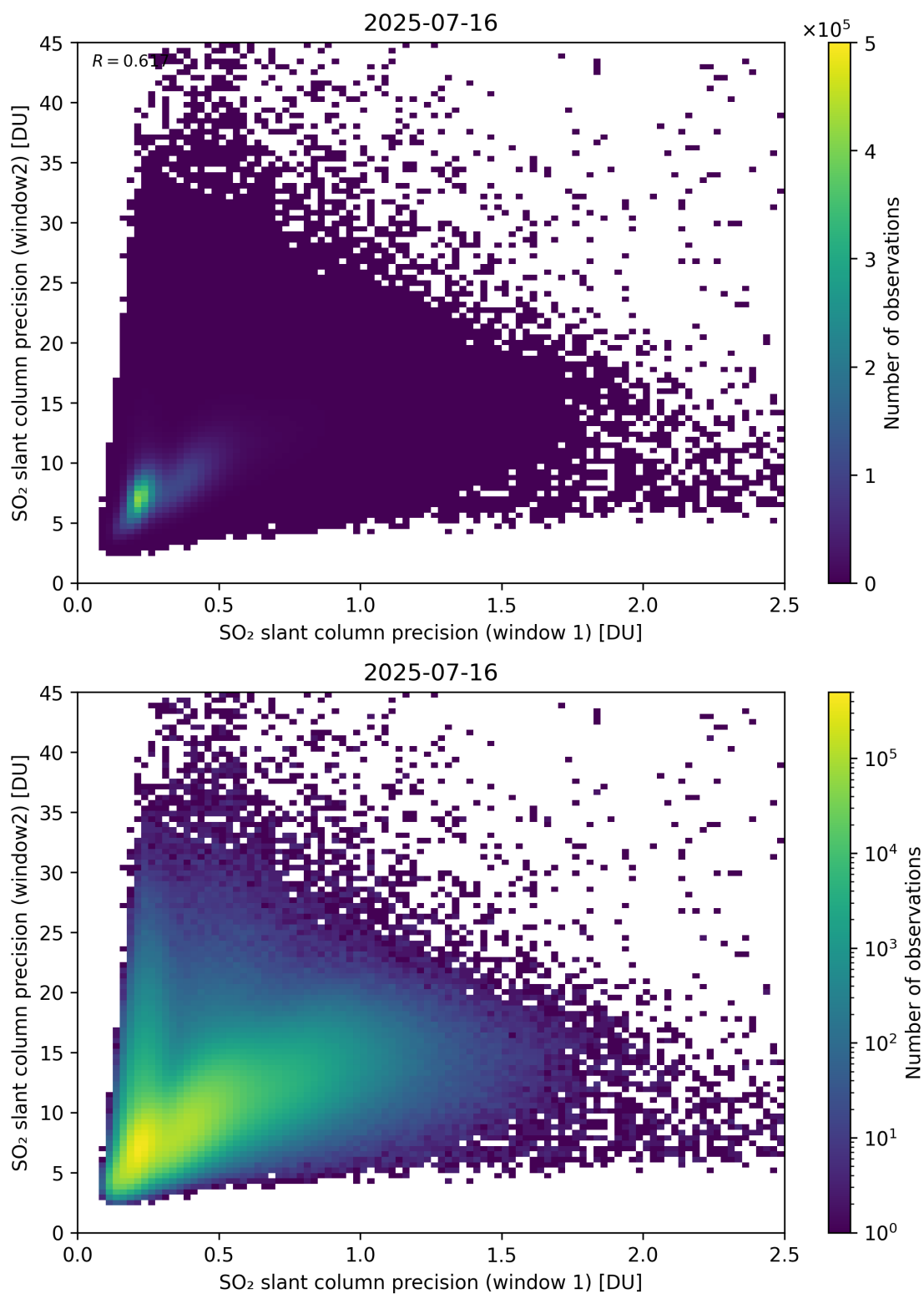
Figure 277: Scatter density plot of “SO 2 slant column precision (window 1)” against “SO 2 slant column precision (window2)” for 2025-07-15 to 2025-07-17.
