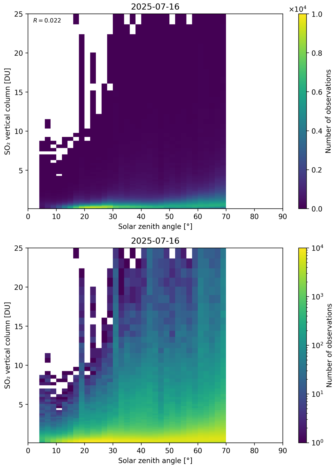
Figure 191: Scatter density plot of “Solar zenith angle” against “SO 2 vertical column” for 2025-07-15 to 2025-07-17.
