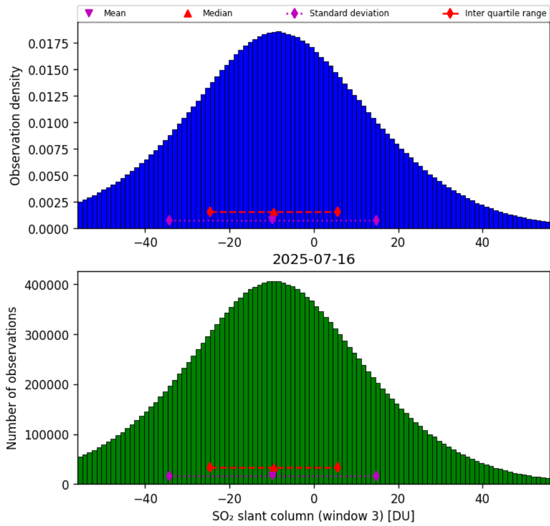
Figure 71: Histogram of “SO 2 slant column (window 3)” for 2025-07-15 to 2025-07-17
