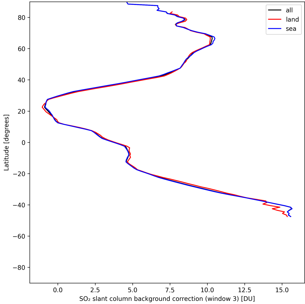
Figure 48: Zonal average of “SO 2 slant column background correction (window 3)” for 2025-07-15 to 2025-07-17.
