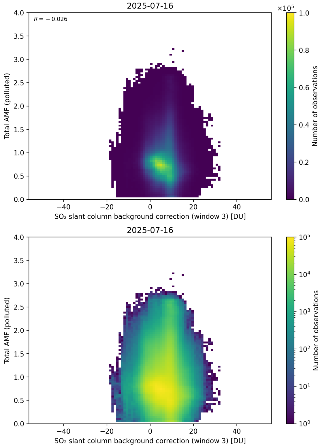
Figure 136: Scatter density plot of “SO 2 slant column background correction (window 3)” against “Total AMF (polluted)” for 2025-07-15 to 2025-07-17.
