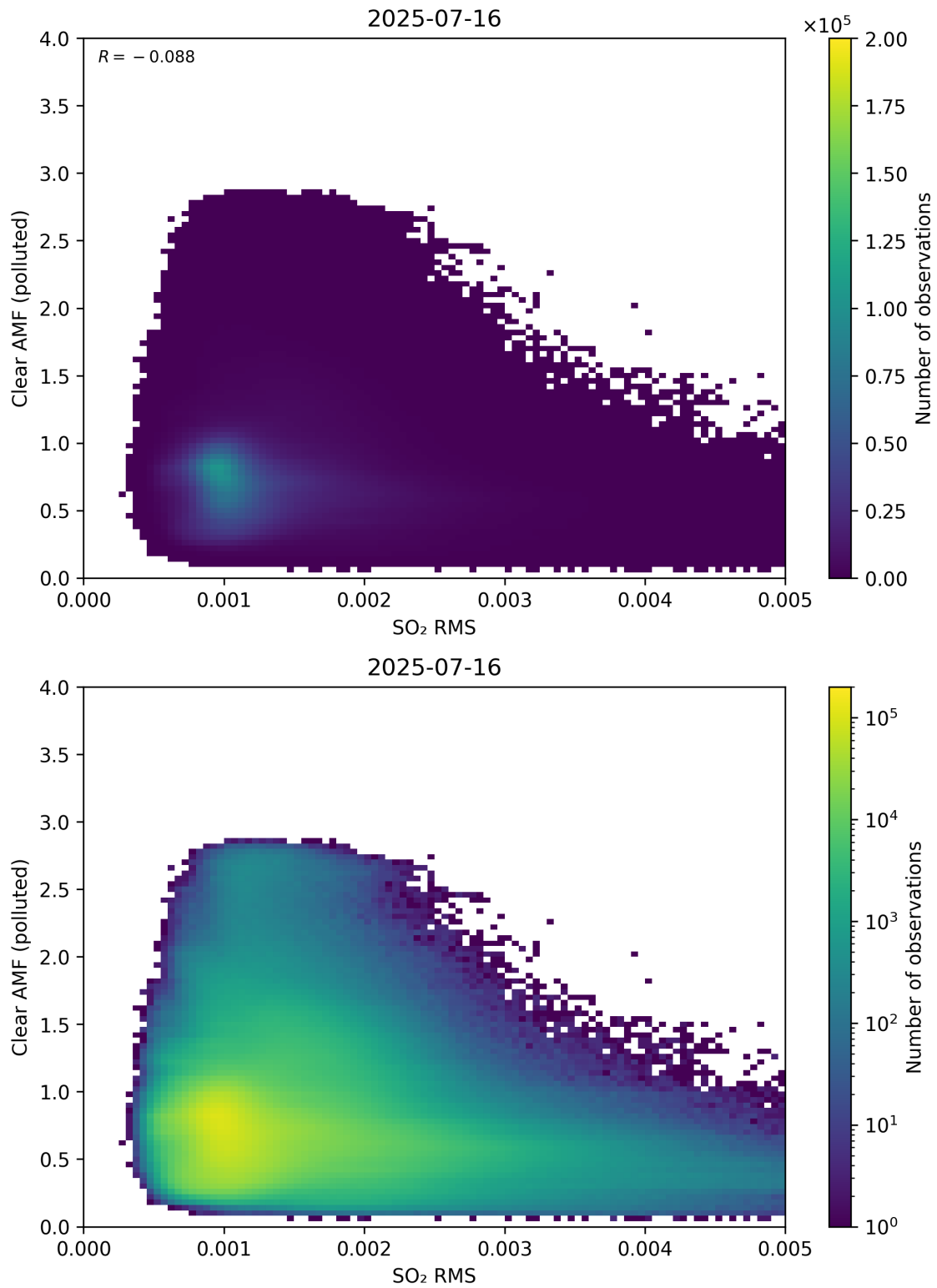
Figure 147: Scatter density plot of “SO 2 RMS” against “Clear AMF (polluted)” for 2025-07-15 to 2025-07-17.
