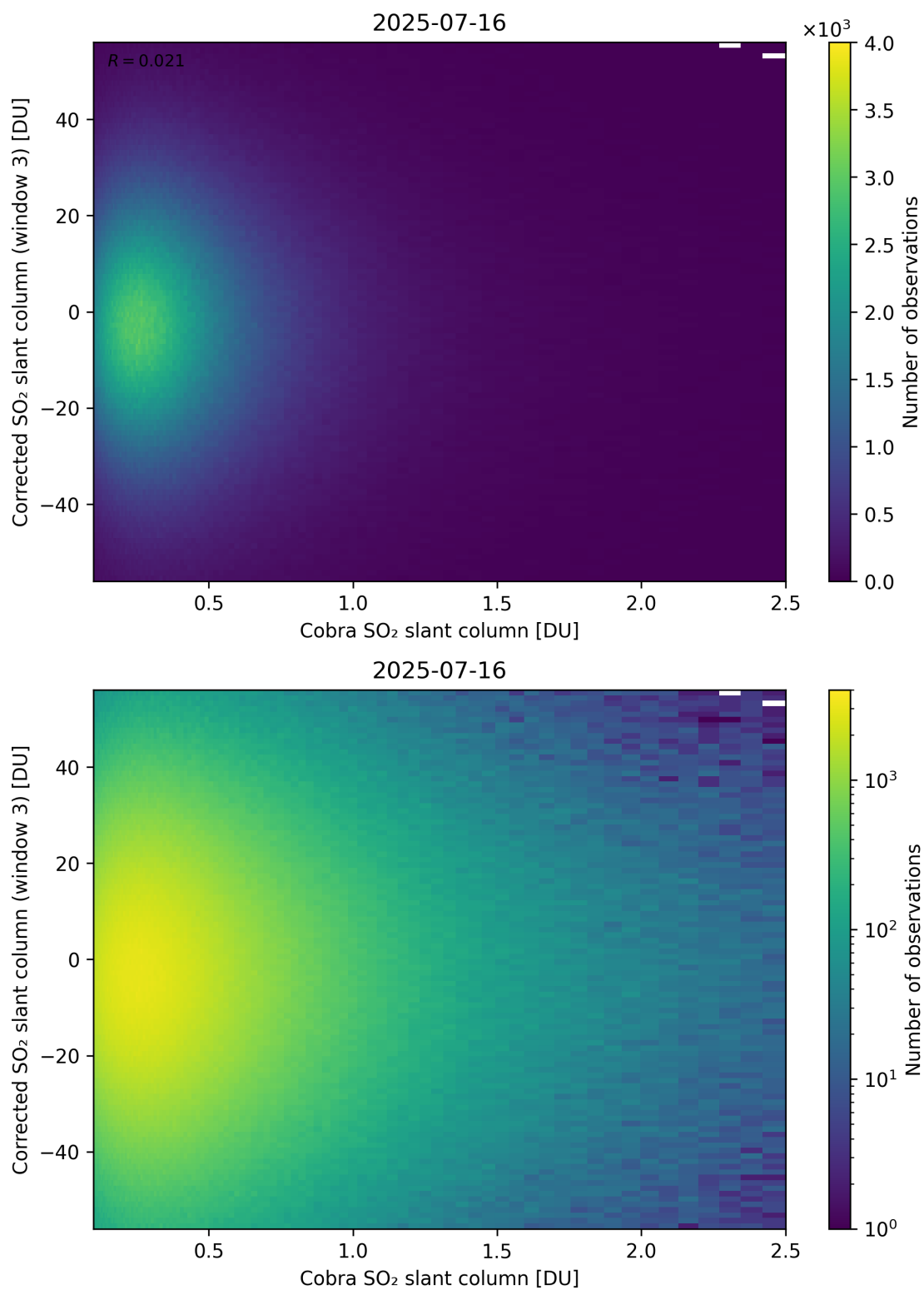
Figure 218: Scatter density plot of “Cobra SO 2 slant column” against “Corrected SO 2 slant column (window 3)” for 2025-07-15 to 2025-07-17.
