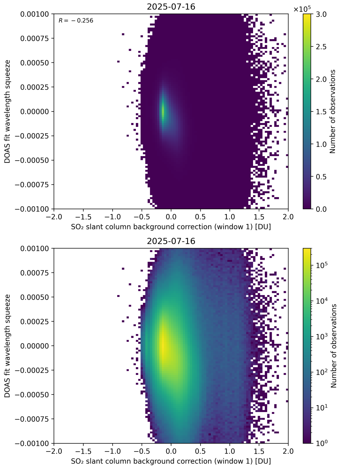
Figure 112: Scatter density plot of “SO 2 slant column background correction (window 1)” against “DOAS fit wavelength squeeze” for 2025-07-15 to 2025-07-17.
