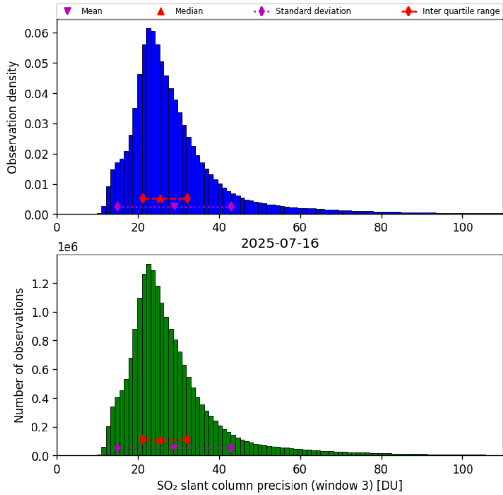
Figure 72: Histogram of “SO 2 slant column precision (window 3)” for 2025-07-15 to 2025-07-17
