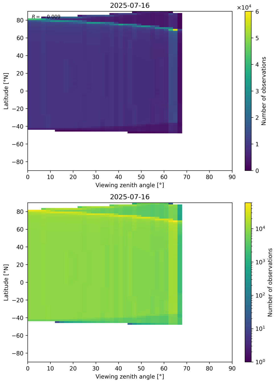
Figure 368: Scatter density plot of “Viewing zenith angle” against “Latitude” for 2025-07-15 to 2025-07-17.
