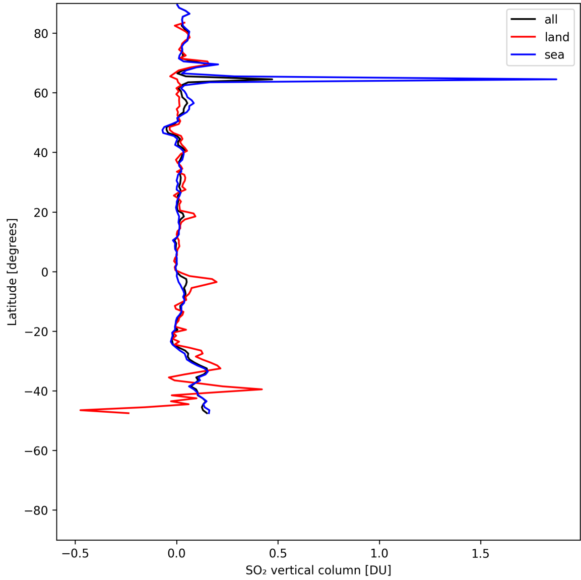
Figure 32: Zonal average of “SO 2 vertical column” for 2025-07-15 to 2025-07-17.
