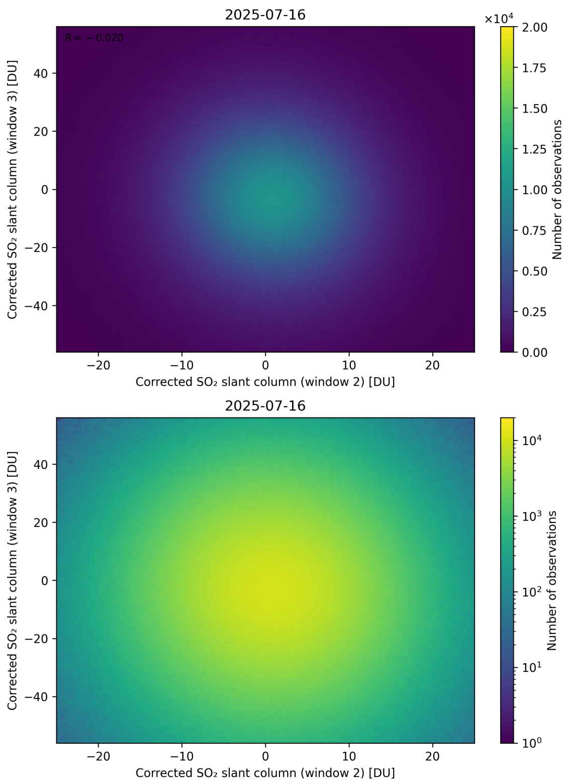
Figure 250: Scatter density plot of “Corrected SO 2 slant column (window 2)” against “Corrected SO 2 slant column (window 3)” for 2025-07-15 to 2025-07-17.
