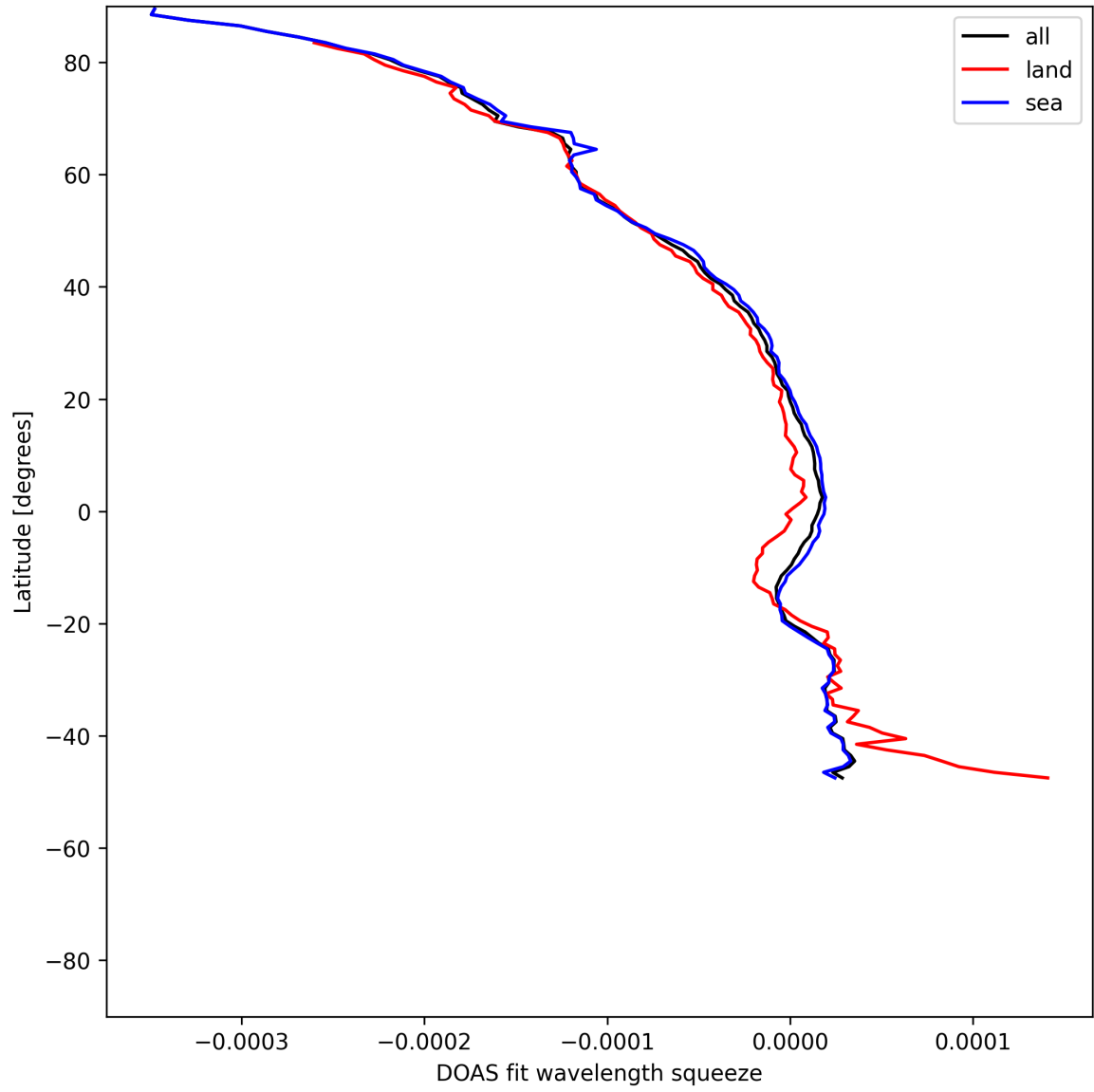
Figure 51: Zonal average of “DOAS fit wavelength squeeze” for 2025-07-15 to 2025-07-17.
