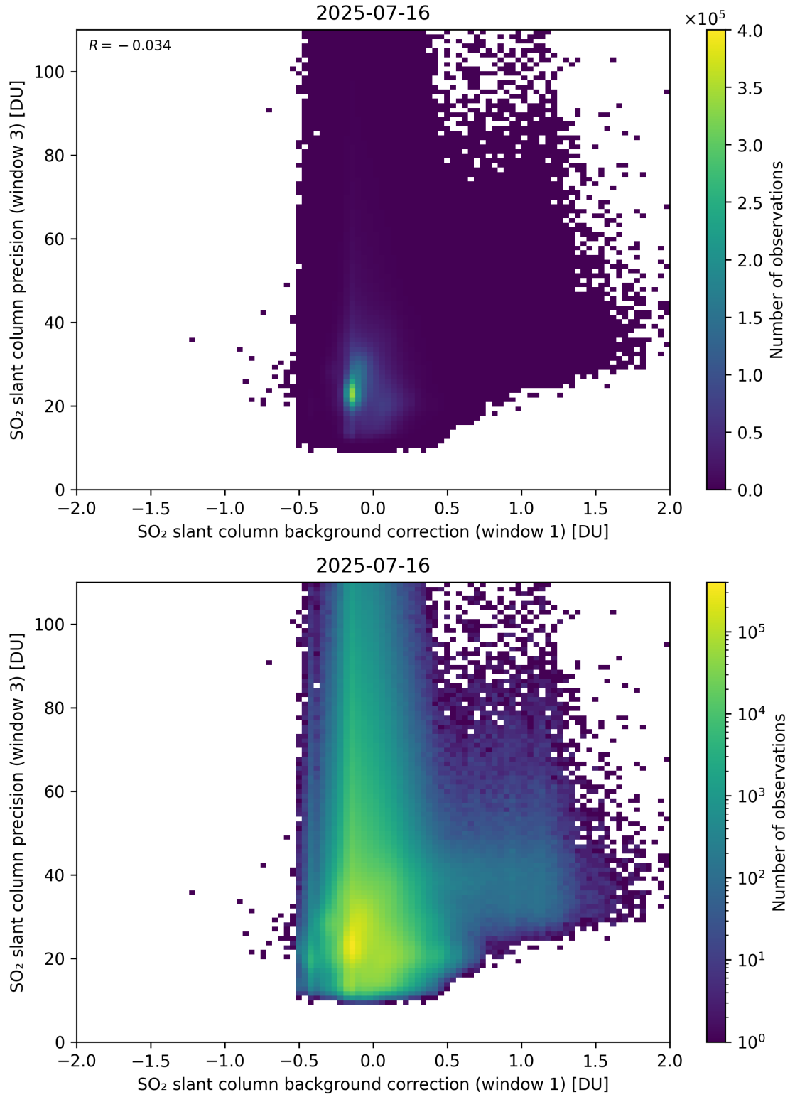
Figure 119: Scatter density plot of “SO 2 slant column background correction (window 1)” against “SO 2 slant column precision (window 3)” for 2025-07-15 to 2025-07-17.
