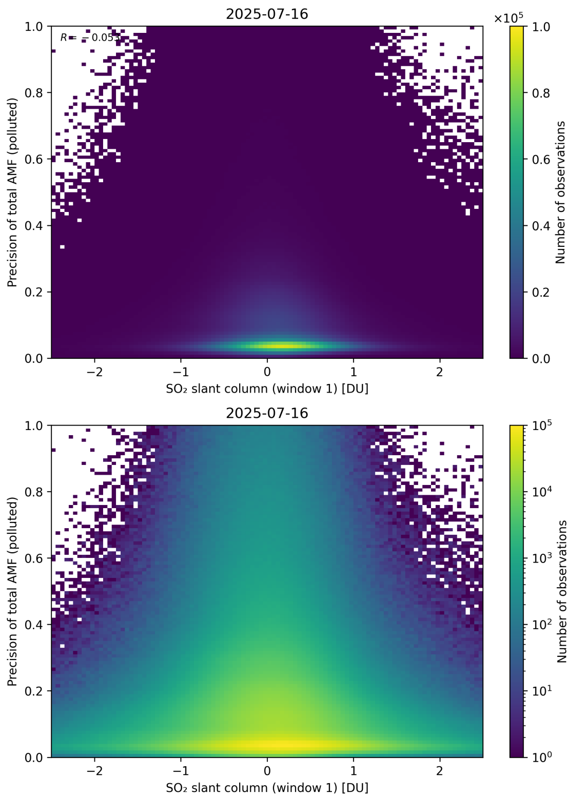
Figure 290: Scatter density plot of “SO 2 slant column (window 1)” against “Precision of total AMF (polluted)” for 2025-07-15 to 2025-07-17.
