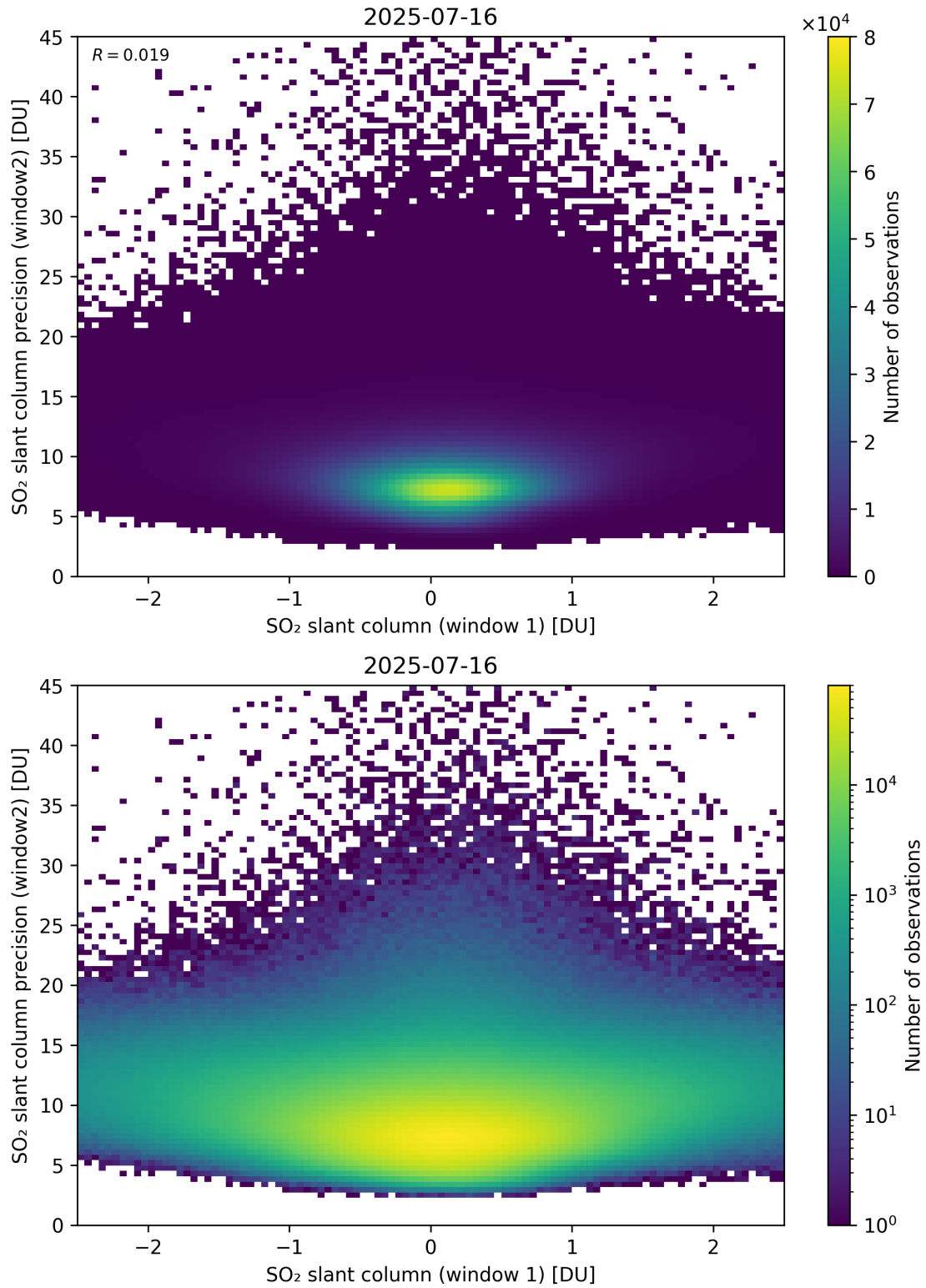
Figure 286: Scatter density plot of “SO 2 slant column (window 1)” against “SO 2 slant column precision (window2)” for 2025-07-15 to 2025-07-17.
