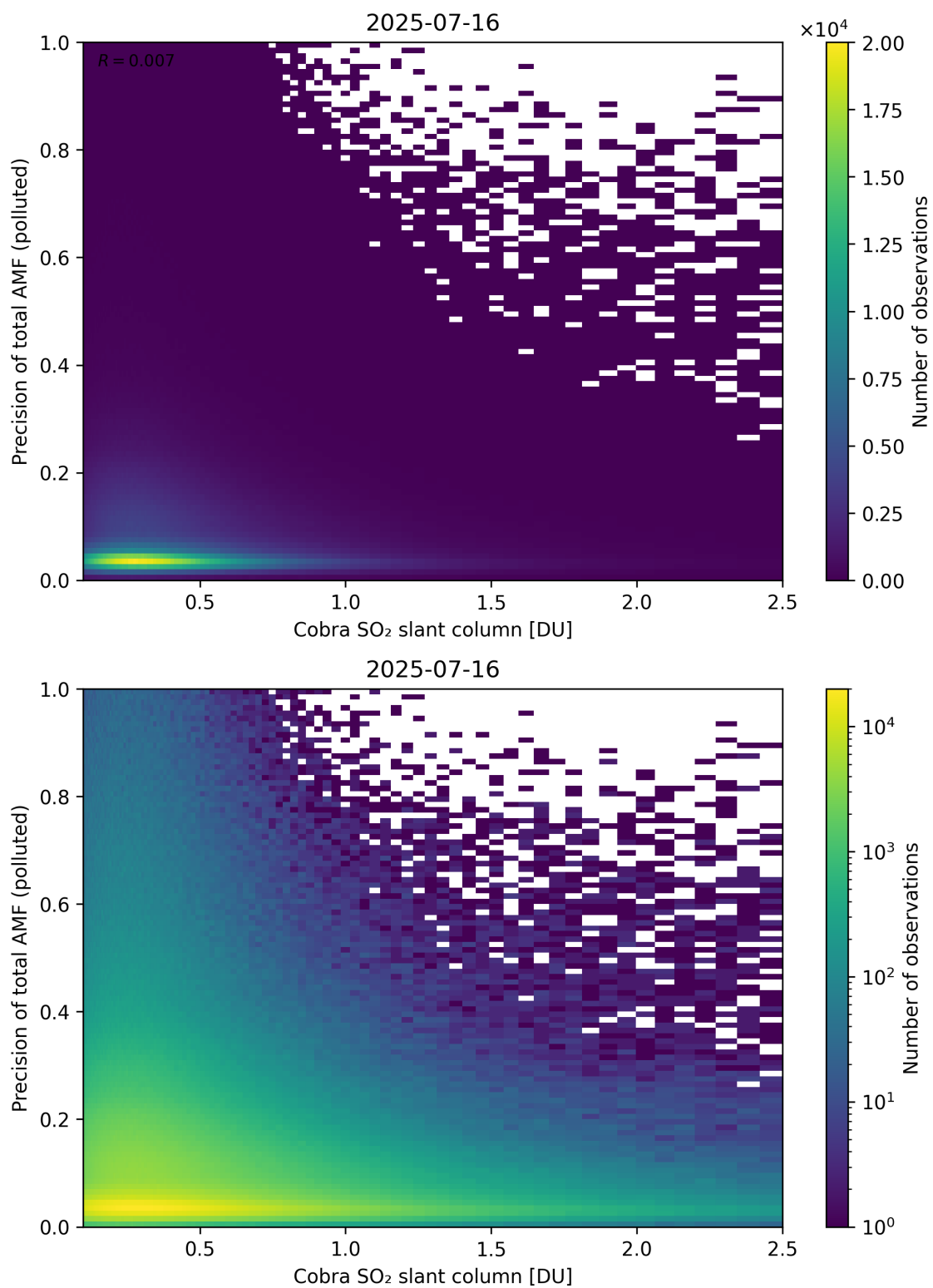
Figure 225: Scatter density plot of “Cobra SO 2 slant column” against “Precision of total AMF (polluted)” for 2025-07-15 to 2025-07-17.
