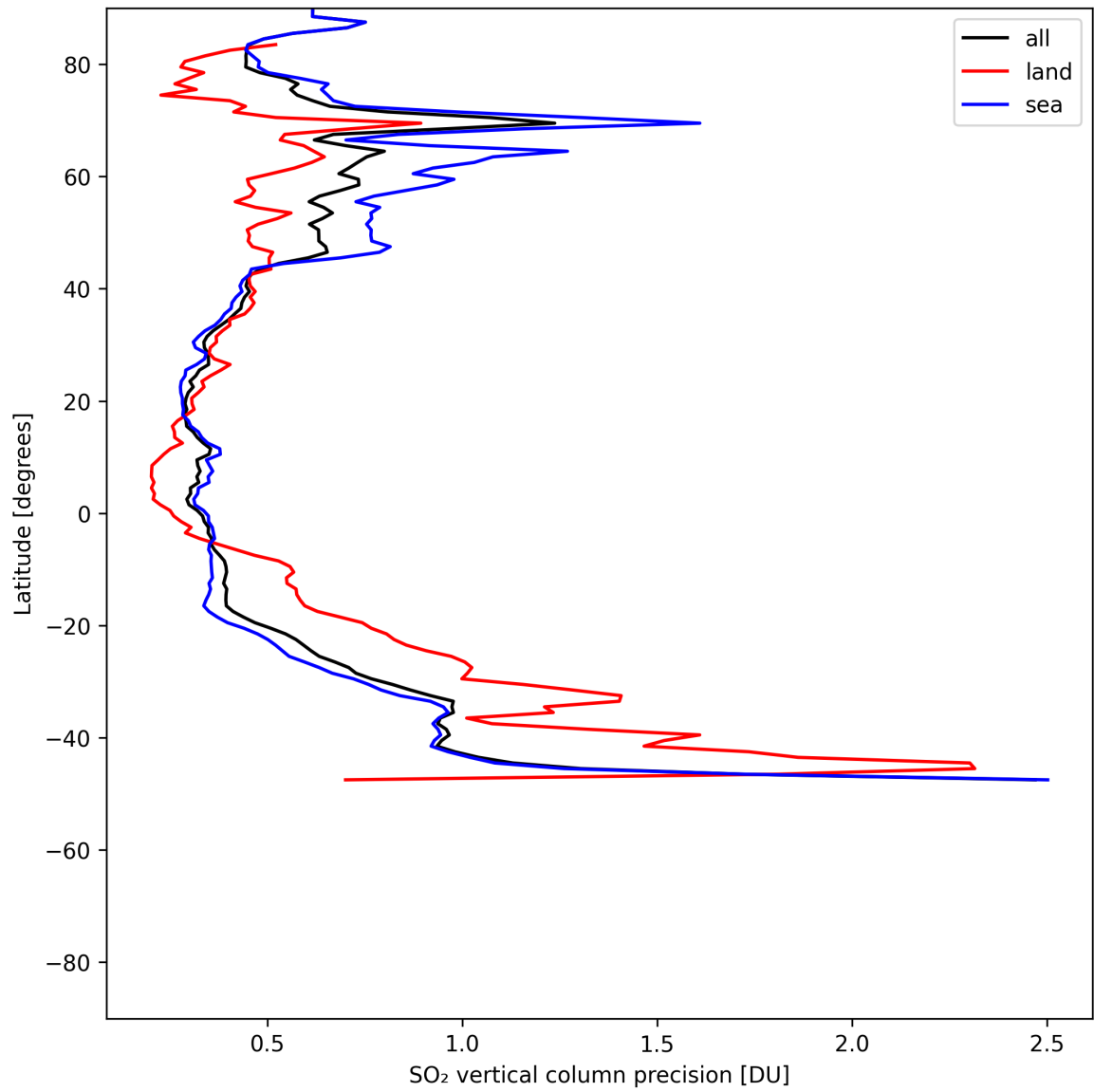
Figure 33: Zonal average of “SO 2 vertical column precision” for 2025-07-15 to 2025-07-17.
