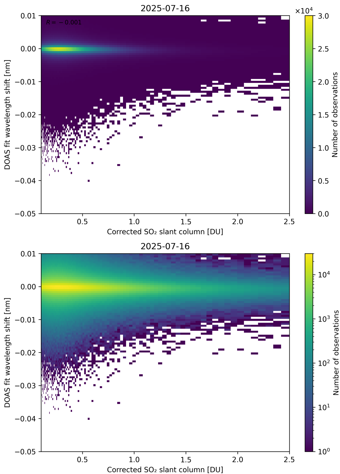
Figure 229: Scatter density plot of “Corrected SO 2 slant column” against “DOAS fit wavelength shift” for 2025-07-15 to 2025-07-17.
