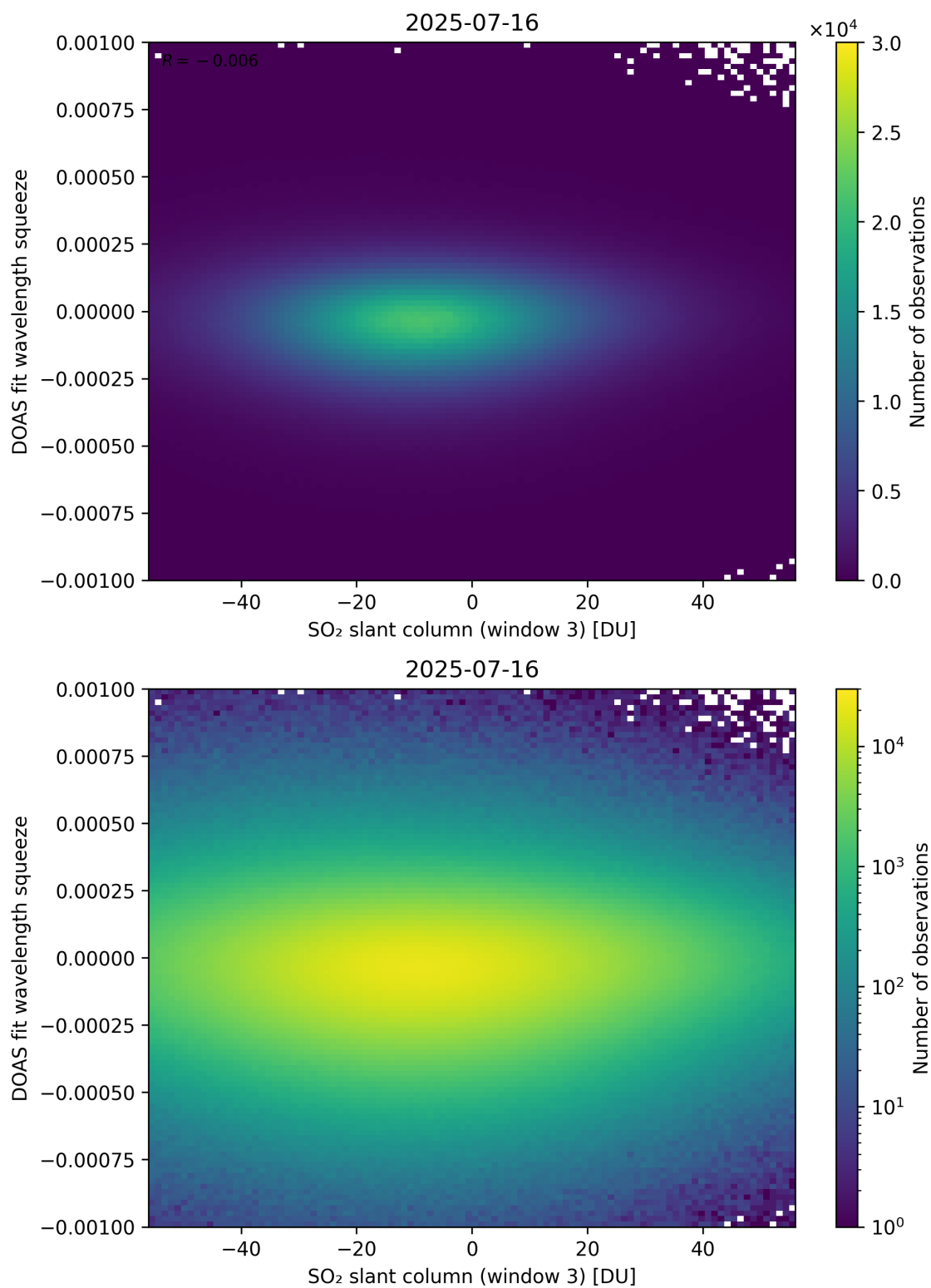
Figure 305: Scatter density plot of “SO 2 slant column (window 3)” against “DOAS fit wavelength squeeze” for 2025-07-15 to 2025-07-17.
