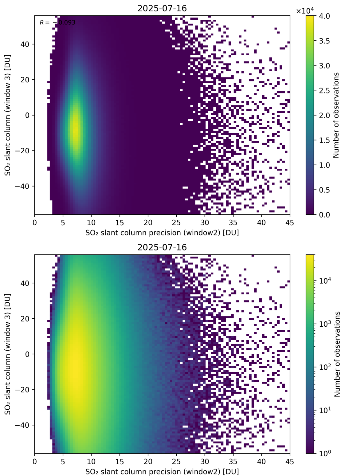
Figure 299: Scatter density plot of “SO 2 slant column precision (window2)” against “SO 2 slant column (window 3)” for 2025-07-15 to 2025-07-17.
