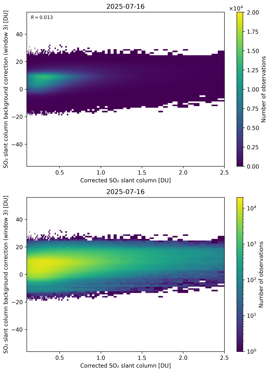
Figure 228: Scatter density plot of “Corrected SO 2 slant column” against “SO 2 slant column background correction (window 3)” for 2025-07-15 to 2025-07-17.
