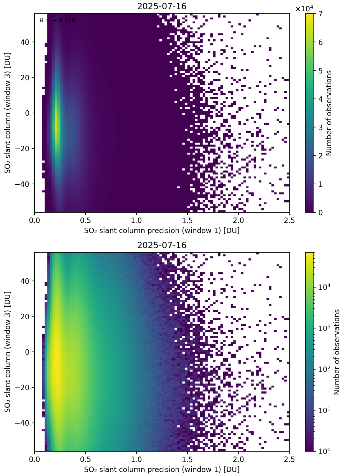
Figure 278: Scatter density plot of “SO 2 slant column precision (window 1)” against “SO 2 slant column (window 3)” for 2025-07-15 to 2025-07-17.
