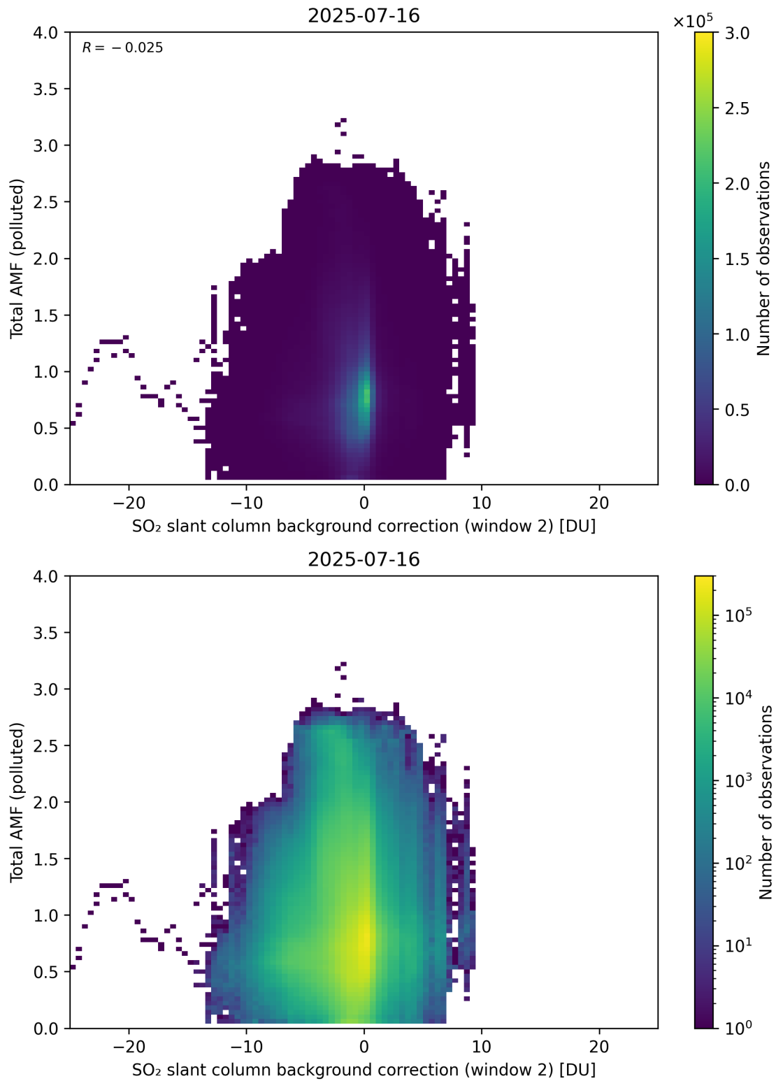
Figure 130: Scatter density plot of “SO 2 slant column background correction (window 2)” against “Total AMF (polluted)” for 2025-07-15 to 2025-07-17.
