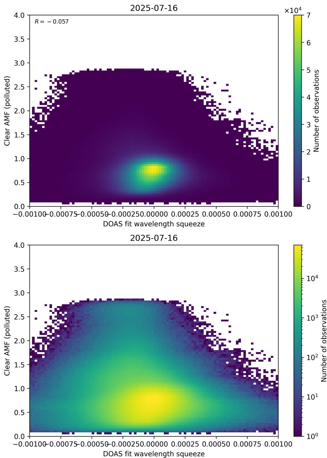
Figure 144: Scatter density plot of “DOAS fit wavelength squeeze” against “Clear AMF (polluted)” for 2025-07-15 to 2025-07-17.
