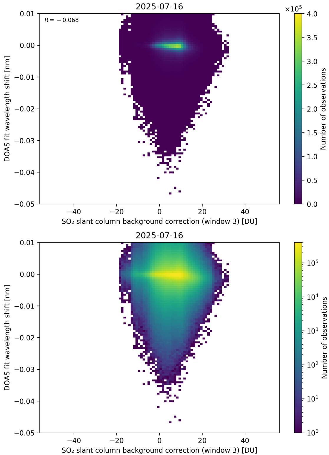
Figure 132: Scatter density plot of “SO 2 slant column background correction (window 3)” against “DOAS fit wavelength shift” for 2025-07-15 to 2025-07-17.
