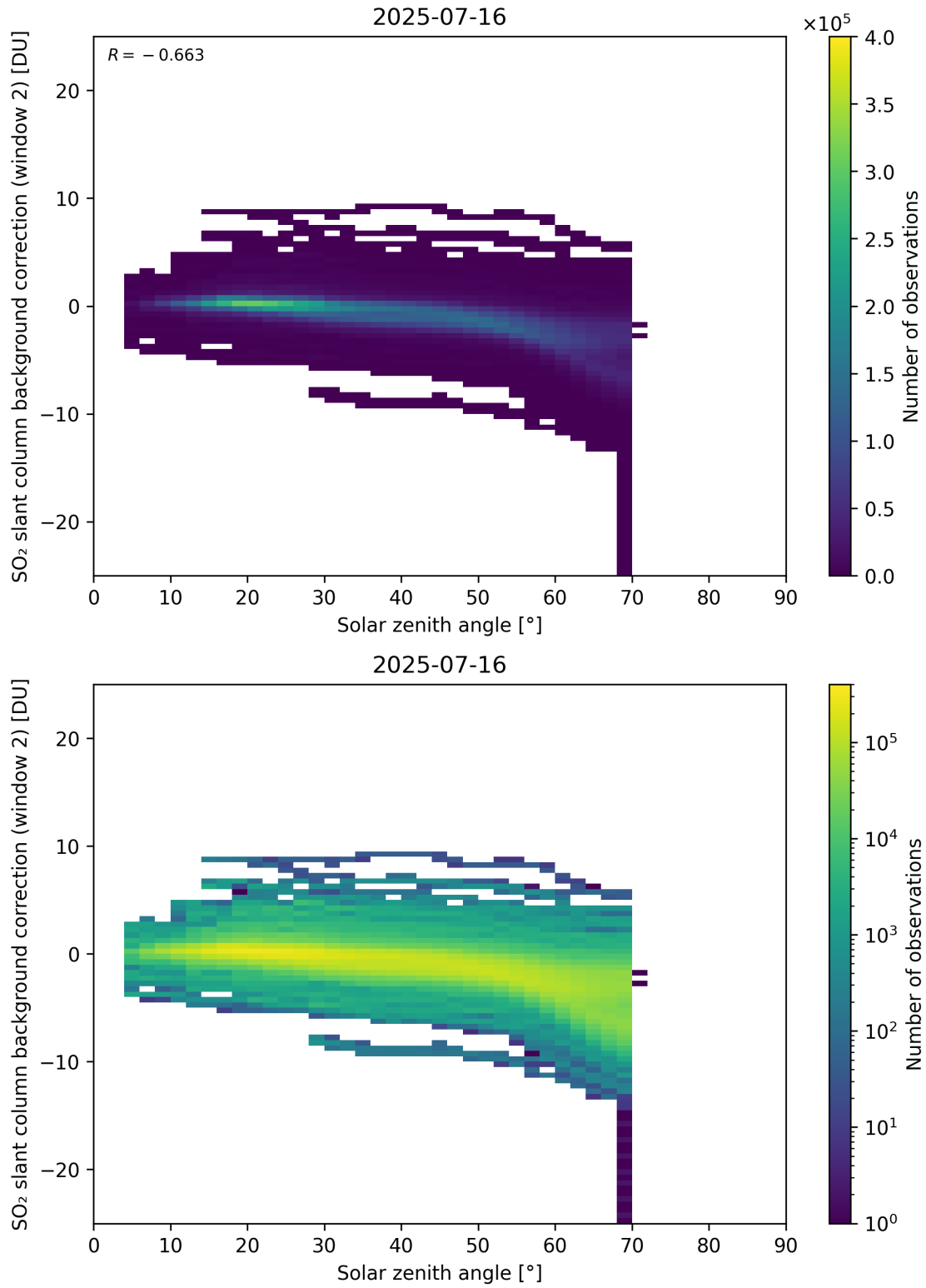
Figure 172: Scatter density plot of “Solar zenith angle” against “SO 2 slant column background correction (window 2)” for 2025-07-15 to 2025-07-17.
