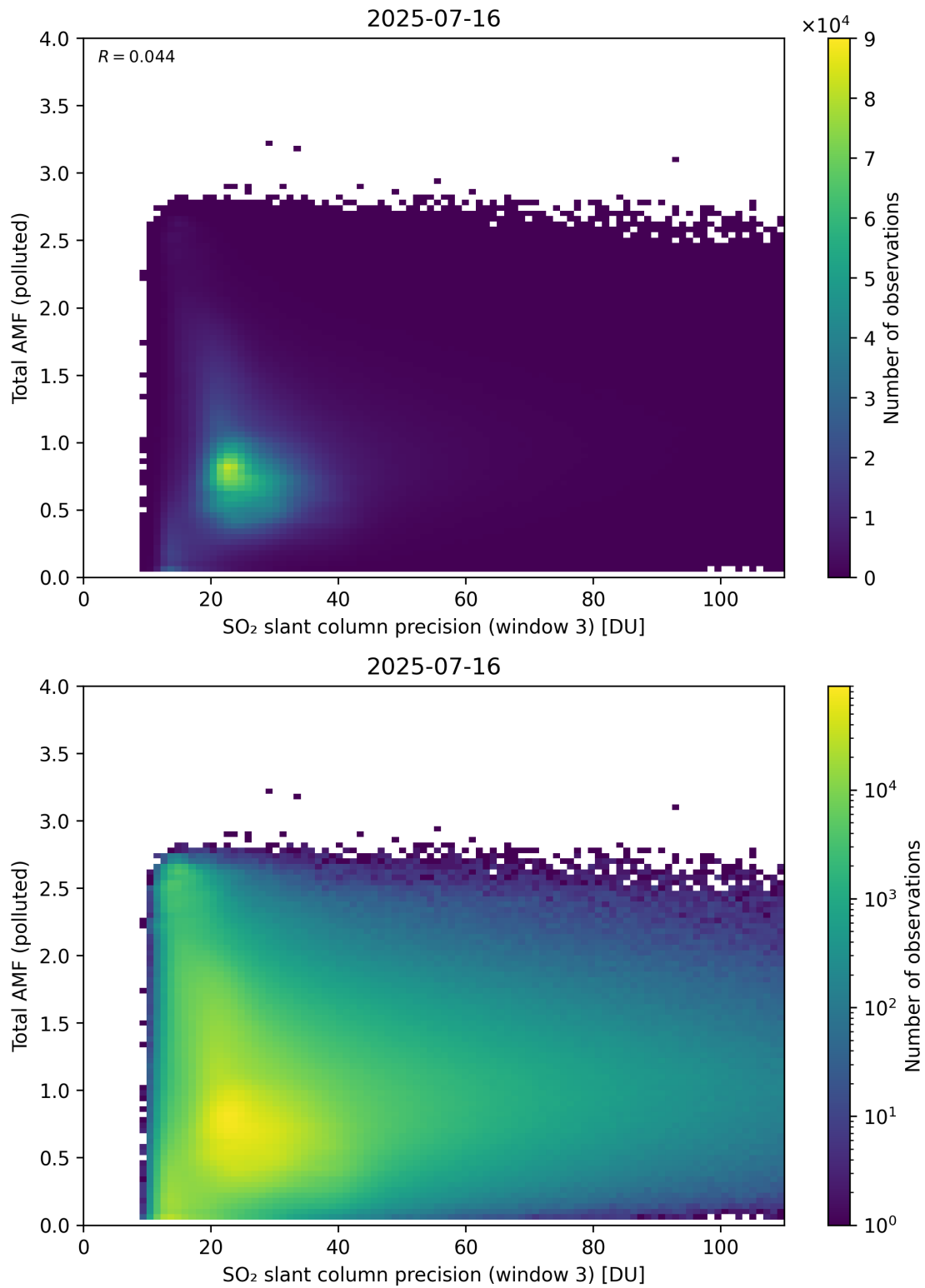
Figure 313: Scatter density plot of “SO 2 slant column precision (window 3)” against “Total AMF (polluted)” for 2025-07-15 to 2025-07-17.
