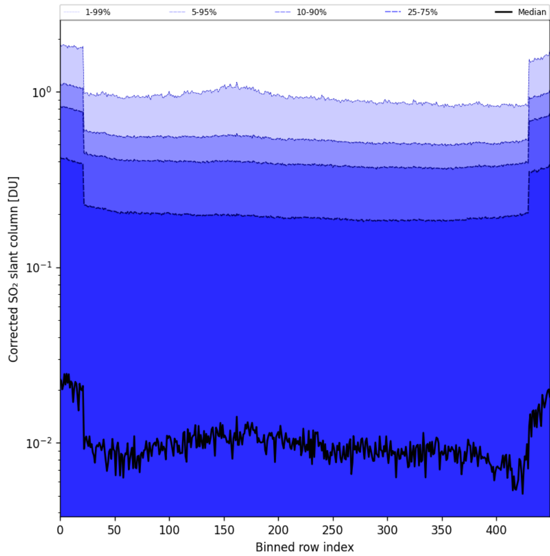
Figure 86: Along track statistics of “Corrected SO 2 slant column” for 2025-07-15 to 2025-07-17
