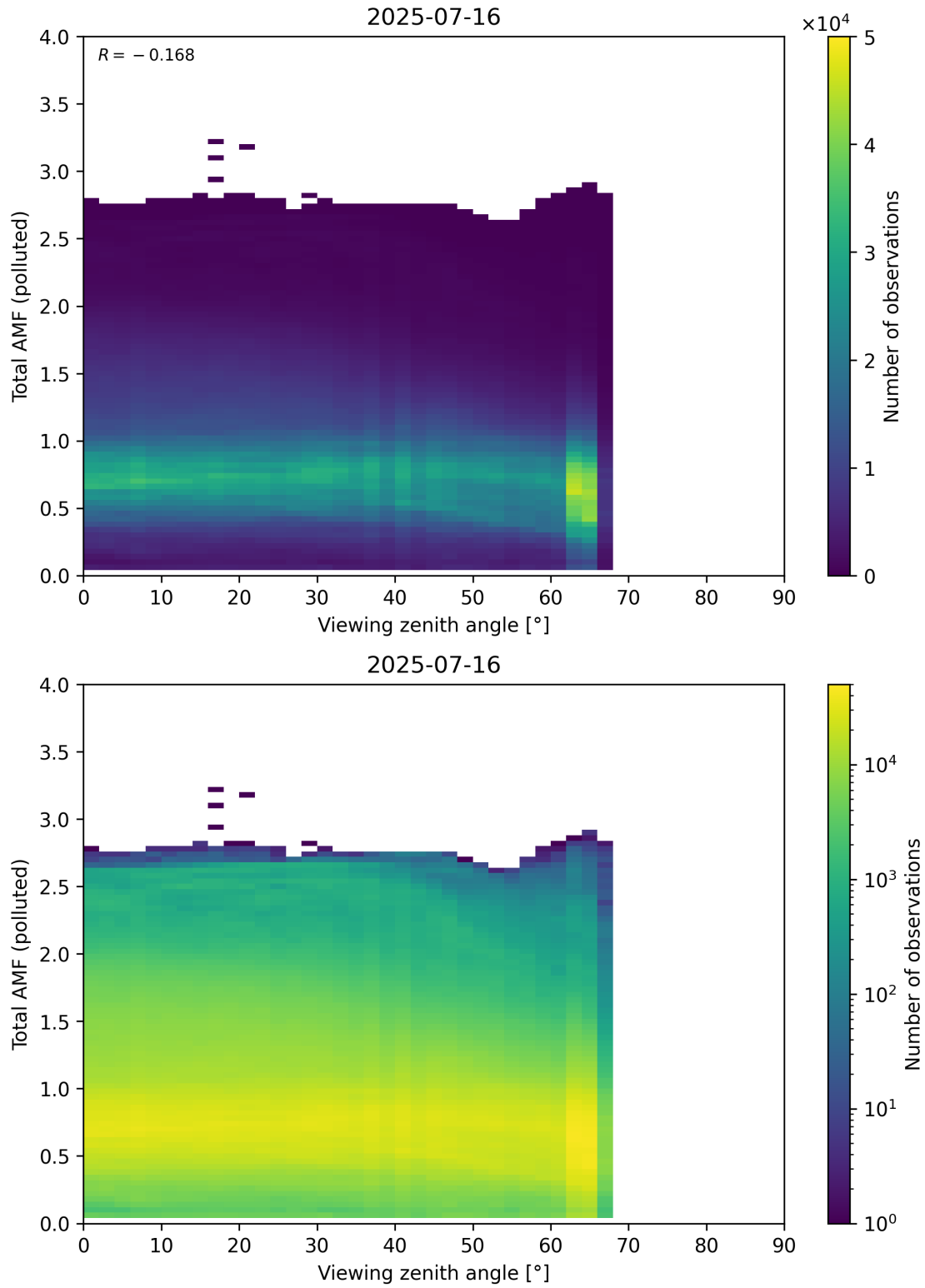
Figure 381: Scatter density plot of “Viewing zenith angle” against “Total AMF (polluted)” for 2025-07-15 to 2025-07-17.
