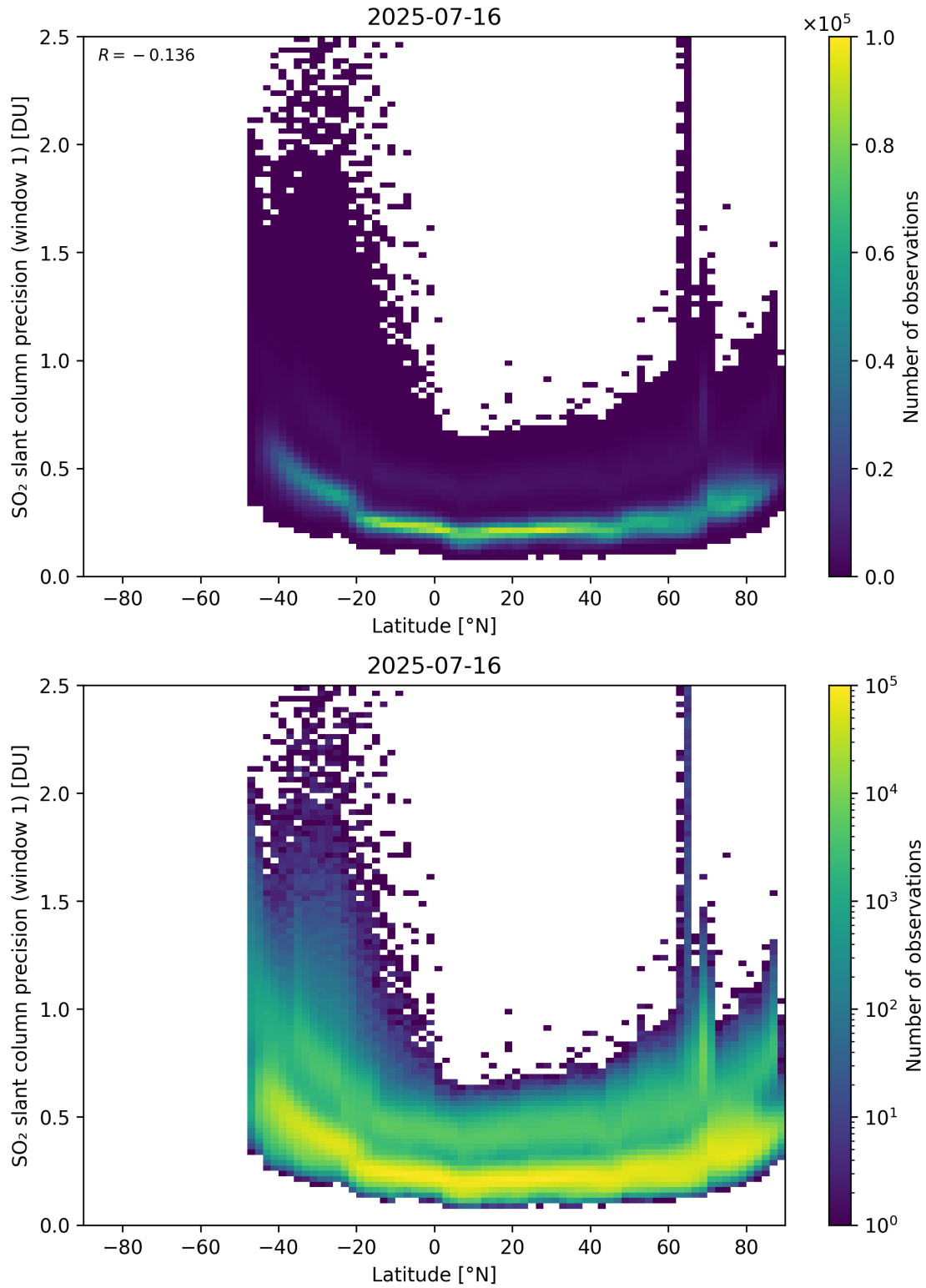
Figure 163: Scatter density plot of “Latitude” against “SO 2 slant column precision (window 1)” for 2025-07-15 to 2025-07-17.
