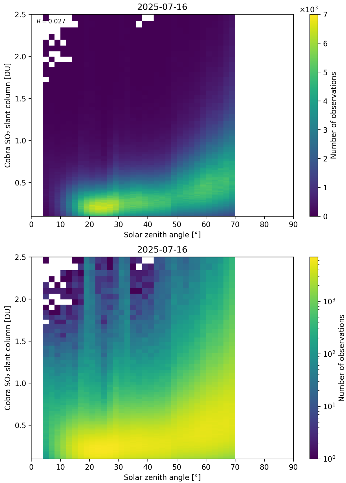
Figure 179: Scatter density plot of “Solar zenith angle” against “Cobra SO 2 slant column” for 2025-07-15 to 2025-07-17.
