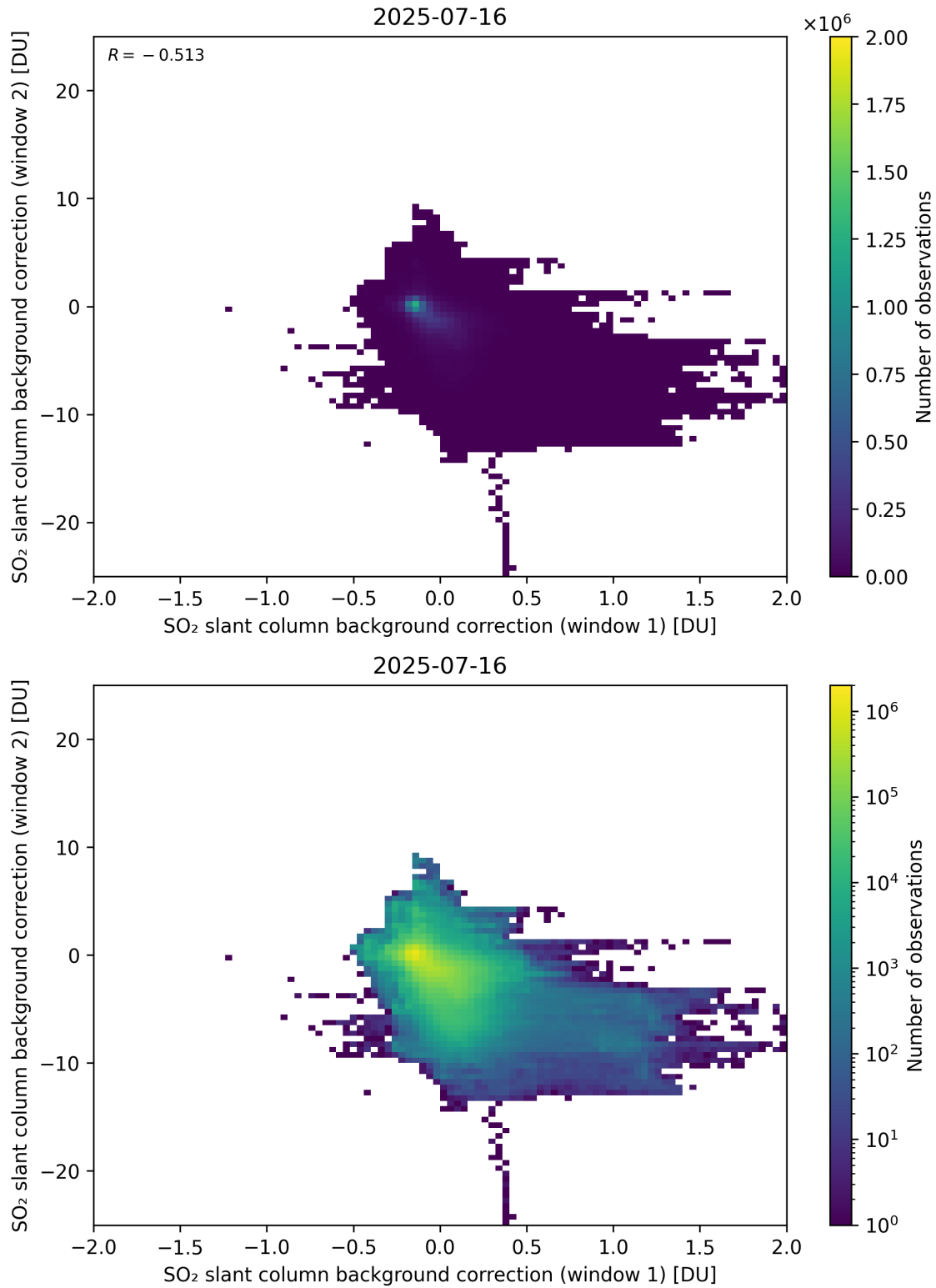
Figure 109: Scatter density plot of “SO 2 slant column background correction (window 1)” against “SO 2 slant column background correction (window 2)” for 2025-07-15 to 2025-07-17.
