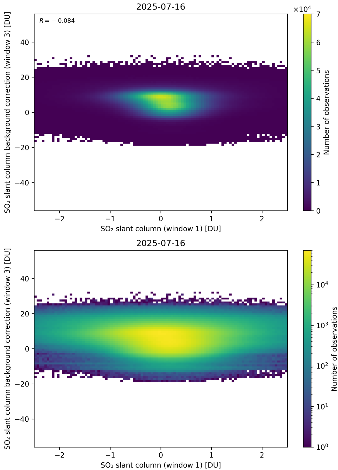
Figure 264: Scatter density plot of “SO 2 slant column (window 1)” against “SO 2 slant column background correction (window 3)” for 2025-07-15 to 2025-07-17.
