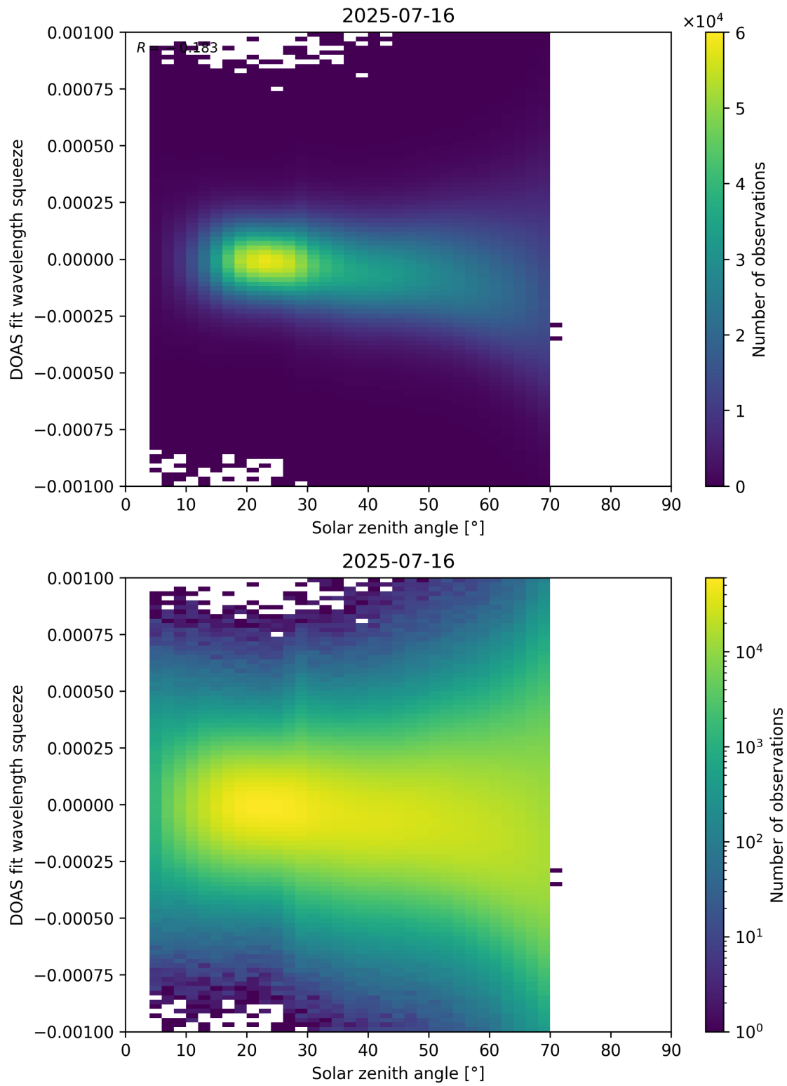
Figure 175: Scatter density plot of “Solar zenith angle” against “DOAS fit wavelength squeeze” for 2025-07-15 to 2025-07-17.
