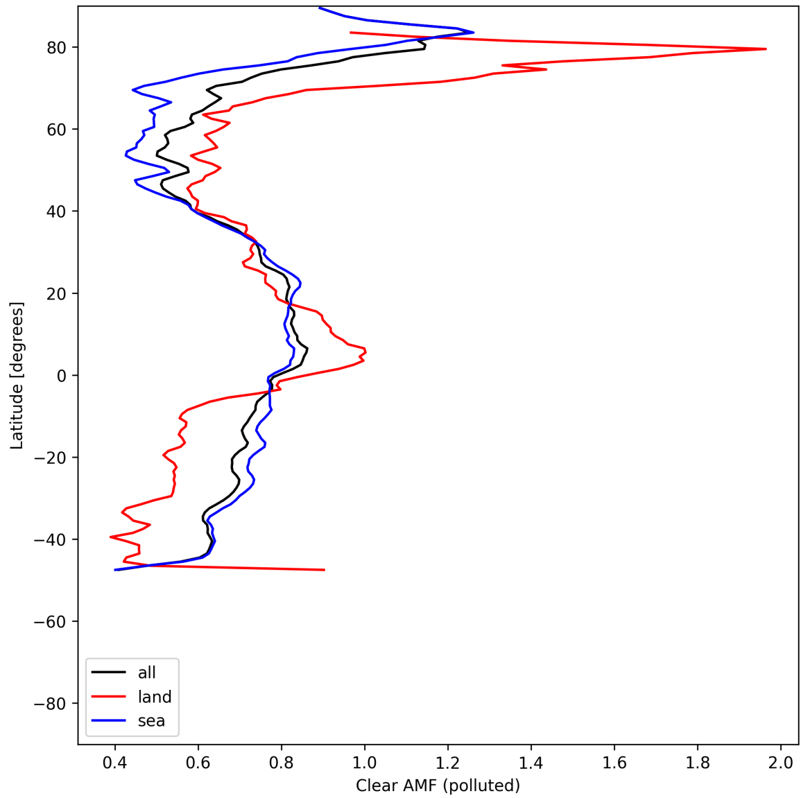
Figure 55: Zonal average of “Clear AMF (polluted)” for 2025-07-15 to 2025-07-17.
