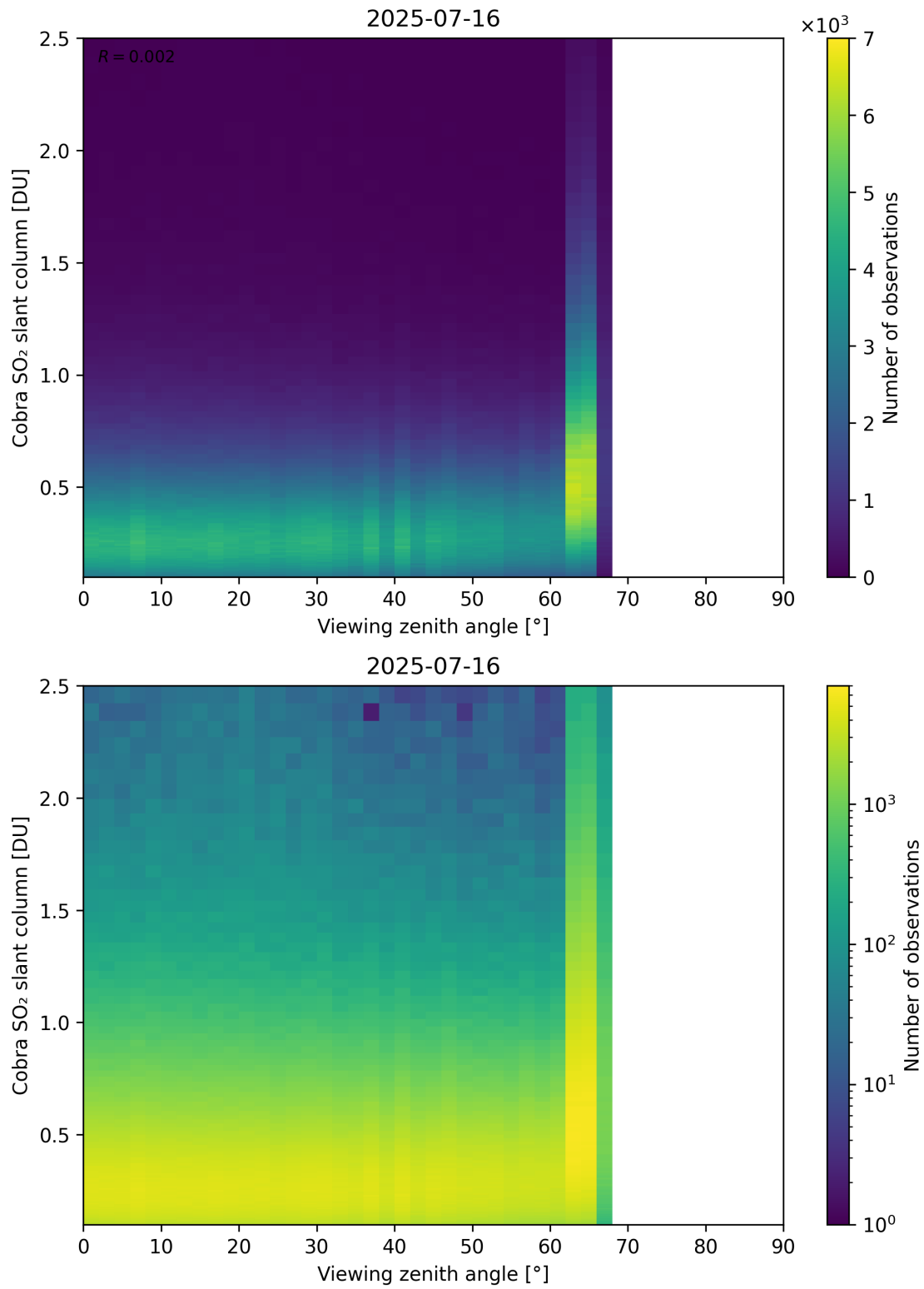
Figure 371: Scatter density plot of “Viewing zenith angle” against “Cobra SO 2 slant column” for 2025-07-15 to 2025-07-17.
