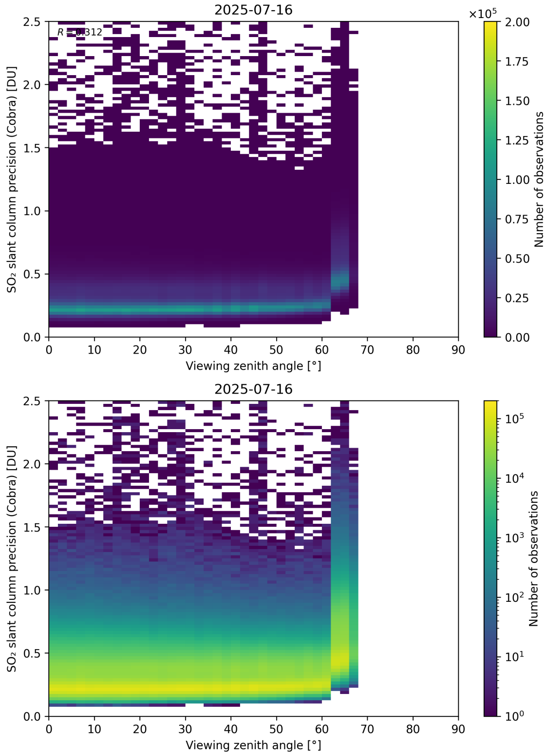
Figure 372: Scatter density plot of “Viewing zenith angle” against “SO 2 slant column precision (Cobra)” for 2025-07-15 to 2025-07-17.
