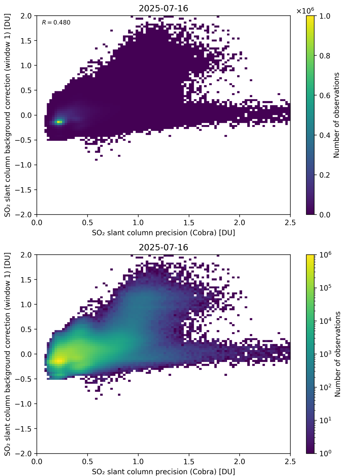
Figure 199: Scatter density plot of “SO 2 slant column precision (Cobra)” against “SO 2 slant column background correction (window 1)” for 2025-07-15 to 2025-07-17.
