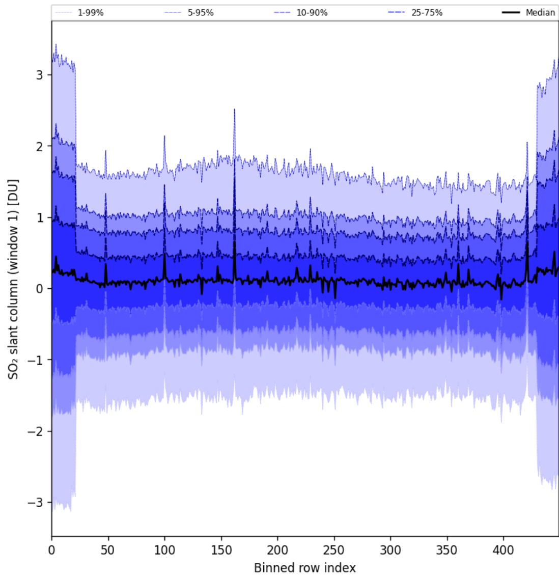
Figure 89: Along track statistics of “SO 2 slant column (window 1)” for 2025-07-15 to 2025-07-17
