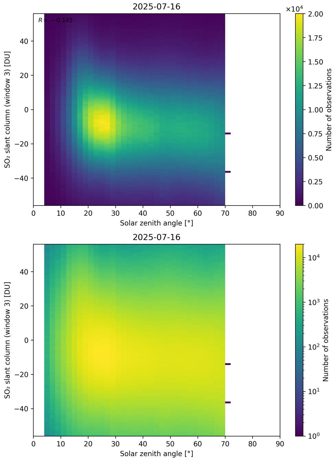
Figure 187: Scatter density plot of “Solar zenith angle” against “SO 2 slant column (window 3)” for 2025-07-15 to 2025-07-17.
