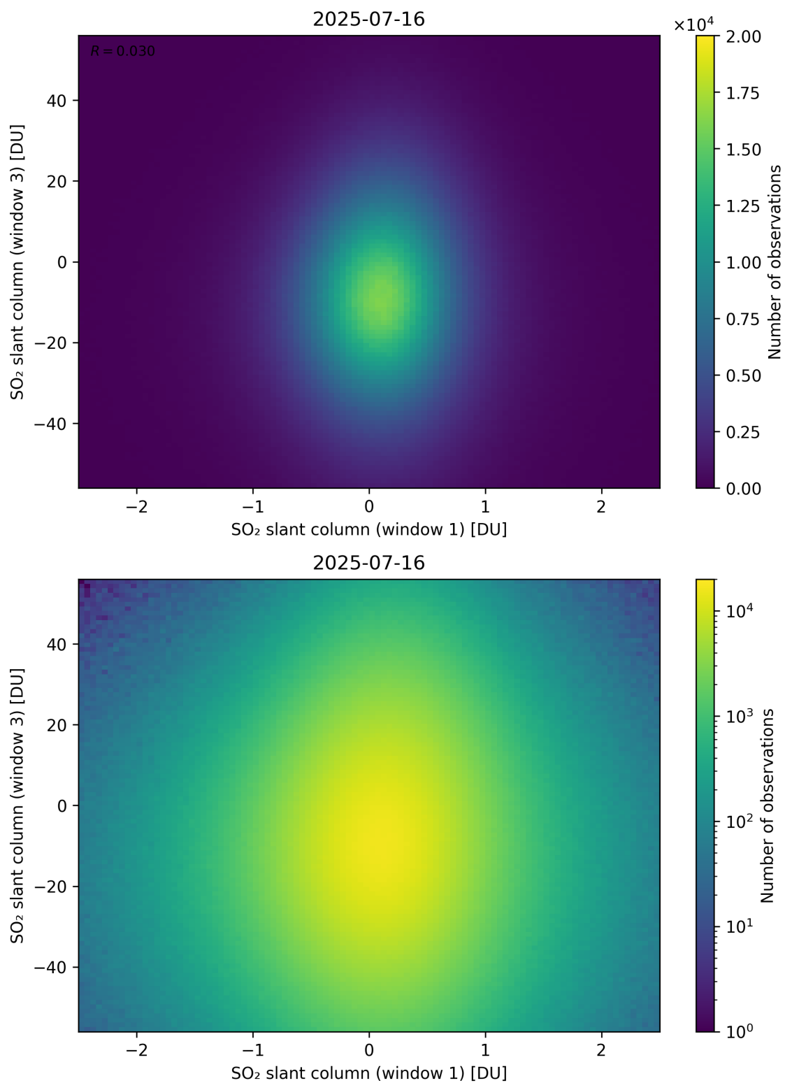
Figure 287: Scatter density plot of “SO 2 slant column (window 1)” against “SO 2 slant column (window 3)” for 2025-07-15 to 2025-07-17.
