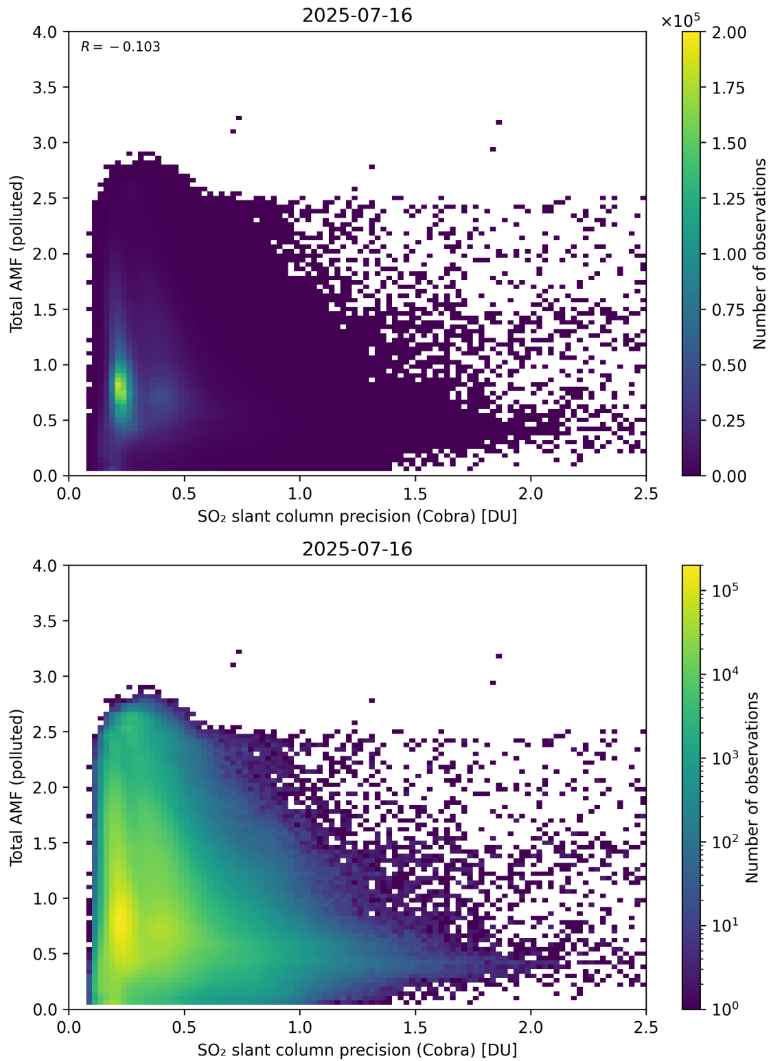
Figure 213: Scatter density plot of “SO 2 slant column precision (Cobra)” against “Total AMF (polluted)” for 2025-07-15 to 2025-07-17.
