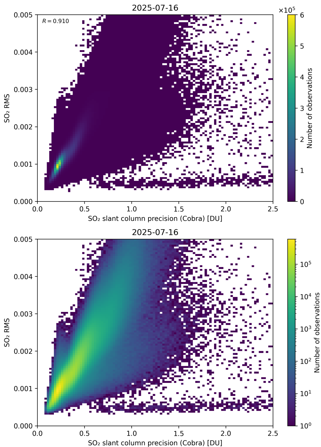
Figure 204: Scatter density plot of “SO 2 slant column precision (Cobra)” against “SO 2 RMS” for 2025-07-15 to 2025-07-17.
