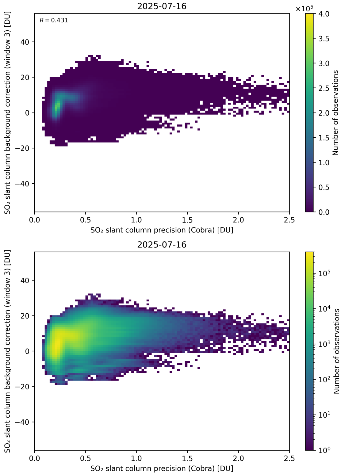
Figure 201: Scatter density plot of “SO 2 slant column precision (Cobra)” against “SO 2 slant column background correction (window 3)” for 2025-07-15 to 2025-07-17.
