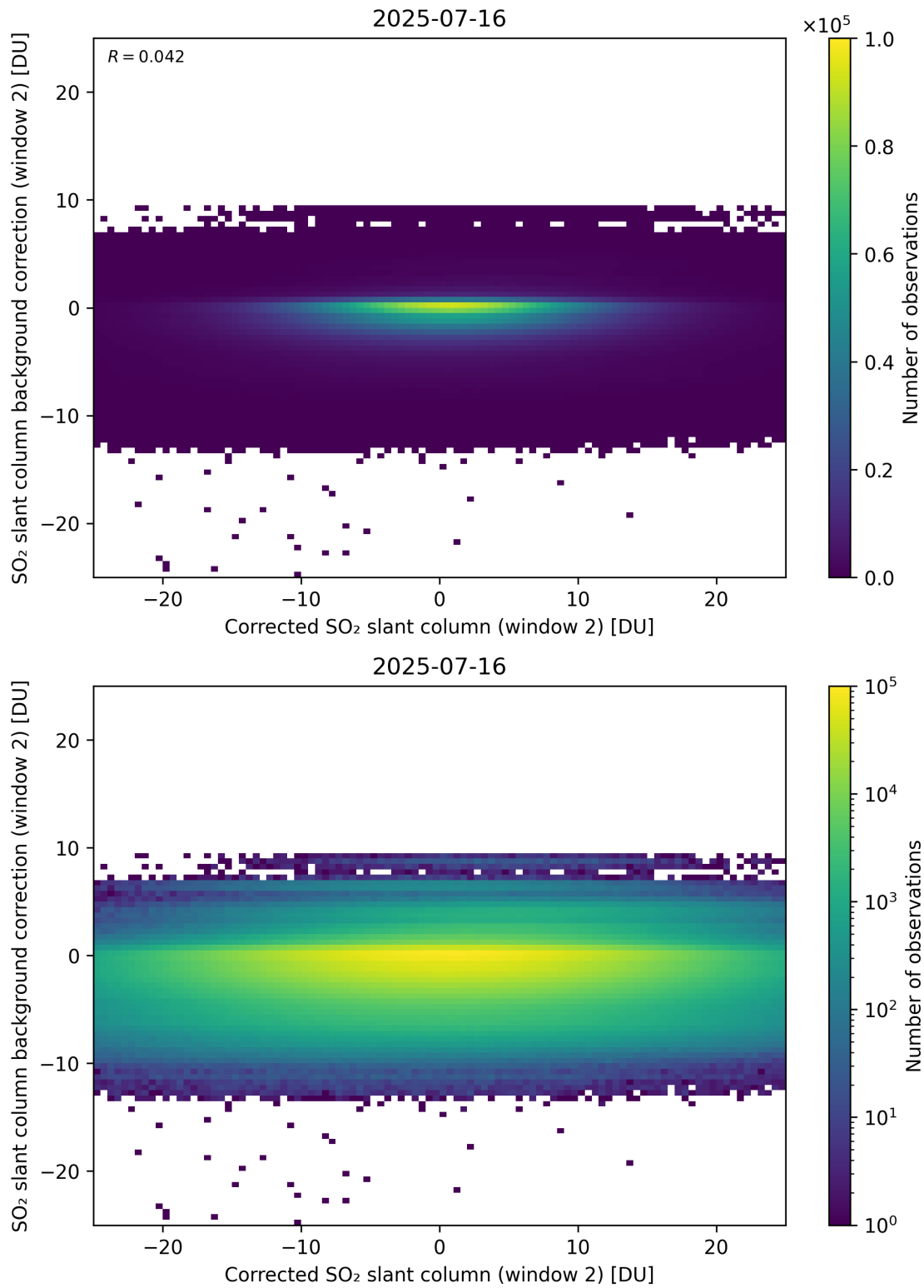
Figure 244: Scatter density plot of “Corrected SO 2 slant column (window 2)” against “SO 2 slant column background correction (window 2)” for 2025-07-15 to 2025-07-17.
