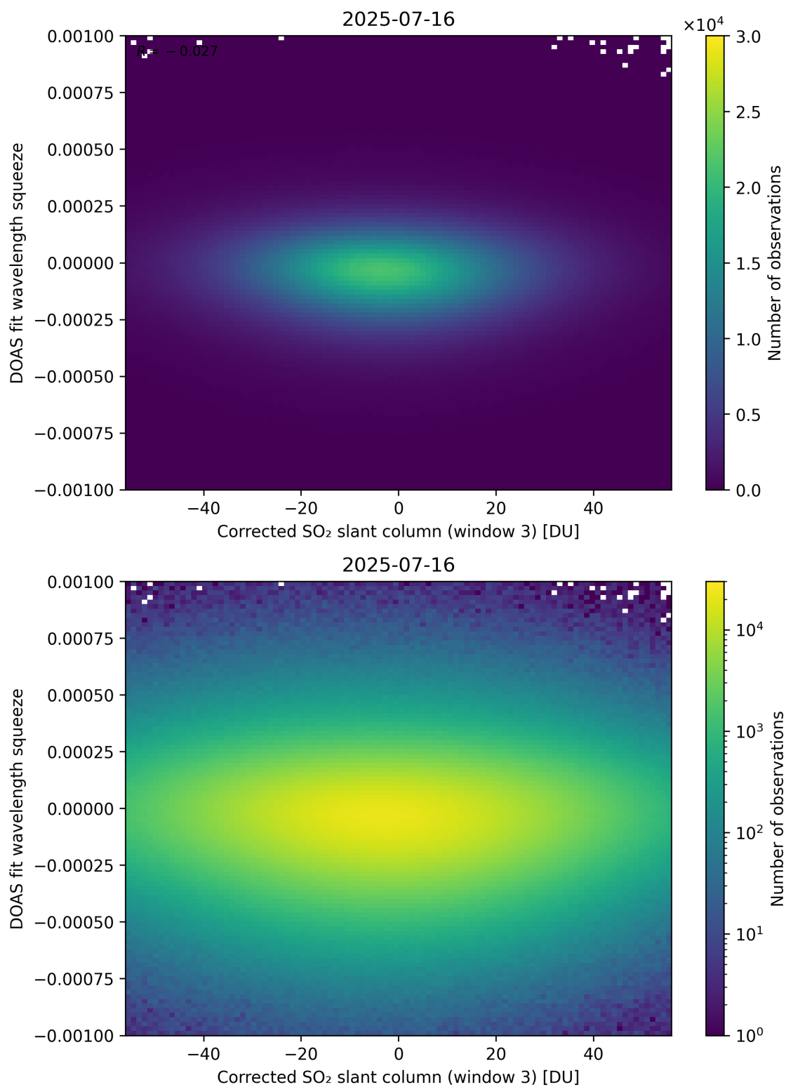
Figure 257: Scatter density plot of “Corrected SO 2 slant column (window 3)” against “DOAS fit wavelength squeeze” for 2025-07-15 to 2025-07-17.
