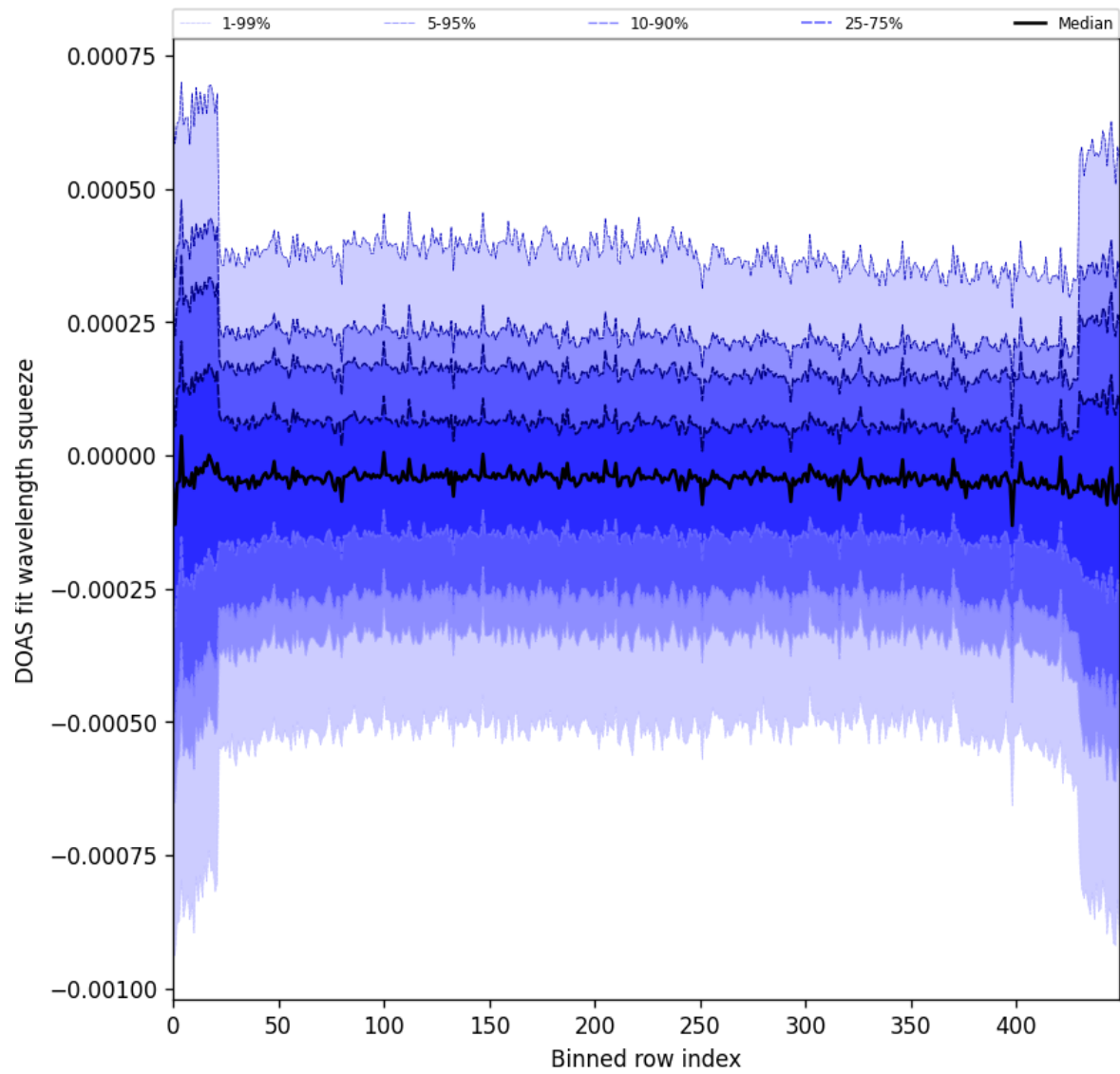
Figure 103: Along track statistics of “DOAS fit wavelength squeeze” for 2025-07-15 to 2025-07-17
