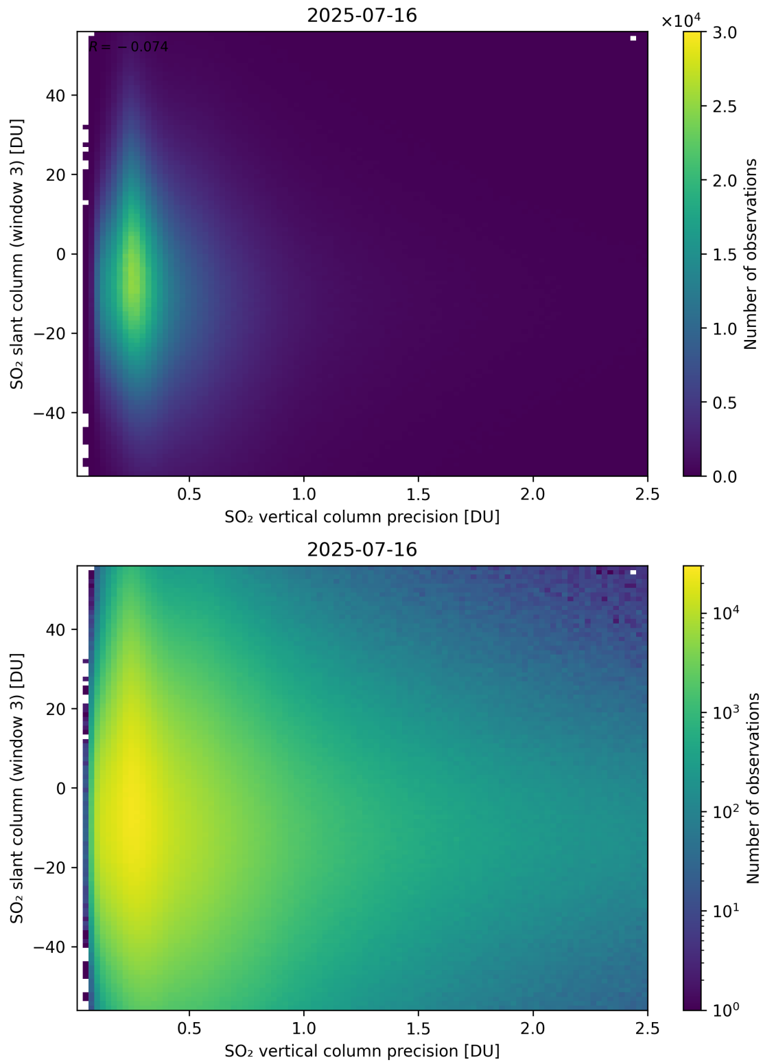
Figure 344: Scatter density plot of “SO 2 vertical column precision” against “SO 2 slant column (window 3)” for 2025-07-15 to 2025-07-17.
