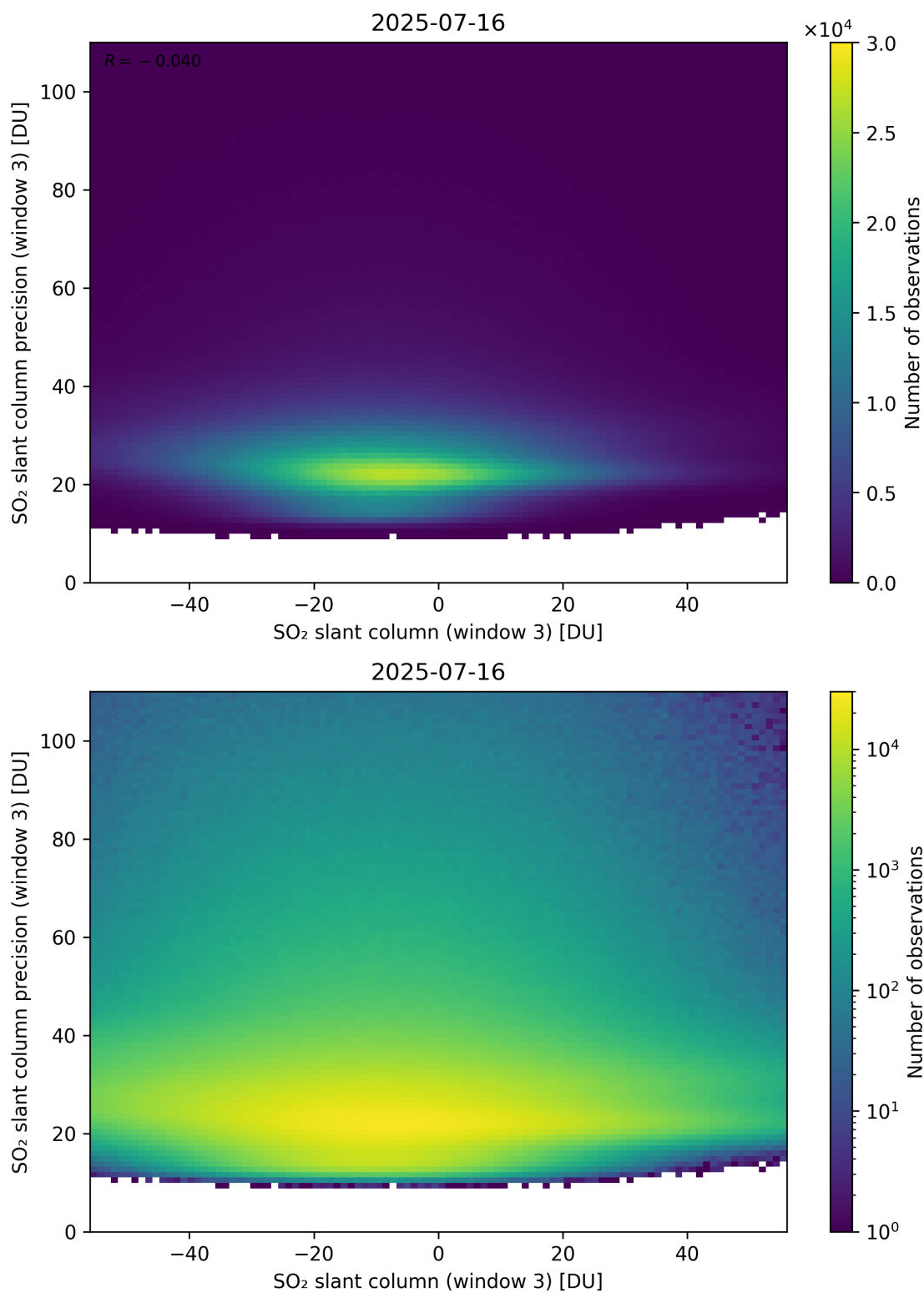
Figure 317: Scatter density plot of “SO 2 slant column (window 3)” against “SO 2 slant column precision (window 3)” for 2025-07-15 to 2025-07-17.
