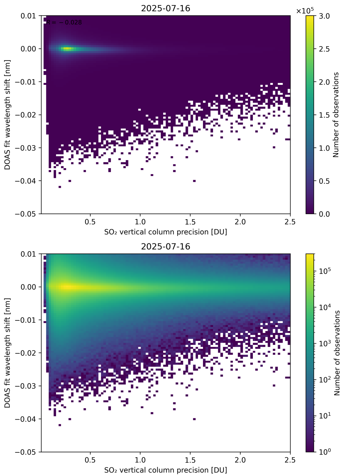
Figure 332: Scatter density plot of “SO 2 vertical column precision” against “DOAS fit wavelength shift” for 2025-07-15 to 2025-07-17.
