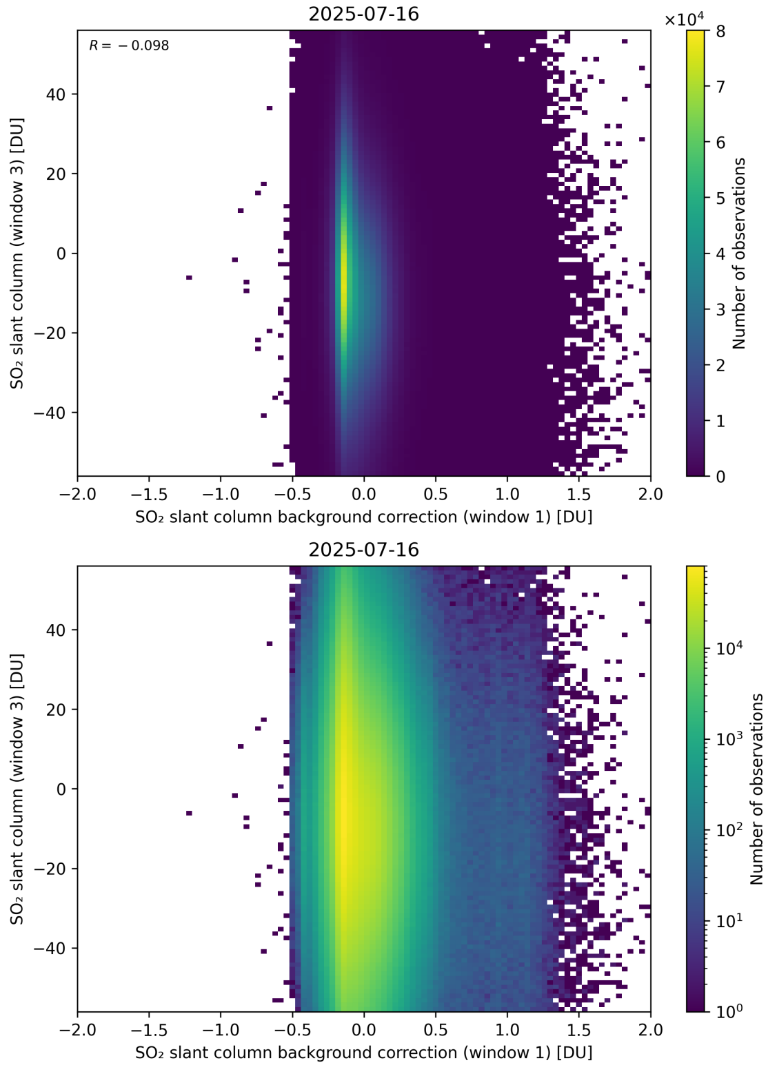
Figure 118: Scatter density plot of “SO 2 slant column background correction (window 1)” against “SO 2 slant column (window 3)” for 2025-07-15 to 2025-07-17.
