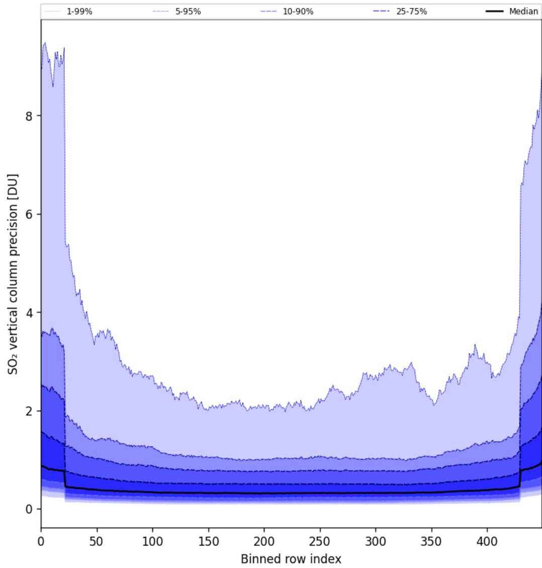
Figure 85: Along track statistics of “SO 2 vertical column precision” for 2025-07-15 to 2025-07-17
