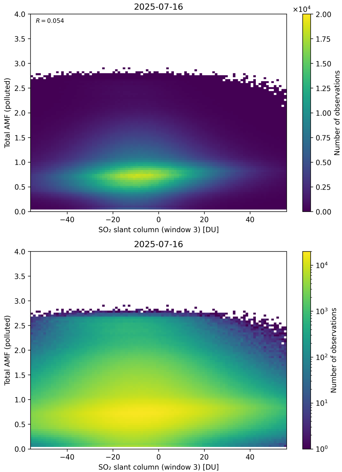
Figure 318: Scatter density plot of “SO 2 slant column (window 3)” against “Total AMF (polluted)” for 2025-07-15 to 2025-07-17.
