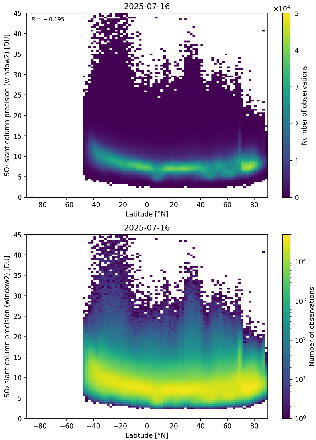
Figure 164: Scatter density plot of “Latitude” against “SO 2 slant column precision (window2)” for 2025-07-15 to 2025-07-17.
