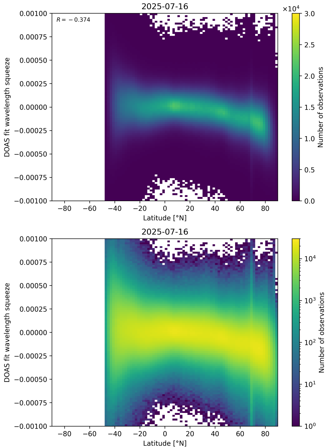
Figure 154: Scatter density plot of “Latitude” against “DOAS fit wavelength squeeze” for 2025-07-15 to 2025-07-17.
