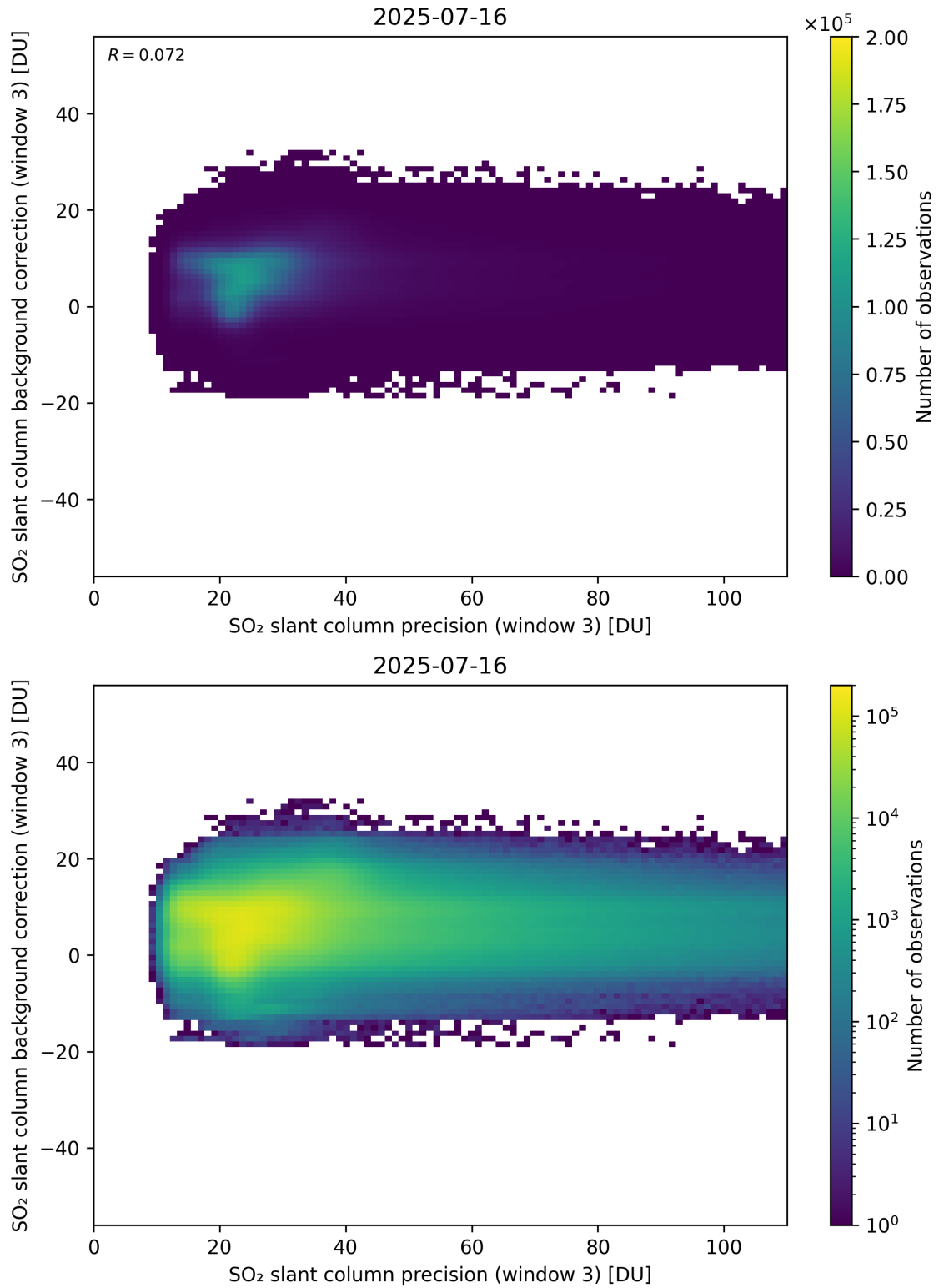
Figure 307: Scatter density plot of “SO 2 slant column precision (window 3)” against “SO 2 slant column background correction (window 3)” for 2025-07-15 to 2025-07-17.
