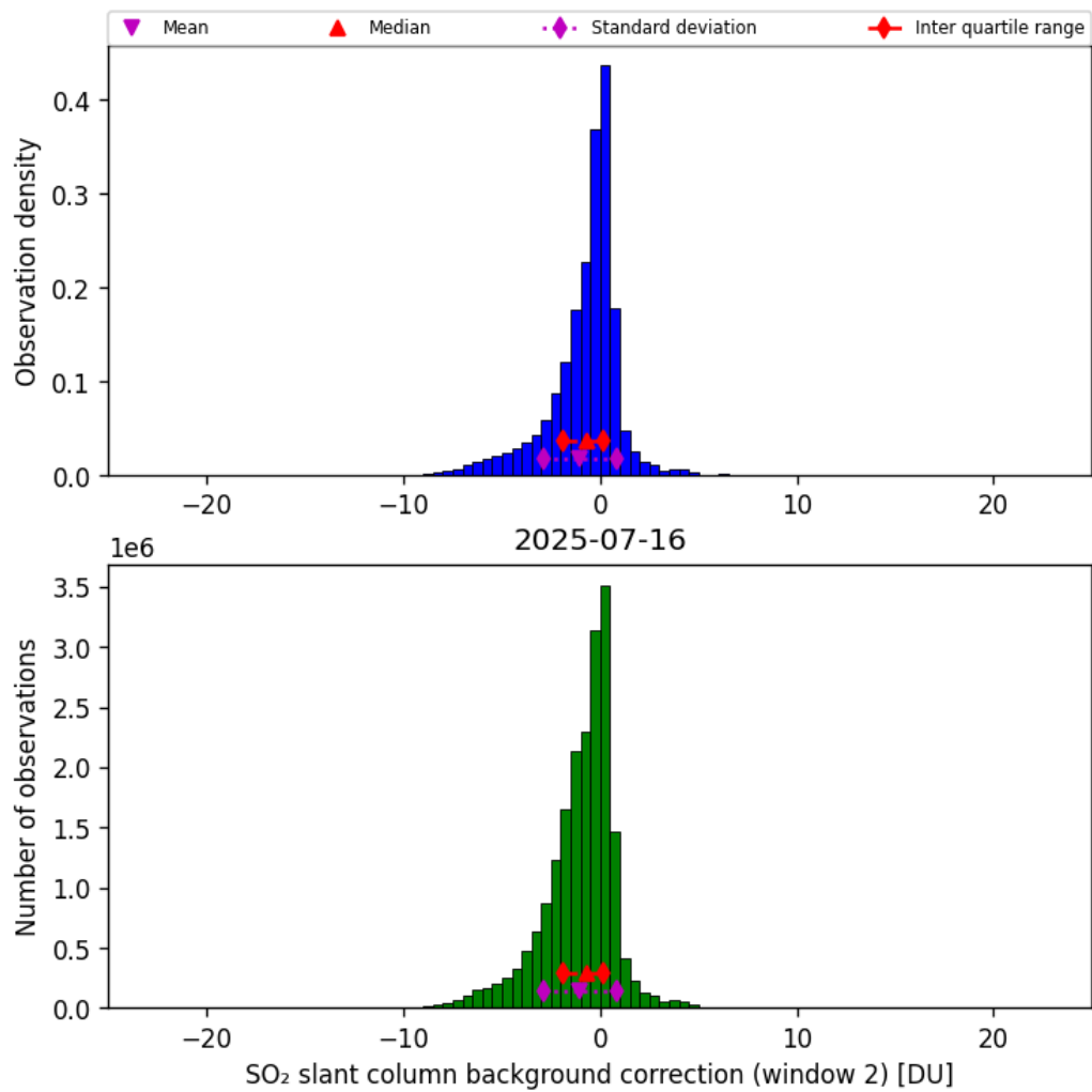
Figure 70: Histogram of “SO 2 slant column background correction (window 2)” for 2025-07-15 to 2025-07-17
