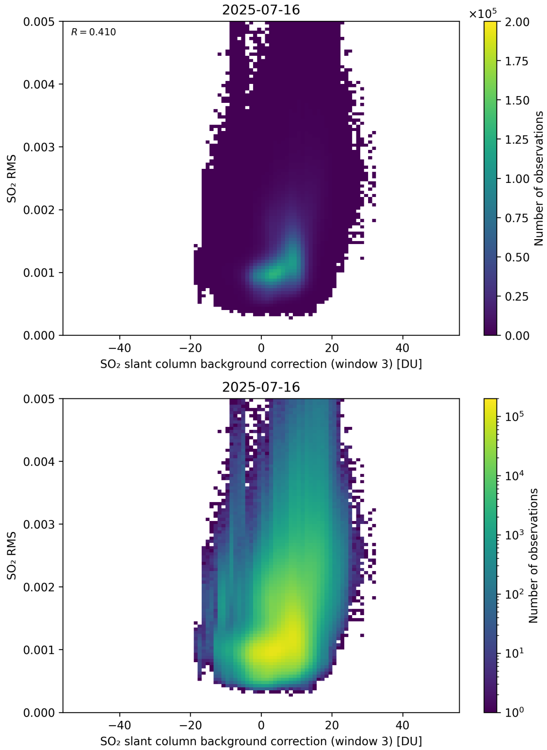
Figure 134: Scatter density plot of “SO 2 slant column background correction (window 3)” against “SO 2 RMS” for 2025-07-15 to 2025-07-17.
