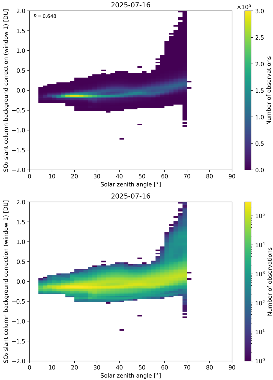
Figure 171: Scatter density plot of “Solar zenith angle” against “SO 2 slant column background correction (window 1)” for 2025-07-15 to 2025-07-17.
