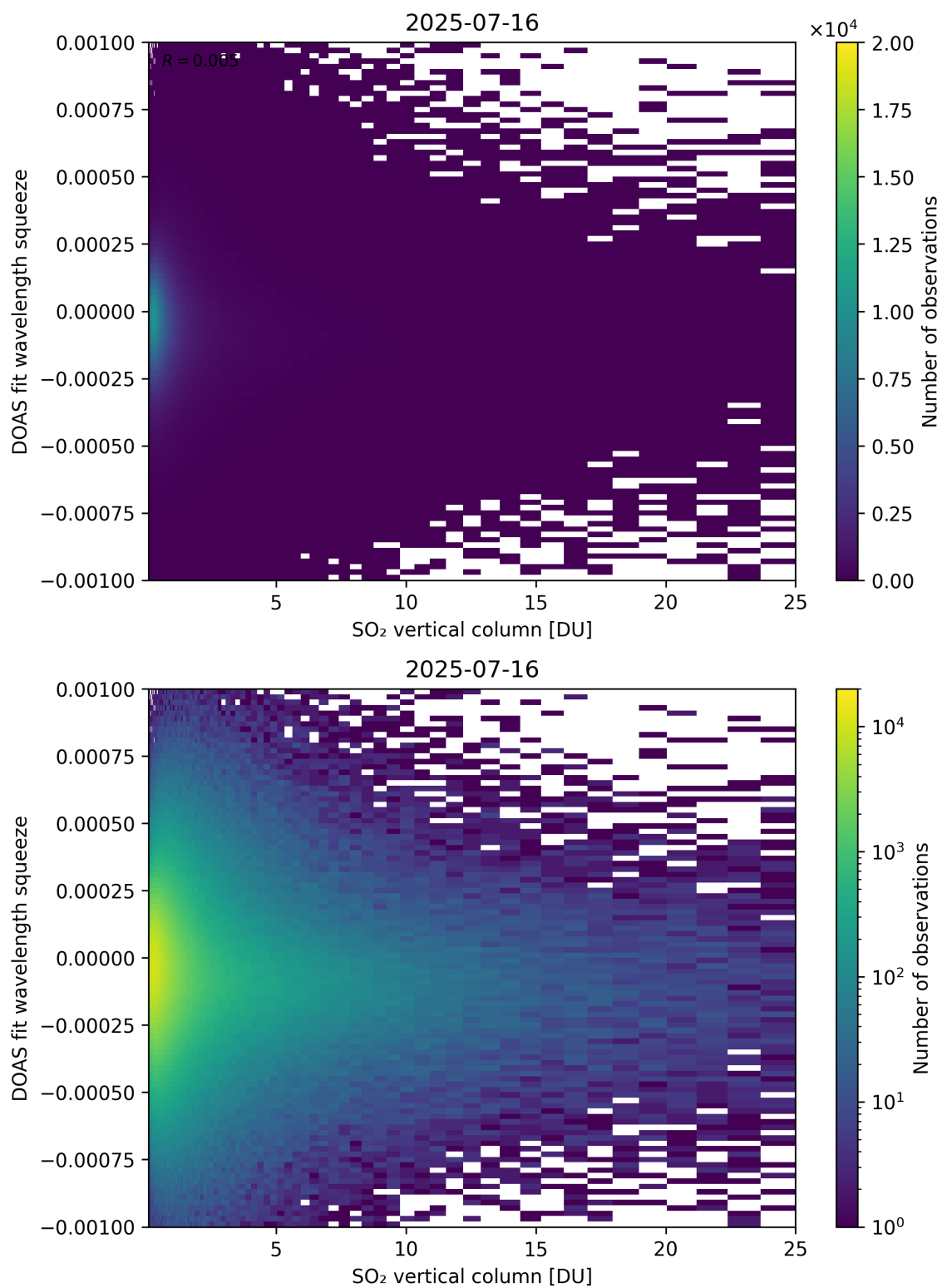
Figure 327: Scatter density plot of “SO 2 vertical column” against “DOAS fit wavelength squeeze” for 2025-07-15 to 2025-07-17.
