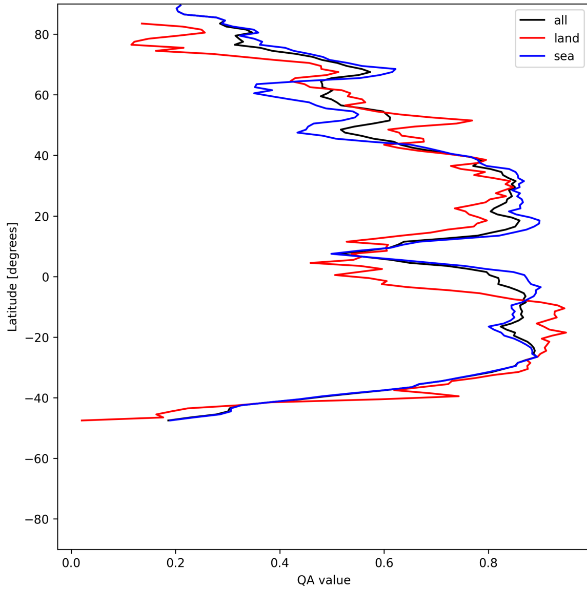
Figure 31: Zonal average of “QA value” for 2025-07-15 to 2025-07-17.
