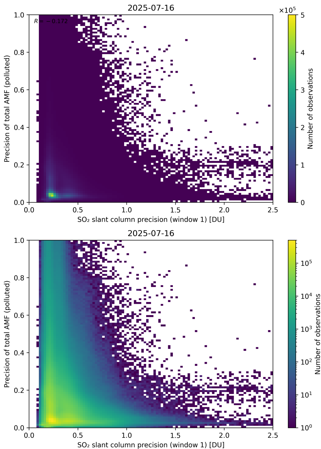
Figure 281: Scatter density plot of “SO 2 slant column precision (window 1)” against “Precision of total AMF (polluted)” for 2025-07-15 to 2025-07-17.
