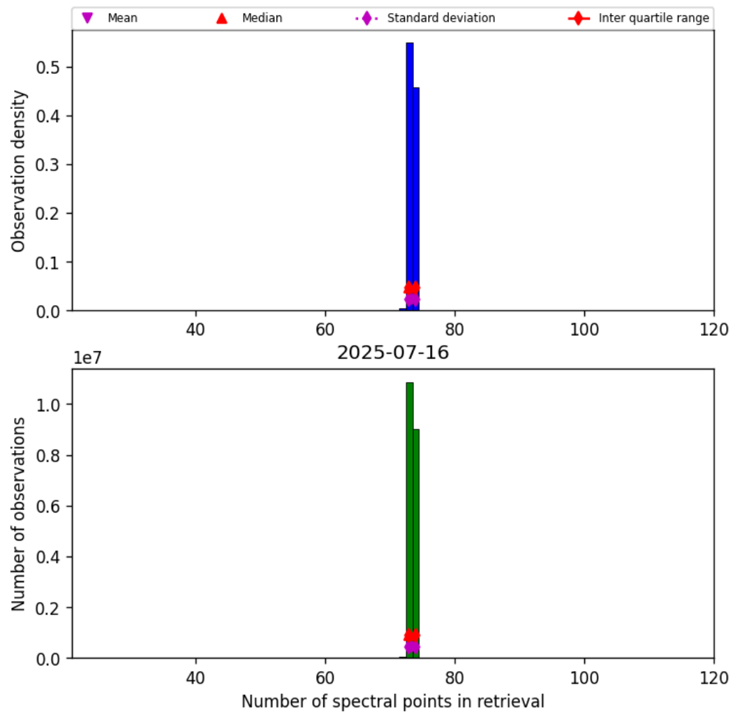
Figure 82: Histogram of “Number of spectral points in retrieval” for 2025-07-15 to 2025-07-17
