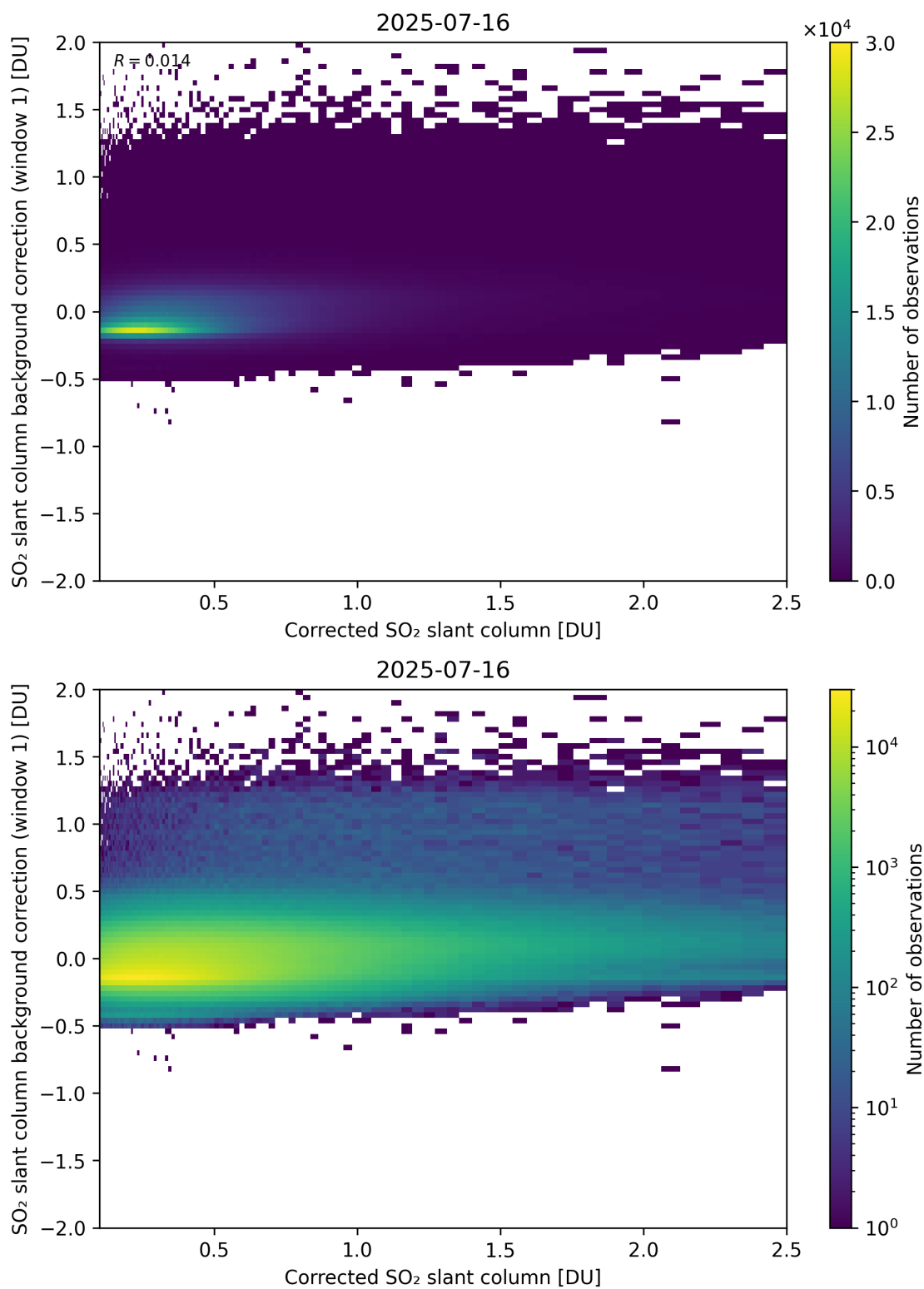
Figure 226: Scatter density plot of “Corrected SO 2 slant column” against “SO 2 slant column background correction (window 1)” for 2025-07-15 to 2025-07-17.
