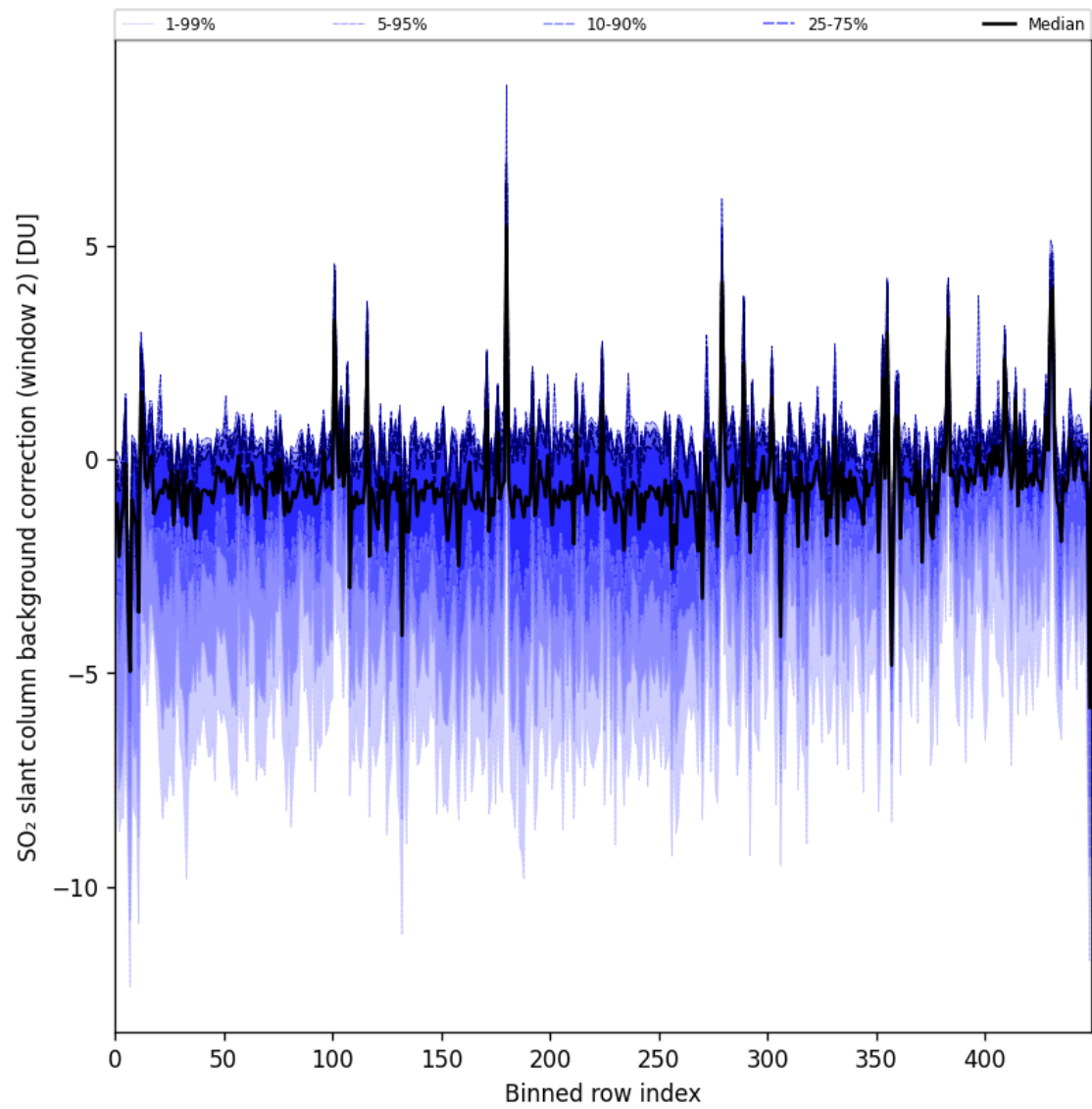
Figure 96: Along track statistics of “SO 2 slant column background correction (window 2)” for 2025-07-15 to 2025-07-17
