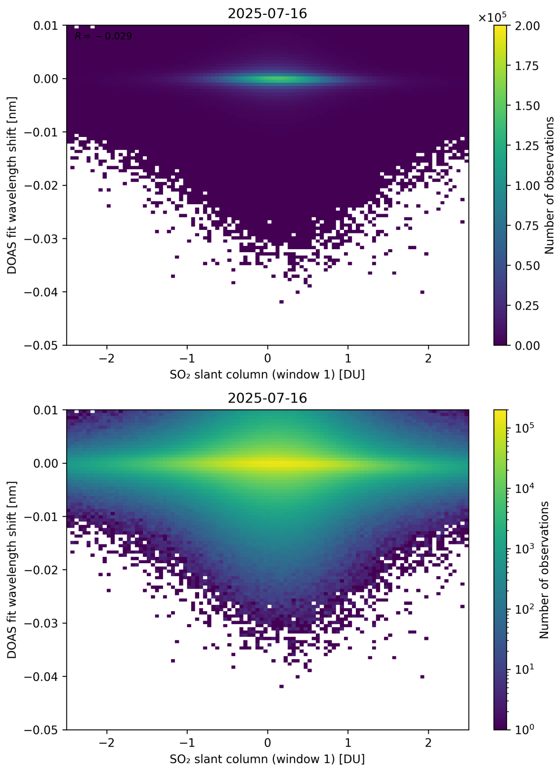
Figure 265: Scatter density plot of “SO 2 slant column (window 1)” against “DOAS fit wavelength shift” for 2025-07-15 to 2025-07-17.
