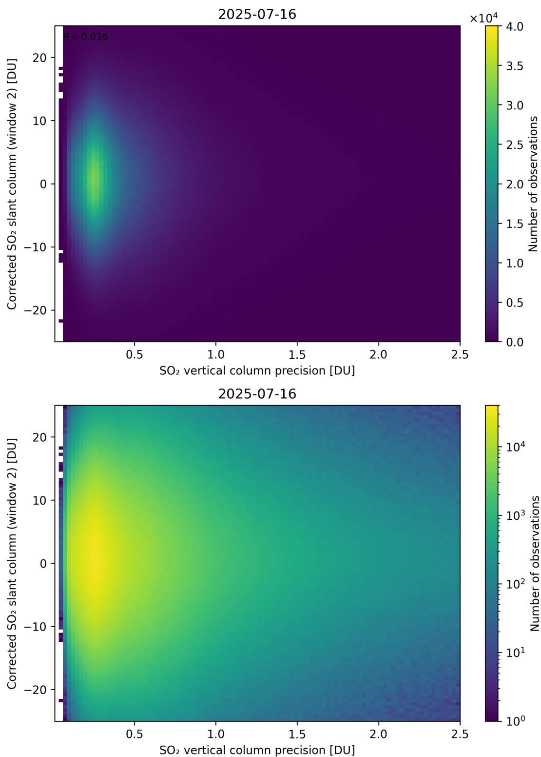
Figure 339: Scatter density plot of “SO 2 vertical column precision” against “Corrected SO 2 slant column (window 2)” for 2025-07-15 to 2025-07-17.
