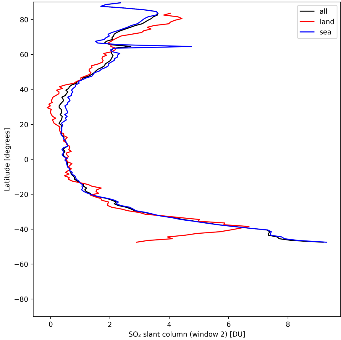
Figure 41: Zonal average of “SO 2 slant column (window 2)” for 2025-07-15 to 2025-07-17.
