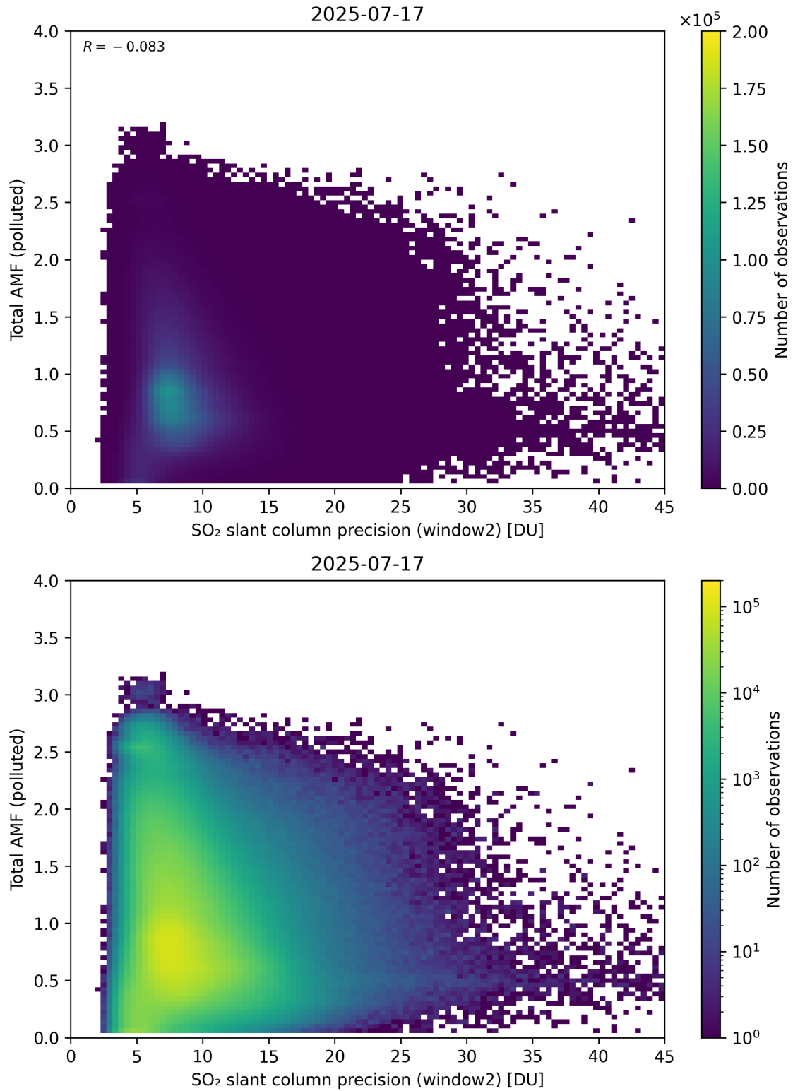
Figure 301: Scatter density plot of “SO 2 slant column precision (window2)” against “Total AMF (polluted)” for 2025-07-16 to 2025-07-18.
