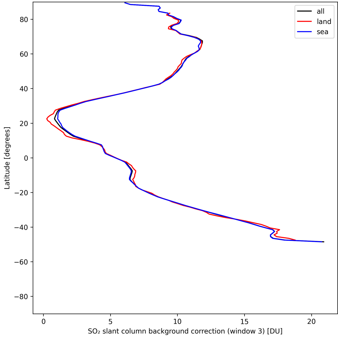
Figure 48: Zonal average of “SO 2 slant column background correction (window 3)” for 2025-07-16 to 2025-07-18.
