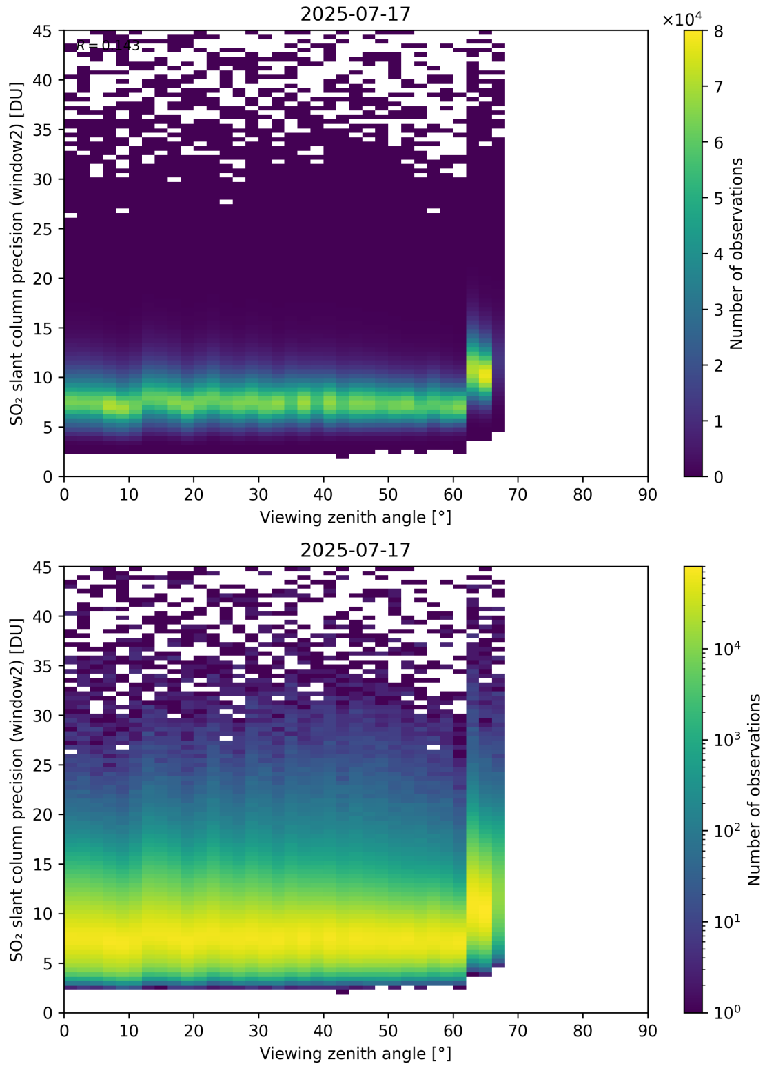
Figure 378: Scatter density plot of “Viewing zenith angle” against “SO 2 slant column precision (window2)” for 2025-07-16 to 2025-07-18.
