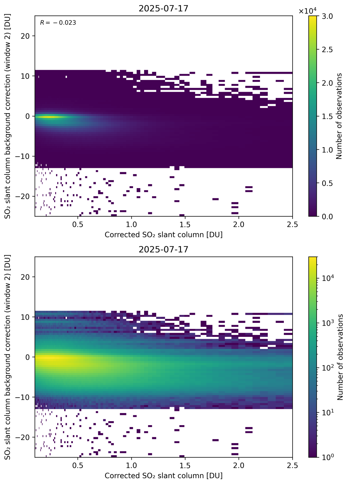
Figure 227: Scatter density plot of “Corrected SO 2 slant column” against “SO 2 slant column background correction (window 2)” for 2025-07-16 to 2025-07-18.
