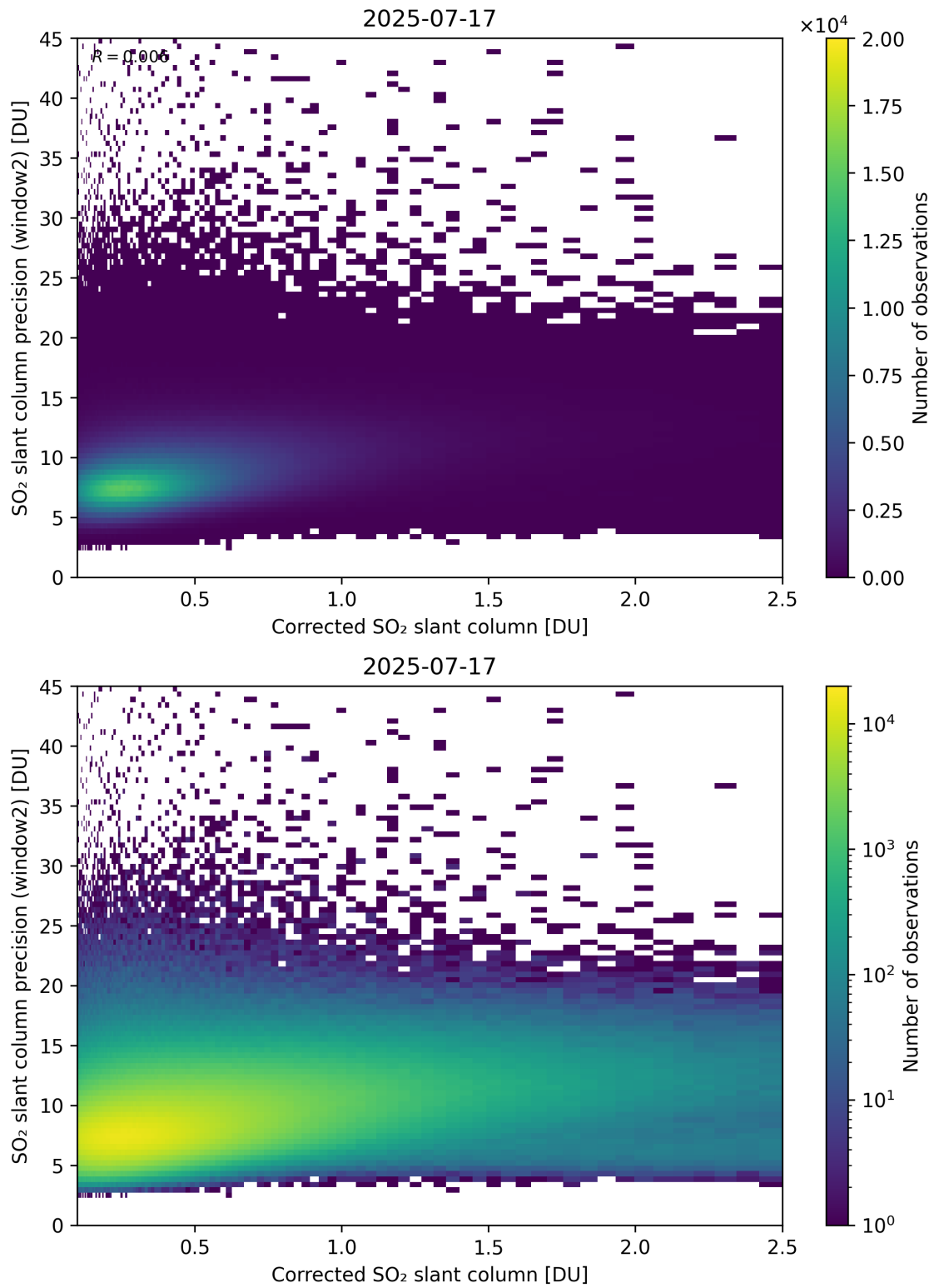
Figure 239: Scatter density plot of “Corrected SO 2 slant column” against “SO 2 slant column precision (window2)” for 2025-07-16 to 2025-07-18.
