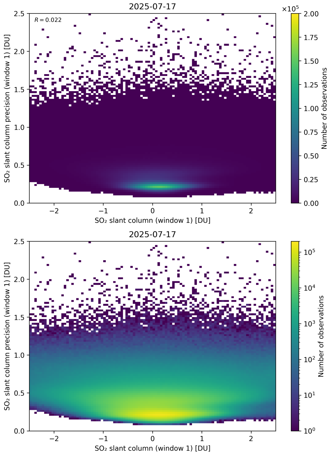
Figure 285: Scatter density plot of “SO 2 slant column (window 1)” against “SO 2 slant column precision (window 1)” for 2025-07-16 to 2025-07-18.
