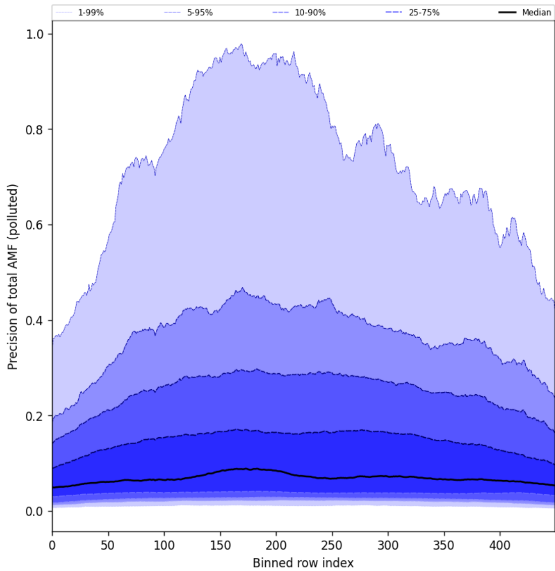
Figure 106: Along track statistics of “Precision of total AMF (polluted)” for 2025-07-16 to 2025-07-18
