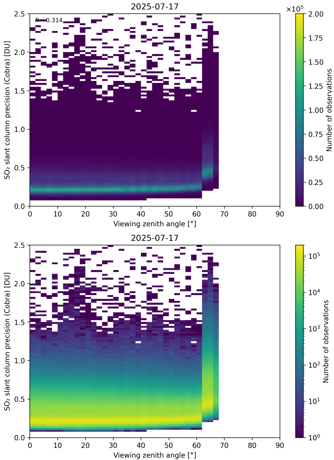
Figure 372: Scatter density plot of “Viewing zenith angle” against “SO 2 slant column precision (Cobra)” for 2025-07-16 to 2025-07-18.
