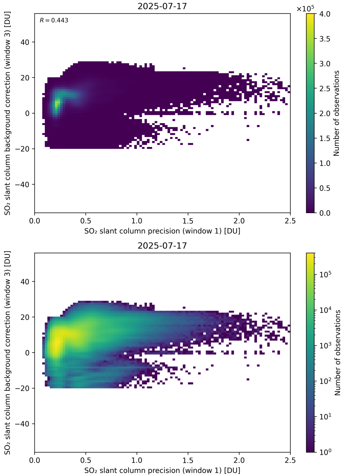
Figure 270: Scatter density plot of “SO 2 slant column precision (window 1)” against “SO 2 slant column background correction (window 3)” for 2025-07-16 to 2025-07-18.
