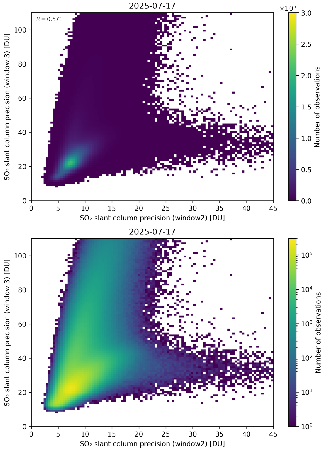
Figure 300: Scatter density plot of “SO 2 slant column precision (window2)” against “SO 2 slant column precision (window 3)” for 2025-07-16 to 2025-07-18.
