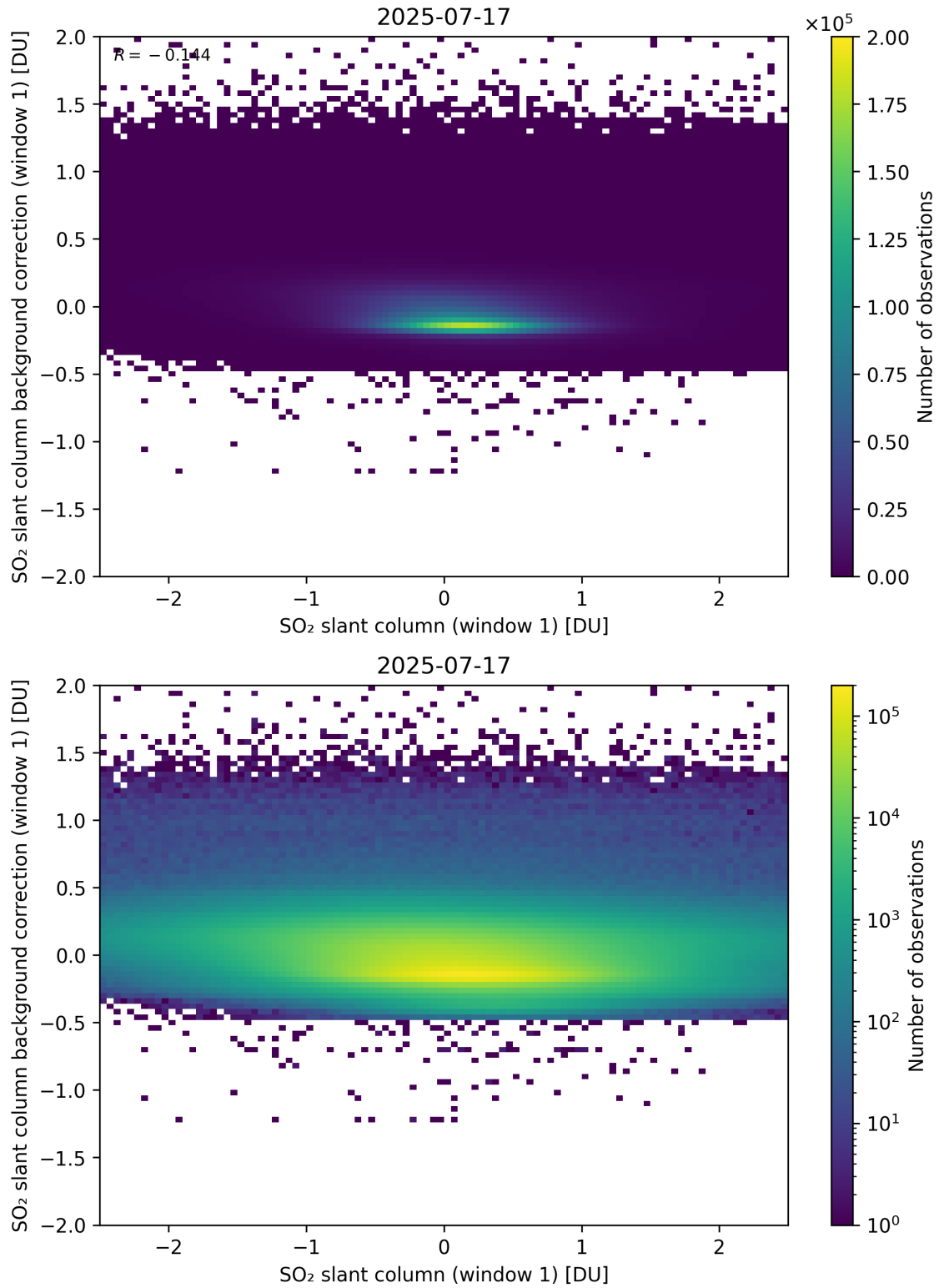
Figure 262: Scatter density plot of “SO 2 slant column (window 1)” against “SO 2 slant column background correction (window 1)” for 2025-07-16 to 2025-07-18.
