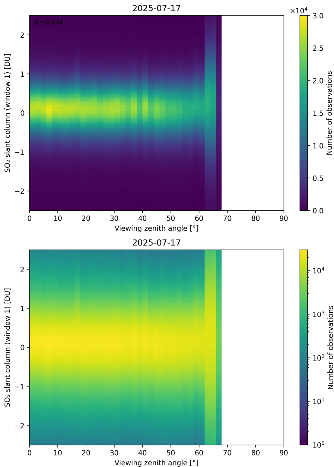
Figure 376: Scatter density plot of “Viewing zenith angle” against “SO 2 slant column (window 1)” for 2025-07-16 to 2025-07-18.
