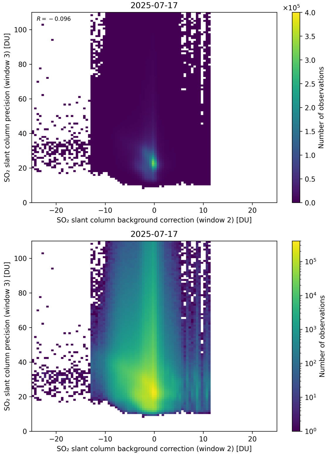
Figure 129: Scatter density plot of “SO 2 slant column background correction (window 2)” against “SO 2 slant column precision (window 3)” for 2025-07-16 to 2025-07-18.
