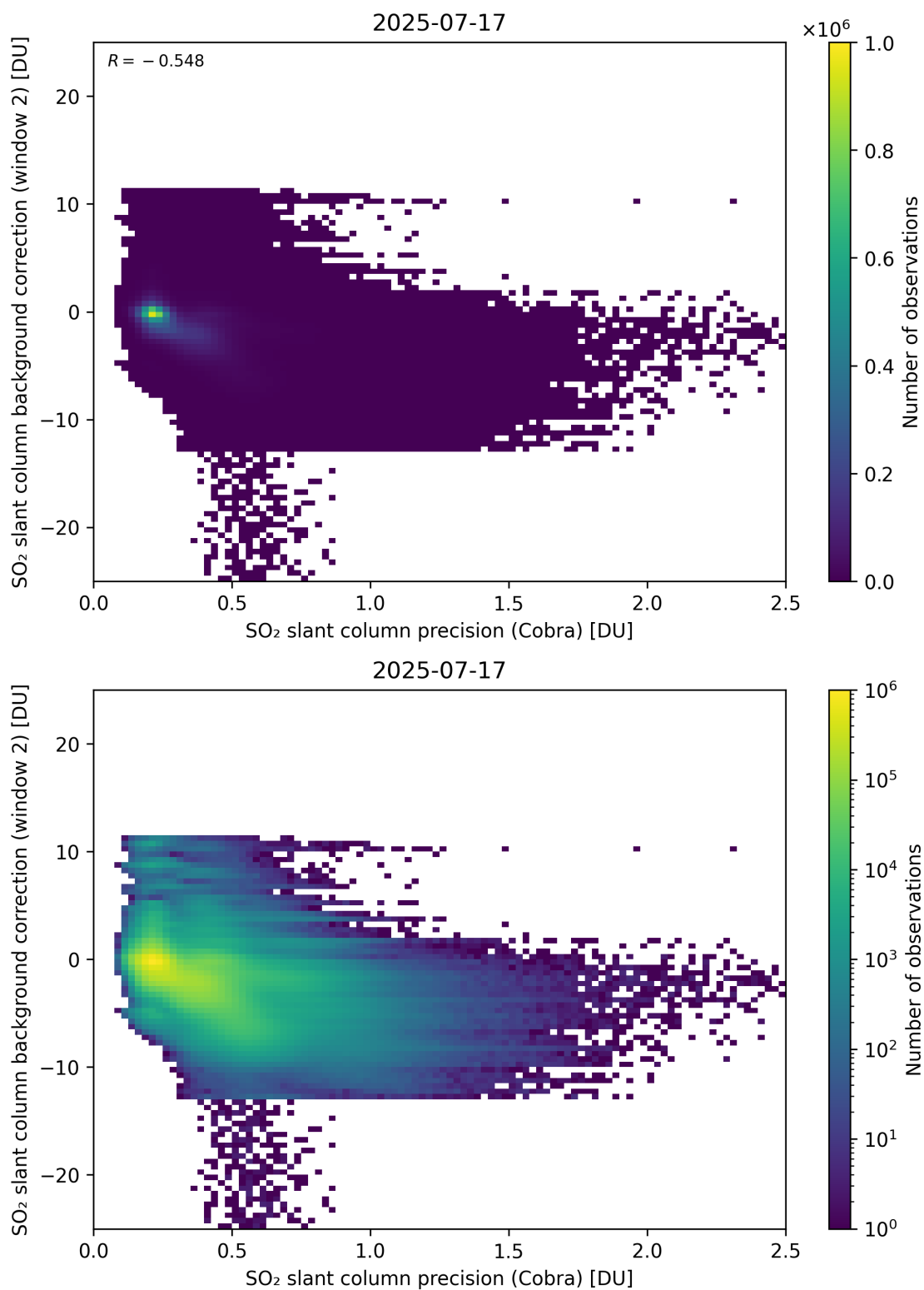
Figure 200: Scatter density plot of “SO 2 slant column precision (Cobra)” against “SO 2 slant column background correction (window 2)” for 2025-07-16 to 2025-07-18.
