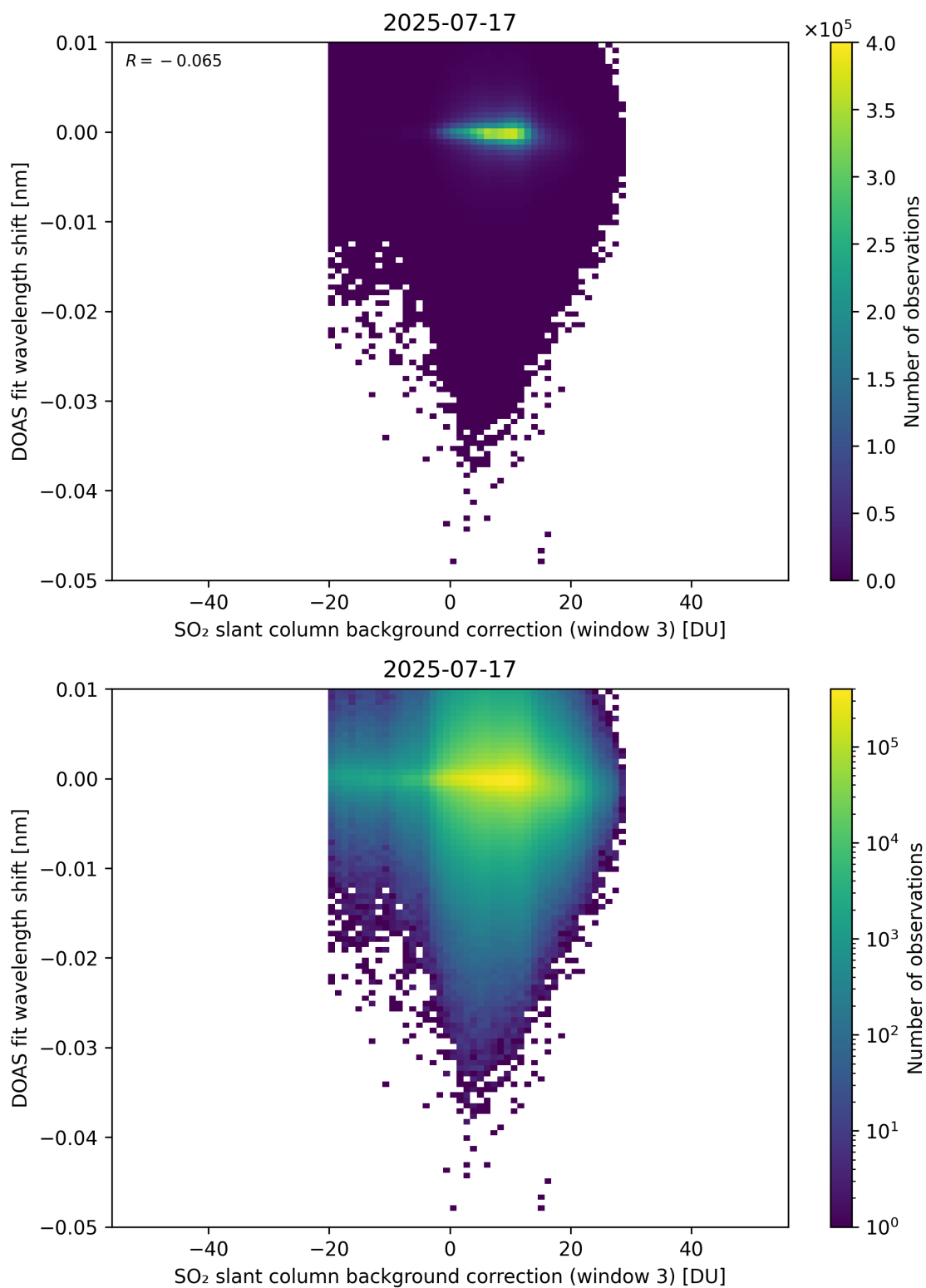
Figure 132: Scatter density plot of “SO 2 slant column background correction (window 3)” against “DOAS fit wavelength shift” for 2025-07-16 to 2025-07-18.
