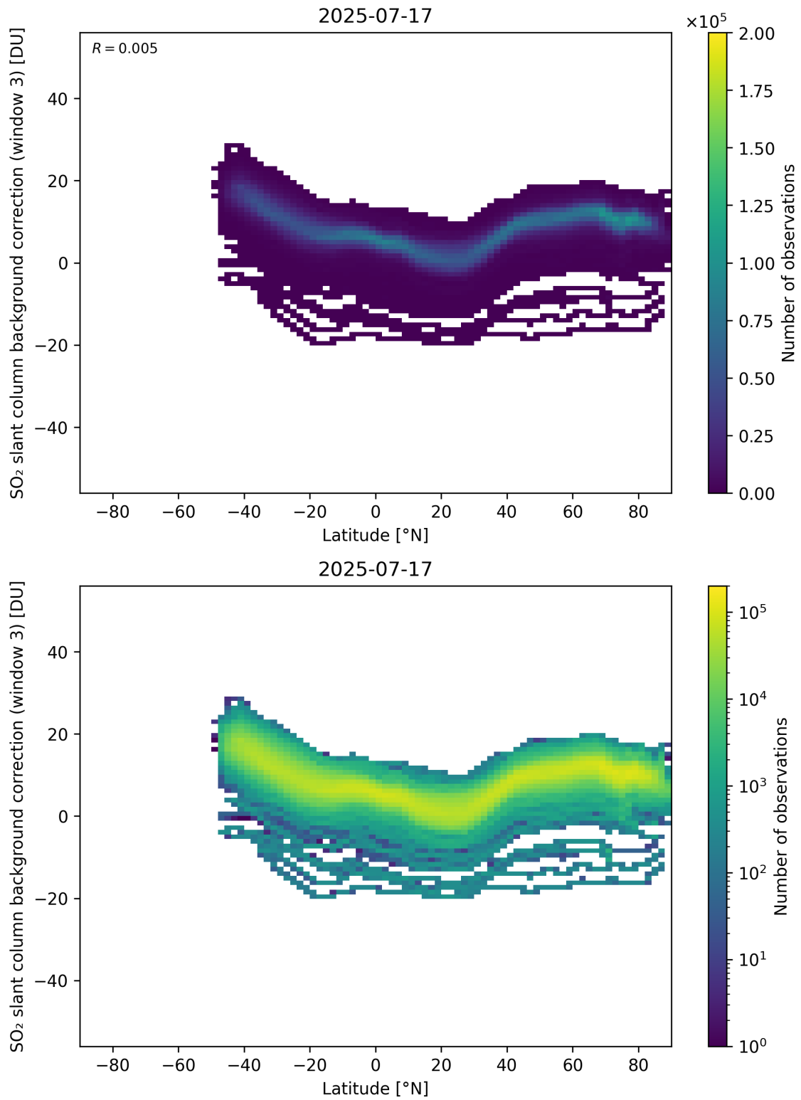
Figure 152: Scatter density plot of “Latitude” against “SO 2 slant column background correction (window 3)” for 2025-07-16 to 2025-07-18.
