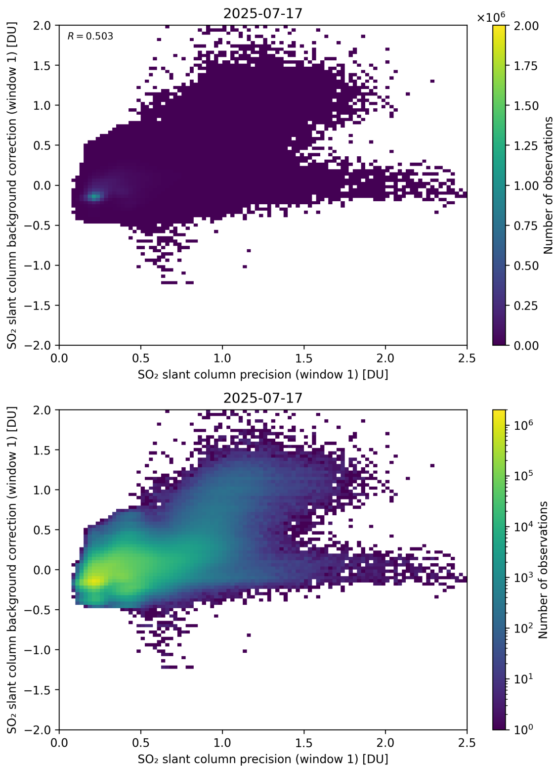
Figure 268: Scatter density plot of “SO 2 slant column precision (window 1)” against “SO 2 slant column background correction (window 1)” for 2025-07-16 to 2025-07-18.
