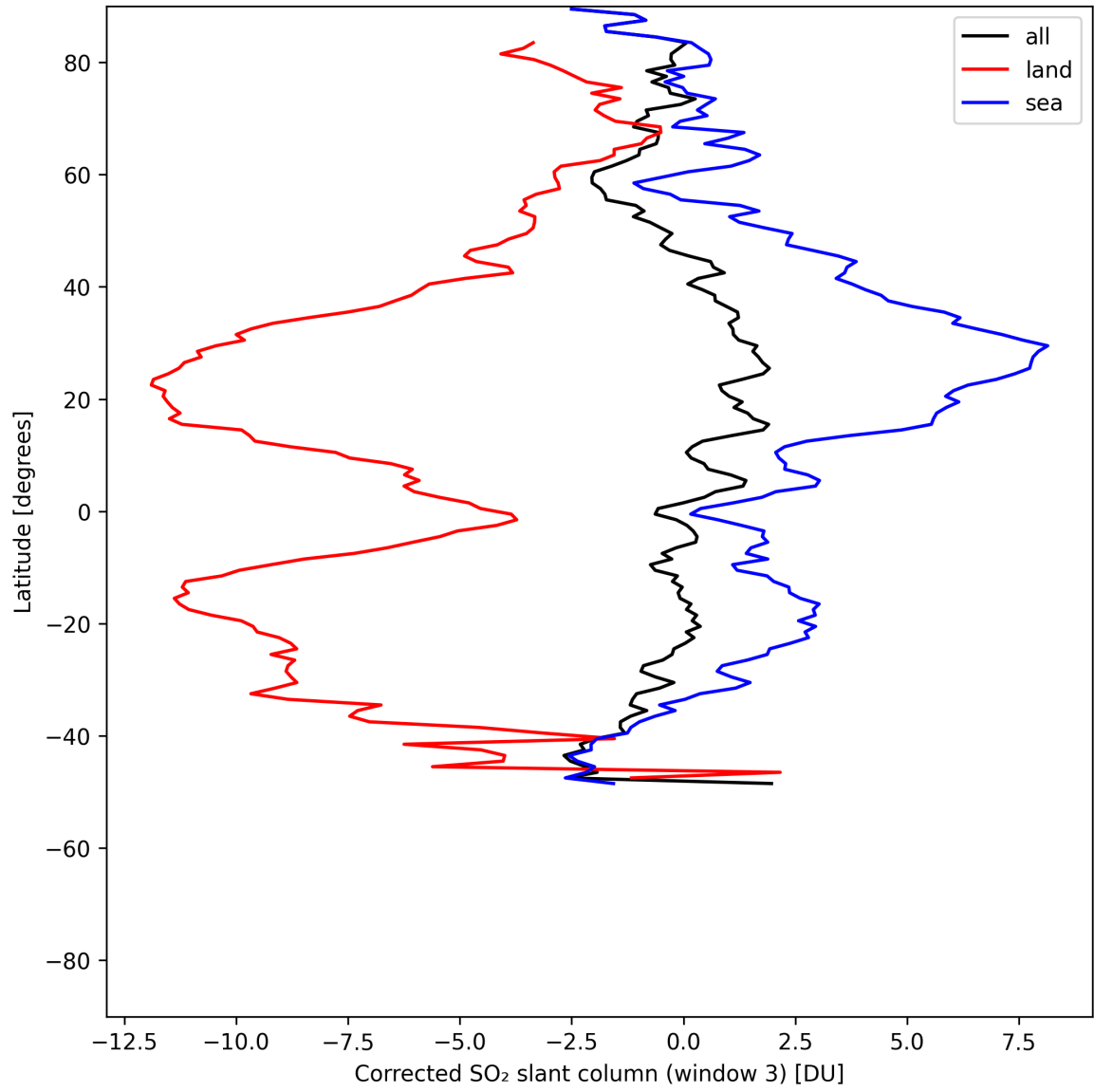
Figure 47: Zonal average of “Corrected SO 2 slant column (window 3)” for 2025-07-16 to 2025-07-18.
