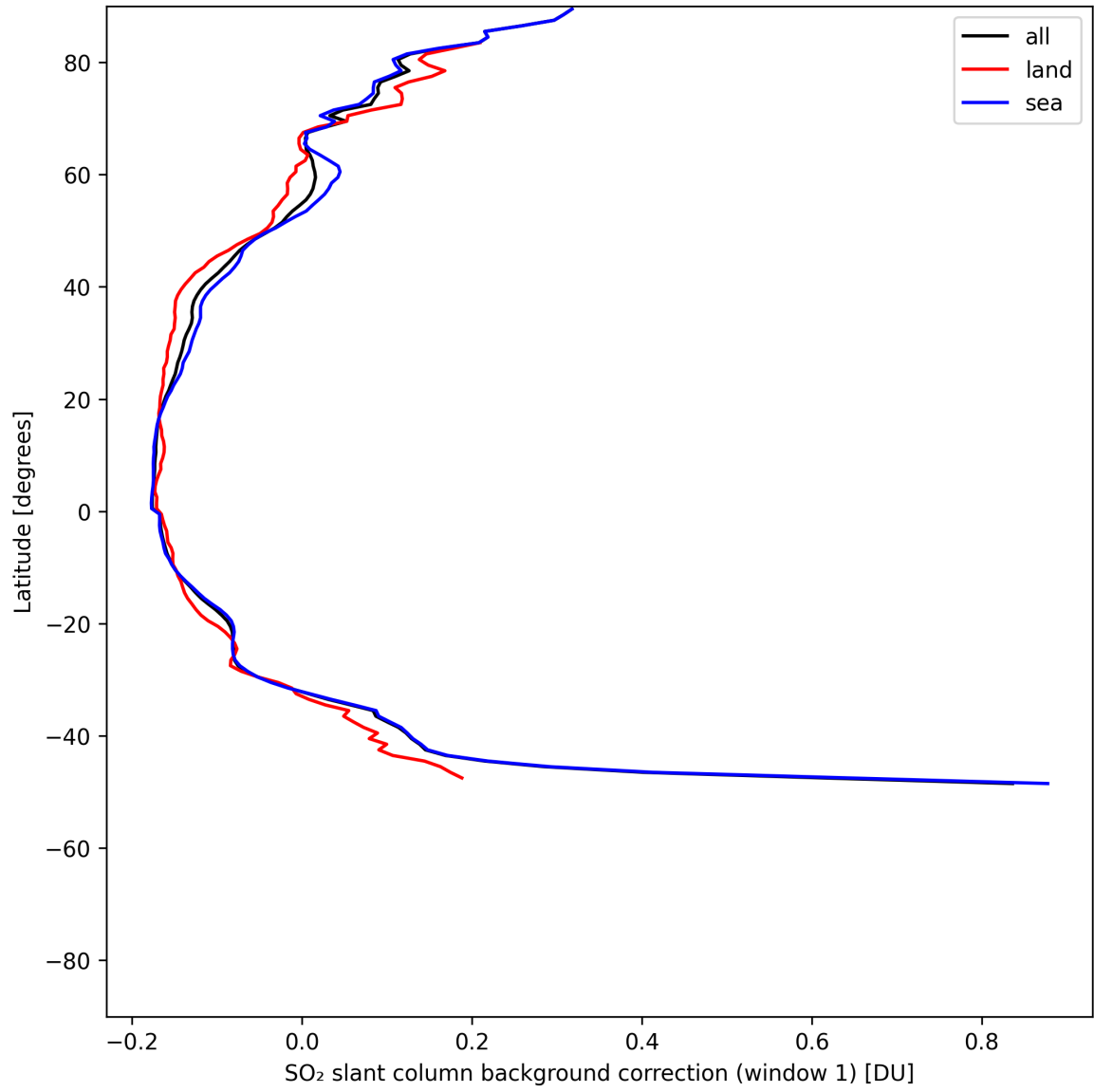
Figure 40: Zonal average of “SO 2 slant column background correction (window 1)” for 2025-07-16 to 2025-07-18.
