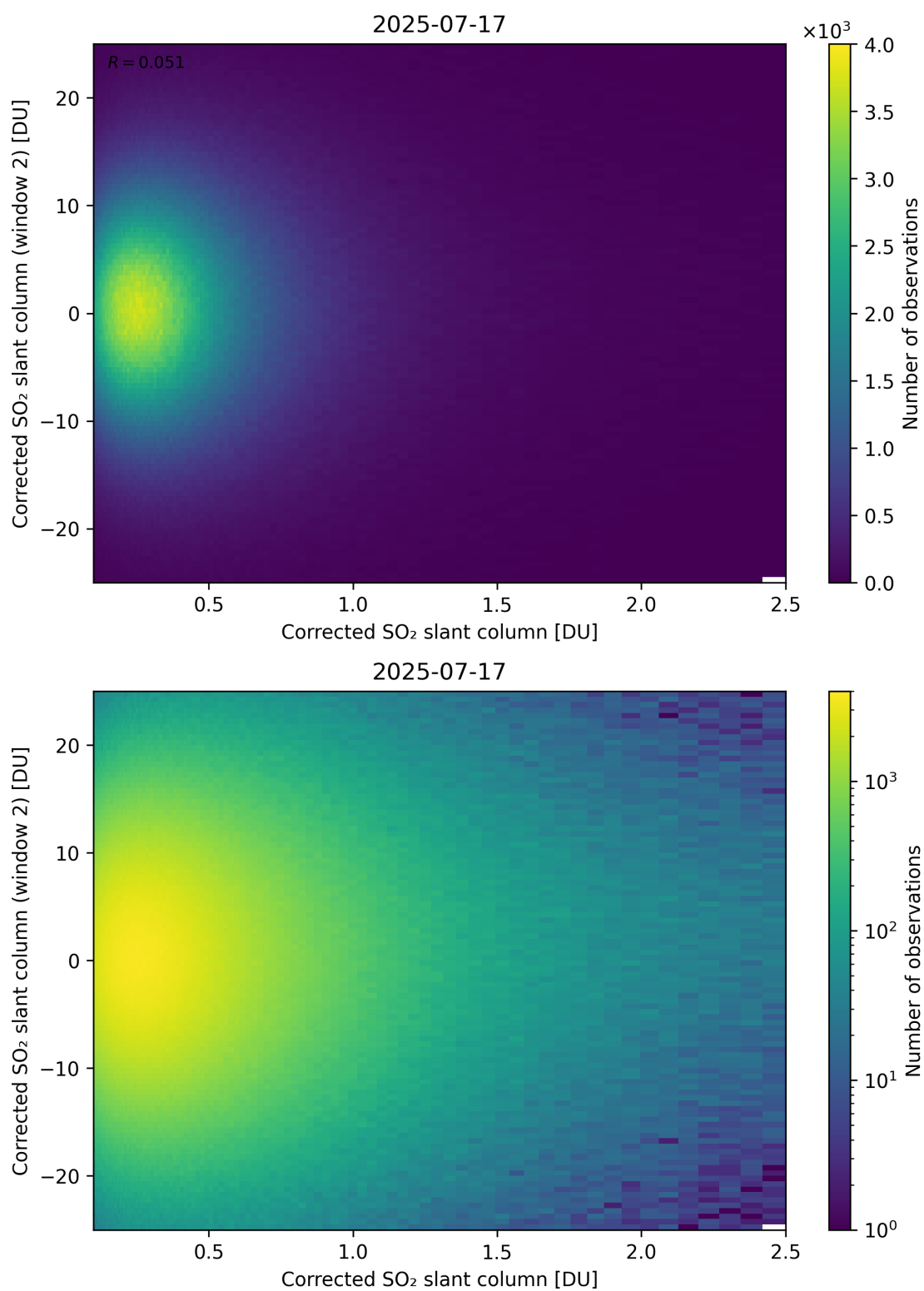
Figure 235: Scatter density plot of “Corrected SO 2 slant column” against “Corrected SO 2 slant column (window 2)” for 2025-07-16 to 2025-07-18.
