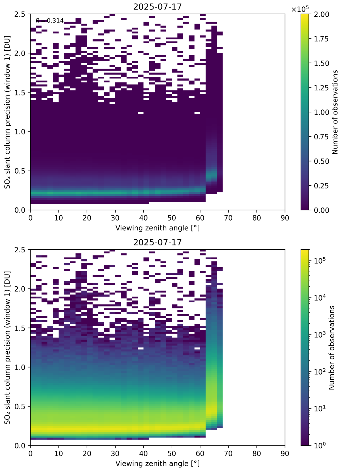
Figure 377: Scatter density plot of “Viewing zenith angle” against “SO 2 slant column precision (window 1)” for 2025-07-16 to 2025-07-18.
