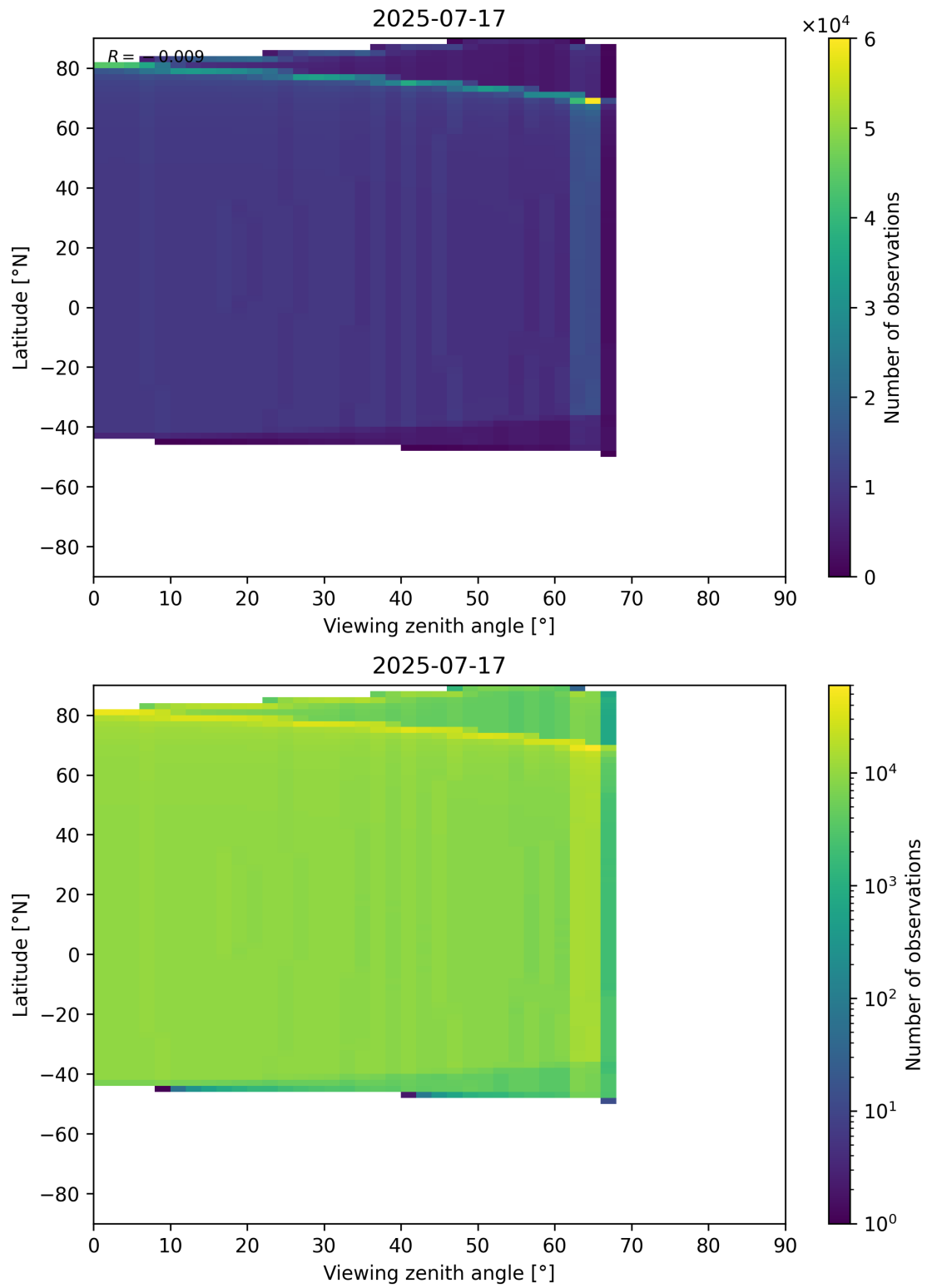
Figure 368: Scatter density plot of “Viewing zenith angle” against “Latitude” for 2025-07-16 to 2025-07-18.
