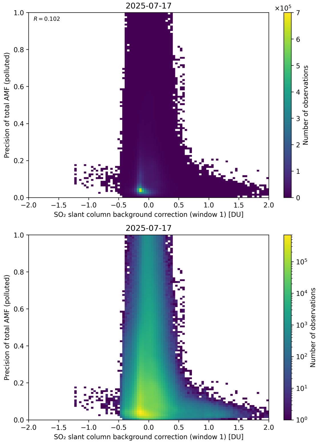
Figure 121: Scatter density plot of “SO 2 slant column background correction (window 1)” against “Precision of total AMF (polluted)” for 2025-07-16 to 2025-07-18.
