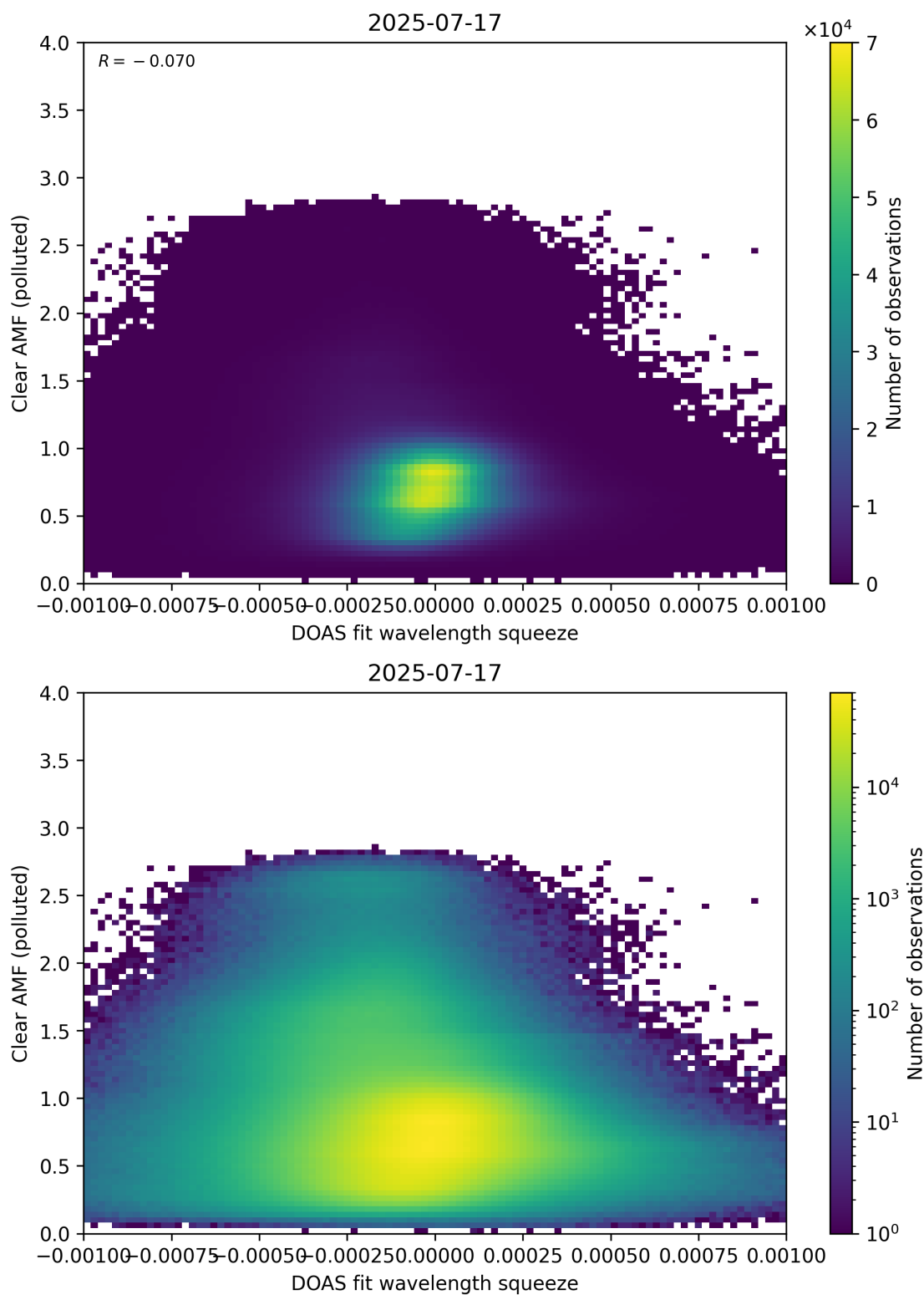
Figure 144: Scatter density plot of “DOAS fit wavelength squeeze” against “Clear AMF (polluted)” for 2025-07-16 to 2025-07-18.
