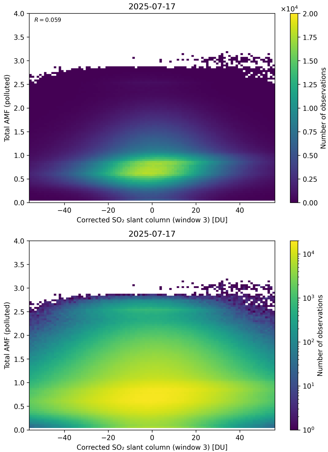
Figure 260: Scatter density plot of “Corrected SO 2 slant column (window 3)” against “Total AMF (polluted)” for 2025-07-16 to 2025-07-18.
