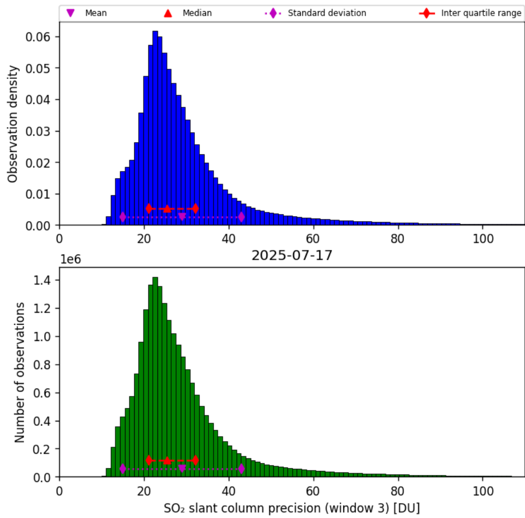
Figure 72: Histogram of “SO 2 slant column precision (window 3)” for 2025-07-16 to 2025-07-18
