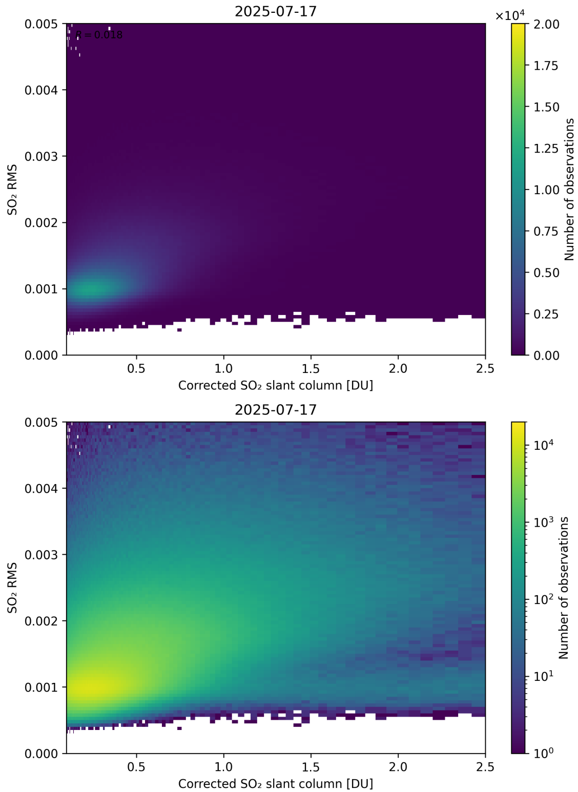
Figure 231: Scatter density plot of “Corrected SO 2 slant column” against “SO 2 RMS” for 2025-07-16 to 2025-07-18.
