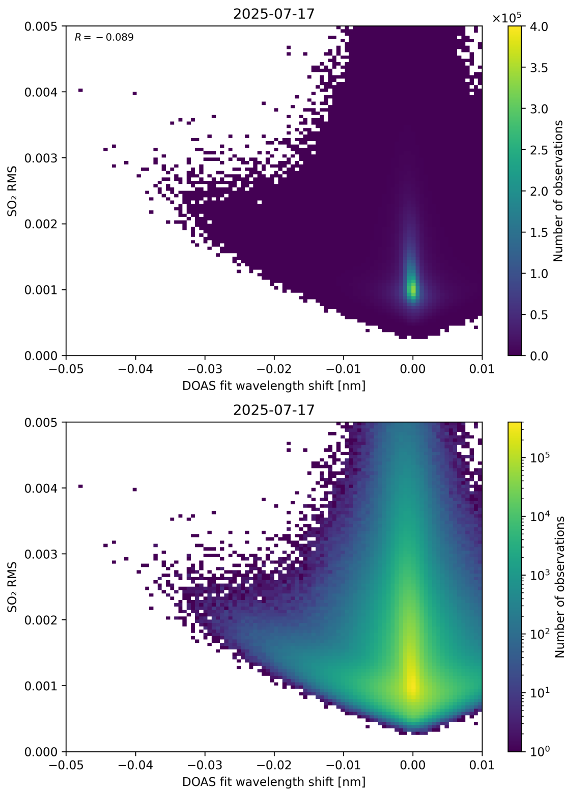
Figure 139: Scatter density plot of “DOAS fit wavelength shift” against “SO 2 RMS” for 2025-07-16 to 2025-07-18.
