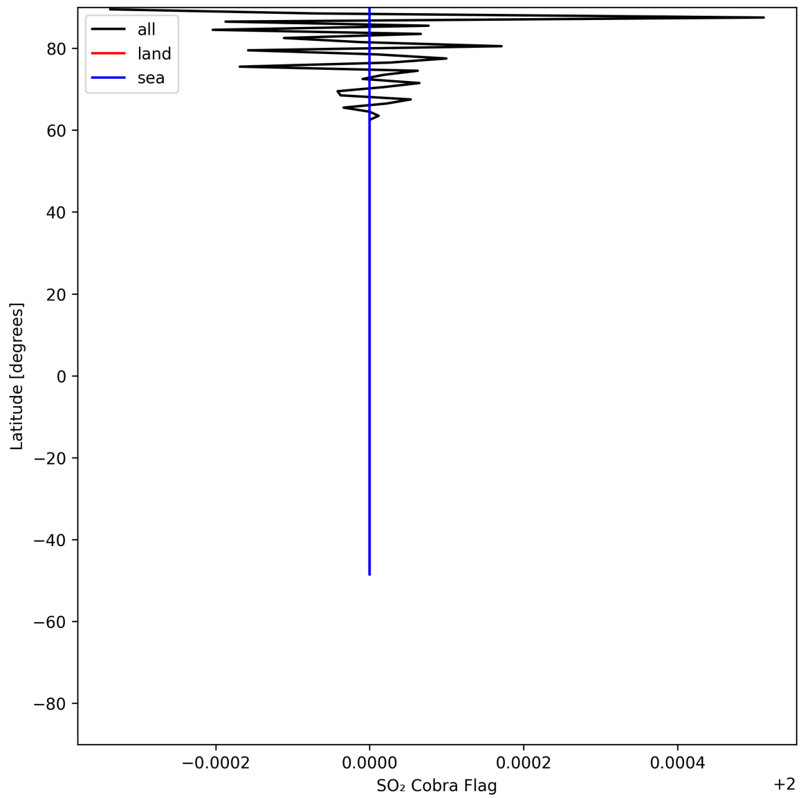
Figure 49: Zonal average of “SO 2 Cobra Flag” for 2025-07-16 to 2025-07-18.
