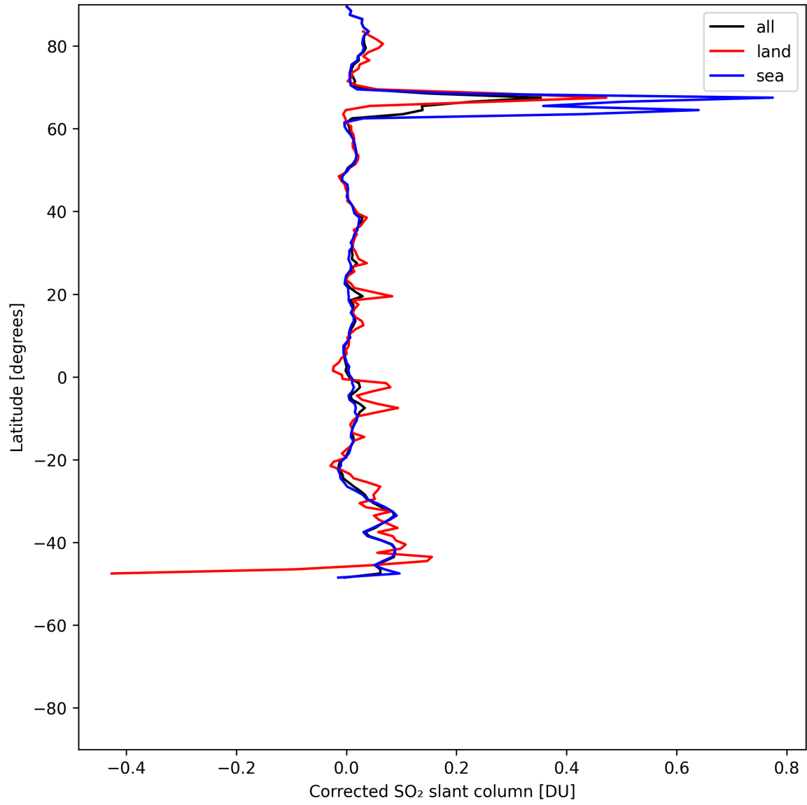
Figure 34: Zonal average of “Corrected SO 2 slant column” for 2025-07-16 to 2025-07-18.
