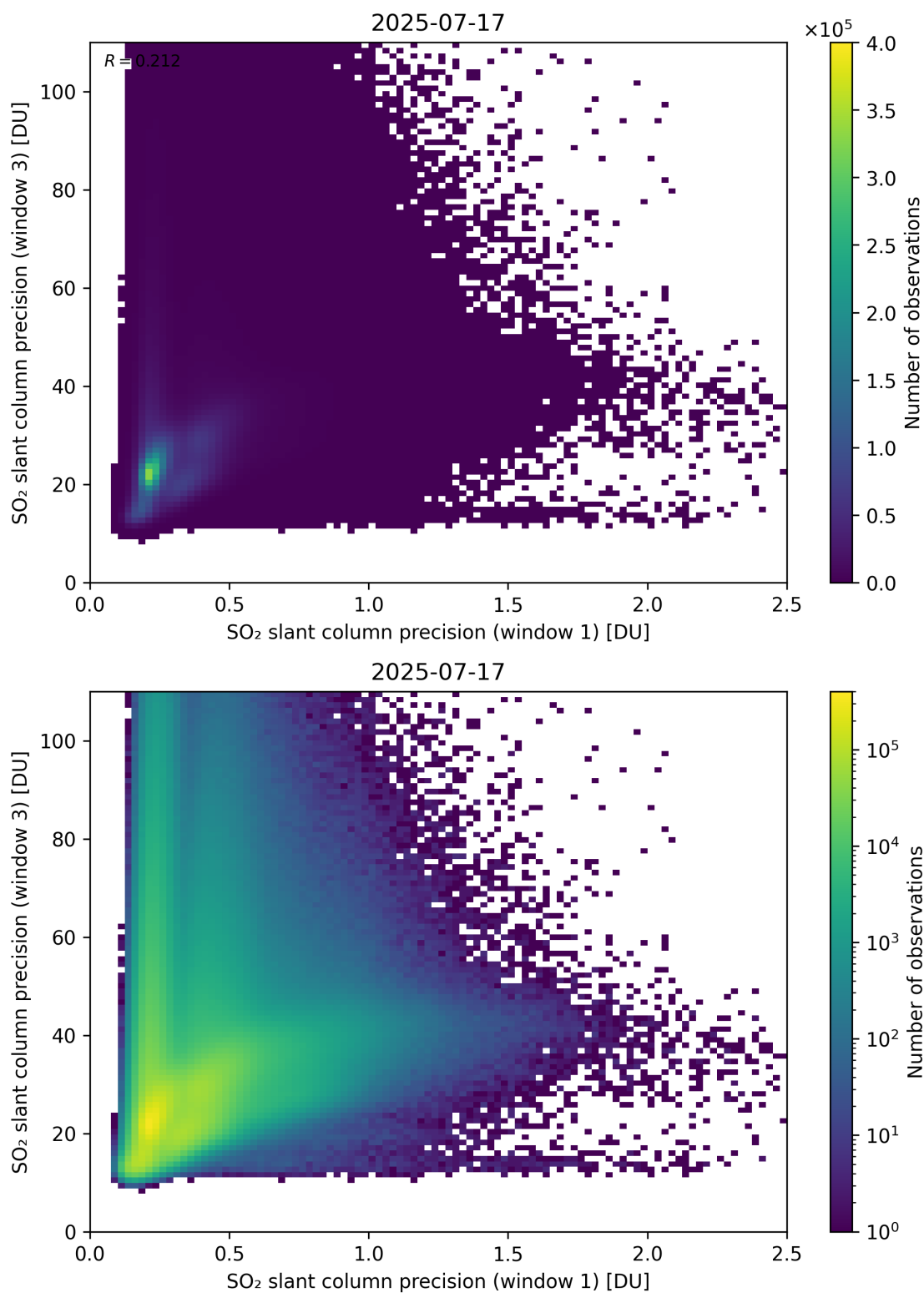
Figure 279: Scatter density plot of “SO 2 slant column precision (window 1)” against “SO 2 slant column precision (window 3)” for 2025-07-16 to 2025-07-18.
