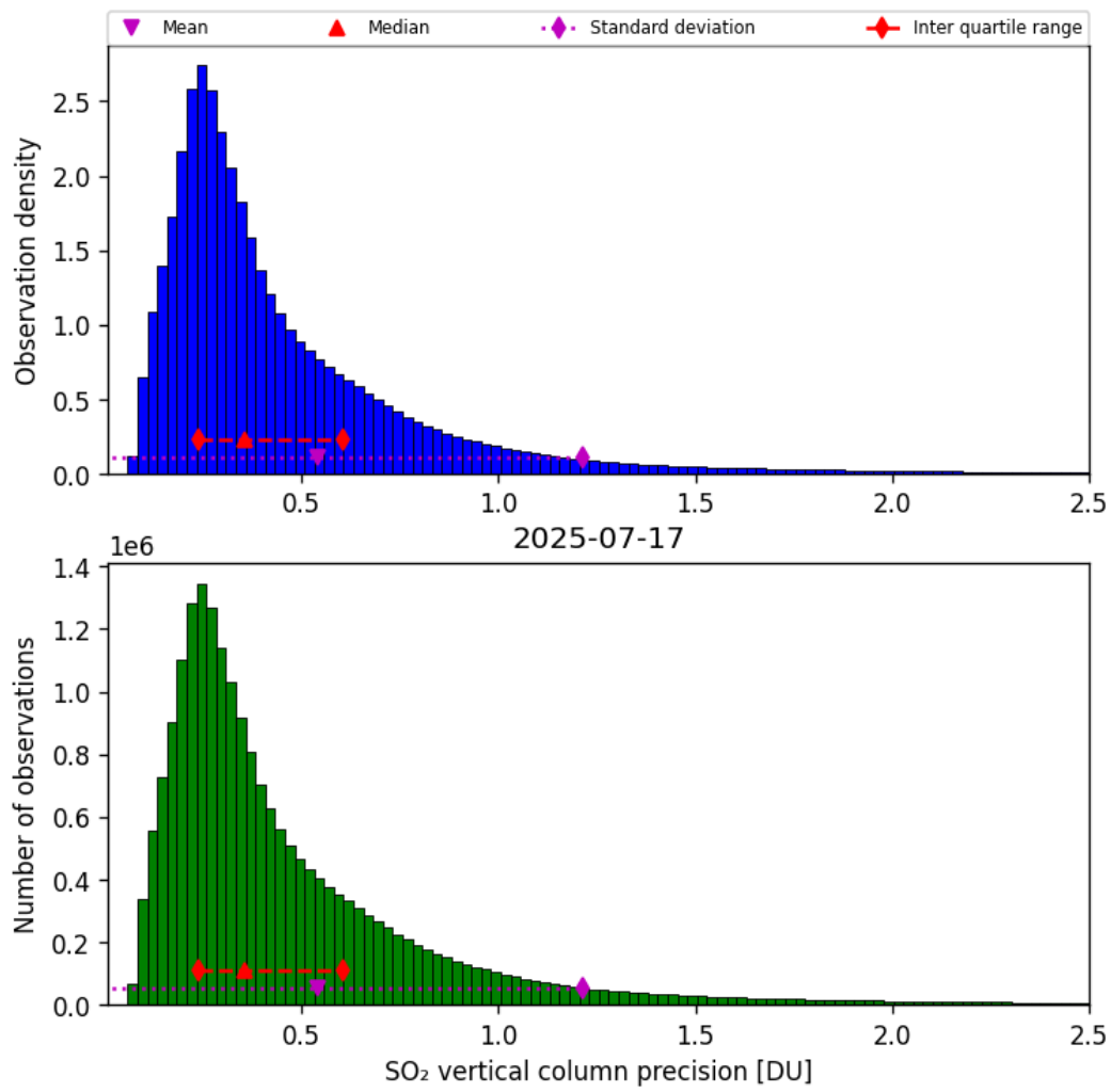
Figure 59: Histogram of “SO 2 vertical column precision” for 2025-07-16 to 2025-07-18
