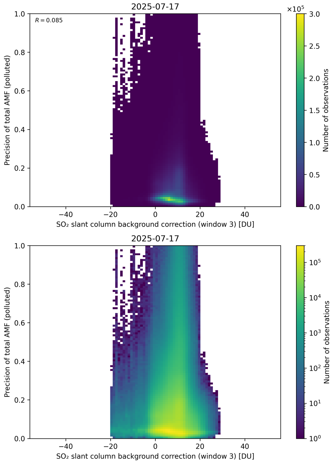
Figure 137: Scatter density plot of “SO 2 slant column background correction (window 3)” against “Precision of total AMF (polluted)” for 2025-07-16 to 2025-07-18.
