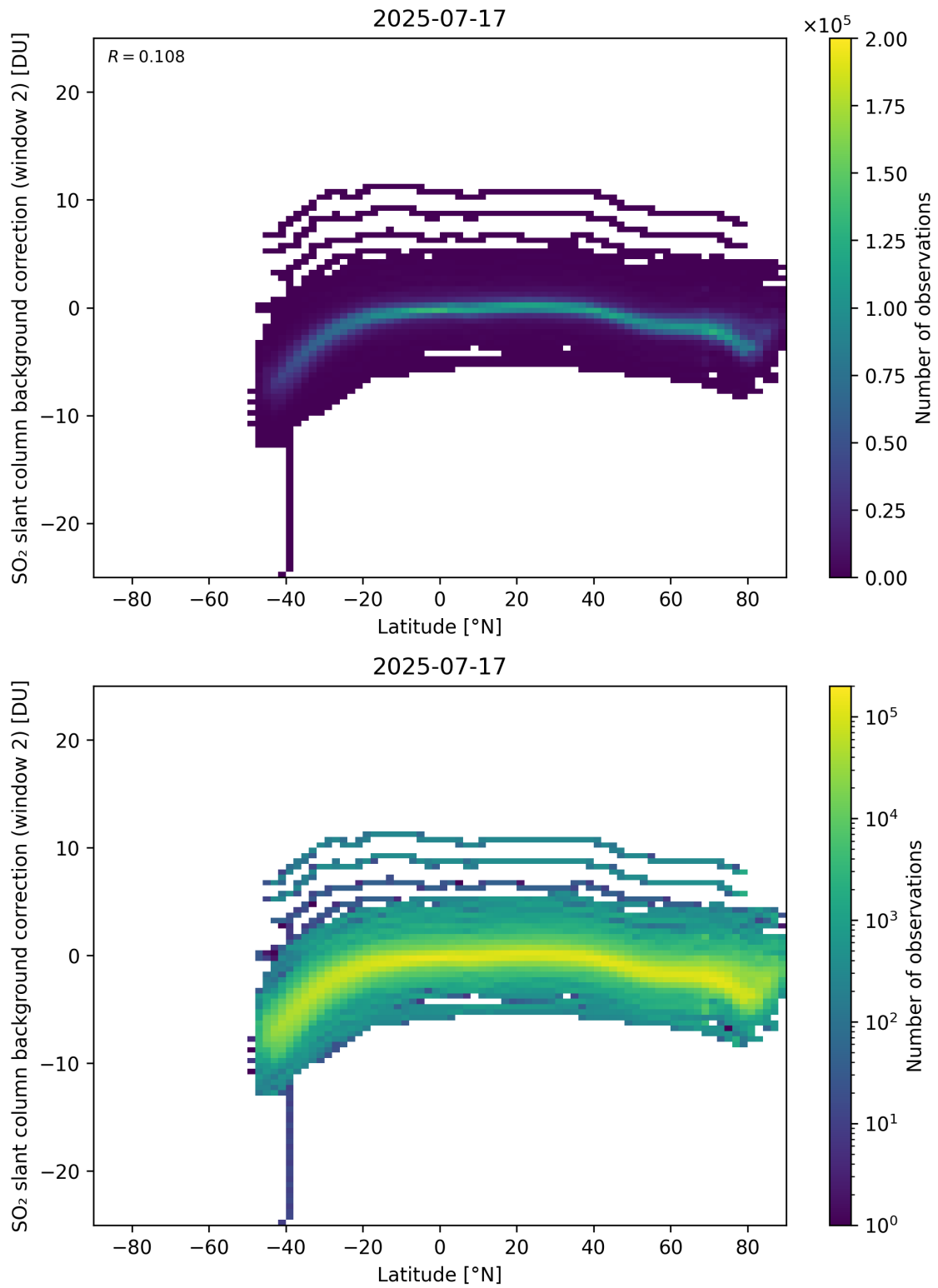
Figure 151: Scatter density plot of “Latitude” against “SO 2 slant column background correction (window 2)” for 2025-07-16 to 2025-07-18.
