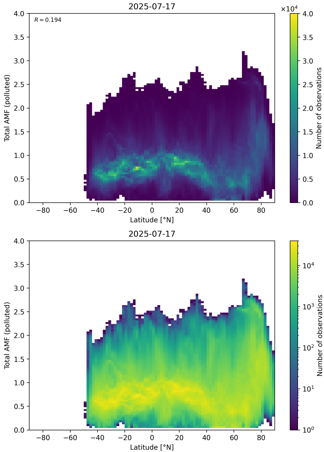
Figure 167: Scatter density plot of “Latitude” against “Total AMF (polluted)” for 2025-07-16 to 2025-07-18.
