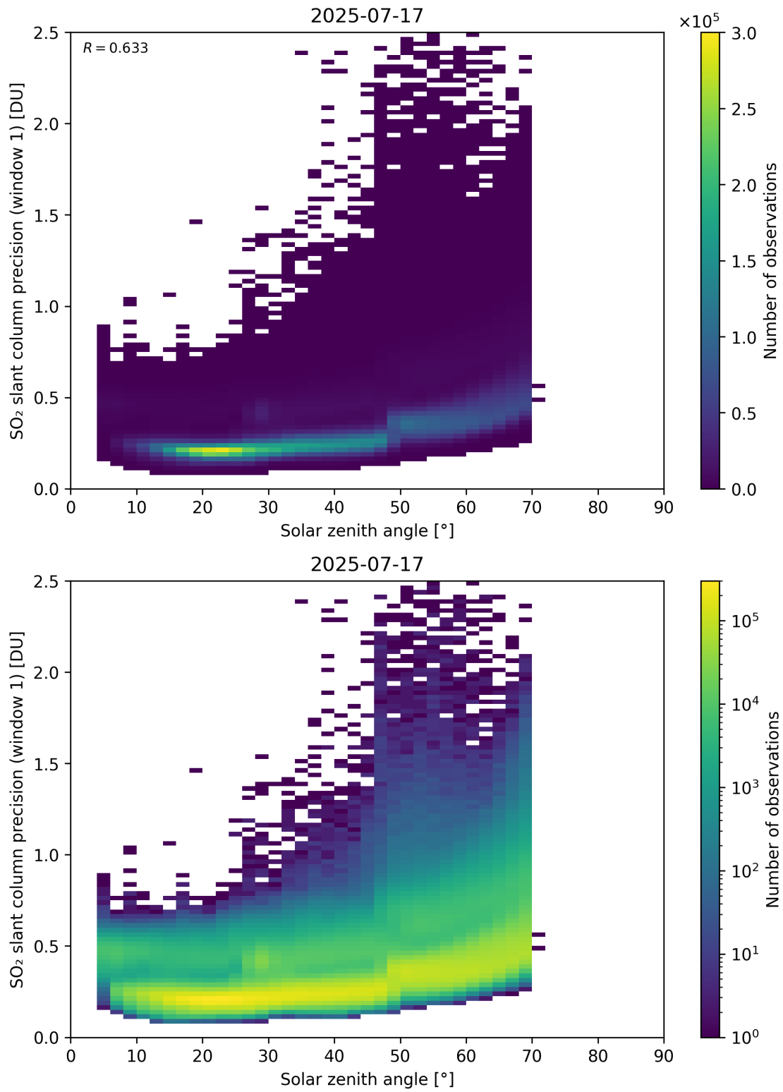
Figure 185: Scatter density plot of “Solar zenith angle” against “SO 2 slant column precision (window 1)” for 2025-07-16 to 2025-07-18.
