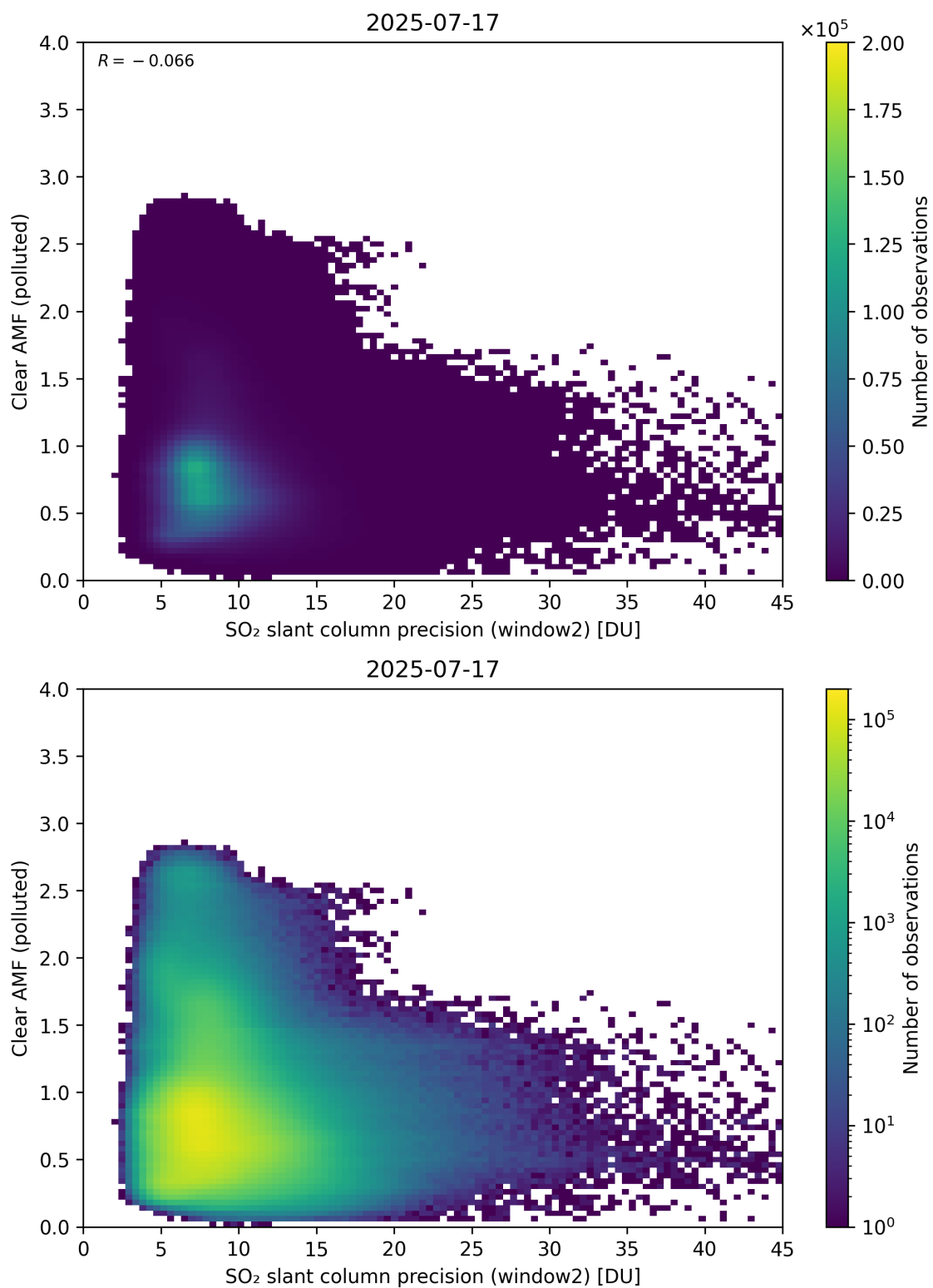
Figure 296: Scatter density plot of “SO 2 slant column precision (window2)” against “Clear AMF (polluted)” for 2025-07-16 to 2025-07-18.
