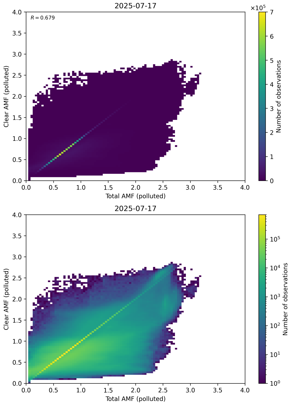
Figure 321: Scatter density plot of “Total AMF (polluted)” against “Clear AMF (polluted)” for 2025-07-16 to 2025-07-18.
