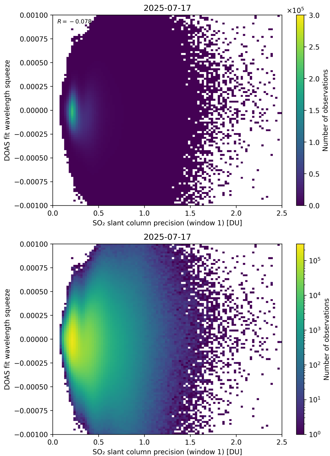
Figure 272: Scatter density plot of “SO 2 slant column precision (window 1)” against “DOAS fit wavelength squeeze” for 2025-07-16 to 2025-07-18.
