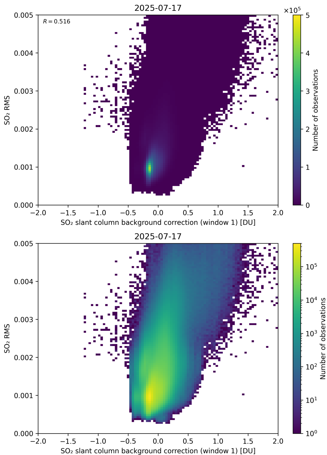
Figure 113: Scatter density plot of “SO 2 slant column background correction (window 1)” against “SO 2 RMS” for 2025-07-16 to 2025-07-18.
