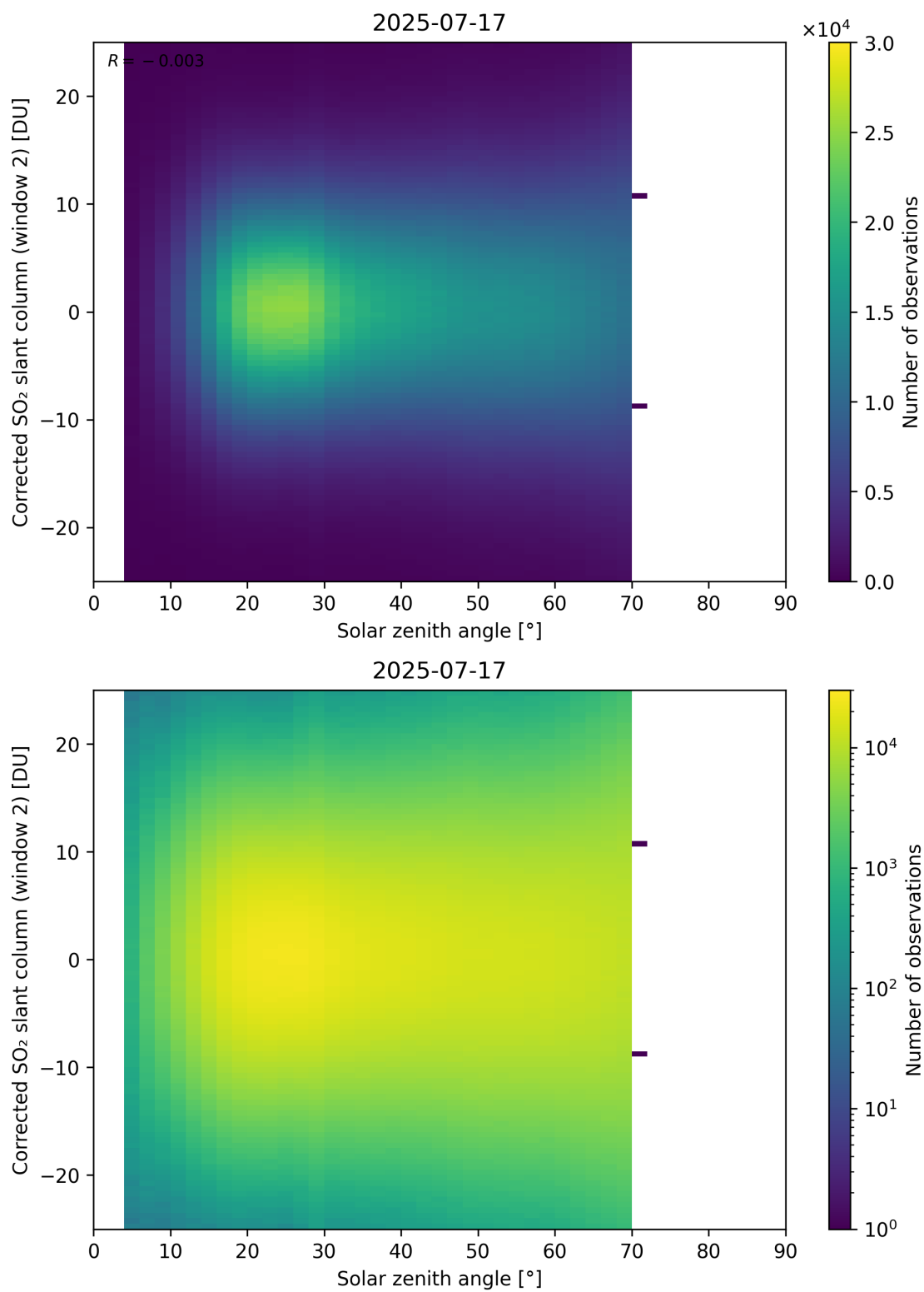
Figure 182: Scatter density plot of “Solar zenith angle” against “Corrected SO 2 slant column (window 2)” for 2025-07-16 to 2025-07-18.
