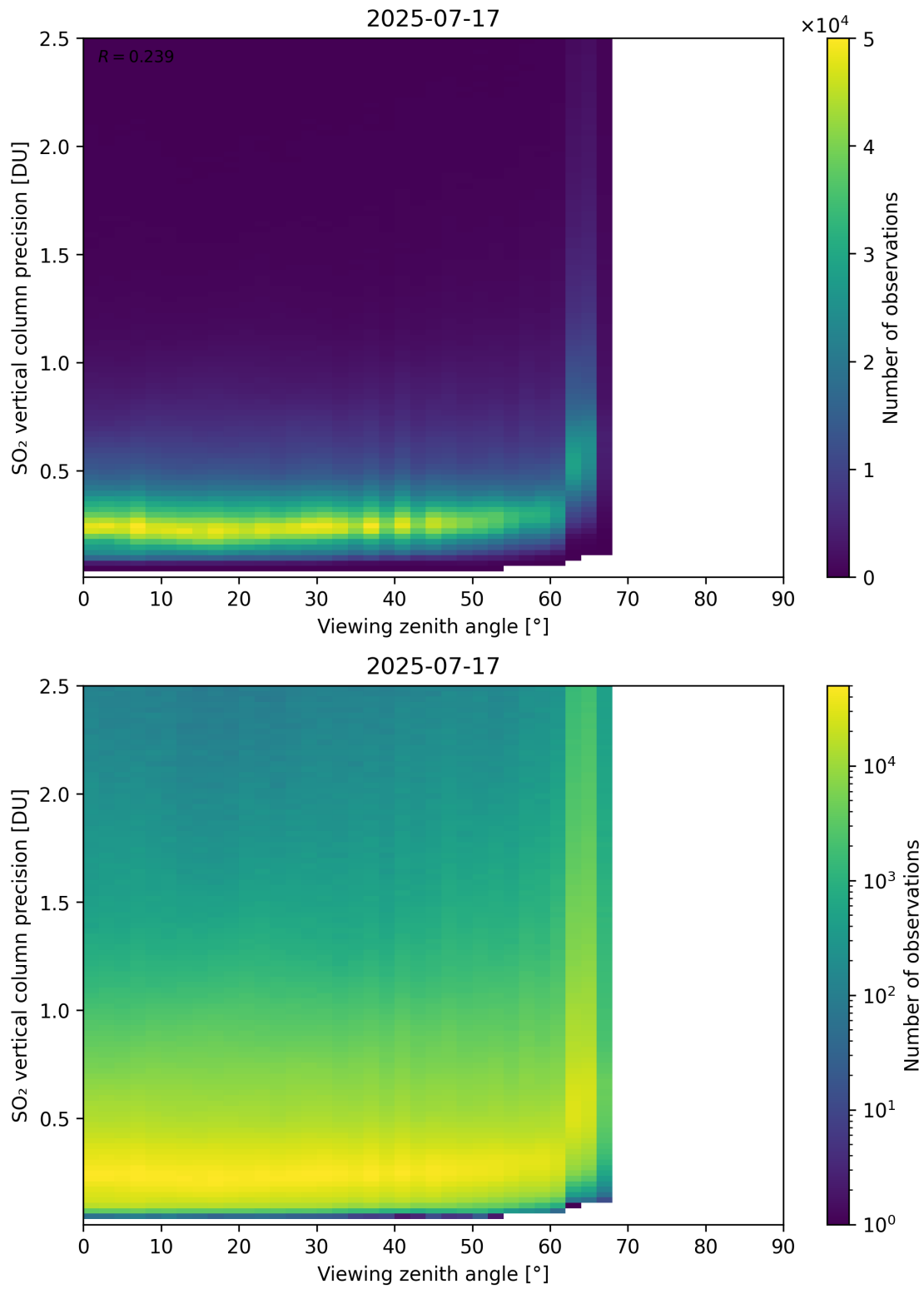
Figure 384: Scatter density plot of “Viewing zenith angle” against “SO 2 vertical column precision” for 2025-07-16 to 2025-07-18.
