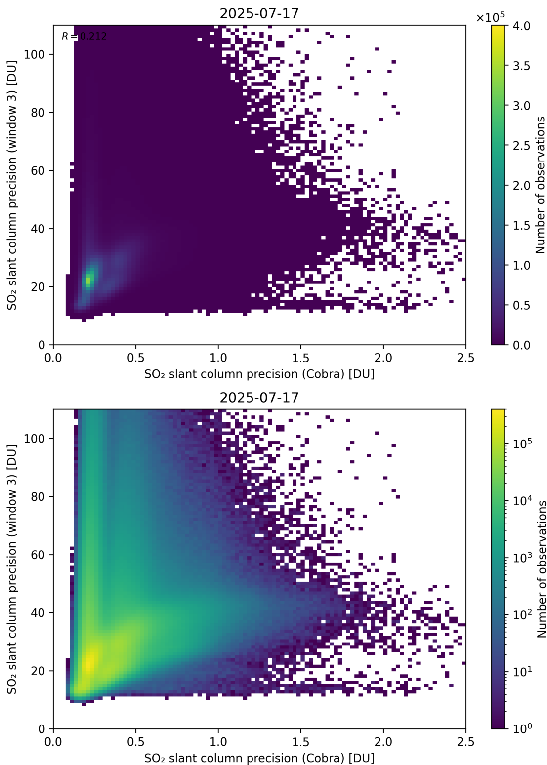
Figure 212: Scatter density plot of “SO 2 slant column precision (Cobra)” against “SO 2 slant column precision (window 3)” for 2025-07-16 to 2025-07-18.
