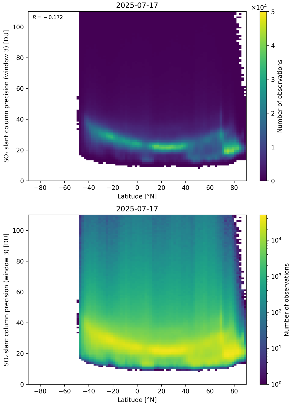
Figure 166: Scatter density plot of “Latitude” against “SO 2 slant column precision (window 3)” for 2025-07-16 to 2025-07-18.
