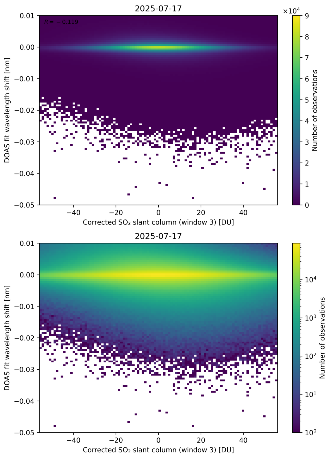
Figure 256: Scatter density plot of “Corrected SO 2 slant column (window 3)” against “DOAS fit wavelength shift” for 2025-07-16 to 2025-07-18.
