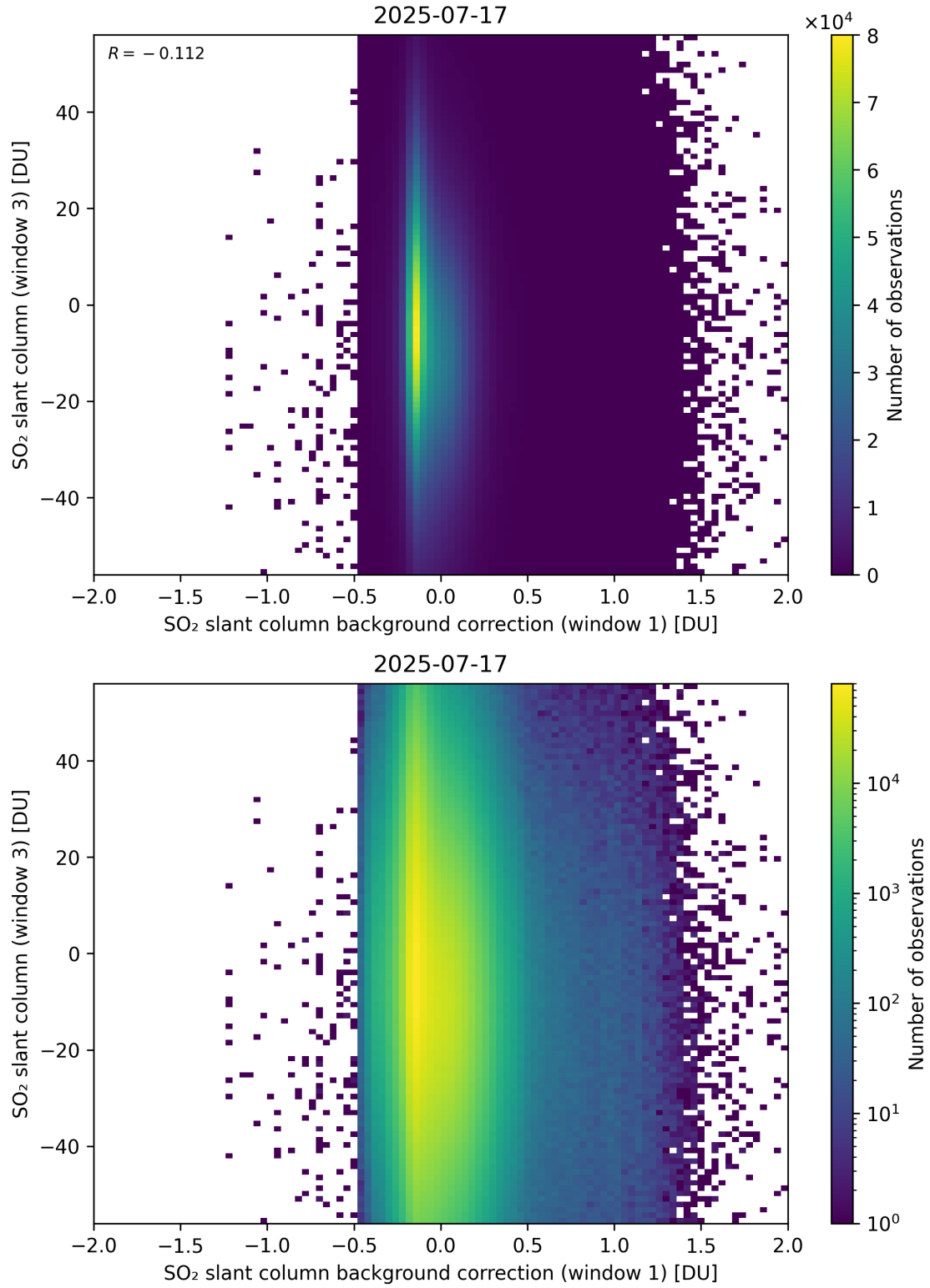
Figure 118: Scatter density plot of “SO 2 slant column background correction (window 1)” against “SO 2 slant column (window 3)” for 2025-07-16 to 2025-07-18.
