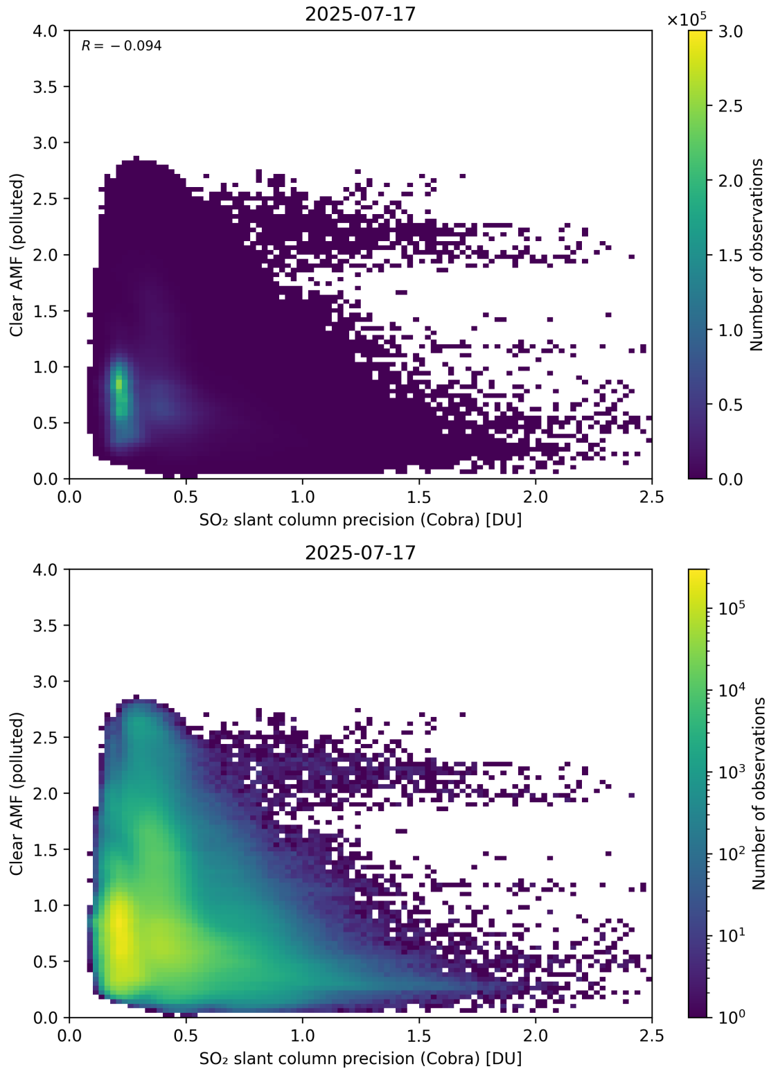
Figure 205: Scatter density plot of “SO 2 slant column precision (Cobra)” against “Clear AMF (polluted)” for 2025-07-16 to 2025-07-18.
