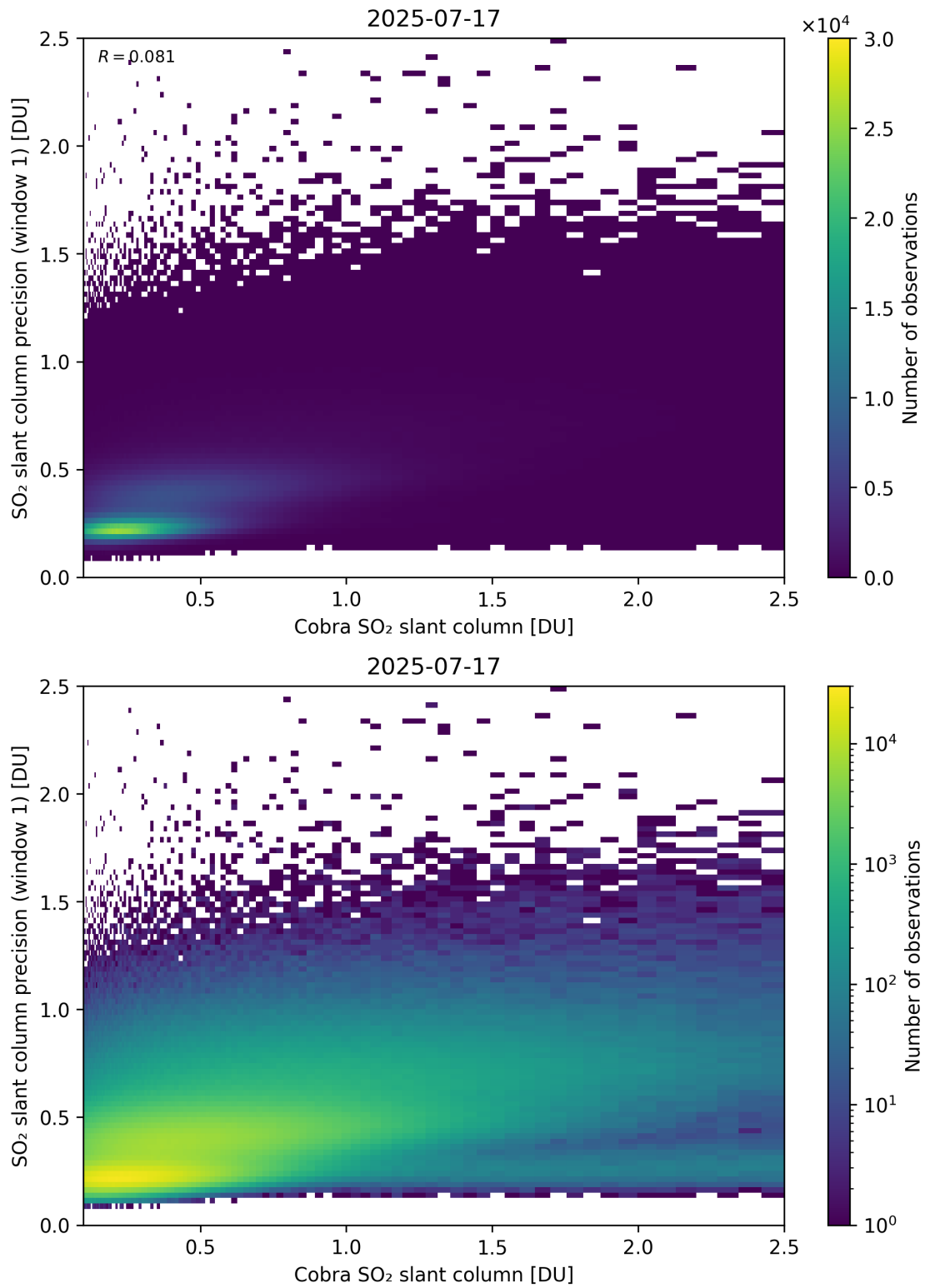
Figure 220: Scatter density plot of “Cobra SO 2 slant column” against “SO 2 slant column precision (window 1)” for 2025-07-16 to 2025-07-18.
