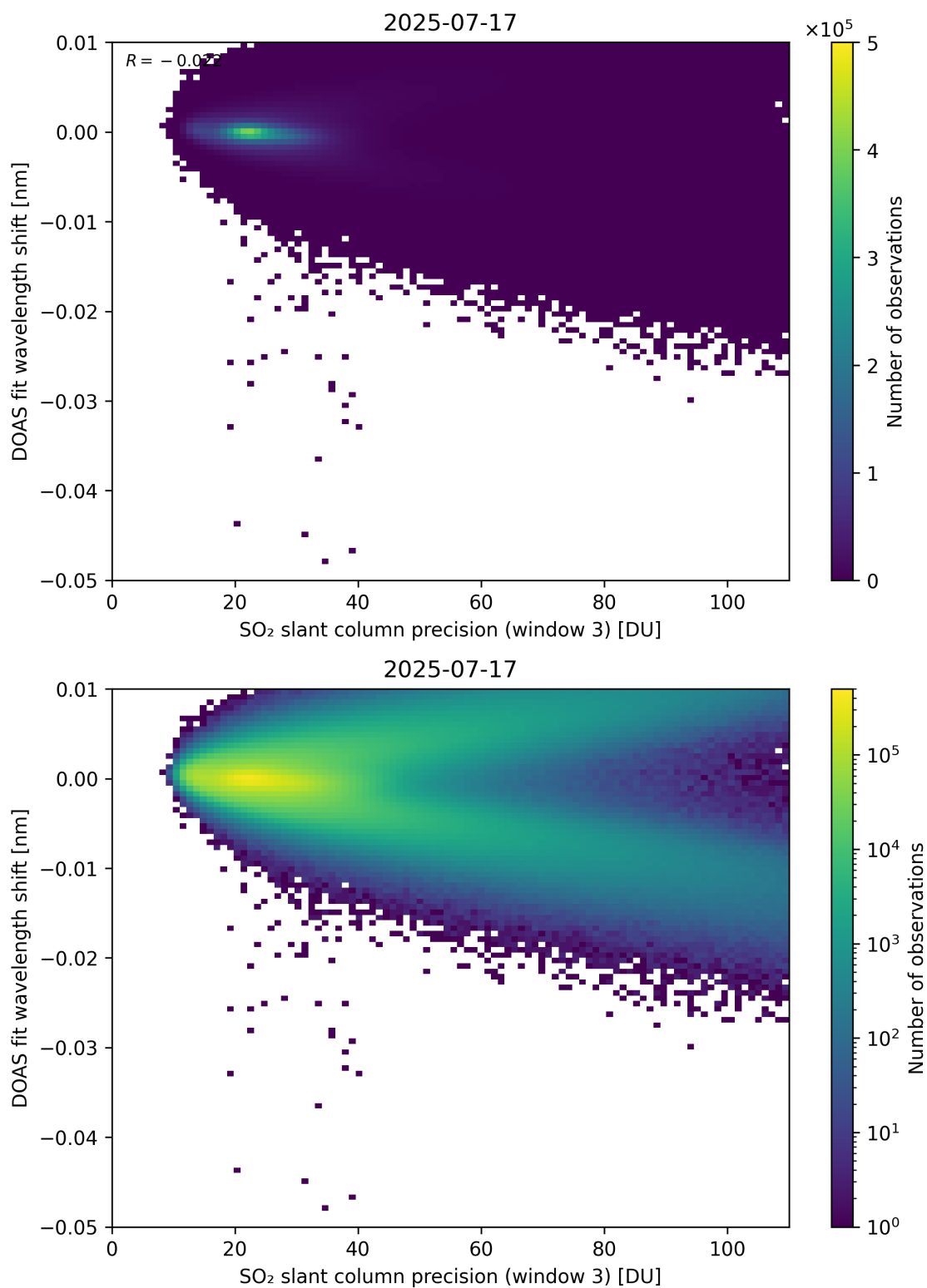
Figure 308: Scatter density plot of “SO 2 slant column precision (window 3)” against “DOAS fit wavelength shift” for 2025-07-16 to 2025-07-18.
