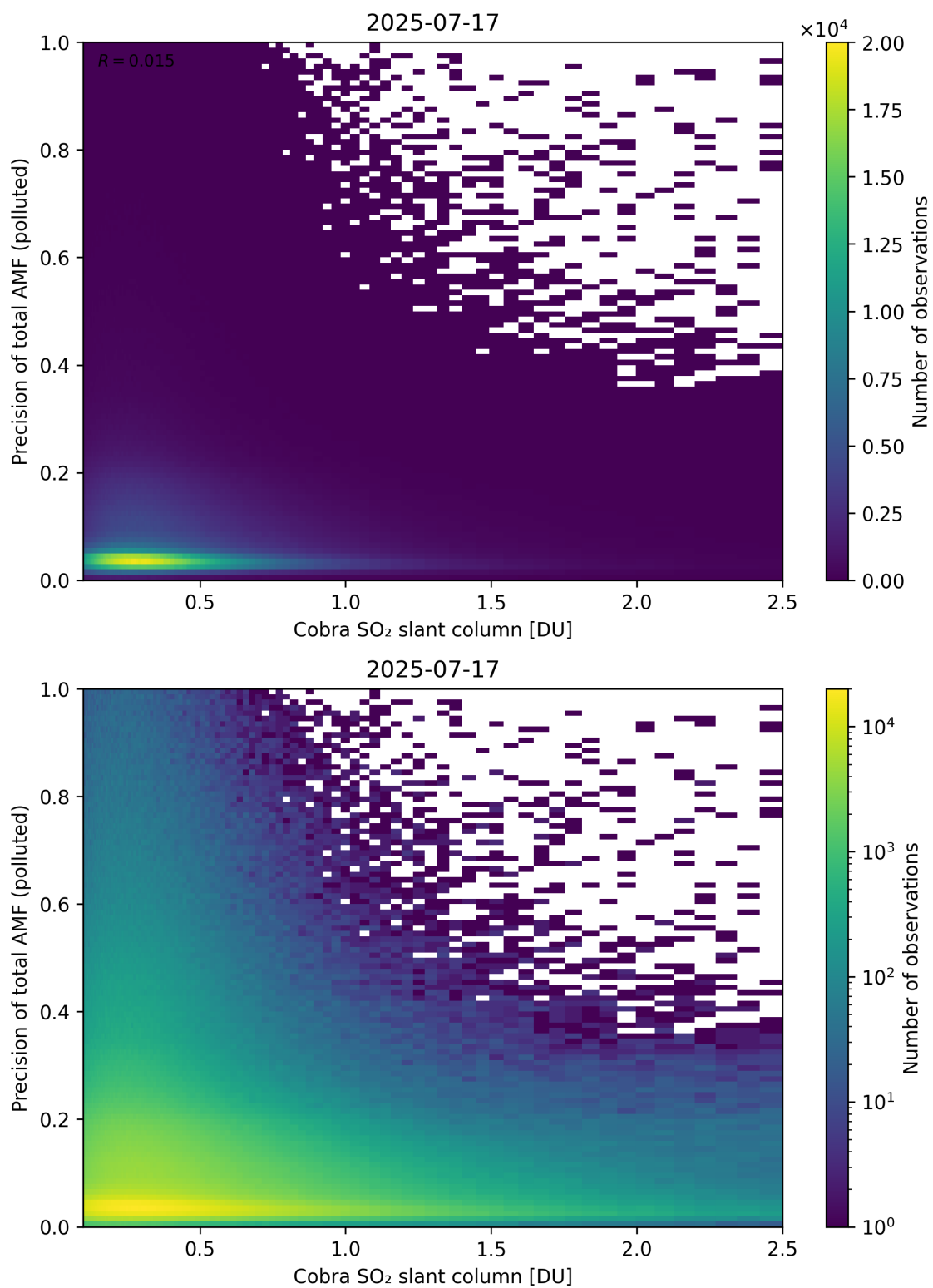
Figure 225: Scatter density plot of “Cobra SO 2 slant column” against “Precision of total AMF (polluted)” for 2025-07-16 to 2025-07-18.
