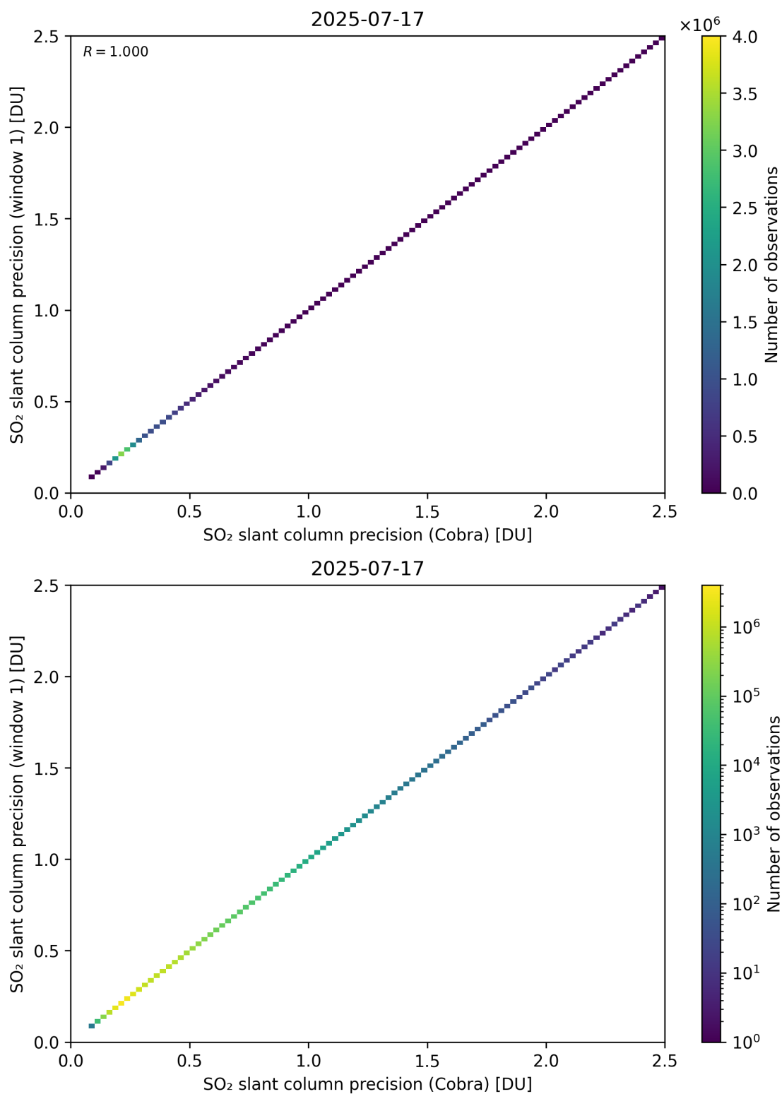
Figure 209: Scatter density plot of “SO 2 slant column precision (Cobra)” against “SO 2 slant column precision (window 1)” for 2025-07-16 to 2025-07-18.
