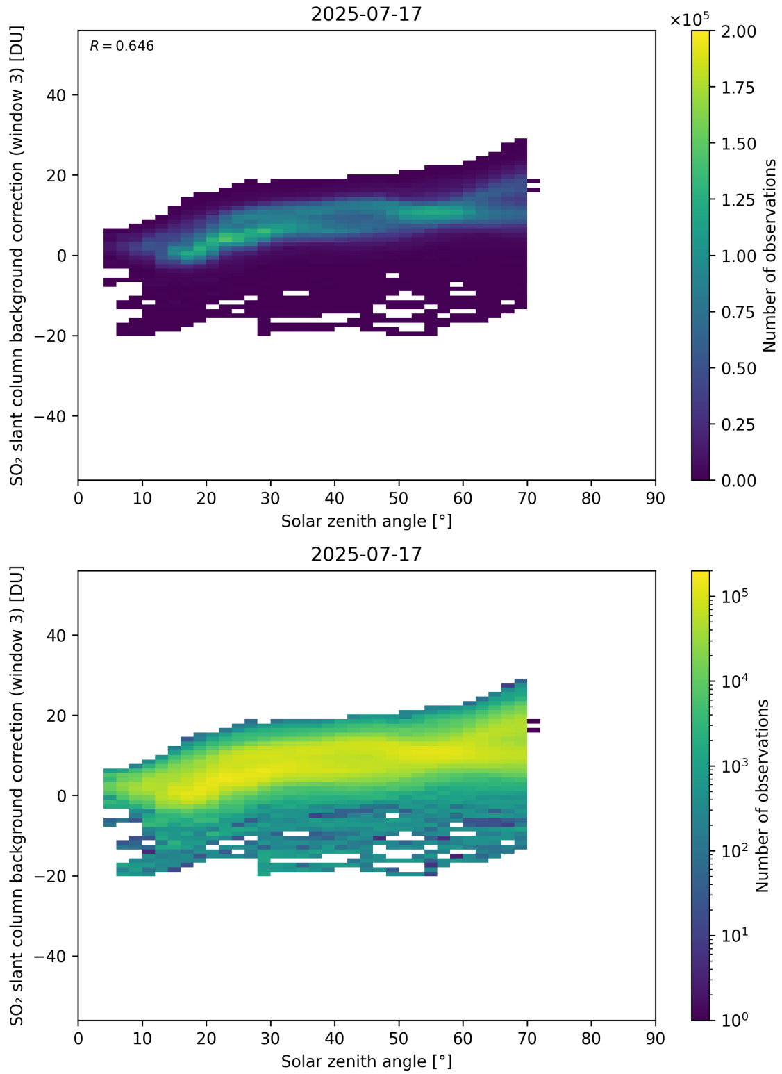
Figure 173: Scatter density plot of “Solar zenith angle” against “SO 2 slant column background correction (window 3)” for 2025-07-16 to 2025-07-18.
