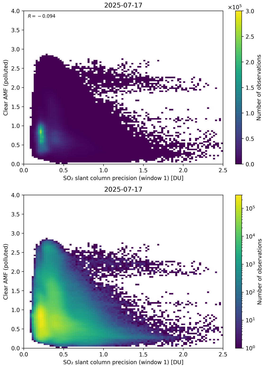
Figure 274: Scatter density plot of “SO 2 slant column precision (window 1)” against “Clear AMF (polluted)” for 2025-07-16 to 2025-07-18.
