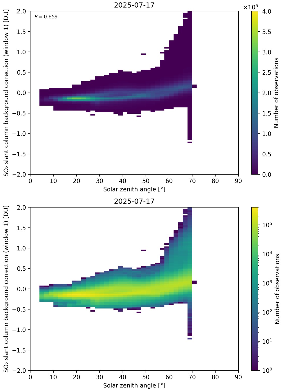
Figure 171: Scatter density plot of “Solar zenith angle” against “SO 2 slant column background correction (window 1)” for 2025-07-16 to 2025-07-18.
