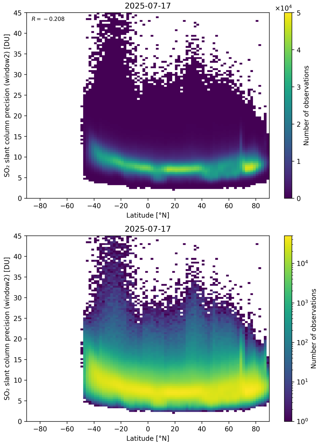
Figure 164: Scatter density plot of “Latitude” against “SO 2 slant column precision (window2)” for 2025-07-16 to 2025-07-18.
