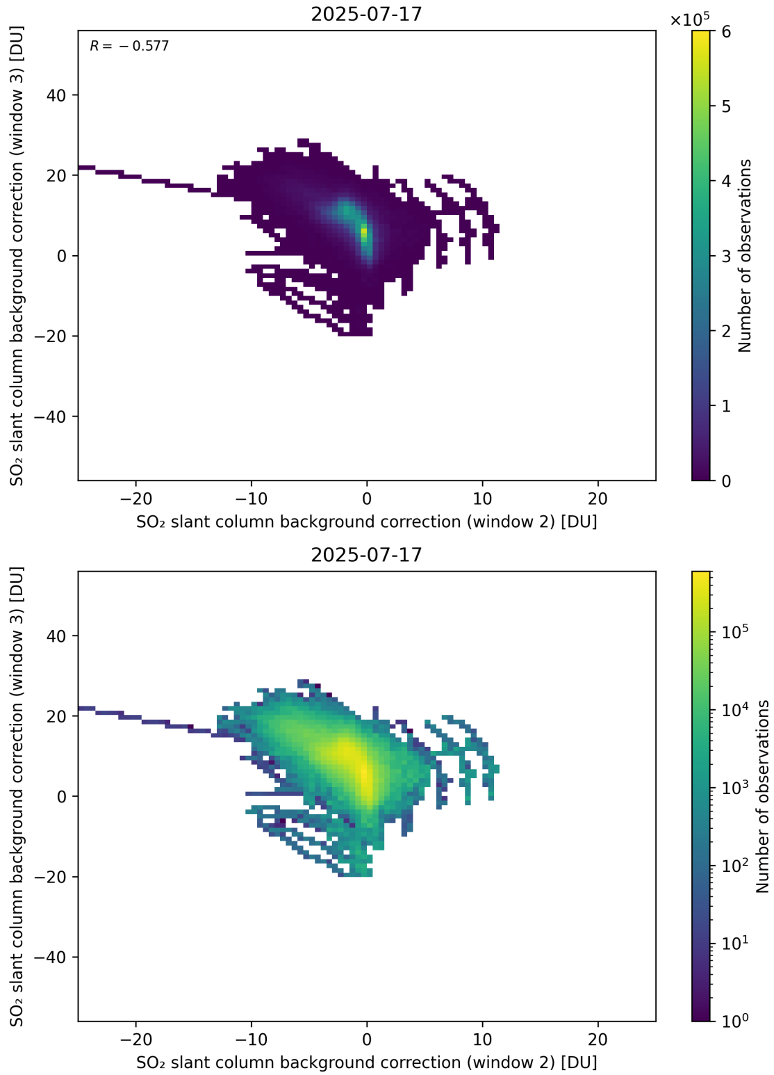
Figure 122: Scatter density plot of “SO 2 slant column background correction (window 2)” against “SO 2 slant column background correction (window 3)” for 2025-07-16 to 2025-07-18.
