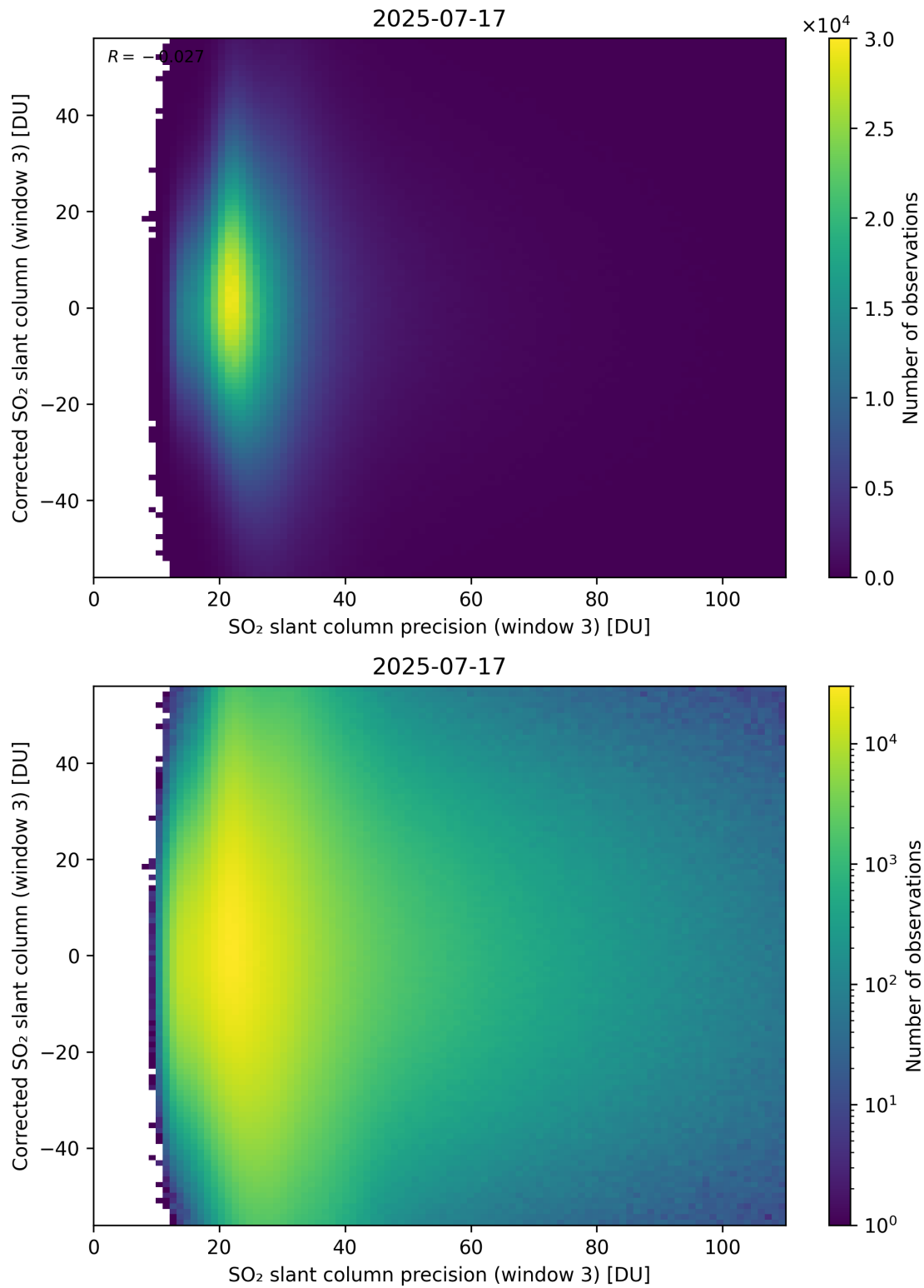
Figure 312: Scatter density plot of “SO 2 slant column precision (window 3)” against “Corrected SO 2 slant column (window 3)” for 2025-07-16 to 2025-07-18.
