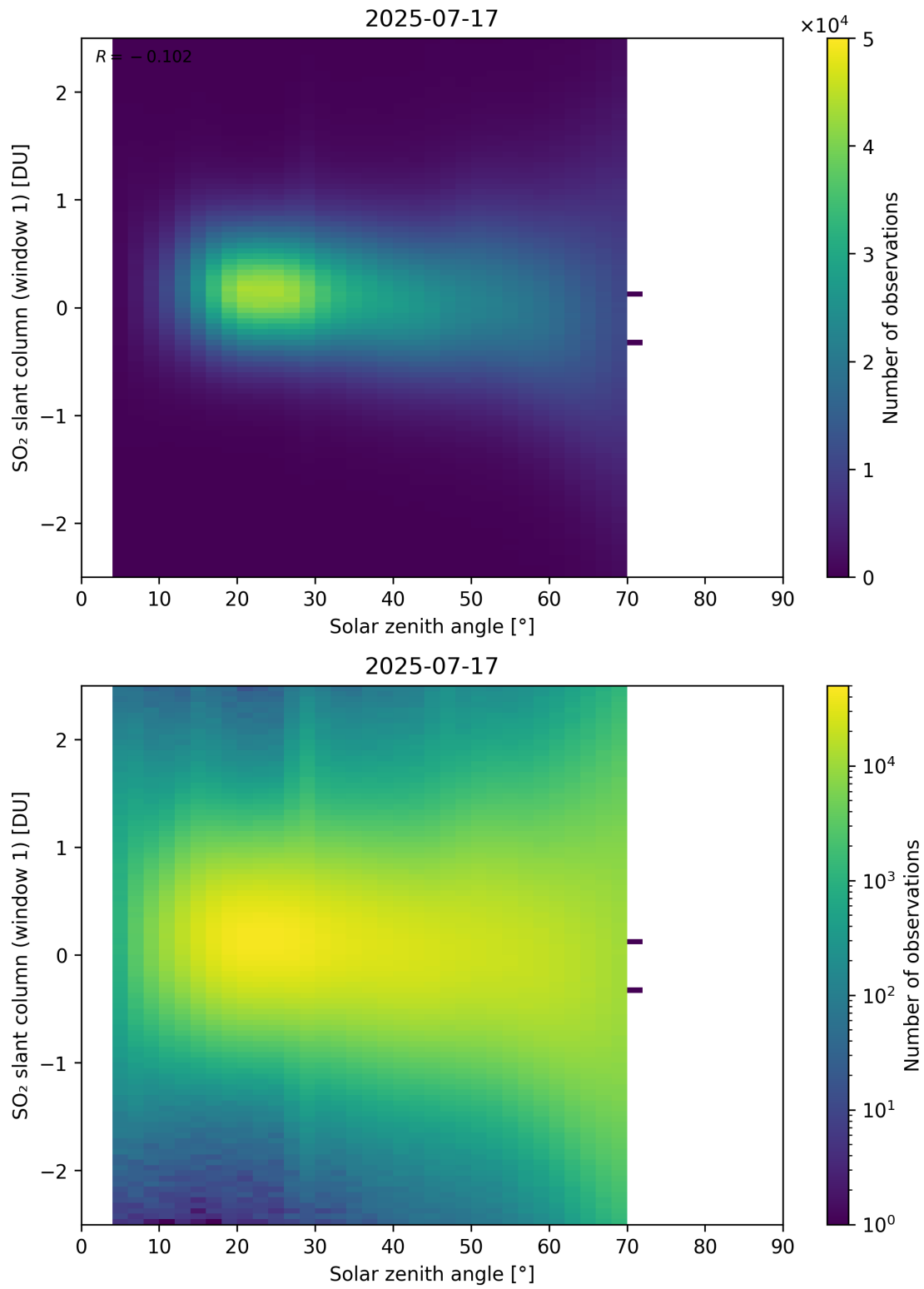
Figure 184: Scatter density plot of “Solar zenith angle” against “SO 2 slant column (window 1)” for 2025-07-16 to 2025-07-18.
