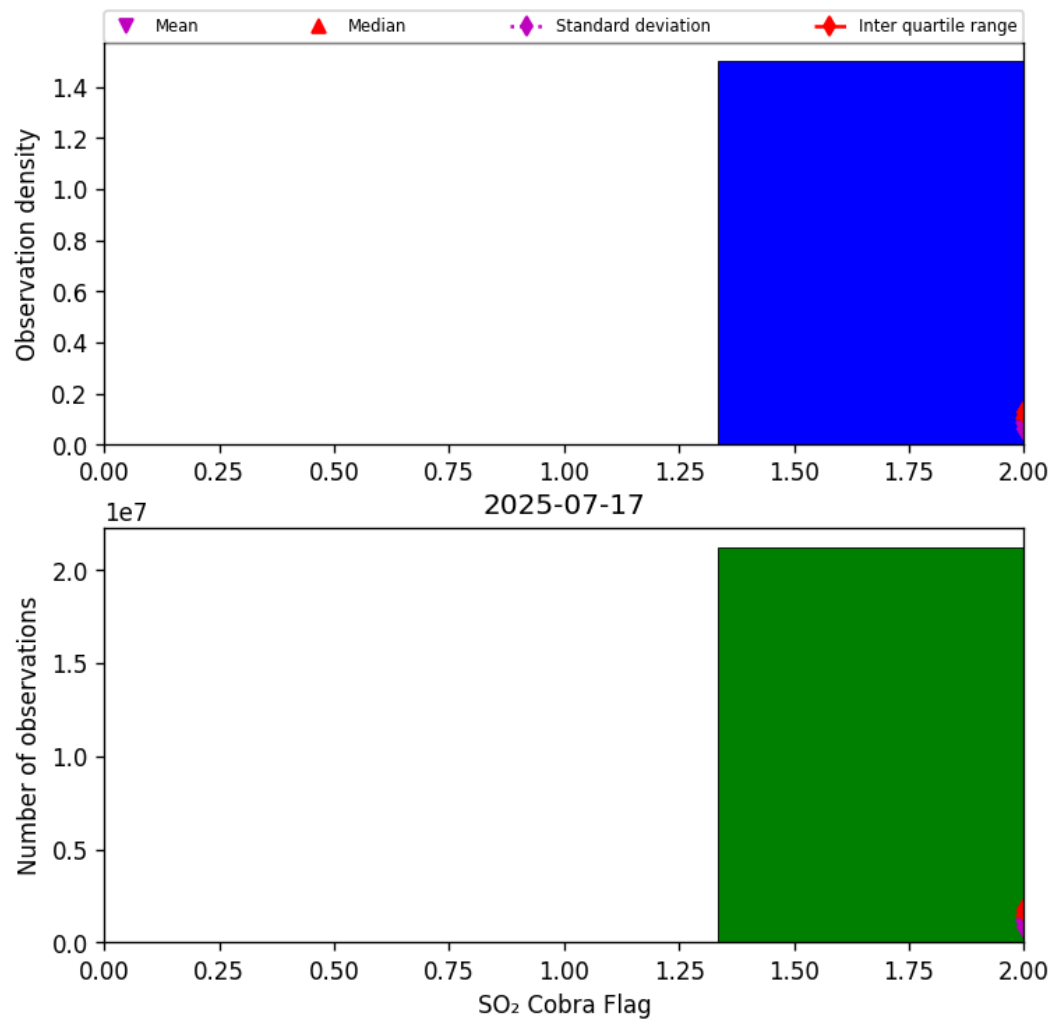
Figure 75: Histogram of “SO 2 Cobra Flag” for 2025-07-16 to 2025-07-18
