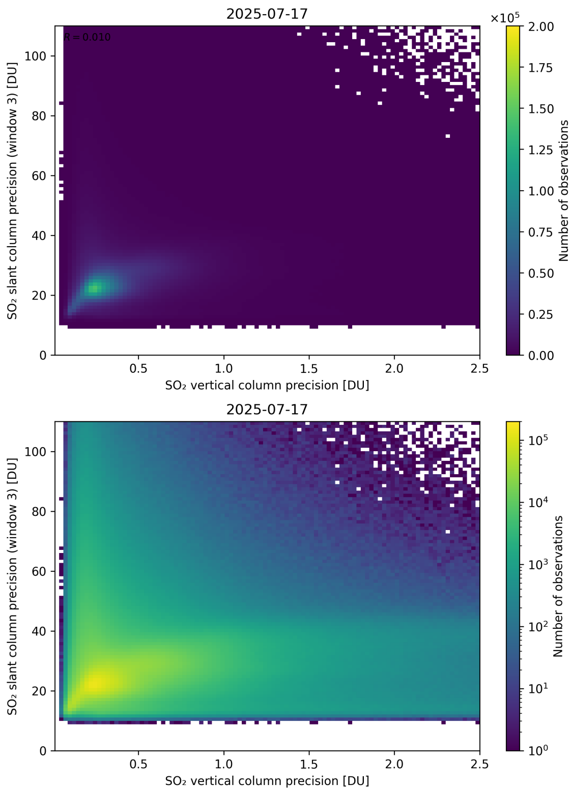
Figure 345: Scatter density plot of “SO 2 vertical column precision” against “SO 2 slant column precision (window 3)” for 2025-07-16 to 2025-07-18.
