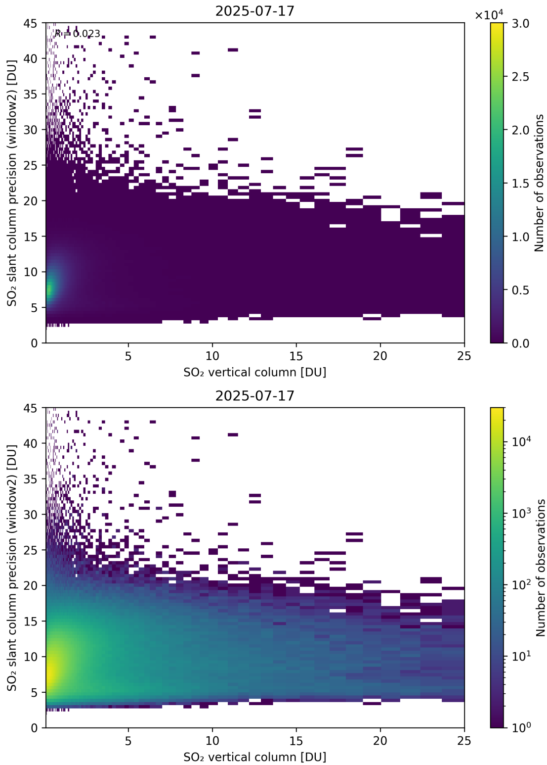
Figure 356: Scatter density plot of “SO 2 vertical column” against “SO 2 slant column precision (window2)” for 2025-07-16 to 2025-07-18.
