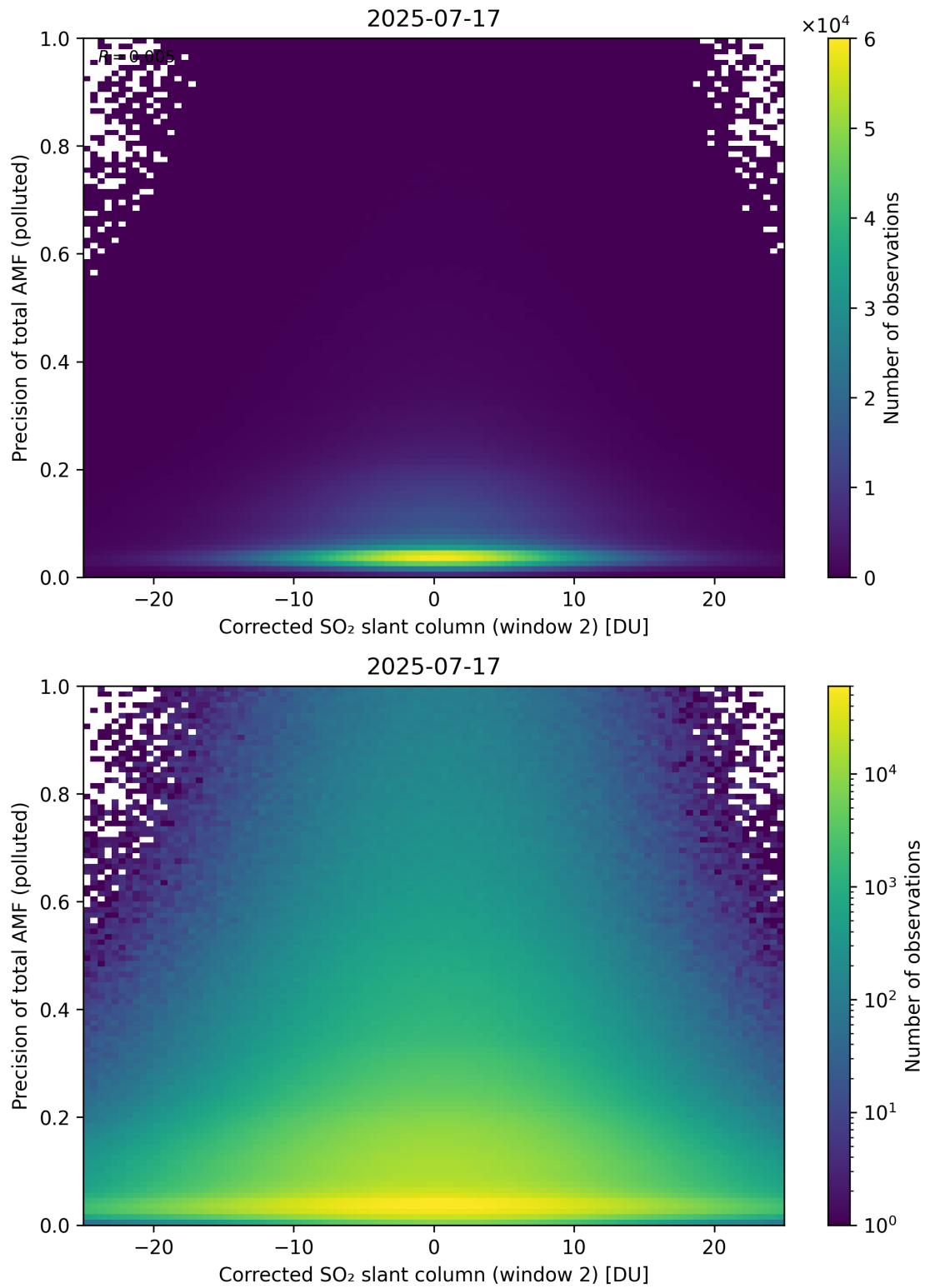
Figure 254: Scatter density plot of “Corrected SO 2 slant column (window 2)” against “Precision of total AMF (polluted)” for 2025-07-16 to 2025-07-18.
