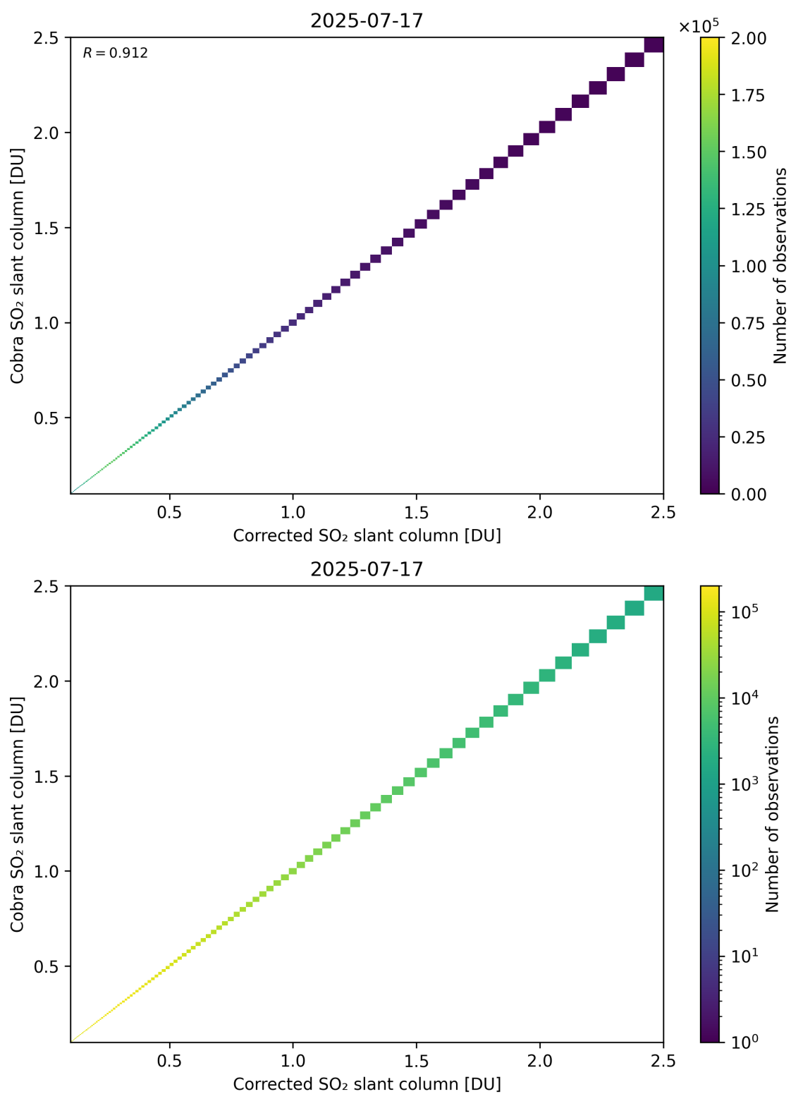
Figure 233: Scatter density plot of “Corrected SO 2 slant column” against “Cobra SO 2 slant column” for 2025-07-16 to 2025-07-18.
