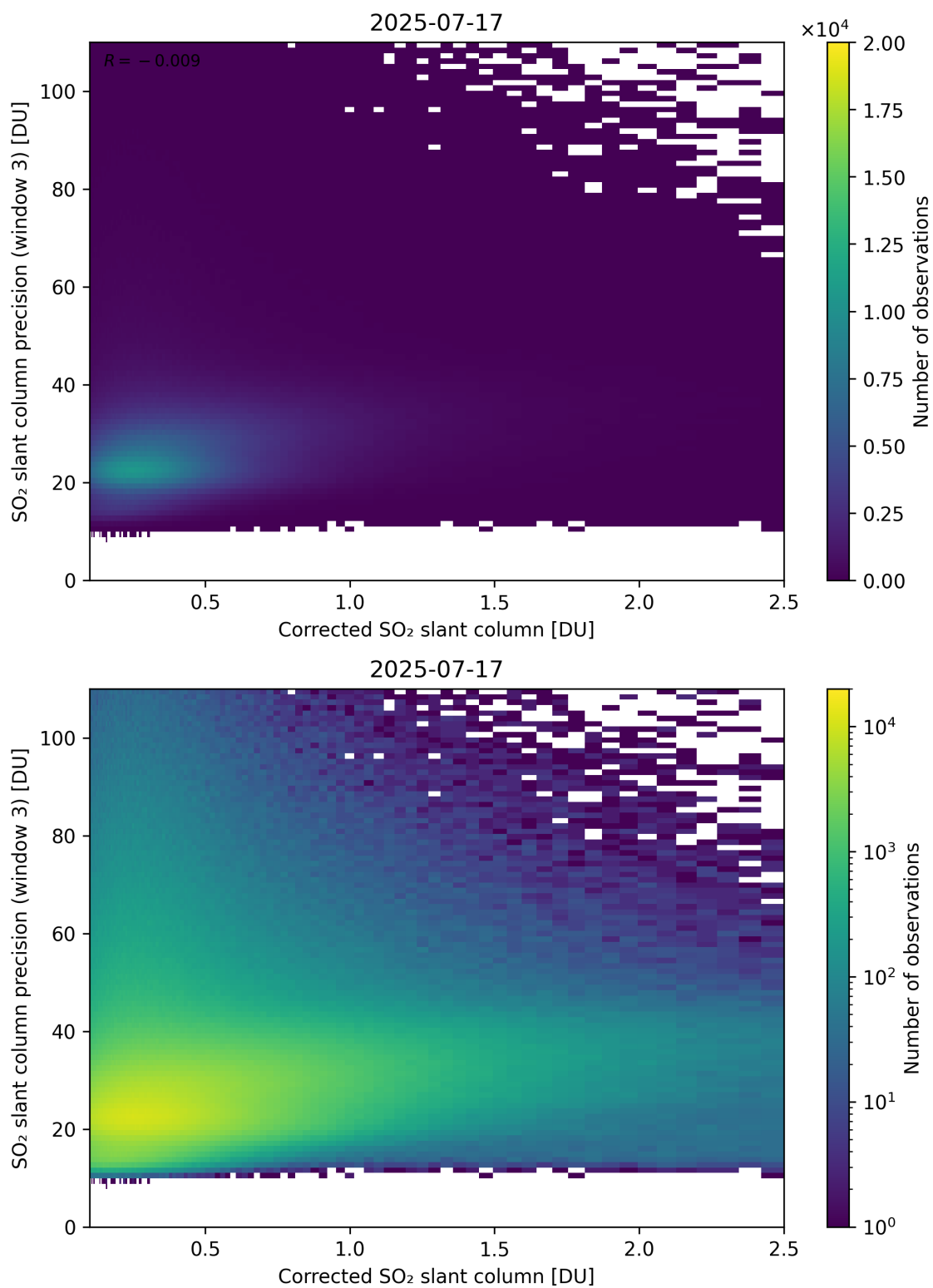
Figure 241: Scatter density plot of “Corrected SO 2 slant column” against “SO 2 slant column precision (window 3)” for 2025-07-16 to 2025-07-18.
