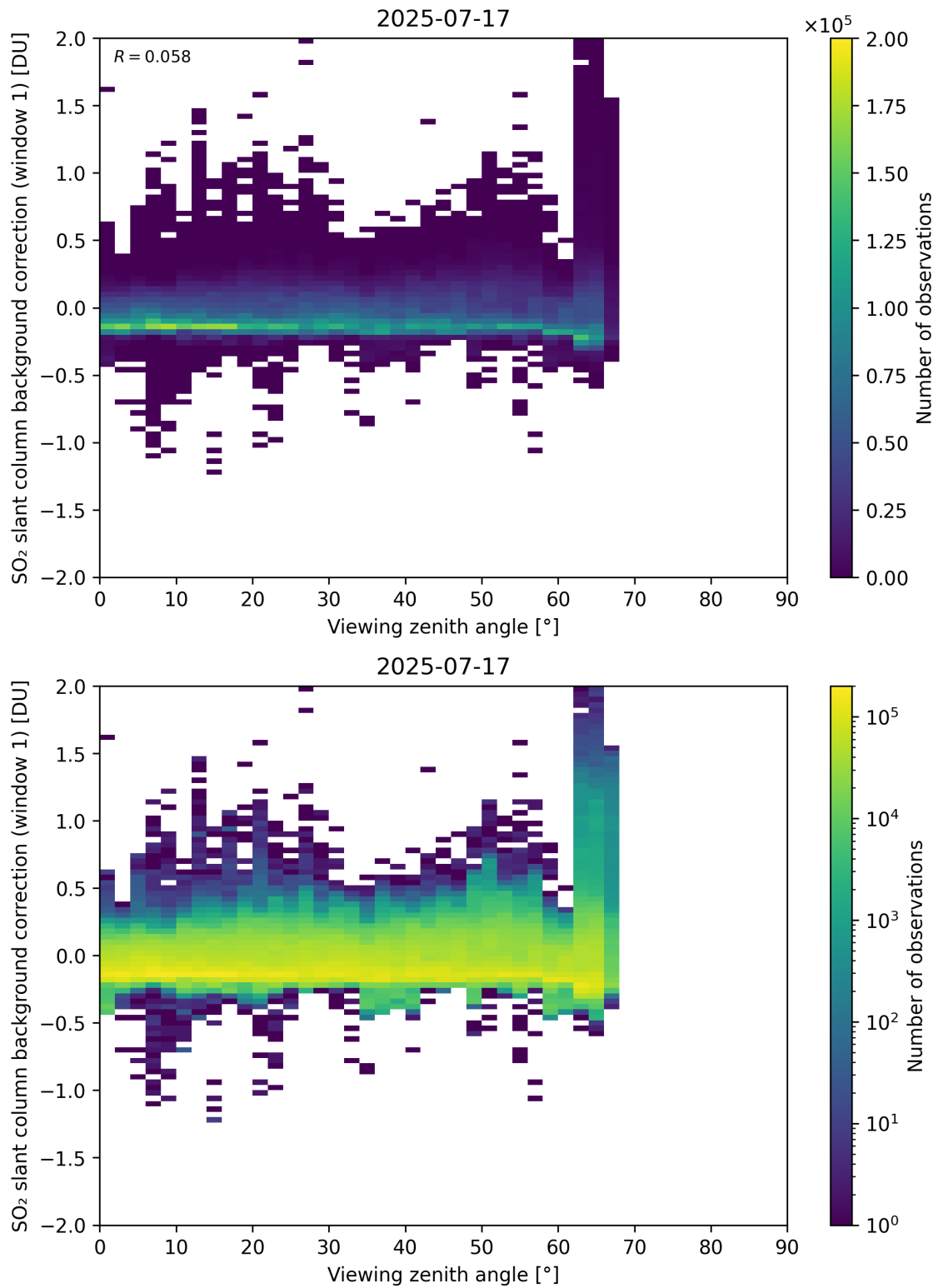
Figure 362: Scatter density plot of “Viewing zenith angle” against “SO 2 slant column background correction (window 1)” for 2025-07-16 to 2025-07-18.
