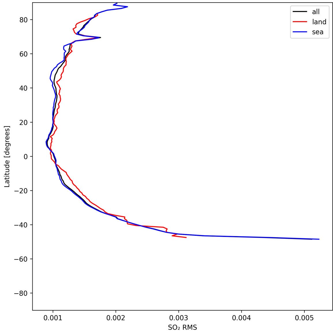
Figure 52: Zonal average of “SO 2 RMS” for 2025-07-16 to 2025-07-18.
