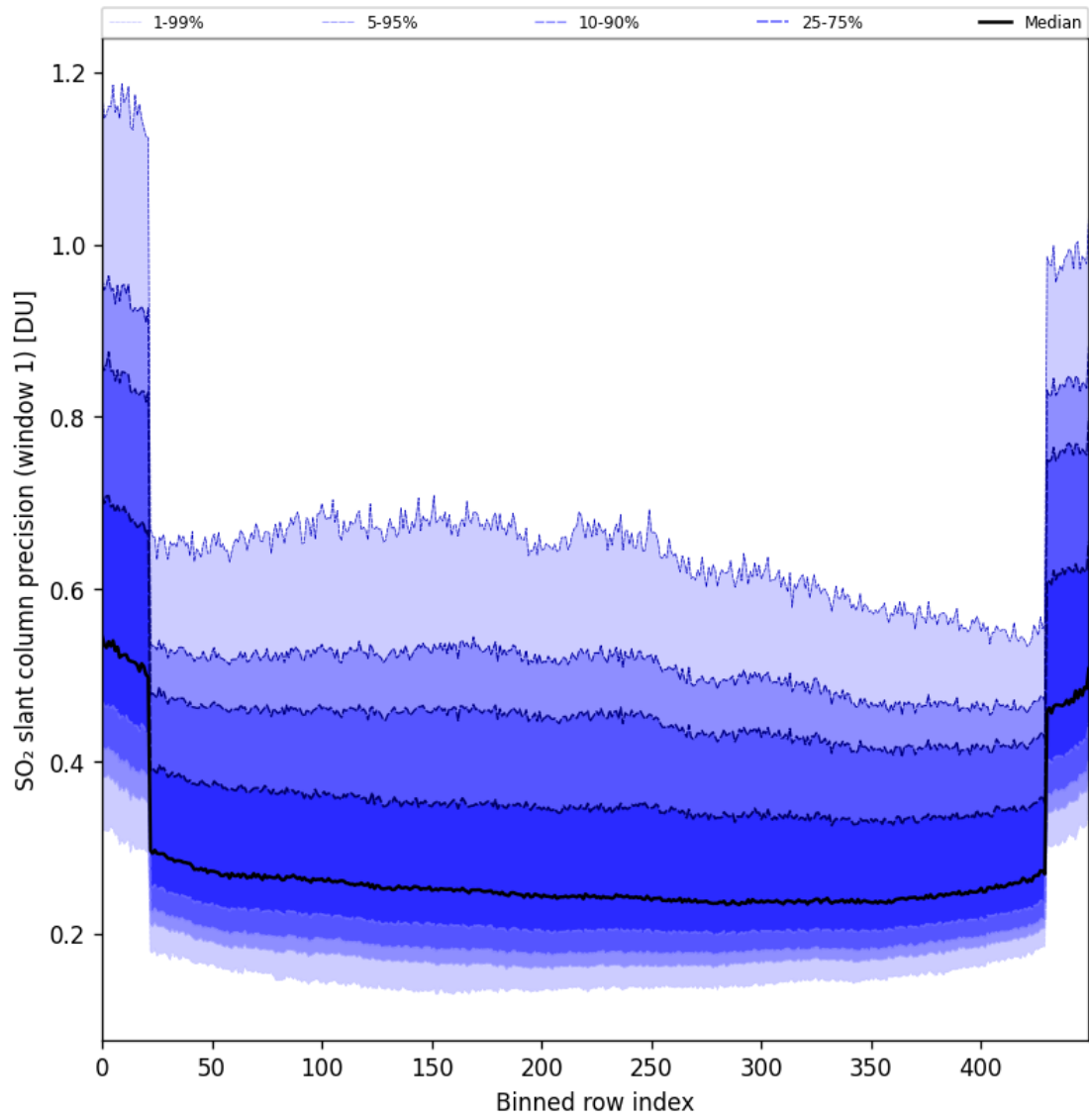
Figure 90: Along track statistics of “SO 2 slant column precision (window 1)” for 2025-07-16 to 2025-07-18
