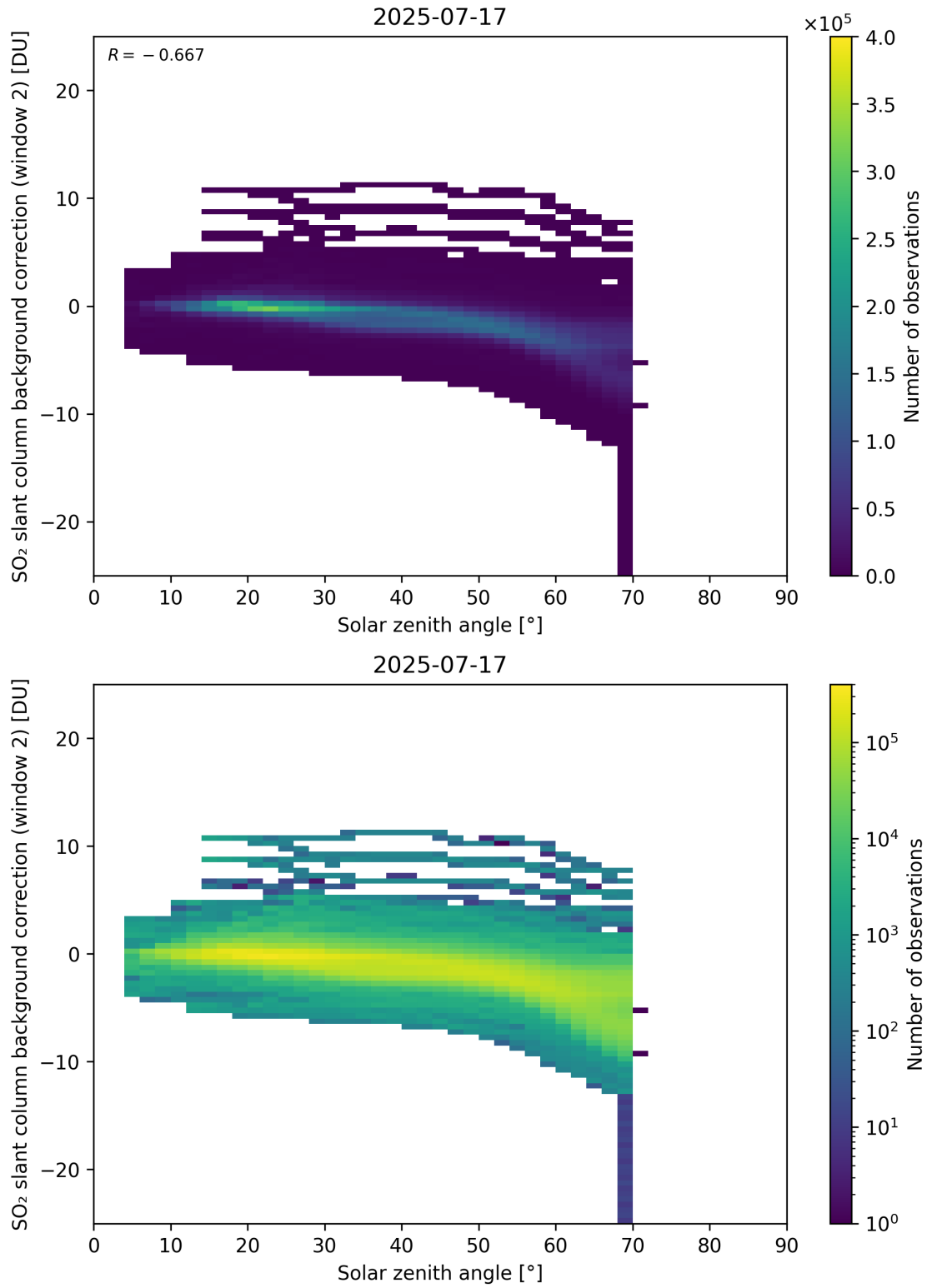
Figure 172: Scatter density plot of “Solar zenith angle” against “SO 2 slant column background correction (window 2)” for 2025-07-16 to 2025-07-18.
