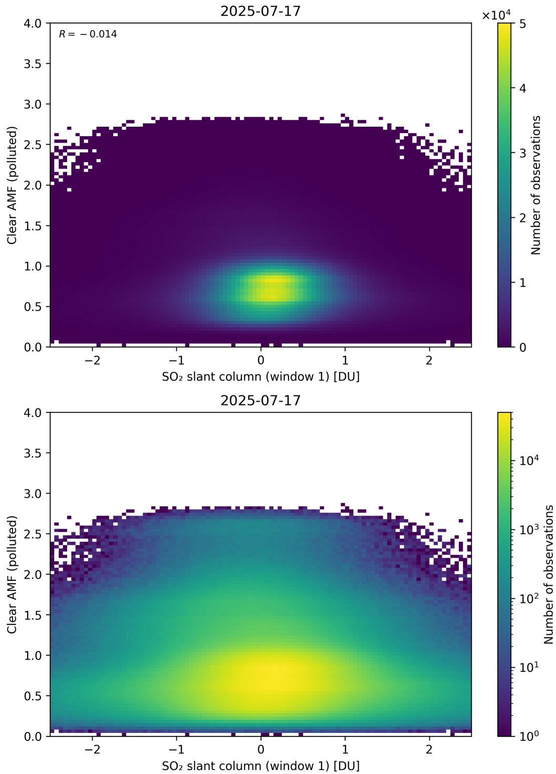
Figure 282: Scatter density plot of “SO 2 slant column (window 1)” against “Clear AMF (polluted)” for 2025-07-16 to 2025-07-18.
