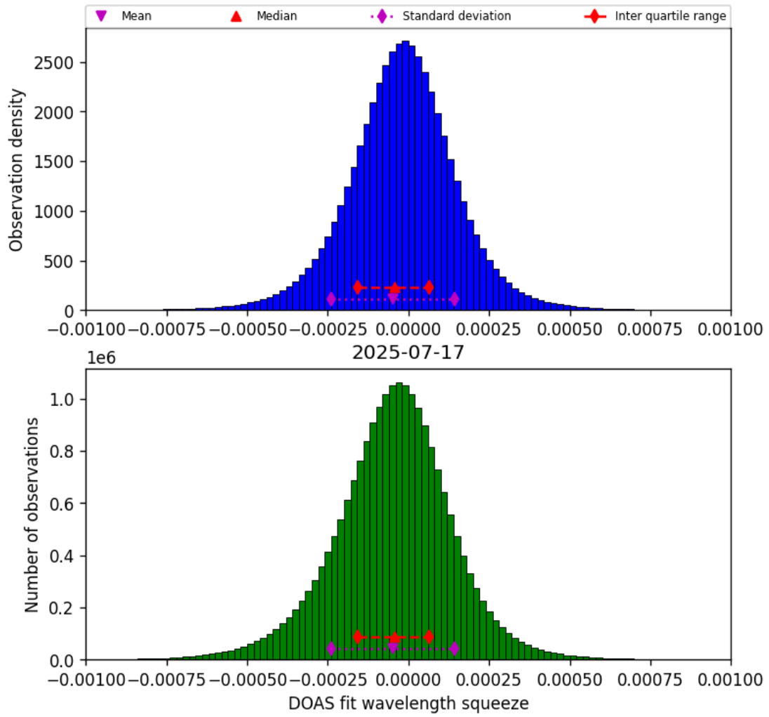
Figure 77: Histogram of “DOAS fit wavelength squeeze” for 2025-07-16 to 2025-07-18
