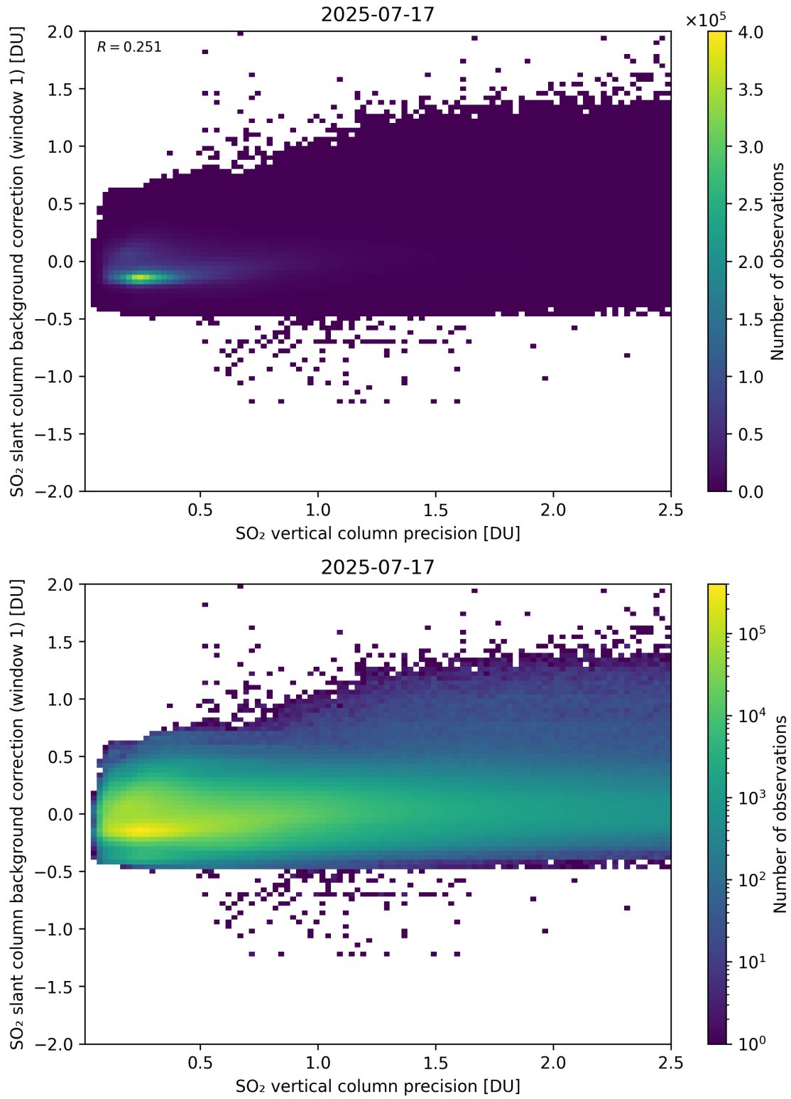
Figure 329: Scatter density plot of “SO 2 vertical column precision” against “SO 2 slant column background correction (window 1)” for 2025-07-16 to 2025-07-18.
