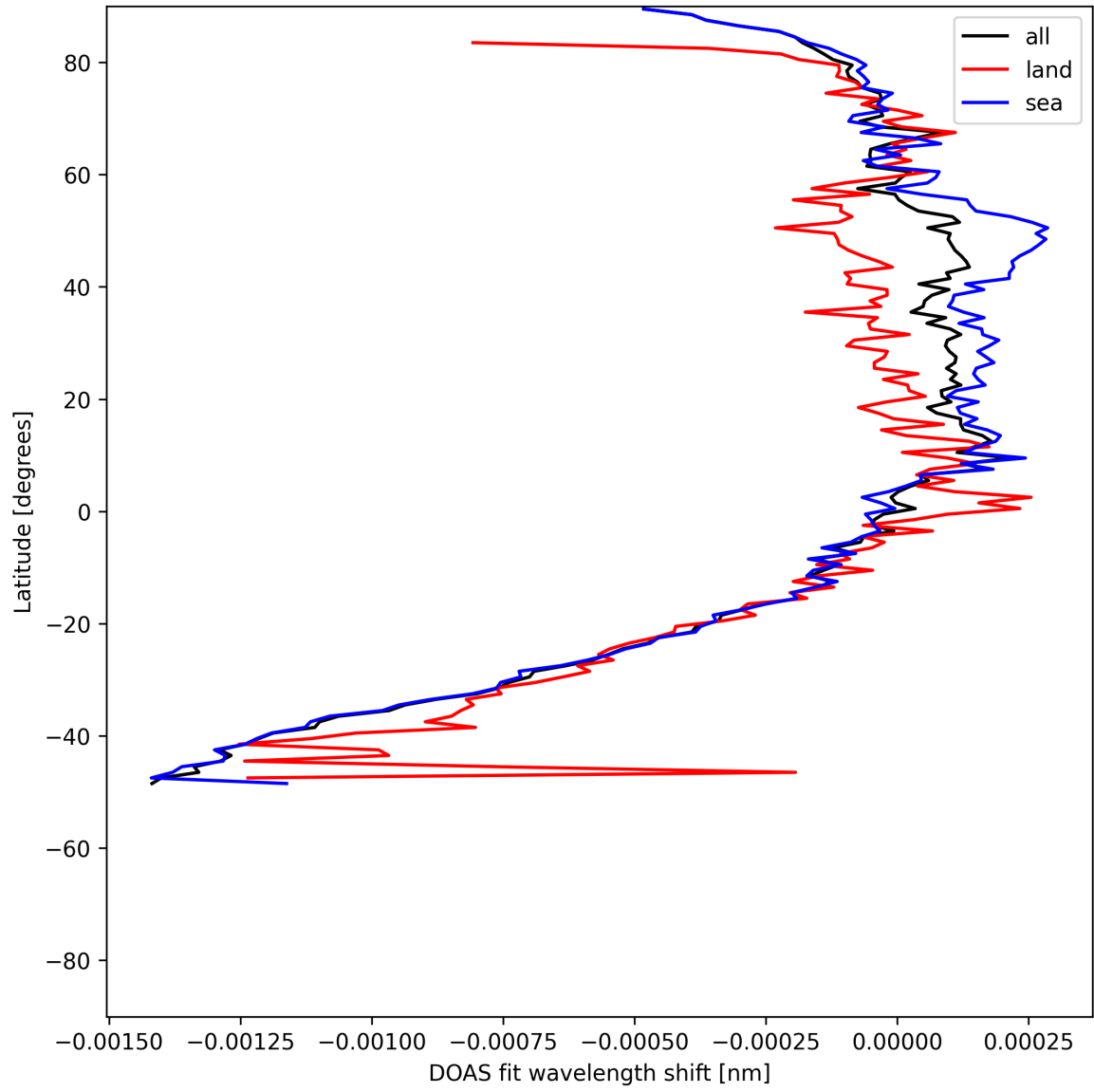
Figure 50: Zonal average of “DOAS fit wavelength shift” for 2025-07-16 to 2025-07-18.
