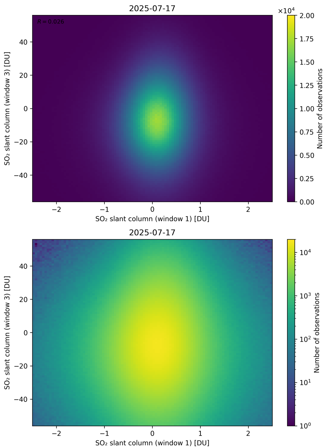
Figure 287: Scatter density plot of “SO 2 slant column (window 1)” against “SO 2 slant column (window 3)” for 2025-07-16 to 2025-07-18.
