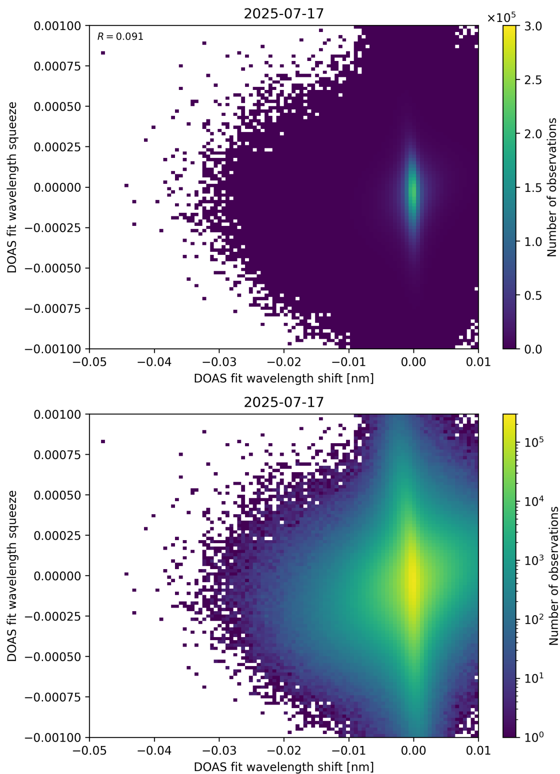
Figure 138: Scatter density plot of “DOAS fit wavelength shift” against “DOAS fit wavelength squeeze” for 2025-07-16 to 2025-07-18.
