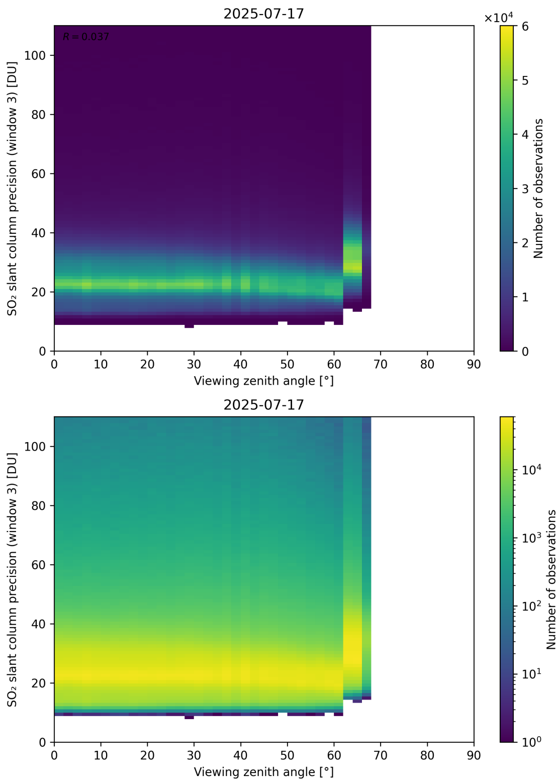
Figure 380: Scatter density plot of “Viewing zenith angle” against “SO 2 slant column precision (window 3)” for 2025-07-16 to 2025-07-18.
