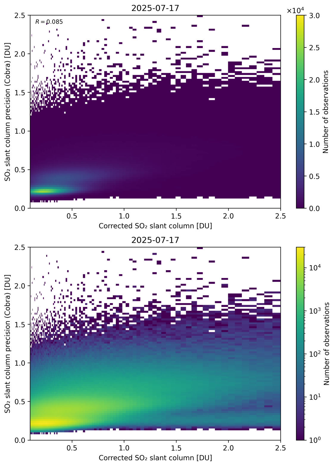
Figure 234: Scatter density plot of “Corrected SO 2 slant column” against “SO 2 slant column precision (Cobra)” for 2025-07-16 to 2025-07-18.
