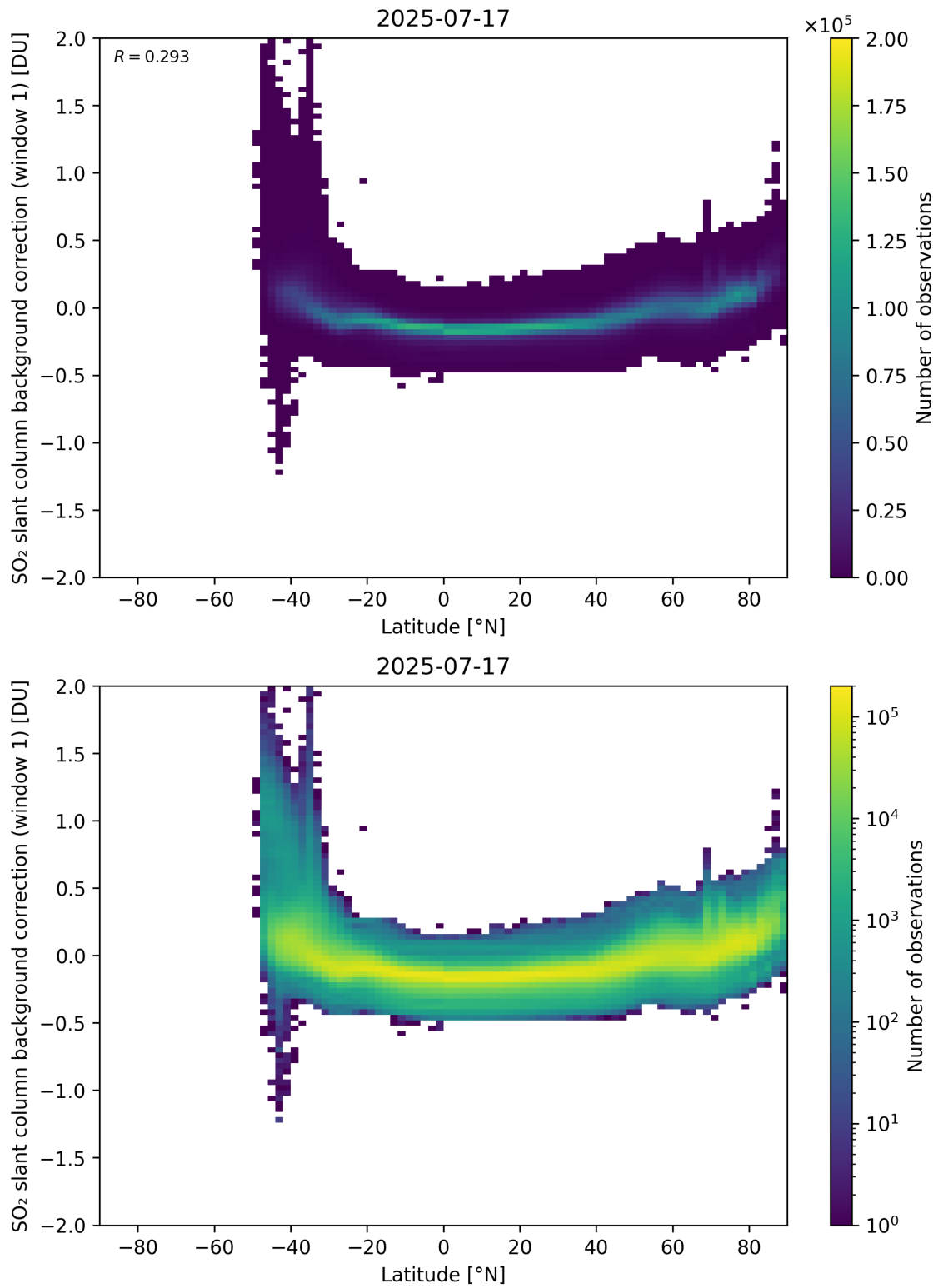
Figure 150: Scatter density plot of “Latitude” against “SO 2 slant column background correction (window 1)” for 2025-07-16 to 2025-07-18.
