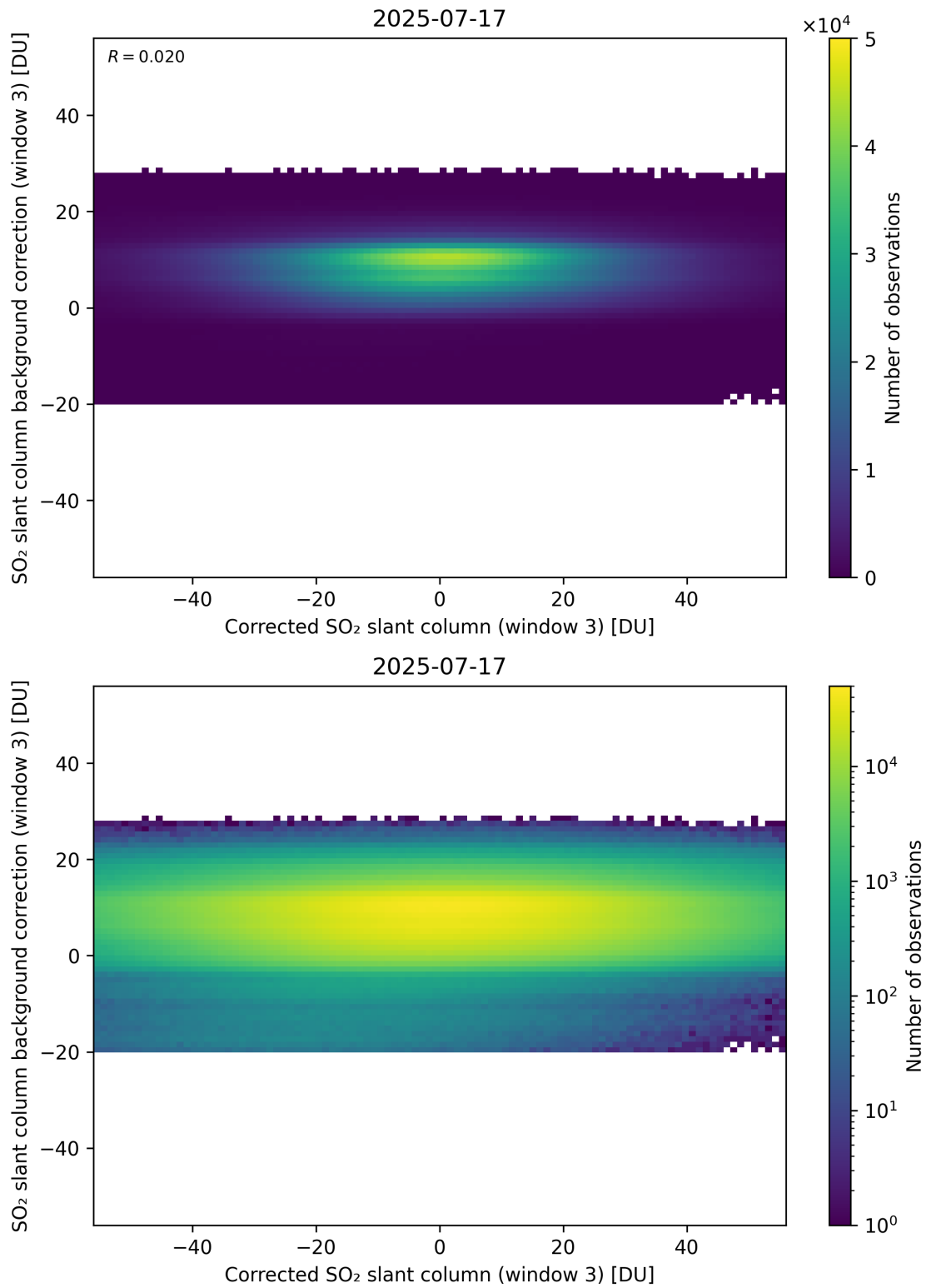
Figure 255: Scatter density plot of “Corrected SO 2 slant column (window 3)” against “SO 2 slant column background correction (window 3)” for 2025-07-16 to 2025-07-18.
