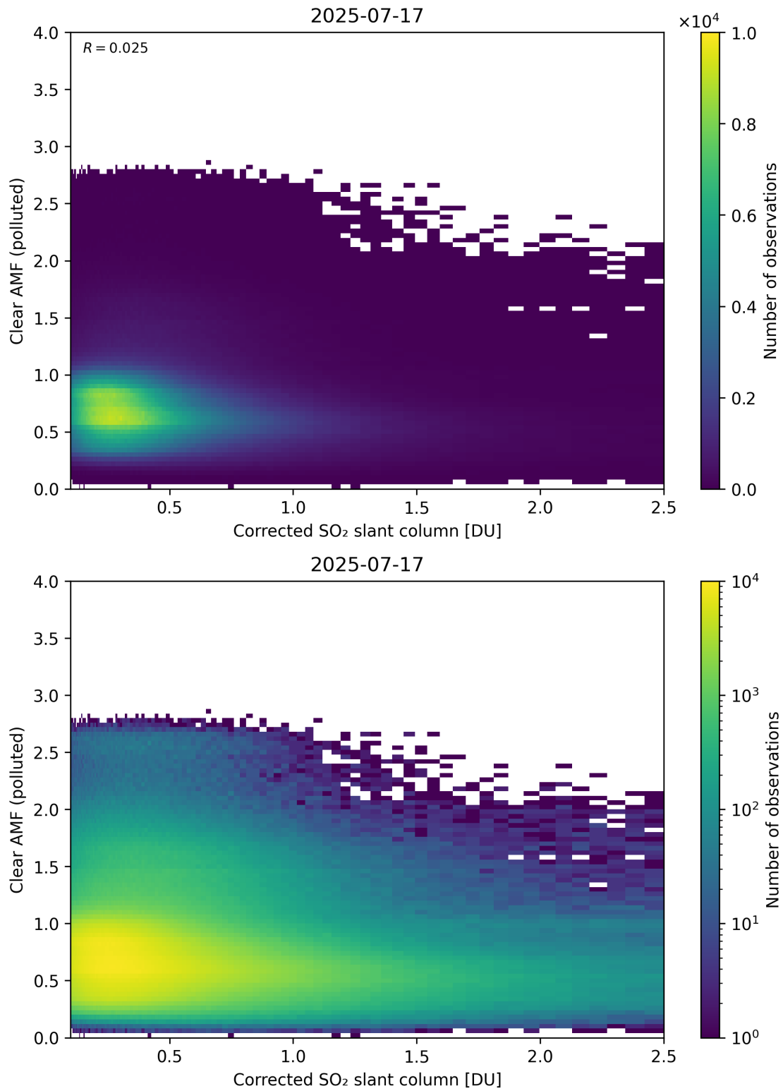
Figure 232: Scatter density plot of “Corrected SO 2 slant column” against “Clear AMF (polluted)” for 2025-07-16 to 2025-07-18.
