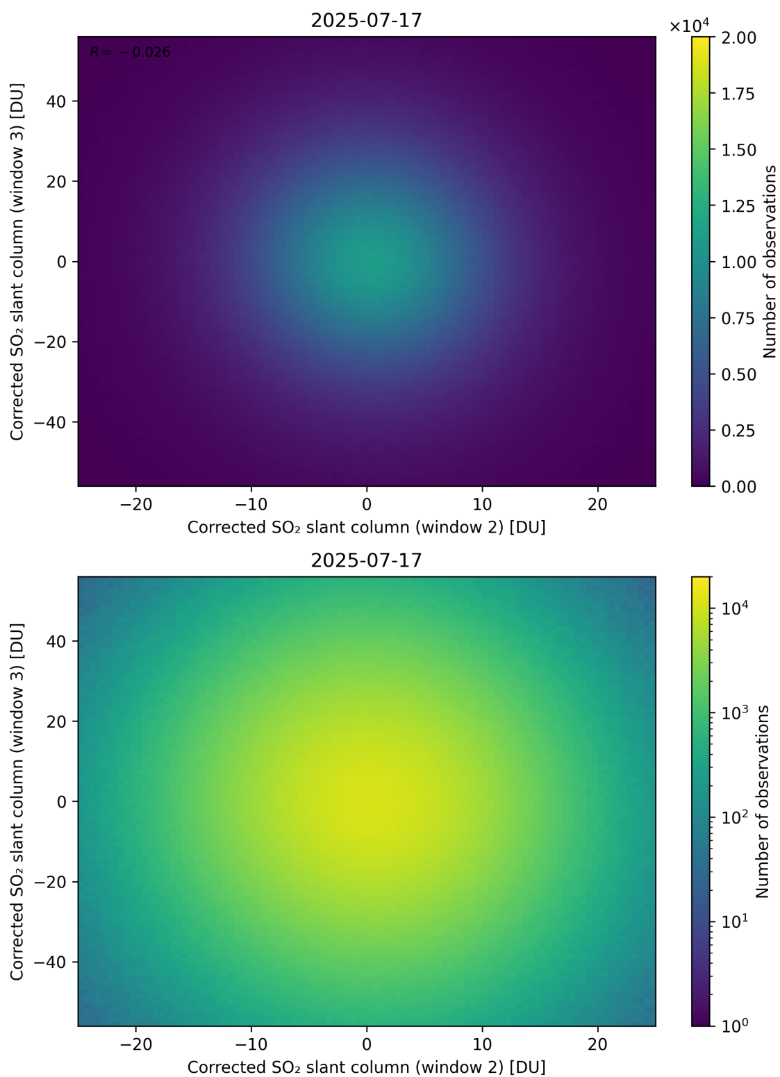
Figure 250: Scatter density plot of “Corrected SO 2 slant column (window 2)” against “Corrected SO 2 slant column (window 3)” for 2025-07-16 to 2025-07-18.
