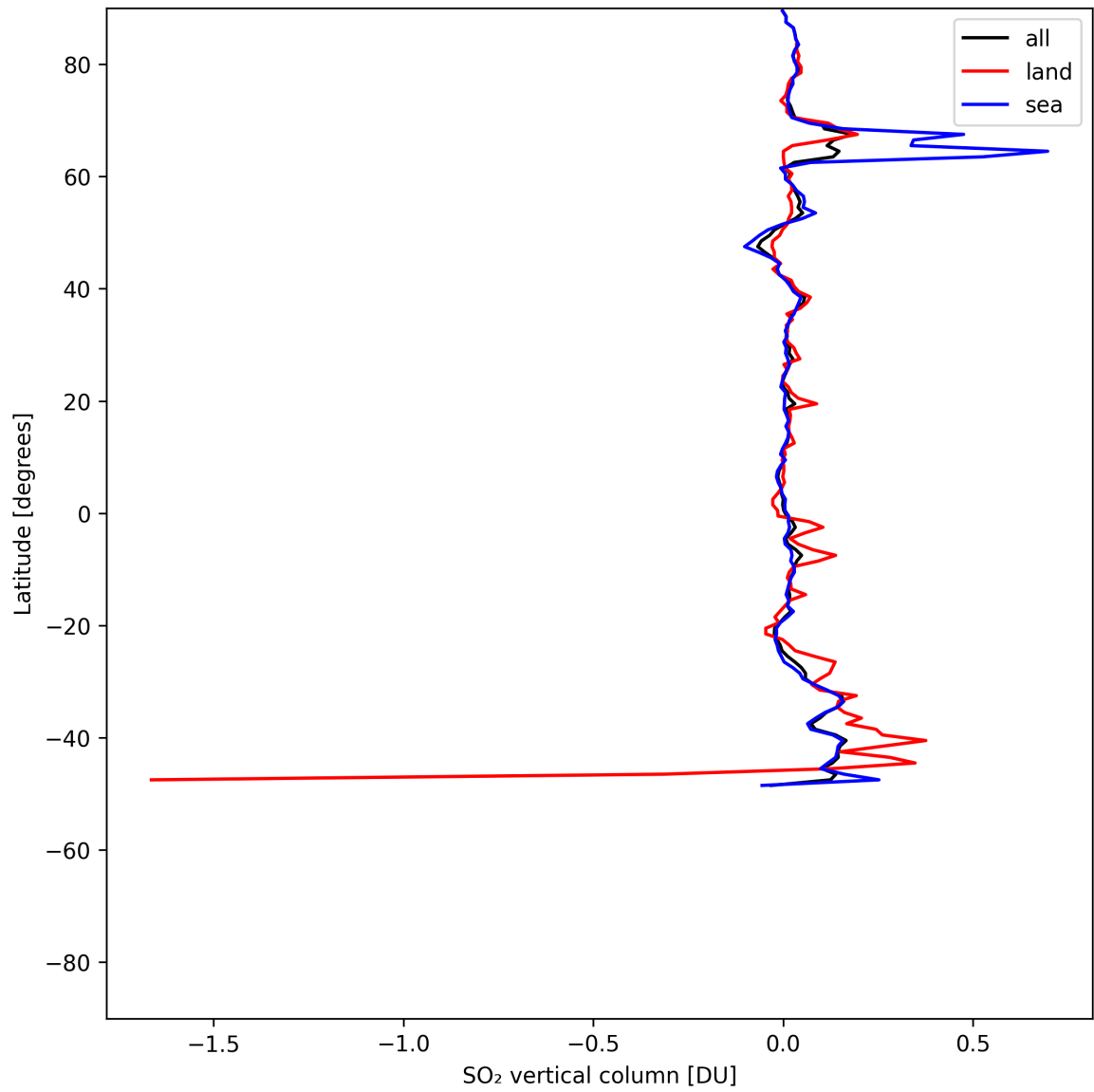
Figure 32: Zonal average of “SO 2 vertical column” for 2025-07-16 to 2025-07-18.
