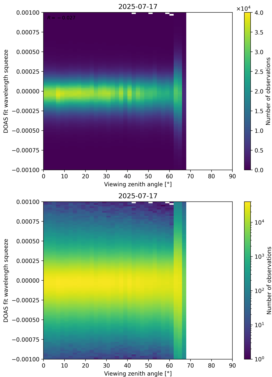
Figure 366: Scatter density plot of “Viewing zenith angle” against “DOAS fit wavelength squeeze” for 2025-07-16 to 2025-07-18.
