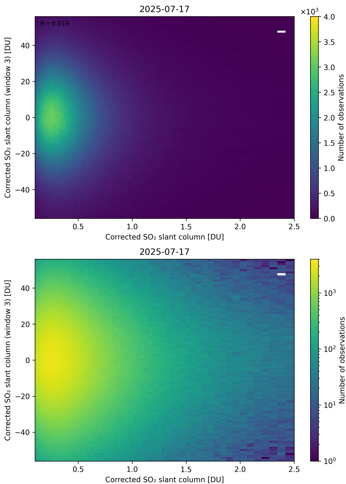
Figure 236: Scatter density plot of “Corrected SO 2 slant column” against “Corrected SO 2 slant column (window 3)” for 2025-07-16 to 2025-07-18.
