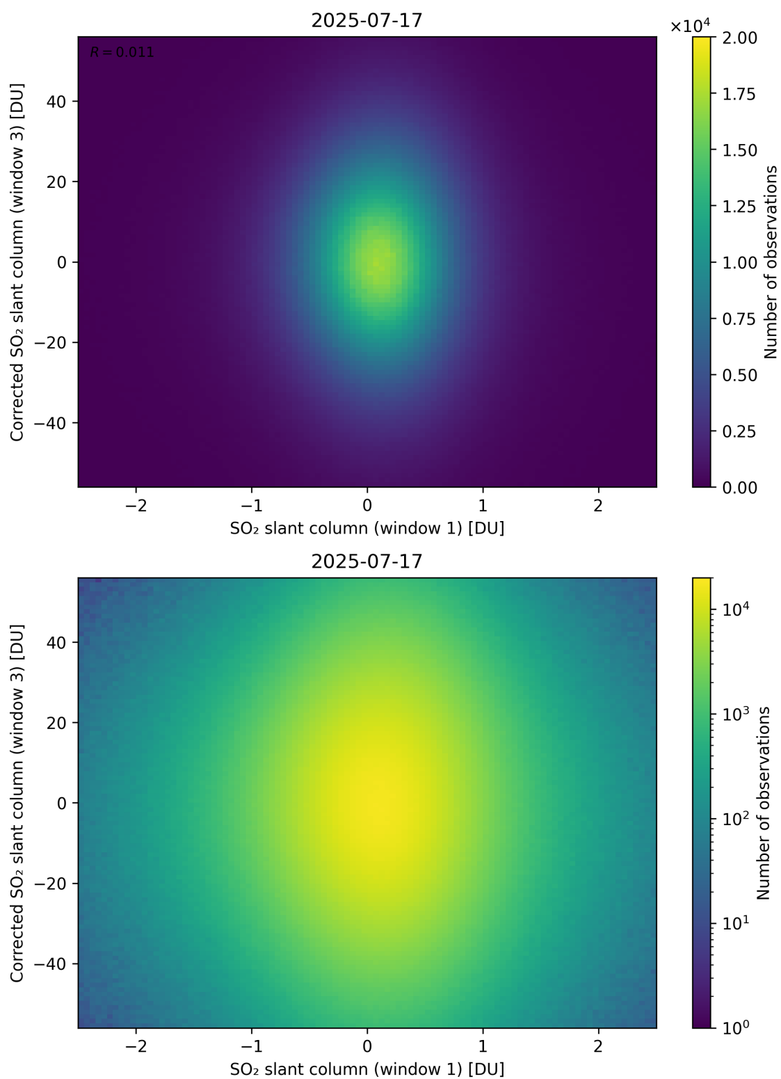
Figure 284: Scatter density plot of “SO 2 slant column (window 1)” against “Corrected SO 2 slant column (window 3)” for 2025-07-16 to 2025-07-18.
