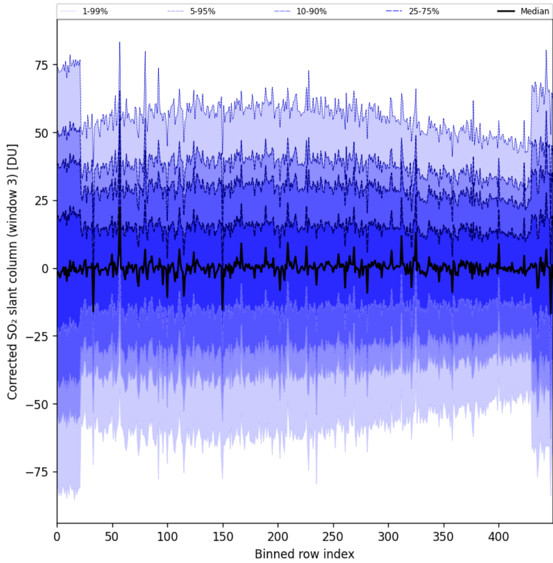
Figure 99: Along track statistics of “Corrected SO 2 slant column (window 3)” for 2025-07-16 to 2025-07-18
