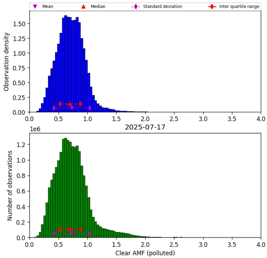
Figure 81: Histogram of “Clear AMF (polluted)” for 2025-07-16 to 2025-07-18
