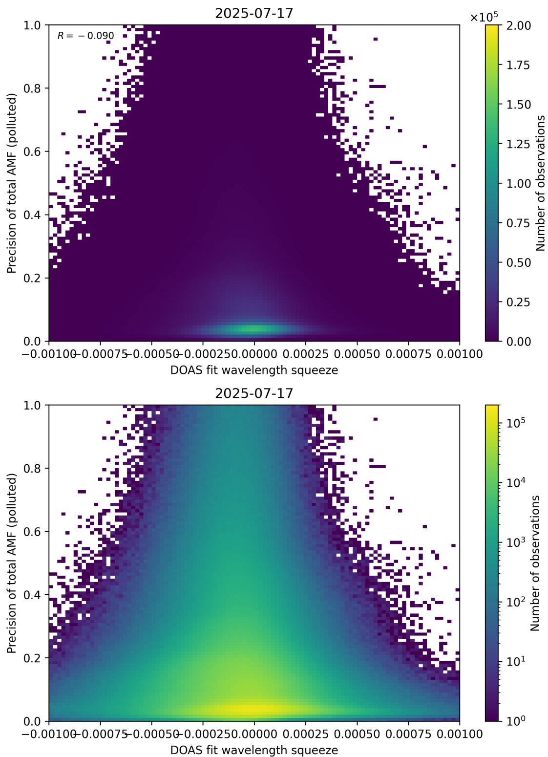
Figure 146: Scatter density plot of “DOAS fit wavelength squeeze” against “Precision of total AMF (polluted)” for 2025-07-16 to 2025-07-18.
