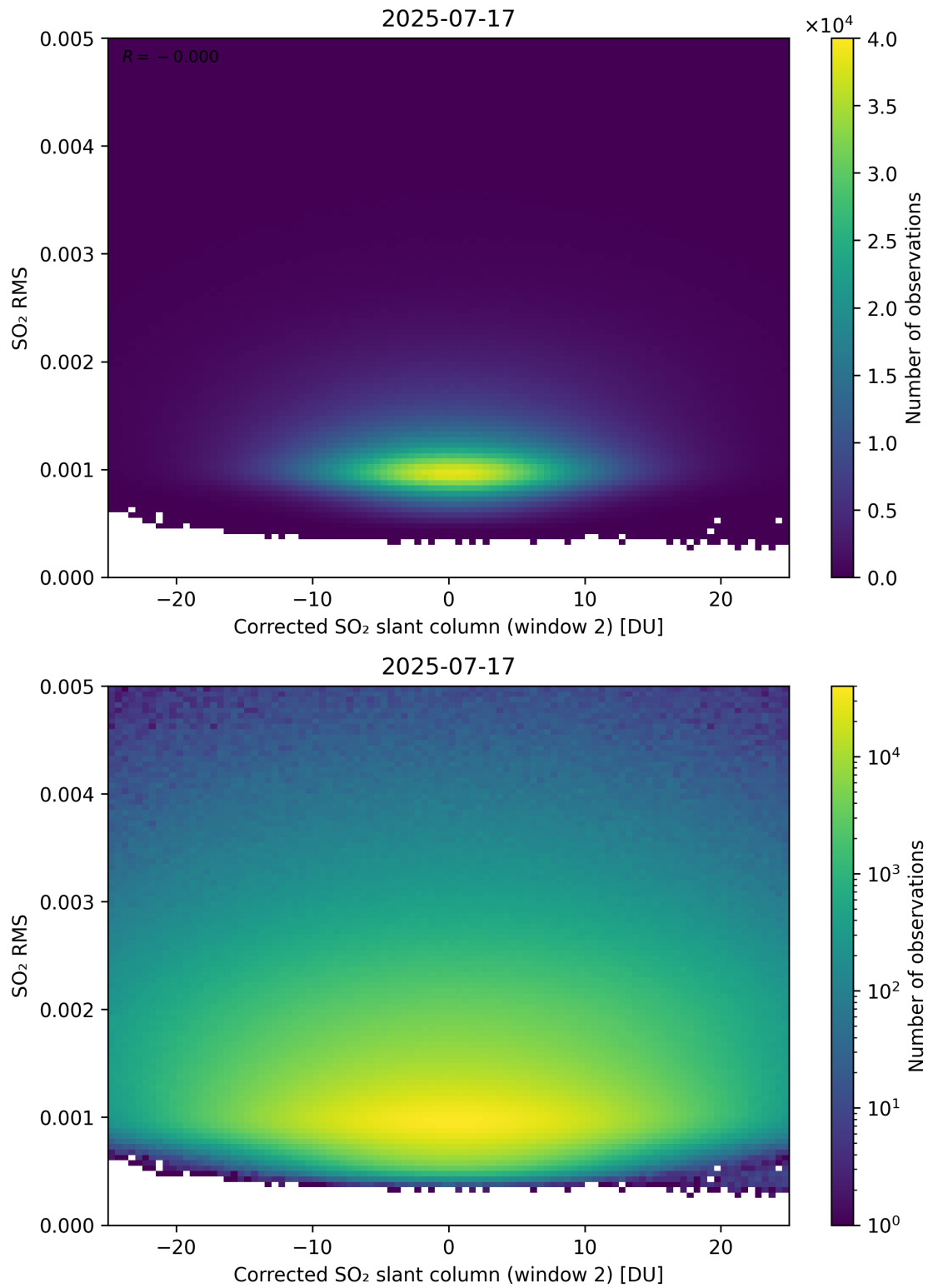
Figure 248: Scatter density plot of “Corrected SO 2 slant column (window 2)” against “SO 2 RMS” for 2025-07-16 to 2025-07-18.
