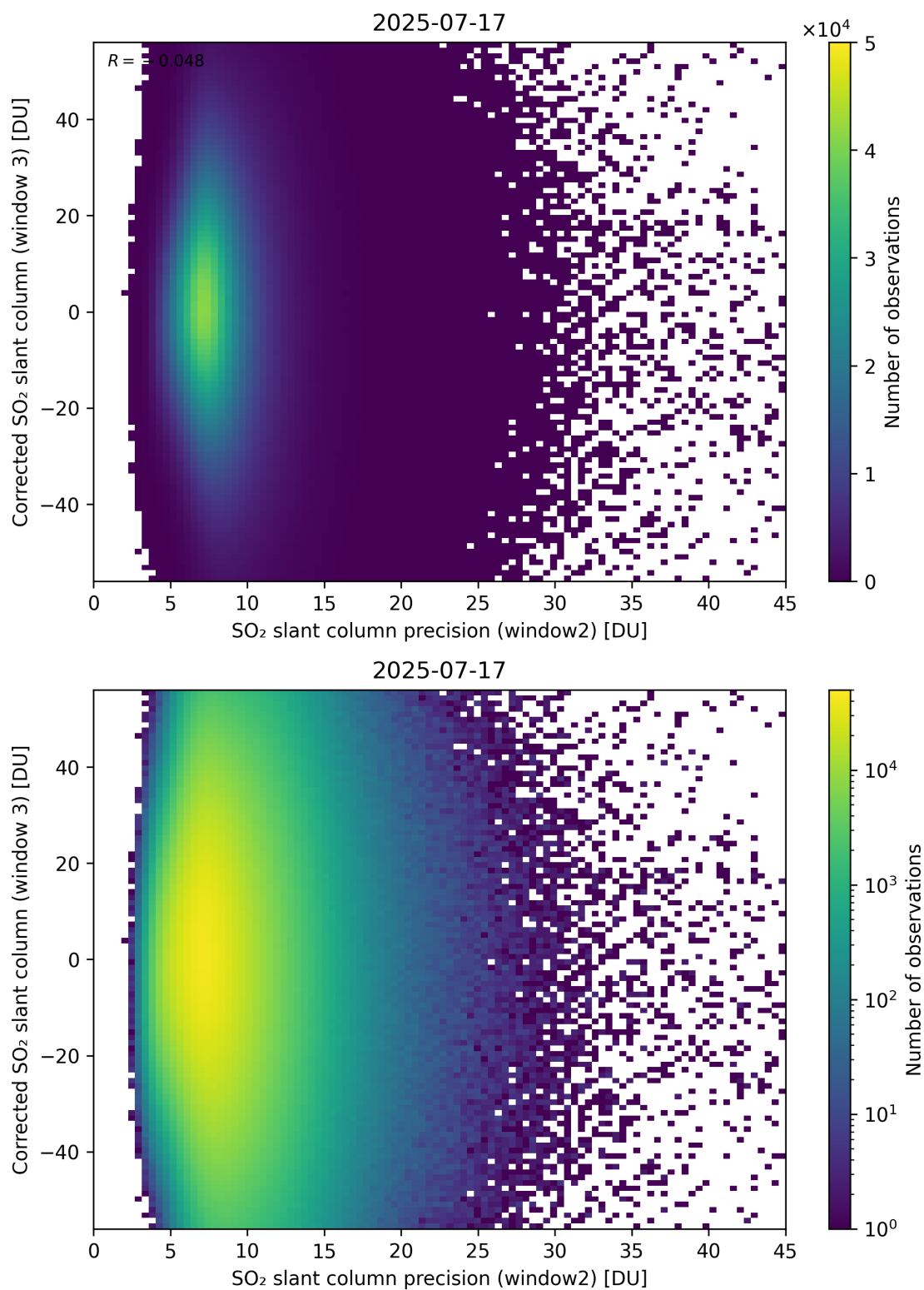
Figure 298: Scatter density plot of “SO 2 slant column precision (window2)” against “Corrected SO 2 slant column (window 3)” for 2025-07-16 to 2025-07-18.
