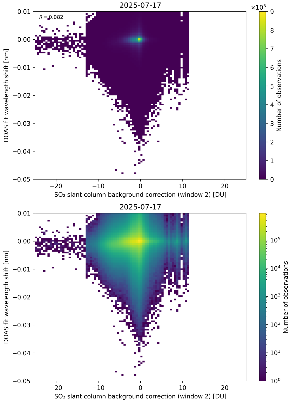
Figure 123: Scatter density plot of “SO 2 slant column background correction (window 2)” against “DOAS fit wavelength shift” for 2025-07-16 to 2025-07-18.
