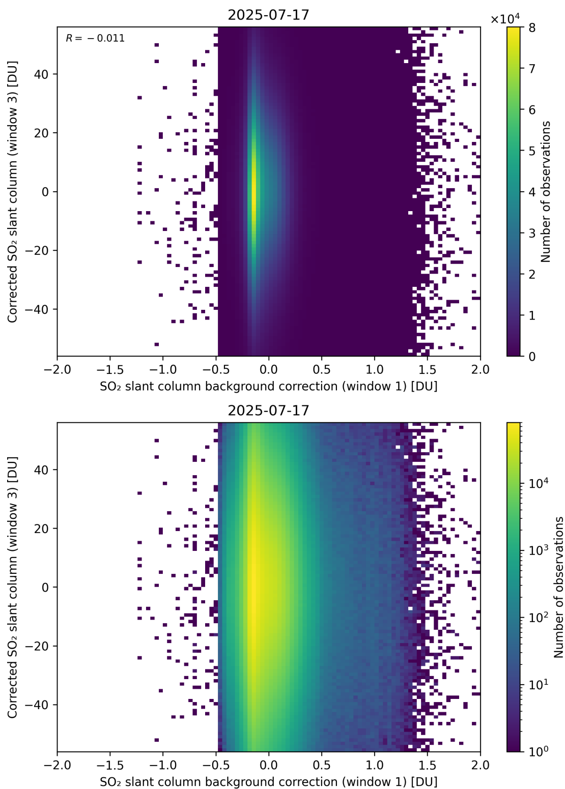
Figure 116: Scatter density plot of “SO 2 slant column background correction (window 1)” against “Corrected SO 2 slant column (window 3)” for 2025-07-16 to 2025-07-18.
