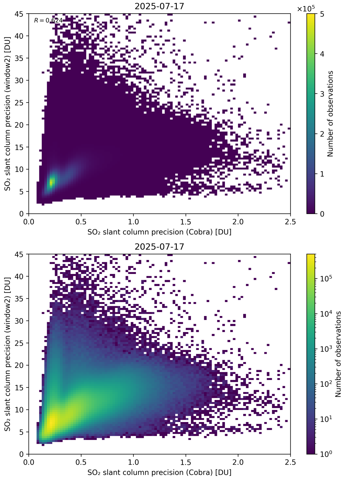
Figure 210: Scatter density plot of “SO 2 slant column precision (Cobra)” against “SO 2 slant column precision (window2)” for 2025-07-16 to 2025-07-18.
