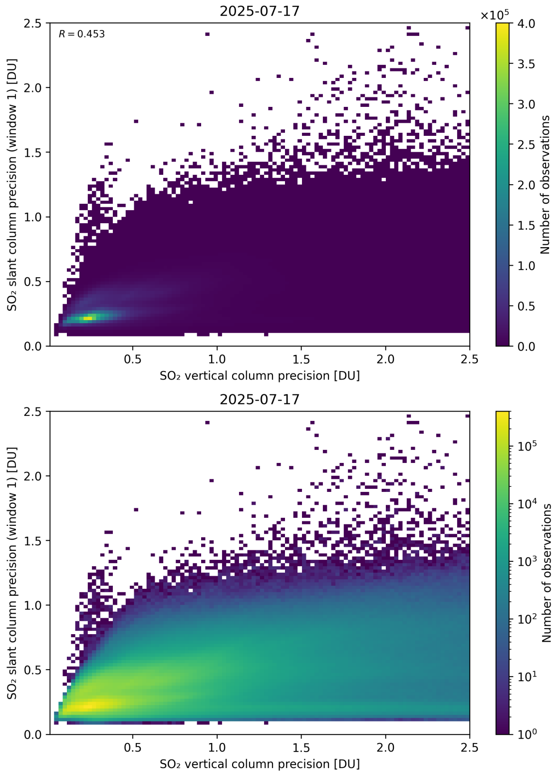
Figure 342: Scatter density plot of “SO 2 vertical column precision” against “SO 2 slant column precision (window 1)” for 2025-07-16 to 2025-07-18.
