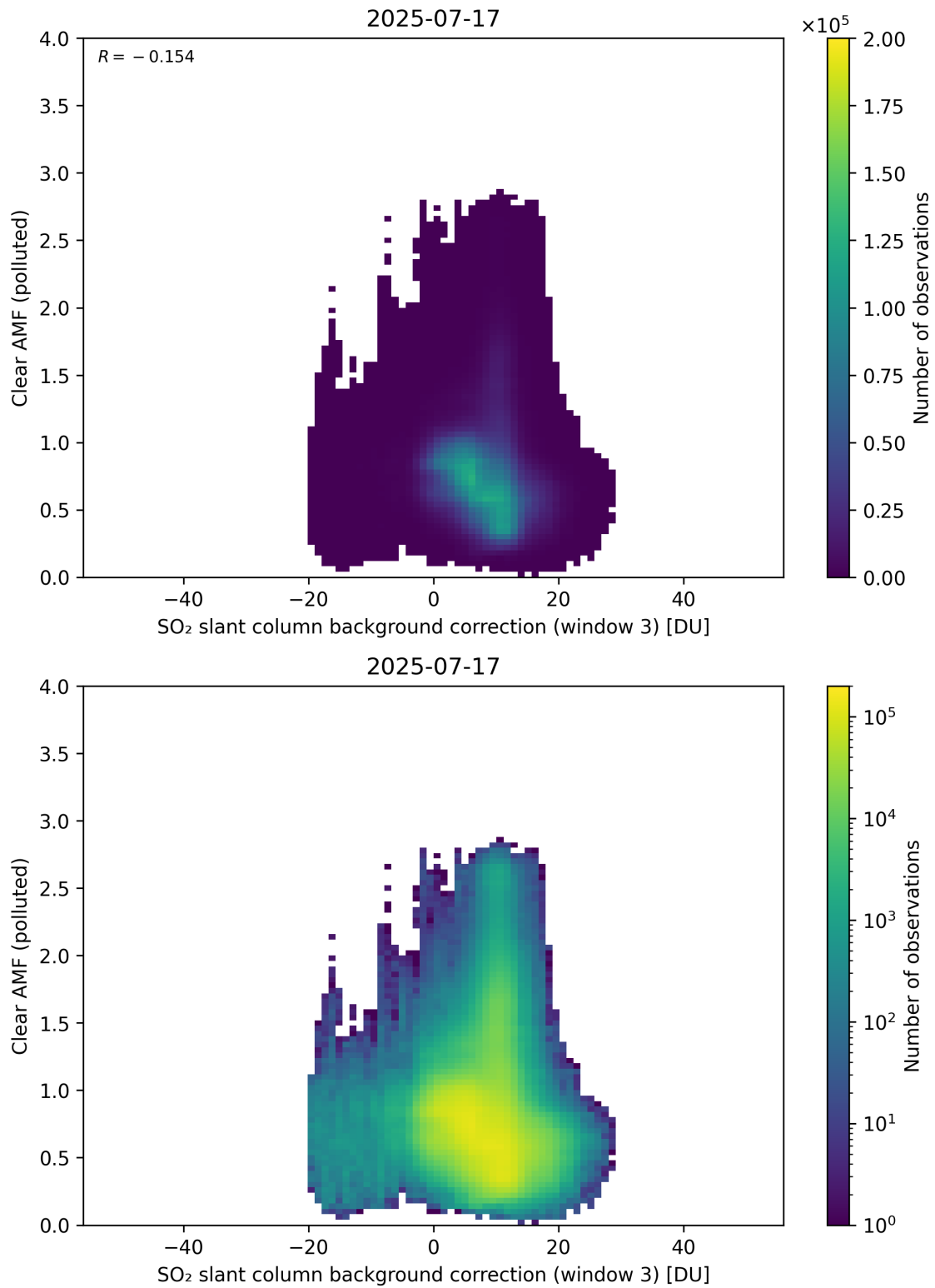
Figure 135: Scatter density plot of “SO 2 slant column background correction (window 3)” against “Clear AMF (polluted)” for 2025-07-16 to 2025-07-18.
