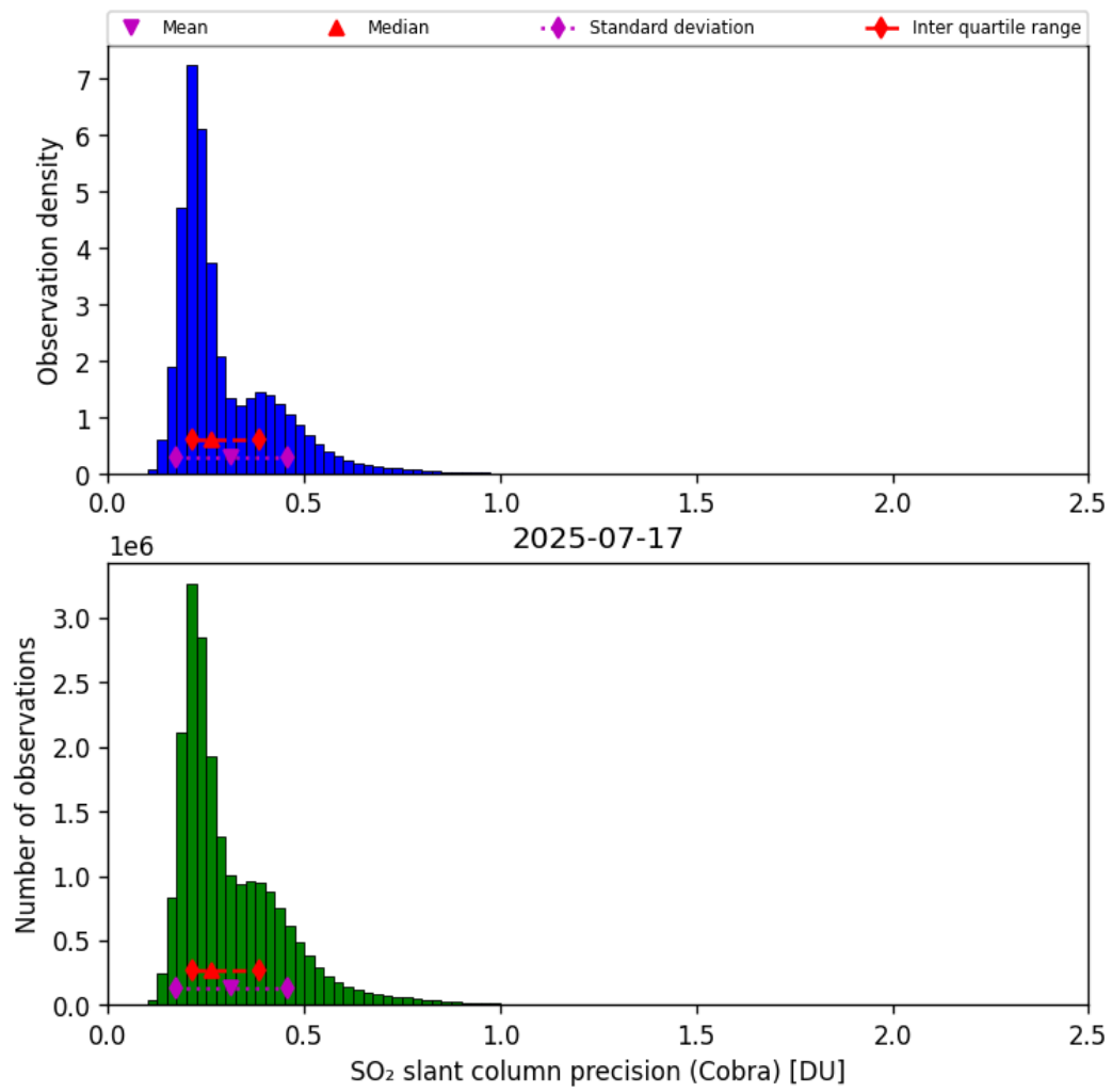
Figure 62: Histogram of “SO 2 slant column precision (Cobra)” for 2025-07-16 to 2025-07-18
