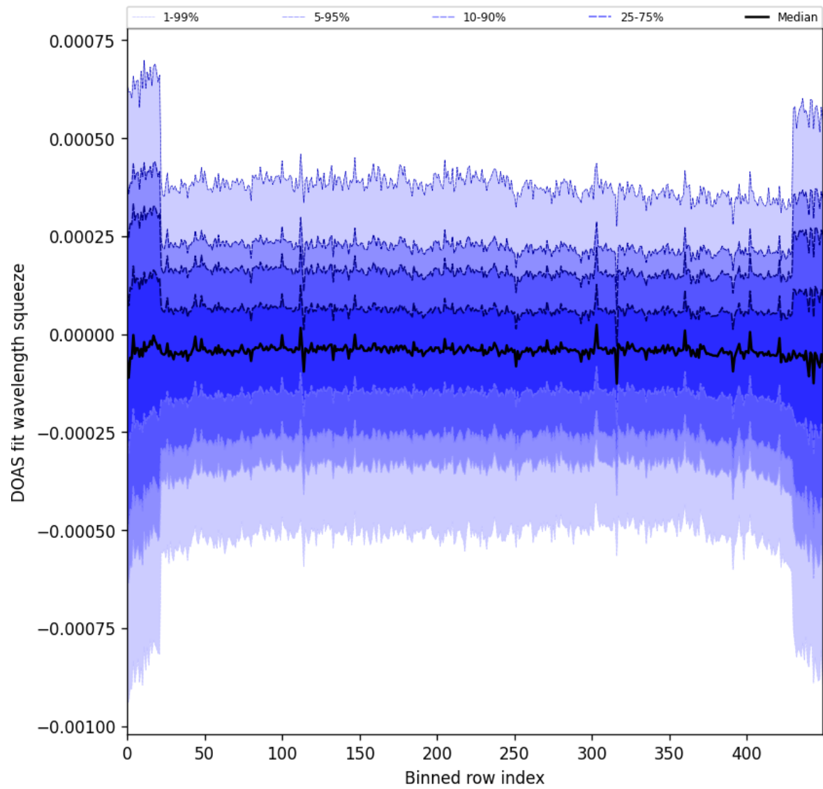
Figure 103: Along track statistics of “DOAS fit wavelength squeeze” for 2025-07-16 to 2025-07-18
