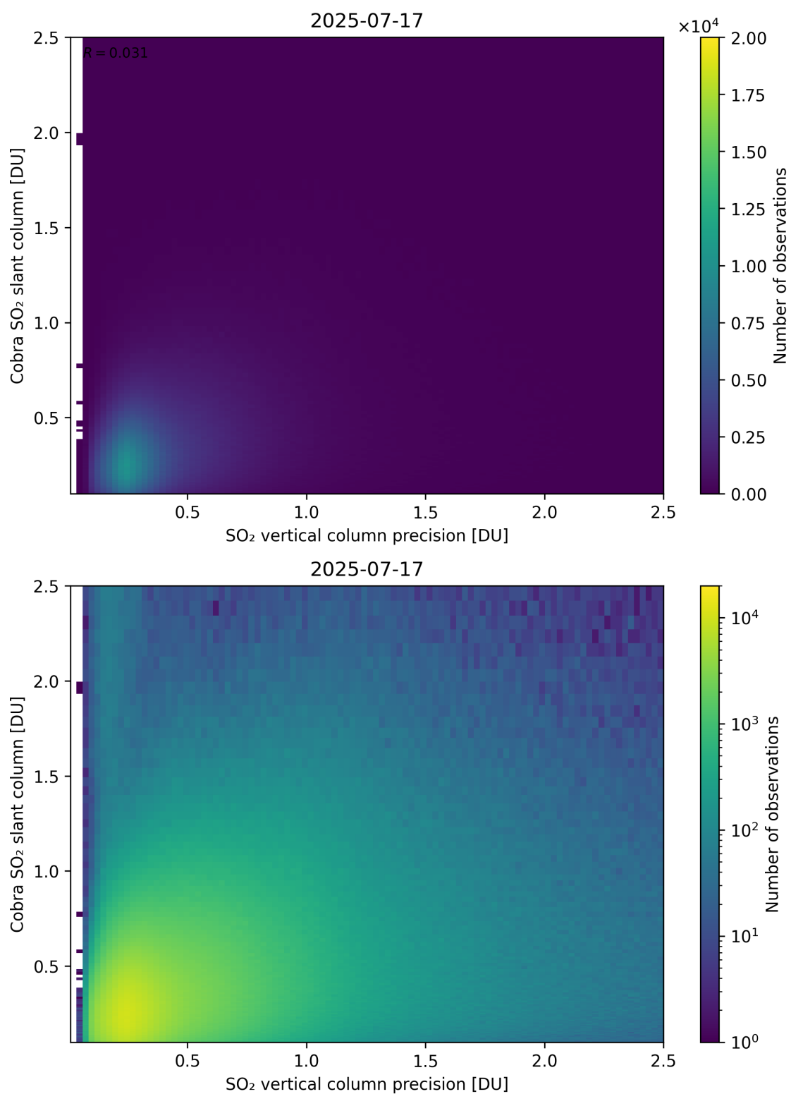
Figure 336: Scatter density plot of “SO 2 vertical column precision” against “Cobra SO 2 slant column” for 2025-07-16 to 2025-07-18.
