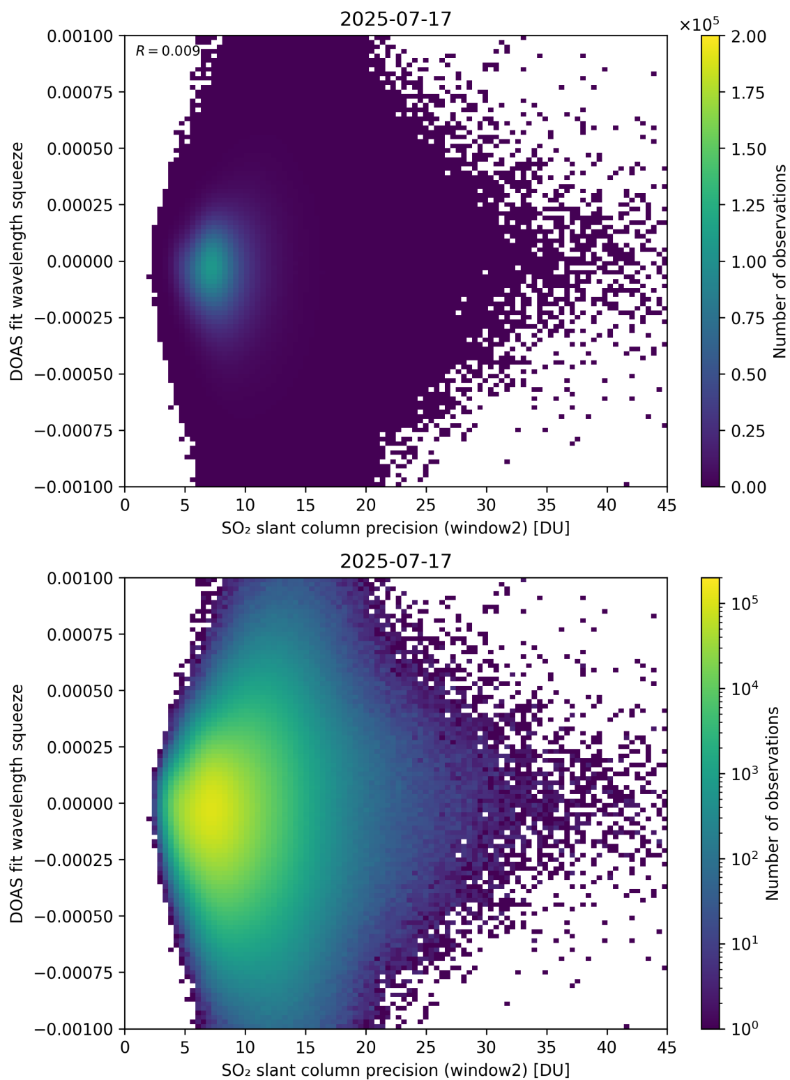
Figure 294: Scatter density plot of “SO 2 slant column precision (window2)” against “DOAS fit wavelength squeeze” for 2025-07-16 to 2025-07-18.
