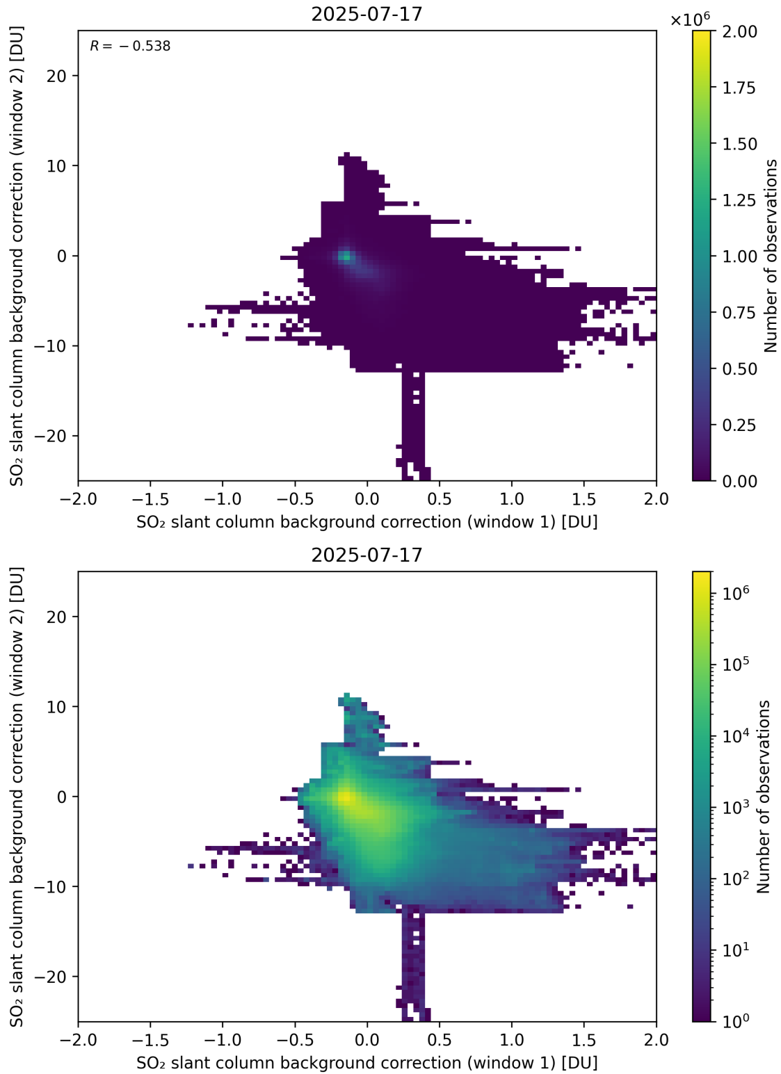
Figure 109: Scatter density plot of “SO 2 slant column background correction (window 1)” against “SO 2 slant column background correction (window 2)” for 2025-07-16 to 2025-07-18.
