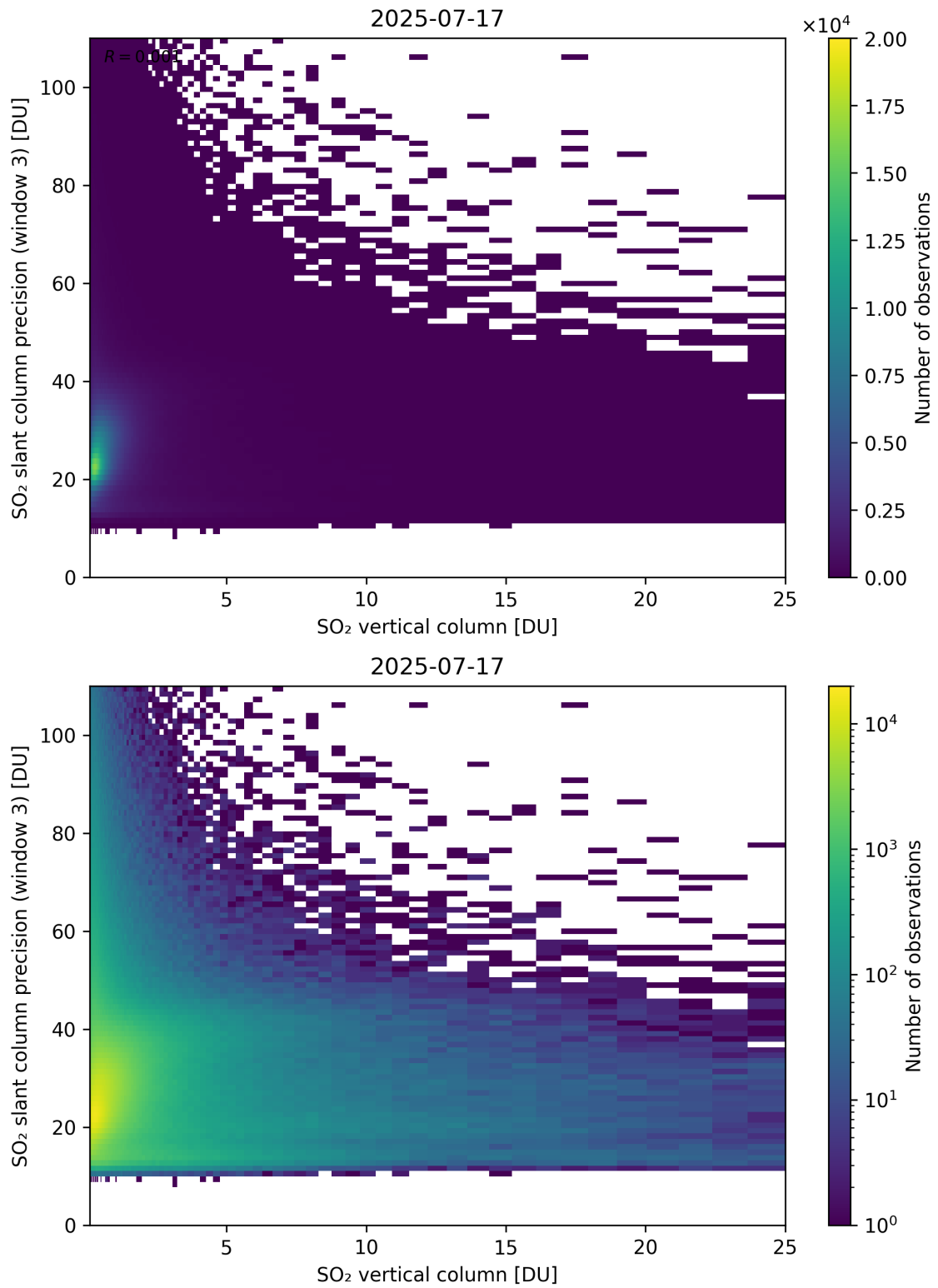
Figure 358: Scatter density plot of “SO 2 vertical column” against “SO 2 slant column precision (window 3)” for 2025-07-16 to 2025-07-18.
