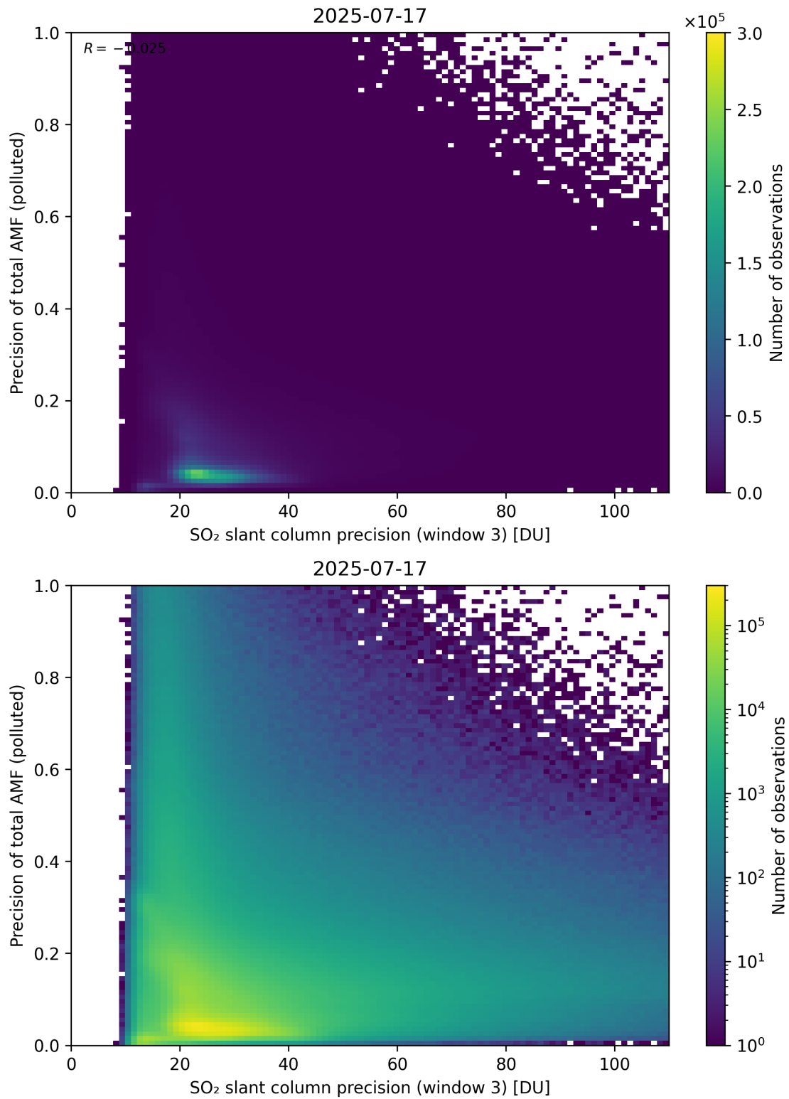
Figure 314: Scatter density plot of “SO 2 slant column precision (window 3)” against “Precision of total AMF (polluted)” for 2025-07-16 to 2025-07-18.
