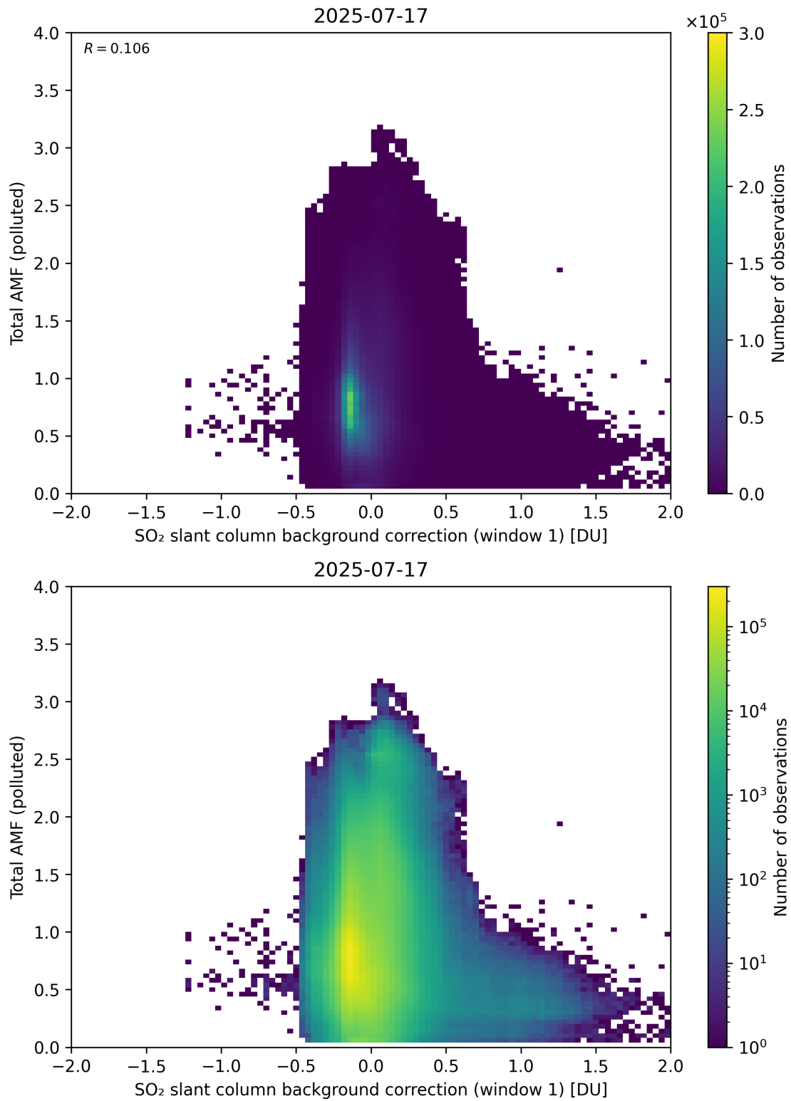
Figure 120: Scatter density plot of “SO 2 slant column background correction (window 1)” against “Total AMF (polluted)” for 2025-07-16 to 2025-07-18.
