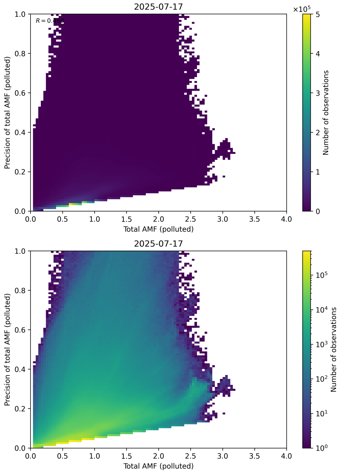
Figure 322: Scatter density plot of “Total AMF (polluted)” against “Precision of total AMF (polluted)” for 2025-07-16 to 2025-07-18.
