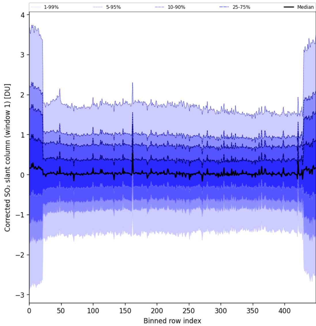
Figure 91: Along track statistics of “Corrected SO 2 slant column (window 1)” for 2025-07-16 to 2025-07-18
