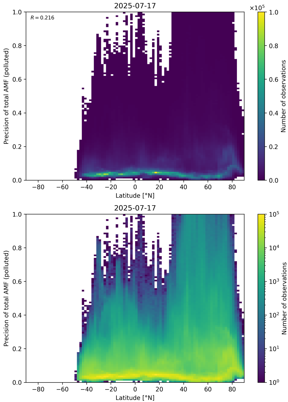
Figure 168: Scatter density plot of “Latitude” against “Precision of total AMF (polluted)” for 2025-07-16 to 2025-07-18.
