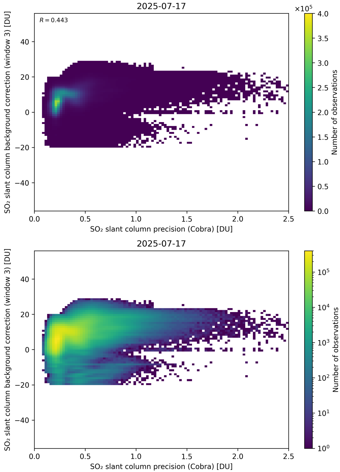
Figure 201: Scatter density plot of “SO 2 slant column precision (Cobra)” against “SO 2 slant column background correction (window 3)” for 2025-07-16 to 2025-07-18.
