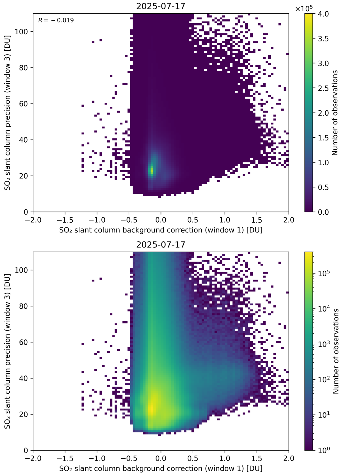
Figure 119: Scatter density plot of “SO 2 slant column background correction (window 1)” against “SO 2 slant column precision (window 3)” for 2025-07-16 to 2025-07-18.
