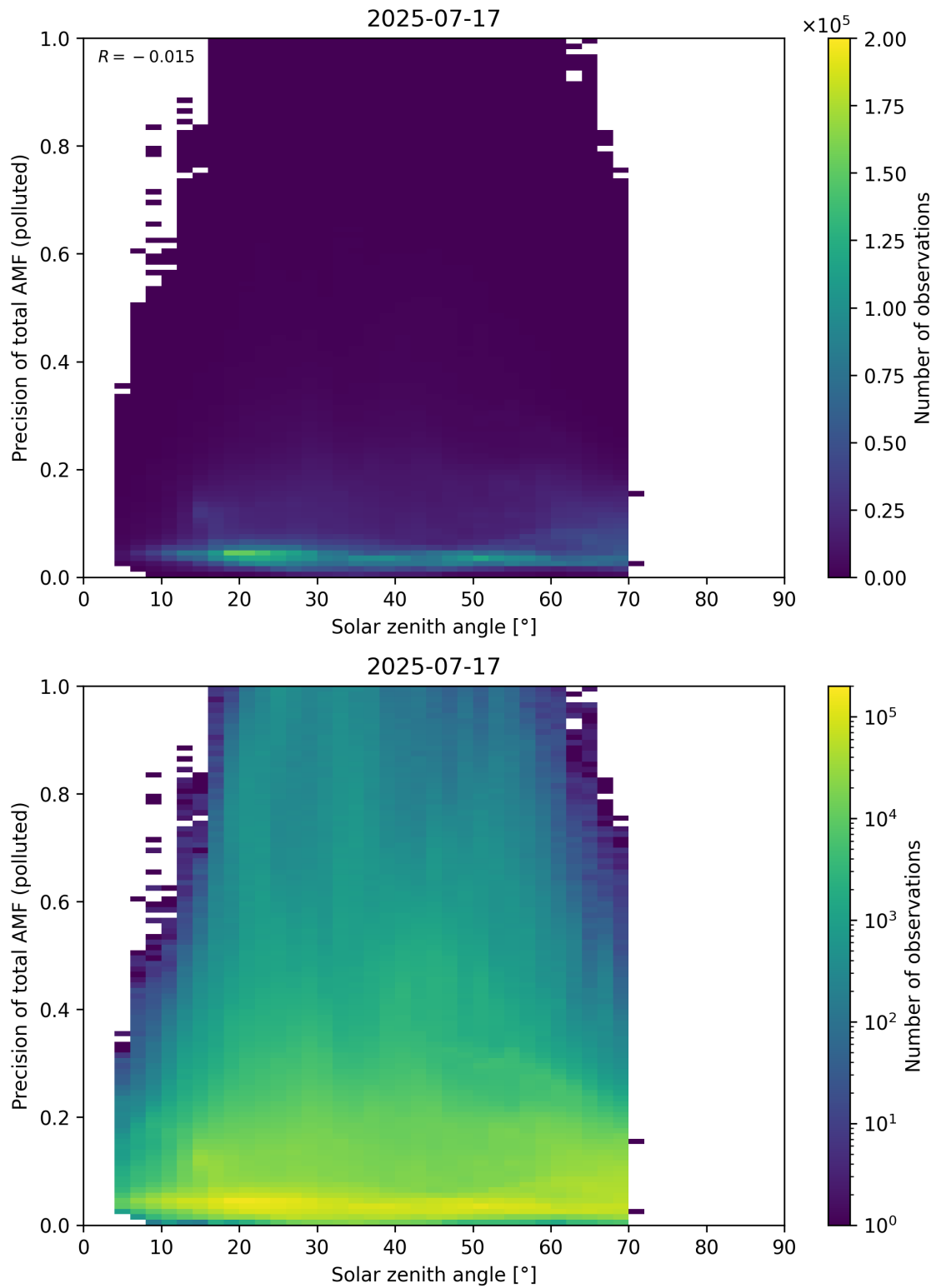
Figure 190: Scatter density plot of “Solar zenith angle” against “Precision of total AMF (polluted)” for 2025-07-16 to 2025-07-18.
