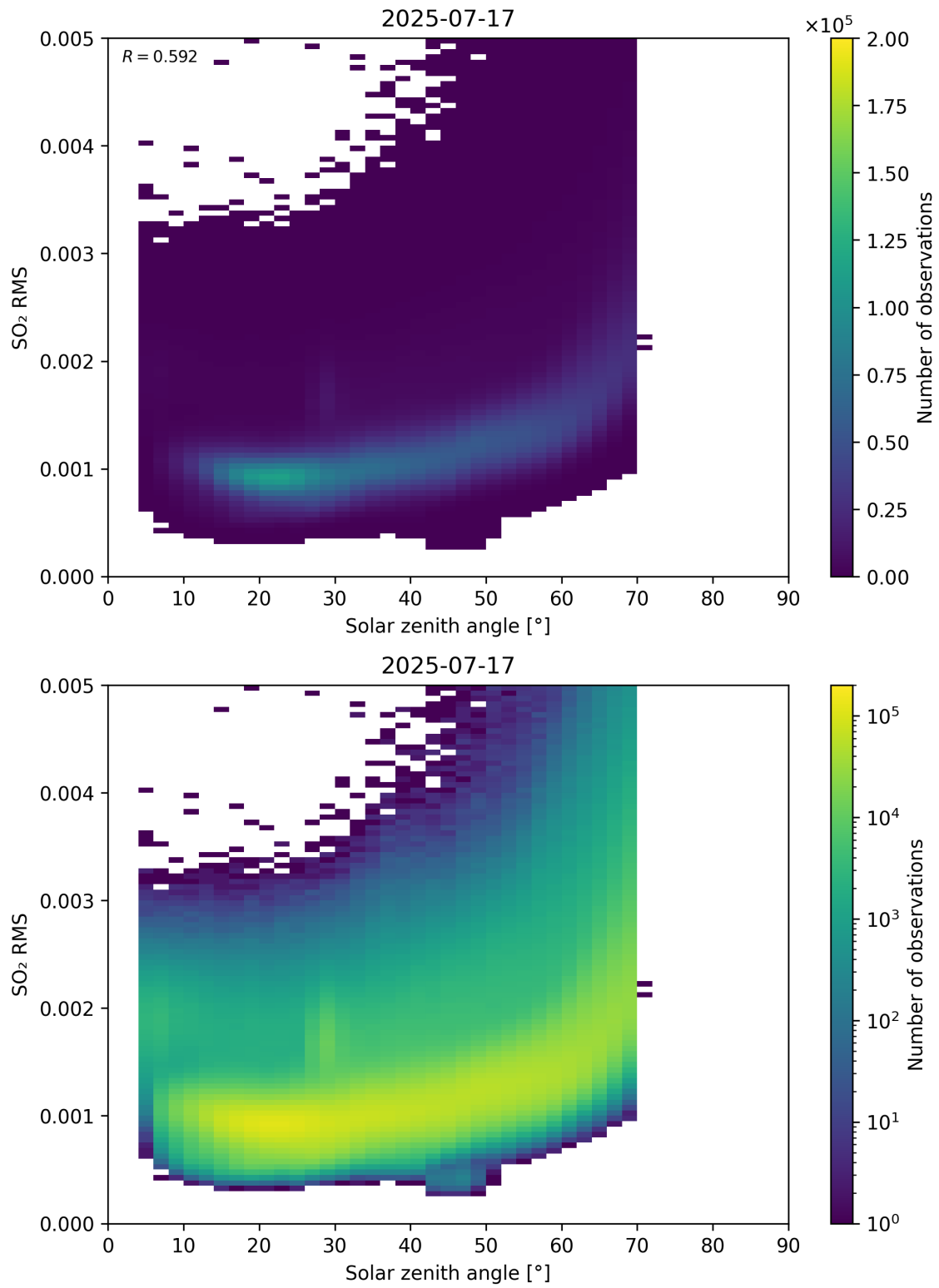
Figure 176: Scatter density plot of “Solar zenith angle” against “SO 2 RMS” for 2025-07-16 to 2025-07-18.
