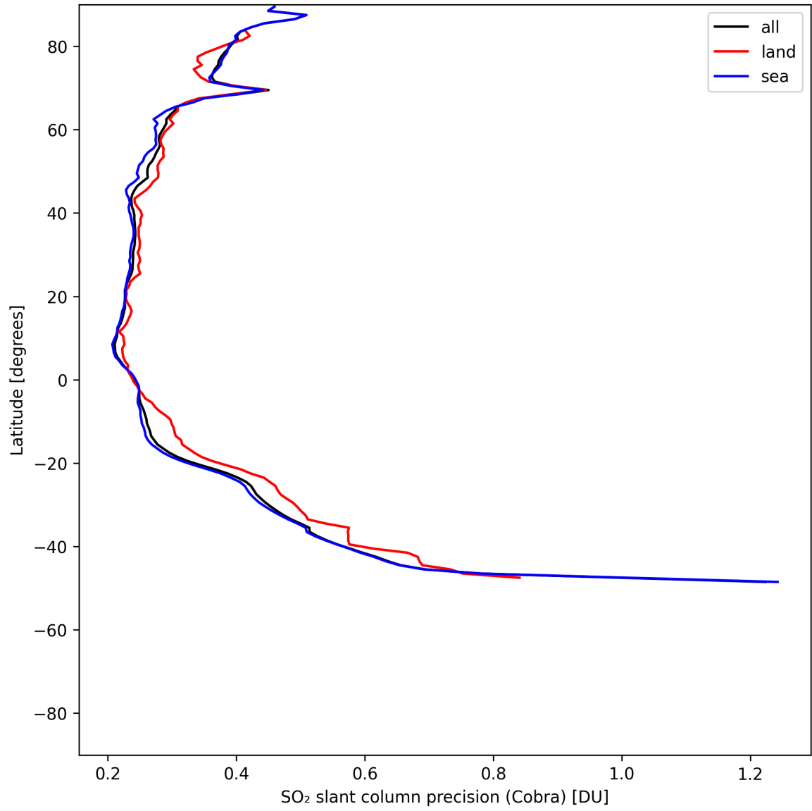
Figure 36: Zonal average of “SO 2 slant column precision (Cobra)” for 2025-07-16 to 2025-07-18.
