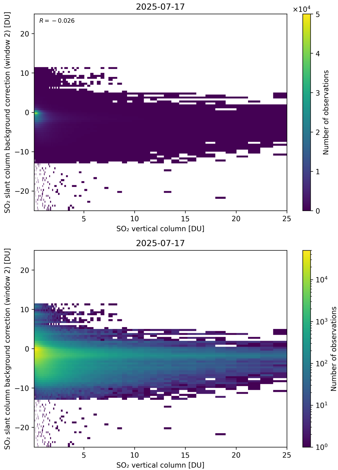
Figure 324: Scatter density plot of “SO 2 vertical column” against “SO 2 slant column background correction (window 2)” for 2025-07-16 to 2025-07-18.
