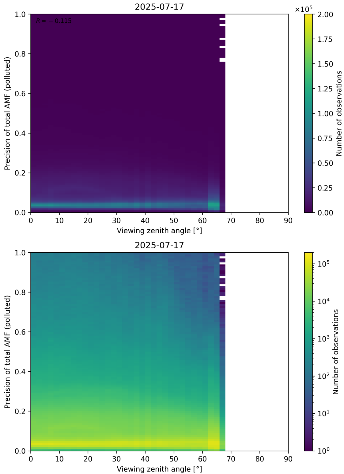
Figure 382: Scatter density plot of “Viewing zenith angle” against “Precision of total AMF (polluted)” for 2025-07-16 to 2025-07-18.
