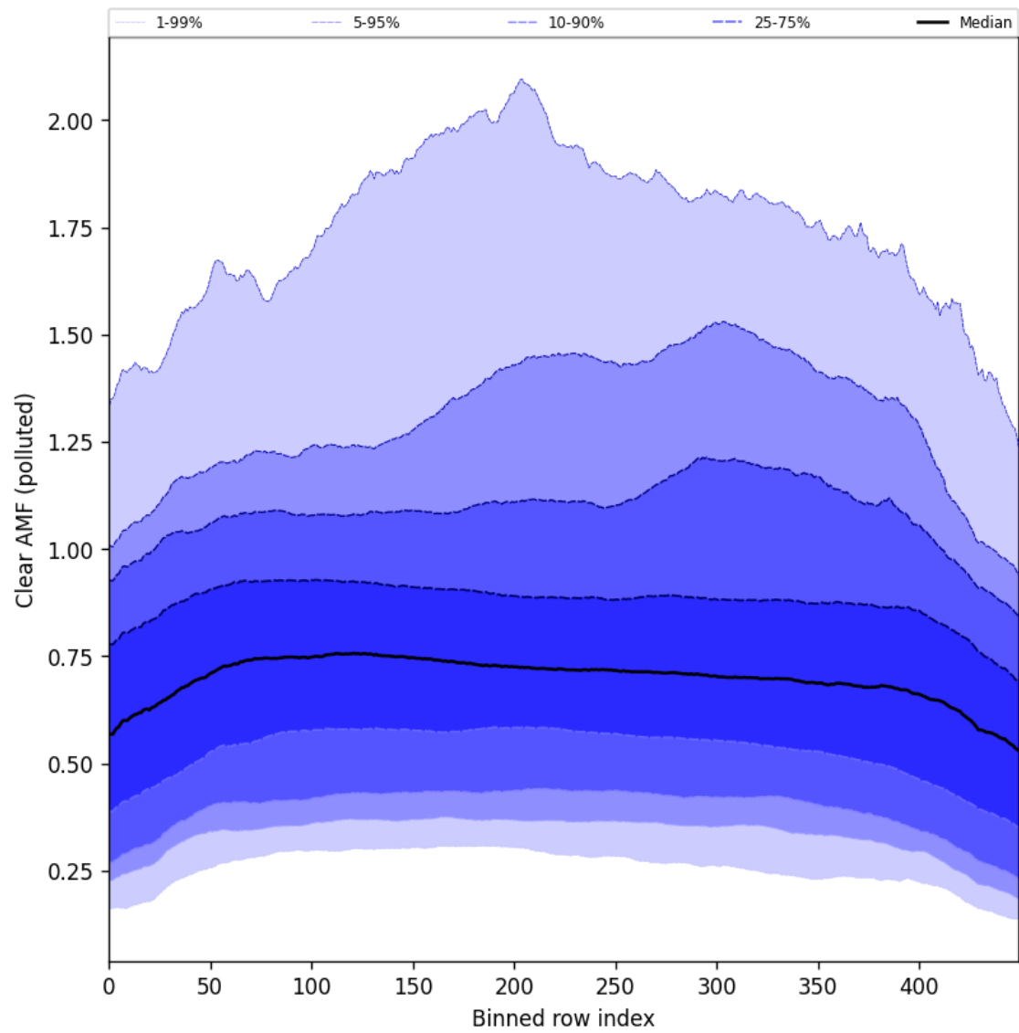
Figure 107: Along track statistics of “Clear AMF (polluted)” for 2025-07-16 to 2025-07-18
