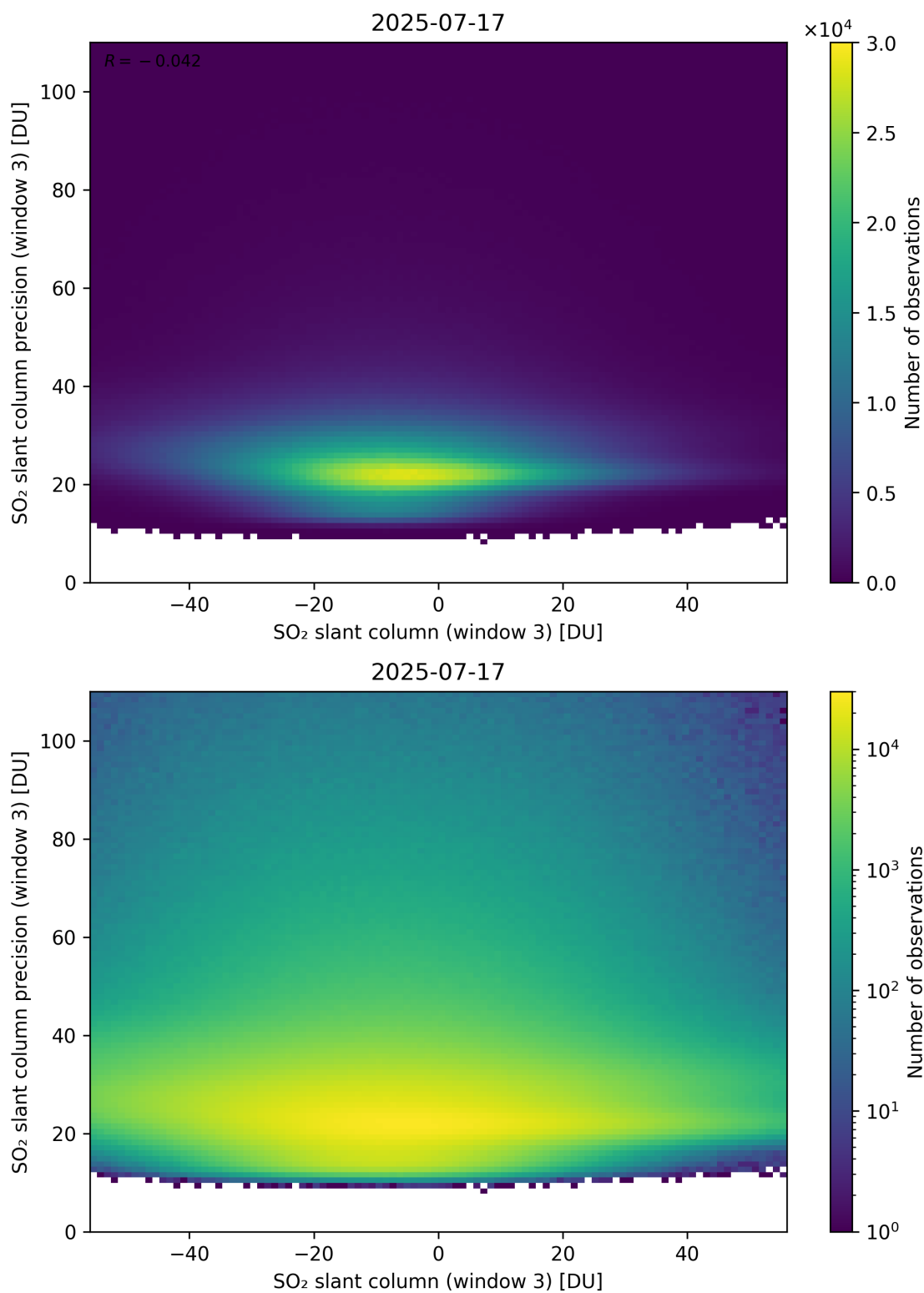
Figure 317: Scatter density plot of “SO 2 slant column (window 3)” against “SO 2 slant column precision (window 3)” for 2025-07-16 to 2025-07-18.
