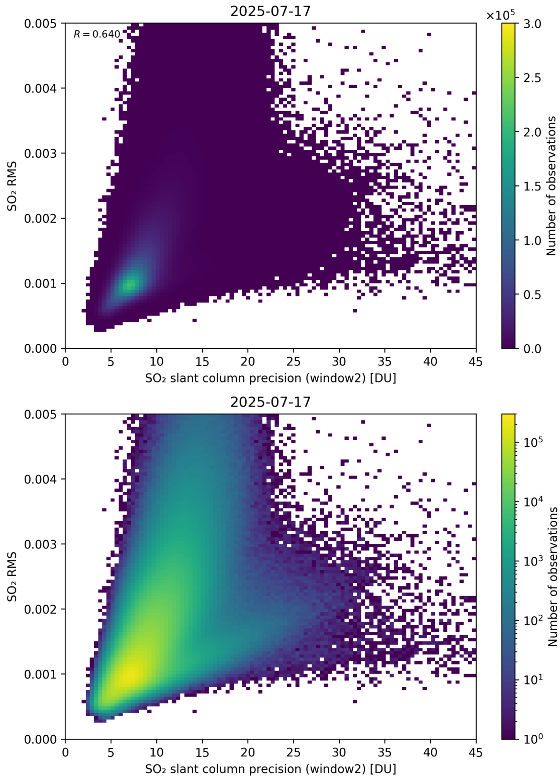
Figure 295: Scatter density plot of “SO 2 slant column precision (window2)” against “SO 2 RMS” for 2025-07-16 to 2025-07-18.
