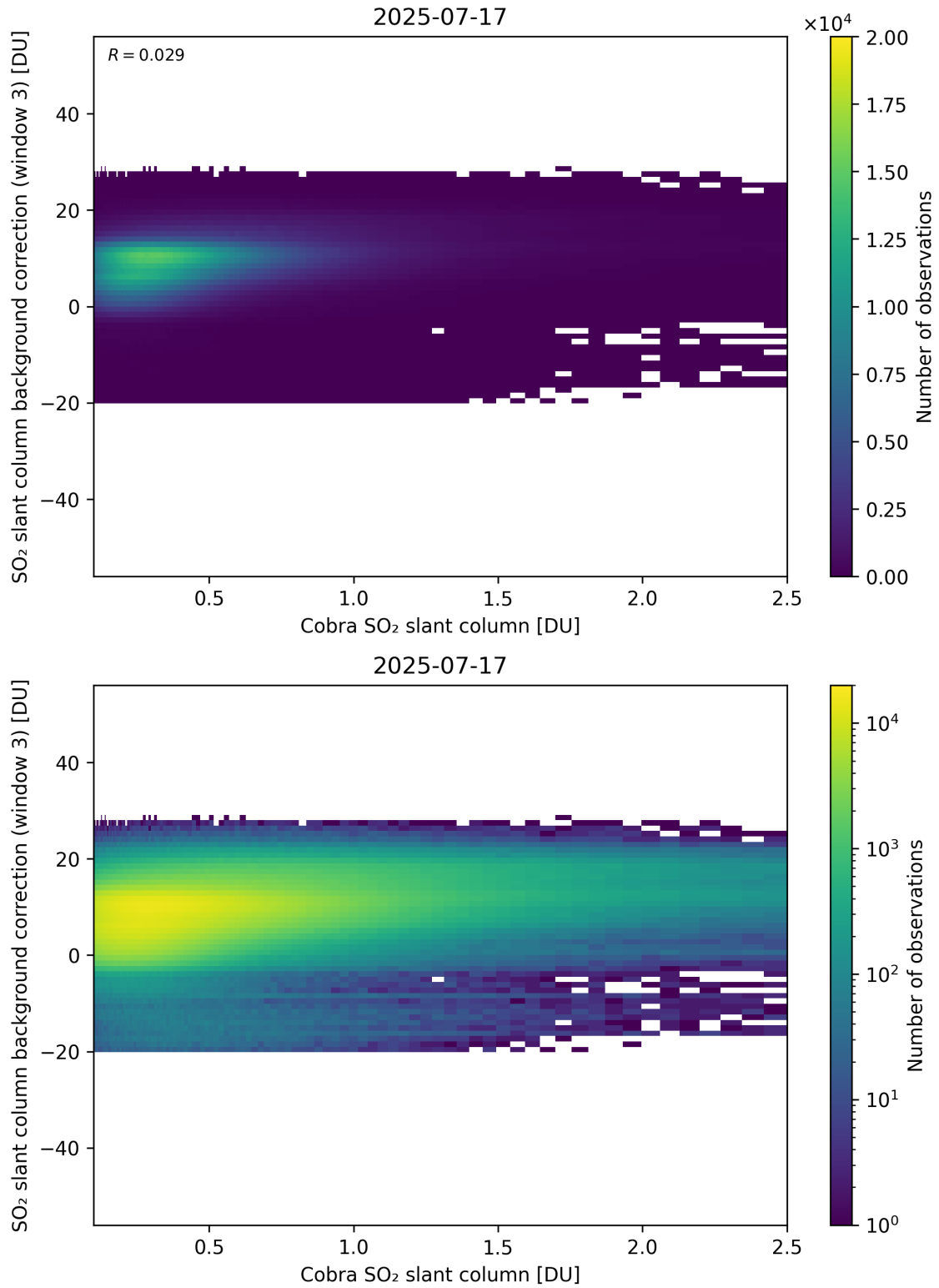
Figure 195: Scatter density plot of “Cobra SO 2 slant column” against “SO 2 slant column background correction (window 3)” for 2025-07-16 to 2025-07-18.
