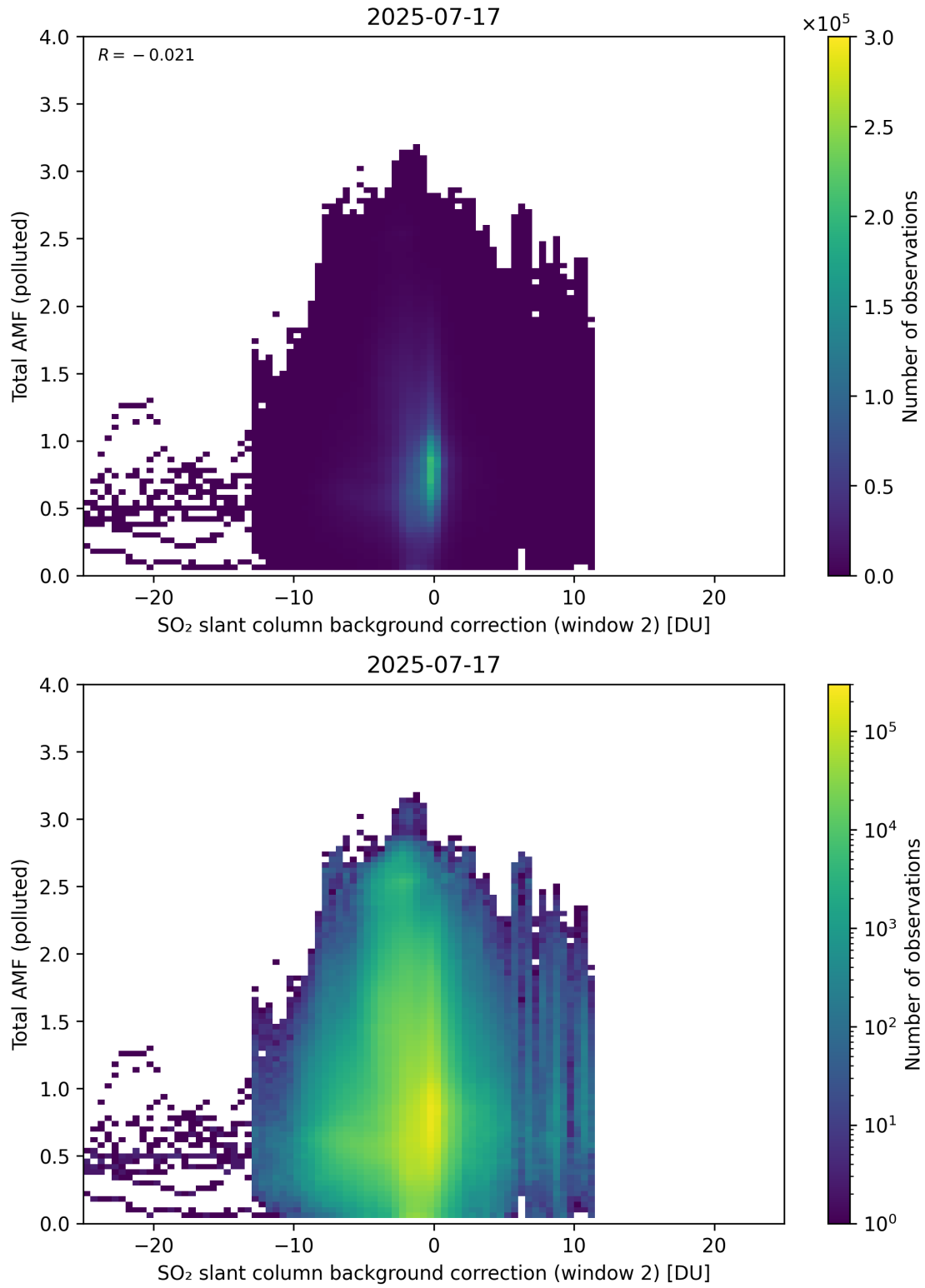
Figure 130: Scatter density plot of “SO 2 slant column background correction (window 2)” against “Total AMF (polluted)” for 2025-07-16 to 2025-07-18.
