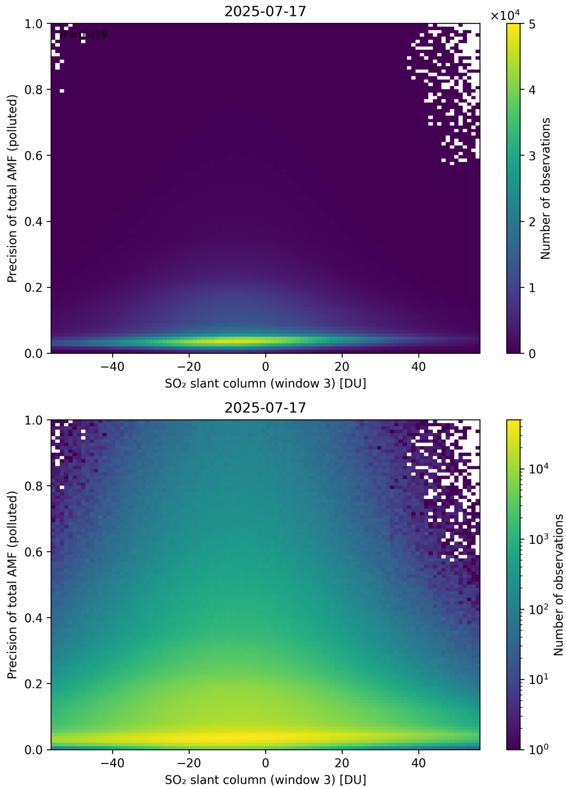
Figure 319: Scatter density plot of “SO 2 slant column (window 3)” against “Precision of total AMF (polluted)” for 2025-07-16 to 2025-07-18.
