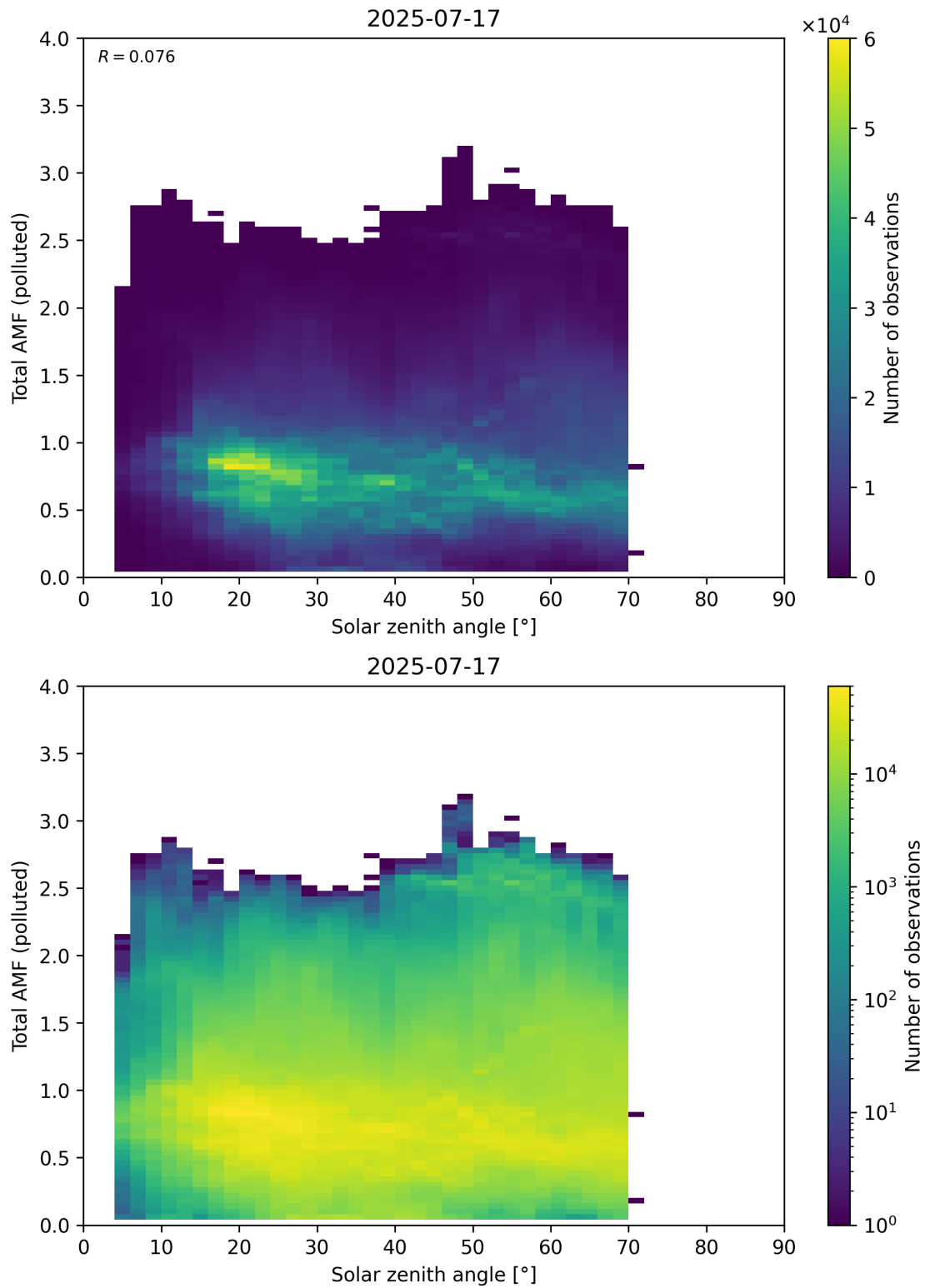
Figure 189: Scatter density plot of “Solar zenith angle” against “Total AMF (polluted)” for 2025-07-16 to 2025-07-18.
