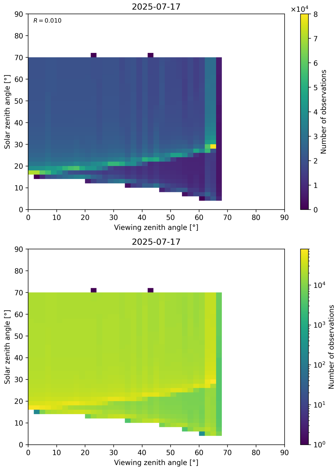
Figure 369: Scatter density plot of “Viewing zenith angle” against “Solar zenith angle” for 2025-07-16 to 2025-07-18.
