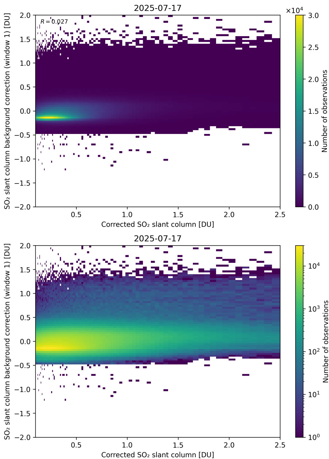
Figure 226: Scatter density plot of “Corrected SO 2 slant column” against “SO 2 slant column background correction (window 1)” for 2025-07-16 to 2025-07-18.
