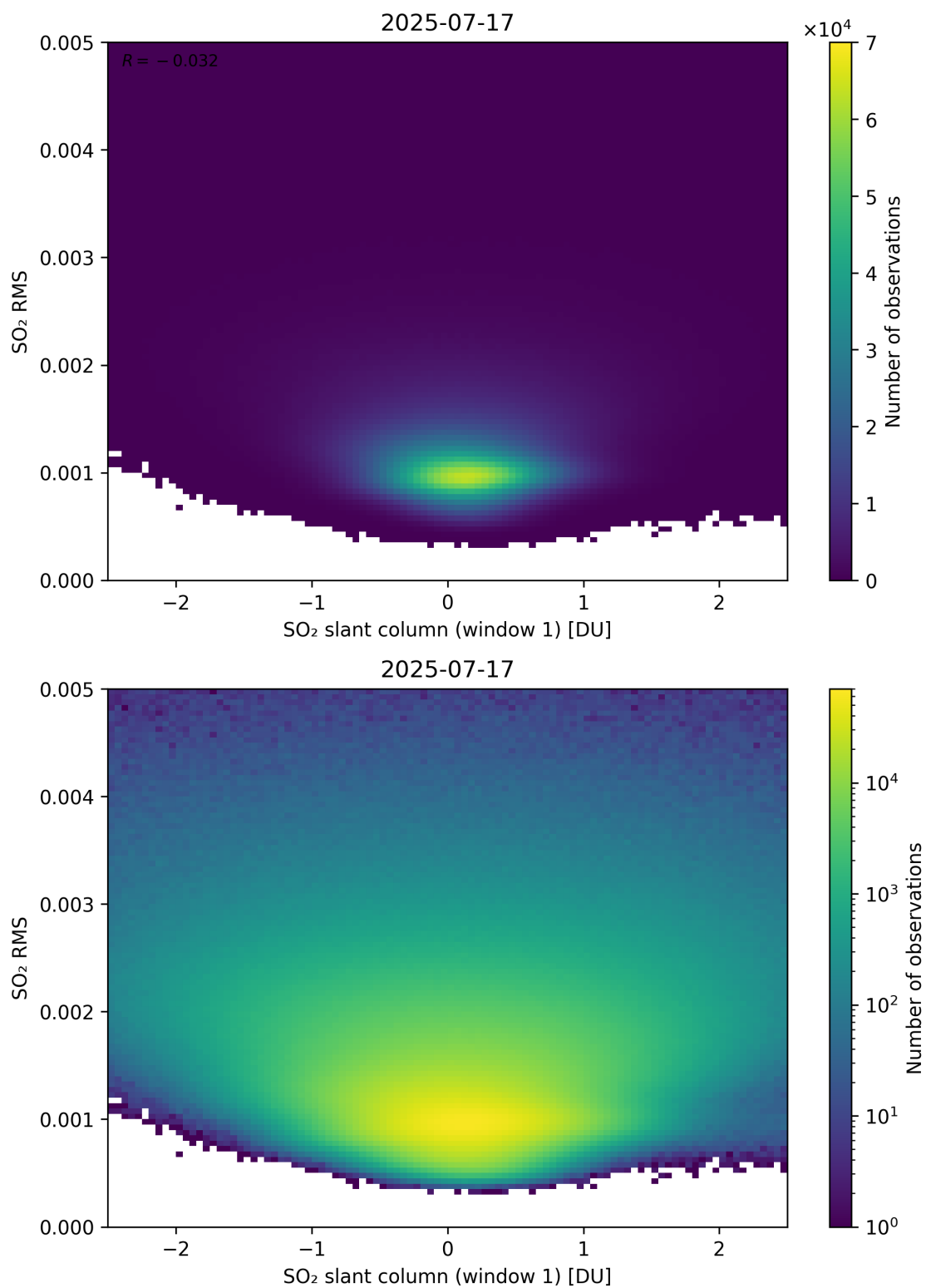
Figure 267: Scatter density plot of “SO 2 slant column (window 1)” against “SO 2 RMS” for 2025-07-16 to 2025-07-18.
