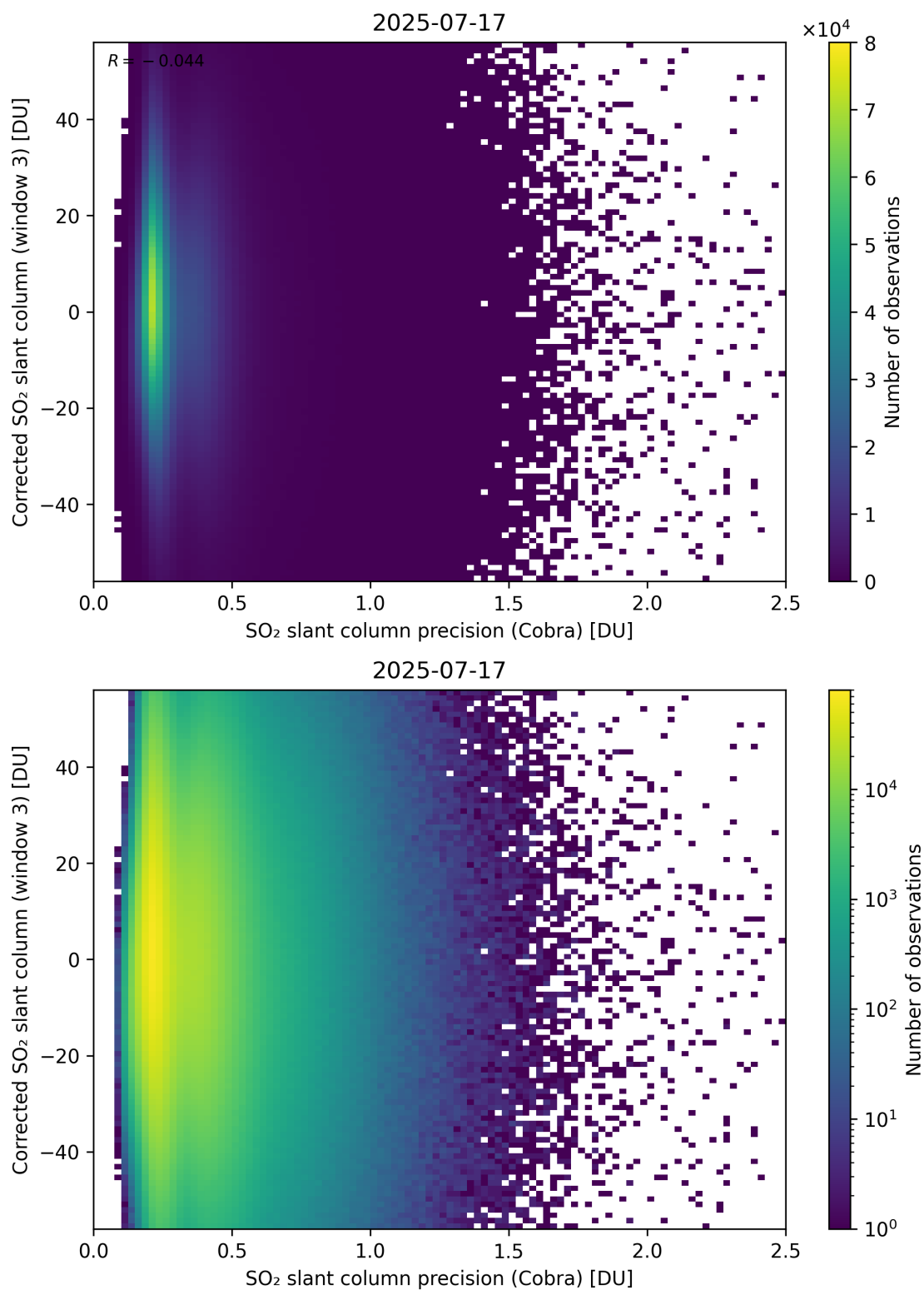
Figure 207: Scatter density plot of “SO 2 slant column precision (Cobra)” against “Corrected SO 2 slant column (window 3)” for 2025-07-16 to 2025-07-18.
