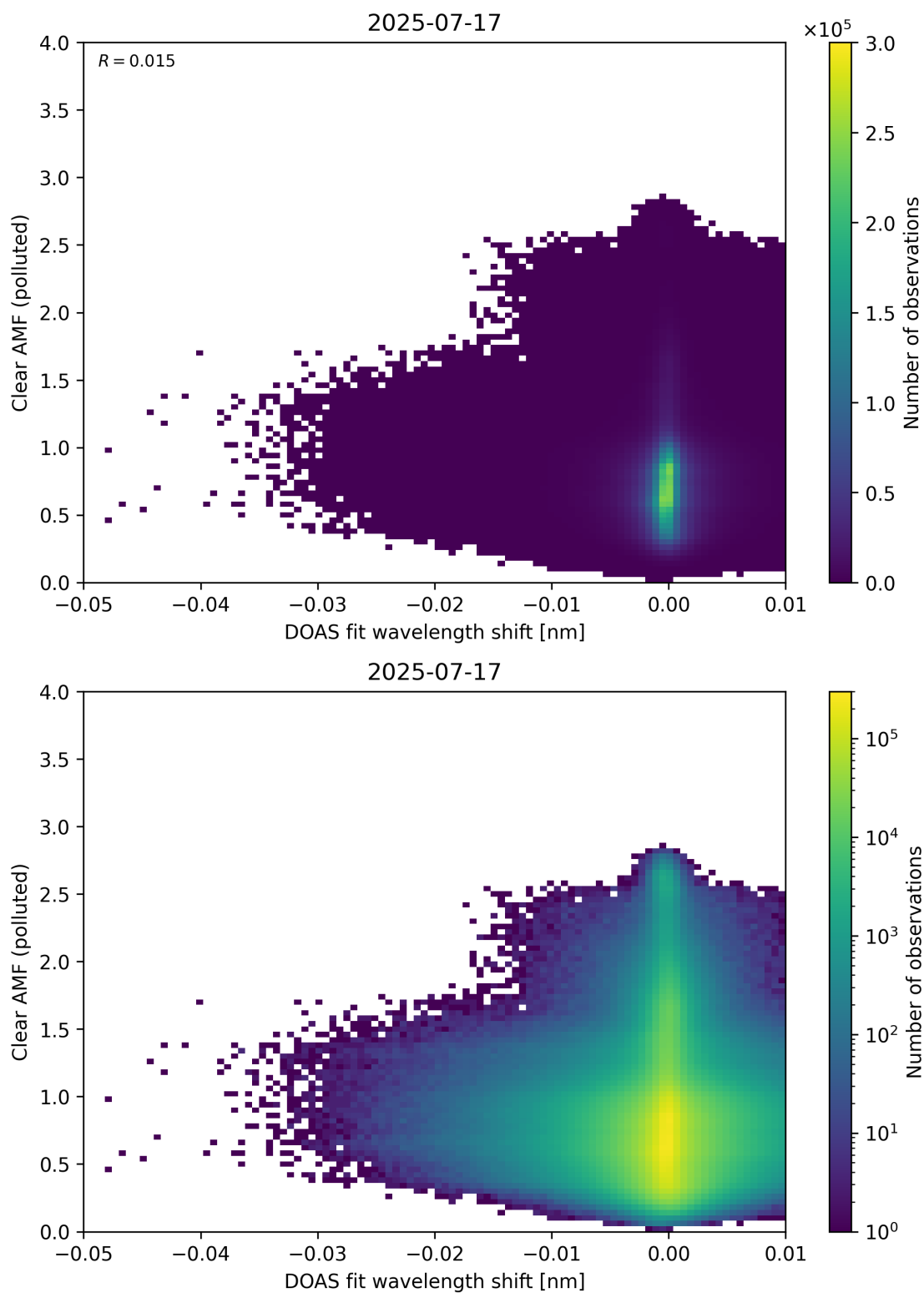
Figure 140: Scatter density plot of “DOAS fit wavelength shift” against “Clear AMF (polluted)” for 2025-07-16 to 2025-07-18.
