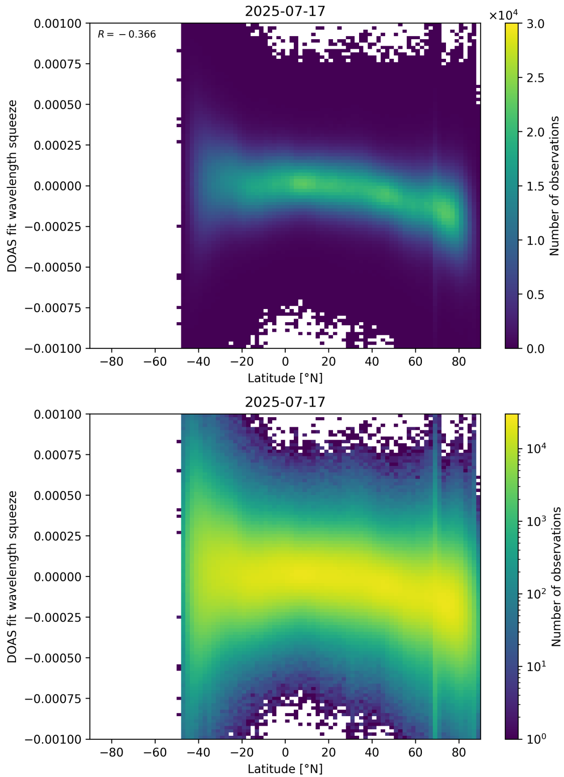
Figure 154: Scatter density plot of “Latitude” against “DOAS fit wavelength squeeze” for 2025-07-16 to 2025-07-18.
