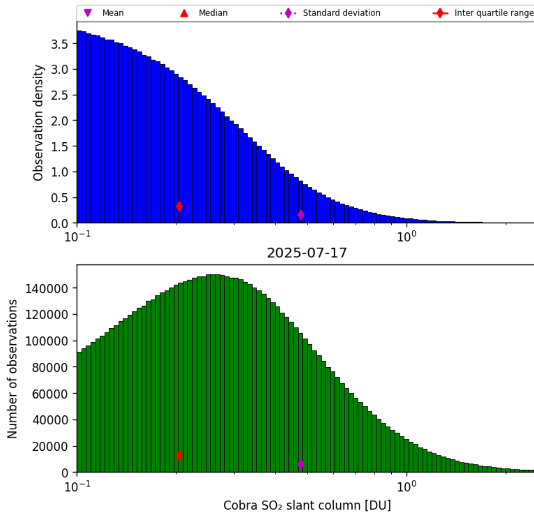
Figure 61: Histogram of “Cobra SO 2 slant column” for 2025-07-16 to 2025-07-18
