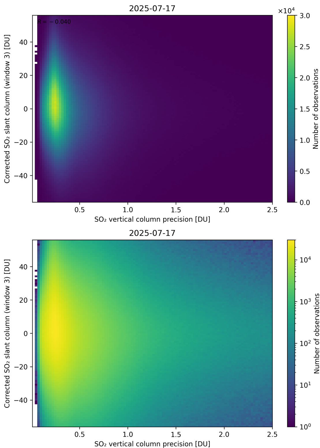
Figure 340: Scatter density plot of “SO 2 vertical column precision” against “Corrected SO 2 slant column (window 3)” for 2025-07-16 to 2025-07-18.
