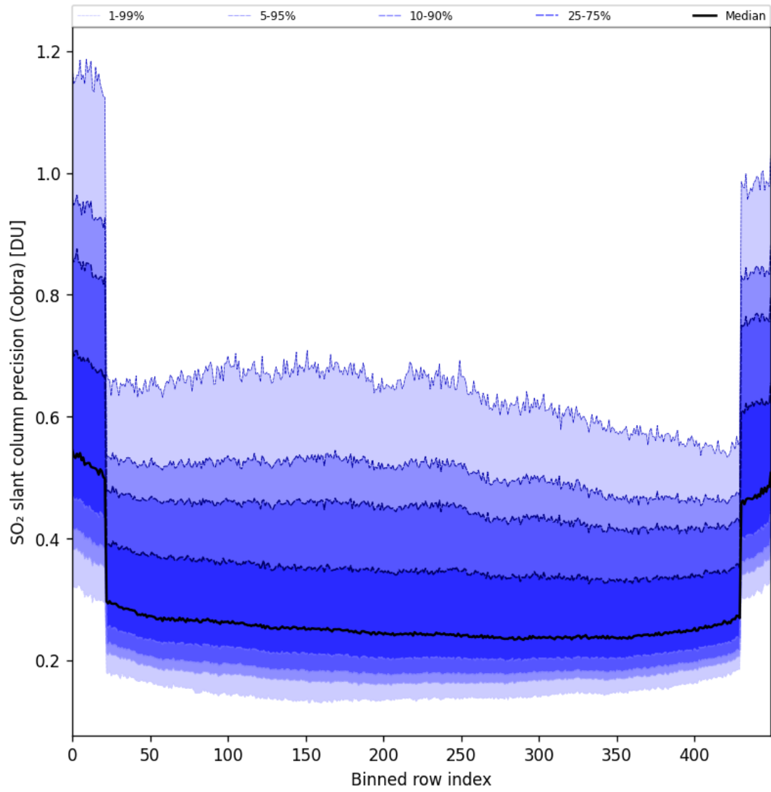
Figure 88: Along track statistics of “SO 2 slant column precision (Cobra)” for 2025-07-16 to 2025-07-18
