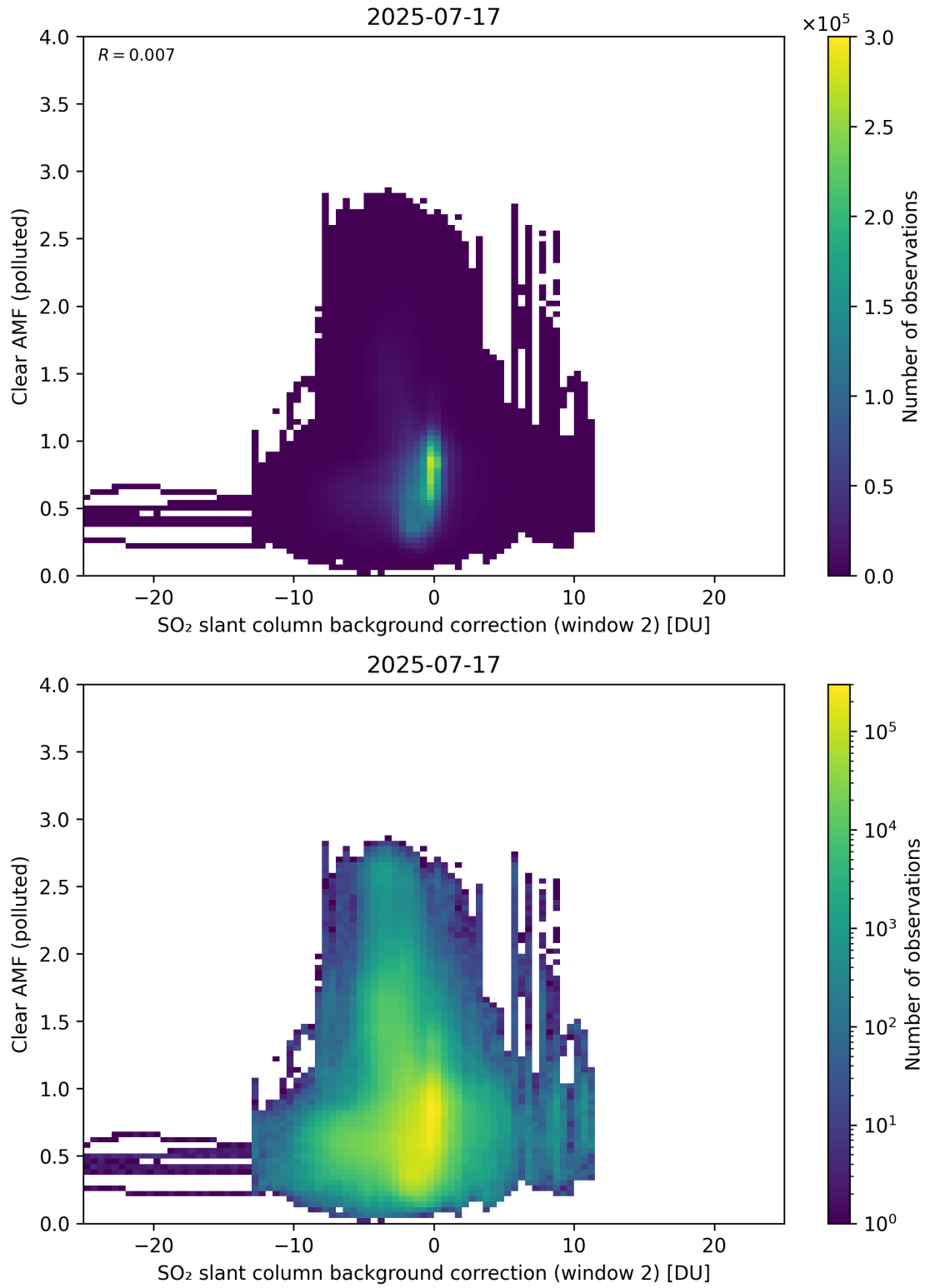
Figure 126: Scatter density plot of “SO 2 slant column background correction (window 2)” against “Clear AMF (polluted)” for 2025-07-16 to 2025-07-18.
