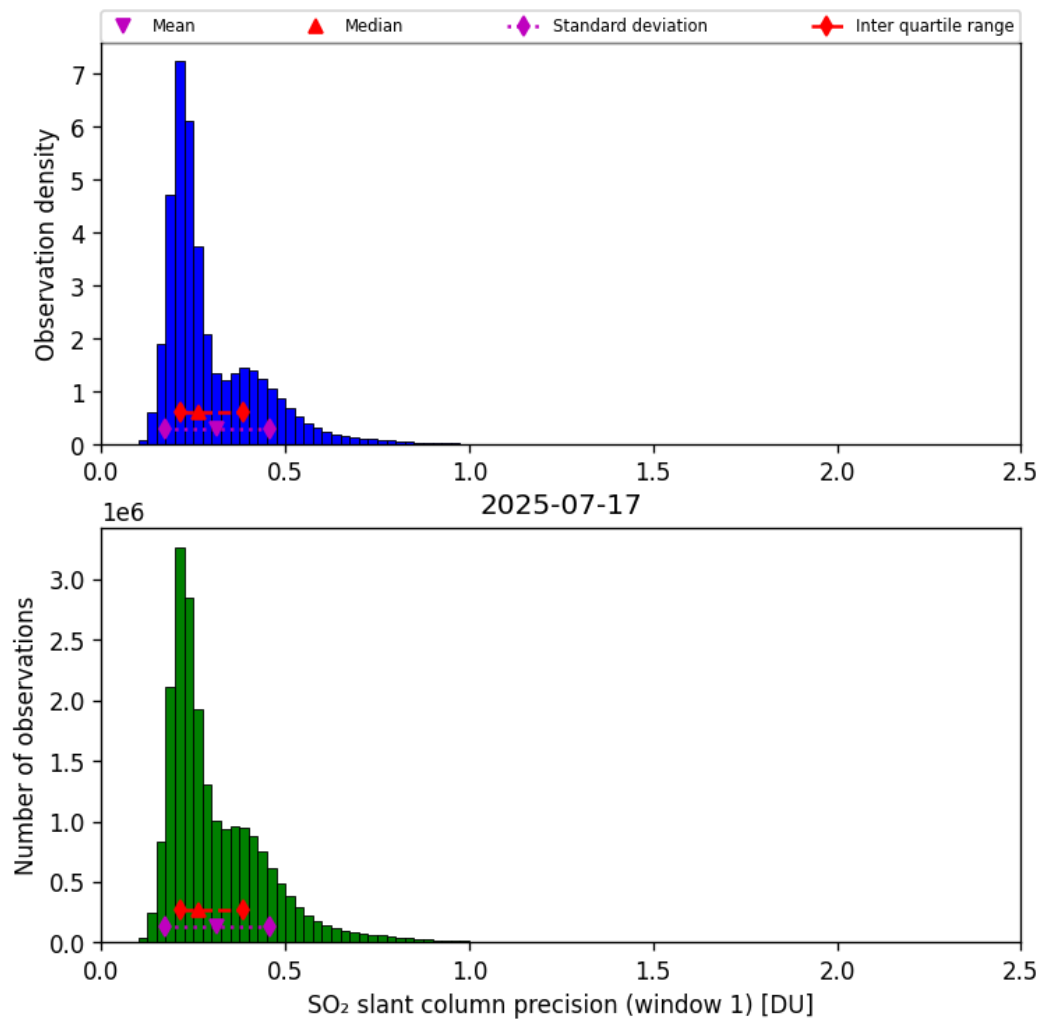
Figure 64: Histogram of “SO 2 slant column precision (window 1)” for 2025-07-16 to 2025-07-18
