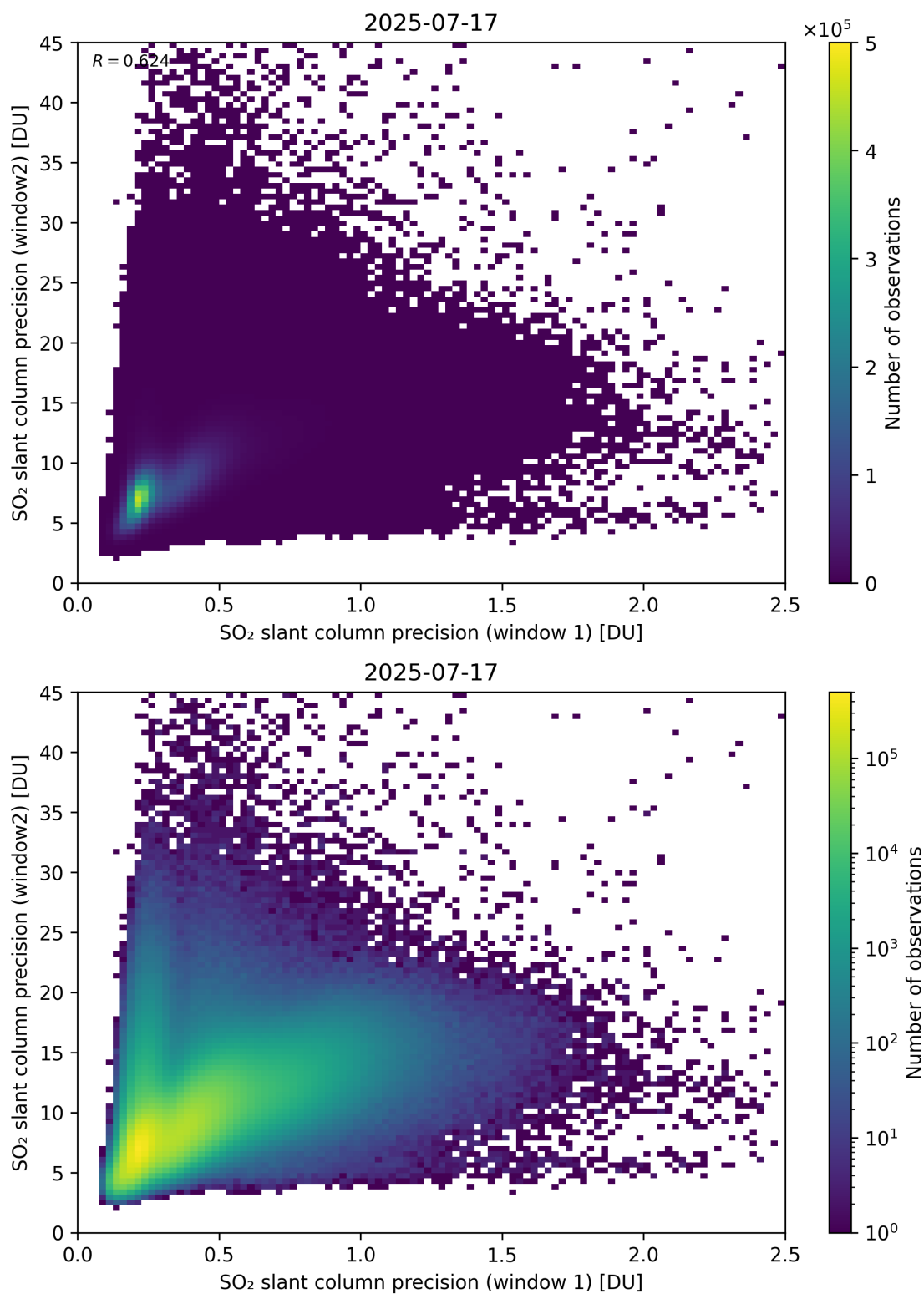
Figure 277: Scatter density plot of “SO 2 slant column precision (window 1)” against “SO 2 slant column precision (window2)” for 2025-07-16 to 2025-07-18.
