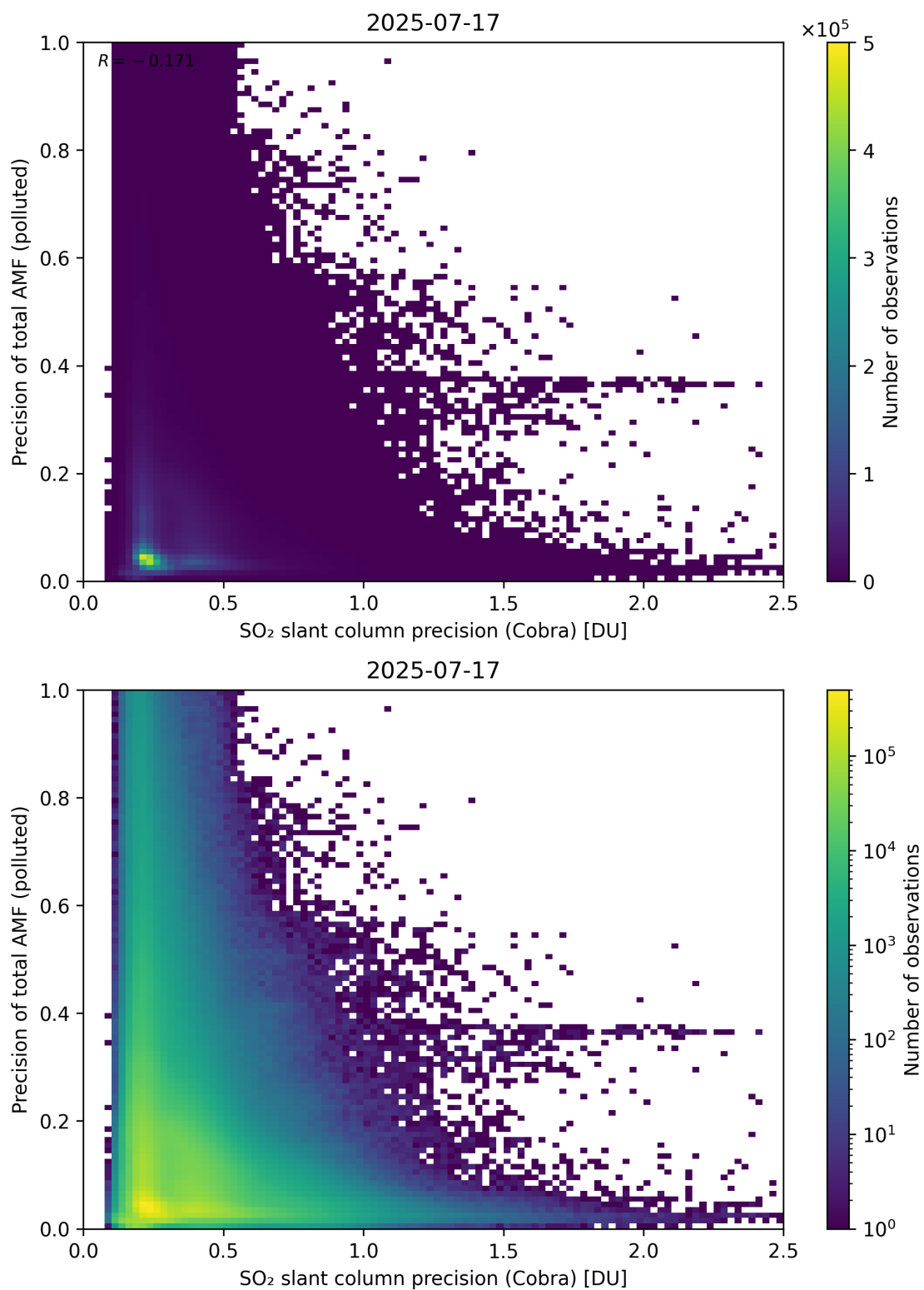
Figure 214: Scatter density plot of “SO 2 slant column precision (Cobra)” against “Precision of total AMF (polluted)” for 2025-07-16 to 2025-07-18.
