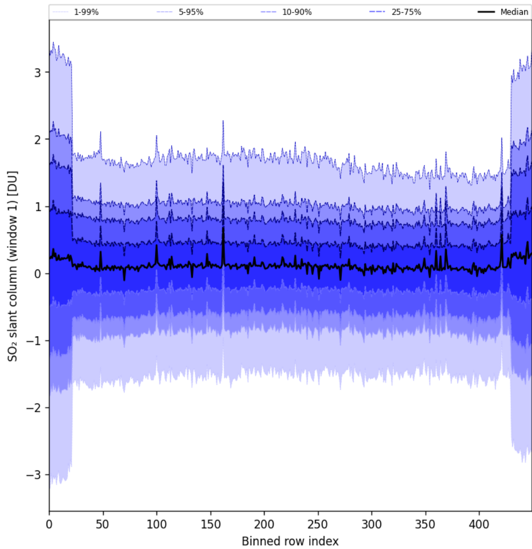
Figure 89: Along track statistics of “SO 2 slant column (window 1)” for 2025-07-16 to 2025-07-18
