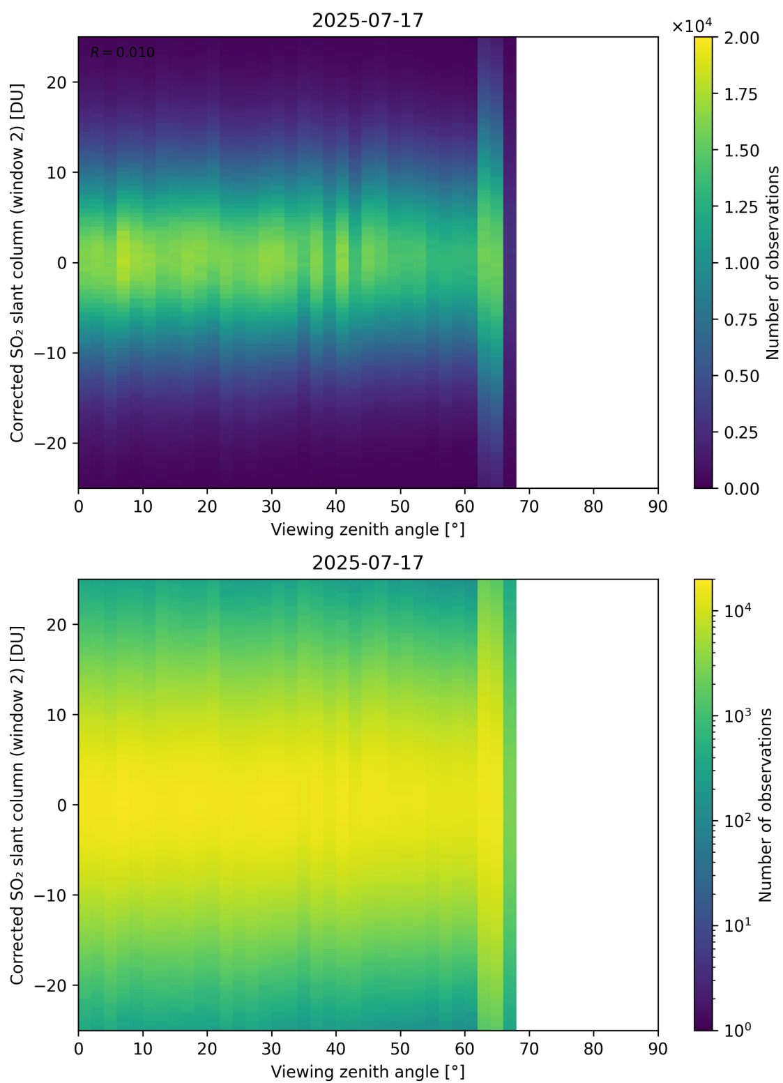
Figure 374: Scatter density plot of “Viewing zenith angle” against “Corrected SO 2 slant column (window 2)” for 2025-07-16 to 2025-07-18.
