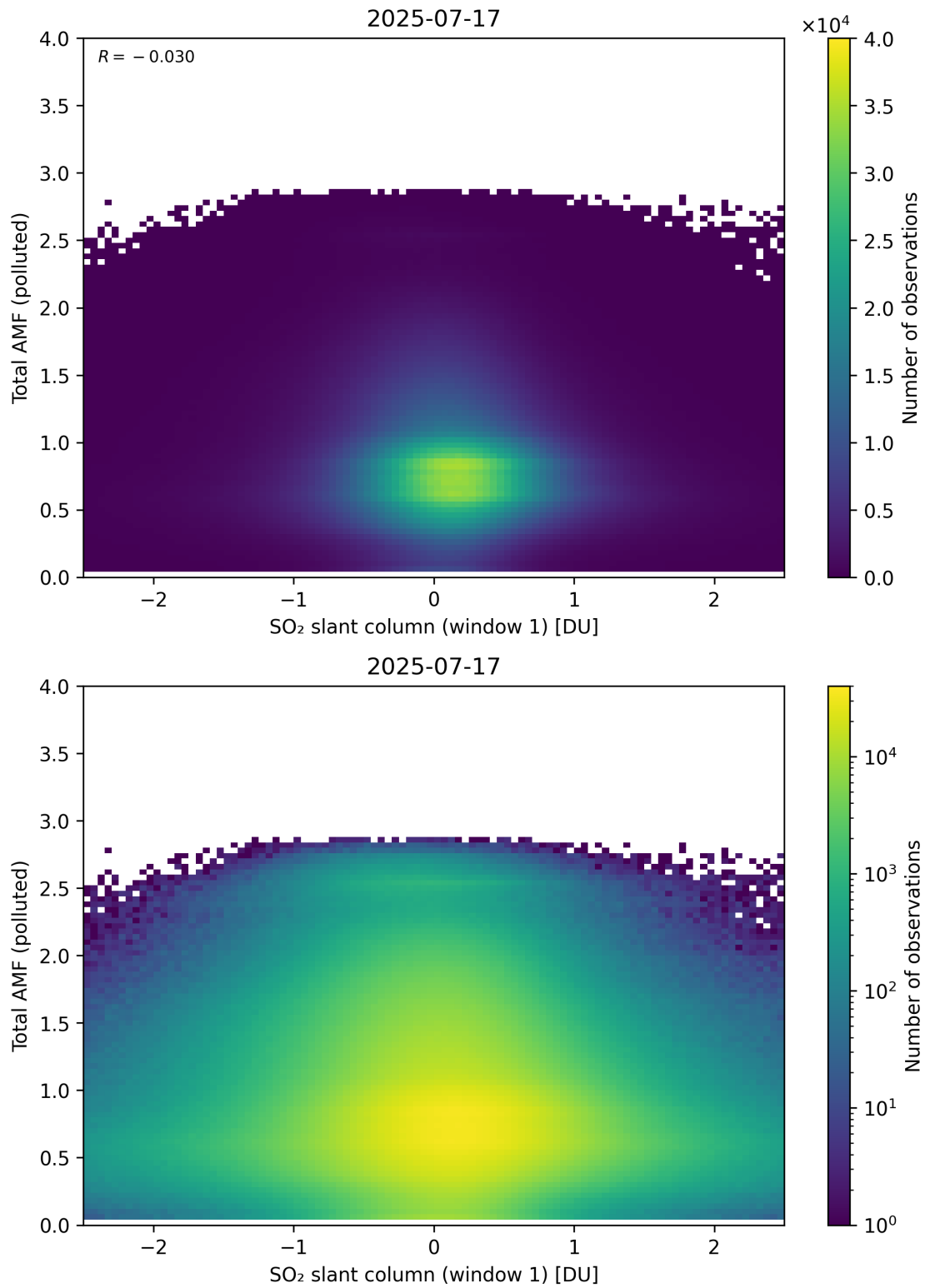
Figure 289: Scatter density plot of “SO 2 slant column (window 1)” against “Total AMF (polluted)” for 2025-07-16 to 2025-07-18.
