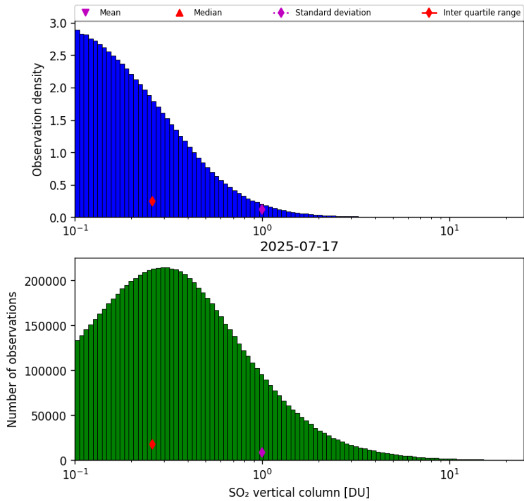
Figure 58: Histogram of “SO 2 vertical column” for 2025-07-16 to 2025-07-18
