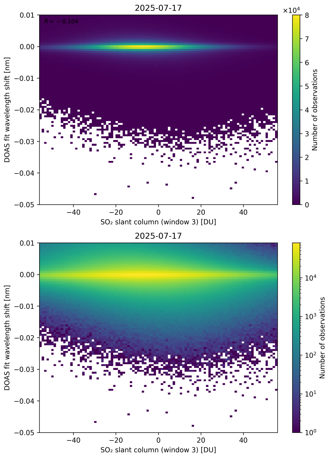
Figure 304: Scatter density plot of “SO 2 slant column (window 3)” against “DOAS fit wavelength shift” for 2025-07-16 to 2025-07-18.
