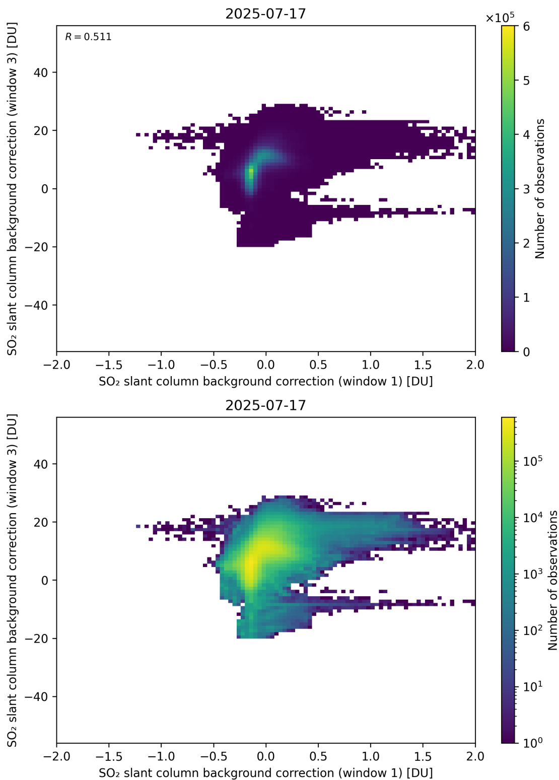
Figure 110: Scatter density plot of “SO 2 slant column background correction (window 1)” against “SO 2 slant column background correction (window 3)” for 2025-07-16 to 2025-07-18.
