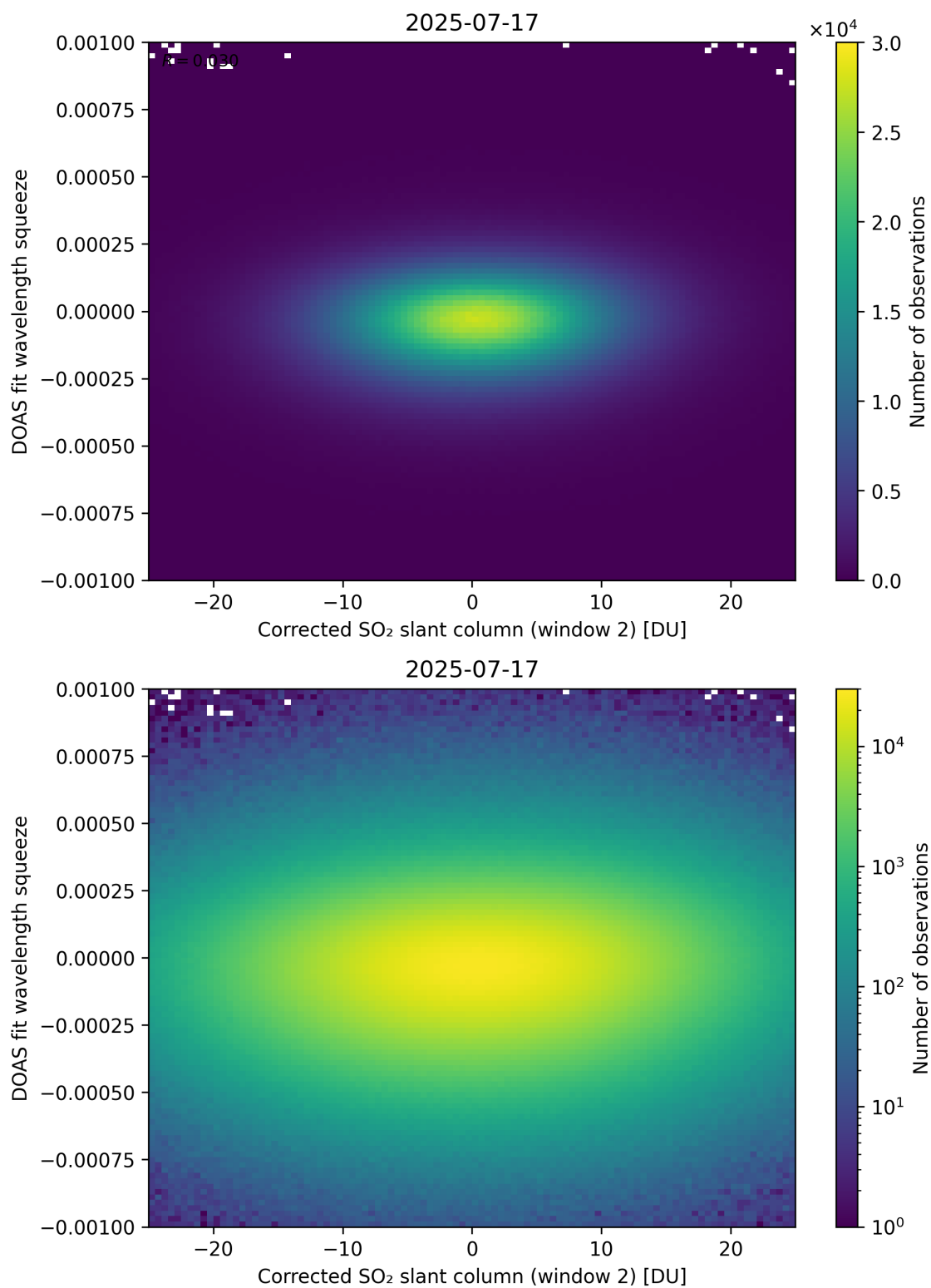
Figure 247: Scatter density plot of “Corrected SO 2 slant column (window 2)” against “DOAS fit wavelength squeeze” for 2025-07-16 to 2025-07-18.
