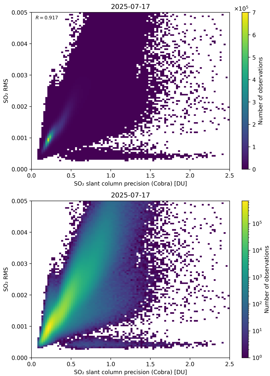
Figure 204: Scatter density plot of “SO 2 slant column precision (Cobra)” against “SO 2 RMS” for 2025-07-16 to 2025-07-18.
