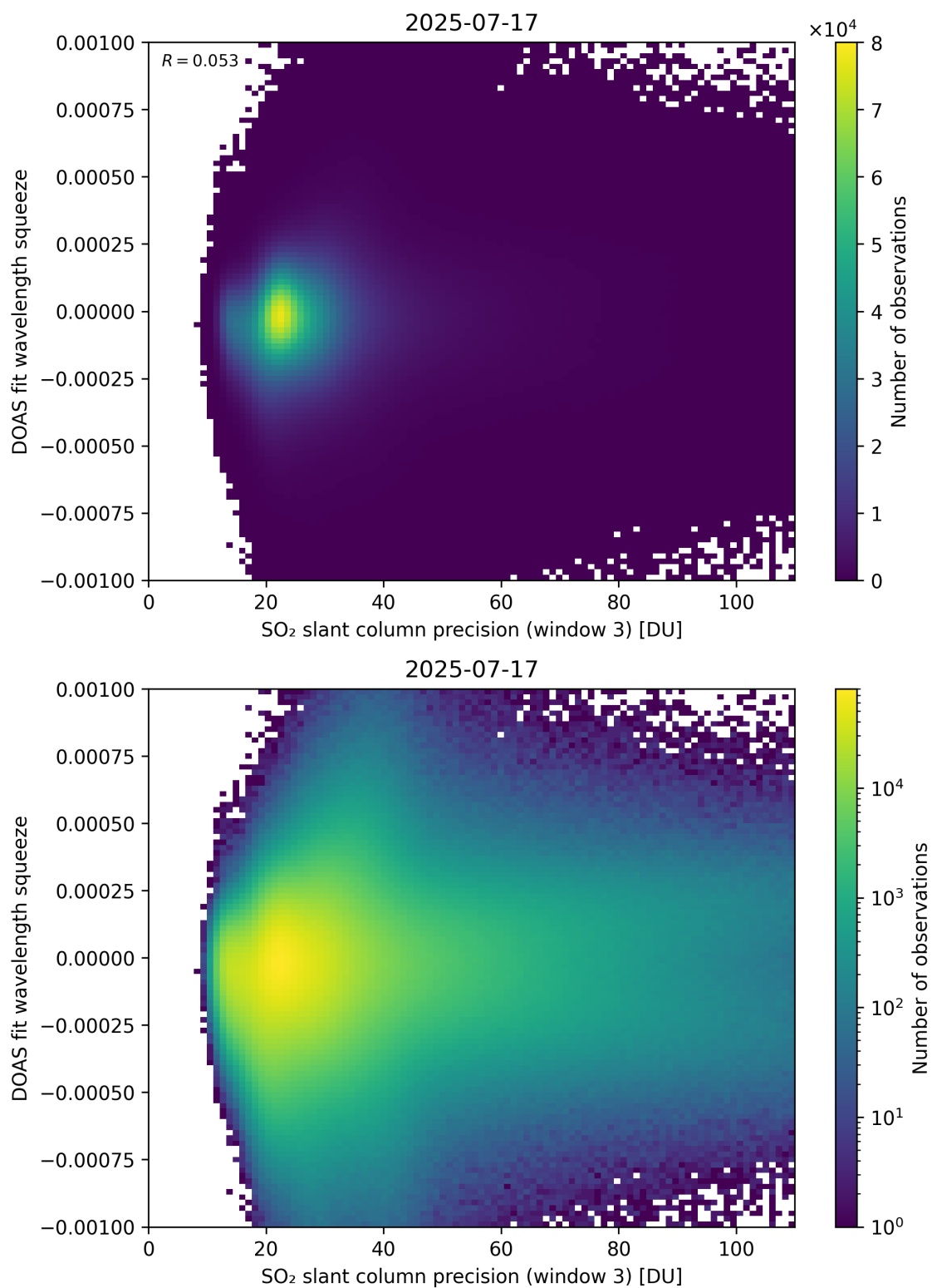
Figure 309: Scatter density plot of “SO 2 slant column precision (window 3)” against “DOAS fit wavelength squeeze” for 2025-07-16 to 2025-07-18.
