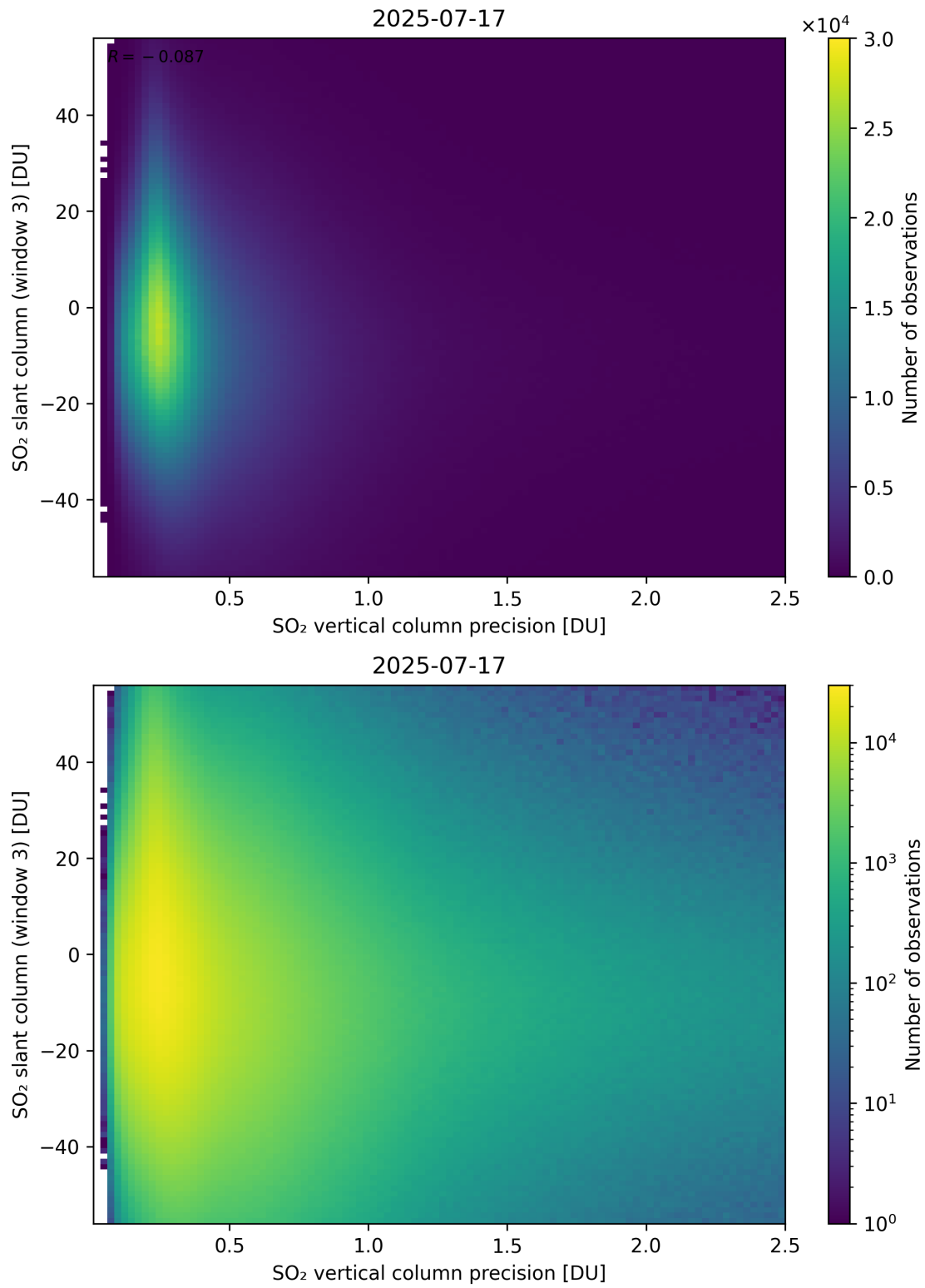
Figure 344: Scatter density plot of “SO 2 vertical column precision” against “SO 2 slant column (window 3)” for 2025-07-16 to 2025-07-18.
