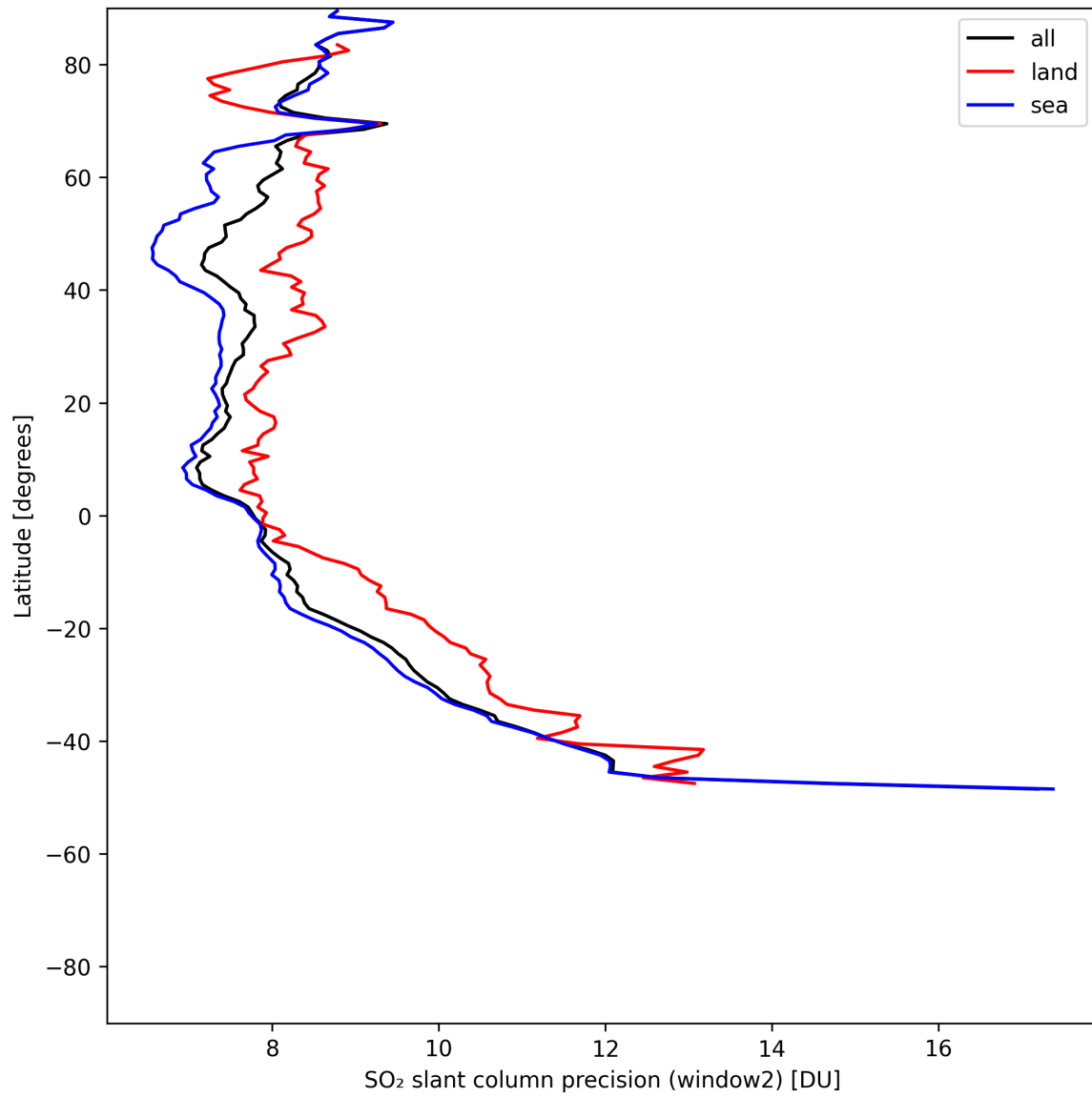
Figure 42: Zonal average of “SO 2 slant column precision (window2)” for 2025-07-16 to 2025-07-18.
