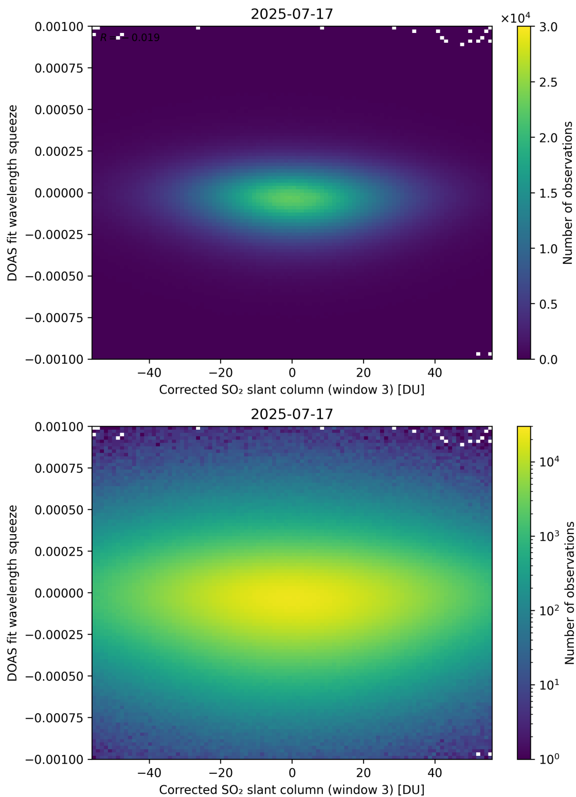
Figure 257: Scatter density plot of “Corrected SO 2 slant column (window 3)” against “DOAS fit wavelength squeeze” for 2025-07-16 to 2025-07-18.
