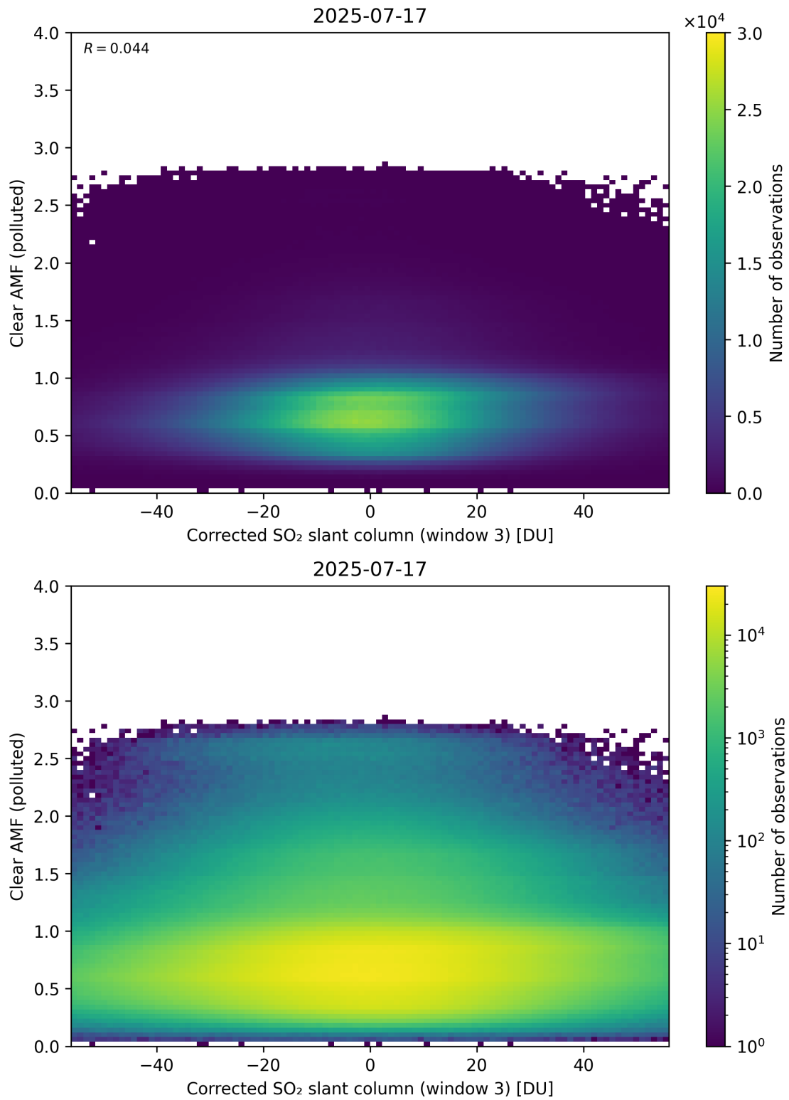
Figure 259: Scatter density plot of “Corrected SO 2 slant column (window 3)” against “Clear AMF (polluted)” for 2025-07-16 to 2025-07-18.
