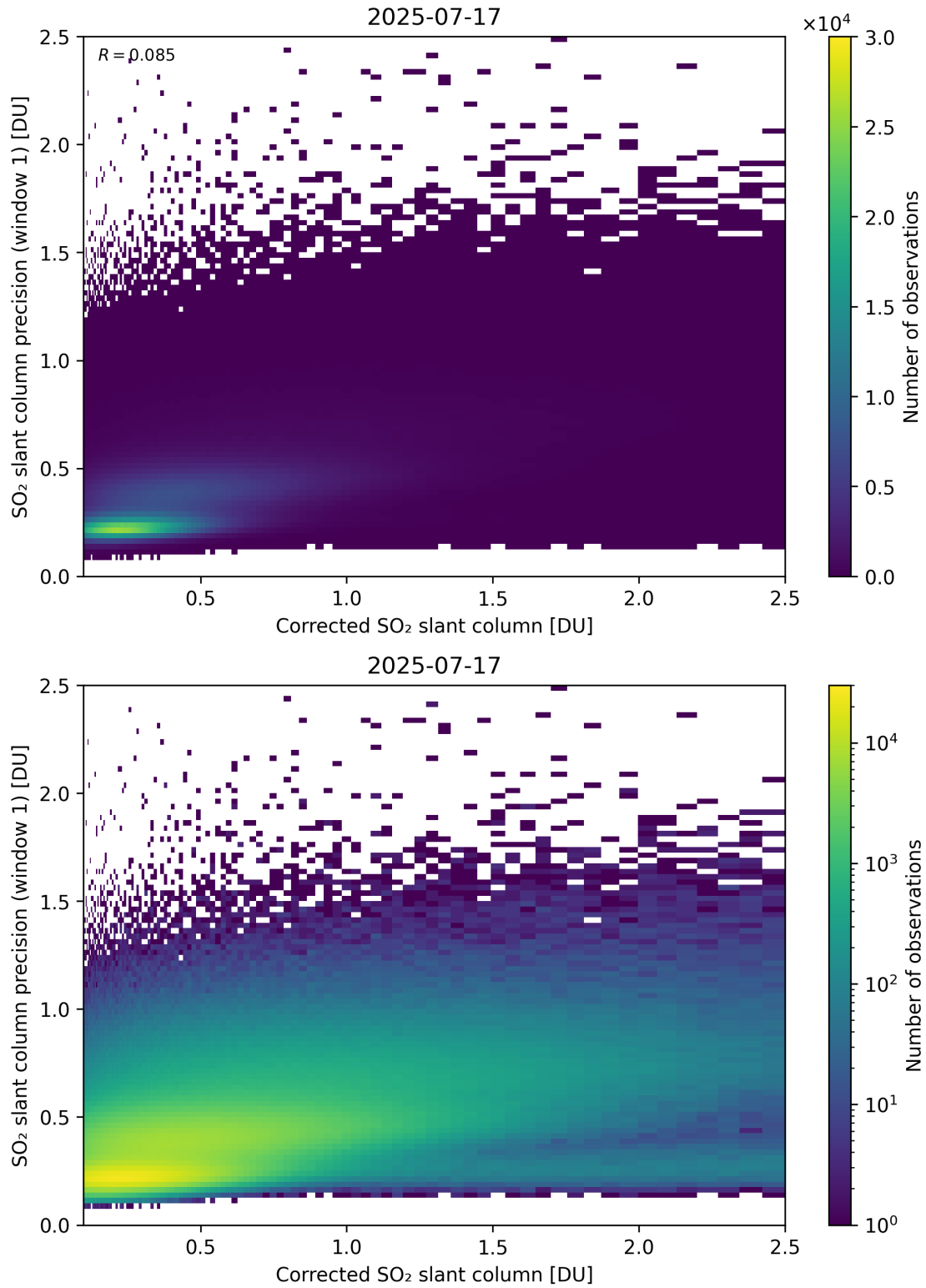
Figure 238: Scatter density plot of “Corrected SO 2 slant column” against “SO 2 slant column precision (window 1)” for 2025-07-16 to 2025-07-18.
