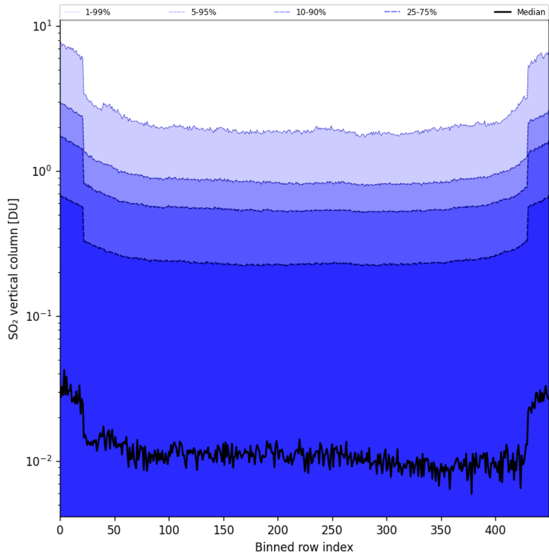
Figure 84: Along track statistics of “SO 2 vertical column” for 2025-07-16 to 2025-07-18
