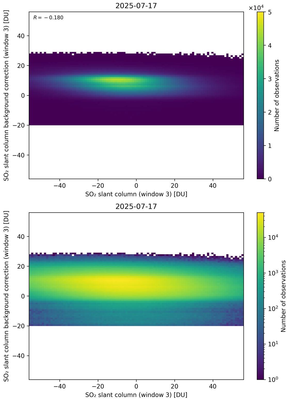
Figure 303: Scatter density plot of “SO 2 slant column (window 3)” against “SO 2 slant column background correction (window 3)” for 2025-07-16 to 2025-07-18.
