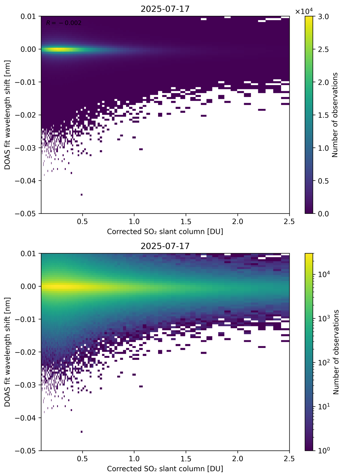
Figure 229: Scatter density plot of “Corrected SO 2 slant column” against “DOAS fit wavelength shift” for 2025-07-16 to 2025-07-18.
