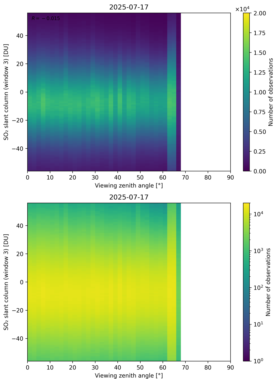
Figure 379: Scatter density plot of “Viewing zenith angle” against “SO 2 slant column (window 3)” for 2025-07-16 to 2025-07-18.
