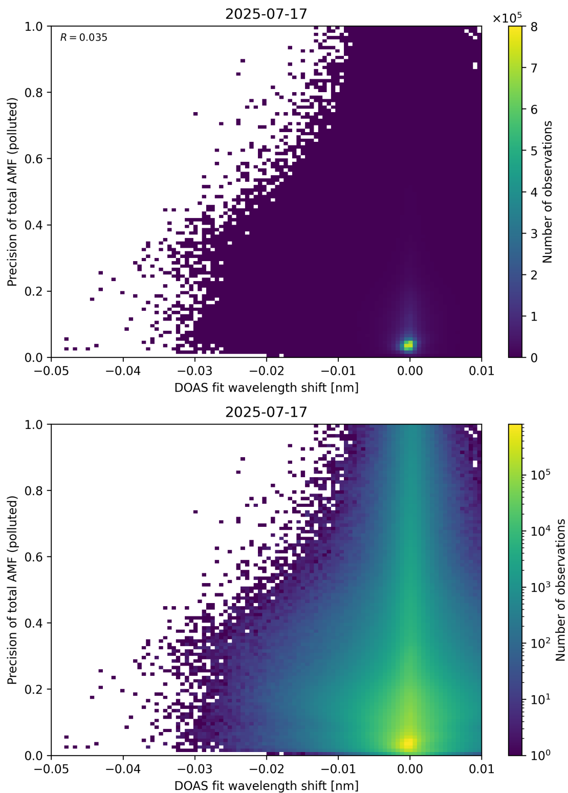
Figure 142: Scatter density plot of “DOAS fit wavelength shift” against “Precision of total AMF (polluted)” for 2025-07-16 to 2025-07-18.
