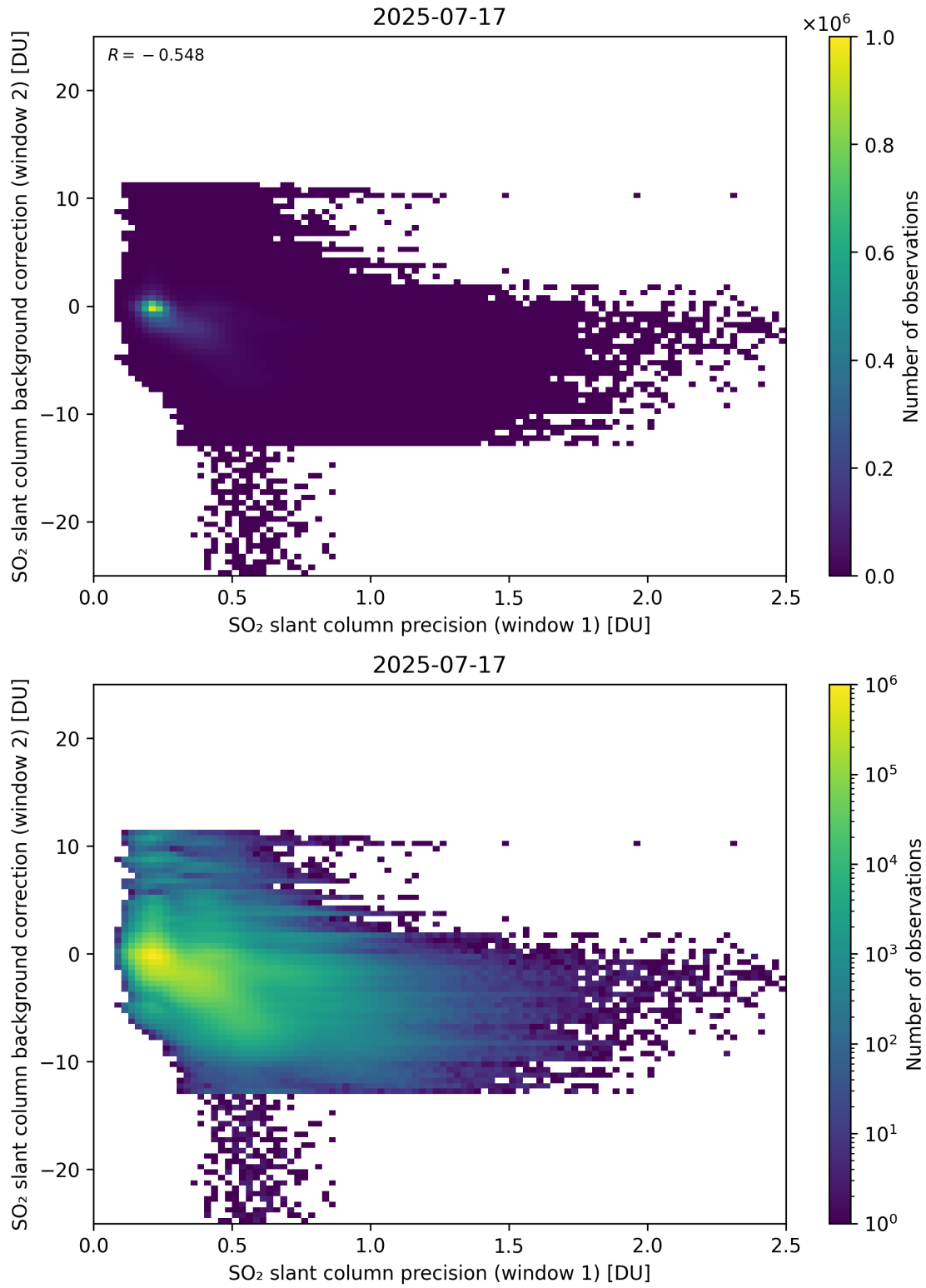
Figure 269: Scatter density plot of “SO 2 slant column precision (window 1)” against “SO 2 slant column background correction (window 2)” for 2025-07-16 to 2025-07-18.
