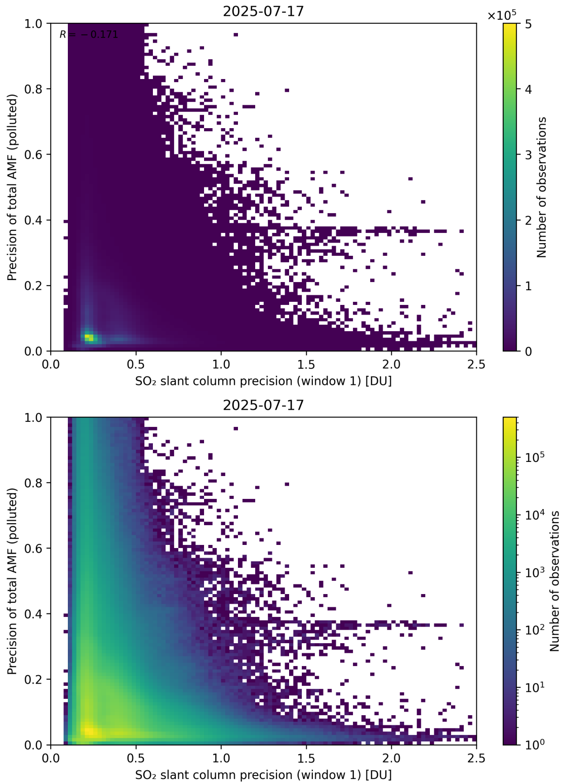
Figure 281: Scatter density plot of “SO 2 slant column precision (window 1)” against “Precision of total AMF (polluted)” for 2025-07-16 to 2025-07-18.
