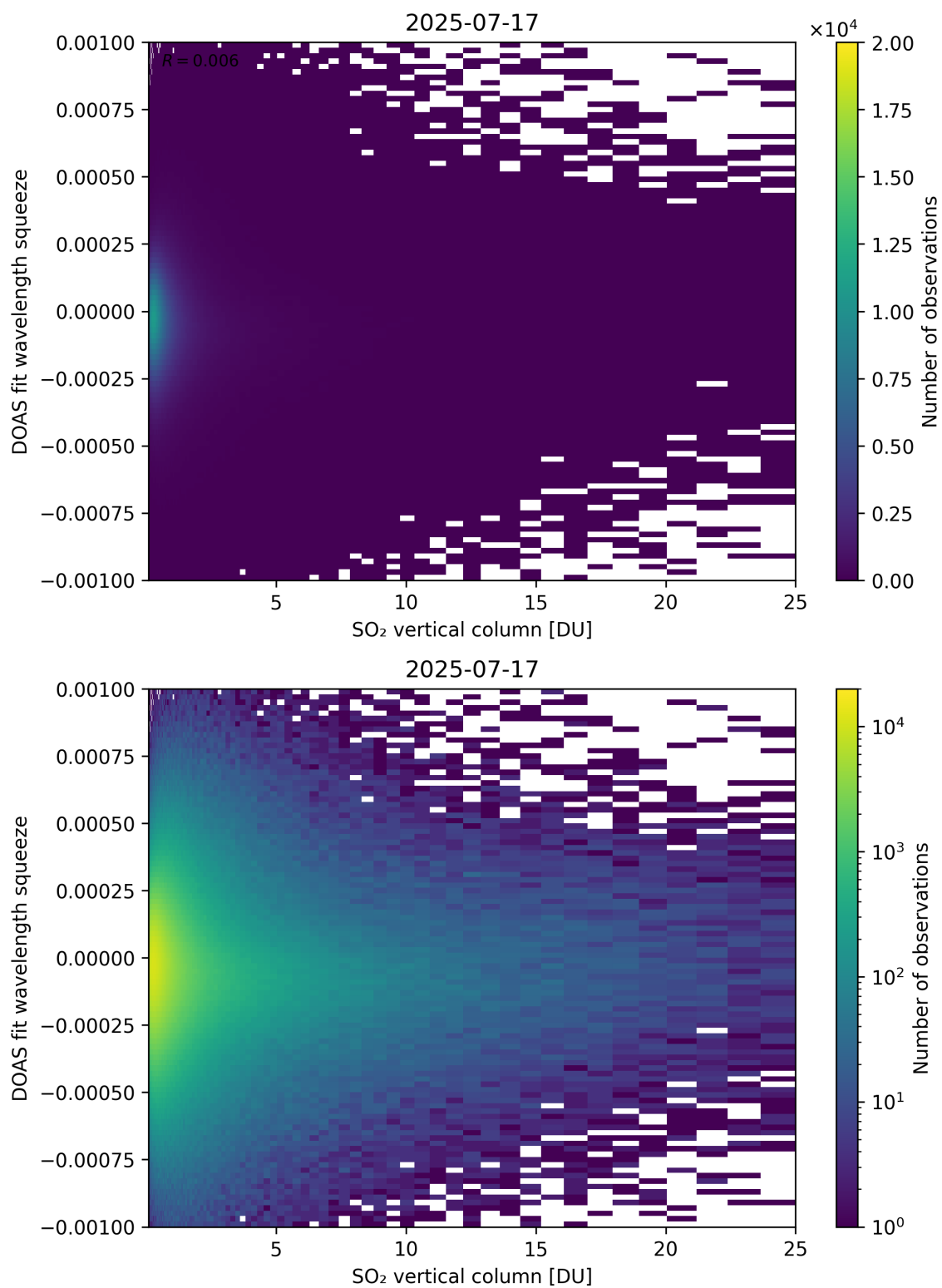
Figure 327: Scatter density plot of “SO 2 vertical column” against “DOAS fit wavelength squeeze” for 2025-07-16 to 2025-07-18.
