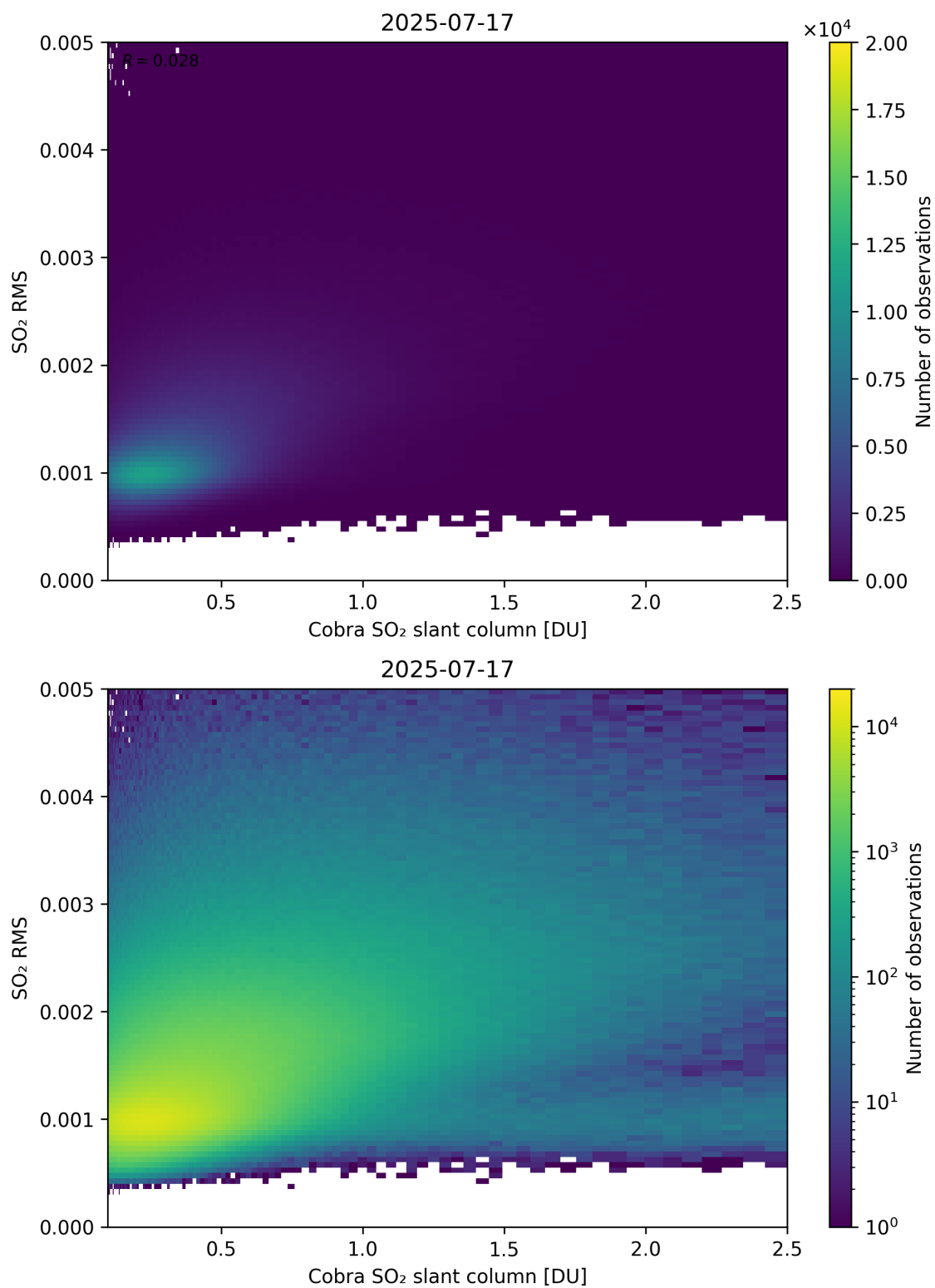
Figure 198: Scatter density plot of “Cobra SO 2 slant column” against “SO 2 RMS” for 2025-07-16 to 2025-07-18.
