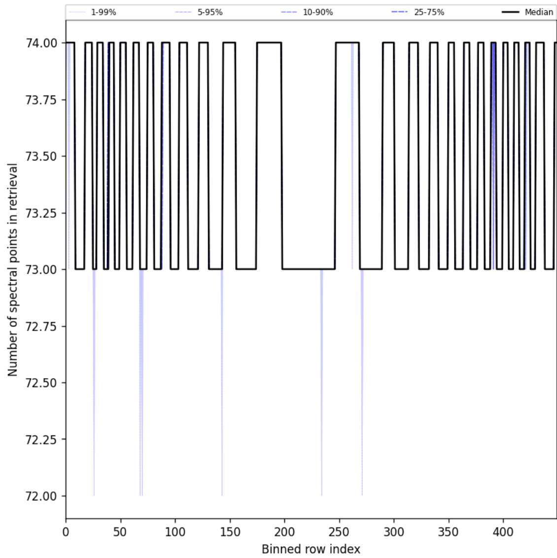
Figure 108: Along track statistics of “Number of spectral points in retrieval” for 2025-07-16 to 2025-07-18
