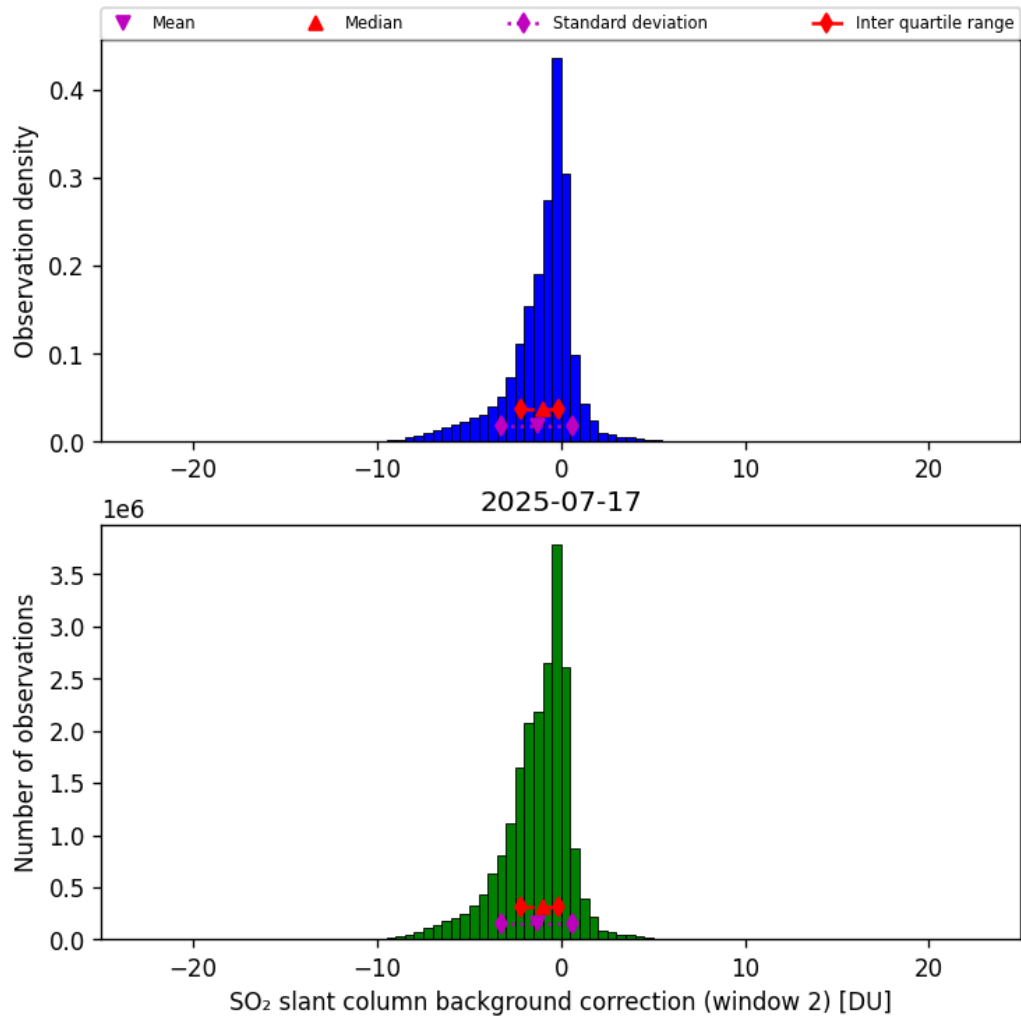
Figure 70: Histogram of “SO 2 slant column background correction (window 2)” for 2025-07-16 to 2025-07-18
