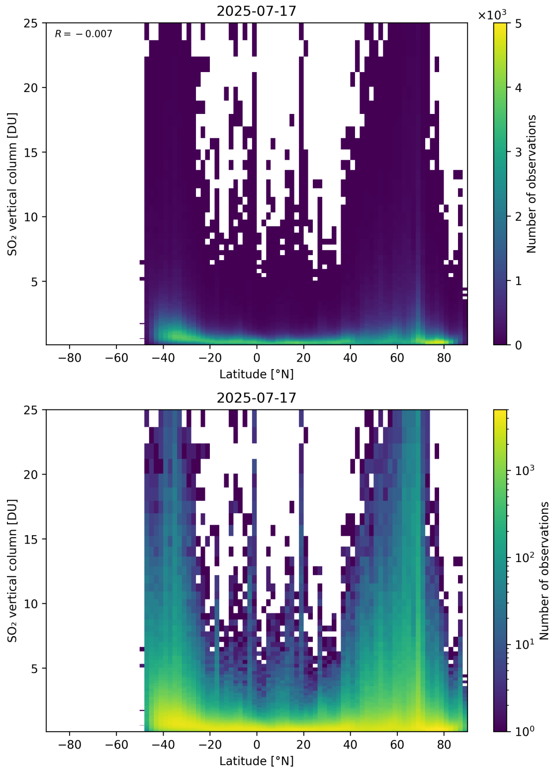
Figure 169: Scatter density plot of “Latitude” against “SO 2 vertical column” for 2025-07-16 to 2025-07-18.
