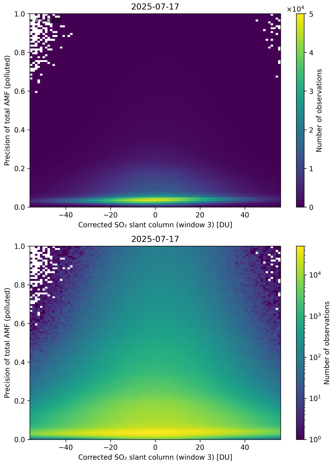
Figure 261: Scatter density plot of “Corrected SO 2 slant column (window 3)” against “Precision of total AMF (polluted)” for 2025-07-16 to 2025-07-18.
