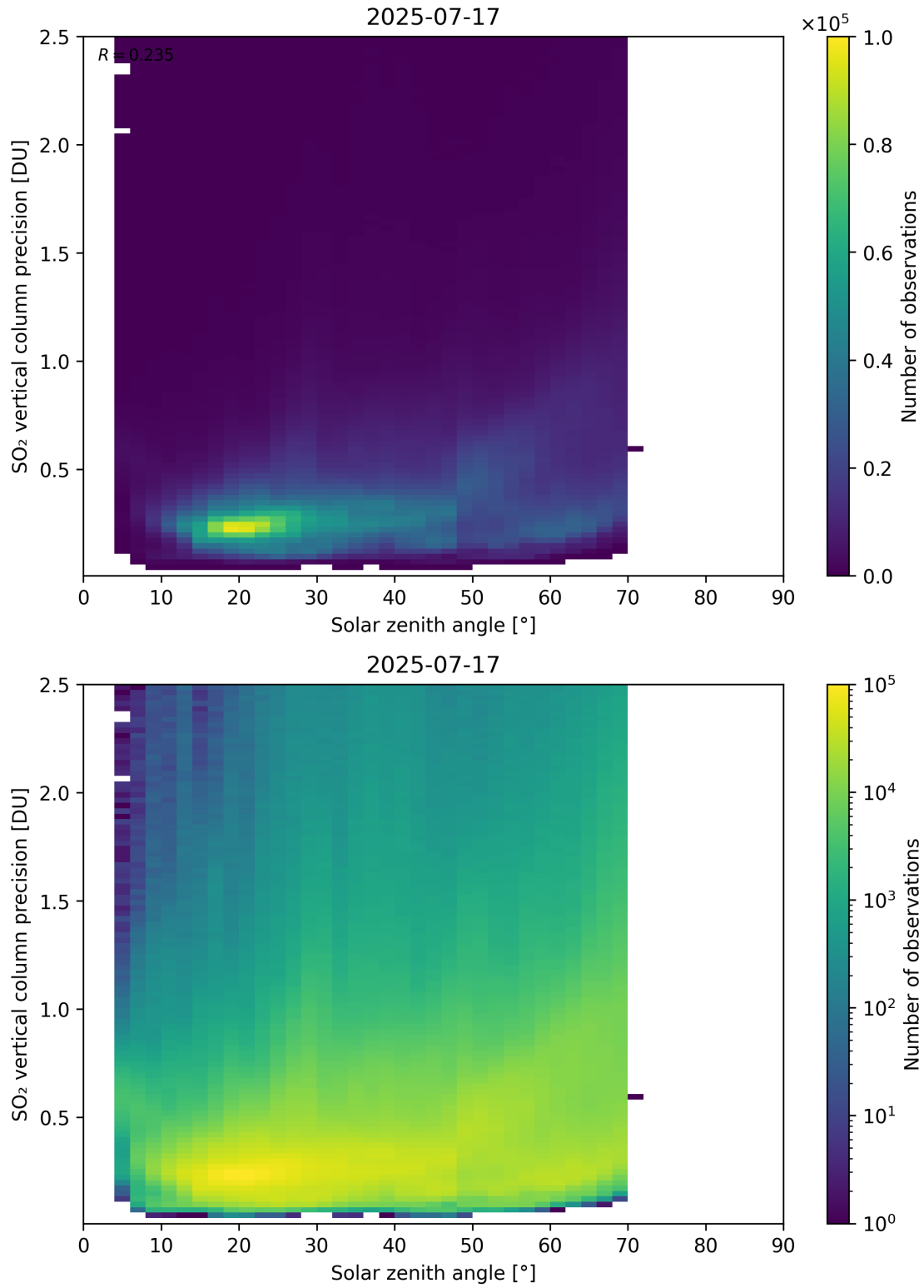
Figure 192: Scatter density plot of “Solar zenith angle” against “SO 2 vertical column precision” for 2025-07-16 to 2025-07-18.
