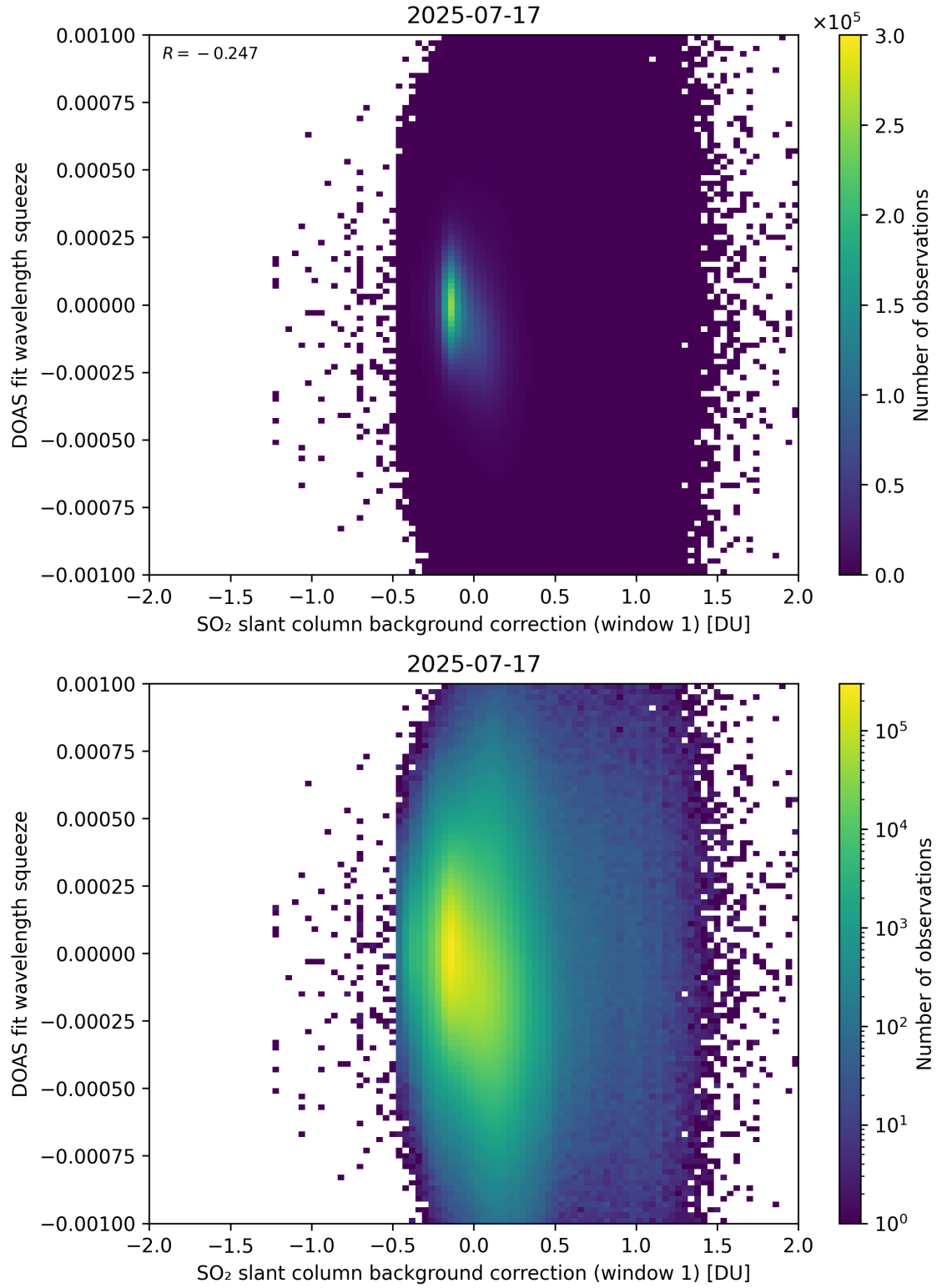
Figure 112: Scatter density plot of “SO 2 slant column background correction (window 1)” against “DOAS fit wavelength squeeze” for 2025-07-16 to 2025-07-18.
