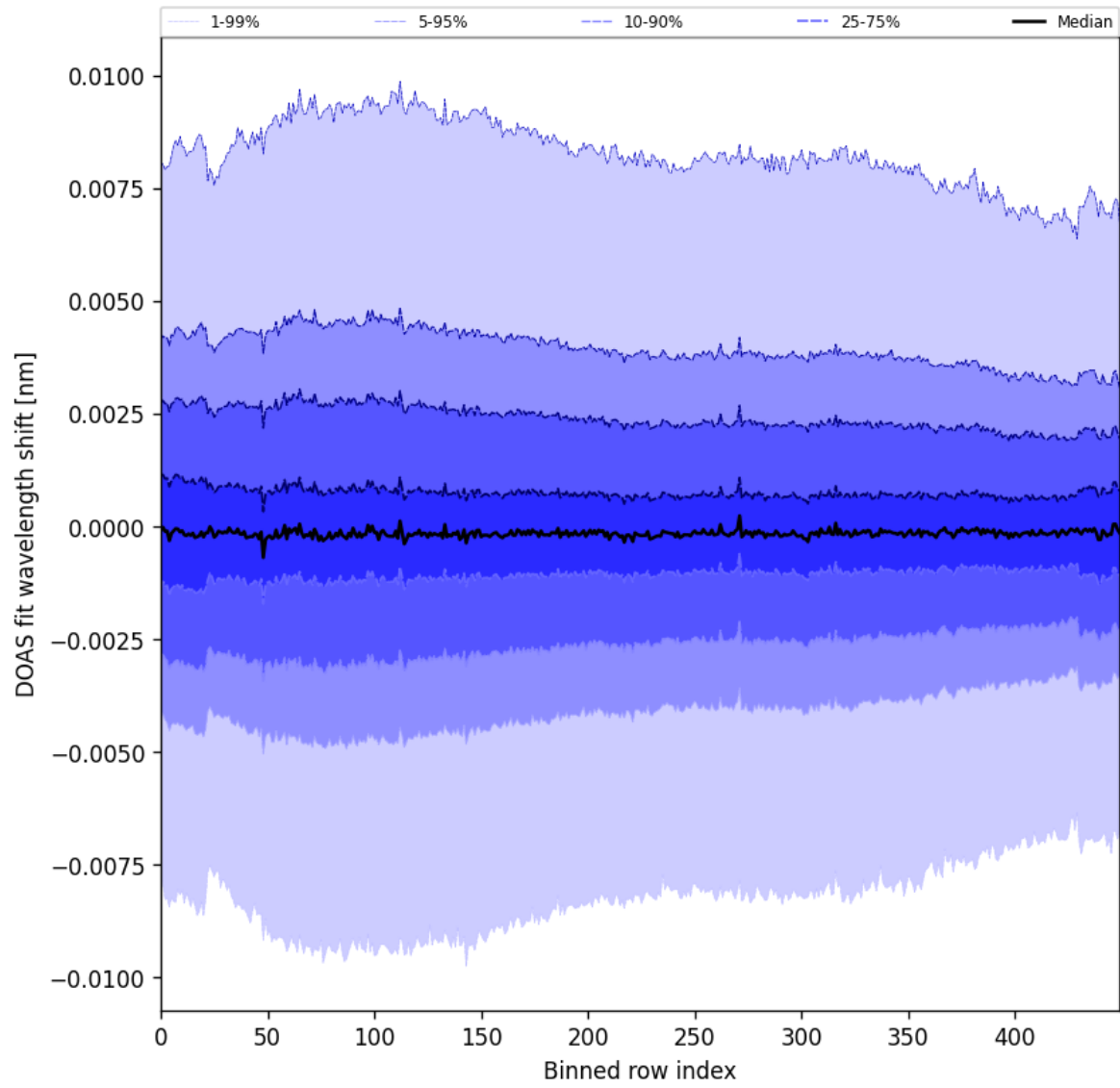
Figure 102: Along track statistics of “DOAS fit wavelength shift” for 2025-07-16 to 2025-07-18
