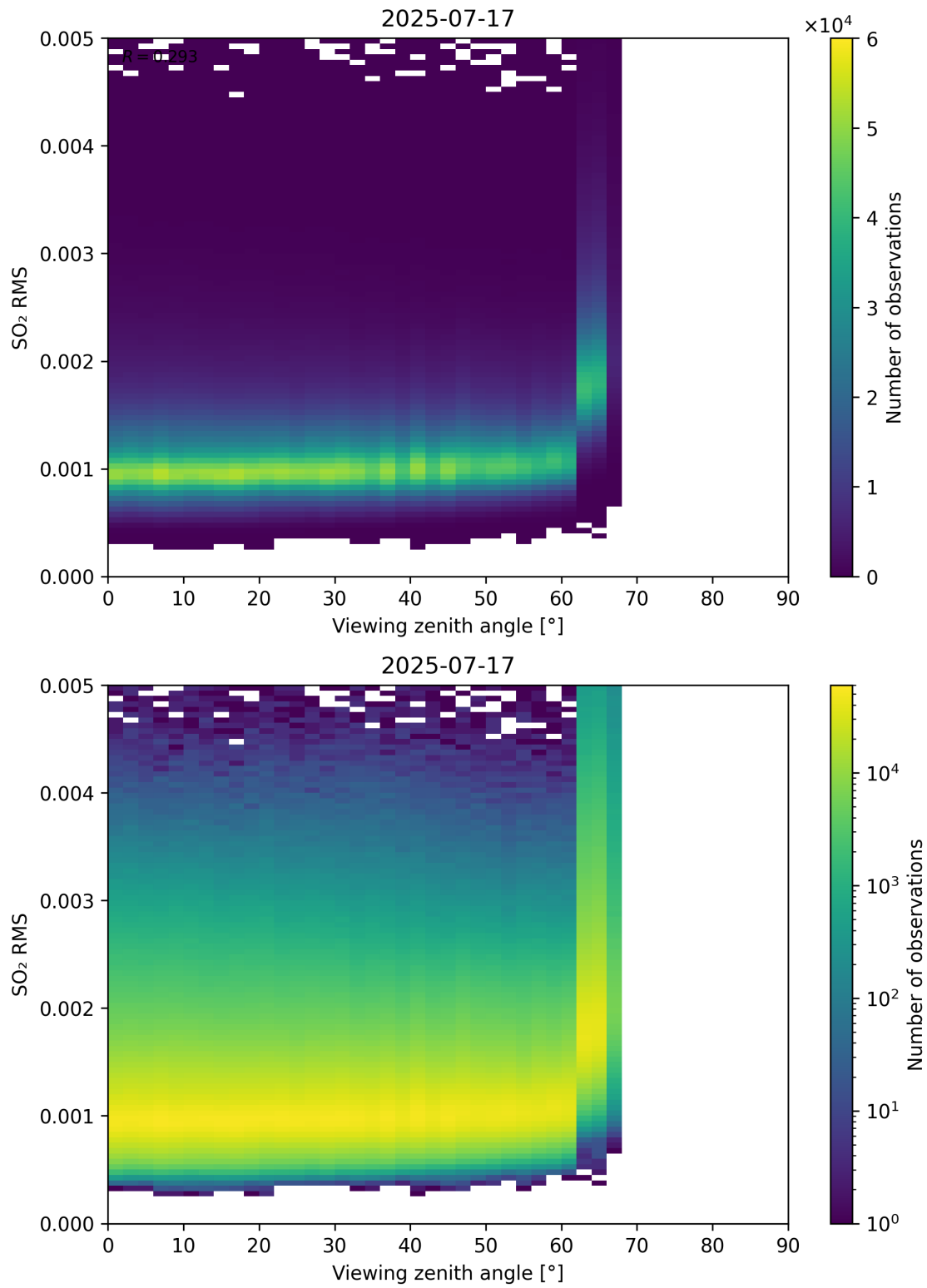
Figure 367: Scatter density plot of “Viewing zenith angle” against “SO 2 RMS” for 2025-07-16 to 2025-07-18.
