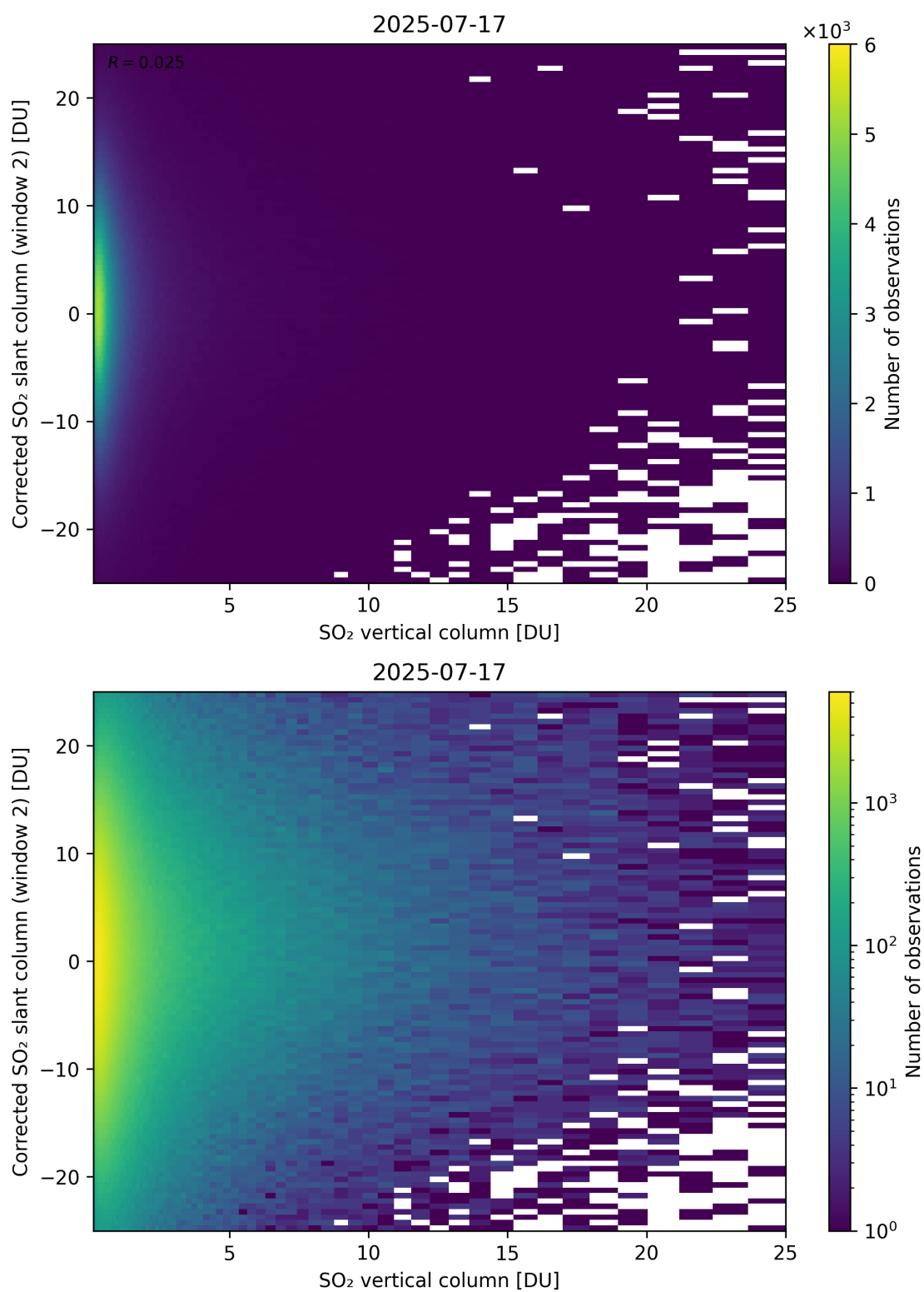
Figure 352: Scatter density plot of “SO 2 vertical column” against “Corrected SO 2 slant column (window 2)” for 2025-07-16 to 2025-07-18.
