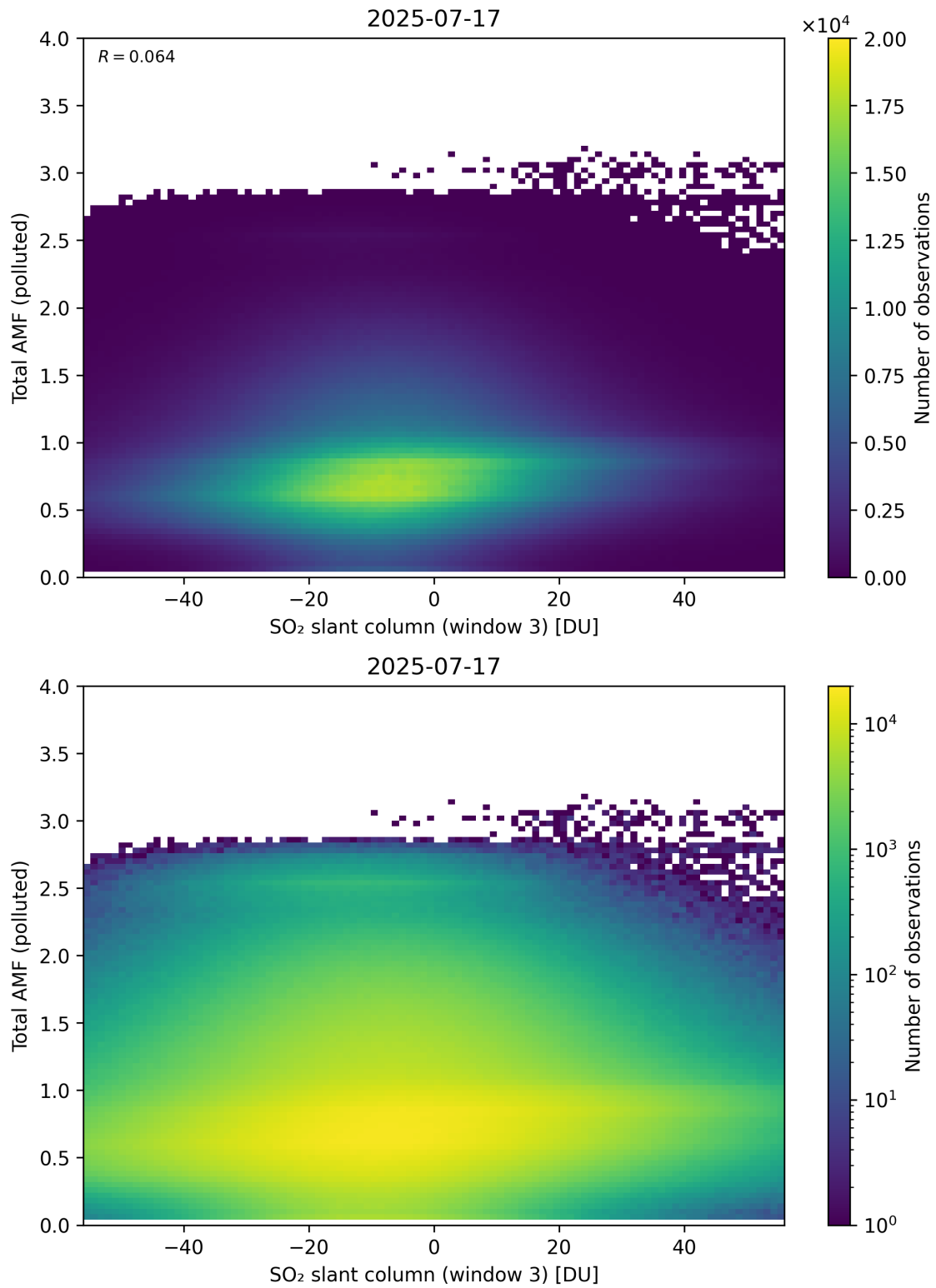
Figure 318: Scatter density plot of “SO 2 slant column (window 3)” against “Total AMF (polluted)” for 2025-07-16 to 2025-07-18.
