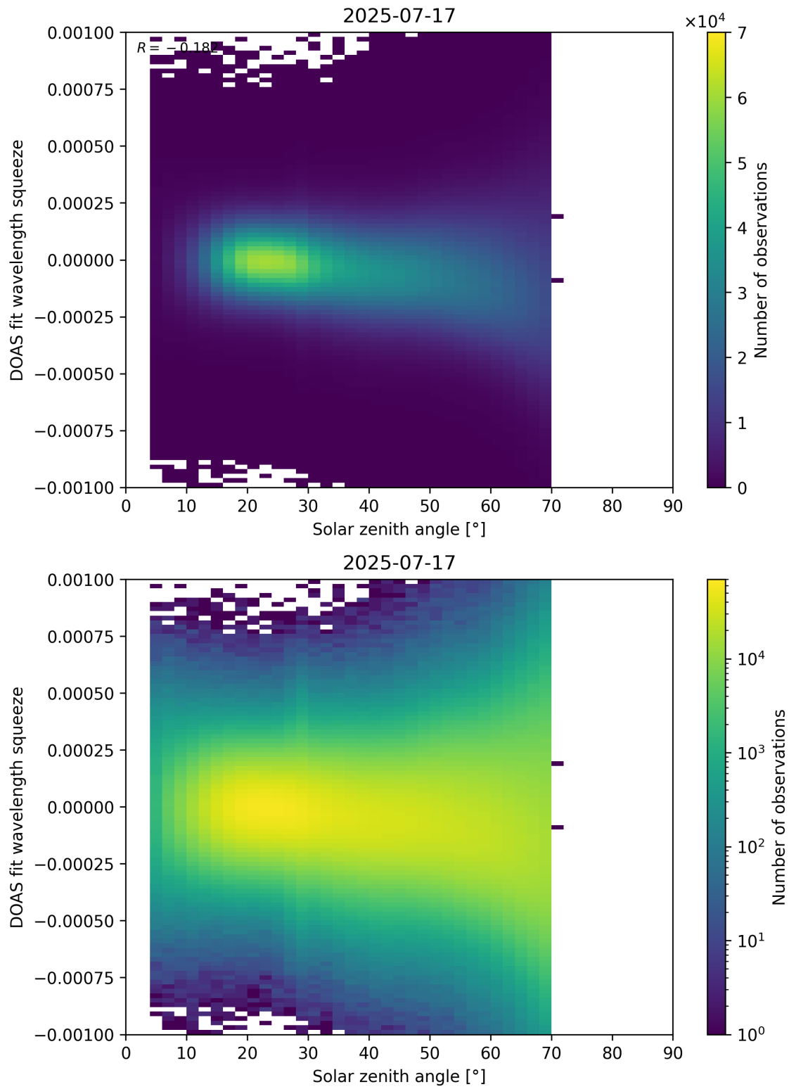
Figure 175: Scatter density plot of “Solar zenith angle” against “DOAS fit wavelength squeeze” for 2025-07-16 to 2025-07-18.
