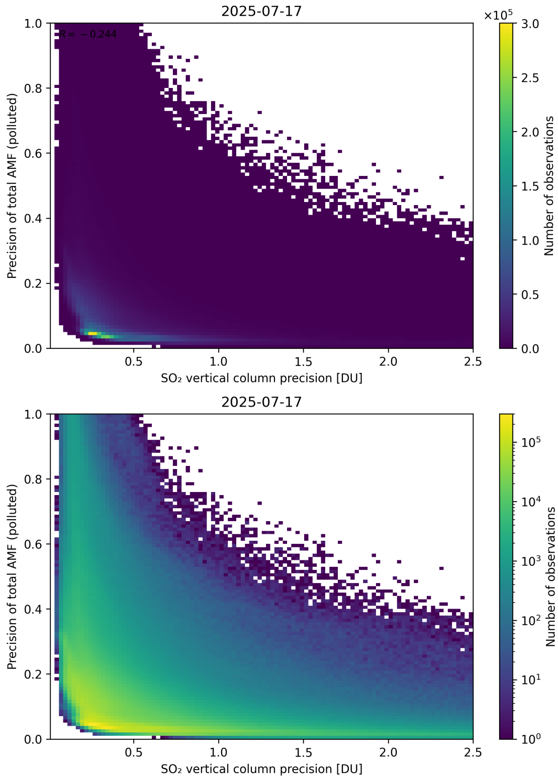
Figure 347: Scatter density plot of “SO 2 vertical column precision” against “Precision of total AMF (polluted)” for 2025-07-16 to 2025-07-18.
