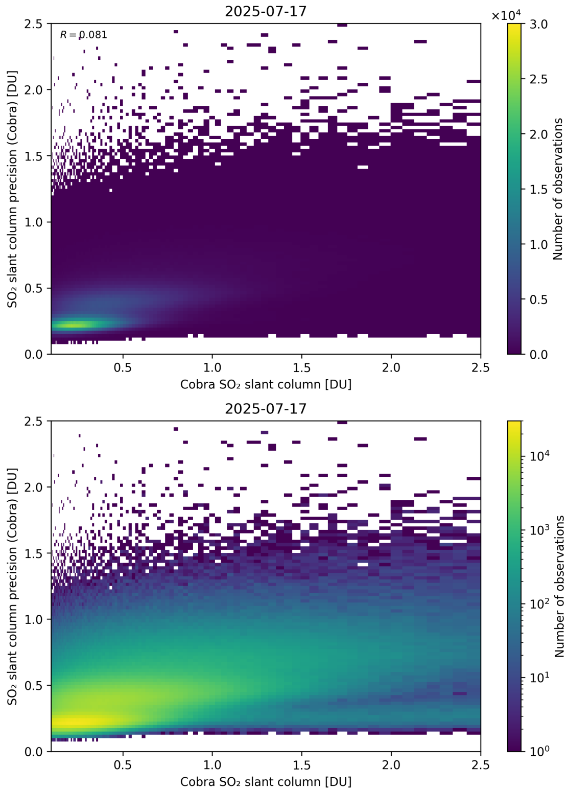
Figure 216: Scatter density plot of “Cobra SO 2 slant column” against “SO 2 slant column precision (Cobra)” for 2025-07-16 to 2025-07-18.
