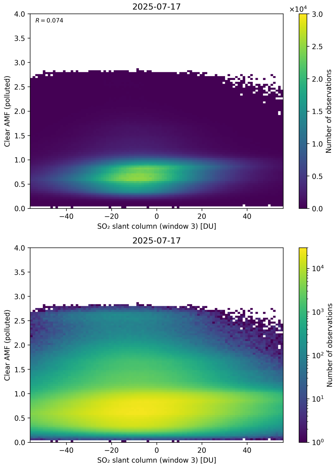
Figure 315: Scatter density plot of “SO 2 slant column (window 3)” against “Clear AMF (polluted)” for 2025-07-16 to 2025-07-18.
