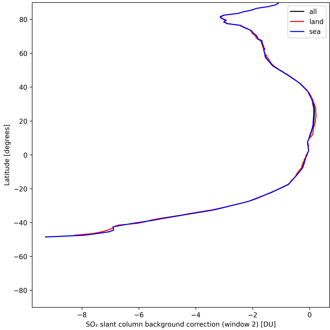
Figure 44: Zonal average of “SO 2 slant column background correction (window 2)” for 2025-07-16 to 2025-07-18.
