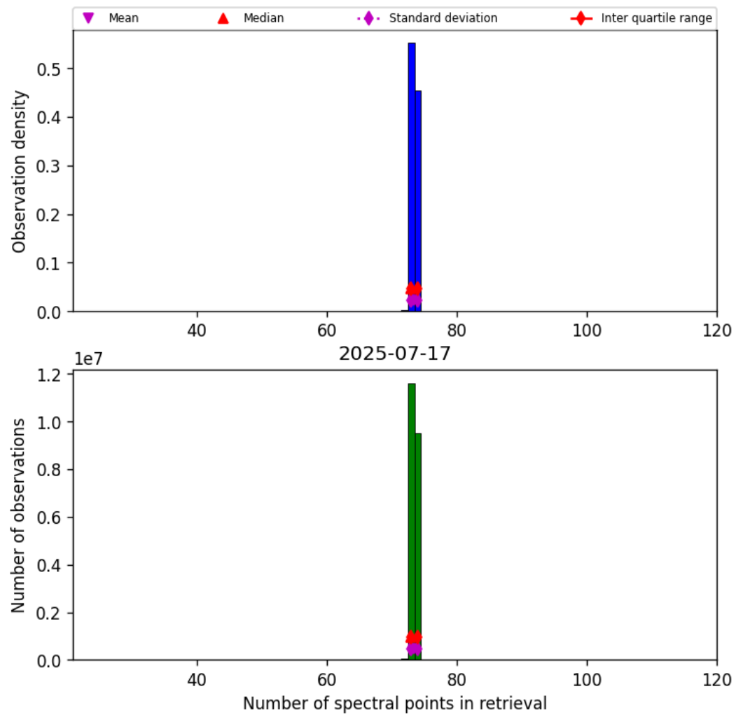
Figure 82: Histogram of “Number of spectral points in retrieval” for 2025-07-16 to 2025-07-18
