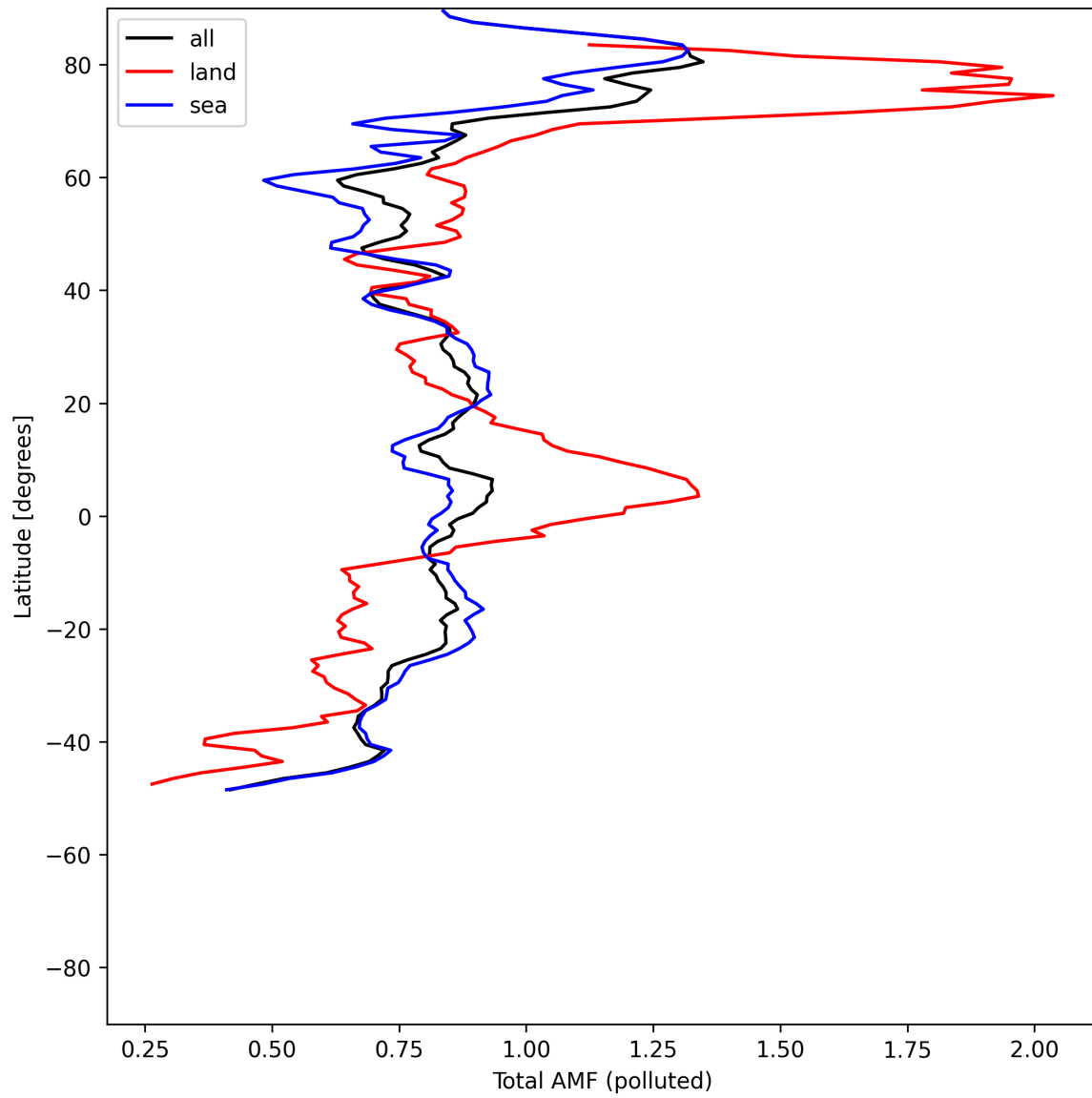
Figure 53: Zonal average of “Total AMF (polluted)” for 2025-07-16 to 2025-07-18.
