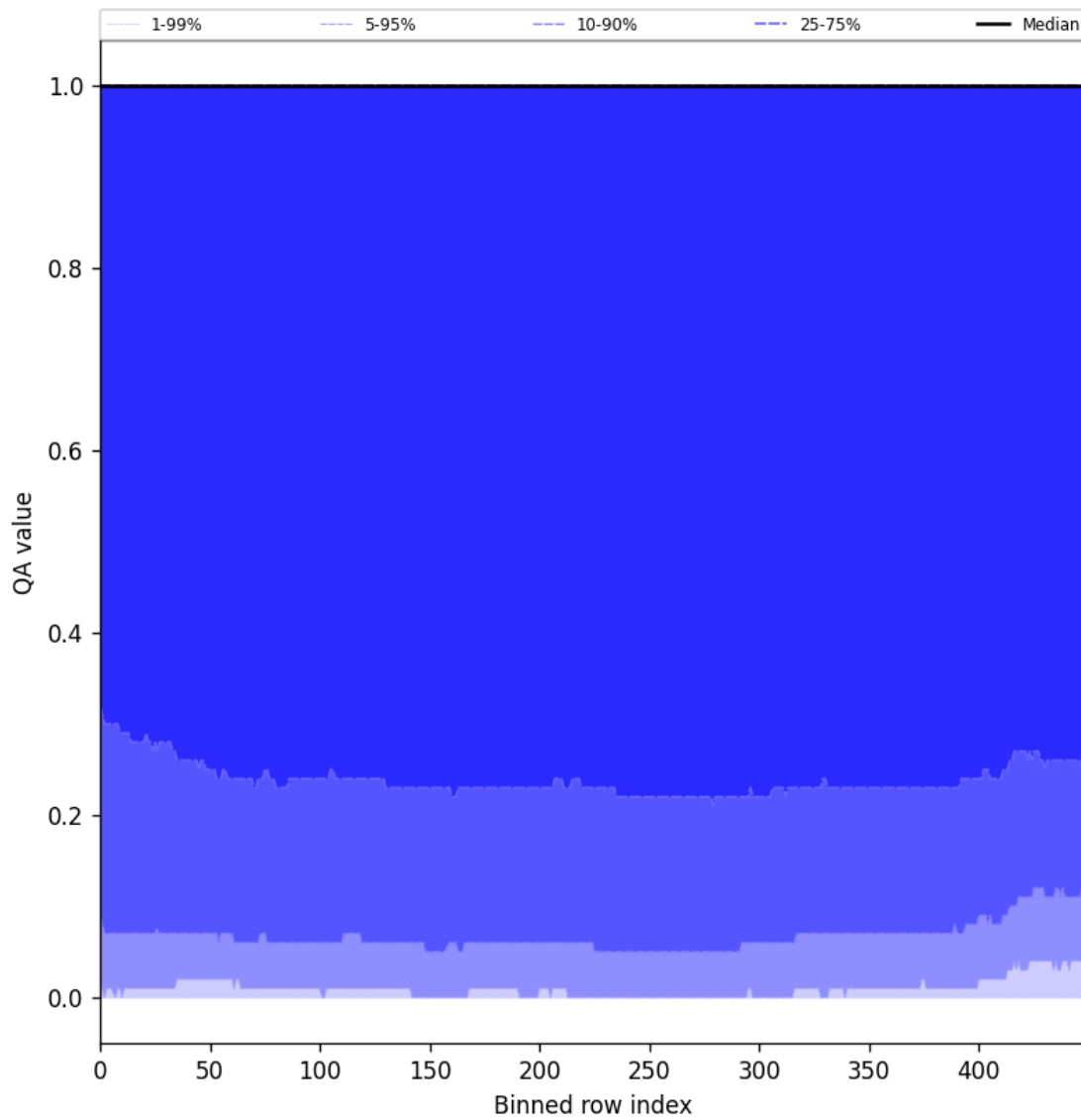
Figure 83: Along track statistics of “QA value” for 2025-07-16 to 2025-07-18
