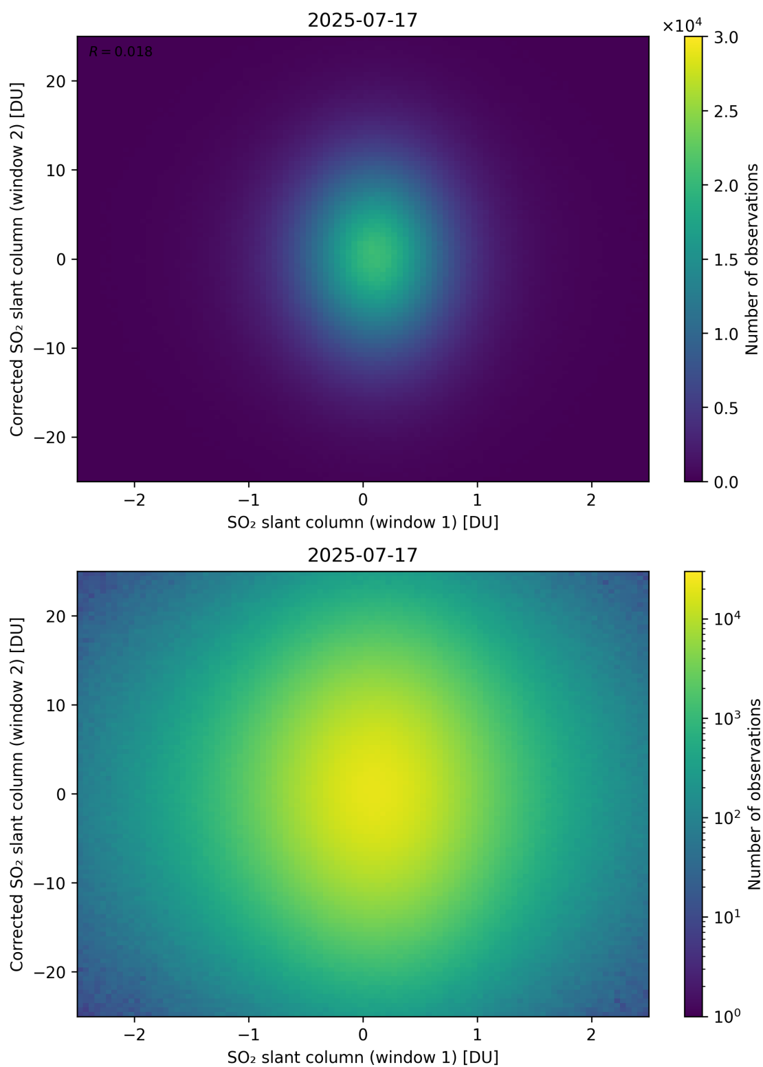
Figure 283: Scatter density plot of “SO 2 slant column (window 1)” against “Corrected SO 2 slant column (window 2)” for 2025-07-16 to 2025-07-18.
