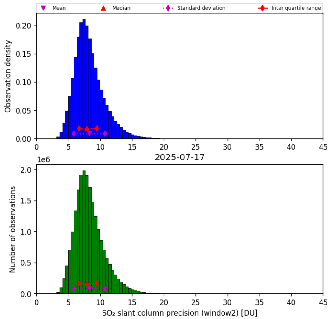
Figure 68: Histogram of “SO 2 slant column precision (window2)” for 2025-07-16 to 2025-07-18
