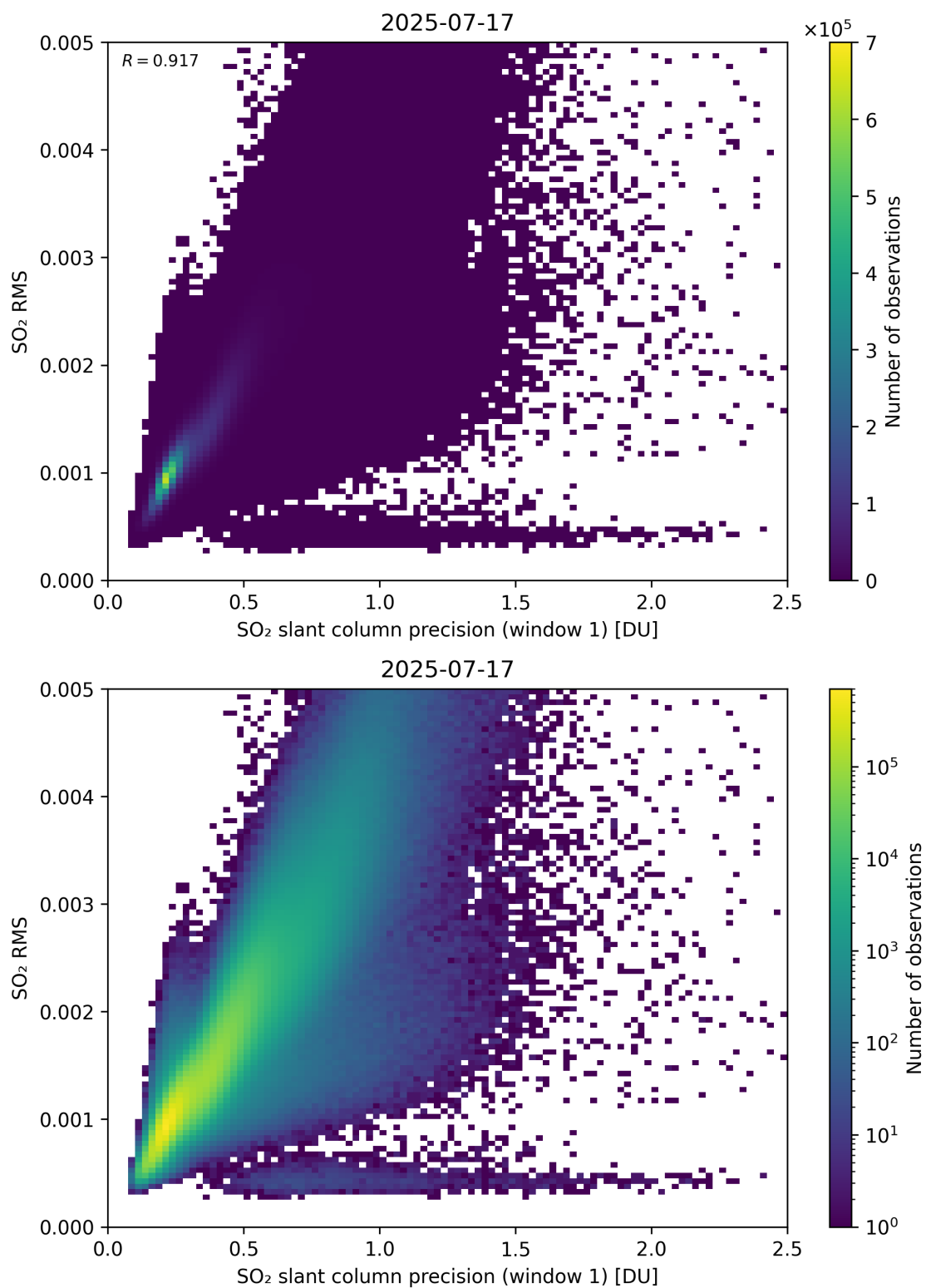
Figure 273: Scatter density plot of “SO 2 slant column precision (window 1)” against “SO 2 RMS” for 2025-07-16 to 2025-07-18.
