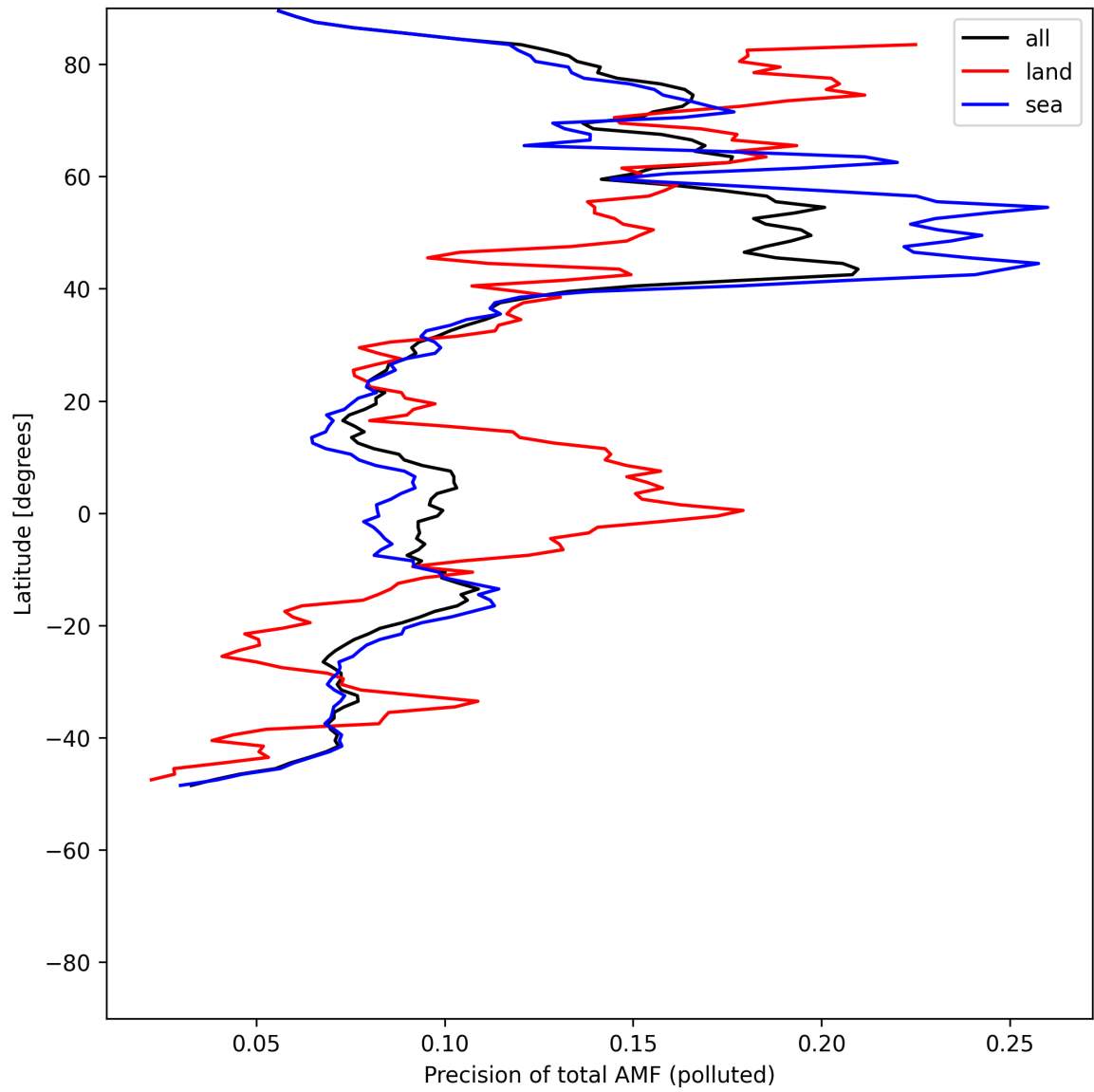
Figure 54: Zonal average of “Precision of total AMF (polluted)” for 2025-07-16 to 2025-07-18.
