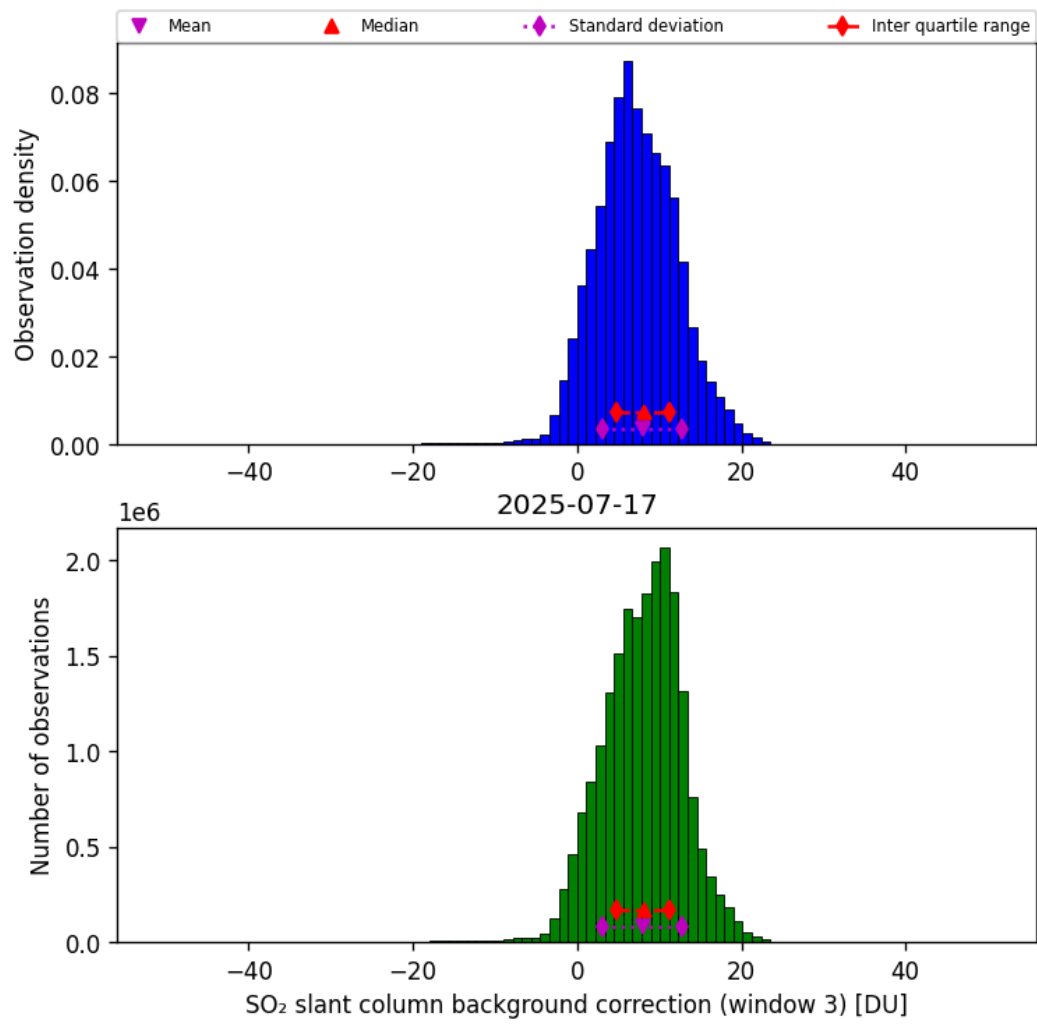
Figure 74: Histogram of “SO 2 slant column background correction (window 3)” for 2025-07-16 to 2025-07-18
