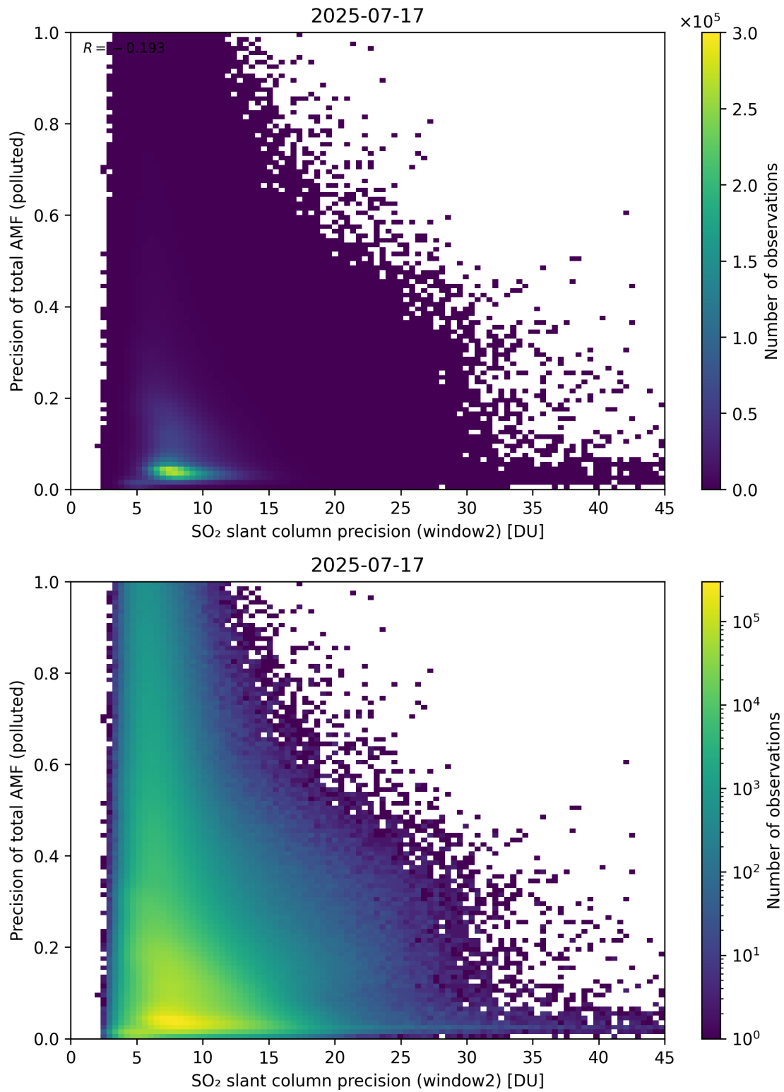
Figure 302: Scatter density plot of “SO 2 slant column precision (window2)” against “Precision of total AMF (polluted)” for 2025-07-16 to 2025-07-18.
