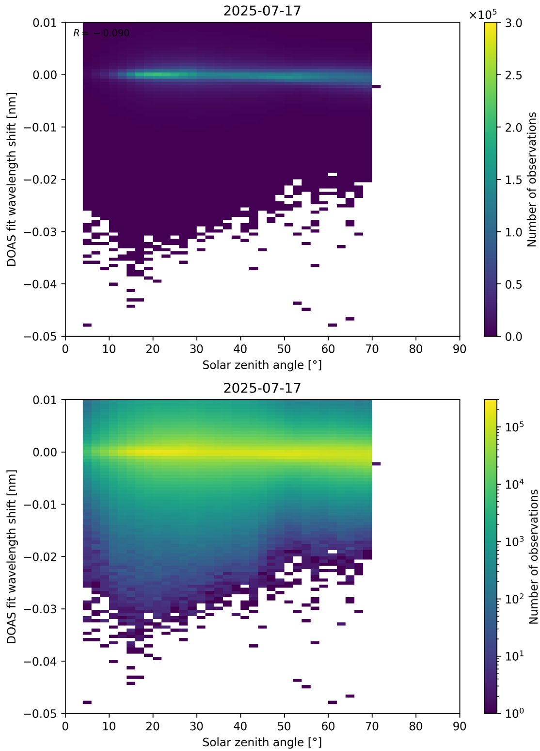
Figure 174: Scatter density plot of “Solar zenith angle” against “DOAS fit wavelength shift” for 2025-07-16 to 2025-07-18.
