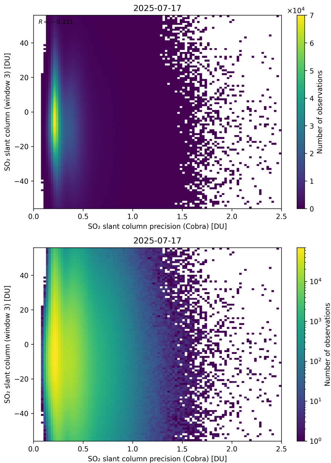
Figure 211: Scatter density plot of “SO 2 slant column precision (Cobra)” against “SO 2 slant column (window 3)” for 2025-07-16 to 2025-07-18.
