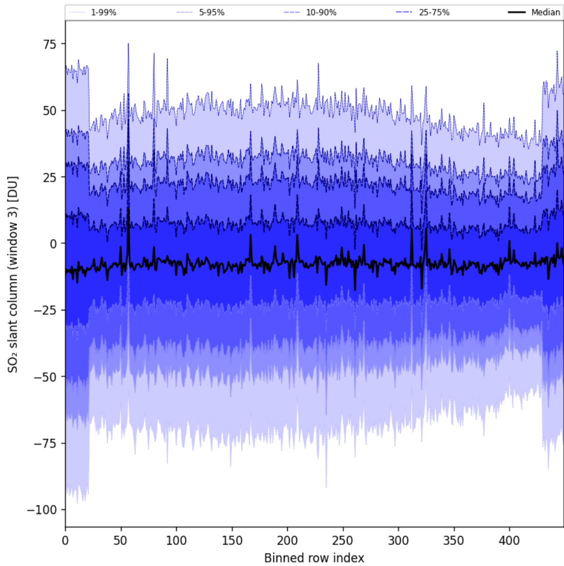
Figure 97: Along track statistics of “SO 2 slant column (window 3)” for 2025-07-16 to 2025-07-18
