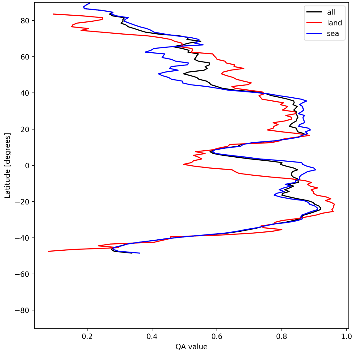
Figure 31: Zonal average of “QA value” for 2025-07-16 to 2025-07-18.
