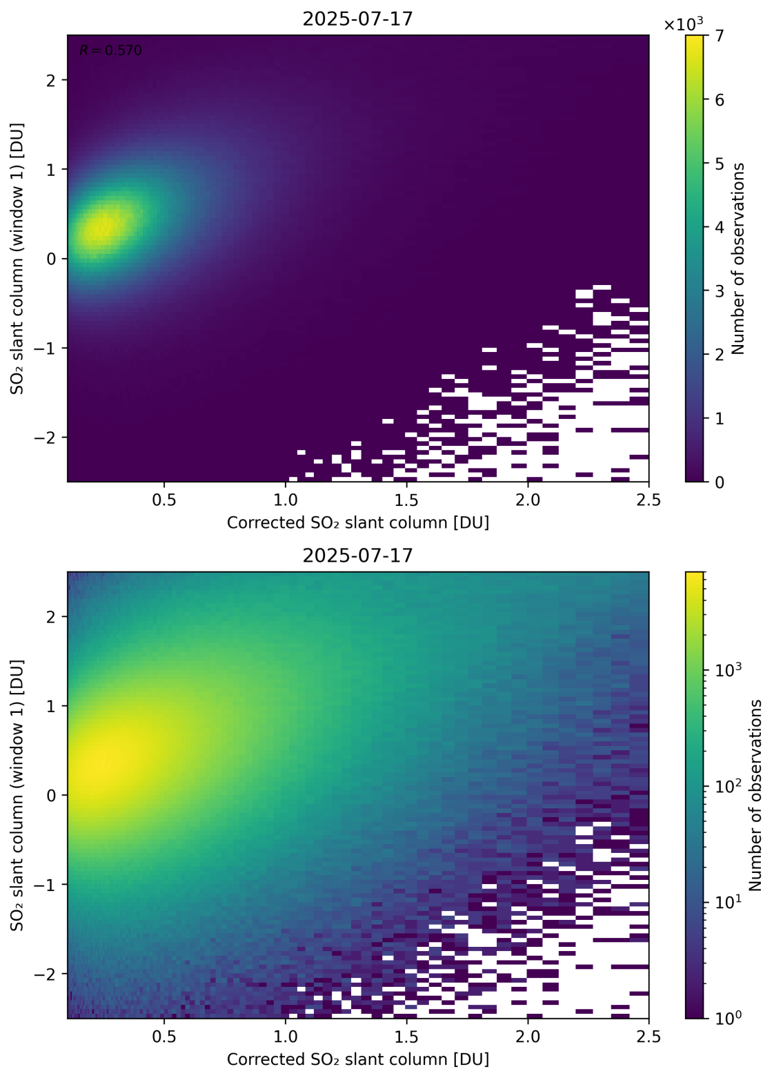
Figure 237: Scatter density plot of “Corrected SO 2 slant column” against “SO 2 slant column (window 1)” for 2025-07-16 to 2025-07-18.
