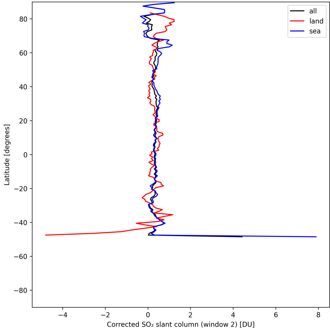
Figure 43: Zonal average of “Corrected SO 2 slant column (window 2)” for 2025-07-16 to 2025-07-18.
