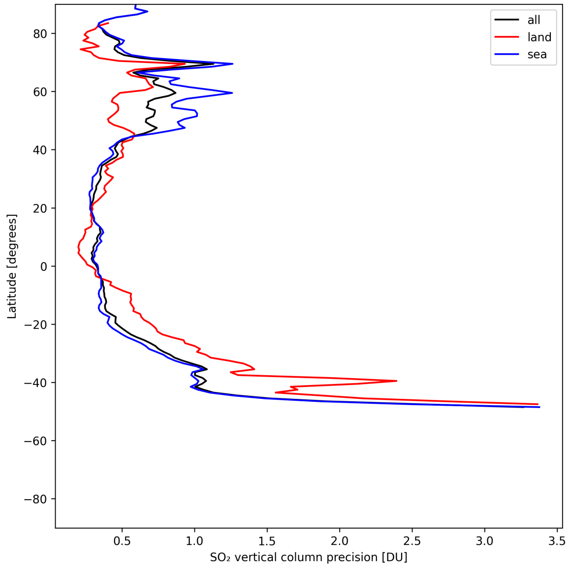
Figure 33: Zonal average of “SO 2 vertical column precision” for 2025-07-16 to 2025-07-18.
