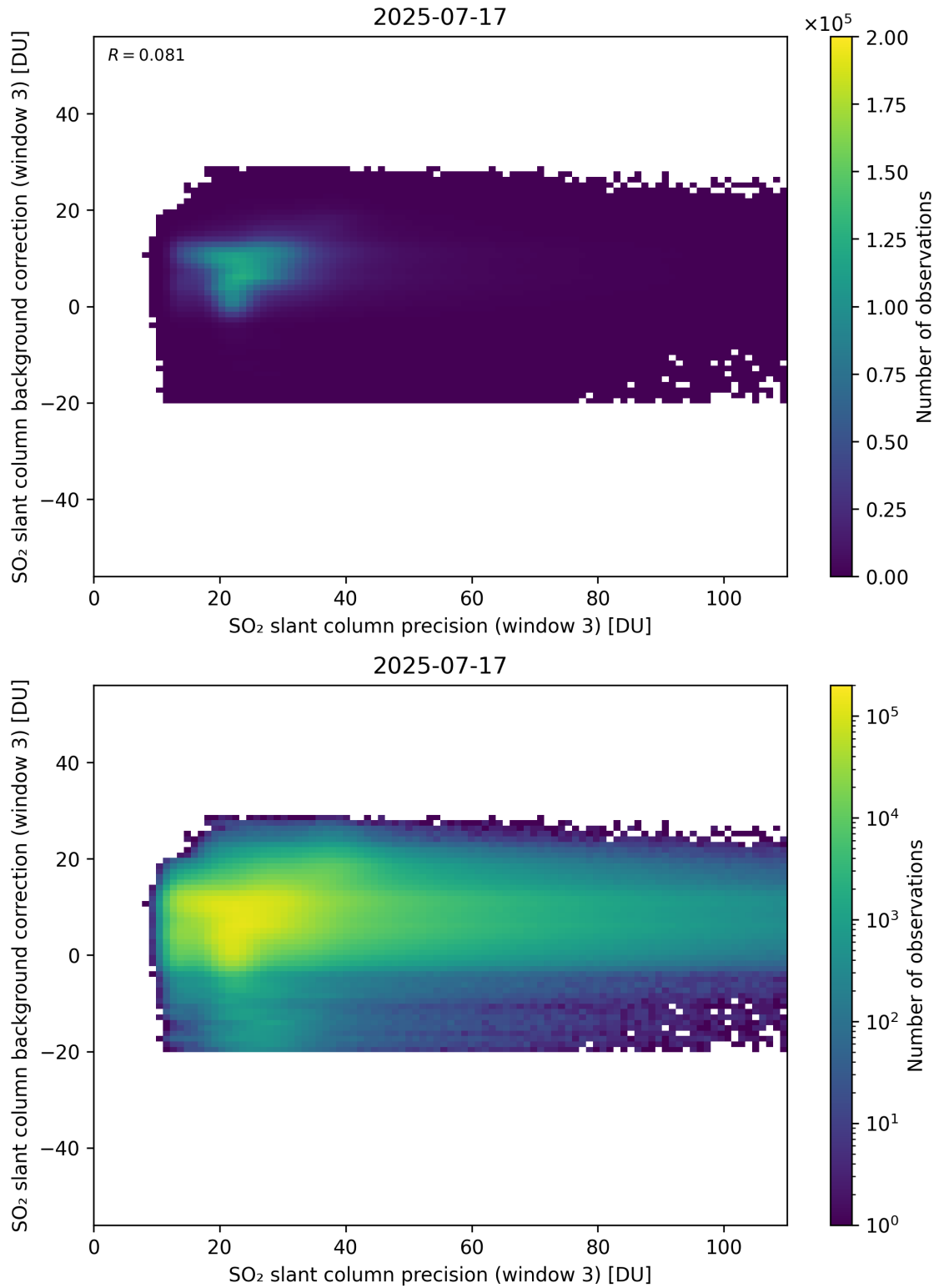
Figure 307: Scatter density plot of “SO 2 slant column precision (window 3)” against “SO 2 slant column background correction (window 3)” for 2025-07-16 to 2025-07-18.
