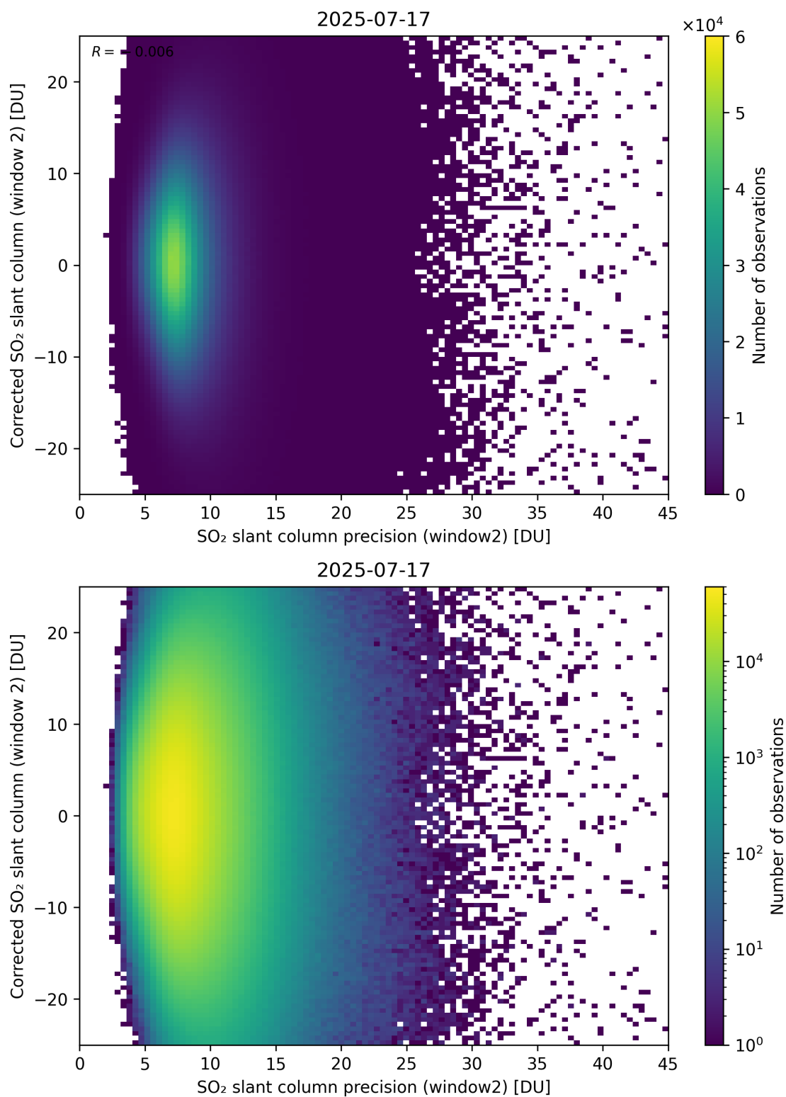
Figure 297: Scatter density plot of “SO 2 slant column precision (window2)” against “Corrected SO 2 slant column (window 2)” for 2025-07-16 to 2025-07-18.
