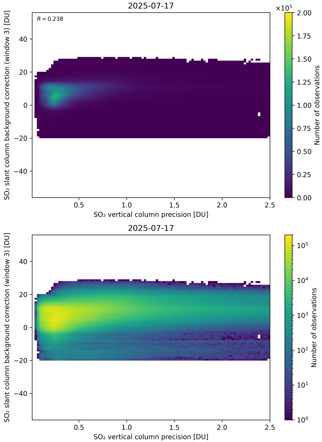
Figure 331: Scatter density plot of “SO 2 vertical column precision” against “SO 2 slant column background correction (window 3)” for 2025-07-16 to 2025-07-18.
