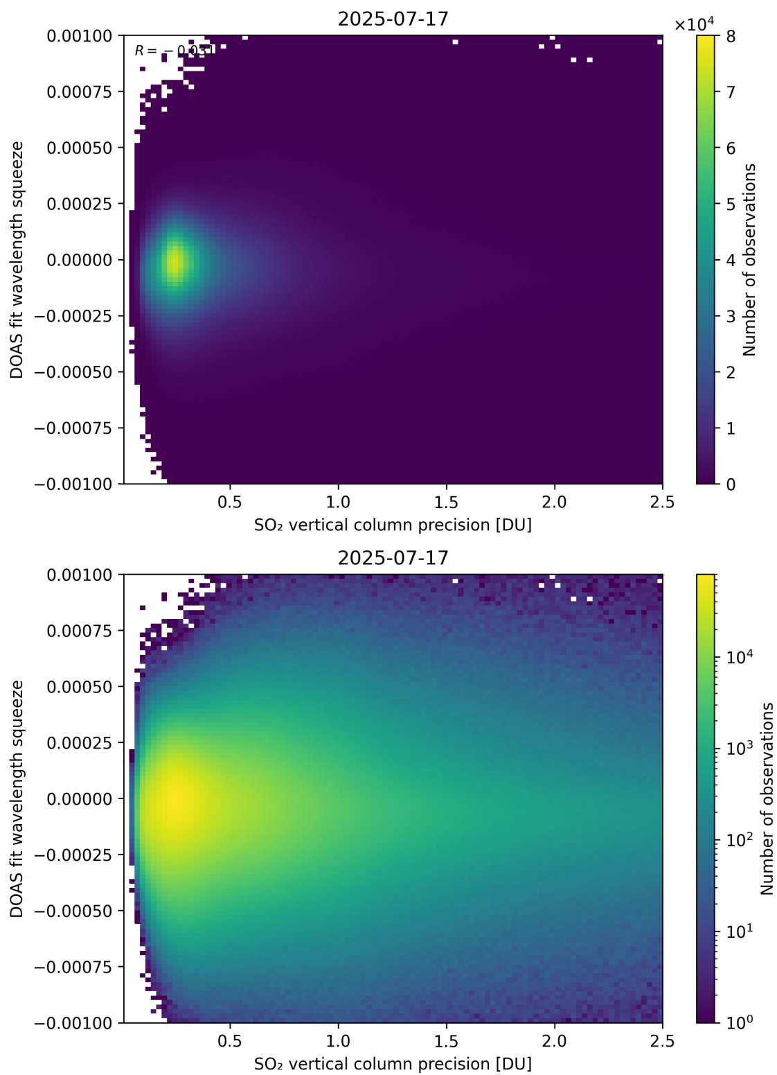
Figure 333: Scatter density plot of “SO 2 vertical column precision” against “DOAS fit wavelength squeeze” for 2025-07-16 to 2025-07-18.
