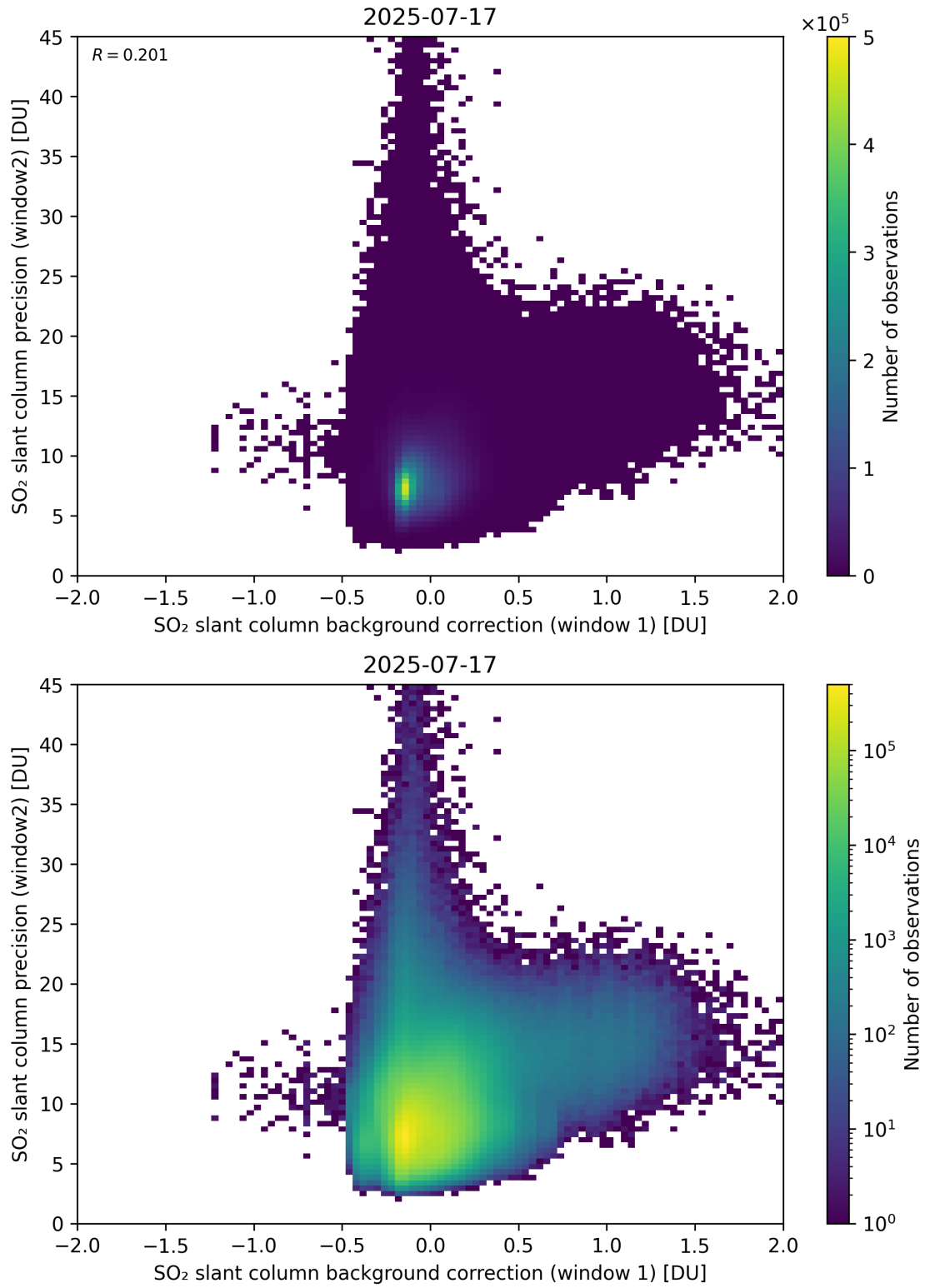
Figure 117: Scatter density plot of “SO 2 slant column background correction (window 1)” against “SO 2 slant column precision (window2)” for 2025-07-16 to 2025-07-18.
