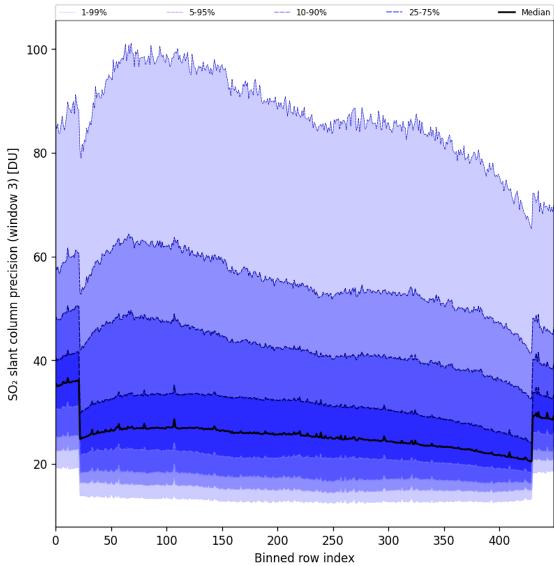
Figure 98: Along track statistics of “SO 2 slant column precision (window 3)” for 2025-07-16 to 2025-07-18
