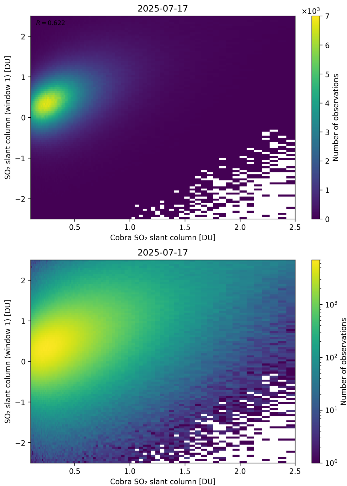
Figure 219: Scatter density plot of “Cobra SO 2 slant column” against “SO 2 slant column (window 1)” for 2025-07-16 to 2025-07-18.
