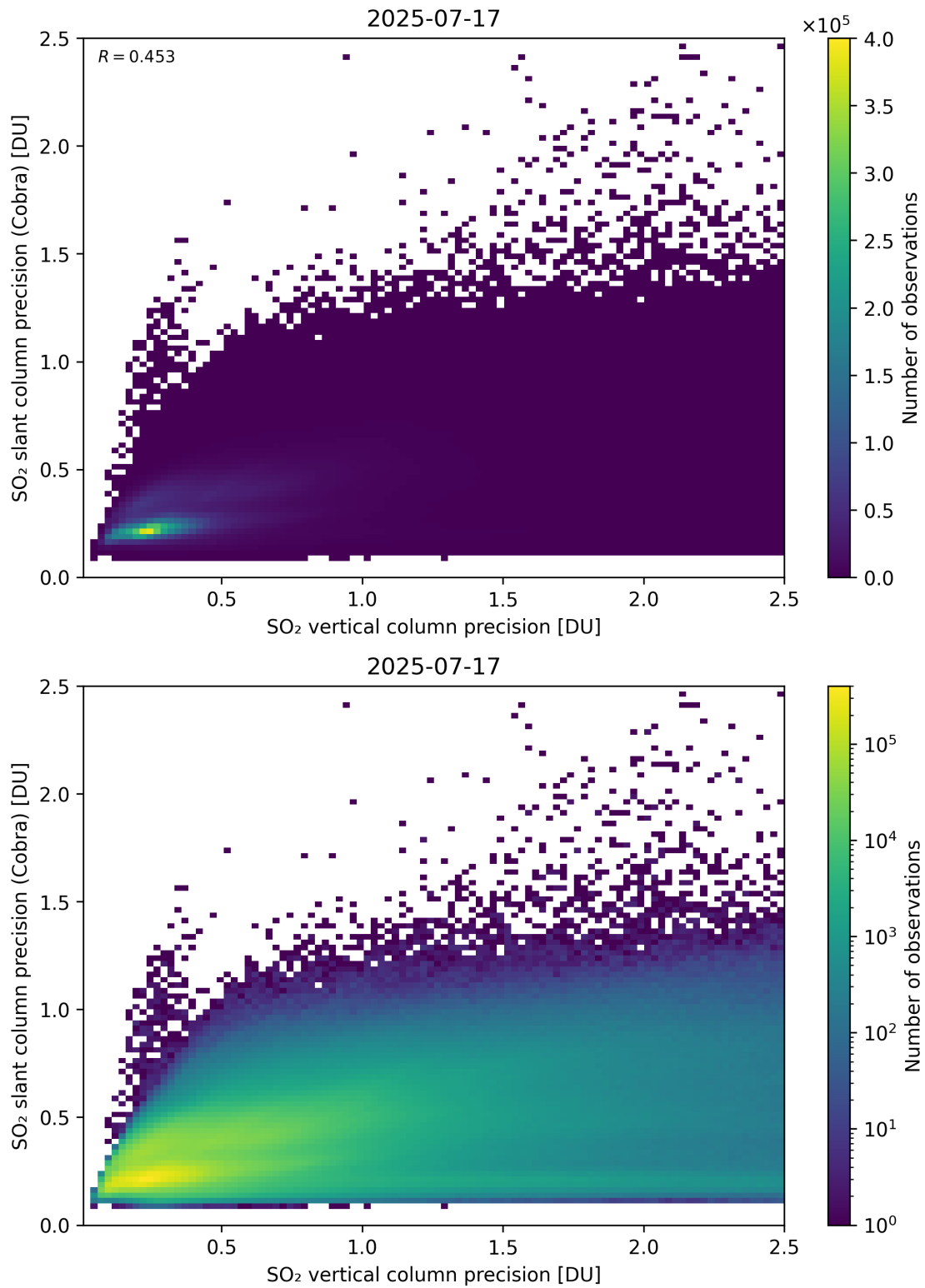
Figure 337: Scatter density plot of “SO 2 vertical column precision” against “SO 2 slant column precision (Cobra)” for 2025-07-16 to 2025-07-18.
