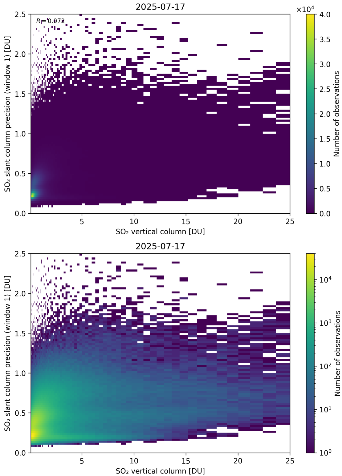
Figure 355: Scatter density plot of “SO 2 vertical column” against “SO 2 slant column precision (window 1)” for 2025-07-16 to 2025-07-18.
