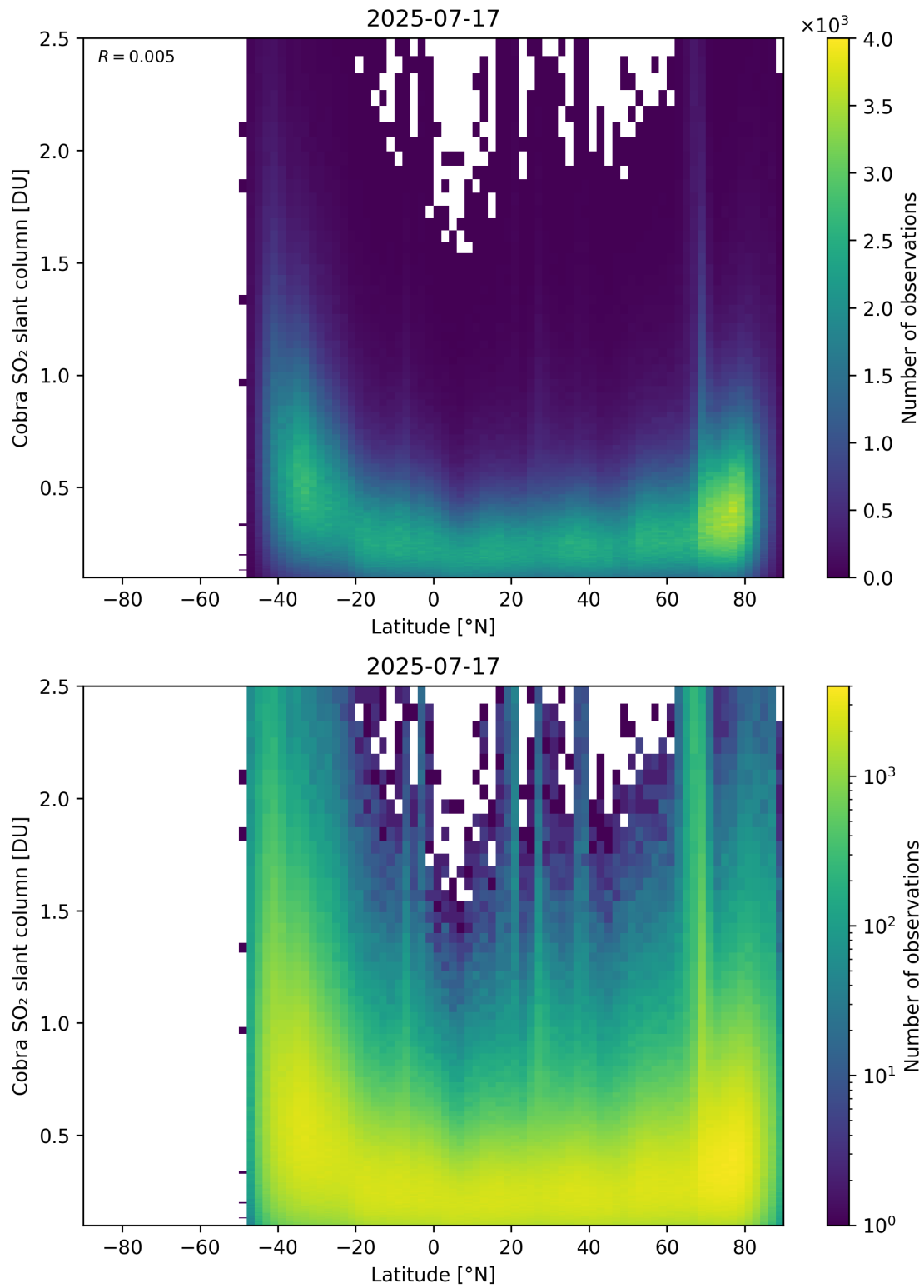
Figure 157: Scatter density plot of “Latitude” against “Cobra SO 2 slant column” for 2025-07-16 to 2025-07-18.
