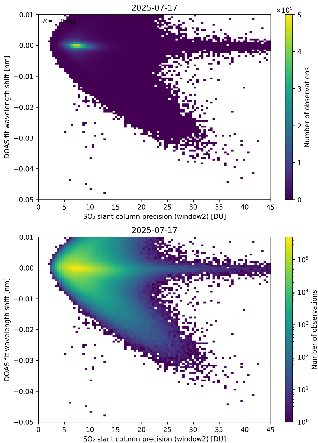
Figure 293: Scatter density plot of “SO 2 slant column precision (window2)” against “DOAS fit wavelength shift” for 2025-07-16 to 2025-07-18.
