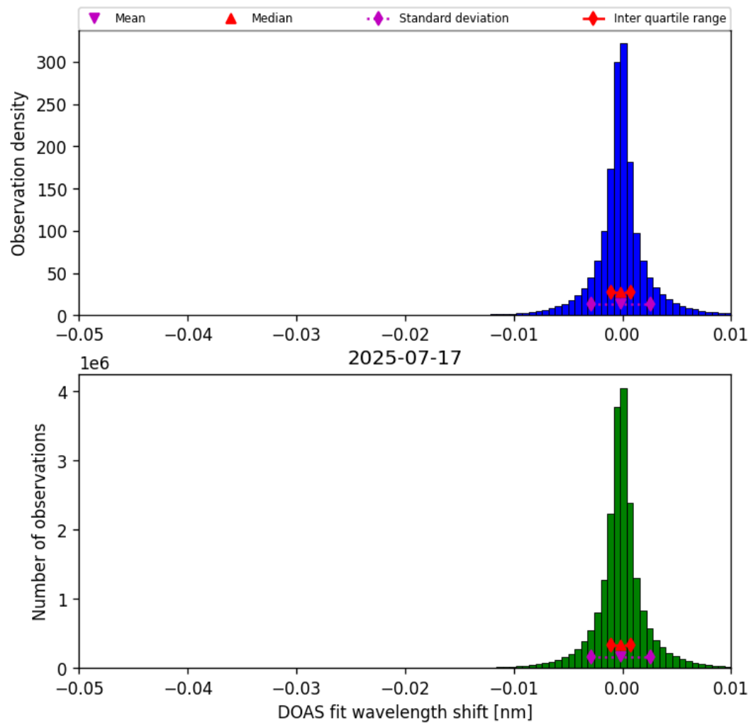
Figure 76: Histogram of “DOAS fit wavelength shift” for 2025-07-16 to 2025-07-18
