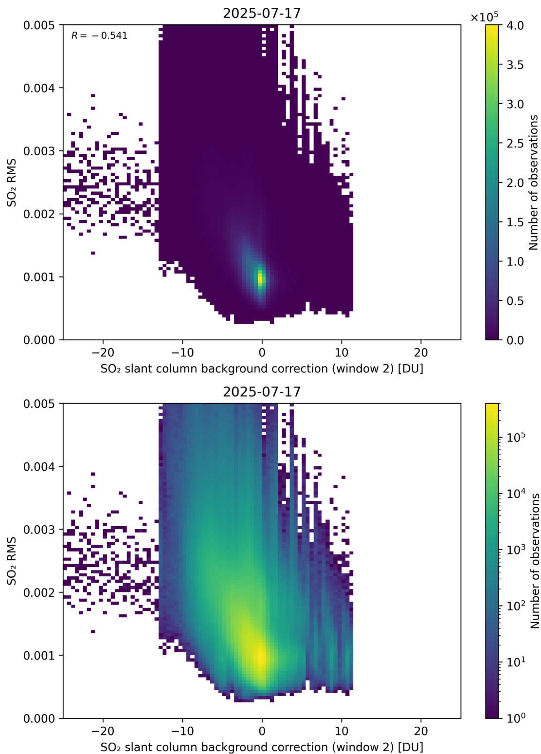
Figure 125: Scatter density plot of “SO 2 slant column background correction (window 2)” against “SO 2 RMS” for 2025-07-16 to 2025-07-18.
