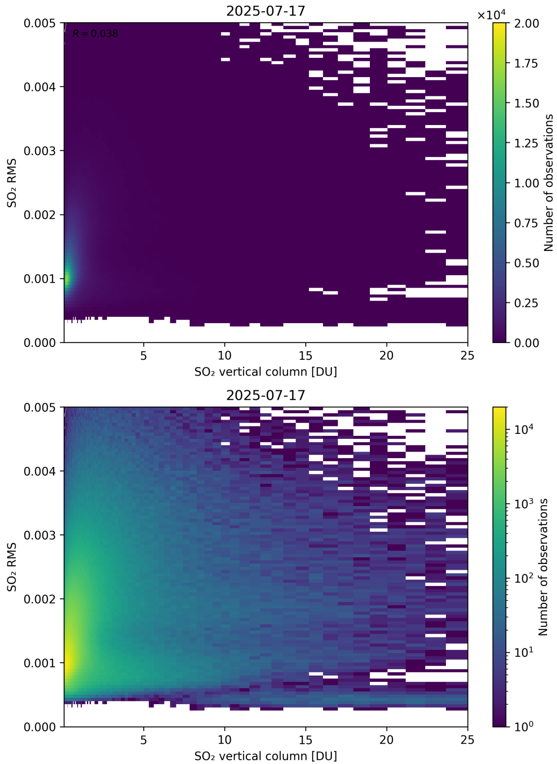
Figure 328: Scatter density plot of “SO 2 vertical column” against “SO 2 RMS” for 2025-07-16 to 2025-07-18.
