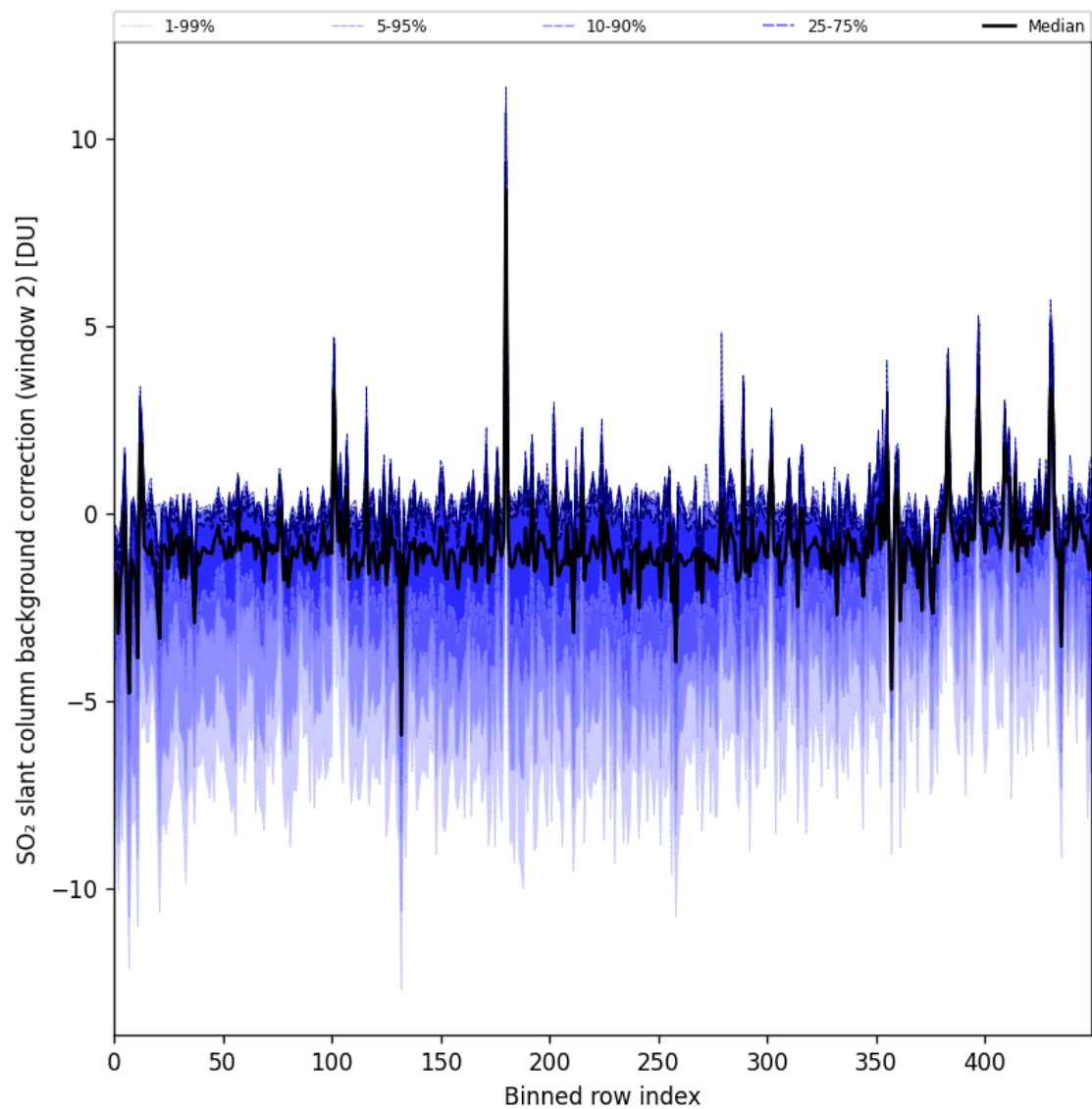
Figure 96: Along track statistics of “SO 2 slant column background correction (window 2)” for 2025-07-16 to 2025-07-18
