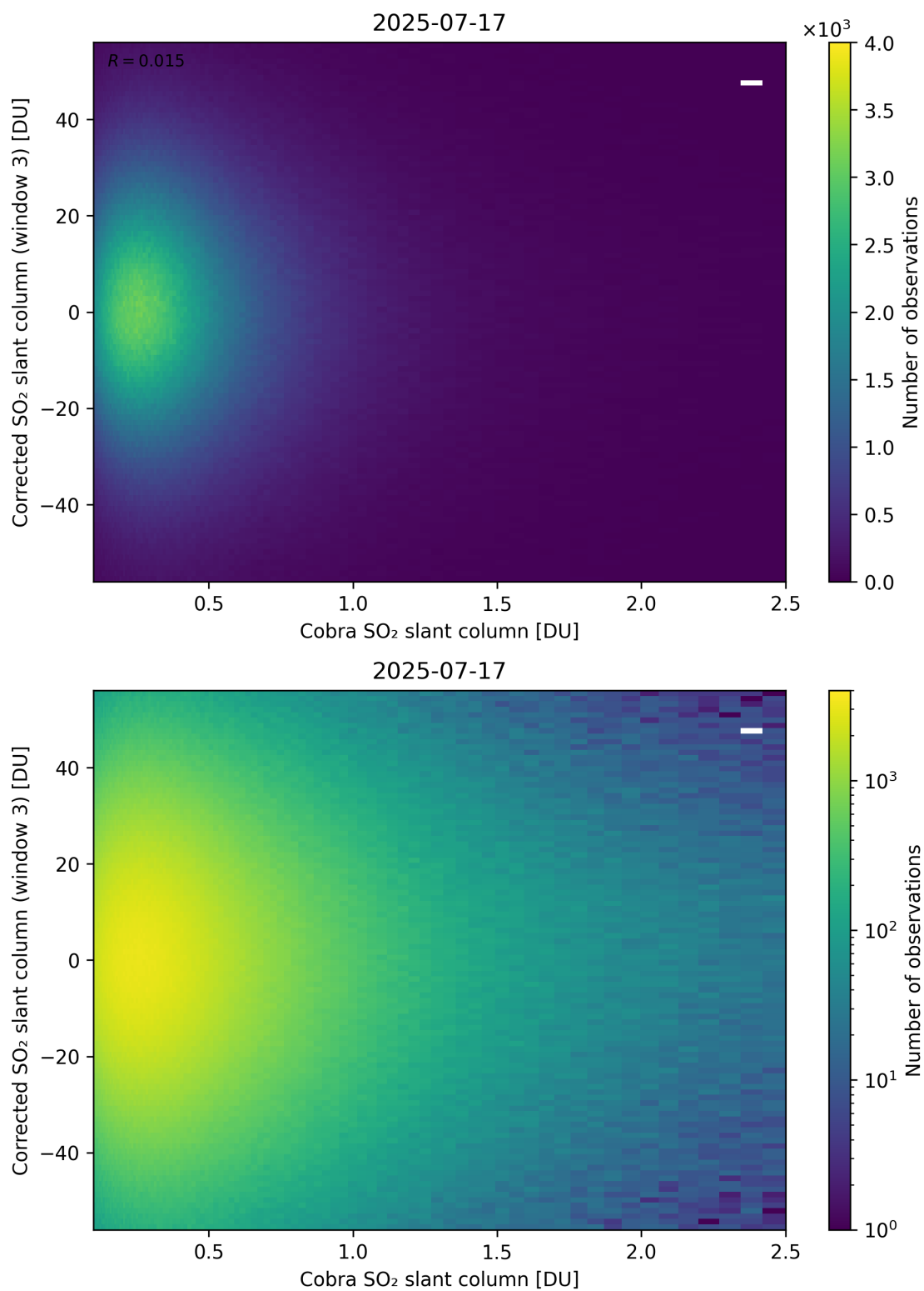
Figure 218: Scatter density plot of “Cobra SO 2 slant column” against “Corrected SO 2 slant column (window 3)” for 2025-07-16 to 2025-07-18.
