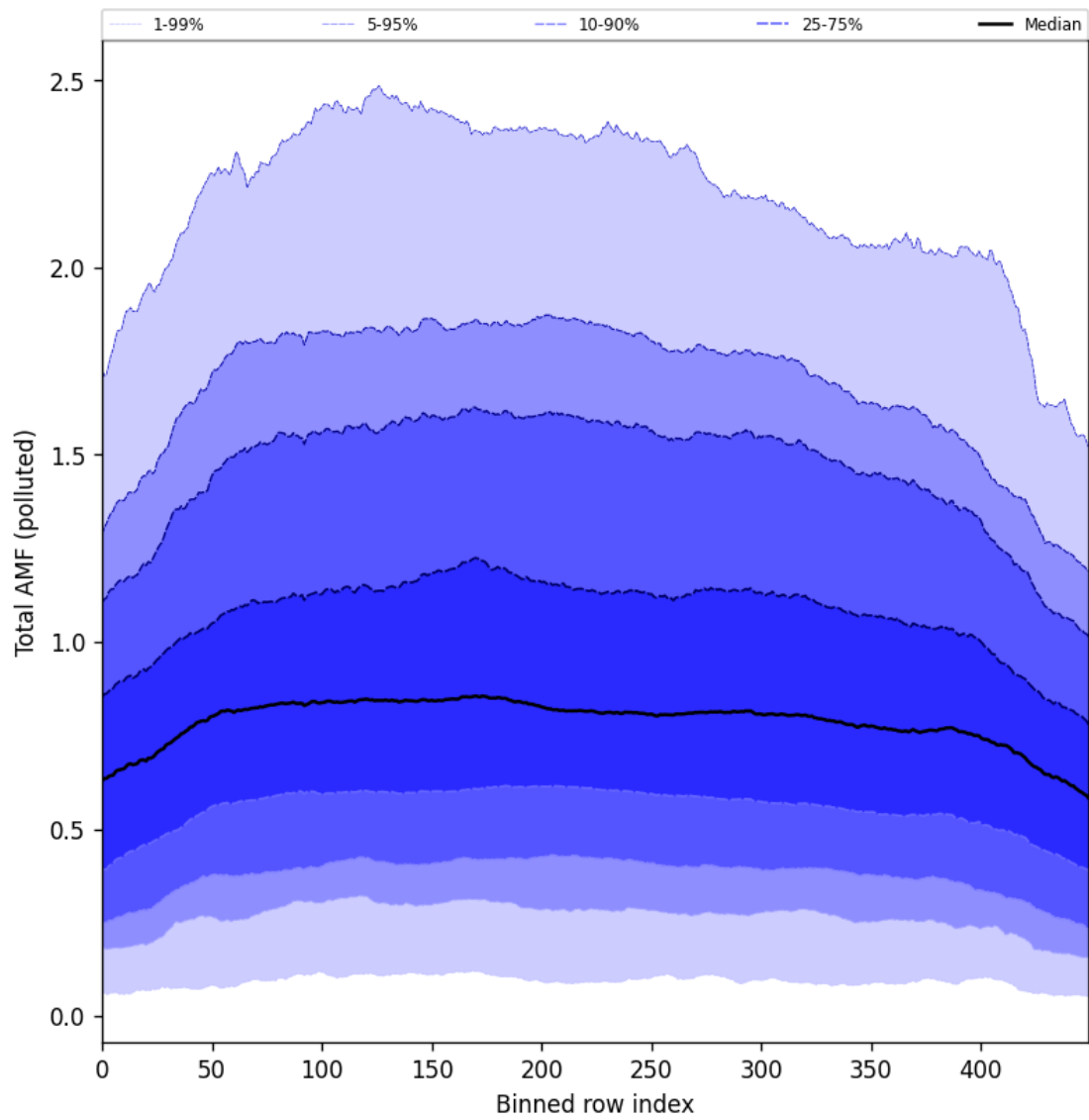
Figure 105: Along track statistics of “Total AMF (polluted)” for 2025-07-16 to 2025-07-18
