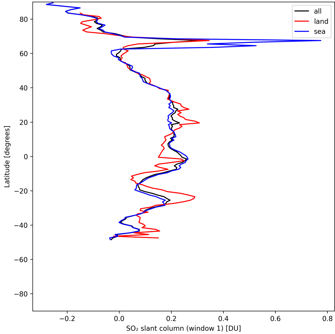
Figure 37: Zonal average of “SO 2 slant column (window 1)” for 2025-07-16 to 2025-07-18.
