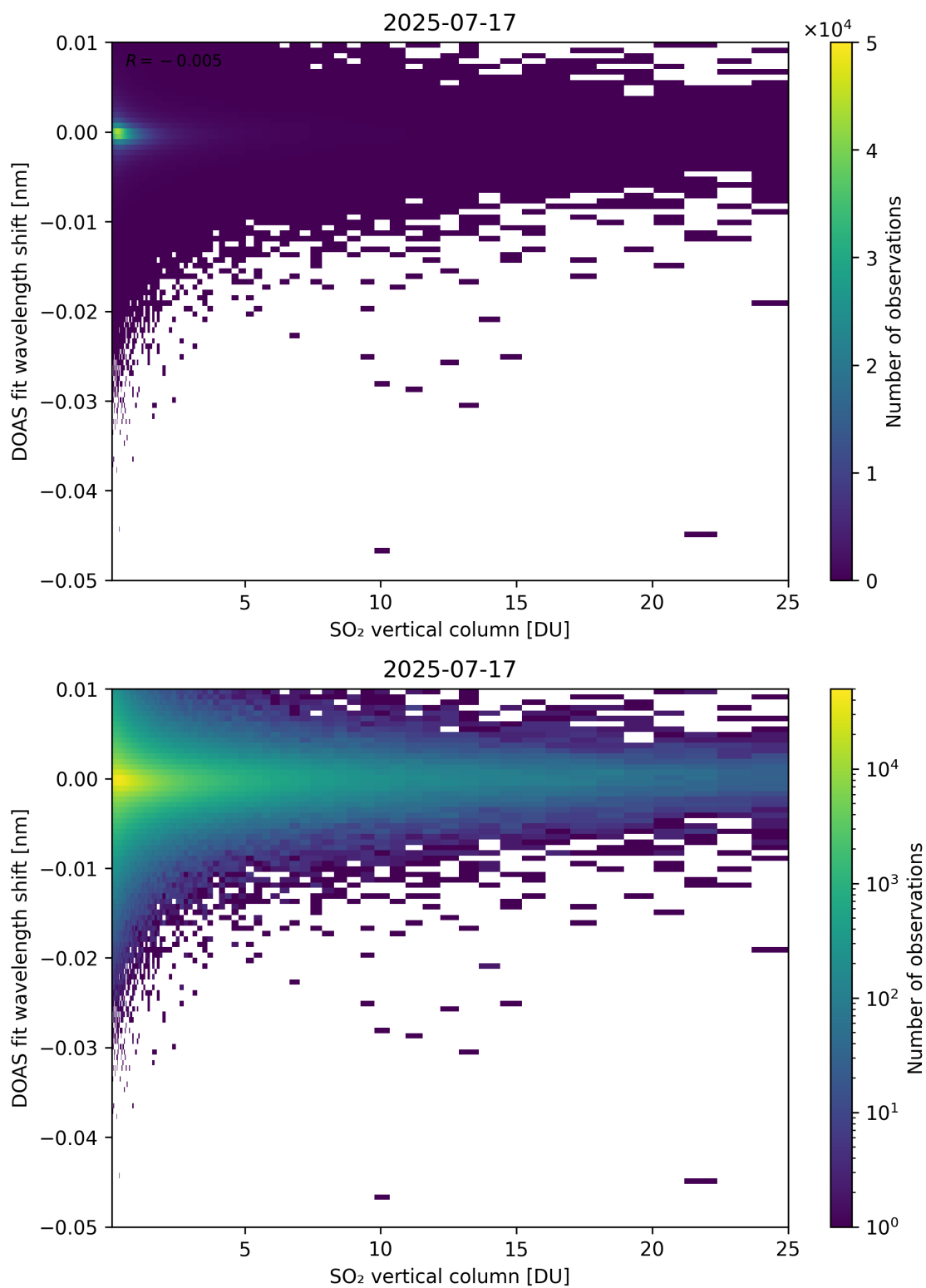
Figure 326: Scatter density plot of “SO 2 vertical column” against “DOAS fit wavelength shift” for 2025-07-16 to 2025-07-18.
