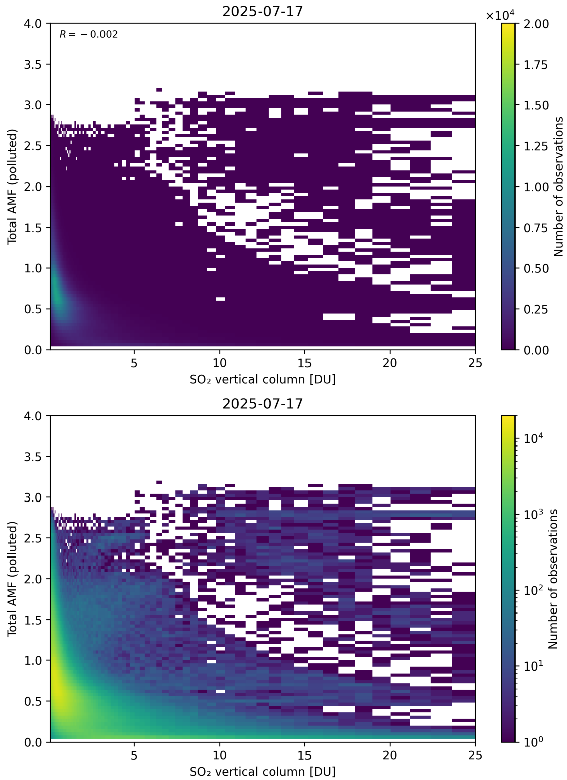
Figure 359: Scatter density plot of “SO 2 vertical column” against “Total AMF (polluted)” for 2025-07-16 to 2025-07-18.
