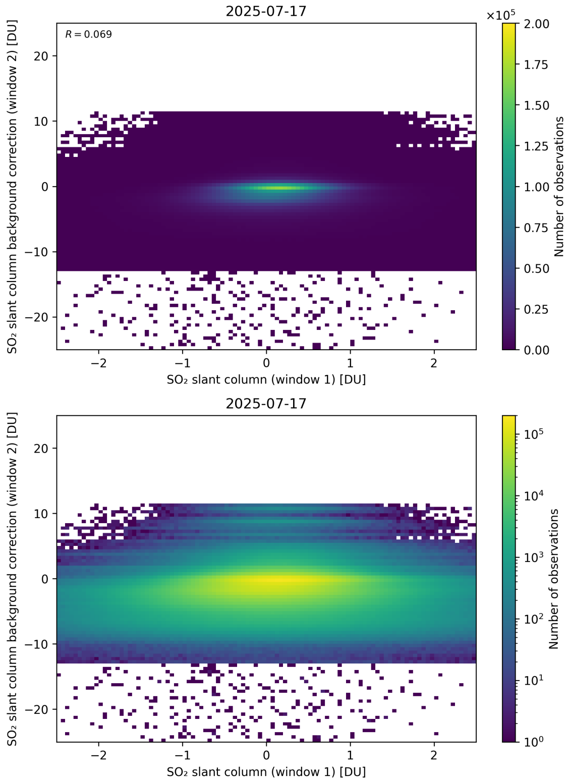
Figure 263: Scatter density plot of “SO 2 slant column (window 1)” against “SO 2 slant column background correction (window 2)” for 2025-07-16 to 2025-07-18.
