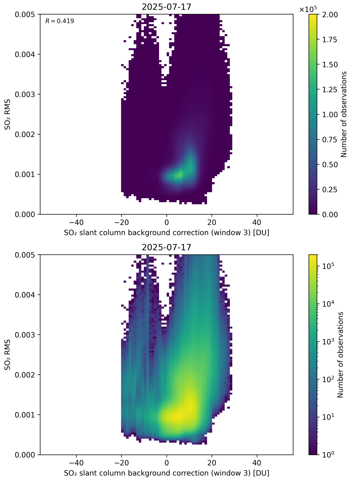
Figure 134: Scatter density plot of “SO 2 slant column background correction (window 3)” against “SO 2 RMS” for 2025-07-16 to 2025-07-18.
