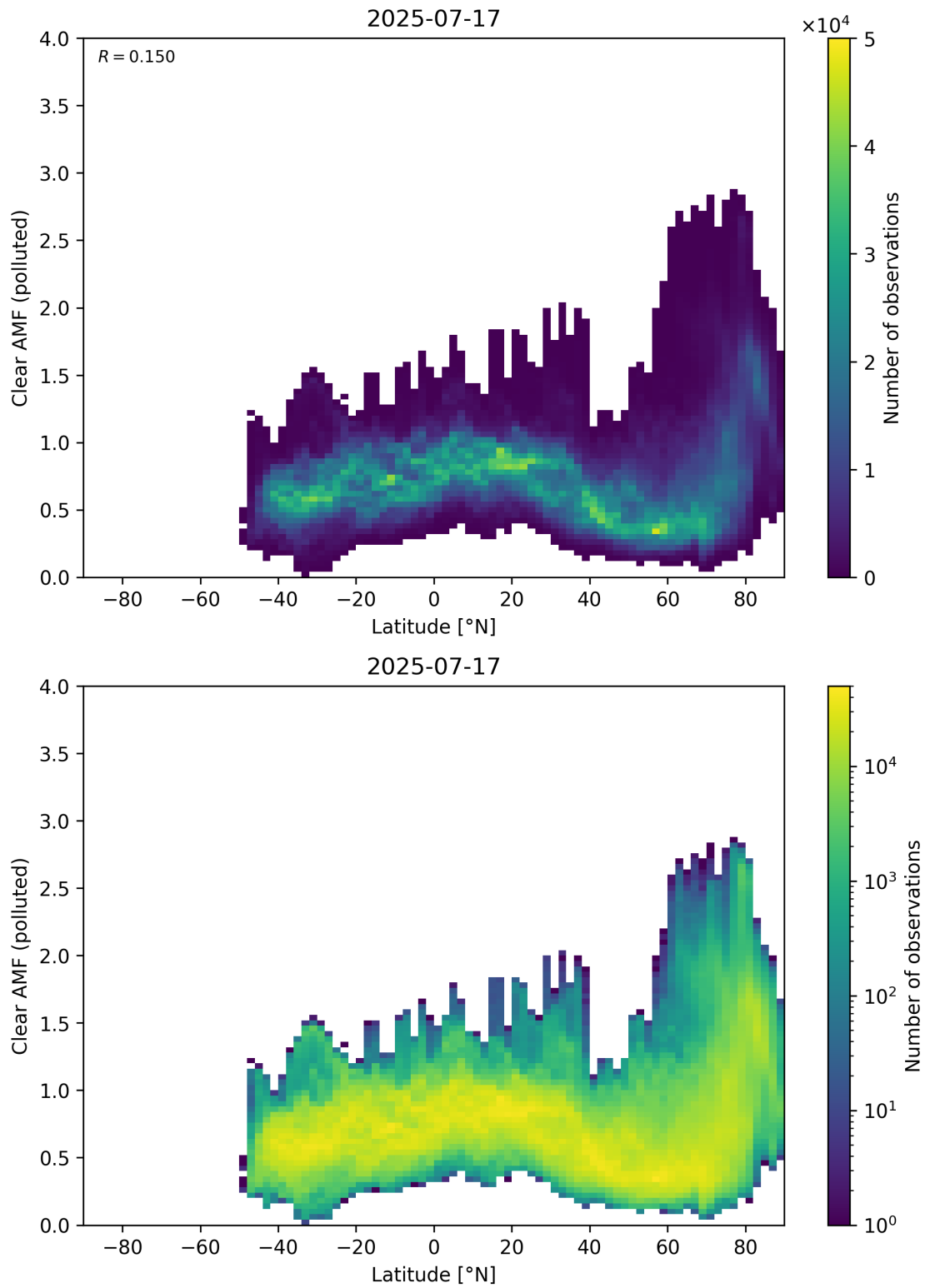
Figure 156: Scatter density plot of “Latitude” against “Clear AMF (polluted)” for 2025-07-16 to 2025-07-18.
