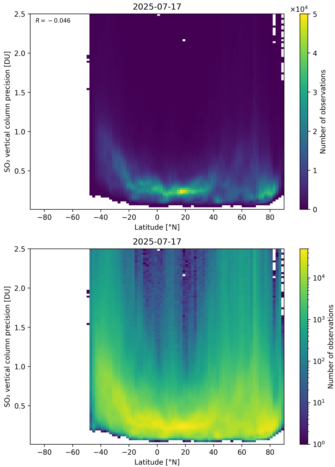
Figure 170: Scatter density plot of “Latitude” against “SO 2 vertical column precision” for 2025-07-16 to 2025-07-18.
