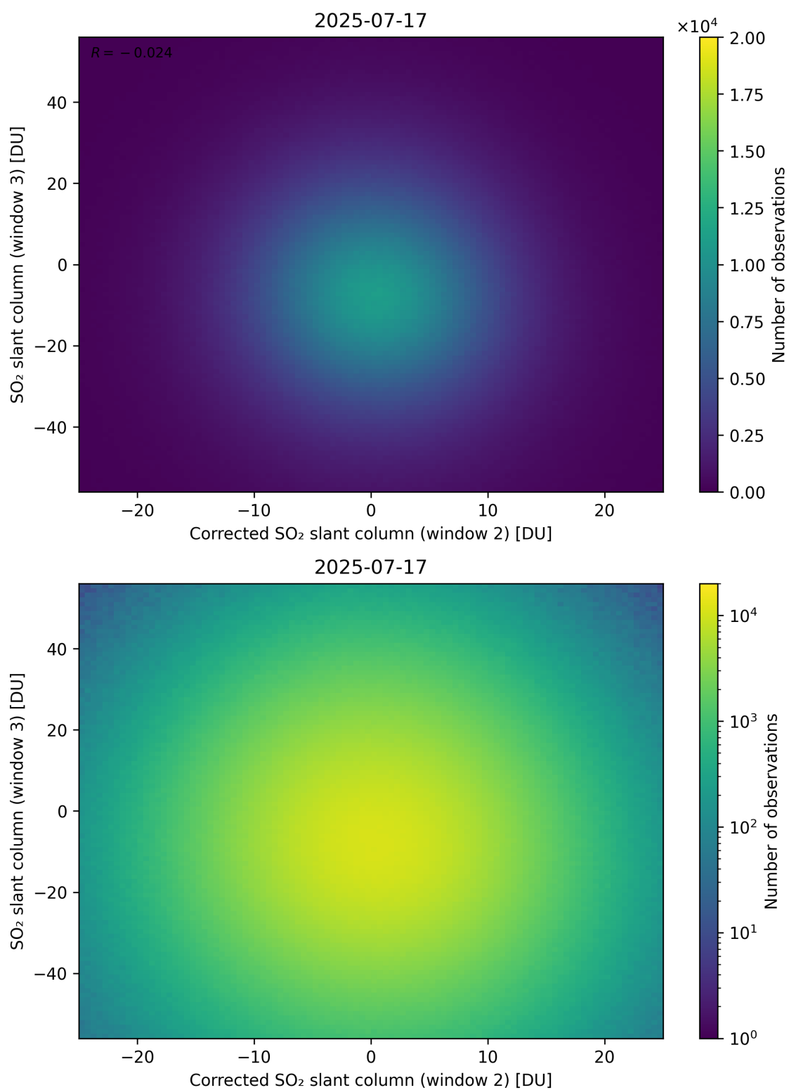
Figure 251: Scatter density plot of “Corrected SO 2 slant column (window 2)” against “SO 2 slant column (window 3)” for 2025-07-16 to 2025-07-18.
