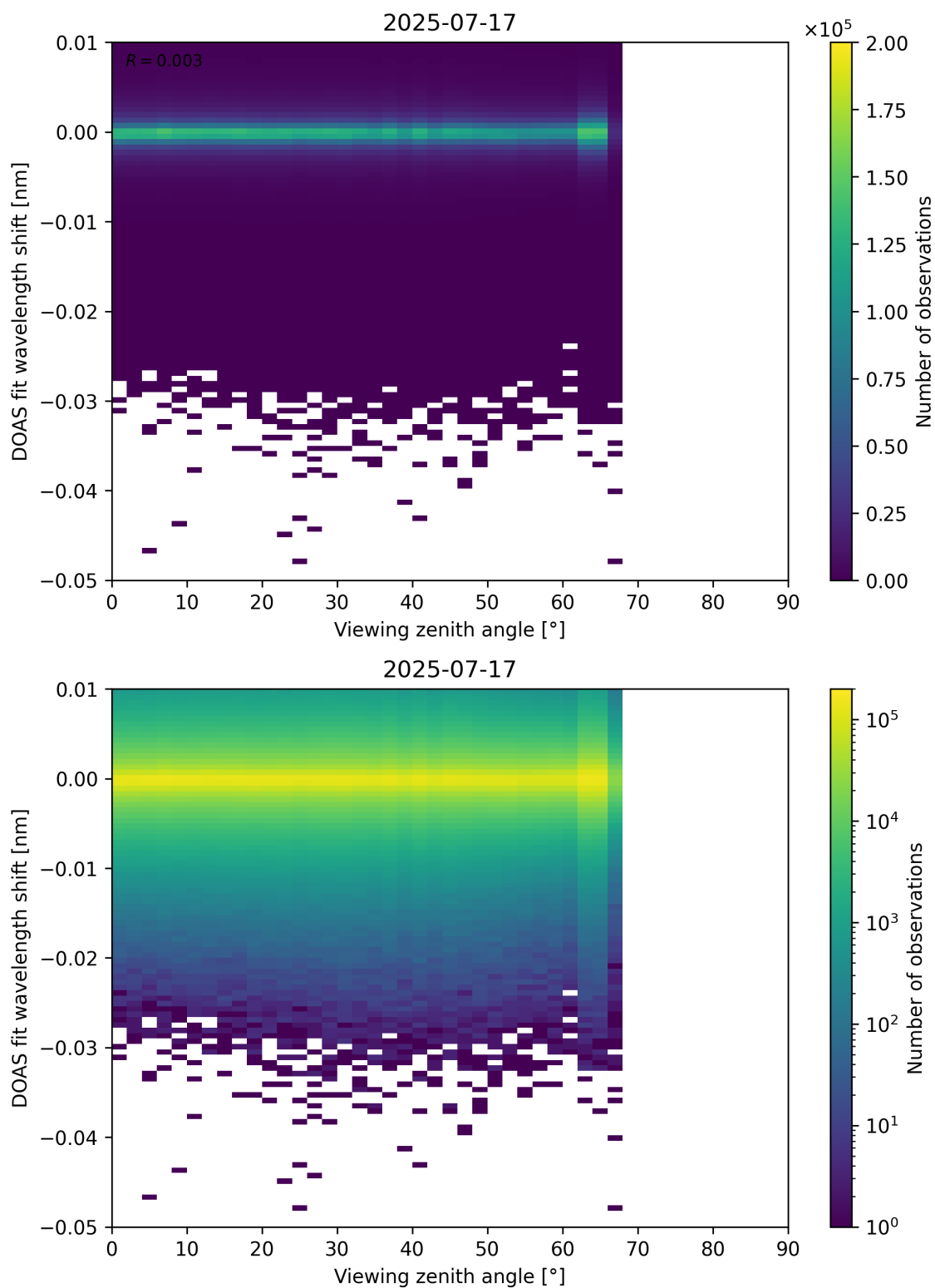
Figure 365: Scatter density plot of “Viewing zenith angle” against “DOAS fit wavelength shift” for 2025-07-16 to 2025-07-18.
