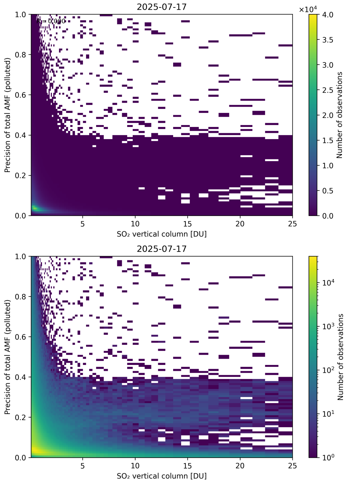
Figure 360: Scatter density plot of “SO 2 vertical column” against “Precision of total AMF (polluted)” for 2025-07-16 to 2025-07-18.
