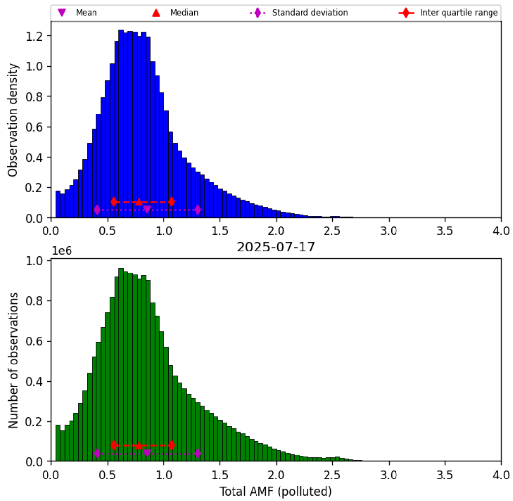
Figure 79: Histogram of “Total AMF (polluted)” for 2025-07-16 to 2025-07-18
