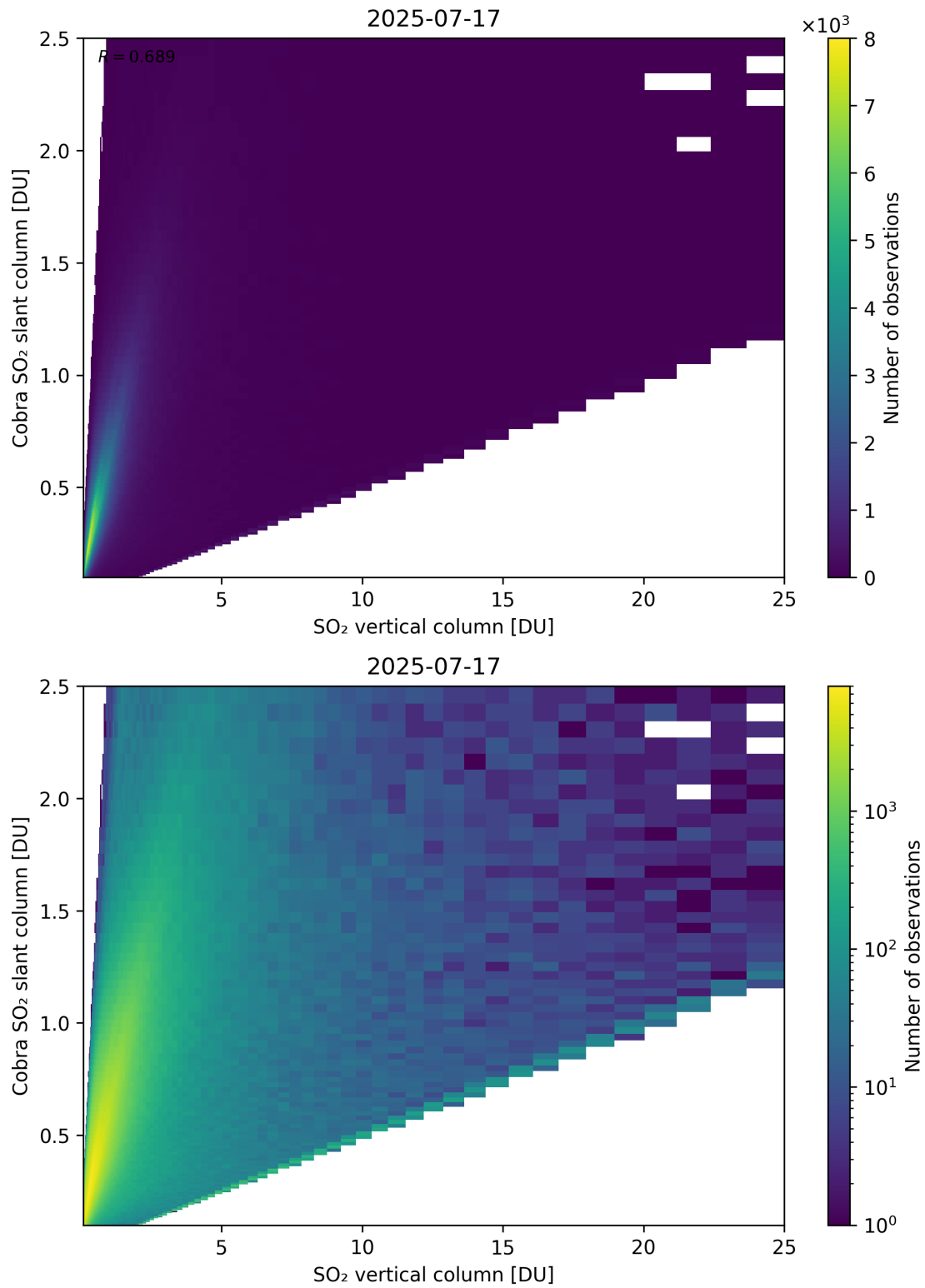
Figure 349: Scatter density plot of “SO 2 vertical column” against “Cobra SO 2 slant column” for 2025-07-16 to 2025-07-18.
