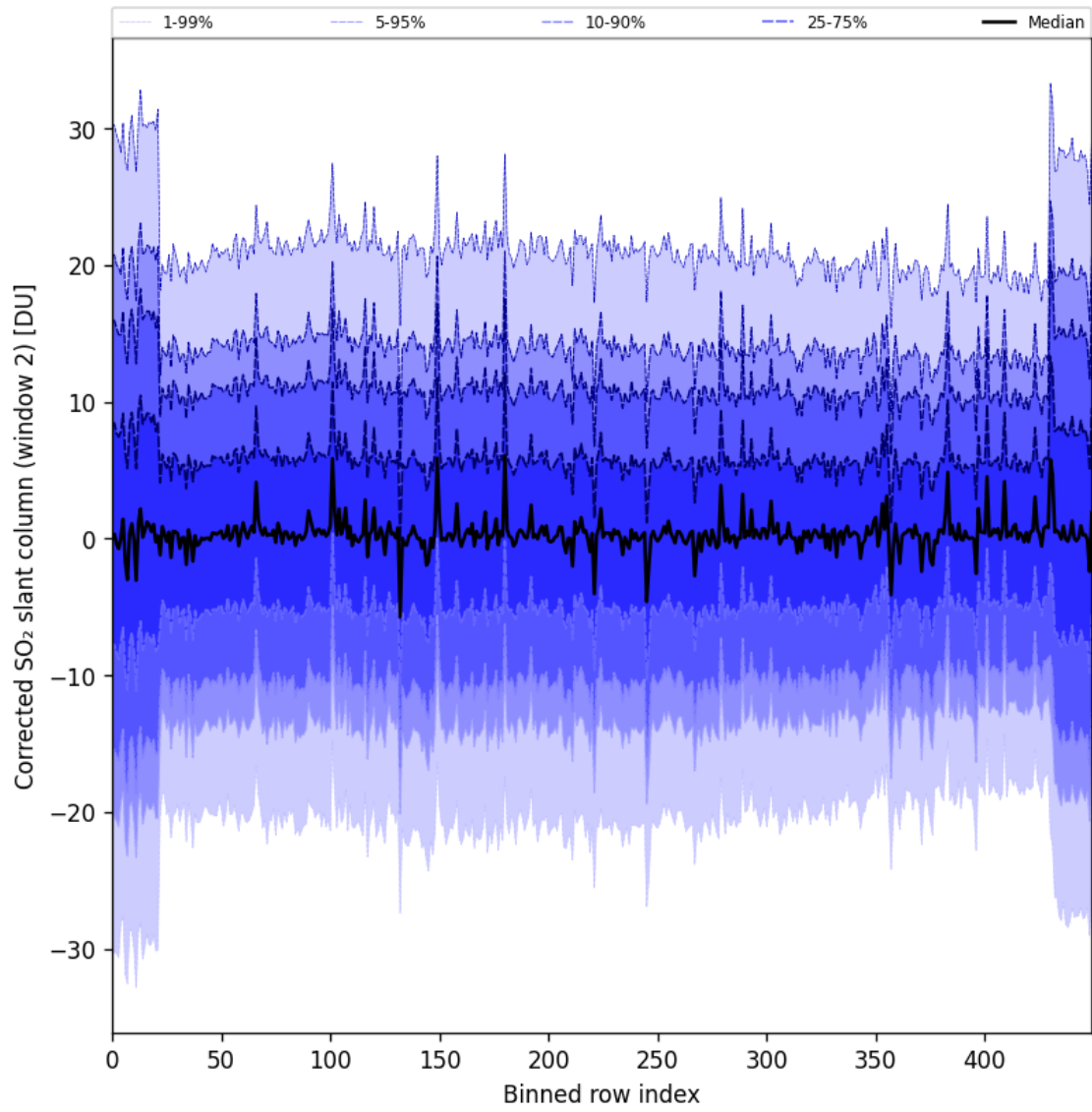
Figure 95: Along track statistics of “Corrected SO 2 slant column (window 2)” for 2025-07-16 to 2025-07-18
