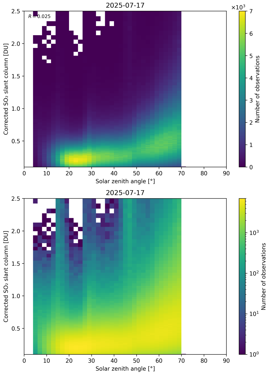
Figure 181: Scatter density plot of “Solar zenith angle” against “Corrected SO 2 slant column” for 2025-07-16 to 2025-07-18.
