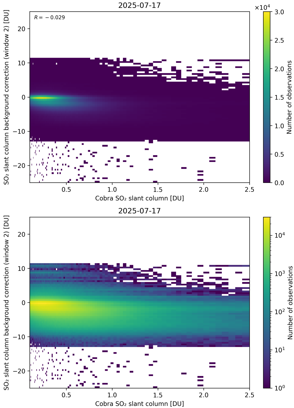
Figure 194: Scatter density plot of “Cobra SO 2 slant column” against “SO 2 slant column background correction (window 2)” for 2025-07-16 to 2025-07-18.
