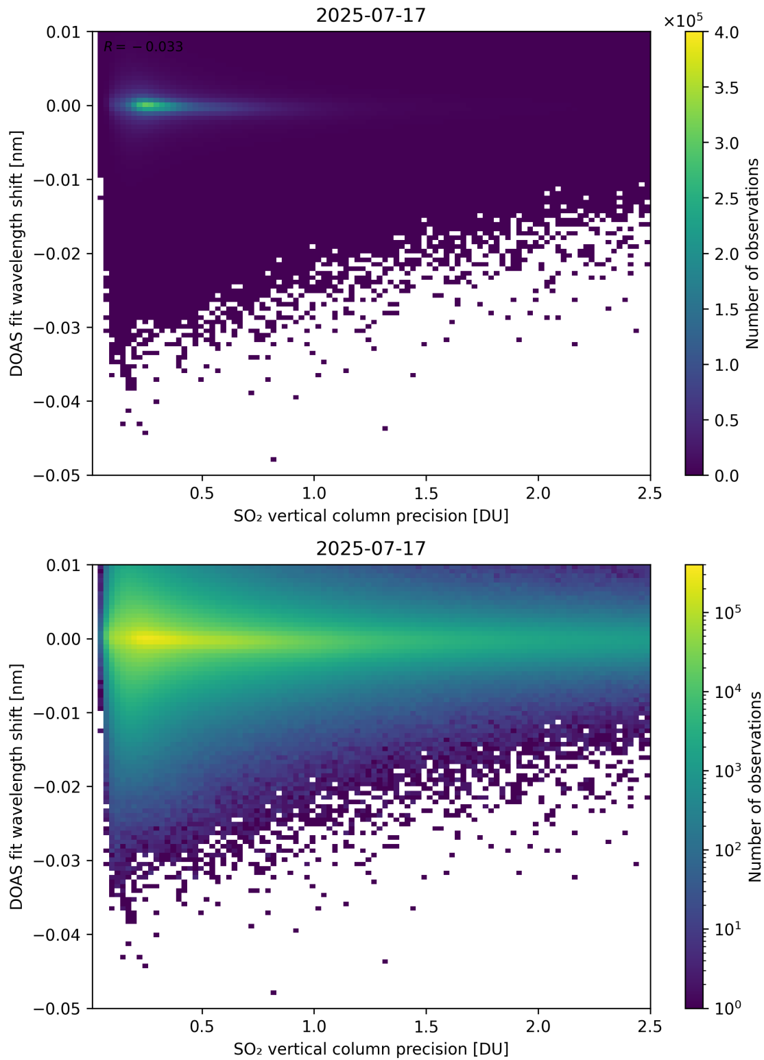
Figure 332: Scatter density plot of “SO 2 vertical column precision” against “DOAS fit wavelength shift” for 2025-07-16 to 2025-07-18.
