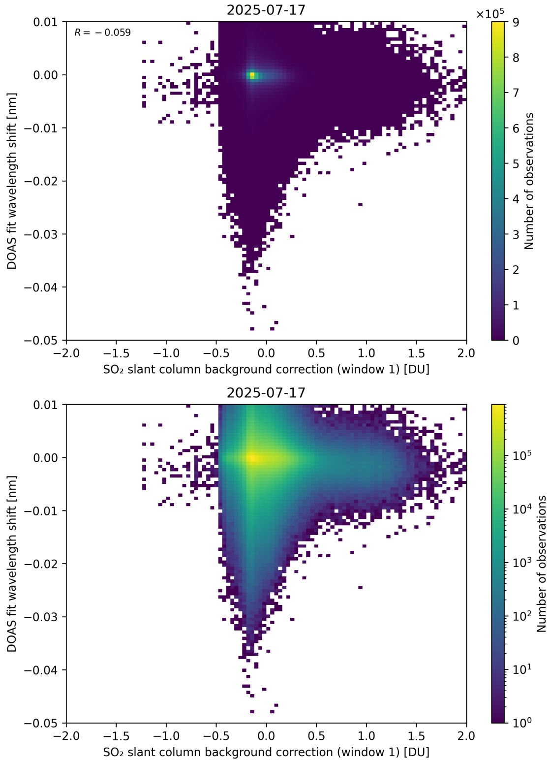
Figure 111: Scatter density plot of “SO 2 slant column background correction (window 1)” against “DOAS fit wavelength shift” for 2025-07-16 to 2025-07-18.
