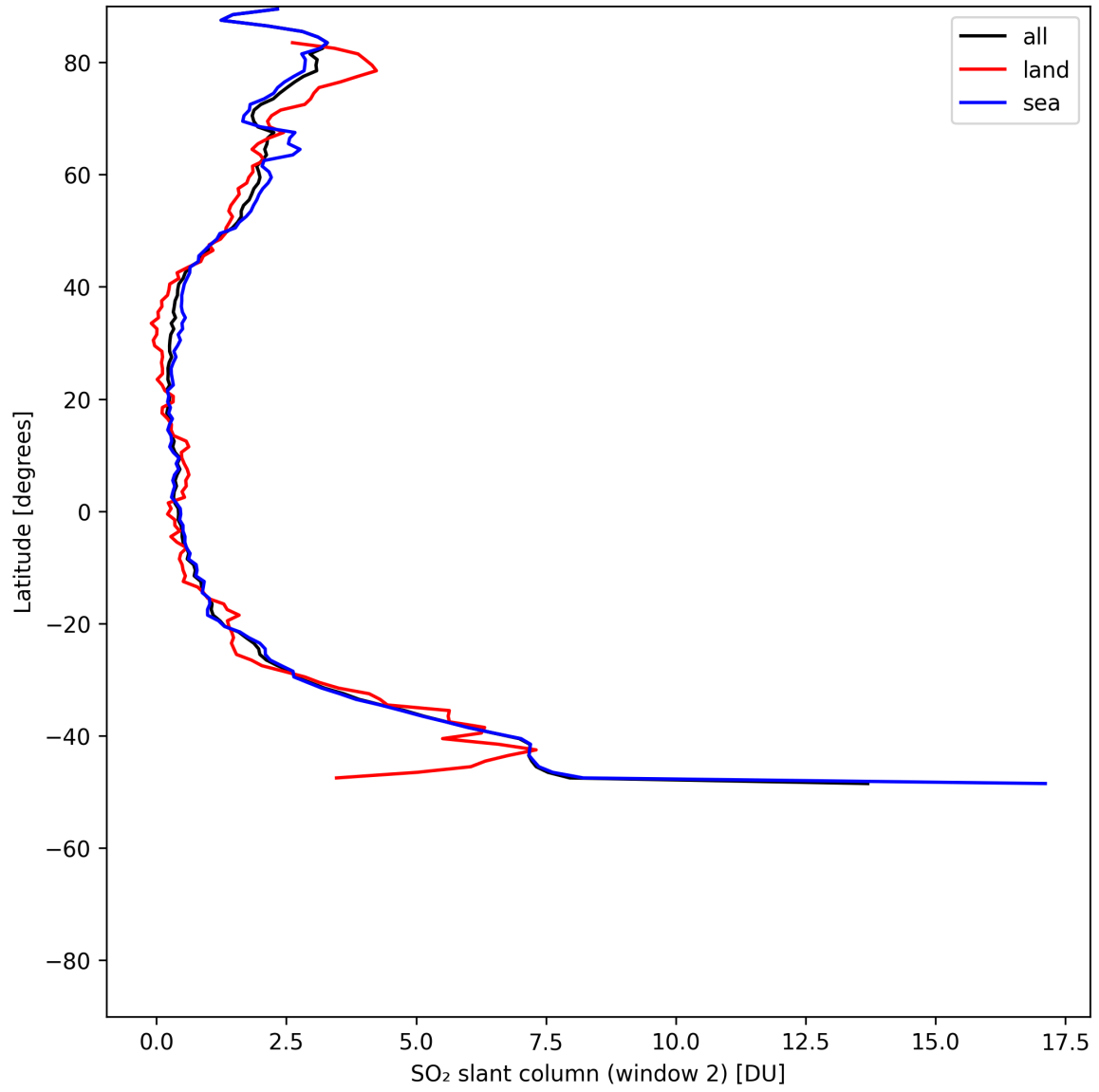
Figure 41: Zonal average of “SO 2 slant column (window 2)” for 2025-07-16 to 2025-07-18.
