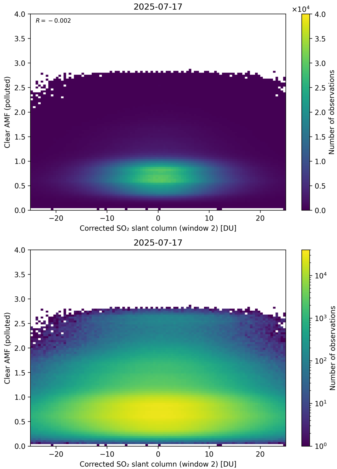
Figure 249: Scatter density plot of “Corrected SO 2 slant column (window 2)” against “Clear AMF (polluted)” for 2025-07-16 to 2025-07-18.
