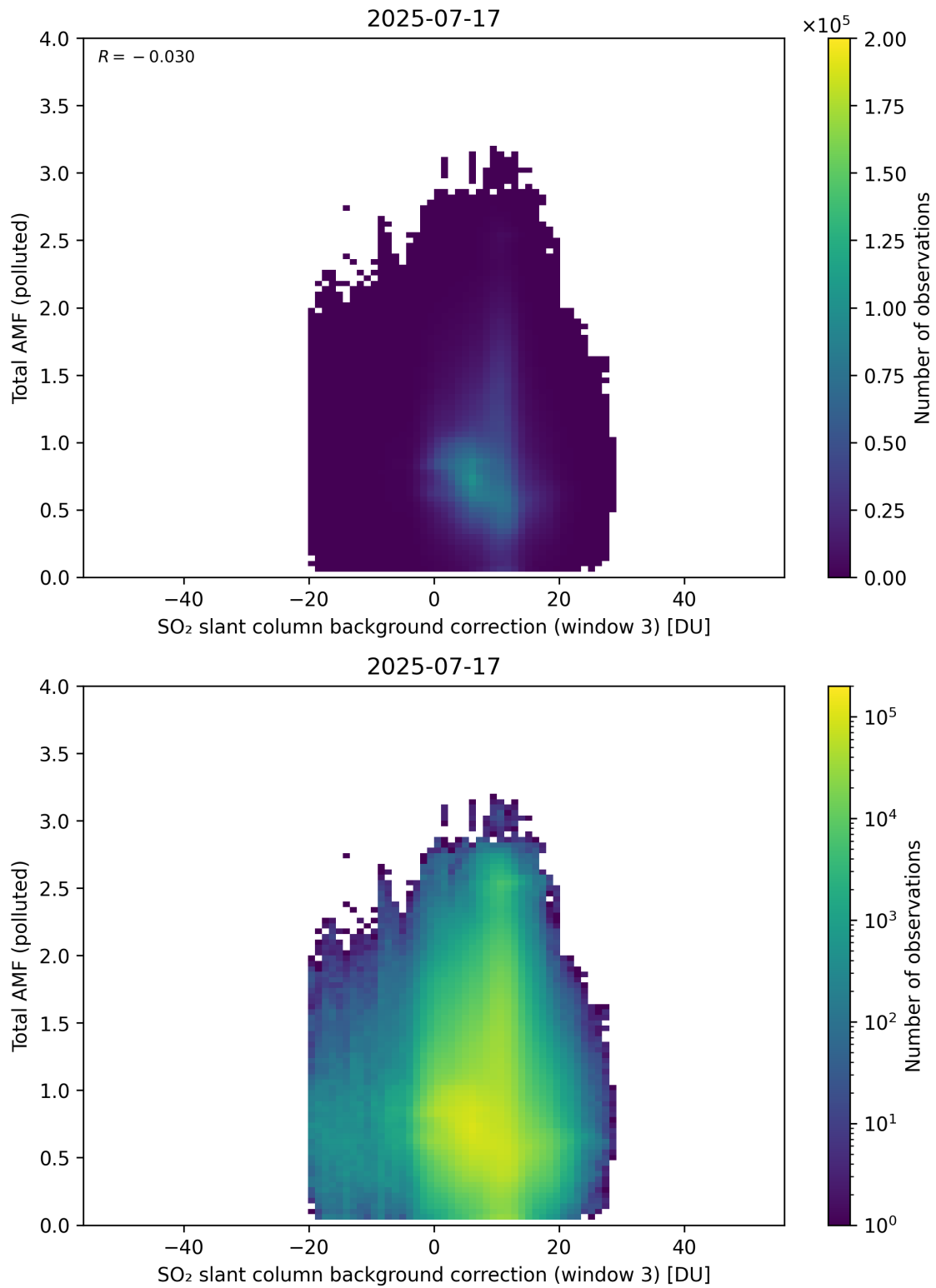
Figure 136: Scatter density plot of “SO 2 slant column background correction (window 3)” against “Total AMF (polluted)” for 2025-07-16 to 2025-07-18.
