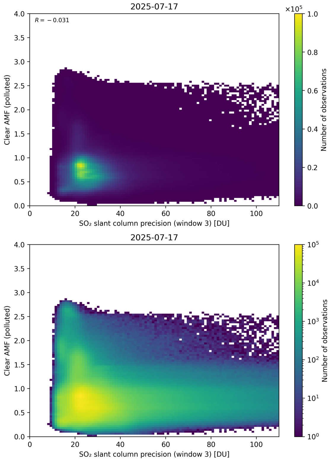
Figure 311: Scatter density plot of “SO 2 slant column precision (window 3)” against “Clear AMF (polluted)” for 2025-07-16 to 2025-07-18.
