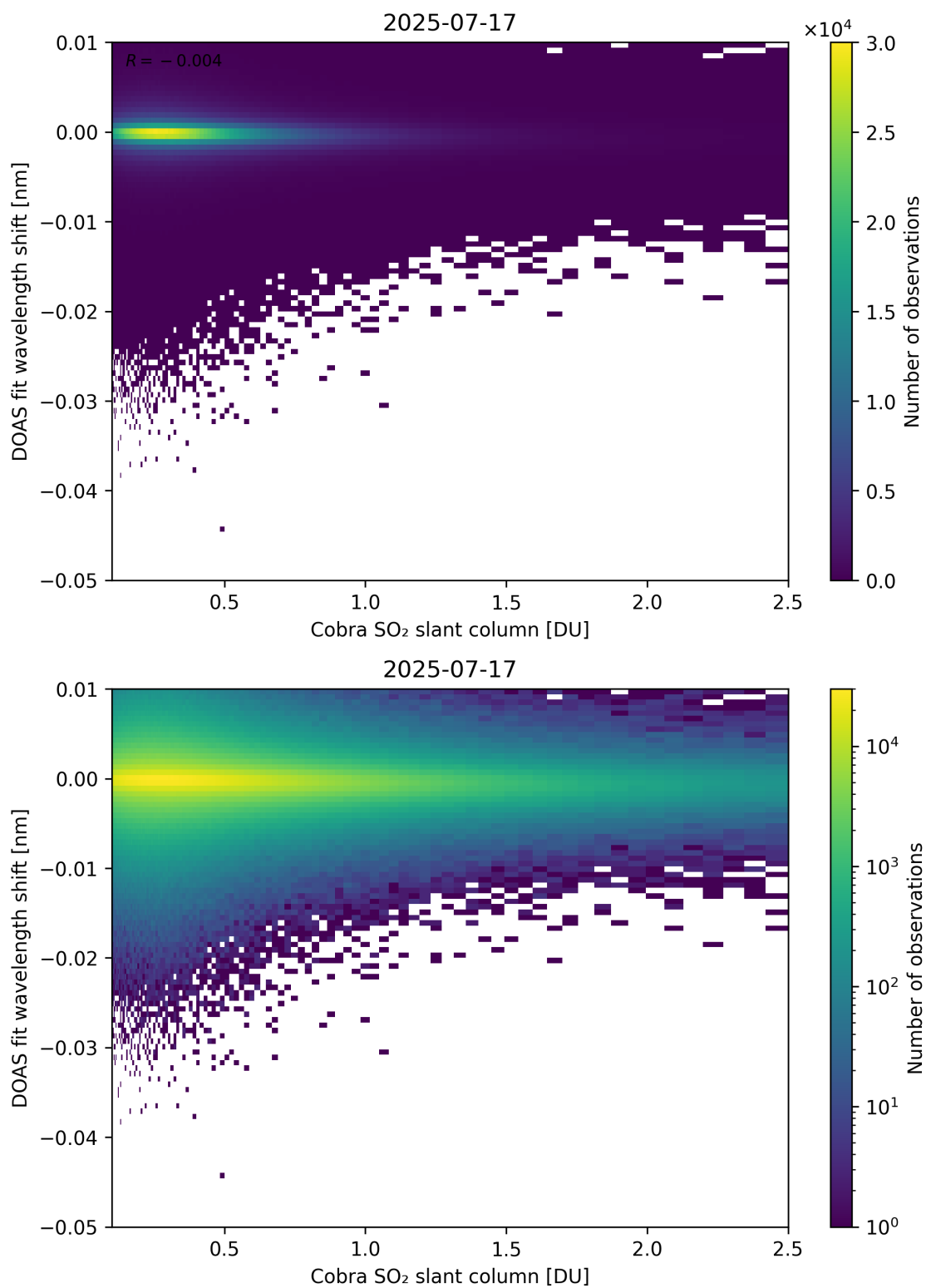
Figure 196: Scatter density plot of “Cobra SO 2 slant column” against “DOAS fit wavelength shift” for 2025-07-16 to 2025-07-18.
