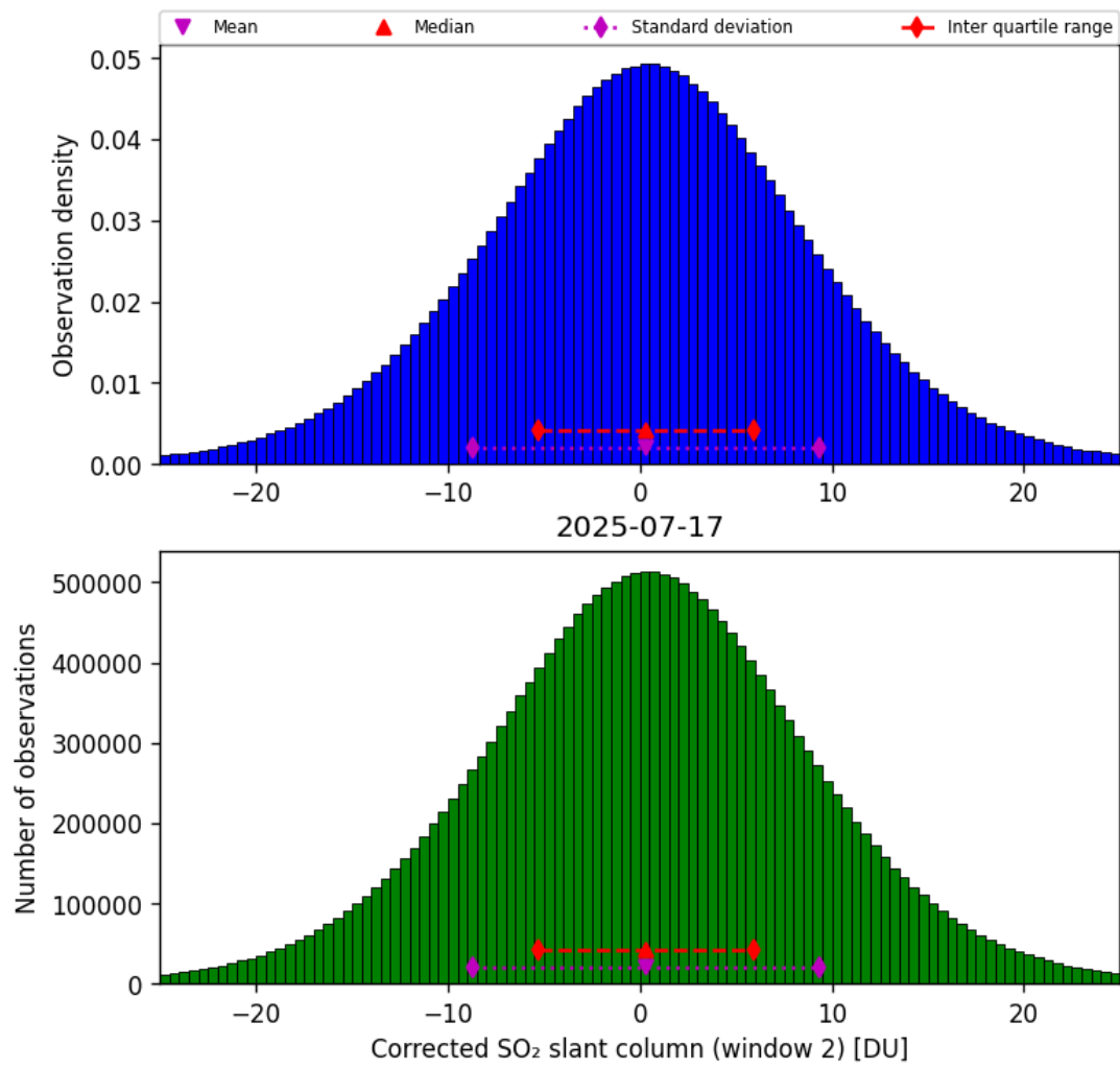
Figure 69: Histogram of “Corrected SO 2 slant column (window 2)” for 2025-07-16 to 2025-07-18
