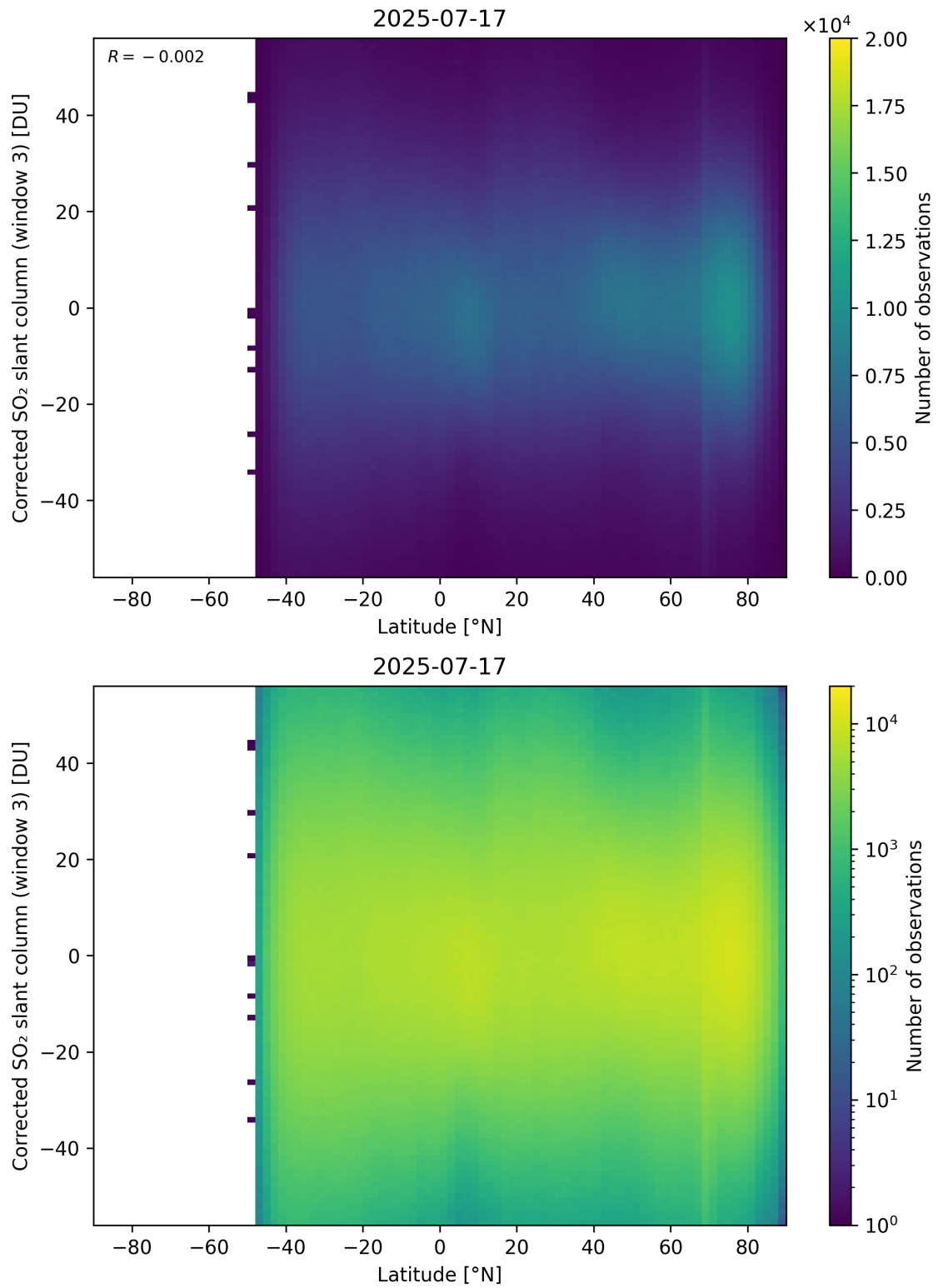
Figure 161: Scatter density plot of “Latitude” against “Corrected SO 2 slant column (window 3)” for 2025-07-16 to 2025-07-18.
