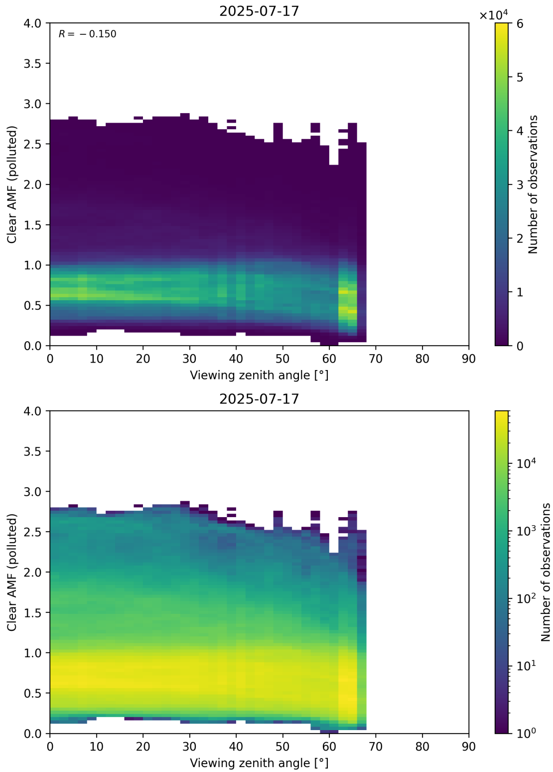
Figure 370: Scatter density plot of “Viewing zenith angle” against “Clear AMF (polluted)” for 2025-07-16 to 2025-07-18.
