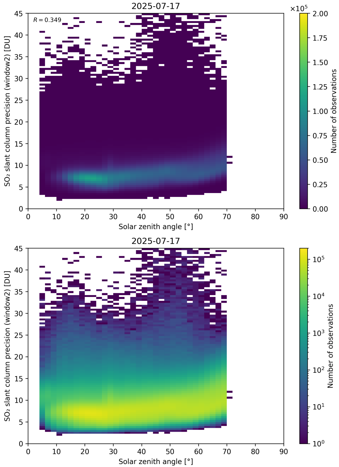
Figure 186: Scatter density plot of “Solar zenith angle” against “SO 2 slant column precision (window2)” for 2025-07-16 to 2025-07-18.
