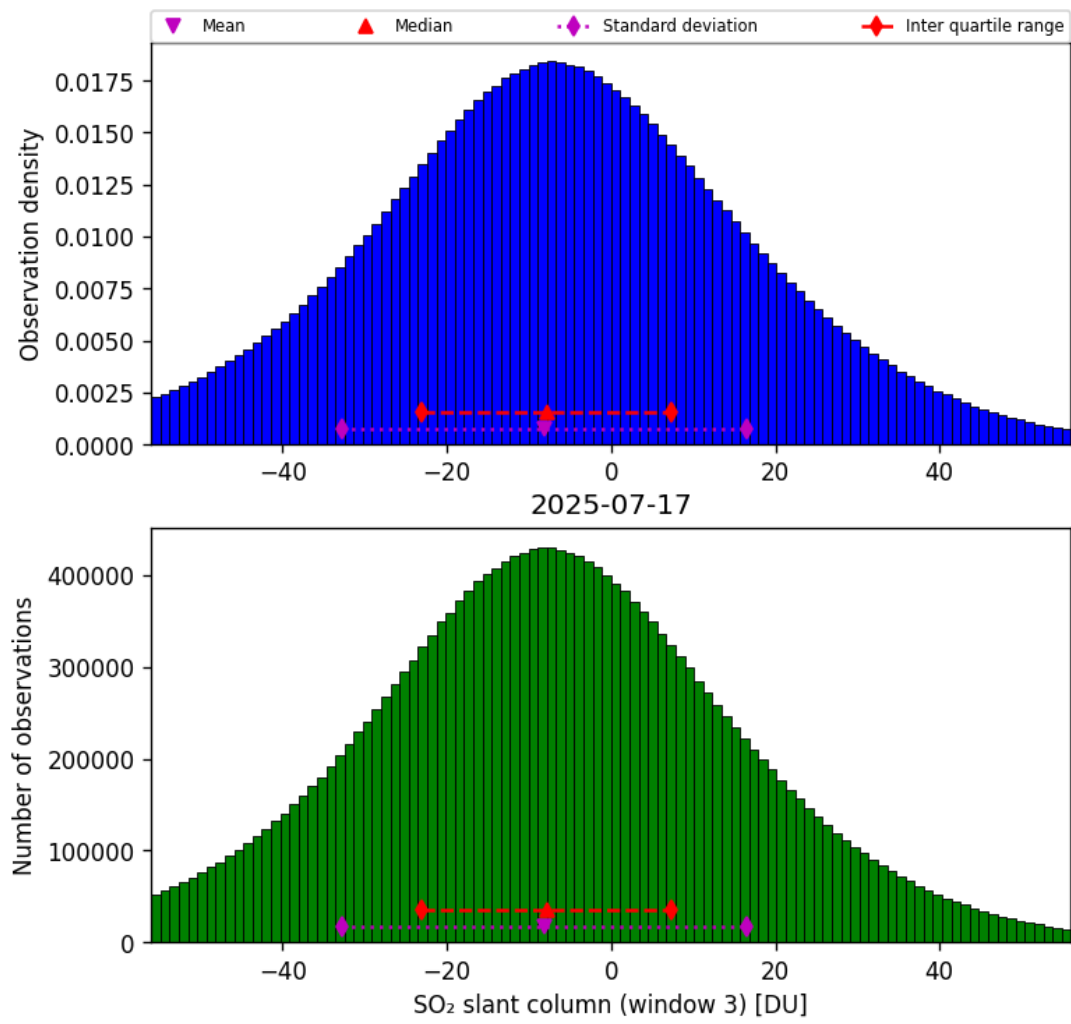
Figure 71: Histogram of “SO 2 slant column (window 3)” for 2025-07-16 to 2025-07-18
