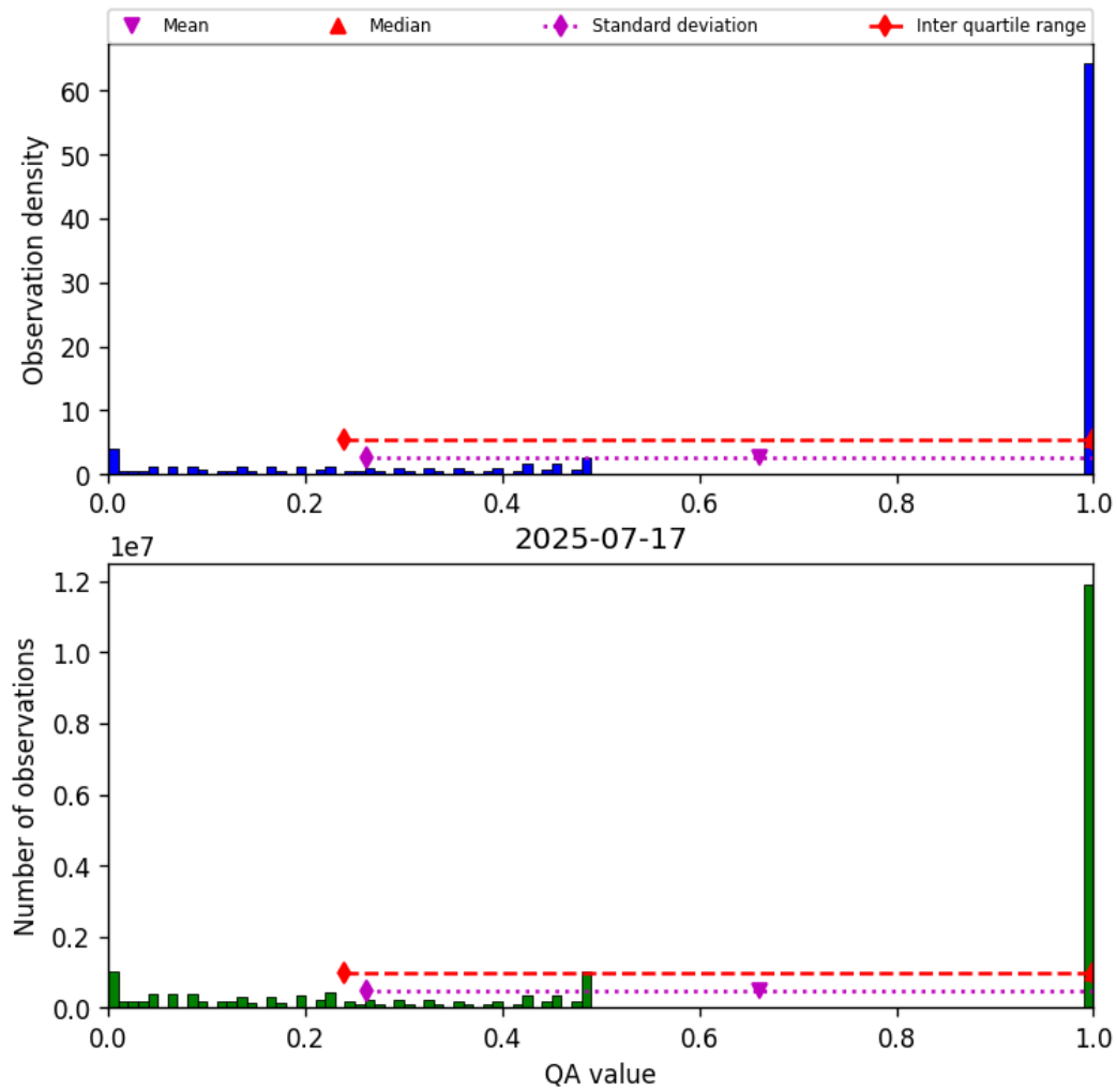
Figure 57: Histogram of “QA value” for 2025-07-16 to 2025-07-18
