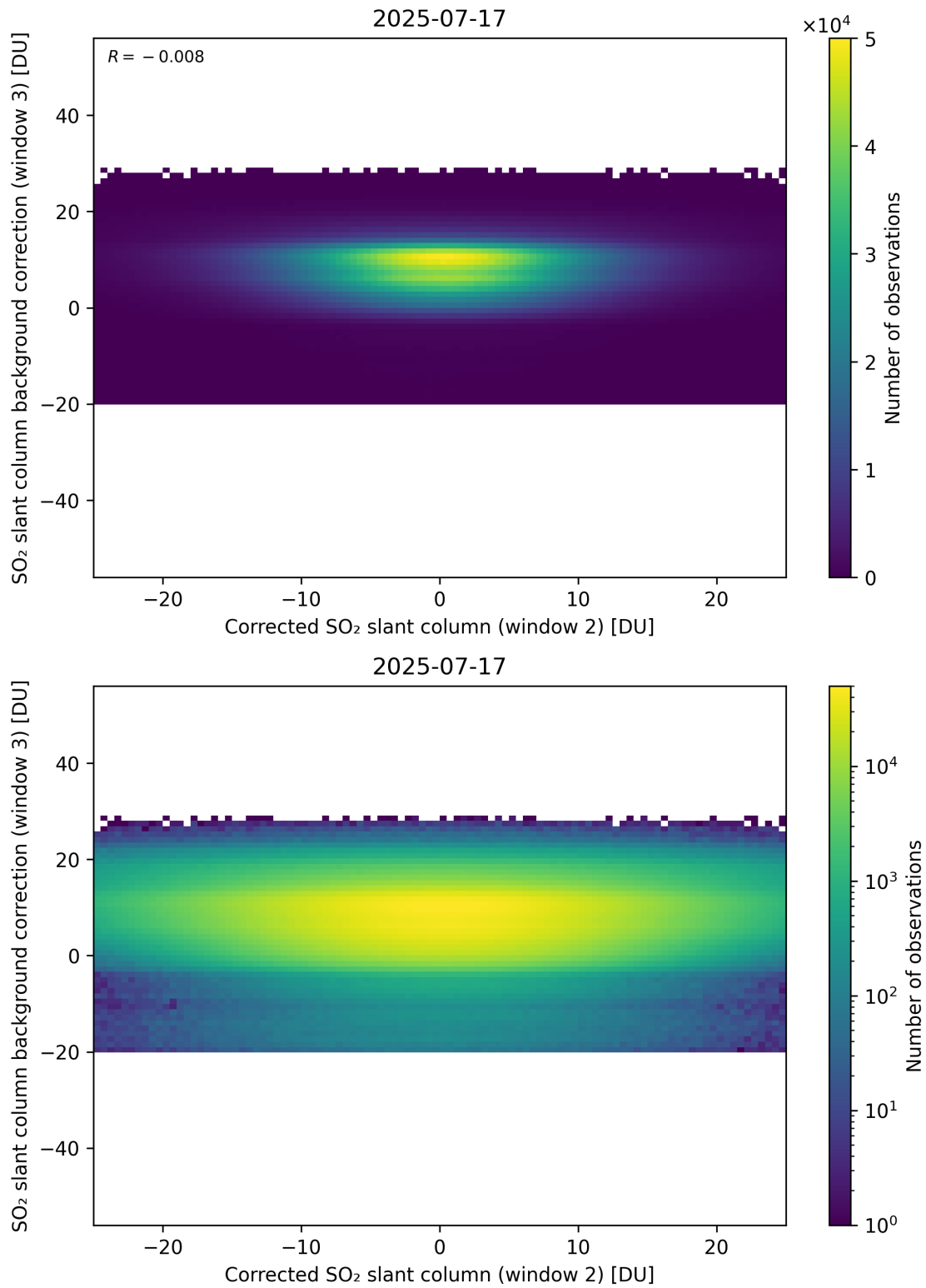
Figure 245: Scatter density plot of “Corrected SO 2 slant column (window 2)” against “SO 2 slant column background correction (window 3)” for 2025-07-16 to 2025-07-18.
