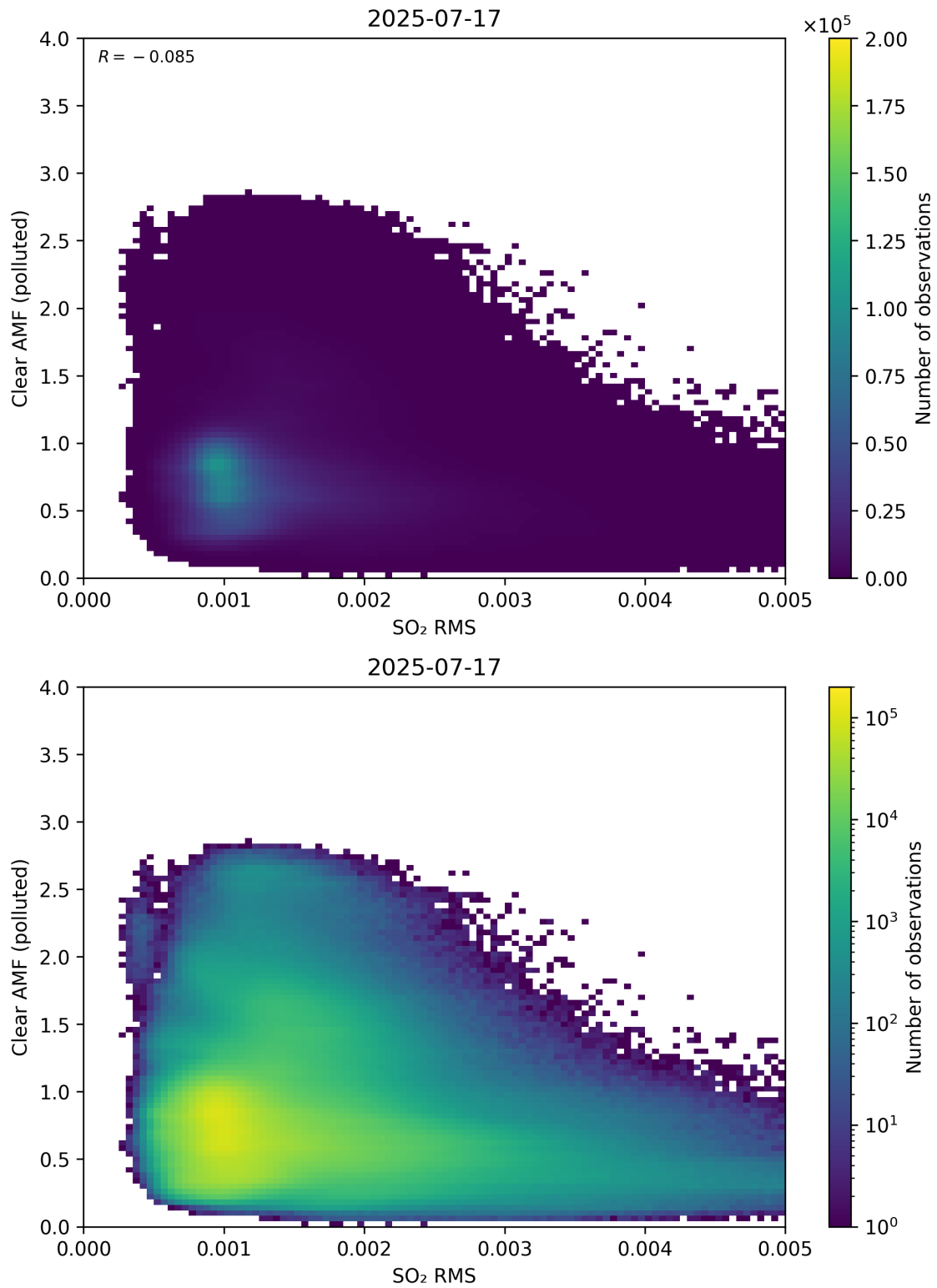
Figure 147: Scatter density plot of “SO 2 RMS” against “Clear AMF (polluted)” for 2025-07-16 to 2025-07-18.
