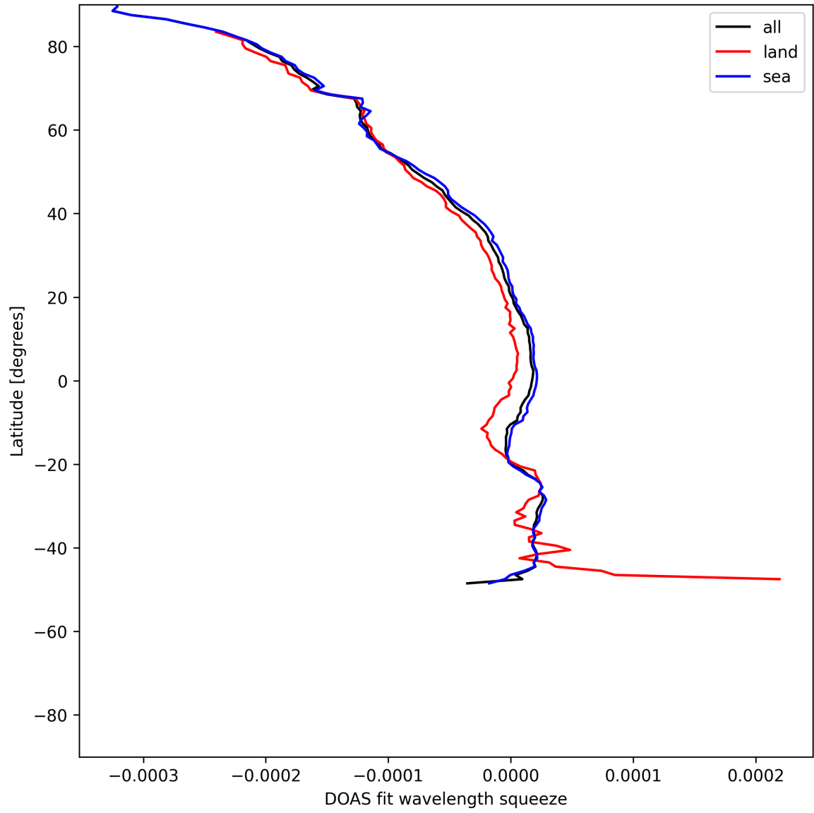
Figure 51: Zonal average of “DOAS fit wavelength squeeze” for 2025-07-16 to 2025-07-18.
