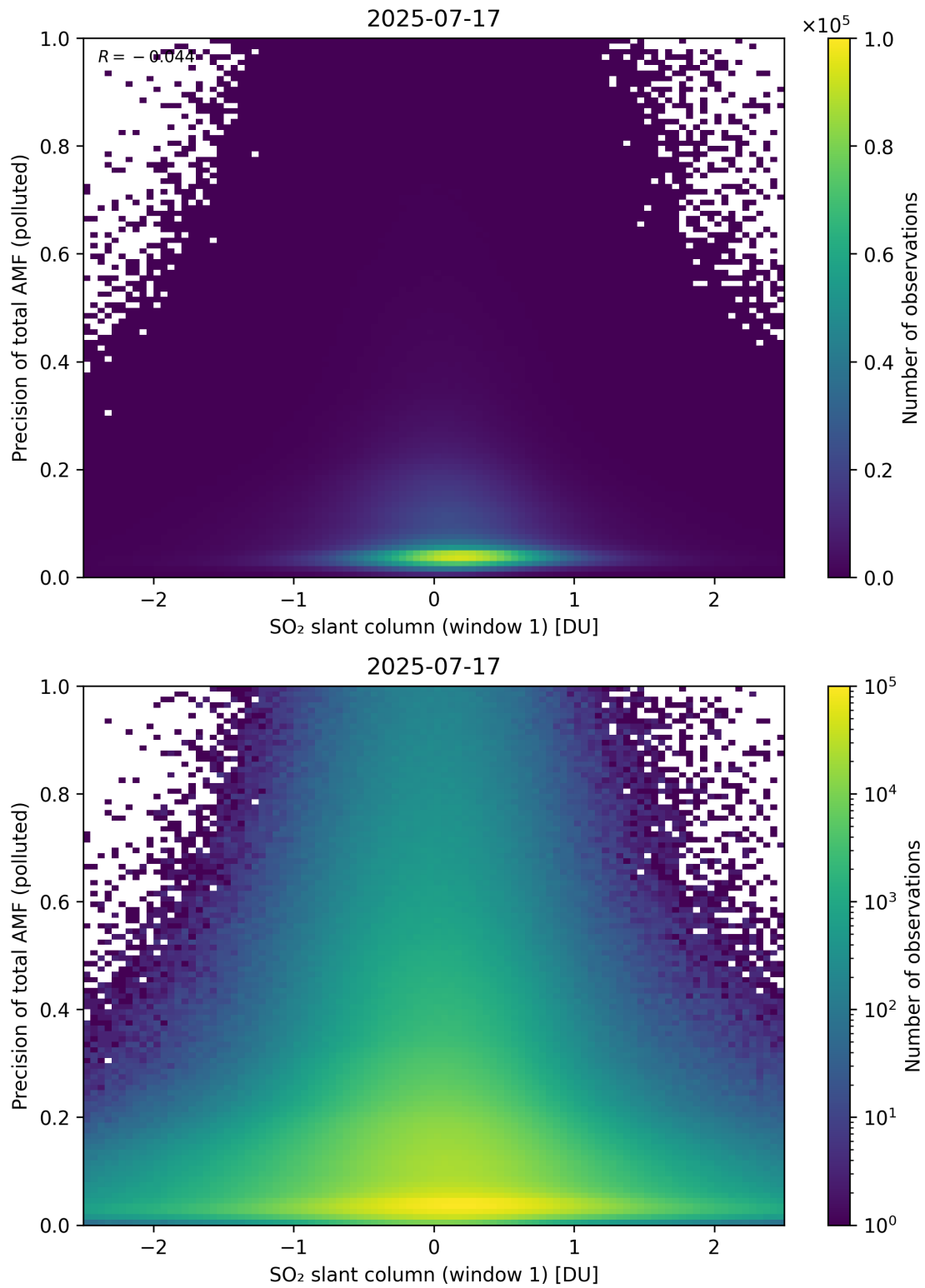
Figure 290: Scatter density plot of “SO 2 slant column (window 1)” against “Precision of total AMF (polluted)” for 2025-07-16 to 2025-07-18.
