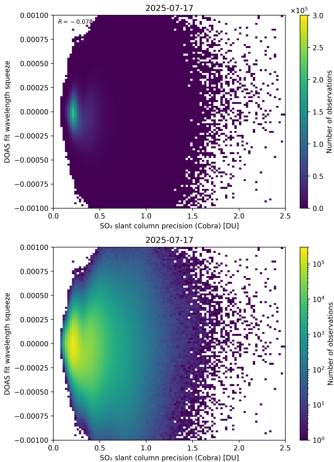
Figure 203: Scatter density plot of “SO 2 slant column precision (Cobra)” against “DOAS fit wavelength squeeze” for 2025-07-16 to 2025-07-18.
