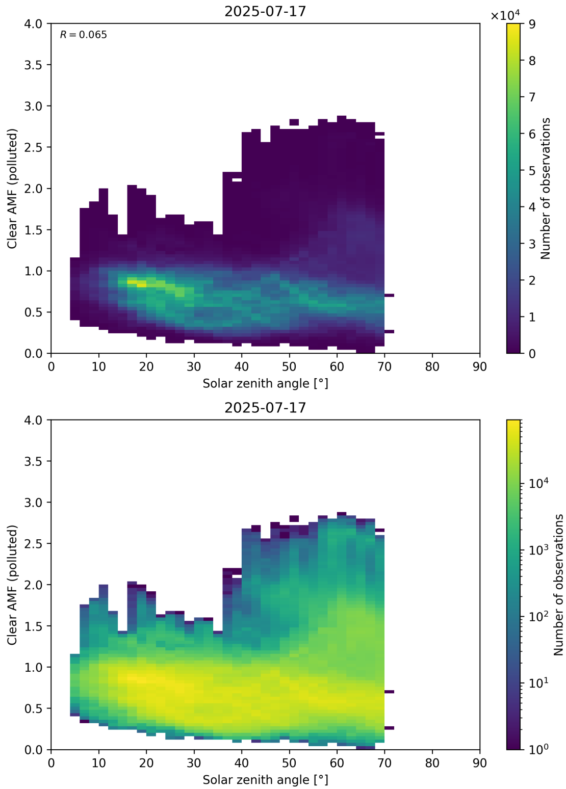
Figure 178: Scatter density plot of “Solar zenith angle” against “Clear AMF (polluted)” for 2025-07-16 to 2025-07-18.
