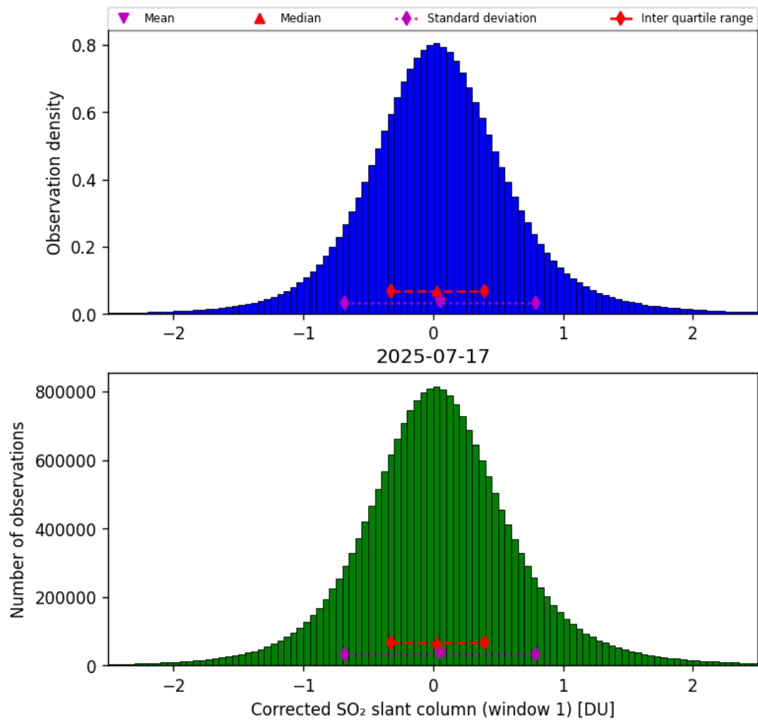
Figure 65: Histogram of “Corrected SO 2 slant column (window 1)” for 2025-07-16 to 2025-07-18
