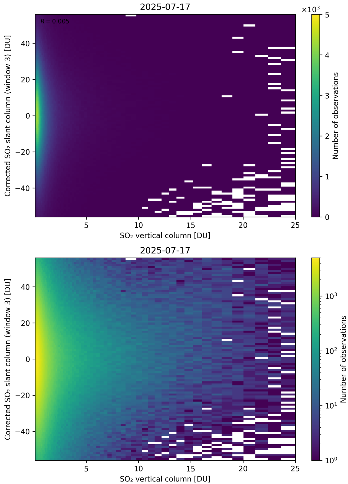
Figure 353: Scatter density plot of “SO 2 vertical column” against “Corrected SO 2 slant column (window 3)” for 2025-07-16 to 2025-07-18.
