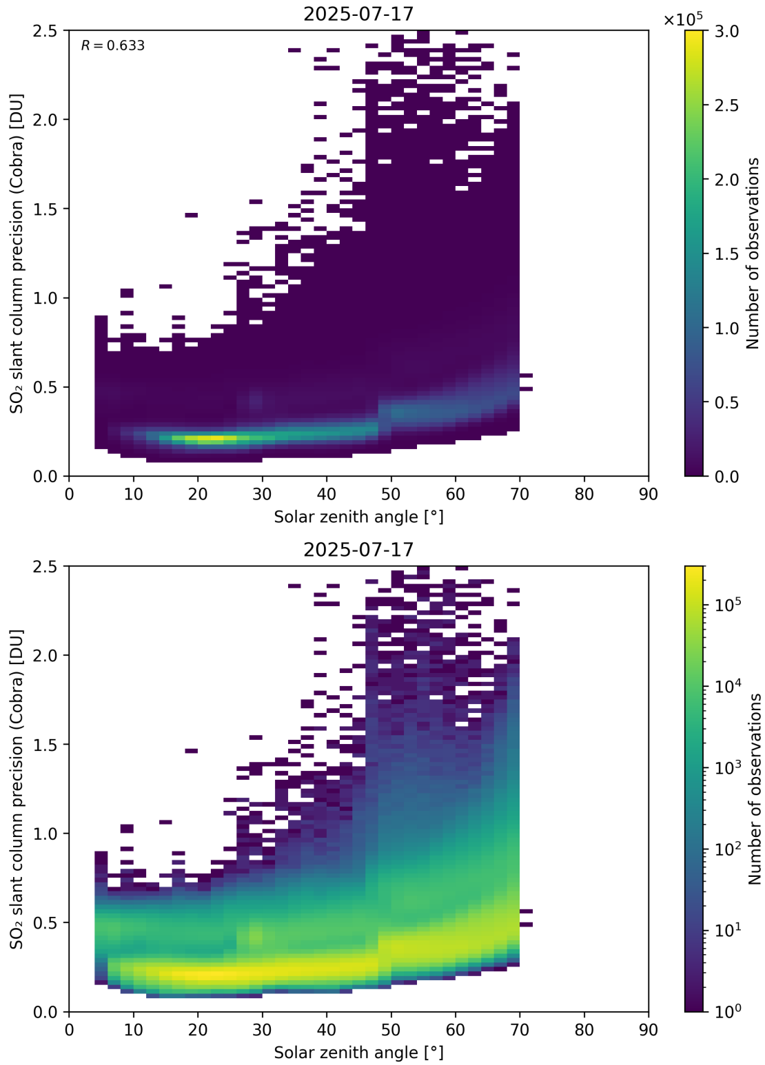
Figure 180: Scatter density plot of “Solar zenith angle” against “SO 2 slant column precision (Cobra)” for 2025-07-16 to 2025-07-18.
