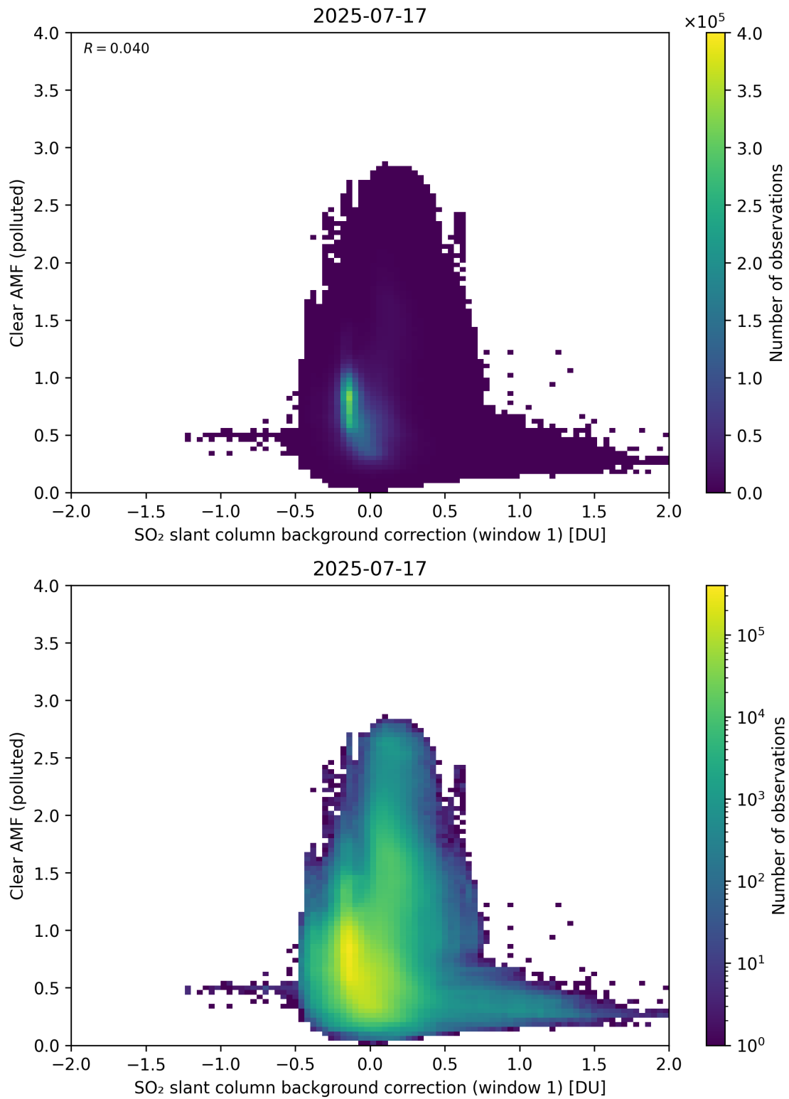
Figure 114: Scatter density plot of “SO 2 slant column background correction (window 1)” against “Clear AMF (polluted)” for 2025-07-16 to 2025-07-18.
