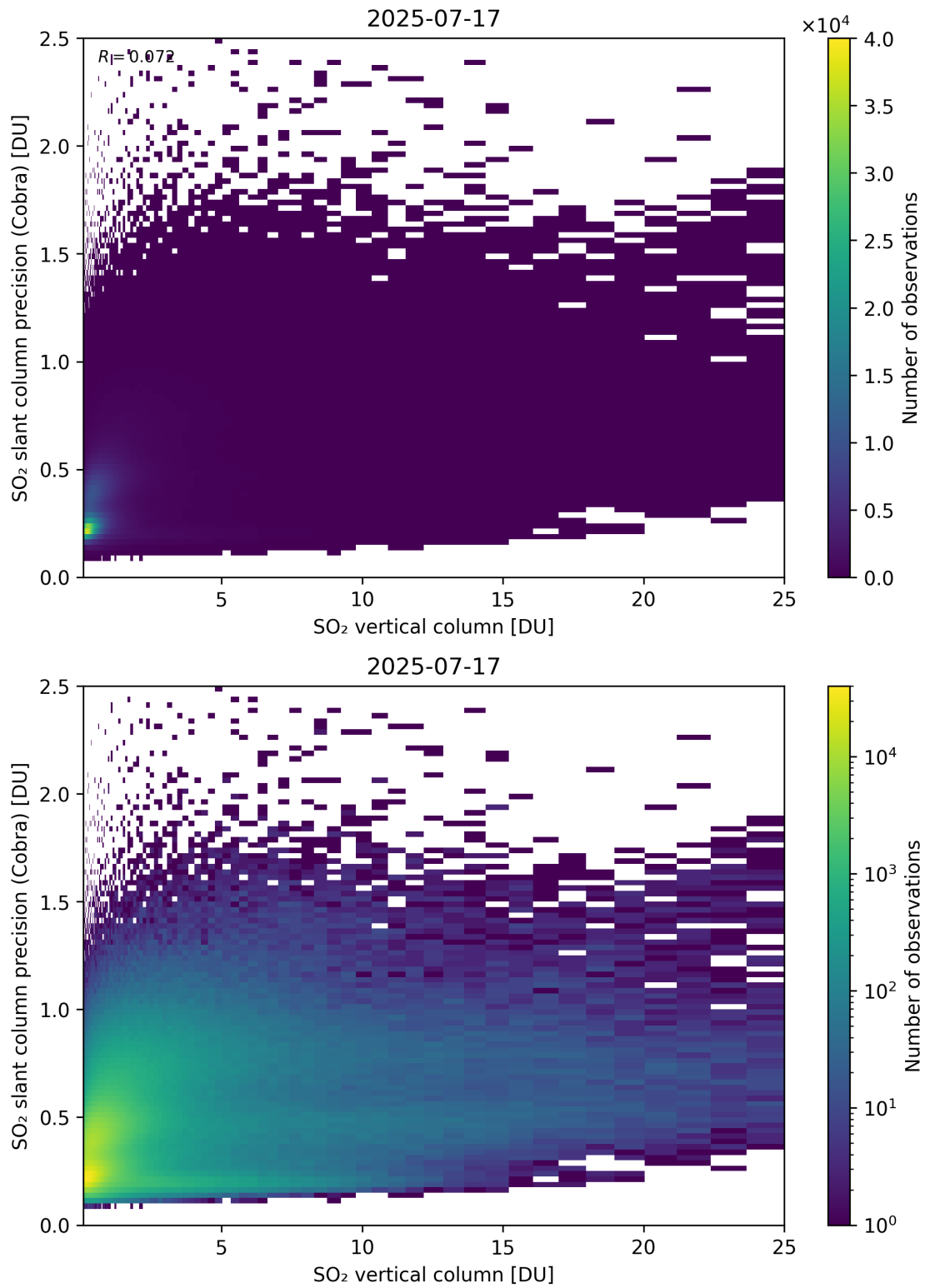
Figure 350: Scatter density plot of “SO 2 vertical column” against “SO 2 slant column precision (Cobra)” for 2025-07-16 to 2025-07-18.
