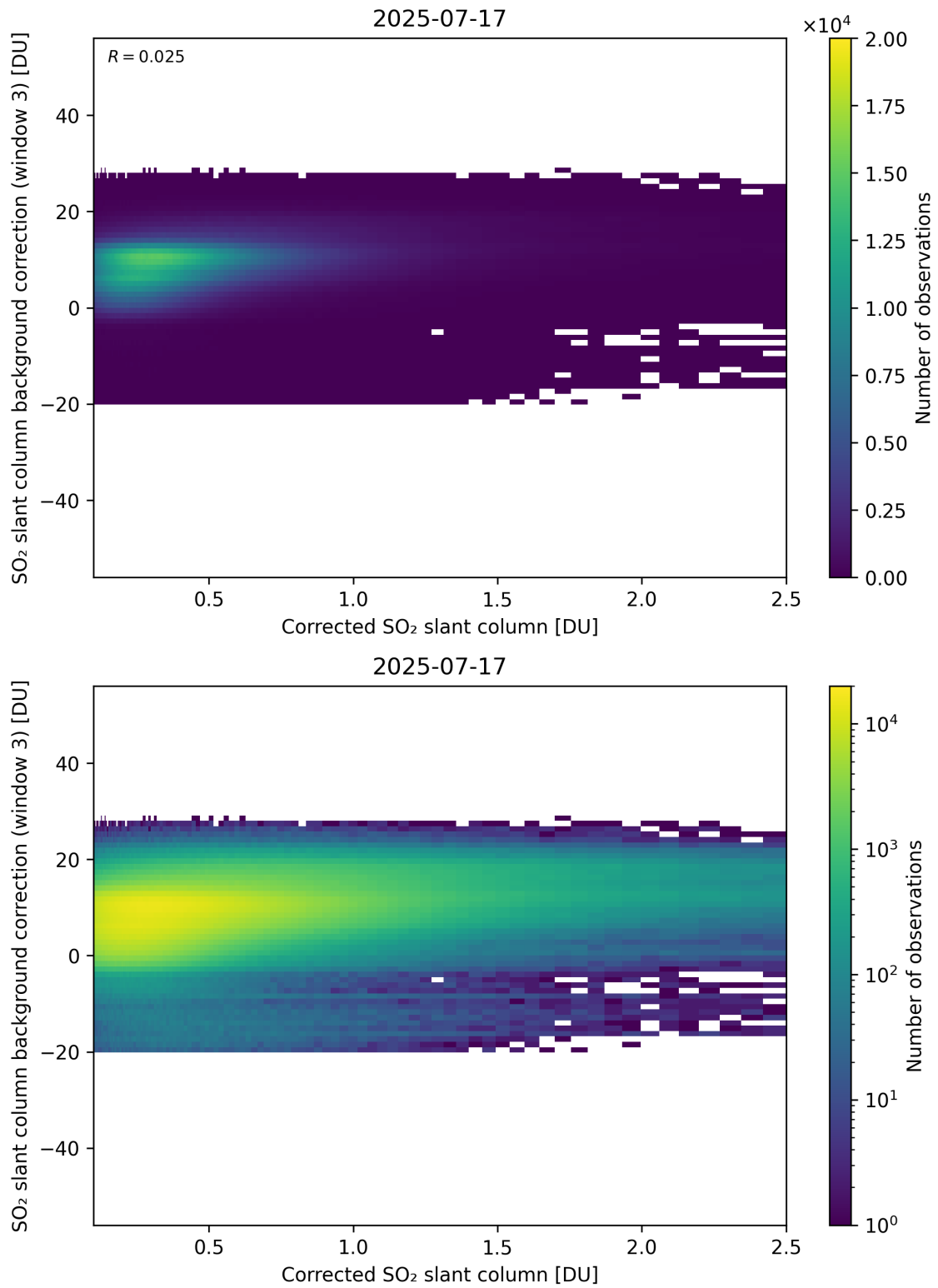
Figure 228: Scatter density plot of “Corrected SO 2 slant column” against “SO 2 slant column background correction (window 3)” for 2025-07-16 to 2025-07-18.
