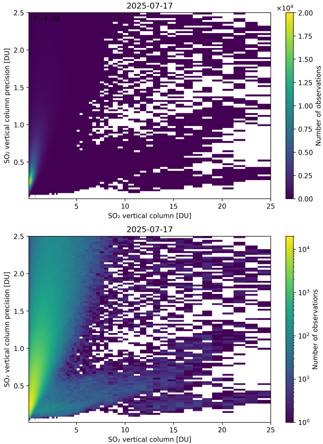
Figure 361: Scatter density plot of “SO 2 vertical column” against “SO 2 vertical column precision” for 2025-07-16 to 2025-07-18.
