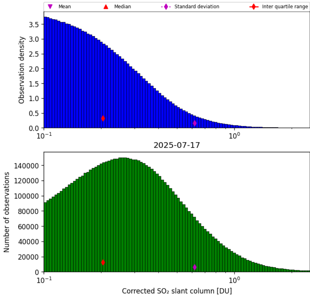
Figure 60: Histogram of “Corrected SO 2 slant column” for 2025-07-16 to 2025-07-18
