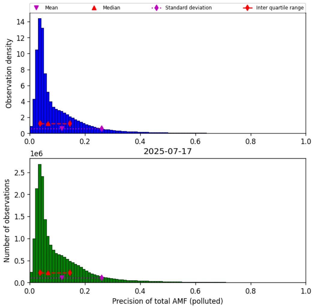
Figure 80: Histogram of “Precision of total AMF (polluted)” for 2025-07-16 to 2025-07-18
