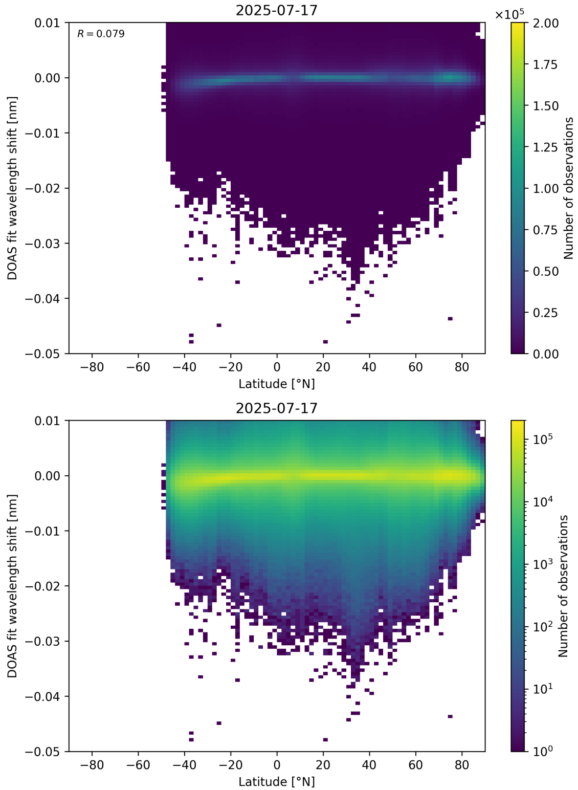
Figure 153: Scatter density plot of “Latitude” against “DOAS fit wavelength shift” for 2025-07-16 to 2025-07-18.
