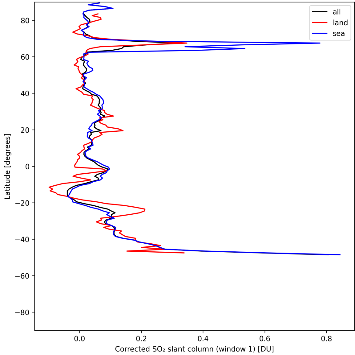
Figure 39: Zonal average of “Corrected SO 2 slant column (window 1)” for 2025-07-16 to 2025-07-18.
