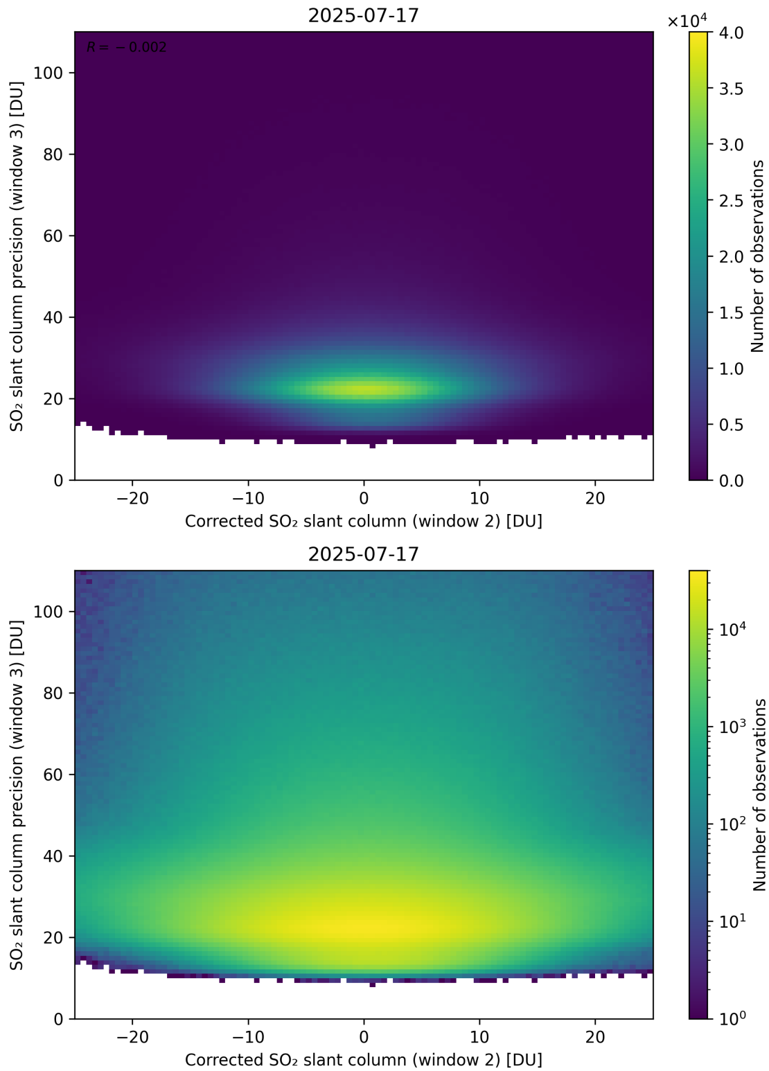
Figure 252: Scatter density plot of “Corrected SO 2 slant column (window 2)” against “SO 2 slant column precision (window 3)” for 2025-07-16 to 2025-07-18.
