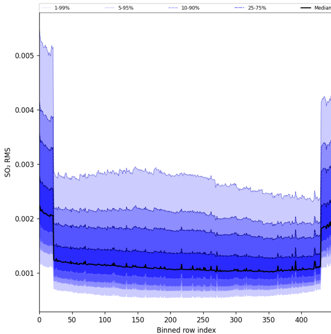
Figure 104: Along track statistics of “SO 2 RMS” for 2025-07-16 to 2025-07-18
