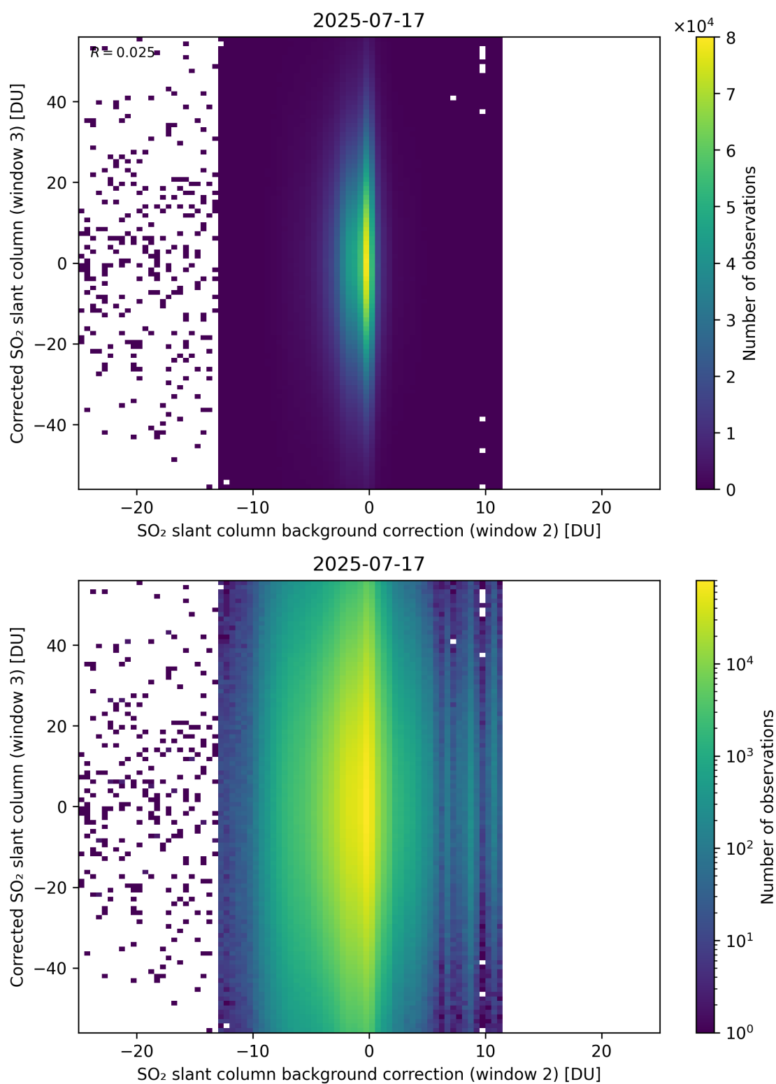
Figure 127: Scatter density plot of “SO 2 slant column background correction (window 2)” against “Corrected SO 2 slant column (window 3)” for 2025-07-16 to 2025-07-18.
