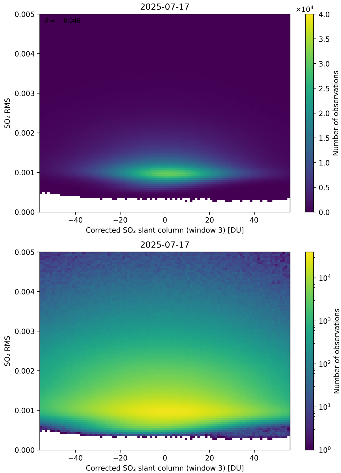
Figure 258: Scatter density plot of “Corrected SO 2 slant column (window 3)” against “SO 2 RMS” for 2025-07-16 to 2025-07-18.
