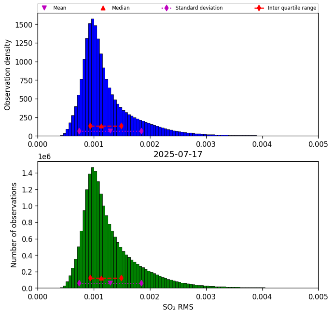
Figure 78: Histogram of “SO 2 RMS” for 2025-07-16 to 2025-07-18
