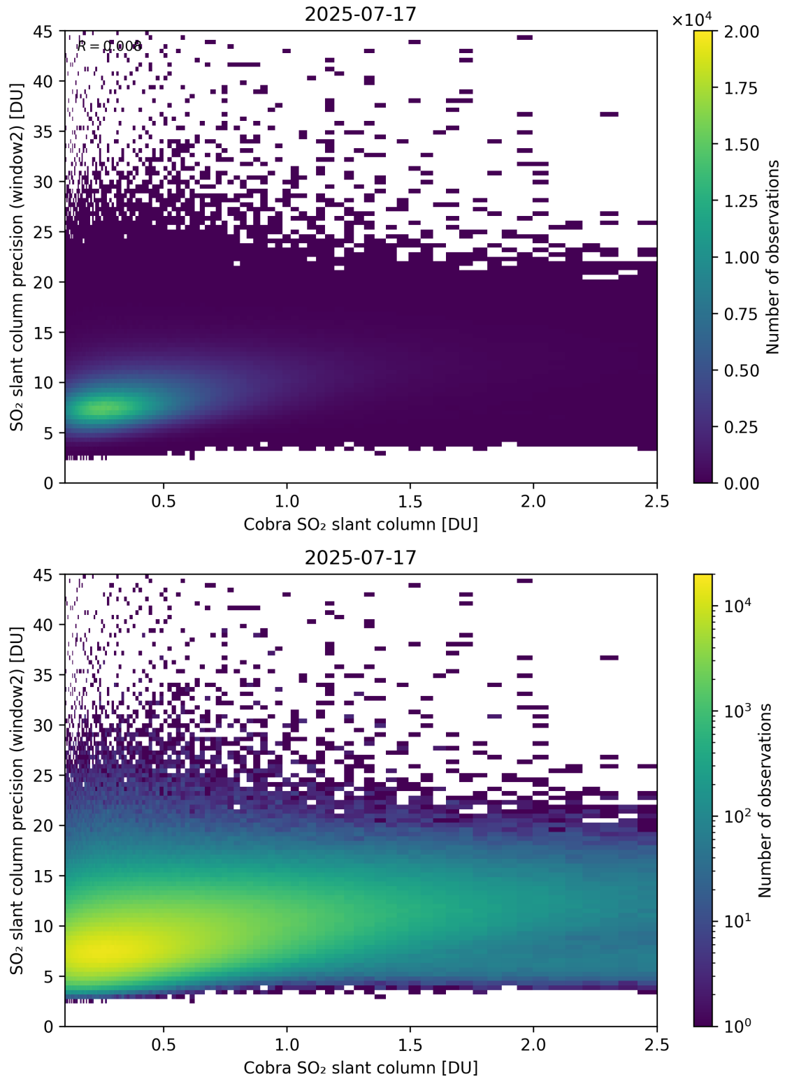
Figure 221: Scatter density plot of “Cobra SO 2 slant column” against “SO 2 slant column precision (window2)” for 2025-07-16 to 2025-07-18.
