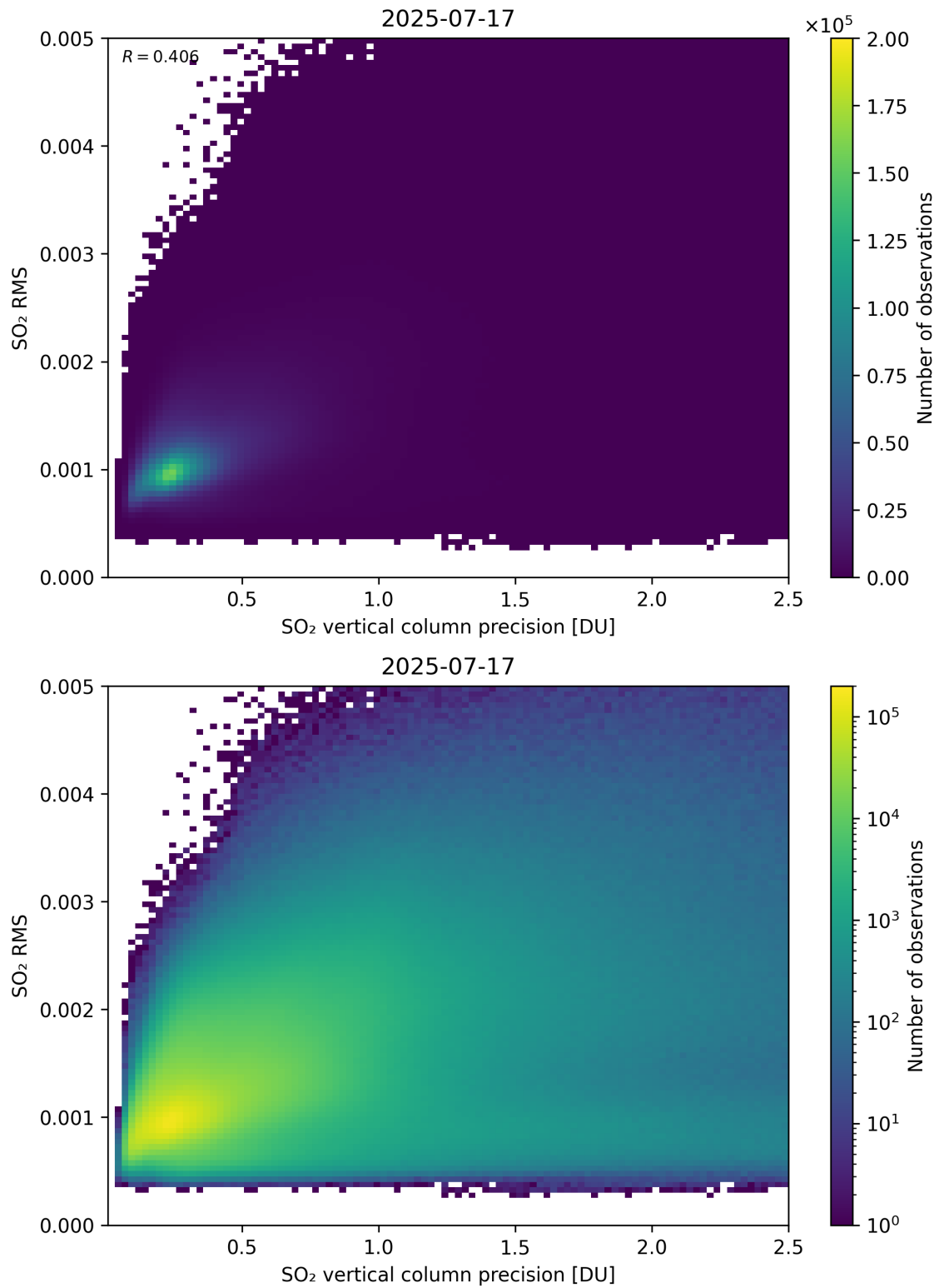
Figure 334: Scatter density plot of “SO 2 vertical column precision” against “SO 2 RMS” for 2025-07-16 to 2025-07-18.
