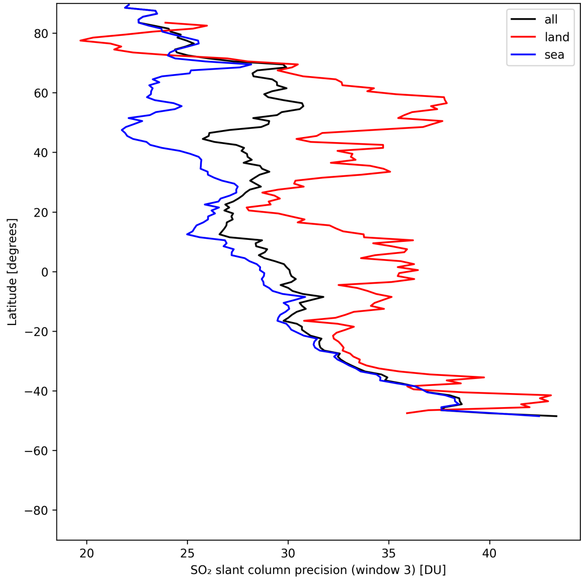
Figure 46: Zonal average of “SO 2 slant column precision (window 3)” for 2025-07-16 to 2025-07-18.
