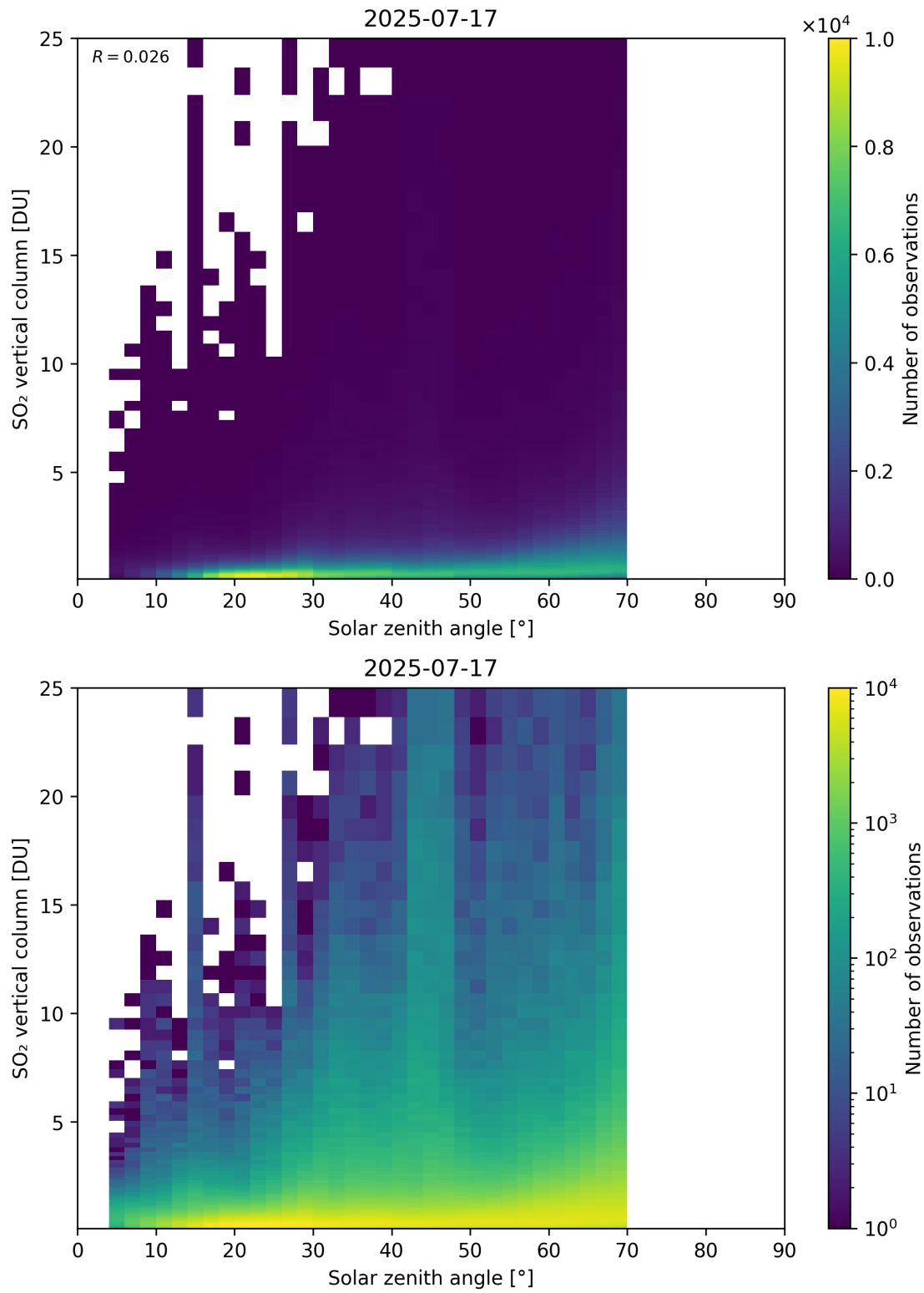
Figure 191: Scatter density plot of “Solar zenith angle” against “SO 2 vertical column” for 2025-07-16 to 2025-07-18.
