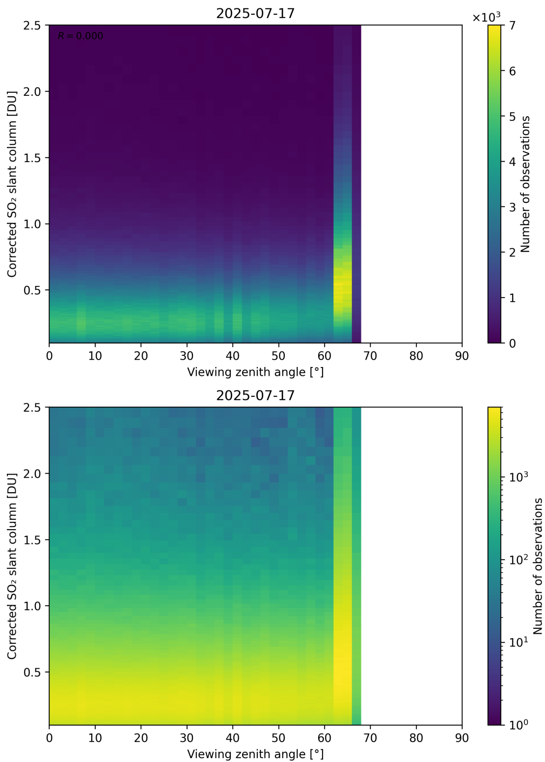
Figure 373: Scatter density plot of “Viewing zenith angle” against “Corrected SO 2 slant column” for 2025-07-16 to 2025-07-18.
