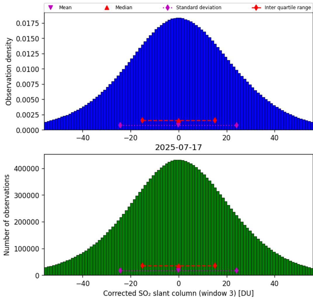
Figure 73: Histogram of “Corrected SO 2 slant column (window 3)” for 2025-07-16 to 2025-07-18
