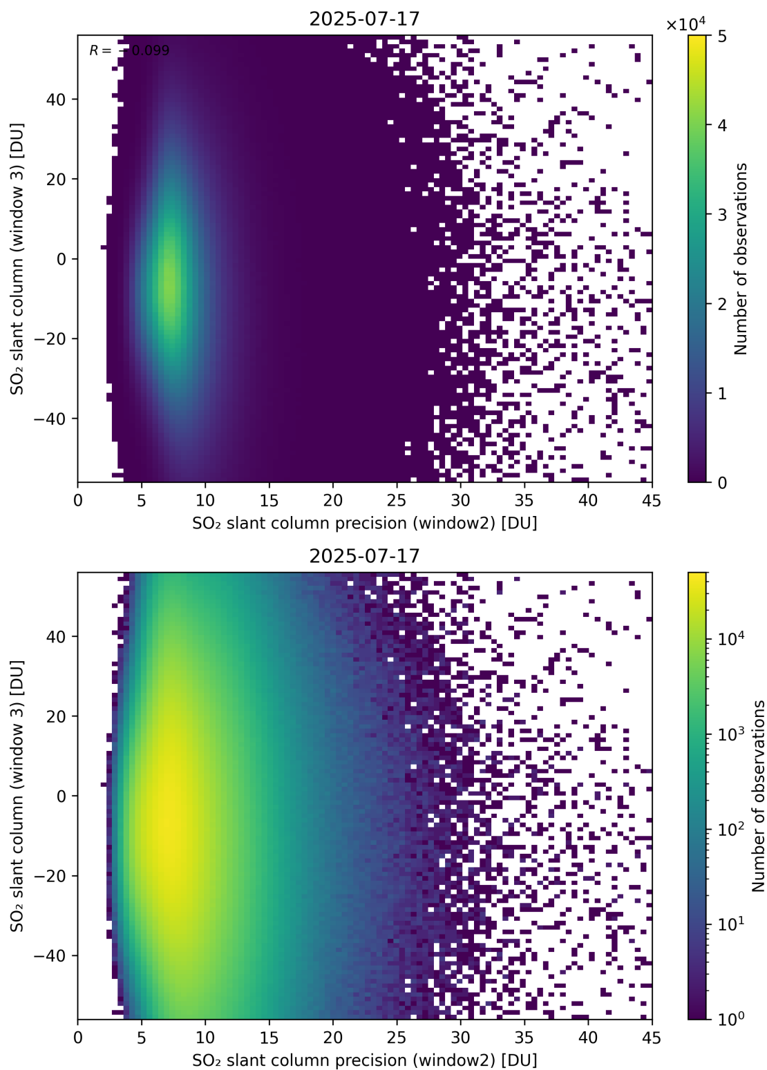
Figure 299: Scatter density plot of “SO 2 slant column precision (window2)” against “SO 2 slant column (window 3)” for 2025-07-16 to 2025-07-18.
