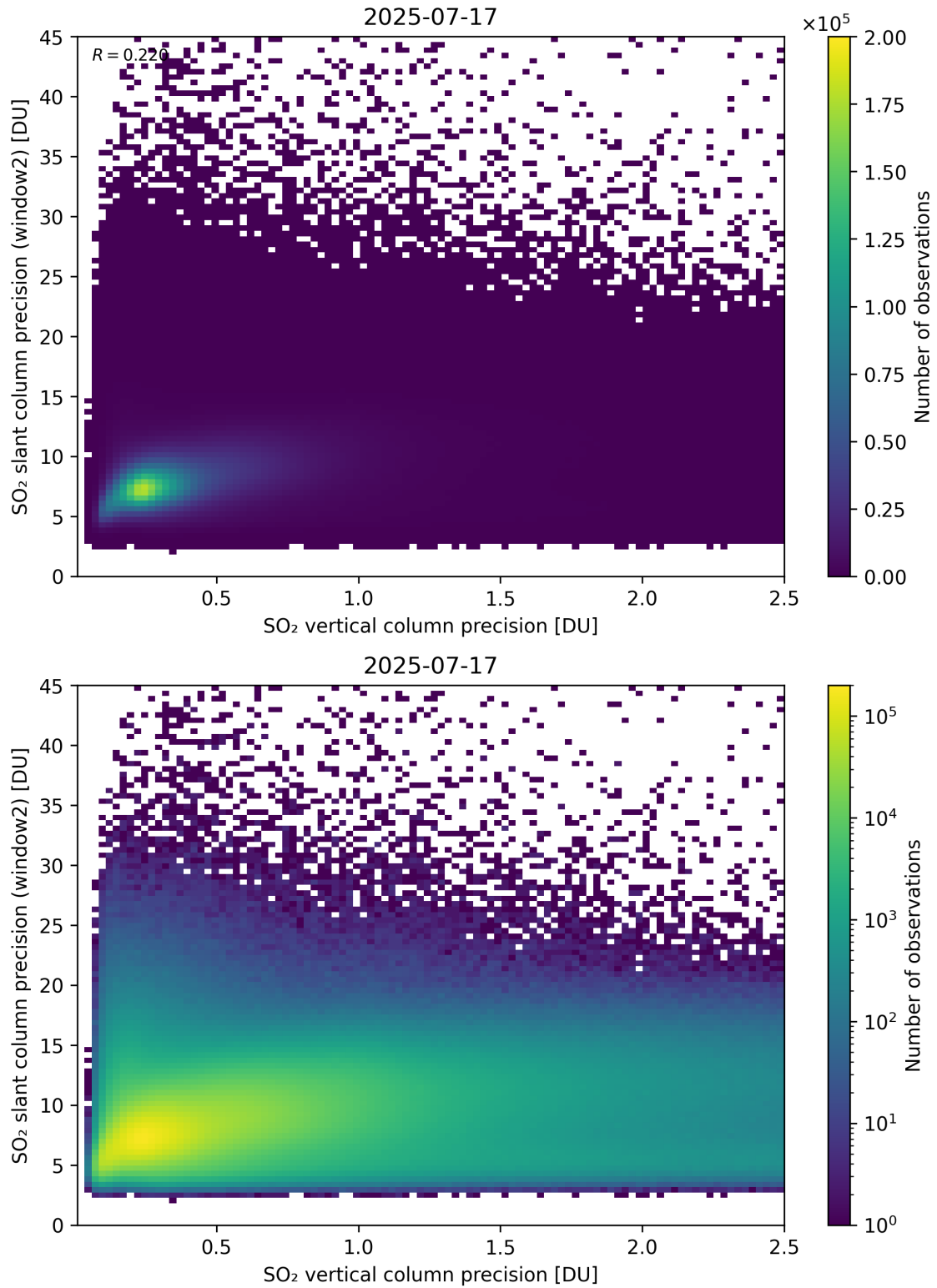
Figure 343: Scatter density plot of “SO 2 vertical column precision” against “SO 2 slant column precision (window2)” for 2025-07-16 to 2025-07-18.
