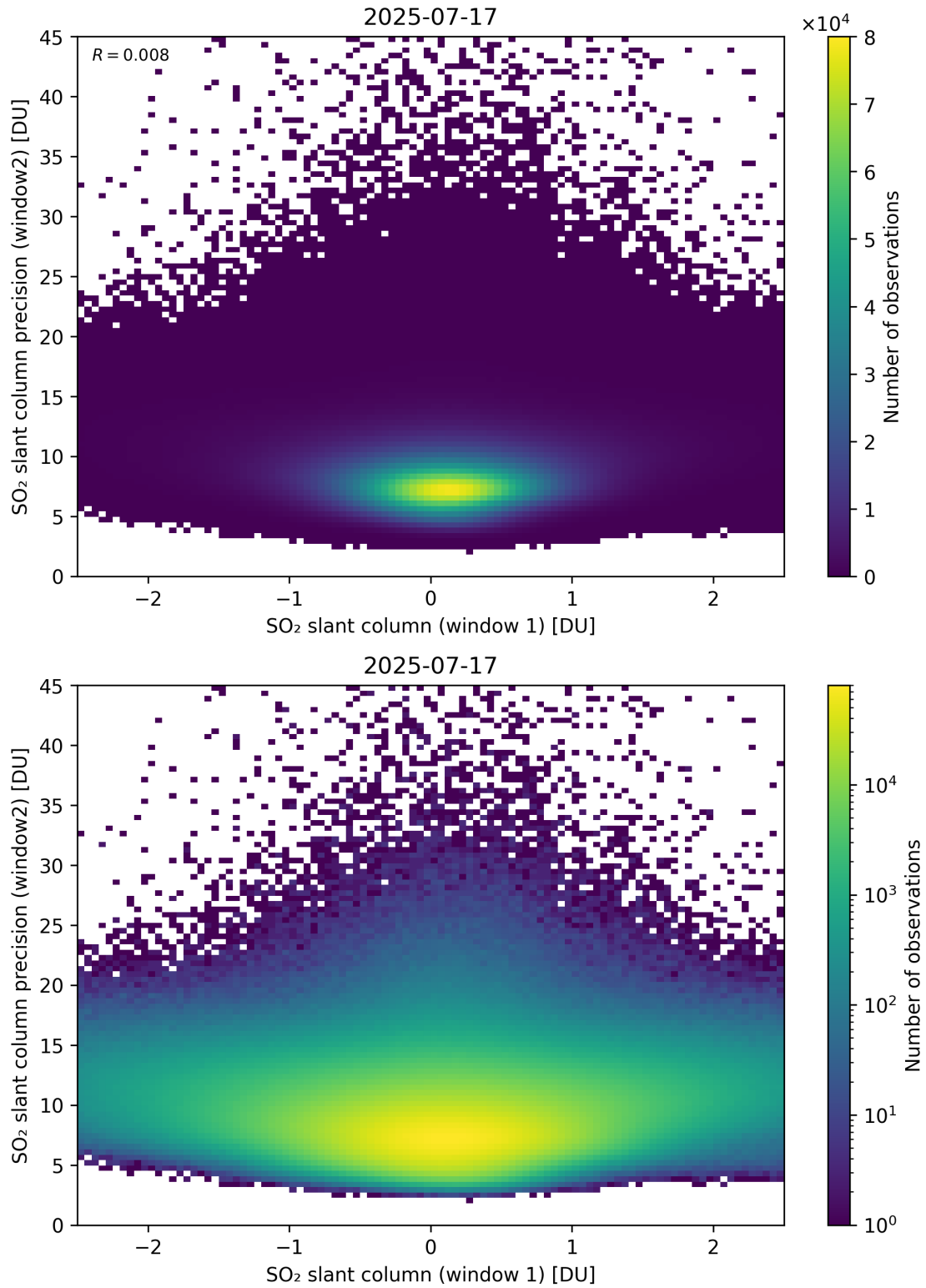
Figure 286: Scatter density plot of “SO 2 slant column (window 1)” against “SO 2 slant column precision (window2)” for 2025-07-16 to 2025-07-18.
