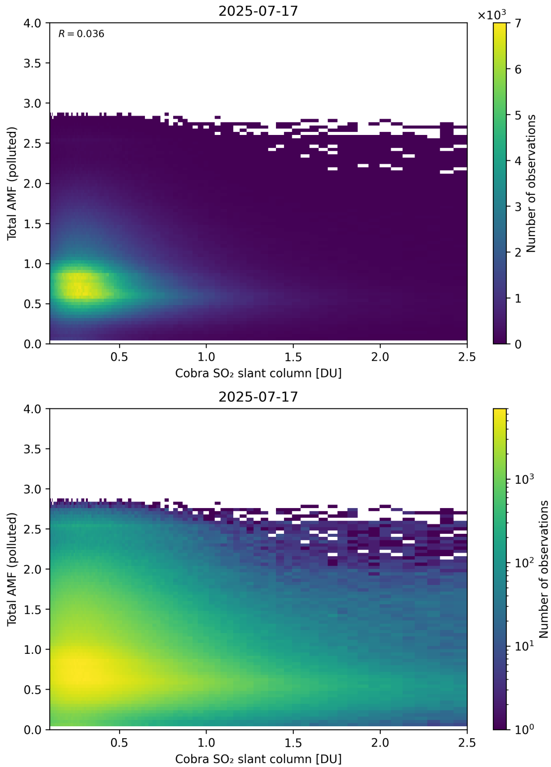
Figure 224: Scatter density plot of “Cobra SO 2 slant column” against “Total AMF (polluted)” for 2025-07-16 to 2025-07-18.
