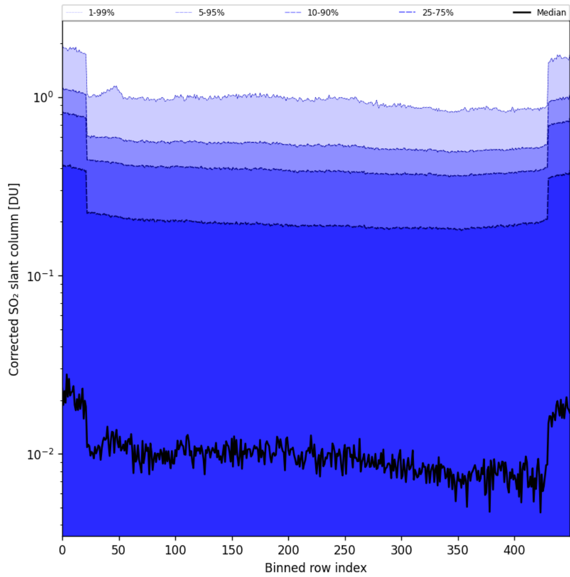
Figure 86: Along track statistics of “Corrected SO 2 slant column” for 2025-07-16 to 2025-07-18
