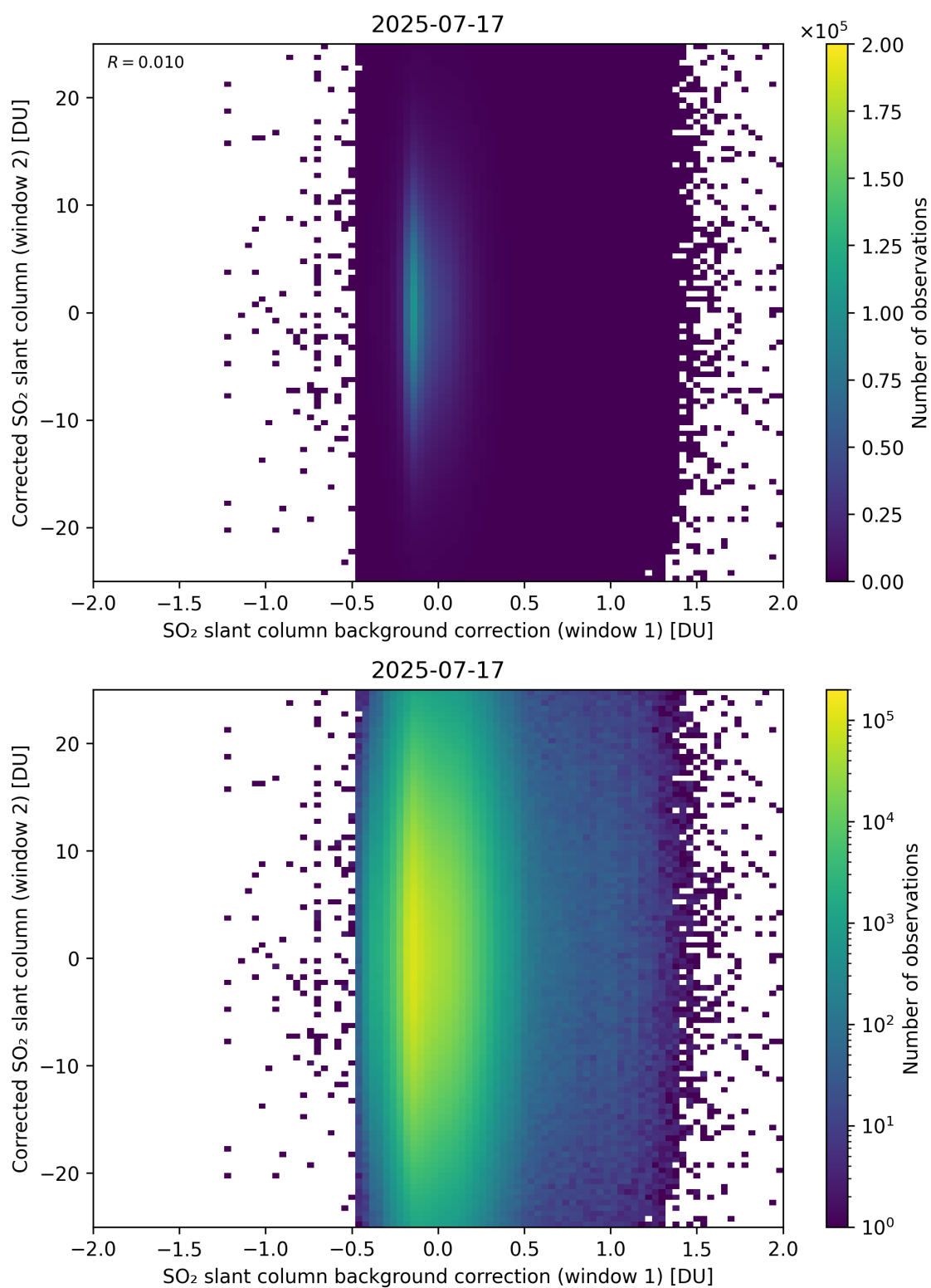
Figure 115: Scatter density plot of “SO 2 slant column background correction (window 1)” against “Corrected SO 2 slant column (window 2)” for 2025-07-16 to 2025-07-18.
