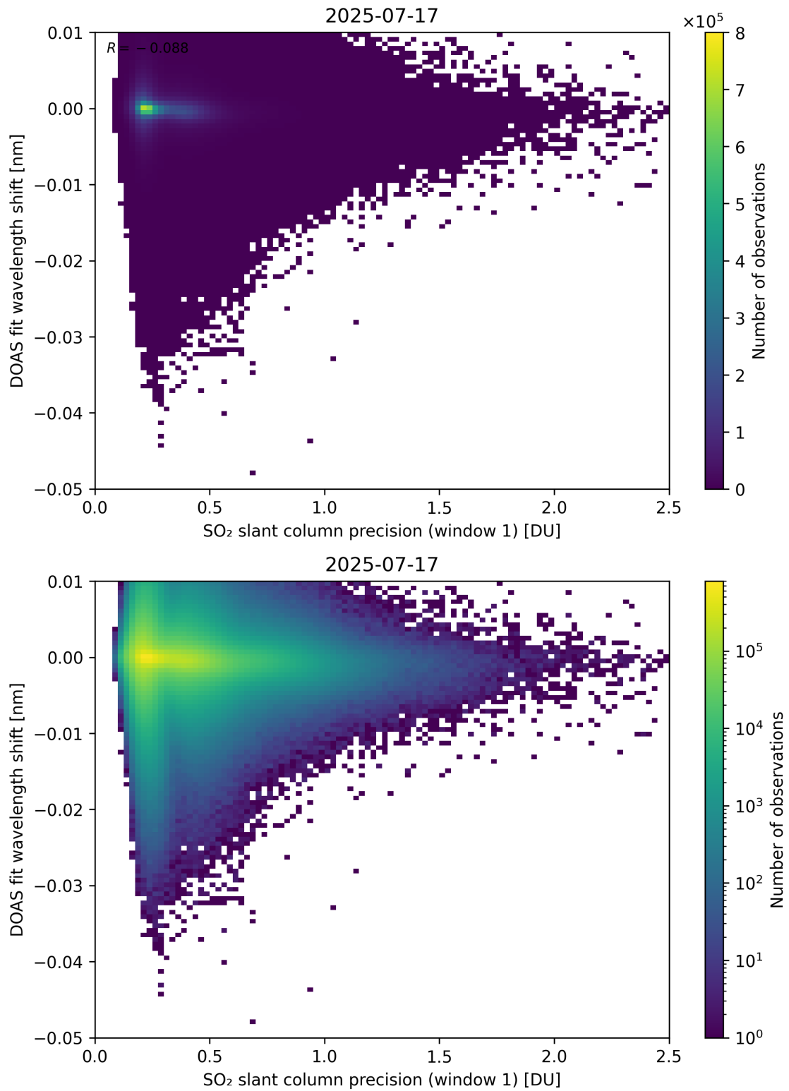
Figure 271: Scatter density plot of “SO 2 slant column precision (window 1)” against “DOAS fit wavelength shift” for 2025-07-16 to 2025-07-18.
