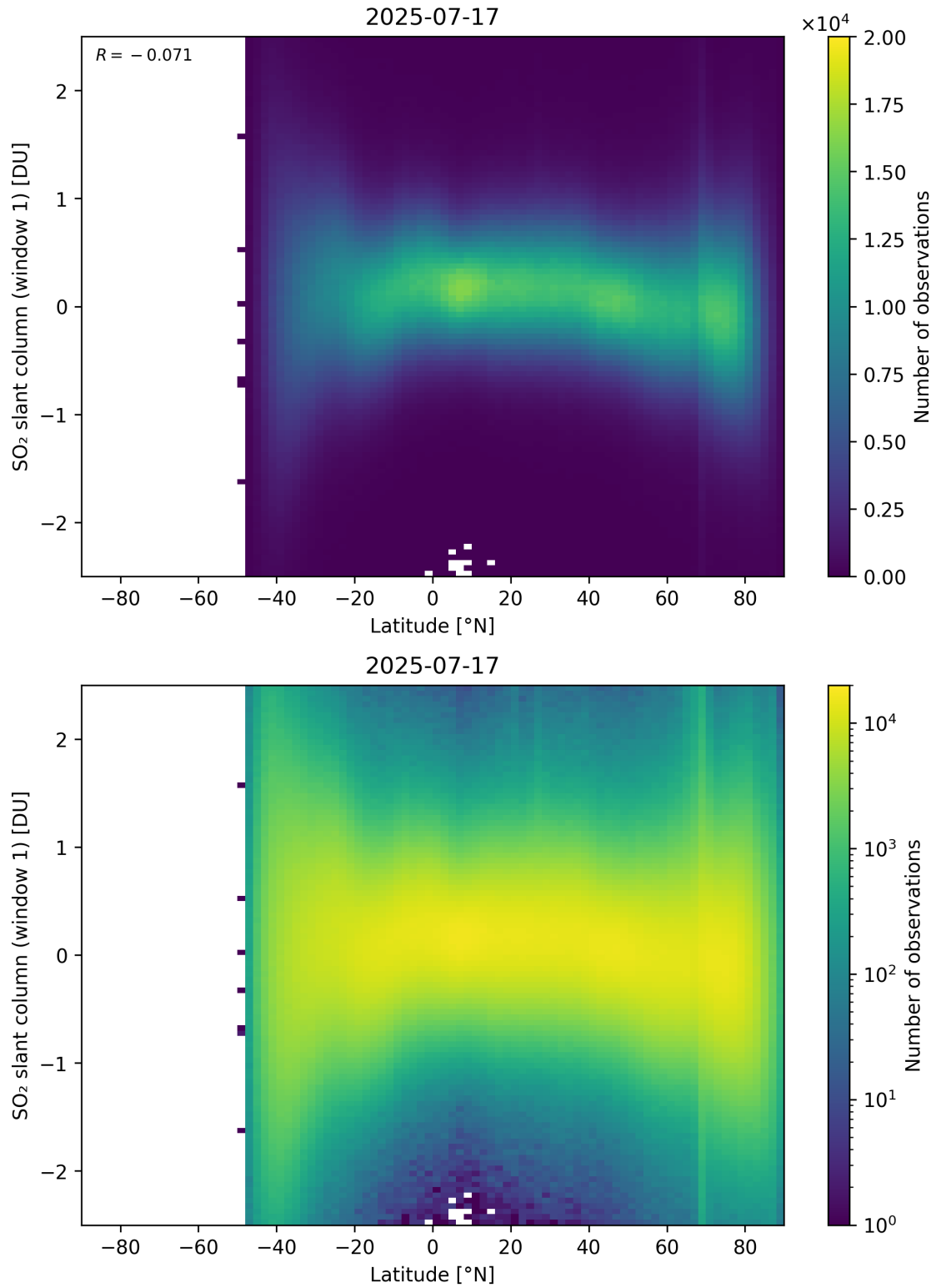
Figure 162: Scatter density plot of “Latitude” against “SO 2 slant column (window 1)” for 2025-07-16 to 2025-07-18.
