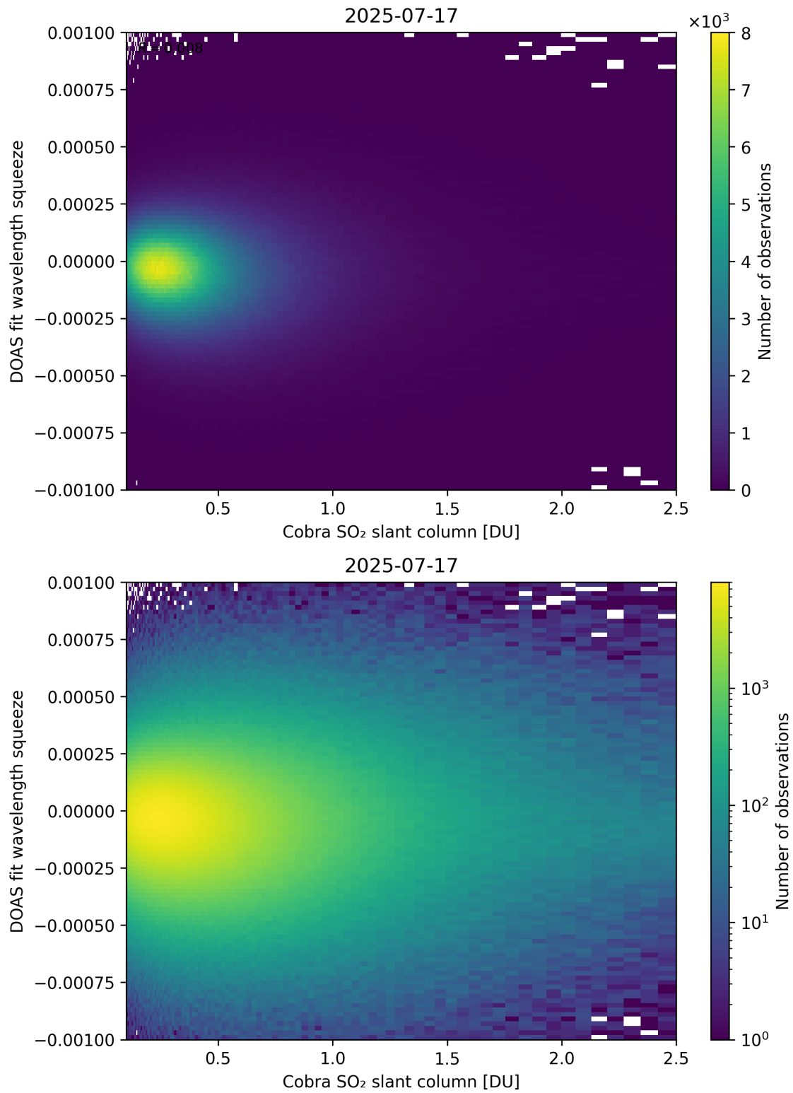
Figure 197: Scatter density plot of “Cobra SO 2 slant column” against “DOAS fit wavelength squeeze” for 2025-07-16 to 2025-07-18.
