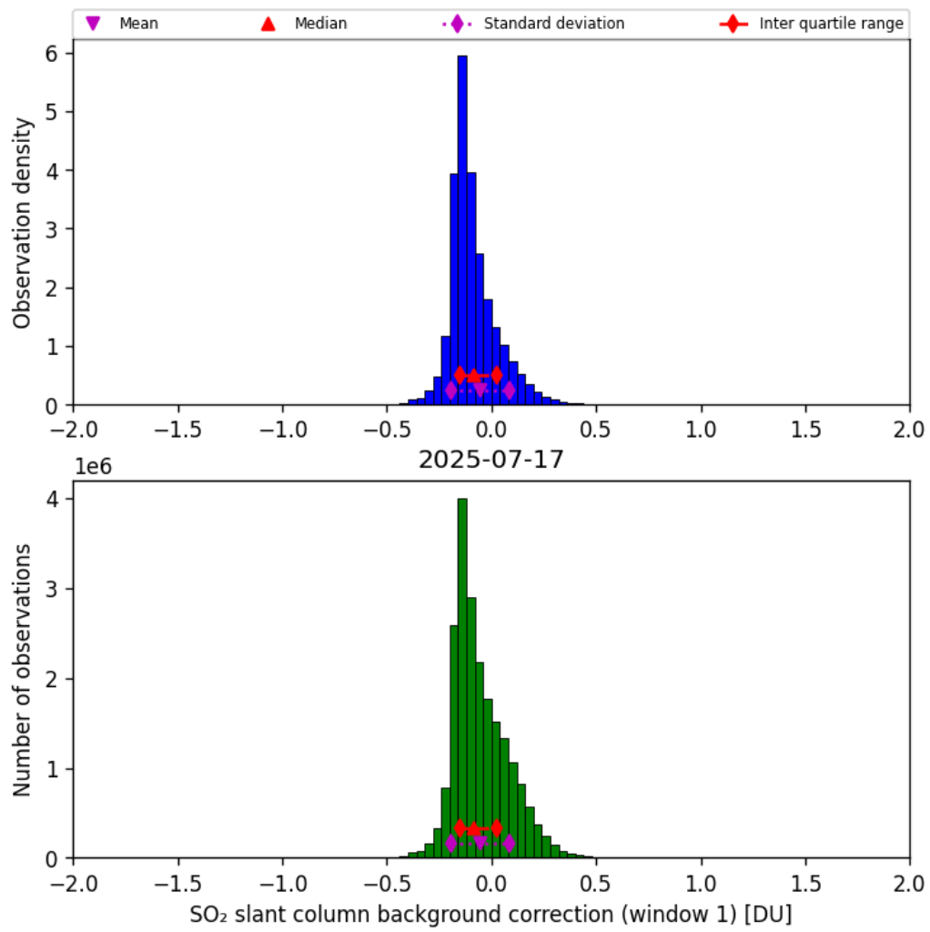
Figure 66: Histogram of “SO 2 slant column background correction (window 1)” for 2025-07-16 to 2025-07-18
