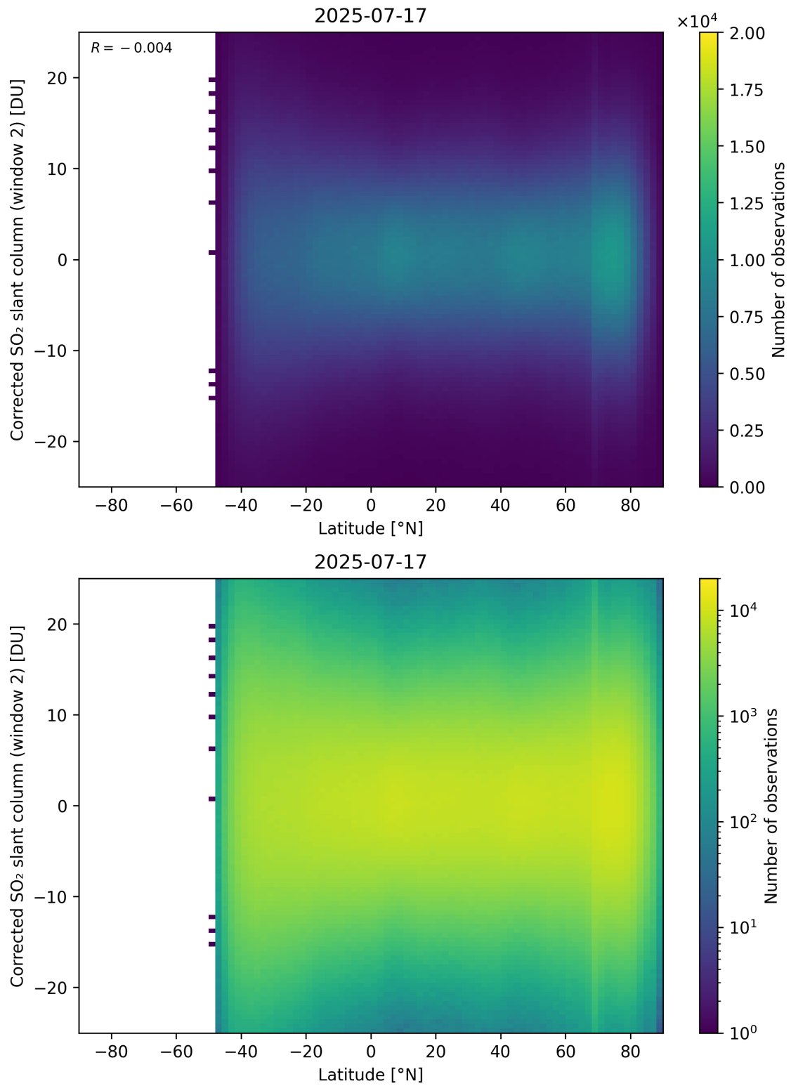
Figure 160: Scatter density plot of “Latitude” against “Corrected SO 2 slant column (window 2)” for 2025-07-16 to 2025-07-18.
