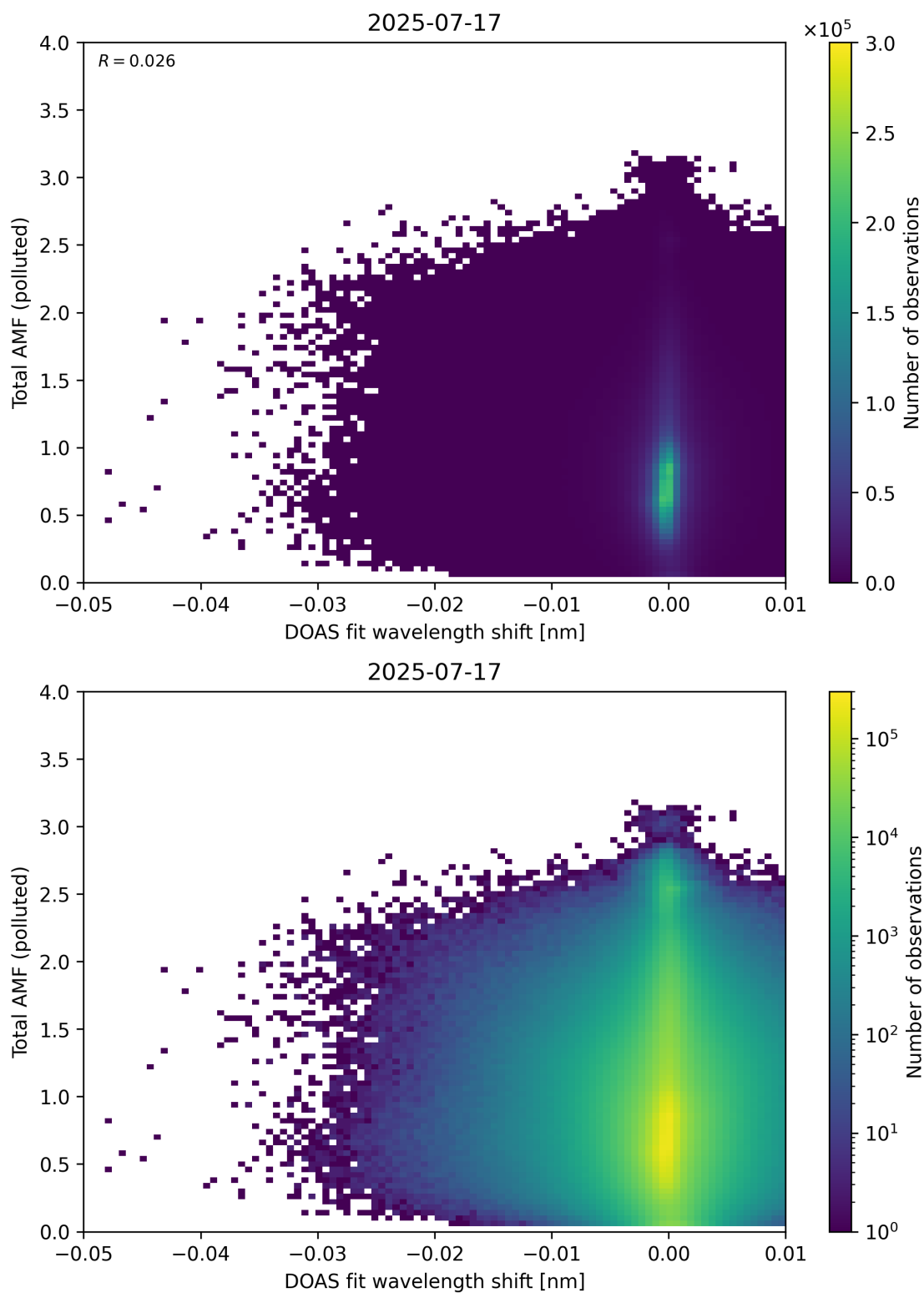
Figure 141: Scatter density plot of “DOAS fit wavelength shift” against “Total AMF (polluted)” for 2025-07-16 to 2025-07-18.
