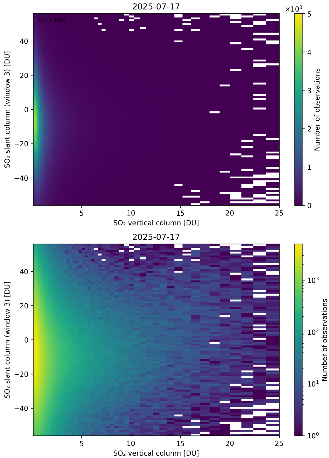
Figure 357: Scatter density plot of “SO 2 vertical column” against “SO 2 slant column (window 3)” for 2025-07-16 to 2025-07-18.
