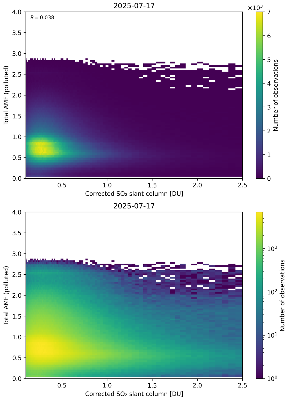
Figure 242: Scatter density plot of “Corrected SO 2 slant column” against “Total AMF (polluted)” for 2025-07-16 to 2025-07-18.
