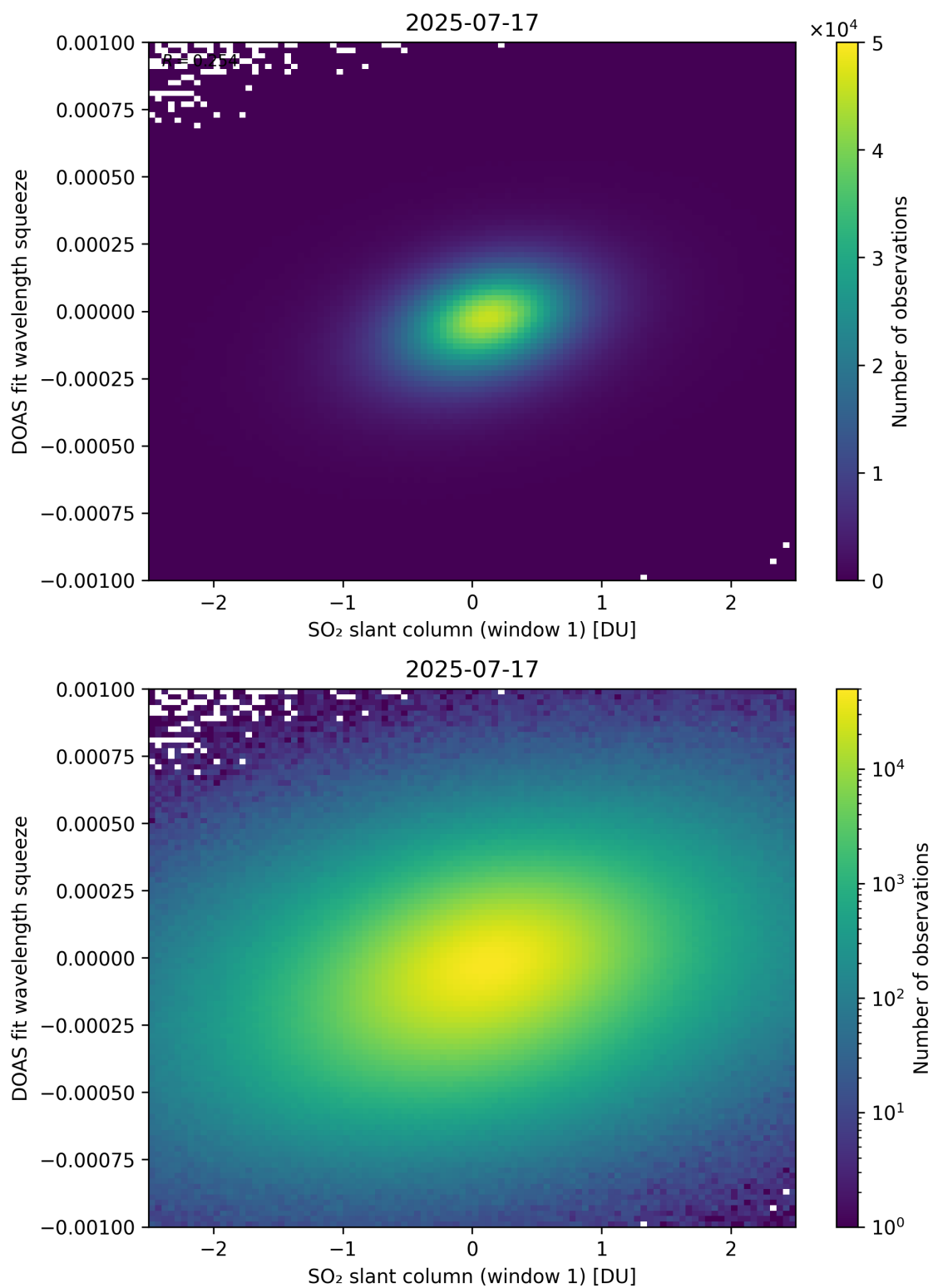
Figure 266: Scatter density plot of “SO 2 slant column (window 1)” against “DOAS fit wavelength squeeze” for 2025-07-16 to 2025-07-18.
