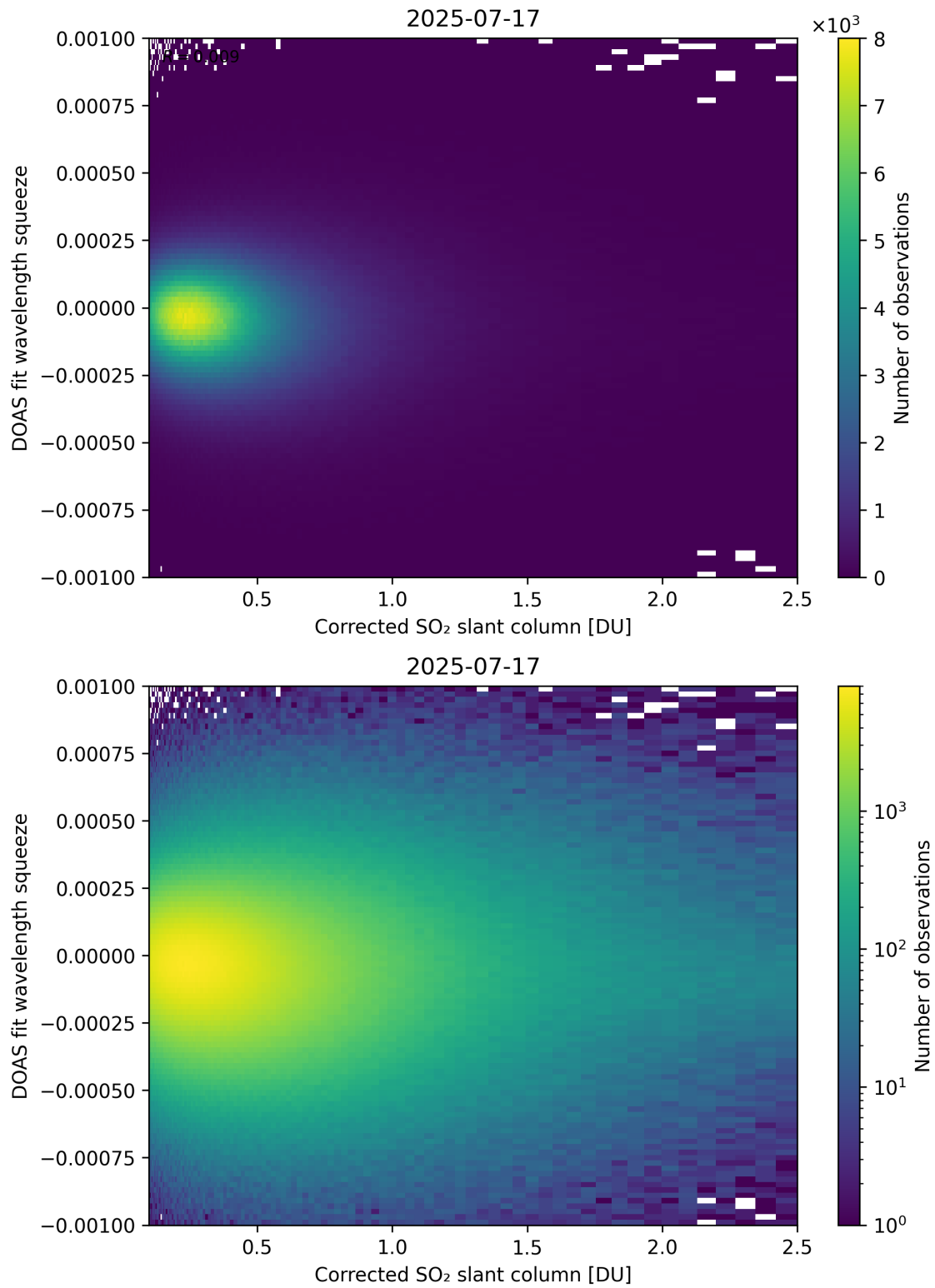
Figure 230: Scatter density plot of “Corrected SO 2 slant column” against “DOAS fit wavelength squeeze” for 2025-07-16 to 2025-07-18.
