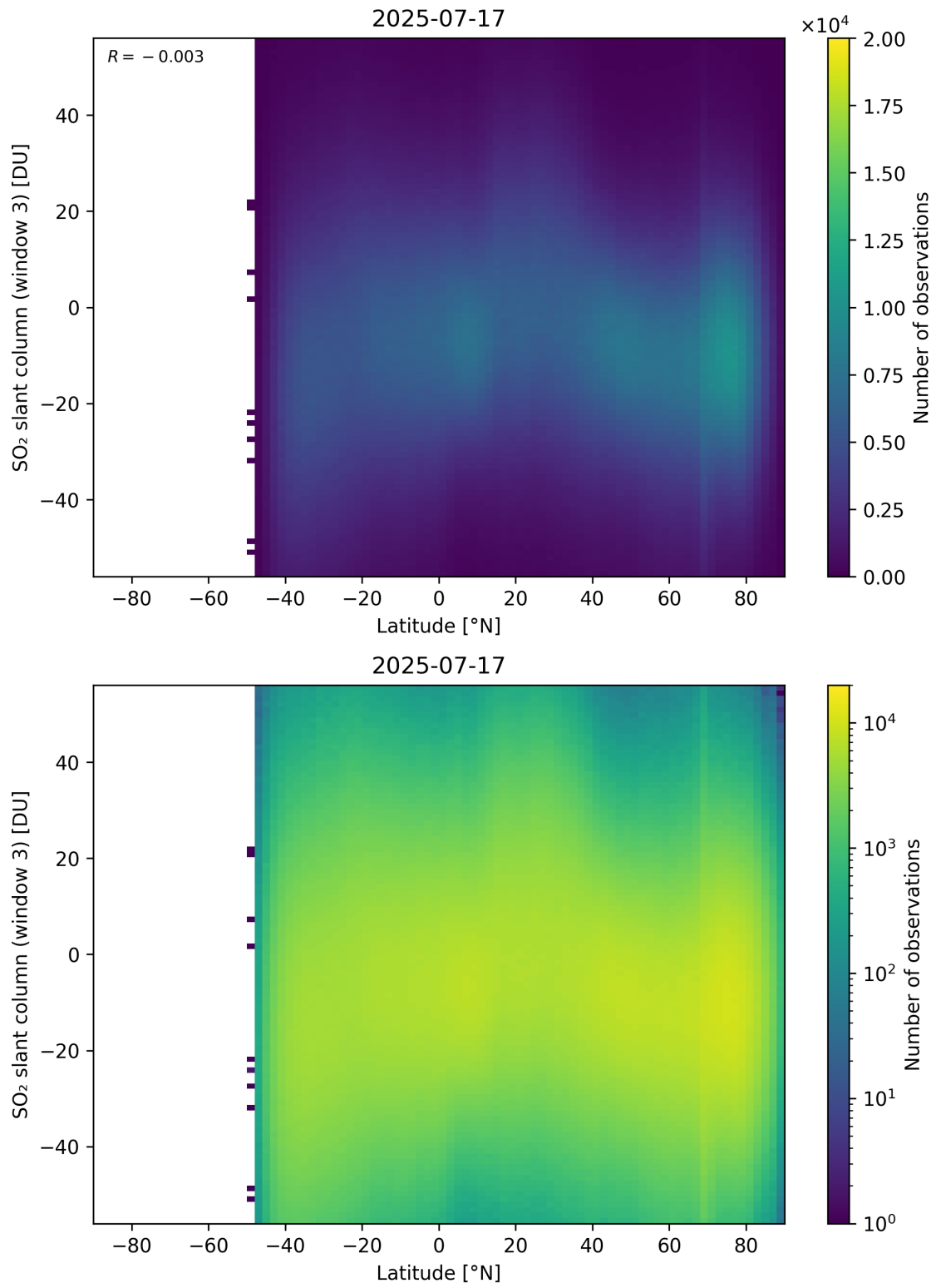
Figure 165: Scatter density plot of “Latitude” against “SO 2 slant column (window 3)” for 2025-07-16 to 2025-07-18.
