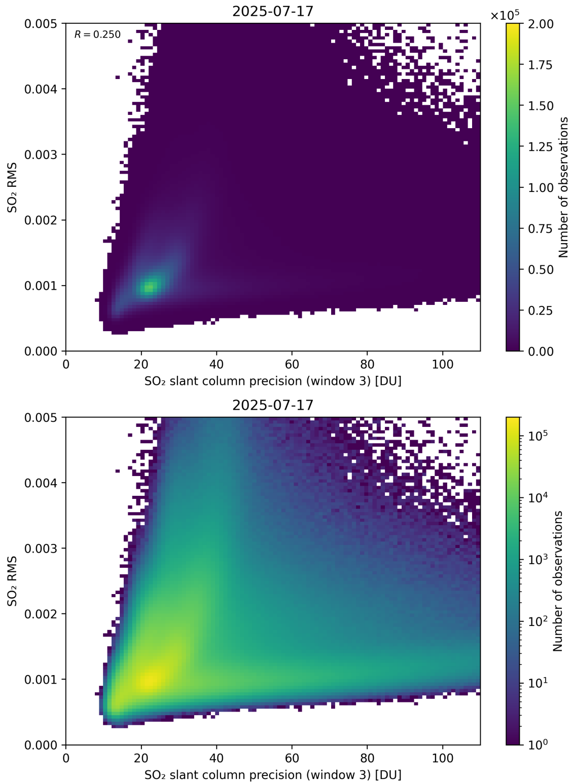
Figure 310: Scatter density plot of “SO 2 slant column precision (window 3)” against “SO 2 RMS” for 2025-07-16 to 2025-07-18.
