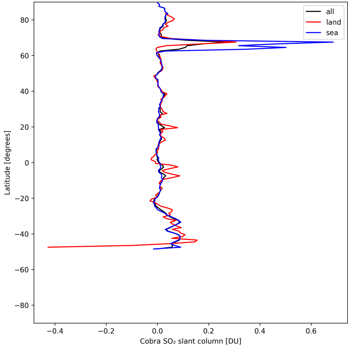
Figure 35: Zonal average of “Cobra SO 2 slant column” for 2025-07-16 to 2025-07-18.
