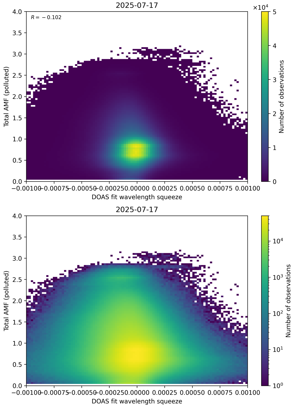
Figure 145: Scatter density plot of “DOAS fit wavelength squeeze” against “Total AMF (polluted)” for 2025-07-16 to 2025-07-18.
