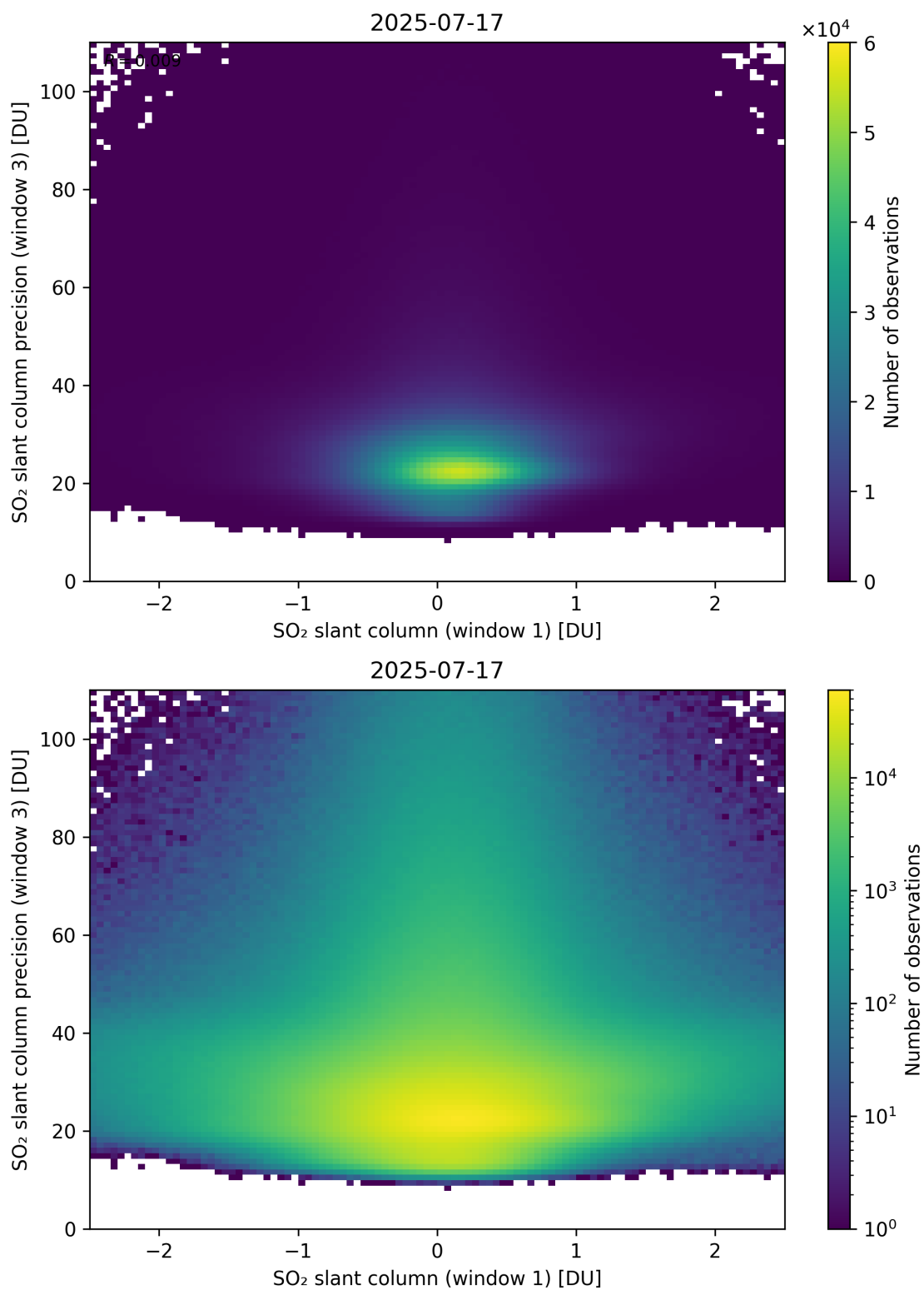
Figure 288: Scatter density plot of “SO 2 slant column (window 1)” against “SO 2 slant column precision (window 3)” for 2025-07-16 to 2025-07-18.
