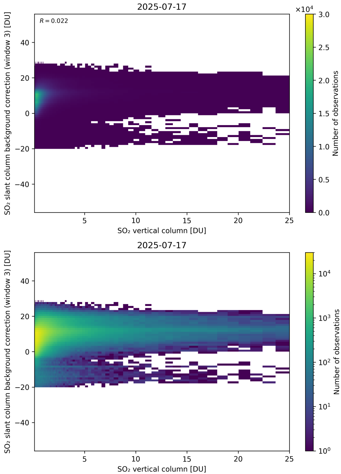
Figure 325: Scatter density plot of “SO 2 vertical column” against “SO 2 slant column background correction (window 3)” for 2025-07-16 to 2025-07-18.
