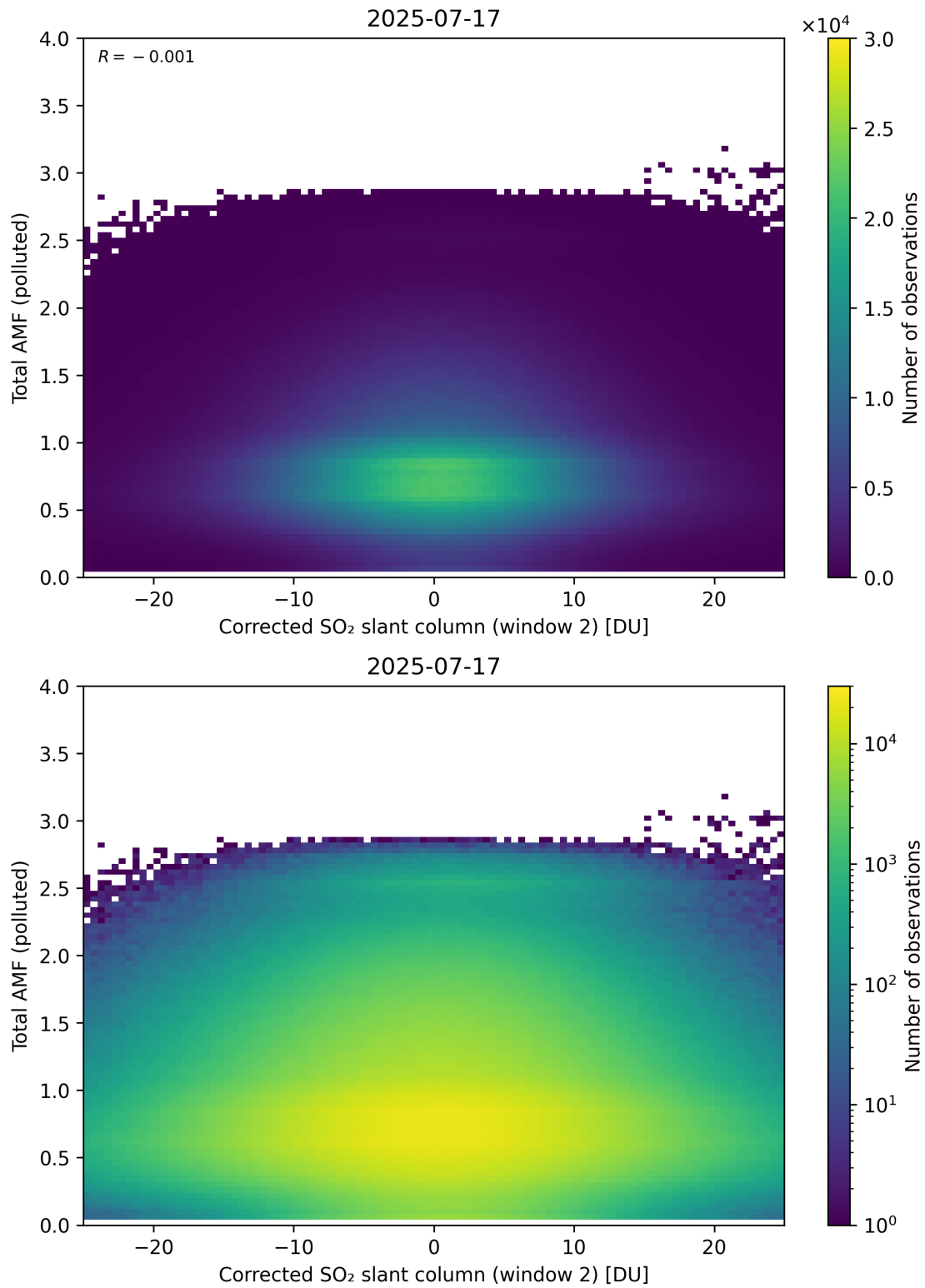
Figure 253: Scatter density plot of “Corrected SO 2 slant column (window 2)” against “Total AMF (polluted)” for 2025-07-16 to 2025-07-18.
