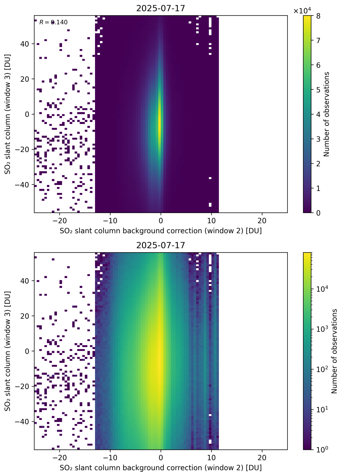
Figure 128: Scatter density plot of “SO 2 slant column background correction (window 2)” against “SO 2 slant column (window 3)” for 2025-07-16 to 2025-07-18.
