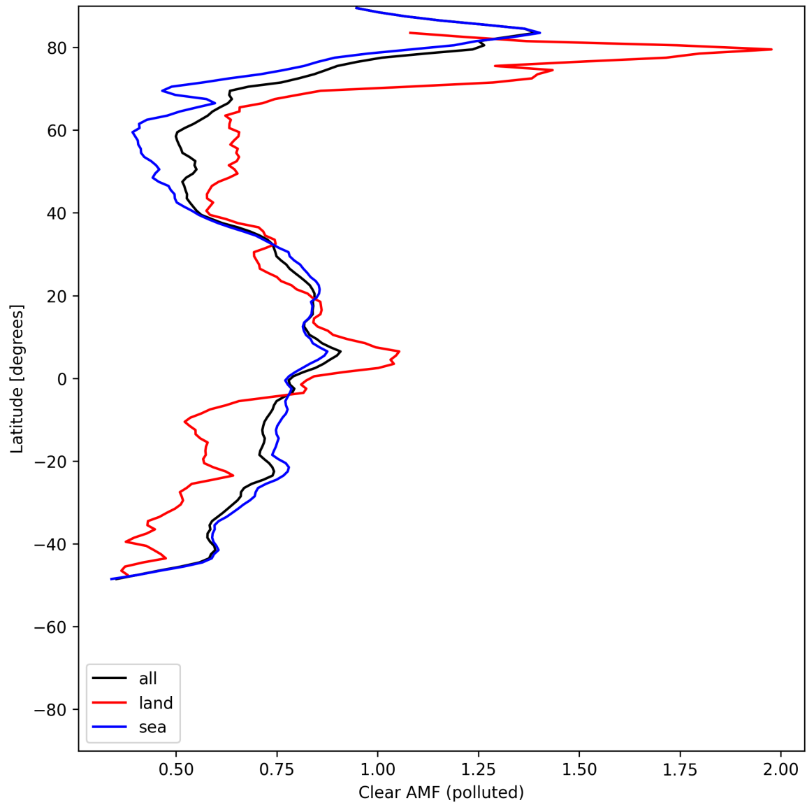
Figure 55: Zonal average of “Clear AMF (polluted)” for 2025-07-16 to 2025-07-18.
