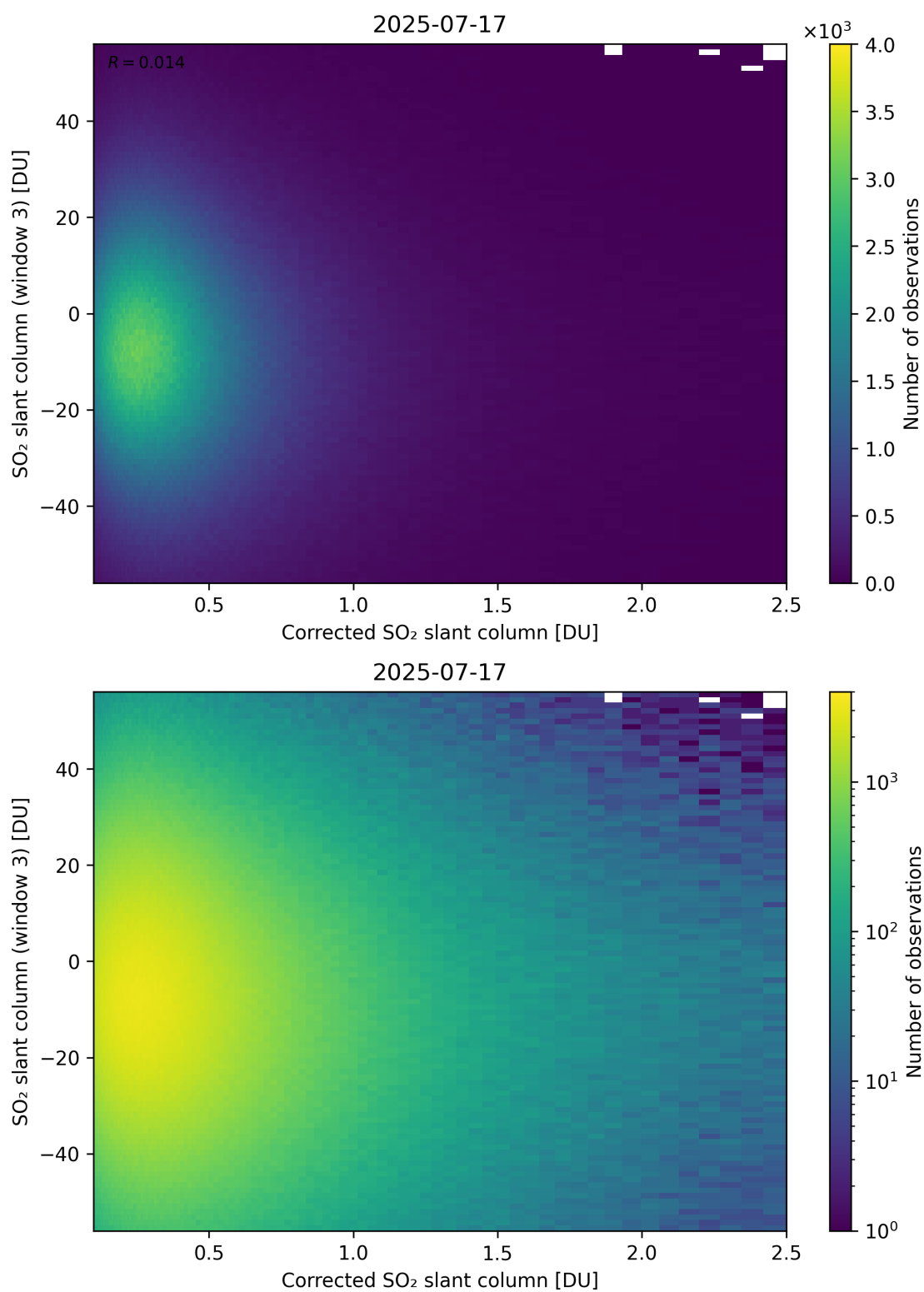
Figure 240: Scatter density plot of “Corrected SO 2 slant column” against “SO 2 slant column (window 3)” for 2025-07-16 to 2025-07-18.
