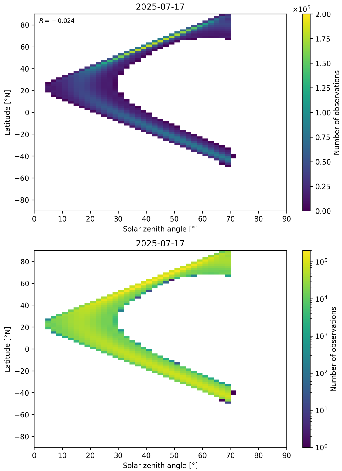
Figure 177: Scatter density plot of “Solar zenith angle” against “Latitude” for 2025-07-16 to 2025-07-18.
