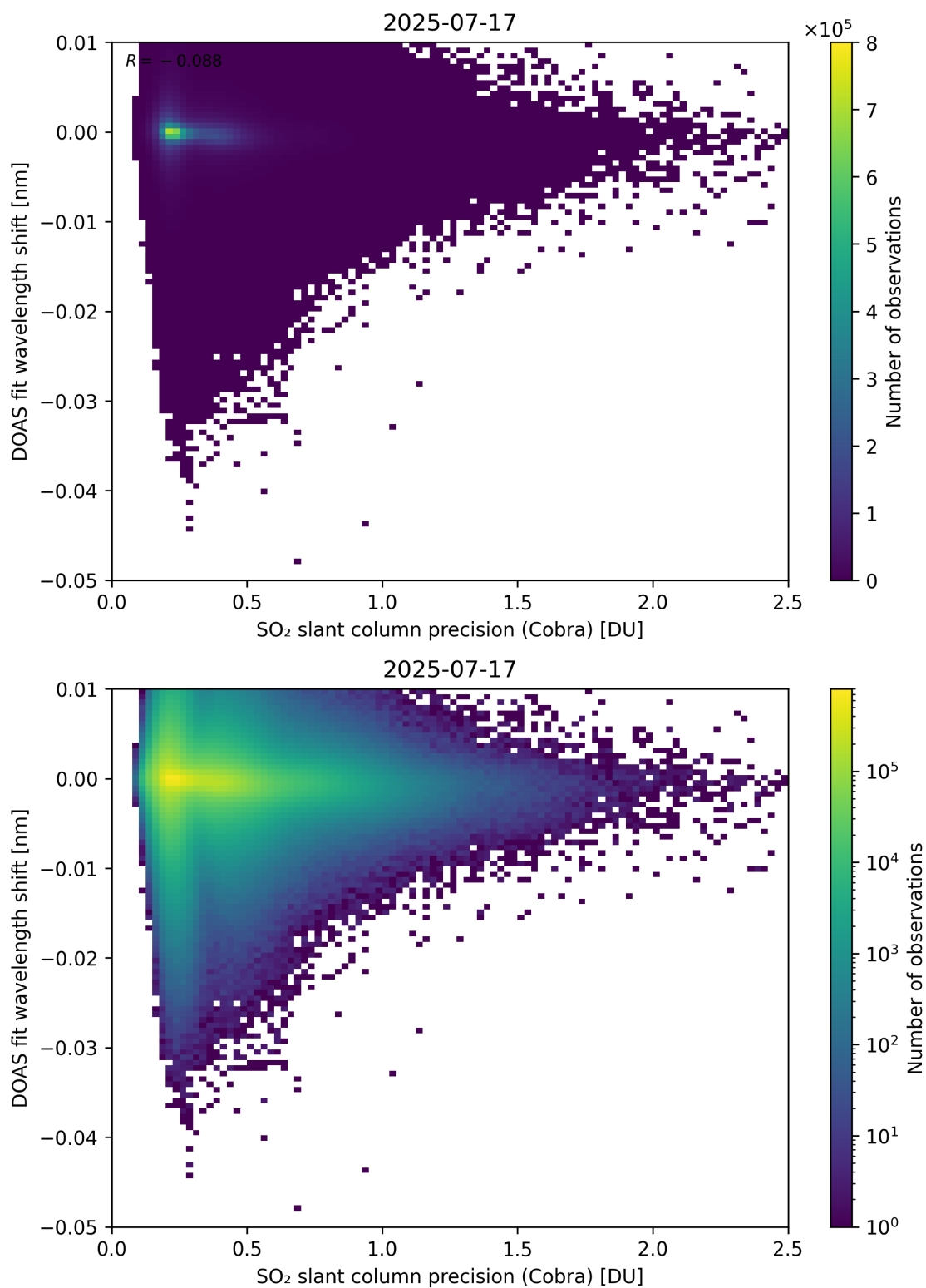
Figure 202: Scatter density plot of “SO 2 slant column precision (Cobra)” against “DOAS fit wavelength shift” for 2025-07-16 to 2025-07-18.
