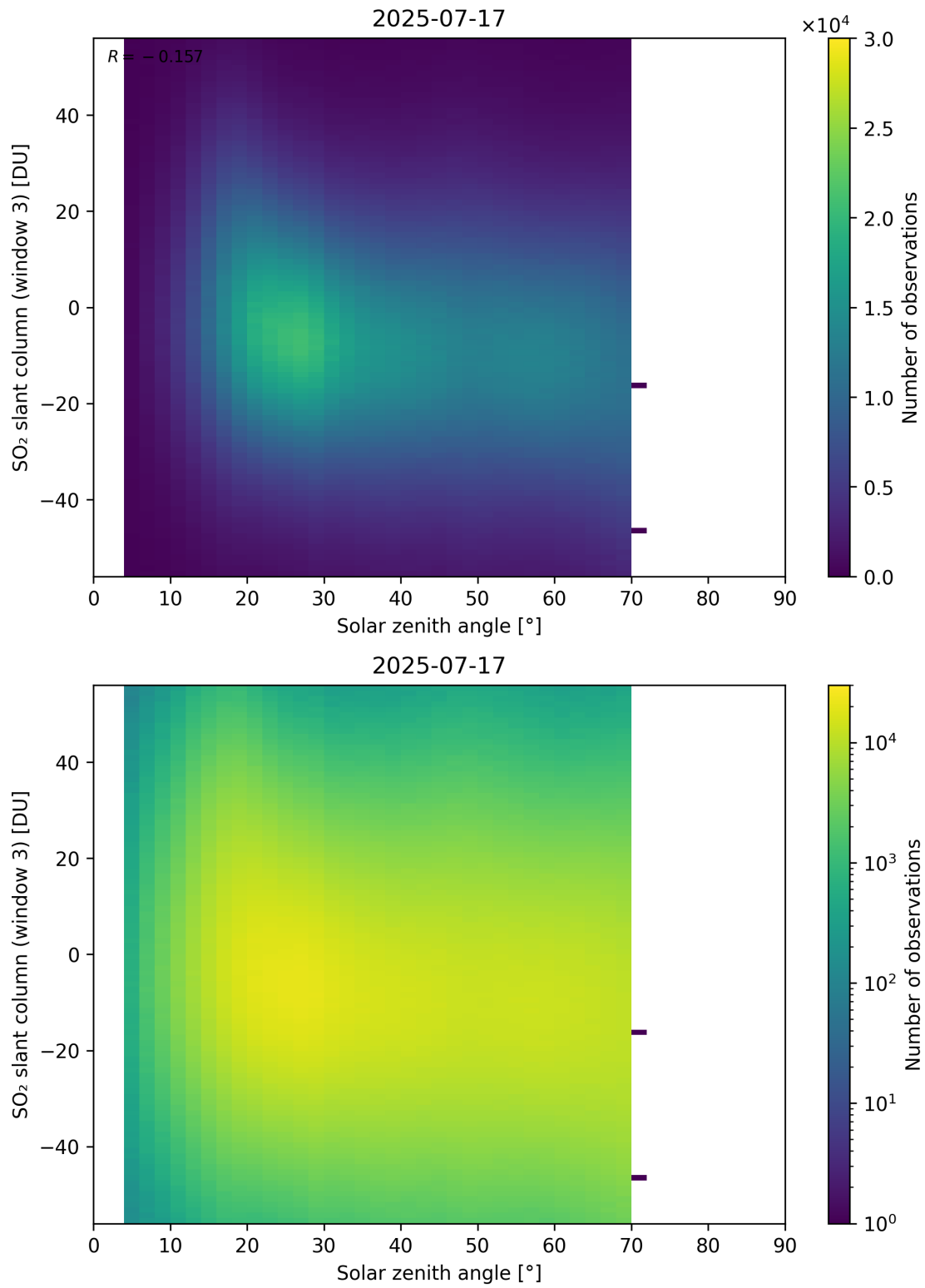
Figure 187: Scatter density plot of “Solar zenith angle” against “SO 2 slant column (window 3)” for 2025-07-16 to 2025-07-18.
