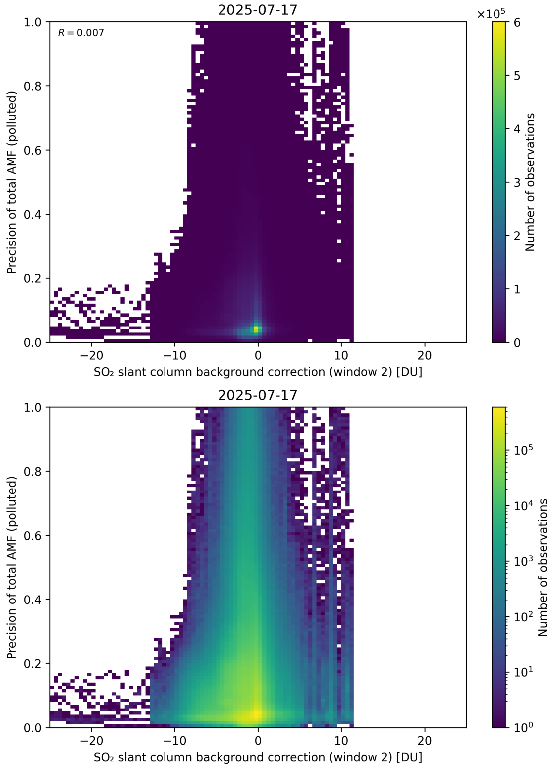
Figure 131: Scatter density plot of “SO 2 slant column background correction (window 2)” against “Precision of total AMF (polluted)” for 2025-07-16 to 2025-07-18.
