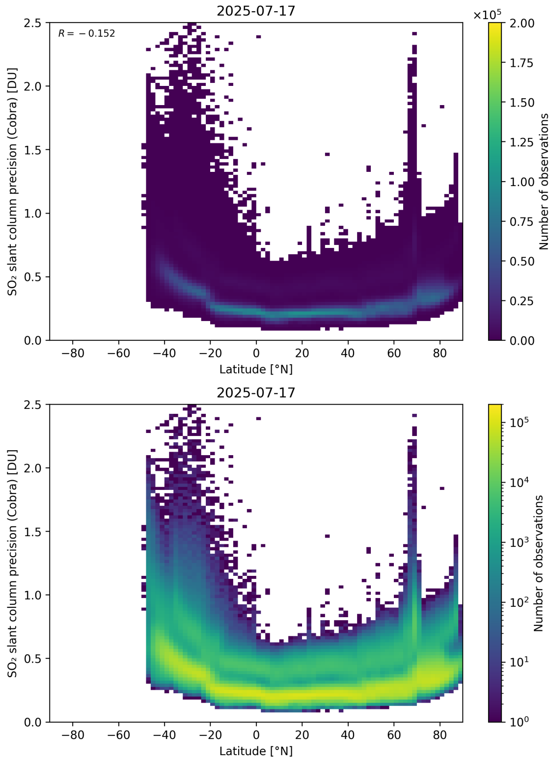
Figure 158: Scatter density plot of “Latitude” against “SO 2 slant column precision (Cobra)” for 2025-07-16 to 2025-07-18.
