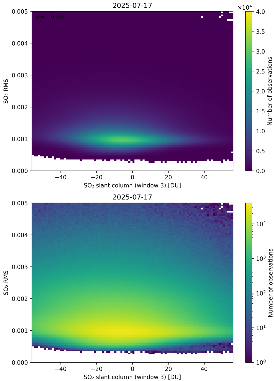
Figure 306: Scatter density plot of “SO 2 slant column (window 3)” against “SO 2 RMS” for 2025-07-16 to 2025-07-18.
