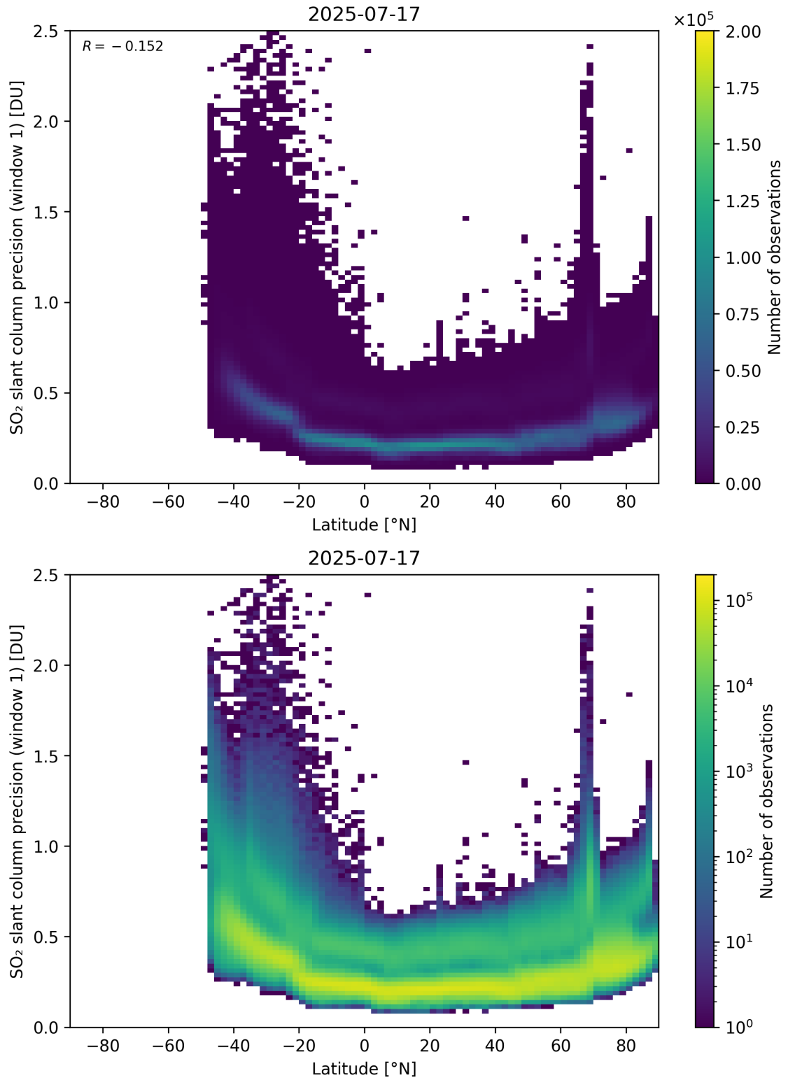
Figure 163: Scatter density plot of “Latitude” against “SO 2 slant column precision (window 1)” for 2025-07-16 to 2025-07-18.
