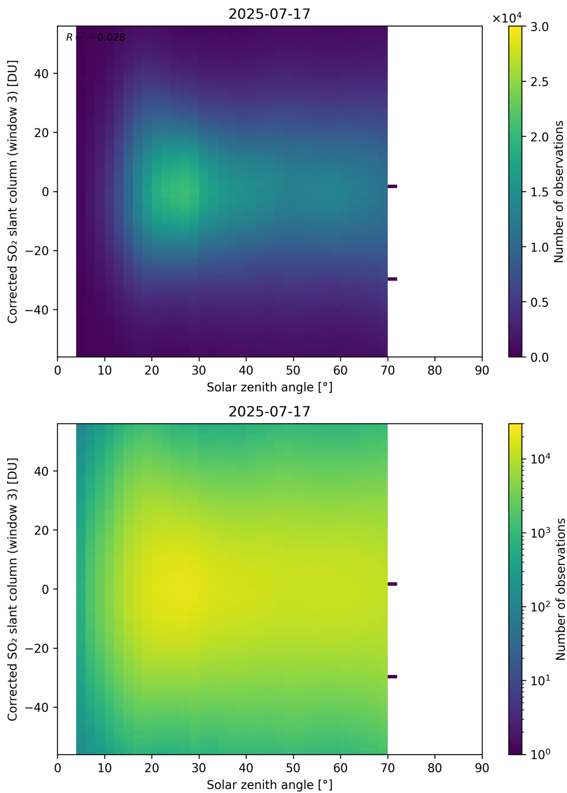
Figure 183: Scatter density plot of “Solar zenith angle” against “Corrected SO 2 slant column (window 3)” for 2025-07-16 to 2025-07-18.
