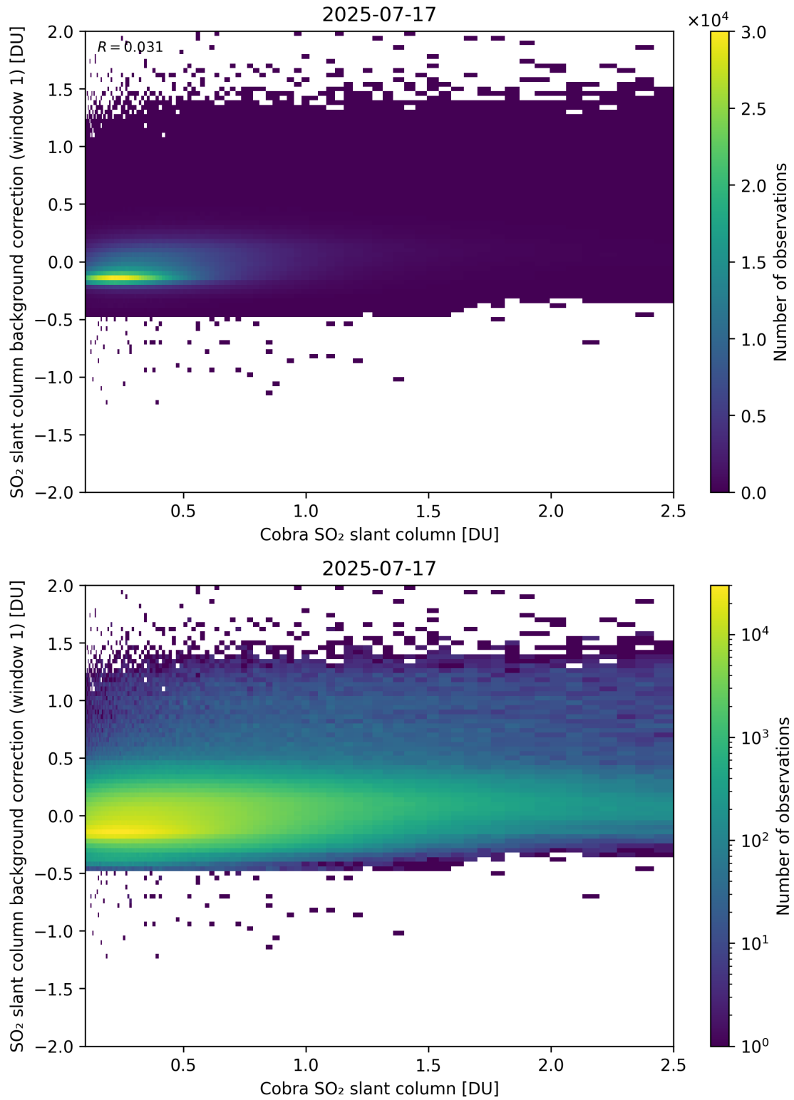
Figure 193: Scatter density plot of “Cobra SO 2 slant column” against “SO 2 slant column background correction (window 1)” for 2025-07-16 to 2025-07-18.
