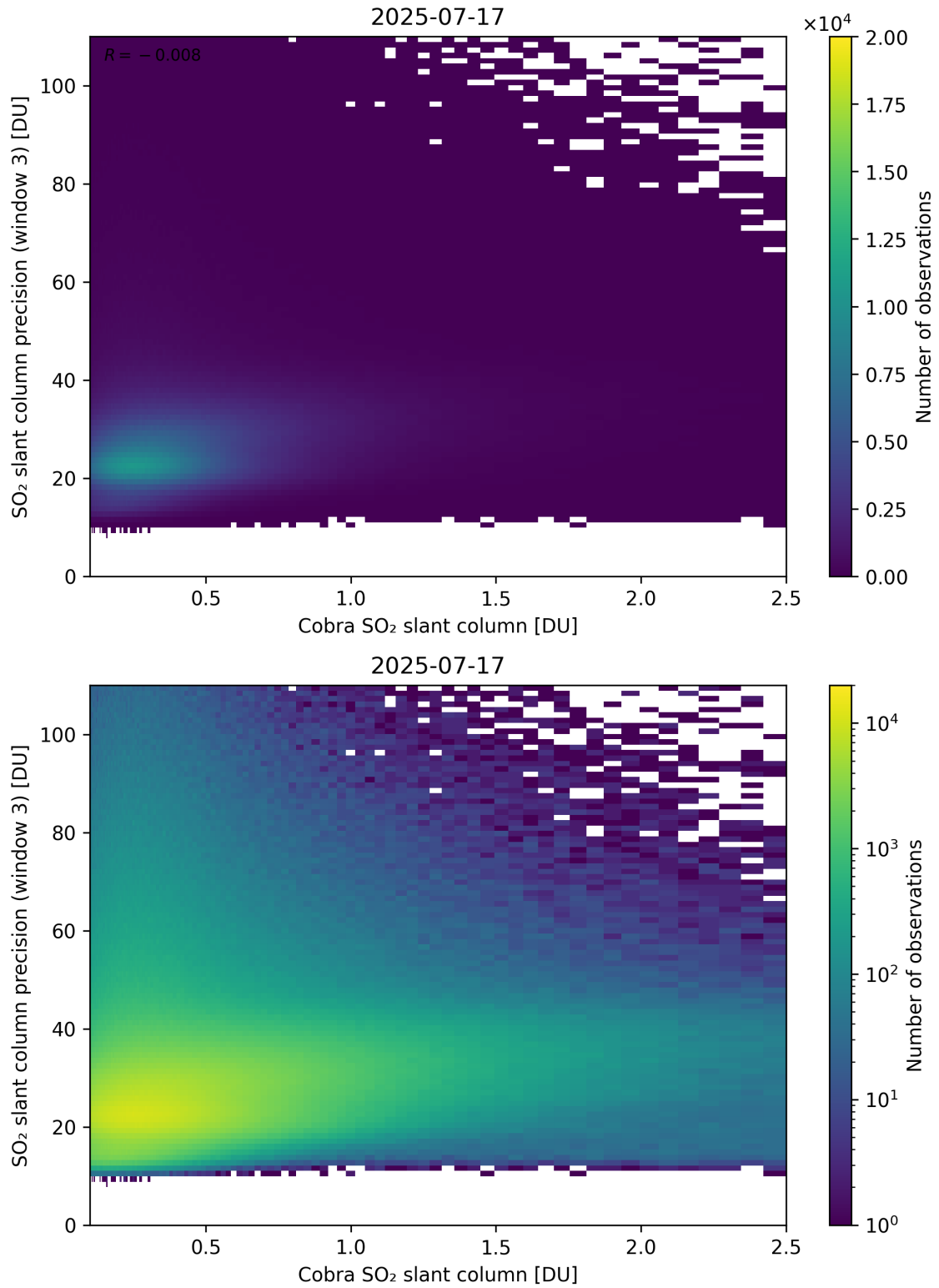
Figure 223: Scatter density plot of “Cobra SO 2 slant column” against “SO 2 slant column precision (window 3)” for 2025-07-16 to 2025-07-18.
