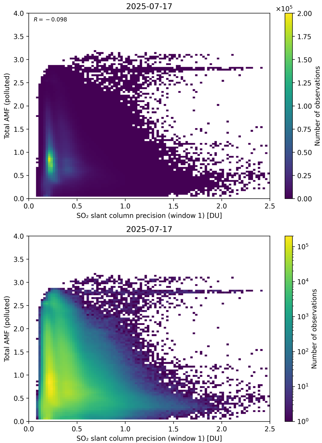
Figure 280: Scatter density plot of “SO 2 slant column precision (window 1)” against “Total AMF (polluted)” for 2025-07-16 to 2025-07-18.
