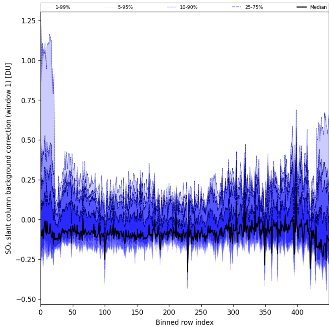
Figure 92: Along track statistics of “SO 2 slant column background correction (window 1)” for 2025-07-16 to 2025-07-18
