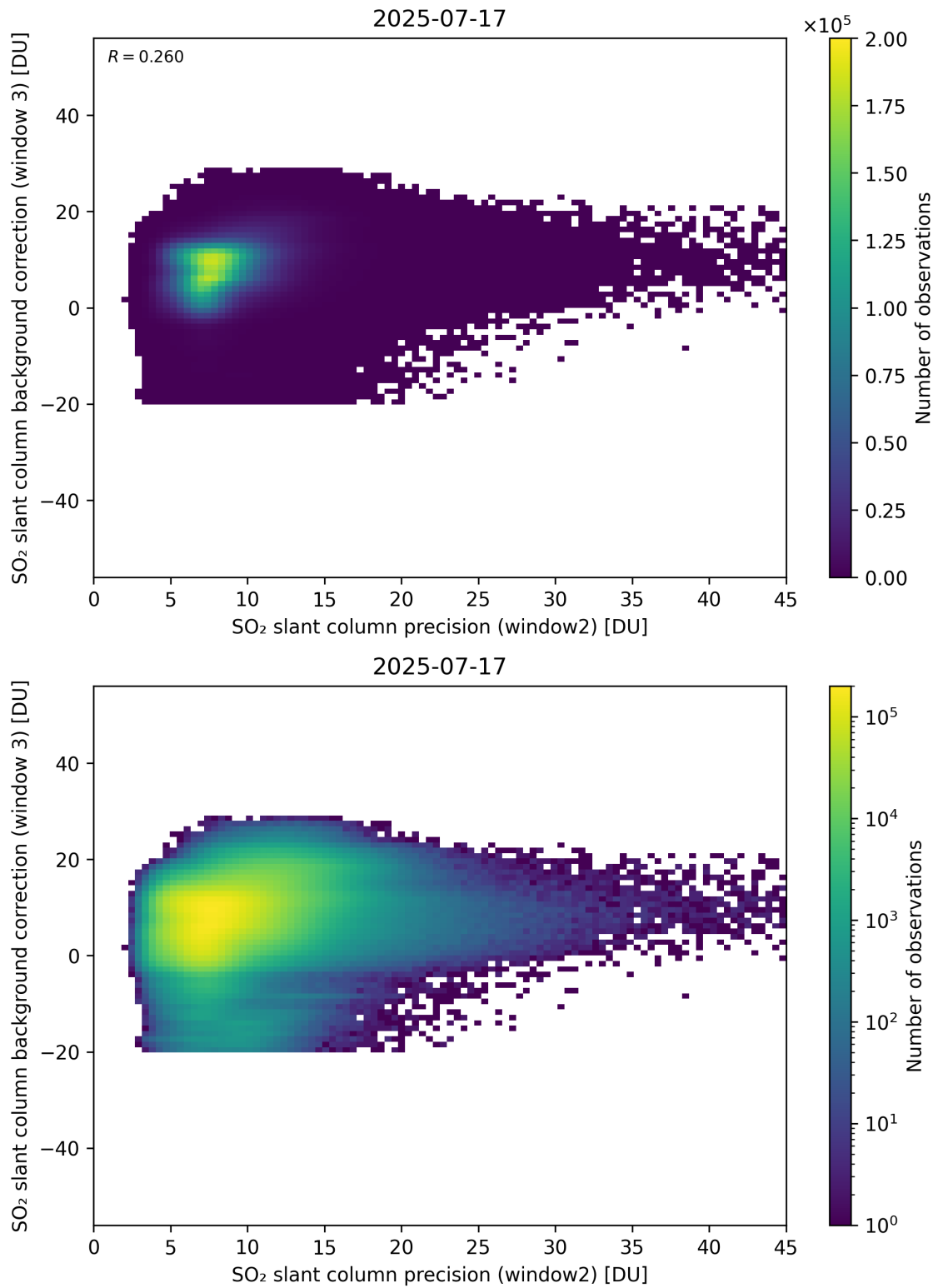
Figure 292: Scatter density plot of “SO 2 slant column precision (window2)” against “SO 2 slant column background correction (window 3)” for 2025-07-16 to 2025-07-18.
