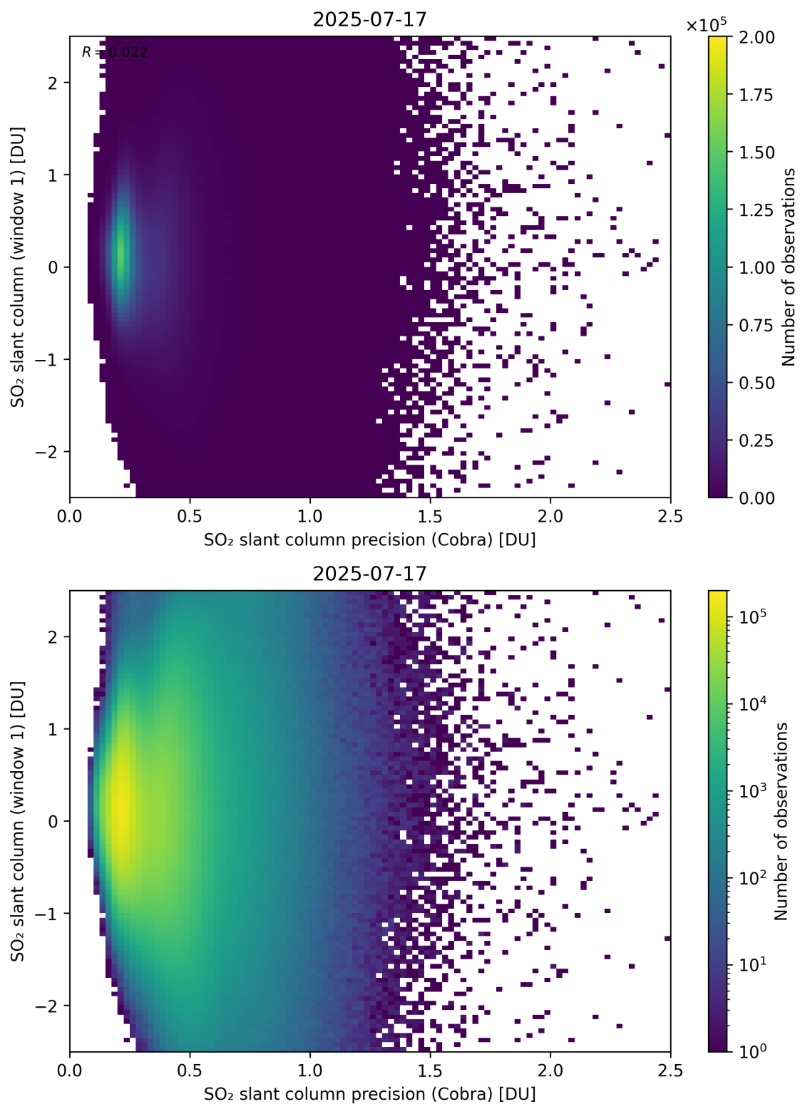
Figure 208: Scatter density plot of “SO 2 slant column precision (Cobra)” against “SO 2 slant column (window 1)” for 2025-07-16 to 2025-07-18.
