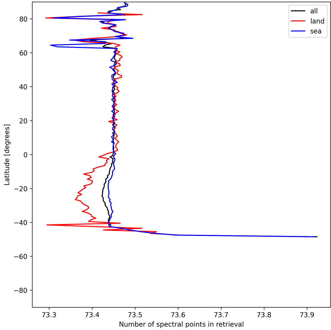
Figure 56: Zonal average of “Number of spectral points in retrieval” for 2025-07-16 to 2025-07-18.
