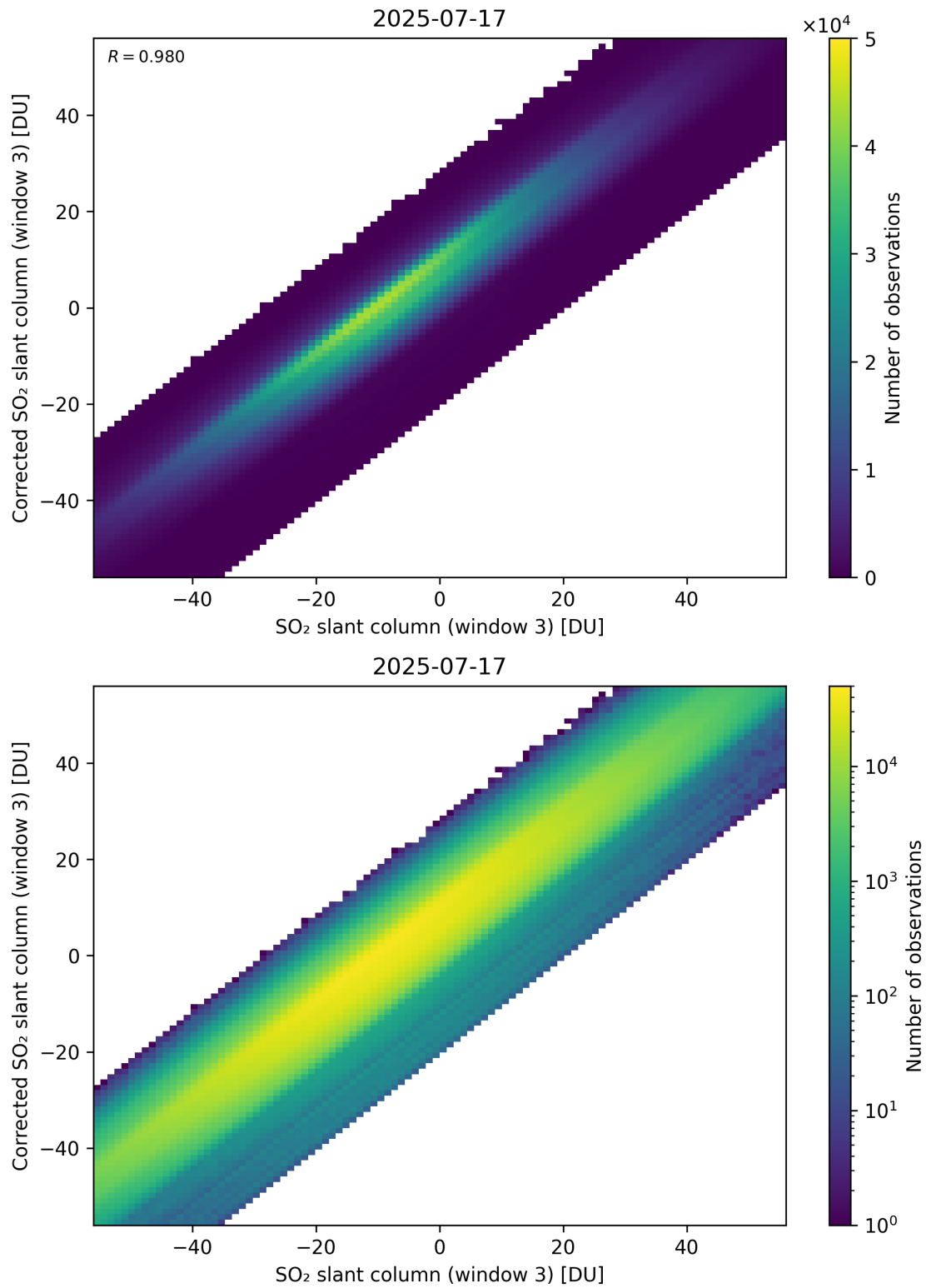
Figure 316: Scatter density plot of “SO 2 slant column (window 3)” against “Corrected SO 2 slant column (window 3)” for 2025-07-16 to 2025-07-18.
