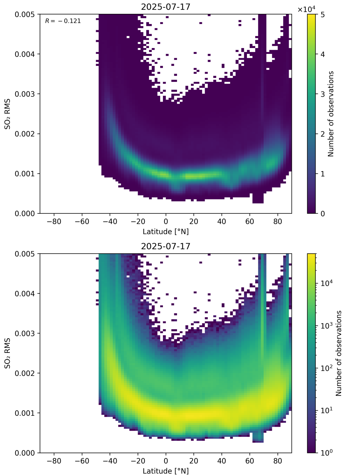
Figure 155: Scatter density plot of “Latitude” against “SO 2 RMS” for 2025-07-16 to 2025-07-18.
