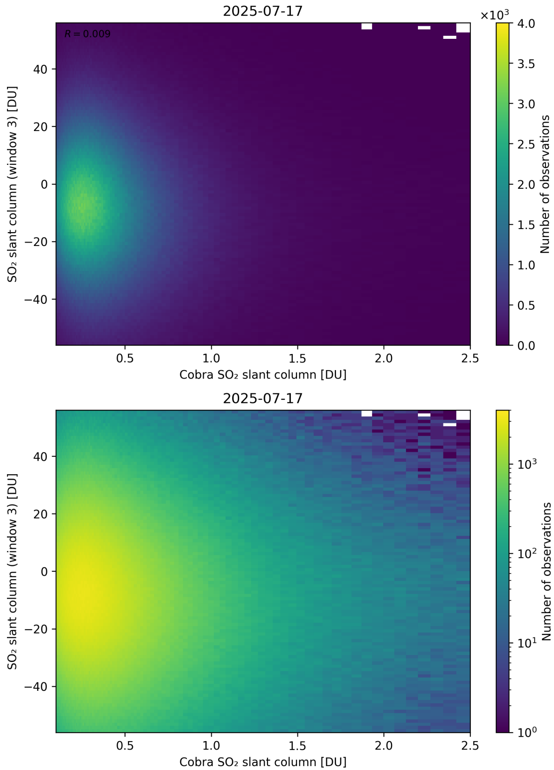
Figure 222: Scatter density plot of “Cobra SO 2 slant column” against “SO 2 slant column (window 3)” for 2025-07-16 to 2025-07-18.
