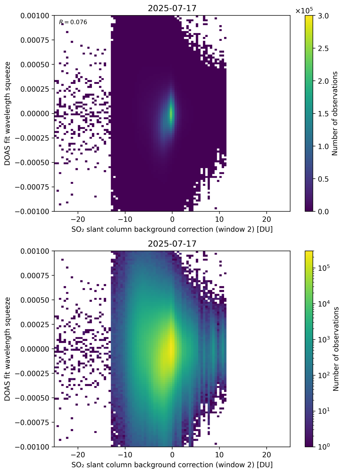
Figure 124: Scatter density plot of “SO 2 slant column background correction (window 2)” against “DOAS fit wavelength squeeze” for 2025-07-16 to 2025-07-18.
