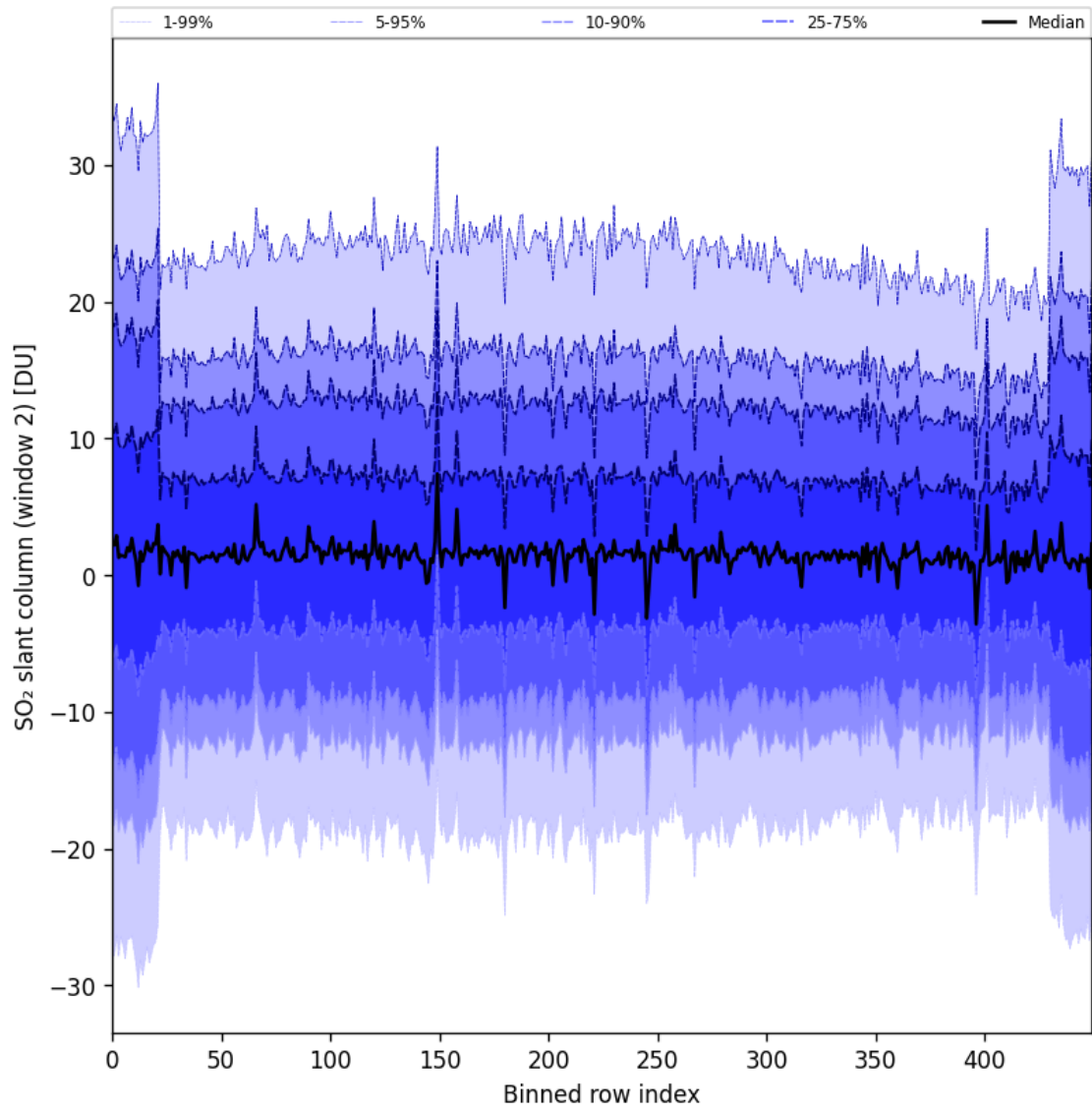
Figure 93: Along track statistics of “SO 2 slant column (window 2)” for 2025-07-16 to 2025-07-18
