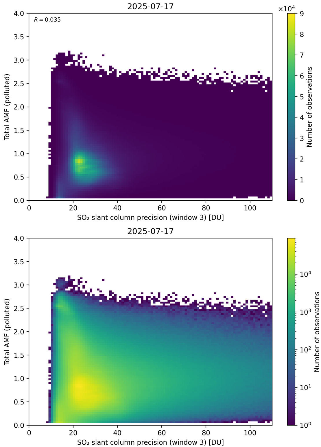
Figure 313: Scatter density plot of “SO 2 slant column precision (window 3)” against “Total AMF (polluted)” for 2025-07-16 to 2025-07-18.
