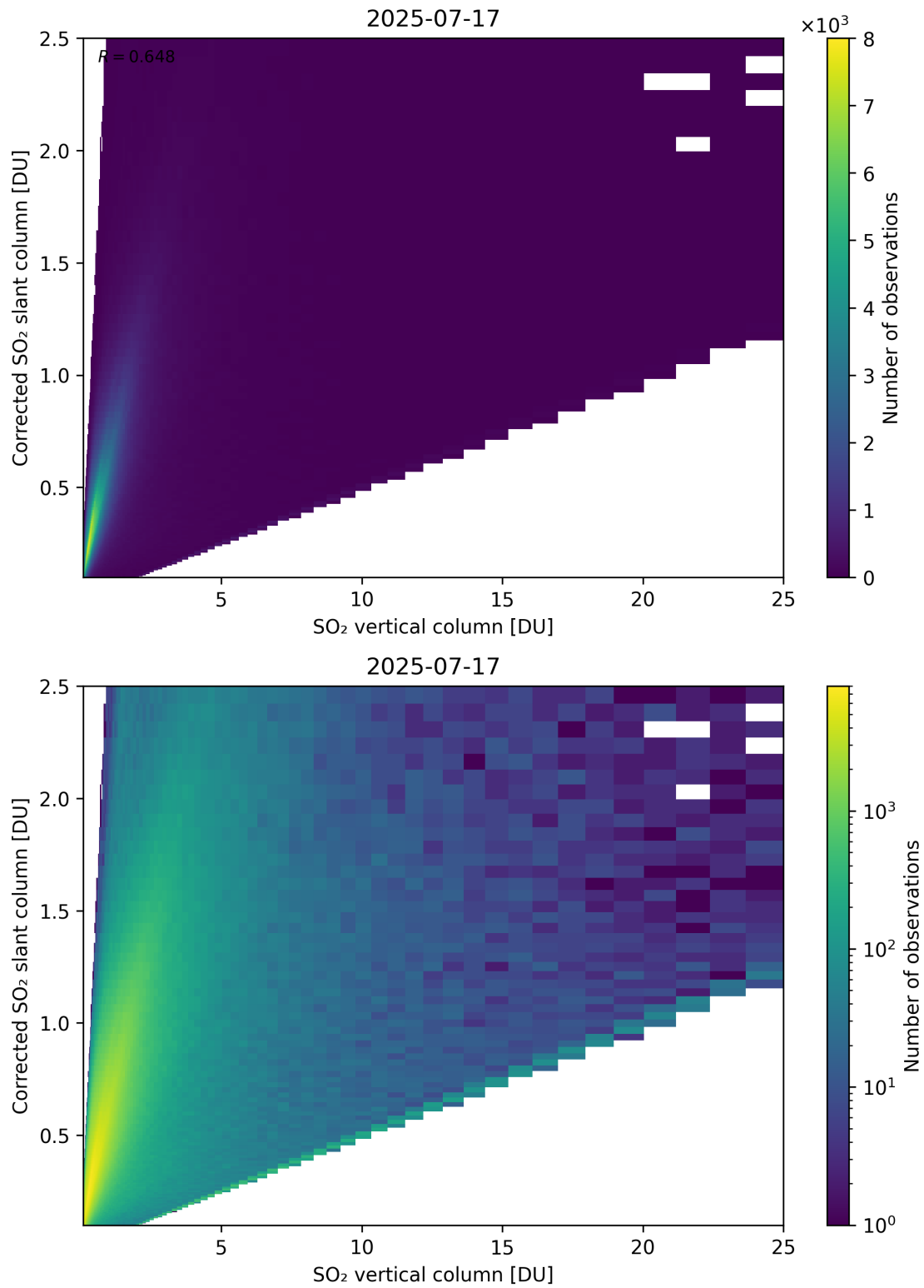
Figure 351: Scatter density plot of “SO 2 vertical column” against “Corrected SO 2 slant column” for 2025-07-16 to 2025-07-18.
