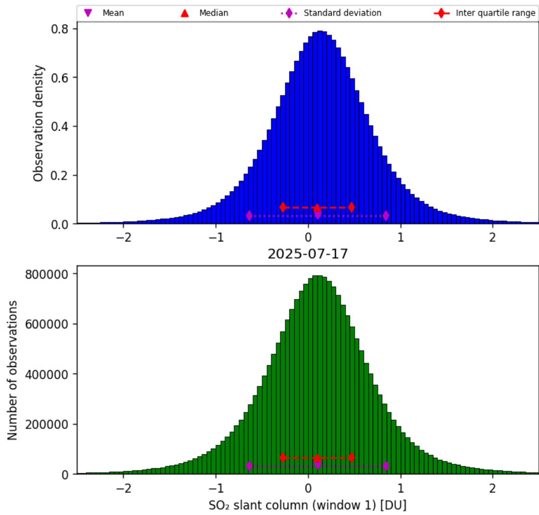
Figure 63: Histogram of “SO 2 slant column (window 1)” for 2025-07-16 to 2025-07-18
