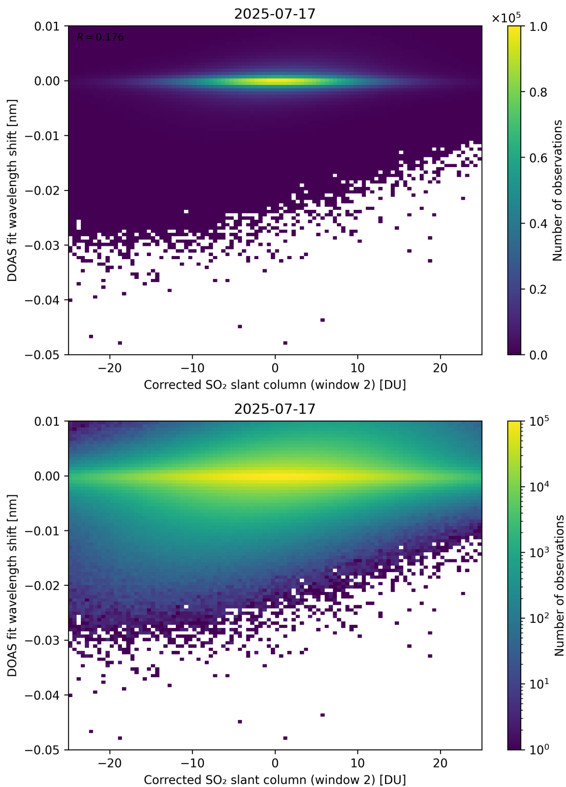
Figure 246: Scatter density plot of “Corrected SO 2 slant column (window 2)” against “DOAS fit wavelength shift” for 2025-07-16 to 2025-07-18.
