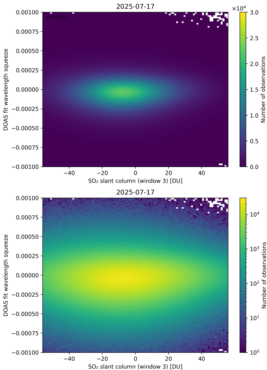
Figure 305: Scatter density plot of “SO 2 slant column (window 3)” against “DOAS fit wavelength squeeze” for 2025-07-16 to 2025-07-18.
