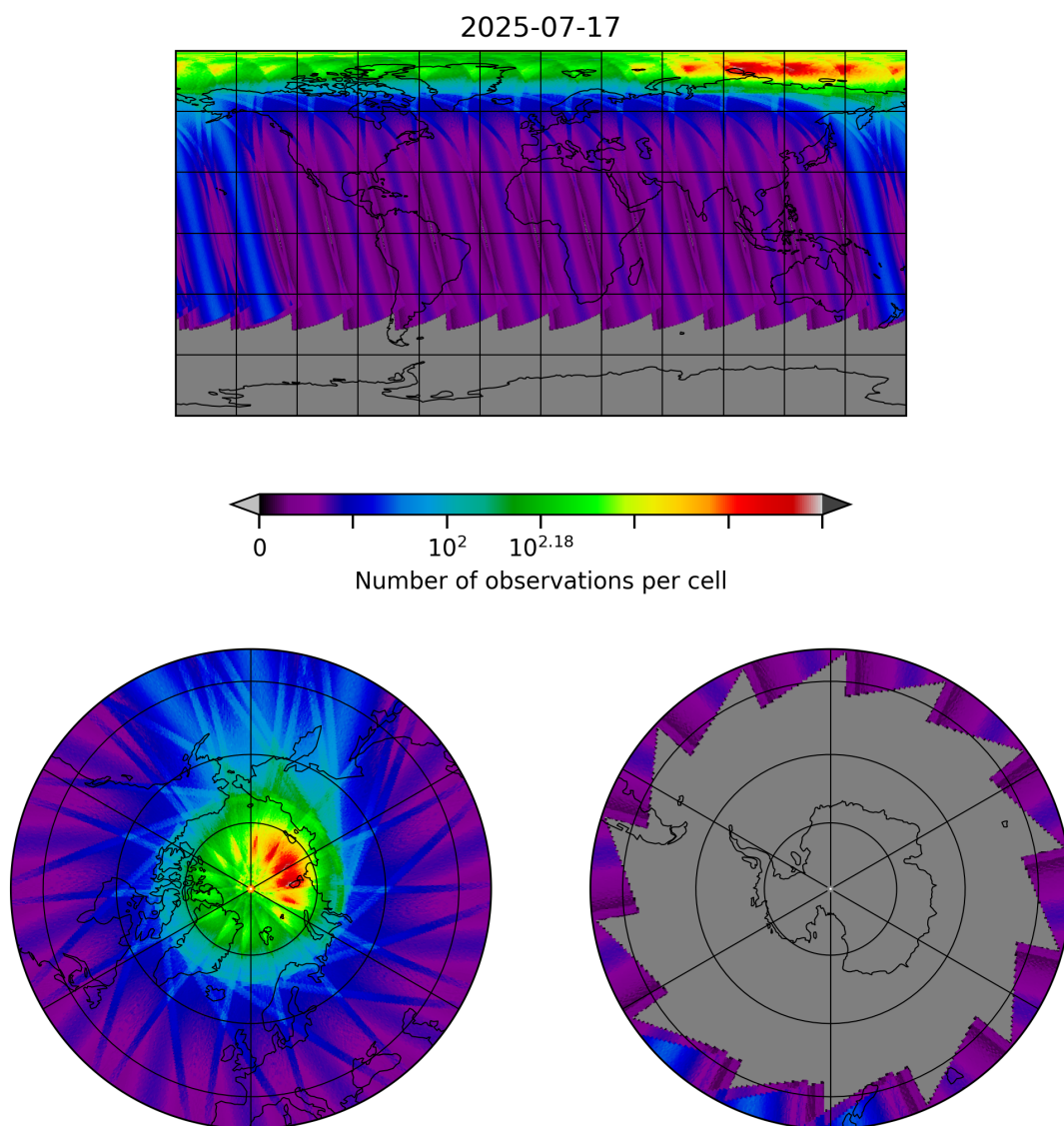
Figure 30: Map of the number of observations for 2025-07-16 to 2025-07-18
