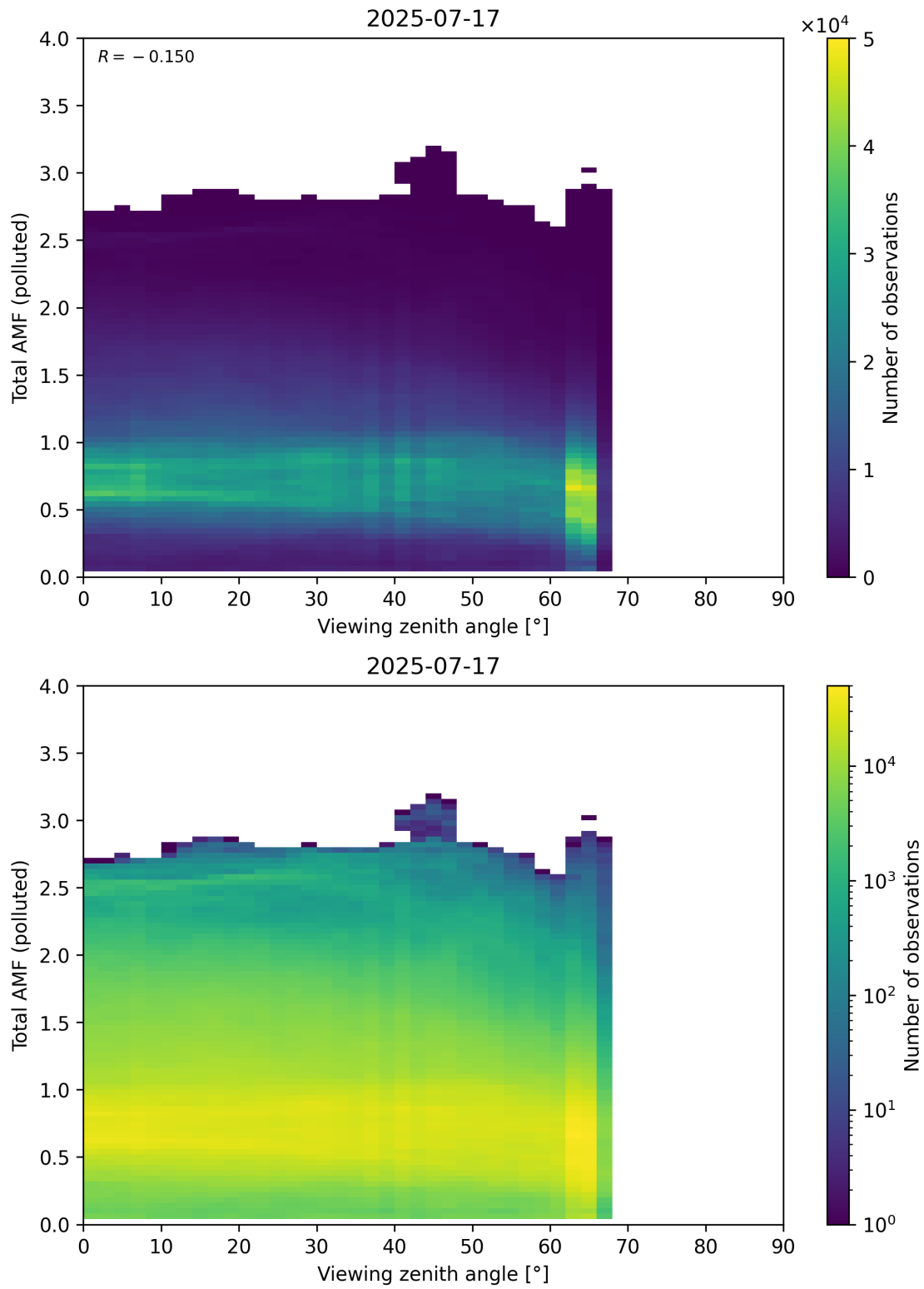
Figure 381: Scatter density plot of “Viewing zenith angle” against “Total AMF (polluted)” for 2025-07-16 to 2025-07-18.
