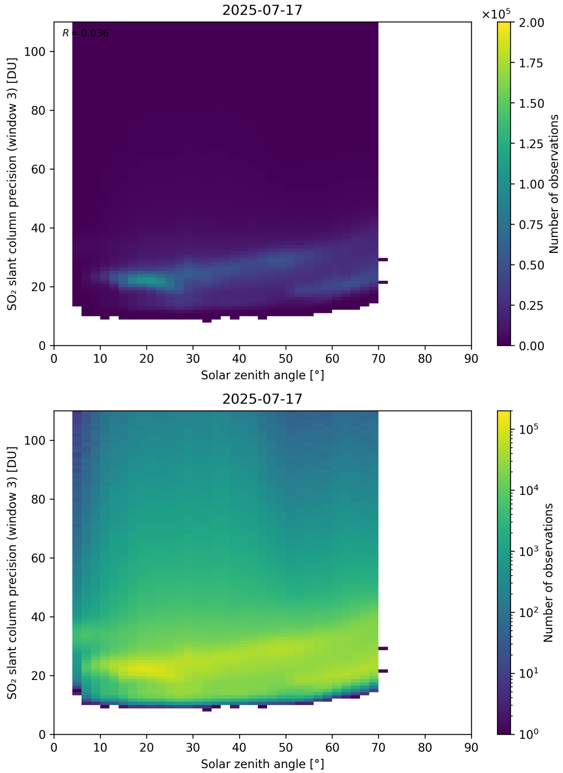
Figure 188: Scatter density plot of “Solar zenith angle” against “SO 2 slant column precision (window 3)” for 2025-07-16 to 2025-07-18.
