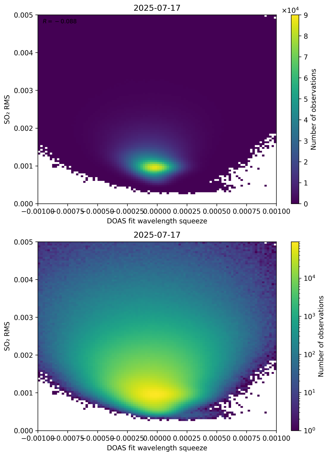
Figure 143: Scatter density plot of “DOAS fit wavelength squeeze” against “SO 2 RMS” for 2025-07-16 to 2025-07-18.
