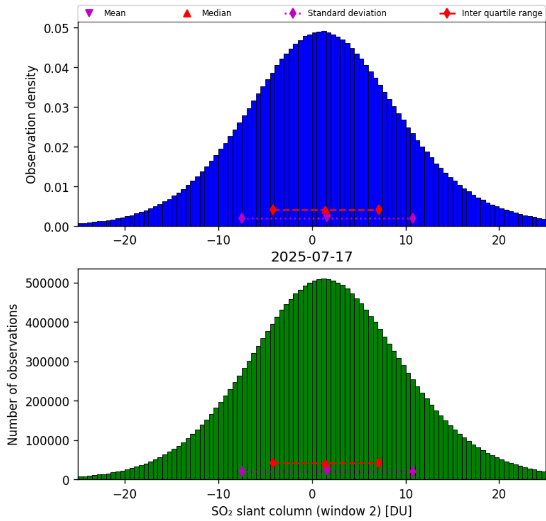
Figure 67: Histogram of “SO 2 slant column (window 2)” for 2025-07-16 to 2025-07-18
