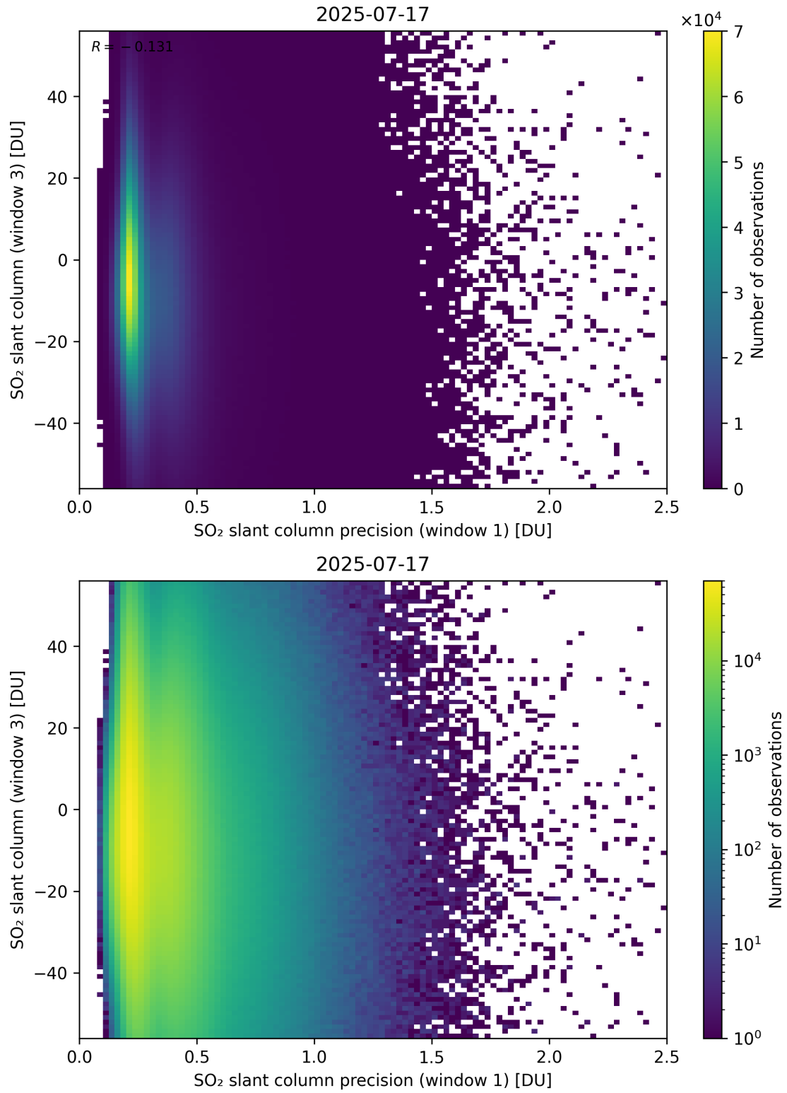
Figure 278: Scatter density plot of “SO 2 slant column precision (window 1)” against “SO 2 slant column (window 3)” for 2025-07-16 to 2025-07-18.
