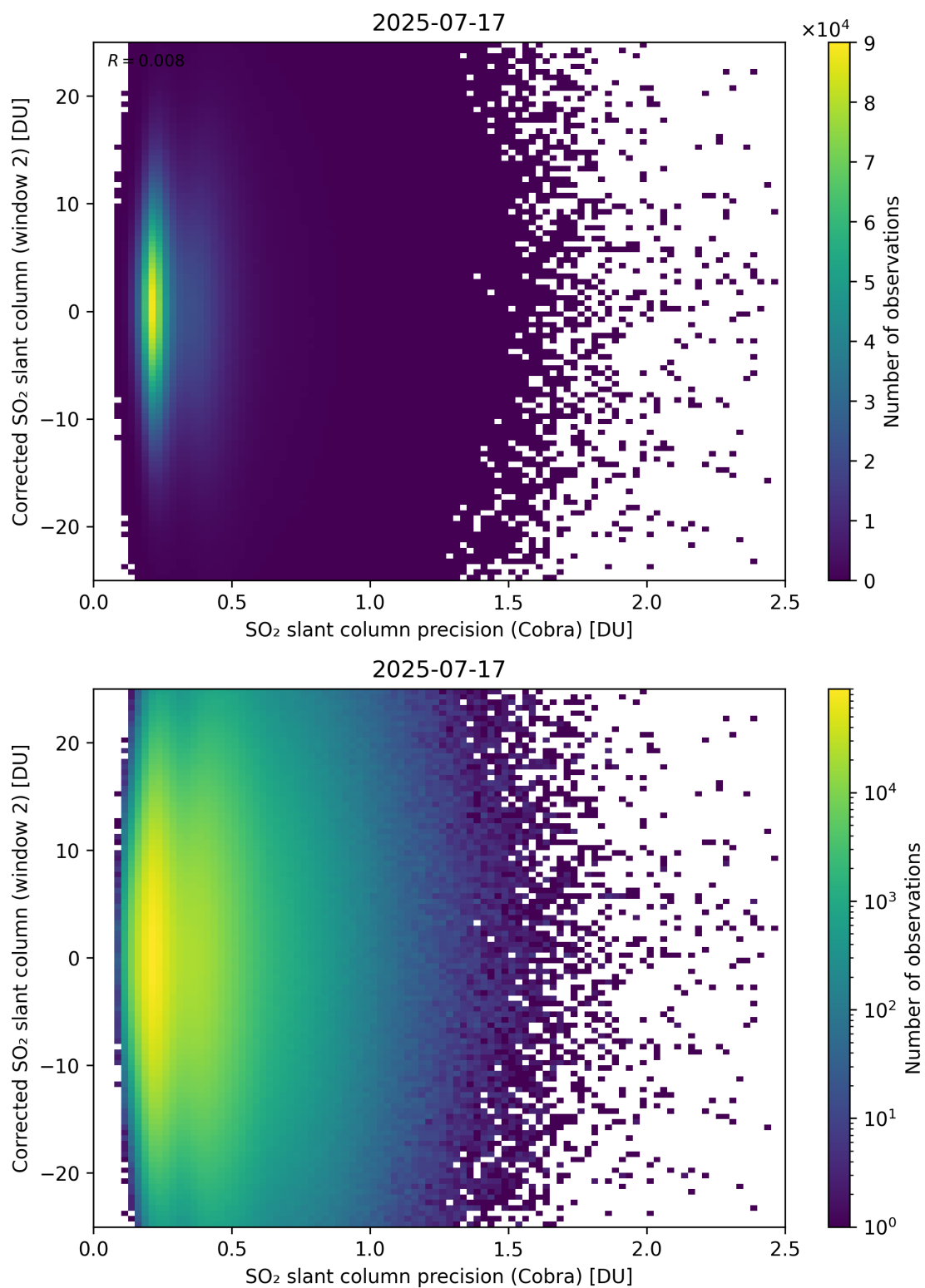
Figure 206: Scatter density plot of “SO 2 slant column precision (Cobra)” against “Corrected SO 2 slant column (window 2)” for 2025-07-16 to 2025-07-18.
