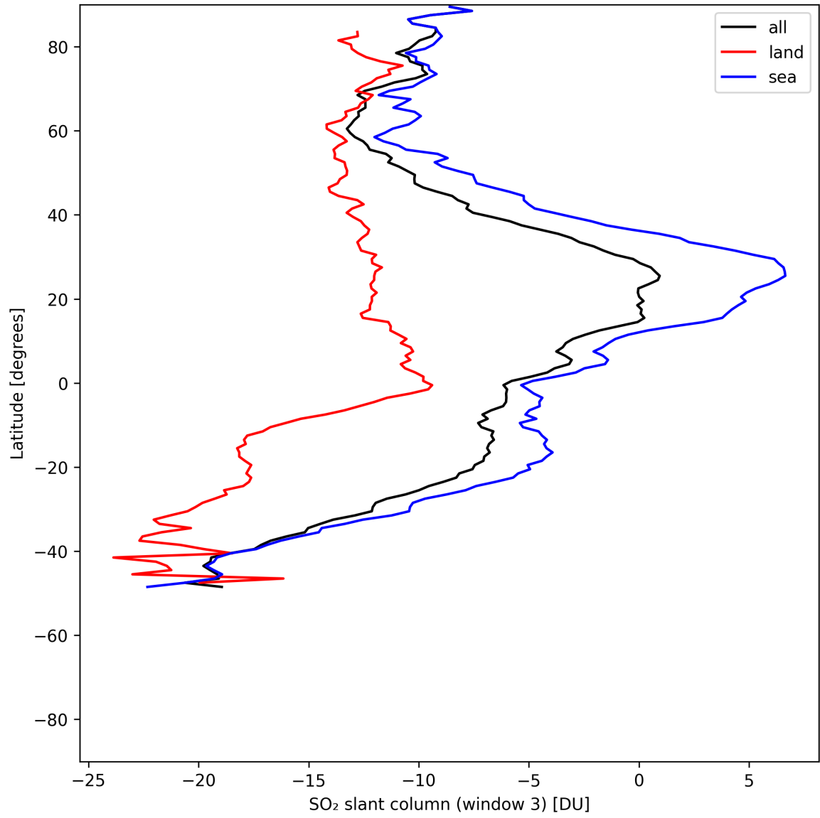
Figure 45: Zonal average of “SO 2 slant column (window 3)” for 2025-07-16 to 2025-07-18.
