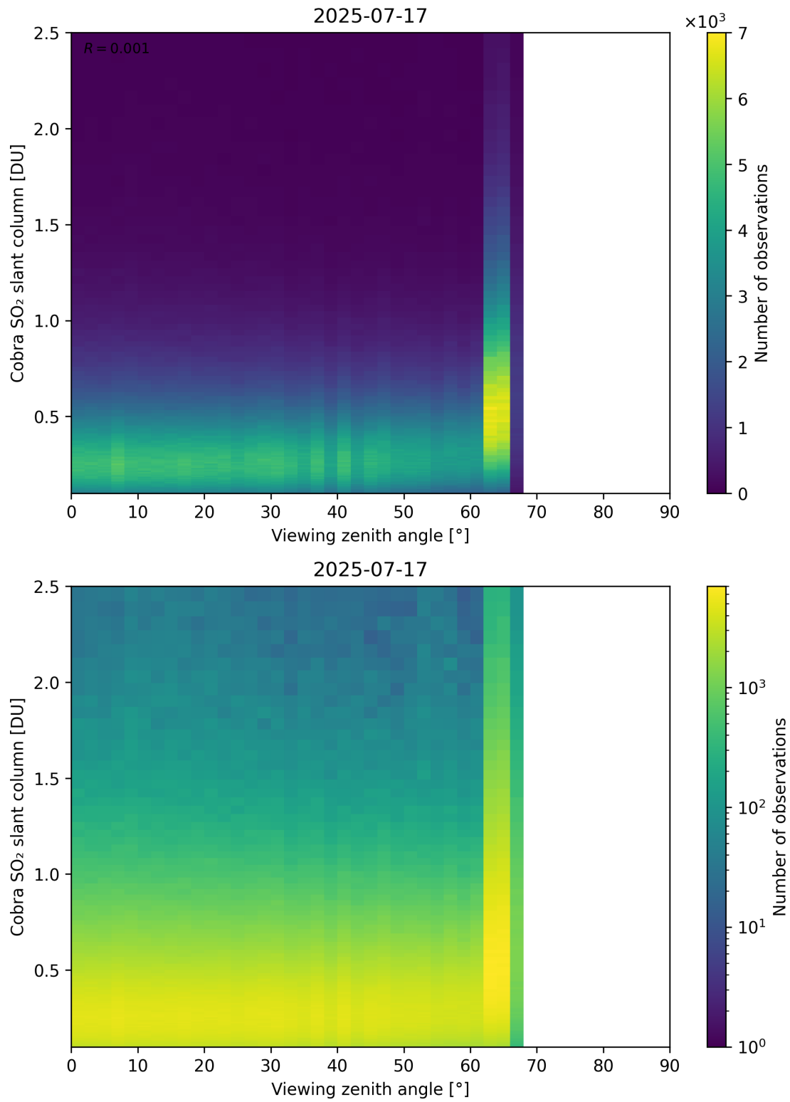
Figure 371: Scatter density plot of “Viewing zenith angle” against “Cobra SO 2 slant column” for 2025-07-16 to 2025-07-18.
