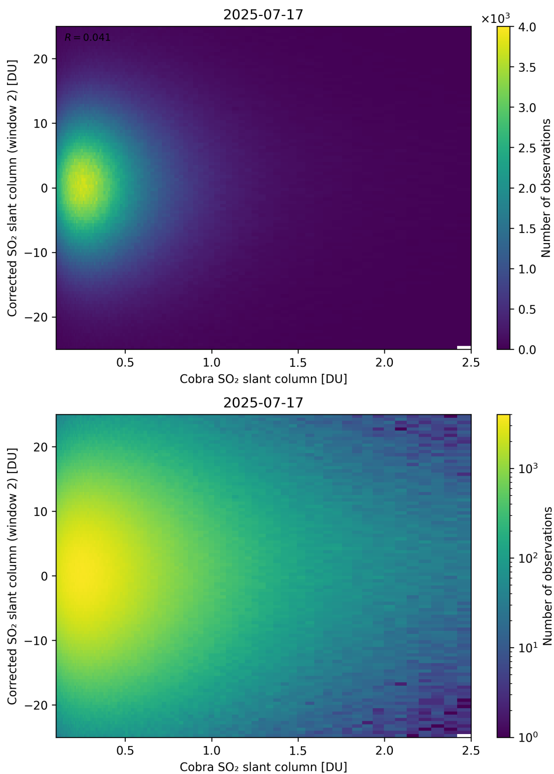
Figure 217: Scatter density plot of “Cobra SO 2 slant column” against “Corrected SO 2 slant column (window 2)” for 2025-07-16 to 2025-07-18.
