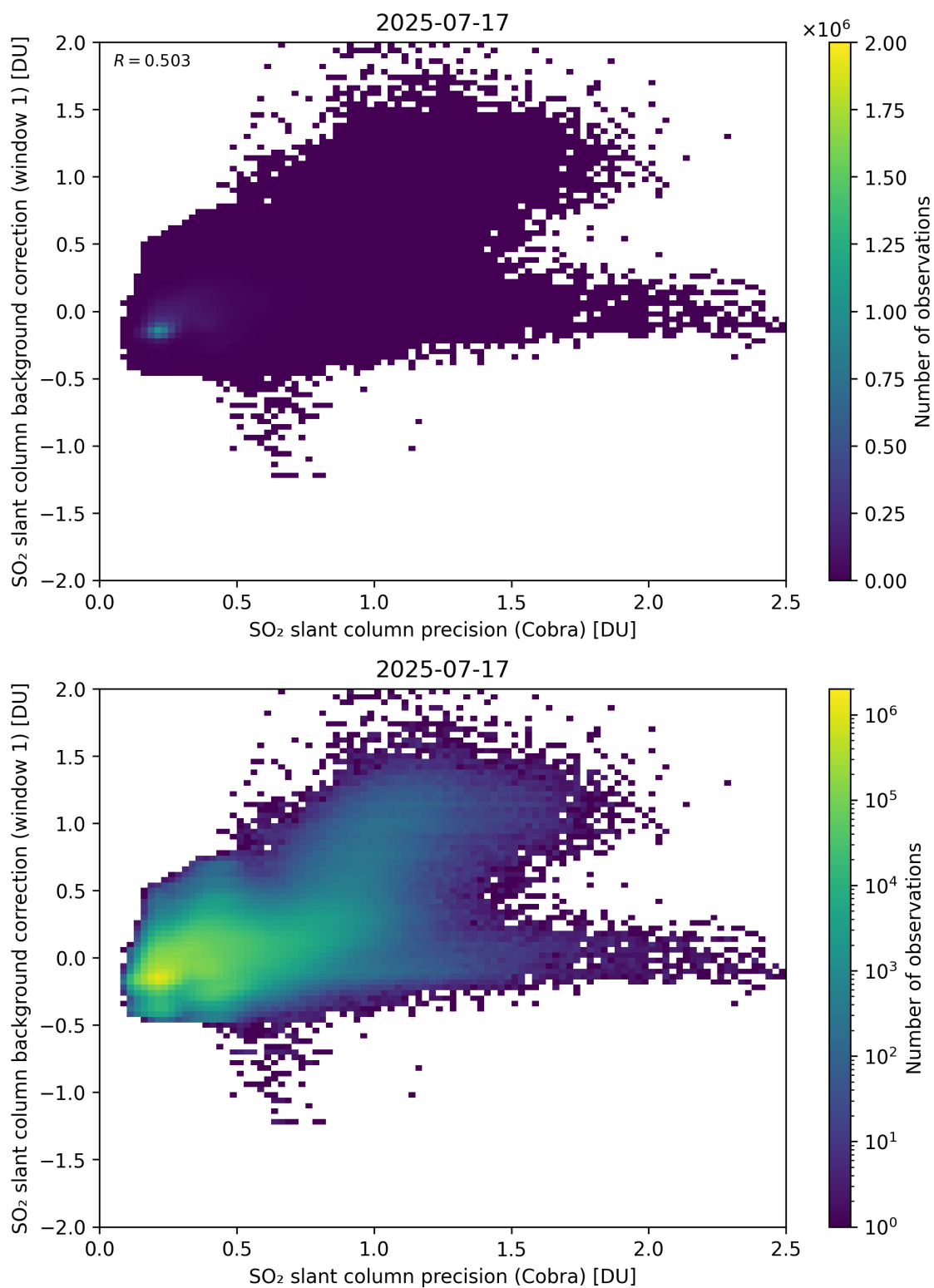
Figure 199: Scatter density plot of “SO 2 slant column precision (Cobra)” against “SO 2 slant column background correction (window 1)” for 2025-07-16 to 2025-07-18.
