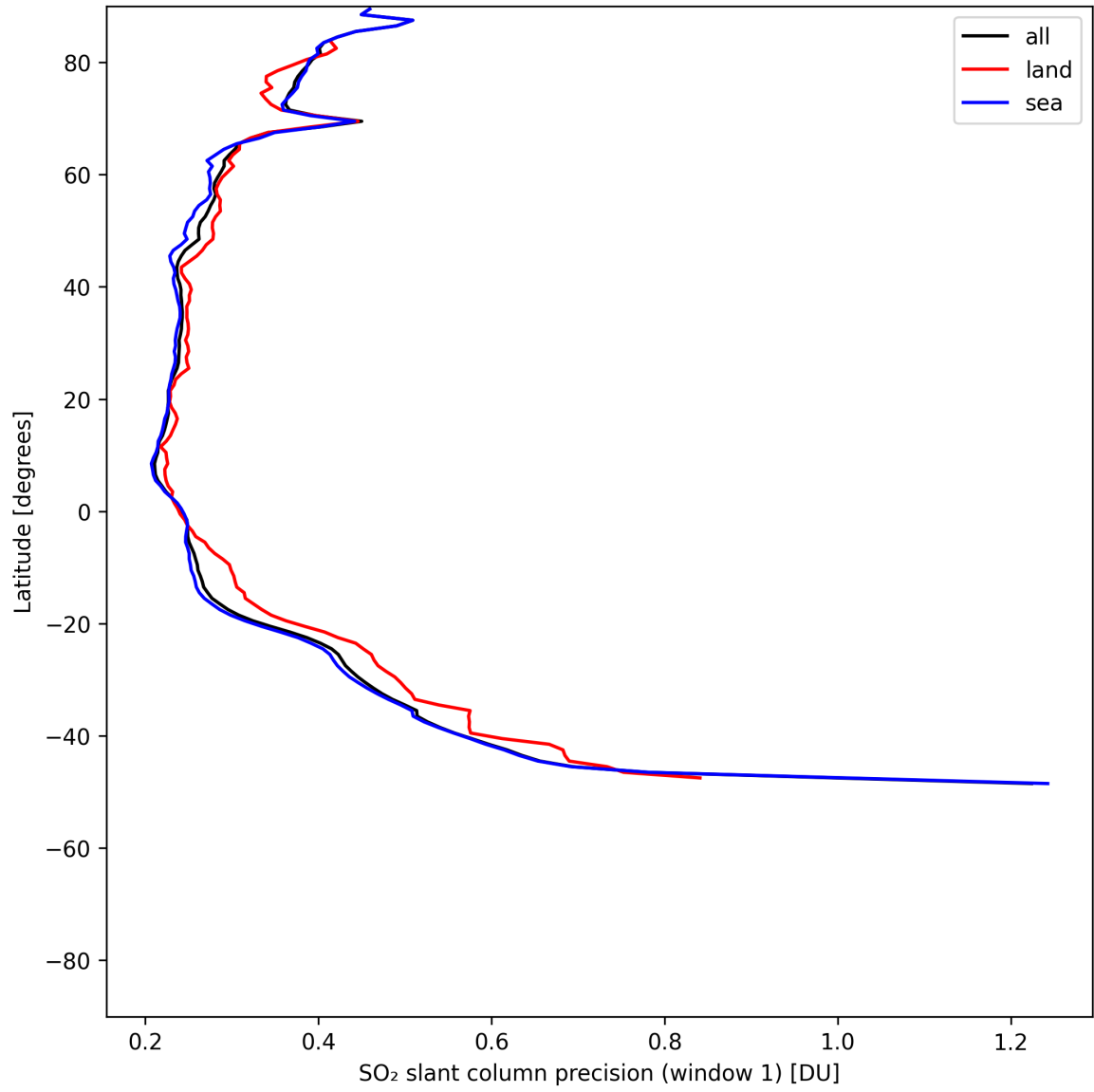
Figure 38: Zonal average of “SO 2 slant column precision (window 1)” for 2025-07-16 to 2025-07-18.
