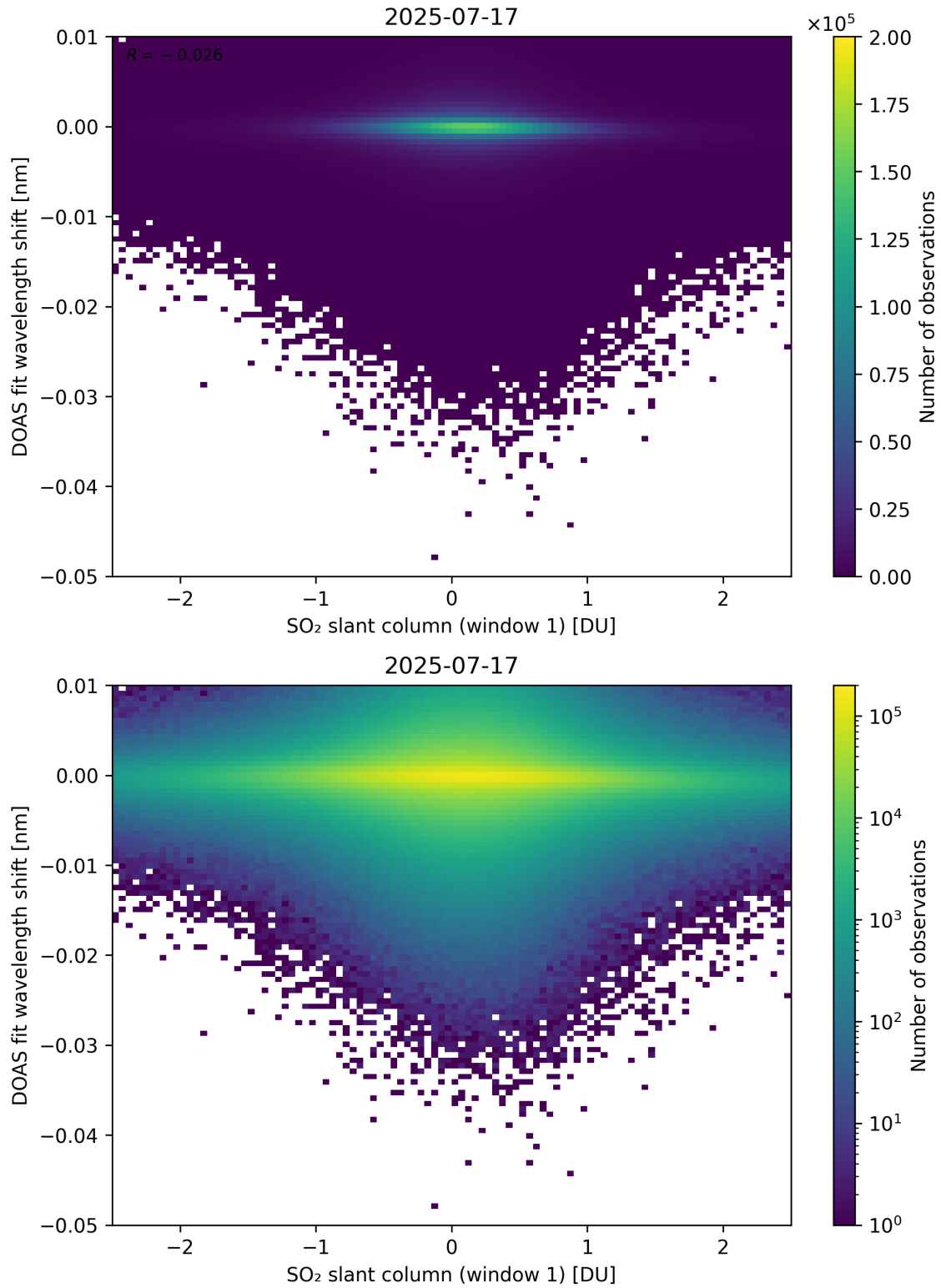
Figure 265: Scatter density plot of “SO 2 slant column (window 1)” against “DOAS fit wavelength shift” for 2025-07-16 to 2025-07-18.
