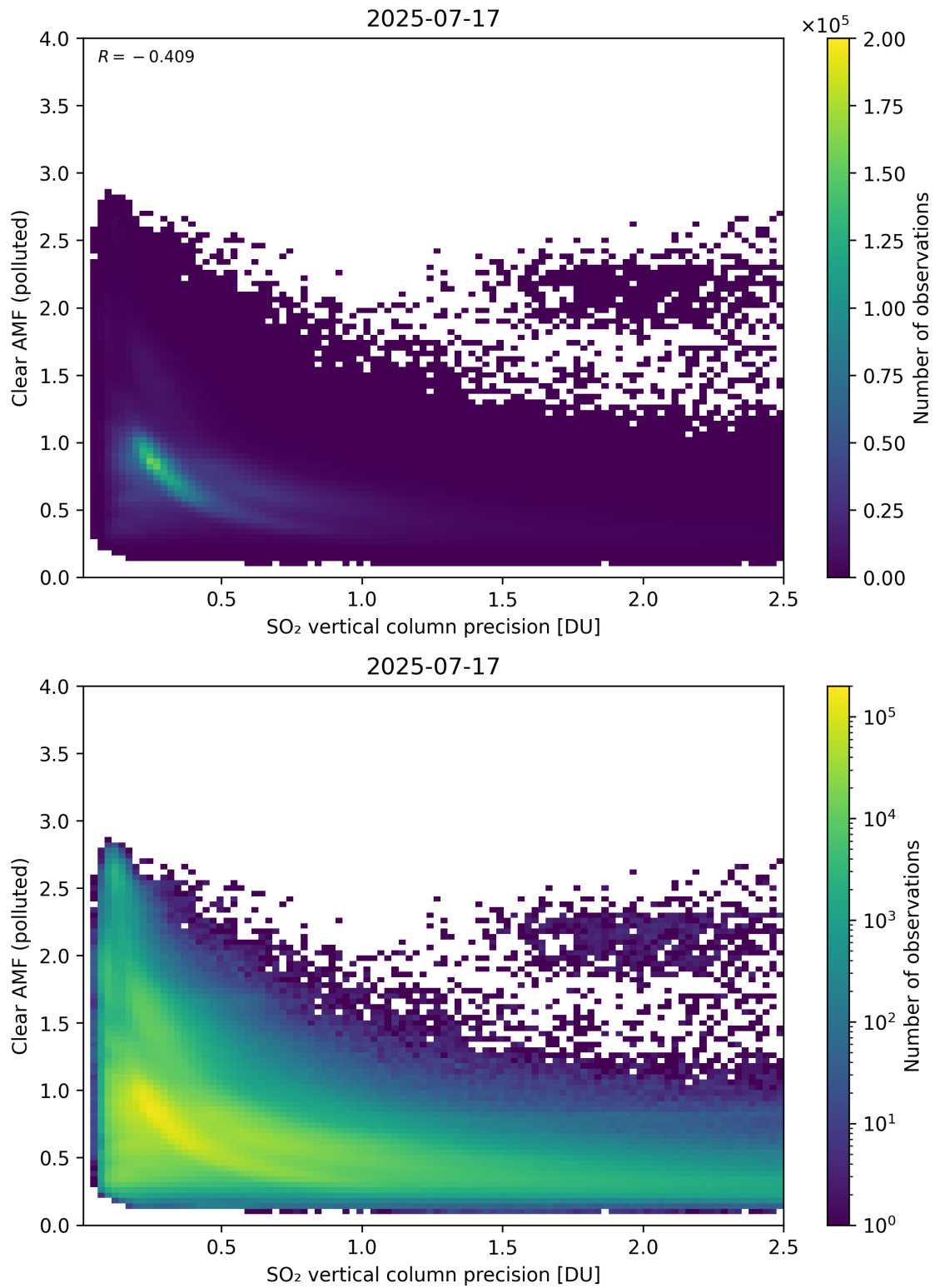
Figure 335: Scatter density plot of “SO 2 vertical column precision” against “Clear AMF (polluted)” for 2025-07-16 to 2025-07-18.
