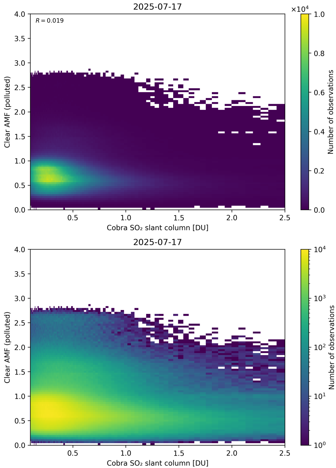
Figure 215: Scatter density plot of “Cobra SO 2 slant column” against “Clear AMF (polluted)” for 2025-07-16 to 2025-07-18.
