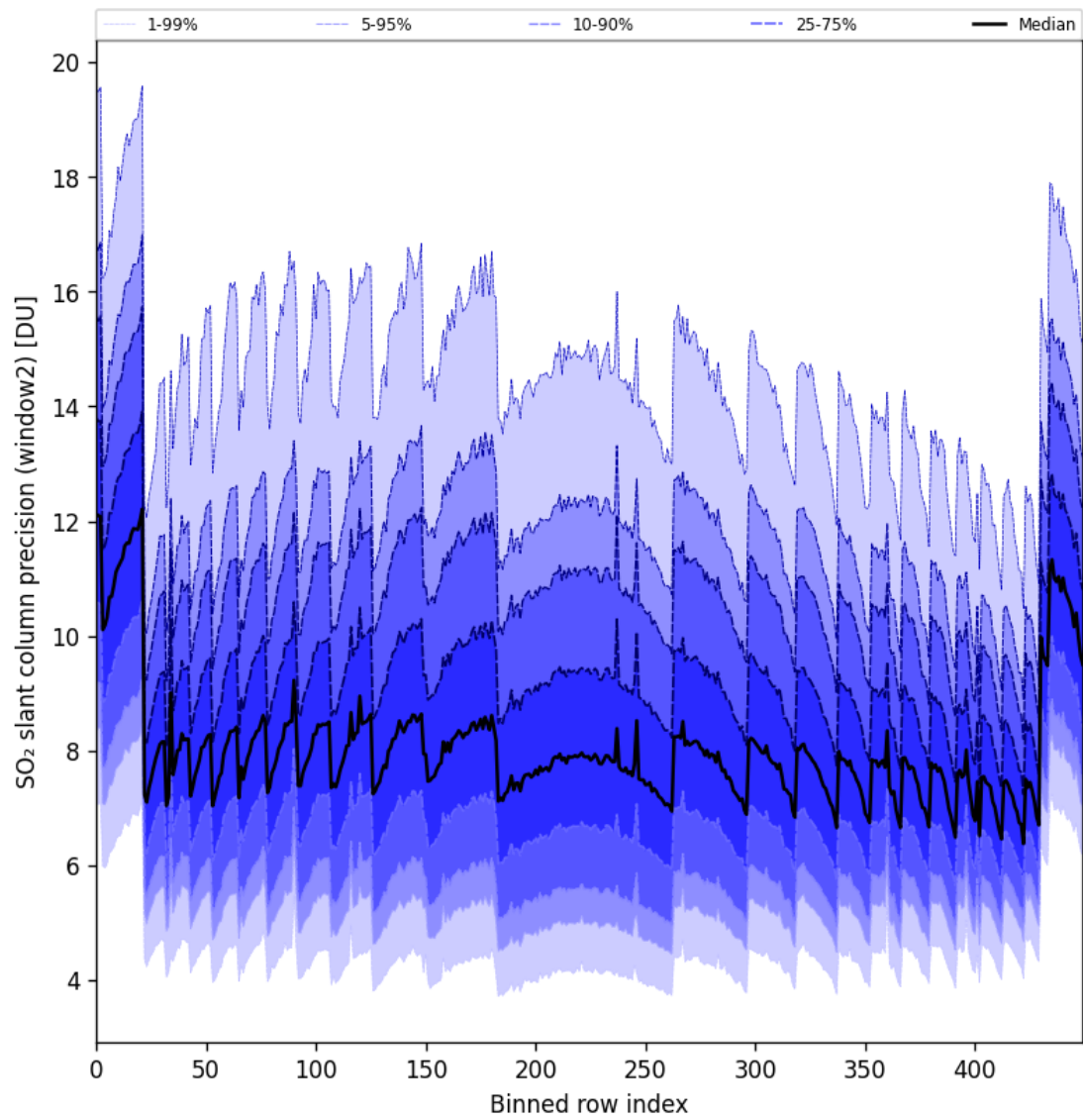
Figure 94: Along track statistics of “SO 2 slant column precision (window2)” for 2025-07-16 to 2025-07-18
