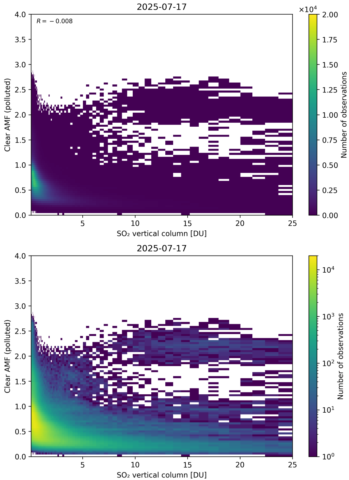
Figure 348: Scatter density plot of “SO 2 vertical column” against “Clear AMF (polluted)” for 2025-07-16 to 2025-07-18.
