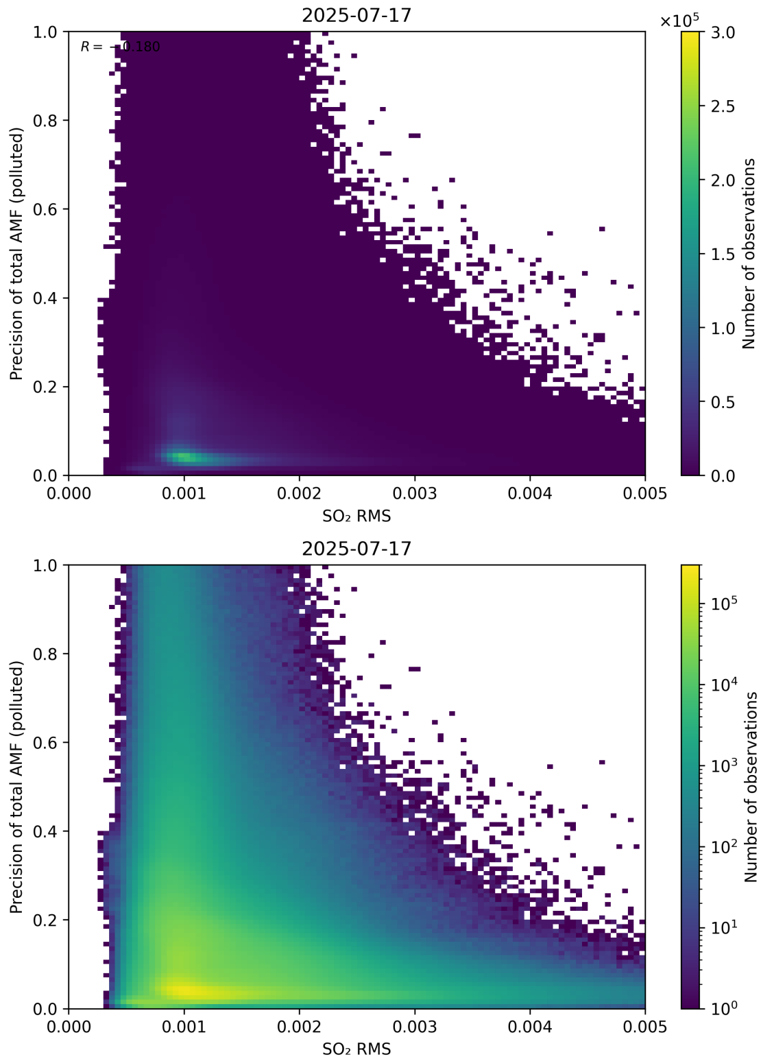
Figure 149: Scatter density plot of “SO 2 RMS” against “Precision of total AMF (polluted)” for 2025-07-16 to 2025-07-18.
