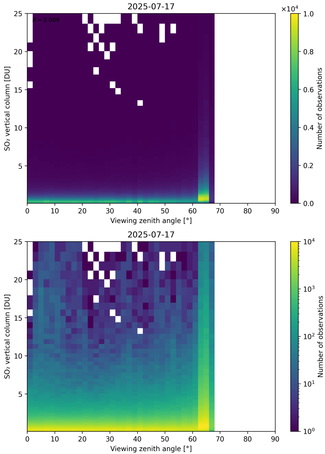
Figure 383: Scatter density plot of “Viewing zenith angle” against “SO 2 vertical column” for 2025-07-16 to 2025-07-18.
