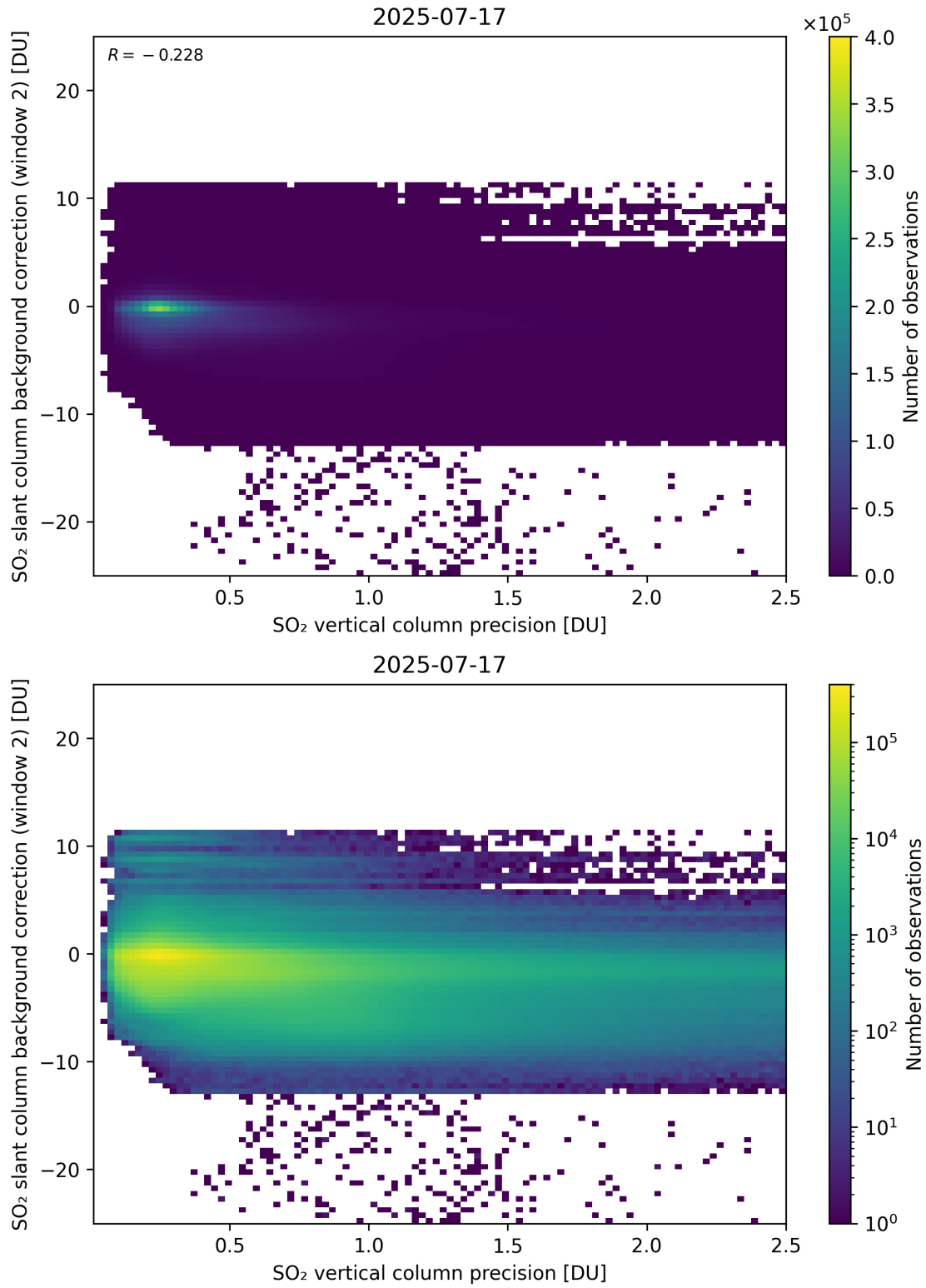
Figure 330: Scatter density plot of “SO 2 vertical column precision” against “SO 2 slant column background correction (window 2)” for 2025-07-16 to 2025-07-18.
