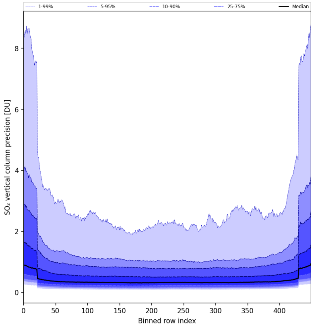
Figure 85: Along track statistics of “SO 2 vertical column precision” for 2025-07-16 to 2025-07-18
