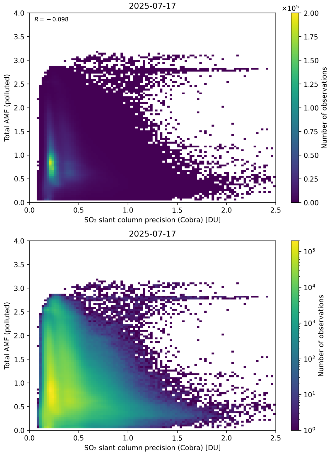
Figure 213: Scatter density plot of “SO 2 slant column precision (Cobra)” against “Total AMF (polluted)” for 2025-07-16 to 2025-07-18.
