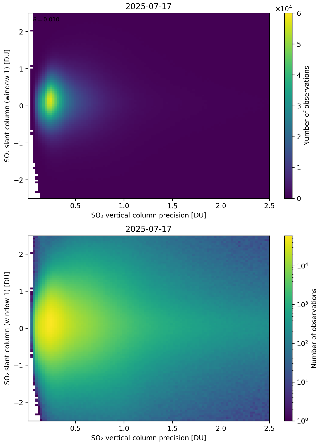
Figure 341: Scatter density plot of “SO 2 vertical column precision” against “SO 2 slant column (window 1)” for 2025-07-16 to 2025-07-18.
