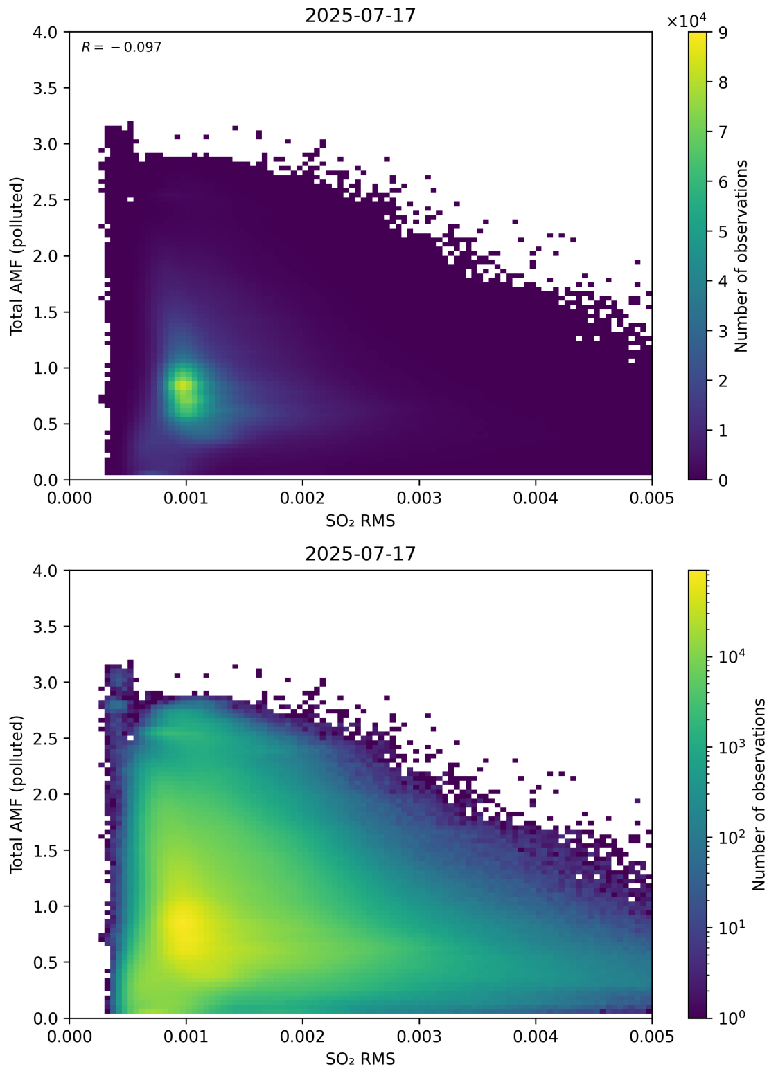
Figure 148: Scatter density plot of “SO 2 RMS” against “Total AMF (polluted)” for 2025-07-16 to 2025-07-18.
