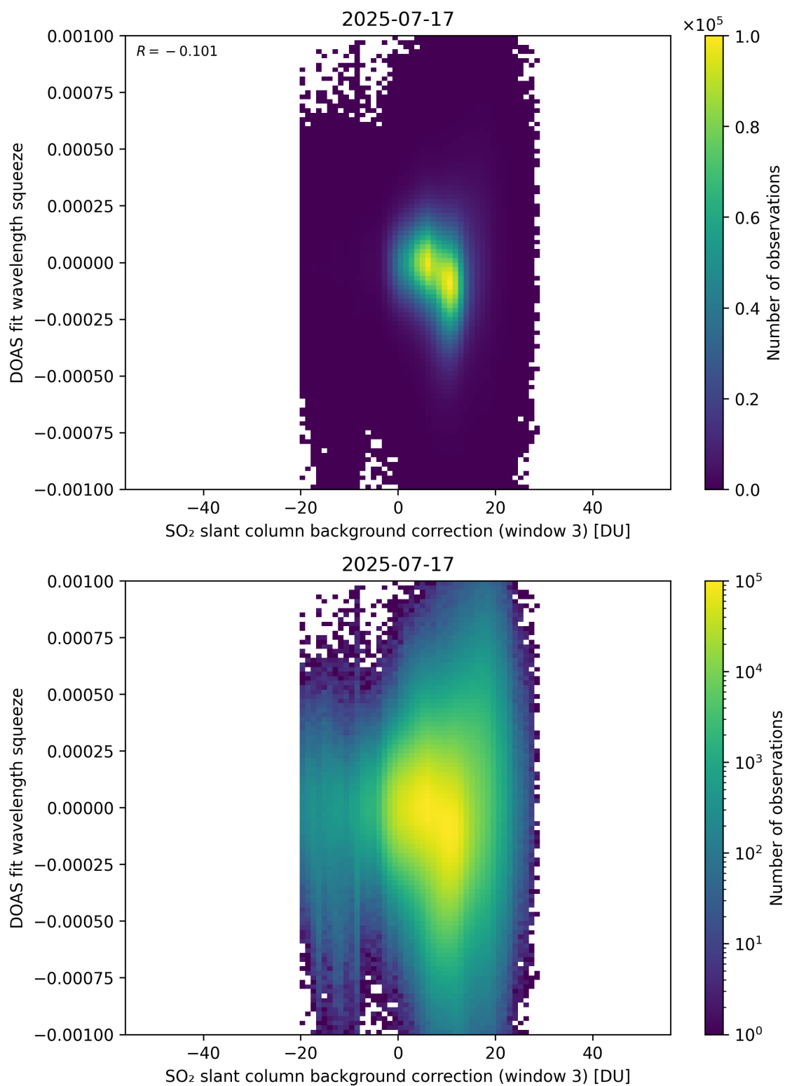
Figure 133: Scatter density plot of “SO 2 slant column background correction (window 3)” against “DOAS fit wavelength squeeze” for 2025-07-16 to 2025-07-18.
