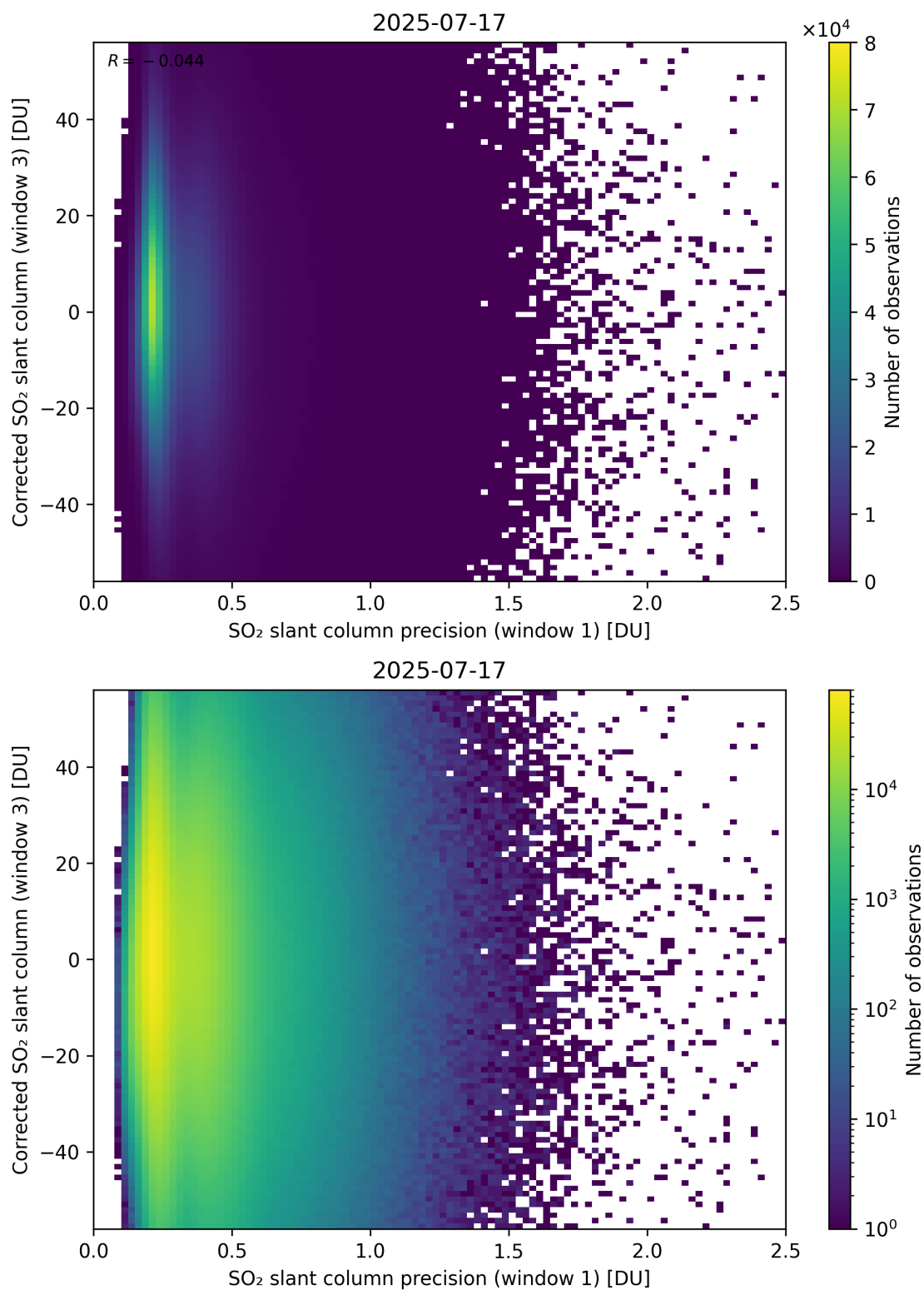
Figure 276: Scatter density plot of “SO 2 slant column precision (window 1)” against “Corrected SO 2 slant column (window 3)” for 2025-07-16 to 2025-07-18.
