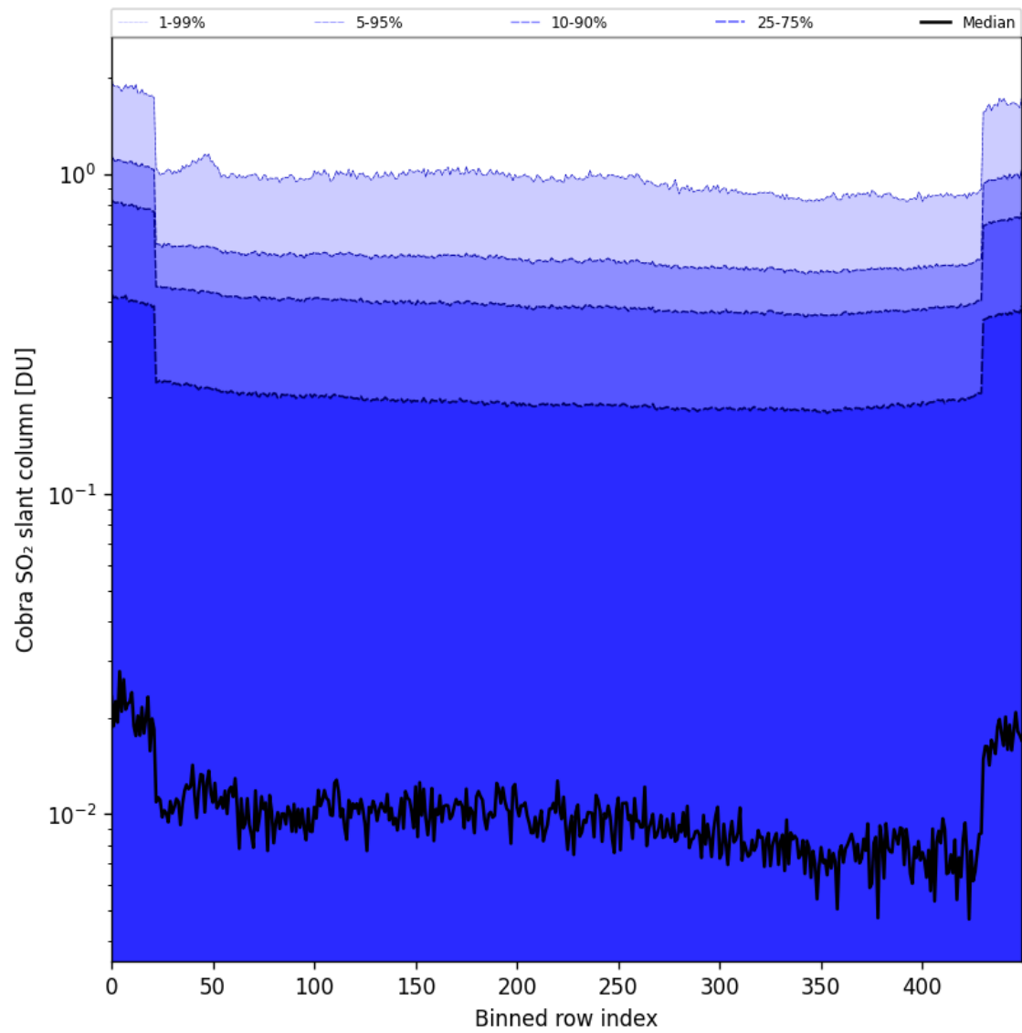
Figure 87: Along track statistics of “Cobra SO 2 slant column” for 2025-07-16 to 2025-07-18
