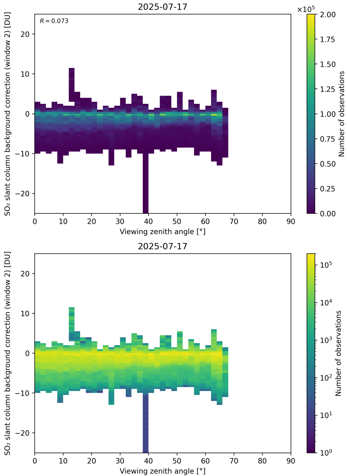
Figure 363: Scatter density plot of “Viewing zenith angle” against “SO 2 slant column background correction (window 2)” for 2025-07-16 to 2025-07-18.
