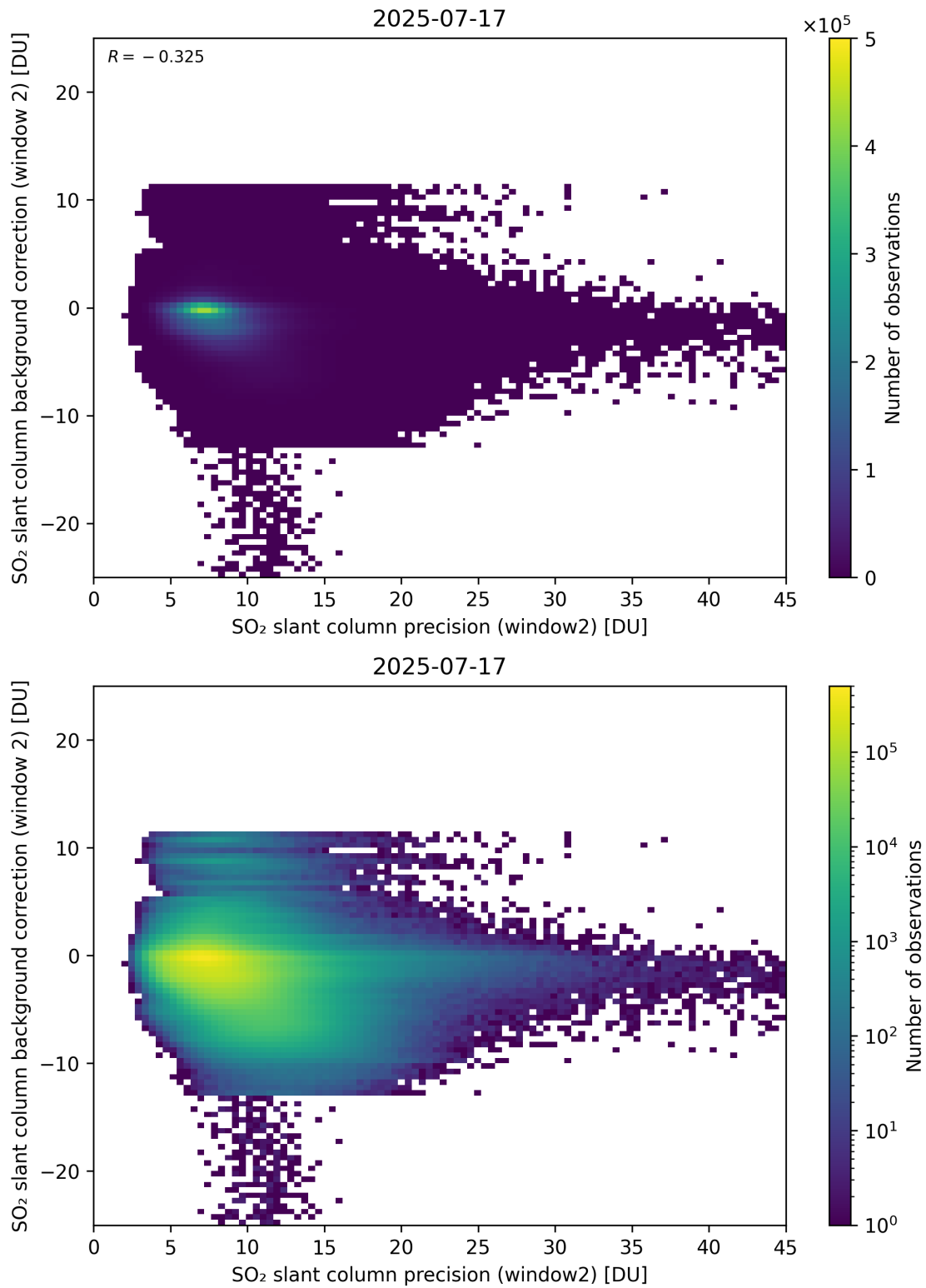
Figure 291: Scatter density plot of “SO 2 slant column precision (window2)” against “SO 2 slant column background correction (window 2)” for 2025-07-16 to 2025-07-18.
