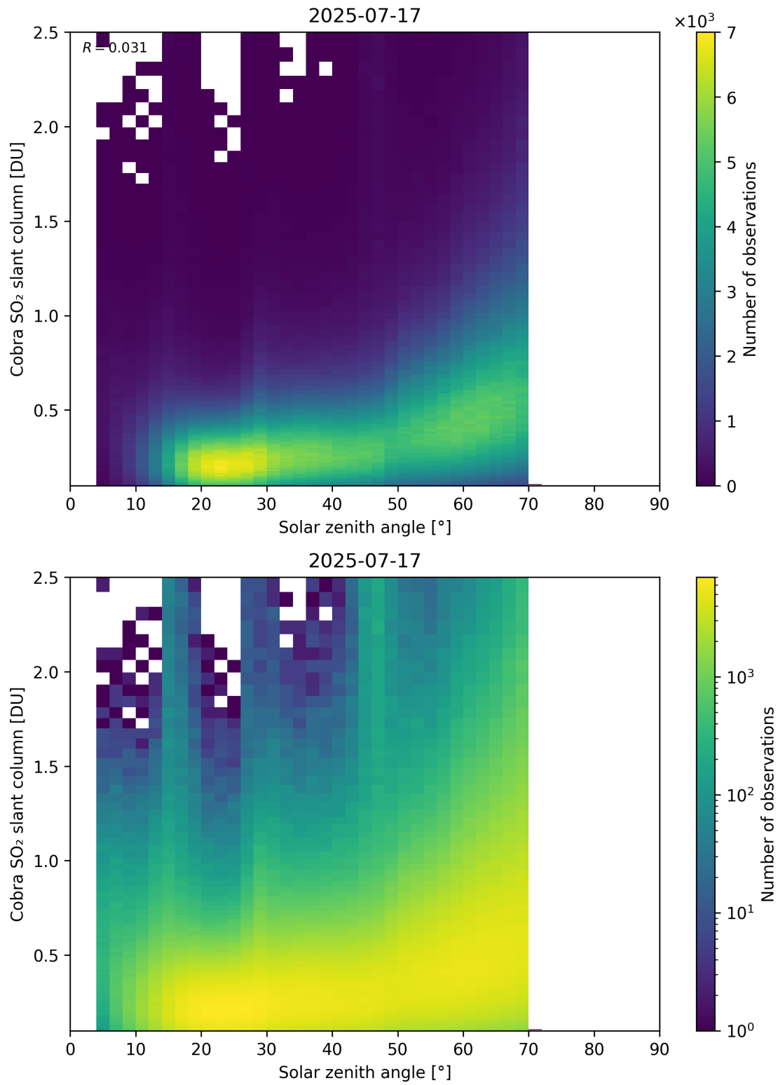
Figure 179: Scatter density plot of “Solar zenith angle” against “Cobra SO 2 slant column” for 2025-07-16 to 2025-07-18.
