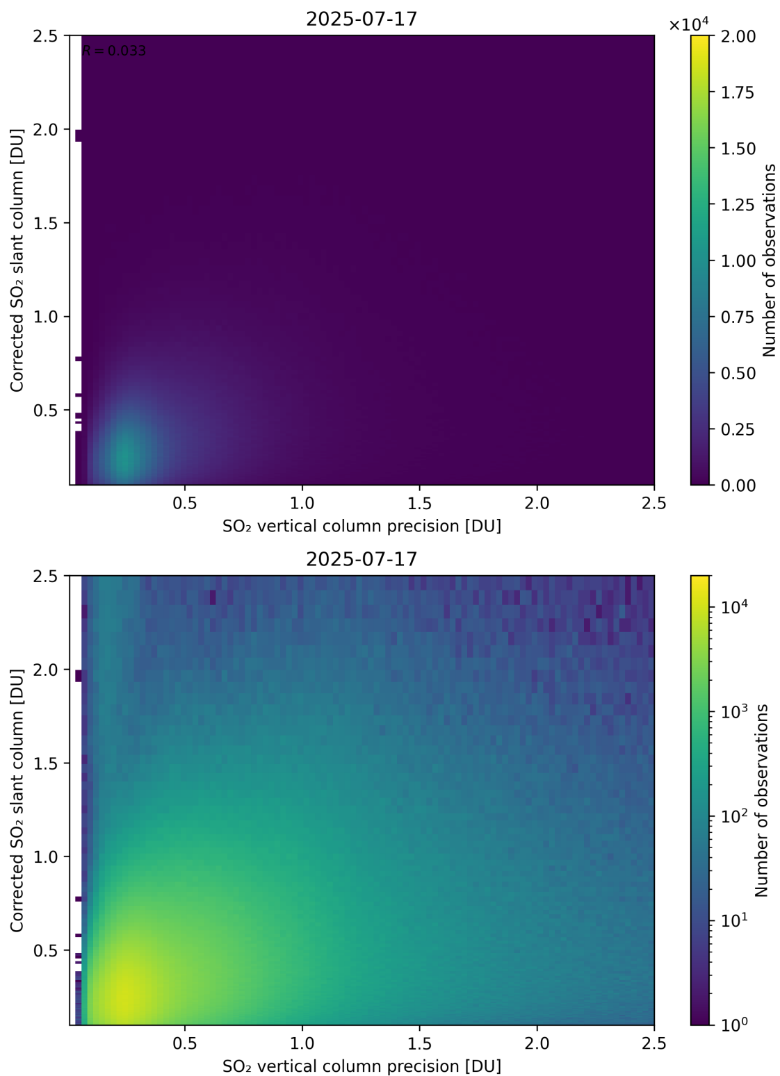
Figure 338: Scatter density plot of “SO 2 vertical column precision” against “Corrected SO 2 slant column” for 2025-07-16 to 2025-07-18.
