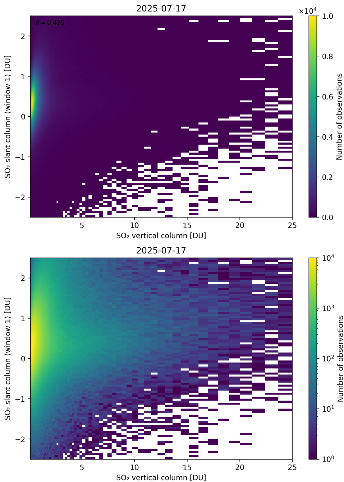
Figure 354: Scatter density plot of “SO 2 vertical column” against “SO 2 slant column (window 1)” for 2025-07-16 to 2025-07-18.
