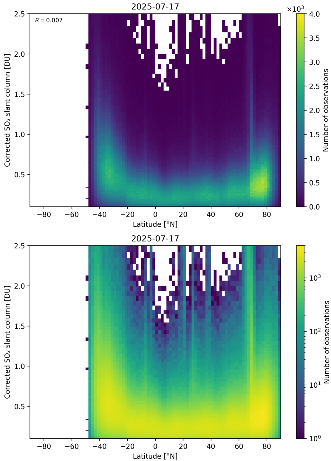
Figure 159: Scatter density plot of “Latitude” against “Corrected SO 2 slant column” for 2025-07-16 to 2025-07-18.
