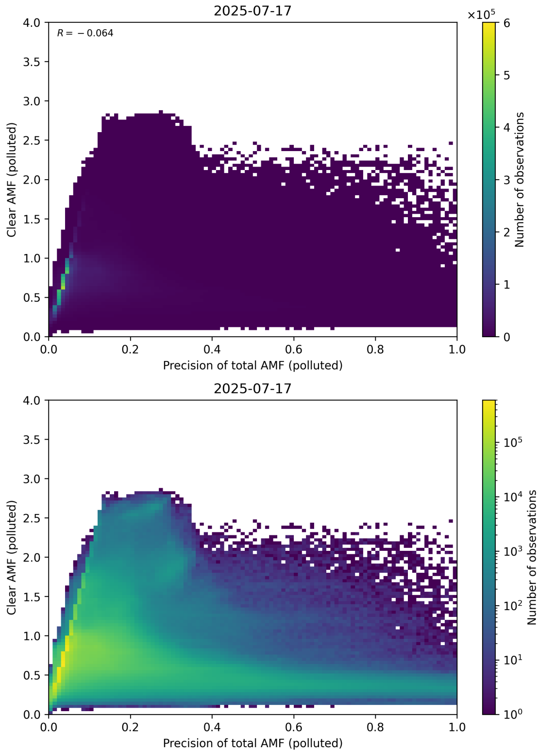
Figure 320: Scatter density plot of “Precision of total AMF (polluted)” against “Clear AMF (polluted)” for 2025-07-16 to 2025-07-18.
