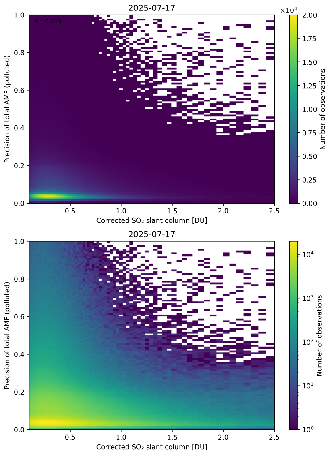
Figure 243: Scatter density plot of “Corrected SO 2 slant column” against “Precision of total AMF (polluted)” for 2025-07-16 to 2025-07-18.
