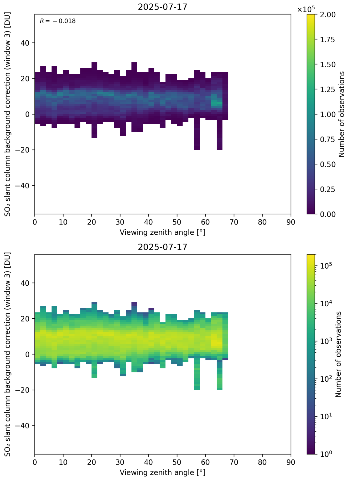
Figure 364: Scatter density plot of “Viewing zenith angle” against “SO 2 slant column background correction (window 3)” for 2025-07-16 to 2025-07-18.
