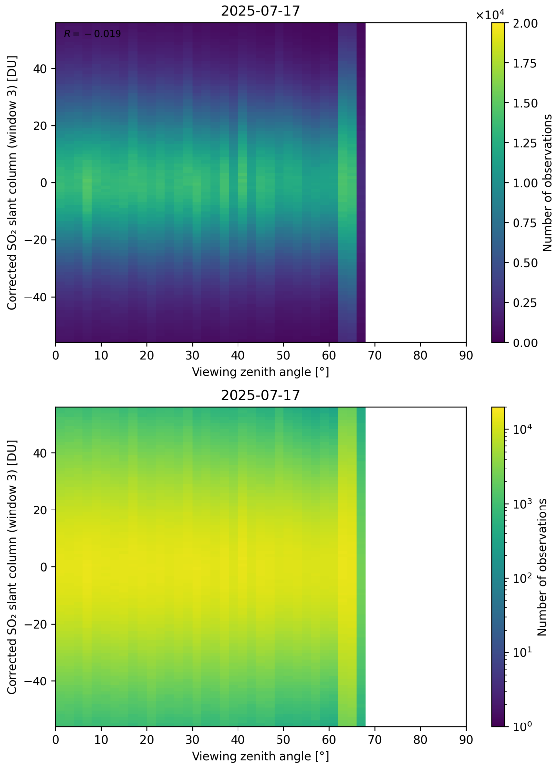
Figure 375: Scatter density plot of “Viewing zenith angle” against “Corrected SO 2 slant column (window 3)” for 2025-07-16 to 2025-07-18.
