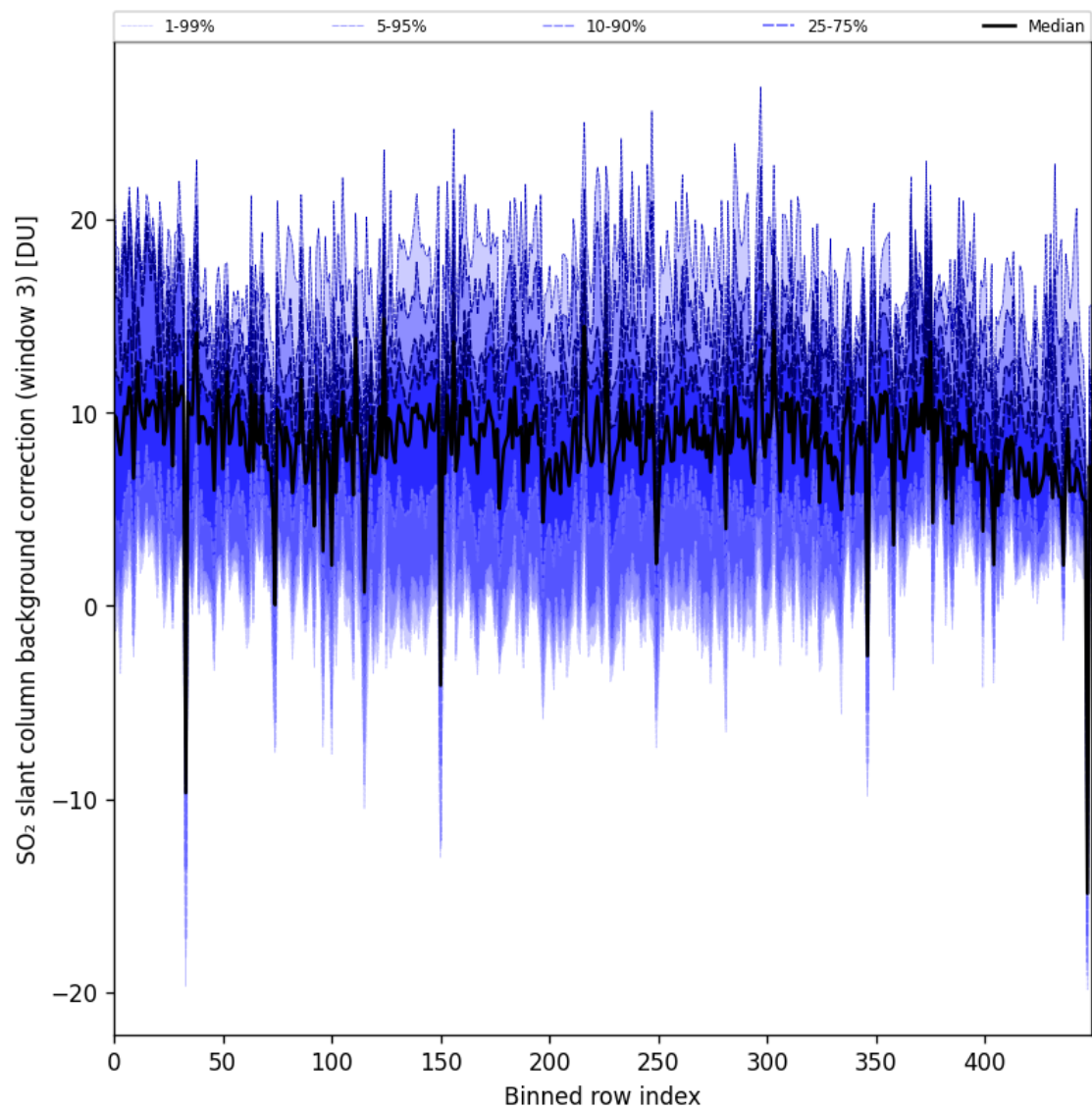
Figure 100: Along track statistics of “SO 2 slant column background correction (window 3)” for 2025-07-16 to 2025-07-18
