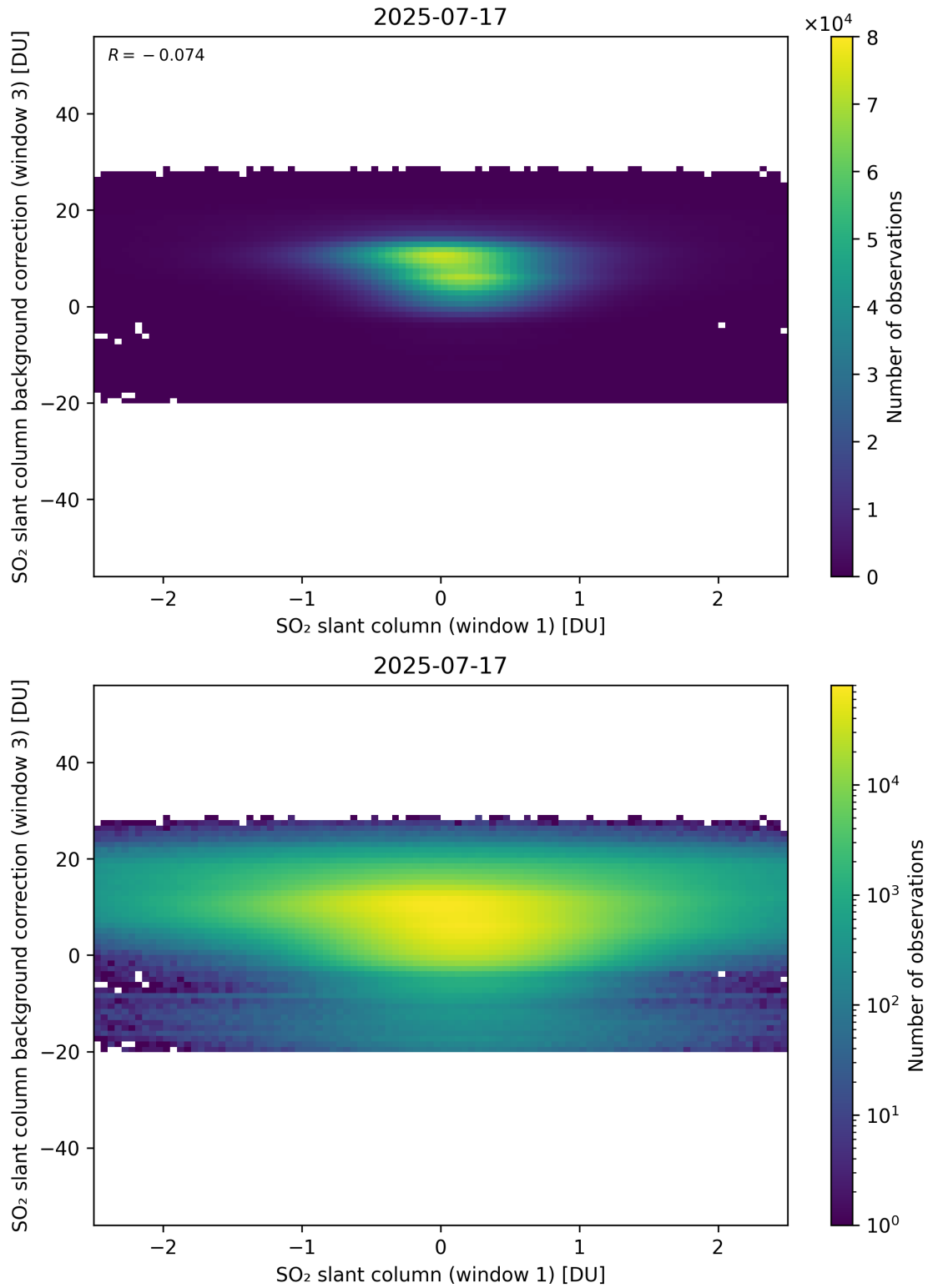
Figure 264: Scatter density plot of “SO 2 slant column (window 1)” against “SO 2 slant column background correction (window 3)” for 2025-07-16 to 2025-07-18.
