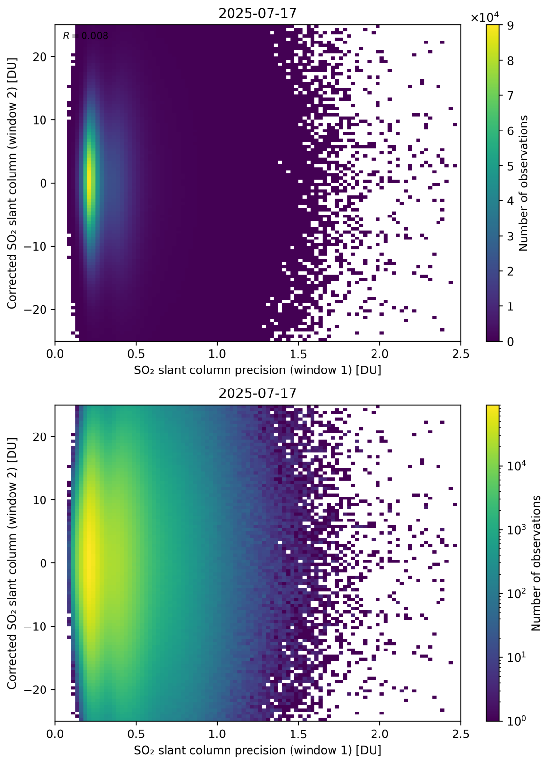
Figure 275: Scatter density plot of “SO 2 slant column precision (window 1)” against “Corrected SO 2 slant column (window 2)” for 2025-07-16 to 2025-07-18.
