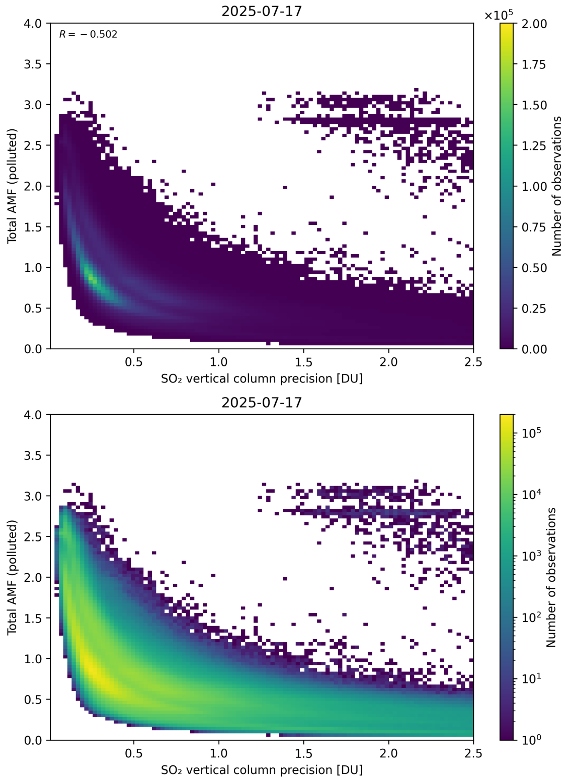
Figure 346: Scatter density plot of “SO 2 vertical column precision” against “Total AMF (polluted)” for 2025-07-16 to 2025-07-18.
