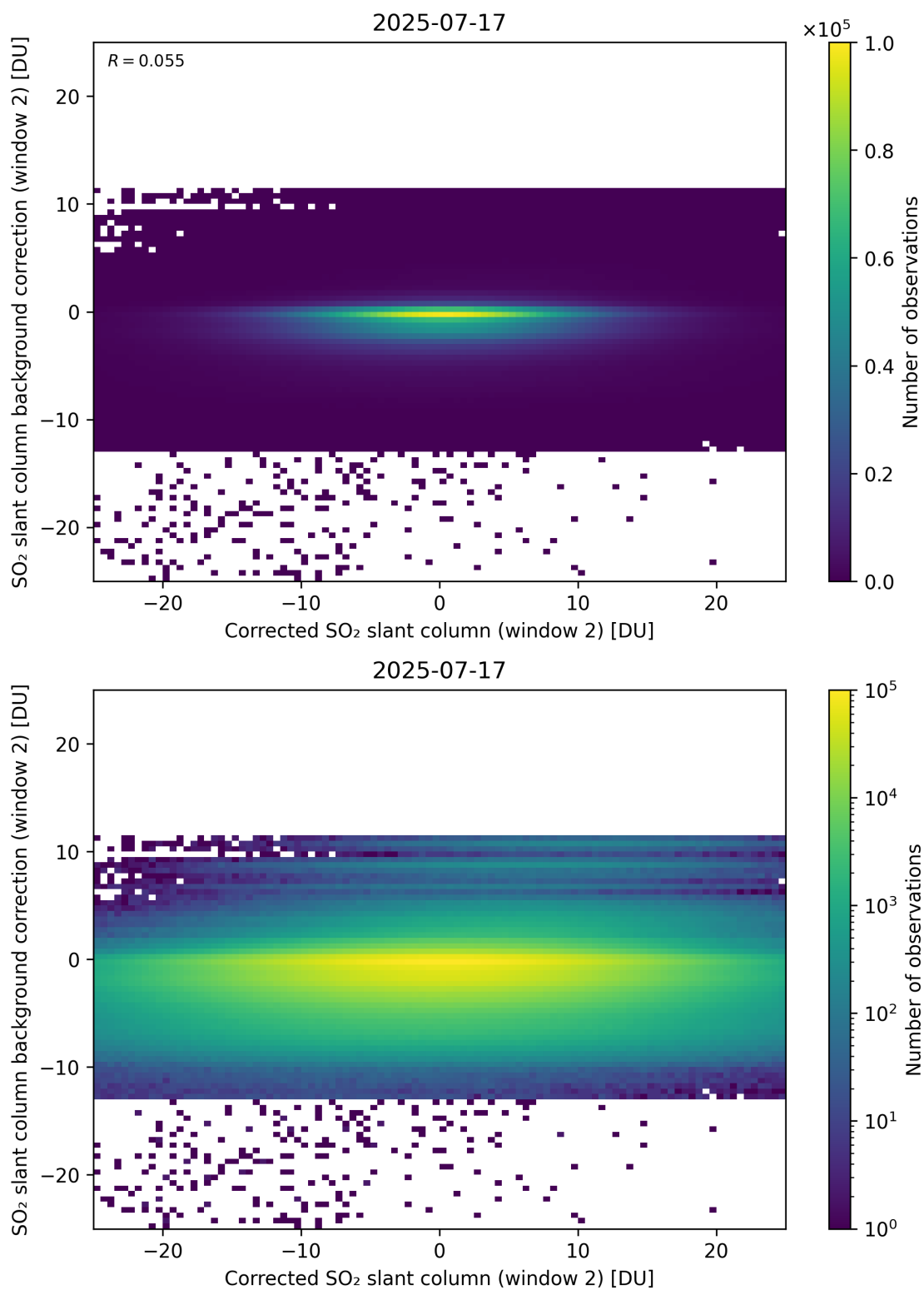
Figure 244: Scatter density plot of “Corrected SO 2 slant column (window 2)” against “SO 2 slant column background correction (window 2)” for 2025-07-16 to 2025-07-18.
