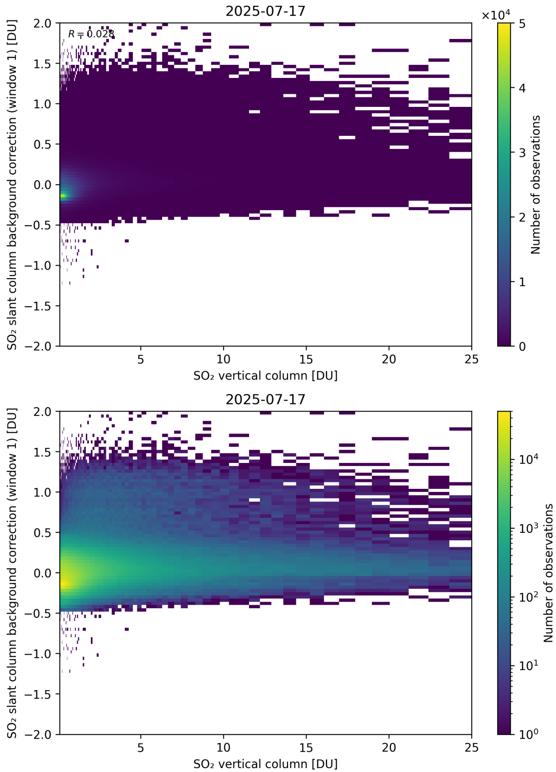
Figure 323: Scatter density plot of “SO 2 vertical column” against “SO 2 slant column background correction (window 1)” for 2025-07-16 to 2025-07-18.
