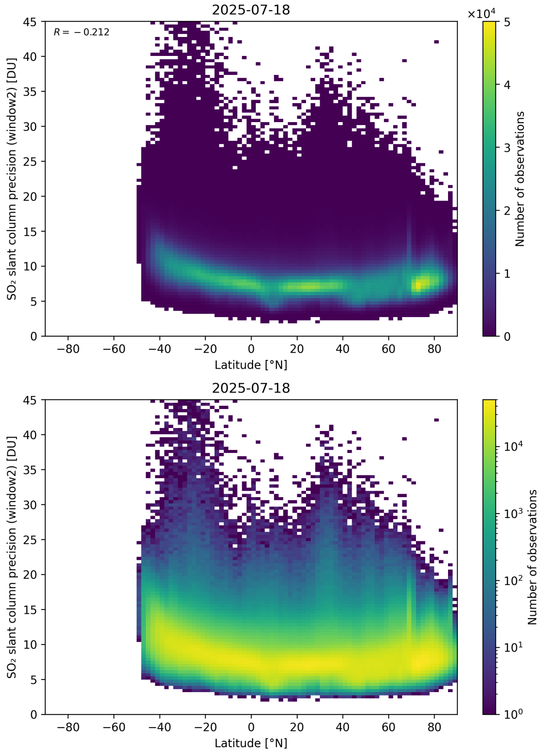
Figure 164: Scatter density plot of “Latitude” against “SO 2 slant column precision (window2)” for 2025-07-18 to 2025-07-19.
