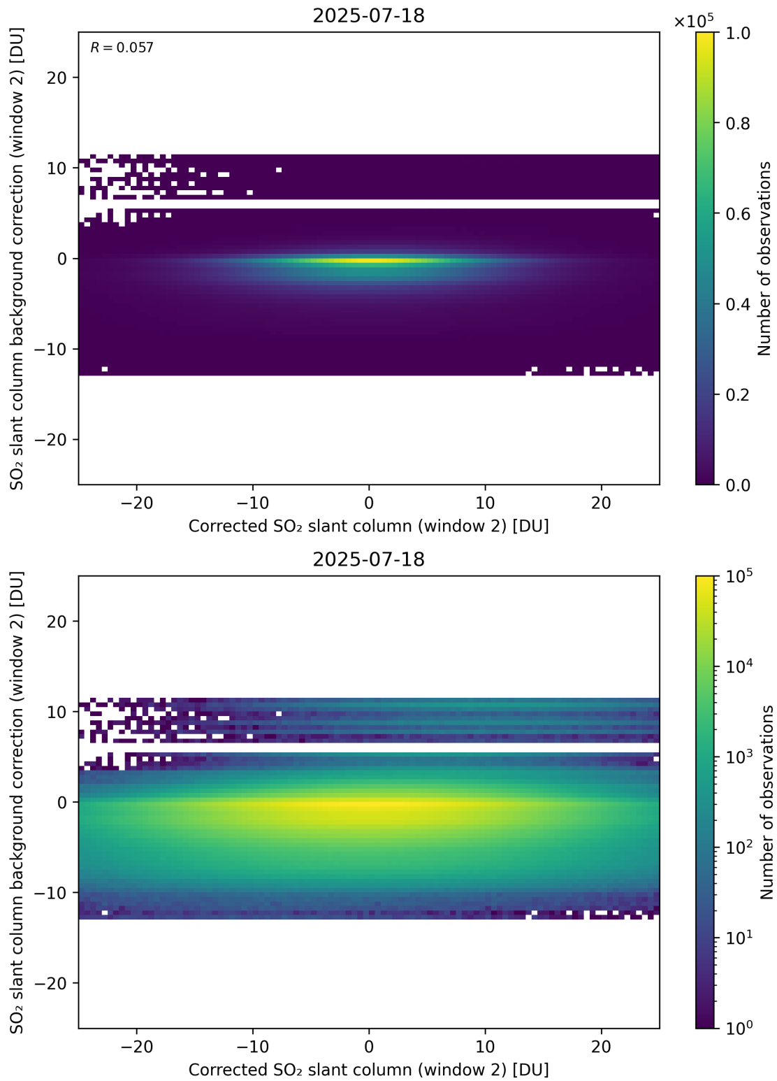
Figure 244: Scatter density plot of “Corrected SO 2 slant column (window 2)” against “SO 2 slant column background correction (window 2)” for 2025-07-18 to 2025-07-19.
