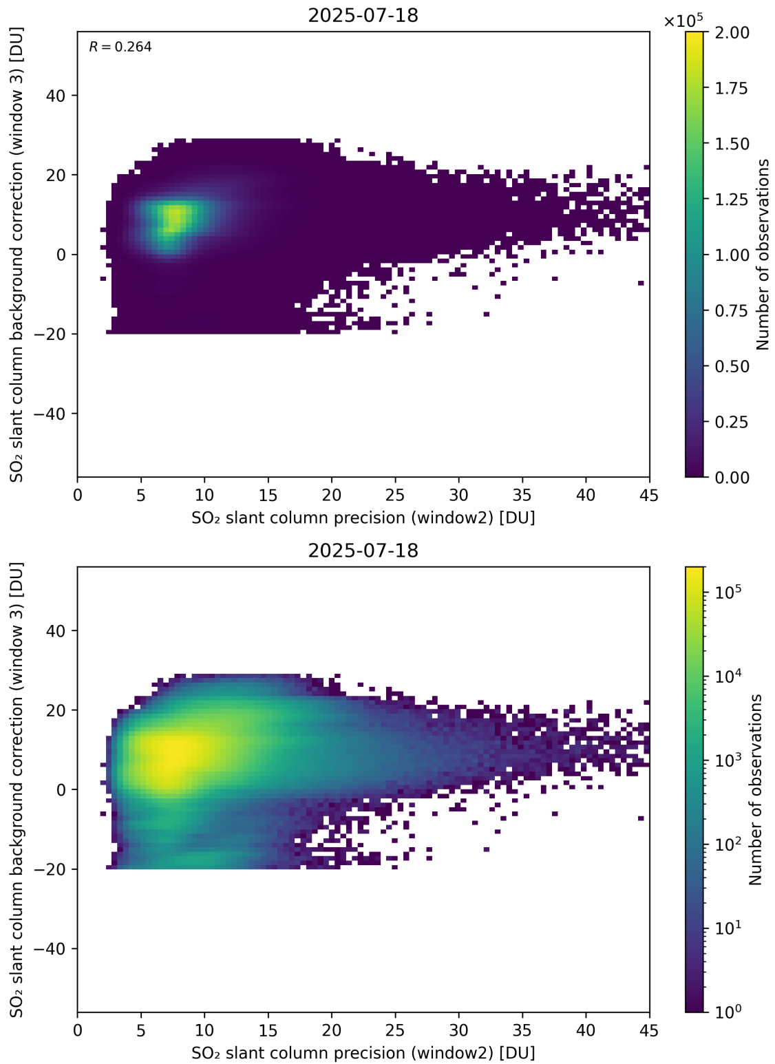
Figure 292: Scatter density plot of “SO 2 slant column precision (window2)” against “SO 2 slant column background correction (window 3)” for 2025-07-18 to 2025-07-19.
