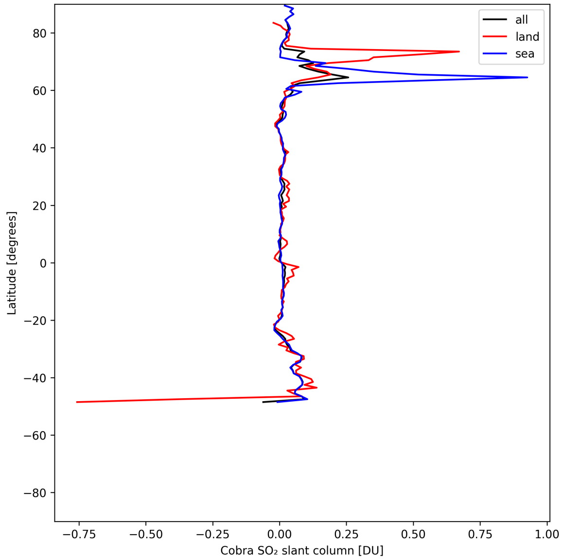
Figure 35: Zonal average of “Cobra SO 2 slant column” for 2025-07-18 to 2025-07-19.
