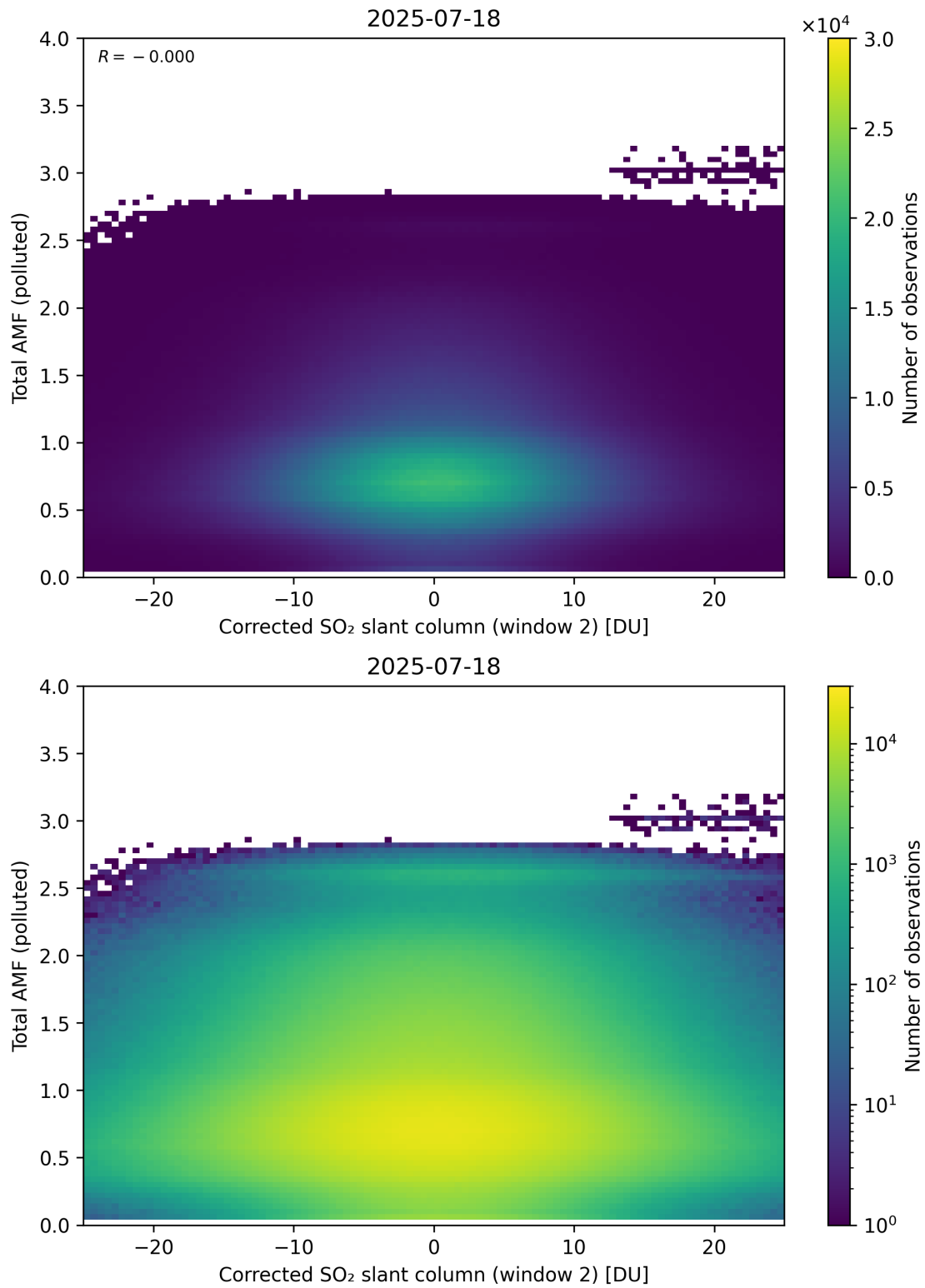
Figure 253: Scatter density plot of “Corrected SO 2 slant column (window 2)” against “Total AMF (polluted)” for 2025-07-18 to 2025-07-19.
