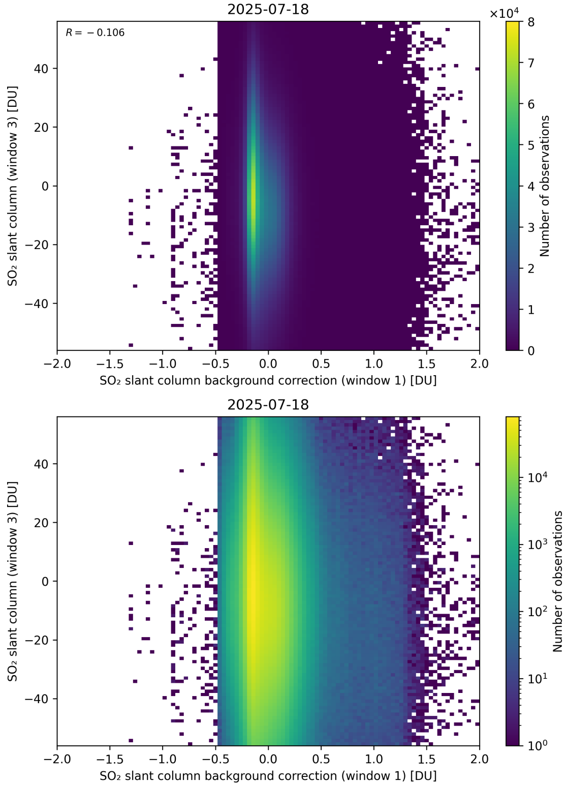
Figure 118: Scatter density plot of “SO 2 slant column background correction (window 1)” against “SO 2 slant column (window 3)” for 2025-07-18 to 2025-07-19.
