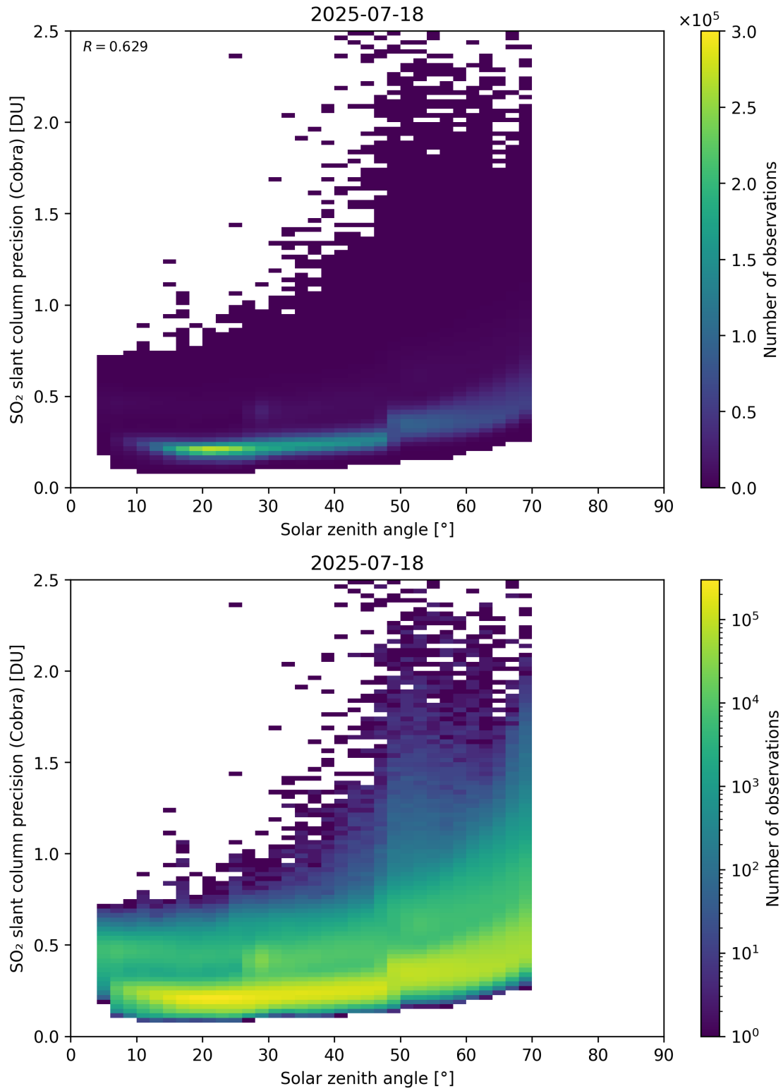
Figure 180: Scatter density plot of “Solar zenith angle” against “SO 2 slant column precision (Cobra)” for 2025-07-18 to 2025-07-19.
