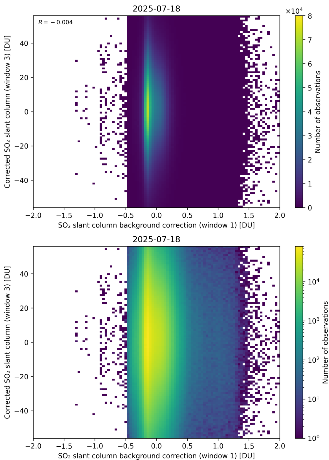
Figure 116: Scatter density plot of “SO 2 slant column background correction (window 1)” against “Corrected SO 2 slant column (window 3)” for 2025-07-18 to 2025-07-19.
