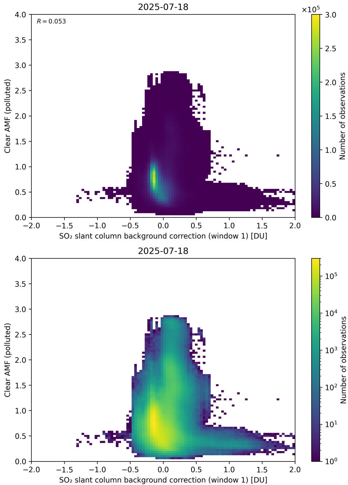
Figure 114: Scatter density plot of “SO 2 slant column background correction (window 1)” against “Clear AMF (polluted)” for 2025-07-18 to 2025-07-19.
