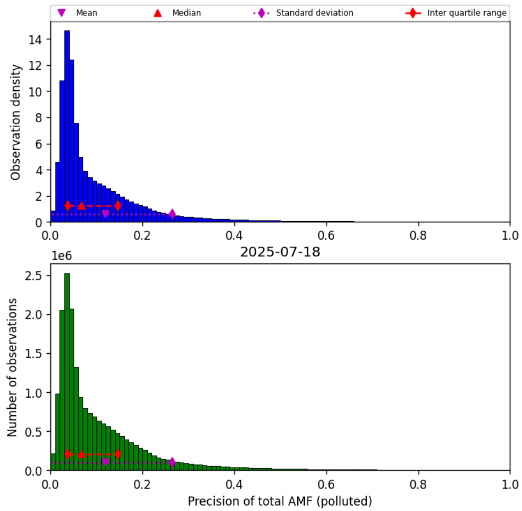
Figure 80: Histogram of “Precision of total AMF (polluted)” for 2025-07-18 to 2025-07-19
