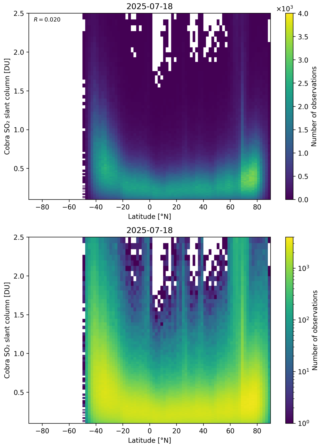
Figure 157: Scatter density plot of “Latitude” against “Cobra SO 2 slant column” for 2025-07-18 to 2025-07-19.
