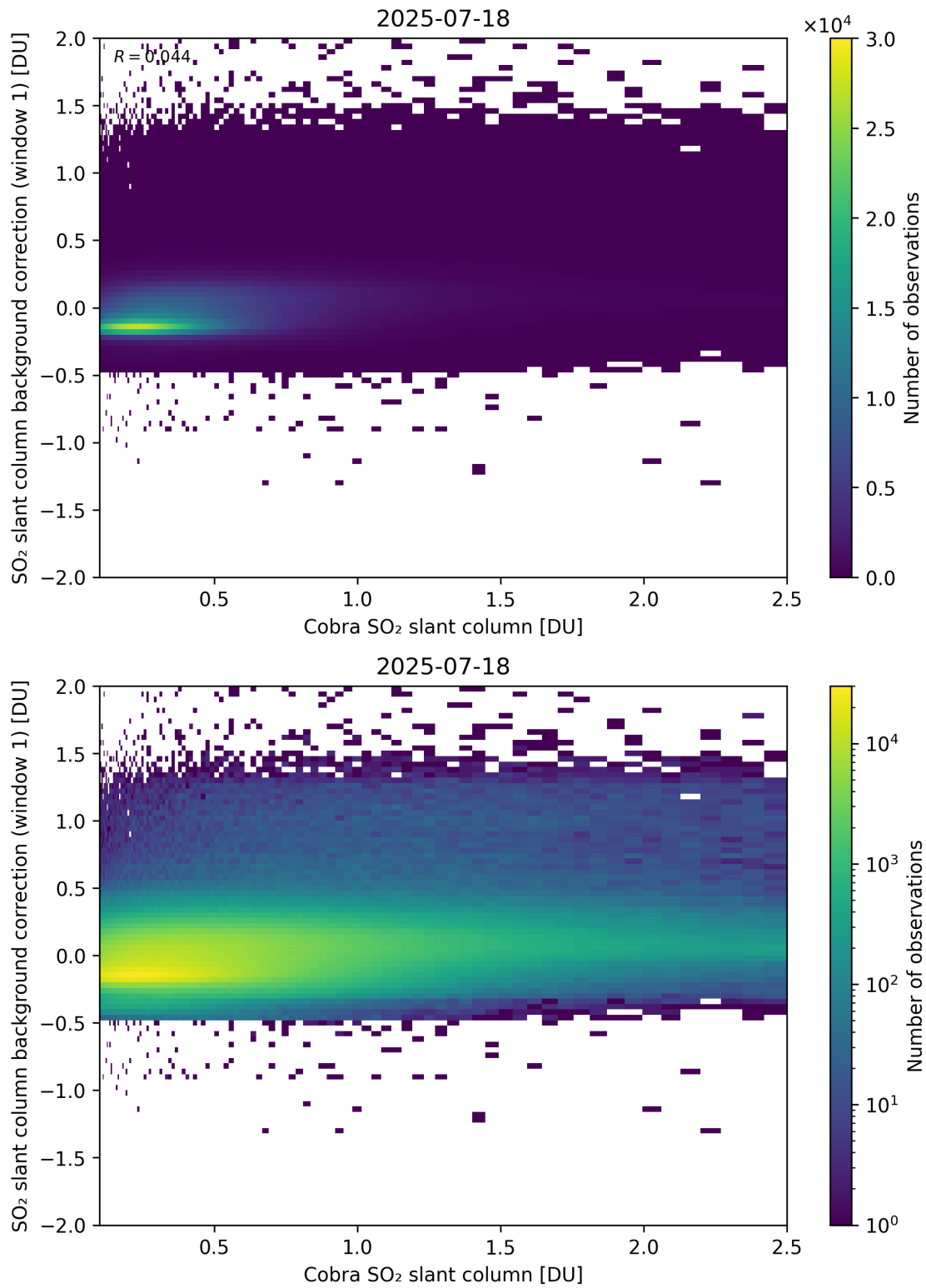
Figure 193: Scatter density plot of “Cobra SO 2 slant column” against “SO 2 slant column background correction (window 1)” for 2025-07-18 to 2025-07-19.
