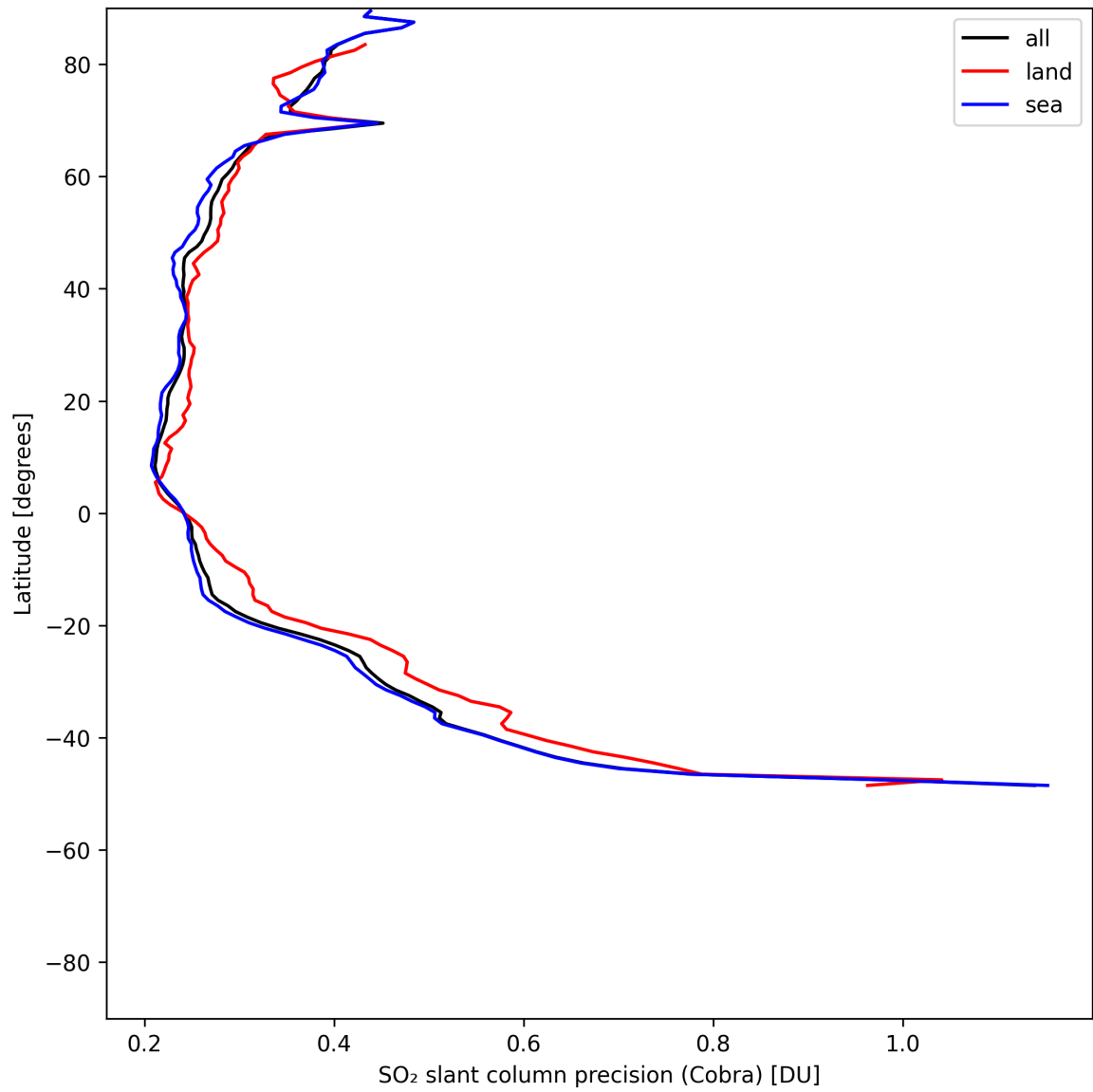
Figure 36: Zonal average of “SO 2 slant column precision (Cobra)” for 2025-07-18 to 2025-07-19.
