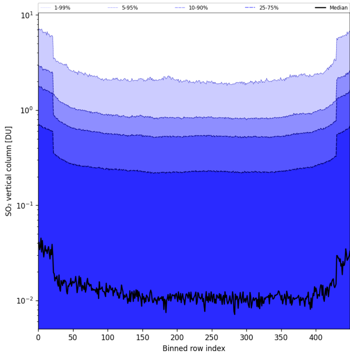
Figure 84: Along track statistics of “SO 2 vertical column” for 2025-07-18 to 2025-07-19
