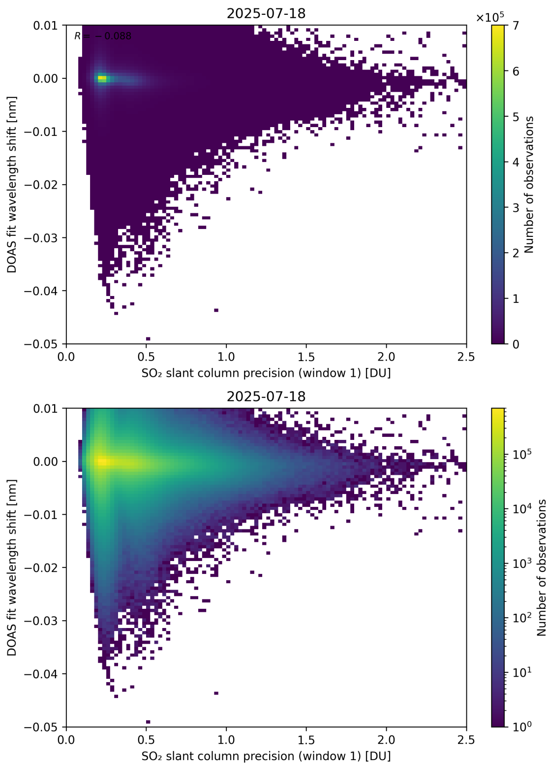
Figure 271: Scatter density plot of “SO 2 slant column precision (window 1)” against “DOAS fit wavelength shift” for 2025-07-18 to 2025-07-19.
