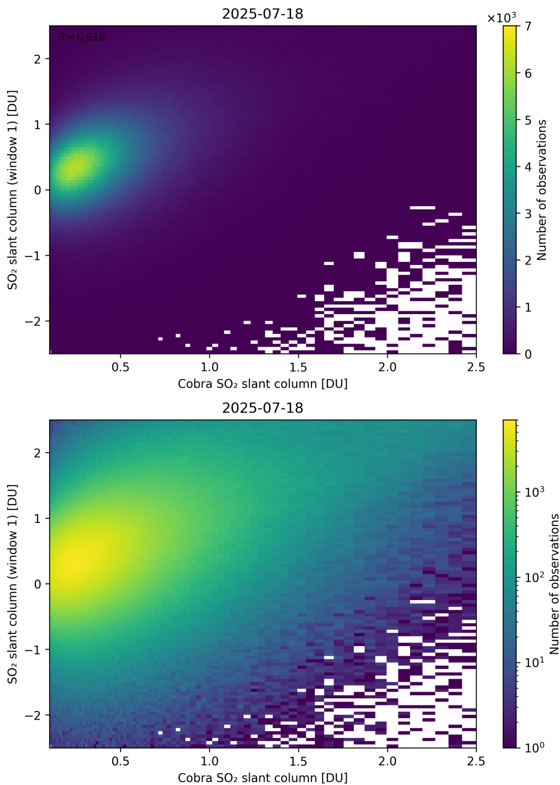
Figure 219: Scatter density plot of “Cobra SO 2 slant column” against “SO 2 slant column (window 1)” for 2025-07-18 to 2025-07-19.
