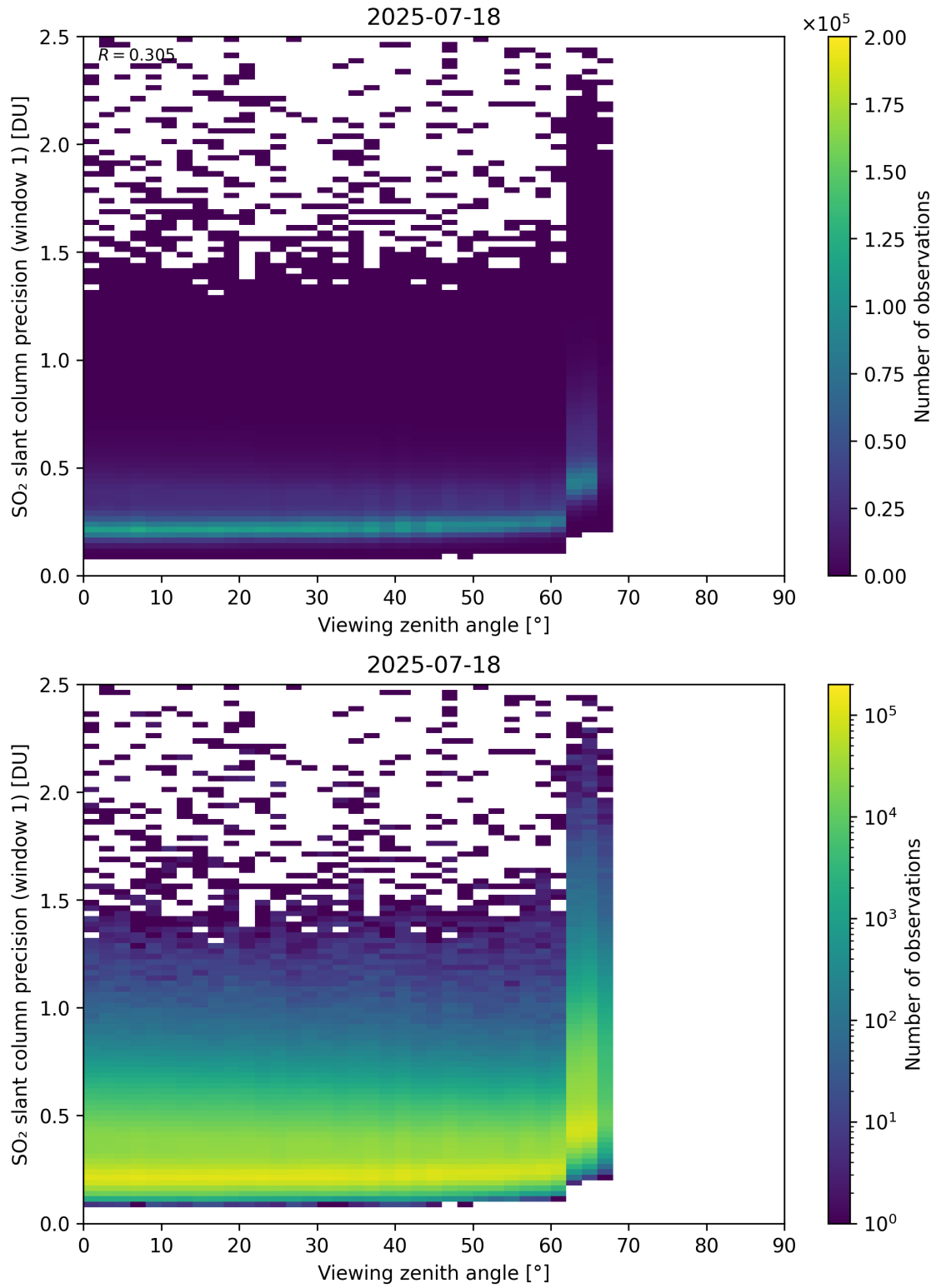
Figure 377: Scatter density plot of “Viewing zenith angle” against “SO 2 slant column precision (window 1)” for 2025-07-18 to 2025-07-19.
