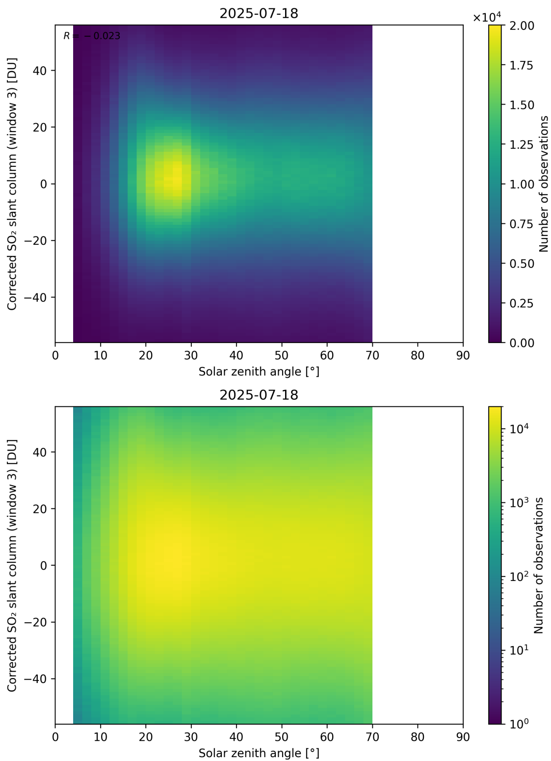
Figure 183: Scatter density plot of “Solar zenith angle” against “Corrected SO 2 slant column (window 3)” for 2025-07-18 to 2025-07-19.
