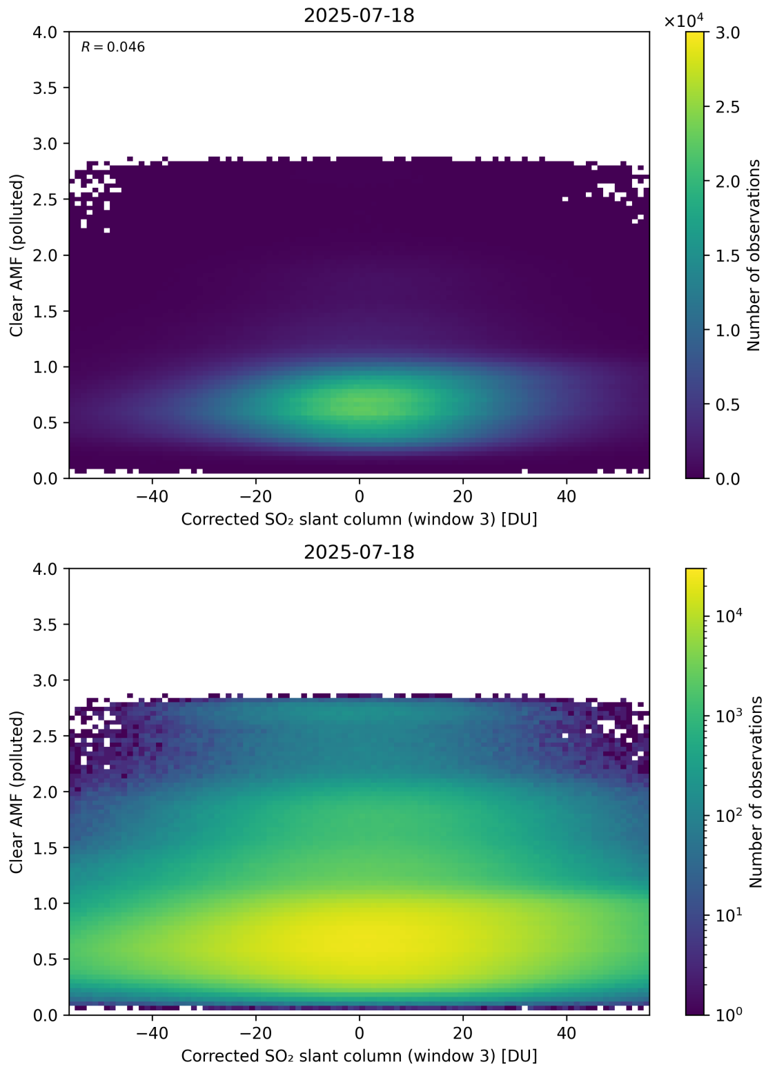
Figure 259: Scatter density plot of “Corrected SO 2 slant column (window 3)” against “Clear AMF (polluted)” for 2025-07-18 to 2025-07-19.
