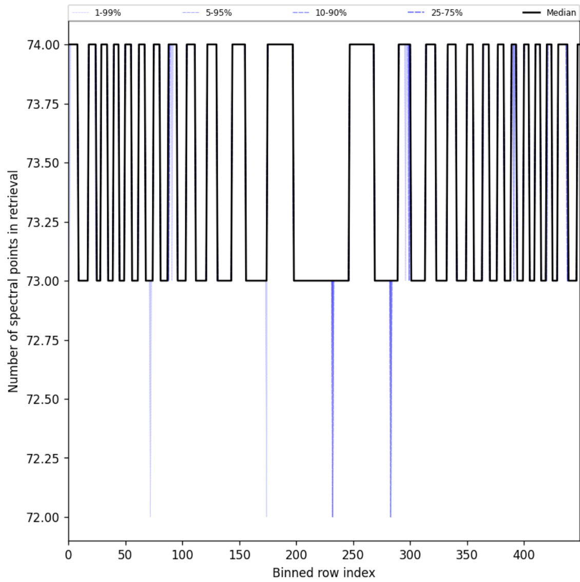
Figure 108: Along track statistics of “Number of spectral points in retrieval” for 2025-07-18 to 2025-07-19
