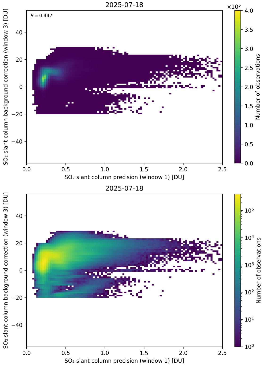
Figure 270: Scatter density plot of “SO 2 slant column precision (window 1)” against “SO 2 slant column background correction (window 3)” for 2025-07-18 to 2025-07-19.
