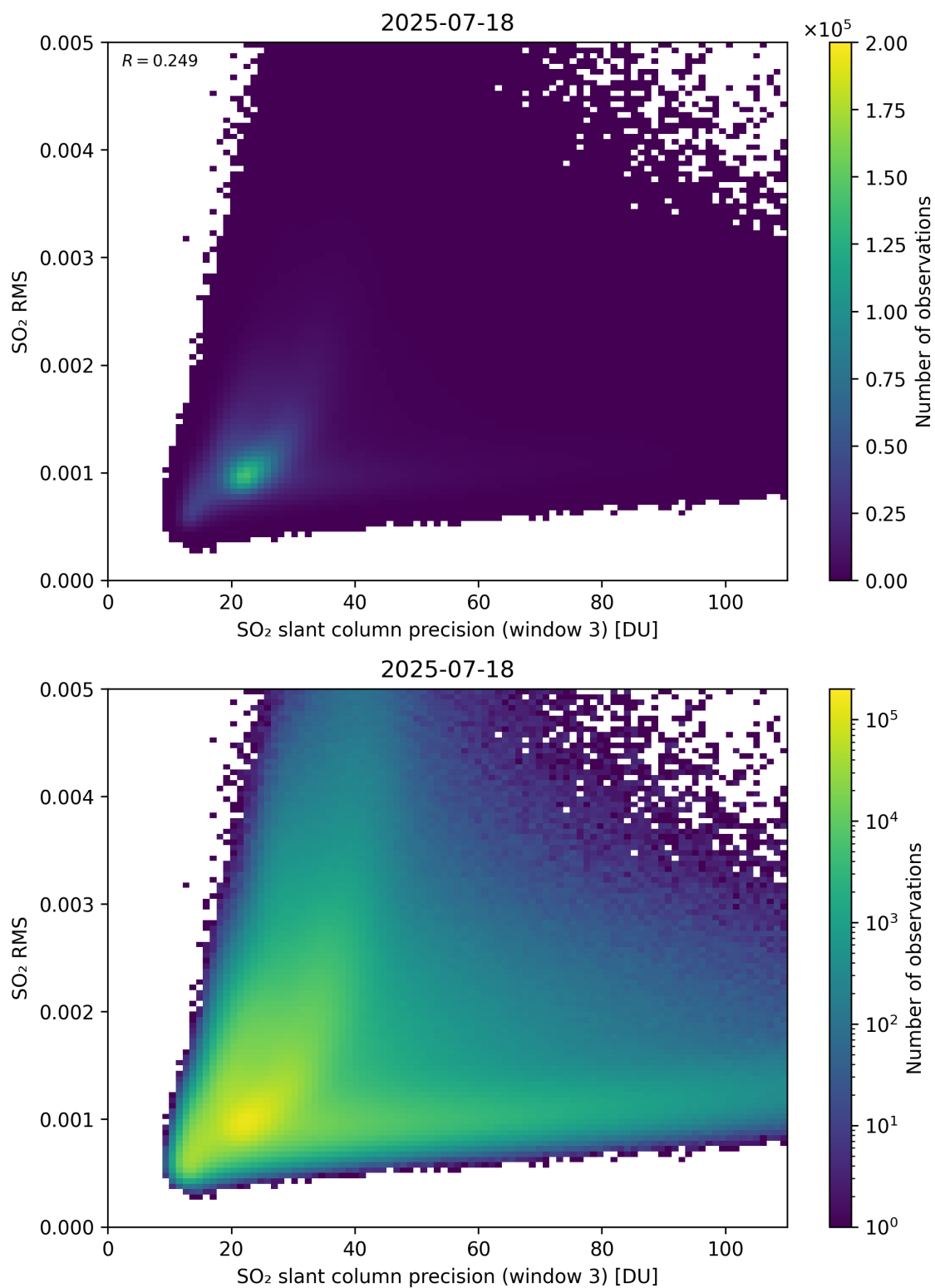
Figure 310: Scatter density plot of “SO 2 slant column precision (window 3)” against “SO 2 RMS” for 2025-07-18 to 2025-07-19.
