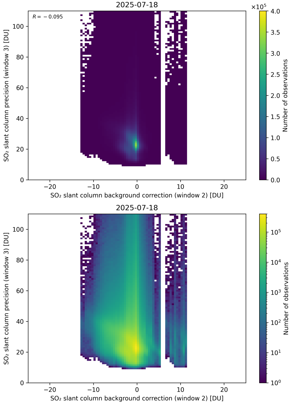
Figure 129: Scatter density plot of “SO 2 slant column background correction (window 2)” against “SO 2 slant column precision (window 3)” for 2025-07-18 to 2025-07-19.
