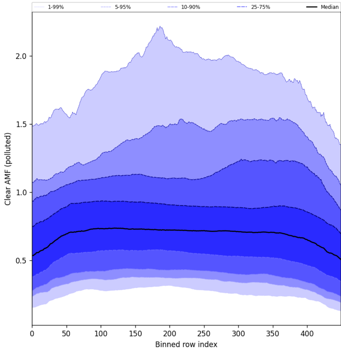
Figure 107: Along track statistics of “Clear AMF (polluted)” for 2025-07-18 to 2025-07-19
