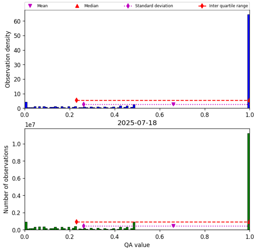
Figure 57: Histogram of “QA value” for 2025-07-18 to 2025-07-19
