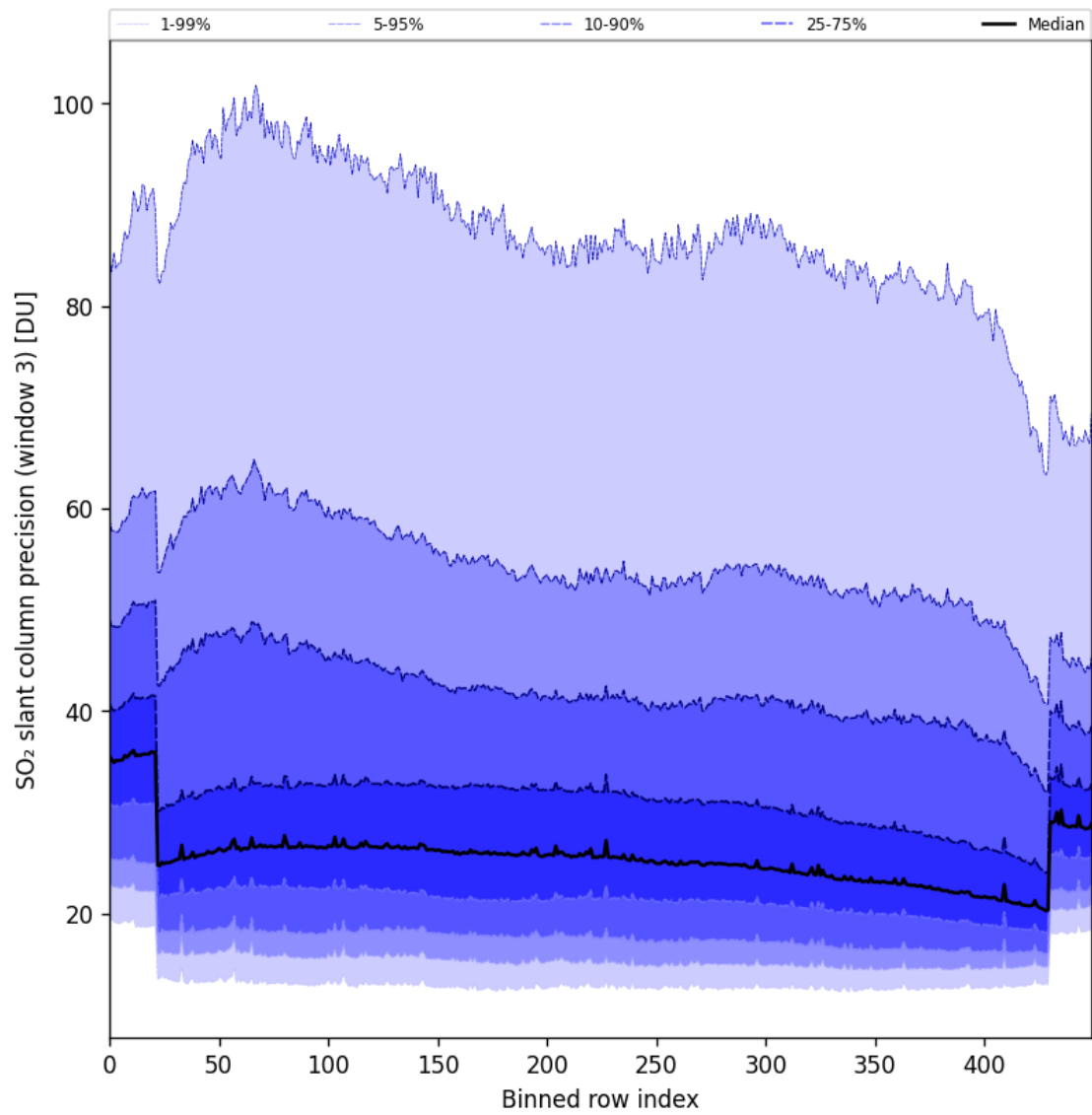
Figure 98: Along track statistics of “SO 2 slant column precision (window 3)” for 2025-07-18 to 2025-07-19
