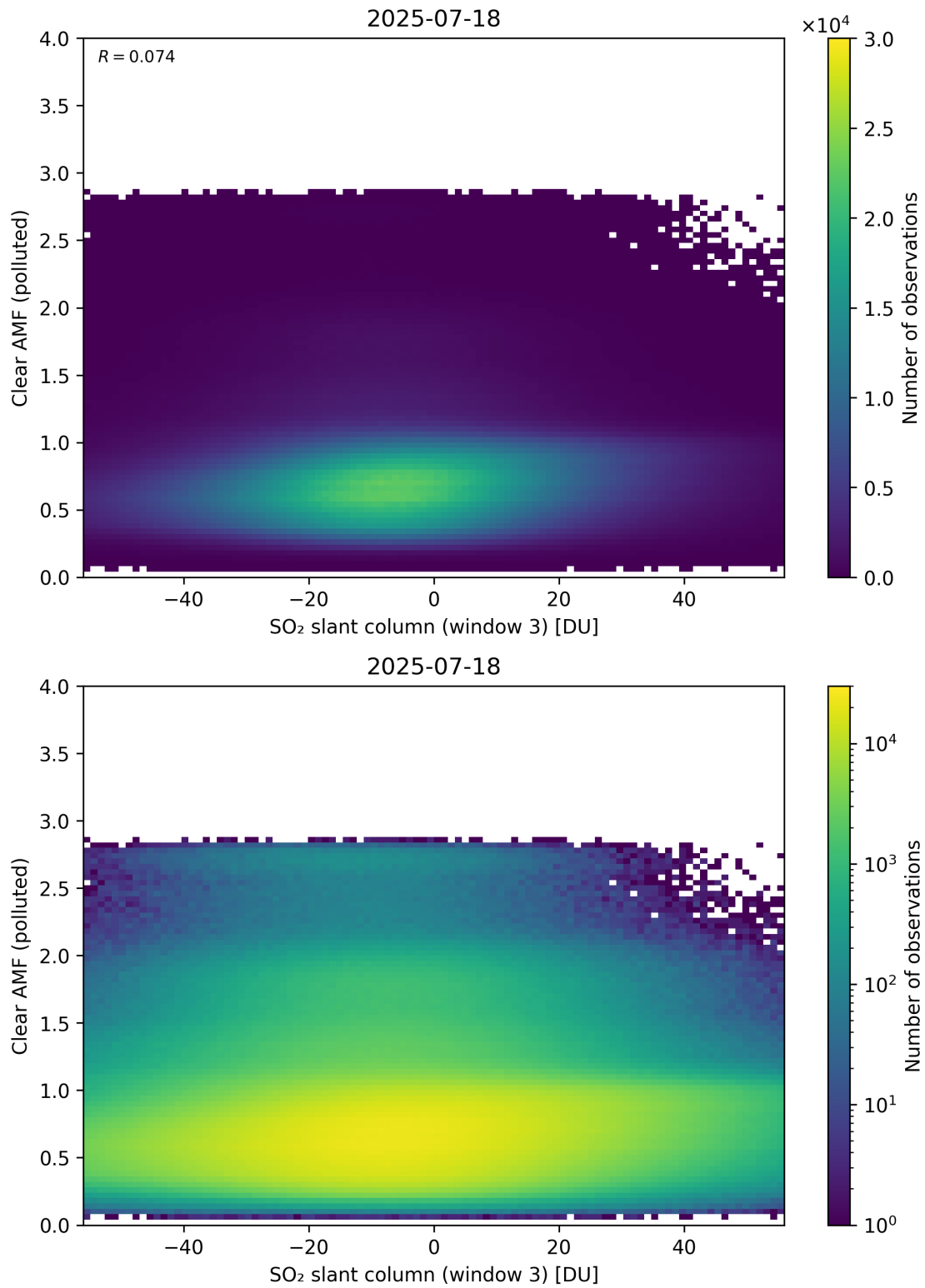
Figure 315: Scatter density plot of “SO 2 slant column (window 3)” against “Clear AMF (polluted)” for 2025-07-18 to 2025-07-19.
