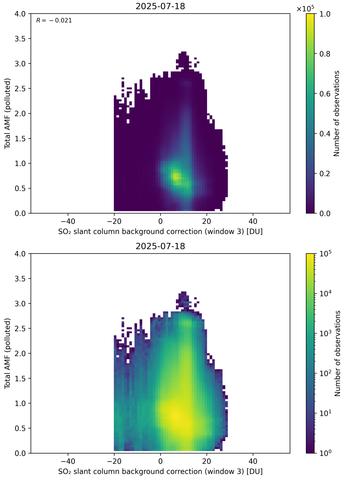
Figure 136: Scatter density plot of “SO 2 slant column background correction (window 3)” against “Total AMF (polluted)” for 2025-07-18 to 2025-07-19.
