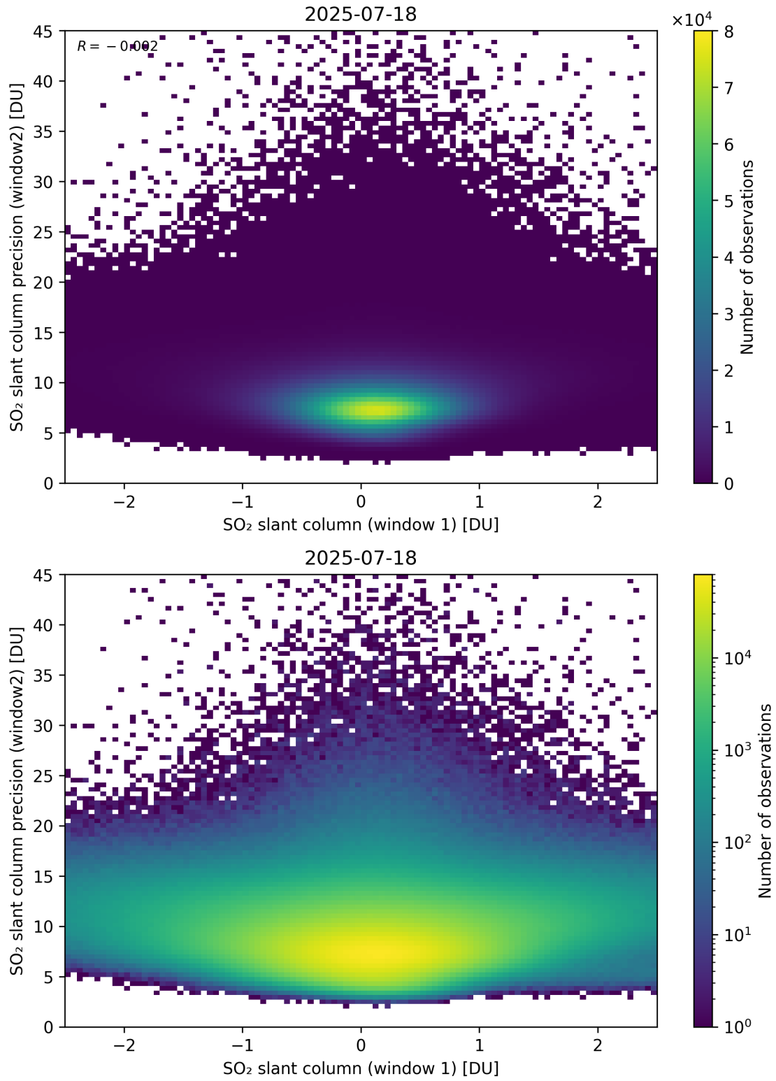
Figure 286: Scatter density plot of “SO 2 slant column (window 1)” against “SO 2 slant column precision (window2)” for 2025-07-18 to 2025-07-19.
