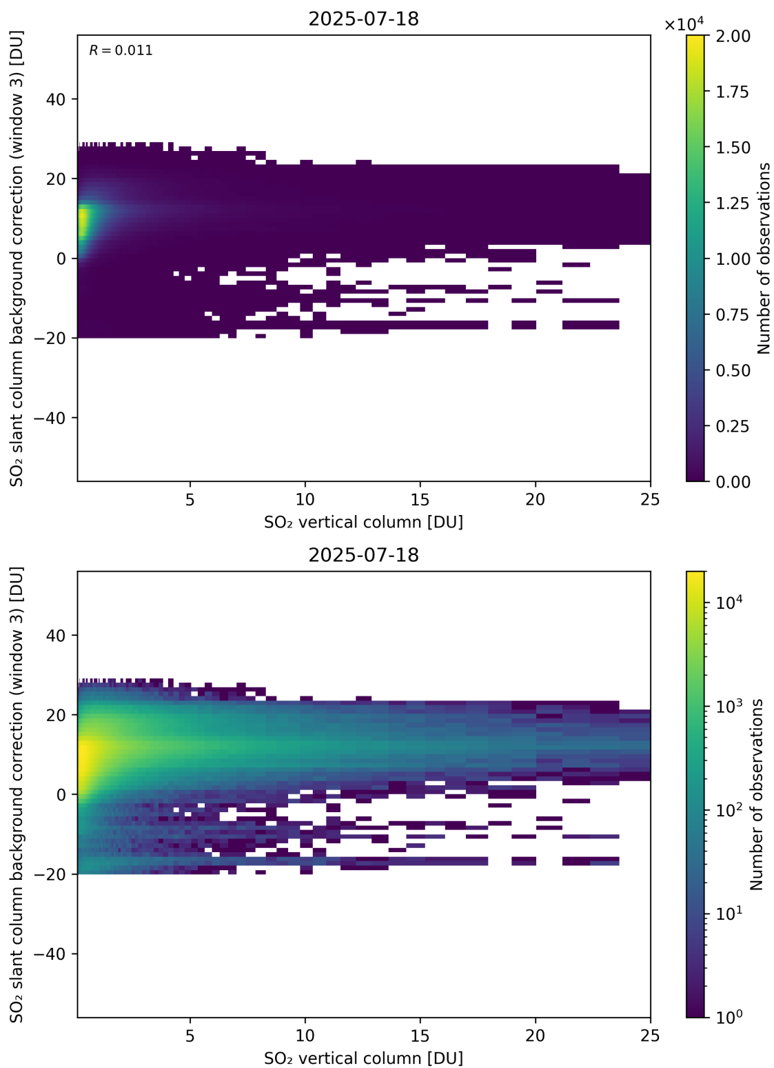
Figure 325: Scatter density plot of “SO 2 vertical column” against “SO 2 slant column background correction (window 3)” for 2025-07-18 to 2025-07-19.
