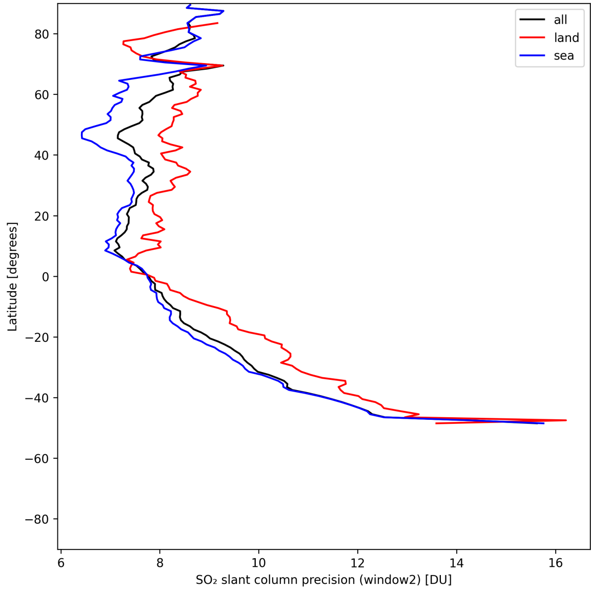
Figure 42: Zonal average of “SO 2 slant column precision (window2)” for 2025-07-18 to 2025-07-19.
