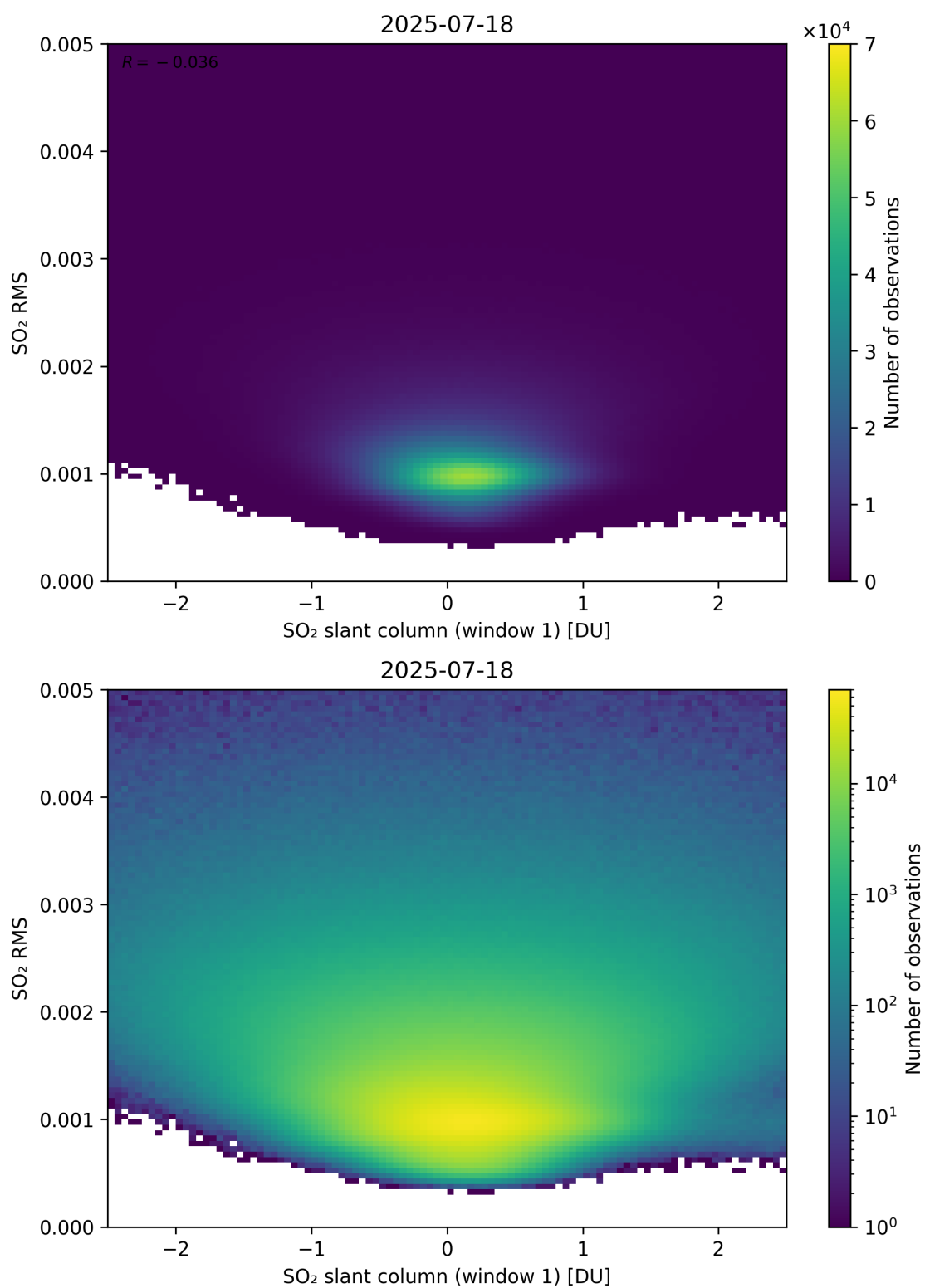
Figure 267: Scatter density plot of “SO 2 slant column (window 1)” against “SO 2 RMS” for 2025-07-18 to 2025-07-19.
