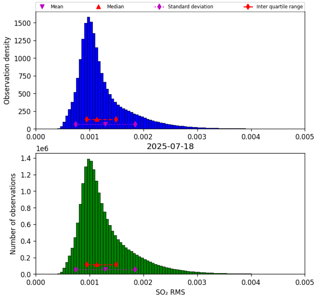
Figure 78: Histogram of “SO 2 RMS” for 2025-07-18 to 2025-07-19
