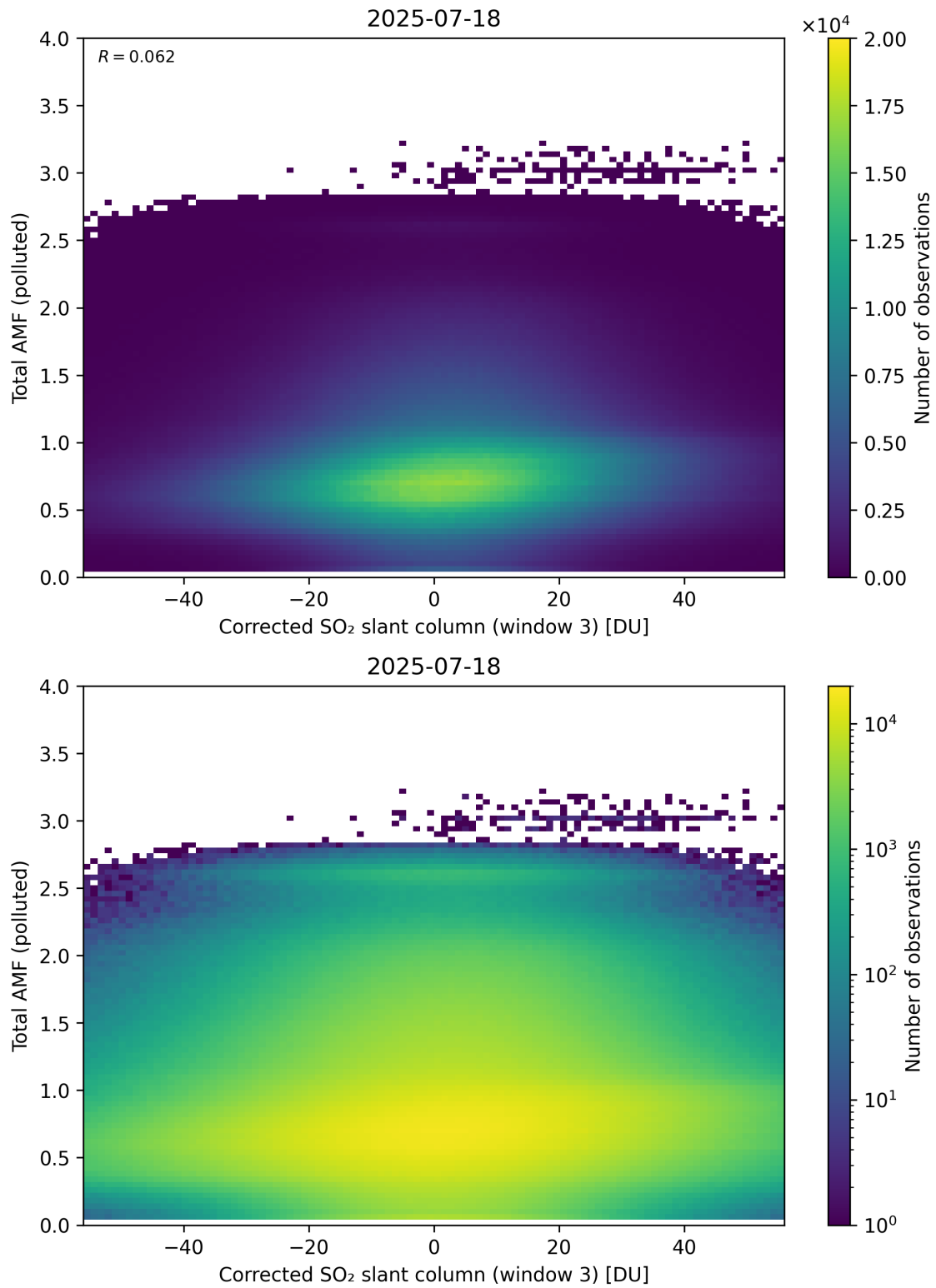
Figure 260: Scatter density plot of “Corrected SO 2 slant column (window 3)” against “Total AMF (polluted)” for 2025-07-18 to 2025-07-19.
