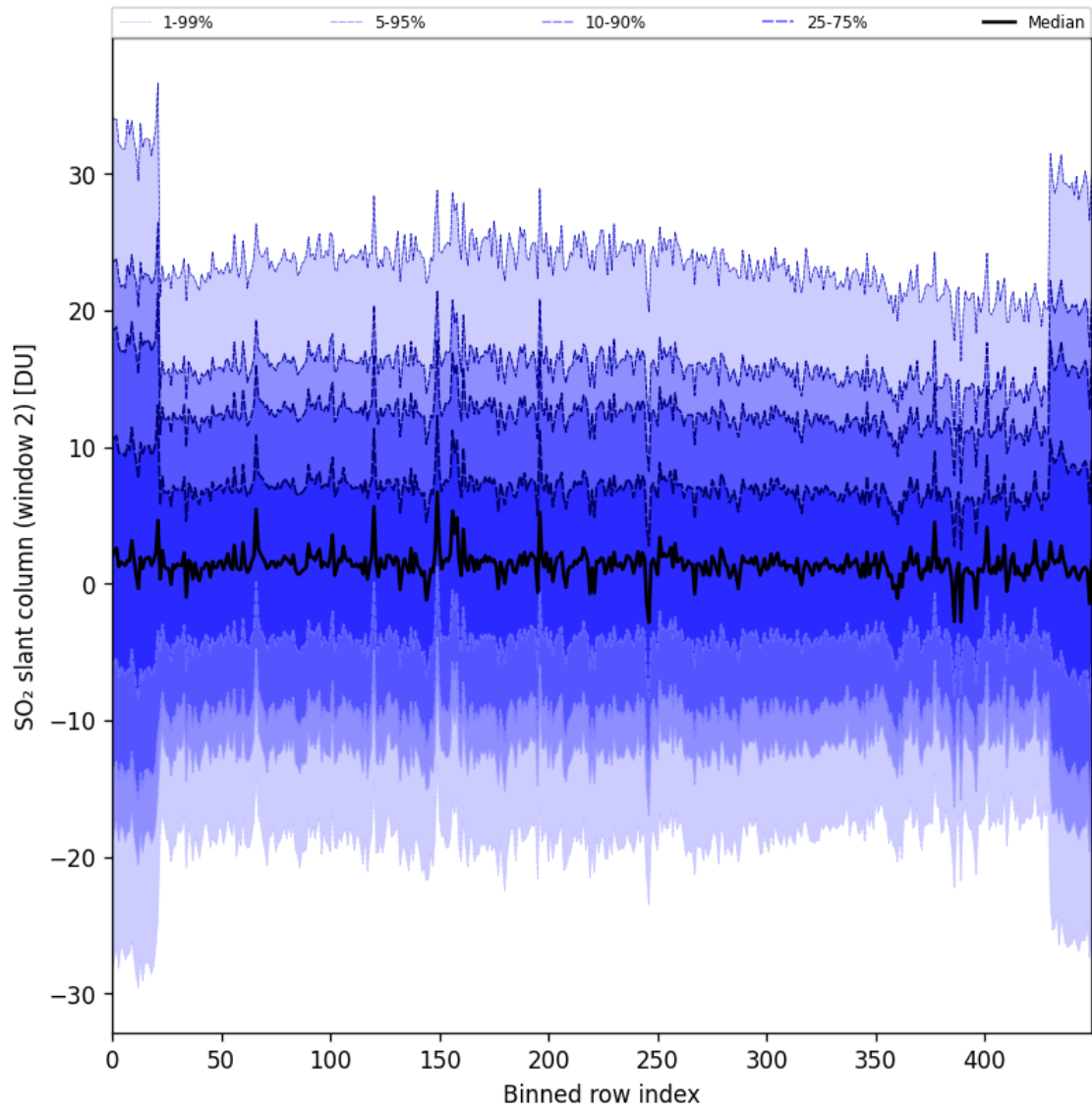
Figure 93: Along track statistics of “SO 2 slant column (window 2)” for 2025-07-18 to 2025-07-19
