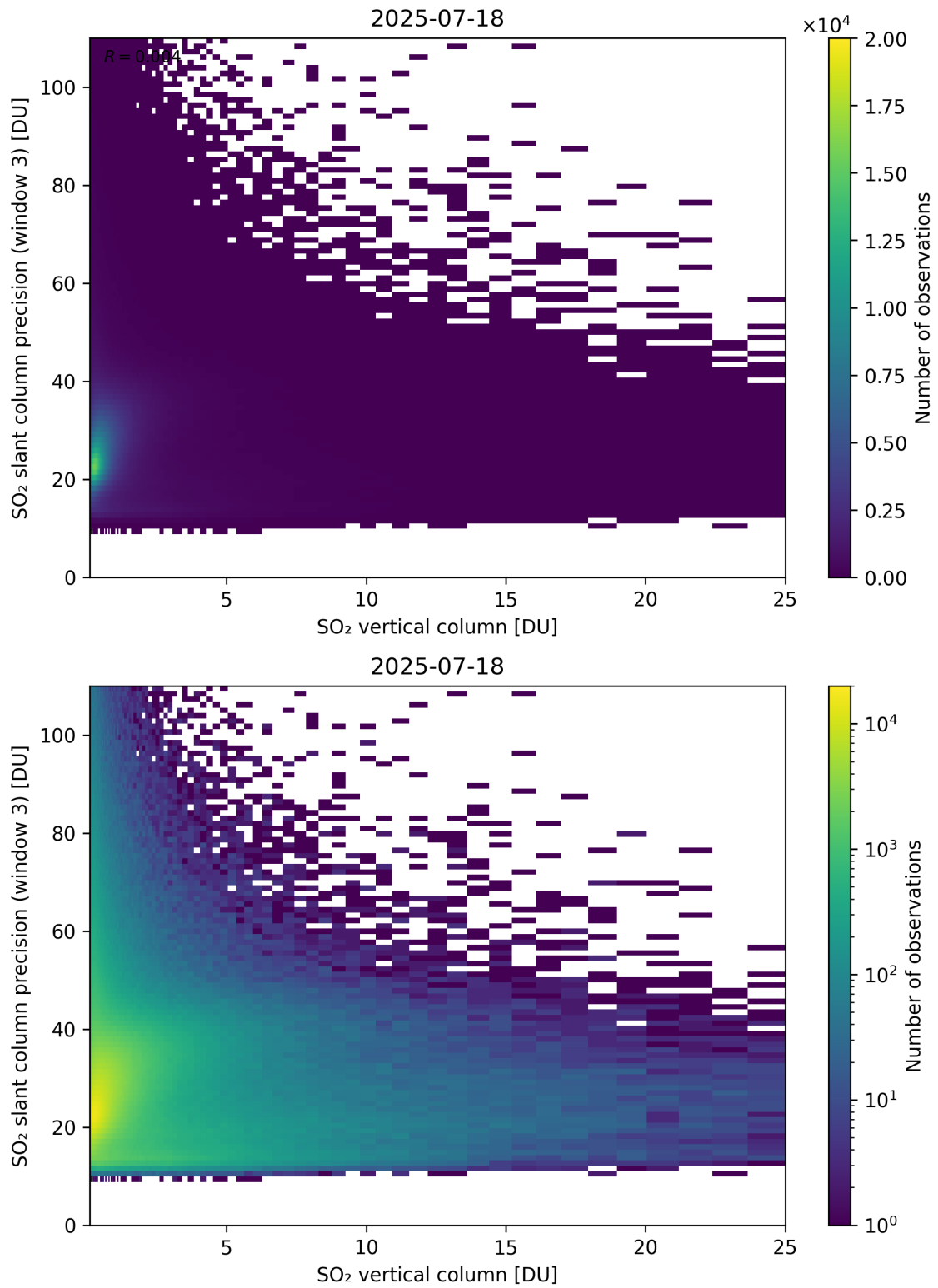
Figure 358: Scatter density plot of “SO 2 vertical column” against “SO 2 slant column precision (window 3)” for 2025-07-18 to 2025-07-19.
