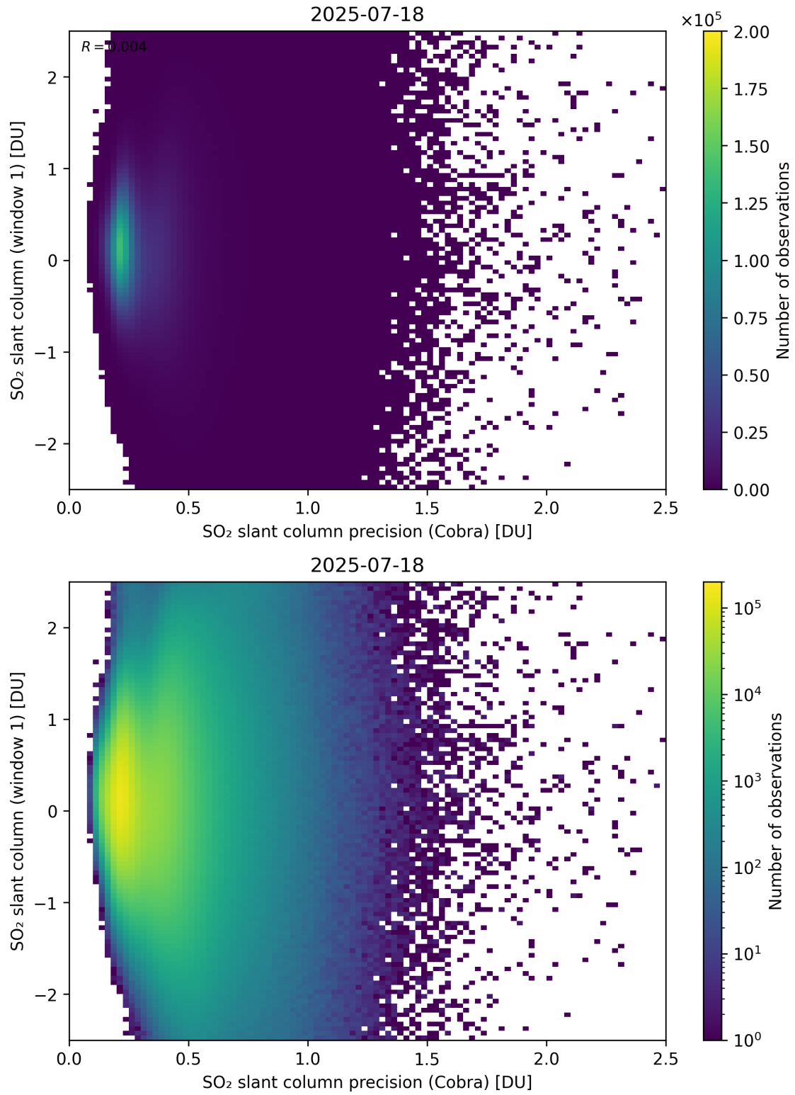
Figure 208: Scatter density plot of “SO 2 slant column precision (Cobra)” against “SO 2 slant column (window 1)” for 2025-07-18 to 2025-07-19.
