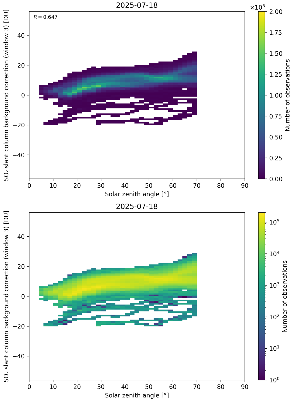
Figure 173: Scatter density plot of “Solar zenith angle” against “SO 2 slant column background correction (window 3)” for 2025-07-18 to 2025-07-19.
