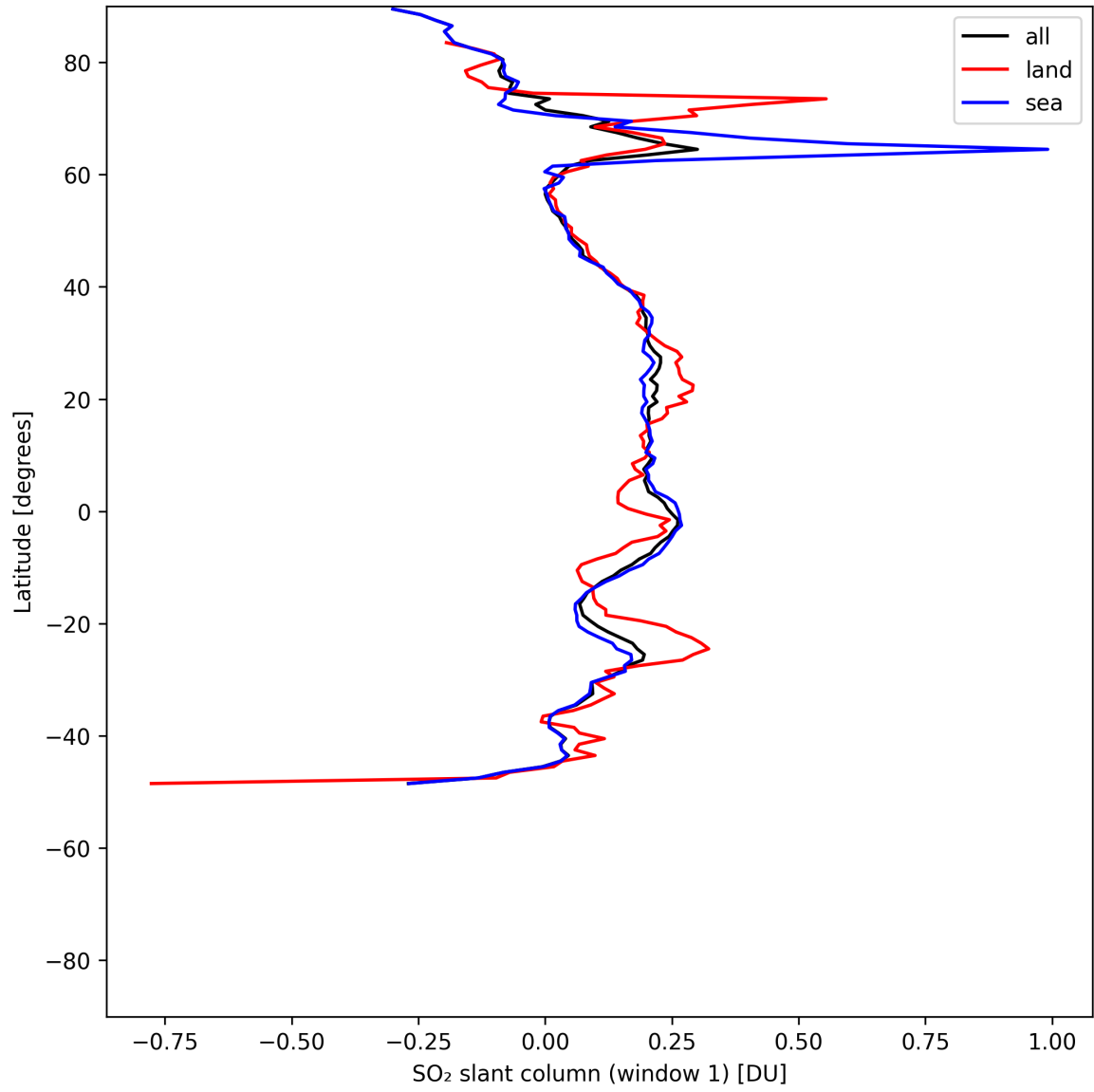
Figure 37: Zonal average of “SO 2 slant column (window 1)” for 2025-07-18 to 2025-07-19.
