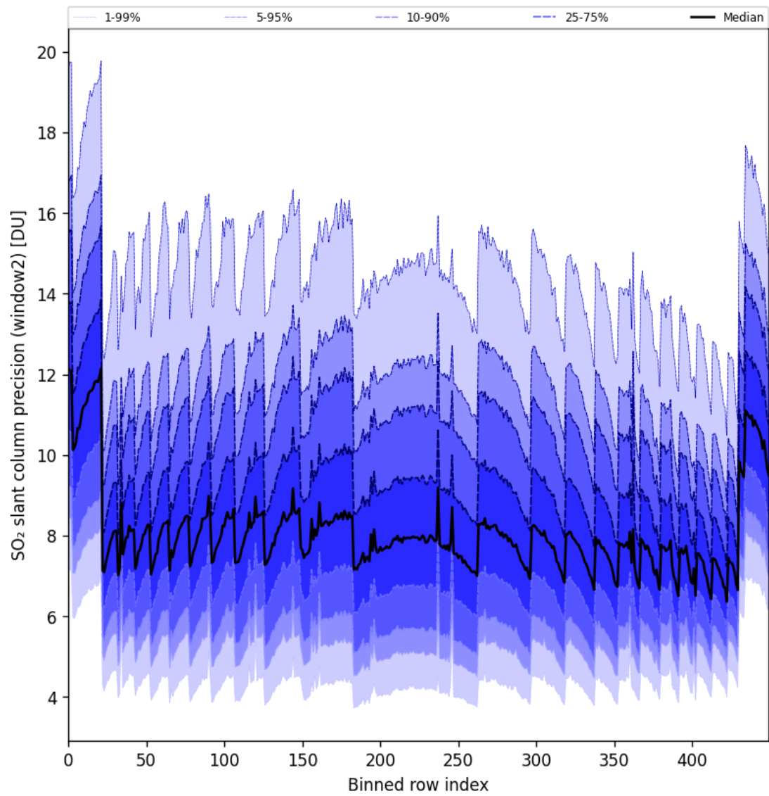
Figure 94: Along track statistics of “SO 2 slant column precision (window2)” for 2025-07-18 to 2025-07-19
