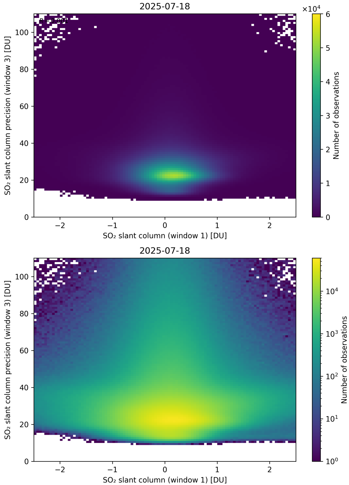
Figure 288: Scatter density plot of “SO 2 slant column (window 1)” against “SO 2 slant column precision (window 3)” for 2025-07-18 to 2025-07-19.
