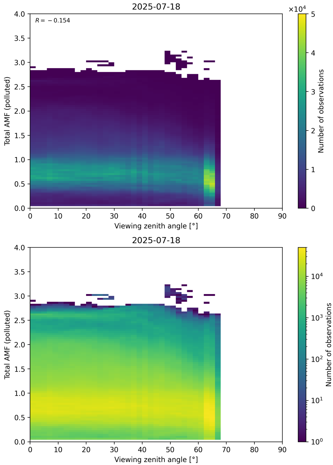
Figure 381: Scatter density plot of “Viewing zenith angle” against “Total AMF (polluted)” for 2025-07-18 to 2025-07-19.
