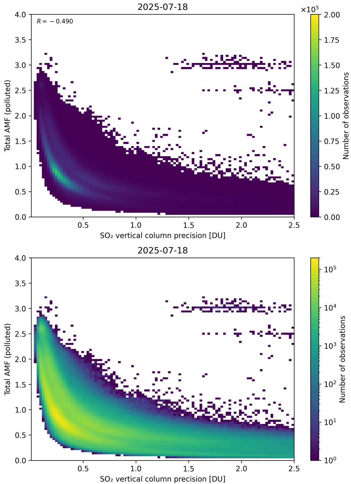
Figure 346: Scatter density plot of “SO 2 vertical column precision” against “Total AMF (polluted)” for 2025-07-18 to 2025-07-19.
