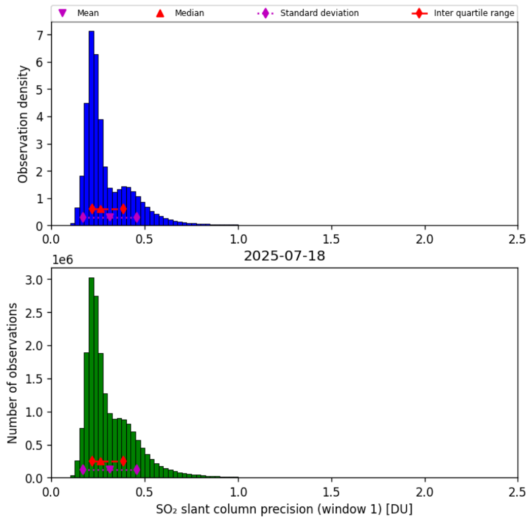
Figure 64: Histogram of “SO 2 slant column precision (window 1)” for 2025-07-18 to 2025-07-19
