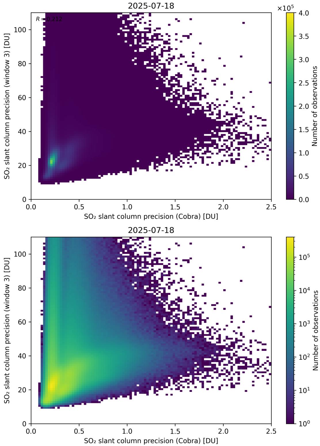
Figure 212: Scatter density plot of “SO 2 slant column precision (Cobra)” against “SO 2 slant column precision (window 3)” for 2025-07-18 to 2025-07-19.
