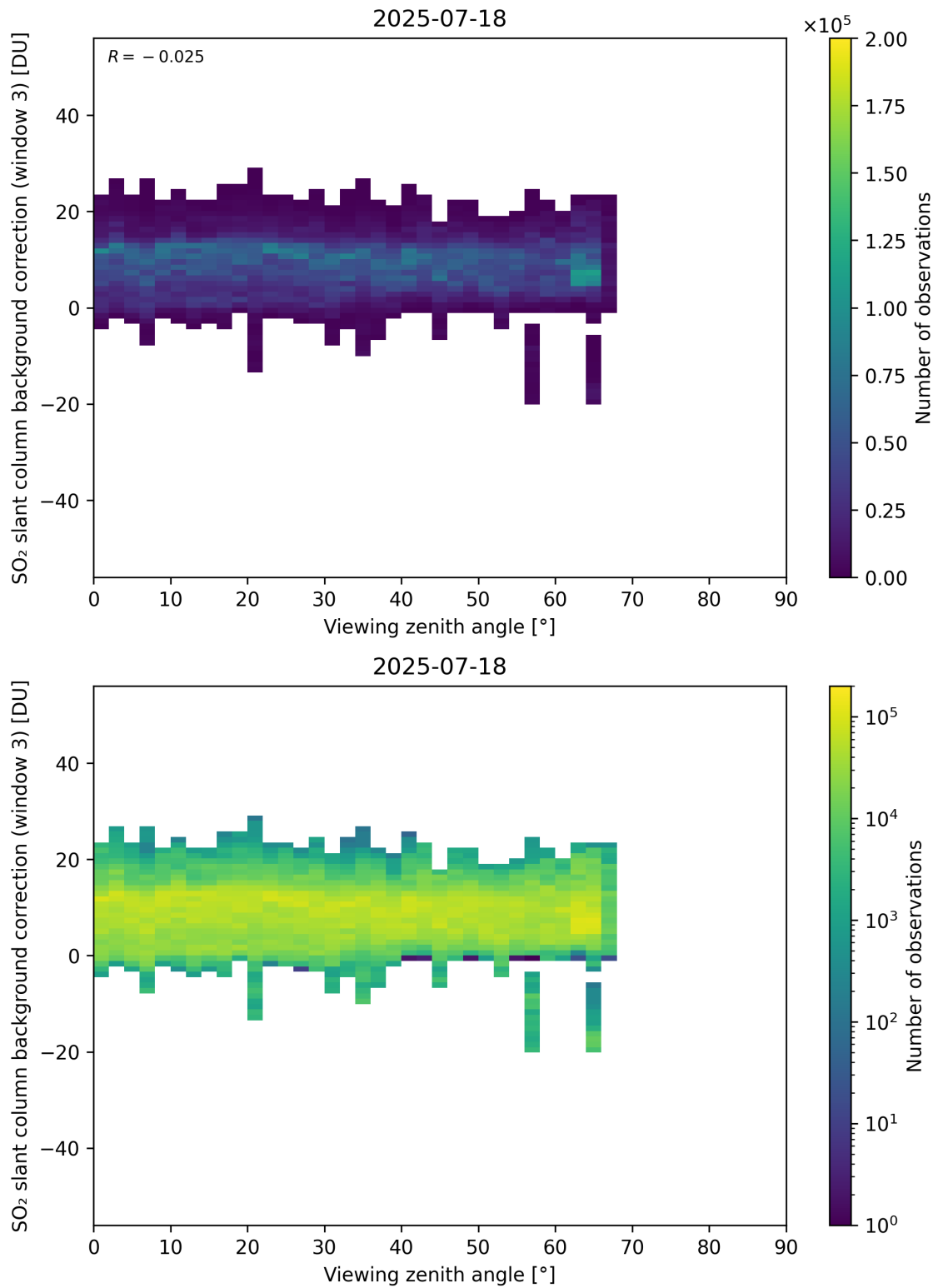
Figure 364: Scatter density plot of “Viewing zenith angle” against “SO 2 slant column background correction (window 3)” for 2025-07-18 to 2025-07-19.
