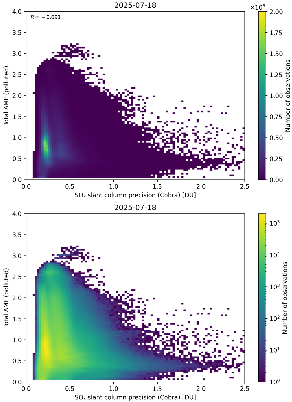
Figure 213: Scatter density plot of “SO 2 slant column precision (Cobra)” against “Total AMF (polluted)” for 2025-07-18 to 2025-07-19.
