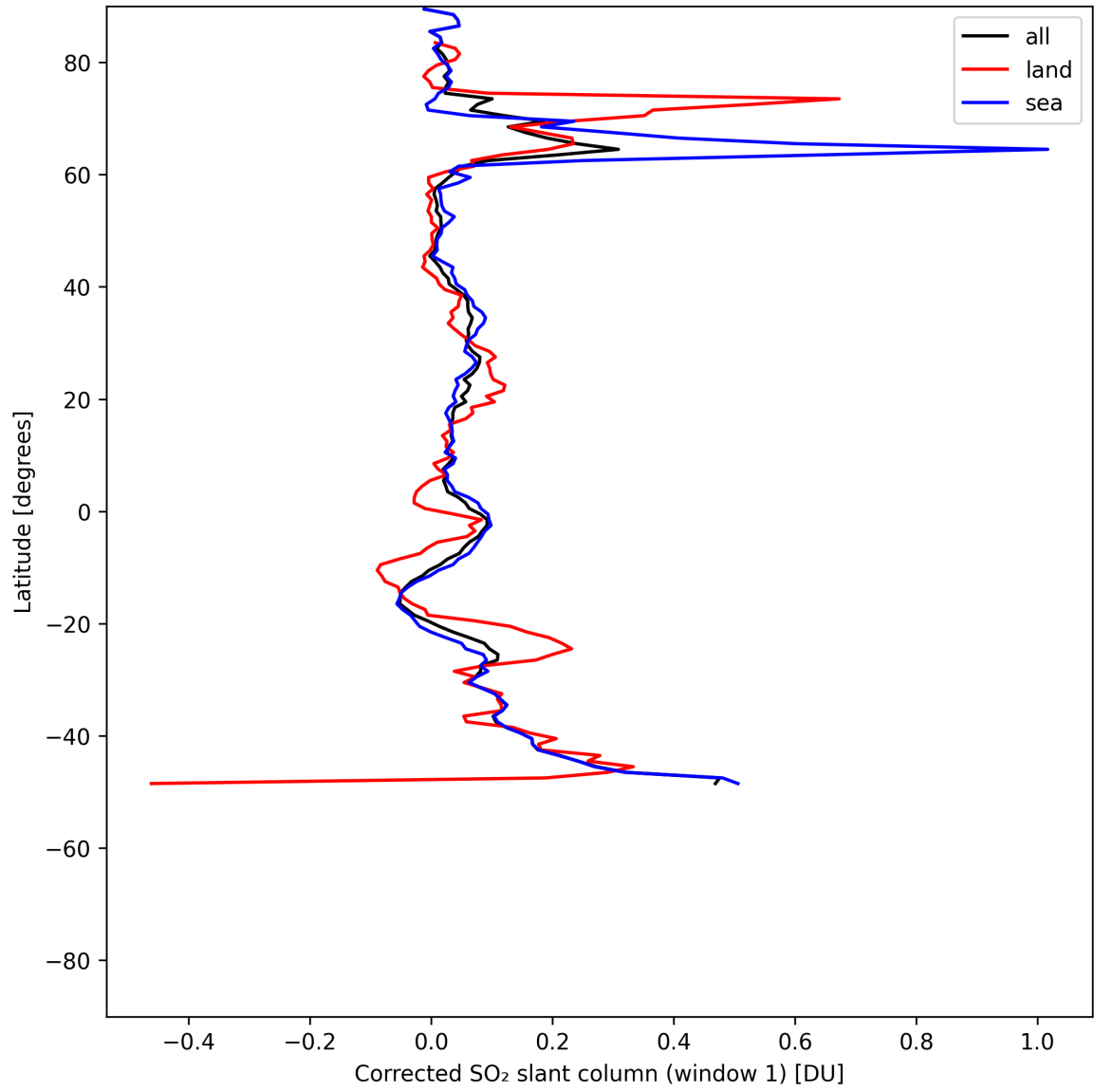
Figure 39: Zonal average of “Corrected SO 2 slant column (window 1)” for 2025-07-18 to 2025-07-19.
