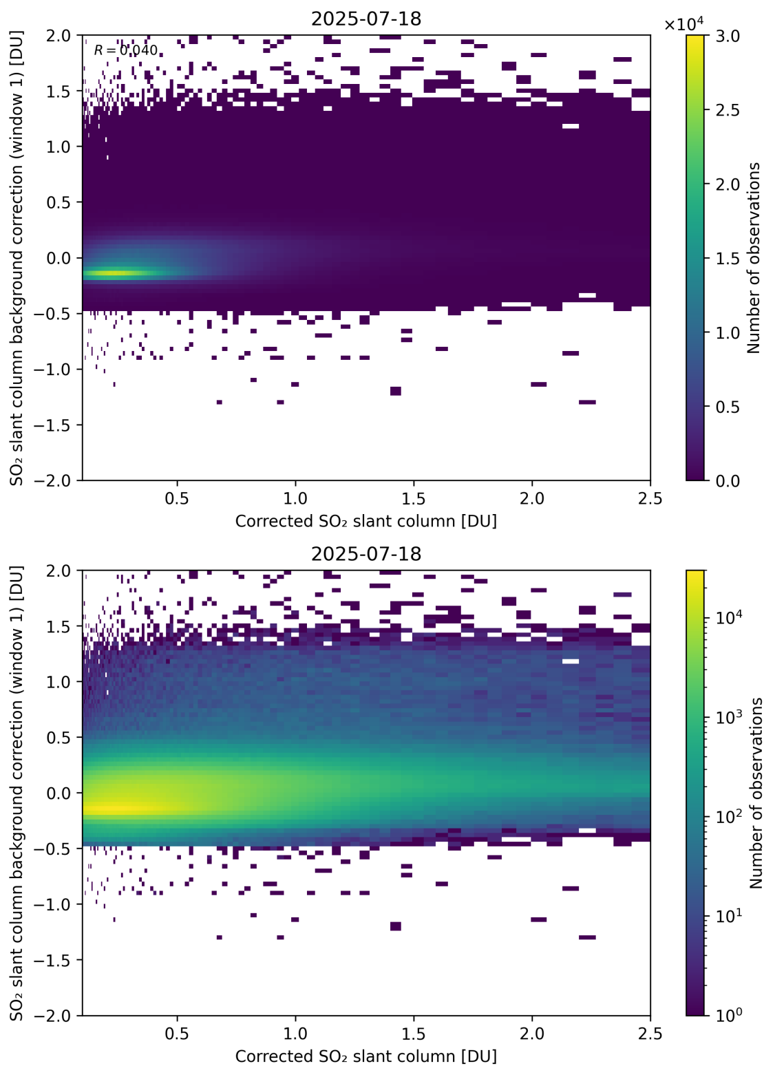
Figure 226: Scatter density plot of “Corrected SO 2 slant column” against “SO 2 slant column background correction (window 1)” for 2025-07-18 to 2025-07-19.
