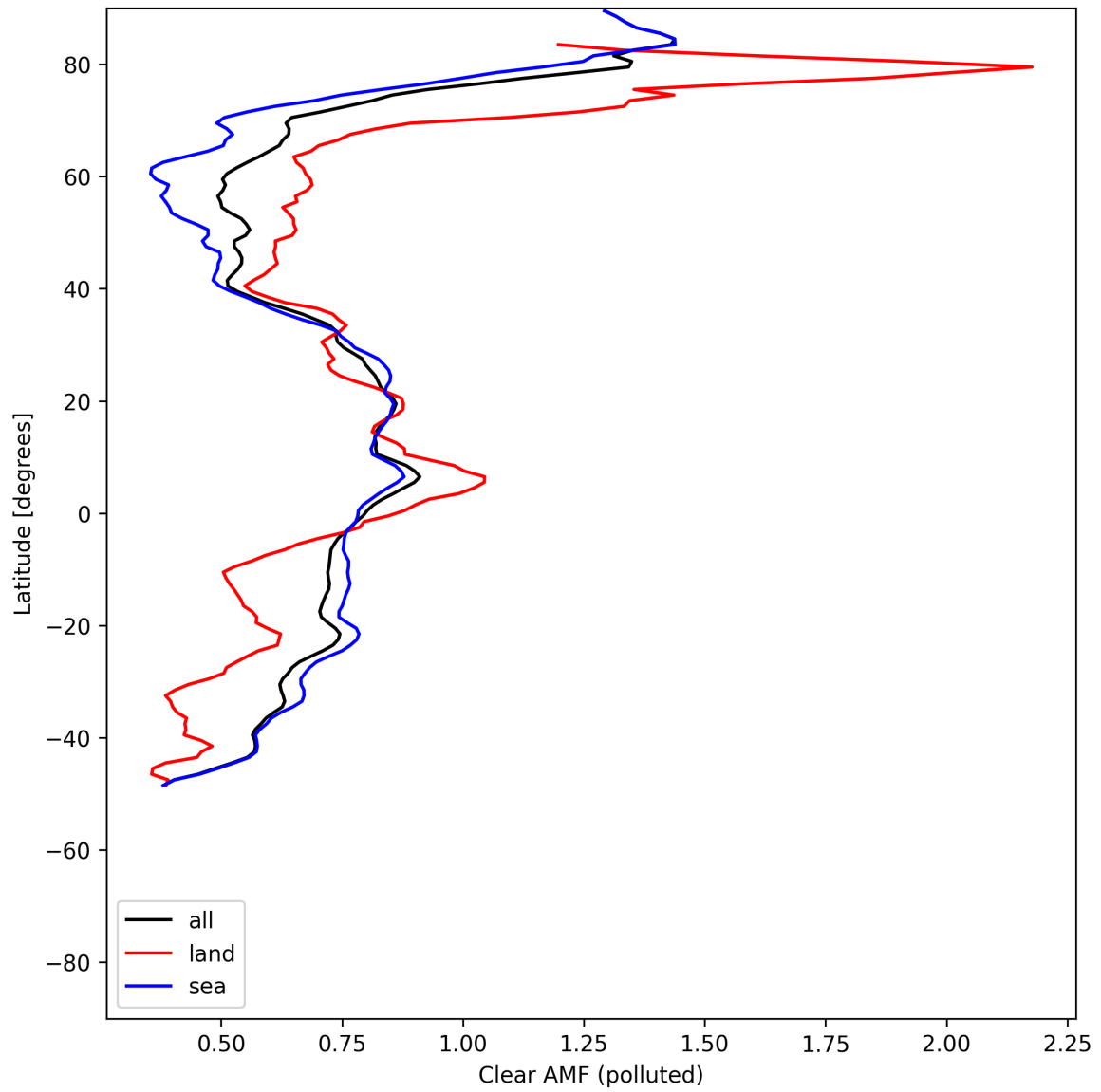
Figure 55: Zonal average of “Clear AMF (polluted)” for 2025-07-18 to 2025-07-19.
