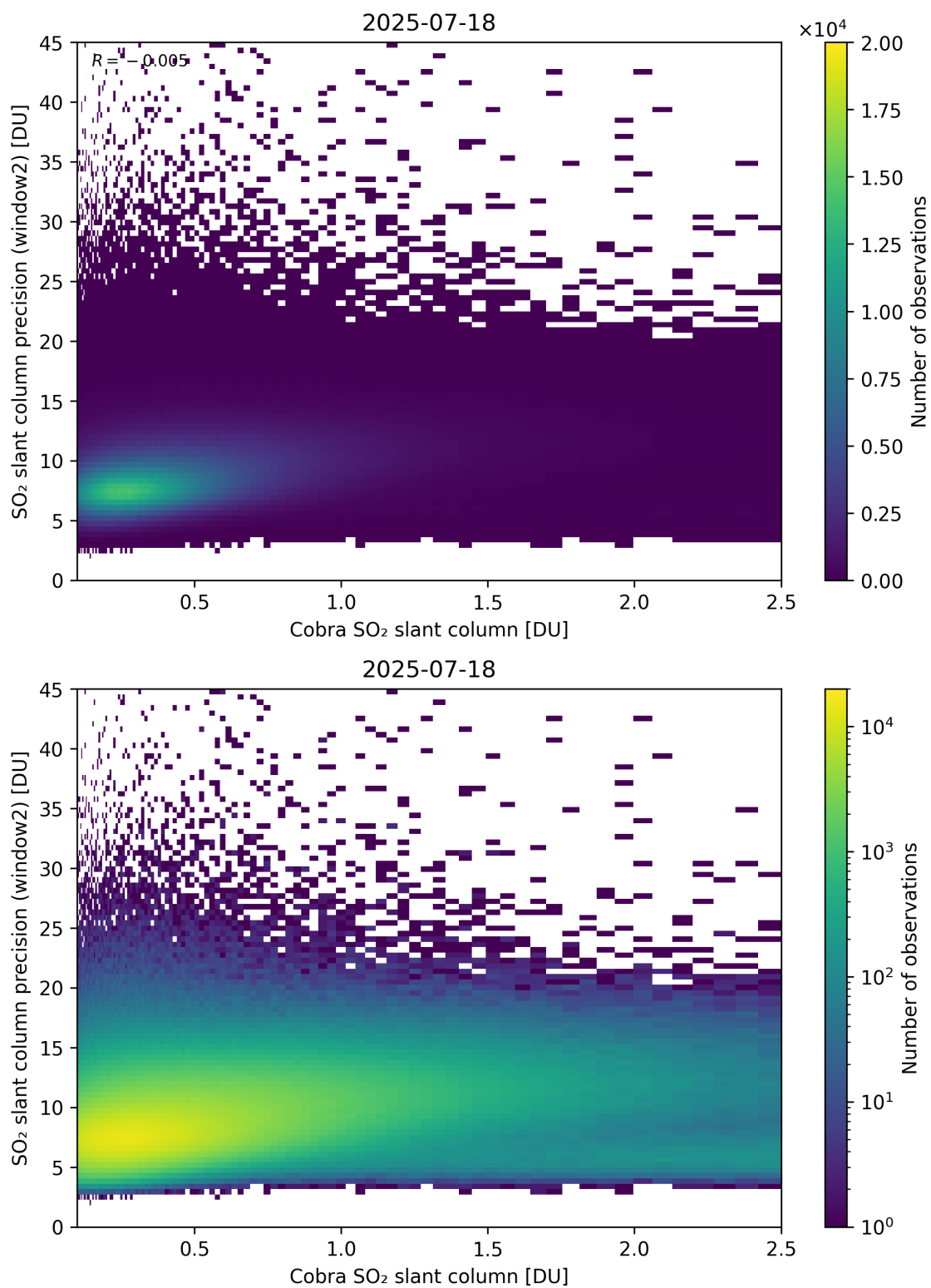
Figure 221: Scatter density plot of “Cobra SO 2 slant column” against “SO 2 slant column precision (window2)” for 2025-07-18 to 2025-07-19.
