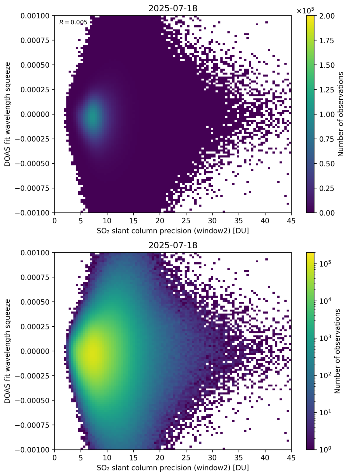
Figure 294: Scatter density plot of “SO 2 slant column precision (window2)” against “DOAS fit wavelength squeeze” for 2025-07-18 to 2025-07-19.
