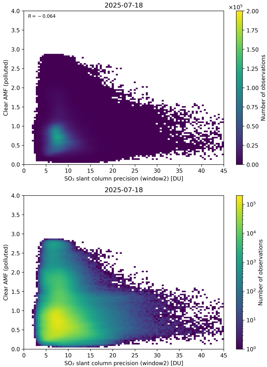
Figure 296: Scatter density plot of “SO 2 slant column precision (window2)” against “Clear AMF (polluted)” for 2025-07-18 to 2025-07-19.
