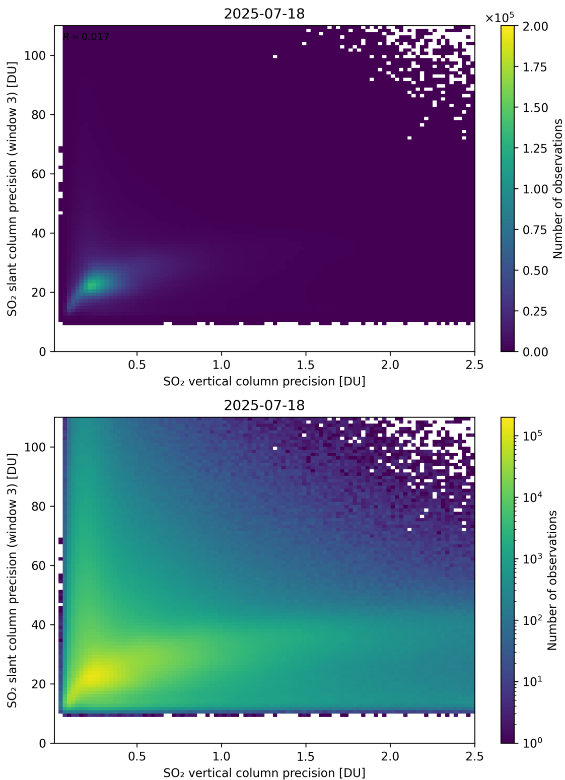
Figure 345: Scatter density plot of “SO 2 vertical column precision” against “SO 2 slant column precision (window 3)” for 2025-07-18 to 2025-07-19.
