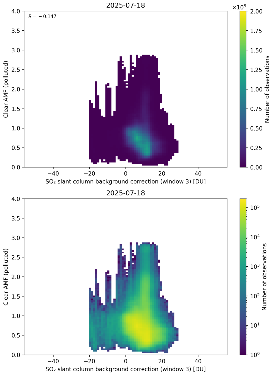
Figure 135: Scatter density plot of “SO 2 slant column background correction (window 3)” against “Clear AMF (polluted)” for 2025-07-18 to 2025-07-19.
