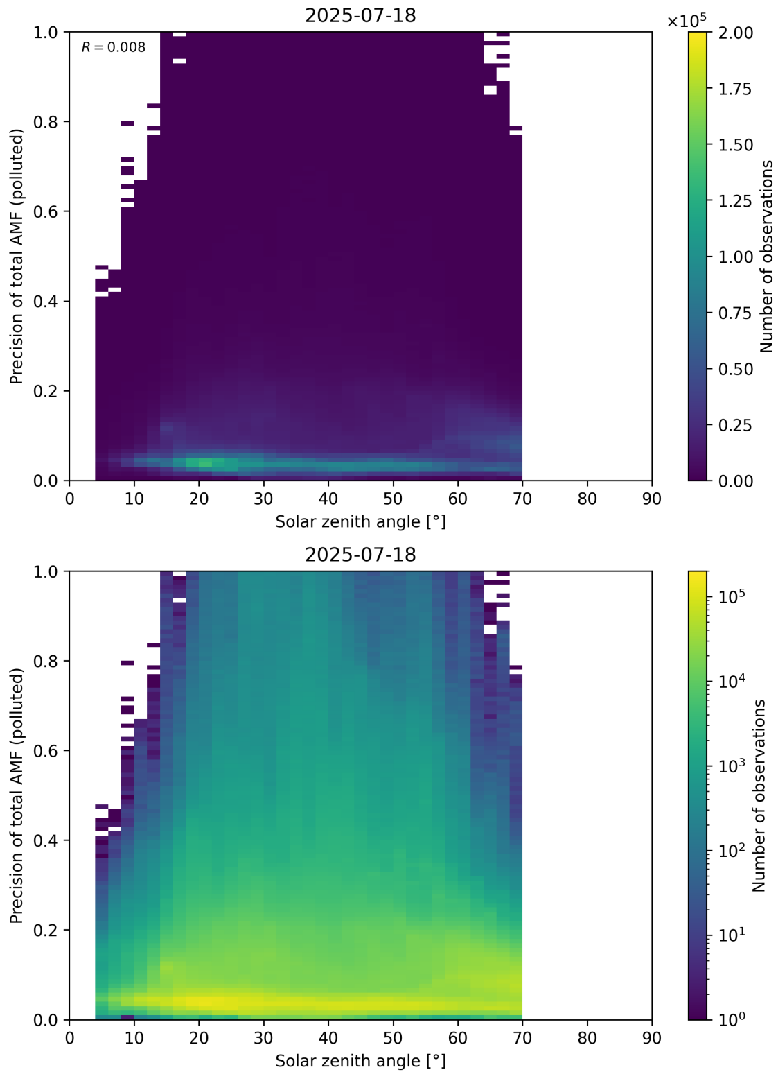
Figure 190: Scatter density plot of “Solar zenith angle” against “Precision of total AMF (polluted)” for 2025-07-18 to 2025-07-19.
