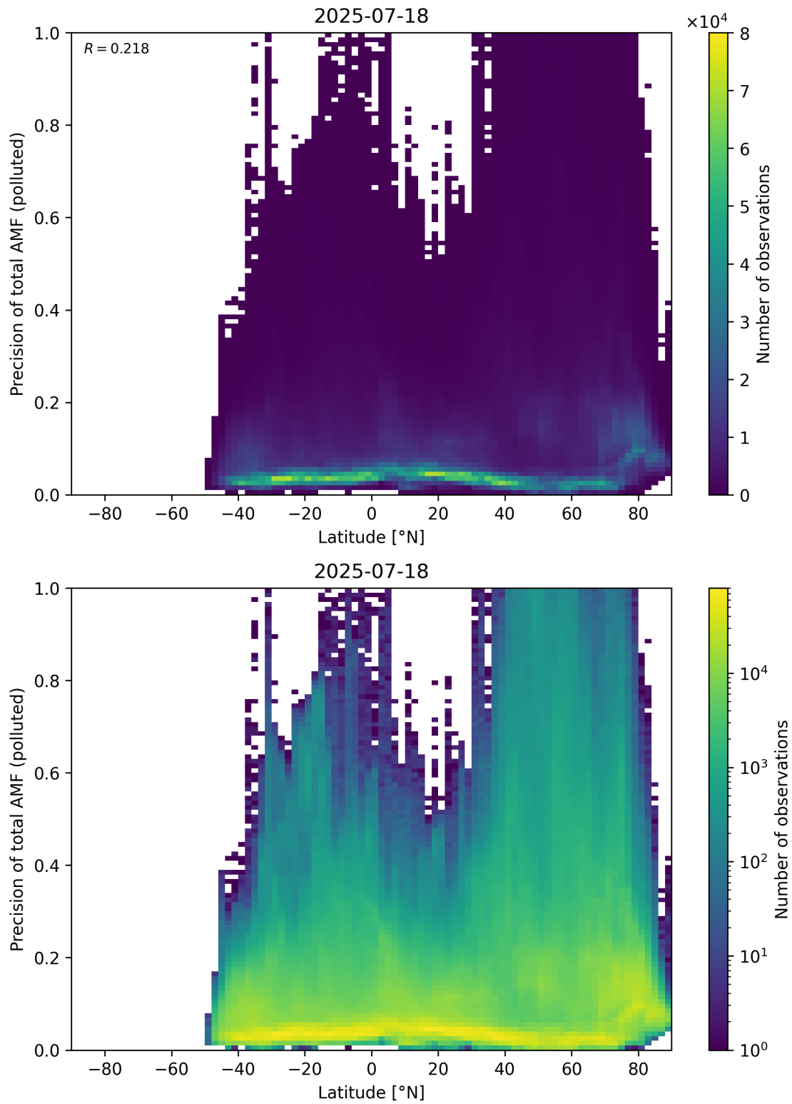
Figure 168: Scatter density plot of “Latitude” against “Precision of total AMF (polluted)” for 2025-07-18 to 2025-07-19.
