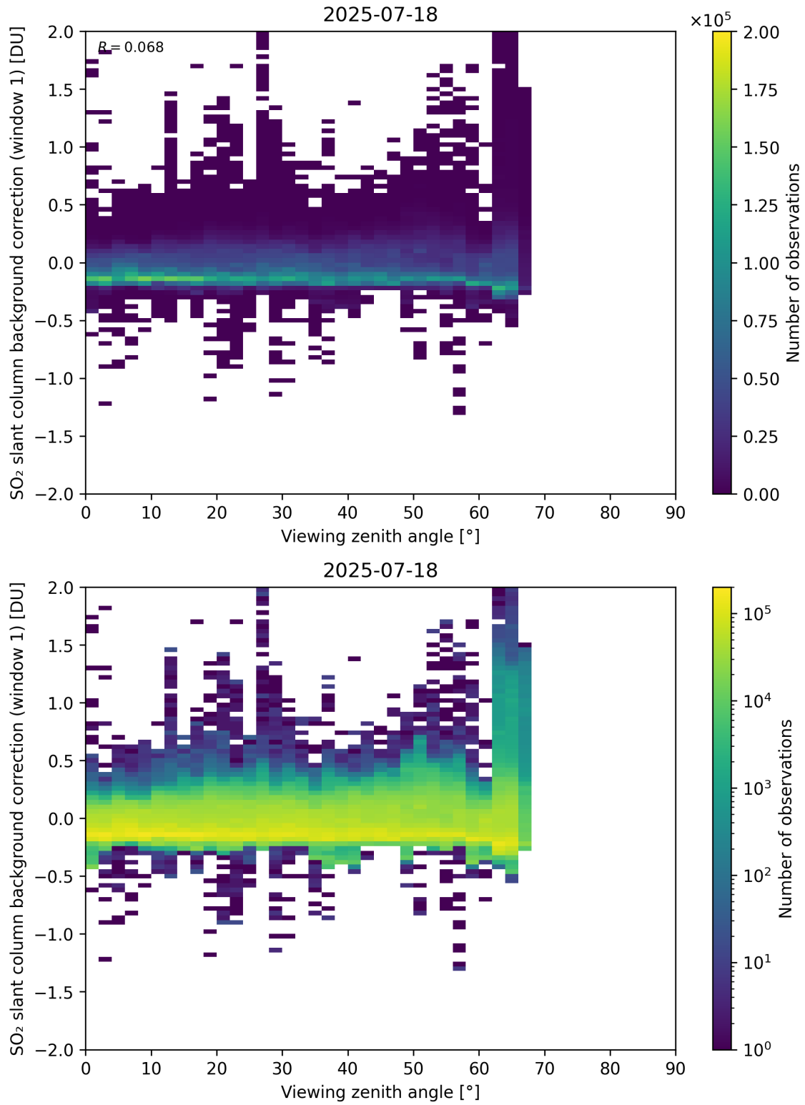
Figure 362: Scatter density plot of “Viewing zenith angle” against “SO 2 slant column background correction (window 1)” for 2025-07-18 to 2025-07-19.
