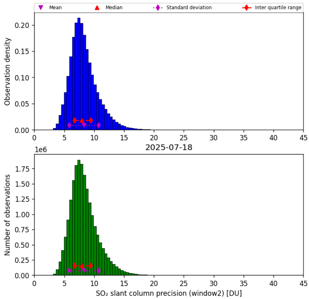
Figure 68: Histogram of “SO 2 slant column precision (window2)” for 2025-07-18 to 2025-07-19
