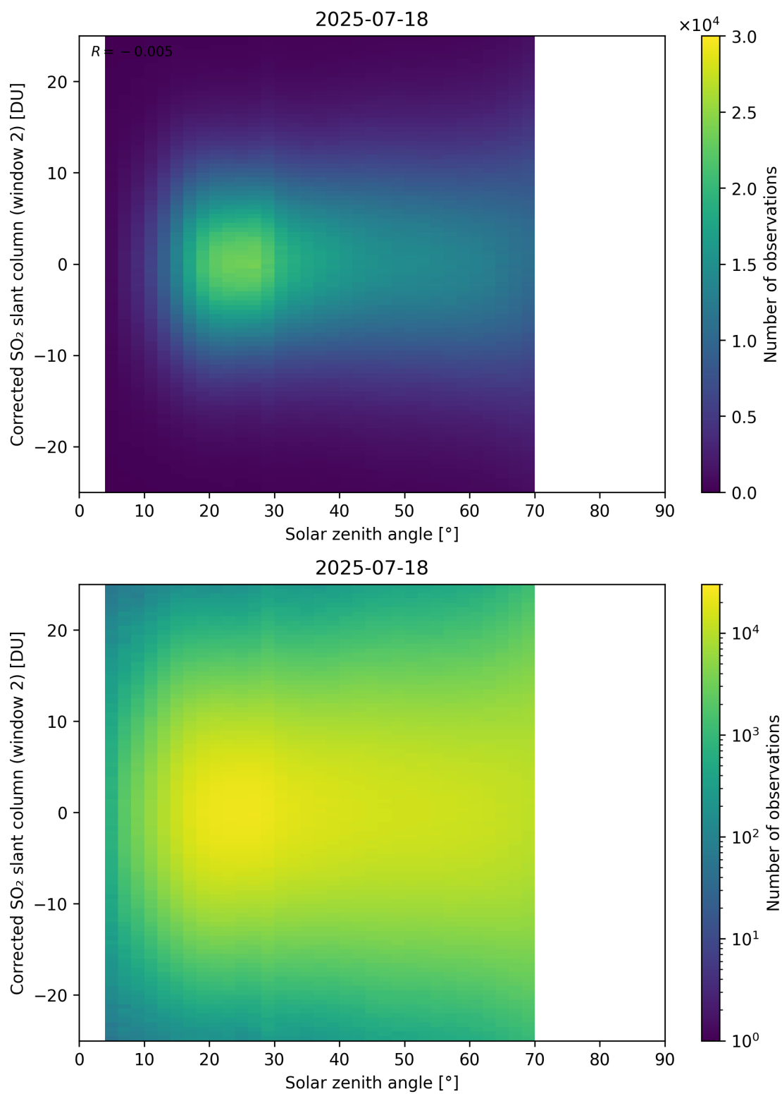
Figure 182: Scatter density plot of “Solar zenith angle” against “Corrected SO 2 slant column (window 2)” for 2025-07-18 to 2025-07-19.
