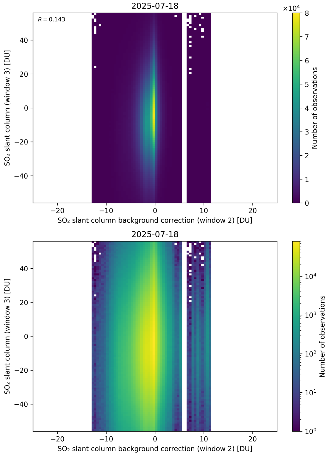
Figure 128: Scatter density plot of “SO 2 slant column background correction (window 2)” against “SO 2 slant column (window 3)” for 2025-07-18 to 2025-07-19.
