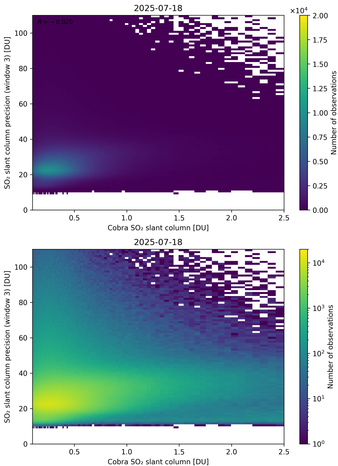
Figure 223: Scatter density plot of “Cobra SO 2 slant column” against “SO 2 slant column precision (window 3)” for 2025-07-18 to 2025-07-19.
