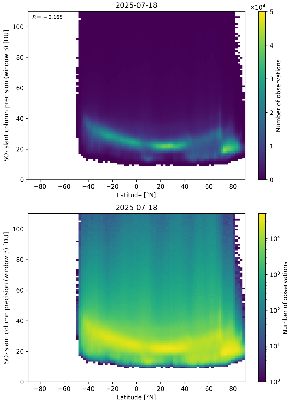
Figure 166: Scatter density plot of “Latitude” against “SO 2 slant column precision (window 3)” for 2025-07-18 to 2025-07-19.
