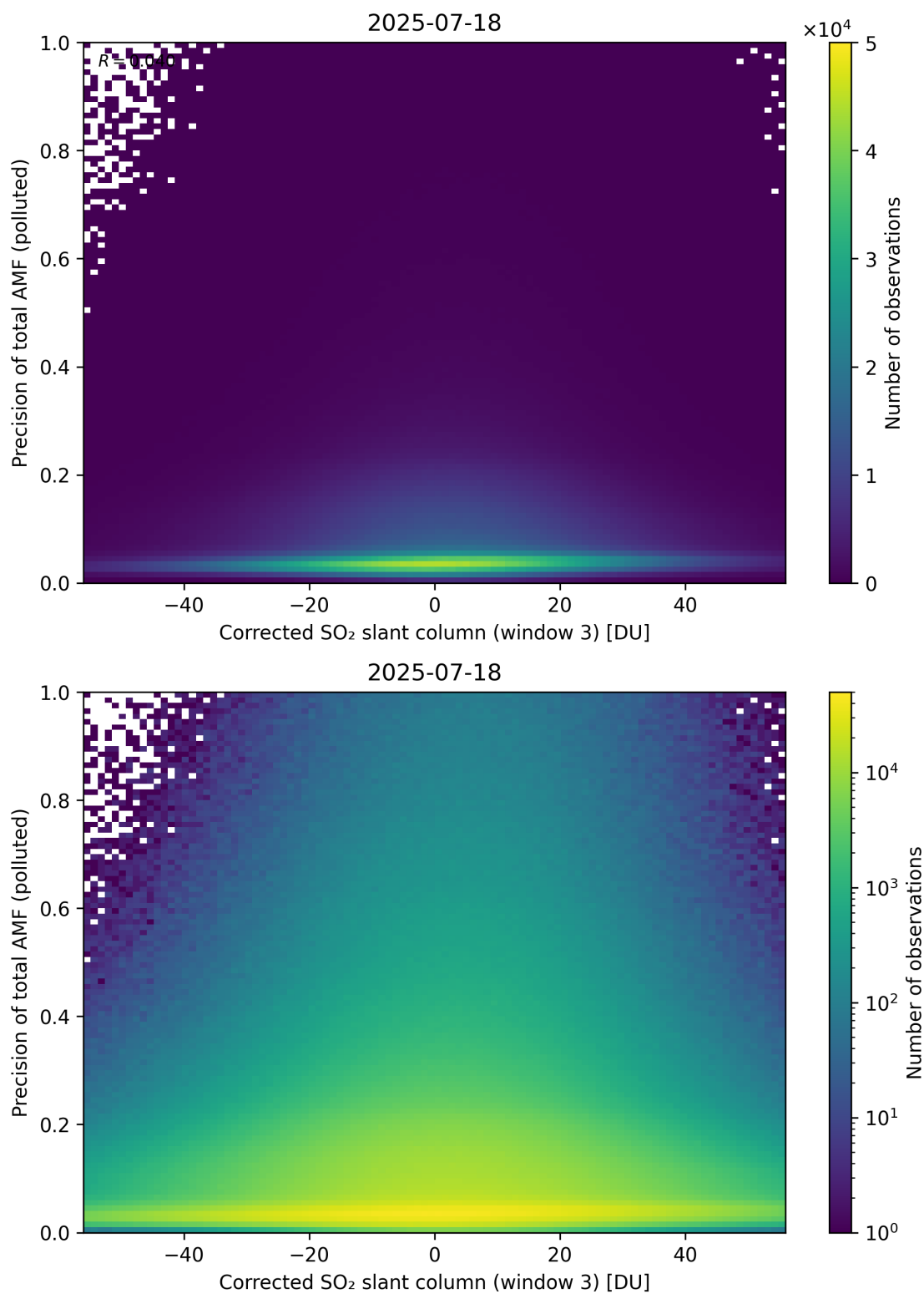
Figure 261: Scatter density plot of “Corrected SO 2 slant column (window 3)” against “Precision of total AMF (polluted)” for 2025-07-18 to 2025-07-19.
