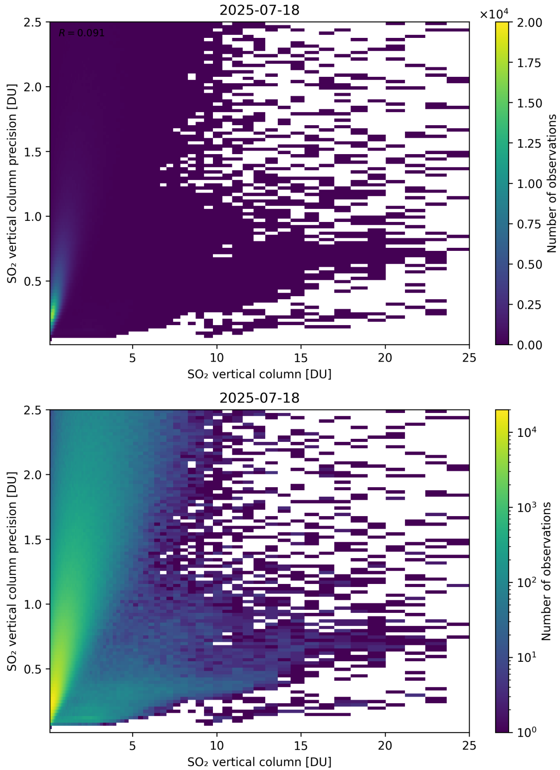
Figure 361: Scatter density plot of “SO 2 vertical column” against “SO 2 vertical column precision” for 2025-07-18 to 2025-07-19.
