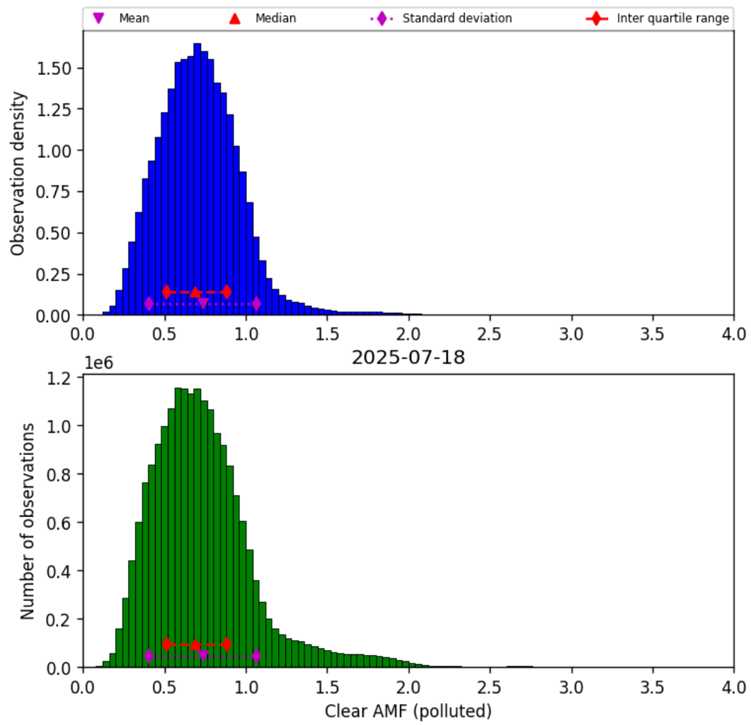
Figure 81: Histogram of “Clear AMF (polluted)” for 2025-07-18 to 2025-07-19
