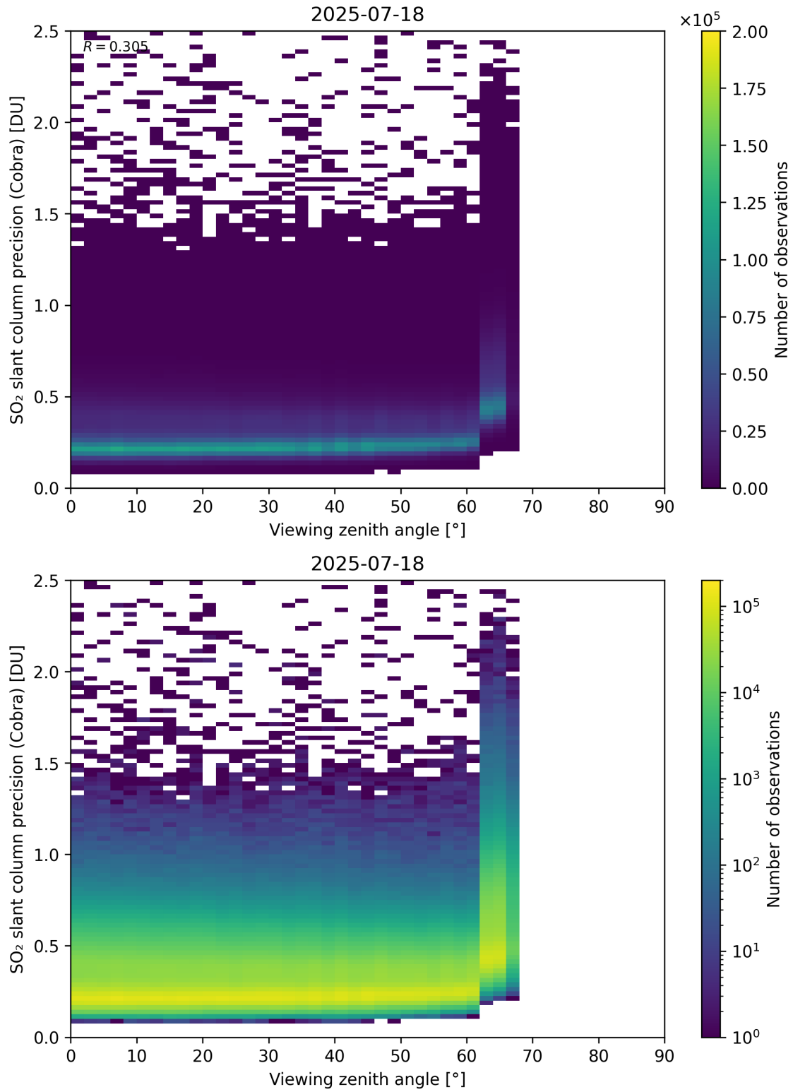
Figure 372: Scatter density plot of “Viewing zenith angle” against “SO 2 slant column precision (Cobra)” for 2025-07-18 to 2025-07-19.
