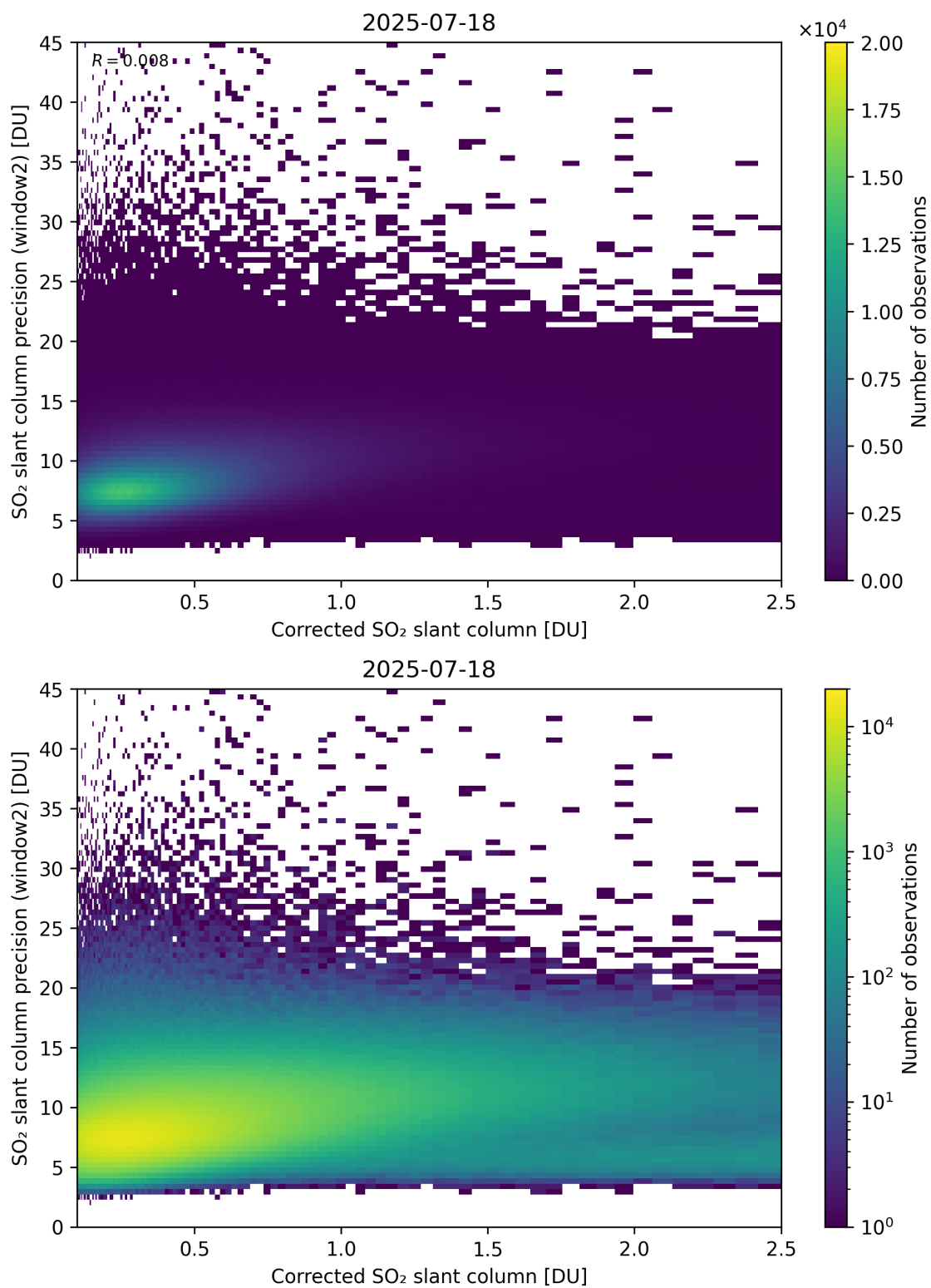
Figure 239: Scatter density plot of “Corrected SO 2 slant column” against “SO 2 slant column precision (window2)” for 2025-07-18 to 2025-07-19.
