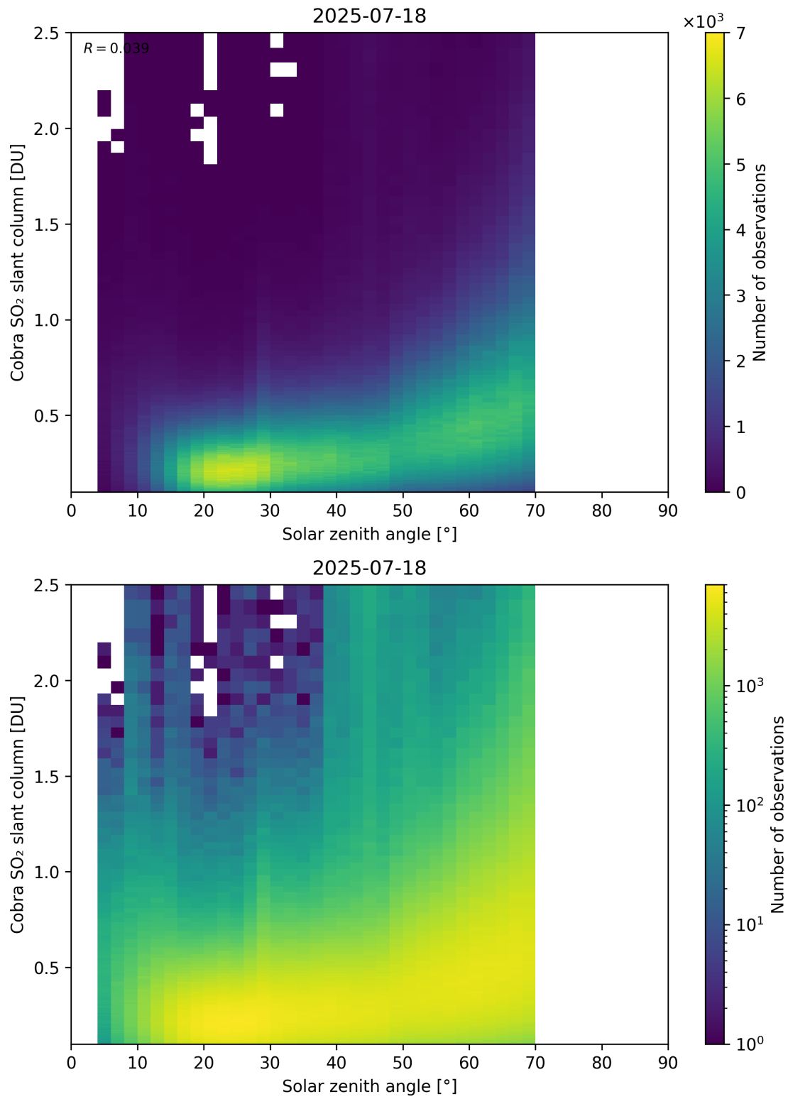
Figure 179: Scatter density plot of “Solar zenith angle” against “Cobra SO 2 slant column” for 2025-07-18 to 2025-07-19.
