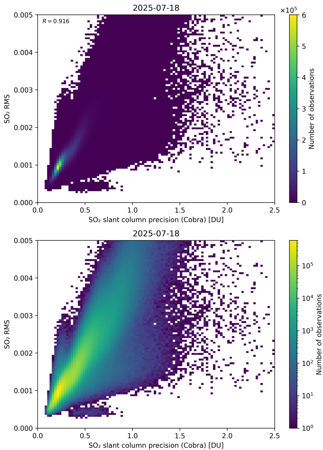
Figure 204: Scatter density plot of “SO 2 slant column precision (Cobra)” against “SO 2 RMS” for 2025-07-18 to 2025-07-19.
