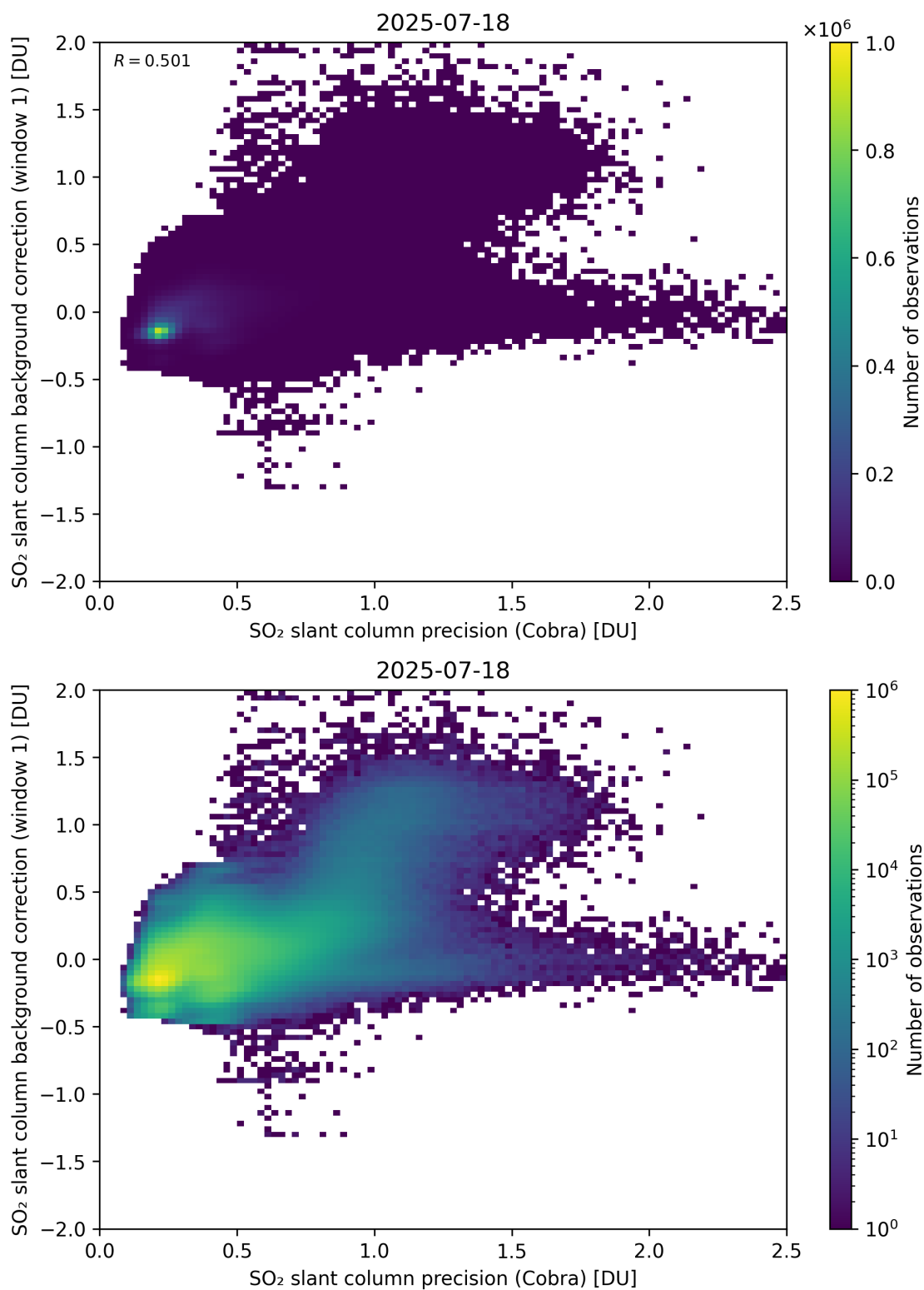
Figure 199: Scatter density plot of “SO 2 slant column precision (Cobra)” against “SO 2 slant column background correction (window 1)” for 2025-07-18 to 2025-07-19.
