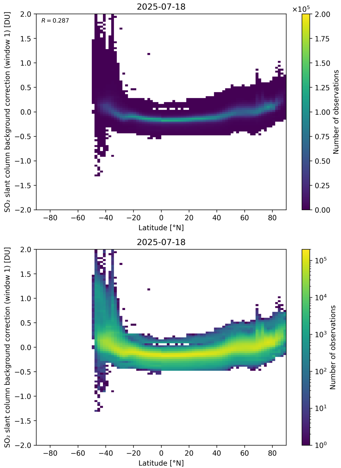
Figure 150: Scatter density plot of “Latitude” against “SO 2 slant column background correction (window 1)” for 2025-07-18 to 2025-07-19.
