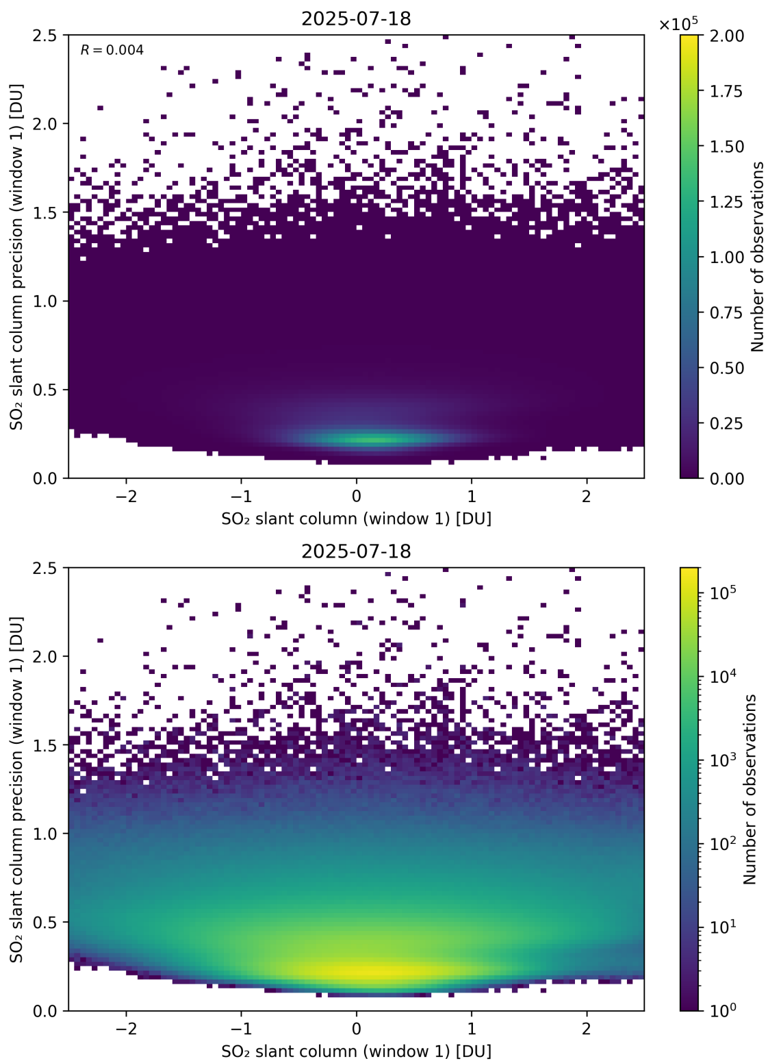
Figure 285: Scatter density plot of “SO 2 slant column (window 1)” against “SO 2 slant column precision (window 1)” for 2025-07-18 to 2025-07-19.
