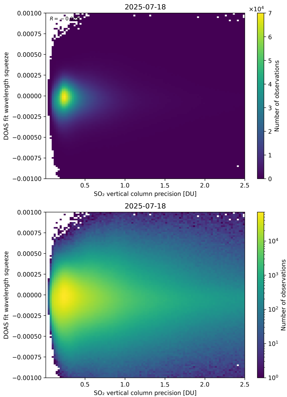
Figure 333: Scatter density plot of “SO 2 vertical column precision” against “DOAS fit wavelength squeeze” for 2025-07-18 to 2025-07-19.
