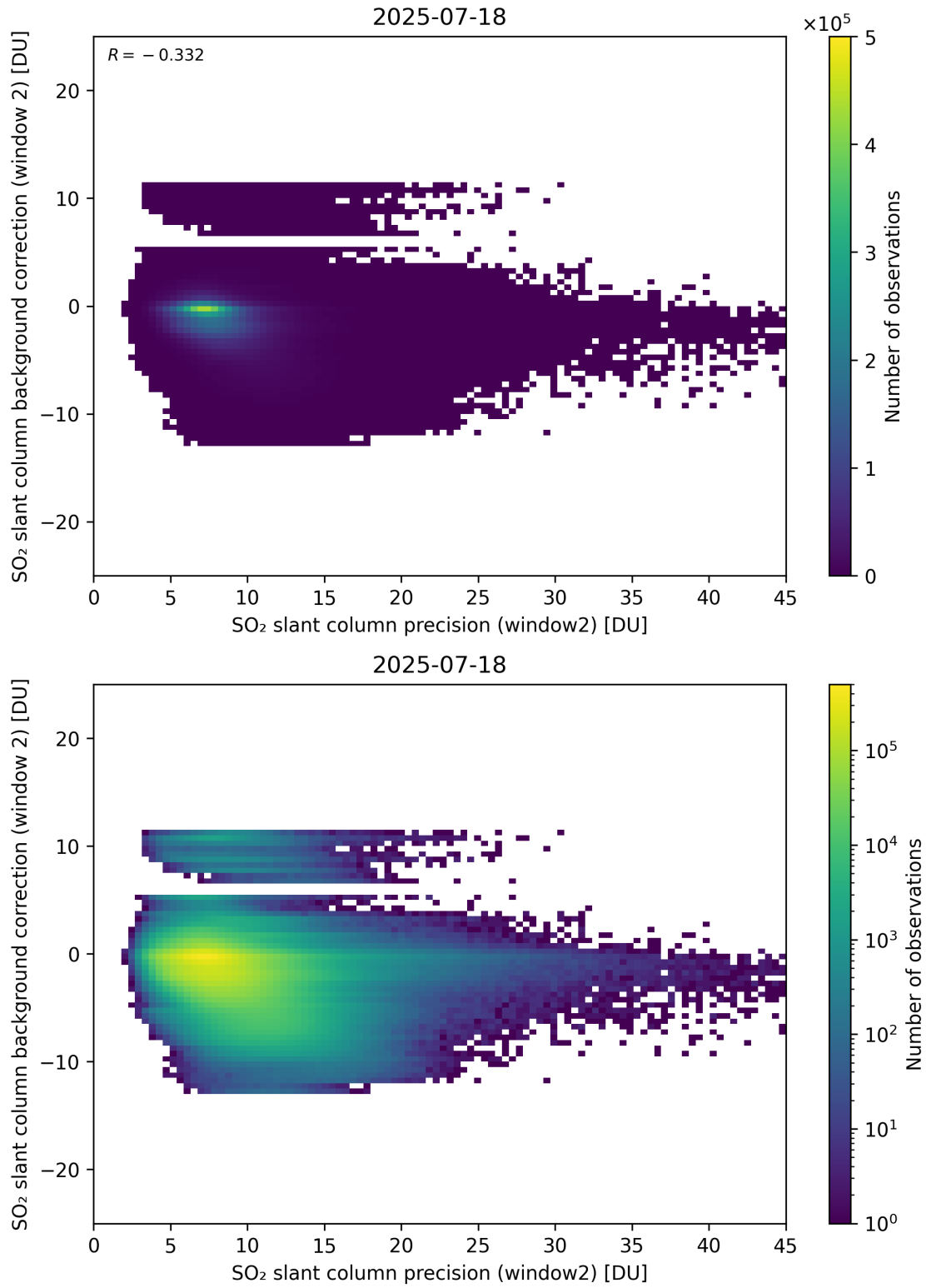
Figure 291: Scatter density plot of “SO 2 slant column precision (window2)” against “SO 2 slant column background correction (window 2)” for 2025-07-18 to 2025-07-19.
