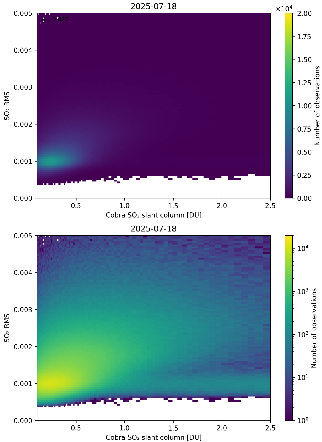
Figure 198: Scatter density plot of “Cobra SO 2 slant column” against “SO 2 RMS” for 2025-07-18 to 2025-07-19.
