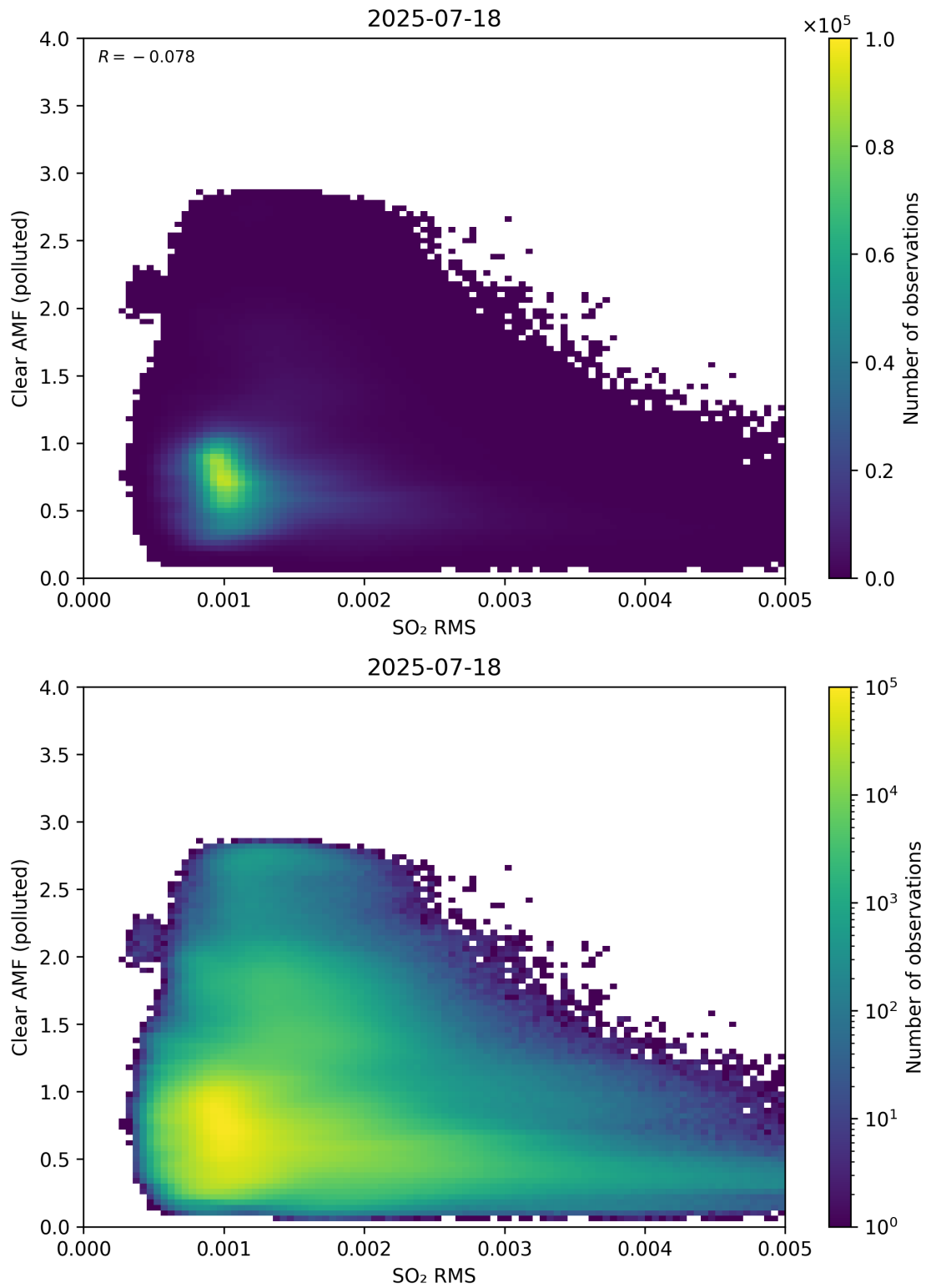
Figure 147: Scatter density plot of “SO 2 RMS” against “Clear AMF (polluted)” for 2025-07-18 to 2025-07-19.
