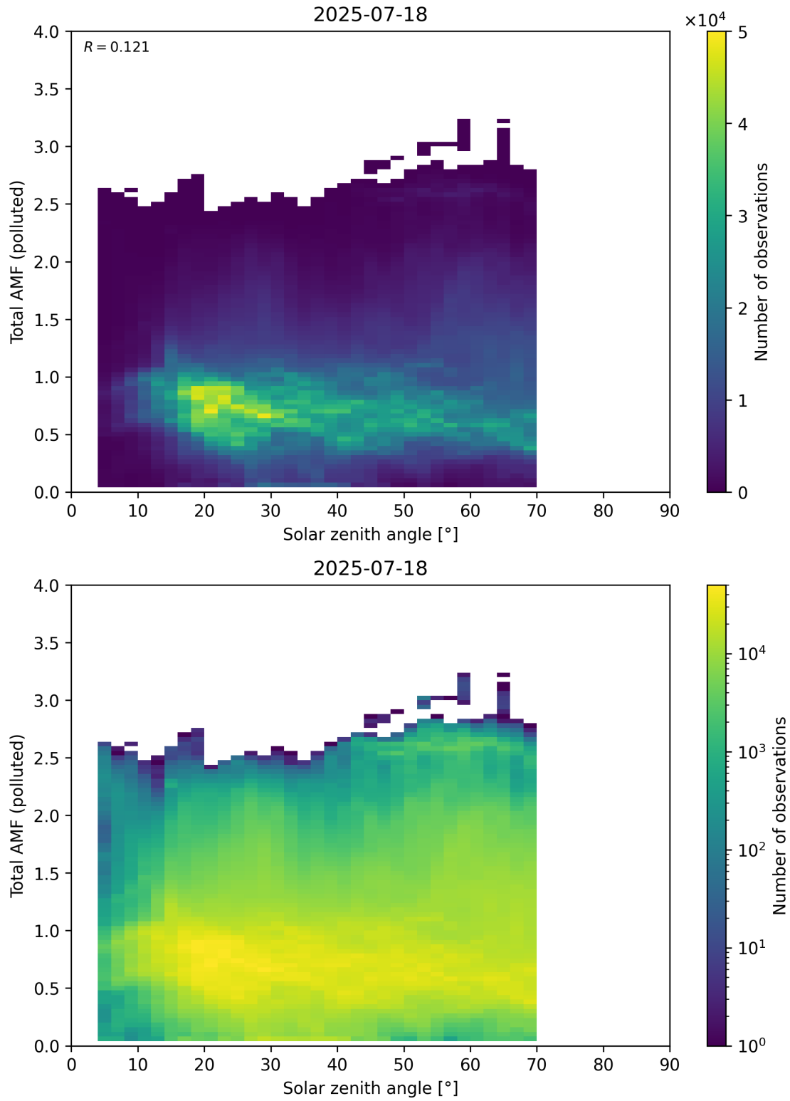
Figure 189: Scatter density plot of “Solar zenith angle” against “Total AMF (polluted)” for 2025-07-18 to 2025-07-19.
