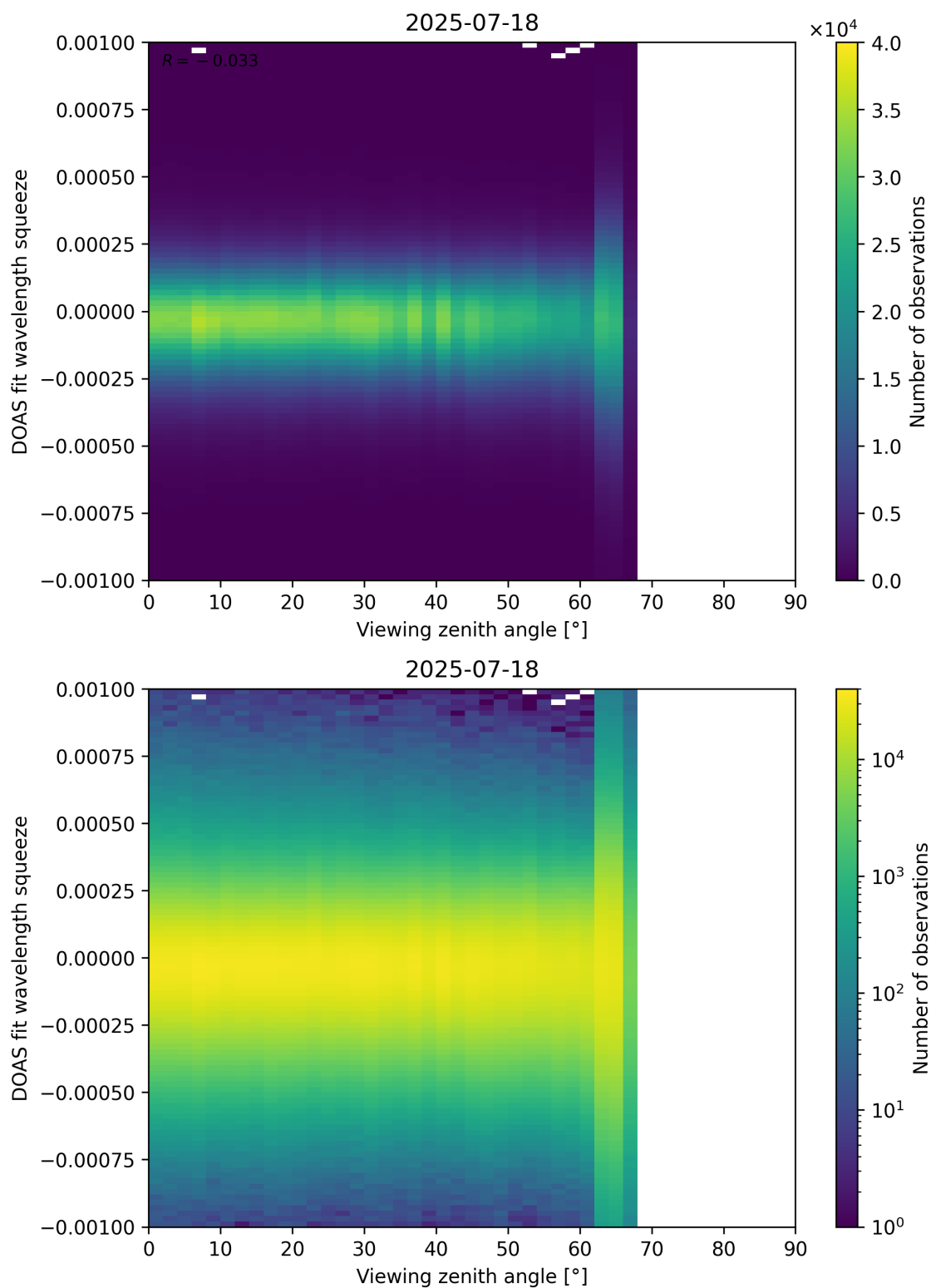
Figure 366: Scatter density plot of “Viewing zenith angle” against “DOAS fit wavelength squeeze” for 2025-07-18 to 2025-07-19.
