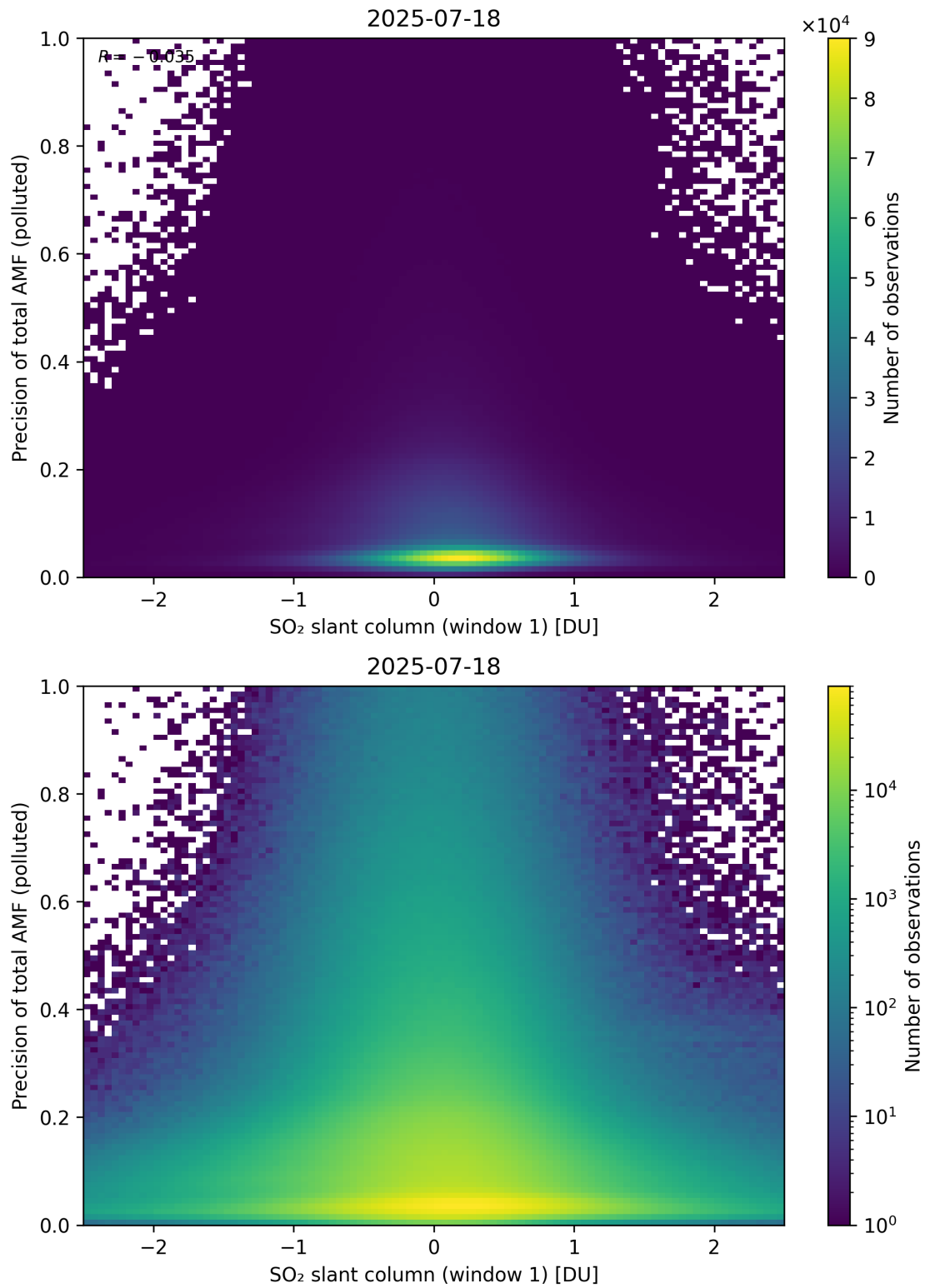
Figure 290: Scatter density plot of “SO 2 slant column (window 1)” against “Precision of total AMF (polluted)” for 2025-07-18 to 2025-07-19.
