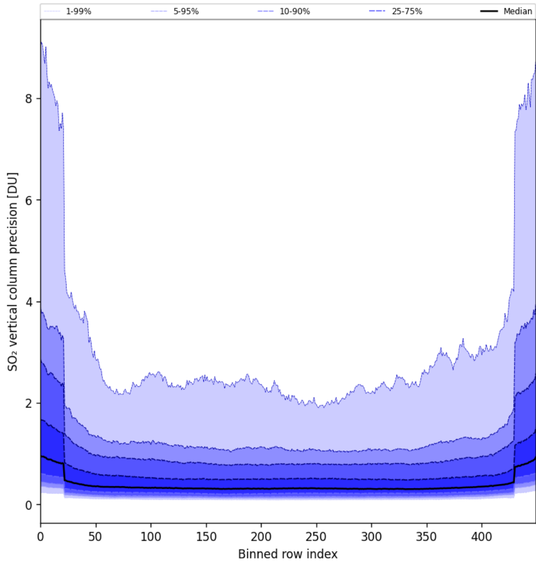
Figure 85: Along track statistics of “SO 2 vertical column precision” for 2025-07-18 to 2025-07-19
