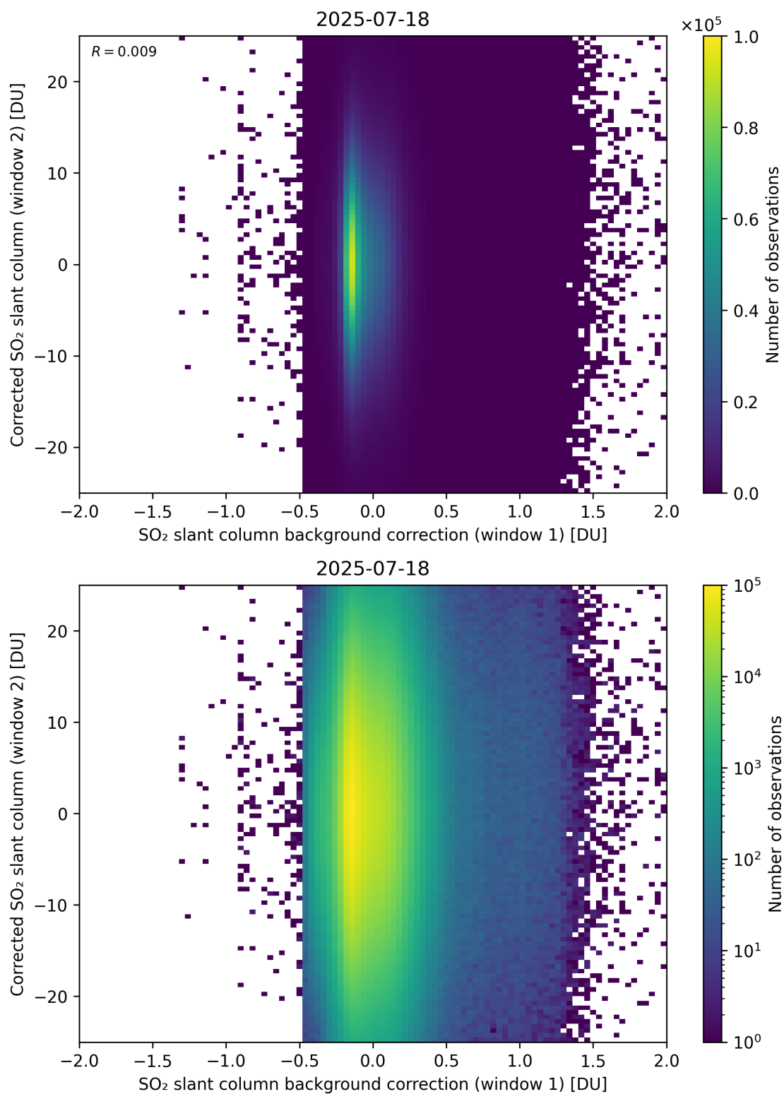
Figure 115: Scatter density plot of “SO 2 slant column background correction (window 1)” against “Corrected SO 2 slant column (window 2)” for 2025-07-18 to 2025-07-19.
