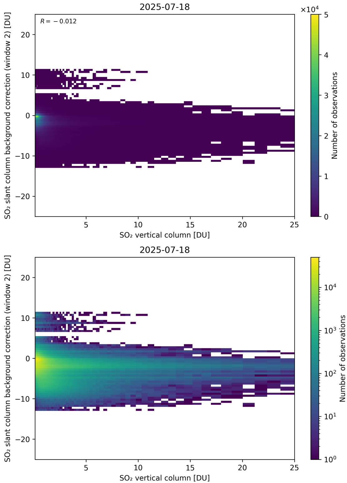
Figure 324: Scatter density plot of “SO 2 vertical column” against “SO 2 slant column background correction (window 2)” for 2025-07-18 to 2025-07-19.
