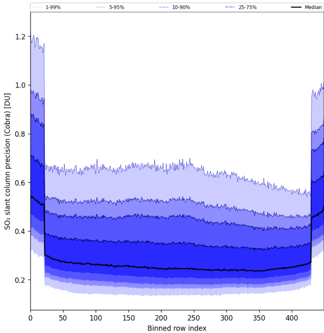
Figure 88: Along track statistics of “SO 2 slant column precision (Cobra)” for 2025-07-18 to 2025-07-19
