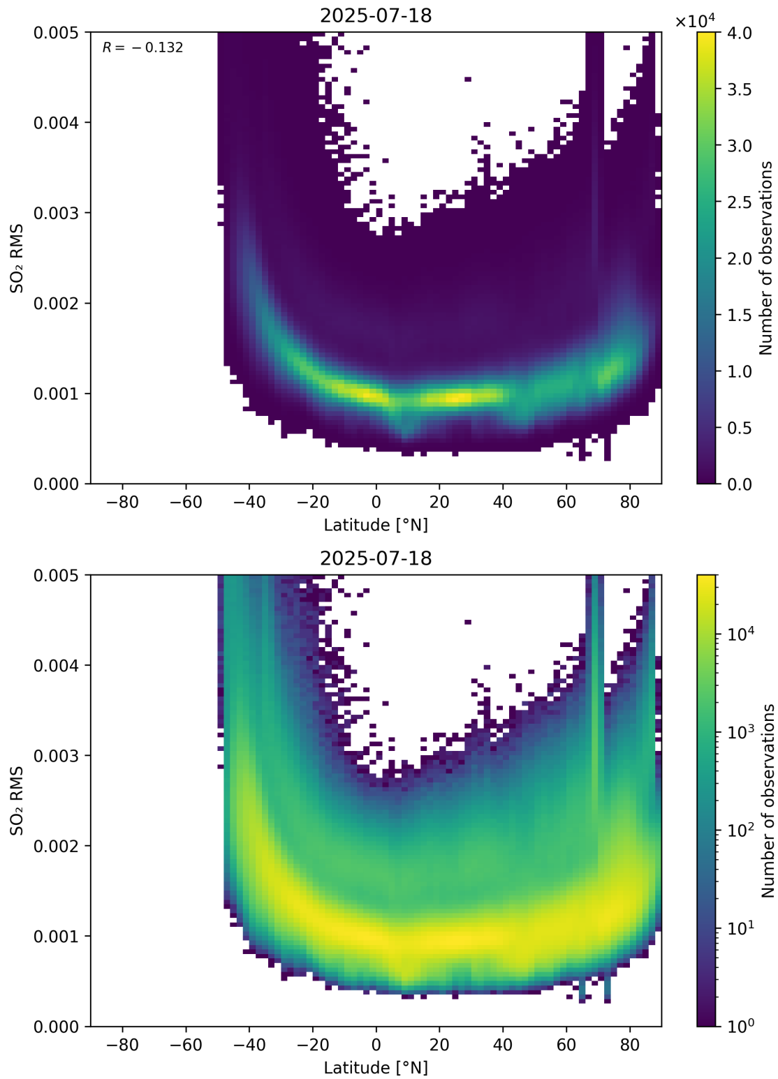
Figure 155: Scatter density plot of “Latitude” against “SO 2 RMS” for 2025-07-18 to 2025-07-19.
