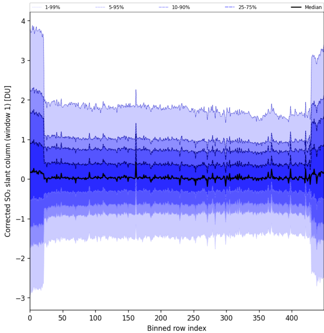
Figure 91: Along track statistics of “Corrected SO 2 slant column (window 1)” for 2025-07-18 to 2025-07-19
