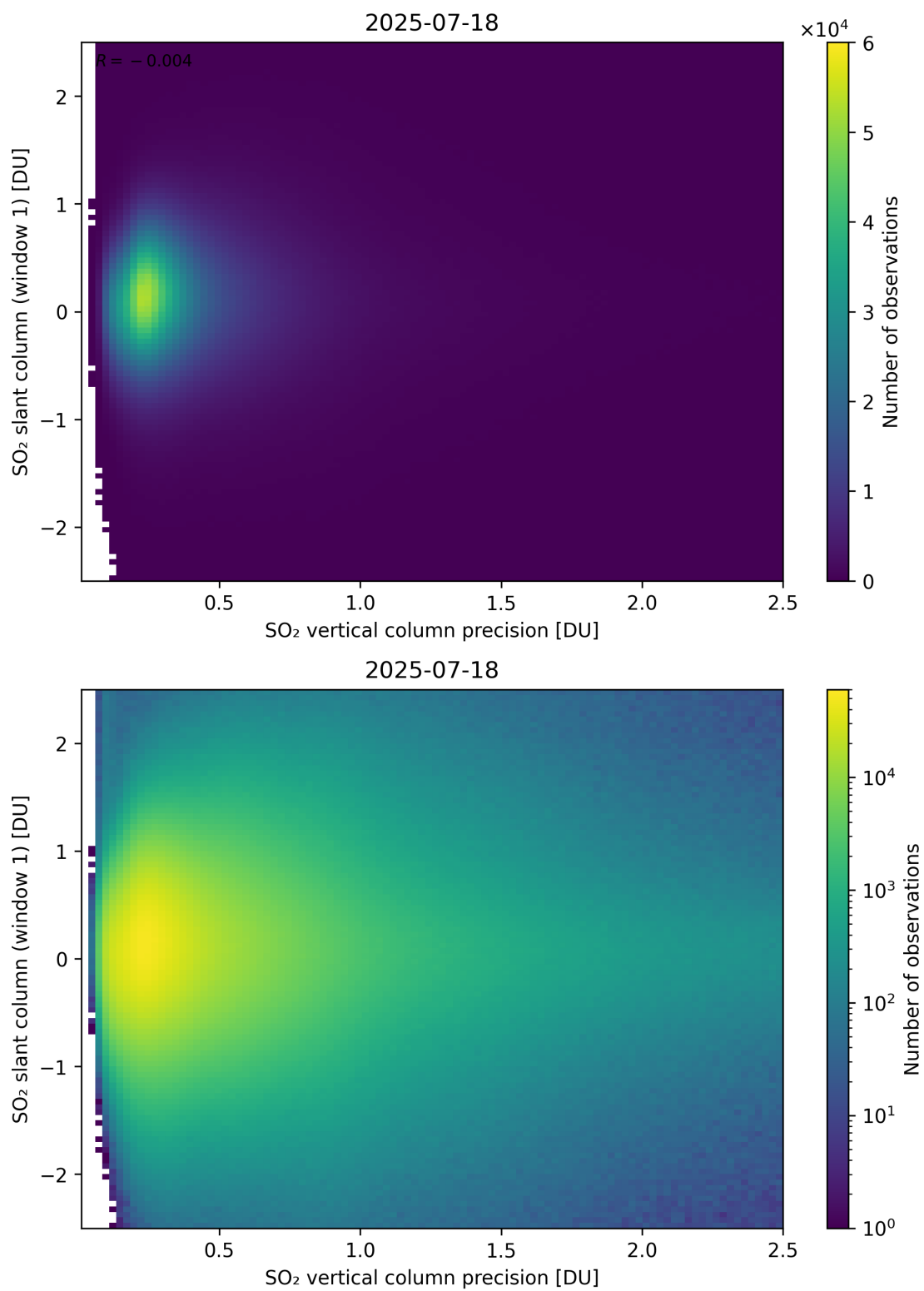
Figure 341: Scatter density plot of “SO 2 vertical column precision” against “SO 2 slant column (window 1)” for 2025-07-18 to 2025-07-19.
