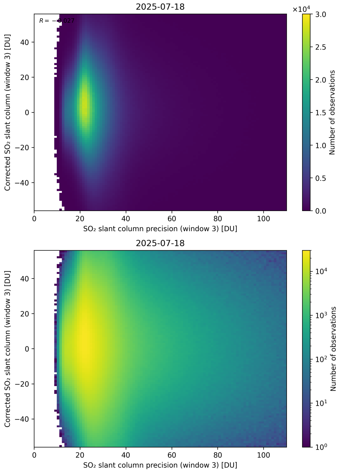
Figure 312: Scatter density plot of “SO 2 slant column precision (window 3)” against “Corrected SO 2 slant column (window 3)” for 2025-07-18 to 2025-07-19.
