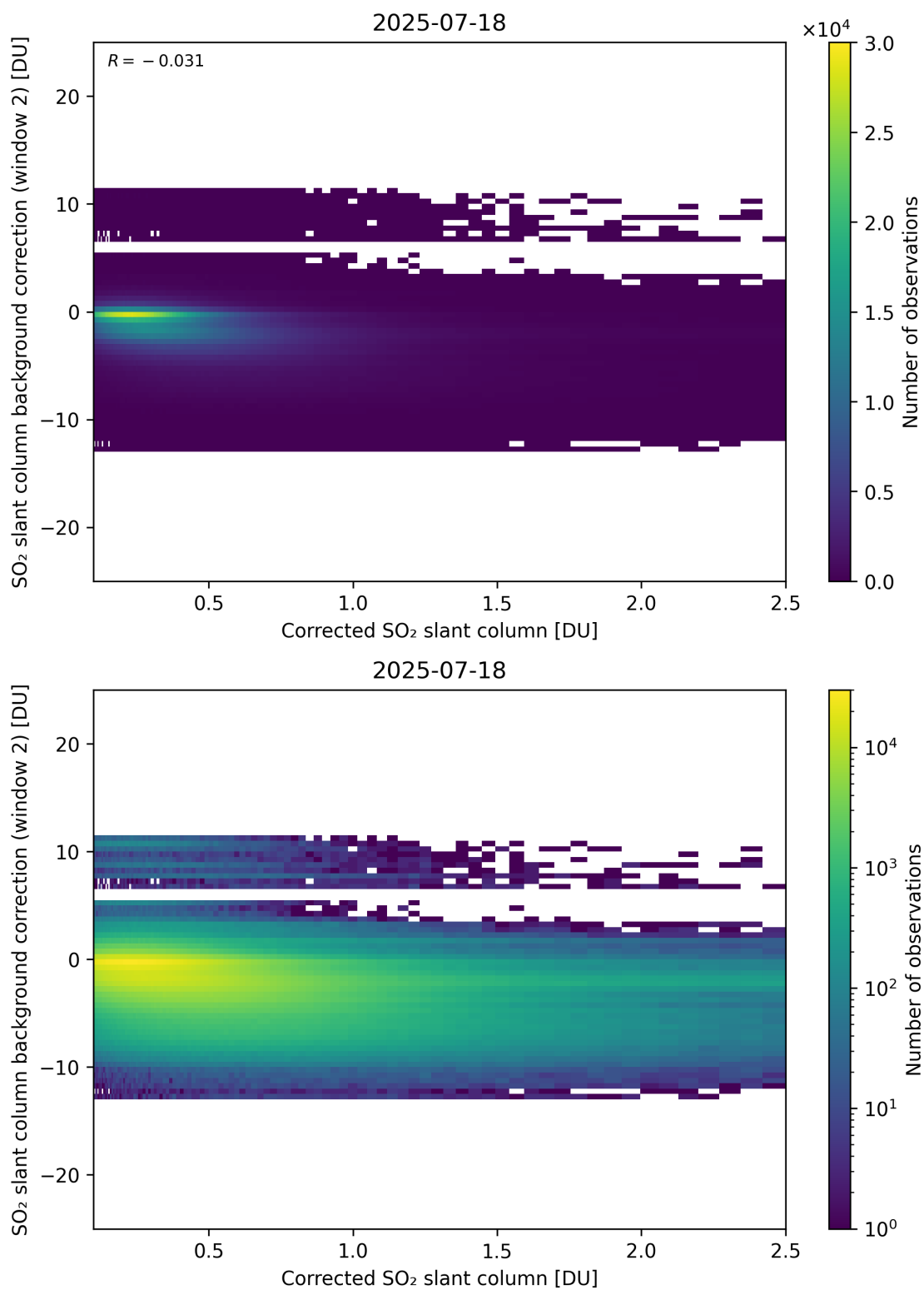
Figure 227: Scatter density plot of “Corrected SO 2 slant column” against “SO 2 slant column background correction (window 2)” for 2025-07-18 to 2025-07-19.
