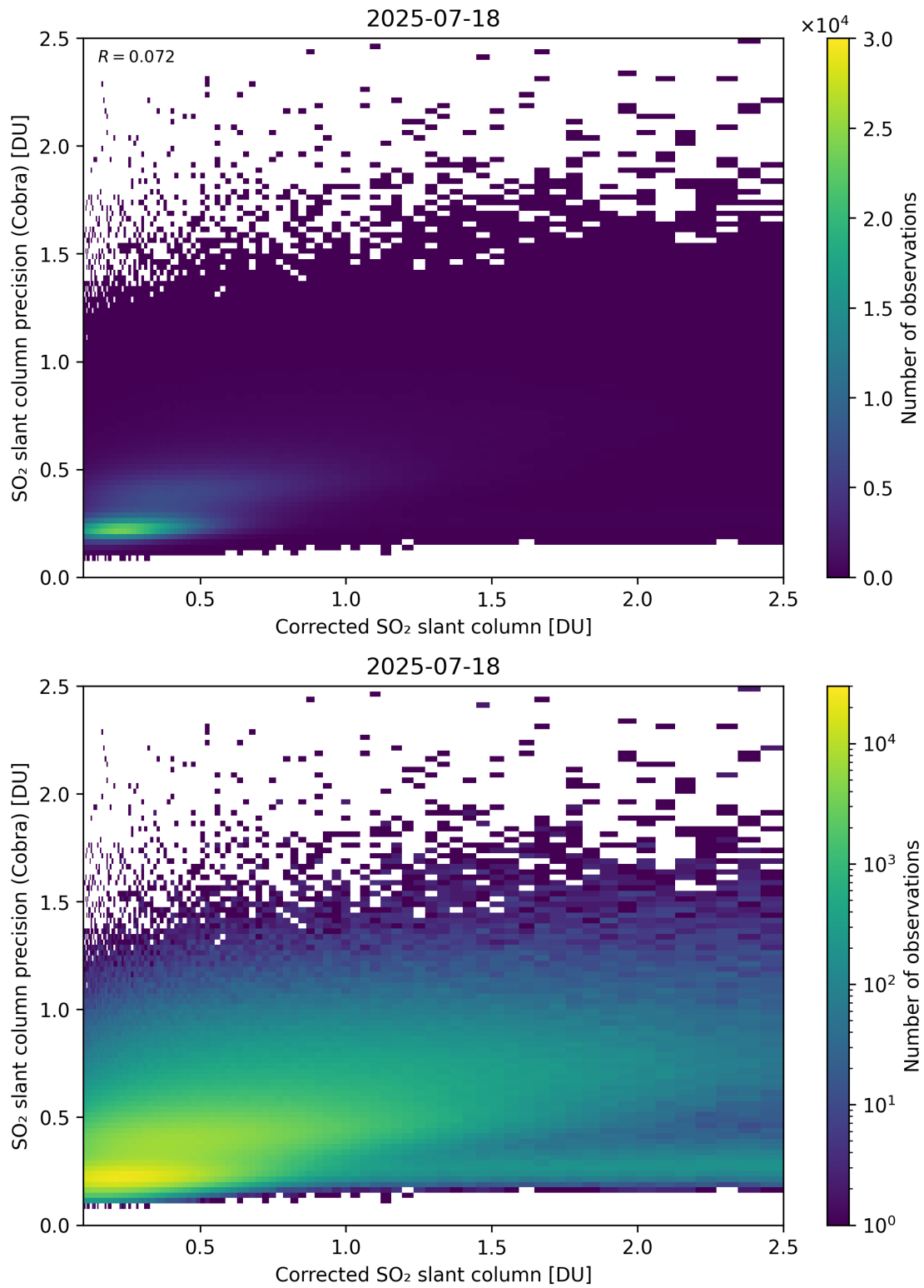
Figure 234: Scatter density plot of “Corrected SO 2 slant column” against “SO 2 slant column precision (Cobra)” for 2025-07-18 to 2025-07-19.
