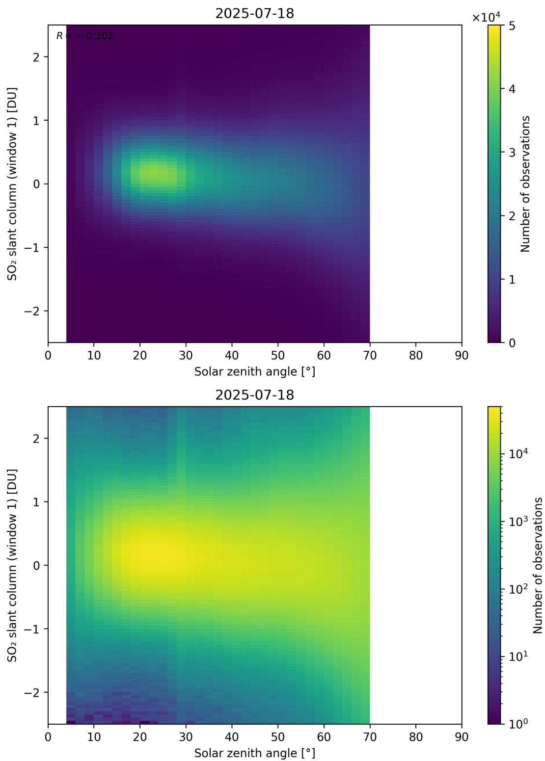
Figure 184: Scatter density plot of “Solar zenith angle” against “SO 2 slant column (window 1)” for 2025-07-18 to 2025-07-19.
