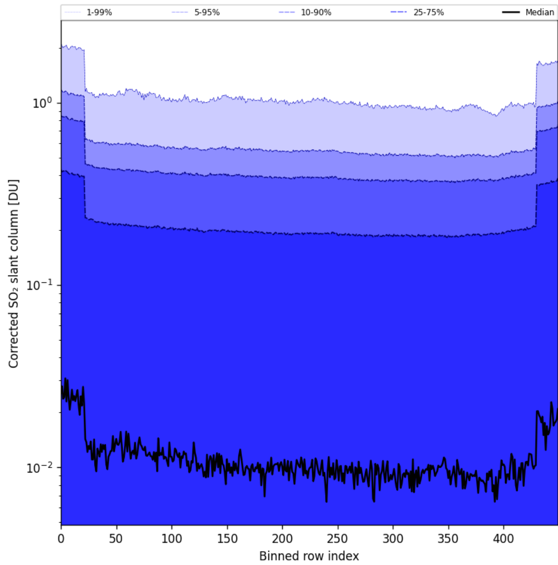
Figure 86: Along track statistics of “Corrected SO 2 slant column” for 2025-07-18 to 2025-07-19
