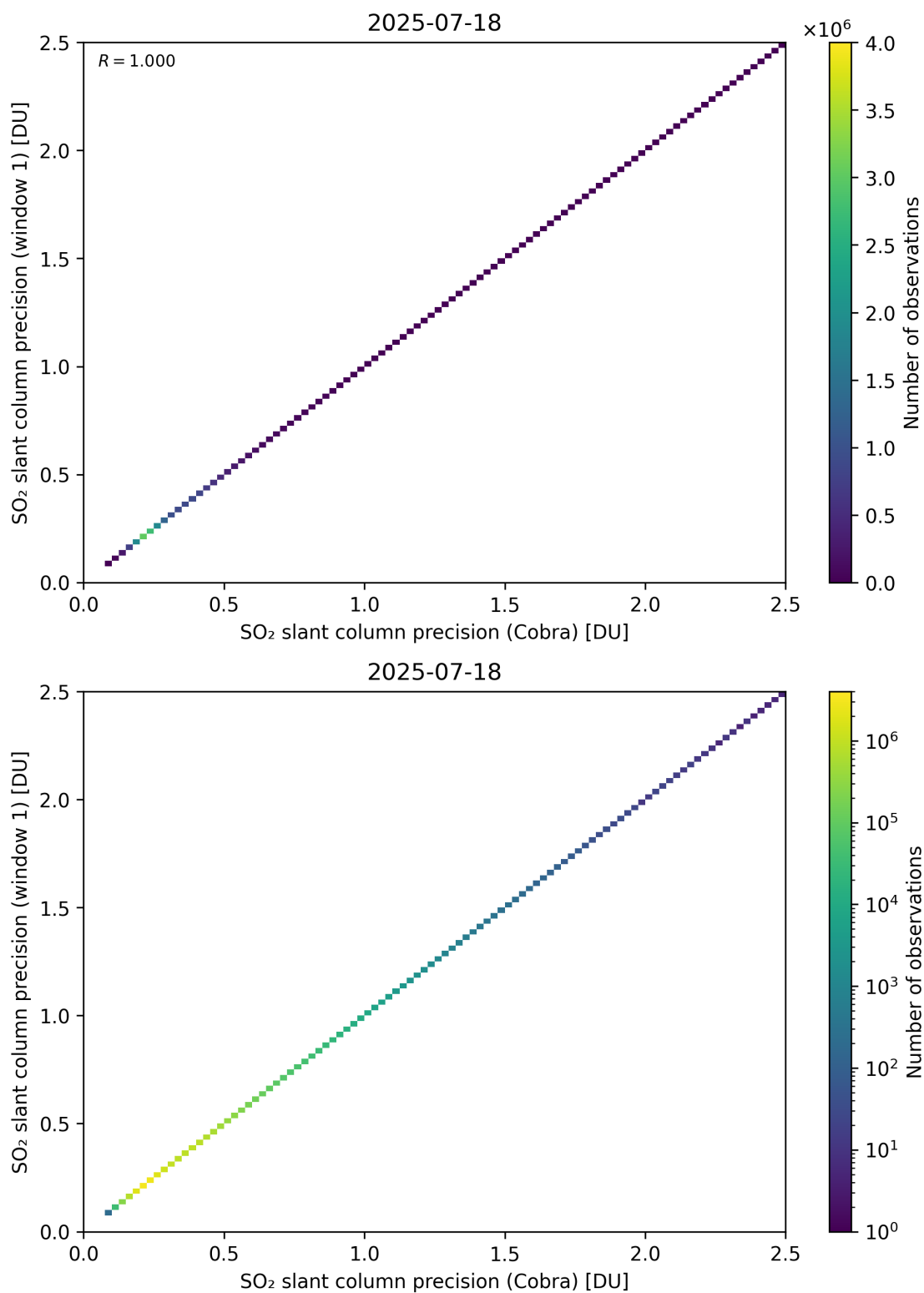
Figure 209: Scatter density plot of “SO 2 slant column precision (Cobra)” against “SO 2 slant column precision (window 1)” for 2025-07-18 to 2025-07-19.
