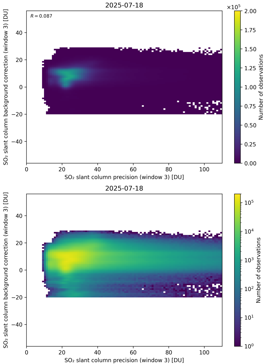
Figure 307: Scatter density plot of “SO 2 slant column precision (window 3)” against “SO 2 slant column background correction (window 3)” for 2025-07-18 to 2025-07-19.
