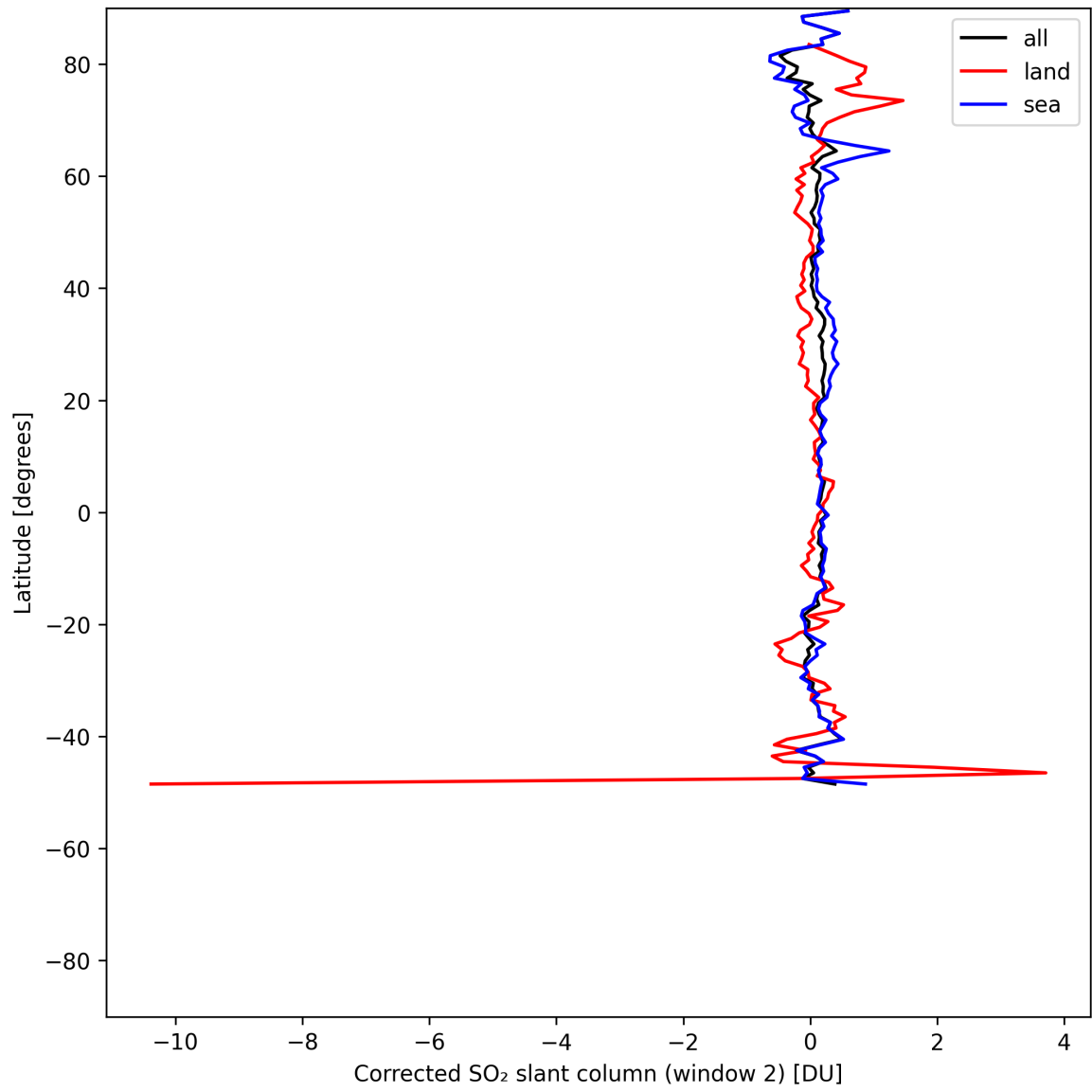
Figure 43: Zonal average of “Corrected SO 2 slant column (window 2)” for 2025-07-18 to 2025-07-19.
