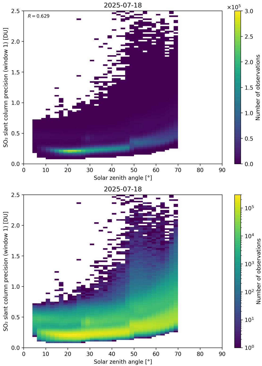
Figure 185: Scatter density plot of “Solar zenith angle” against “SO 2 slant column precision (window 1)” for 2025-07-18 to 2025-07-19.
