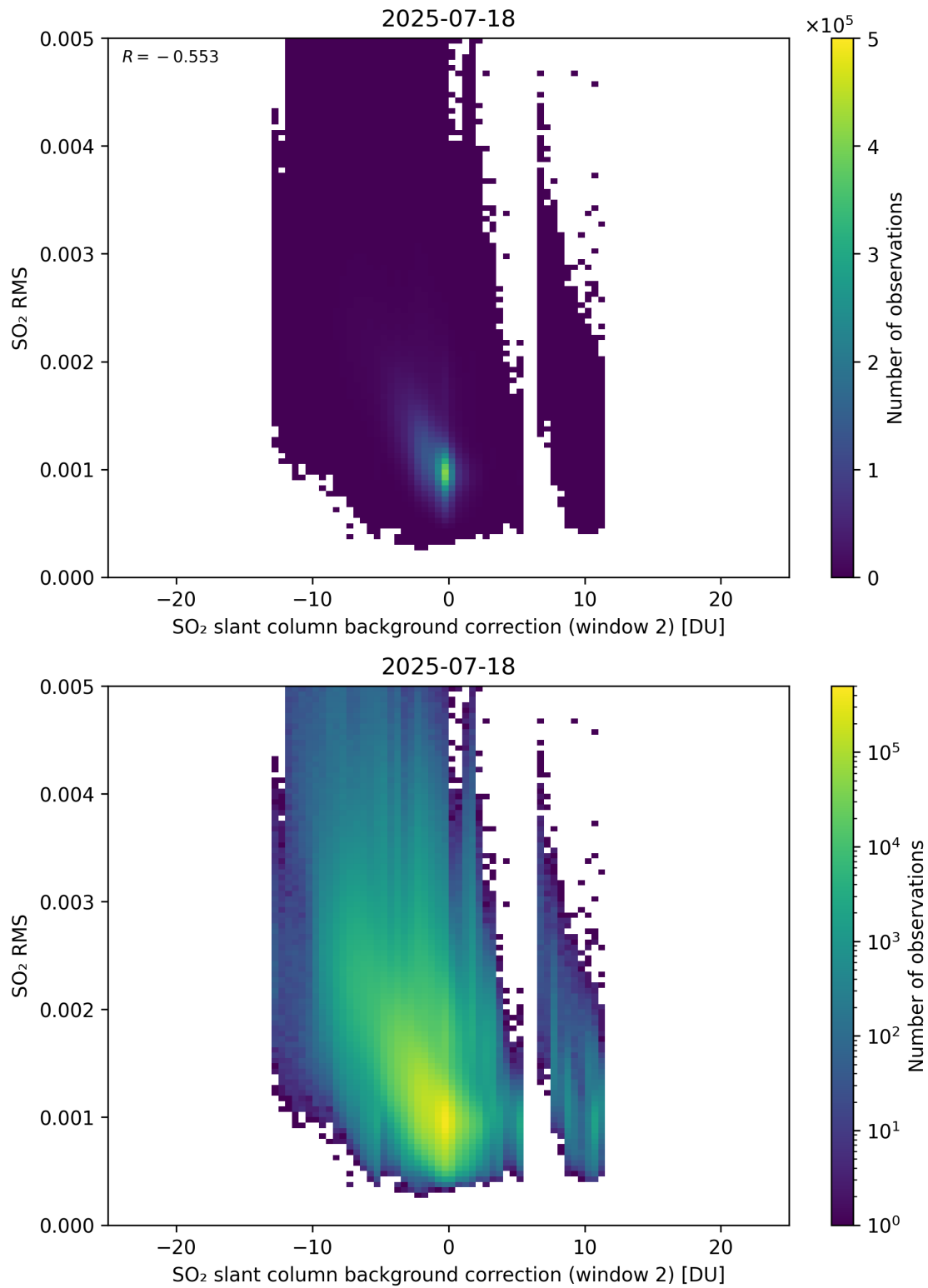
Figure 125: Scatter density plot of “SO 2 slant column background correction (window 2)” against “SO 2 RMS” for 2025-07-18 to 2025-07-19.
