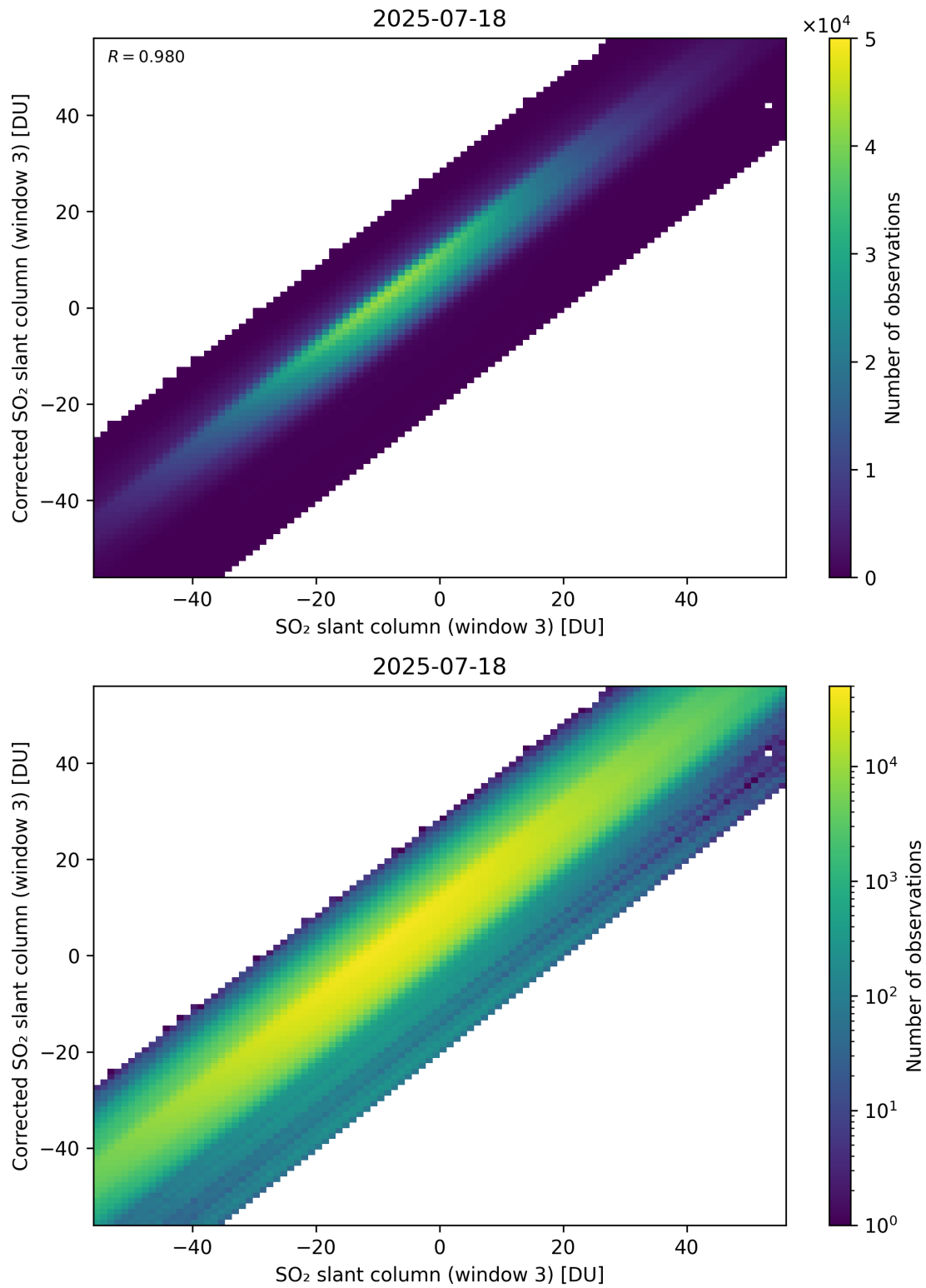
Figure 316: Scatter density plot of “SO 2 slant column (window 3)” against “Corrected SO 2 slant column (window 3)” for 2025-07-18 to 2025-07-19.
