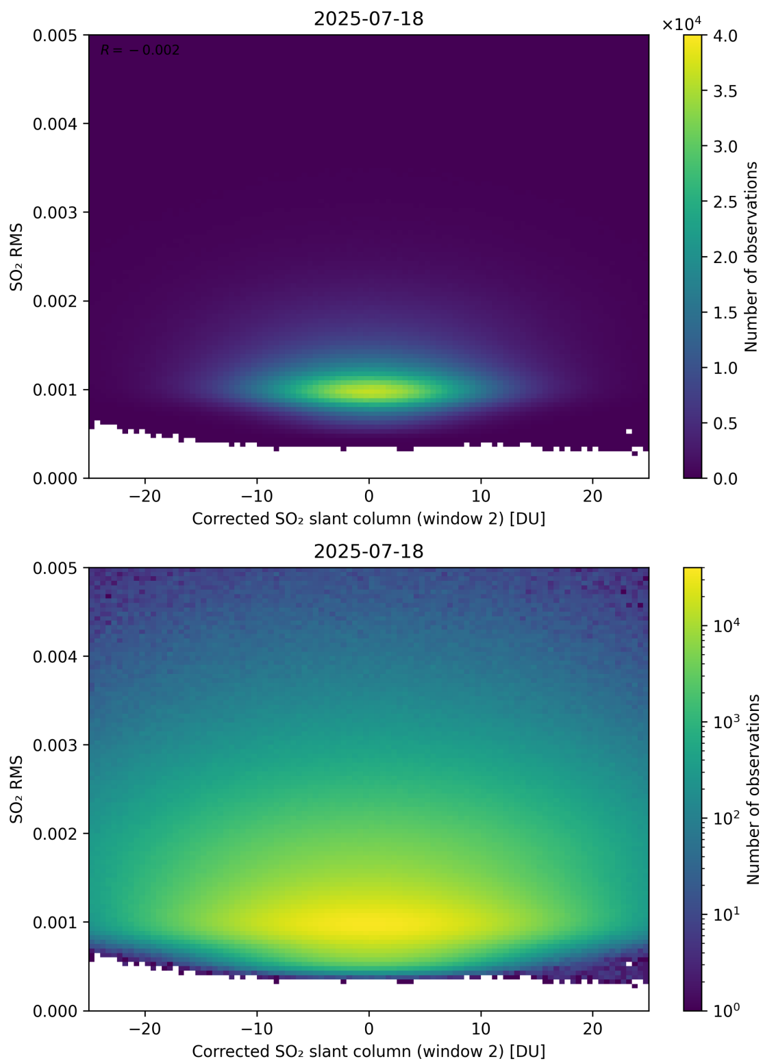
Figure 248: Scatter density plot of “Corrected SO 2 slant column (window 2)” against “SO 2 RMS” for 2025-07-18 to 2025-07-19.
