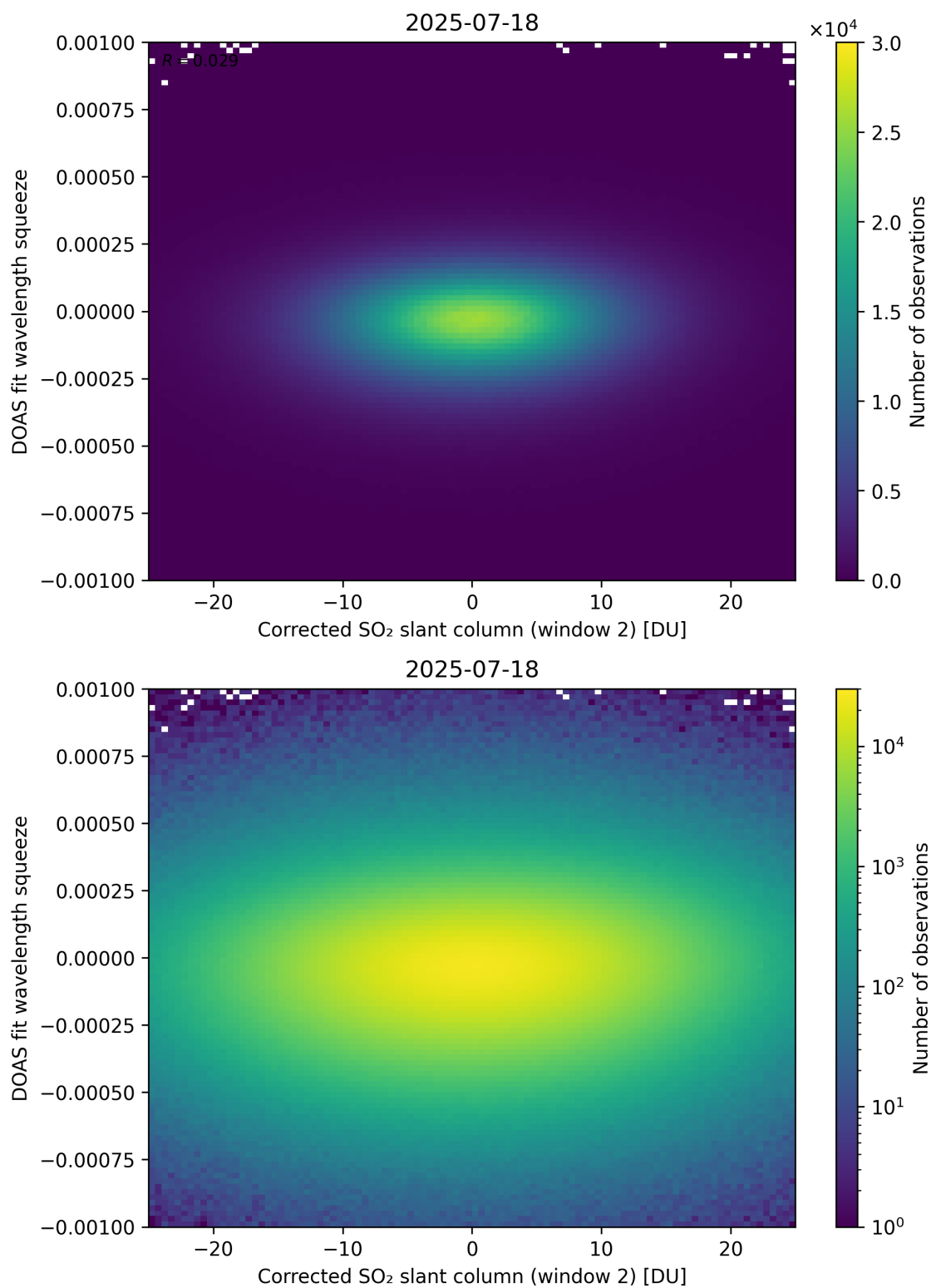
Figure 247: Scatter density plot of “Corrected SO 2 slant column (window 2)” against “DOAS fit wavelength squeeze” for 2025-07-18 to 2025-07-19.
