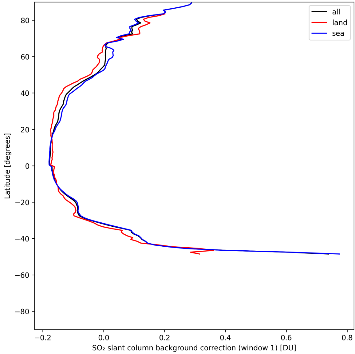
Figure 40: Zonal average of “SO 2 slant column background correction (window 1)” for 2025-07-18 to 2025-07-19.
