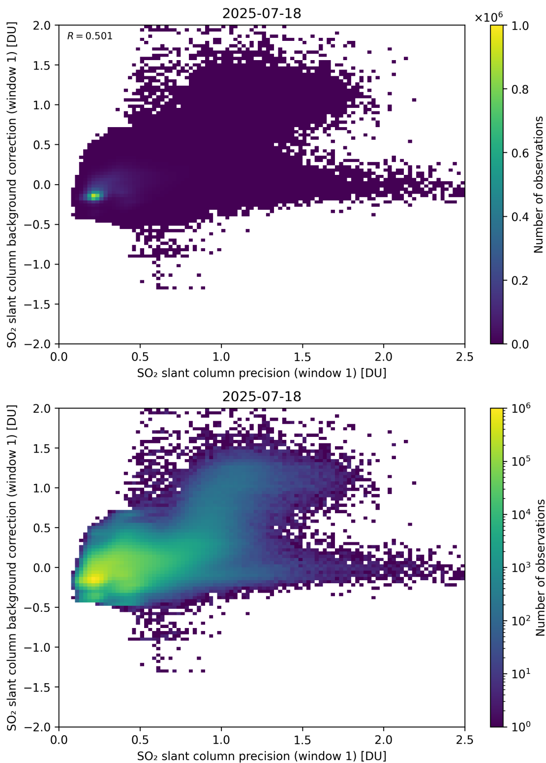
Figure 268: Scatter density plot of “SO 2 slant column precision (window 1)” against “SO 2 slant column background correction (window 1)” for 2025-07-18 to 2025-07-19.
