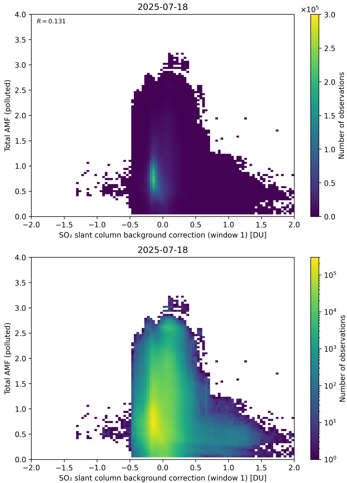
Figure 120: Scatter density plot of “SO 2 slant column background correction (window 1)” against “Total AMF (polluted)” for 2025-07-18 to 2025-07-19.
