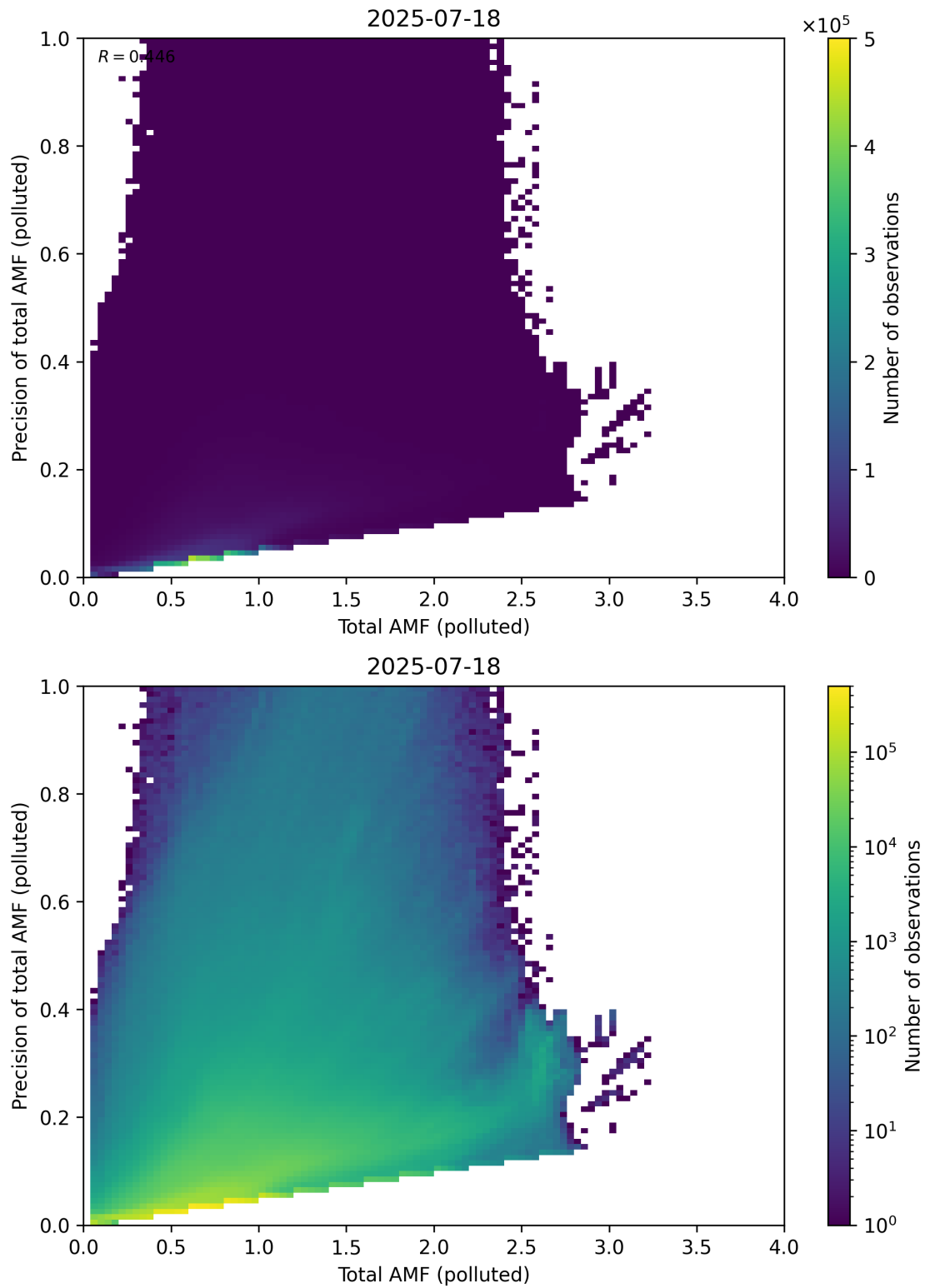
Figure 322: Scatter density plot of “Total AMF (polluted)” against “Precision of total AMF (polluted)” for 2025-07-18 to 2025-07-19.
