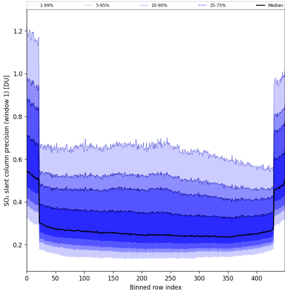
Figure 90: Along track statistics of “SO 2 slant column precision (window 1)” for 2025-07-18 to 2025-07-19
