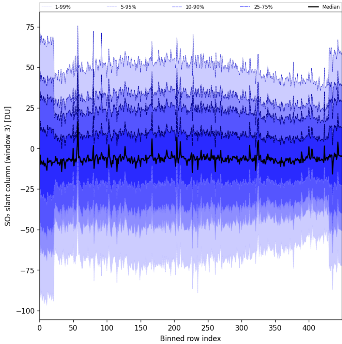
Figure 97: Along track statistics of “SO 2 slant column (window 3)” for 2025-07-18 to 2025-07-19
