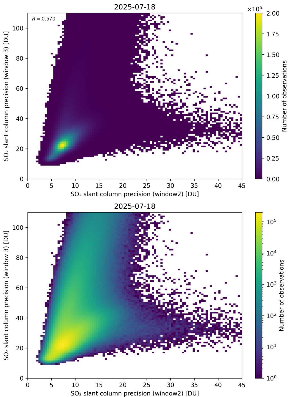
Figure 300: Scatter density plot of “SO 2 slant column precision (window2)” against “SO 2 slant column precision (window 3)” for 2025-07-18 to 2025-07-19.
