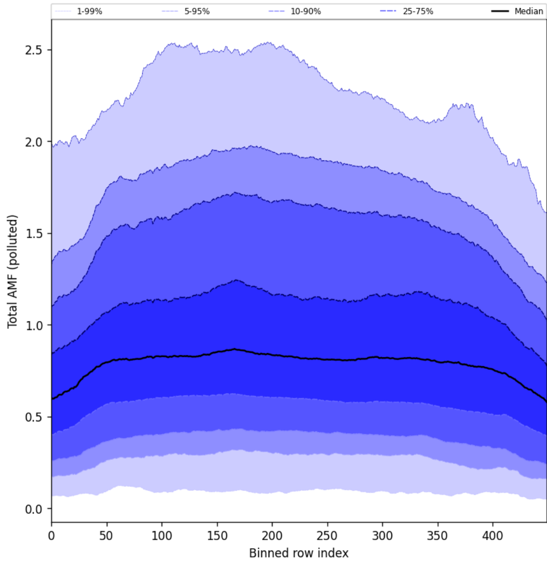
Figure 105: Along track statistics of “Total AMF (polluted)” for 2025-07-18 to 2025-07-19
