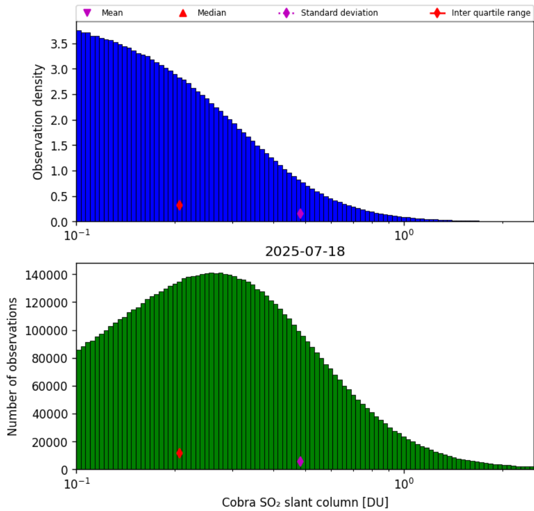
Figure 61: Histogram of “Cobra SO 2 slant column” for 2025-07-18 to 2025-07-19
