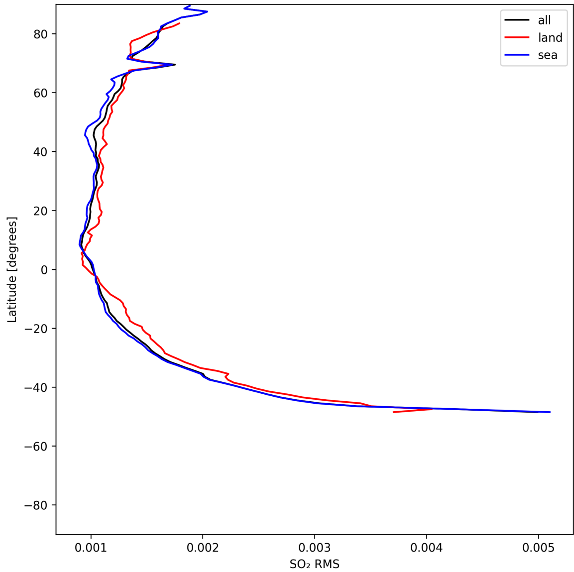
Figure 52: Zonal average of “SO 2 RMS” for 2025-07-18 to 2025-07-19.
