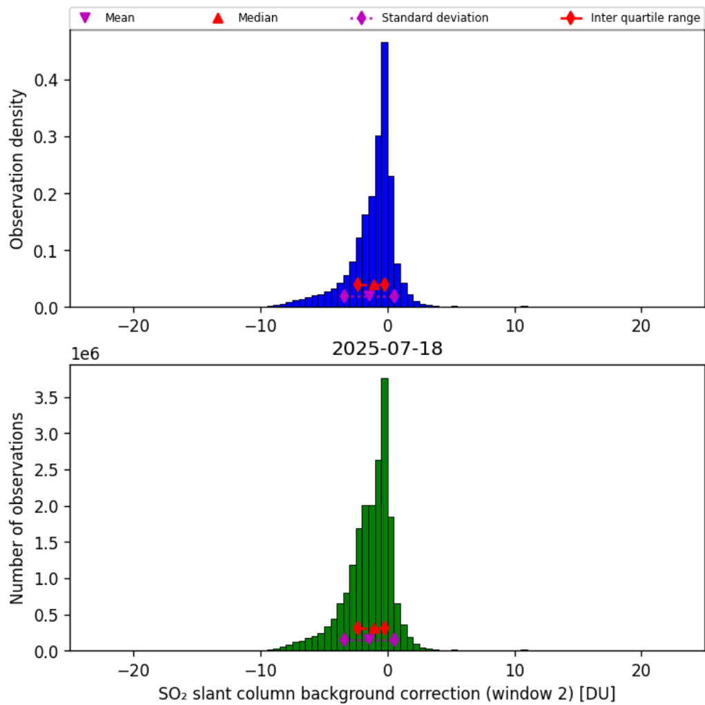
Figure 70: Histogram of “SO 2 slant column background correction (window 2)” for 2025-07-18 to 2025-07-19
