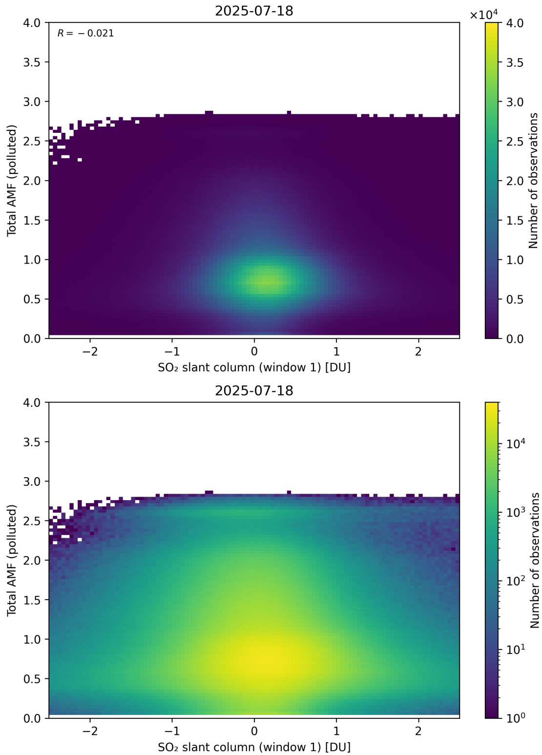
Figure 289: Scatter density plot of “SO 2 slant column (window 1)” against “Total AMF (polluted)” for 2025-07-18 to 2025-07-19.
