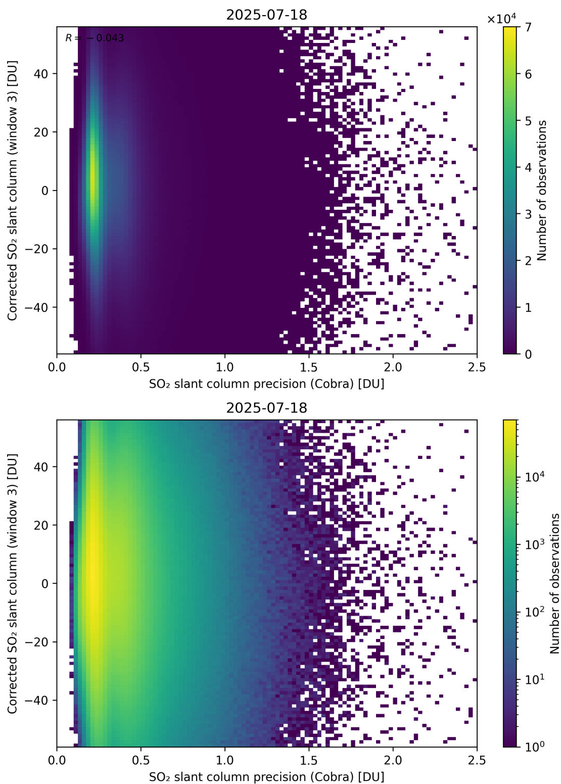
Figure 207: Scatter density plot of “SO 2 slant column precision (Cobra)” against “Corrected SO 2 slant column (window 3)” for 2025-07-18 to 2025-07-19.
