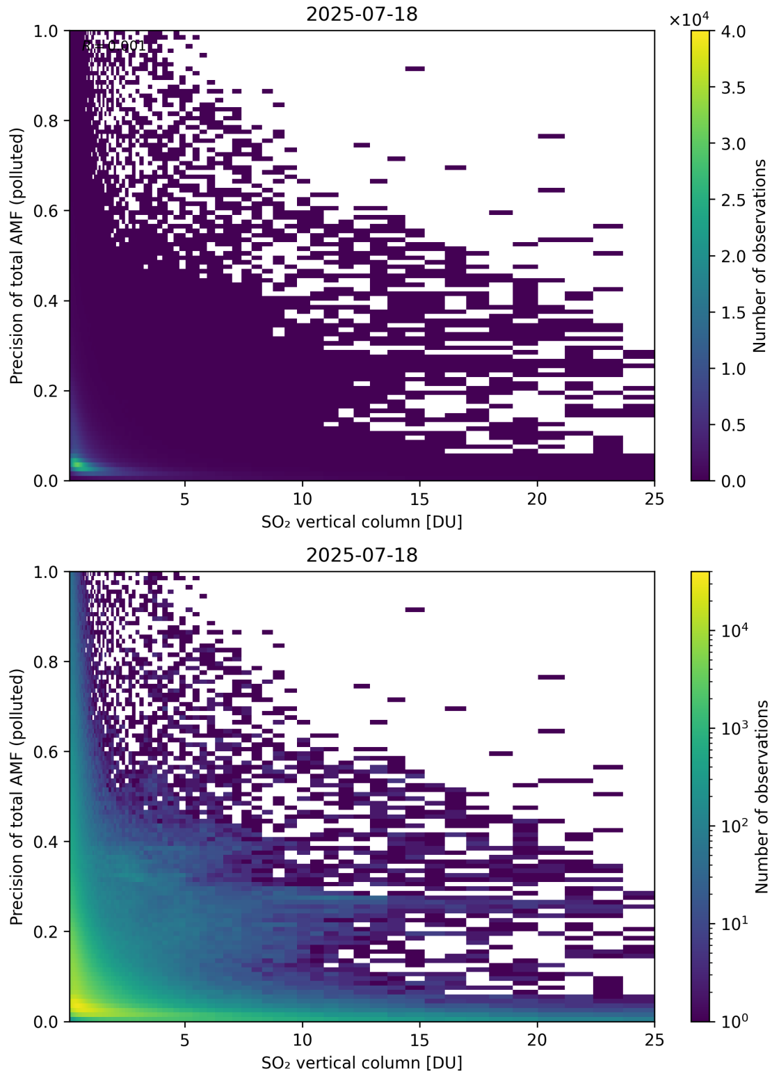
Figure 360: Scatter density plot of “SO 2 vertical column” against “Precision of total AMF (polluted)” for 2025-07-18 to 2025-07-19.
