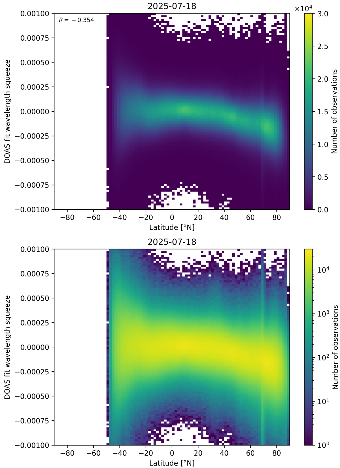
Figure 154: Scatter density plot of “Latitude” against “DOAS fit wavelength squeeze” for 2025-07-18 to 2025-07-19.
