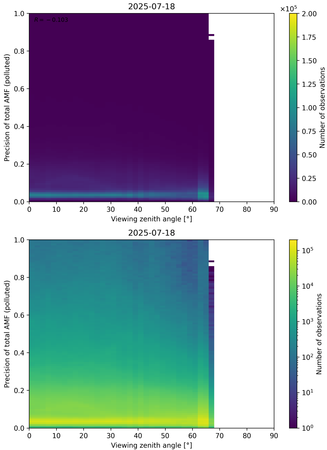
Figure 382: Scatter density plot of “Viewing zenith angle” against “Precision of total AMF (polluted)” for 2025-07-18 to 2025-07-19.
