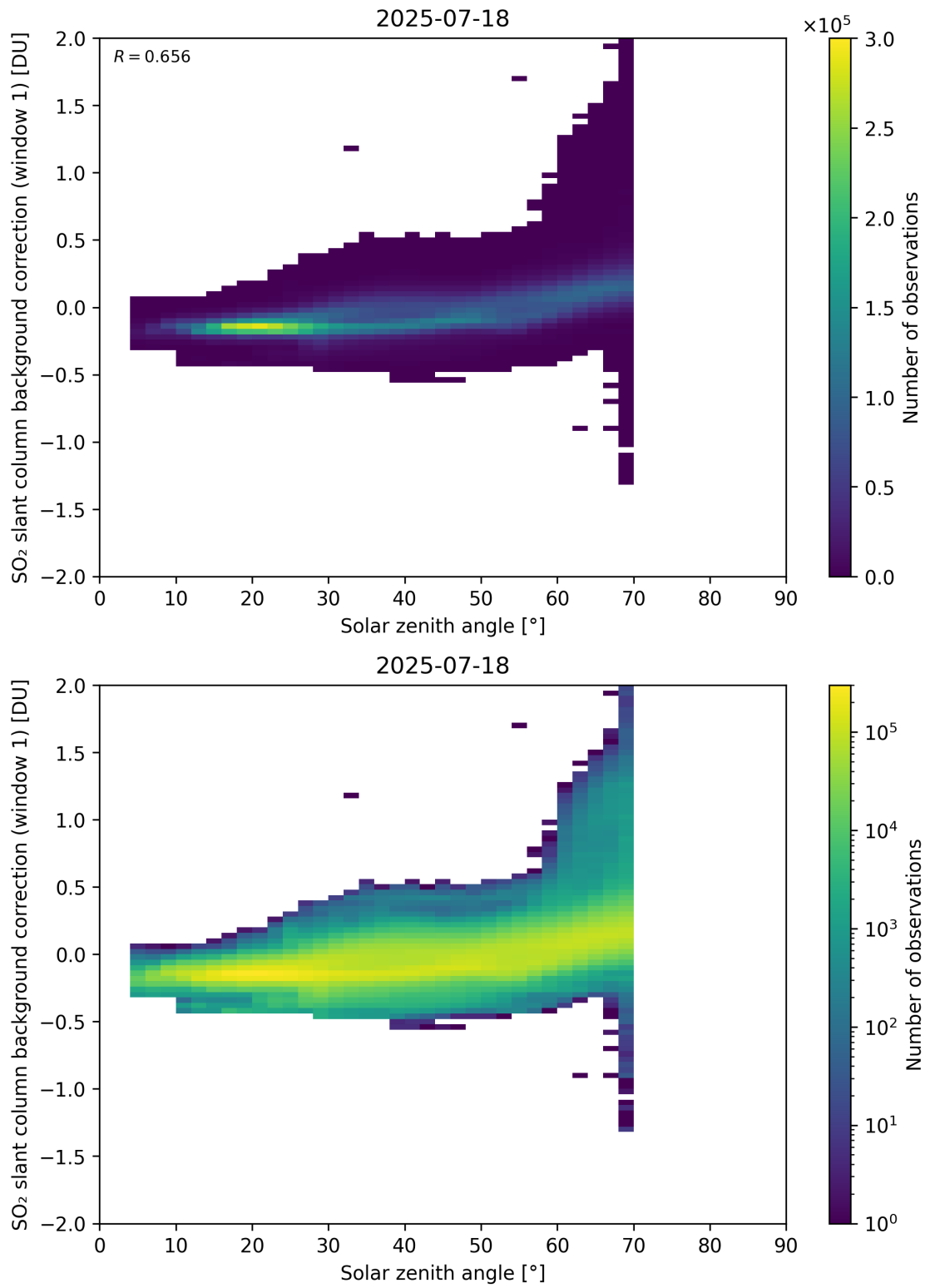
Figure 171: Scatter density plot of “Solar zenith angle” against “SO 2 slant column background correction (window 1)” for 2025-07-18 to 2025-07-19.
