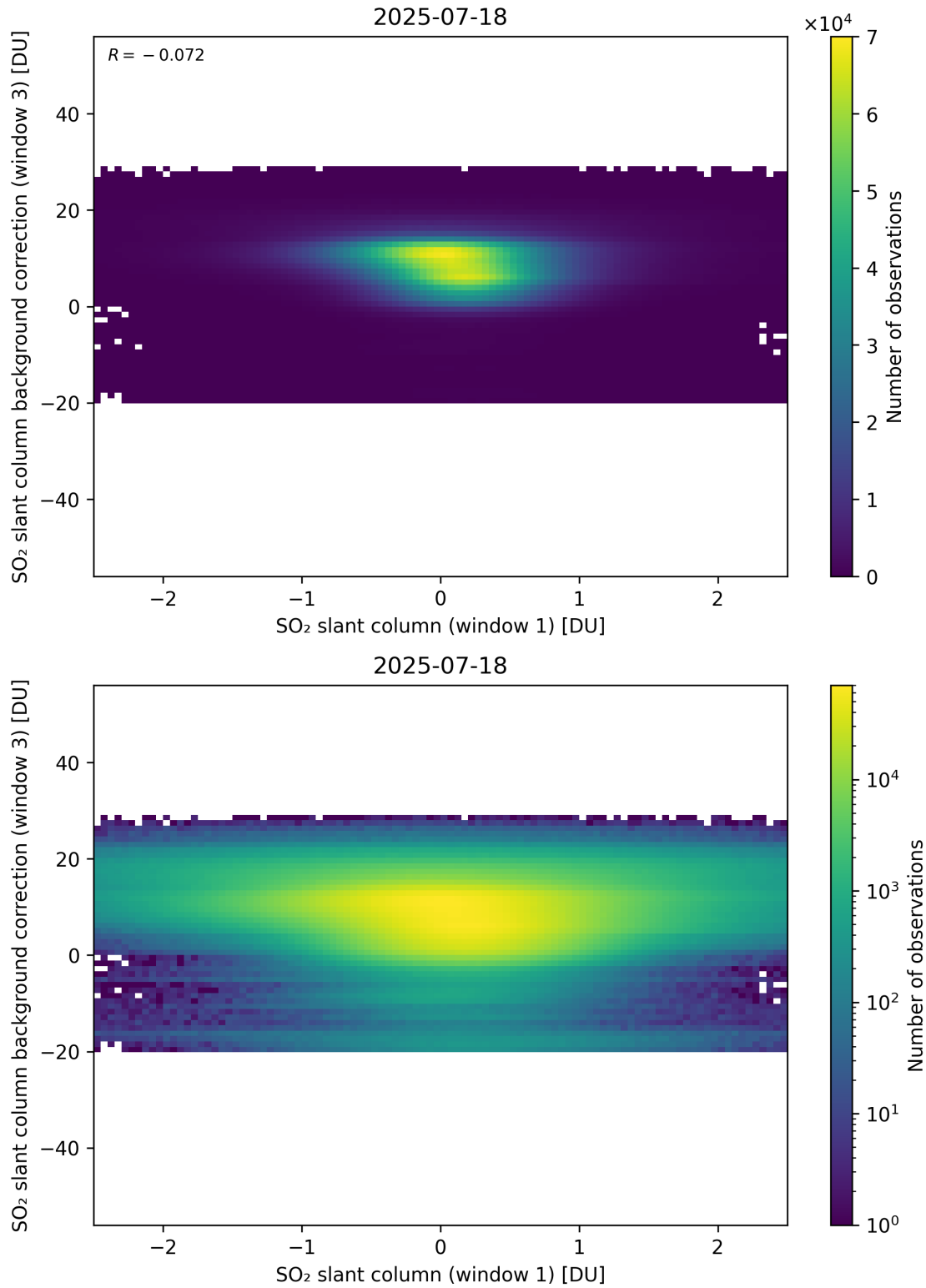
Figure 264: Scatter density plot of “SO 2 slant column (window 1)” against “SO 2 slant column background correction (window 3)” for 2025-07-18 to 2025-07-19.
