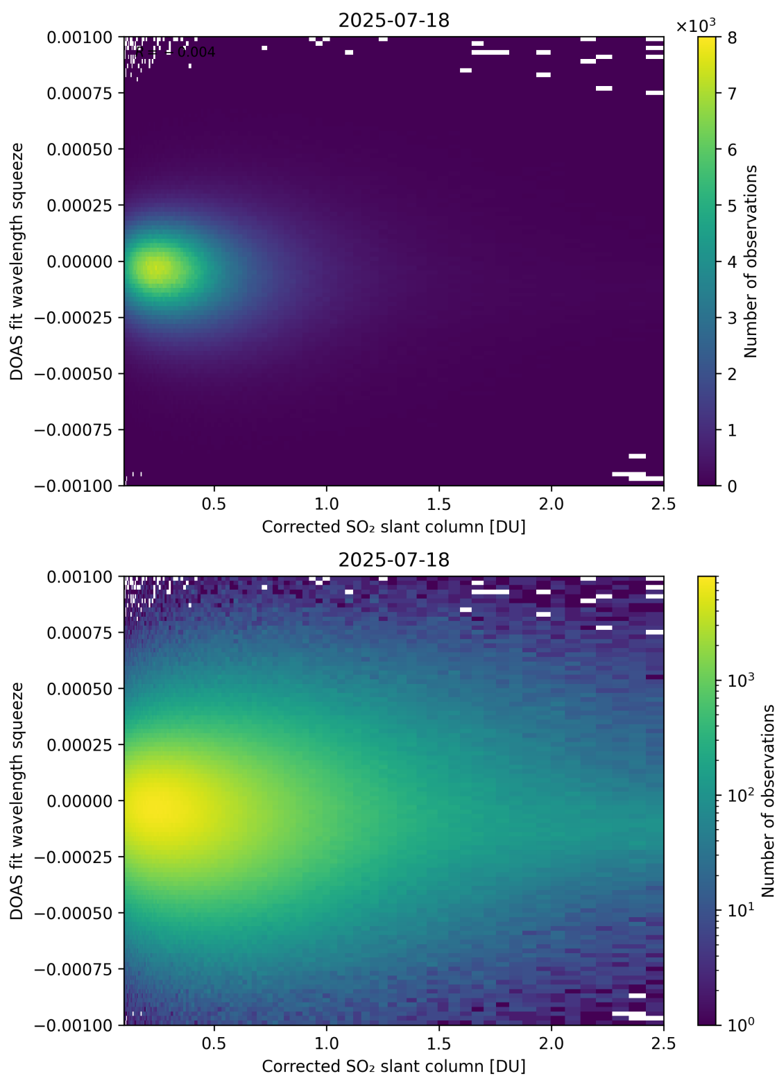
Figure 230: Scatter density plot of “Corrected SO 2 slant column” against “DOAS fit wavelength squeeze” for 2025-07-18 to 2025-07-19.
