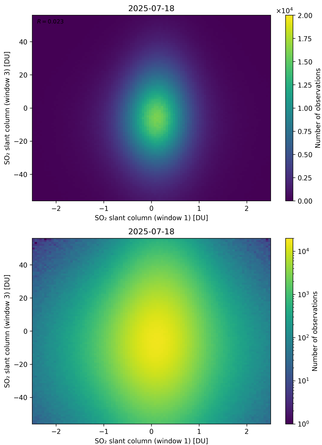
Figure 287: Scatter density plot of “SO 2 slant column (window 1)” against “SO 2 slant column (window 3)” for 2025-07-18 to 2025-07-19.
