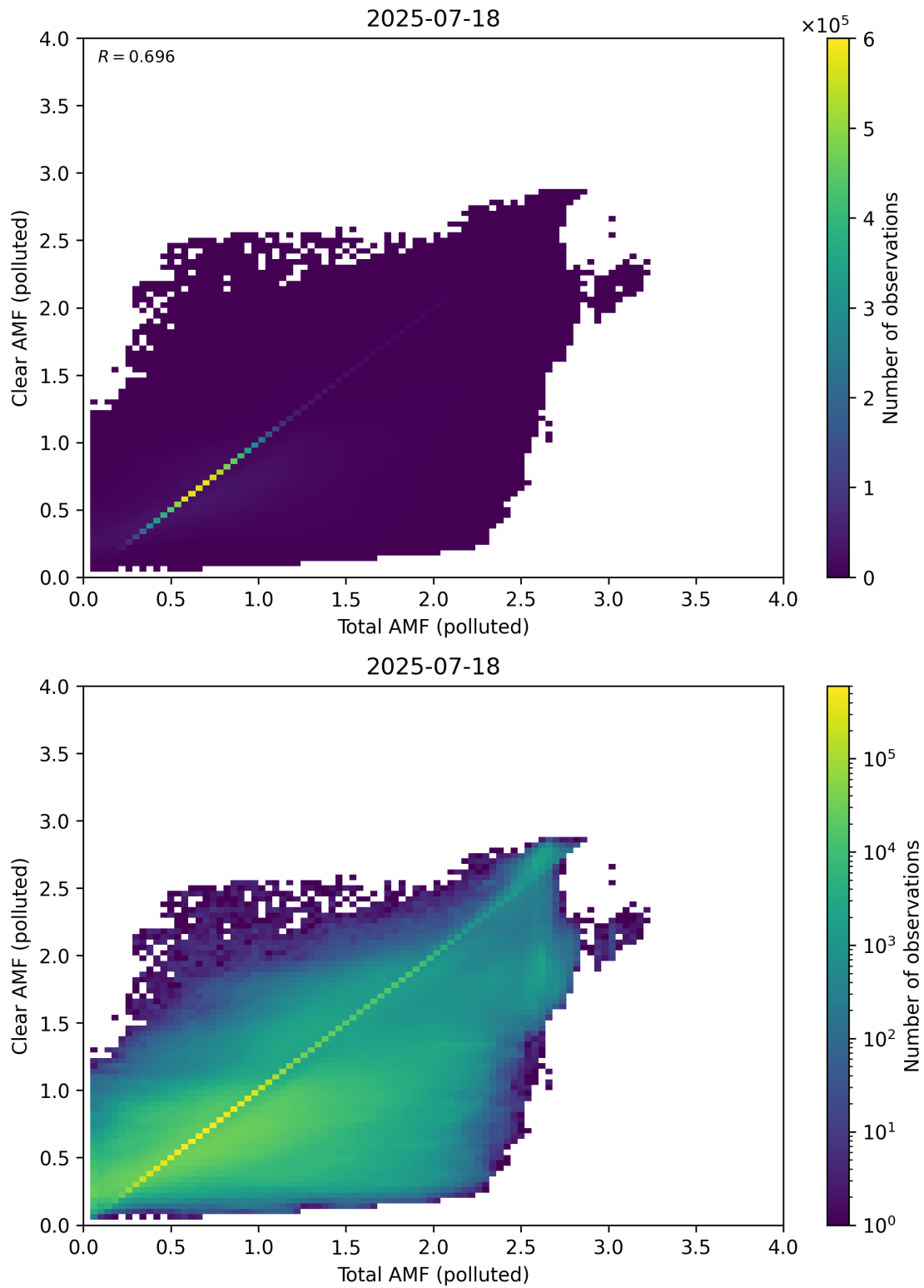
Figure 321: Scatter density plot of “Total AMF (polluted)” against “Clear AMF (polluted)” for 2025-07-18 to 2025-07-19.
