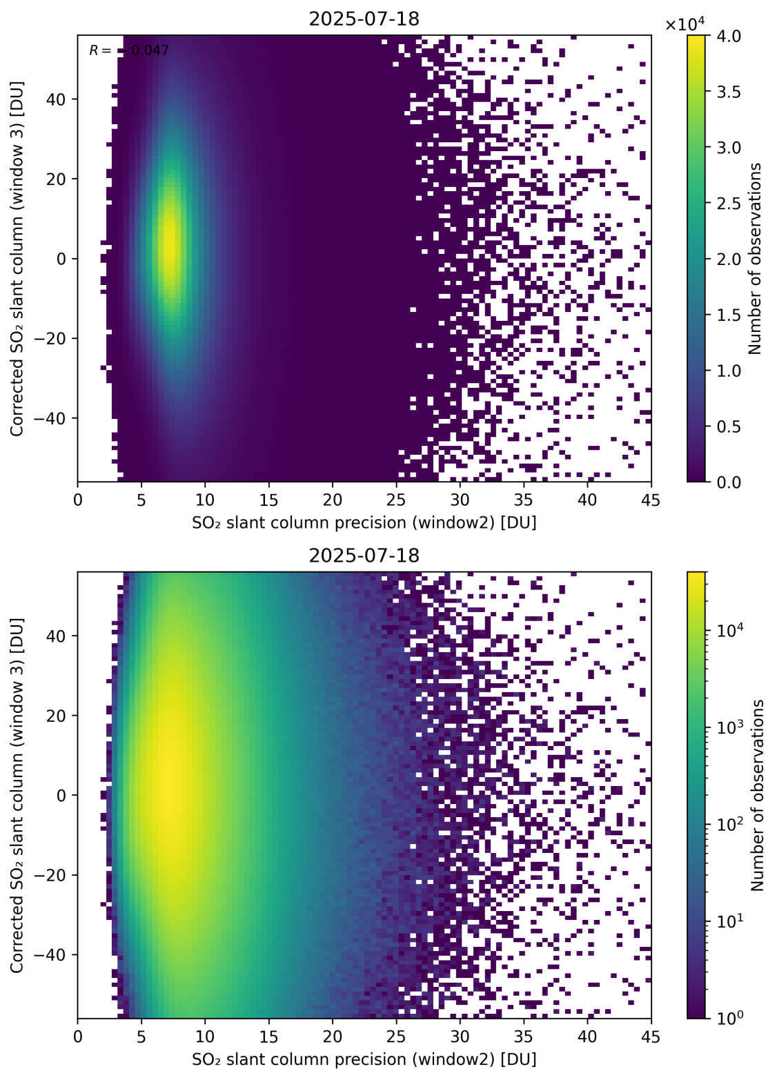
Figure 298: Scatter density plot of “SO 2 slant column precision (window2)” against “Corrected SO 2 slant column (window 3)” for 2025-07-18 to 2025-07-19.
