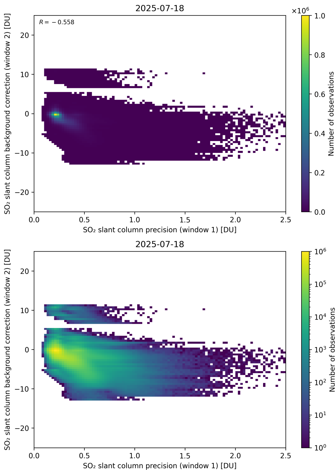
Figure 269: Scatter density plot of “SO 2 slant column precision (window 1)” against “SO 2 slant column background correction (window 2)” for 2025-07-18 to 2025-07-19.
