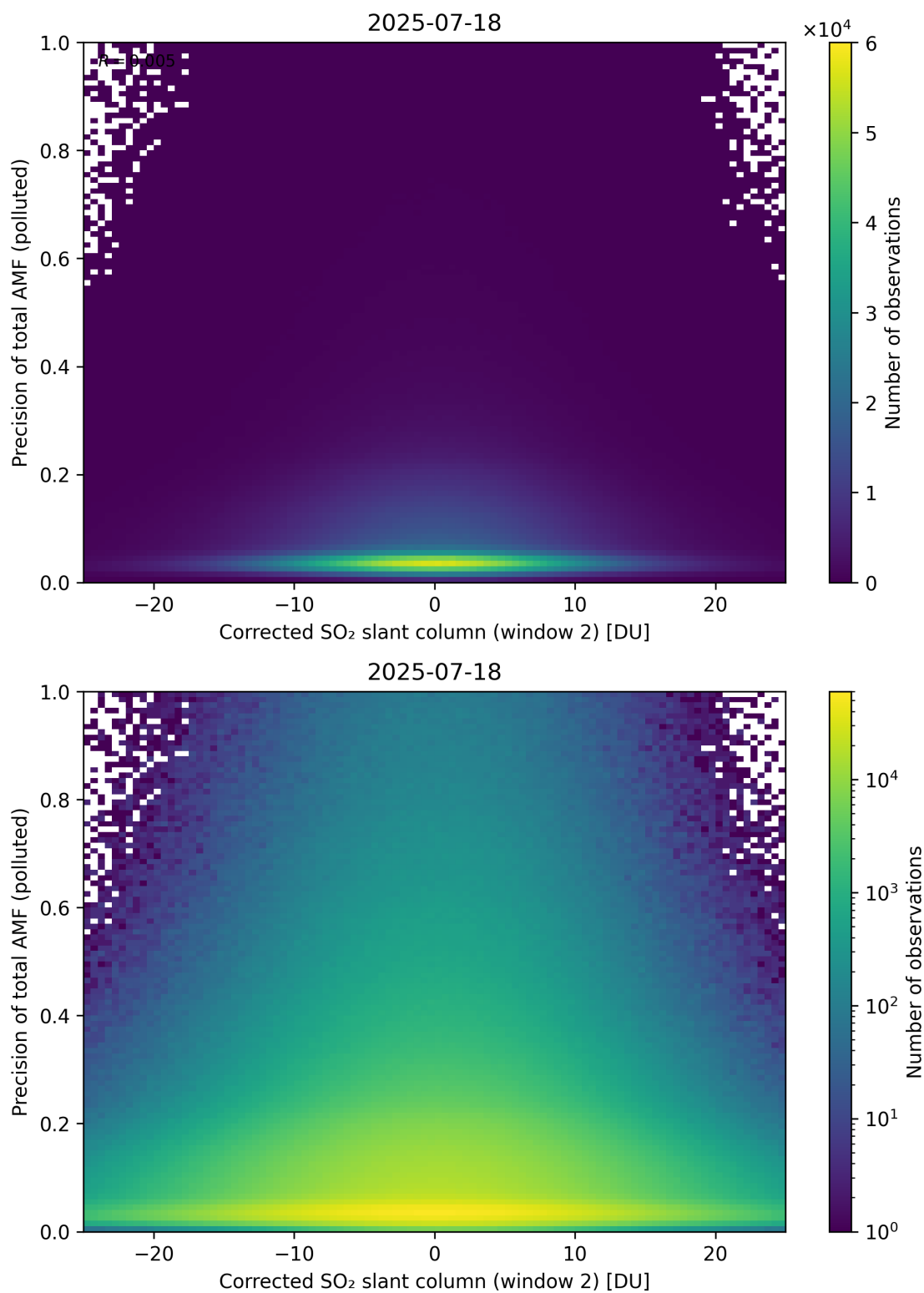
Figure 254: Scatter density plot of “Corrected SO 2 slant column (window 2)” against “Precision of total AMF (polluted)” for 2025-07-18 to 2025-07-19.
