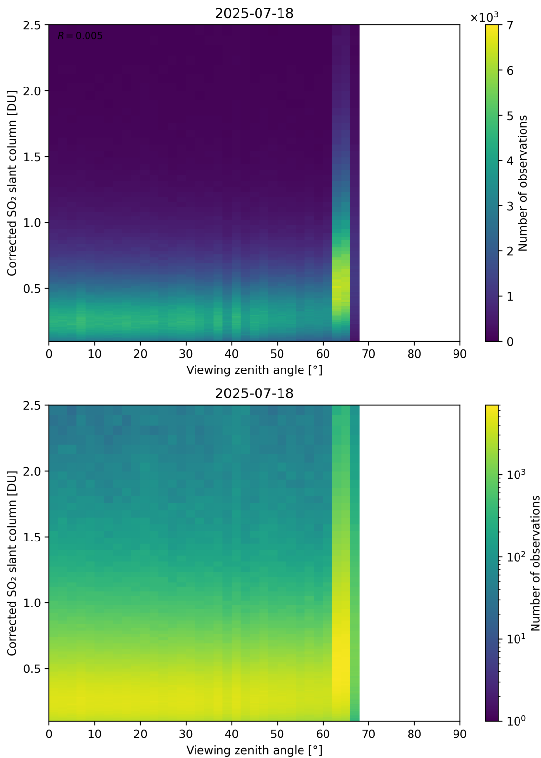
Figure 373: Scatter density plot of “Viewing zenith angle” against “Corrected SO 2 slant column” for 2025-07-18 to 2025-07-19.
