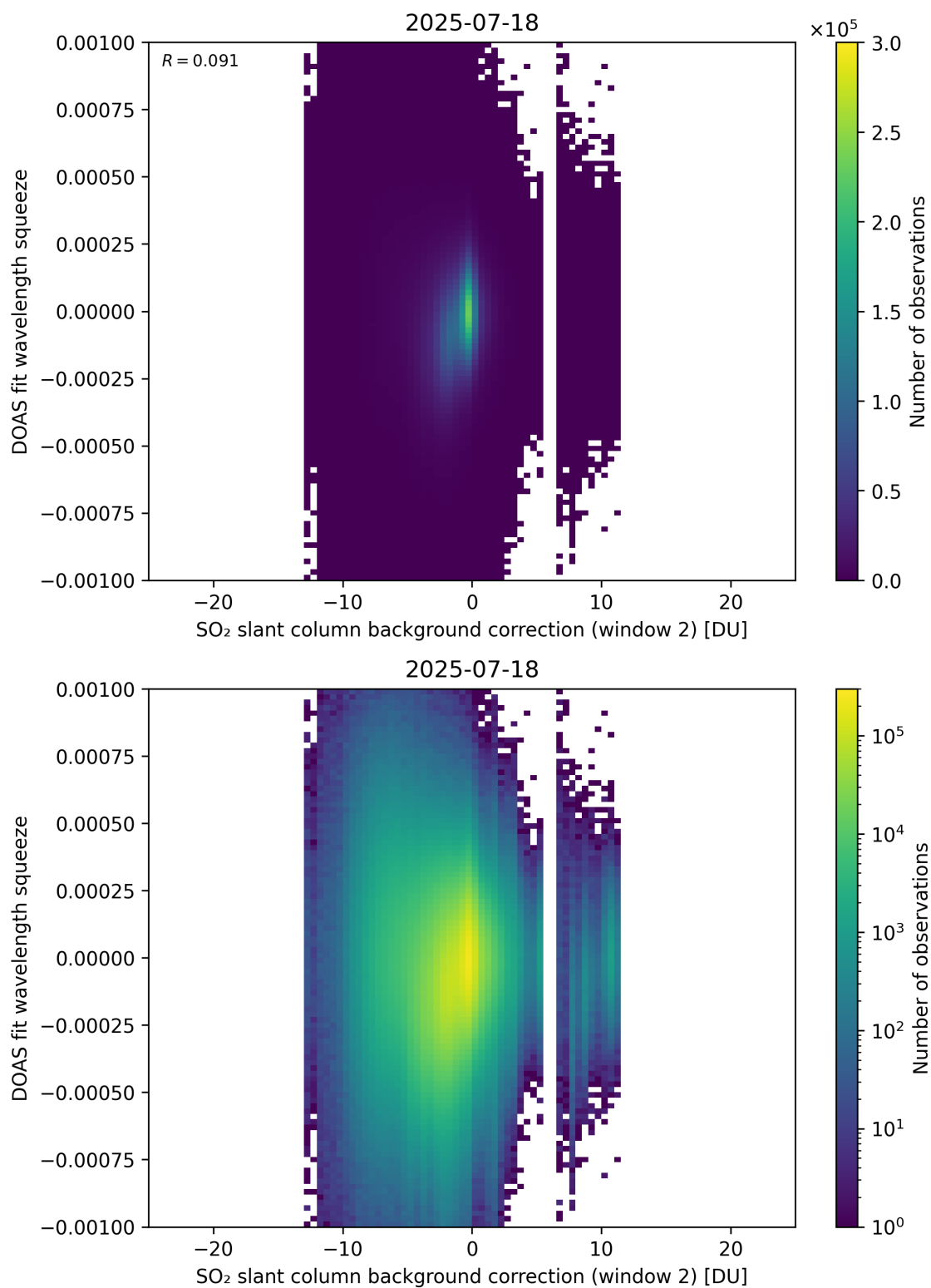
Figure 124: Scatter density plot of “SO 2 slant column background correction (window 2)” against “DOAS fit wavelength squeeze” for 2025-07-18 to 2025-07-19.
