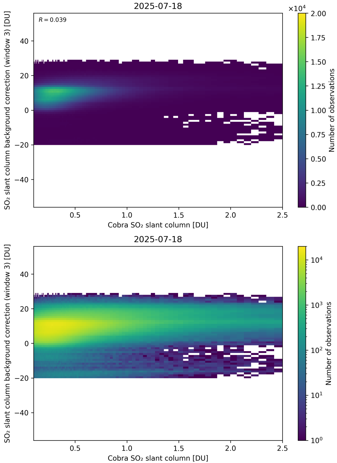
Figure 195: Scatter density plot of “Cobra SO 2 slant column” against “SO 2 slant column background correction (window 3)” for 2025-07-18 to 2025-07-19.
