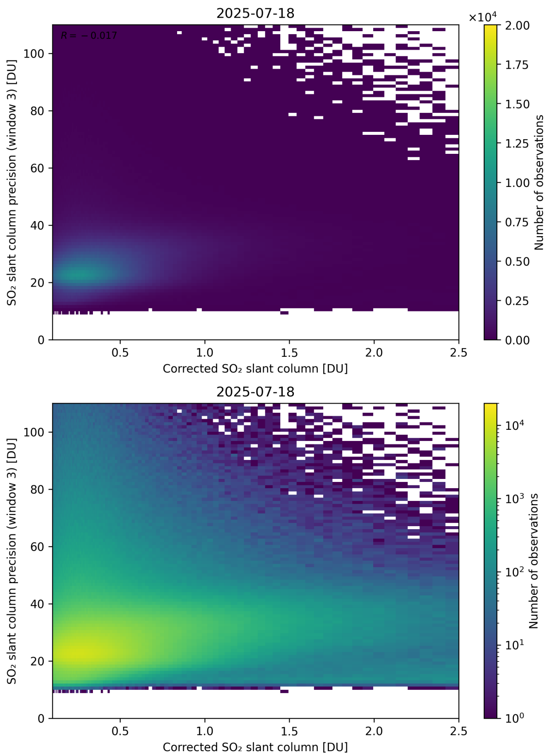
Figure 241: Scatter density plot of “Corrected SO 2 slant column” against “SO 2 slant column precision (window 3)” for 2025-07-18 to 2025-07-19.
