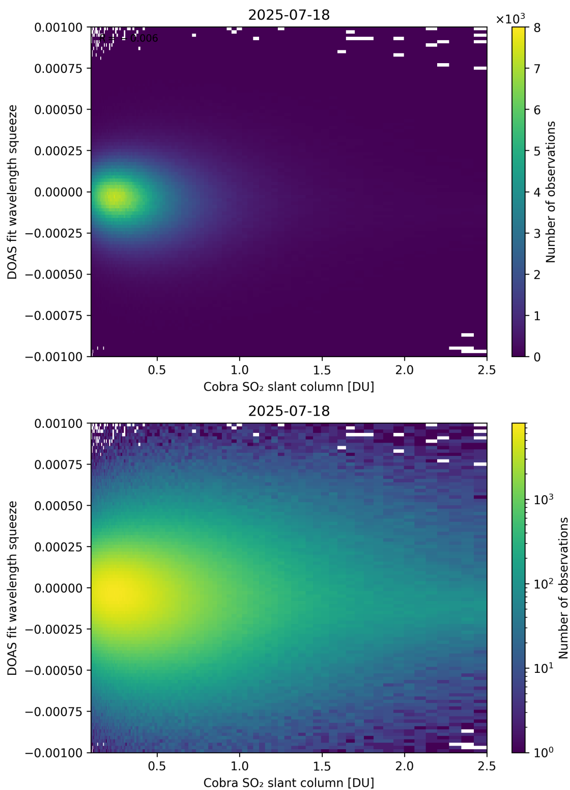
Figure 197: Scatter density plot of “Cobra SO 2 slant column” against “DOAS fit wavelength squeeze” for 2025-07-18 to 2025-07-19.
