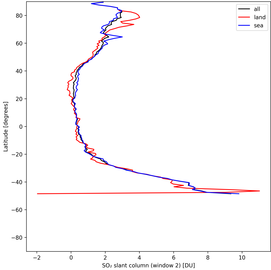
Figure 41: Zonal average of “SO 2 slant column (window 2)” for 2025-07-18 to 2025-07-19.
