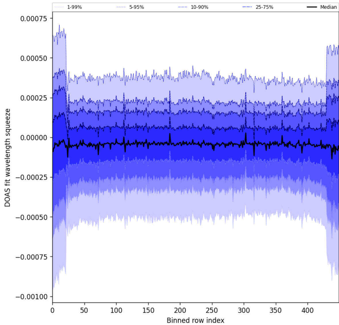
Figure 103: Along track statistics of “DOAS fit wavelength squeeze” for 2025-07-18 to 2025-07-19
