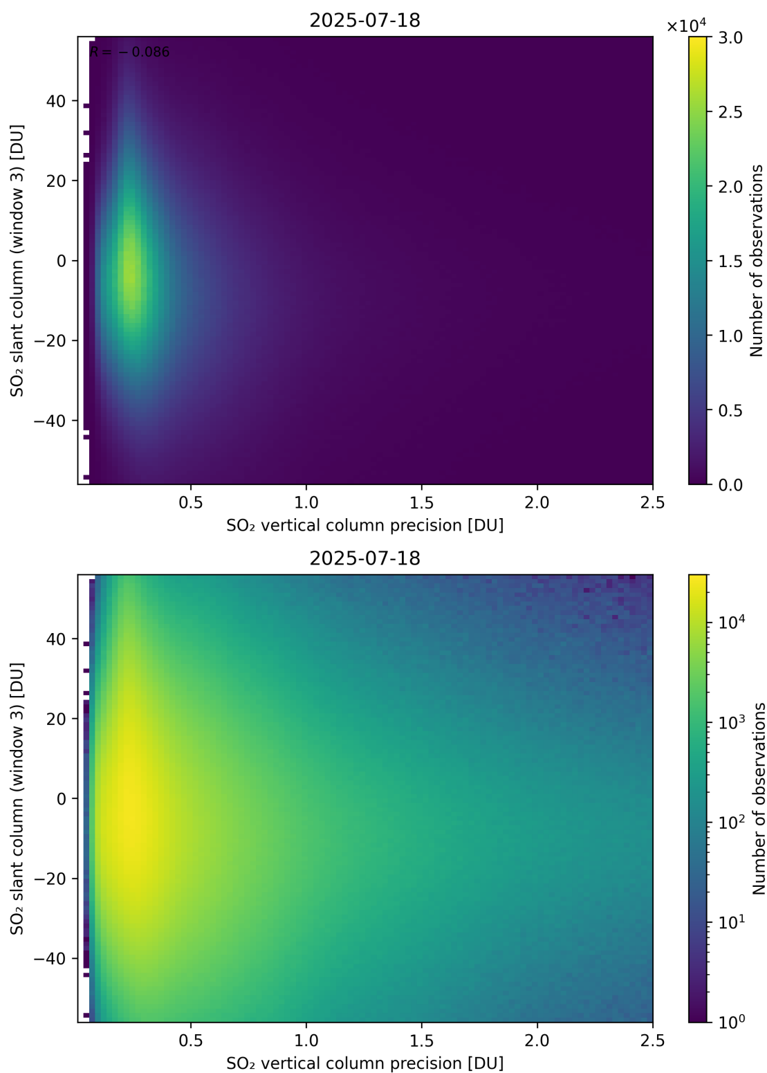
Figure 344: Scatter density plot of “SO 2 vertical column precision” against “SO 2 slant column (window 3)” for 2025-07-18 to 2025-07-19.
