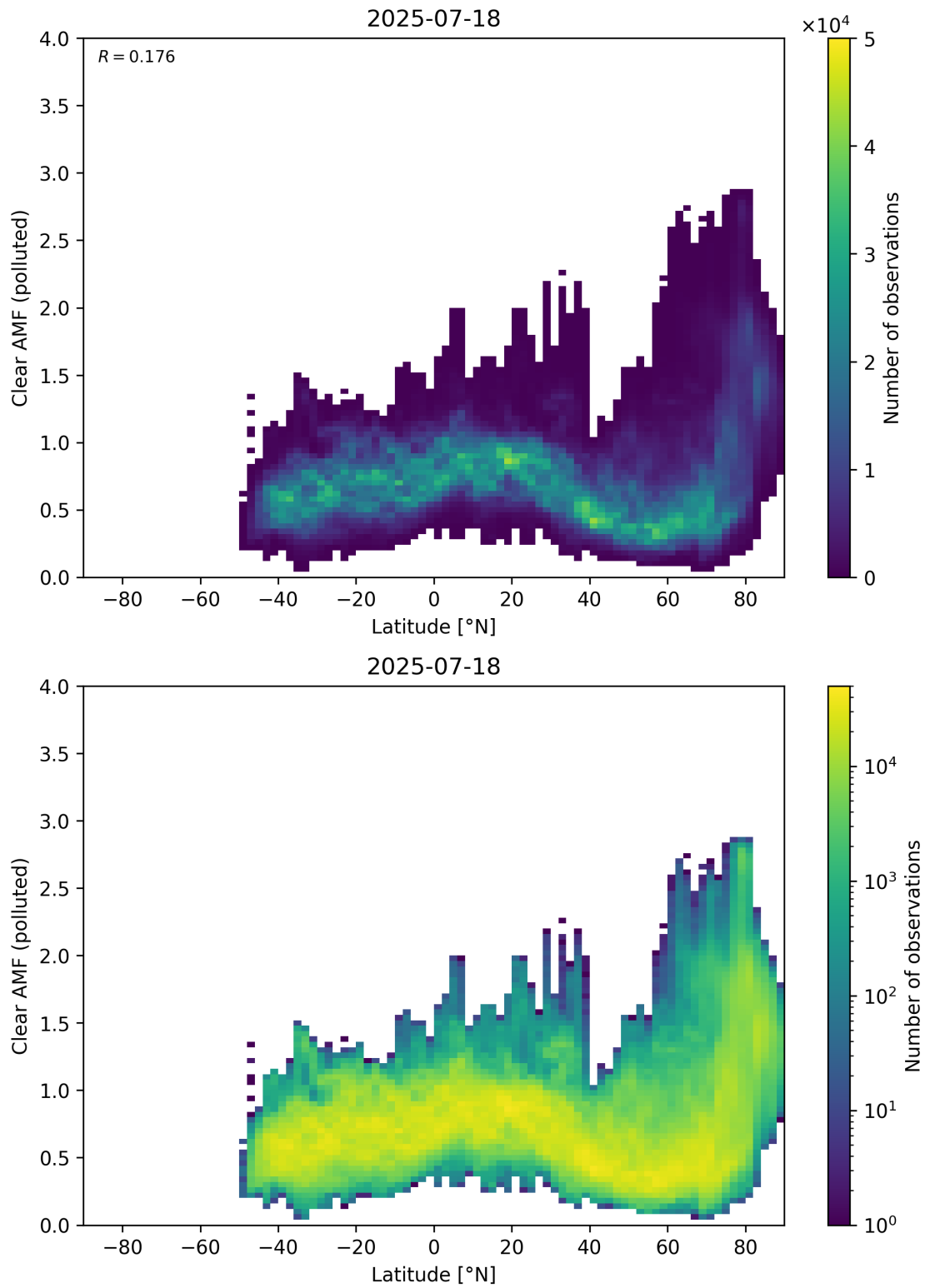
Figure 156: Scatter density plot of “Latitude” against “Clear AMF (polluted)” for 2025-07-18 to 2025-07-19.
