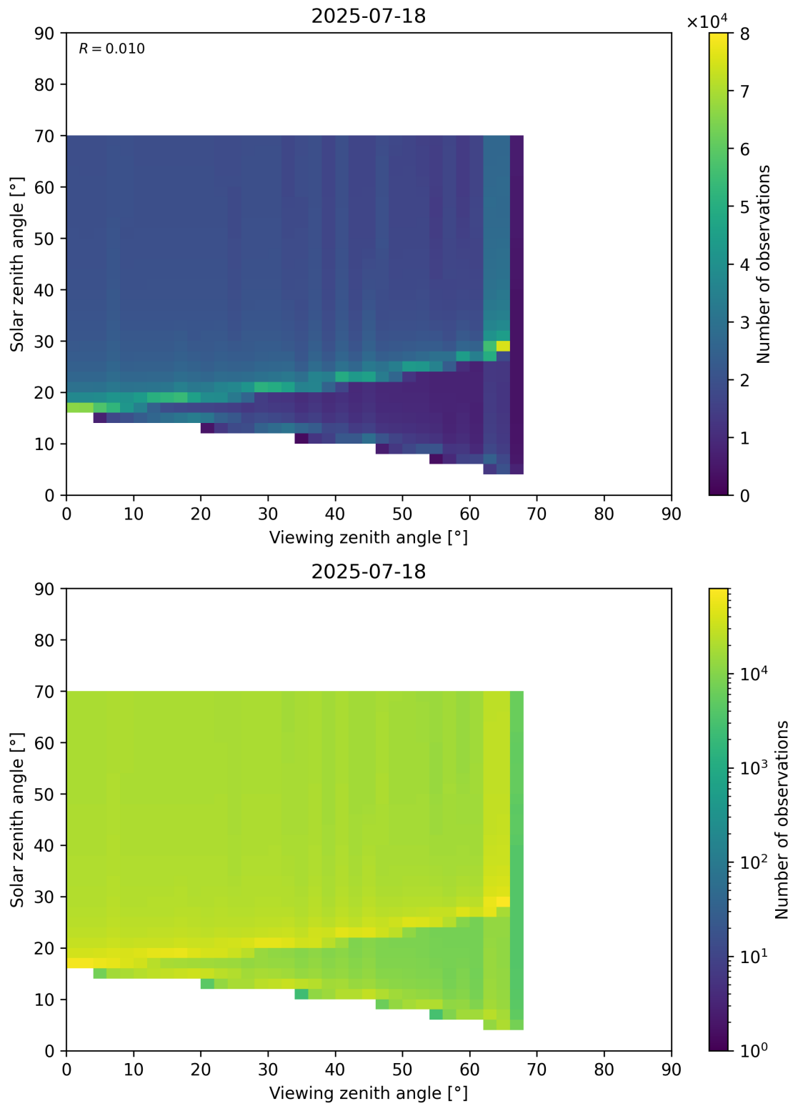
Figure 369: Scatter density plot of “Viewing zenith angle” against “Solar zenith angle” for 2025-07-18 to 2025-07-19.
