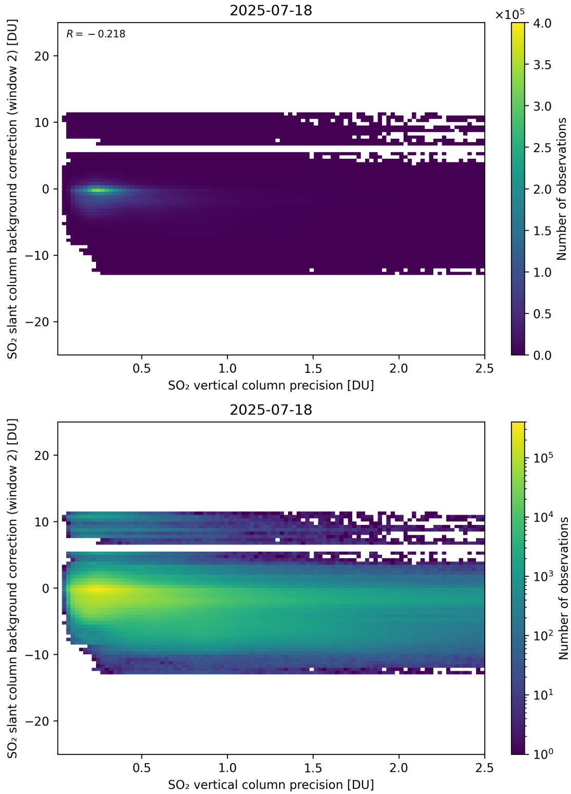
Figure 330: Scatter density plot of “SO 2 vertical column precision” against “SO 2 slant column background correction (window 2)” for 2025-07-18 to 2025-07-19.
