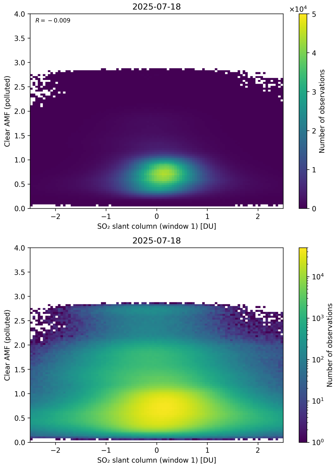
Figure 282: Scatter density plot of “SO 2 slant column (window 1)” against “Clear AMF (polluted)” for 2025-07-18 to 2025-07-19.
