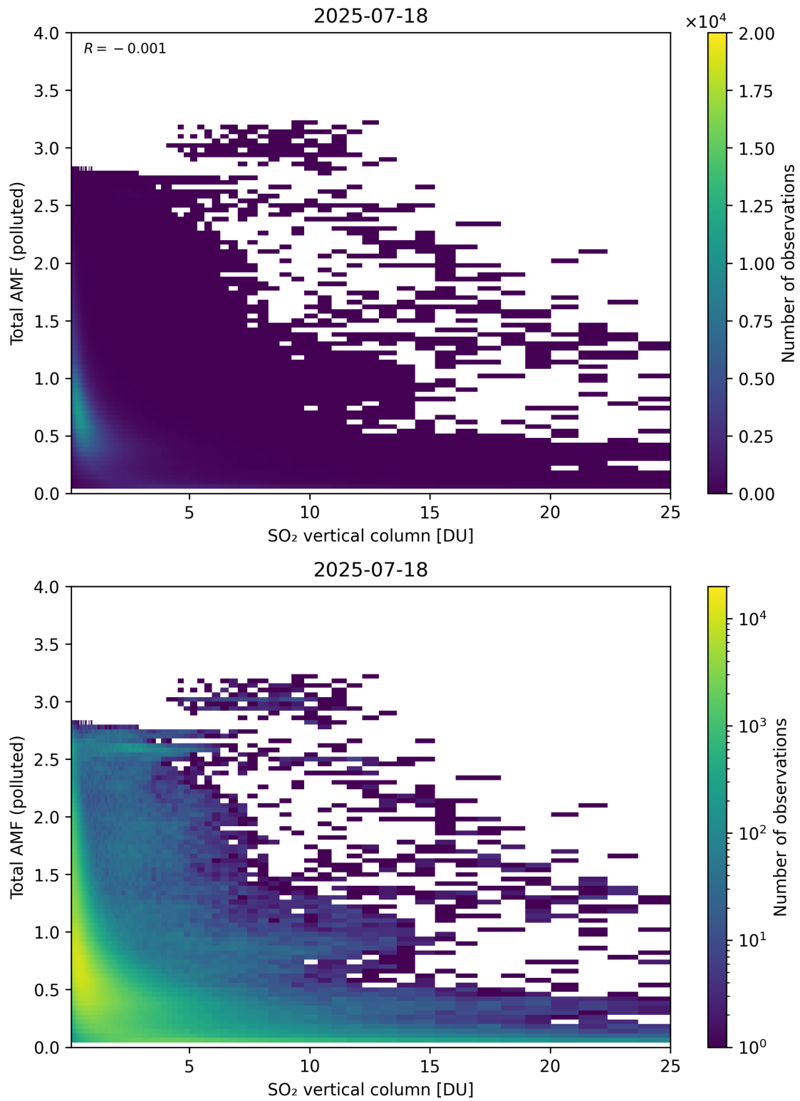
Figure 359: Scatter density plot of “SO 2 vertical column” against “Total AMF (polluted)” for 2025-07-18 to 2025-07-19.
