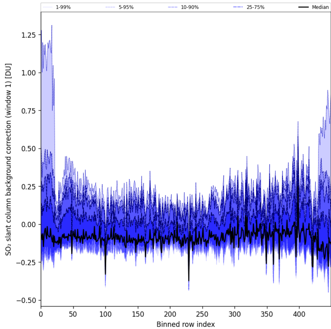
Figure 92: Along track statistics of “SO 2 slant column background correction (window 1)” for 2025-07-18 to 2025-07-19
