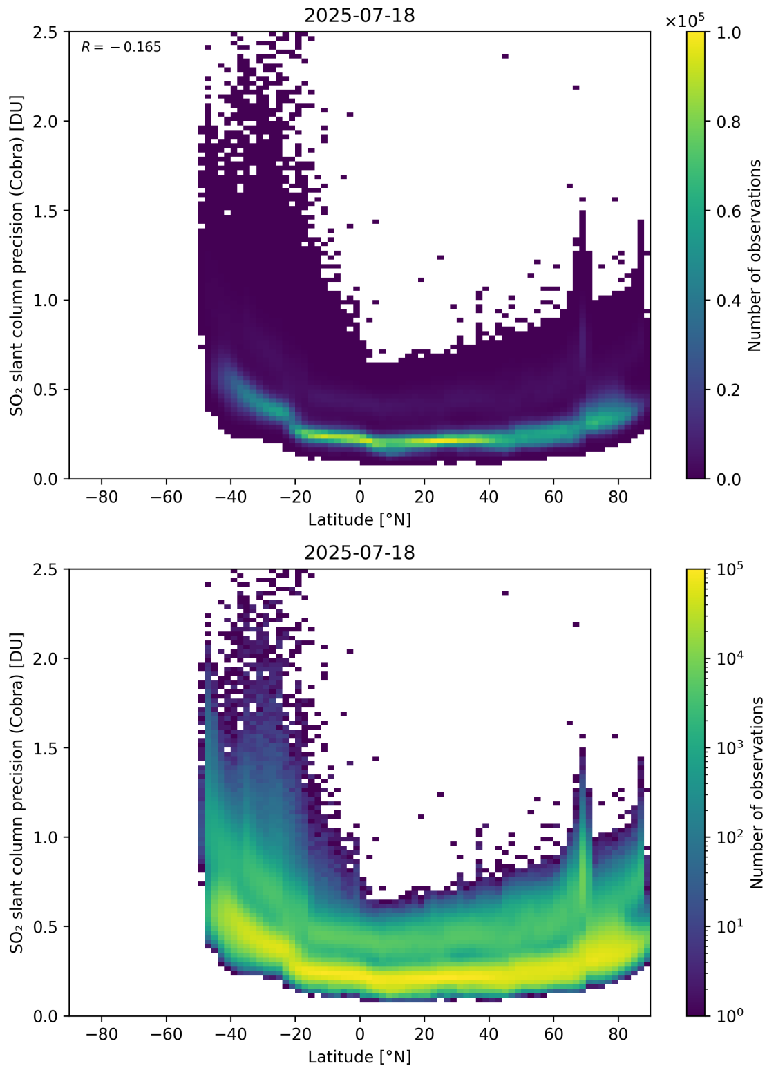
Figure 158: Scatter density plot of “Latitude” against “SO 2 slant column precision (Cobra)” for 2025-07-18 to 2025-07-19.
