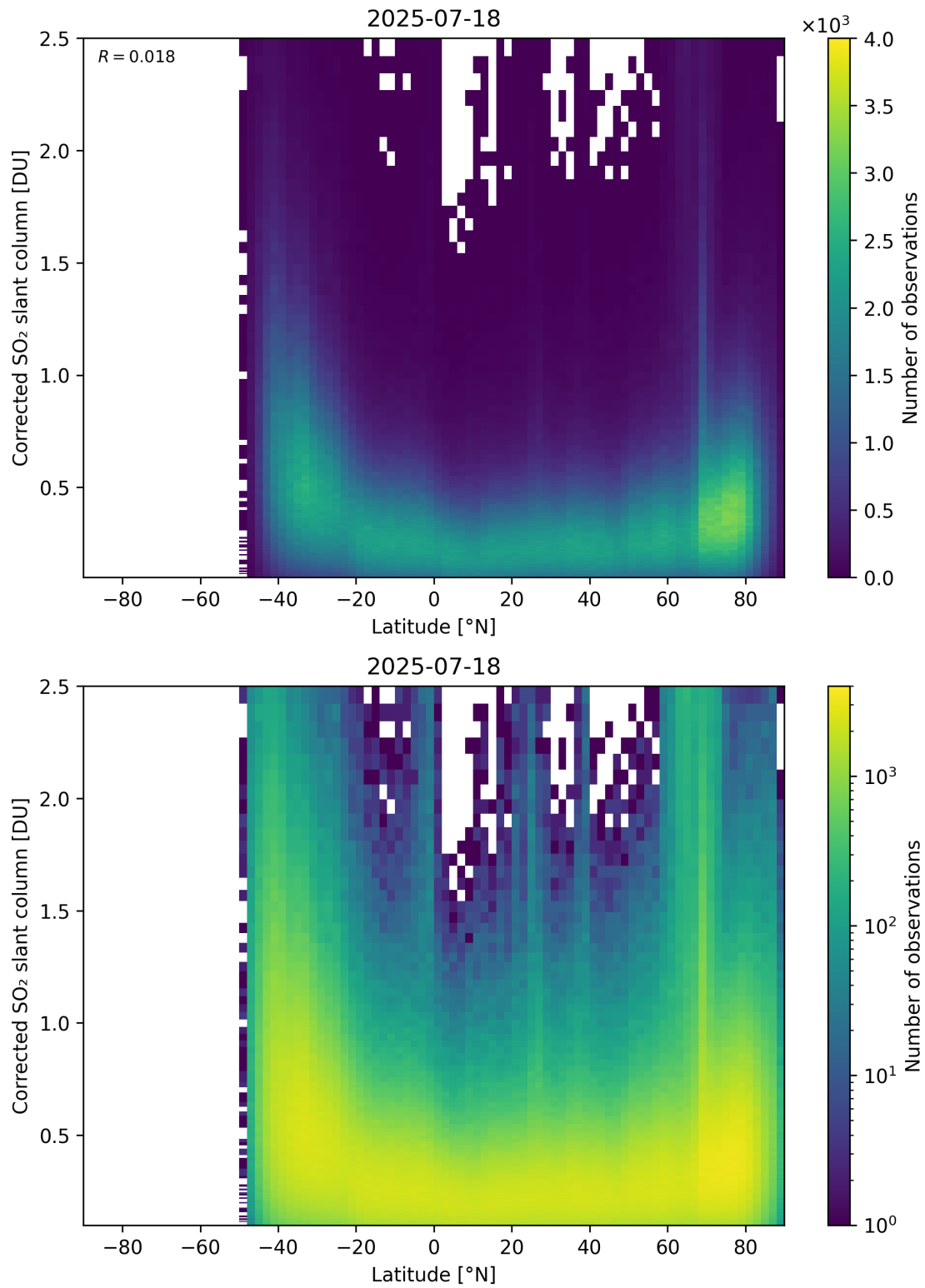
Figure 159: Scatter density plot of “Latitude” against “Corrected SO 2 slant column” for 2025-07-18 to 2025-07-19.
