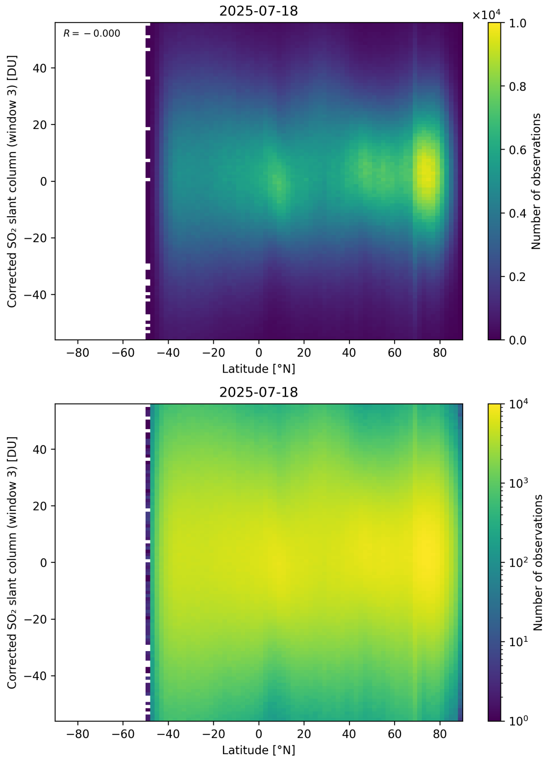
Figure 161: Scatter density plot of “Latitude” against “Corrected SO 2 slant column (window 3)” for 2025-07-18 to 2025-07-19.
