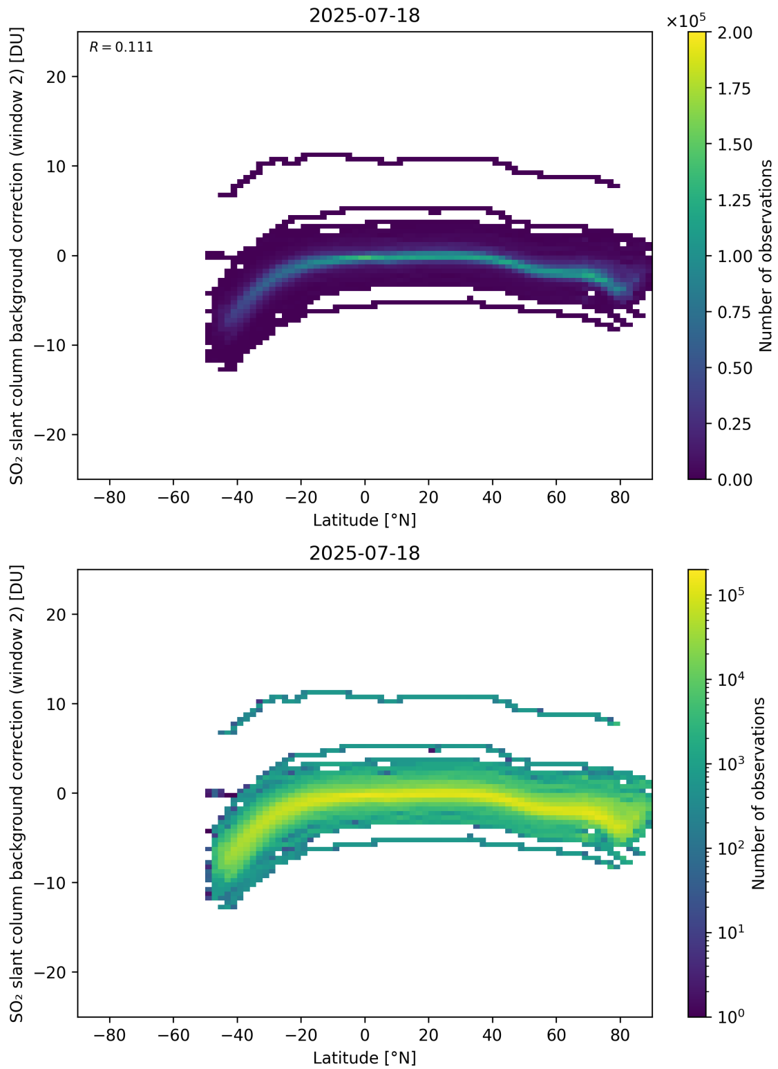
Figure 151: Scatter density plot of “Latitude” against “SO 2 slant column background correction (window 2)” for 2025-07-18 to 2025-07-19.
