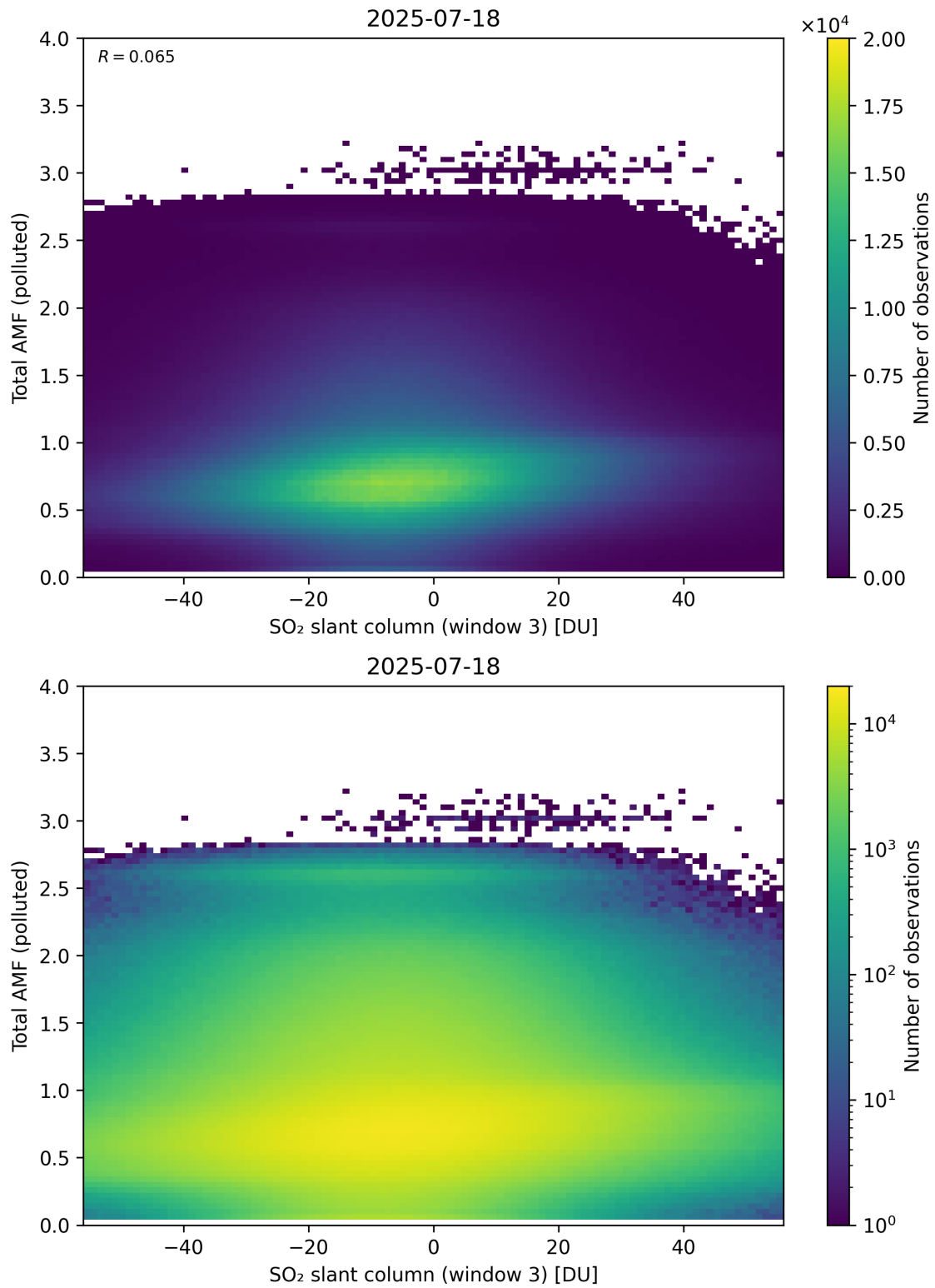
Figure 318: Scatter density plot of “SO 2 slant column (window 3)” against “Total AMF (polluted)” for 2025-07-18 to 2025-07-19.
