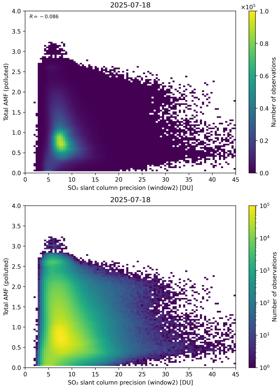
Figure 301: Scatter density plot of “SO 2 slant column precision (window2)” against “Total AMF (polluted)” for 2025-07-18 to 2025-07-19.
