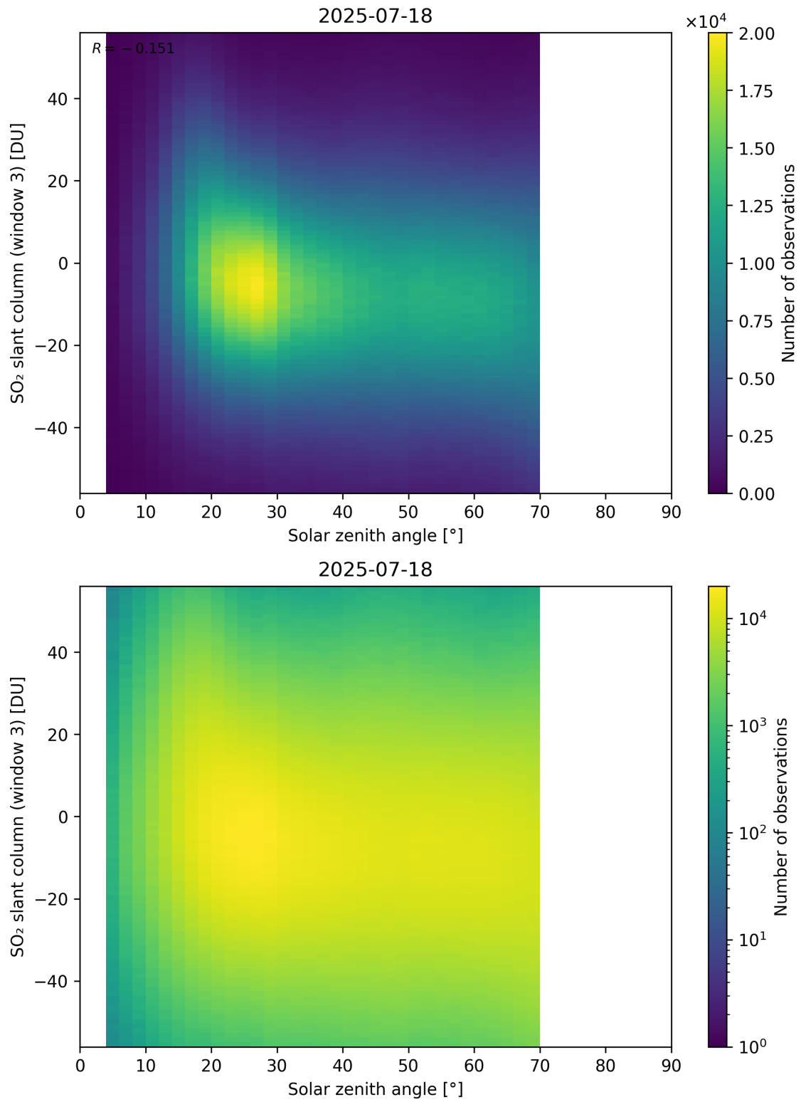
Figure 187: Scatter density plot of “Solar zenith angle” against “SO 2 slant column (window 3)” for 2025-07-18 to 2025-07-19.
