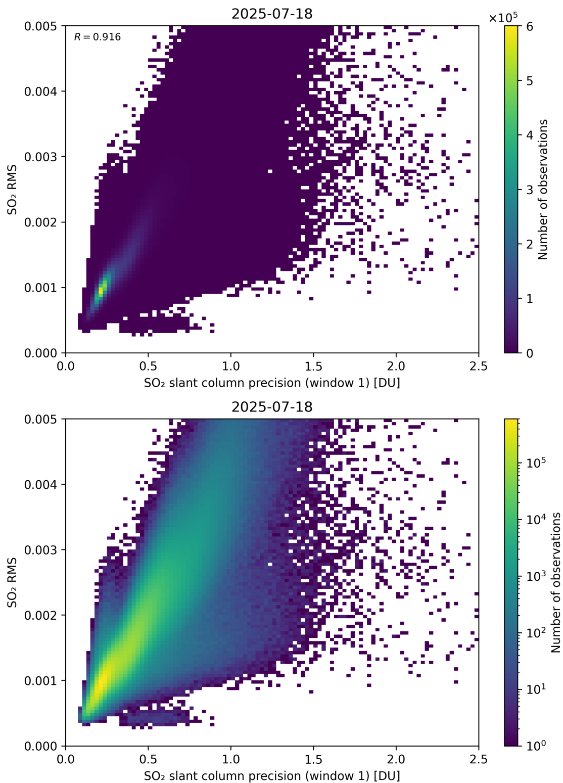
Figure 273: Scatter density plot of “SO 2 slant column precision (window 1)” against “SO 2 RMS” for 2025-07-18 to 2025-07-19.
