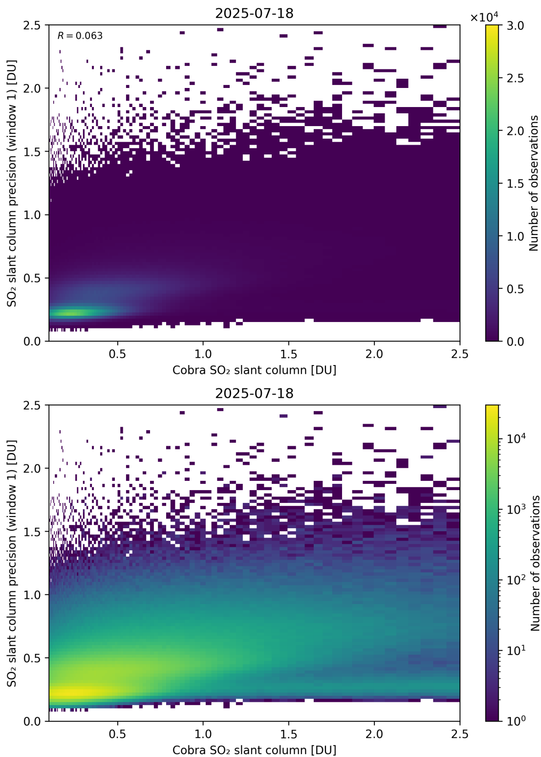
Figure 220: Scatter density plot of “Cobra SO 2 slant column” against “SO 2 slant column precision (window 1)” for 2025-07-18 to 2025-07-19.
