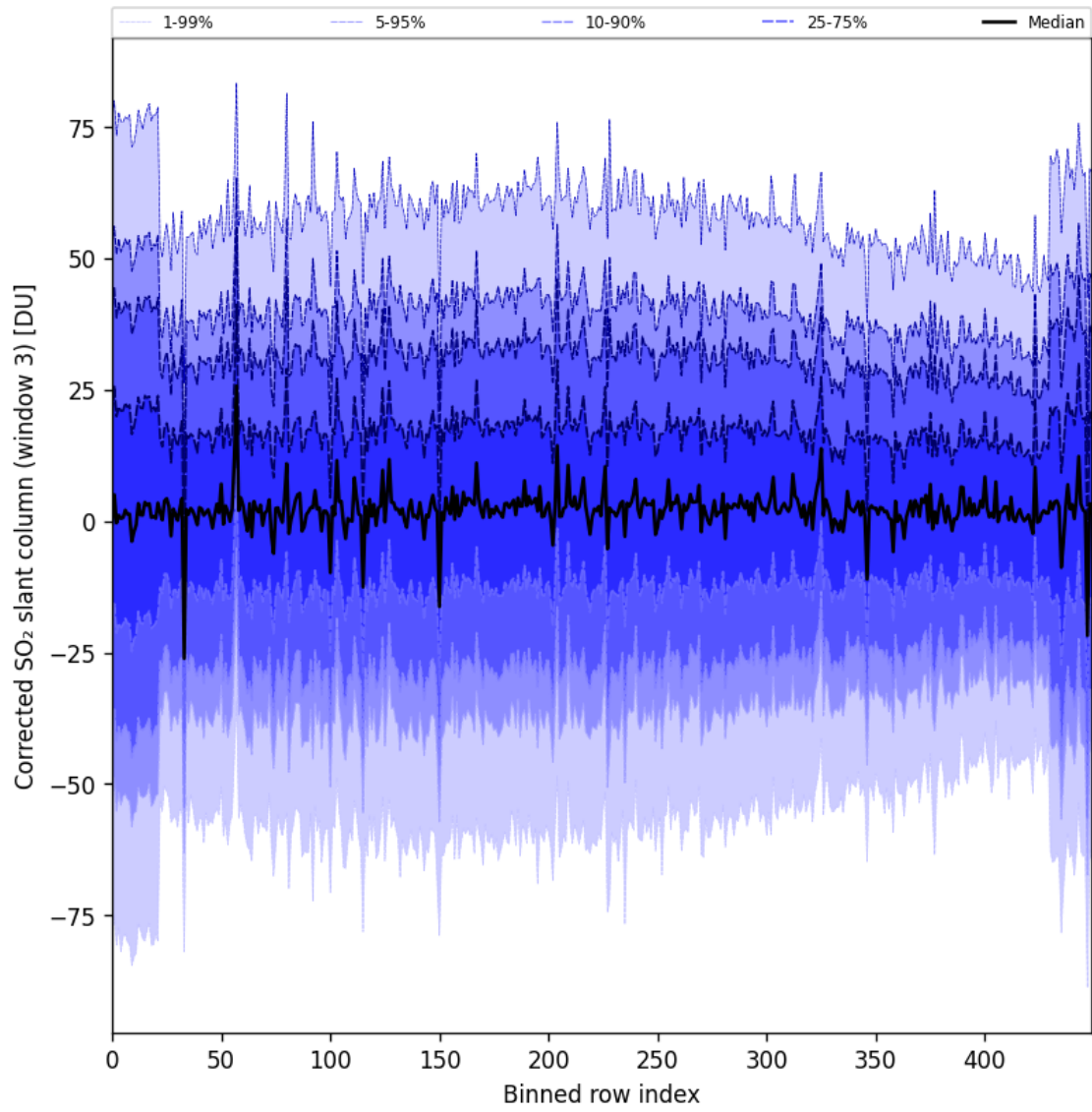
Figure 99: Along track statistics of “Corrected SO 2 slant column (window 3)” for 2025-07-18 to 2025-07-19
