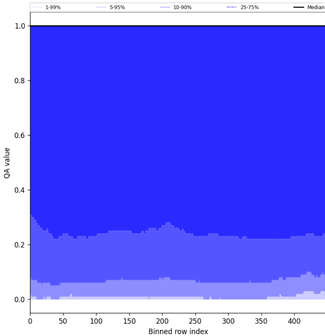
Figure 83: Along track statistics of “QA value” for 2025-07-18 to 2025-07-19
