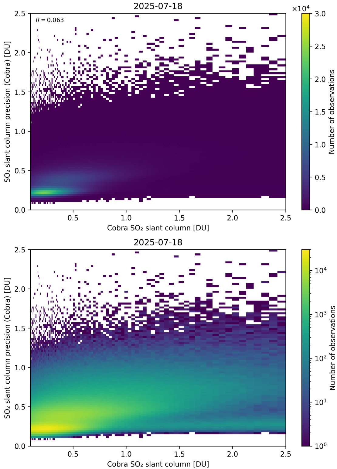
Figure 216: Scatter density plot of “Cobra SO 2 slant column” against “SO 2 slant column precision (Cobra)” for 2025-07-18 to 2025-07-19.
