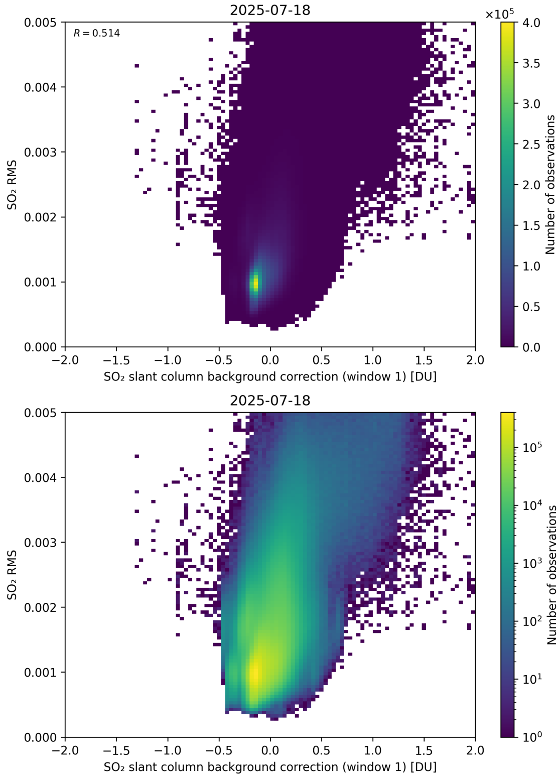
Figure 113: Scatter density plot of “SO 2 slant column background correction (window 1)” against “SO 2 RMS” for 2025-07-18 to 2025-07-19.
