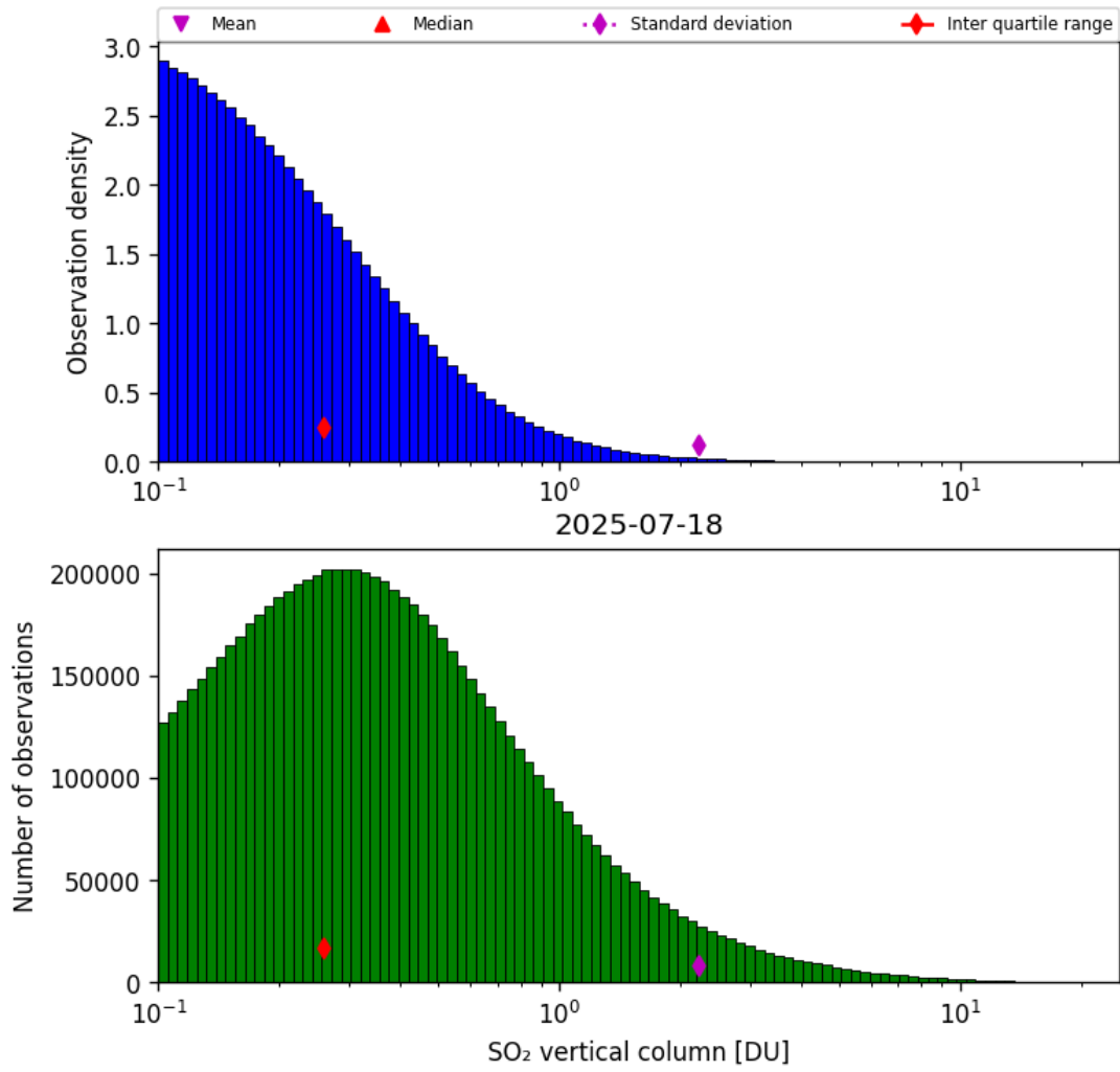
Figure 58: Histogram of “SO 2 vertical column” for 2025-07-18 to 2025-07-19
