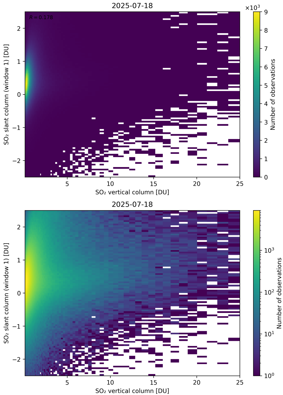
Figure 354: Scatter density plot of “SO 2 vertical column” against “SO 2 slant column (window 1)” for 2025-07-18 to 2025-07-19.
