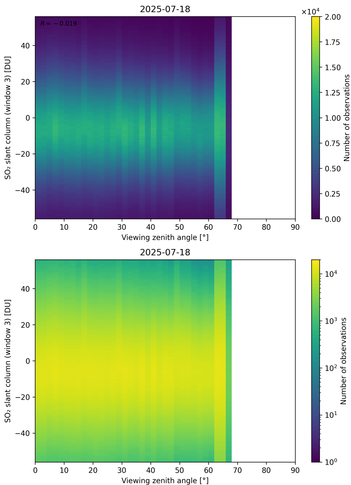
Figure 379: Scatter density plot of “Viewing zenith angle” against “SO 2 slant column (window 3)” for 2025-07-18 to 2025-07-19.
