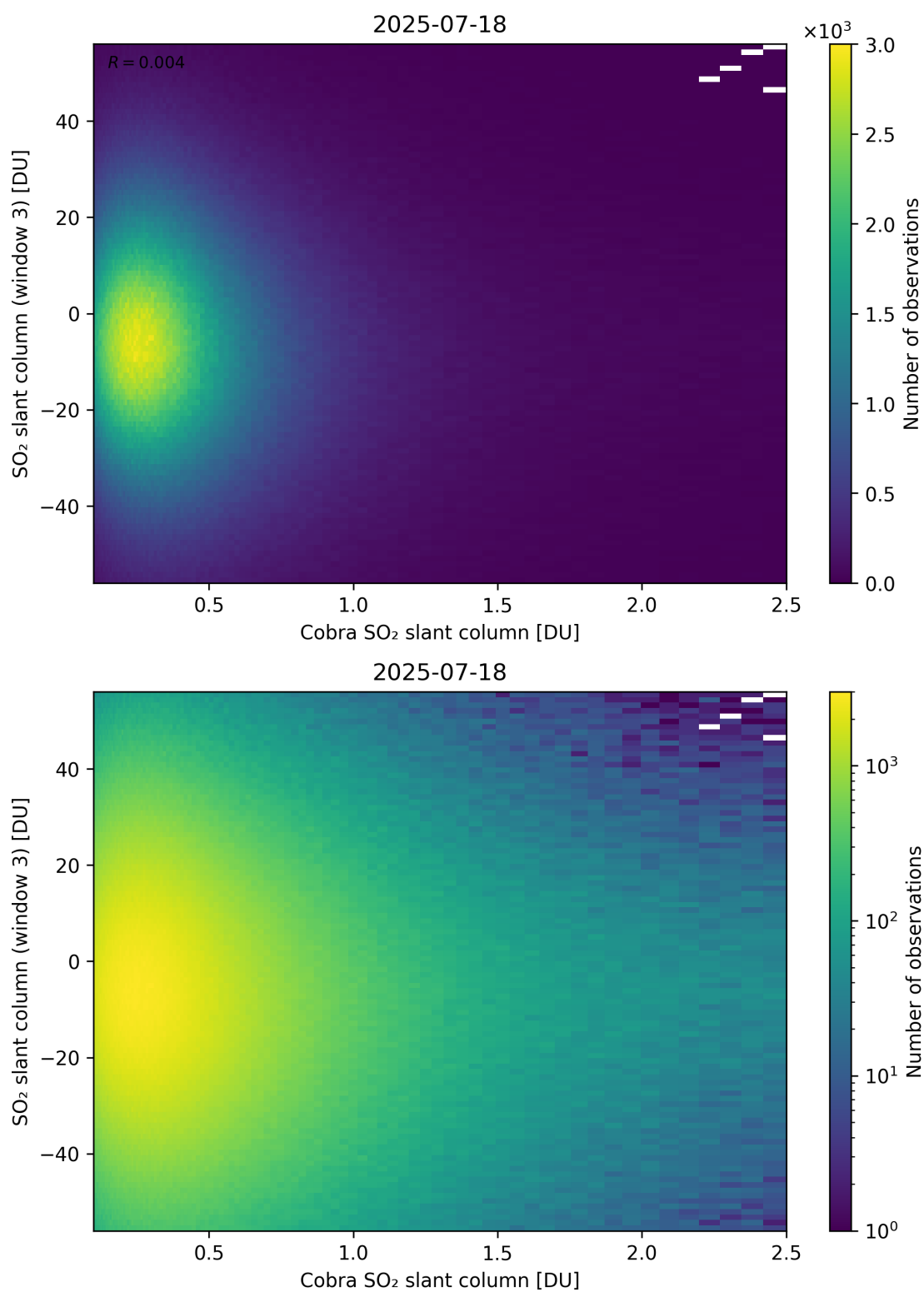
Figure 222: Scatter density plot of “Cobra SO 2 slant column” against “SO 2 slant column (window 3)” for 2025-07-18 to 2025-07-19.
