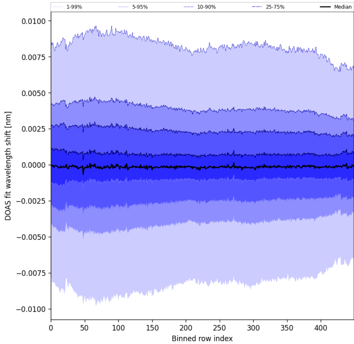
Figure 102: Along track statistics of “DOAS fit wavelength shift” for 2025-07-18 to 2025-07-19
