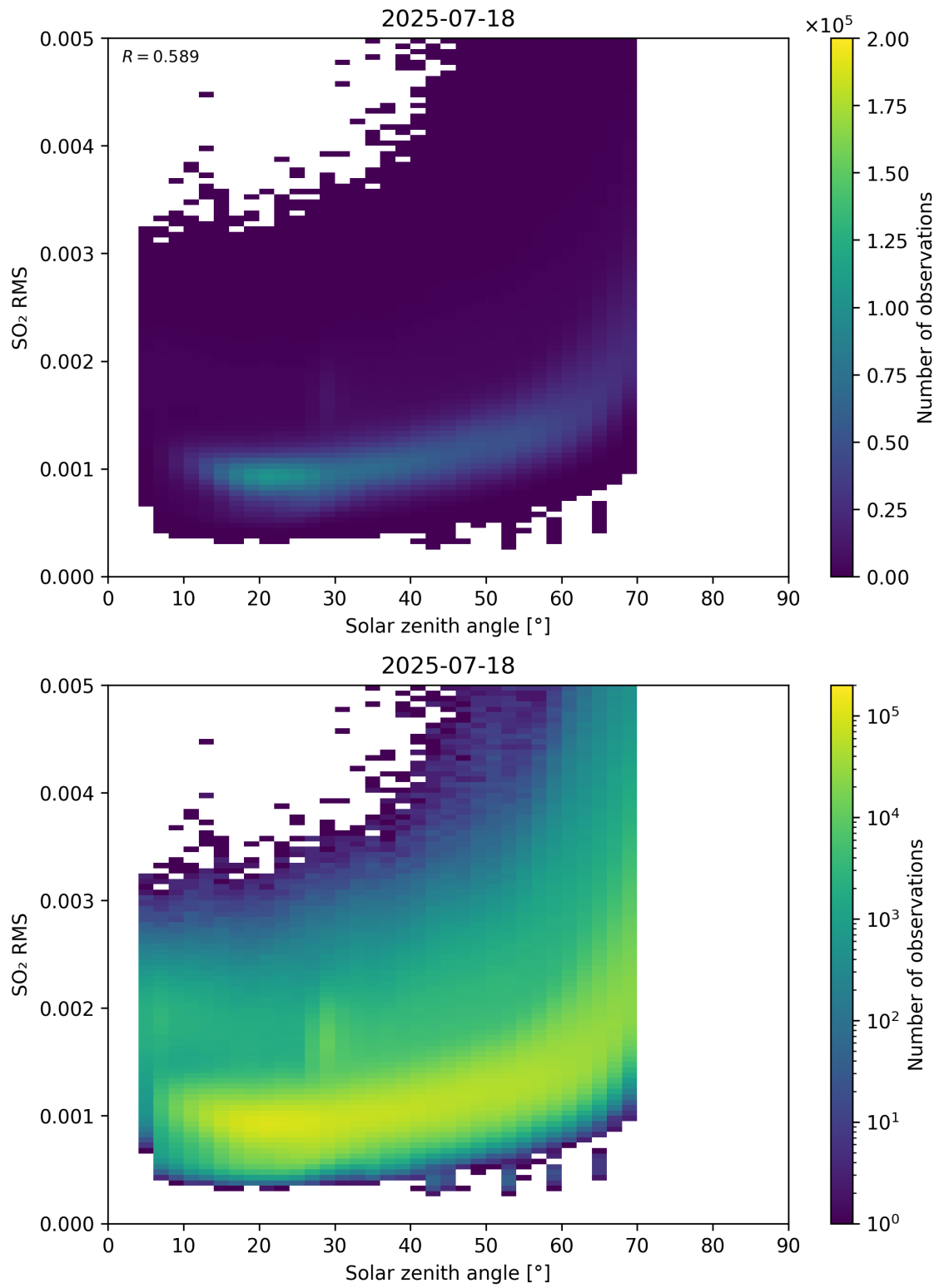
Figure 176: Scatter density plot of “Solar zenith angle” against “SO 2 RMS” for 2025-07-18 to 2025-07-19.
