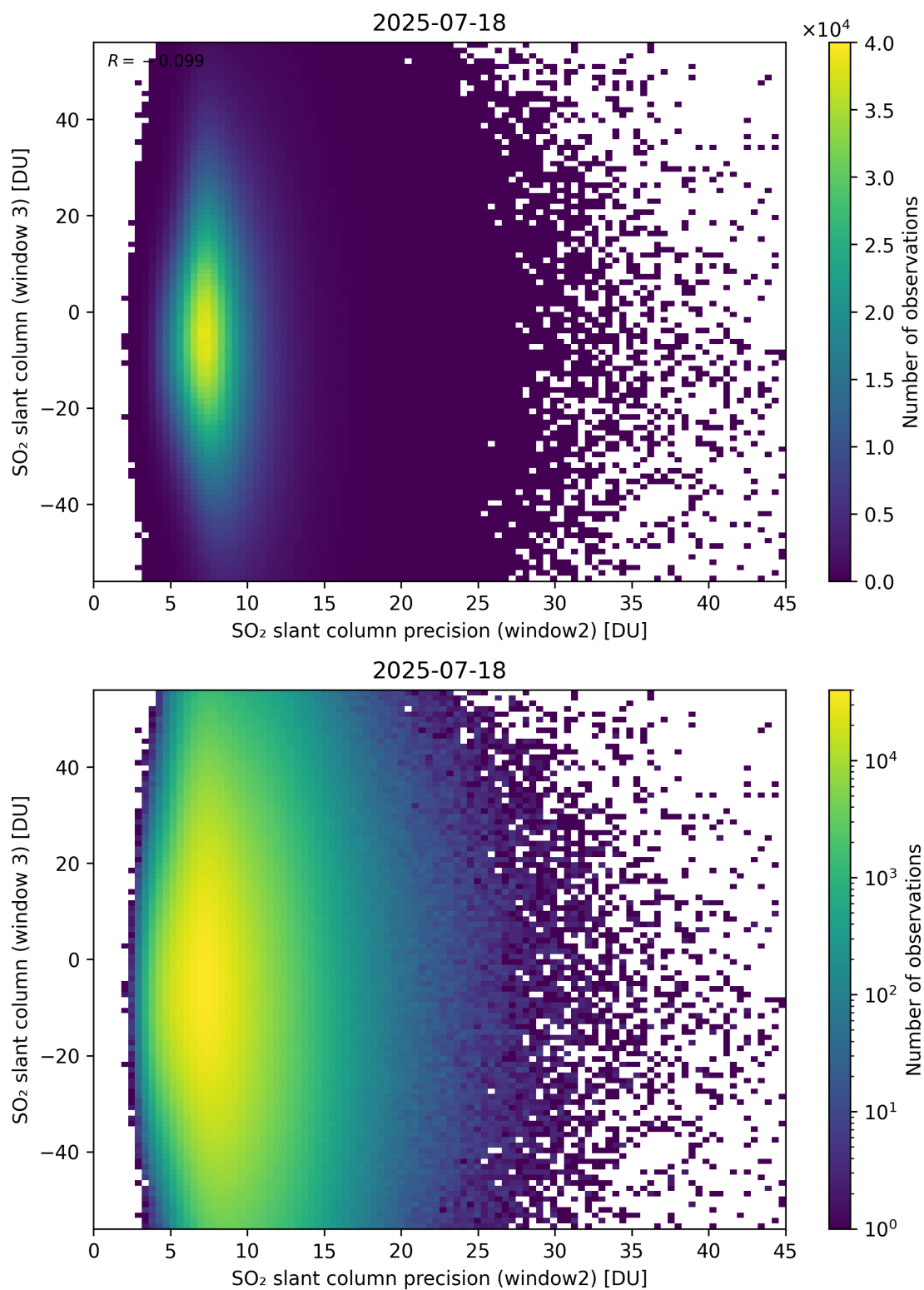
Figure 299: Scatter density plot of “SO 2 slant column precision (window2)” against “SO 2 slant column (window 3)” for 2025-07-18 to 2025-07-19.
