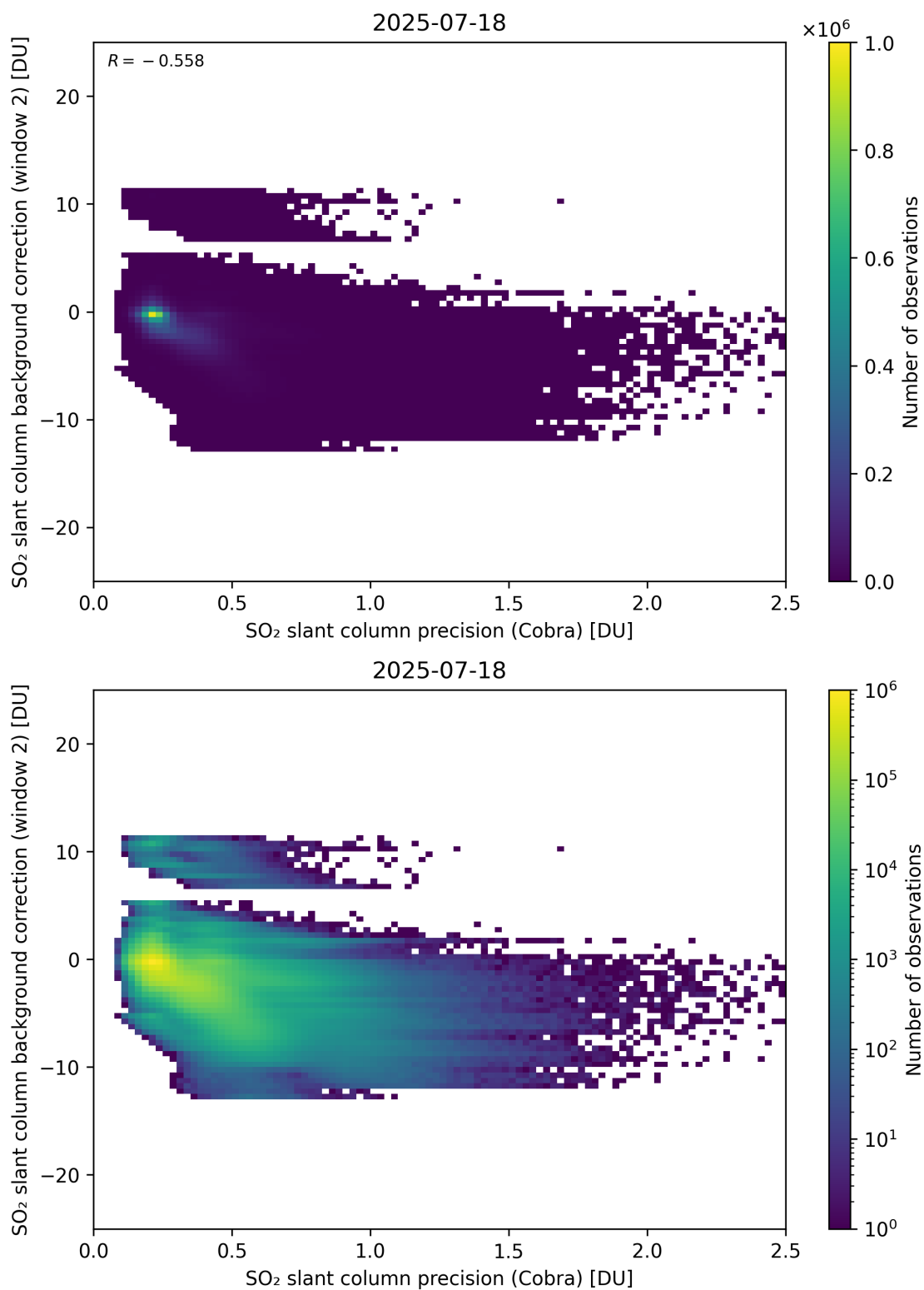
Figure 200: Scatter density plot of “SO 2 slant column precision (Cobra)” against “SO 2 slant column background correction (window 2)” for 2025-07-18 to 2025-07-19.
