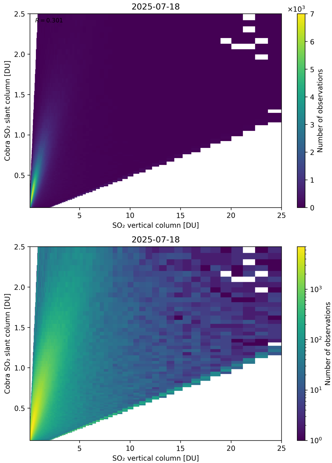
Figure 349: Scatter density plot of “SO 2 vertical column” against “Cobra SO 2 slant column” for 2025-07-18 to 2025-07-19.
