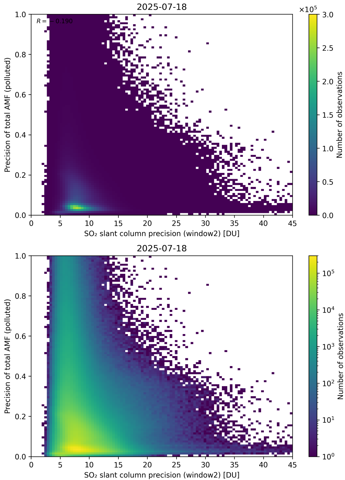
Figure 302: Scatter density plot of “SO 2 slant column precision (window2)” against “Precision of total AMF (polluted)” for 2025-07-18 to 2025-07-19.
