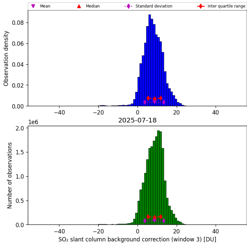
Figure 74: Histogram of “SO 2 slant column background correction (window 3)” for 2025-07-18 to 2025-07-19
