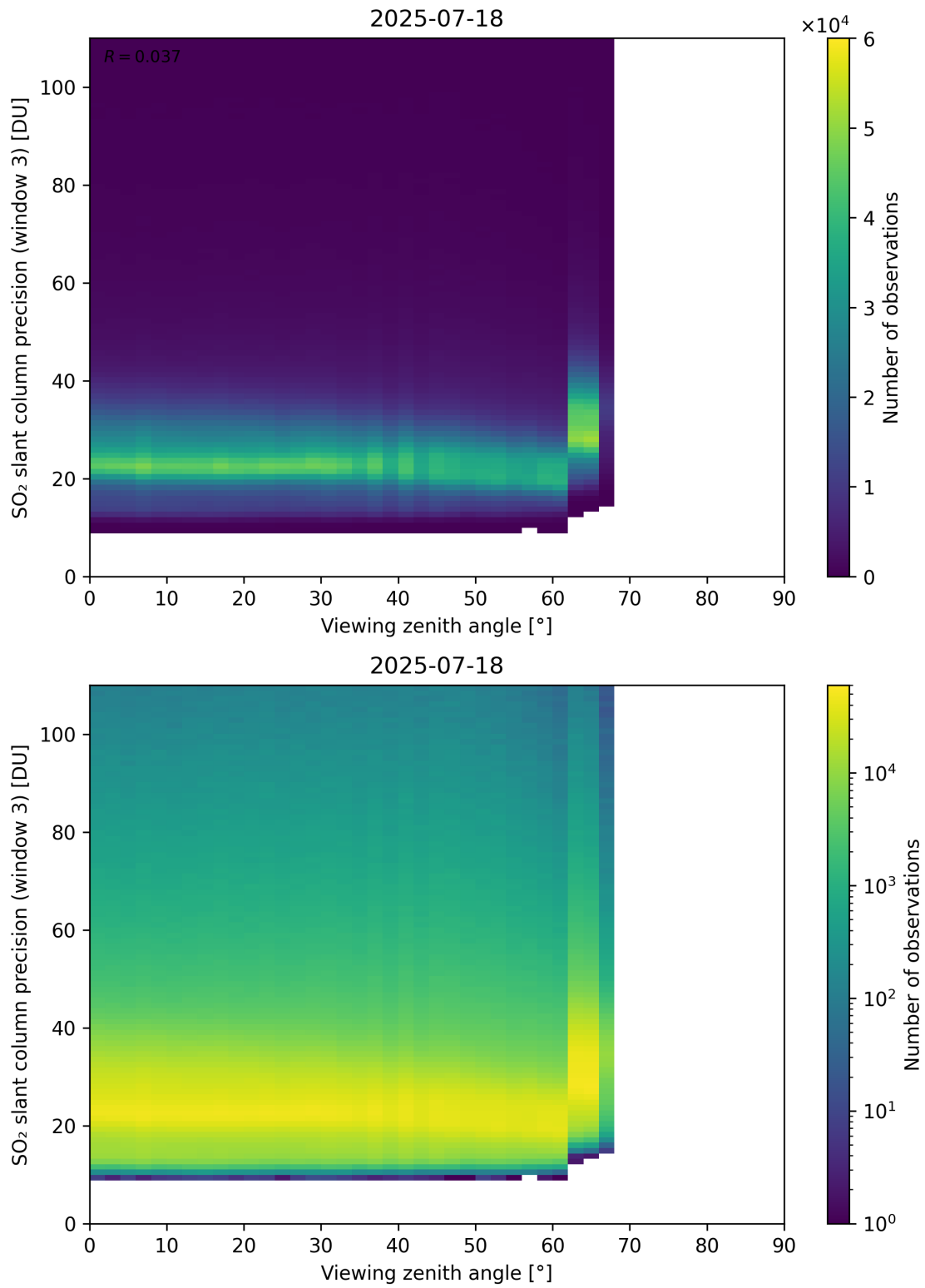
Figure 380: Scatter density plot of “Viewing zenith angle” against “SO 2 slant column precision (window 3)” for 2025-07-18 to 2025-07-19.
