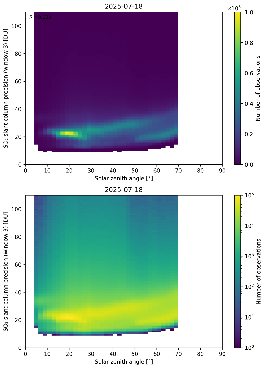
Figure 188: Scatter density plot of “Solar zenith angle” against “SO 2 slant column precision (window 3)” for 2025-07-18 to 2025-07-19.
