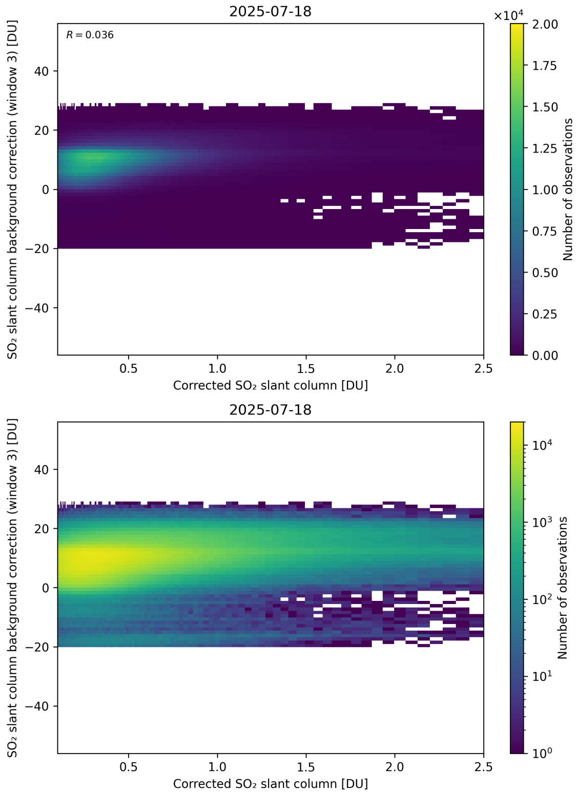
Figure 228: Scatter density plot of “Corrected SO 2 slant column” against “SO 2 slant column background correction (window 3)” for 2025-07-18 to 2025-07-19.
