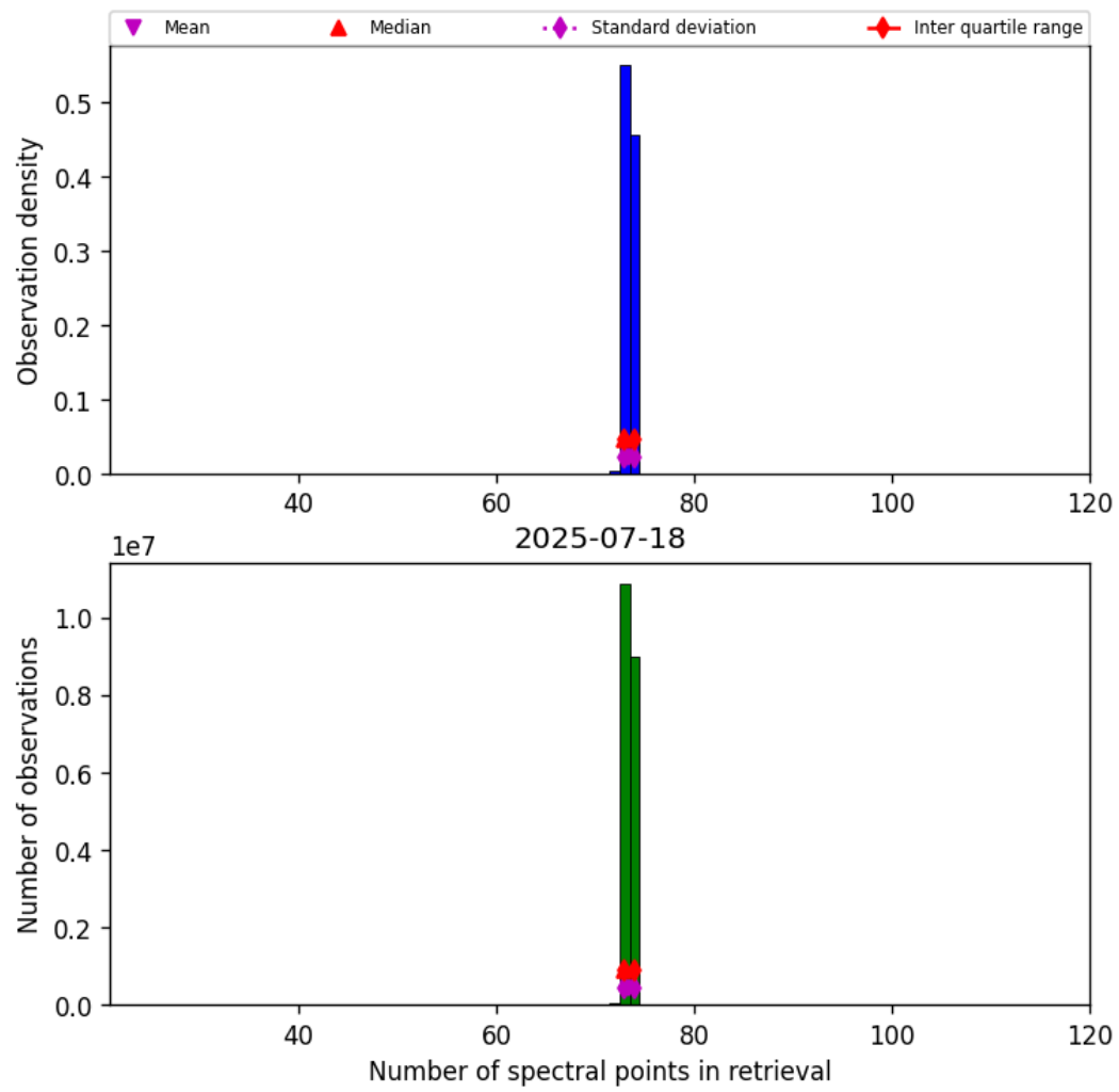
Figure 82: Histogram of “Number of spectral points in retrieval” for 2025-07-18 to 2025-07-19
