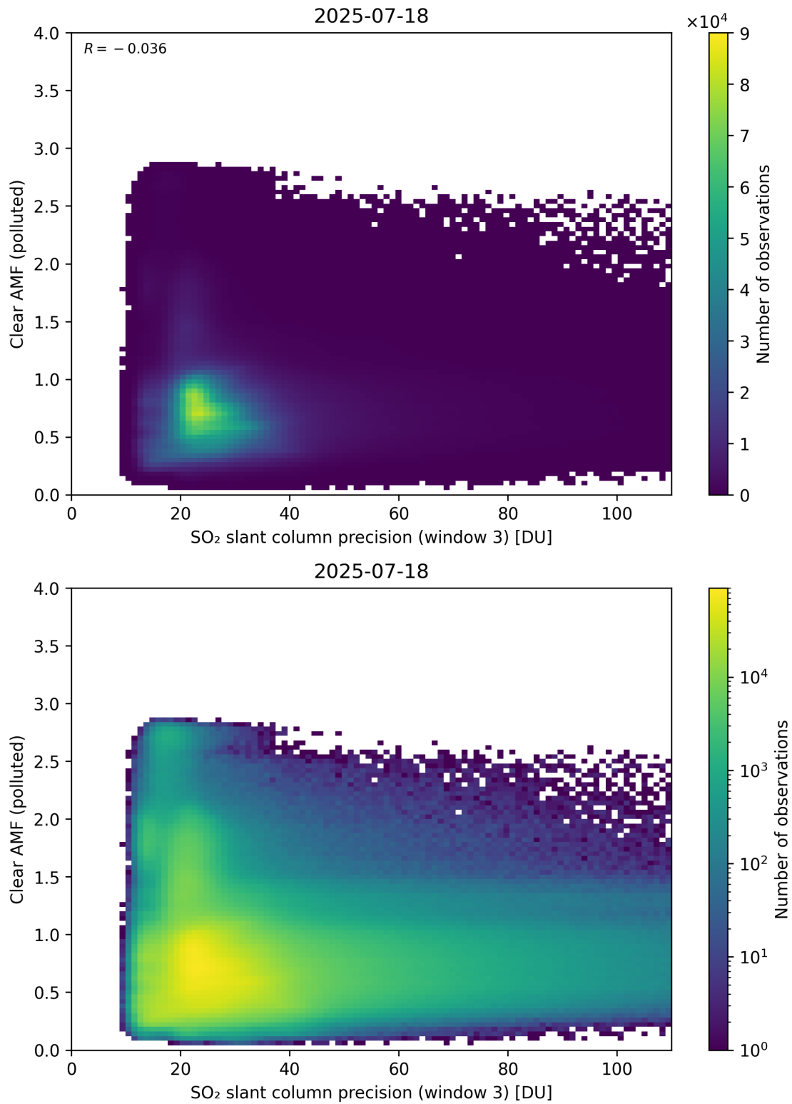
Figure 311: Scatter density plot of “SO 2 slant column precision (window 3)” against “Clear AMF (polluted)” for 2025-07-18 to 2025-07-19.
