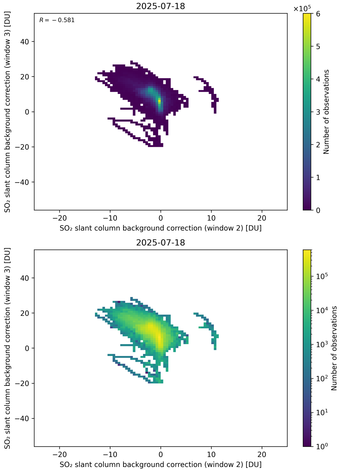
Figure 122: Scatter density plot of “SO 2 slant column background correction (window 2)” against “SO 2 slant column background correction (window 3)” for 2025-07-18 to 2025-07-19.
