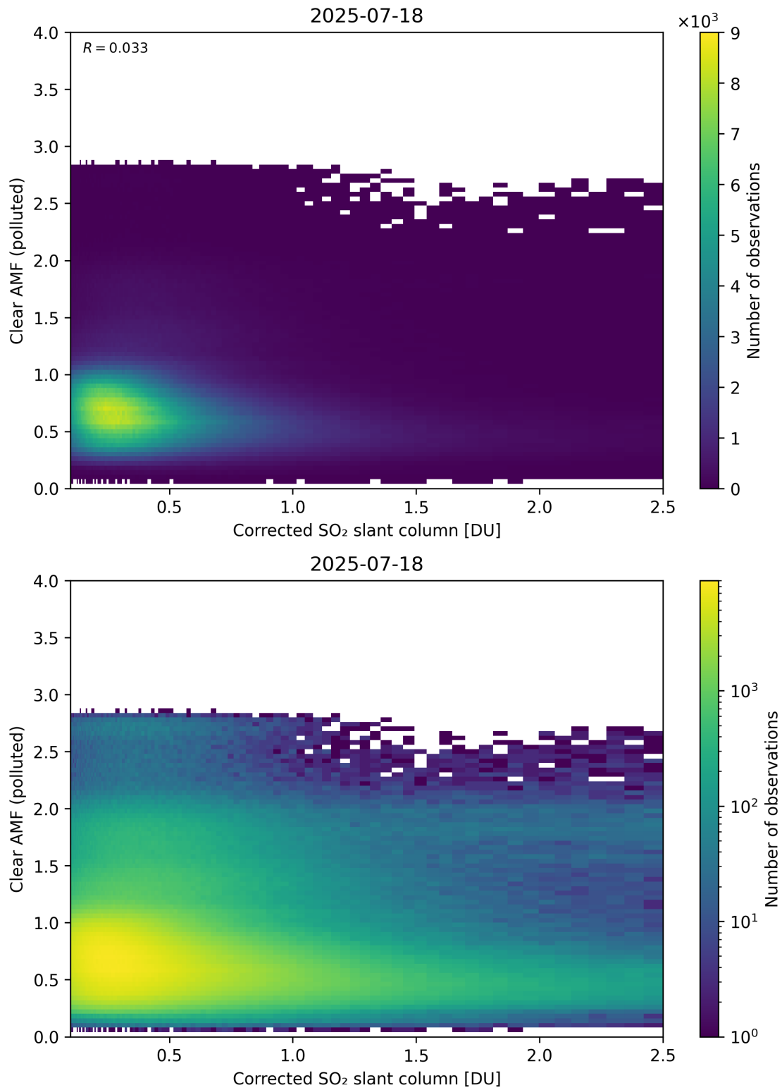
Figure 232: Scatter density plot of “Corrected SO 2 slant column” against “Clear AMF (polluted)” for 2025-07-18 to 2025-07-19.
