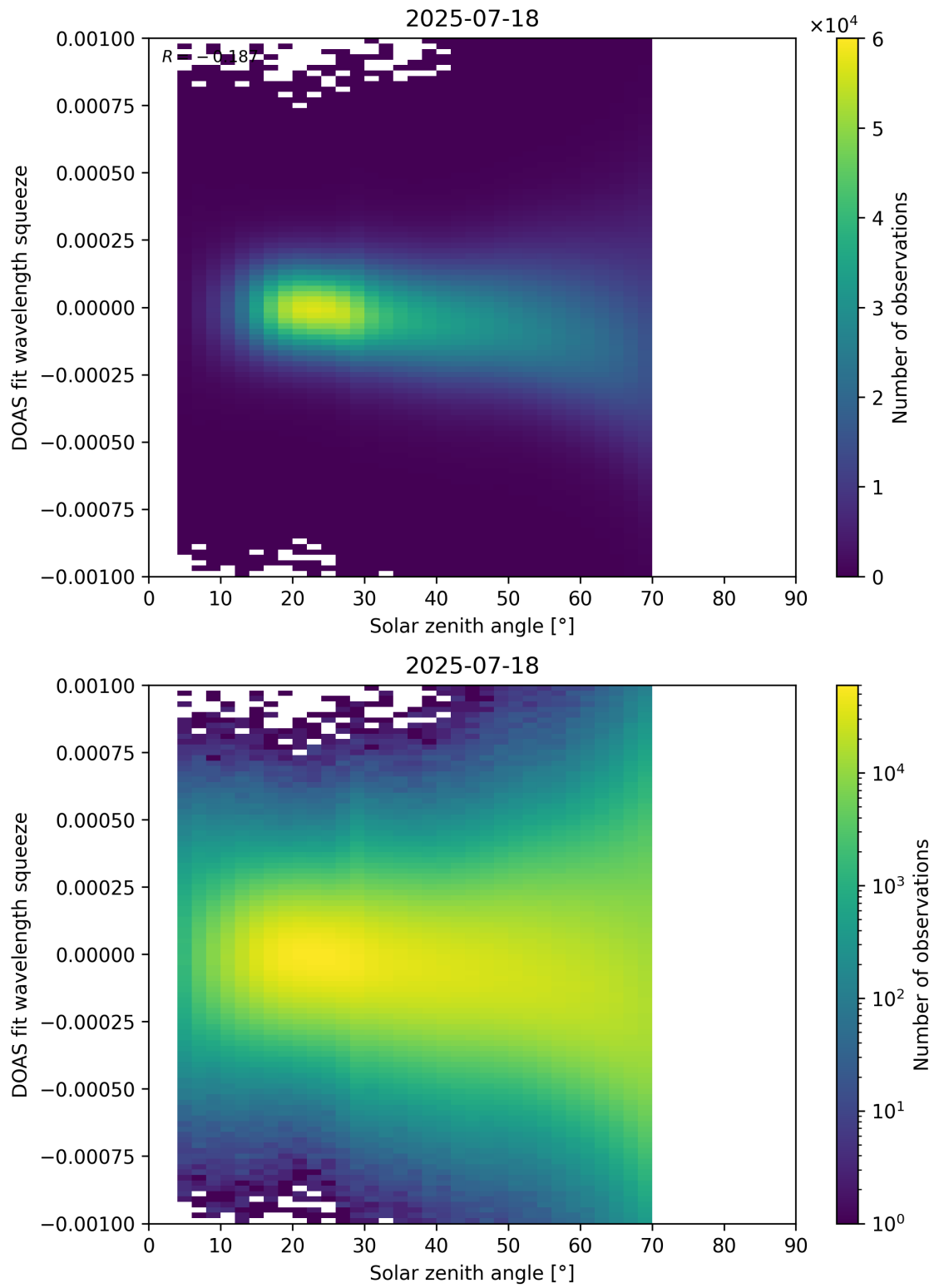
Figure 175: Scatter density plot of “Solar zenith angle” against “DOAS fit wavelength squeeze” for 2025-07-18 to 2025-07-19.
