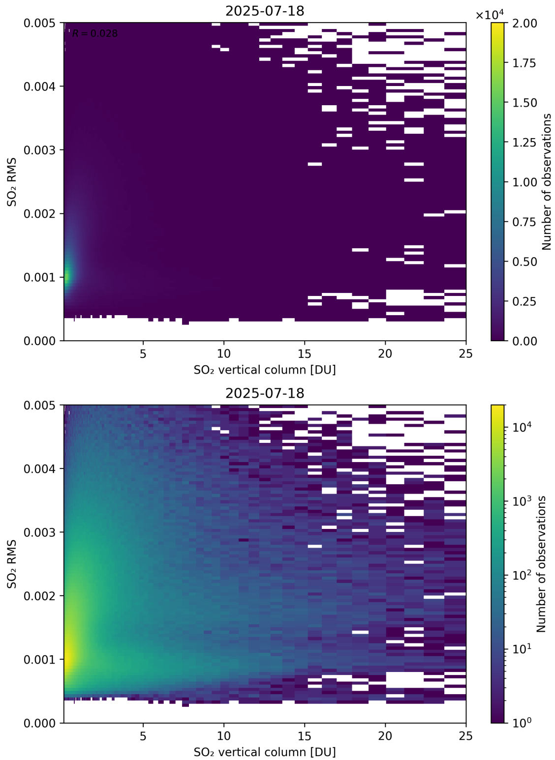
Figure 328: Scatter density plot of “SO 2 vertical column” against “SO 2 RMS” for 2025-07-18 to 2025-07-19.
