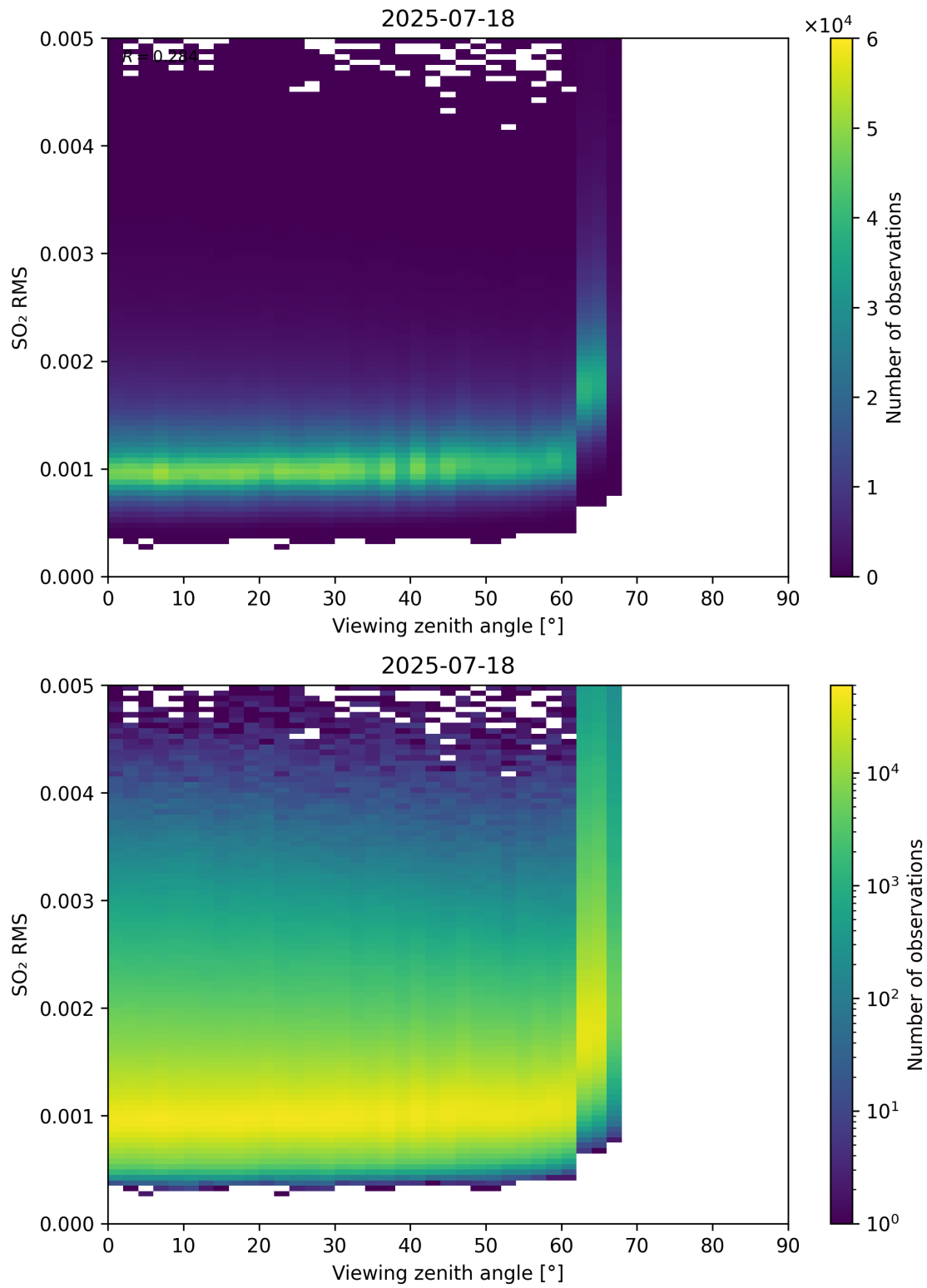
Figure 367: Scatter density plot of “Viewing zenith angle” against “SO 2 RMS” for 2025-07-18 to 2025-07-19.
