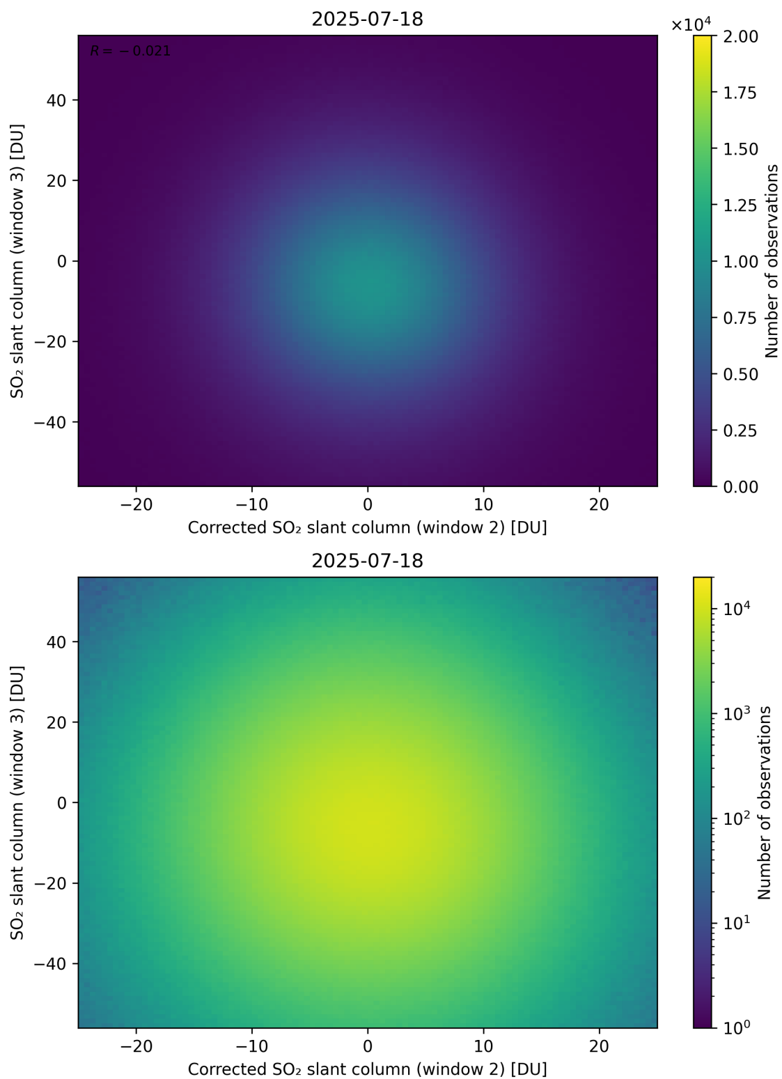
Figure 251: Scatter density plot of “Corrected SO 2 slant column (window 2)” against “SO 2 slant column (window 3)” for 2025-07-18 to 2025-07-19.
