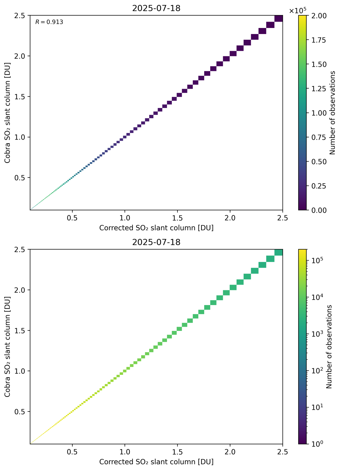
Figure 233: Scatter density plot of “Corrected SO 2 slant column” against “Cobra SO 2 slant column” for 2025-07-18 to 2025-07-19.
