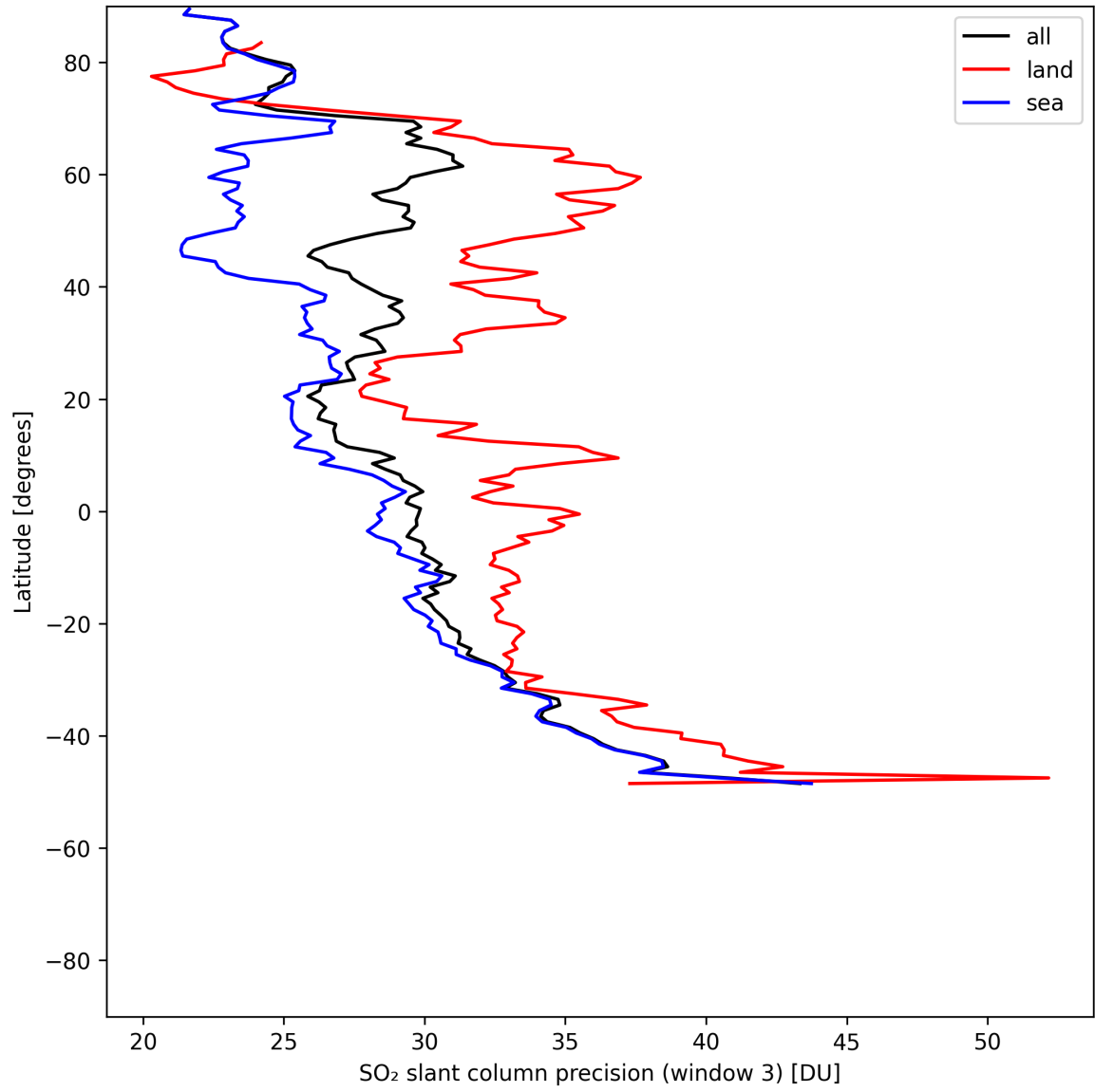
Figure 46: Zonal average of “SO 2 slant column precision (window 3)” for 2025-07-18 to 2025-07-19.
