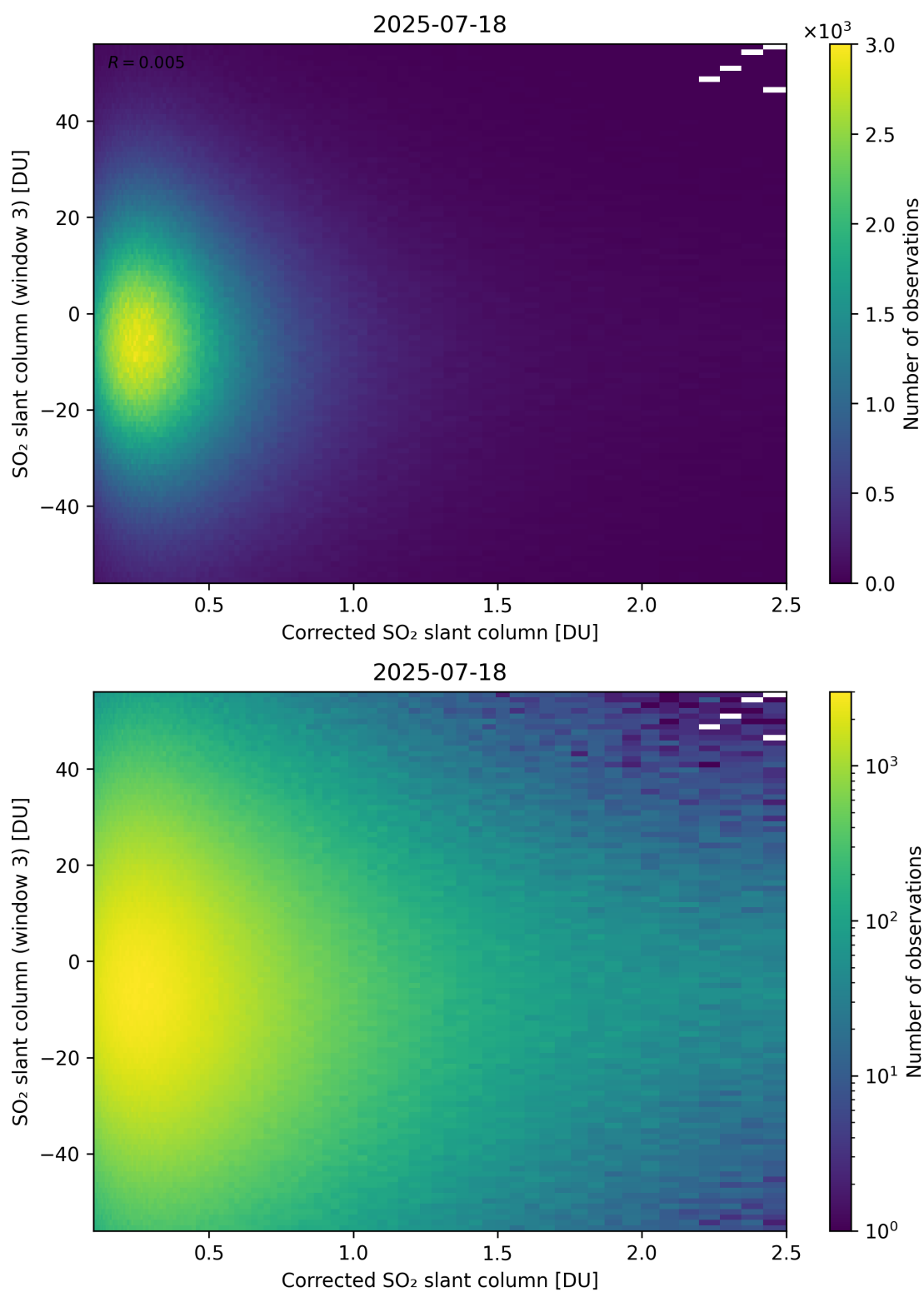
Figure 240: Scatter density plot of “Corrected SO 2 slant column” against “SO 2 slant column (window 3)” for 2025-07-18 to 2025-07-19.
