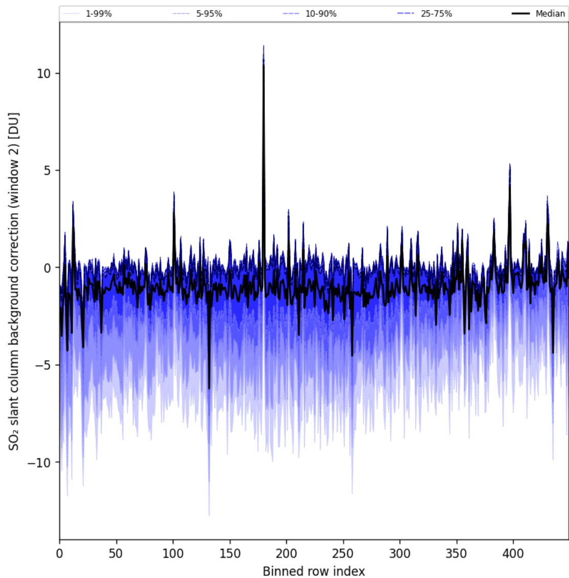
Figure 96: Along track statistics of “SO 2 slant column background correction (window 2)” for 2025-07-18 to 2025-07-19
