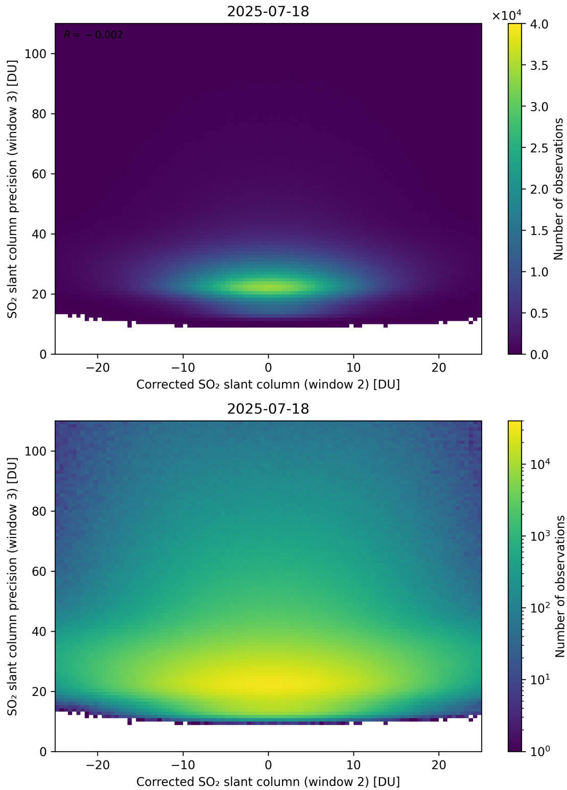
Figure 252: Scatter density plot of “Corrected SO 2 slant column (window 2)” against “SO 2 slant column precision (window 3)” for 2025-07-18 to 2025-07-19.
