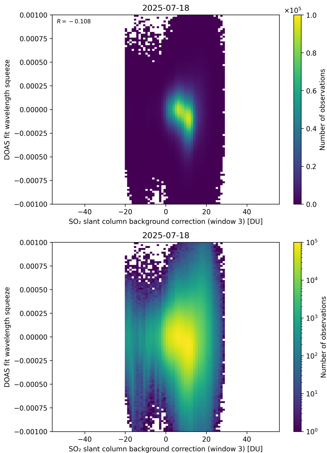
Figure 133: Scatter density plot of “SO 2 slant column background correction (window 3)” against “DOAS fit wavelength squeeze” for 2025-07-18 to 2025-07-19.
