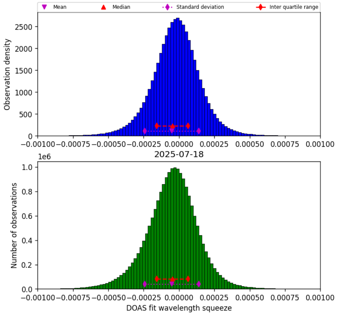
Figure 77: Histogram of “DOAS fit wavelength squeeze” for 2025-07-18 to 2025-07-19
