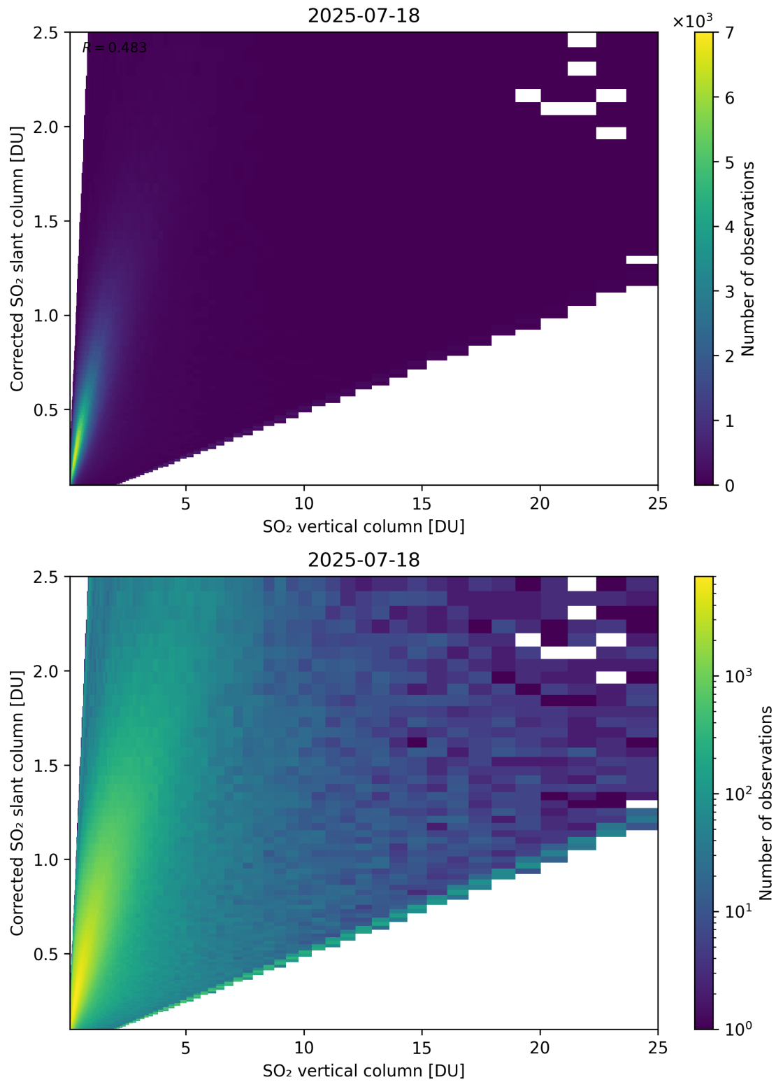
Figure 351: Scatter density plot of “SO 2 vertical column” against “Corrected SO 2 slant column” for 2025-07-18 to 2025-07-19.
