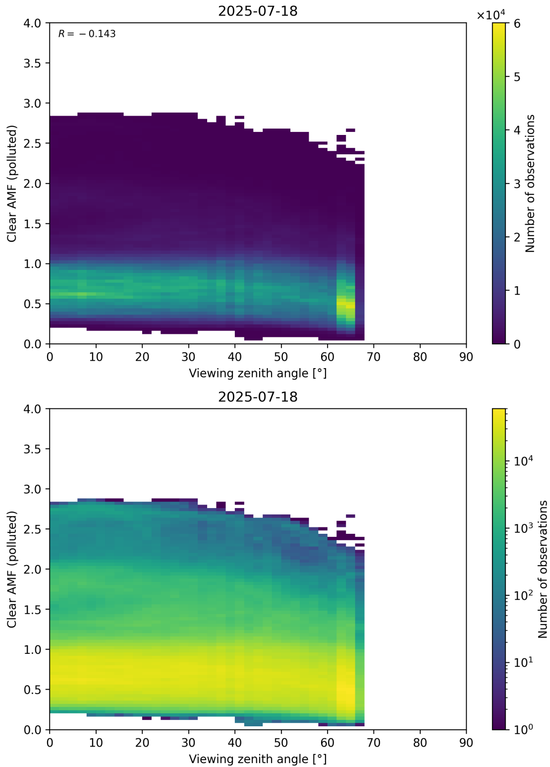
Figure 370: Scatter density plot of “Viewing zenith angle” against “Clear AMF (polluted)” for 2025-07-18 to 2025-07-19.
