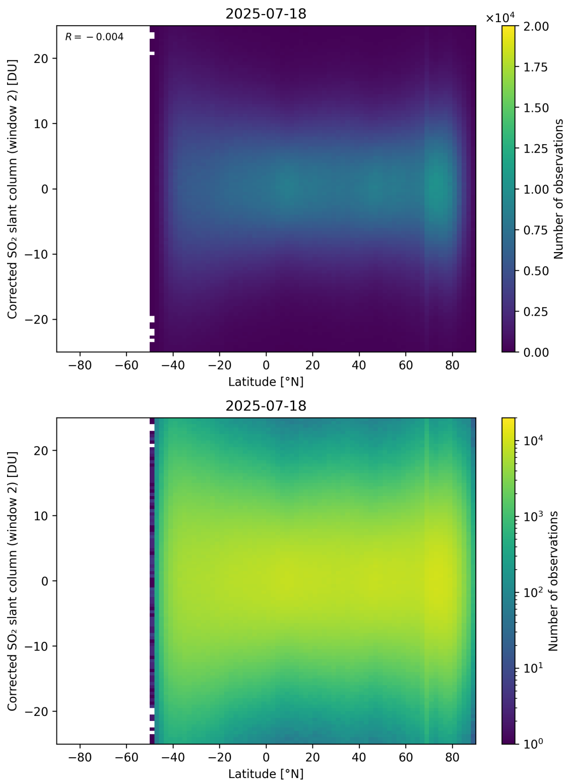
Figure 160: Scatter density plot of “Latitude” against “Corrected SO 2 slant column (window 2)” for 2025-07-18 to 2025-07-19.
