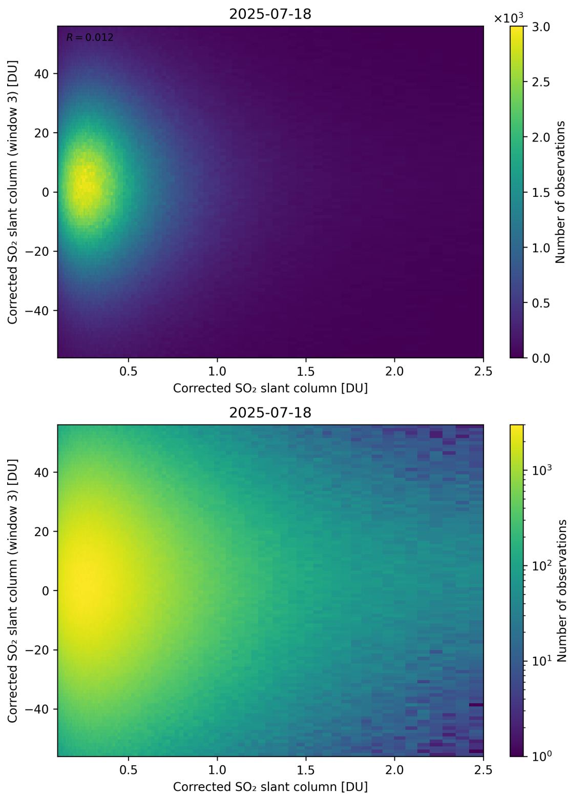
Figure 236: Scatter density plot of “Corrected SO 2 slant column” against “Corrected SO 2 slant column (window 3)” for 2025-07-18 to 2025-07-19.
