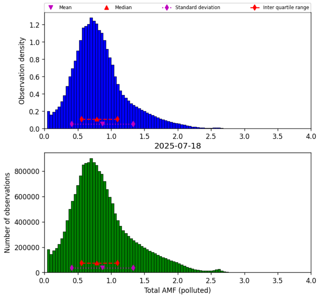
Figure 79: Histogram of “Total AMF (polluted)” for 2025-07-18 to 2025-07-19
