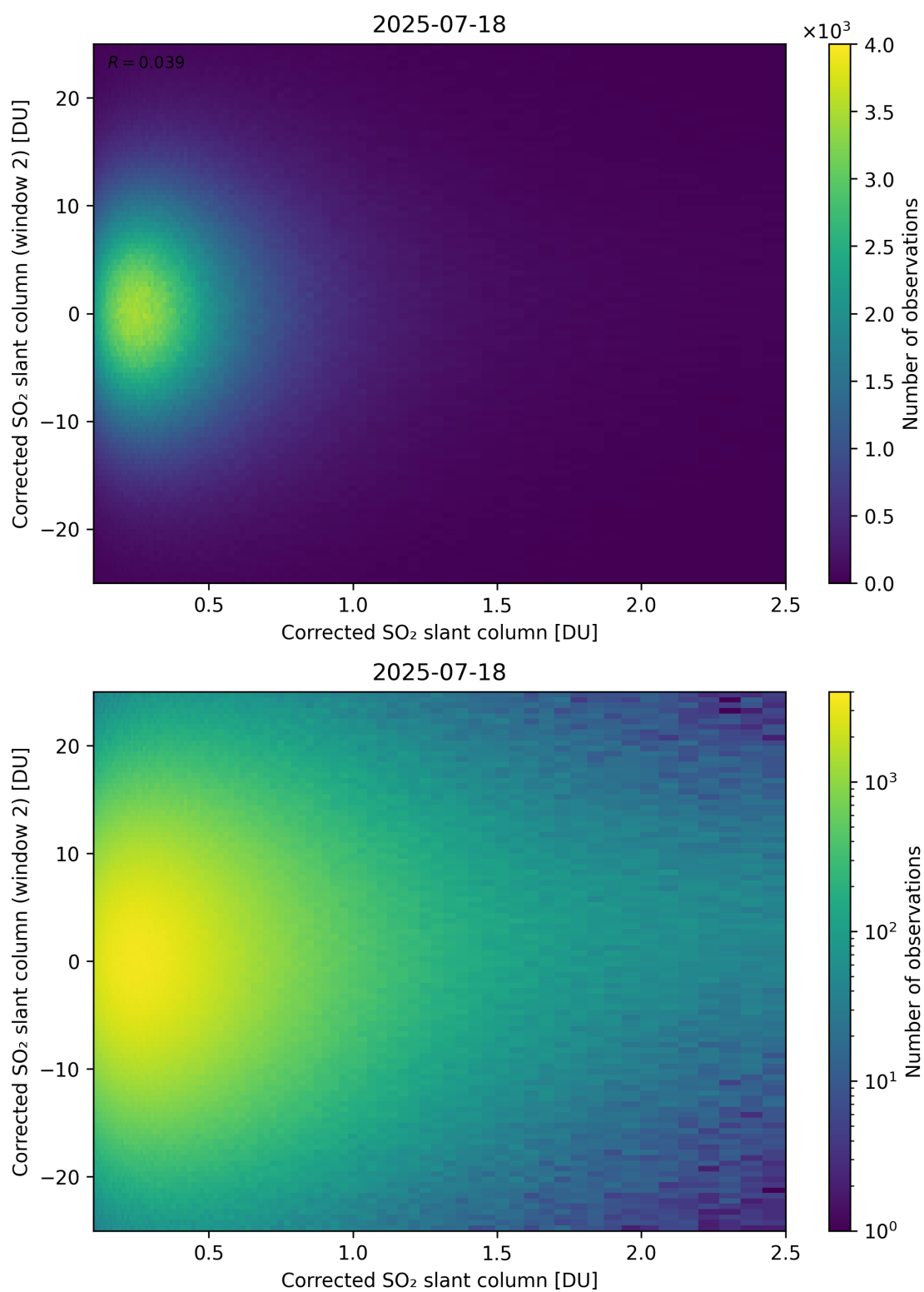
Figure 235: Scatter density plot of “Corrected SO 2 slant column” against “Corrected SO 2 slant column (window 2)” for 2025-07-18 to 2025-07-19.
