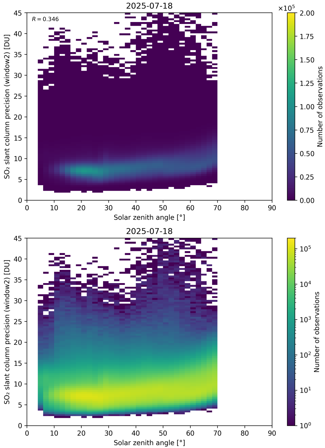
Figure 186: Scatter density plot of “Solar zenith angle” against “SO 2 slant column precision (window2)” for 2025-07-18 to 2025-07-19.
