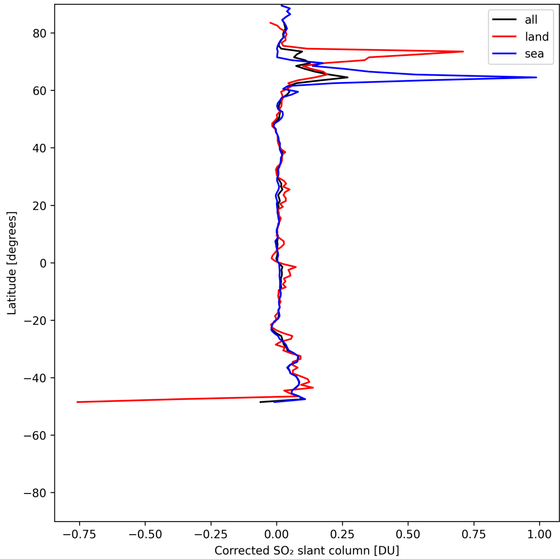
Figure 34: Zonal average of “Corrected SO 2 slant column” for 2025-07-18 to 2025-07-19.
