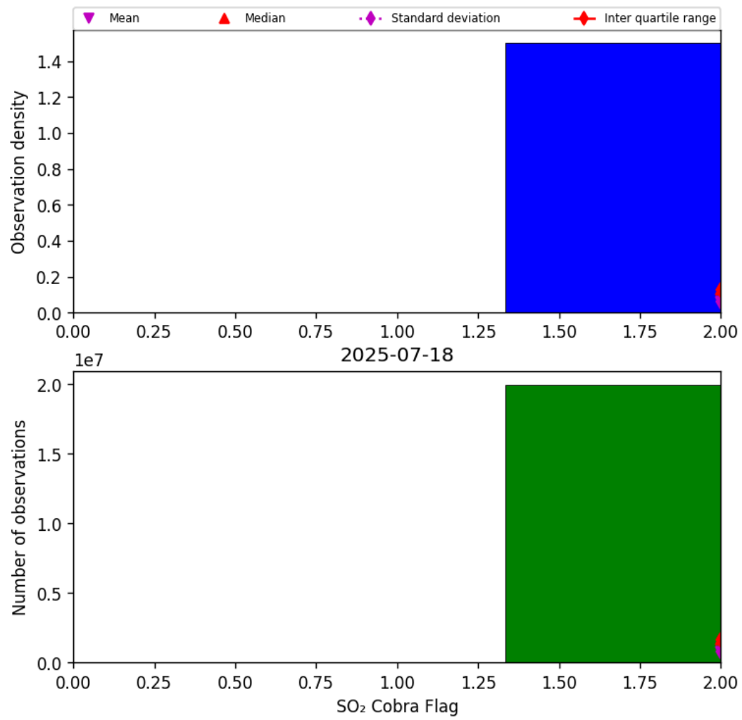
Figure 75: Histogram of “SO 2 Cobra Flag” for 2025-07-18 to 2025-07-19
