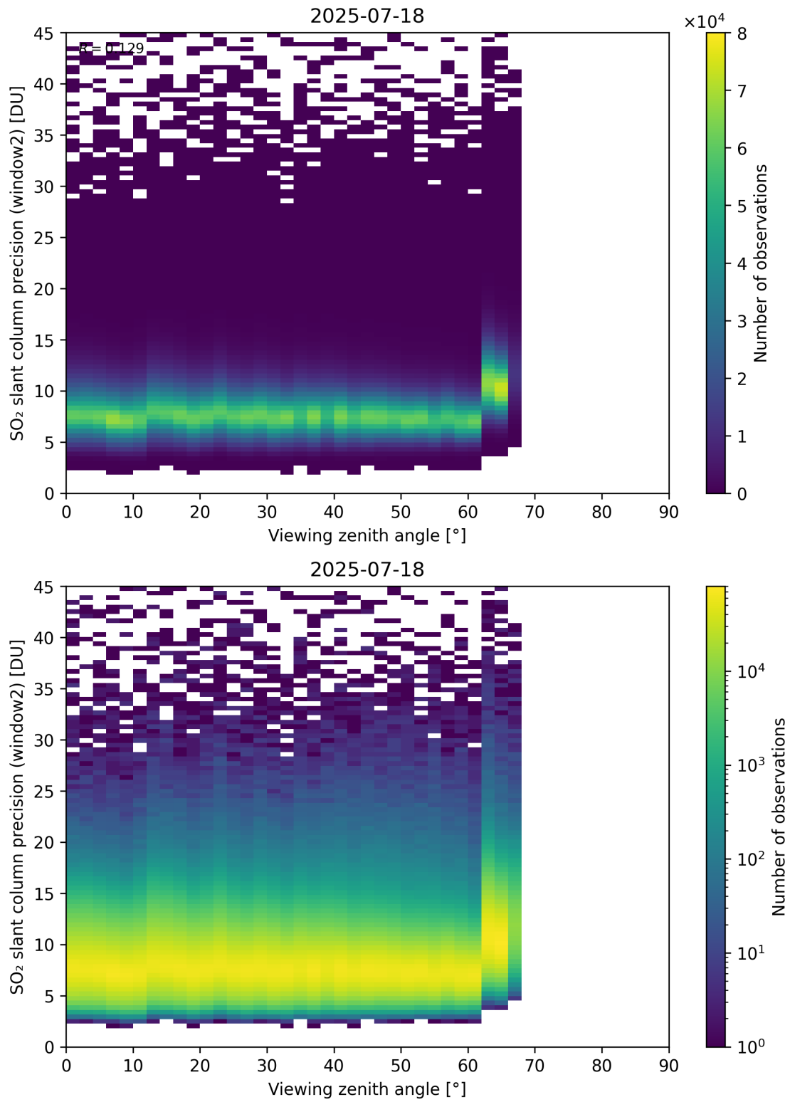
Figure 378: Scatter density plot of “Viewing zenith angle” against “SO 2 slant column precision (window2)” for 2025-07-18 to 2025-07-19.
