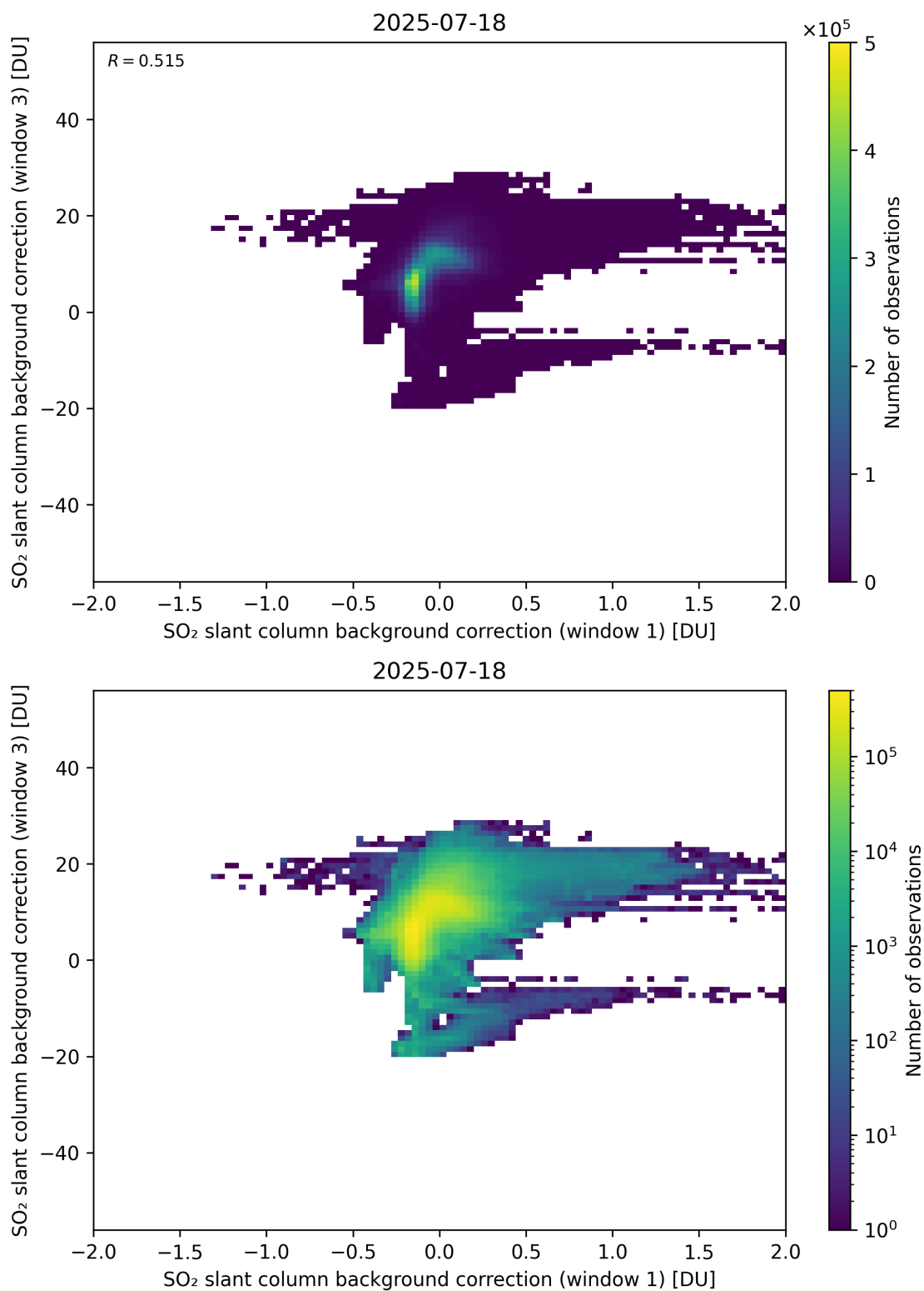
Figure 110: Scatter density plot of “SO 2 slant column background correction (window 1)” against “SO 2 slant column background correction (window 3)” for 2025-07-18 to 2025-07-19.
