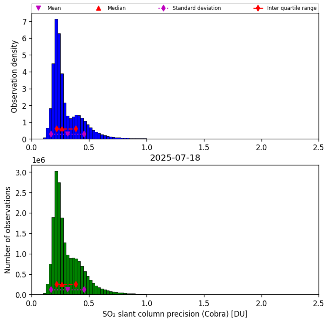
Figure 62: Histogram of “SO 2 slant column precision (Cobra)” for 2025-07-18 to 2025-07-19
