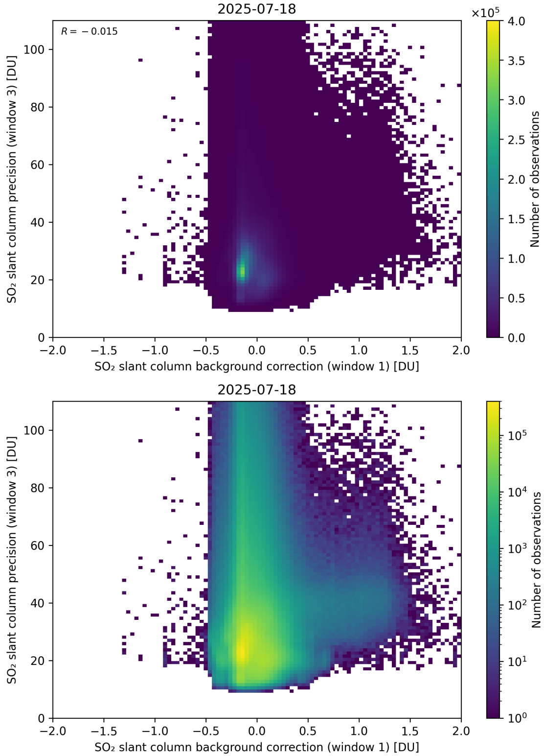
Figure 119: Scatter density plot of “SO 2 slant column background correction (window 1)” against “SO 2 slant column precision (window 3)” for 2025-07-18 to 2025-07-19.
