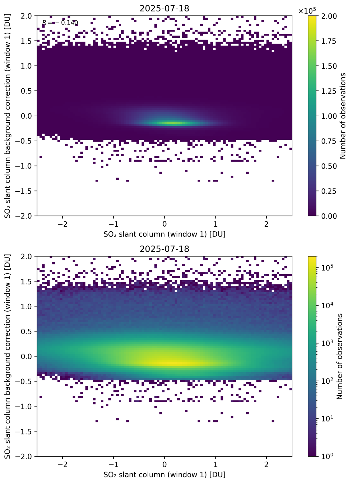
Figure 262: Scatter density plot of “SO 2 slant column (window 1)” against “SO 2 slant column background correction (window 1)” for 2025-07-18 to 2025-07-19.
