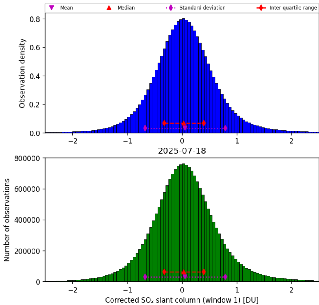
Figure 65: Histogram of “Corrected SO 2 slant column (window 1)” for 2025-07-18 to 2025-07-19
