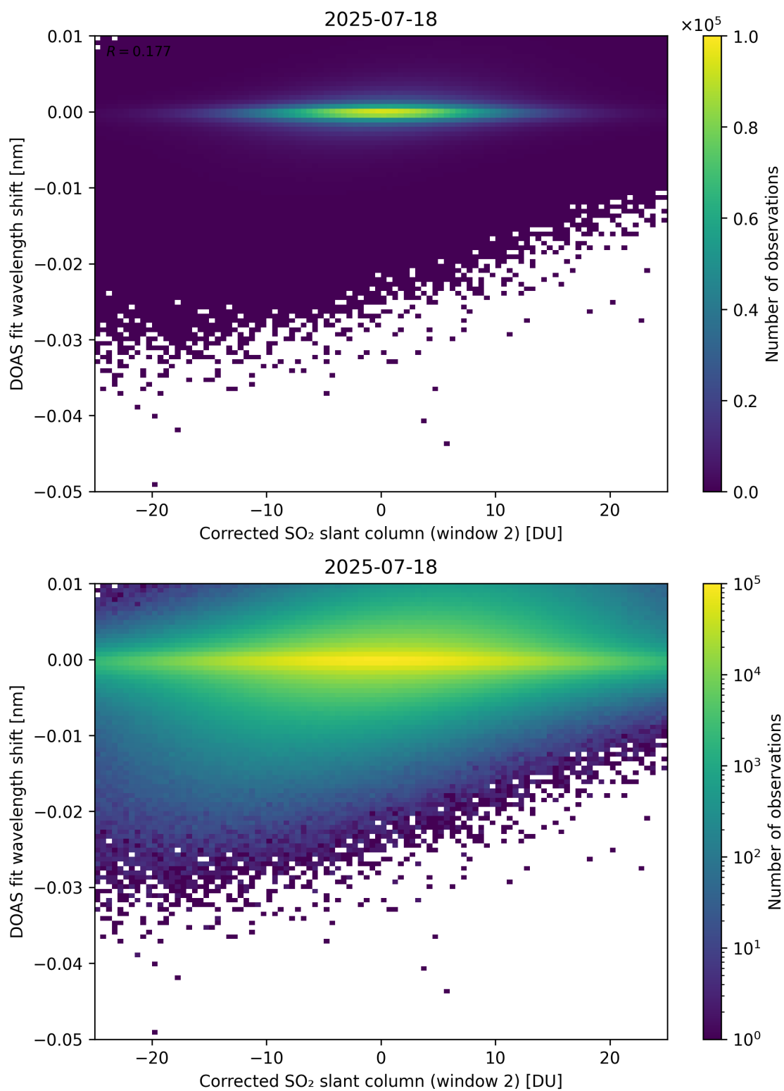
Figure 246: Scatter density plot of “Corrected SO 2 slant column (window 2)” against “DOAS fit wavelength shift” for 2025-07-18 to 2025-07-19.
