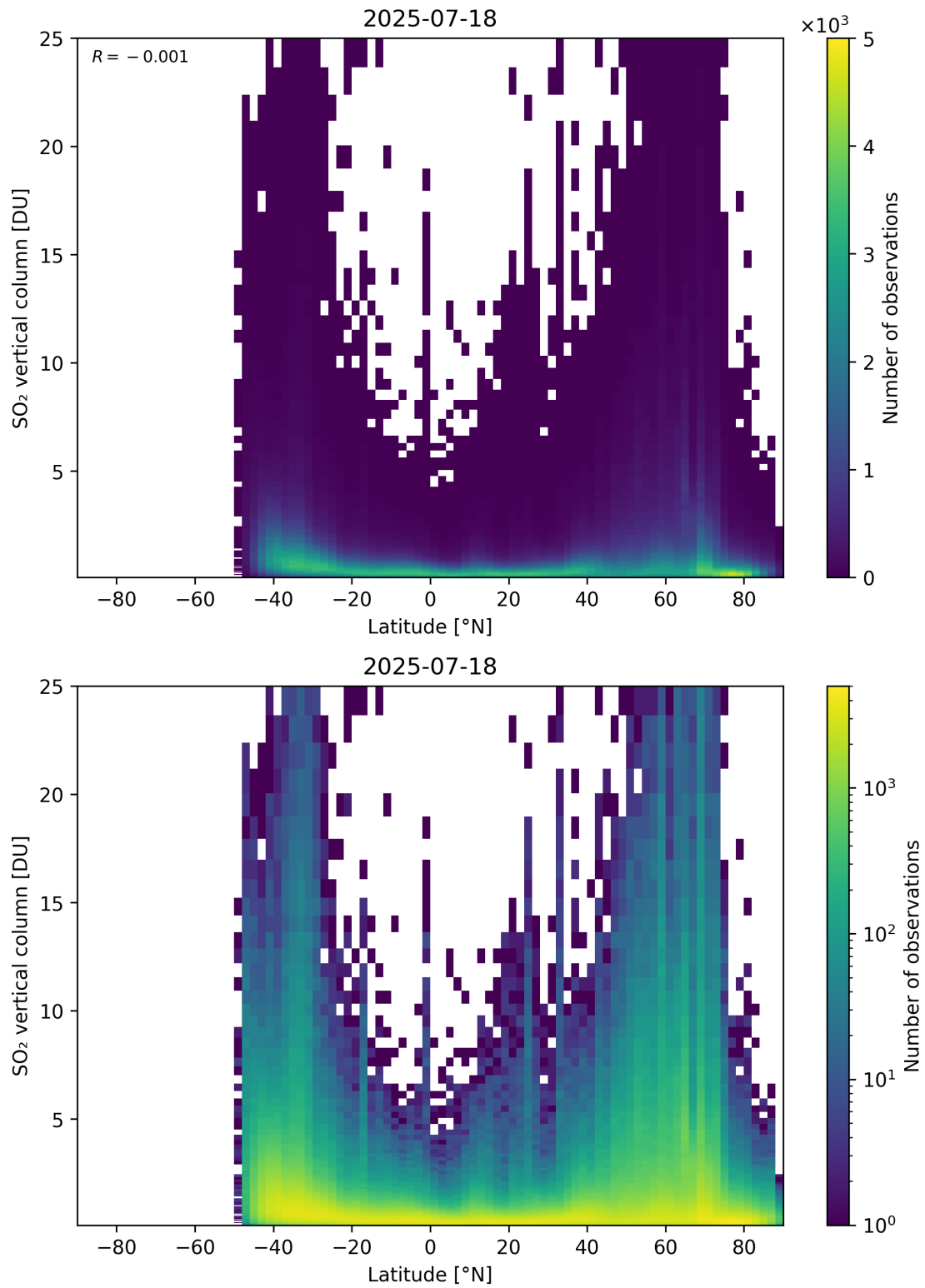
Figure 169: Scatter density plot of “Latitude” against “SO 2 vertical column” for 2025-07-18 to 2025-07-19.
