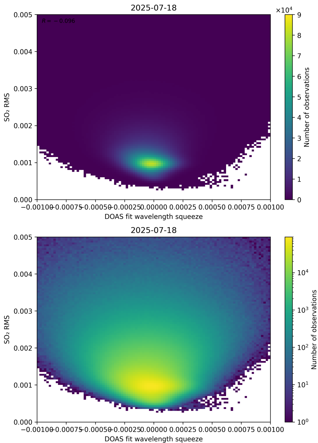
Figure 143: Scatter density plot of “DOAS fit wavelength squeeze” against “SO 2 RMS” for 2025-07-18 to 2025-07-19.
