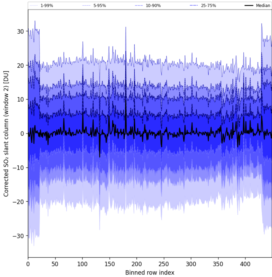
Figure 95: Along track statistics of “Corrected SO 2 slant column (window 2)” for 2025-07-18 to 2025-07-19
