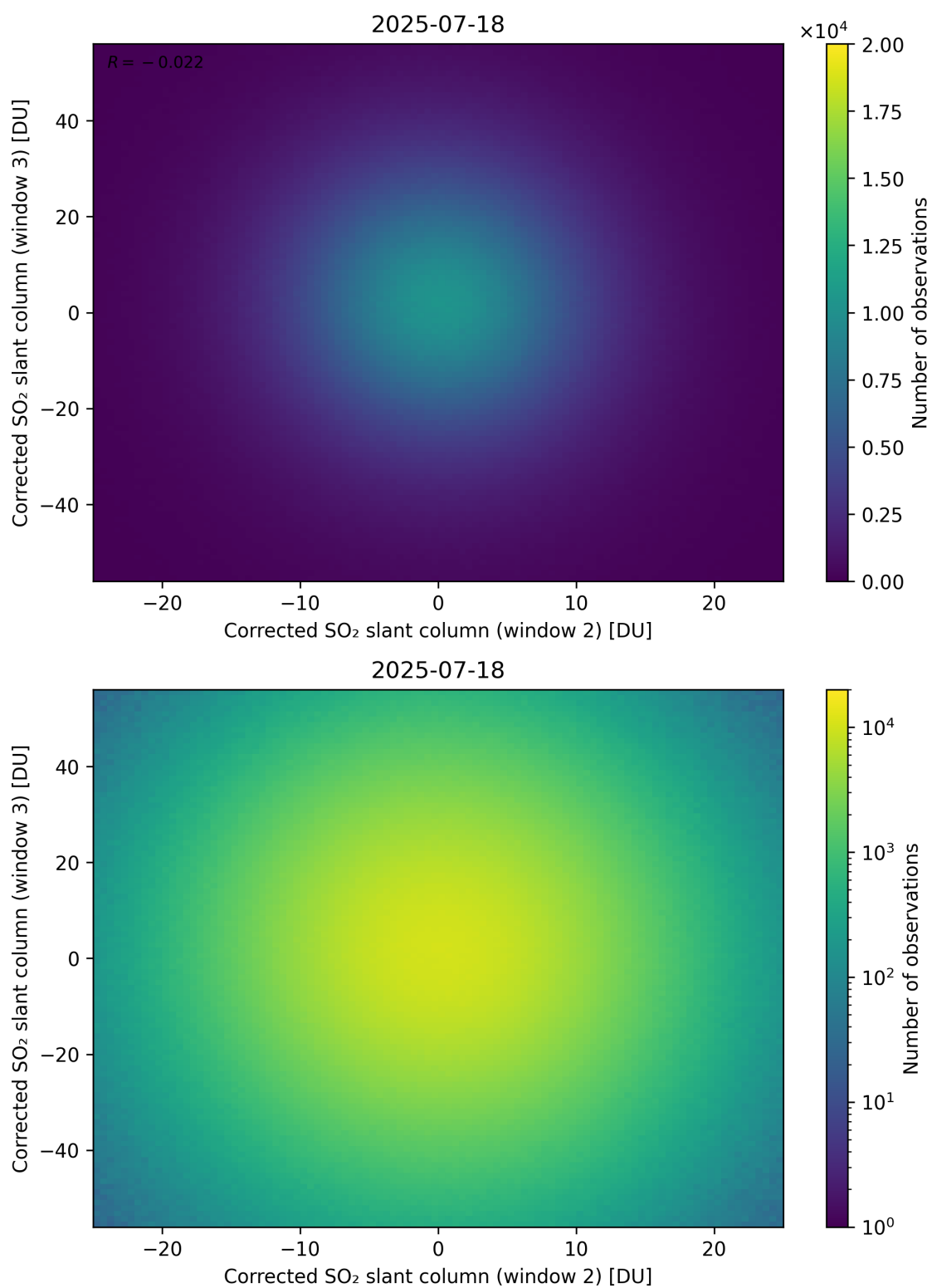
Figure 250: Scatter density plot of “Corrected SO 2 slant column (window 2)” against “Corrected SO 2 slant column (window 3)” for 2025-07-18 to 2025-07-19.
