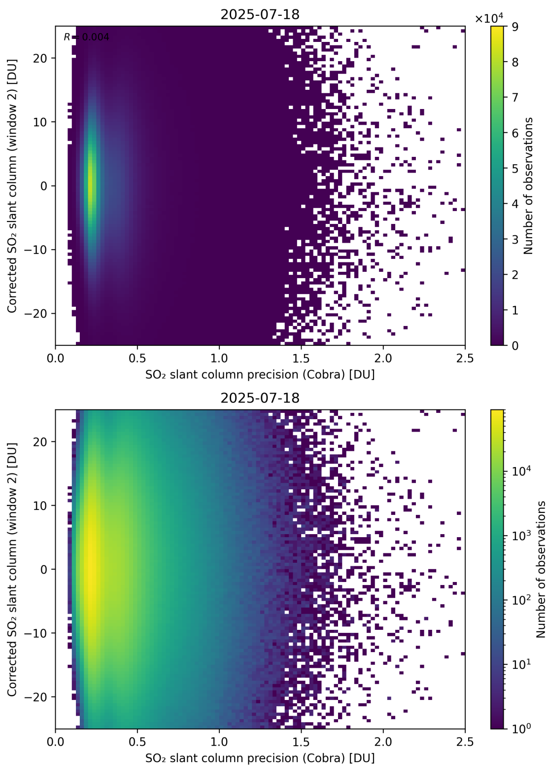
Figure 206: Scatter density plot of “SO 2 slant column precision (Cobra)” against “Corrected SO 2 slant column (window 2)” for 2025-07-18 to 2025-07-19.
