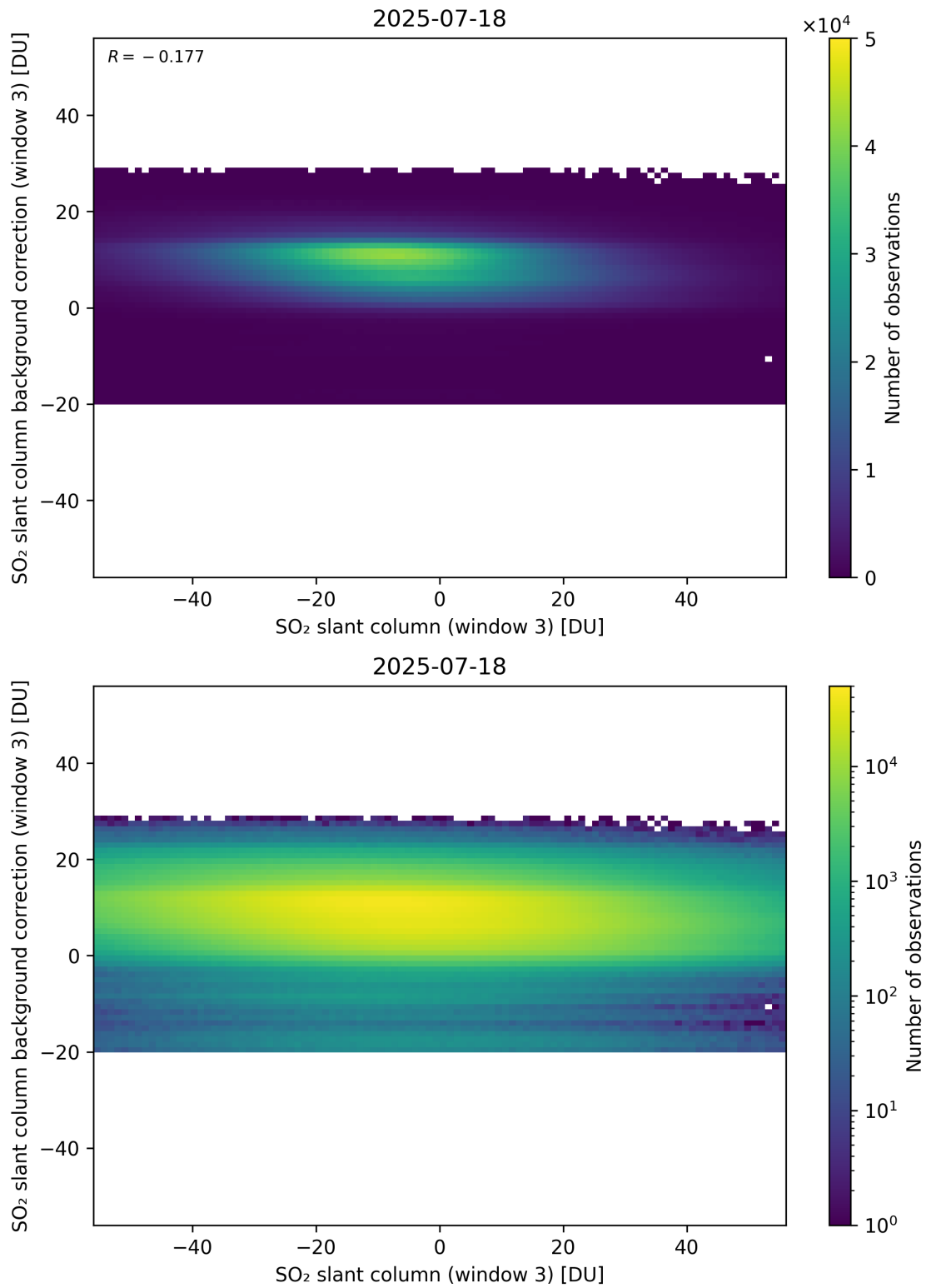
Figure 303: Scatter density plot of “SO 2 slant column (window 3)” against “SO 2 slant column background correction (window 3)” for 2025-07-18 to 2025-07-19.
