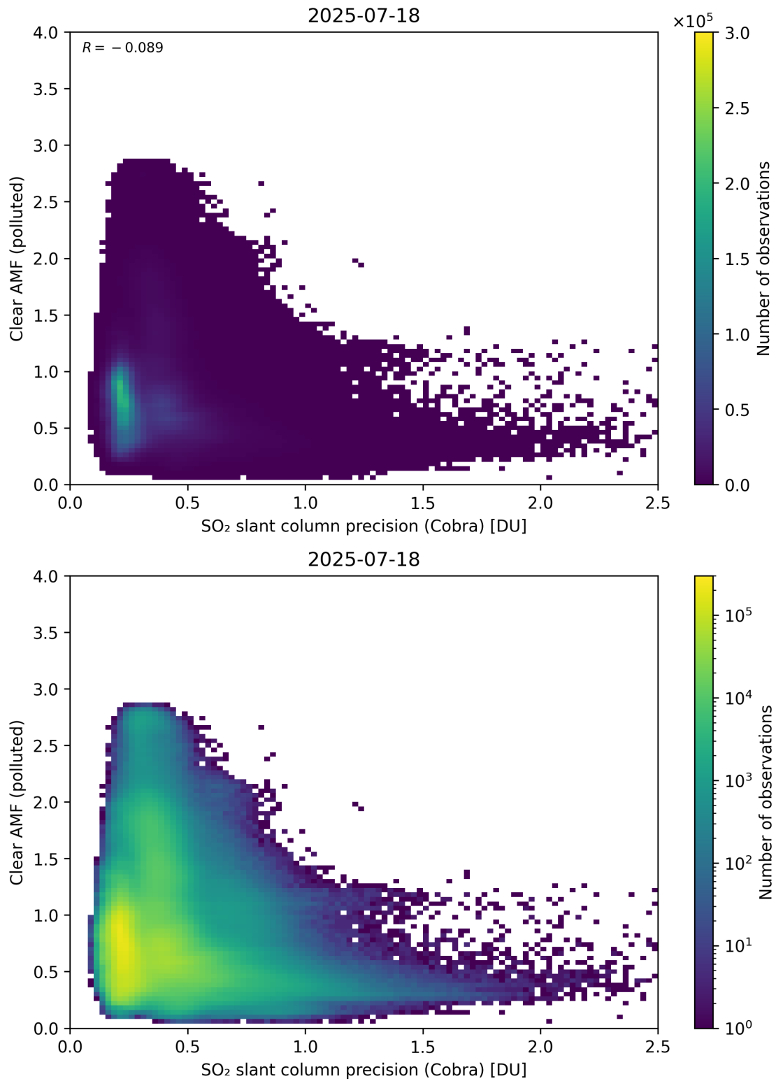
Figure 205: Scatter density plot of “SO 2 slant column precision (Cobra)” against “Clear AMF (polluted)” for 2025-07-18 to 2025-07-19.
