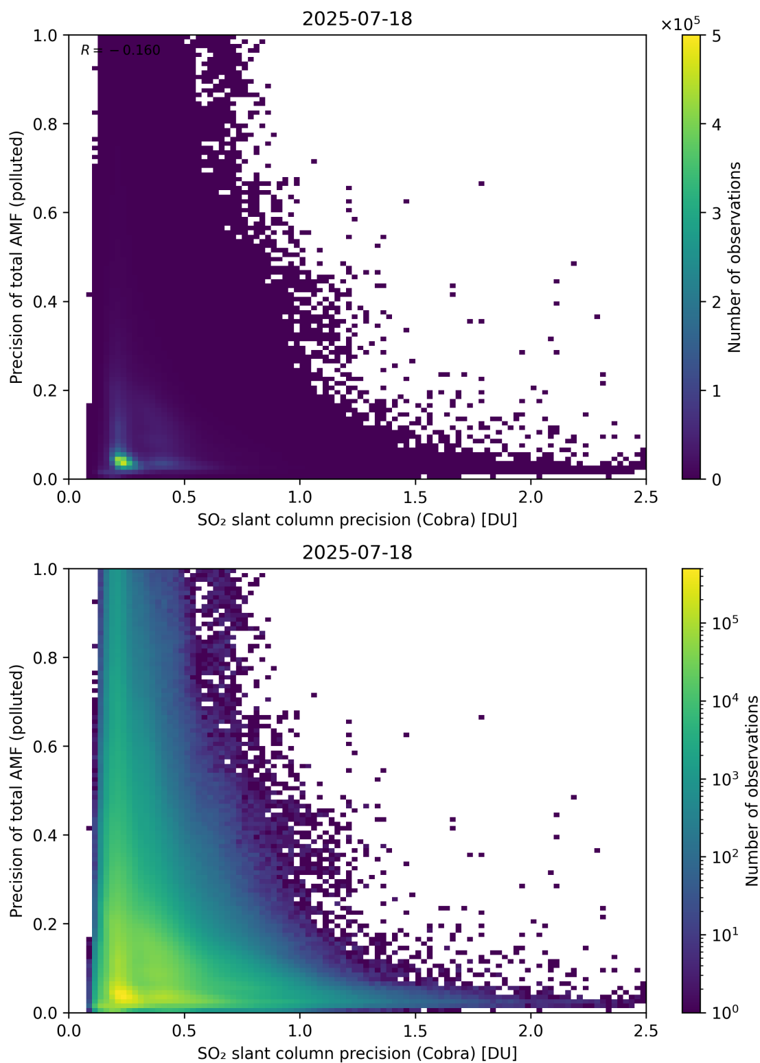
Figure 214: Scatter density plot of “SO 2 slant column precision (Cobra)” against “Precision of total AMF (polluted)” for 2025-07-18 to 2025-07-19.
