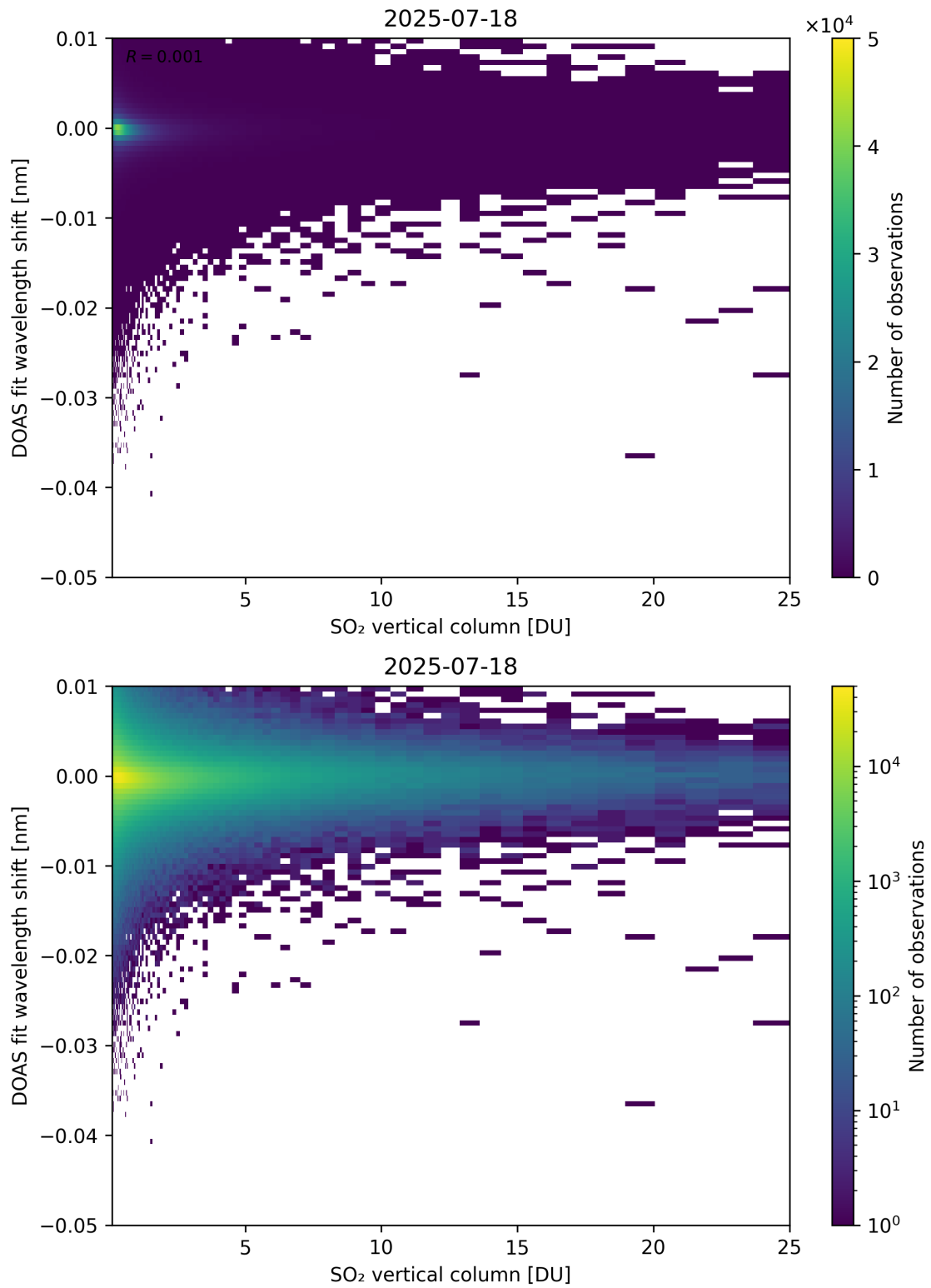
Figure 326: Scatter density plot of “SO 2 vertical column” against “DOAS fit wavelength shift” for 2025-07-18 to 2025-07-19.
