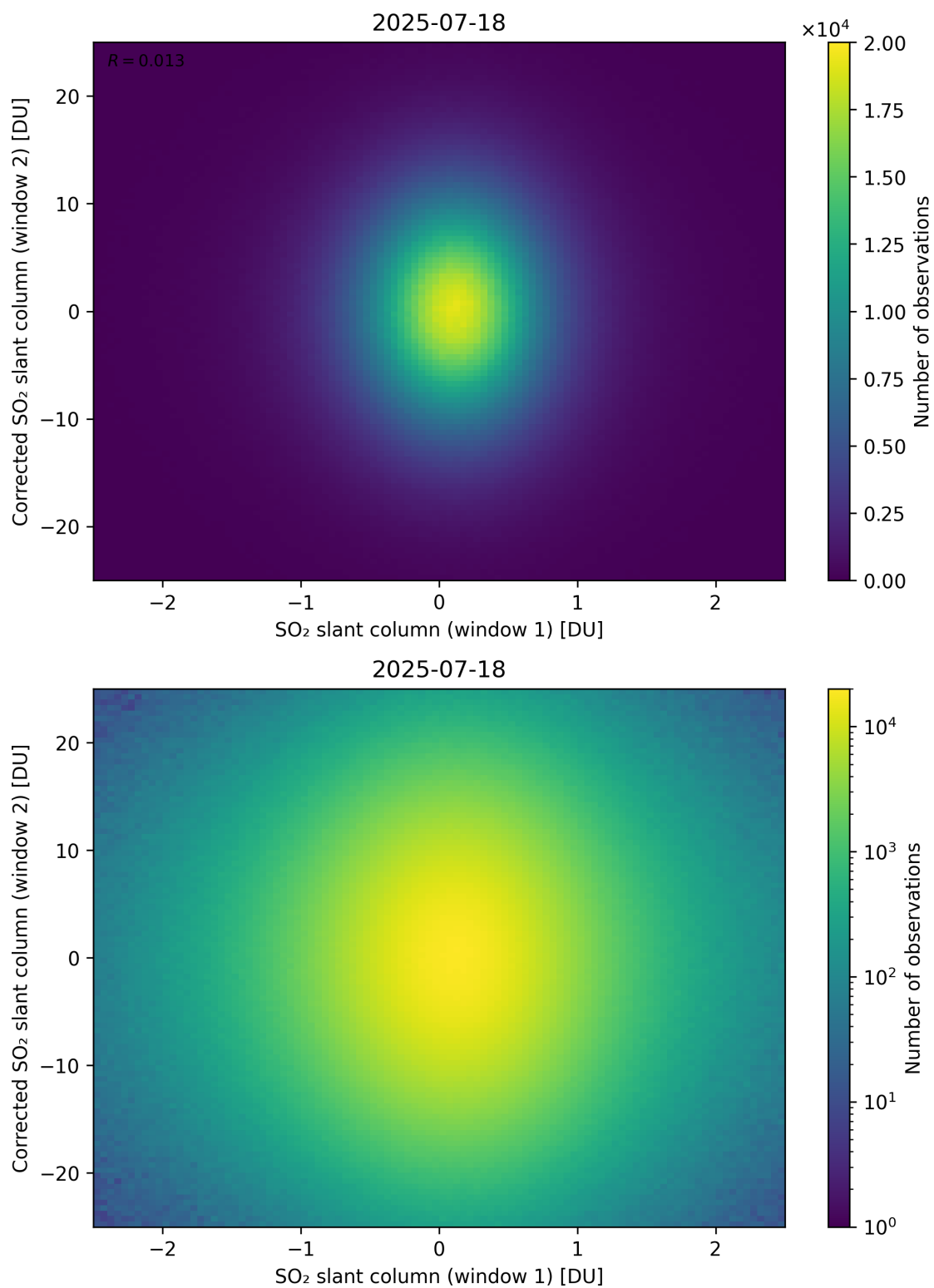
Figure 283: Scatter density plot of “SO 2 slant column (window 1)” against “Corrected SO 2 slant column (window 2)” for 2025-07-18 to 2025-07-19.
