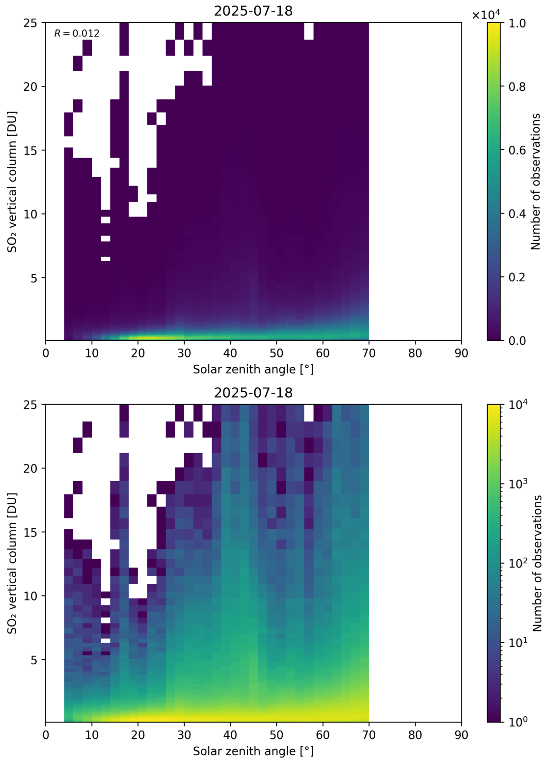
Figure 191: Scatter density plot of “Solar zenith angle” against “SO 2 vertical column” for 2025-07-18 to 2025-07-19.
