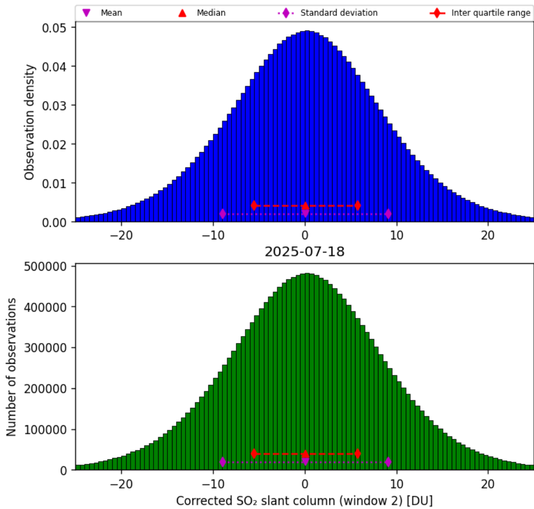
Figure 69: Histogram of “Corrected SO 2 slant column (window 2)” for 2025-07-18 to 2025-07-19
