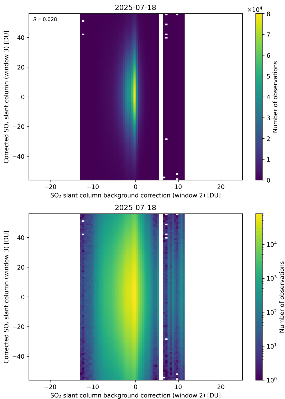
Figure 127: Scatter density plot of “SO 2 slant column background correction (window 2)” against “Corrected SO 2 slant column (window 3)” for 2025-07-18 to 2025-07-19.
