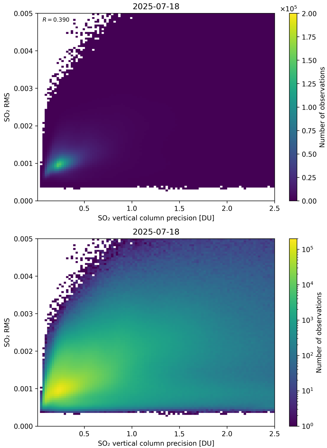
Figure 334: Scatter density plot of “SO 2 vertical column precision” against “SO 2 RMS” for 2025-07-18 to 2025-07-19.
