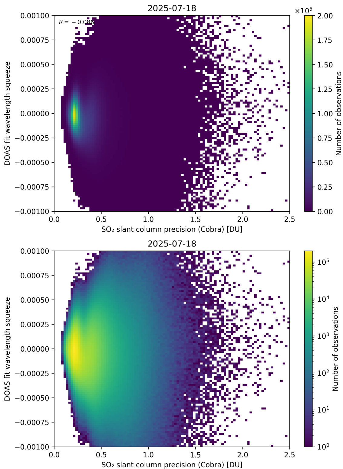
Figure 203: Scatter density plot of “SO 2 slant column precision (Cobra)” against “DOAS fit wavelength squeeze” for 2025-07-18 to 2025-07-19.
