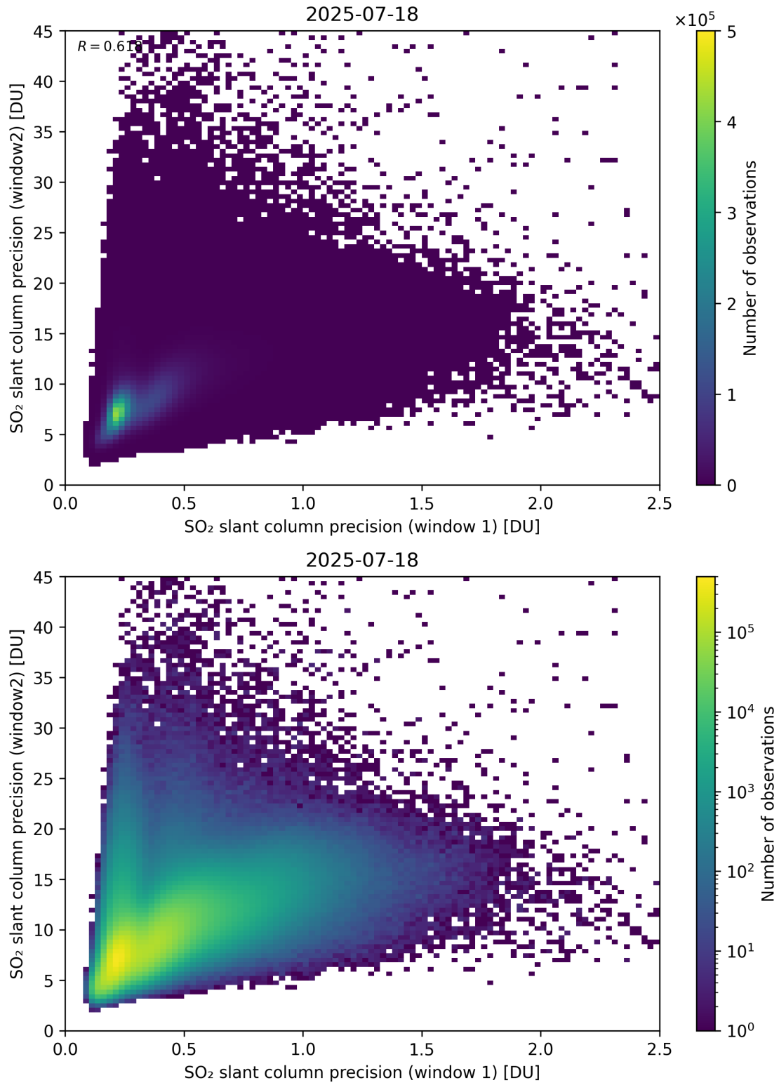
Figure 277: Scatter density plot of “SO 2 slant column precision (window 1)” against “SO 2 slant column precision (window2)” for 2025-07-18 to 2025-07-19.
