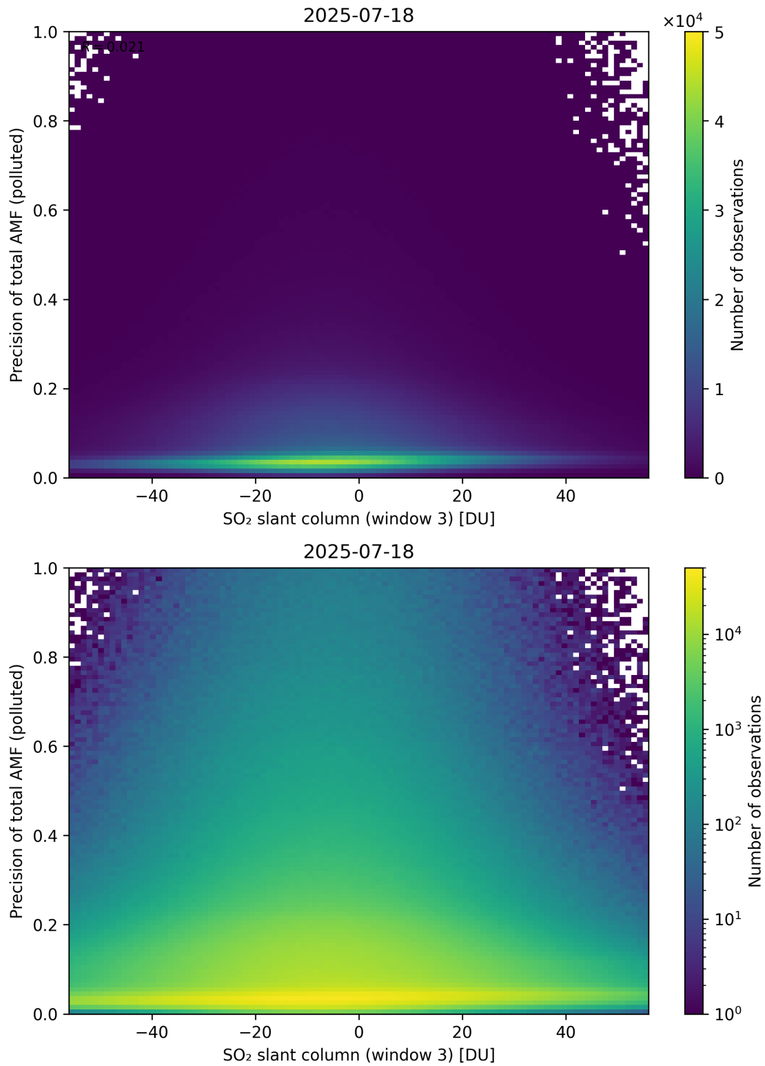
Figure 319: Scatter density plot of “SO 2 slant column (window 3)” against “Precision of total AMF (polluted)” for 2025-07-18 to 2025-07-19.
