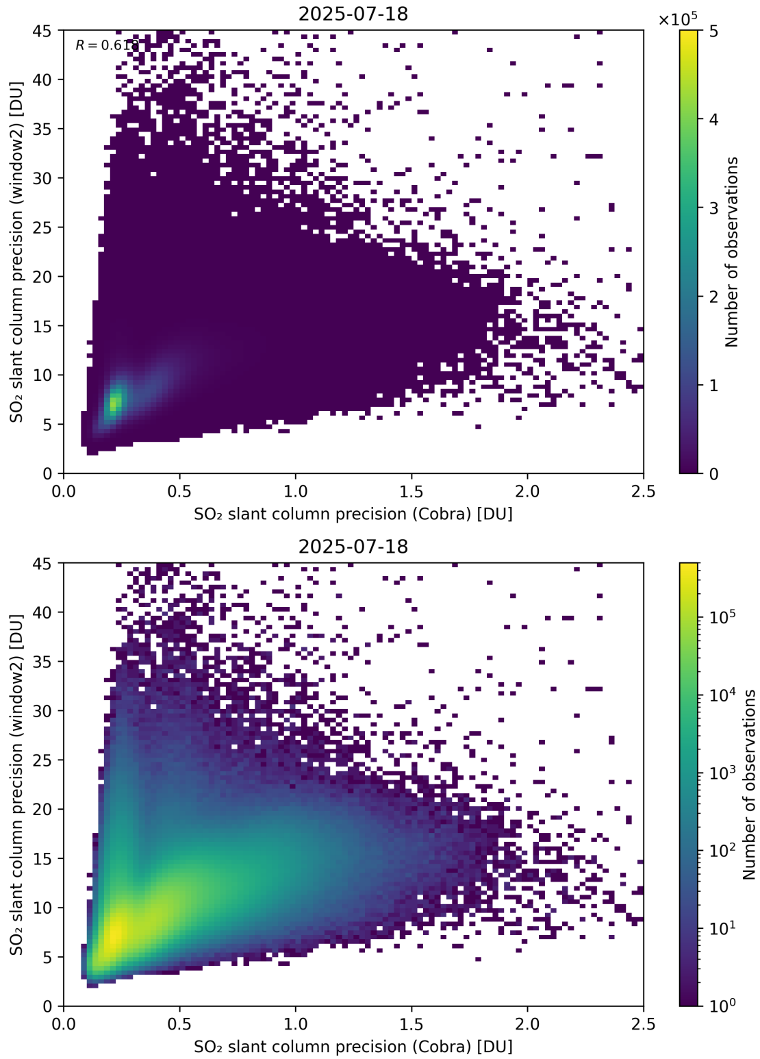
Figure 210: Scatter density plot of “SO 2 slant column precision (Cobra)” against “SO 2 slant column precision (window2)” for 2025-07-18 to 2025-07-19.
