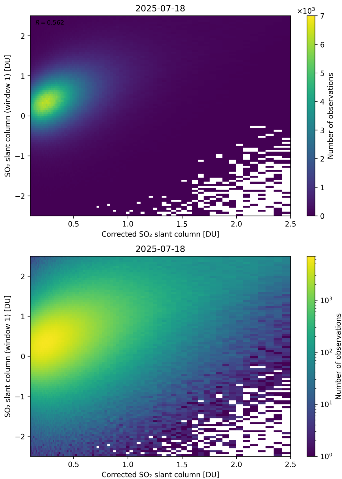
Figure 237: Scatter density plot of “Corrected SO 2 slant column” against “SO 2 slant column (window 1)” for 2025-07-18 to 2025-07-19.
