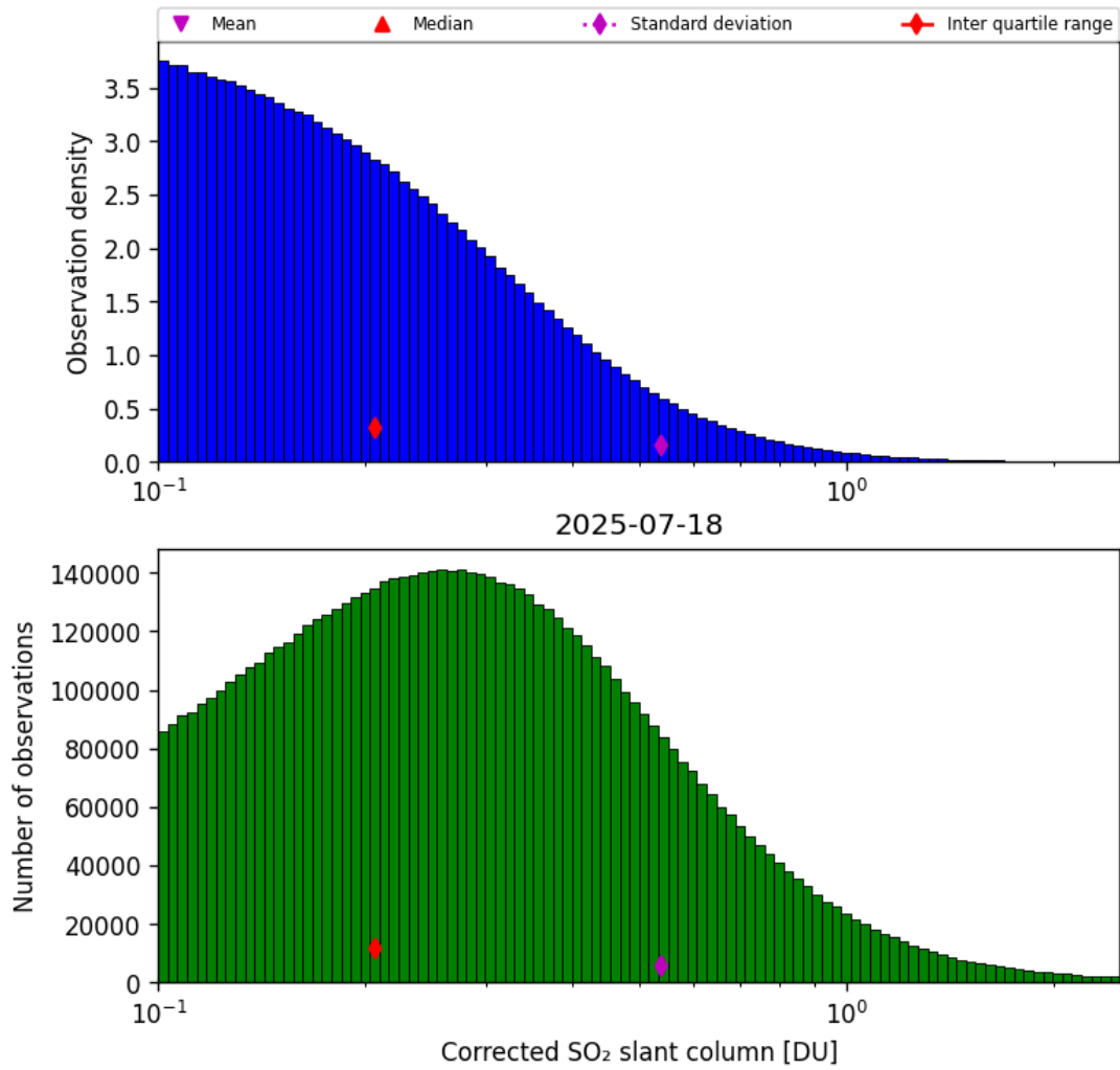
Figure 60: Histogram of "Corrected SO 2 slant column" for 2025-07-18 to 2025-07-19
