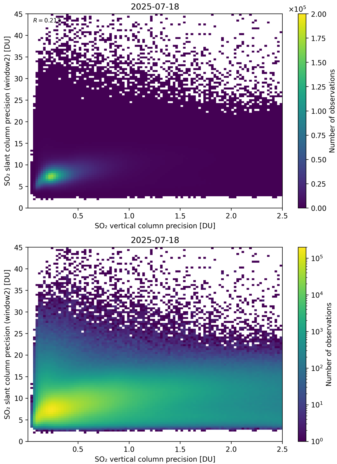
Figure 343: Scatter density plot of “SO 2 vertical column precision” against “SO 2 slant column precision (window2)” for 2025-07-18 to 2025-07-19.
