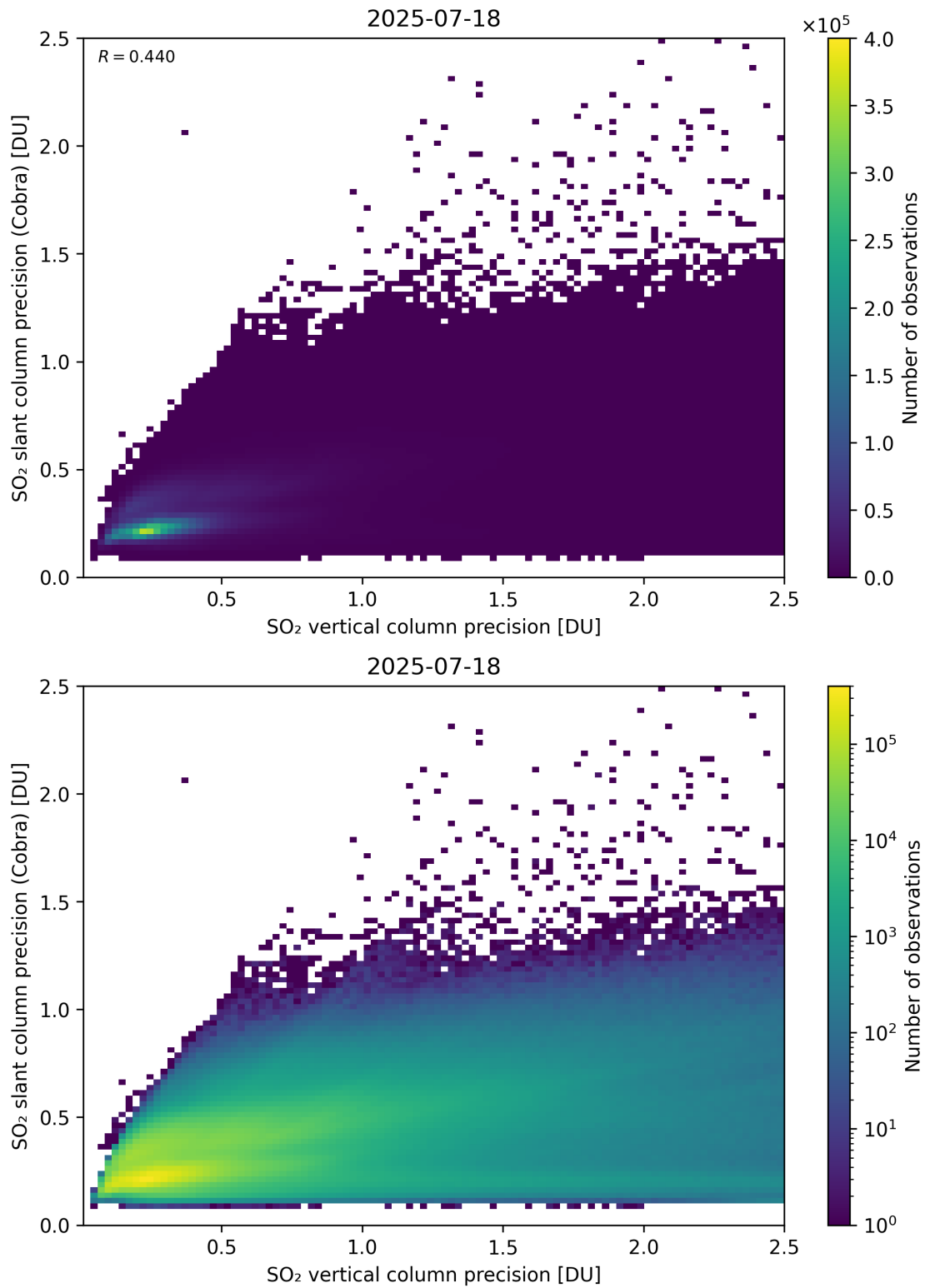
Figure 337: Scatter density plot of “SO 2 vertical column precision” against “SO 2 slant column precision (Cobra)” for 2025-07-18 to 2025-07-19.
