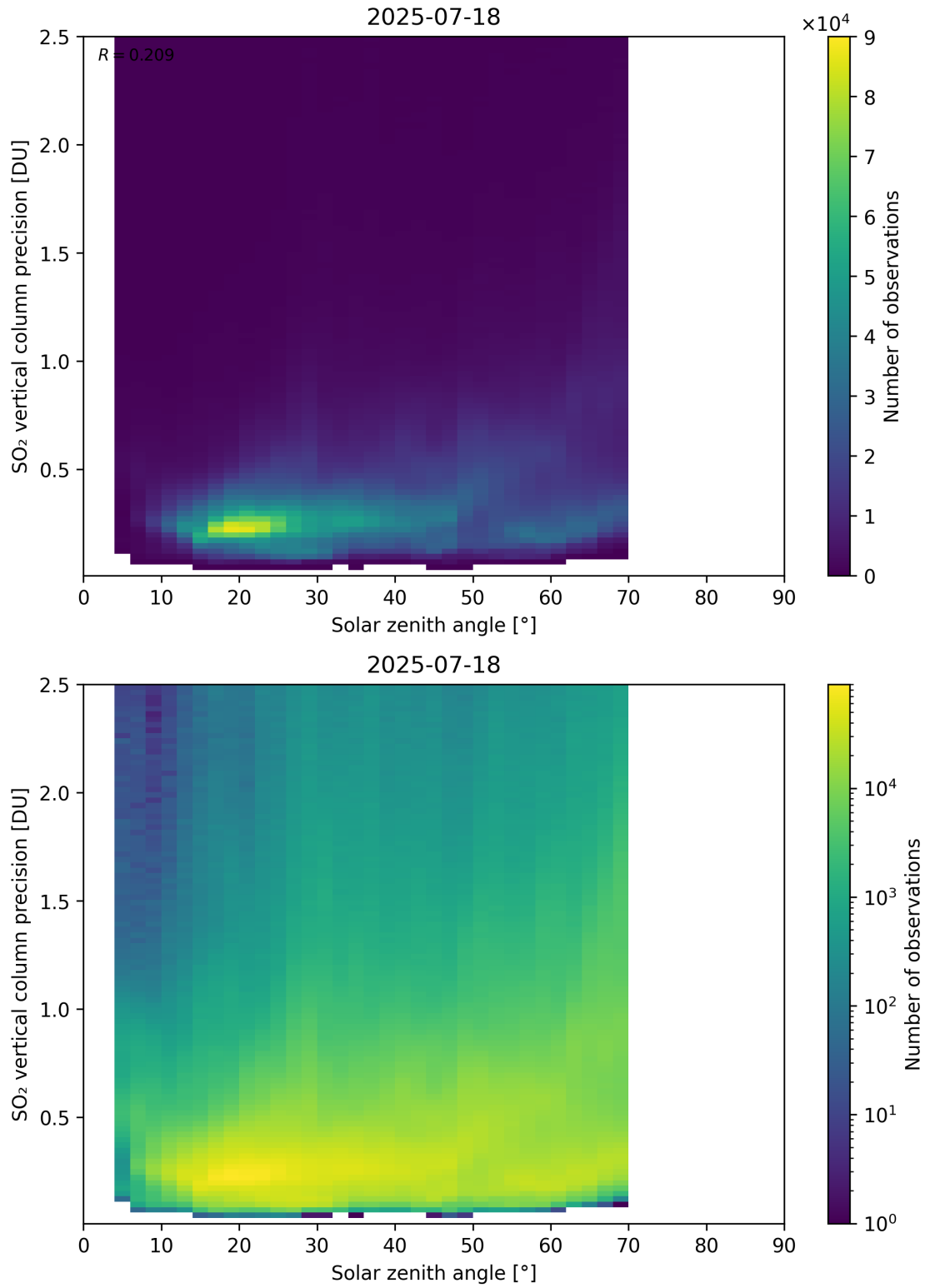
Figure 192: Scatter density plot of “Solar zenith angle” against “SO 2 vertical column precision” for 2025-07-18 to 2025-07-19.
