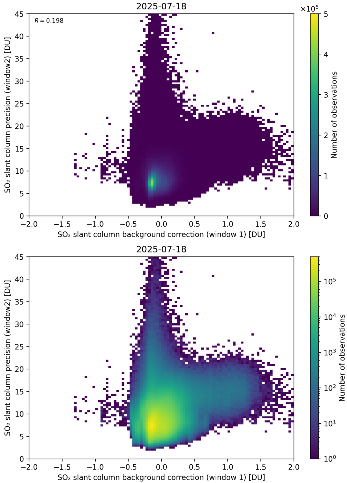
Figure 117: Scatter density plot of “SO 2 slant column background correction (window 1)” against “SO 2 slant column precision (window2)” for 2025-07-18 to 2025-07-19.
