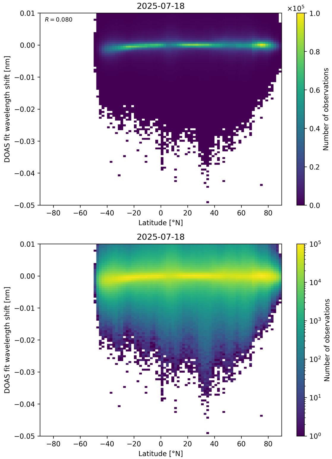
Figure 153: Scatter density plot of “Latitude” against “DOAS fit wavelength shift” for 2025-07-18 to 2025-07-19.
