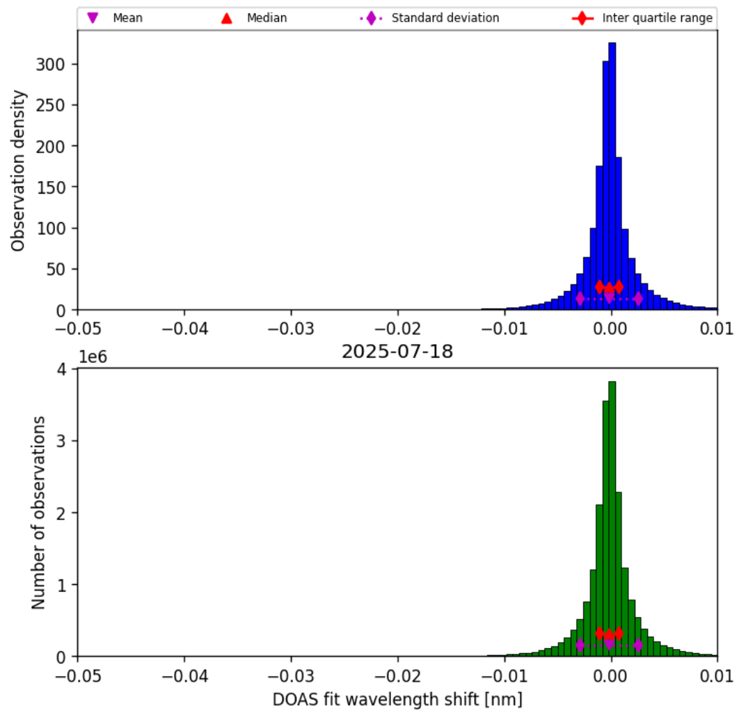
Figure 76: Histogram of “DOAS fit wavelength shift” for 2025-07-18 to 2025-07-19
