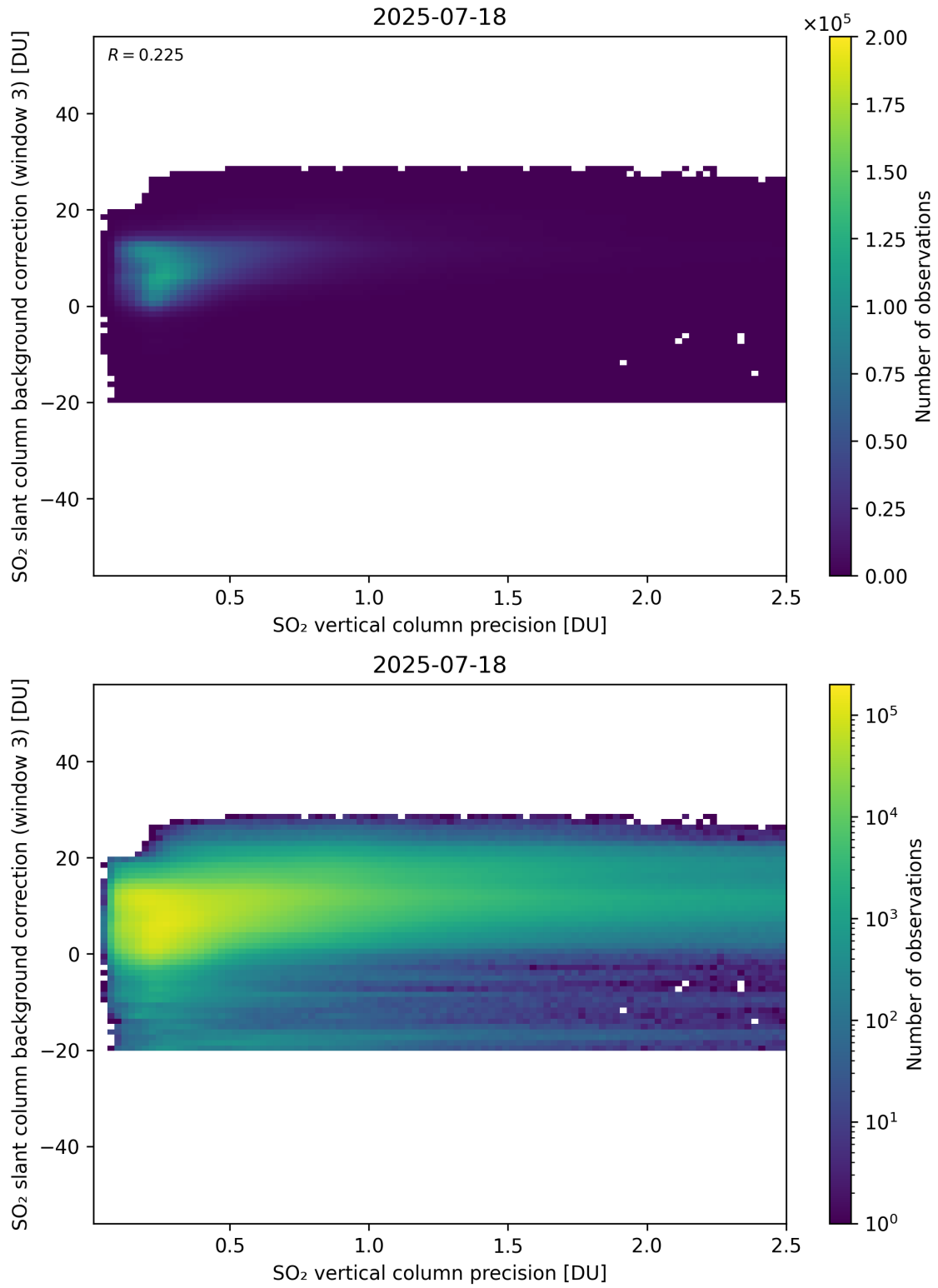
Figure 331: Scatter density plot of “SO 2 vertical column precision” against “SO 2 slant column background correction (window 3)” for 2025-07-18 to 2025-07-19.
