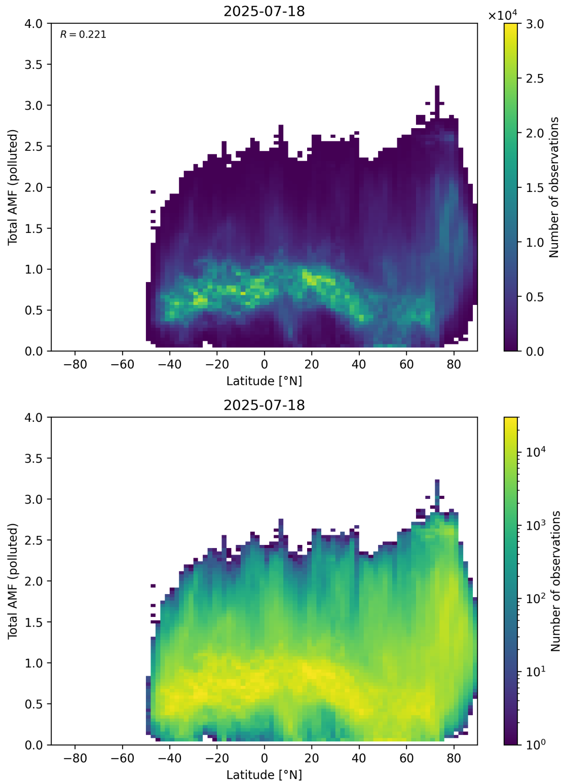
Figure 167: Scatter density plot of “Latitude” against “Total AMF (polluted)” for 2025-07-18 to 2025-07-19.
