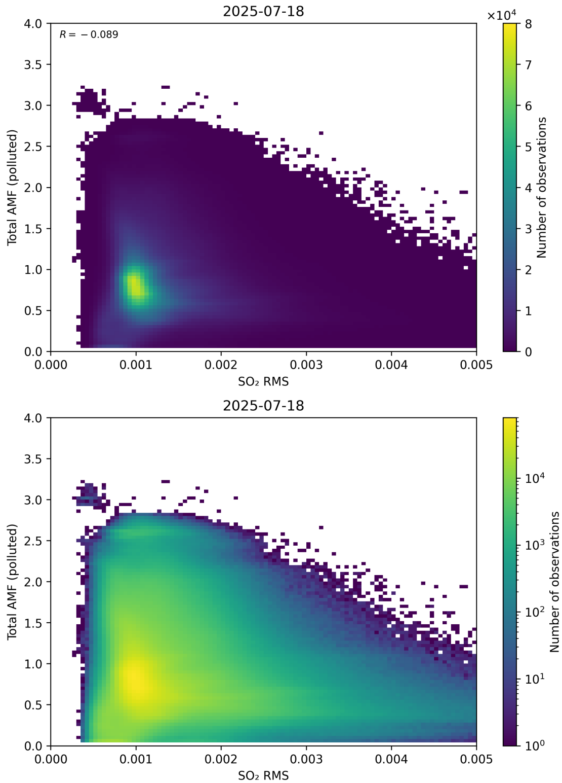
Figure 148: Scatter density plot of “SO 2 RMS” against “Total AMF (polluted)” for 2025-07-18 to 2025-07-19.
