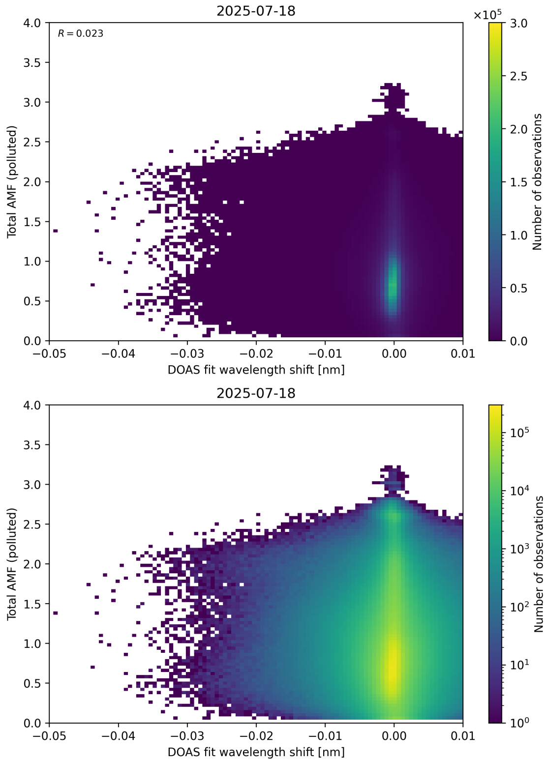
Figure 141: Scatter density plot of “DOAS fit wavelength shift” against “Total AMF (polluted)” for 2025-07-18 to 2025-07-19.
