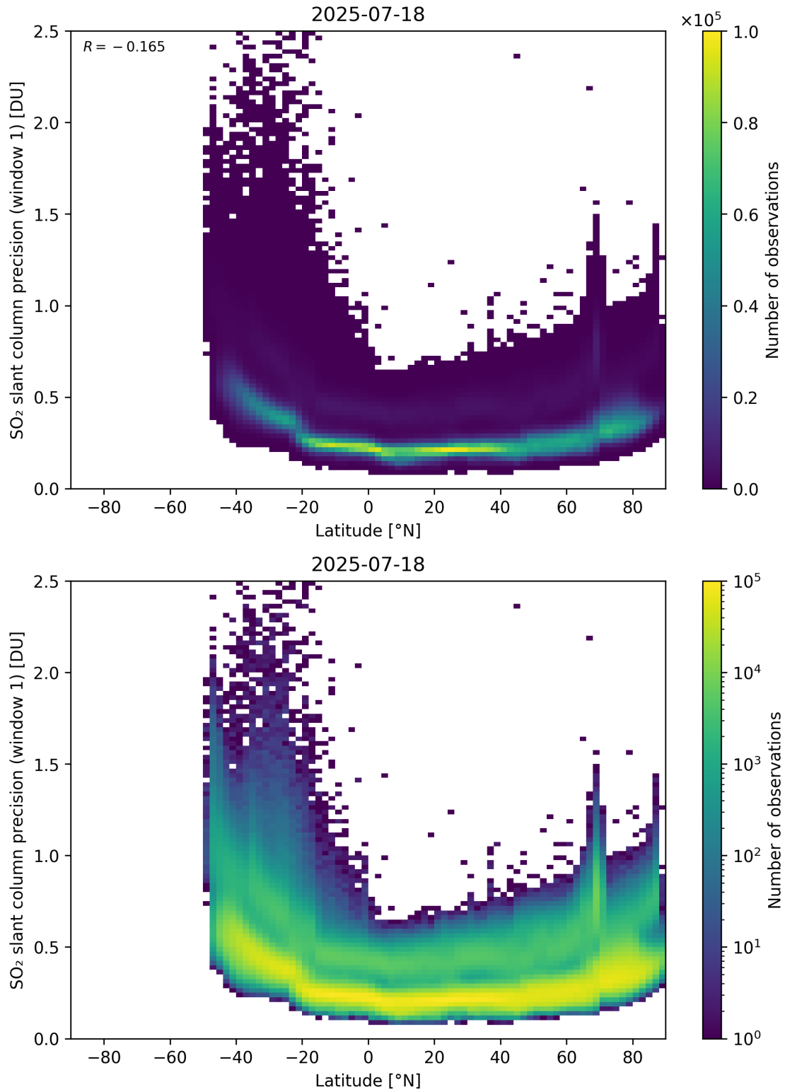
Figure 163: Scatter density plot of “Latitude” against “SO 2 slant column precision (window 1)” for 2025-07-18 to 2025-07-19.
