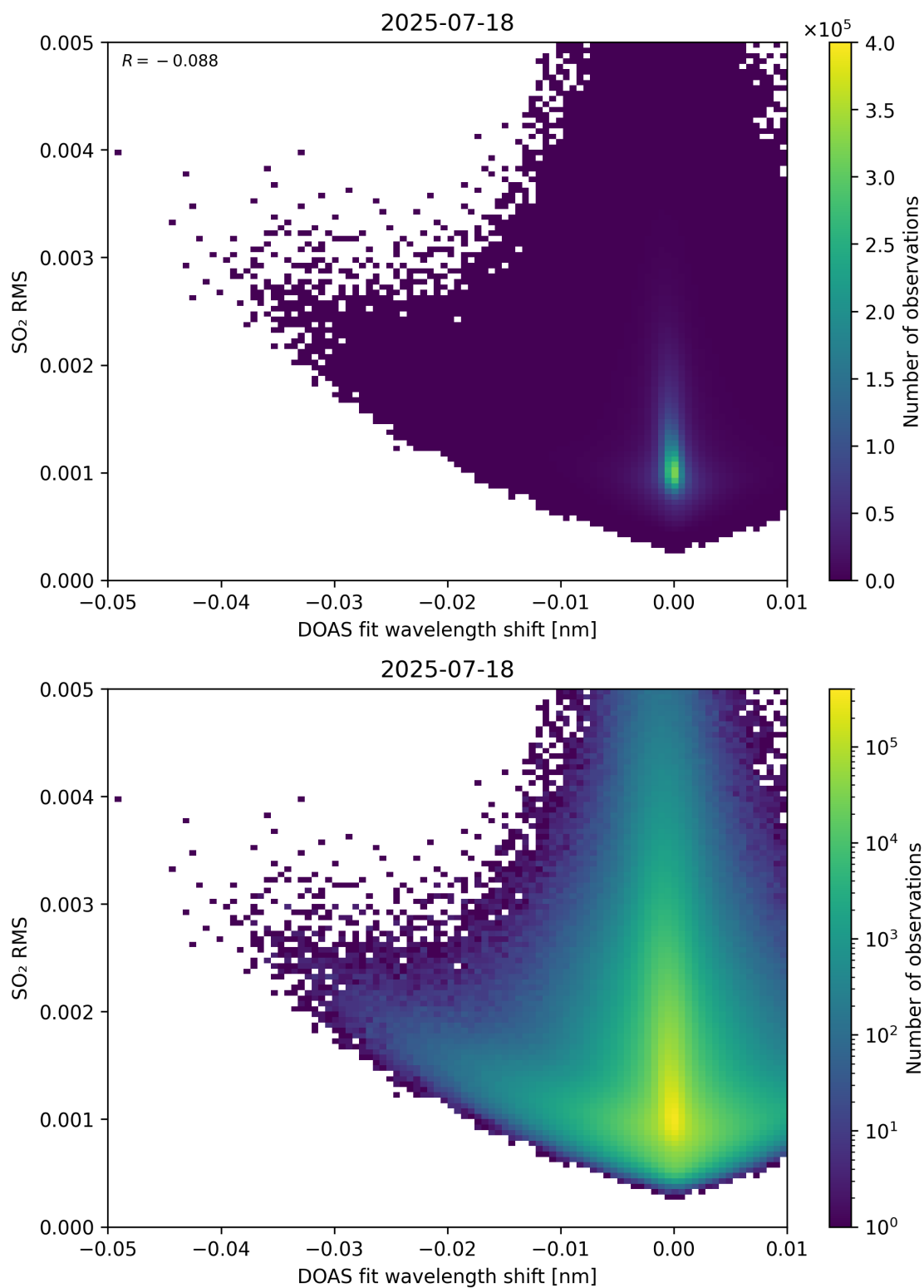
Figure 139: Scatter density plot of “DOAS fit wavelength shift” against “SO 2 RMS” for 2025-07-18 to 2025-07-19.
