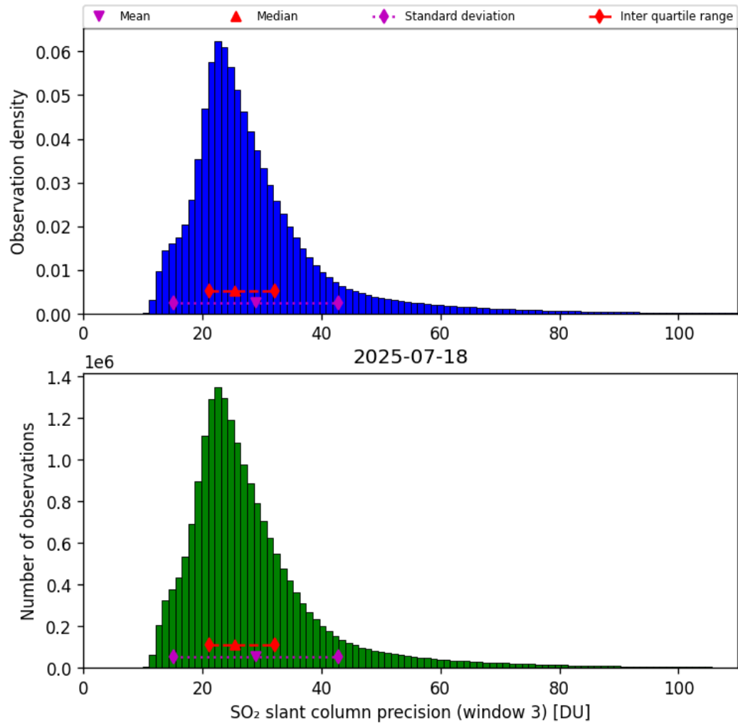
Figure 72: Histogram of “SO 2 slant column precision (window 3)” for 2025-07-18 to 2025-07-19
