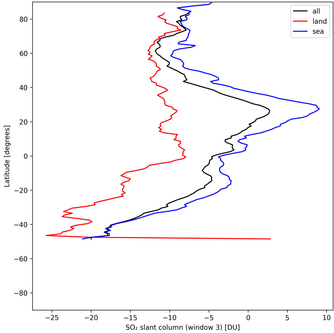
Figure 45: Zonal average of “SO 2 slant column (window 3)” for 2025-07-18 to 2025-07-19.
