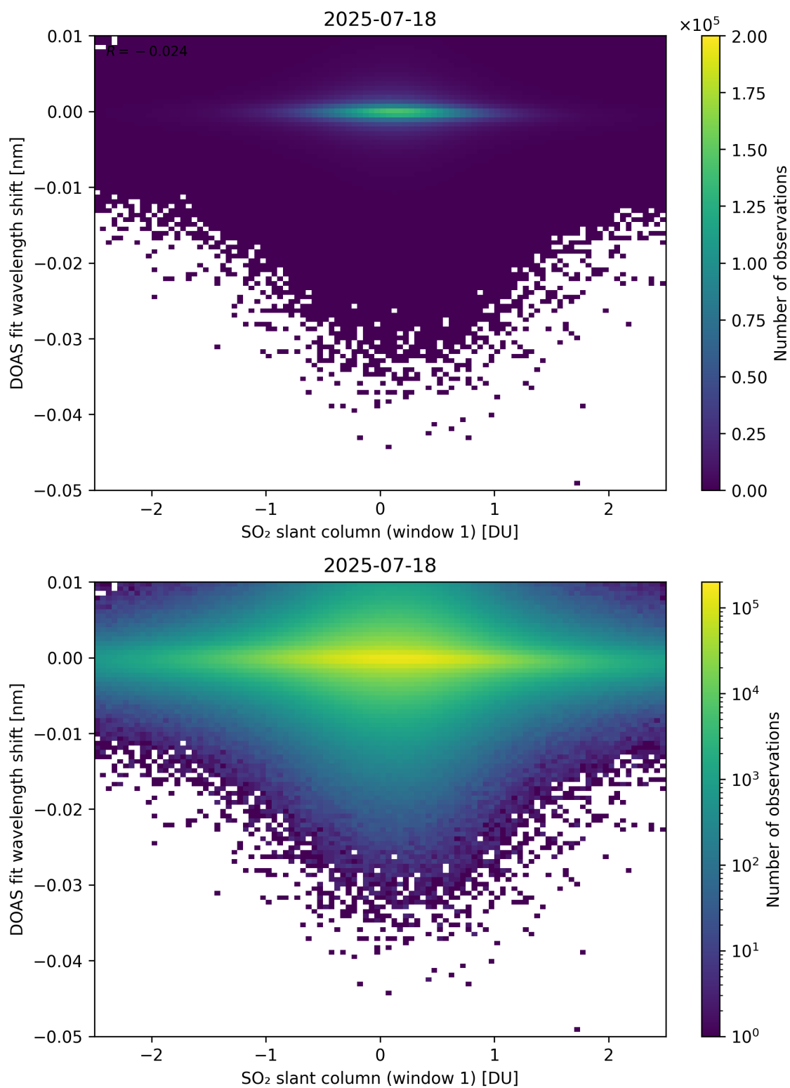
Figure 265: Scatter density plot of “SO 2 slant column (window 1)” against “DOAS fit wavelength shift” for 2025-07-18 to 2025-07-19.
