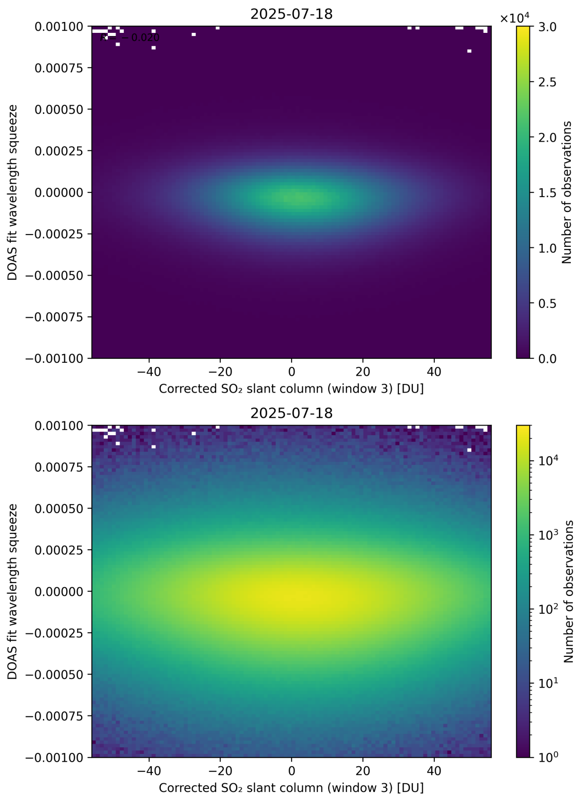
Figure 257: Scatter density plot of “Corrected SO 2 slant column (window 3)” against “DOAS fit wavelength squeeze” for 2025-07-18 to 2025-07-19.
