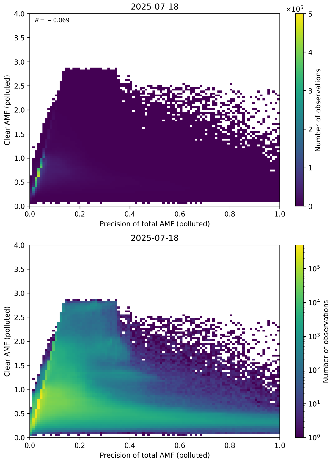
Figure 320: Scatter density plot of “Precision of total AMF (polluted)” against “Clear AMF (polluted)” for 2025-07-18 to 2025-07-19.
