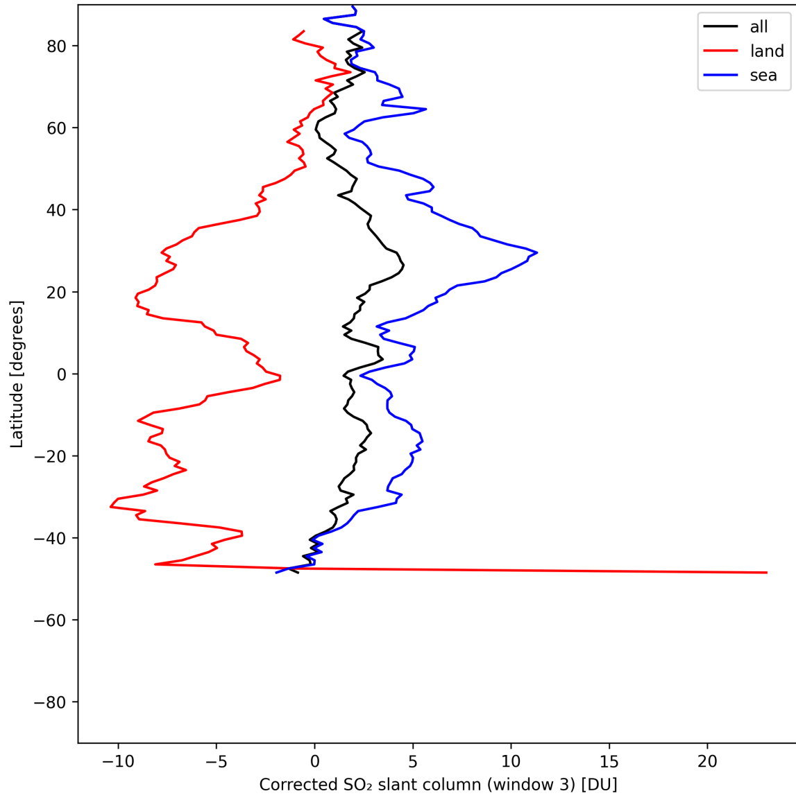
Figure 47: Zonal average of “Corrected SO 2 slant column (window 3)” for 2025-07-18 to 2025-07-19.
