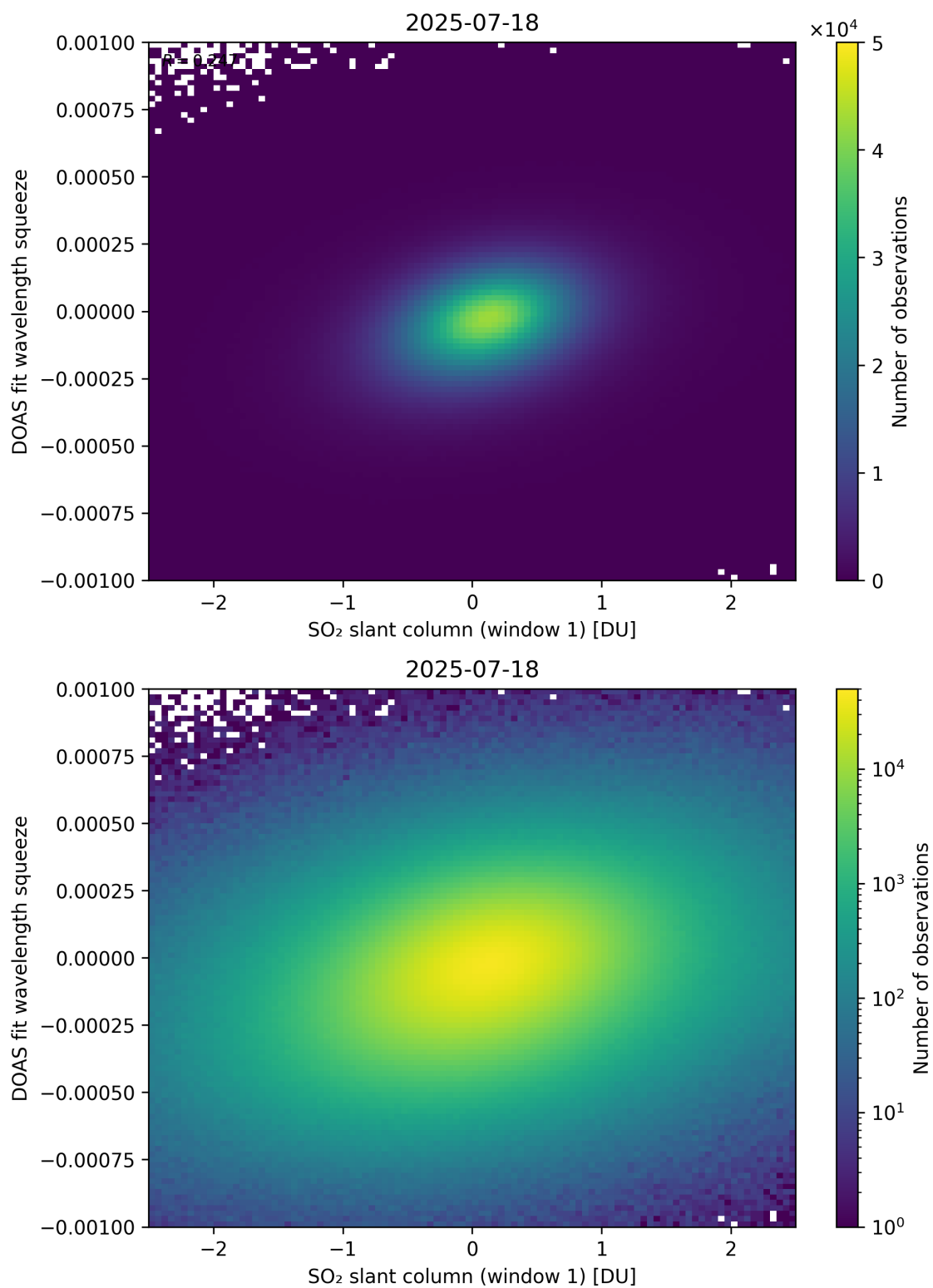
Figure 266: Scatter density plot of “SO 2 slant column (window 1)” against “DOAS fit wavelength squeeze” for 2025-07-18 to 2025-07-19.
