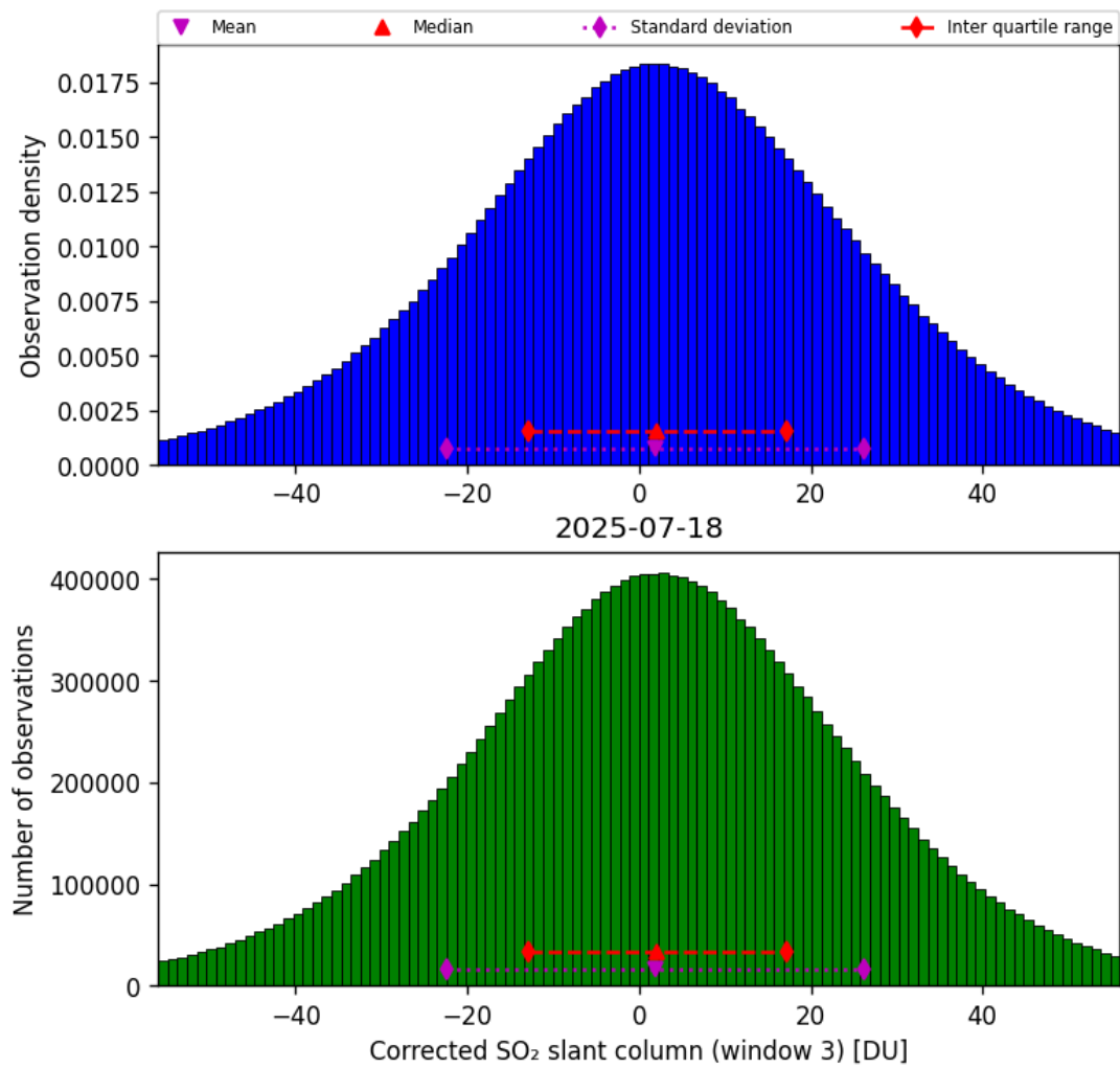
Figure 73: Histogram of “Corrected SO 2 slant column (window 3)” for 2025-07-18 to 2025-07-19
