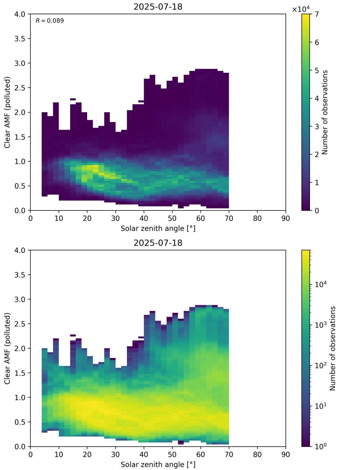
Figure 178: Scatter density plot of “Solar zenith angle” against “Clear AMF (polluted)” for 2025-07-18 to 2025-07-19.
