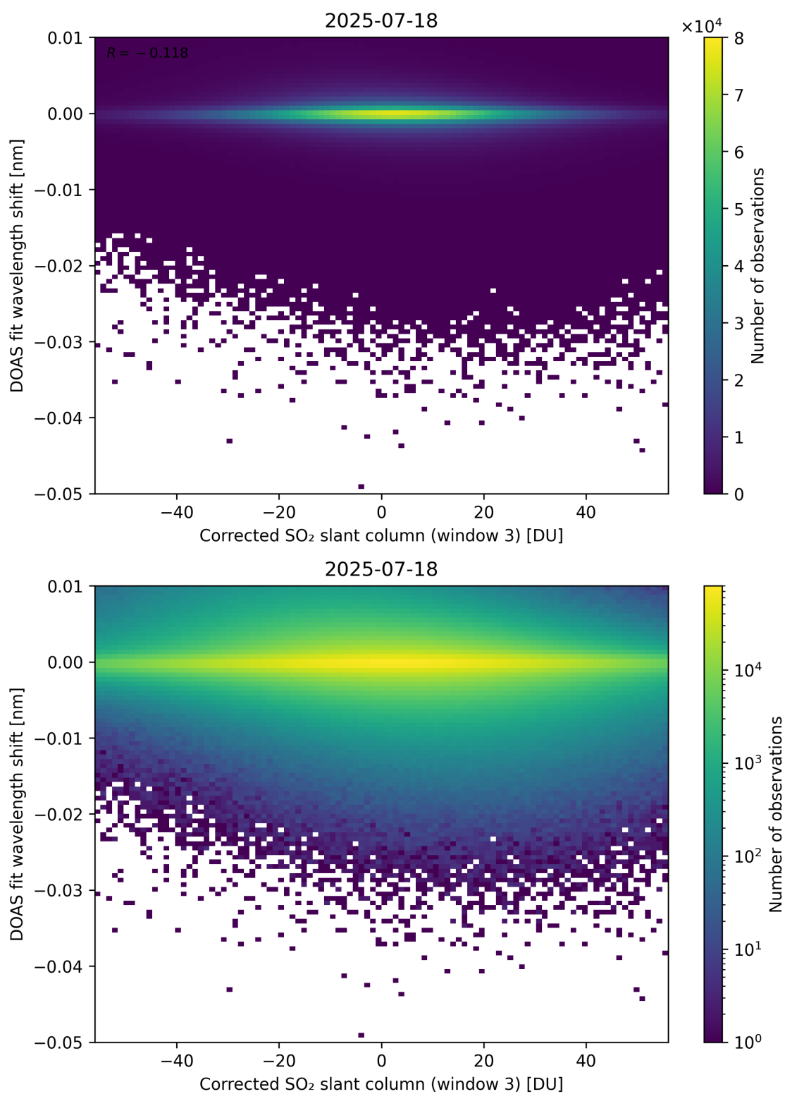
Figure 256: Scatter density plot of “Corrected SO 2 slant column (window 3)” against “DOAS fit wavelength shift” for 2025-07-18 to 2025-07-19.
