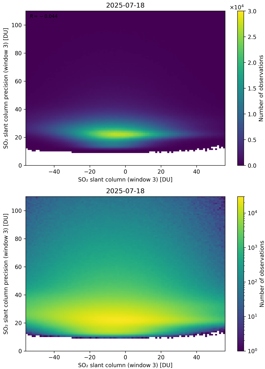
Figure 317: Scatter density plot of “SO 2 slant column (window 3)” against “SO 2 slant column precision (window 3)” for 2025-07-18 to 2025-07-19.
