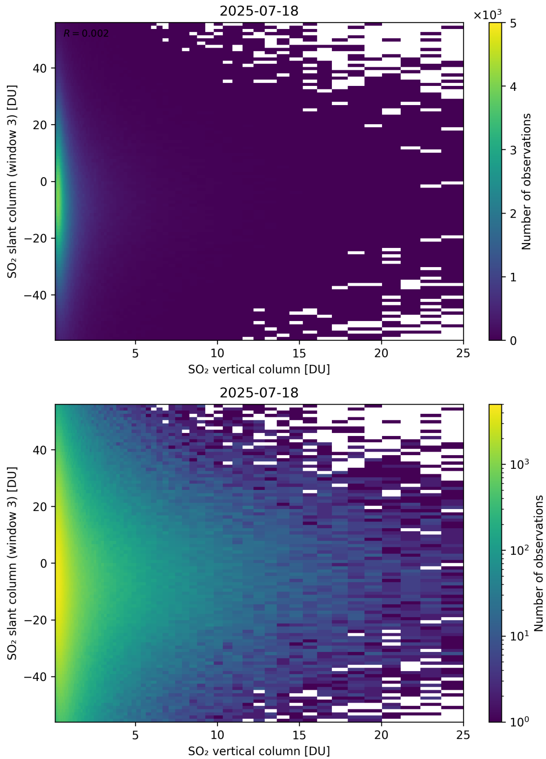
Figure 357: Scatter density plot of “SO 2 vertical column” against “SO 2 slant column (window 3)” for 2025-07-18 to 2025-07-19.
