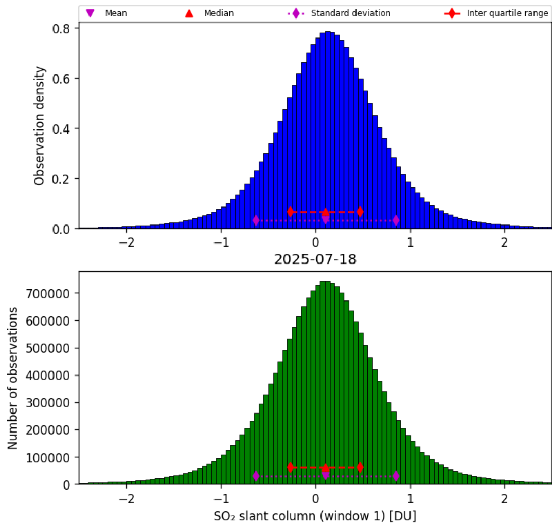
Figure 63: Histogram of “SO 2 slant column (window 1)” for 2025-07-18 to 2025-07-19
