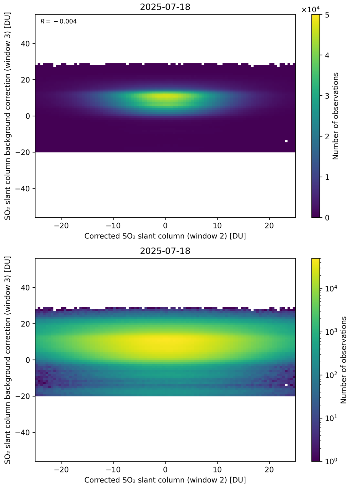
Figure 245: Scatter density plot of “Corrected SO 2 slant column (window 2)” against “SO 2 slant column background correction (window 3)” for 2025-07-18 to 2025-07-19.
