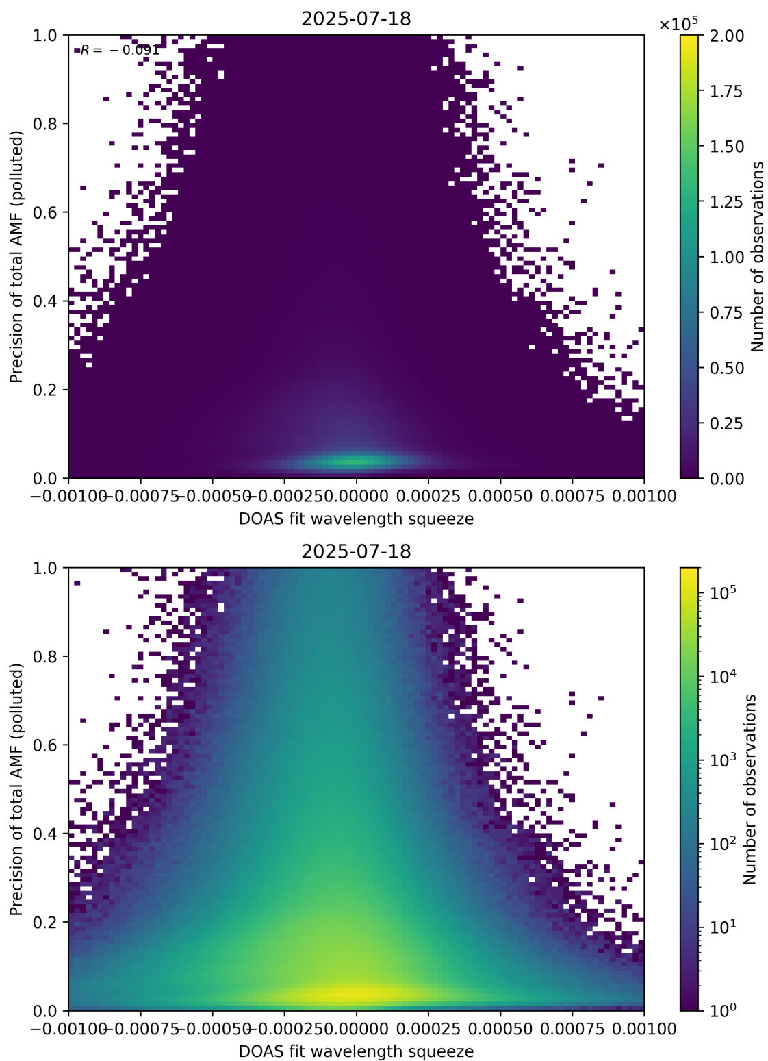
Figure 146: Scatter density plot of “DOAS fit wavelength squeeze” against “Precision of total AMF (polluted)” for 2025-07-18 to 2025-07-19.
