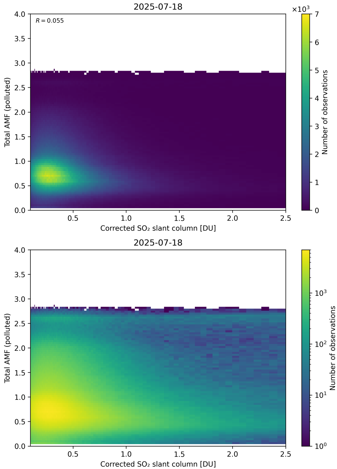
Figure 242: Scatter density plot of “Corrected SO 2 slant column” against “Total AMF (polluted)” for 2025-07-18 to 2025-07-19.
