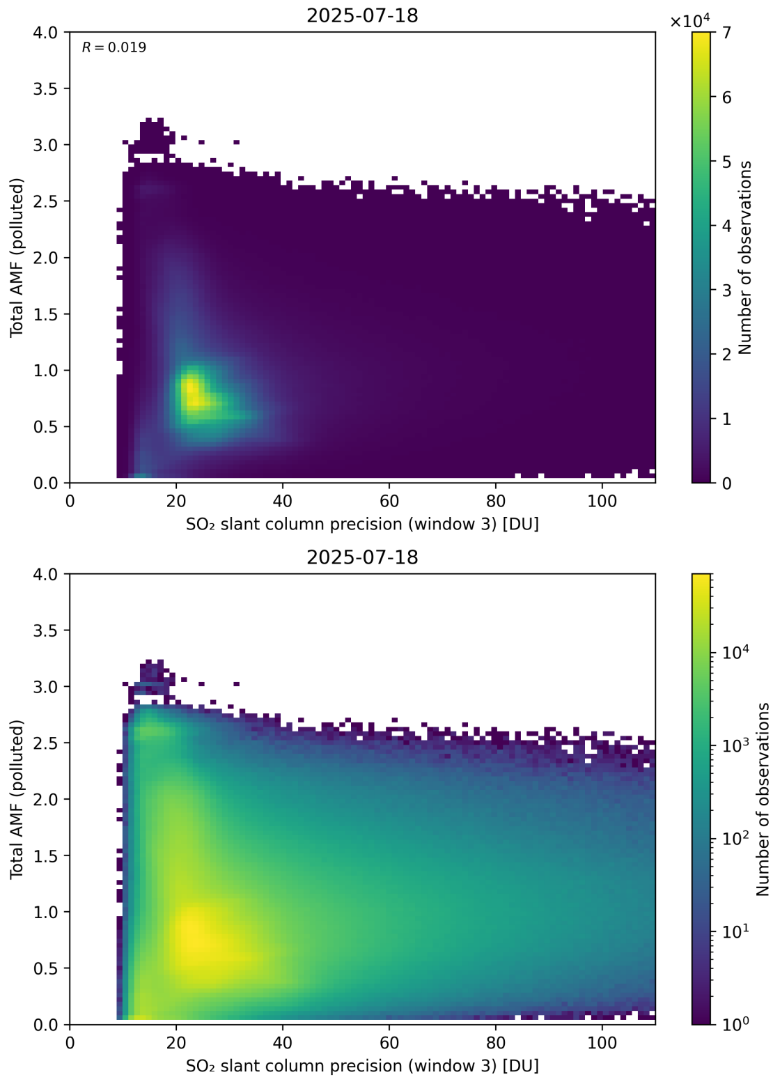
Figure 313: Scatter density plot of “SO 2 slant column precision (window 3)” against “Total AMF (polluted)” for 2025-07-18 to 2025-07-19.
