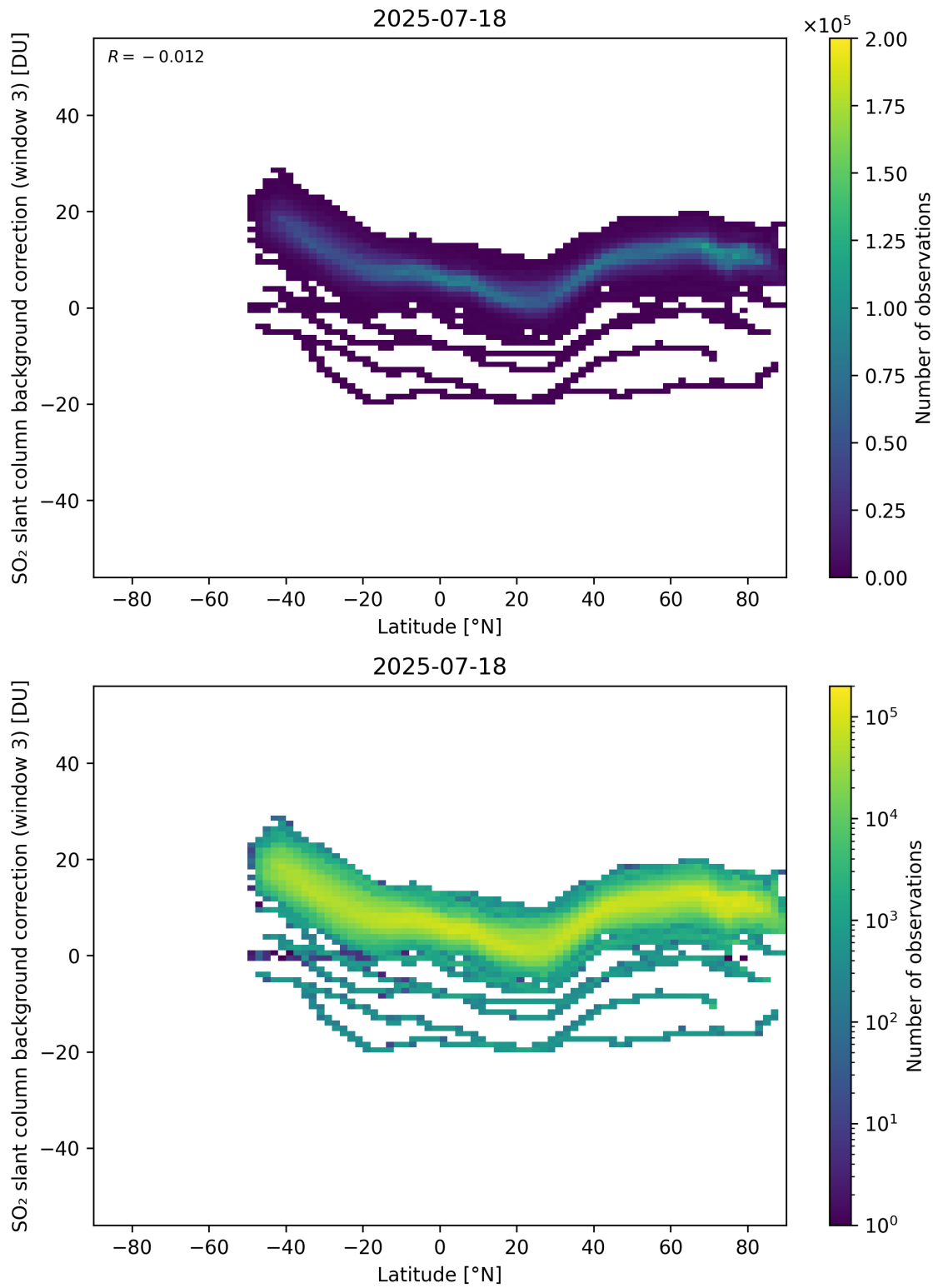
Figure 152: Scatter density plot of “Latitude” against “SO 2 slant column background correction (window 3)” for 2025-07-18 to 2025-07-19.
