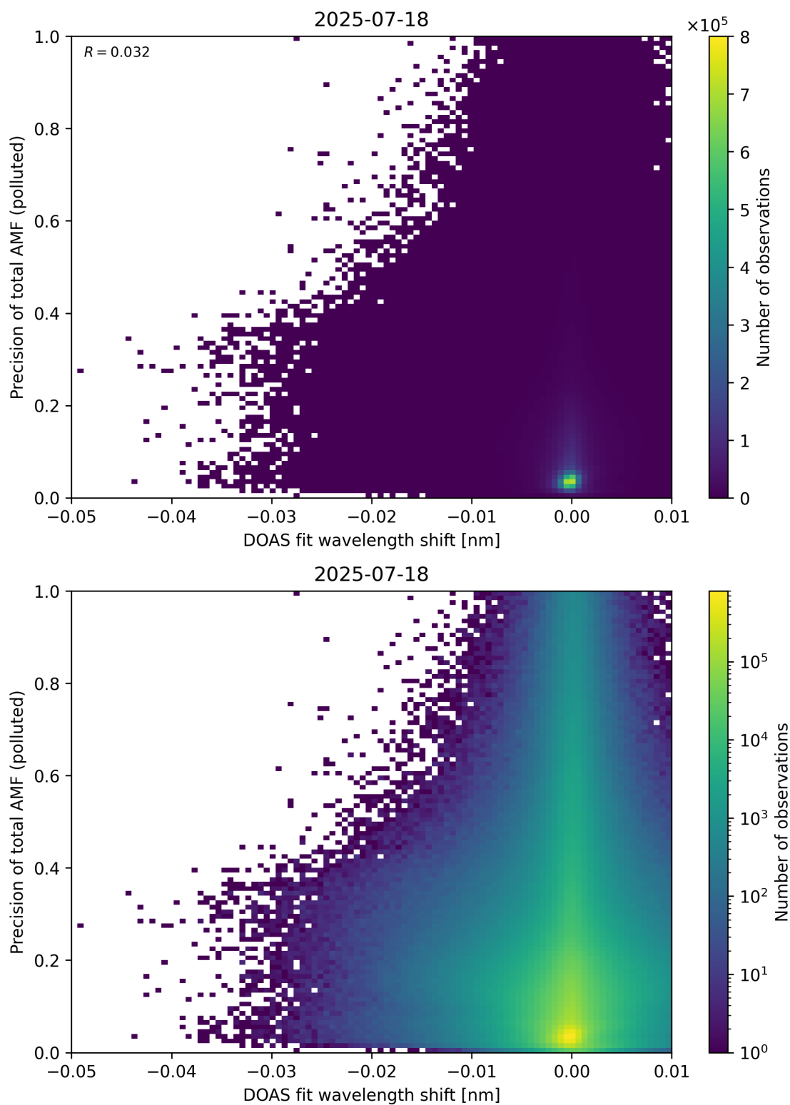
Figure 142: Scatter density plot of “DOAS fit wavelength shift” against “Precision of total AMF (polluted)” for 2025-07-18 to 2025-07-19.
