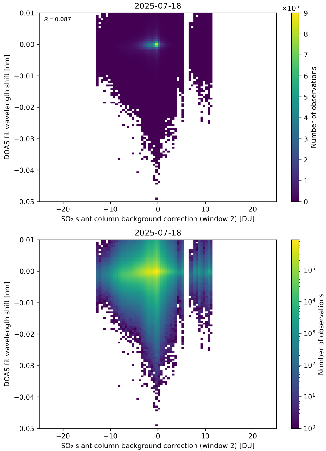
Figure 123: Scatter density plot of “SO 2 slant column background correction (window 2)” against “DOAS fit wavelength shift” for 2025-07-18 to 2025-07-19.
