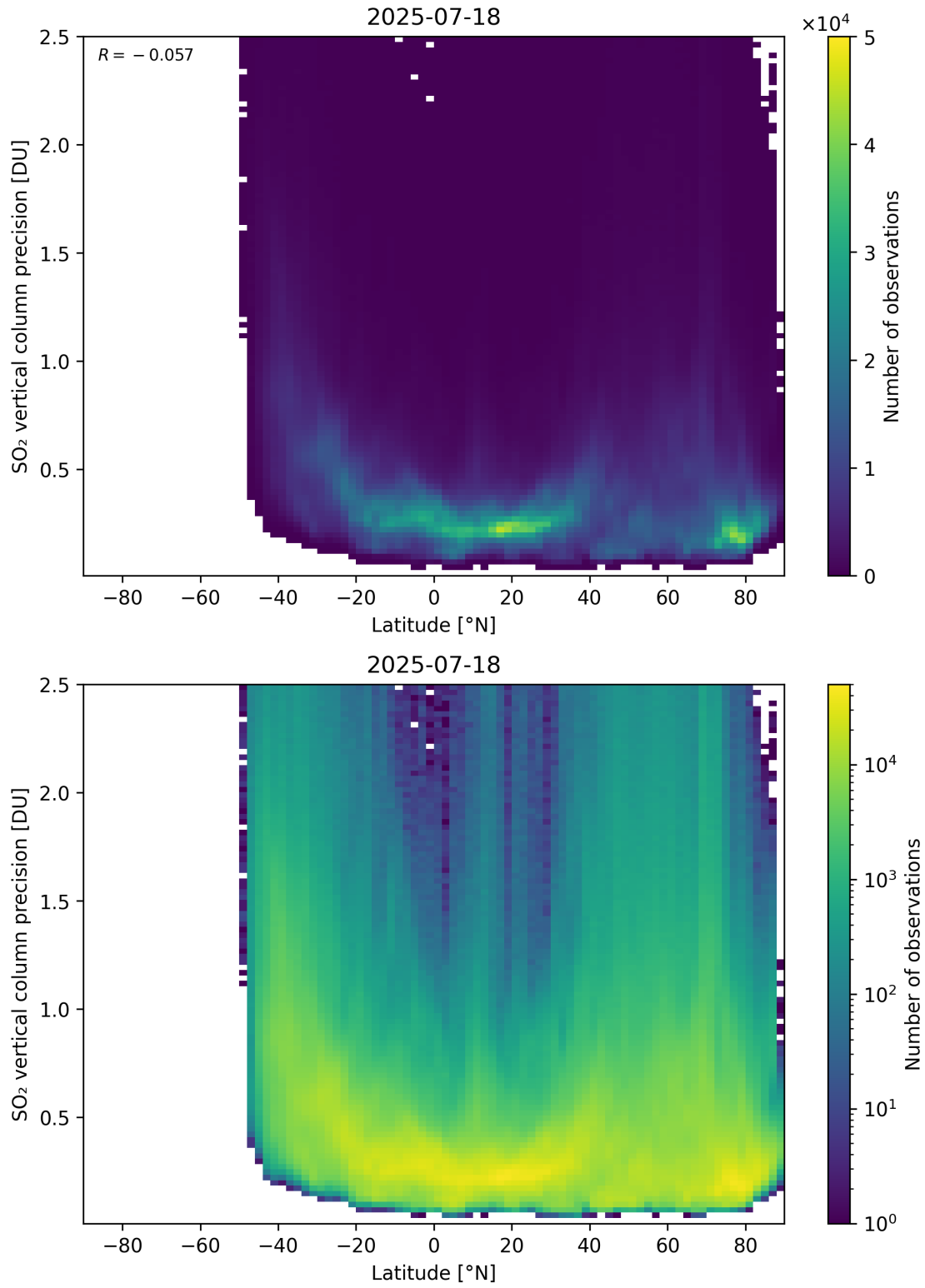
Figure 170: Scatter density plot of “Latitude” against “SO 2 vertical column precision” for 2025-07-18 to 2025-07-19.
