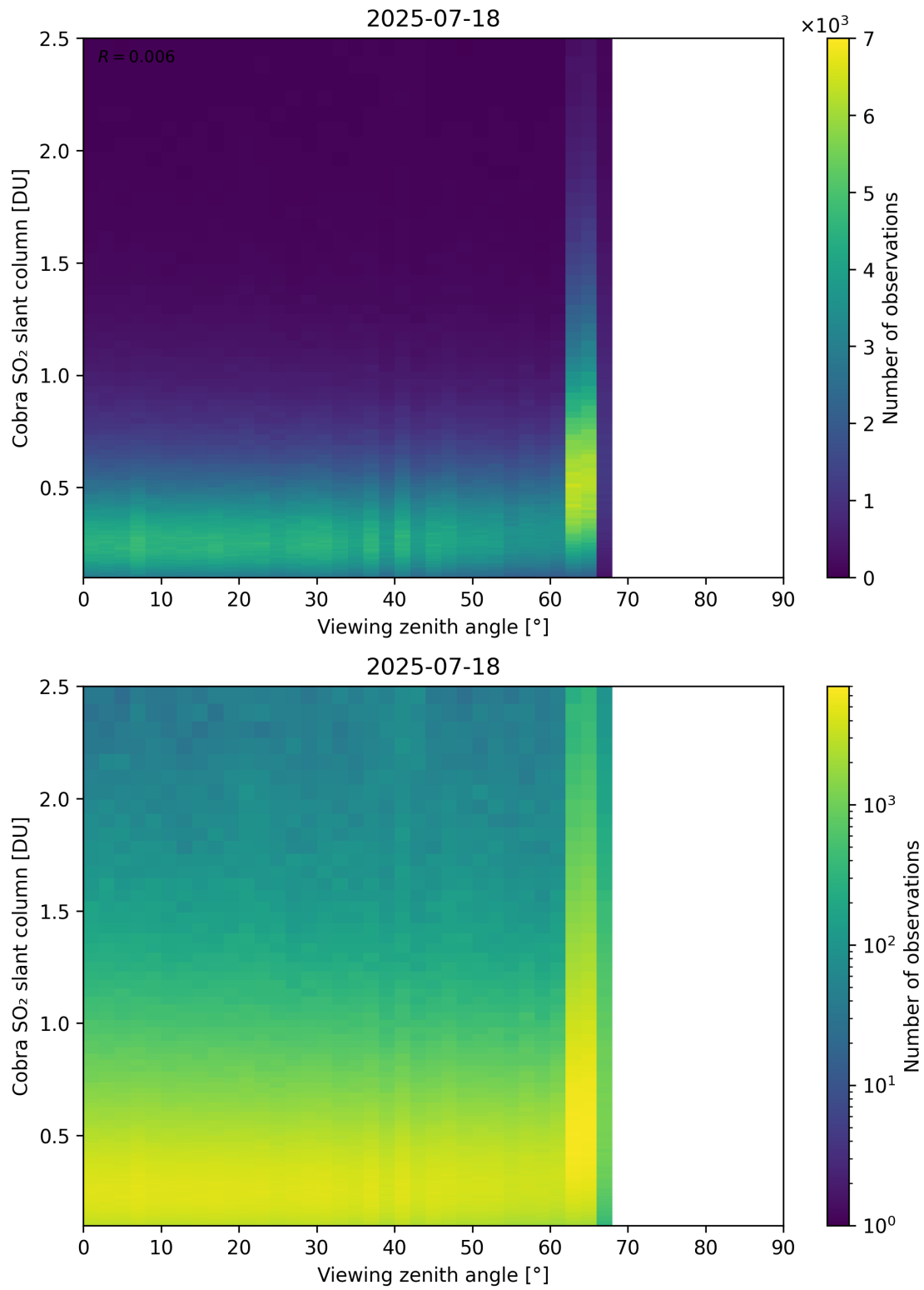
Figure 371: Scatter density plot of “Viewing zenith angle” against “Cobra SO 2 slant column” for 2025-07-18 to 2025-07-19.
