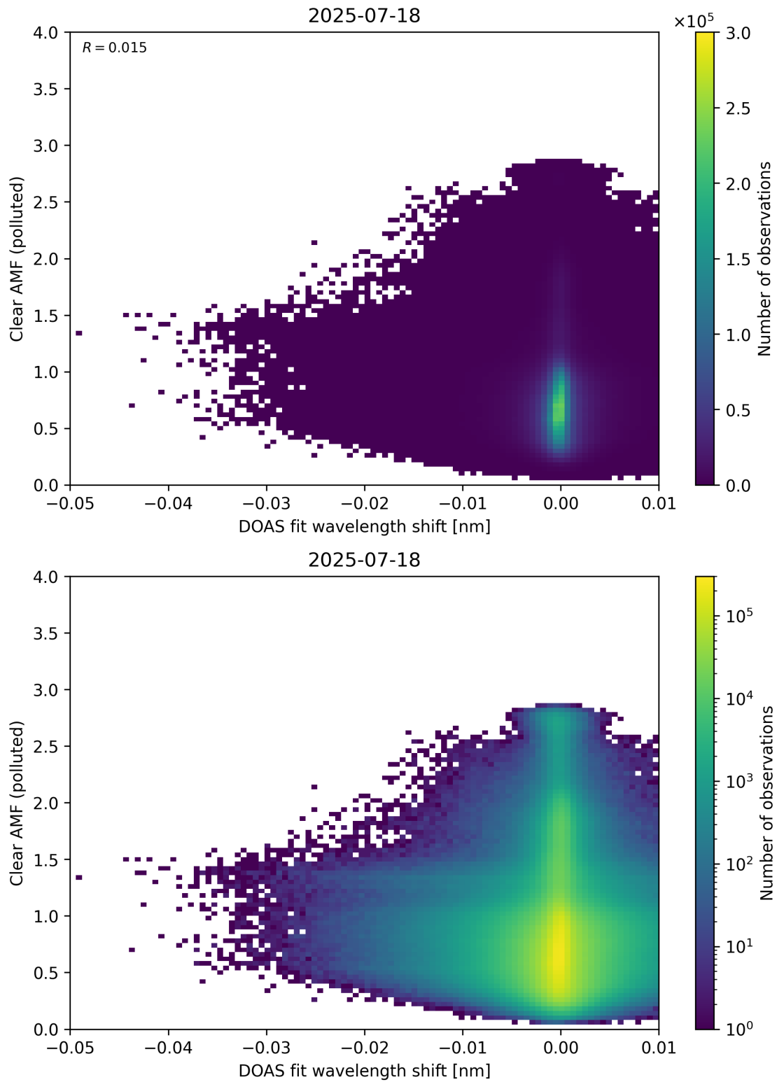
Figure 140: Scatter density plot of “DOAS fit wavelength shift” against “Clear AMF (polluted)” for 2025-07-18 to 2025-07-19.
