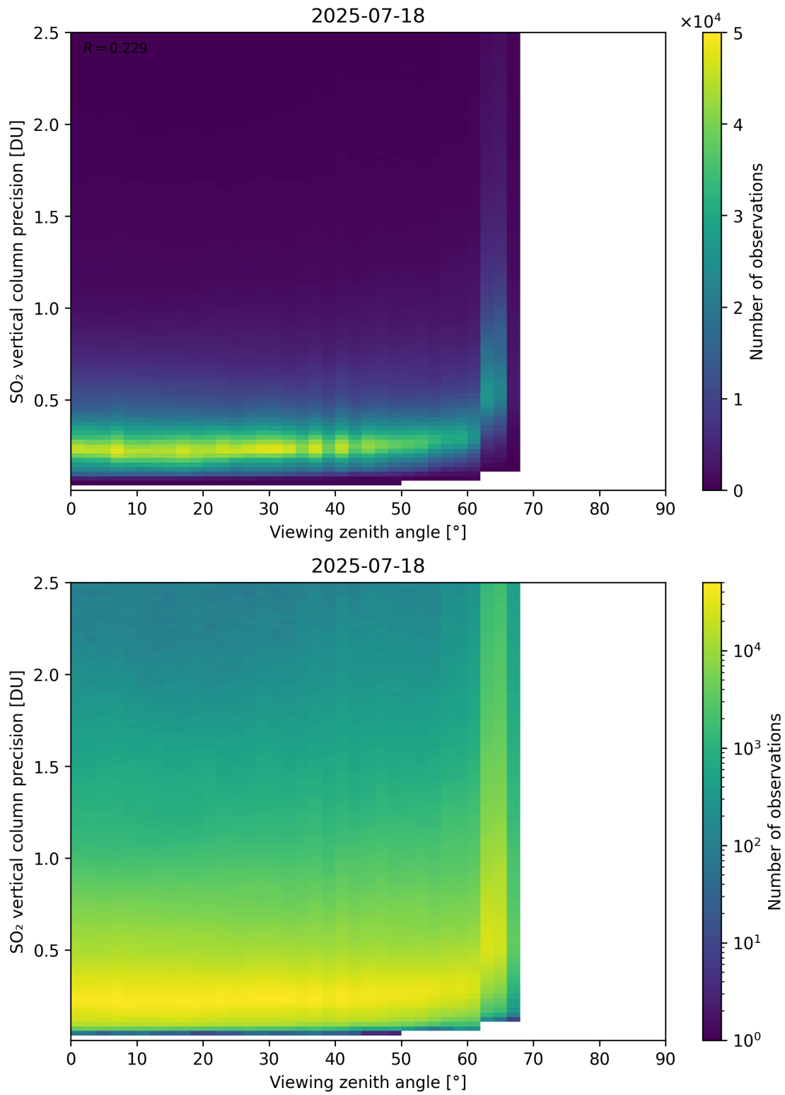
Figure 384: Scatter density plot of “Viewing zenith angle” against “SO 2 vertical column precision” for 2025-07-18 to 2025-07-19.
