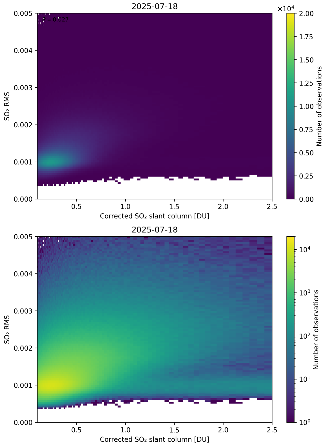
Figure 231: Scatter density plot of “Corrected SO 2 slant column” against “SO 2 RMS” for 2025-07-18 to 2025-07-19.
