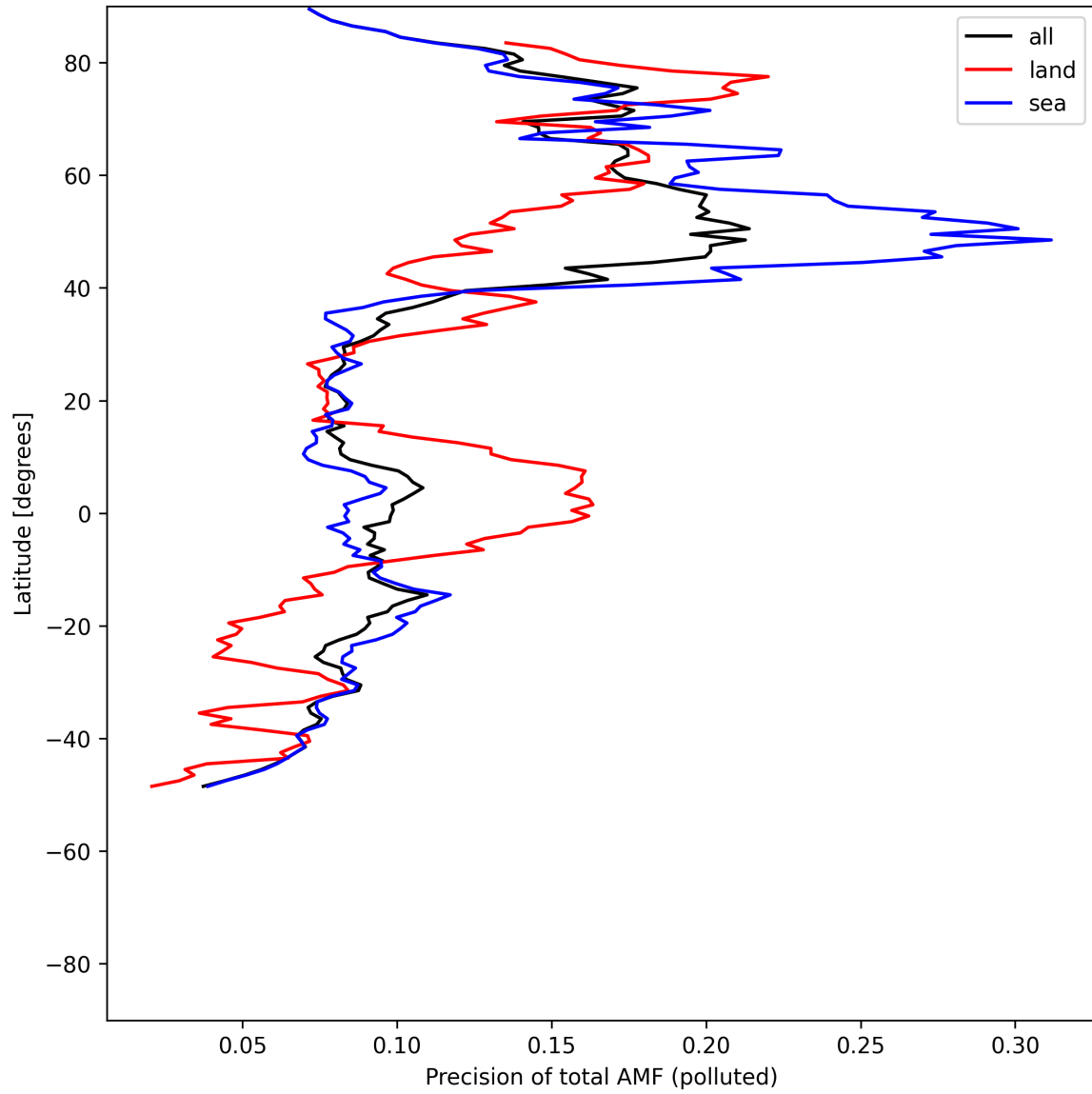
Figure 54: Zonal average of “Precision of total AMF (polluted)” for 2025-07-18 to 2025-07-19.
