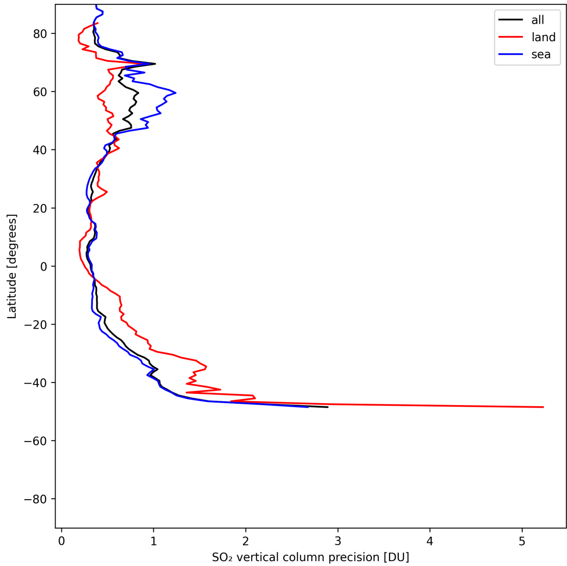
Figure 33: Zonal average of “SO 2 vertical column precision” for 2025-07-18 to 2025-07-19.
