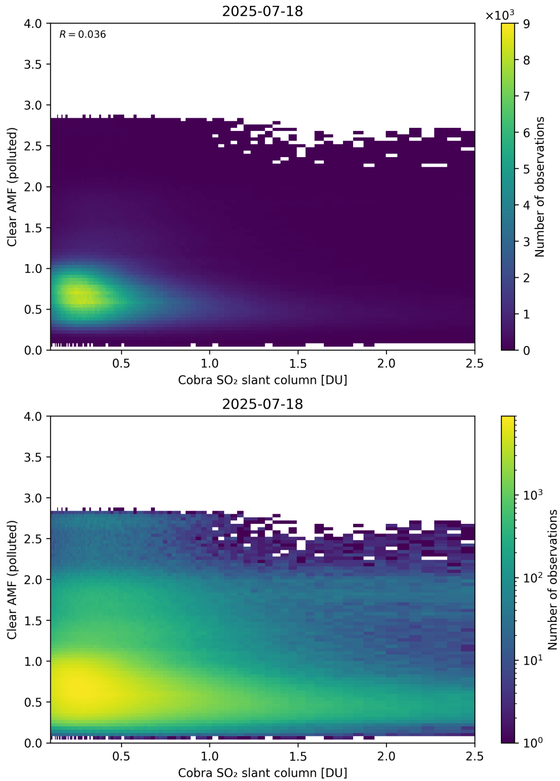
Figure 215: Scatter density plot of “Cobra SO 2 slant column” against “Clear AMF (polluted)” for 2025-07-18 to 2025-07-19.
