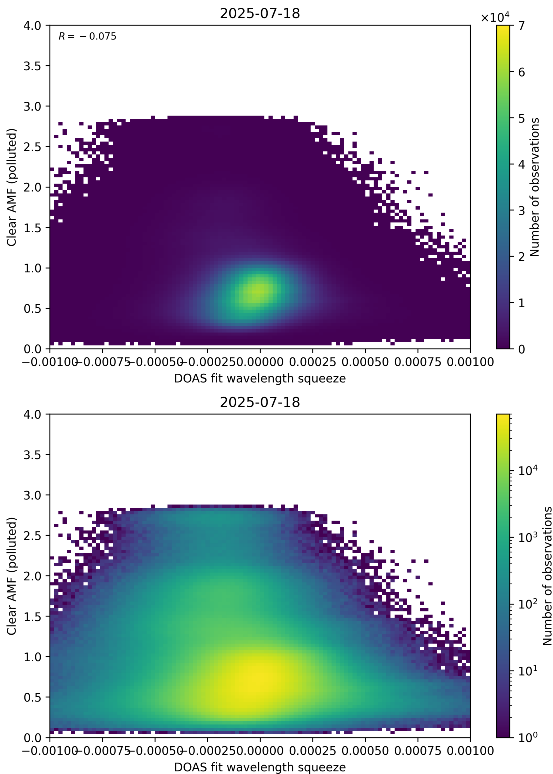
Figure 144: Scatter density plot of “DOAS fit wavelength squeeze” against “Clear AMF (polluted)” for 2025-07-18 to 2025-07-19.
