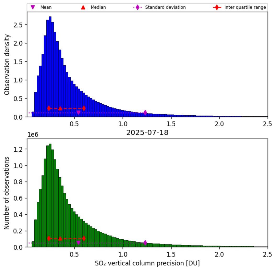
Figure 59: Histogram of “SO 2 vertical column precision” for 2025-07-18 to 2025-07-19
