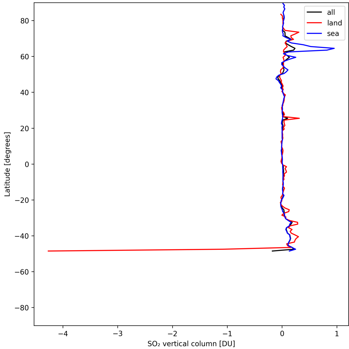
Figure 32: Zonal average of “SO 2 vertical column” for 2025-07-18 to 2025-07-19.
