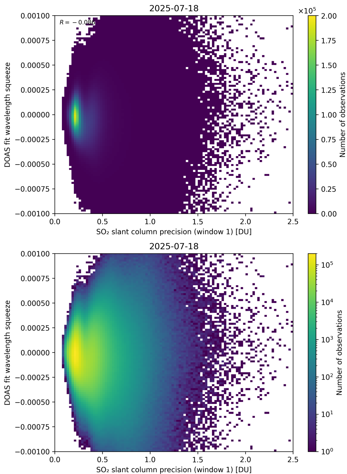
Figure 272: Scatter density plot of “SO 2 slant column precision (window 1)” against “DOAS fit wavelength squeeze” for 2025-07-18 to 2025-07-19.
