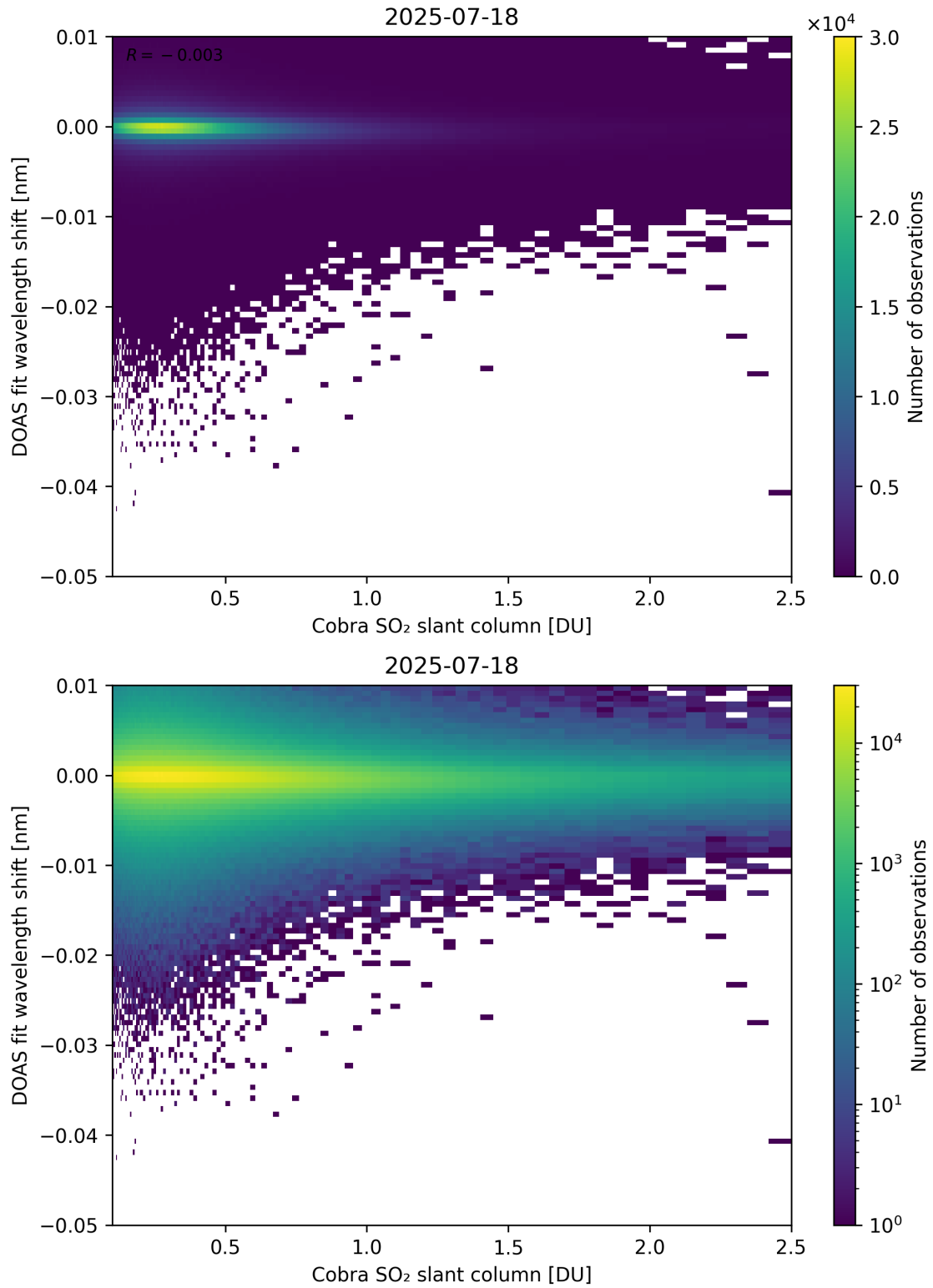
Figure 196: Scatter density plot of “Cobra SO 2 slant column” against “DOAS fit wavelength shift” for 2025-07-18 to 2025-07-19.
