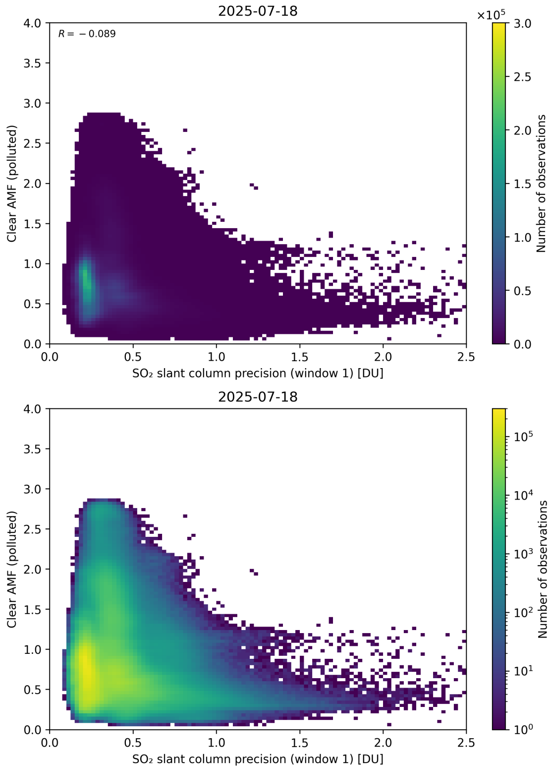
Figure 274: Scatter density plot of “SO 2 slant column precision (window 1)” against “Clear AMF (polluted)” for 2025-07-18 to 2025-07-19.
