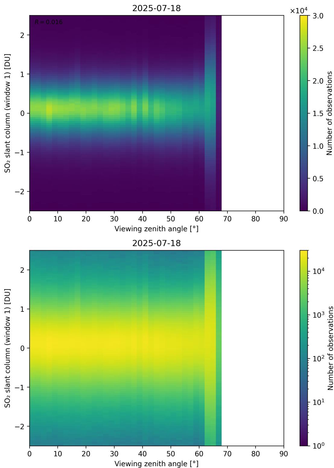
Figure 376: Scatter density plot of “Viewing zenith angle” against “SO 2 slant column (window 1)” for 2025-07-18 to 2025-07-19.
