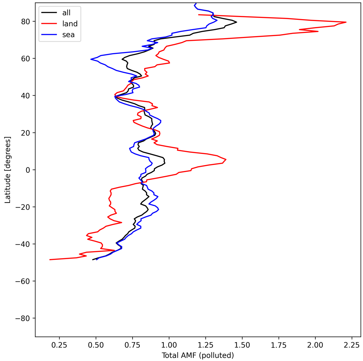
Figure 53: Zonal average of “Total AMF (polluted)” for 2025-07-18 to 2025-07-19.
