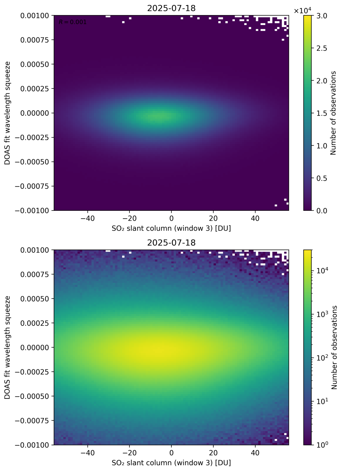
Figure 305: Scatter density plot of “SO 2 slant column (window 3)” against “DOAS fit wavelength squeeze” for 2025-07-18 to 2025-07-19.
