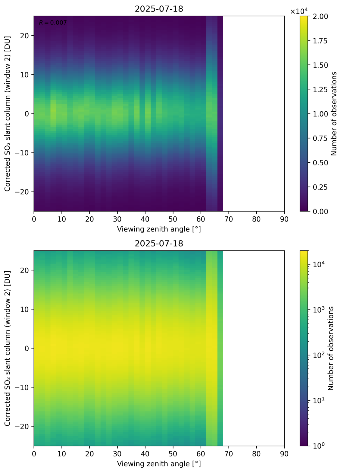
Figure 374: Scatter density plot of “Viewing zenith angle” against “Corrected SO 2 slant column (window 2)” for 2025-07-18 to 2025-07-19.
