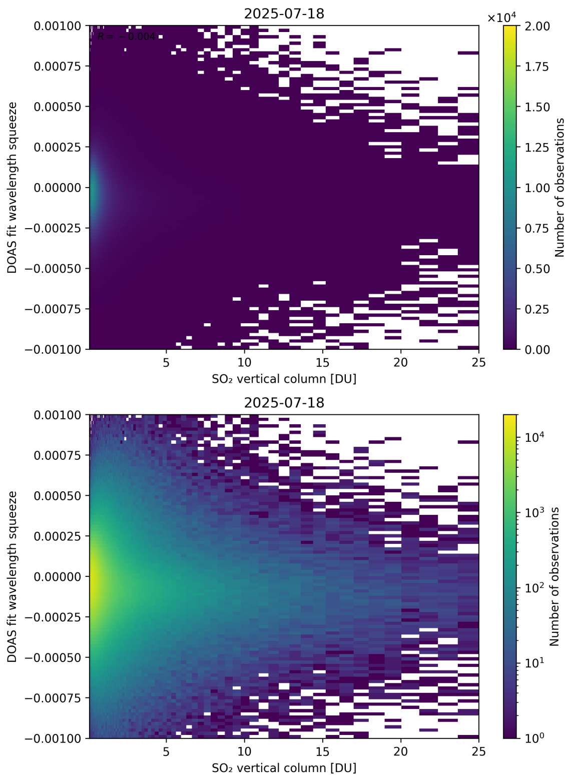
Figure 327: Scatter density plot of “SO 2 vertical column” against “DOAS fit wavelength squeeze” for 2025-07-18 to 2025-07-19.
