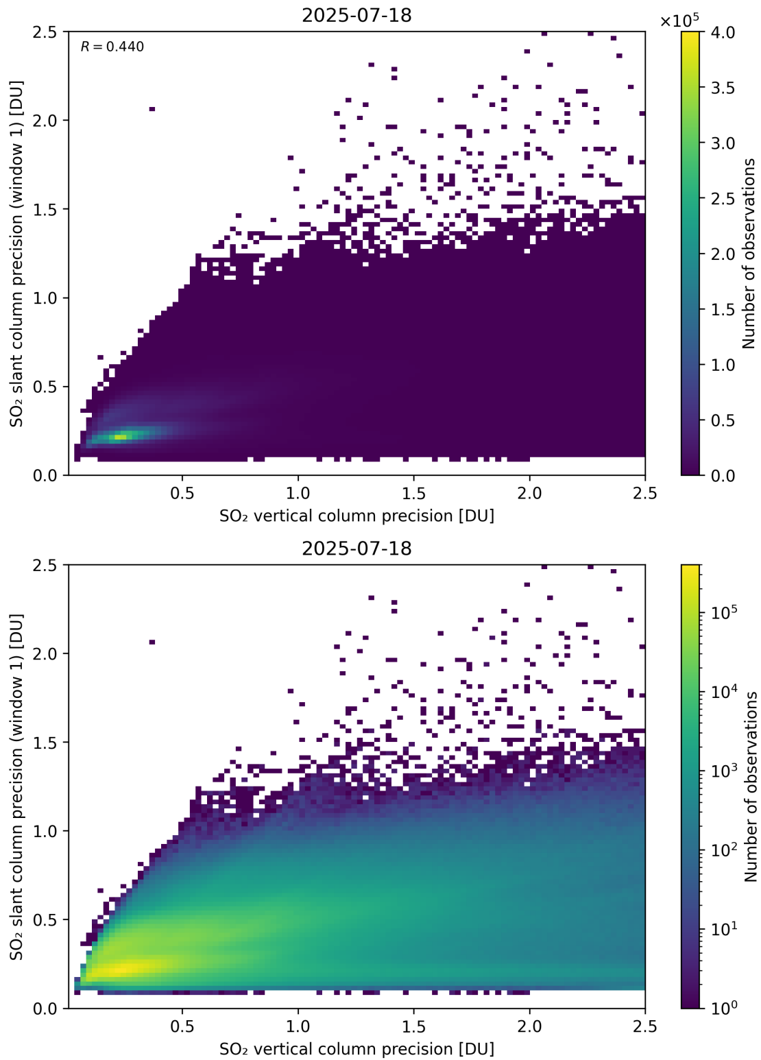
Figure 342: Scatter density plot of “SO 2 vertical column precision” against “SO 2 slant column precision (window 1)” for 2025-07-18 to 2025-07-19.
