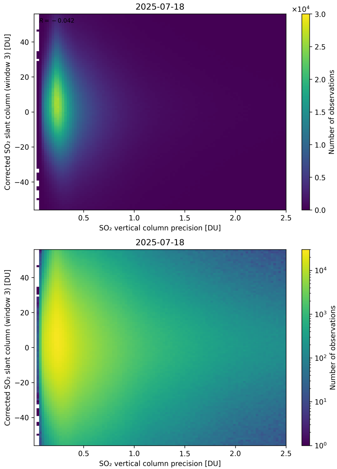
Figure 340: Scatter density plot of “SO 2 vertical column precision” against “Corrected SO 2 slant column (window 3)” for 2025-07-18 to 2025-07-19.
