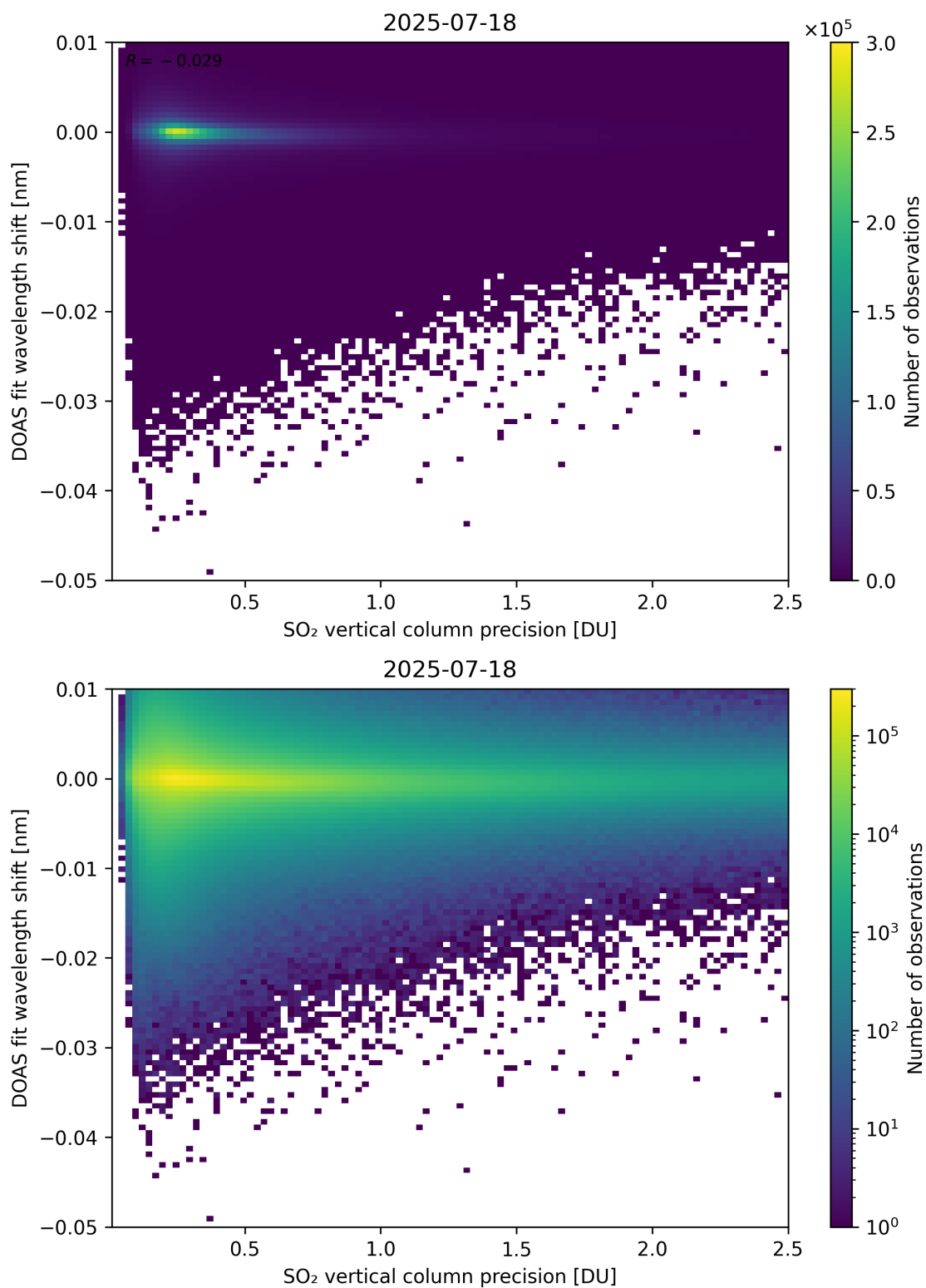
Figure 332: Scatter density plot of “SO 2 vertical column precision” against “DOAS fit wavelength shift” for 2025-07-18 to 2025-07-19.
