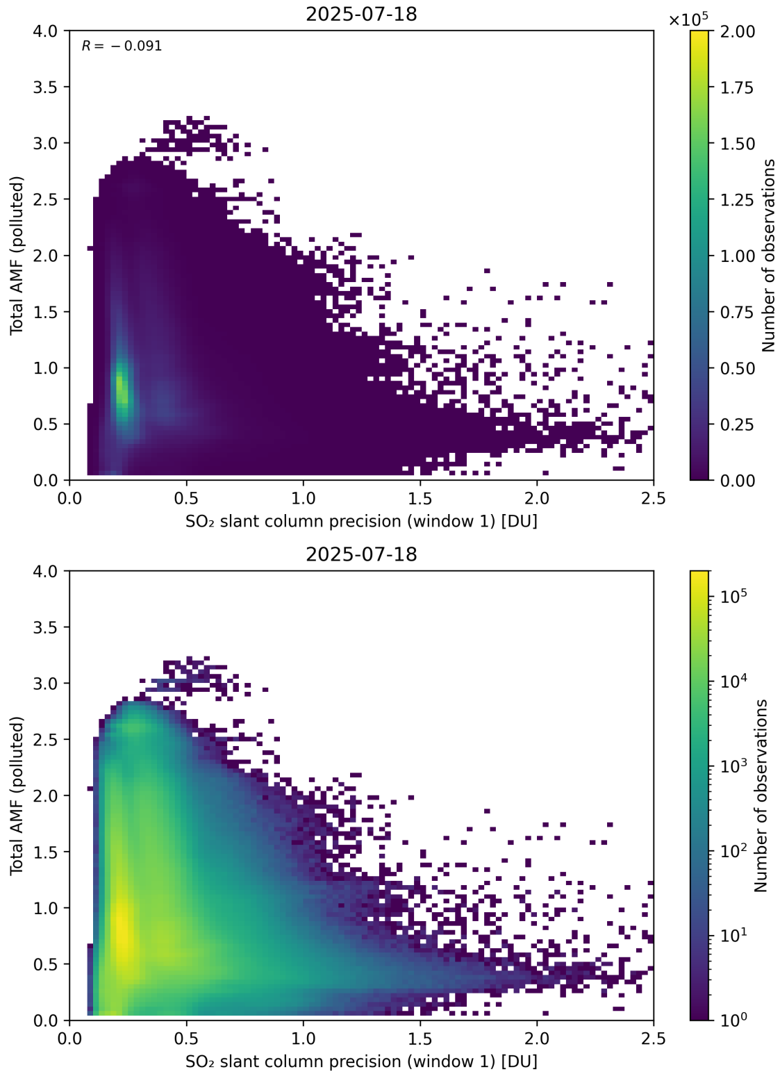
Figure 280: Scatter density plot of “SO 2 slant column precision (window 1)” against “Total AMF (polluted)” for 2025-07-18 to 2025-07-19.
