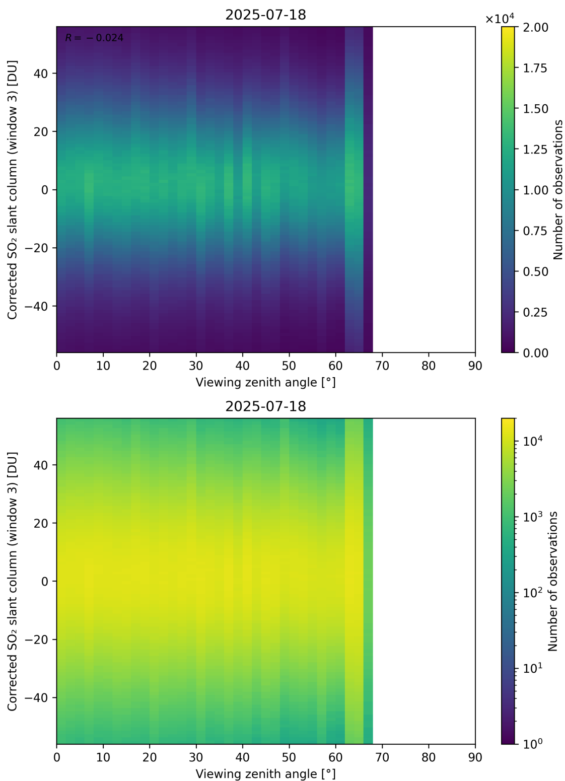
Figure 375: Scatter density plot of “Viewing zenith angle” against “Corrected SO 2 slant column (window 3)” for 2025-07-18 to 2025-07-19.
