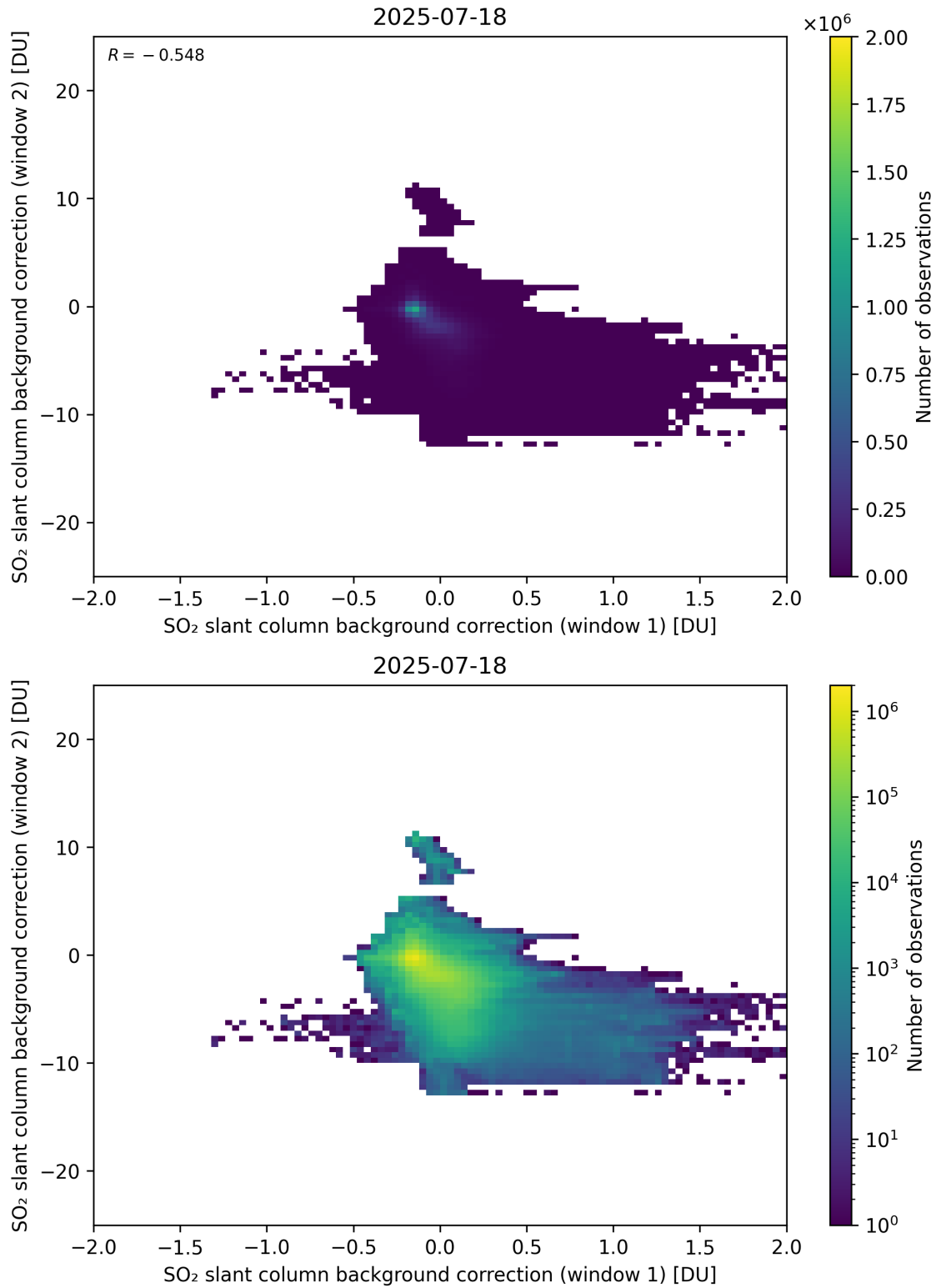
Figure 109: Scatter density plot of “SO 2 slant column background correction (window 1)” against “SO 2 slant column background correction (window 2)” for 2025-07-18 to 2025-07-19.
