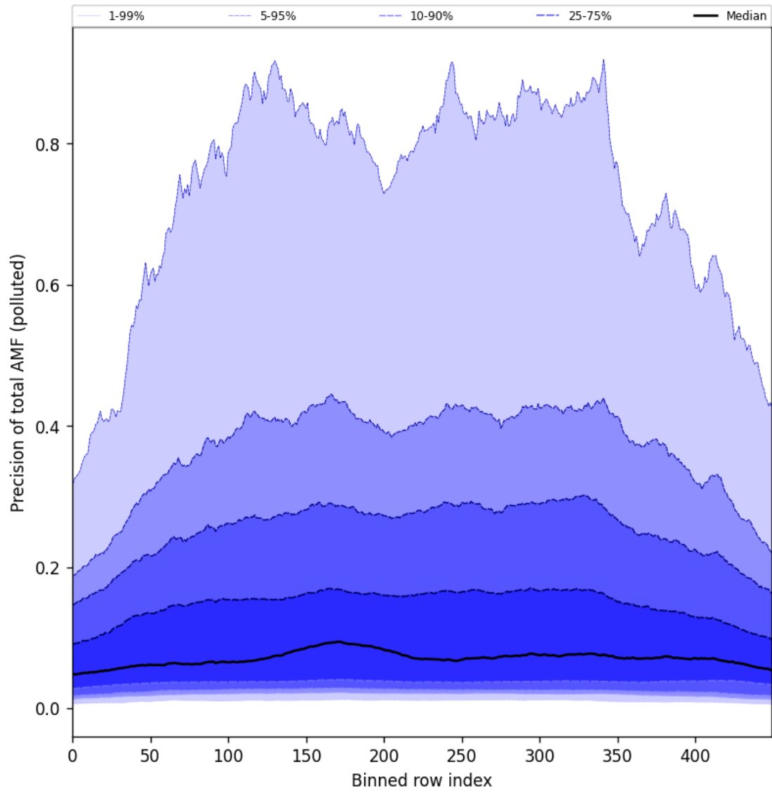
Figure 106: Along track statistics of “Precision of total AMF (polluted)” for 2025-07-18 to 2025-07-19
