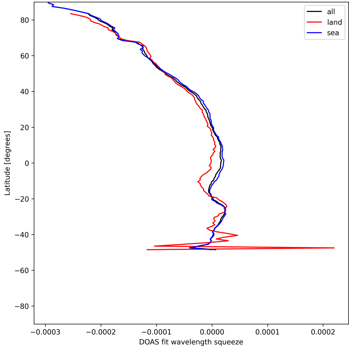
Figure 51: Zonal average of “DOAS fit wavelength squeeze” for 2025-07-18 to 2025-07-19.
