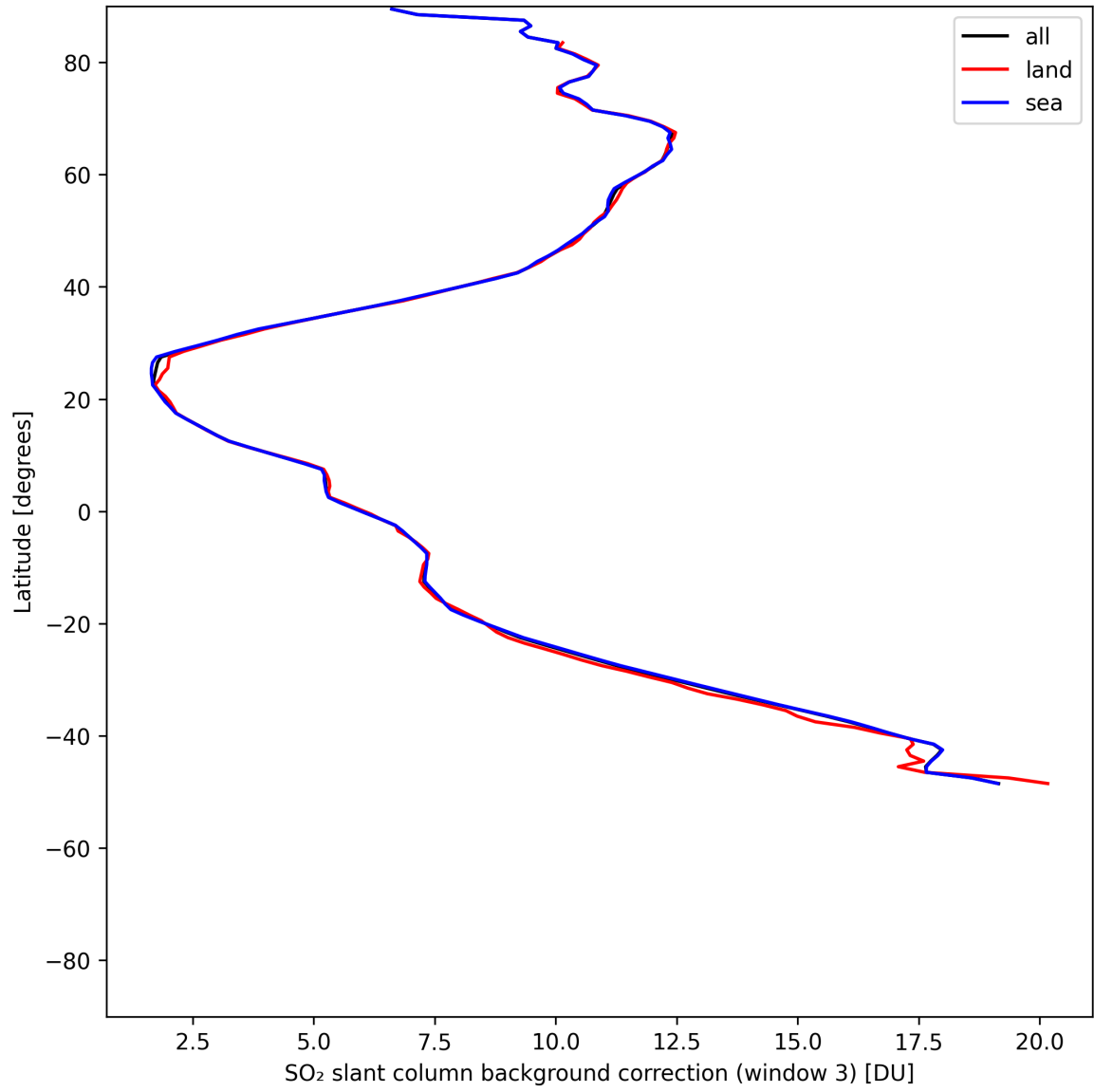
Figure 48: Zonal average of “SO 2 slant column background correction (window 3)” for 2025-07-18 to 2025-07-19.
