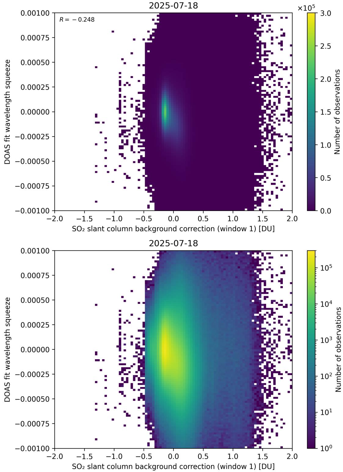
Figure 112: Scatter density plot of “SO 2 slant column background correction (window 1)” against “DOAS fit wavelength squeeze” for 2025-07-18 to 2025-07-19.
