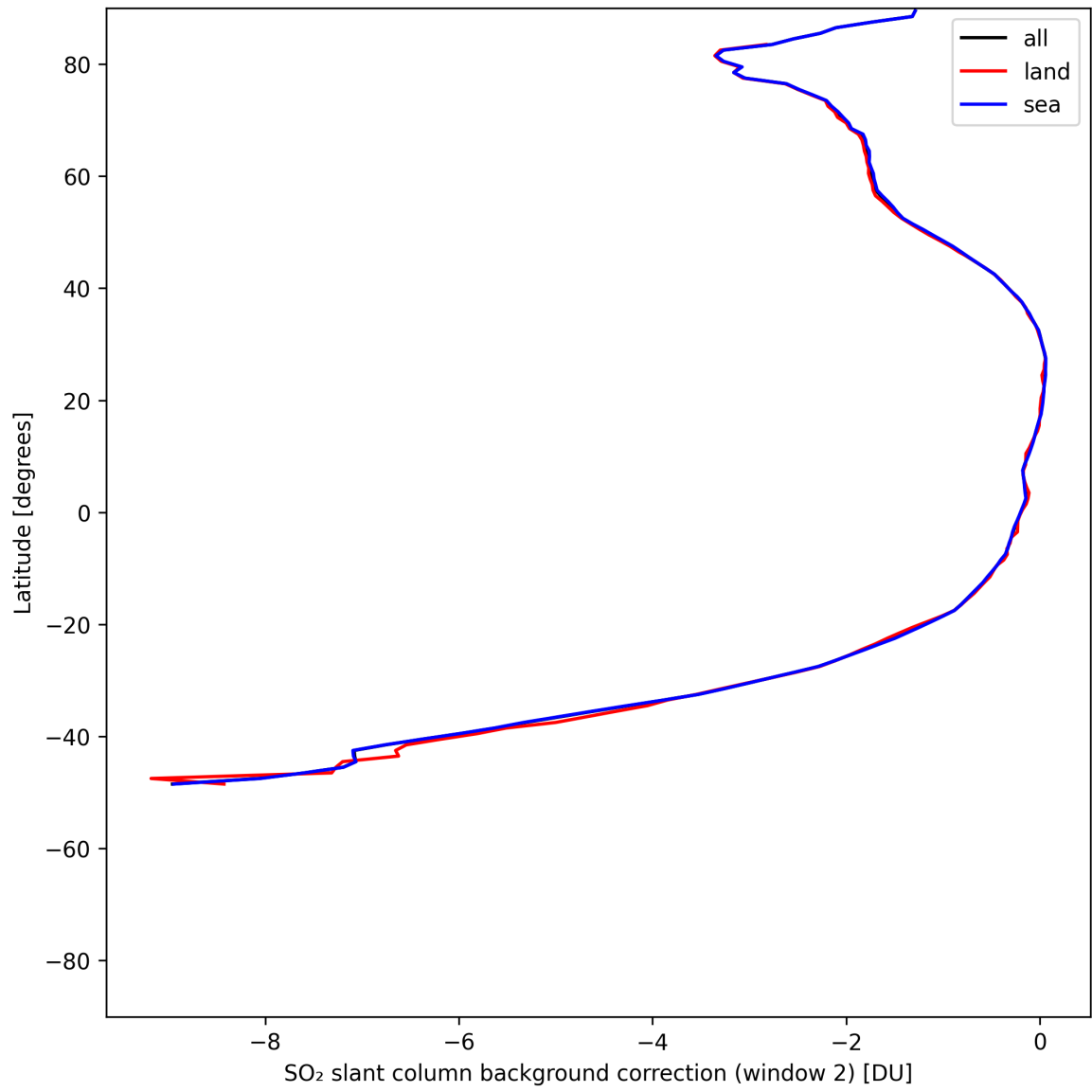
Figure 44: Zonal average of “SO 2 slant column background correction (window 2)” for 2025-07-18 to 2025-07-19.
