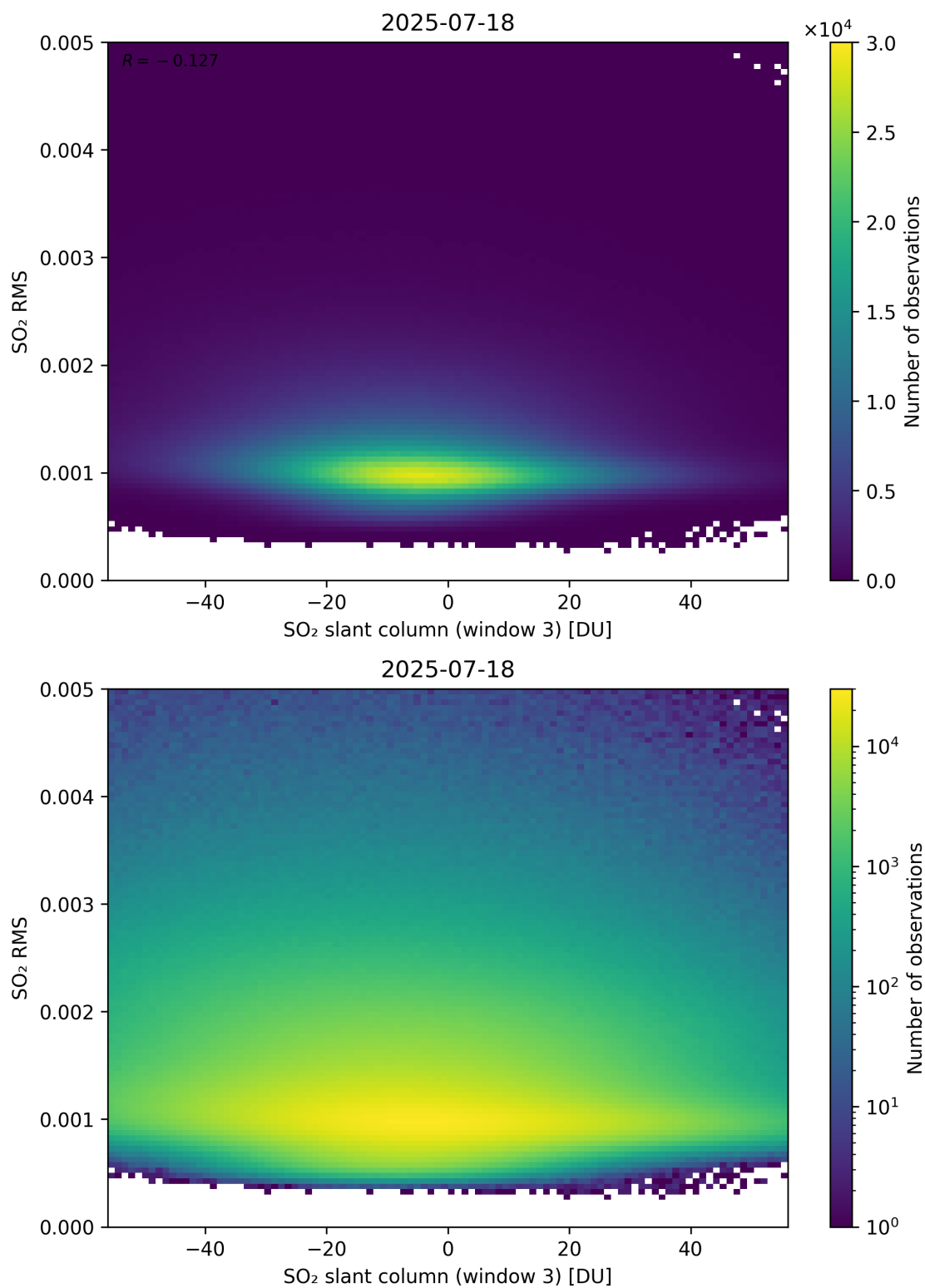
Figure 306: Scatter density plot of “SO 2 slant column (window 3)” against “SO 2 RMS” for 2025-07-18 to 2025-07-19.
