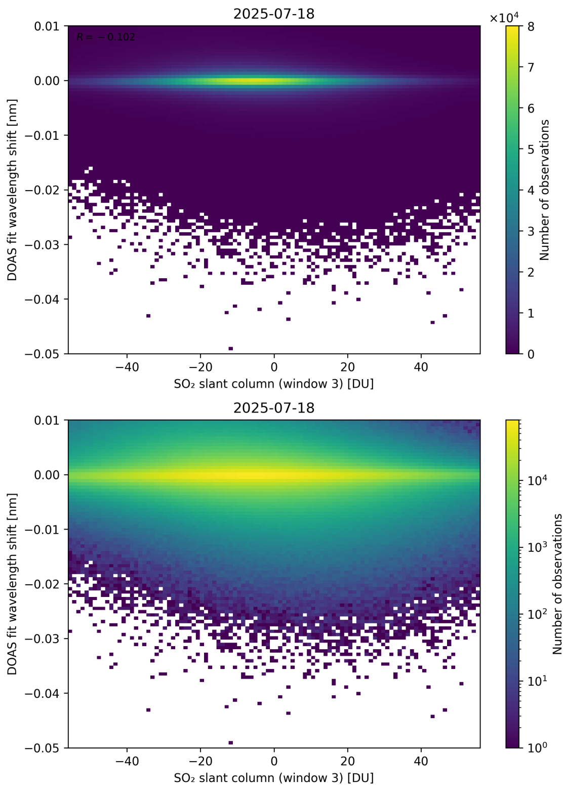
Figure 304: Scatter density plot of “SO 2 slant column (window 3)” against “DOAS fit wavelength shift” for 2025-07-18 to 2025-07-19.
