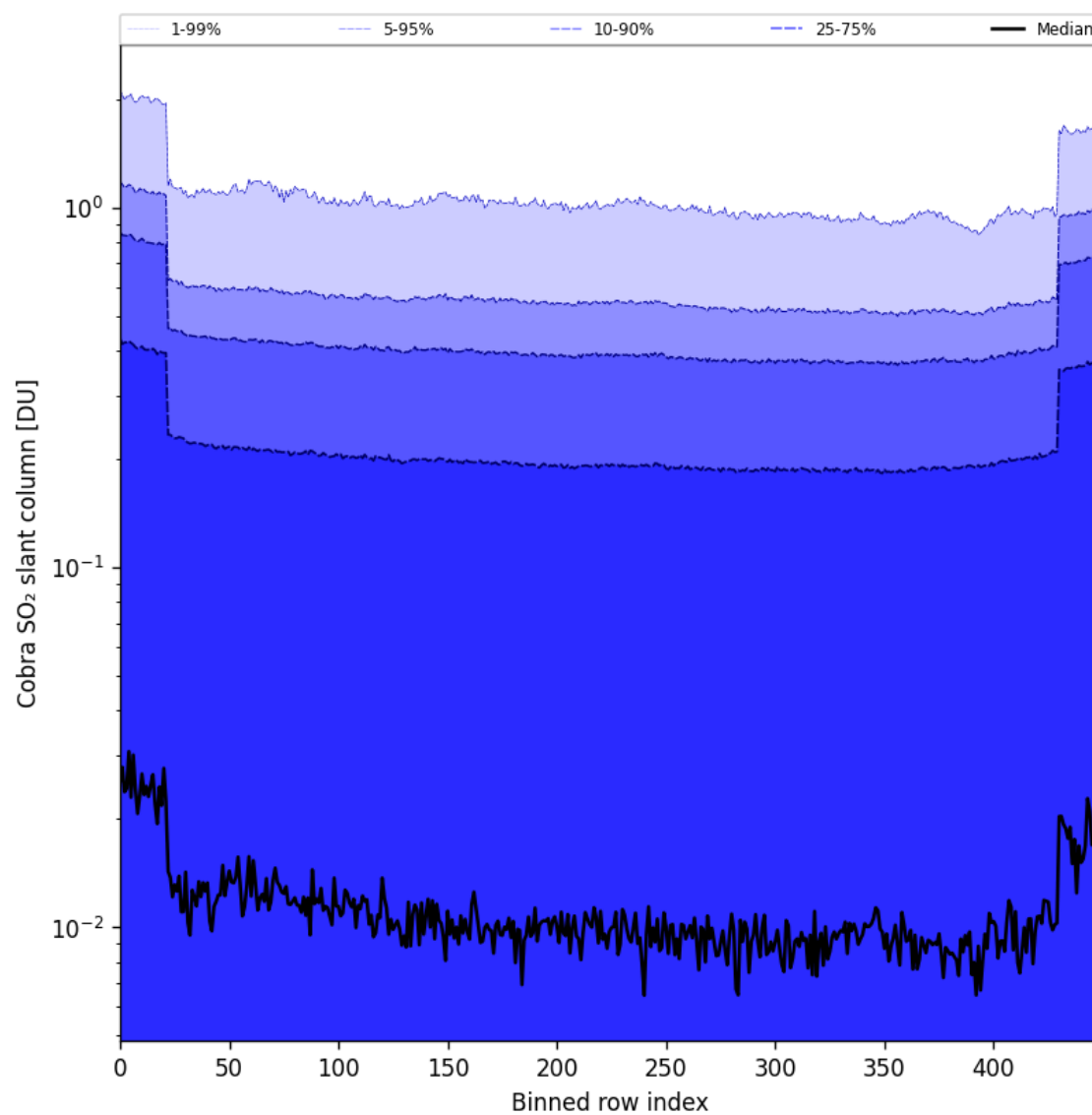
Figure 87: Along track statistics of “Cobra SO 2 slant column” for 2025-07-18 to 2025-07-19
