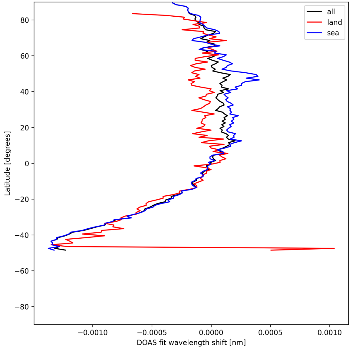
Figure 50: Zonal average of “DOAS fit wavelength shift” for 2025-07-18 to 2025-07-19.
