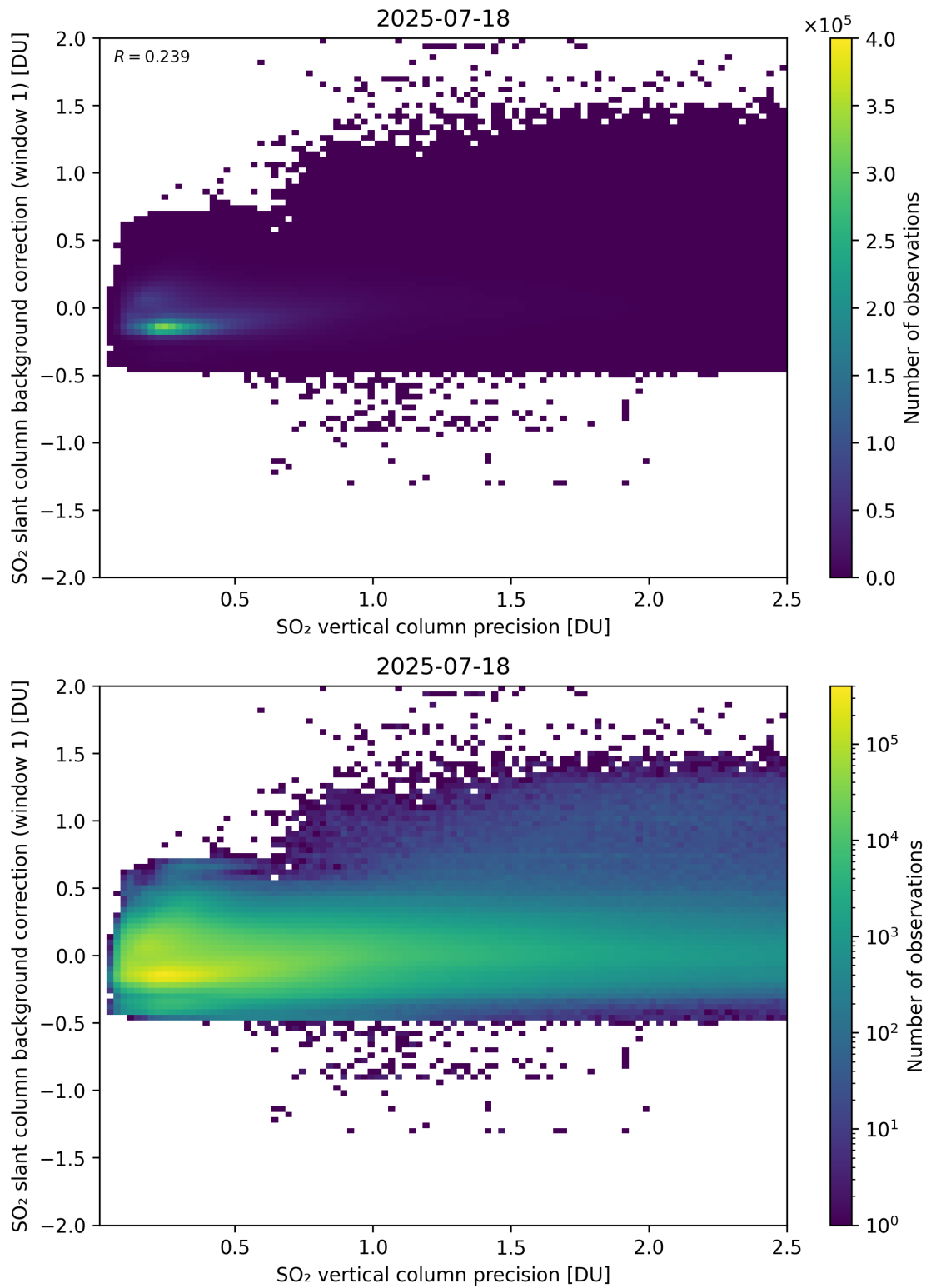
Figure 329: Scatter density plot of “SO 2 vertical column precision” against “SO 2 slant column background correction (window 1)” for 2025-07-18 to 2025-07-19.
