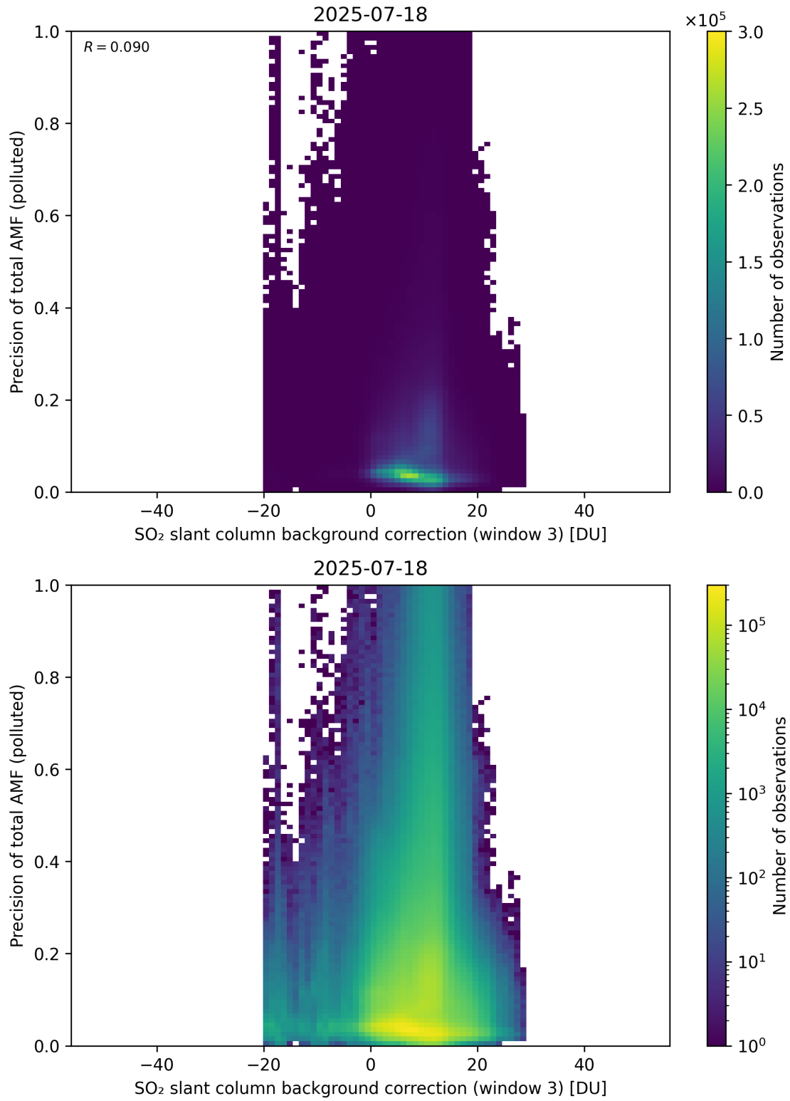
Figure 137: Scatter density plot of “SO 2 slant column background correction (window 3)” against “Precision of total AMF (polluted)” for 2025-07-18 to 2025-07-19.
