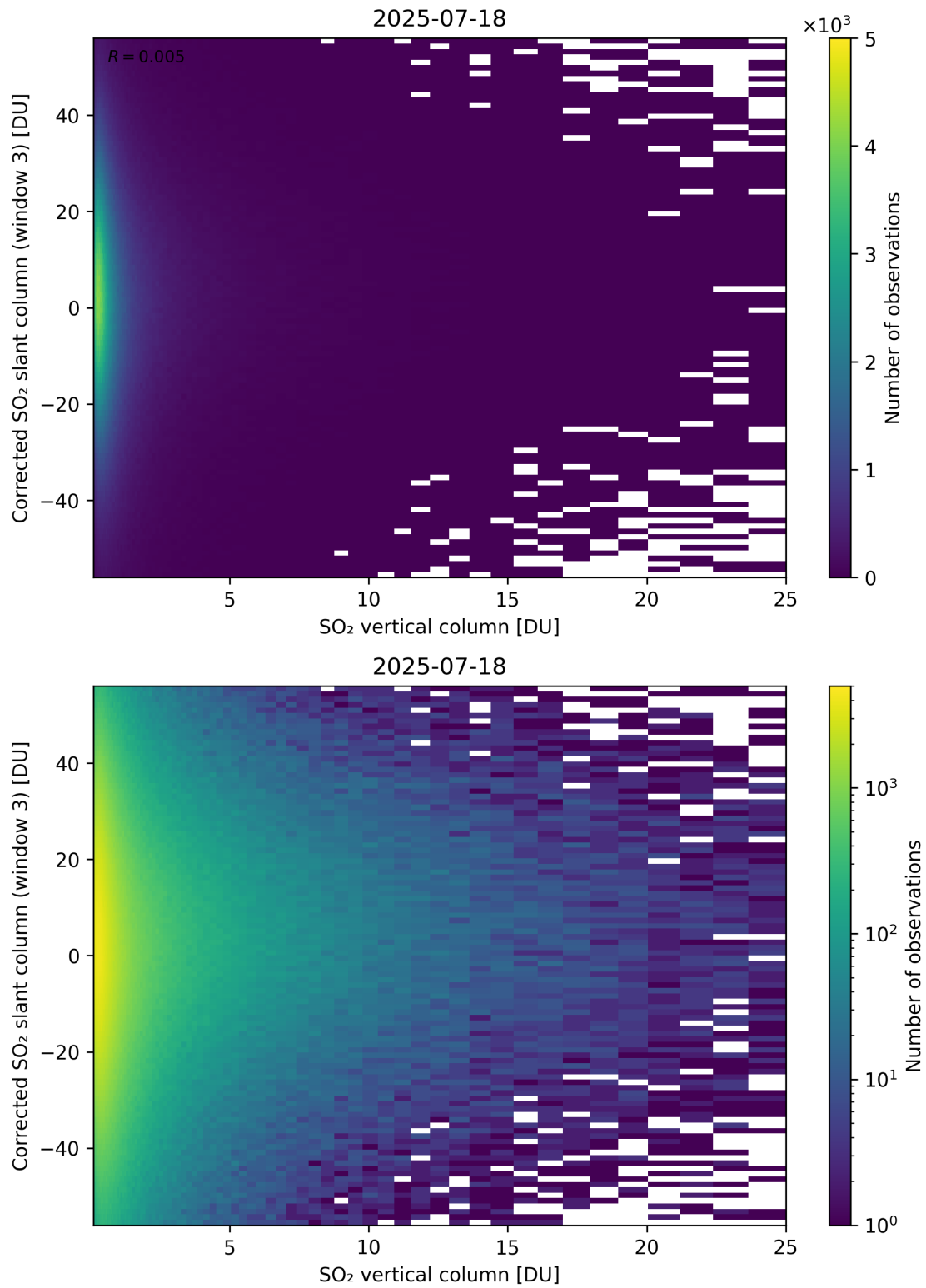
Figure 353: Scatter density plot of “SO 2 vertical column” against “Corrected SO 2 slant column (window 3)” for 2025-07-18 to 2025-07-19.
