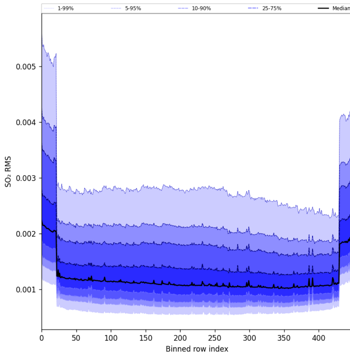
Figure 104: Along track statistics of “SO 2 RMS” for 2025-07-18 to 2025-07-19
