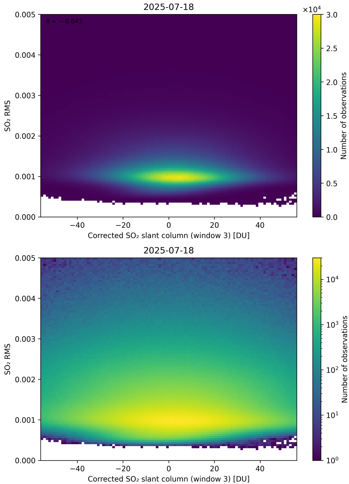
Figure 258: Scatter density plot of “Corrected SO 2 slant column (window 3)” against “SO 2 RMS” for 2025-07-18 to 2025-07-19.
