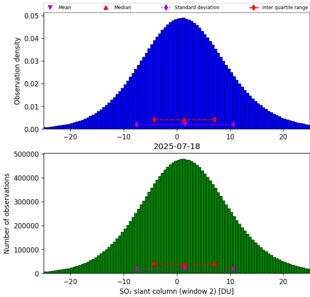
Figure 67: Histogram of “SO 2 slant column (window 2)” for 2025-07-18 to 2025-07-19
