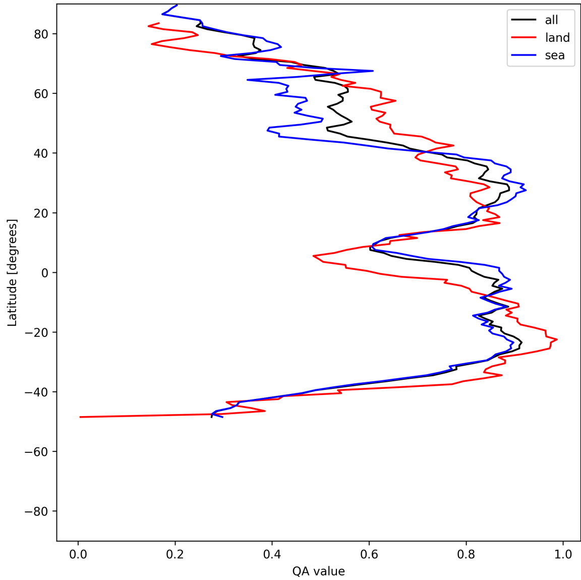
Figure 31: Zonal average of “QA value” for 2025-07-18 to 2025-07-19.
