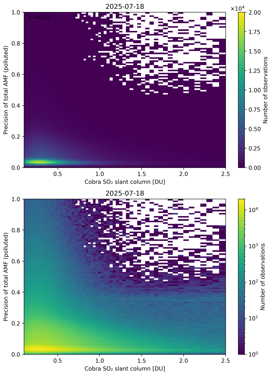
Figure 225: Scatter density plot of “Cobra SO 2 slant column” against “Precision of total AMF (polluted)” for 2025-07-18 to 2025-07-19.
