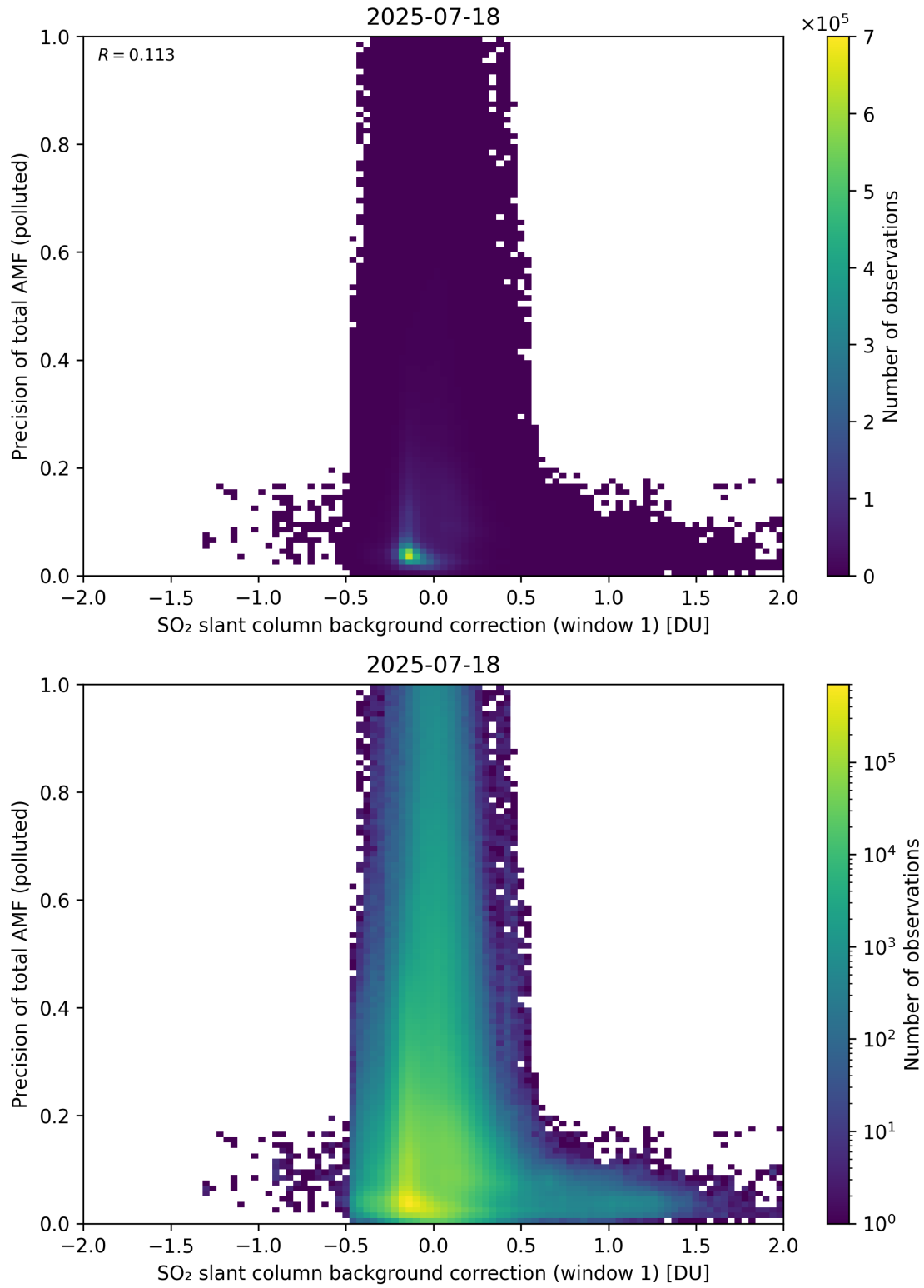
Figure 121: Scatter density plot of “SO 2 slant column background correction (window 1)” against “Precision of total AMF (polluted)” for 2025-07-18 to 2025-07-19.
