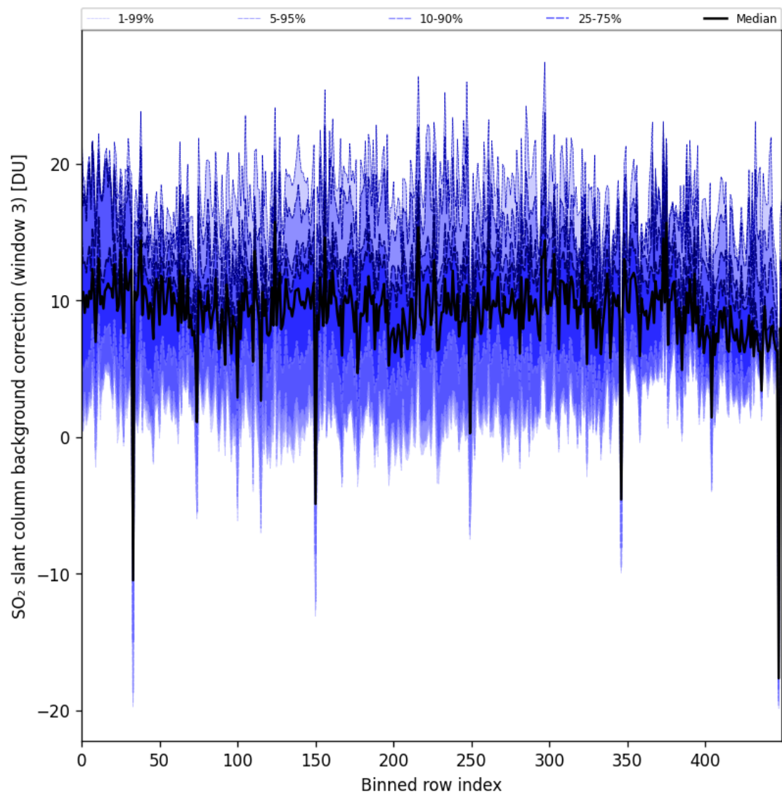
Figure 100: Along track statistics of “SO 2 slant column background correction (window 3)” for 2025-07-18 to 2025-07-19
