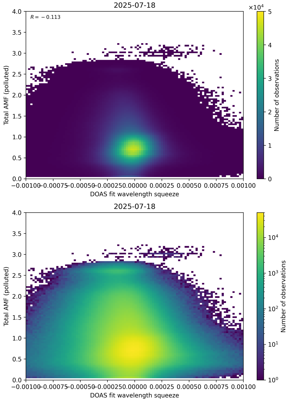
Figure 145: Scatter density plot of “DOAS fit wavelength squeeze” against “Total AMF (polluted)” for 2025-07-18 to 2025-07-19.
