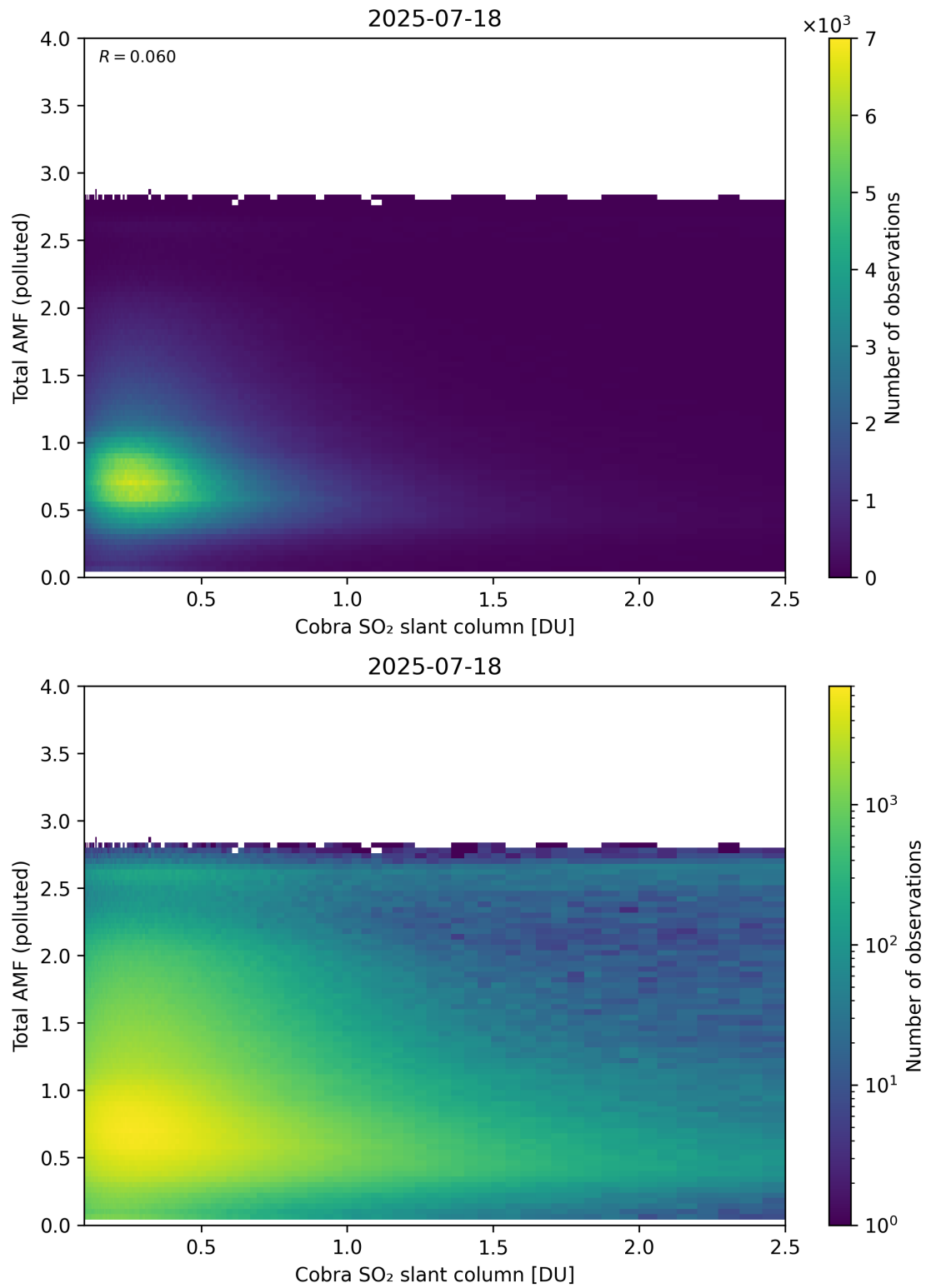
Figure 224: Scatter density plot of “Cobra SO 2 slant column” against “Total AMF (polluted)” for 2025-07-18 to 2025-07-19.
