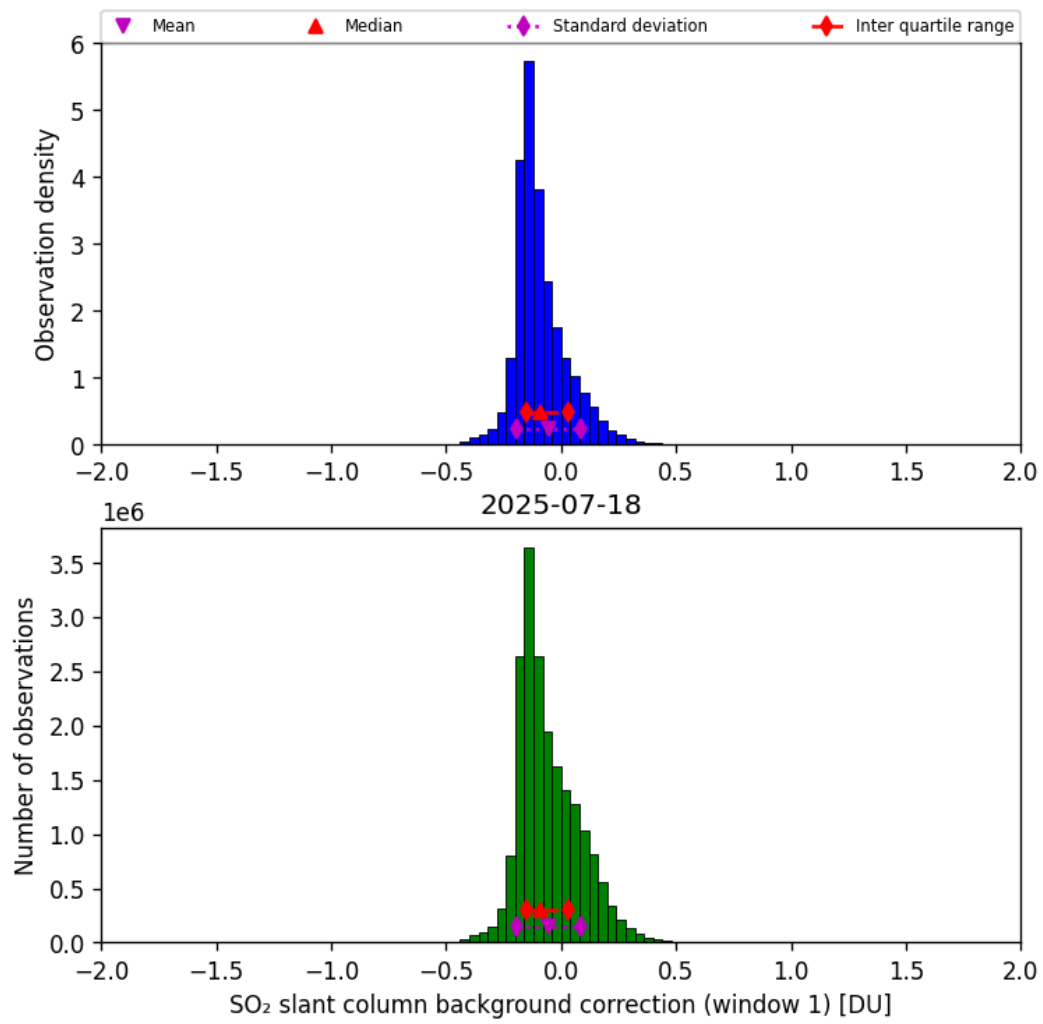
Figure 66: Histogram of “SO 2 slant column background correction (window 1)” for 2025-07-18 to 2025-07-19
