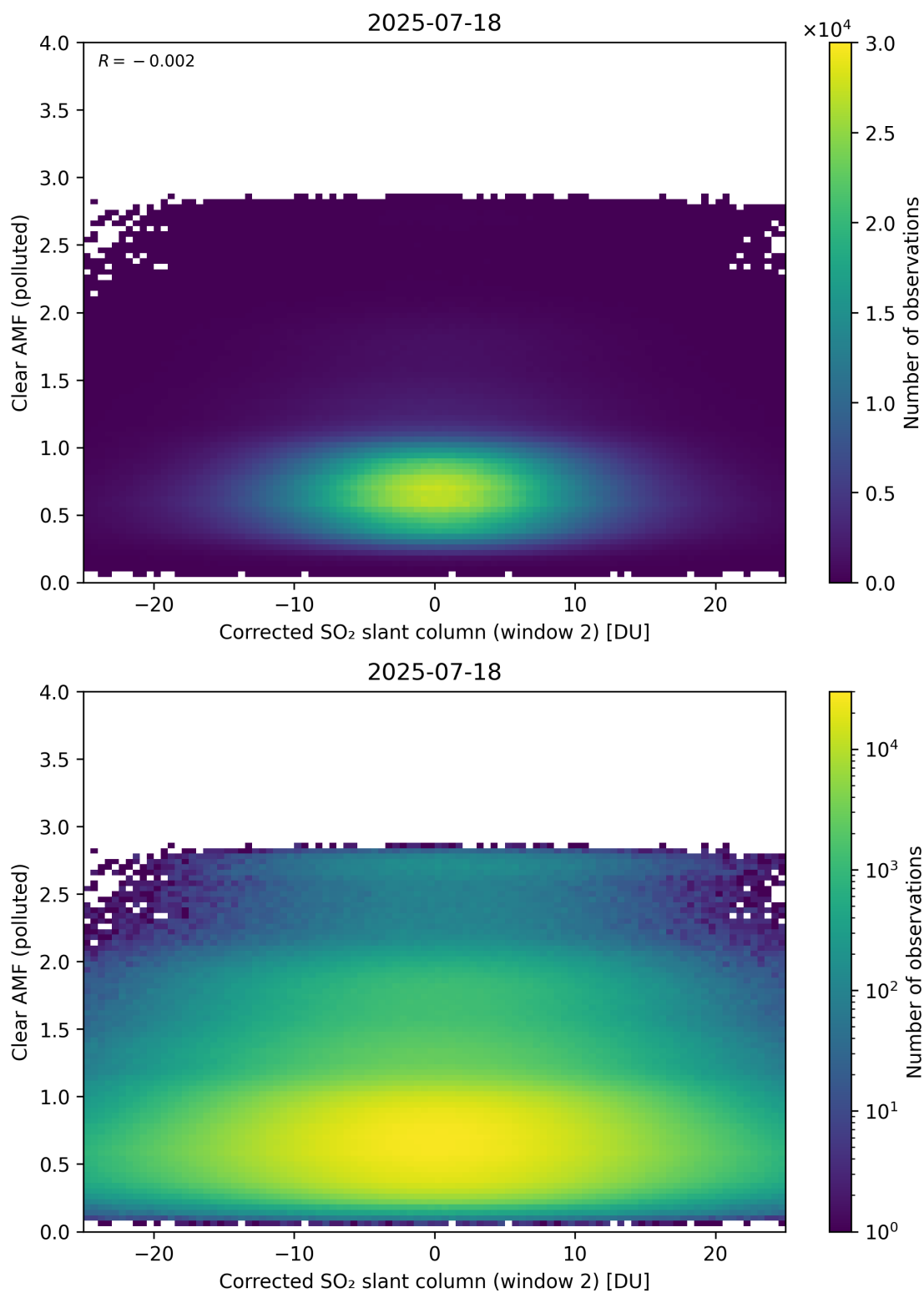
Figure 249: Scatter density plot of “Corrected SO 2 slant column (window 2)” against “Clear AMF (polluted)” for 2025-07-18 to 2025-07-19.
