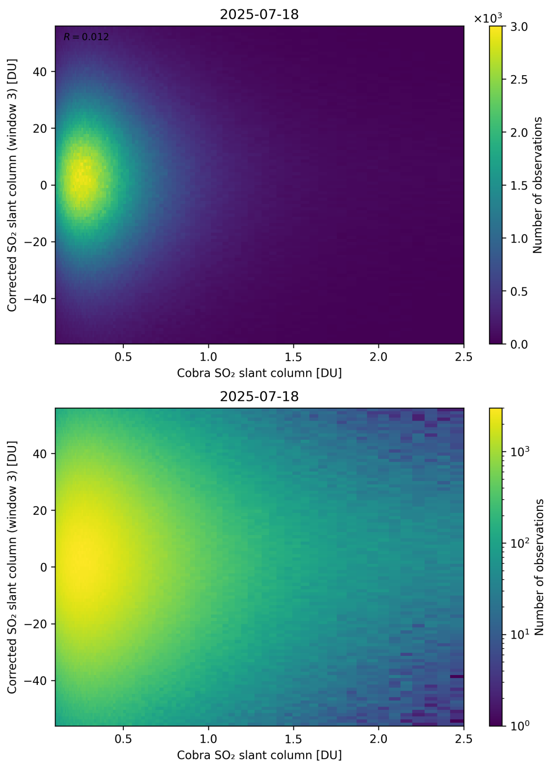
Figure 218: Scatter density plot of “Cobra SO 2 slant column” against “Corrected SO 2 slant column (window 3)” for 2025-07-18 to 2025-07-19.
