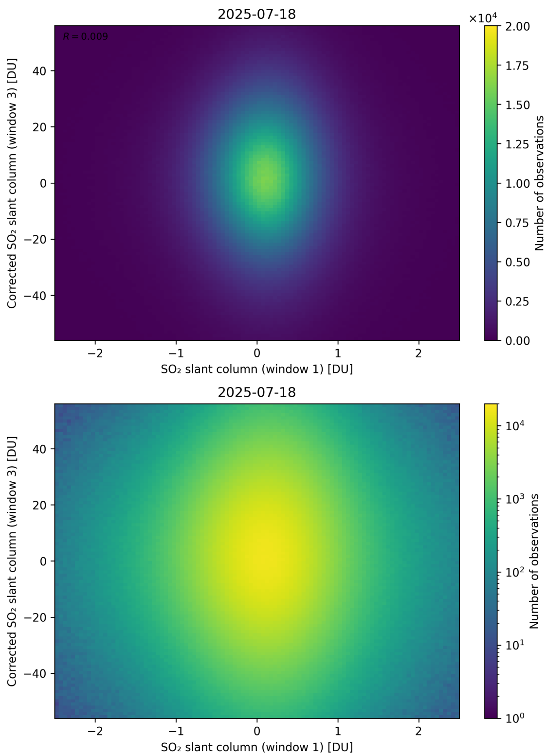
Figure 284: Scatter density plot of “SO 2 slant column (window 1)” against “Corrected SO 2 slant column (window 3)” for 2025-07-18 to 2025-07-19.
