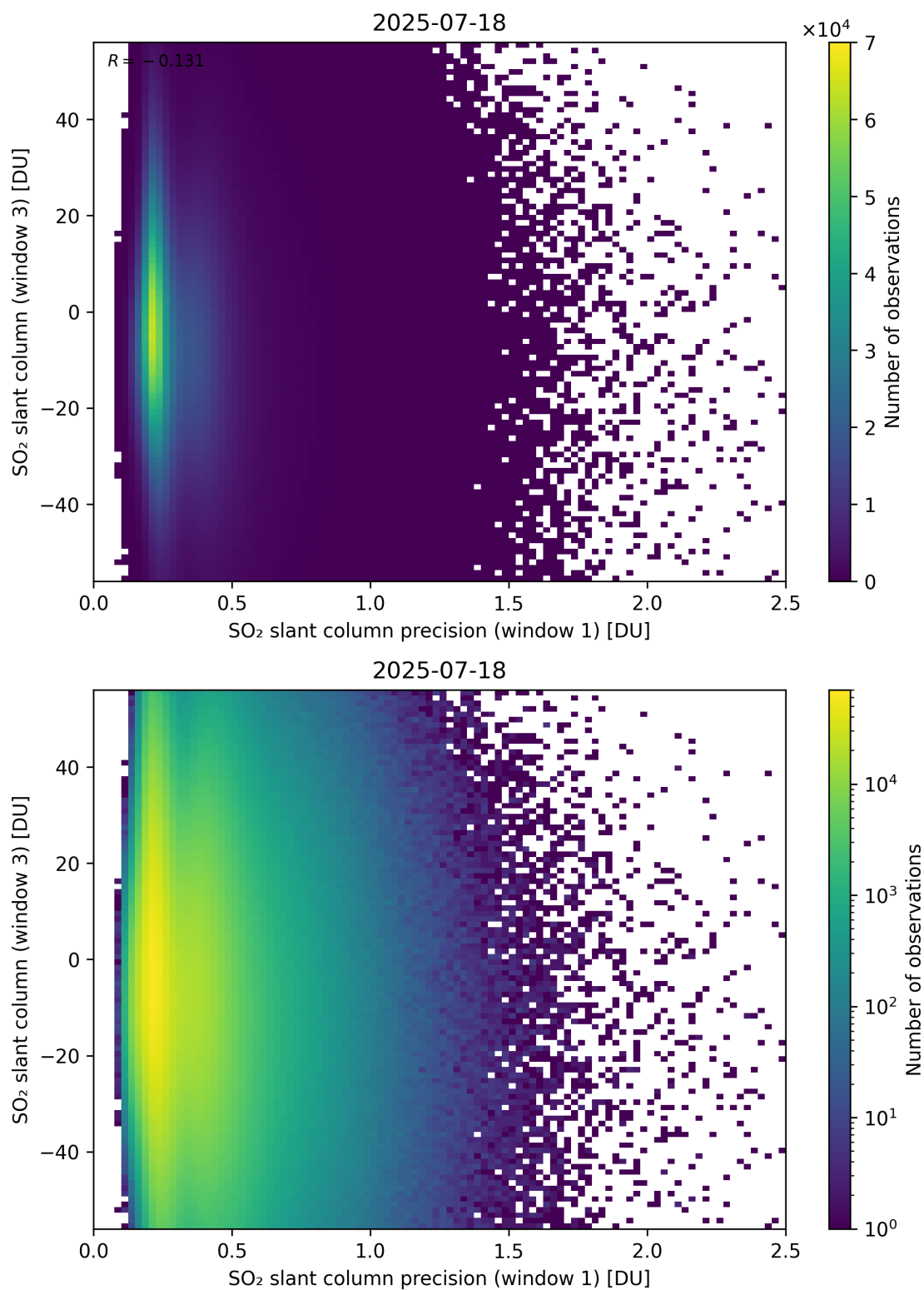
Figure 278: Scatter density plot of “SO 2 slant column precision (window 1)” against “SO 2 slant column (window 3)” for 2025-07-18 to 2025-07-19.
