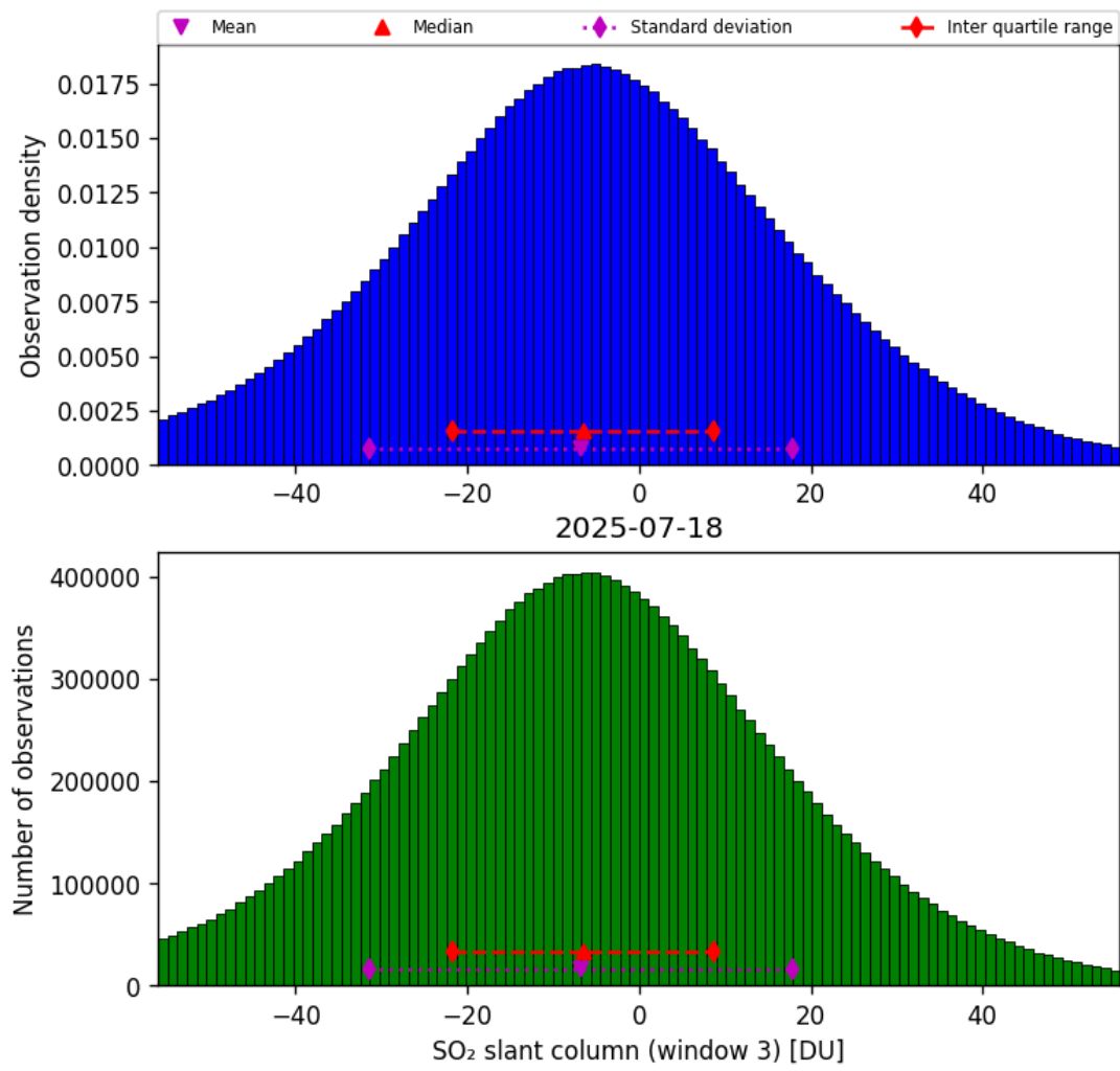
Figure 71: Histogram of “SO 2 slant column (window 3)” for 2025-07-18 to 2025-07-19
