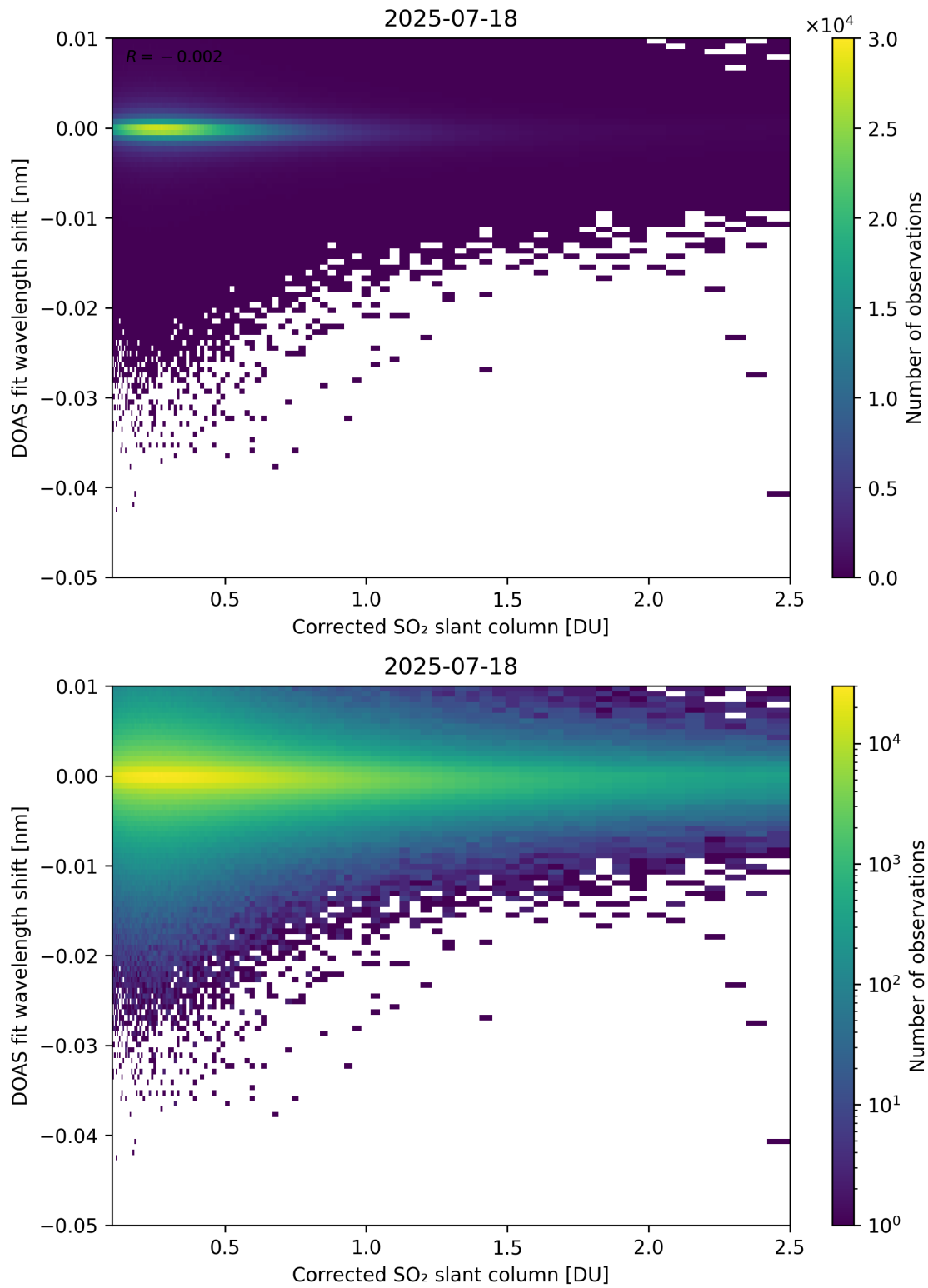
Figure 229: Scatter density plot of “Corrected SO 2 slant column” against “DOAS fit wavelength shift” for 2025-07-18 to 2025-07-19.
