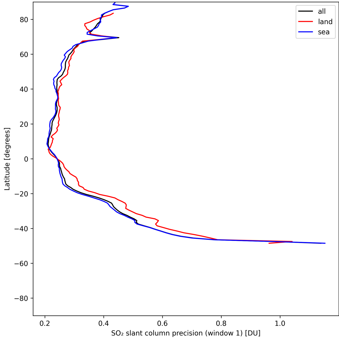
Figure 38: Zonal average of “SO 2 slant column precision (window 1)” for 2025-07-18 to 2025-07-19.
