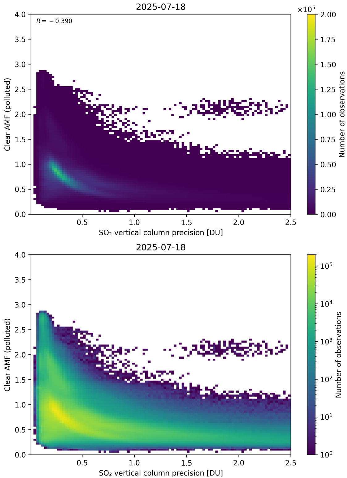
Figure 335: Scatter density plot of “SO 2 vertical column precision” against “Clear AMF (polluted)” for 2025-07-18 to 2025-07-19.
