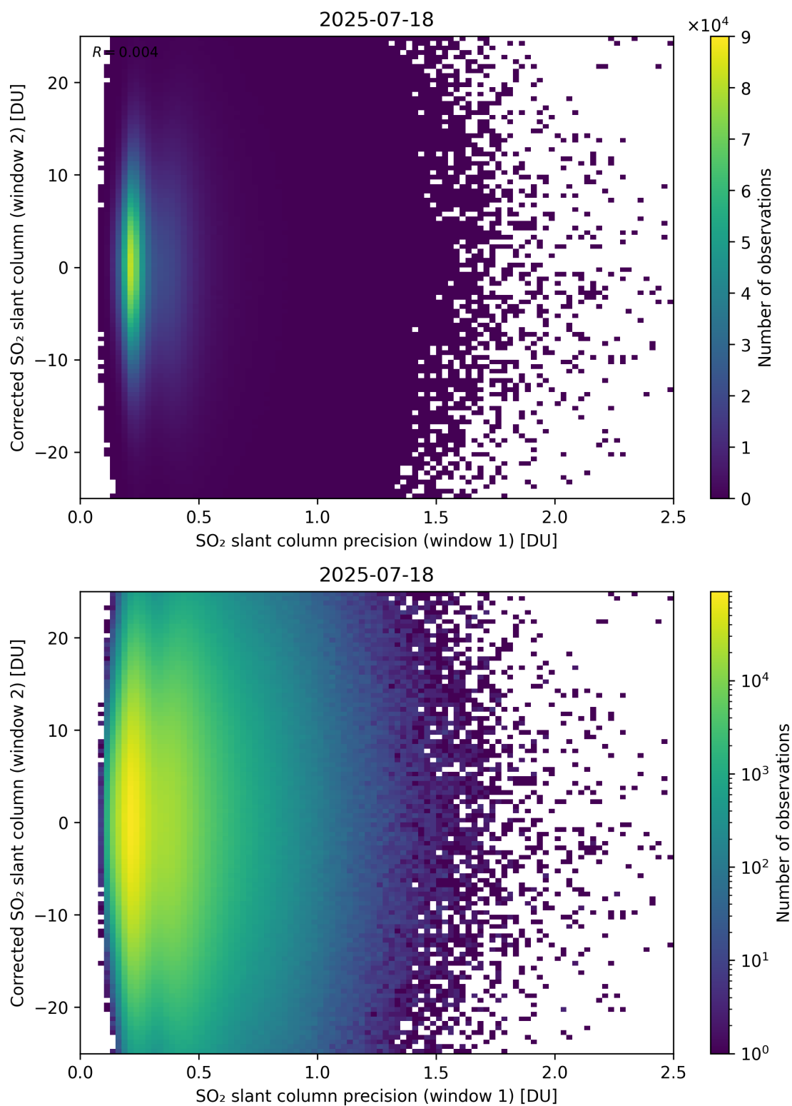
Figure 275: Scatter density plot of “SO 2 slant column precision (window 1)” against “Corrected SO 2 slant column (window 2)” for 2025-07-18 to 2025-07-19.
