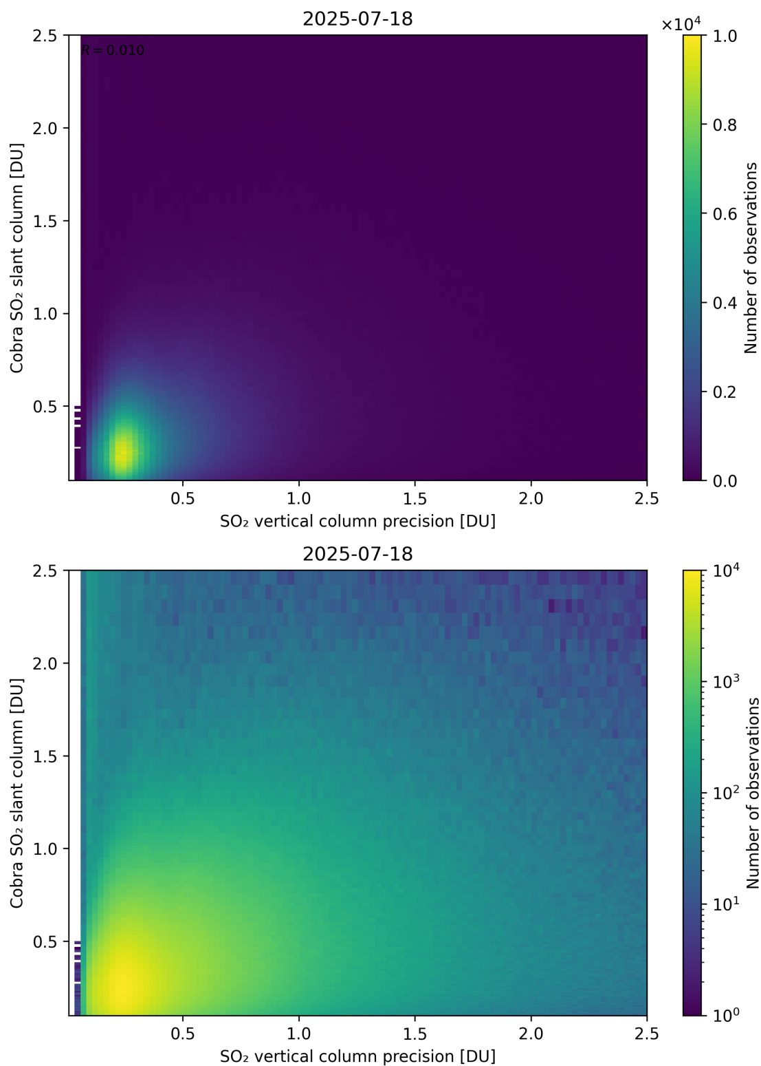
Figure 336: Scatter density plot of “SO 2 vertical column precision” against “Cobra SO 2 slant column” for 2025-07-18 to 2025-07-19.
