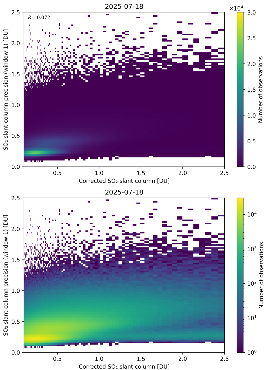
Figure 238: Scatter density plot of “Corrected SO 2 slant column” against “SO 2 slant column precision (window 1)” for 2025-07-18 to 2025-07-19.
