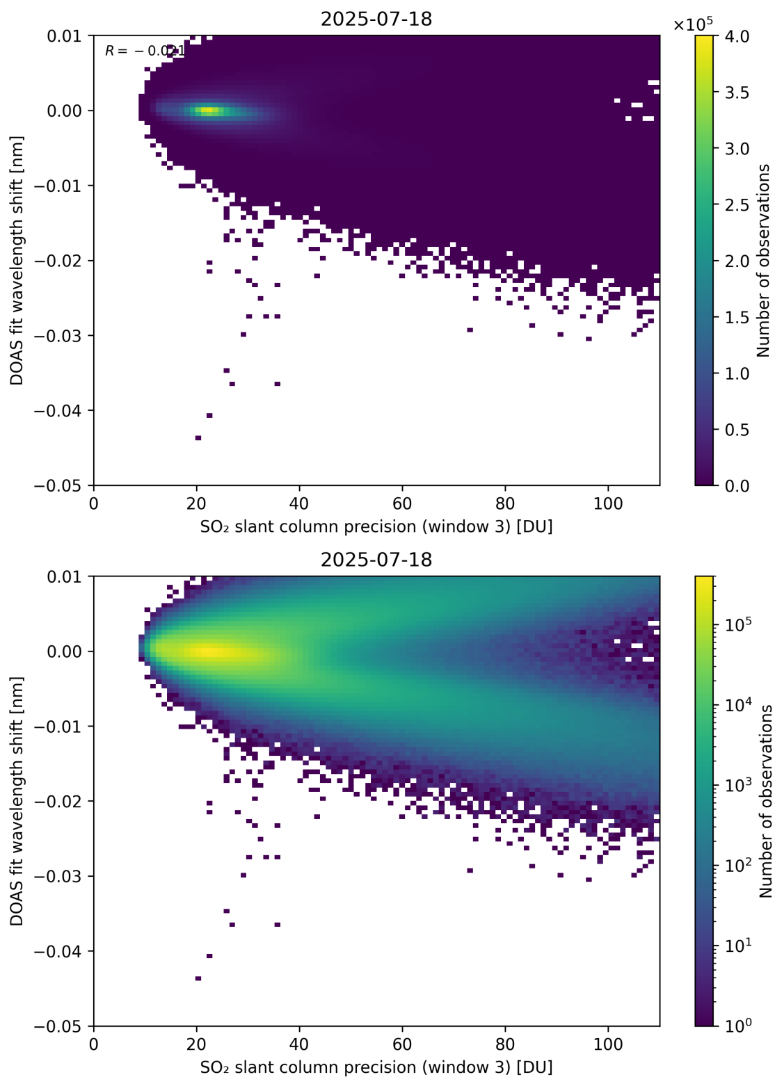
Figure 308: Scatter density plot of “SO 2 slant column precision (window 3)” against “DOAS fit wavelength shift” for 2025-07-18 to 2025-07-19.
