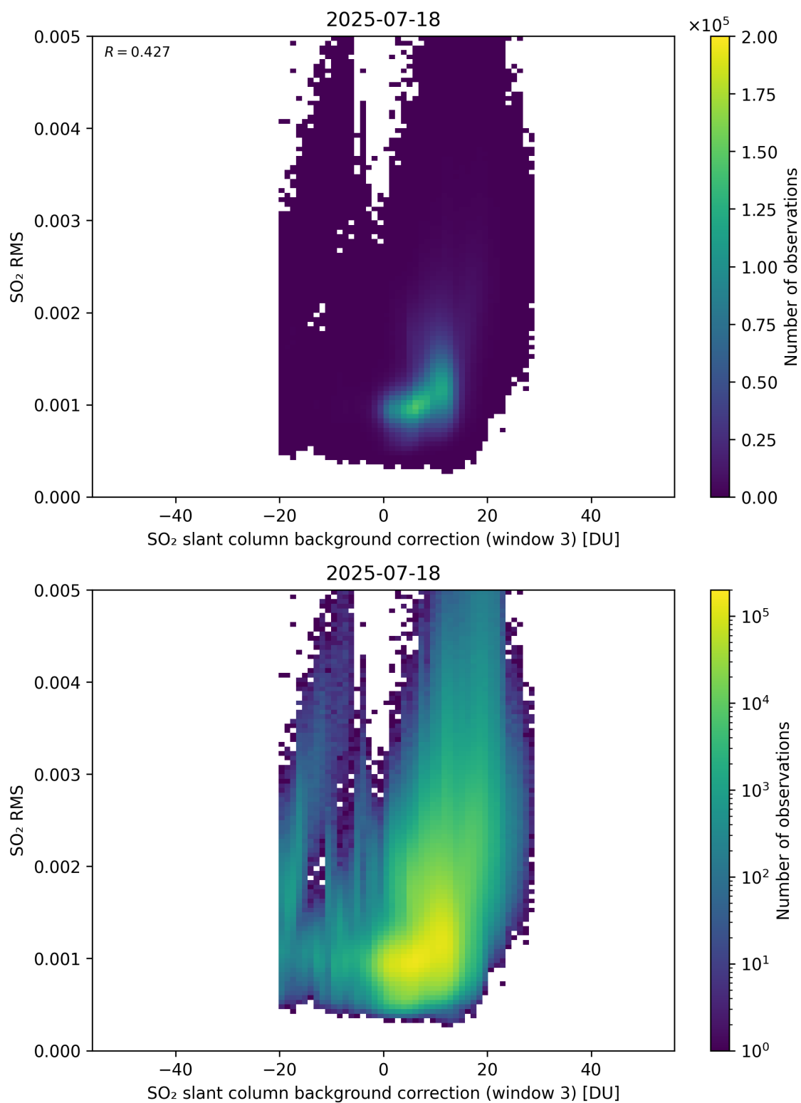
Figure 134: Scatter density plot of “SO 2 slant column background correction (window 3)” against “SO 2 RMS” for 2025-07-18 to 2025-07-19.
