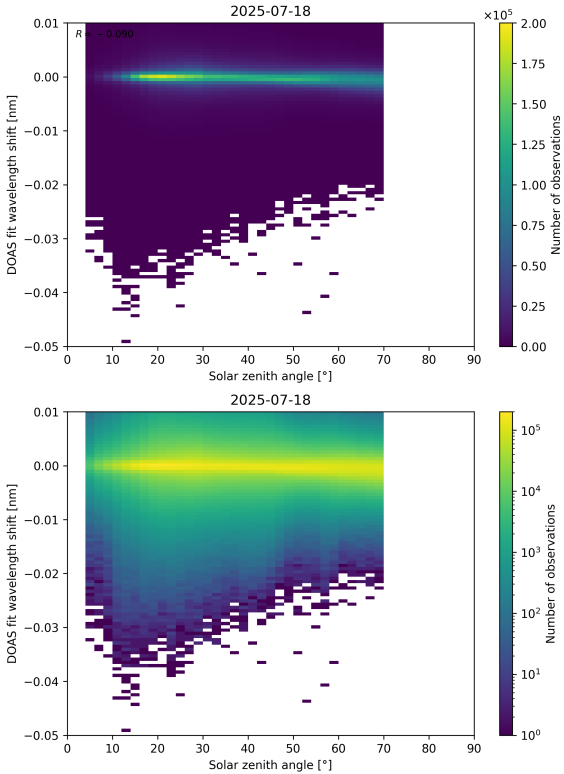
Figure 174: Scatter density plot of “Solar zenith angle” against “DOAS fit wavelength shift” for 2025-07-18 to 2025-07-19.
