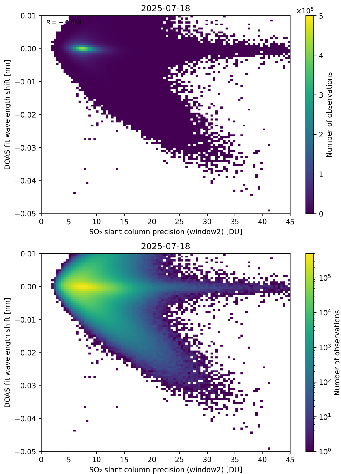
Figure 293: Scatter density plot of “SO 2 slant column precision (window2)” against “DOAS fit wavelength shift” for 2025-07-18 to 2025-07-19.
