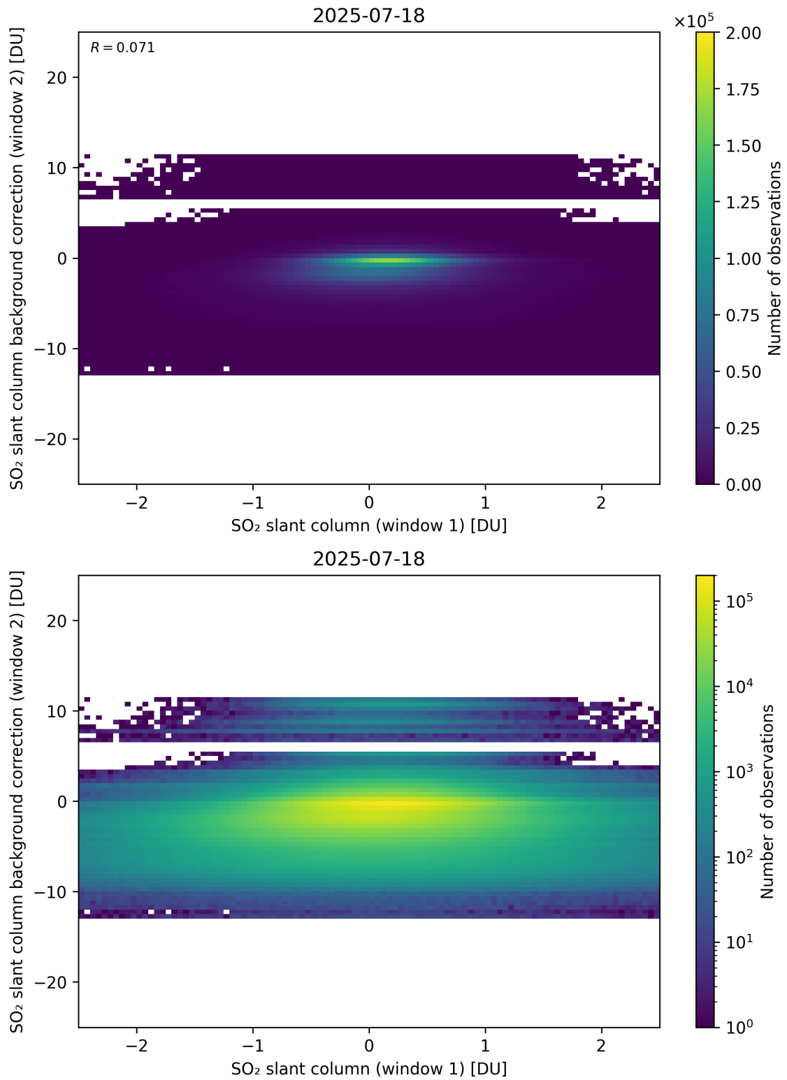
Figure 263: Scatter density plot of “SO 2 slant column (window 1)” against “SO 2 slant column background correction (window 2)” for 2025-07-18 to 2025-07-19.
