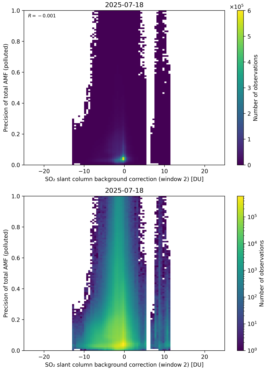
Figure 131: Scatter density plot of “SO 2 slant column background correction (window 2)” against “Precision of total AMF (polluted)” for 2025-07-18 to 2025-07-19.
