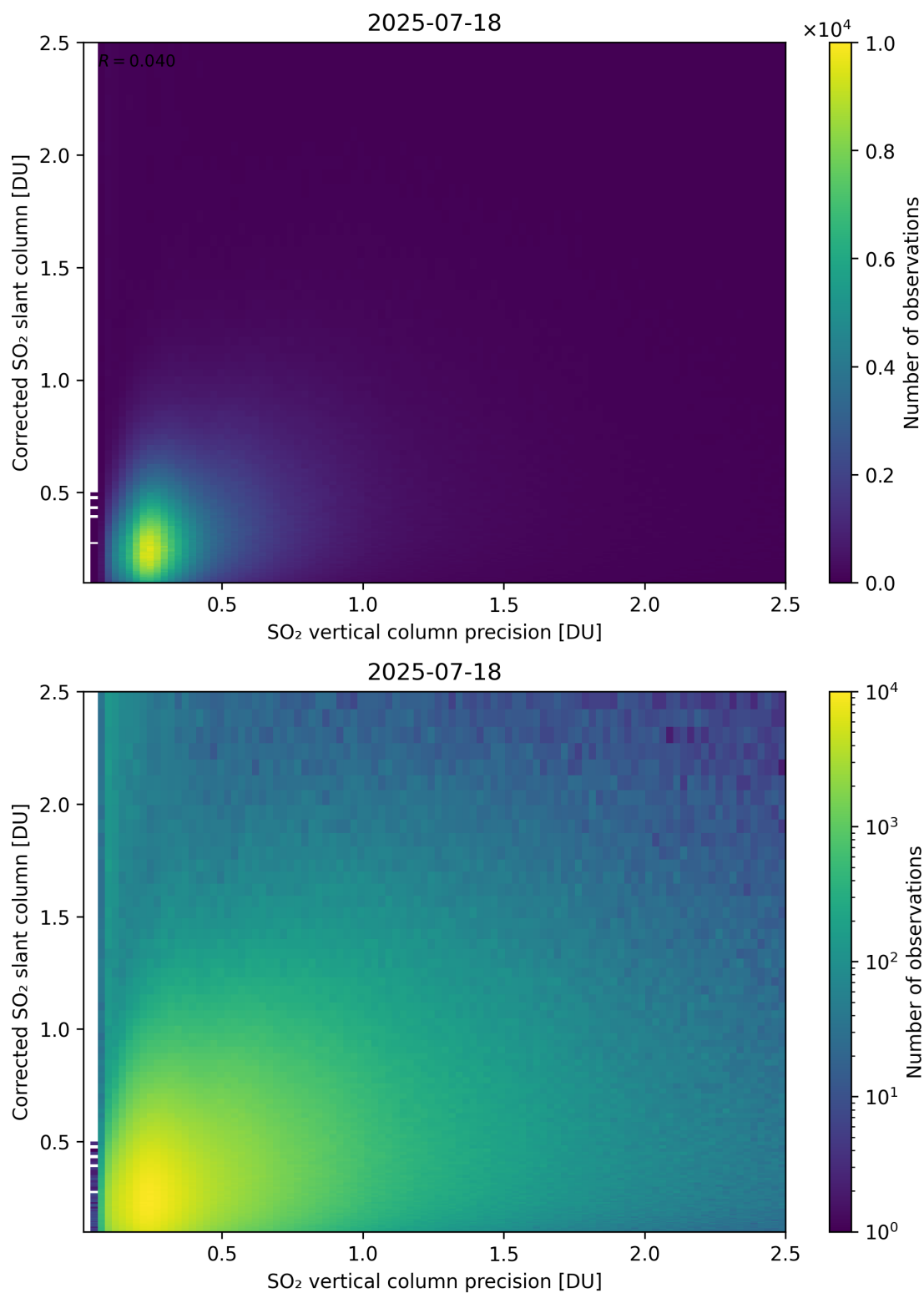
Figure 338: Scatter density plot of “SO 2 vertical column precision” against “Corrected SO 2 slant column” for 2025-07-18 to 2025-07-19.
