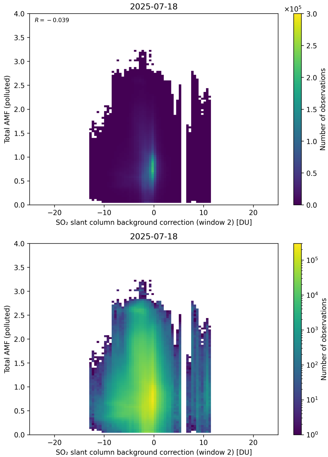
Figure 130: Scatter density plot of “SO 2 slant column background correction (window 2)” against “Total AMF (polluted)” for 2025-07-18 to 2025-07-19.
