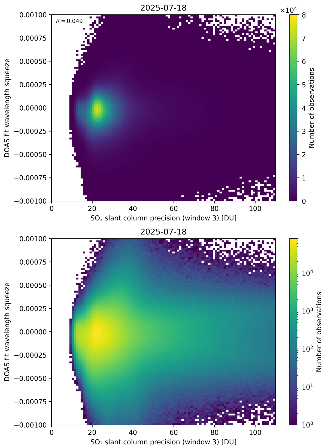
Figure 309: Scatter density plot of “SO 2 slant column precision (window 3)” against “DOAS fit wavelength squeeze” for 2025-07-18 to 2025-07-19.
