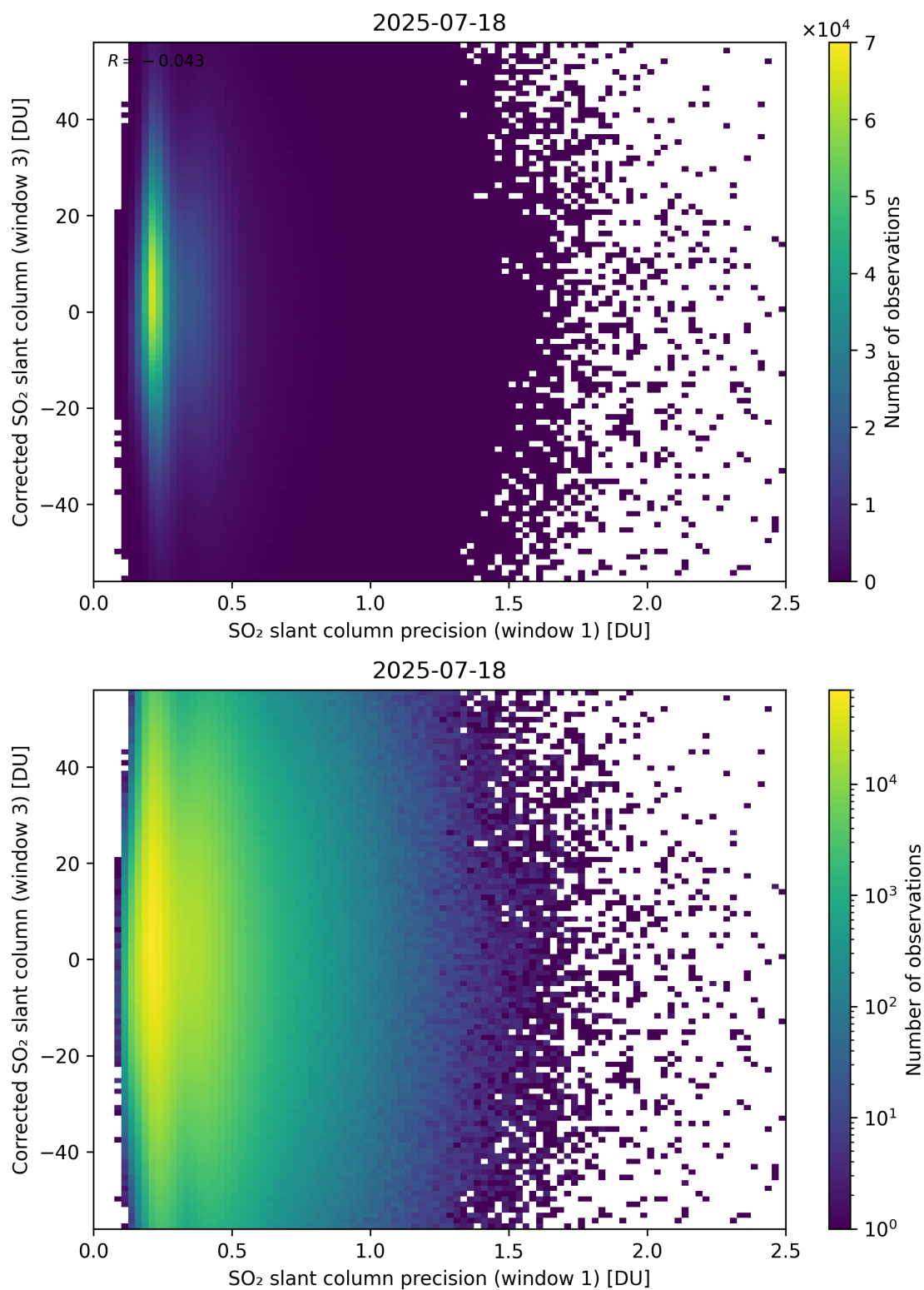
Figure 276: Scatter density plot of “SO 2 slant column precision (window 1)” against “Corrected SO 2 slant column (window 3)” for 2025-07-18 to 2025-07-19.
