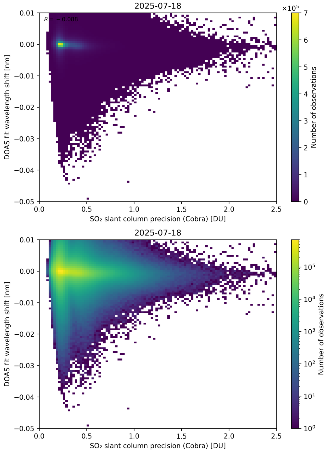
Figure 202: Scatter density plot of “SO 2 slant column precision (Cobra)” against “DOAS fit wavelength shift” for 2025-07-18 to 2025-07-19.
