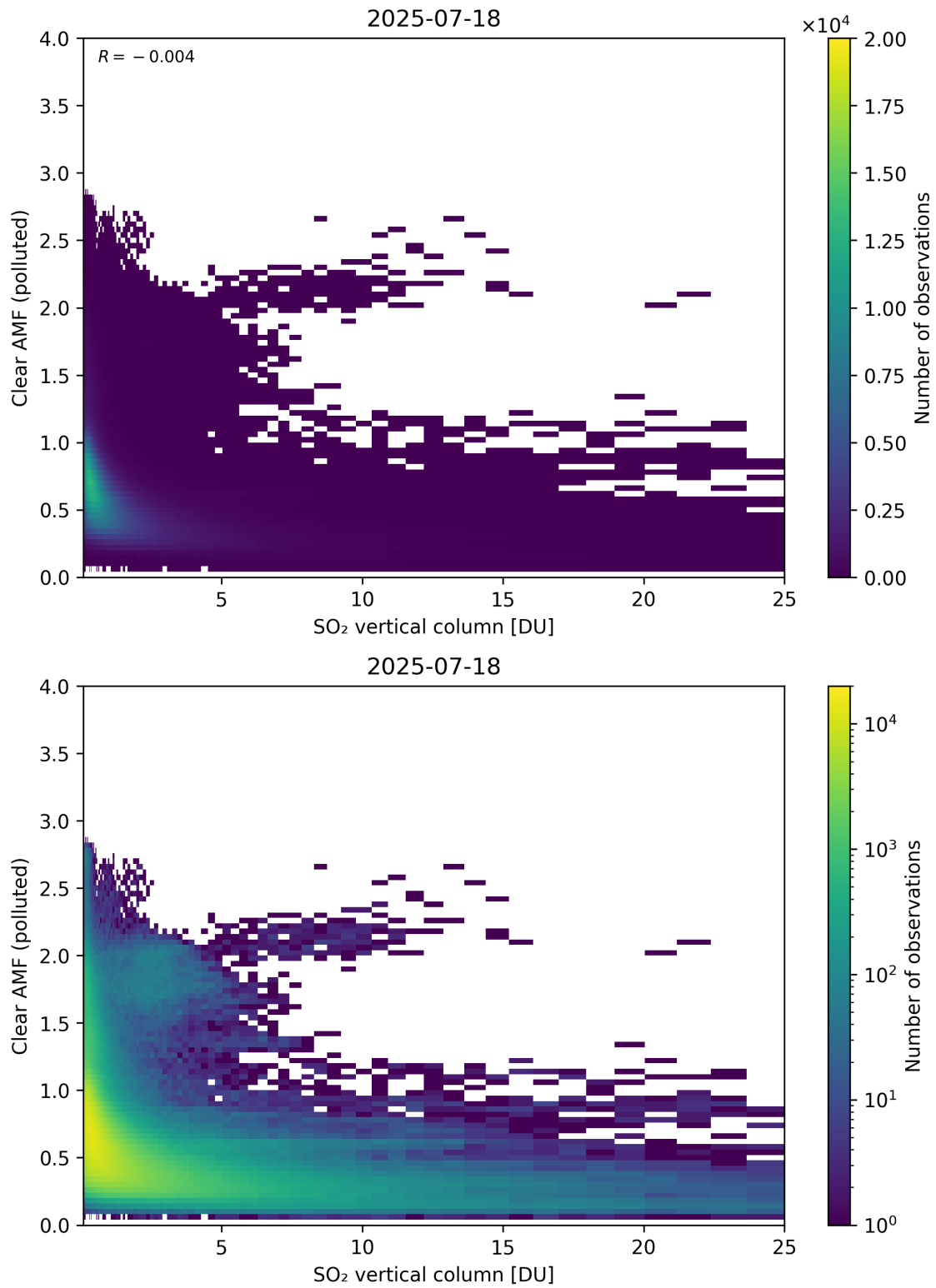
Figure 348: Scatter density plot of “SO 2 vertical column” against “Clear AMF (polluted)” for 2025-07-18 to 2025-07-19.
