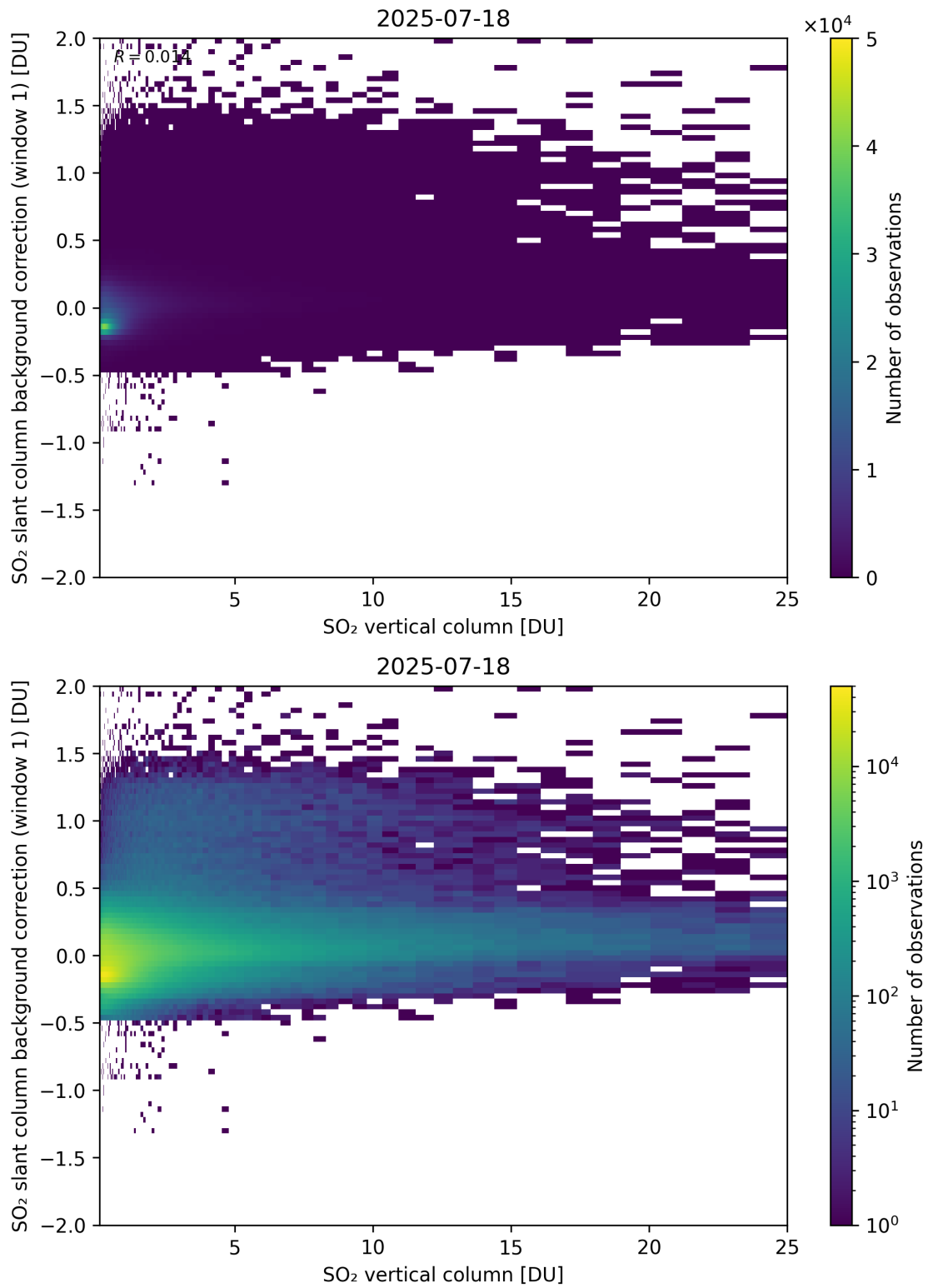
Figure 323: Scatter density plot of “SO 2 vertical column” against “SO 2 slant column background correction (window 1)” for 2025-07-18 to 2025-07-19.
