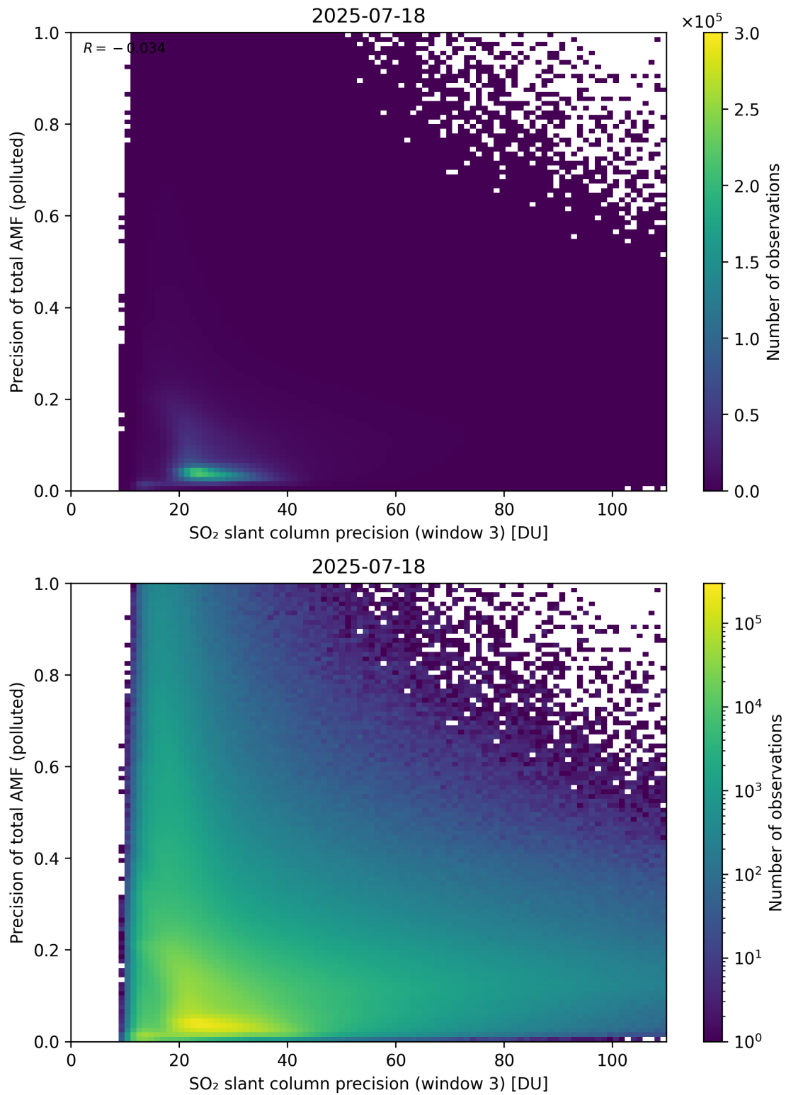
Figure 314: Scatter density plot of “SO 2 slant column precision (window 3)” against “Precision of total AMF (polluted)” for 2025-07-18 to 2025-07-19.
