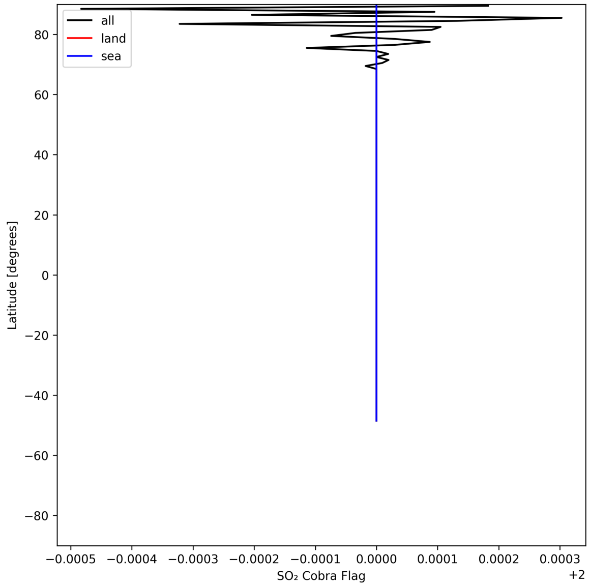
Figure 49: Zonal average of "SO 2 Cobra Flag" for 2025-07-18 to 2025-07-19.
