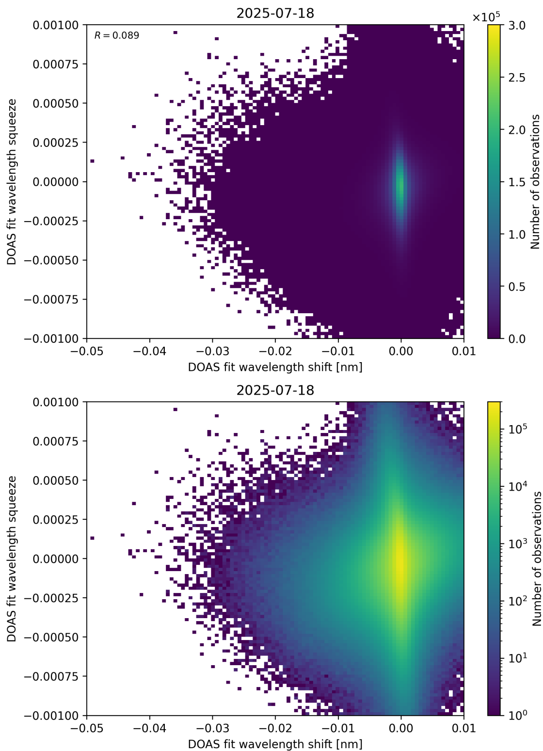
Figure 138: Scatter density plot of “DOAS fit wavelength shift” against “DOAS fit wavelength squeeze” for 2025-07-18 to 2025-07-19.
