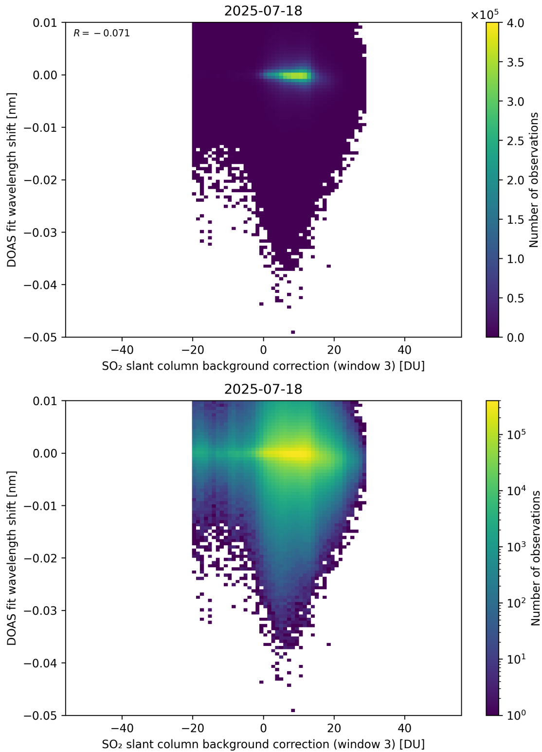
Figure 132: Scatter density plot of “SO 2 slant column background correction (window 3)” against “DOAS fit wavelength shift” for 2025-07-18 to 2025-07-19.
