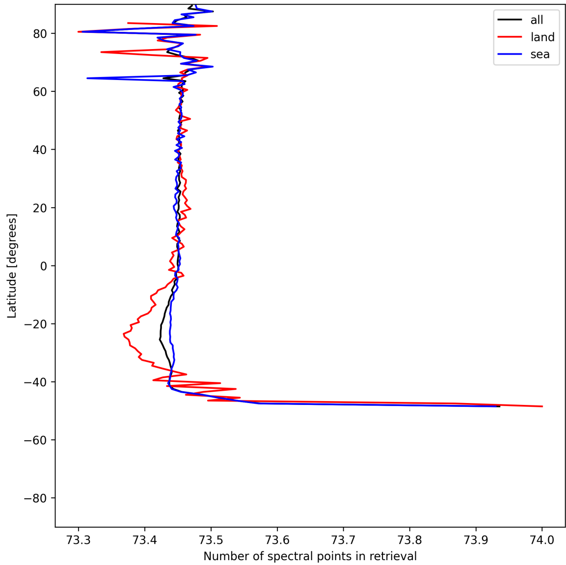
Figure 56: Zonal average of “Number of spectral points in retrieval” for 2025-07-18 to 2025-07-19.
