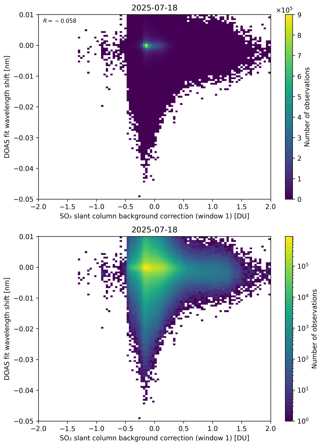
Figure 111: Scatter density plot of “SO 2 slant column background correction (window 1)” against “DOAS fit wavelength shift” for 2025-07-18 to 2025-07-19.
