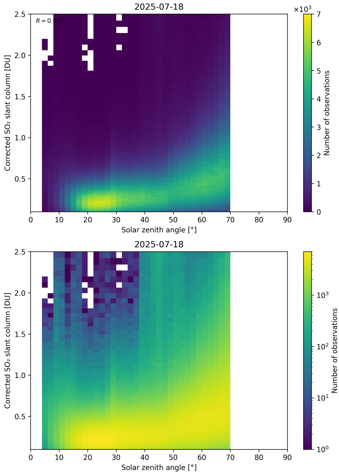
Figure 181: Scatter density plot of “Solar zenith angle” against “Corrected SO 2 slant column” for 2025-07-18 to 2025-07-19.
