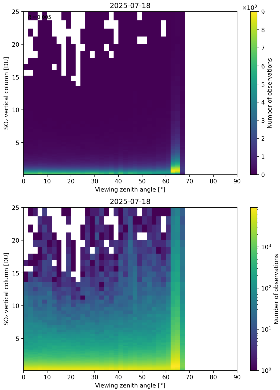
Figure 383: Scatter density plot of “Viewing zenith angle” against “SO 2 vertical column” for 2025-07-18 to 2025-07-19.
