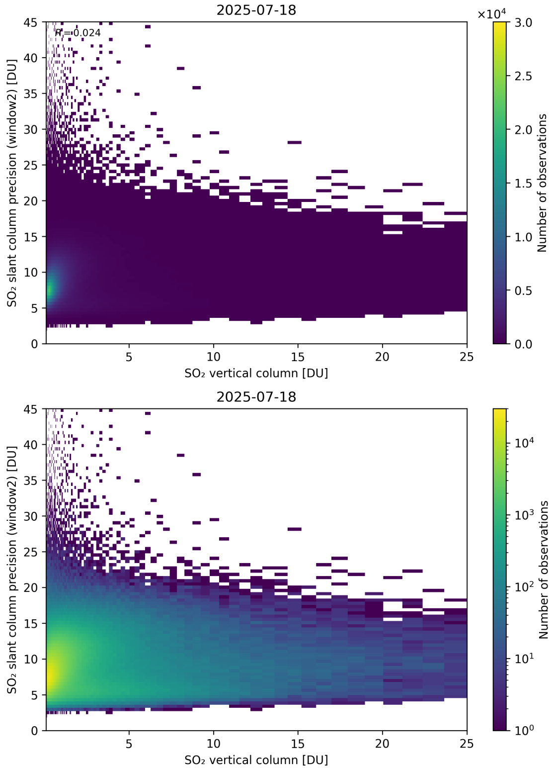
Figure 356: Scatter density plot of “SO 2 vertical column” against “SO 2 slant column precision (window2)” for 2025-07-18 to 2025-07-19.
