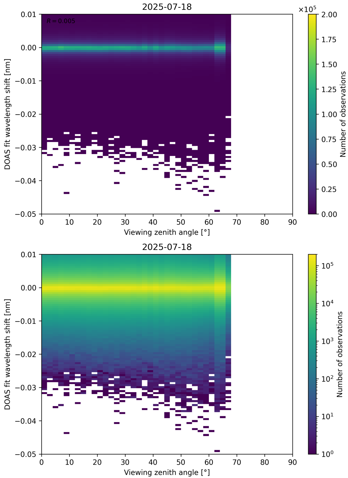
Figure 365: Scatter density plot of “Viewing zenith angle” against “DOAS fit wavelength shift” for 2025-07-18 to 2025-07-19.
