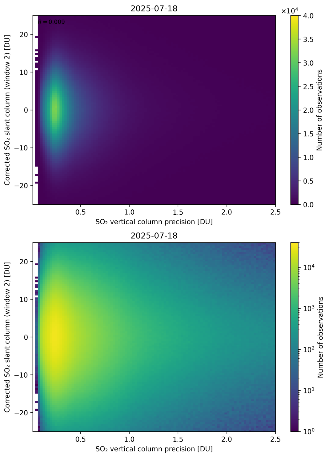
Figure 339: Scatter density plot of “SO 2 vertical column precision” against “Corrected SO 2 slant column (window 2)” for 2025-07-18 to 2025-07-19.
