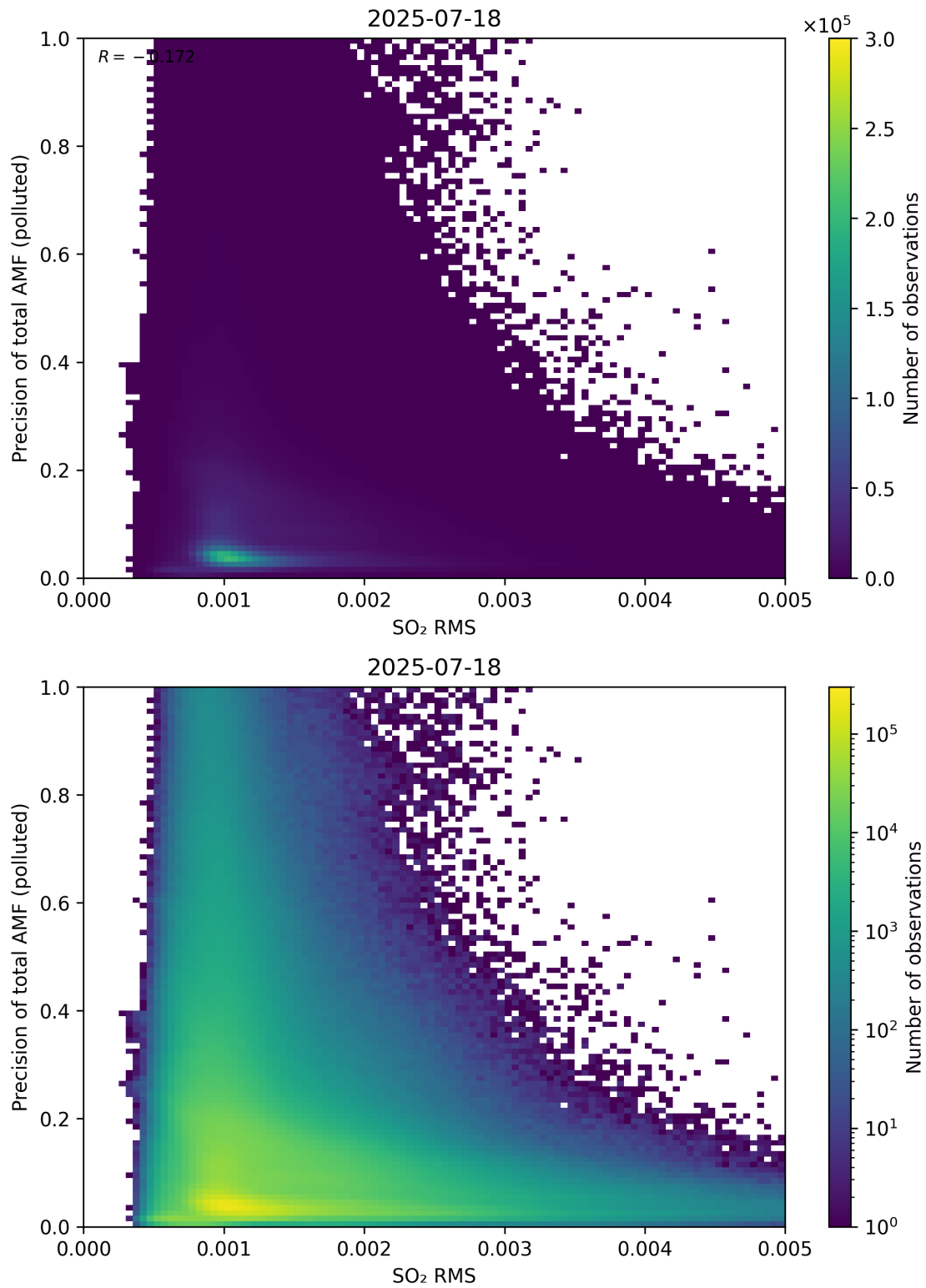
Figure 149: Scatter density plot of “SO 2 RMS” against “Precision of total AMF (polluted)” for 2025-07-18 to 2025-07-19.
