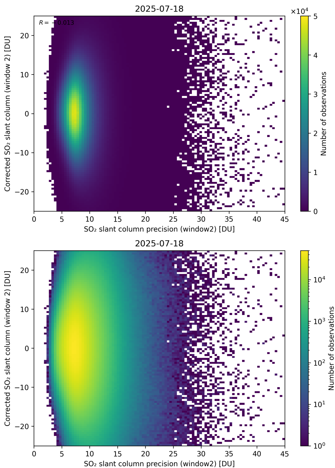
Figure 297: Scatter density plot of “SO 2 slant column precision (window2)” against “Corrected SO 2 slant column (window 2)” for 2025-07-18 to 2025-07-19.
