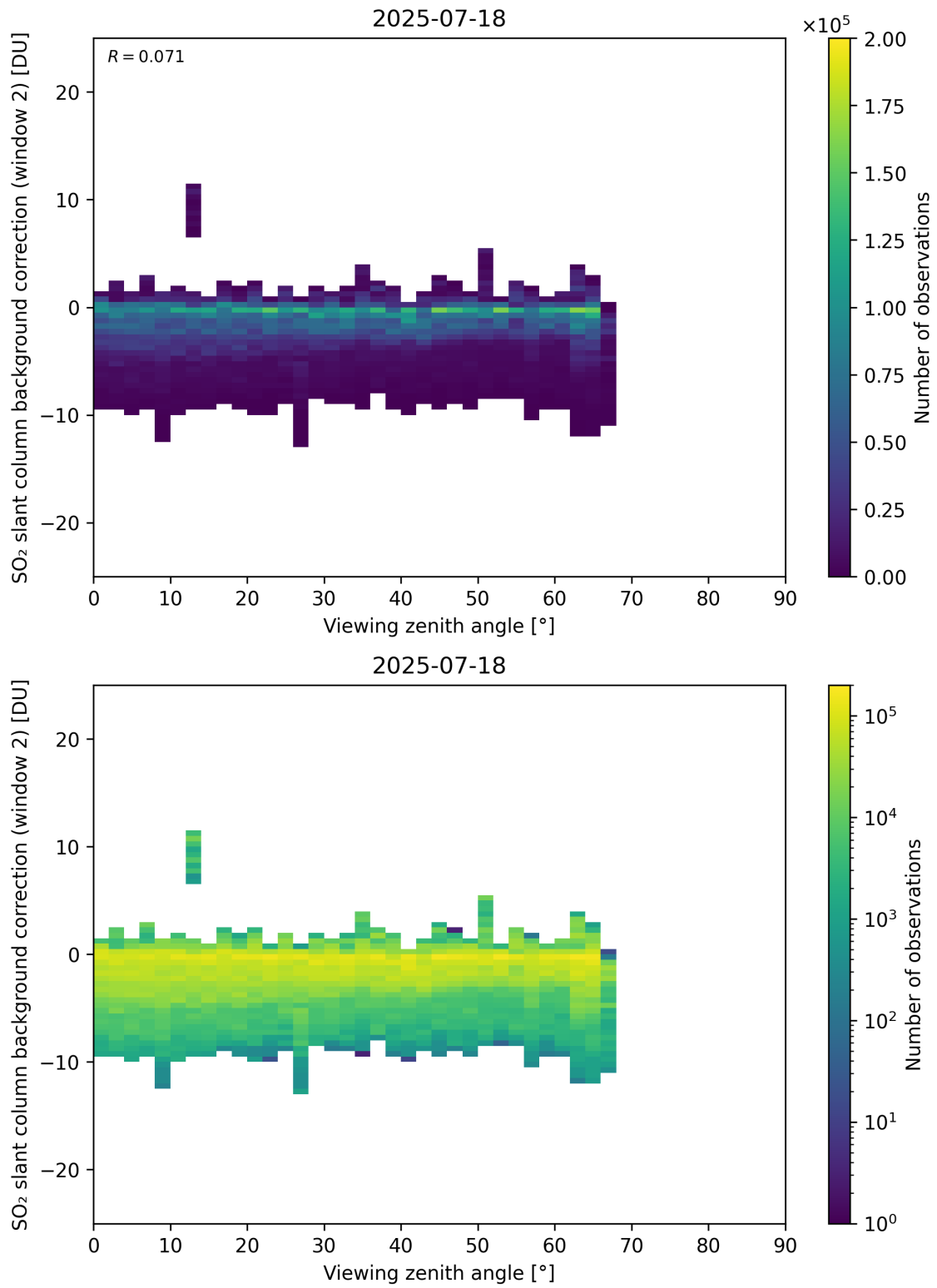
Figure 363: Scatter density plot of “Viewing zenith angle” against “SO 2 slant column background correction (window 2)” for 2025-07-18 to 2025-07-19.
