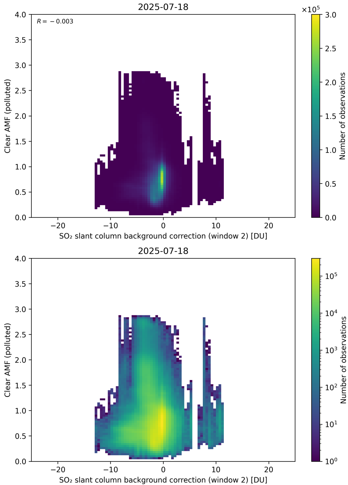
Figure 126: Scatter density plot of “SO 2 slant column background correction (window 2)” against “Clear AMF (polluted)” for 2025-07-18 to 2025-07-19.
