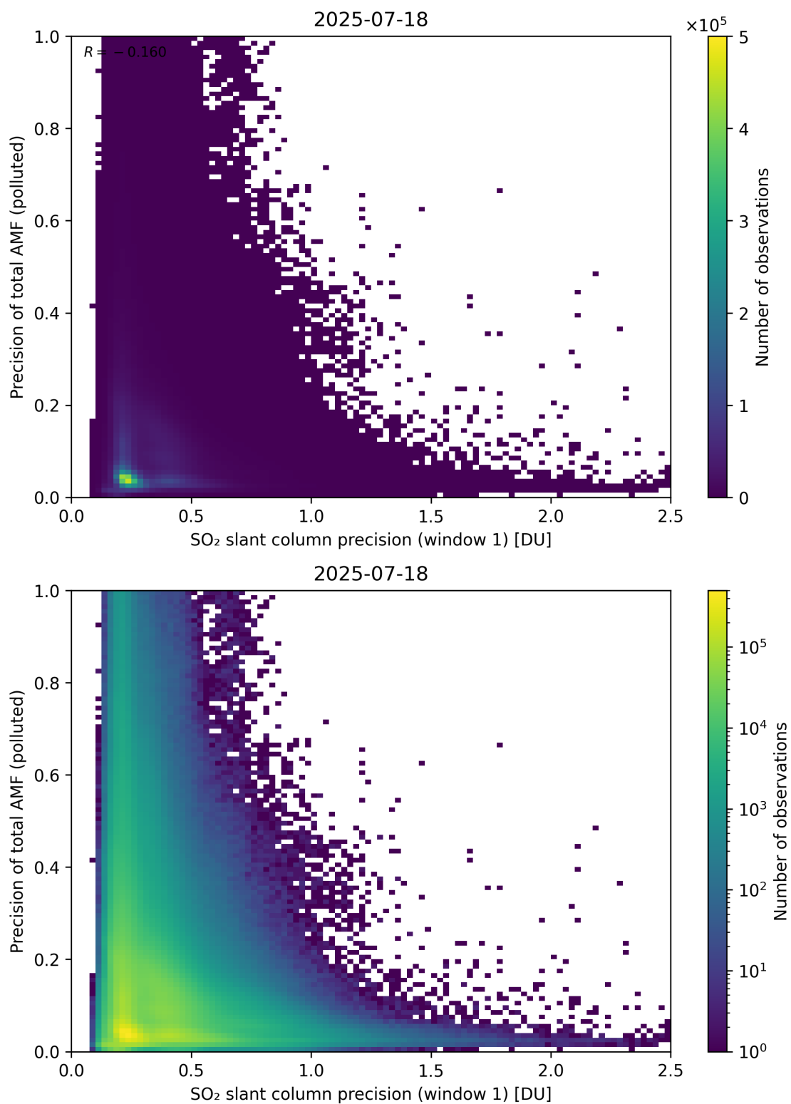
Figure 281: Scatter density plot of “SO 2 slant column precision (window 1)” against “Precision of total AMF (polluted)” for 2025-07-18 to 2025-07-19.
