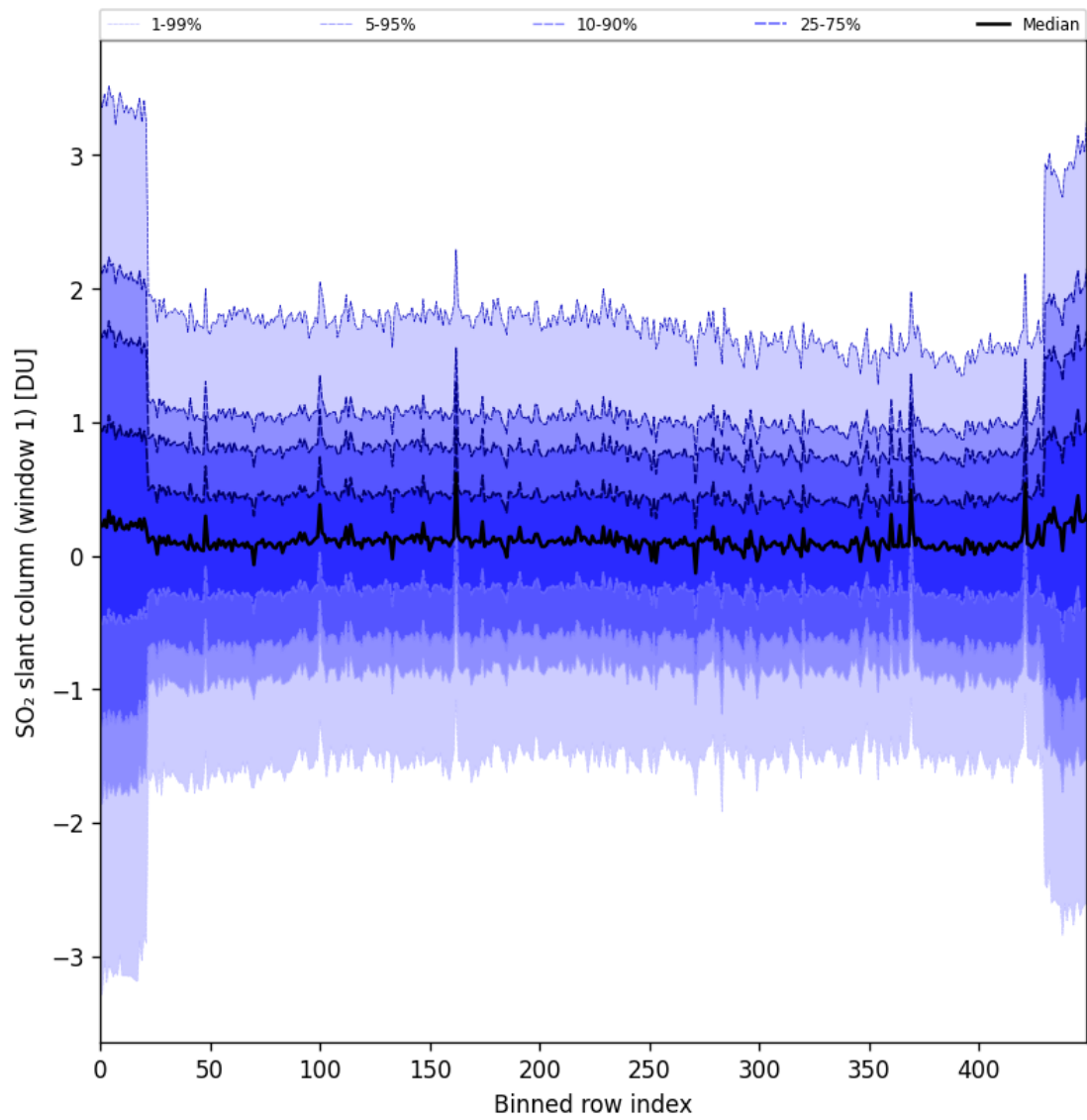
Figure 89: Along track statistics of “SO 2 slant column (window 1)” for 2025-07-18 to 2025-07-19
