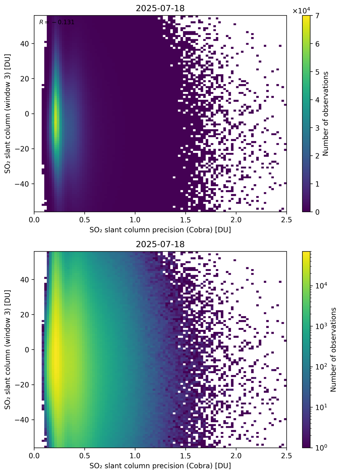
Figure 211: Scatter density plot of “SO 2 slant column precision (Cobra)” against “SO 2 slant column (window 3)” for 2025-07-18 to 2025-07-19.
