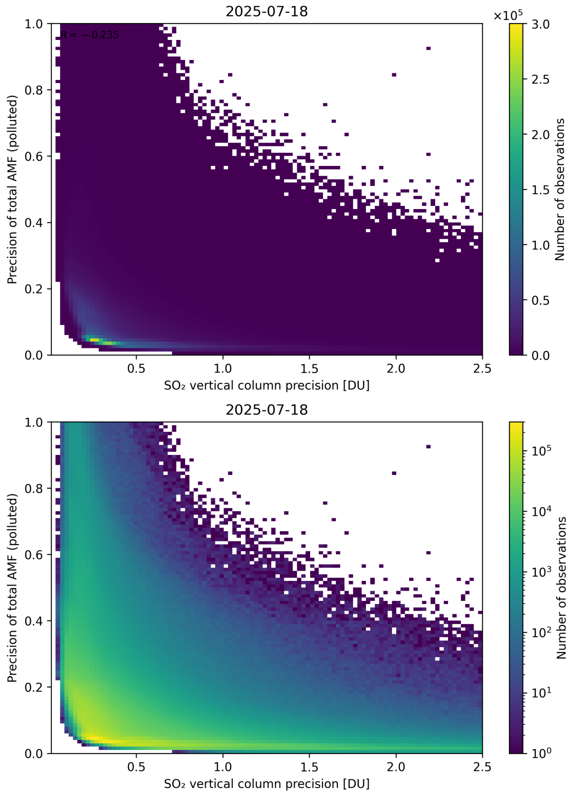
Figure 347: Scatter density plot of “SO 2 vertical column precision” against “Precision of total AMF (polluted)” for 2025-07-18 to 2025-07-19.
