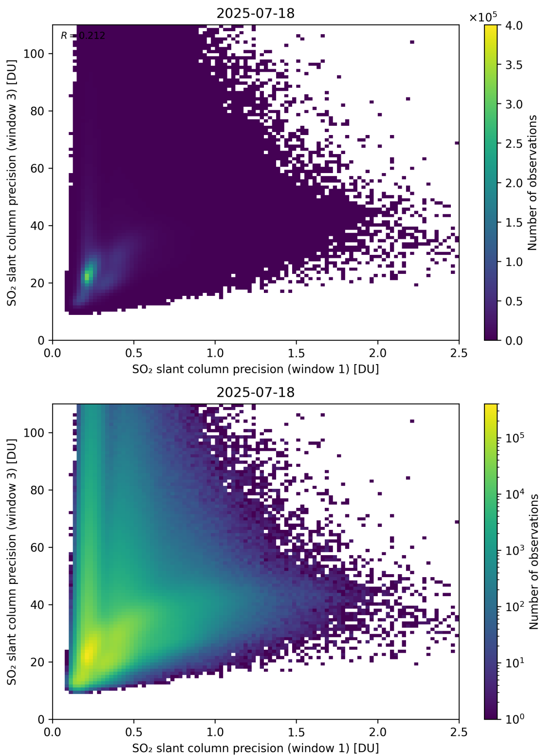
Figure 279: Scatter density plot of “SO 2 slant column precision (window 1)” against “SO 2 slant column precision (window 3)” for 2025-07-18 to 2025-07-19.
