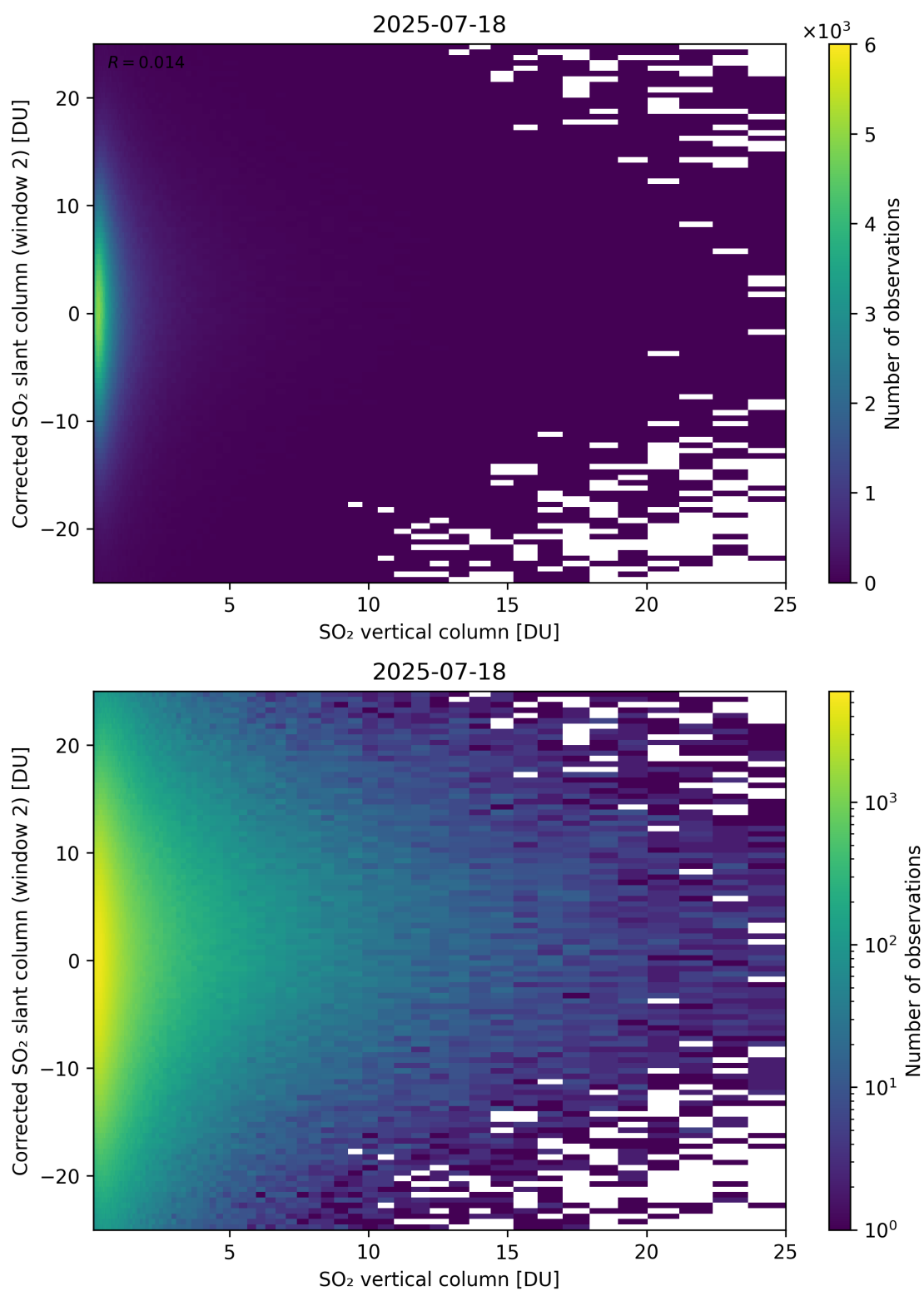
Figure 352: Scatter density plot of “SO 2 vertical column” against “Corrected SO 2 slant column (window 2)” for 2025-07-18 to 2025-07-19.
