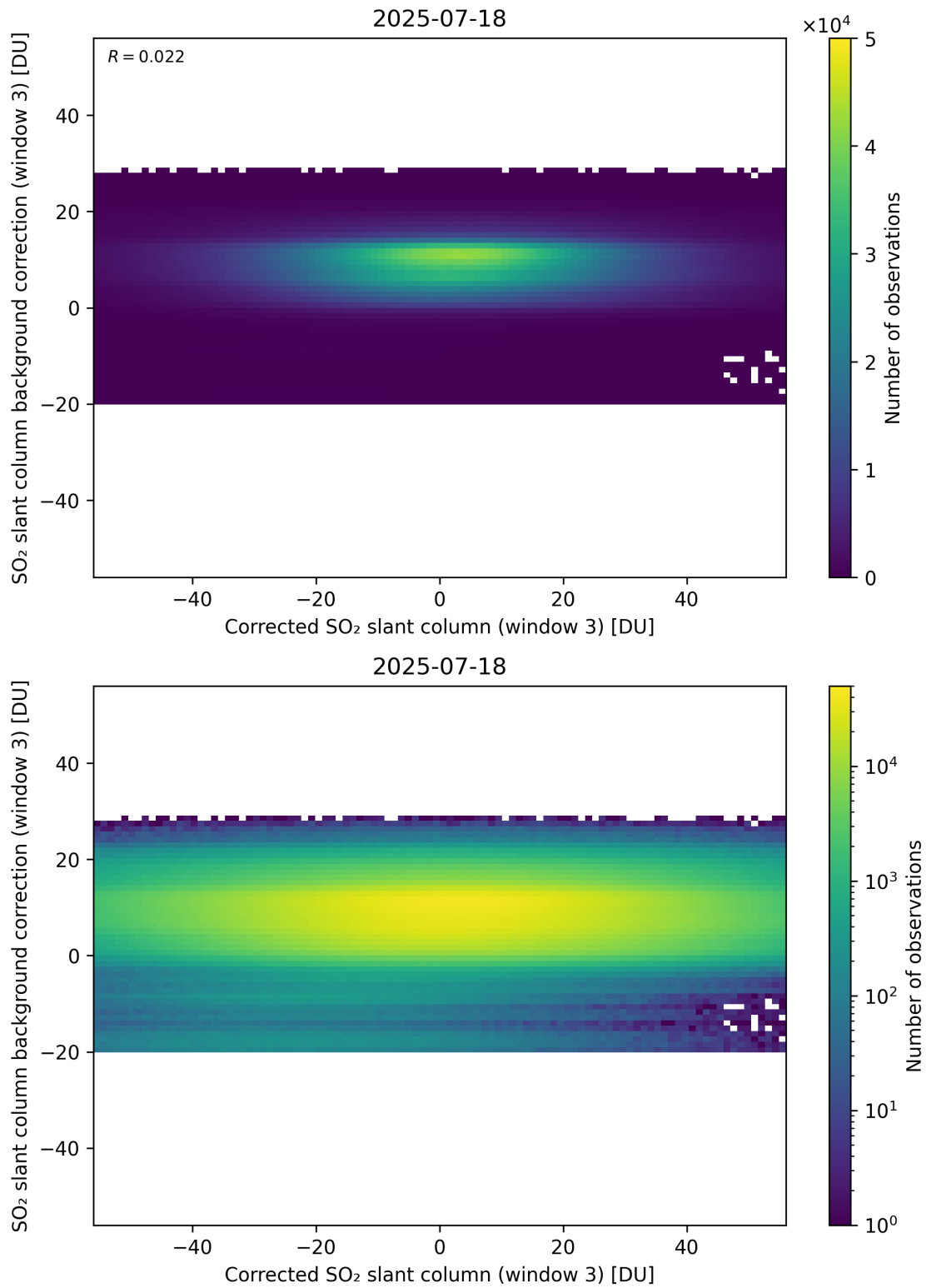
Figure 255: Scatter density plot of “Corrected SO 2 slant column (window 3)” against “SO 2 slant column background correction (window 3)” for 2025-07-18 to 2025-07-19.
