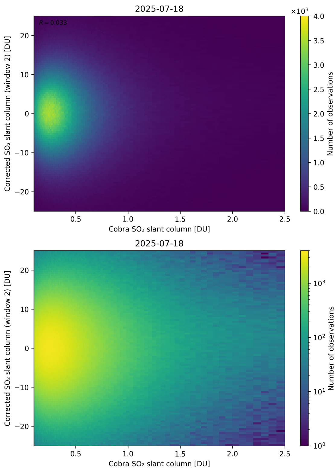
Figure 217: Scatter density plot of “Cobra SO 2 slant column” against “Corrected SO 2 slant column (window 2)” for 2025-07-18 to 2025-07-19.
