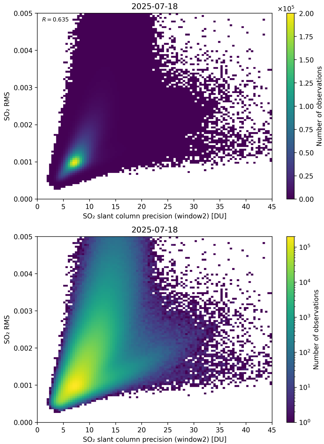
Figure 295: Scatter density plot of “SO 2 slant column precision (window2)” against “SO 2 RMS” for 2025-07-18 to 2025-07-19.
