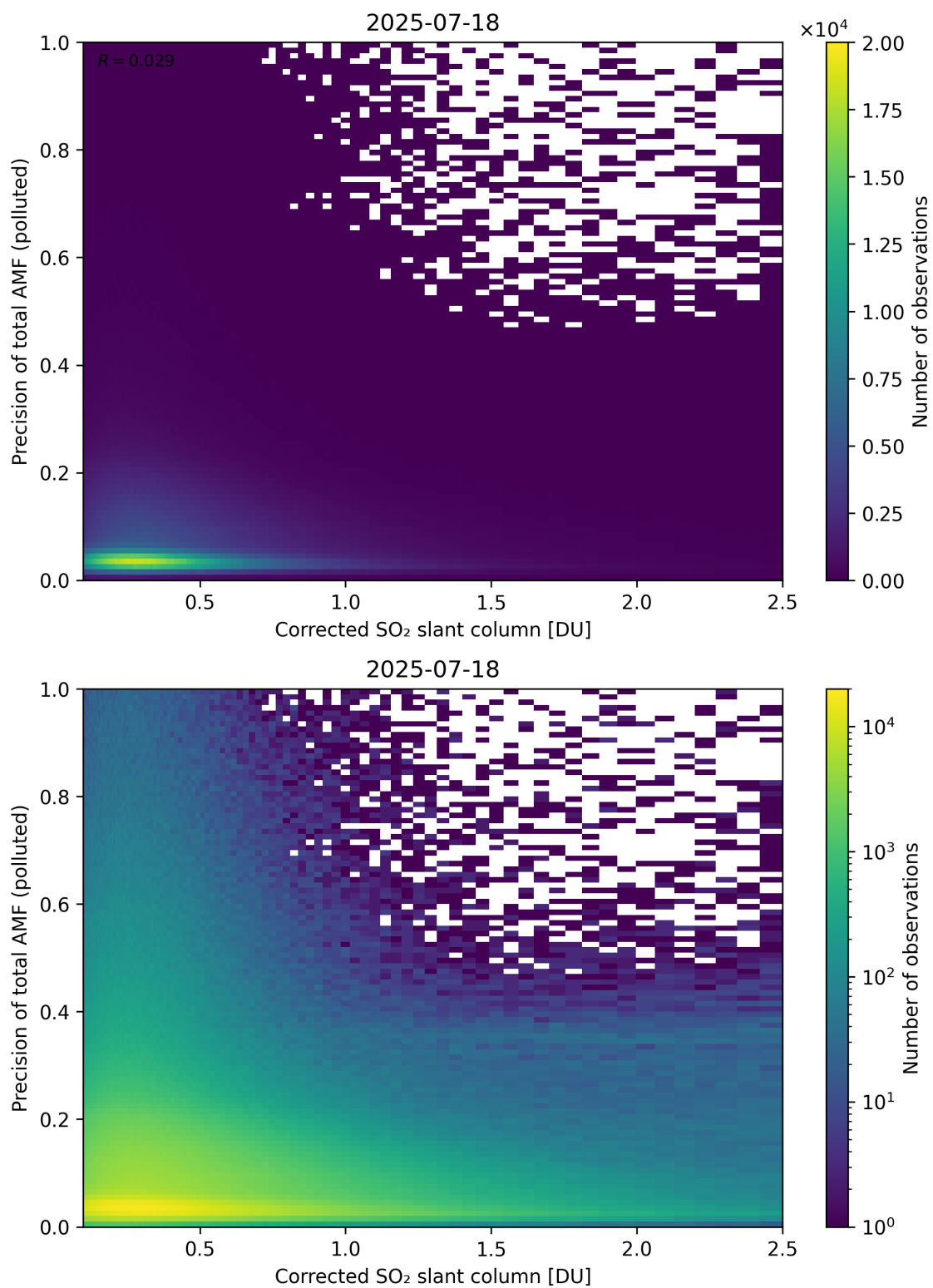
Figure 243: Scatter density plot of “Corrected SO 2 slant column” against “Precision of total AMF (polluted)” for 2025-07-18 to 2025-07-19.
