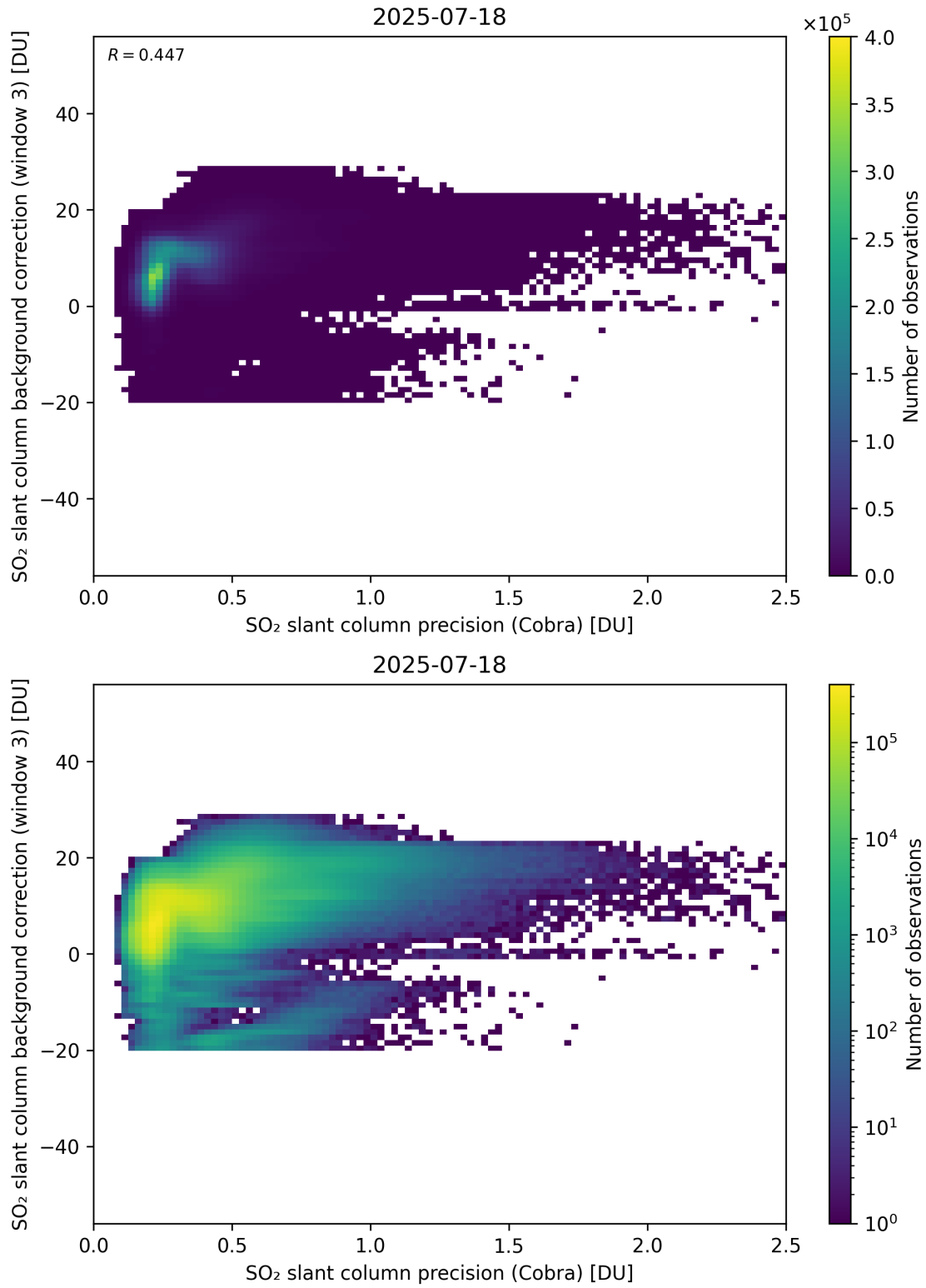
Figure 201: Scatter density plot of “SO 2 slant column precision (Cobra)” against “SO 2 slant column background correction (window 3)” for 2025-07-18 to 2025-07-19.
