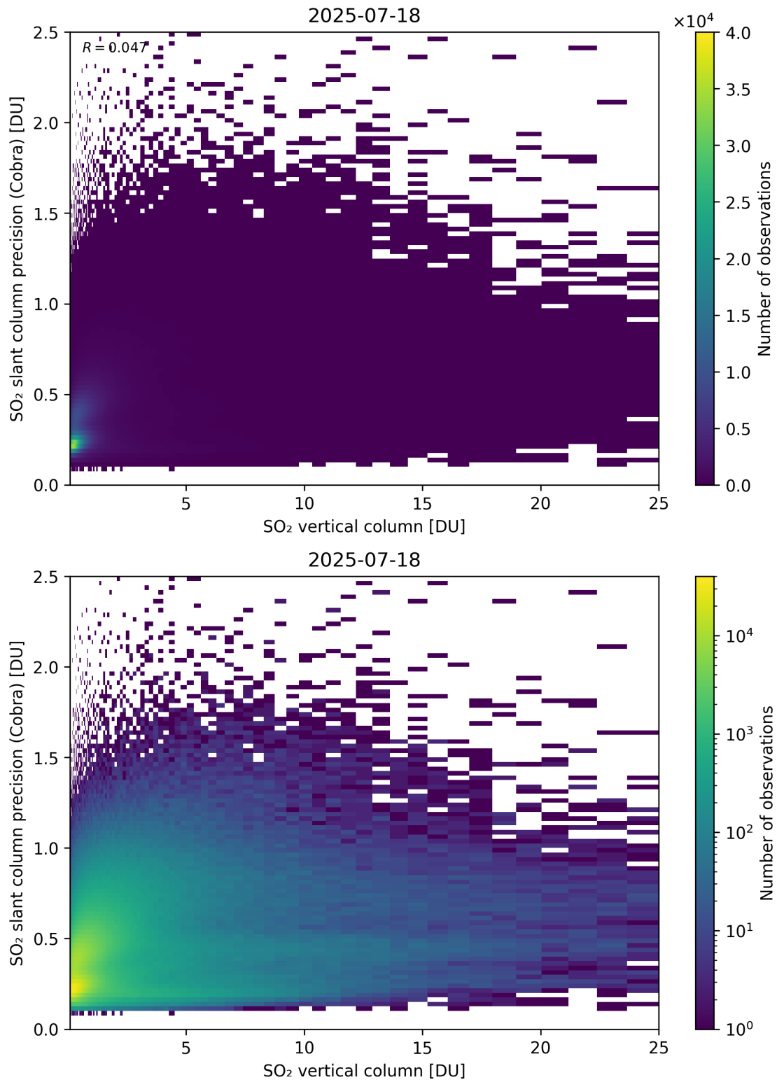
Figure 350: Scatter density plot of “SO 2 vertical column” against “SO 2 slant column precision (Cobra)” for 2025-07-18 to 2025-07-19.
