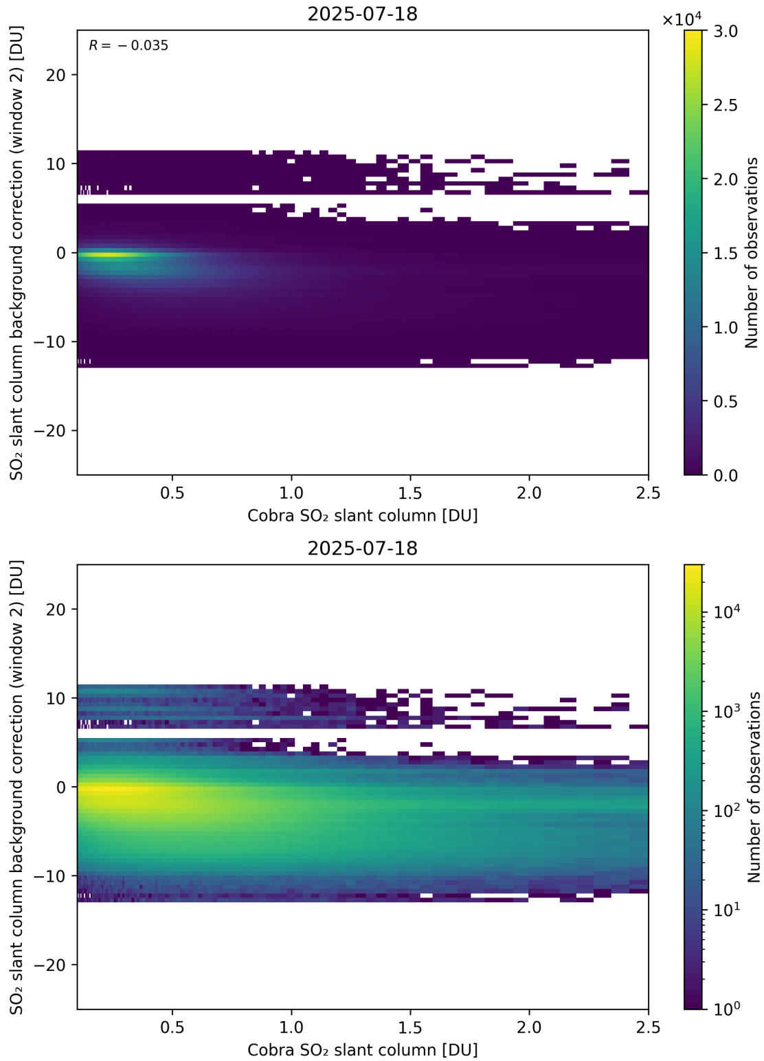
Figure 194: Scatter density plot of “Cobra SO 2 slant column” against “SO 2 slant column background correction (window 2)” for 2025-07-18 to 2025-07-19.
