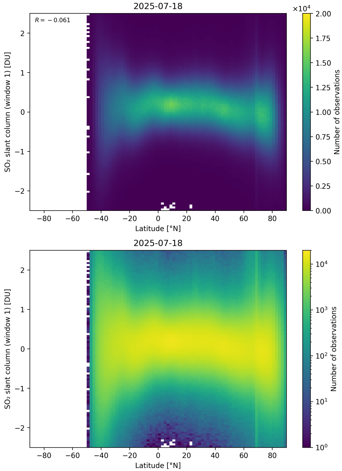
Figure 162: Scatter density plot of “Latitude” against “SO 2 slant column (window 1)” for 2025-07-18 to 2025-07-19.
