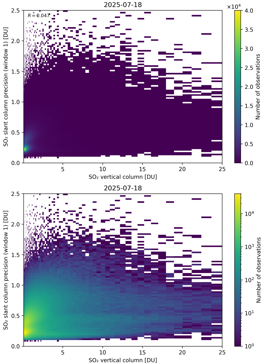
Figure 355: Scatter density plot of “SO 2 vertical column” against “SO 2 slant column precision (window 1)” for 2025-07-18 to 2025-07-19.
