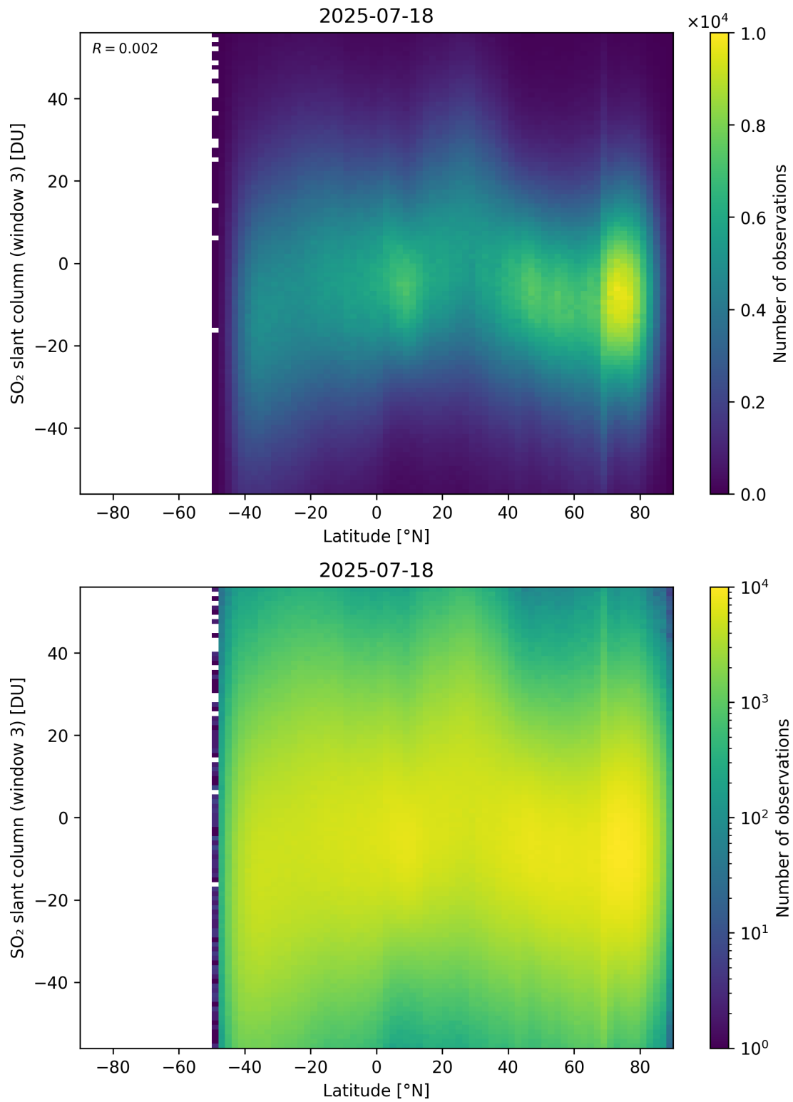
Figure 165: Scatter density plot of “Latitude” against “SO 2 slant column (window 3)” for 2025-07-18 to 2025-07-19.
