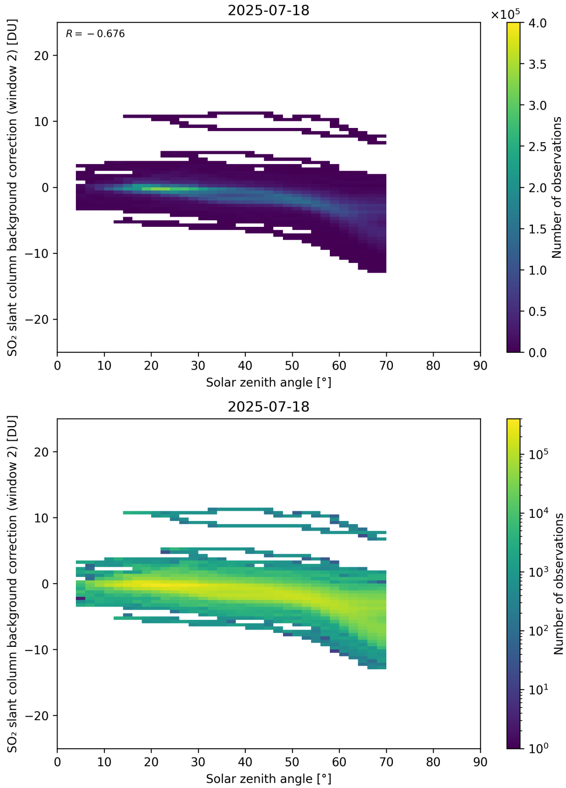
Figure 172: Scatter density plot of “Solar zenith angle” against “SO 2 slant column background correction (window 2)” for 2025-07-18 to 2025-07-19.
