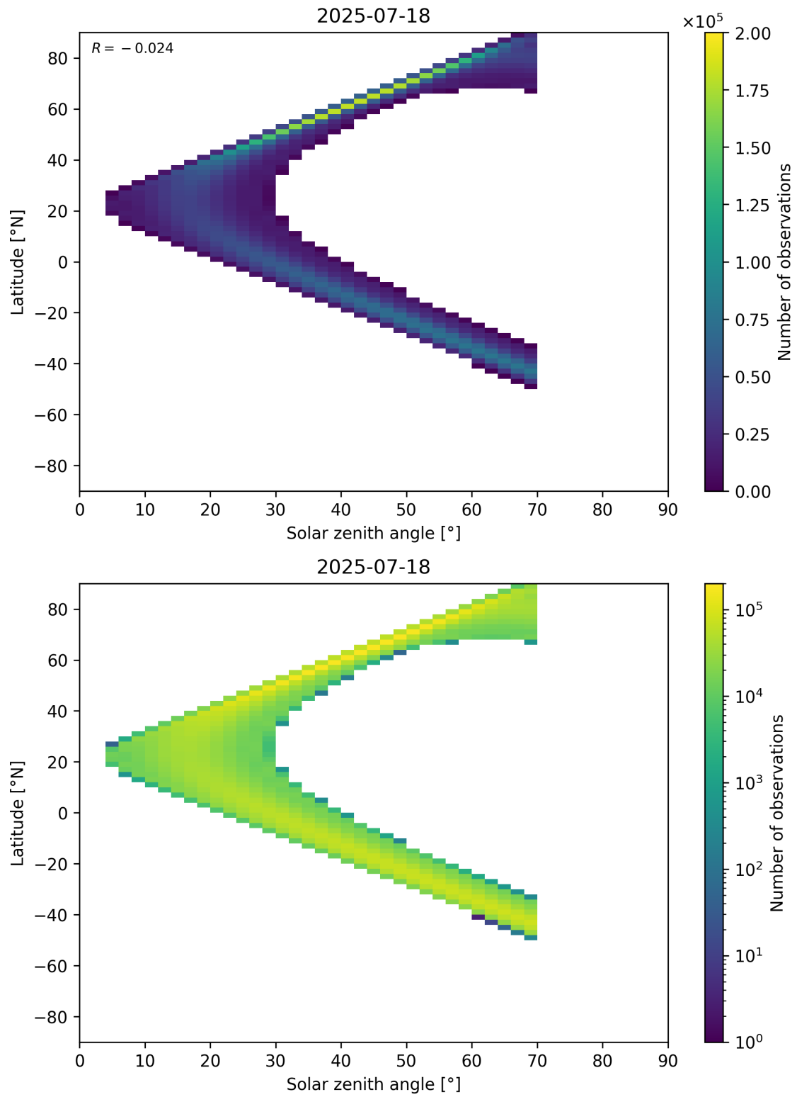
Figure 177: Scatter density plot of “Solar zenith angle” against “Latitude” for 2025-07-18 to 2025-07-19.
