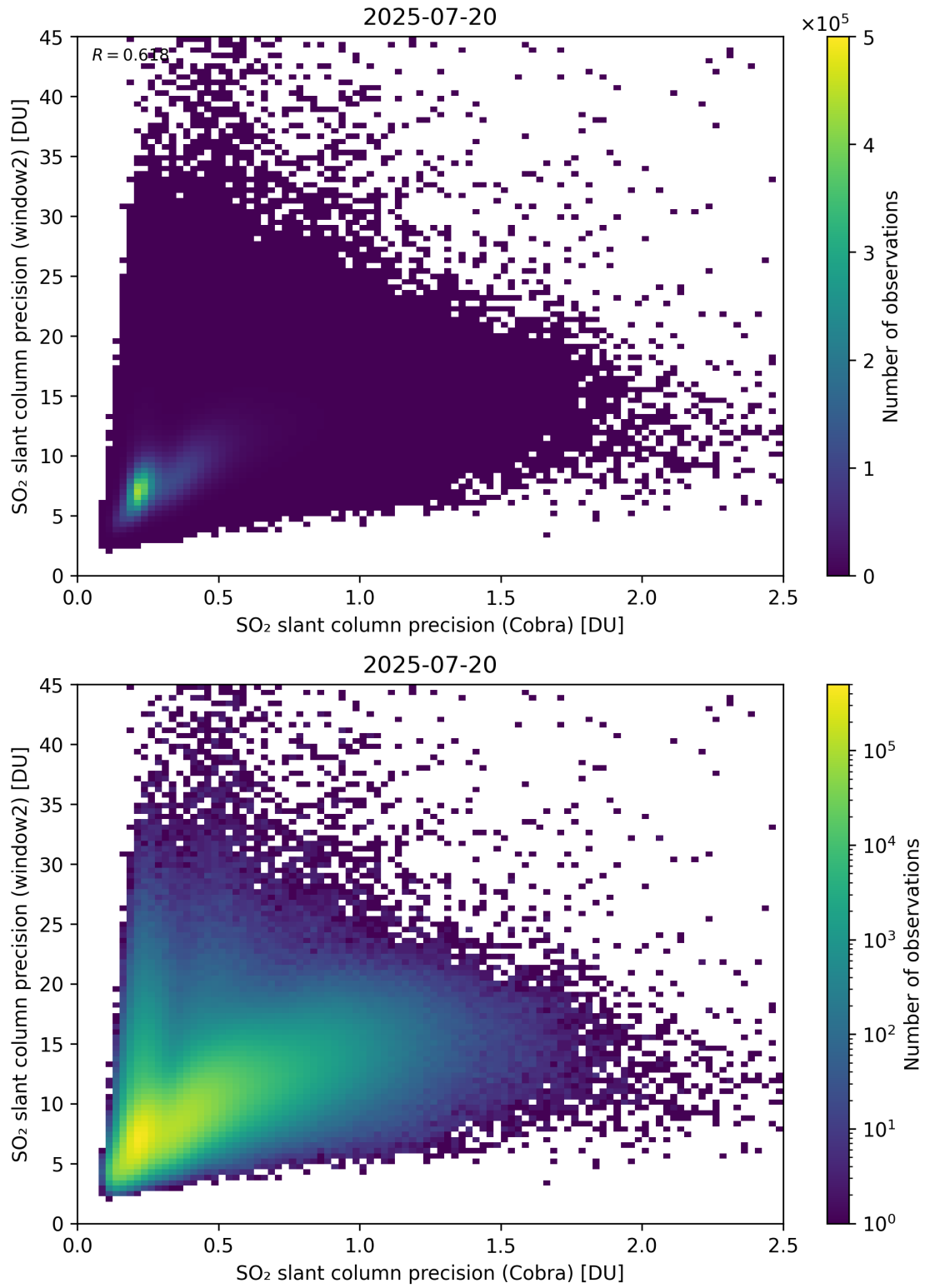
Figure 210: Scatter density plot of “SO 2 slant column precision (Cobra)” against “SO 2 slant column precision (window2)” for 2025-07-19 to 2025-07-21.
