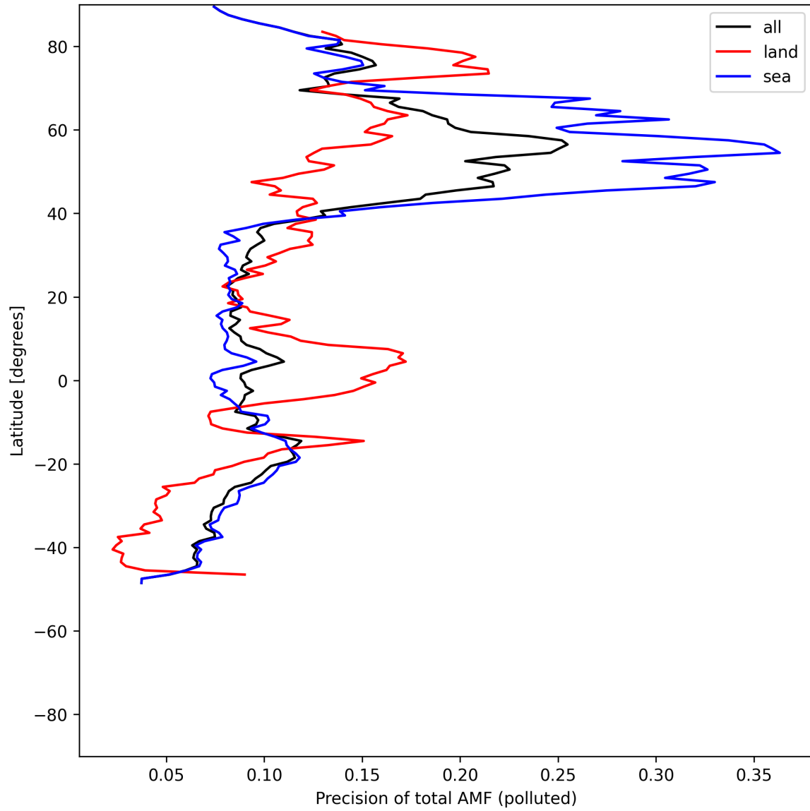
Figure 54: Zonal average of “Precision of total AMF (polluted)” for 2025-07-19 to 2025-07-21.
