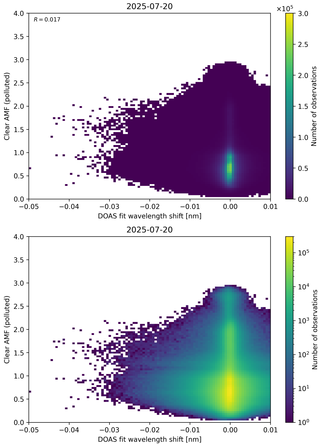
Figure 140: Scatter density plot of “DOAS fit wavelength shift” against “Clear AMF (polluted)” for 2025-07-19 to 2025-07-21.
