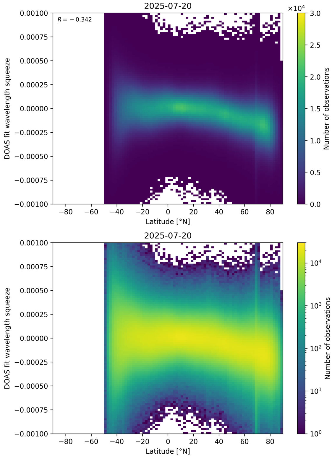
Figure 154: Scatter density plot of “Latitude” against “DOAS fit wavelength squeeze” for 2025-07-19 to 2025-07-21.
