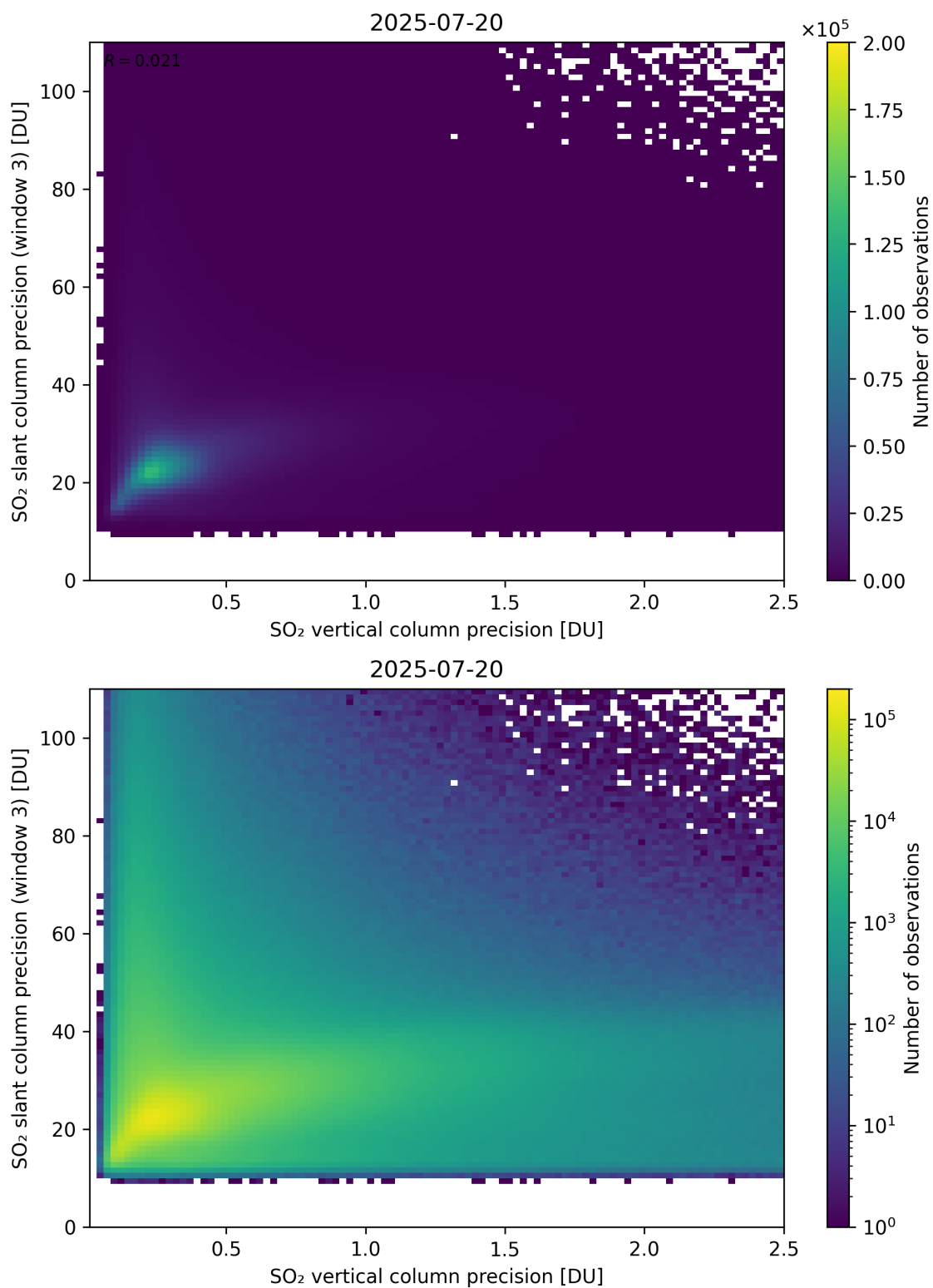
Figure 345: Scatter density plot of “SO 2 vertical column precision” against “SO 2 slant column precision (window 3)” for 2025-07-19 to 2025-07-21.
