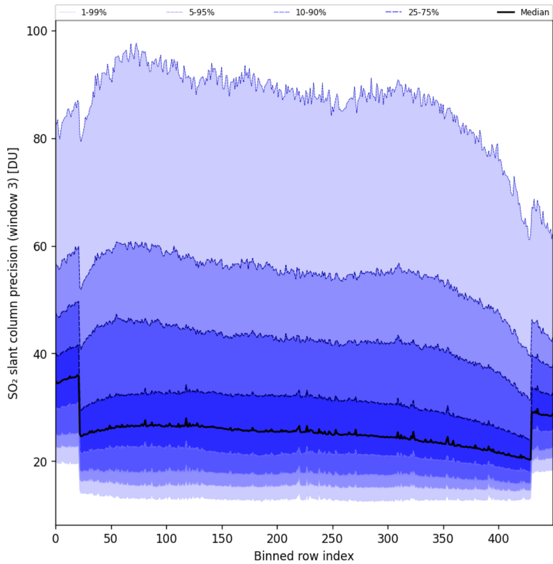
Figure 98: Along track statistics of “SO 2 slant column precision (window 3)” for 2025-07-19 to 2025-07-21
