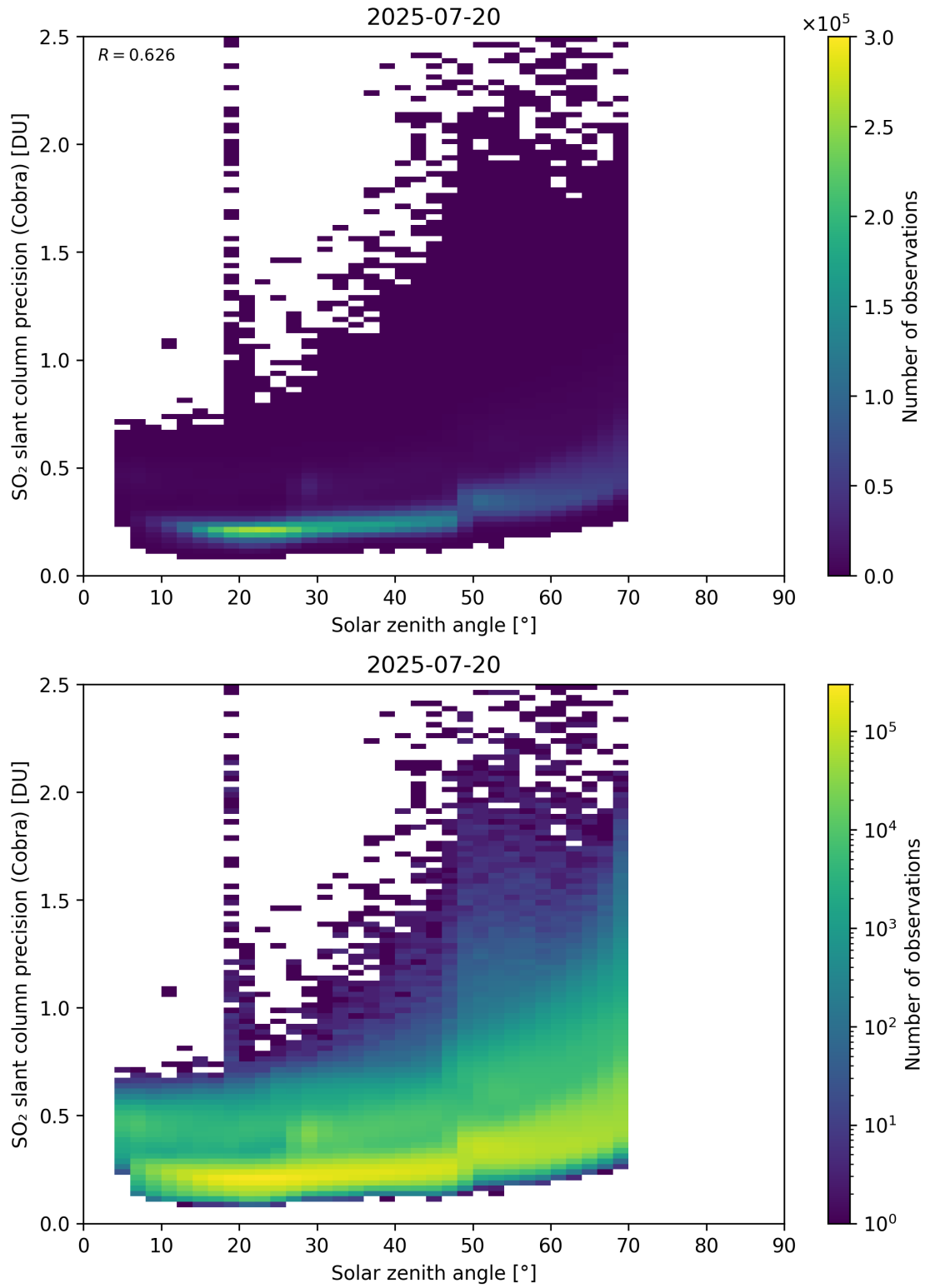
Figure 180: Scatter density plot of “Solar zenith angle” against “SO 2 slant column precision (Cobra)” for 2025-07-19 to 2025-07-21.
