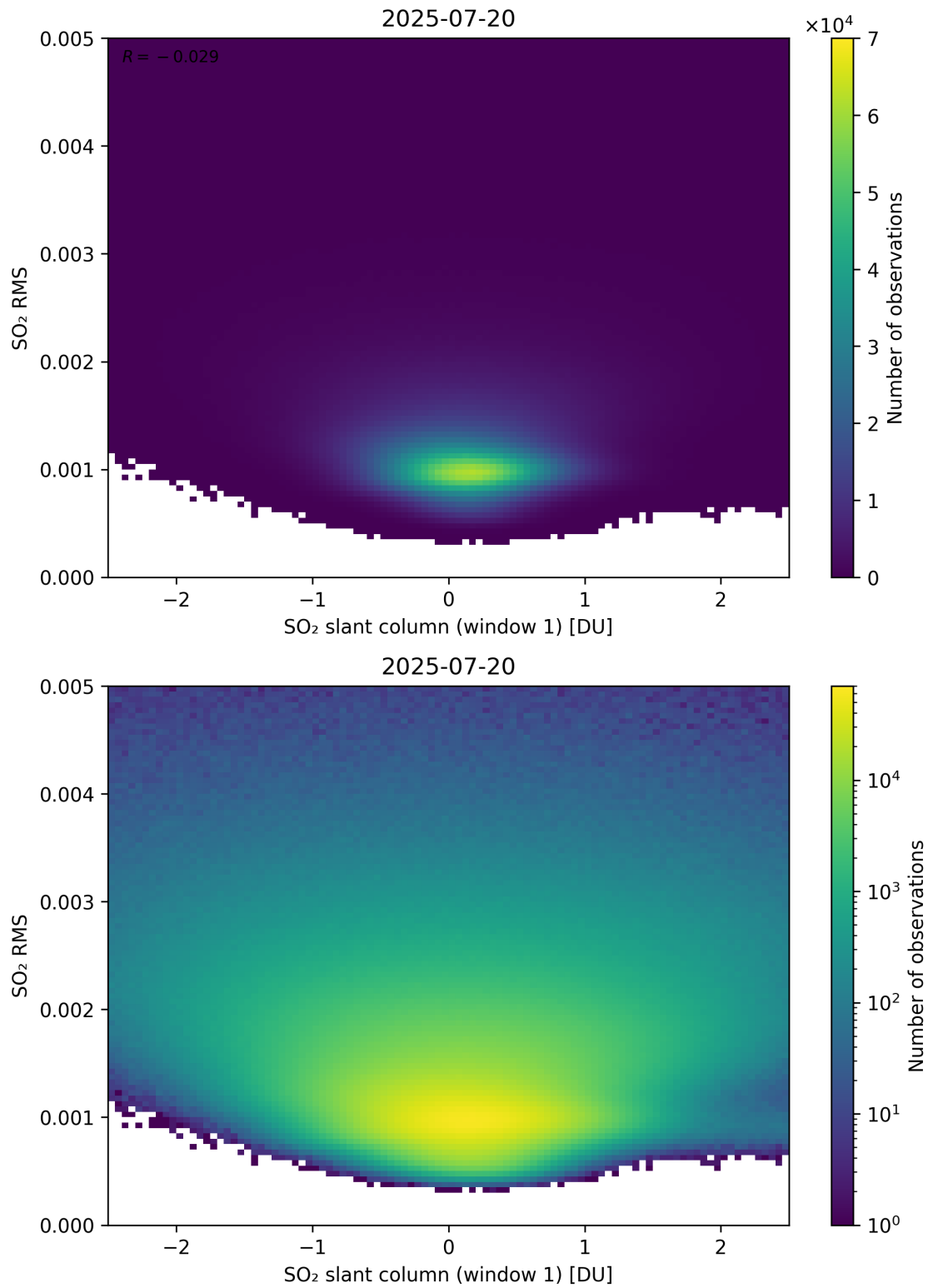
Figure 267: Scatter density plot of “SO 2 slant column (window 1)” against “SO 2 RMS” for 2025-07-19 to 2025-07-21.
