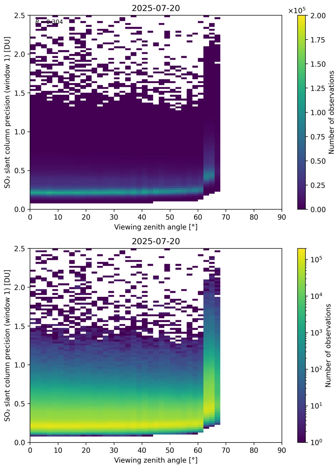
Figure 377: Scatter density plot of “Viewing zenith angle” against “SO 2 slant column precision (window 1)” for 2025-07-19 to 2025-07-21.
