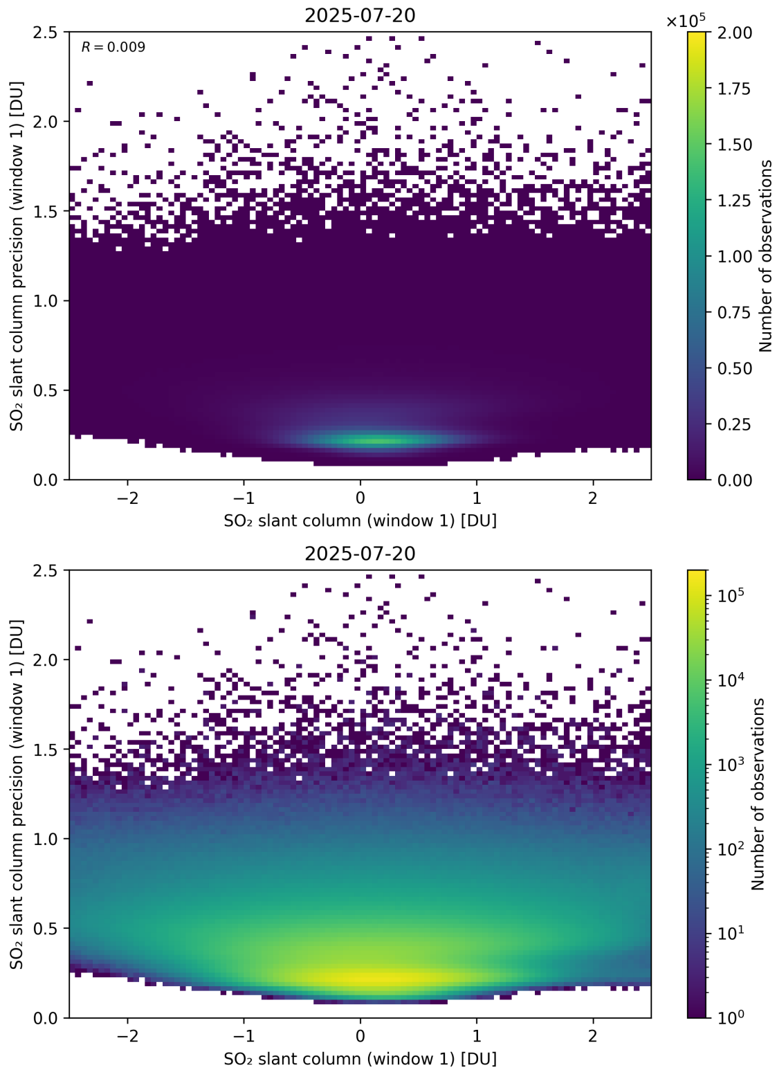
Figure 285: Scatter density plot of “SO 2 slant column (window 1)” against “SO 2 slant column precision (window 1)” for 2025-07-19 to 2025-07-21.
