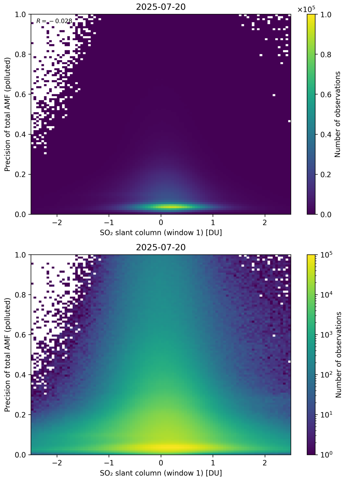
Figure 290: Scatter density plot of “SO 2 slant column (window 1)” against “Precision of total AMF (polluted)” for 2025-07-19 to 2025-07-21.
