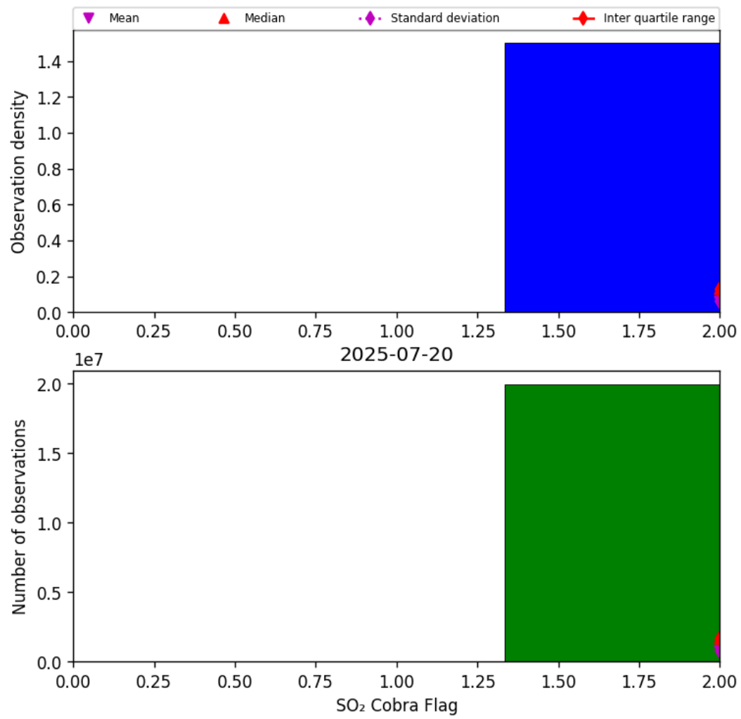
Figure 75: Histogram of “SO 2 Cobra Flag” for 2025-07-19 to 2025-07-21
