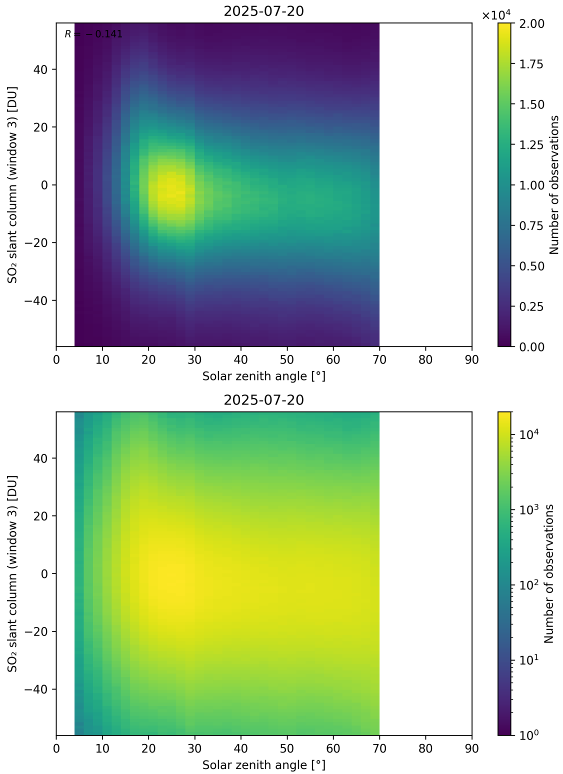
Figure 187: Scatter density plot of “Solar zenith angle” against “SO 2 slant column (window 3)” for 2025-07-19 to 2025-07-21.
