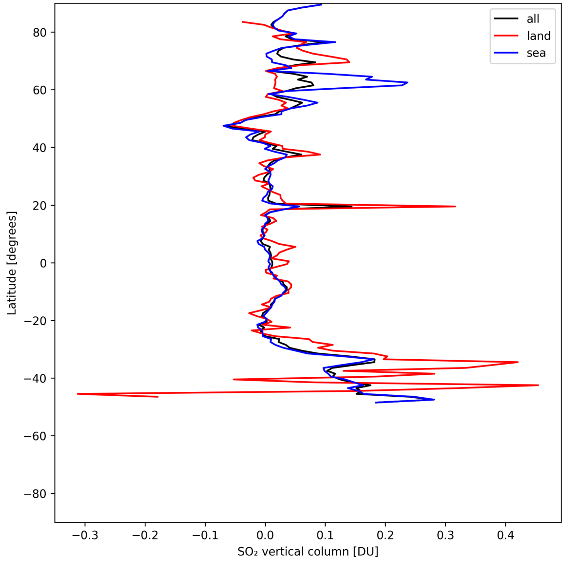
Figure 32: Zonal average of “SO 2 vertical column” for 2025-07-19 to 2025-07-21.
