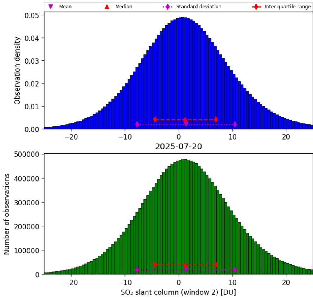
Figure 67: Histogram of “SO 2 slant column (window 2)” for 2025-07-19 to 2025-07-21
