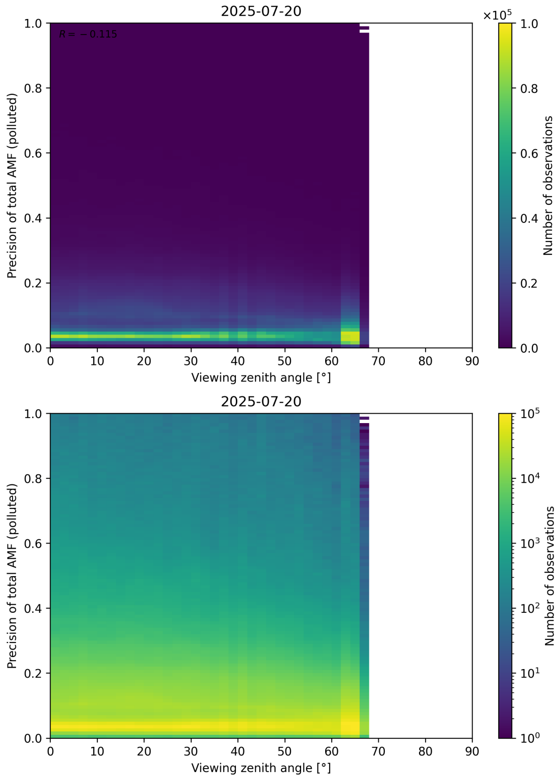
Figure 382: Scatter density plot of “Viewing zenith angle” against “Precision of total AMF (polluted)” for 2025-07-19 to 2025-07-21.
