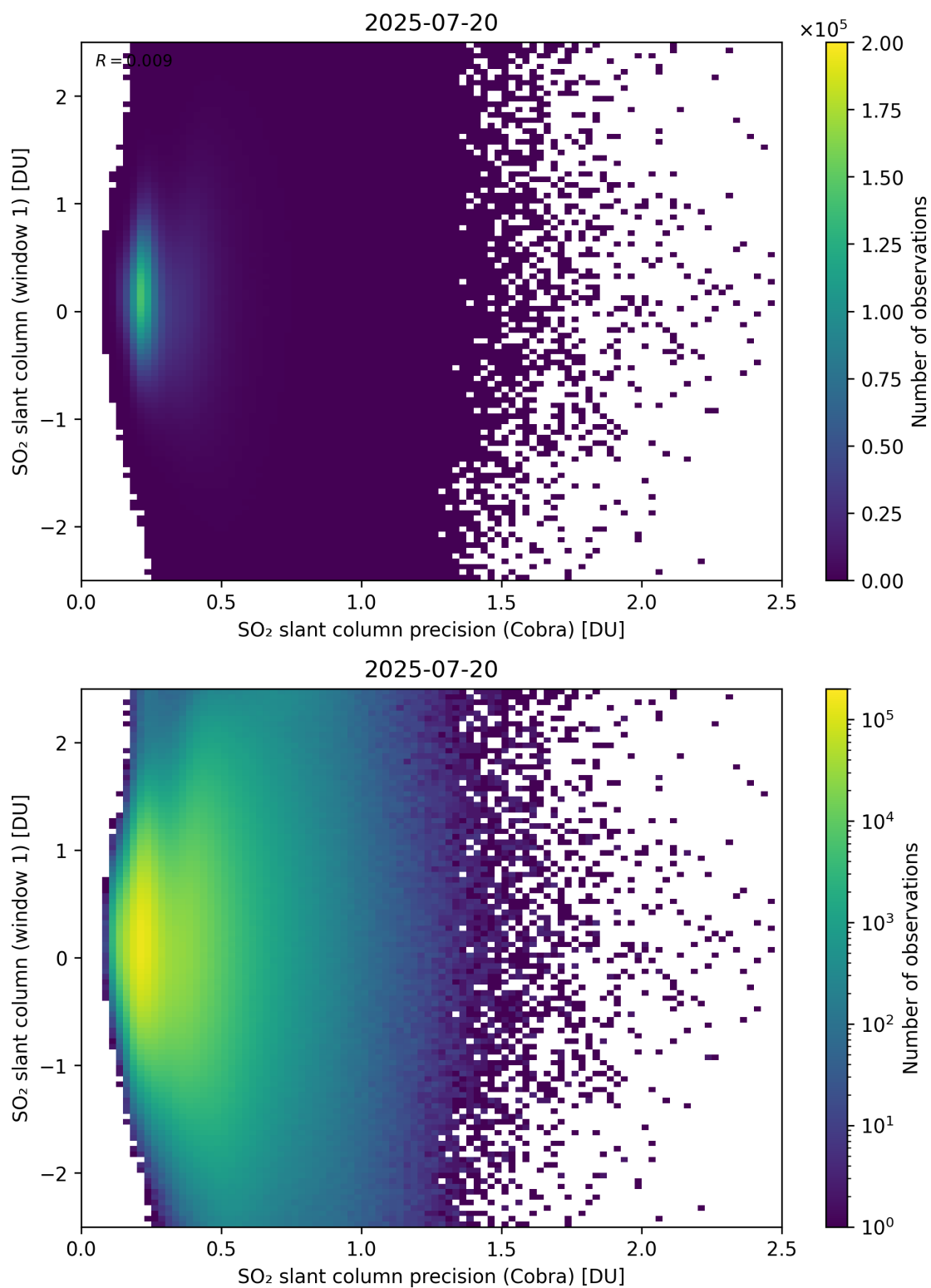
Figure 208: Scatter density plot of “SO 2 slant column precision (Cobra)” against “SO 2 slant column (window 1)” for 2025-07-19 to 2025-07-21.
