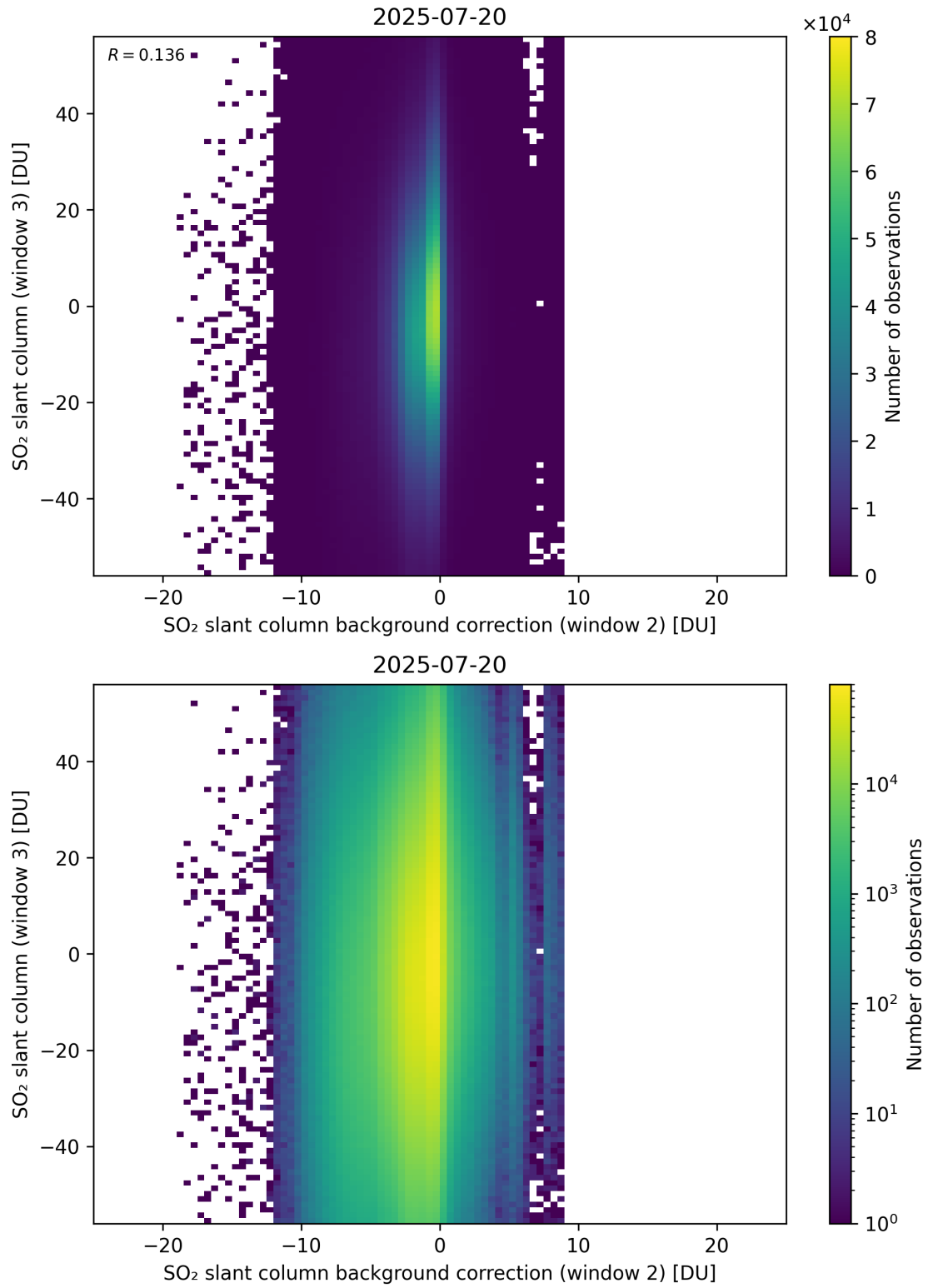
Figure 128: Scatter density plot of “SO 2 slant column background correction (window 2)” against “SO 2 slant column (window 3)” for 2025-07-19 to 2025-07-21.
