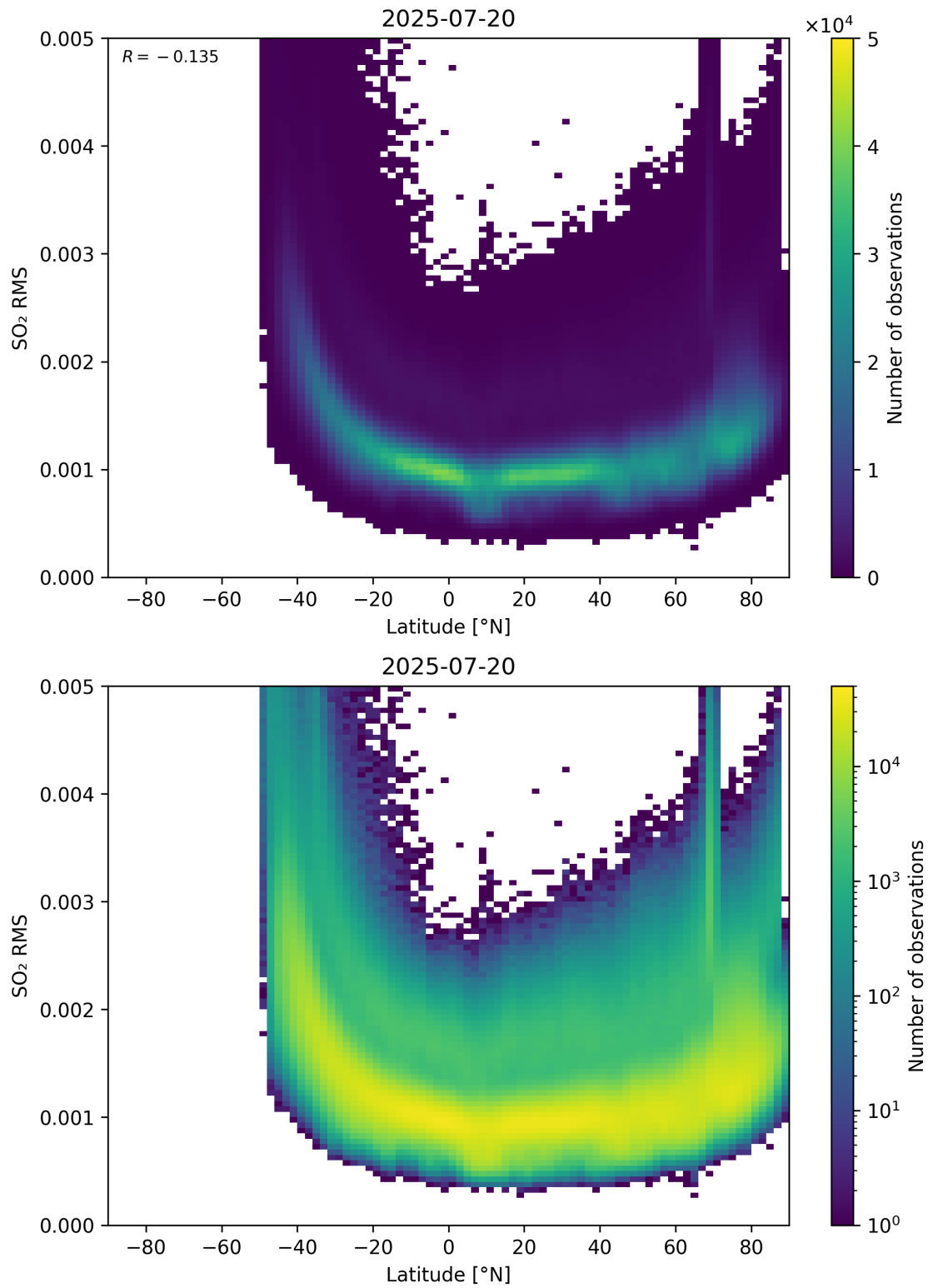
Figure 155: Scatter density plot of “Latitude” against “SO 2 RMS” for 2025-07-19 to 2025-07-21.
