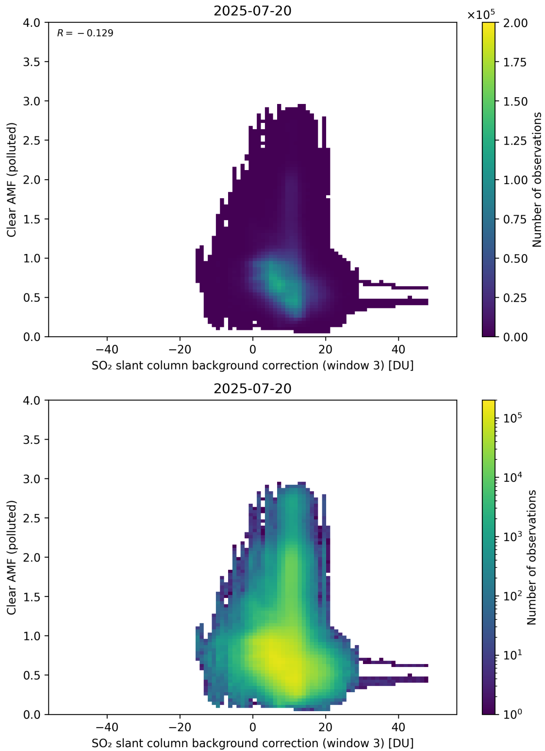
Figure 135: Scatter density plot of “SO 2 slant column background correction (window 3)” against “Clear AMF (polluted)” for 2025-07-19 to 2025-07-21.
