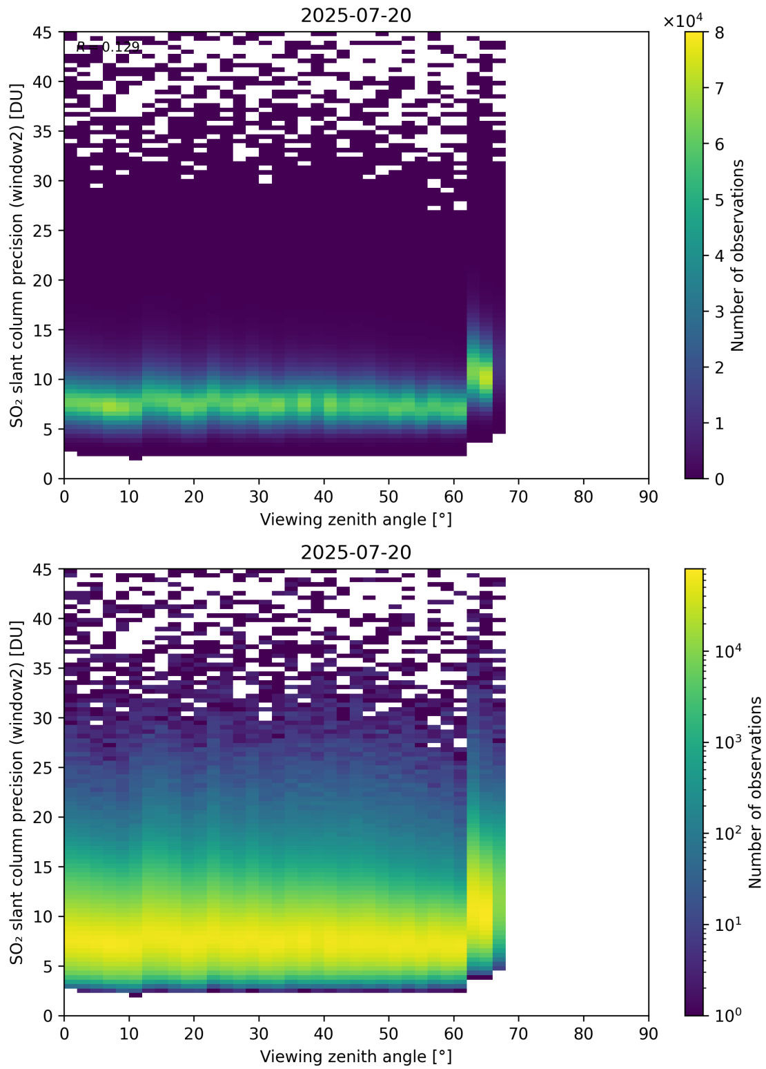
Figure 378: Scatter density plot of “Viewing zenith angle” against “SO 2 slant column precision (window2)” for 2025-07-19 to 2025-07-21.
