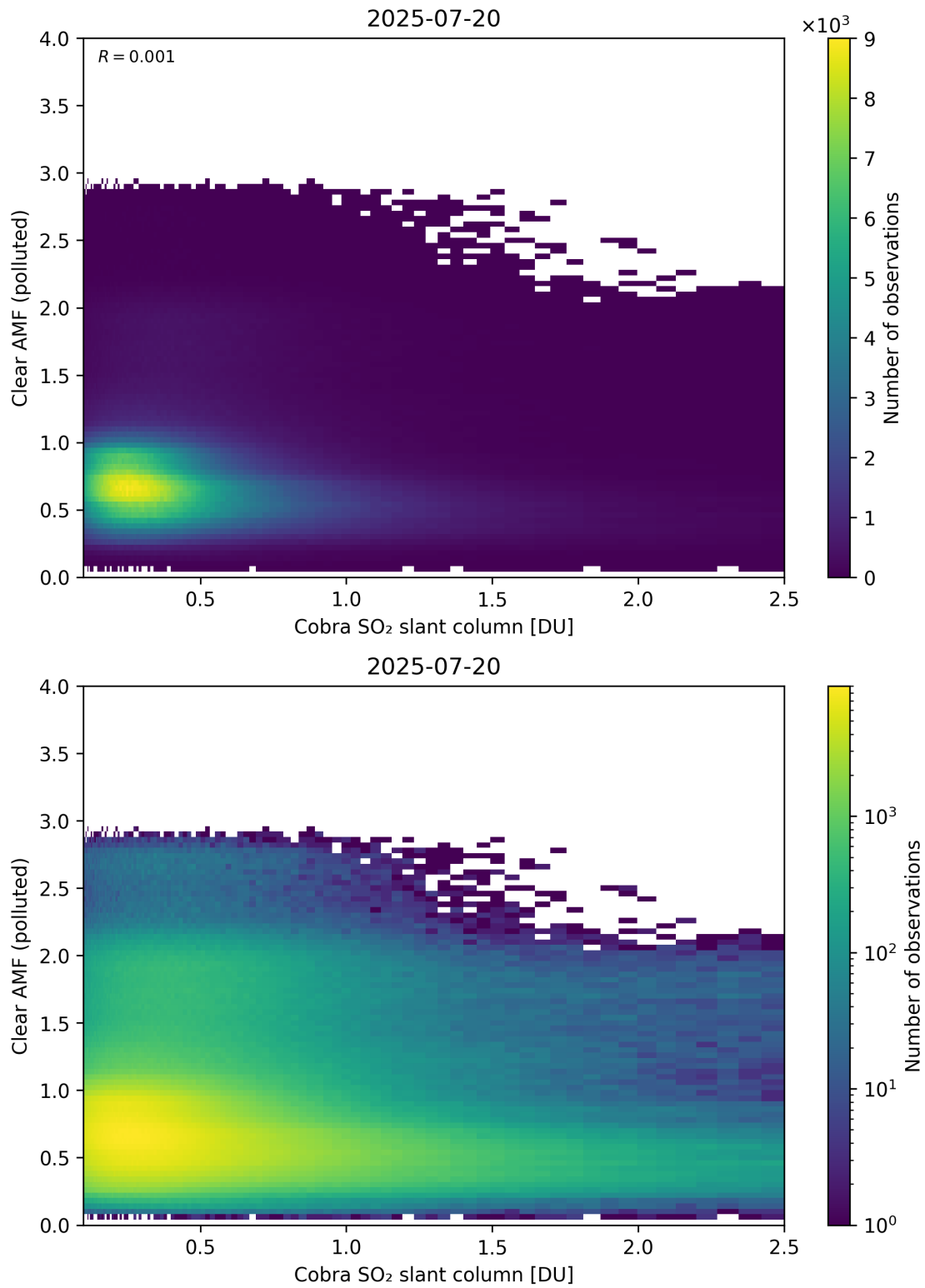
Figure 215: Scatter density plot of “Cobra SO 2 slant column” against “Clear AMF (polluted)” for 2025-07-19 to 2025-07-21.
