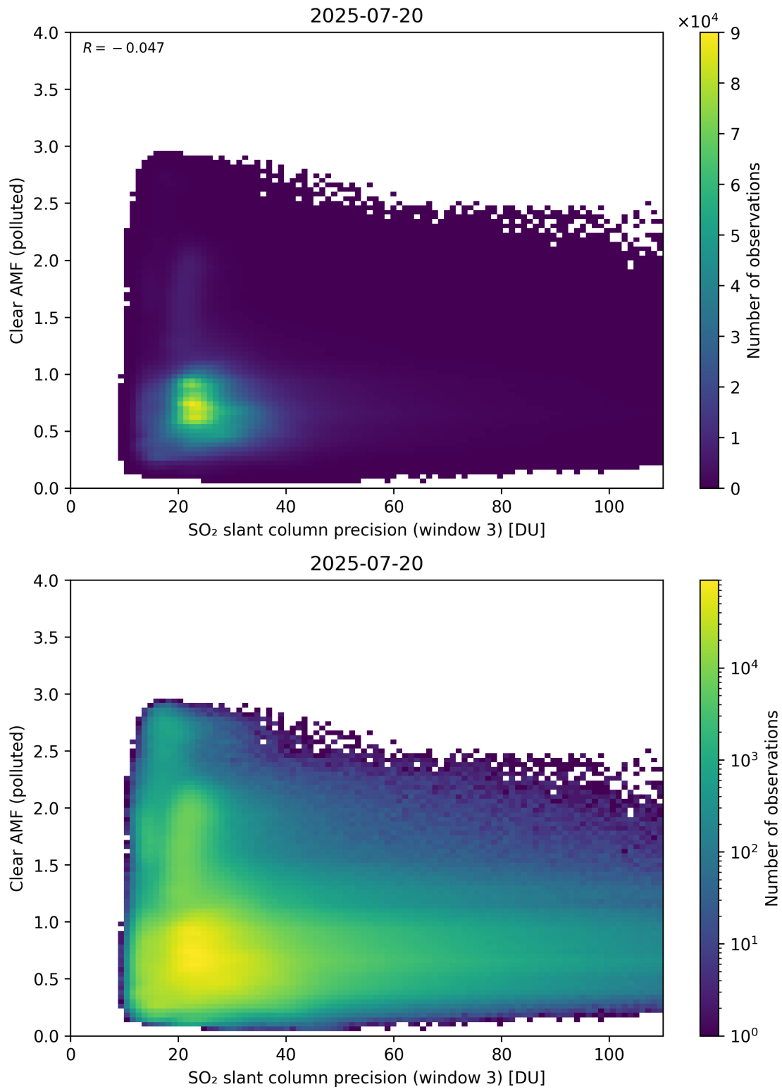
Figure 311: Scatter density plot of “SO 2 slant column precision (window 3)” against “Clear AMF (polluted)” for 2025-07-19 to 2025-07-21.
