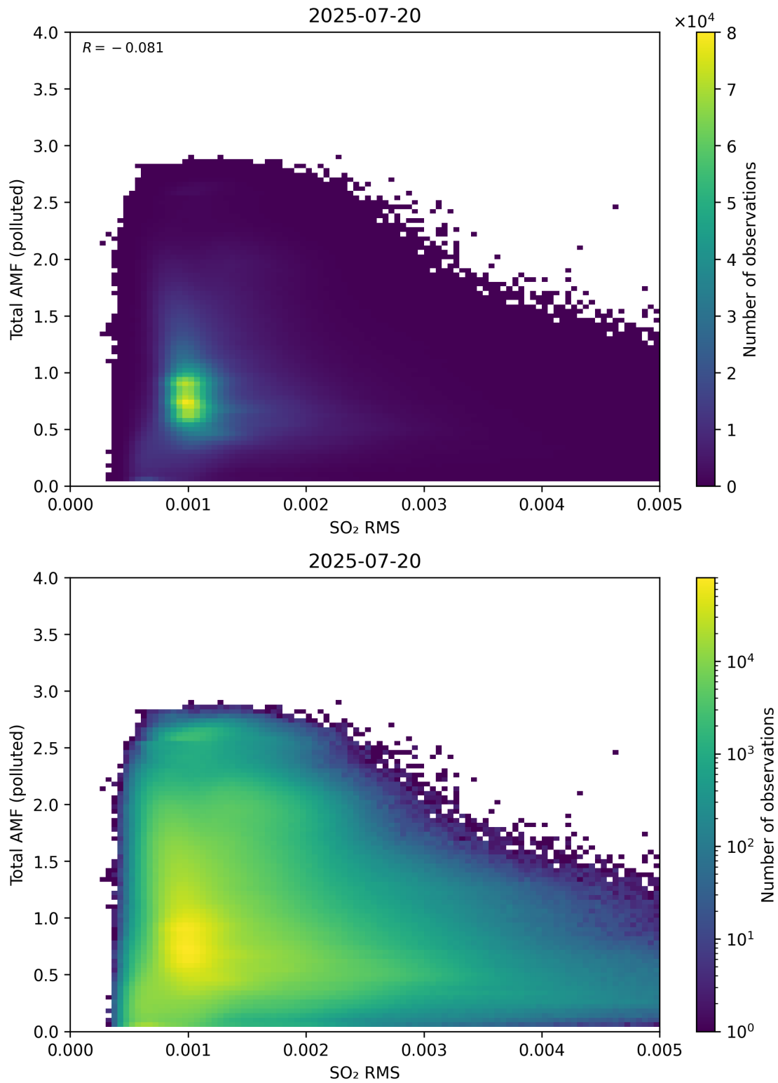
Figure 148: Scatter density plot of “SO 2 RMS” against “Total AMF (polluted)” for 2025-07-19 to 2025-07-21.
