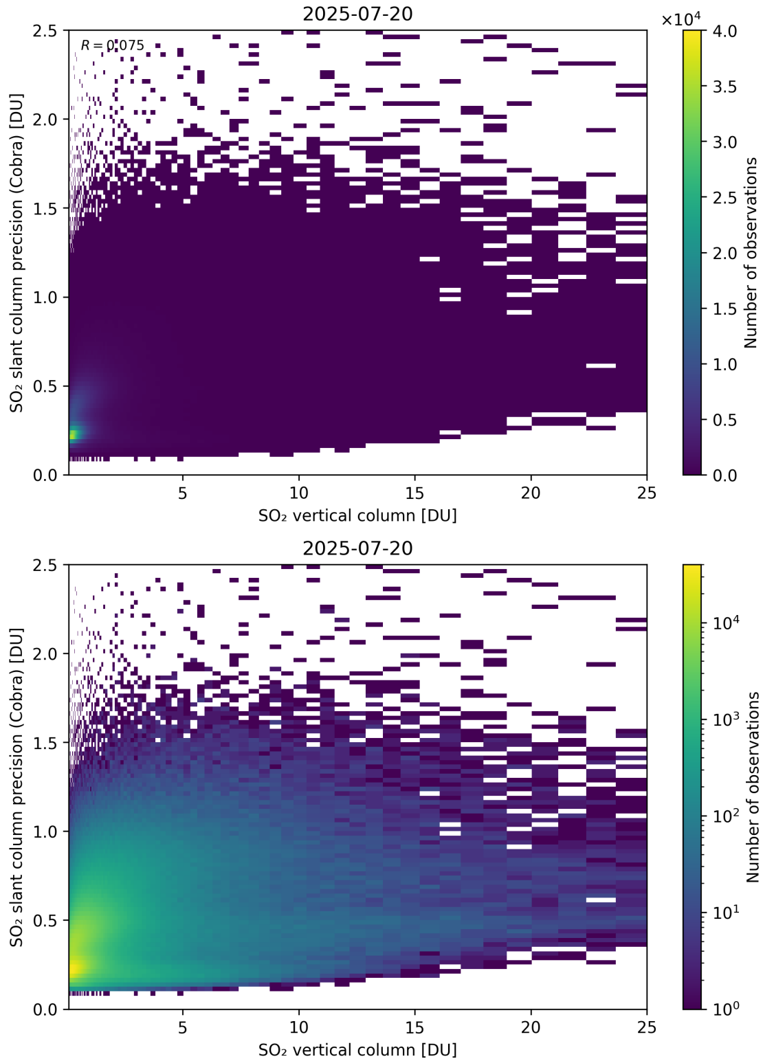
Figure 350: Scatter density plot of “SO 2 vertical column” against “SO 2 slant column precision (Cobra)” for 2025-07-19 to 2025-07-21.
