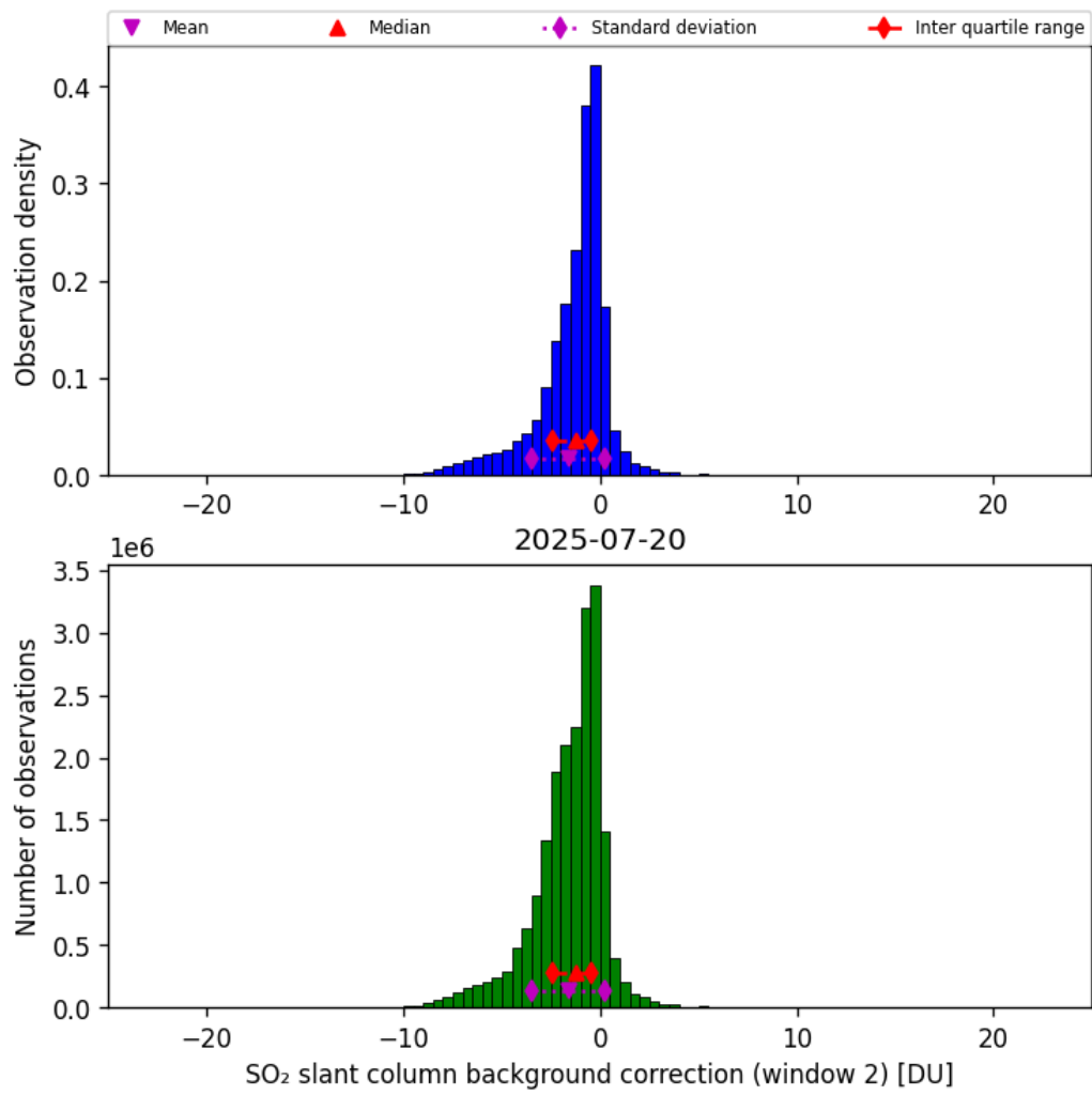
Figure 70: Histogram of “SO 2 slant column background correction (window 2)” for 2025-07-19 to 2025-07-21
