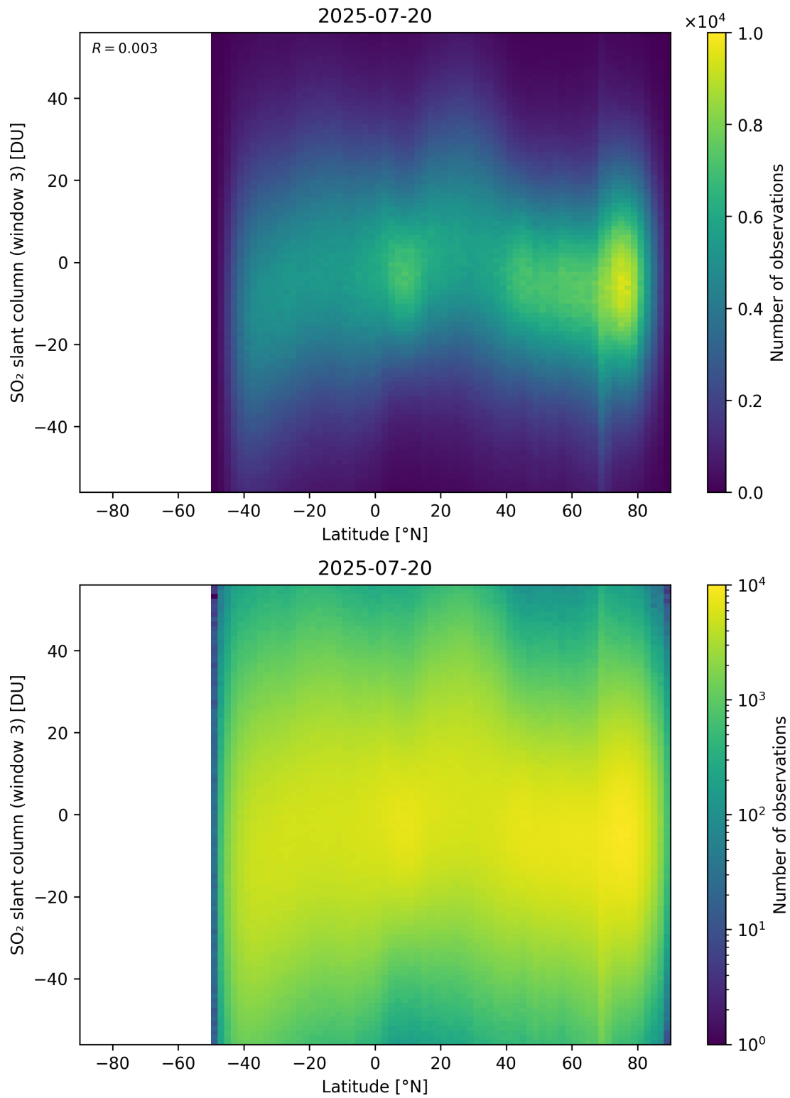
Figure 165: Scatter density plot of “Latitude” against “SO 2 slant column (window 3)” for 2025-07-19 to 2025-07-21.
