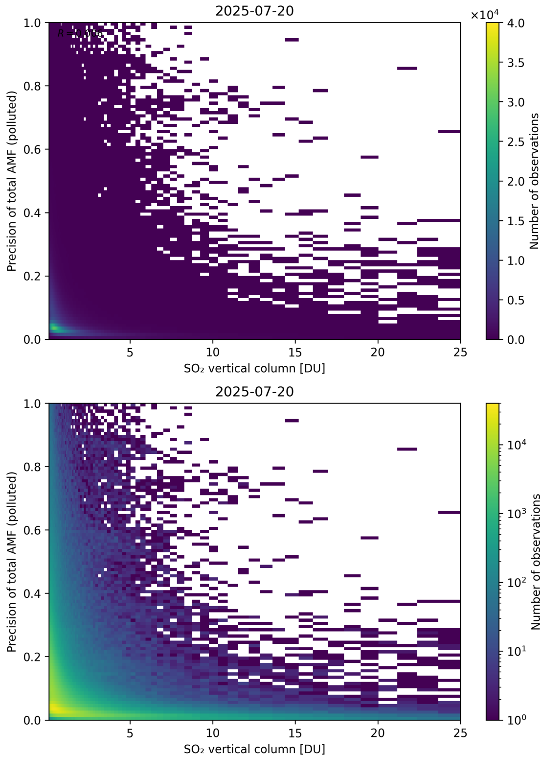
Figure 360: Scatter density plot of “SO 2 vertical column” against “Precision of total AMF (polluted)” for 2025-07-19 to 2025-07-21.
