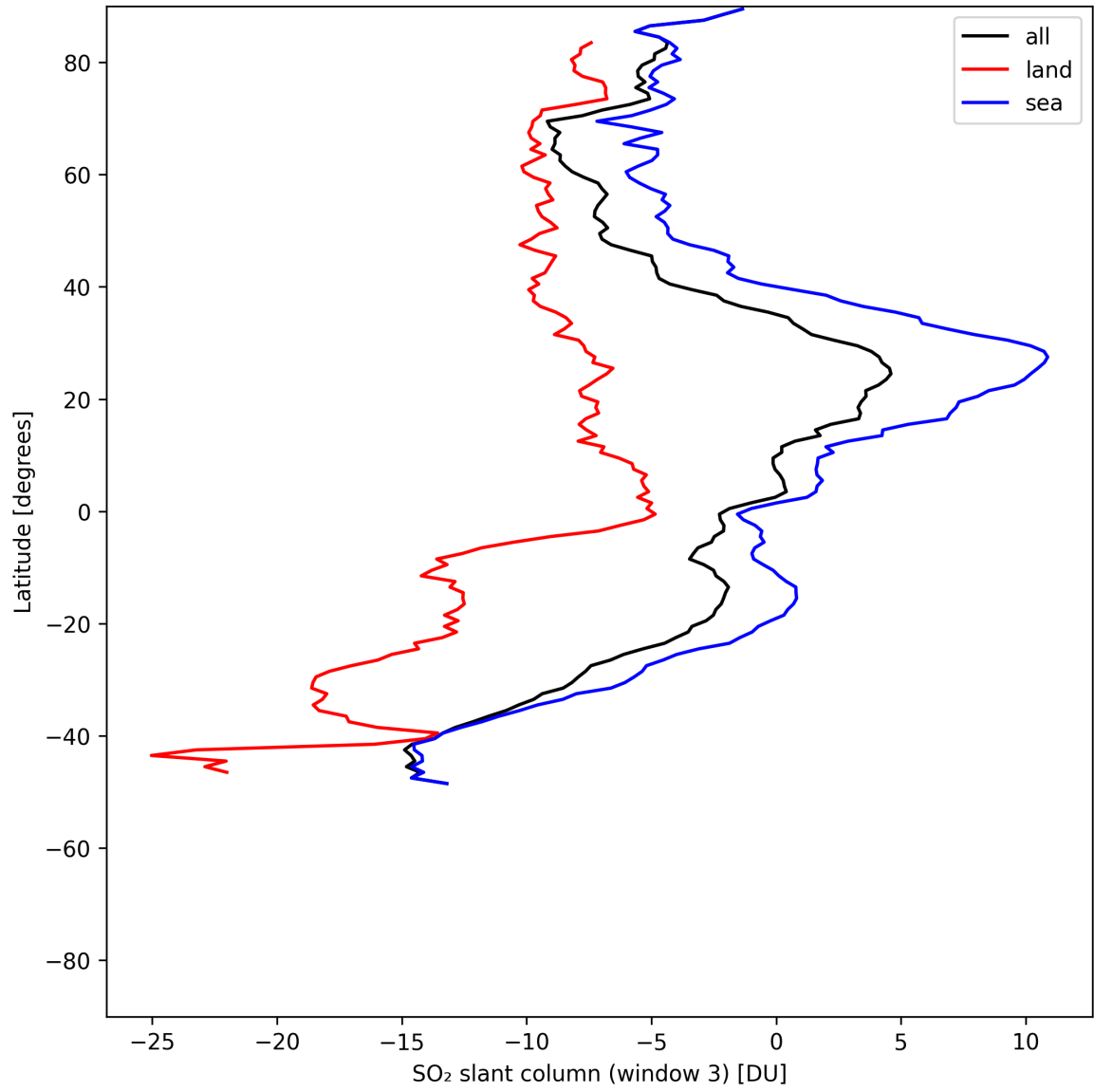
Figure 45: Zonal average of “SO 2 slant column (window 3)” for 2025-07-19 to 2025-07-21.
