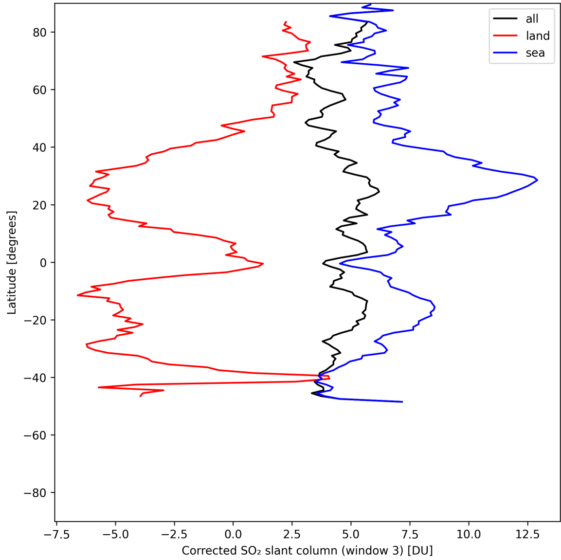
Figure 47: Zonal average of “Corrected SO 2 slant column (window 3)” for 2025-07-19 to 2025-07-21.
