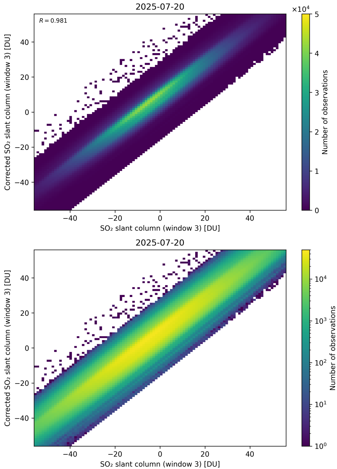
Figure 316: Scatter density plot of “SO 2 slant column (window 3)” against “Corrected SO 2 slant column (window 3)” for 2025-07-19 to 2025-07-21.
