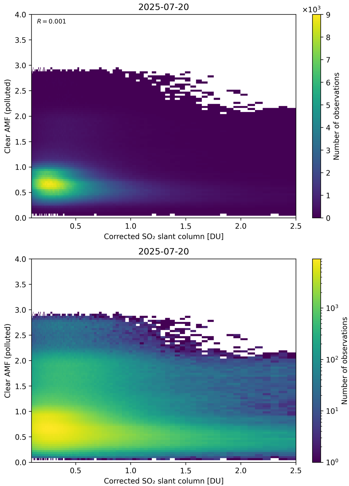
Figure 232: Scatter density plot of “Corrected SO 2 slant column” against “Clear AMF (polluted)” for 2025-07-19 to 2025-07-21.
