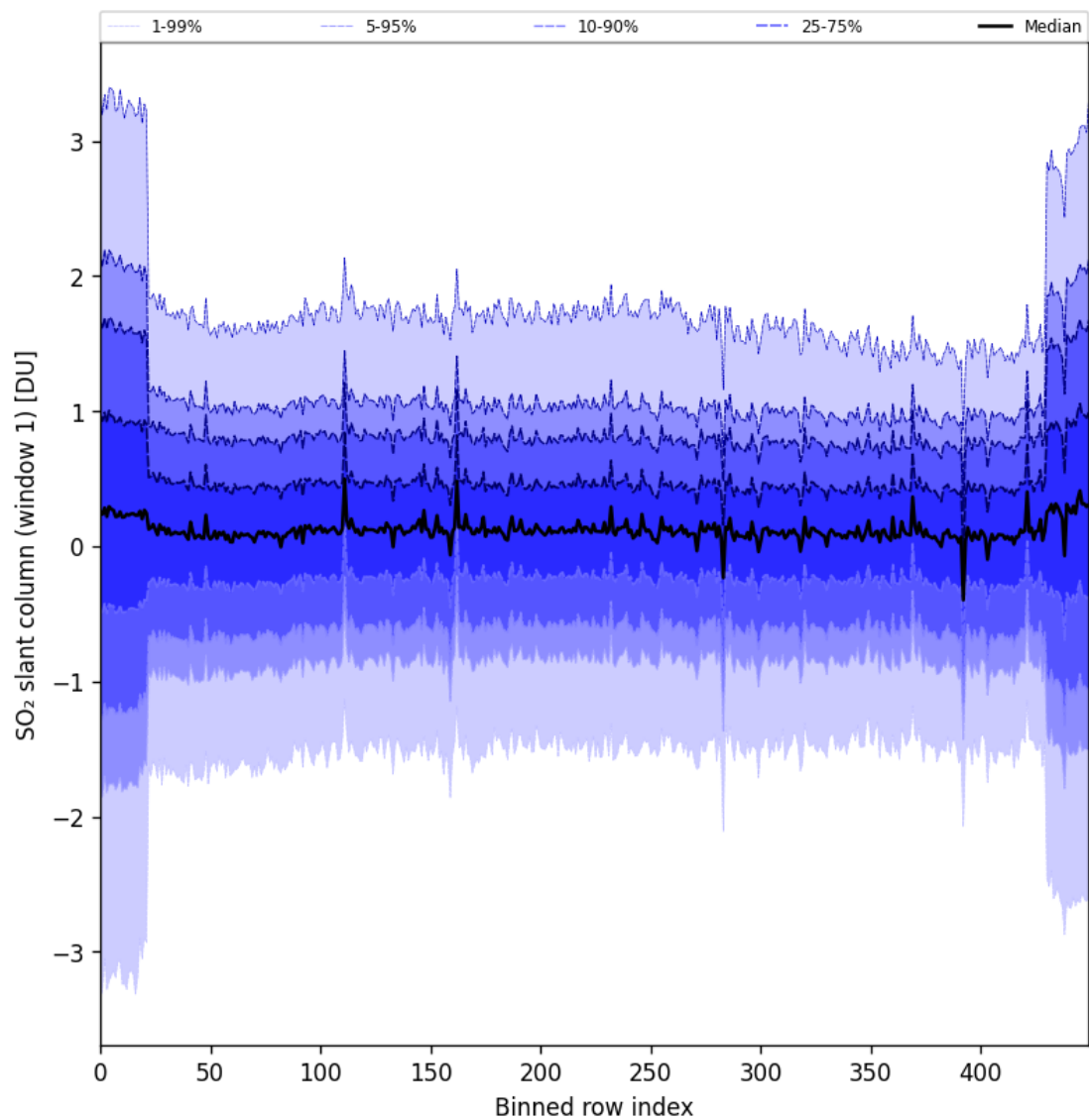
Figure 89: Along track statistics of “SO 2 slant column (window 1)” for 2025-07-19 to 2025-07-21
