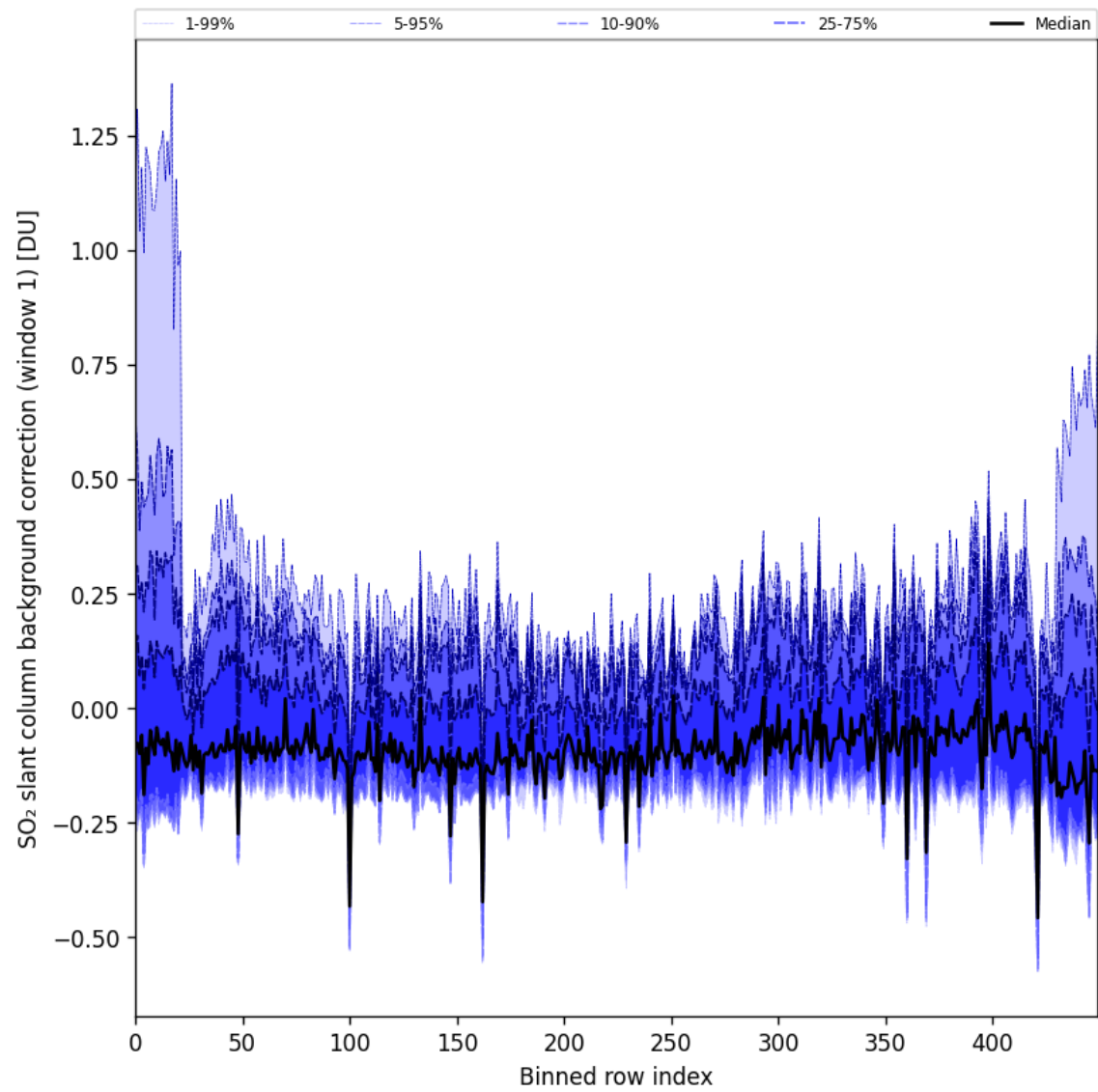
Figure 92: Along track statistics of “SO 2 slant column background correction (window 1)” for 2025-07-19 to 2025-07-21
