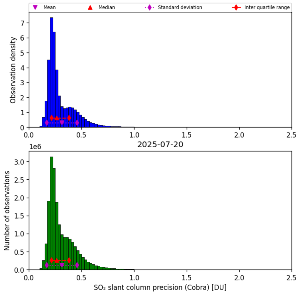
Figure 62: Histogram of “SO 2 slant column precision (Cobra)” for 2025-07-19 to 2025-07-21
