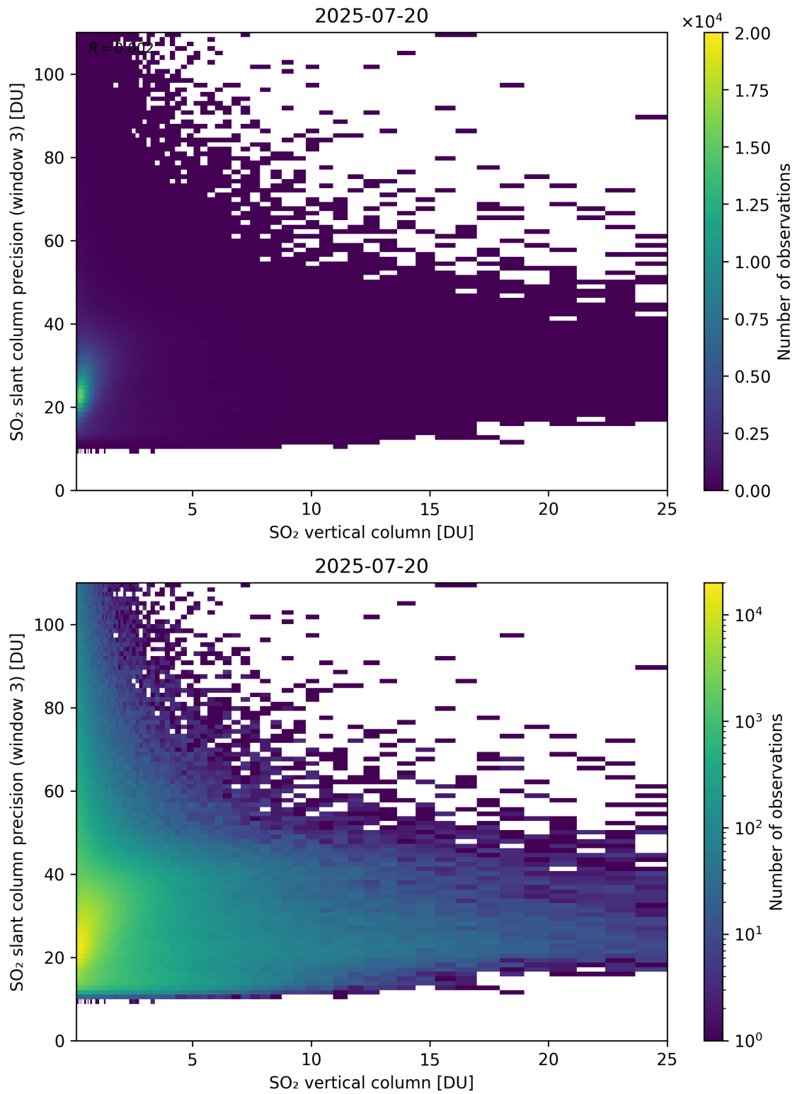
Figure 358: Scatter density plot of “SO 2 vertical column” against “SO 2 slant column precision (window 3)” for 2025-07-19 to 2025-07-21.
