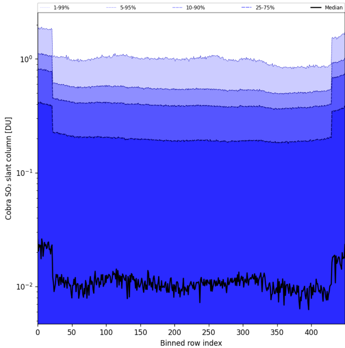
Figure 87: Along track statistics of “Cobra SO 2 slant column” for 2025-07-19 to 2025-07-21
