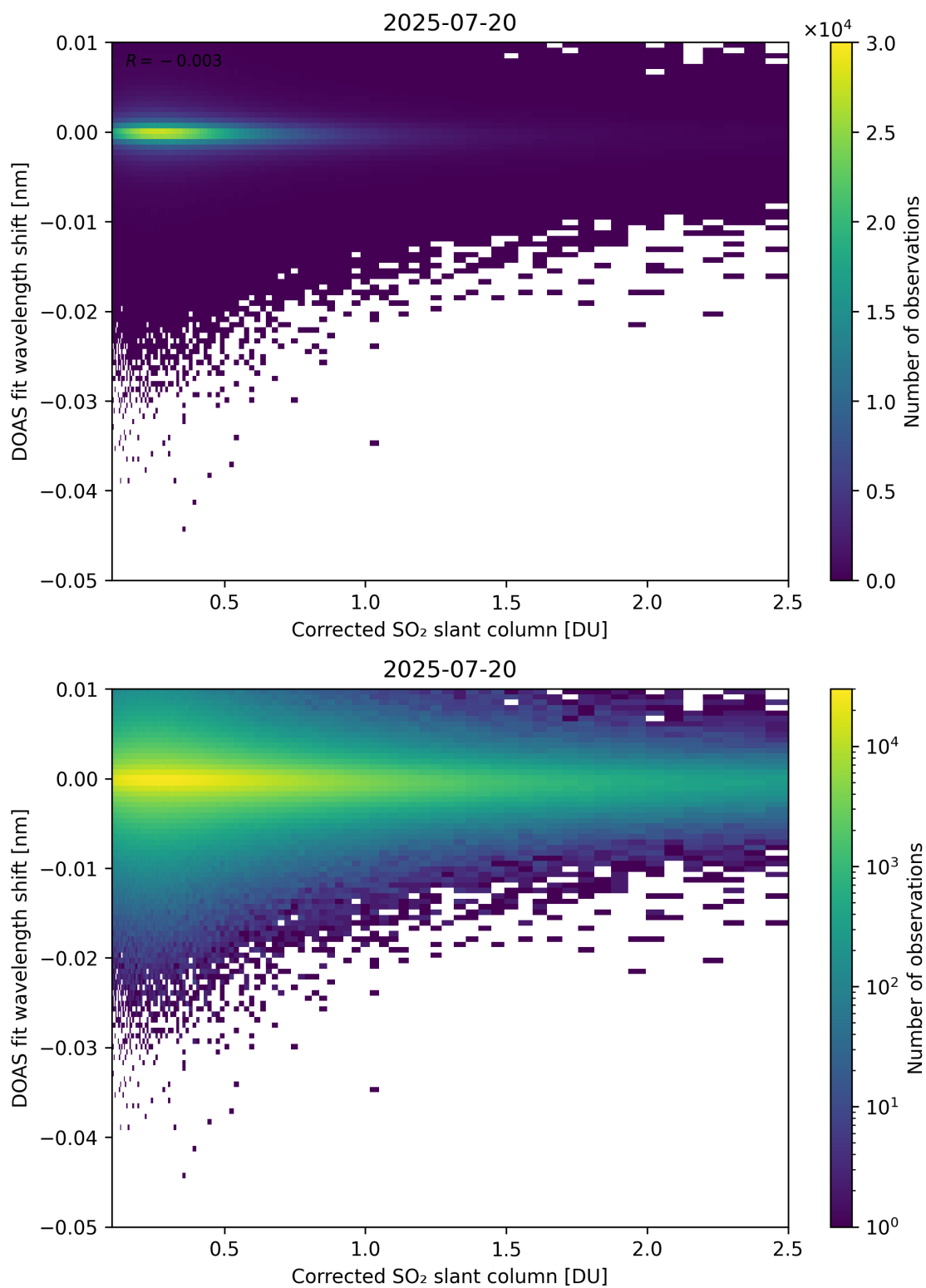
Figure 229: Scatter density plot of “Corrected SO 2 slant column” against “DOAS fit wavelength shift” for 2025-07-19 to 2025-07-21.
