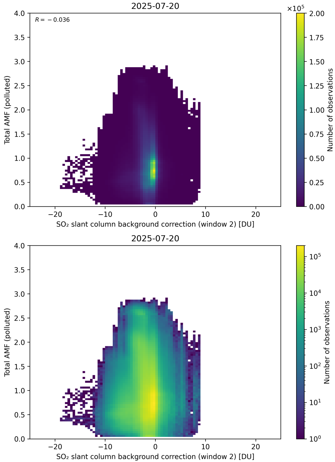
Figure 130: Scatter density plot of “SO 2 slant column background correction (window 2)” against “Total AMF (polluted)” for 2025-07-19 to 2025-07-21.
