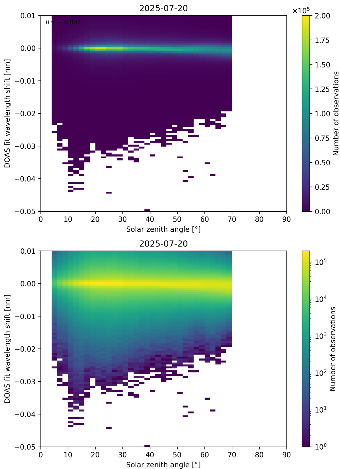
Figure 174: Scatter density plot of “Solar zenith angle” against “DOAS fit wavelength shift” for 2025-07-19 to 2025-07-21.
