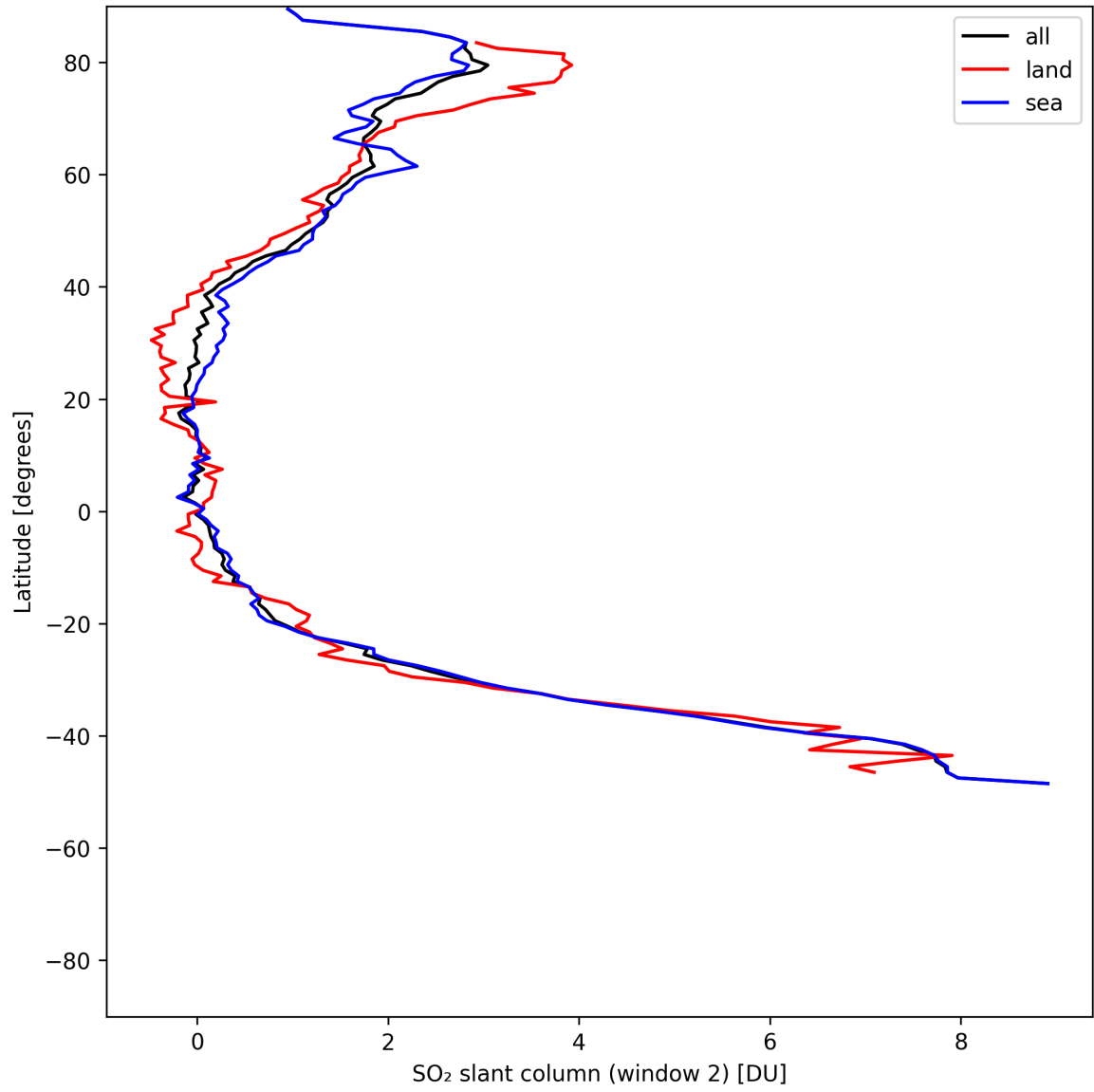
Figure 41: Zonal average of “SO 2 slant column (window 2)” for 2025-07-19 to 2025-07-21.
