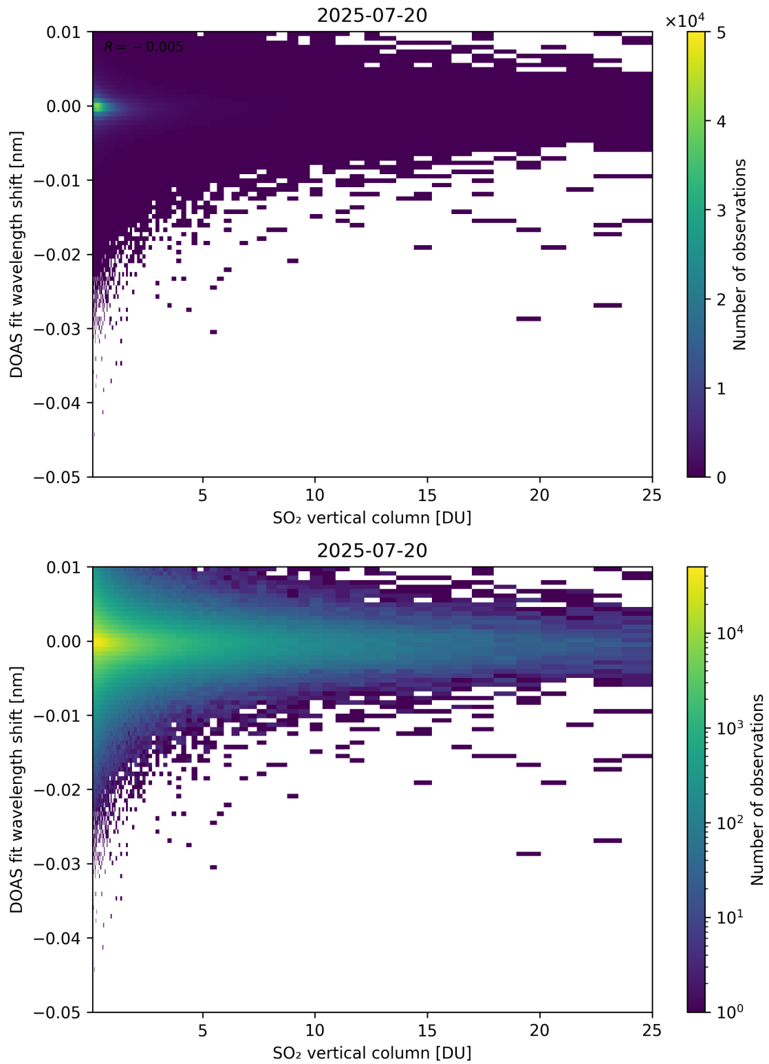
Figure 326: Scatter density plot of “SO 2 vertical column” against “DOAS fit wavelength shift” for 2025-07-19 to 2025-07-21.
