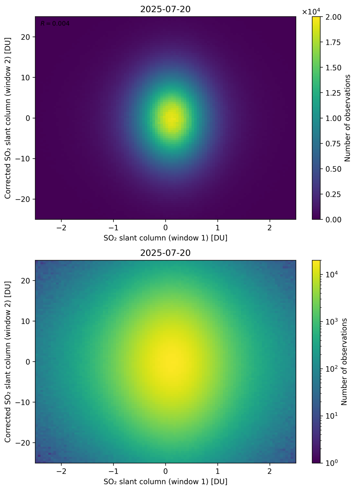
Figure 283: Scatter density plot of “SO 2 slant column (window 1)” against “Corrected SO 2 slant column (window 2)” for 2025-07-19 to 2025-07-21.
