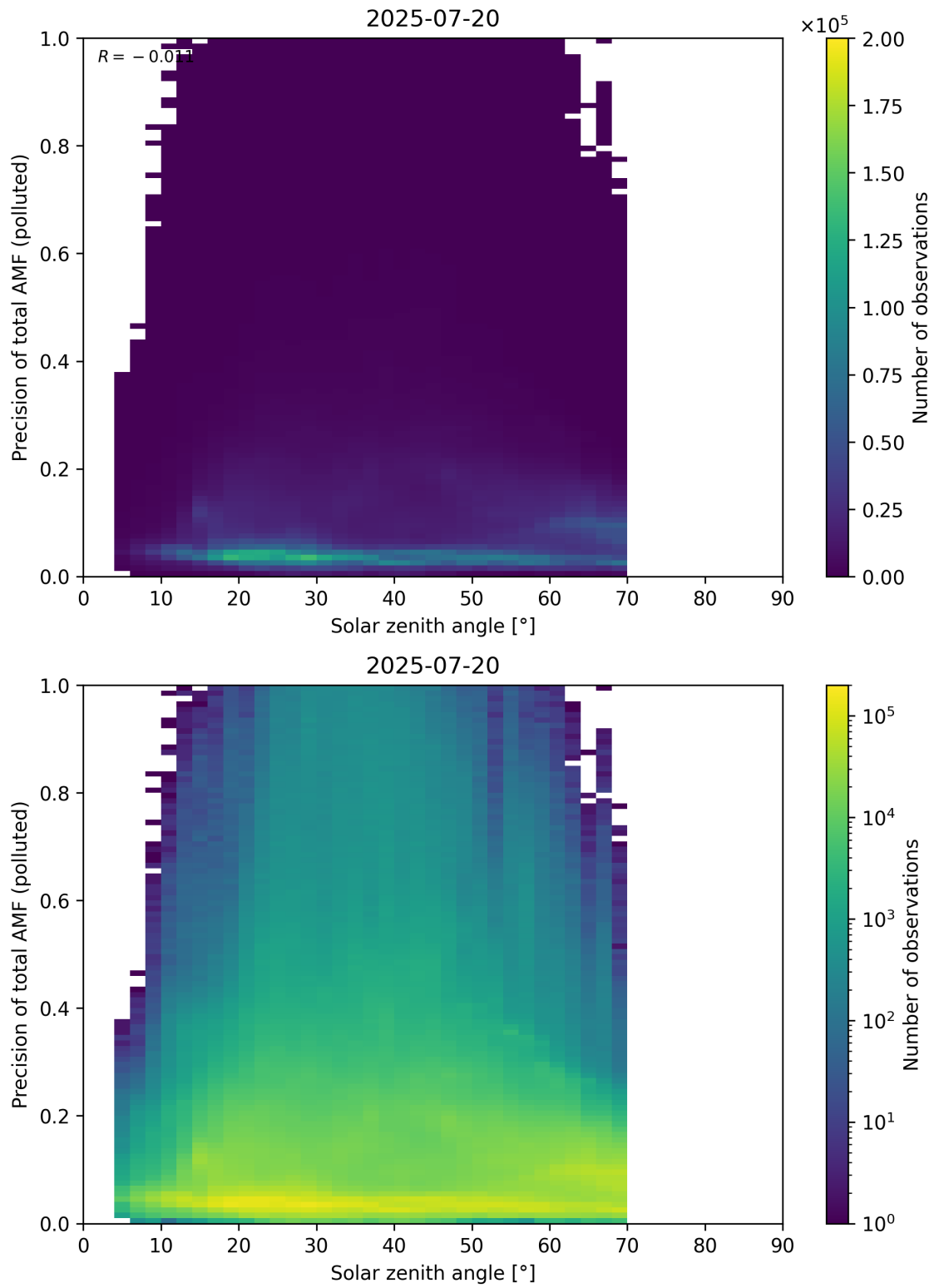
Figure 190: Scatter density plot of “Solar zenith angle” against “Precision of total AMF (polluted)” for 2025-07-19 to 2025-07-21.
