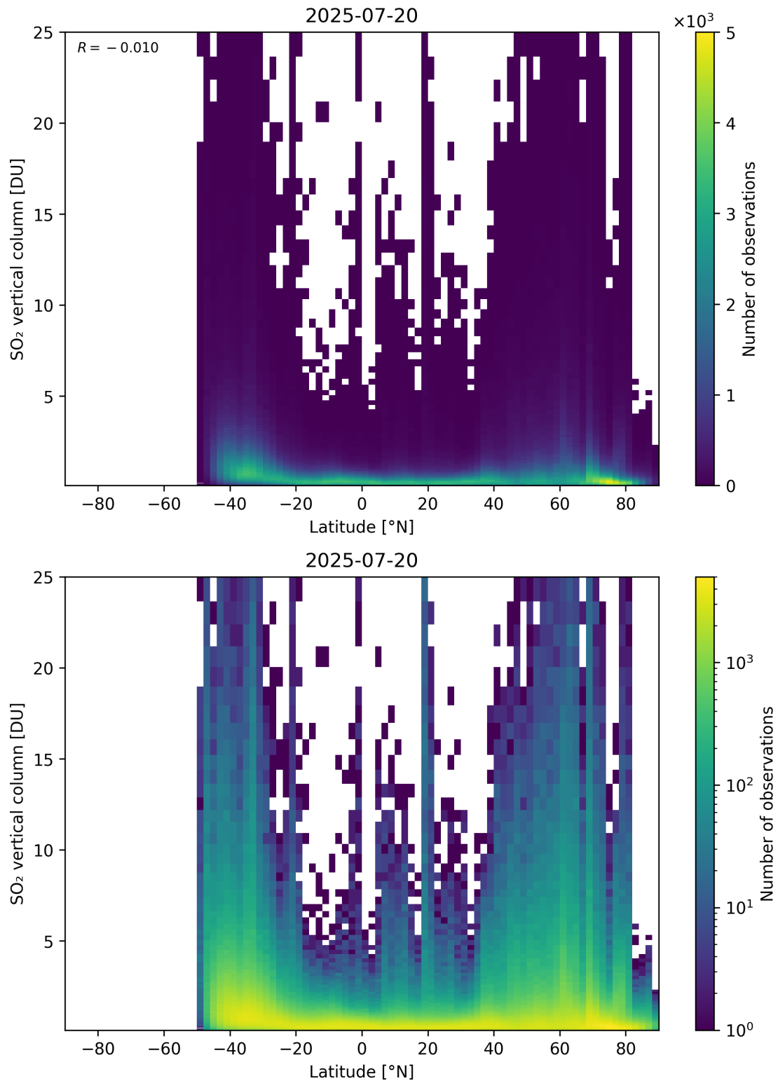
Figure 169: Scatter density plot of “Latitude” against “SO 2 vertical column” for 2025-07-19 to 2025-07-21.
