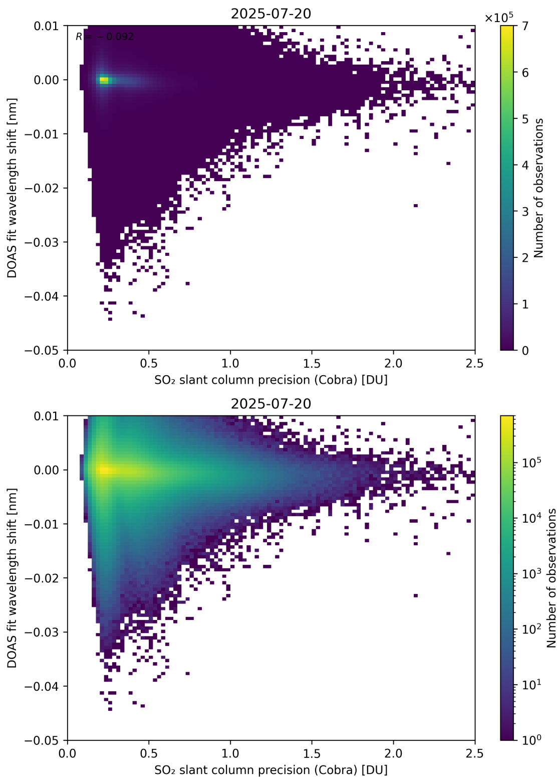
Figure 202: Scatter density plot of “SO 2 slant column precision (Cobra)” against “DOAS fit wavelength shift” for 2025-07-19 to 2025-07-21.
