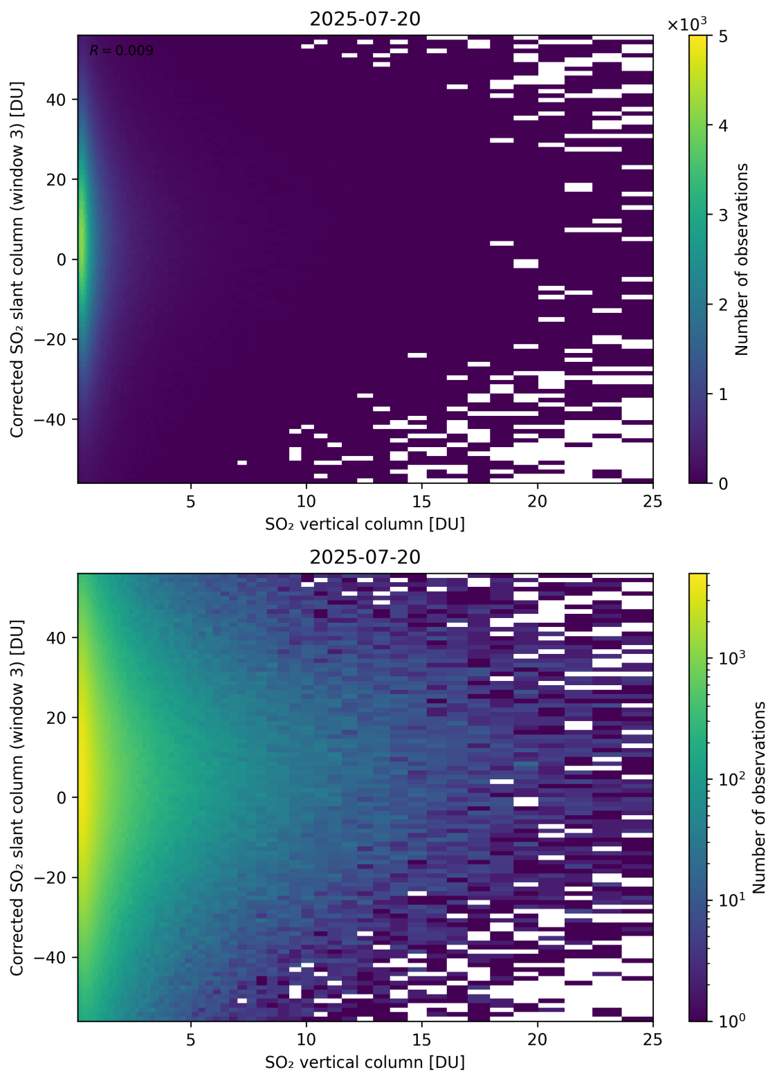
Figure 353: Scatter density plot of “SO 2 vertical column” against “Corrected SO 2 slant column (window 3)” for 2025-07-19 to 2025-07-21.
