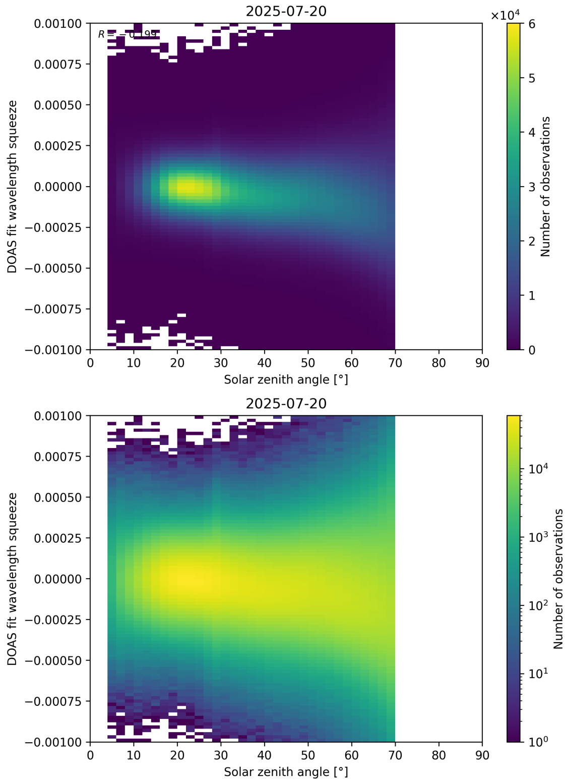
Figure 175: Scatter density plot of “Solar zenith angle” against “DOAS fit wavelength squeeze” for 2025-07-19 to 2025-07-21.
