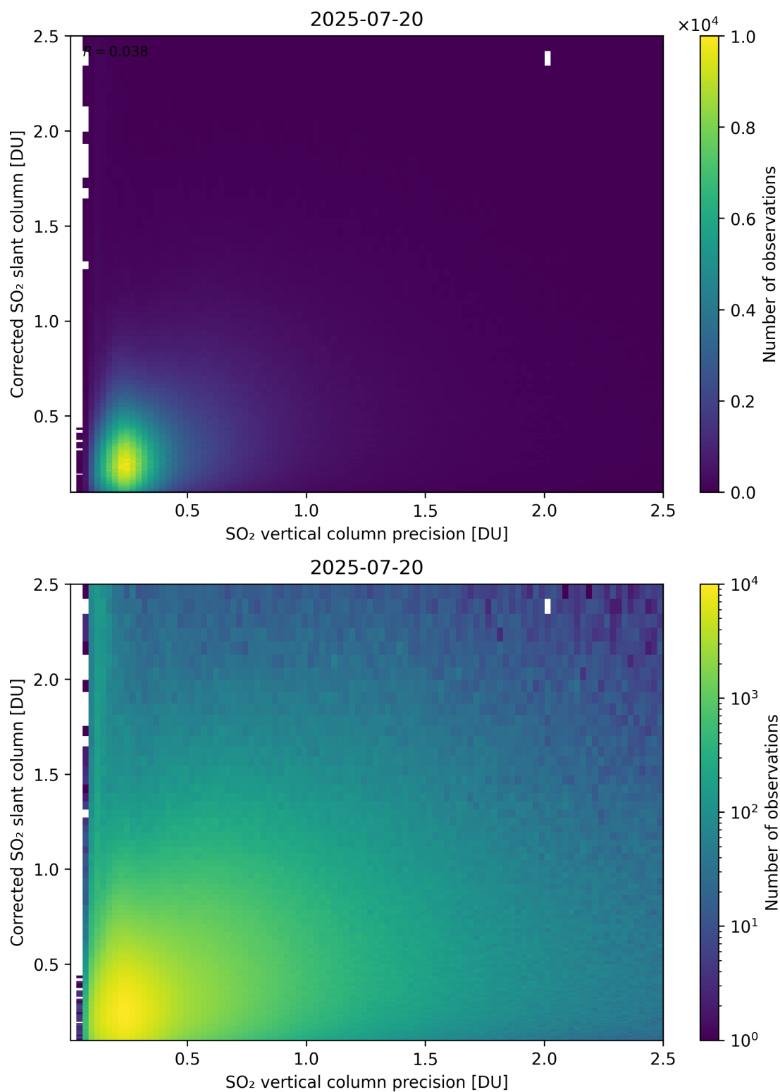
Figure 338: Scatter density plot of “SO 2 vertical column precision” against “Corrected SO 2 slant column” for 2025-07-19 to 2025-07-21.
