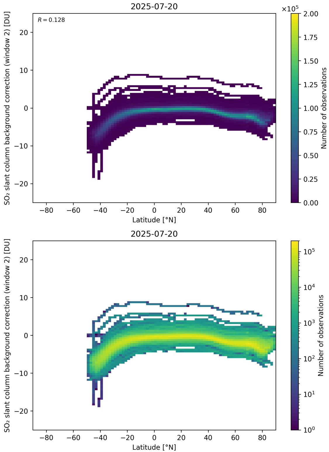
Figure 151: Scatter density plot of “Latitude” against “SO 2 slant column background correction (window 2)” for 2025-07-19 to 2025-07-21.
