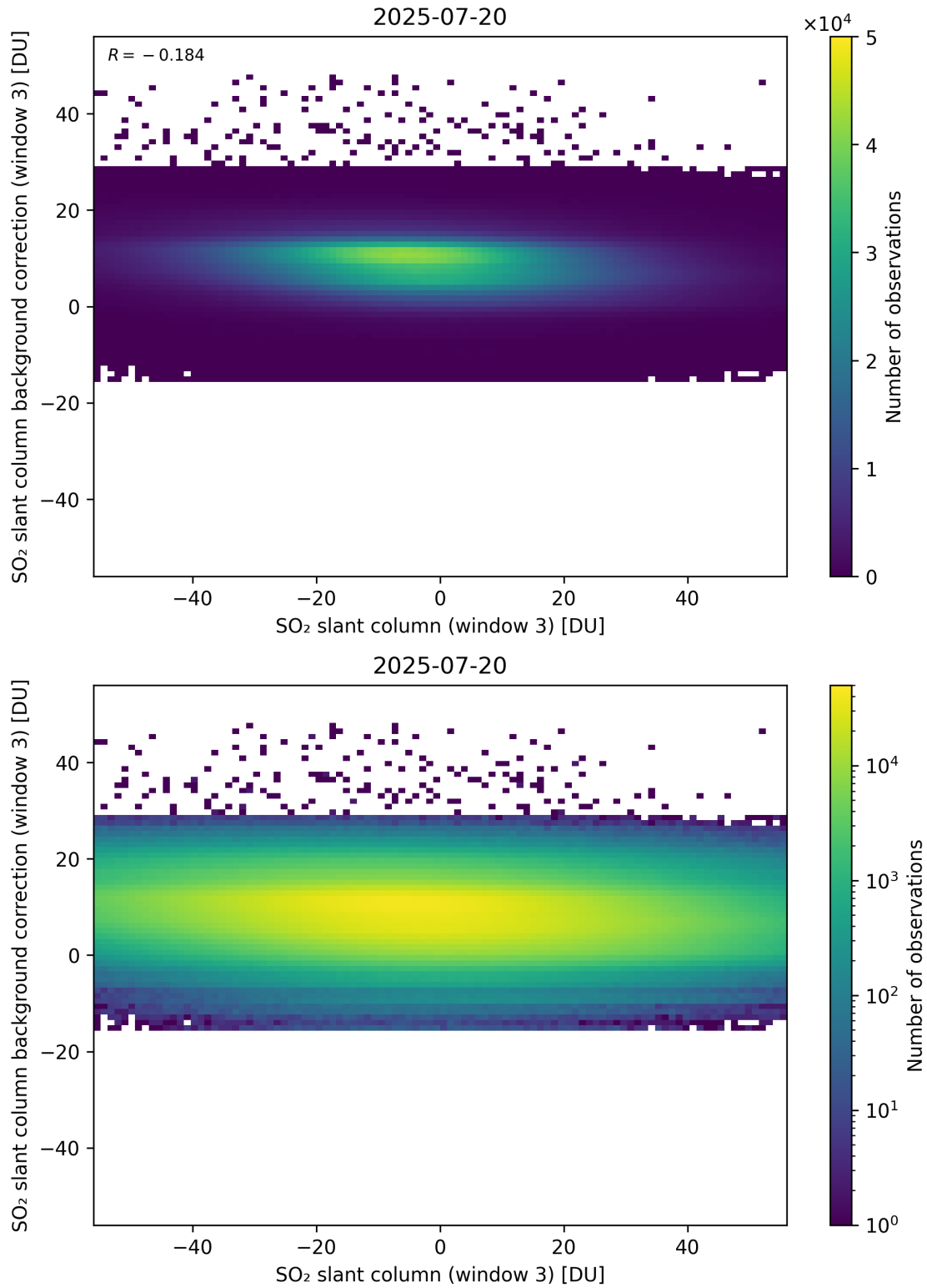
Figure 303: Scatter density plot of “SO 2 slant column (window 3)” against “SO 2 slant column background correction (window 3)” for 2025-07-19 to 2025-07-21.
