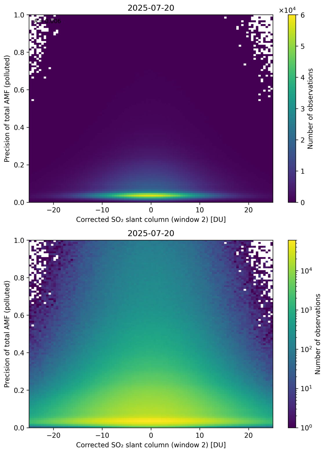
Figure 254: Scatter density plot of “Corrected SO 2 slant column (window 2)” against “Precision of total AMF (polluted)” for 2025-07-19 to 2025-07-21.
