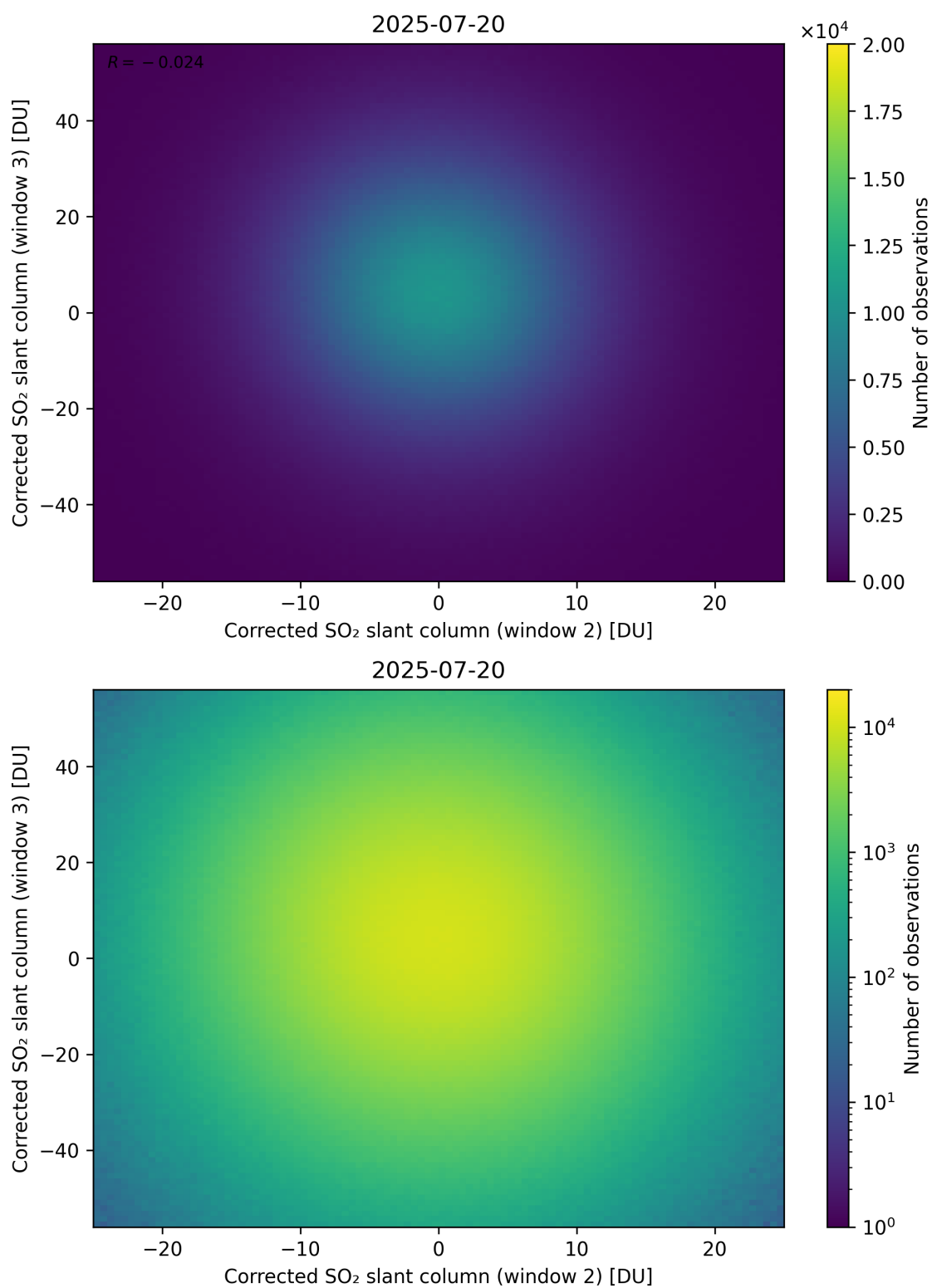
Figure 250: Scatter density plot of “Corrected SO 2 slant column (window 2)” against “Corrected SO 2 slant column (window 3)” for 2025-07-19 to 2025-07-21.
