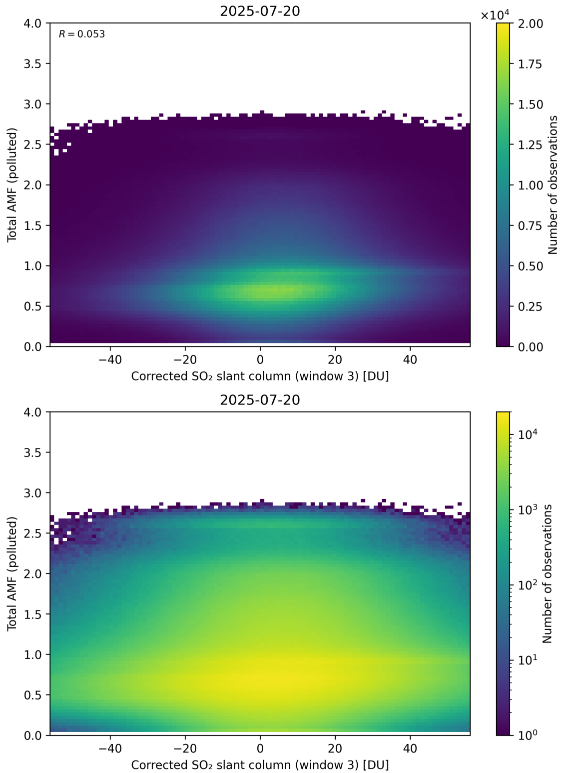
Figure 260: Scatter density plot of “Corrected SO 2 slant column (window 3)” against “Total AMF (polluted)” for 2025-07-19 to 2025-07-21.
