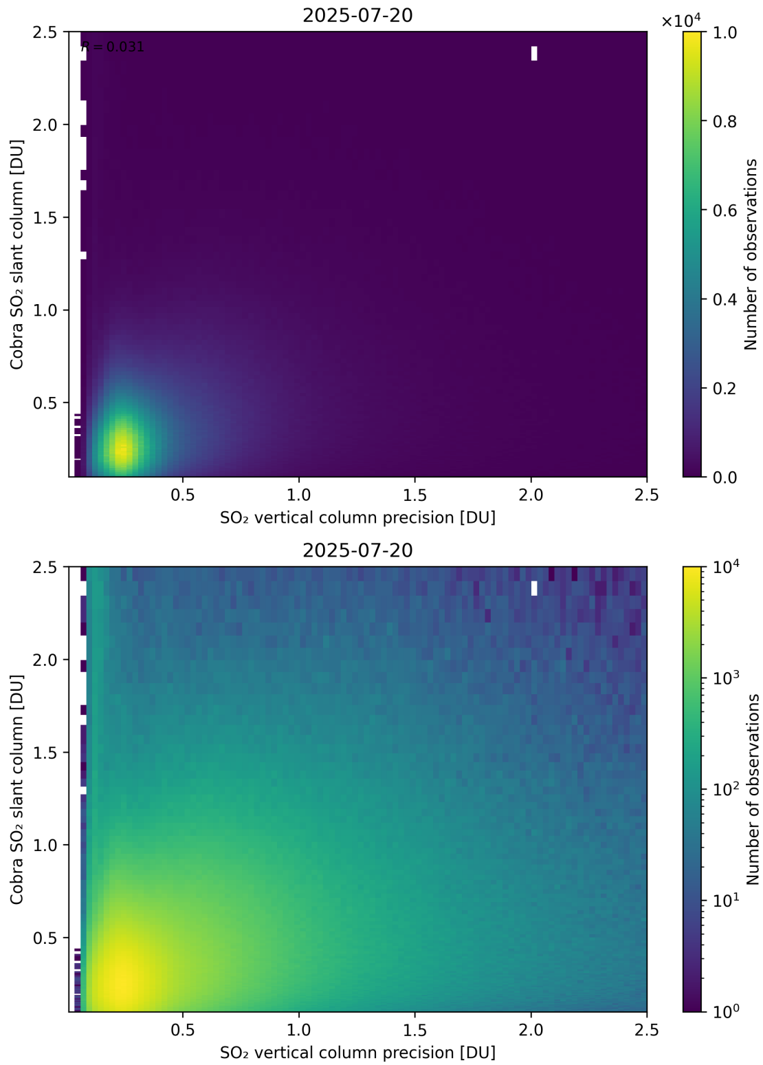
Figure 336: Scatter density plot of “SO 2 vertical column precision” against “Cobra SO 2 slant column” for 2025-07-19 to 2025-07-21.
