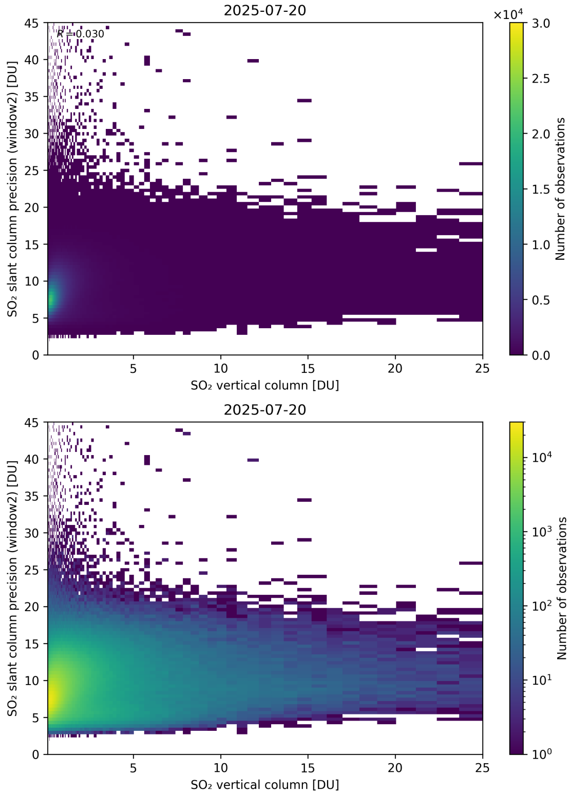
Figure 356: Scatter density plot of “SO 2 vertical column” against “SO 2 slant column precision (window2)” for 2025-07-19 to 2025-07-21.
