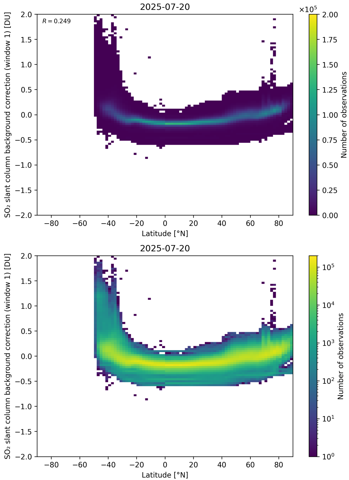
Figure 150: Scatter density plot of “Latitude” against “SO 2 slant column background correction (window 1)” for 2025-07-19 to 2025-07-21.
