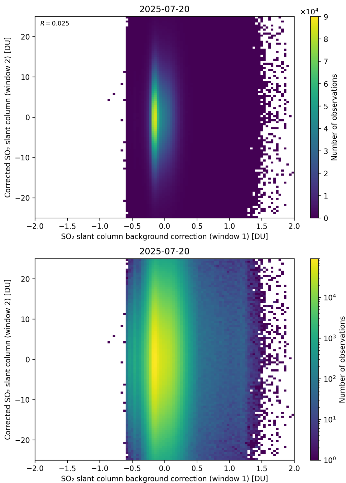
Figure 115: Scatter density plot of “SO 2 slant column background correction (window 1)” against “Corrected SO 2 slant column (window 2)” for 2025-07-19 to 2025-07-21.
