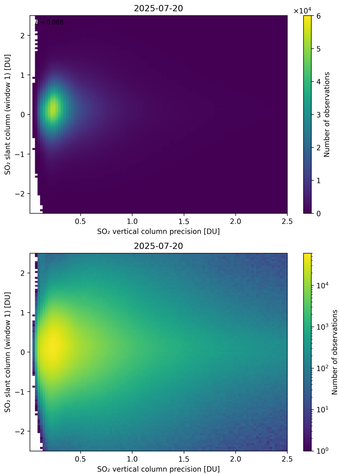
Figure 341: Scatter density plot of “SO 2 vertical column precision” against “SO 2 slant column (window 1)” for 2025-07-19 to 2025-07-21.
