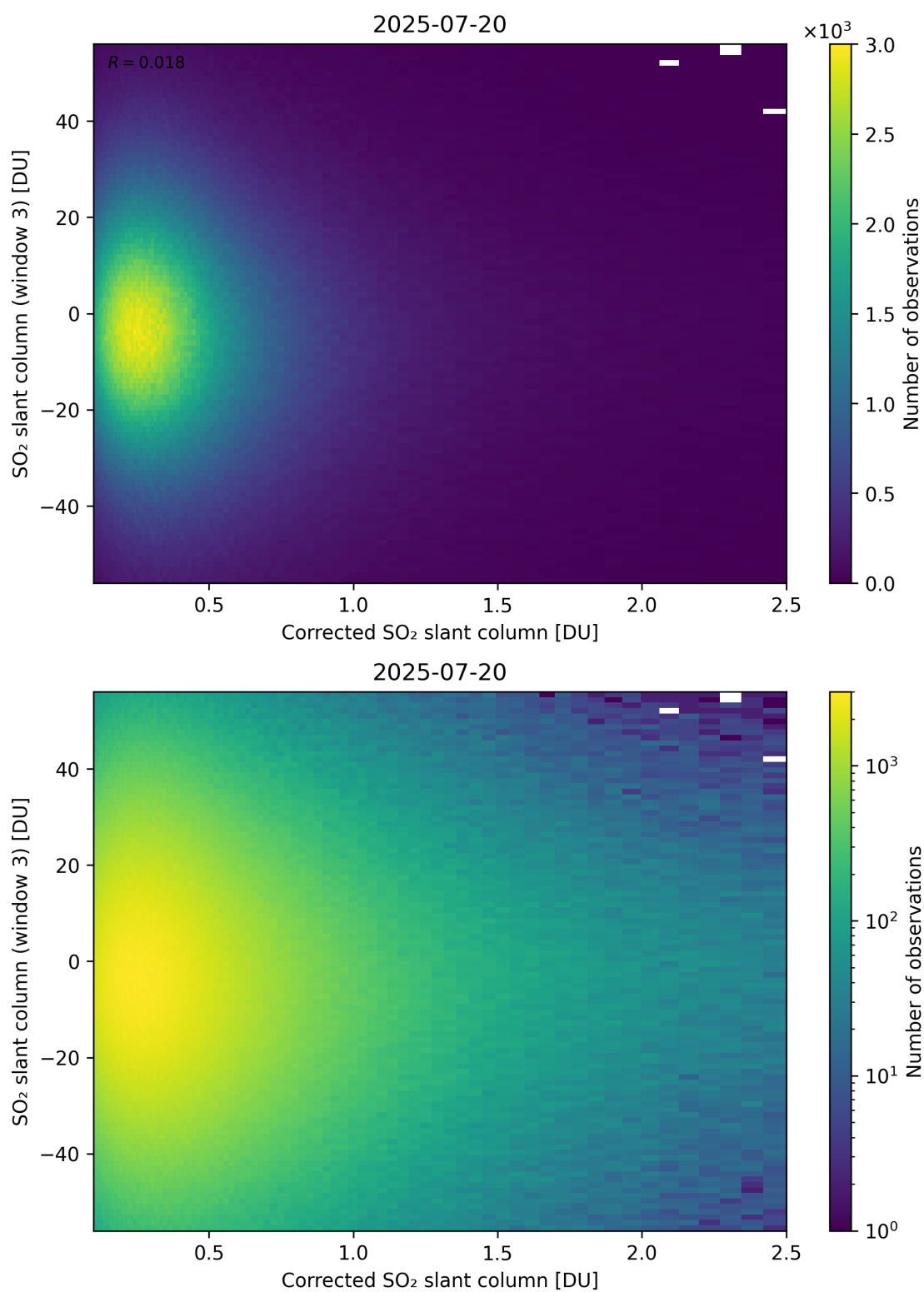
Figure 240: Scatter density plot of “Corrected SO 2 slant column” against “SO 2 slant column (window 3)” for 2025-07-19 to 2025-07-21.
