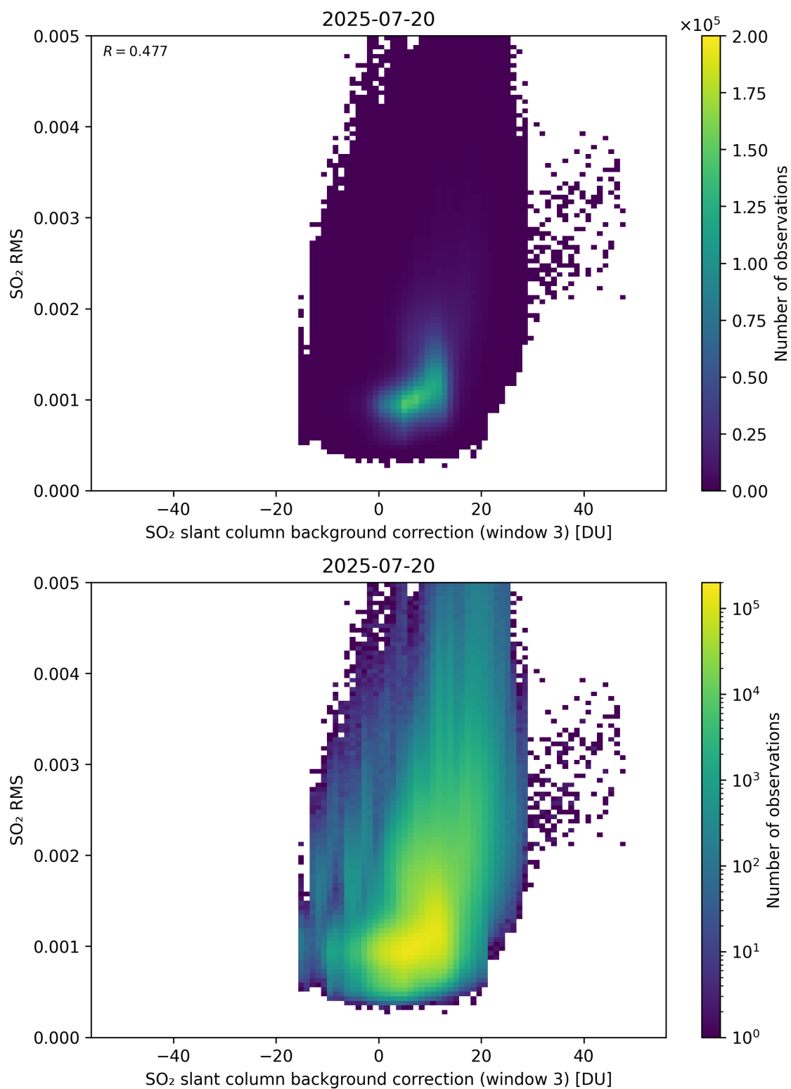
Figure 134: Scatter density plot of “SO 2 slant column background correction (window 3)” against “SO 2 RMS” for 2025-07-19 to 2025-07-21.
