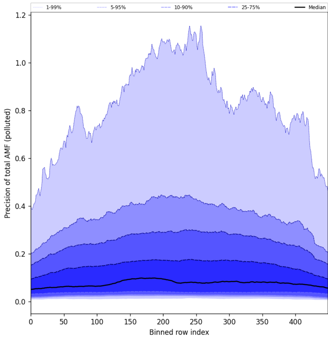
Figure 106: Along track statistics of “Precision of total AMF (polluted)” for 2025-07-19 to 2025-07-21
