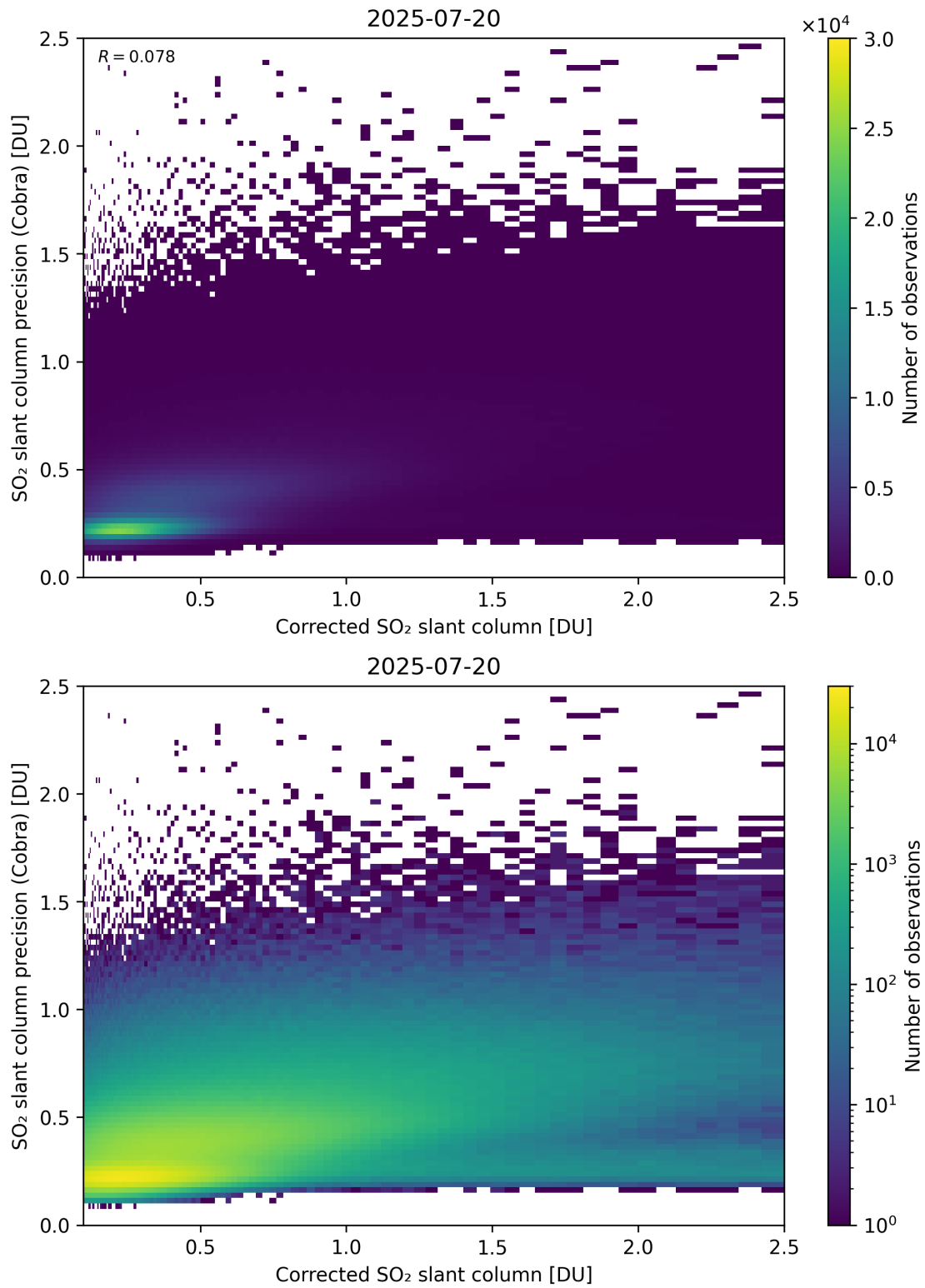
Figure 234: Scatter density plot of “Corrected SO 2 slant column” against “SO 2 slant column precision (Cobra)” for 2025-07-19 to 2025-07-21.
