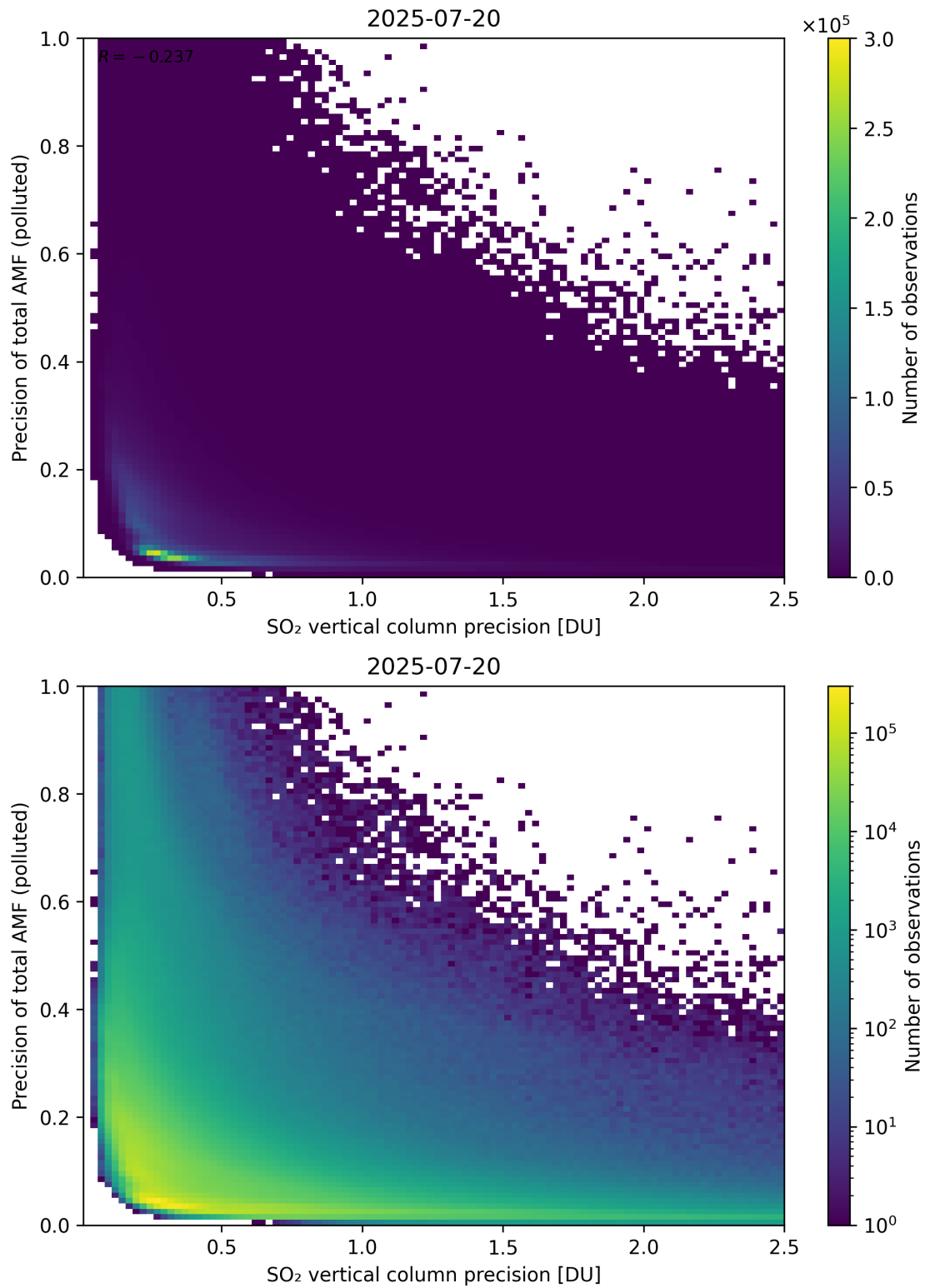
Figure 347: Scatter density plot of “SO 2 vertical column precision” against “Precision of total AMF (polluted)” for 2025-07-19 to 2025-07-21.
