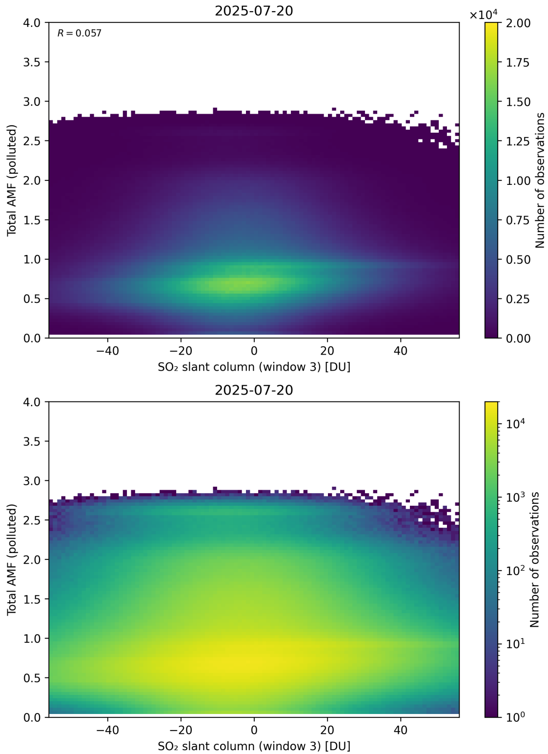
Figure 318: Scatter density plot of “SO 2 slant column (window 3)” against “Total AMF (polluted)” for 2025-07-19 to 2025-07-21.
