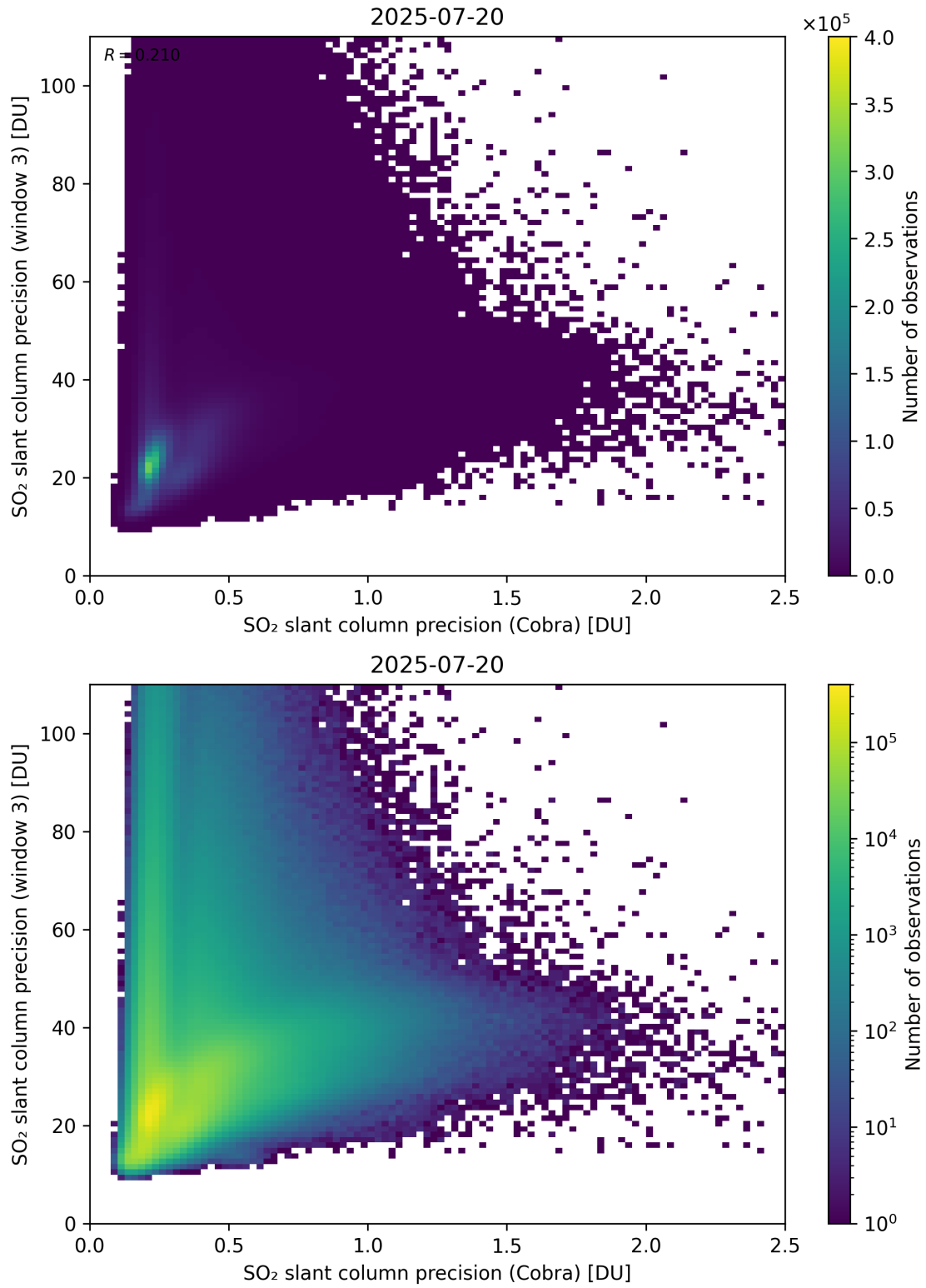
Figure 212: Scatter density plot of “SO 2 slant column precision (Cobra)” against “SO 2 slant column precision (window 3)” for 2025-07-19 to 2025-07-21.
