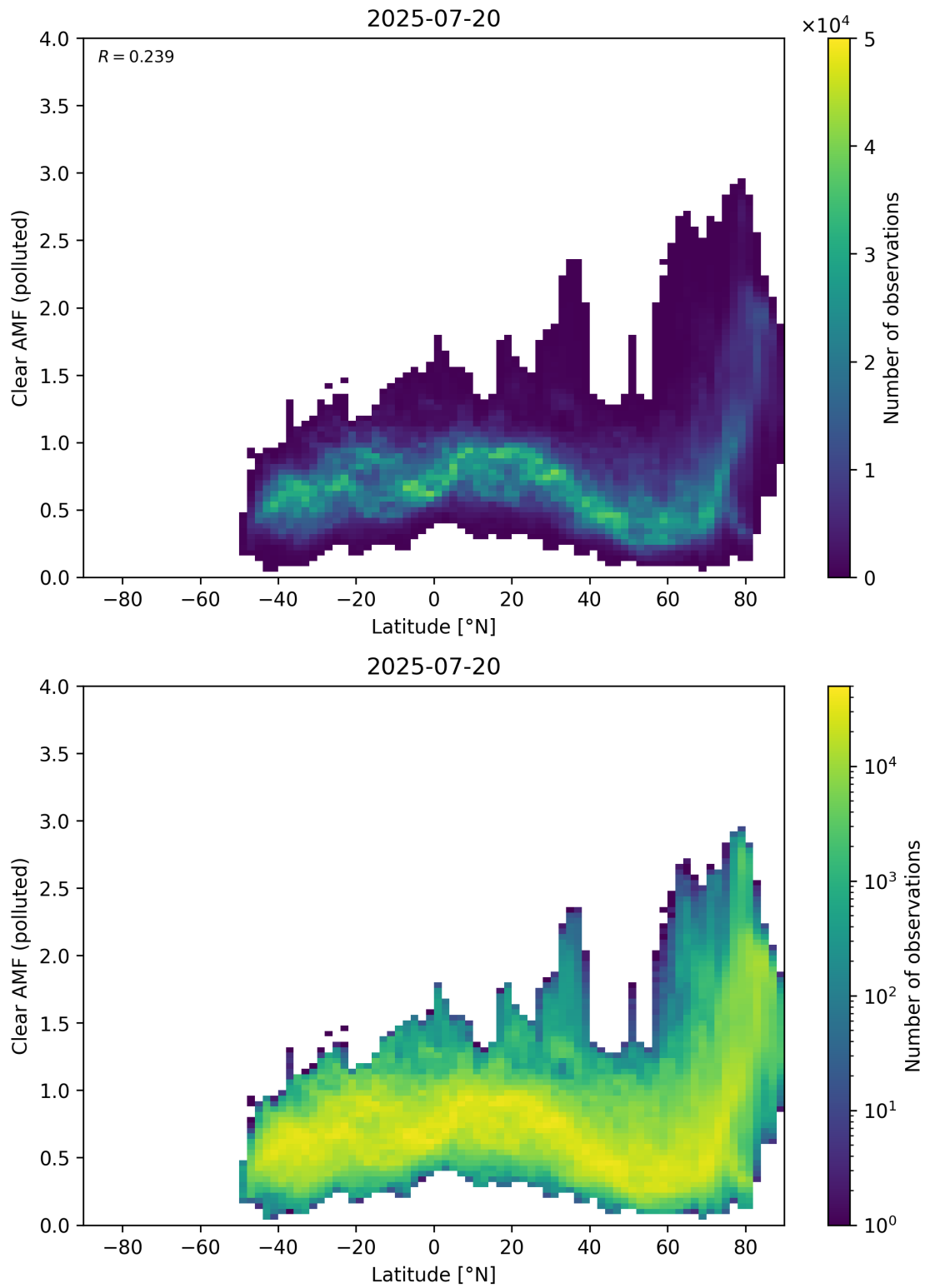
Figure 156: Scatter density plot of “Latitude” against “Clear AMF (polluted)” for 2025-07-19 to 2025-07-21.
