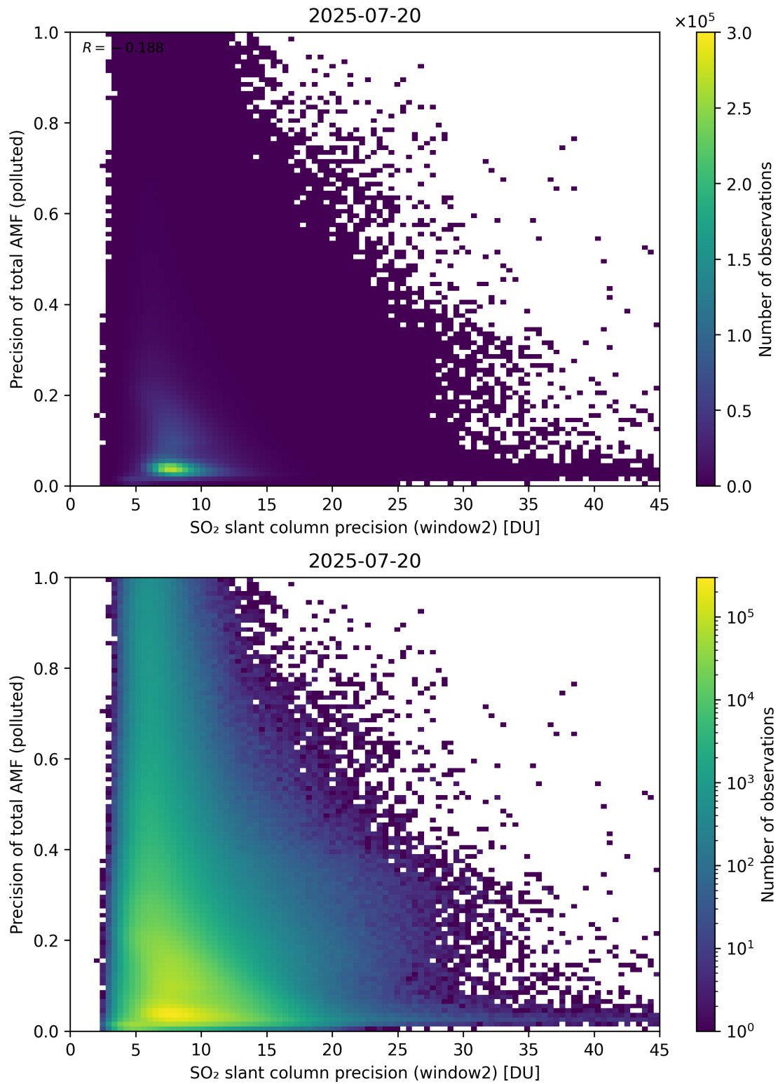
Figure 302: Scatter density plot of “SO 2 slant column precision (window2)” against “Precision of total AMF (polluted)” for 2025-07-19 to 2025-07-21.
