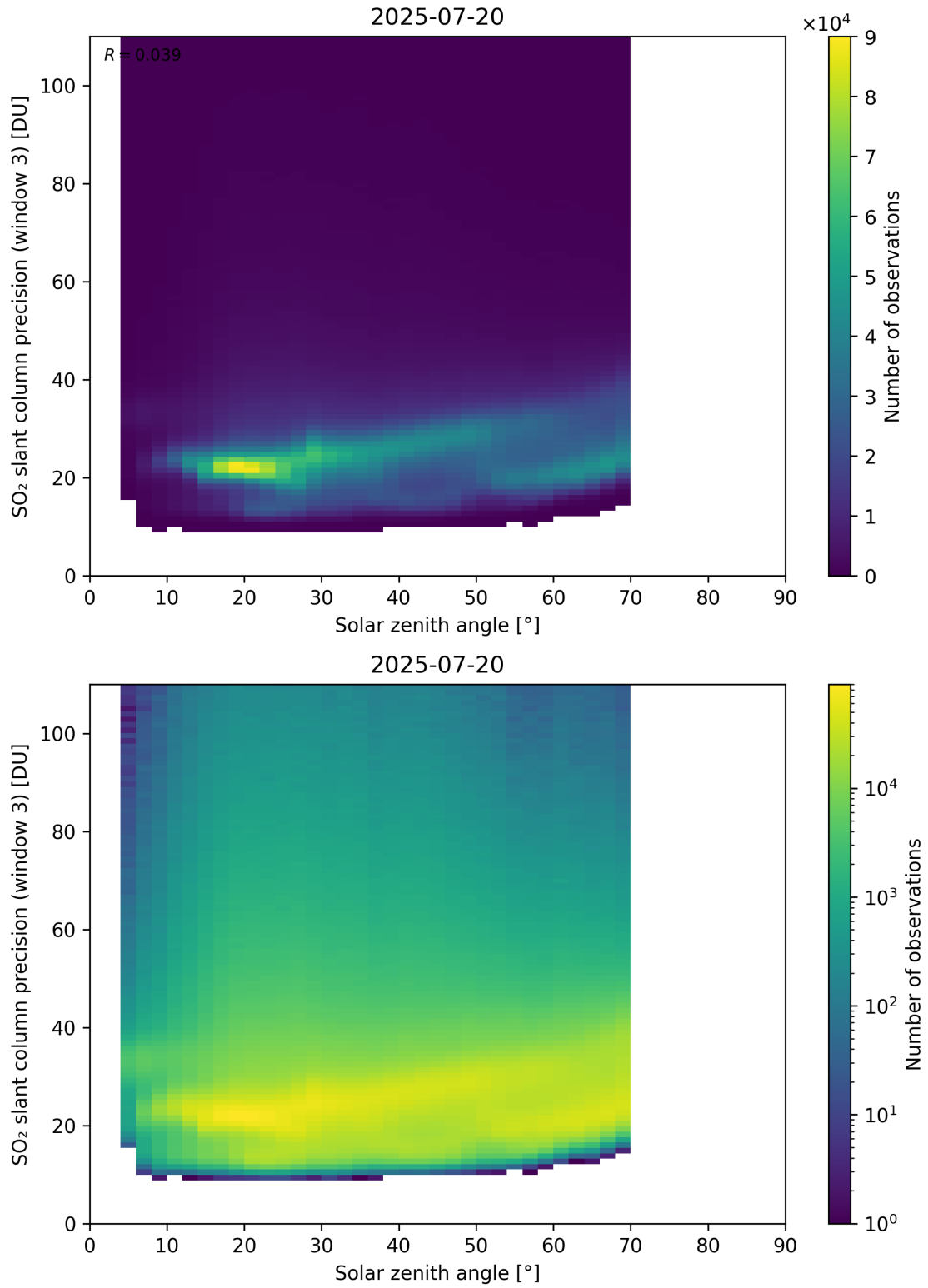
Figure 188: Scatter density plot of “Solar zenith angle” against “SO 2 slant column precision (window 3)” for 2025-07-19 to 2025-07-21.
