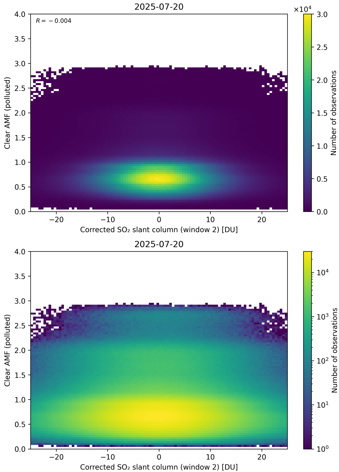
Figure 249: Scatter density plot of “Corrected SO 2 slant column (window 2)” against “Clear AMF (polluted)” for 2025-07-19 to 2025-07-21.
