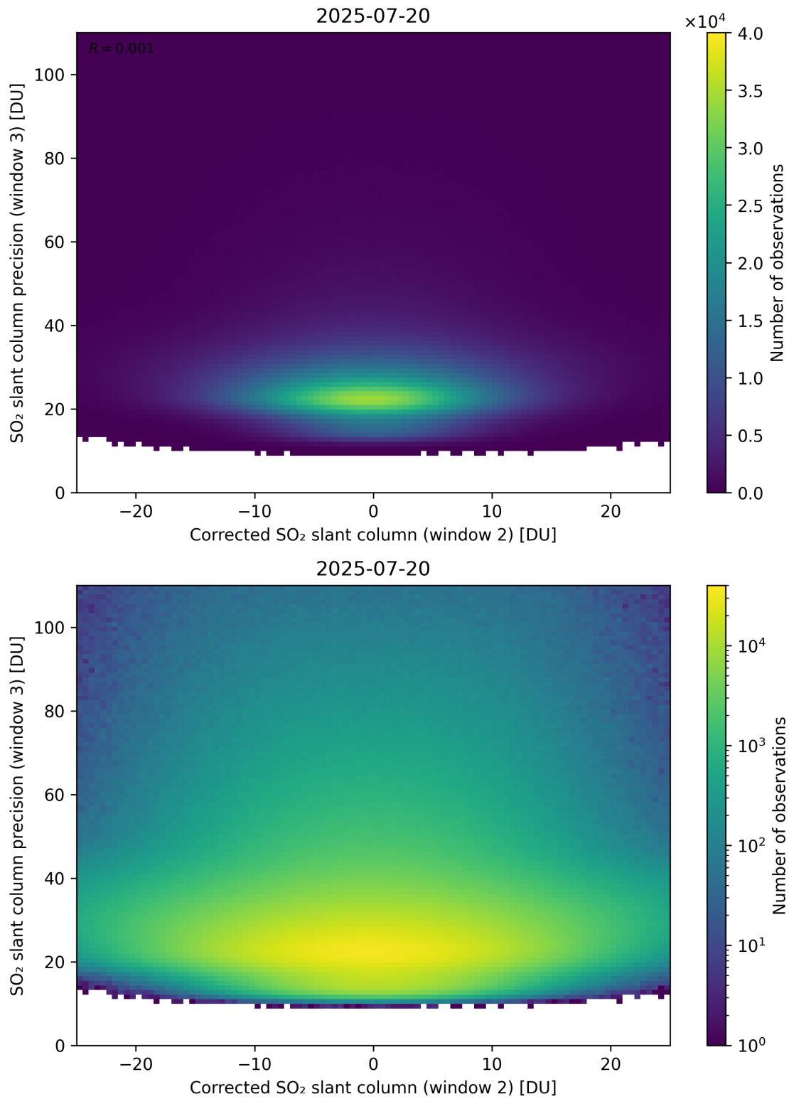
Figure 252: Scatter density plot of “Corrected SO 2 slant column (window 2)” against “SO 2 slant column precision (window 3)” for 2025-07-19 to 2025-07-21.
