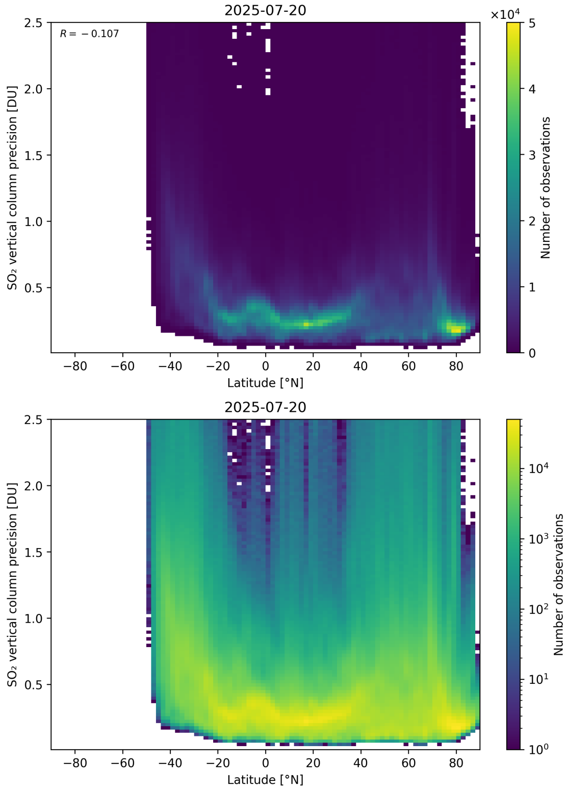
Figure 170: Scatter density plot of “Latitude” against “SO 2 vertical column precision” for 2025-07-19 to 2025-07-21.
