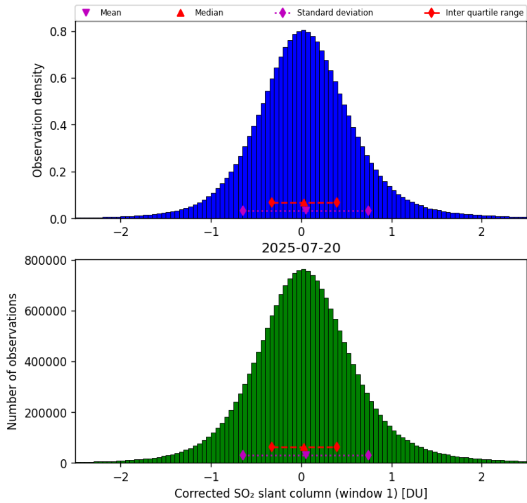
Figure 65: Histogram of “Corrected SO 2 slant column (window 1)” for 2025-07-19 to 2025-07-21
