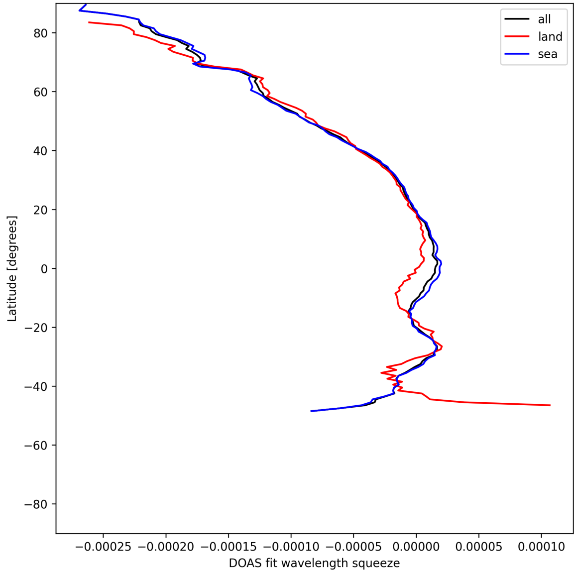
Figure 51: Zonal average of “DOAS fit wavelength squeeze” for 2025-07-19 to 2025-07-21.
