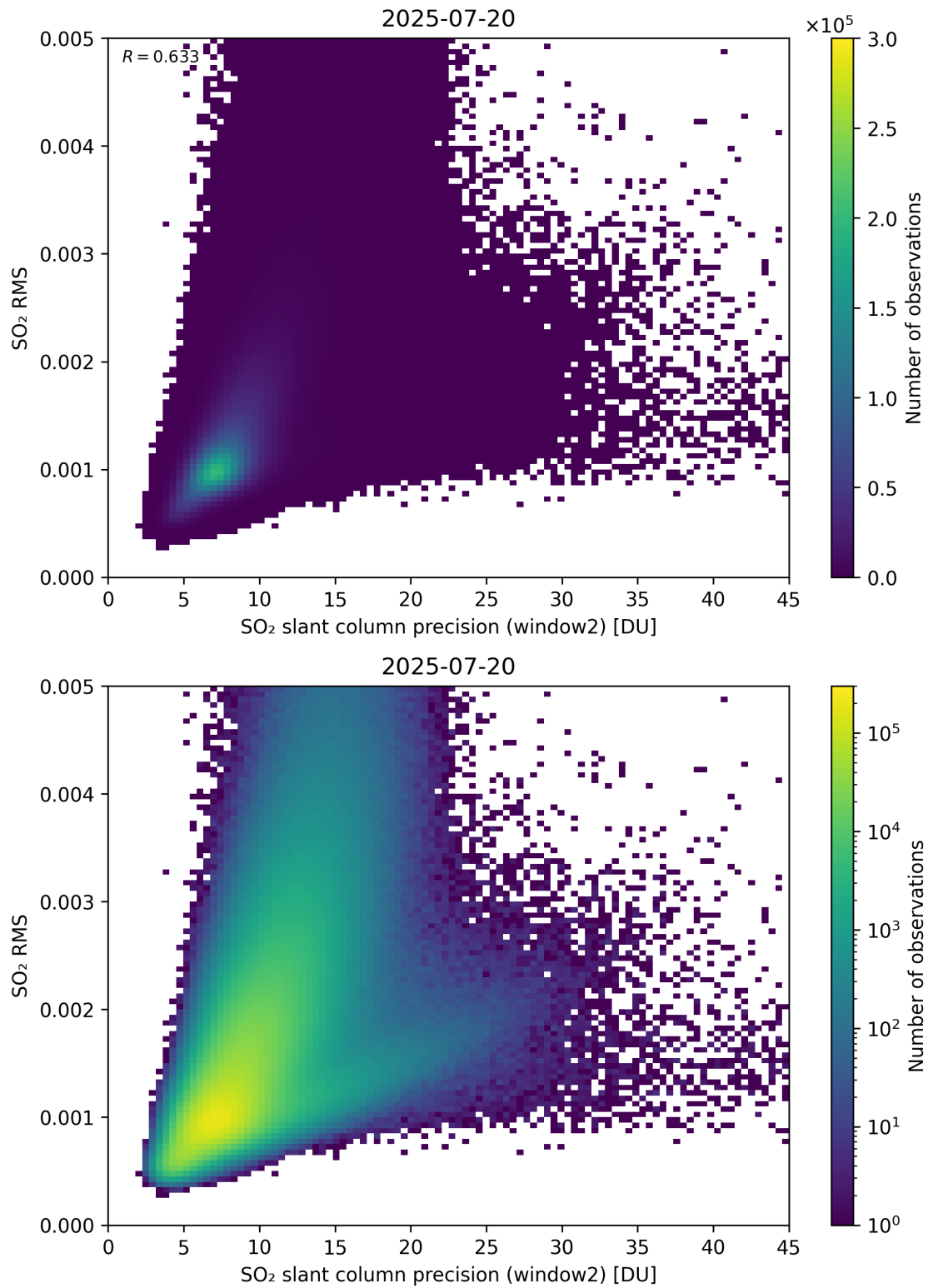
Figure 295: Scatter density plot of “SO 2 slant column precision (window2)” against “SO 2 RMS” for 2025-07-19 to 2025-07-21.
