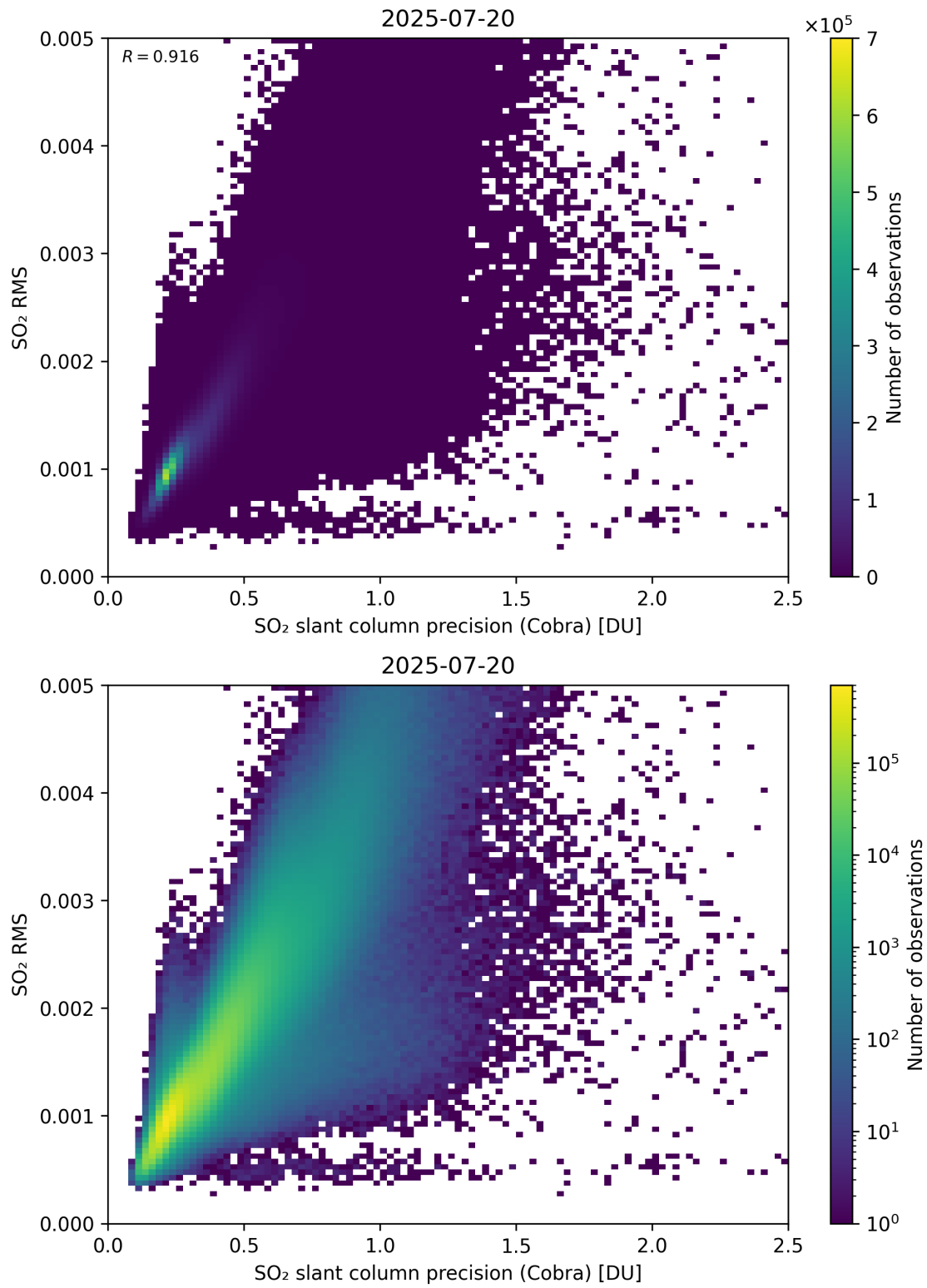
Figure 204: Scatter density plot of “SO 2 slant column precision (Cobra)” against “SO 2 RMS” for 2025-07-19 to 2025-07-21.
