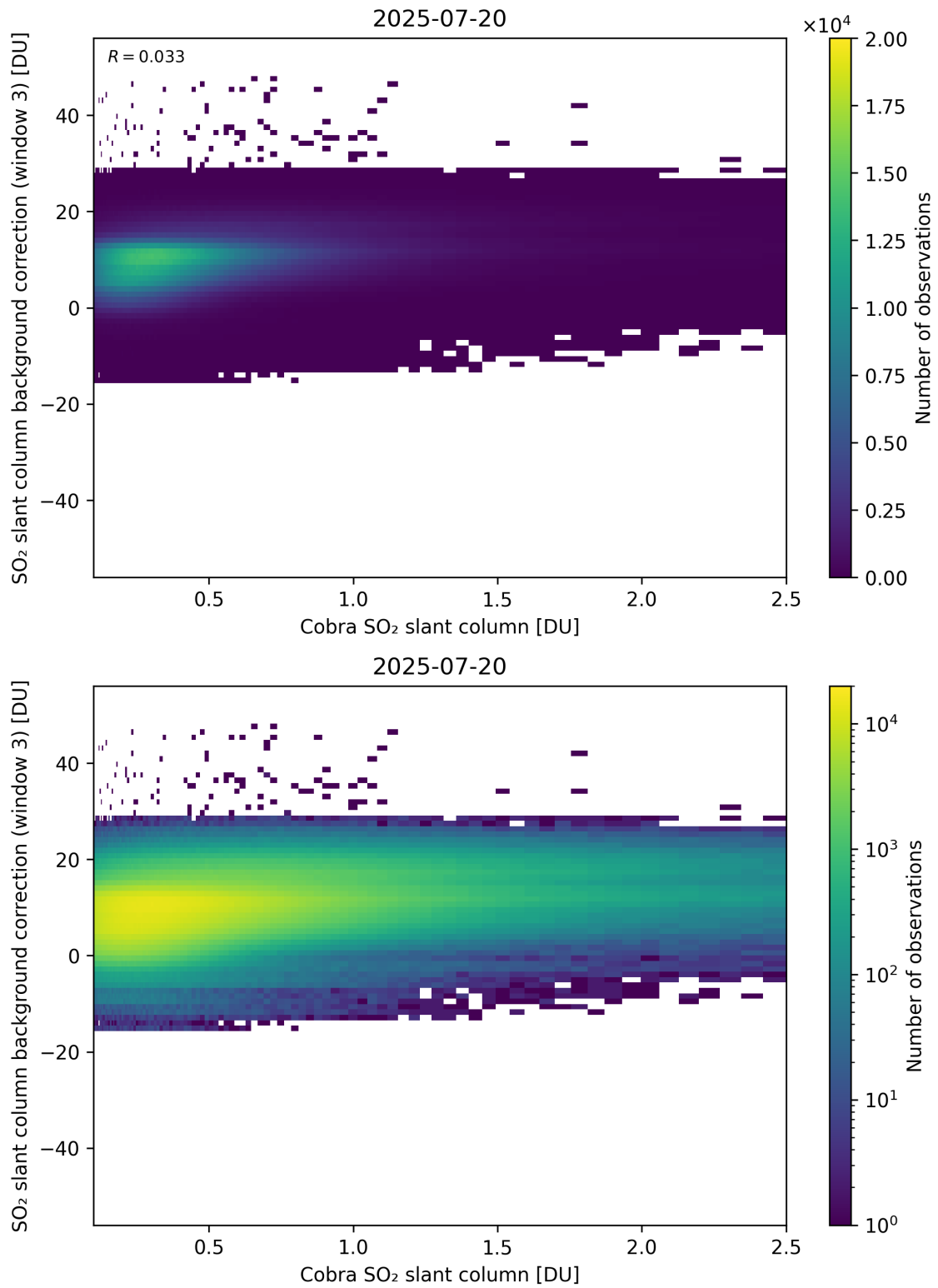
Figure 195: Scatter density plot of “Cobra SO 2 slant column” against “SO 2 slant column background correction (window 3)” for 2025-07-19 to 2025-07-21.
