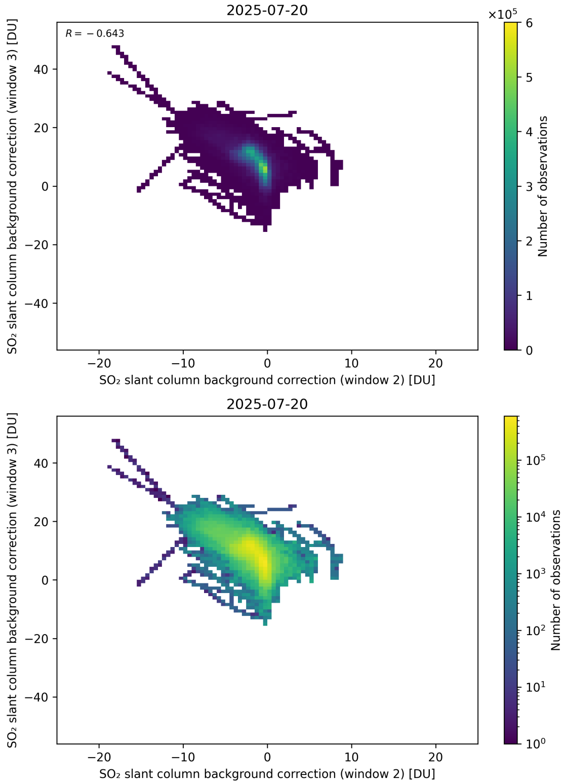
Figure 122: Scatter density plot of “SO 2 slant column background correction (window 2)” against “SO 2 slant column background correction (window 3)” for 2025-07-19 to 2025-07-21.
