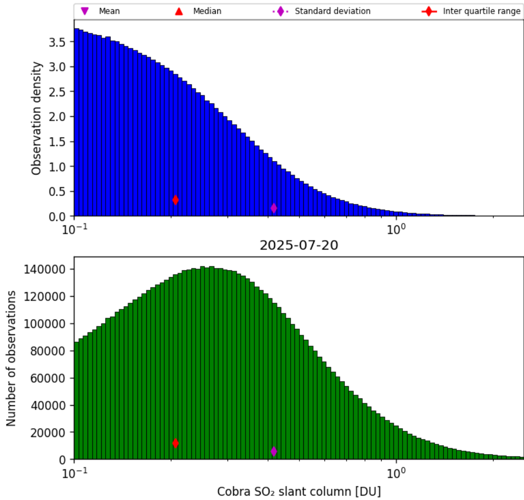
Figure 61: Histogram of “Cobra SO 2 slant column” for 2025-07-19 to 2025-07-21
