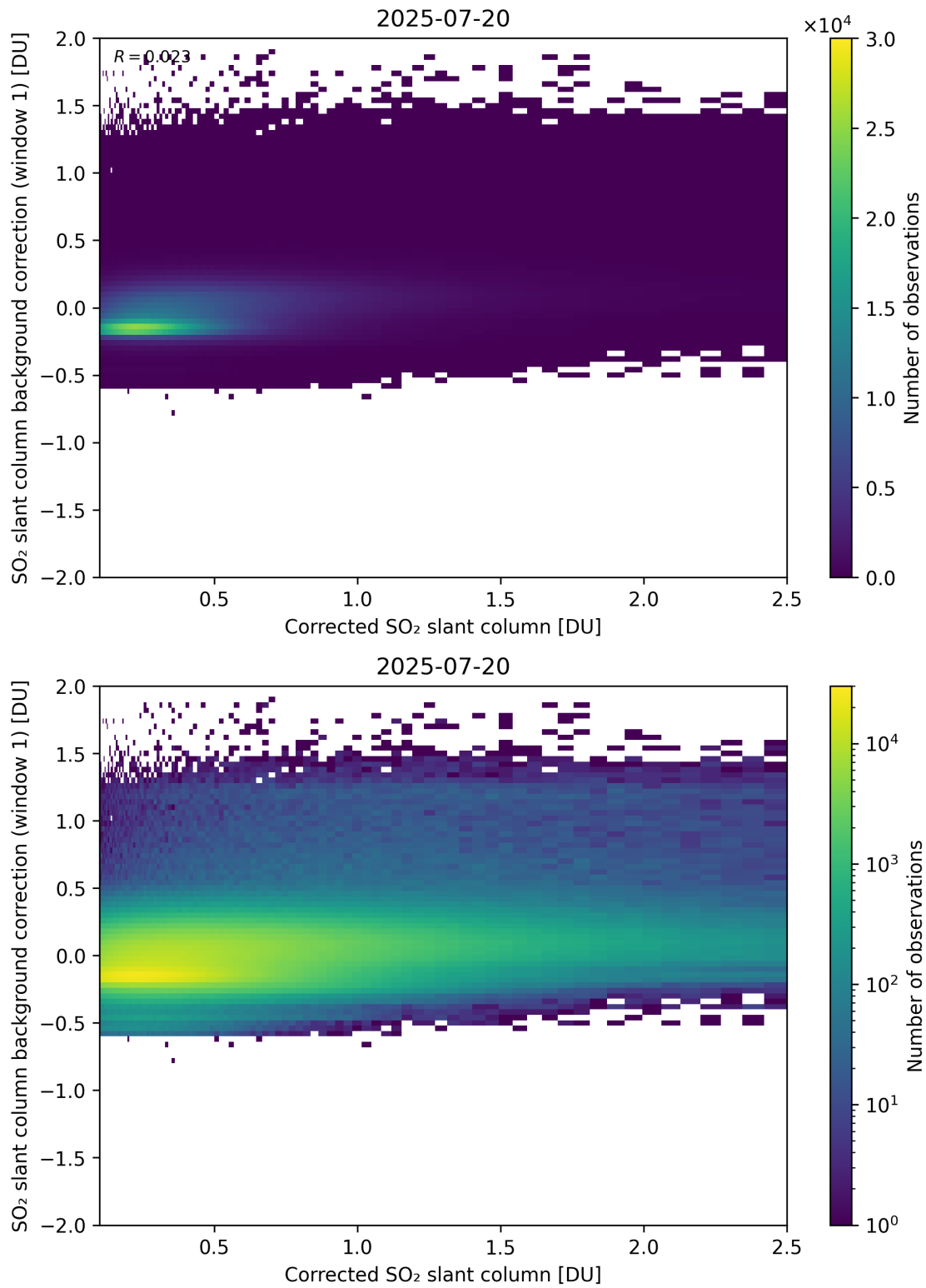
Figure 226: Scatter density plot of “Corrected SO 2 slant column” against “SO 2 slant column background correction (window 1)” for 2025-07-19 to 2025-07-21.
