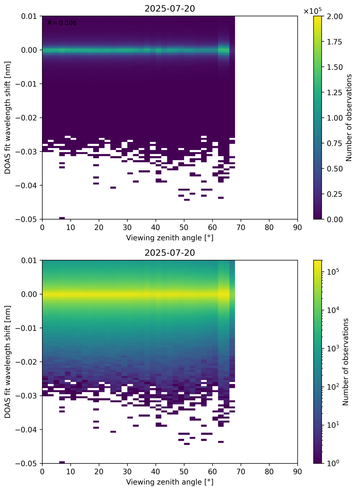
Figure 365: Scatter density plot of “Viewing zenith angle” against “DOAS fit wavelength shift” for 2025-07-19 to 2025-07-21.
