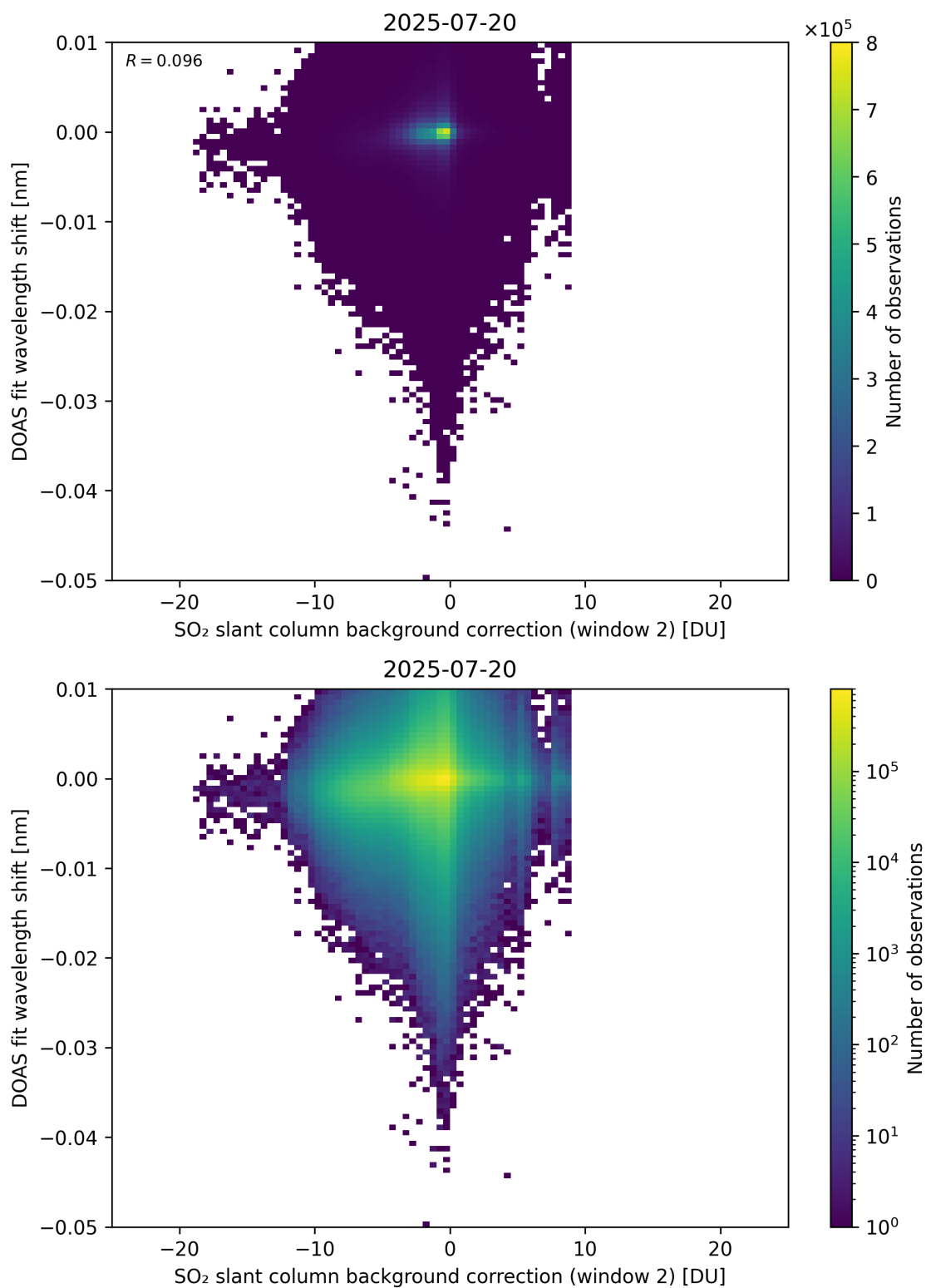
Figure 123: Scatter density plot of “SO 2 slant column background correction (window 2)” against “DOAS fit wavelength shift” for 2025-07-19 to 2025-07-21.
