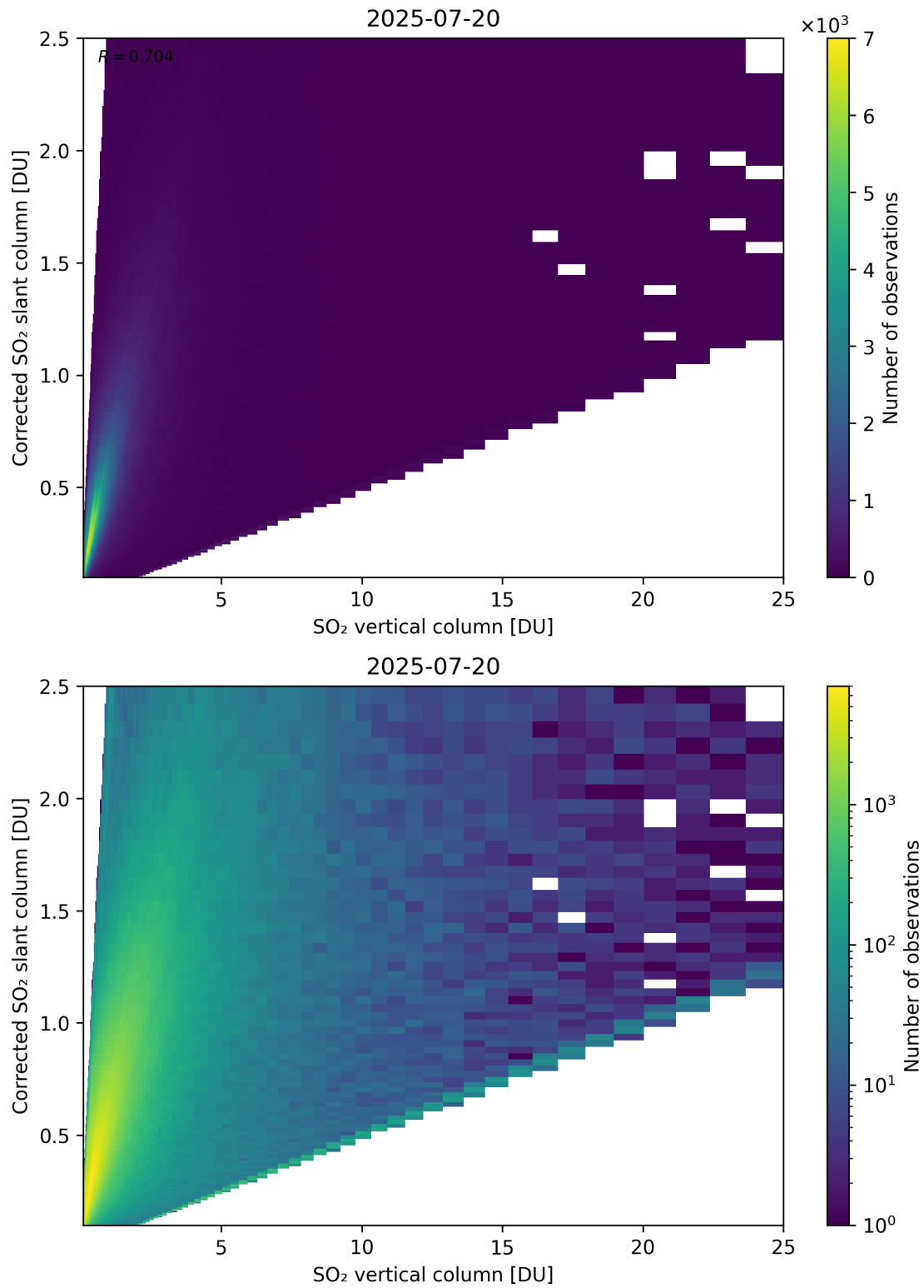
Figure 351: Scatter density plot of “SO 2 vertical column” against “Corrected SO 2 slant column” for 2025-07-19 to 2025-07-21.
