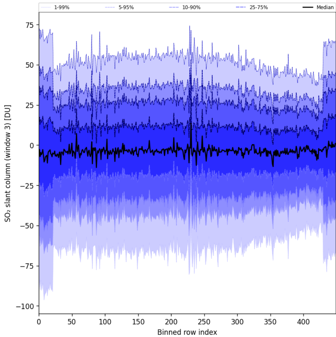
Figure 97: Along track statistics of “SO 2 slant column (window 3)” for 2025-07-19 to 2025-07-21
