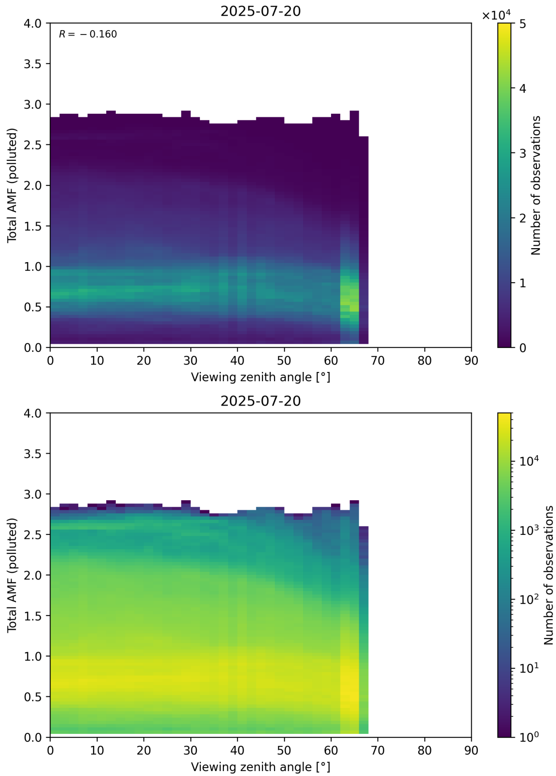
Figure 381: Scatter density plot of “Viewing zenith angle” against “Total AMF (polluted)” for 2025-07-19 to 2025-07-21.
