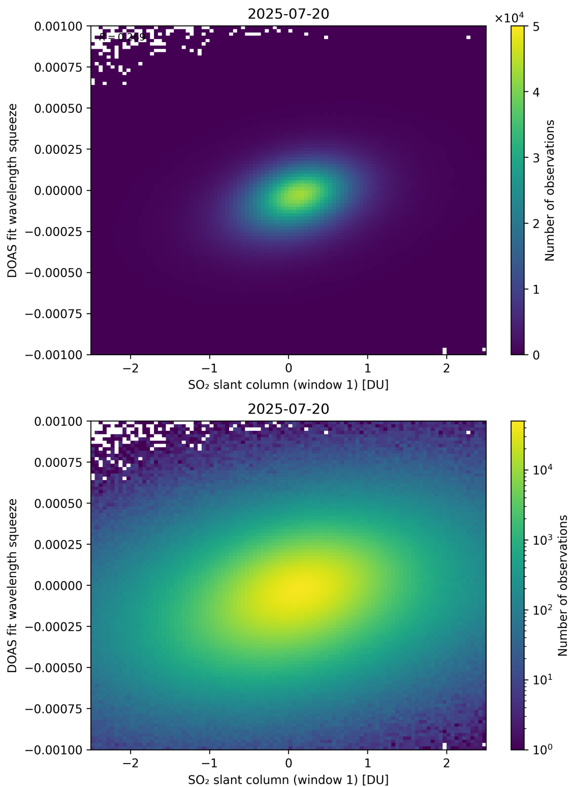
Figure 266: Scatter density plot of “SO 2 slant column (window 1)” against “DOAS fit wavelength squeeze” for 2025-07-19 to 2025-07-21.
