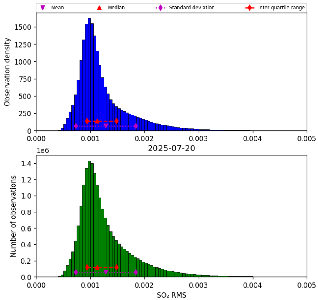
Figure 78: Histogram of “SO 2 RMS” for 2025-07-19 to 2025-07-21
