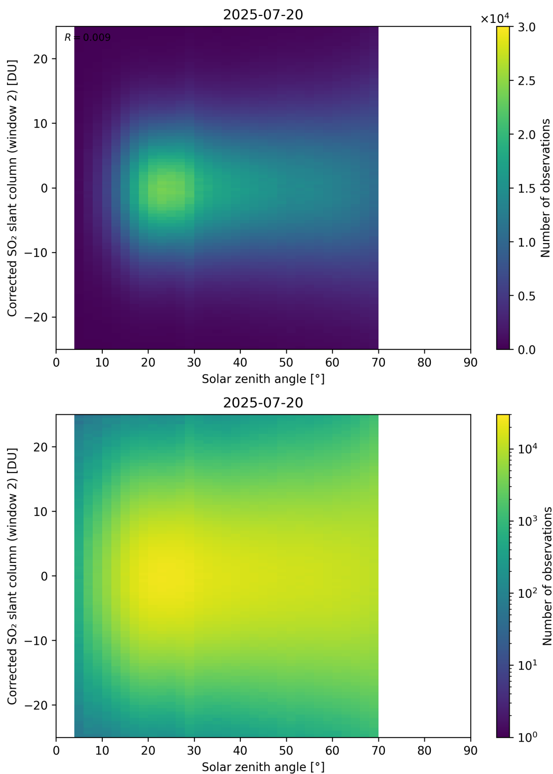
Figure 182: Scatter density plot of “Solar zenith angle” against “Corrected SO 2 slant column (window 2)” for 2025-07-19 to 2025-07-21.
