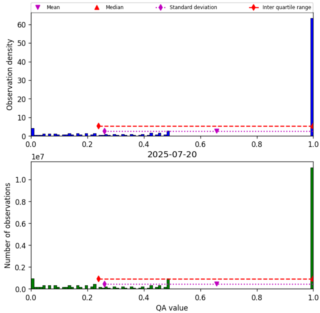
Figure 57: Histogram of “QA value” for 2025-07-19 to 2025-07-21
