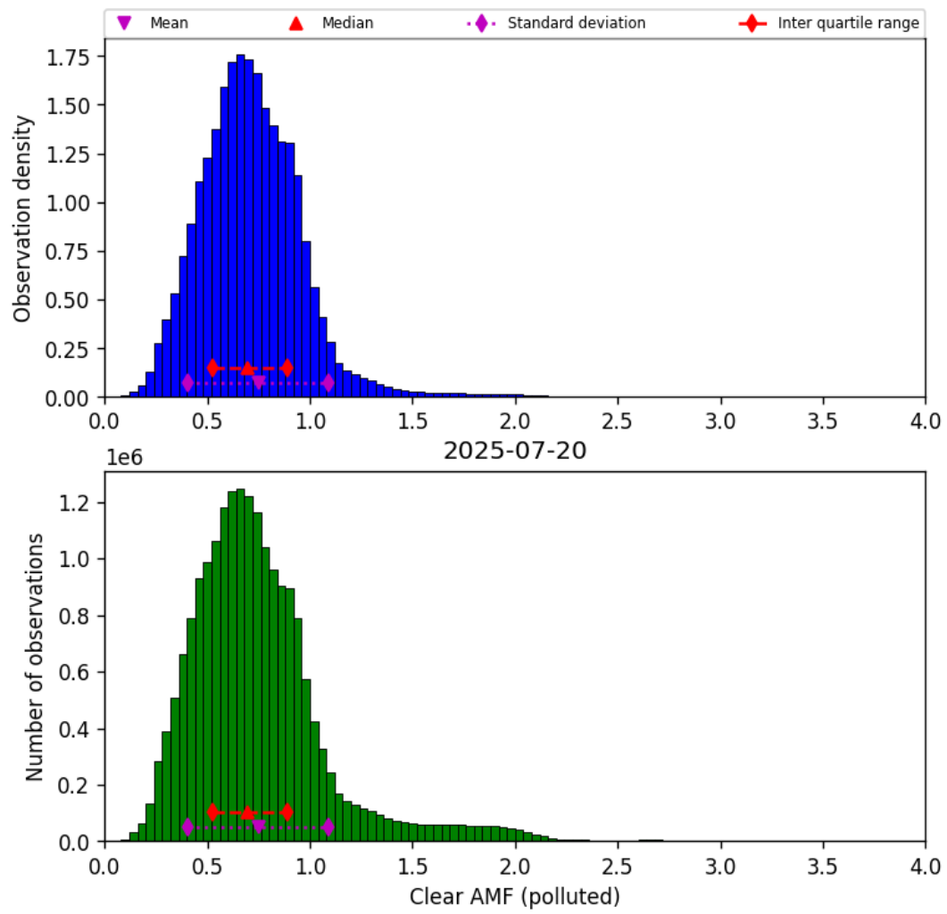
Figure 81: Histogram of “Clear AMF (polluted)” for 2025-07-19 to 2025-07-21
