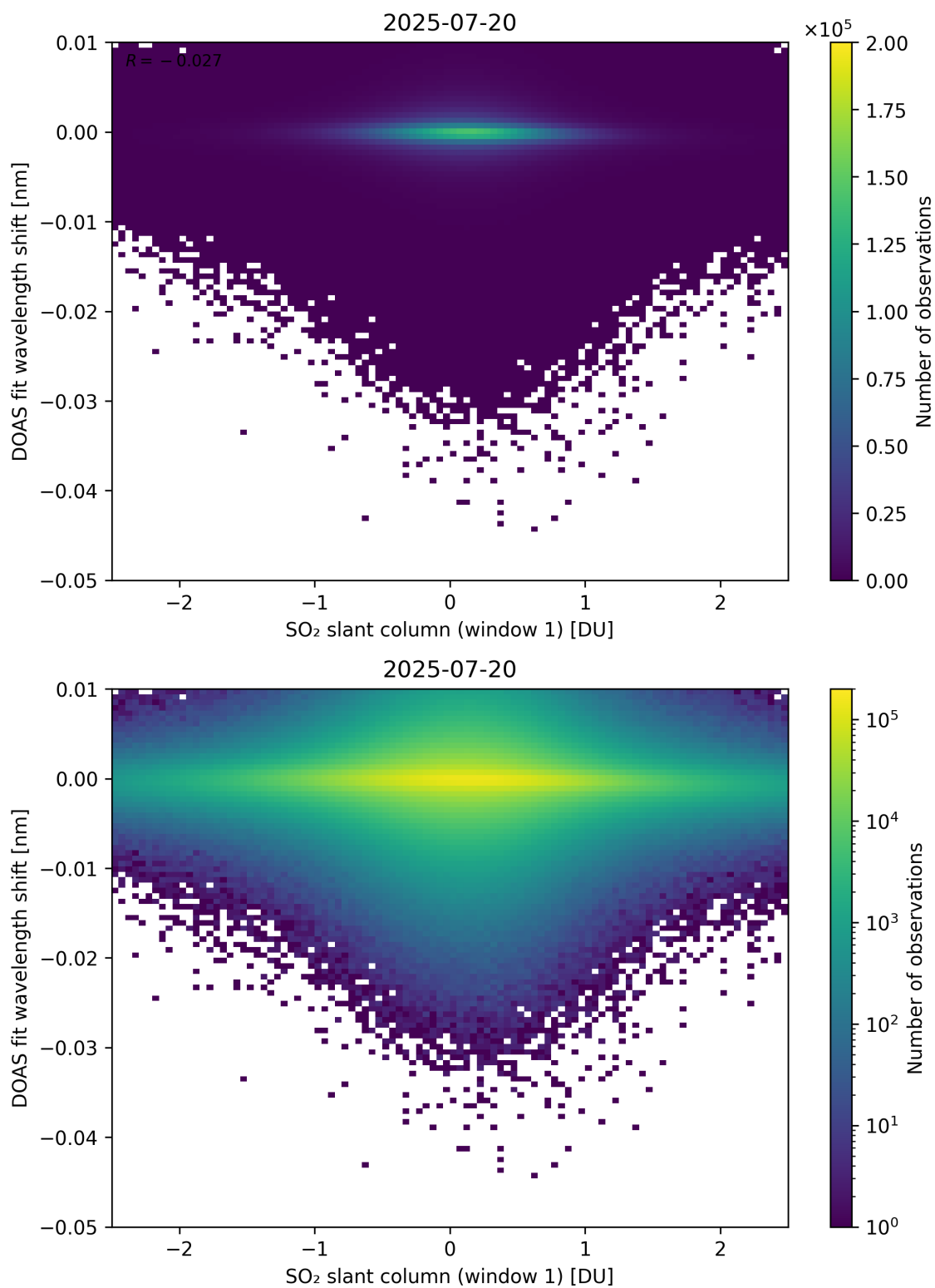
Figure 265: Scatter density plot of “SO 2 slant column (window 1)” against “DOAS fit wavelength shift” for 2025-07-19 to 2025-07-21.
