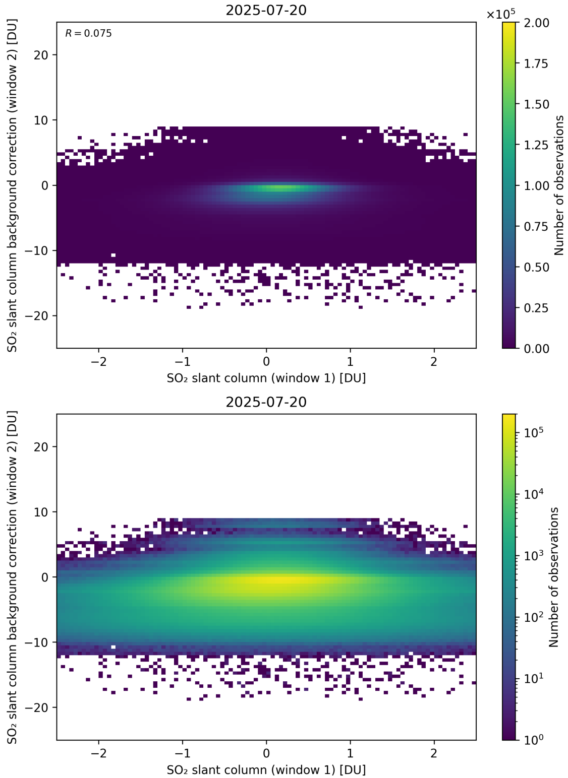
Figure 263: Scatter density plot of “SO 2 slant column (window 1)” against “SO 2 slant column background correction (window 2)” for 2025-07-19 to 2025-07-21.
