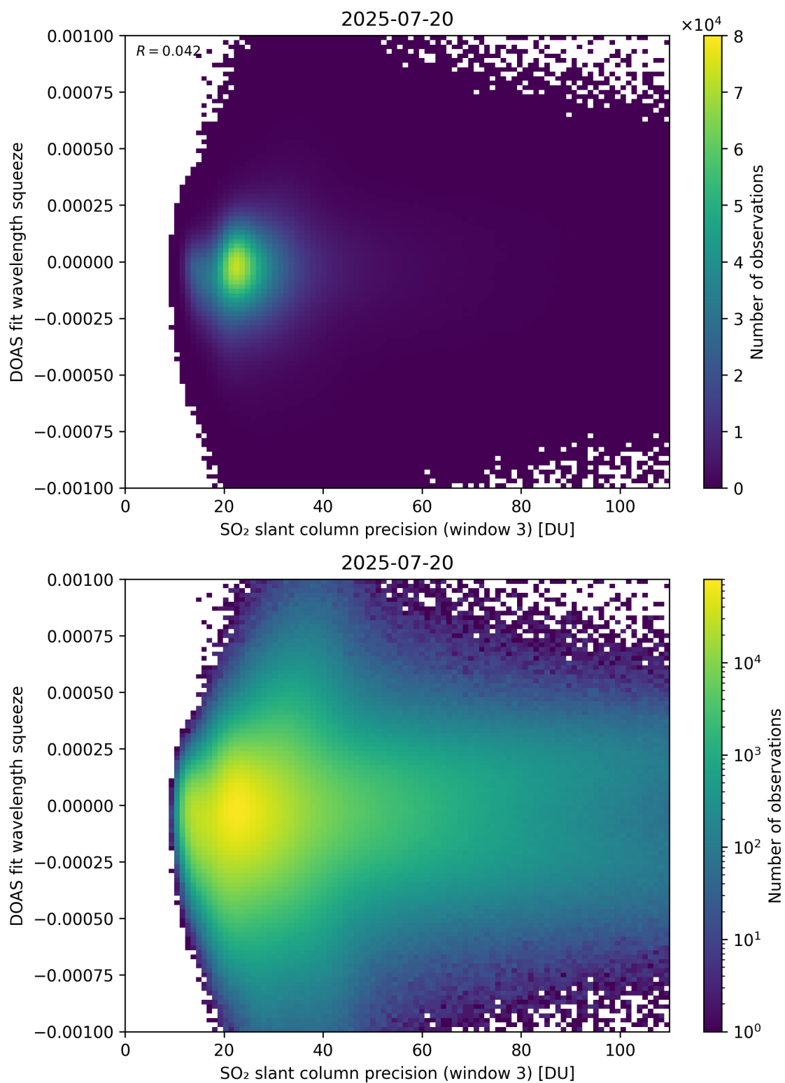
Figure 309: Scatter density plot of “SO 2 slant column precision (window 3)” against “DOAS fit wavelength squeeze” for 2025-07-19 to 2025-07-21.
