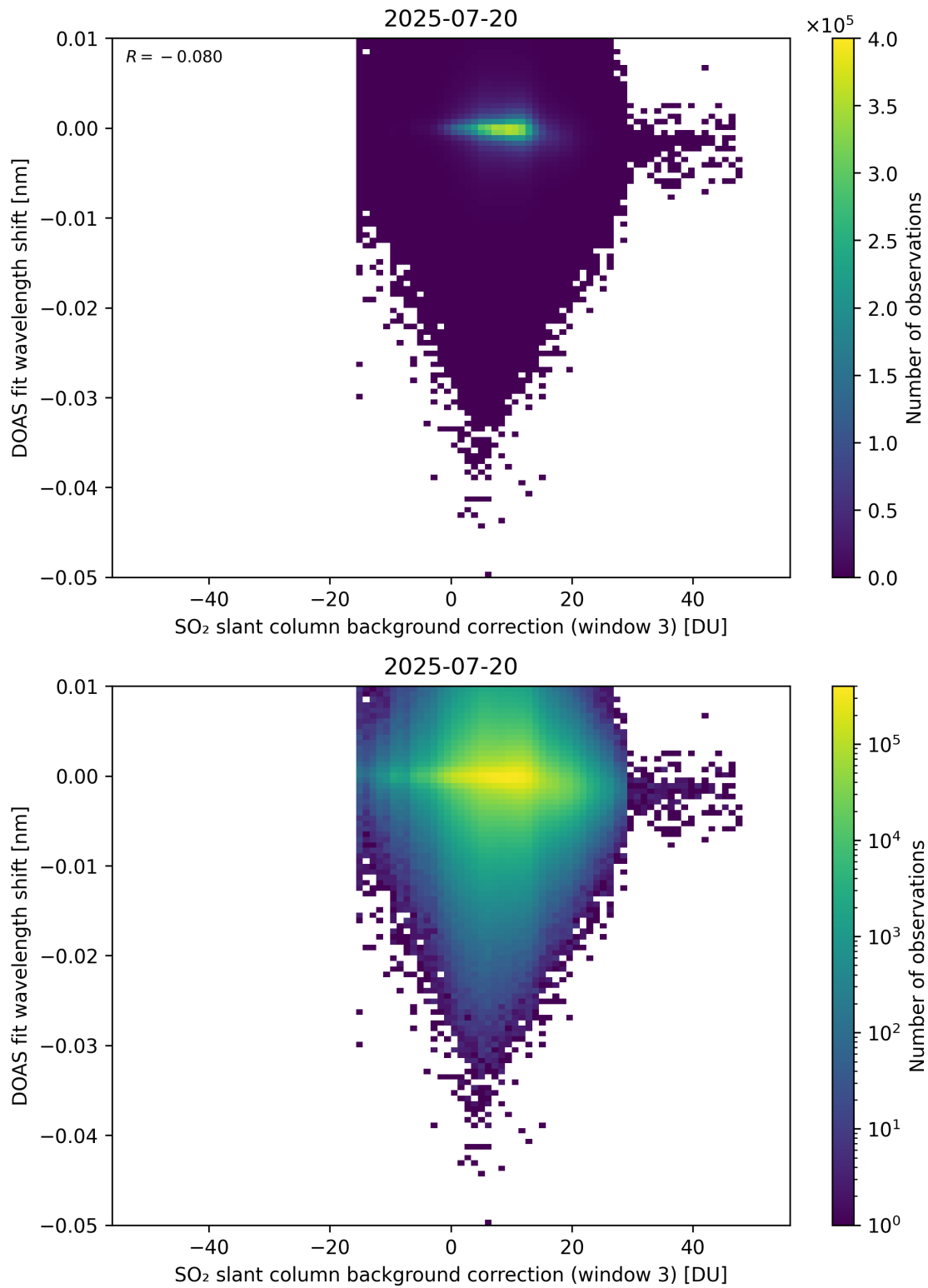
Figure 132: Scatter density plot of “SO 2 slant column background correction (window 3)” against “DOAS fit wavelength shift” for 2025-07-19 to 2025-07-21.
