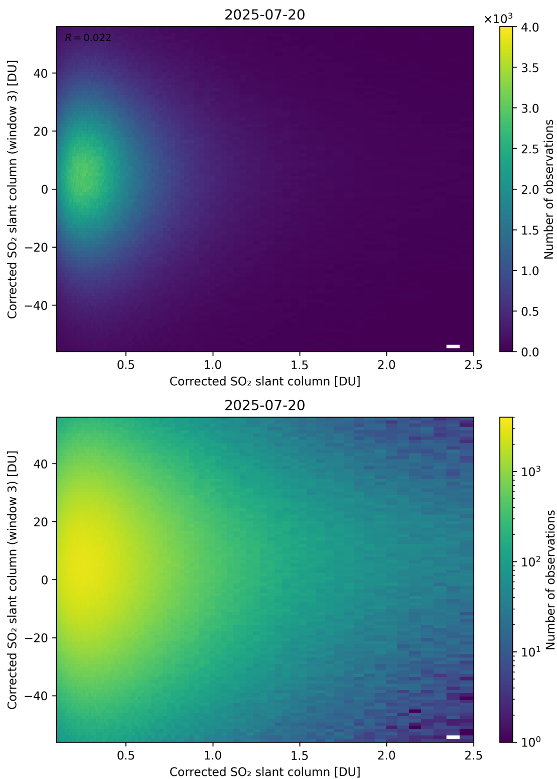
Figure 236: Scatter density plot of “Corrected SO 2 slant column” against “Corrected SO 2 slant column (window 3)” for 2025-07-19 to 2025-07-21.
