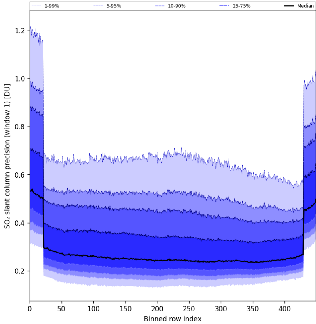
Figure 90: Along track statistics of “SO 2 slant column precision (window 1)” for 2025-07-19 to 2025-07-21
