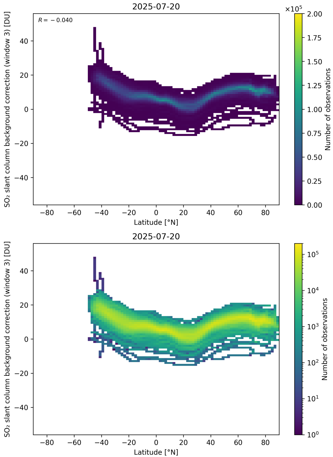
Figure 152: Scatter density plot of “Latitude” against “SO 2 slant column background correction (window 3)” for 2025-07-19 to 2025-07-21.
