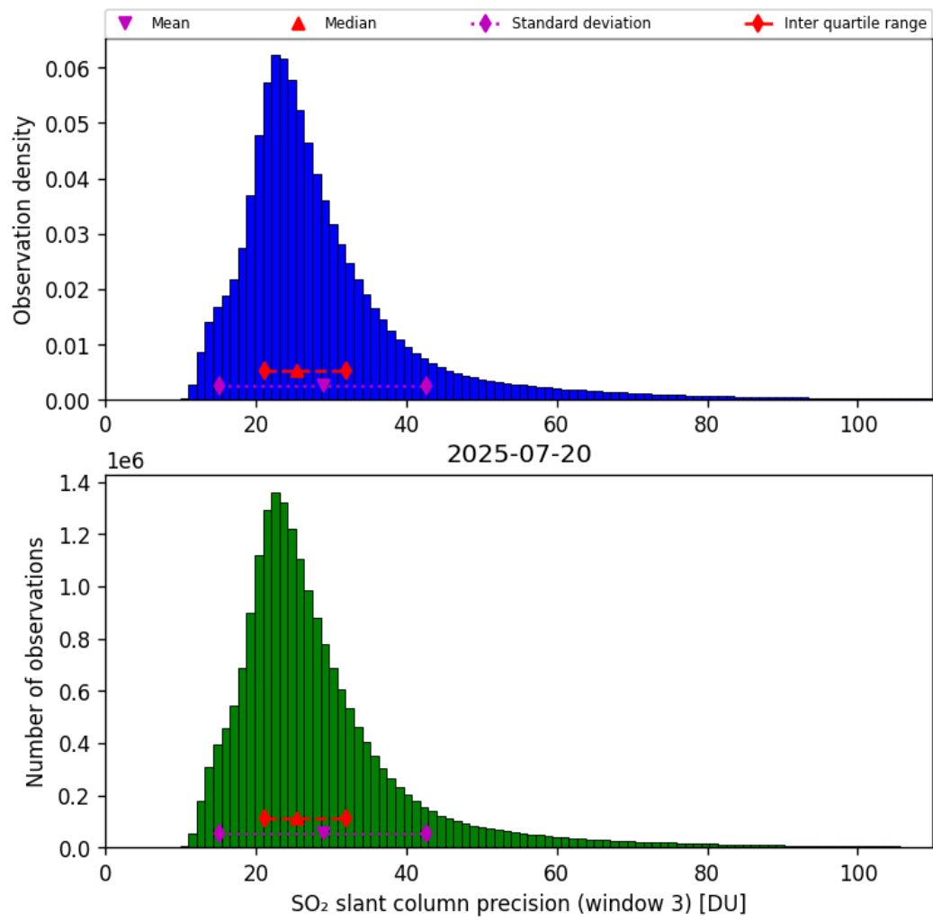
Figure 72: Histogram of “SO 2 slant column precision (window 3)” for 2025-07-19 to 2025-07-21
