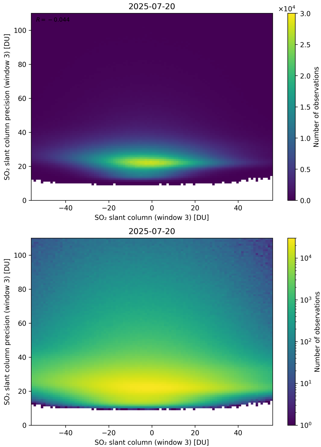
Figure 317: Scatter density plot of “SO 2 slant column (window 3)” against “SO 2 slant column precision (window 3)” for 2025-07-19 to 2025-07-21.
