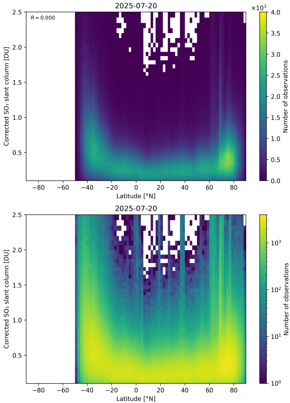
Figure 159: Scatter density plot of “Latitude” against “Corrected SO 2 slant column” for 2025-07-19 to 2025-07-21.
