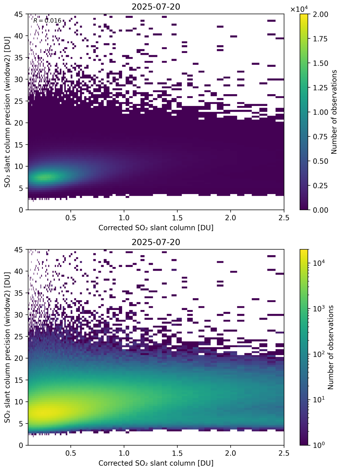
Figure 239: Scatter density plot of “Corrected SO 2 slant column” against “SO 2 slant column precision (window2)” for 2025-07-19 to 2025-07-21.
