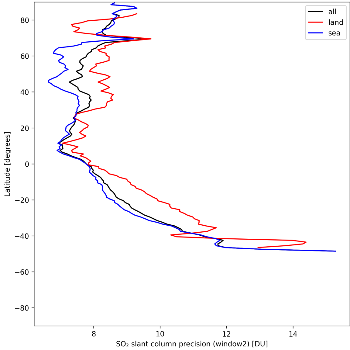
Figure 42: Zonal average of “SO 2 slant column precision (window2)” for 2025-07-19 to 2025-07-21.
