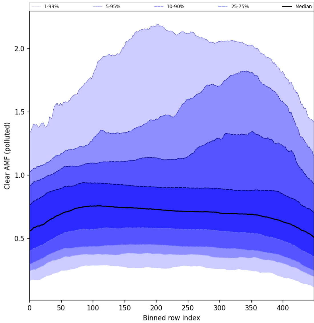
Figure 107: Along track statistics of “Clear AMF (polluted)” for 2025-07-19 to 2025-07-21
