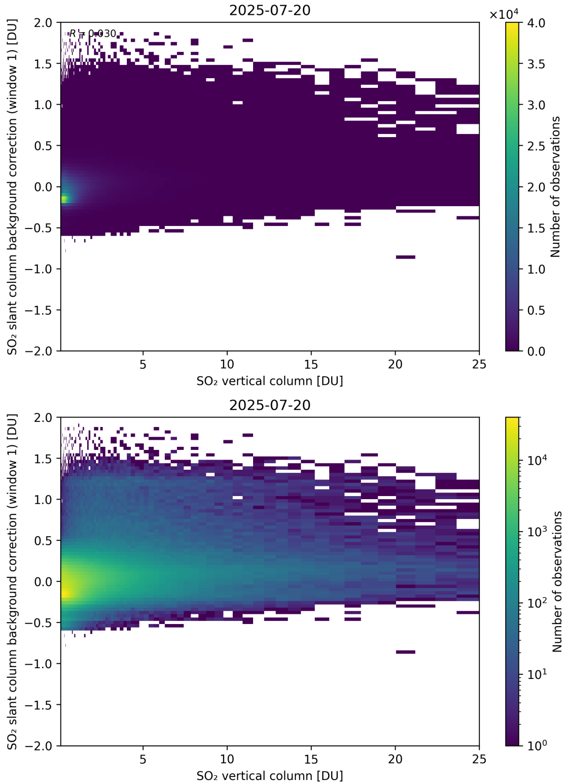
Figure 323: Scatter density plot of “SO 2 vertical column” against “SO 2 slant column background correction (window 1)” for 2025-07-19 to 2025-07-21.
