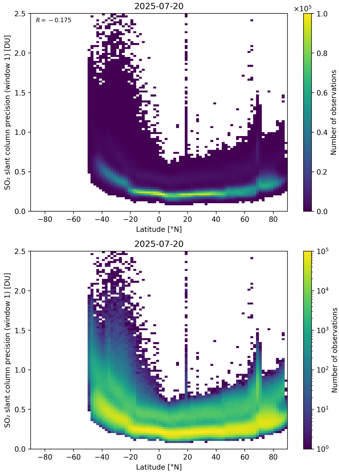
Figure 163: Scatter density plot of “Latitude” against “SO 2 slant column precision (window 1)” for 2025-07-19 to 2025-07-21.
