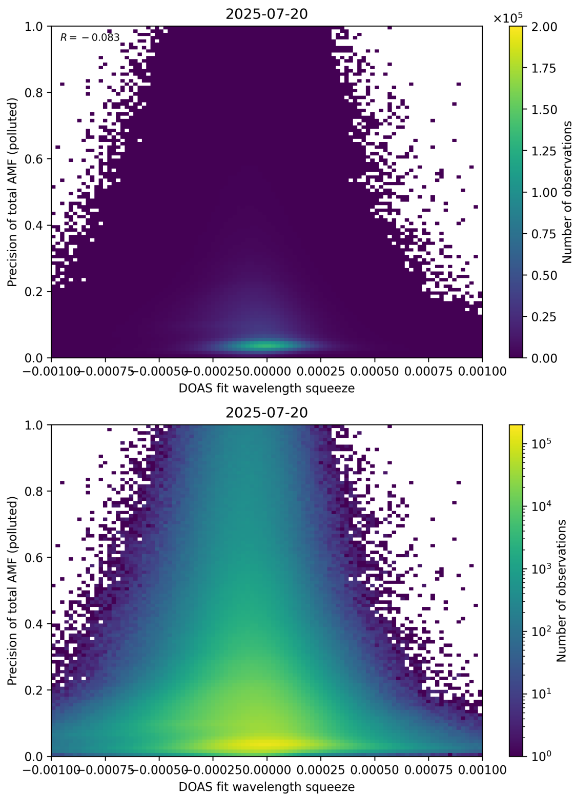
Figure 146: Scatter density plot of “DOAS fit wavelength squeeze” against “Precision of total AMF (polluted)” for 2025-07-19 to 2025-07-21.
