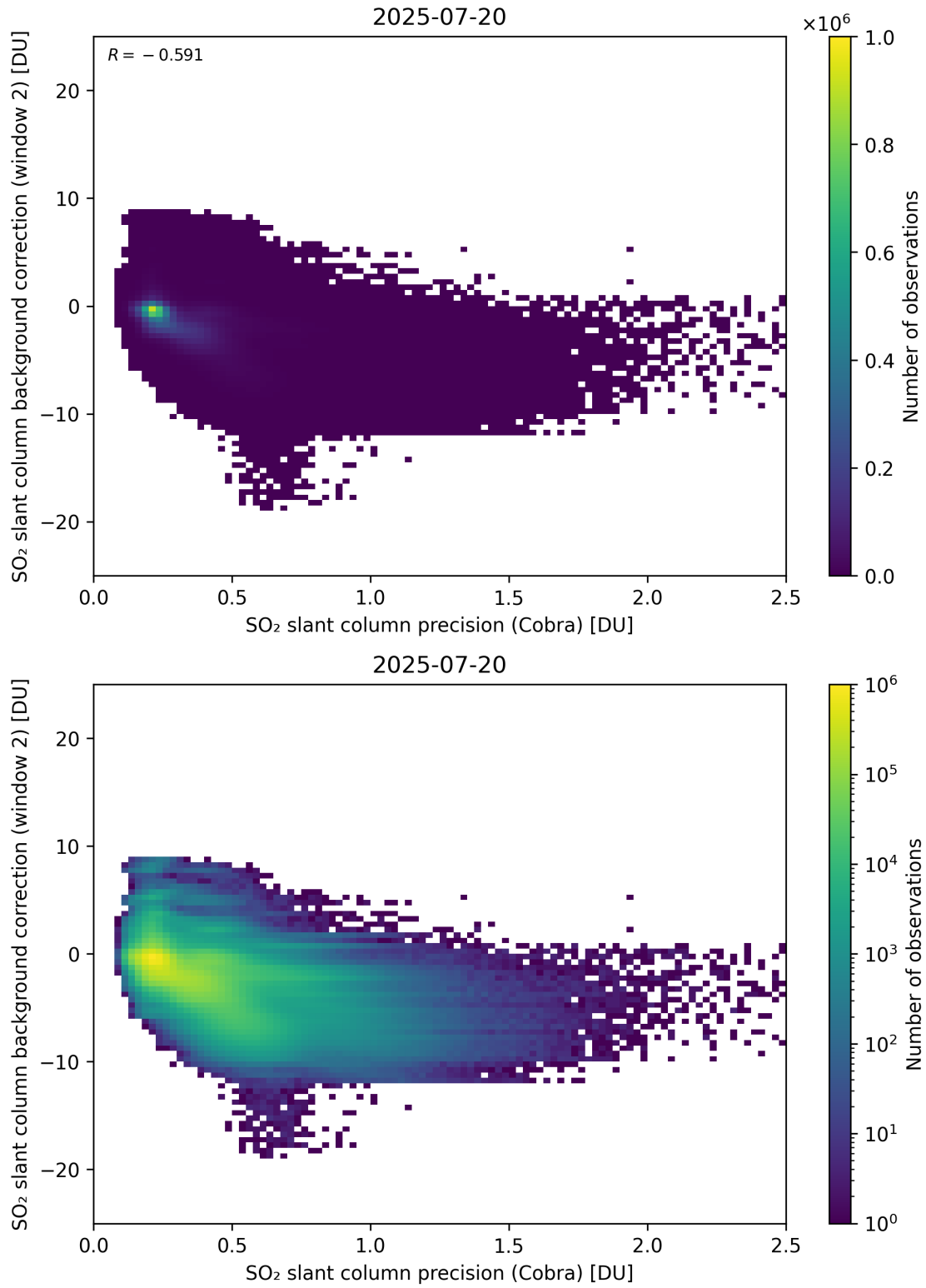
Figure 200: Scatter density plot of “SO 2 slant column precision (Cobra)” against “SO 2 slant column background correction (window 2)” for 2025-07-19 to 2025-07-21.
