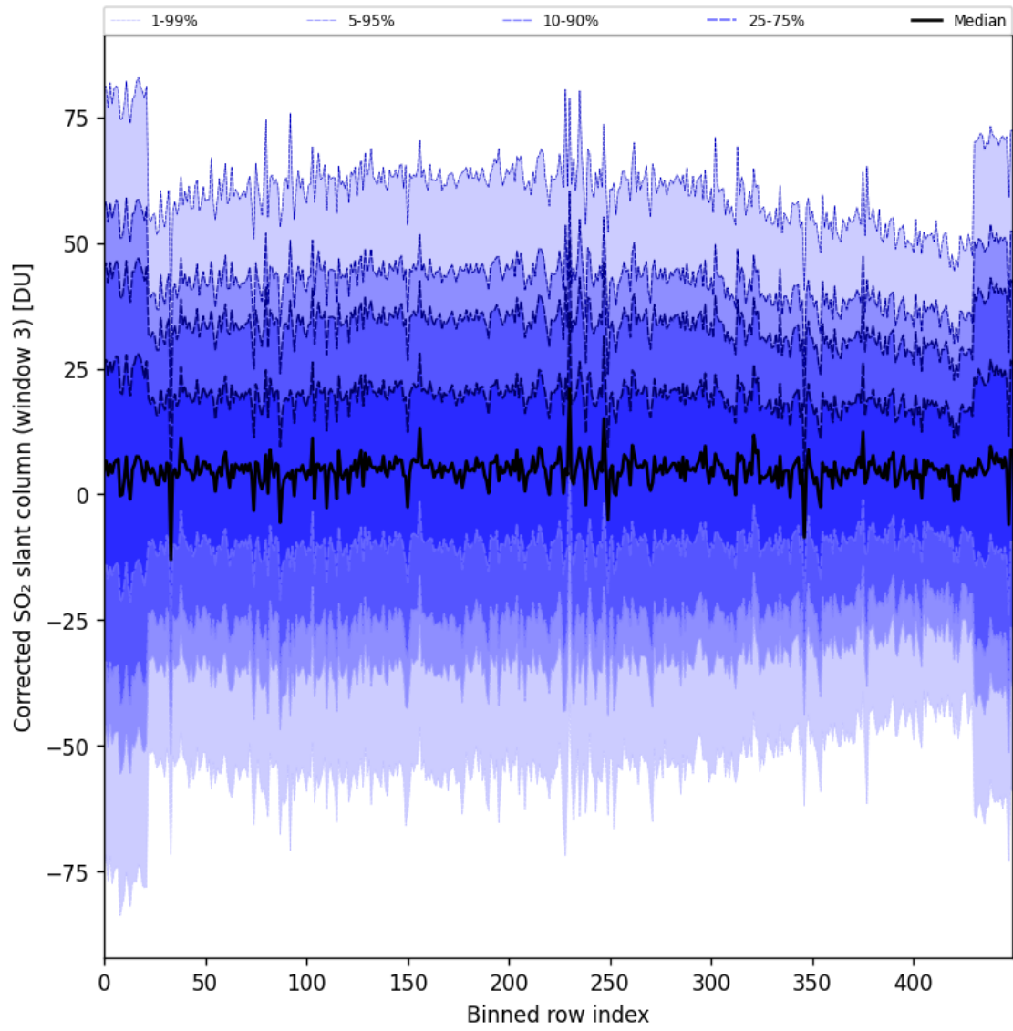
Figure 99: Along track statistics of “Corrected SO 2 slant column (window 3)” for 2025-07-19 to 2025-07-21
