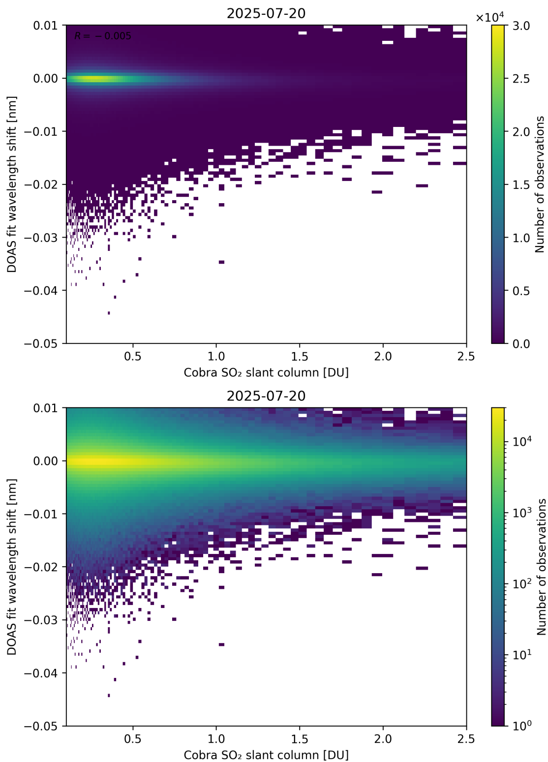
Figure 196: Scatter density plot of “Cobra SO 2 slant column” against “DOAS fit wavelength shift” for 2025-07-19 to 2025-07-21.
