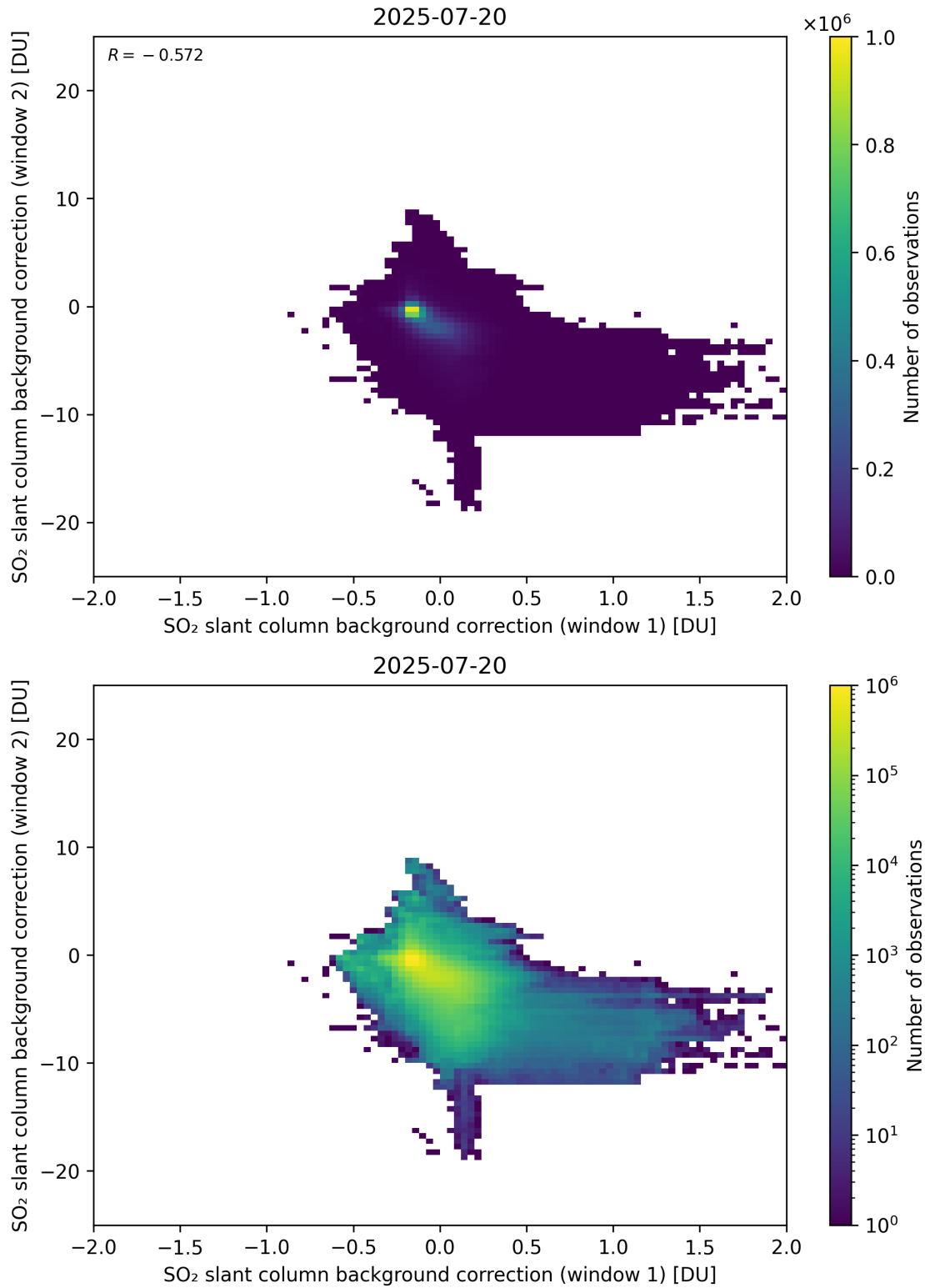
Figure 109: Scatter density plot of “SO 2 slant column background correction (window 1)” against “SO 2 slant column background correction (window 2)” for 2025-07-19 to 2025-07-21.
