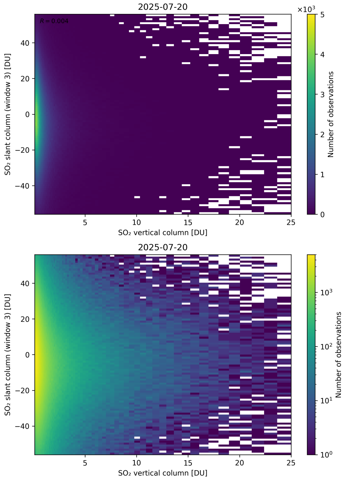
Figure 357: Scatter density plot of “SO 2 vertical column” against “SO 2 slant column (window 3)” for 2025-07-19 to 2025-07-21.
