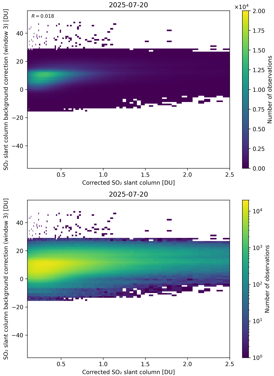
Figure 228: Scatter density plot of “Corrected SO 2 slant column” against “SO 2 slant column background correction (window 3)” for 2025-07-19 to 2025-07-21.
