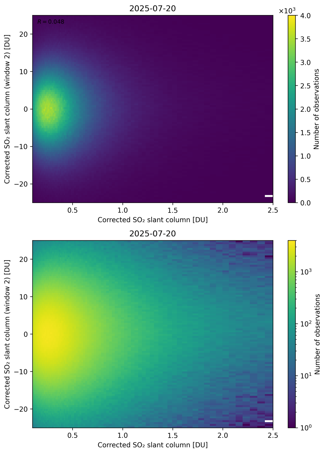
Figure 235: Scatter density plot of “Corrected SO 2 slant column” against “Corrected SO 2 slant column (window 2)” for 2025-07-19 to 2025-07-21.
