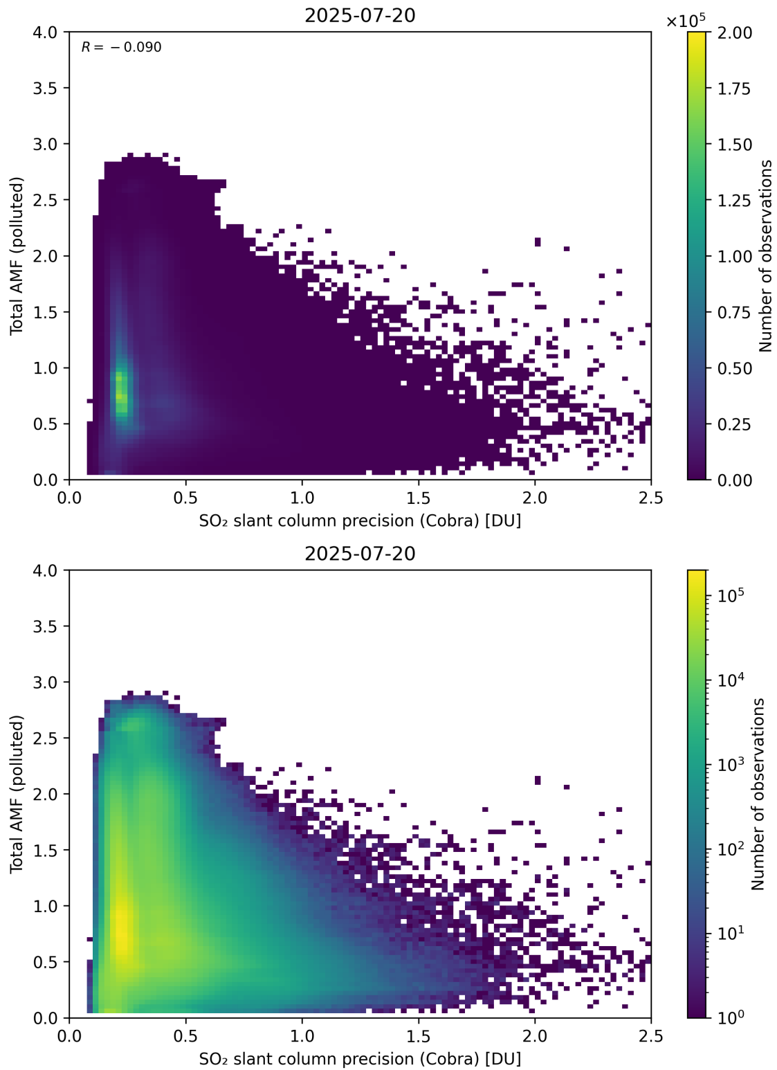
Figure 213: Scatter density plot of “SO 2 slant column precision (Cobra)” against “Total AMF (polluted)” for 2025-07-19 to 2025-07-21.
