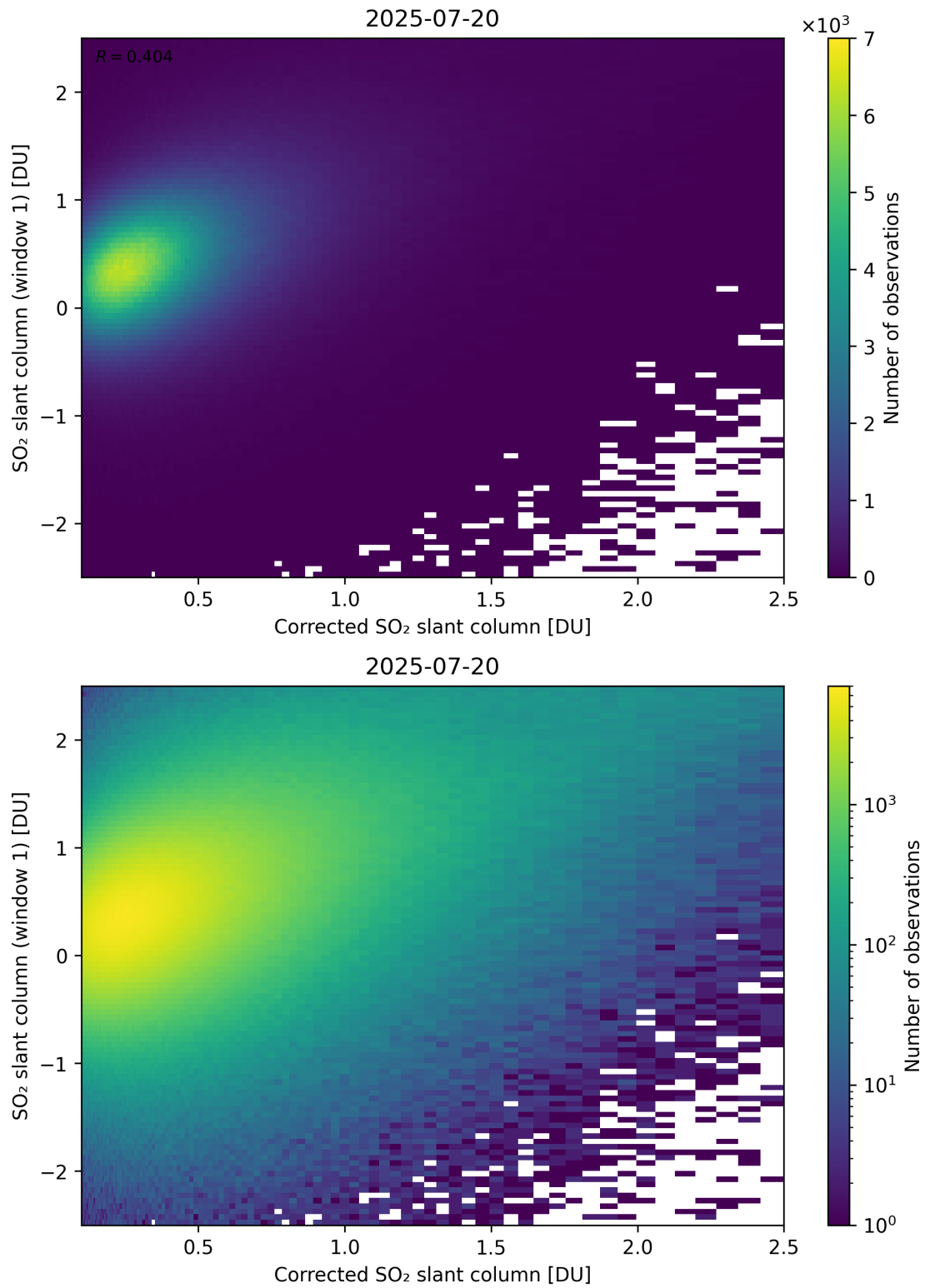
Figure 237: Scatter density plot of “Corrected SO 2 slant column” against “SO 2 slant column (window 1)” for 2025-07-19 to 2025-07-21.
