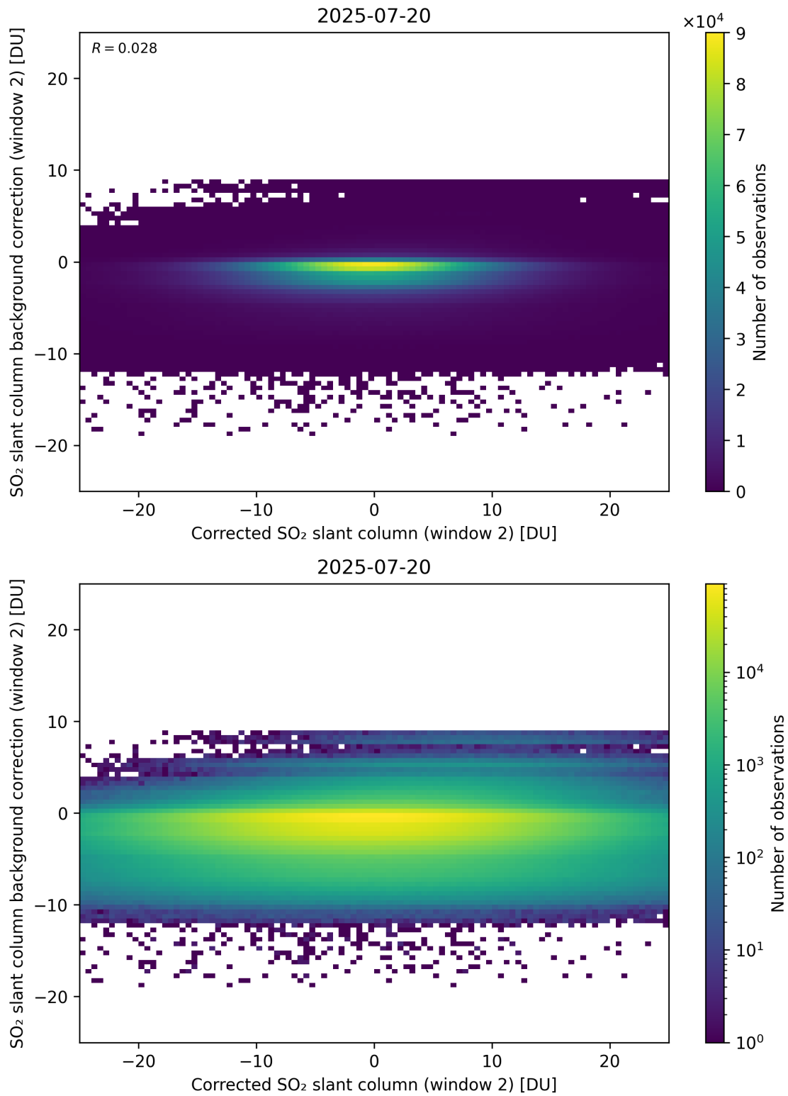
Figure 244: Scatter density plot of “Corrected SO 2 slant column (window 2)” against “SO 2 slant column background correction (window 2)” for 2025-07-19 to 2025-07-21.
