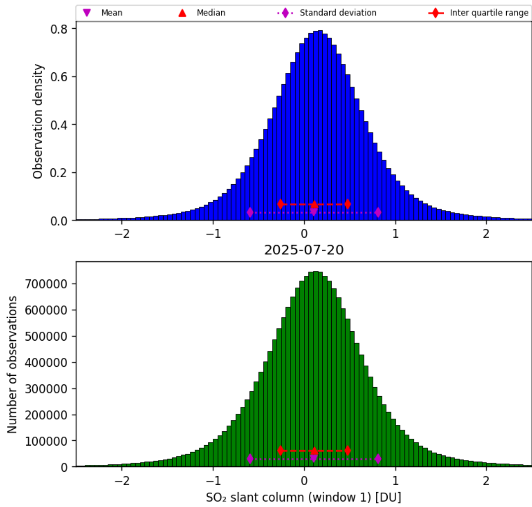
Figure 63: Histogram of “SO 2 slant column (window 1)” for 2025-07-19 to 2025-07-21
