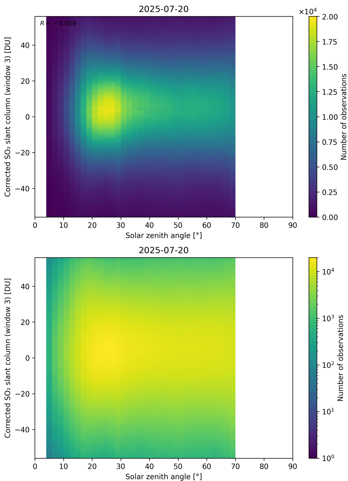
Figure 183: Scatter density plot of “Solar zenith angle” against “Corrected SO 2 slant column (window 3)” for 2025-07-19 to 2025-07-21.
