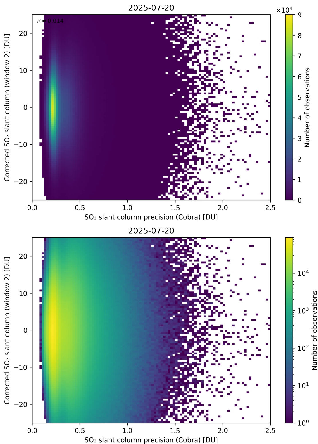
Figure 206: Scatter density plot of “SO 2 slant column precision (Cobra)” against “Corrected SO 2 slant column (window 2)” for 2025-07-19 to 2025-07-21.
