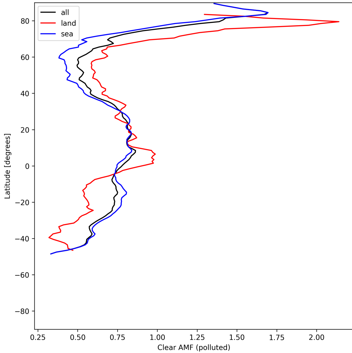
Figure 55: Zonal average of “Clear AMF (polluted)” for 2025-07-19 to 2025-07-21.
