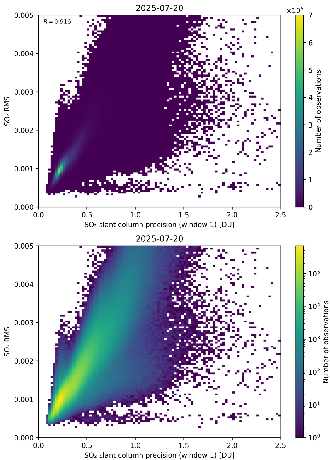
Figure 273: Scatter density plot of “SO 2 slant column precision (window 1)” against “SO 2 RMS” for 2025-07-19 to 2025-07-21.
