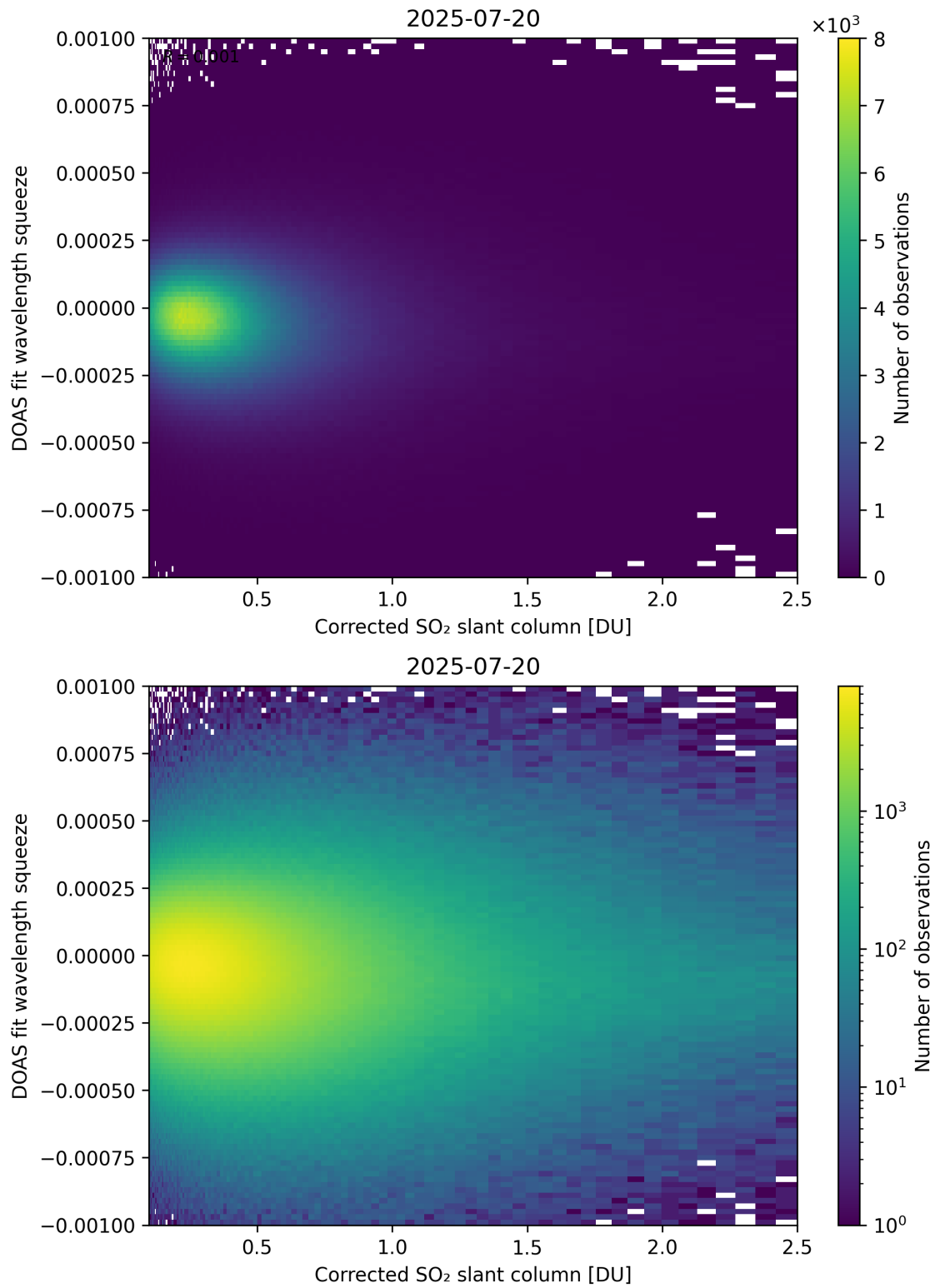
Figure 230: Scatter density plot of “Corrected SO 2 slant column” against “DOAS fit wavelength squeeze” for 2025-07-19 to 2025-07-21.
