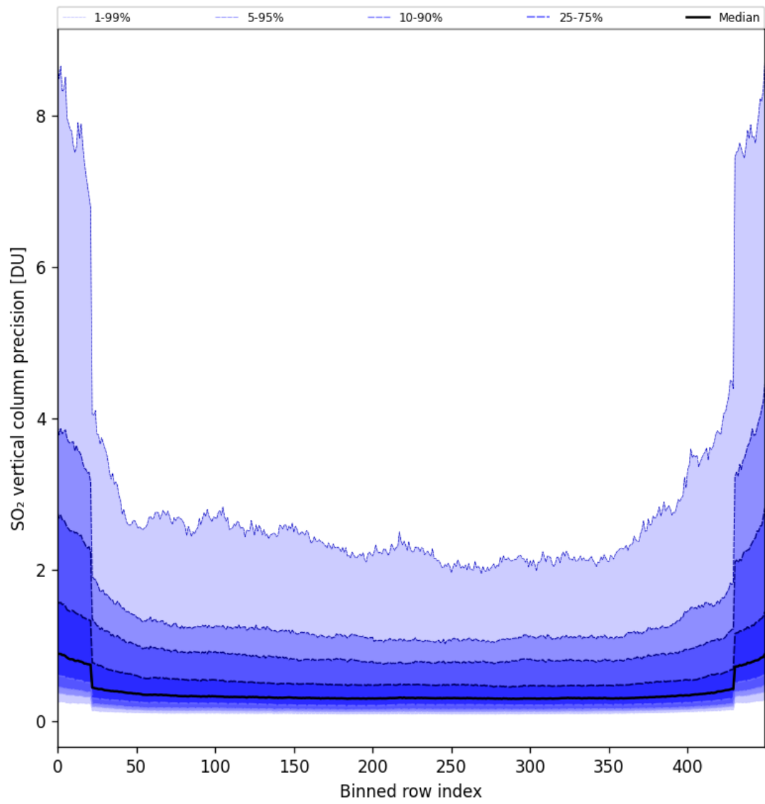
Figure 85: Along track statistics of “SO 2 vertical column precision” for 2025-07-19 to 2025-07-21
