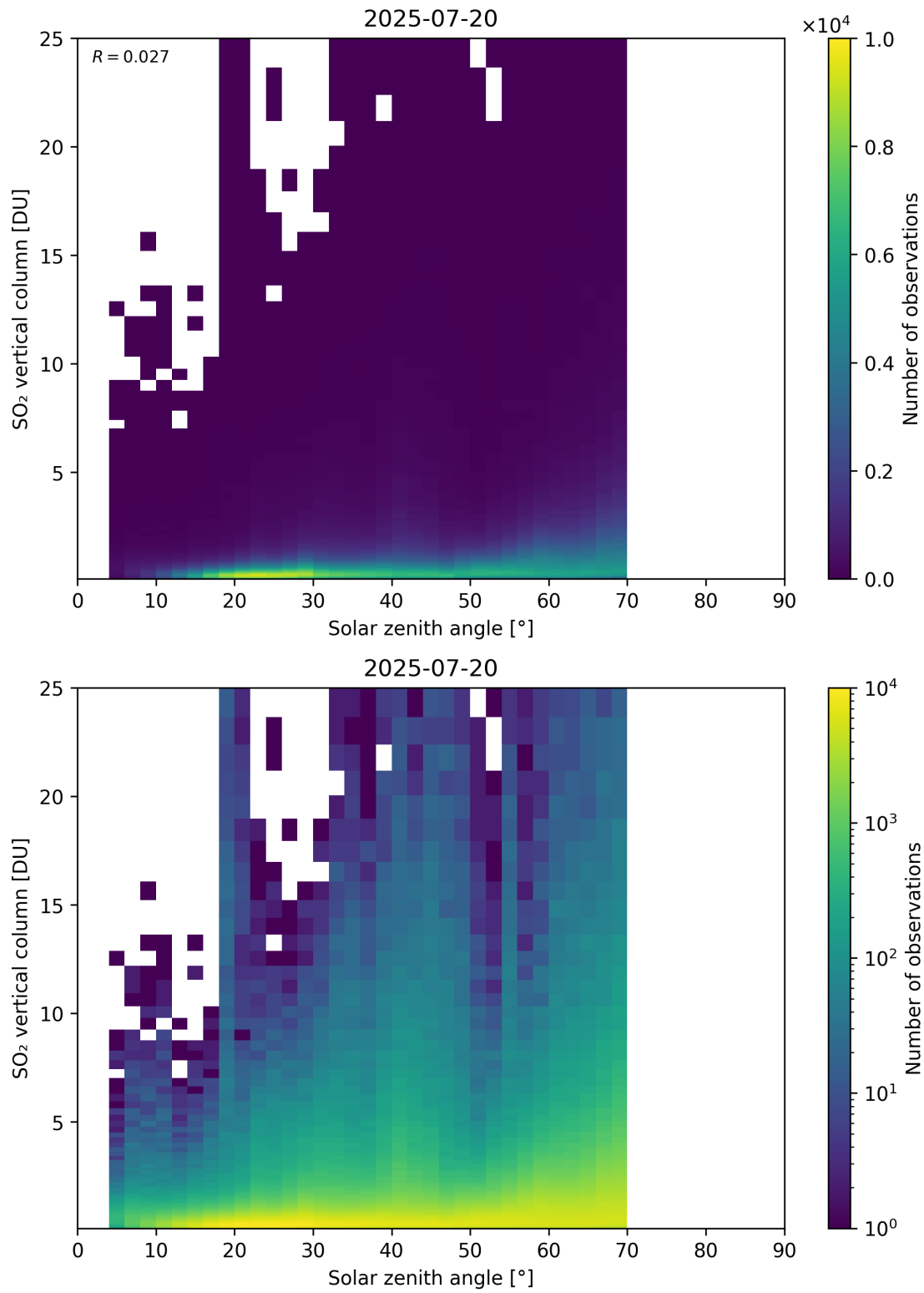
Figure 191: Scatter density plot of “Solar zenith angle” against “SO 2 vertical column” for 2025-07-19 to 2025-07-21.
