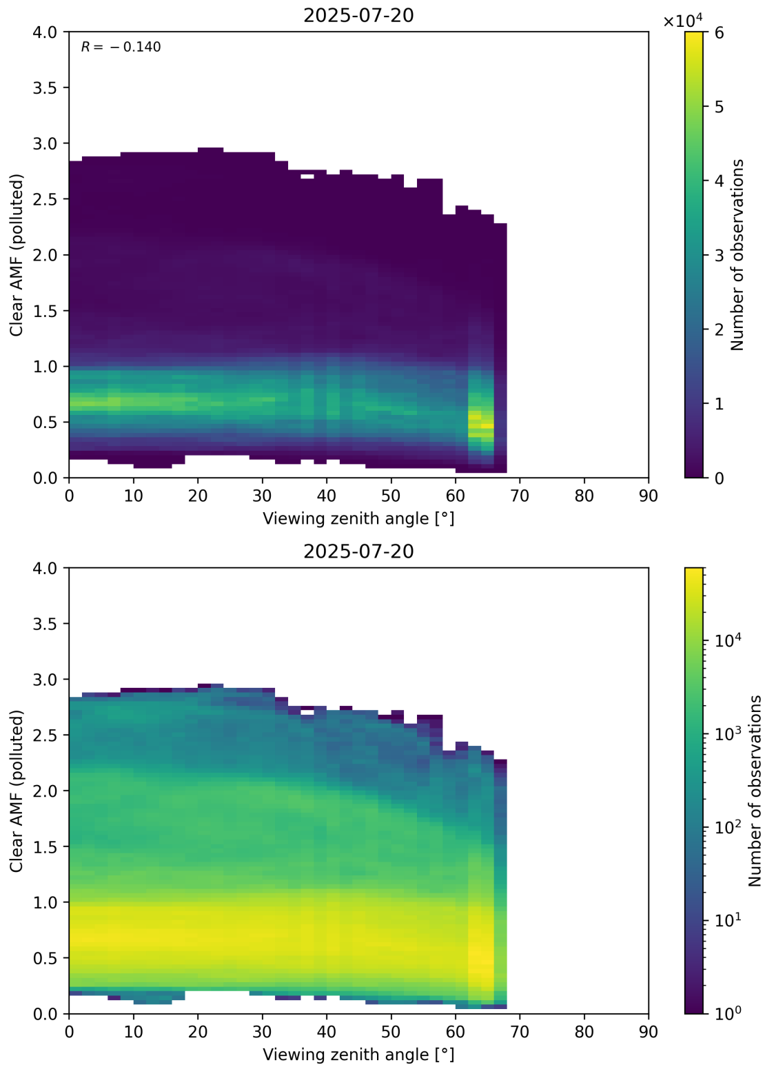
Figure 370: Scatter density plot of “Viewing zenith angle” against “Clear AMF (polluted)” for 2025-07-19 to 2025-07-21.
