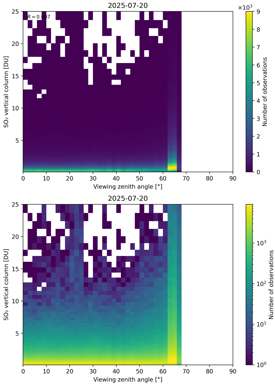
Figure 383: Scatter density plot of “Viewing zenith angle” against “SO 2 vertical column” for 2025-07-19 to 2025-07-21.
