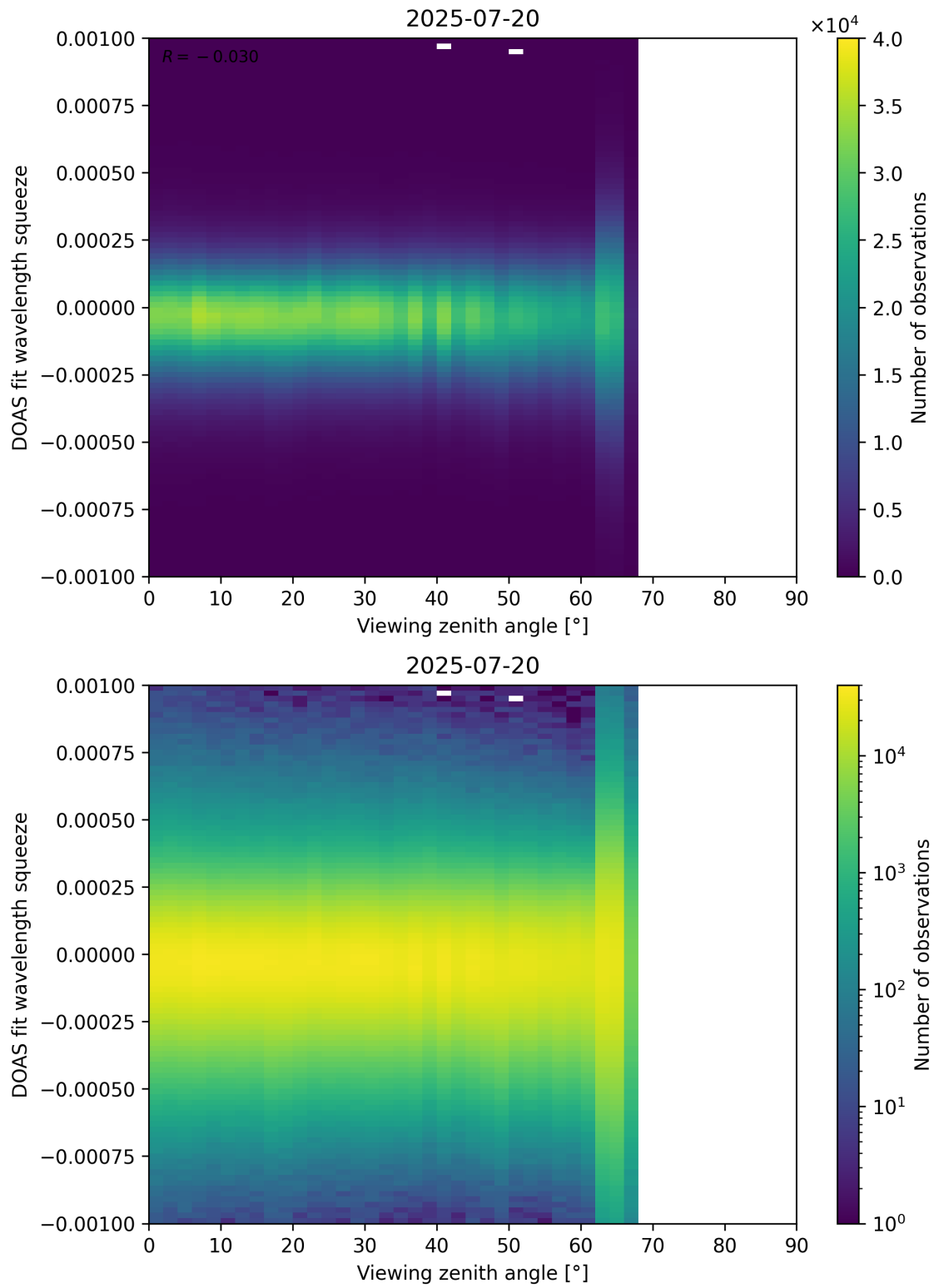
Figure 366: Scatter density plot of “Viewing zenith angle” against “DOAS fit wavelength squeeze” for 2025-07-19 to 2025-07-21.
