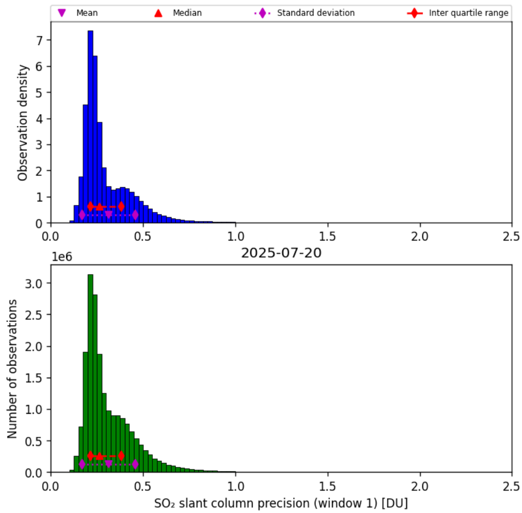
Figure 64: Histogram of “SO 2 slant column precision (window 1)” for 2025-07-19 to 2025-07-21
