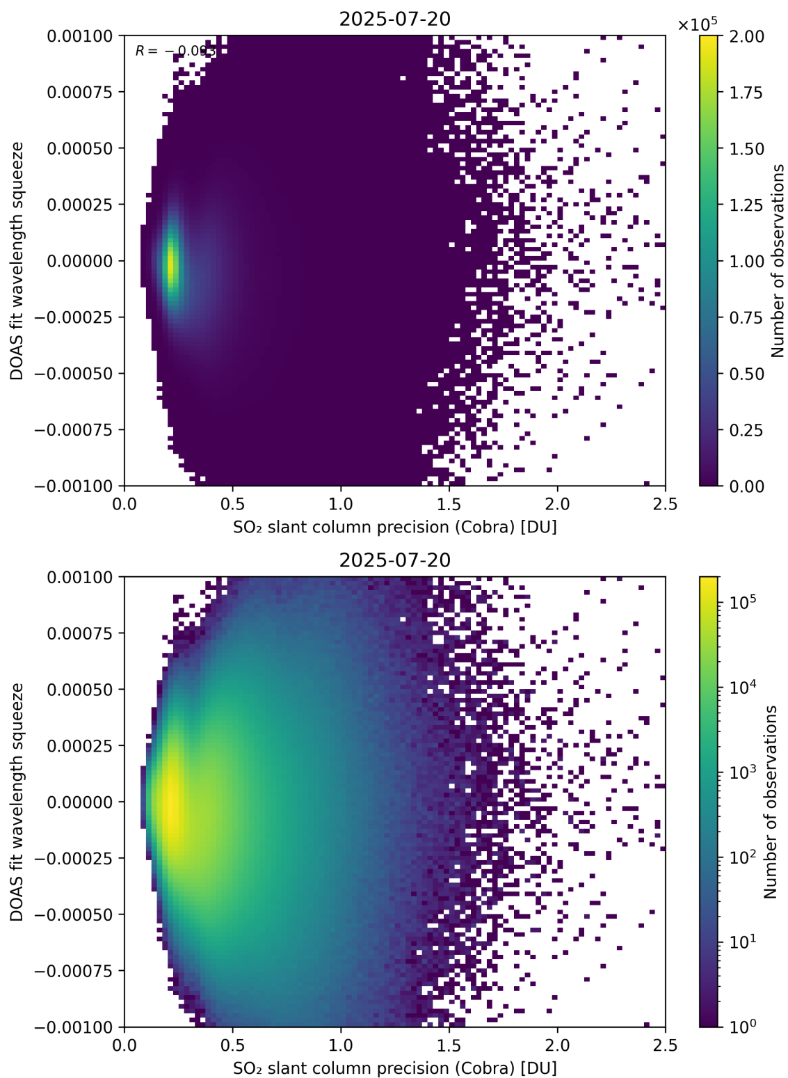
Figure 203: Scatter density plot of “SO 2 slant column precision (Cobra)” against “DOAS fit wavelength squeeze” for 2025-07-19 to 2025-07-21.
