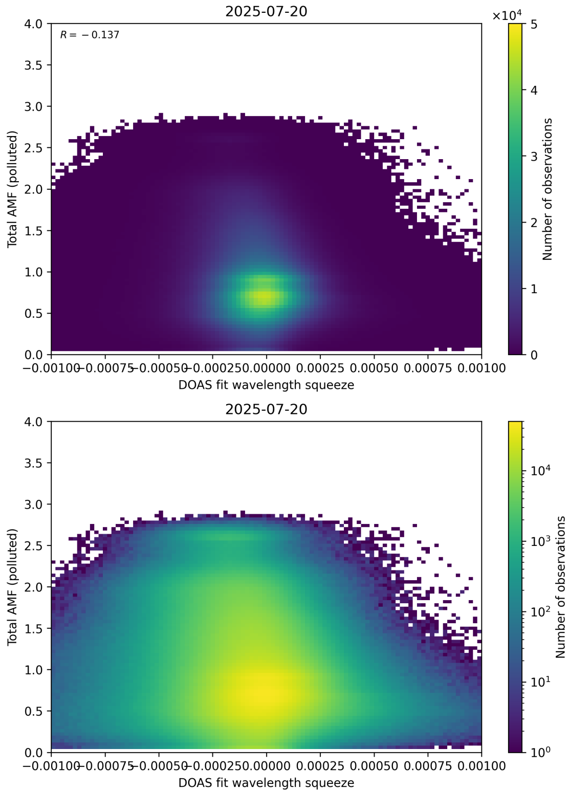
Figure 145: Scatter density plot of “DOAS fit wavelength squeeze” against “Total AMF (polluted)” for 2025-07-19 to 2025-07-21.
