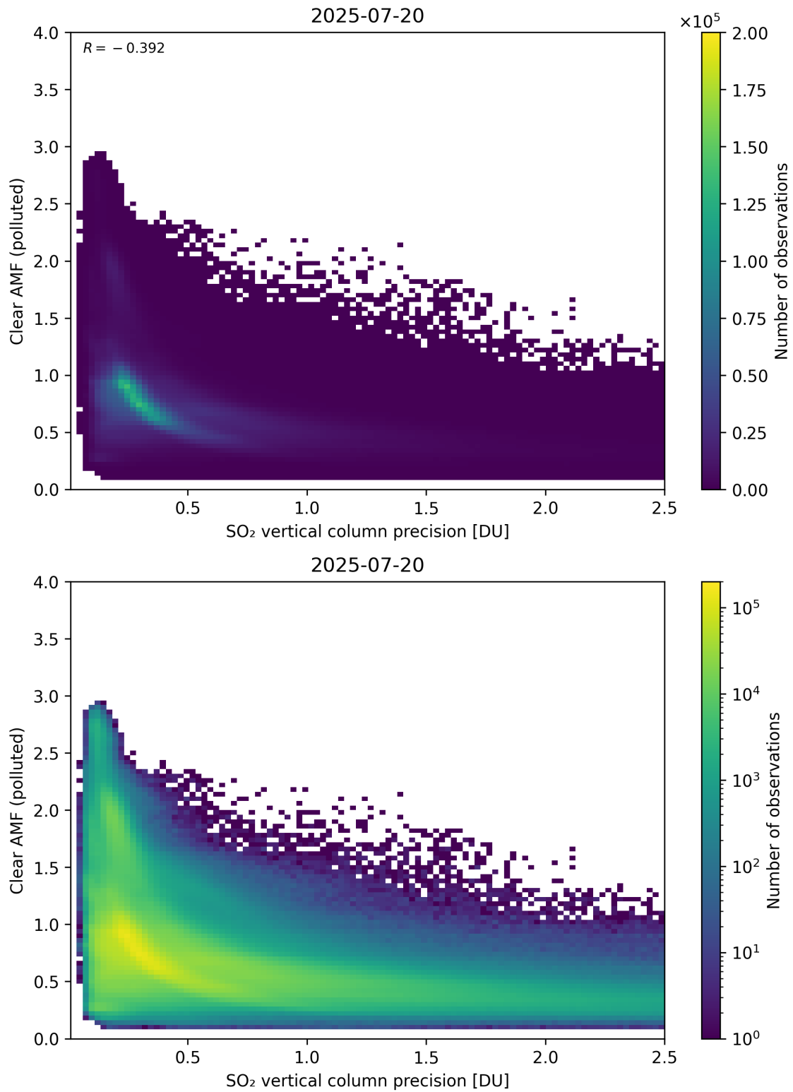
Figure 335: Scatter density plot of “SO 2 vertical column precision” against “Clear AMF (polluted)” for 2025-07-19 to 2025-07-21.
