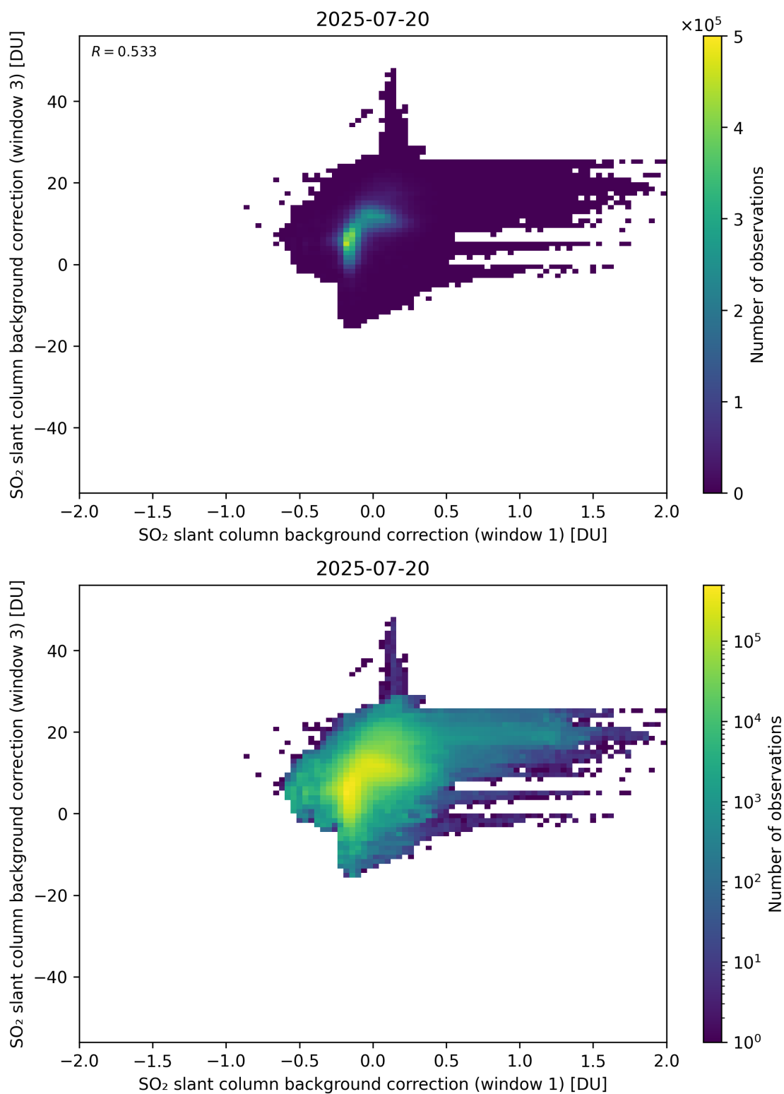
Figure 110: Scatter density plot of “SO 2 slant column background correction (window 1)” against “SO 2 slant column background correction (window 3)” for 2025-07-19 to 2025-07-21.
