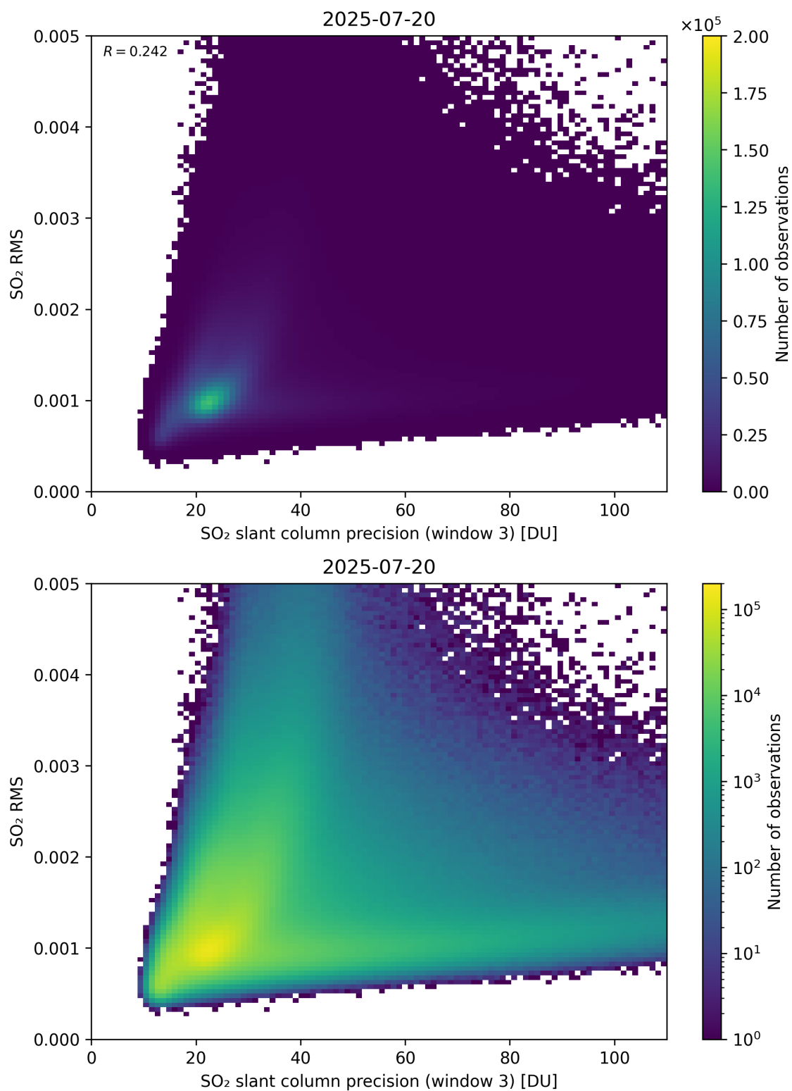
Figure 310: Scatter density plot of “SO 2 slant column precision (window 3)” against “SO 2 RMS” for 2025-07-19 to 2025-07-21.
