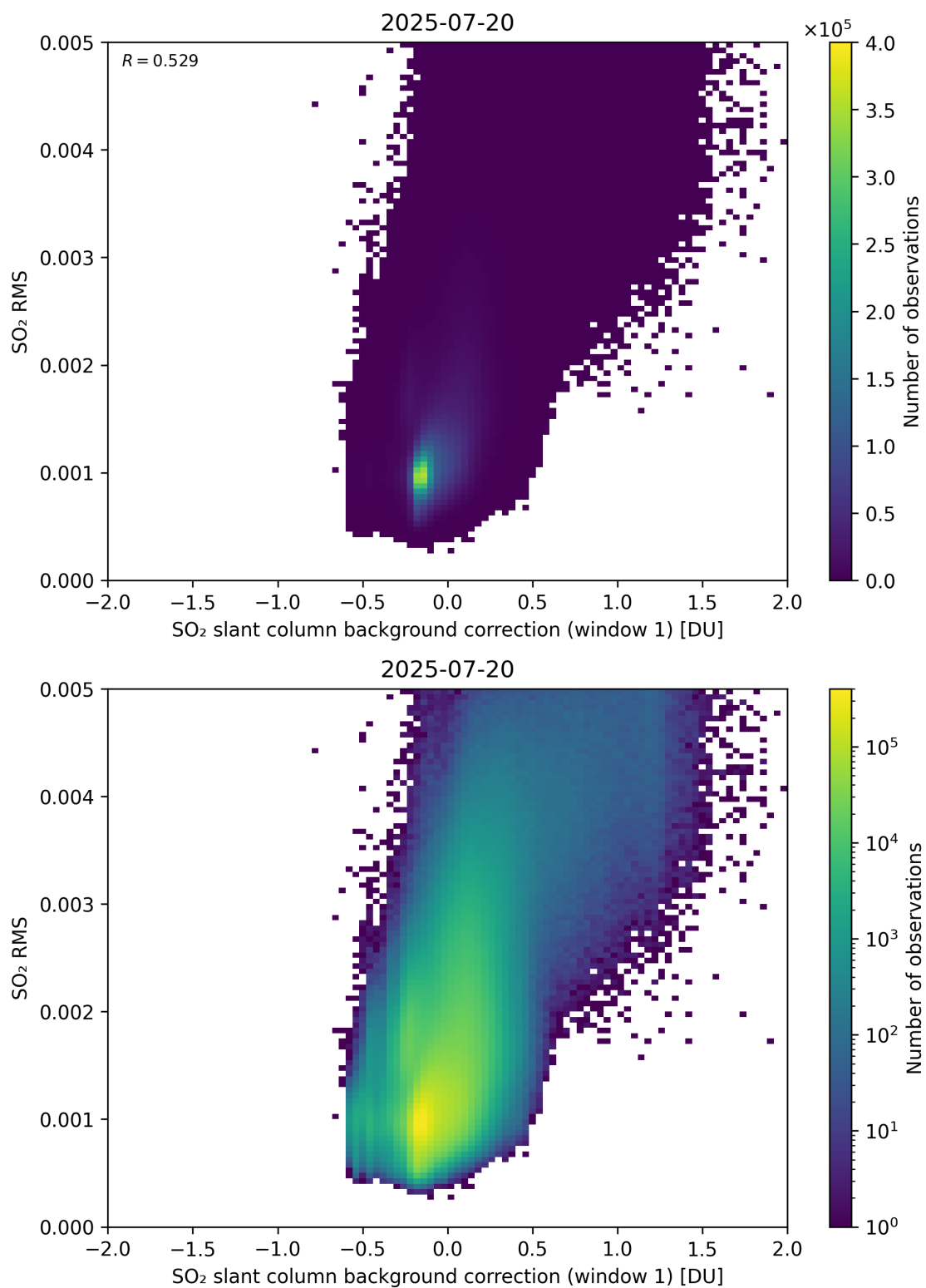
Figure 113: Scatter density plot of “SO 2 slant column background correction (window 1)” against “SO 2 RMS” for 2025-07-19 to 2025-07-21.
