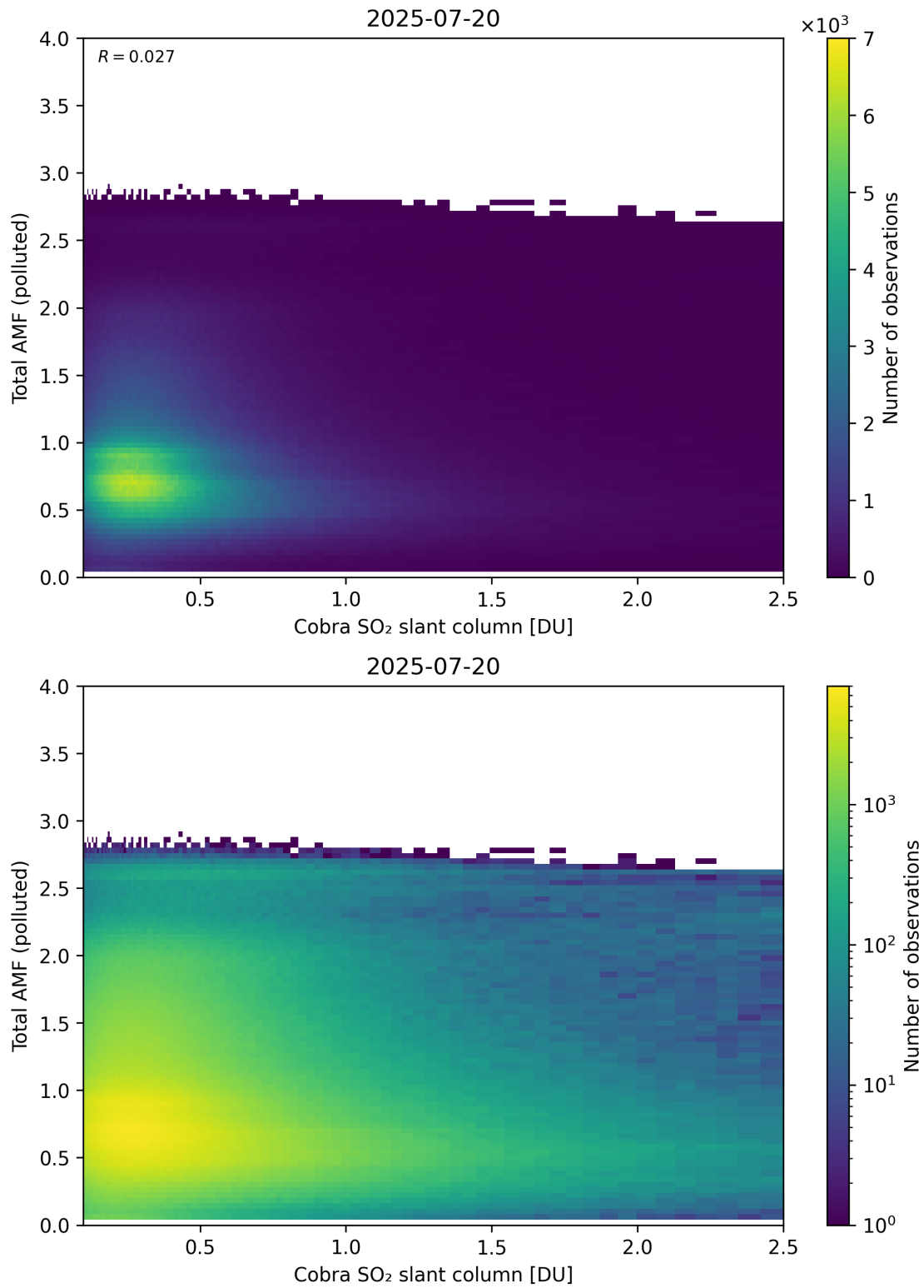
Figure 224: Scatter density plot of “Cobra SO 2 slant column” against “Total AMF (polluted)” for 2025-07-19 to 2025-07-21.
