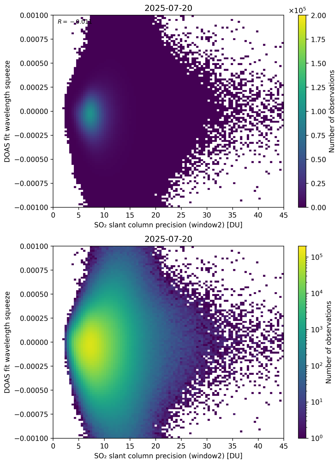
Figure 294: Scatter density plot of “SO 2 slant column precision (window2)” against “DOAS fit wavelength squeeze” for 2025-07-19 to 2025-07-21.
