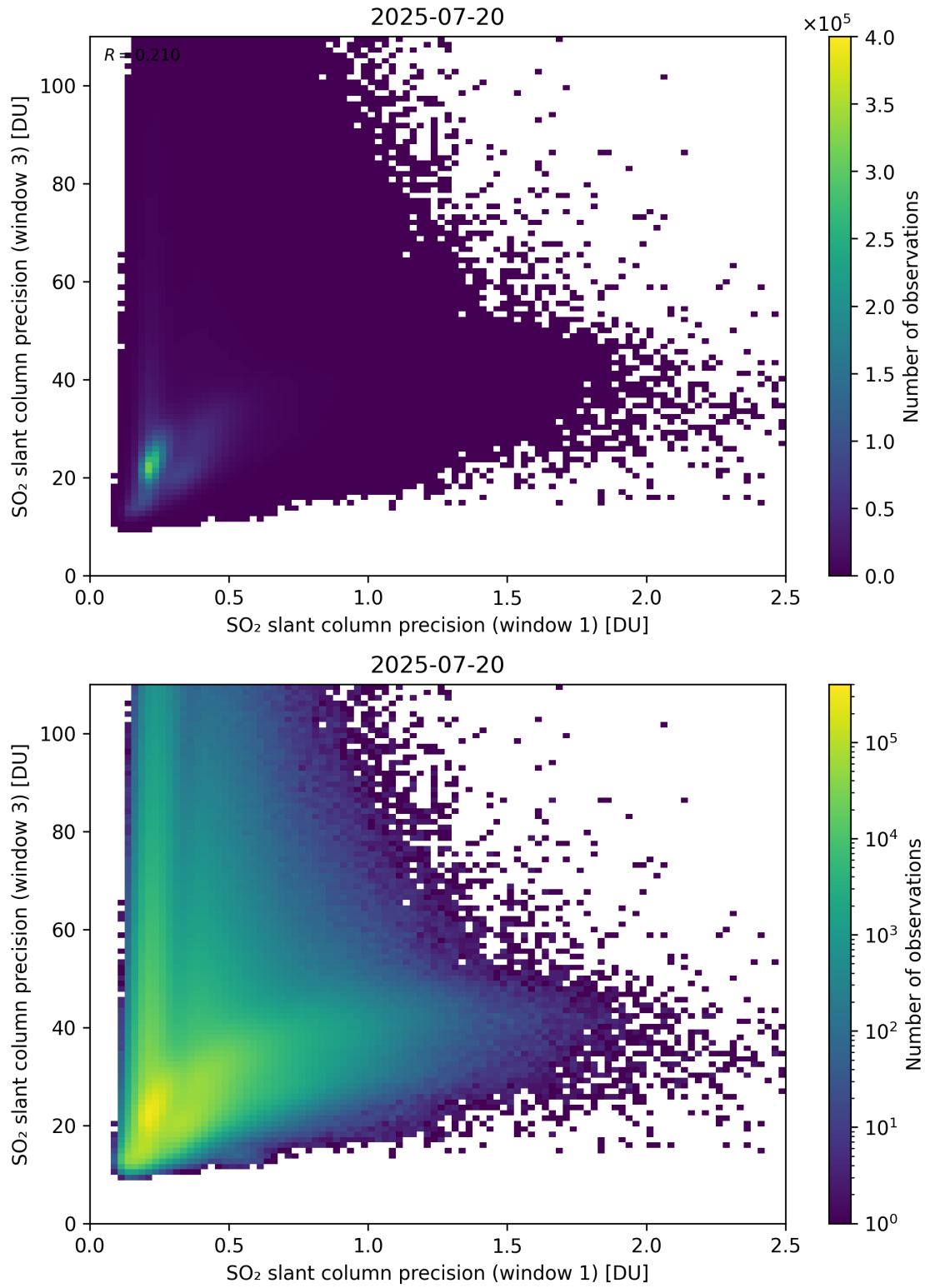
Figure 279: Scatter density plot of “SO 2 slant column precision (window 1)” against “SO 2 slant column precision (window 3)” for 2025-07-19 to 2025-07-21.
