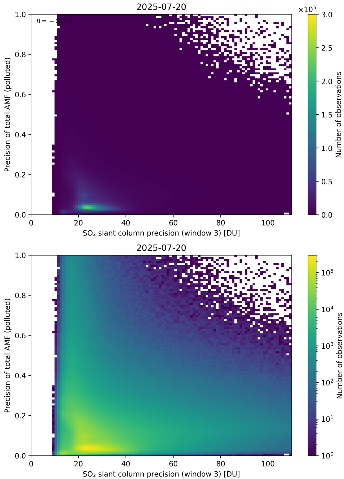
Figure 314: Scatter density plot of “SO 2 slant column precision (window 3)” against “Precision of total AMF (polluted)” for 2025-07-19 to 2025-07-21.
