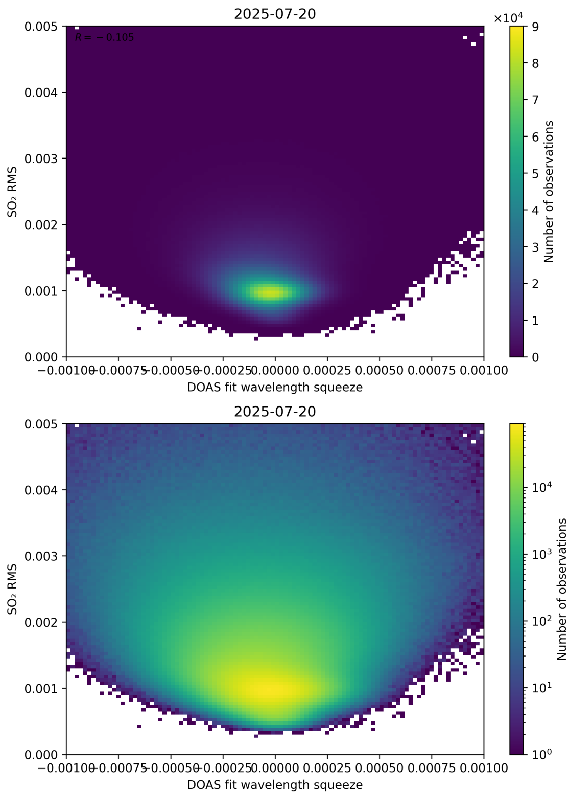
Figure 143: Scatter density plot of “DOAS fit wavelength squeeze” against “SO 2 RMS” for 2025-07-19 to 2025-07-21.
