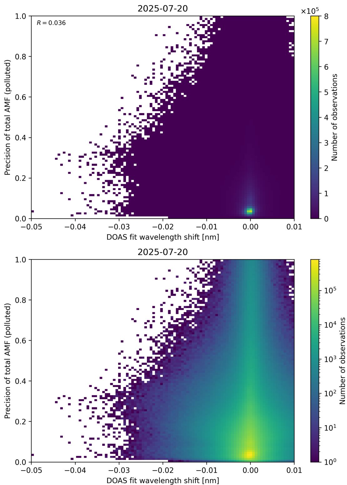
Figure 142: Scatter density plot of “DOAS fit wavelength shift” against “Precision of total AMF (polluted)” for 2025-07-19 to 2025-07-21.
