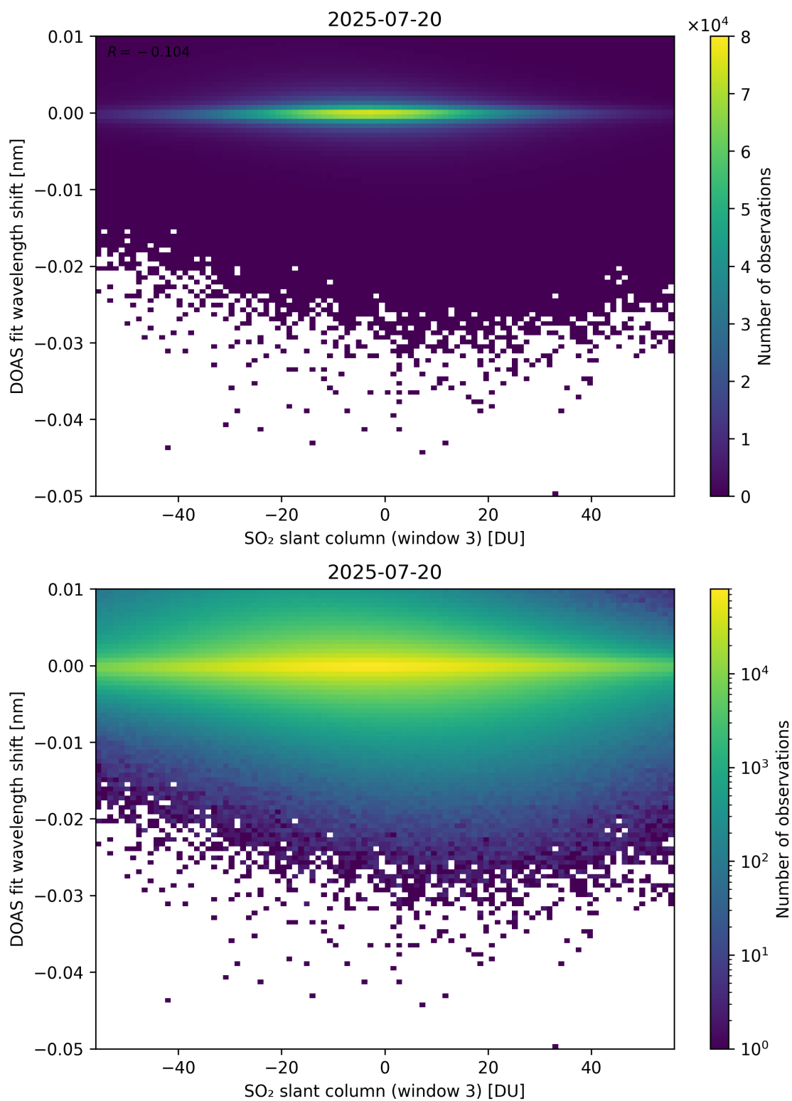
Figure 304: Scatter density plot of “SO 2 slant column (window 3)” against “DOAS fit wavelength shift” for 2025-07-19 to 2025-07-21.
