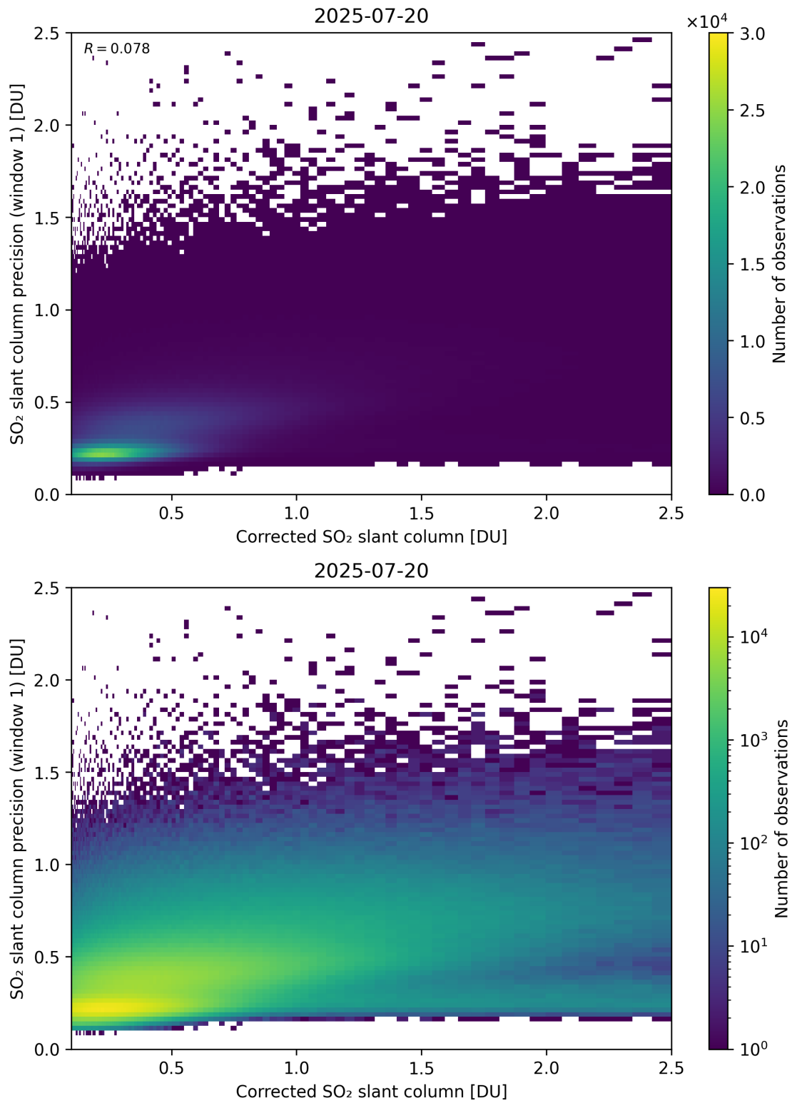
Figure 238: Scatter density plot of “Corrected SO 2 slant column” against “SO 2 slant column precision (window 1)” for 2025-07-19 to 2025-07-21.
