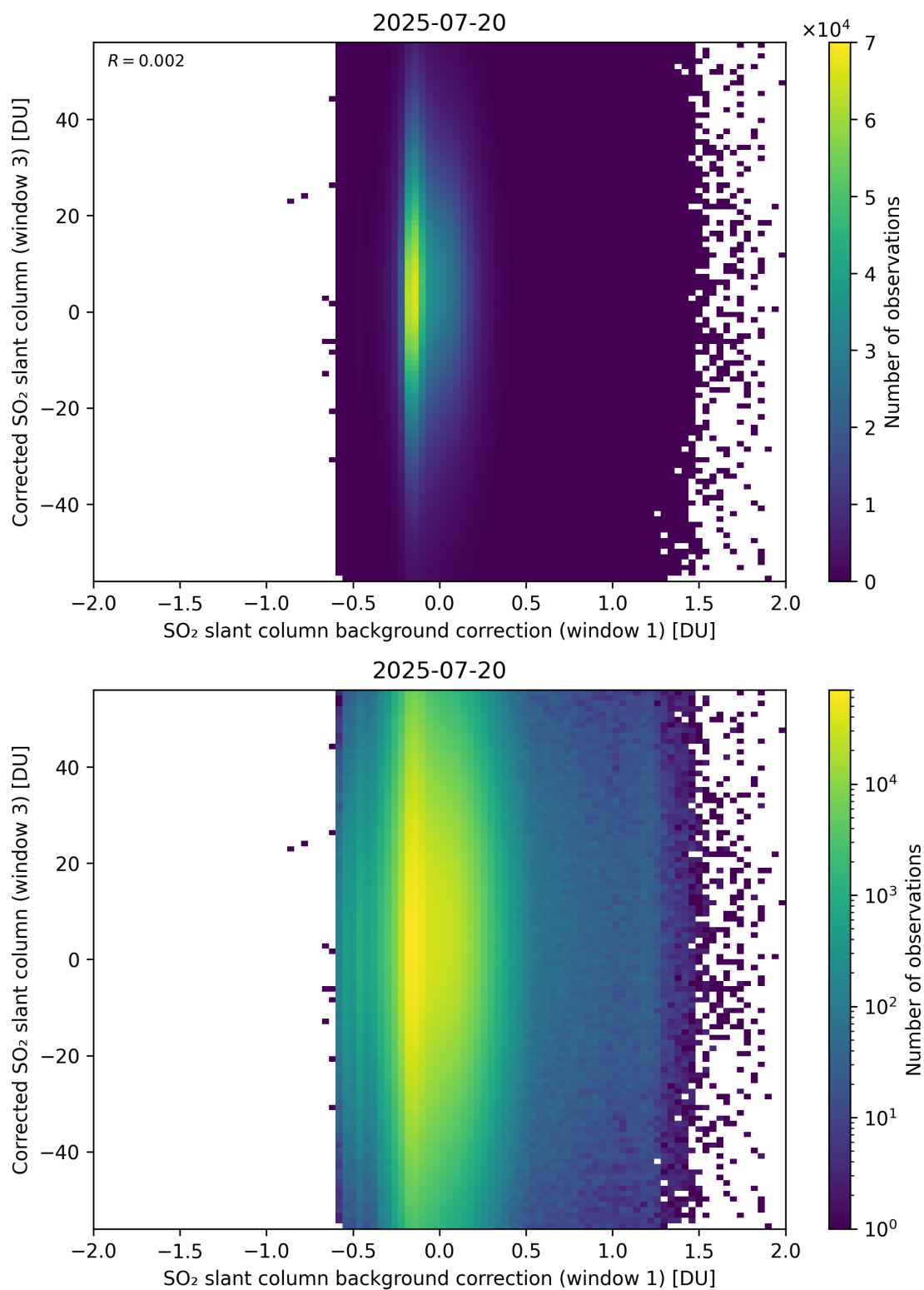
Figure 116: Scatter density plot of “SO 2 slant column background correction (window 1)” against “Corrected SO 2 slant column (window 3)” for 2025-07-19 to 2025-07-21.
