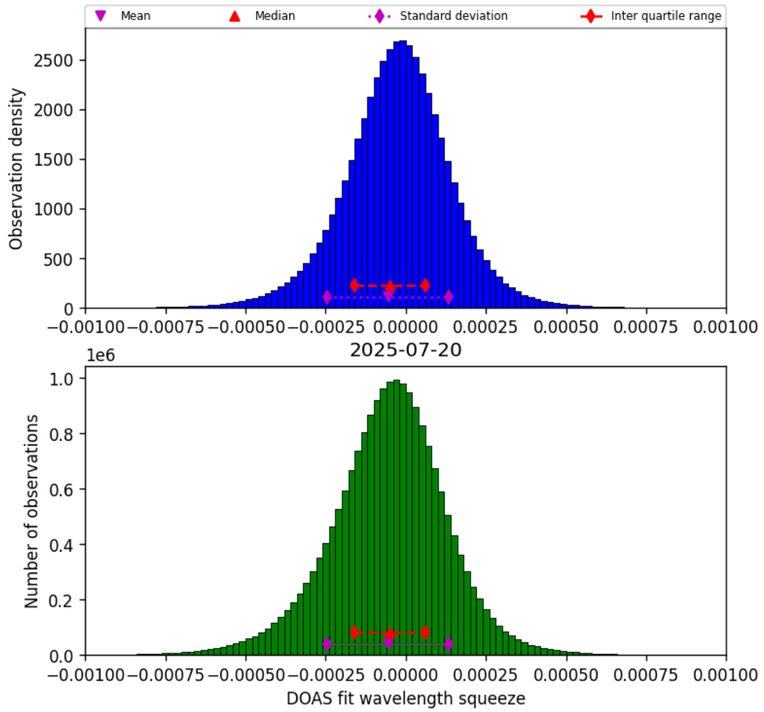
Figure 77: Histogram of “DOAS fit wavelength squeeze” for 2025-07-19 to 2025-07-21
