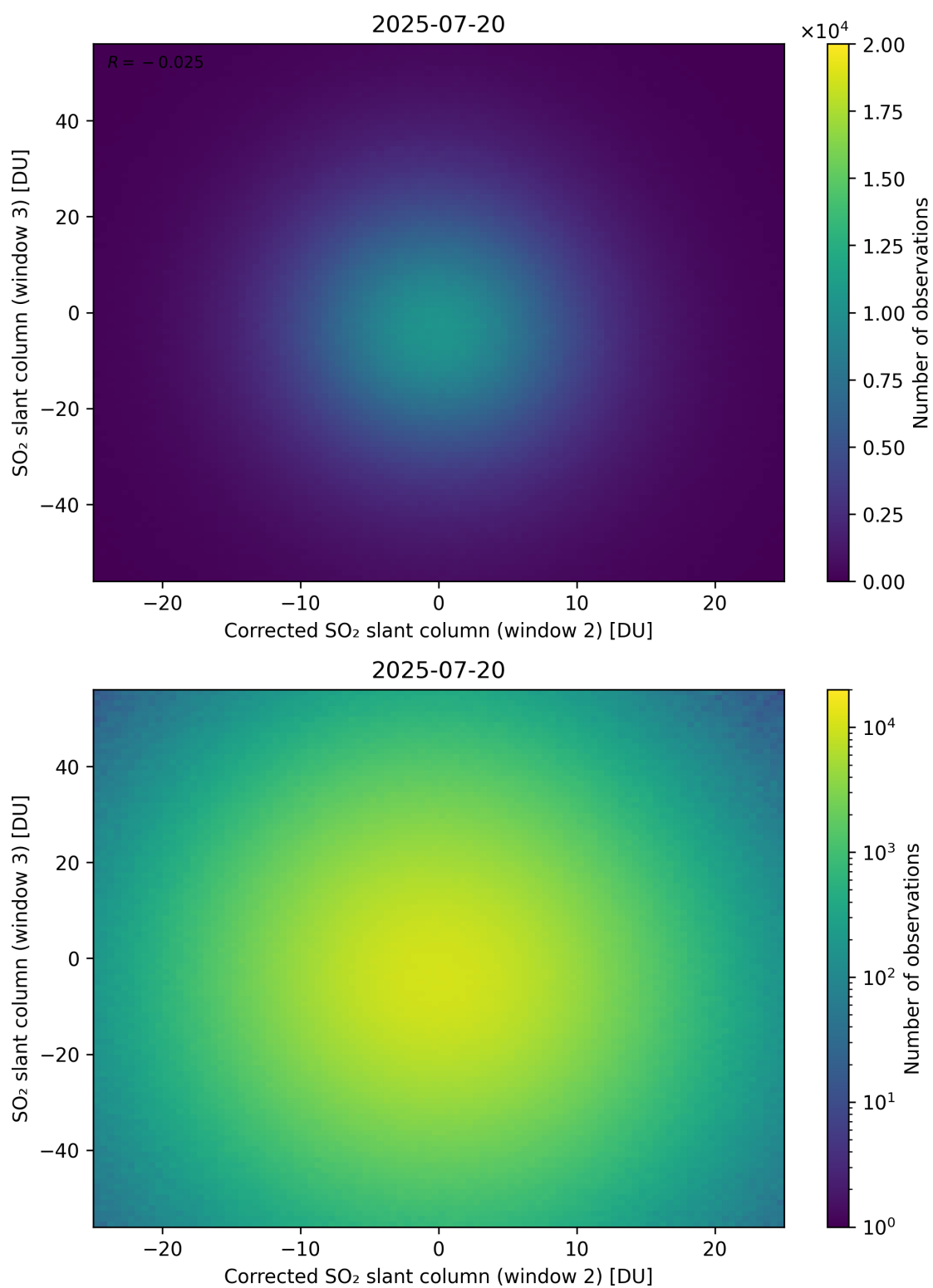
Figure 251: Scatter density plot of “Corrected SO 2 slant column (window 2)” against “SO 2 slant column (window 3)” for 2025-07-19 to 2025-07-21.
