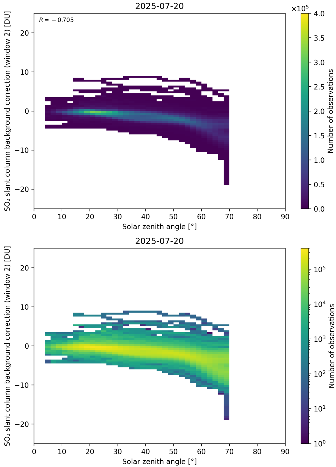
Figure 172: Scatter density plot of “Solar zenith angle” against “SO 2 slant column background correction (window 2)” for 2025-07-19 to 2025-07-21.
