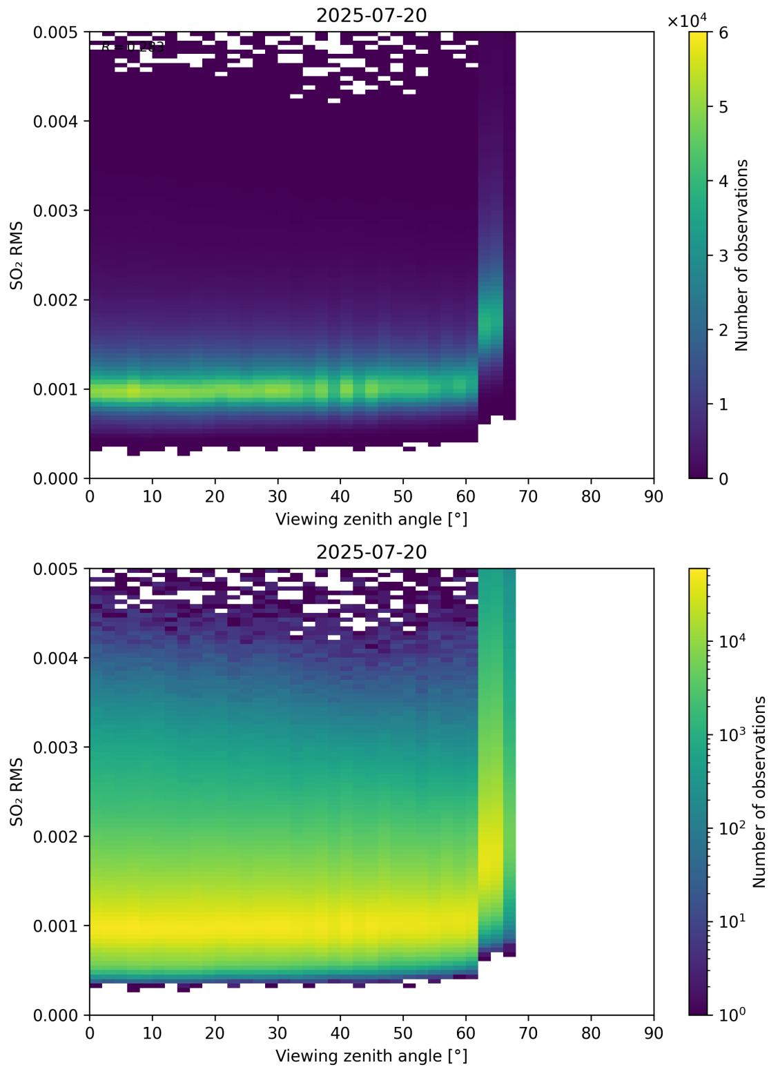
Figure 367: Scatter density plot of “Viewing zenith angle” against “SO 2 RMS” for 2025-07-19 to 2025-07-21.
