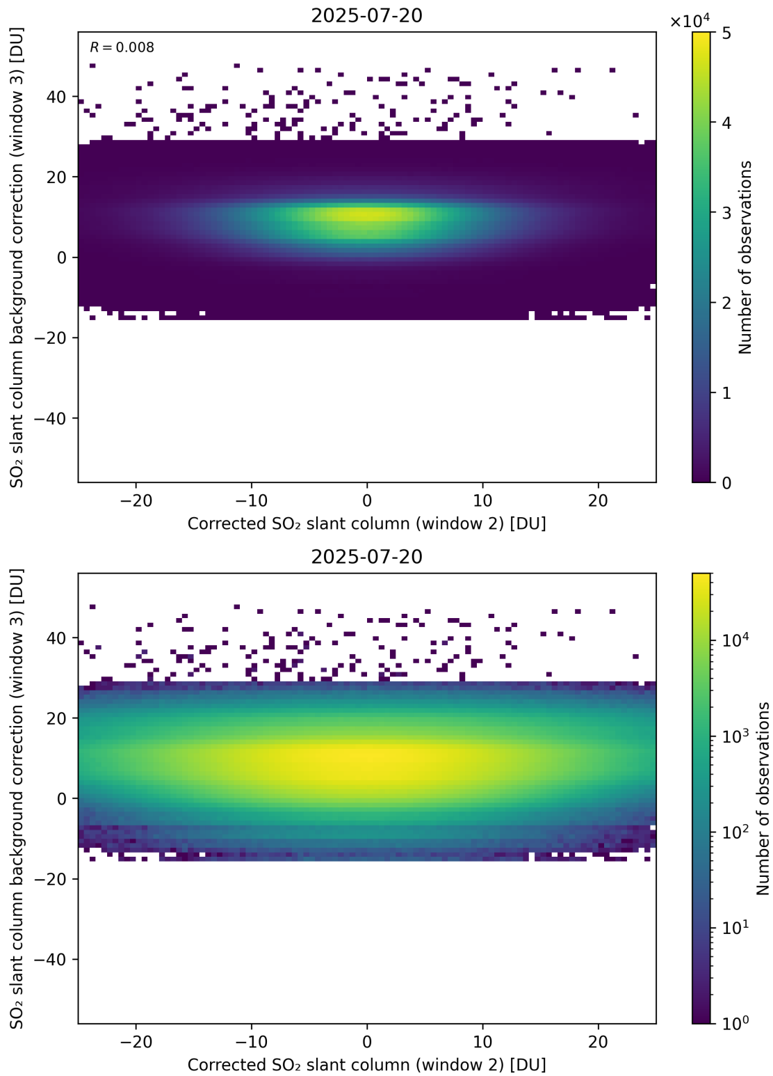
Figure 245: Scatter density plot of “Corrected SO 2 slant column (window 2)” against “SO 2 slant column background correction (window 3)” for 2025-07-19 to 2025-07-21.
