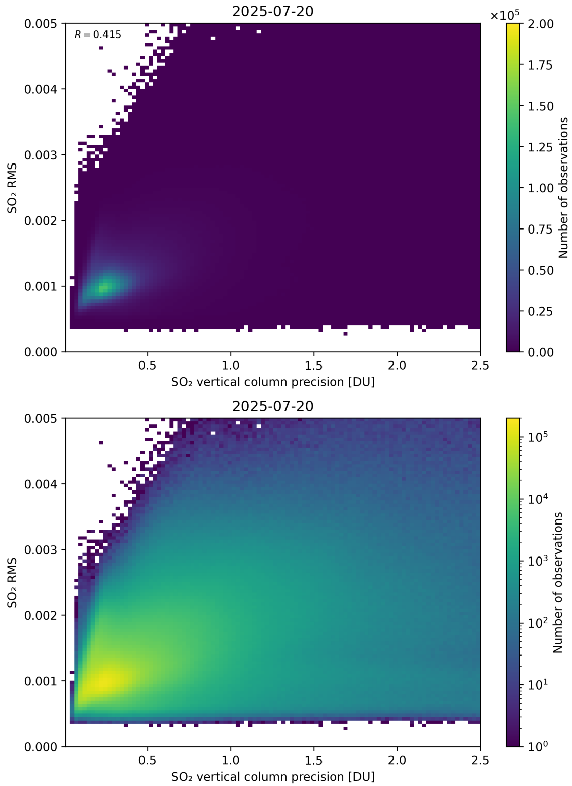
Figure 334: Scatter density plot of “SO 2 vertical column precision” against “SO 2 RMS” for 2025-07-19 to 2025-07-21.
