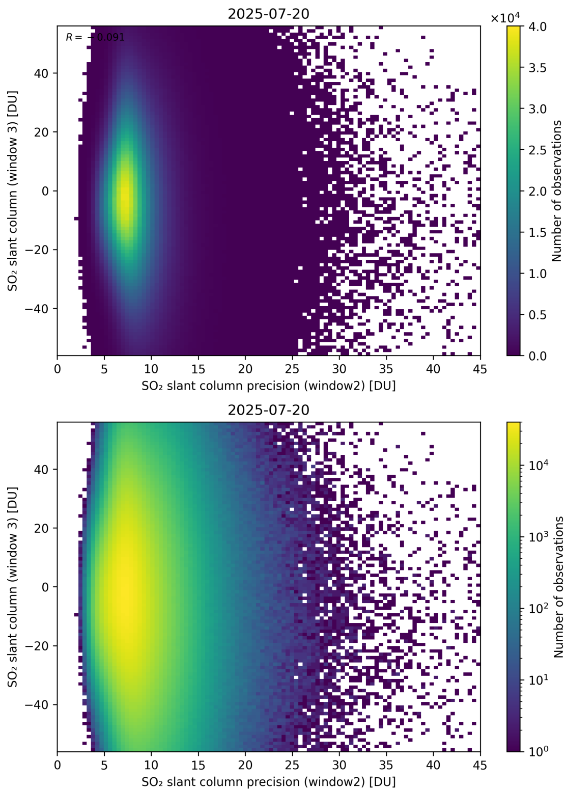
Figure 299: Scatter density plot of “SO 2 slant column precision (window2)” against “SO 2 slant column (window 3)” for 2025-07-19 to 2025-07-21.
