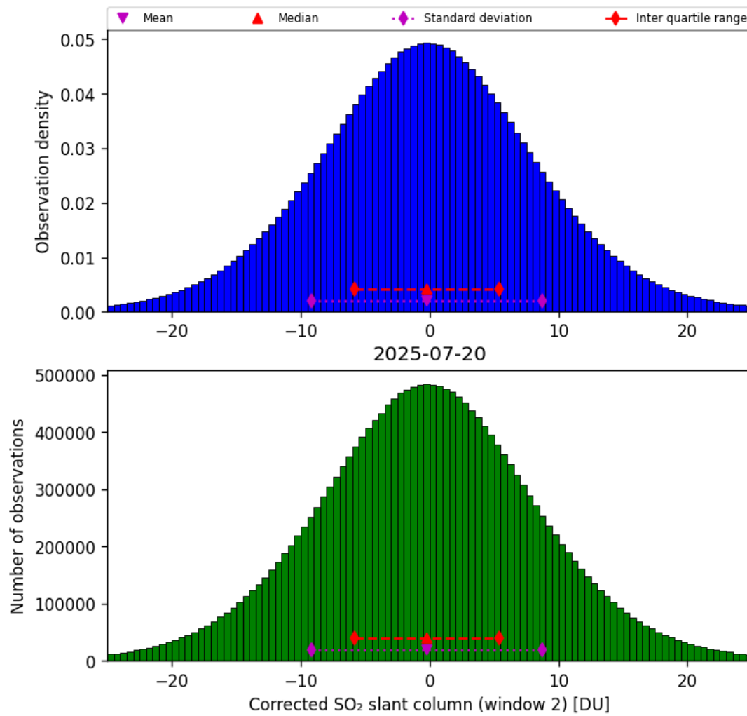
Figure 69: Histogram of “Corrected SO 2 slant column (window 2)” for 2025-07-19 to 2025-07-21
