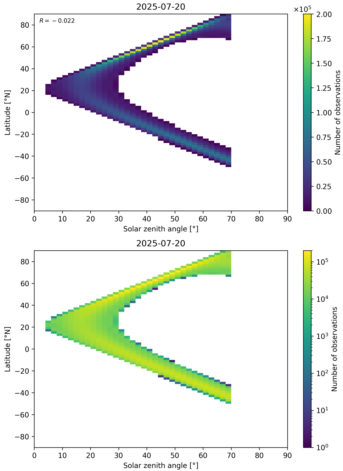
Figure 177: Scatter density plot of “Solar zenith angle” against “Latitude” for 2025-07-19 to 2025-07-21.
