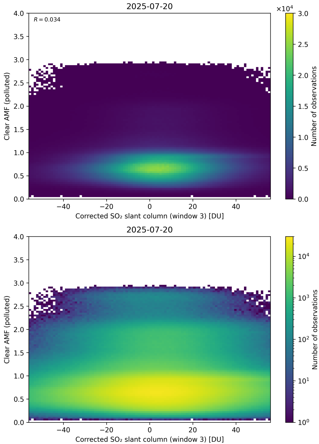
Figure 259: Scatter density plot of “Corrected SO 2 slant column (window 3)” against “Clear AMF (polluted)” for 2025-07-19 to 2025-07-21.
