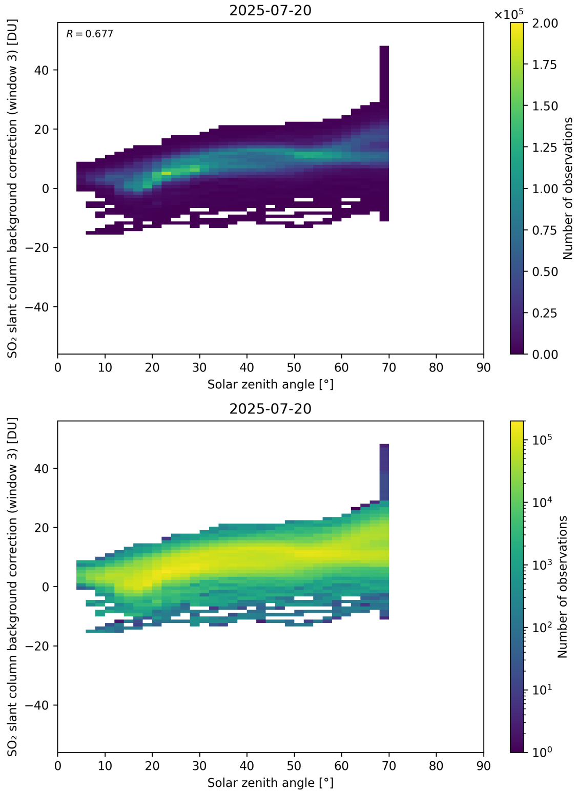
Figure 173: Scatter density plot of “Solar zenith angle” against “SO 2 slant column background correction (window 3)” for 2025-07-19 to 2025-07-21.
