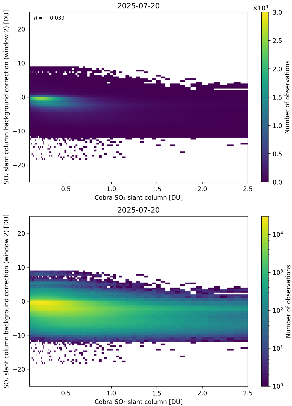
Figure 194: Scatter density plot of “Cobra SO 2 slant column” against “SO 2 slant column background correction (window 2)” for 2025-07-19 to 2025-07-21.
