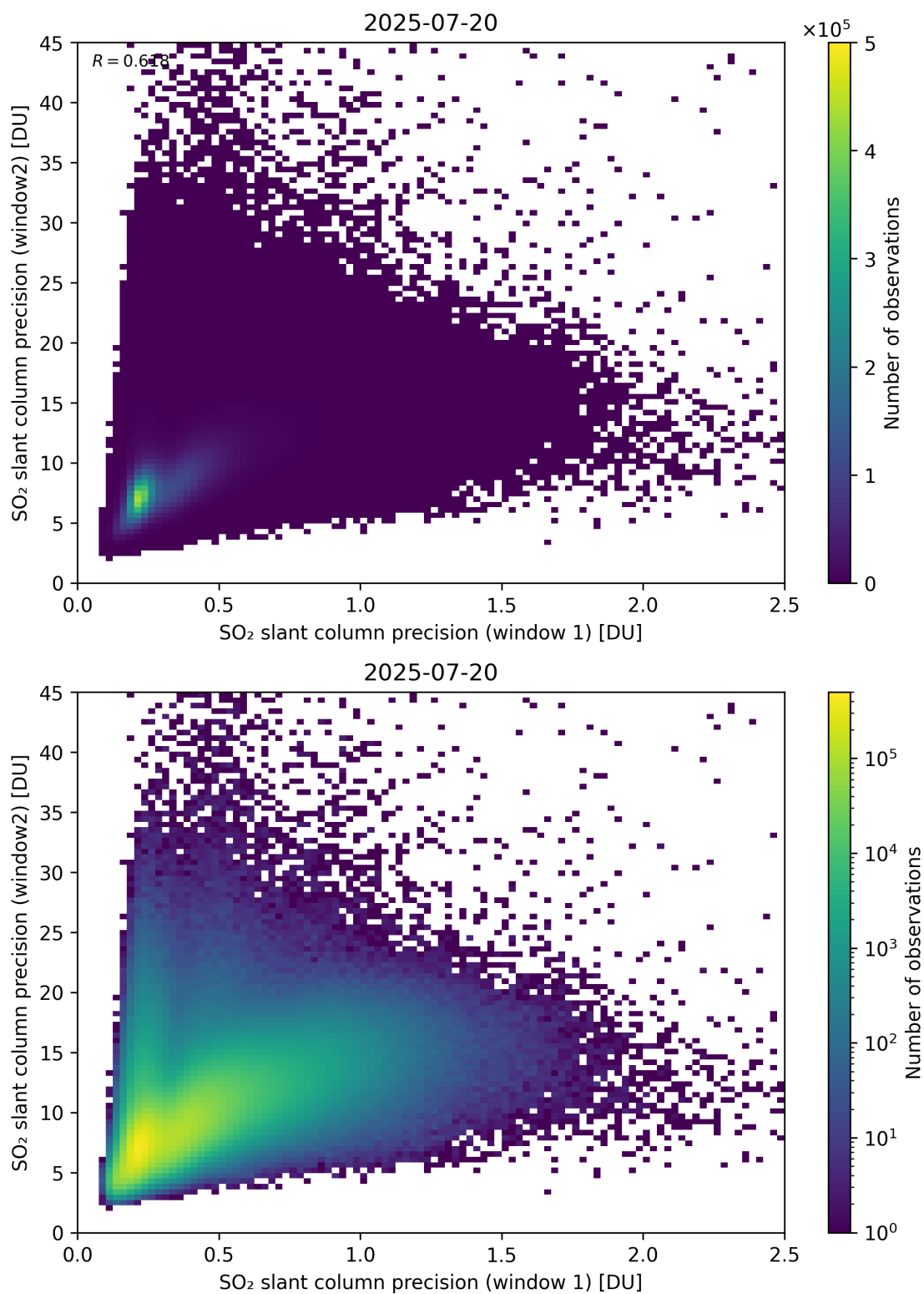
Figure 277: Scatter density plot of “SO 2 slant column precision (window 1)” against “SO 2 slant column precision (window2)” for 2025-07-19 to 2025-07-21.
