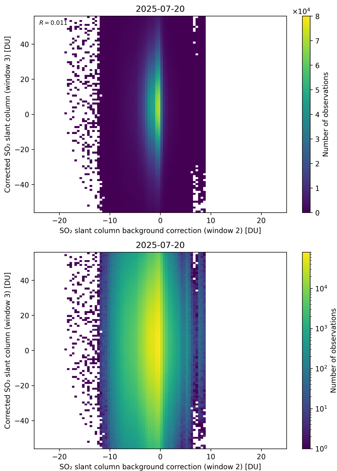
Figure 127: Scatter density plot of “SO 2 slant column background correction (window 2)” against “Corrected SO 2 slant column (window 3)” for 2025-07-19 to 2025-07-21.
