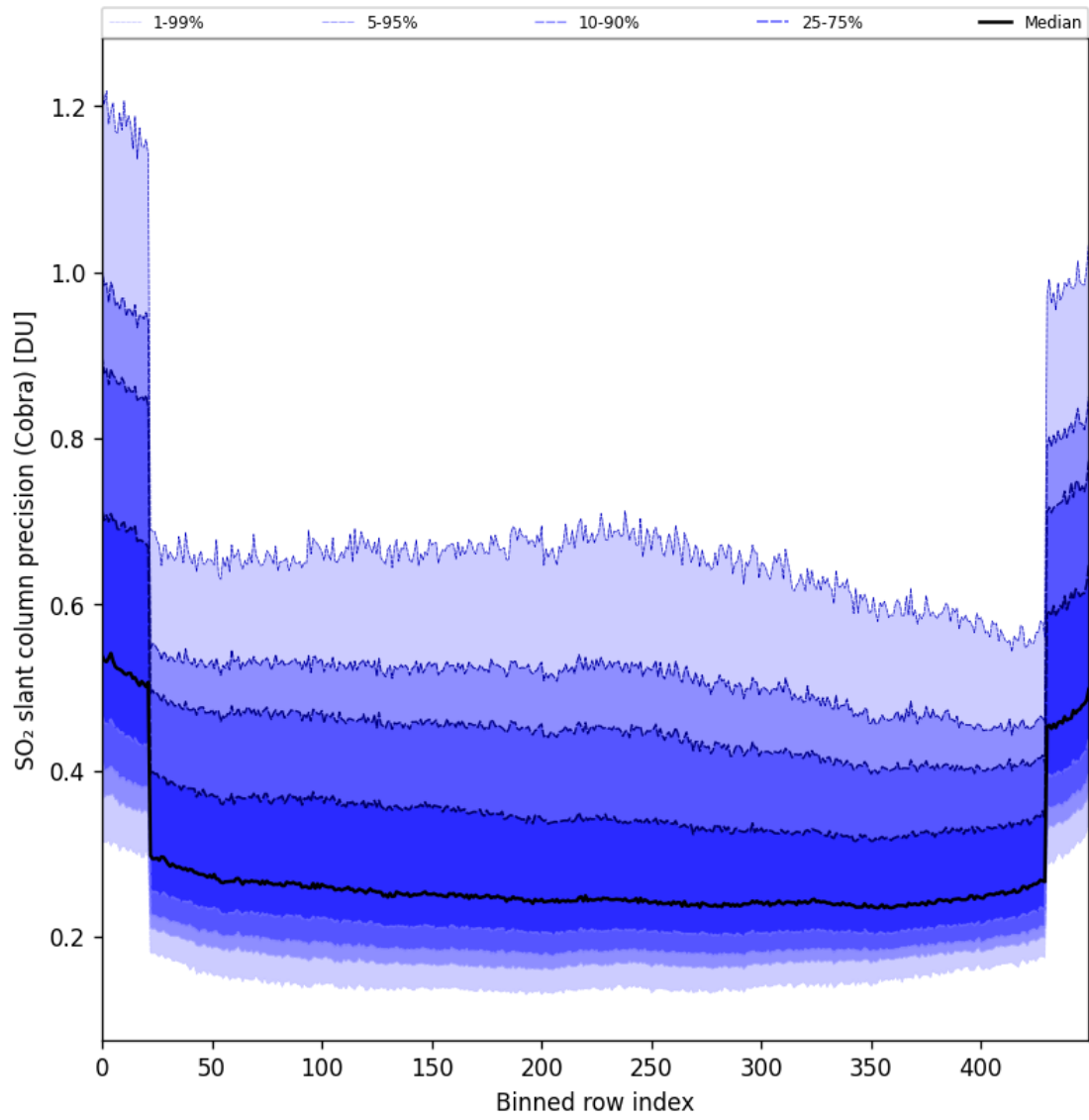
Figure 88: Along track statistics of “SO 2 slant column precision (Cobra)” for 2025-07-19 to 2025-07-21
