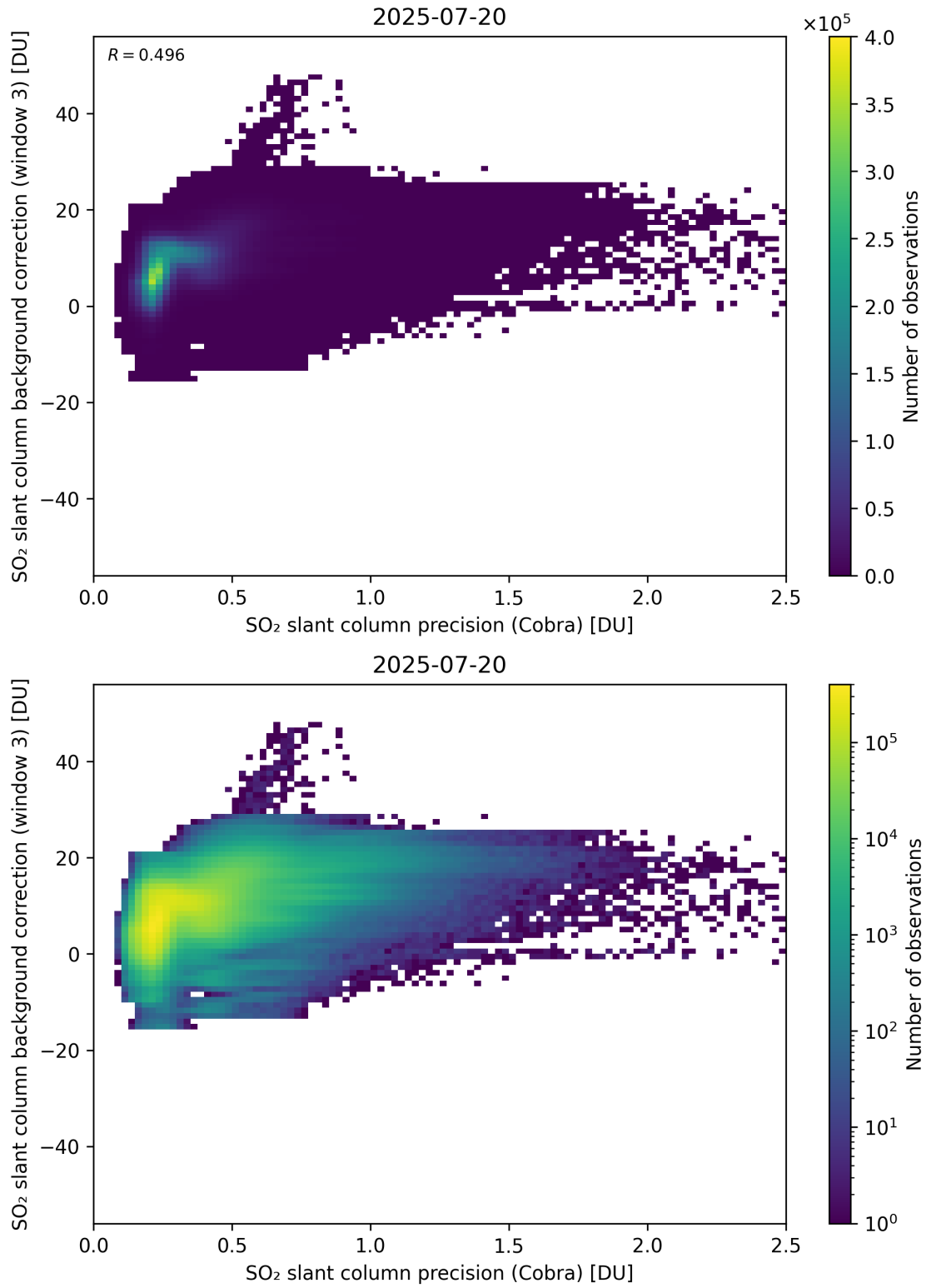
Figure 201: Scatter density plot of “SO 2 slant column precision (Cobra)” against “SO 2 slant column background correction (window 3)” for 2025-07-19 to 2025-07-21.
