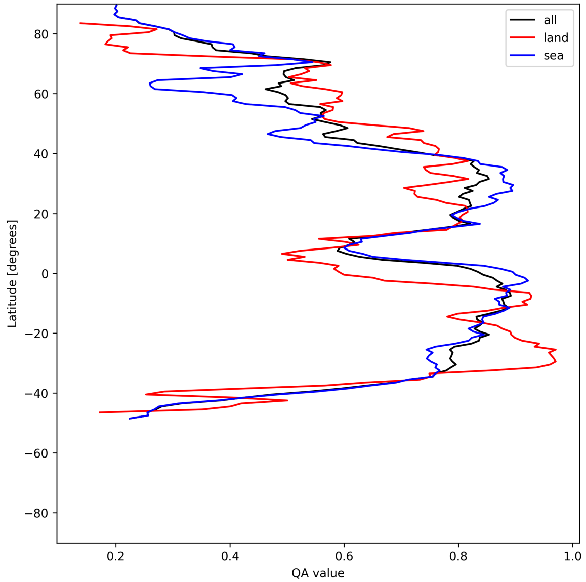
Figure 31: Zonal average of “QA value” for 2025-07-19 to 2025-07-21.
