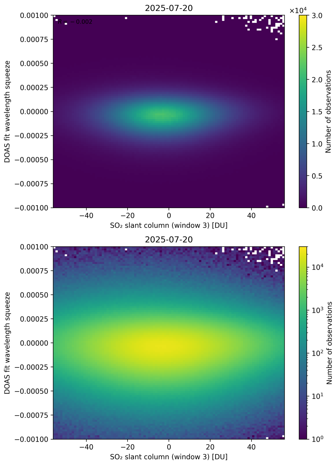
Figure 305: Scatter density plot of “SO 2 slant column (window 3)” against “DOAS fit wavelength squeeze” for 2025-07-19 to 2025-07-21.
