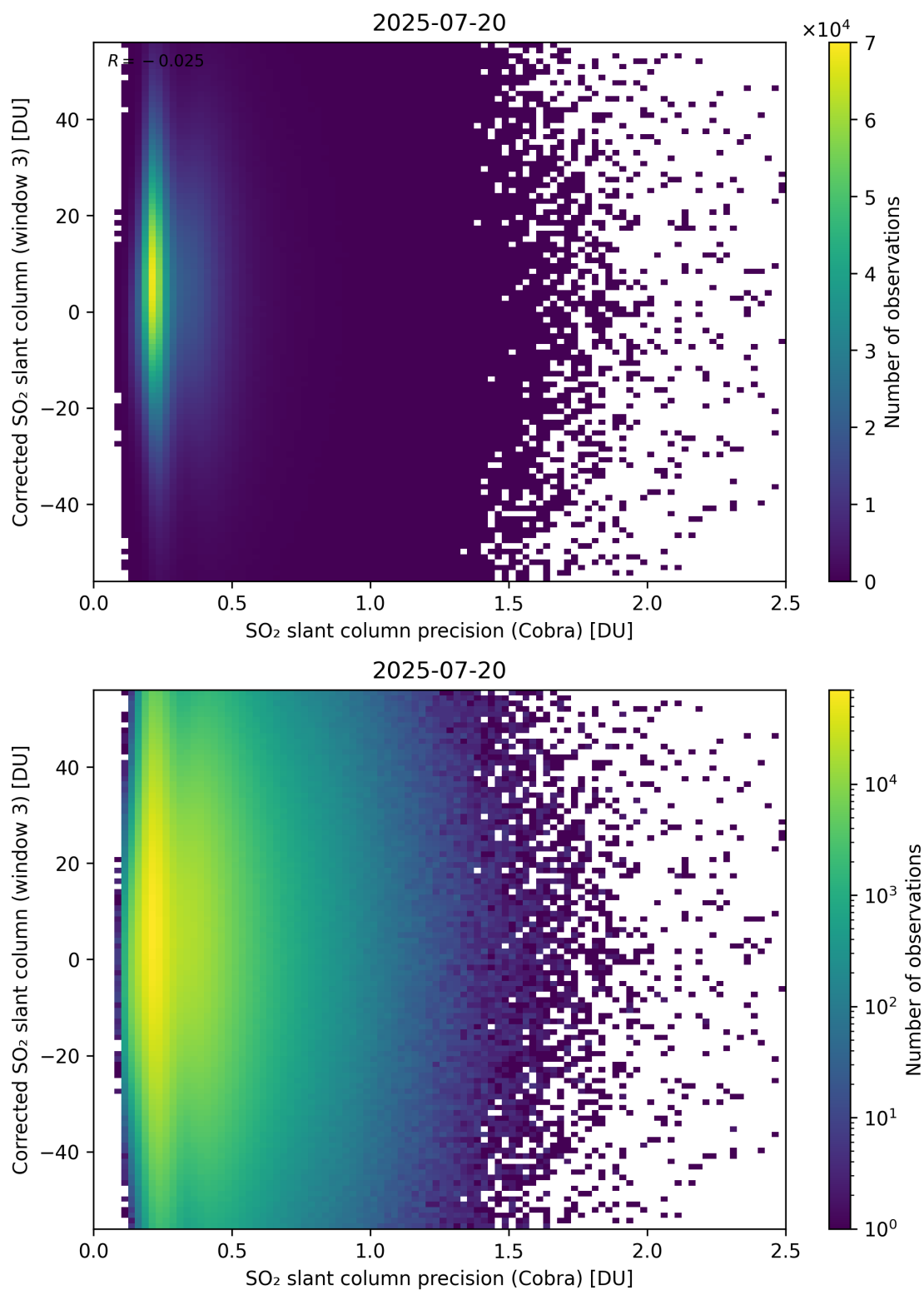
Figure 207: Scatter density plot of “SO 2 slant column precision (Cobra)” against “Corrected SO 2 slant column (window 3)” for 2025-07-19 to 2025-07-21.
