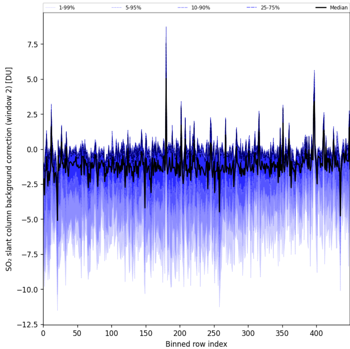
Figure 96: Along track statistics of “SO 2 slant column background correction (window 2)” for 2025-07-19 to 2025-07-21
