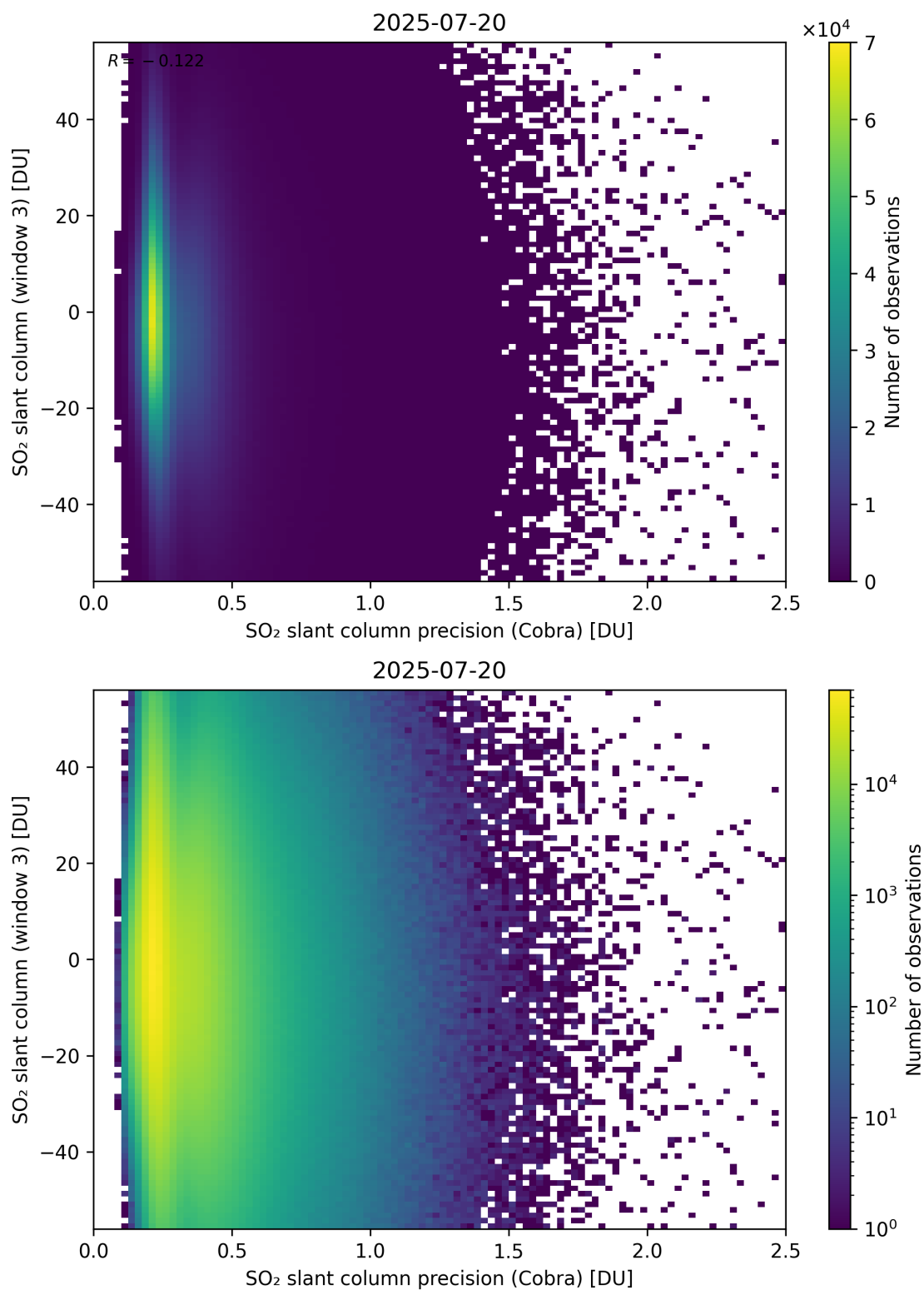
Figure 211: Scatter density plot of “SO 2 slant column precision (Cobra)” against “SO 2 slant column (window 3)” for 2025-07-19 to 2025-07-21.
