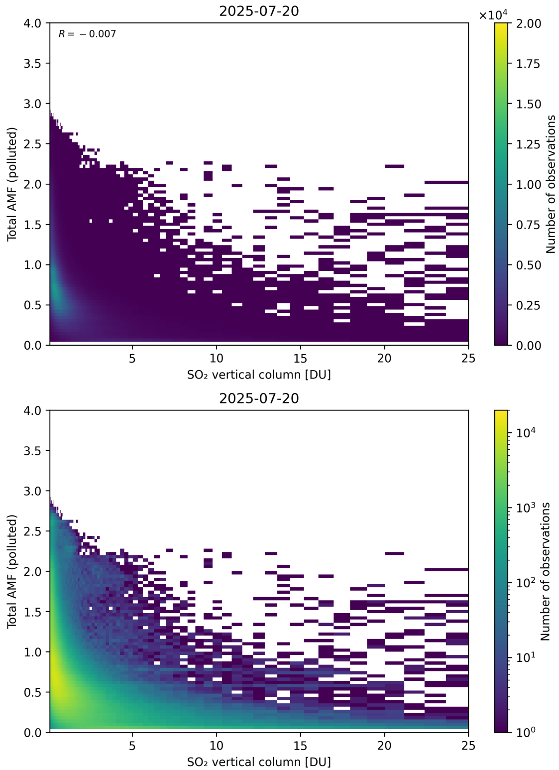
Figure 359: Scatter density plot of “SO 2 vertical column” against “Total AMF (polluted)” for 2025-07-19 to 2025-07-21.
