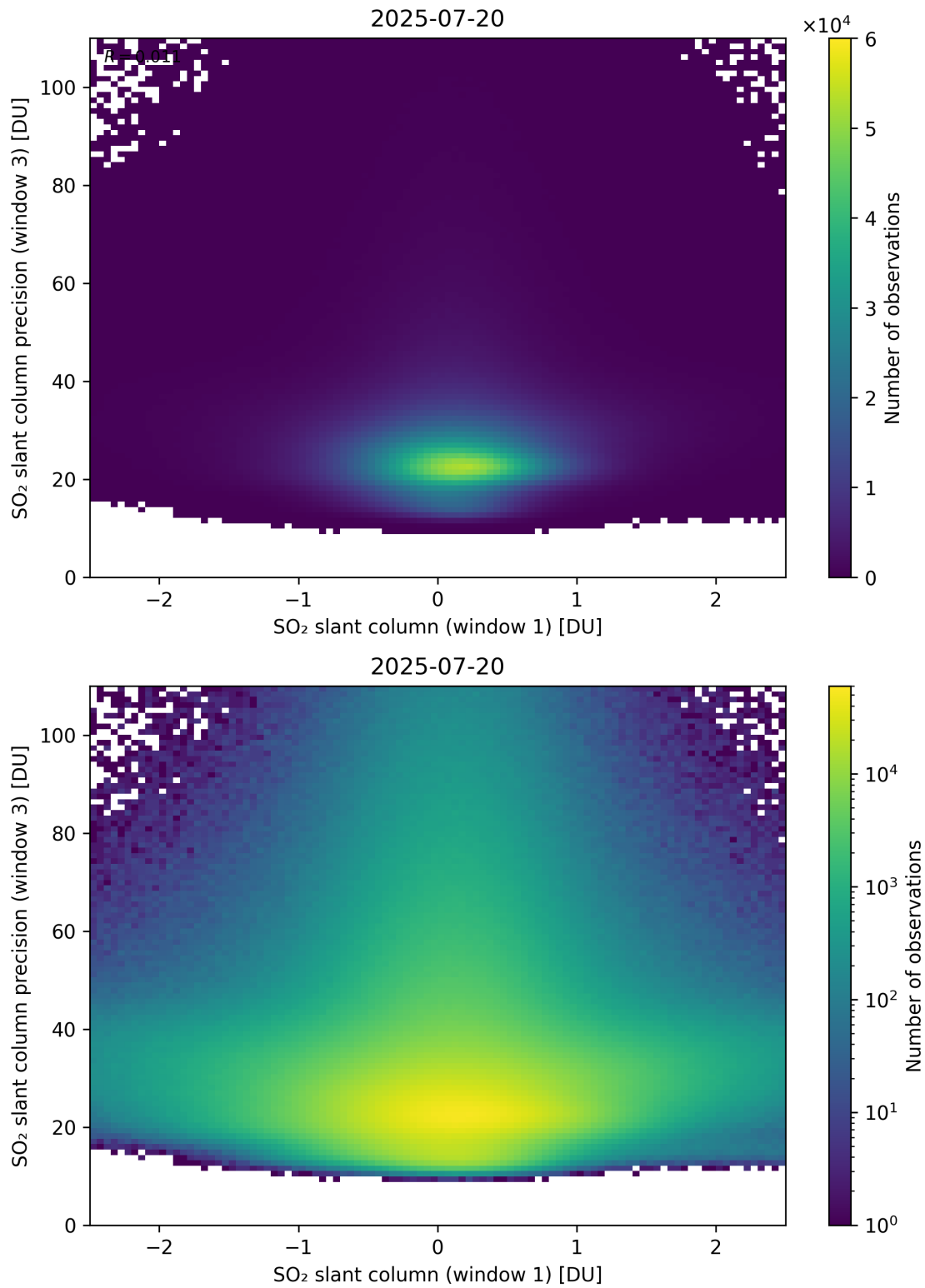
Figure 288: Scatter density plot of “SO 2 slant column (window 1)” against “SO 2 slant column precision (window 3)” for 2025-07-19 to 2025-07-21.
