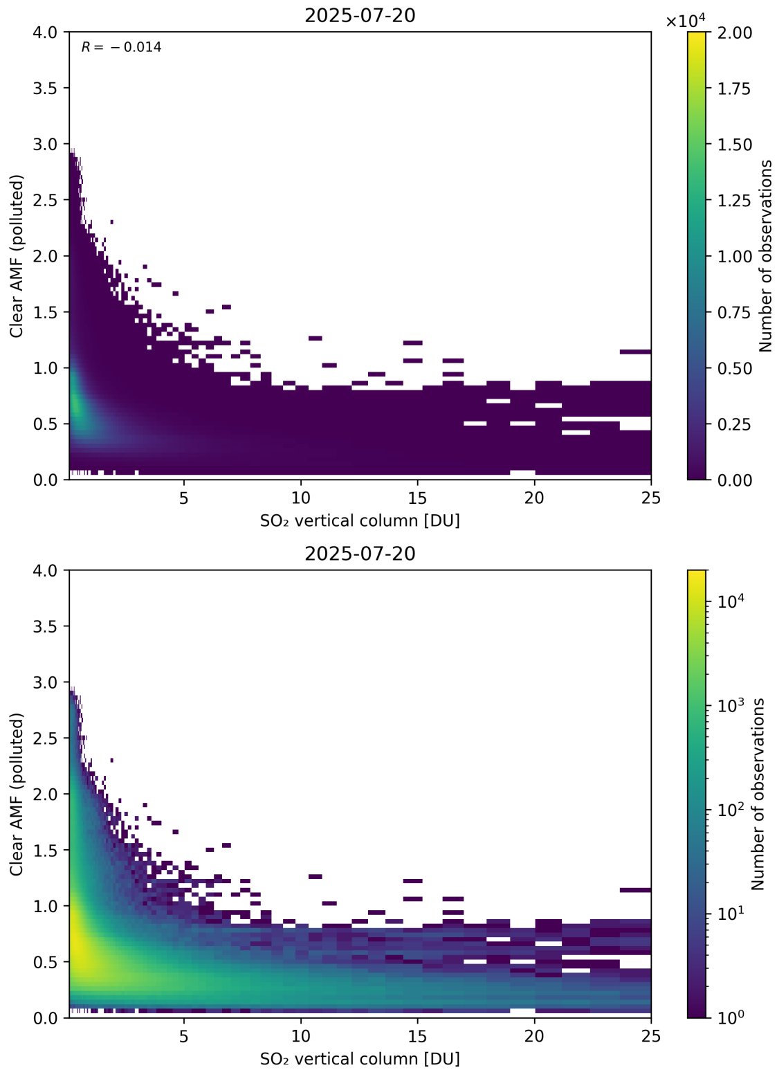
Figure 348: Scatter density plot of “SO 2 vertical column” against “Clear AMF (polluted)” for 2025-07-19 to 2025-07-21.
