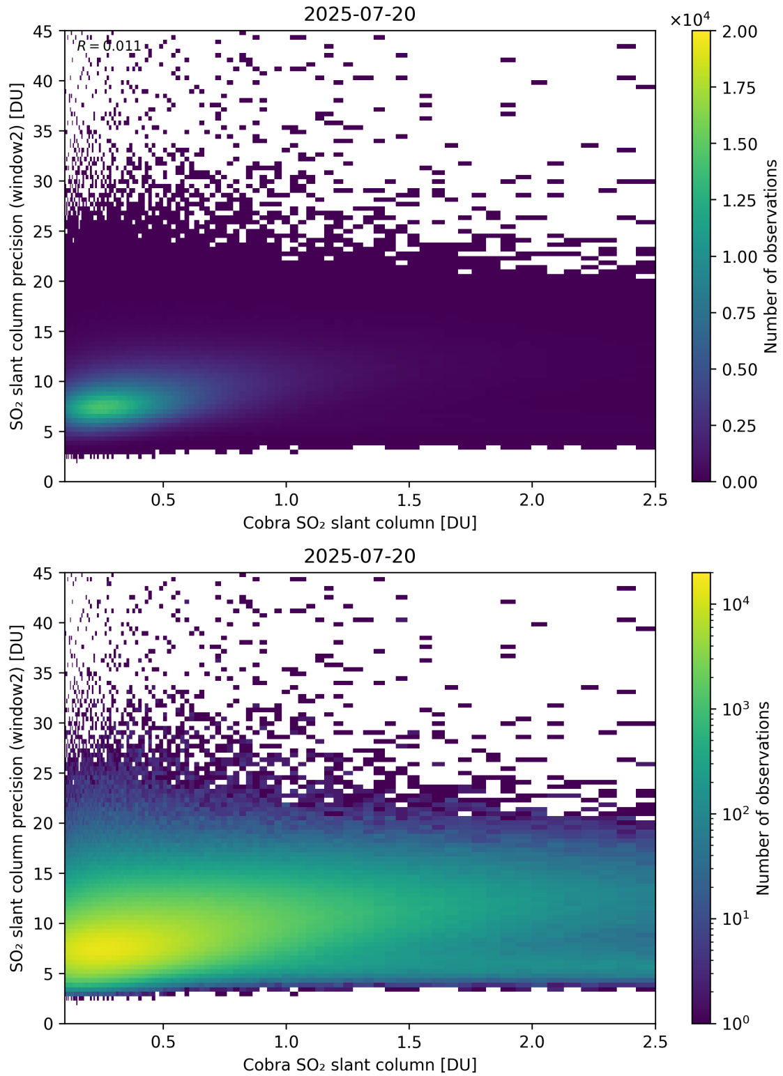
Figure 221: Scatter density plot of “Cobra SO 2 slant column” against “SO 2 slant column precision (window2)” for 2025-07-19 to 2025-07-21.
