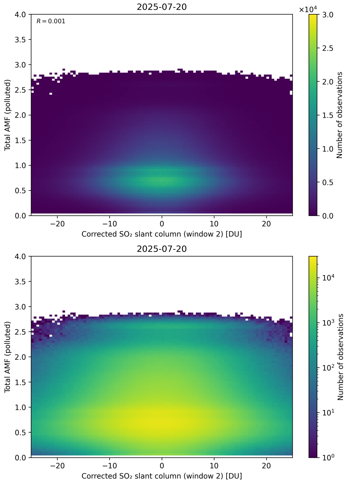
Figure 253: Scatter density plot of “Corrected SO 2 slant column (window 2)” against “Total AMF (polluted)” for 2025-07-19 to 2025-07-21.
