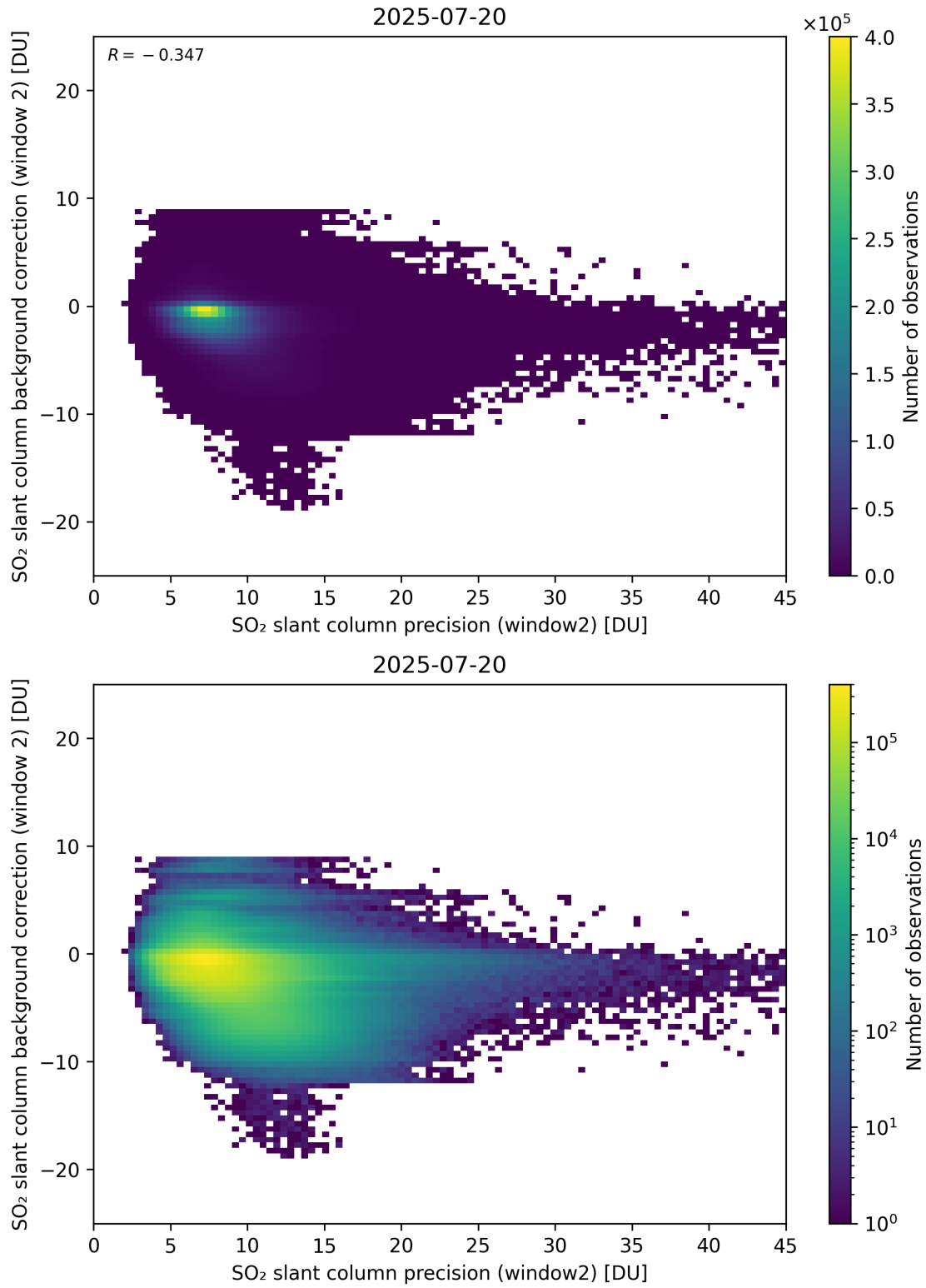
Figure 291: Scatter density plot of “SO 2 slant column precision (window2)” against “SO 2 slant column background correction (window 2)” for 2025-07-19 to 2025-07-21.
