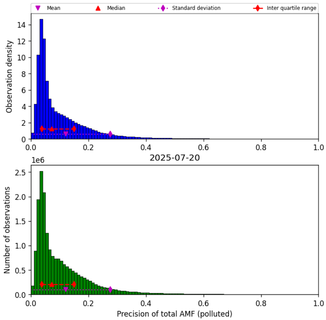
Figure 80: Histogram of “Precision of total AMF (polluted)” for 2025-07-19 to 2025-07-21
