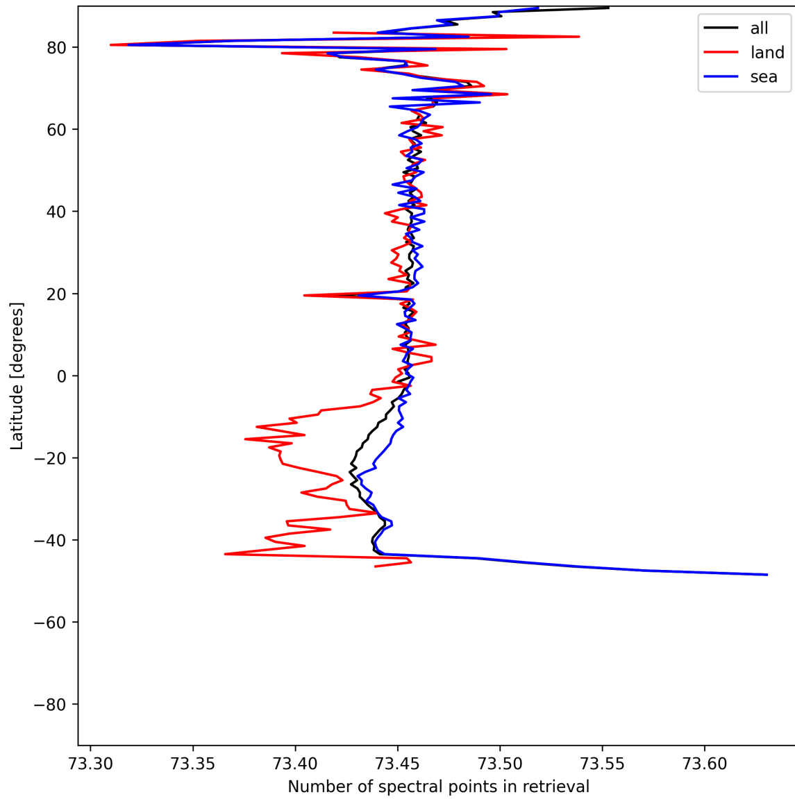
Figure 56: Zonal average of “Number of spectral points in retrieval” for 2025-07-19 to 2025-07-21.
