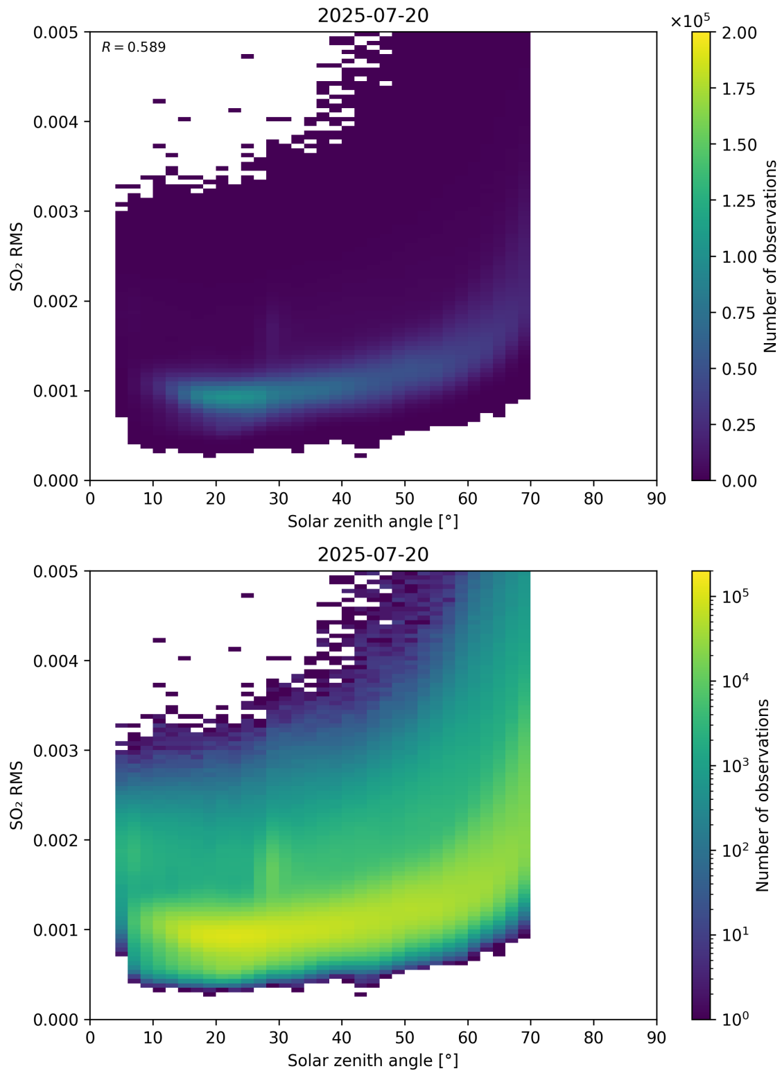
Figure 176: Scatter density plot of “Solar zenith angle” against “SO 2 RMS” for 2025-07-19 to 2025-07-21.
