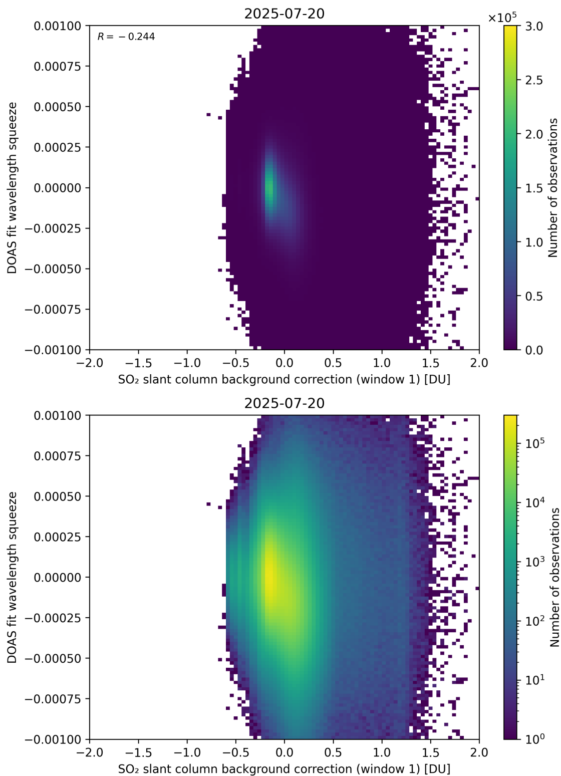
Figure 112: Scatter density plot of “SO 2 slant column background correction (window 1)” against “DOAS fit wavelength squeeze” for 2025-07-19 to 2025-07-21.
