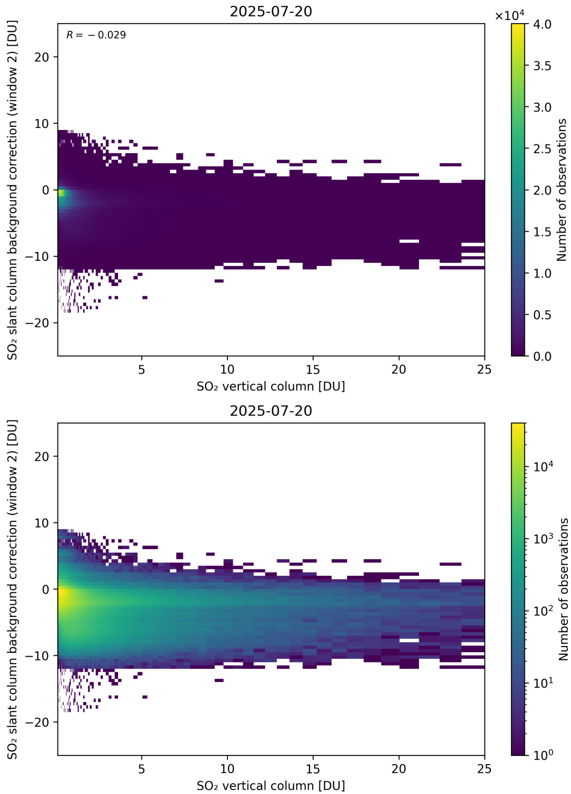
Figure 324: Scatter density plot of “SO 2 vertical column” against “SO 2 slant column background correction (window 2)” for 2025-07-19 to 2025-07-21.
