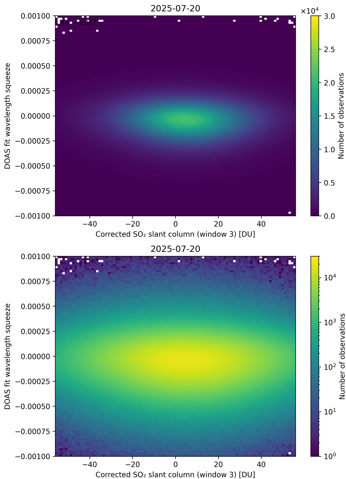
Figure 257: Scatter density plot of “Corrected SO 2 slant column (window 3)” against “DOAS fit wavelength squeeze” for 2025-07-19 to 2025-07-21.
