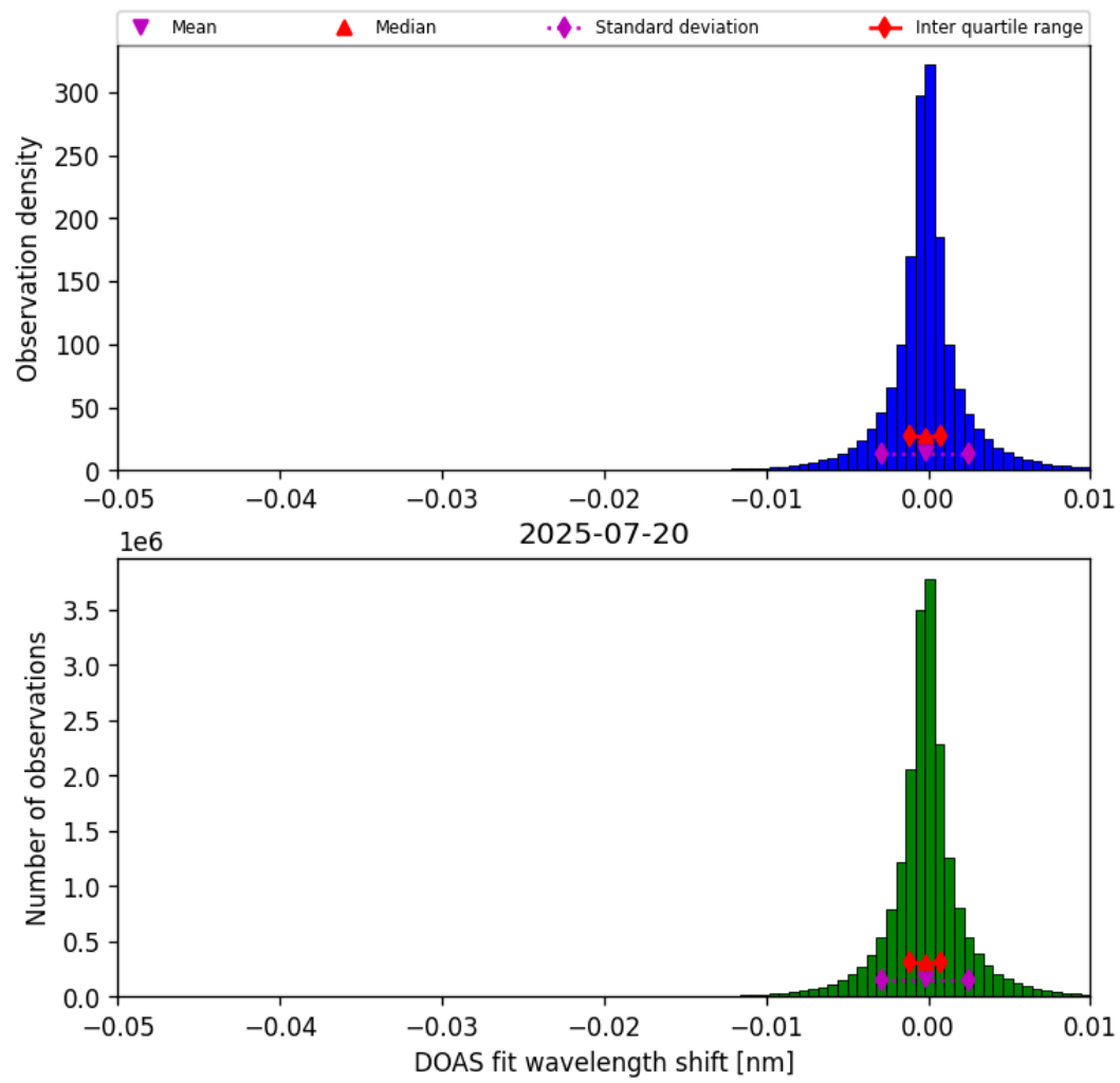
Figure 76: Histogram of “DOAS fit wavelength shift” for 2025-07-19 to 2025-07-21
