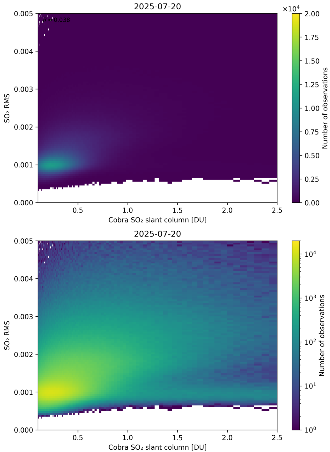
Figure 198: Scatter density plot of “Cobra SO 2 slant column” against “SO 2 RMS” for 2025-07-19 to 2025-07-21.
