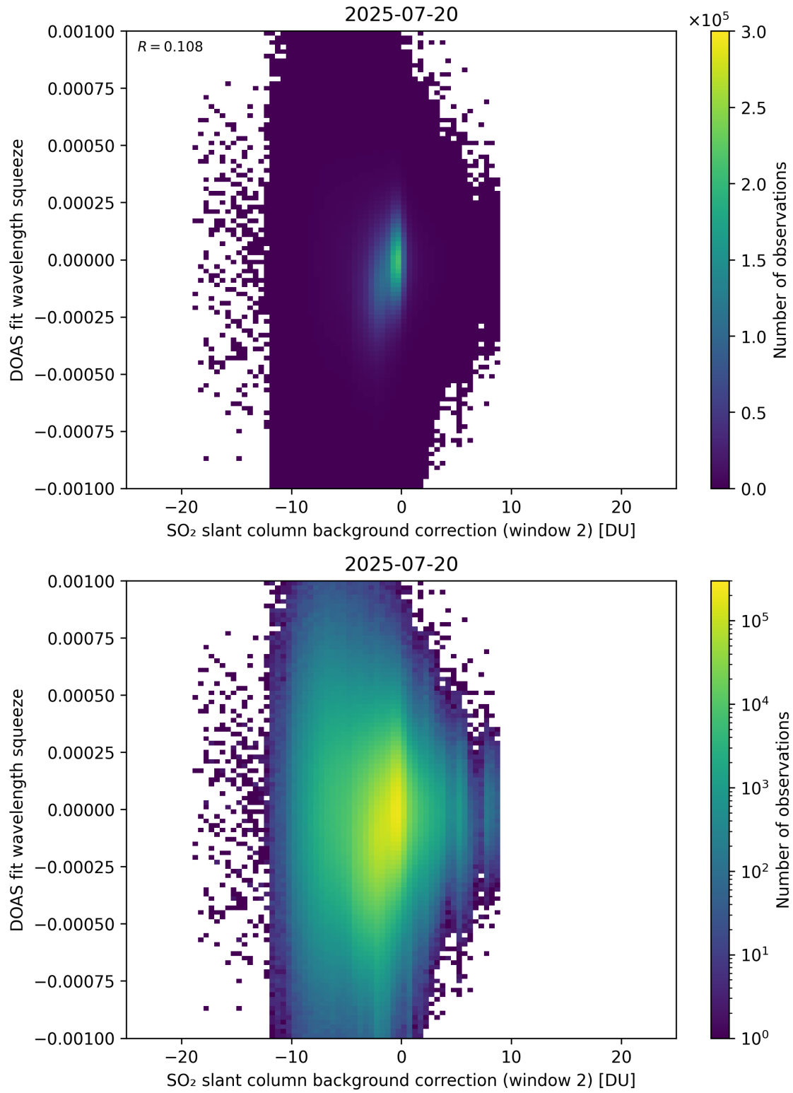
Figure 124: Scatter density plot of “SO 2 slant column background correction (window 2)” against “DOAS fit wavelength squeeze” for 2025-07-19 to 2025-07-21.
