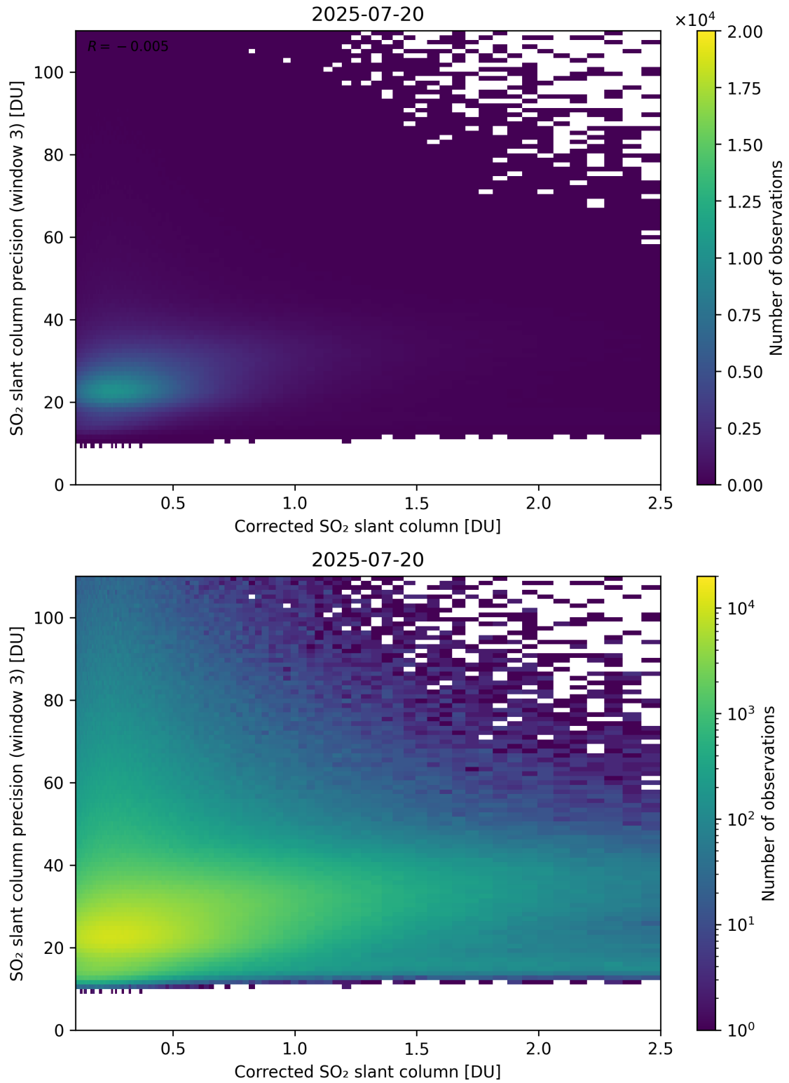
Figure 241: Scatter density plot of “Corrected SO 2 slant column” against “SO 2 slant column precision (window 3)” for 2025-07-19 to 2025-07-21.
