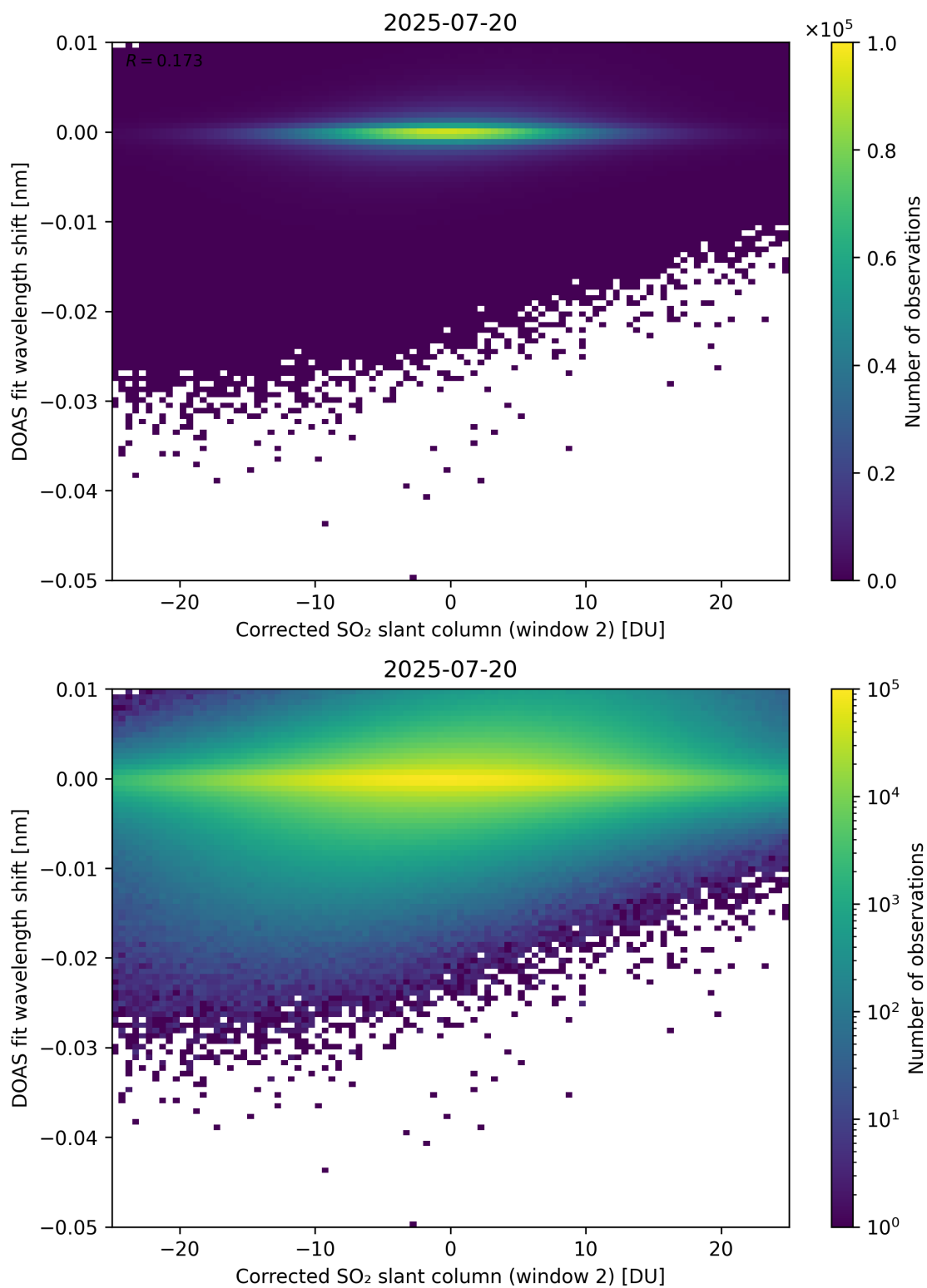
Figure 246: Scatter density plot of “Corrected SO 2 slant column (window 2)” against “DOAS fit wavelength shift” for 2025-07-19 to 2025-07-21.
