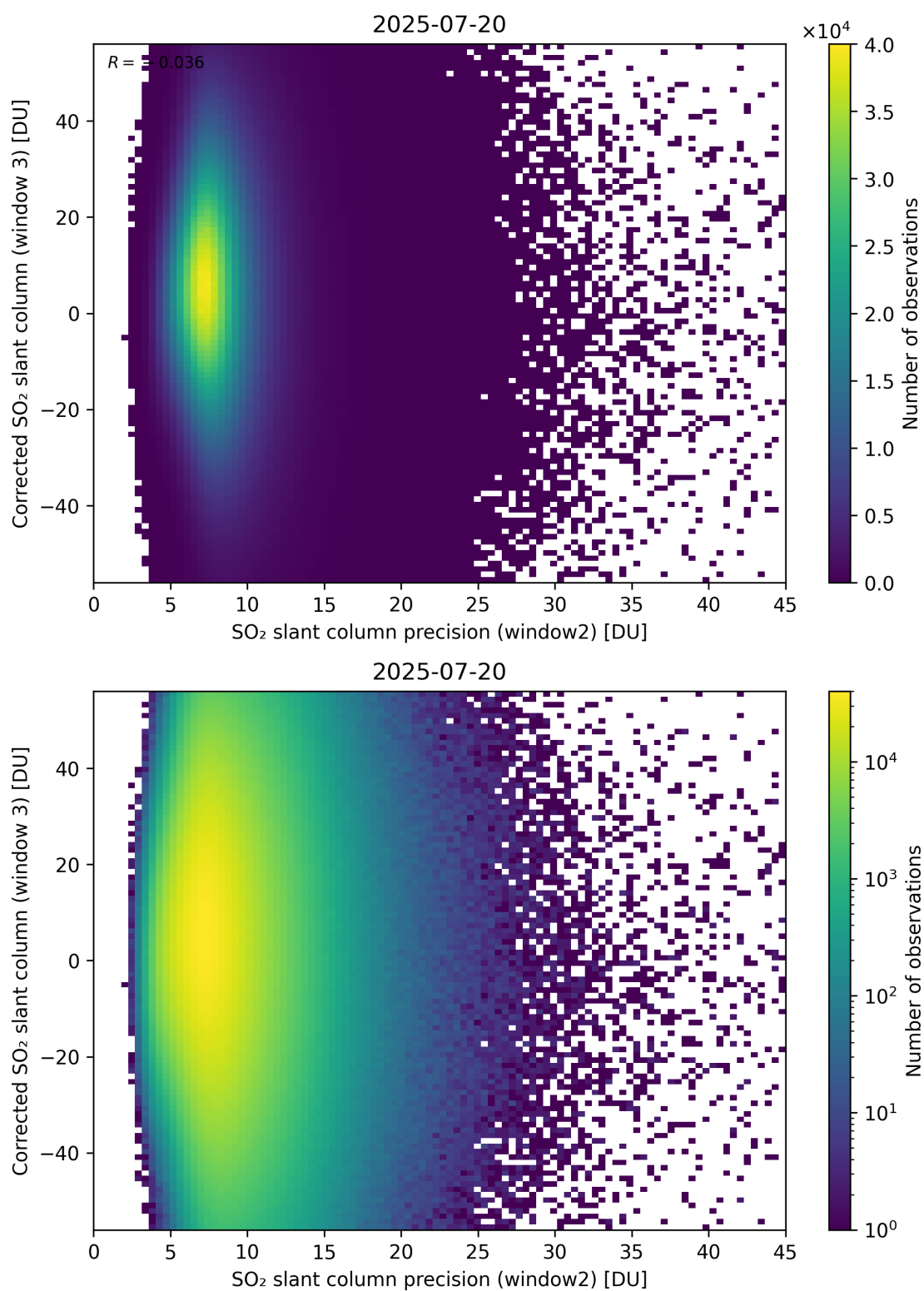
Figure 298: Scatter density plot of “SO 2 slant column precision (window2)” against “Corrected SO 2 slant column (window 3)” for 2025-07-19 to 2025-07-21.
