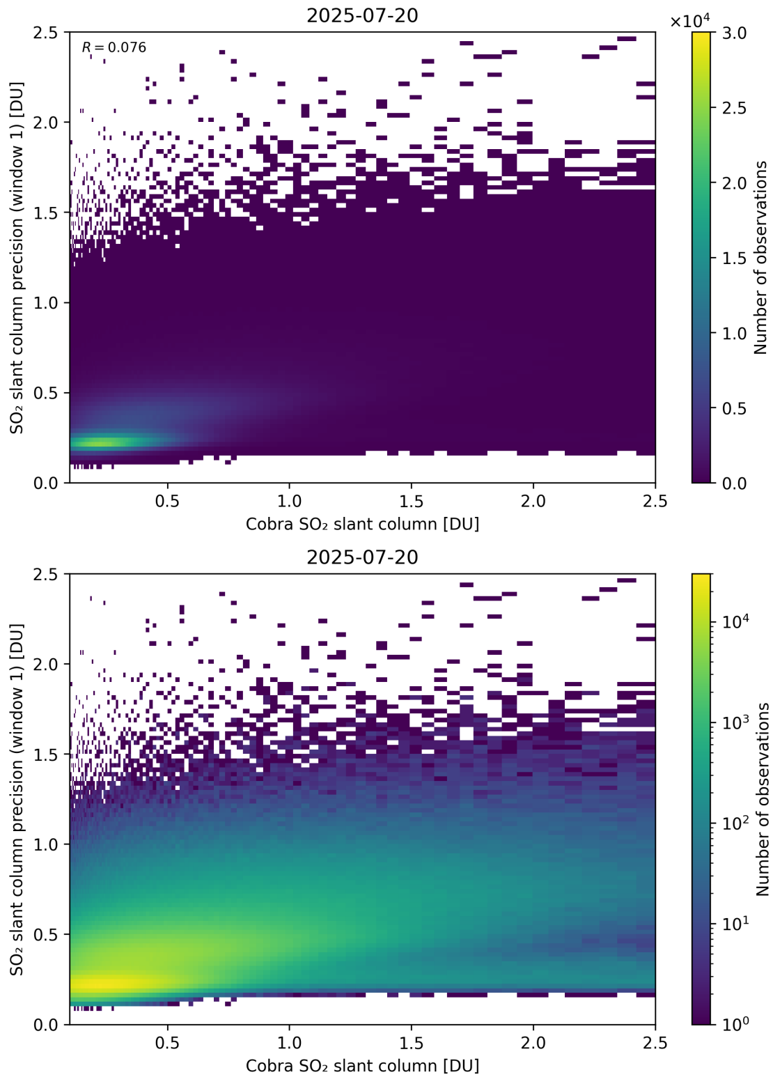
Figure 220: Scatter density plot of “Cobra SO 2 slant column” against “SO 2 slant column precision (window 1)” for 2025-07-19 to 2025-07-21.
