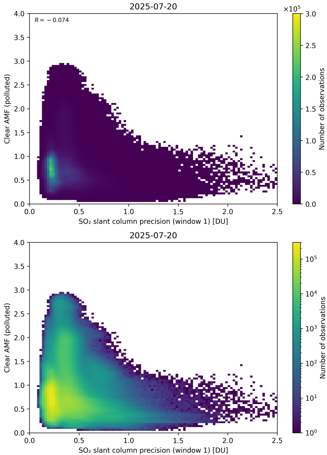
Figure 274: Scatter density plot of “SO 2 slant column precision (window 1)” against “Clear AMF (polluted)” for 2025-07-19 to 2025-07-21.
