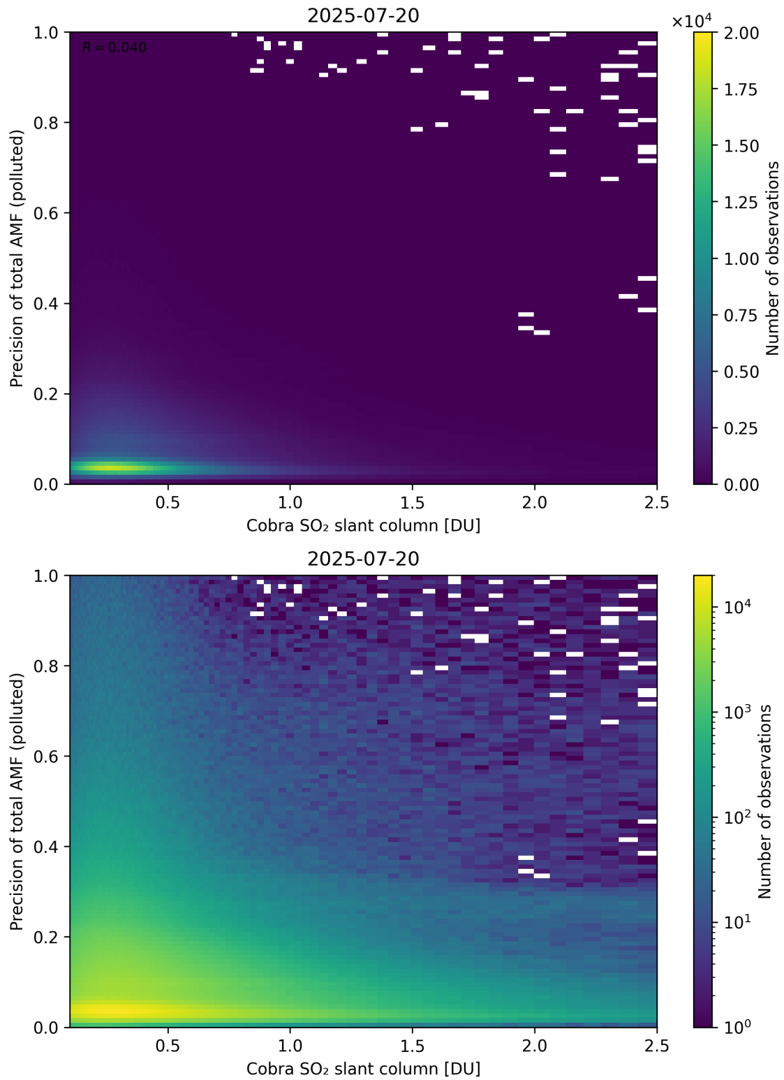
Figure 225: Scatter density plot of “Cobra SO 2 slant column” against “Precision of total AMF (polluted)” for 2025-07-19 to 2025-07-21.
