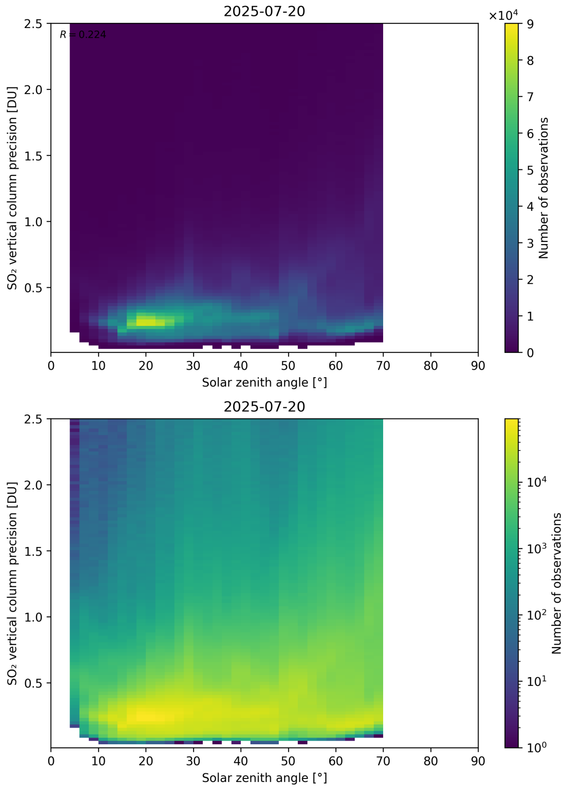
Figure 192: Scatter density plot of “Solar zenith angle” against “SO 2 vertical column precision” for 2025-07-19 to 2025-07-21.
