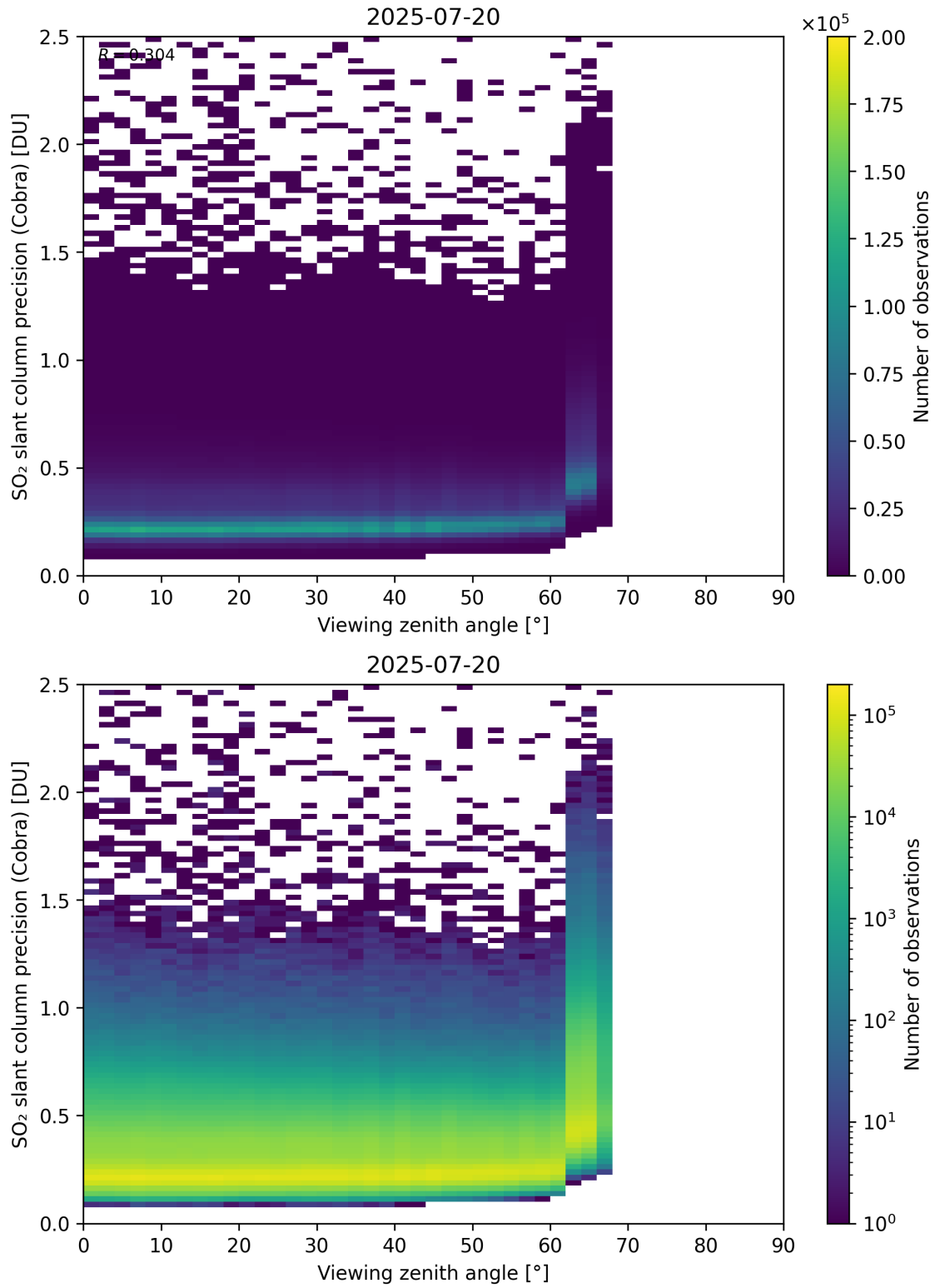
Figure 372: Scatter density plot of “Viewing zenith angle” against “SO 2 slant column precision (Cobra)” for 2025-07-19 to 2025-07-21.
