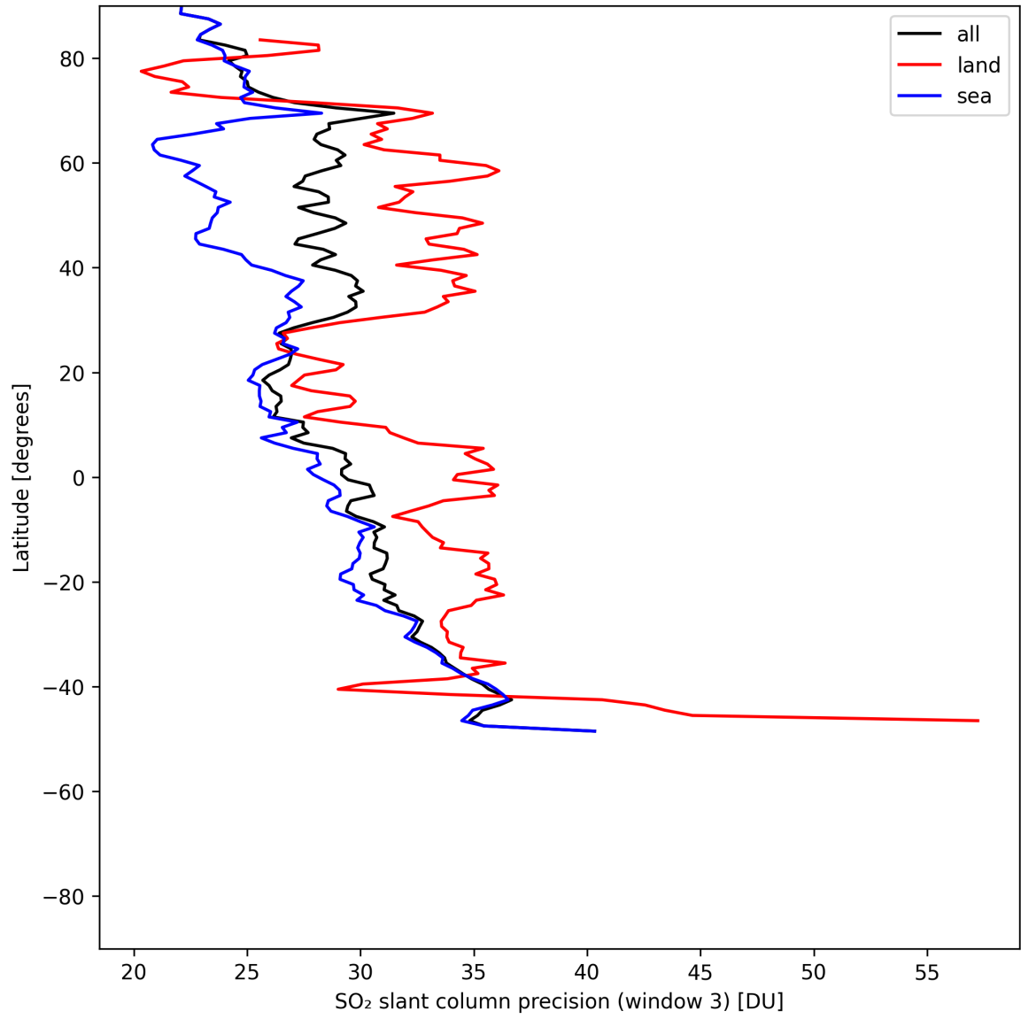
Figure 46: Zonal average of “SO 2 slant column precision (window 3)” for 2025-07-19 to 2025-07-21.
