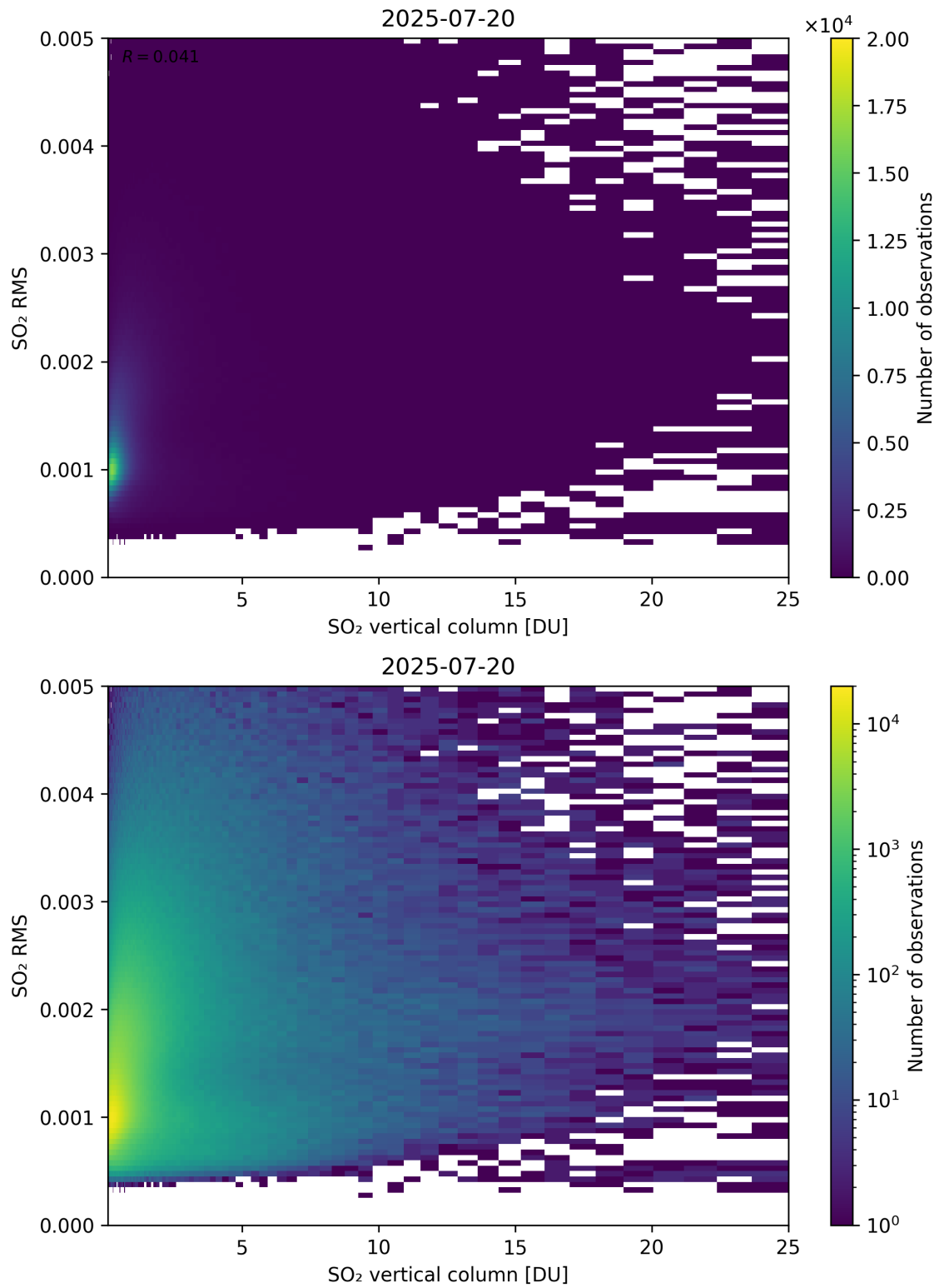
Figure 328: Scatter density plot of “SO 2 vertical column” against “SO 2 RMS” for 2025-07-19 to 2025-07-21.
