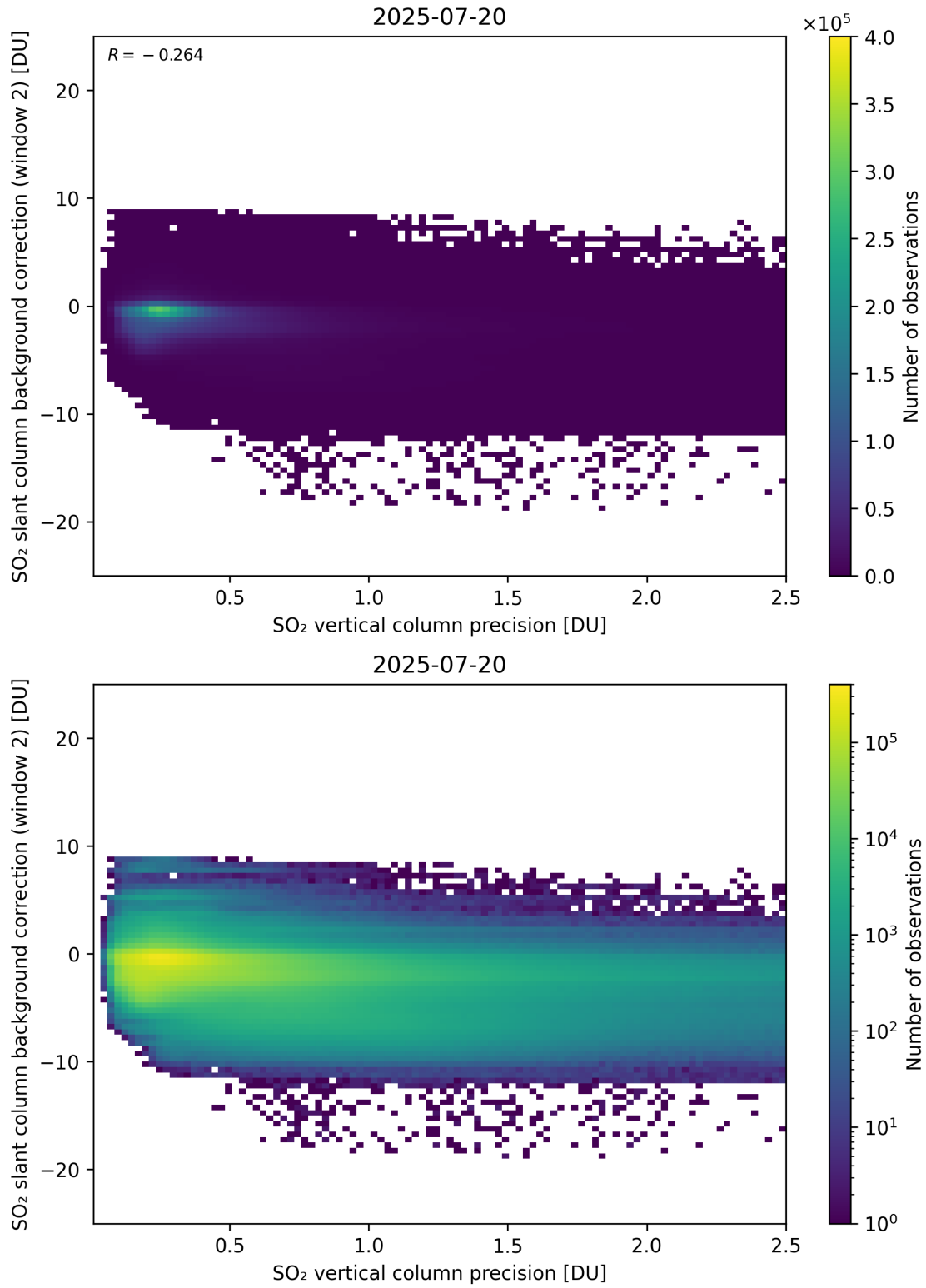
Figure 330: Scatter density plot of “SO 2 vertical column precision” against “SO 2 slant column background correction (window 2)” for 2025-07-19 to 2025-07-21.
