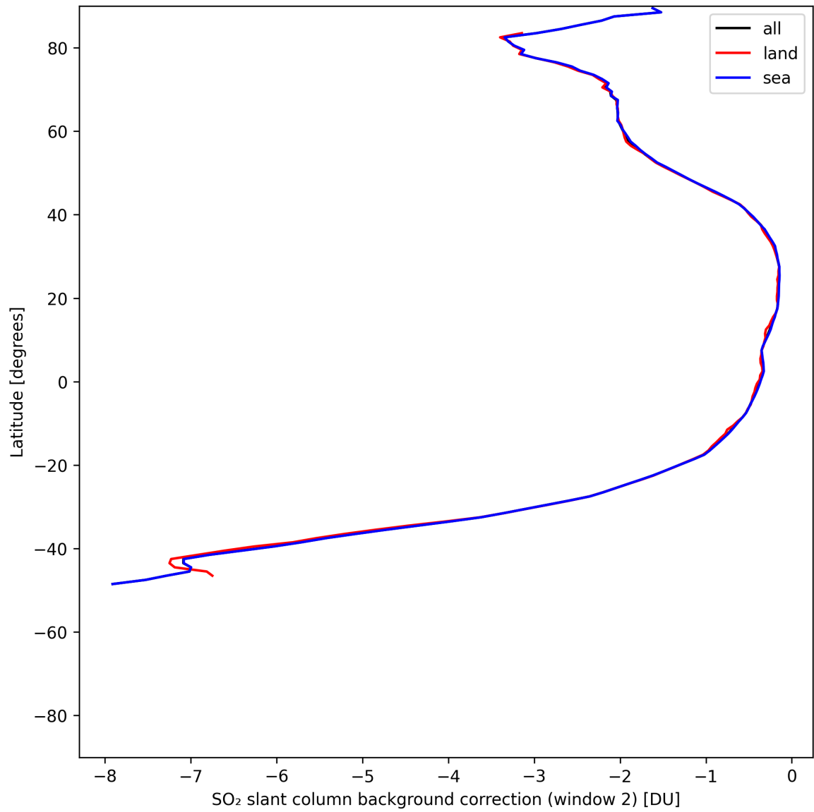
Figure 44: Zonal average of “SO 2 slant column background correction (window 2)” for 2025-07-19 to 2025-07-21.
