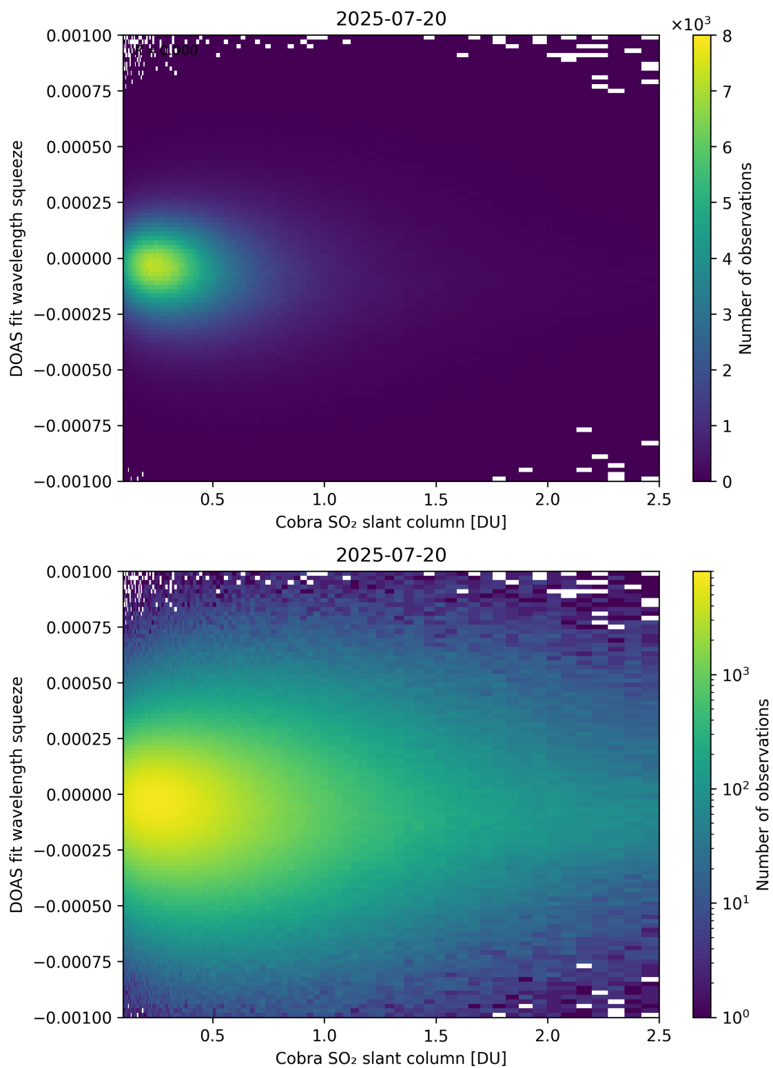
Figure 197: Scatter density plot of “Cobra SO 2 slant column” against “DOAS fit wavelength squeeze” for 2025-07-19 to 2025-07-21.
