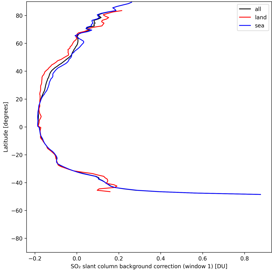
Figure 40: Zonal average of “SO 2 slant column background correction (window 1)” for 2025-07-19 to 2025-07-21.
