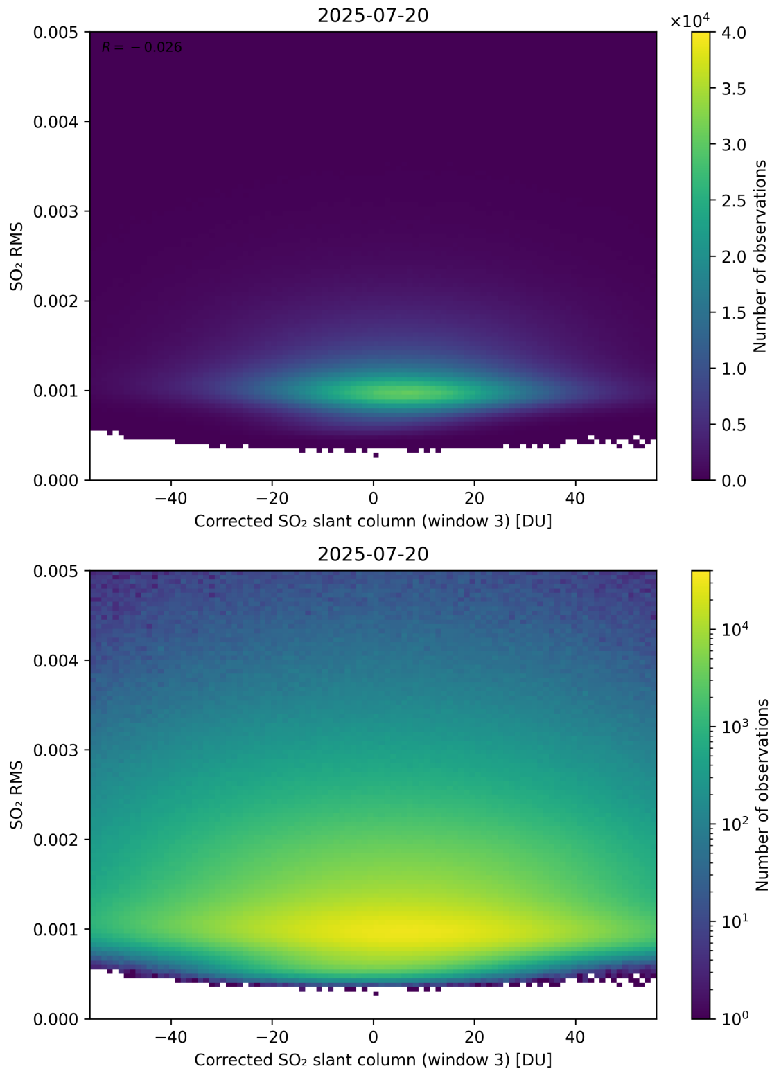
Figure 258: Scatter density plot of “Corrected SO 2 slant column (window 3)” against “SO 2 RMS” for 2025-07-19 to 2025-07-21.
