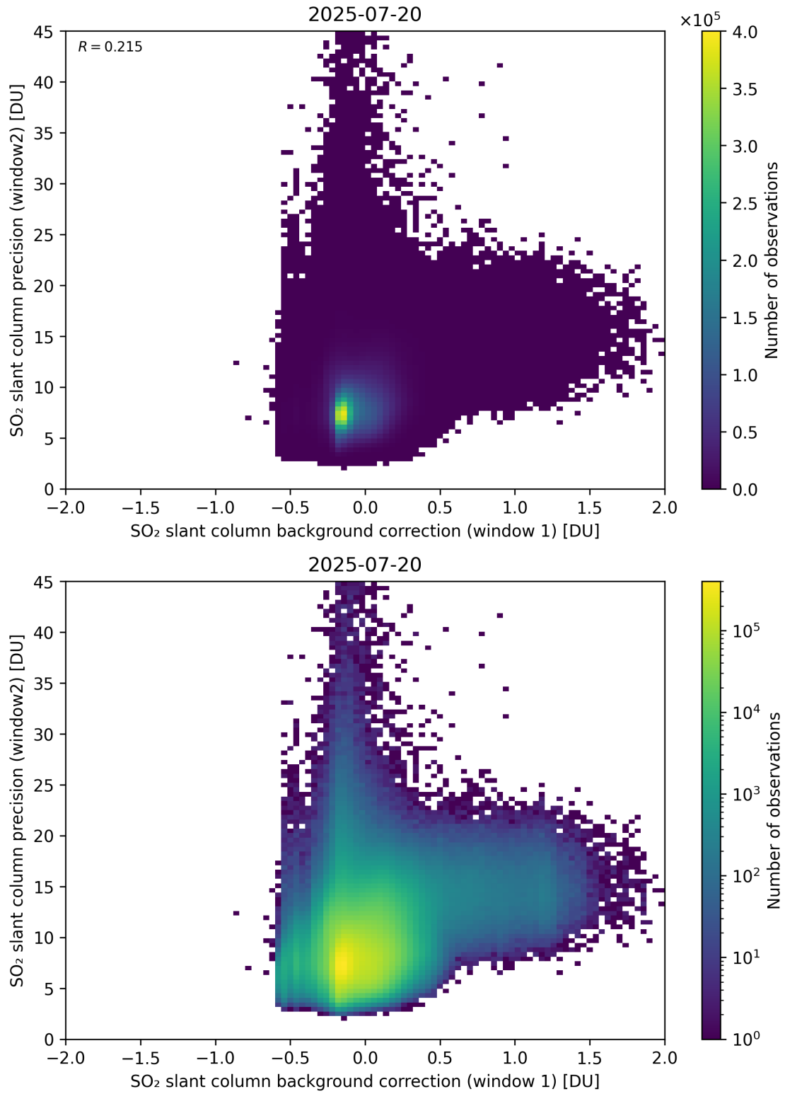
Figure 117: Scatter density plot of “SO 2 slant column background correction (window 1)” against “SO 2 slant column precision (window2)” for 2025-07-19 to 2025-07-21.
