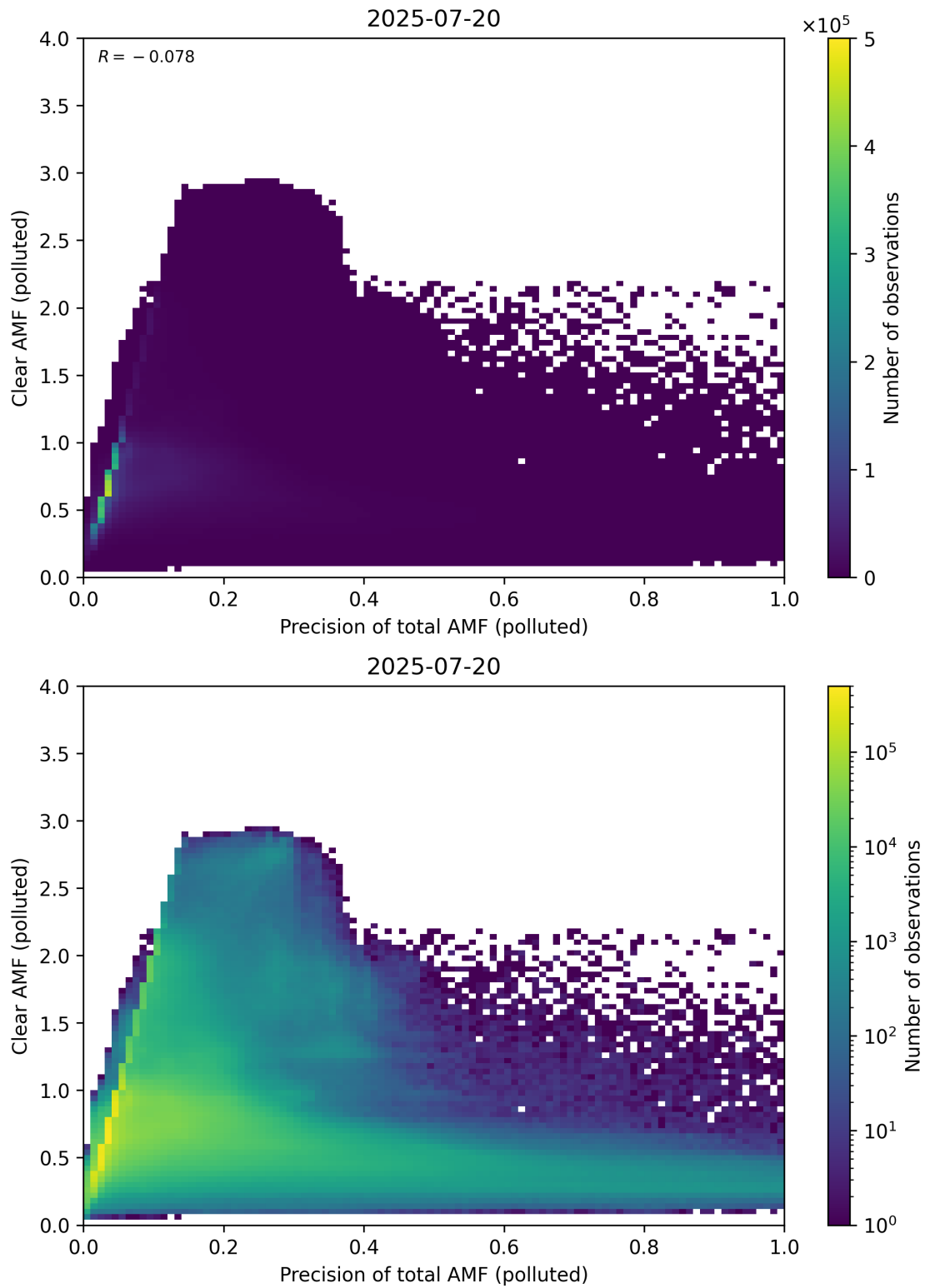
Figure 320: Scatter density plot of “Precision of total AMF (polluted)” against “Clear AMF (polluted)” for 2025-07-19 to 2025-07-21.
