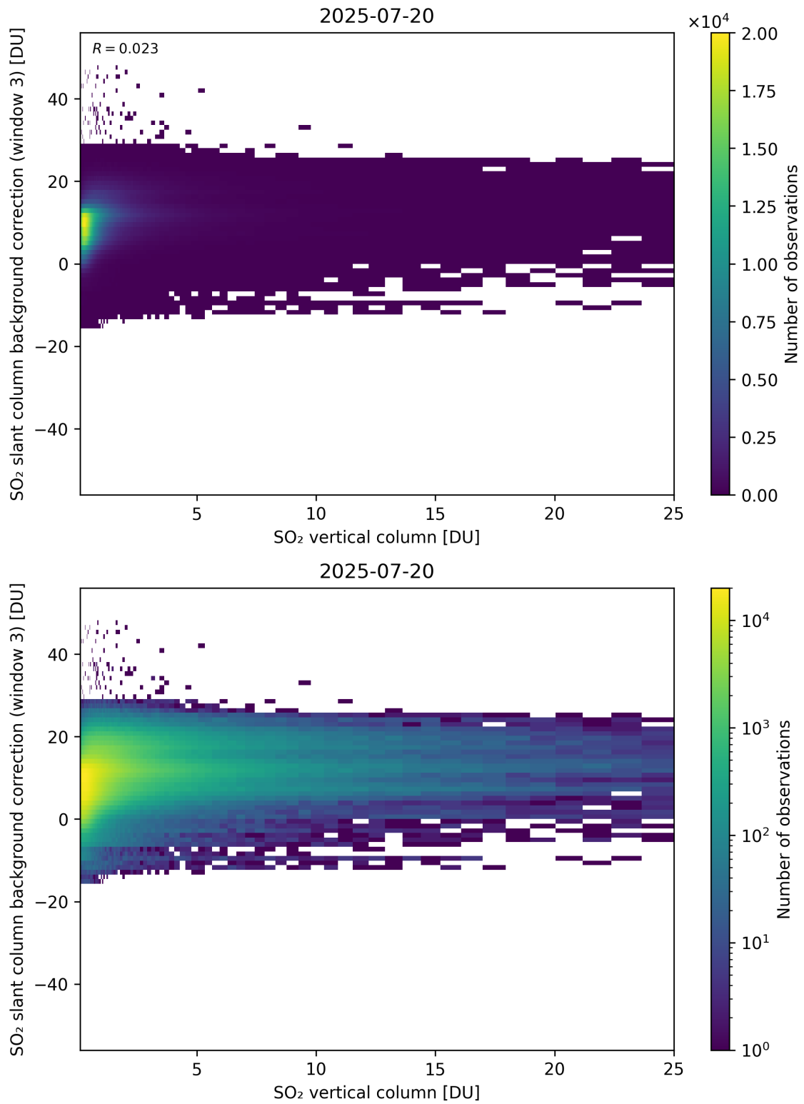
Figure 325: Scatter density plot of “SO 2 vertical column” against “SO 2 slant column background correction (window 3)” for 2025-07-19 to 2025-07-21.
