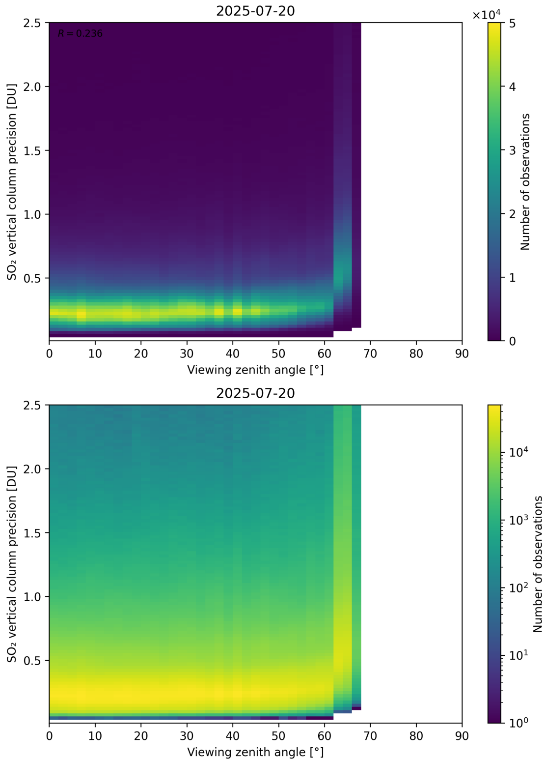
Figure 384: Scatter density plot of “Viewing zenith angle” against “SO 2 vertical column precision” for 2025-07-19 to 2025-07-21.
