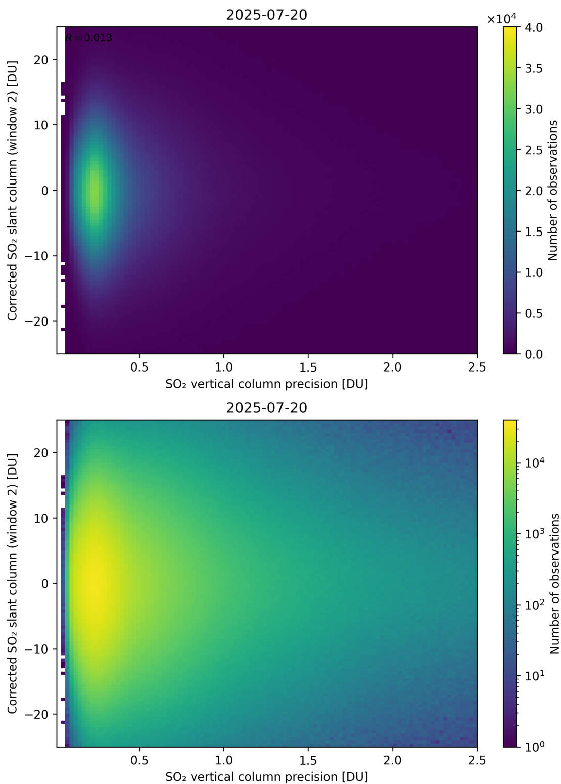
Figure 339: Scatter density plot of “SO 2 vertical column precision” against “Corrected SO 2 slant column (window 2)” for 2025-07-19 to 2025-07-21.
