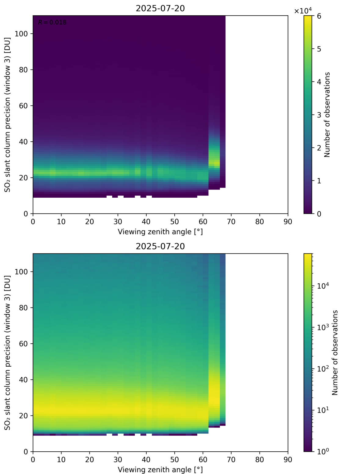
Figure 380: Scatter density plot of “Viewing zenith angle” against “SO 2 slant column precision (window 3)” for 2025-07-19 to 2025-07-21.
