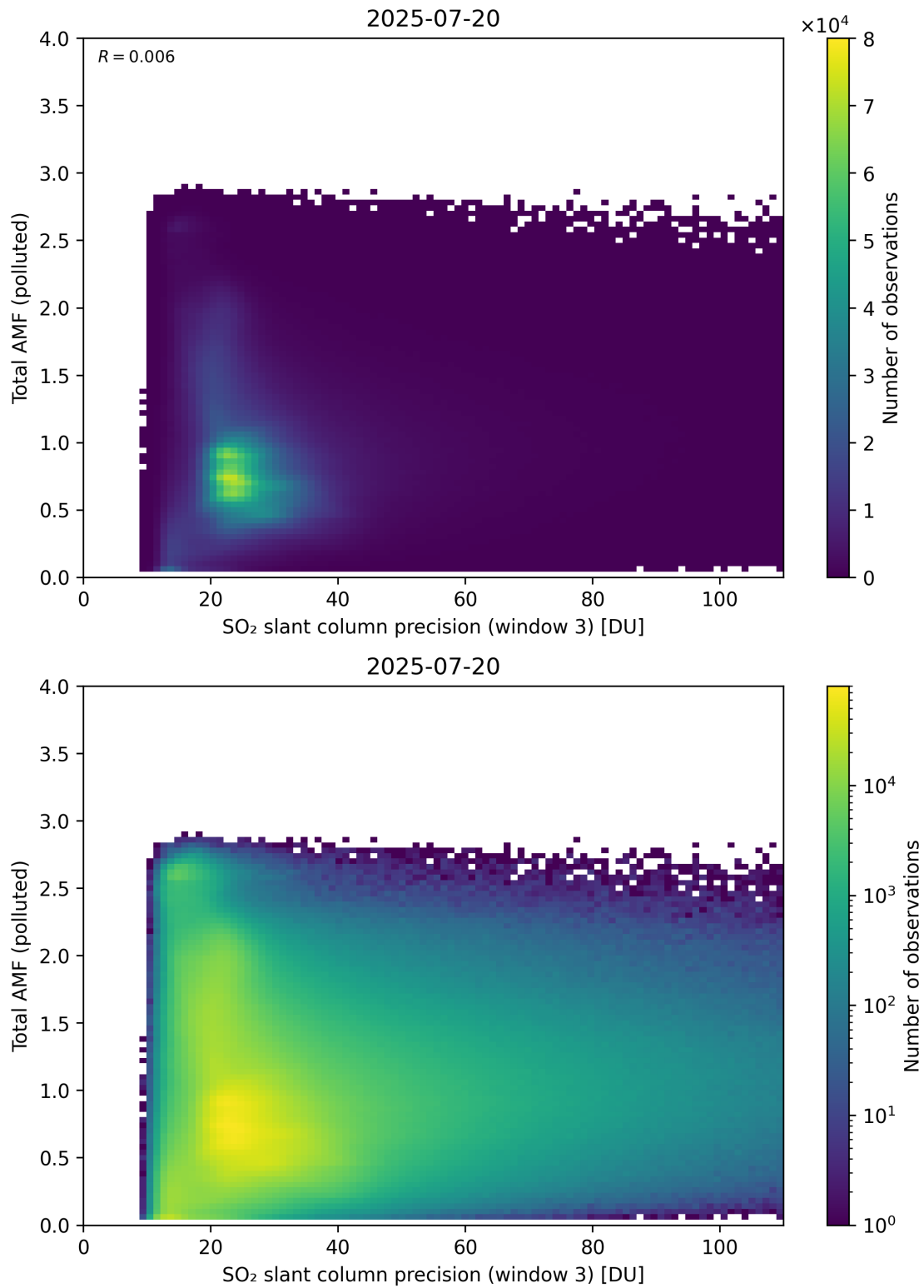
Figure 313: Scatter density plot of “SO 2 slant column precision (window 3)” against “Total AMF (polluted)” for 2025-07-19 to 2025-07-21.
