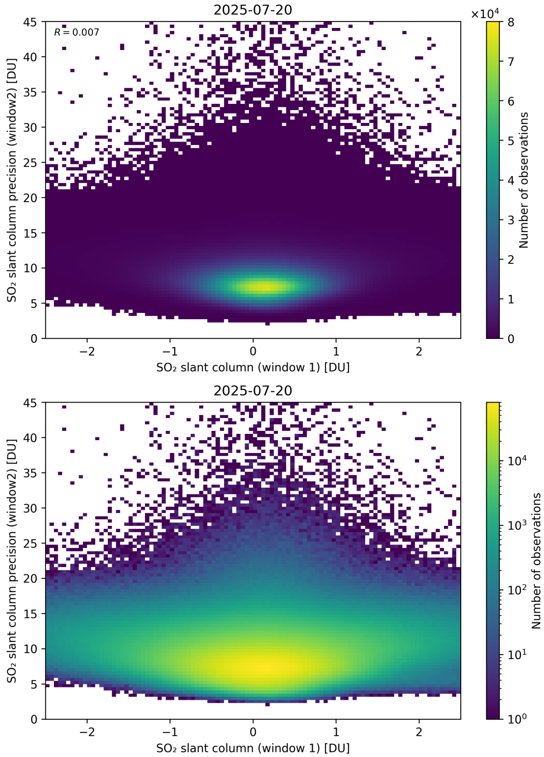
Figure 286: Scatter density plot of “SO 2 slant column (window 1)” against “SO 2 slant column precision (window2)” for 2025-07-19 to 2025-07-21.
