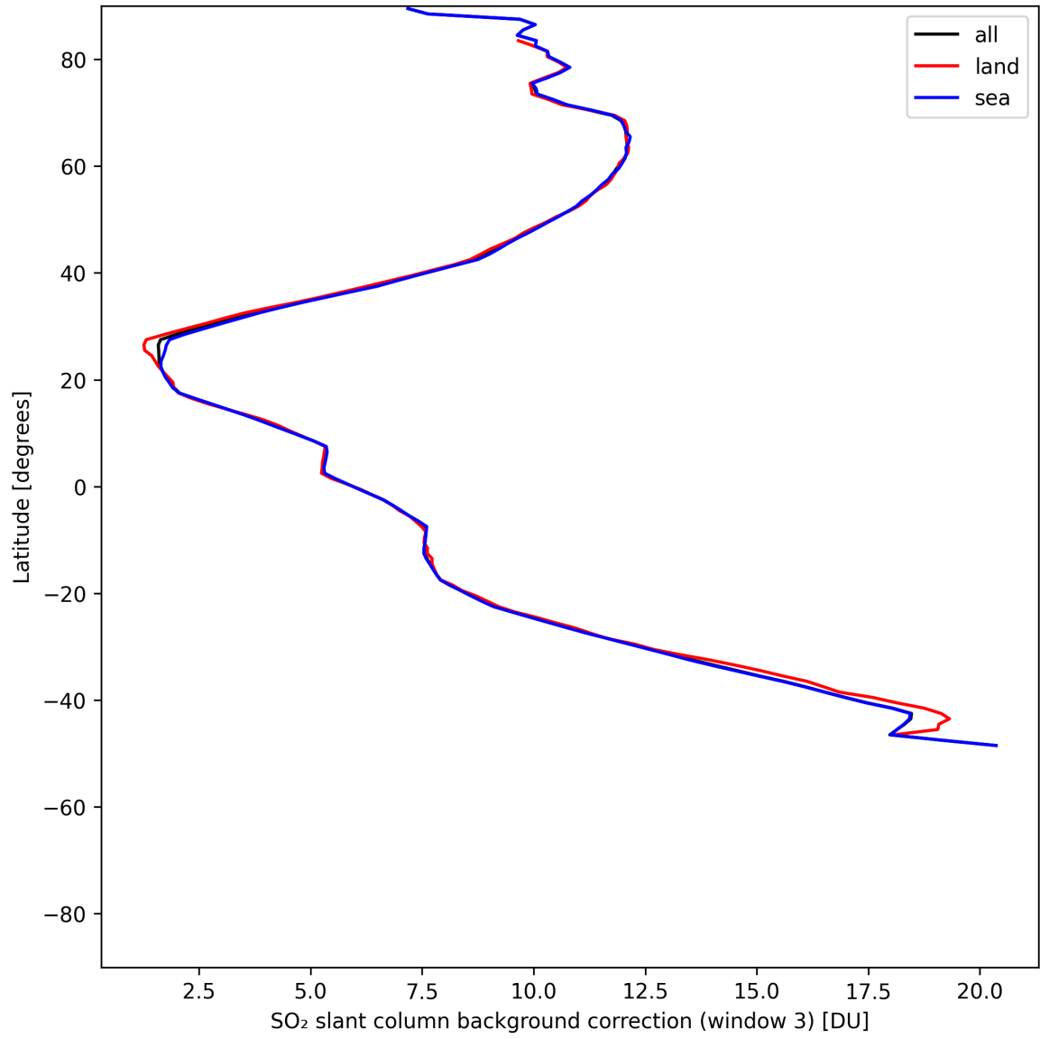
Figure 48: Zonal average of “SO 2 slant column background correction (window 3)” for 2025-07-19 to 2025-07-21.
