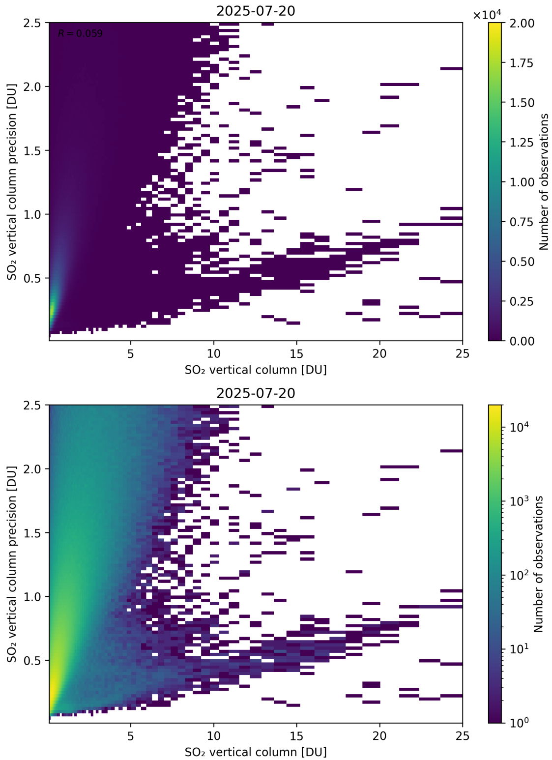
Figure 361: Scatter density plot of “SO 2 vertical column” against “SO 2 vertical column precision” for 2025-07-19 to 2025-07-21.
