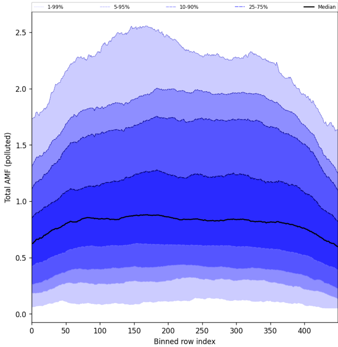
Figure 105: Along track statistics of “Total AMF (polluted)” for 2025-07-19 to 2025-07-21
