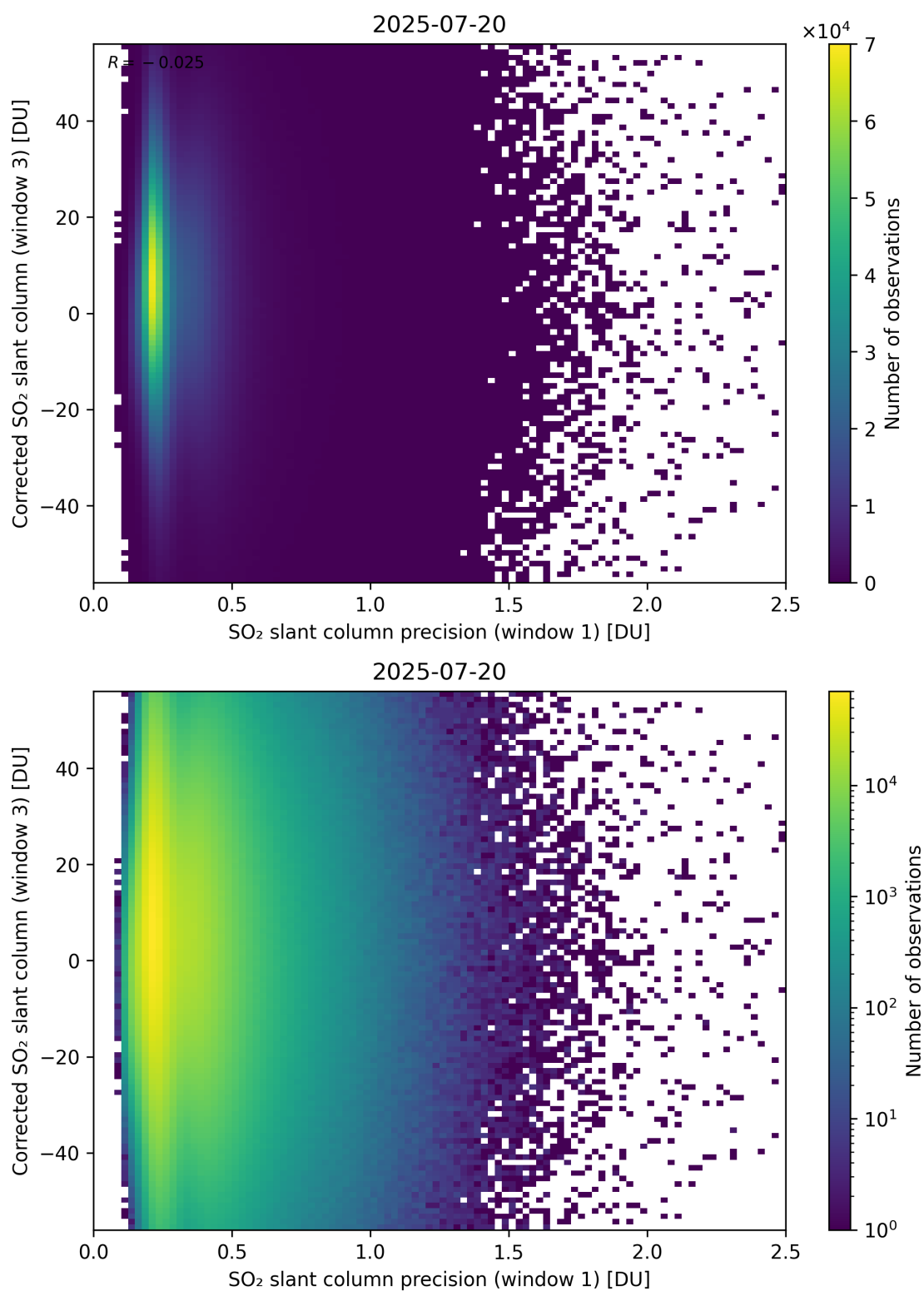
Figure 276: Scatter density plot of “SO 2 slant column precision (window 1)” against “Corrected SO 2 slant column (window 3)” for 2025-07-19 to 2025-07-21.
