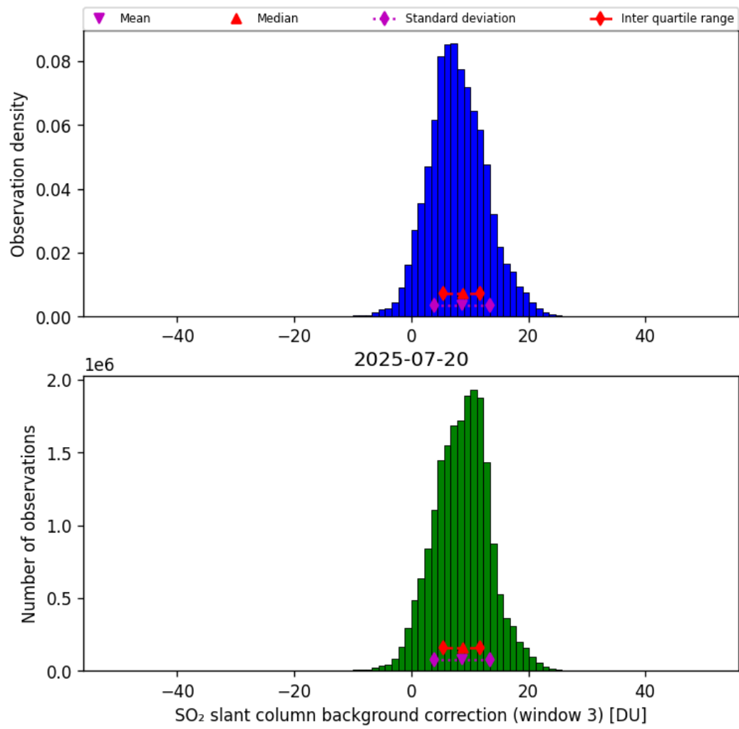
Figure 74: Histogram of “SO 2 slant column background correction (window 3)” for 2025-07-19 to 2025-07-21
