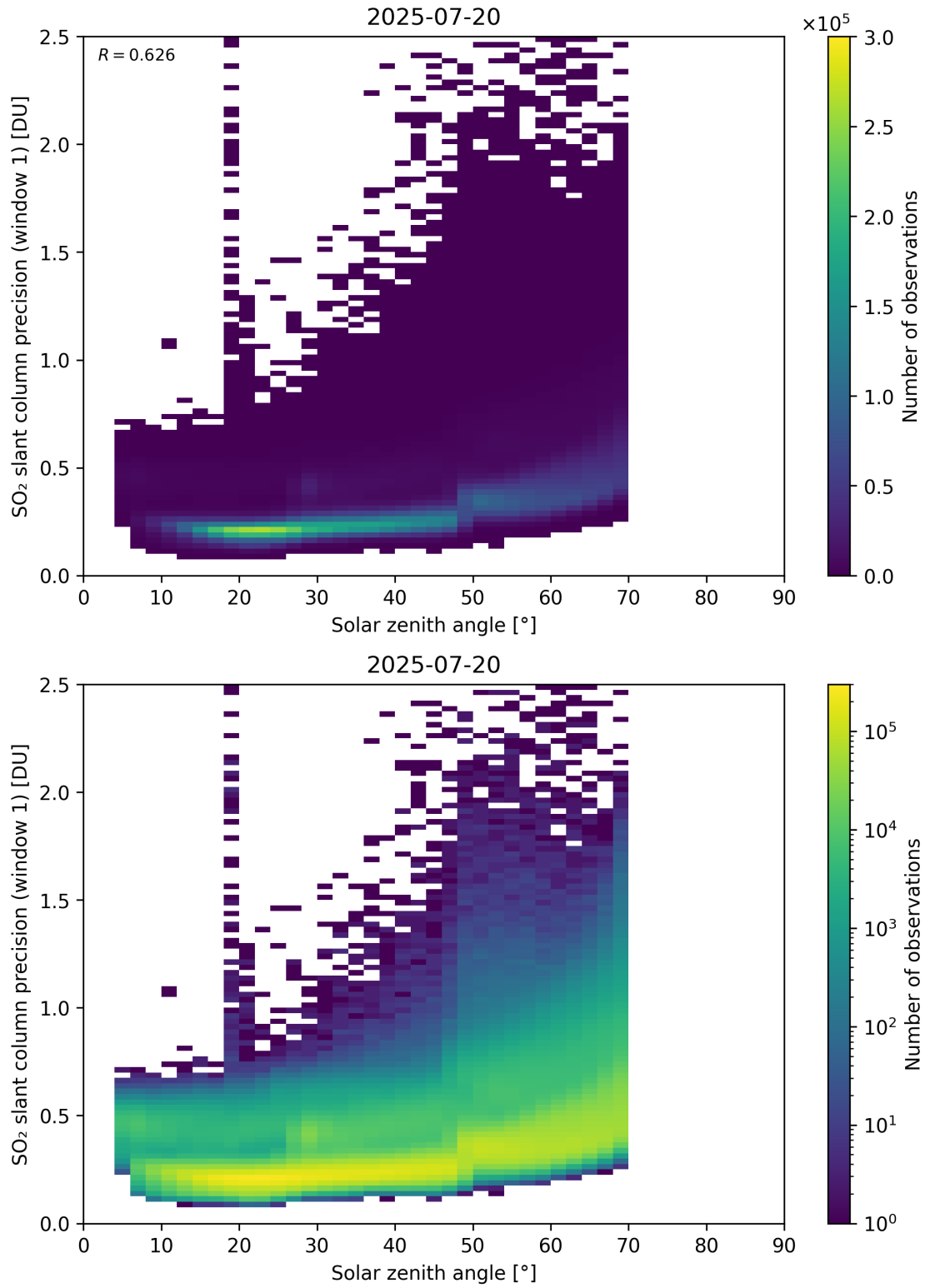
Figure 185: Scatter density plot of “Solar zenith angle” against “SO 2 slant column precision (window 1)” for 2025-07-19 to 2025-07-21.
