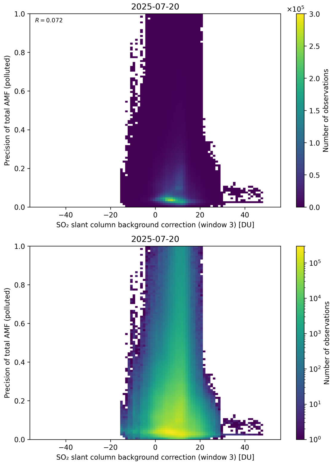
Figure 137: Scatter density plot of “SO 2 slant column background correction (window 3)” against “Precision of total AMF (polluted)” for 2025-07-19 to 2025-07-21.
