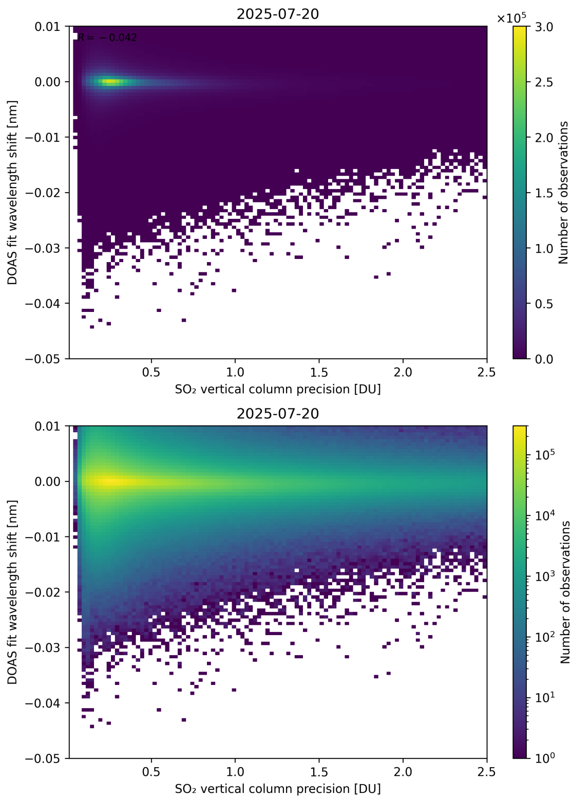
Figure 332: Scatter density plot of “SO 2 vertical column precision” against “DOAS fit wavelength shift” for 2025-07-19 to 2025-07-21.
