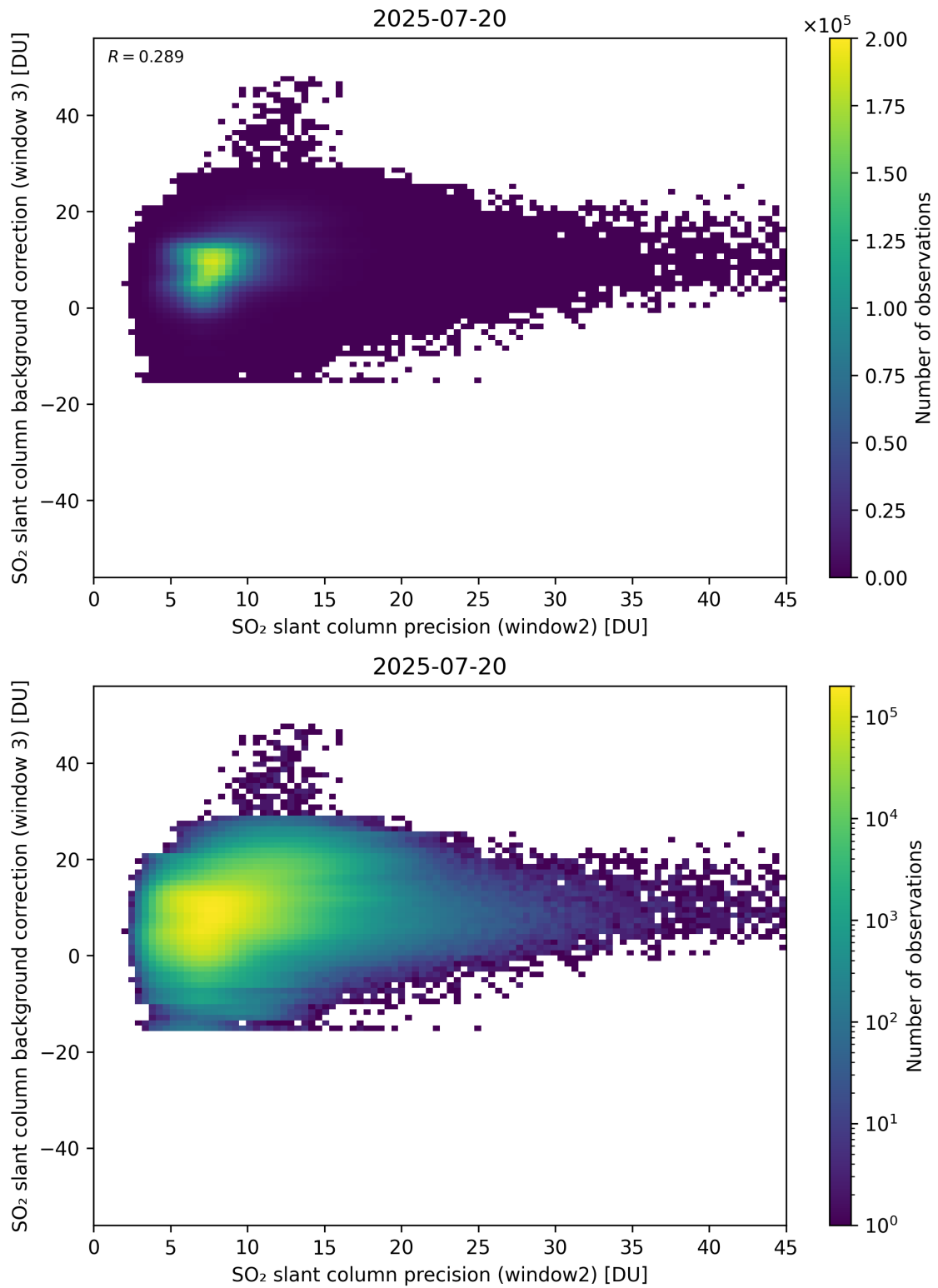
Figure 292: Scatter density plot of “SO 2 slant column precision (window2)” against “SO 2 slant column background correction (window 3)” for 2025-07-19 to 2025-07-21.
