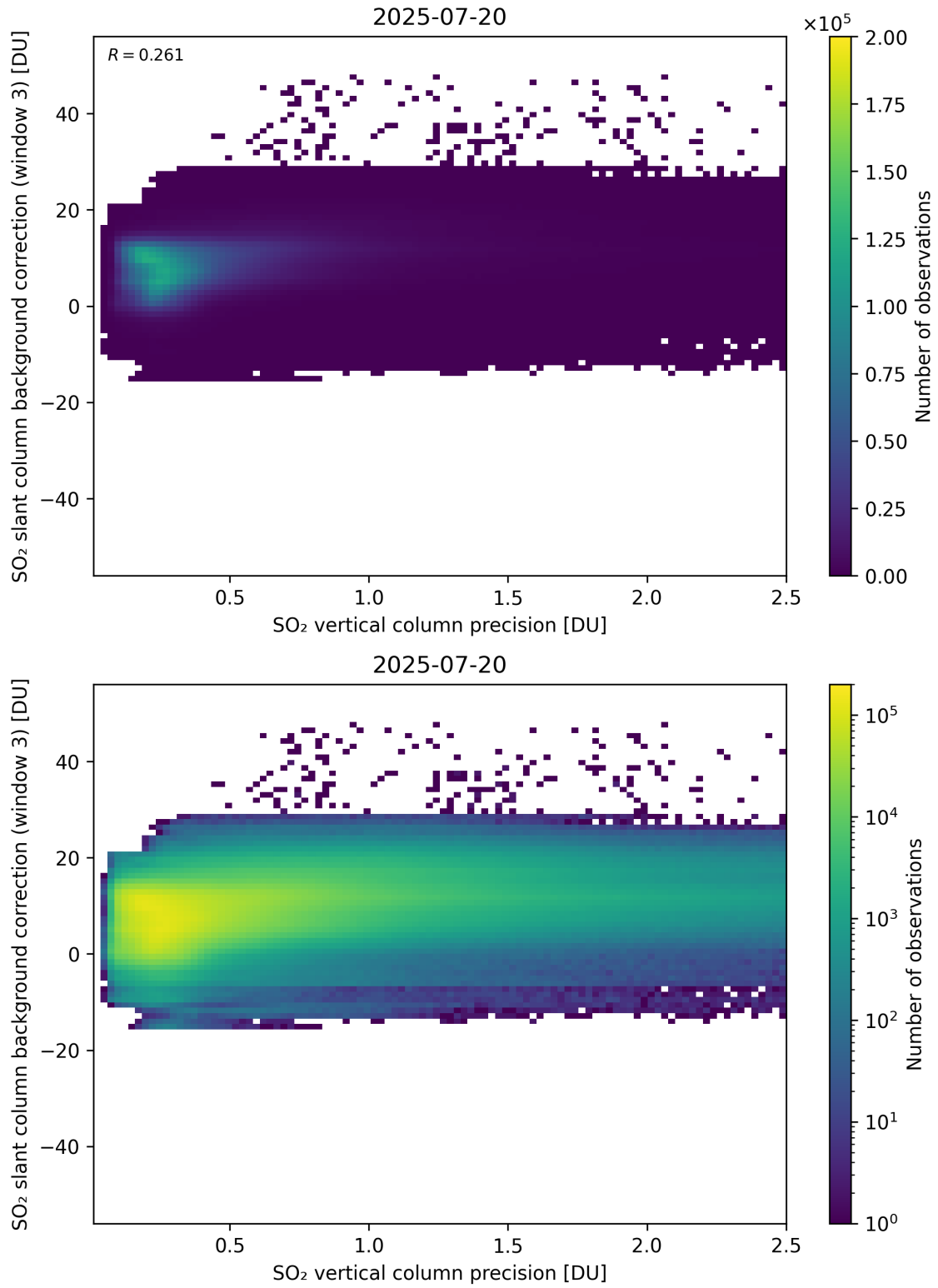
Figure 331: Scatter density plot of “SO 2 vertical column precision” against “SO 2 slant column background correction (window 3)” for 2025-07-19 to 2025-07-21.
