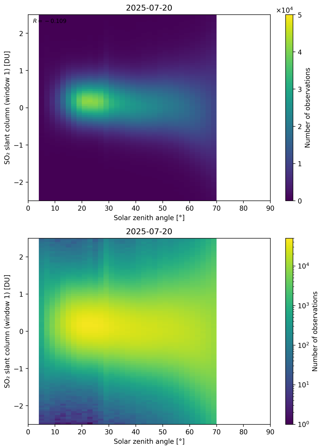
Figure 184: Scatter density plot of “Solar zenith angle” against “SO 2 slant column (window 1)” for 2025-07-19 to 2025-07-21.
