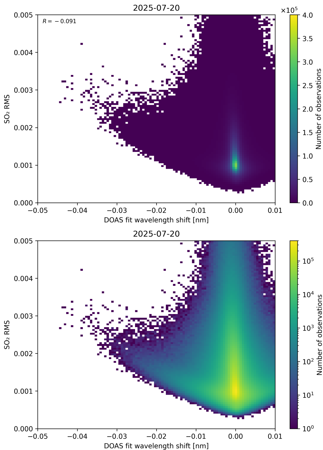
Figure 139: Scatter density plot of “DOAS fit wavelength shift” against “SO 2 RMS” for 2025-07-19 to 2025-07-21.
