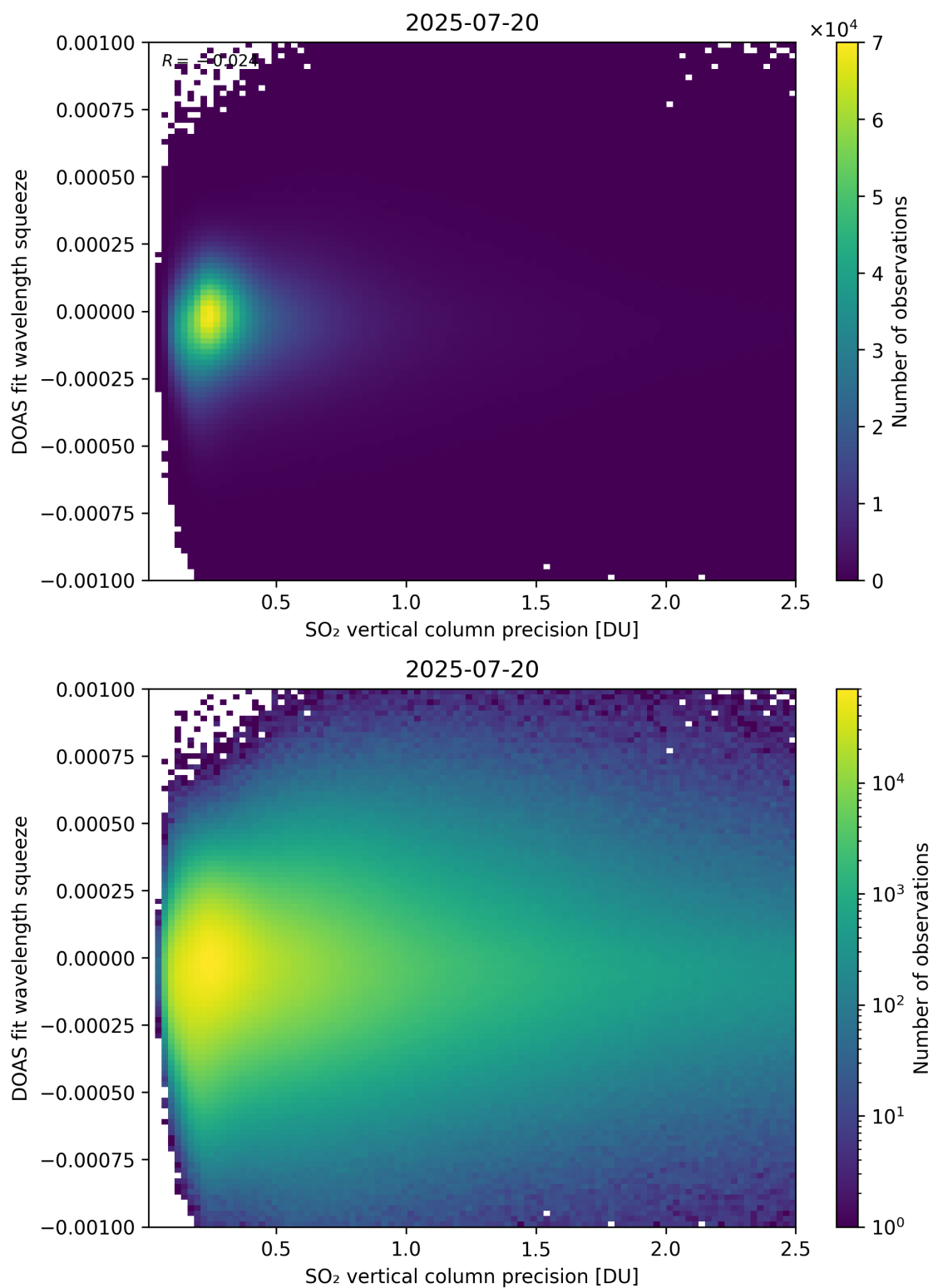
Figure 333: Scatter density plot of “SO 2 vertical column precision” against “DOAS fit wavelength squeeze” for 2025-07-19 to 2025-07-21.
