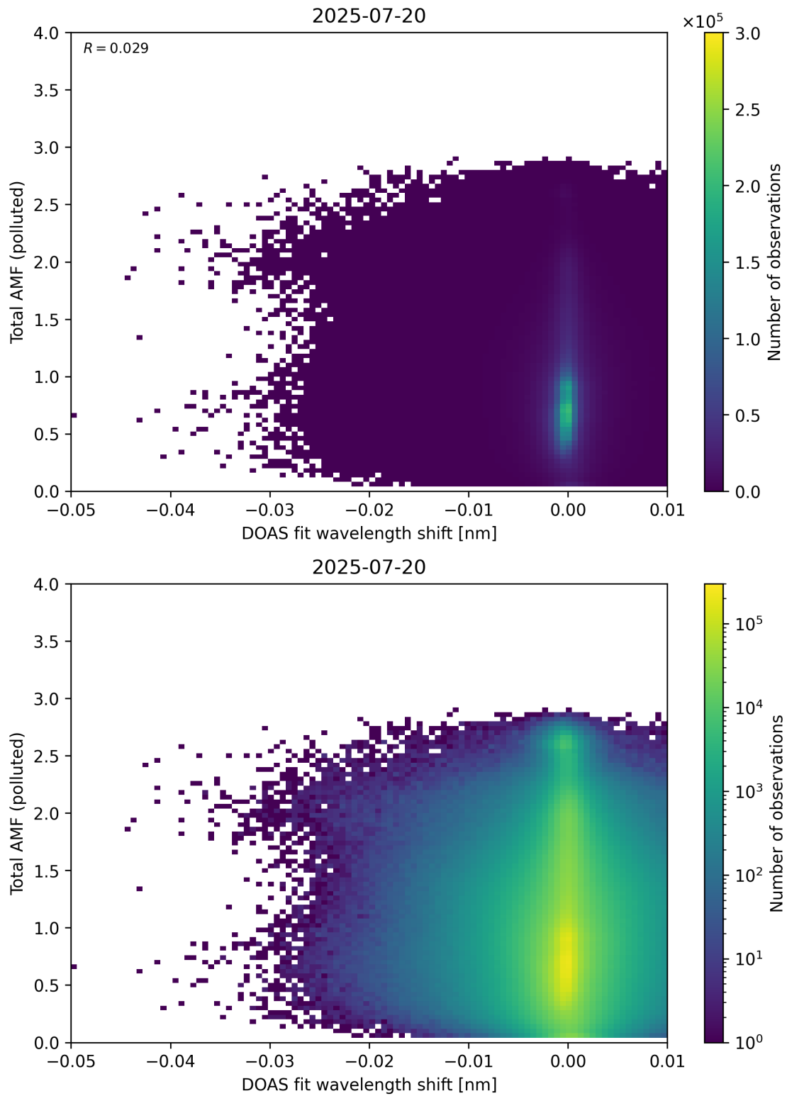
Figure 141: Scatter density plot of “DOAS fit wavelength shift” against “Total AMF (polluted)” for 2025-07-19 to 2025-07-21.
