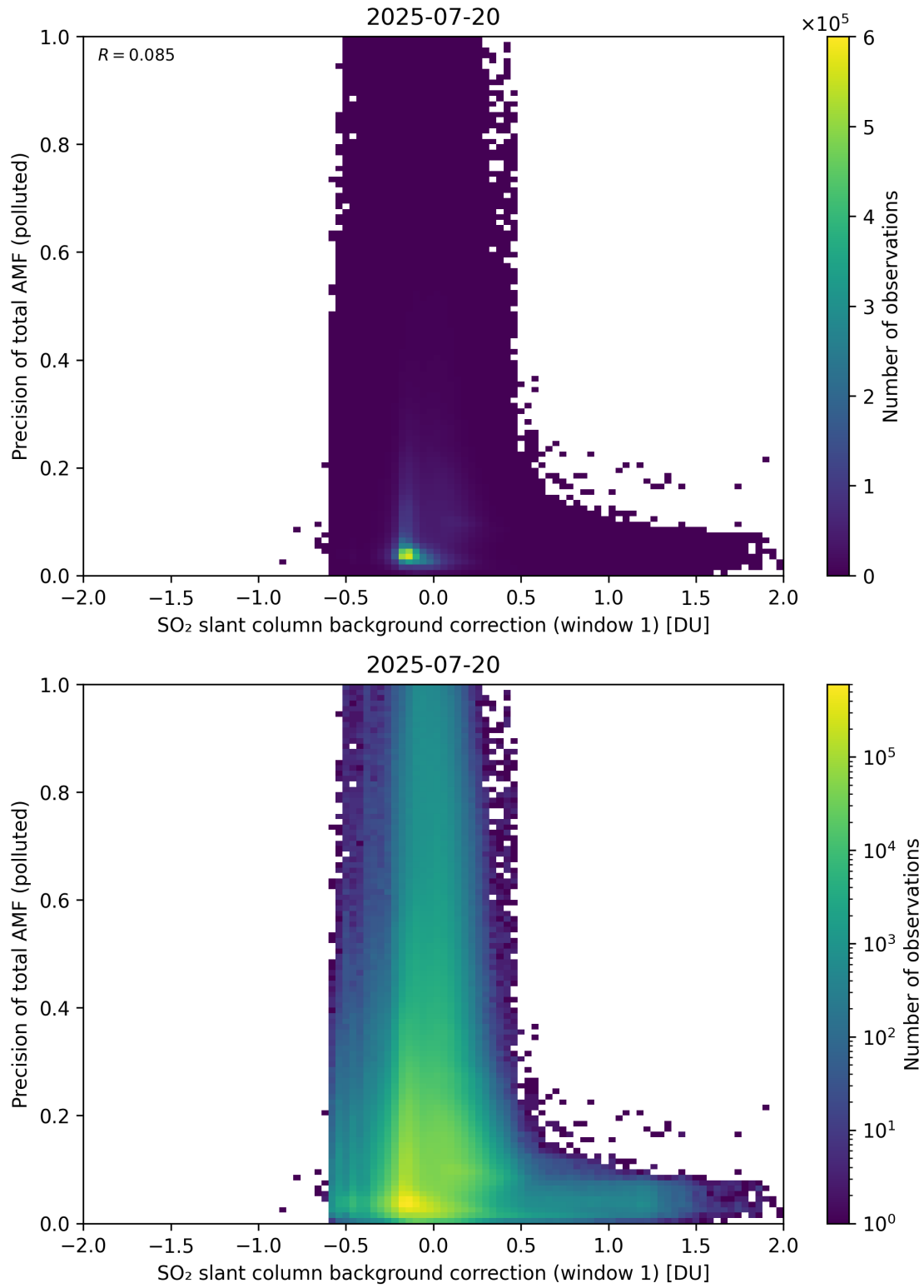
Figure 121: Scatter density plot of “SO 2 slant column background correction (window 1)” against “Precision of total AMF (polluted)” for 2025-07-19 to 2025-07-21.
