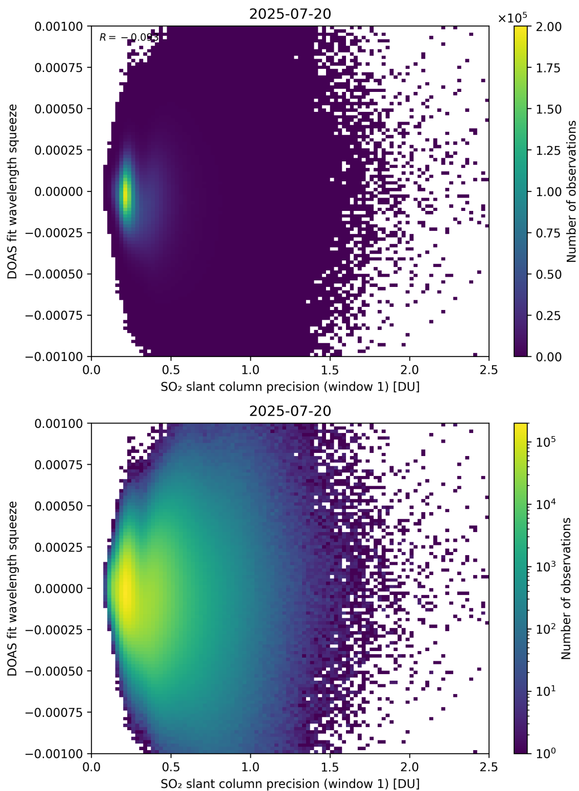
Figure 272: Scatter density plot of “SO 2 slant column precision (window 1)” against “DOAS fit wavelength squeeze” for 2025-07-19 to 2025-07-21.
