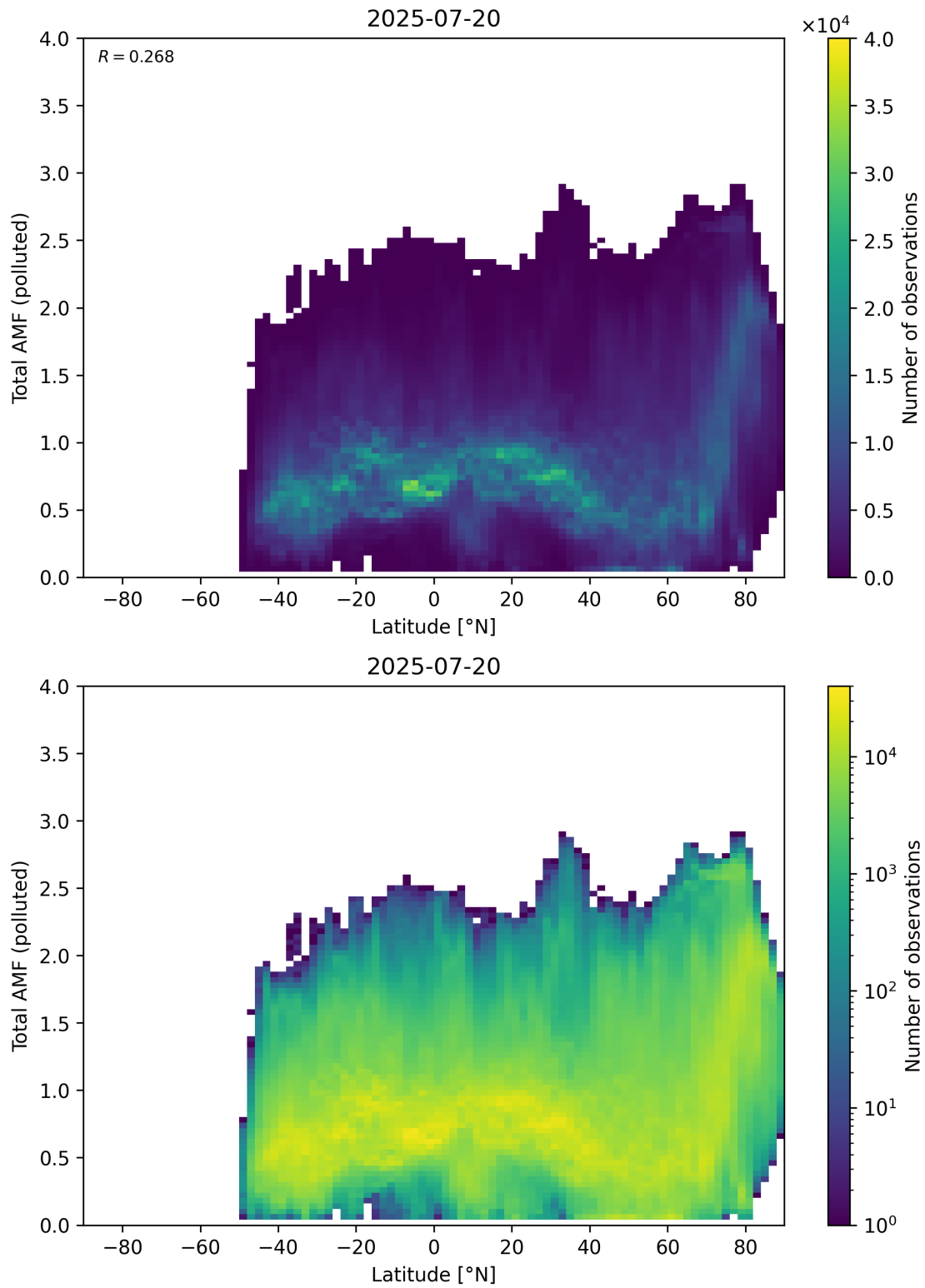
Figure 167: Scatter density plot of “Latitude” against “Total AMF (polluted)” for 2025-07-19 to 2025-07-21.
