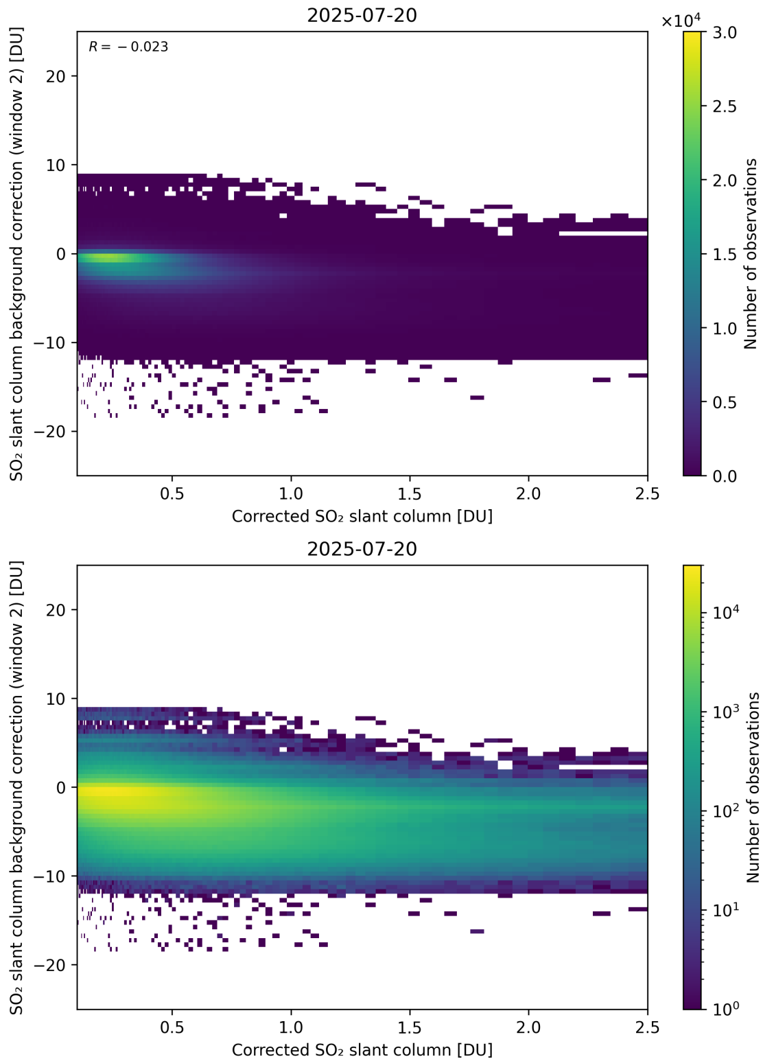
Figure 227: Scatter density plot of “Corrected SO 2 slant column” against “SO 2 slant column background correction (window 2)” for 2025-07-19 to 2025-07-21.
