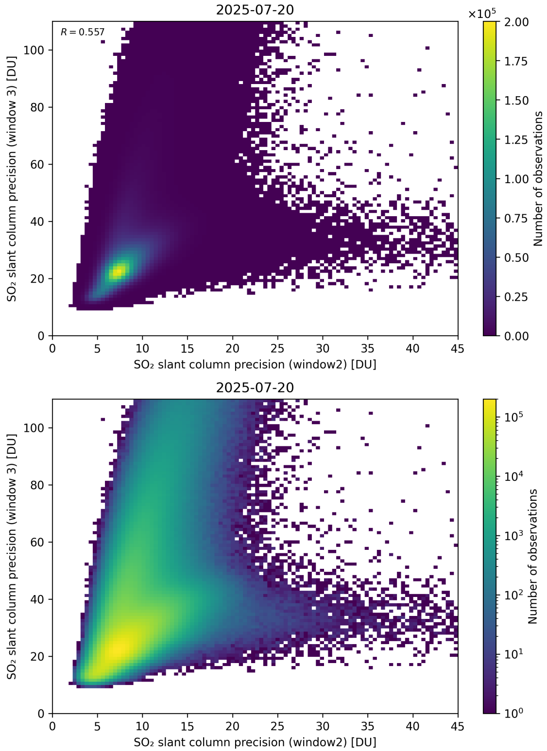
Figure 300: Scatter density plot of “SO 2 slant column precision (window2)” against “SO 2 slant column precision (window 3)” for 2025-07-19 to 2025-07-21.
