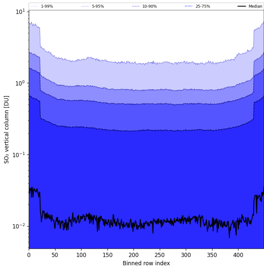
Figure 84: Along track statistics of “SO 2 vertical column” for 2025-07-19 to 2025-07-21
