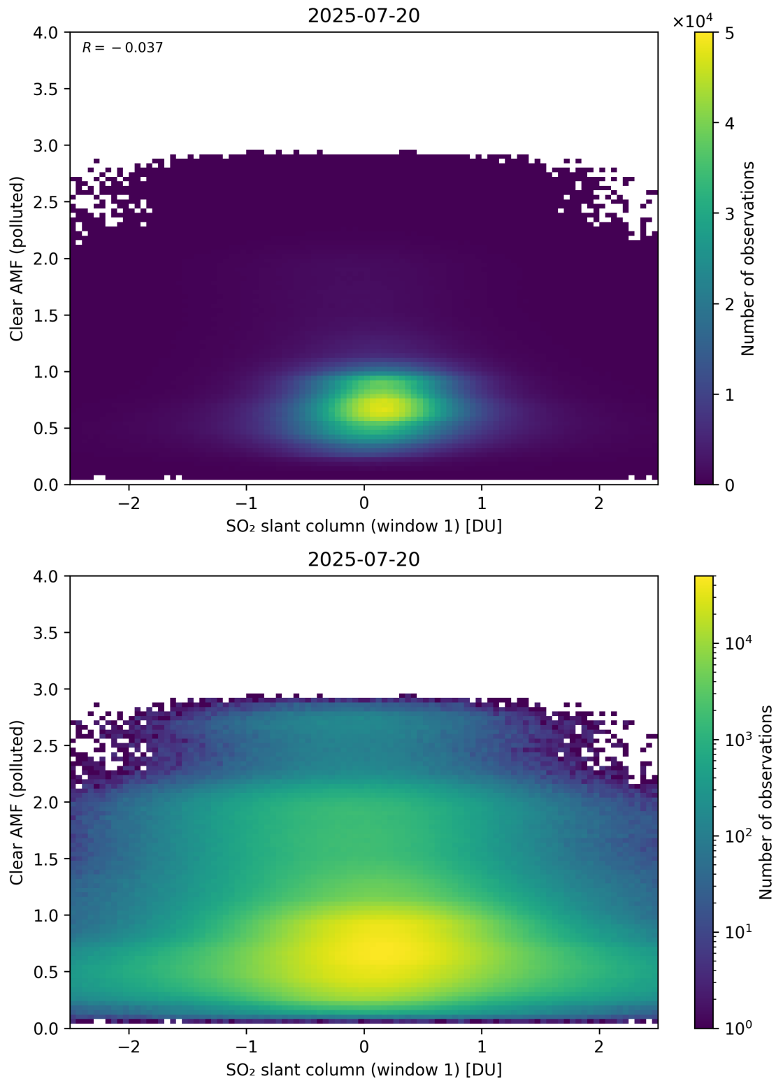
Figure 282: Scatter density plot of “SO 2 slant column (window 1)” against “Clear AMF (polluted)” for 2025-07-19 to 2025-07-21.
