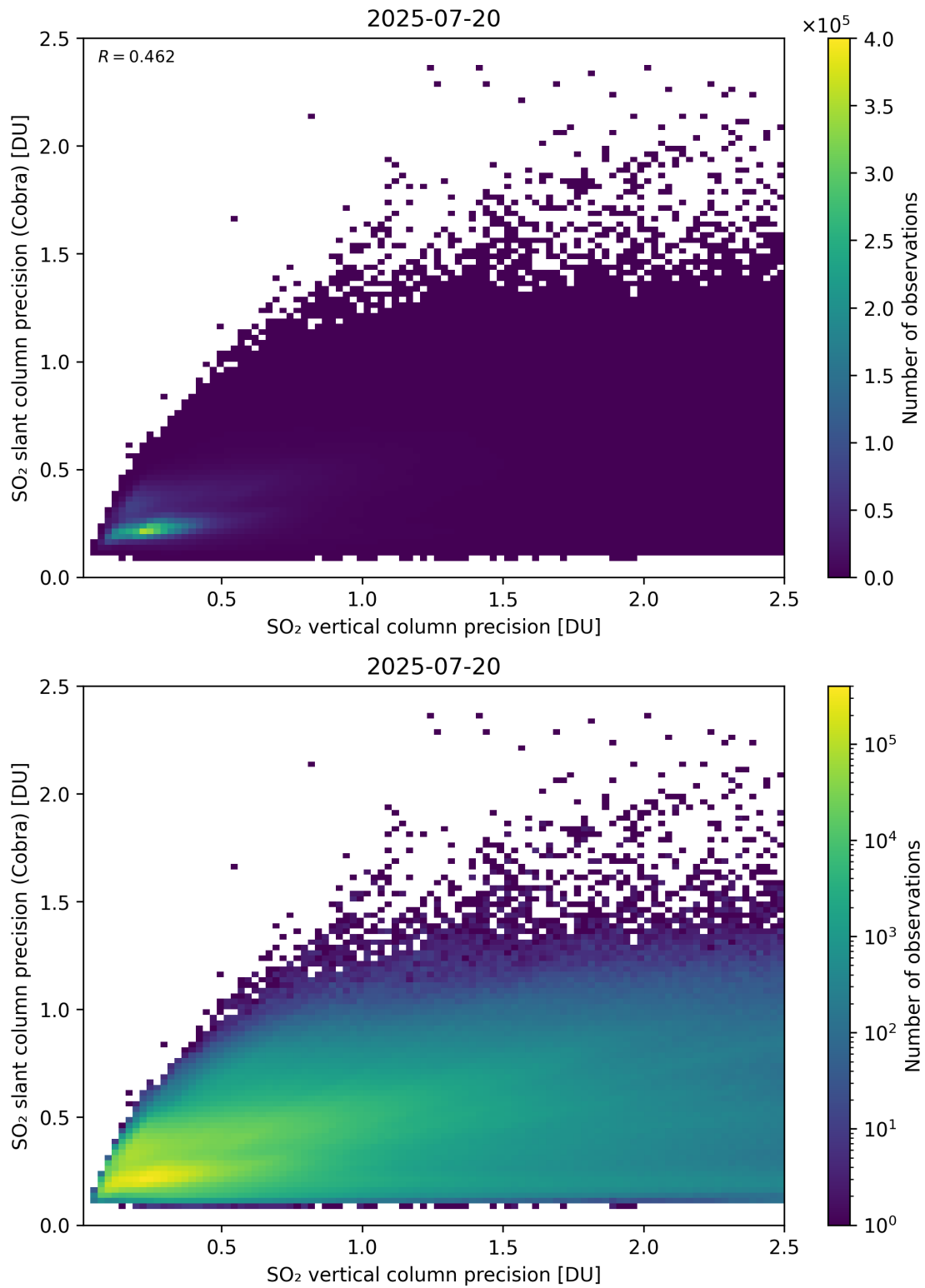
Figure 337: Scatter density plot of “SO 2 vertical column precision” against “SO 2 slant column precision (Cobra)” for 2025-07-19 to 2025-07-21.
