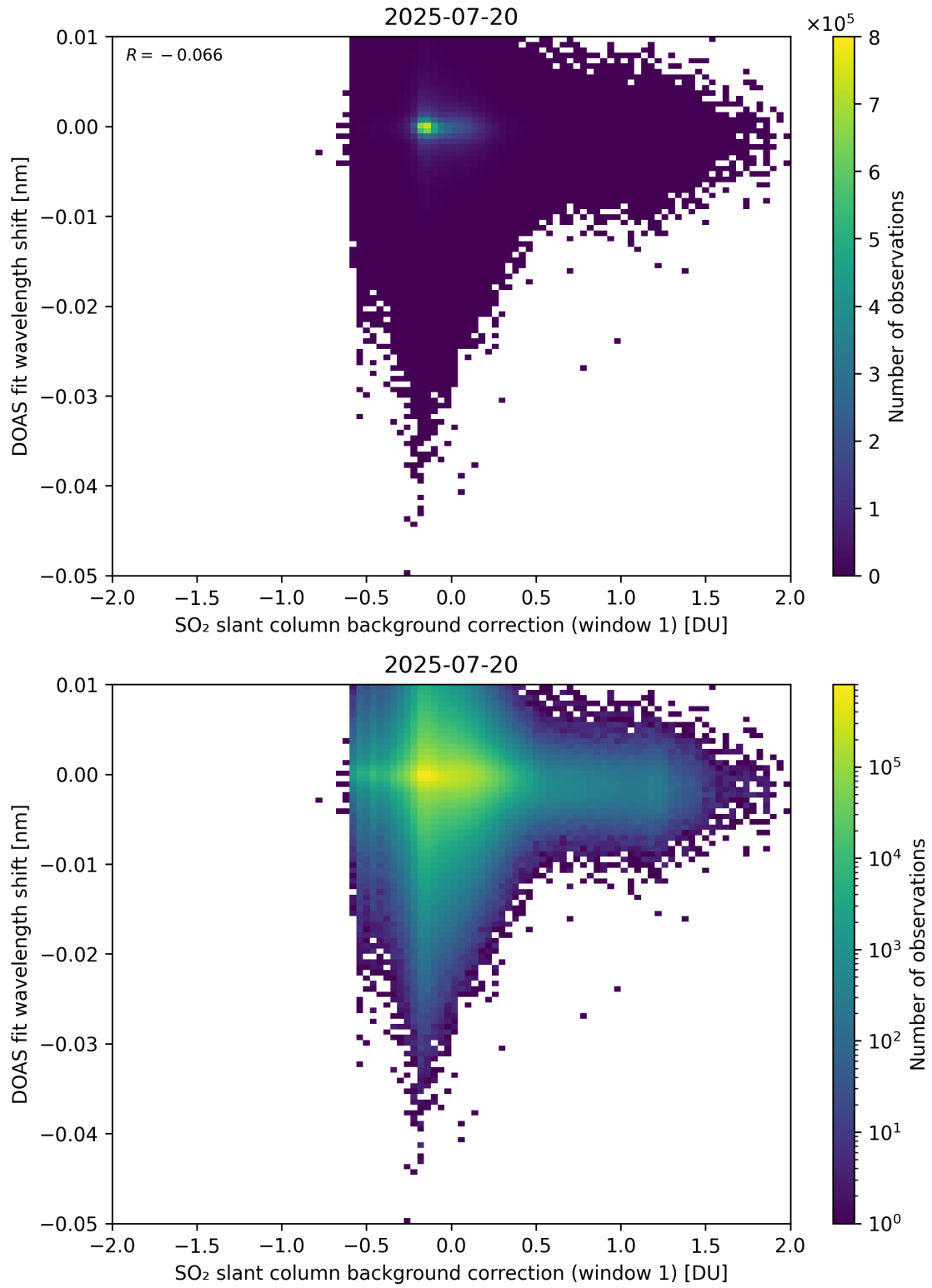
Figure 111: Scatter density plot of “SO 2 slant column background correction (window 1)” against “DOAS fit wavelength shift” for 2025-07-19 to 2025-07-21.
