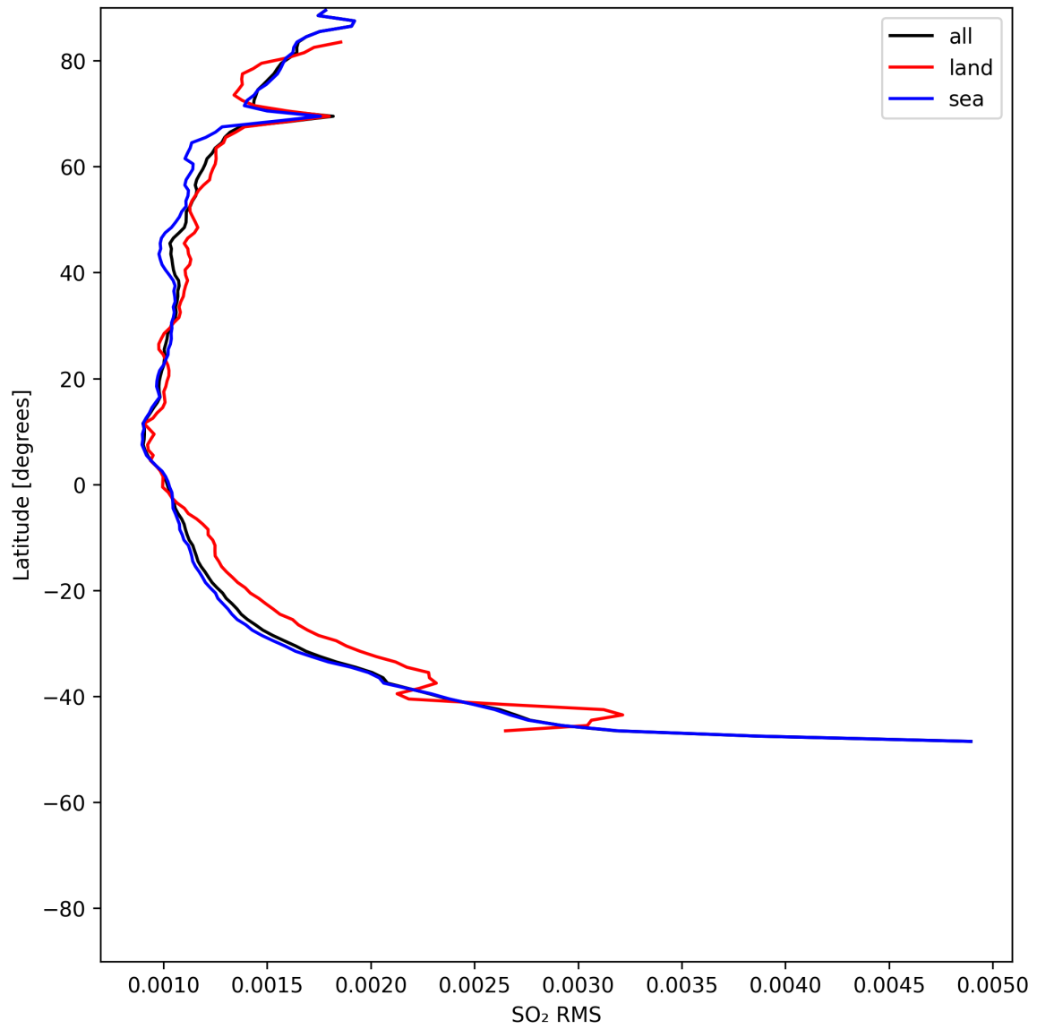
Figure 52: Zonal average of “SO 2 RMS” for 2025-07-19 to 2025-07-21.
