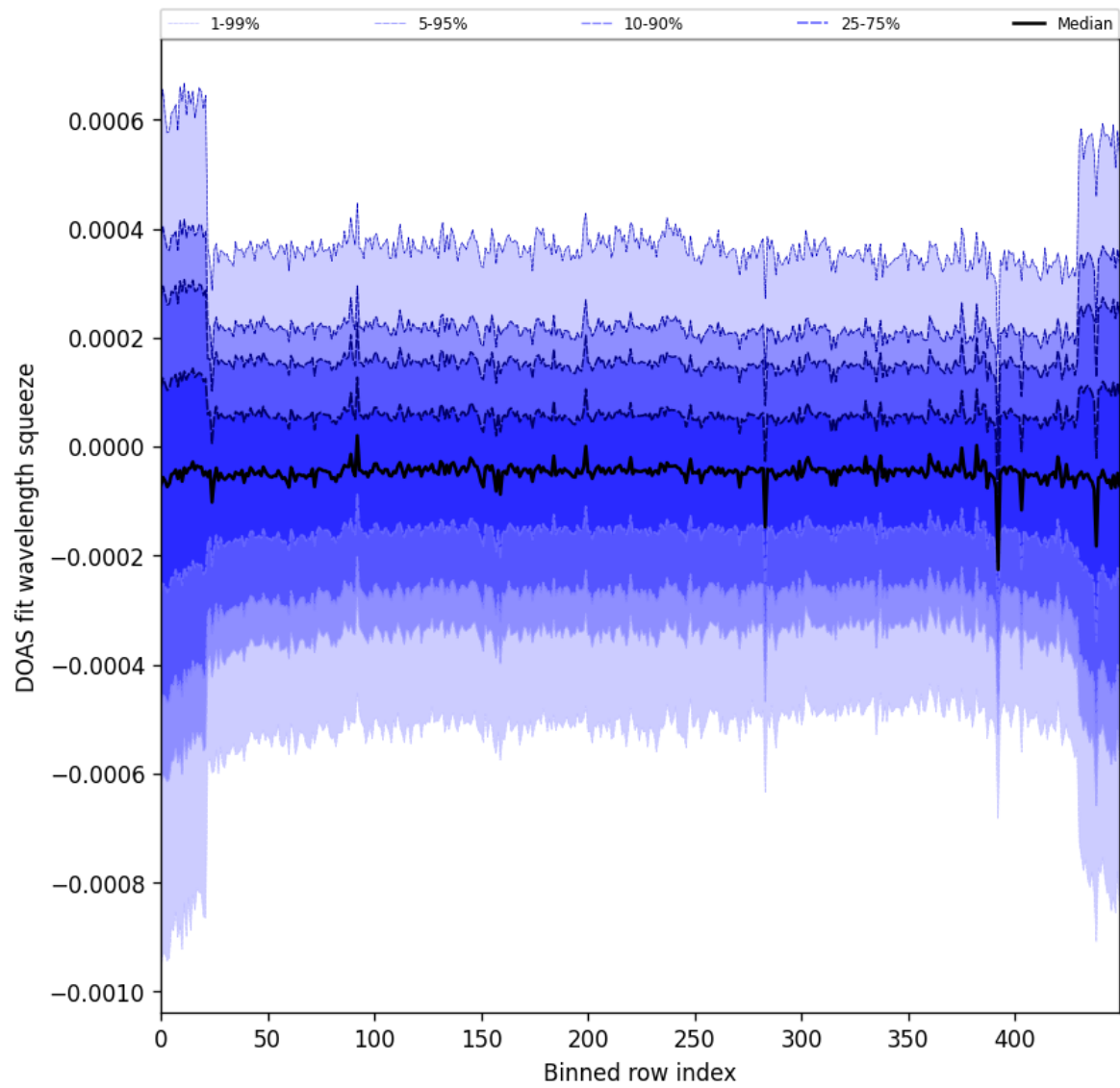
Figure 103: Along track statistics of “DOAS fit wavelength squeeze” for 2025-07-19 to 2025-07-21
