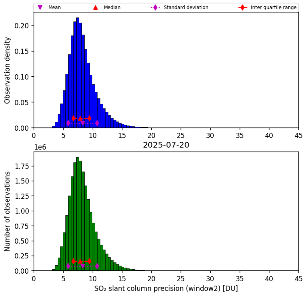
Figure 68: Histogram of “SO 2 slant column precision (window2)” for 2025-07-19 to 2025-07-21
