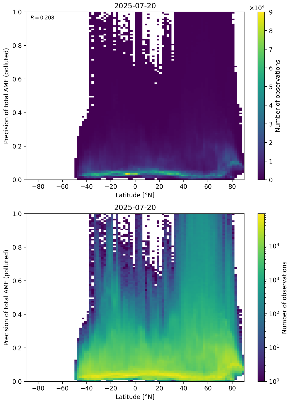
Figure 168: Scatter density plot of “Latitude” against “Precision of total AMF (polluted)” for 2025-07-19 to 2025-07-21.
