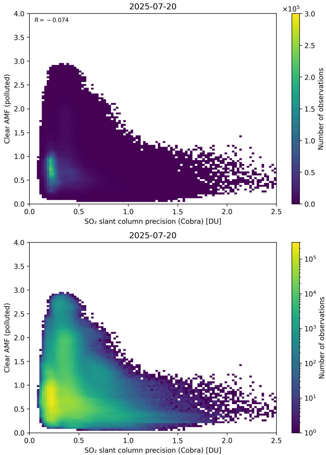
Figure 205: Scatter density plot of “SO 2 slant column precision (Cobra)” against “Clear AMF (polluted)” for 2025-07-19 to 2025-07-21.
