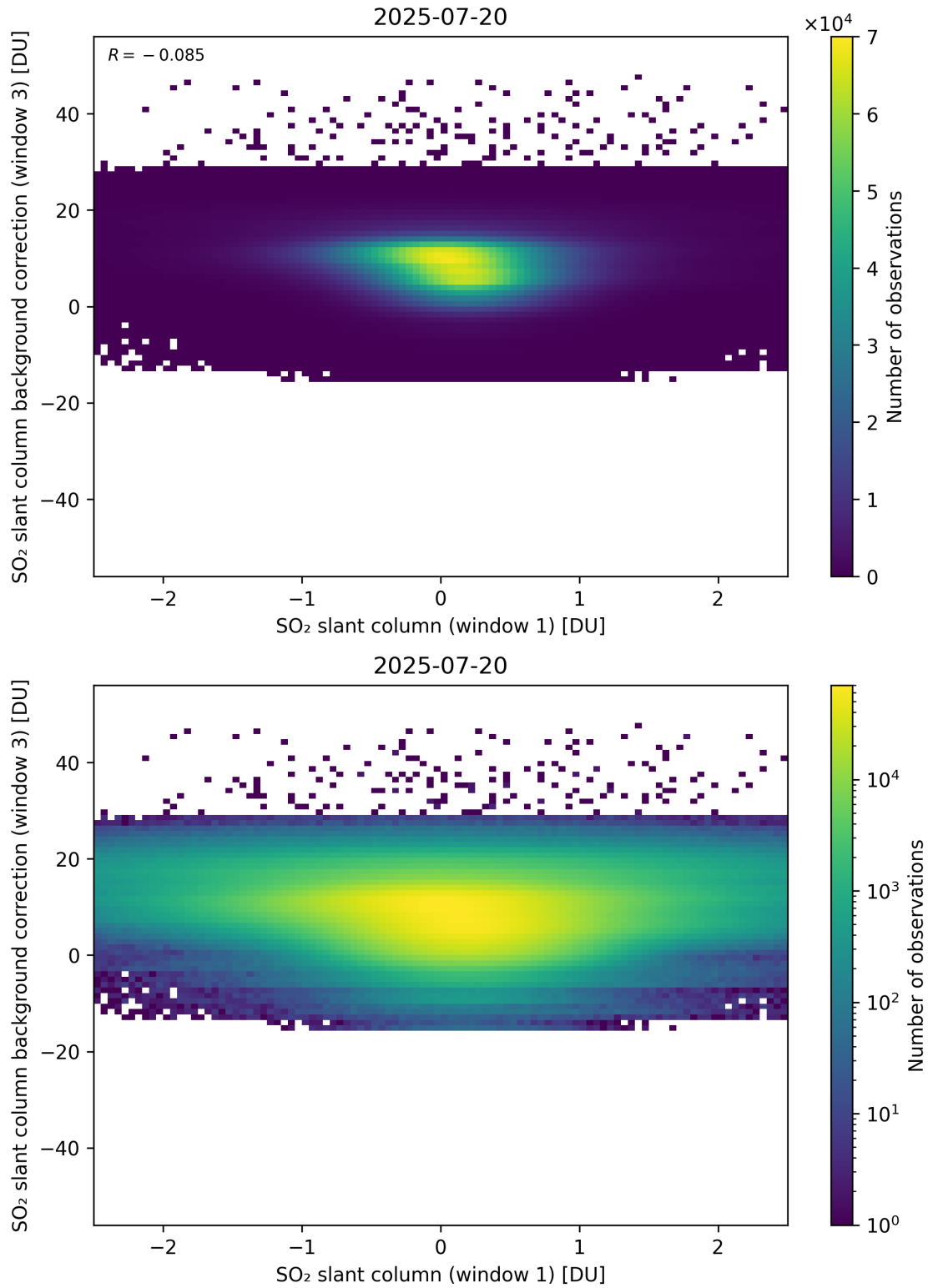
Figure 264: Scatter density plot of “SO 2 slant column (window 1)” against “SO 2 slant column background correction (window 3)” for 2025-07-19 to 2025-07-21.
