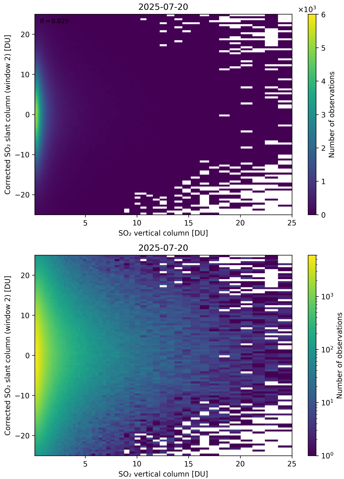
Figure 352: Scatter density plot of “SO 2 vertical column” against “Corrected SO 2 slant column (window 2)” for 2025-07-19 to 2025-07-21.
