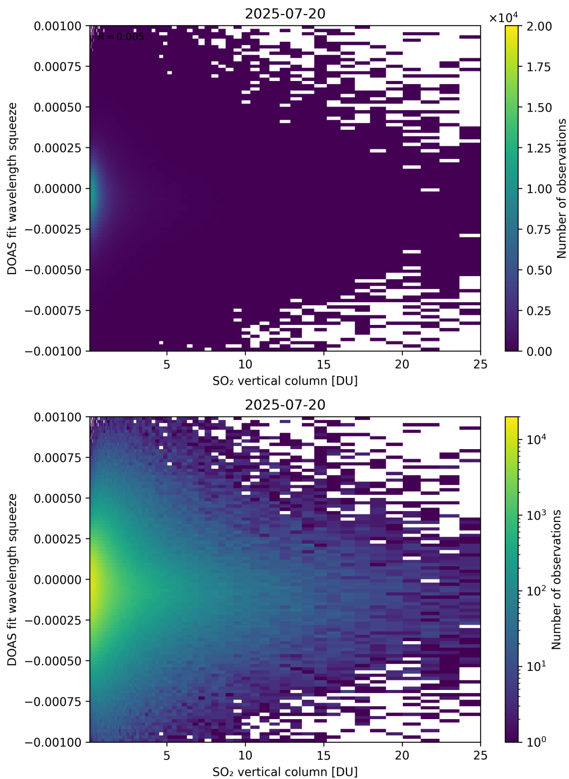
Figure 327: Scatter density plot of “SO 2 vertical column” against “DOAS fit wavelength squeeze” for 2025-07-19 to 2025-07-21.
