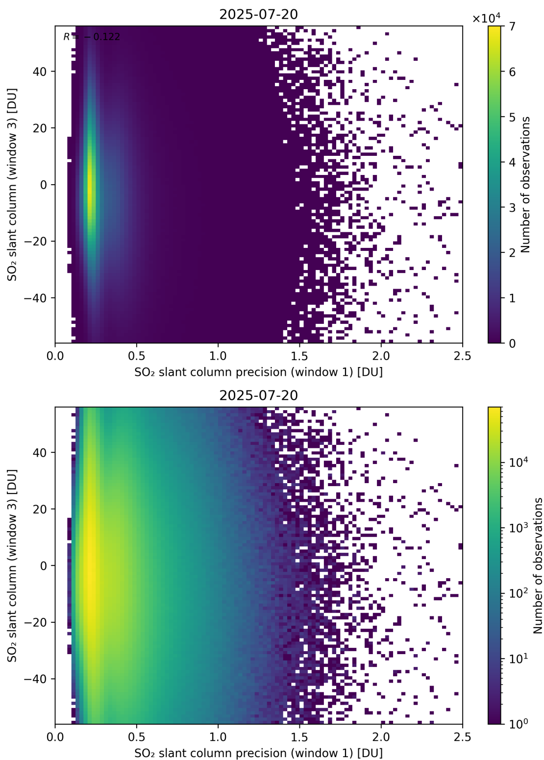
Figure 278: Scatter density plot of “SO 2 slant column precision (window 1)” against “SO 2 slant column (window 3)” for 2025-07-19 to 2025-07-21.
