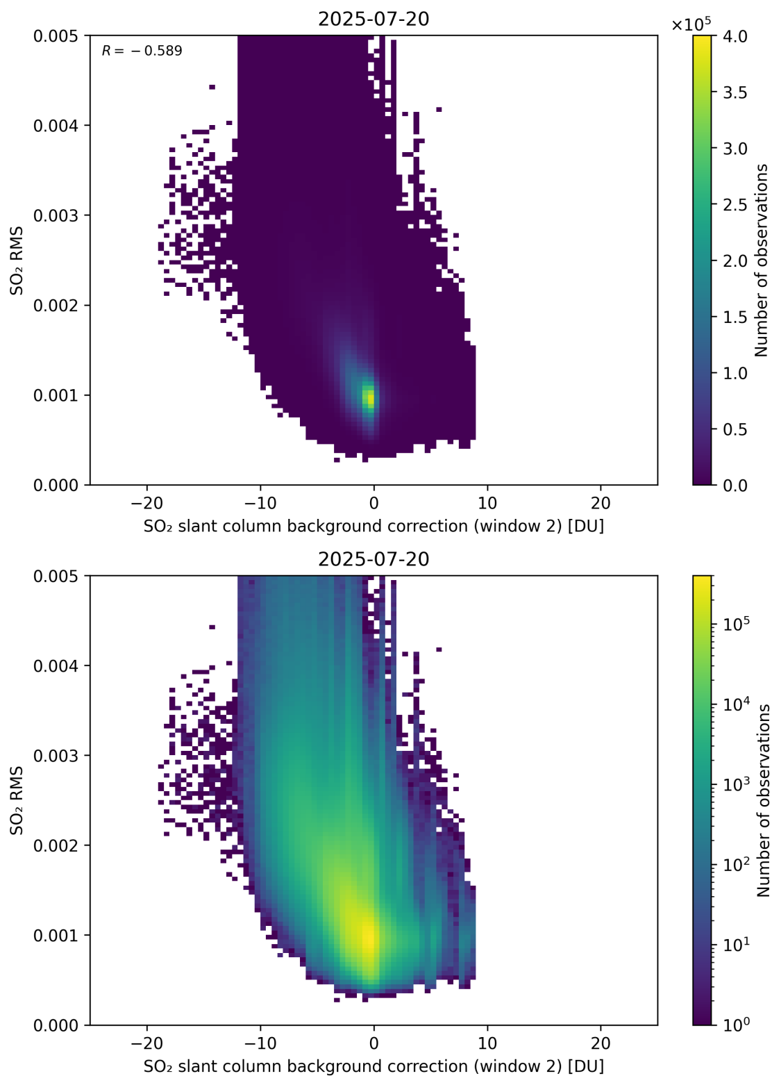
Figure 125: Scatter density plot of “SO 2 slant column background correction (window 2)” against “SO 2 RMS” for 2025-07-19 to 2025-07-21.
