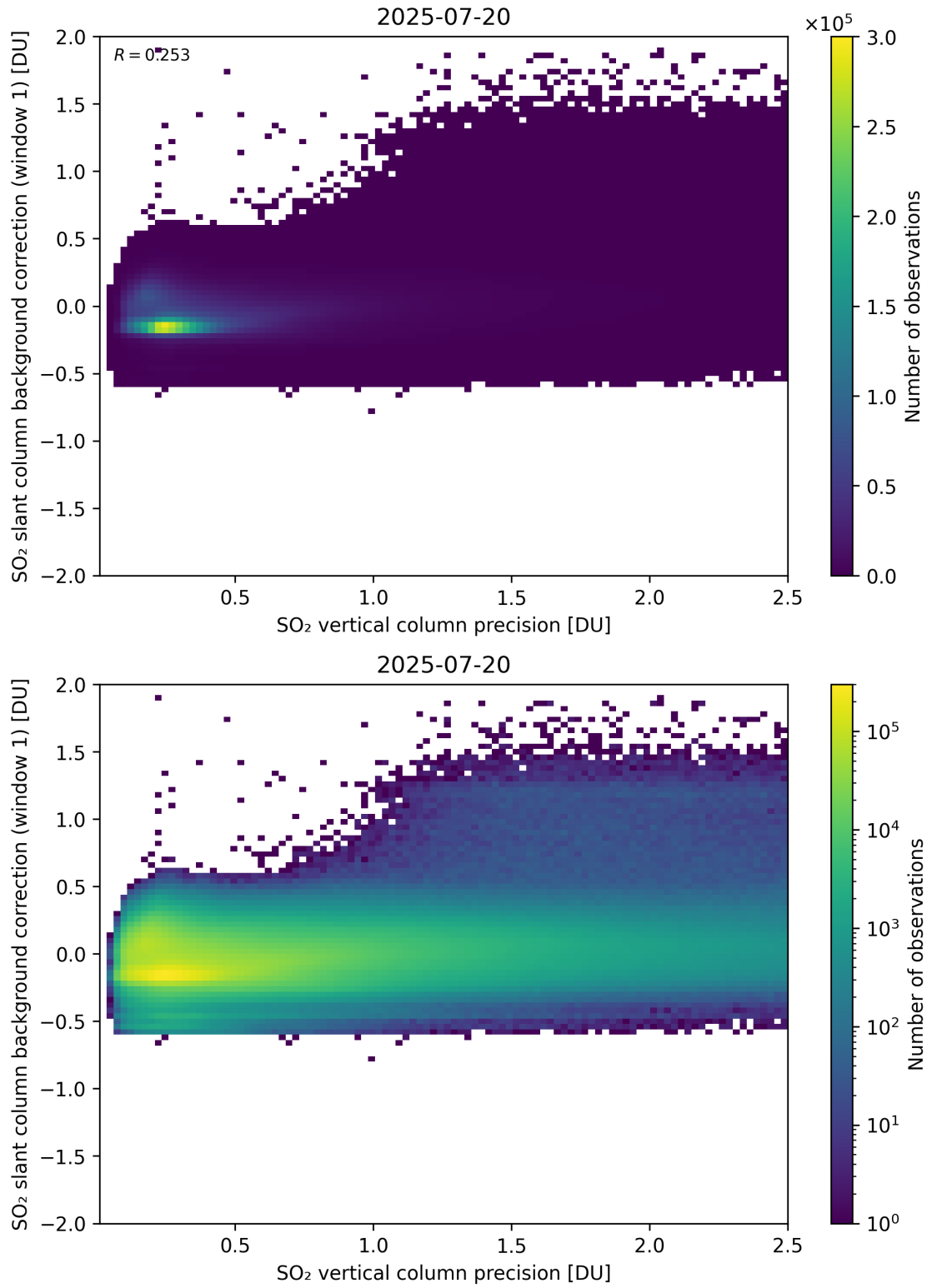
Figure 329: Scatter density plot of “SO 2 vertical column precision” against “SO 2 slant column background correction (window 1)” for 2025-07-19 to 2025-07-21.
