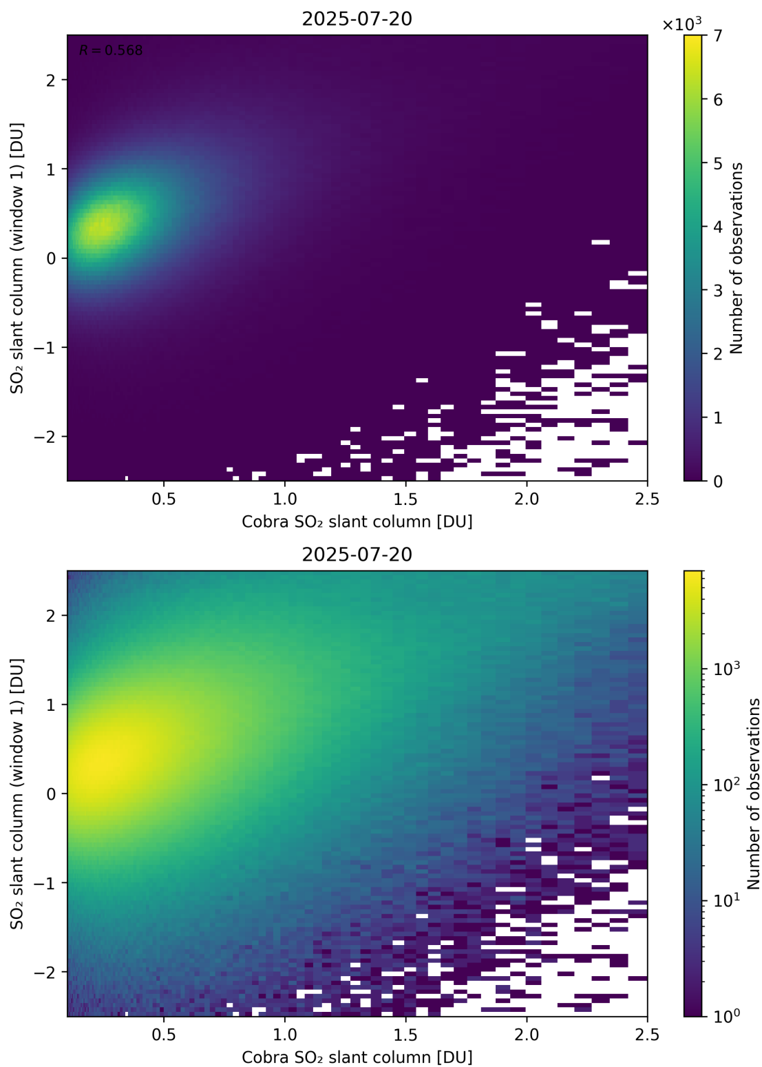
Figure 219: Scatter density plot of “Cobra SO 2 slant column” against “SO 2 slant column (window 1)” for 2025-07-19 to 2025-07-21.
