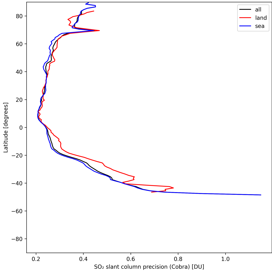
Figure 36: Zonal average of “SO 2 slant column precision (Cobra)” for 2025-07-19 to 2025-07-21.
