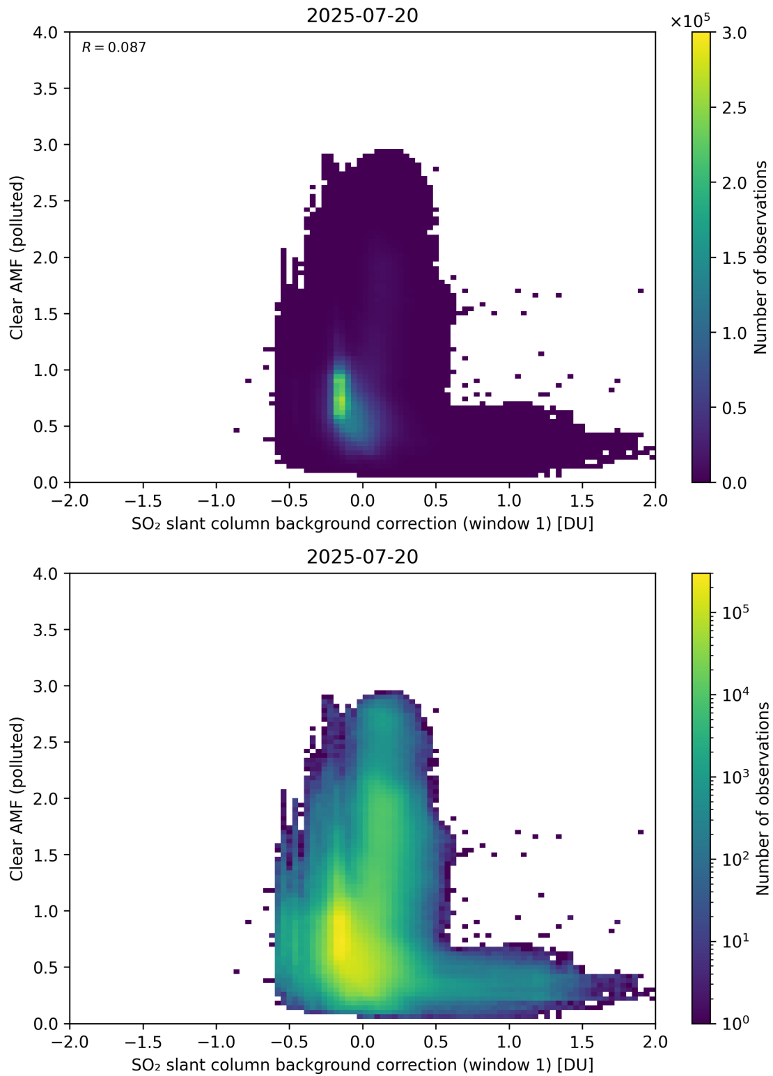
Figure 114: Scatter density plot of “SO 2 slant column background correction (window 1)” against “Clear AMF (polluted)” for 2025-07-19 to 2025-07-21.
