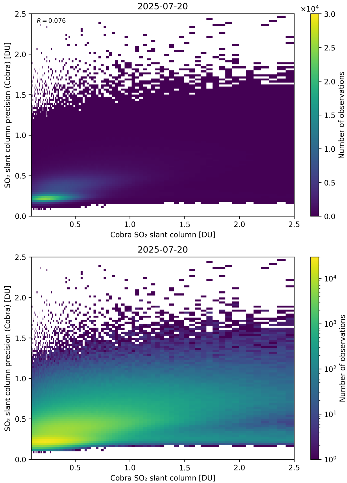
Figure 216: Scatter density plot of “Cobra SO 2 slant column” against “SO 2 slant column precision (Cobra)” for 2025-07-19 to 2025-07-21.
