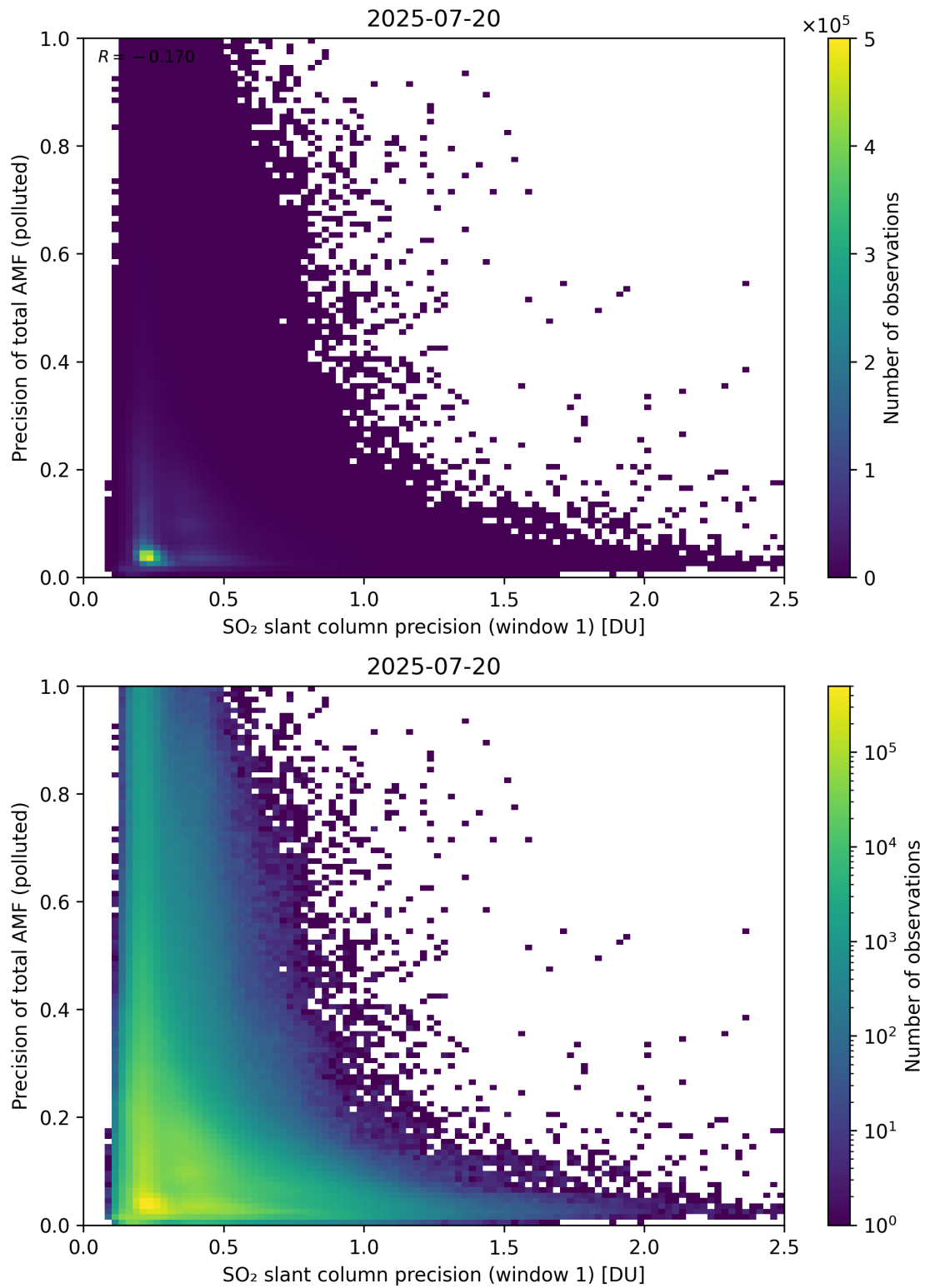
Figure 281: Scatter density plot of “SO 2 slant column precision (window 1)” against “Precision of total AMF (polluted)” for 2025-07-19 to 2025-07-21.
