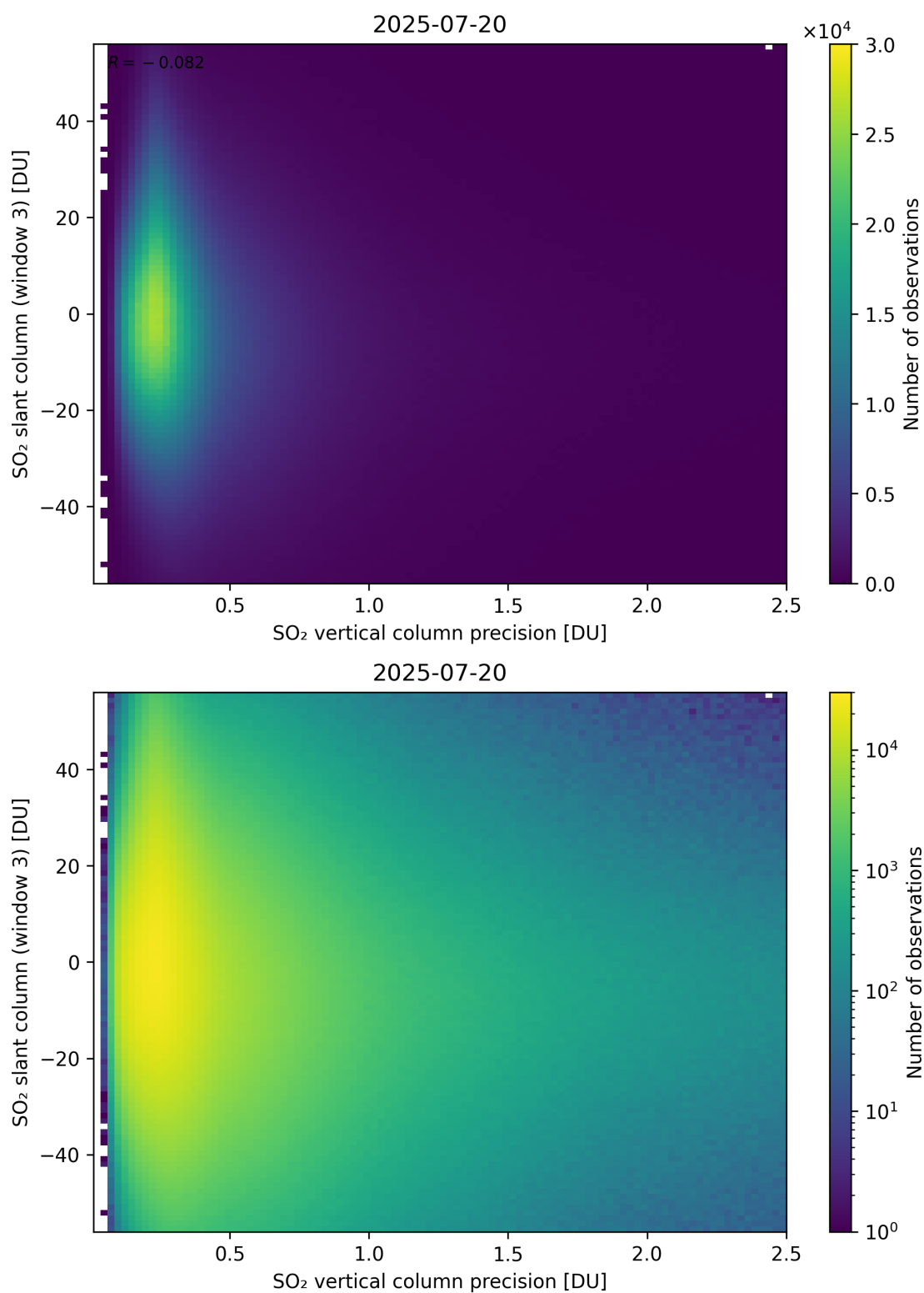
Figure 344: Scatter density plot of “SO 2 vertical column precision” against “SO 2 slant column (window 3)” for 2025-07-19 to 2025-07-21.
