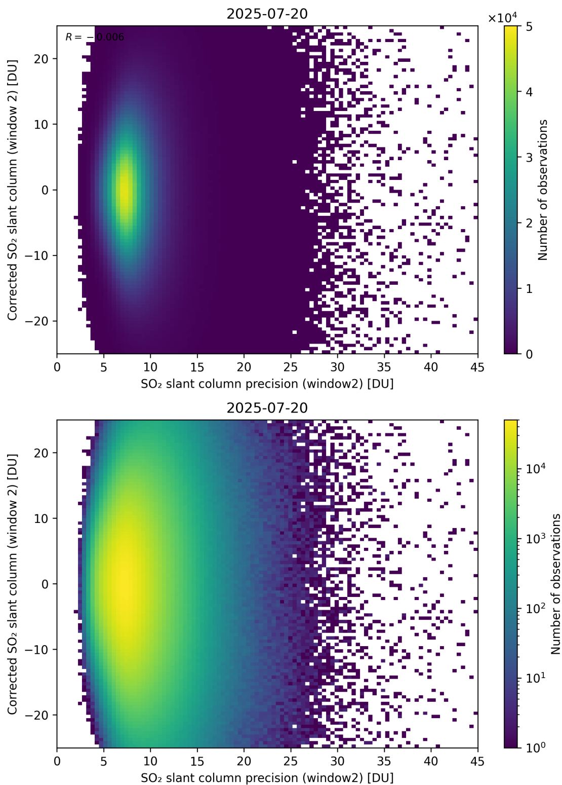
Figure 297: Scatter density plot of “SO 2 slant column precision (window2)” against “Corrected SO 2 slant column (window 2)” for 2025-07-19 to 2025-07-21.
