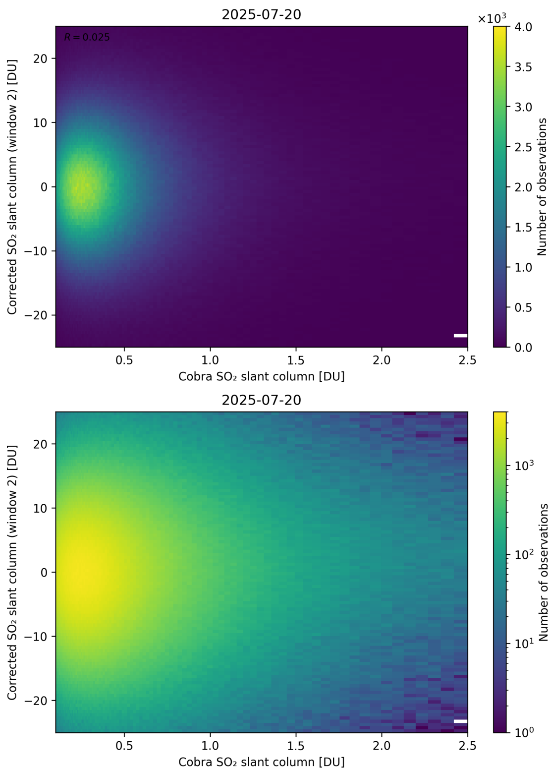
Figure 217: Scatter density plot of “Cobra SO 2 slant column” against “Corrected SO 2 slant column (window 2)” for 2025-07-19 to 2025-07-21.
