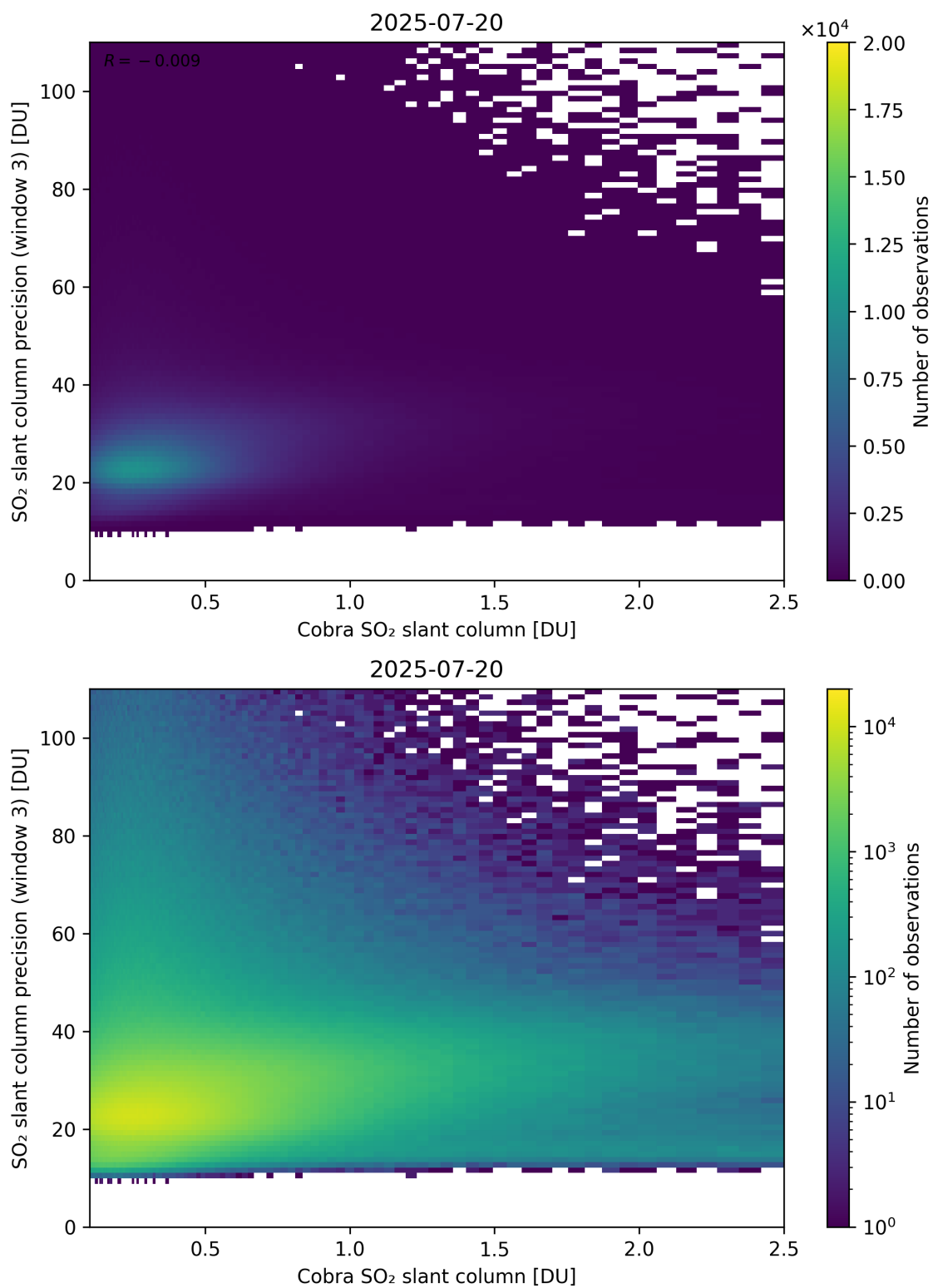
Figure 223: Scatter density plot of “Cobra SO 2 slant column” against “SO 2 slant column precision (window 3)” for 2025-07-19 to 2025-07-21.
