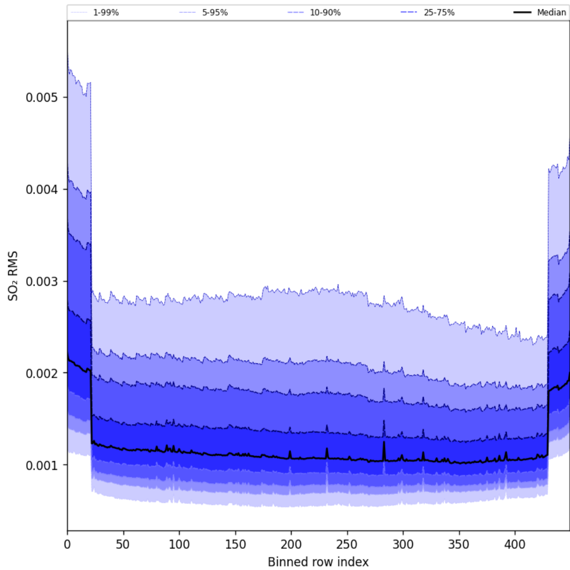
Figure 104: Along track statistics of “SO 2 RMS” for 2025-07-19 to 2025-07-21
