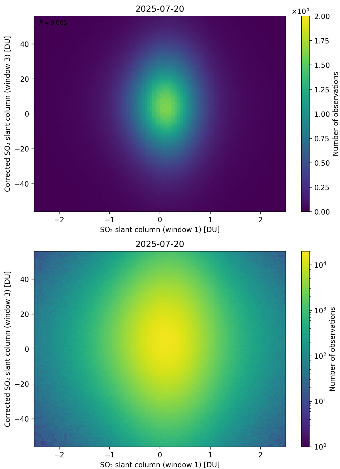
Figure 284: Scatter density plot of “SO 2 slant column (window 1)” against “Corrected SO 2 slant column (window 3)” for 2025-07-19 to 2025-07-21.
