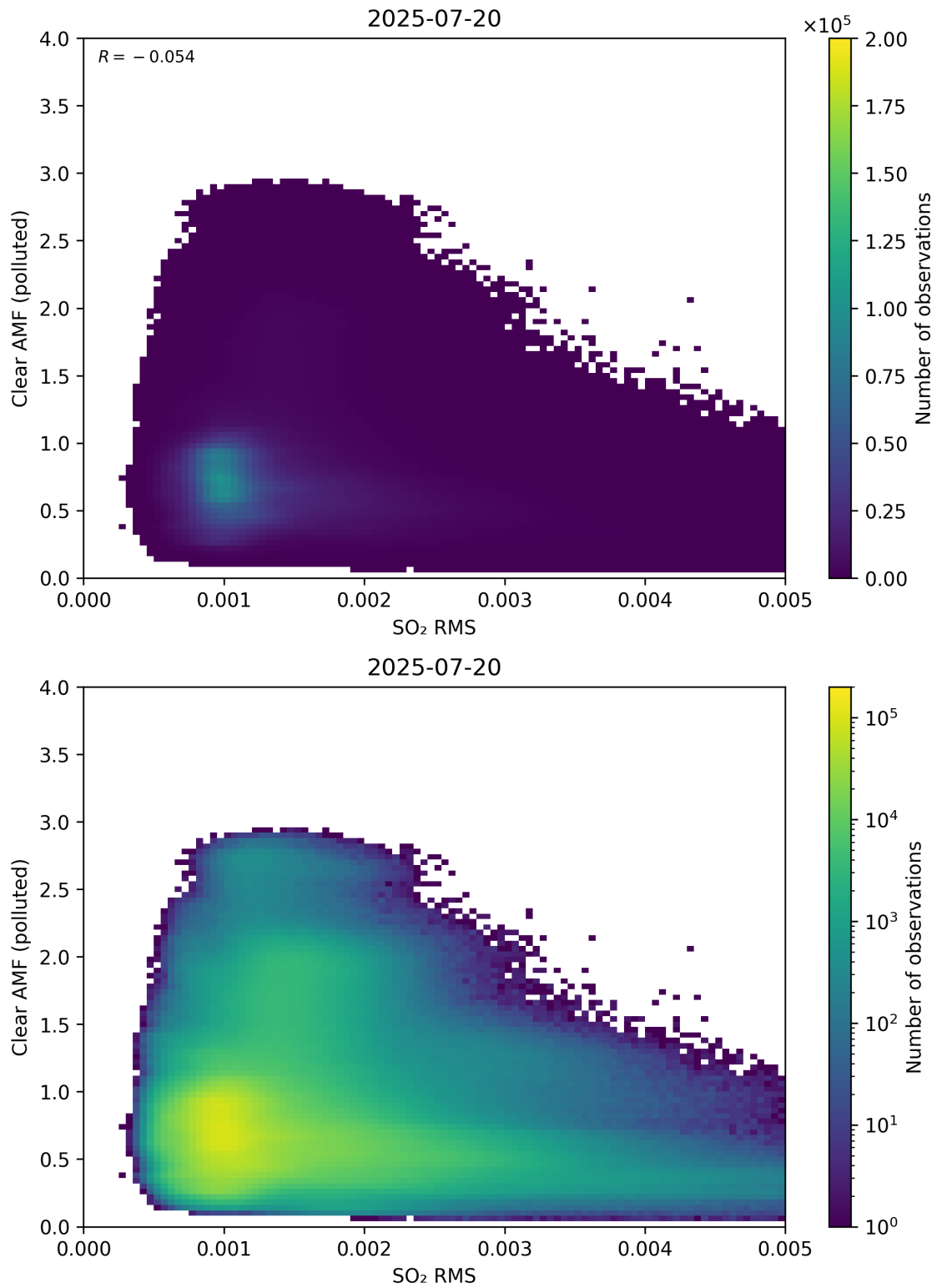
Figure 147: Scatter density plot of “SO 2 RMS” against “Clear AMF (polluted)” for 2025-07-19 to 2025-07-21.
