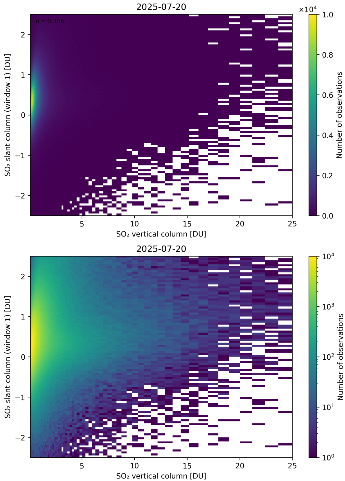
Figure 354: Scatter density plot of “SO 2 vertical column” against “SO 2 slant column (window 1)” for 2025-07-19 to 2025-07-21.
