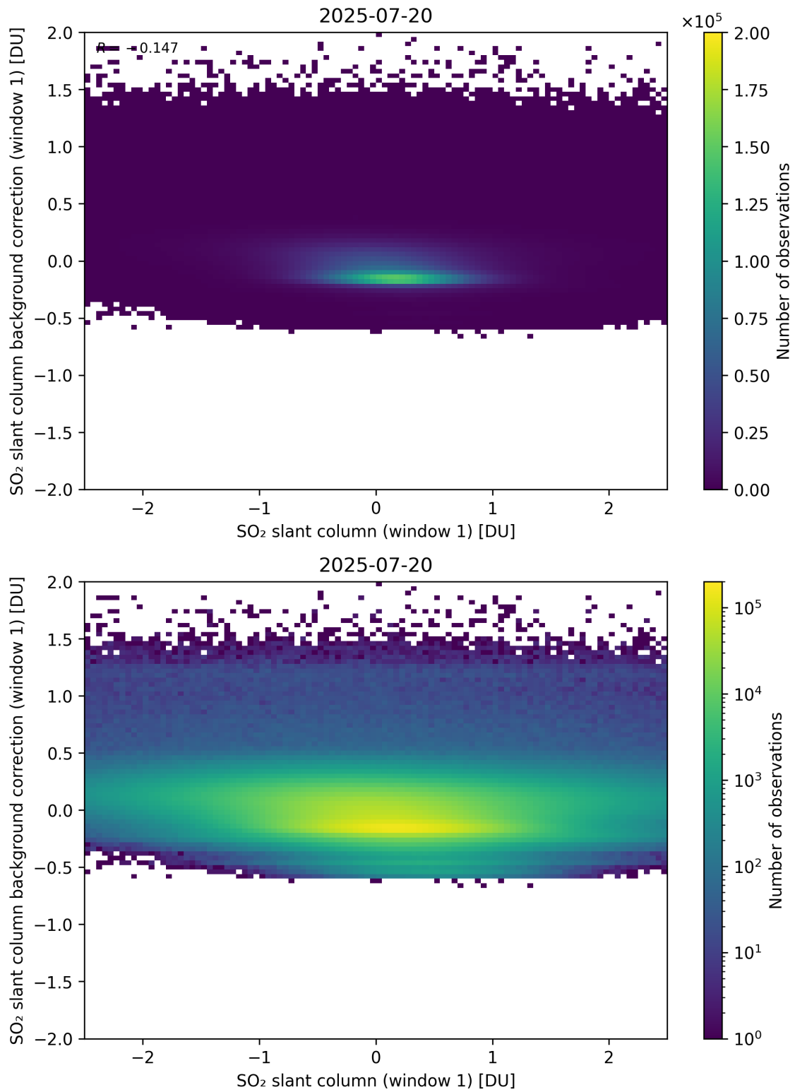
Figure 262: Scatter density plot of “SO 2 slant column (window 1)” against “SO 2 slant column background correction (window 1)” for 2025-07-19 to 2025-07-21.
