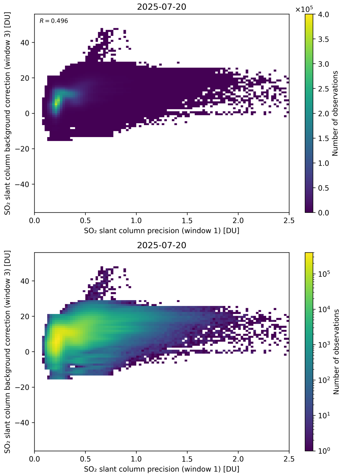
Figure 270: Scatter density plot of “SO 2 slant column precision (window 1)” against “SO 2 slant column background correction (window 3)” for 2025-07-19 to 2025-07-21.
