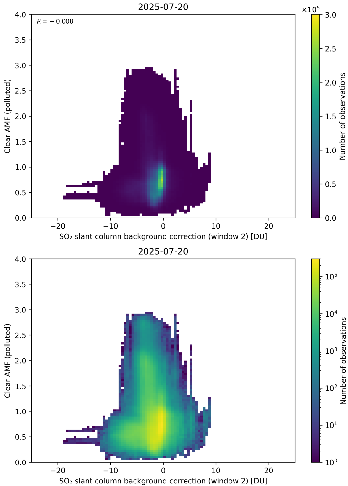
Figure 126: Scatter density plot of “SO 2 slant column background correction (window 2)” against “Clear AMF (polluted)” for 2025-07-19 to 2025-07-21.
