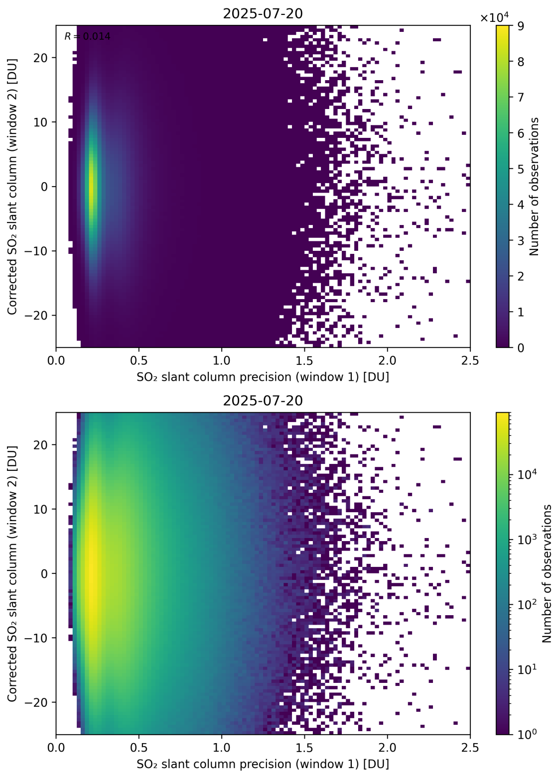
Figure 275: Scatter density plot of “SO 2 slant column precision (window 1)” against “Corrected SO 2 slant column (window 2)” for 2025-07-19 to 2025-07-21.
