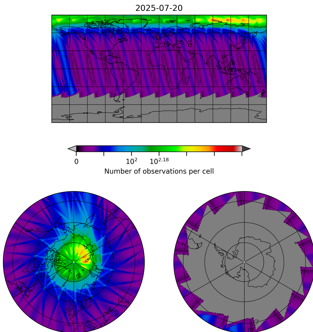
Figure 30: Map of the number of observations for 2025-07-19 to 2025-07-21
