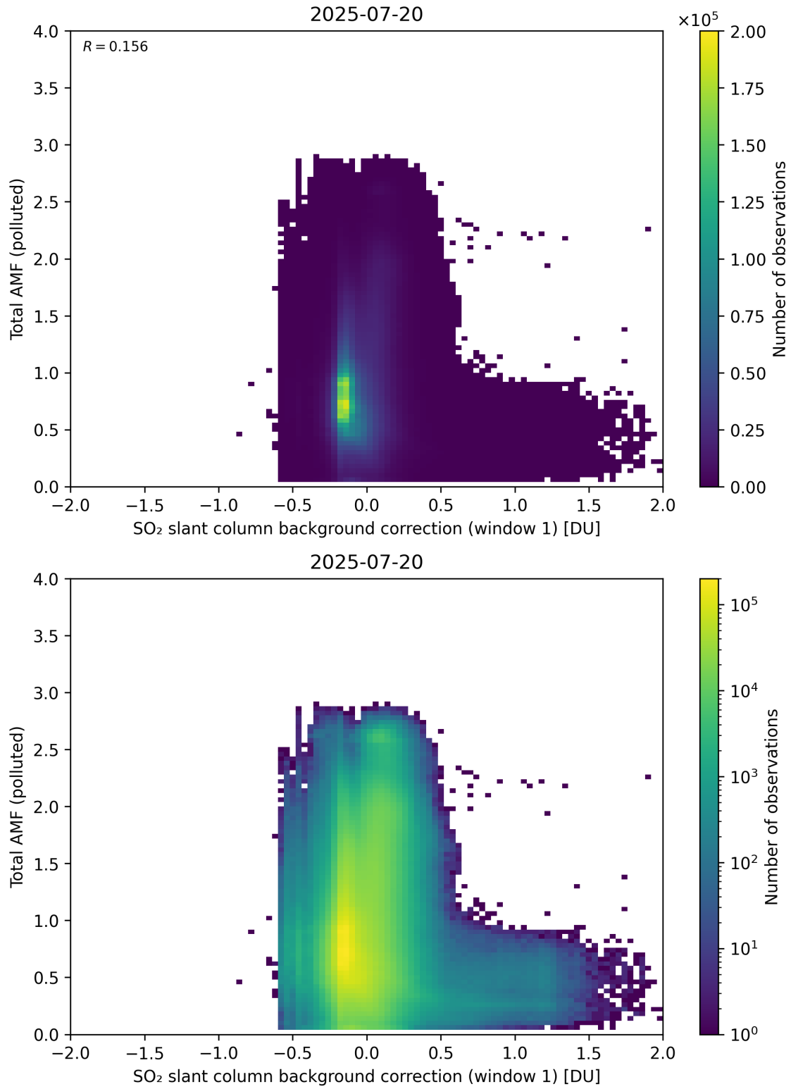
Figure 120: Scatter density plot of “SO 2 slant column background correction (window 1)” against “Total AMF (polluted)” for 2025-07-19 to 2025-07-21.
