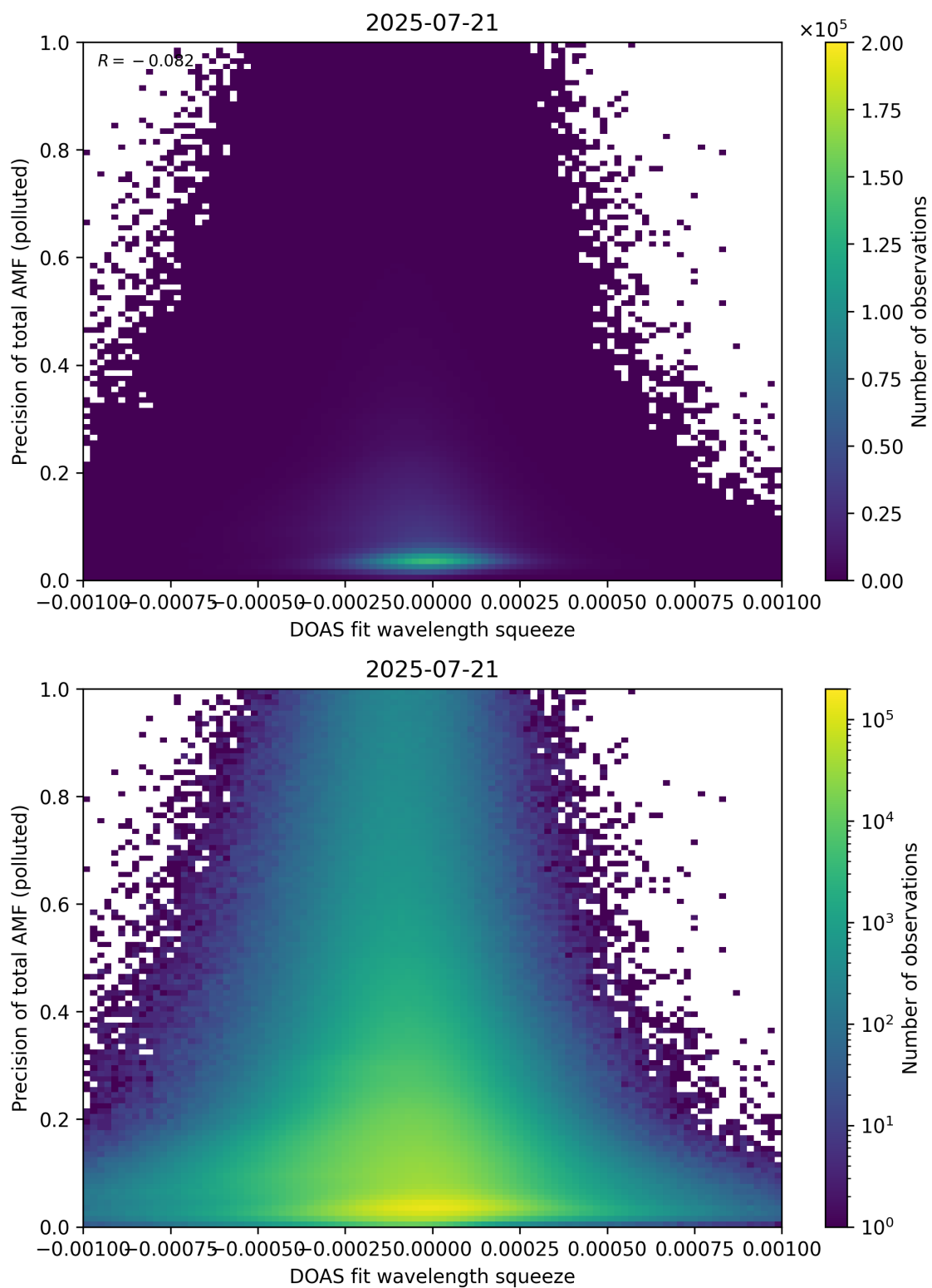
Figure 146: Scatter density plot of “DOAS fit wavelength squeeze” against “Precision of total AMF (polluted)” for 2025-07-20 to 2025-07-22.
