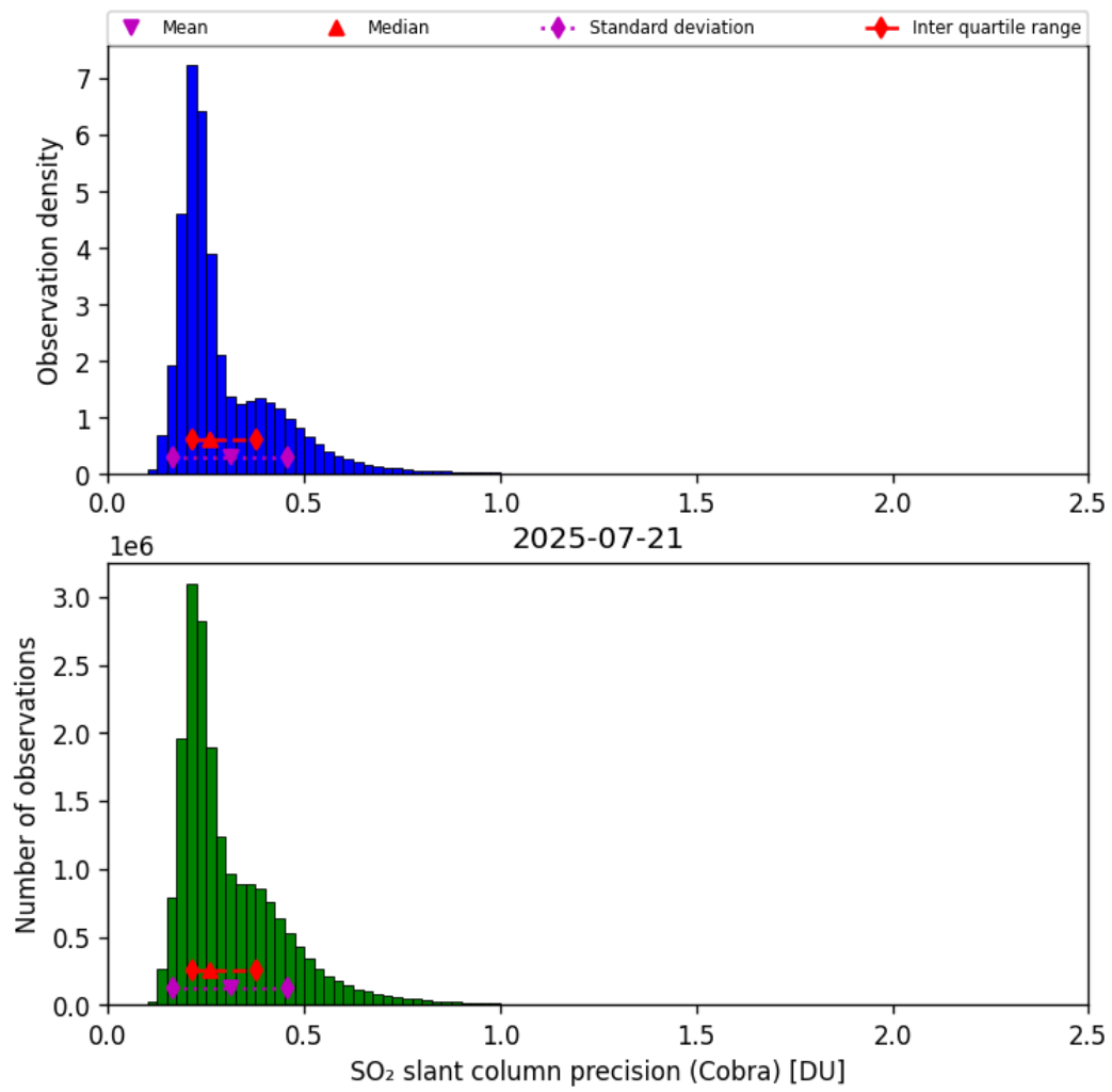
Figure 62: Histogram of “SO 2 slant column precision (Cobra)” for 2025-07-20 to 2025-07-22
