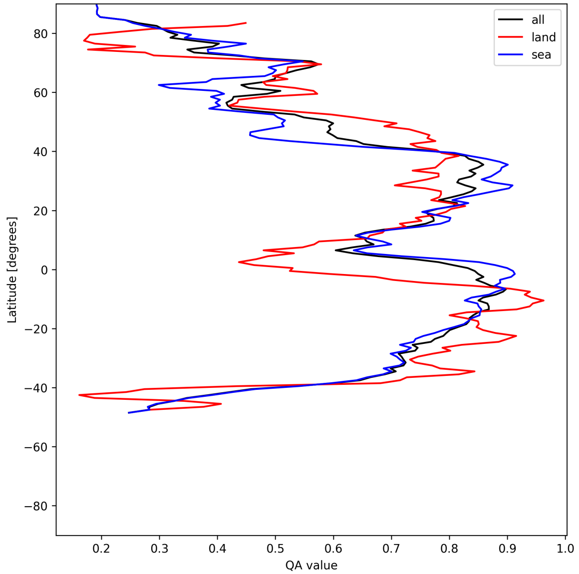
Figure 31: Zonal average of “QA value” for 2025-07-20 to 2025-07-22.
