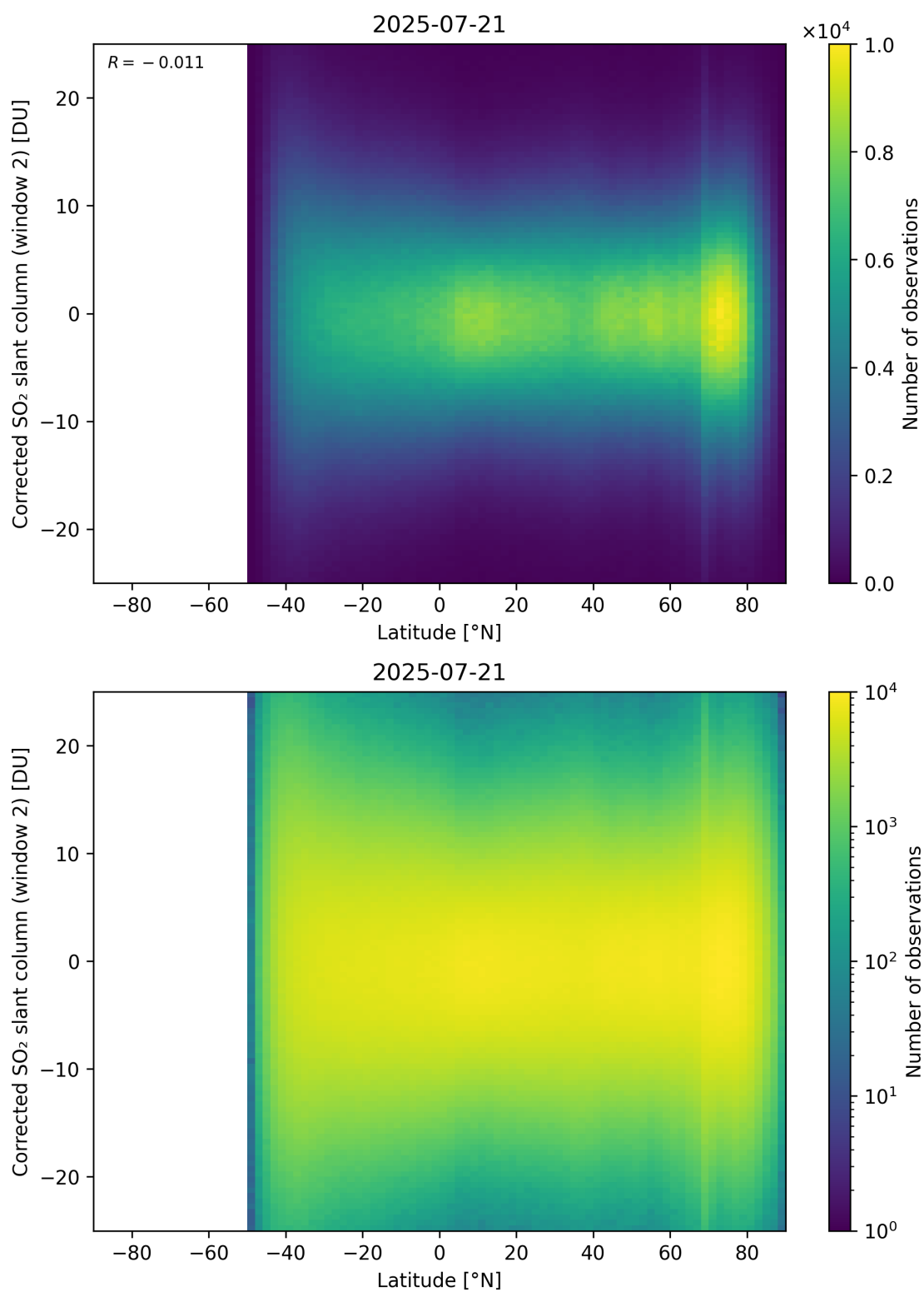
Figure 160: Scatter density plot of “Latitude” against “Corrected SO 2 slant column (window 2)” for 2025-07-20 to 2025-07-22.
