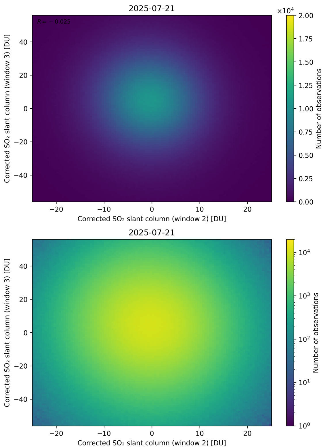
Figure 250: Scatter density plot of “Corrected SO 2 slant column (window 2)” against “Corrected SO 2 slant column (window 3)” for 2025-07-20 to 2025-07-22.
