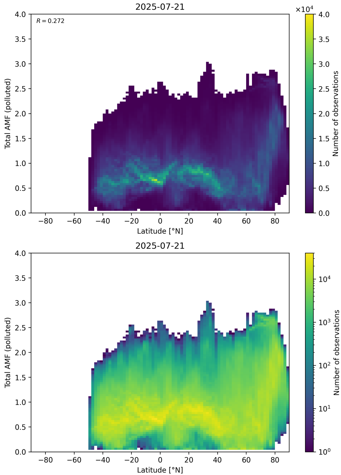
Figure 167: Scatter density plot of “Latitude” against “Total AMF (polluted)” for 2025-07-20 to 2025-07-22.
