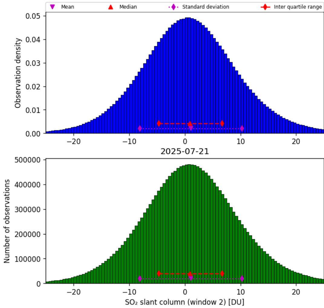
Figure 67: Histogram of “SO 2 slant column (window 2)” for 2025-07-20 to 2025-07-22
