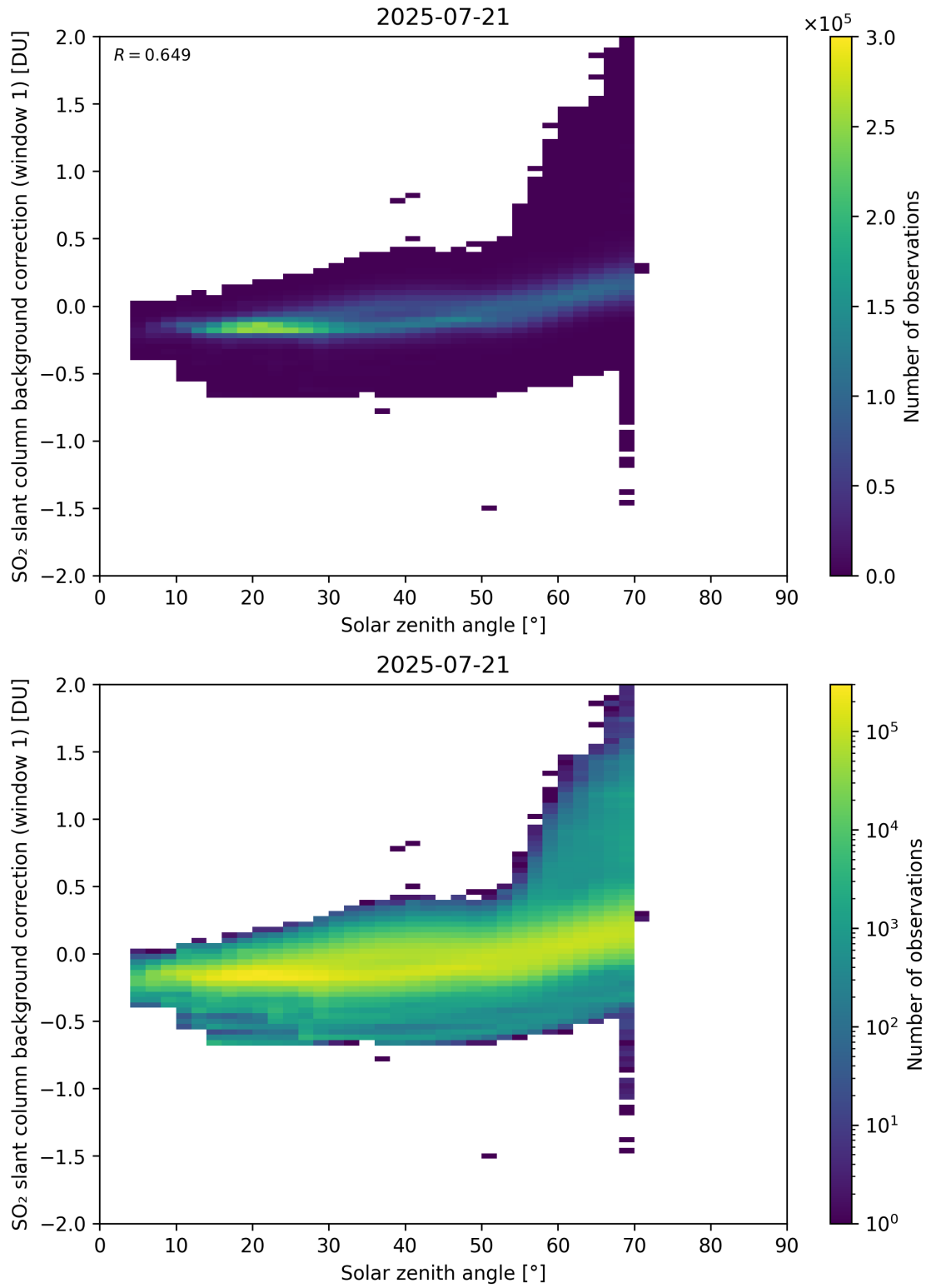
Figure 171: Scatter density plot of “Solar zenith angle” against “SO 2 slant column background correction (window 1)” for 2025-07-20 to 2025-07-22.
