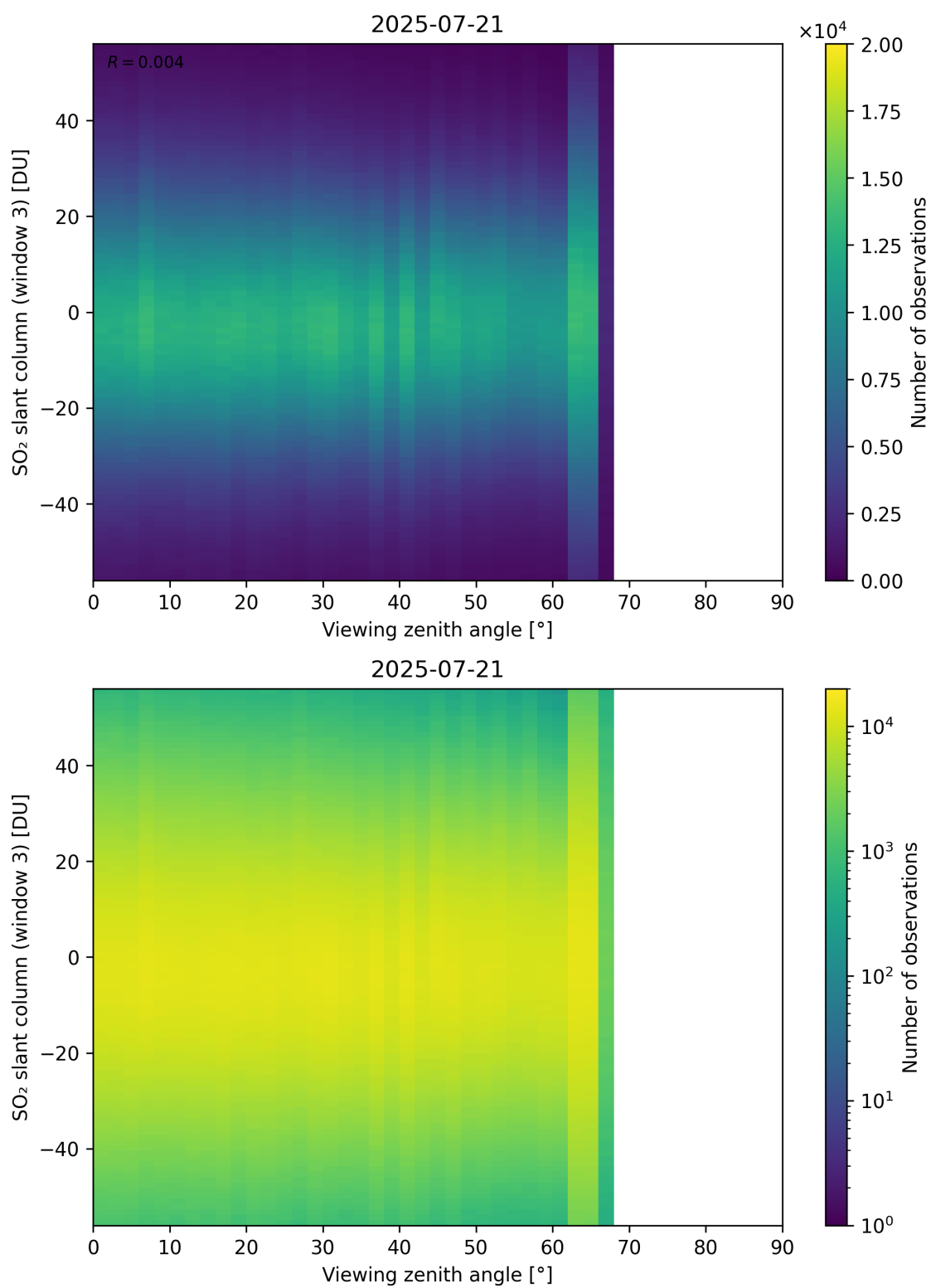
Figure 379: Scatter density plot of “Viewing zenith angle” against “SO 2 slant column (window 3)” for 2025-07-20 to 2025-07-22.
