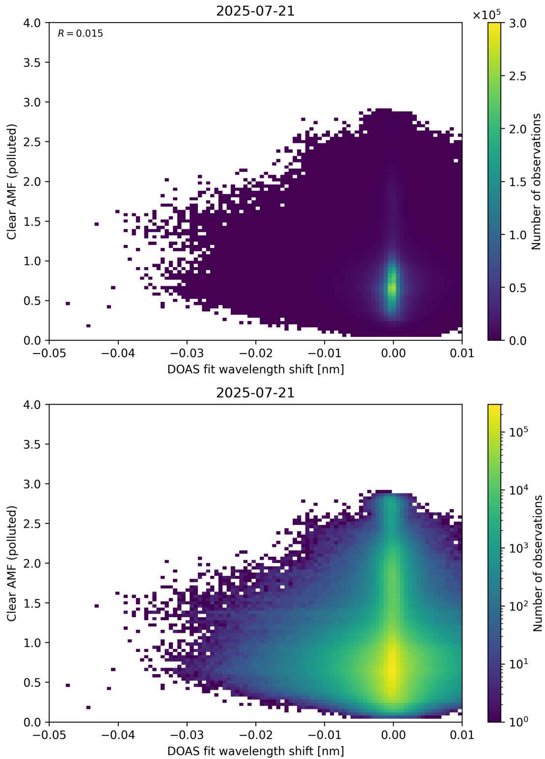
Figure 140: Scatter density plot of “DOAS fit wavelength shift” against “Clear AMF (polluted)” for 2025-07-20 to 2025-07-22.
