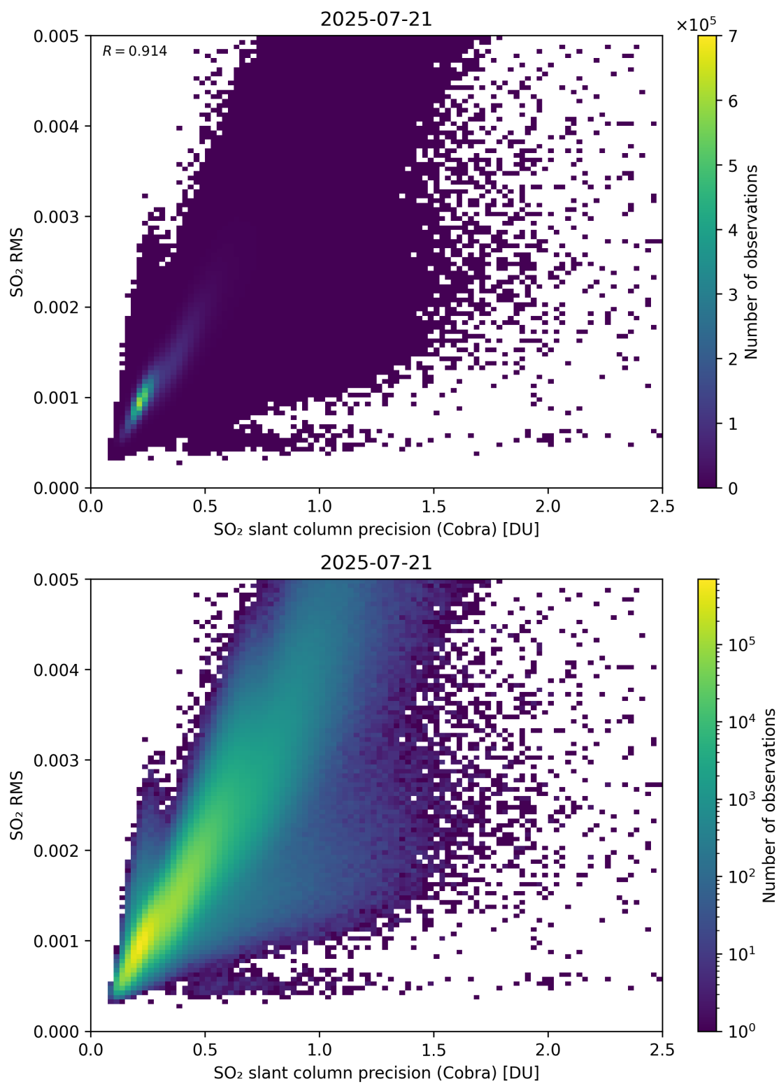
Figure 204: Scatter density plot of “SO 2 slant column precision (Cobra)” against “SO 2 RMS” for 2025-07-20 to 2025-07-22.
