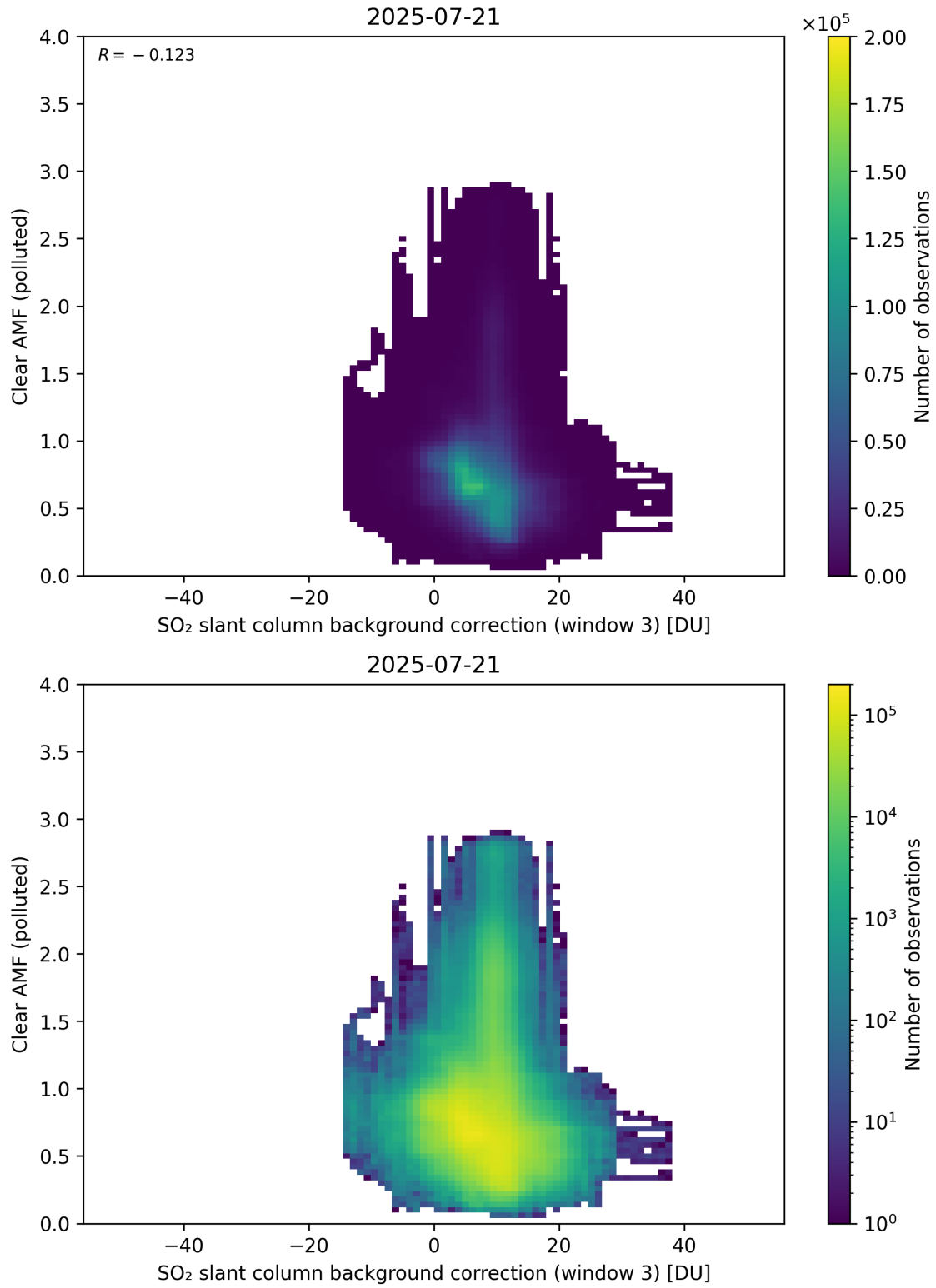
Figure 135: Scatter density plot of “SO 2 slant column background correction (window 3)” against “Clear AMF (polluted)” for 2025-07-20 to 2025-07-22.
