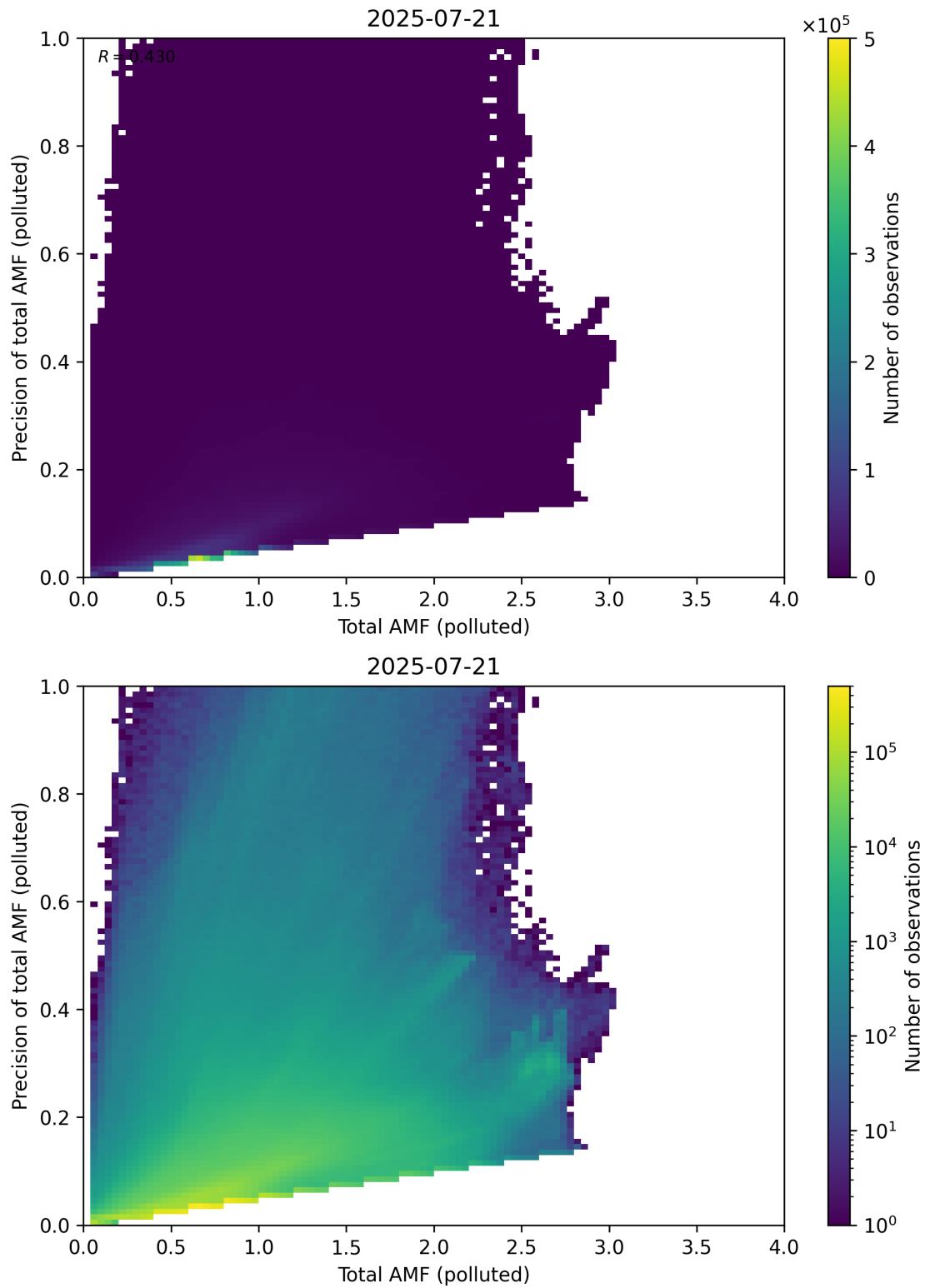
Figure 322: Scatter density plot of “Total AMF (polluted)” against “Precision of total AMF (polluted)” for 2025-07-20 to 2025-07-22.
