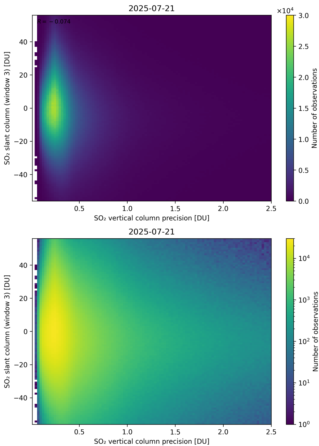
Figure 344: Scatter density plot of “SO 2 vertical column precision” against “SO 2 slant column (window 3)” for 2025-07-20 to 2025-07-22.
