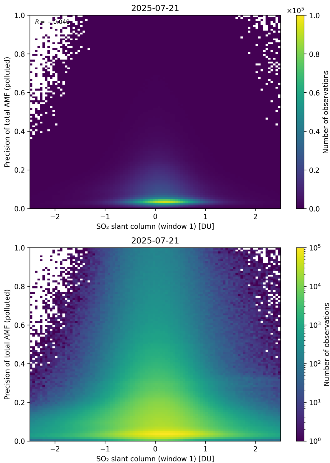
Figure 290: Scatter density plot of “SO 2 slant column (window 1)” against “Precision of total AMF (polluted)” for 2025-07-20 to 2025-07-22.
