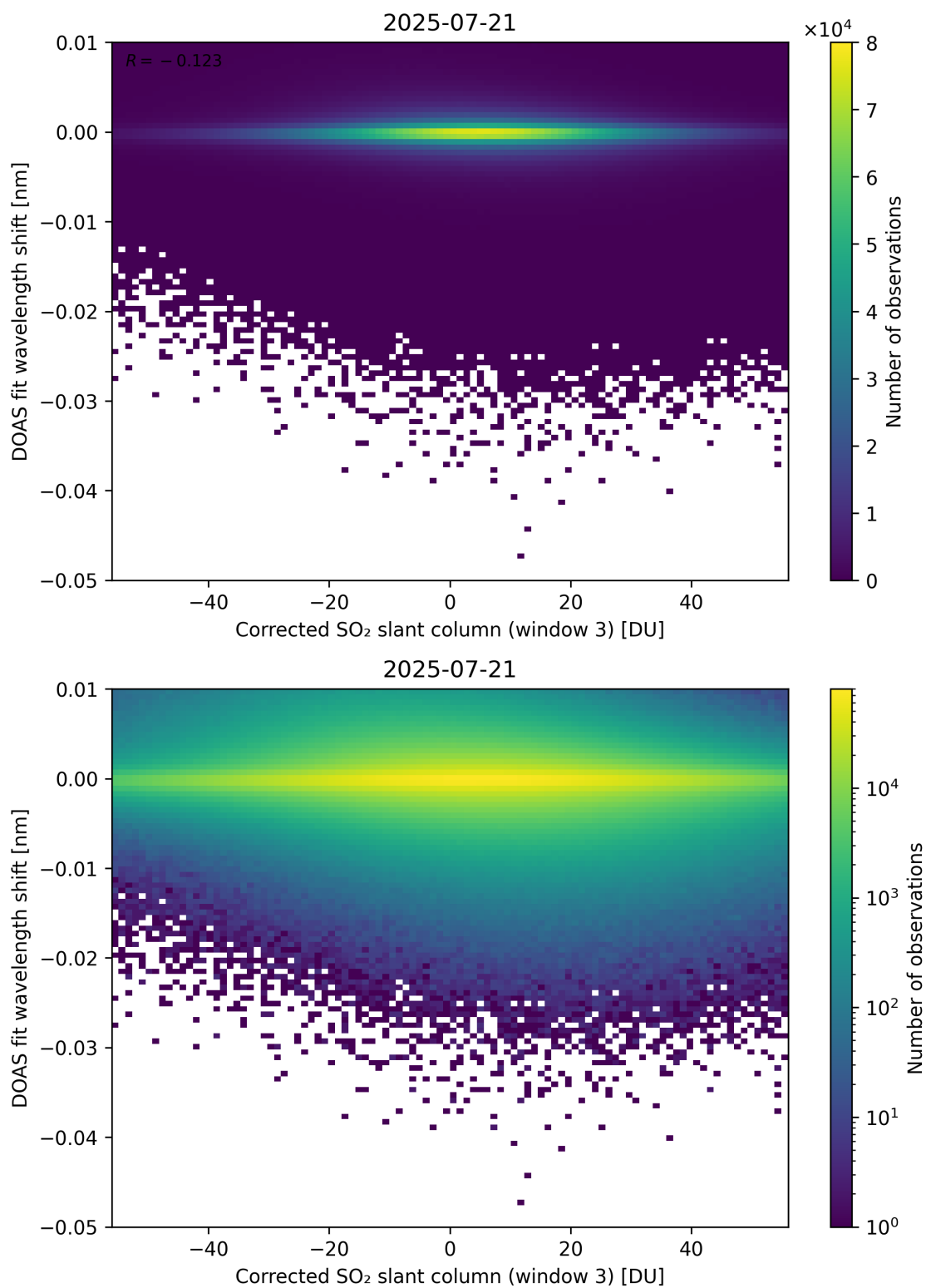
Figure 256: Scatter density plot of “Corrected SO 2 slant column (window 3)” against “DOAS fit wavelength shift” for 2025-07-20 to 2025-07-22.
