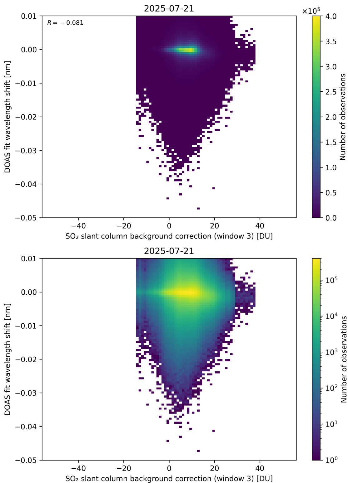
Figure 132: Scatter density plot of “SO 2 slant column background correction (window 3)” against “DOAS fit wavelength shift” for 2025-07-20 to 2025-07-22.
