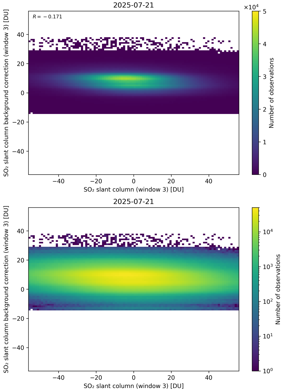
Figure 303: Scatter density plot of “SO 2 slant column (window 3)” against “SO 2 slant column background correction (window 3)” for 2025-07-20 to 2025-07-22.
