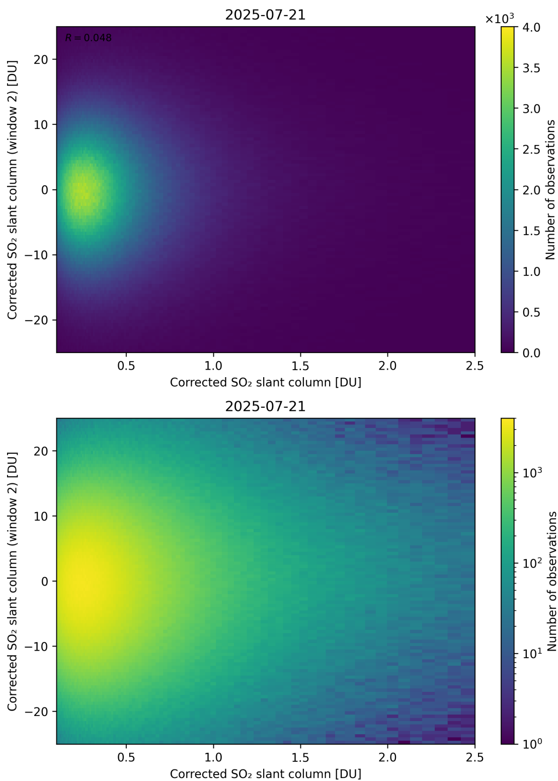
Figure 235: Scatter density plot of “Corrected SO 2 slant column” against “Corrected SO 2 slant column (window 2)” for 2025-07-20 to 2025-07-22.
