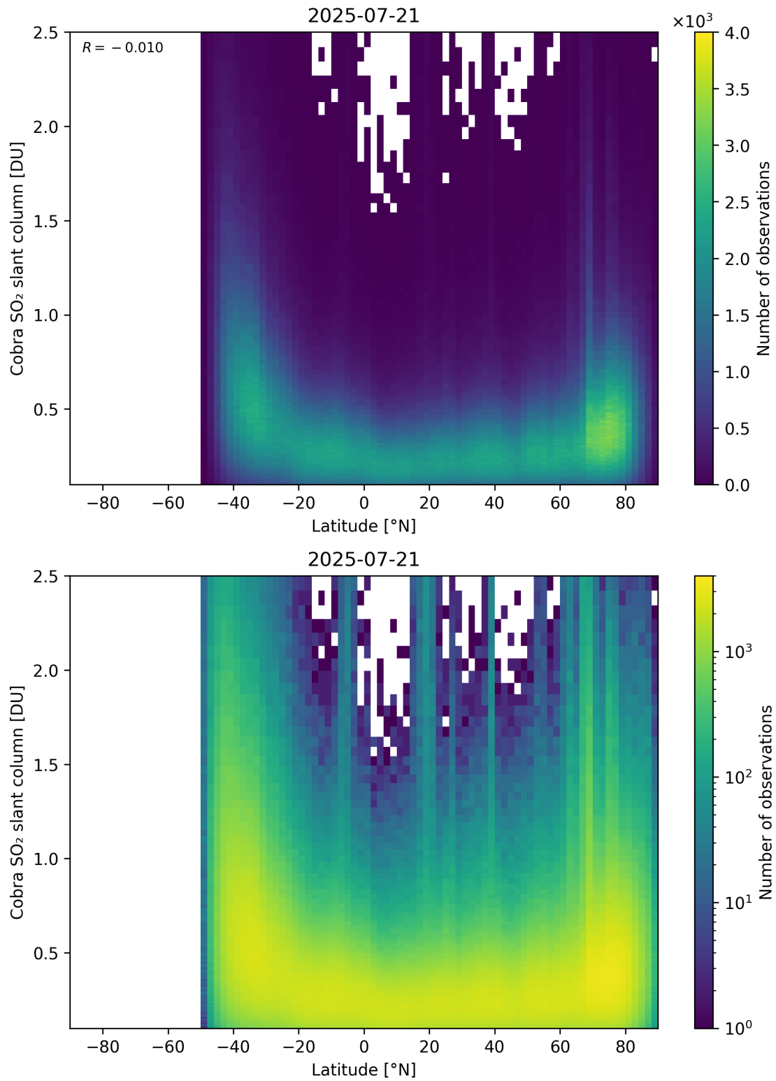
Figure 157: Scatter density plot of “Latitude” against “Cobra SO 2 slant column” for 2025-07-20 to 2025-07-22.
