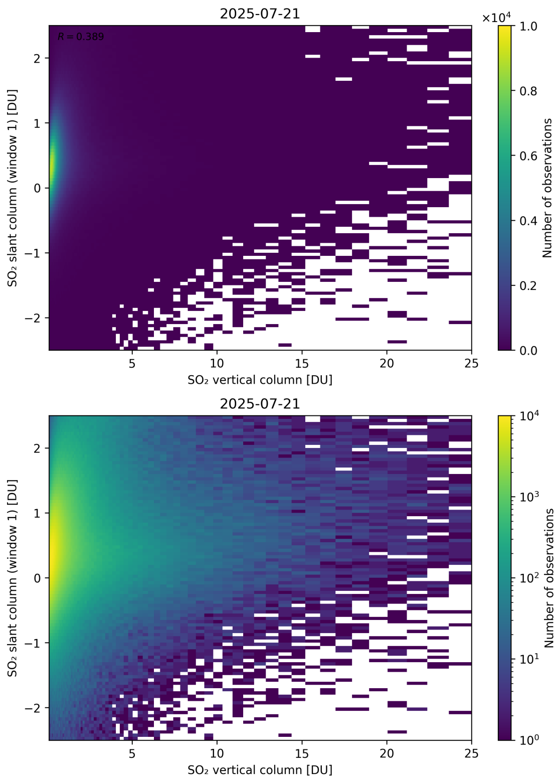
Figure 354: Scatter density plot of “SO 2 vertical column” against “SO 2 slant column (window 1)” for 2025-07-20 to 2025-07-22.
