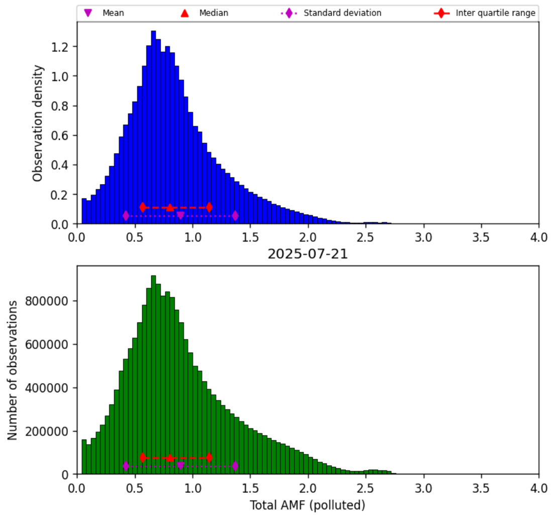
Figure 79: Histogram of “Total AMF (polluted)” for 2025-07-20 to 2025-07-22
