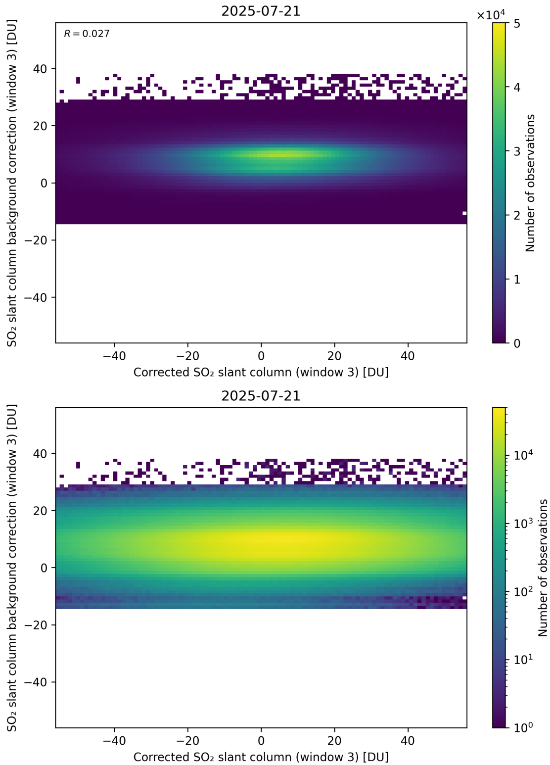
Figure 255: Scatter density plot of “Corrected SO 2 slant column (window 3)” against “SO 2 slant column background correction (window 3)” for 2025-07-20 to 2025-07-22.
