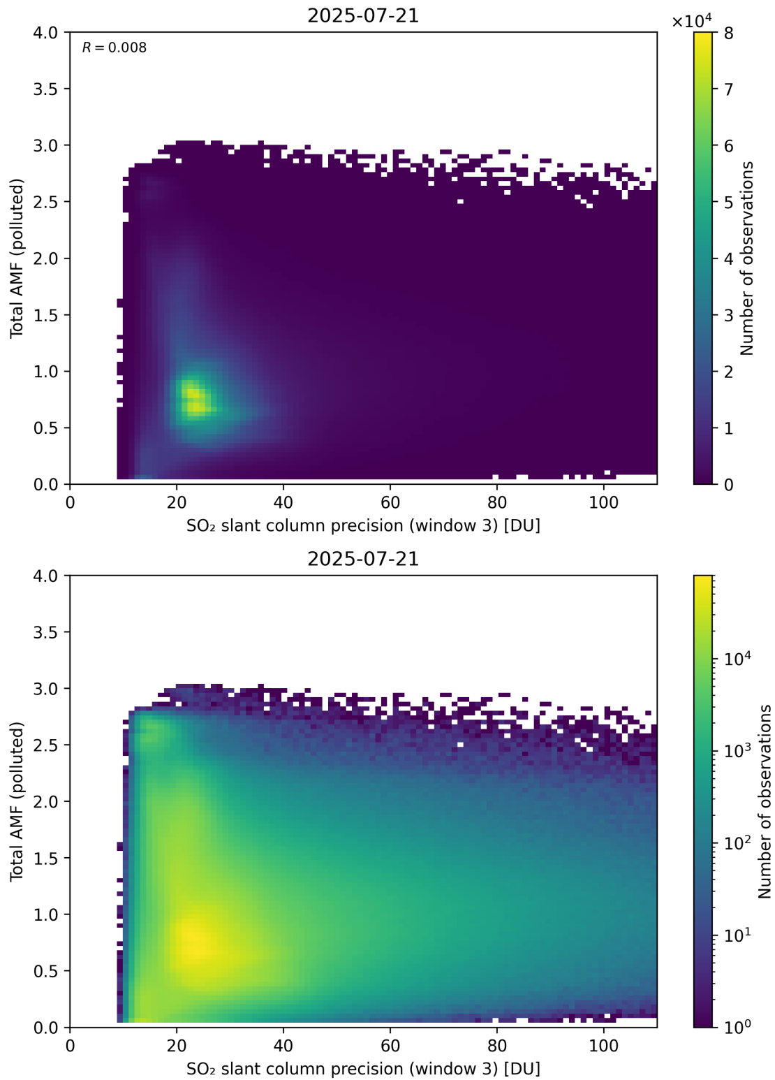
Figure 313: Scatter density plot of “SO 2 slant column precision (window 3)” against “Total AMF (polluted)” for 2025-07-20 to 2025-07-22.
