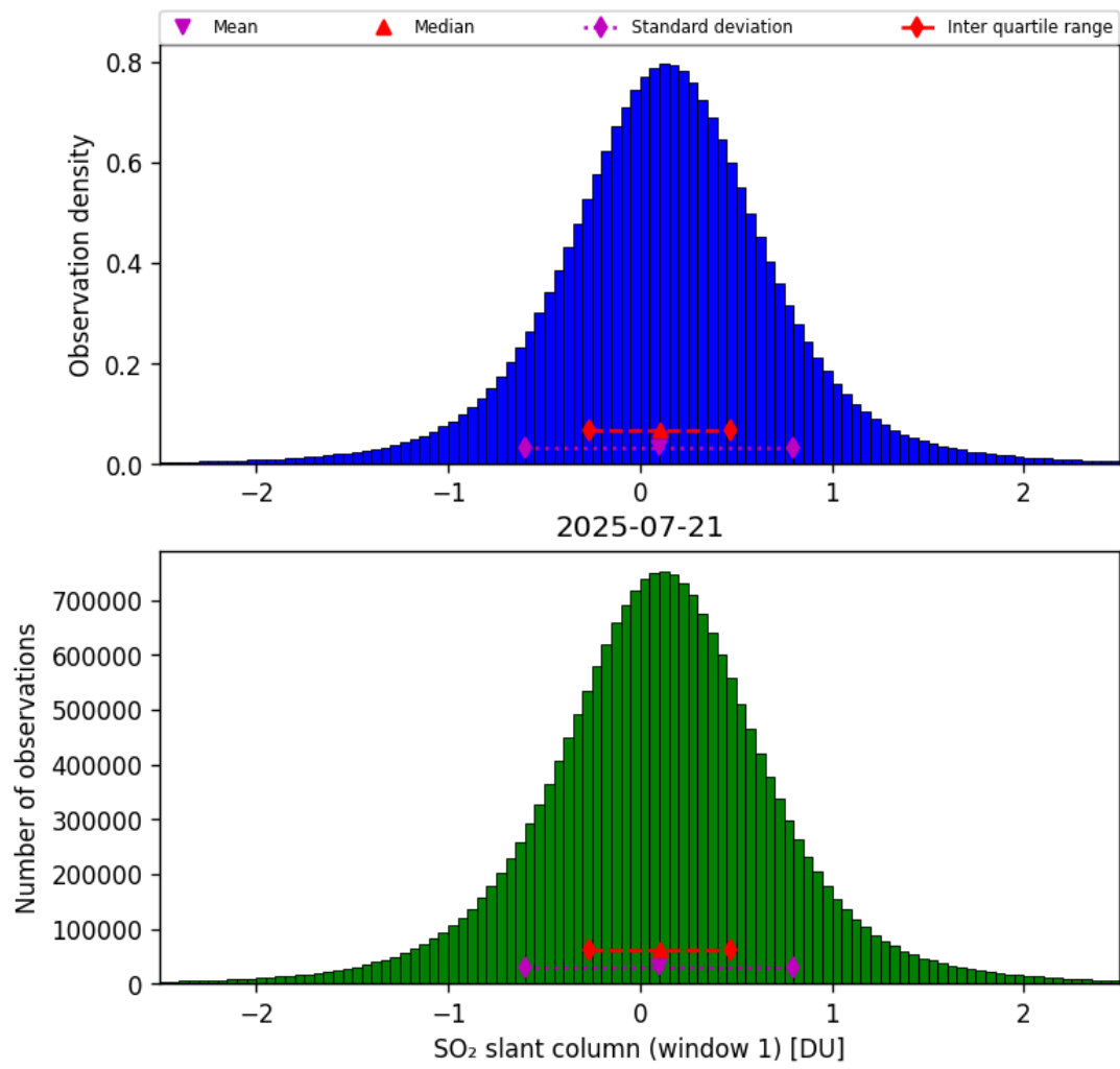
Figure 63: Histogram of “SO 2 slant column (window 1)” for 2025-07-20 to 2025-07-22
