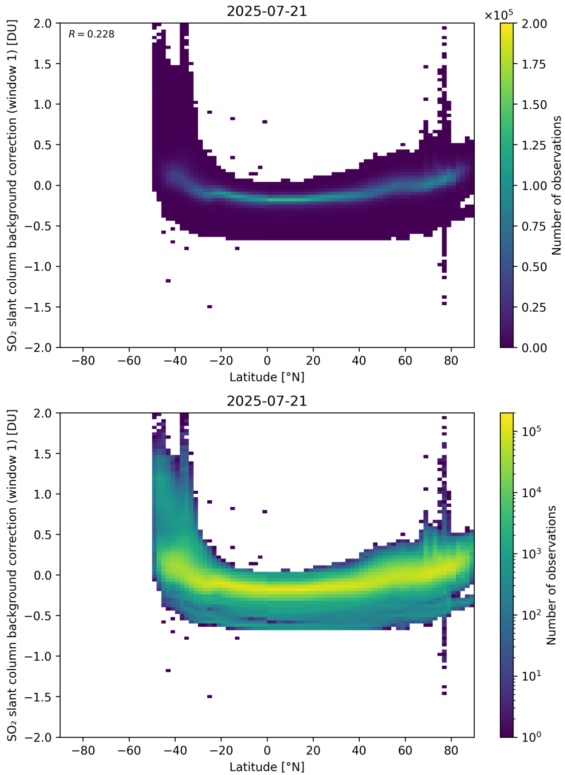
Figure 150: Scatter density plot of “Latitude” against “SO 2 slant column background correction (window 1)” for 2025-07-20 to 2025-07-22.
