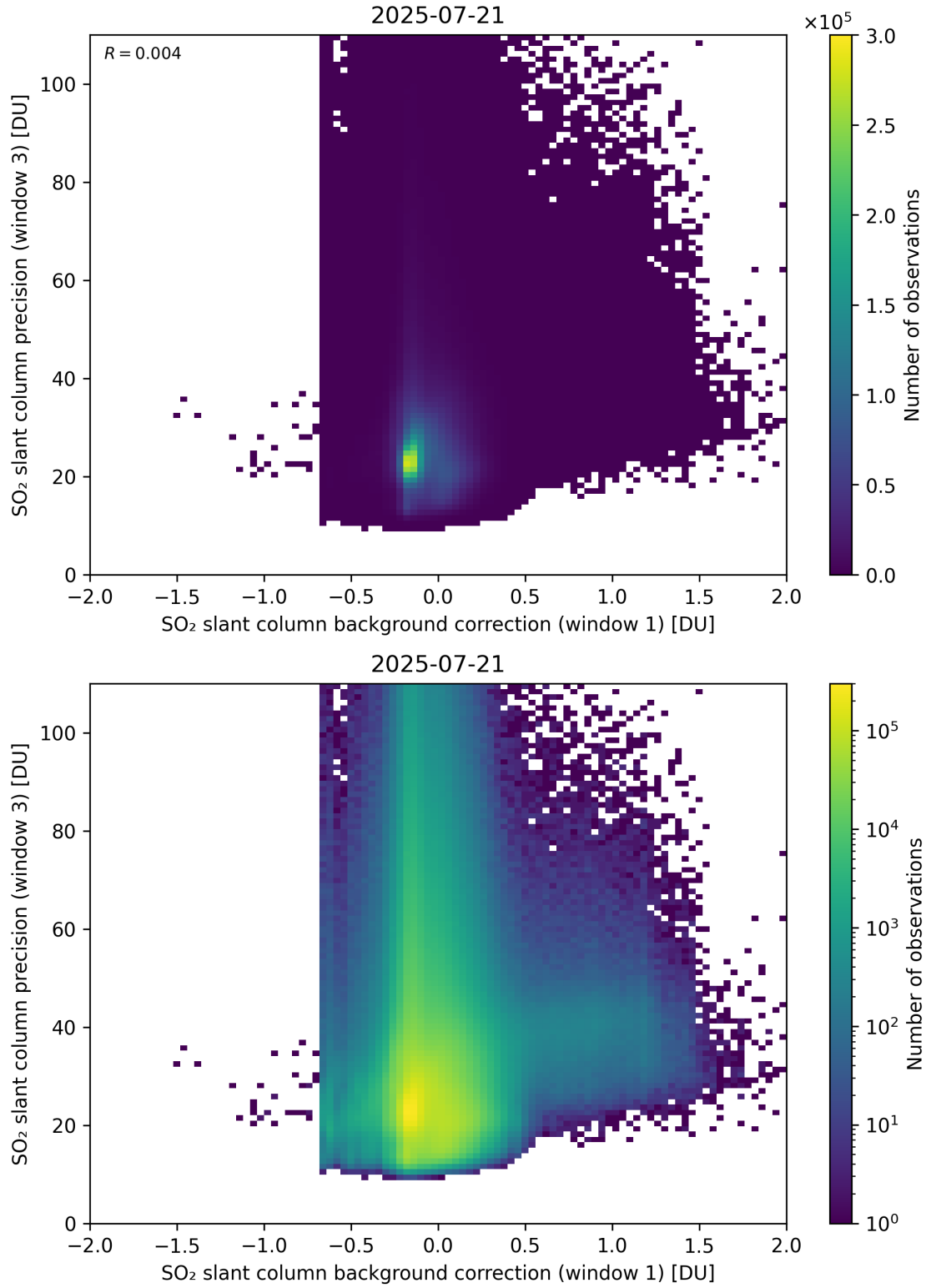
Figure 119: Scatter density plot of “SO 2 slant column background correction (window 1)” against “SO 2 slant column precision (window 3)” for 2025-07-20 to 2025-07-22.
