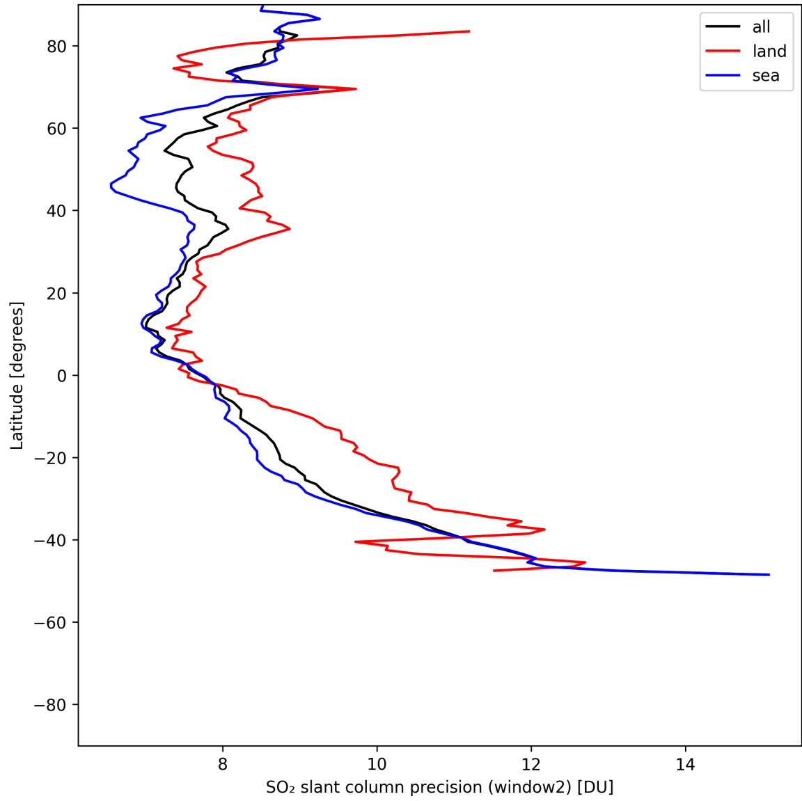
Figure 42: Zonal average of “SO 2 slant column precision (window2)” for 2025-07-20 to 2025-07-22.
