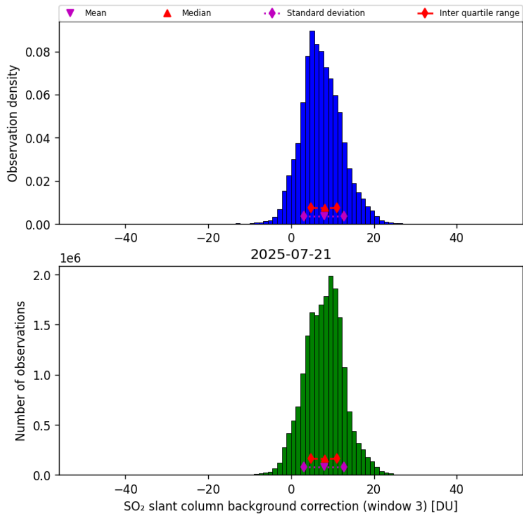
Figure 74: Histogram of “SO 2 slant column background correction (window 3)” for 2025-07-20 to 2025-07-22
