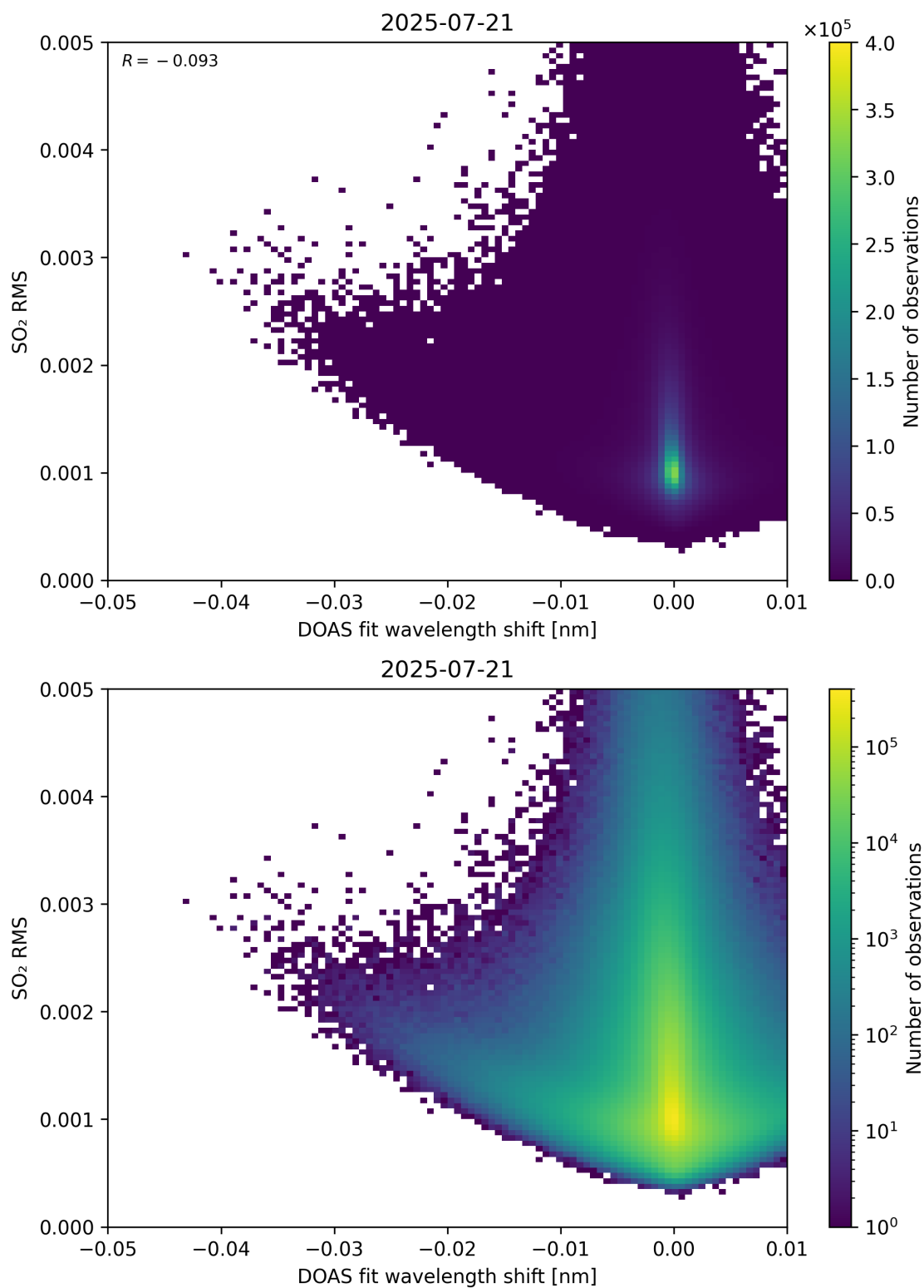
Figure 139: Scatter density plot of “DOAS fit wavelength shift” against “SO 2 RMS” for 2025-07-20 to 2025-07-22.
