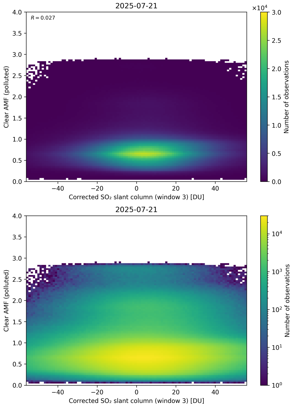
Figure 259: Scatter density plot of “Corrected SO 2 slant column (window 3)” against “Clear AMF (polluted)” for 2025-07-20 to 2025-07-22.
