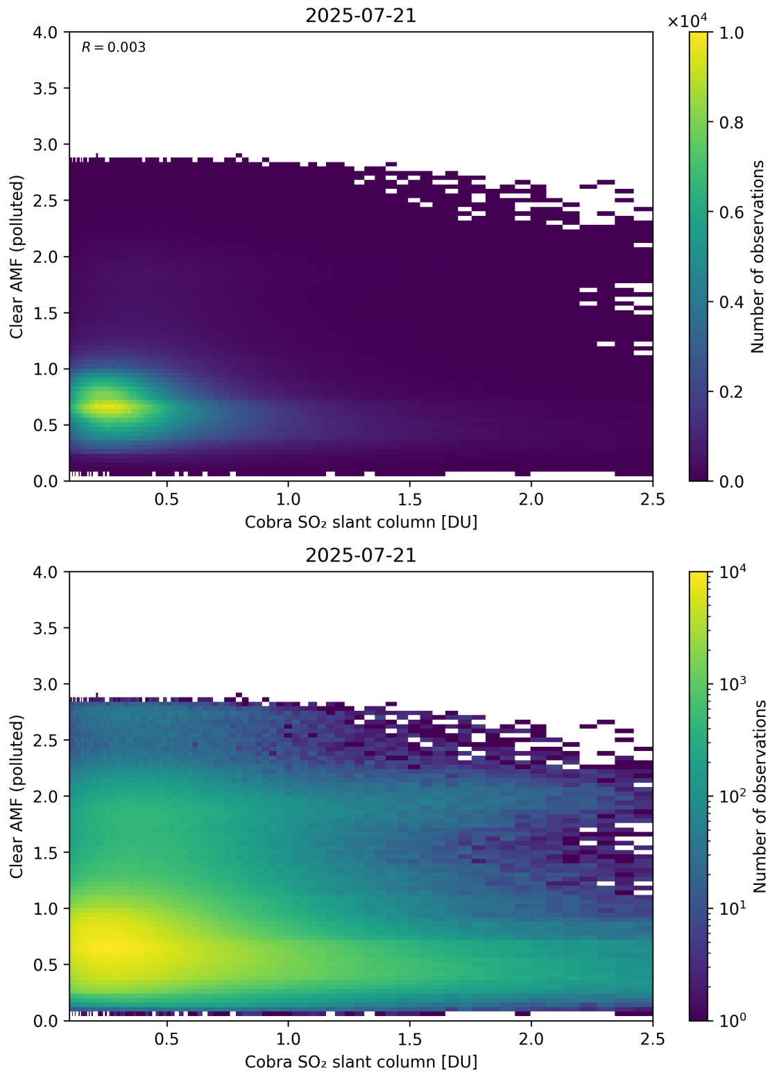
Figure 215: Scatter density plot of “Cobra SO 2 slant column” against “Clear AMF (polluted)” for 2025-07-20 to 2025-07-22.
