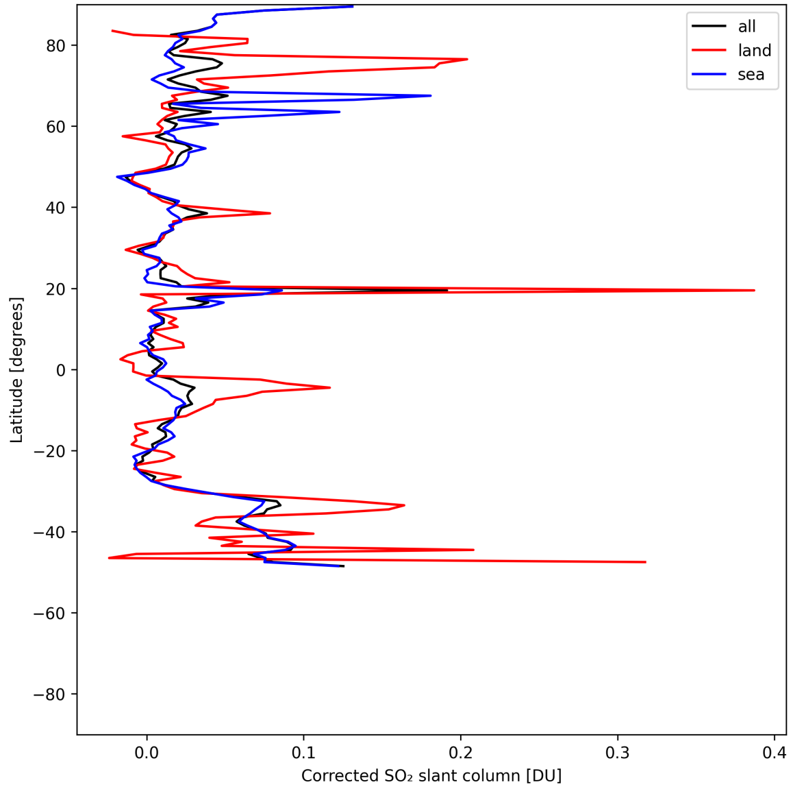
Figure 34: Zonal average of “Corrected SO 2 slant column” for 2025-07-20 to 2025-07-22.
