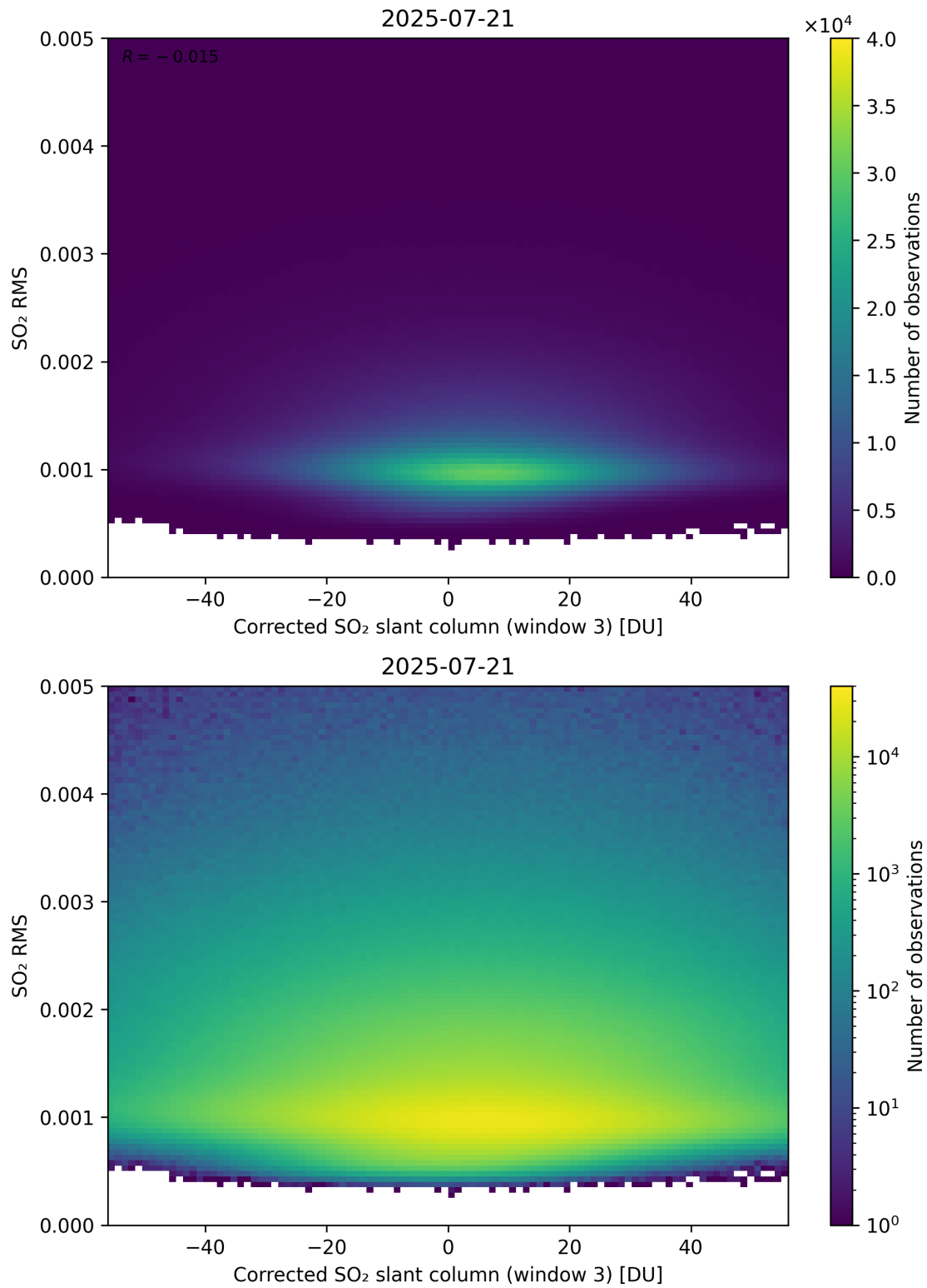
Figure 258: Scatter density plot of “Corrected SO 2 slant column (window 3)” against “SO 2 RMS” for 2025-07-20 to 2025-07-22.
