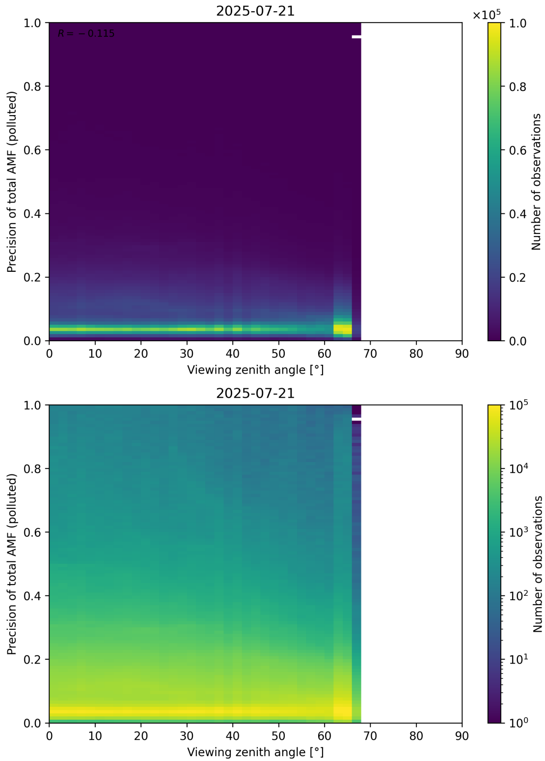
Figure 382: Scatter density plot of “Viewing zenith angle” against “Precision of total AMF (polluted)” for 2025-07-20 to 2025-07-22.
