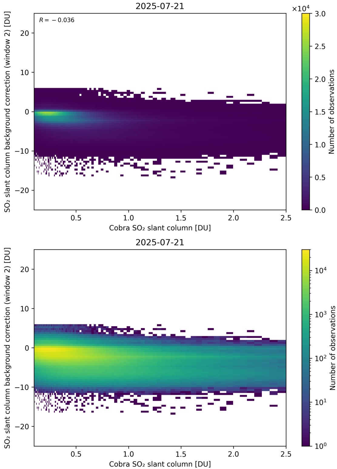
Figure 194: Scatter density plot of “Cobra SO 2 slant column” against “SO 2 slant column background correction (window 2)” for 2025-07-20 to 2025-07-22.
