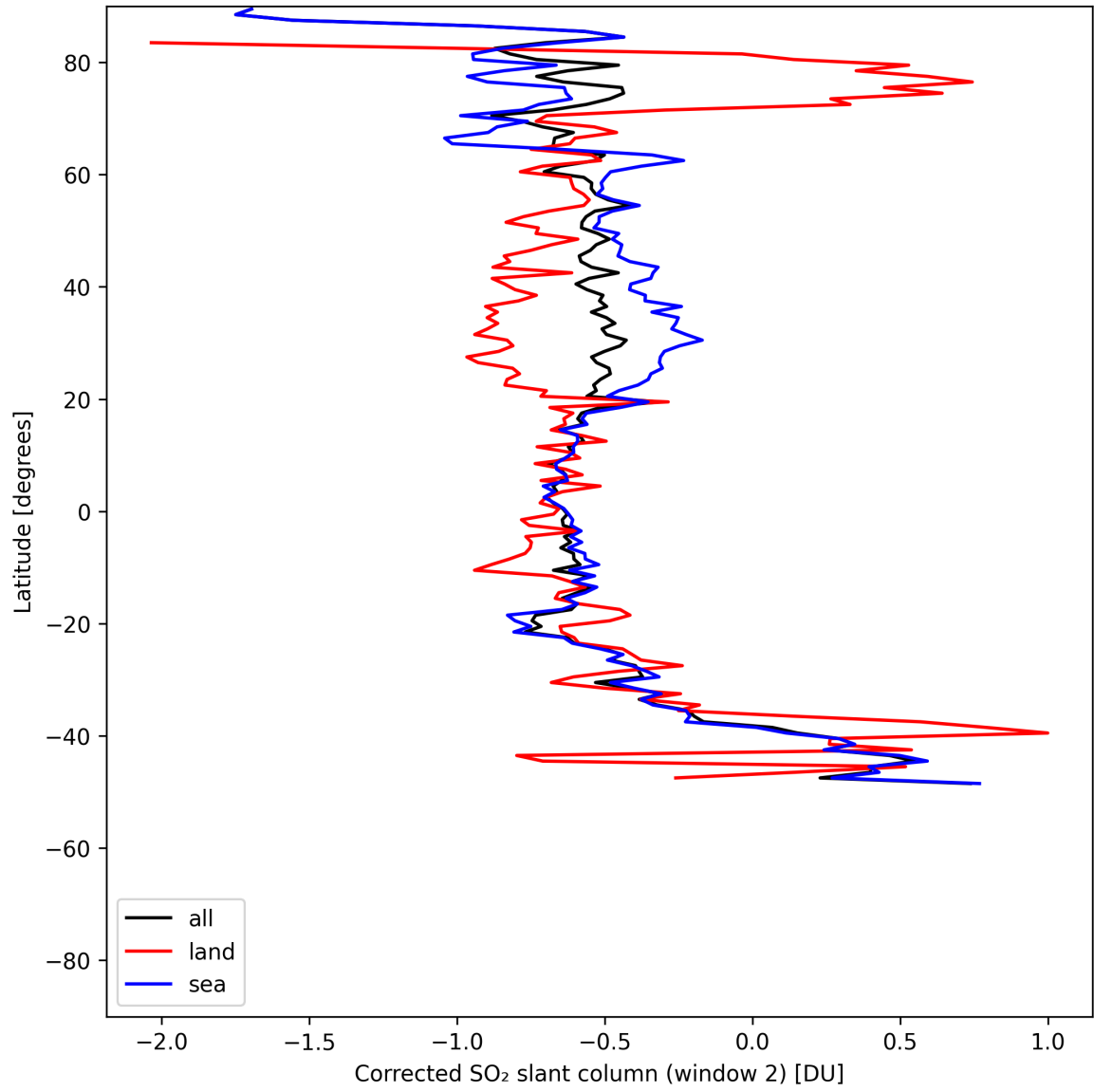
Figure 43: Zonal average of “Corrected SO 2 slant column (window 2)” for 2025-07-20 to 2025-07-22.
