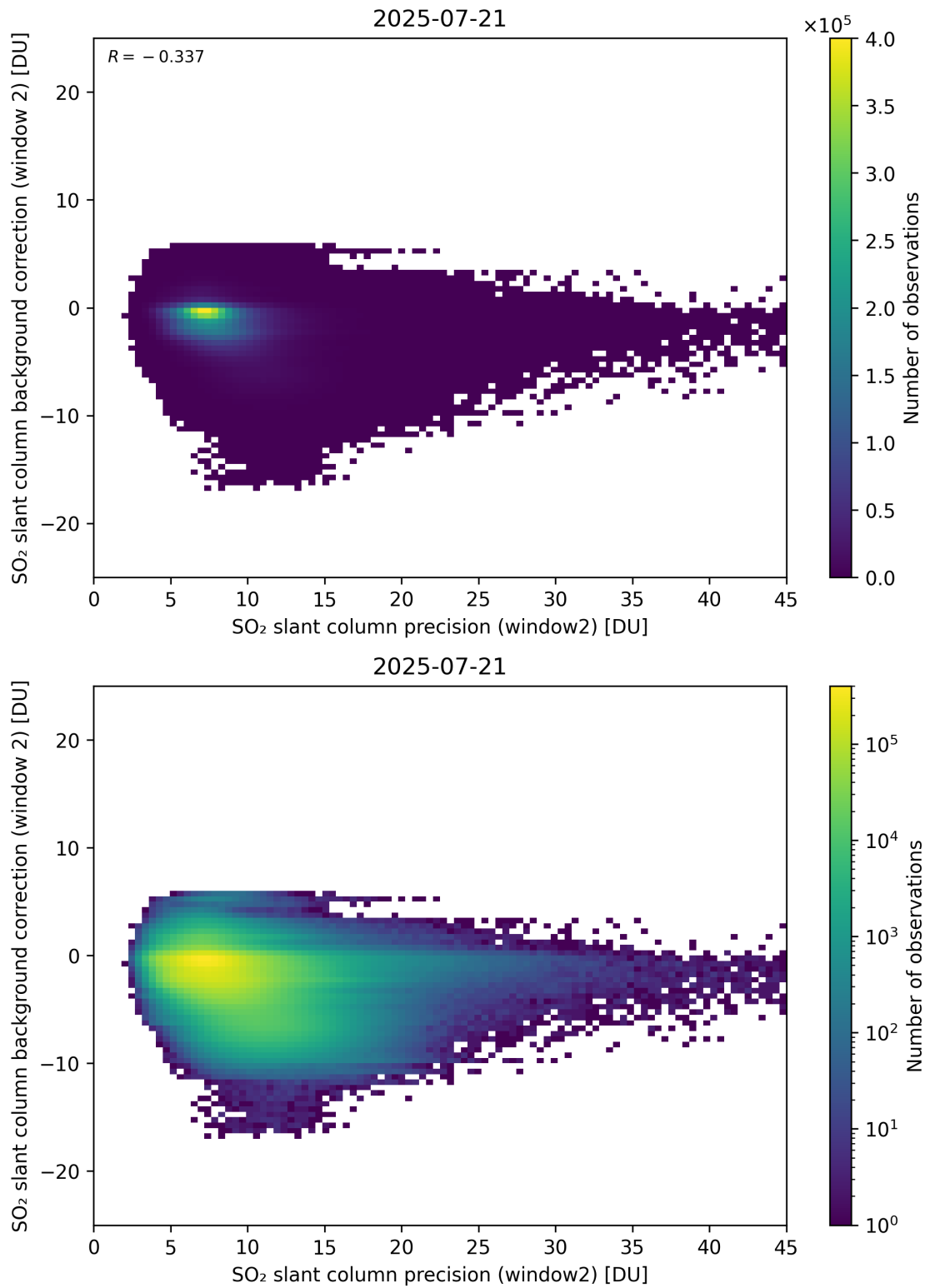
Figure 291: Scatter density plot of “SO 2 slant column precision (window2)” against “SO 2 slant column background correction (window 2)” for 2025-07-20 to 2025-07-22.
