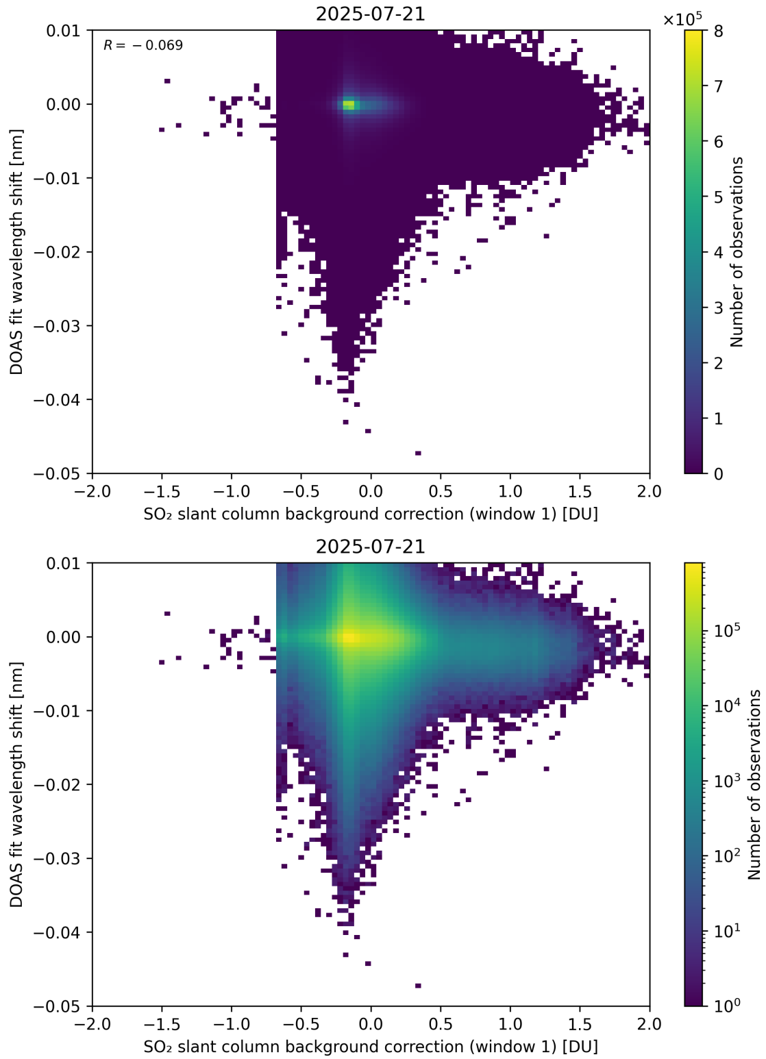
Figure 111: Scatter density plot of “SO 2 slant column background correction (window 1)” against “DOAS fit wavelength shift” for 2025-07-20 to 2025-07-22.
