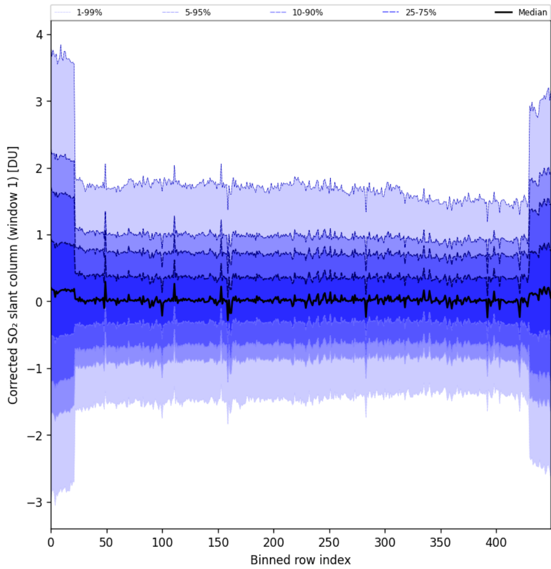
Figure 91: Along track statistics of “Corrected SO 2 slant column (window 1)” for 2025-07-20 to 2025-07-22
