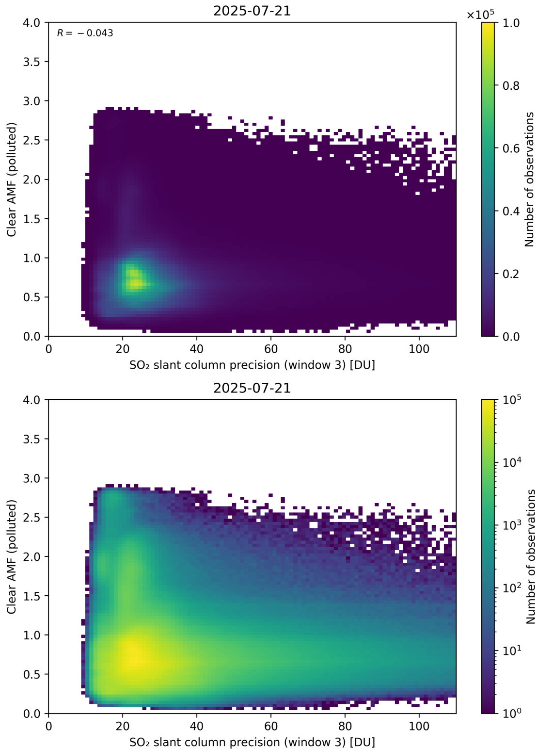
Figure 311: Scatter density plot of “SO 2 slant column precision (window 3)” against “Clear AMF (polluted)” for 2025-07-20 to 2025-07-22.
