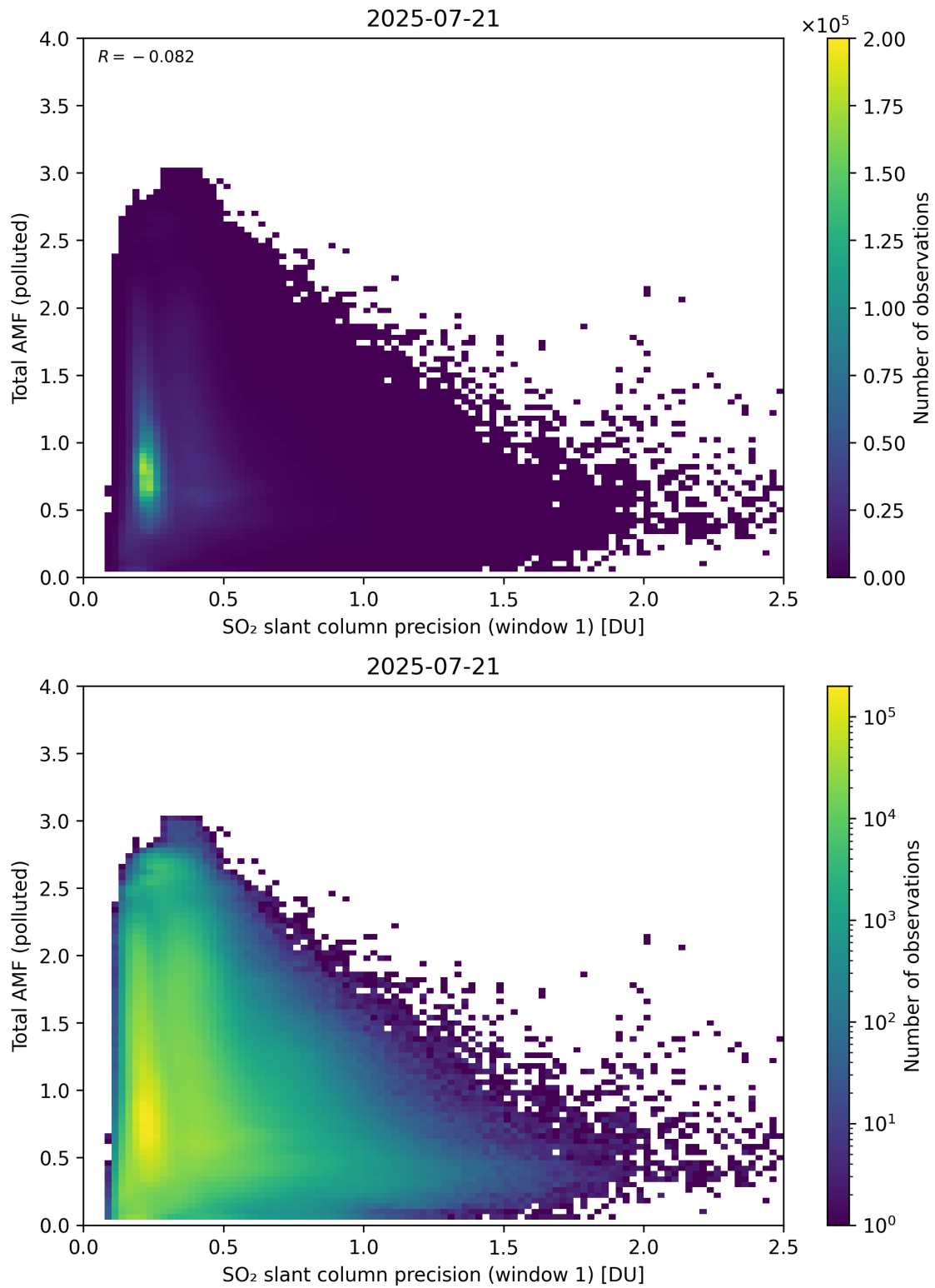
Figure 280: Scatter density plot of “SO 2 slant column precision (window 1)” against “Total AMF (polluted)” for 2025-07-20 to 2025-07-22.
