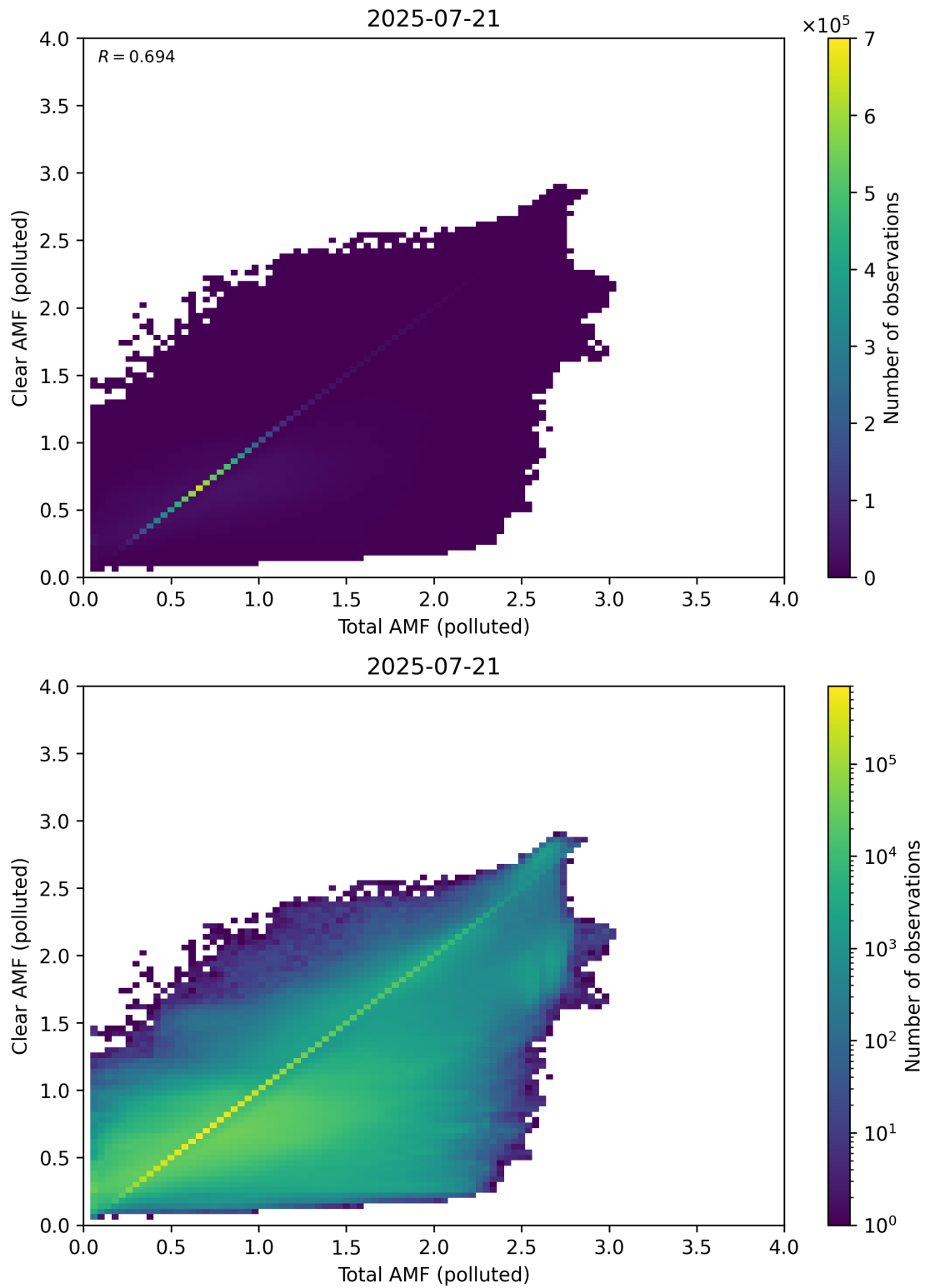
Figure 321: Scatter density plot of “Total AMF (polluted)” against “Clear AMF (polluted)” for 2025-07-20 to 2025-07-22.
