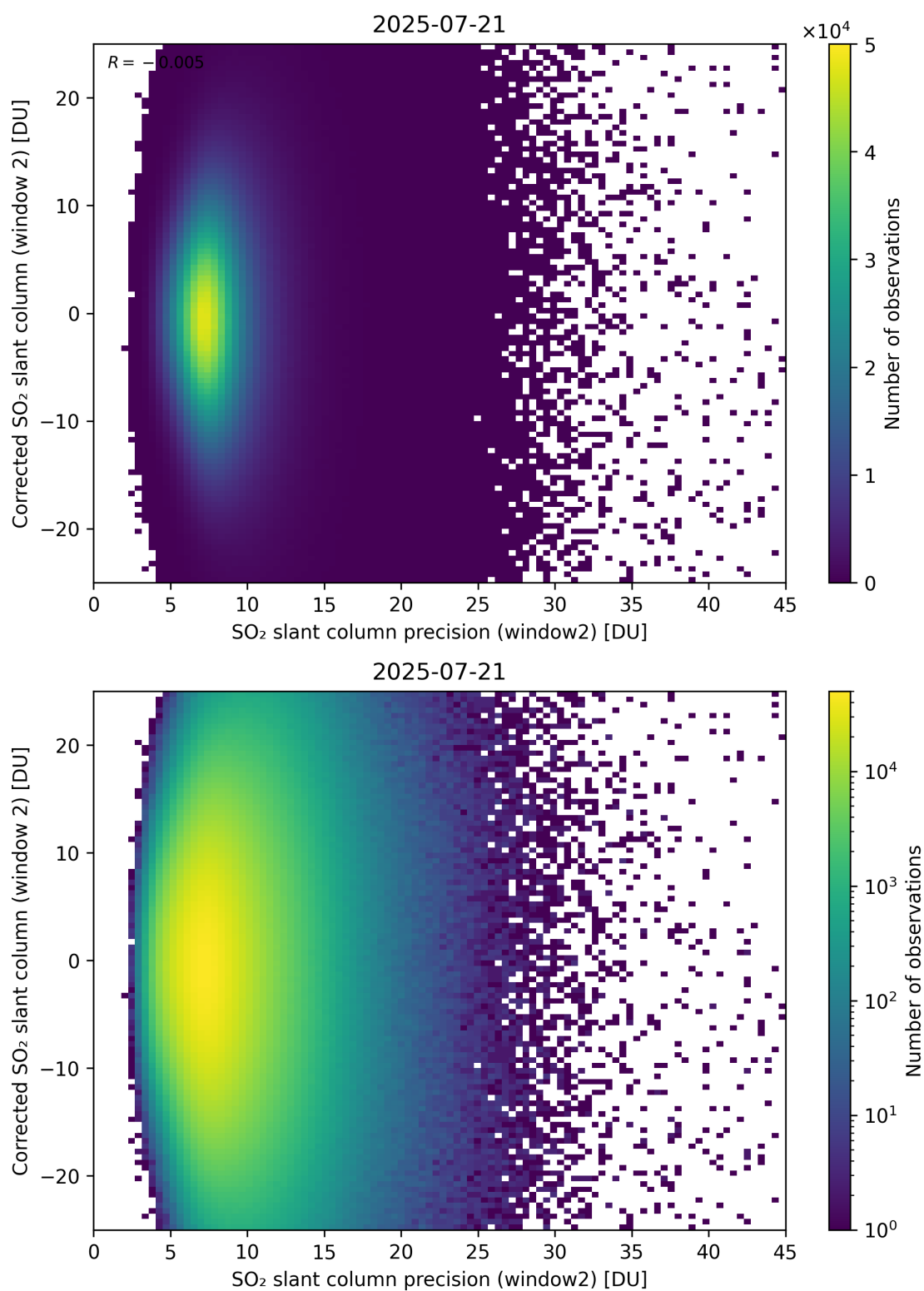
Figure 297: Scatter density plot of “SO 2 slant column precision (window2)” against “Corrected SO 2 slant column (window 2)” for 2025-07-20 to 2025-07-22.
