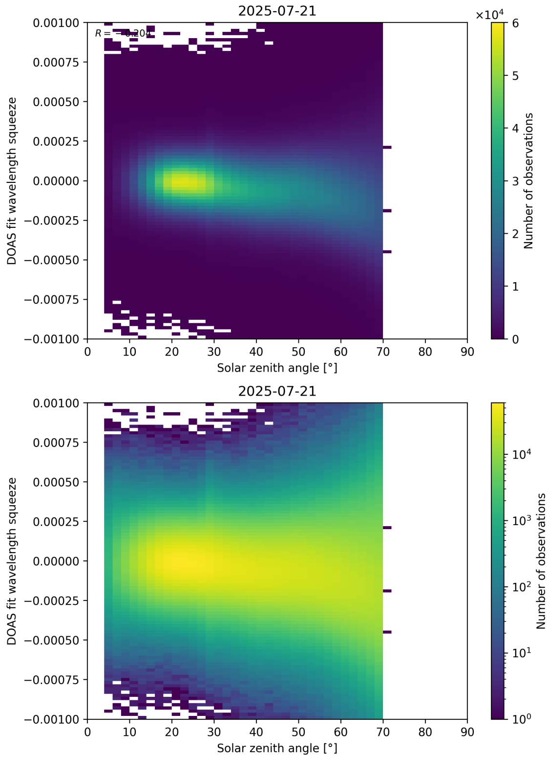
Figure 175: Scatter density plot of “Solar zenith angle” against “DOAS fit wavelength squeeze” for 2025-07-20 to 2025-07-22.
