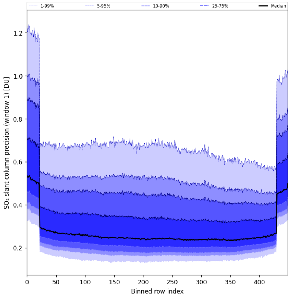
Figure 90: Along track statistics of “SO 2 slant column precision (window 1)” for 2025-07-20 to 2025-07-22
