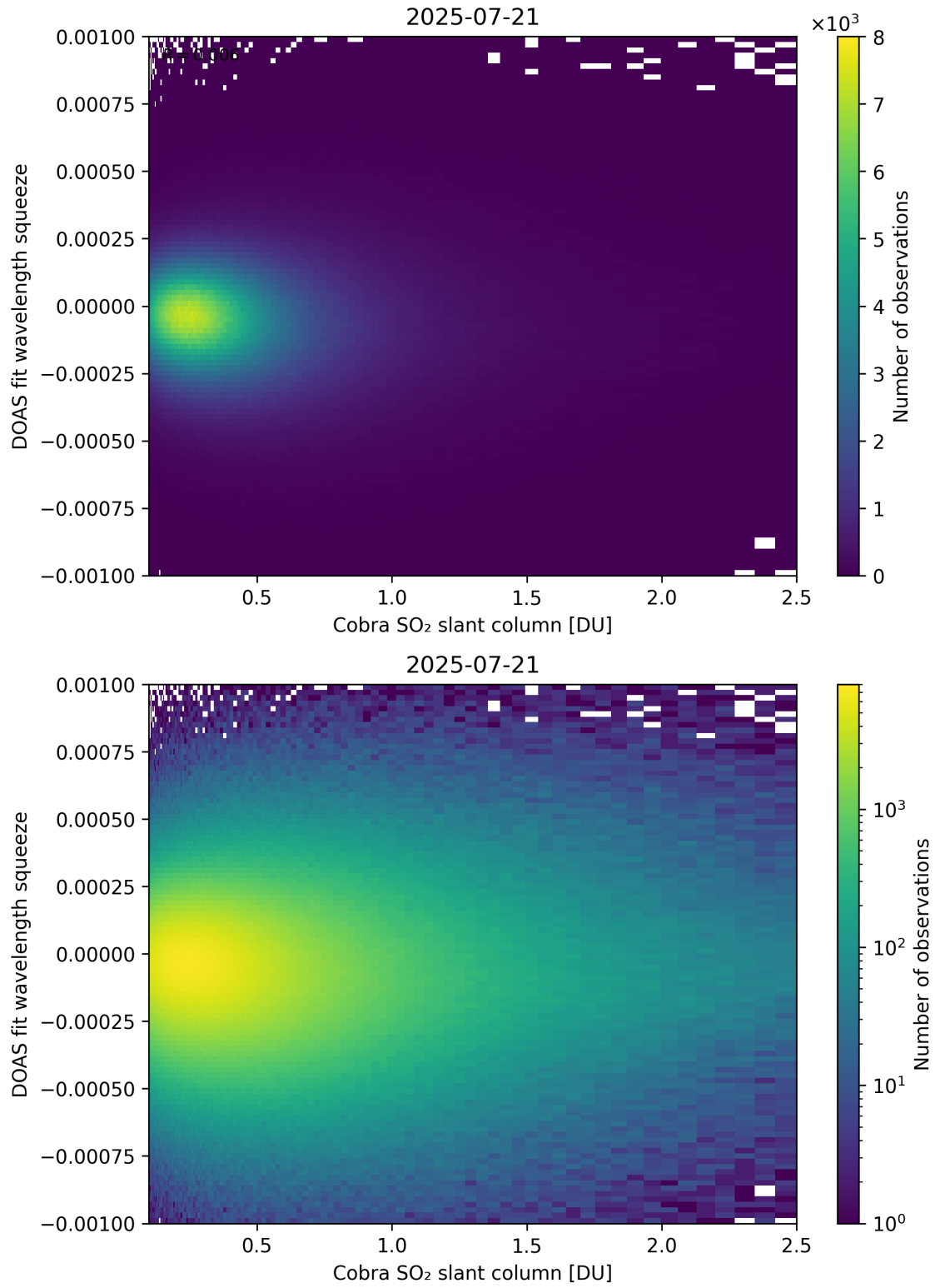
Figure 197: Scatter density plot of “Cobra SO 2 slant column” against “DOAS fit wavelength squeeze” for 2025-07-20 to 2025-07-22.
