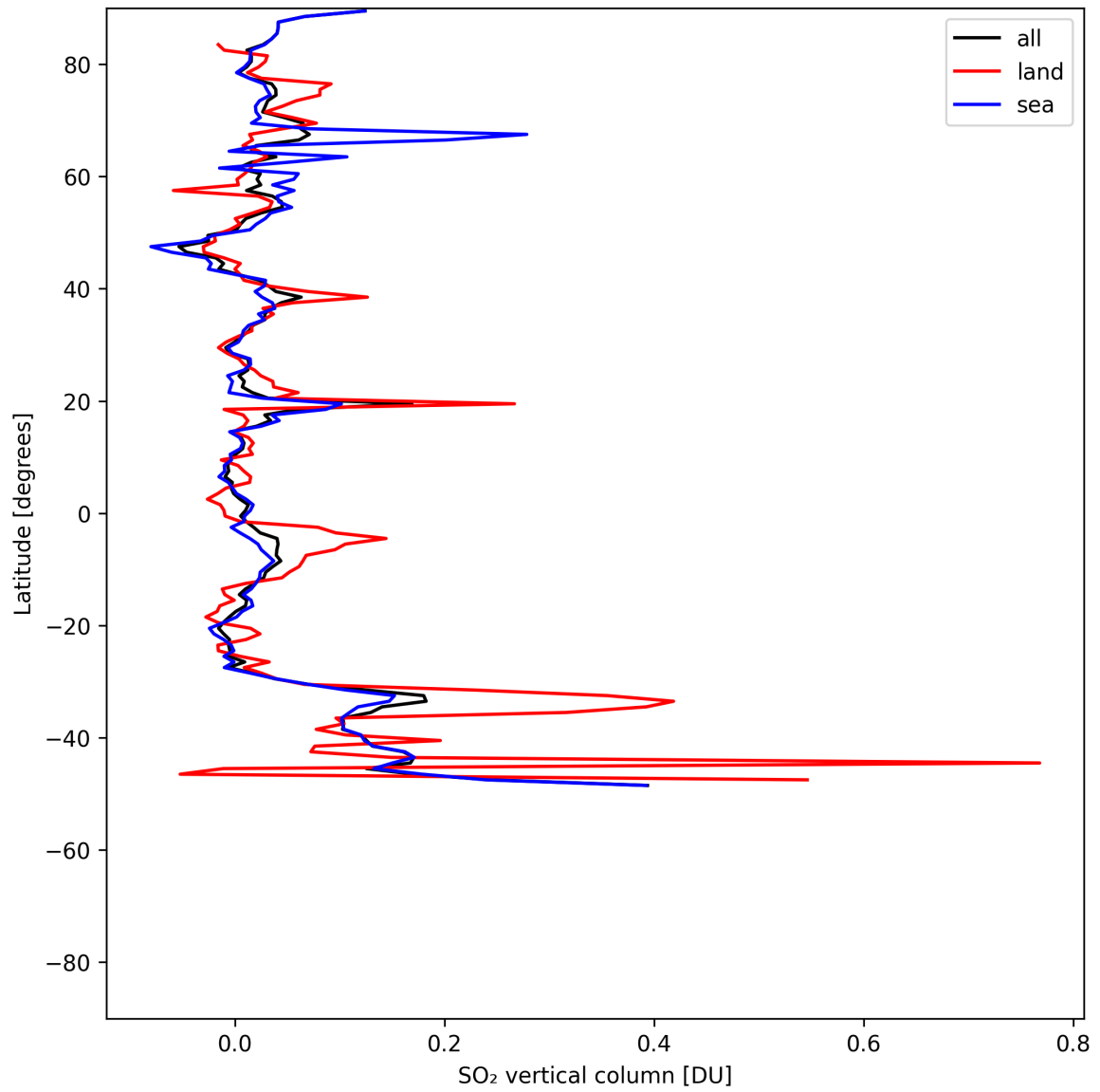
Figure 32: Zonal average of “SO 2 vertical column” for 2025-07-20 to 2025-07-22.
