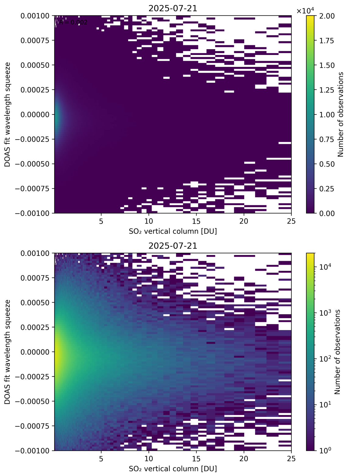
Figure 327: Scatter density plot of “SO 2 vertical column” against “DOAS fit wavelength squeeze” for 2025-07-20 to 2025-07-22.
