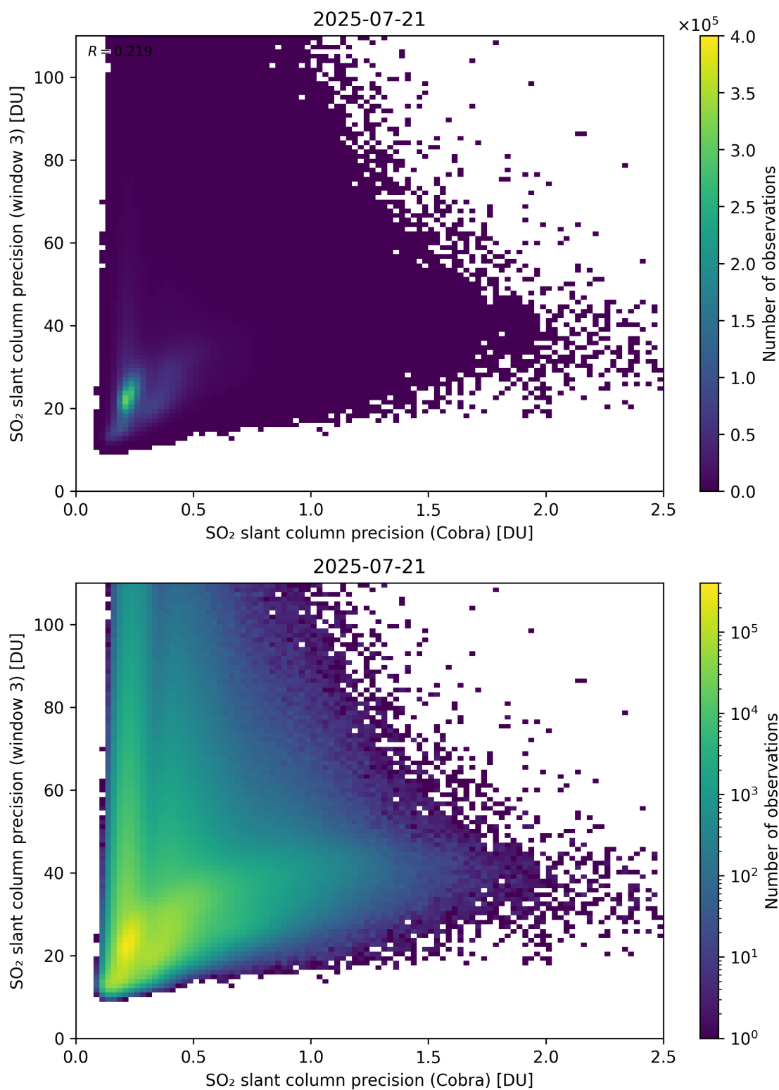
Figure 212: Scatter density plot of “SO 2 slant column precision (Cobra)” against “SO 2 slant column precision (window 3)” for 2025-07-20 to 2025-07-22.
