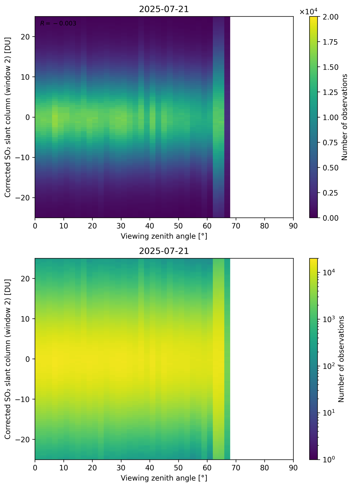
Figure 374: Scatter density plot of “Viewing zenith angle” against “Corrected SO 2 slant column (window 2)” for 2025-07-20 to 2025-07-22.
