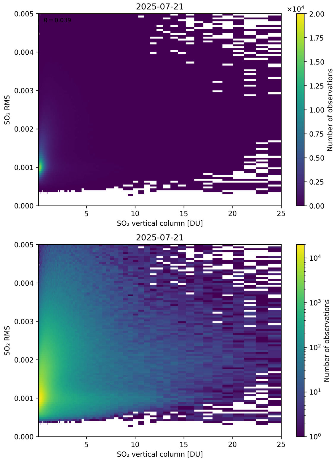
Figure 328: Scatter density plot of “SO 2 vertical column” against “SO 2 RMS” for 2025-07-20 to 2025-07-22.
