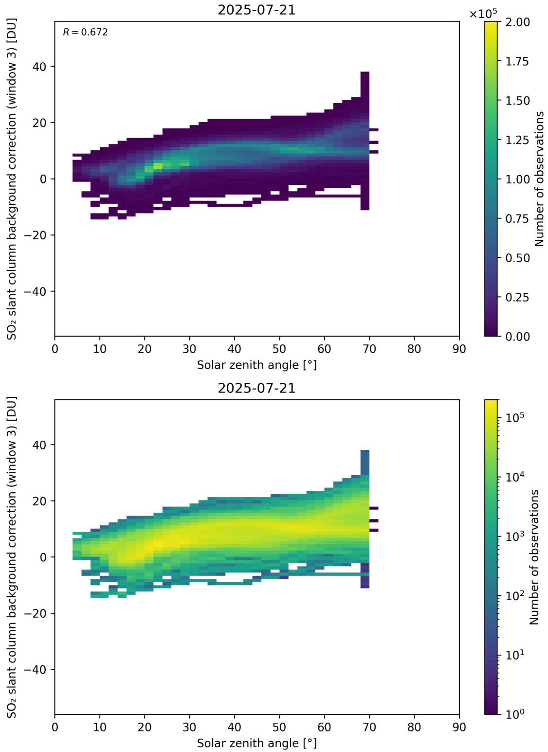
Figure 173: Scatter density plot of “Solar zenith angle” against “SO 2 slant column background correction (window 3)” for 2025-07-20 to 2025-07-22.
