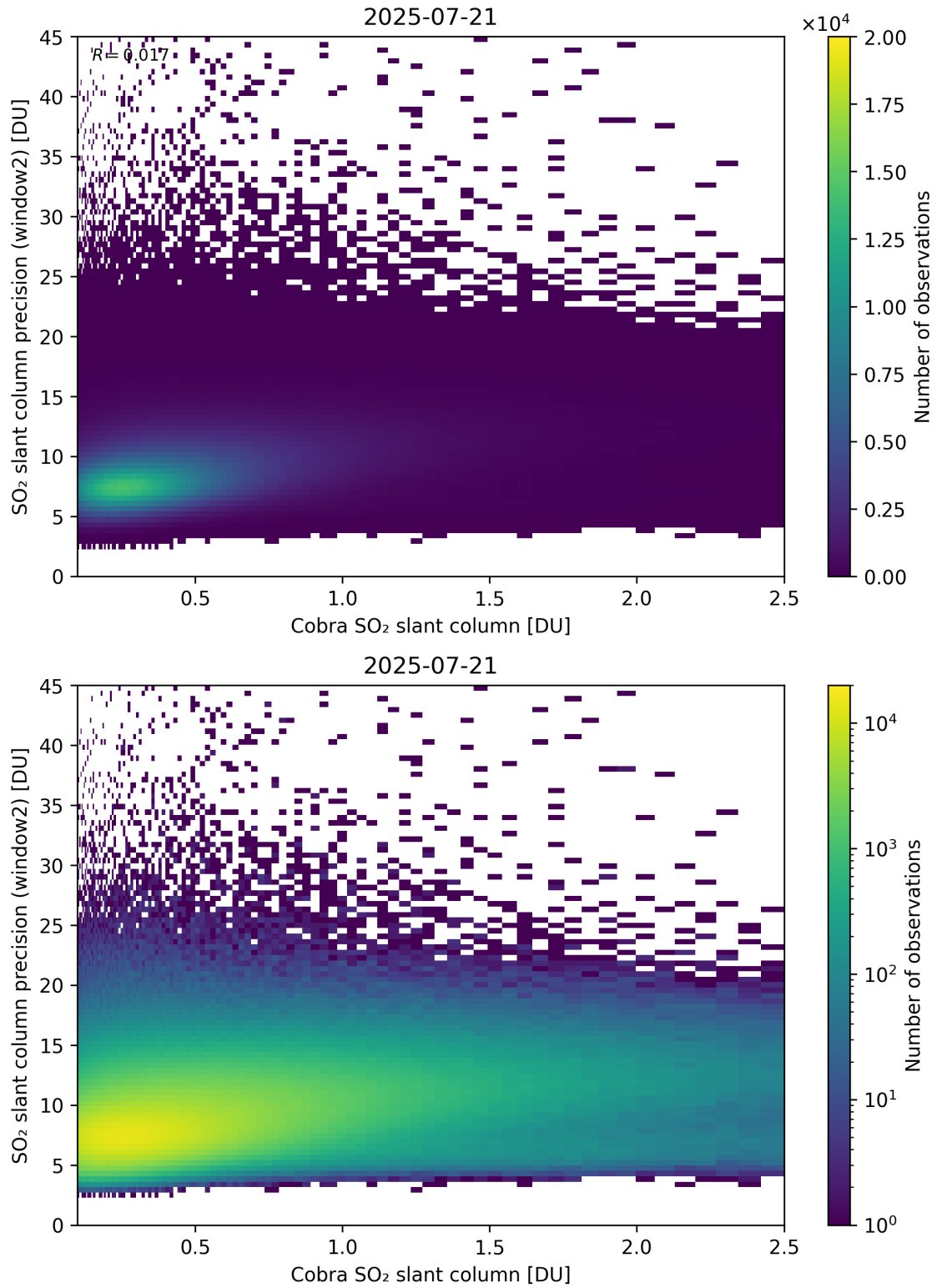
Figure 221: Scatter density plot of “Cobra SO 2 slant column” against “SO 2 slant column precision (window2)” for 2025-07-20 to 2025-07-22.
