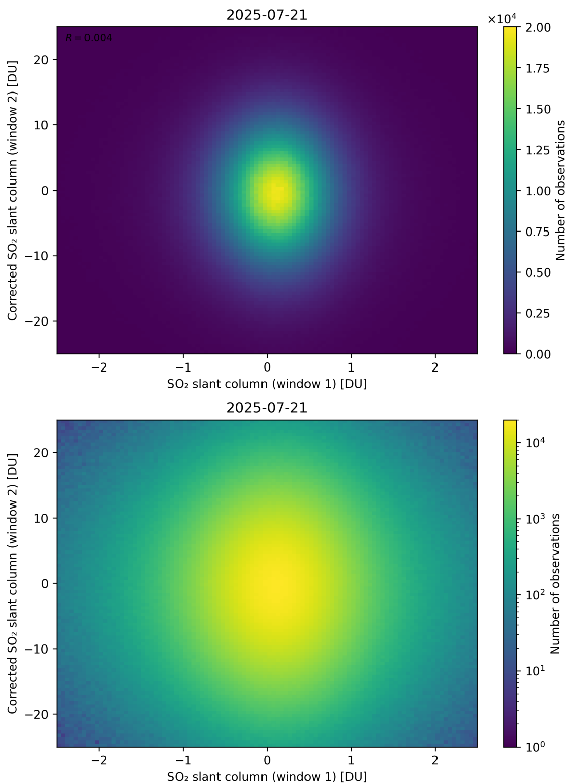
Figure 283: Scatter density plot of “SO 2 slant column (window 1)” against “Corrected SO 2 slant column (window 2)” for 2025-07-20 to 2025-07-22.
