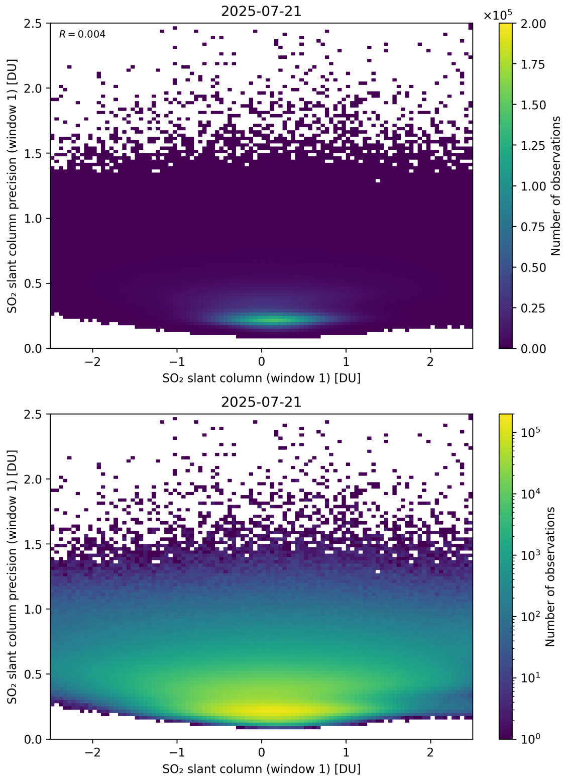
Figure 285: Scatter density plot of “SO 2 slant column (window 1)” against “SO 2 slant column precision (window 1)” for 2025-07-20 to 2025-07-22.
