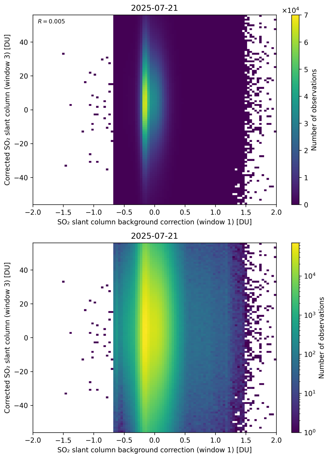
Figure 116: Scatter density plot of “SO 2 slant column background correction (window 1)” against “Corrected SO 2 slant column (window 3)” for 2025-07-20 to 2025-07-22.
