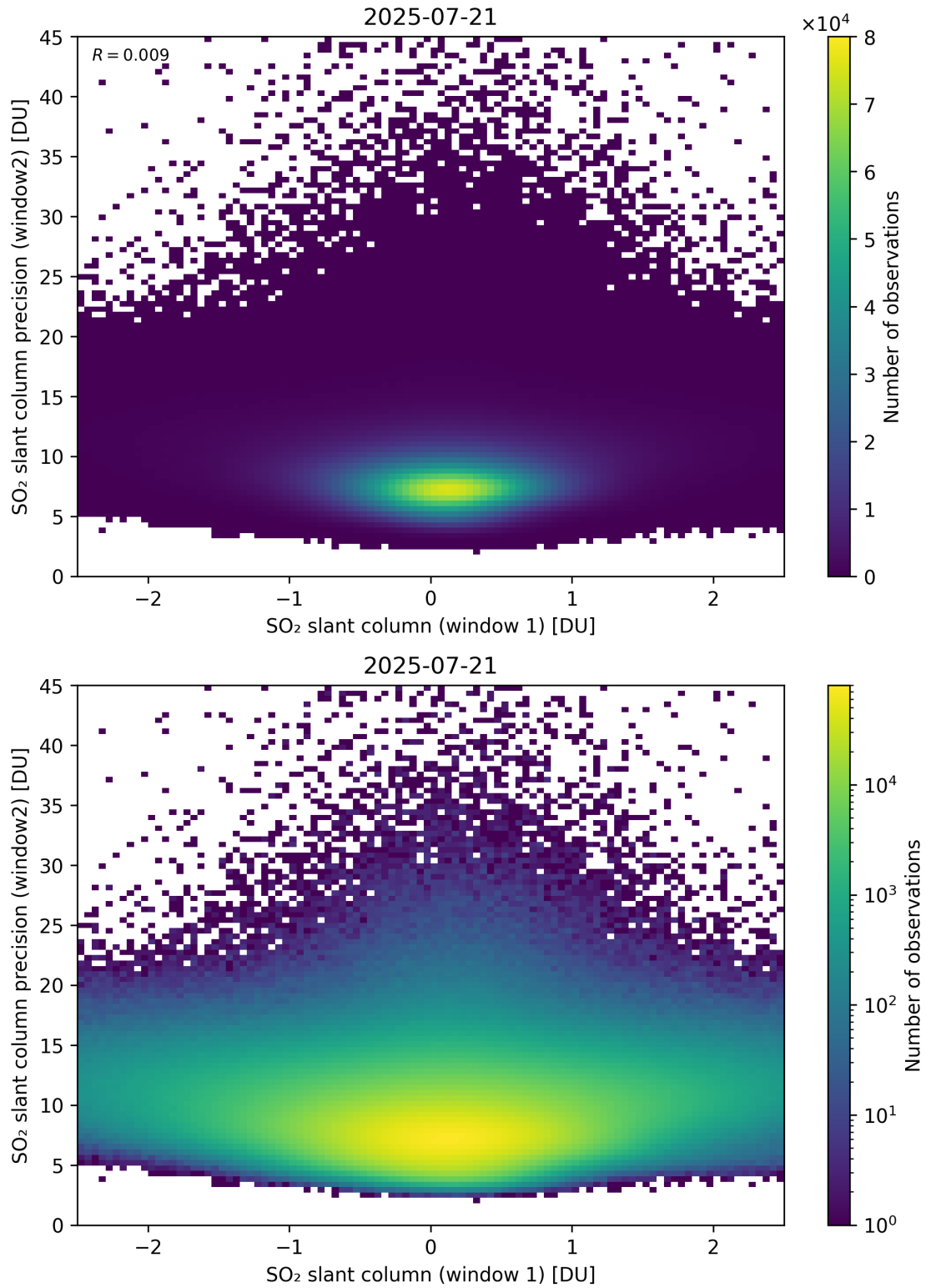
Figure 286: Scatter density plot of “SO 2 slant column (window 1)” against “SO 2 slant column precision (window2)” for 2025-07-20 to 2025-07-22.
