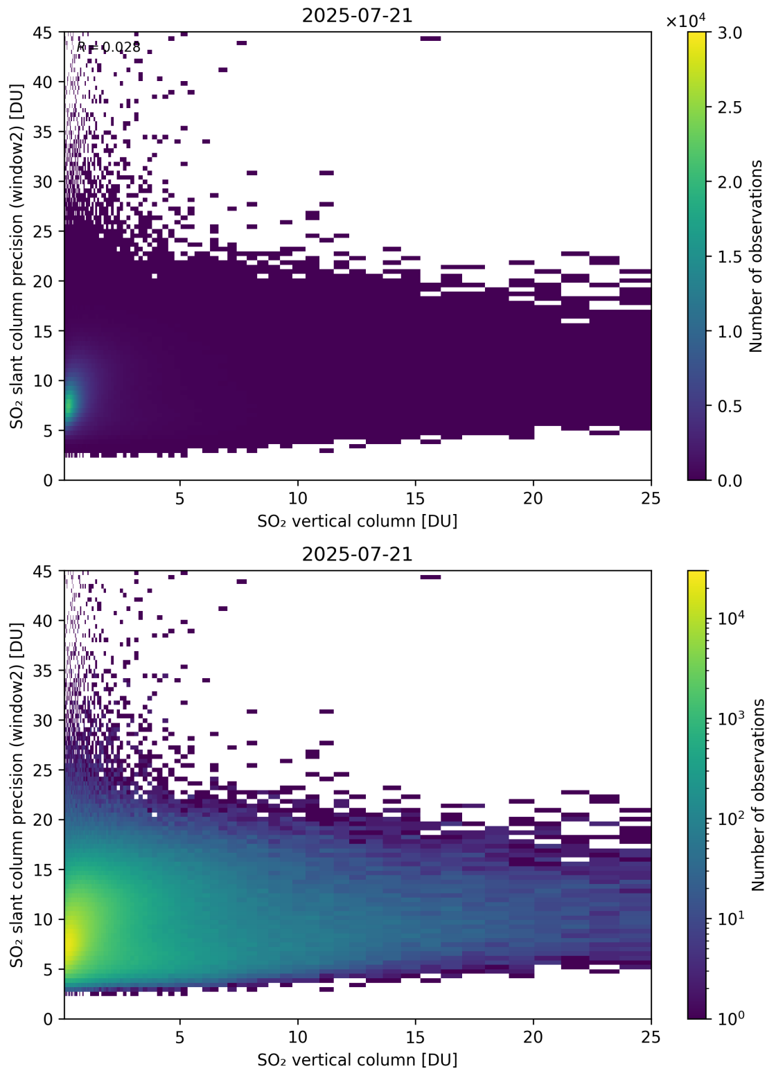
Figure 356: Scatter density plot of “SO 2 vertical column” against “SO 2 slant column precision (window2)” for 2025-07-20 to 2025-07-22.
