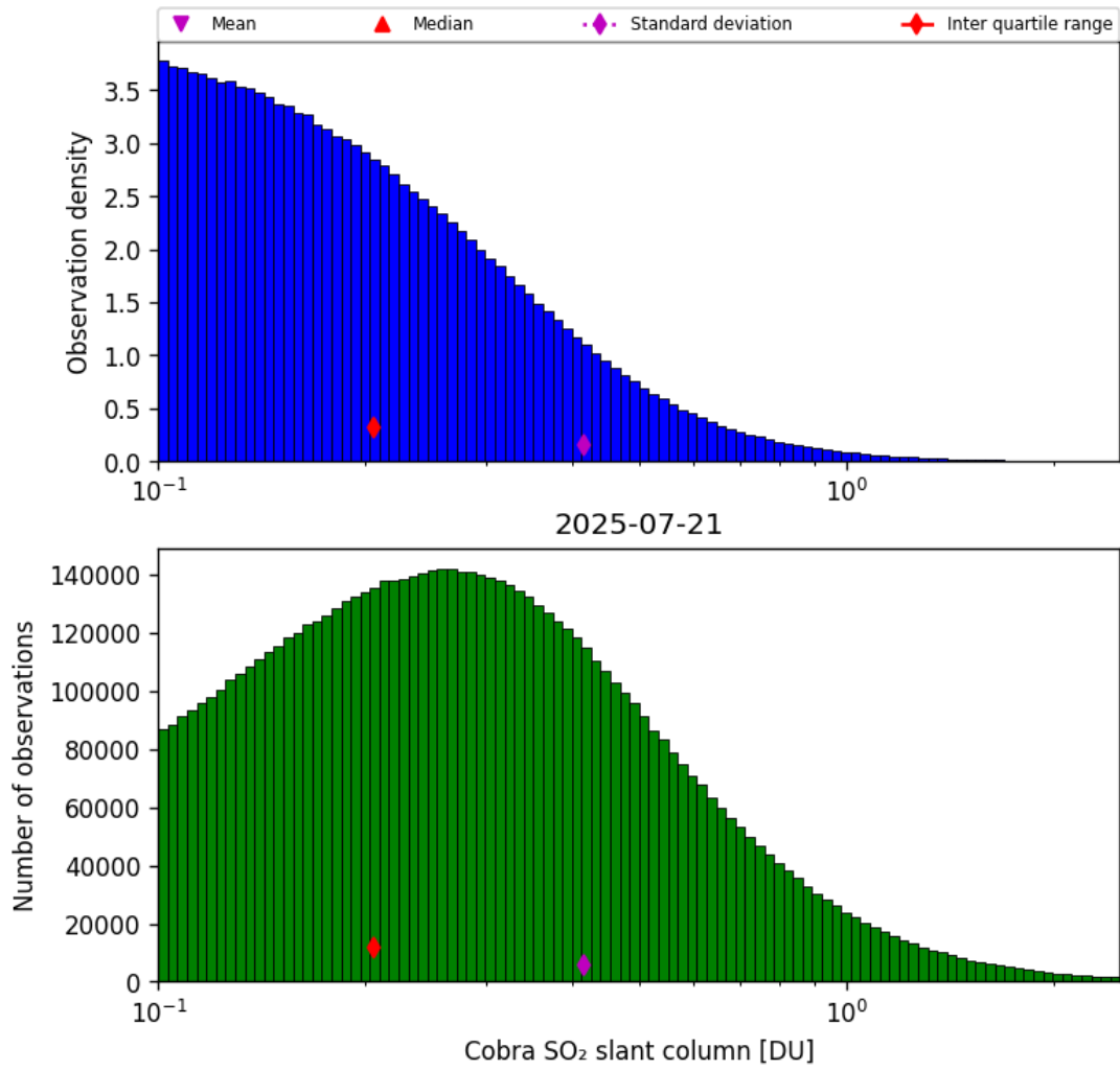
Figure 61: Histogram of “Cobra SO 2 slant column” for 2025-07-20 to 2025-07-22
