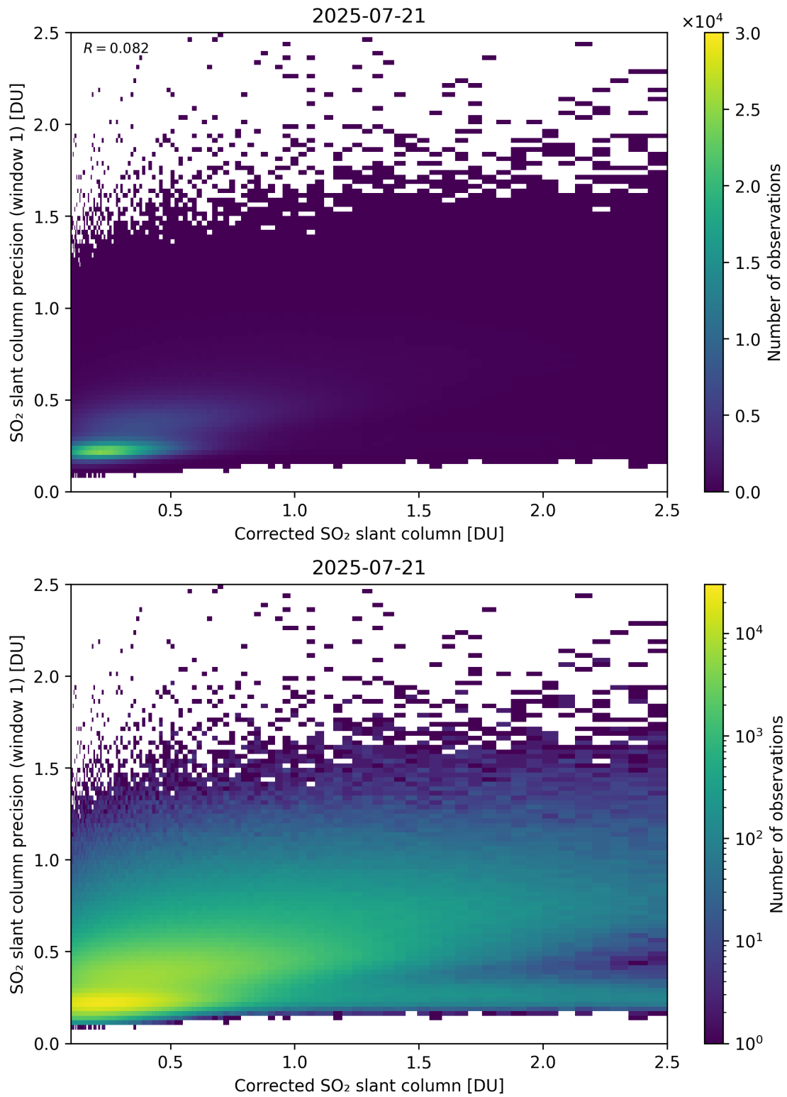
Figure 238: Scatter density plot of “Corrected SO 2 slant column” against “SO 2 slant column precision (window 1)” for 2025-07-20 to 2025-07-22.
