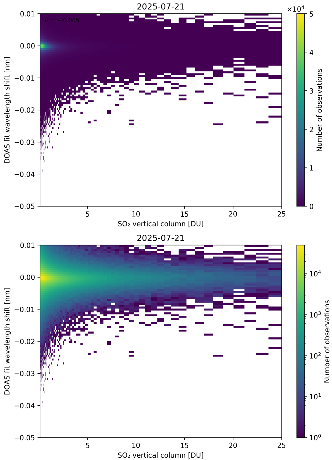
Figure 326: Scatter density plot of “SO 2 vertical column” against “DOAS fit wavelength shift” for 2025-07-20 to 2025-07-22.
