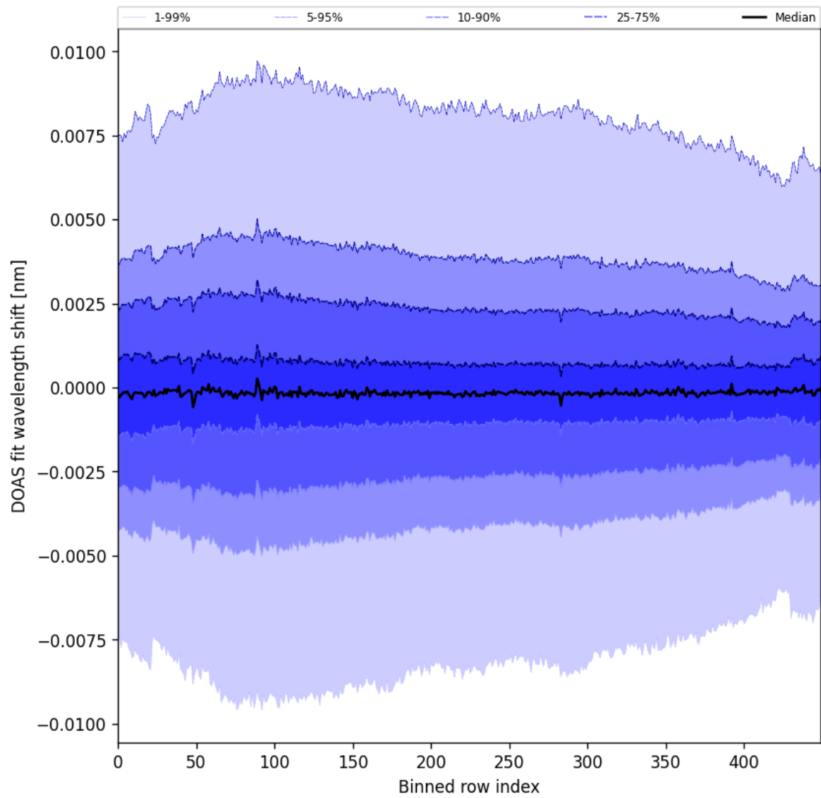
Figure 102: Along track statistics of “DOAS fit wavelength shift” for 2025-07-20 to 2025-07-22
