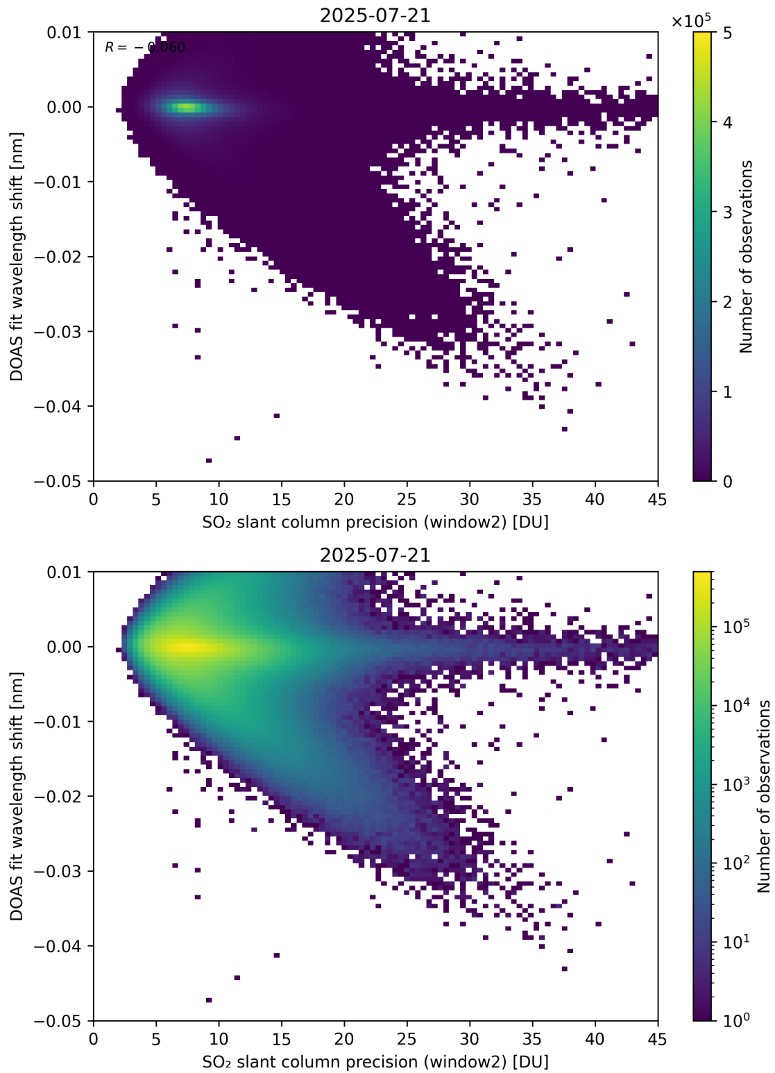
Figure 293: Scatter density plot of “SO 2 slant column precision (window2)” against “DOAS fit wavelength shift” for 2025-07-20 to 2025-07-22.
