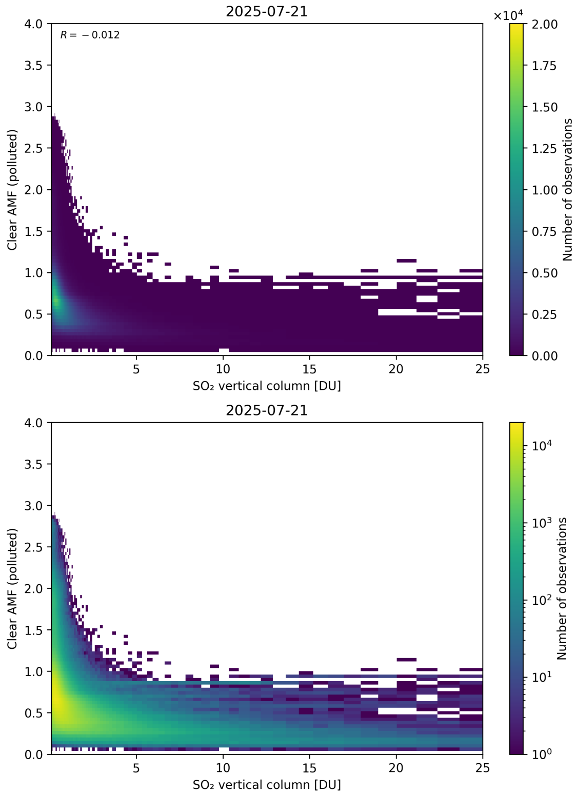
Figure 348: Scatter density plot of “SO 2 vertical column” against “Clear AMF (polluted)” for 2025-07-20 to 2025-07-22.
