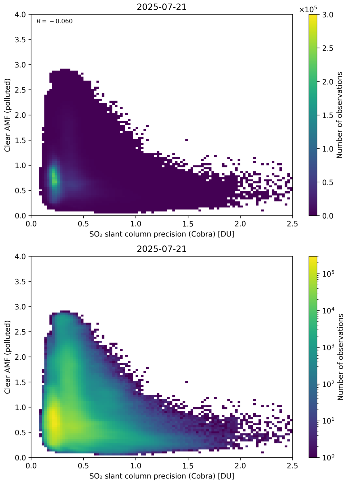
Figure 205: Scatter density plot of “SO 2 slant column precision (Cobra)” against “Clear AMF (polluted)” for 2025-07-20 to 2025-07-22.
