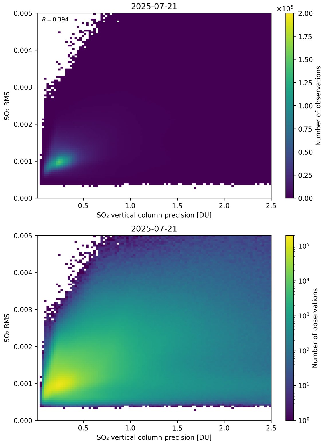
Figure 334: Scatter density plot of “SO 2 vertical column precision” against “SO 2 RMS” for 2025-07-20 to 2025-07-22.
