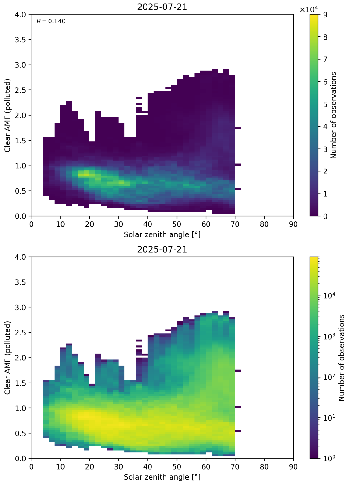
Figure 178: Scatter density plot of “Solar zenith angle” against “Clear AMF (polluted)” for 2025-07-20 to 2025-07-22.
