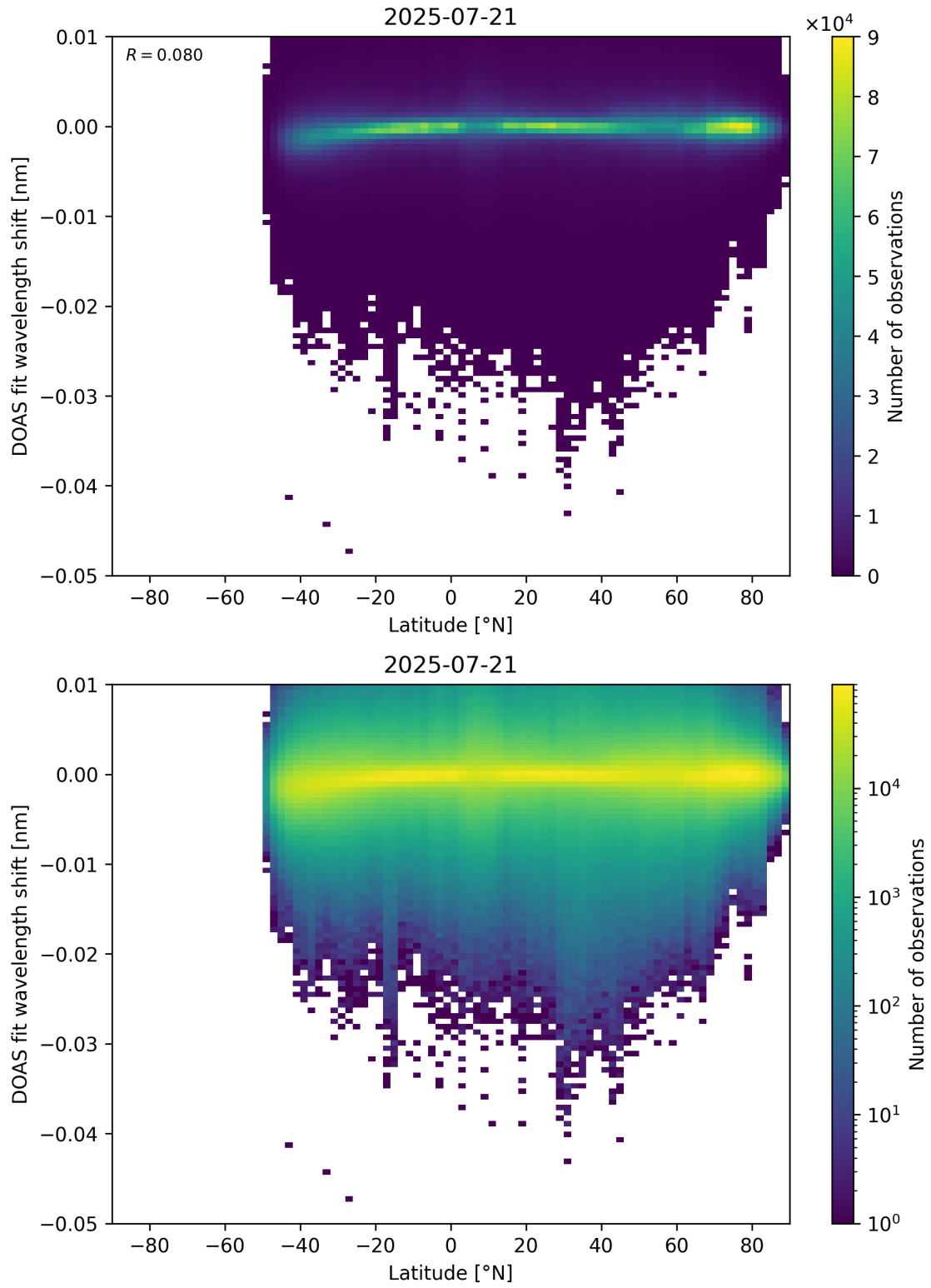
Figure 153: Scatter density plot of “Latitude” against “DOAS fit wavelength shift” for 2025-07-20 to 2025-07-22.
