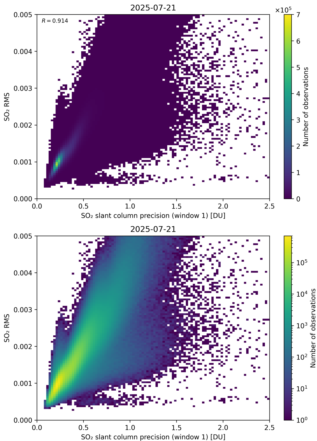
Figure 273: Scatter density plot of “SO 2 slant column precision (window 1)” against “SO 2 RMS” for 2025-07-20 to 2025-07-22.
