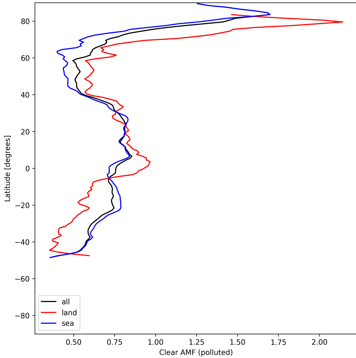
Figure 55: Zonal average of “Clear AMF (polluted)” for 2025-07-20 to 2025-07-22.
