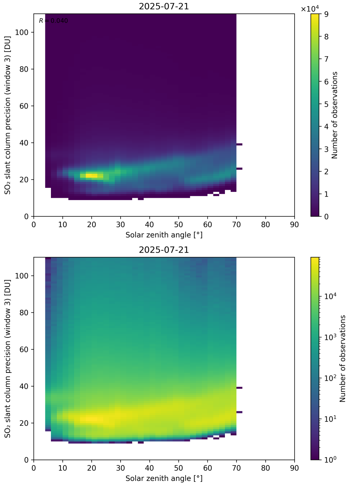
Figure 188: Scatter density plot of “Solar zenith angle” against “SO 2 slant column precision (window 3)” for 2025-07-20 to 2025-07-22.
