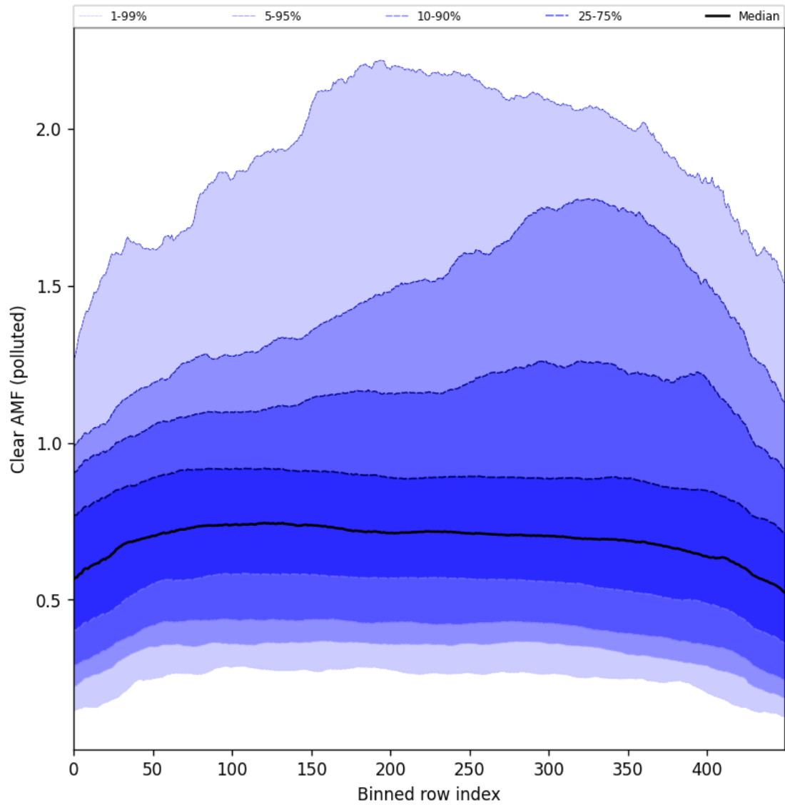
Figure 107: Along track statistics of “Clear AMF (polluted)” for 2025-07-20 to 2025-07-22
