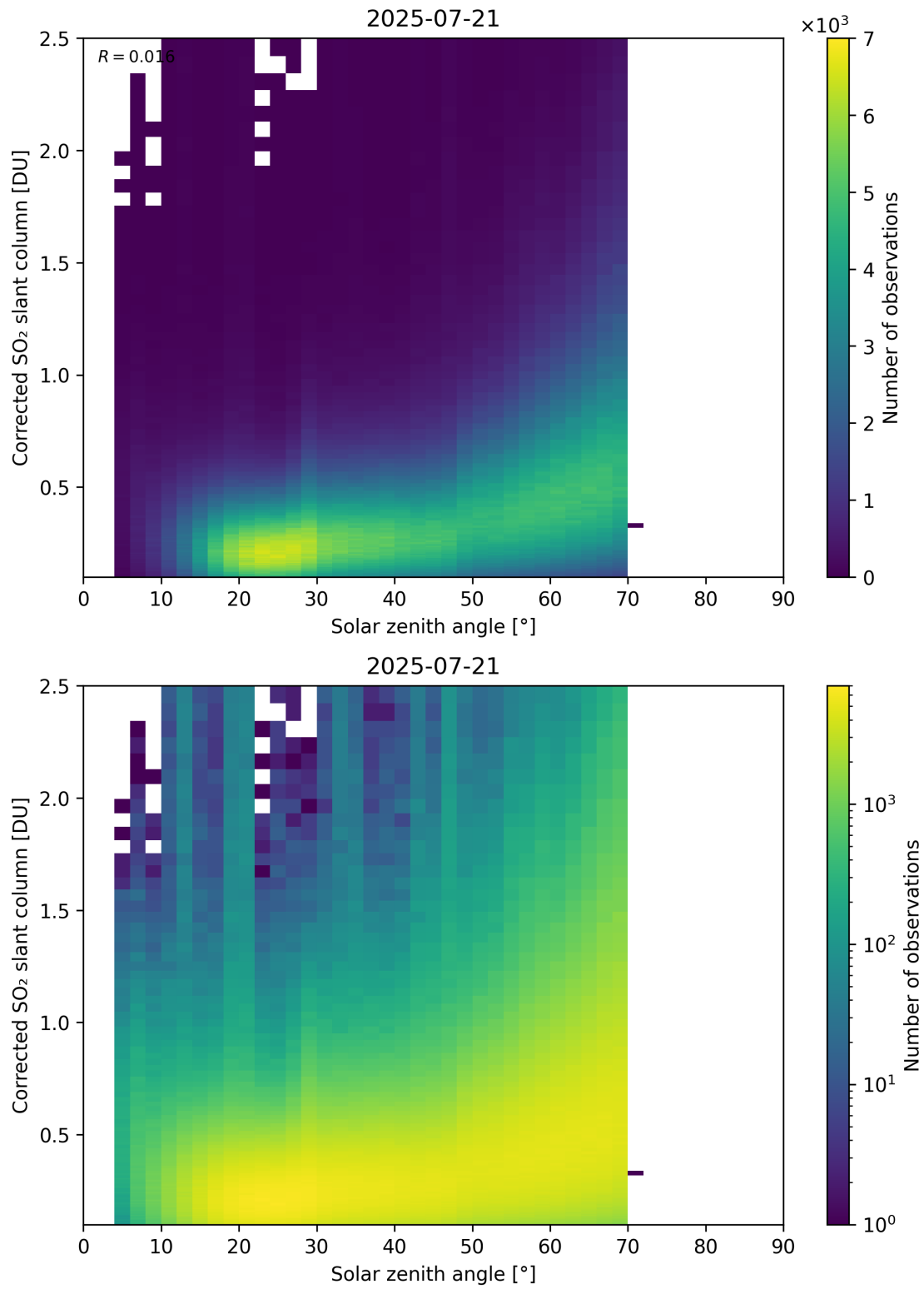
Figure 181: Scatter density plot of “Solar zenith angle” against “Corrected SO 2 slant column” for 2025-07-20 to 2025-07-22.
