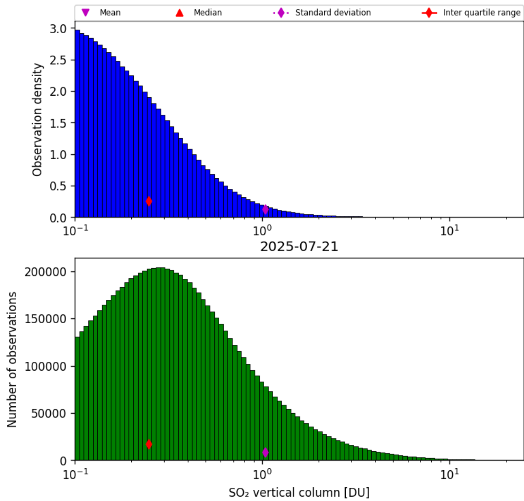
Figure 58: Histogram of “SO 2 vertical column” for 2025-07-20 to 2025-07-22
