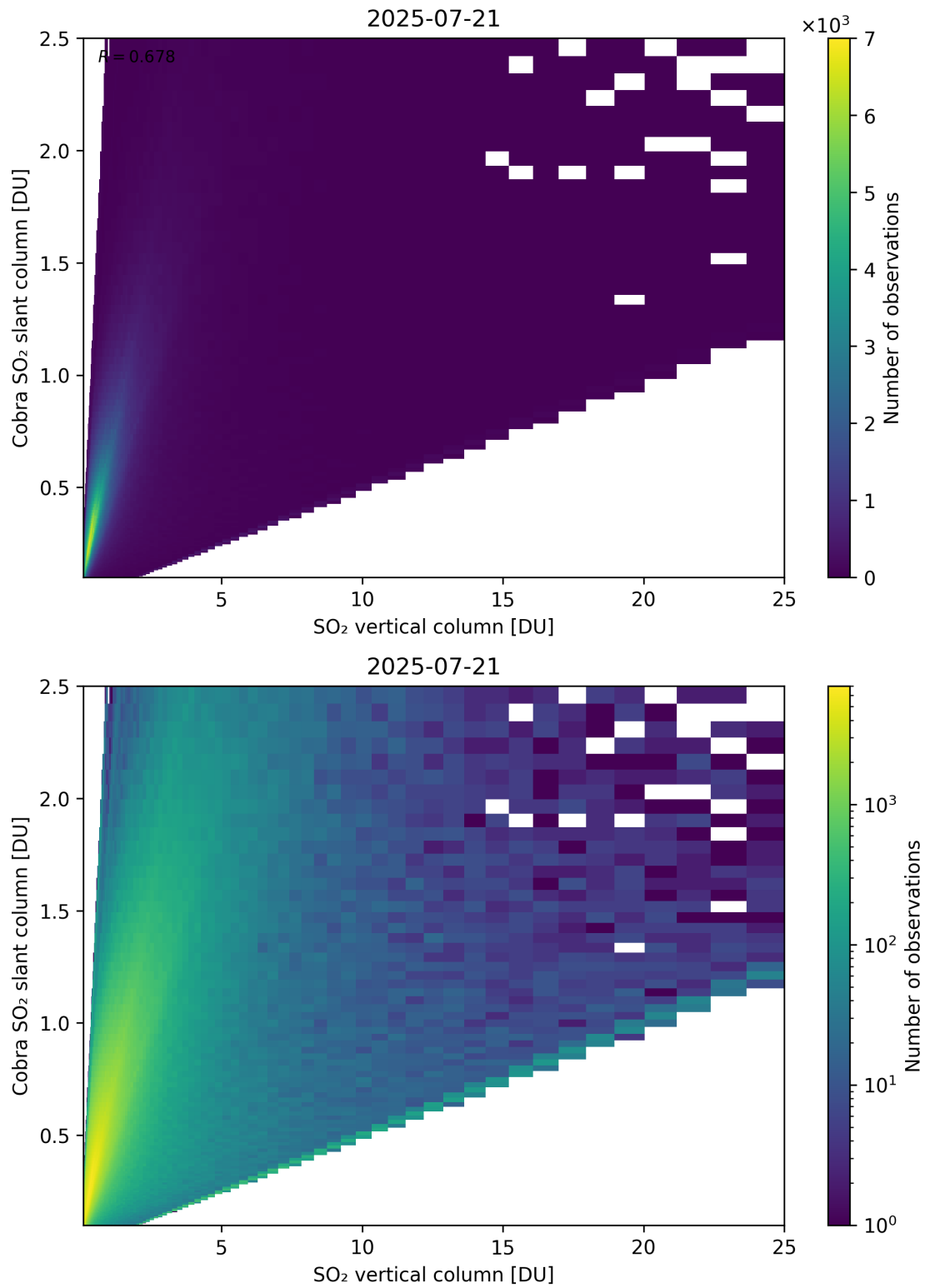
Figure 349: Scatter density plot of “SO 2 vertical column” against “Cobra SO 2 slant column” for 2025-07-20 to 2025-07-22.
