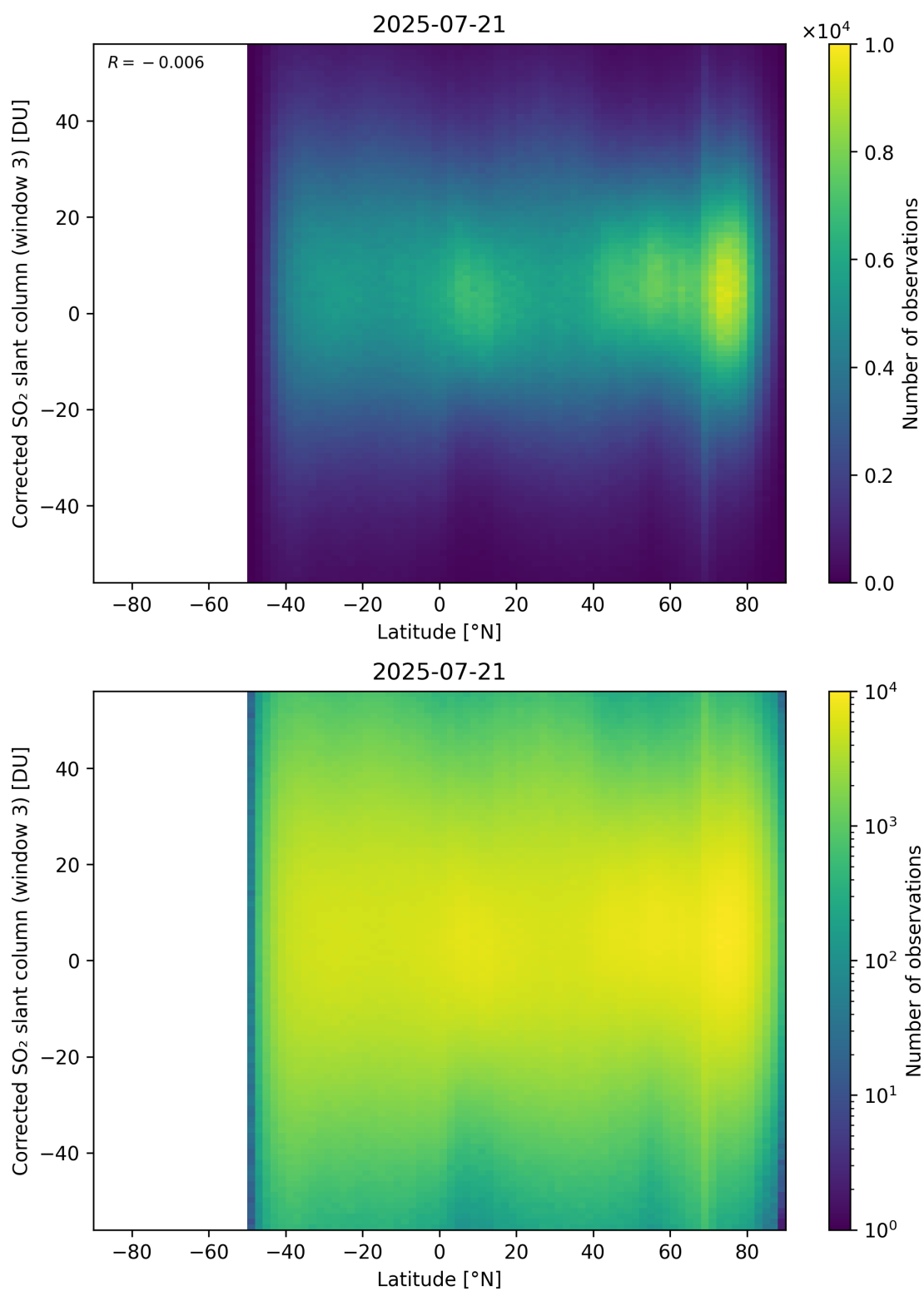
Figure 161: Scatter density plot of “Latitude” against “Corrected SO 2 slant column (window 3)” for 2025-07-20 to 2025-07-22.
