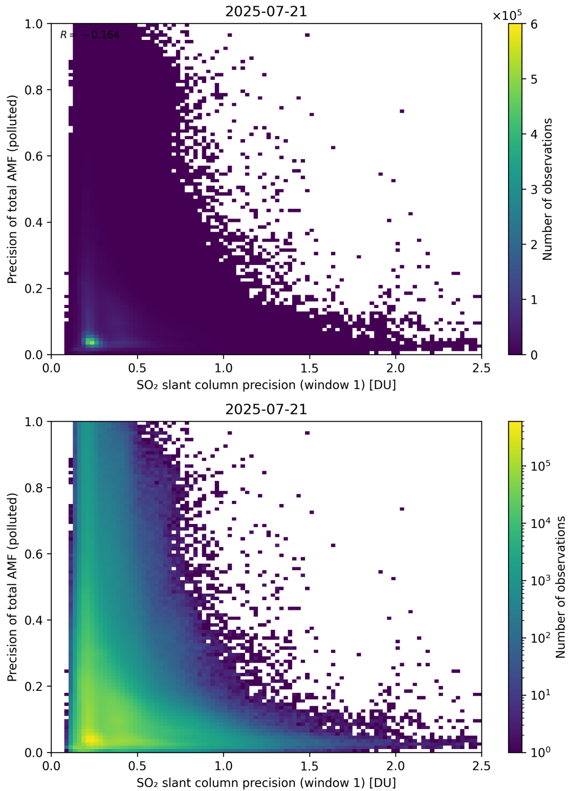
Figure 281: Scatter density plot of “SO 2 slant column precision (window 1)” against “Precision of total AMF (polluted)” for 2025-07-20 to 2025-07-22.
