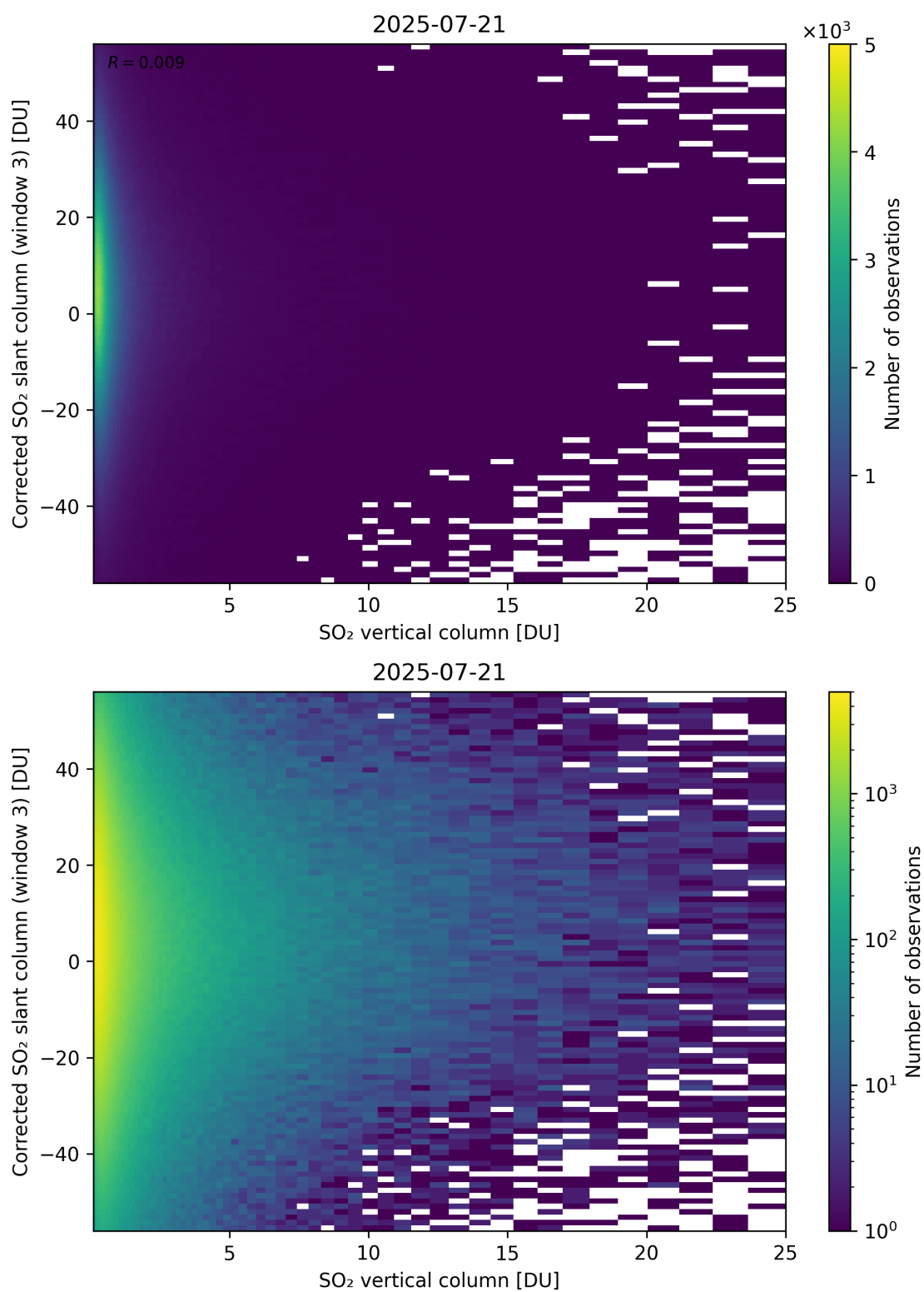
Figure 353: Scatter density plot of “SO 2 vertical column” against “Corrected SO 2 slant column (window 3)” for 2025-07-20 to 2025-07-22.
