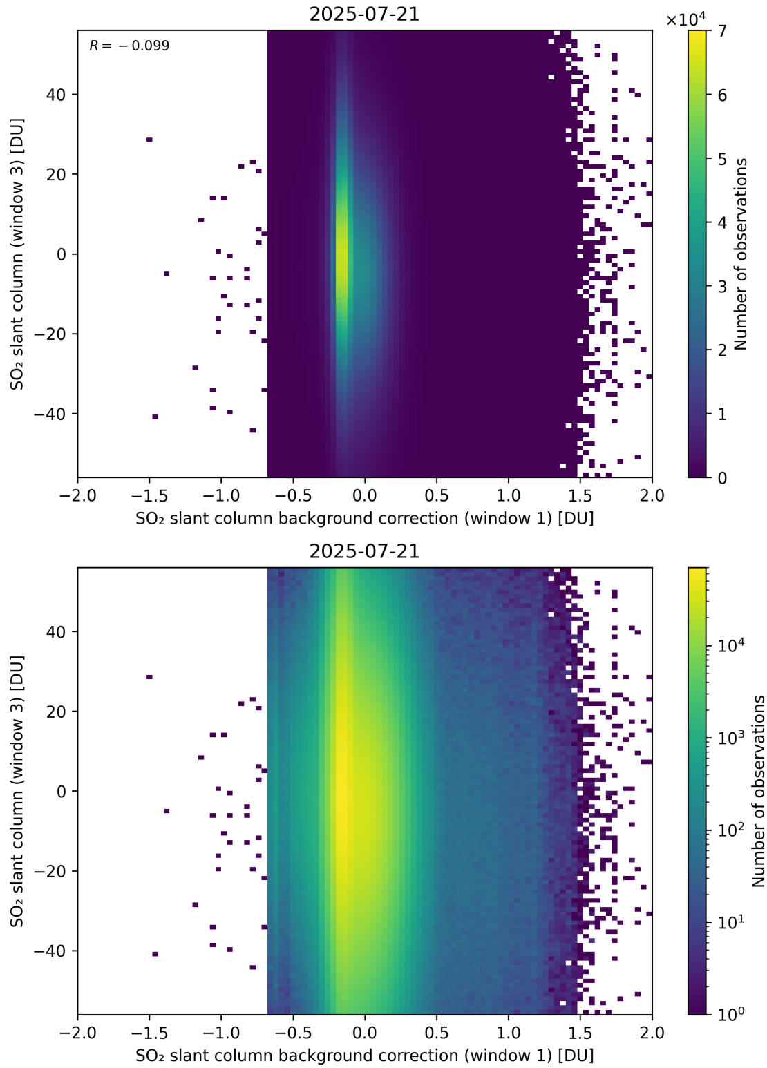
Figure 118: Scatter density plot of “SO 2 slant column background correction (window 1)” against “SO 2 slant column (window 3)” for 2025-07-20 to 2025-07-22.
