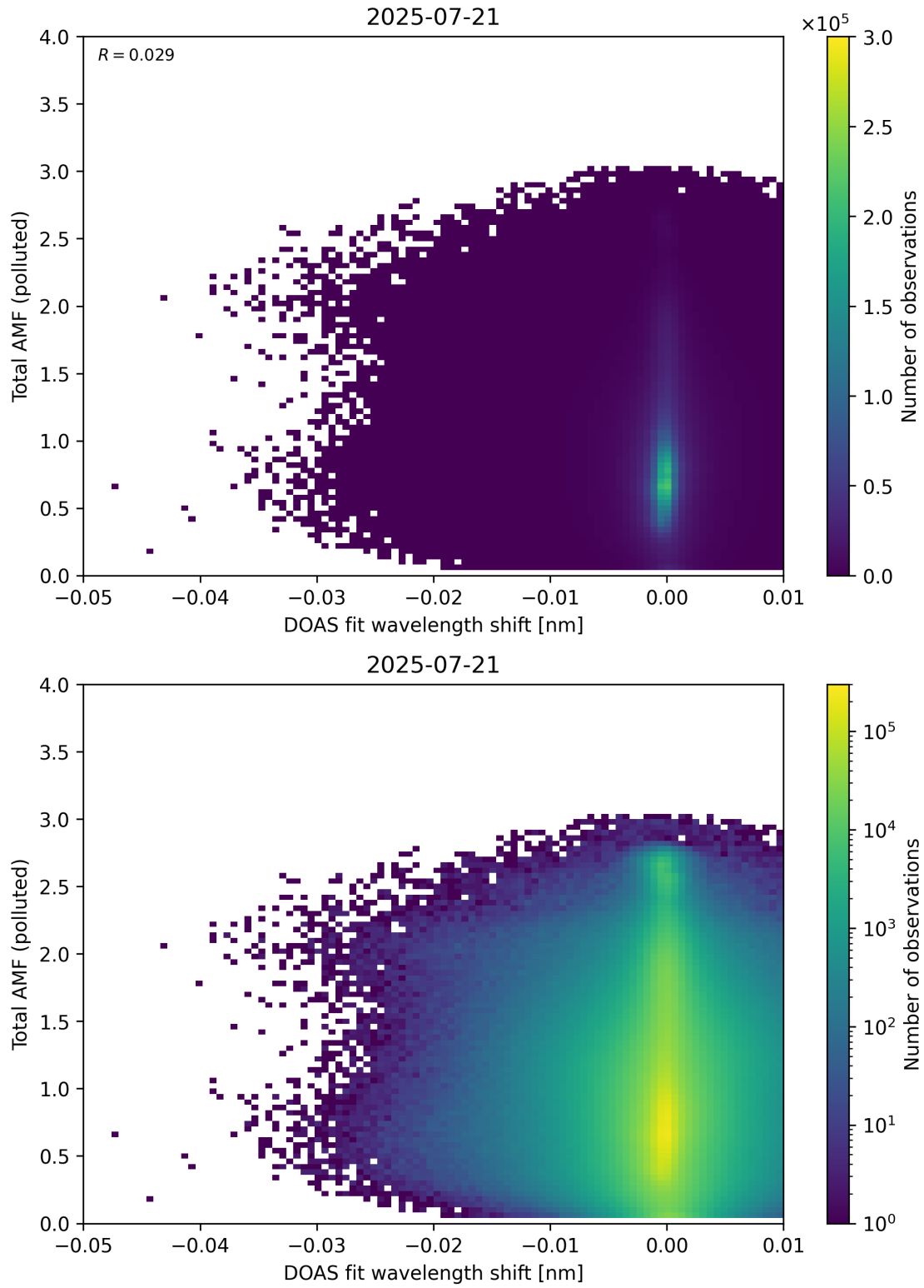
Figure 141: Scatter density plot of “DOAS fit wavelength shift” against “Total AMF (polluted)” for 2025-07-20 to 2025-07-22.
