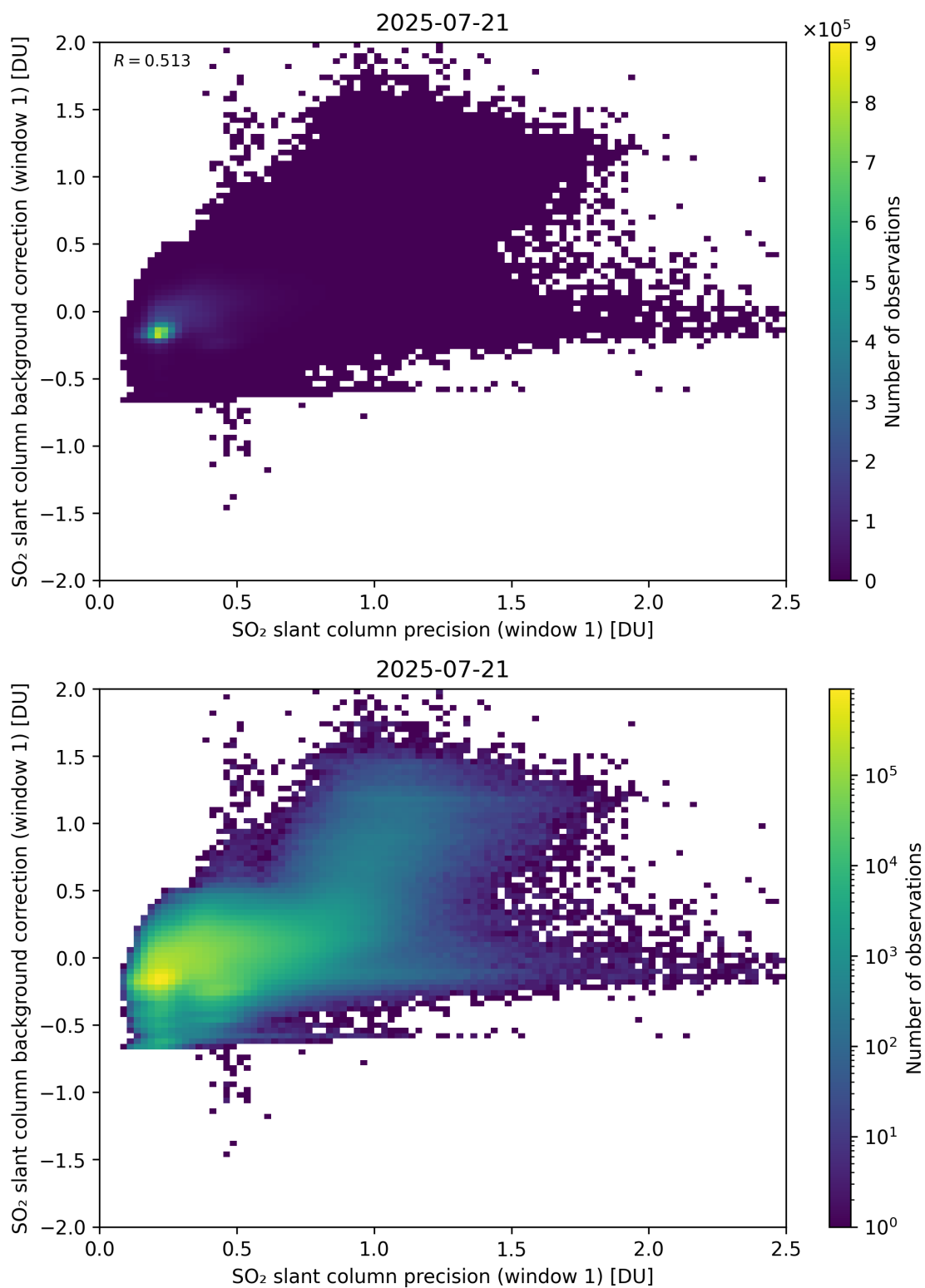
Figure 268: Scatter density plot of “SO 2 slant column precision (window 1)” against “SO 2 slant column background correction (window 1)” for 2025-07-20 to 2025-07-22.
