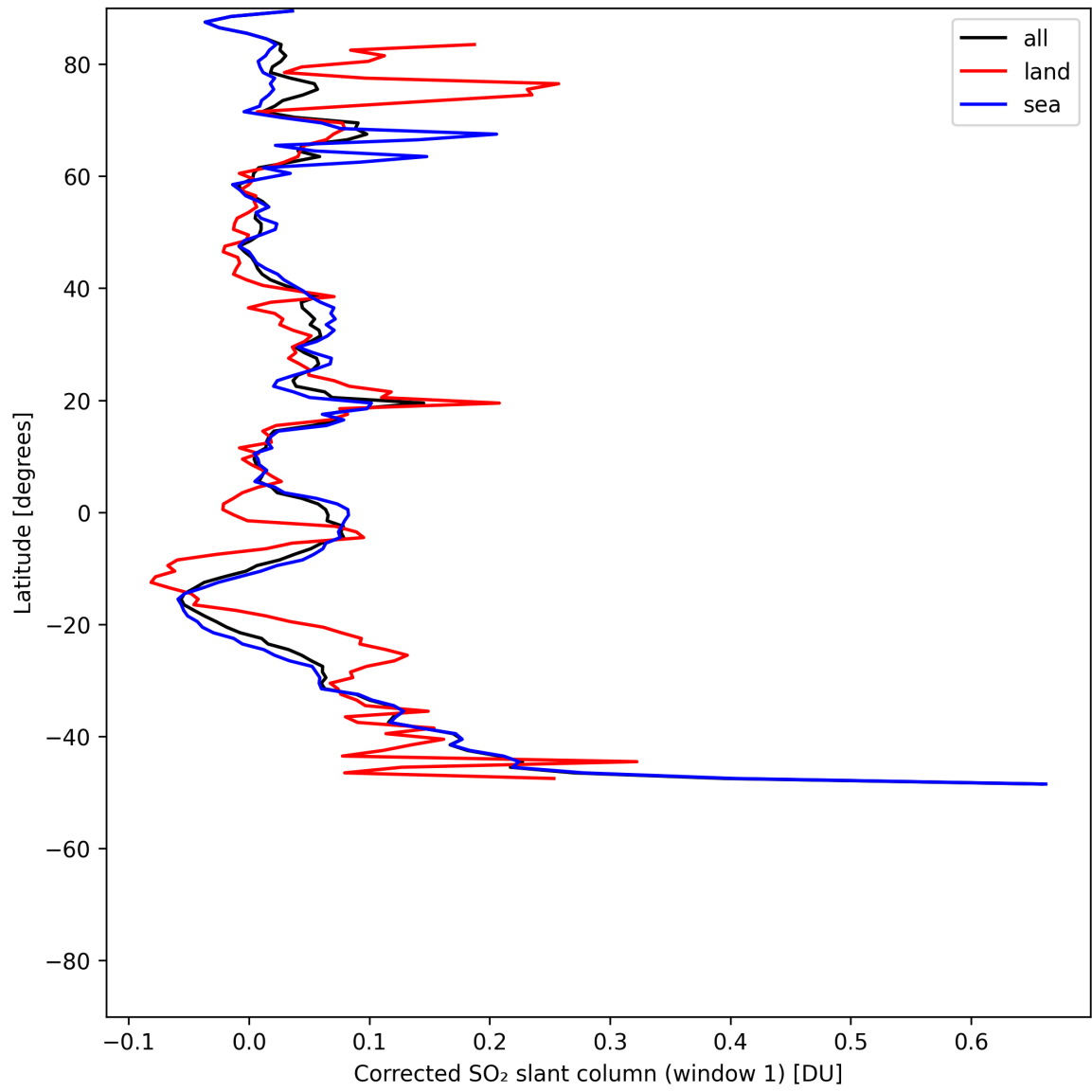
Figure 39: Zonal average of “Corrected SO 2 slant column (window 1)” for 2025-07-20 to 2025-07-22.
