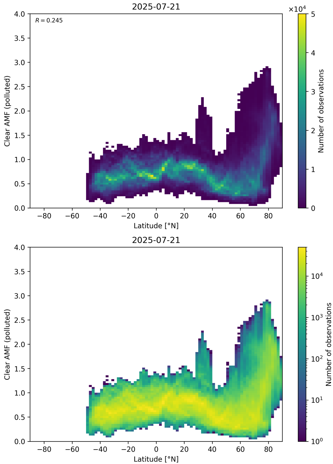
Figure 156: Scatter density plot of “Latitude” against “Clear AMF (polluted)” for 2025-07-20 to 2025-07-22.
