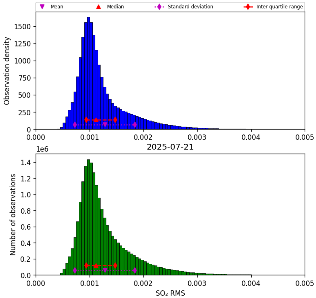
Figure 78: Histogram of “SO 2 RMS” for 2025-07-20 to 2025-07-22
