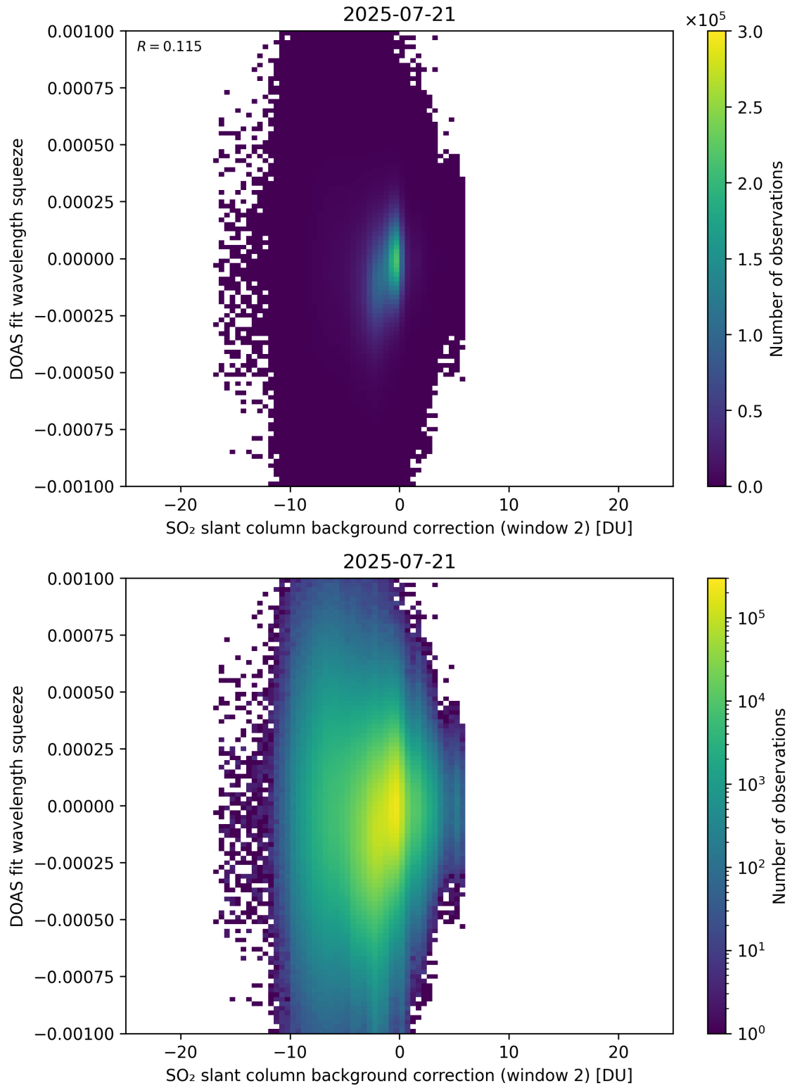
Figure 124: Scatter density plot of “SO 2 slant column background correction (window 2)” against “DOAS fit wavelength squeeze” for 2025-07-20 to 2025-07-22.
