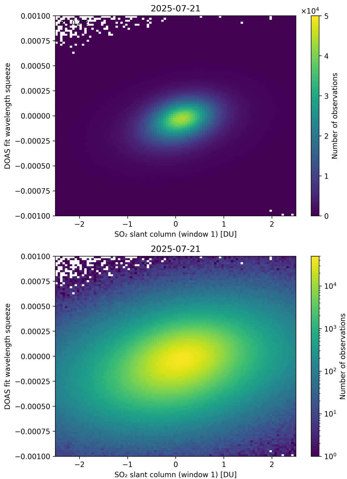
Figure 266: Scatter density plot of “SO 2 slant column (window 1)” against “DOAS fit wavelength squeeze” for 2025-07-20 to 2025-07-22.
