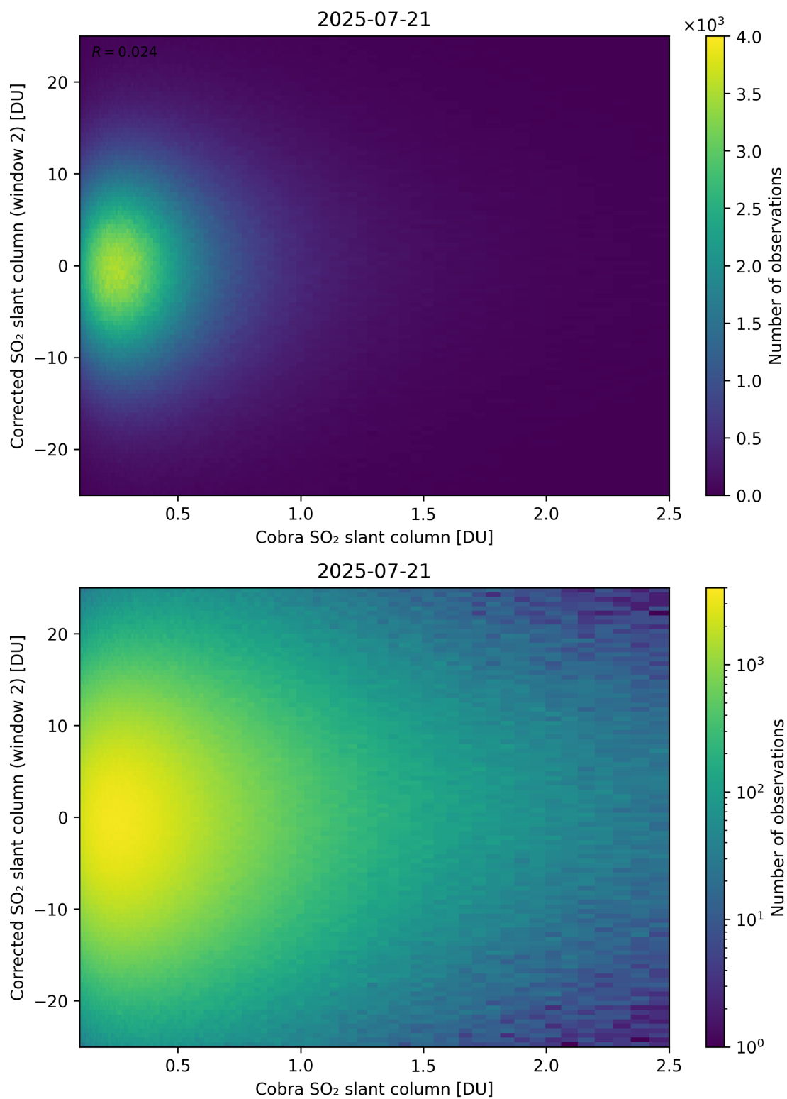
Figure 217: Scatter density plot of “Cobra SO 2 slant column” against “Corrected SO 2 slant column (window 2)” for 2025-07-20 to 2025-07-22.
