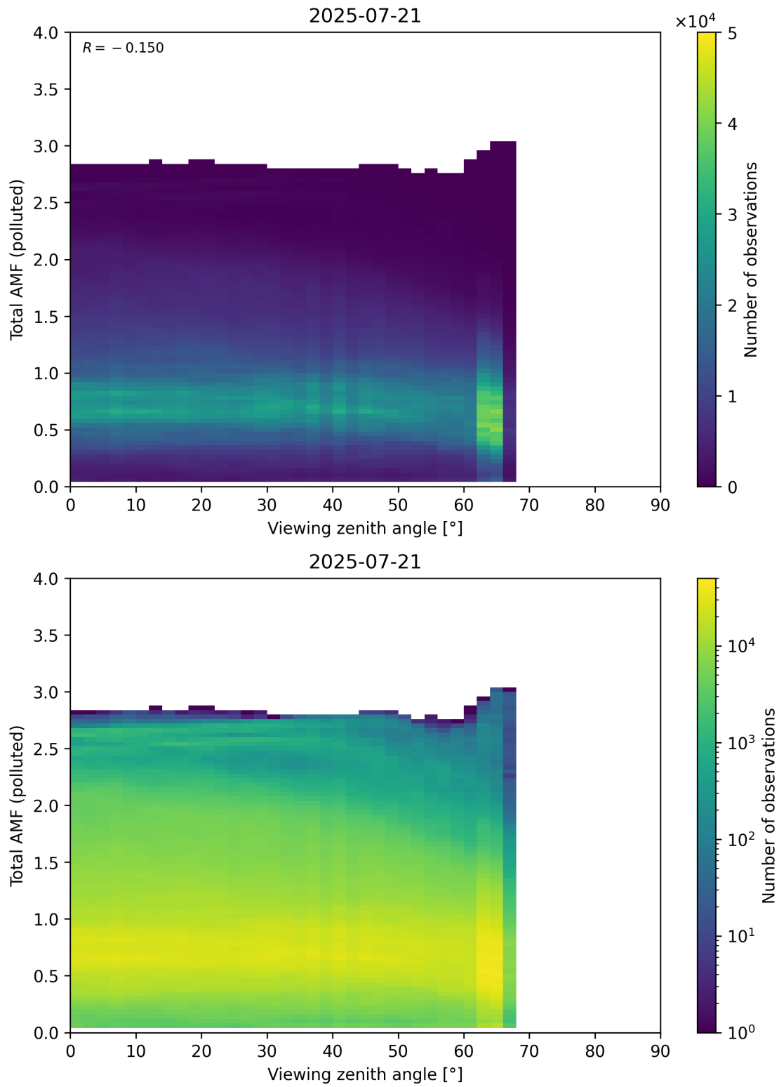
Figure 381: Scatter density plot of “Viewing zenith angle” against “Total AMF (polluted)” for 2025-07-20 to 2025-07-22.
