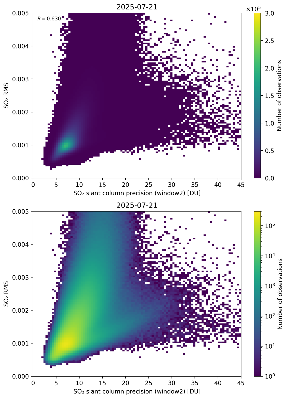
Figure 295: Scatter density plot of “SO 2 slant column precision (window2)” against “SO 2 RMS” for 2025-07-20 to 2025-07-22.
