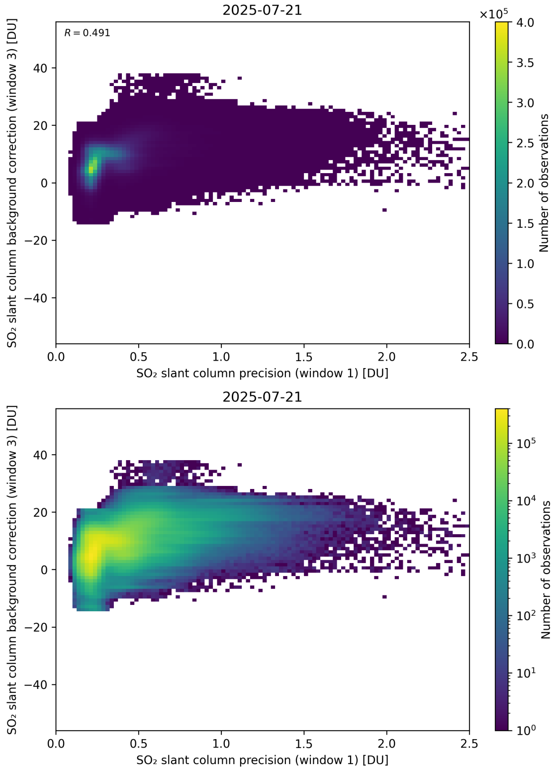
Figure 270: Scatter density plot of “SO 2 slant column precision (window 1)” against “SO 2 slant column background correction (window 3)” for 2025-07-20 to 2025-07-22.
