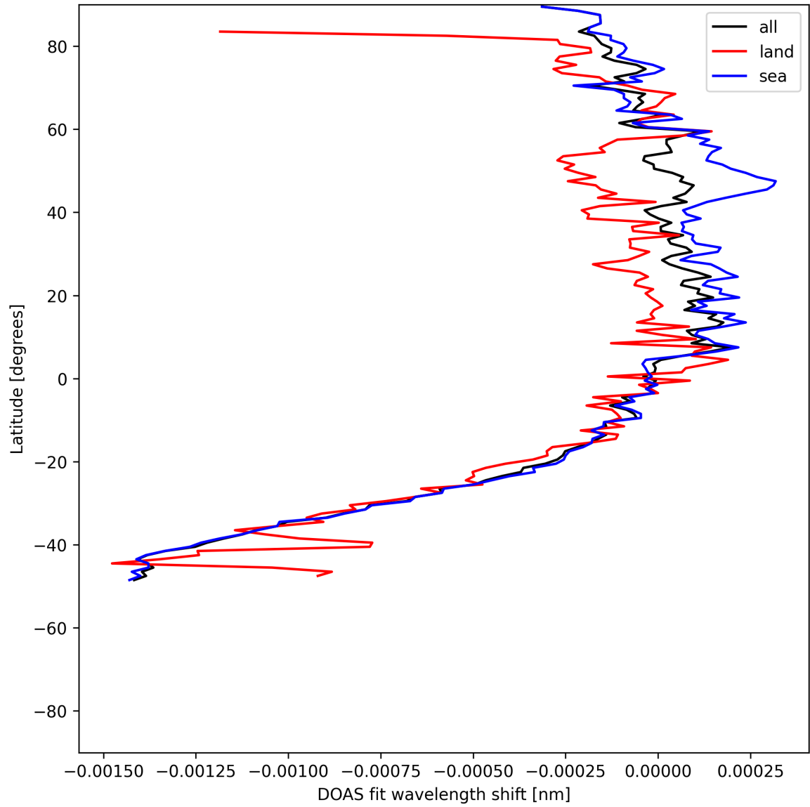
Figure 50: Zonal average of “DOAS fit wavelength shift” for 2025-07-20 to 2025-07-22.
