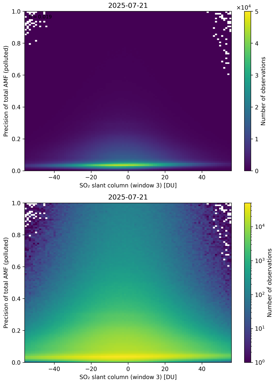
Figure 319: Scatter density plot of “SO 2 slant column (window 3)” against “Precision of total AMF (polluted)” for 2025-07-20 to 2025-07-22.
