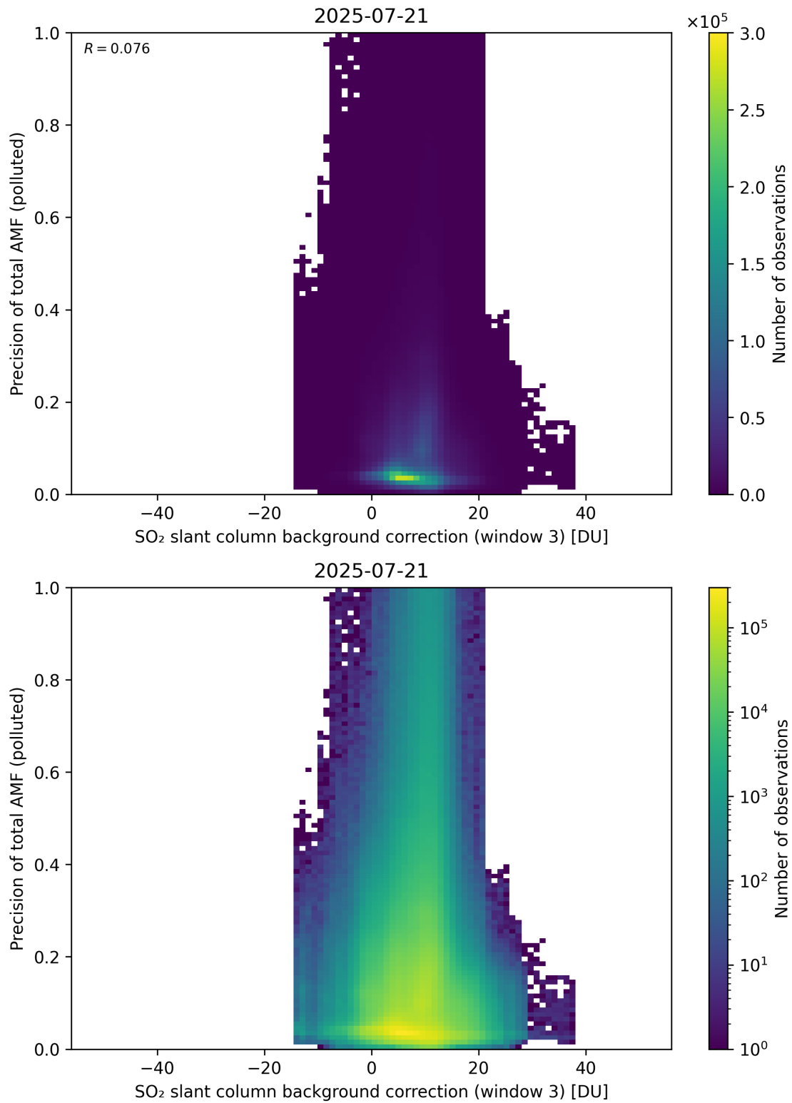
Figure 137: Scatter density plot of “SO 2 slant column background correction (window 3)” against “Precision of total AMF (polluted)” for 2025-07-20 to 2025-07-22.
