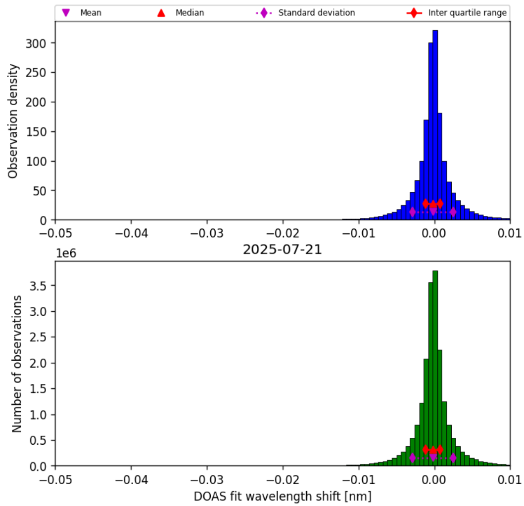
Figure 76: Histogram of “DOAS fit wavelength shift” for 2025-07-20 to 2025-07-22
