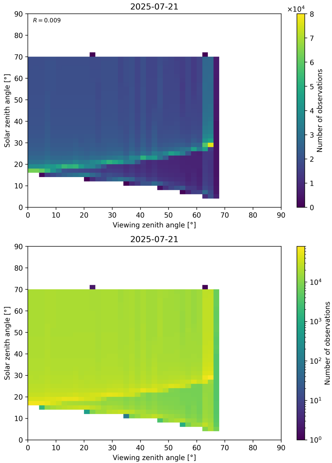
Figure 369: Scatter density plot of “Viewing zenith angle” against “Solar zenith angle” for 2025-07-20 to 2025-07-22.
