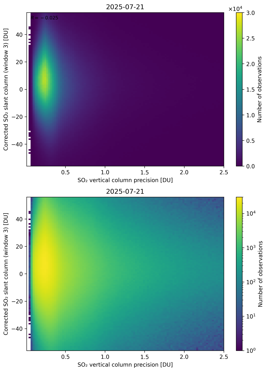
Figure 340: Scatter density plot of “SO 2 vertical column precision” against “Corrected SO 2 slant column (window 3)” for 2025-07-20 to 2025-07-22.
