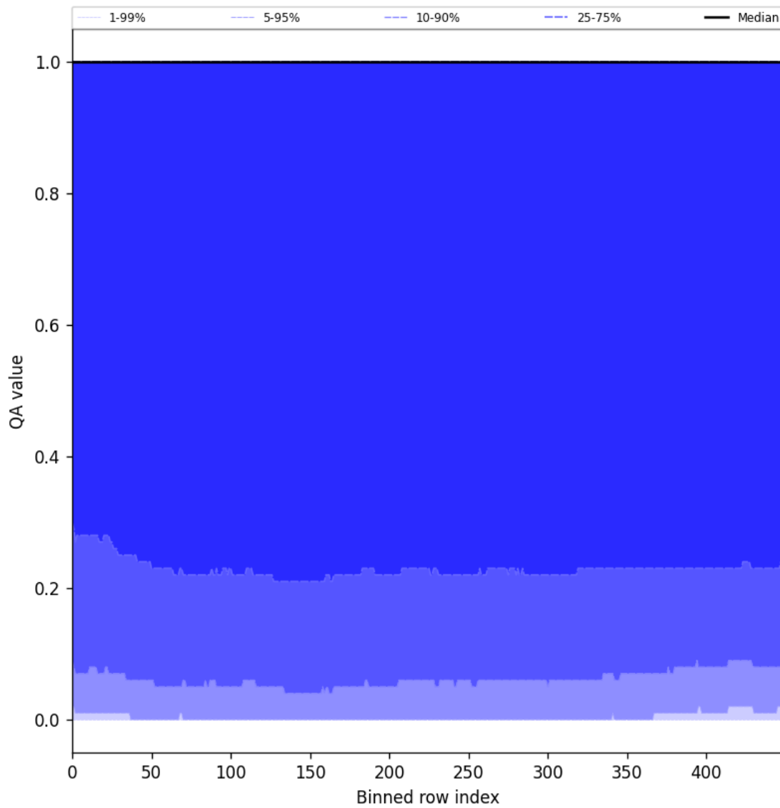
Figure 83: Along track statistics of “QA value” for 2025-07-20 to 2025-07-22
