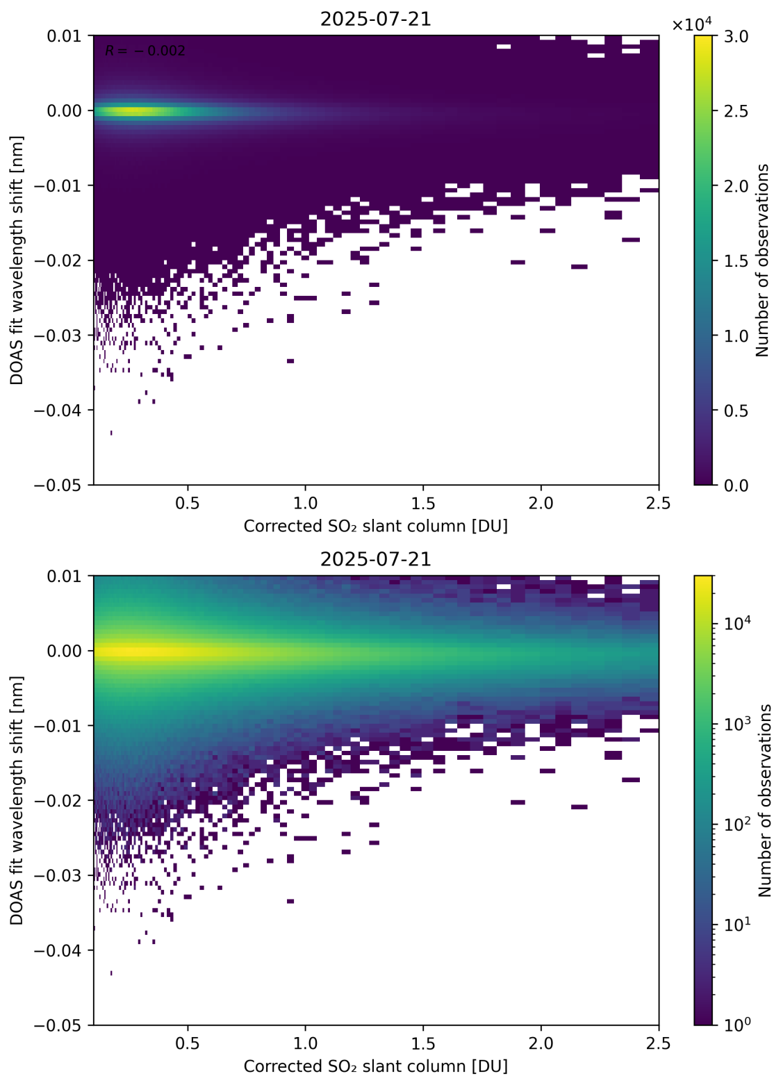
Figure 229: Scatter density plot of “Corrected SO 2 slant column” against “DOAS fit wavelength shift” for 2025-07-20 to 2025-07-22.
