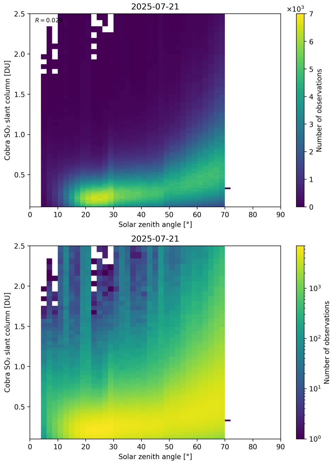
Figure 179: Scatter density plot of “Solar zenith angle” against “Cobra SO 2 slant column” for 2025-07-20 to 2025-07-22.
