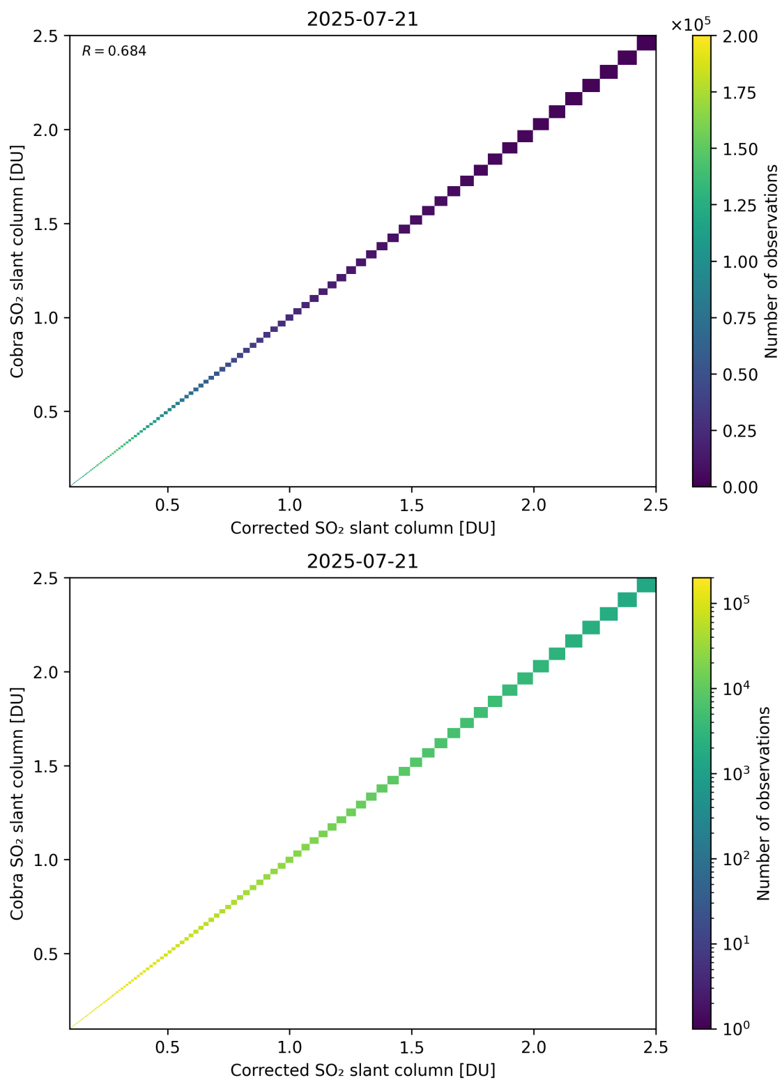
Figure 233: Scatter density plot of “Corrected SO 2 slant column” against “Cobra SO 2 slant column” for 2025-07-20 to 2025-07-22.
