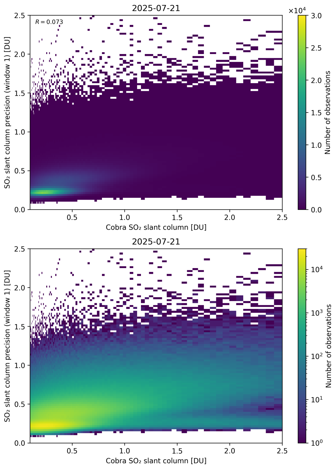
Figure 220: Scatter density plot of “Cobra SO 2 slant column” against “SO 2 slant column precision (window 1)” for 2025-07-20 to 2025-07-22.
