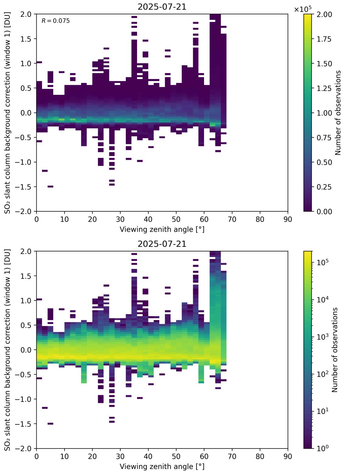
Figure 362: Scatter density plot of “Viewing zenith angle” against “SO 2 slant column background correction (window 1)” for 2025-07-20 to 2025-07-22.
