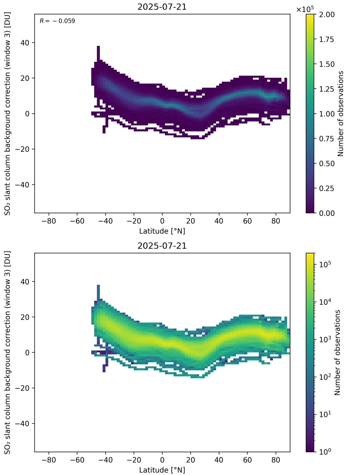
Figure 152: Scatter density plot of “Latitude” against “SO 2 slant column background correction (window 3)” for 2025-07-20 to 2025-07-22.
