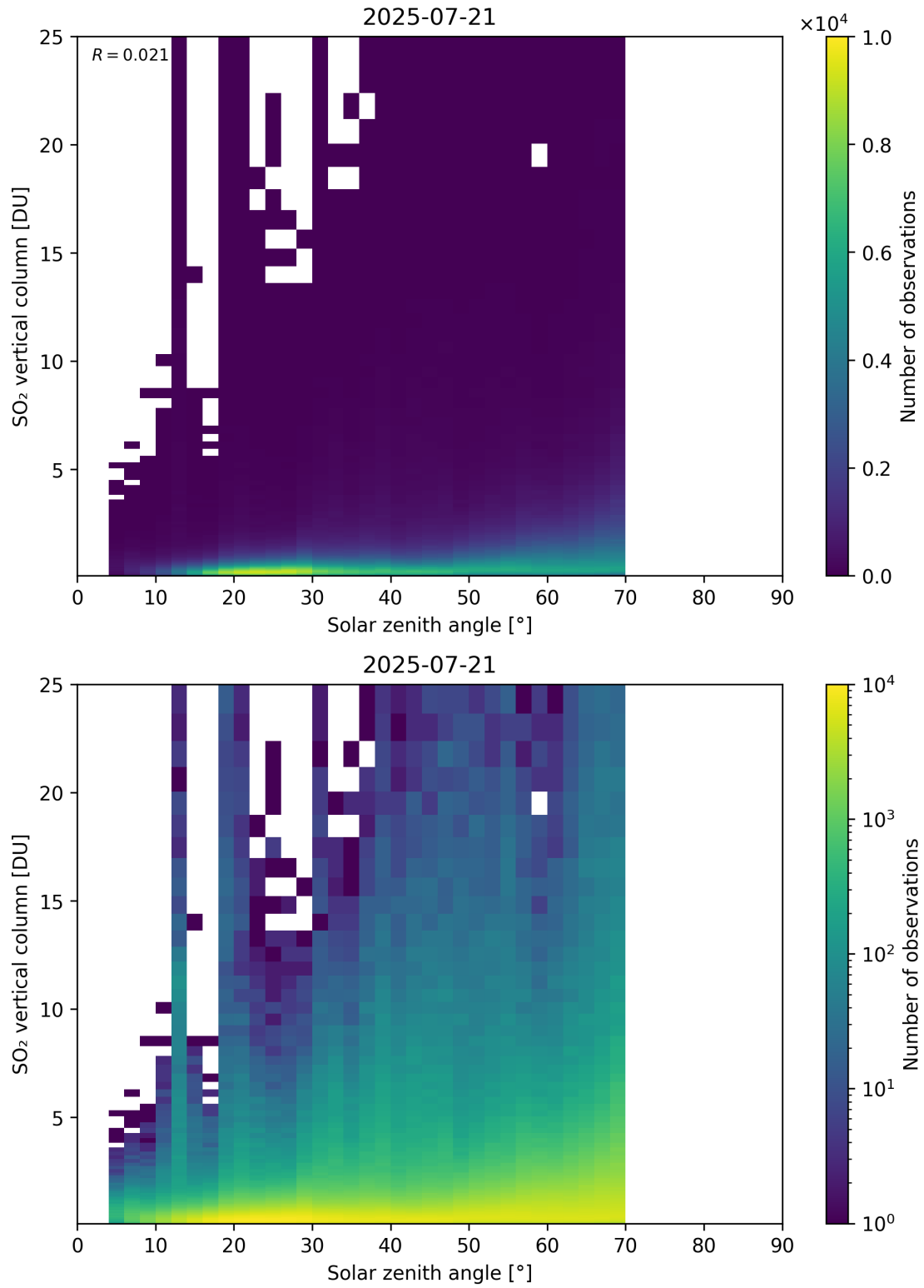
Figure 191: Scatter density plot of “Solar zenith angle” against “SO 2 vertical column” for 2025-07-20 to 2025-07-22.
