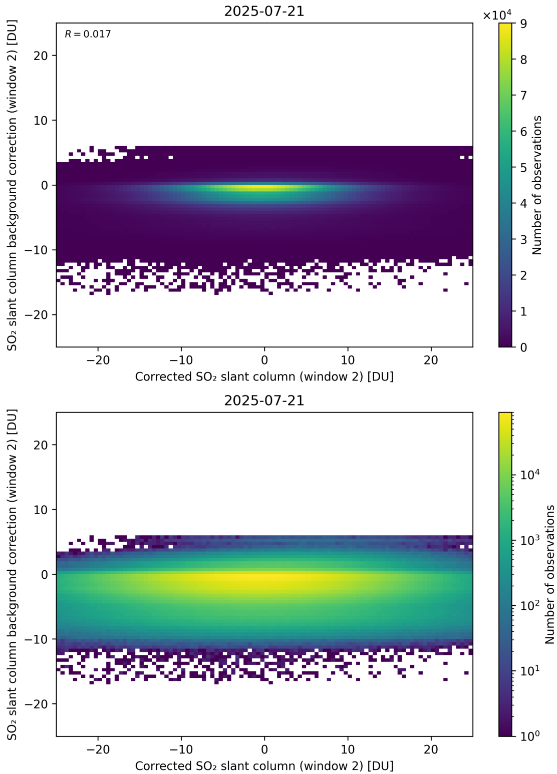
Figure 244: Scatter density plot of “Corrected SO 2 slant column (window 2)” against “SO 2 slant column background correction (window 2)” for 2025-07-20 to 2025-07-22.
