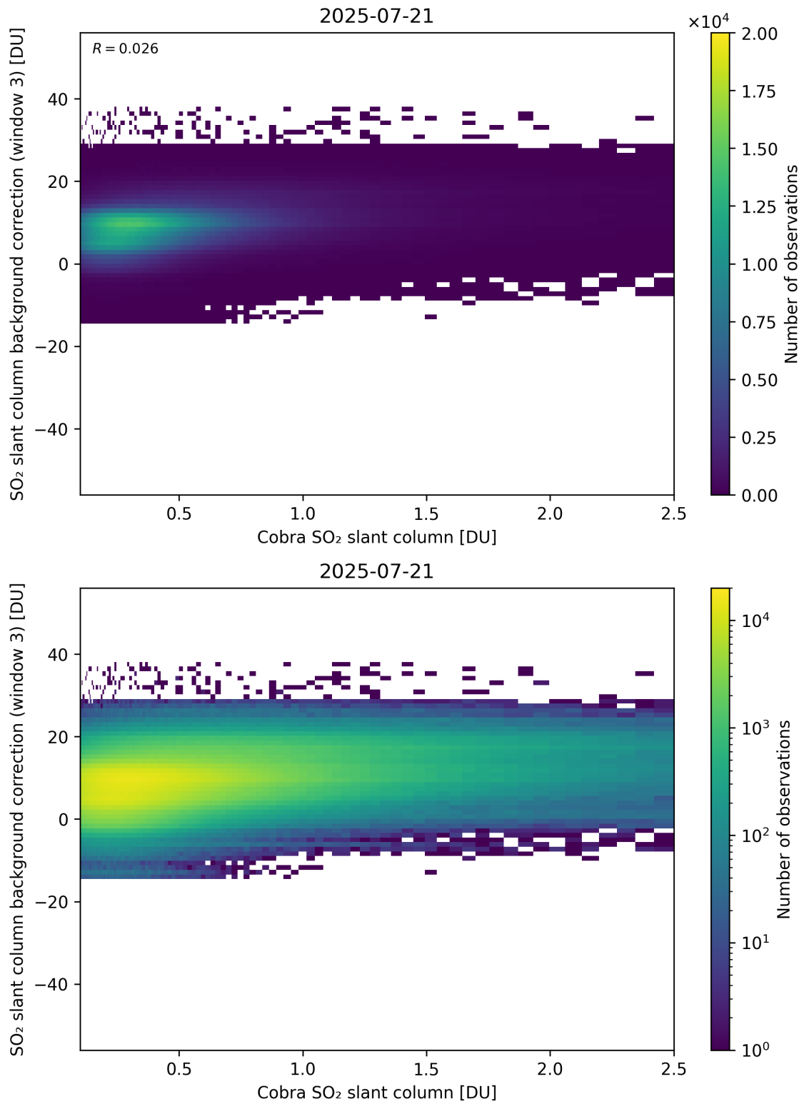
Figure 195: Scatter density plot of “Cobra SO 2 slant column” against “SO 2 slant column background correction (window 3)” for 2025-07-20 to 2025-07-22.
