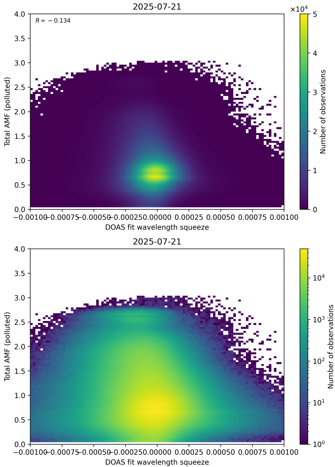
Figure 145: Scatter density plot of “DOAS fit wavelength squeeze” against “Total AMF (polluted)” for 2025-07-20 to 2025-07-22.
