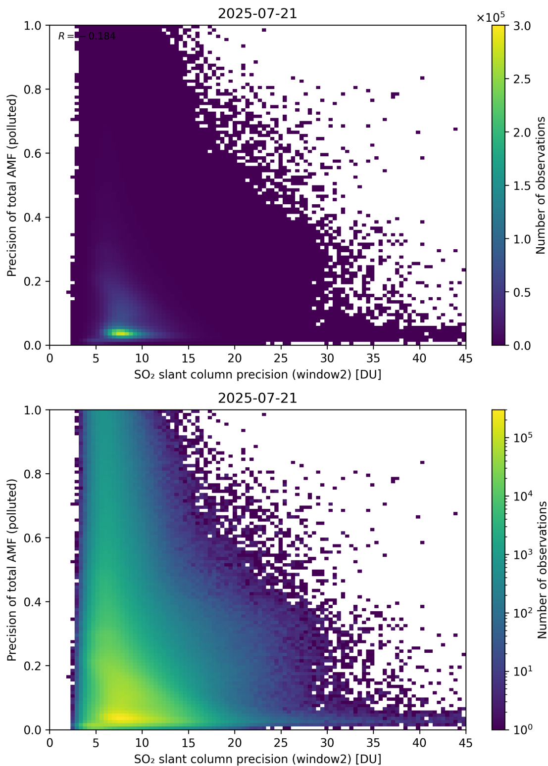
Figure 302: Scatter density plot of “SO 2 slant column precision (window2)” against “Precision of total AMF (polluted)” for 2025-07-20 to 2025-07-22.
