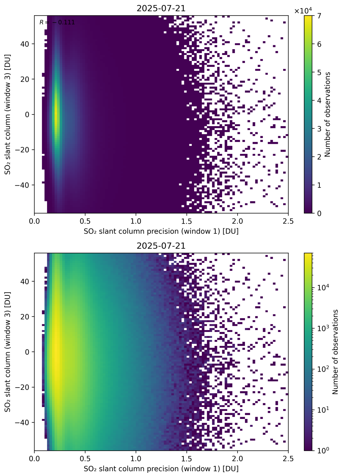
Figure 278: Scatter density plot of “SO 2 slant column precision (window 1)” against “SO 2 slant column (window 3)” for 2025-07-20 to 2025-07-22.
