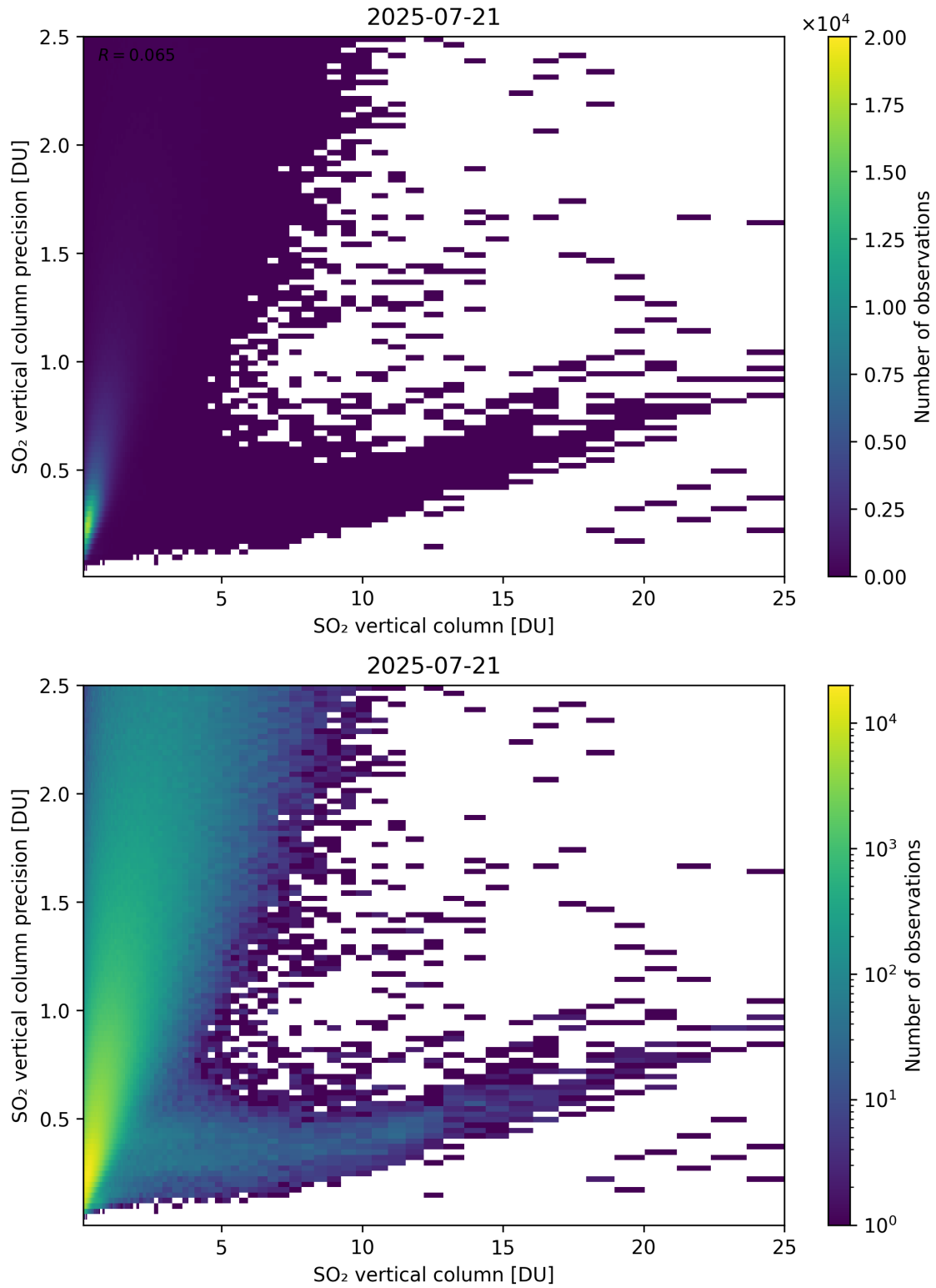
Figure 361: Scatter density plot of “SO 2 vertical column” against “SO 2 vertical column precision” for 2025-07-20 to 2025-07-22.
