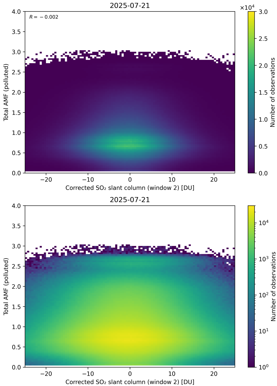
Figure 253: Scatter density plot of “Corrected SO 2 slant column (window 2)” against “Total AMF (polluted)” for 2025-07-20 to 2025-07-22.
