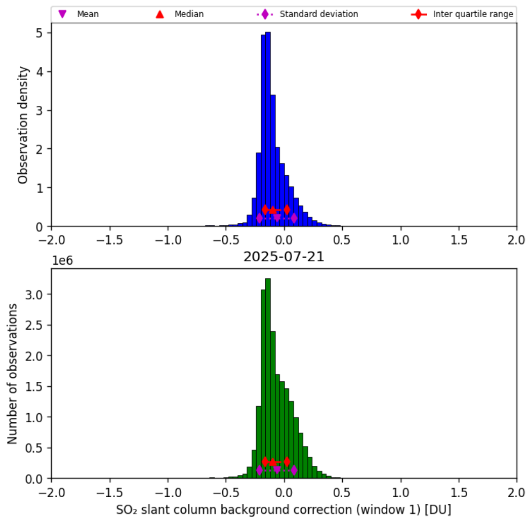
Figure 66: Histogram of “SO 2 slant column background correction (window 1)” for 2025-07-20 to 2025-07-22
