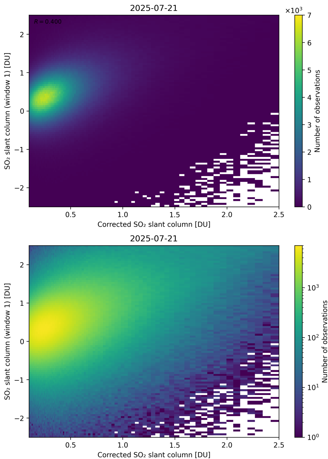
Figure 237: Scatter density plot of “Corrected SO 2 slant column” against “SO 2 slant column (window 1)” for 2025-07-20 to 2025-07-22.
