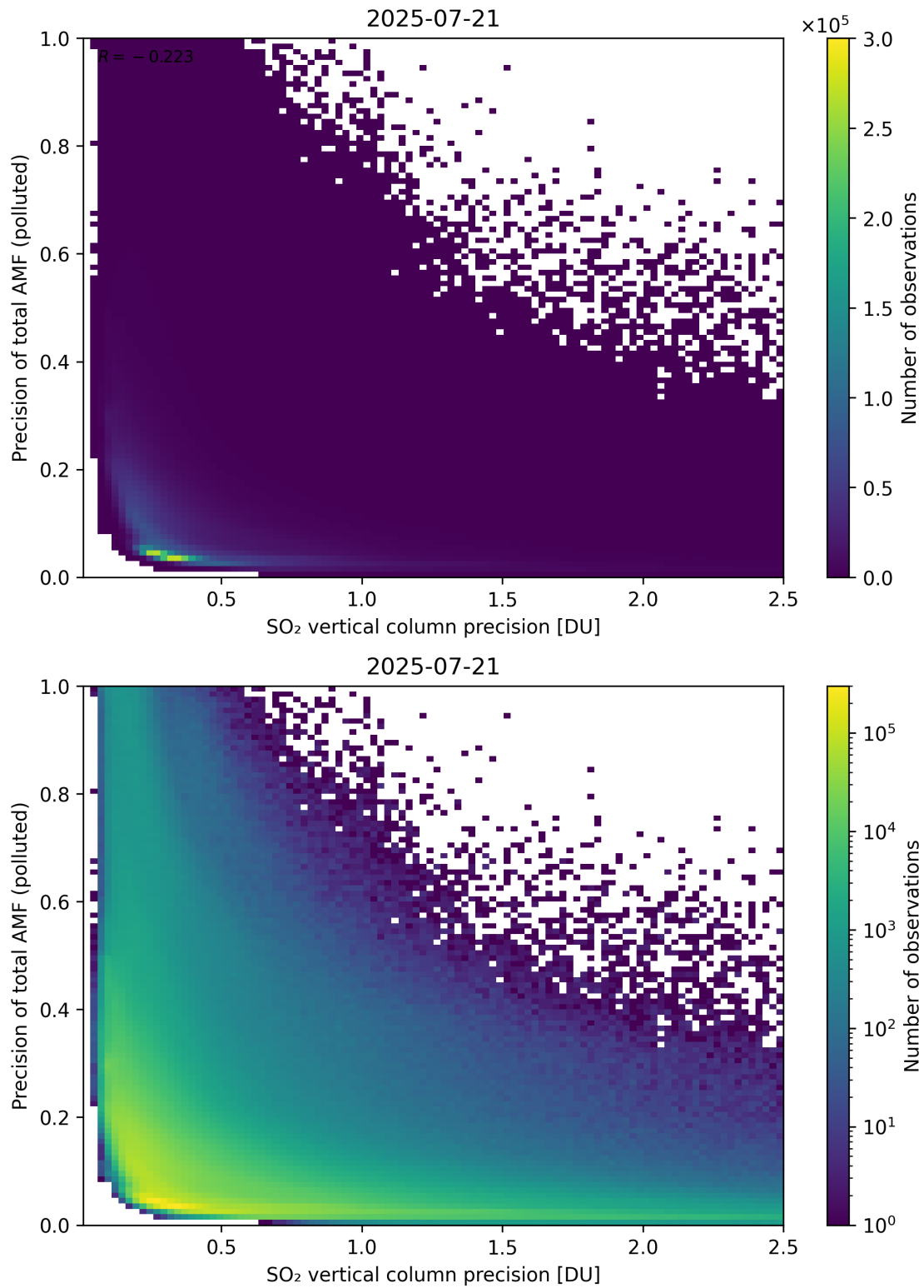
Figure 347: Scatter density plot of “SO 2 vertical column precision” against “Precision of total AMF (polluted)” for 2025-07-20 to 2025-07-22.
