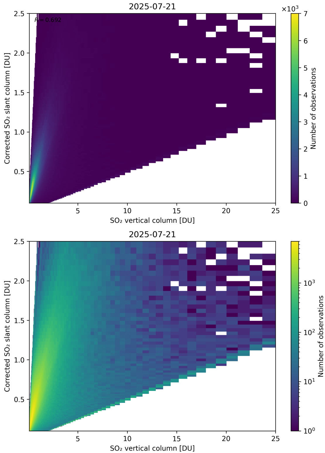
Figure 351: Scatter density plot of “SO 2 vertical column” against “Corrected SO 2 slant column” for 2025-07-20 to 2025-07-22.
