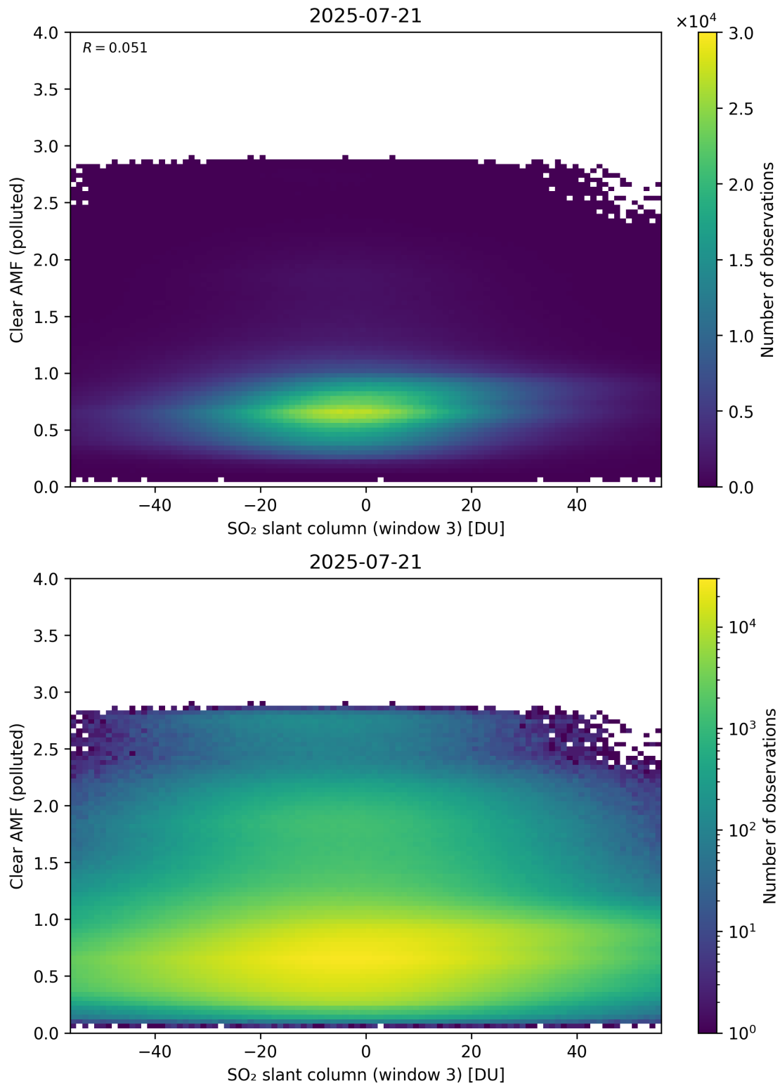
Figure 315: Scatter density plot of “SO 2 slant column (window 3)” against “Clear AMF (polluted)” for 2025-07-20 to 2025-07-22.
