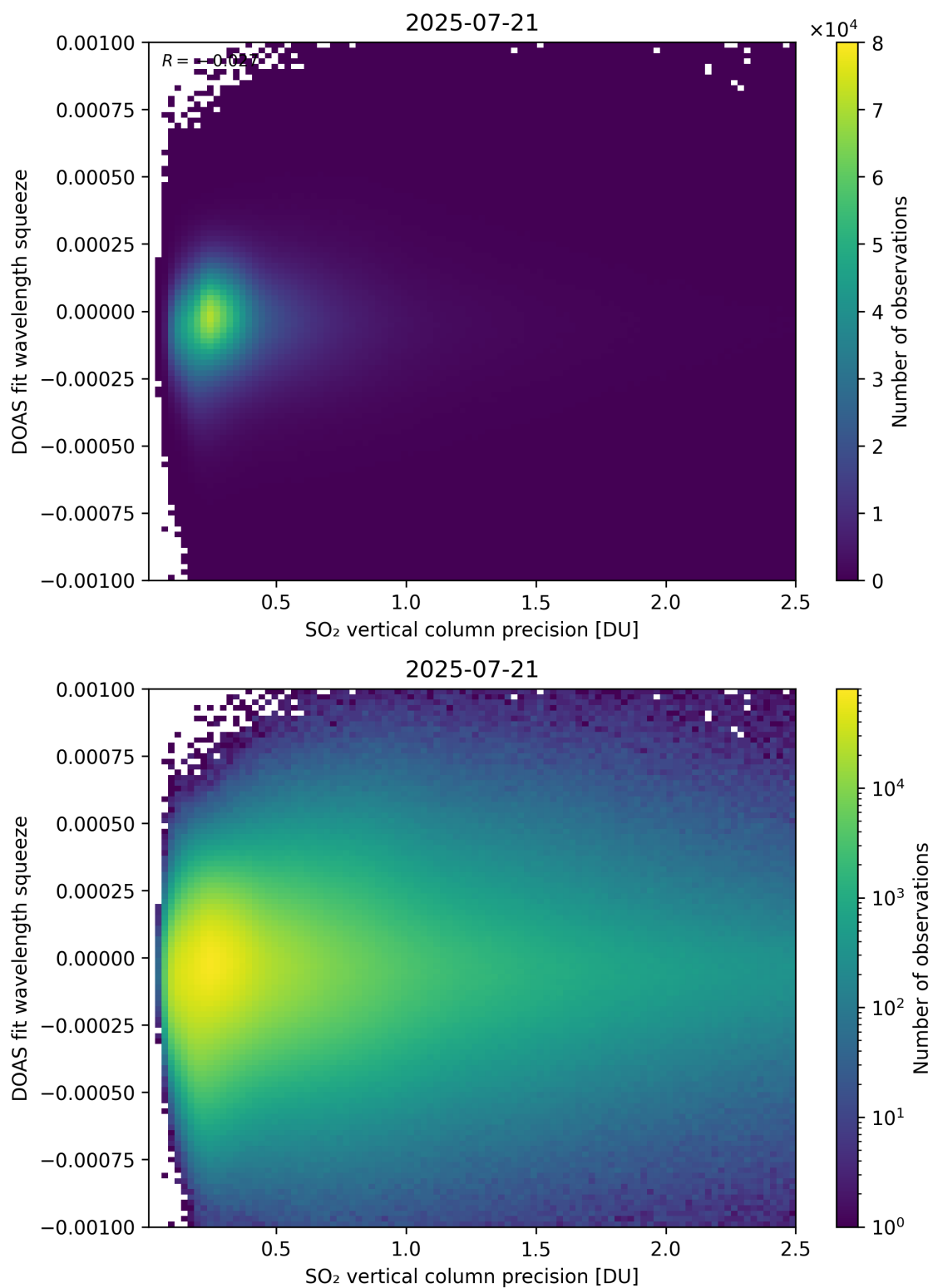
Figure 333: Scatter density plot of “SO 2 vertical column precision” against “DOAS fit wavelength squeeze” for 2025-07-20 to 2025-07-22.
