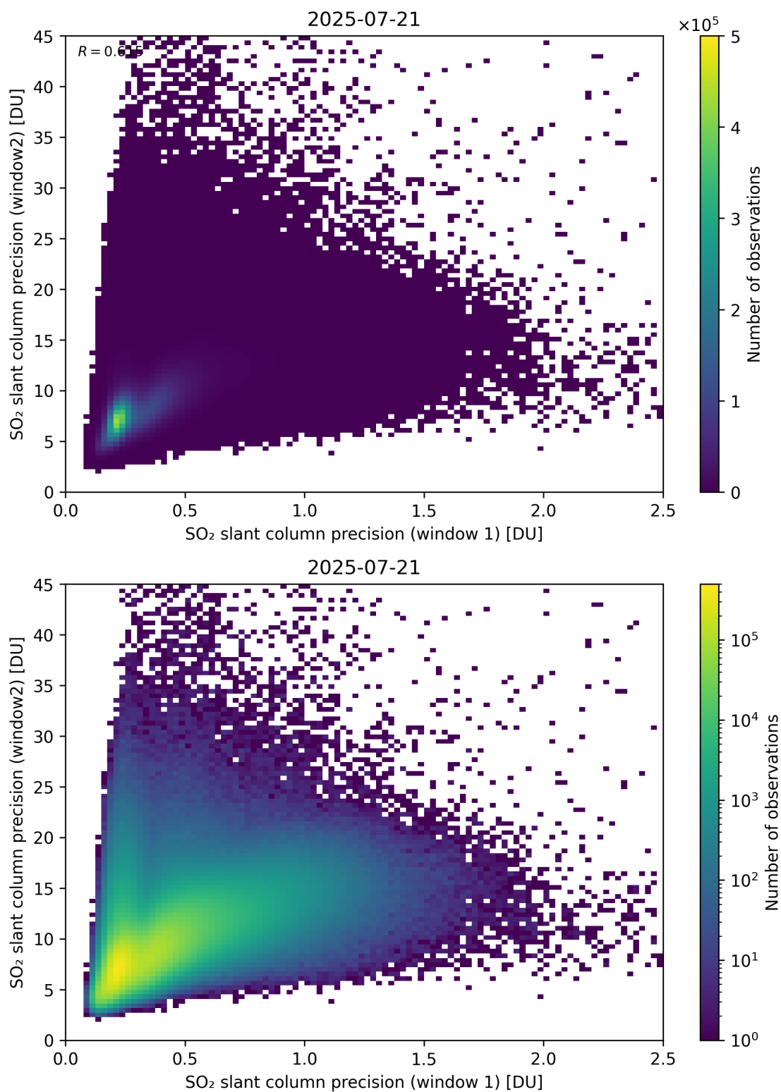
Figure 277: Scatter density plot of “SO 2 slant column precision (window 1)” against “SO 2 slant column precision (window2)” for 2025-07-20 to 2025-07-22.
