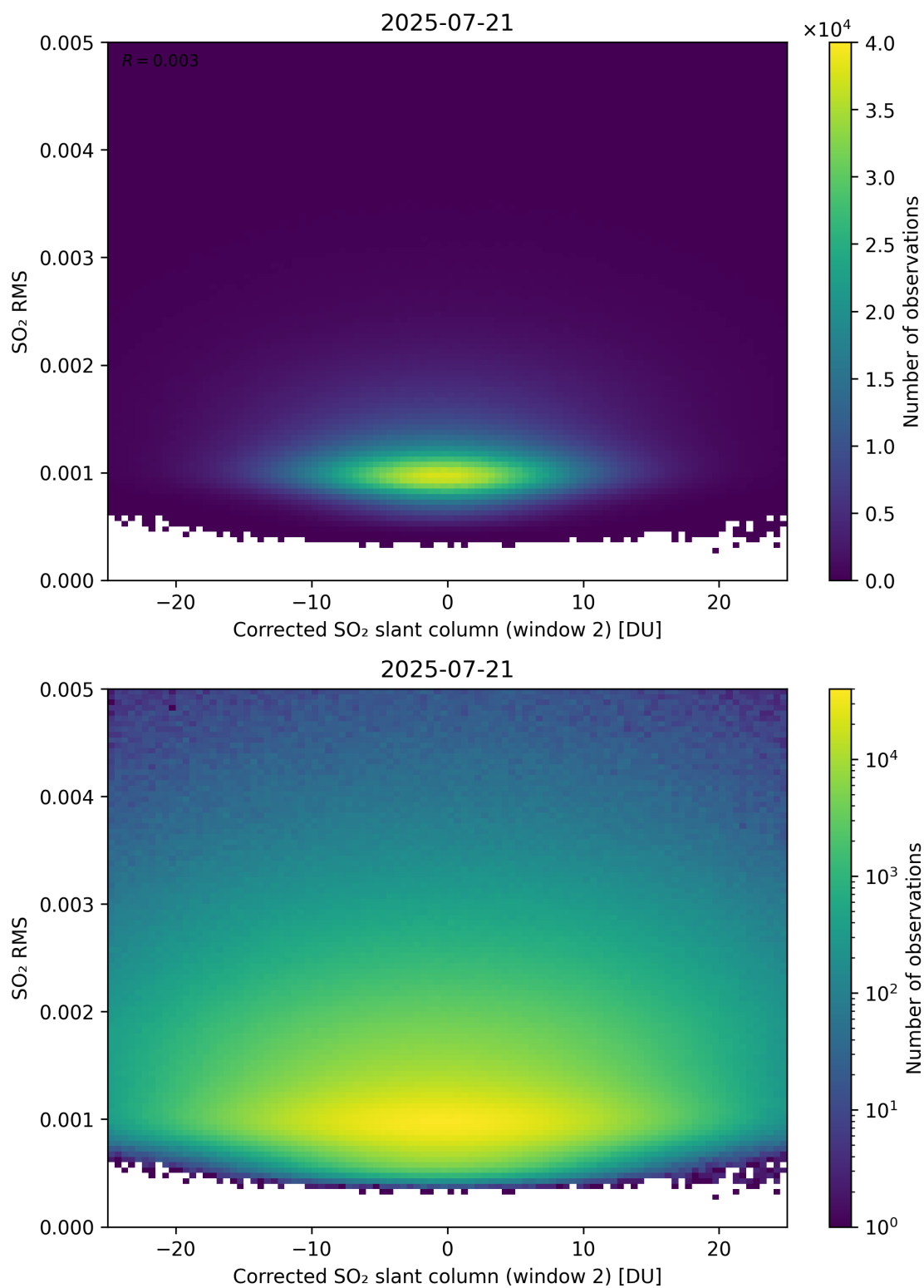
Figure 248: Scatter density plot of “Corrected SO 2 slant column (window 2)” against “SO 2 RMS” for 2025-07-20 to 2025-07-22.
