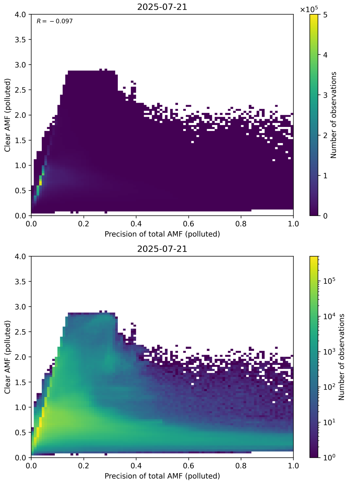
Figure 320: Scatter density plot of “Precision of total AMF (polluted)” against “Clear AMF (polluted)” for 2025-07-20 to 2025-07-22.
