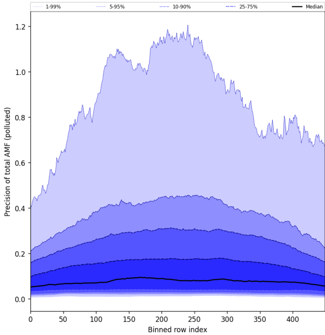
Figure 106: Along track statistics of “Precision of total AMF (polluted)” for 2025-07-20 to 2025-07-22
