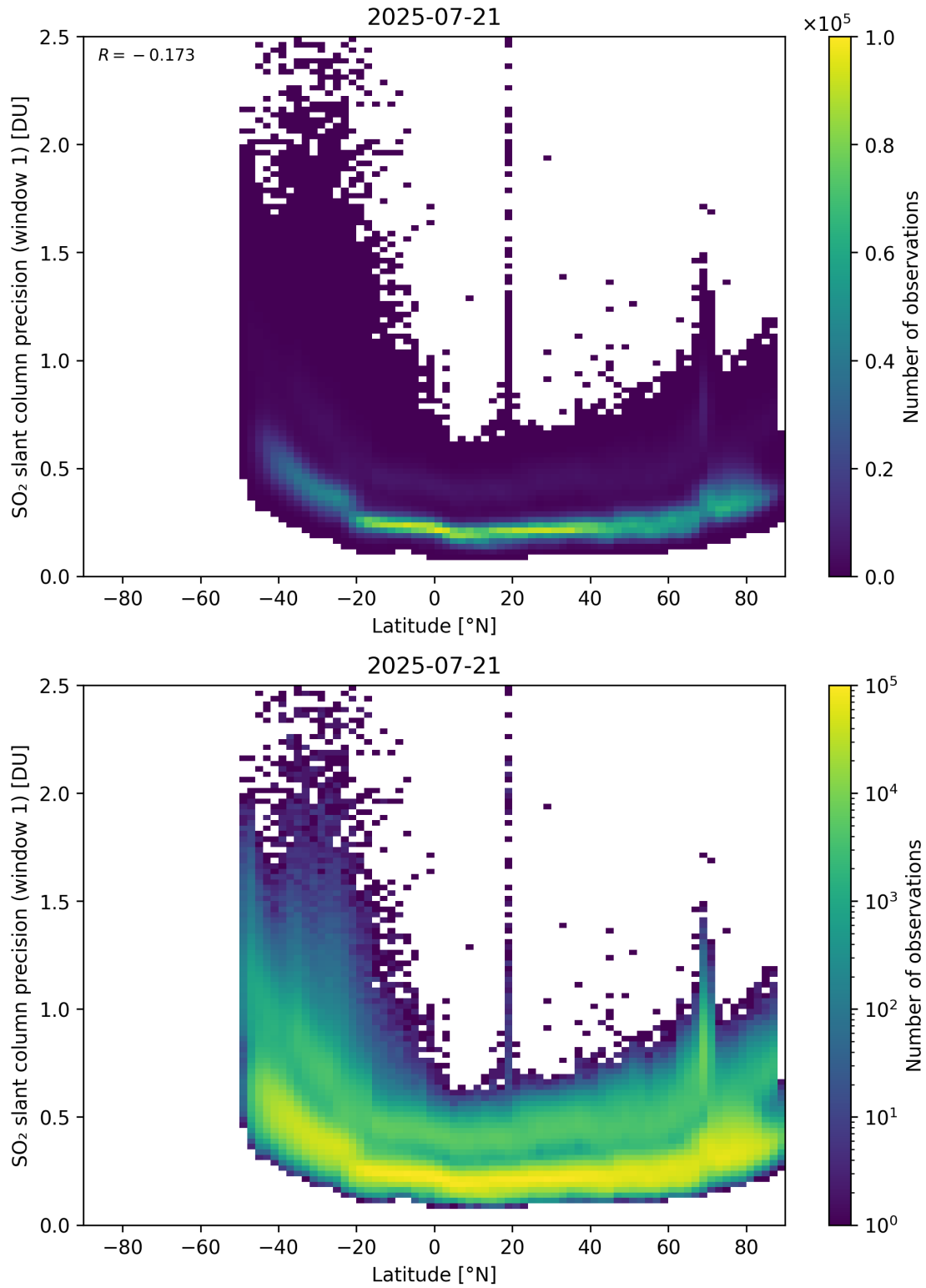
Figure 163: Scatter density plot of “Latitude” against “SO 2 slant column precision (window 1)” for 2025-07-20 to 2025-07-22.
