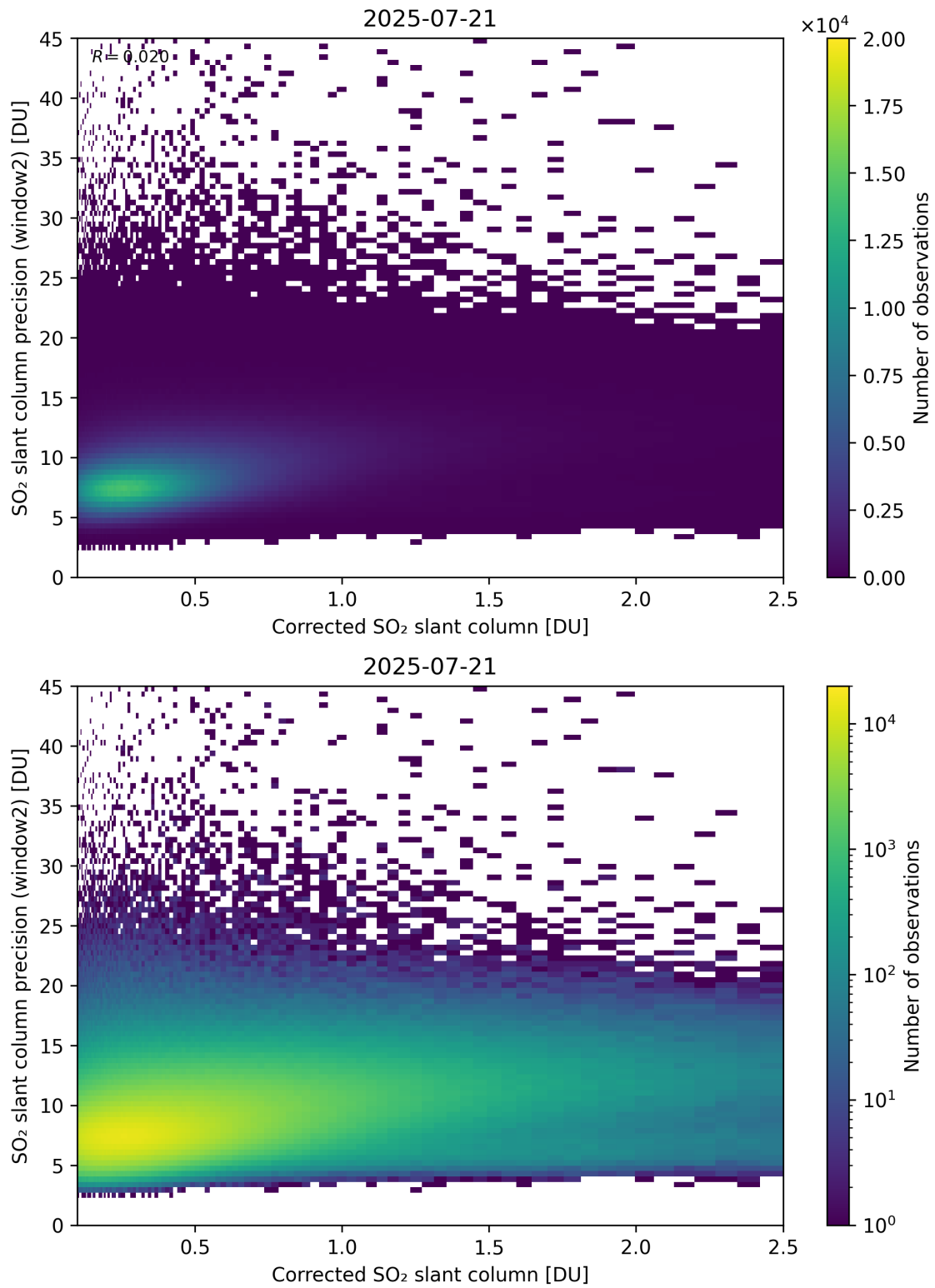
Figure 239: Scatter density plot of “Corrected SO 2 slant column” against “SO 2 slant column precision (window2)” for 2025-07-20 to 2025-07-22.
