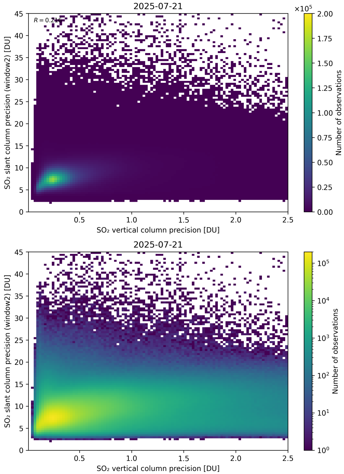
Figure 343: Scatter density plot of “SO 2 vertical column precision” against “SO 2 slant column precision (window2)” for 2025-07-20 to 2025-07-22.
