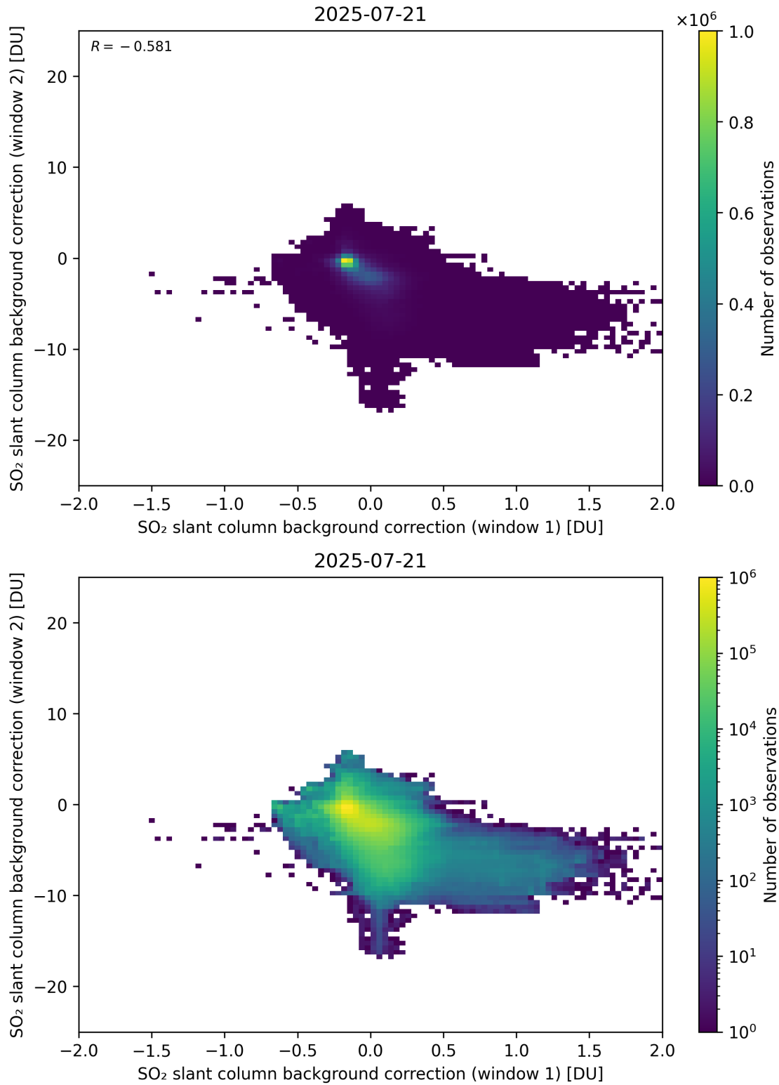
Figure 109: Scatter density plot of “SO 2 slant column background correction (window 1)” against “SO 2 slant column background correction (window 2)” for 2025-07-20 to 2025-07-22.
