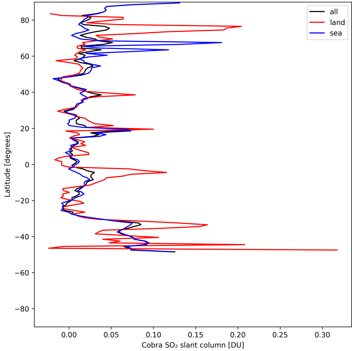
Figure 35: Zonal average of “Cobra SO 2 slant column” for 2025-07-20 to 2025-07-22.
