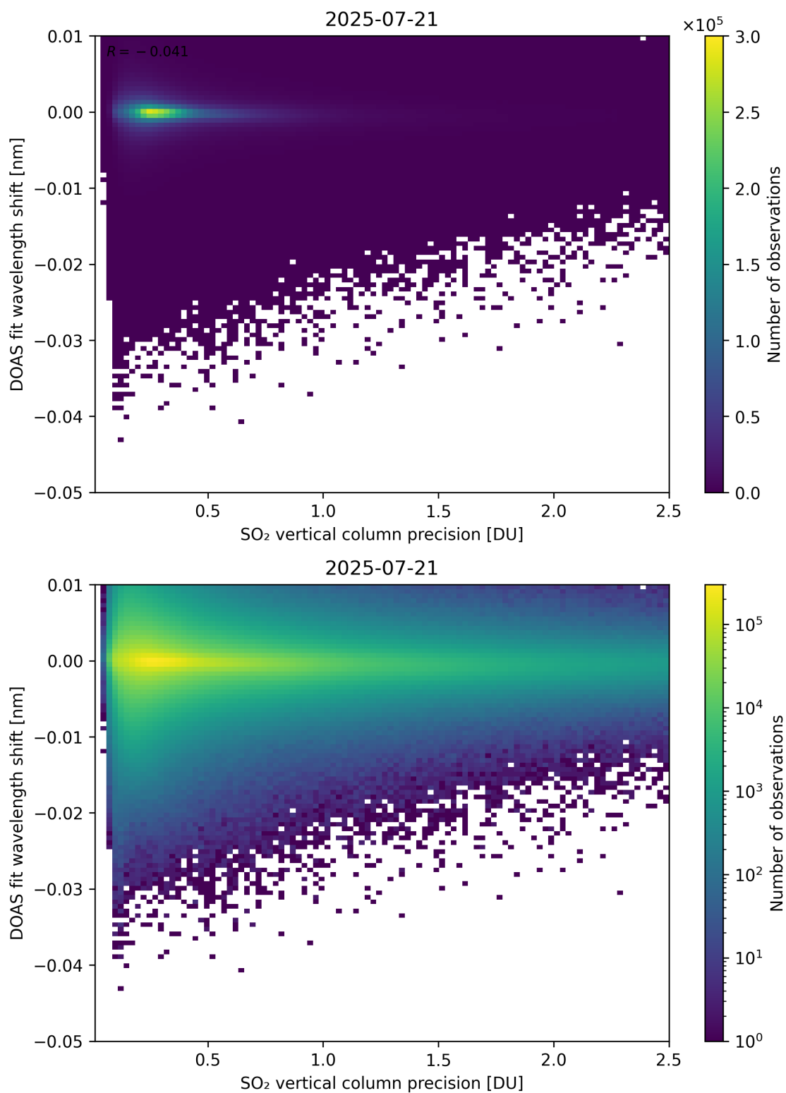
Figure 332: Scatter density plot of “SO 2 vertical column precision” against “DOAS fit wavelength shift” for 2025-07-20 to 2025-07-22.
