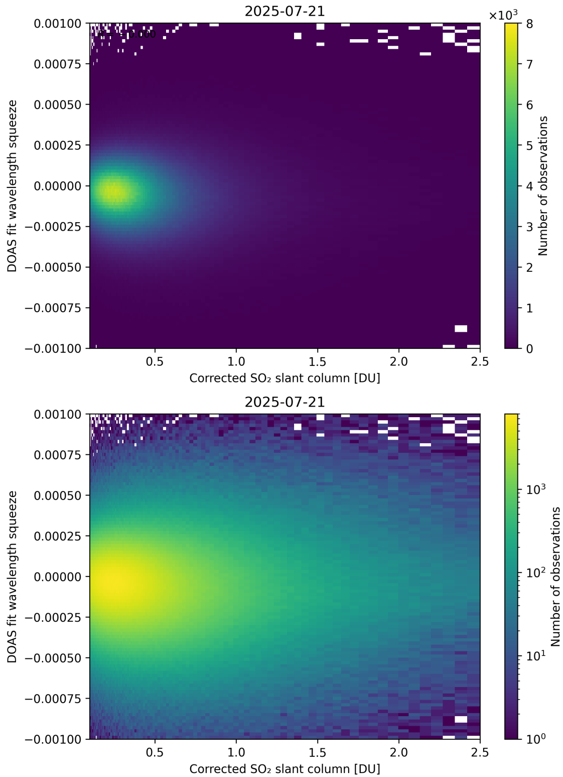
Figure 230: Scatter density plot of “Corrected SO 2 slant column” against “DOAS fit wavelength squeeze” for 2025-07-20 to 2025-07-22.
