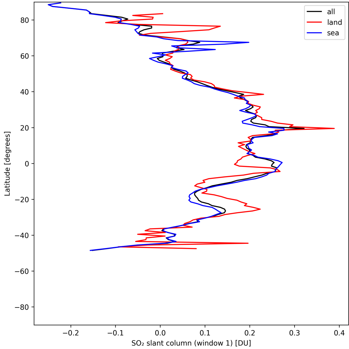
Figure 37: Zonal average of “SO 2 slant column (window 1)” for 2025-07-20 to 2025-07-22.
