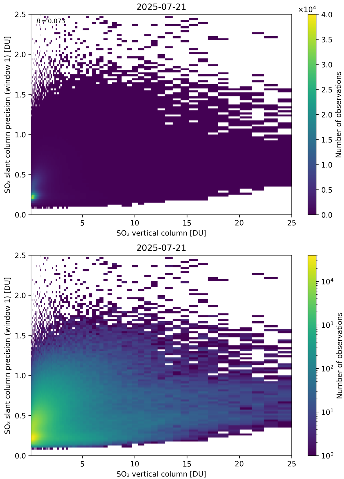
Figure 355: Scatter density plot of “SO 2 vertical column” against “SO 2 slant column precision (window 1)” for 2025-07-20 to 2025-07-22.
