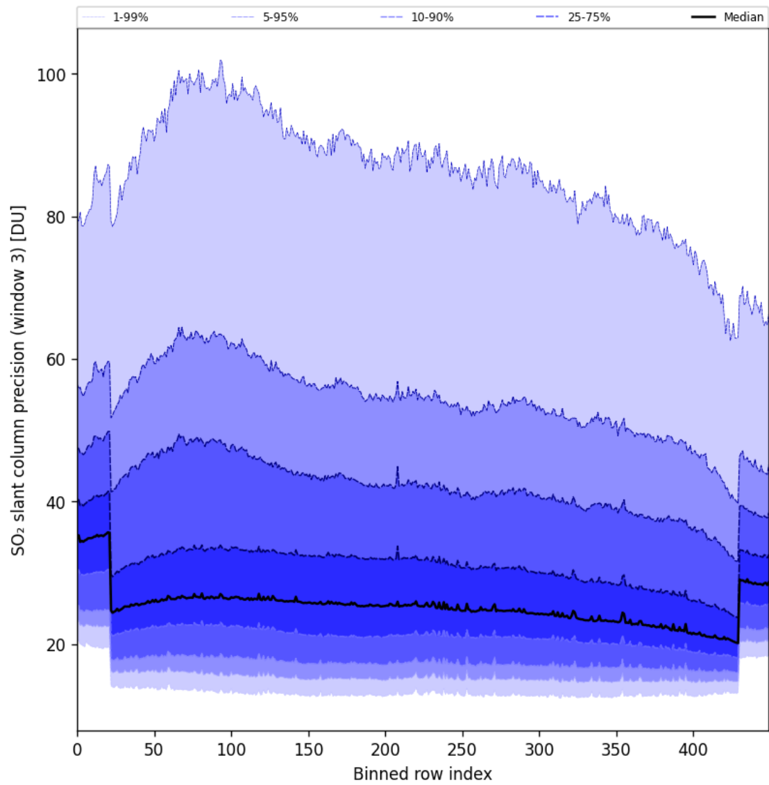
Figure 98: Along track statistics of “SO 2 slant column precision (window 3)” for 2025-07-20 to 2025-07-22
