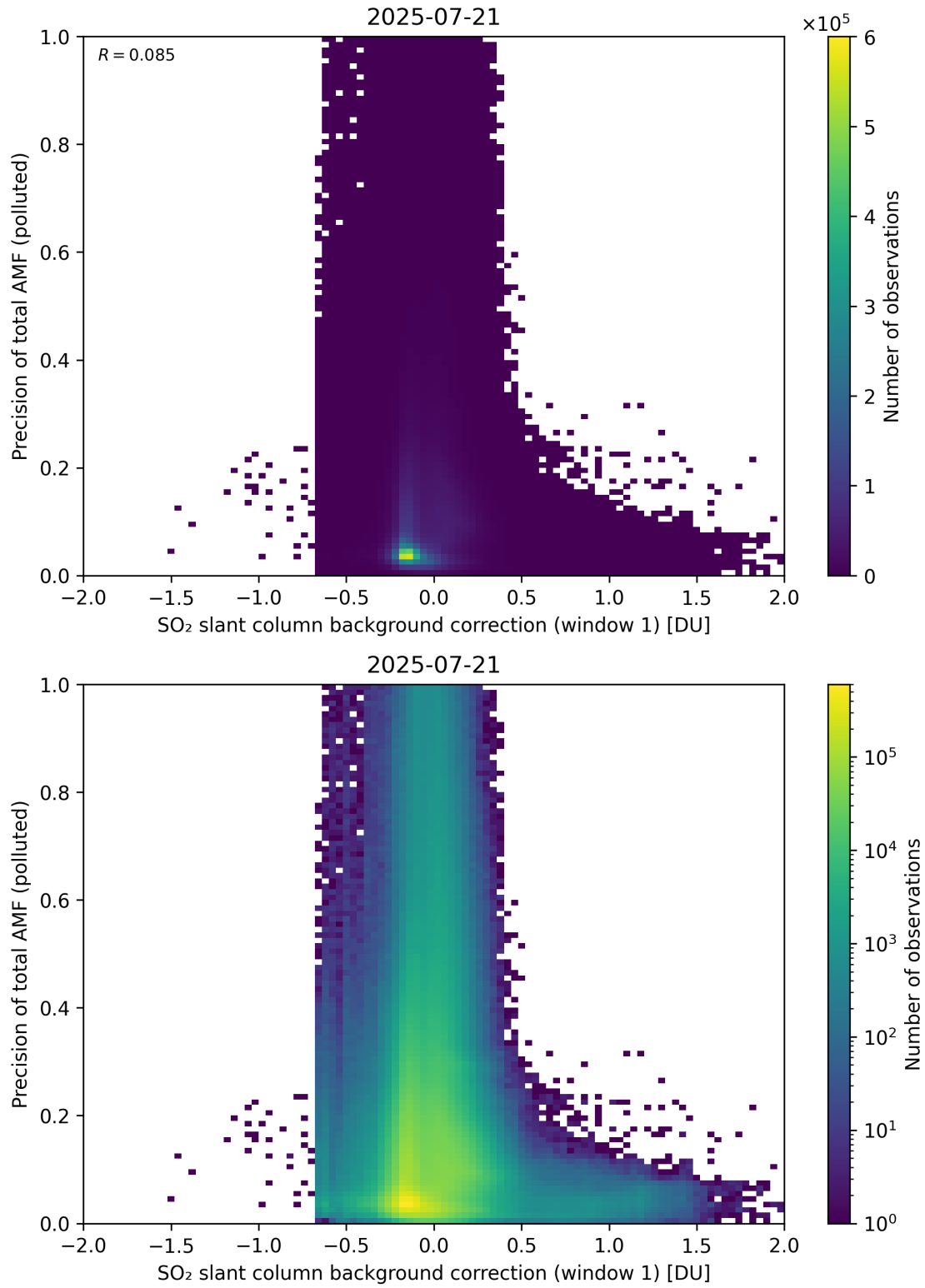
Figure 121: Scatter density plot of “SO 2 slant column background correction (window 1)” against “Precision of total AMF (polluted)” for 2025-07-20 to 2025-07-22.
