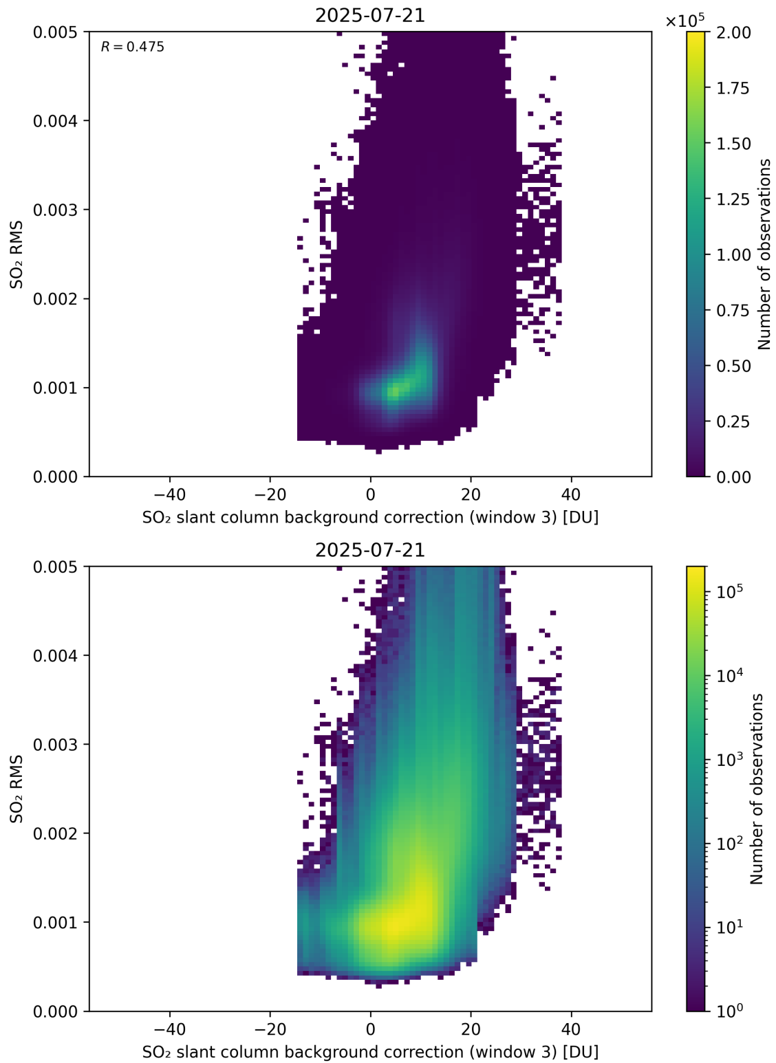
Figure 134: Scatter density plot of “SO 2 slant column background correction (window 3)” against “SO 2 RMS” for 2025-07-20 to 2025-07-22.
