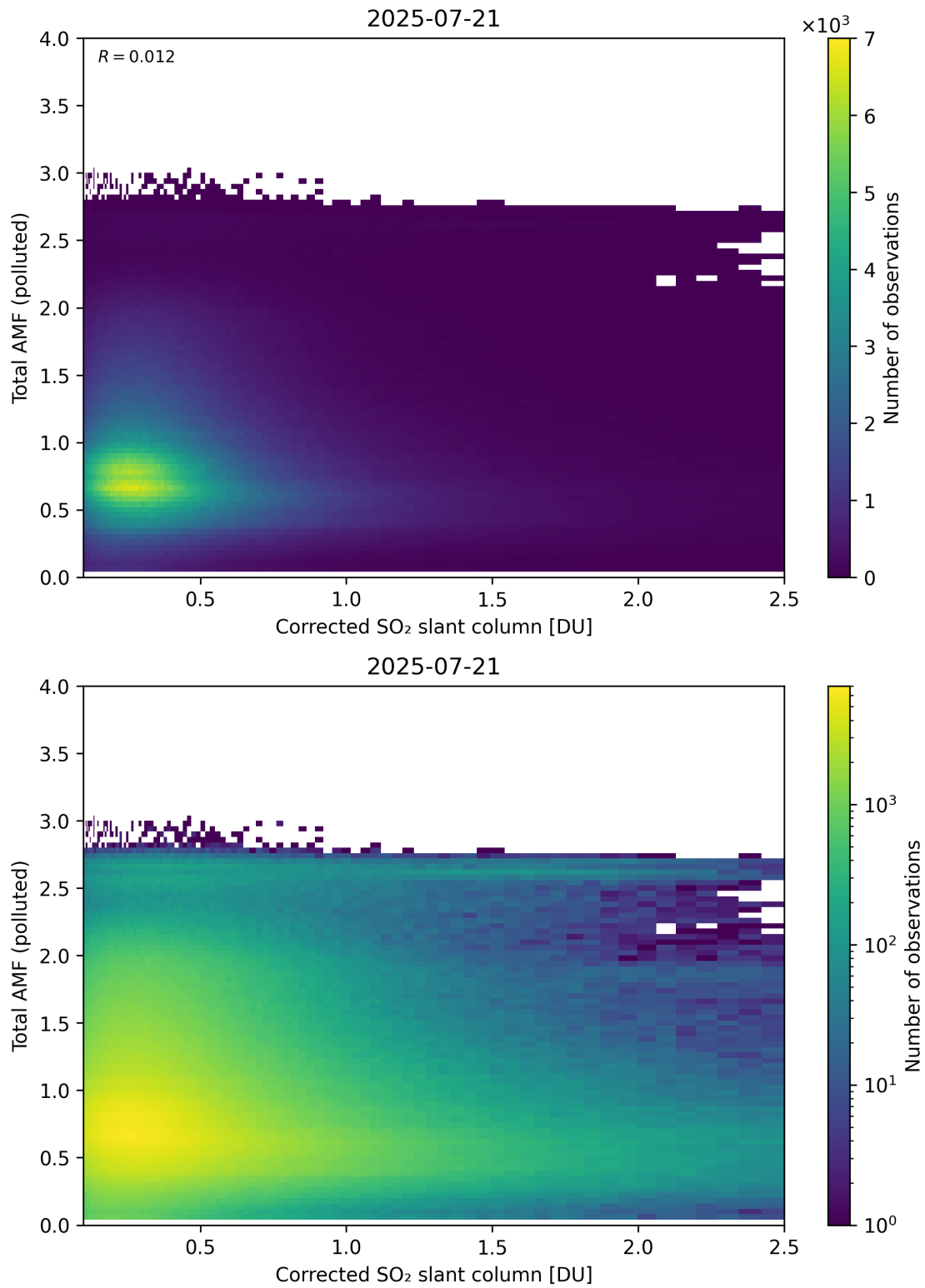
Figure 242: Scatter density plot of “Corrected SO 2 slant column” against “Total AMF (polluted)” for 2025-07-20 to 2025-07-22.
