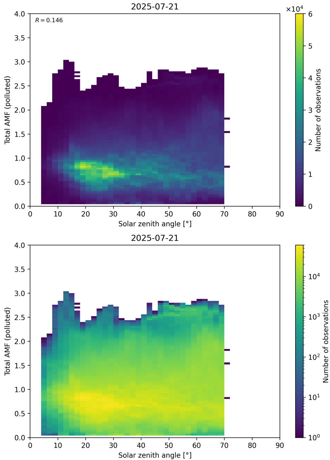
Figure 189: Scatter density plot of “Solar zenith angle” against “Total AMF (polluted)” for 2025-07-20 to 2025-07-22.
