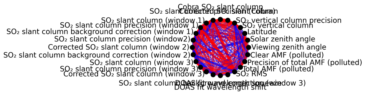
Figure 1: Map of correlation graph for 2025-07-20 to 2025-07-22.
