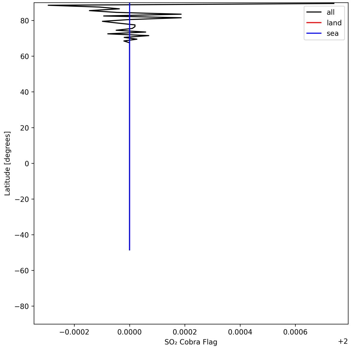
Figure 49: Zonal average of "SO 2 Cobra Flag" for 2025-07-20 to 2025-07-22.
