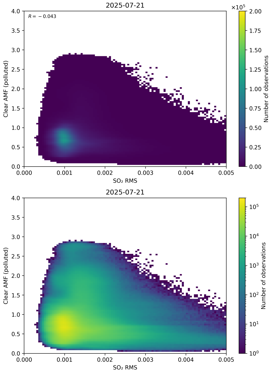
Figure 147: Scatter density plot of “SO 2 RMS” against “Clear AMF (polluted)” for 2025-07-20 to 2025-07-22.
