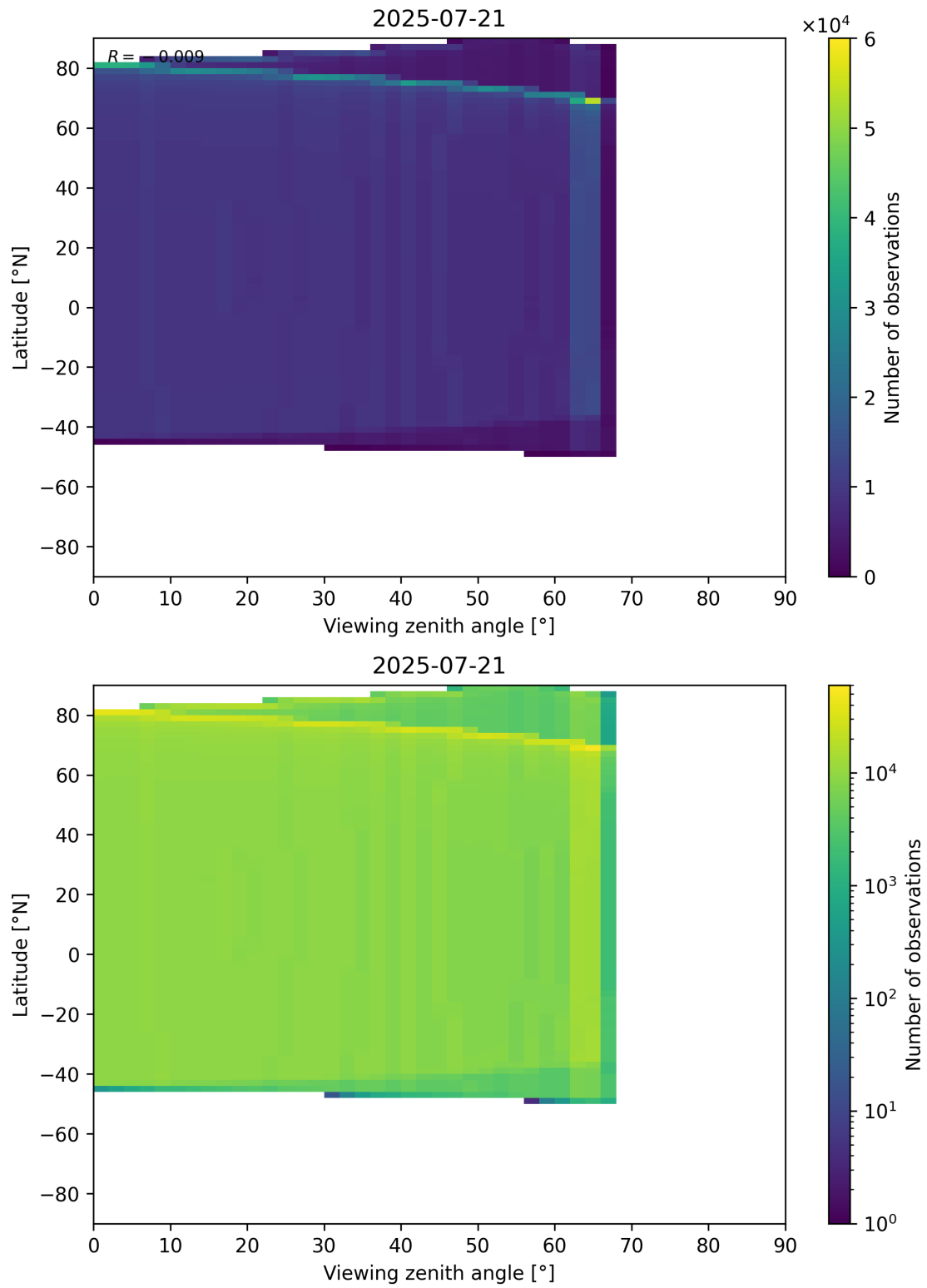
Figure 368: Scatter density plot of “Viewing zenith angle” against “Latitude” for 2025-07-20 to 2025-07-22.
