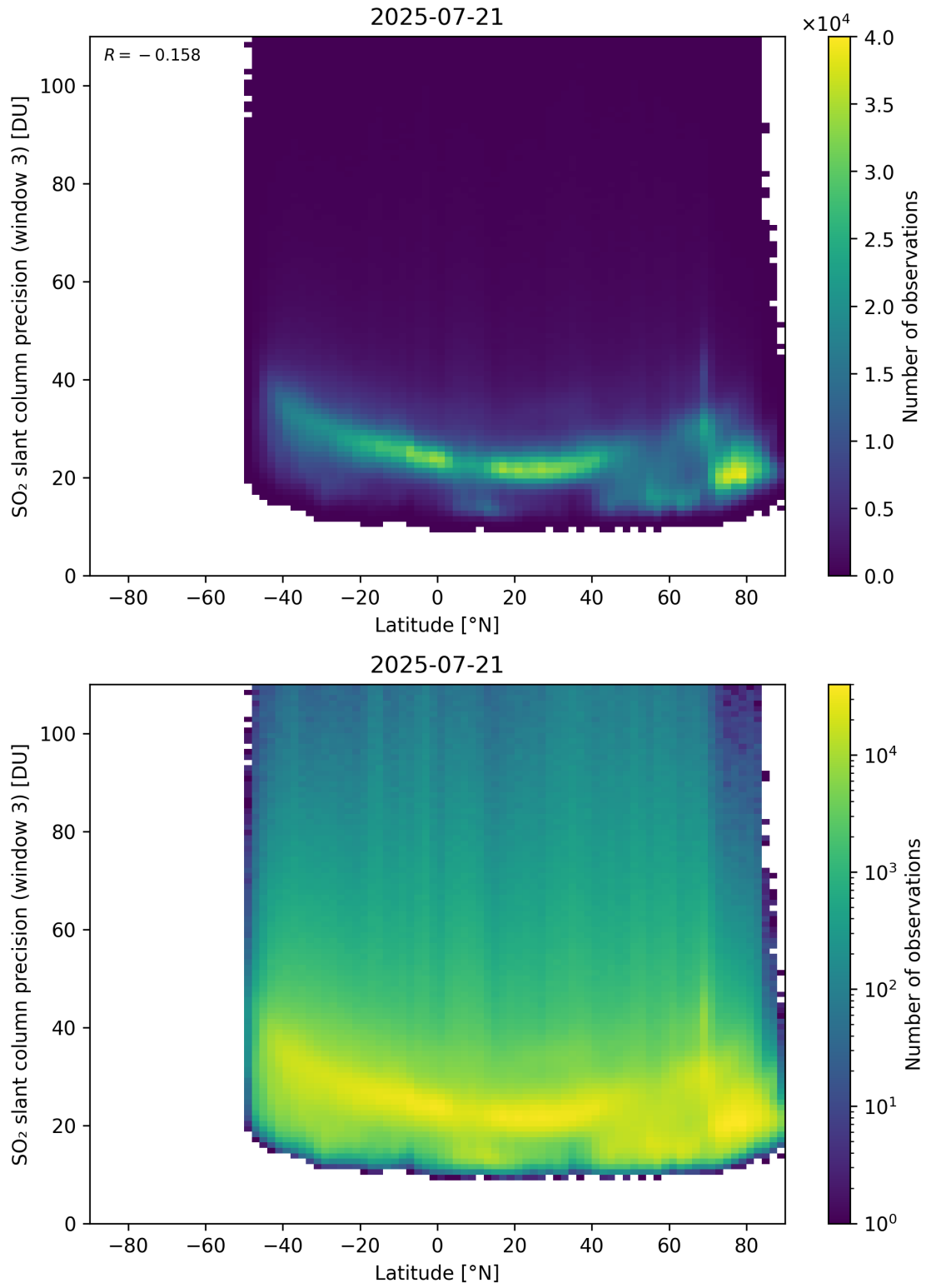
Figure 166: Scatter density plot of “Latitude” against “SO 2 slant column precision (window 3)” for 2025-07-20 to 2025-07-22.
