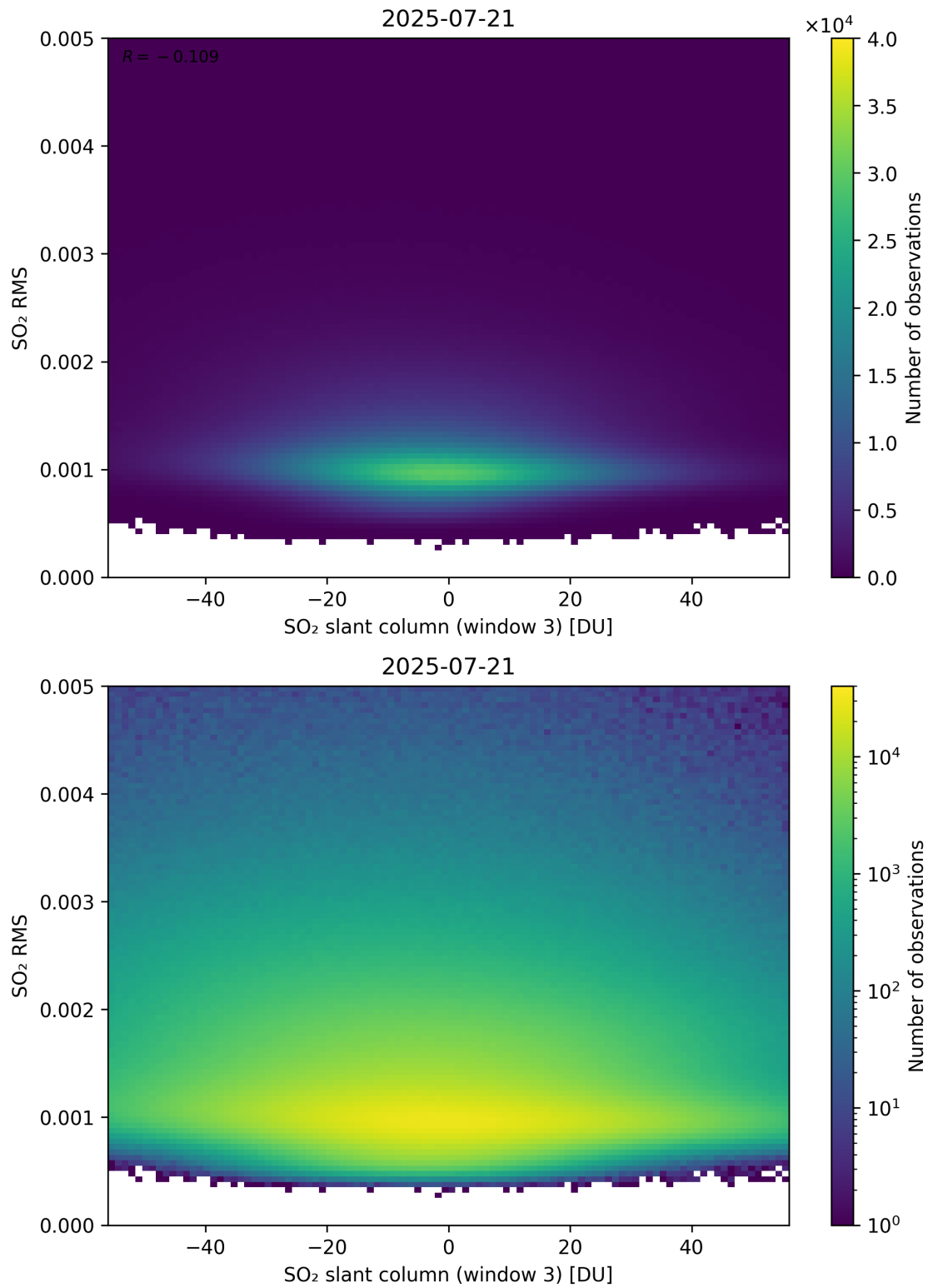
Figure 306: Scatter density plot of “SO 2 slant column (window 3)” against “SO 2 RMS” for 2025-07-20 to 2025-07-22.
