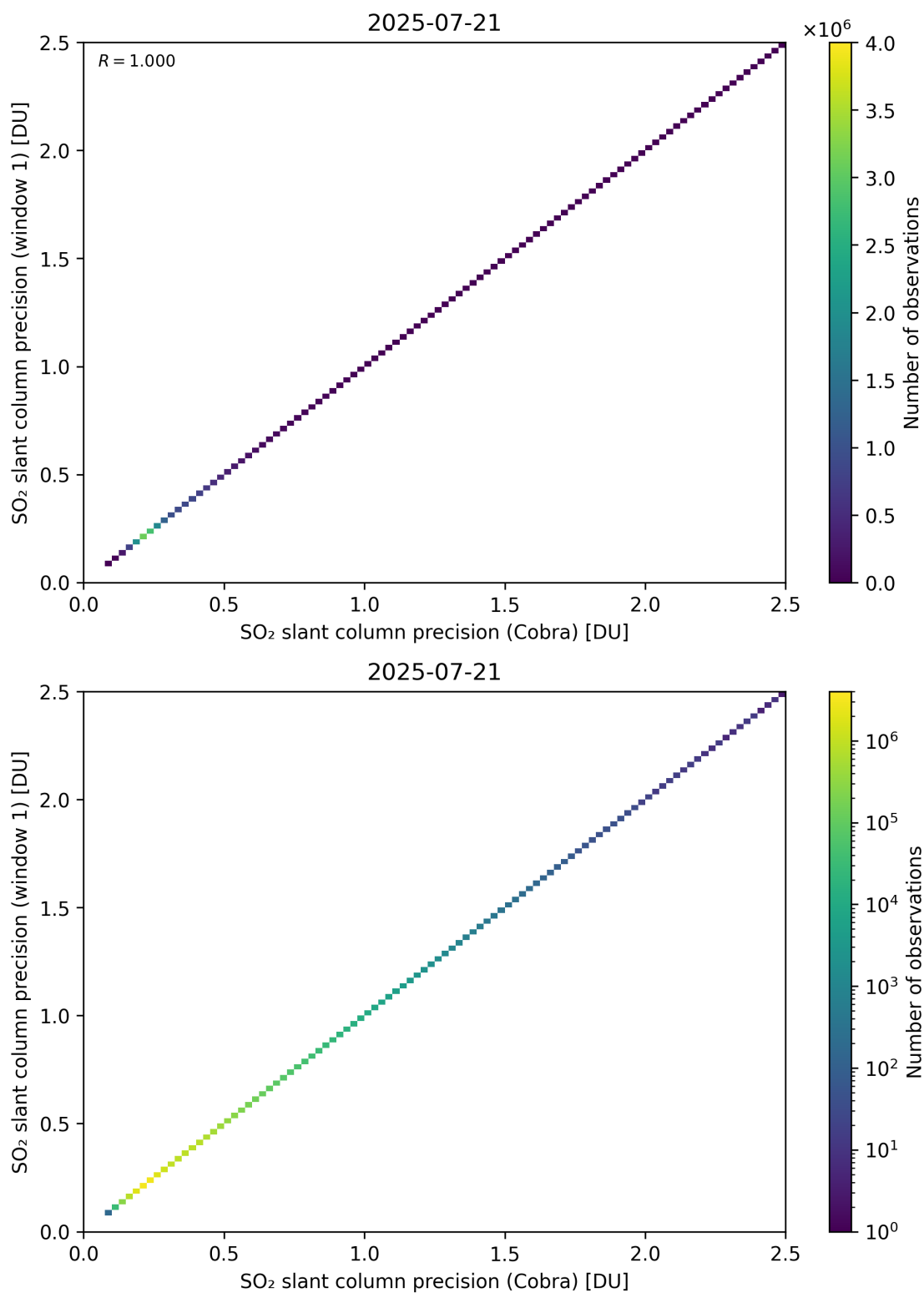
Figure 209: Scatter density plot of “SO 2 slant column precision (Cobra)” against “SO 2 slant column precision (window 1)” for 2025-07-20 to 2025-07-22.
