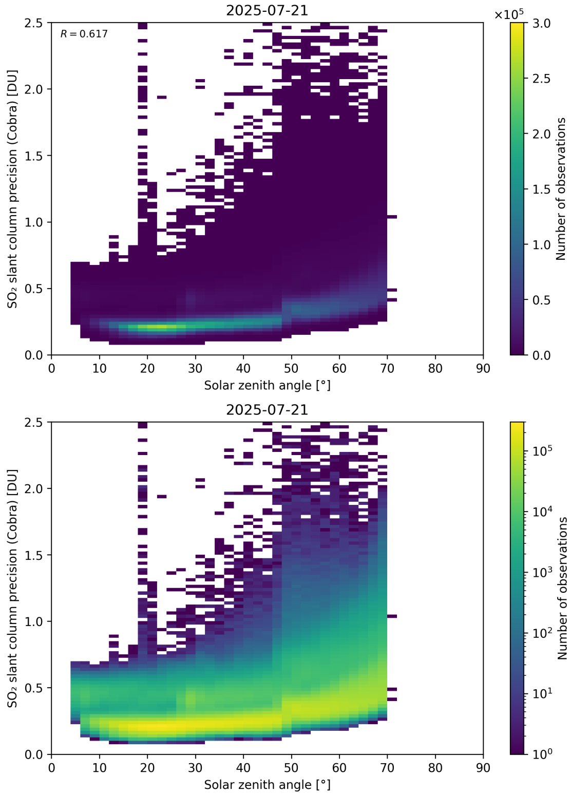
Figure 180: Scatter density plot of “Solar zenith angle” against “SO 2 slant column precision (Cobra)” for 2025-07-20 to 2025-07-22.
