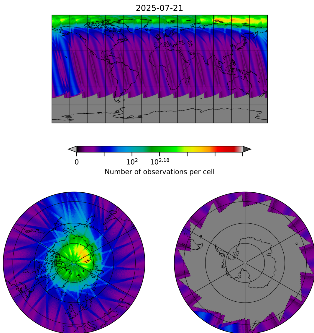
Figure 30: Map of the number of observations for 2025-07-20 to 2025-07-22
