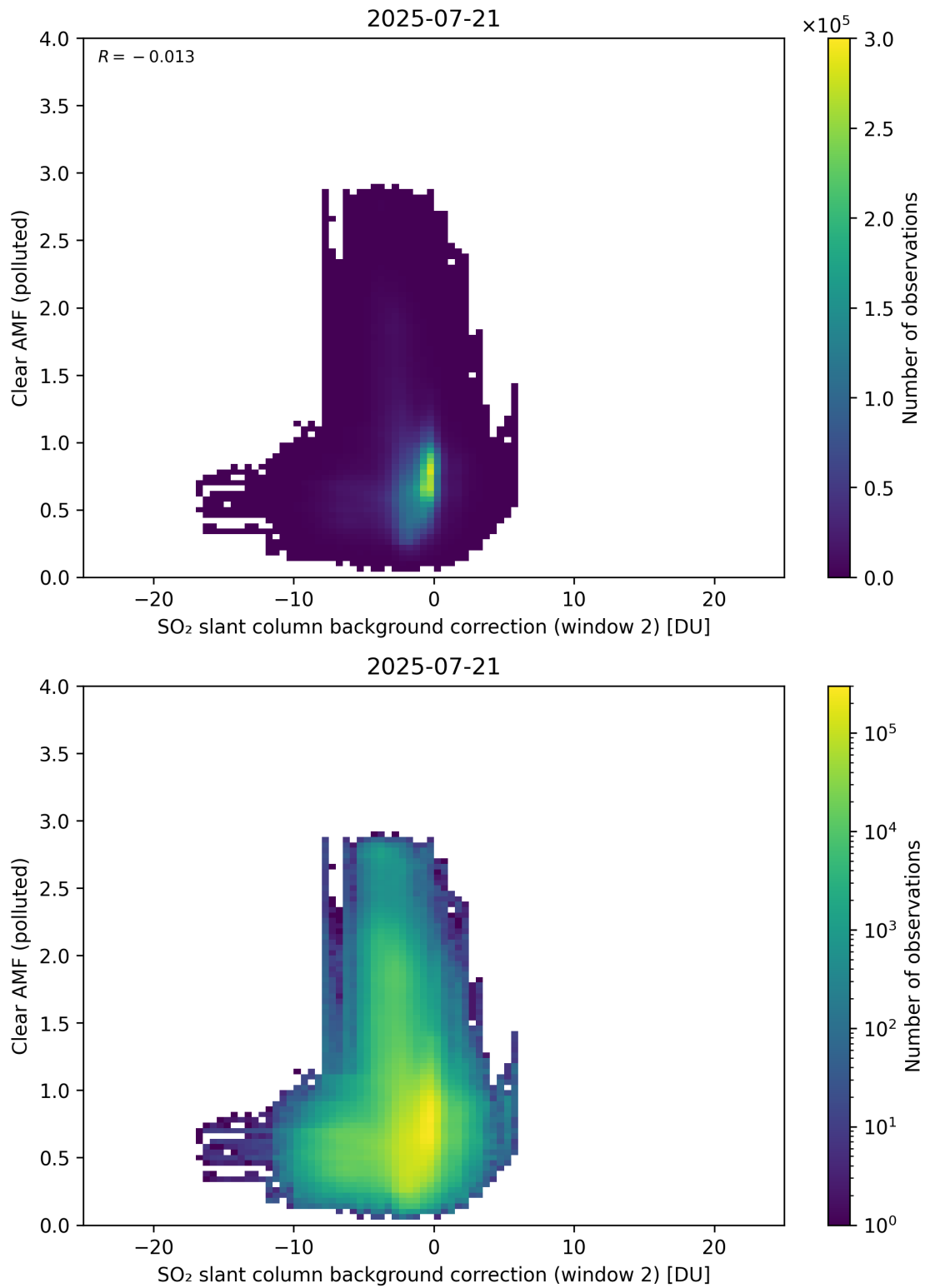
Figure 126: Scatter density plot of “SO 2 slant column background correction (window 2)” against “Clear AMF (polluted)” for 2025-07-20 to 2025-07-22.
