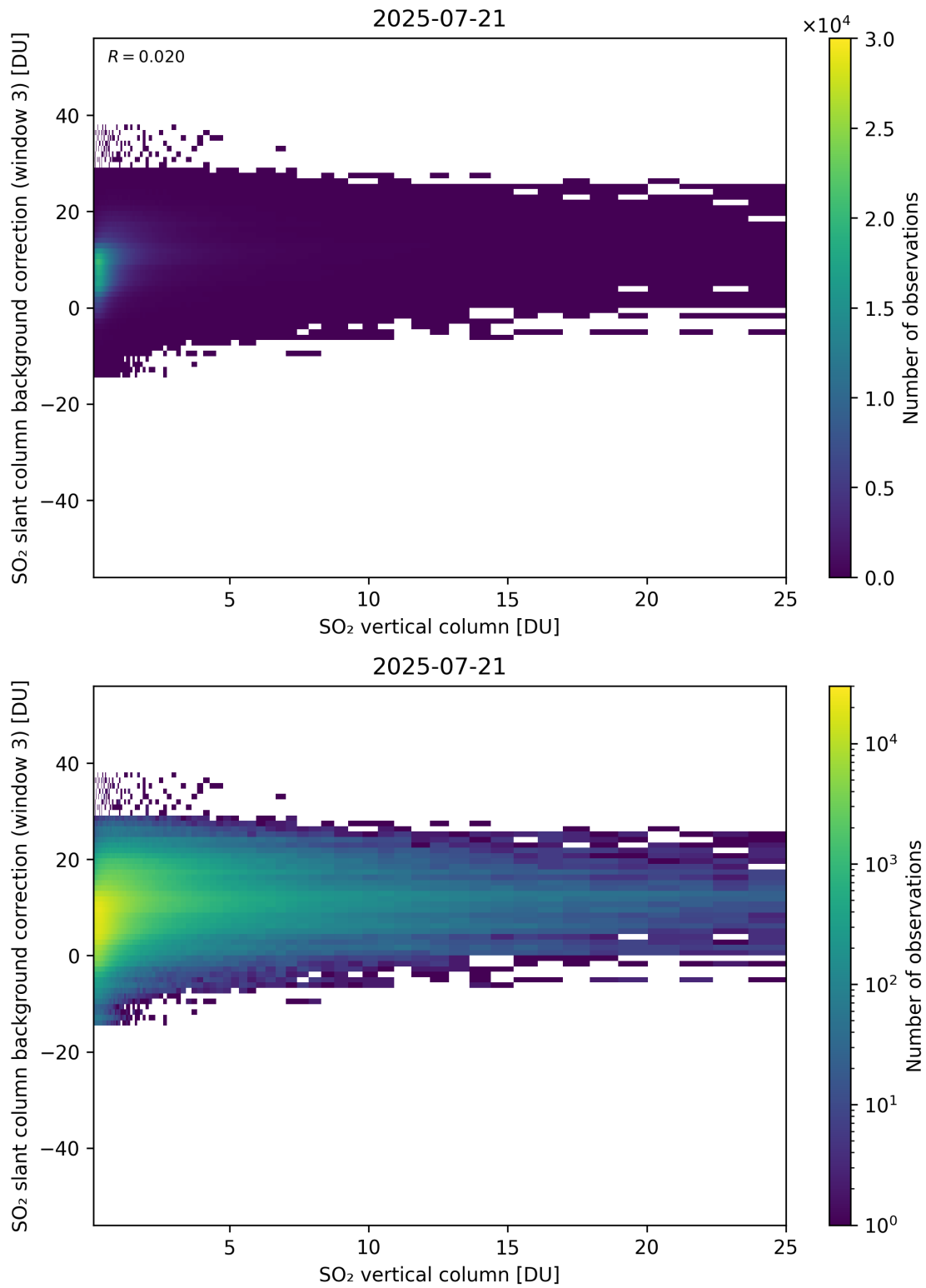
Figure 325: Scatter density plot of “SO 2 vertical column” against “SO 2 slant column background correction (window 3)” for 2025-07-20 to 2025-07-22.
