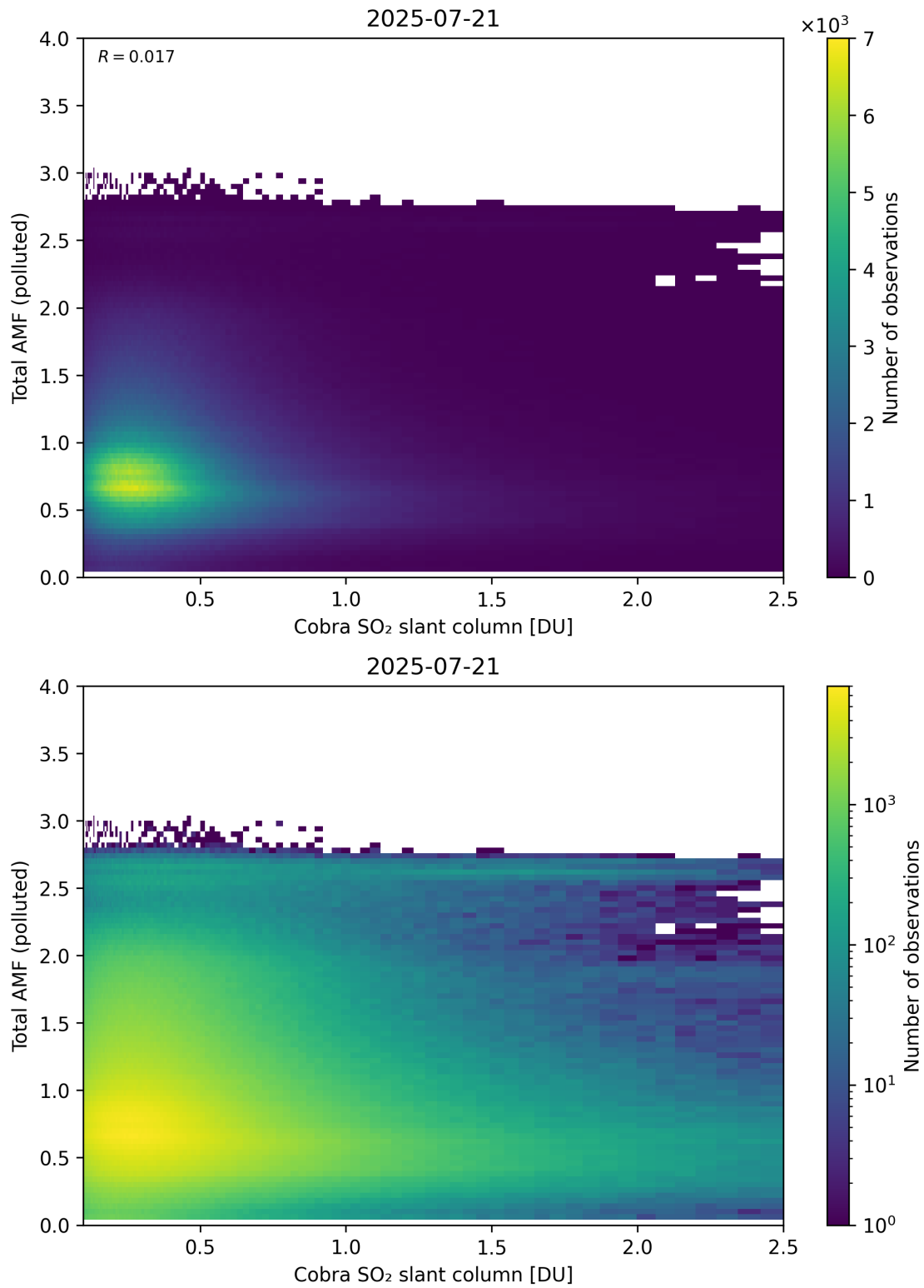
Figure 224: Scatter density plot of “Cobra SO 2 slant column” against “Total AMF (polluted)” for 2025-07-20 to 2025-07-22.
