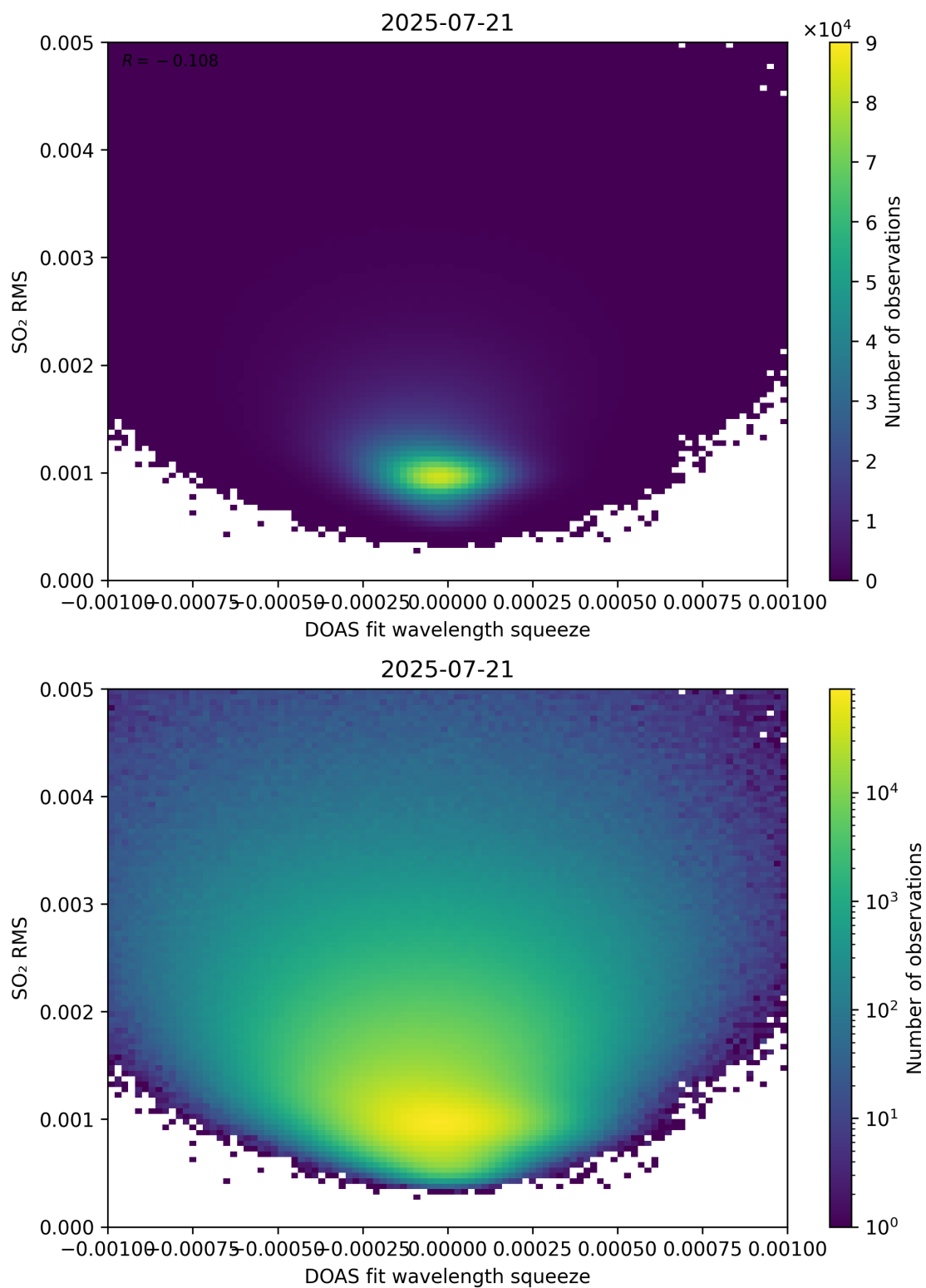
Figure 143: Scatter density plot of “DOAS fit wavelength squeeze” against “SO 2 RMS” for 2025-07-20 to 2025-07-22.
