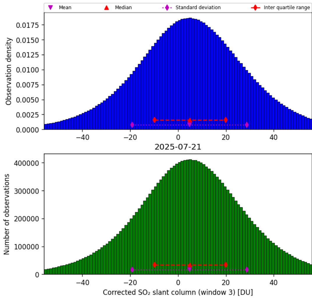
Figure 73: Histogram of “Corrected SO 2 slant column (window 3)” for 2025-07-20 to 2025-07-22
