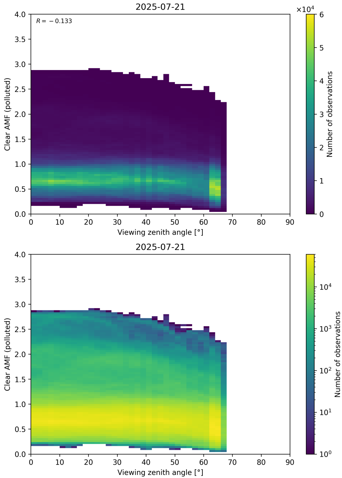
Figure 370: Scatter density plot of “Viewing zenith angle” against “Clear AMF (polluted)” for 2025-07-20 to 2025-07-22.
