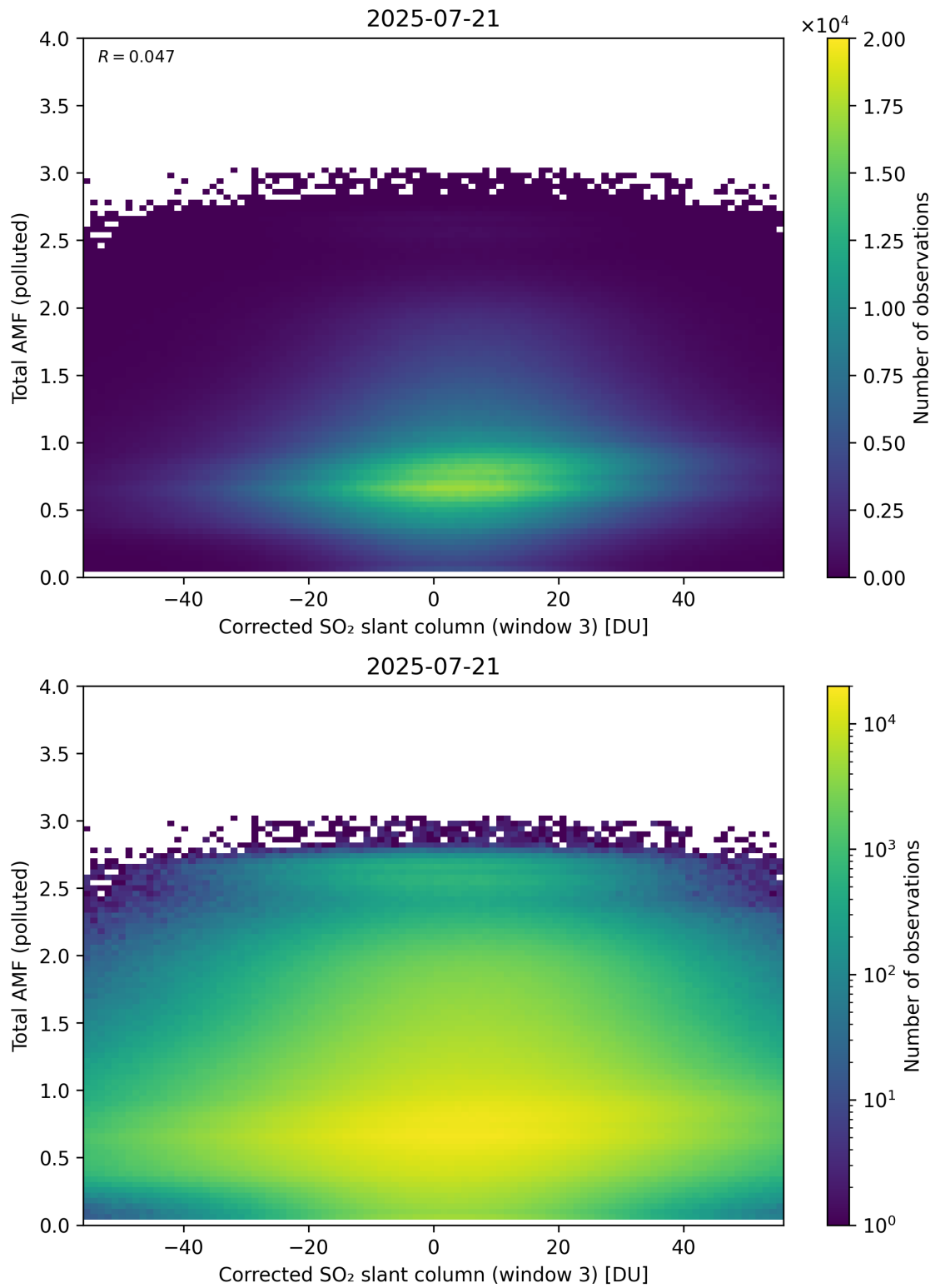
Figure 260: Scatter density plot of “Corrected SO 2 slant column (window 3)” against “Total AMF (polluted)” for 2025-07-20 to 2025-07-22.
