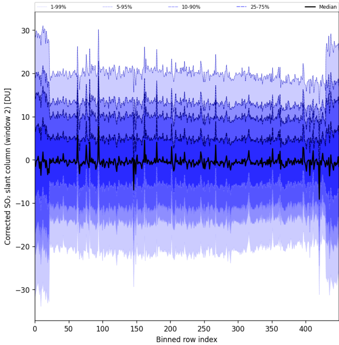
Figure 95: Along track statistics of “Corrected SO 2 slant column (window 2)” for 2025-07-20 to 2025-07-22
