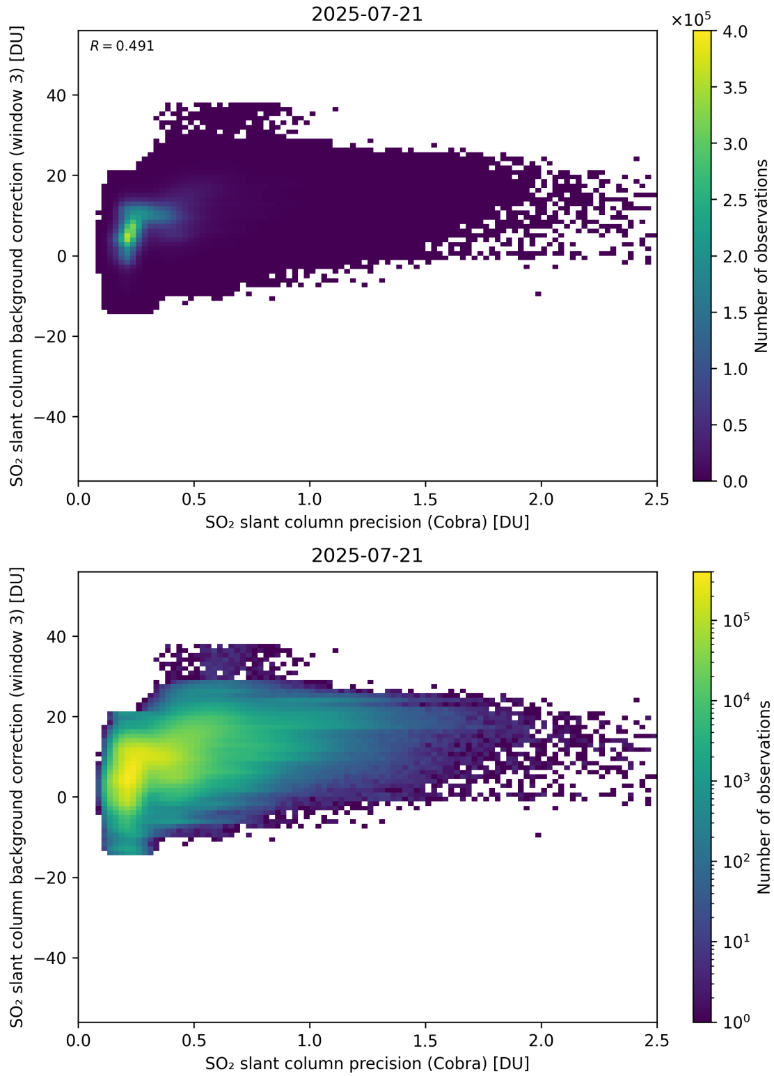
Figure 201: Scatter density plot of “SO 2 slant column precision (Cobra)” against “SO 2 slant column background correction (window 3)” for 2025-07-20 to 2025-07-22.
