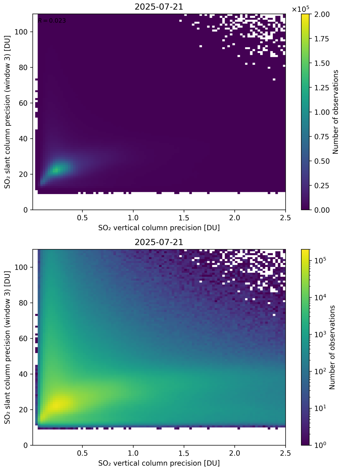
Figure 345: Scatter density plot of “SO 2 vertical column precision” against “SO 2 slant column precision (window 3)” for 2025-07-20 to 2025-07-22.
