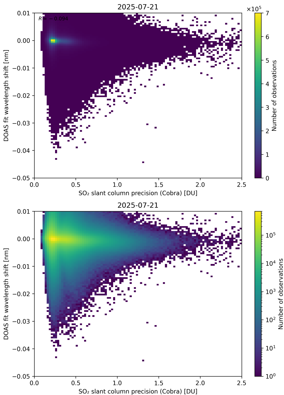
Figure 202: Scatter density plot of “SO 2 slant column precision (Cobra)” against “DOAS fit wavelength shift” for 2025-07-20 to 2025-07-22.
