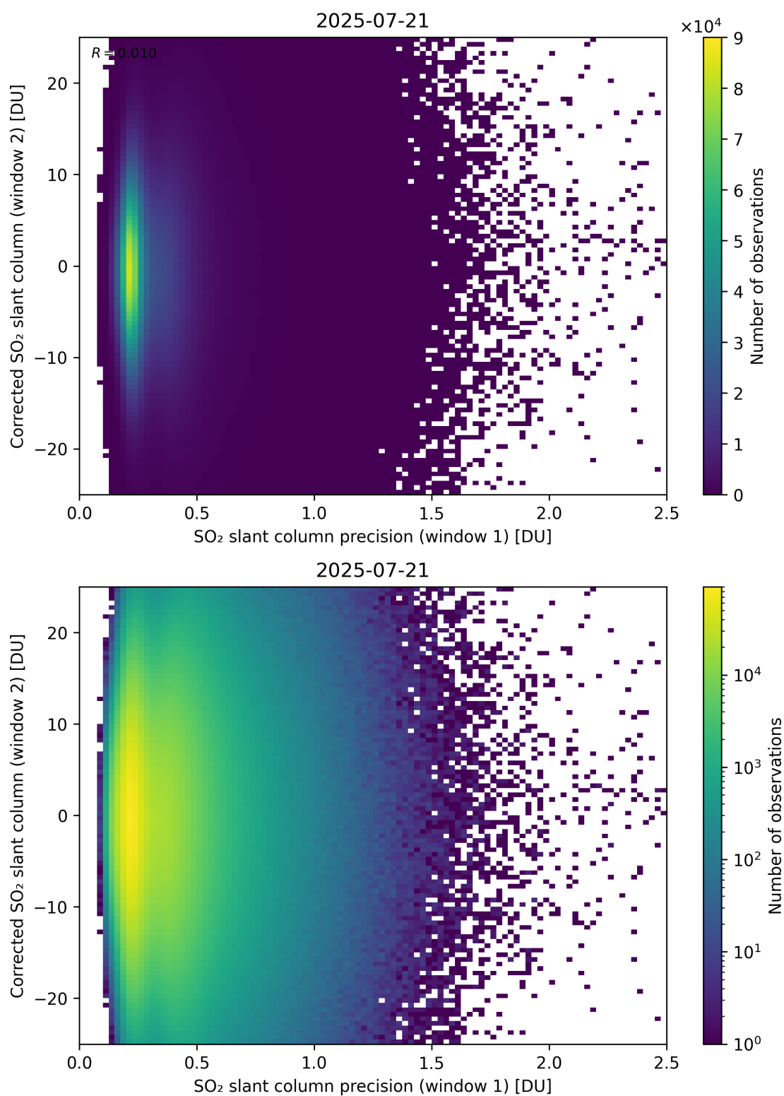
Figure 275: Scatter density plot of “SO 2 slant column precision (window 1)” against “Corrected SO 2 slant column (window 2)” for 2025-07-20 to 2025-07-22.
