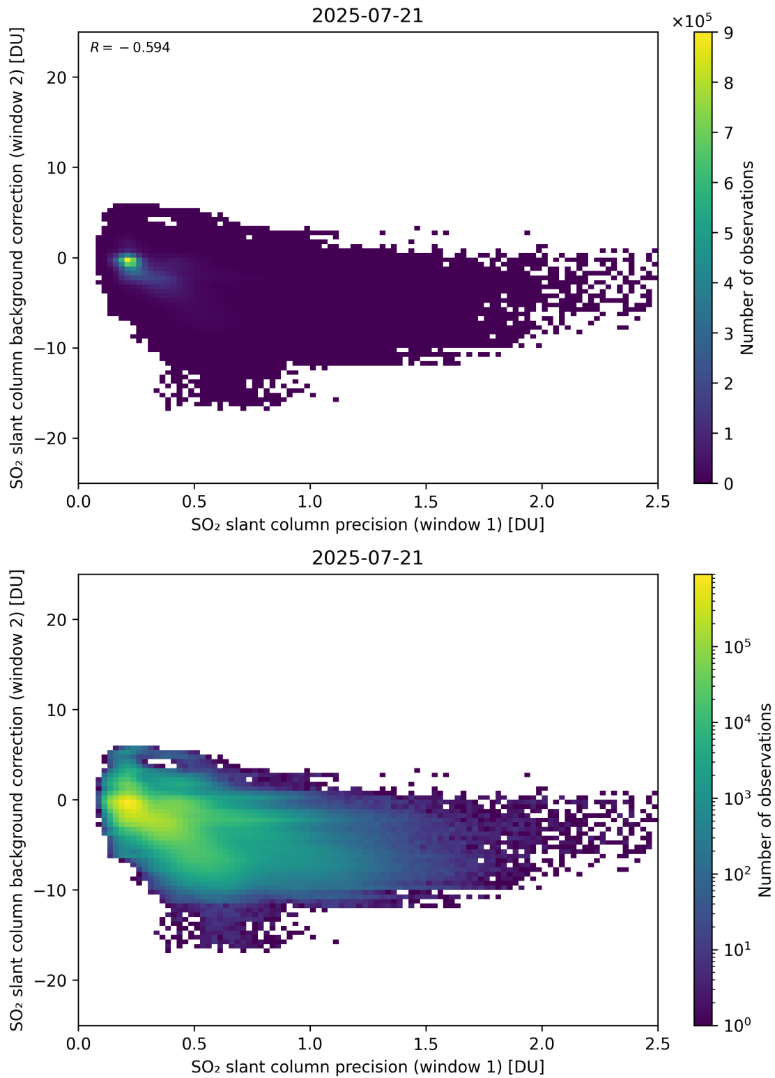
Figure 269: Scatter density plot of “SO 2 slant column precision (window 1)” against “SO 2 slant column background correction (window 2)” for 2025-07-20 to 2025-07-22.
