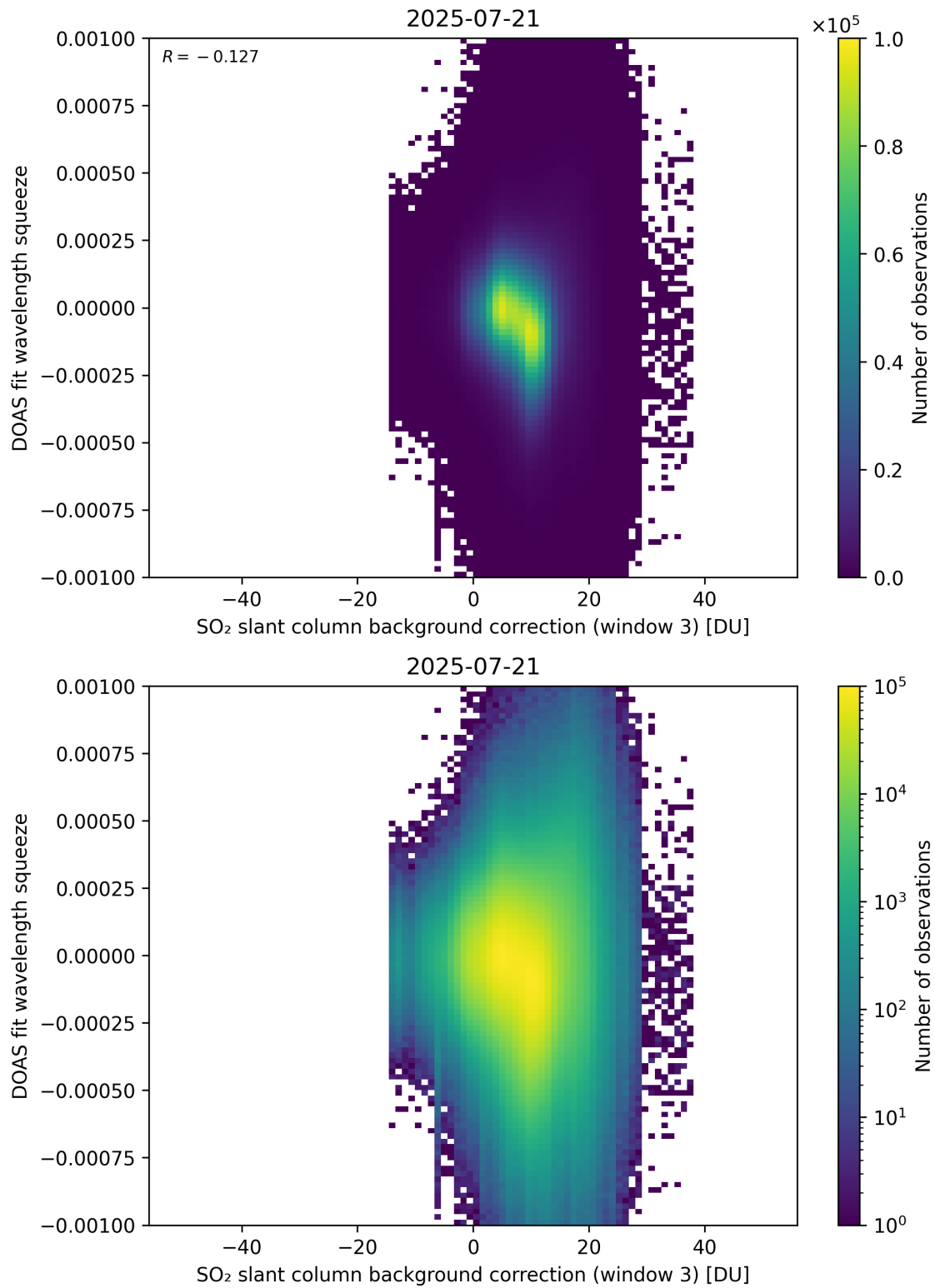
Figure 133: Scatter density plot of “SO 2 slant column background correction (window 3)” against “DOAS fit wavelength squeeze” for 2025-07-20 to 2025-07-22.
