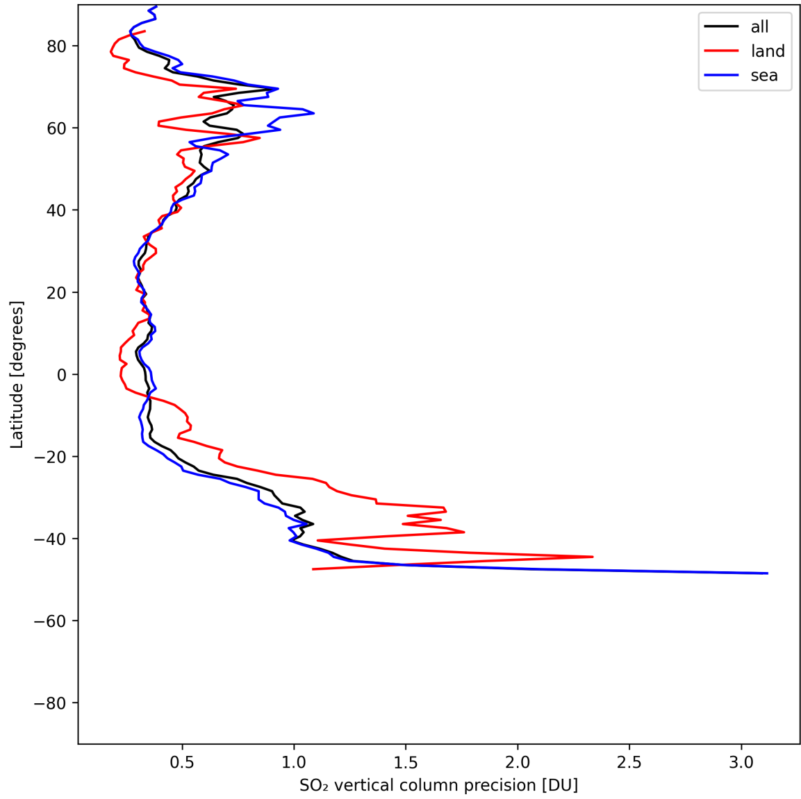
Figure 33: Zonal average of “SO 2 vertical column precision” for 2025-07-20 to 2025-07-22.
