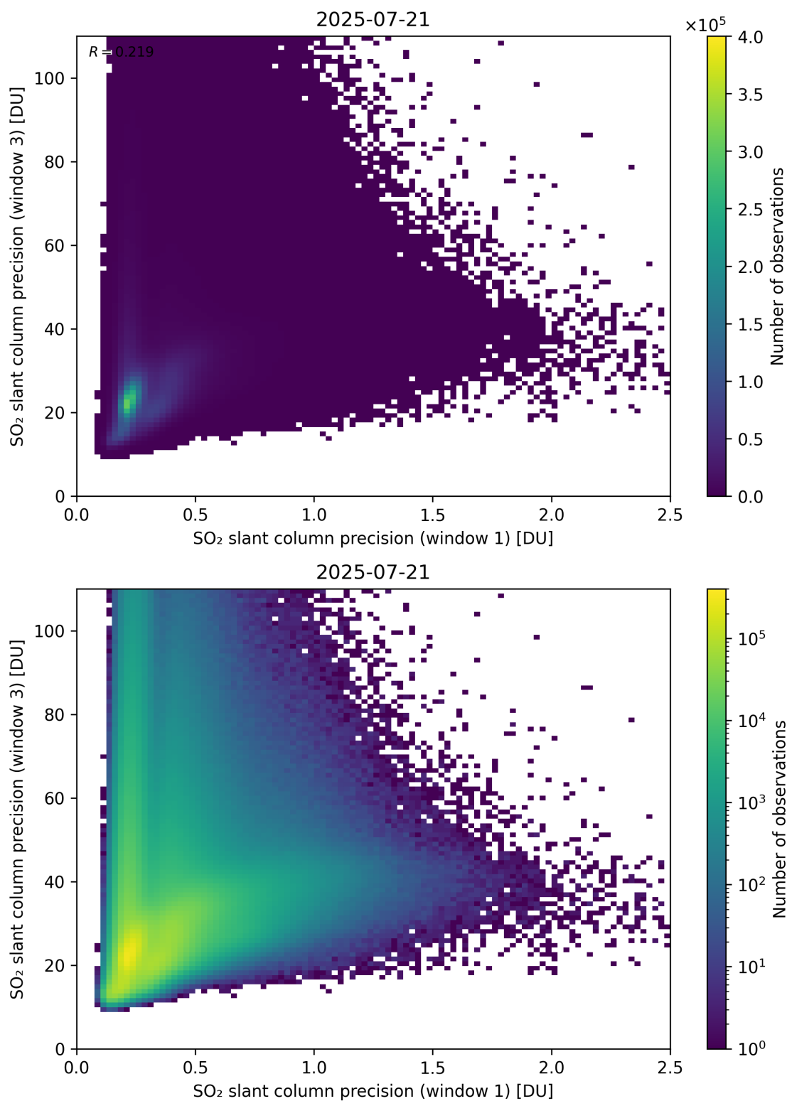
Figure 279: Scatter density plot of “SO 2 slant column precision (window 1)” against “SO 2 slant column precision (window 3)” for 2025-07-20 to 2025-07-22.
