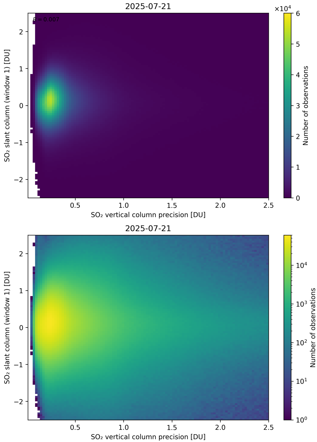
Figure 341: Scatter density plot of “SO 2 vertical column precision” against “SO 2 slant column (window 1)” for 2025-07-20 to 2025-07-22.
