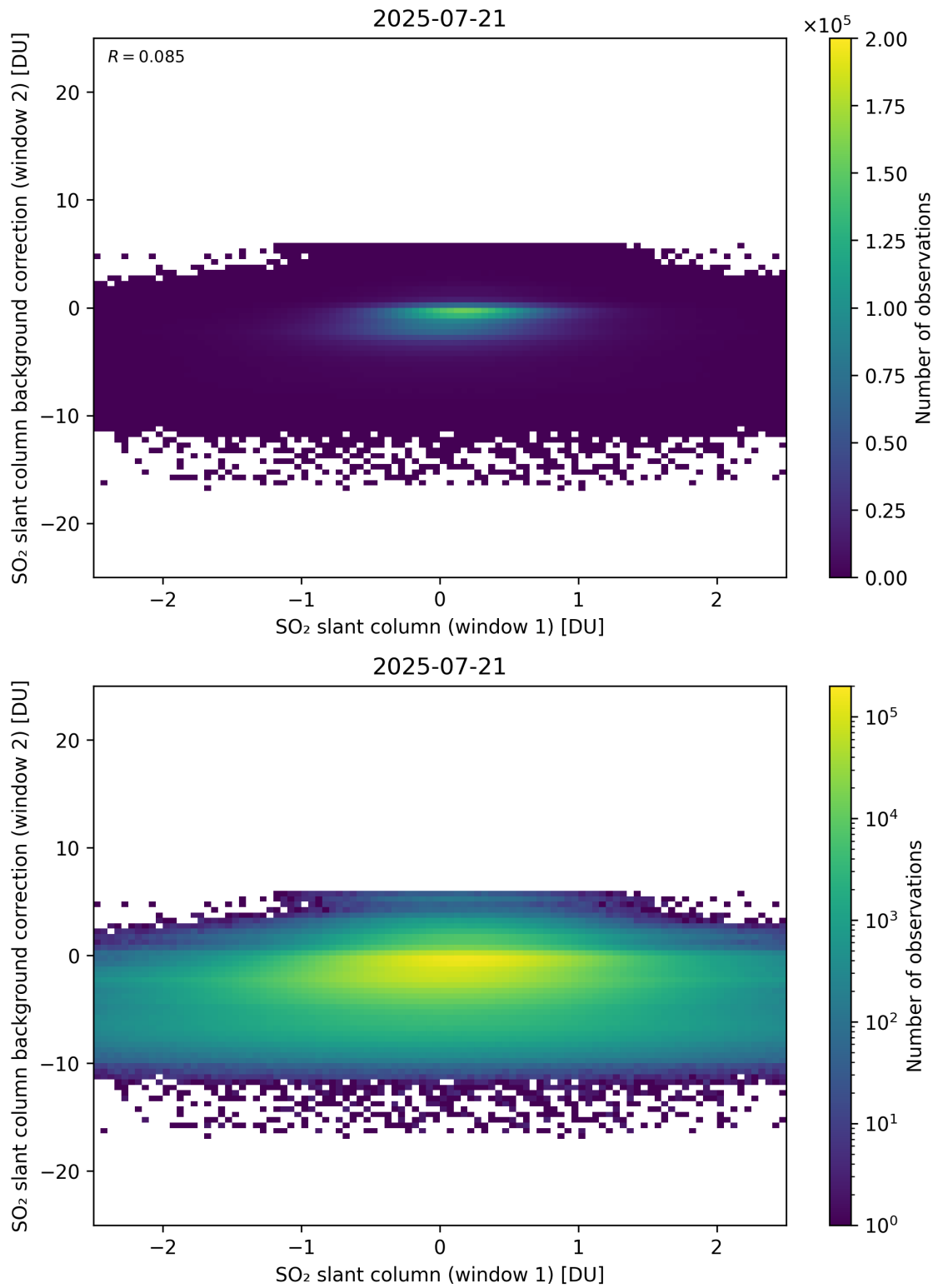
Figure 263: Scatter density plot of “SO 2 slant column (window 1)” against “SO 2 slant column background correction (window 2)” for 2025-07-20 to 2025-07-22.
