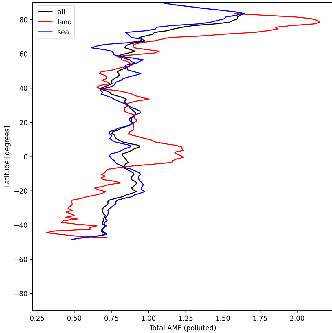
Figure 53: Zonal average of “Total AMF (polluted)” for 2025-07-20 to 2025-07-22.
