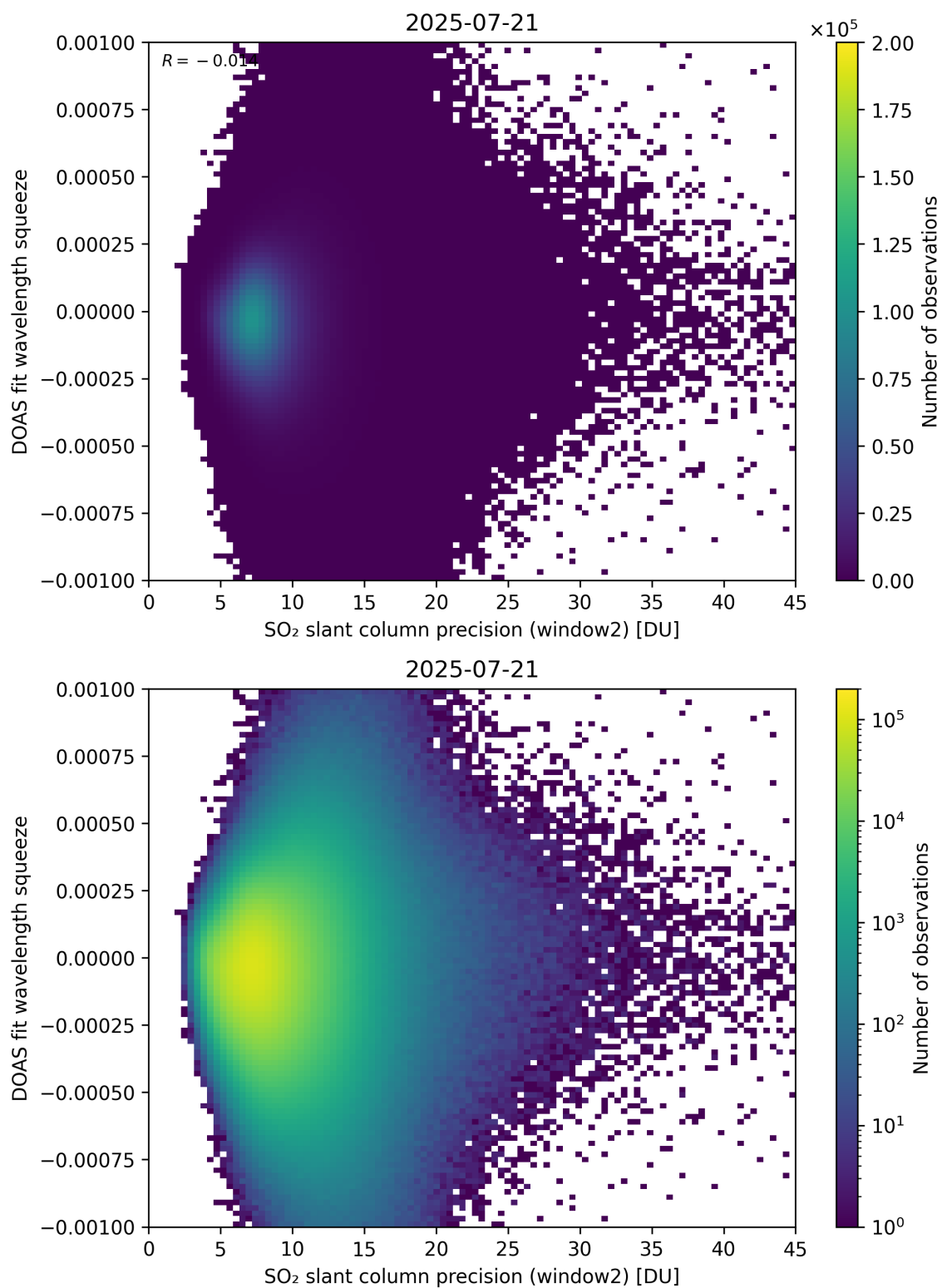
Figure 294: Scatter density plot of “SO 2 slant column precision (window2)” against “DOAS fit wavelength squeeze” for 2025-07-20 to 2025-07-22.
