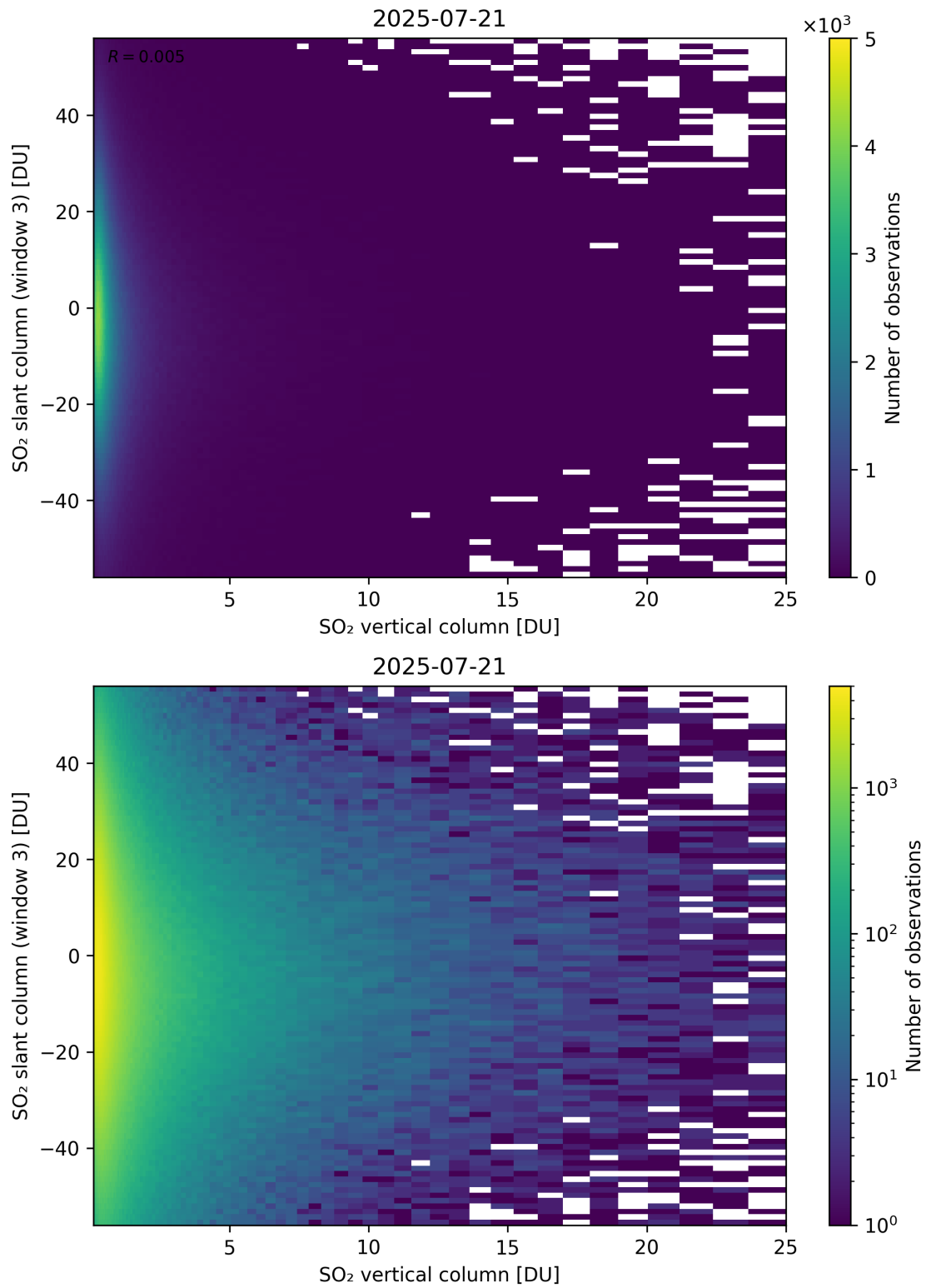
Figure 357: Scatter density plot of “SO 2 vertical column” against “SO 2 slant column (window 3)” for 2025-07-20 to 2025-07-22.
