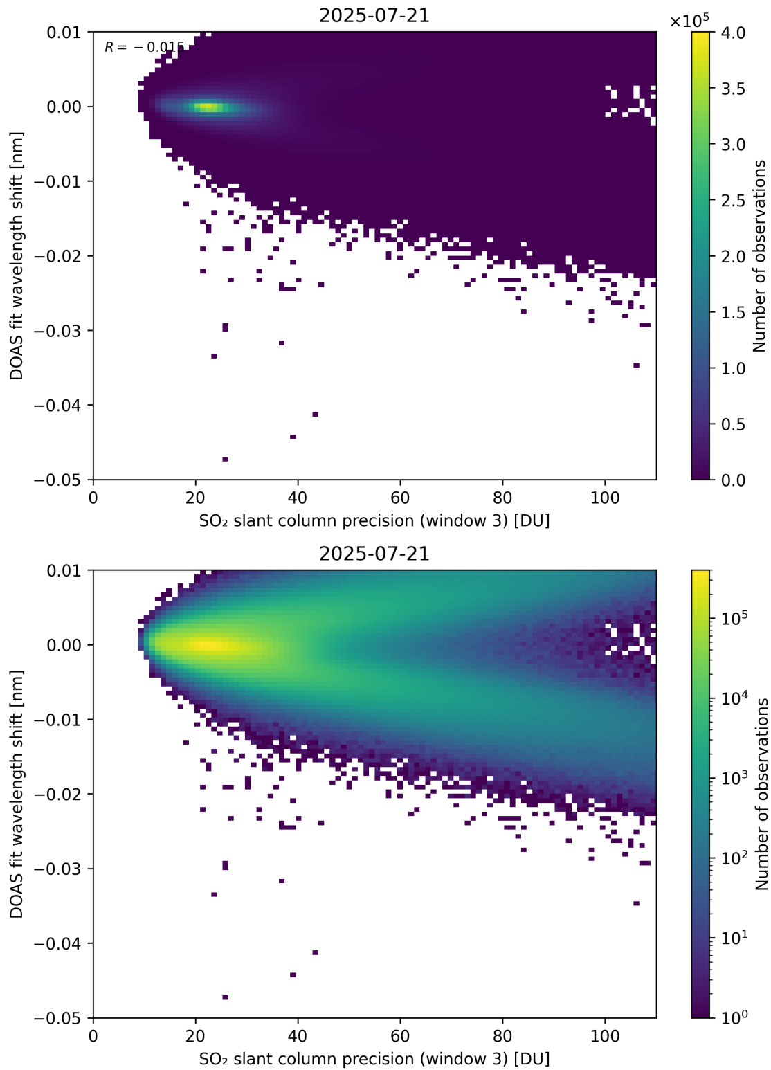
Figure 308: Scatter density plot of “SO 2 slant column precision (window 3)” against “DOAS fit wavelength shift” for 2025-07-20 to 2025-07-22.
