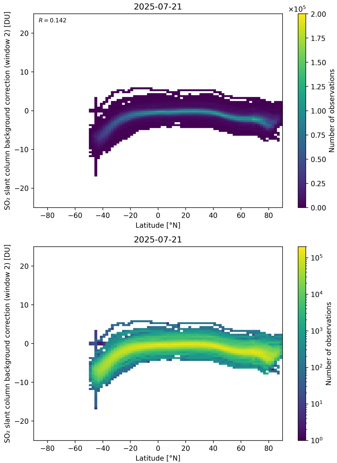
Figure 151: Scatter density plot of “Latitude” against “SO 2 slant column background correction (window 2)” for 2025-07-20 to 2025-07-22.
