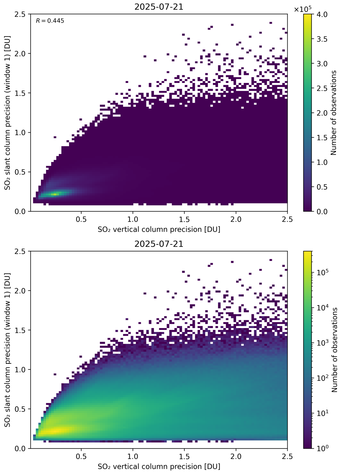
Figure 342: Scatter density plot of “SO 2 vertical column precision” against “SO 2 slant column precision (window 1)” for 2025-07-20 to 2025-07-22.
