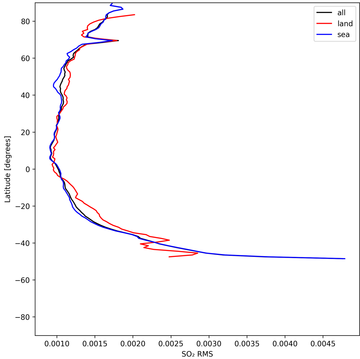
Figure 52: Zonal average of “SO 2 RMS” for 2025-07-20 to 2025-07-22.
