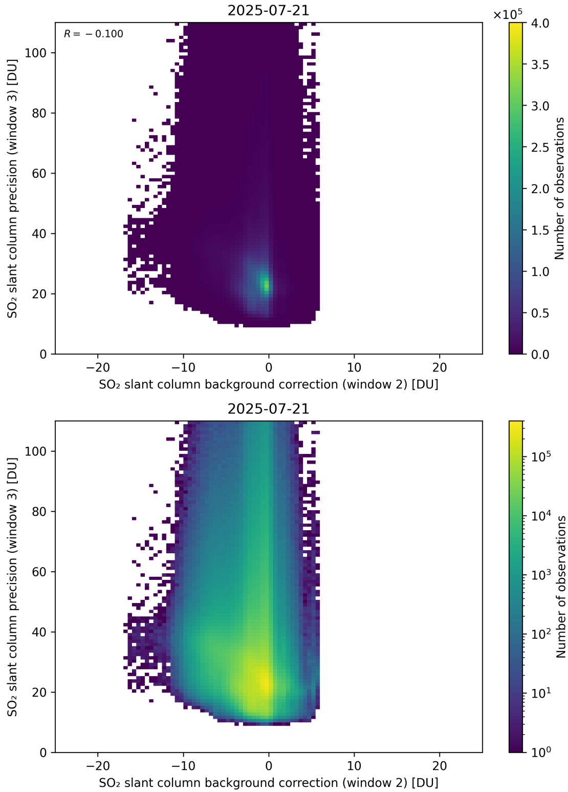
Figure 129: Scatter density plot of “SO 2 slant column background correction (window 2)” against “SO 2 slant column precision (window 3)” for 2025-07-20 to 2025-07-22.
