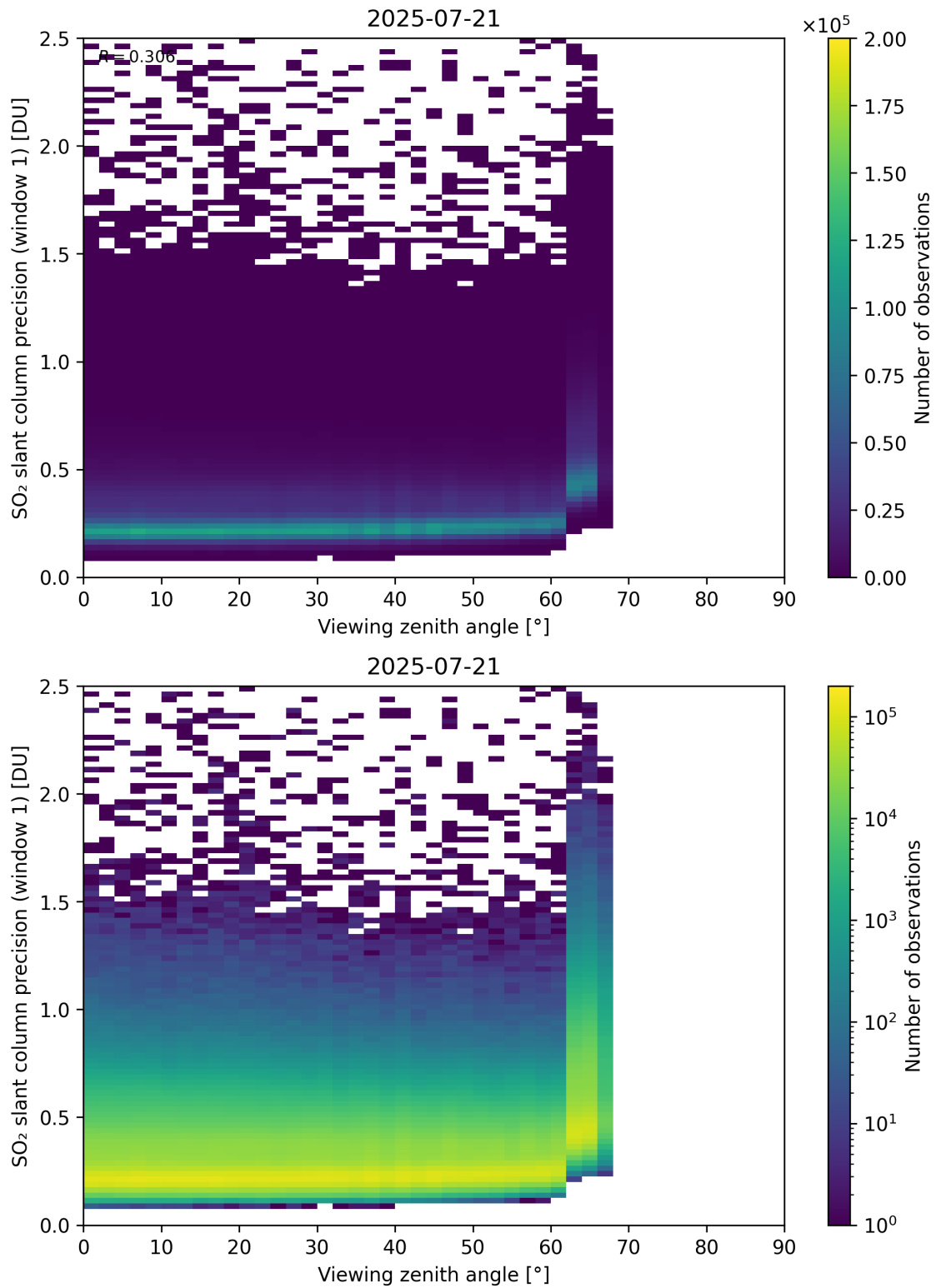
Figure 377: Scatter density plot of “Viewing zenith angle” against “SO 2 slant column precision (window 1)” for 2025-07-20 to 2025-07-22.
