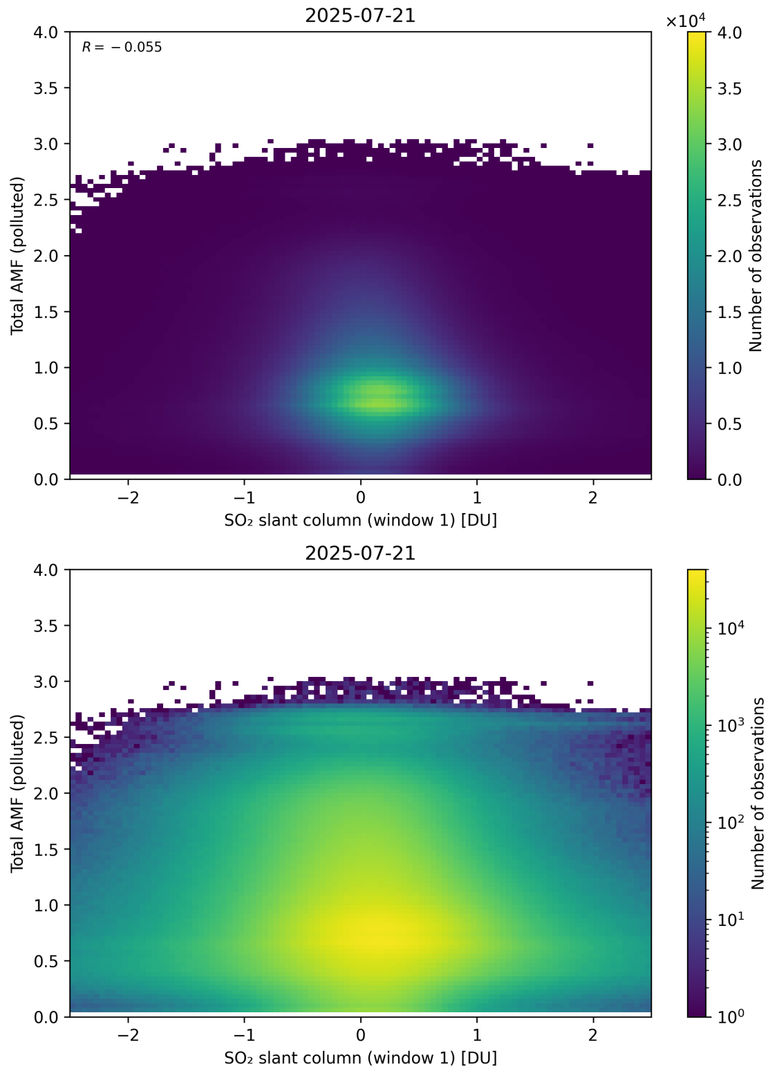
Figure 289: Scatter density plot of “SO 2 slant column (window 1)” against “Total AMF (polluted)” for 2025-07-20 to 2025-07-22.
