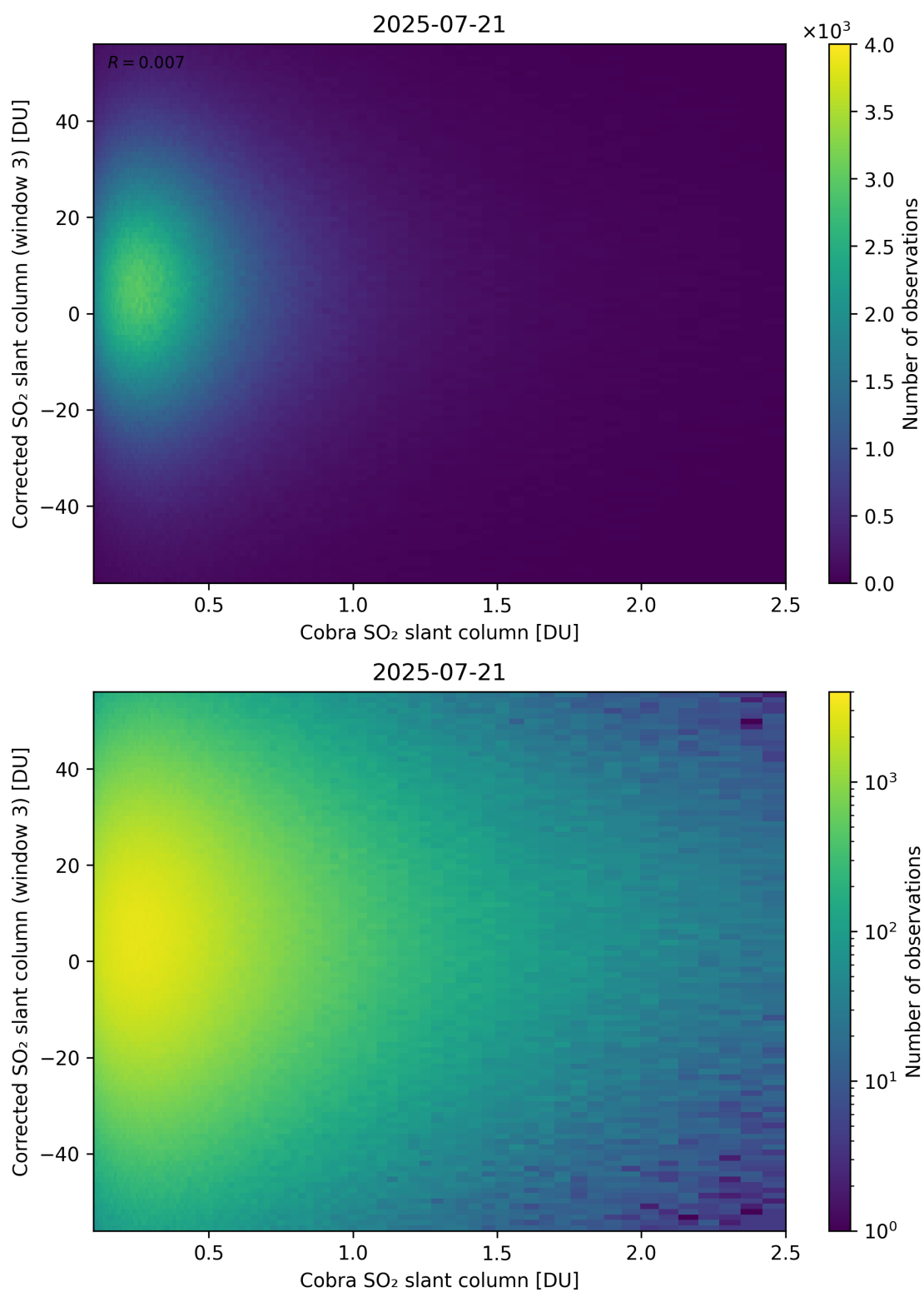
Figure 218: Scatter density plot of “Cobra SO 2 slant column” against “Corrected SO 2 slant column (window 3)” for 2025-07-20 to 2025-07-22.
