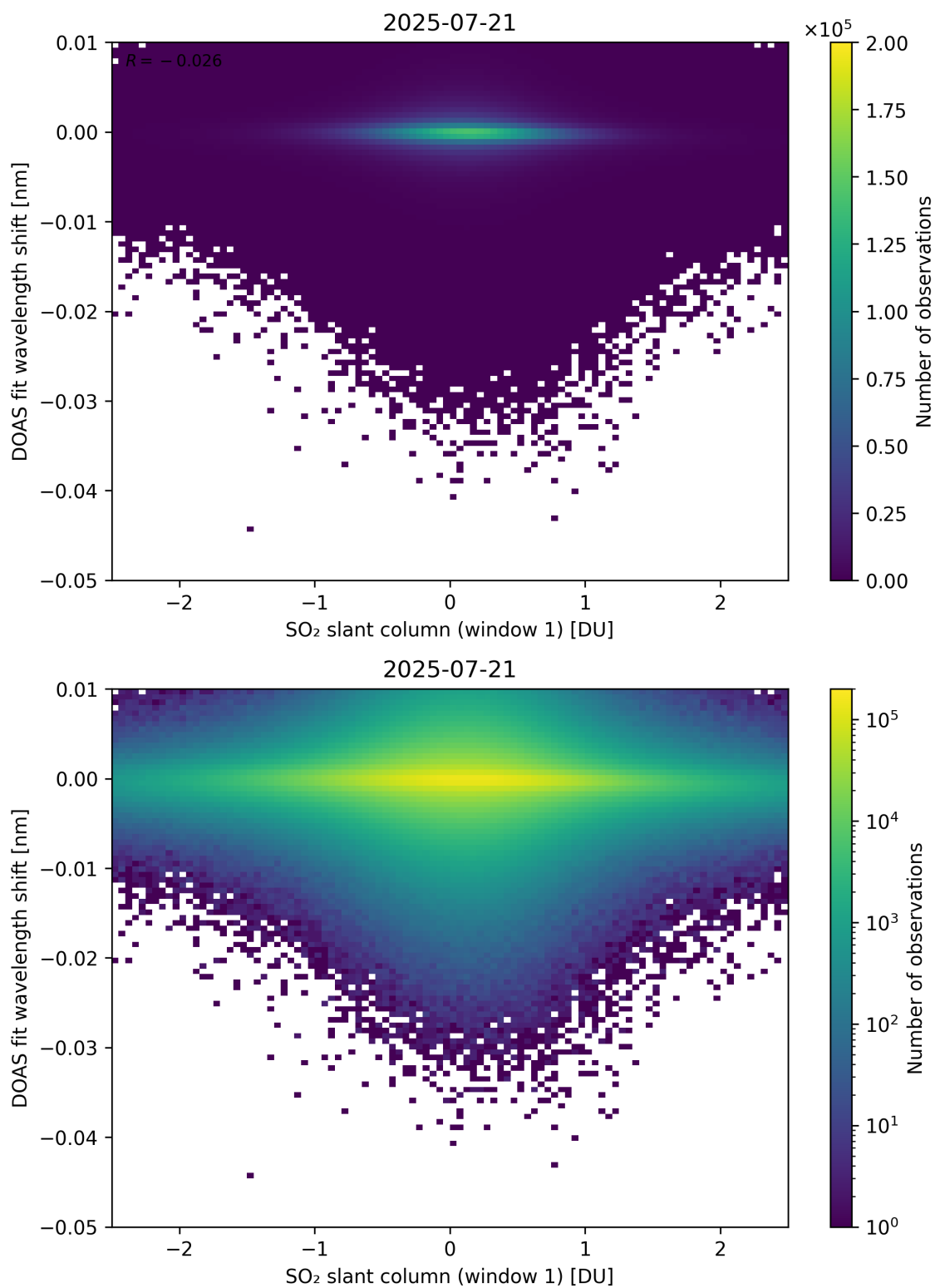
Figure 265: Scatter density plot of “SO 2 slant column (window 1)” against “DOAS fit wavelength shift” for 2025-07-20 to 2025-07-22.
