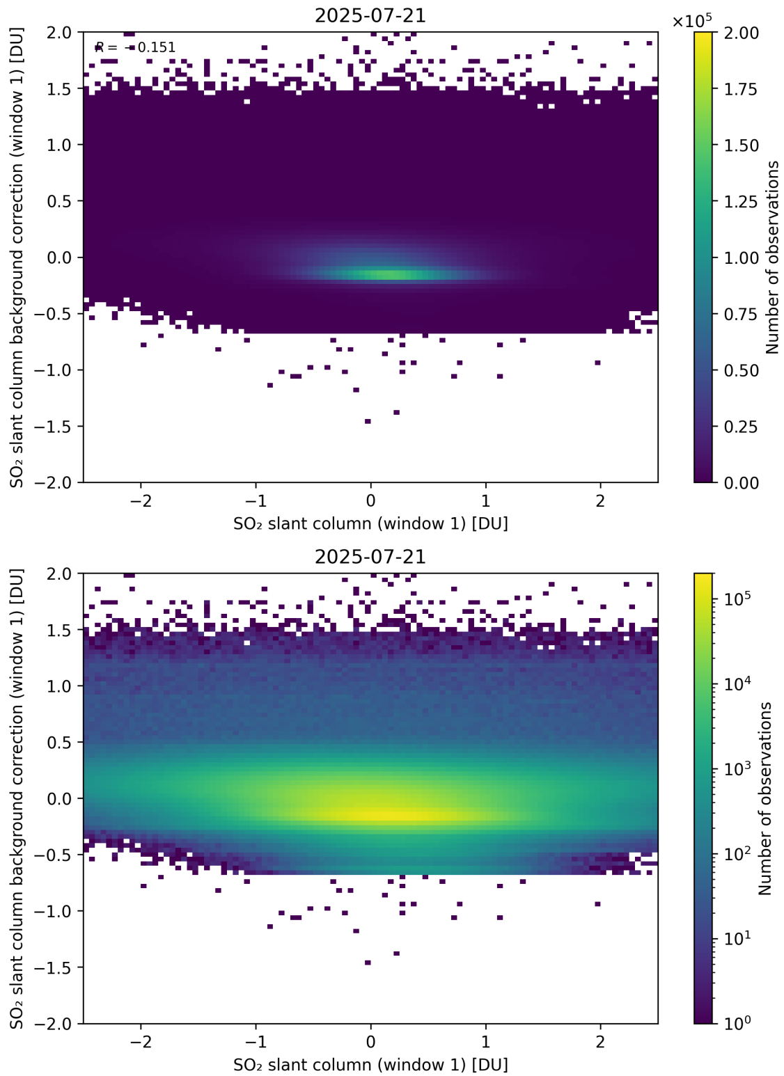
Figure 262: Scatter density plot of “SO 2 slant column (window 1)” against “SO 2 slant column background correction (window 1)” for 2025-07-20 to 2025-07-22.
