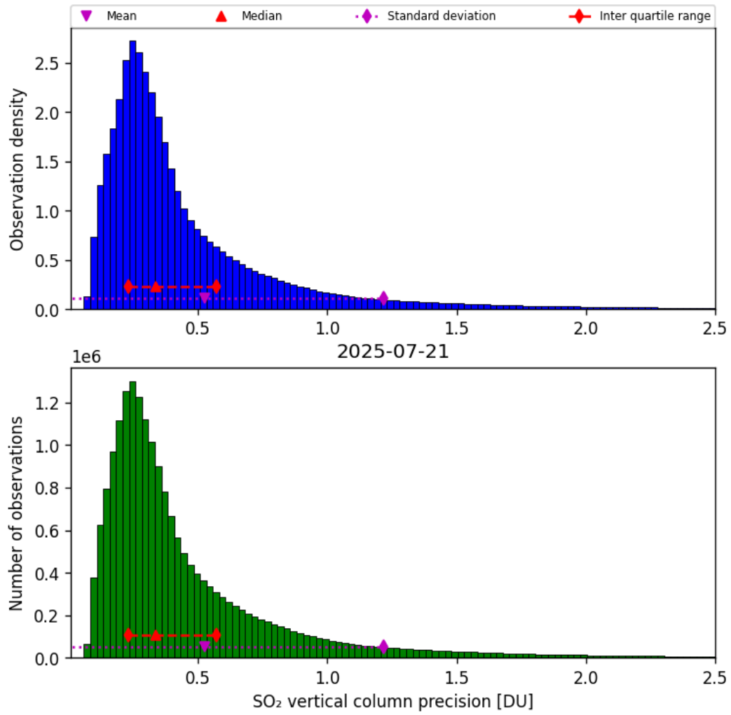
Figure 59: Histogram of “SO 2 vertical column precision” for 2025-07-20 to 2025-07-22
