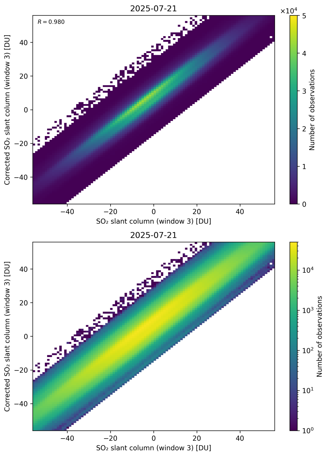
Figure 316: Scatter density plot of “SO 2 slant column (window 3)” against “Corrected SO 2 slant column (window 3)” for 2025-07-20 to 2025-07-22.
