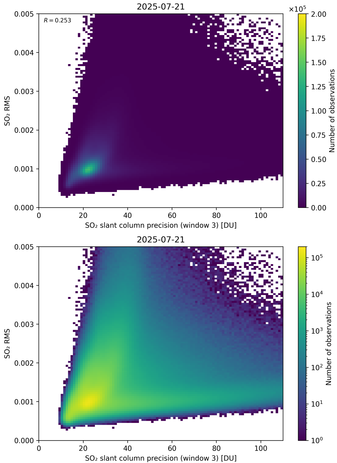
Figure 310: Scatter density plot of “SO 2 slant column precision (window 3)” against “SO 2 RMS” for 2025-07-20 to 2025-07-22.
