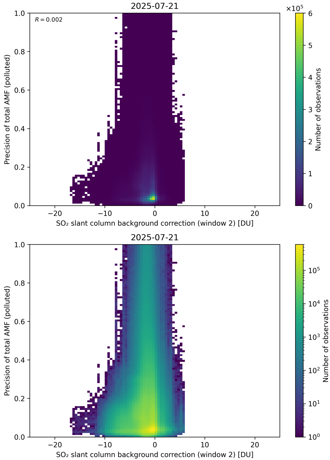
Figure 131: Scatter density plot of “SO 2 slant column background correction (window 2)” against “Precision of total AMF (polluted)” for 2025-07-20 to 2025-07-22.
