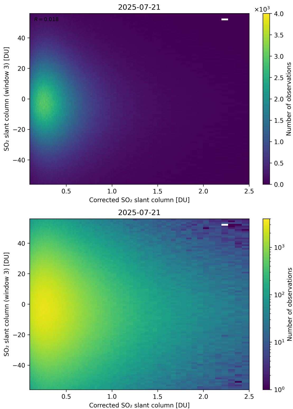
Figure 240: Scatter density plot of “Corrected SO 2 slant column” against “SO 2 slant column (window 3)” for 2025-07-20 to 2025-07-22.
