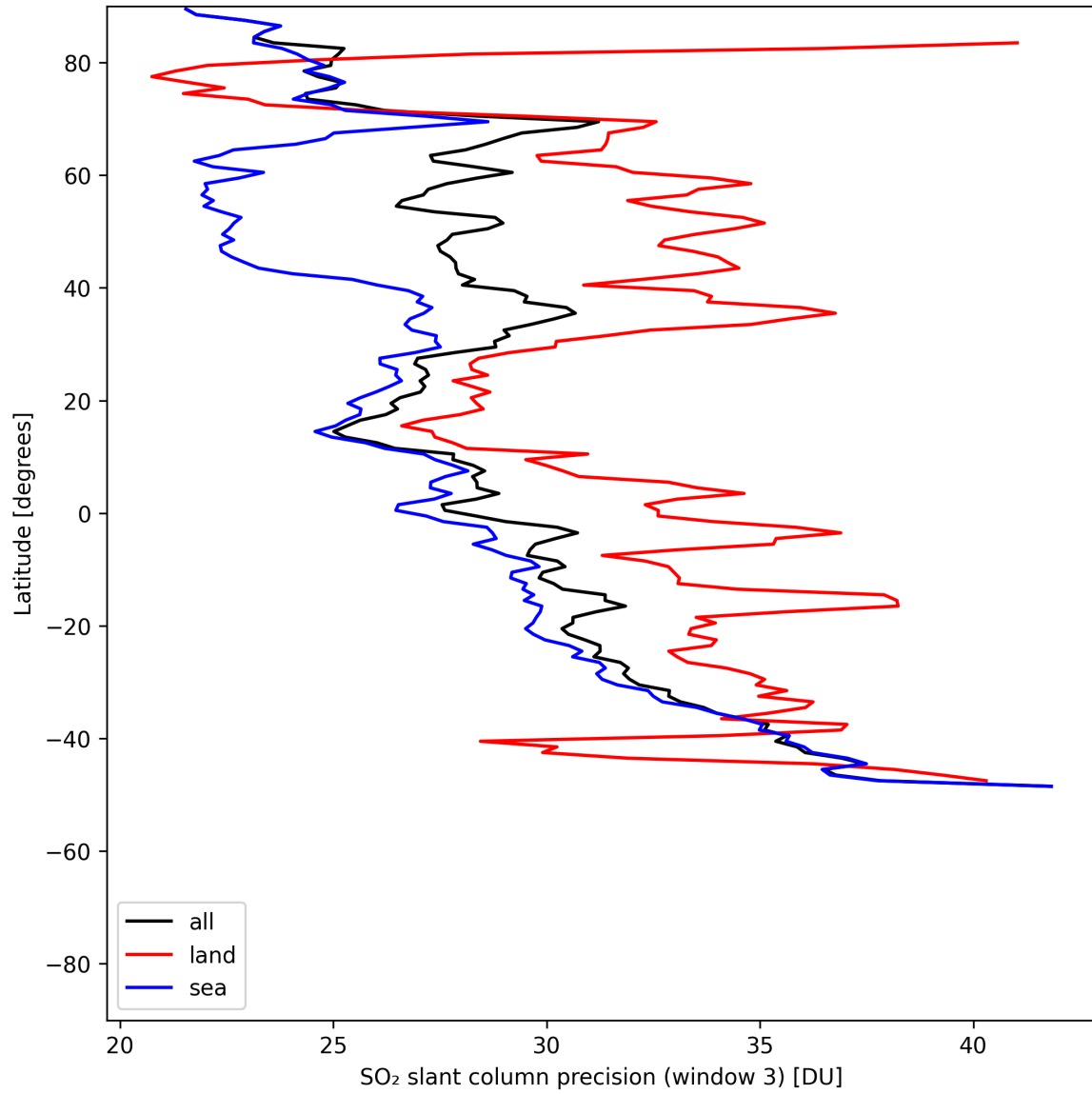
Figure 46: Zonal average of “SO 2 slant column precision (window 3)” for 2025-07-20 to 2025-07-22.
