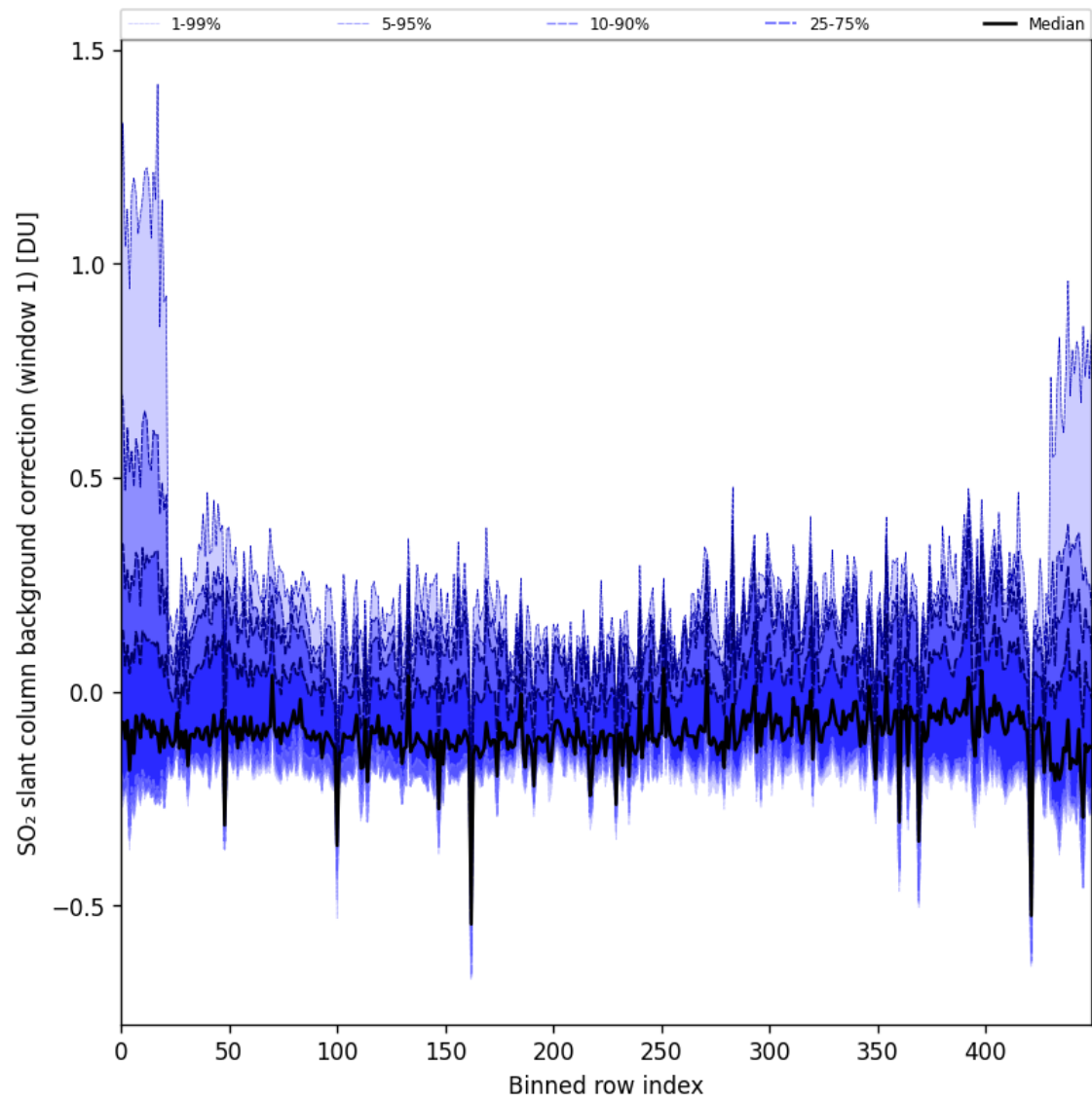
Figure 92: Along track statistics of “SO 2 slant column background correction (window 1)” for 2025-07-20 to 2025-07-22
