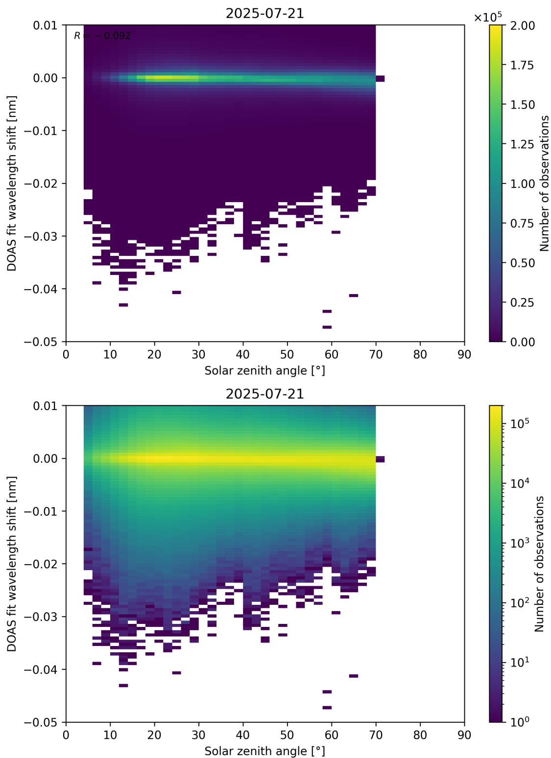
Figure 174: Scatter density plot of “Solar zenith angle” against “DOAS fit wavelength shift” for 2025-07-20 to 2025-07-22.
