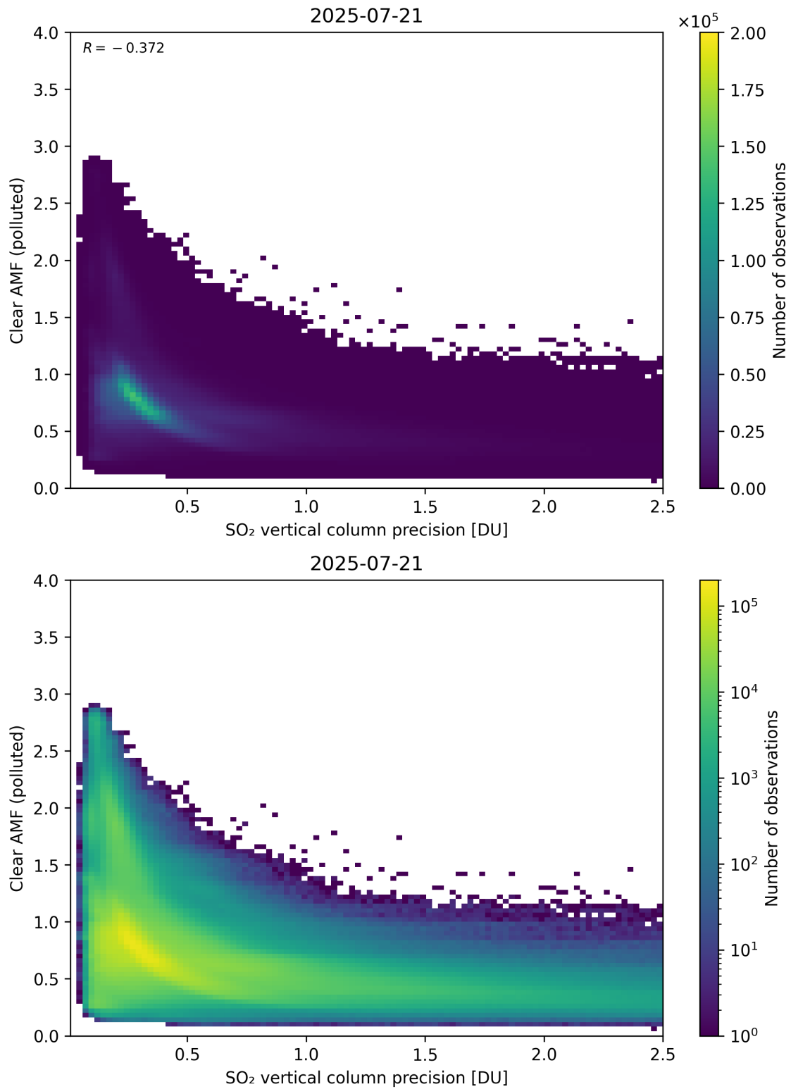
Figure 335: Scatter density plot of “SO 2 vertical column precision” against “Clear AMF (polluted)” for 2025-07-20 to 2025-07-22.
