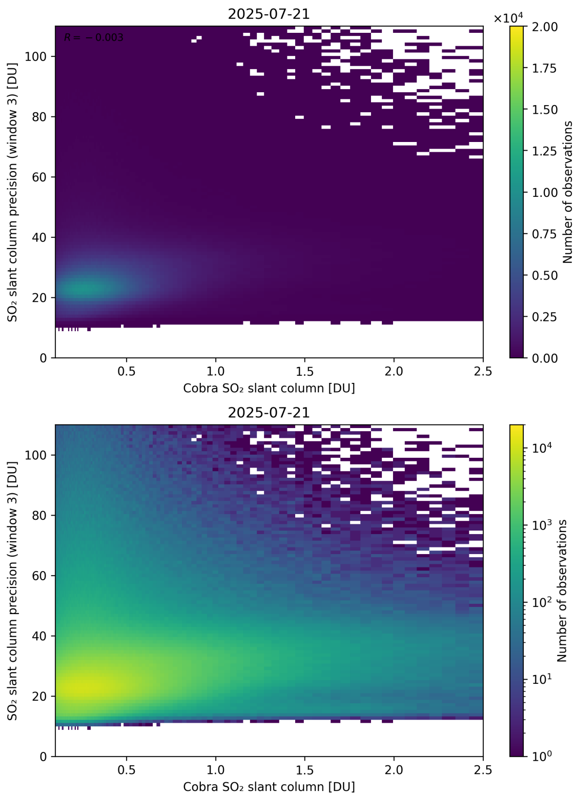
Figure 223: Scatter density plot of “Cobra SO 2 slant column” against “SO 2 slant column precision (window 3)” for 2025-07-20 to 2025-07-22.
