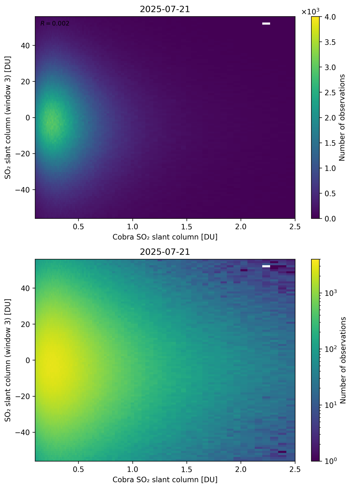
Figure 222: Scatter density plot of “Cobra SO 2 slant column” against “SO 2 slant column (window 3)” for 2025-07-20 to 2025-07-22.
