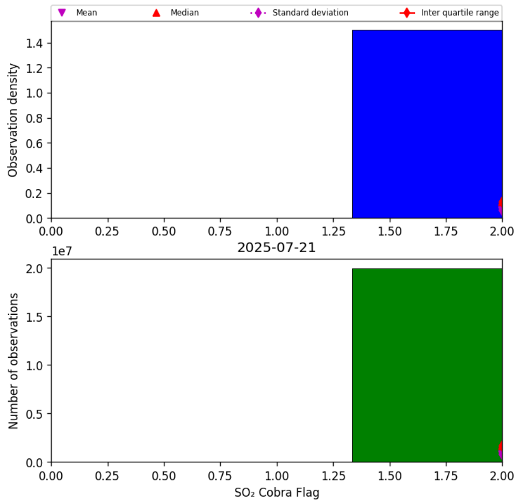
Figure 75: Histogram of “SO 2 Cobra Flag” for 2025-07-20 to 2025-07-22
