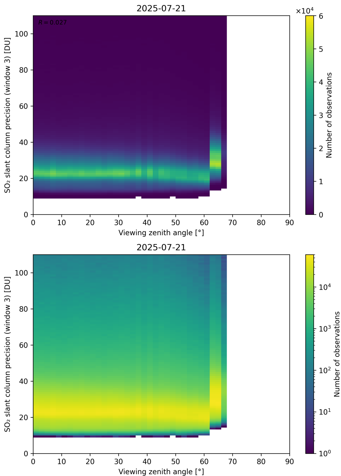
Figure 380: Scatter density plot of “Viewing zenith angle” against “SO 2 slant column precision (window 3)” for 2025-07-20 to 2025-07-22.
