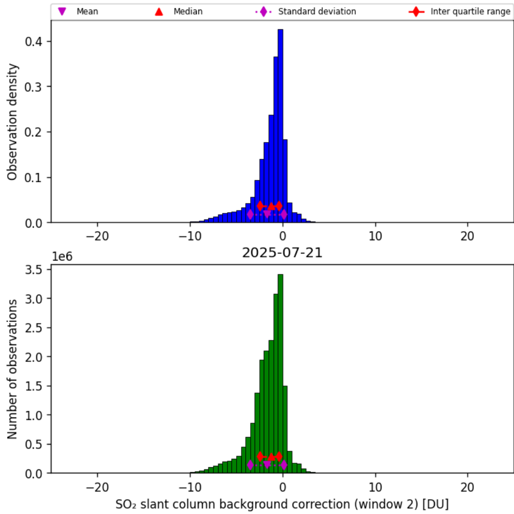
Figure 70: Histogram of “SO 2 slant column background correction (window 2)” for 2025-07-20 to 2025-07-22
