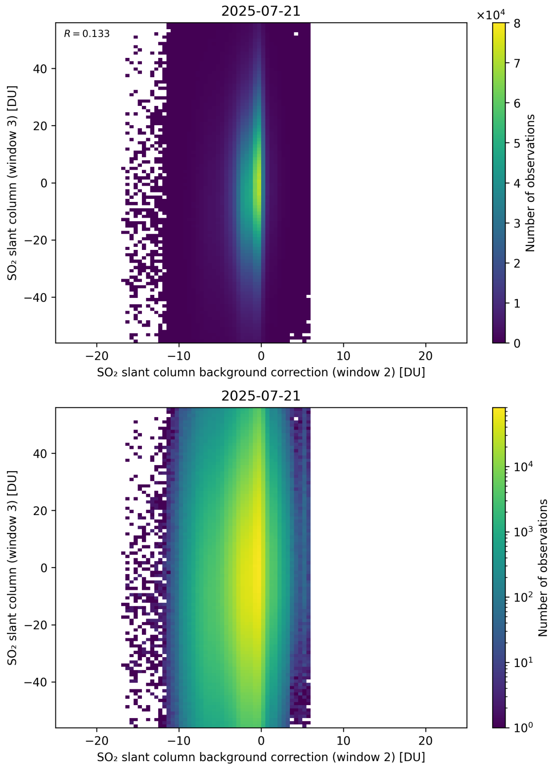
Figure 128: Scatter density plot of “SO 2 slant column background correction (window 2)” against “SO 2 slant column (window 3)” for 2025-07-20 to 2025-07-22.
