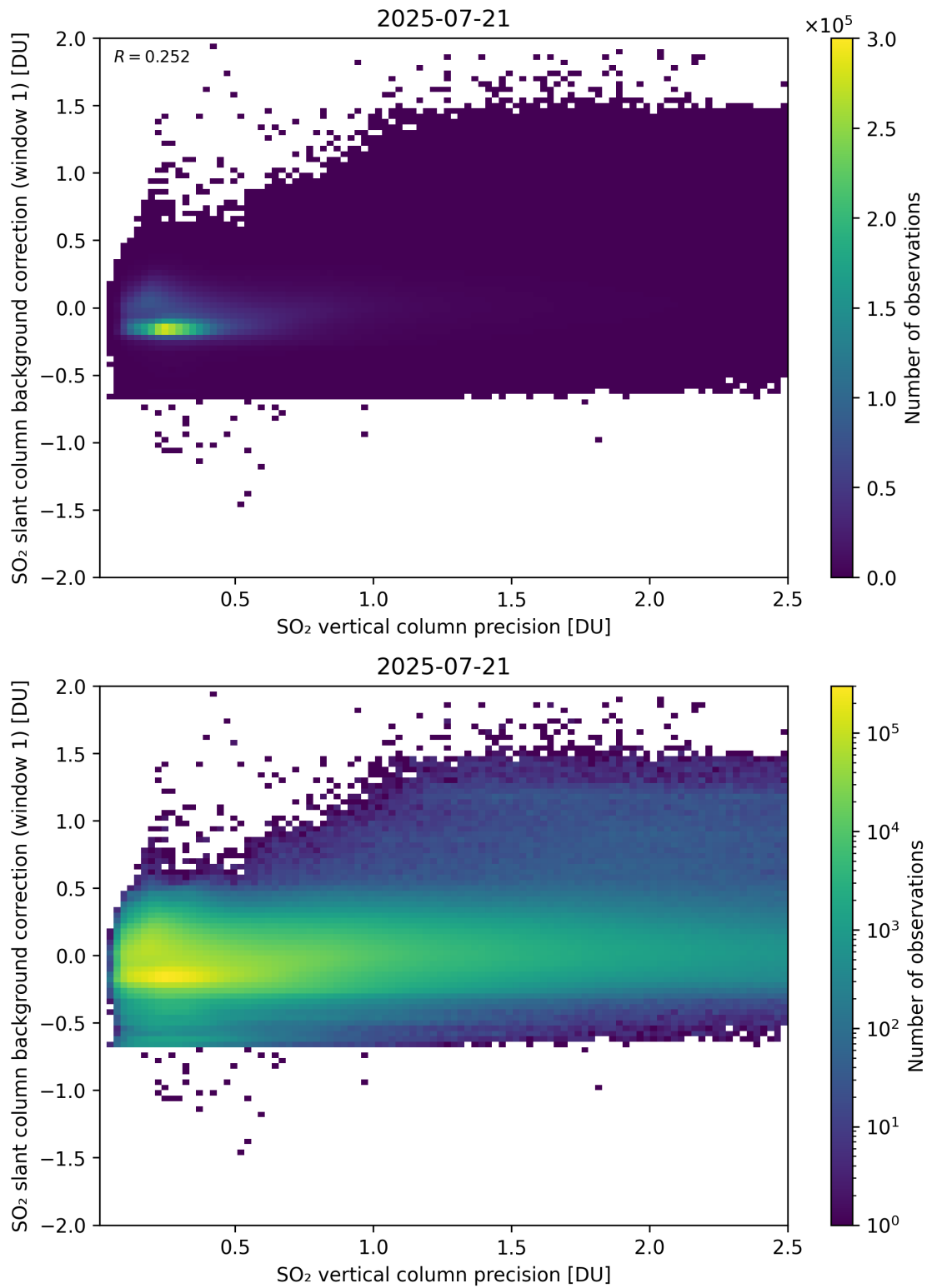
Figure 329: Scatter density plot of “SO 2 vertical column precision” against “SO 2 slant column background correction (window 1)” for 2025-07-20 to 2025-07-22.
