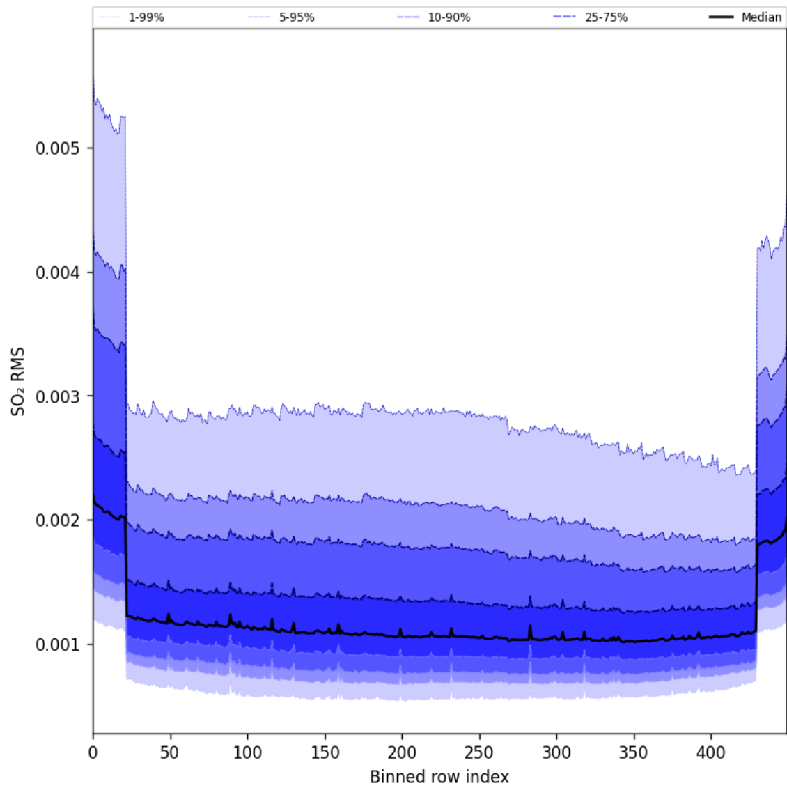
Figure 104: Along track statistics of “SO 2 RMS” for 2025-07-20 to 2025-07-22
