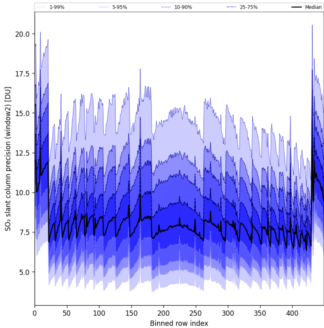
Figure 94: Along track statistics of “SO 2 slant column precision (window2)” for 2025-07-20 to 2025-07-22
