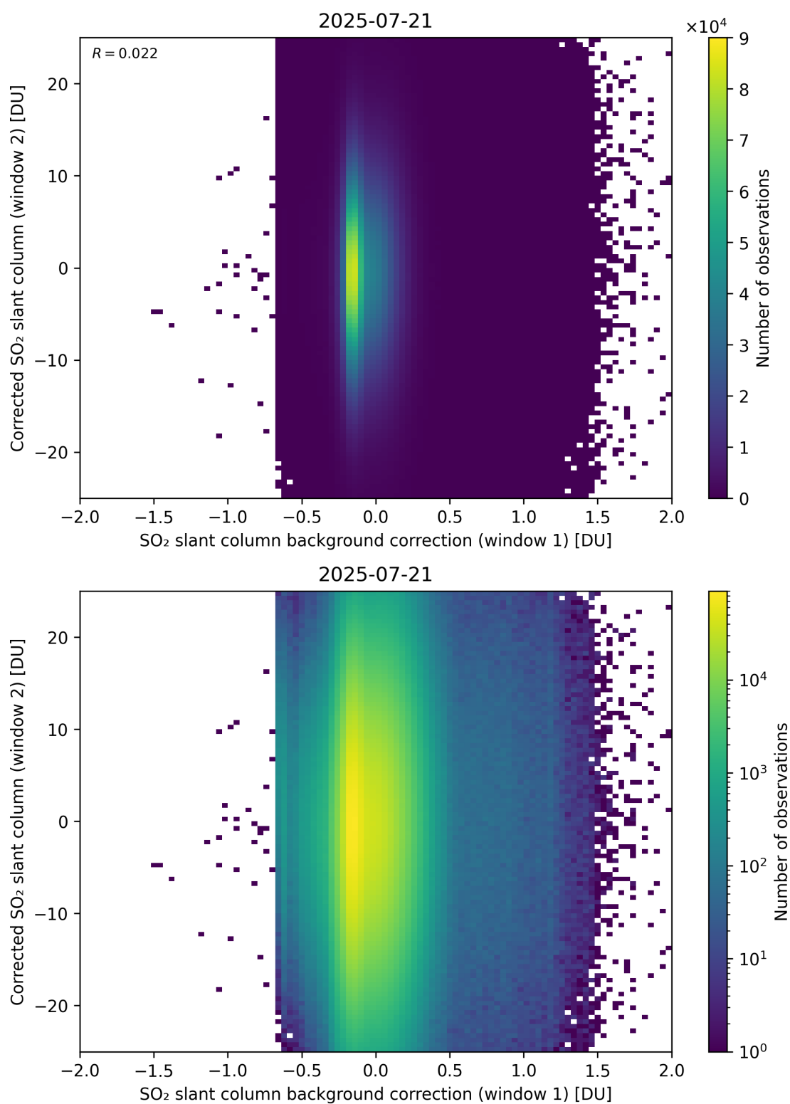
Figure 115: Scatter density plot of “SO 2 slant column background correction (window 1)” against “Corrected SO 2 slant column (window 2)” for 2025-07-20 to 2025-07-22.
