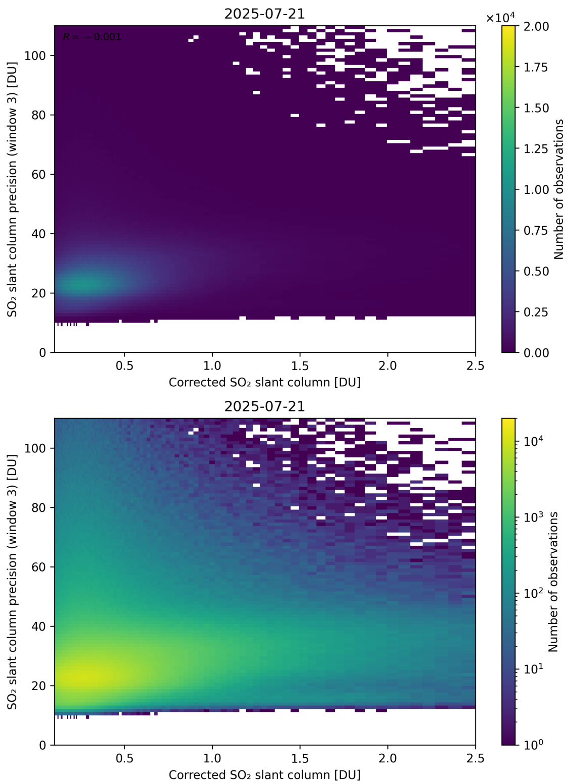
Figure 241: Scatter density plot of “Corrected SO 2 slant column” against “SO 2 slant column precision (window 3)” for 2025-07-20 to 2025-07-22.
