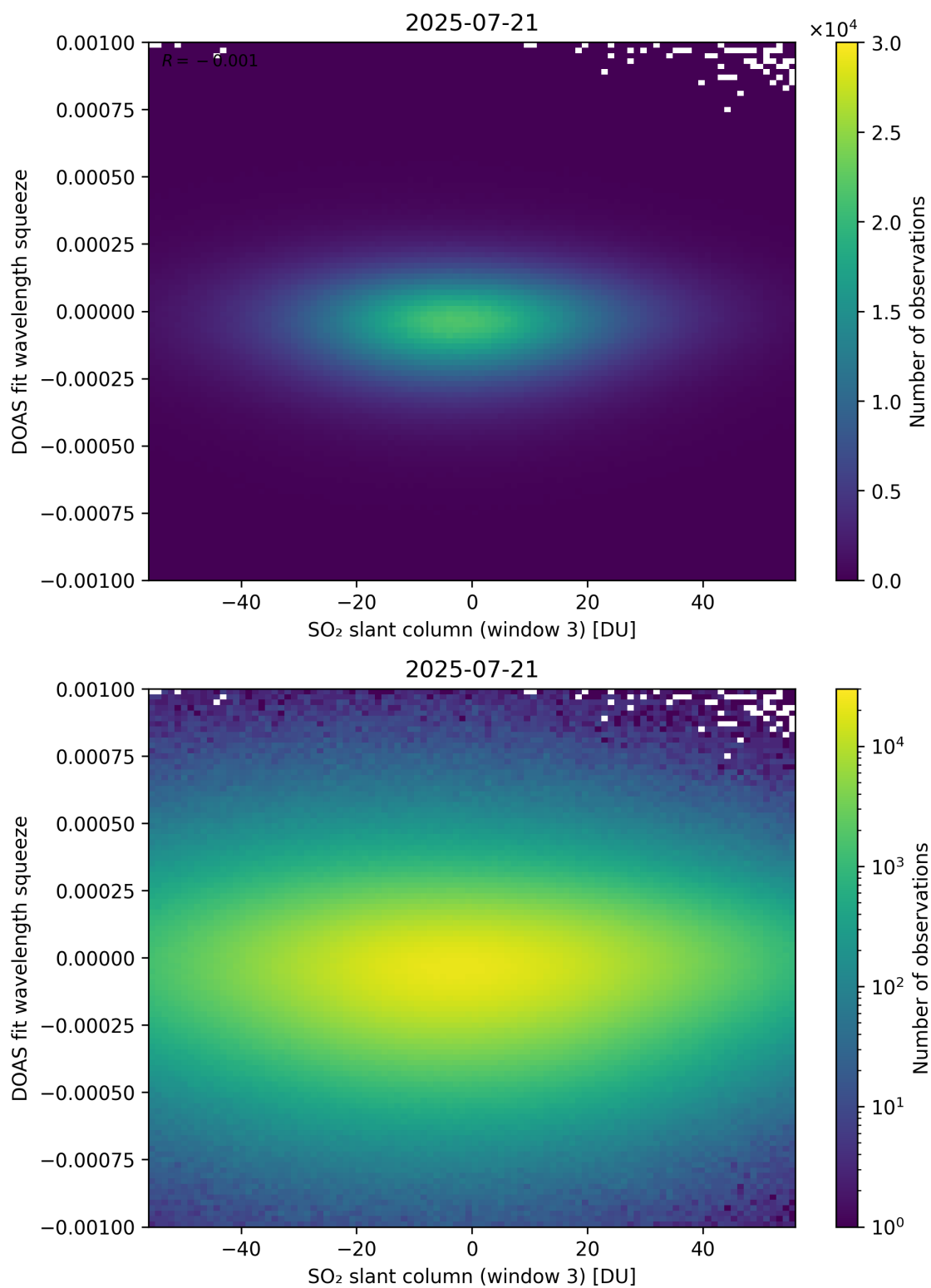
Figure 305: Scatter density plot of “SO 2 slant column (window 3)” against “DOAS fit wavelength squeeze” for 2025-07-20 to 2025-07-22.
