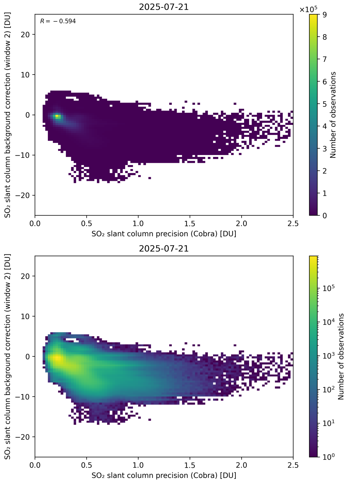
Figure 200: Scatter density plot of “SO 2 slant column precision (Cobra)” against “SO 2 slant column background correction (window 2)” for 2025-07-20 to 2025-07-22.
