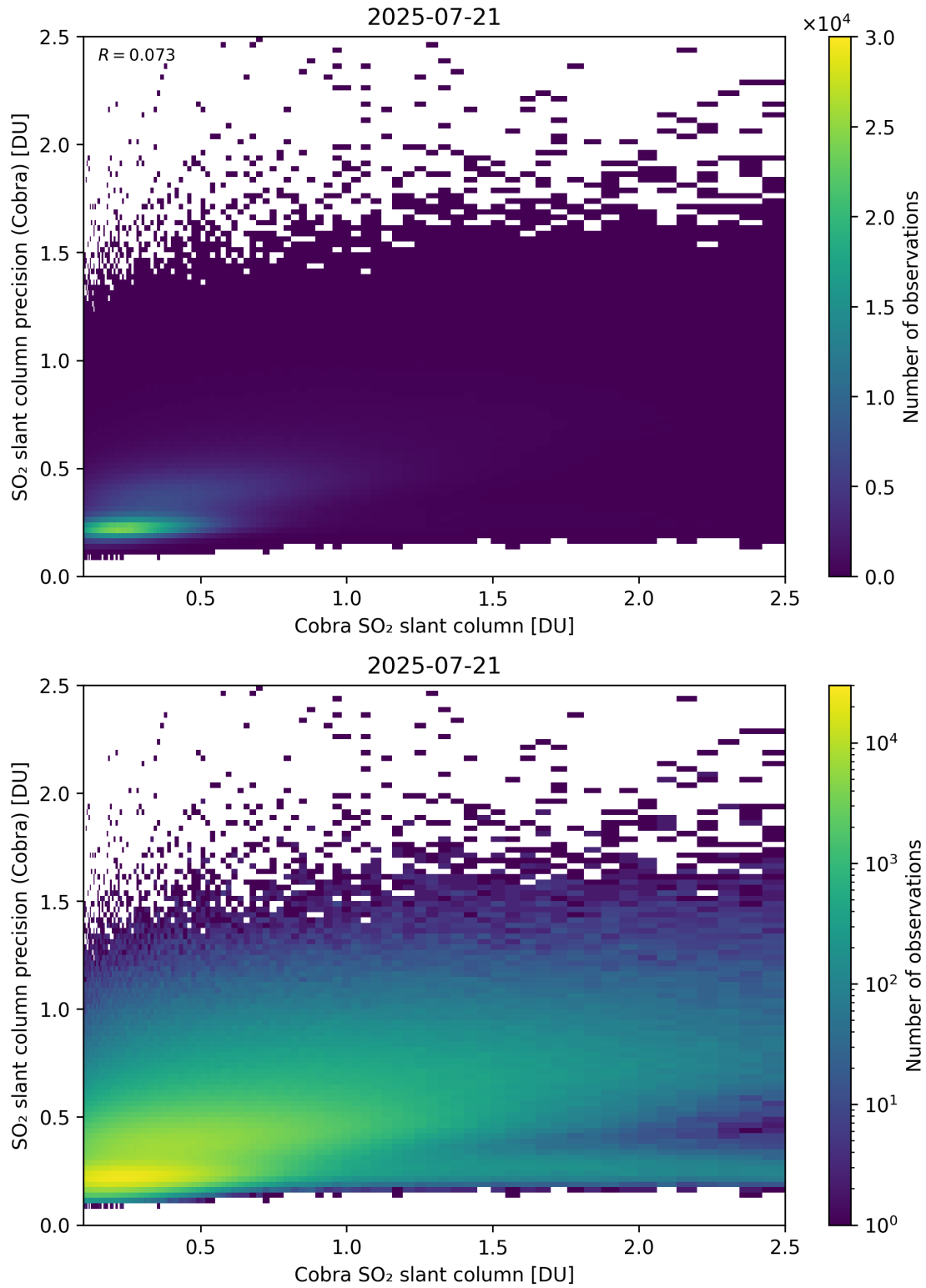
Figure 216: Scatter density plot of “Cobra SO 2 slant column” against “SO 2 slant column precision (Cobra)” for 2025-07-20 to 2025-07-22.
