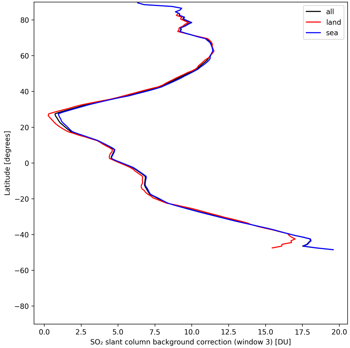
Figure 48: Zonal average of “SO 2 slant column background correction (window 3)” for 2025-07-20 to 2025-07-22.
