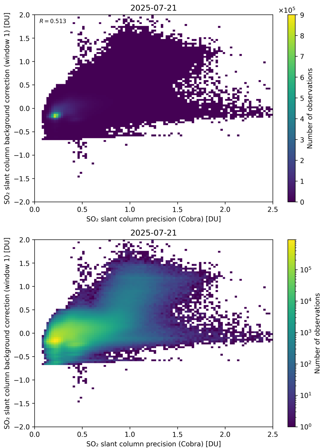
Figure 199: Scatter density plot of “SO 2 slant column precision (Cobra)” against “SO 2 slant column background correction (window 1)” for 2025-07-20 to 2025-07-22.
