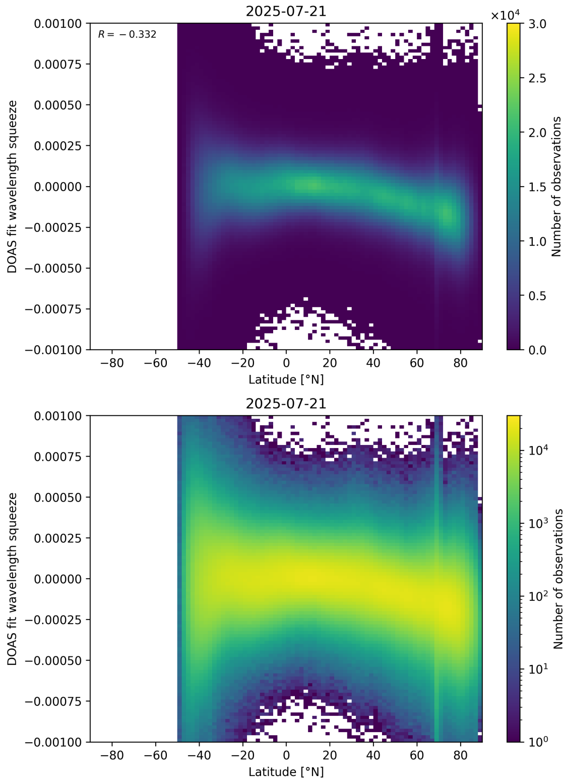
Figure 154: Scatter density plot of “Latitude” against “DOAS fit wavelength squeeze” for 2025-07-20 to 2025-07-22.
