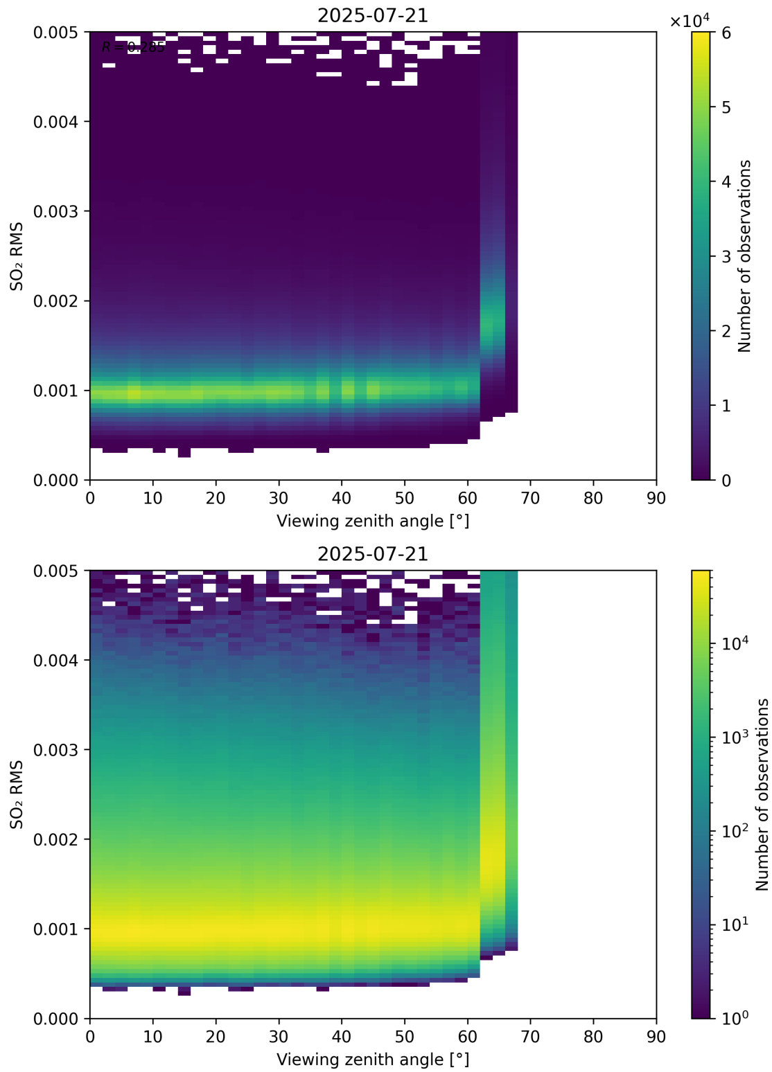
Figure 367: Scatter density plot of “Viewing zenith angle” against “SO 2 RMS” for 2025-07-20 to 2025-07-22.
