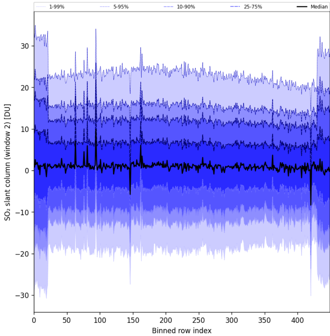
Figure 93: Along track statistics of “SO 2 slant column (window 2)” for 2025-07-20 to 2025-07-22
