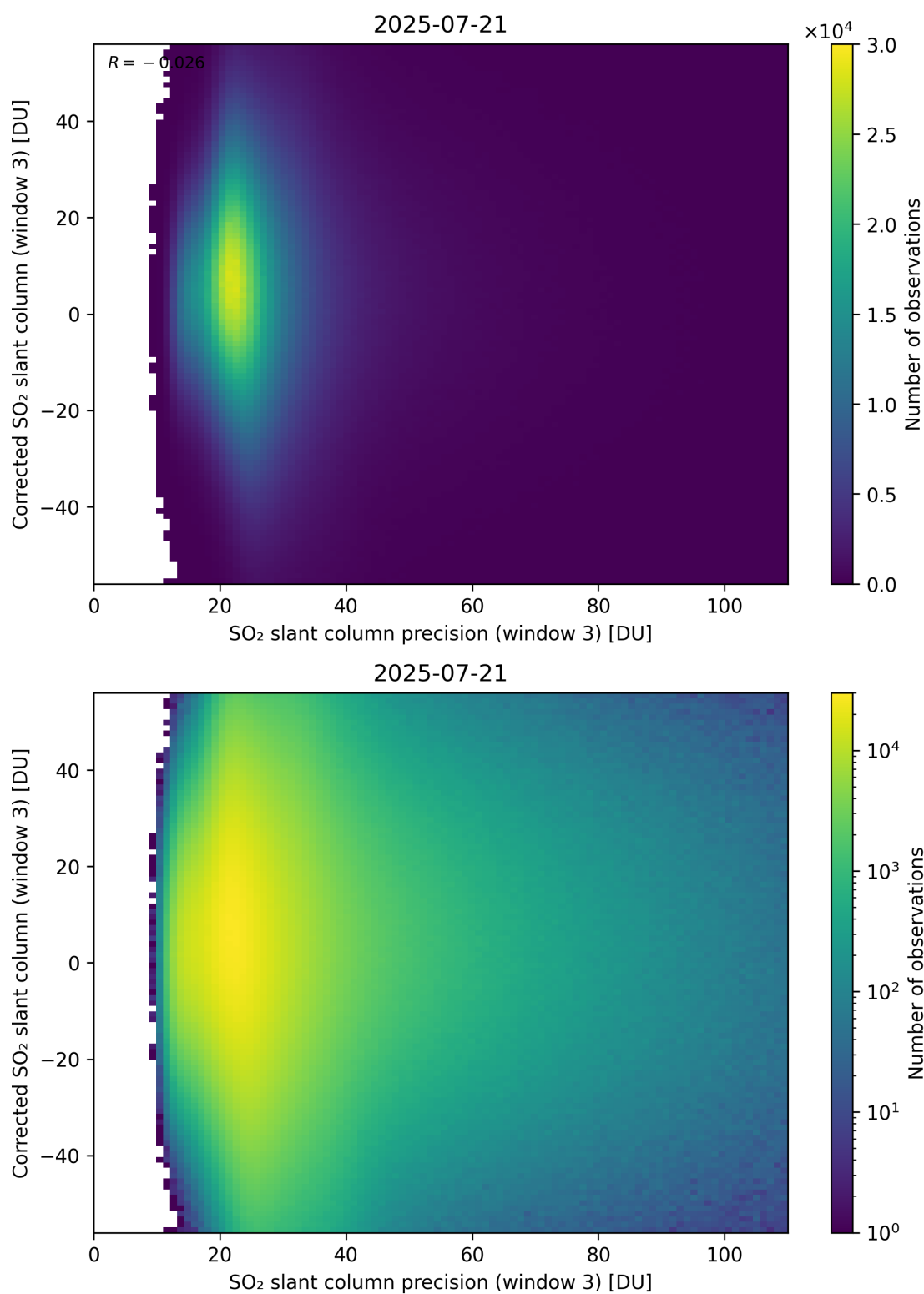
Figure 312: Scatter density plot of “SO 2 slant column precision (window 3)” against “Corrected SO 2 slant column (window 3)” for 2025-07-20 to 2025-07-22.
