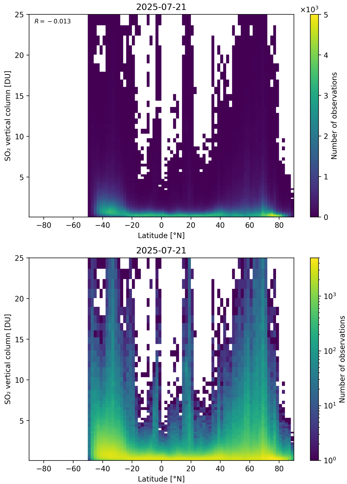
Figure 169: Scatter density plot of “Latitude” against “SO 2 vertical column” for 2025-07-20 to 2025-07-22.
