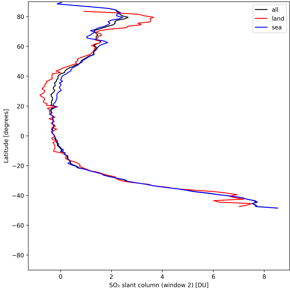
Figure 41: Zonal average of “SO 2 slant column (window 2)” for 2025-07-20 to 2025-07-22.
