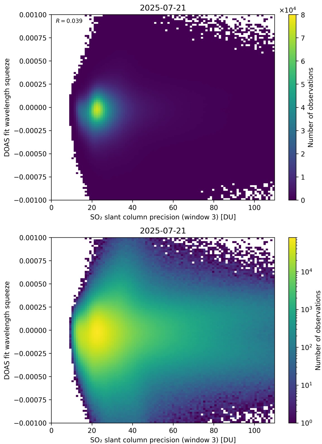
Figure 309: Scatter density plot of “SO 2 slant column precision (window 3)” against “DOAS fit wavelength squeeze” for 2025-07-20 to 2025-07-22.
