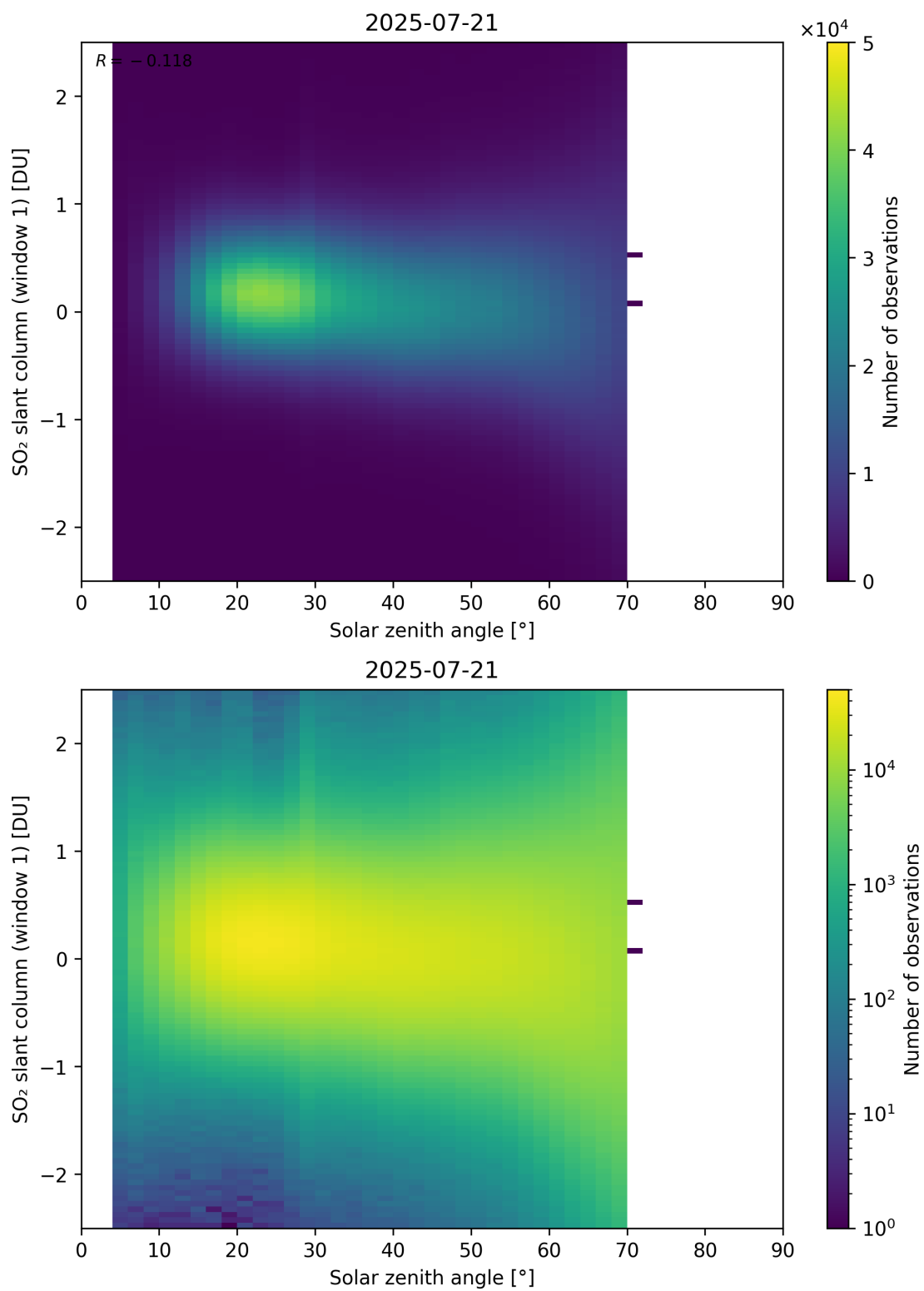
Figure 184: Scatter density plot of “Solar zenith angle” against “SO 2 slant column (window 1)” for 2025-07-20 to 2025-07-22.
