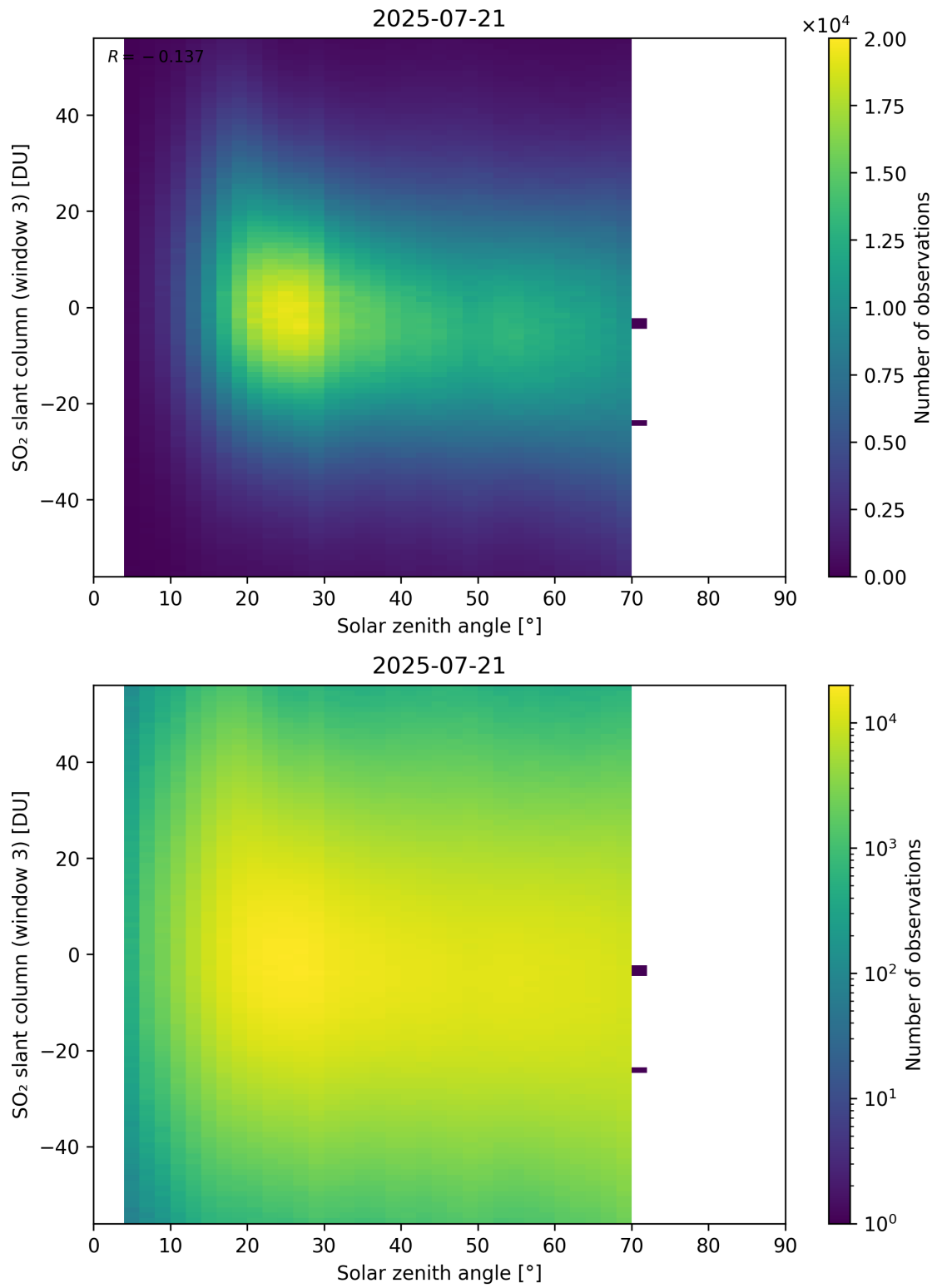
Figure 187: Scatter density plot of “Solar zenith angle” against “SO 2 slant column (window 3)” for 2025-07-20 to 2025-07-22.
