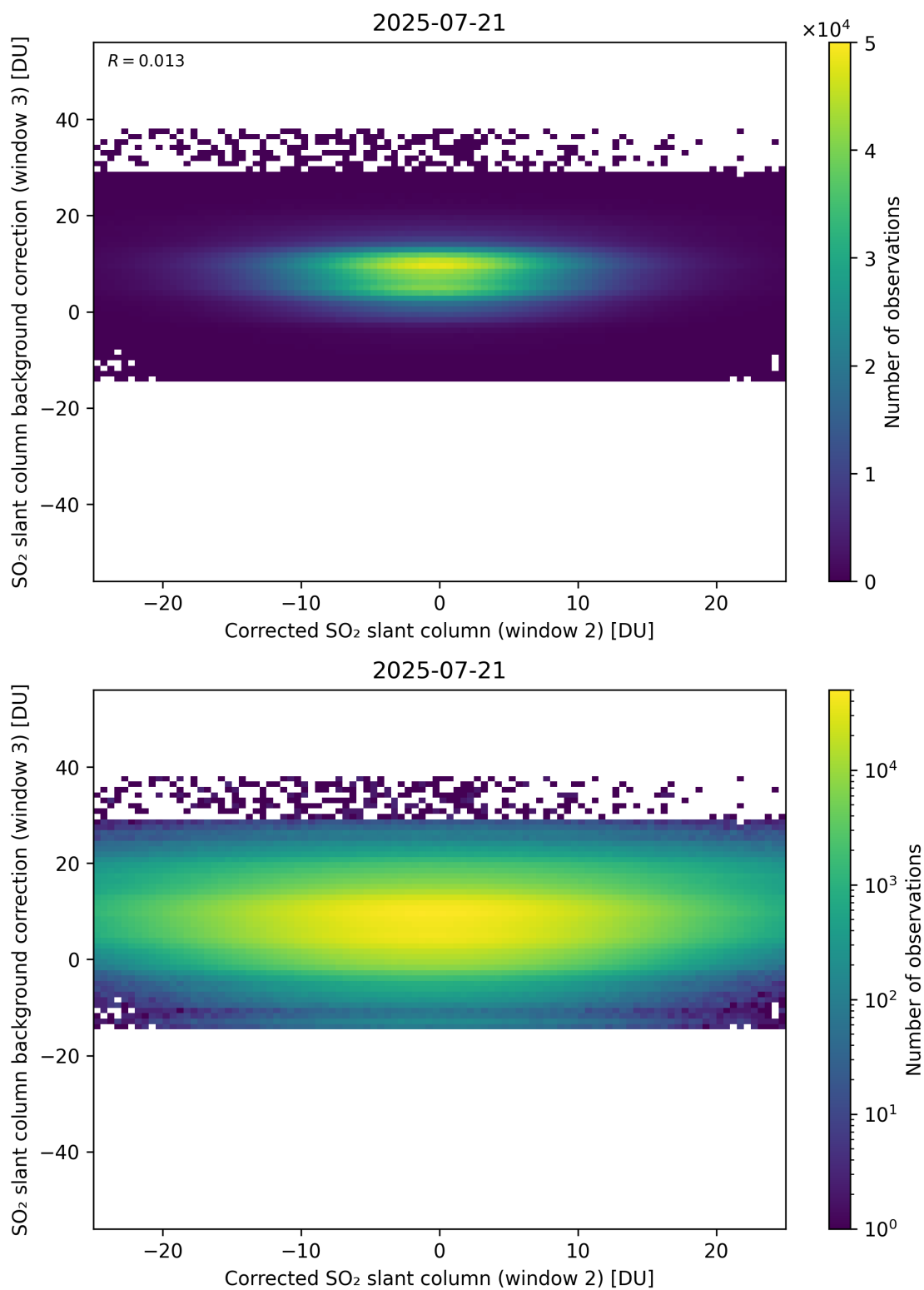
Figure 245: Scatter density plot of “Corrected SO 2 slant column (window 2)” against “SO 2 slant column background correction (window 3)” for 2025-07-20 to 2025-07-22.
