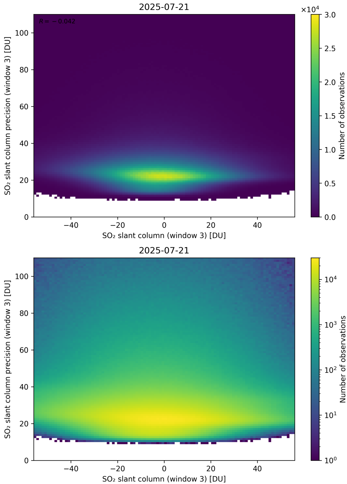
Figure 317: Scatter density plot of “SO 2 slant column (window 3)” against “SO 2 slant column precision (window 3)” for 2025-07-20 to 2025-07-22.
