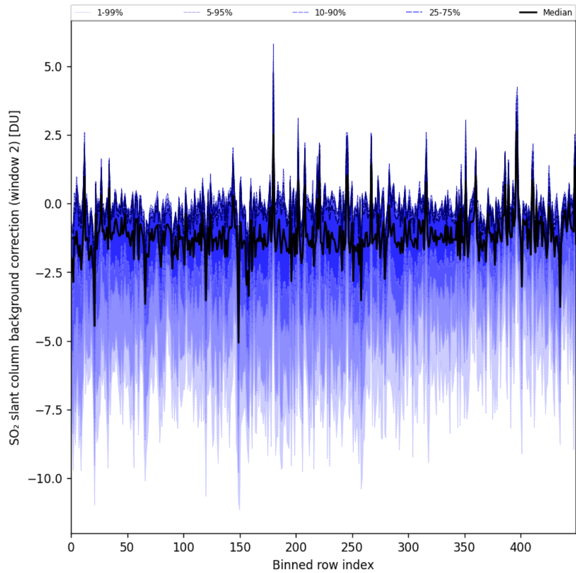
Figure 96: Along track statistics of “SO 2 slant column background correction (window 2)” for 2025-07-20 to 2025-07-22
