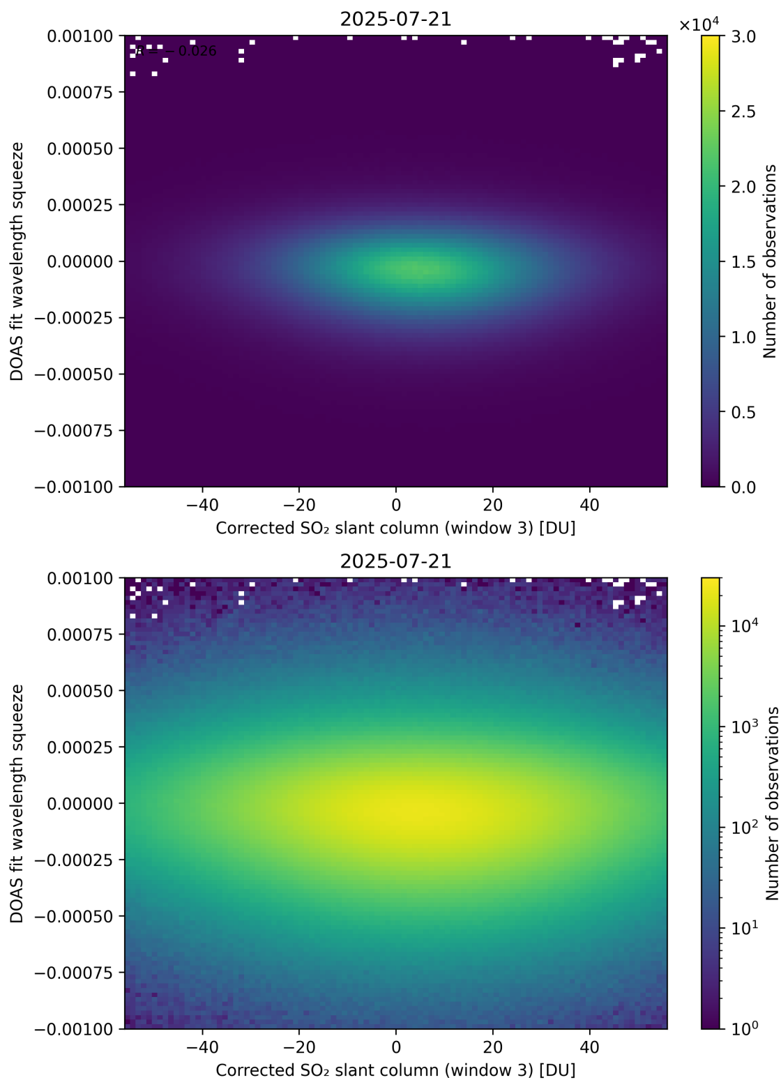
Figure 257: Scatter density plot of “Corrected SO 2 slant column (window 3)” against “DOAS fit wavelength squeeze” for 2025-07-20 to 2025-07-22.
