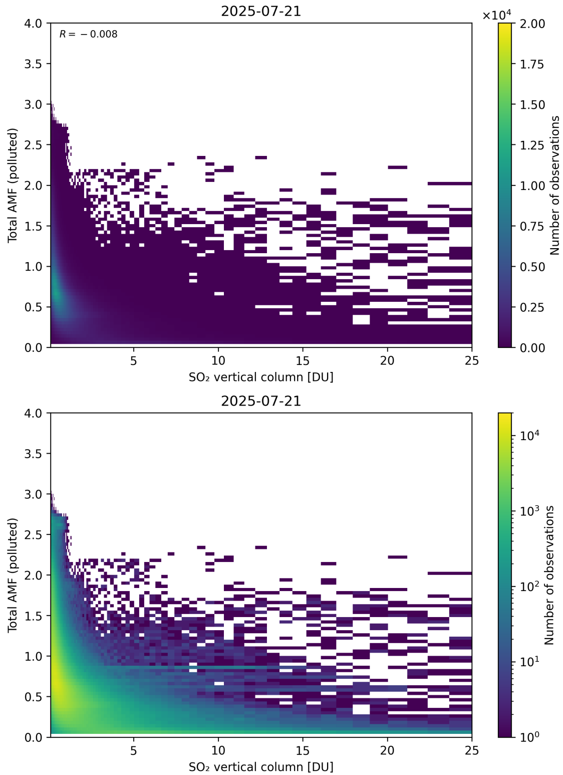
Figure 359: Scatter density plot of “SO 2 vertical column” against “Total AMF (polluted)” for 2025-07-20 to 2025-07-22.
