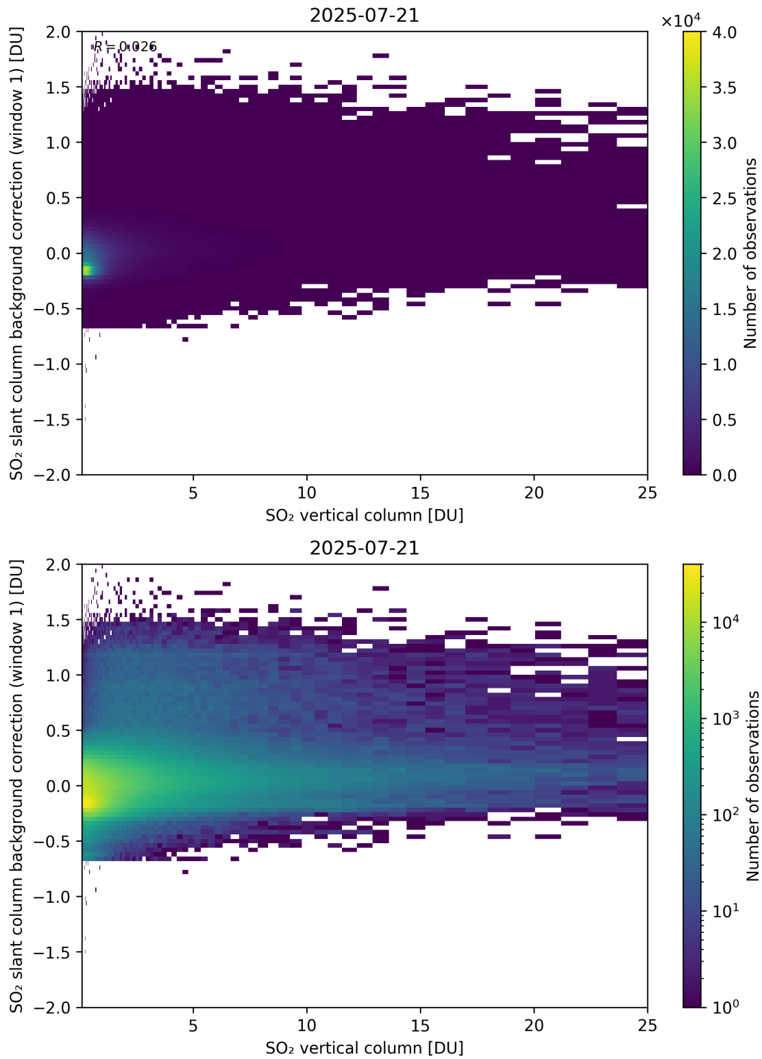
Figure 323: Scatter density plot of “SO 2 vertical column” against “SO 2 slant column background correction (window 1)” for 2025-07-20 to 2025-07-22.
