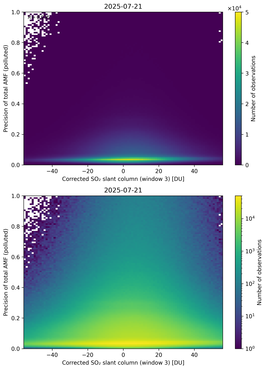
Figure 261: Scatter density plot of “Corrected SO 2 slant column (window 3)” against “Precision of total AMF (polluted)” for 2025-07-20 to 2025-07-22.
