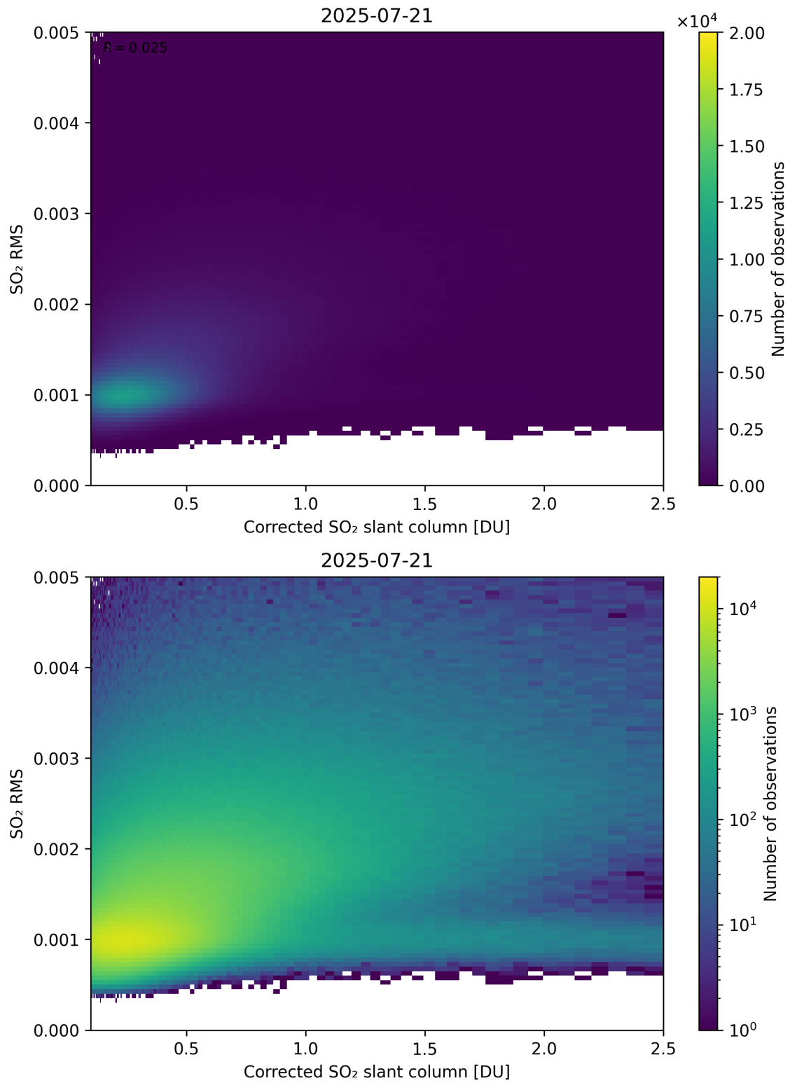
Figure 231: Scatter density plot of “Corrected SO 2 slant column” against “SO 2 RMS” for 2025-07-20 to 2025-07-22.
