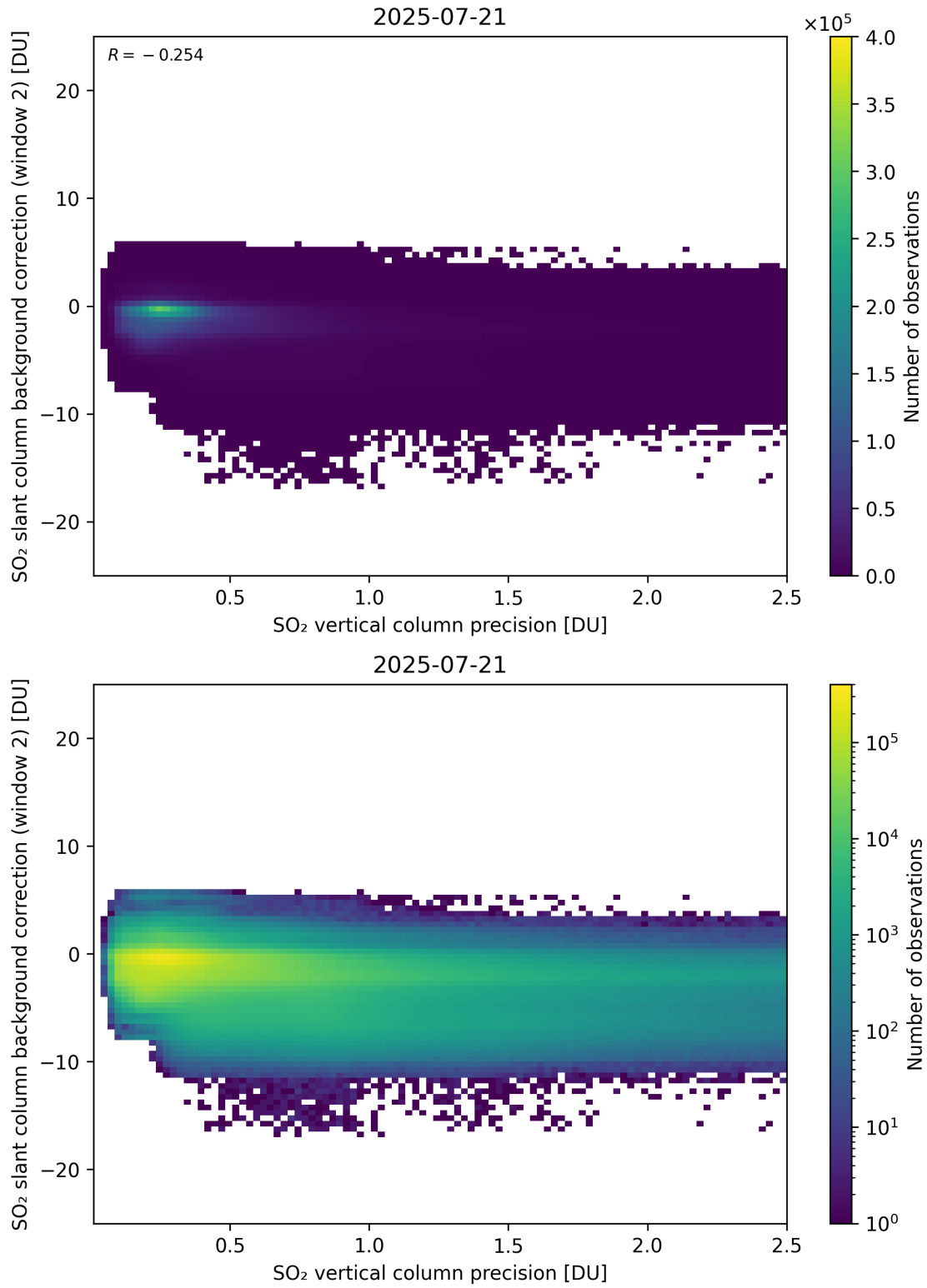
Figure 330: Scatter density plot of “SO 2 vertical column precision” against “SO 2 slant column background correction (window 2)” for 2025-07-20 to 2025-07-22.
