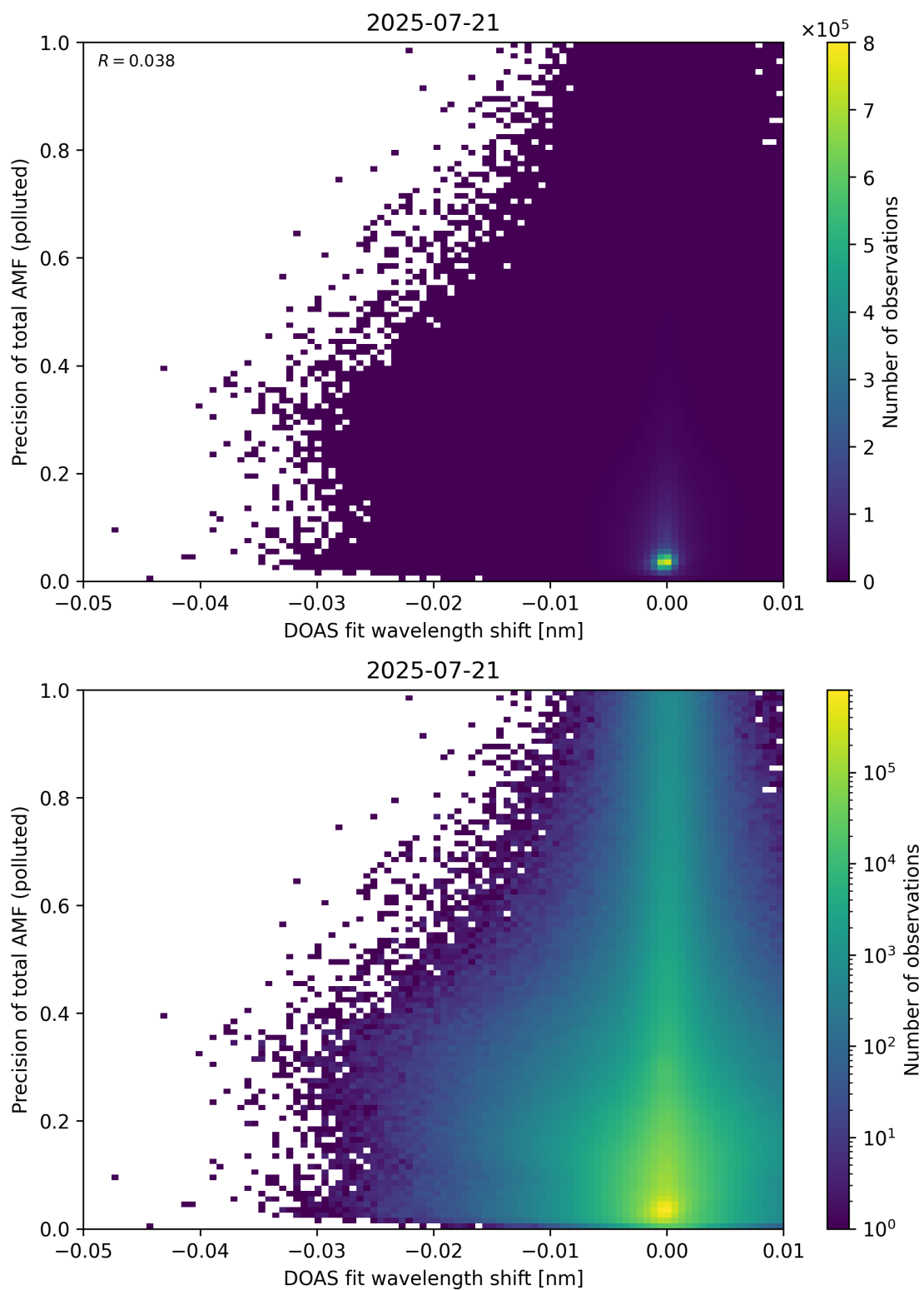
Figure 142: Scatter density plot of “DOAS fit wavelength shift” against “Precision of total AMF (polluted)” for 2025-07-20 to 2025-07-22.
