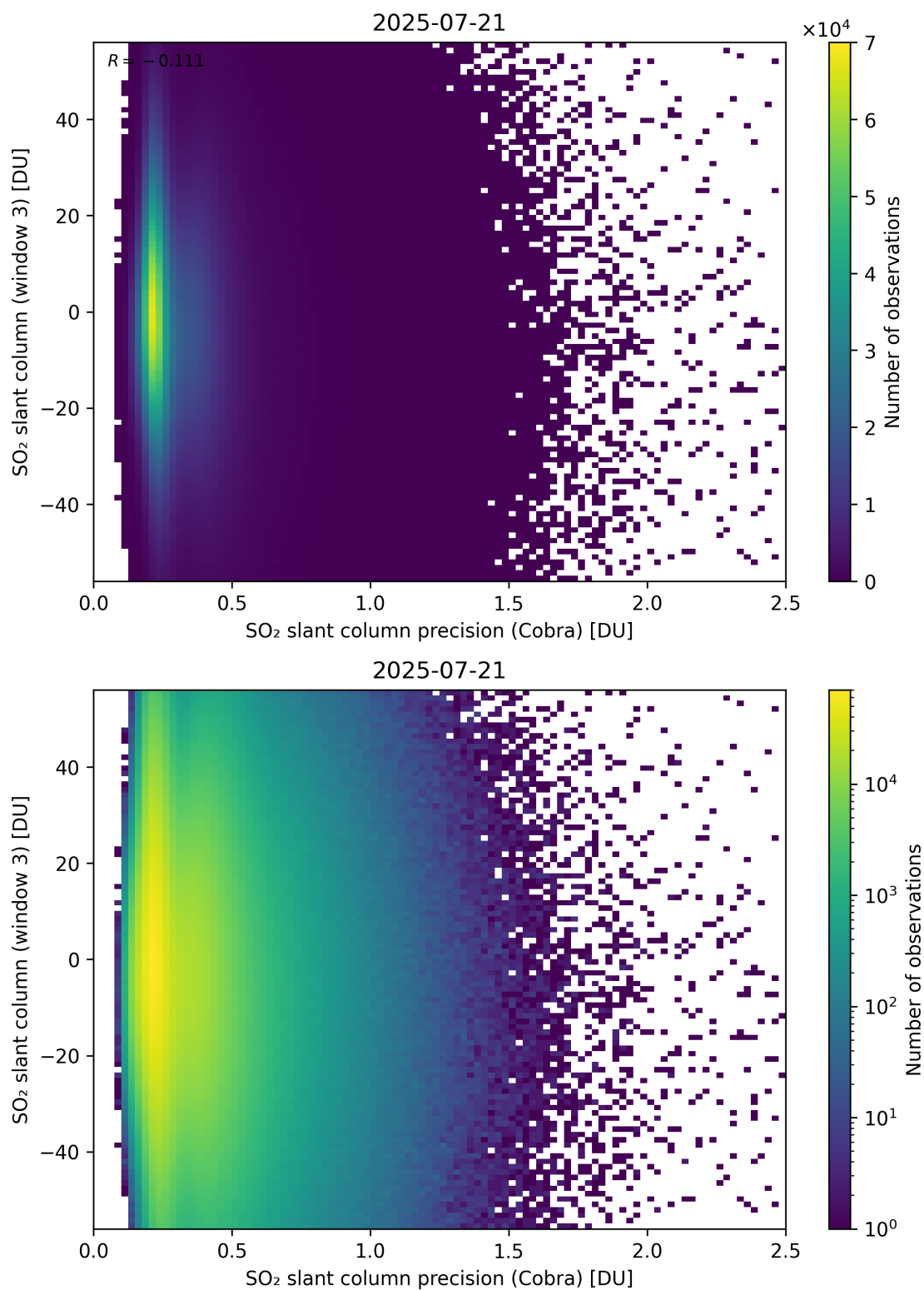
Figure 211: Scatter density plot of “SO 2 slant column precision (Cobra)” against “SO 2 slant column (window 3)” for 2025-07-20 to 2025-07-22.
