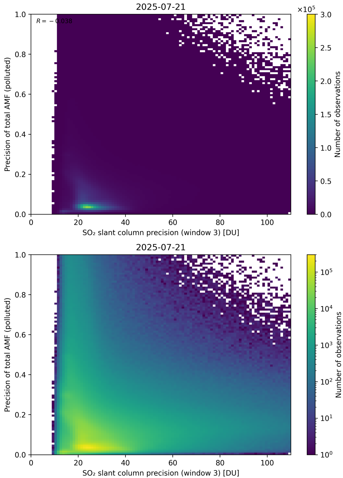
Figure 314: Scatter density plot of “SO 2 slant column precision (window 3)” against “Precision of total AMF (polluted)” for 2025-07-20 to 2025-07-22.
