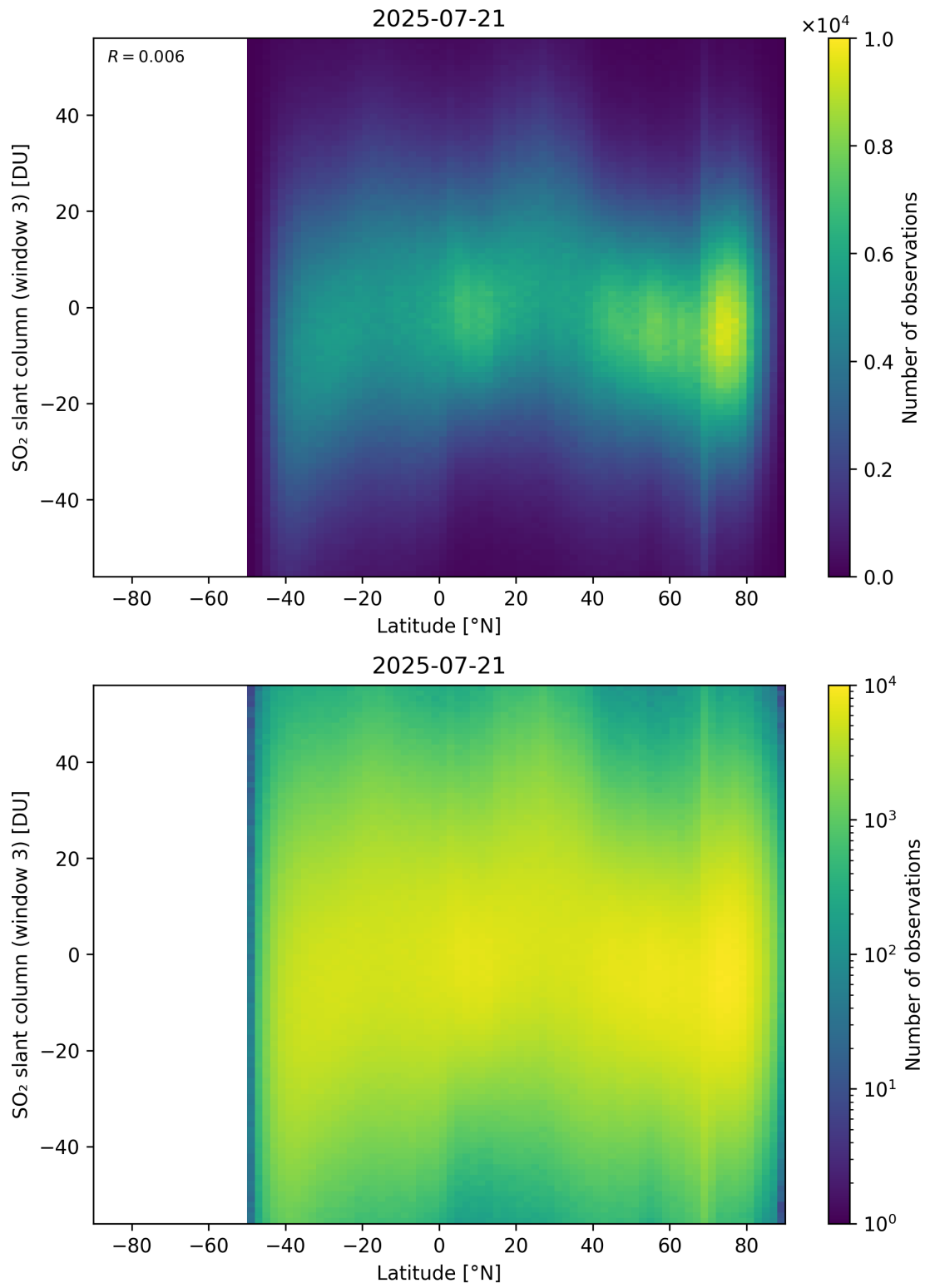
Figure 165: Scatter density plot of “Latitude” against “SO 2 slant column (window 3)” for 2025-07-20 to 2025-07-22.
