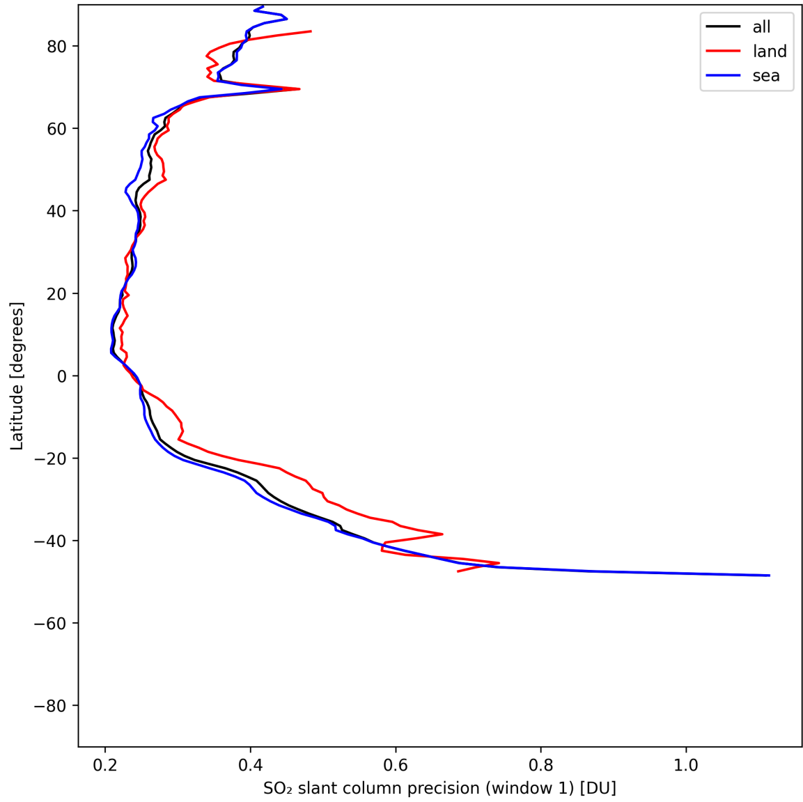
Figure 38: Zonal average of “SO 2 slant column precision (window 1)” for 2025-07-20 to 2025-07-22.
