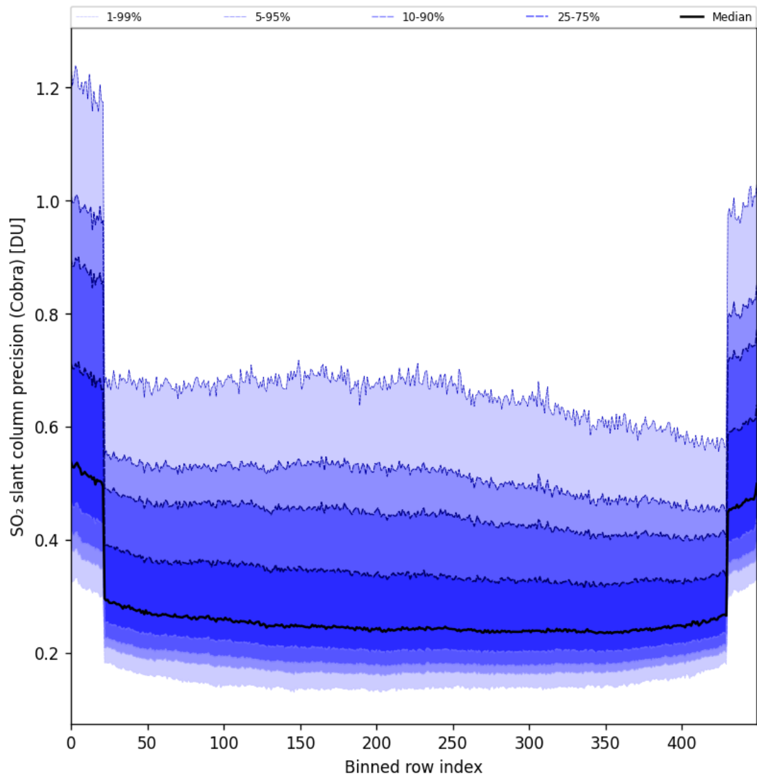
Figure 88: Along track statistics of “SO 2 slant column precision (Cobra)” for 2025-07-20 to 2025-07-22
