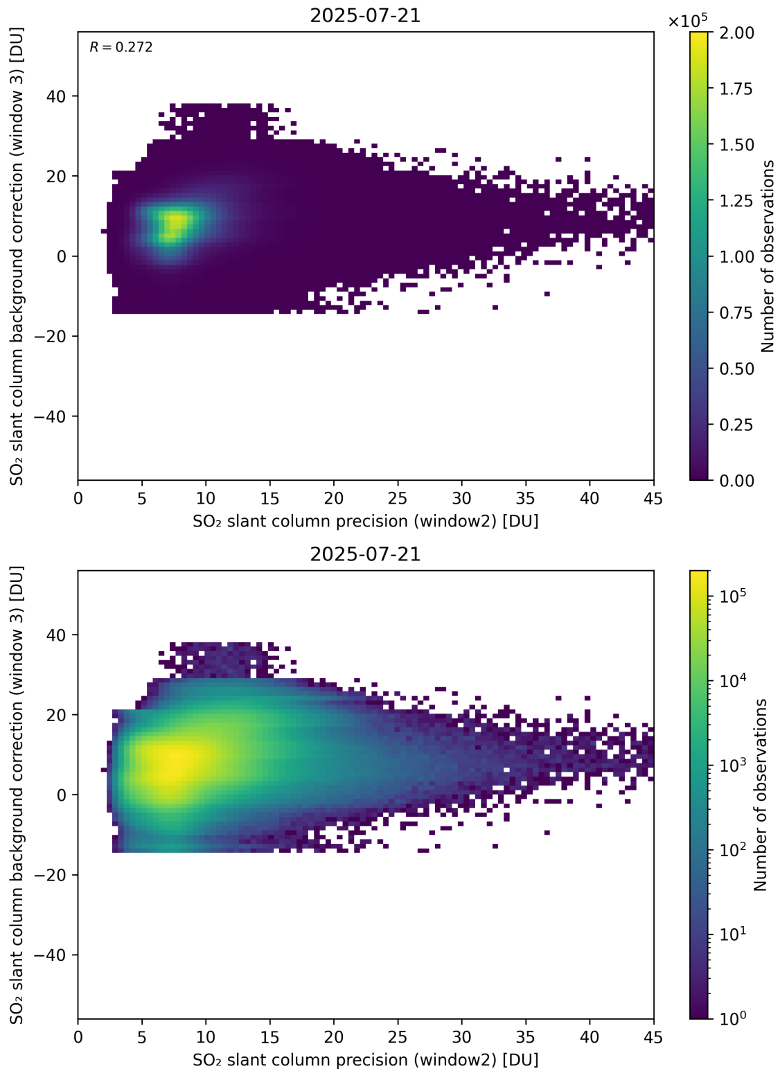
Figure 292: Scatter density plot of “SO 2 slant column precision (window2)” against “SO 2 slant column background correction (window 3)” for 2025-07-20 to 2025-07-22.
