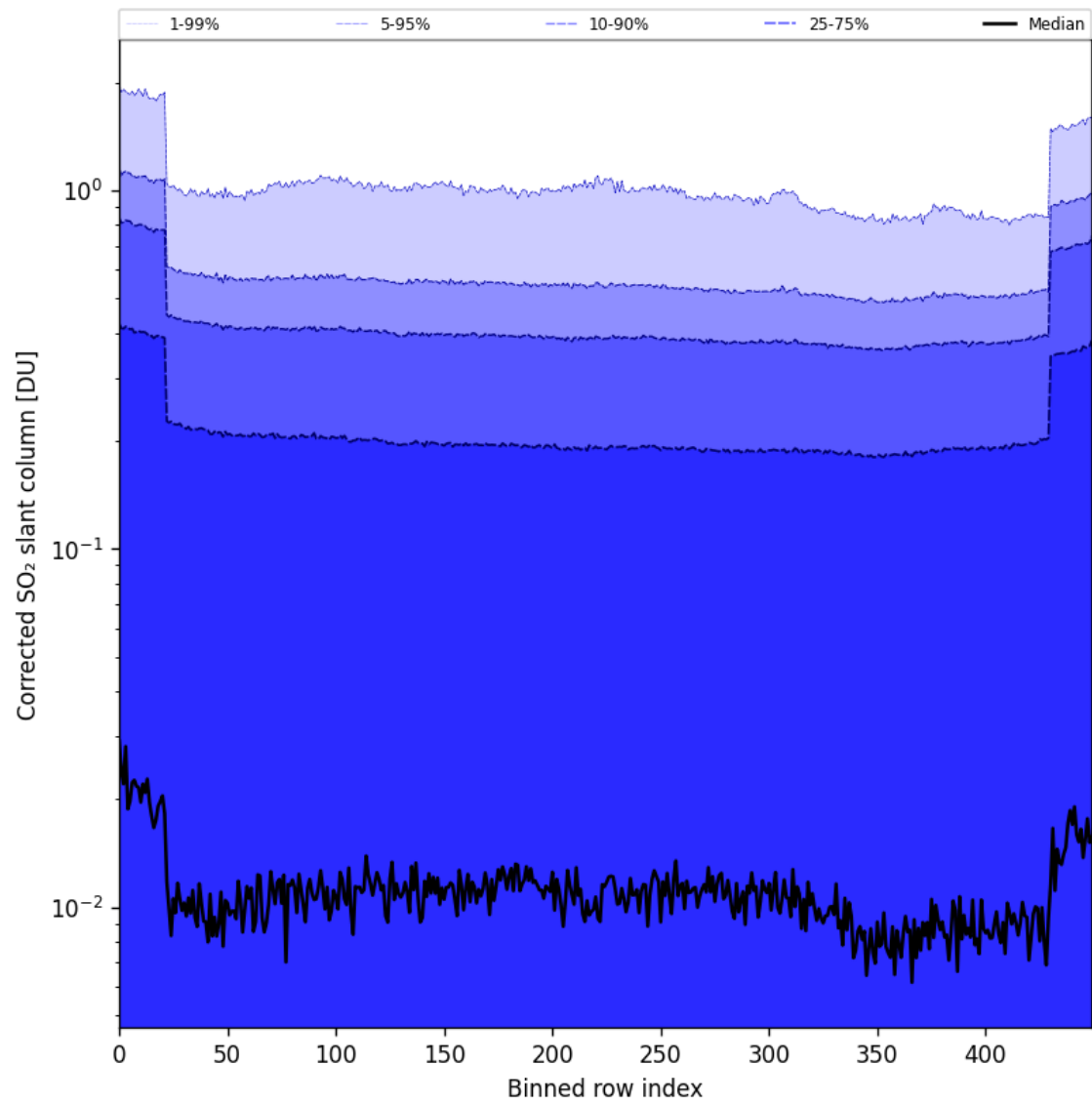
Figure 86: Along track statistics of “Corrected SO 2 slant column” for 2025-07-20 to 2025-07-22
