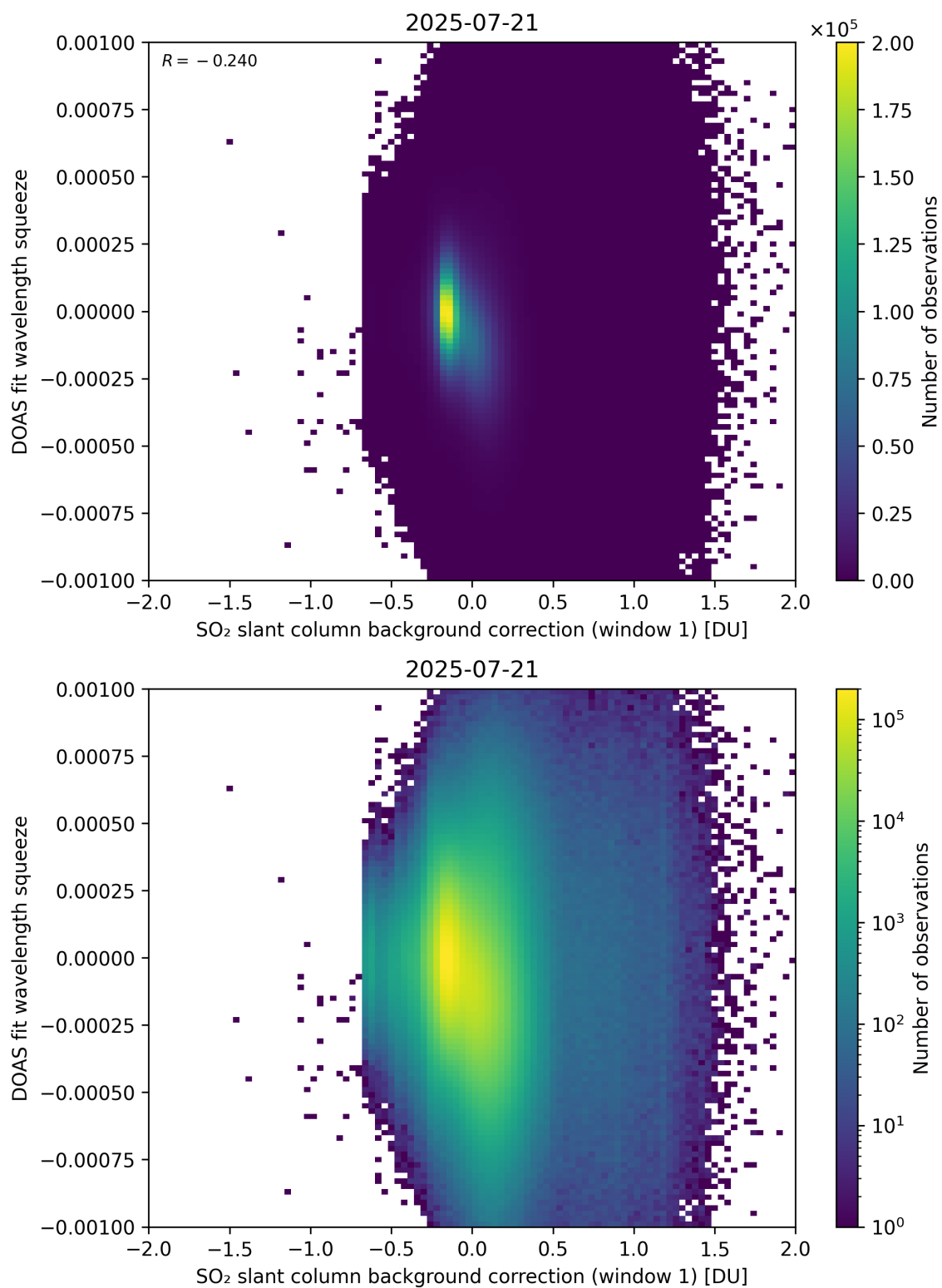
Figure 112: Scatter density plot of “SO 2 slant column background correction (window 1)” against “DOAS fit wavelength squeeze” for 2025-07-20 to 2025-07-22.
