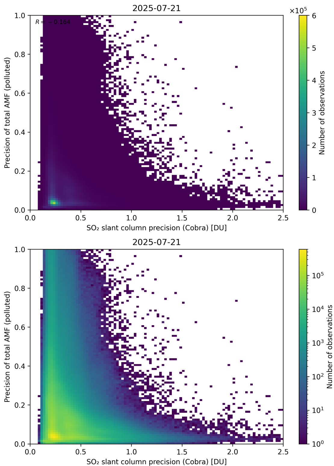
Figure 214: Scatter density plot of “SO 2 slant column precision (Cobra)” against “Precision of total AMF (polluted)” for 2025-07-20 to 2025-07-22.
