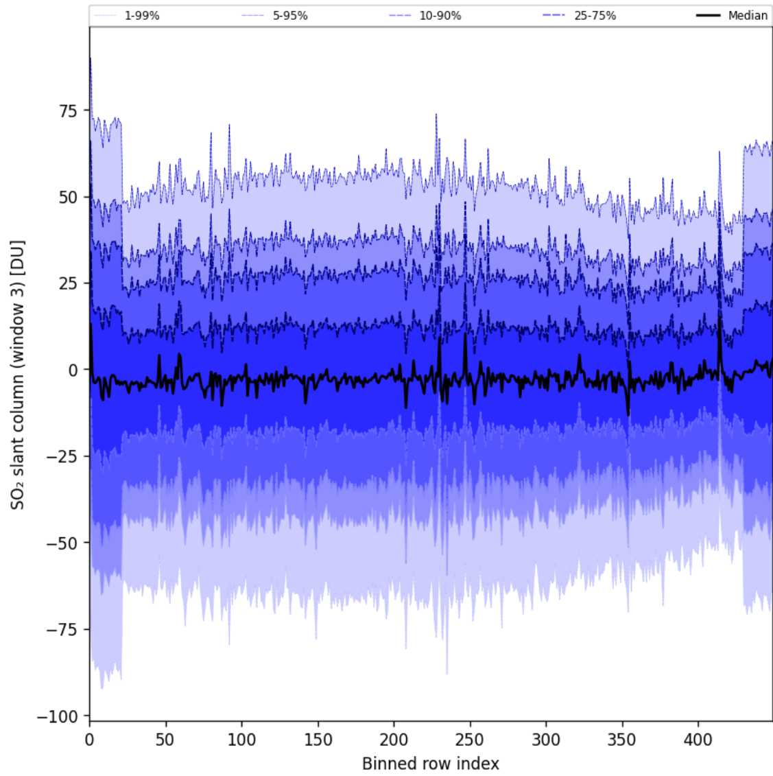
Figure 97: Along track statistics of “SO 2 slant column (window 3)” for 2025-07-20 to 2025-07-22
