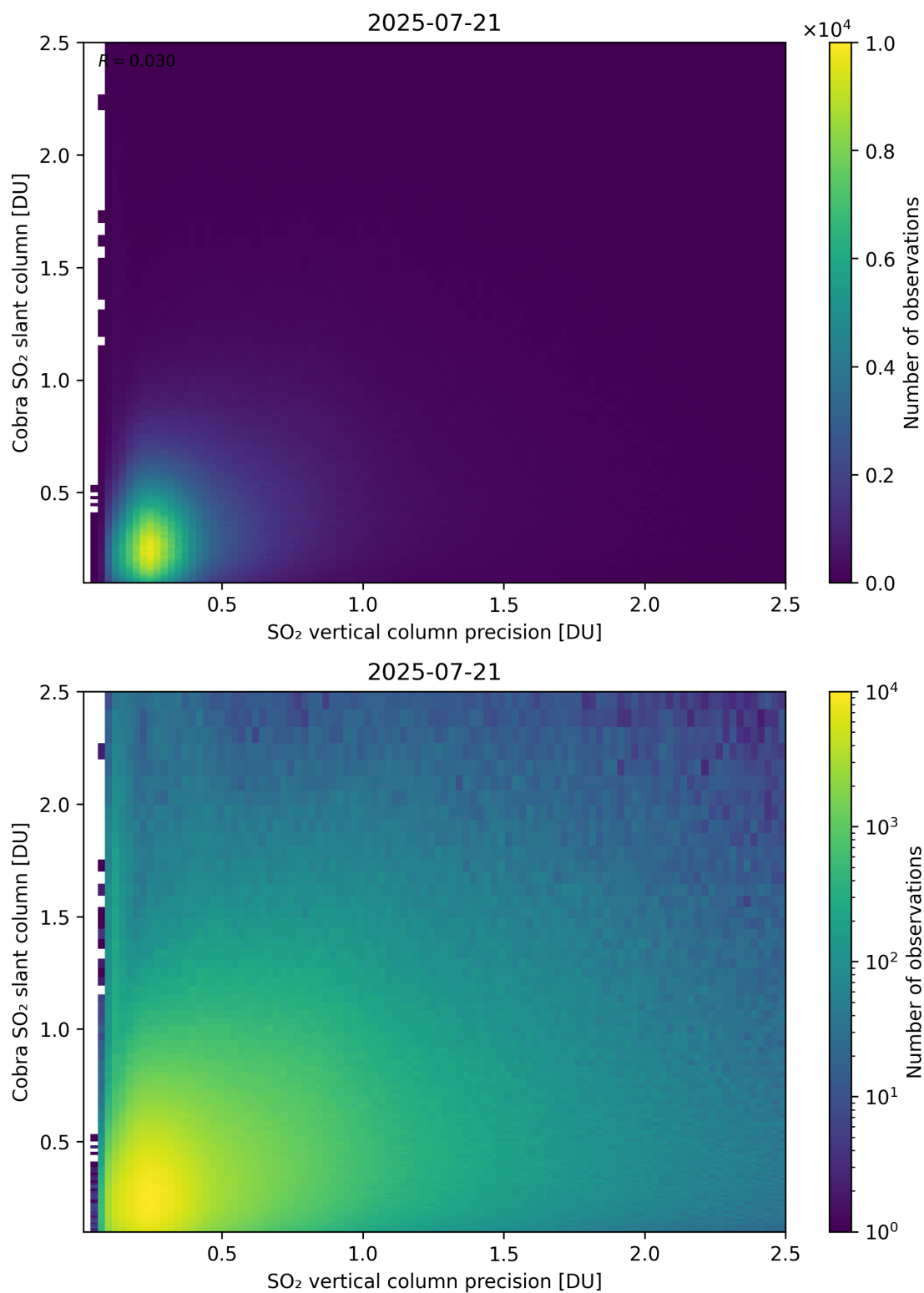
Figure 336: Scatter density plot of “SO 2 vertical column precision” against “Cobra SO 2 slant column” for 2025-07-20 to 2025-07-22.
