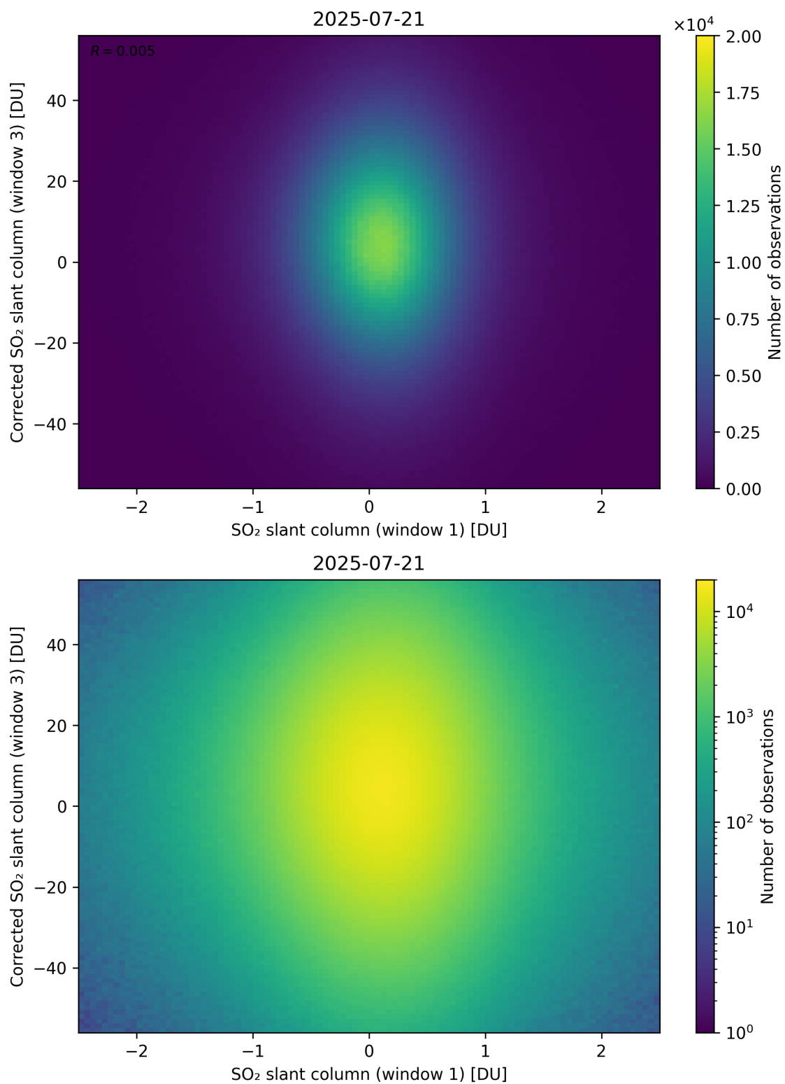
Figure 284: Scatter density plot of “SO 2 slant column (window 1)” against “Corrected SO 2 slant column (window 3)” for 2025-07-20 to 2025-07-22.
