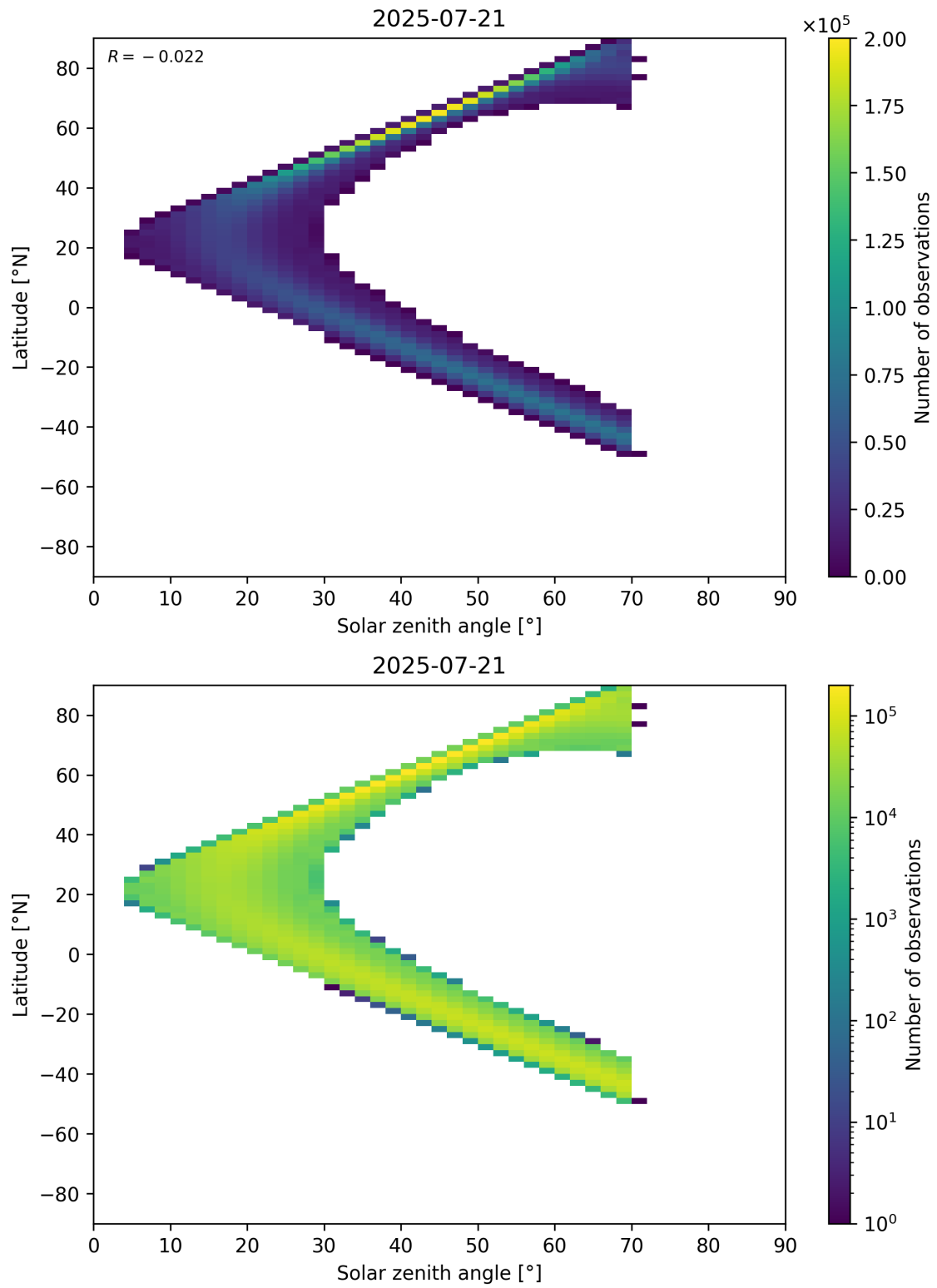
Figure 177: Scatter density plot of “Solar zenith angle” against “Latitude” for 2025-07-20 to 2025-07-22.
