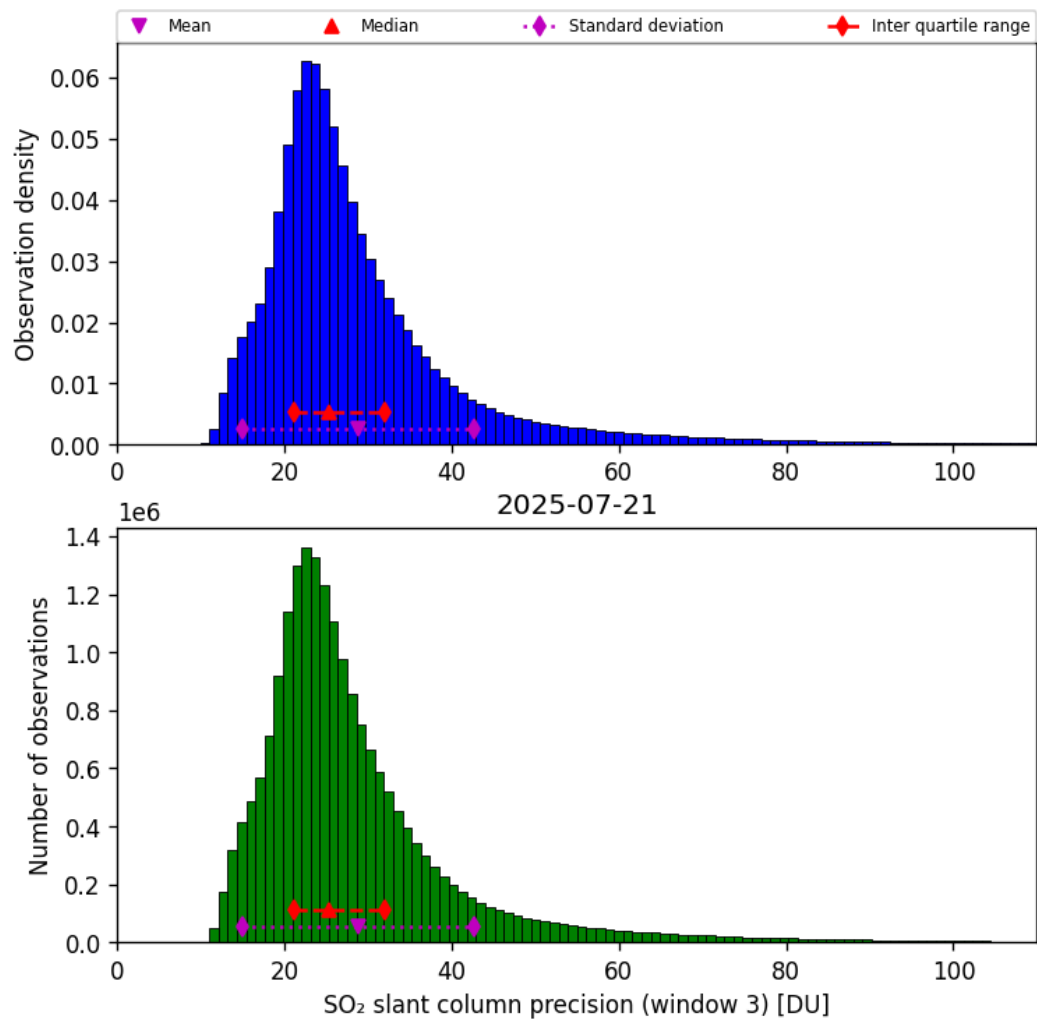
Figure 72: Histogram of “SO 2 slant column precision (window 3)” for 2025-07-20 to 2025-07-22
