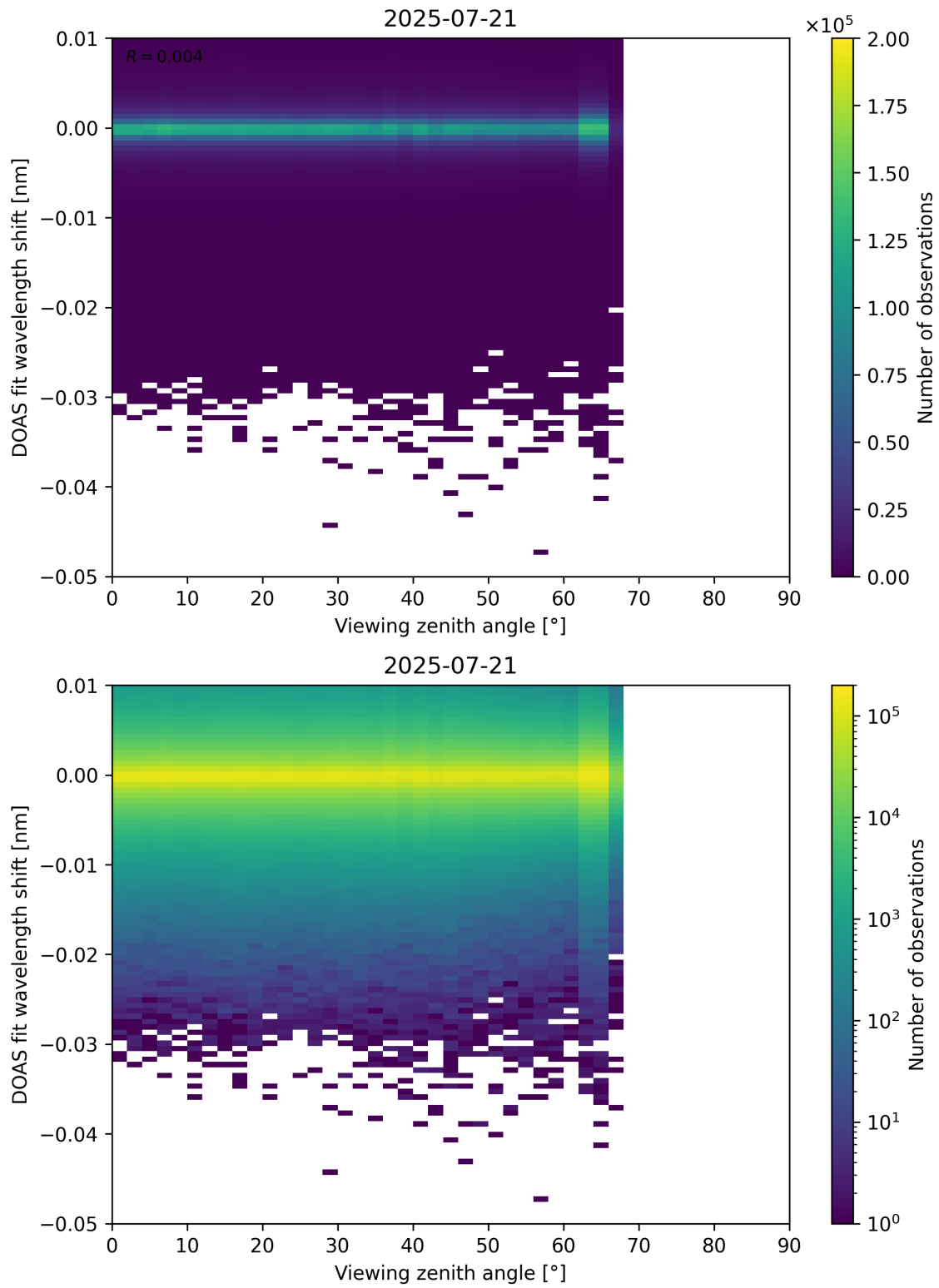
Figure 365: Scatter density plot of “Viewing zenith angle” against “DOAS fit wavelength shift” for 2025-07-20 to 2025-07-22.
