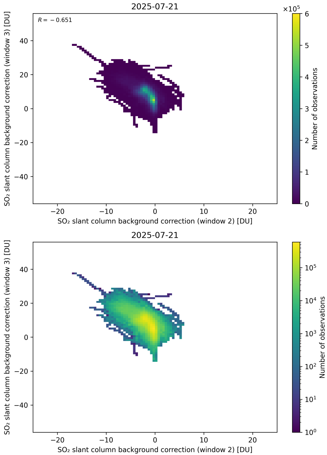
Figure 122: Scatter density plot of “SO 2 slant column background correction (window 2)” against “SO 2 slant column background correction (window 3)” for 2025-07-20 to 2025-07-22.
