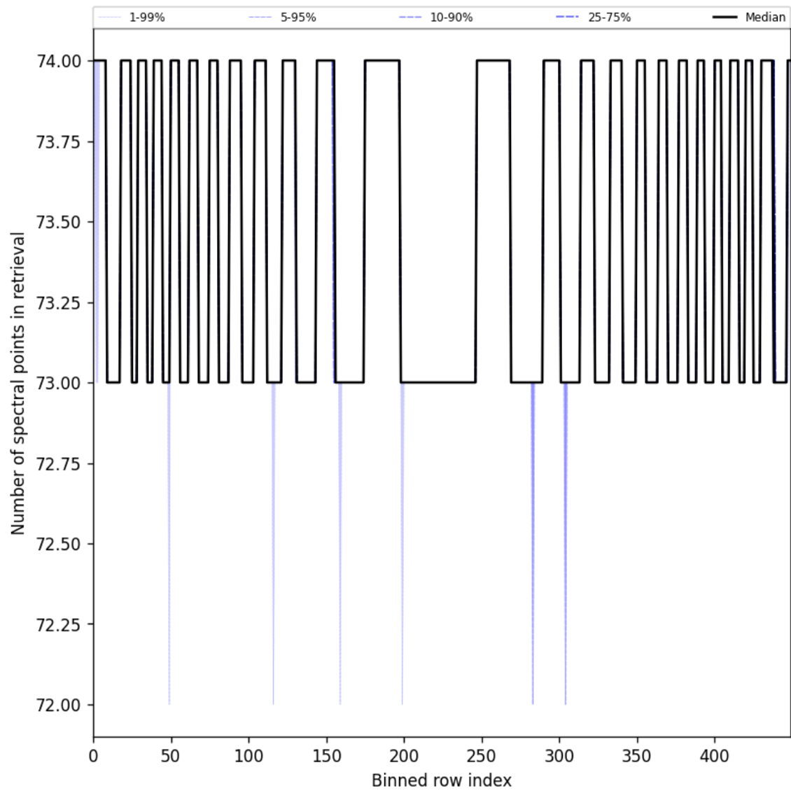
Figure 108: Along track statistics of “Number of spectral points in retrieval” for 2025-07-20 to 2025-07-22
