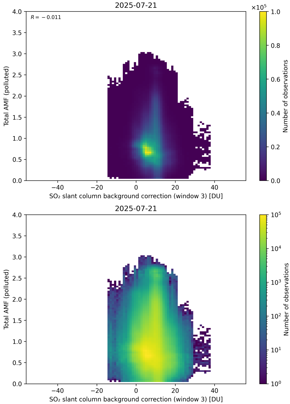
Figure 136: Scatter density plot of “SO 2 slant column background correction (window 3)” against “Total AMF (polluted)” for 2025-07-20 to 2025-07-22.
