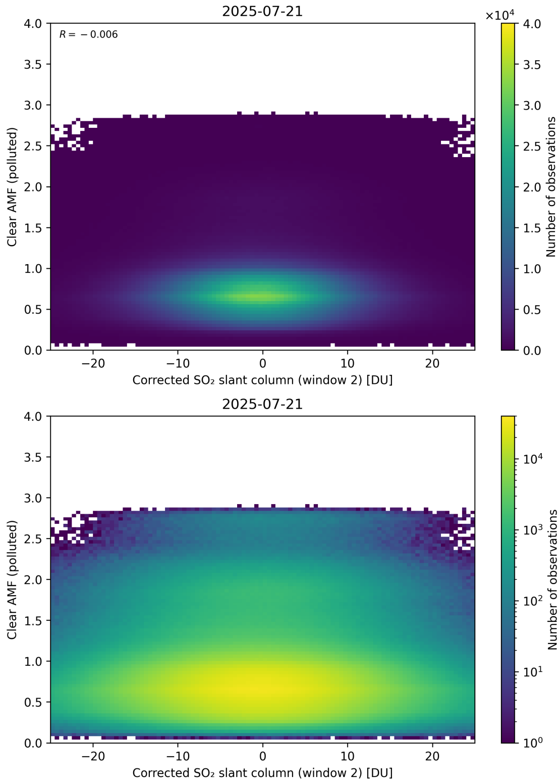
Figure 249: Scatter density plot of “Corrected SO 2 slant column (window 2)” against “Clear AMF (polluted)” for 2025-07-20 to 2025-07-22.
