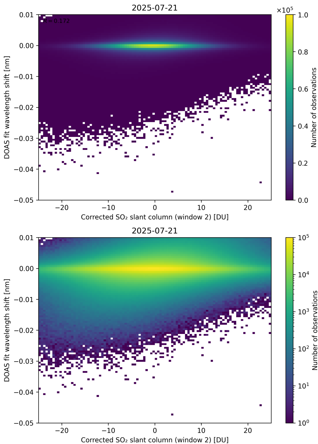
Figure 246: Scatter density plot of “Corrected SO 2 slant column (window 2)” against “DOAS fit wavelength shift” for 2025-07-20 to 2025-07-22.
