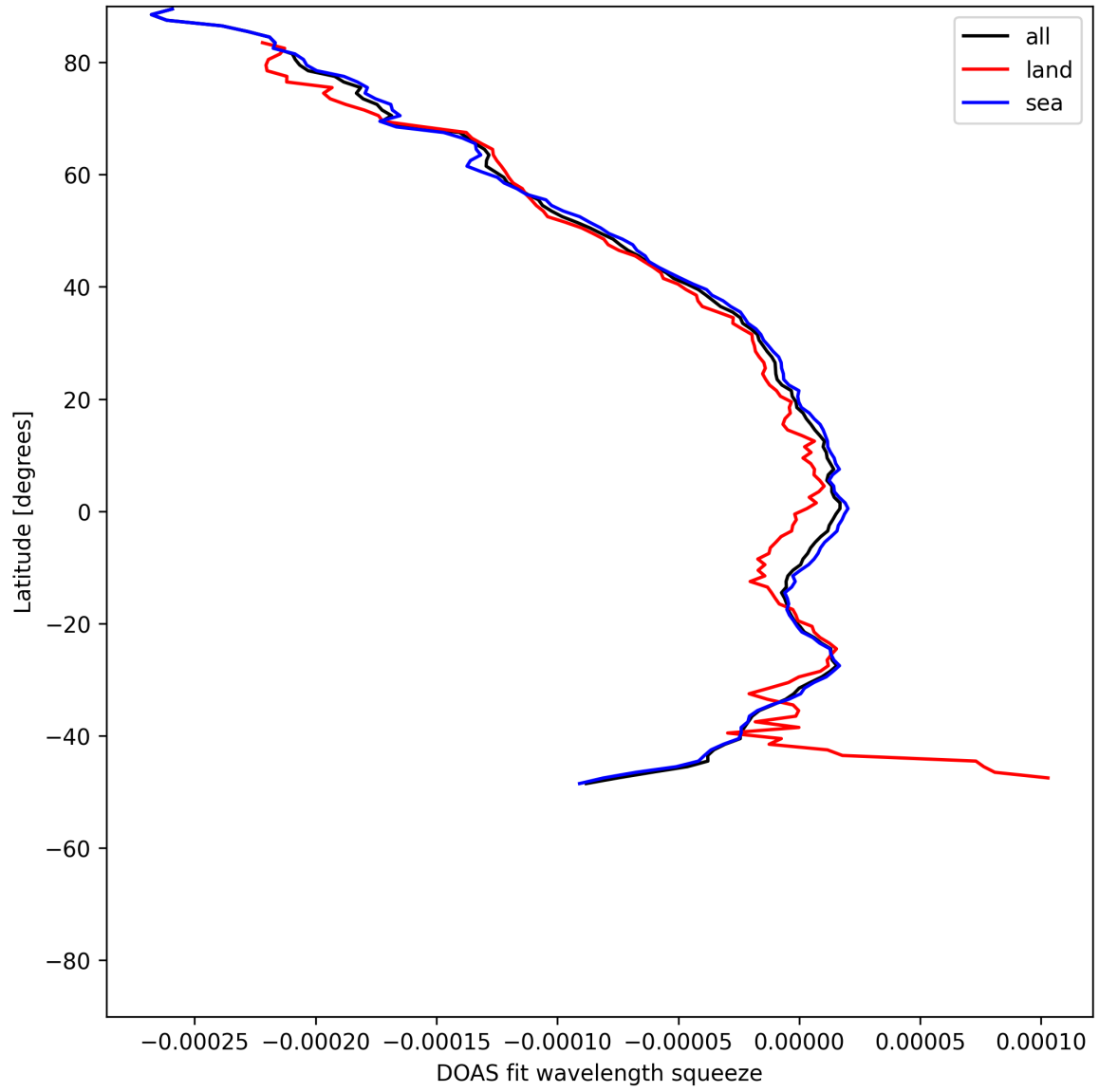
Figure 51: Zonal average of “DOAS fit wavelength squeeze” for 2025-07-20 to 2025-07-22.
