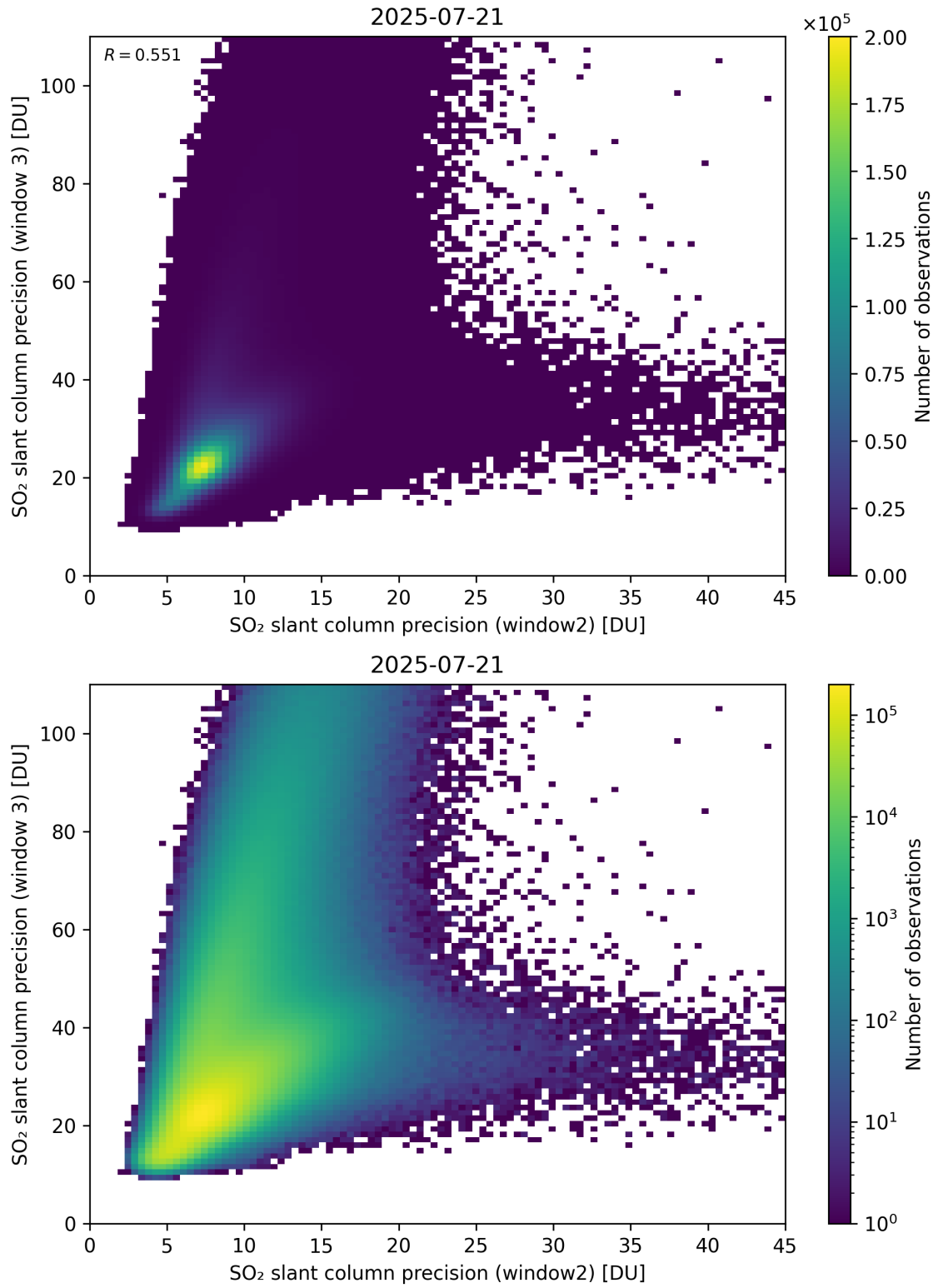
Figure 300: Scatter density plot of “SO 2 slant column precision (window2)” against “SO 2 slant column precision (window 3)” for 2025-07-20 to 2025-07-22.
