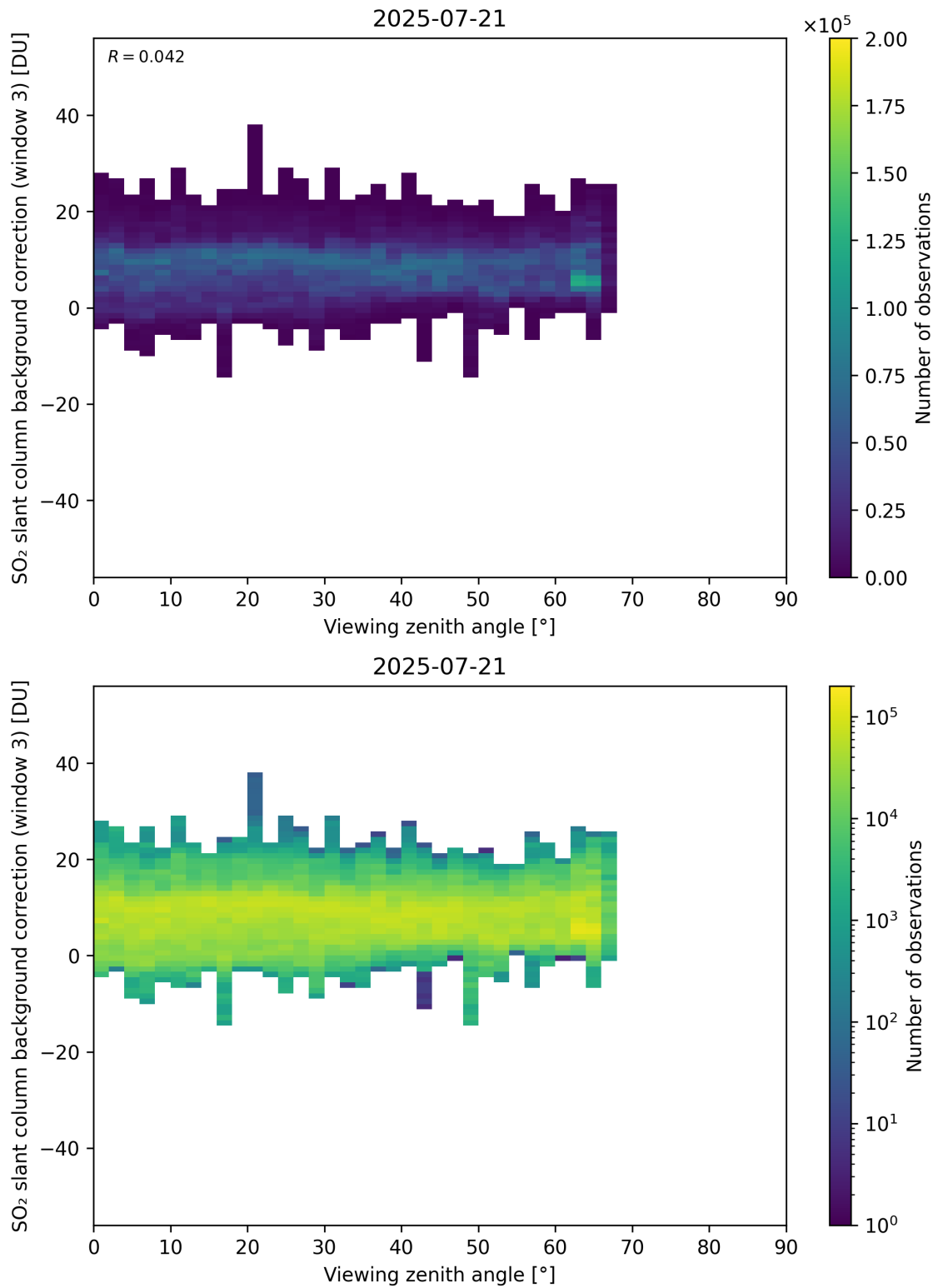
Figure 364: Scatter density plot of “Viewing zenith angle” against “SO 2 slant column background correction (window 3)” for 2025-07-20 to 2025-07-22.
