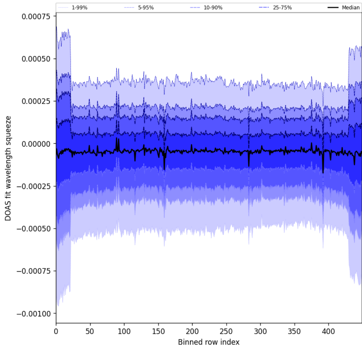
Figure 103: Along track statistics of “DOAS fit wavelength squeeze” for 2025-07-20 to 2025-07-22
