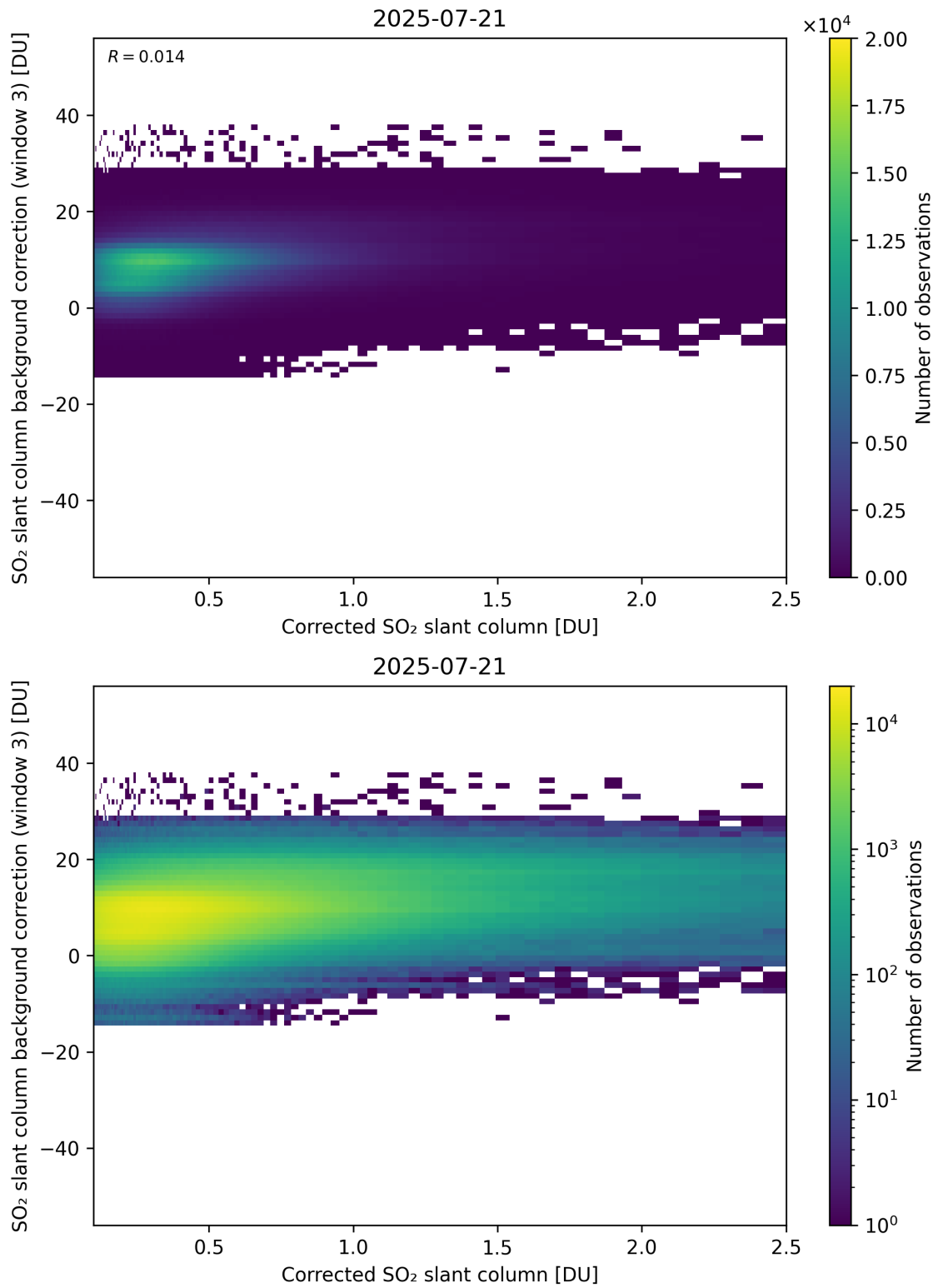
Figure 228: Scatter density plot of “Corrected SO 2 slant column” against “SO 2 slant column background correction (window 3)” for 2025-07-20 to 2025-07-22.
