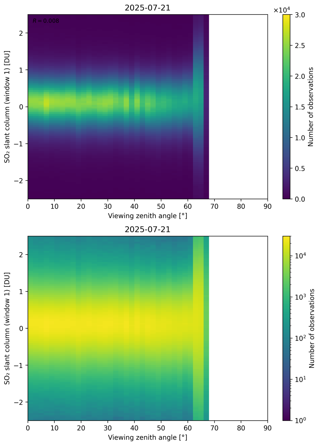
Figure 376: Scatter density plot of “Viewing zenith angle” against “SO 2 slant column (window 1)” for 2025-07-20 to 2025-07-22.
