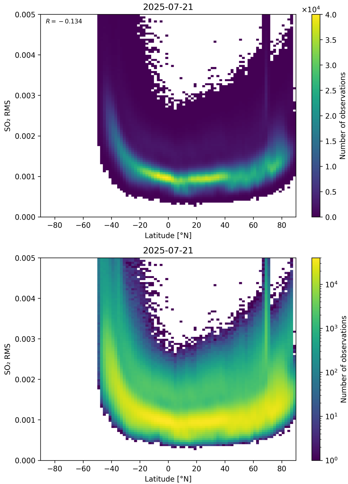
Figure 155: Scatter density plot of “Latitude” against “SO 2 RMS” for 2025-07-20 to 2025-07-22.
