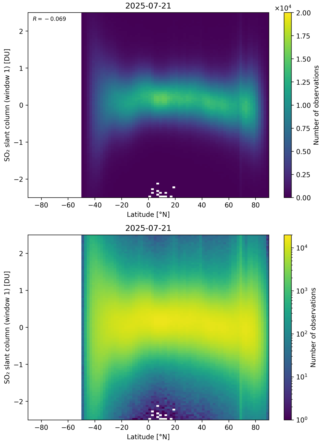
Figure 162: Scatter density plot of “Latitude” against “SO 2 slant column (window 1)” for 2025-07-20 to 2025-07-22.
