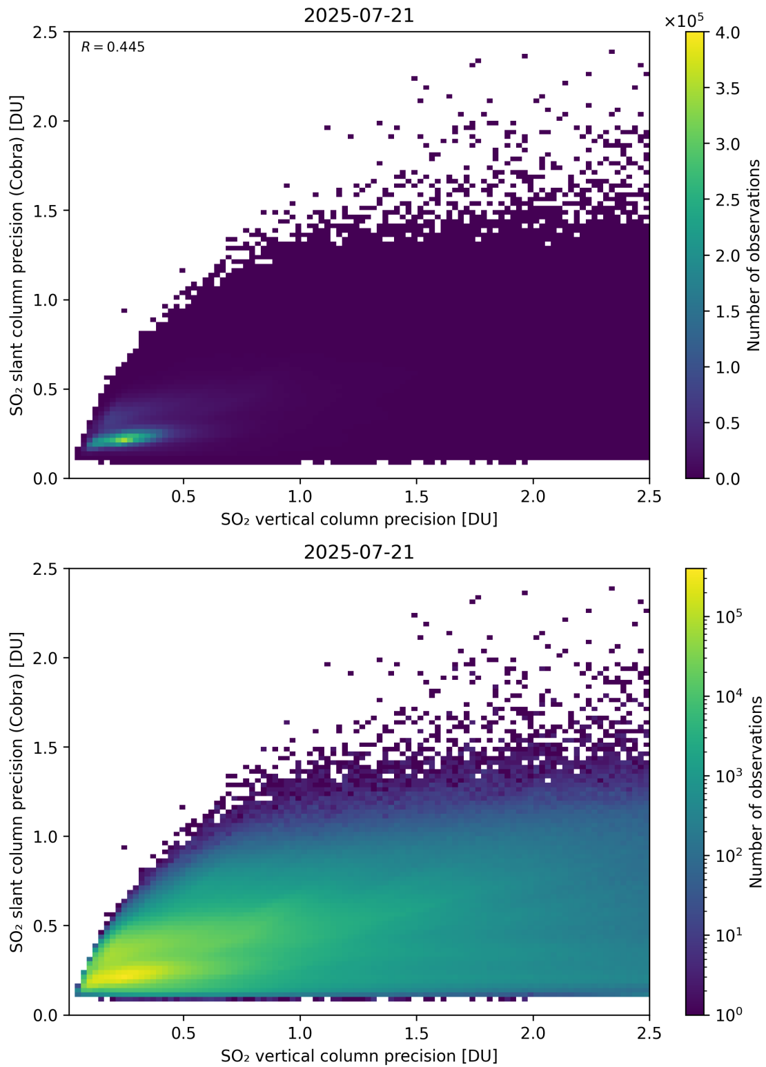
Figure 337: Scatter density plot of “SO 2 vertical column precision” against “SO 2 slant column precision (Cobra)” for 2025-07-20 to 2025-07-22.
