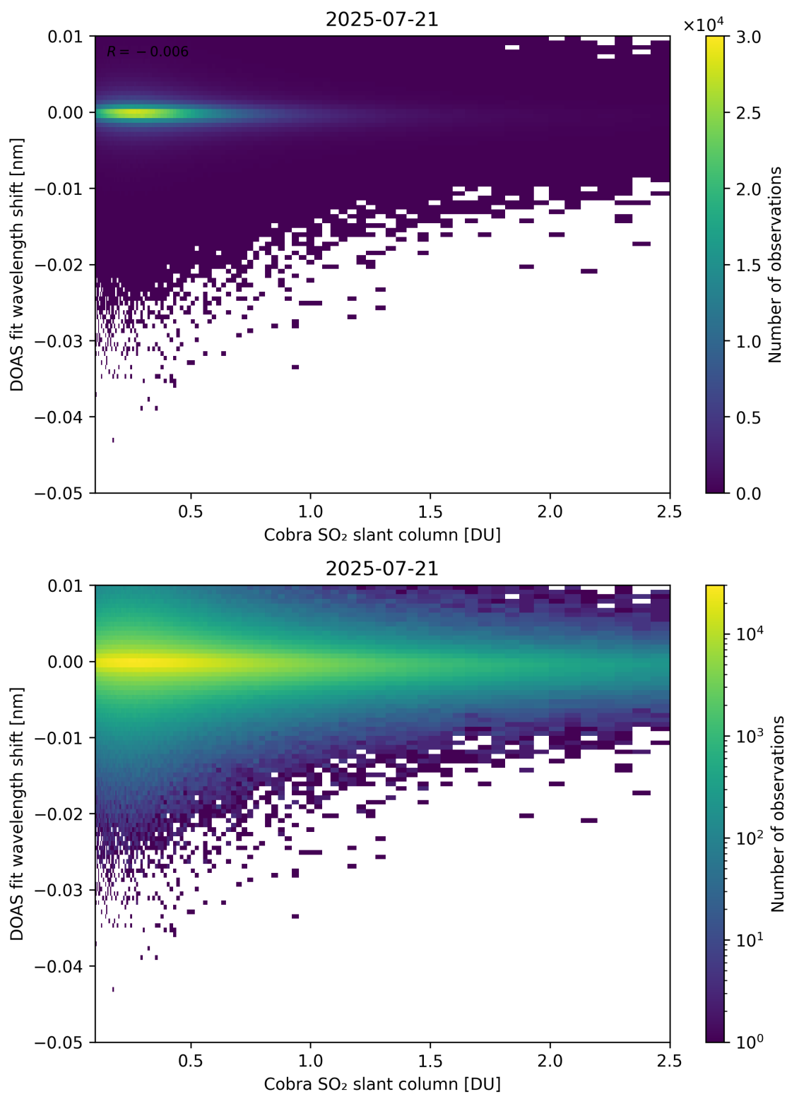
Figure 196: Scatter density plot of “Cobra SO 2 slant column” against “DOAS fit wavelength shift” for 2025-07-20 to 2025-07-22.
