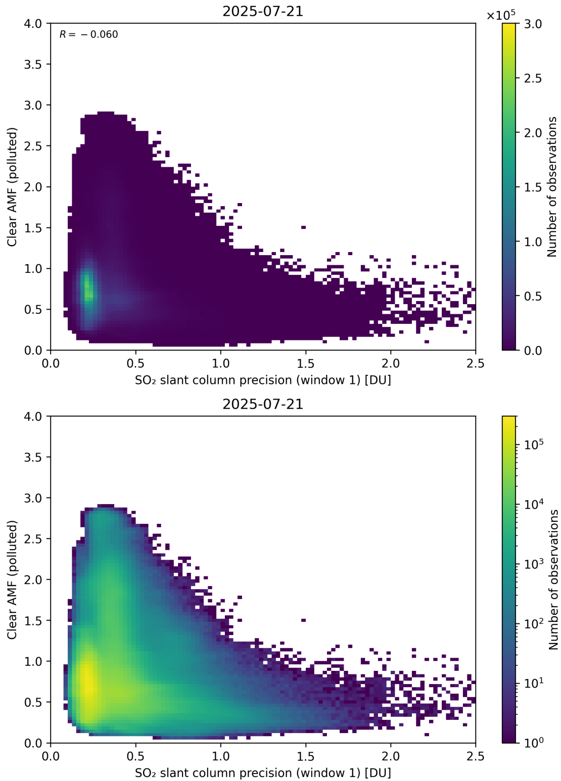
Figure 274: Scatter density plot of “SO 2 slant column precision (window 1)” against “Clear AMF (polluted)” for 2025-07-20 to 2025-07-22.
