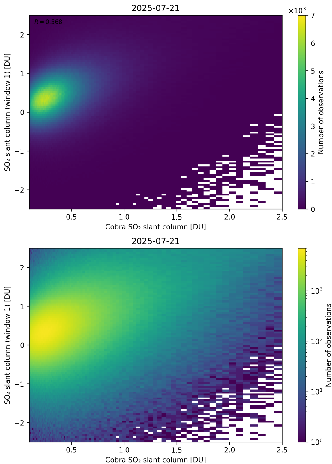
Figure 219: Scatter density plot of “Cobra SO 2 slant column” against “SO 2 slant column (window 1)” for 2025-07-20 to 2025-07-22.
