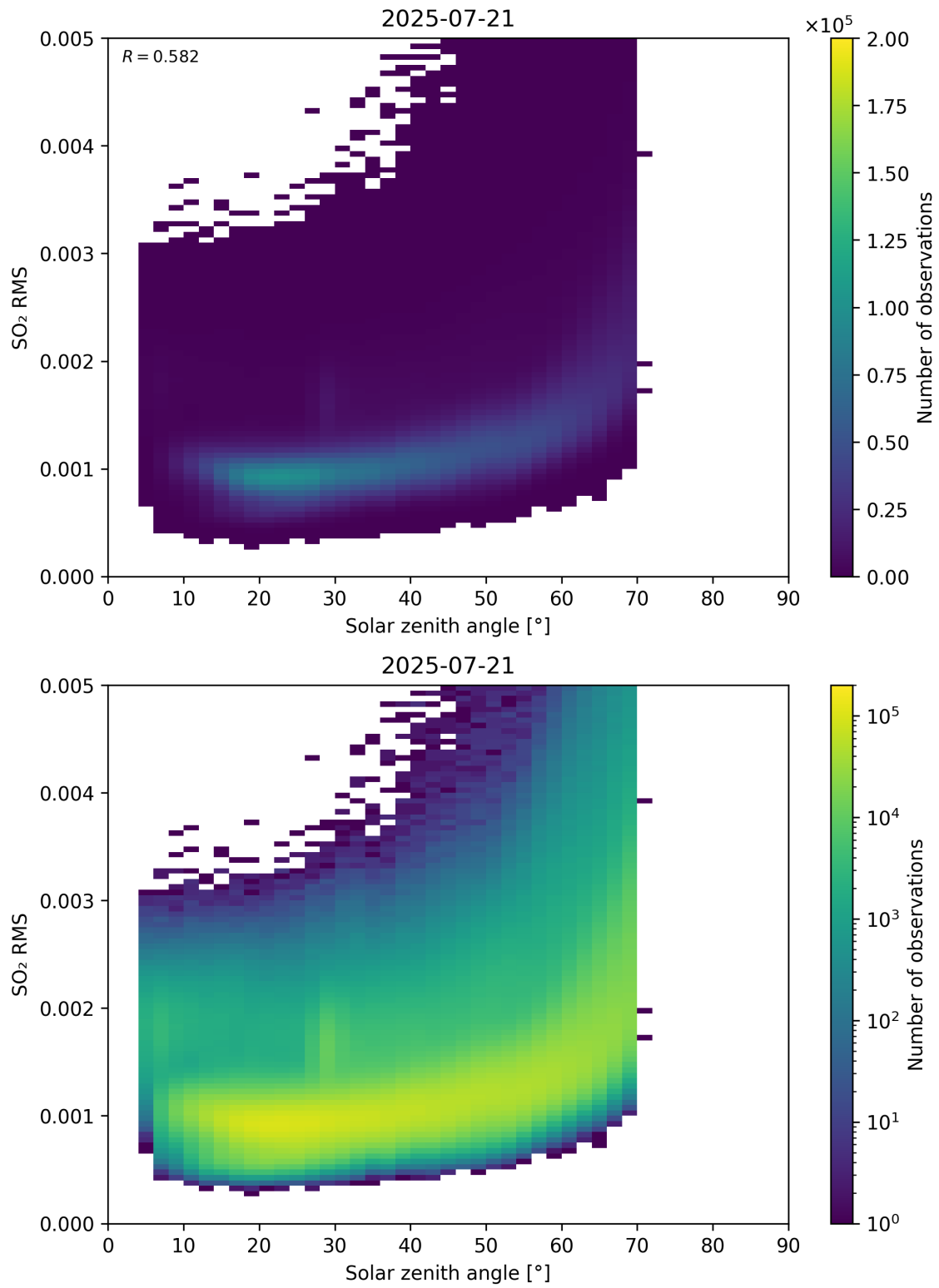
Figure 176: Scatter density plot of “Solar zenith angle” against “SO 2 RMS” for 2025-07-20 to 2025-07-22.
