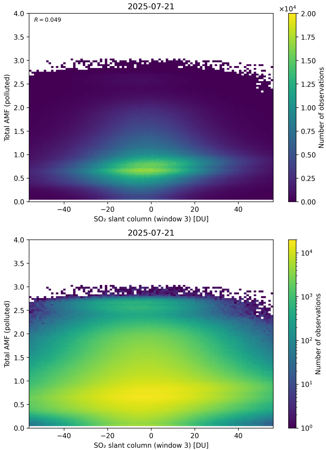
Figure 318: Scatter density plot of “SO 2 slant column (window 3)” against “Total AMF (polluted)” for 2025-07-20 to 2025-07-22.
