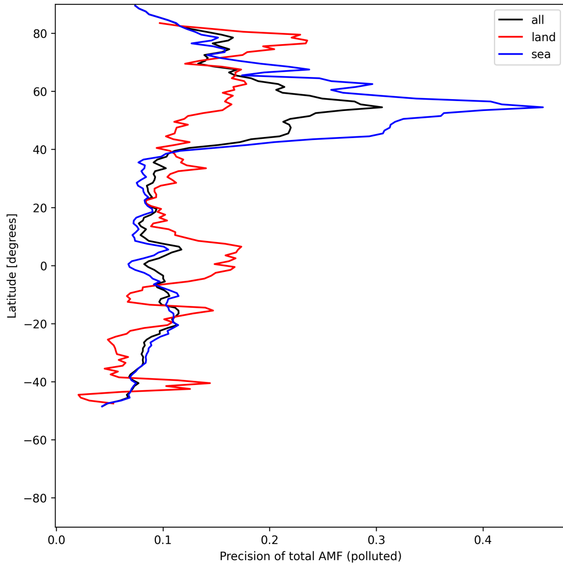
Figure 54: Zonal average of “Precision of total AMF (polluted)” for 2025-07-20 to 2025-07-22.
