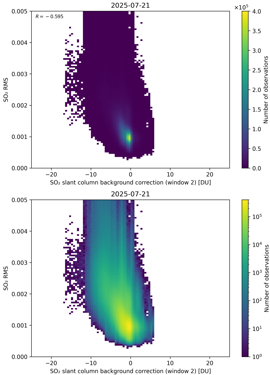
Figure 125: Scatter density plot of “SO 2 slant column background correction (window 2)” against “SO 2 RMS” for 2025-07-20 to 2025-07-22.
