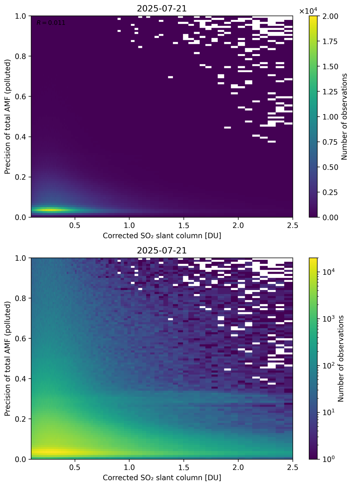
Figure 243: Scatter density plot of “Corrected SO 2 slant column” against “Precision of total AMF (polluted)” for 2025-07-20 to 2025-07-22.
