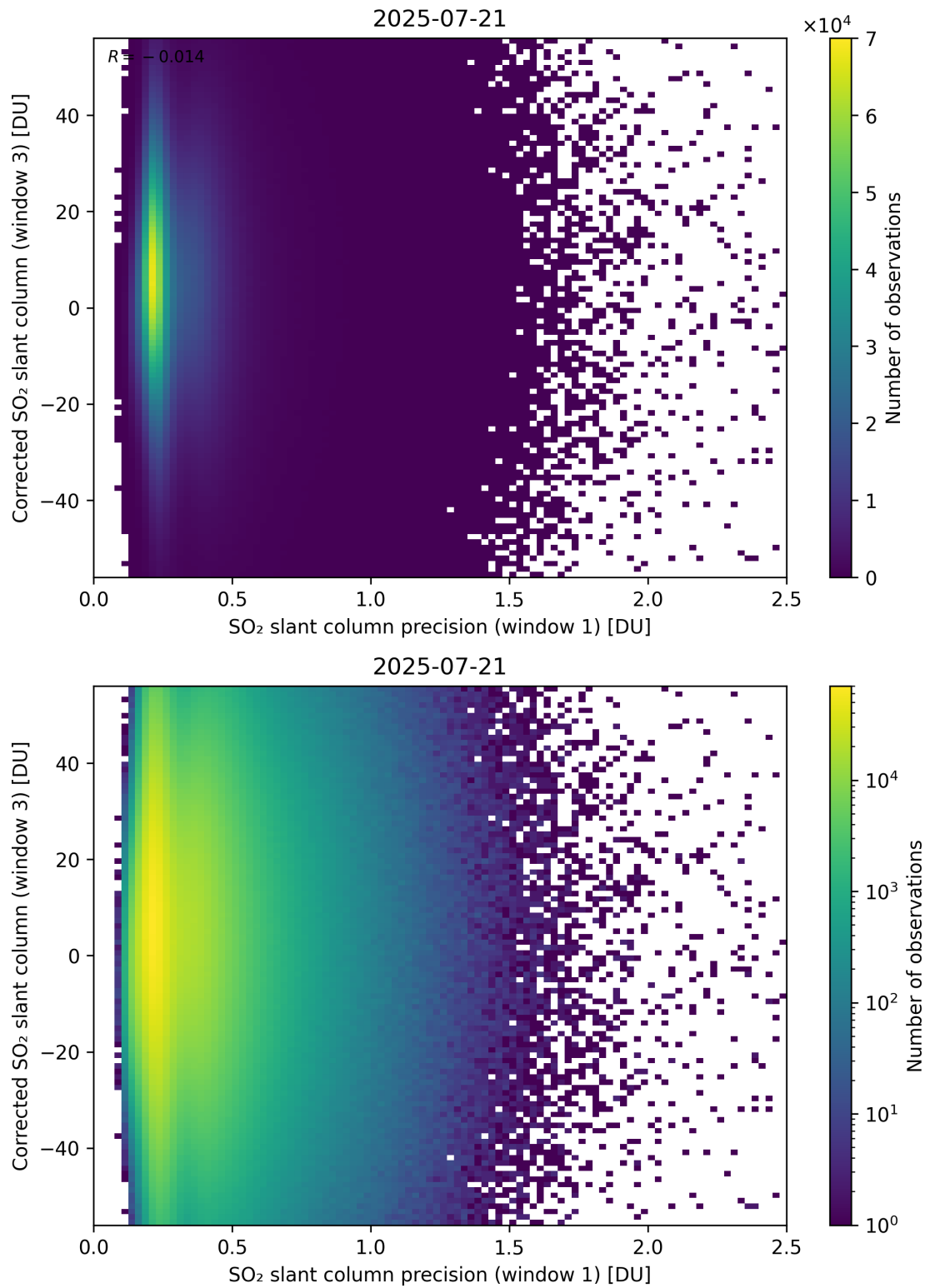
Figure 276: Scatter density plot of “SO 2 slant column precision (window 1)” against “Corrected SO 2 slant column (window 3)” for 2025-07-20 to 2025-07-22.
