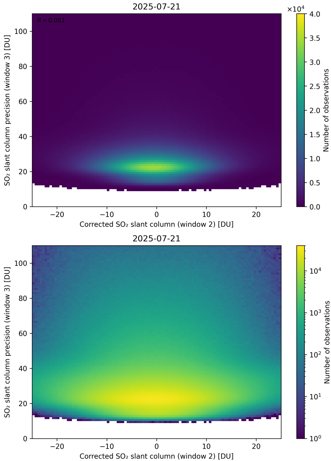
Figure 252: Scatter density plot of “Corrected SO 2 slant column (window 2)” against “SO 2 slant column precision (window 3)” for 2025-07-20 to 2025-07-22.
