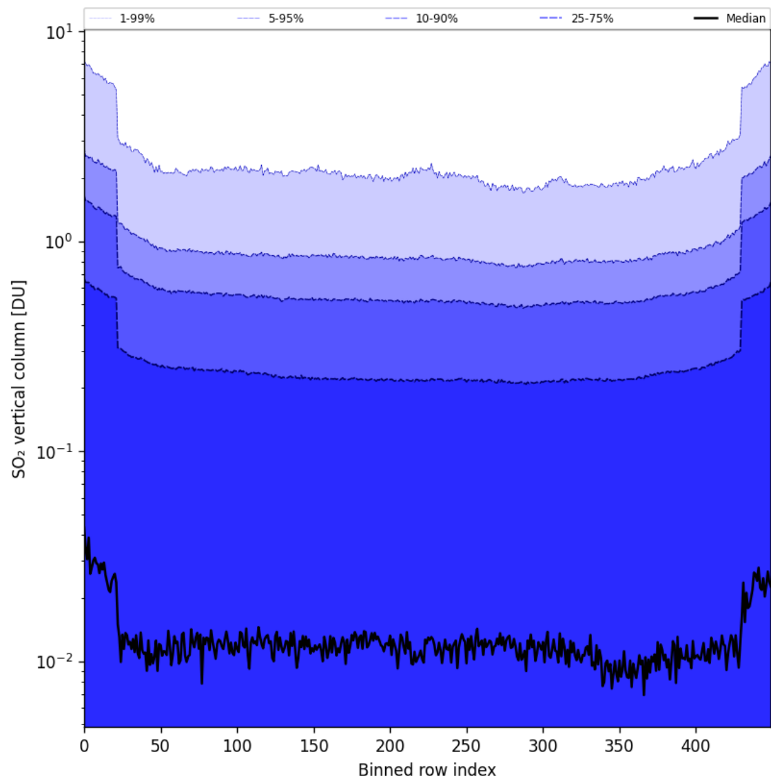
Figure 84: Along track statistics of “SO 2 vertical column” for 2025-07-20 to 2025-07-22
