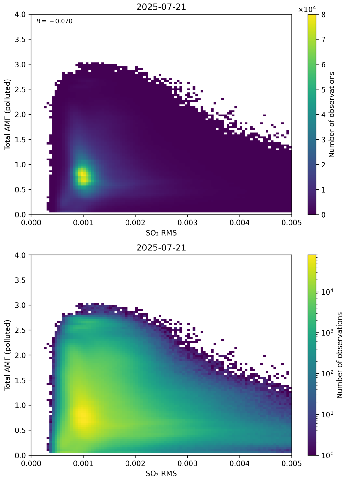
Figure 148: Scatter density plot of “SO 2 RMS” against “Total AMF (polluted)” for 2025-07-20 to 2025-07-22.
