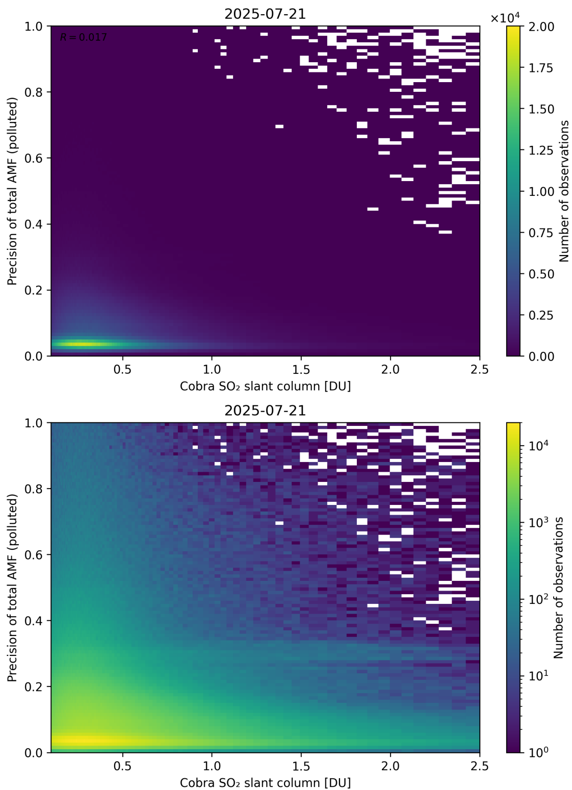
Figure 225: Scatter density plot of “Cobra SO 2 slant column” against “Precision of total AMF (polluted)” for 2025-07-20 to 2025-07-22.
