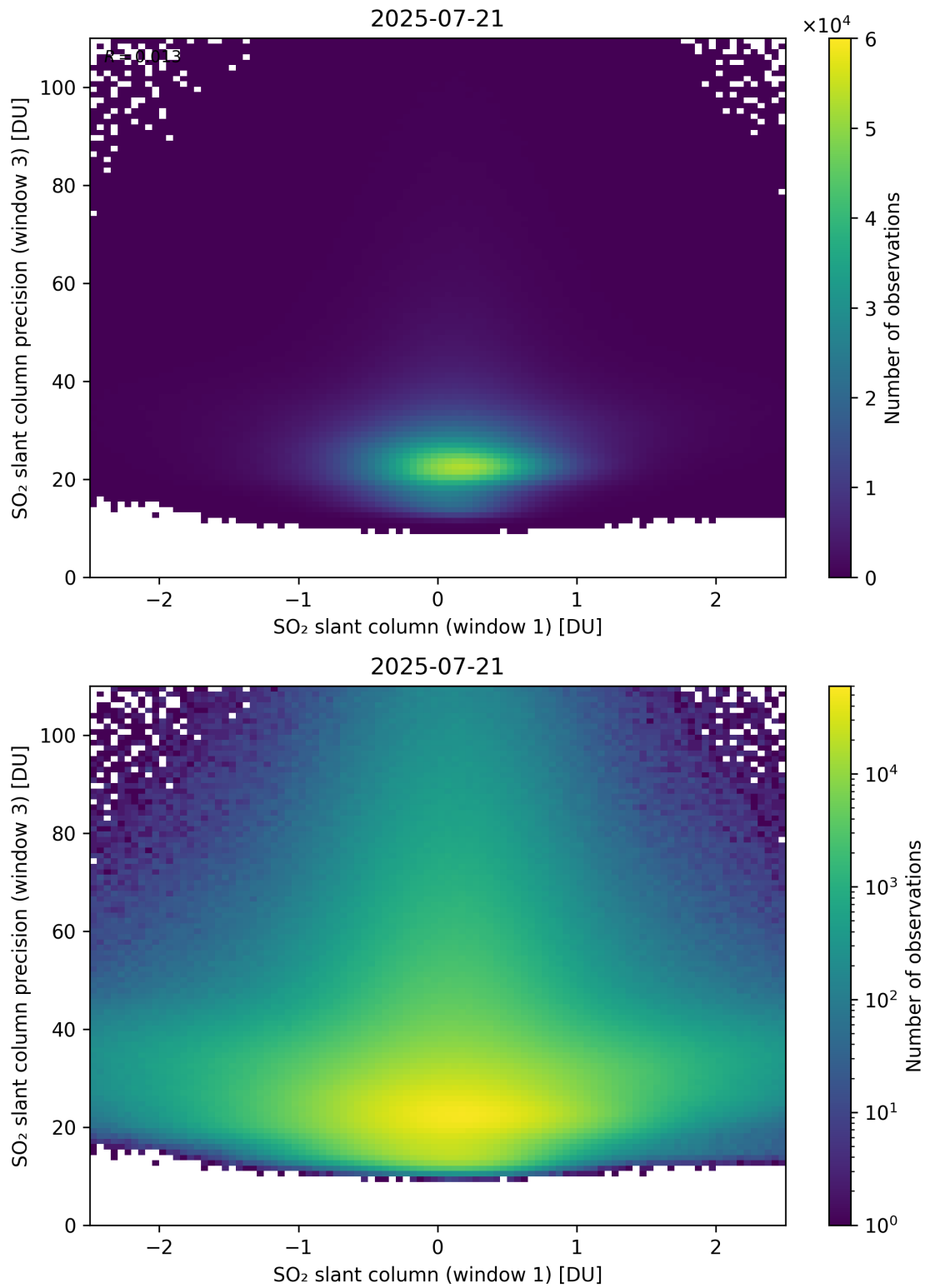
Figure 288: Scatter density plot of “SO 2 slant column (window 1)” against “SO 2 slant column precision (window 3)” for 2025-07-20 to 2025-07-22.
