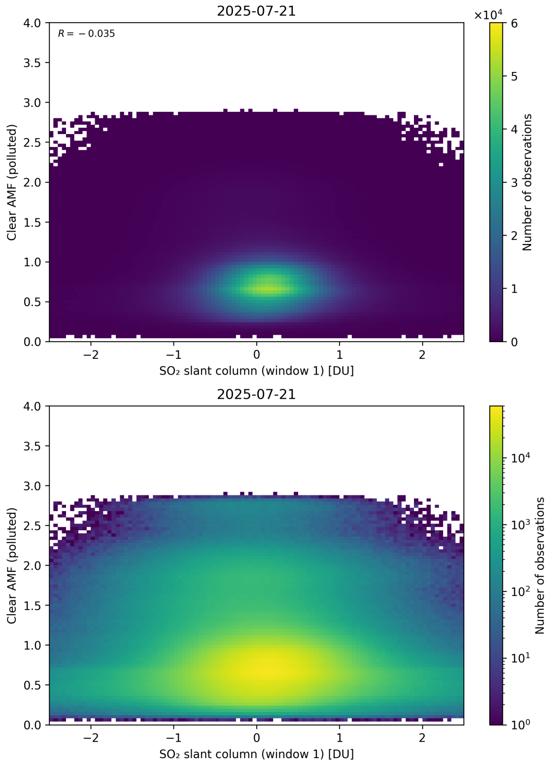
Figure 282: Scatter density plot of “SO 2 slant column (window 1)” against “Clear AMF (polluted)” for 2025-07-20 to 2025-07-22.
