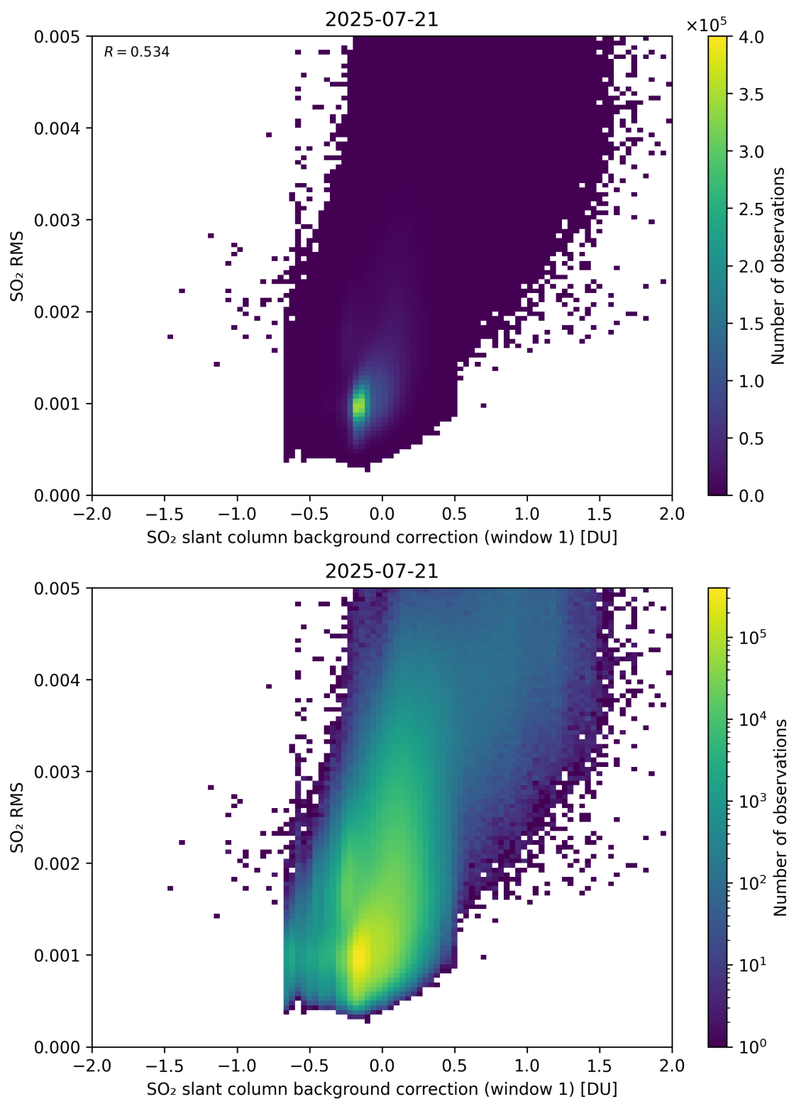
Figure 113: Scatter density plot of “SO 2 slant column background correction (window 1)” against “SO 2 RMS” for 2025-07-20 to 2025-07-22.
