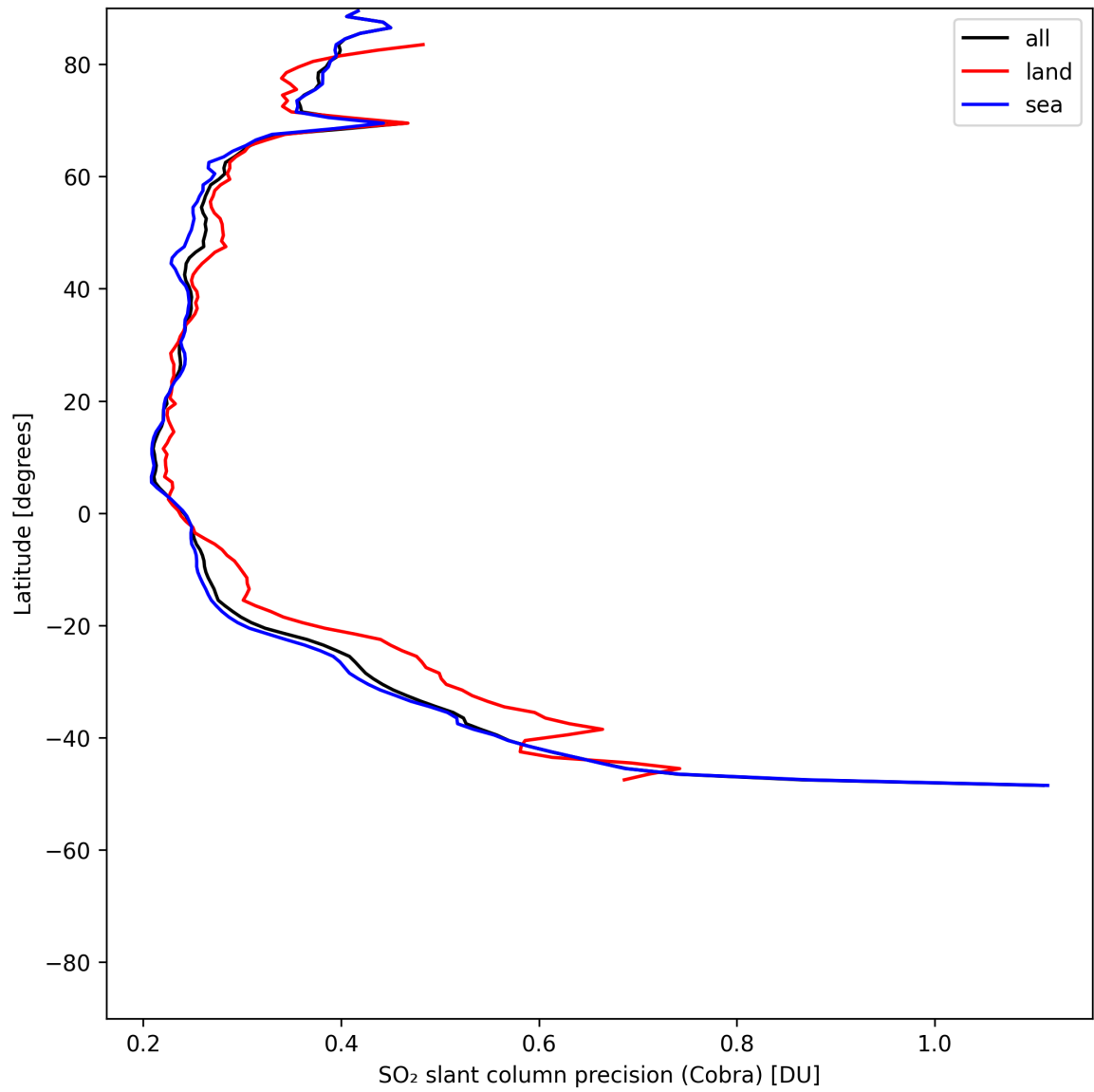
Figure 36: Zonal average of “SO 2 slant column precision (Cobra)” for 2025-07-20 to 2025-07-22.
