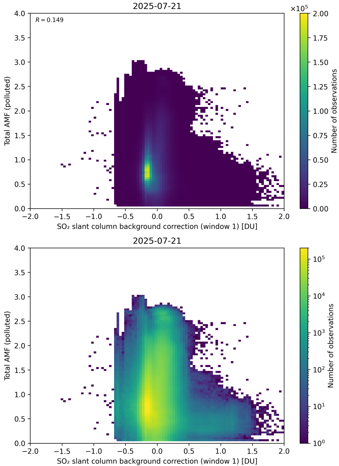
Figure 120: Scatter density plot of “SO 2 slant column background correction (window 1)” against “Total AMF (polluted)” for 2025-07-20 to 2025-07-22.
