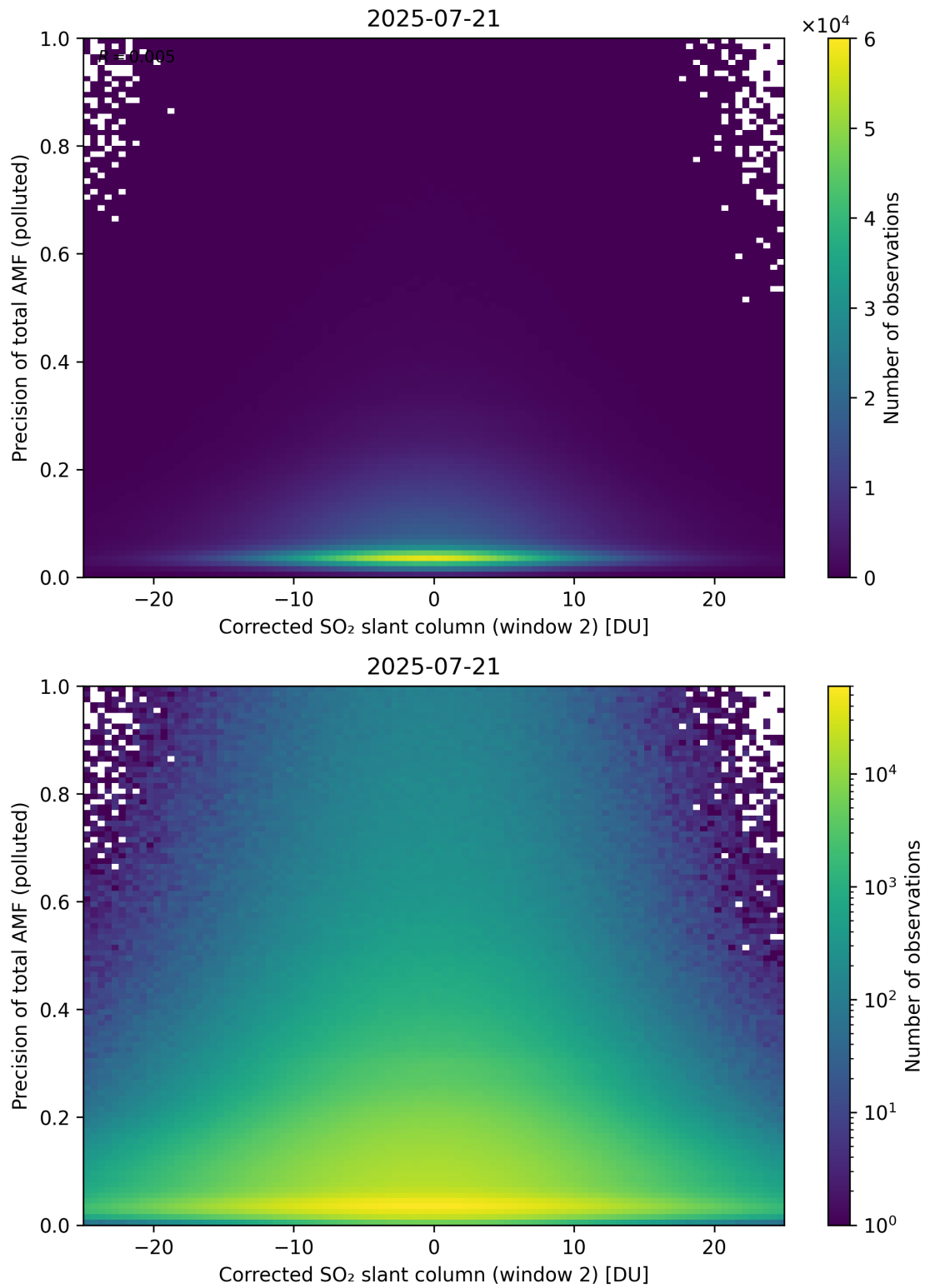
Figure 254: Scatter density plot of “Corrected SO 2 slant column (window 2)” against “Precision of total AMF (polluted)” for 2025-07-20 to 2025-07-22.
