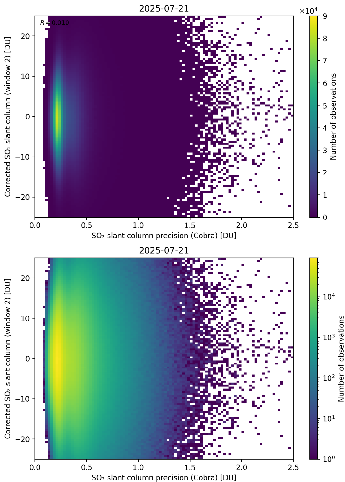
Figure 206: Scatter density plot of “SO 2 slant column precision (Cobra)” against “Corrected SO 2 slant column (window 2)” for 2025-07-20 to 2025-07-22.
