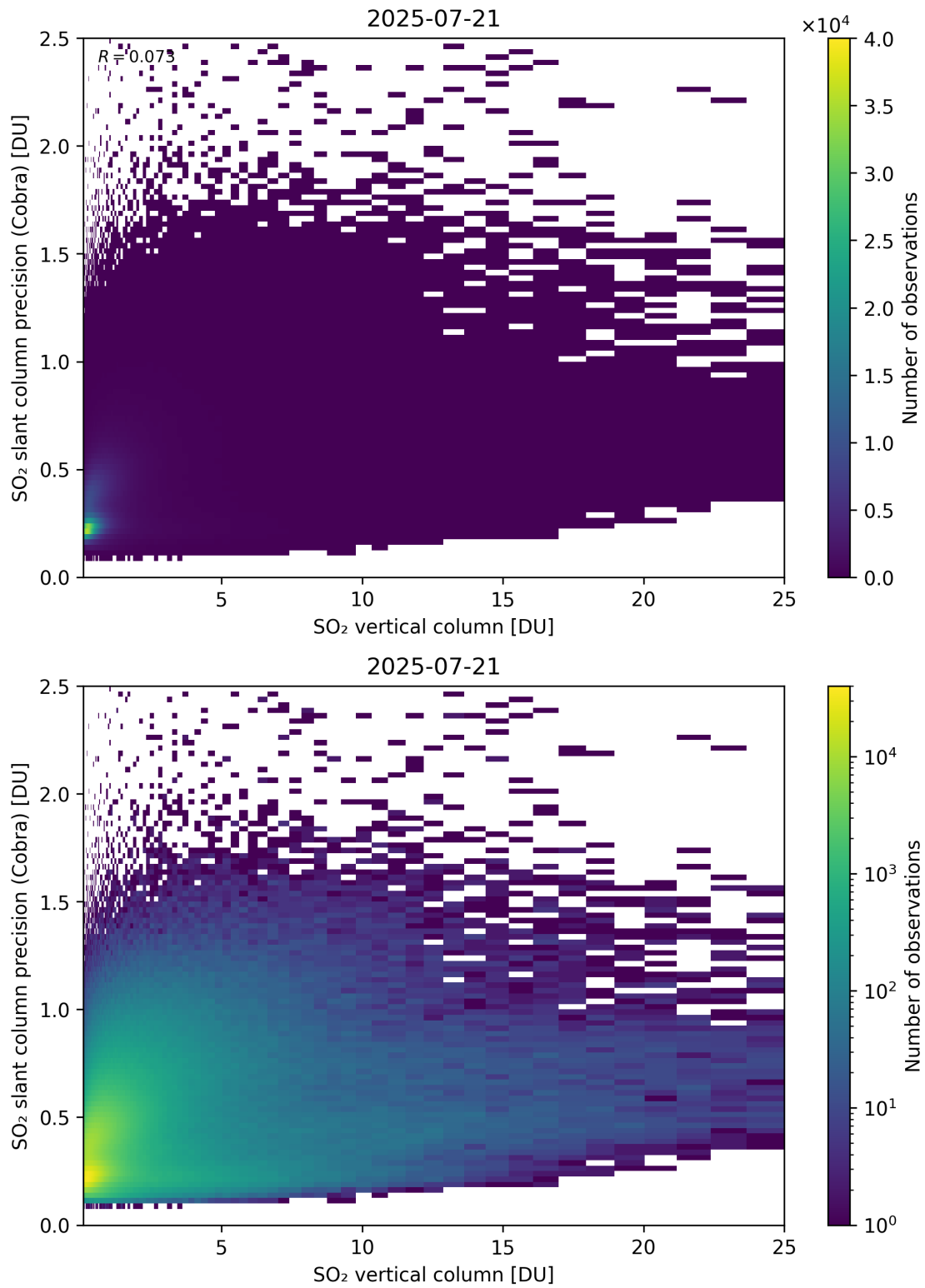
Figure 350: Scatter density plot of “SO 2 vertical column” against “SO 2 slant column precision (Cobra)” for 2025-07-20 to 2025-07-22.
