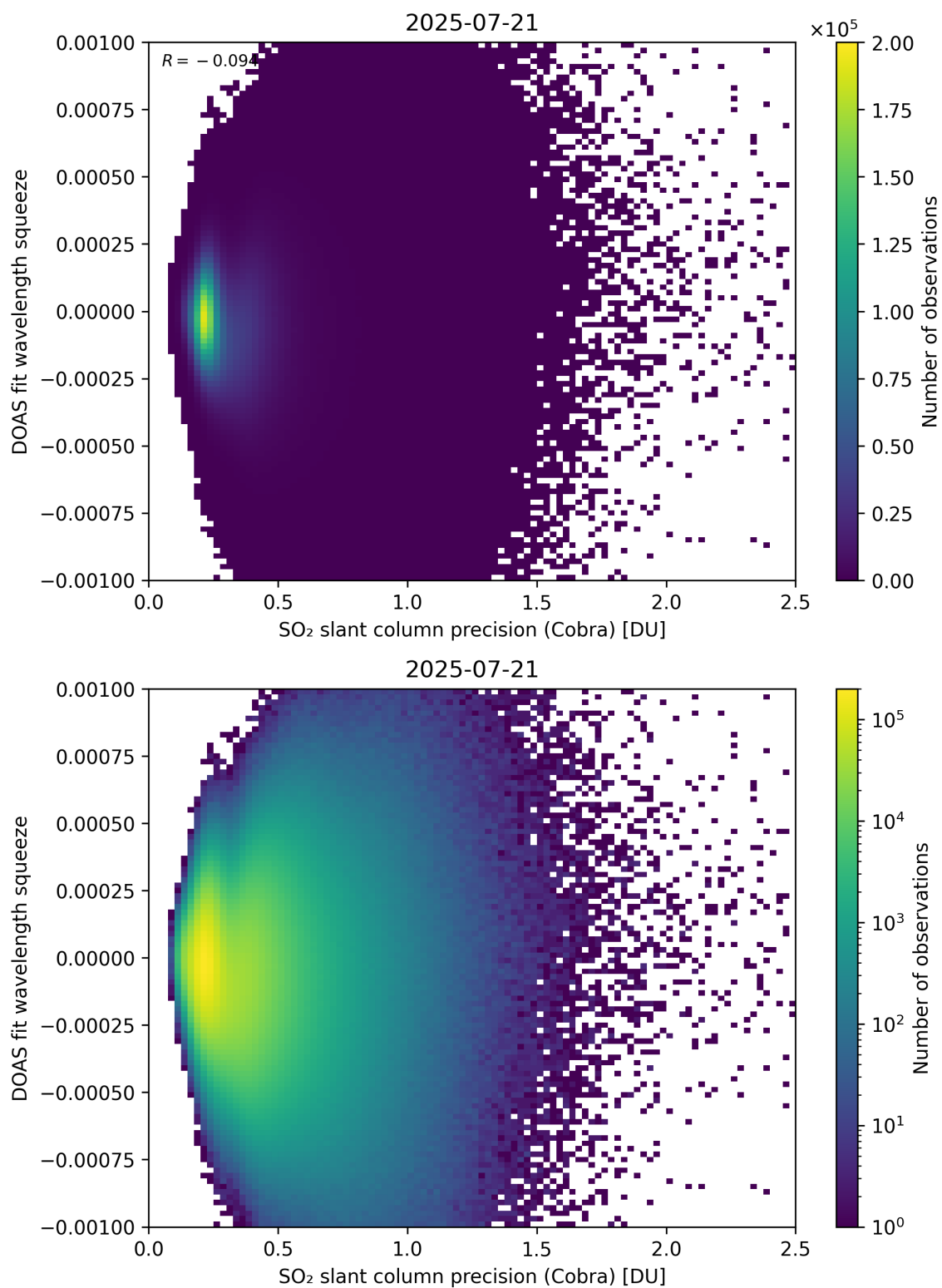
Figure 203: Scatter density plot of “SO 2 slant column precision (Cobra)” against “DOAS fit wavelength squeeze” for 2025-07-20 to 2025-07-22.
