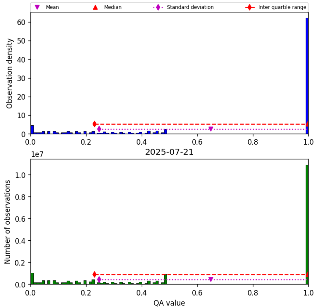
Figure 57: Histogram of “QA value” for 2025-07-20 to 2025-07-22
