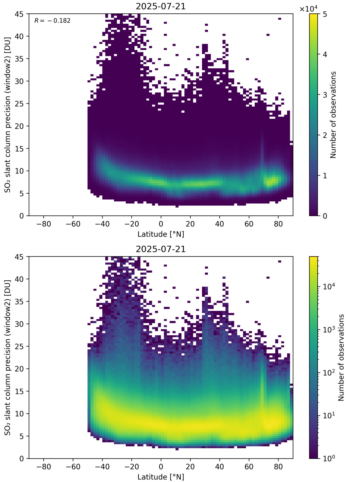
Figure 164: Scatter density plot of “Latitude” against “SO 2 slant column precision (window2)” for 2025-07-20 to 2025-07-22.
