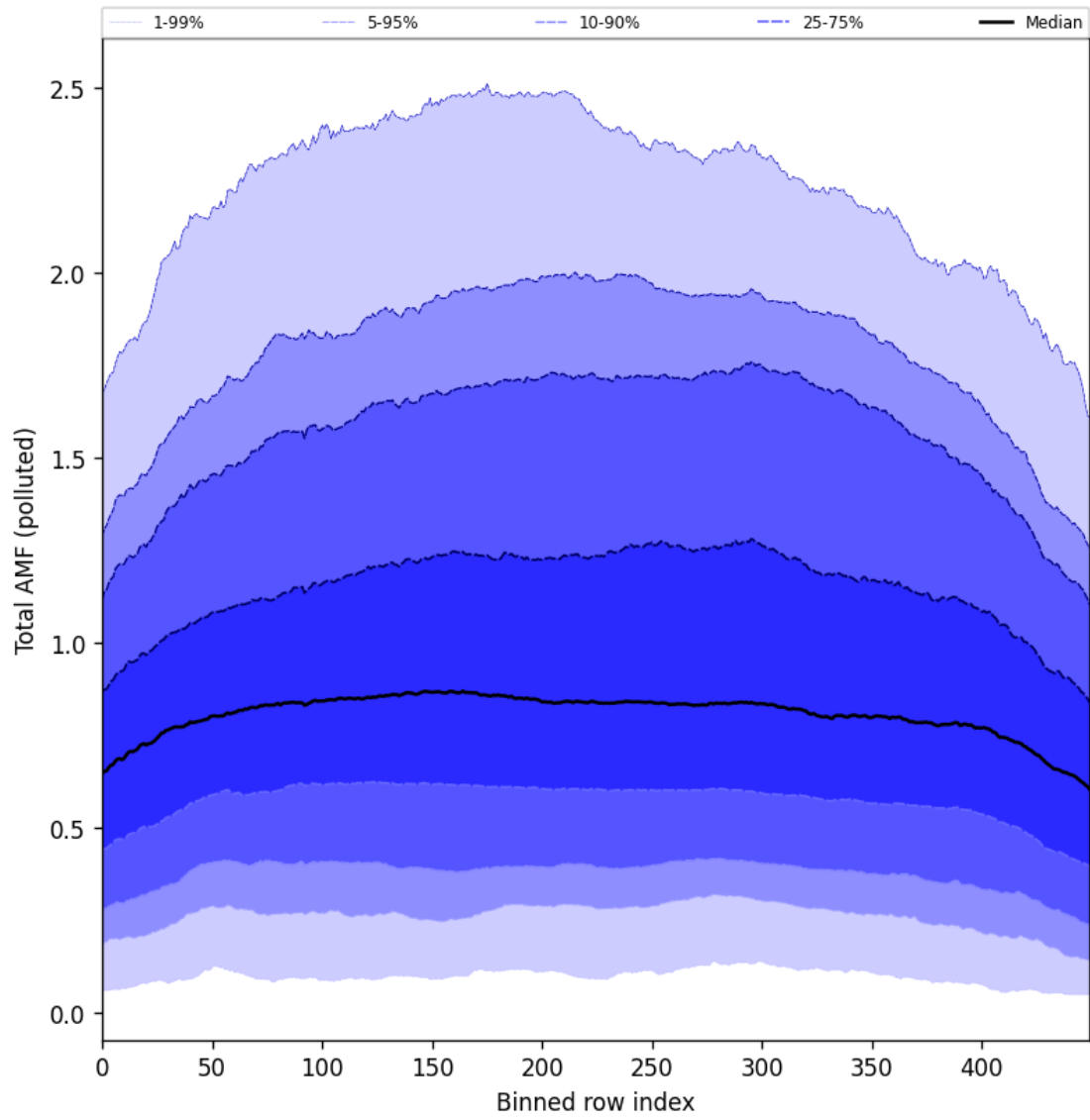
Figure 105: Along track statistics of “Total AMF (polluted)” for 2025-07-20 to 2025-07-22
