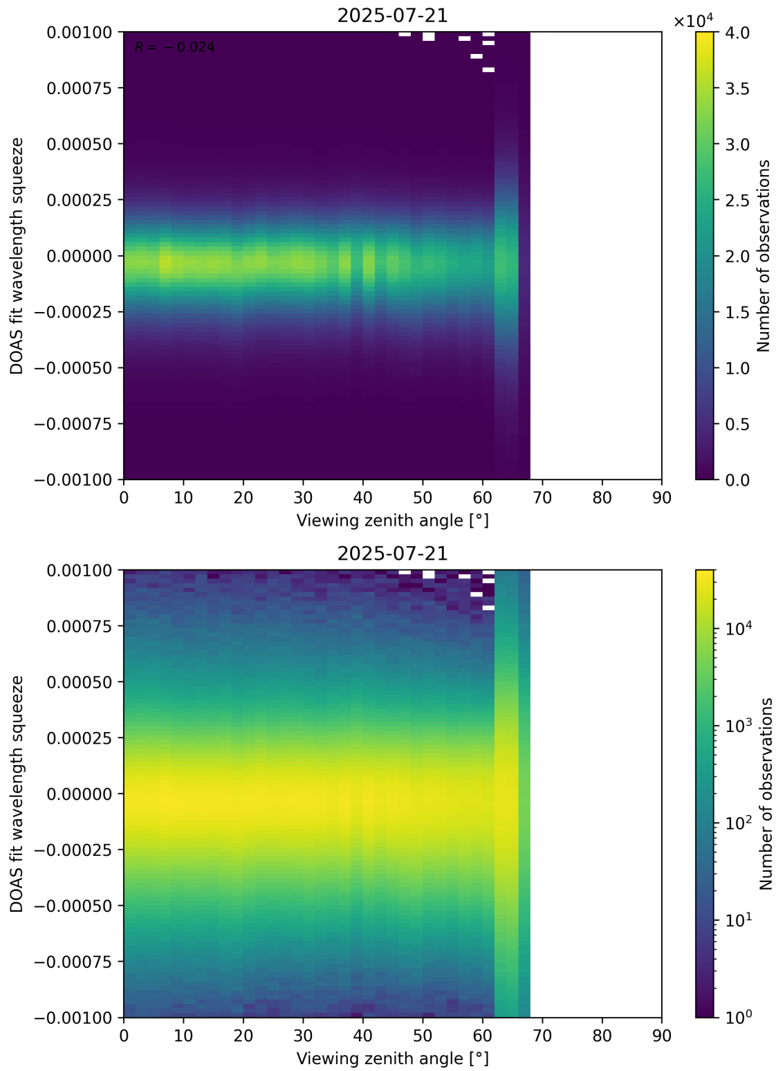
Figure 366: Scatter density plot of “Viewing zenith angle” against “DOAS fit wavelength squeeze” for 2025-07-20 to 2025-07-22.
