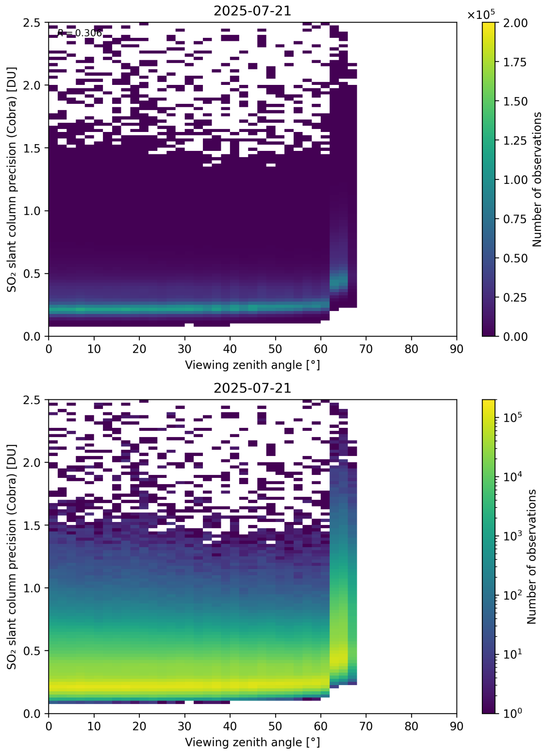
Figure 372: Scatter density plot of “Viewing zenith angle” against “SO 2 slant column precision (Cobra)” for 2025-07-20 to 2025-07-22.
