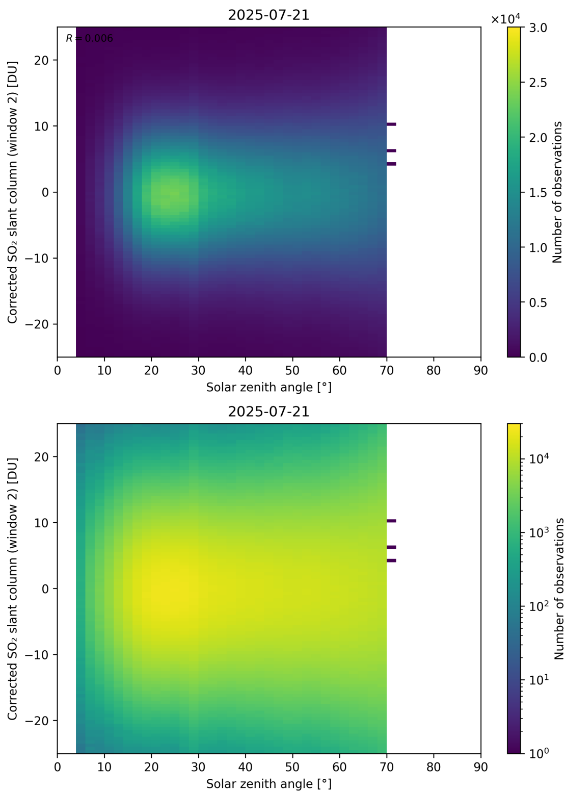
Figure 182: Scatter density plot of “Solar zenith angle” against “Corrected SO 2 slant column (window 2)” for 2025-07-20 to 2025-07-22.
