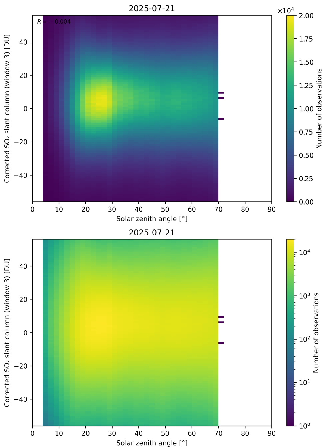
Figure 183: Scatter density plot of “Solar zenith angle” against “Corrected SO 2 slant column (window 3)” for 2025-07-20 to 2025-07-22.
