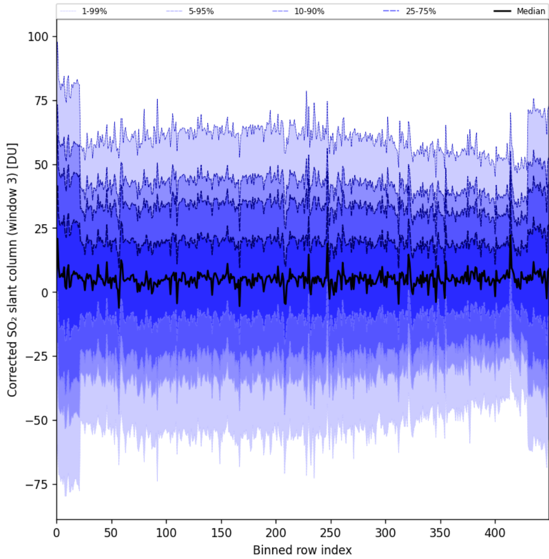
Figure 99: Along track statistics of “Corrected SO 2 slant column (window 3)” for 2025-07-20 to 2025-07-22
