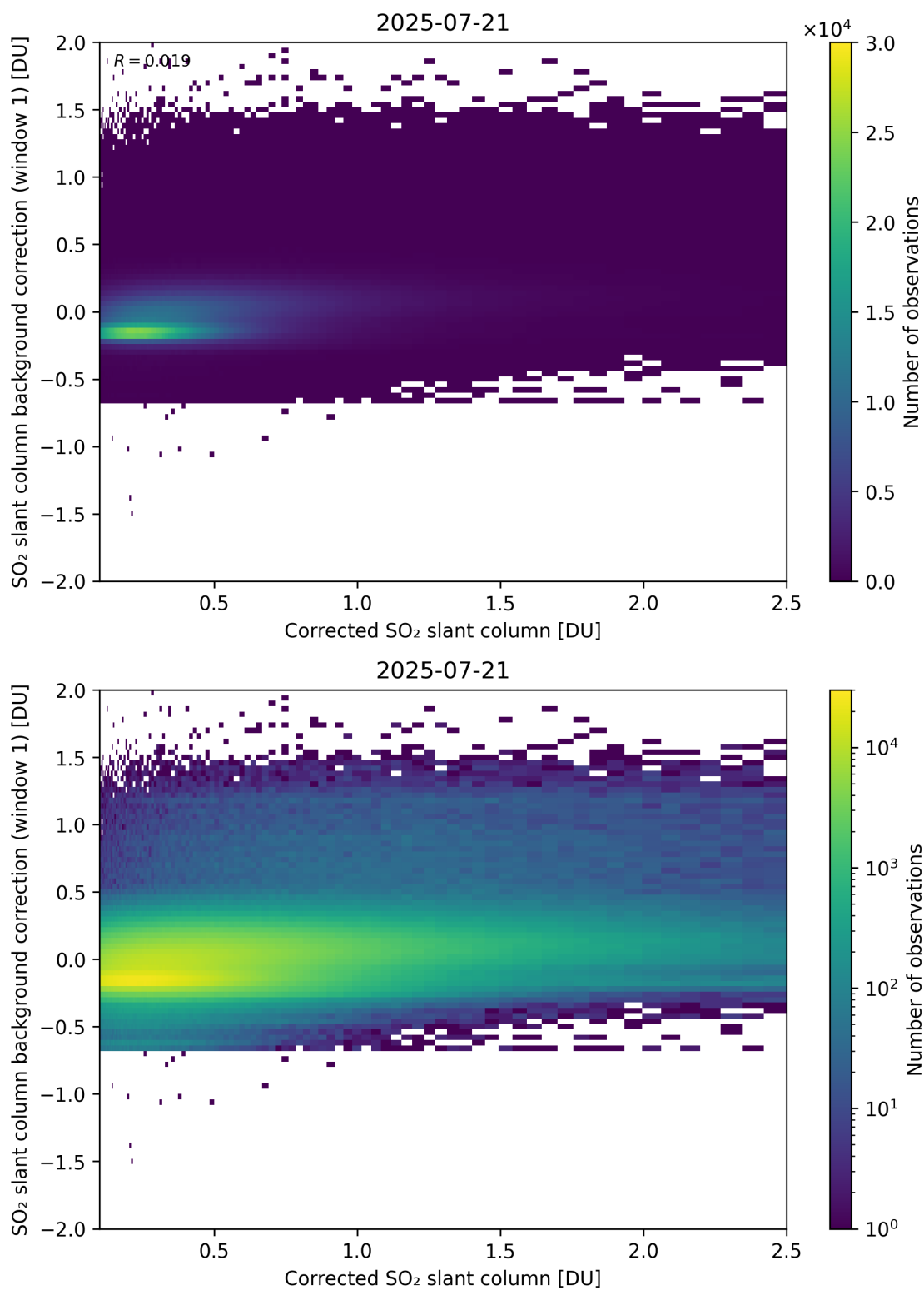
Figure 226: Scatter density plot of “Corrected SO 2 slant column” against “SO 2 slant column background correction (window 1)” for 2025-07-20 to 2025-07-22.
