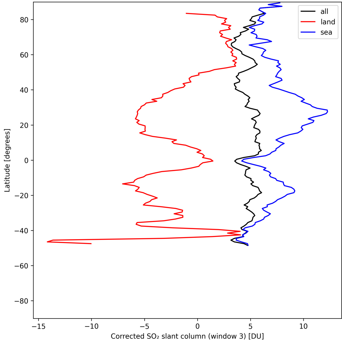
Figure 47: Zonal average of “Corrected SO 2 slant column (window 3)” for 2025-07-20 to 2025-07-22.
