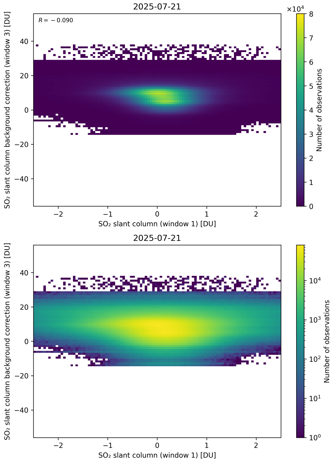
Figure 264: Scatter density plot of “SO 2 slant column (window 1)” against “SO 2 slant column background correction (window 3)” for 2025-07-20 to 2025-07-22.
