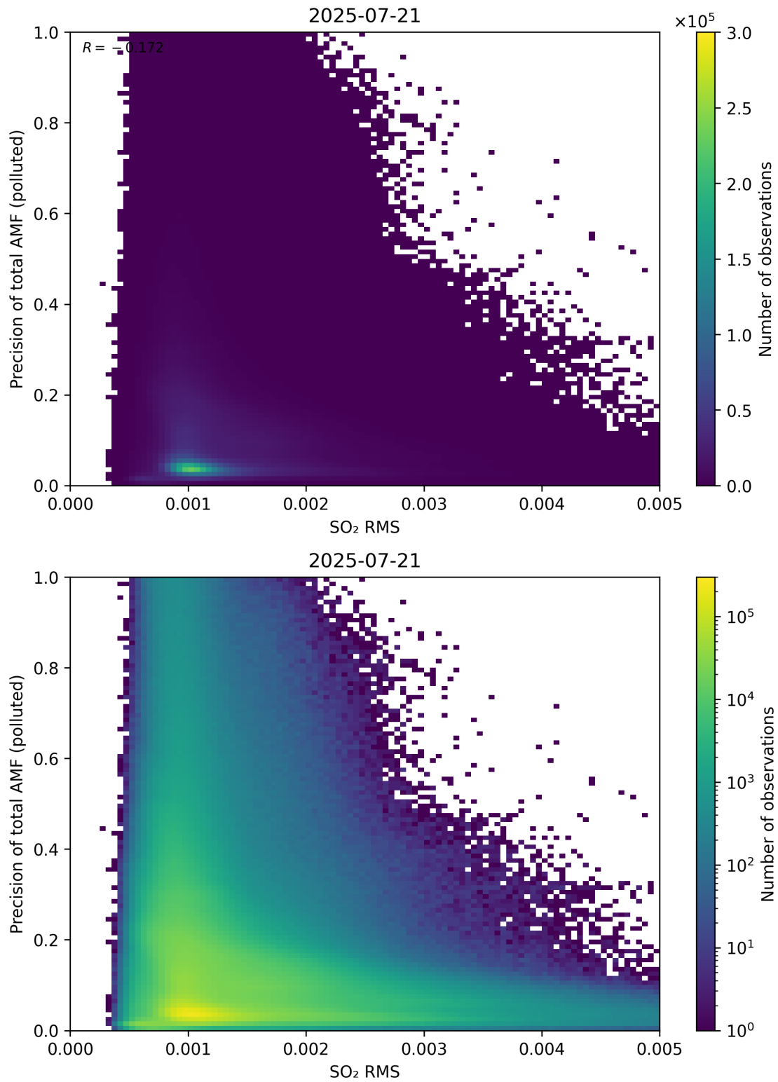
Figure 149: Scatter density plot of “SO 2 RMS” against “Precision of total AMF (polluted)” for 2025-07-20 to 2025-07-22.
