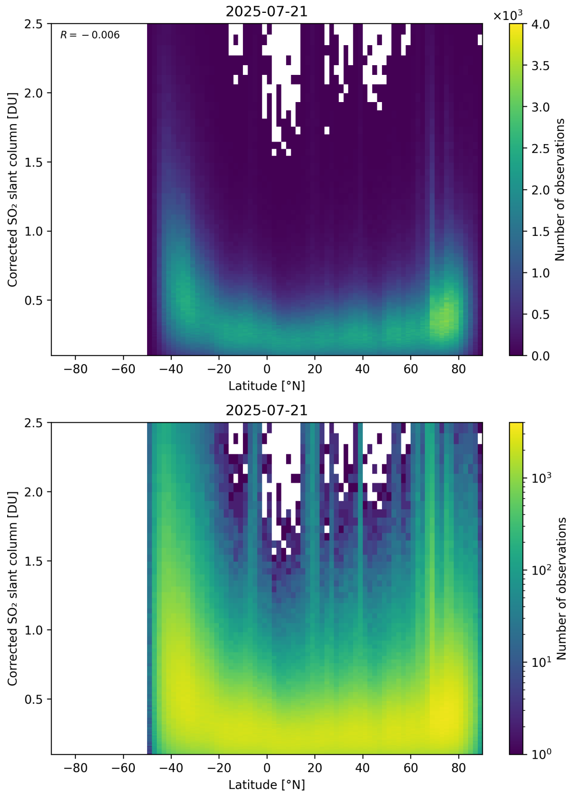
Figure 159: Scatter density plot of “Latitude” against “Corrected SO 2 slant column” for 2025-07-20 to 2025-07-22.
