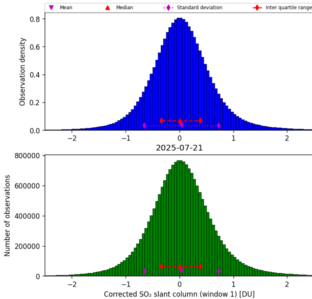
Figure 65: Histogram of “Corrected SO 2 slant column (window 1)” for 2025-07-20 to 2025-07-22
