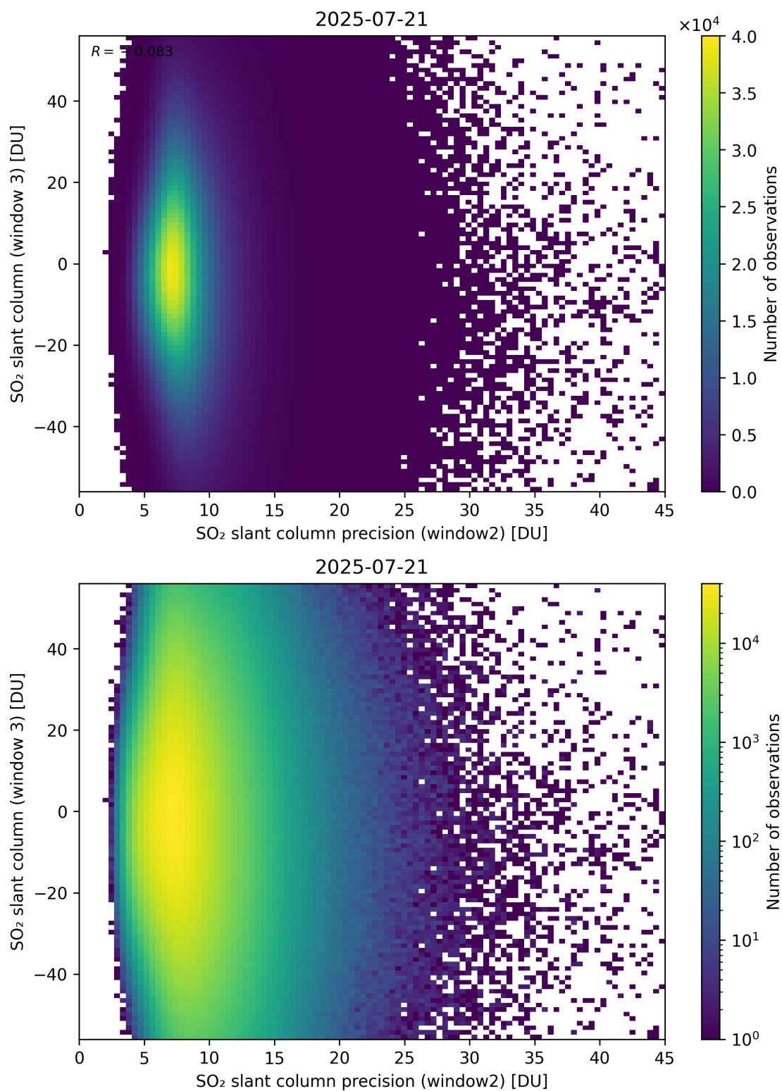
Figure 299: Scatter density plot of “SO 2 slant column precision (window2)” against “SO 2 slant column (window 3)” for 2025-07-20 to 2025-07-22.
