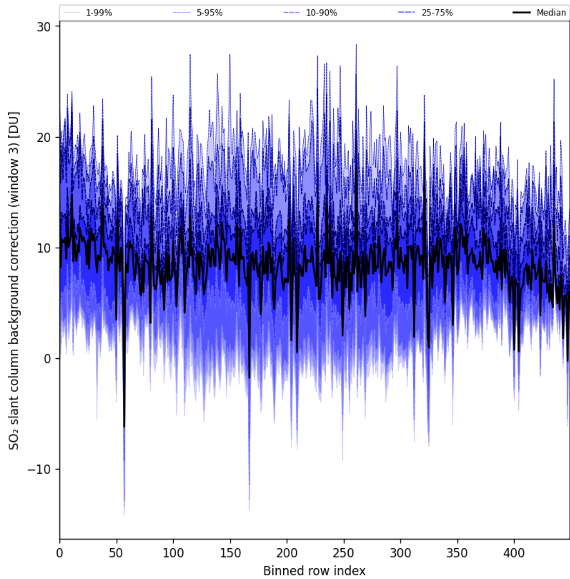
Figure 100: Along track statistics of “SO 2 slant column background correction (window 3)” for 2025-07-20 to 2025-07-22
