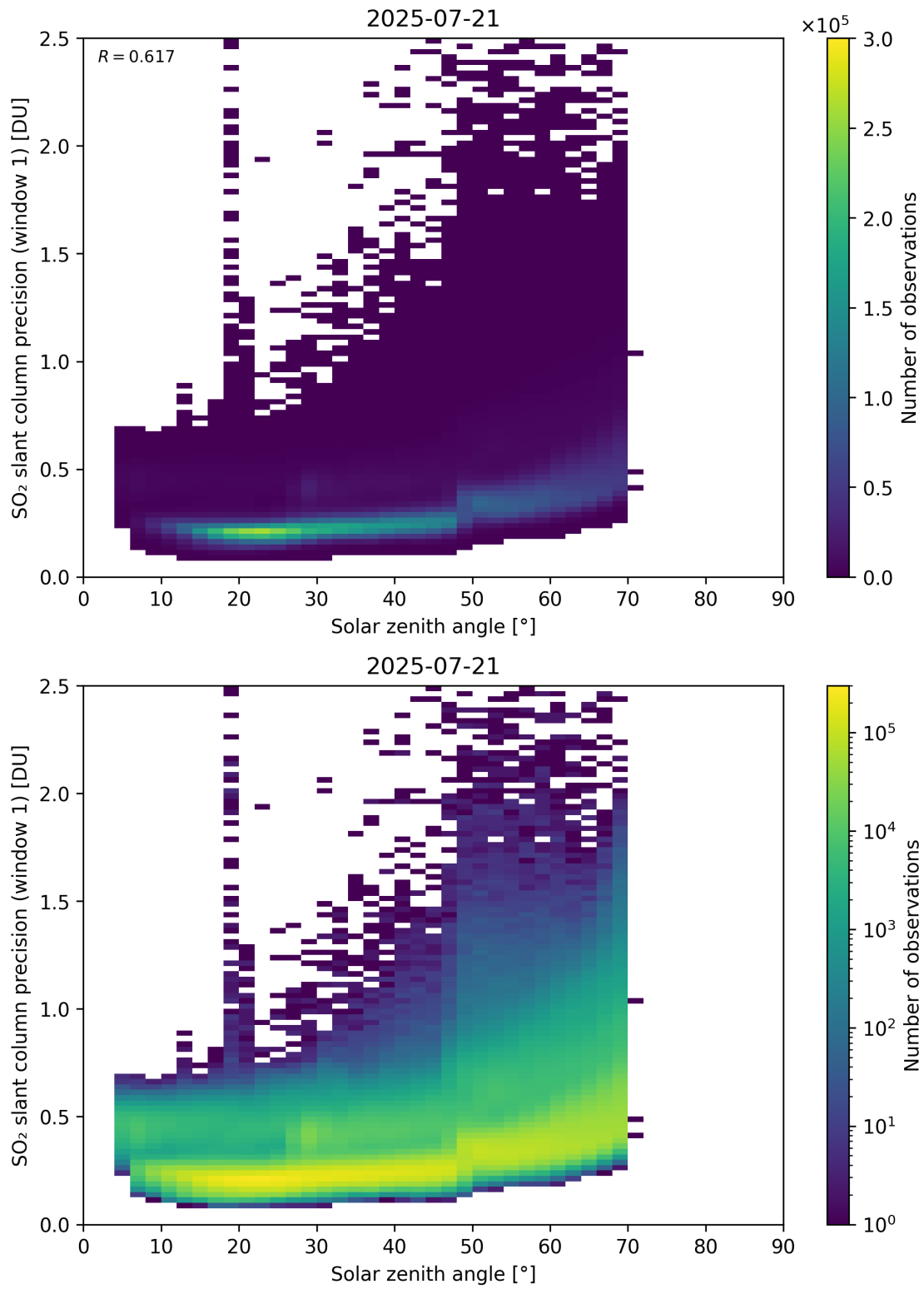
Figure 185: Scatter density plot of “Solar zenith angle” against “SO 2 slant column precision (window 1)” for 2025-07-20 to 2025-07-22.
