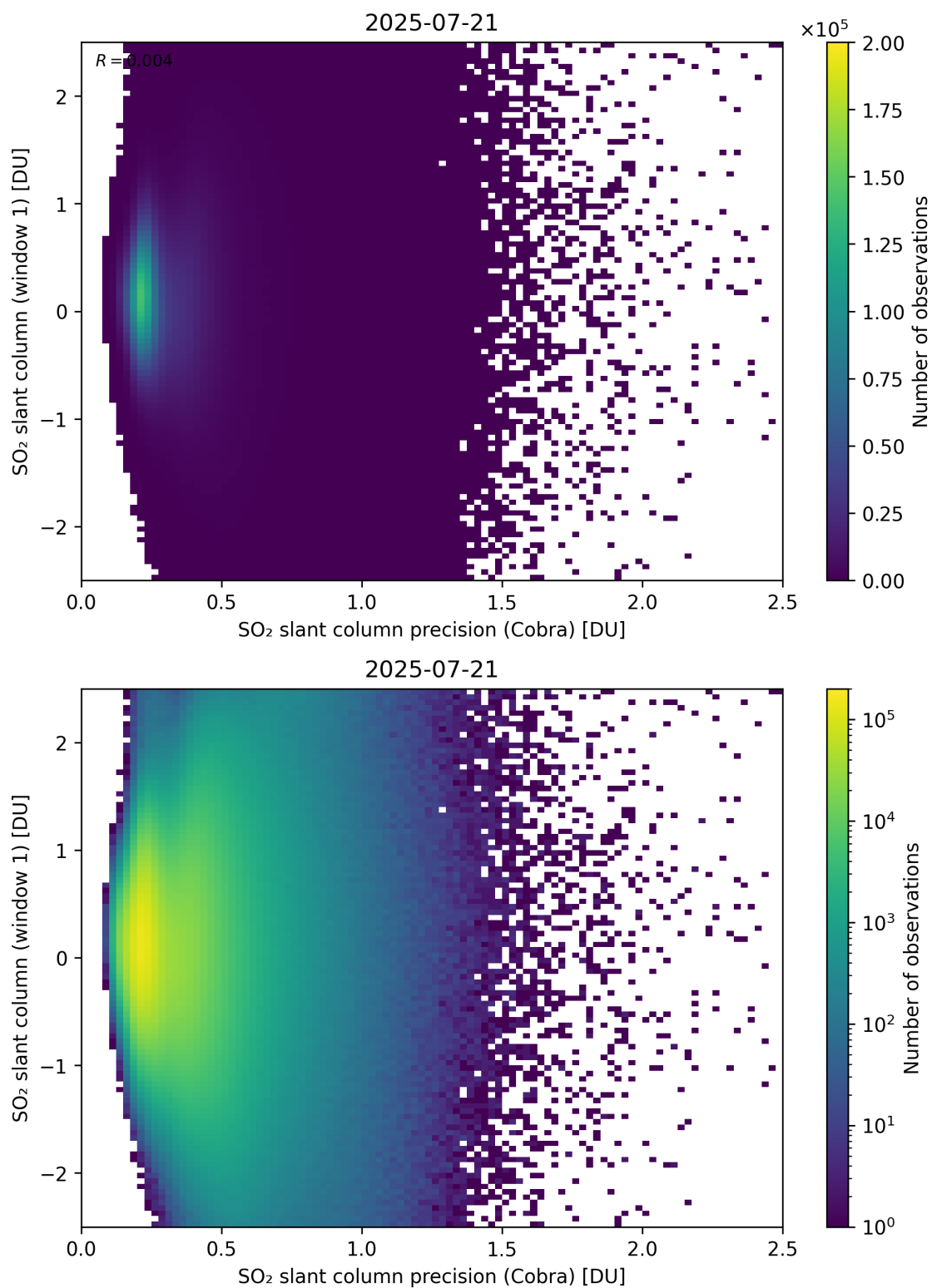
Figure 208: Scatter density plot of “SO 2 slant column precision (Cobra)” against “SO 2 slant column (window 1)” for 2025-07-20 to 2025-07-22.
