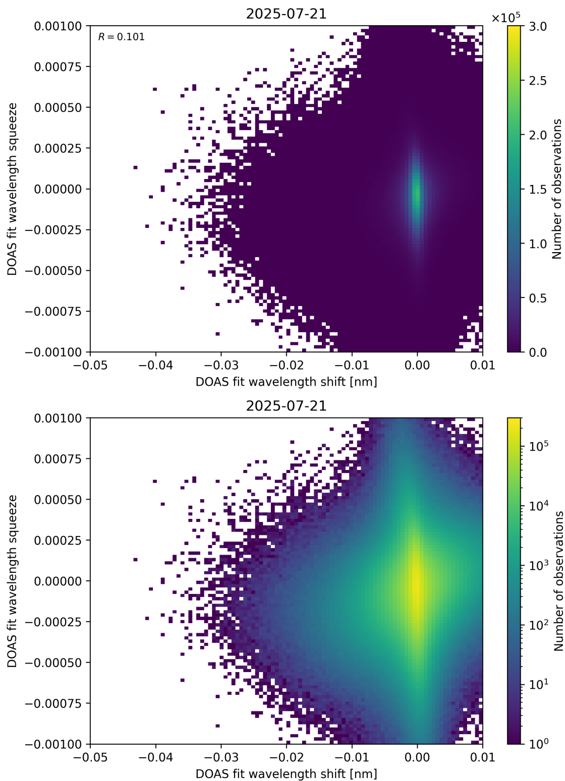
Figure 138: Scatter density plot of “DOAS fit wavelength shift” against “DOAS fit wavelength squeeze” for 2025-07-20 to 2025-07-22.
