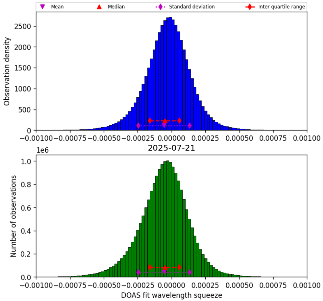
Figure 77: Histogram of “DOAS fit wavelength squeeze” for 2025-07-20 to 2025-07-22
