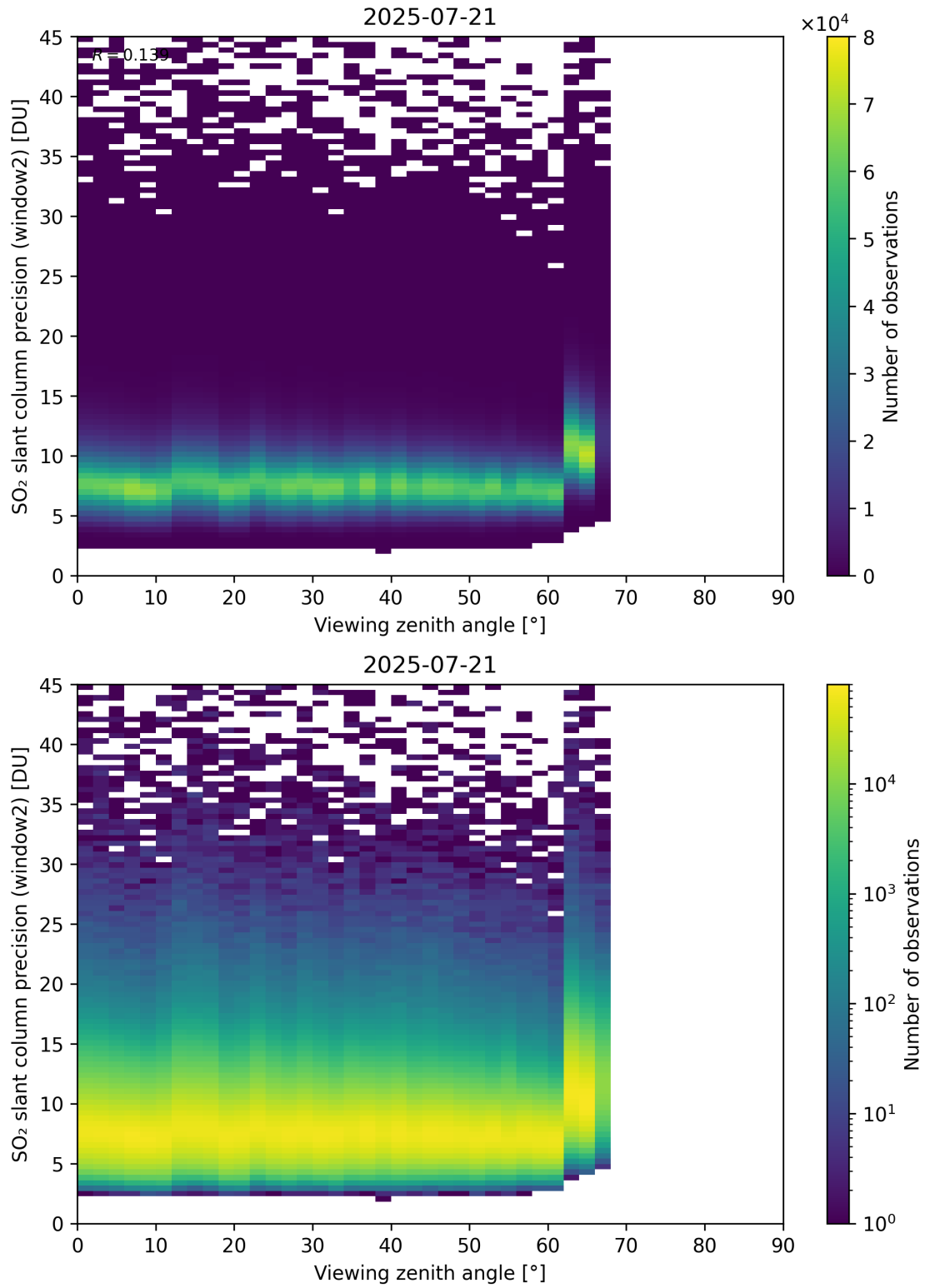
Figure 378: Scatter density plot of “Viewing zenith angle” against “SO 2 slant column precision (window2)” for 2025-07-20 to 2025-07-22.
