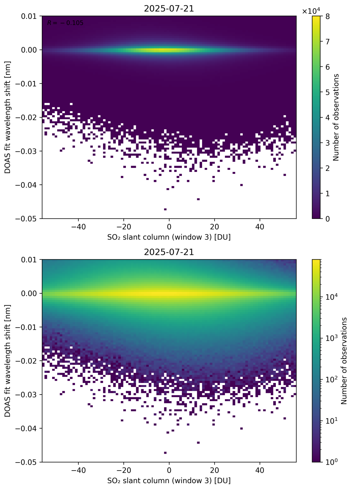
Figure 304: Scatter density plot of “SO 2 slant column (window 3)” against “DOAS fit wavelength shift” for 2025-07-20 to 2025-07-22.
