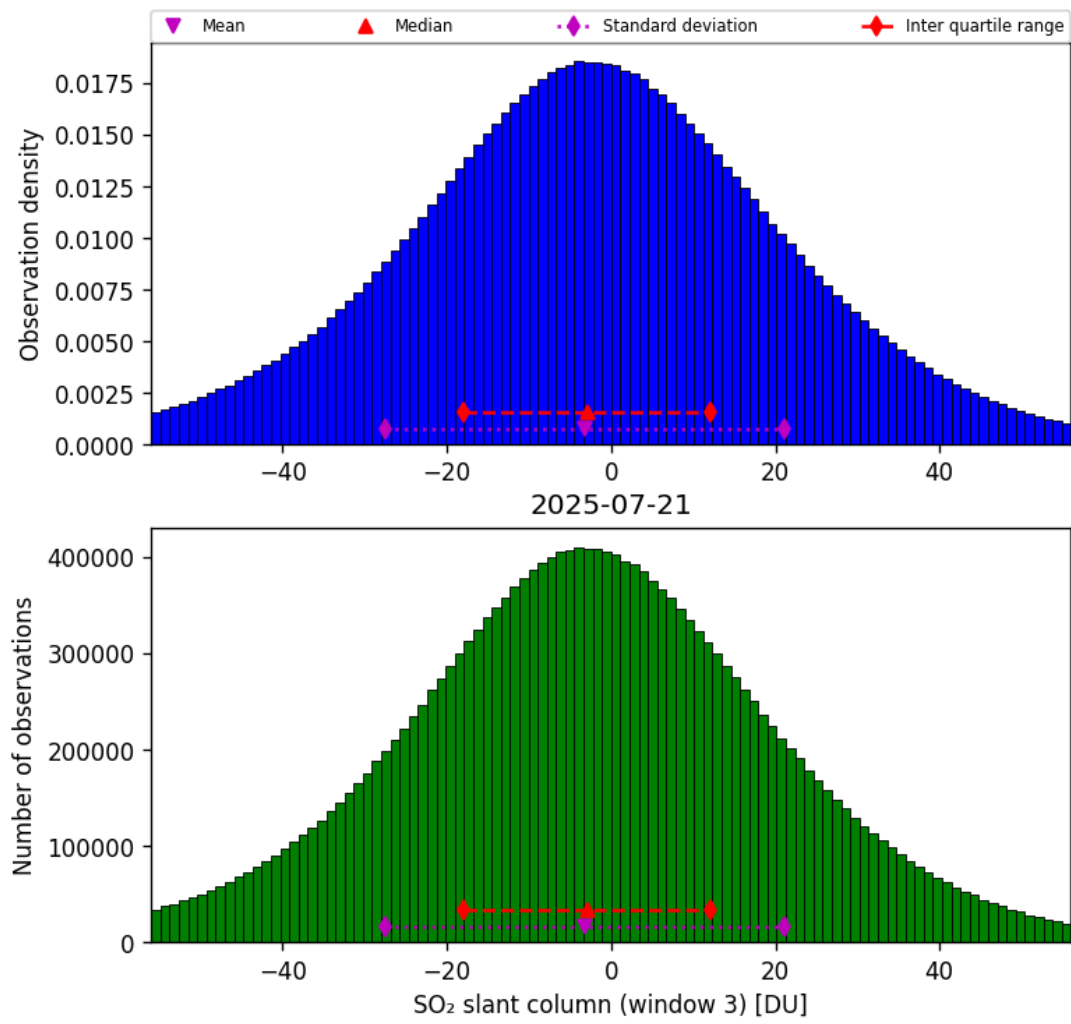
Figure 71: Histogram of “SO 2 slant column (window 3)” for 2025-07-20 to 2025-07-22
