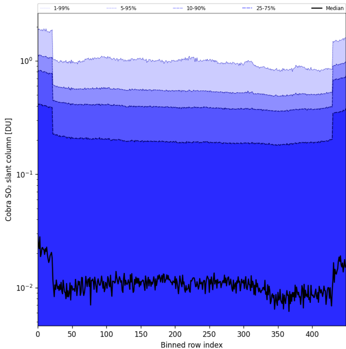
Figure 87: Along track statistics of “Cobra SO 2 slant column” for 2025-07-20 to 2025-07-22
