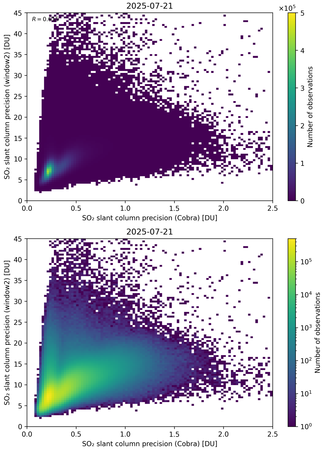
Figure 210: Scatter density plot of “SO 2 slant column precision (Cobra)” against “SO 2 slant column precision (window2)” for 2025-07-20 to 2025-07-22.
