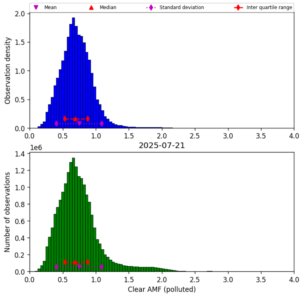
Figure 81: Histogram of “Clear AMF (polluted)” for 2025-07-20 to 2025-07-22
