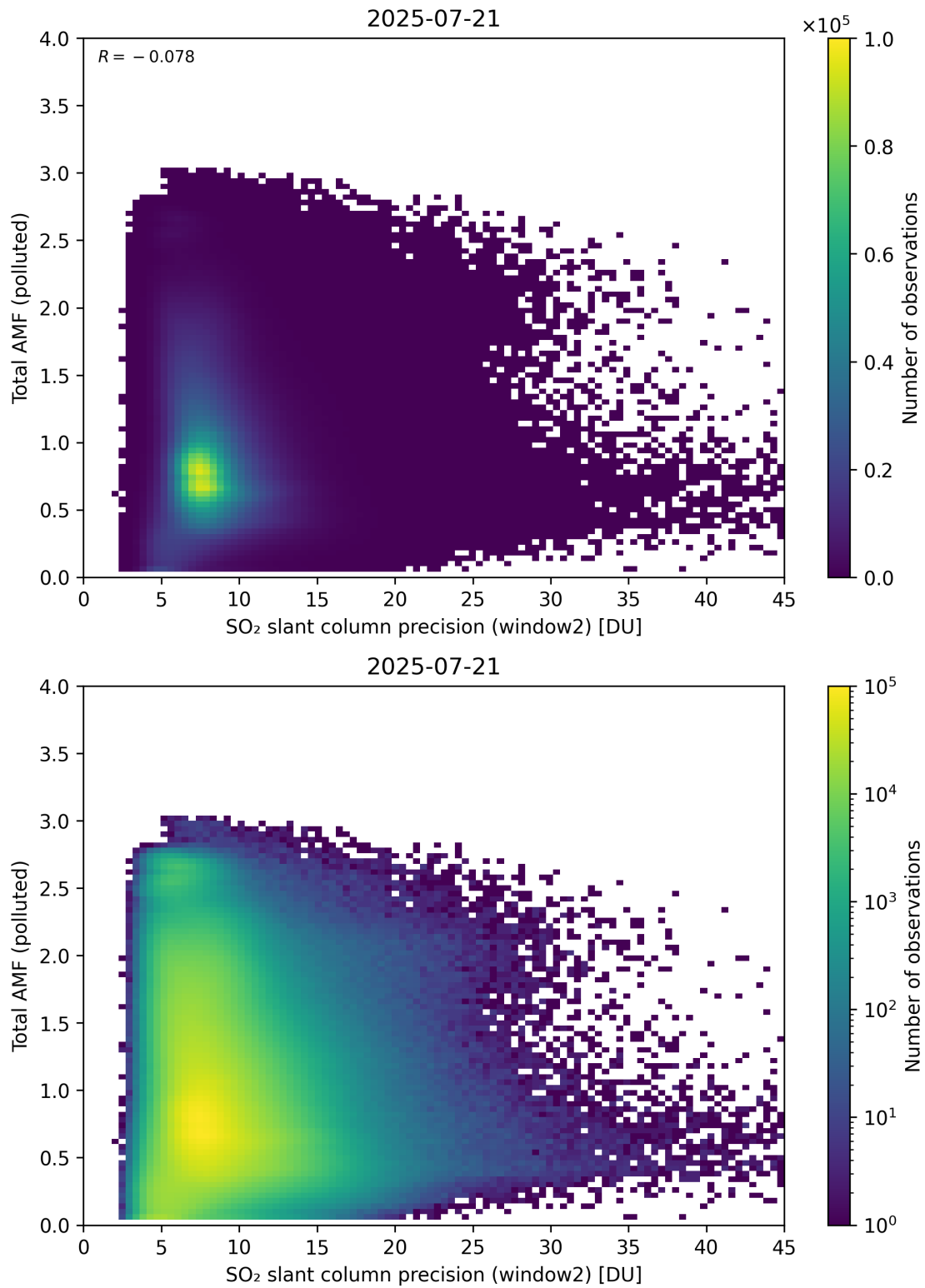
Figure 301: Scatter density plot of “SO 2 slant column precision (window2)” against “Total AMF (polluted)” for 2025-07-20 to 2025-07-22.
