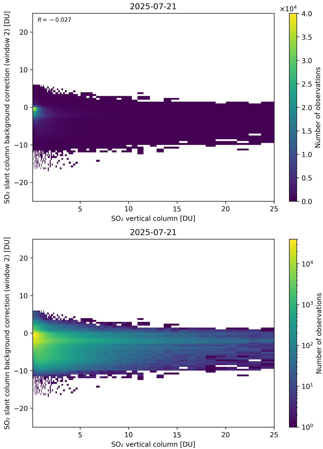
Figure 324: Scatter density plot of “SO 2 vertical column” against “SO 2 slant column background correction (window 2)” for 2025-07-20 to 2025-07-22.
