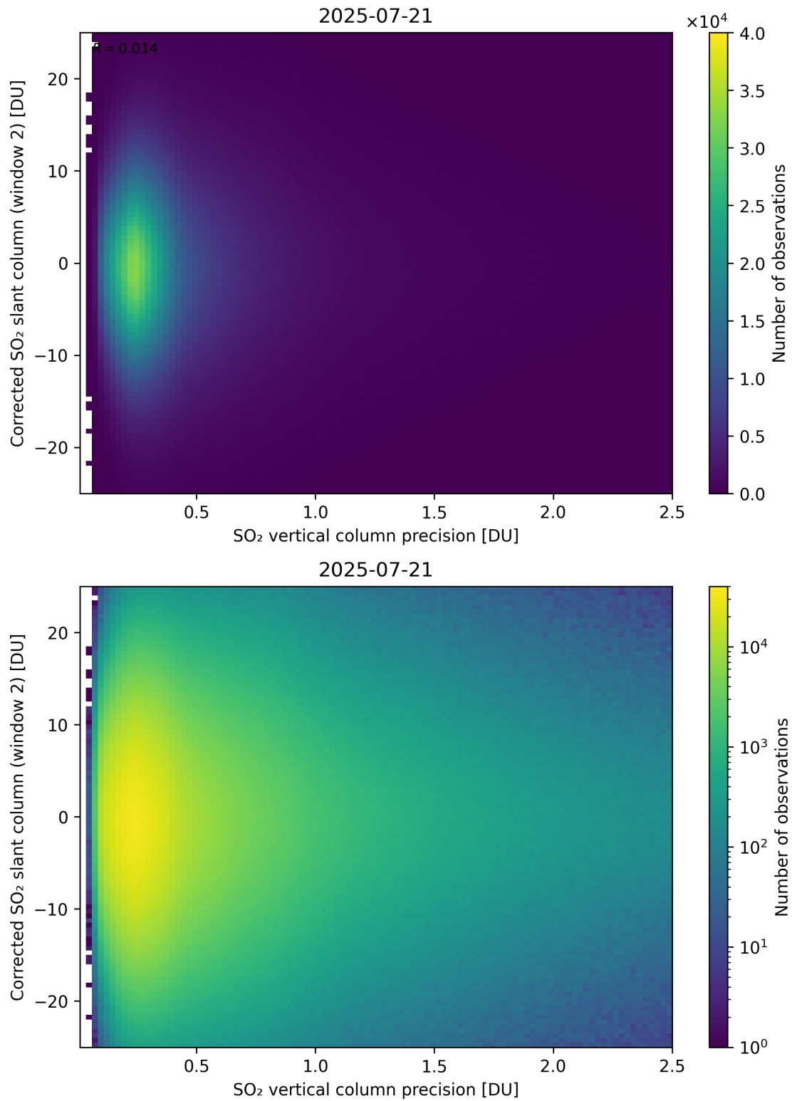
Figure 339: Scatter density plot of “SO 2 vertical column precision” against “Corrected SO 2 slant column (window 2)” for 2025-07-20 to 2025-07-22.
