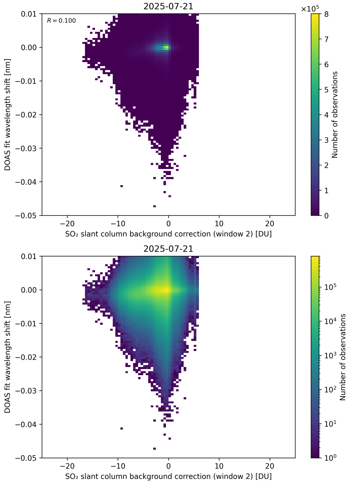
Figure 123: Scatter density plot of “SO 2 slant column background correction (window 2)” against “DOAS fit wavelength shift” for 2025-07-20 to 2025-07-22.
