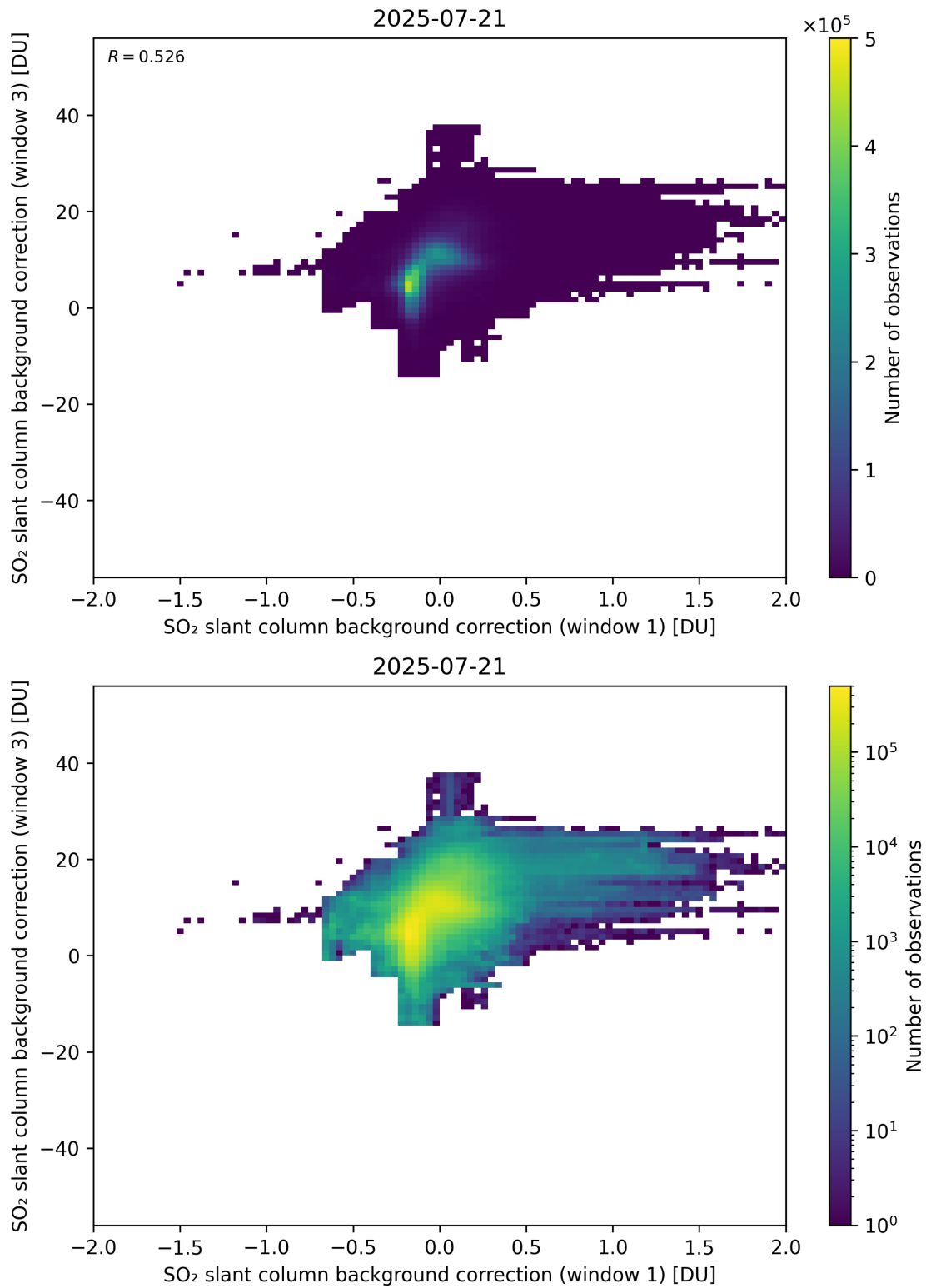
Figure 110: Scatter density plot of “SO 2 slant column background correction (window 1)” against “SO 2 slant column background correction (window 3)” for 2025-07-20 to 2025-07-22.
