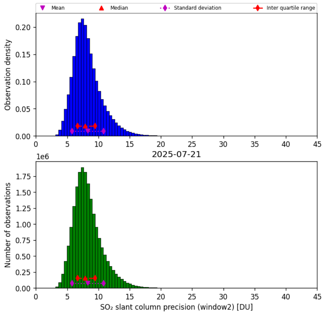
Figure 68: Histogram of “SO 2 slant column precision (window2)” for 2025-07-20 to 2025-07-22
