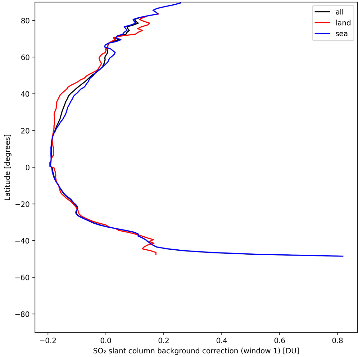
Figure 40: Zonal average of “SO 2 slant column background correction (window 1)” for 2025-07-20 to 2025-07-22.
