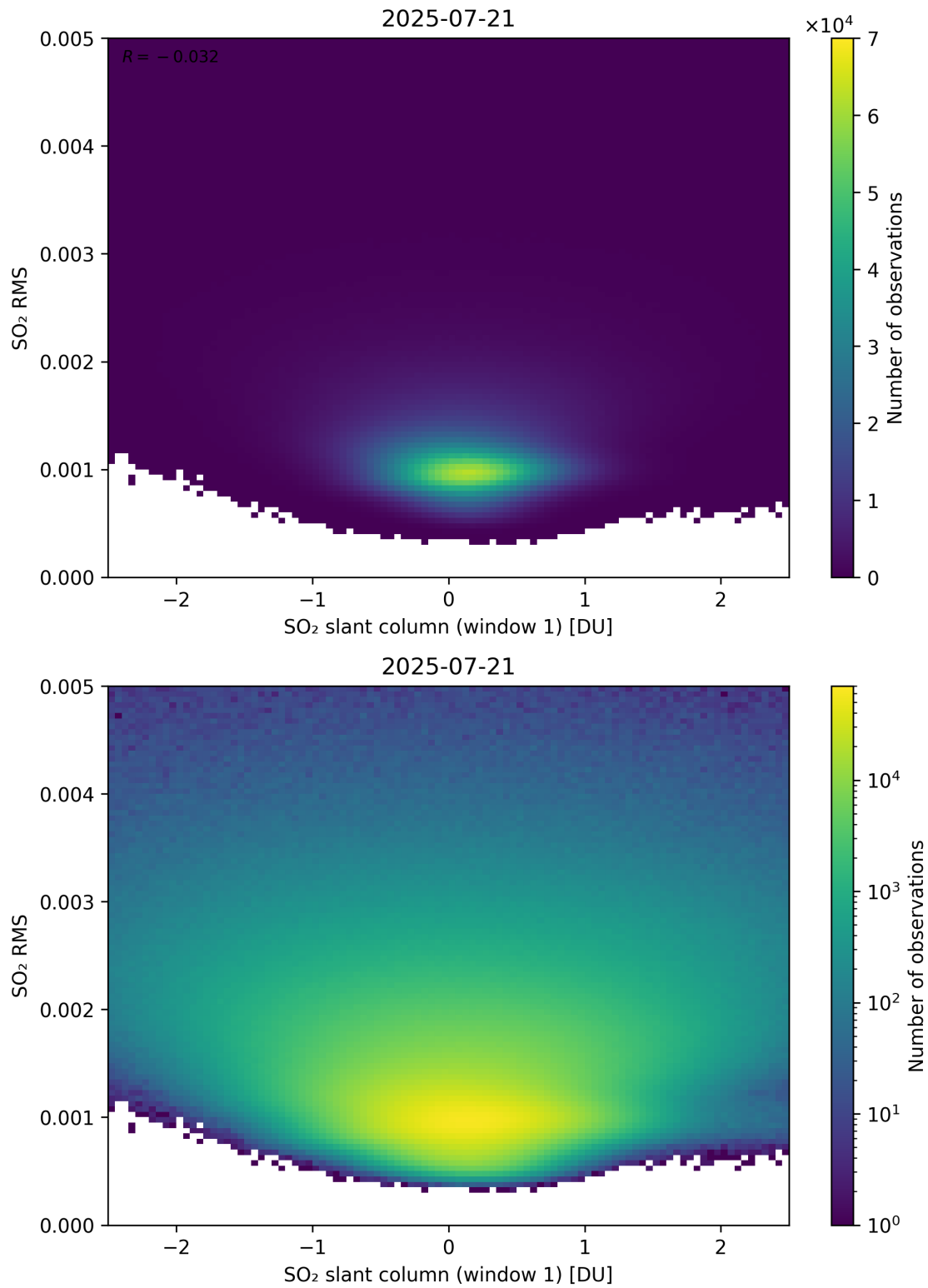
Figure 267: Scatter density plot of “SO 2 slant column (window 1)” against “SO 2 RMS” for 2025-07-20 to 2025-07-22.
