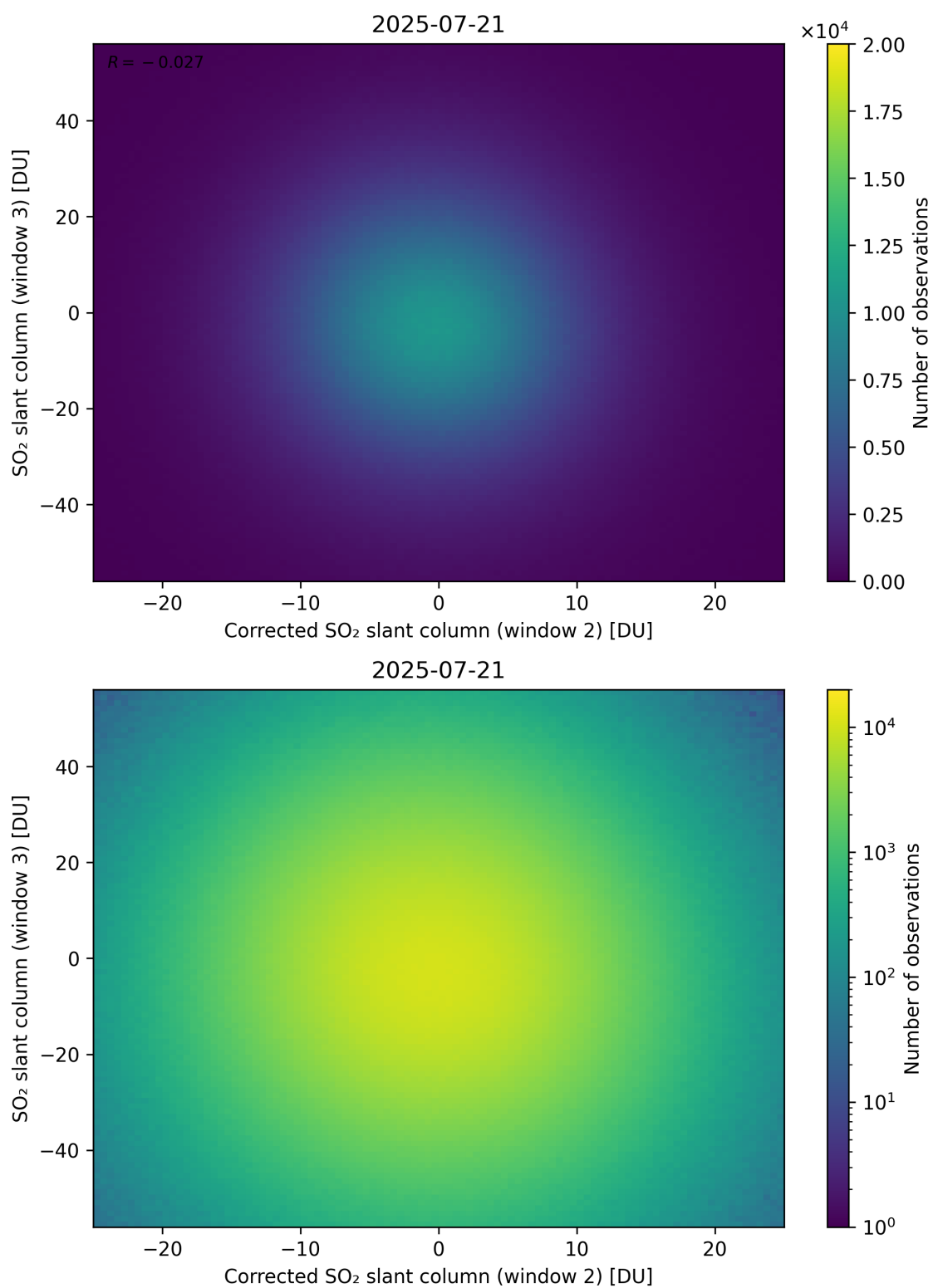
Figure 251: Scatter density plot of “Corrected SO 2 slant column (window 2)” against “SO 2 slant column (window 3)” for 2025-07-20 to 2025-07-22.
