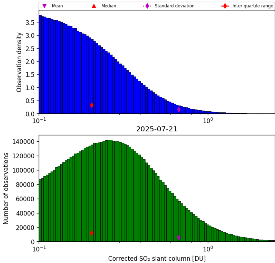
Figure 60: Histogram of “Corrected SO 2 slant column” for 2025-07-20 to 2025-07-22
