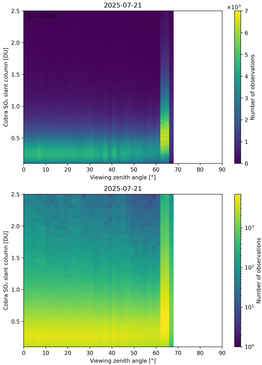
Figure 371: Scatter density plot of “Viewing zenith angle” against “Cobra SO 2 slant column” for 2025-07-20 to 2025-07-22.
