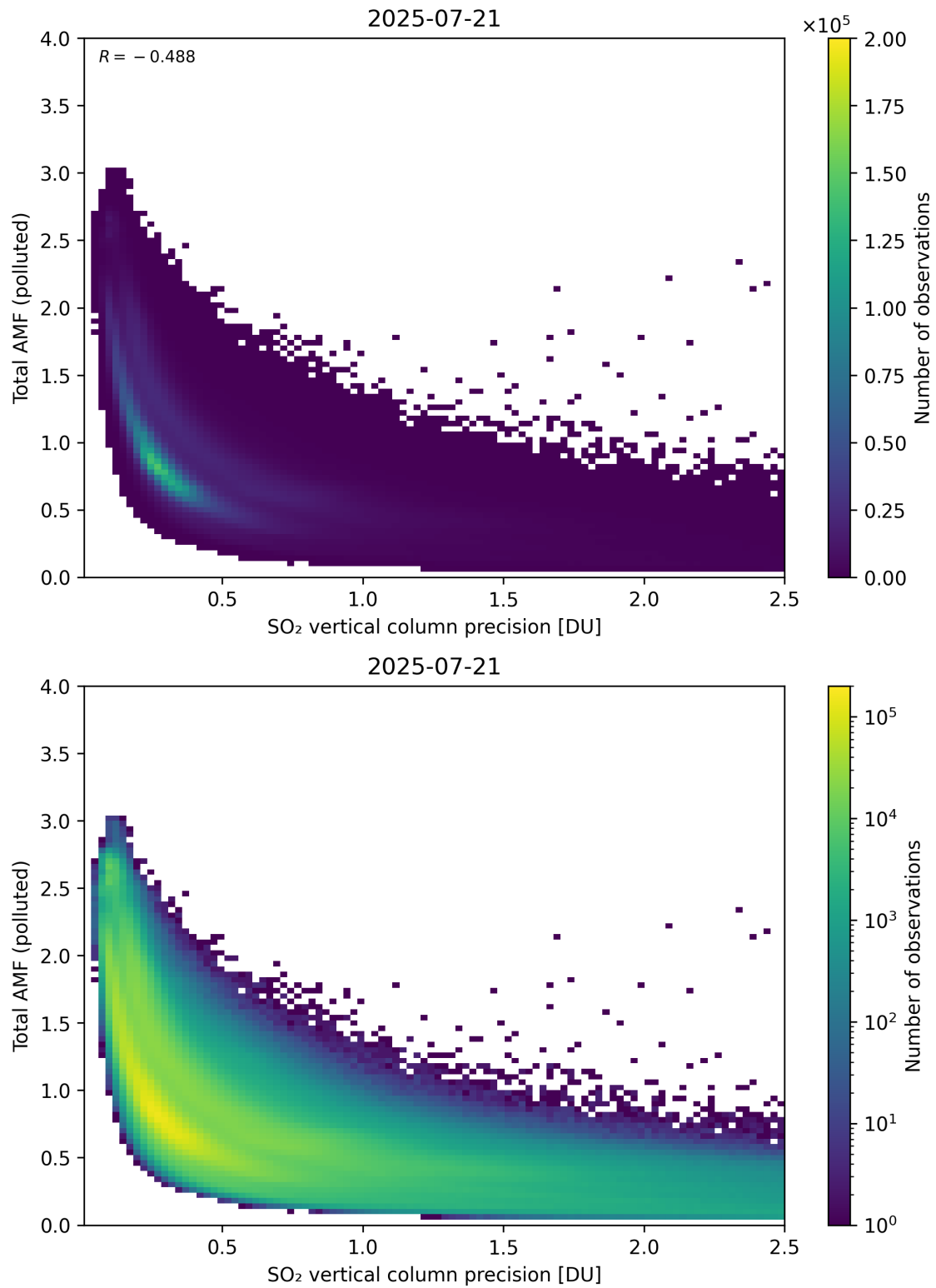
Figure 346: Scatter density plot of “SO 2 vertical column precision” against “Total AMF (polluted)” for 2025-07-20 to 2025-07-22.
