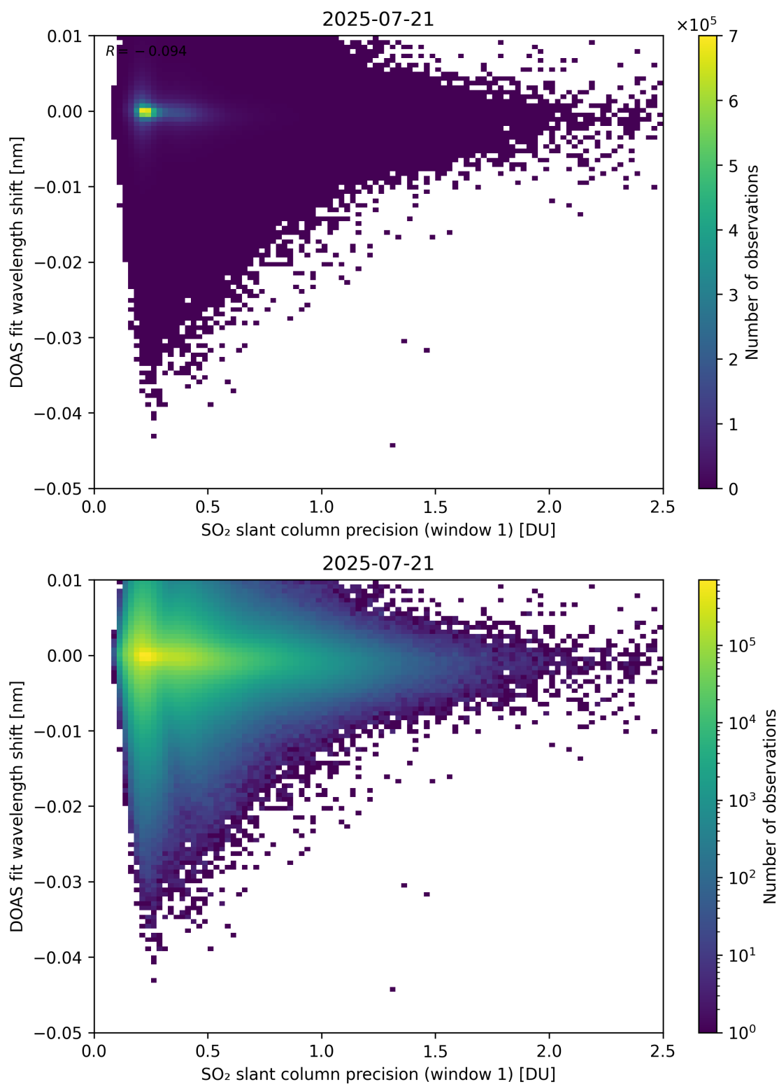
Figure 271: Scatter density plot of “SO 2 slant column precision (window 1)” against “DOAS fit wavelength shift” for 2025-07-20 to 2025-07-22.
