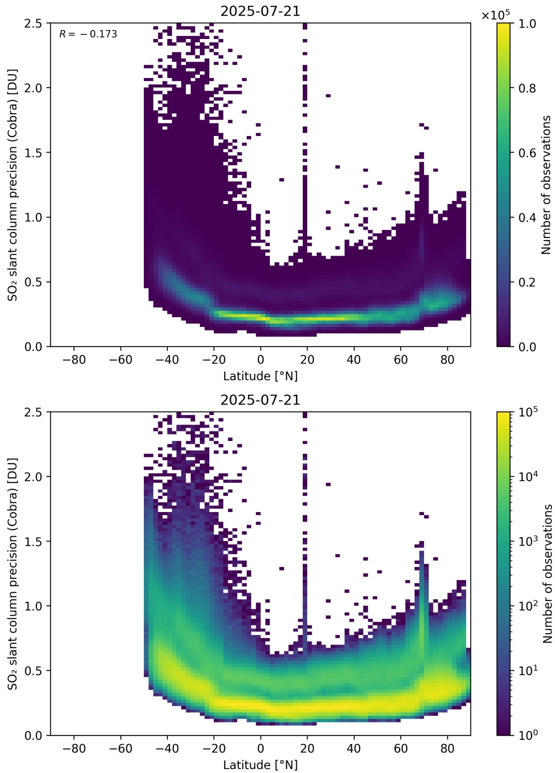
Figure 158: Scatter density plot of “Latitude” against “SO 2 slant column precision (Cobra)” for 2025-07-20 to 2025-07-22.
