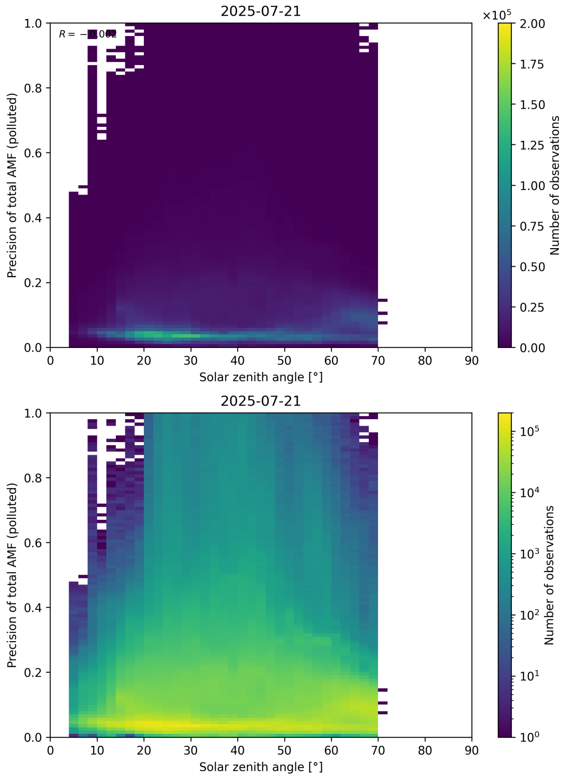
Figure 190: Scatter density plot of “Solar zenith angle” against “Precision of total AMF (polluted)” for 2025-07-20 to 2025-07-22.
