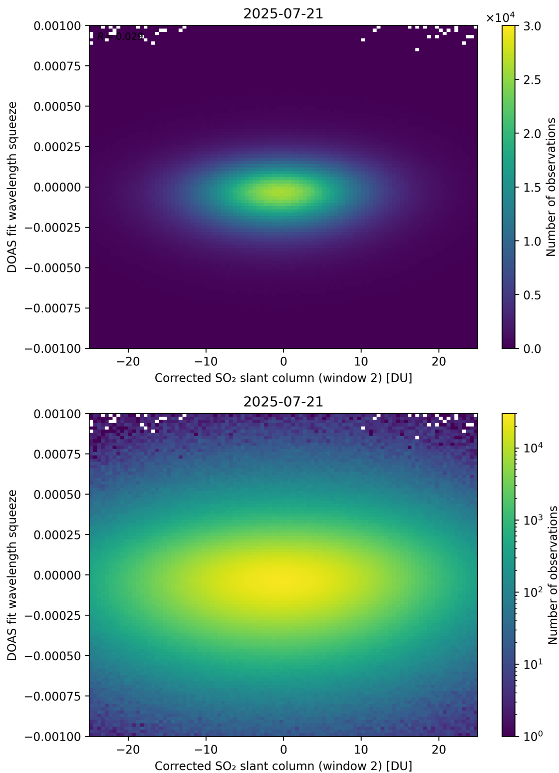
Figure 247: Scatter density plot of “Corrected SO 2 slant column (window 2)” against “DOAS fit wavelength squeeze” for 2025-07-20 to 2025-07-22.
