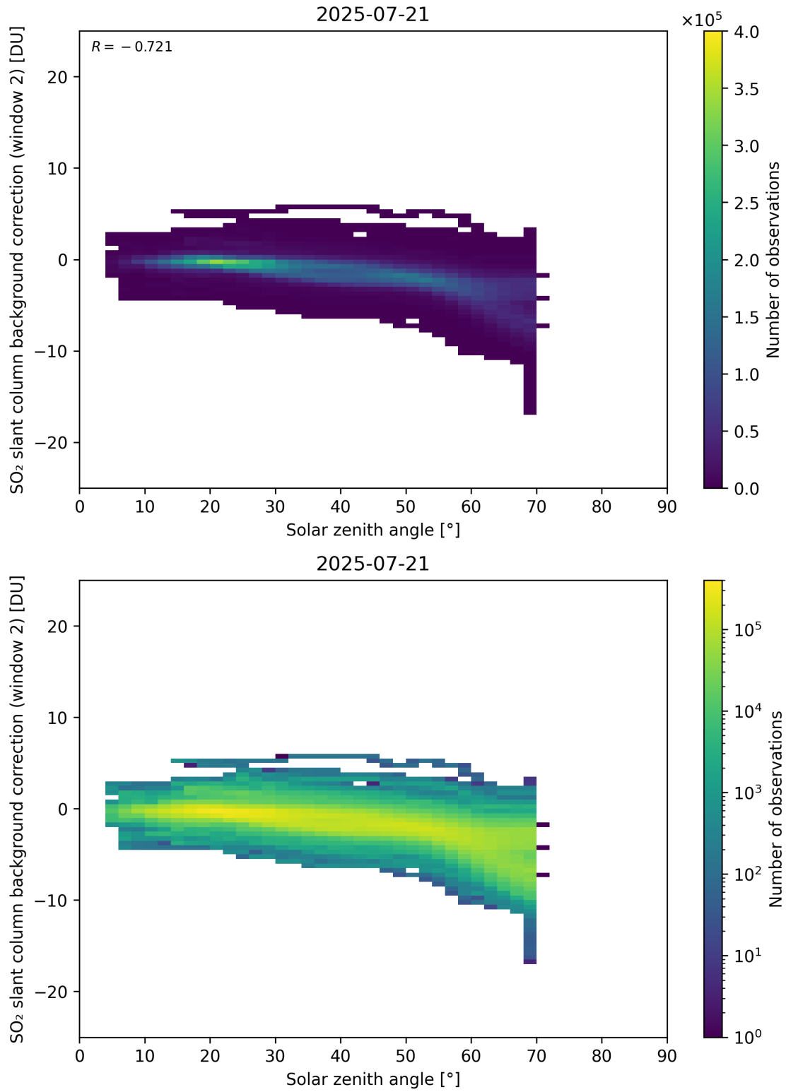
Figure 172: Scatter density plot of “Solar zenith angle” against “SO 2 slant column background correction (window 2)” for 2025-07-20 to 2025-07-22.
