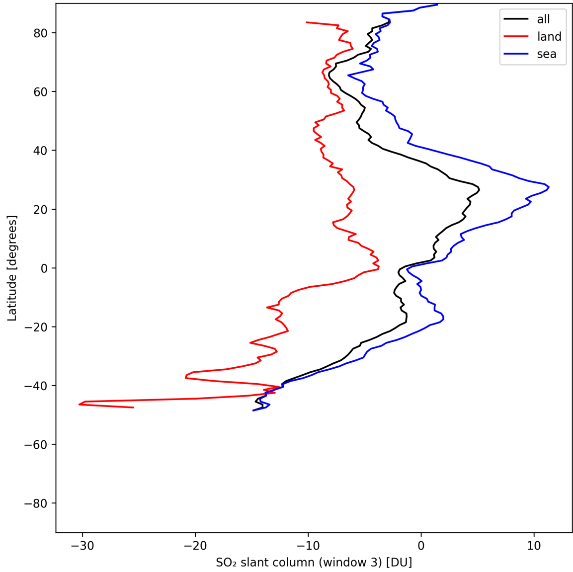
Figure 45: Zonal average of “SO 2 slant column (window 3)” for 2025-07-20 to 2025-07-22.
