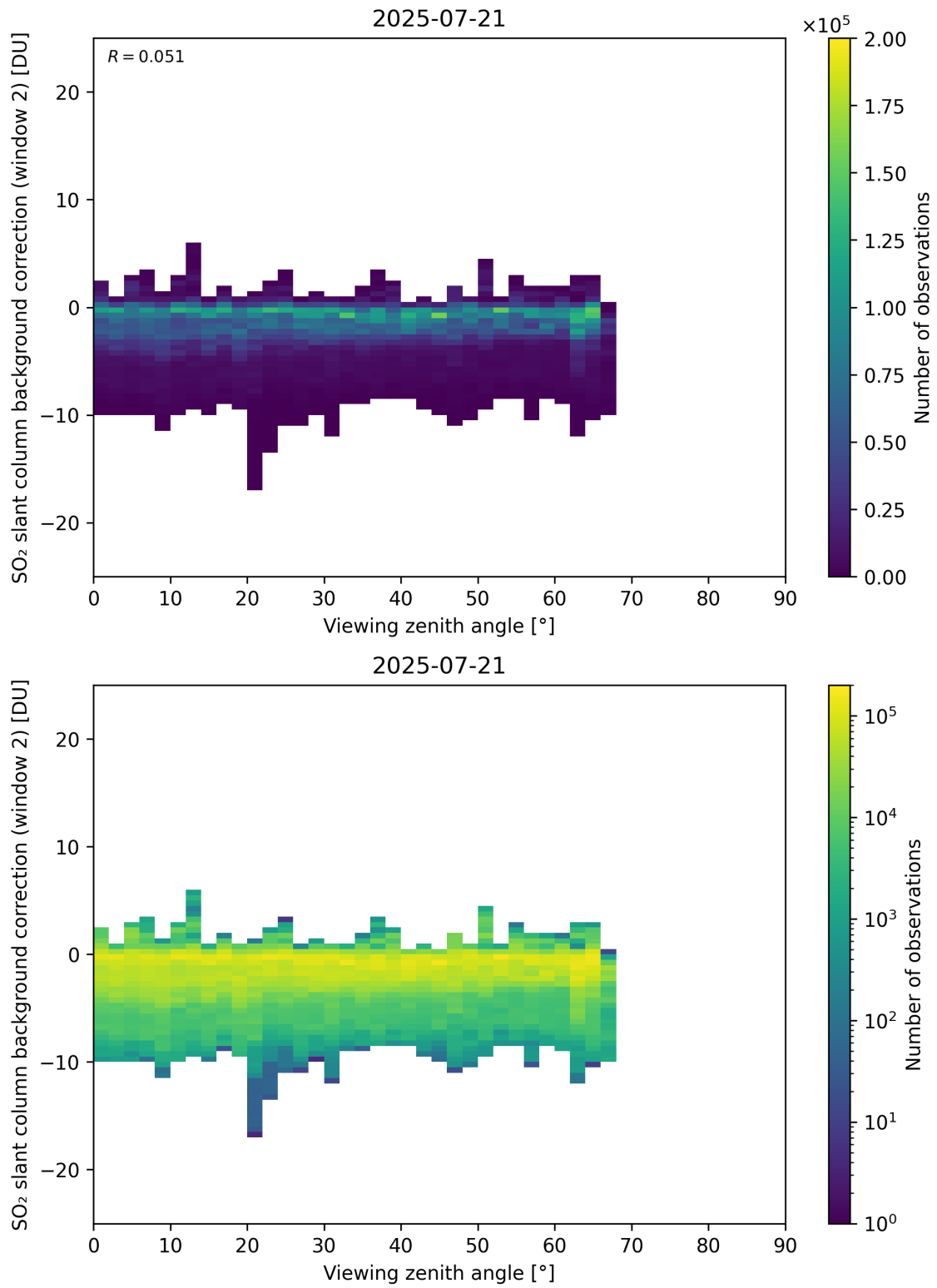
Figure 363: Scatter density plot of “Viewing zenith angle” against “SO 2 slant column background correction (window 2)” for 2025-07-20 to 2025-07-22.
