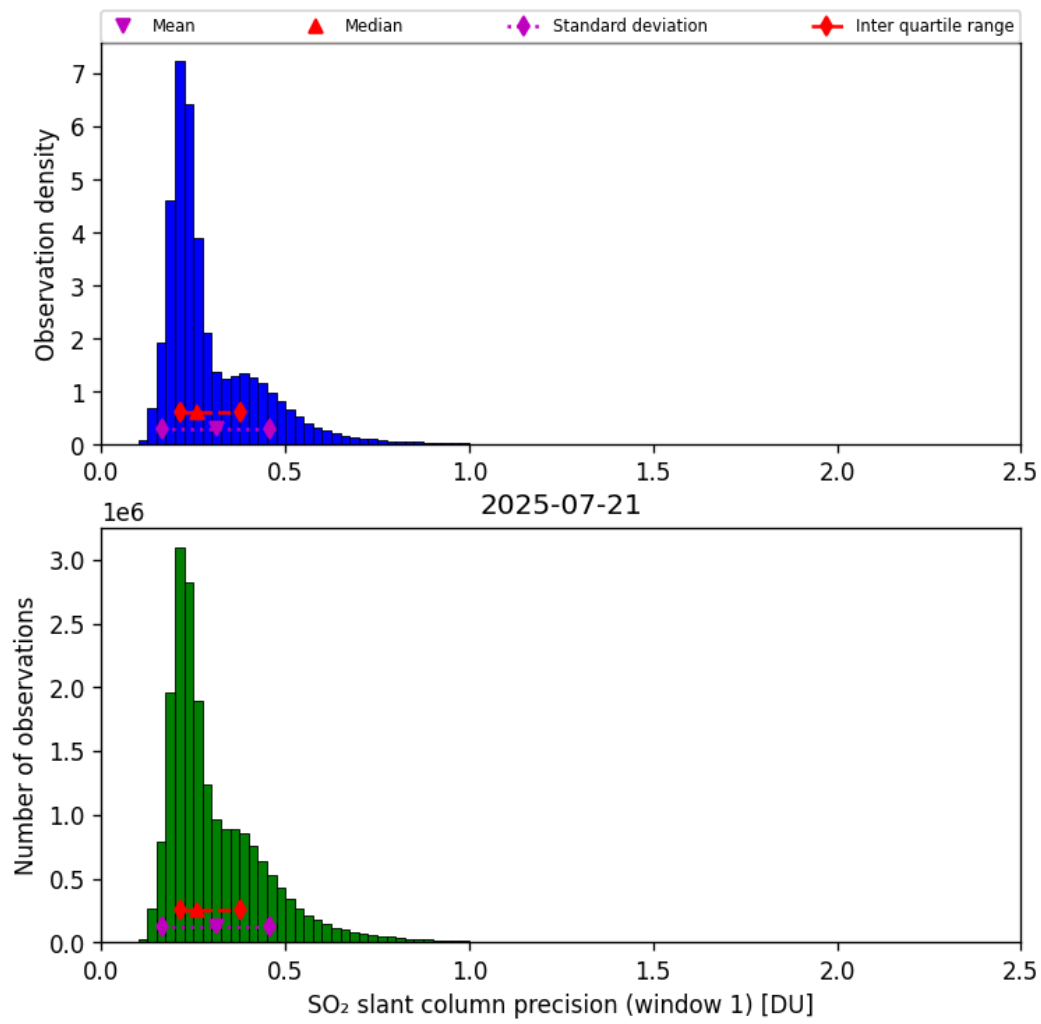
Figure 64: Histogram of “SO 2 slant column precision (window 1)” for 2025-07-20 to 2025-07-22
