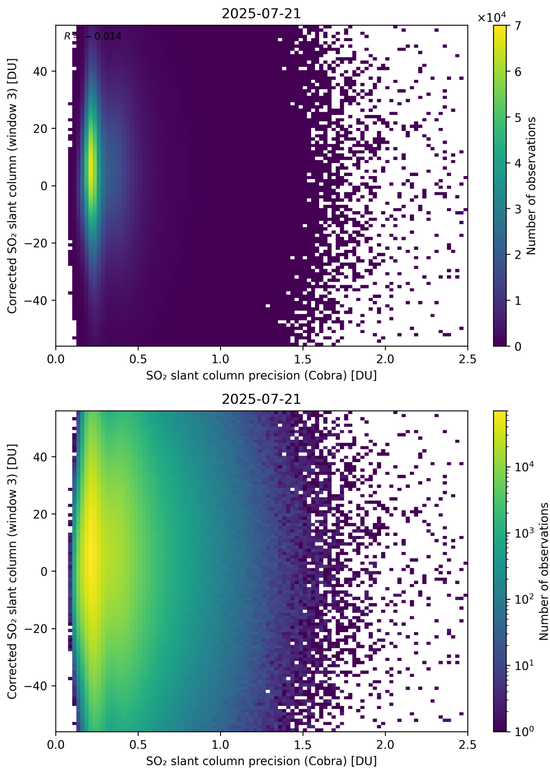
Figure 207: Scatter density plot of “SO 2 slant column precision (Cobra)” against “Corrected SO 2 slant column (window 3)” for 2025-07-20 to 2025-07-22.
