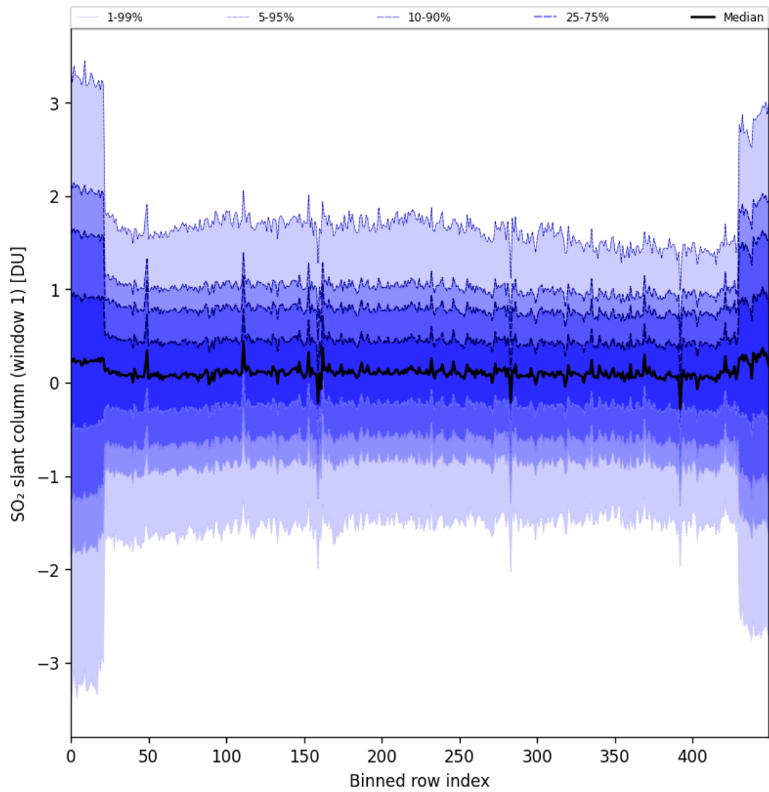
Figure 89: Along track statistics of “SO 2 slant column (window 1)” for 2025-07-20 to 2025-07-22
