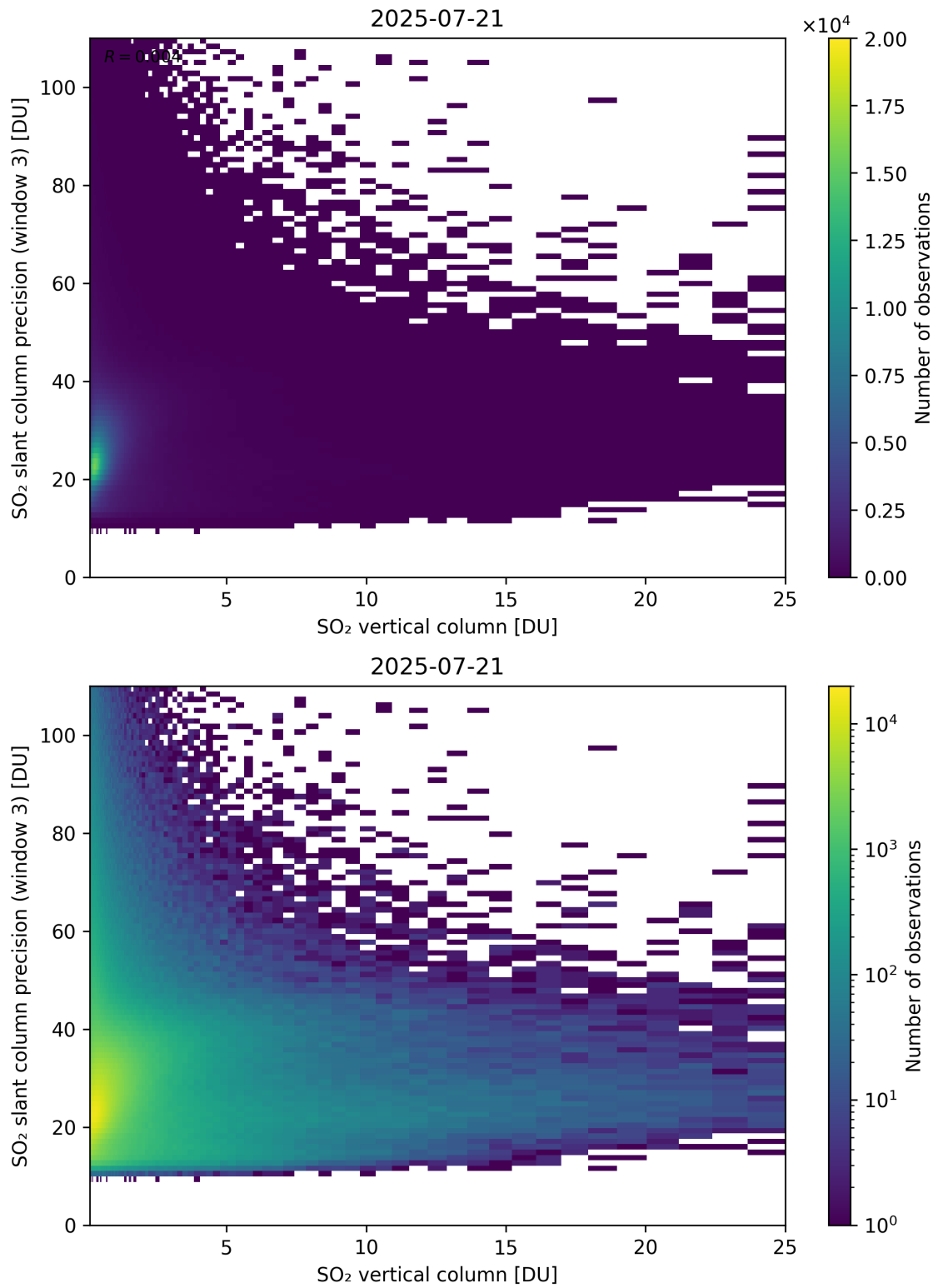
Figure 358: Scatter density plot of “SO 2 vertical column” against “SO 2 slant column precision (window 3)” for 2025-07-20 to 2025-07-22.
