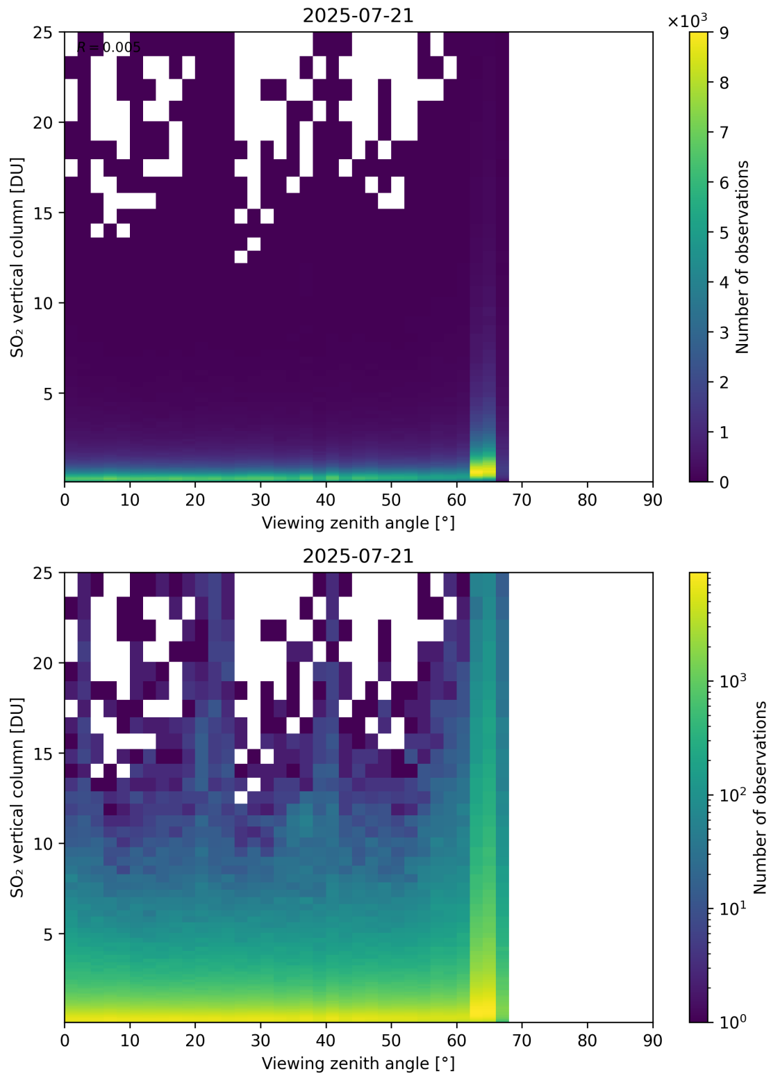
Figure 383: Scatter density plot of “Viewing zenith angle” against “SO 2 vertical column” for 2025-07-20 to 2025-07-22.
