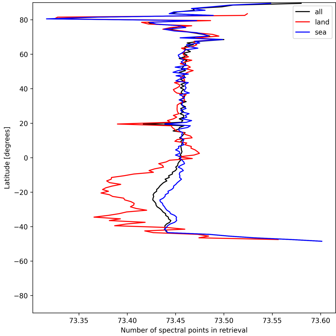
Figure 56: Zonal average of “Number of spectral points in retrieval” for 2025-07-20 to 2025-07-22.
