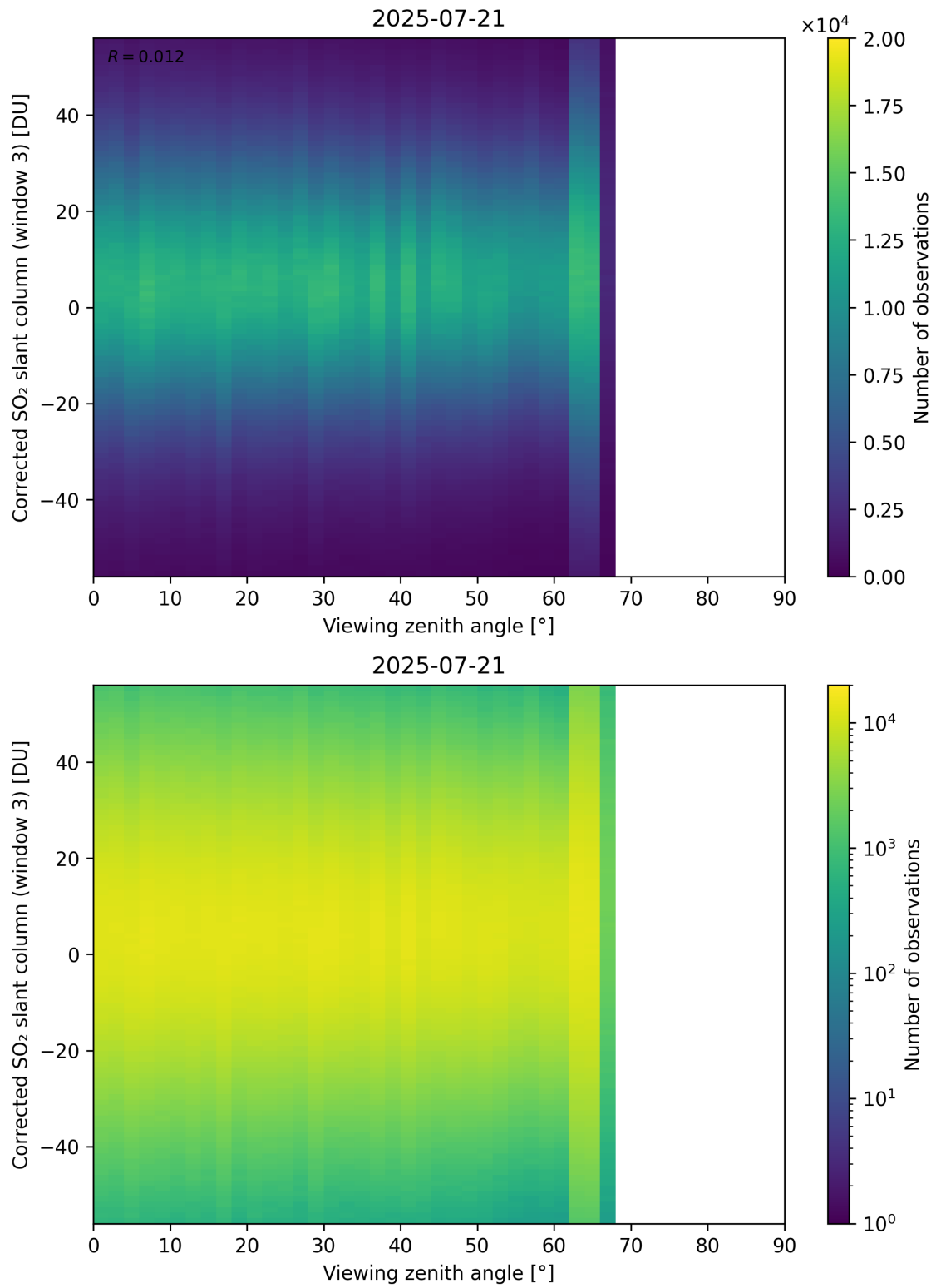
Figure 375: Scatter density plot of “Viewing zenith angle” against “Corrected SO 2 slant column (window 3)” for 2025-07-20 to 2025-07-22.
