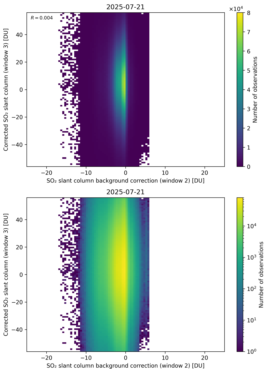
Figure 127: Scatter density plot of “SO 2 slant column background correction (window 2)” against “Corrected SO 2 slant column (window 3)” for 2025-07-20 to 2025-07-22.
