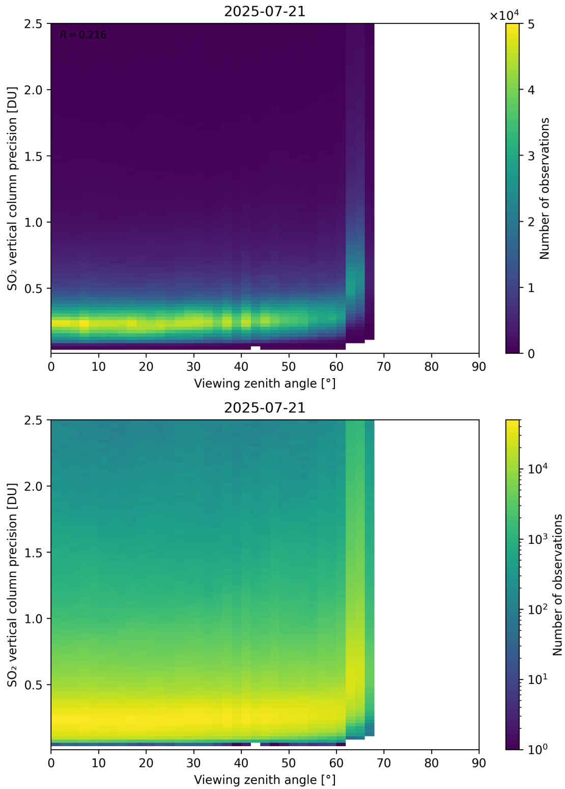
Figure 384: Scatter density plot of “Viewing zenith angle” against “SO 2 vertical column precision” for 2025-07-20 to 2025-07-22.
