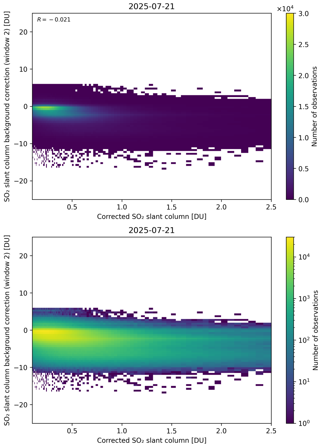
Figure 227: Scatter density plot of “Corrected SO 2 slant column” against “SO 2 slant column background correction (window 2)” for 2025-07-20 to 2025-07-22.
