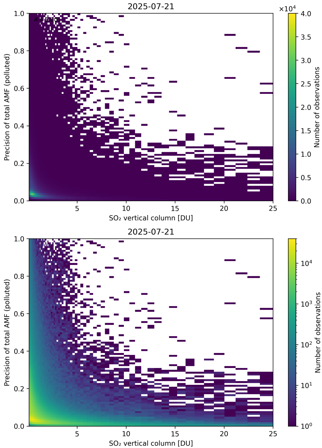
Figure 360: Scatter density plot of “SO 2 vertical column” against “Precision of total AMF (polluted)” for 2025-07-20 to 2025-07-22.
