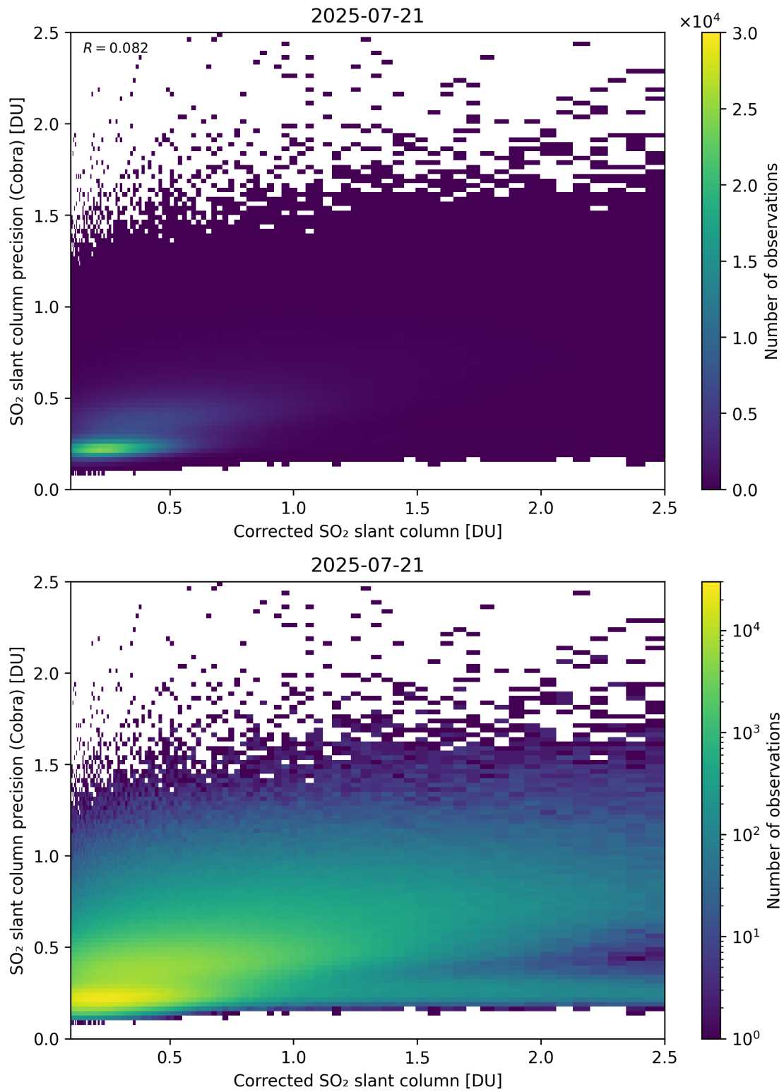
Figure 234: Scatter density plot of “Corrected SO 2 slant column” against “SO 2 slant column precision (Cobra)” for 2025-07-20 to 2025-07-22.
