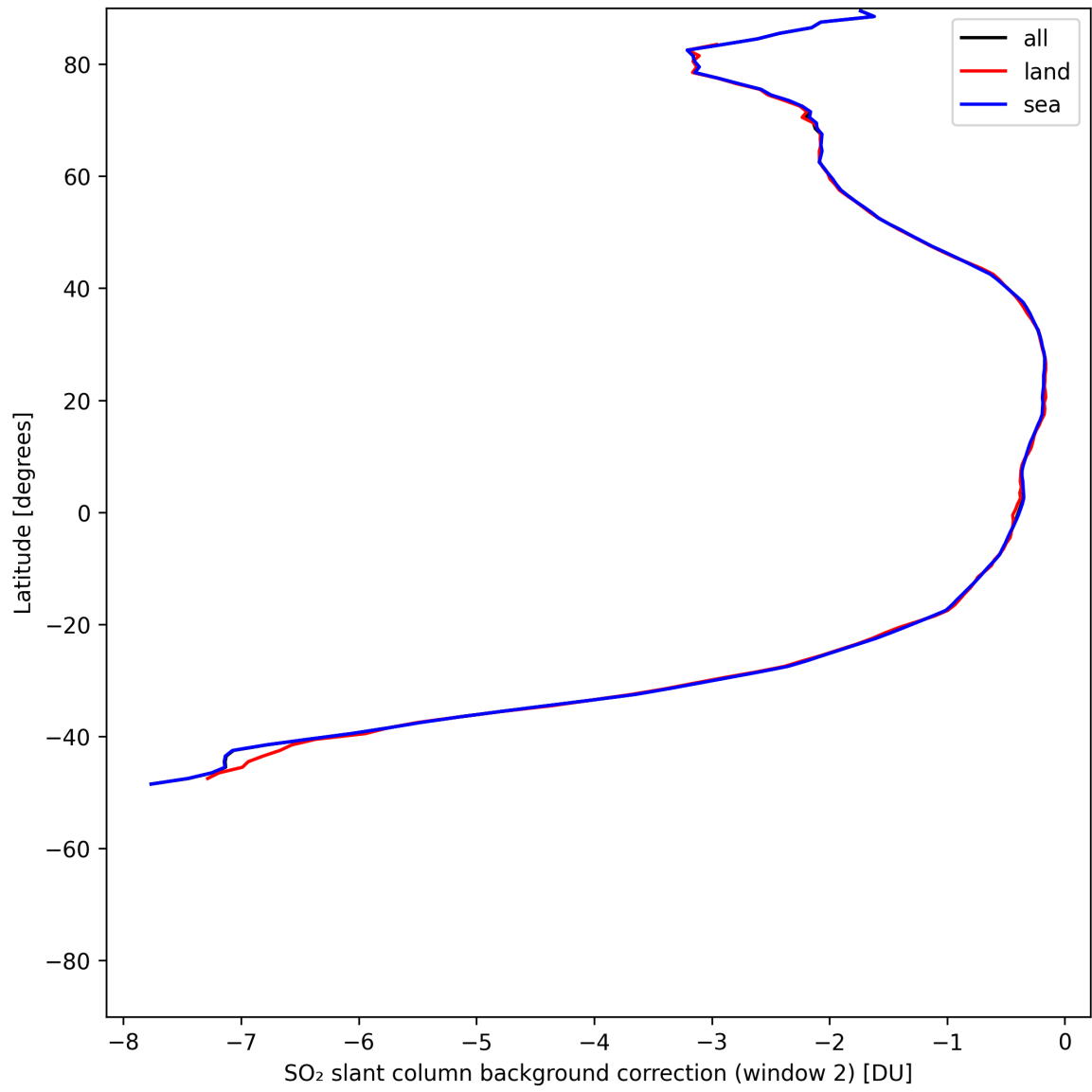
Figure 44: Zonal average of “SO 2 slant column background correction (window 2)” for 2025-07-20 to 2025-07-22.
