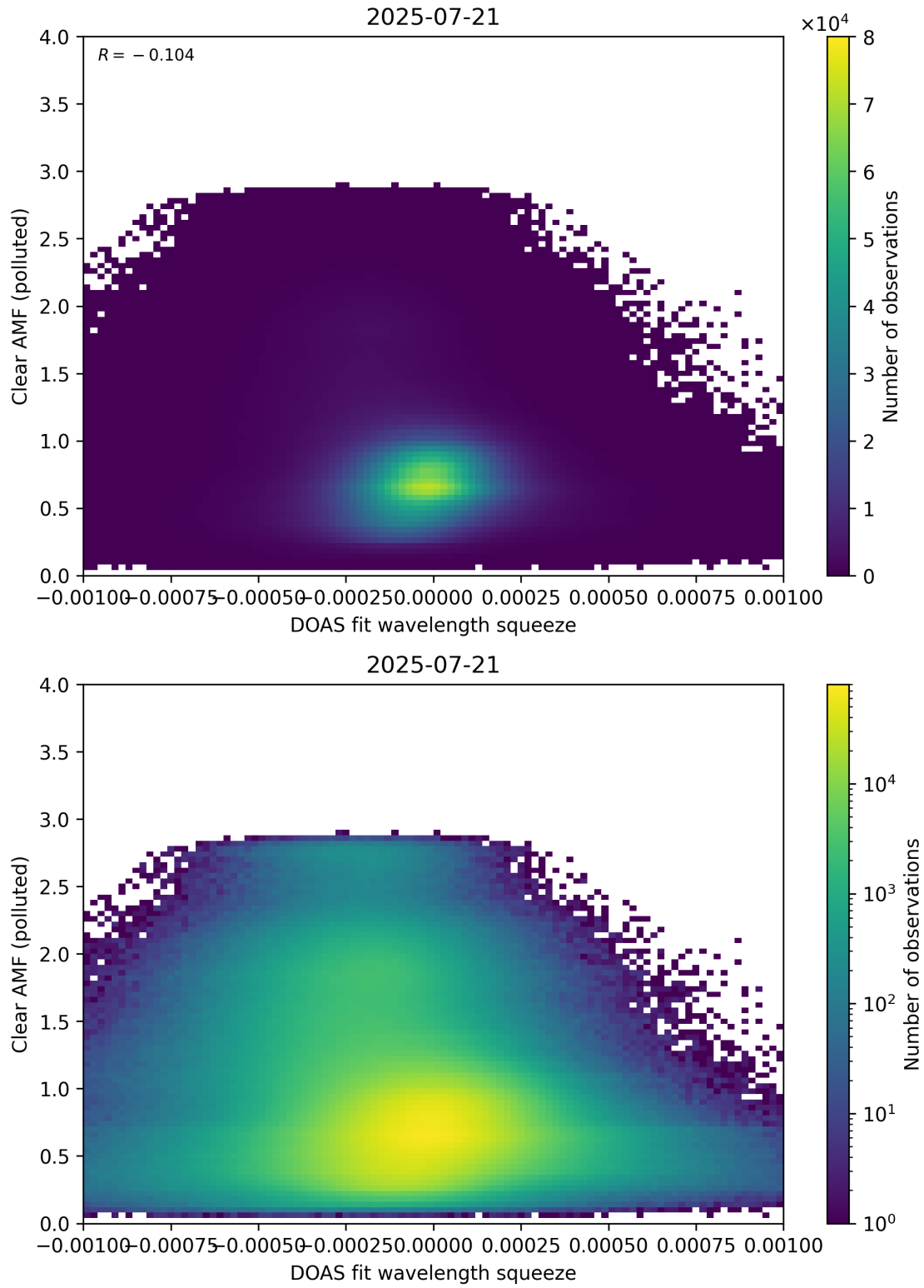
Figure 144: Scatter density plot of “DOAS fit wavelength squeeze” against “Clear AMF (polluted)” for 2025-07-20 to 2025-07-22.
