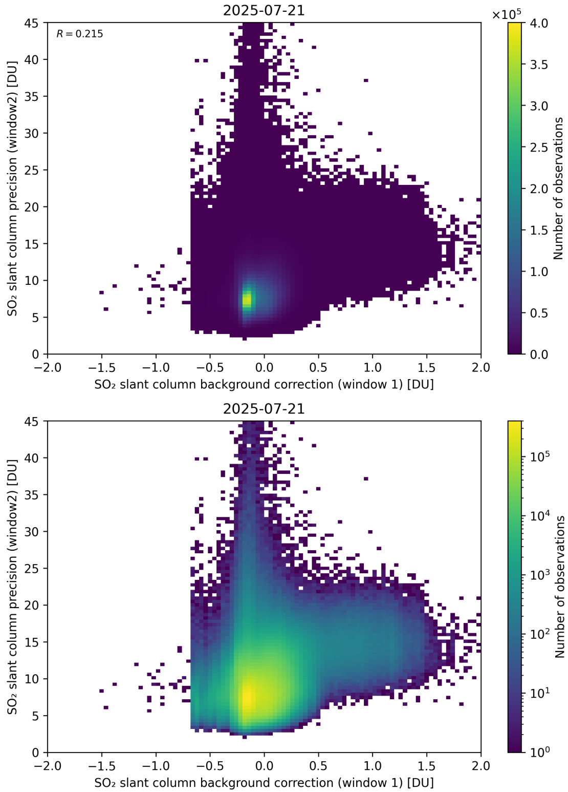
Figure 117: Scatter density plot of “SO 2 slant column background correction (window 1)” against “SO 2 slant column precision (window2)” for 2025-07-20 to 2025-07-22.
