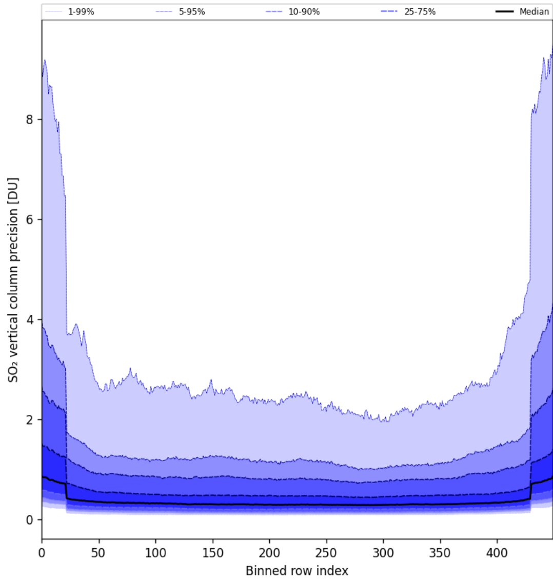
Figure 85: Along track statistics of “SO 2 vertical column precision” for 2025-07-20 to 2025-07-22
