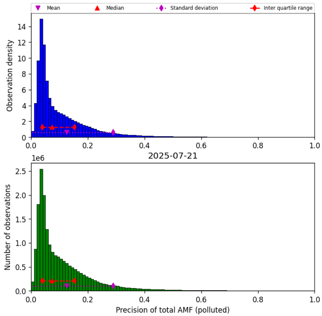
Figure 80: Histogram of “Precision of total AMF (polluted)” for 2025-07-20 to 2025-07-22
