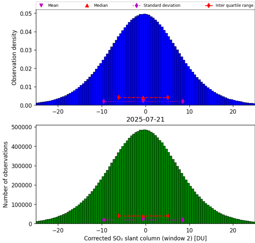
Figure 69: Histogram of “Corrected SO 2 slant column (window 2)” for 2025-07-20 to 2025-07-22
