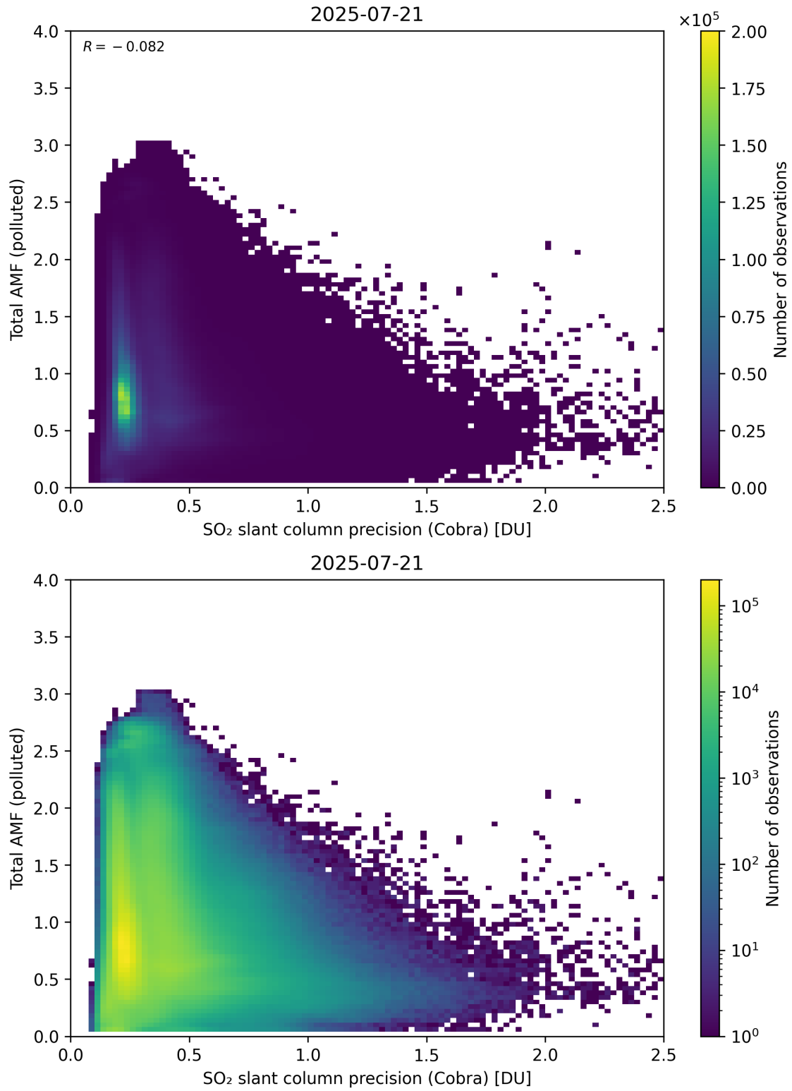
Figure 213: Scatter density plot of “SO 2 slant column precision (Cobra)” against “Total AMF (polluted)” for 2025-07-20 to 2025-07-22.
