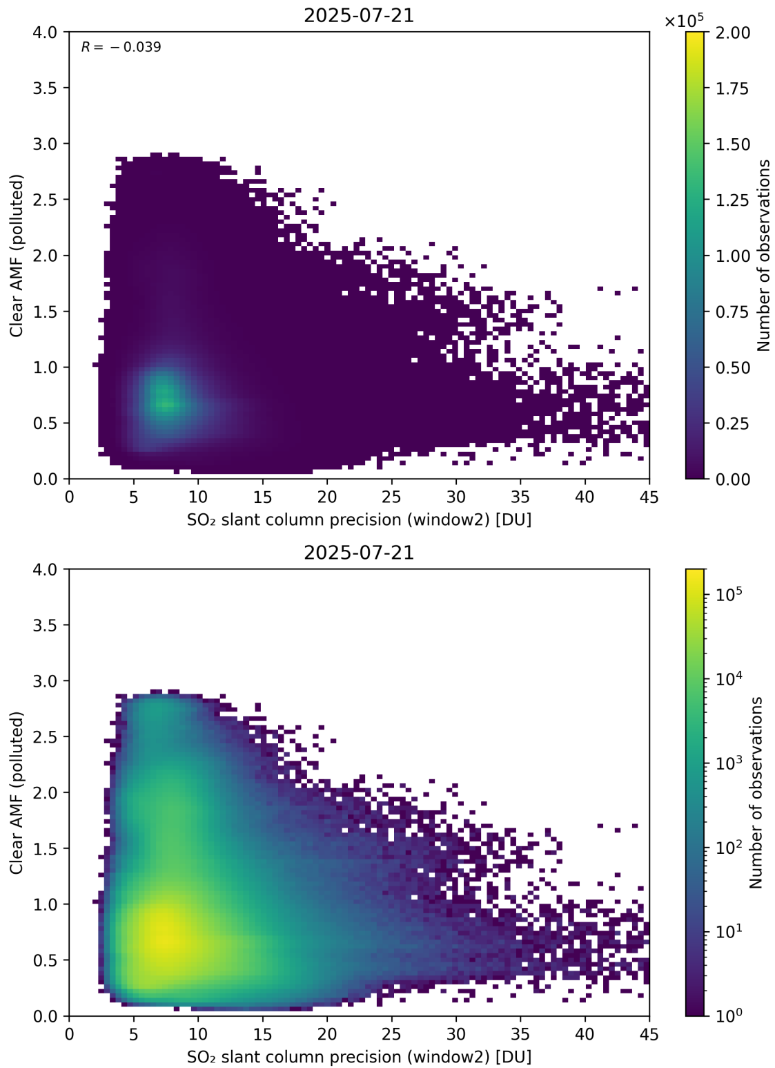
Figure 296: Scatter density plot of “SO 2 slant column precision (window2)” against “Clear AMF (polluted)” for 2025-07-20 to 2025-07-22.
