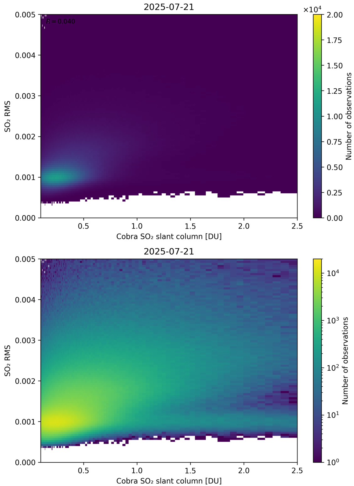
Figure 198: Scatter density plot of “Cobra SO 2 slant column” against “SO 2 RMS” for 2025-07-20 to 2025-07-22.
