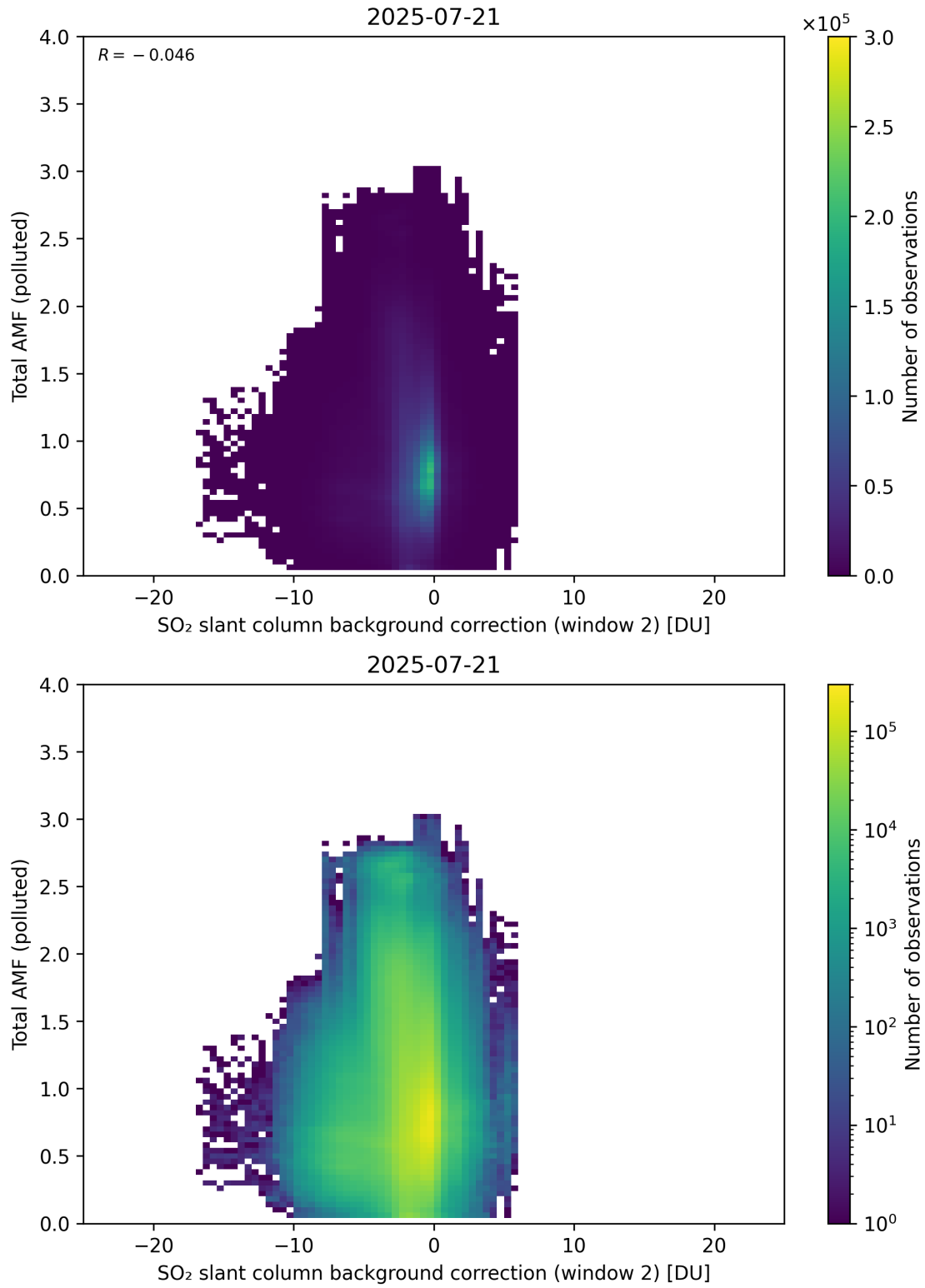
Figure 130: Scatter density plot of “SO 2 slant column background correction (window 2)” against “Total AMF (polluted)” for 2025-07-20 to 2025-07-22.
