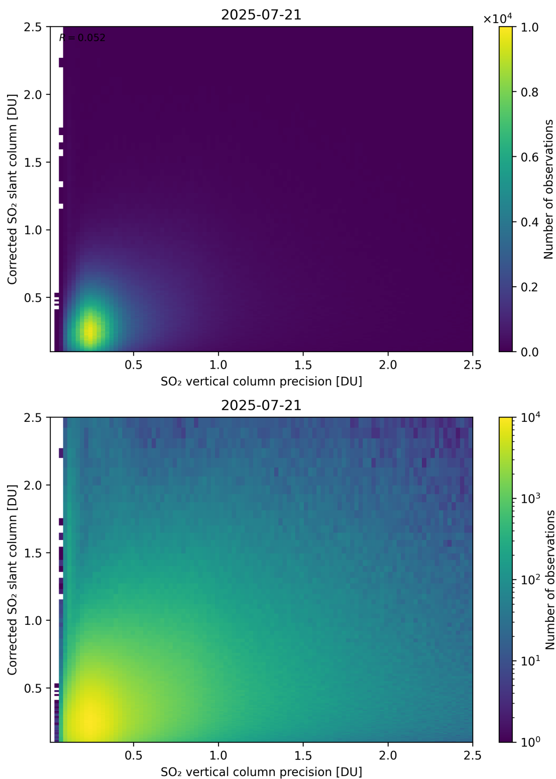
Figure 338: Scatter density plot of “SO 2 vertical column precision” against “Corrected SO 2 slant column” for 2025-07-20 to 2025-07-22.
