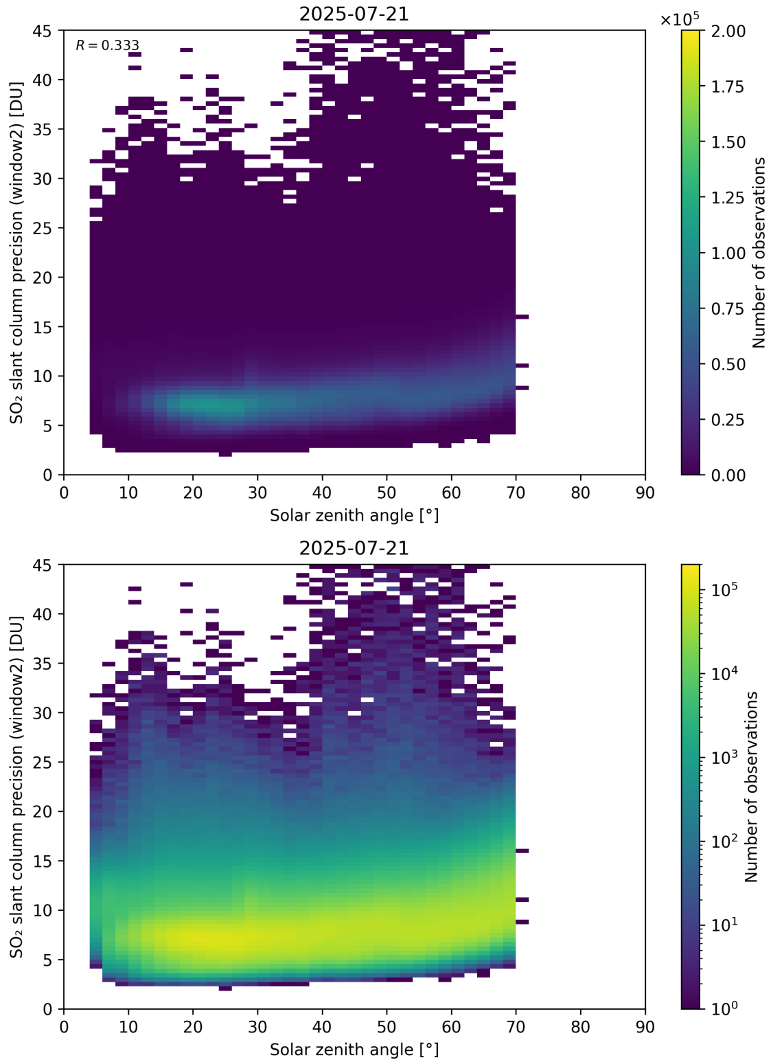
Figure 186: Scatter density plot of “Solar zenith angle” against “SO 2 slant column precision (window2)” for 2025-07-20 to 2025-07-22.
