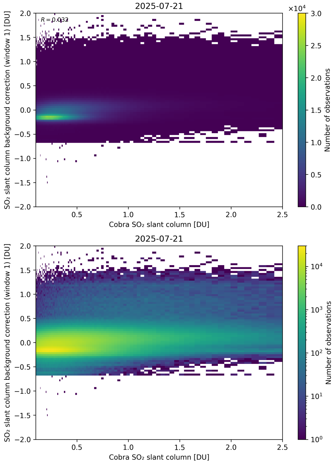
Figure 193: Scatter density plot of “Cobra SO 2 slant column” against “SO 2 slant column background correction (window 1)” for 2025-07-20 to 2025-07-22.
