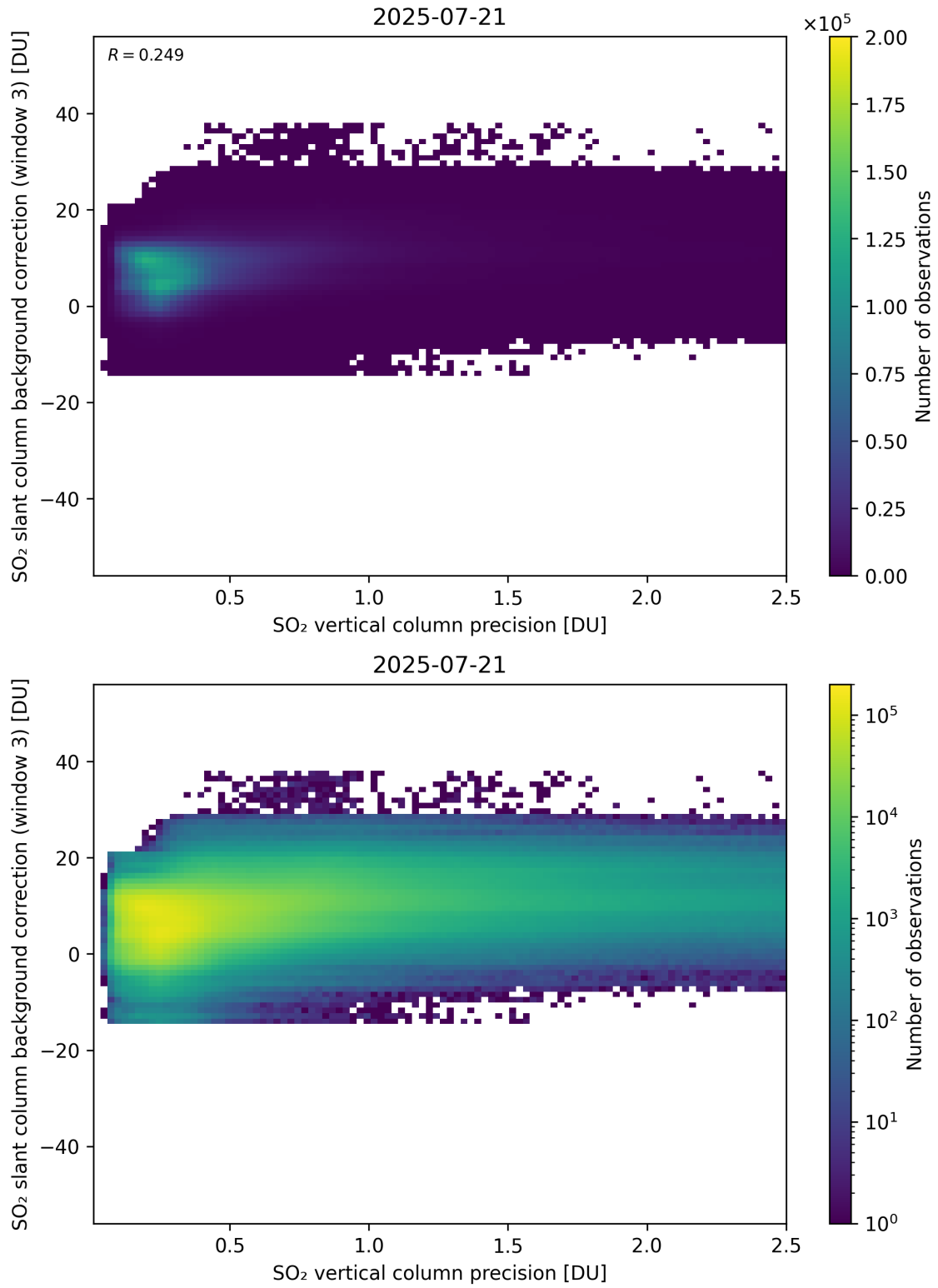
Figure 331: Scatter density plot of “SO 2 vertical column precision” against “SO 2 slant column background correction (window 3)” for 2025-07-20 to 2025-07-22.
