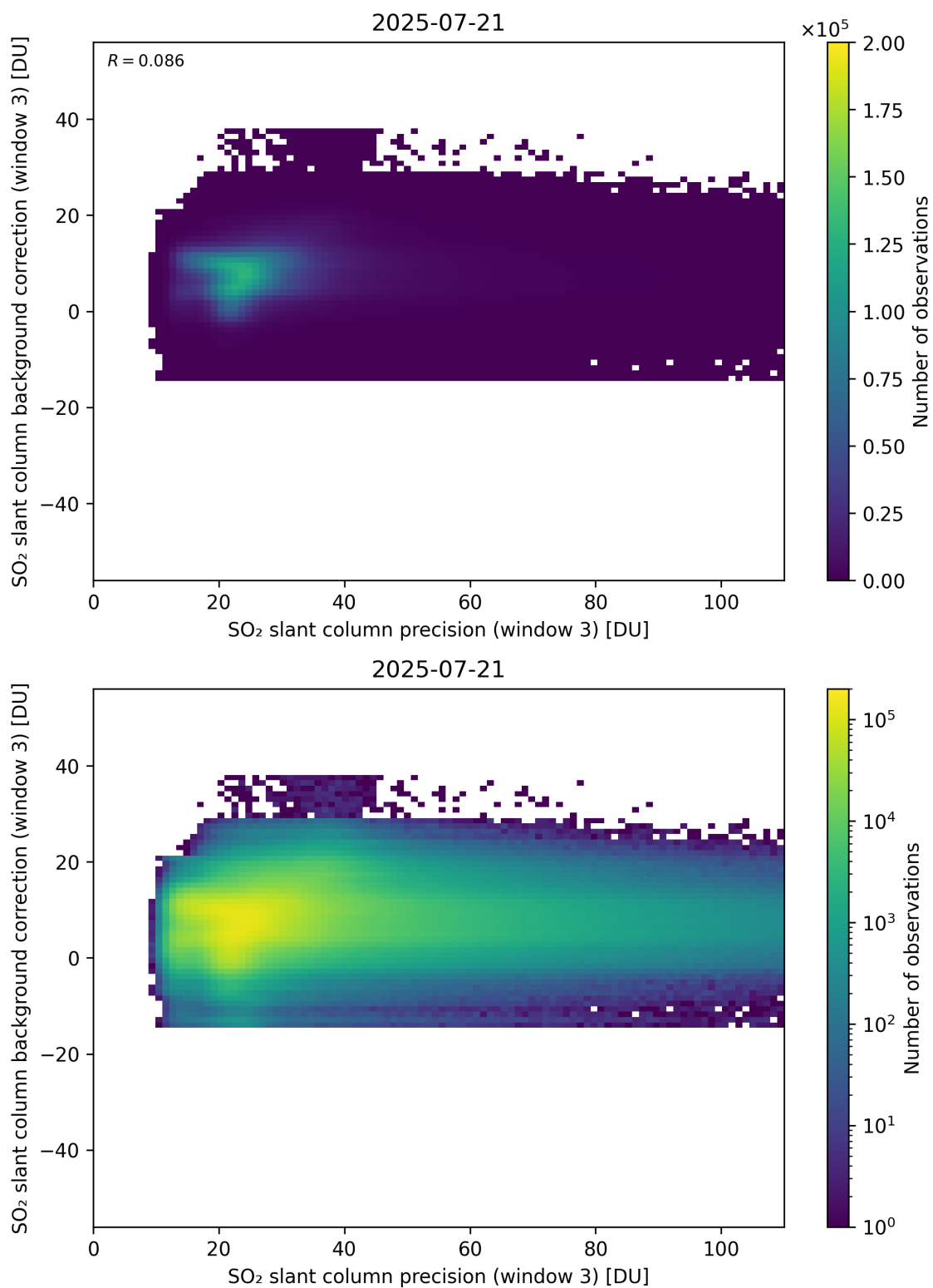
Figure 307: Scatter density plot of “SO 2 slant column precision (window 3)” against “SO 2 slant column background correction (window 3)” for 2025-07-20 to 2025-07-22.
