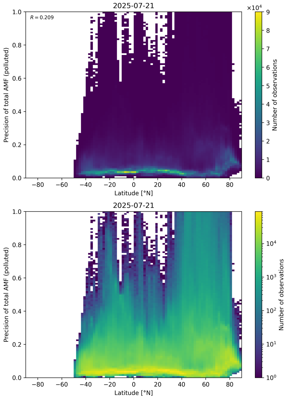
Figure 168: Scatter density plot of “Latitude” against “Precision of total AMF (polluted)” for 2025-07-20 to 2025-07-22.
