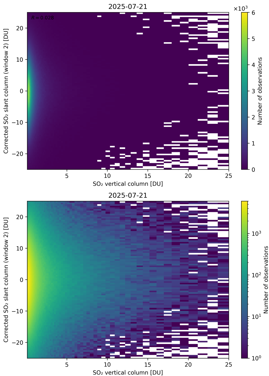
Figure 352: Scatter density plot of “SO 2 vertical column” against “Corrected SO 2 slant column (window 2)” for 2025-07-20 to 2025-07-22.
