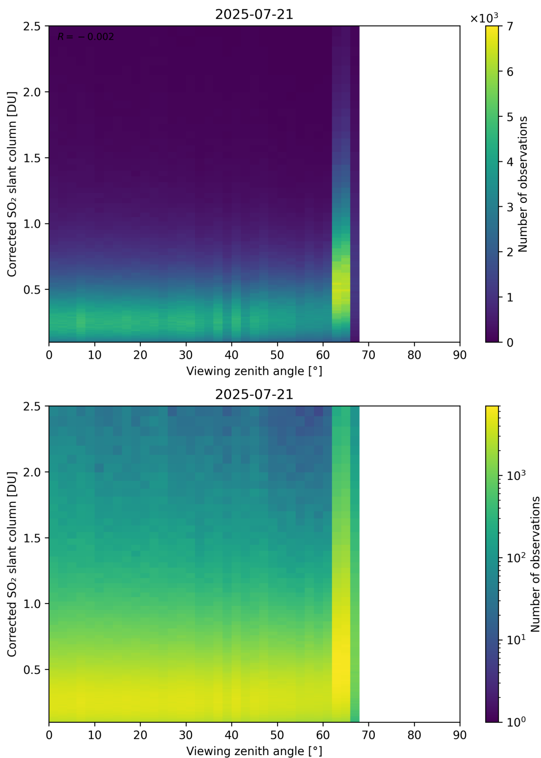
Figure 373: Scatter density plot of “Viewing zenith angle” against “Corrected SO 2 slant column” for 2025-07-20 to 2025-07-22.
