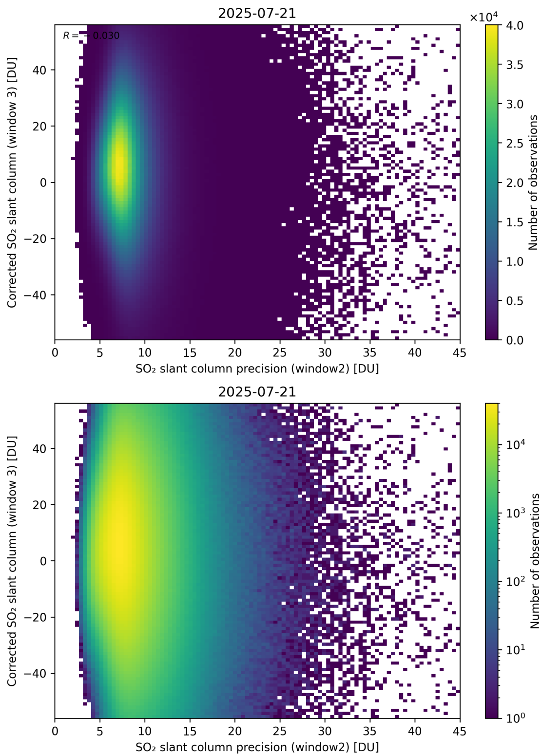
Figure 298: Scatter density plot of “SO 2 slant column precision (window2)” against “Corrected SO 2 slant column (window 3)” for 2025-07-20 to 2025-07-22.
