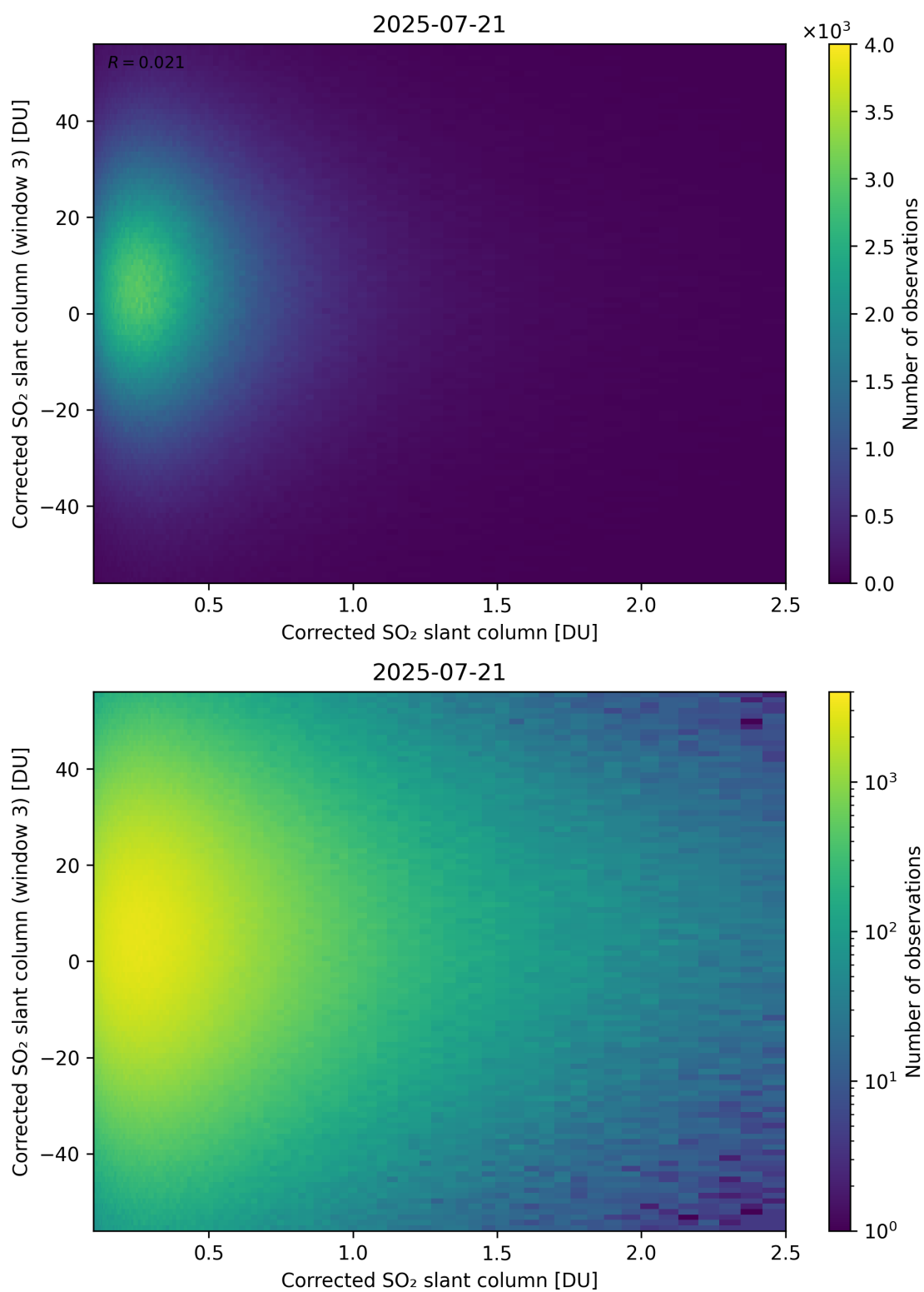
Figure 236: Scatter density plot of “Corrected SO 2 slant column” against “Corrected SO 2 slant column (window 3)” for 2025-07-20 to 2025-07-22.
