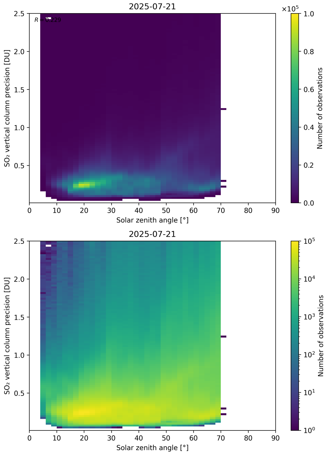
Figure 192: Scatter density plot of “Solar zenith angle” against “SO 2 vertical column precision” for 2025-07-20 to 2025-07-22.
