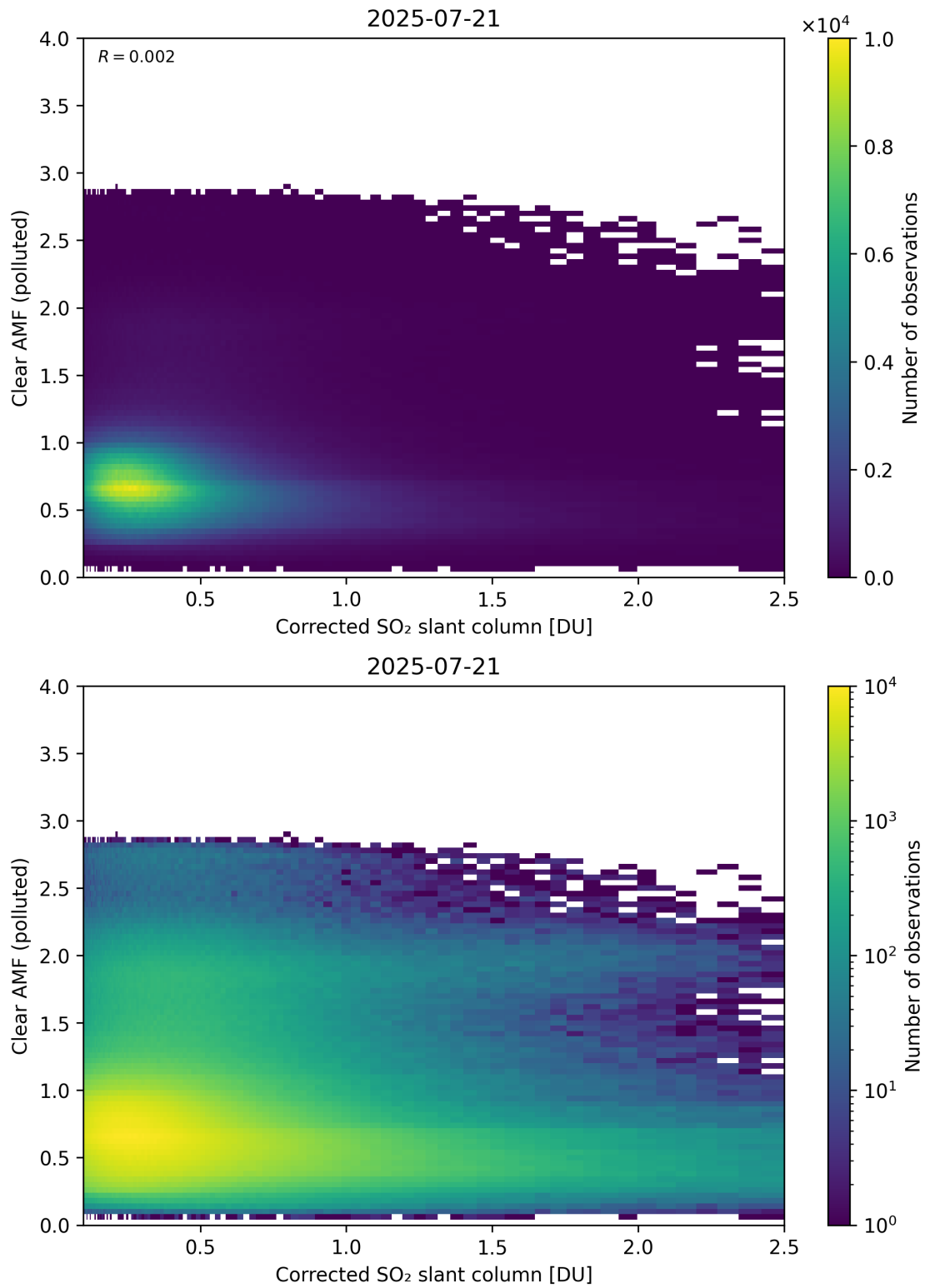
Figure 232: Scatter density plot of “Corrected SO 2 slant column” against “Clear AMF (polluted)” for 2025-07-20 to 2025-07-22.
