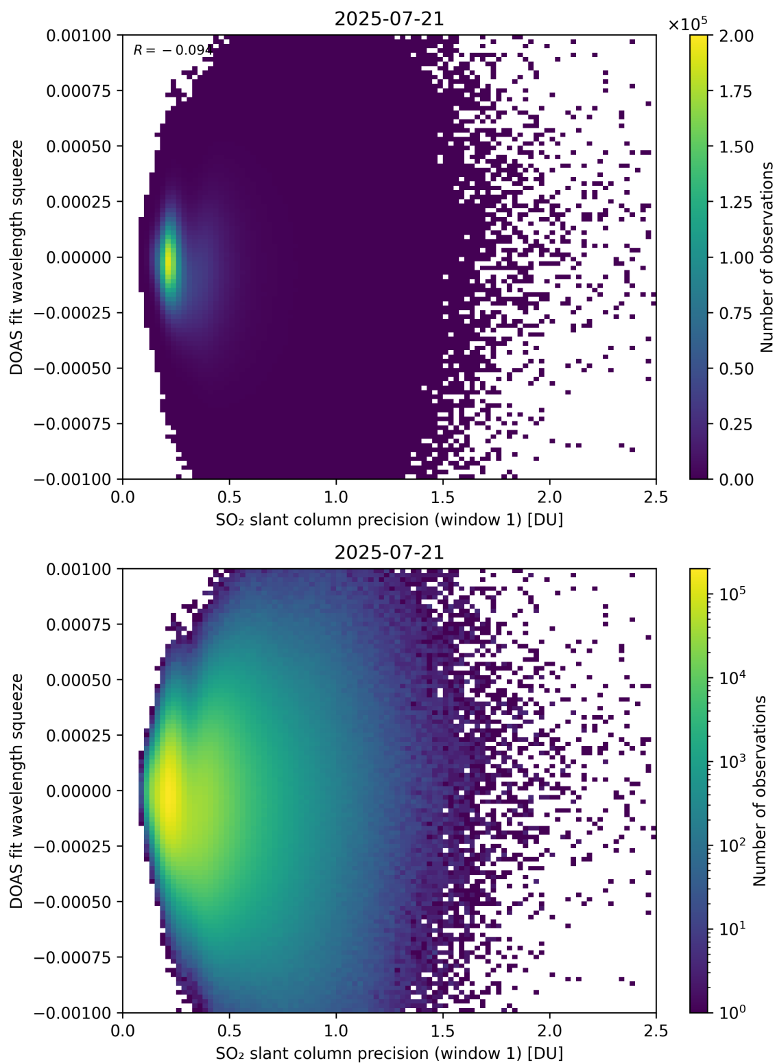
Figure 272: Scatter density plot of “SO 2 slant column precision (window 1)” against “DOAS fit wavelength squeeze” for 2025-07-20 to 2025-07-22.
