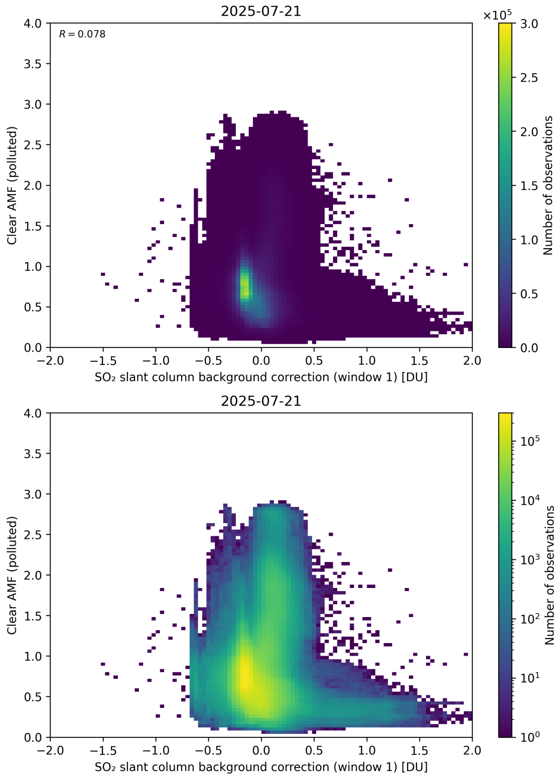
Figure 114: Scatter density plot of “SO 2 slant column background correction (window 1)” against “Clear AMF (polluted)” for 2025-07-20 to 2025-07-22.
