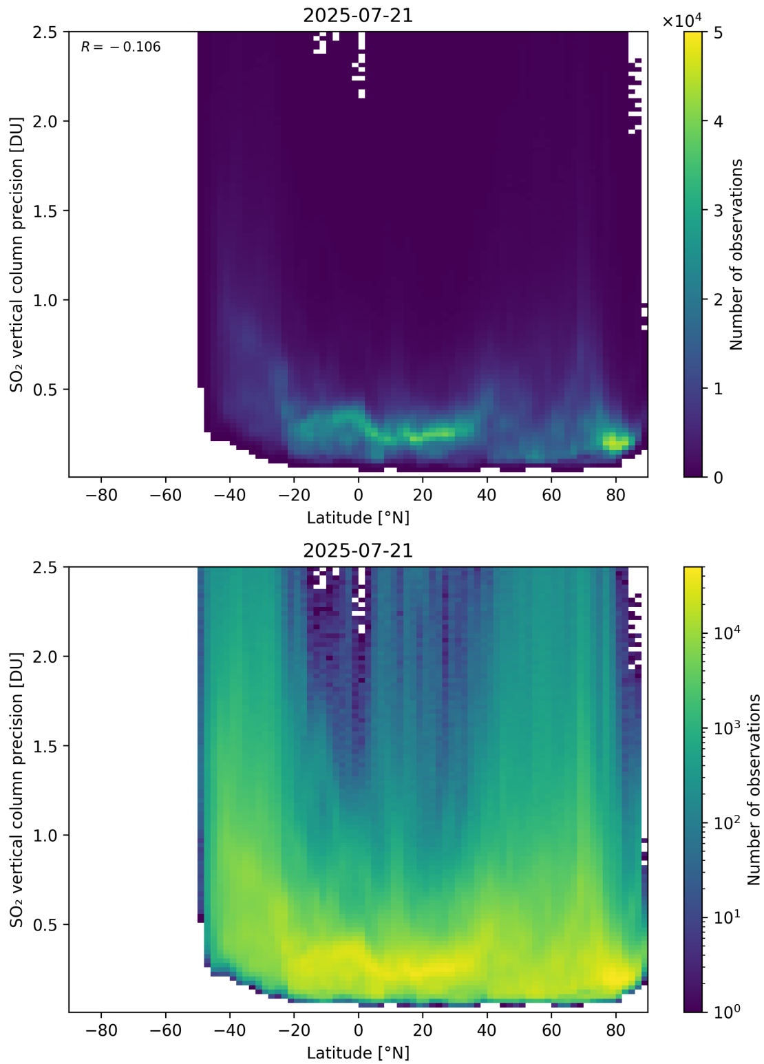
Figure 170: Scatter density plot of “Latitude” against “SO 2 vertical column precision” for 2025-07-20 to 2025-07-22.
