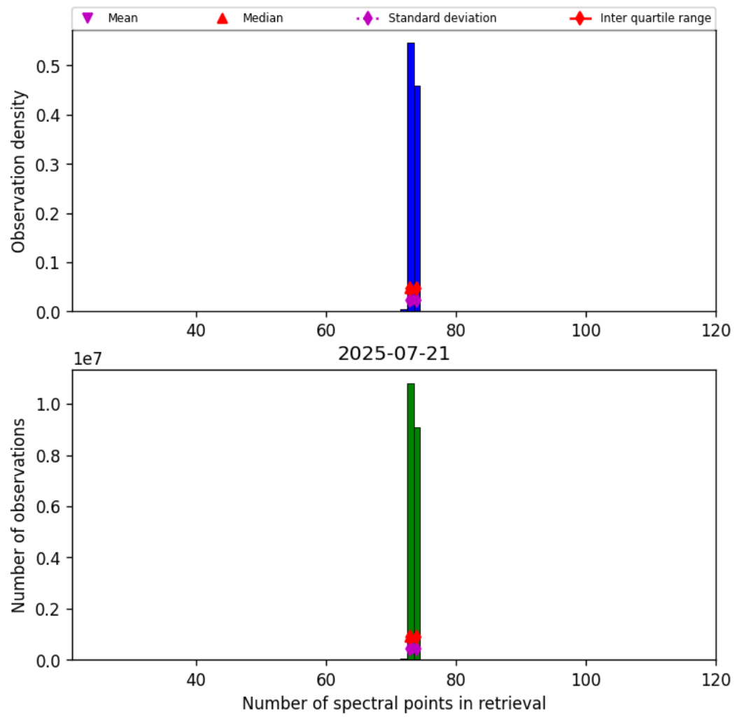
Figure 82: Histogram of “Number of spectral points in retrieval” for 2025-07-20 to 2025-07-22
