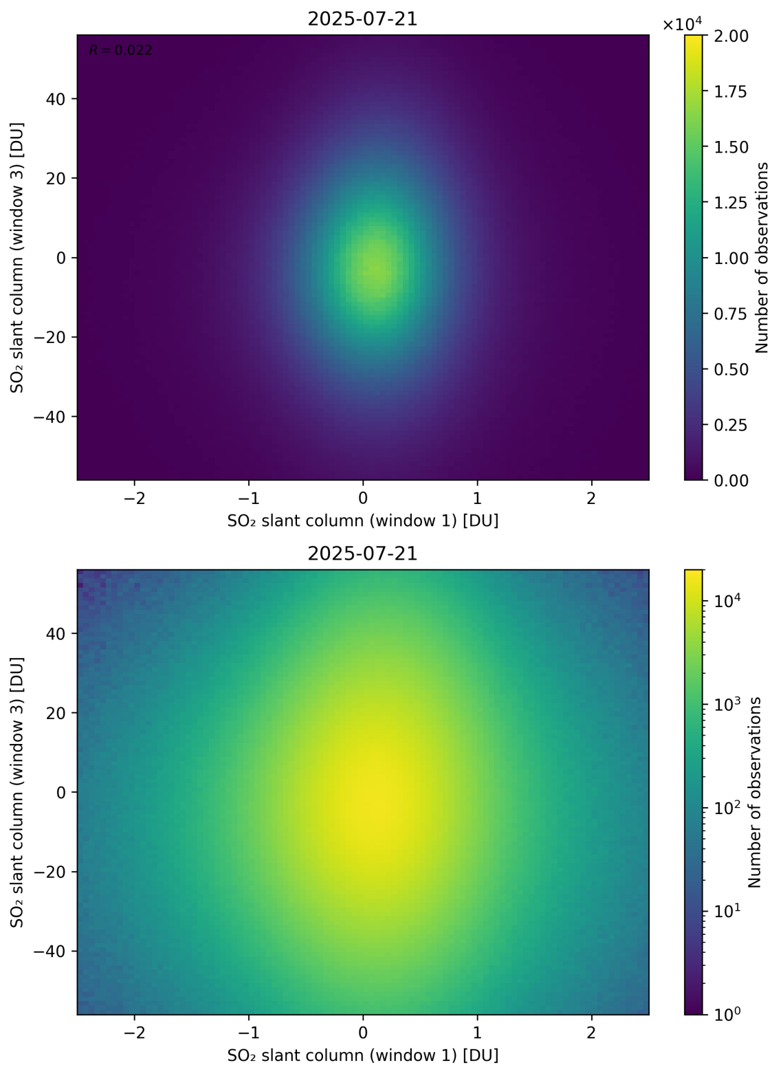
Figure 287: Scatter density plot of “SO 2 slant column (window 1)” against “SO 2 slant column (window 3)” for 2025-07-20 to 2025-07-22.
