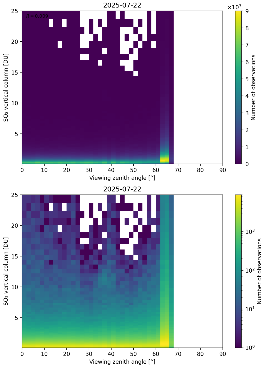
Figure 383: Scatter density plot of “Viewing zenith angle” against “SO 2 vertical column” for 2025-07-21 to 2025-07-23.
