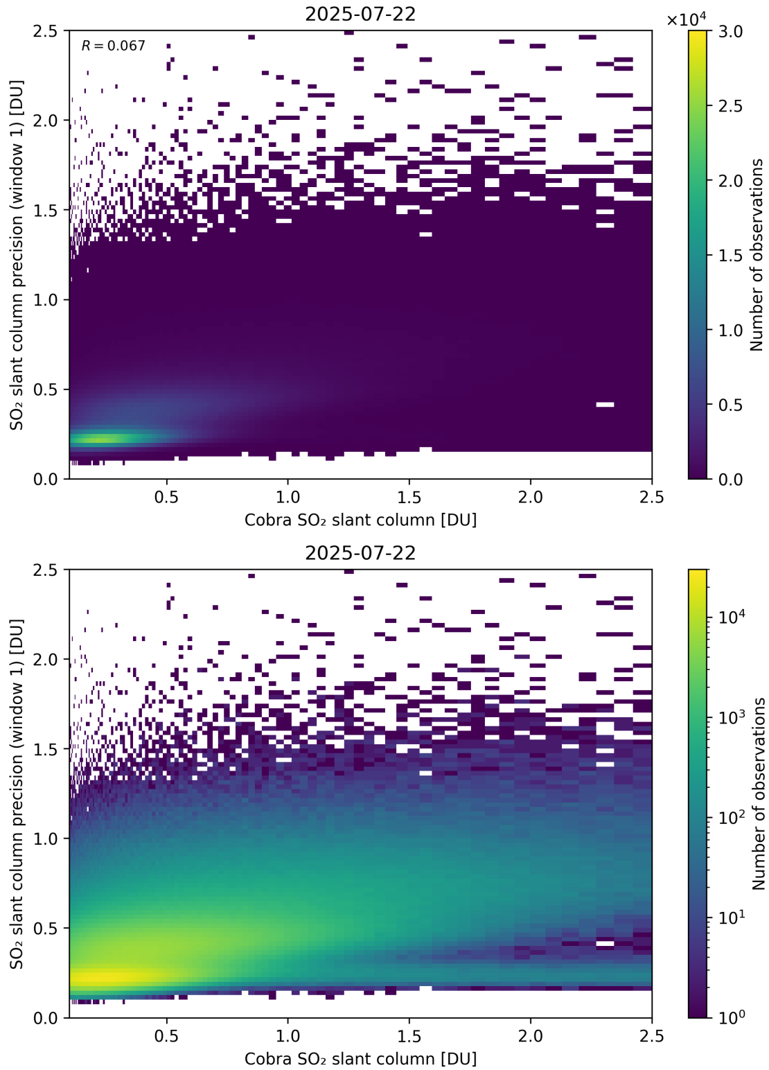
Figure 220: Scatter density plot of “Cobra SO 2 slant column” against “SO 2 slant column precision (window 1)” for 2025-07-21 to 2025-07-23.
