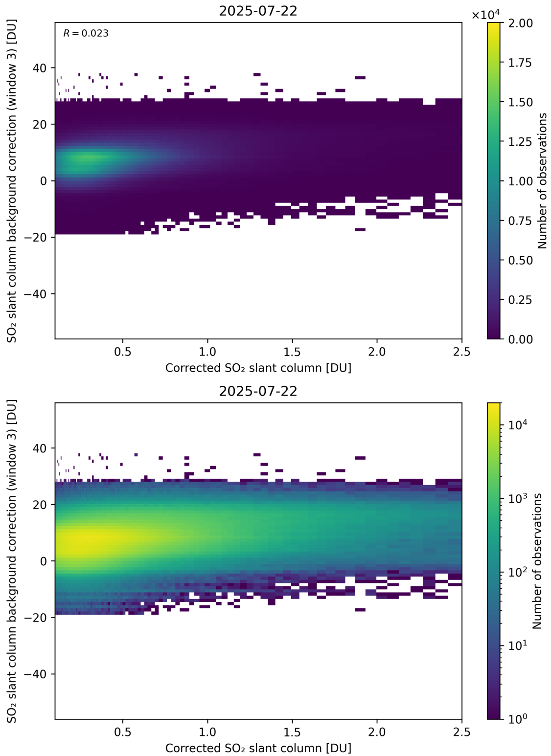
Figure 228: Scatter density plot of “Corrected SO 2 slant column” against “SO 2 slant column background correction (window 3)” for 2025-07-21 to 2025-07-23.
