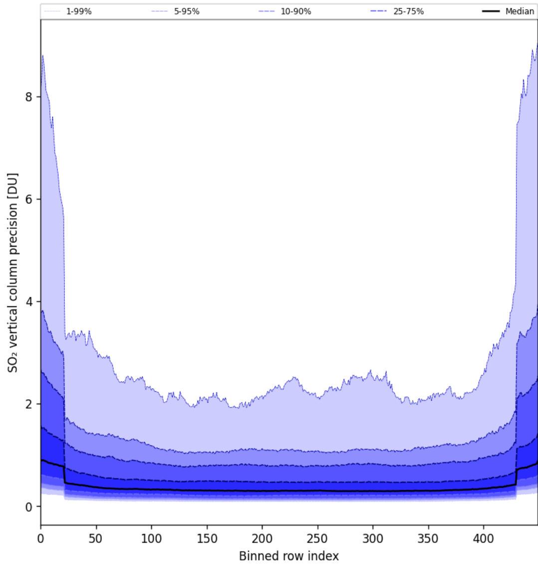
Figure 85: Along track statistics of “SO 2 vertical column precision” for 2025-07-21 to 2025-07-23
