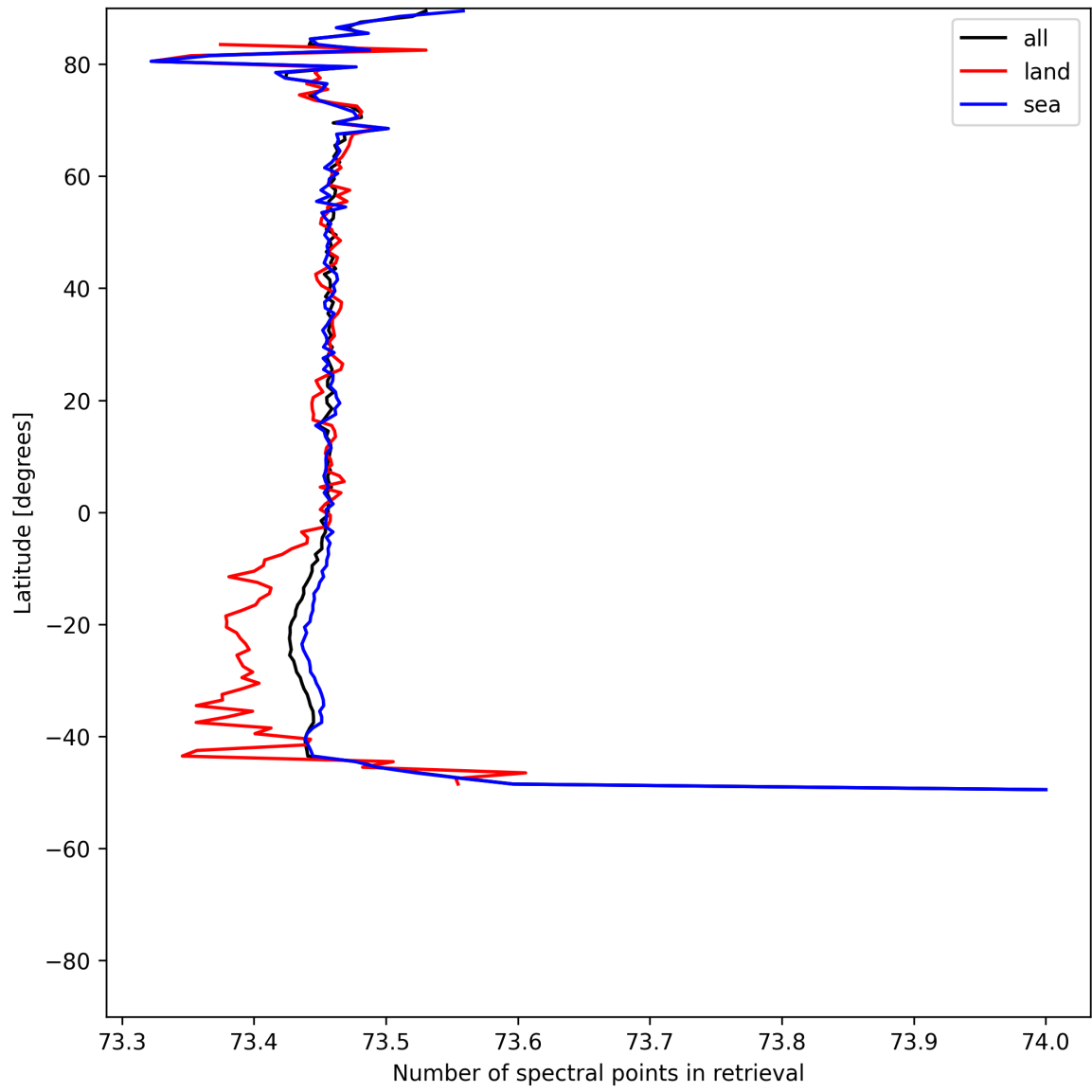
Figure 56: Zonal average of “Number of spectral points in retrieval” for 2025-07-21 to 2025-07-23.
