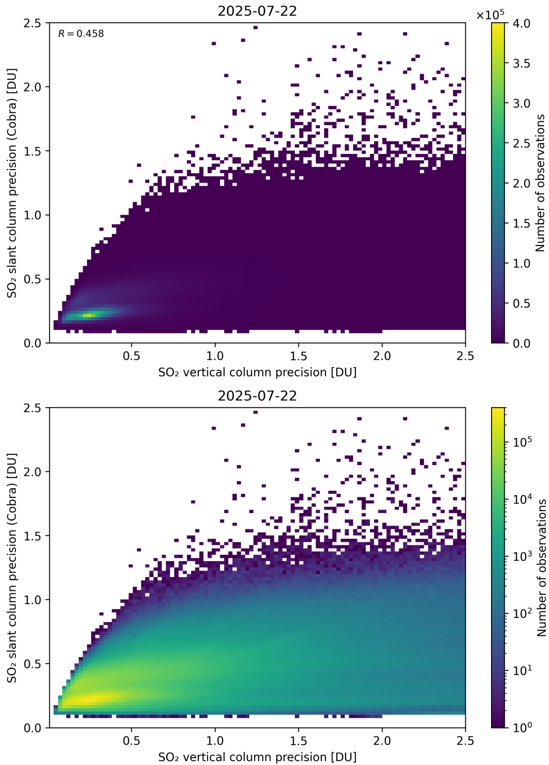
Figure 337: Scatter density plot of “SO 2 vertical column precision” against “SO 2 slant column precision (Cobra)” for 2025-07-21 to 2025-07-23.
