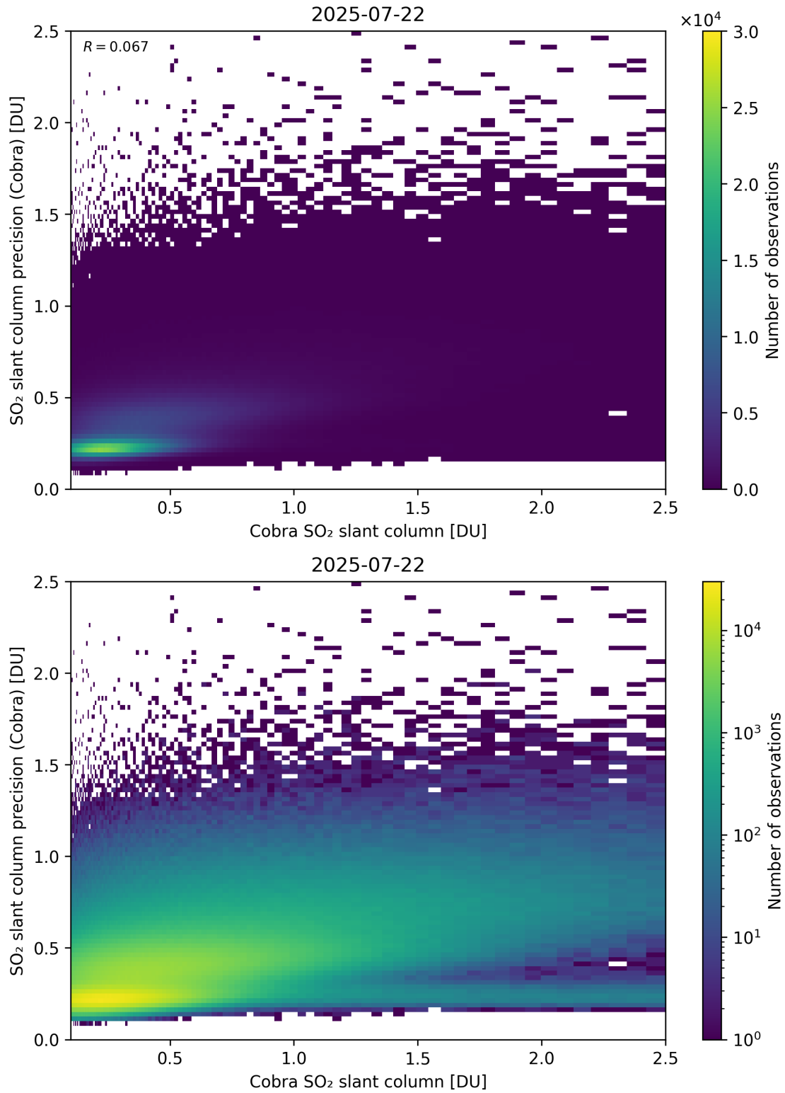
Figure 216: Scatter density plot of “Cobra SO 2 slant column” against “SO 2 slant column precision (Cobra)” for 2025-07-21 to 2025-07-23.
