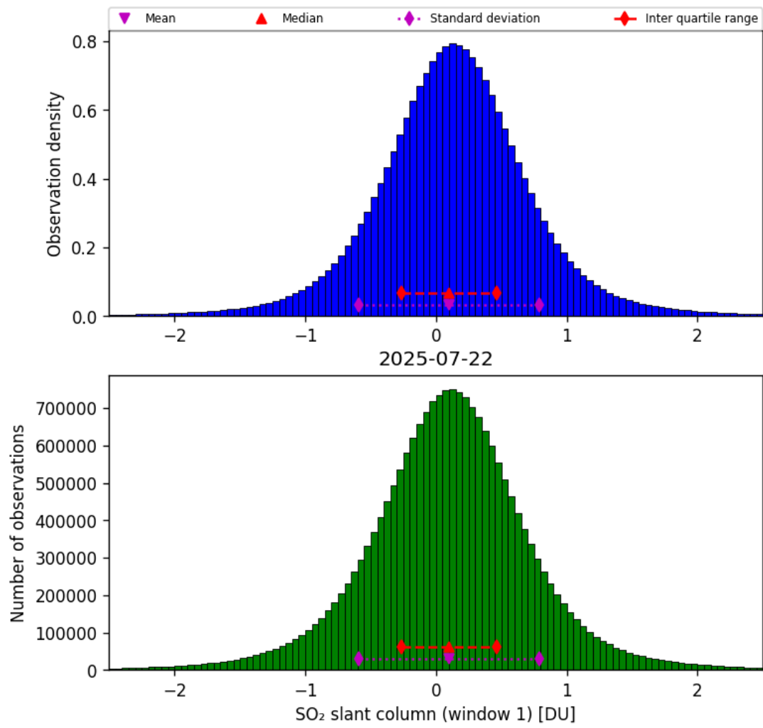
Figure 63: Histogram of “SO 2 slant column (window 1)” for 2025-07-21 to 2025-07-23
