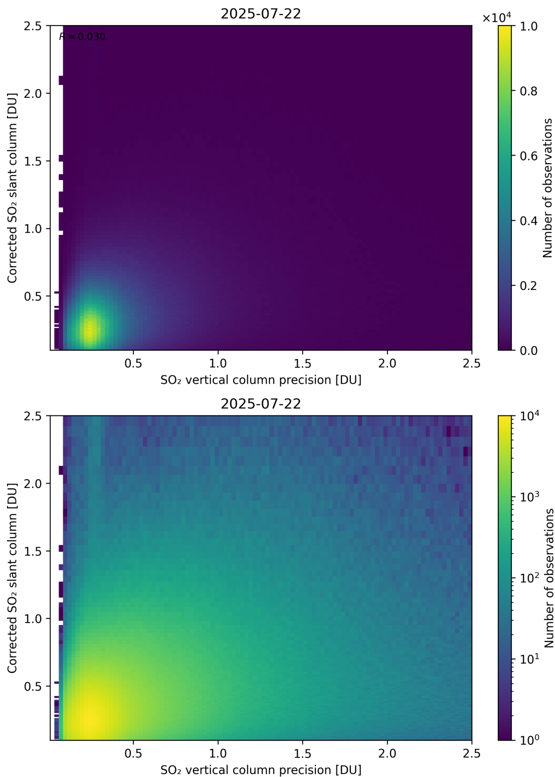
Figure 338: Scatter density plot of “SO 2 vertical column precision” against “Corrected SO 2 slant column” for 2025-07-21 to 2025-07-23.
