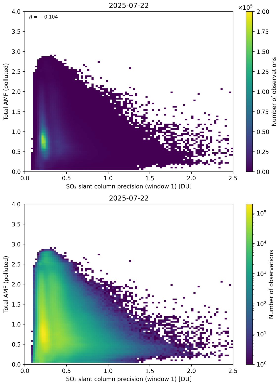
Figure 280: Scatter density plot of “SO 2 slant column precision (window 1)” against “Total AMF (polluted)” for 2025-07-21 to 2025-07-23.
