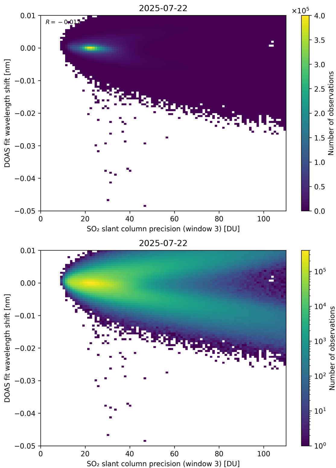
Figure 308: Scatter density plot of “SO 2 slant column precision (window 3)” against “DOAS fit wavelength shift” for 2025-07-21 to 2025-07-23.
