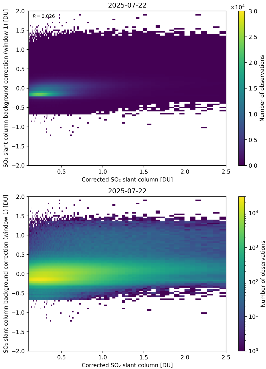
Figure 226: Scatter density plot of “Corrected SO 2 slant column” against “SO 2 slant column background correction (window 1)” for 2025-07-21 to 2025-07-23.
