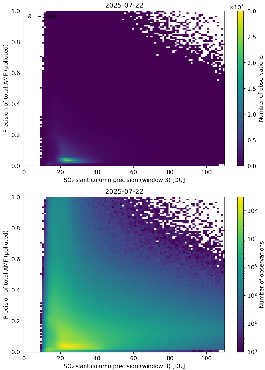
Figure 314: Scatter density plot of “SO 2 slant column precision (window 3)” against “Precision of total AMF (polluted)” for 2025-07-21 to 2025-07-23.
