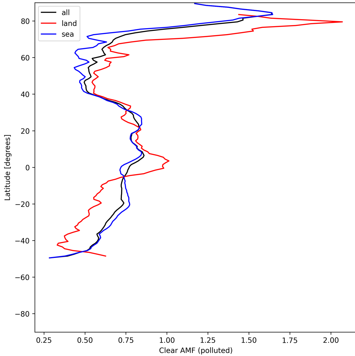
Figure 55: Zonal average of “Clear AMF (polluted)” for 2025-07-21 to 2025-07-23.
