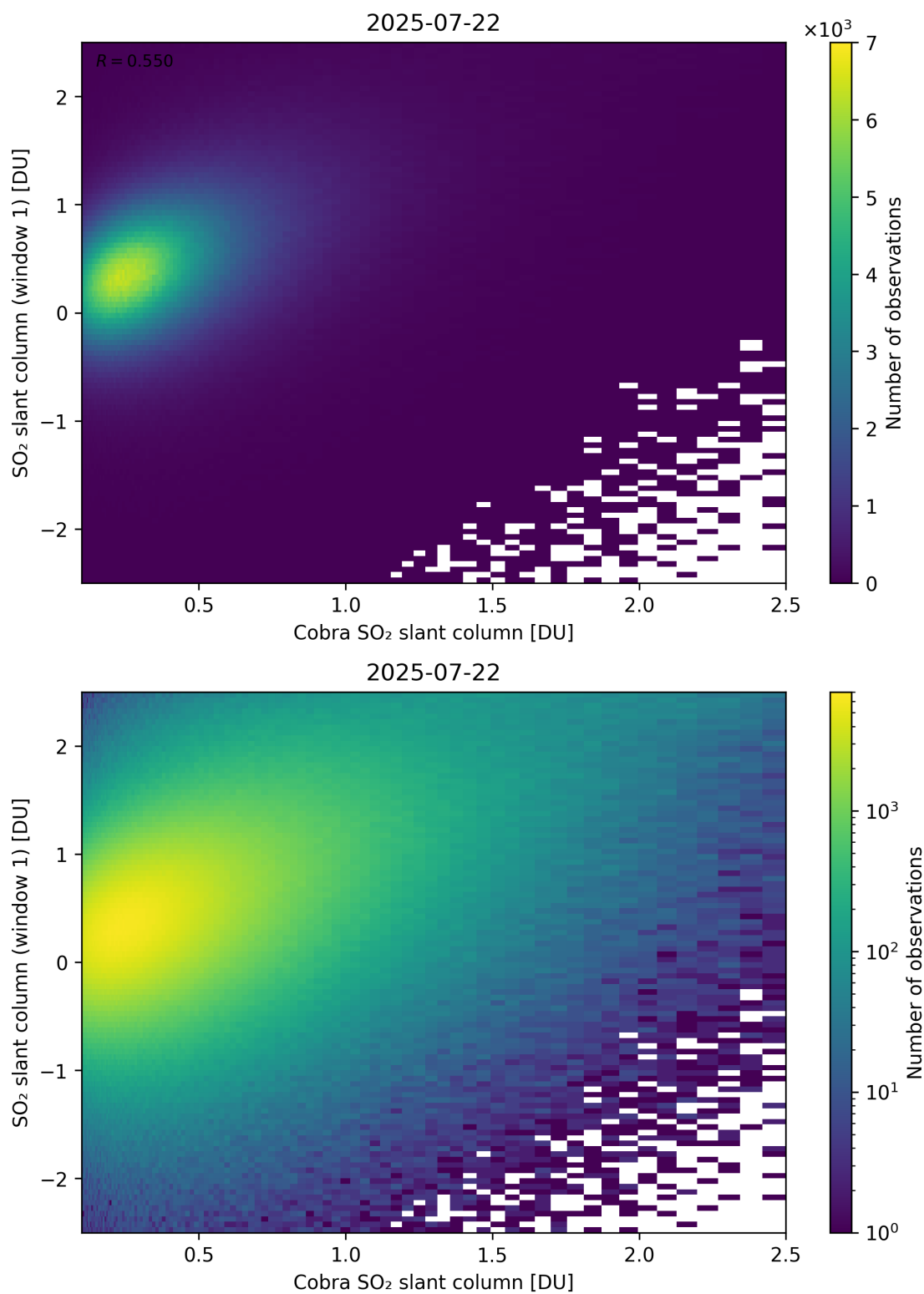
Figure 219: Scatter density plot of “Cobra SO 2 slant column” against “SO 2 slant column (window 1)” for 2025-07-21 to 2025-07-23.
