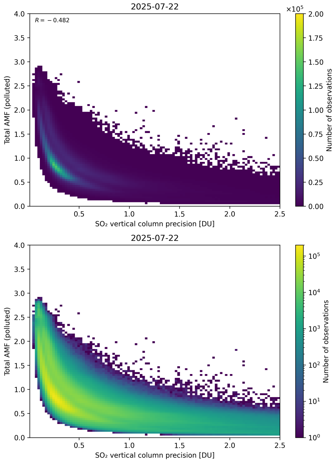
Figure 346: Scatter density plot of “SO 2 vertical column precision” against “Total AMF (polluted)” for 2025-07-21 to 2025-07-23.
