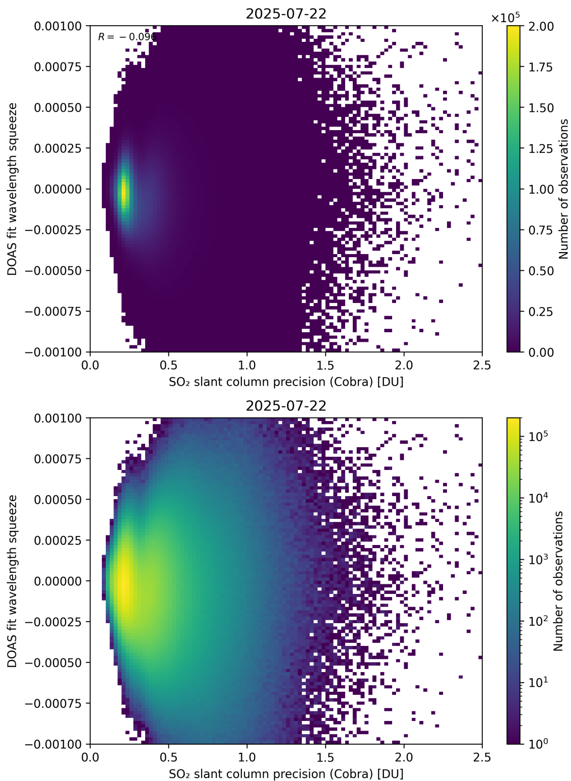
Figure 203: Scatter density plot of “SO 2 slant column precision (Cobra)” against “DOAS fit wavelength squeeze” for 2025-07-21 to 2025-07-23.
