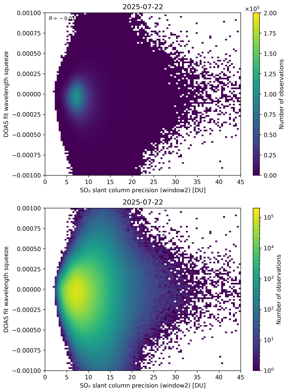
Figure 294: Scatter density plot of “SO 2 slant column precision (window2)” against “DOAS fit wavelength squeeze” for 2025-07-21 to 2025-07-23.
