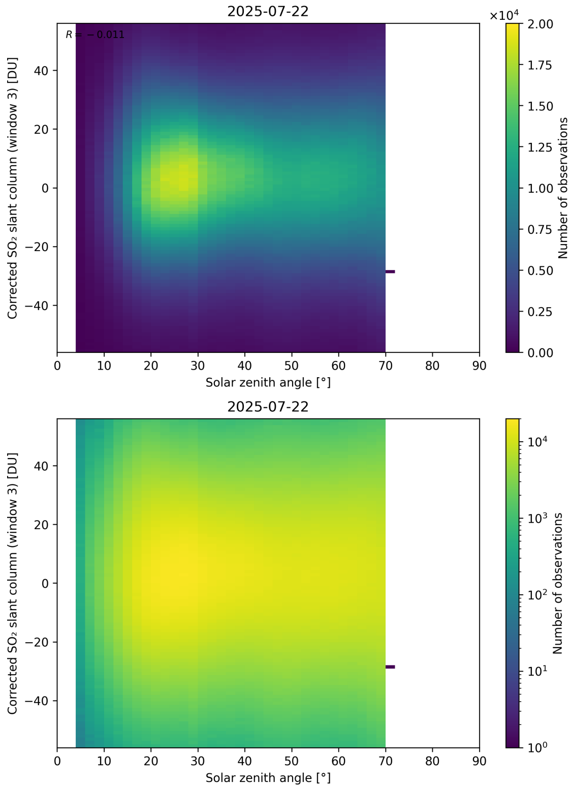
Figure 183: Scatter density plot of “Solar zenith angle” against “Corrected SO 2 slant column (window 3)” for 2025-07-21 to 2025-07-23.
