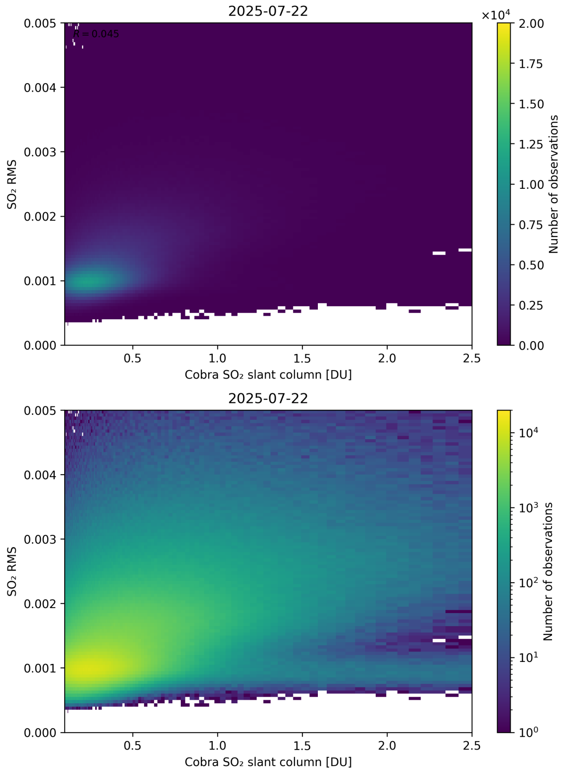
Figure 198: Scatter density plot of “Cobra SO 2 slant column” against “SO 2 RMS” for 2025-07-21 to 2025-07-23.
