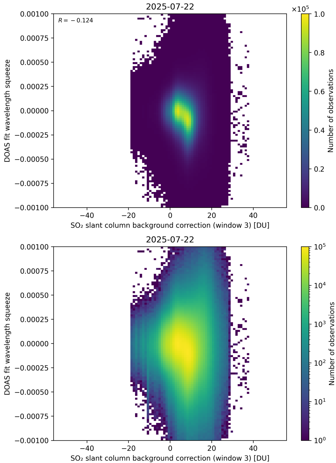
Figure 133: Scatter density plot of “SO 2 slant column background correction (window 3)” against “DOAS fit wavelength squeeze” for 2025-07-21 to 2025-07-23.
