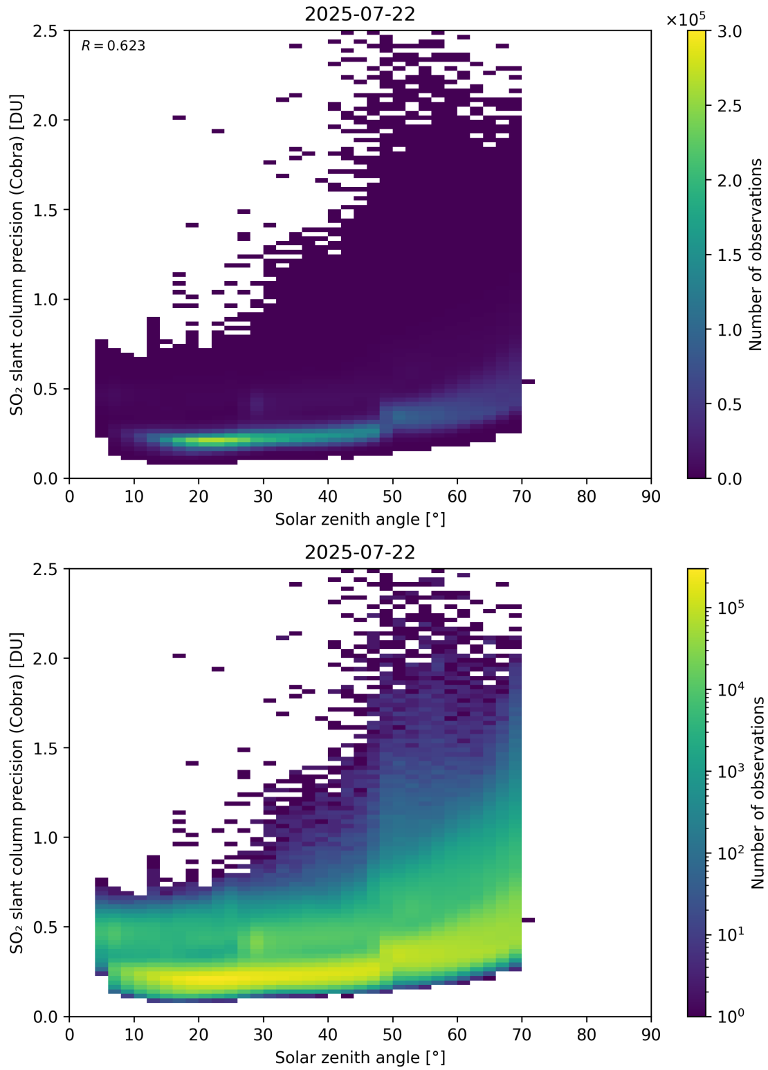
Figure 180: Scatter density plot of “Solar zenith angle” against “SO 2 slant column precision (Cobra)” for 2025-07-21 to 2025-07-23.
