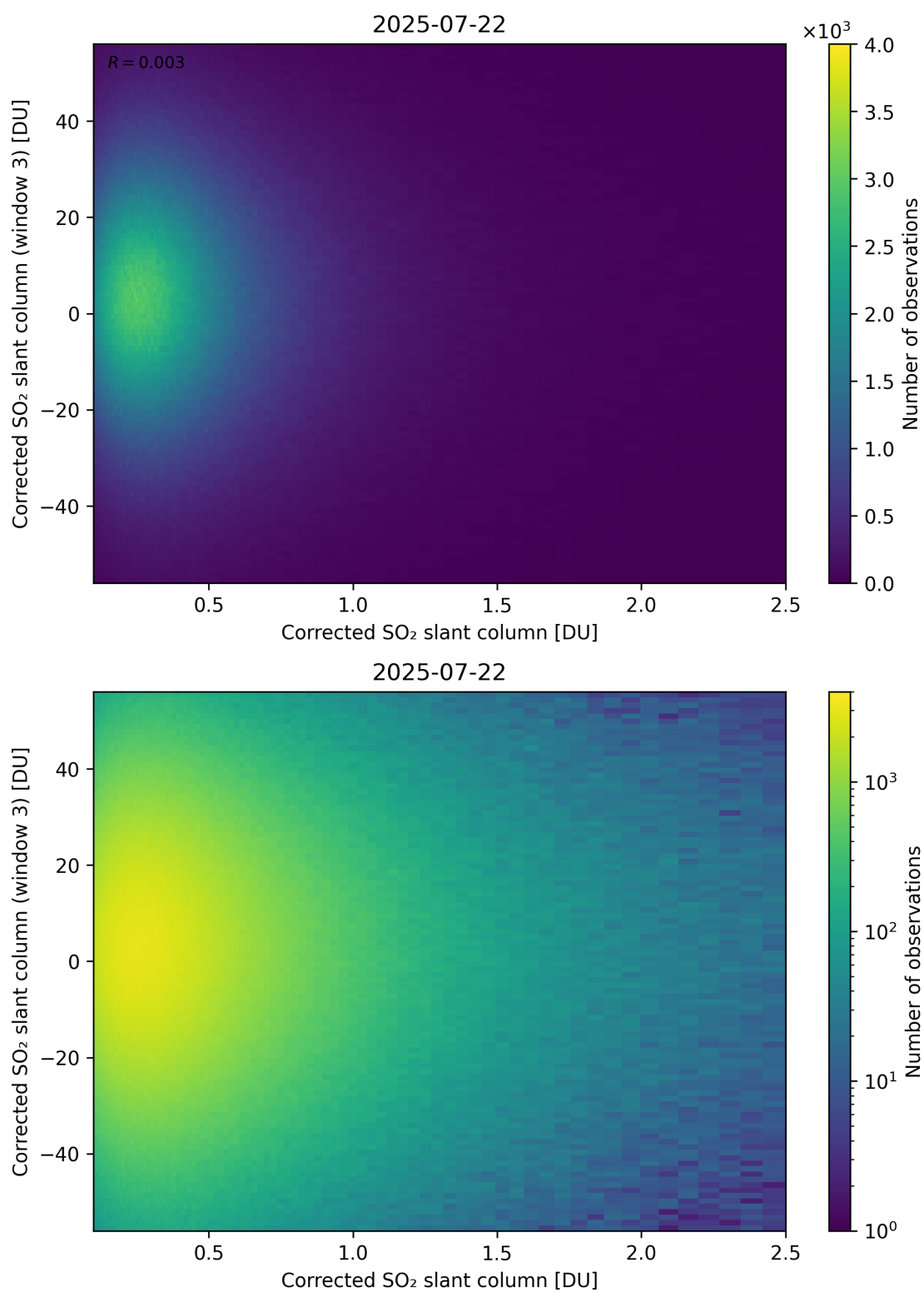
Figure 236: Scatter density plot of “Corrected SO 2 slant column” against “Corrected SO 2 slant column (window 3)” for 2025-07-21 to 2025-07-23.
