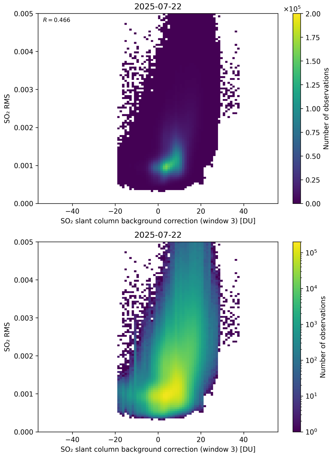
Figure 134: Scatter density plot of “SO 2 slant column background correction (window 3)” against “SO 2 RMS” for 2025-07-21 to 2025-07-23.
