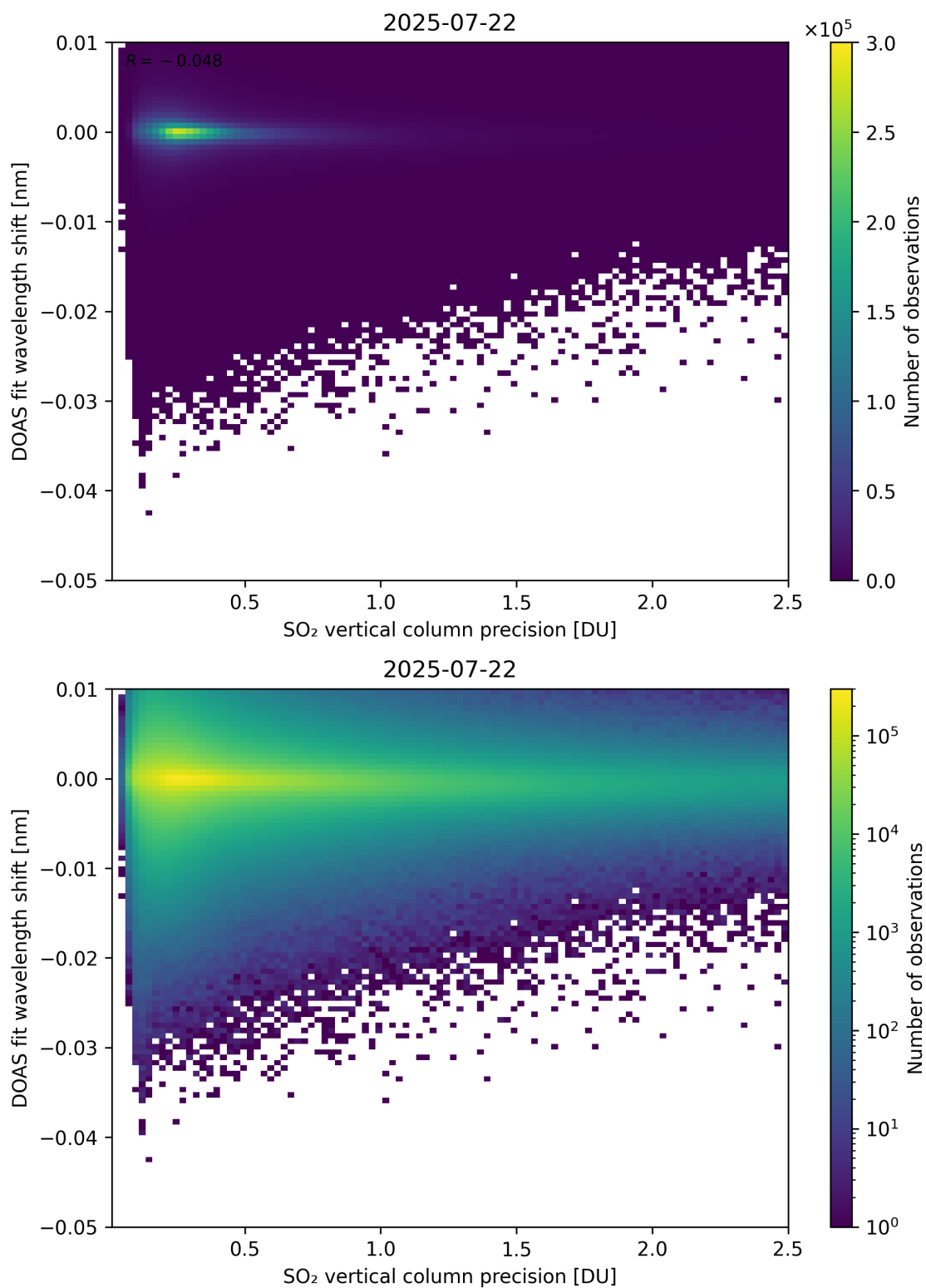
Figure 332: Scatter density plot of “SO 2 vertical column precision” against “DOAS fit wavelength shift” for 2025-07-21 to 2025-07-23.
