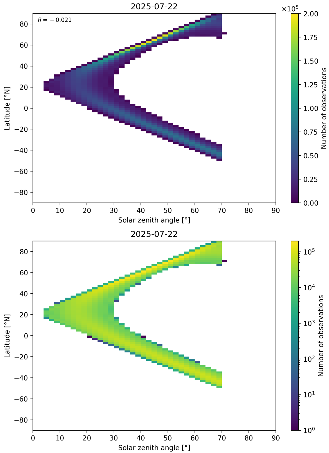
Figure 177: Scatter density plot of “Solar zenith angle” against “Latitude” for 2025-07-21 to 2025-07-23.
