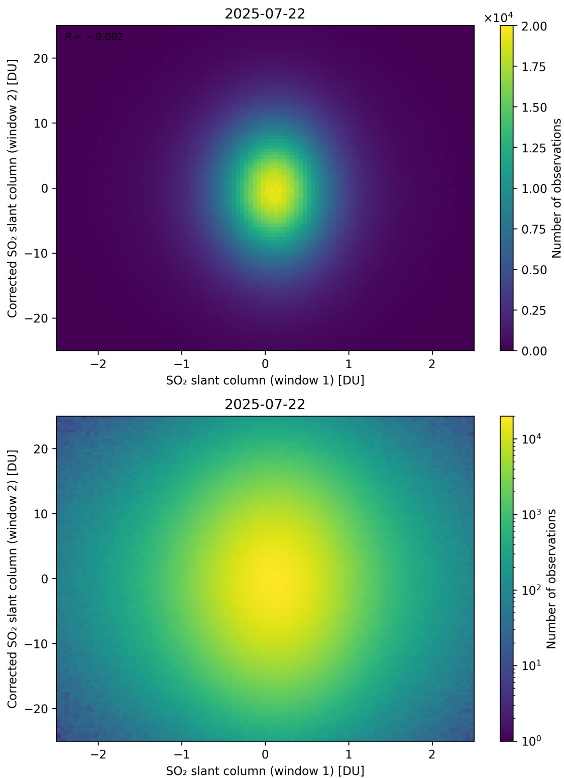
Figure 283: Scatter density plot of “SO 2 slant column (window 1)” against “Corrected SO 2 slant column (window 2)” for 2025-07-21 to 2025-07-23.
