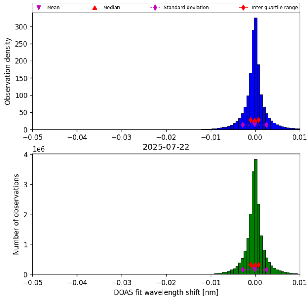
Figure 76: Histogram of “DOAS fit wavelength shift” for 2025-07-21 to 2025-07-23
