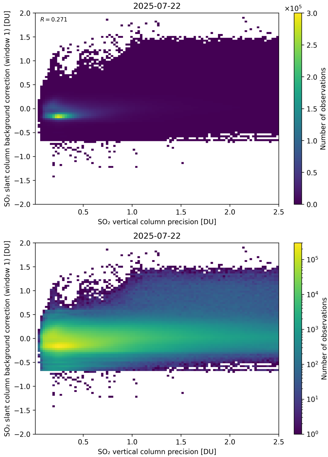
Figure 329: Scatter density plot of “SO 2 vertical column precision” against “SO 2 slant column background correction (window 1)” for 2025-07-21 to 2025-07-23.
