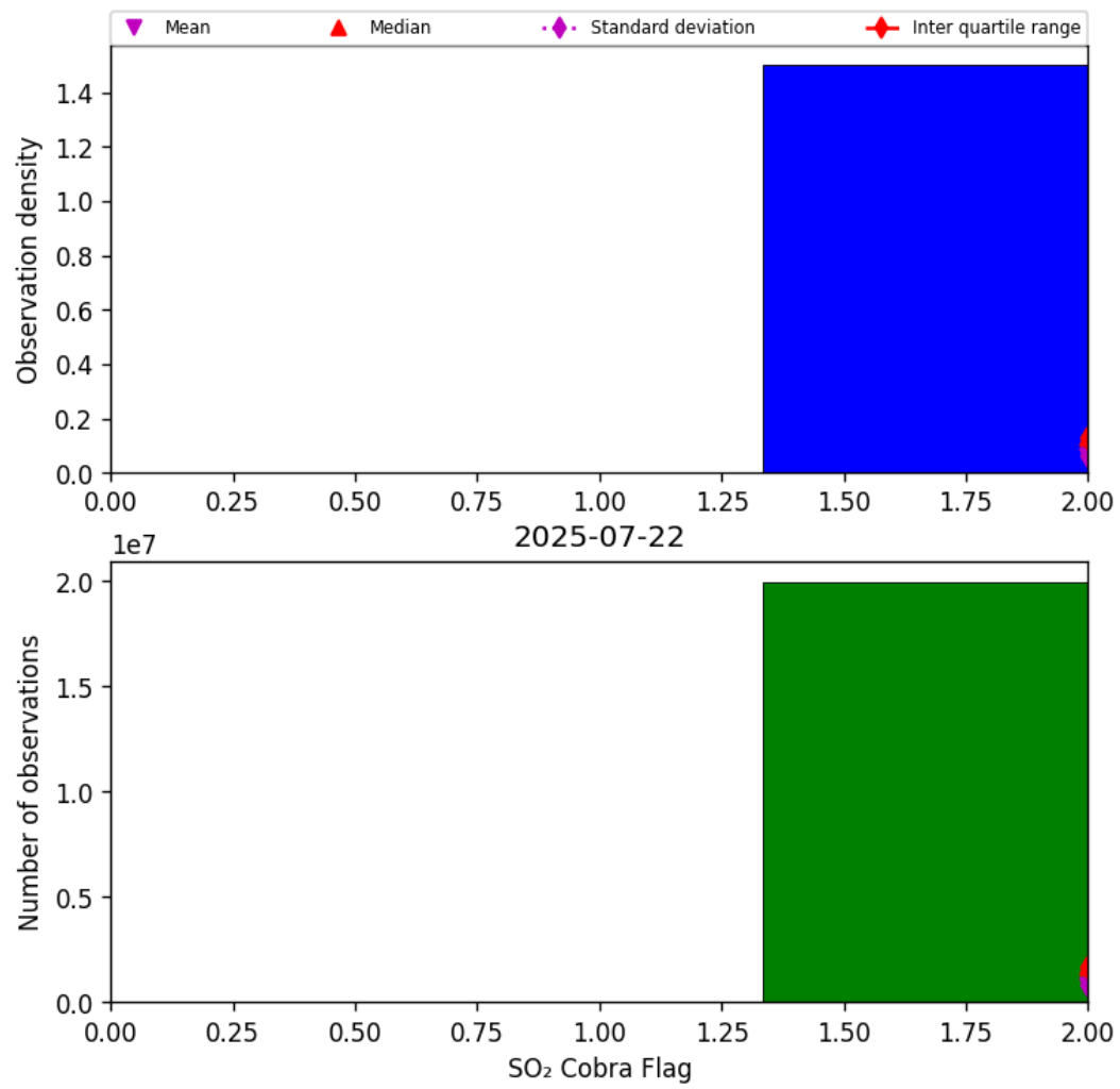
Figure 75: Histogram of “SO 2 Cobra Flag” for 2025-07-21 to 2025-07-23
