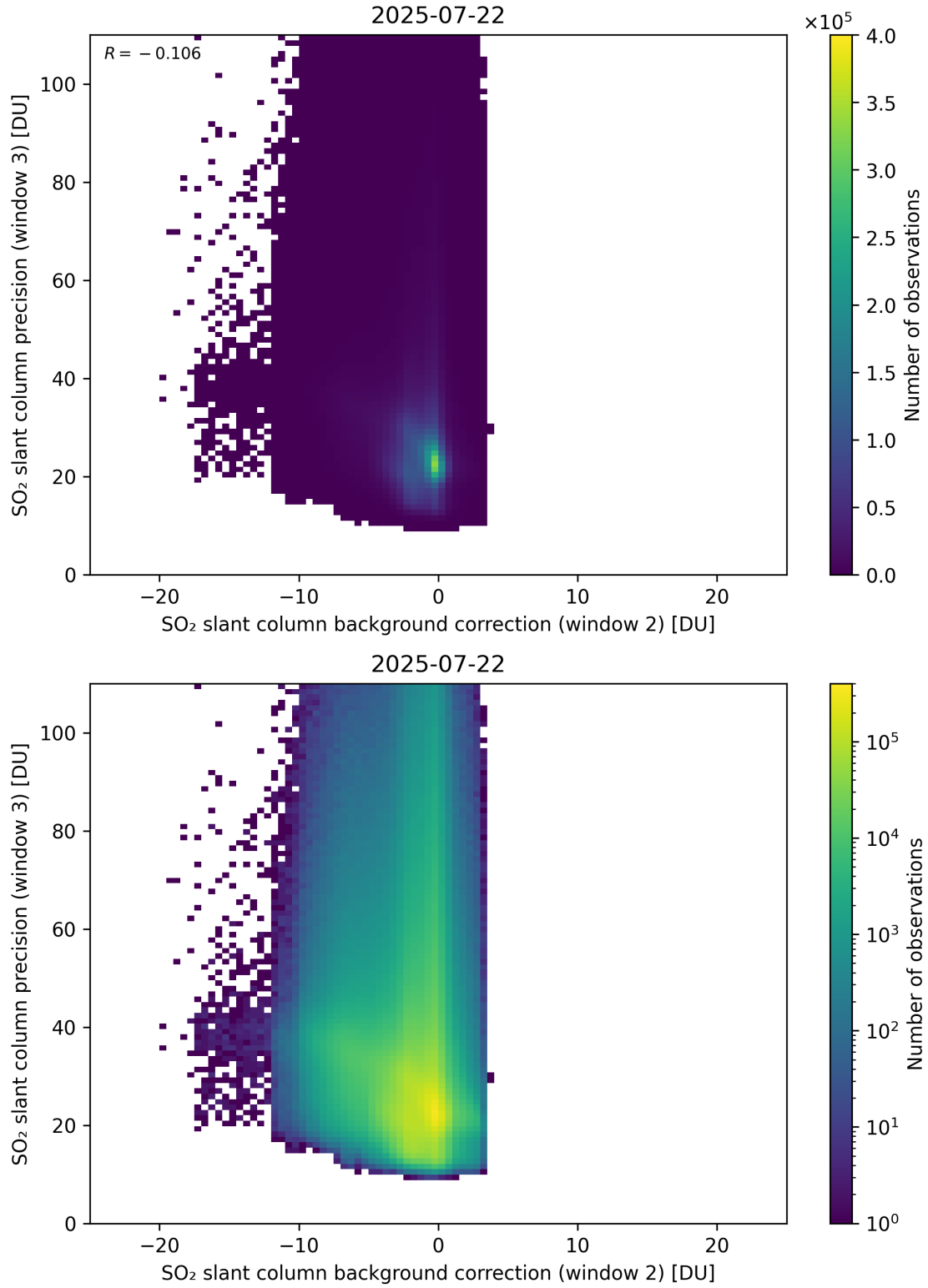
Figure 129: Scatter density plot of “SO 2 slant column background correction (window 2)” against “SO 2 slant column precision (window 3)” for 2025-07-21 to 2025-07-23.
