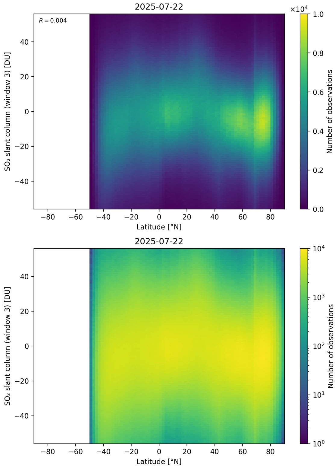
Figure 165: Scatter density plot of “Latitude” against “SO 2 slant column (window 3)” for 2025-07-21 to 2025-07-23.
