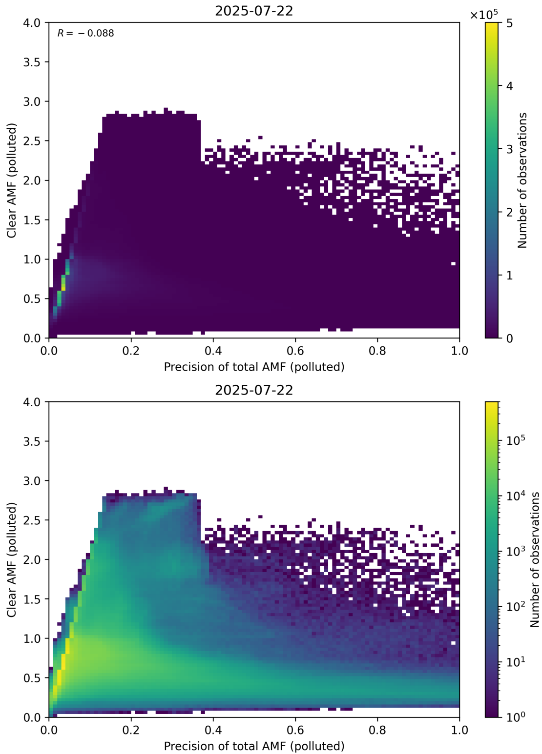
Figure 320: Scatter density plot of “Precision of total AMF (polluted)” against “Clear AMF (polluted)” for 2025-07-21 to 2025-07-23.
