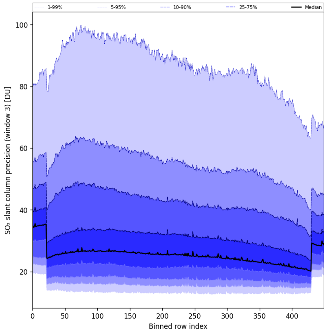
Figure 98: Along track statistics of “SO 2 slant column precision (window 3)” for 2025-07-21 to 2025-07-23
