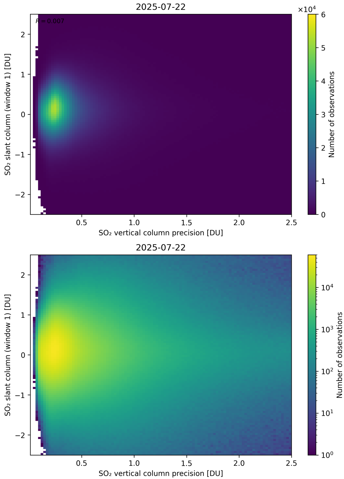
Figure 341: Scatter density plot of “SO 2 vertical column precision” against “SO 2 slant column (window 1)” for 2025-07-21 to 2025-07-23.
