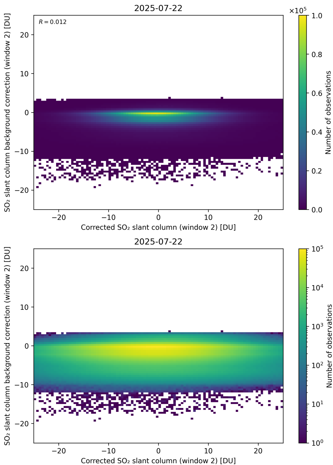
Figure 244: Scatter density plot of “Corrected SO 2 slant column (window 2)” against “SO 2 slant column background correction (window 2)” for 2025-07-21 to 2025-07-23.
