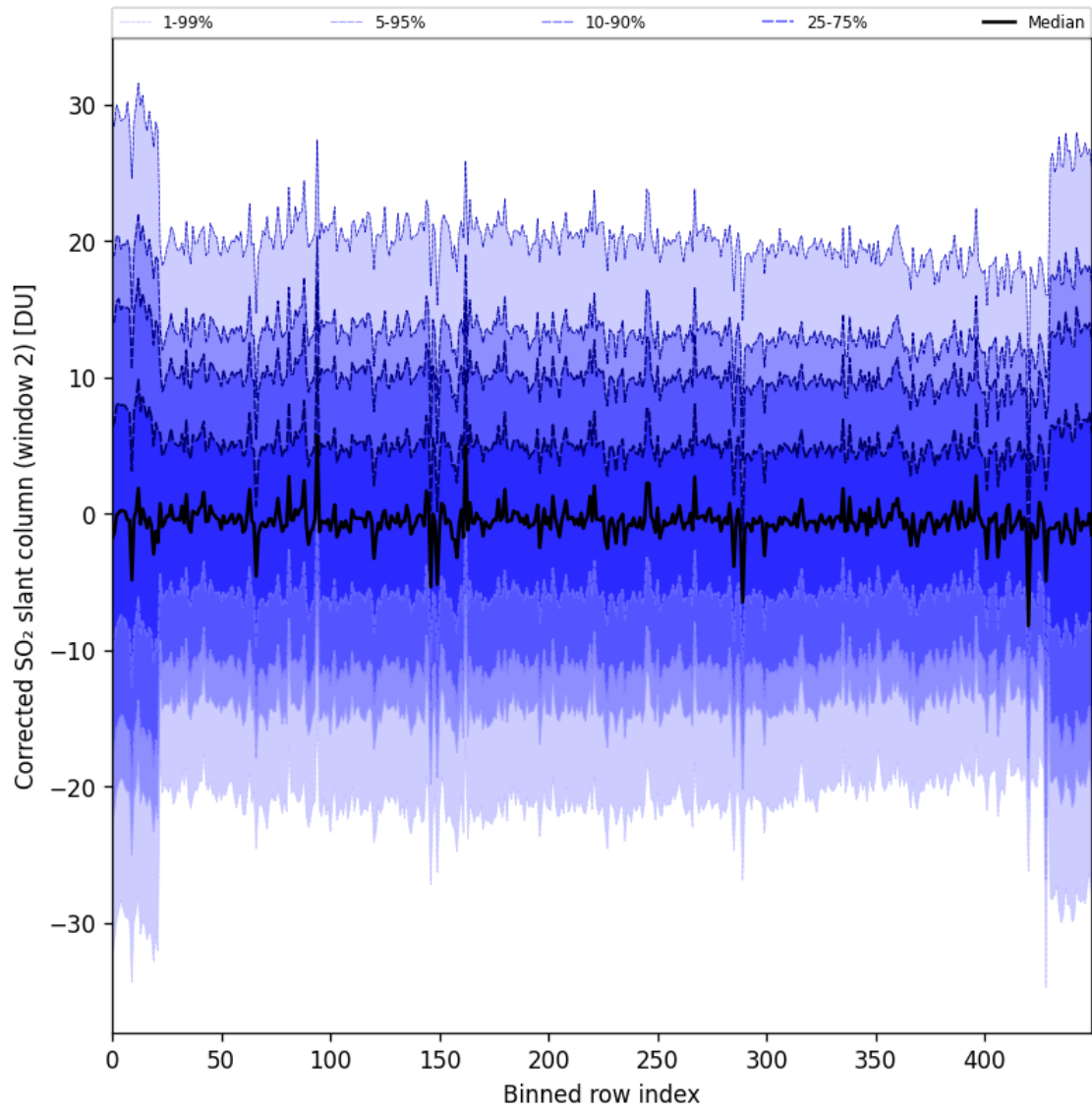
Figure 95: Along track statistics of “Corrected SO 2 slant column (window 2)” for 2025-07-21 to 2025-07-23
