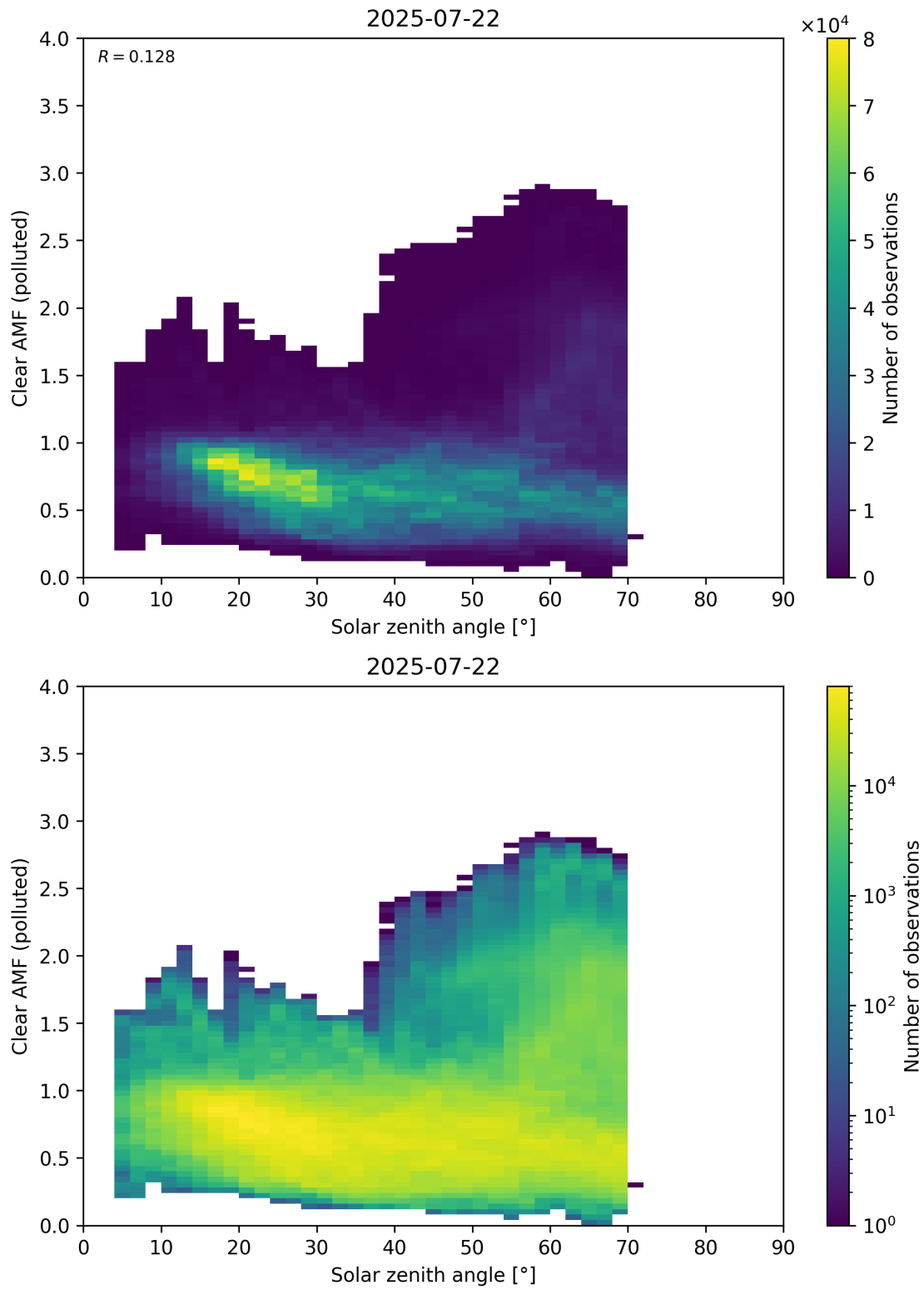
Figure 178: Scatter density plot of “Solar zenith angle” against “Clear AMF (polluted)” for 2025-07-21 to 2025-07-23.
