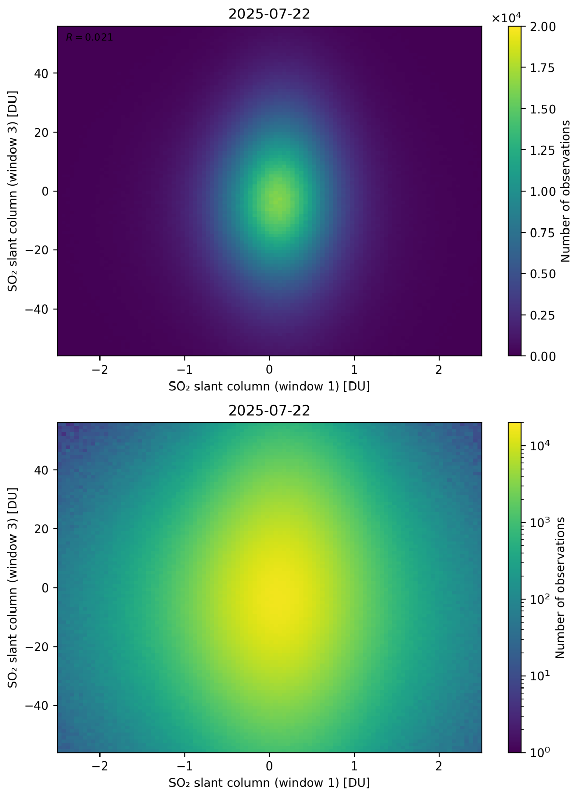
Figure 287: Scatter density plot of “SO 2 slant column (window 1)” against “SO 2 slant column (window 3)” for 2025-07-21 to 2025-07-23.
