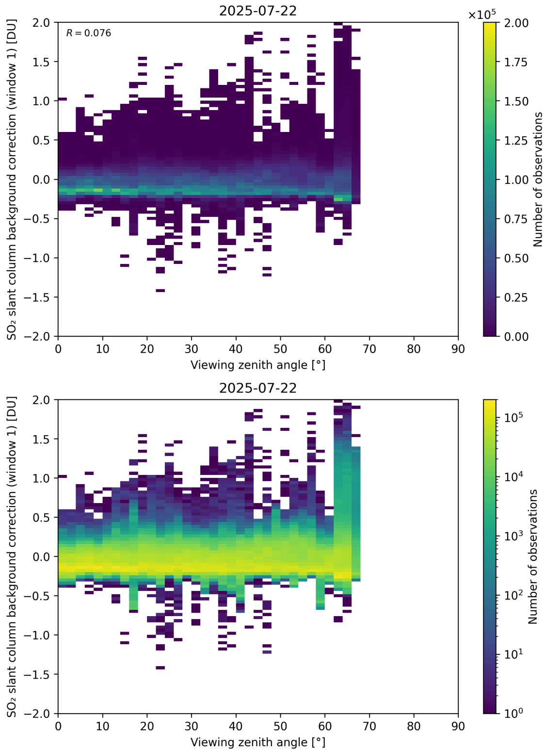
Figure 362: Scatter density plot of “Viewing zenith angle” against “SO 2 slant column background correction (window 1)” for 2025-07-21 to 2025-07-23.
