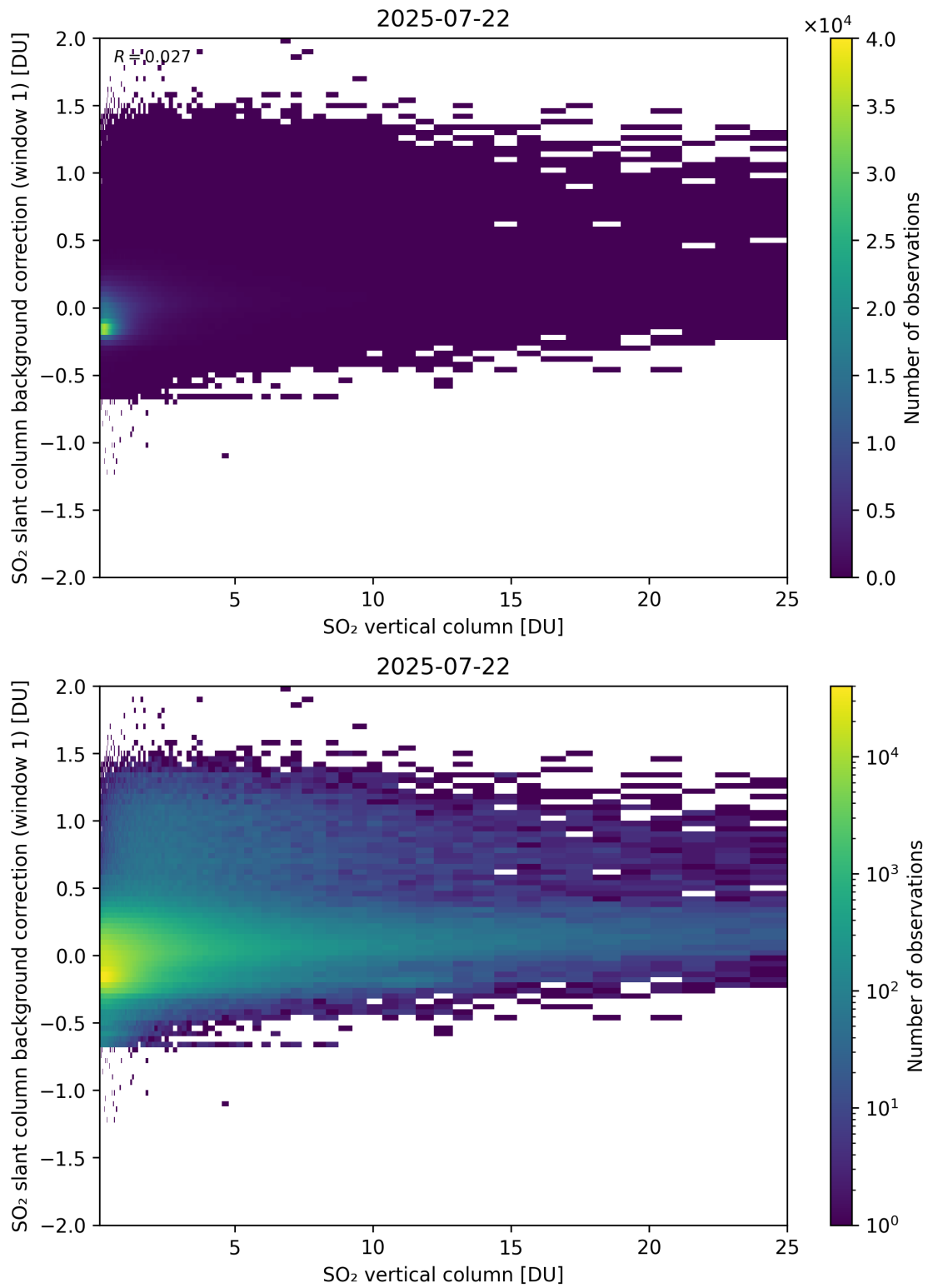
Figure 323: Scatter density plot of “SO 2 vertical column” against “SO 2 slant column background correction (window 1)” for 2025-07-21 to 2025-07-23.
