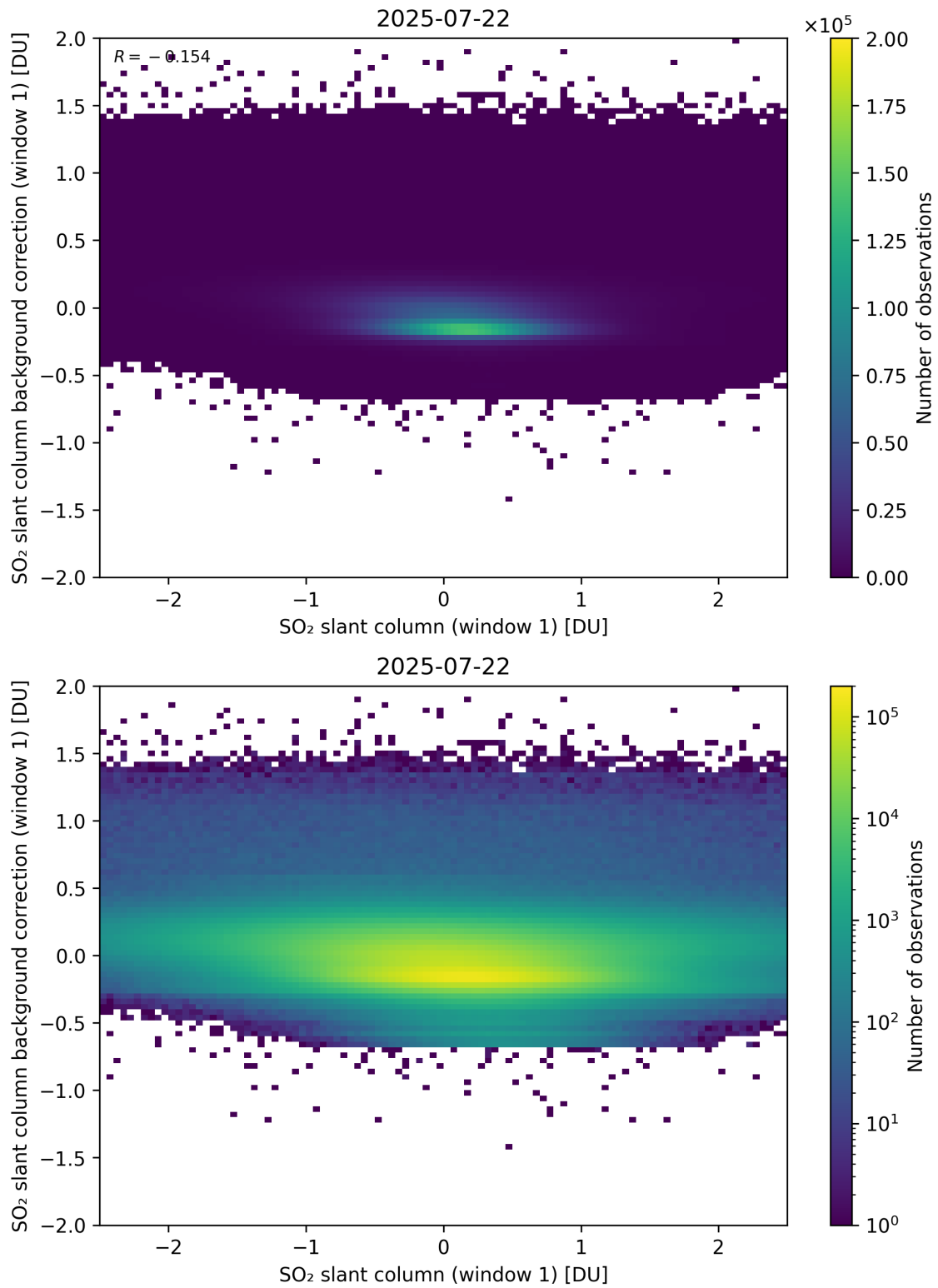
Figure 262: Scatter density plot of “SO 2 slant column (window 1)” against “SO 2 slant column background correction (window 1)” for 2025-07-21 to 2025-07-23.
