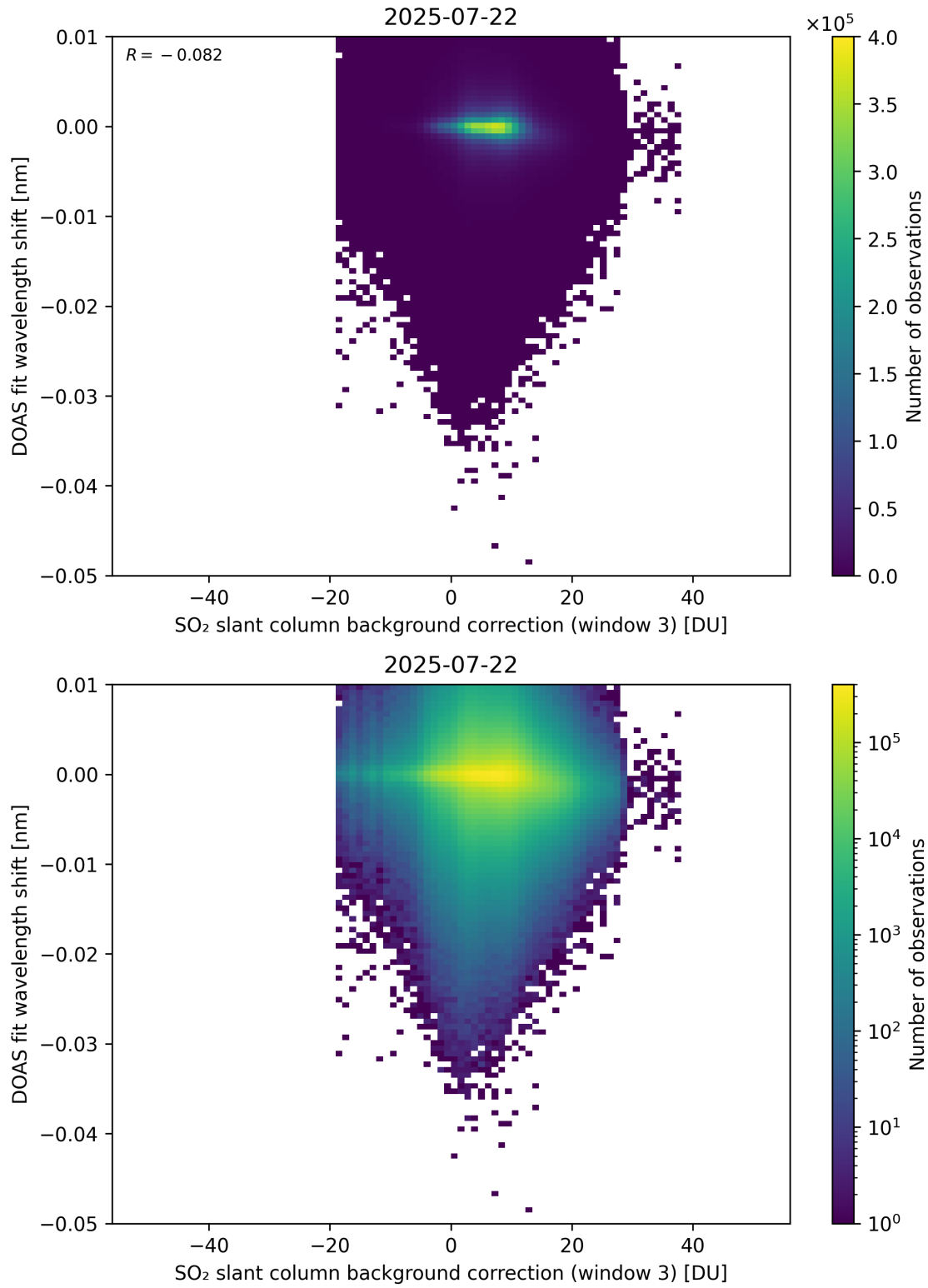
Figure 132: Scatter density plot of “SO 2 slant column background correction (window 3)” against “DOAS fit wavelength shift” for 2025-07-21 to 2025-07-23.
