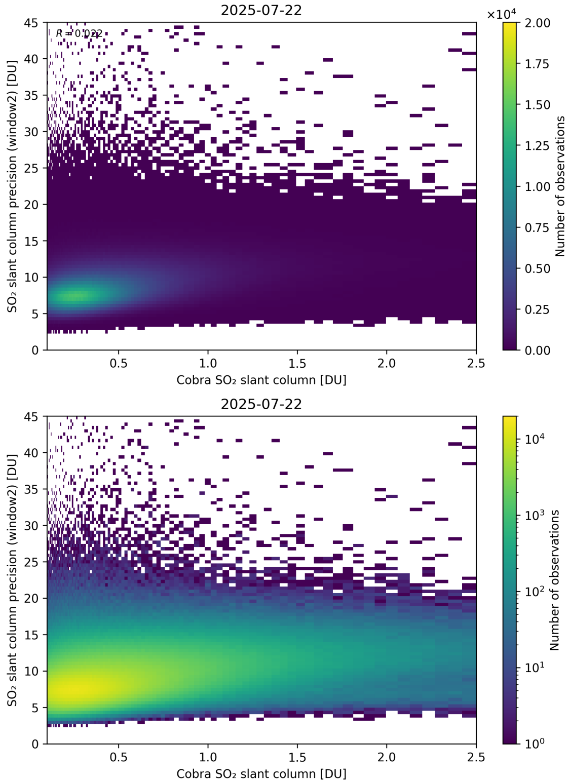
Figure 221: Scatter density plot of “Cobra SO 2 slant column” against “SO 2 slant column precision (window2)” for 2025-07-21 to 2025-07-23.
