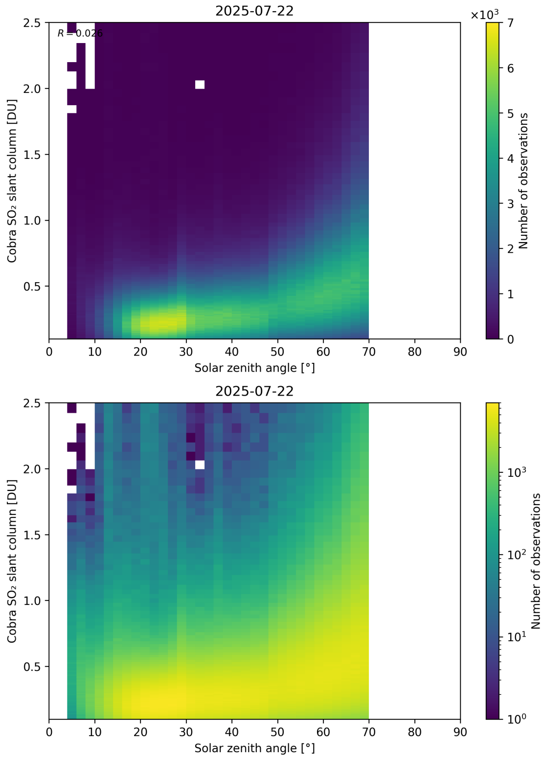
Figure 179: Scatter density plot of “Solar zenith angle” against “Cobra SO 2 slant column” for 2025-07-21 to 2025-07-23.
