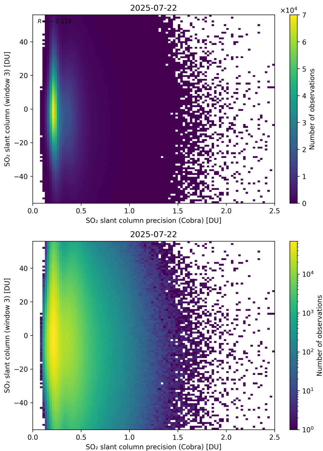
Figure 211: Scatter density plot of “SO 2 slant column precision (Cobra)” against “SO 2 slant column (window 3)” for 2025-07-21 to 2025-07-23.
