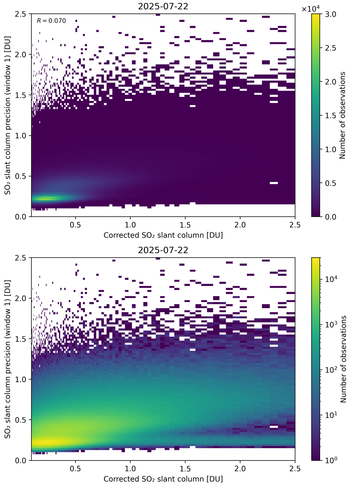
Figure 238: Scatter density plot of “Corrected SO 2 slant column” against “SO 2 slant column precision (window 1)” for 2025-07-21 to 2025-07-23.
