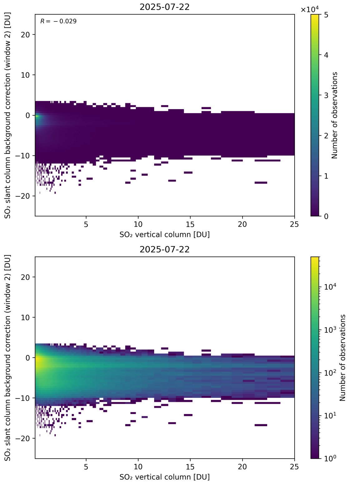
Figure 324: Scatter density plot of “SO 2 vertical column” against “SO 2 slant column background correction (window 2)” for 2025-07-21 to 2025-07-23.
