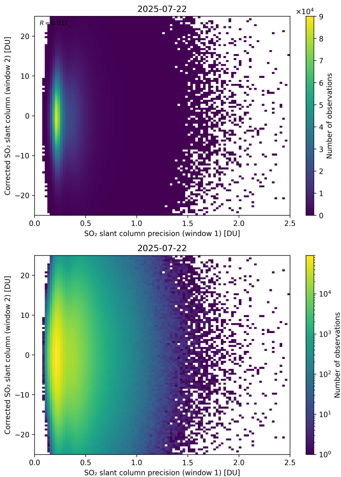
Figure 275: Scatter density plot of “SO 2 slant column precision (window 1)” against “Corrected SO 2 slant column (window 2)” for 2025-07-21 to 2025-07-23.
