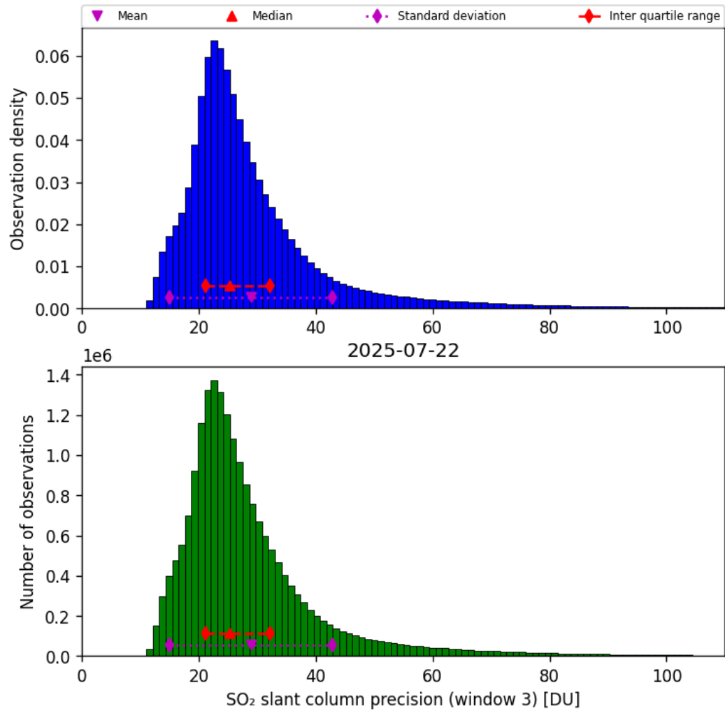
Figure 72: Histogram of “SO 2 slant column precision (window 3)” for 2025-07-21 to 2025-07-23
