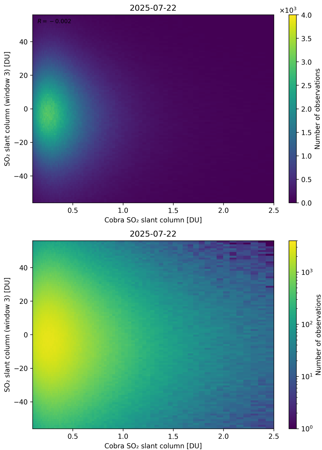
Figure 222: Scatter density plot of “Cobra SO 2 slant column” against “SO 2 slant column (window 3)” for 2025-07-21 to 2025-07-23.
