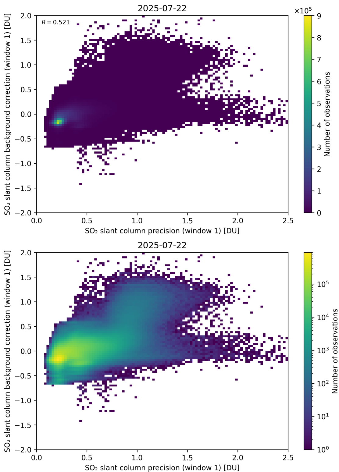
Figure 268: Scatter density plot of “SO 2 slant column precision (window 1)” against “SO 2 slant column background correction (window 1)” for 2025-07-21 to 2025-07-23.
