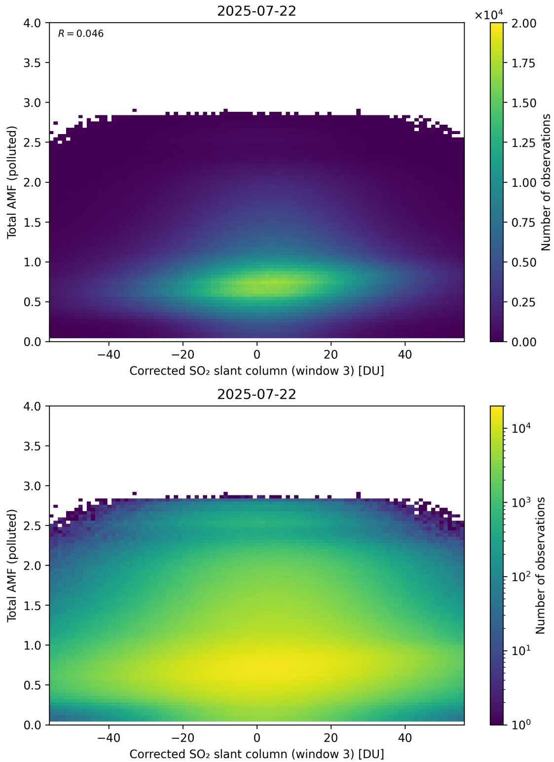
Figure 260: Scatter density plot of “Corrected SO 2 slant column (window 3)” against “Total AMF (polluted)” for 2025-07-21 to 2025-07-23.
