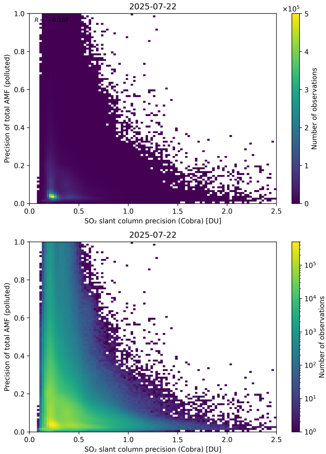
Figure 214: Scatter density plot of “SO 2 slant column precision (Cobra)” against “Precision of total AMF (polluted)” for 2025-07-21 to 2025-07-23.
