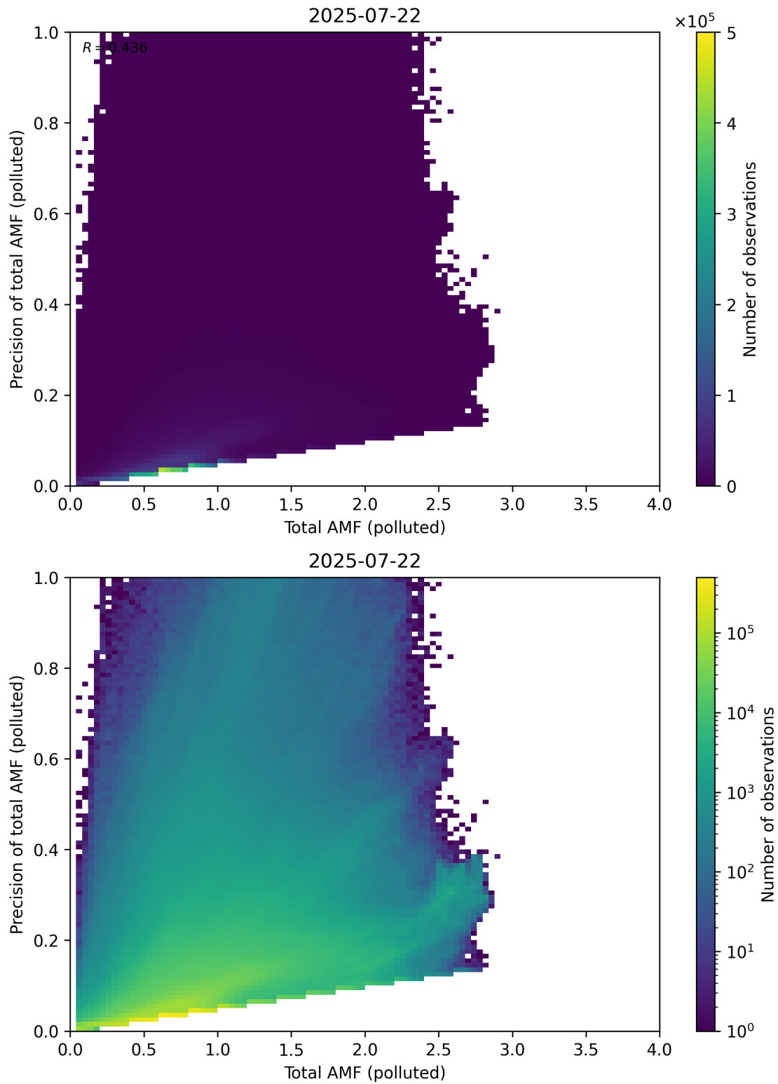
Figure 322: Scatter density plot of “Total AMF (polluted)” against “Precision of total AMF (polluted)” for 2025-07-21 to 2025-07-23.
