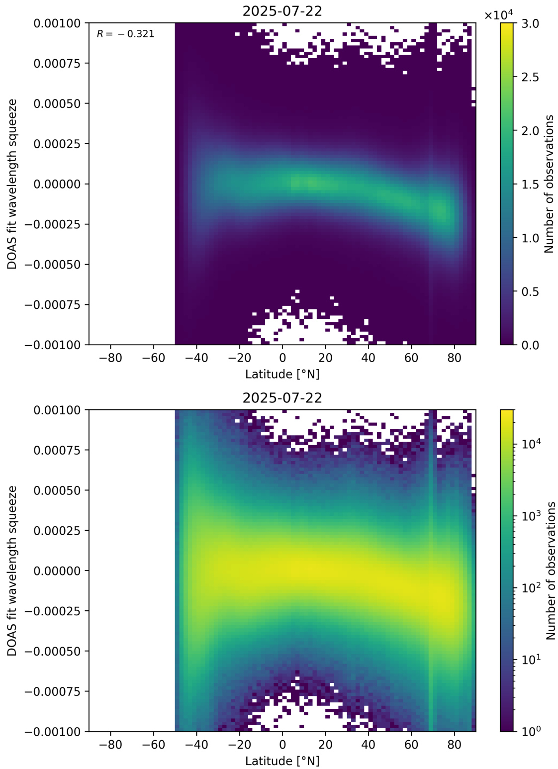
Figure 154: Scatter density plot of “Latitude” against “DOAS fit wavelength squeeze” for 2025-07-21 to 2025-07-23.
