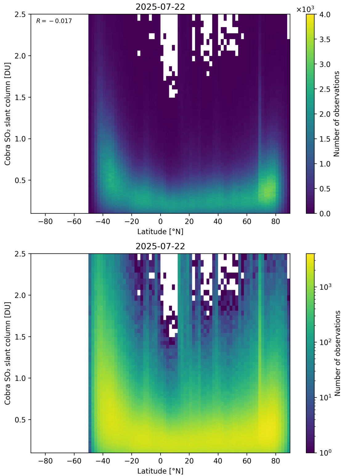
Figure 157: Scatter density plot of “Latitude” against “Cobra SO 2 slant column” for 2025-07-21 to 2025-07-23.
