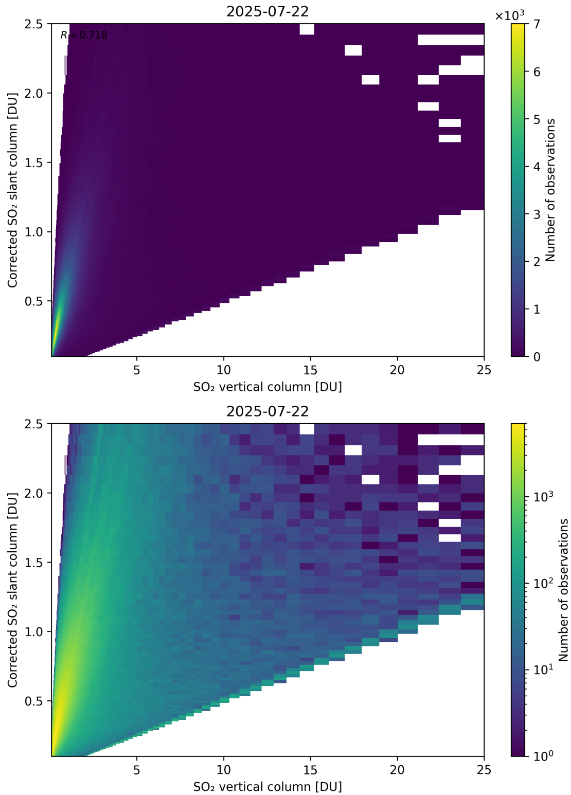
Figure 351: Scatter density plot of “SO 2 vertical column” against “Corrected SO 2 slant column” for 2025-07-21 to 2025-07-23.
