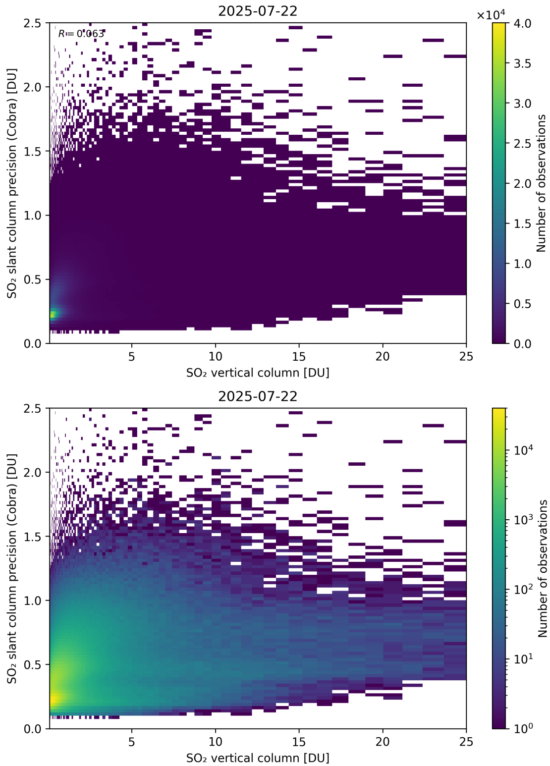
Figure 350: Scatter density plot of “SO 2 vertical column” against “SO 2 slant column precision (Cobra)” for 2025-07-21 to 2025-07-23.
