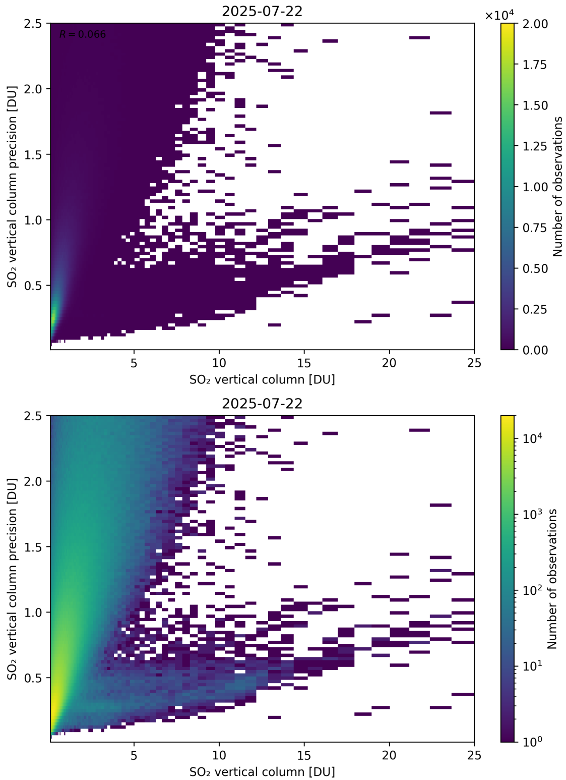
Figure 361: Scatter density plot of “SO 2 vertical column” against “SO 2 vertical column precision” for 2025-07-21 to 2025-07-23.
