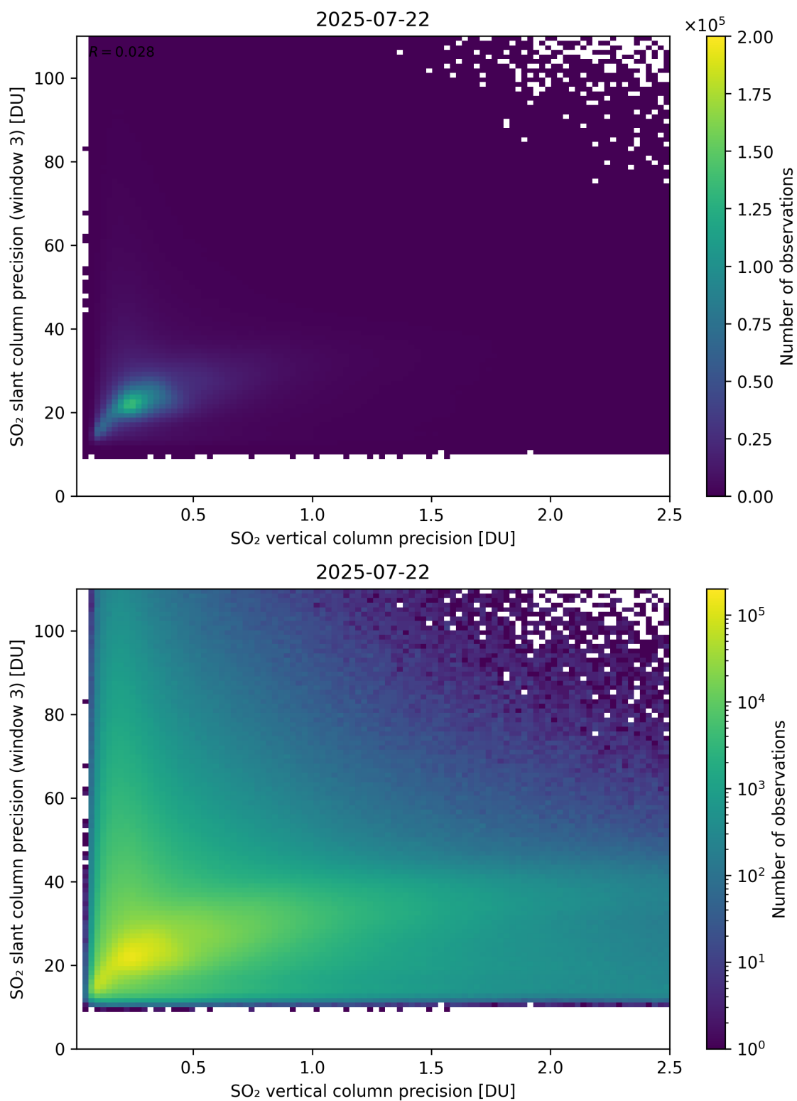
Figure 345: Scatter density plot of “SO 2 vertical column precision” against “SO 2 slant column precision (window 3)” for 2025-07-21 to 2025-07-23.
