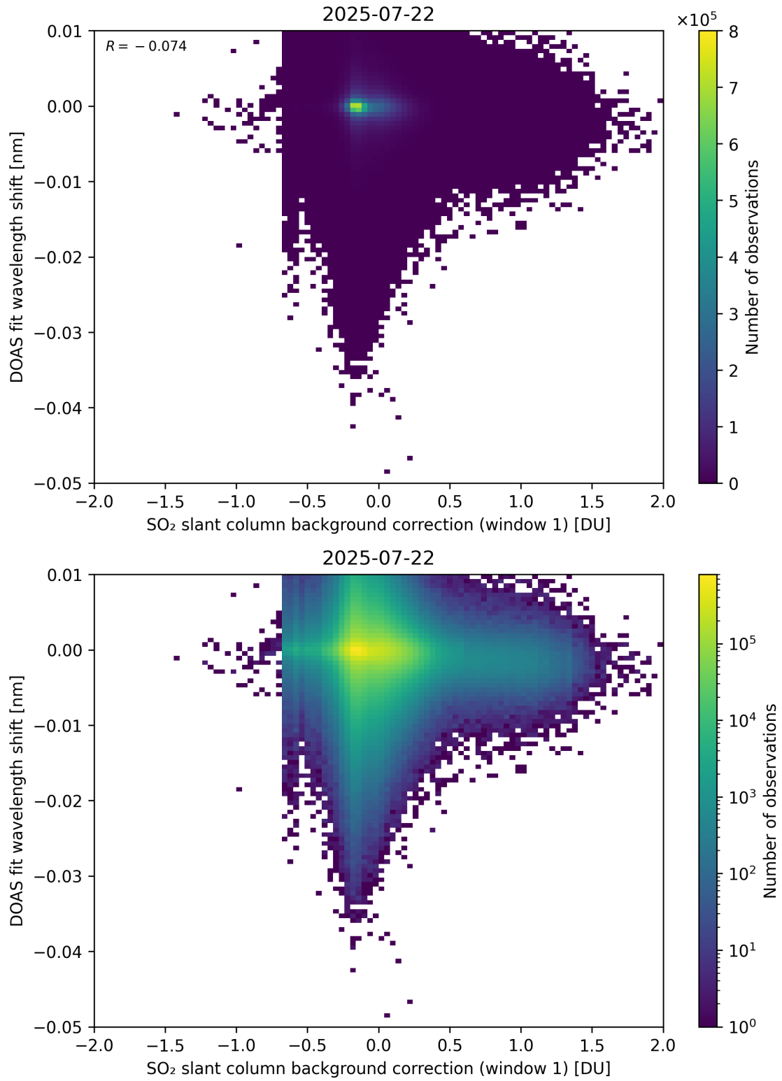
Figure 111: Scatter density plot of “SO 2 slant column background correction (window 1)” against “DOAS fit wavelength shift” for 2025-07-21 to 2025-07-23.
