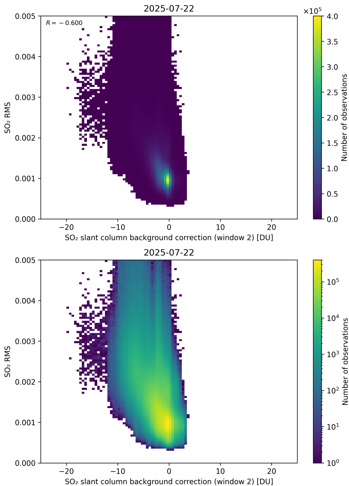
Figure 125: Scatter density plot of “SO 2 slant column background correction (window 2)” against “SO 2 RMS” for 2025-07-21 to 2025-07-23.
