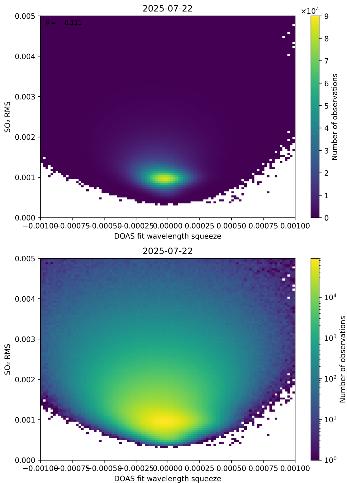
Figure 143: Scatter density plot of “DOAS fit wavelength squeeze” against “SO 2 RMS” for 2025-07-21 to 2025-07-23.
