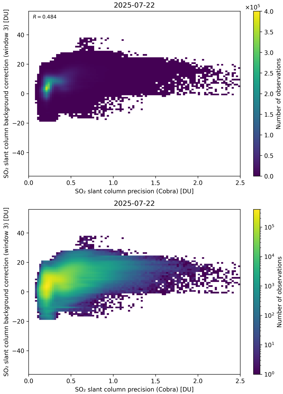
Figure 201: Scatter density plot of “SO 2 slant column precision (Cobra)” against “SO 2 slant column background correction (window 3)” for 2025-07-21 to 2025-07-23.
