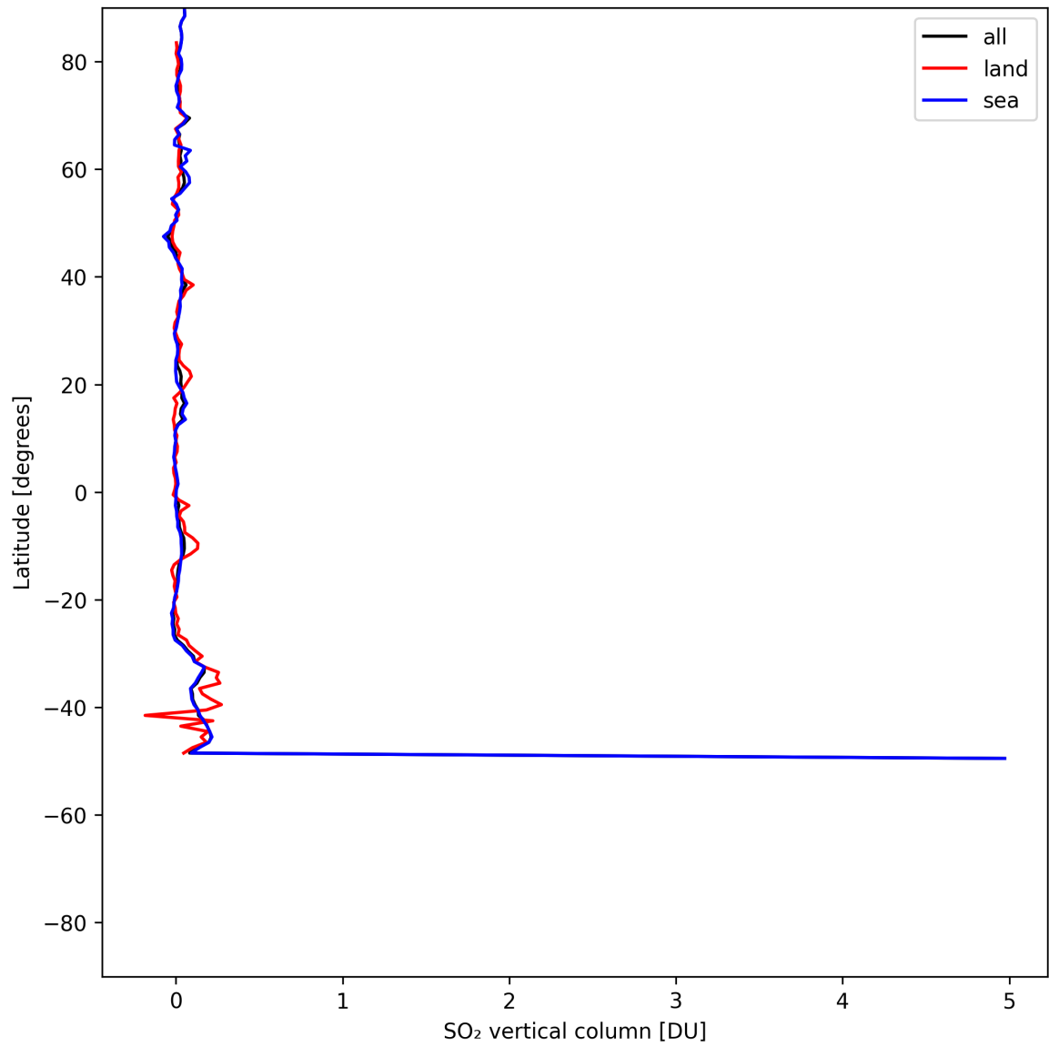
Figure 32: Zonal average of “SO 2 vertical column” for 2025-07-21 to 2025-07-23.
