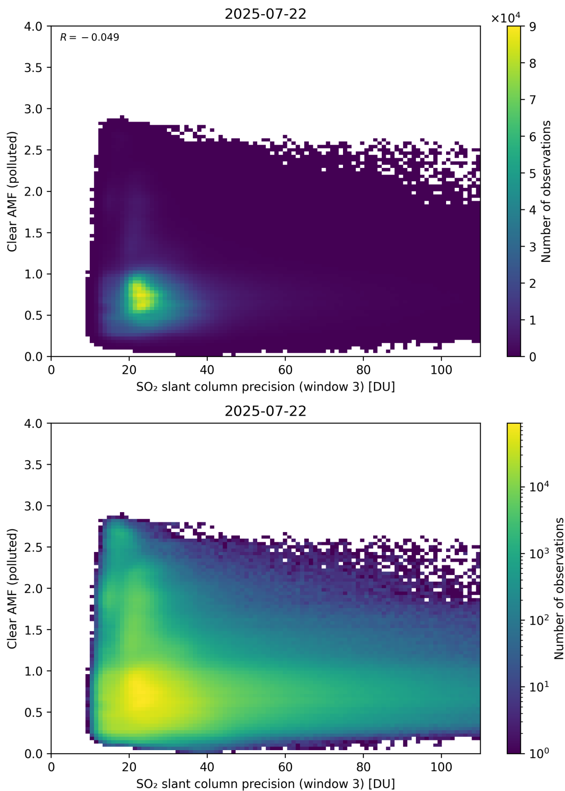
Figure 311: Scatter density plot of “SO 2 slant column precision (window 3)” against “Clear AMF (polluted)” for 2025-07-21 to 2025-07-23.
