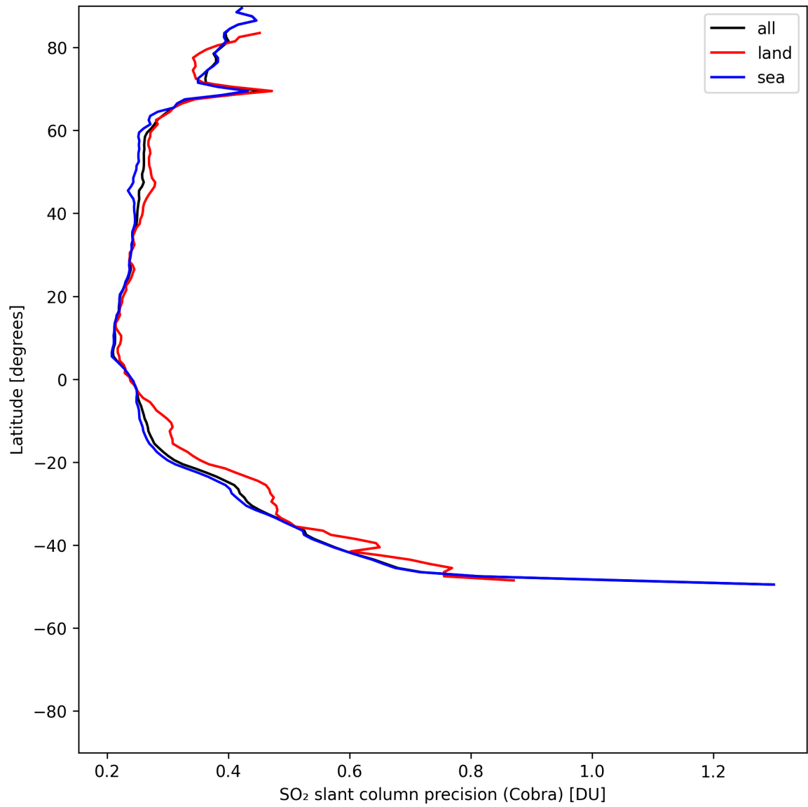
Figure 36: Zonal average of “SO 2 slant column precision (Cobra)” for 2025-07-21 to 2025-07-23.
