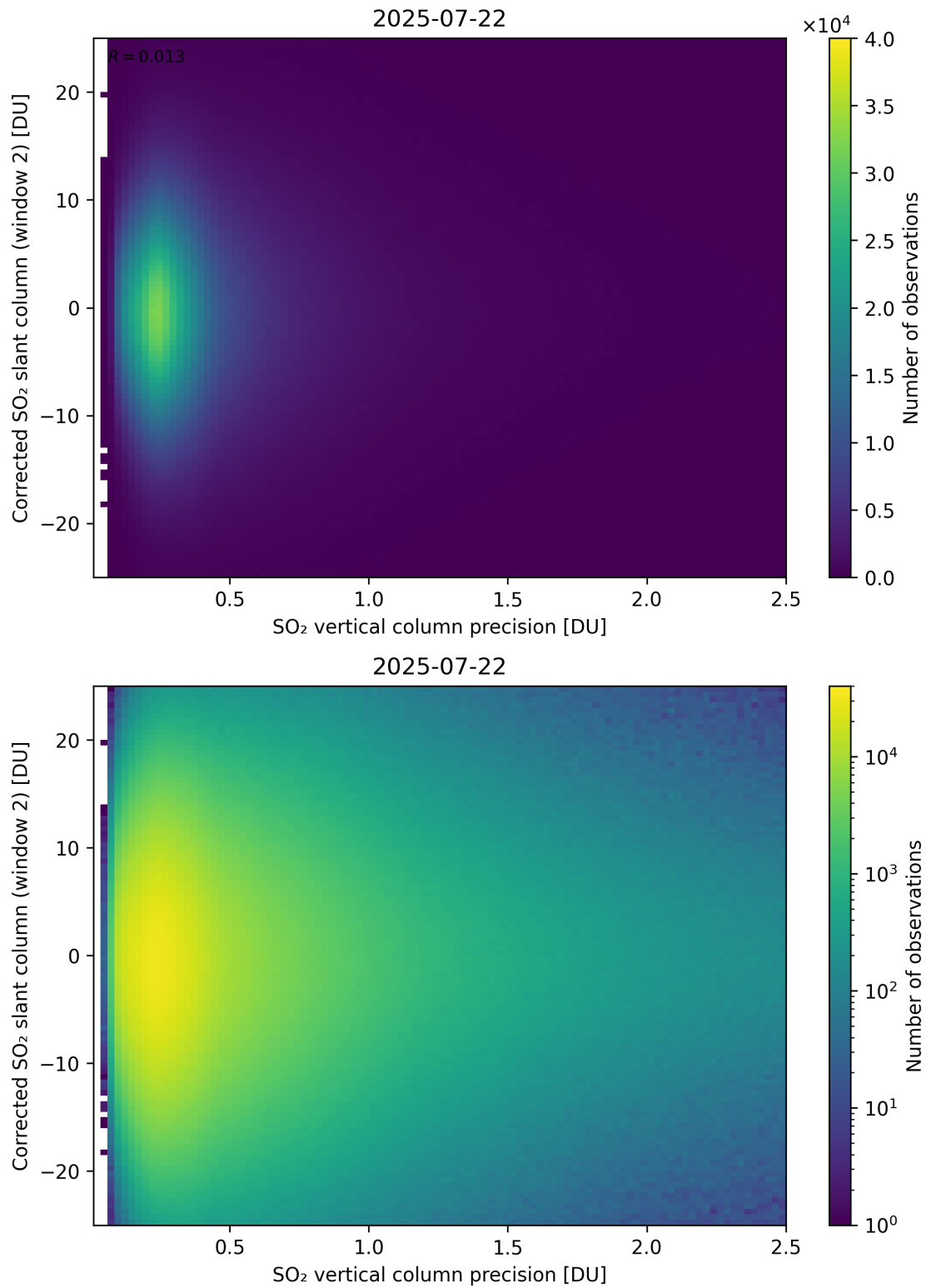
Figure 339: Scatter density plot of “SO 2 vertical column precision” against “Corrected SO 2 slant column (window 2)” for 2025-07-21 to 2025-07-23.
