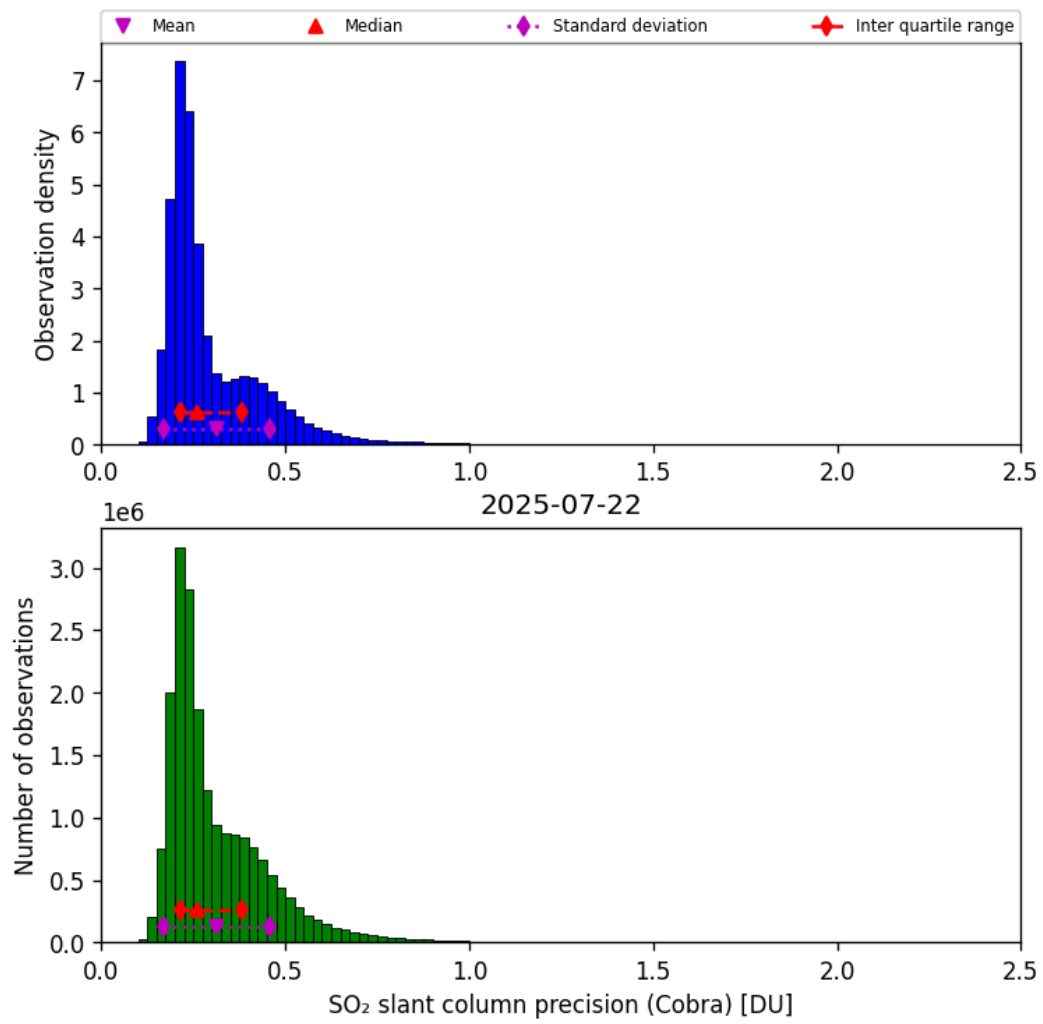
Figure 62: Histogram of “SO 2 slant column precision (Cobra)” for 2025-07-21 to 2025-07-23
