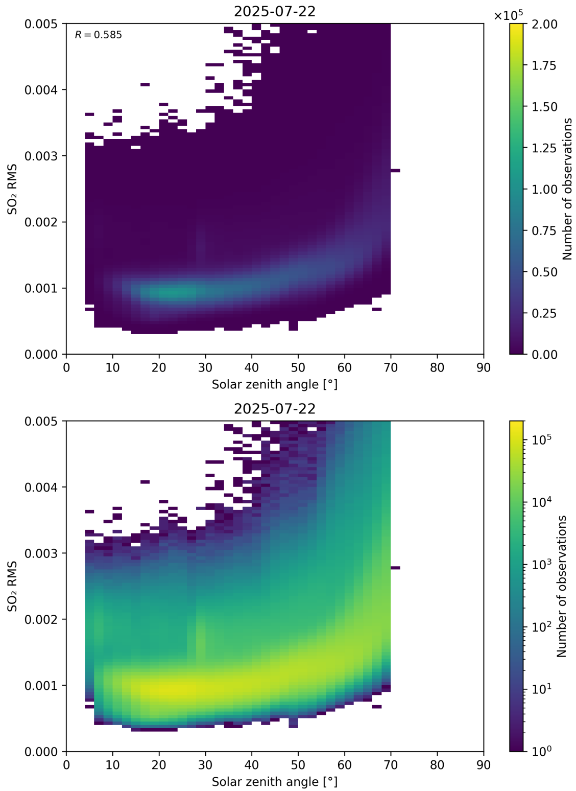
Figure 176: Scatter density plot of “Solar zenith angle” against “SO 2 RMS” for 2025-07-21 to 2025-07-23.
