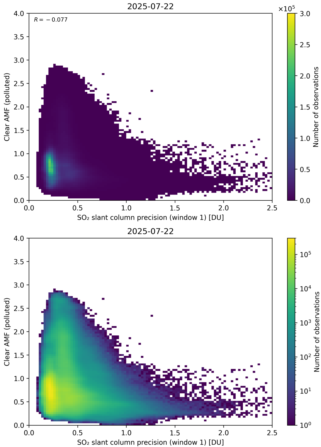
Figure 274: Scatter density plot of “SO 2 slant column precision (window 1)” against “Clear AMF (polluted)” for 2025-07-21 to 2025-07-23.
