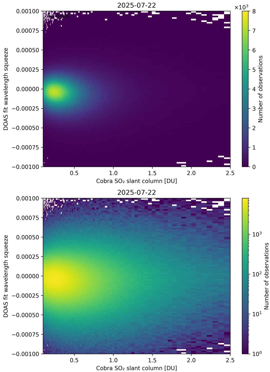
Figure 197: Scatter density plot of “Cobra SO 2 slant column” against “DOAS fit wavelength squeeze” for 2025-07-21 to 2025-07-23.
