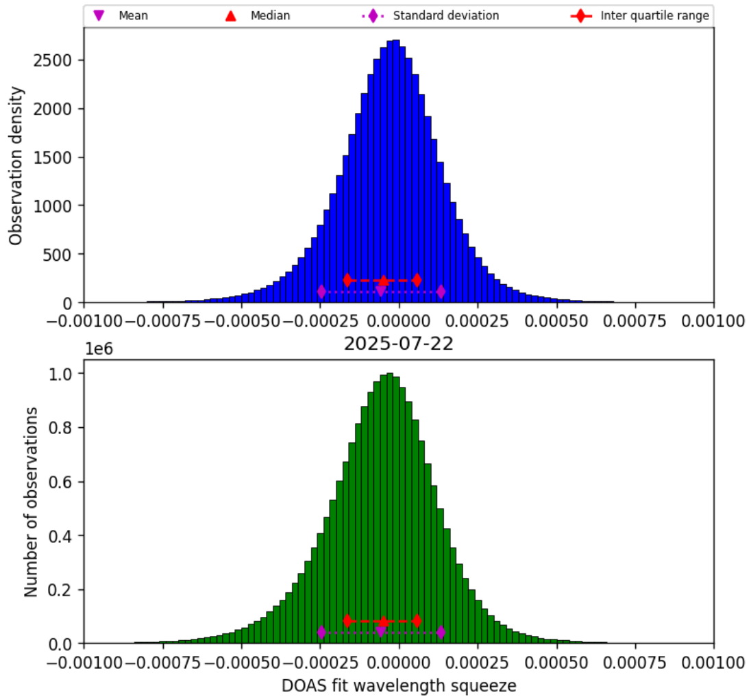
Figure 77: Histogram of “DOAS fit wavelength squeeze” for 2025-07-21 to 2025-07-23
