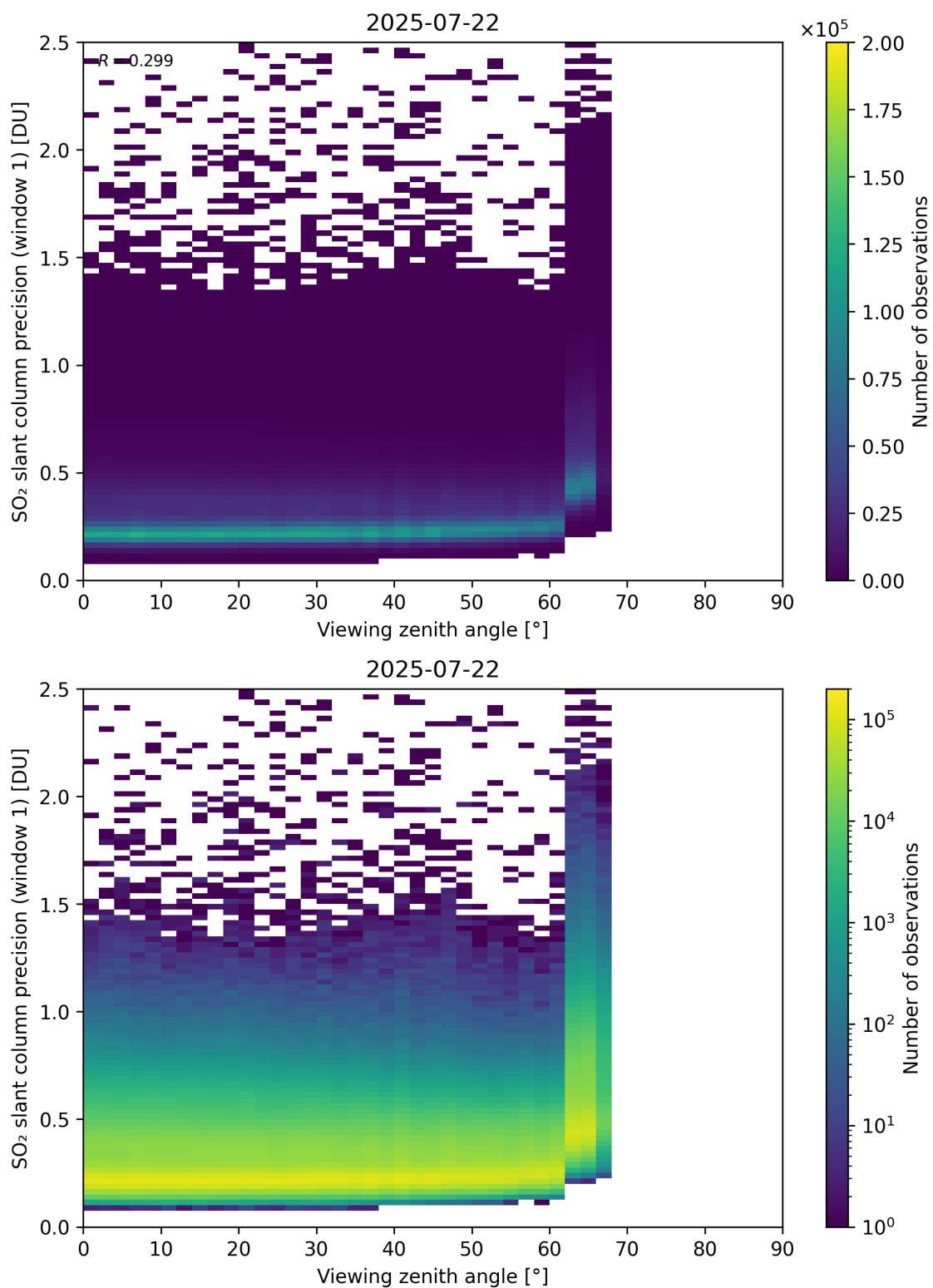
Figure 377: Scatter density plot of “Viewing zenith angle” against “SO 2 slant column precision (window 1)” for 2025-07-21 to 2025-07-23.
