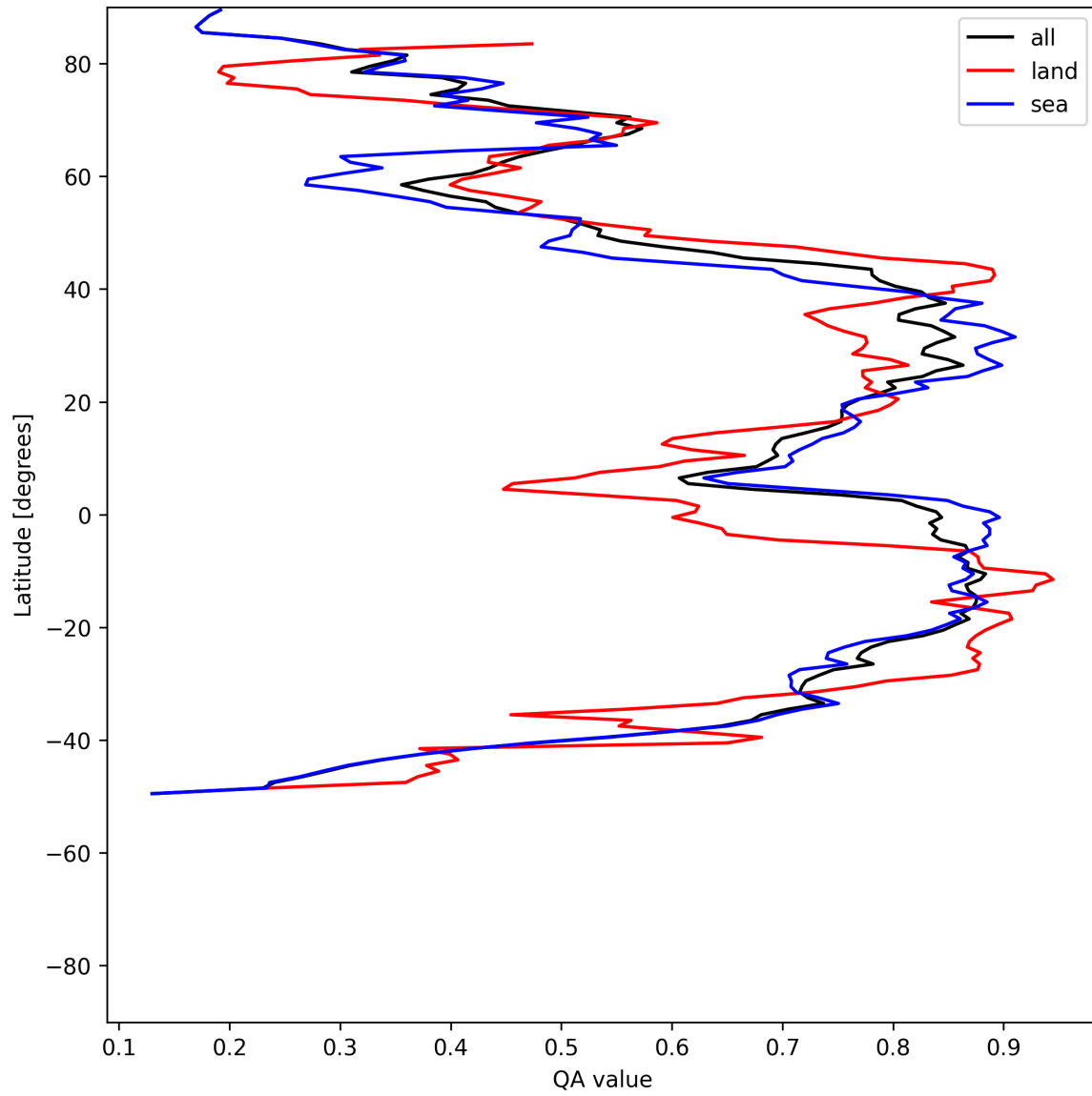
Figure 31: Zonal average of “QA value” for 2025-07-21 to 2025-07-23.
