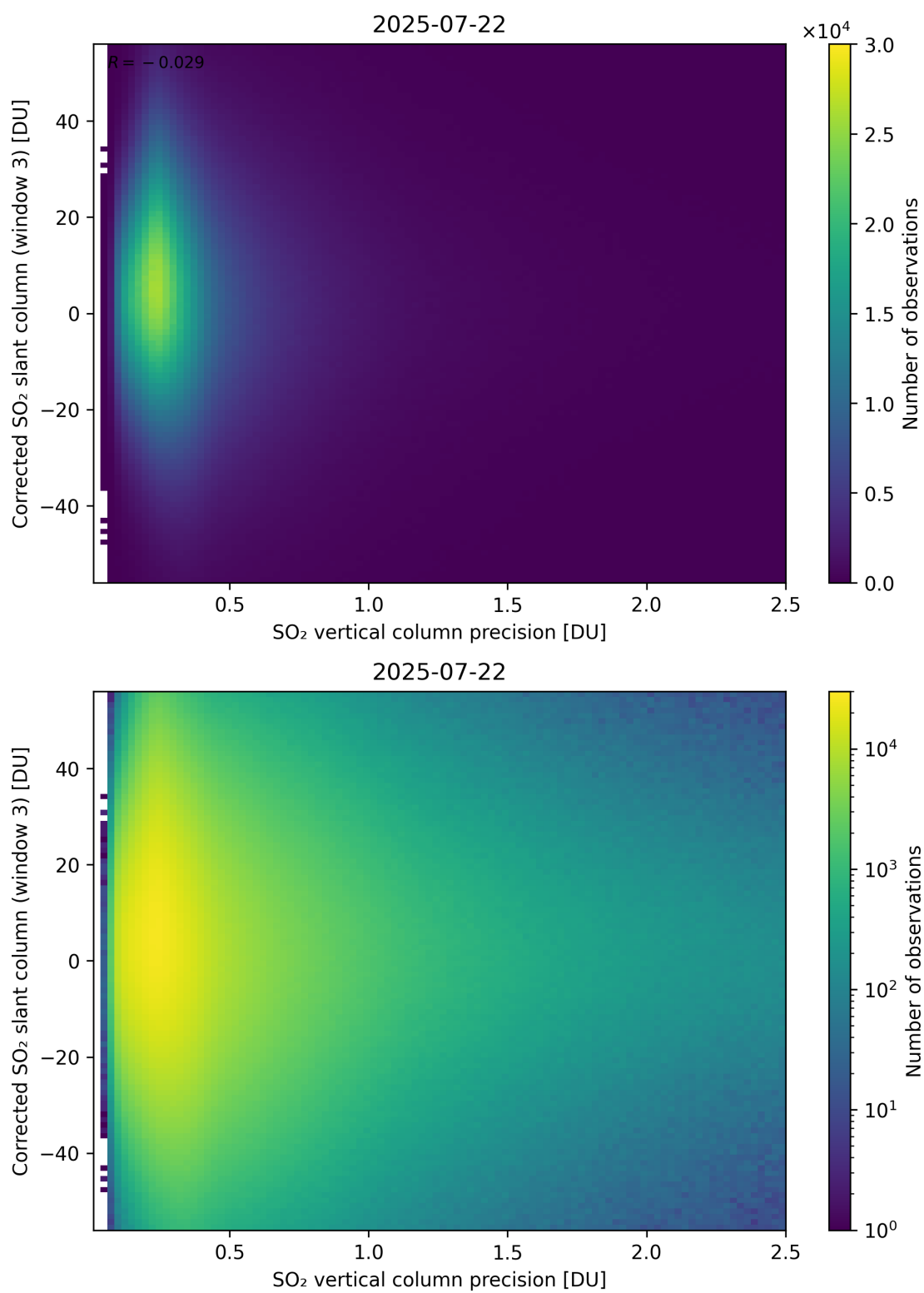
Figure 340: Scatter density plot of “SO 2 vertical column precision” against “Corrected SO 2 slant column (window 3)” for 2025-07-21 to 2025-07-23.
