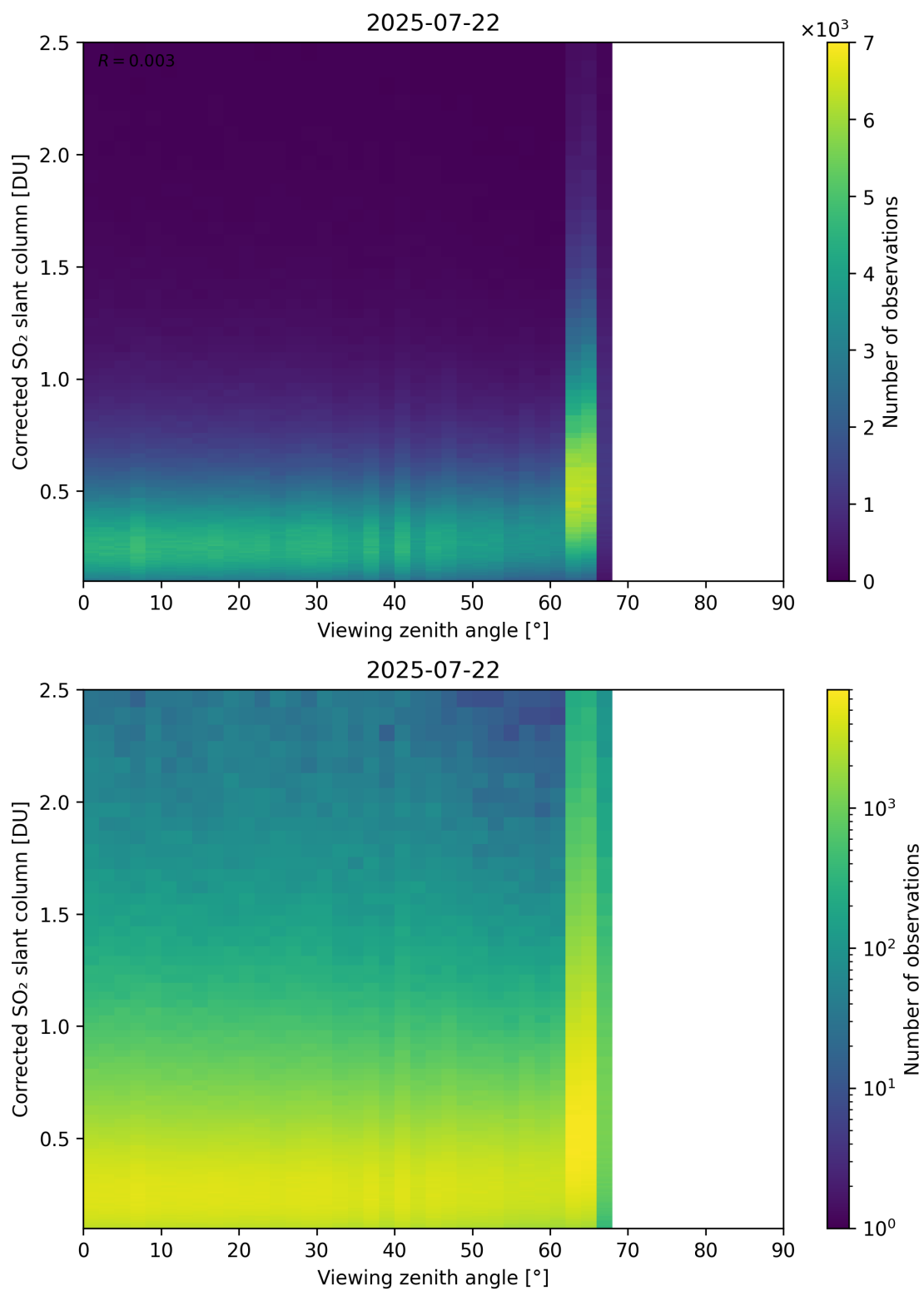
Figure 373: Scatter density plot of “Viewing zenith angle” against “Corrected SO 2 slant column” for 2025-07-21 to 2025-07-23.
