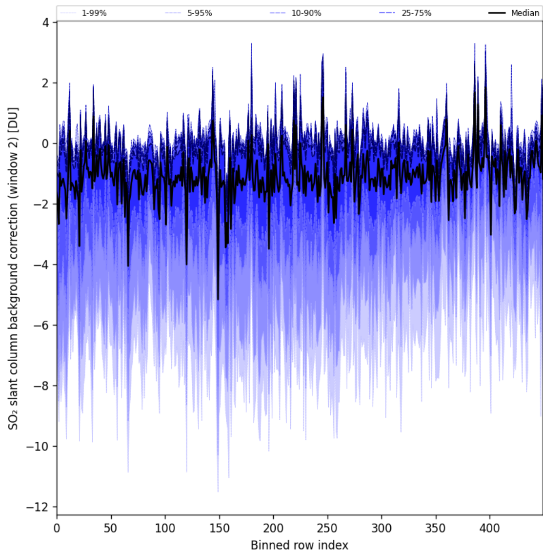
Figure 96: Along track statistics of “SO 2 slant column background correction (window 2)” for 2025-07-21 to 2025-07-23
