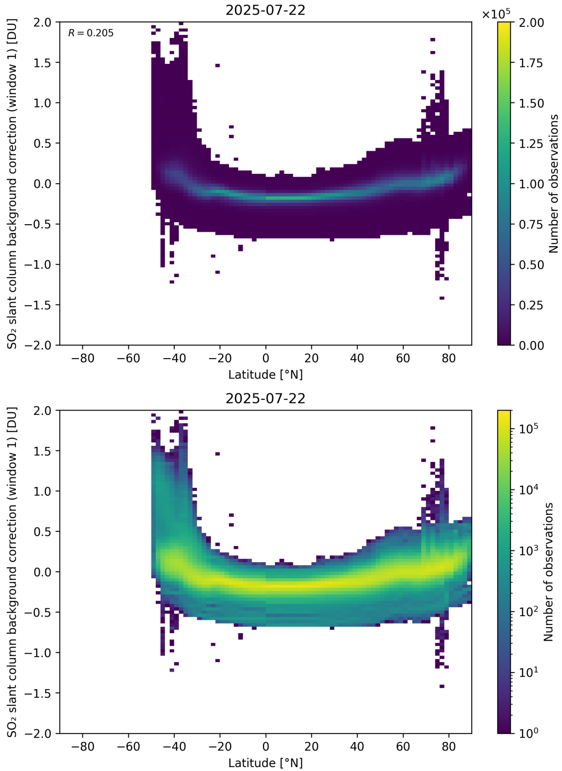
Figure 150: Scatter density plot of “Latitude” against “SO 2 slant column background correction (window 1)” for 2025-07-21 to 2025-07-23.
