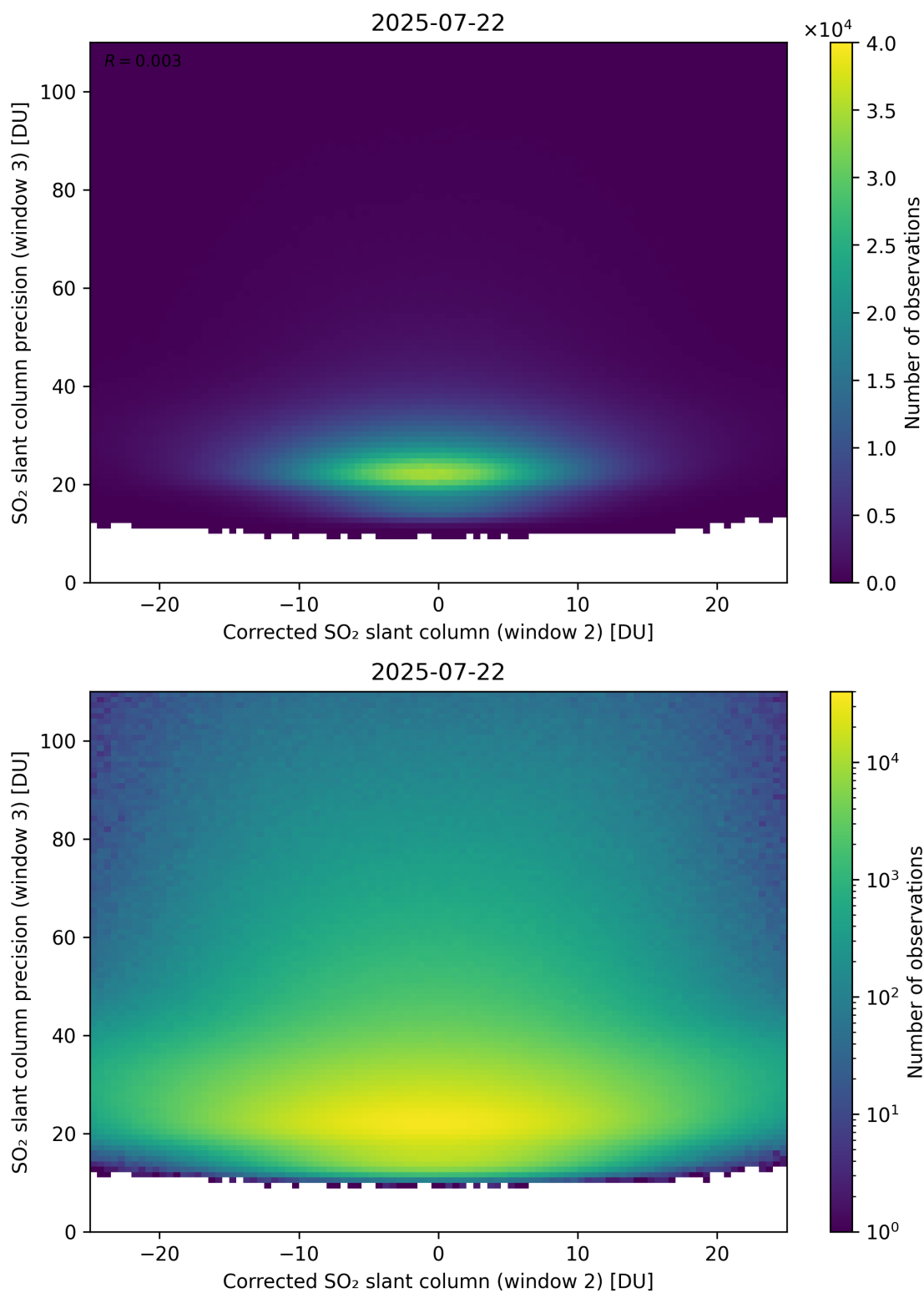
Figure 252: Scatter density plot of “Corrected SO 2 slant column (window 2)” against “SO 2 slant column precision (window 3)” for 2025-07-21 to 2025-07-23.
