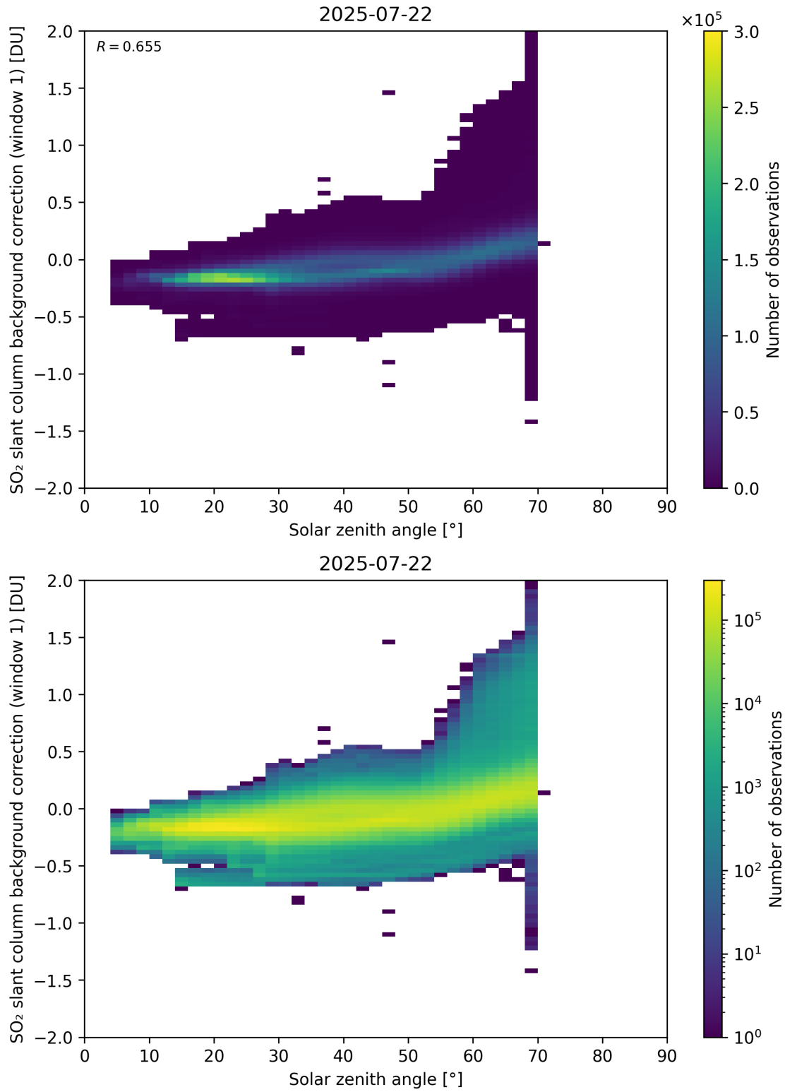
Figure 171: Scatter density plot of “Solar zenith angle” against “SO 2 slant column background correction (window 1)” for 2025-07-21 to 2025-07-23.
