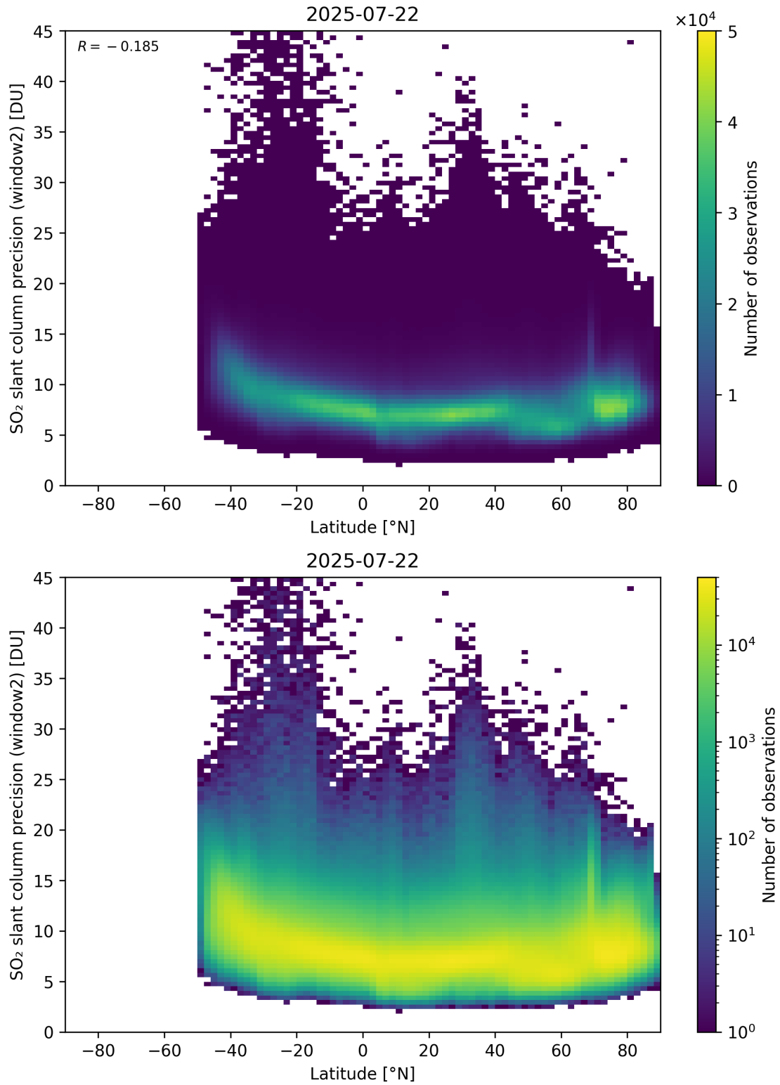
Figure 164: Scatter density plot of “Latitude” against “SO 2 slant column precision (window2)” for 2025-07-21 to 2025-07-23.
