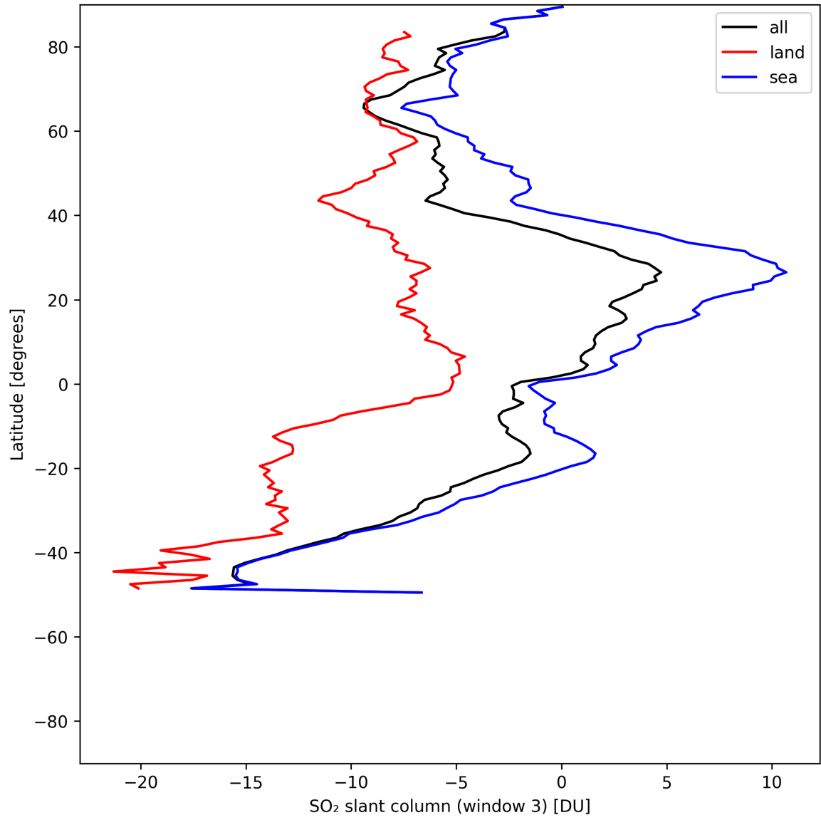
Figure 45: Zonal average of “SO 2 slant column (window 3)” for 2025-07-21 to 2025-07-23.
