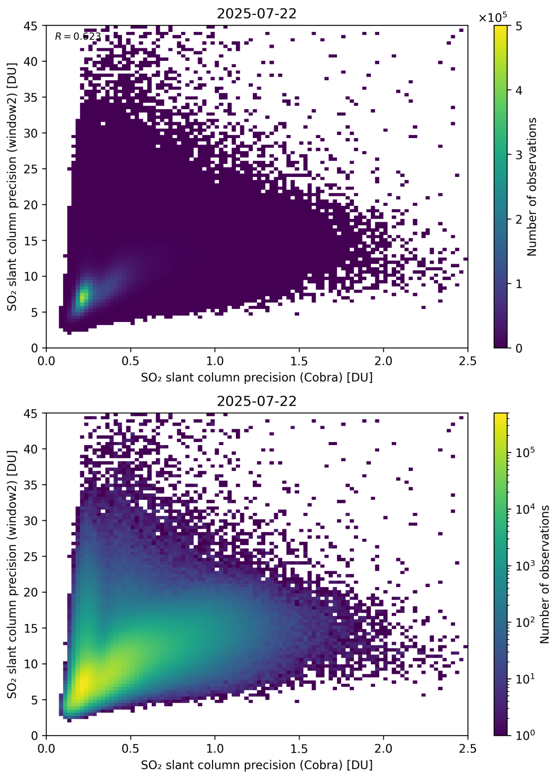
Figure 210: Scatter density plot of “SO 2 slant column precision (Cobra)” against “SO 2 slant column precision (window2)” for 2025-07-21 to 2025-07-23.
