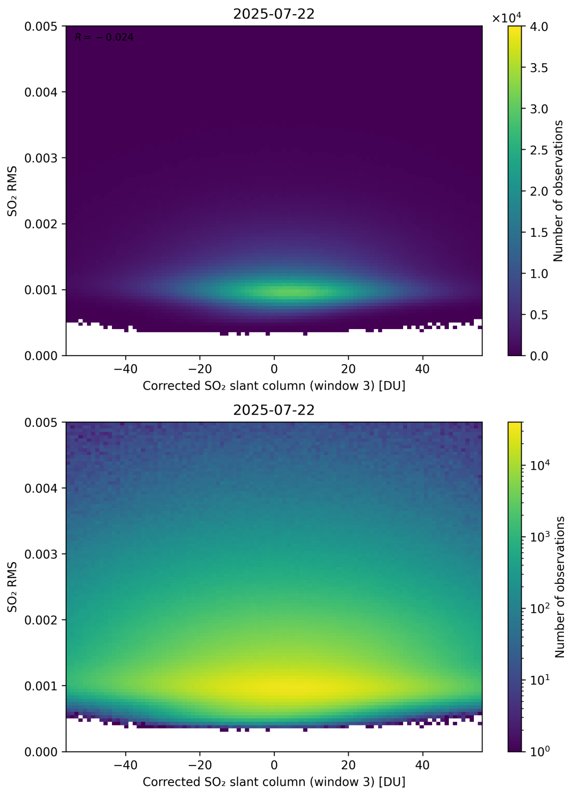
Figure 258: Scatter density plot of “Corrected SO 2 slant column (window 3)” against “SO 2 RMS” for 2025-07-21 to 2025-07-23.
