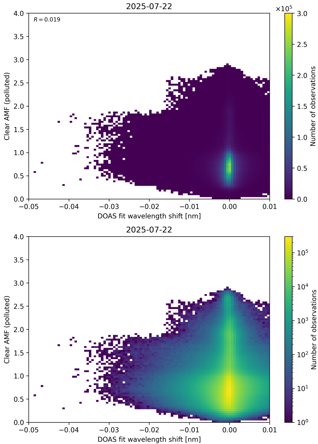
Figure 140: Scatter density plot of “DOAS fit wavelength shift” against “Clear AMF (polluted)” for 2025-07-21 to 2025-07-23.
