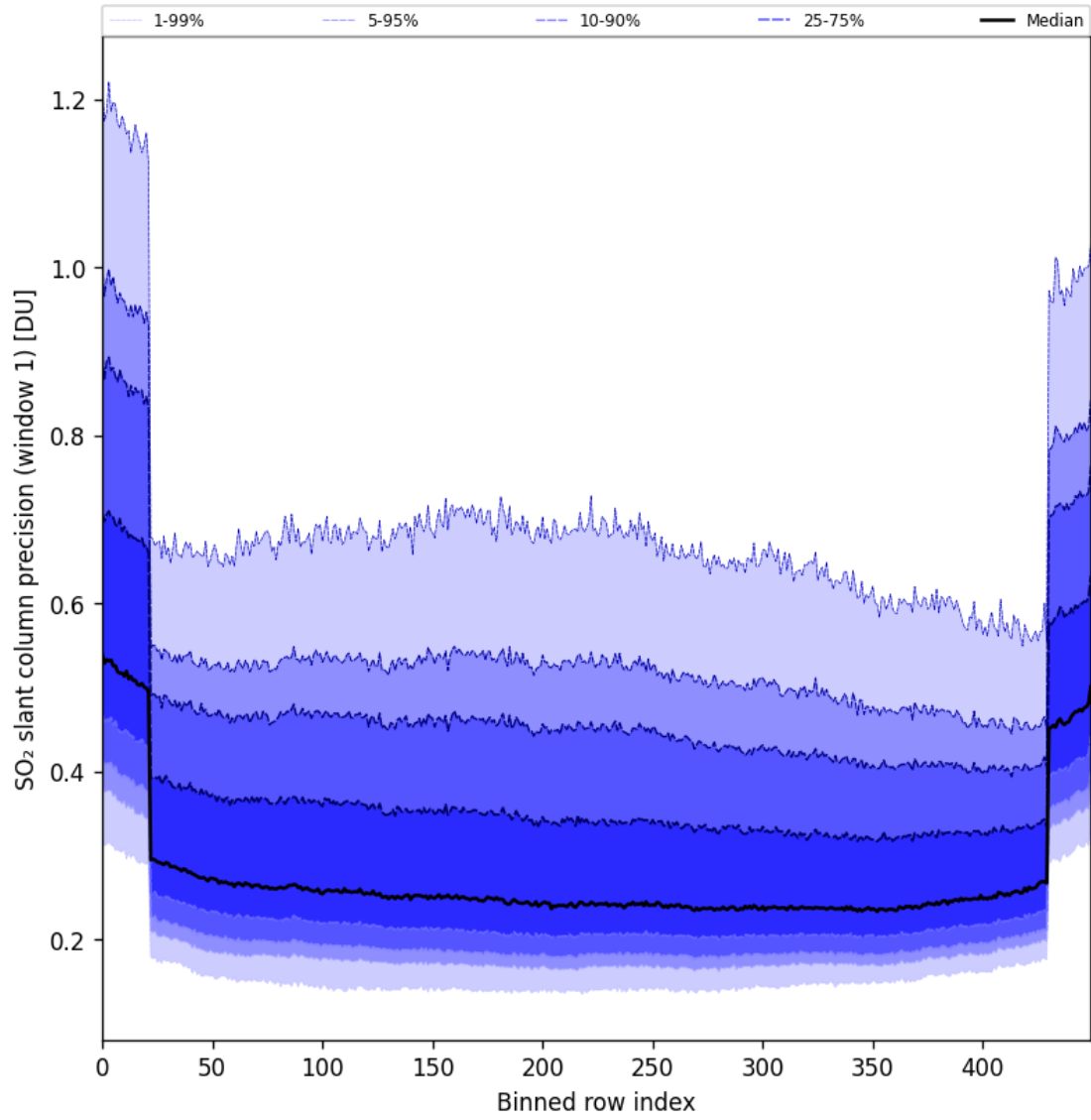
Figure 90: Along track statistics of “SO 2 slant column precision (window 1)” for 2025-07-21 to 2025-07-23
