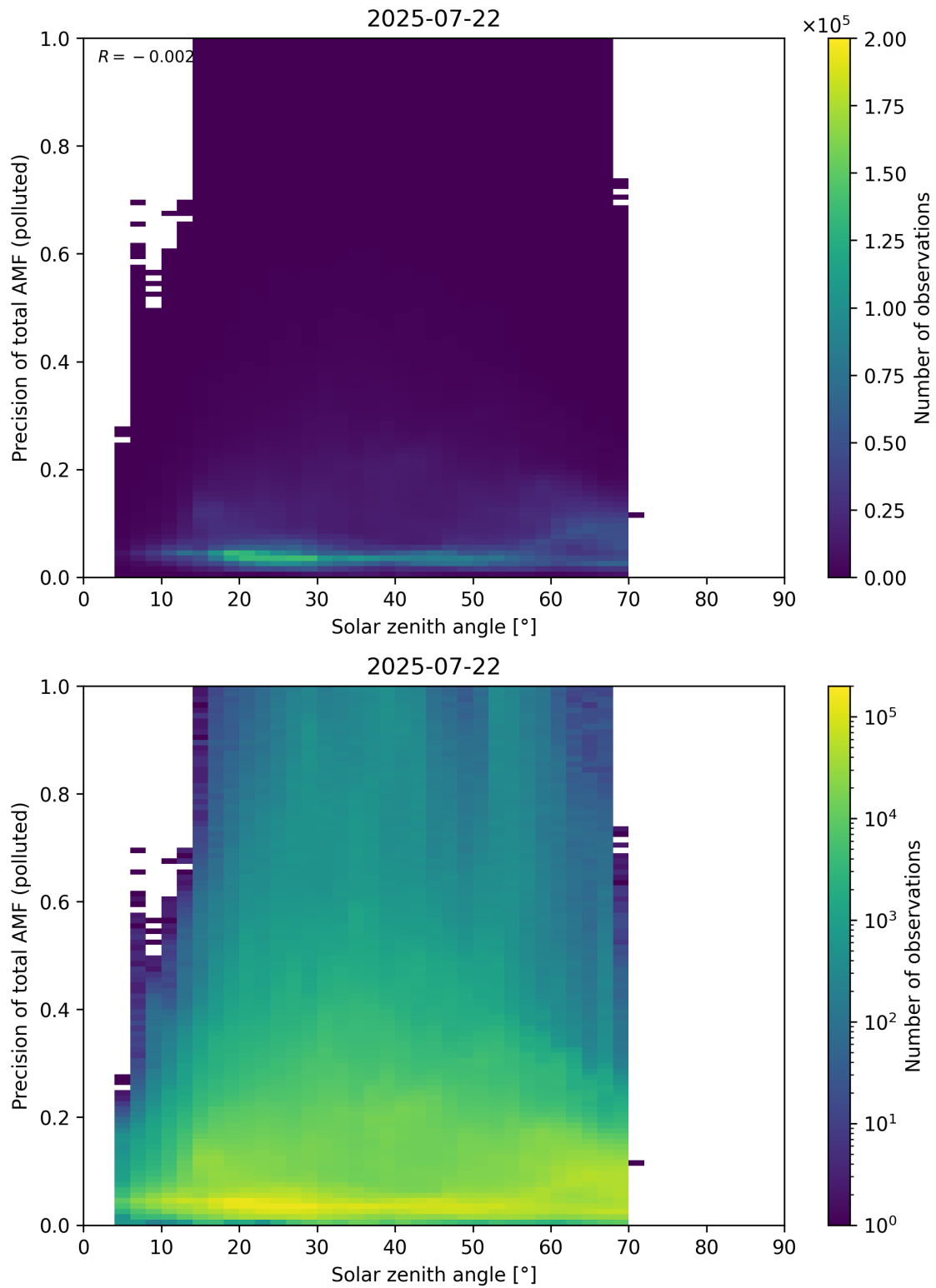
Figure 190: Scatter density plot of “Solar zenith angle” against “Precision of total AMF (polluted)” for 2025-07-21 to 2025-07-23.
