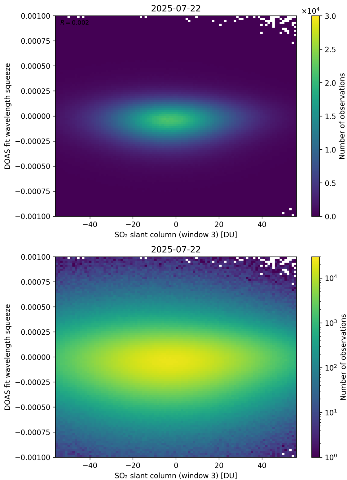
Figure 305: Scatter density plot of “SO 2 slant column (window 3)” against “DOAS fit wavelength squeeze” for 2025-07-21 to 2025-07-23.
