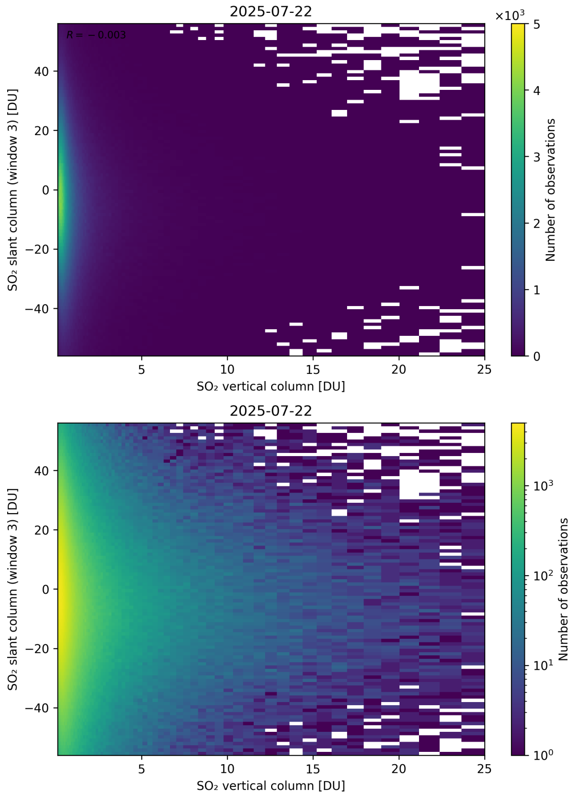
Figure 357: Scatter density plot of “SO 2 vertical column” against “SO 2 slant column (window 3)” for 2025-07-21 to 2025-07-23.
