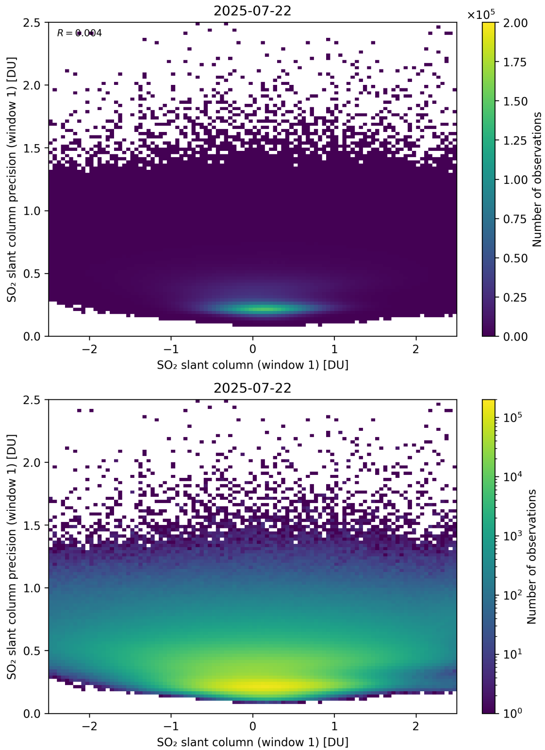
Figure 285: Scatter density plot of “SO 2 slant column (window 1)” against “SO 2 slant column precision (window 1)” for 2025-07-21 to 2025-07-23.
