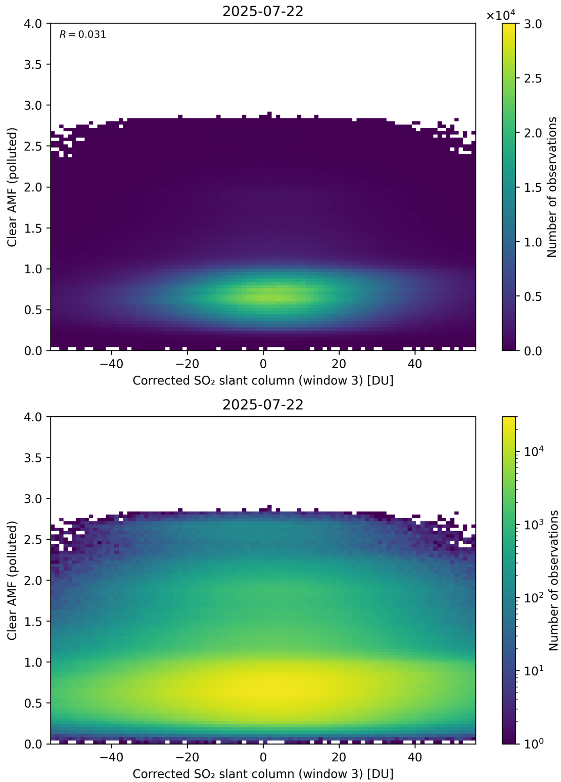
Figure 259: Scatter density plot of “Corrected SO 2 slant column (window 3)” against “Clear AMF (polluted)” for 2025-07-21 to 2025-07-23.
