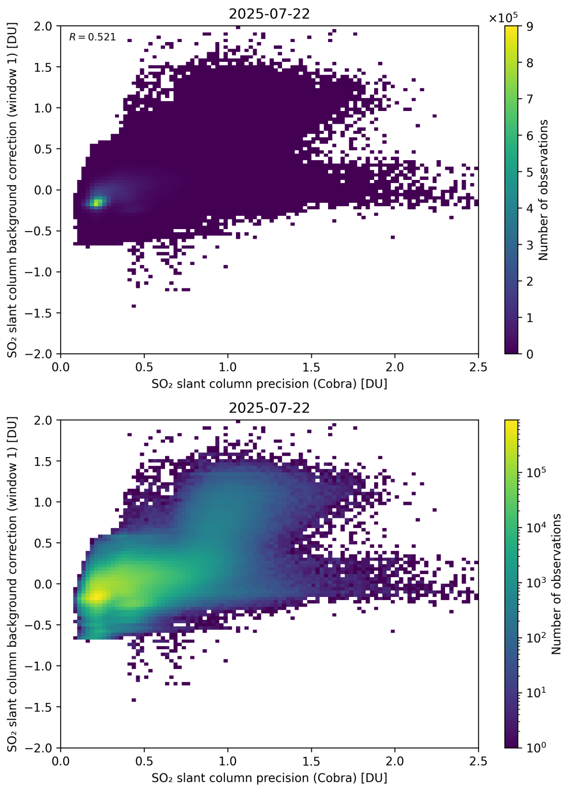
Figure 199: Scatter density plot of “SO 2 slant column precision (Cobra)” against “SO 2 slant column background correction (window 1)” for 2025-07-21 to 2025-07-23.
