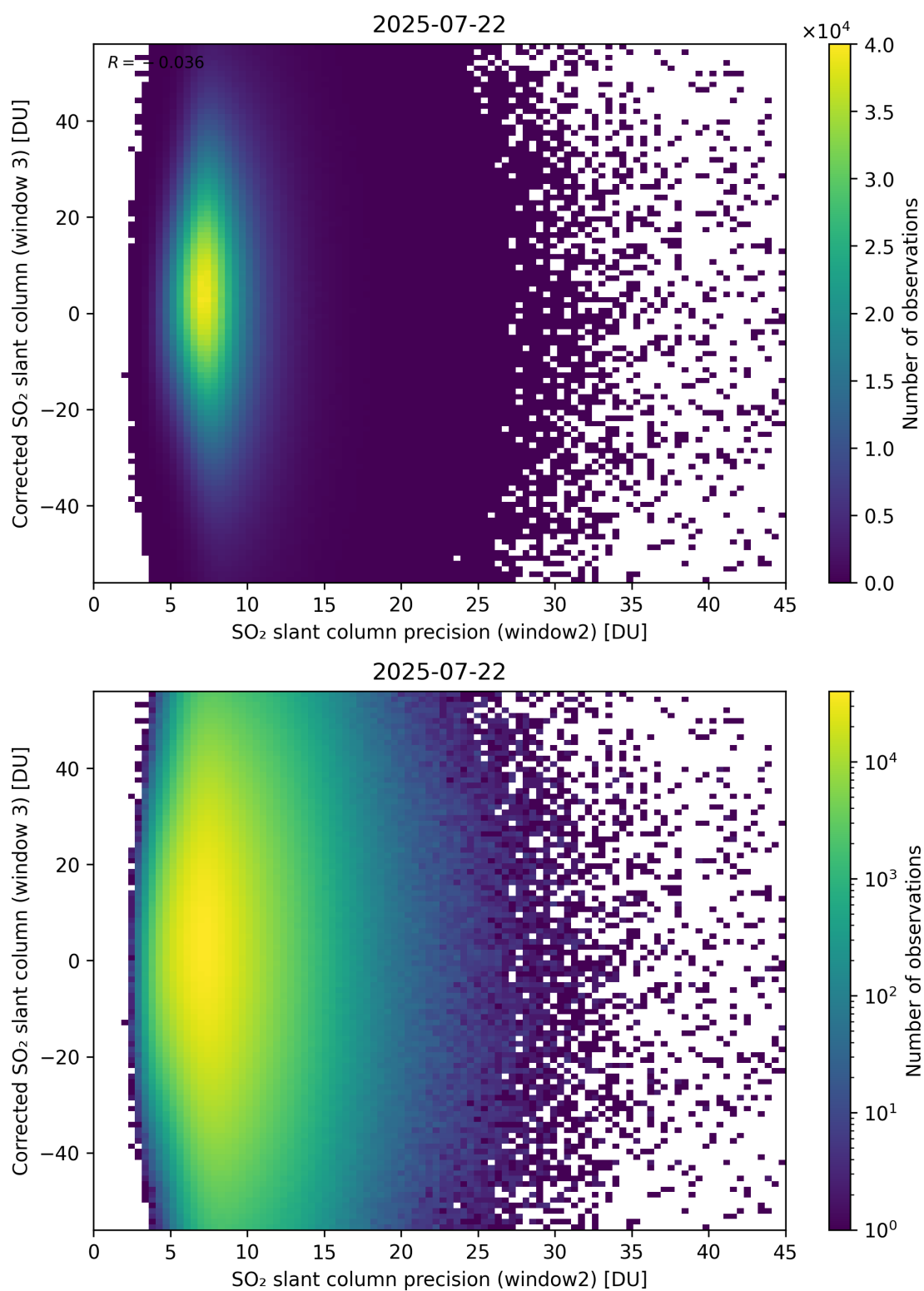
Figure 298: Scatter density plot of “SO 2 slant column precision (window2)” against “Corrected SO 2 slant column (window 3)” for 2025-07-21 to 2025-07-23.
