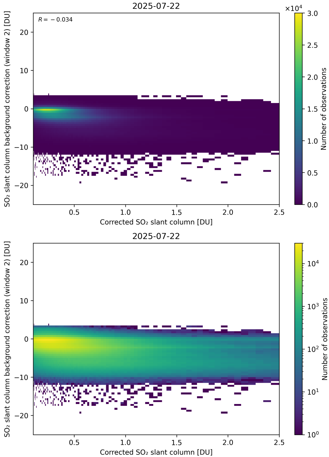
Figure 227: Scatter density plot of “Corrected SO 2 slant column” against “SO 2 slant column background correction (window 2)” for 2025-07-21 to 2025-07-23.
