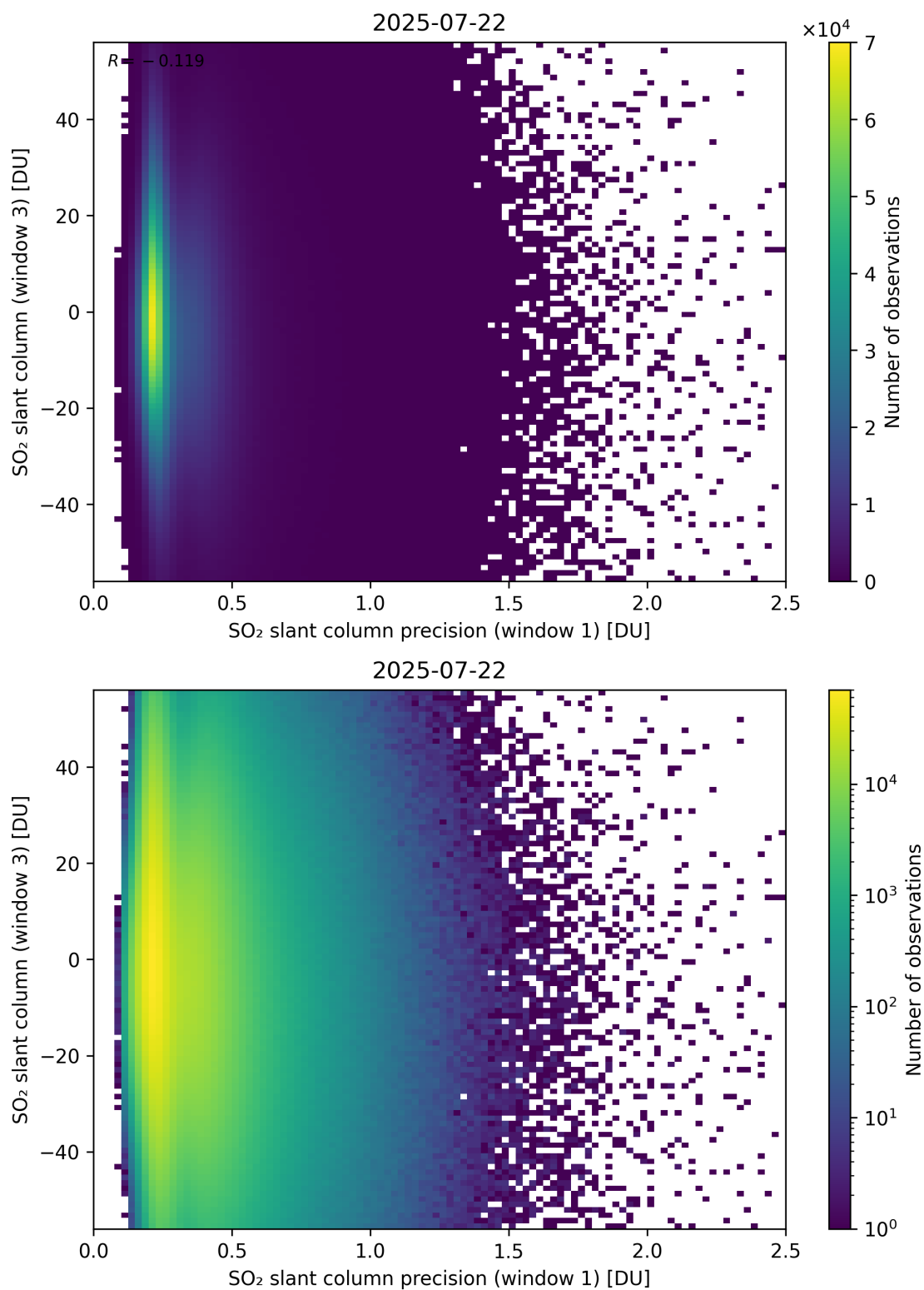
Figure 278: Scatter density plot of “SO 2 slant column precision (window 1)” against “SO 2 slant column (window 3)” for 2025-07-21 to 2025-07-23.
