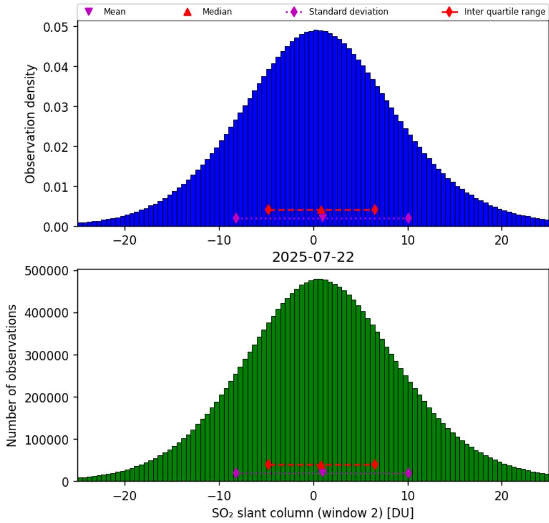
Figure 67: Histogram of “SO 2 slant column (window 2)” for 2025-07-21 to 2025-07-23
