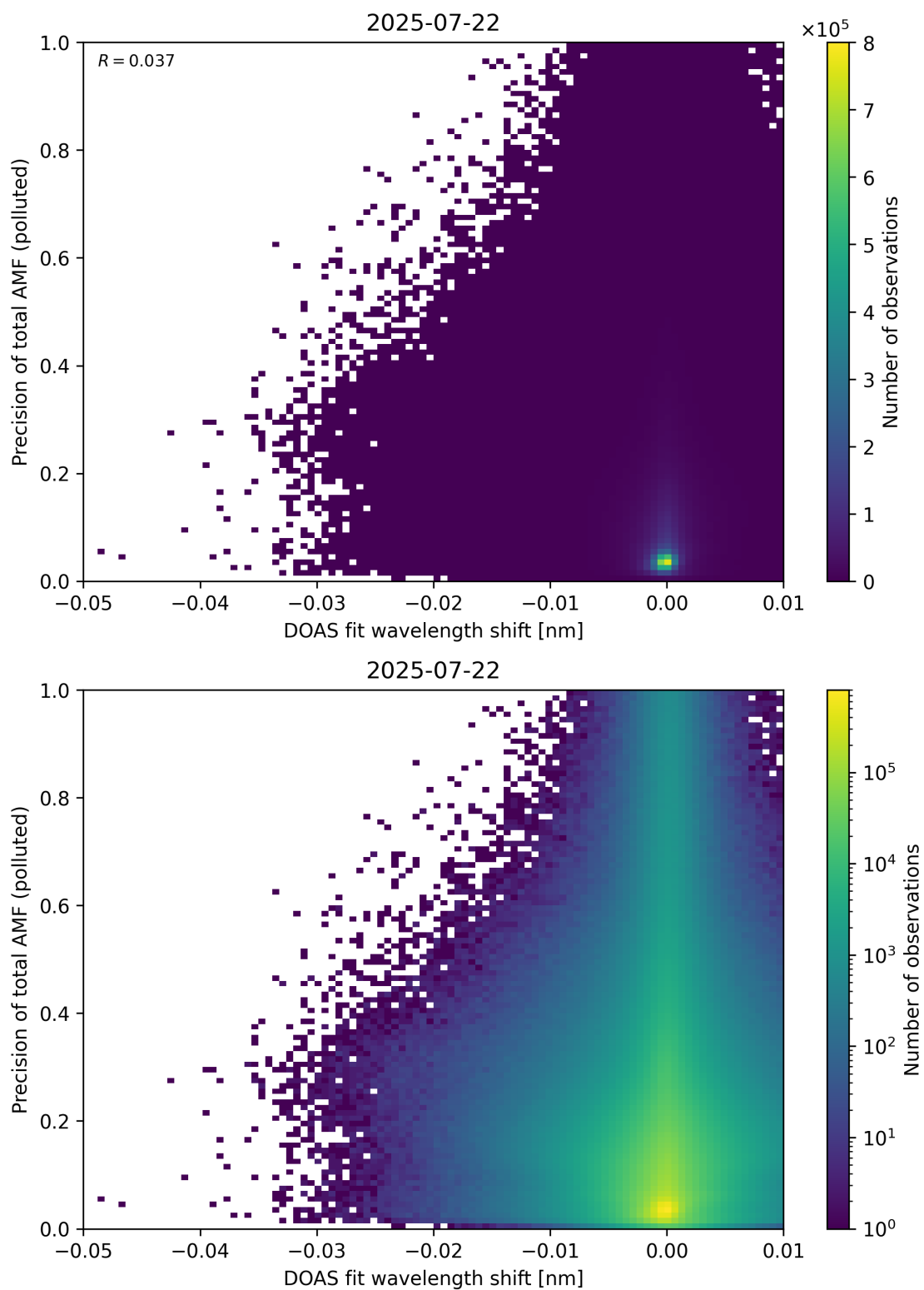
Figure 142: Scatter density plot of “DOAS fit wavelength shift” against “Precision of total AMF (polluted)” for 2025-07-21 to 2025-07-23.
