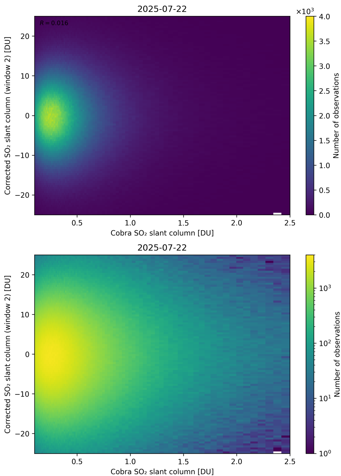
Figure 217: Scatter density plot of “Cobra SO 2 slant column” against “Corrected SO 2 slant column (window 2)” for 2025-07-21 to 2025-07-23.
