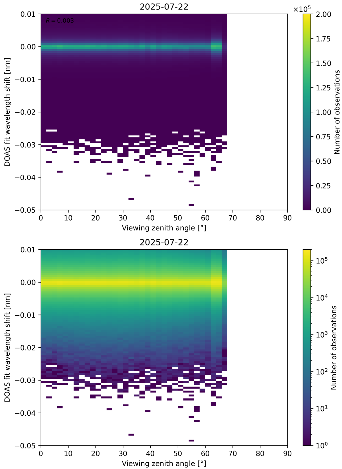
Figure 365: Scatter density plot of “Viewing zenith angle” against “DOAS fit wavelength shift” for 2025-07-21 to 2025-07-23.
