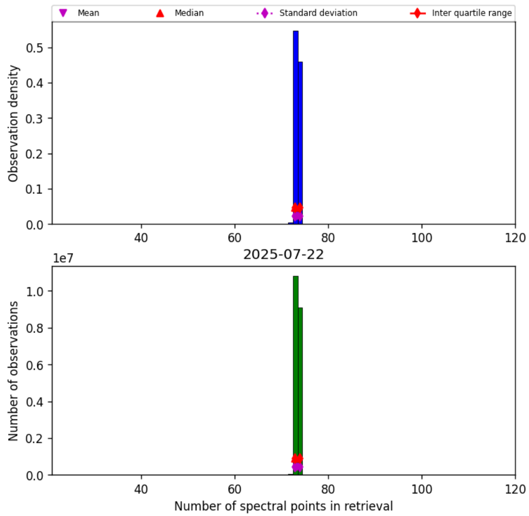
Figure 82: Histogram of “Number of spectral points in retrieval” for 2025-07-21 to 2025-07-23
