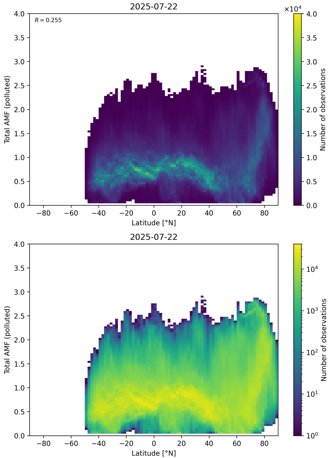
Figure 167: Scatter density plot of “Latitude” against “Total AMF (polluted)” for 2025-07-21 to 2025-07-23.
