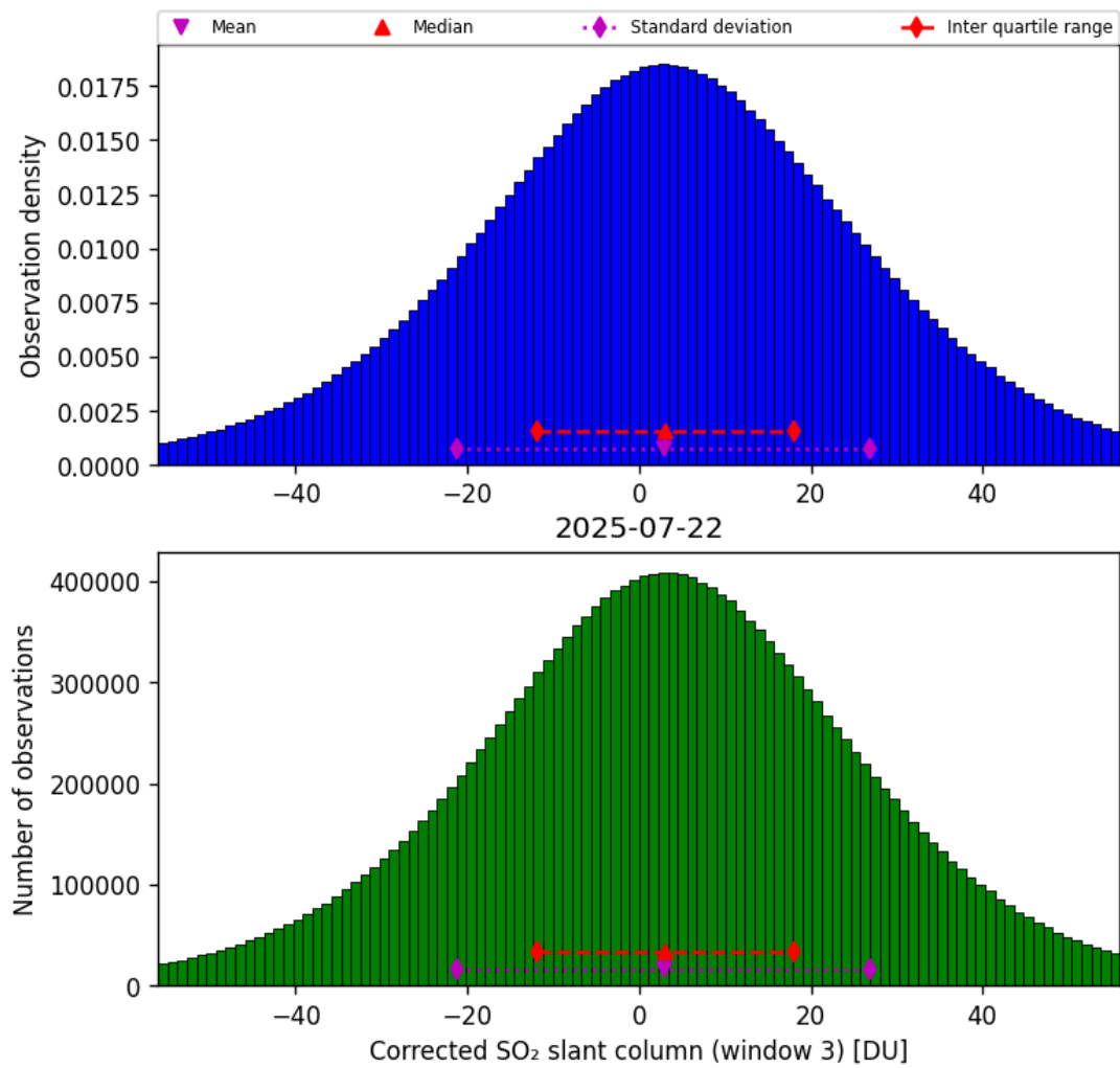
Figure 73: Histogram of “Corrected SO 2 slant column (window 3)” for 2025-07-21 to 2025-07-23
