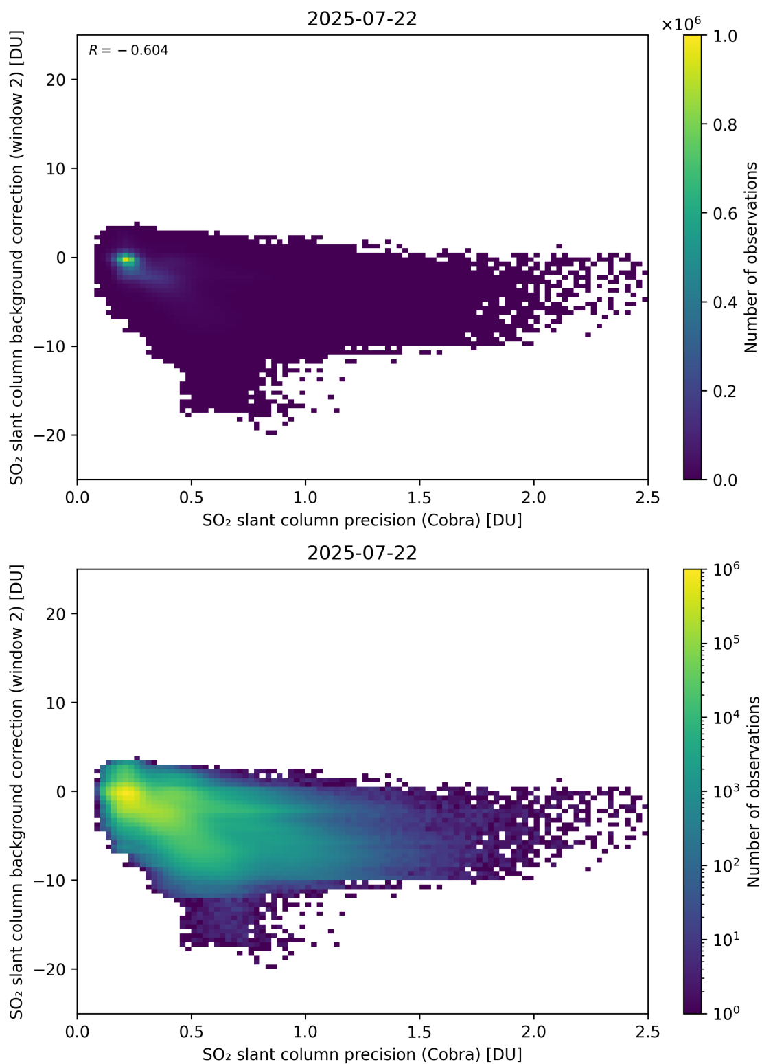
Figure 200: Scatter density plot of “SO 2 slant column precision (Cobra)” against “SO 2 slant column background correction (window 2)” for 2025-07-21 to 2025-07-23.
