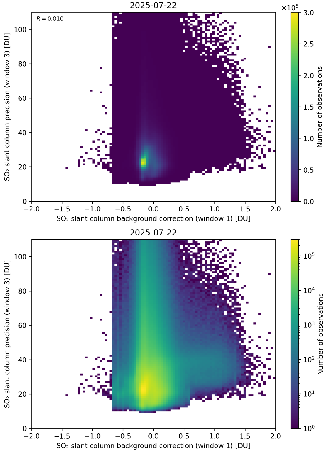
Figure 119: Scatter density plot of “SO 2 slant column background correction (window 1)” against “SO 2 slant column precision (window 3)” for 2025-07-21 to 2025-07-23.
