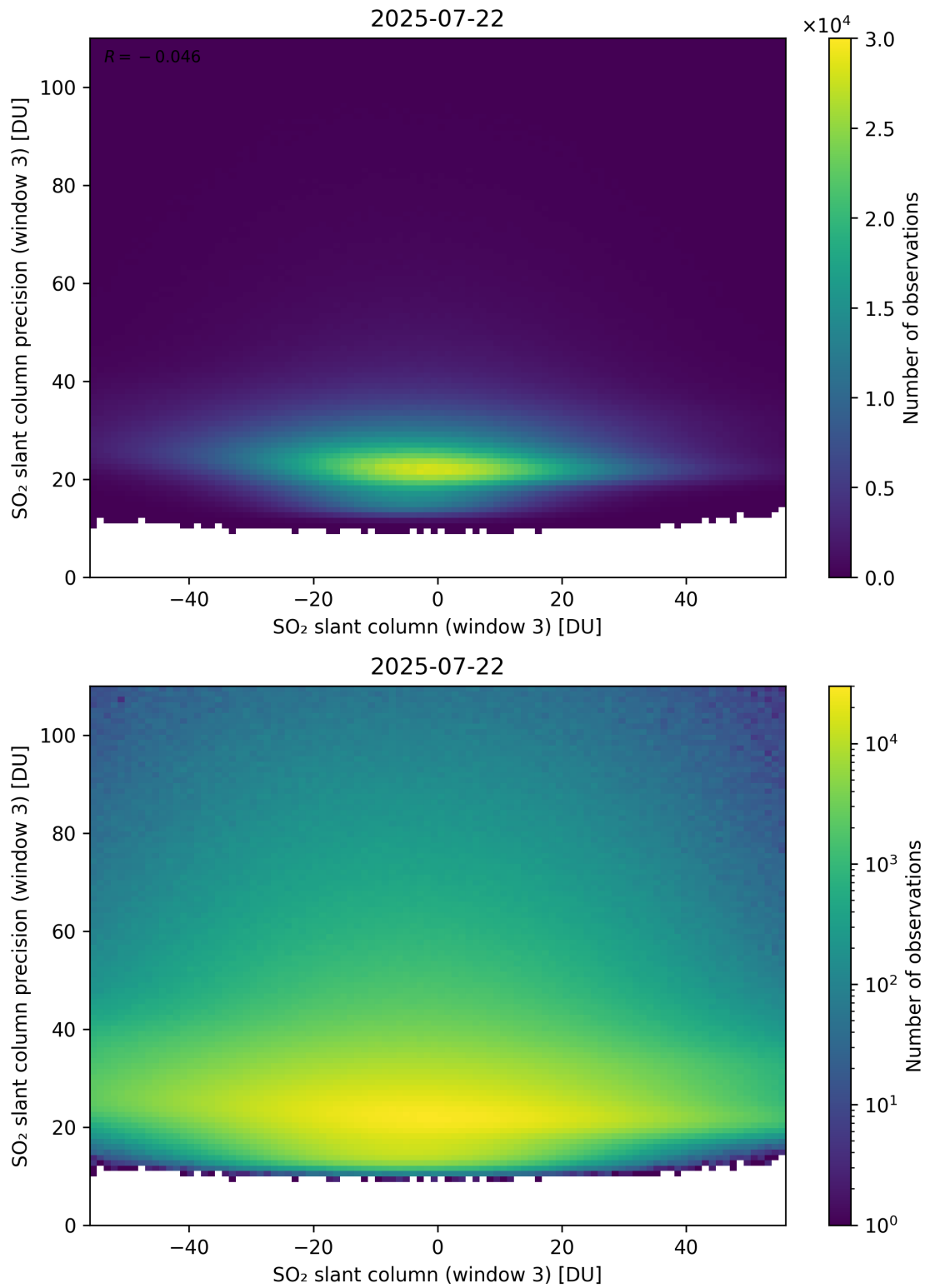
Figure 317: Scatter density plot of “SO 2 slant column (window 3)” against “SO 2 slant column precision (window 3)” for 2025-07-21 to 2025-07-23.
