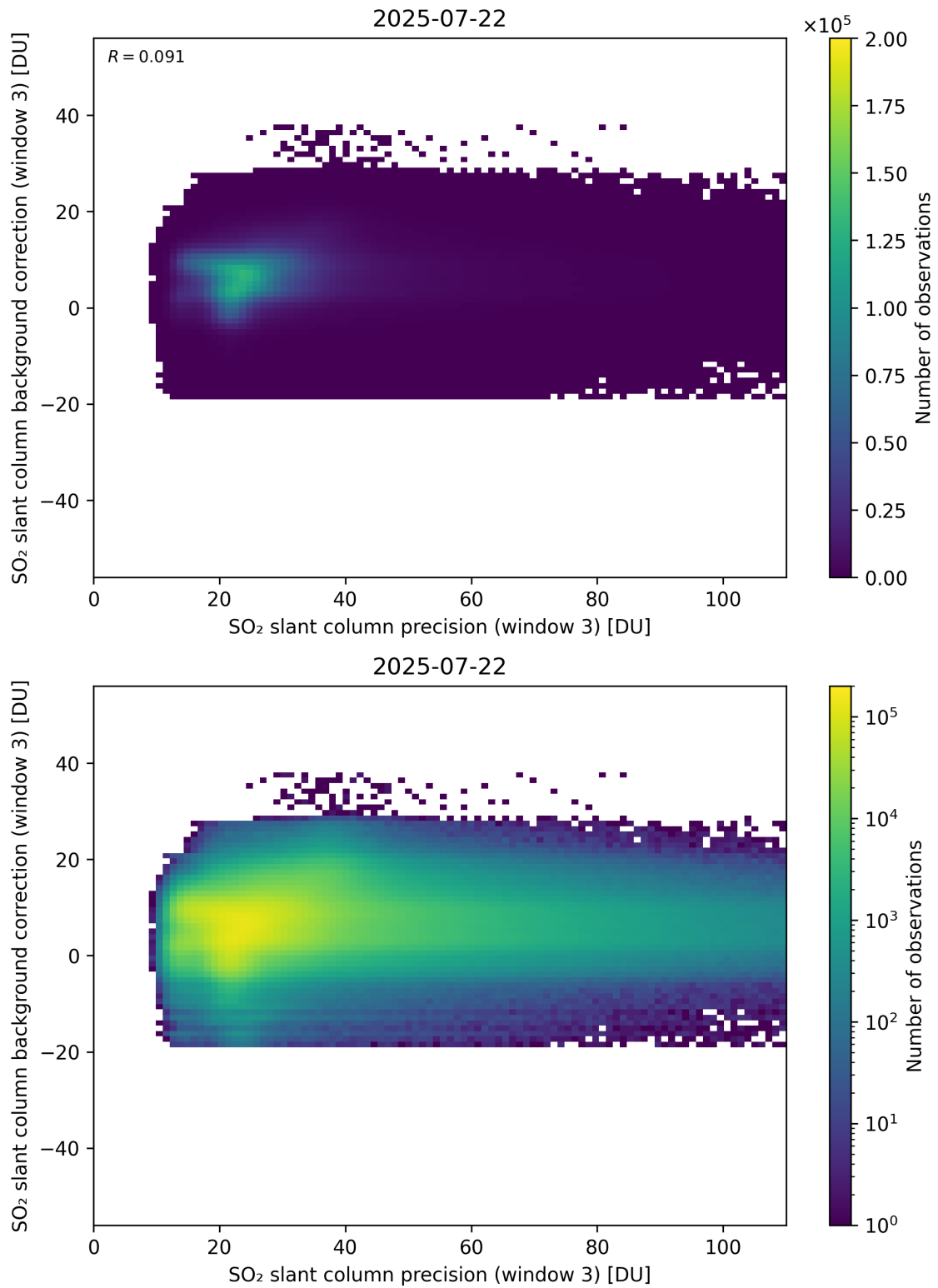
Figure 307: Scatter density plot of “SO 2 slant column precision (window 3)” against “SO 2 slant column background correction (window 3)” for 2025-07-21 to 2025-07-23.
