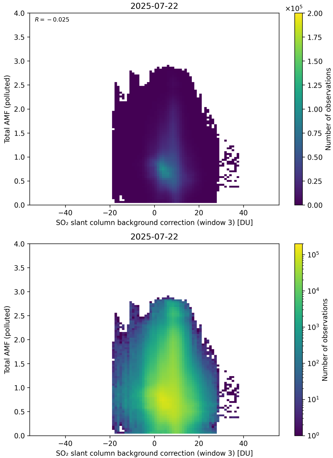
Figure 136: Scatter density plot of “SO 2 slant column background correction (window 3)” against “Total AMF (polluted)” for 2025-07-21 to 2025-07-23.
