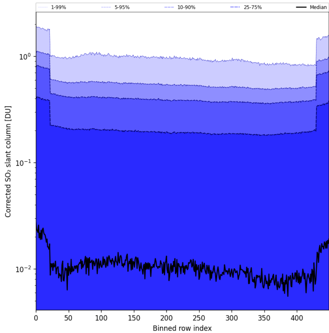
Figure 86: Along track statistics of “Corrected SO 2 slant column” for 2025-07-21 to 2025-07-23
