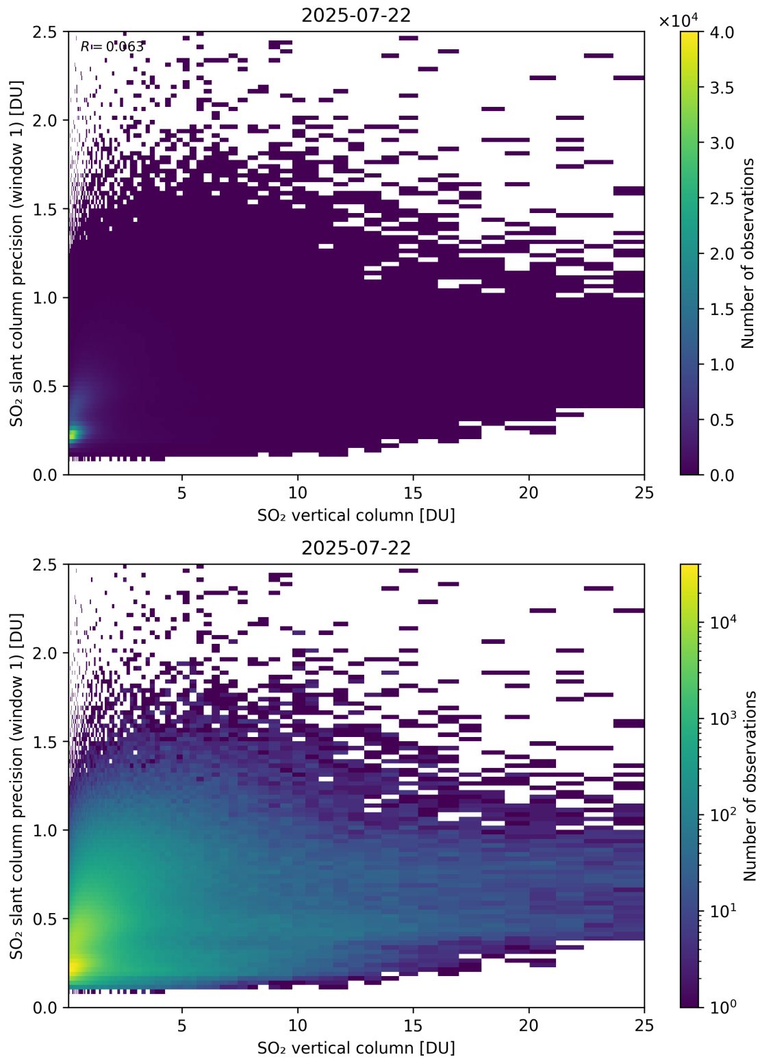
Figure 355: Scatter density plot of “SO 2 vertical column” against “SO 2 slant column precision (window 1)” for 2025-07-21 to 2025-07-23.
