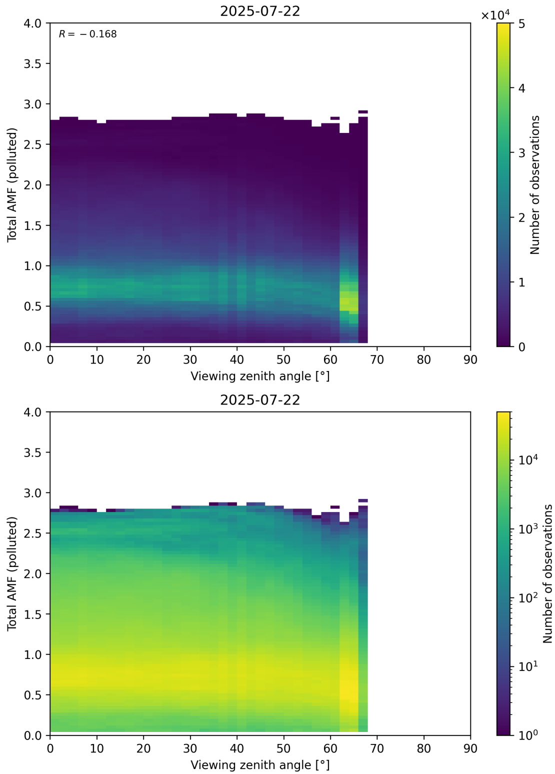
Figure 381: Scatter density plot of “Viewing zenith angle” against “Total AMF (polluted)” for 2025-07-21 to 2025-07-23.
