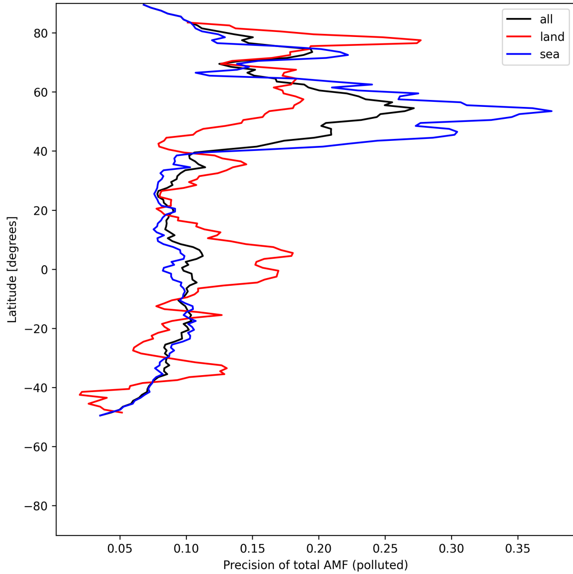
Figure 54: Zonal average of “Precision of total AMF (polluted)” for 2025-07-21 to 2025-07-23.
