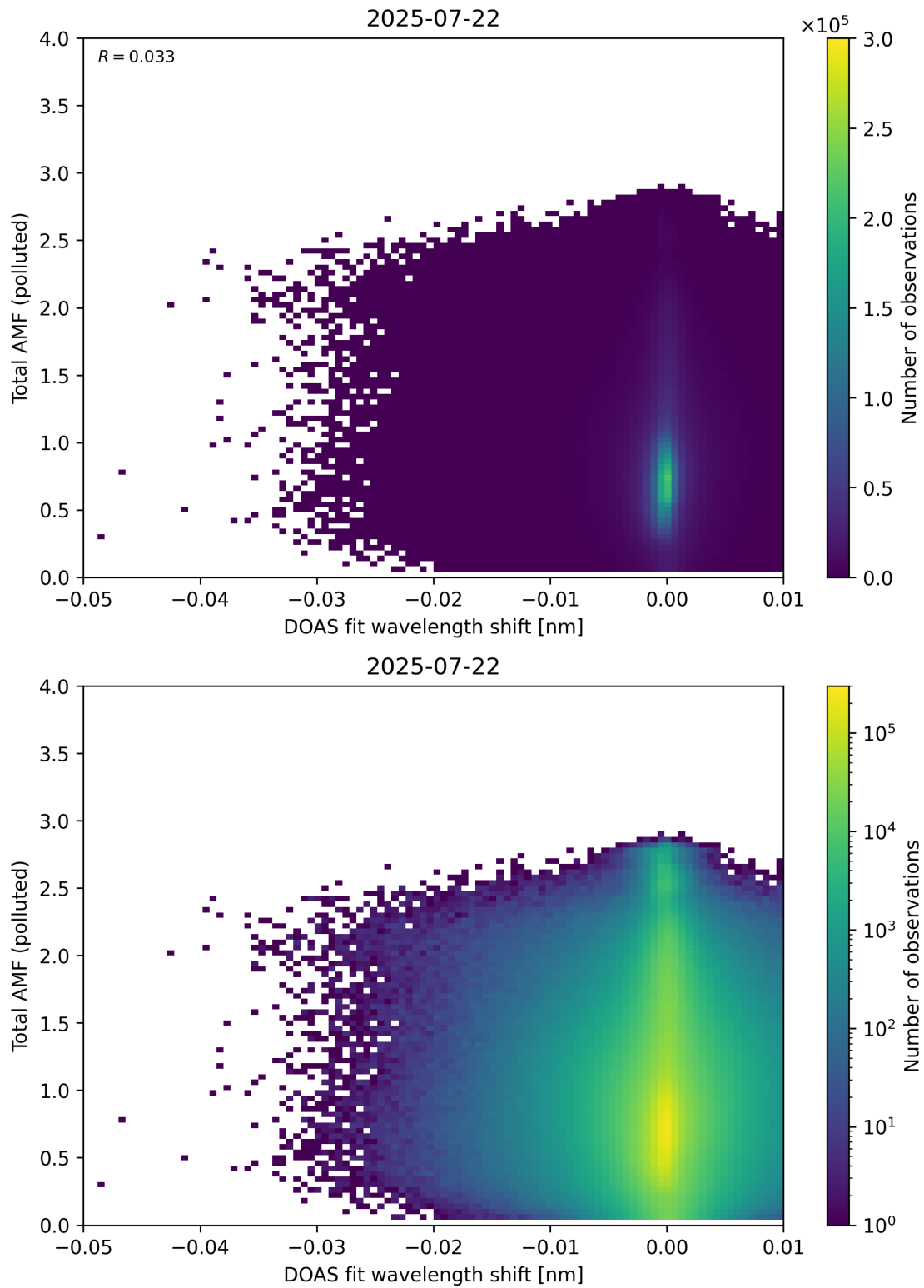
Figure 141: Scatter density plot of “DOAS fit wavelength shift” against “Total AMF (polluted)” for 2025-07-21 to 2025-07-23.
