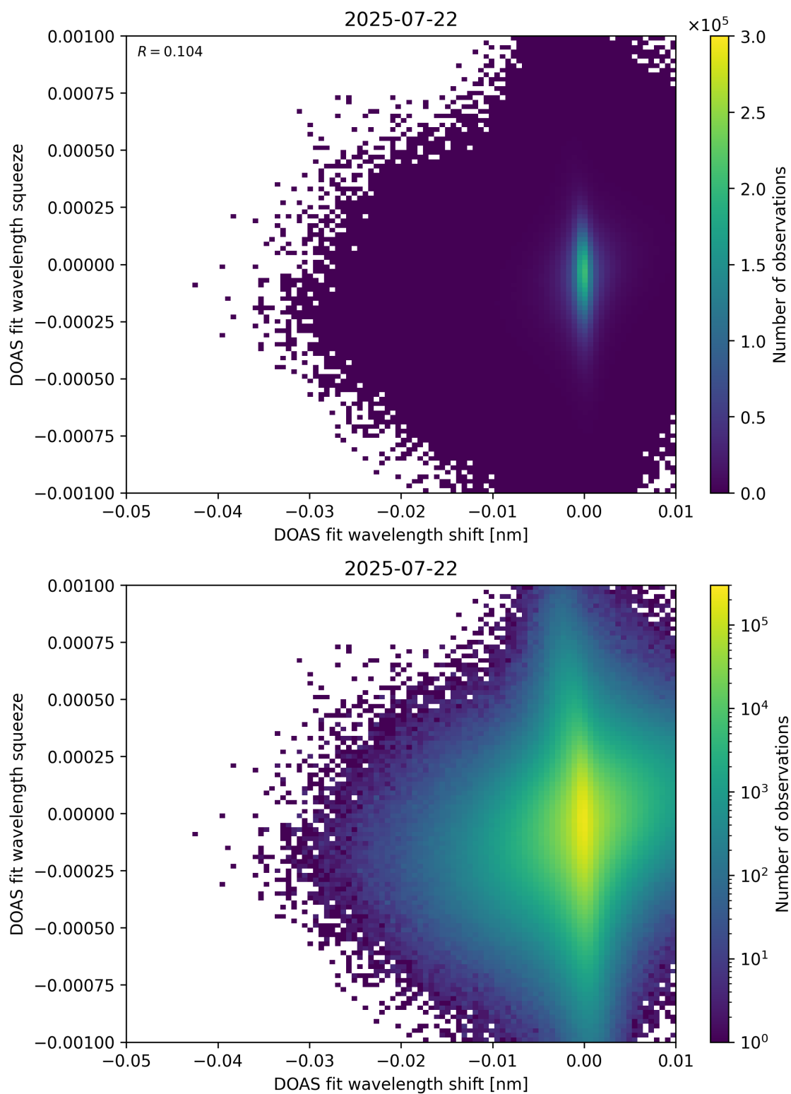
Figure 138: Scatter density plot of “DOAS fit wavelength shift” against “DOAS fit wavelength squeeze” for 2025-07-21 to 2025-07-23.
