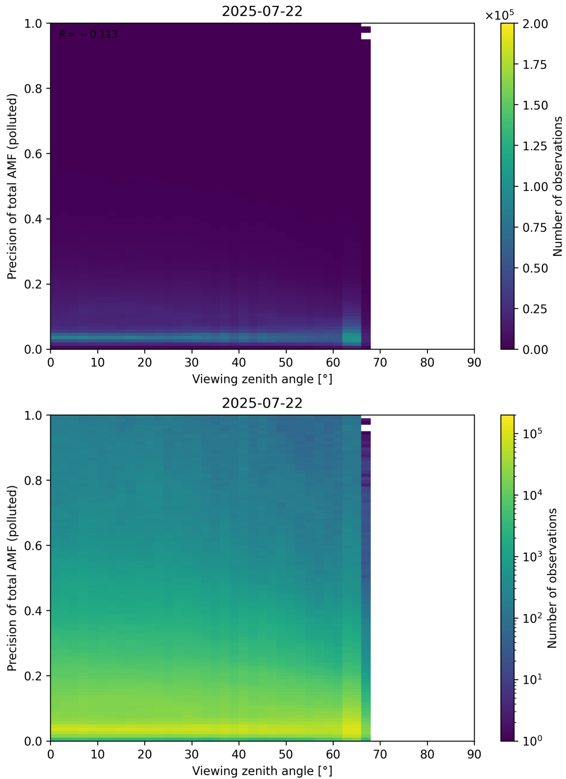
Figure 382: Scatter density plot of “Viewing zenith angle” against “Precision of total AMF (polluted)” for 2025-07-21 to 2025-07-23.
