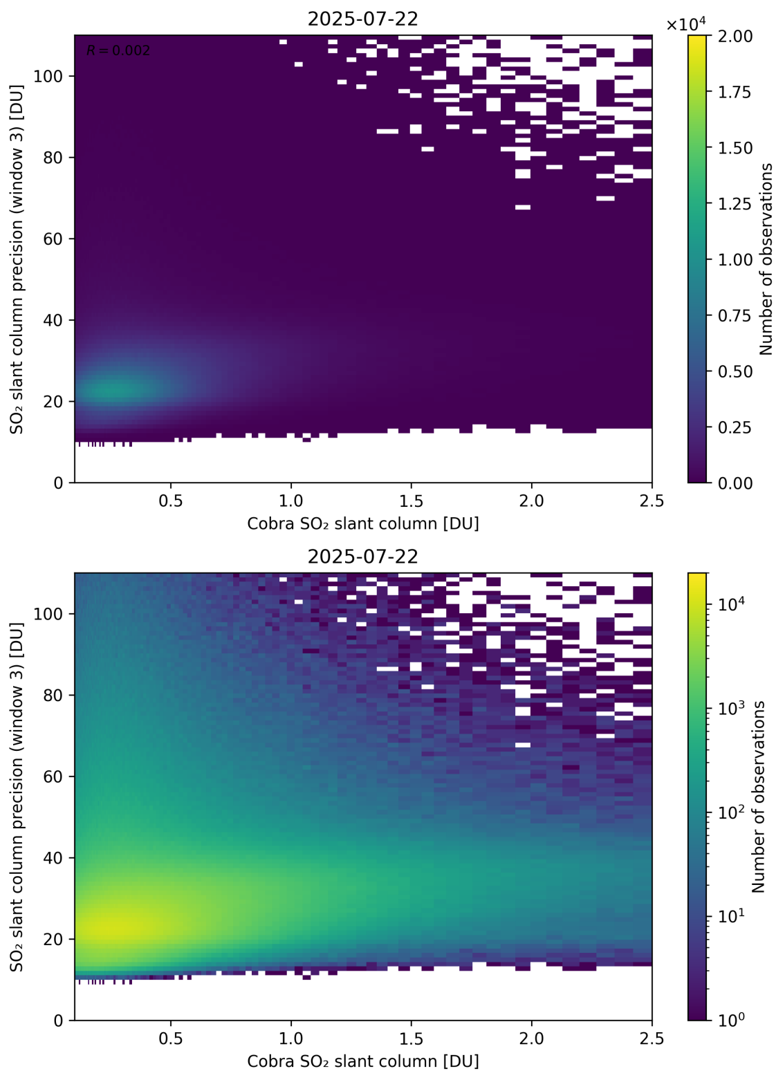
Figure 223: Scatter density plot of “Cobra SO 2 slant column” against “SO 2 slant column precision (window 3)” for 2025-07-21 to 2025-07-23.
