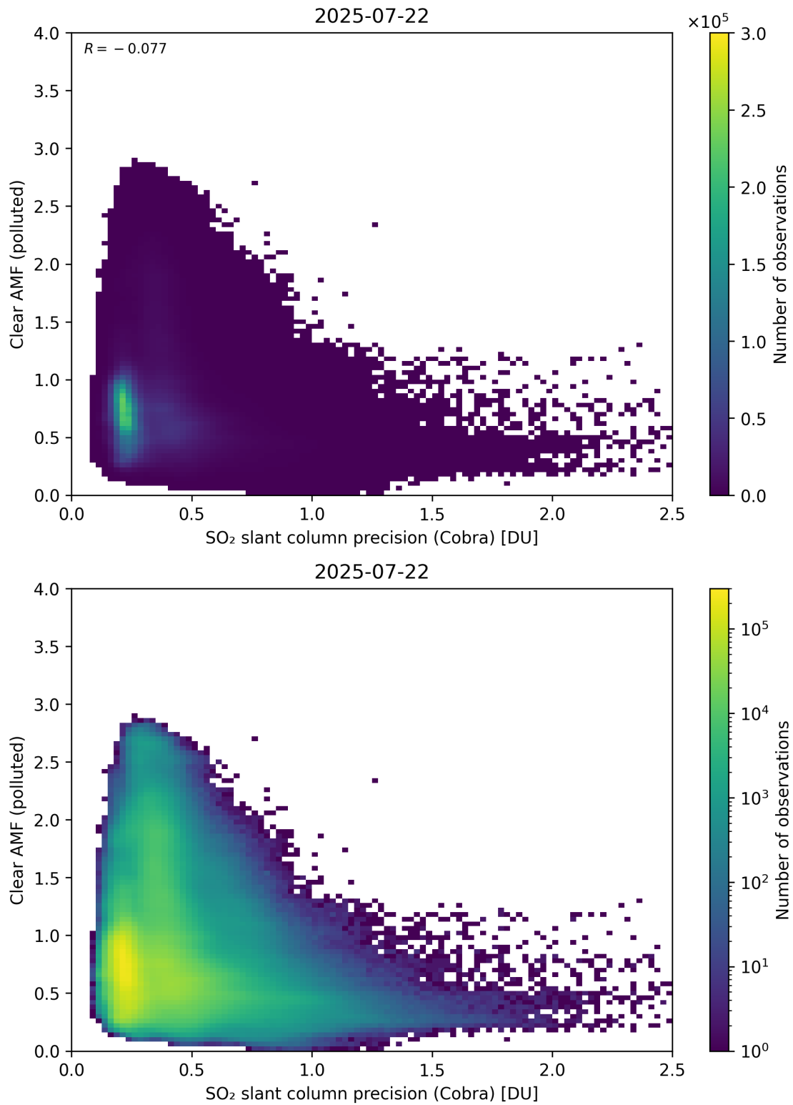
Figure 205: Scatter density plot of “SO 2 slant column precision (Cobra)” against “Clear AMF (polluted)” for 2025-07-21 to 2025-07-23.
