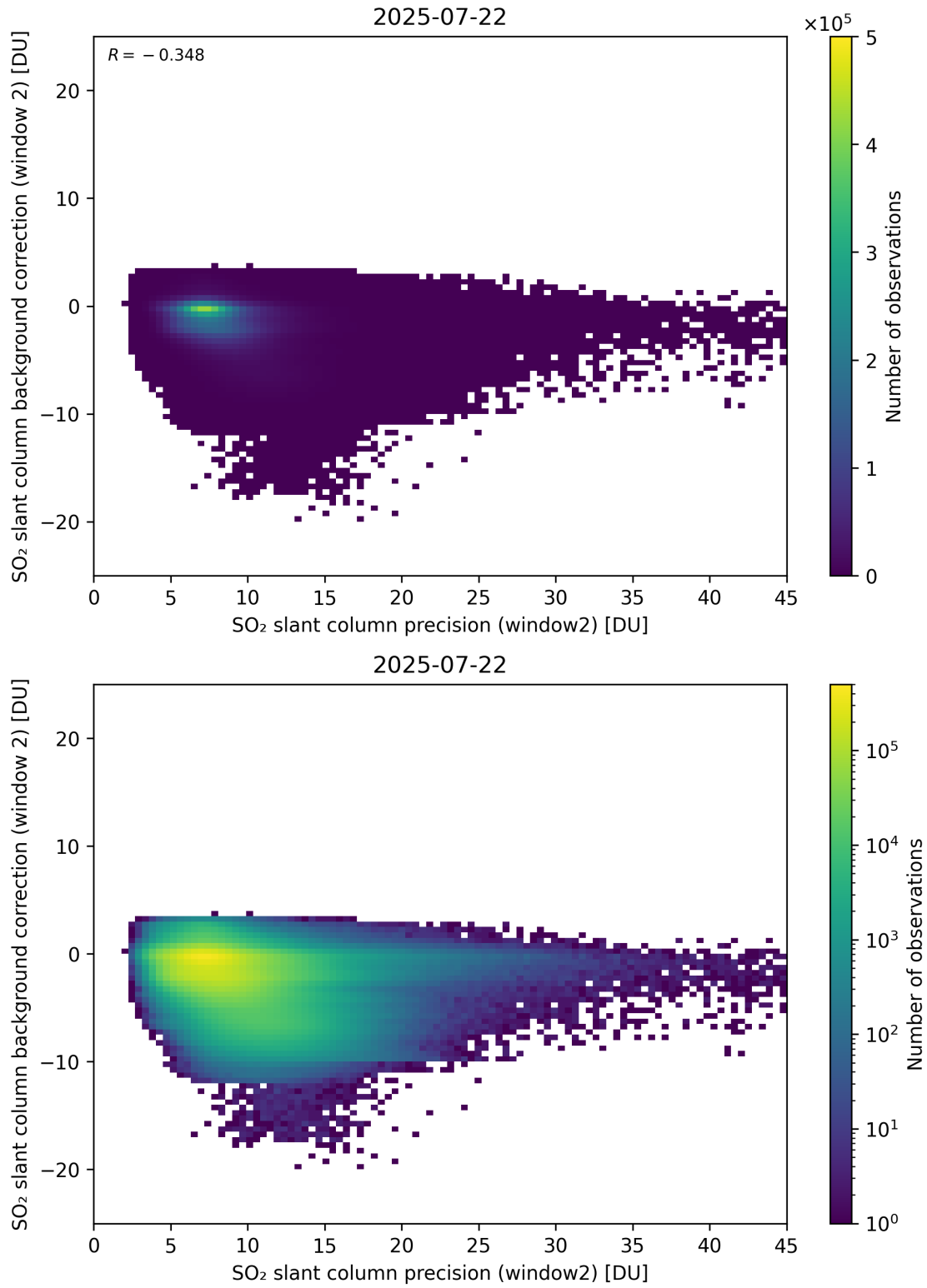
Figure 291: Scatter density plot of “SO 2 slant column precision (window2)” against “SO 2 slant column background correction (window 2)” for 2025-07-21 to 2025-07-23.
