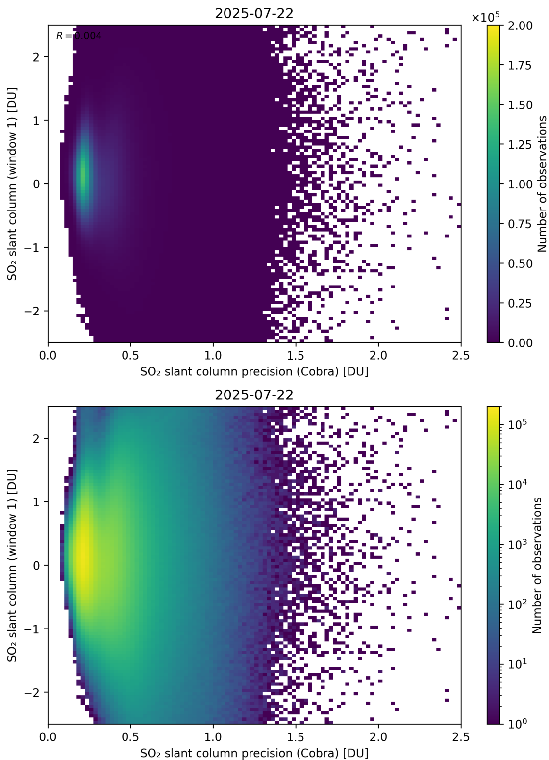
Figure 208: Scatter density plot of “SO 2 slant column precision (Cobra)” against “SO 2 slant column (window 1)” for 2025-07-21 to 2025-07-23.
