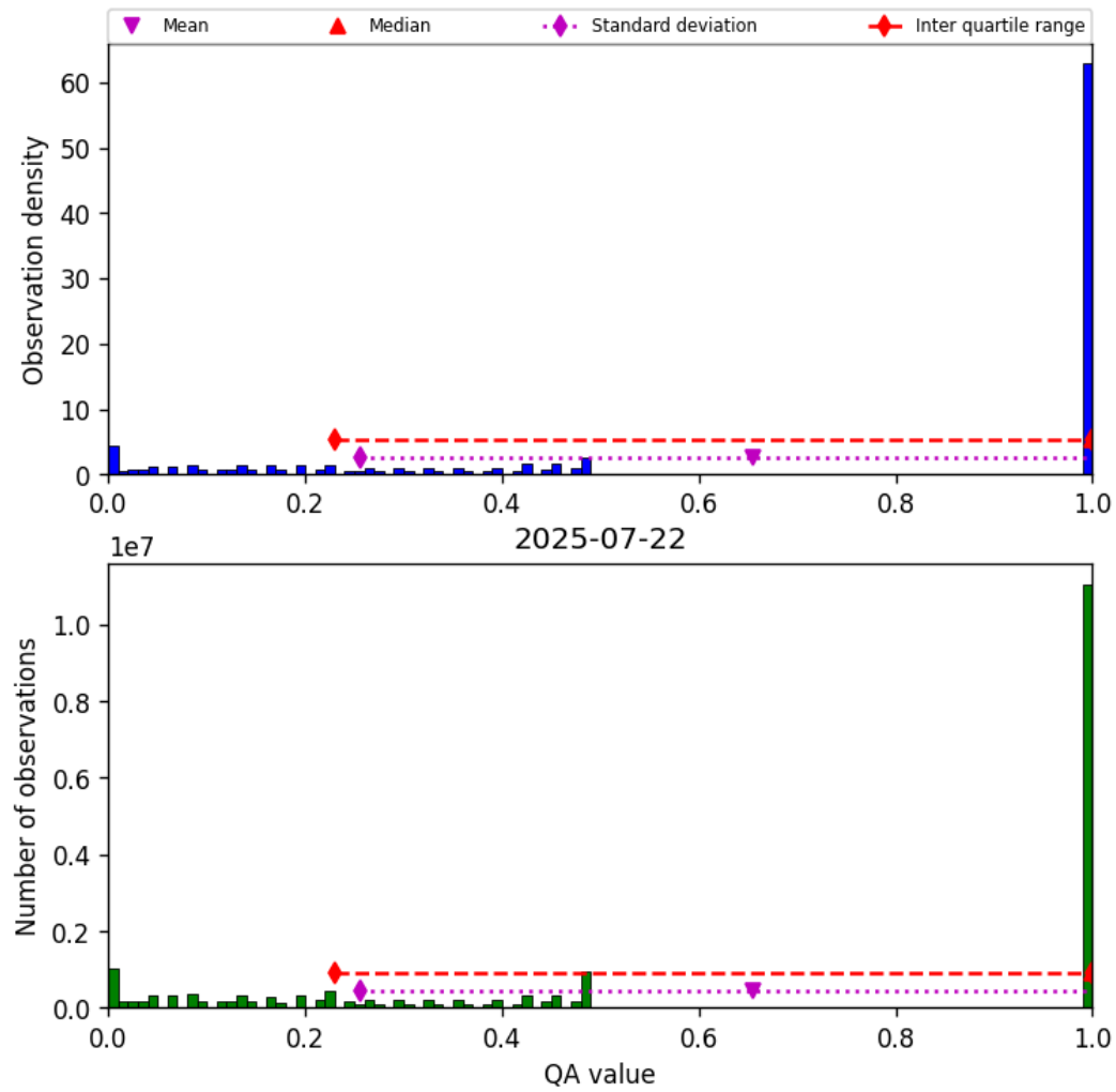
Figure 57: Histogram of “QA value” for 2025-07-21 to 2025-07-23
