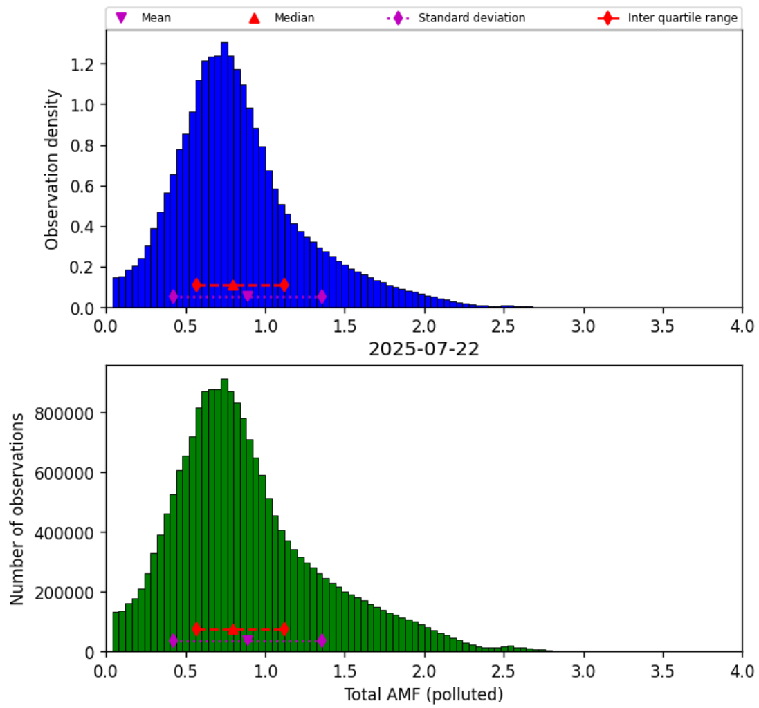
Figure 79: Histogram of “Total AMF (polluted)” for 2025-07-21 to 2025-07-23
