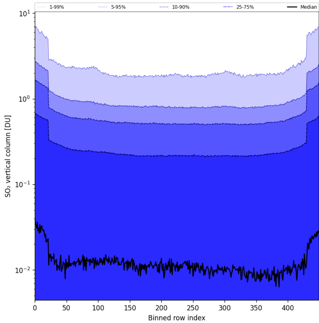
Figure 84: Along track statistics of “SO 2 vertical column” for 2025-07-21 to 2025-07-23
