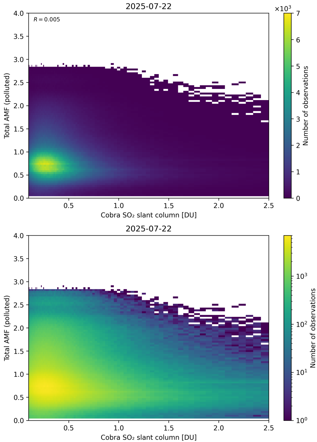
Figure 224: Scatter density plot of “Cobra SO 2 slant column” against “Total AMF (polluted)” for 2025-07-21 to 2025-07-23.
