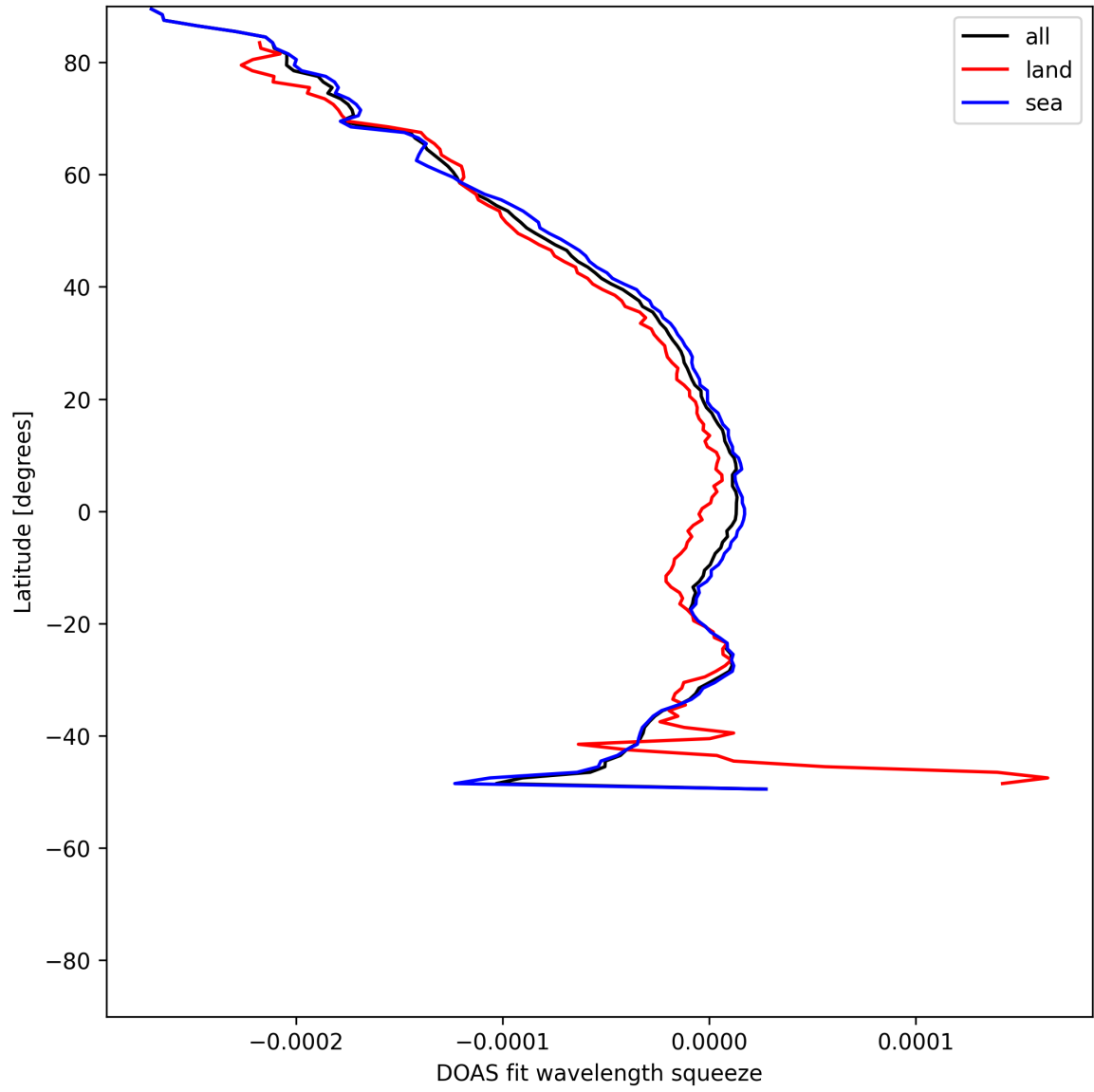
Figure 51: Zonal average of “DOAS fit wavelength squeeze” for 2025-07-21 to 2025-07-23.
