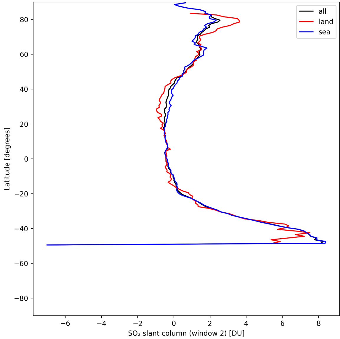
Figure 41: Zonal average of “SO 2 slant column (window 2)” for 2025-07-21 to 2025-07-23.
