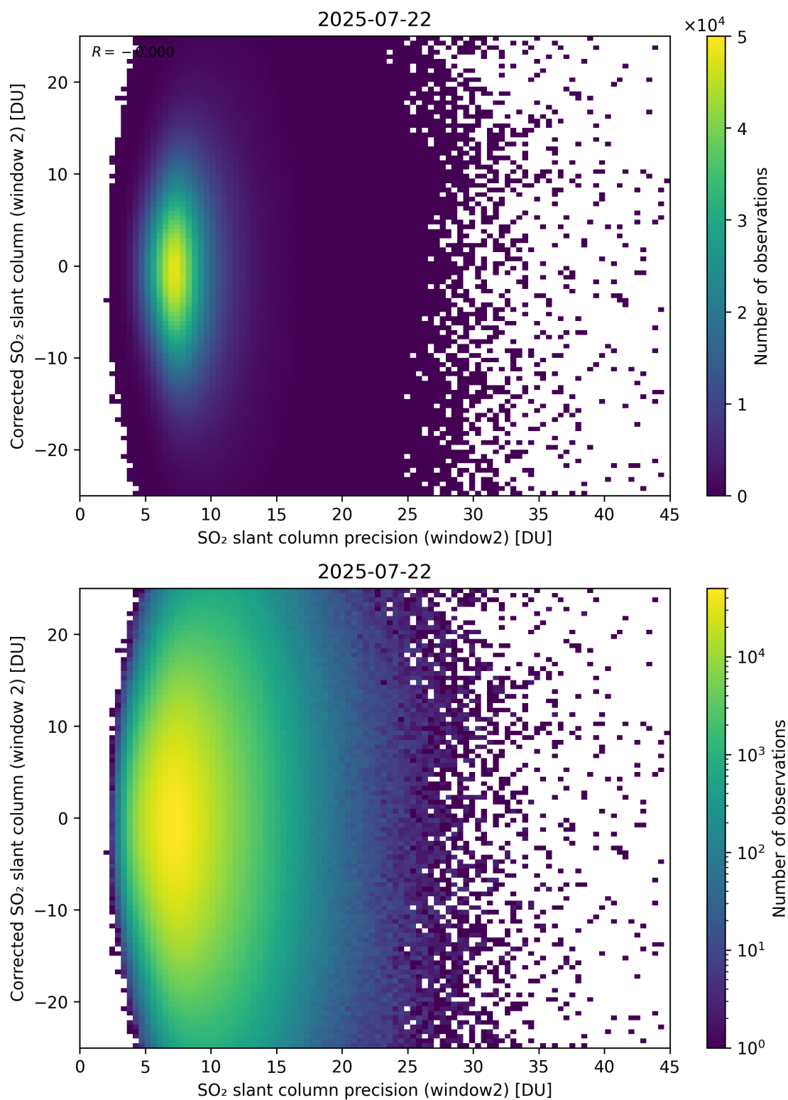
Figure 297: Scatter density plot of “SO 2 slant column precision (window2)” against “Corrected SO 2 slant column (window 2)” for 2025-07-21 to 2025-07-23.
