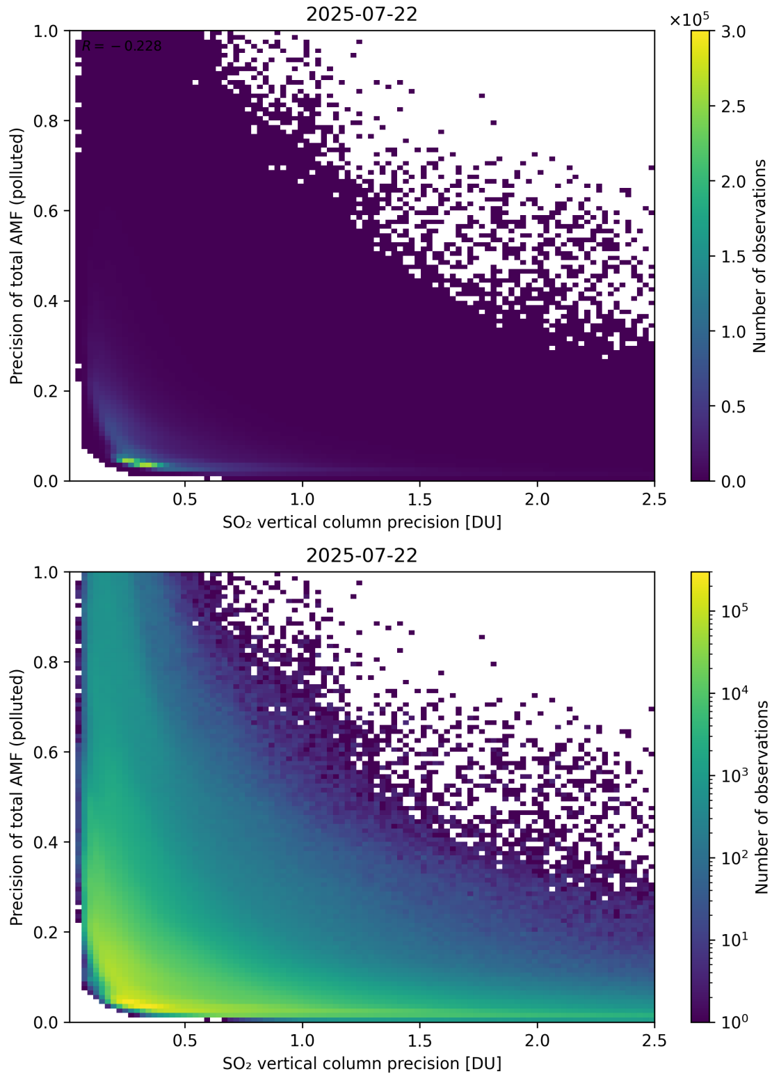
Figure 347: Scatter density plot of “SO 2 vertical column precision” against “Precision of total AMF (polluted)” for 2025-07-21 to 2025-07-23.
