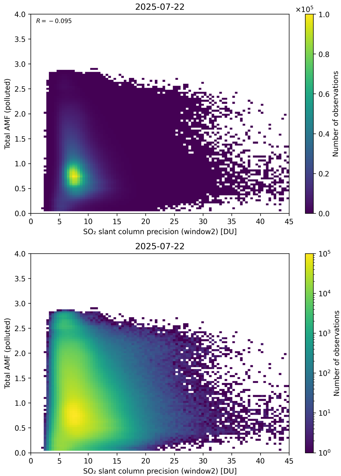
Figure 301: Scatter density plot of “SO 2 slant column precision (window2)” against “Total AMF (polluted)” for 2025-07-21 to 2025-07-23.
