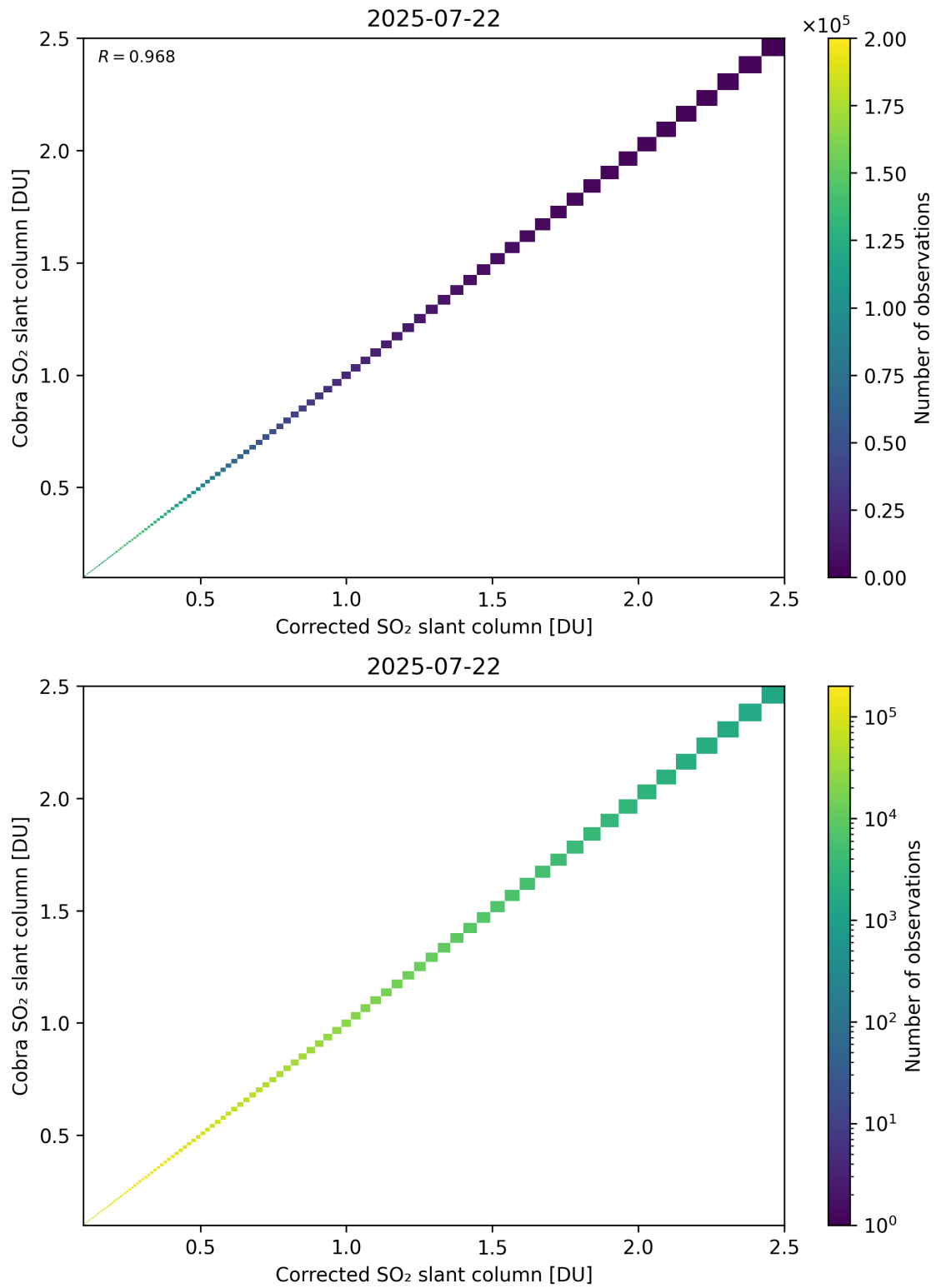
Figure 233: Scatter density plot of “Corrected SO 2 slant column” against “Cobra SO 2 slant column” for 2025-07-21 to 2025-07-23.
