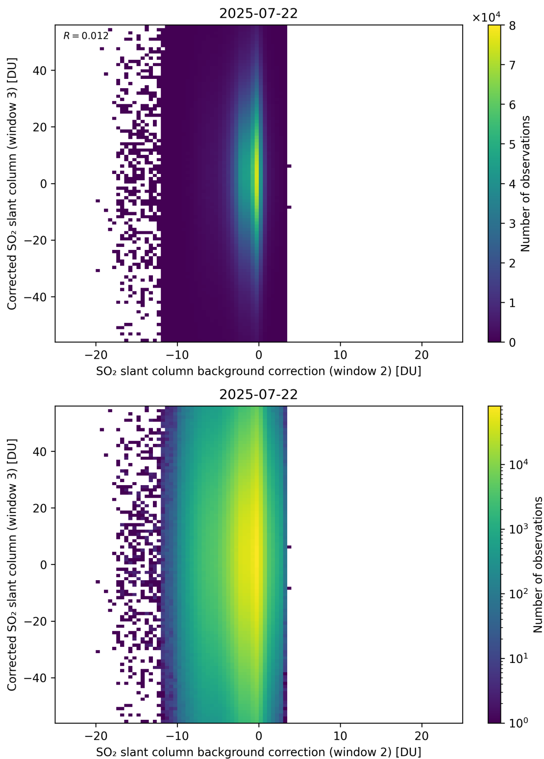
Figure 127: Scatter density plot of “SO 2 slant column background correction (window 2)” against “Corrected SO 2 slant column (window 3)” for 2025-07-21 to 2025-07-23.
