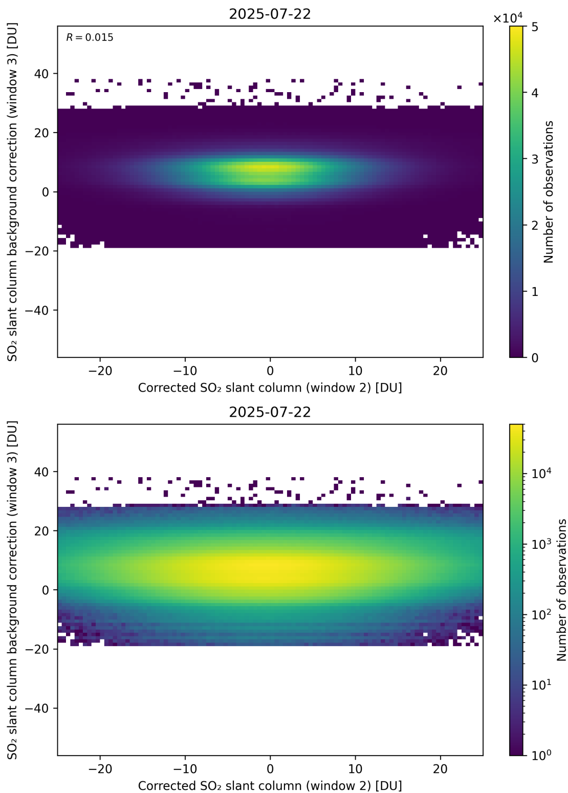
Figure 245: Scatter density plot of “Corrected SO 2 slant column (window 2)” against “SO 2 slant column background correction (window 3)” for 2025-07-21 to 2025-07-23.
