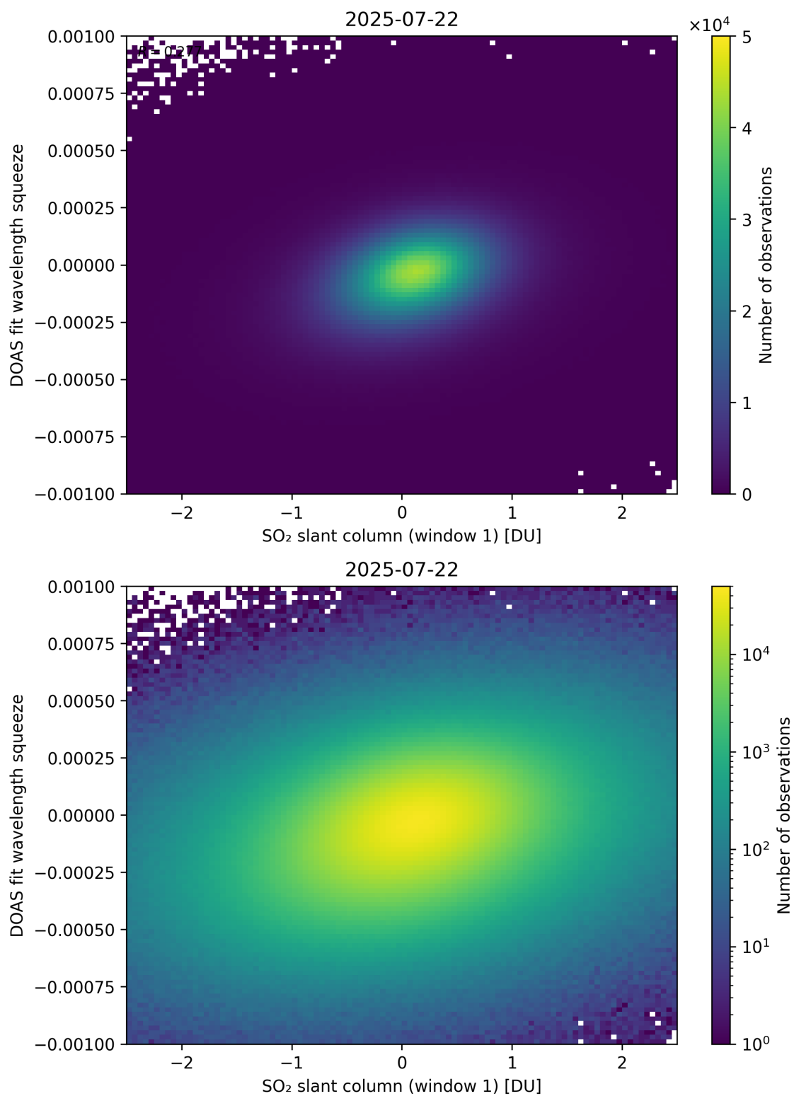
Figure 266: Scatter density plot of “SO 2 slant column (window 1)” against “DOAS fit wavelength squeeze” for 2025-07-21 to 2025-07-23.
