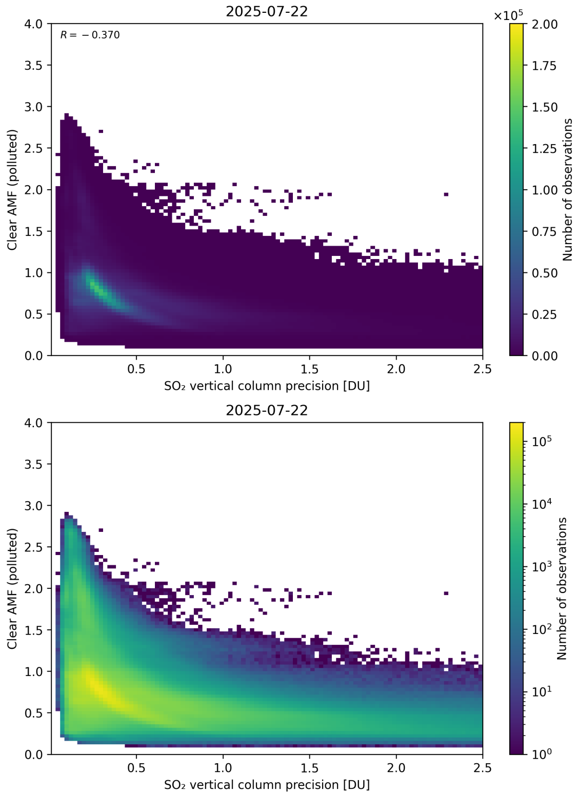
Figure 335: Scatter density plot of “SO 2 vertical column precision” against “Clear AMF (polluted)” for 2025-07-21 to 2025-07-23.
