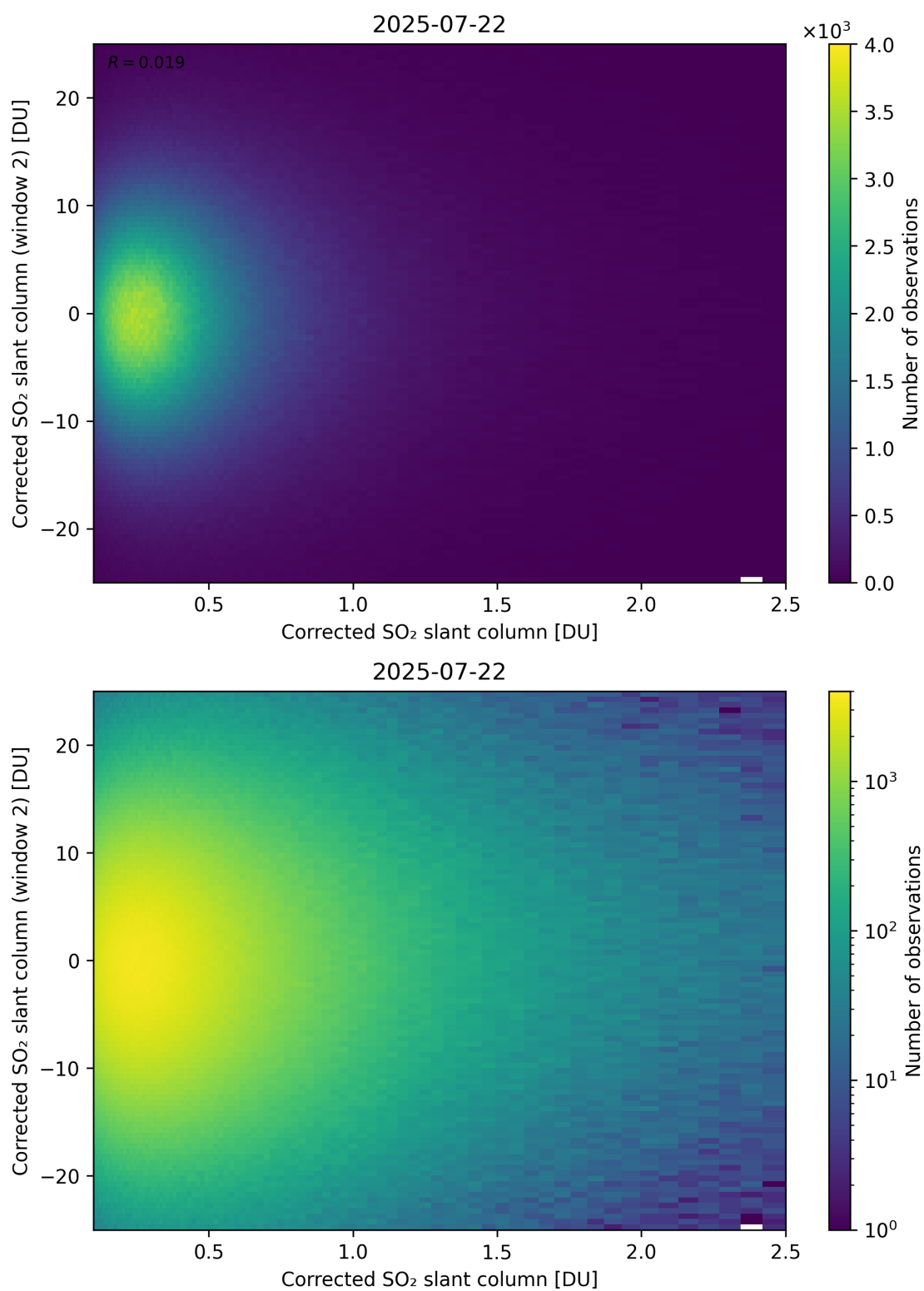
Figure 235: Scatter density plot of “Corrected SO 2 slant column” against “Corrected SO 2 slant column (window 2)” for 2025-07-21 to 2025-07-23.
