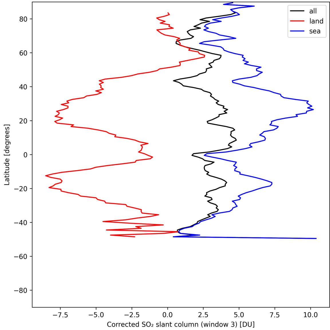
Figure 47: Zonal average of “Corrected SO 2 slant column (window 3)” for 2025-07-21 to 2025-07-23.
