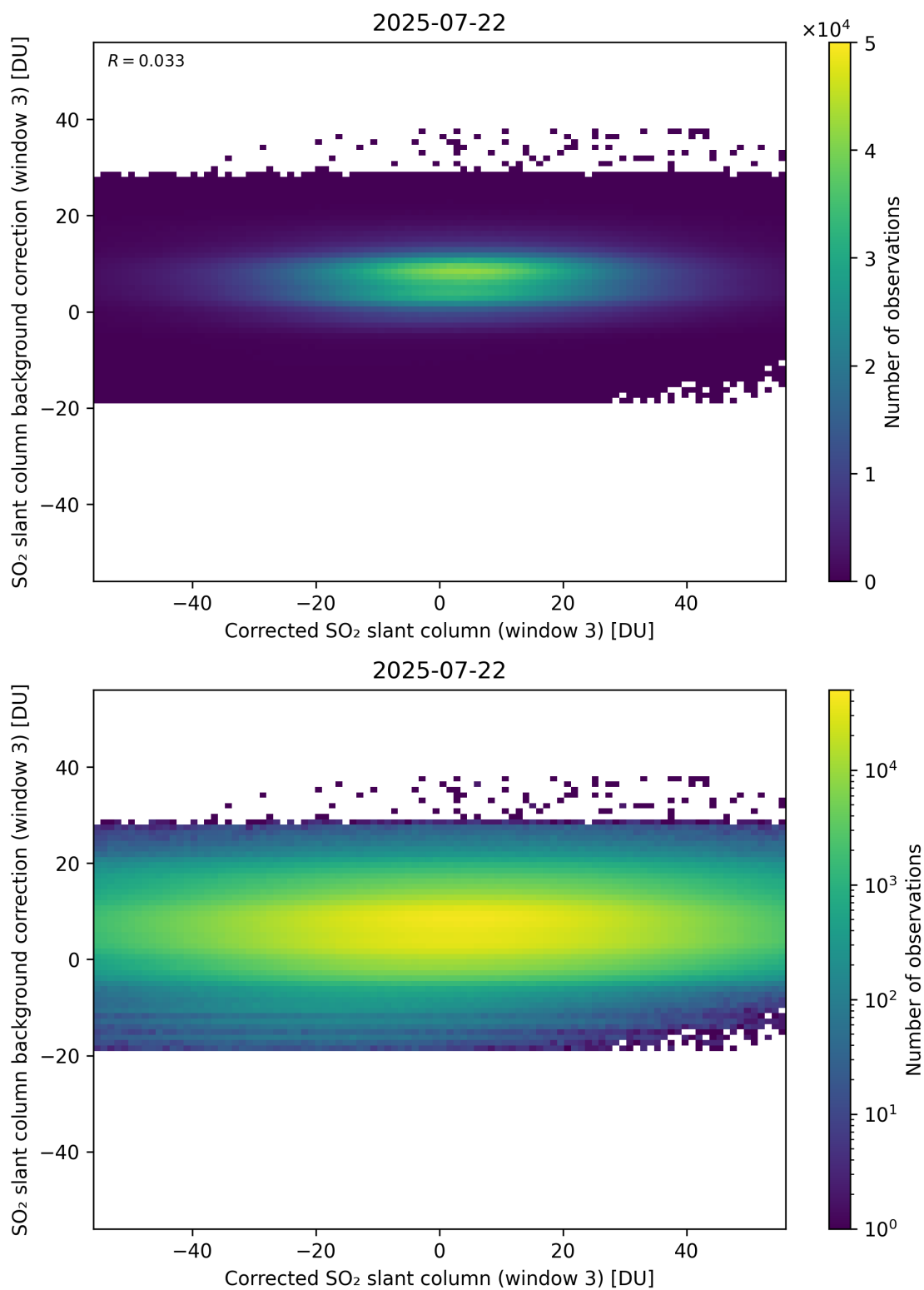
Figure 255: Scatter density plot of “Corrected SO 2 slant column (window 3)” against “SO 2 slant column background correction (window 3)” for 2025-07-21 to 2025-07-23.
