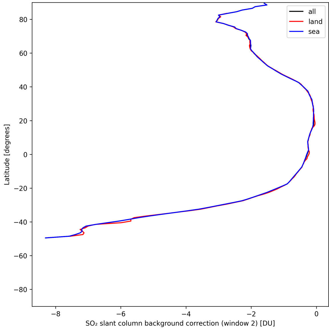
Figure 44: Zonal average of “SO 2 slant column background correction (window 2)” for 2025-07-21 to 2025-07-23.
