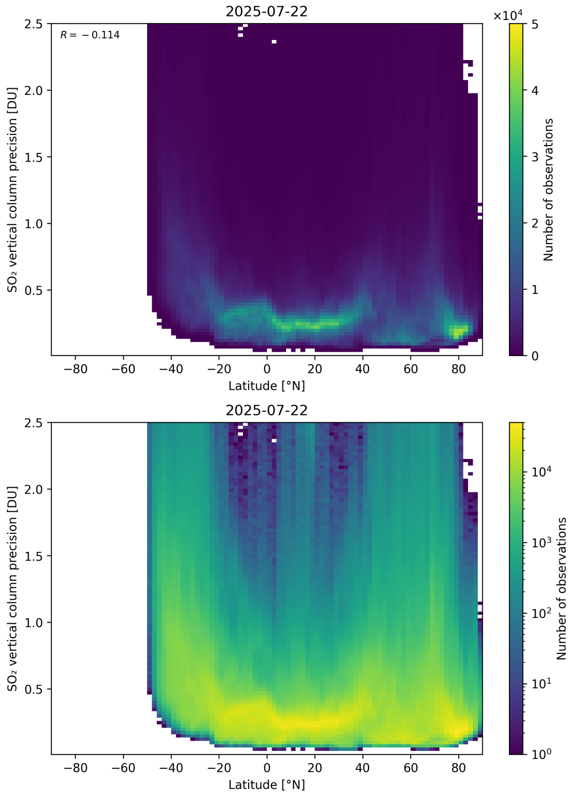
Figure 170: Scatter density plot of “Latitude” against “SO 2 vertical column precision” for 2025-07-21 to 2025-07-23.
