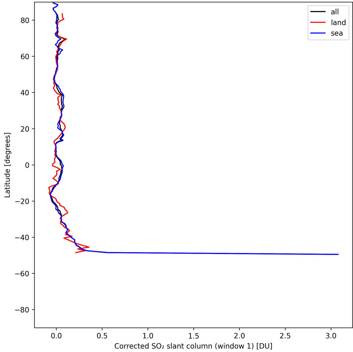
Figure 39: Zonal average of “Corrected SO 2 slant column (window 1)” for 2025-07-21 to 2025-07-23.
