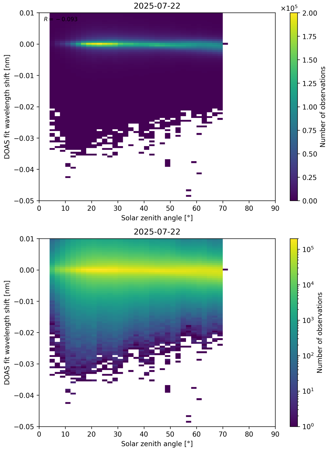
Figure 174: Scatter density plot of “Solar zenith angle” against “DOAS fit wavelength shift” for 2025-07-21 to 2025-07-23.
