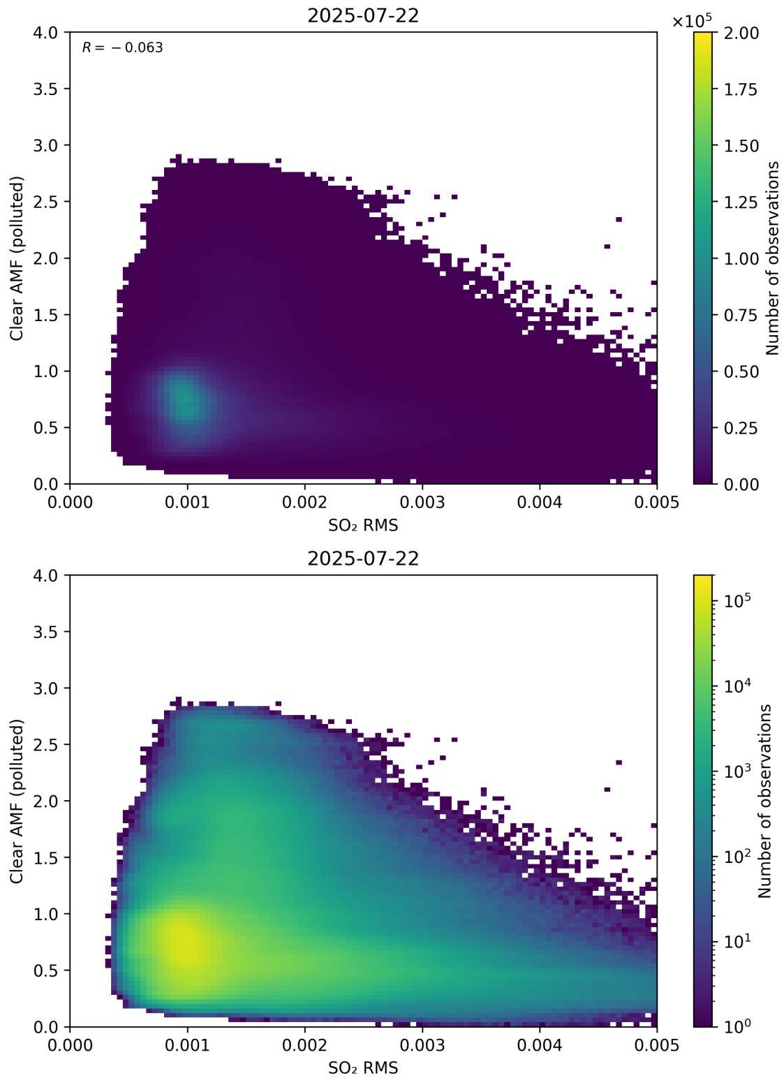
Figure 147: Scatter density plot of “SO 2 RMS” against “Clear AMF (polluted)” for 2025-07-21 to 2025-07-23.
