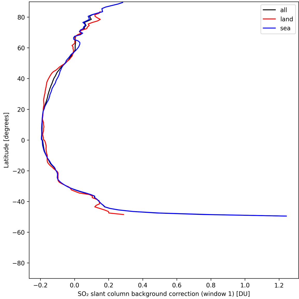
Figure 40: Zonal average of “SO 2 slant column background correction (window 1)” for 2025-07-21 to 2025-07-23.
