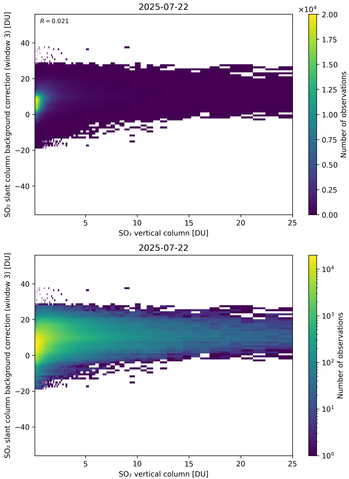
Figure 325: Scatter density plot of “SO 2 vertical column” against “SO 2 slant column background correction (window 3)” for 2025-07-21 to 2025-07-23.
