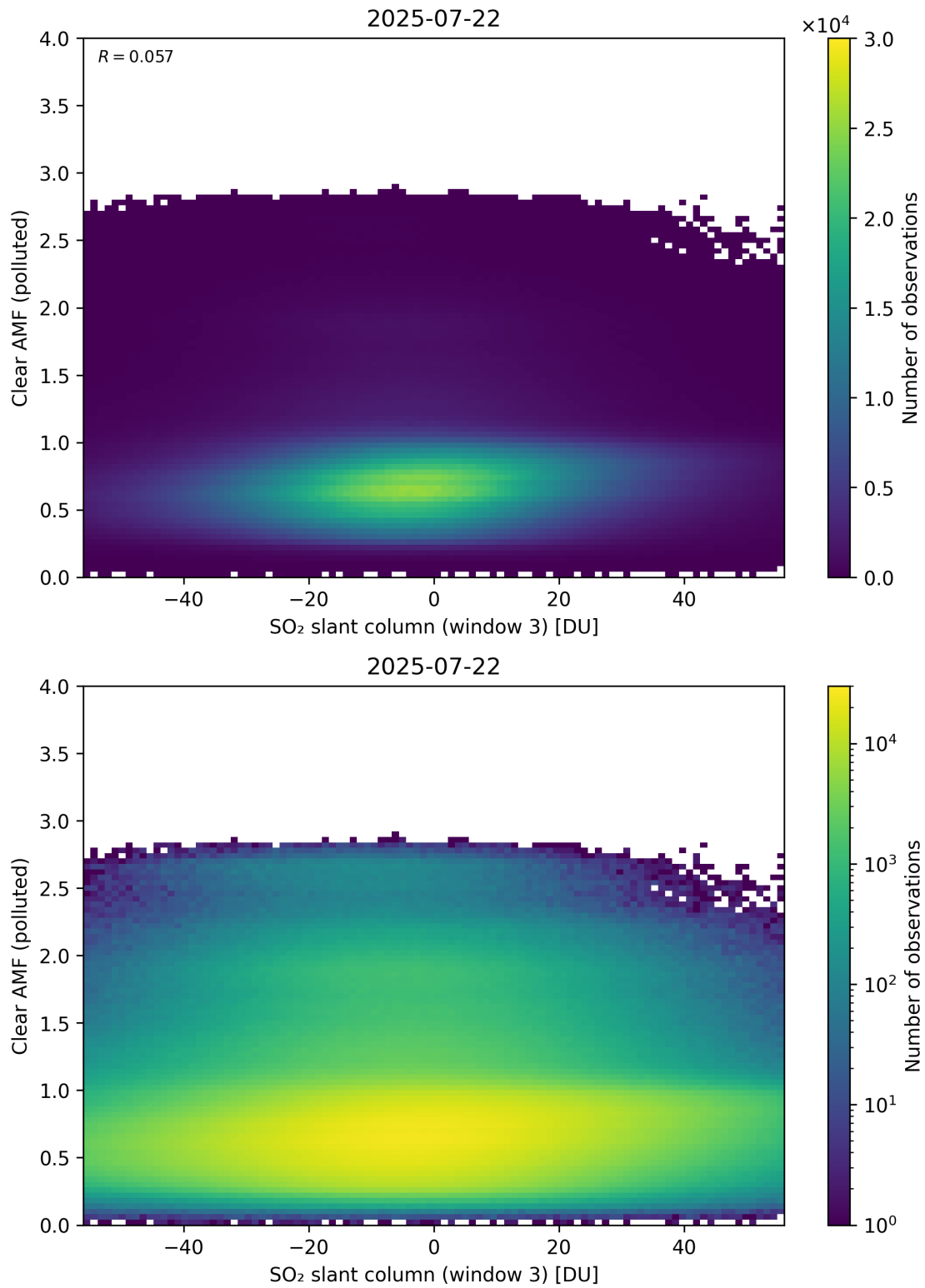
Figure 315: Scatter density plot of “SO 2 slant column (window 3)” against “Clear AMF (polluted)” for 2025-07-21 to 2025-07-23.
