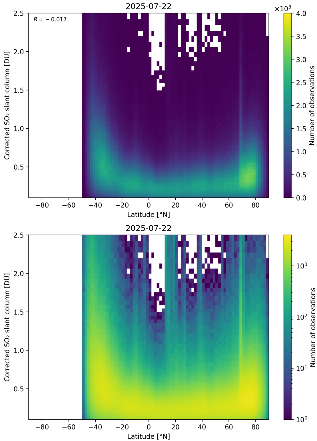
Figure 159: Scatter density plot of “Latitude” against “Corrected SO 2 slant column” for 2025-07-21 to 2025-07-23.
