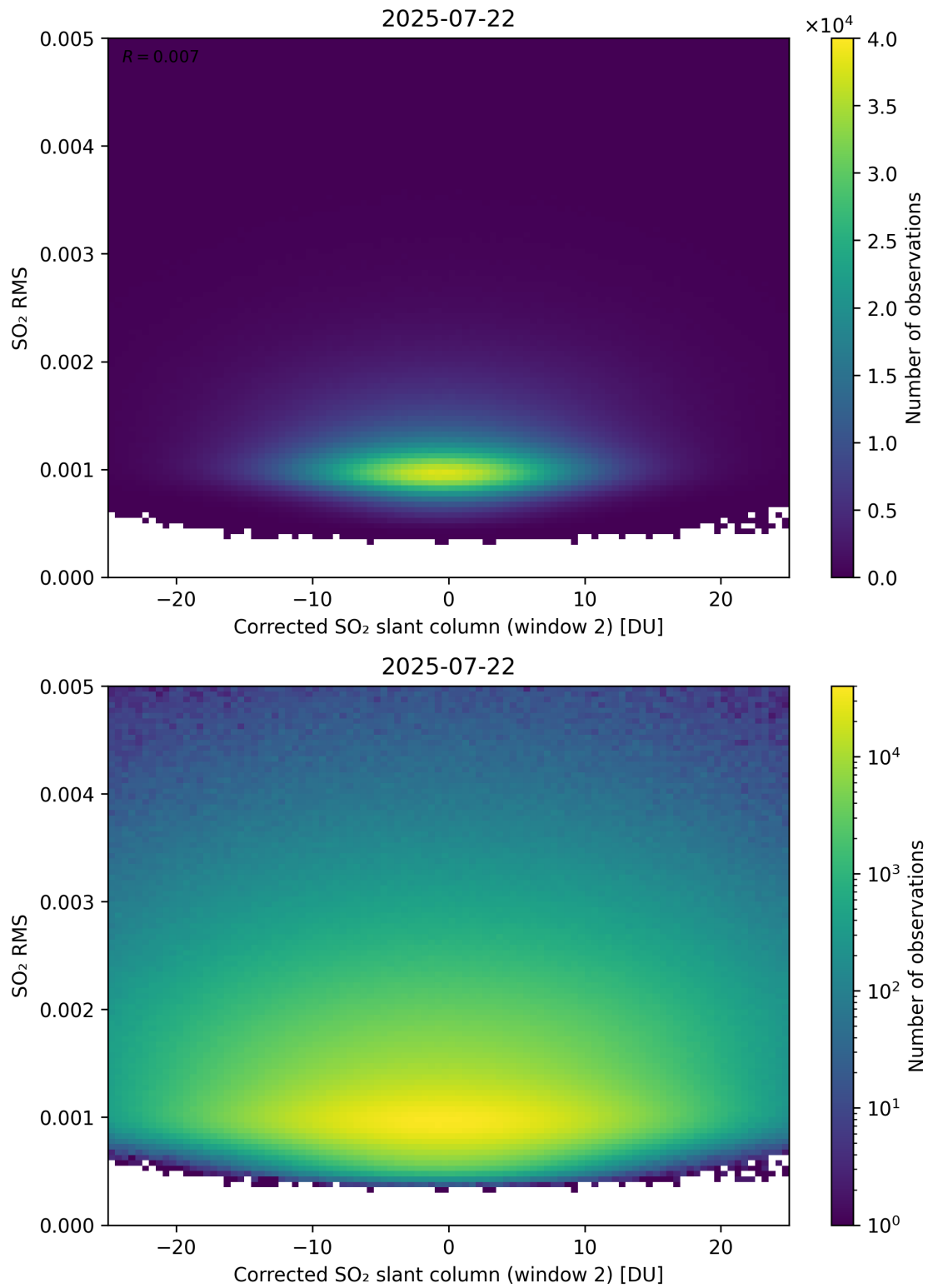
Figure 248: Scatter density plot of “Corrected SO 2 slant column (window 2)” against “SO 2 RMS” for 2025-07-21 to 2025-07-23.
