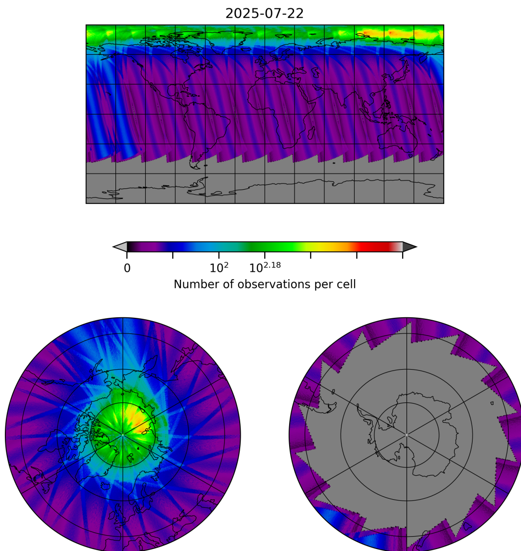
Figure 30: Map of the number of observations for 2025-07-21 to 2025-07-23
