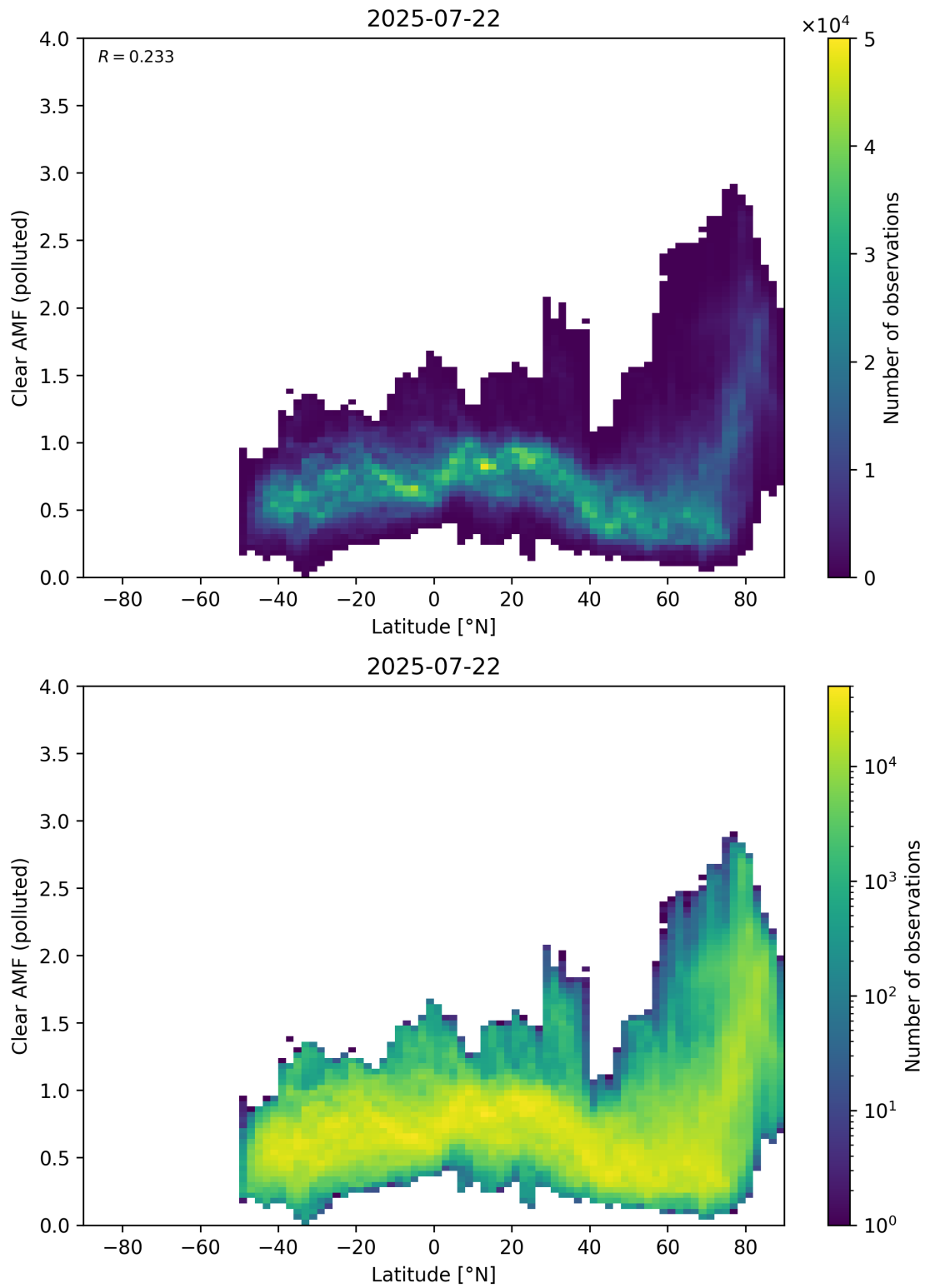
Figure 156: Scatter density plot of “Latitude” against “Clear AMF (polluted)” for 2025-07-21 to 2025-07-23.
