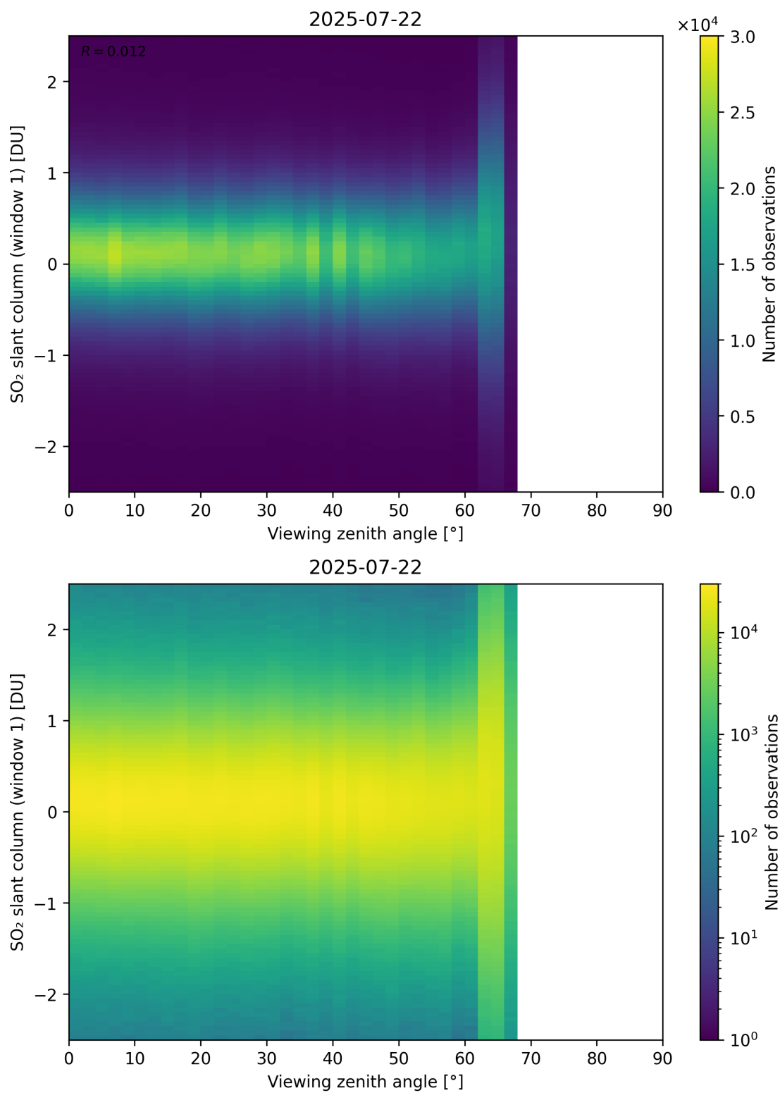
Figure 376: Scatter density plot of “Viewing zenith angle” against “SO 2 slant column (window 1)” for 2025-07-21 to 2025-07-23.
