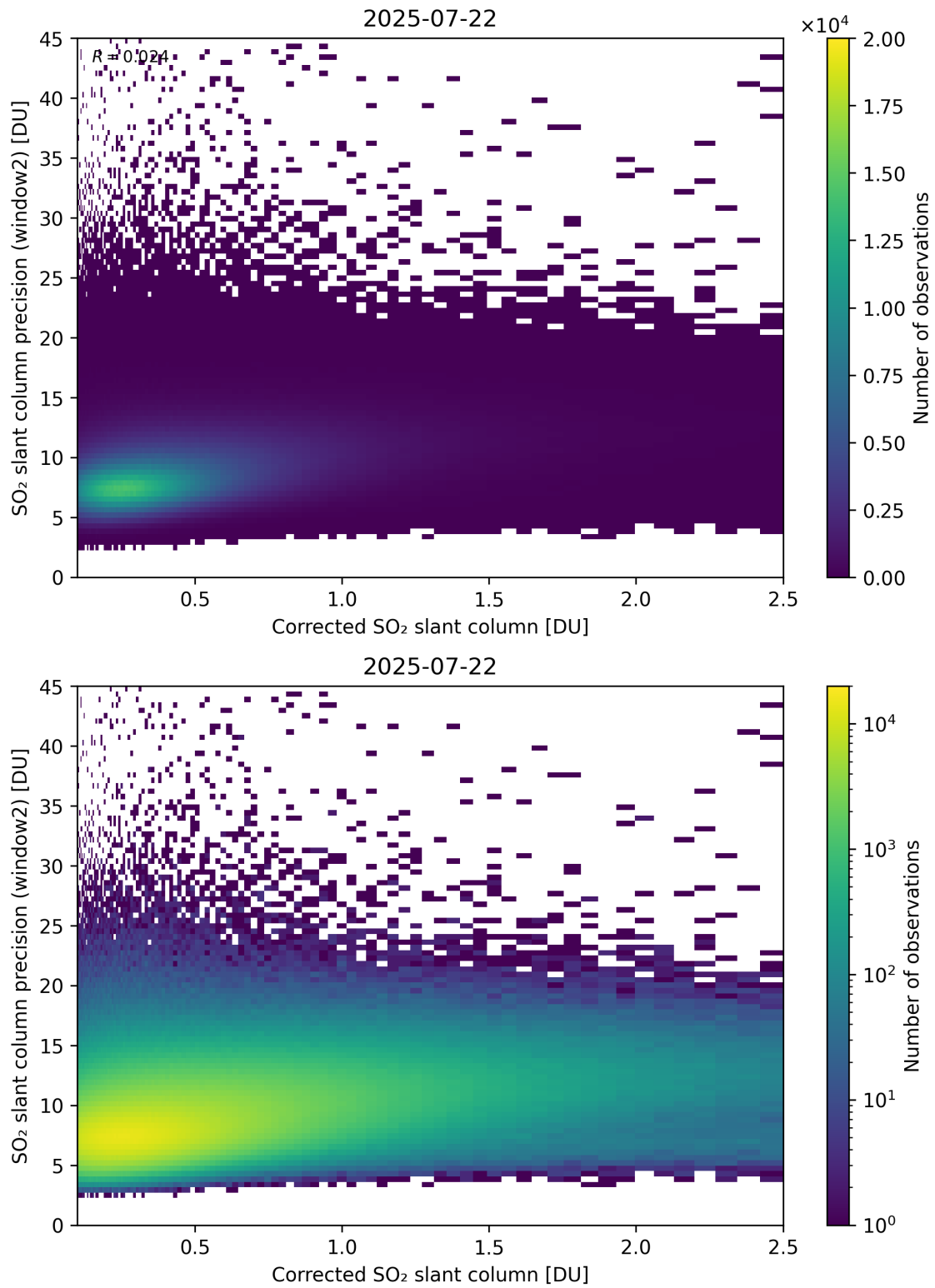
Figure 239: Scatter density plot of “Corrected SO 2 slant column” against “SO 2 slant column precision (window2)” for 2025-07-21 to 2025-07-23.
