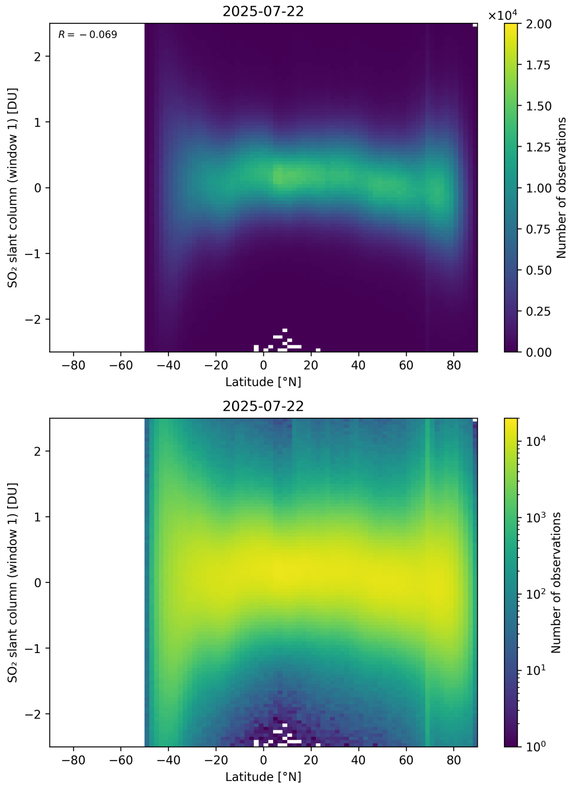
Figure 162: Scatter density plot of “Latitude” against “SO 2 slant column (window 1)” for 2025-07-21 to 2025-07-23.
