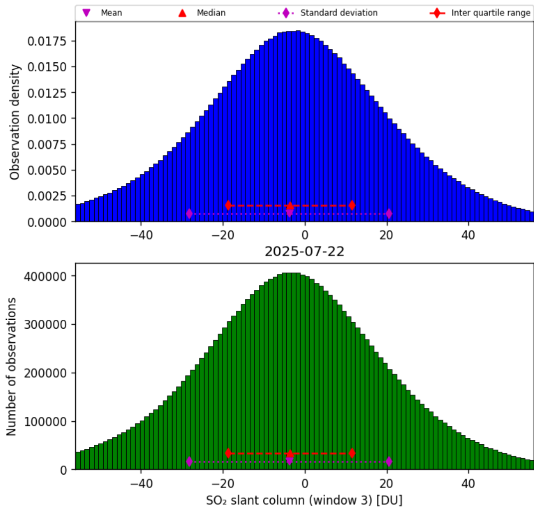
Figure 71: Histogram of “SO 2 slant column (window 3)” for 2025-07-21 to 2025-07-23
