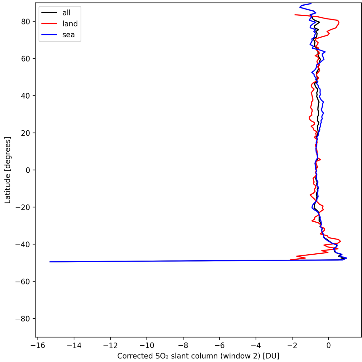
Figure 43: Zonal average of “Corrected SO 2 slant column (window 2)” for 2025-07-21 to 2025-07-23.
