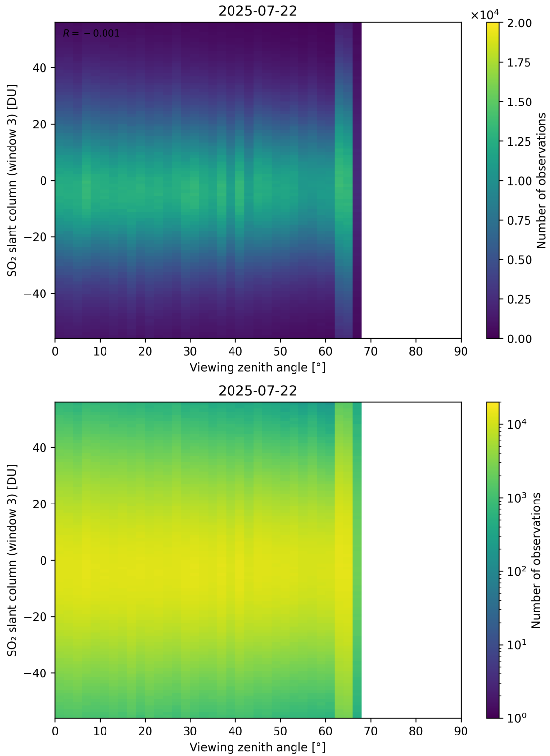
Figure 379: Scatter density plot of “Viewing zenith angle” against “SO 2 slant column (window 3)” for 2025-07-21 to 2025-07-23.
