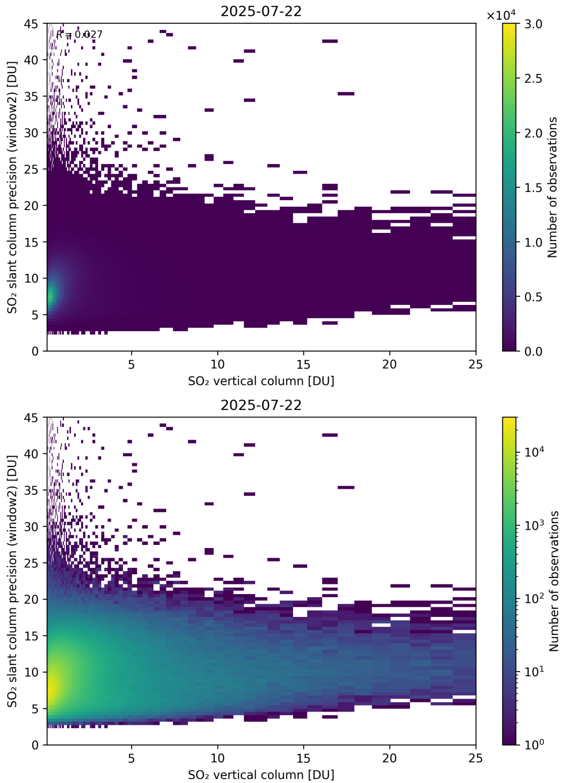
Figure 356: Scatter density plot of “SO 2 vertical column” against “SO 2 slant column precision (window2)” for 2025-07-21 to 2025-07-23.
