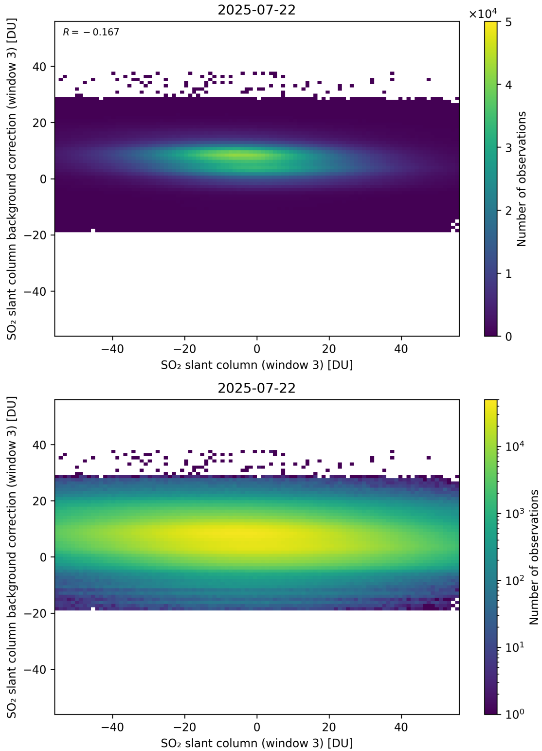
Figure 303: Scatter density plot of “SO 2 slant column (window 3)” against “SO 2 slant column background correction (window 3)” for 2025-07-21 to 2025-07-23.
