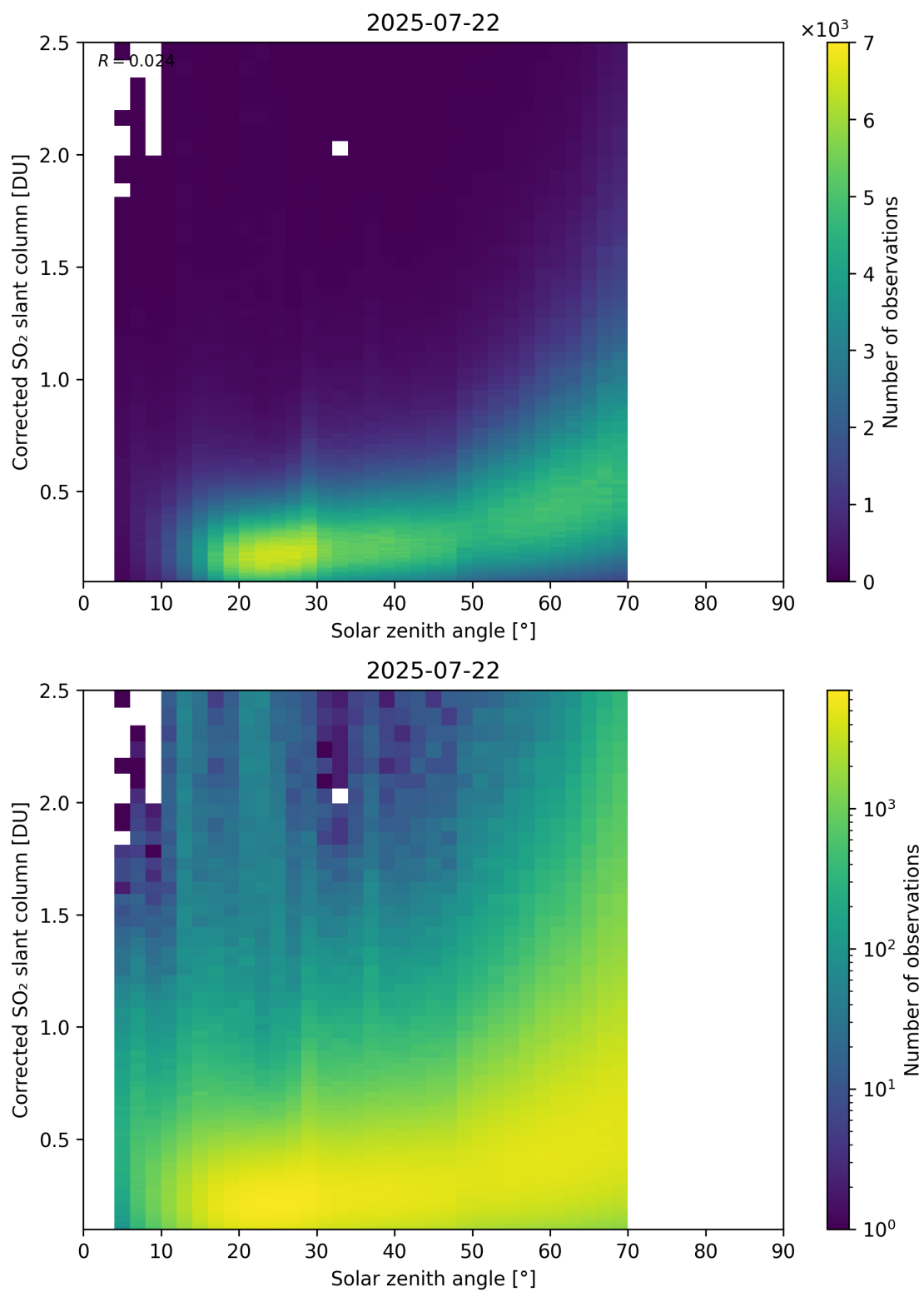
Figure 181: Scatter density plot of “Solar zenith angle” against “Corrected SO 2 slant column” for 2025-07-21 to 2025-07-23.
