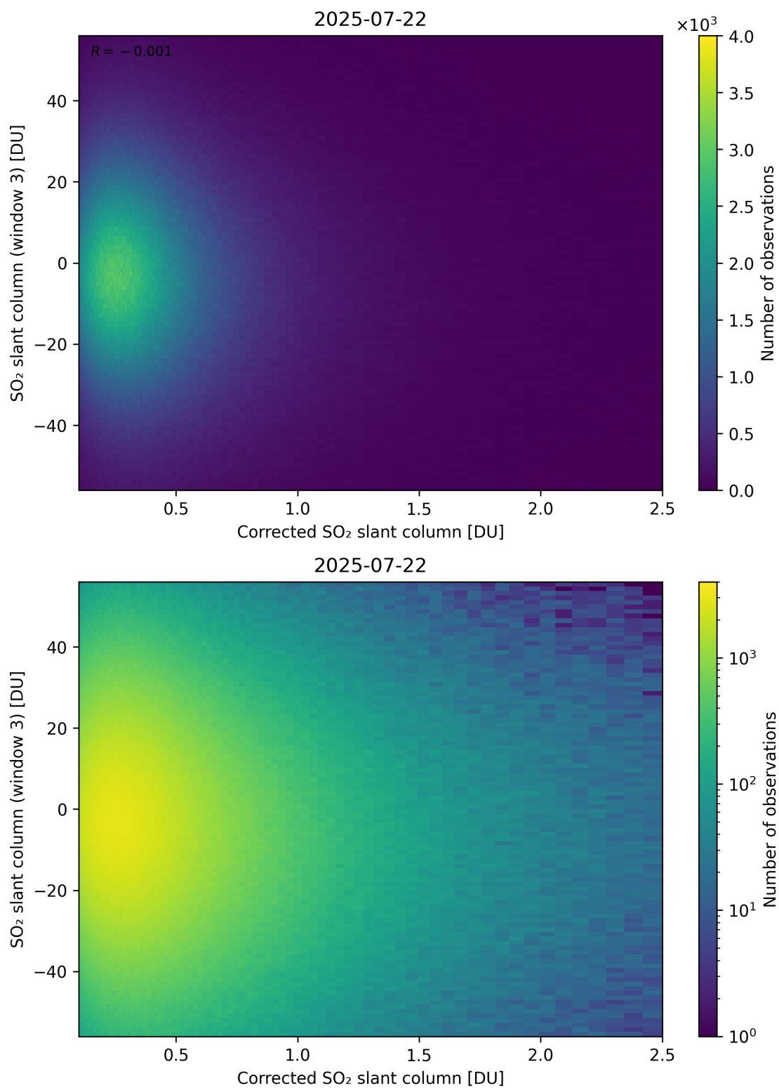
Figure 240: Scatter density plot of “Corrected SO 2 slant column” against “SO 2 slant column (window 3)” for 2025-07-21 to 2025-07-23.
