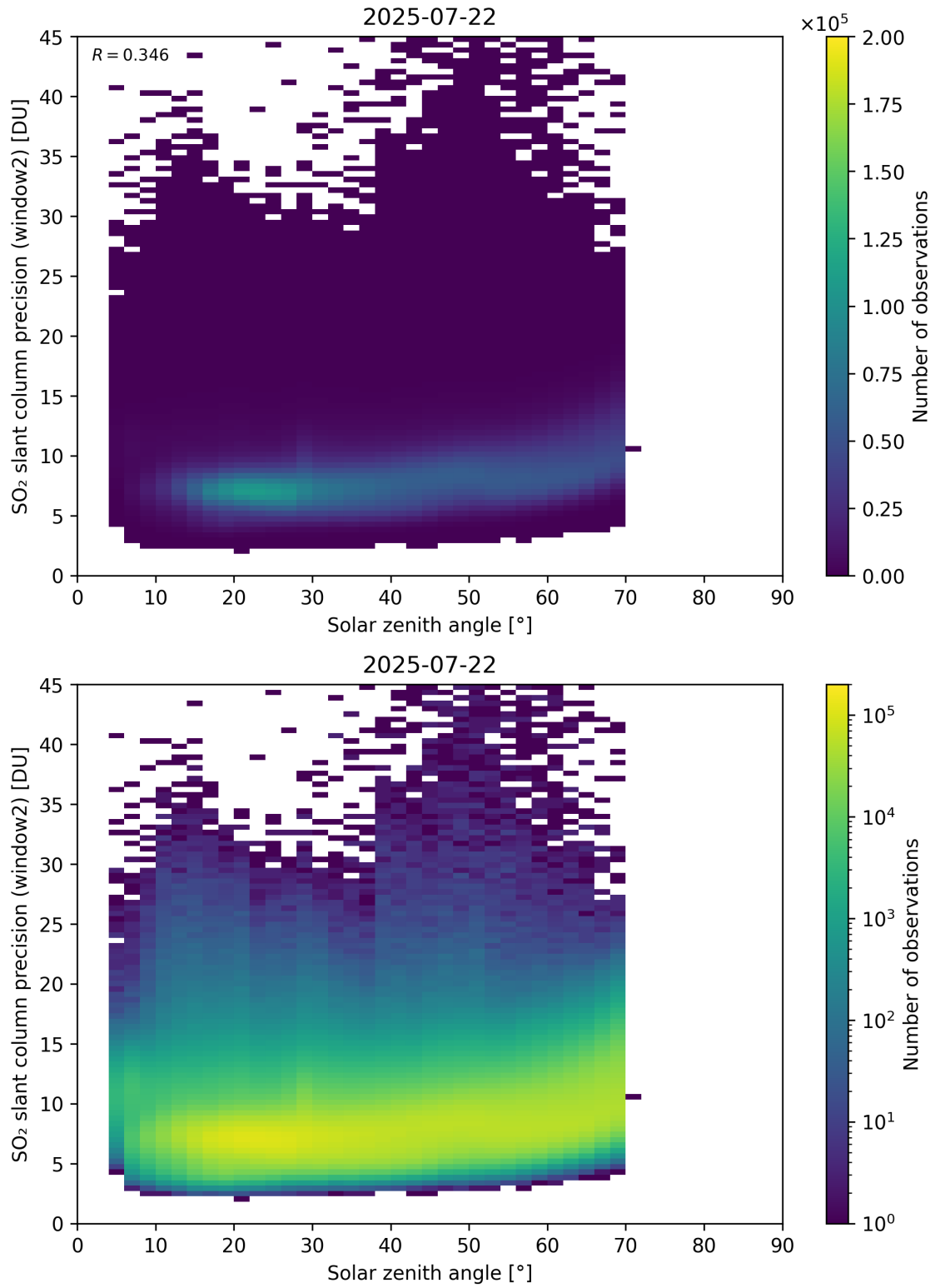
Figure 186: Scatter density plot of “Solar zenith angle” against “SO 2 slant column precision (window2)” for 2025-07-21 to 2025-07-23.
