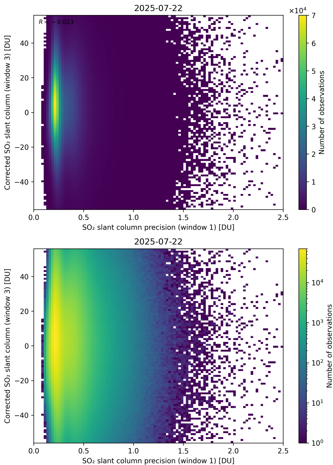
Figure 276: Scatter density plot of “SO 2 slant column precision (window 1)” against “Corrected SO 2 slant column (window 3)” for 2025-07-21 to 2025-07-23.
