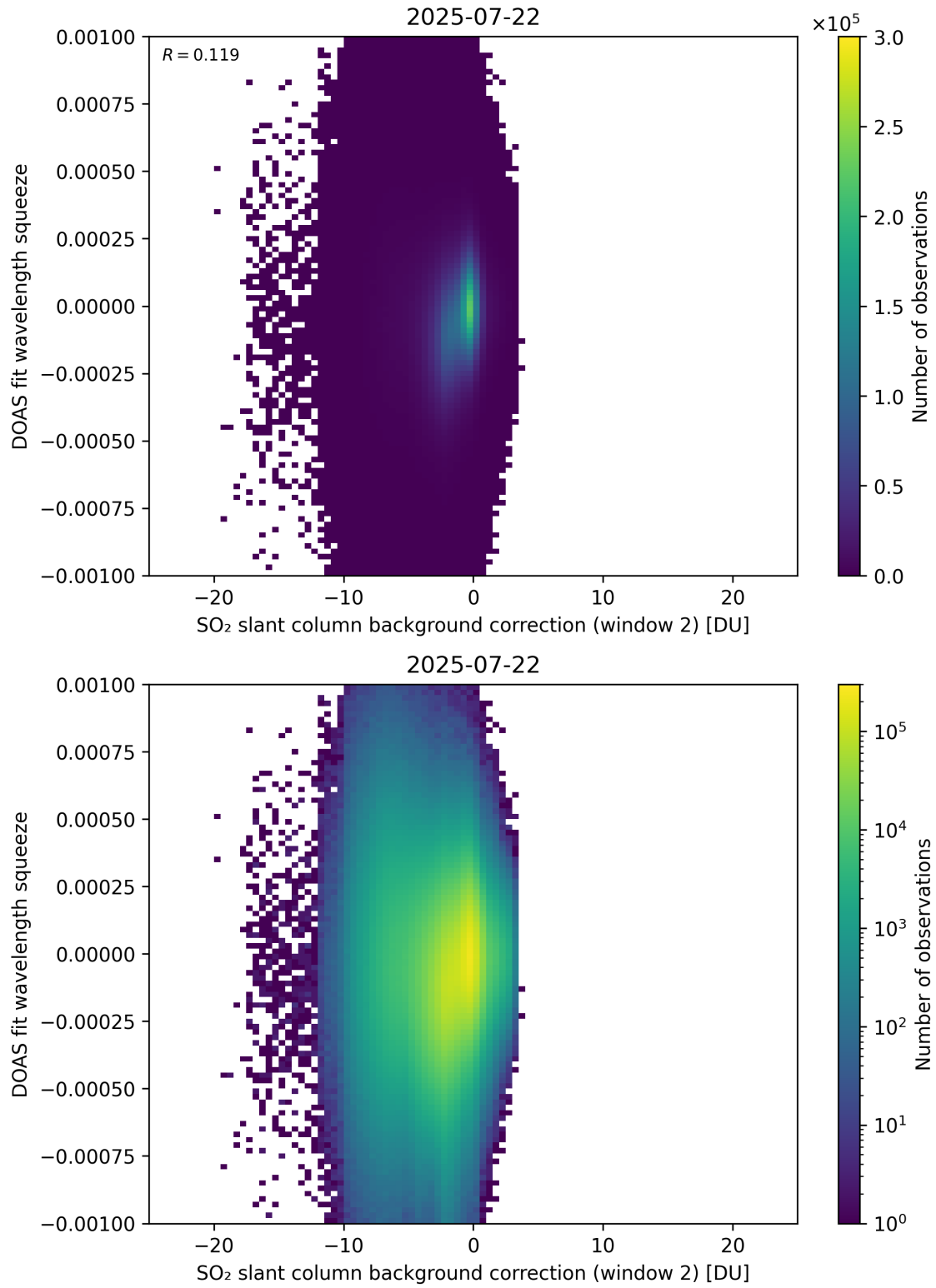
Figure 124: Scatter density plot of “SO 2 slant column background correction (window 2)” against “DOAS fit wavelength squeeze” for 2025-07-21 to 2025-07-23.
