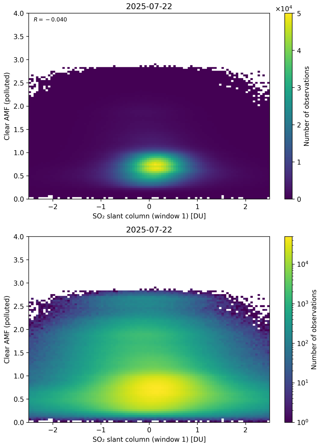
Figure 282: Scatter density plot of “SO 2 slant column (window 1)” against “Clear AMF (polluted)” for 2025-07-21 to 2025-07-23.
