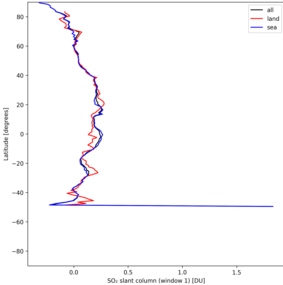
Figure 37: Zonal average of “SO 2 slant column (window 1)” for 2025-07-21 to 2025-07-23.
