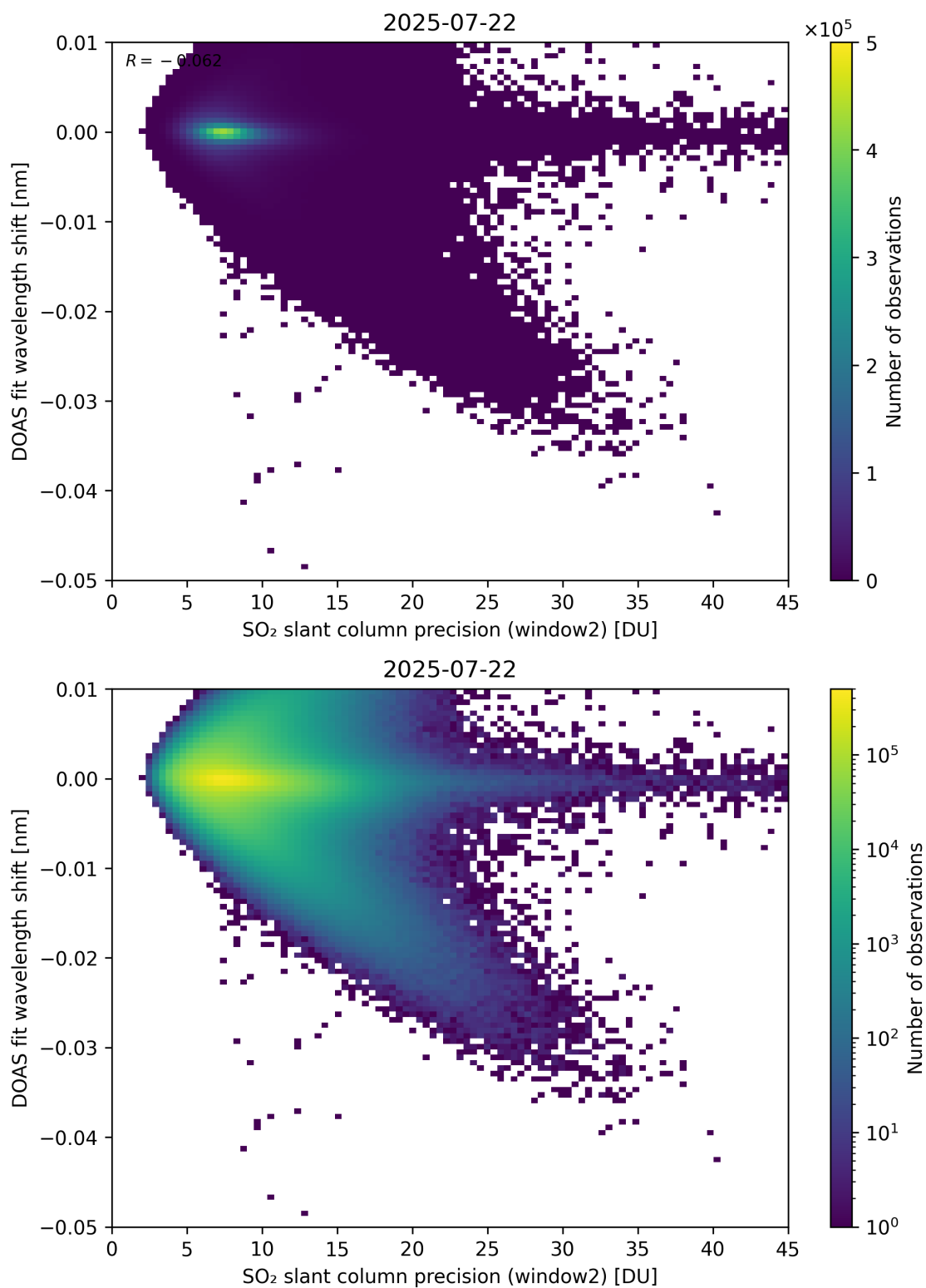
Figure 293: Scatter density plot of “SO 2 slant column precision (window2)” against “DOAS fit wavelength shift” for 2025-07-21 to 2025-07-23.
