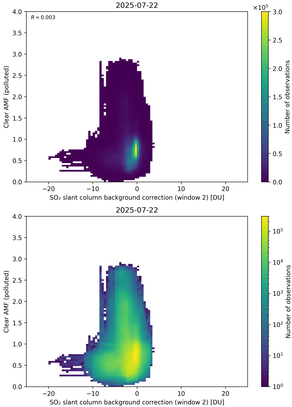
Figure 126: Scatter density plot of “SO 2 slant column background correction (window 2)” against “Clear AMF (polluted)” for 2025-07-21 to 2025-07-23.
