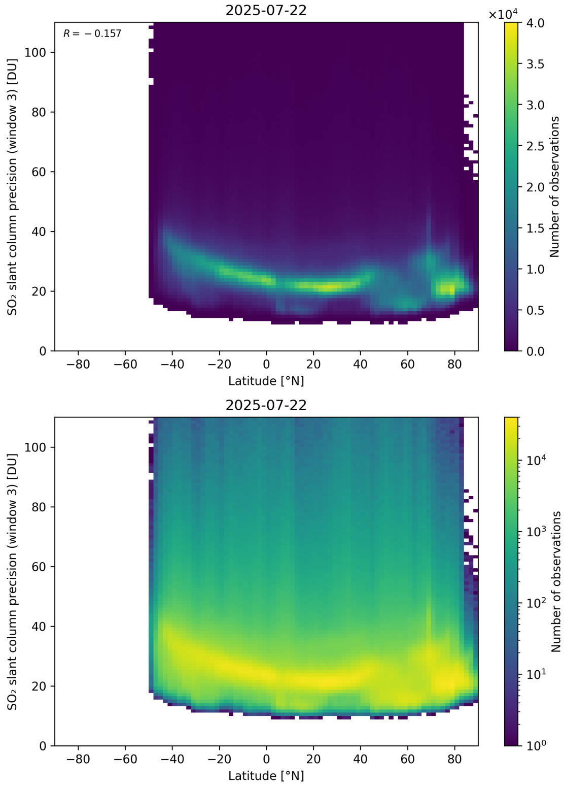
Figure 166: Scatter density plot of “Latitude” against “SO 2 slant column precision (window 3)” for 2025-07-21 to 2025-07-23.
