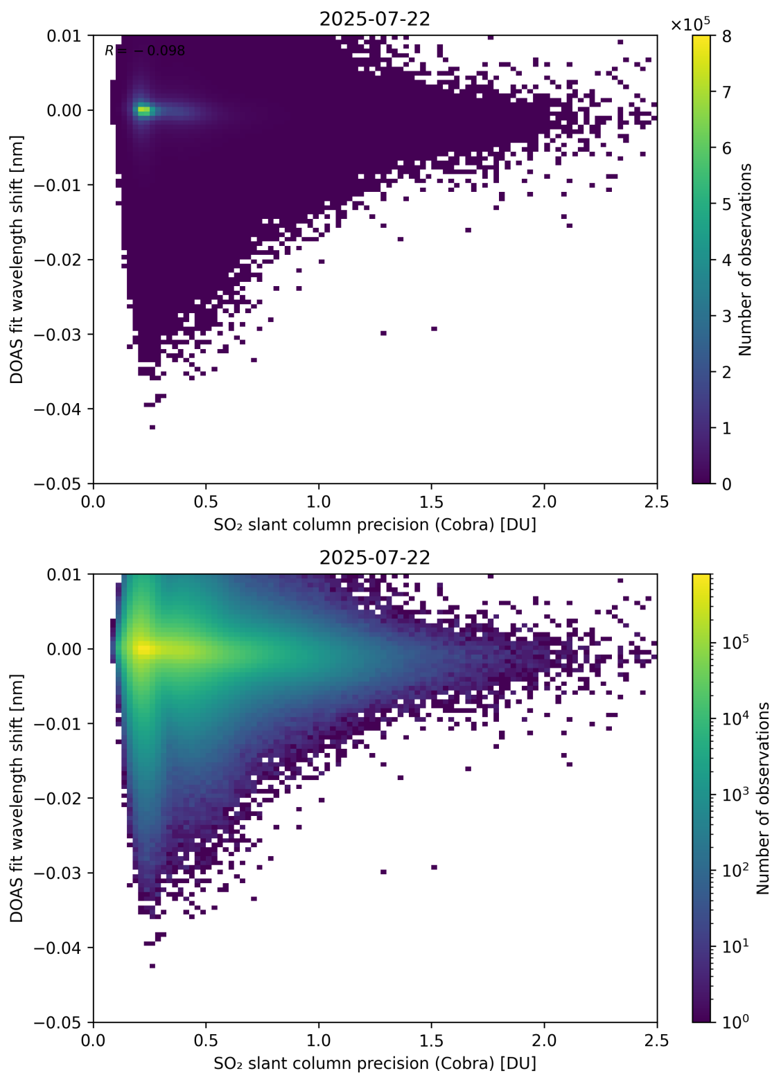
Figure 202: Scatter density plot of “SO 2 slant column precision (Cobra)” against “DOAS fit wavelength shift” for 2025-07-21 to 2025-07-23.
