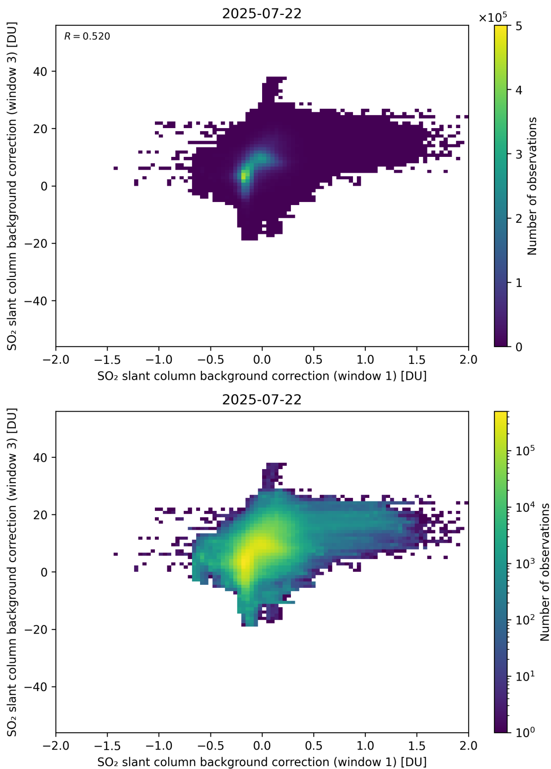
Figure 110: Scatter density plot of “SO 2 slant column background correction (window 1)” against “SO 2 slant column background correction (window 3)” for 2025-07-21 to 2025-07-23.
