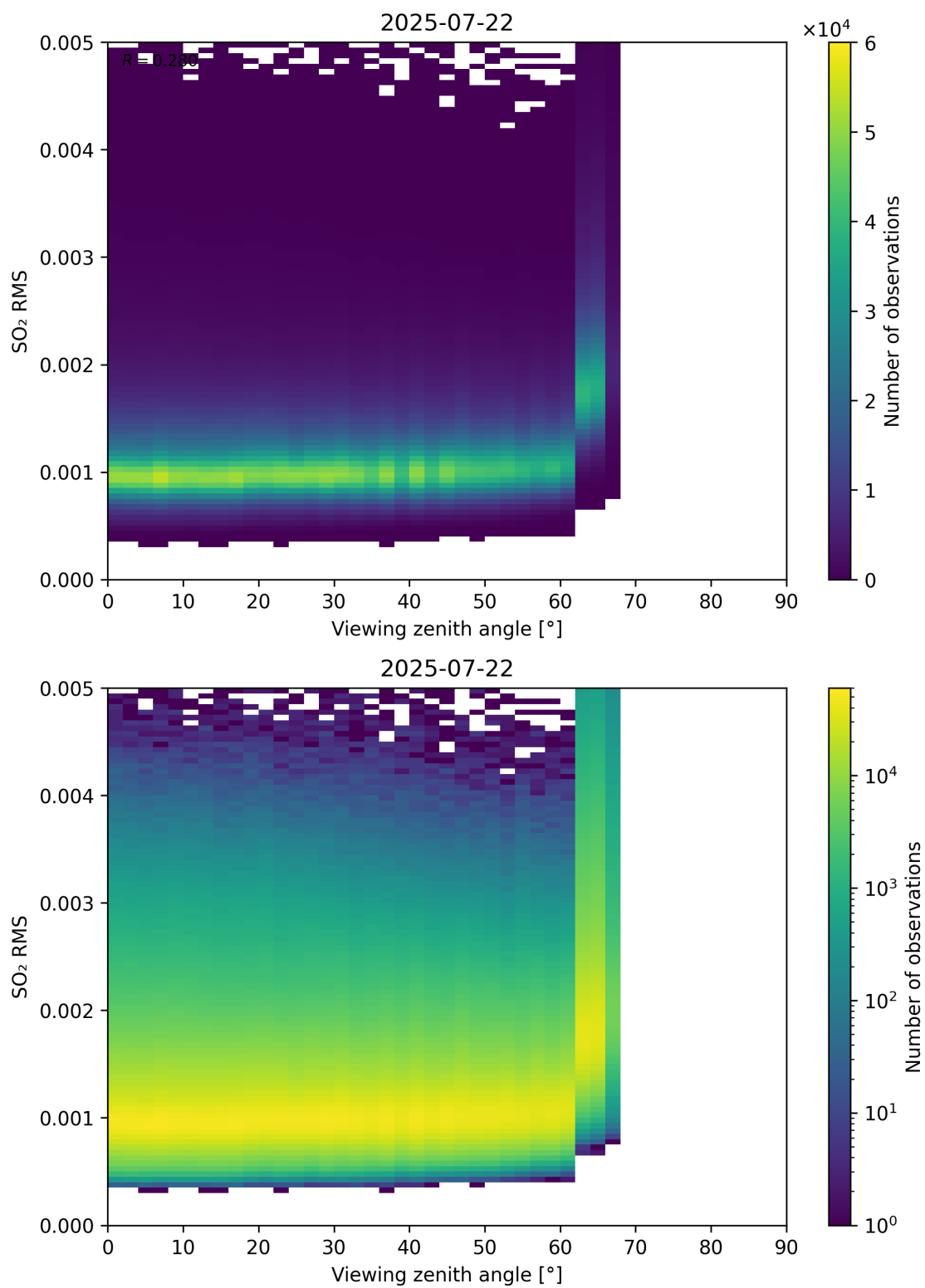
Figure 367: Scatter density plot of “Viewing zenith angle” against “SO 2 RMS” for 2025-07-21 to 2025-07-23.
