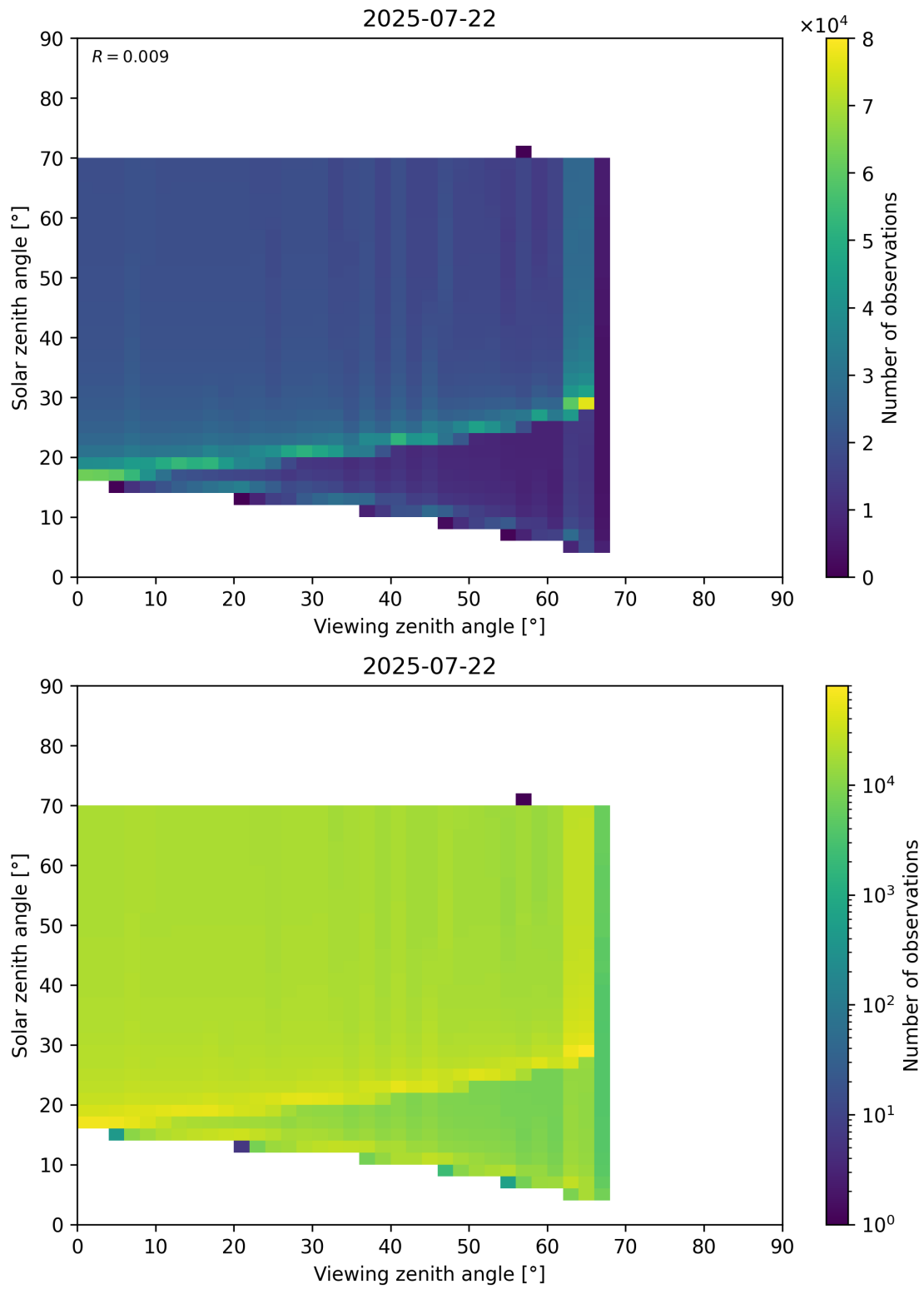
Figure 369: Scatter density plot of “Viewing zenith angle” against “Solar zenith angle” for 2025-07-21 to 2025-07-23.
