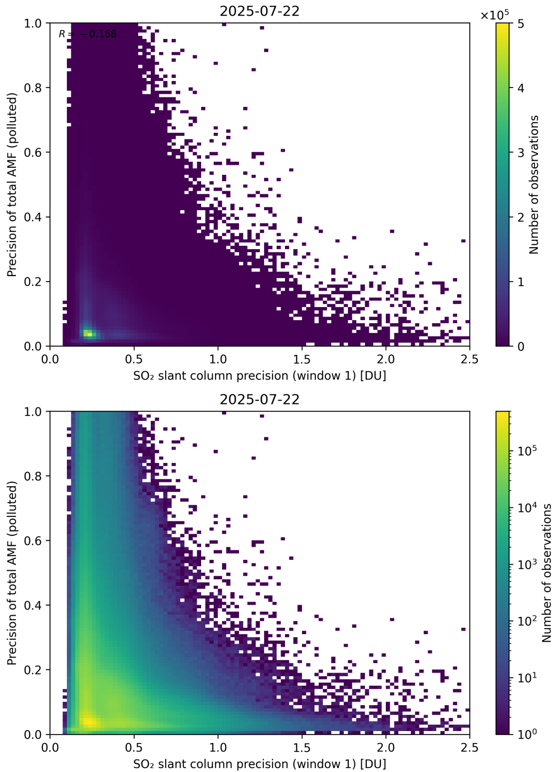
Figure 281: Scatter density plot of “SO 2 slant column precision (window 1)” against “Precision of total AMF (polluted)” for 2025-07-21 to 2025-07-23.
