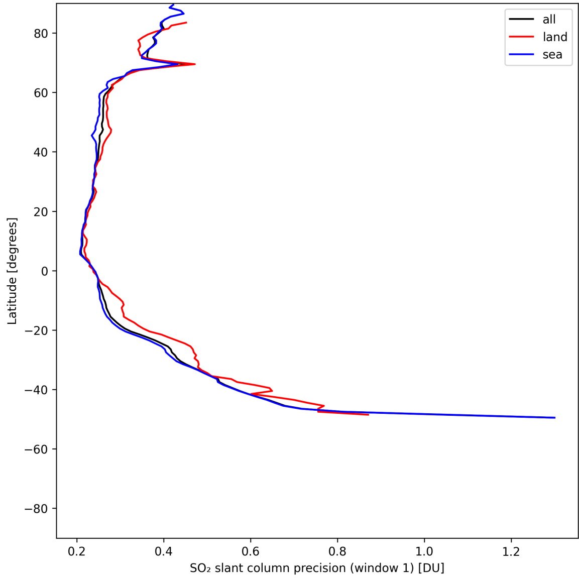
Figure 38: Zonal average of “SO 2 slant column precision (window 1)” for 2025-07-21 to 2025-07-23.
