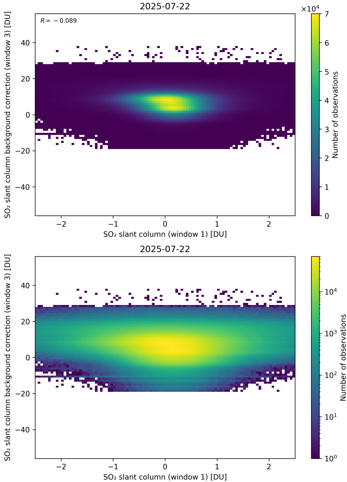
Figure 264: Scatter density plot of “SO 2 slant column (window 1)” against “SO 2 slant column background correction (window 3)” for 2025-07-21 to 2025-07-23.
