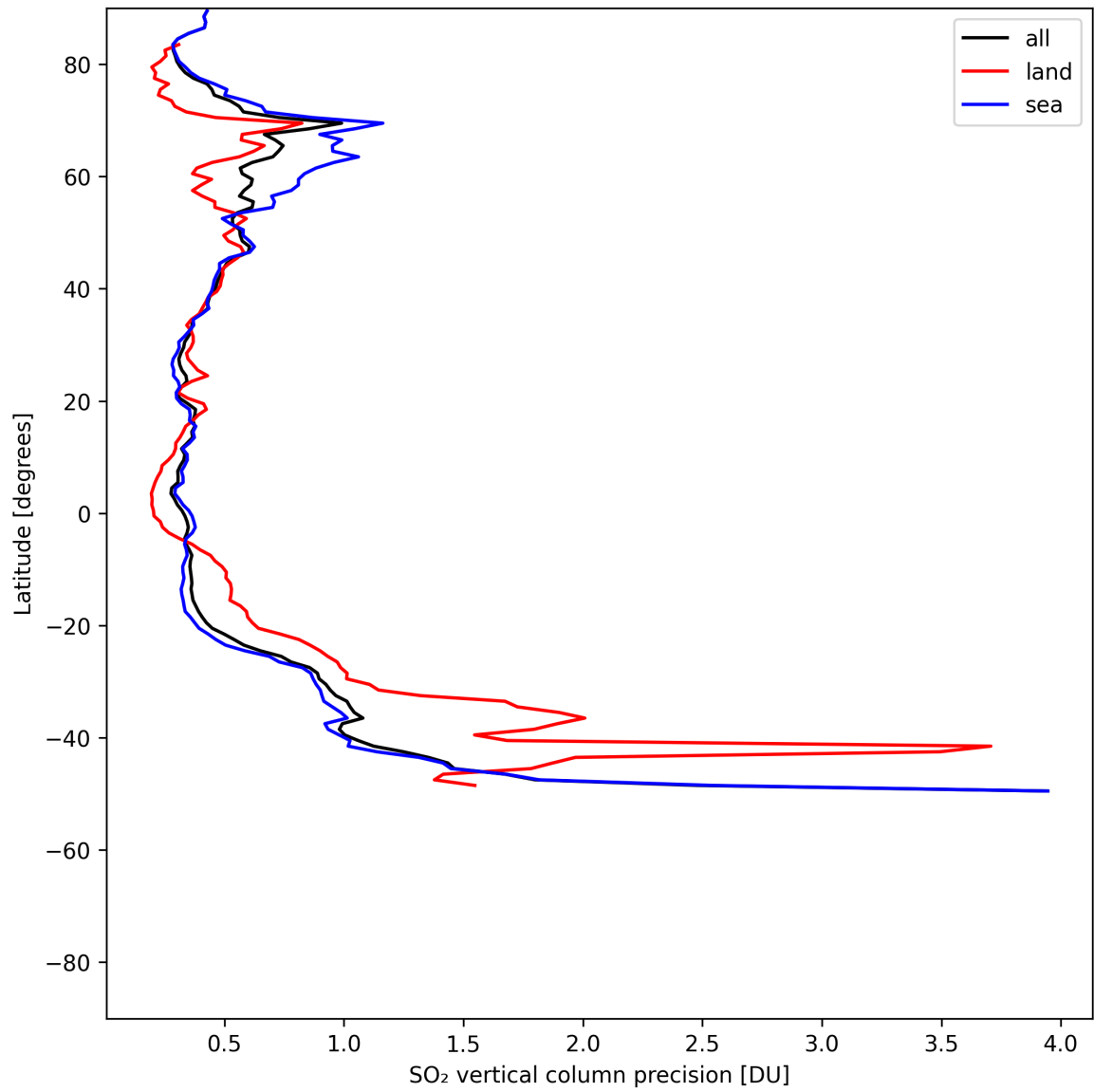
Figure 33: Zonal average of “SO 2 vertical column precision” for 2025-07-21 to 2025-07-23.
