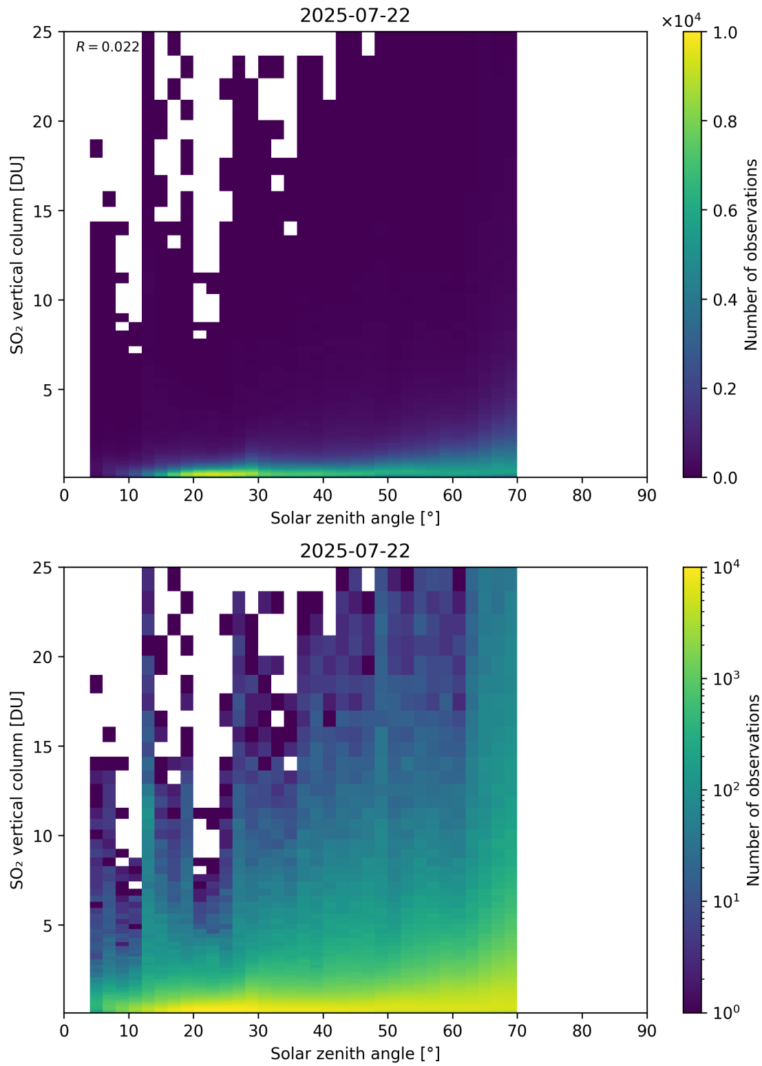
Figure 191: Scatter density plot of “Solar zenith angle” against “SO 2 vertical column” for 2025-07-21 to 2025-07-23.
