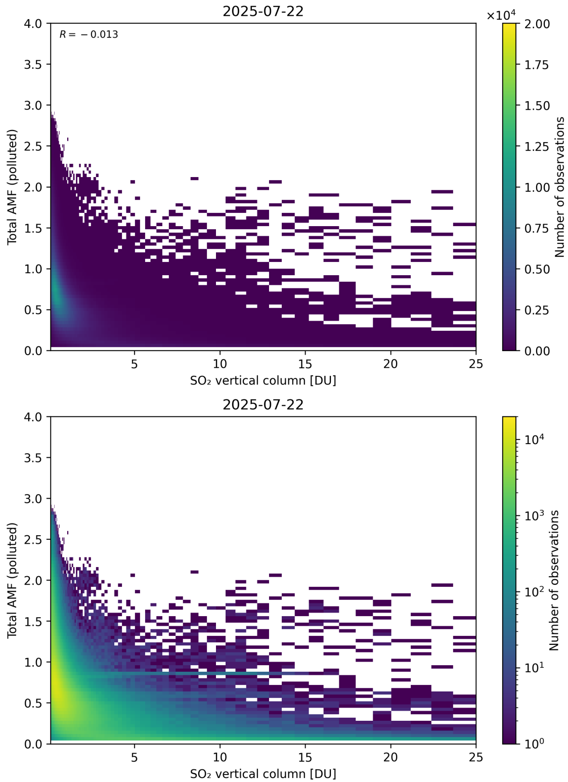
Figure 359: Scatter density plot of “SO 2 vertical column” against “Total AMF (polluted)” for 2025-07-21 to 2025-07-23.
