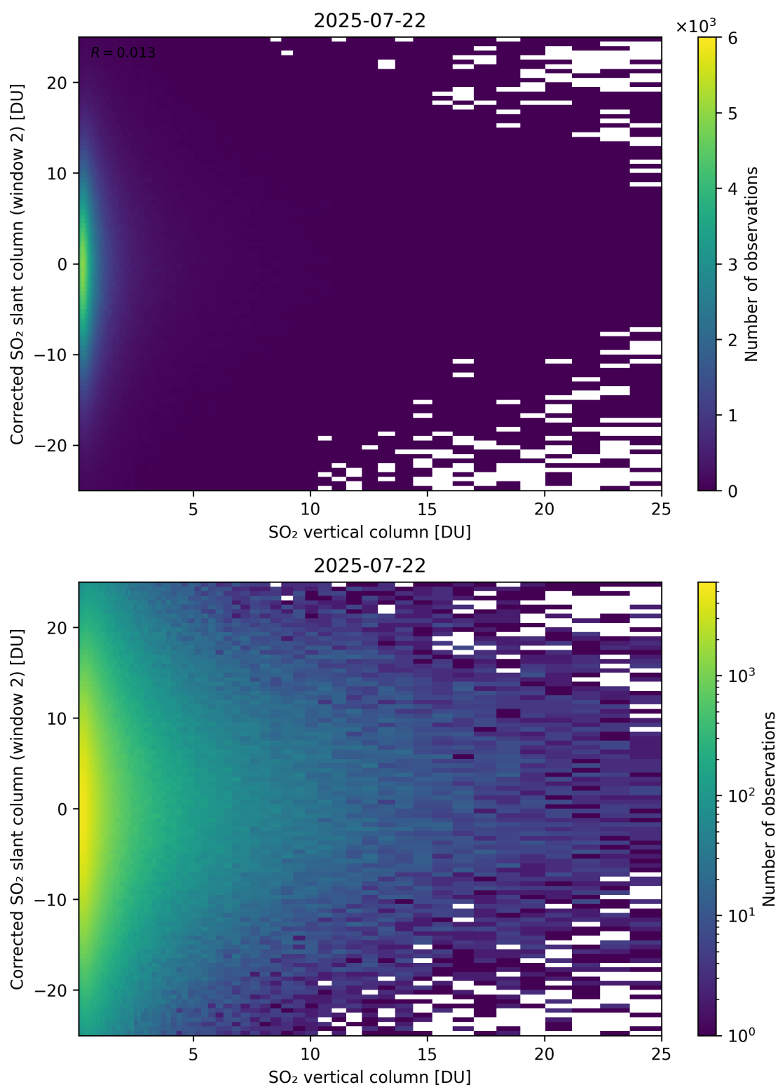
Figure 352: Scatter density plot of “SO 2 vertical column” against “Corrected SO 2 slant column (window 2)” for 2025-07-21 to 2025-07-23.
