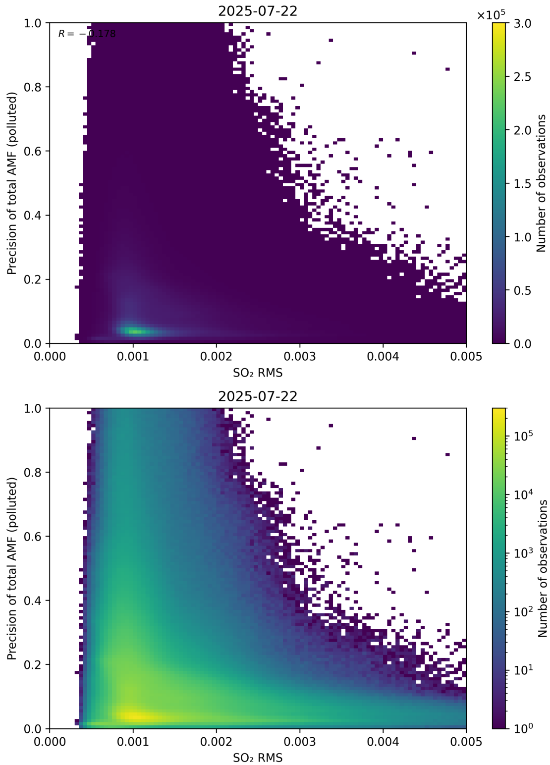
Figure 149: Scatter density plot of “SO 2 RMS” against “Precision of total AMF (polluted)” for 2025-07-21 to 2025-07-23.
