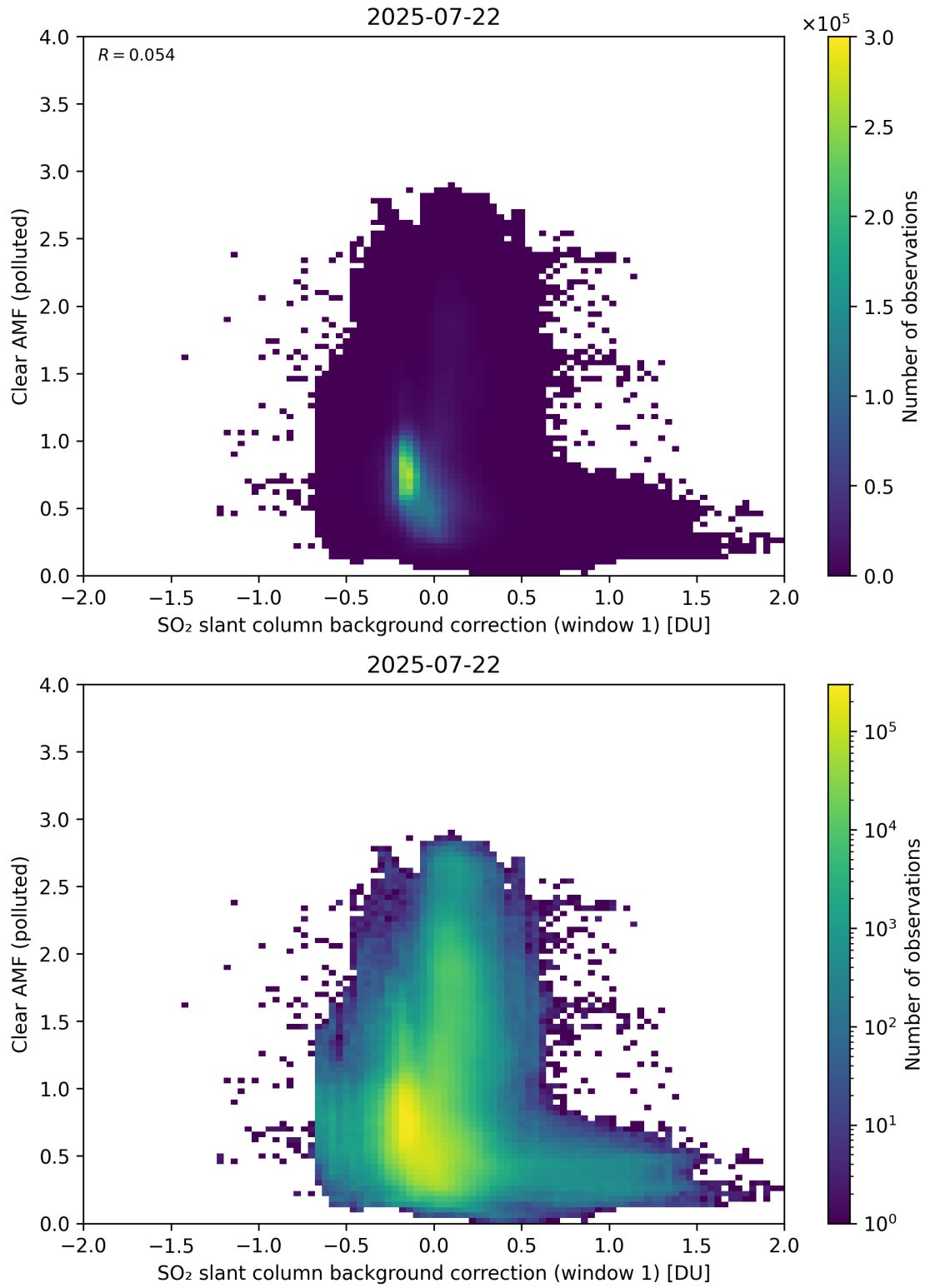
Figure 114: Scatter density plot of “SO 2 slant column background correction (window 1)” against “Clear AMF (polluted)” for 2025-07-21 to 2025-07-23.
