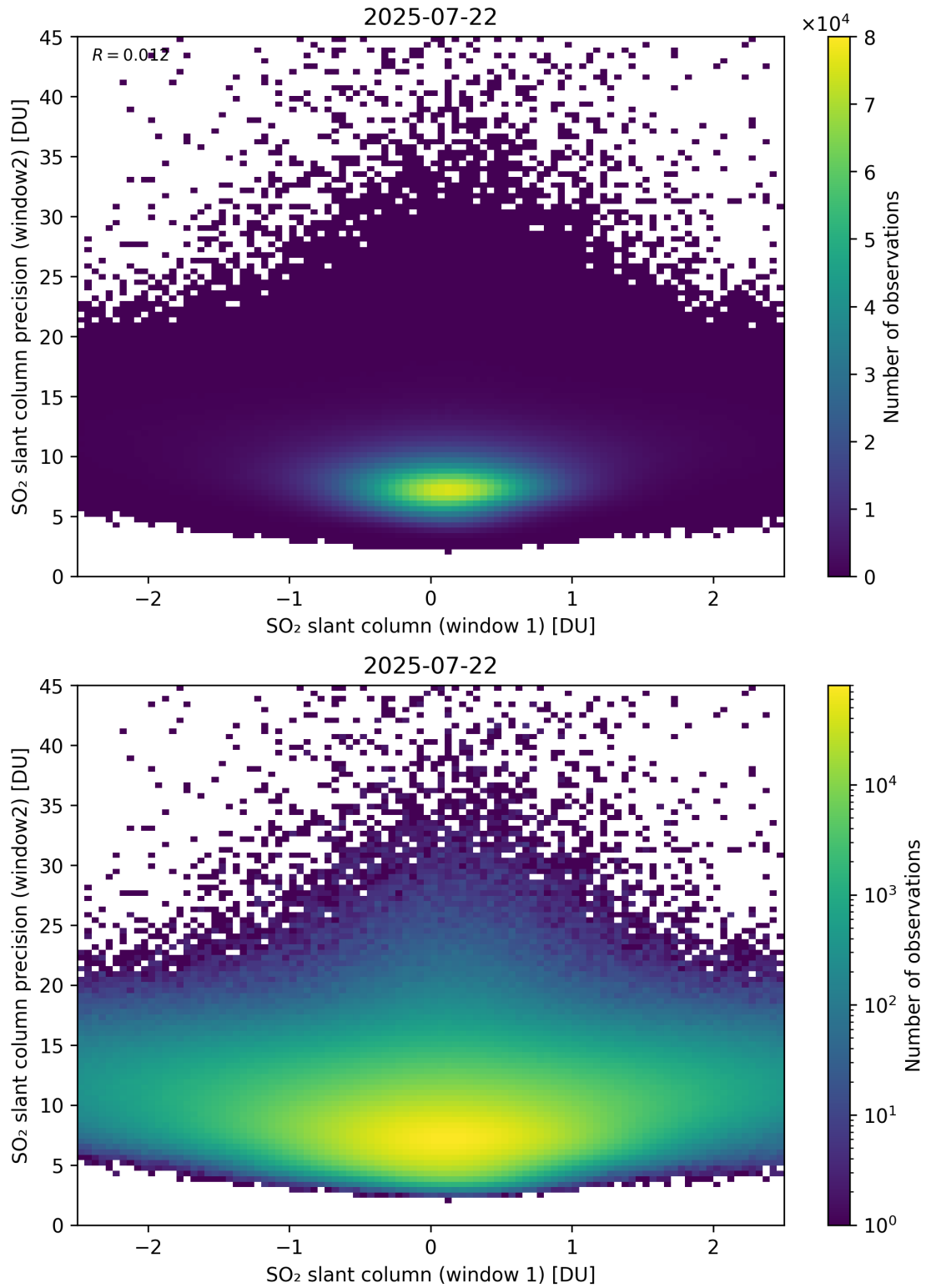
Figure 286: Scatter density plot of “SO 2 slant column (window 1)” against “SO 2 slant column precision (window2)” for 2025-07-21 to 2025-07-23.
