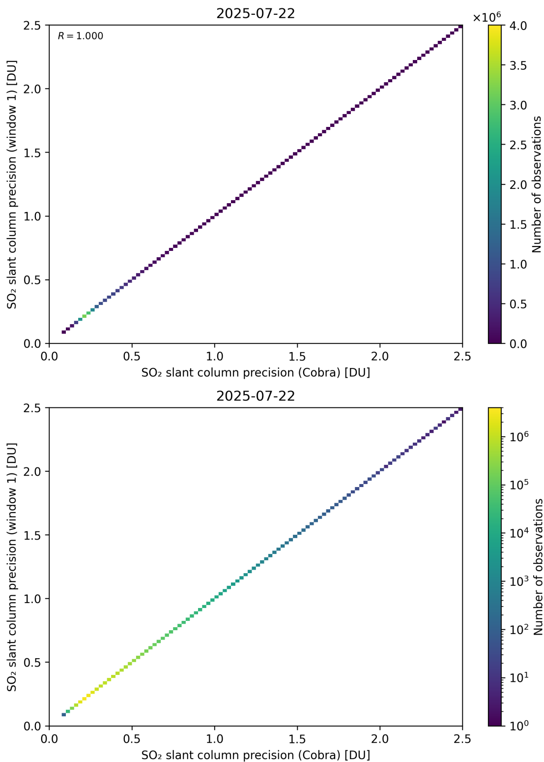
Figure 209: Scatter density plot of “SO 2 slant column precision (Cobra)” against “SO 2 slant column precision (window 1)” for 2025-07-21 to 2025-07-23.
