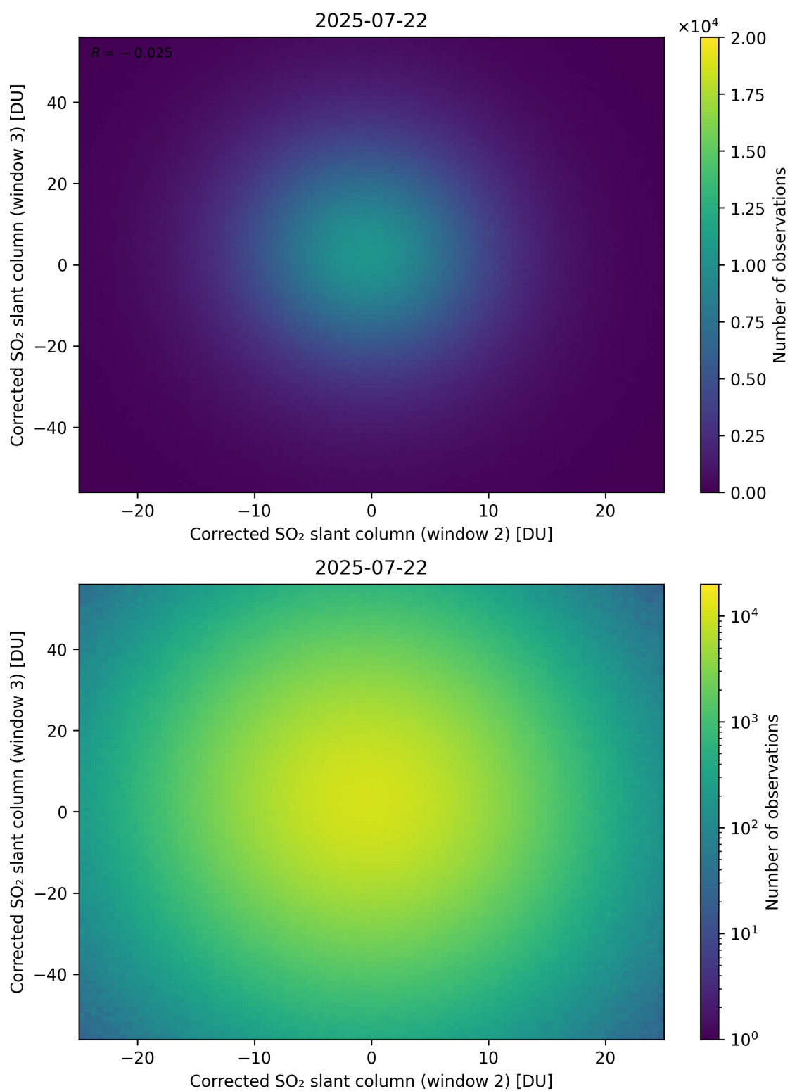
Figure 250: Scatter density plot of “Corrected SO 2 slant column (window 2)” against “Corrected SO 2 slant column (window 3)” for 2025-07-21 to 2025-07-23.
