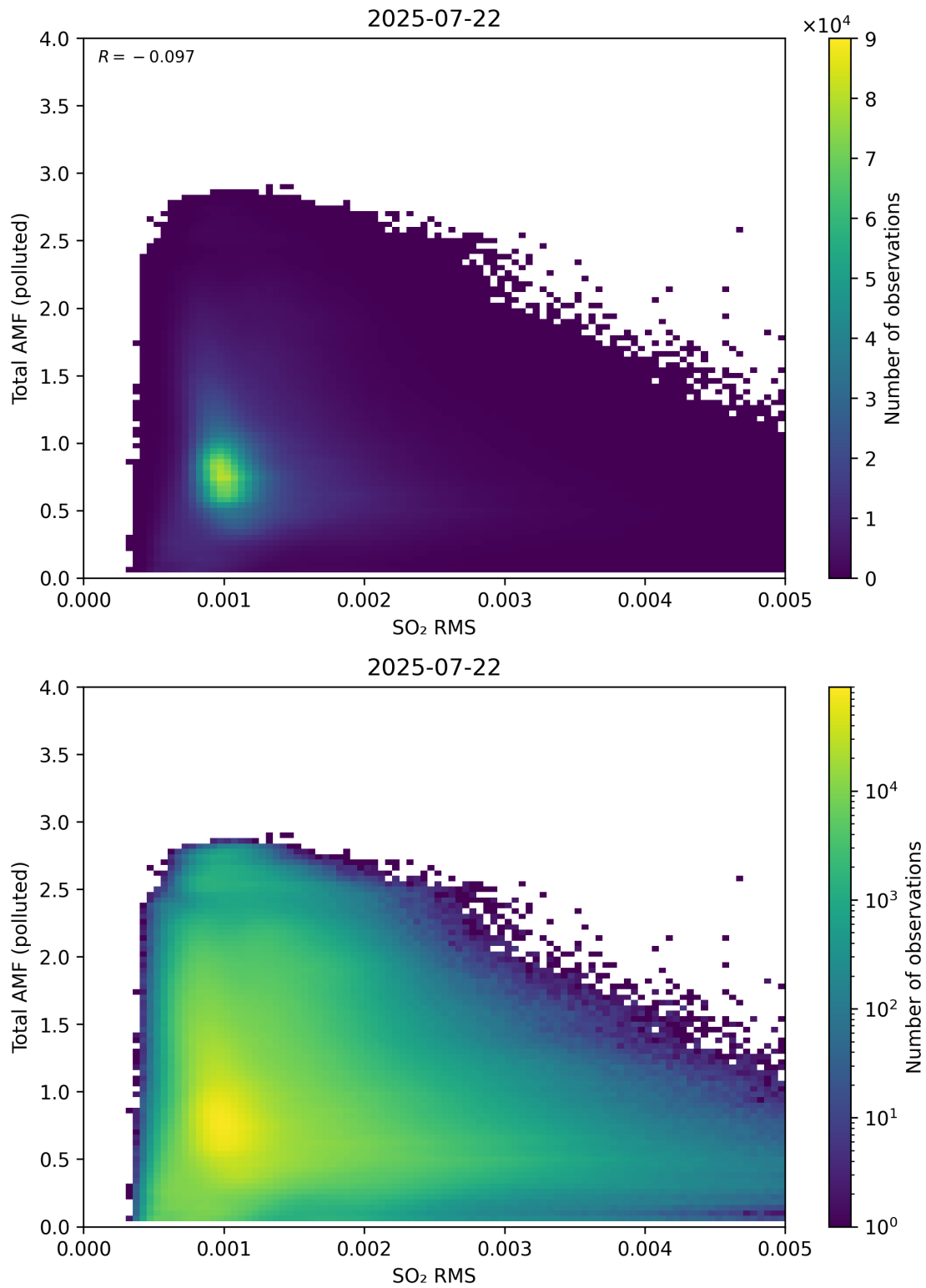
Figure 148: Scatter density plot of “SO 2 RMS” against “Total AMF (polluted)” for 2025-07-21 to 2025-07-23.
