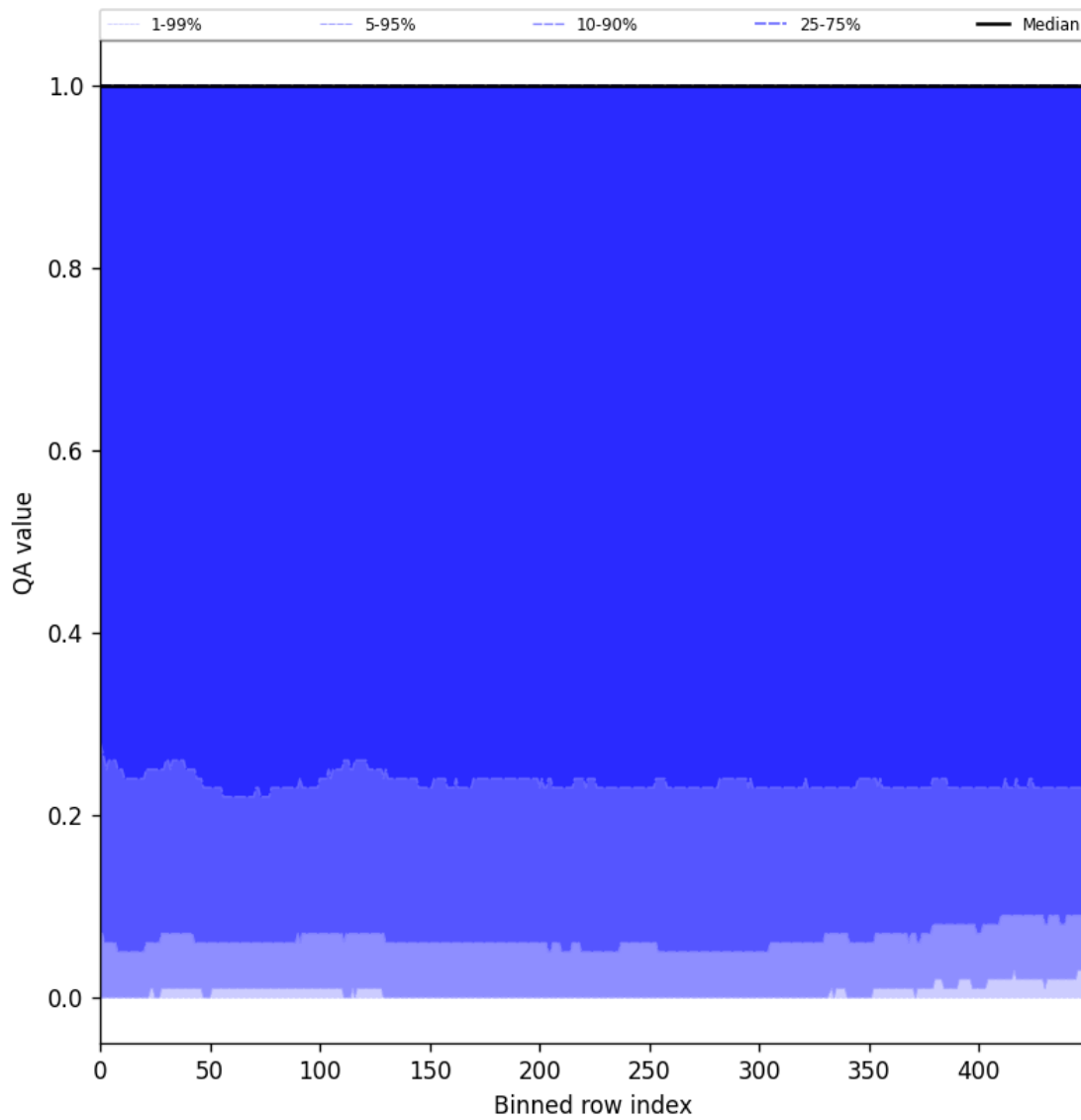
Figure 83: Along track statistics of “QA value” for 2025-07-21 to 2025-07-23
