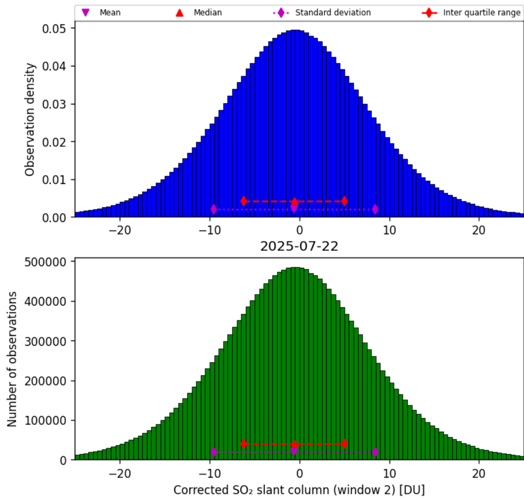
Figure 69: Histogram of “Corrected SO 2 slant column (window 2)” for 2025-07-21 to 2025-07-23
