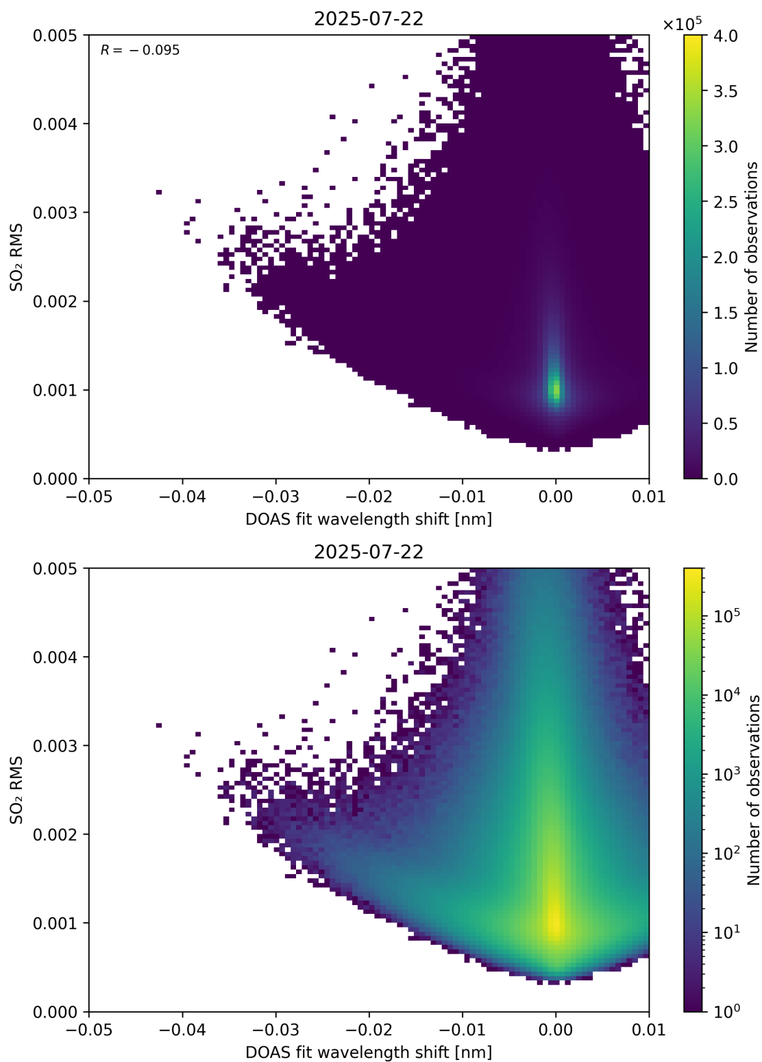
Figure 139: Scatter density plot of “DOAS fit wavelength shift” against “SO 2 RMS” for 2025-07-21 to 2025-07-23.
