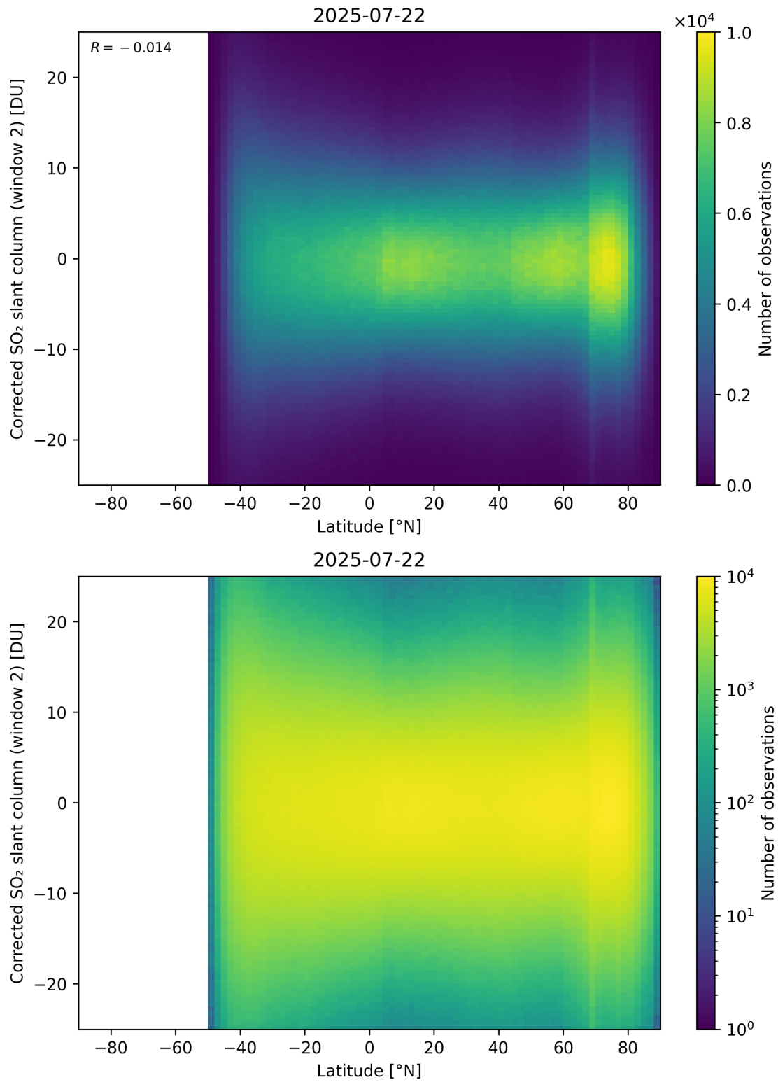
Figure 160: Scatter density plot of “Latitude” against “Corrected SO 2 slant column (window 2)” for 2025-07-21 to 2025-07-23.
