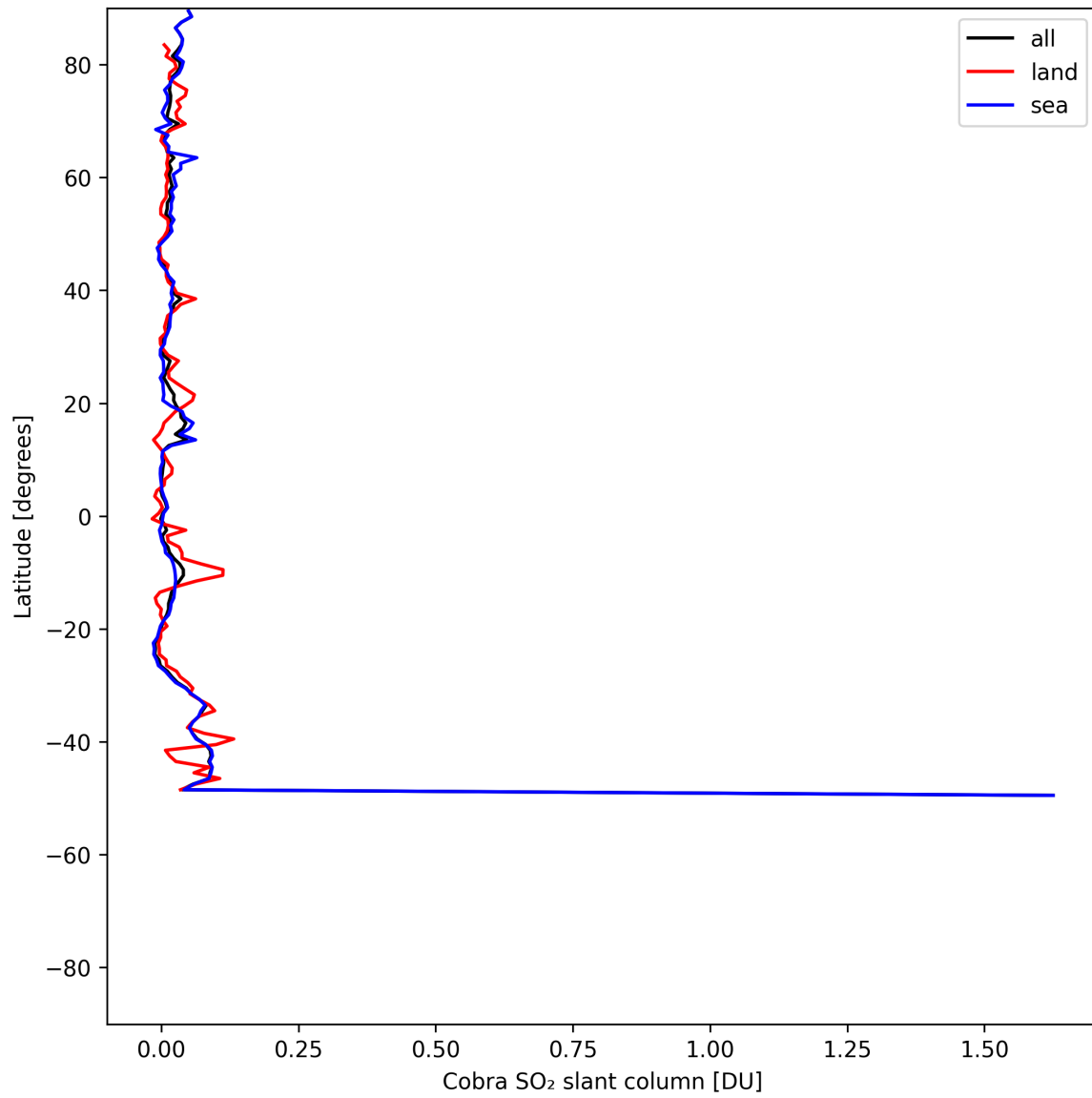
Figure 35: Zonal average of “Cobra SO 2 slant column” for 2025-07-21 to 2025-07-23.
