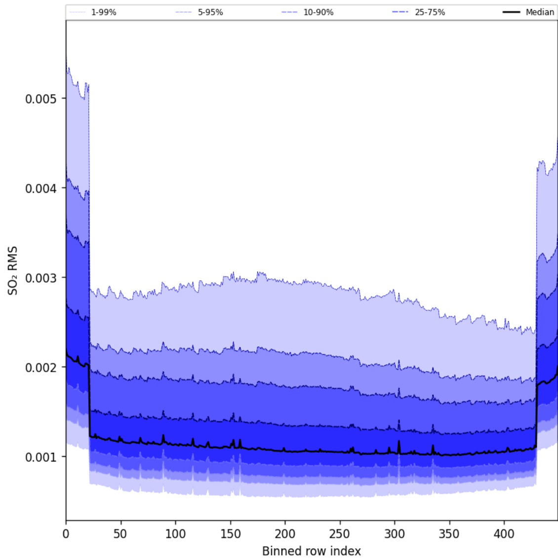
Figure 104: Along track statistics of “SO 2 RMS” for 2025-07-21 to 2025-07-23
