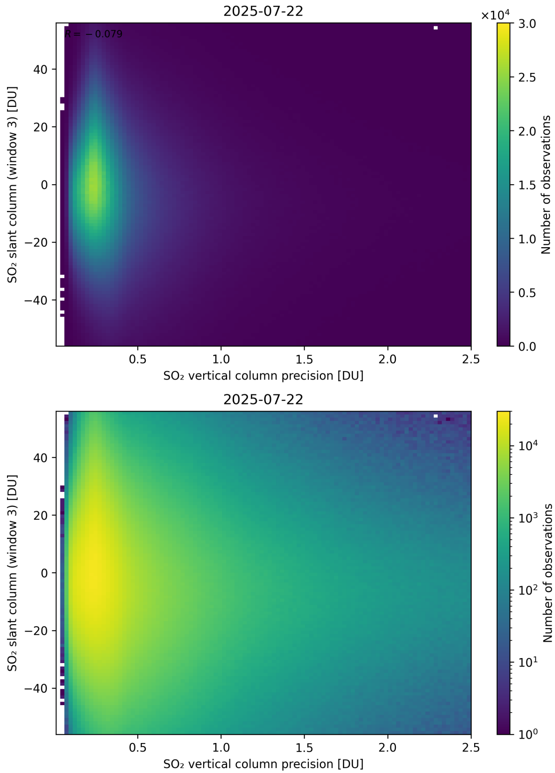
Figure 344: Scatter density plot of “SO 2 vertical column precision” against “SO 2 slant column (window 3)” for 2025-07-21 to 2025-07-23.
