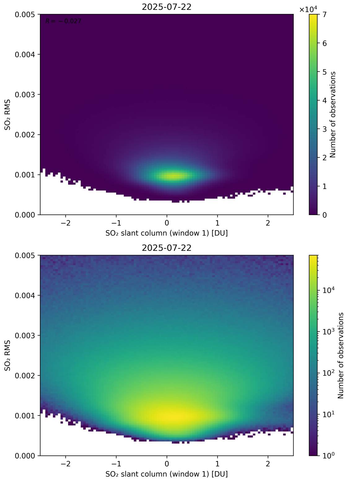
Figure 267: Scatter density plot of “SO 2 slant column (window 1)” against “SO 2 RMS” for 2025-07-21 to 2025-07-23.
