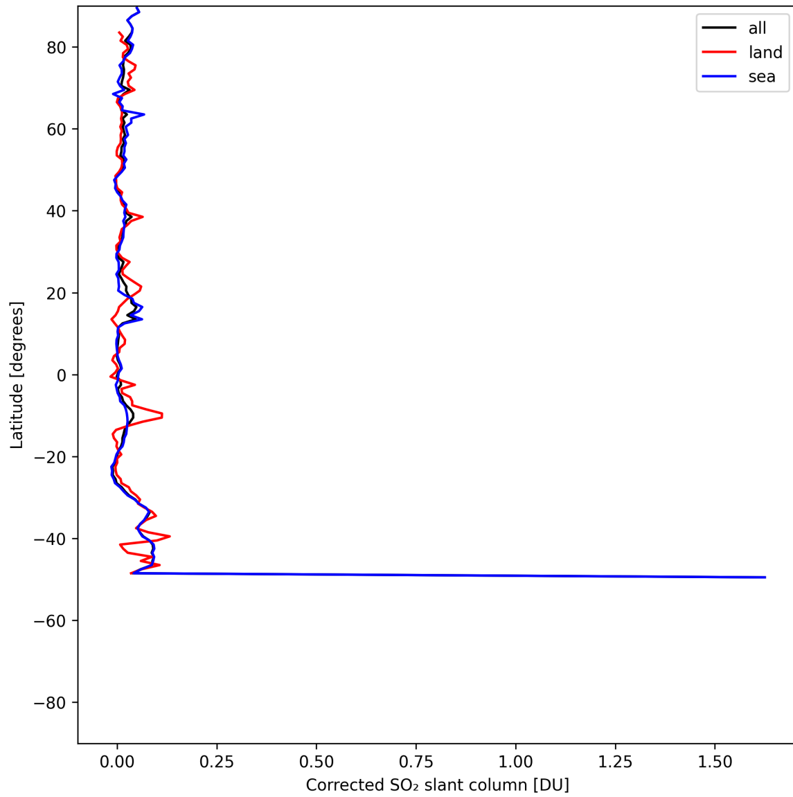
Figure 34: Zonal average of “Corrected SO 2 slant column” for 2025-07-21 to 2025-07-23.
