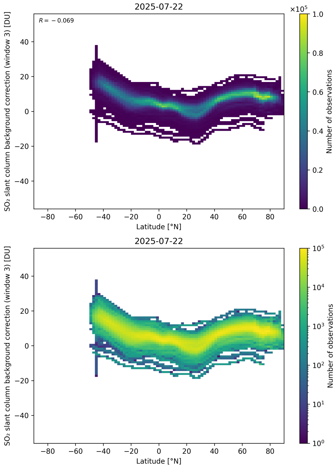
Figure 152: Scatter density plot of “Latitude” against “SO 2 slant column background correction (window 3)” for 2025-07-21 to 2025-07-23.
