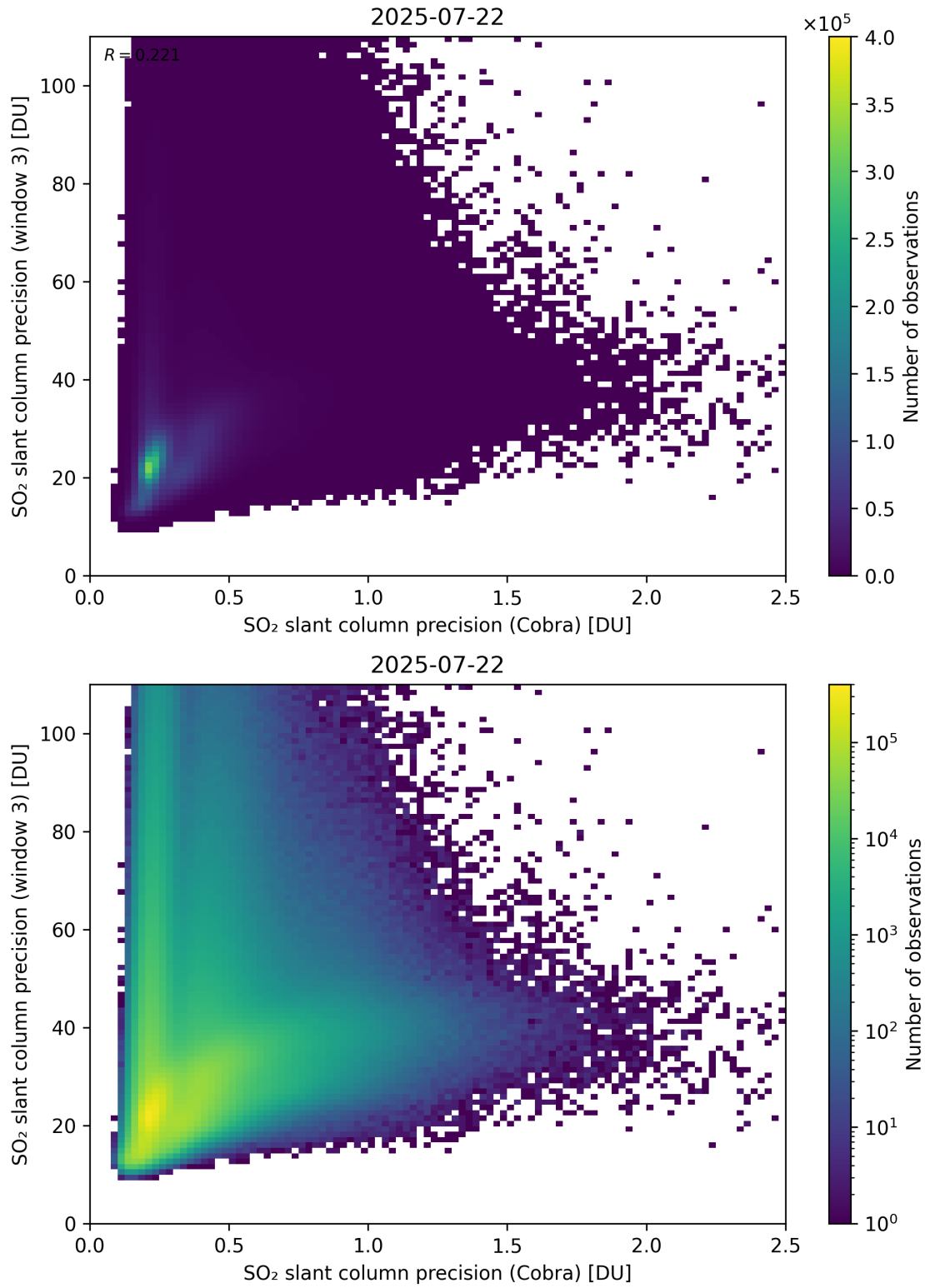
Figure 212: Scatter density plot of “SO 2 slant column precision (Cobra)” against “SO 2 slant column precision (window 3)” for 2025-07-21 to 2025-07-23.
