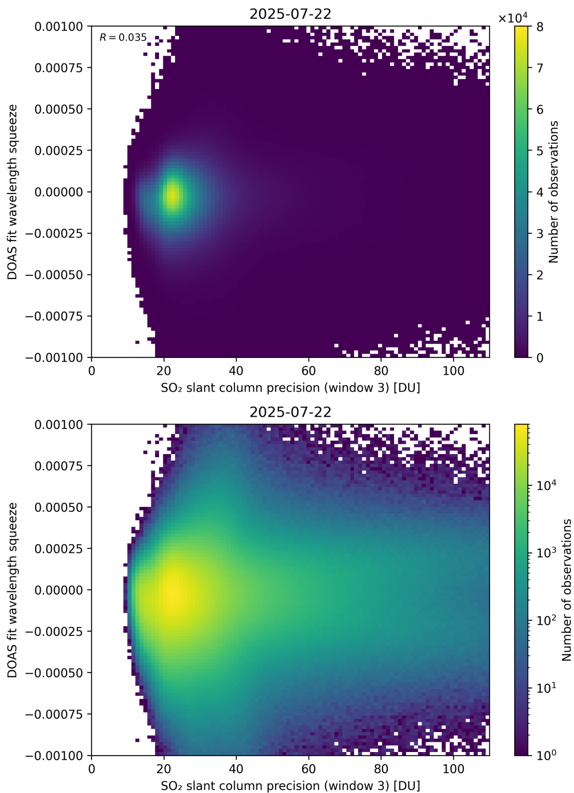
Figure 309: Scatter density plot of “SO 2 slant column precision (window 3)” against “DOAS fit wavelength squeeze” for 2025-07-21 to 2025-07-23.
