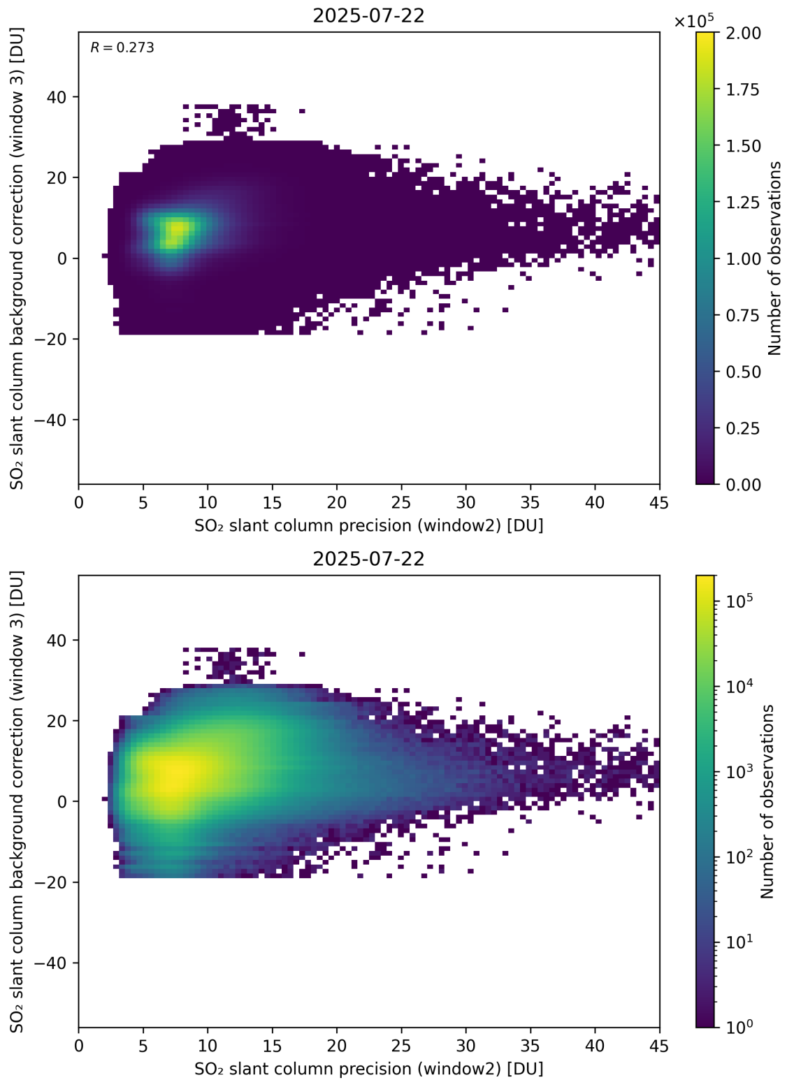
Figure 292: Scatter density plot of “SO 2 slant column precision (window2)” against “SO 2 slant column background correction (window 3)” for 2025-07-21 to 2025-07-23.
