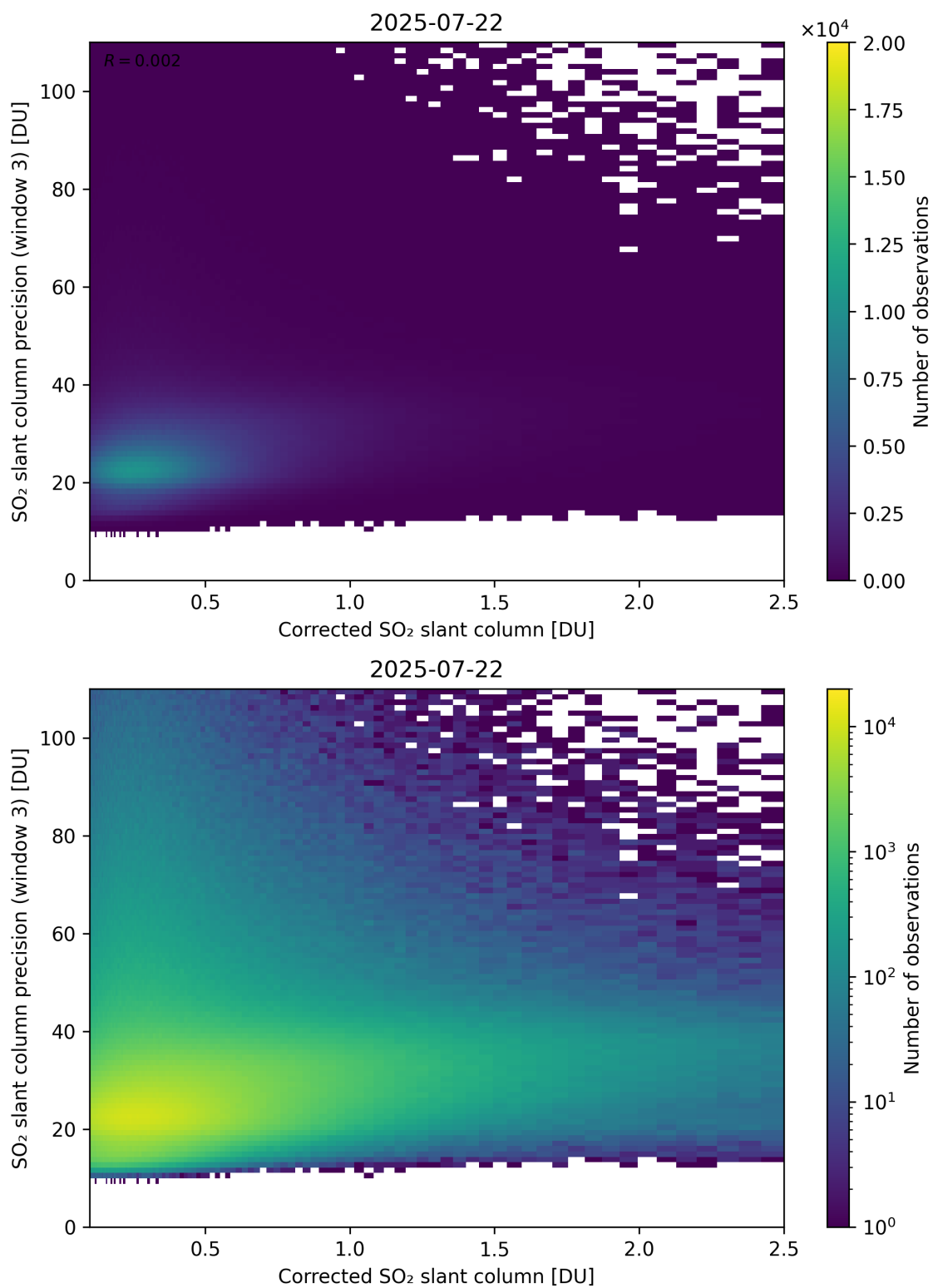
Figure 241: Scatter density plot of “Corrected SO 2 slant column” against “SO 2 slant column precision (window 3)” for 2025-07-21 to 2025-07-23.
