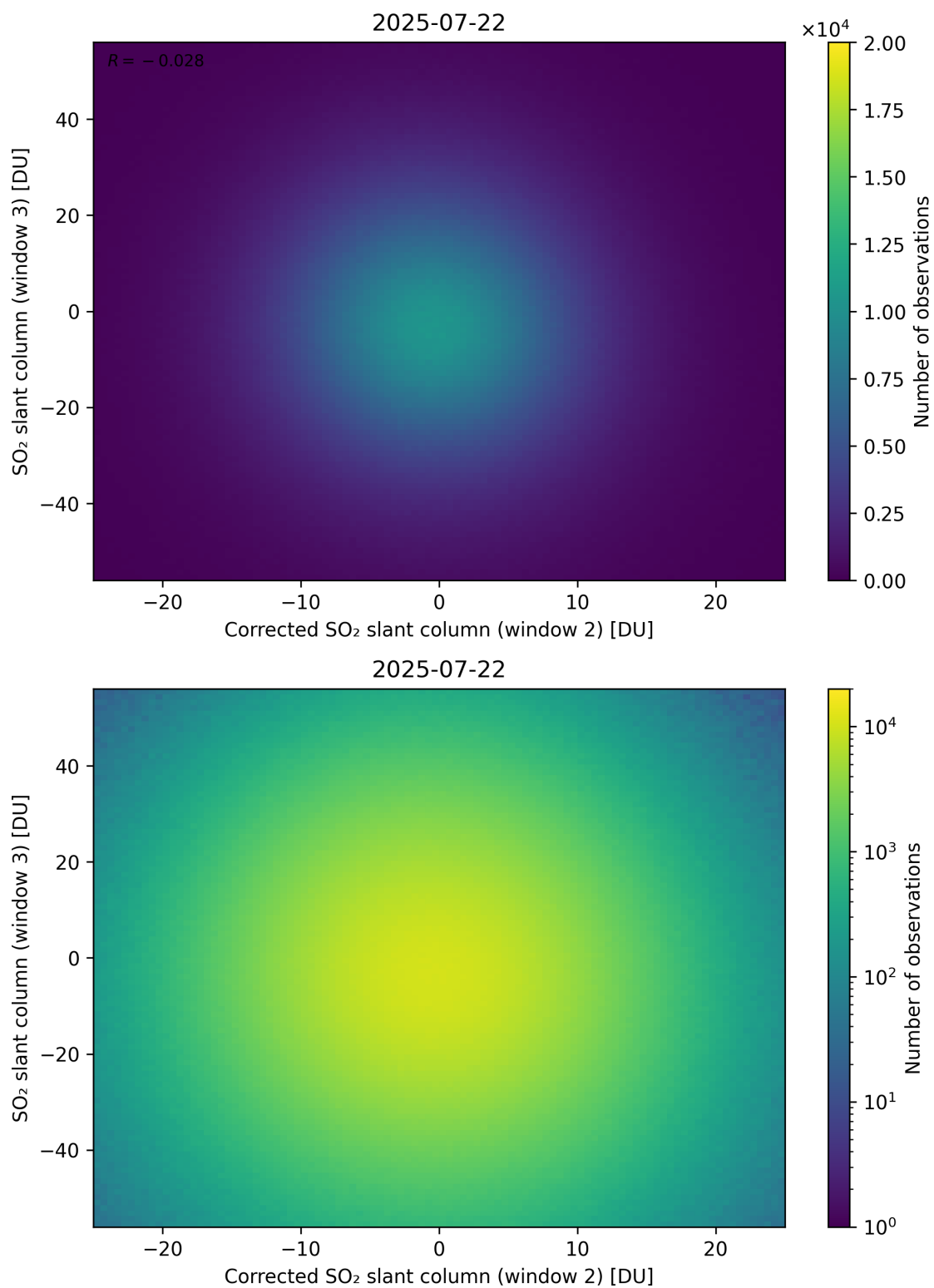
Figure 251: Scatter density plot of “Corrected SO 2 slant column (window 2)” against “SO 2 slant column (window 3)” for 2025-07-21 to 2025-07-23.
