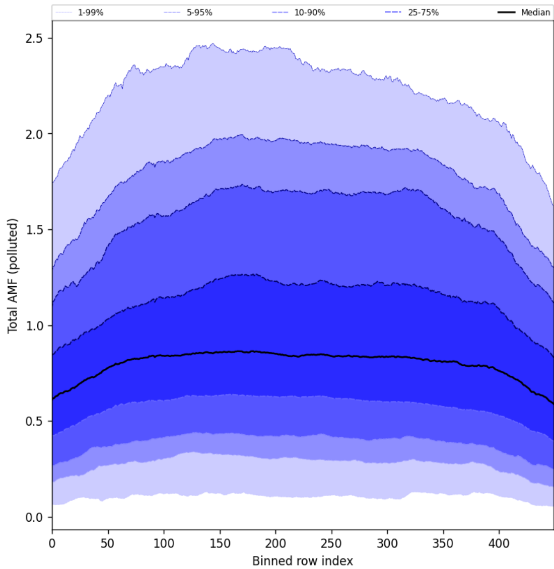
Figure 105: Along track statistics of “Total AMF (polluted)” for 2025-07-21 to 2025-07-23
