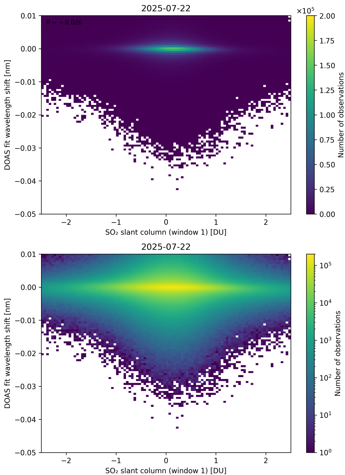
Figure 265: Scatter density plot of “SO 2 slant column (window 1)” against “DOAS fit wavelength shift” for 2025-07-21 to 2025-07-23.
