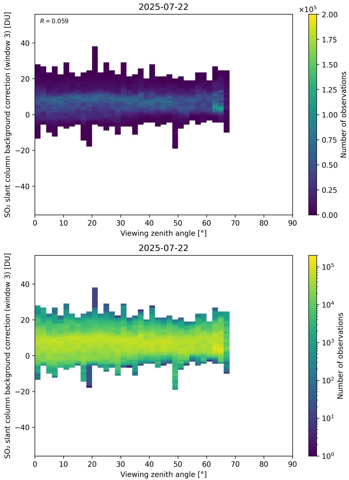
Figure 364: Scatter density plot of “Viewing zenith angle” against “SO 2 slant column background correction (window 3)” for 2025-07-21 to 2025-07-23.
