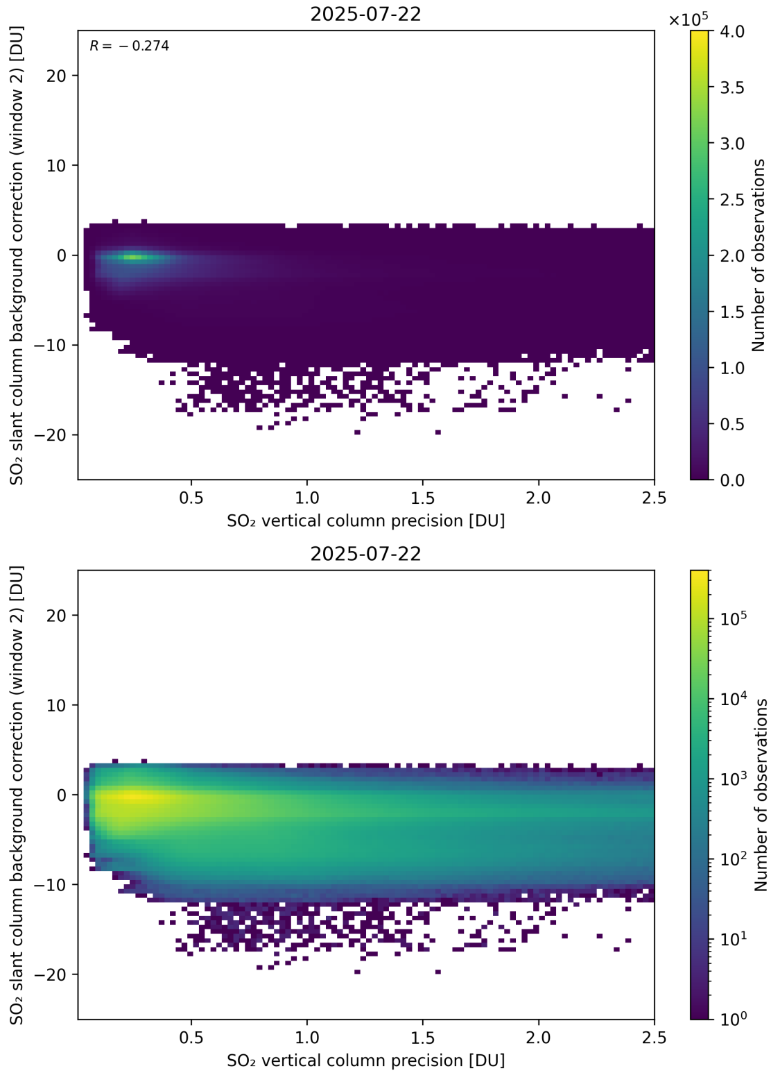
Figure 330: Scatter density plot of “SO 2 vertical column precision” against “SO 2 slant column background correction (window 2)” for 2025-07-21 to 2025-07-23.
