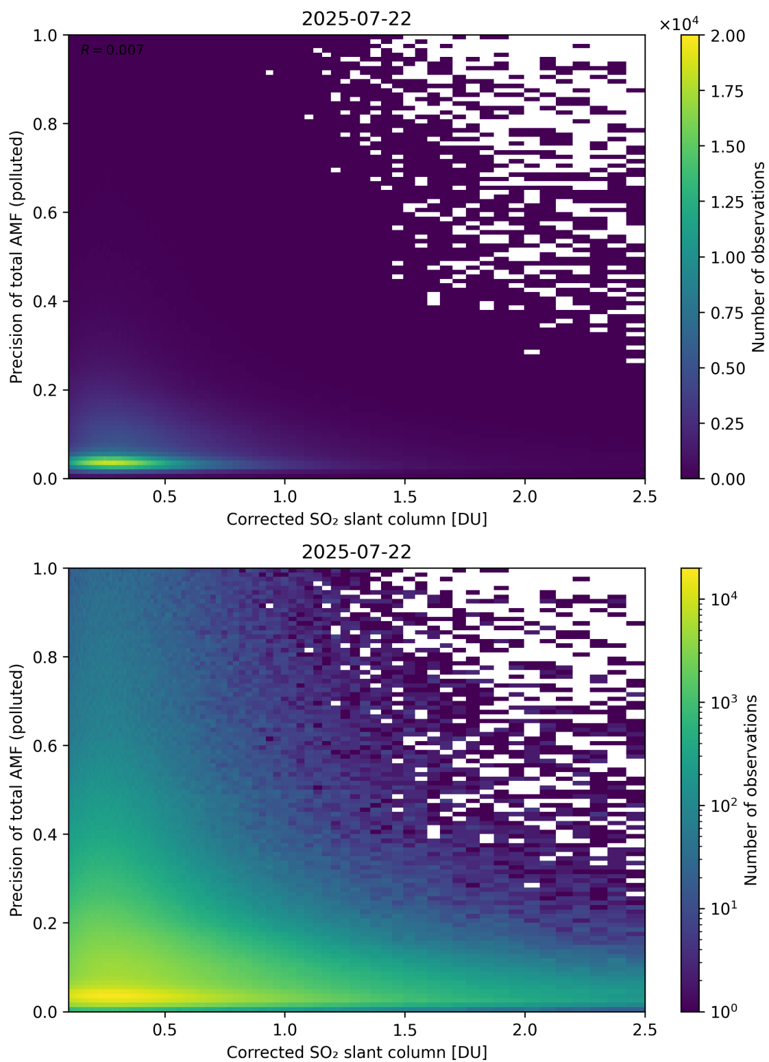
Figure 243: Scatter density plot of “Corrected SO 2 slant column” against “Precision of total AMF (polluted)” for 2025-07-21 to 2025-07-23.
