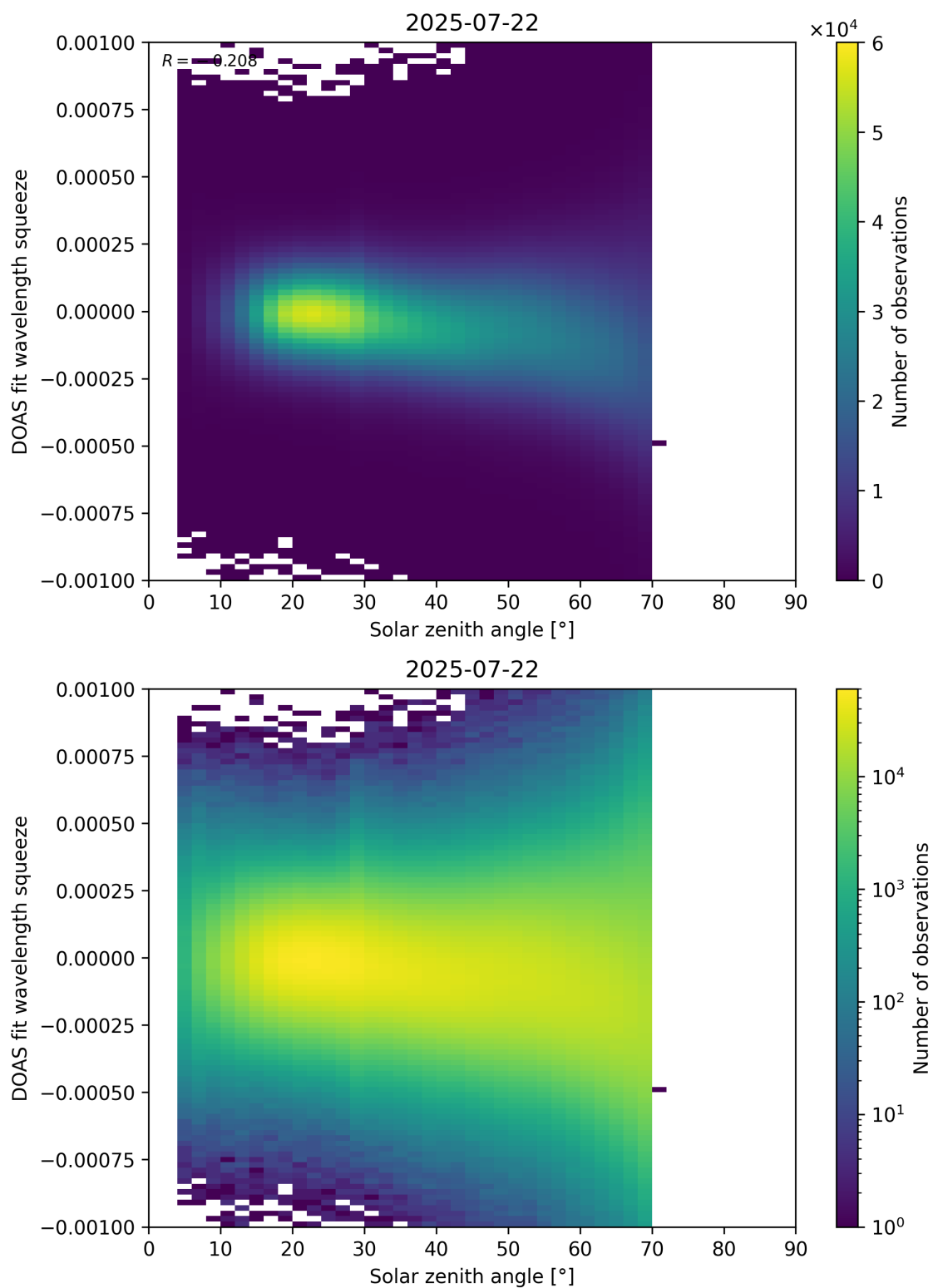
Figure 175: Scatter density plot of “Solar zenith angle” against “DOAS fit wavelength squeeze” for 2025-07-21 to 2025-07-23.
