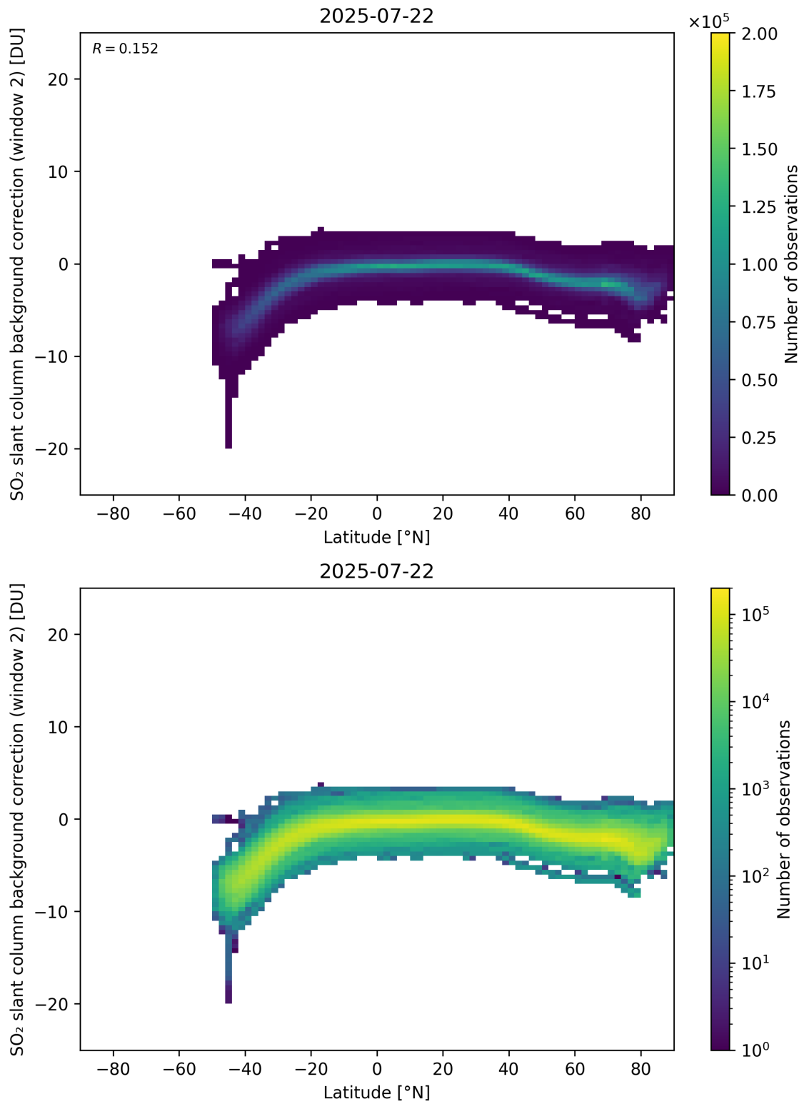
Figure 151: Scatter density plot of “Latitude” against “SO 2 slant column background correction (window 2)” for 2025-07-21 to 2025-07-23.
