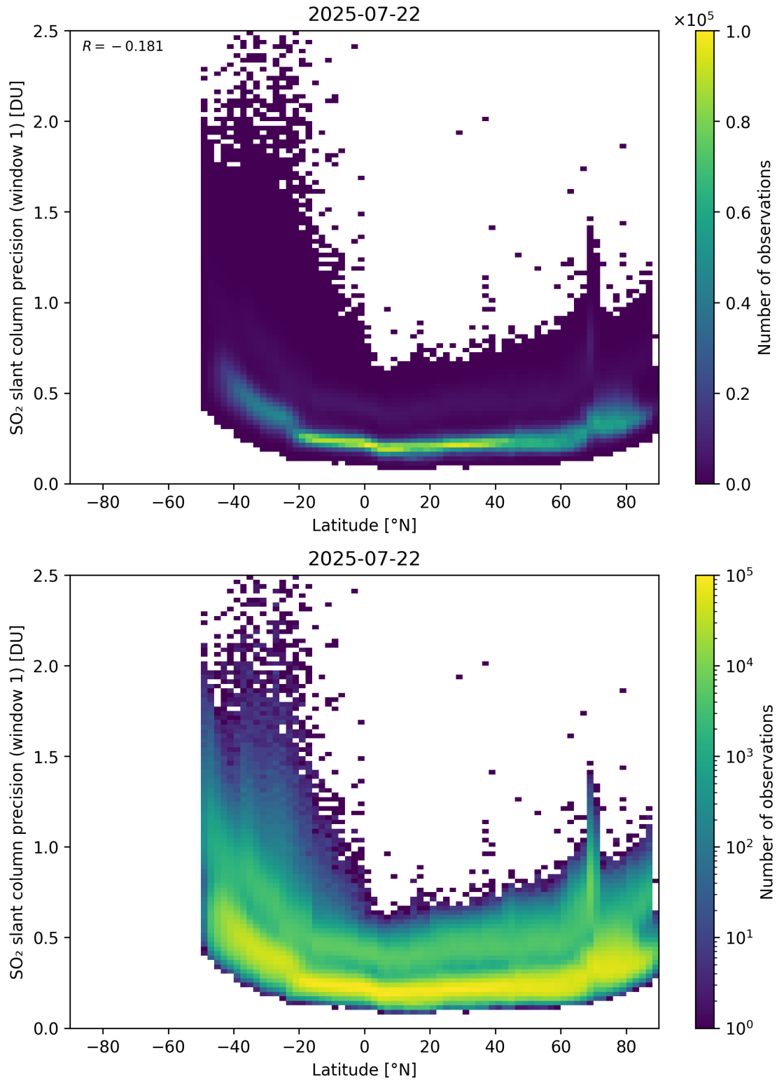
Figure 163: Scatter density plot of “Latitude” against “SO 2 slant column precision (window 1)” for 2025-07-21 to 2025-07-23.
