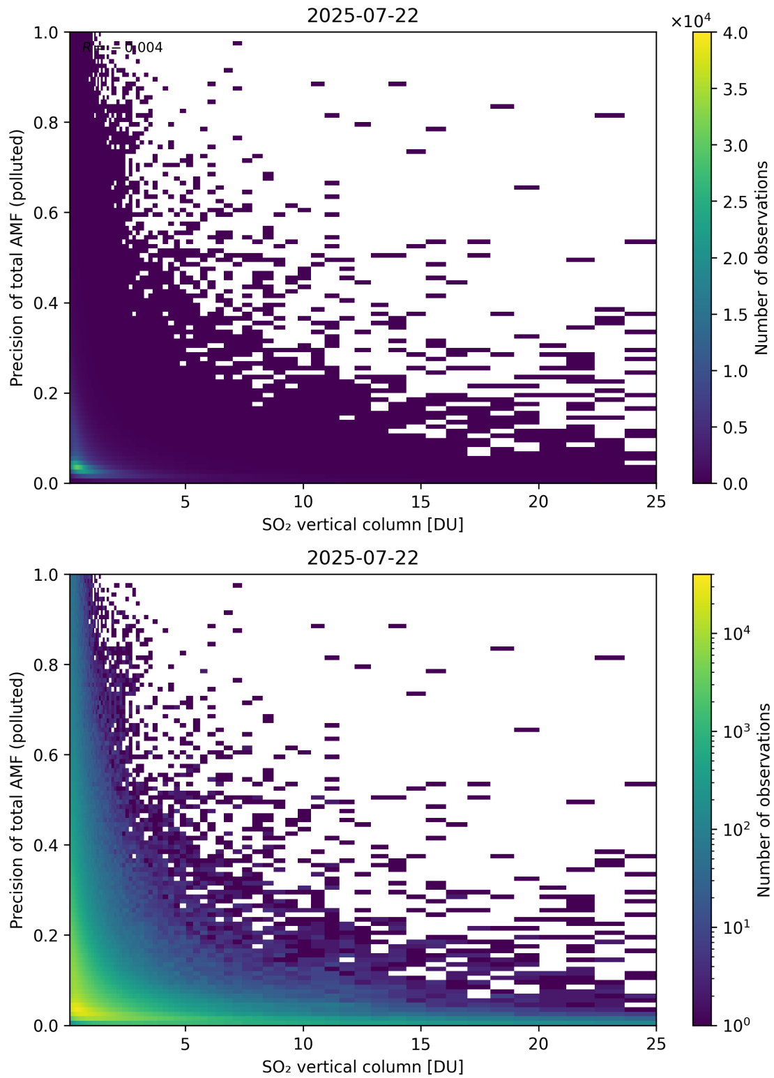
Figure 360: Scatter density plot of “SO 2 vertical column” against “Precision of total AMF (polluted)” for 2025-07-21 to 2025-07-23.
