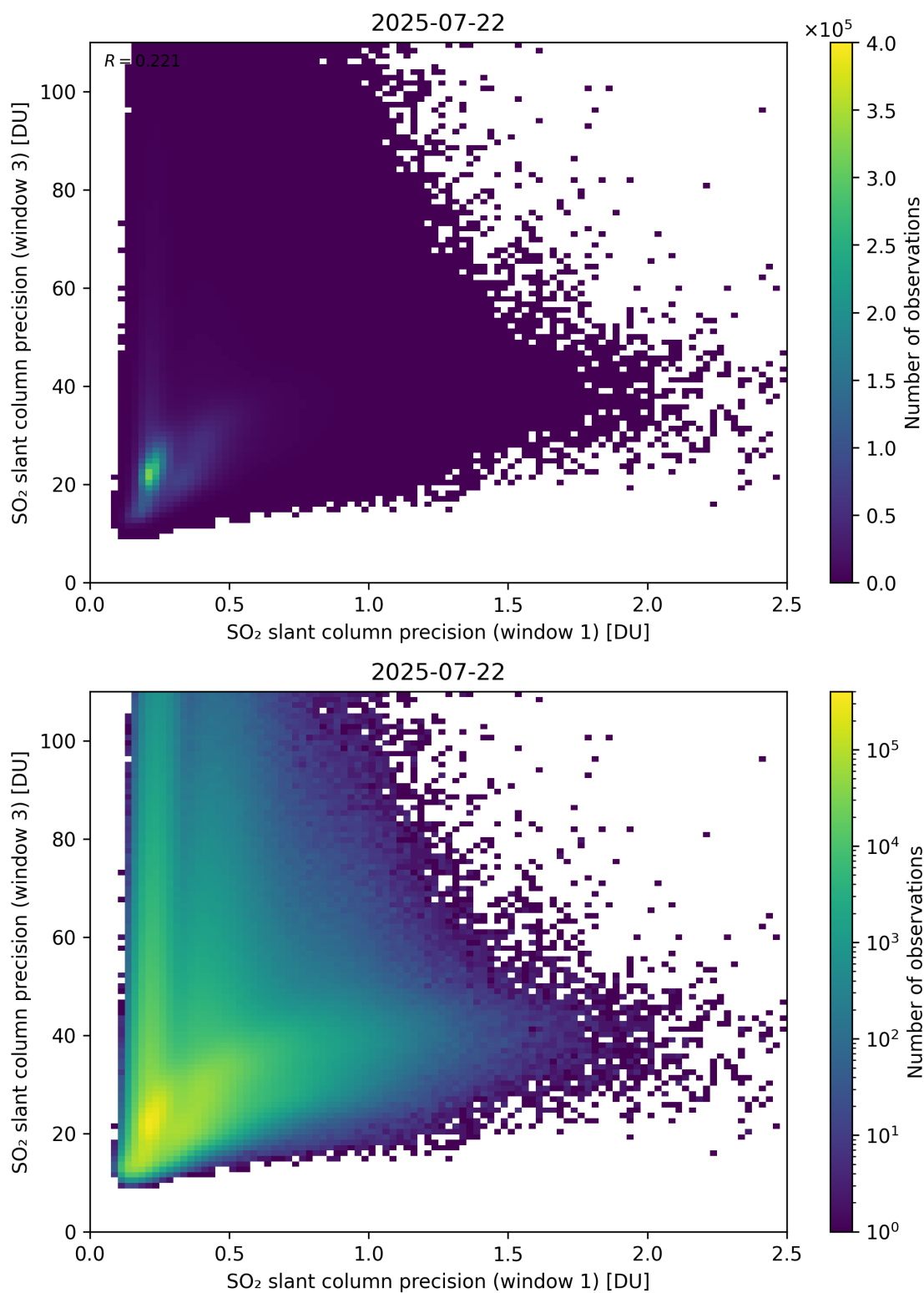
Figure 279: Scatter density plot of “SO 2 slant column precision (window 1)” against “SO 2 slant column precision (window 3)” for 2025-07-21 to 2025-07-23.
