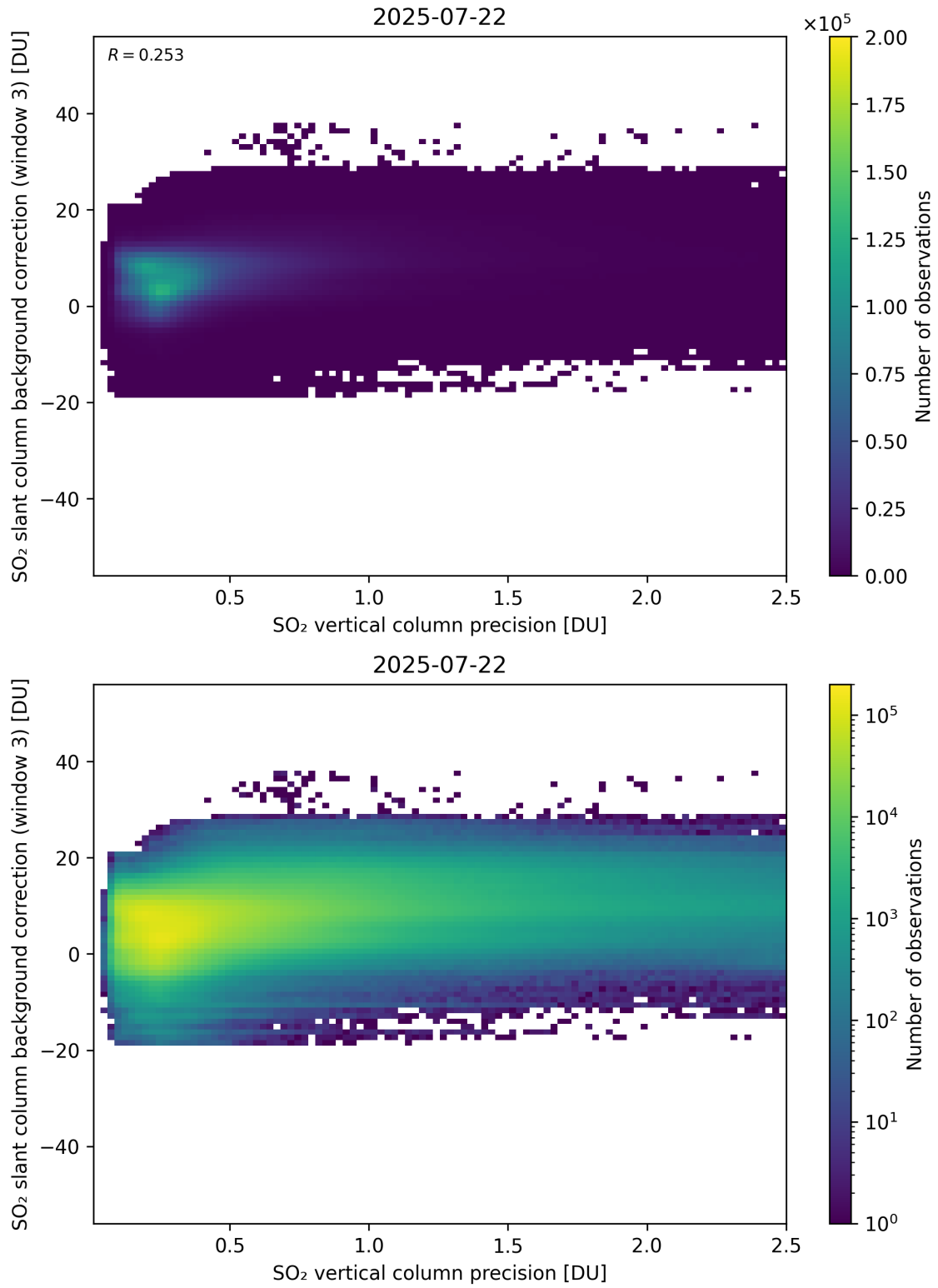
Figure 331: Scatter density plot of “SO 2 vertical column precision” against “SO 2 slant column background correction (window 3)” for 2025-07-21 to 2025-07-23.
