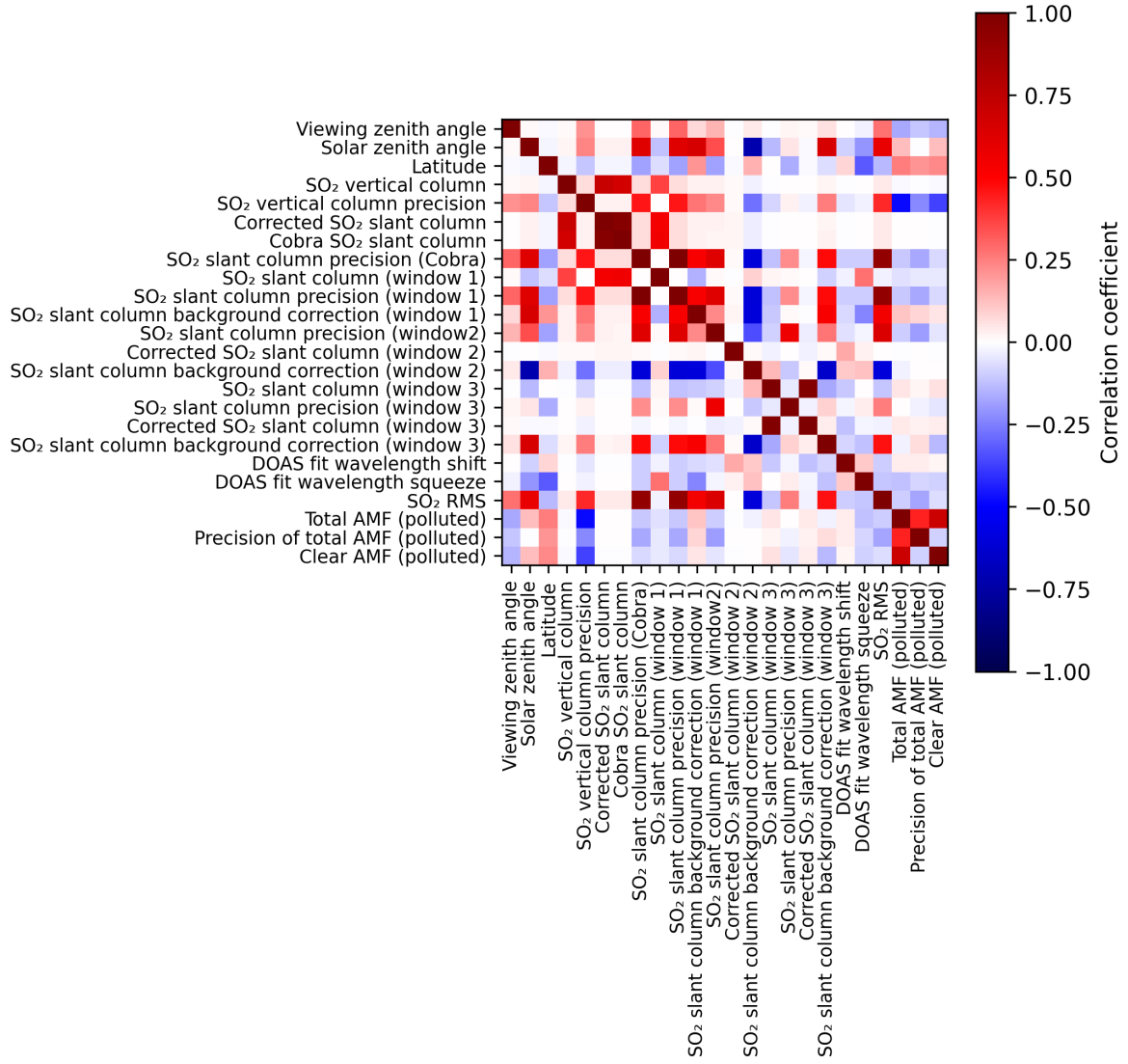
Figure 2: Map of correlation matrix for 2025-07-21 to 2025-07-23.
