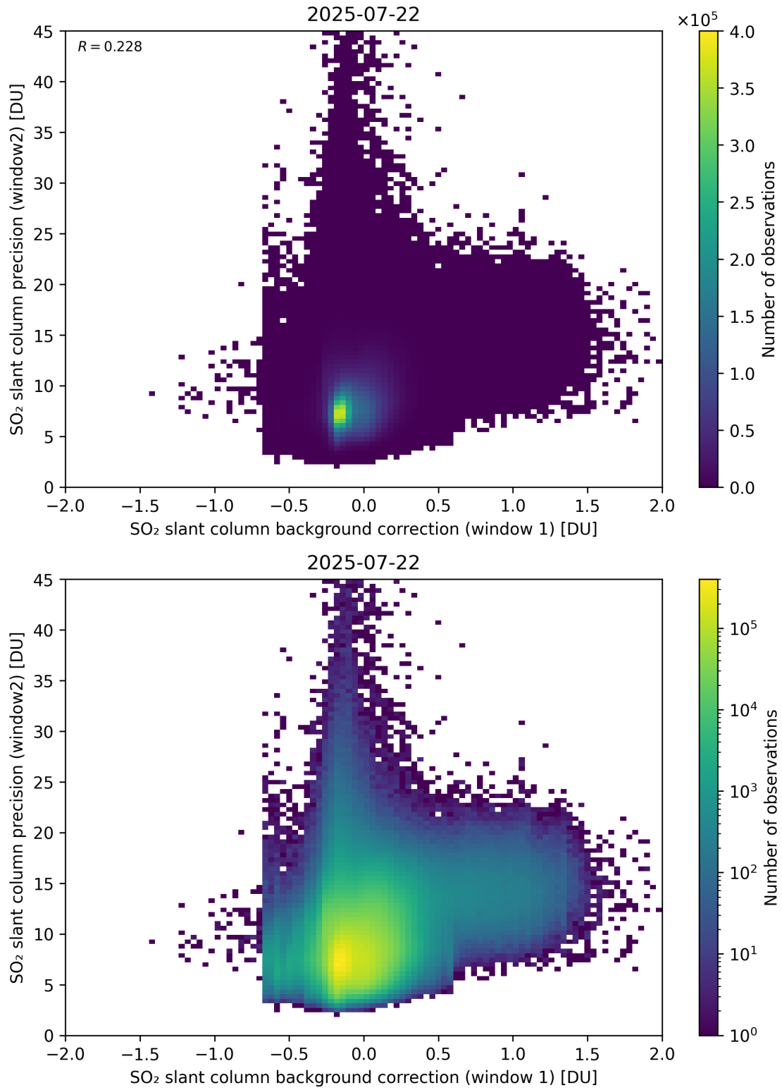
Figure 117: Scatter density plot of “SO 2 slant column background correction (window 1)” against “SO 2 slant column precision (window2)” for 2025-07-21 to 2025-07-23.
