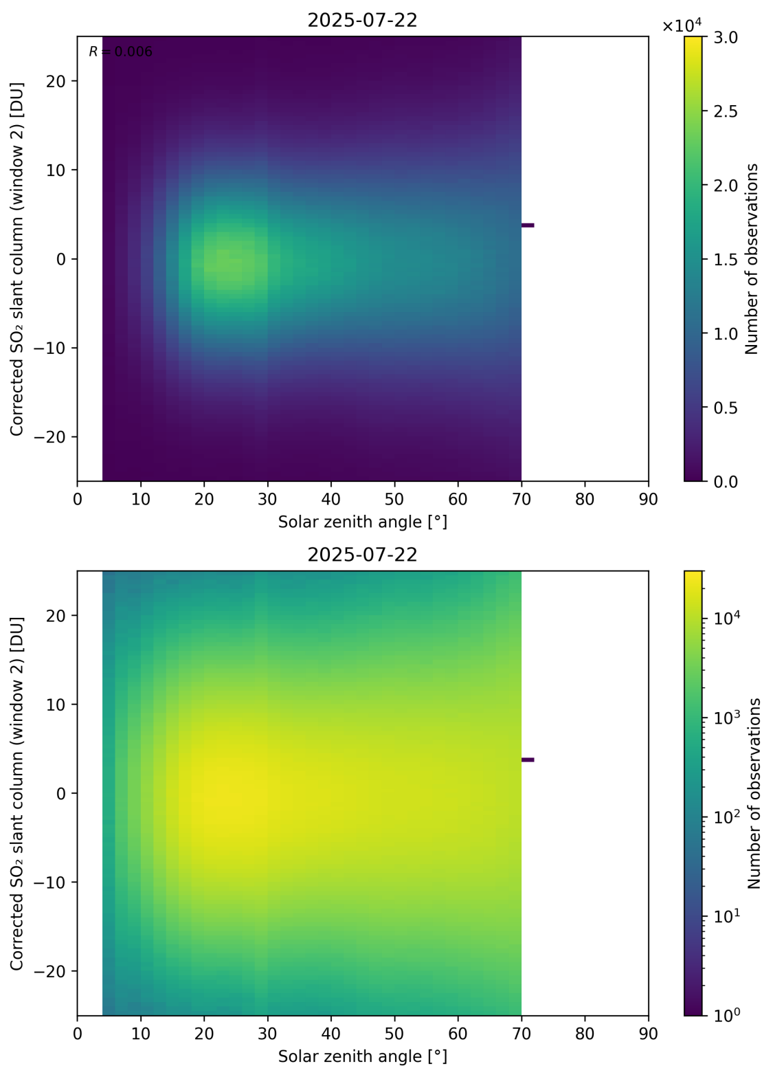
Figure 182: Scatter density plot of “Solar zenith angle” against “Corrected SO 2 slant column (window 2)” for 2025-07-21 to 2025-07-23.
