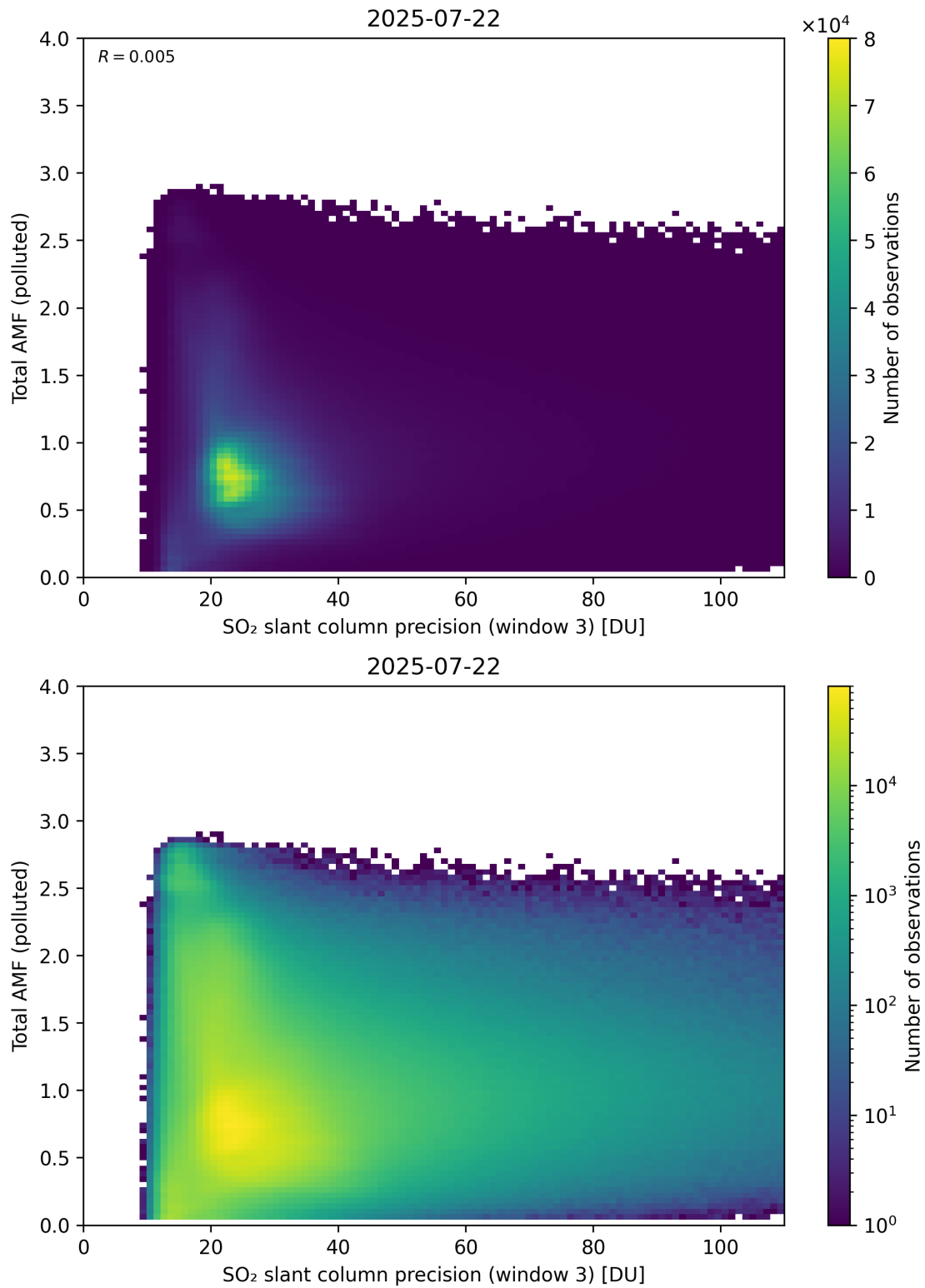
Figure 313: Scatter density plot of “SO 2 slant column precision (window 3)” against “Total AMF (polluted)” for 2025-07-21 to 2025-07-23.
