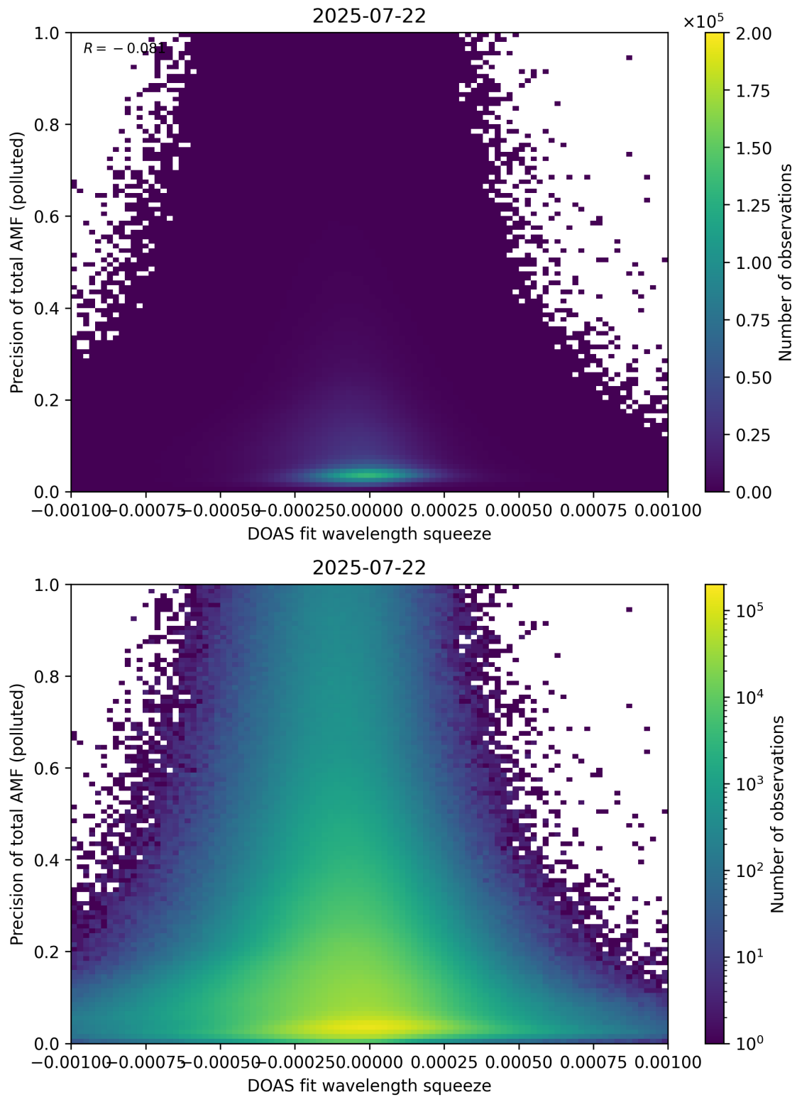
Figure 146: Scatter density plot of “DOAS fit wavelength squeeze” against “Precision of total AMF (polluted)” for 2025-07-21 to 2025-07-23.
