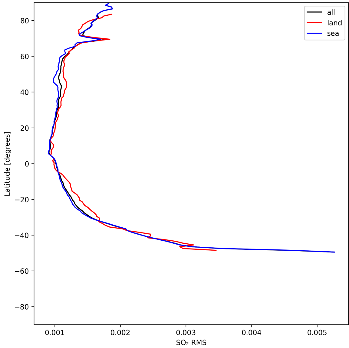
Figure 52: Zonal average of “SO 2 RMS” for 2025-07-21 to 2025-07-23.
