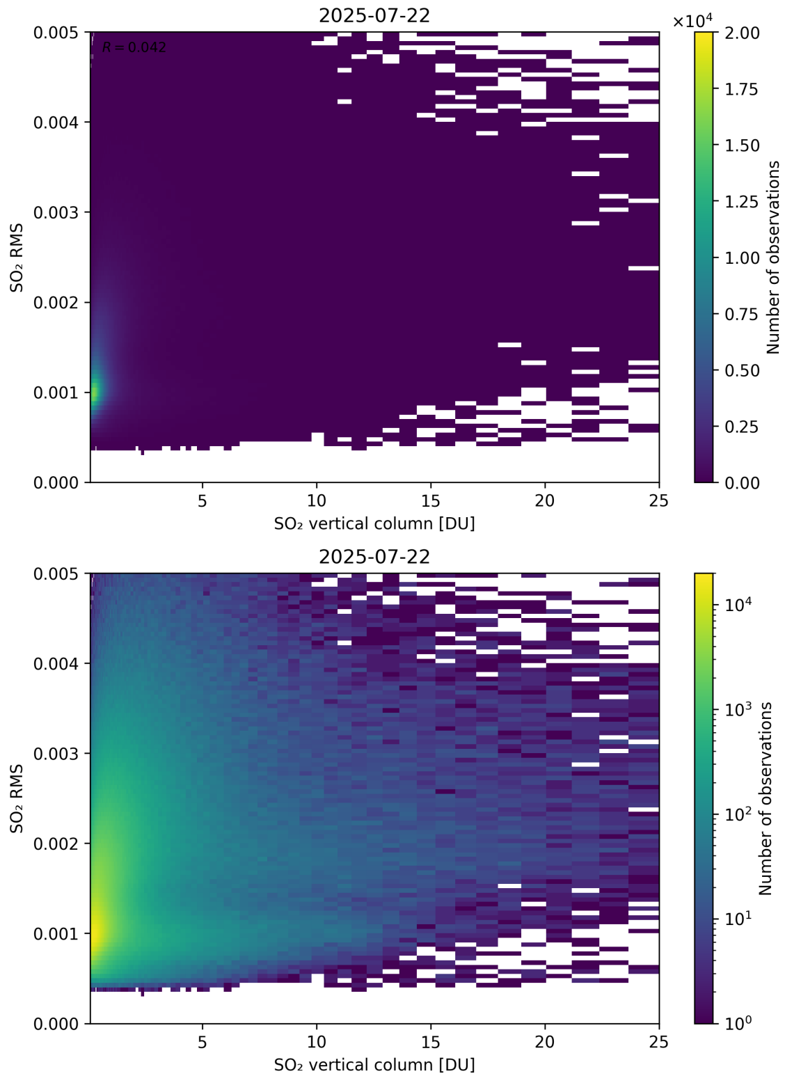
Figure 328: Scatter density plot of “SO 2 vertical column” against “SO 2 RMS” for 2025-07-21 to 2025-07-23.
