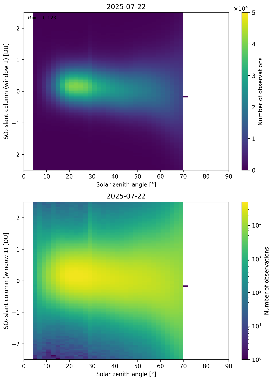
Figure 184: Scatter density plot of “Solar zenith angle” against “SO 2 slant column (window 1)” for 2025-07-21 to 2025-07-23.
