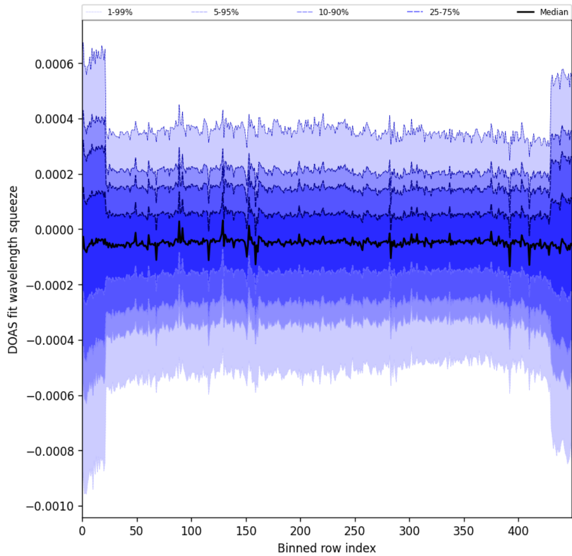
Figure 103: Along track statistics of “DOAS fit wavelength squeeze” for 2025-07-21 to 2025-07-23
