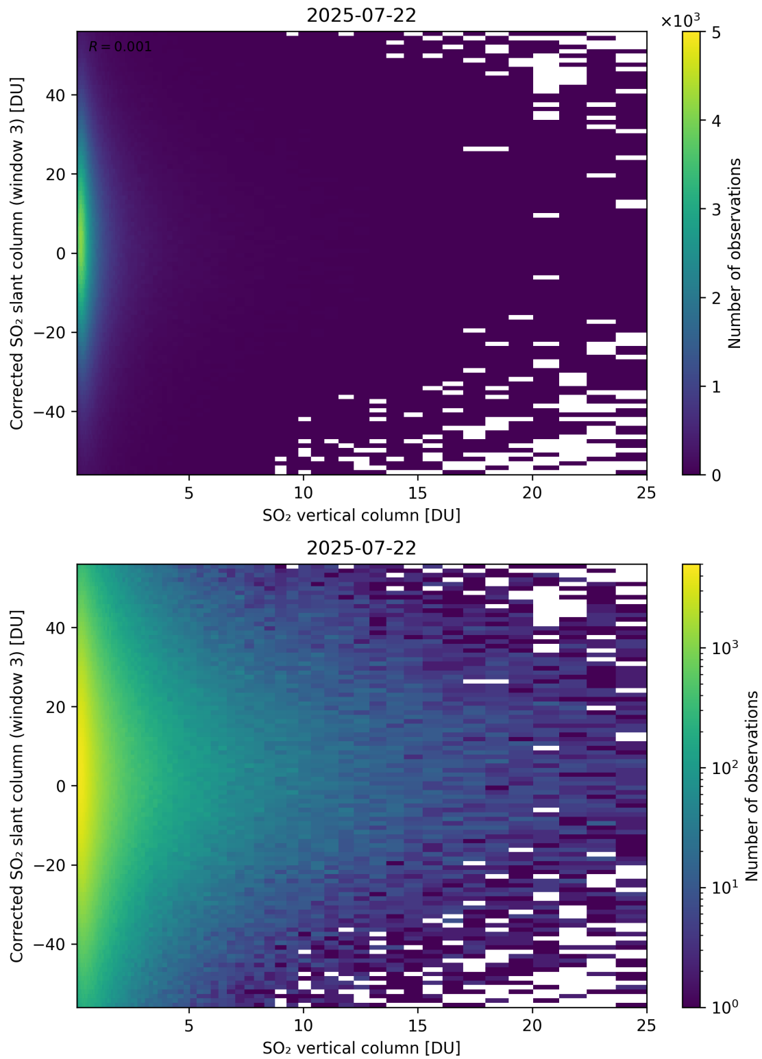
Figure 353: Scatter density plot of “SO 2 vertical column” against “Corrected SO 2 slant column (window 3)” for 2025-07-21 to 2025-07-23.
