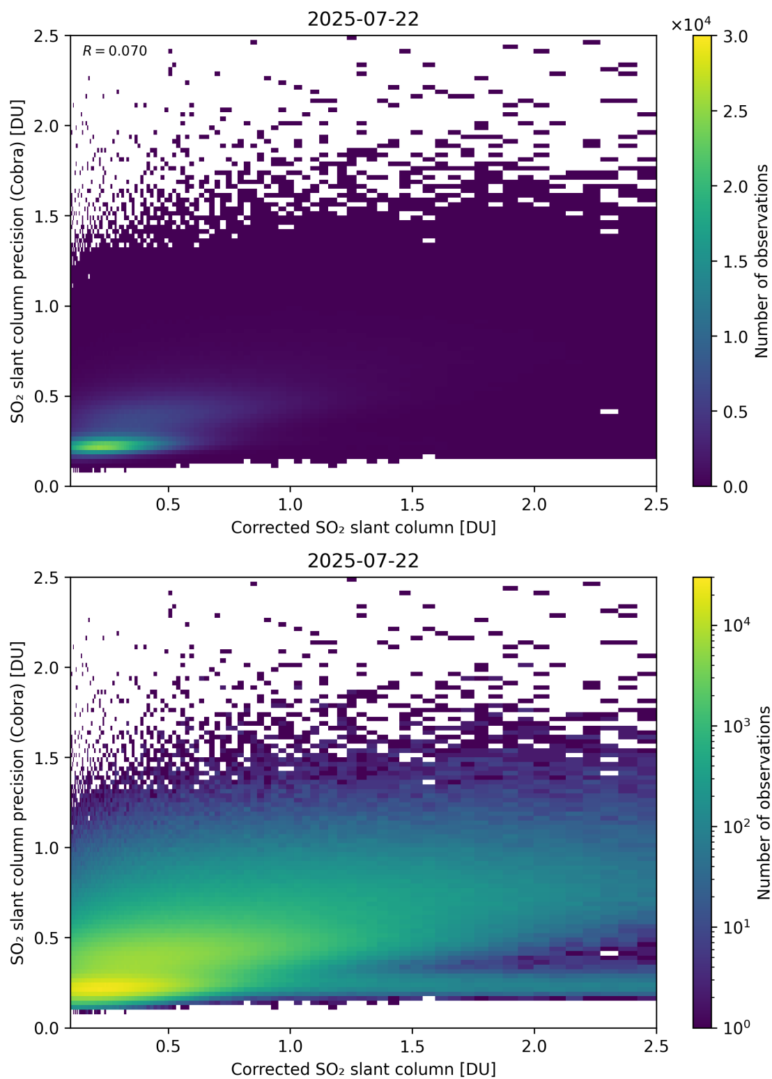
Figure 234: Scatter density plot of “Corrected SO 2 slant column” against “SO 2 slant column precision (Cobra)” for 2025-07-21 to 2025-07-23.
