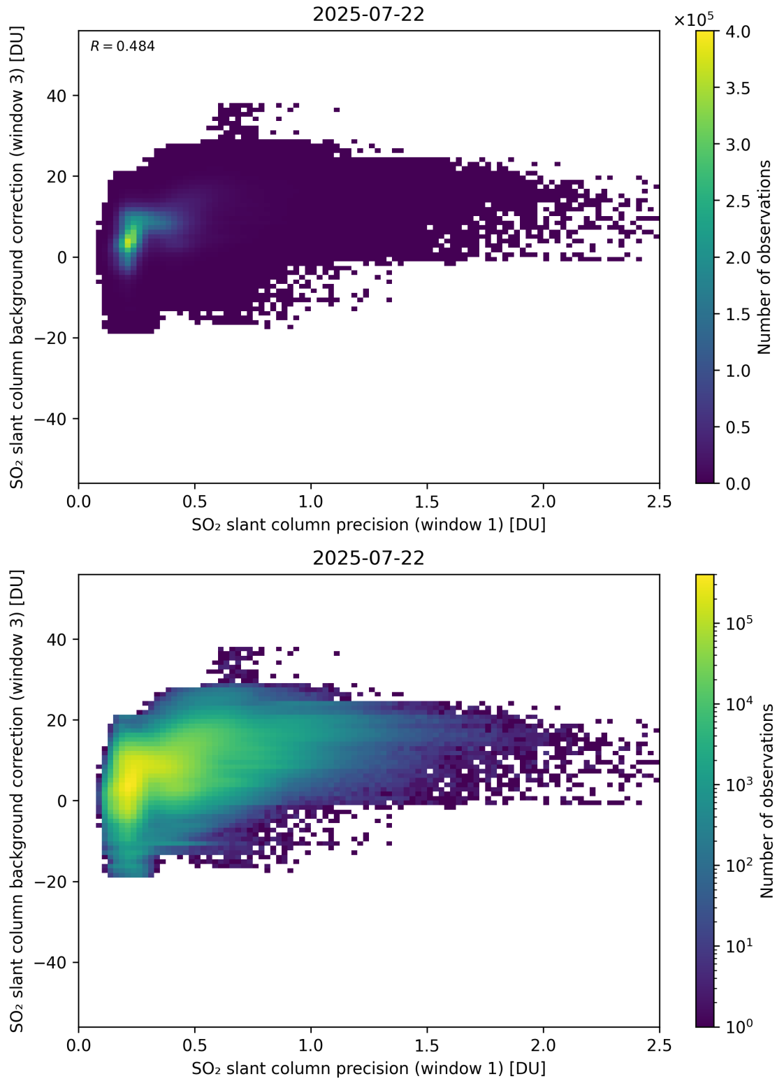
Figure 270: Scatter density plot of “SO 2 slant column precision (window 1)” against “SO 2 slant column background correction (window 3)” for 2025-07-21 to 2025-07-23.
