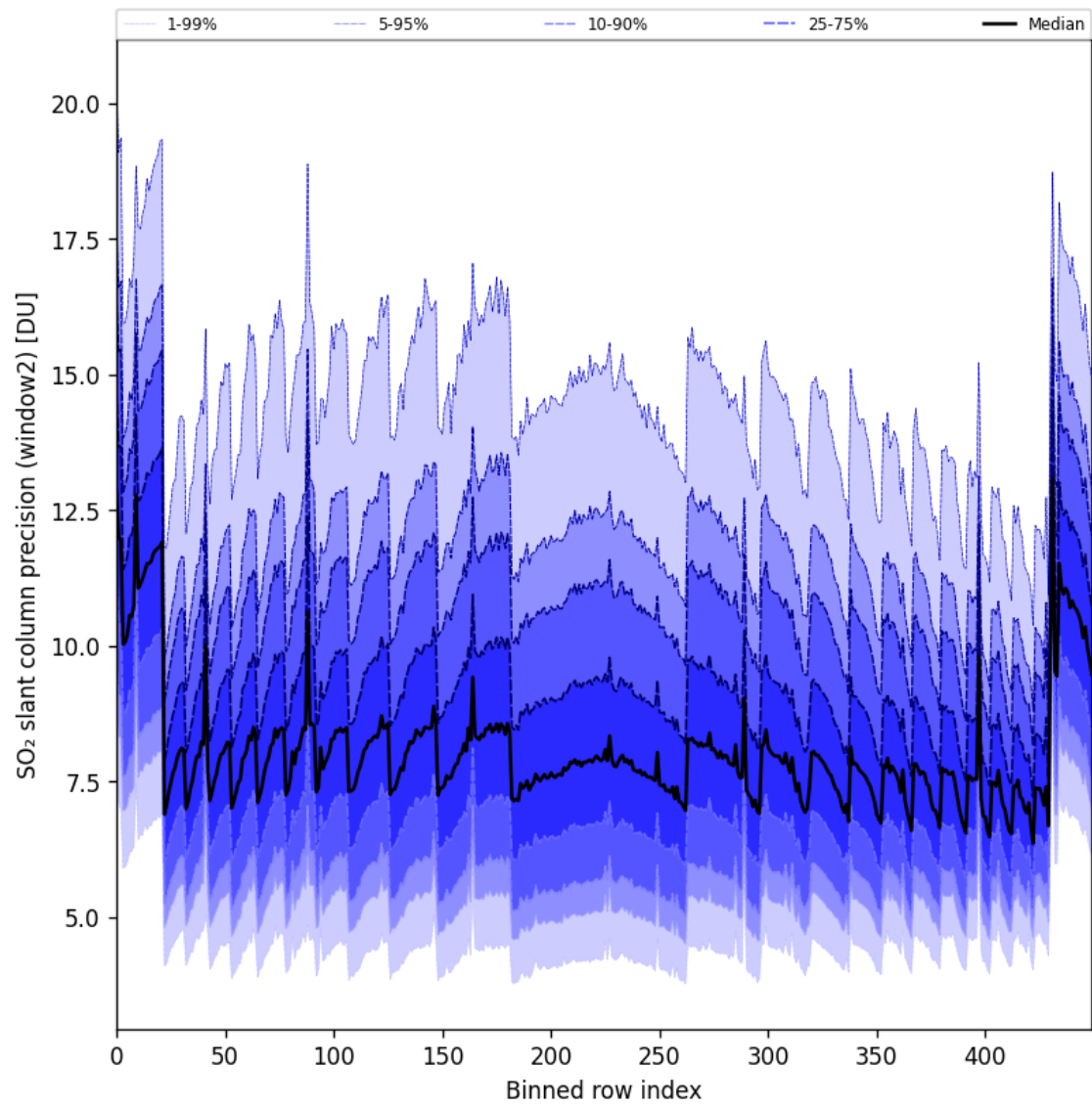
Figure 94: Along track statistics of “SO 2 slant column precision (window2)” for 2025-07-21 to 2025-07-23
