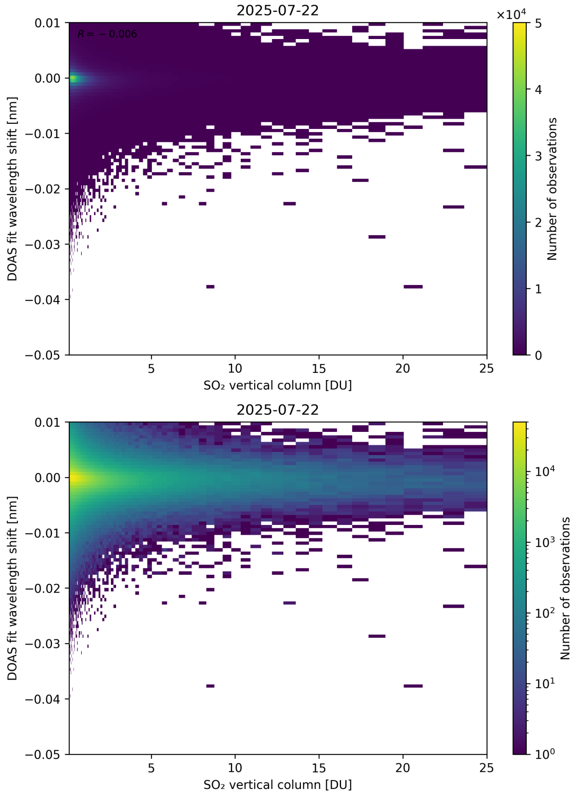
Figure 326: Scatter density plot of “SO 2 vertical column” against “DOAS fit wavelength shift” for 2025-07-21 to 2025-07-23.
