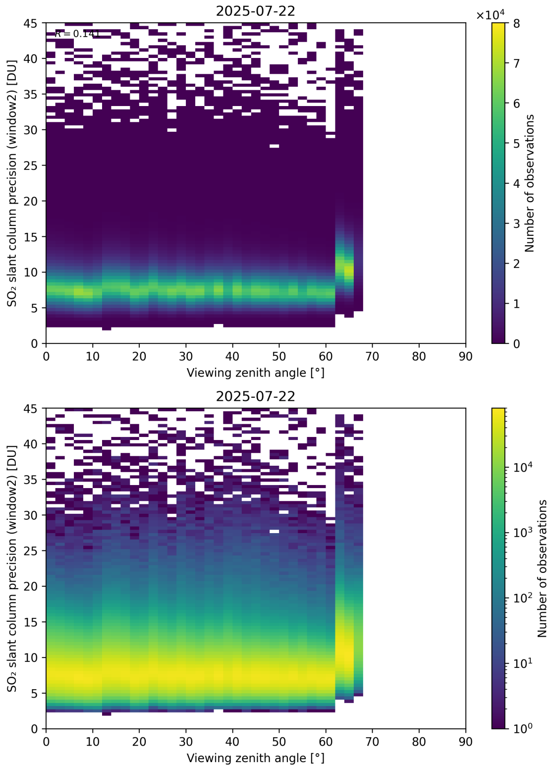
Figure 378: Scatter density plot of “Viewing zenith angle” against “SO 2 slant column precision (window2)” for 2025-07-21 to 2025-07-23.
