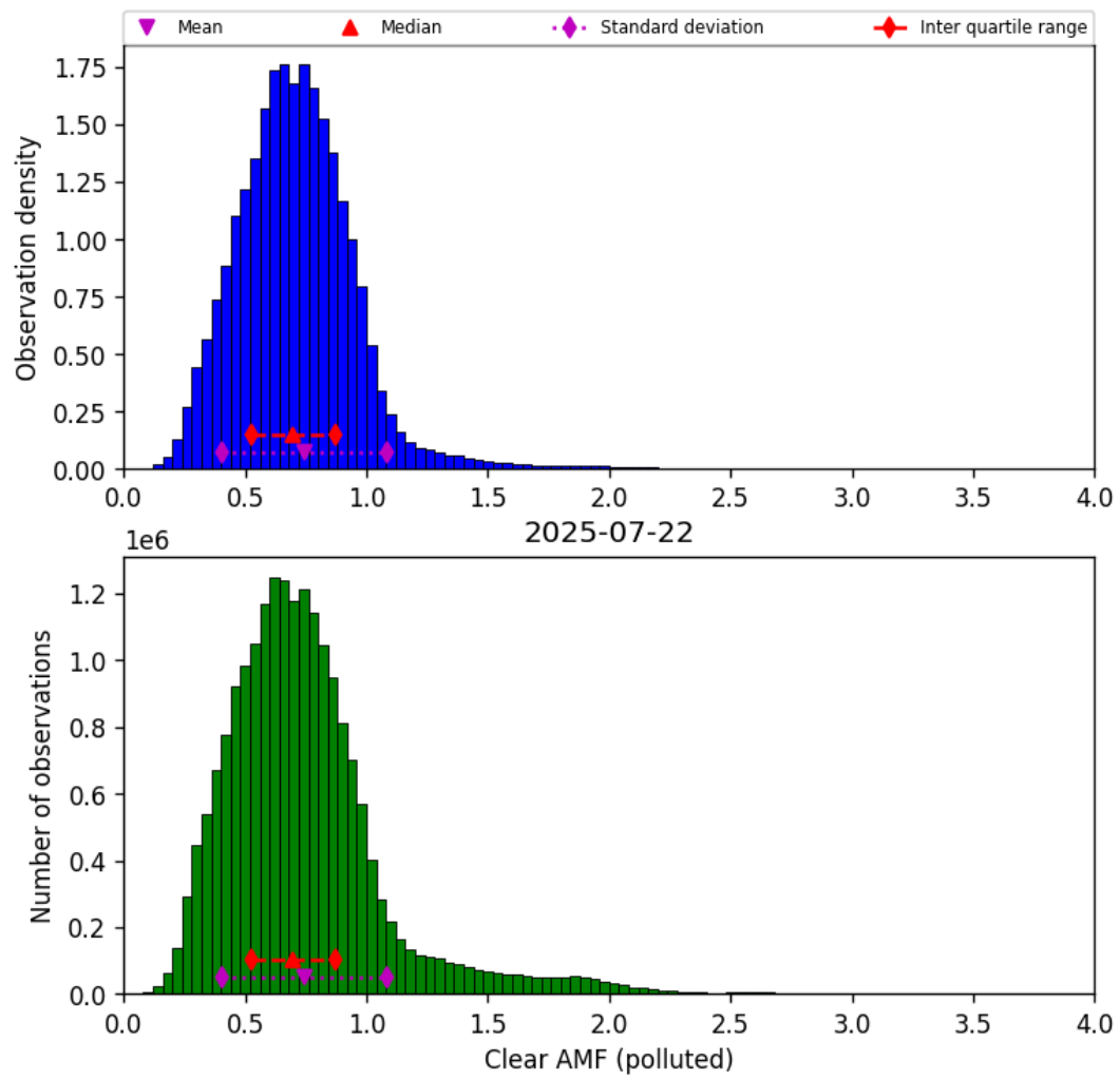
Figure 81: Histogram of “Clear AMF (polluted)” for 2025-07-21 to 2025-07-23
