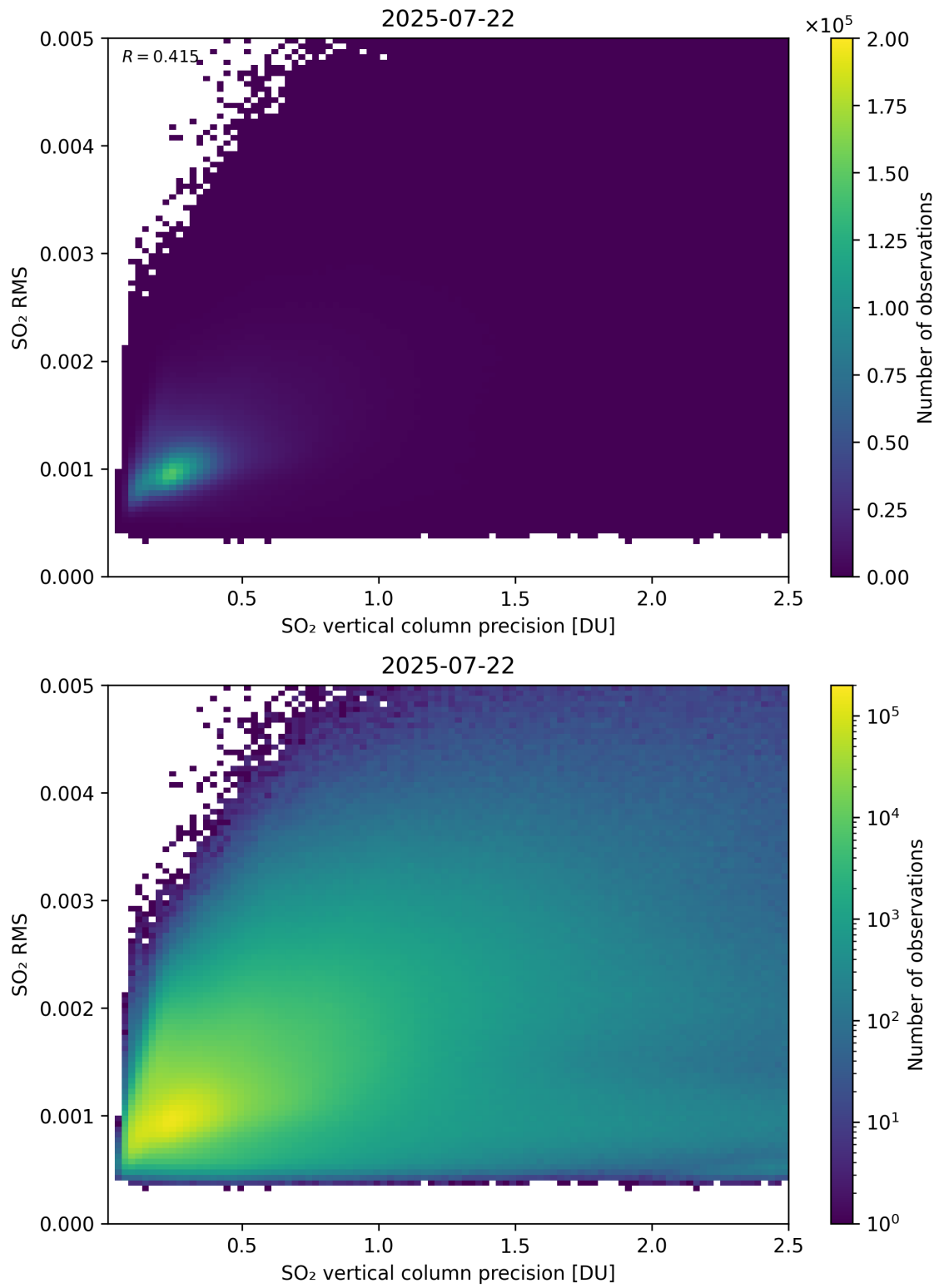
Figure 334: Scatter density plot of “SO 2 vertical column precision” against “SO 2 RMS” for 2025-07-21 to 2025-07-23.
