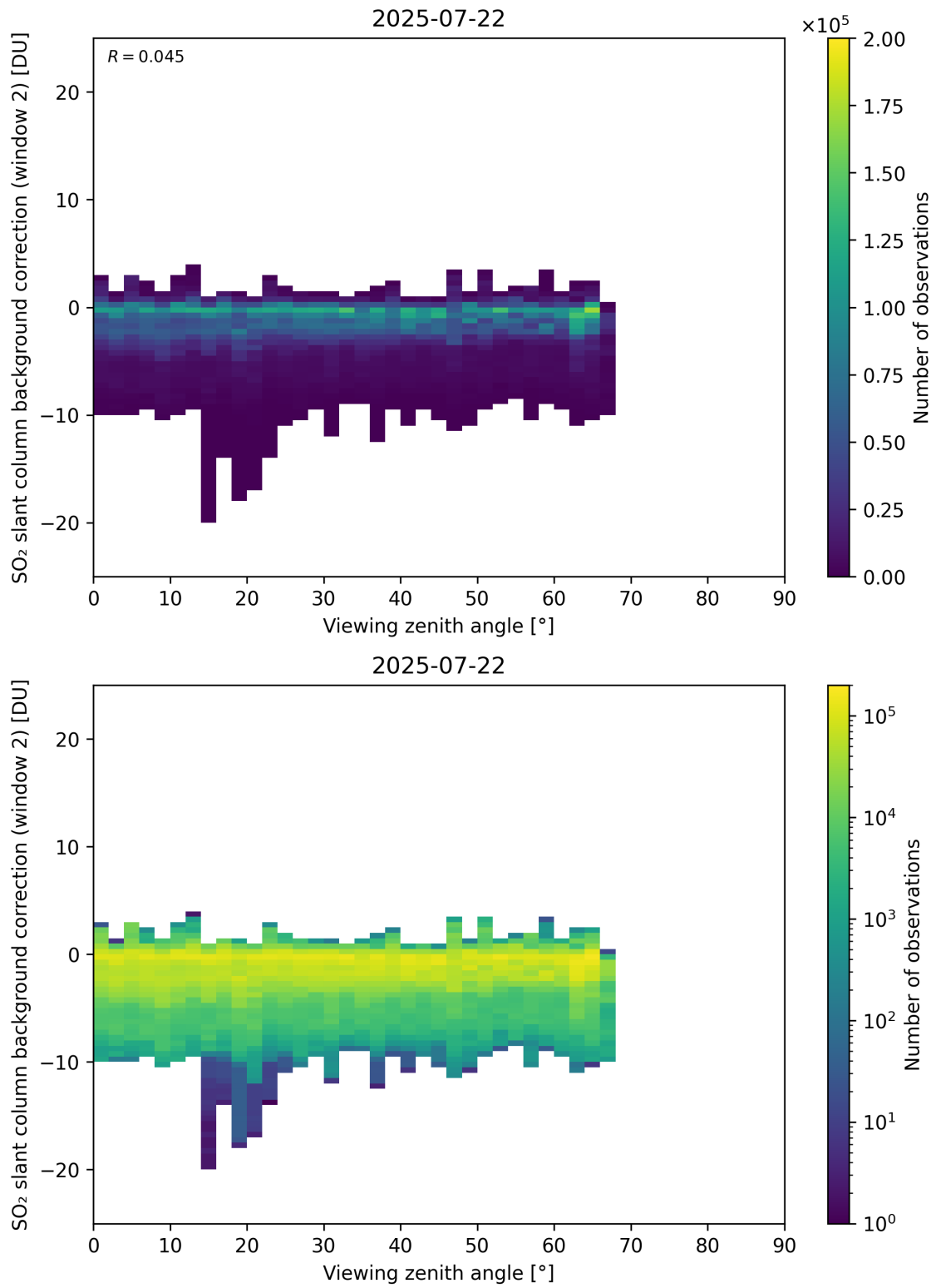
Figure 363: Scatter density plot of “Viewing zenith angle” against “SO 2 slant column background correction (window 2)” for 2025-07-21 to 2025-07-23.
