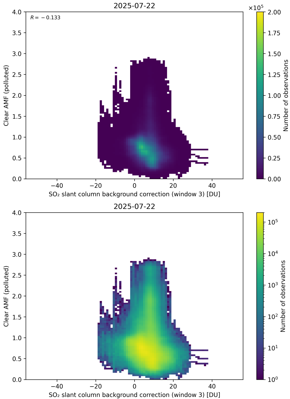
Figure 135: Scatter density plot of “SO 2 slant column background correction (window 3)” against “Clear AMF (polluted)” for 2025-07-21 to 2025-07-23.
