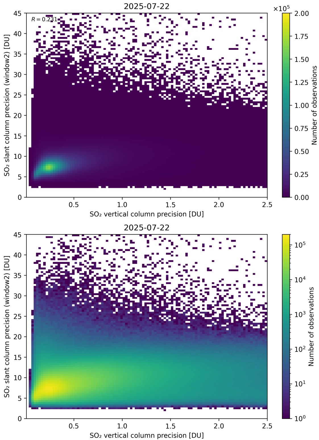
Figure 343: Scatter density plot of “SO 2 vertical column precision” against “SO 2 slant column precision (window2)” for 2025-07-21 to 2025-07-23.
