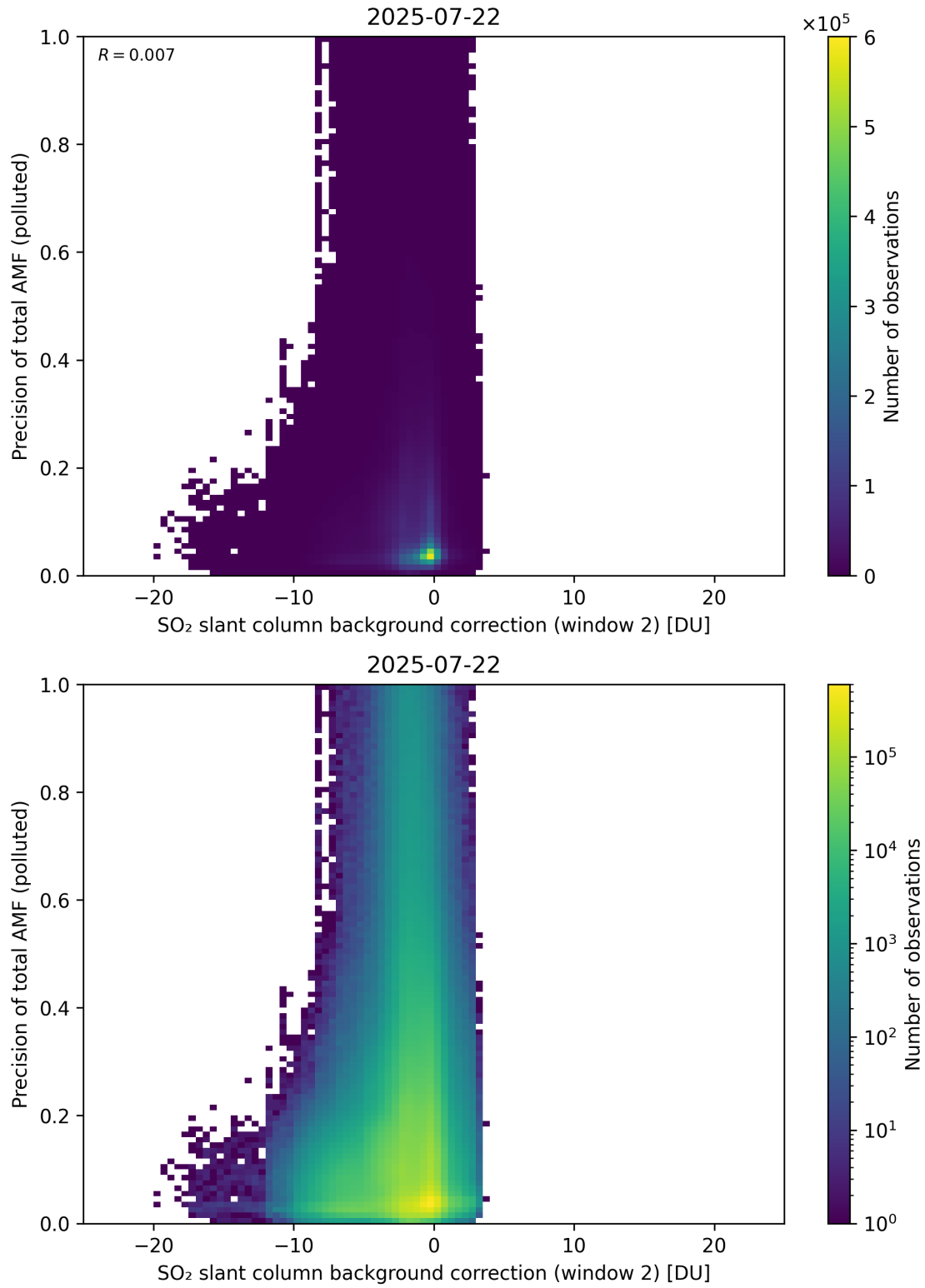
Figure 131: Scatter density plot of “SO 2 slant column background correction (window 2)” against “Precision of total AMF (polluted)” for 2025-07-21 to 2025-07-23.
