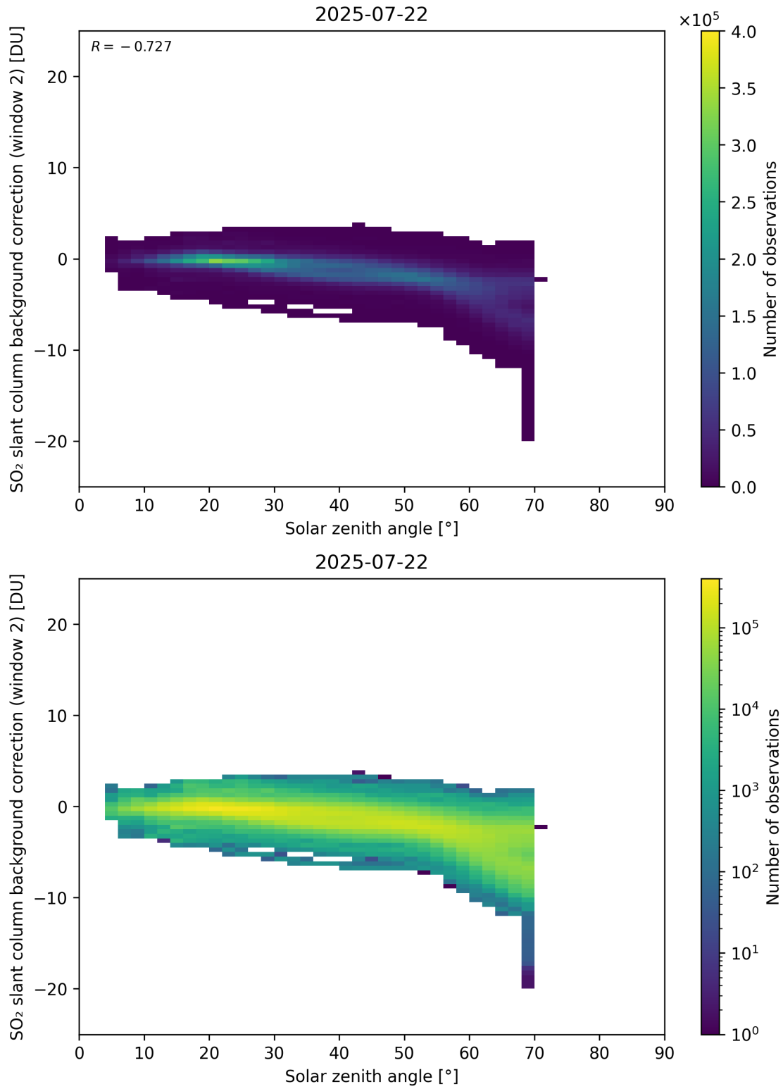
Figure 172: Scatter density plot of “Solar zenith angle” against “SO 2 slant column background correction (window 2)” for 2025-07-21 to 2025-07-23.
