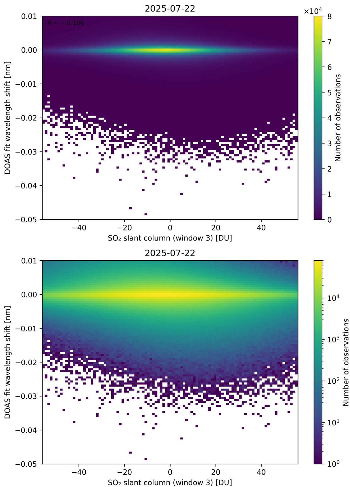
Figure 304: Scatter density plot of “SO 2 slant column (window 3)” against “DOAS fit wavelength shift” for 2025-07-21 to 2025-07-23.
