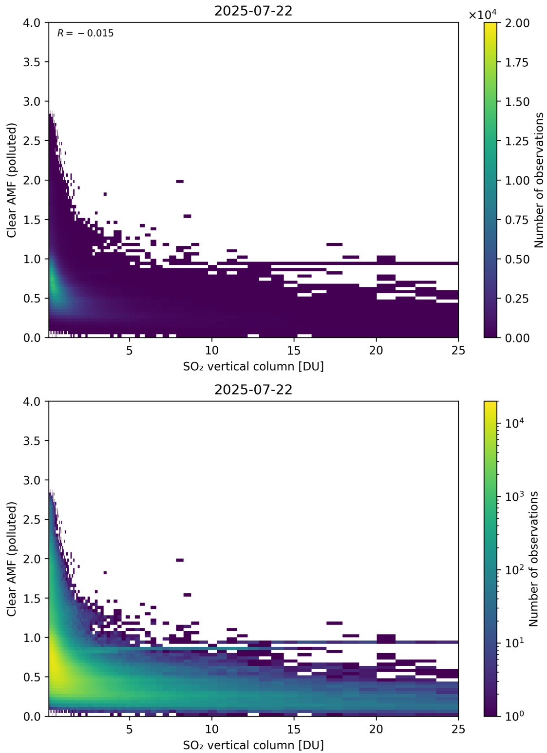
Figure 348: Scatter density plot of “SO 2 vertical column” against “Clear AMF (polluted)” for 2025-07-21 to 2025-07-23.
