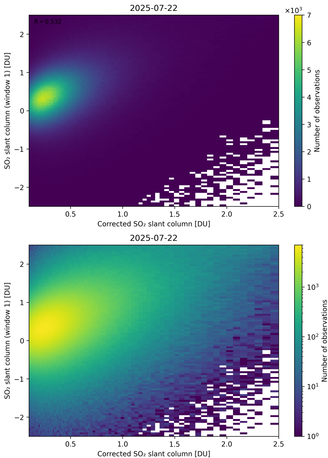
Figure 237: Scatter density plot of “Corrected SO 2 slant column” against “SO 2 slant column (window 1)” for 2025-07-21 to 2025-07-23.
