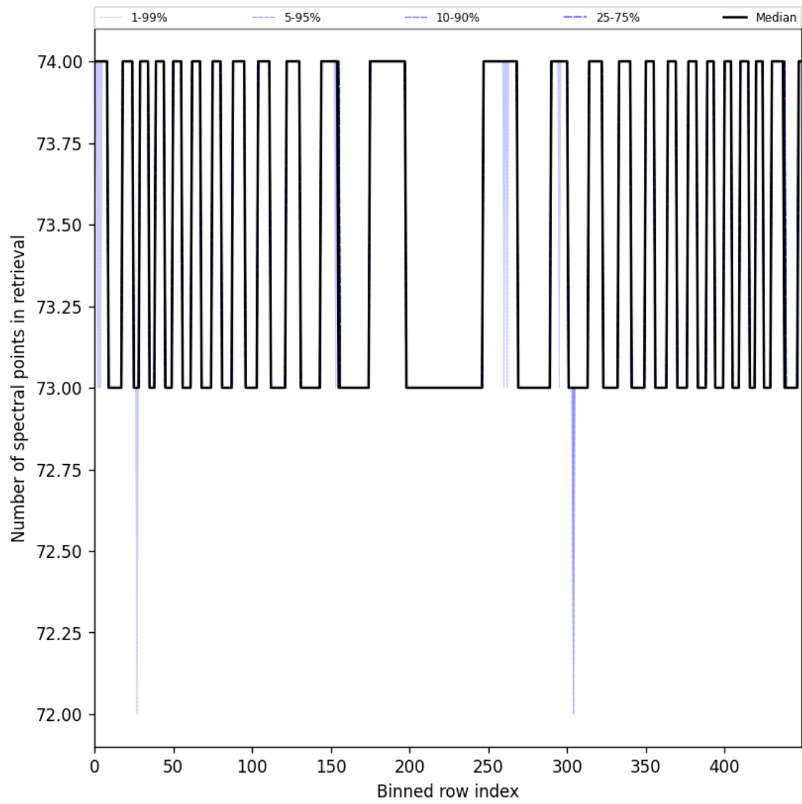
Figure 108: Along track statistics of “Number of spectral points in retrieval” for 2025-07-21 to 2025-07-23
