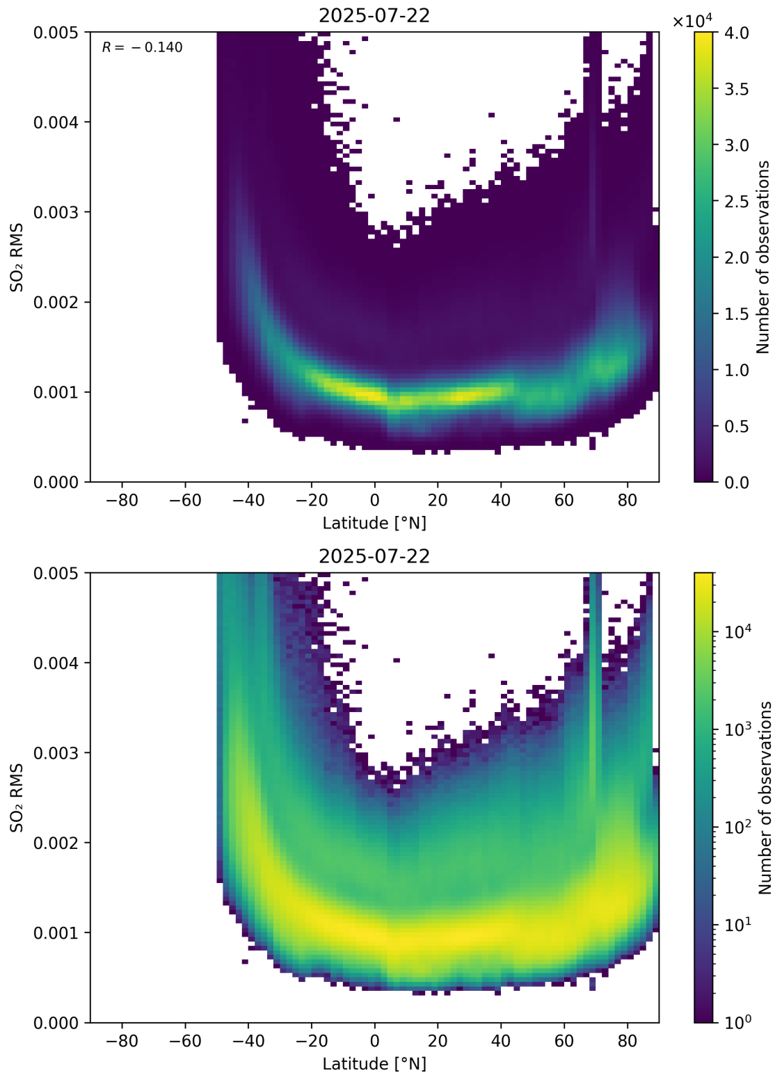
Figure 155: Scatter density plot of “Latitude” against “SO 2 RMS” for 2025-07-21 to 2025-07-23.
