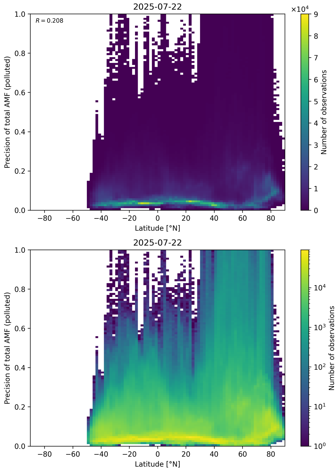
Figure 168: Scatter density plot of “Latitude” against “Precision of total AMF (polluted)” for 2025-07-21 to 2025-07-23.
