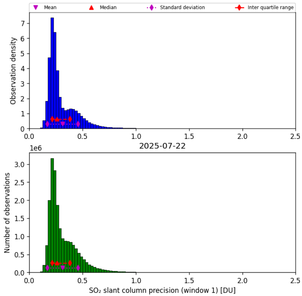
Figure 64: Histogram of “SO 2 slant column precision (window 1)” for 2025-07-21 to 2025-07-23
