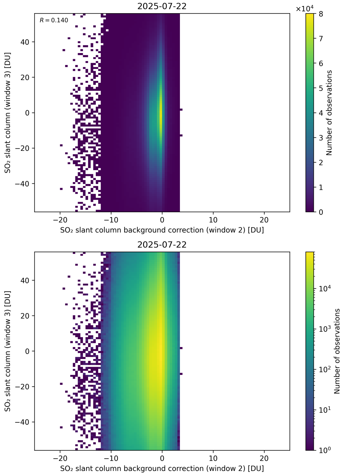
Figure 128: Scatter density plot of “SO 2 slant column background correction (window 2)” against “SO 2 slant column (window 3)” for 2025-07-21 to 2025-07-23.
