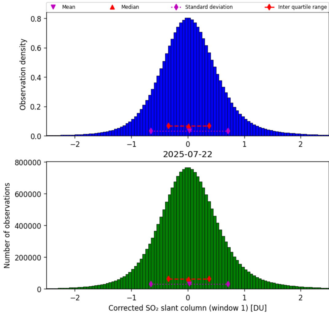
Figure 65: Histogram of “Corrected SO 2 slant column (window 1)” for 2025-07-21 to 2025-07-23
