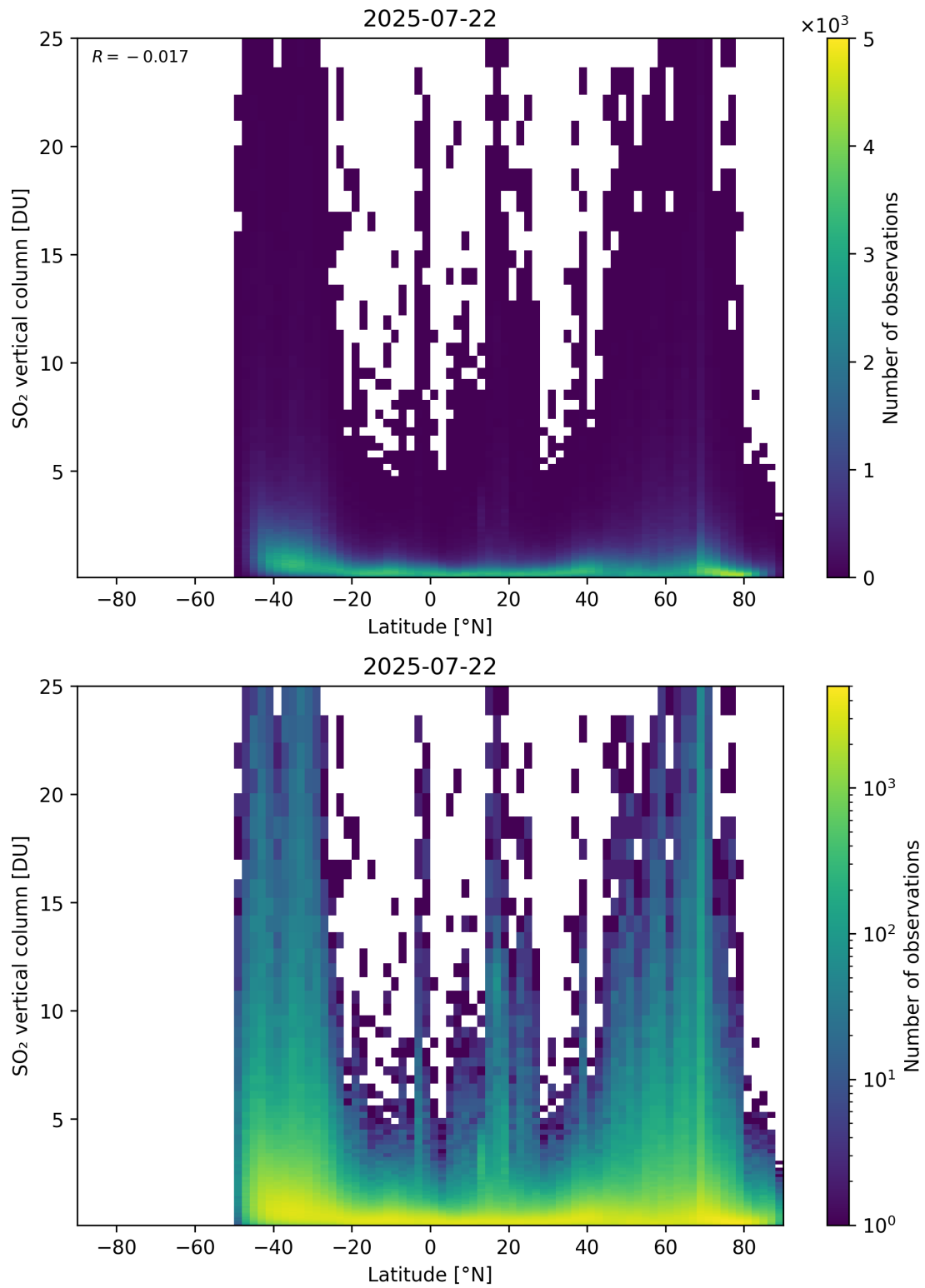
Figure 169: Scatter density plot of “Latitude” against “SO 2 vertical column” for 2025-07-21 to 2025-07-23.
