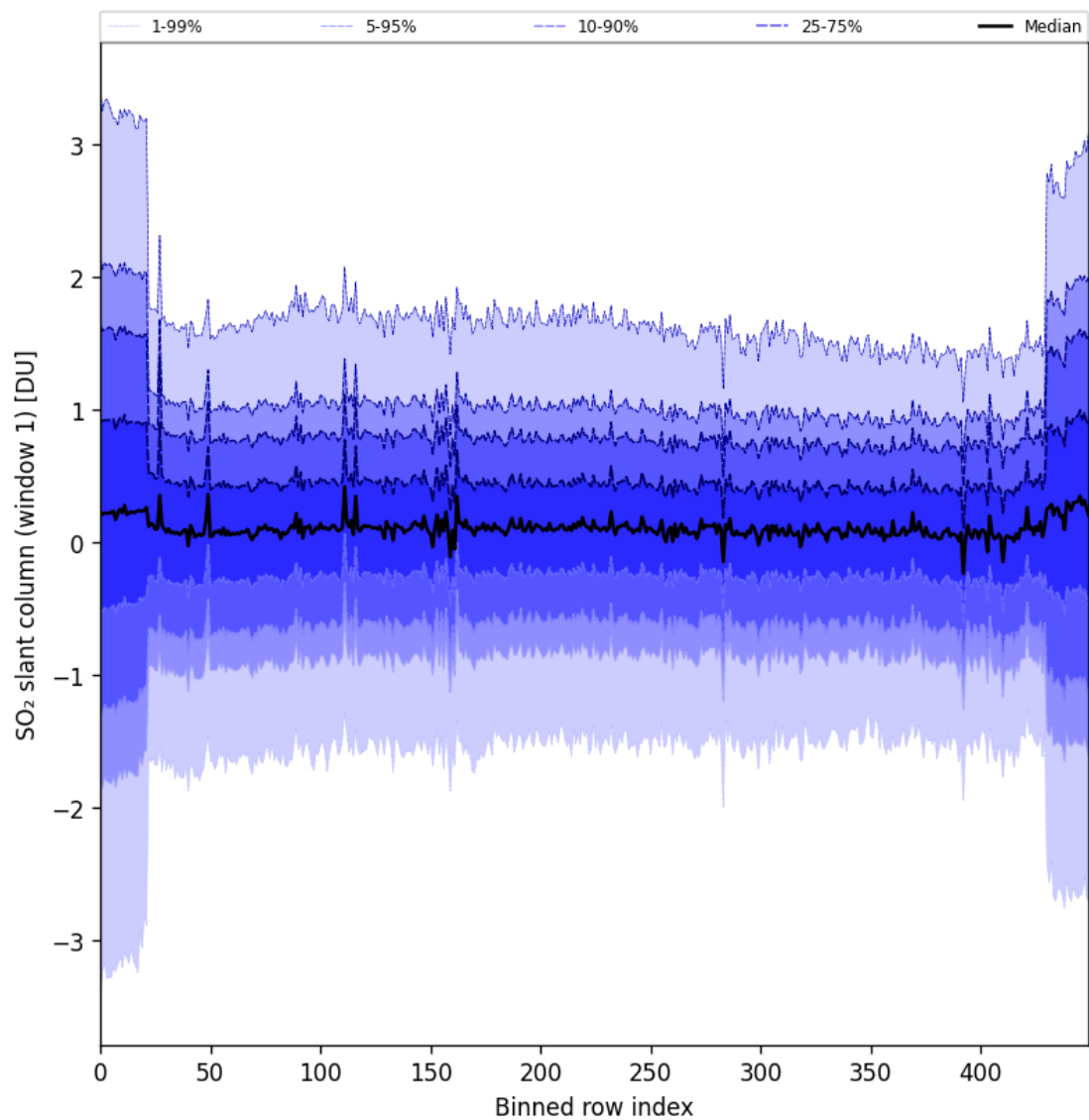
Figure 89: Along track statistics of “SO 2 slant column (window 1)” for 2025-07-21 to 2025-07-23
