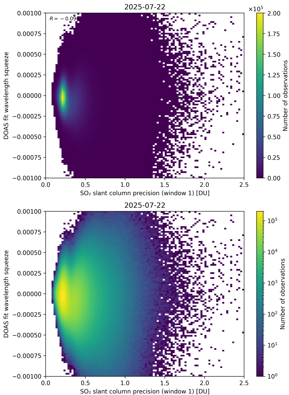
Figure 272: Scatter density plot of “SO 2 slant column precision (window 1)” against “DOAS fit wavelength squeeze” for 2025-07-21 to 2025-07-23.
