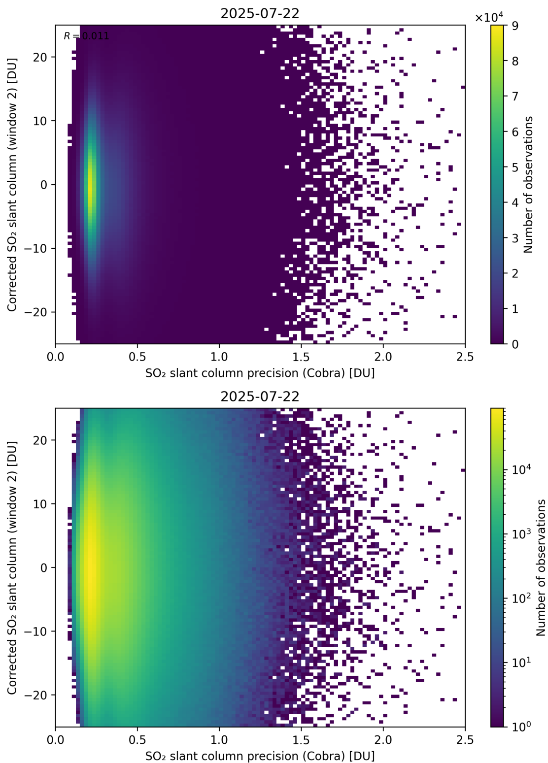
Figure 206: Scatter density plot of “SO 2 slant column precision (Cobra)” against “Corrected SO 2 slant column (window 2)” for 2025-07-21 to 2025-07-23.
