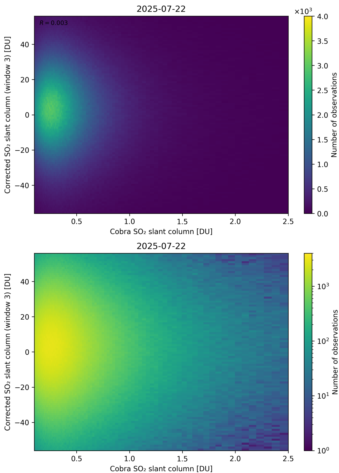
Figure 218: Scatter density plot of “Cobra SO 2 slant column” against “Corrected SO 2 slant column (window 3)” for 2025-07-21 to 2025-07-23.
