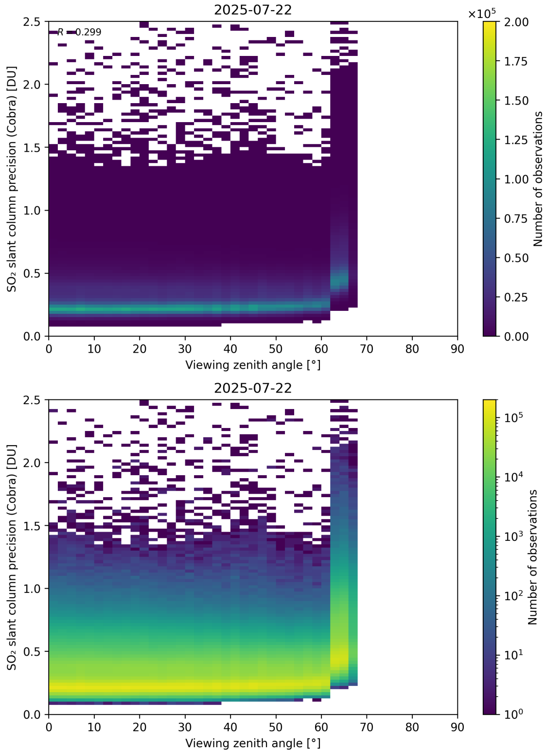
Figure 372: Scatter density plot of “Viewing zenith angle” against “SO 2 slant column precision (Cobra)” for 2025-07-21 to 2025-07-23.
