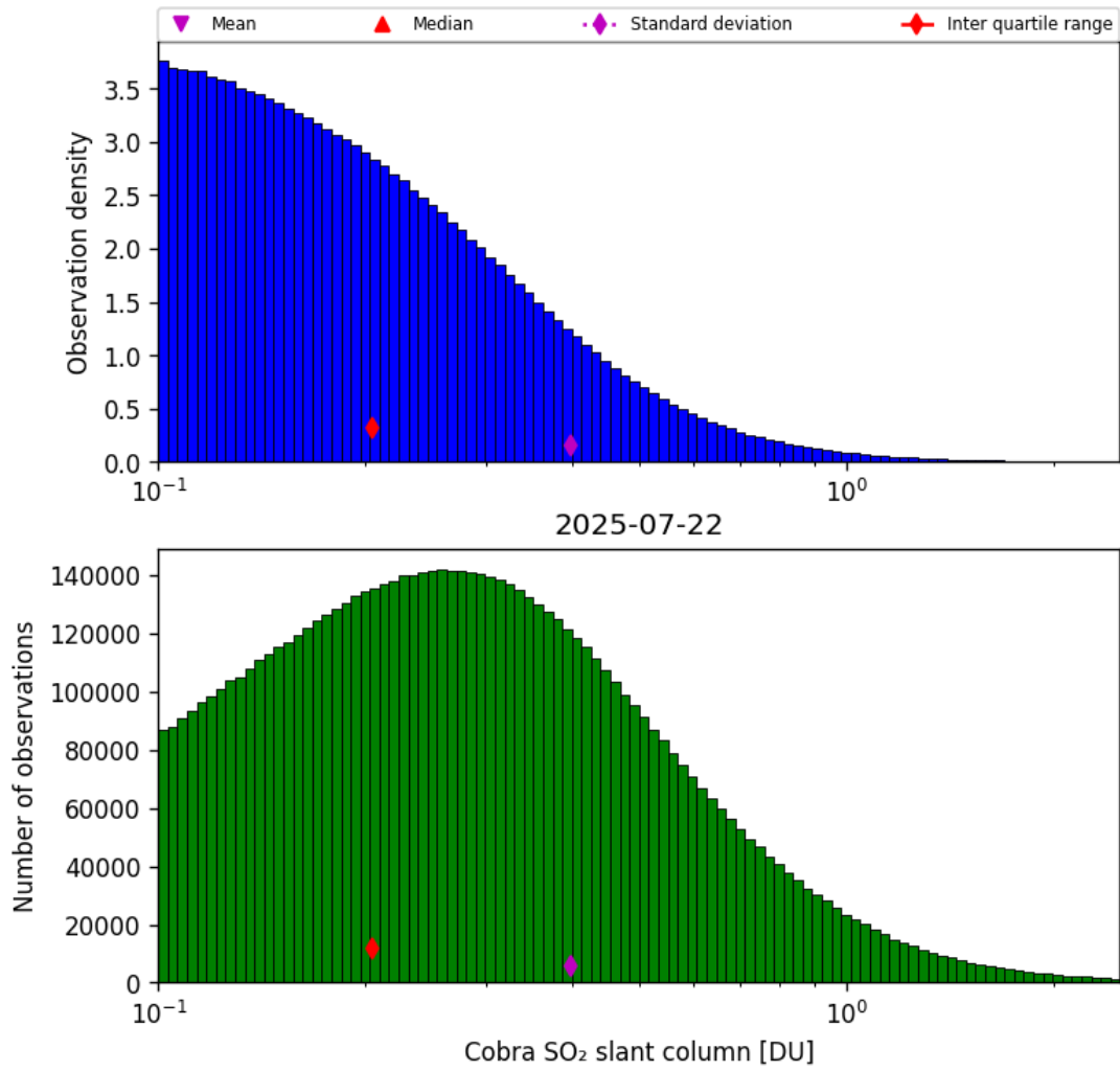
Figure 61: Histogram of “Cobra SO 2 slant column” for 2025-07-21 to 2025-07-23
