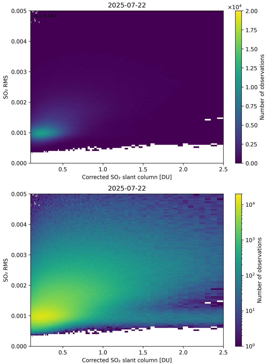
Figure 231: Scatter density plot of “Corrected SO 2 slant column” against “SO 2 RMS” for 2025-07-21 to 2025-07-23.
