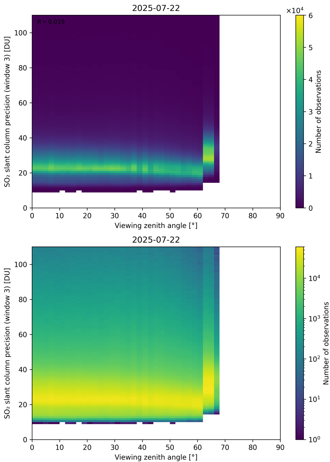
Figure 380: Scatter density plot of “Viewing zenith angle” against “SO 2 slant column precision (window 3)” for 2025-07-21 to 2025-07-23.
