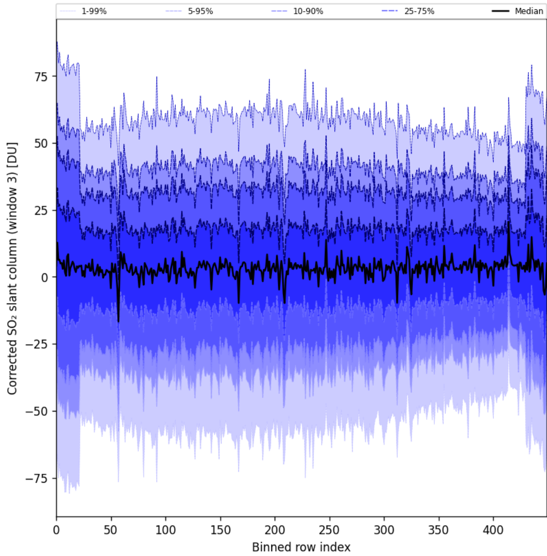
Figure 99: Along track statistics of “Corrected SO 2 slant column (window 3)” for 2025-07-21 to 2025-07-23
