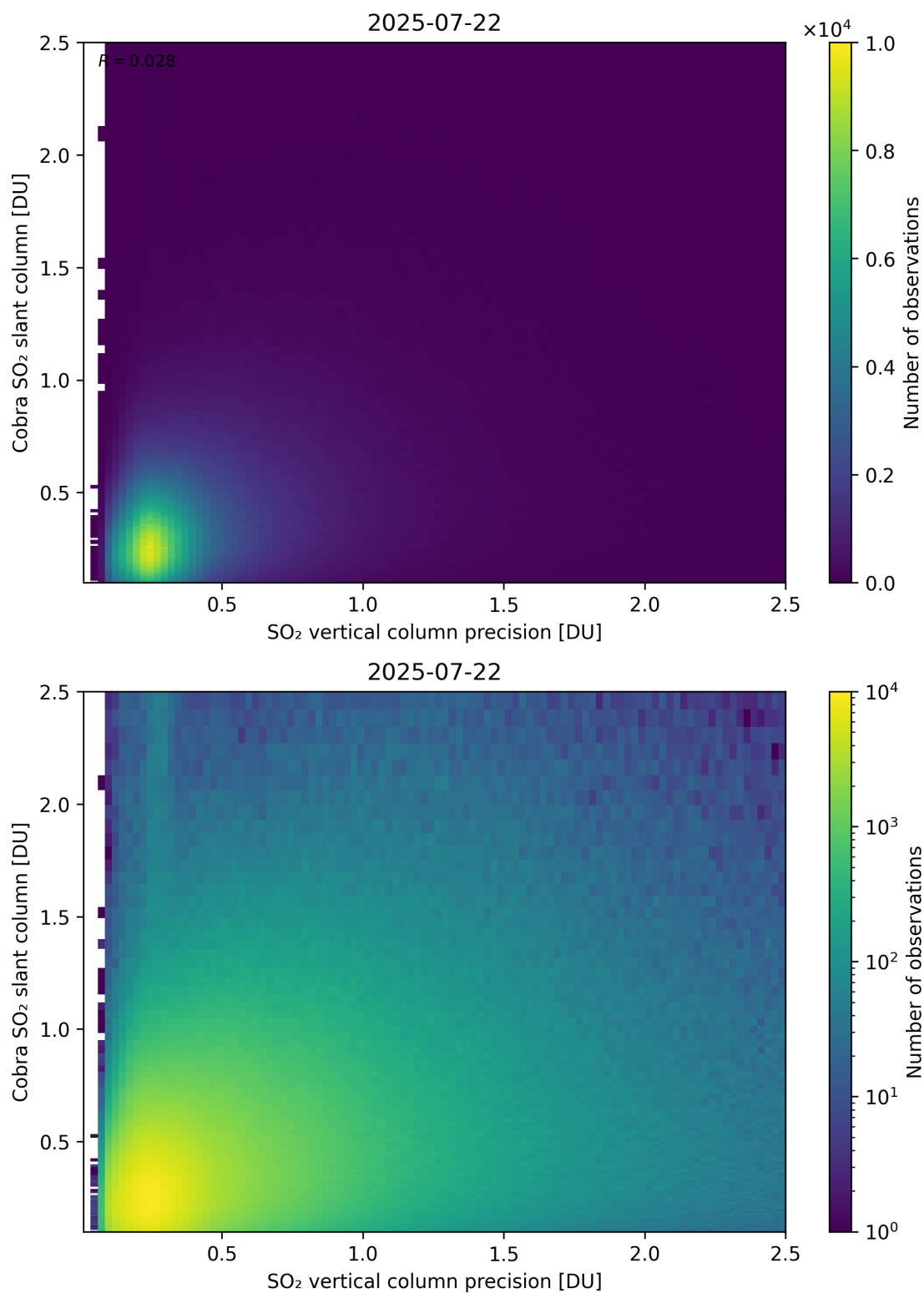
Figure 336: Scatter density plot of “SO 2 vertical column precision” against “Cobra SO 2 slant column” for 2025-07-21 to 2025-07-23.
