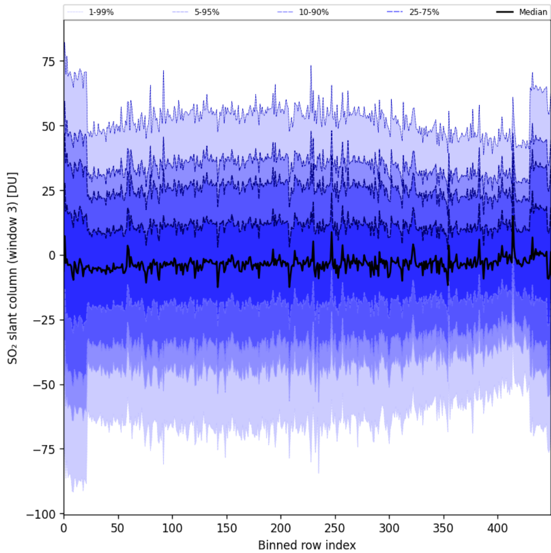
Figure 97: Along track statistics of “SO 2 slant column (window 3)” for 2025-07-21 to 2025-07-23
