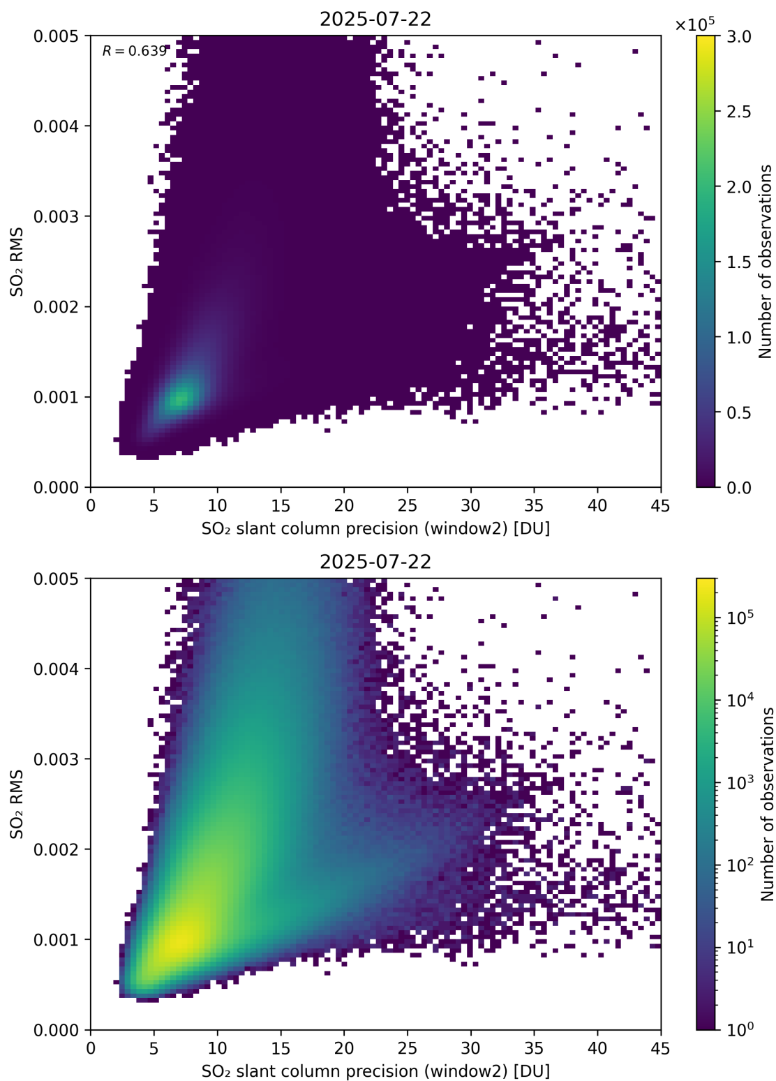
Figure 295: Scatter density plot of “SO 2 slant column precision (window2)” against “SO 2 RMS” for 2025-07-21 to 2025-07-23.
