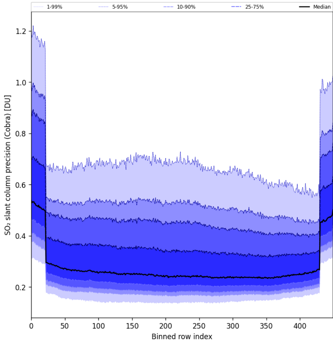
Figure 88: Along track statistics of “SO 2 slant column precision (Cobra)” for 2025-07-21 to 2025-07-23
