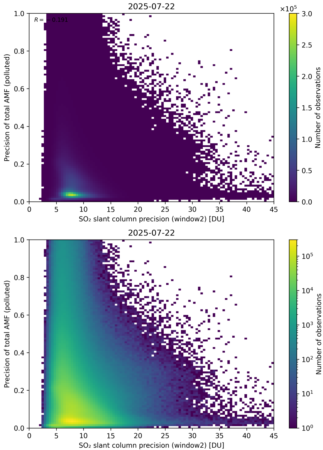
Figure 302: Scatter density plot of “SO 2 slant column precision (window2)” against “Precision of total AMF (polluted)” for 2025-07-21 to 2025-07-23.
