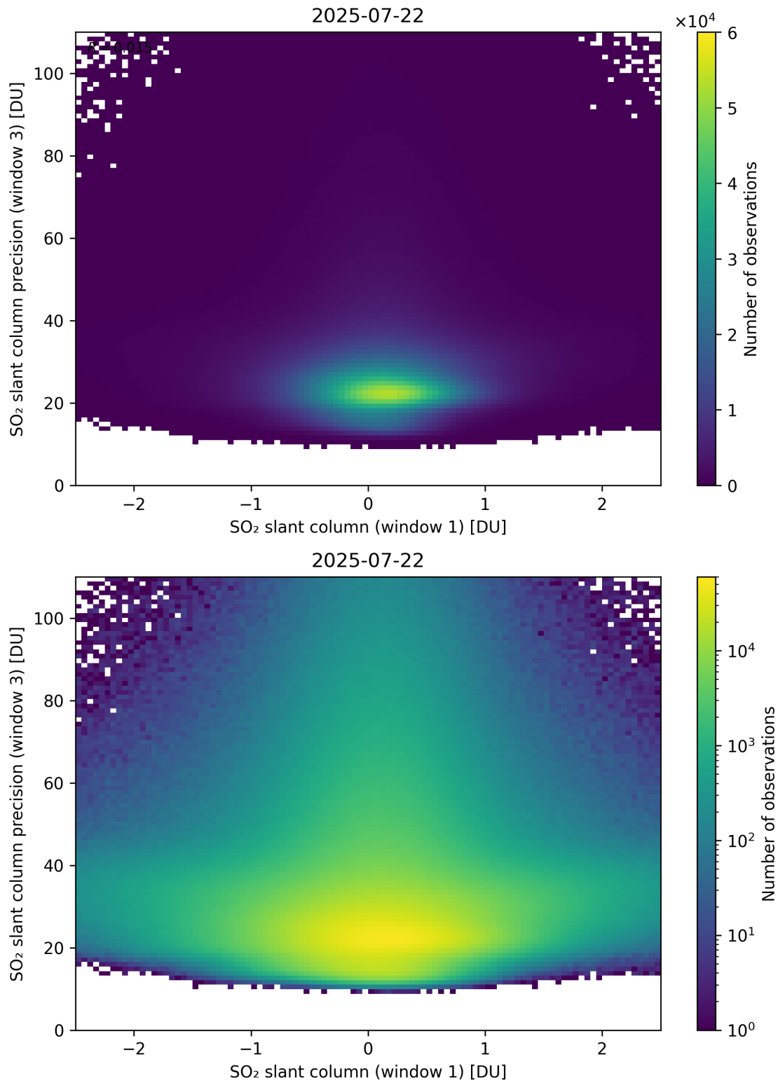
Figure 288: Scatter density plot of “SO 2 slant column (window 1)” against “SO 2 slant column precision (window 3)” for 2025-07-21 to 2025-07-23.
