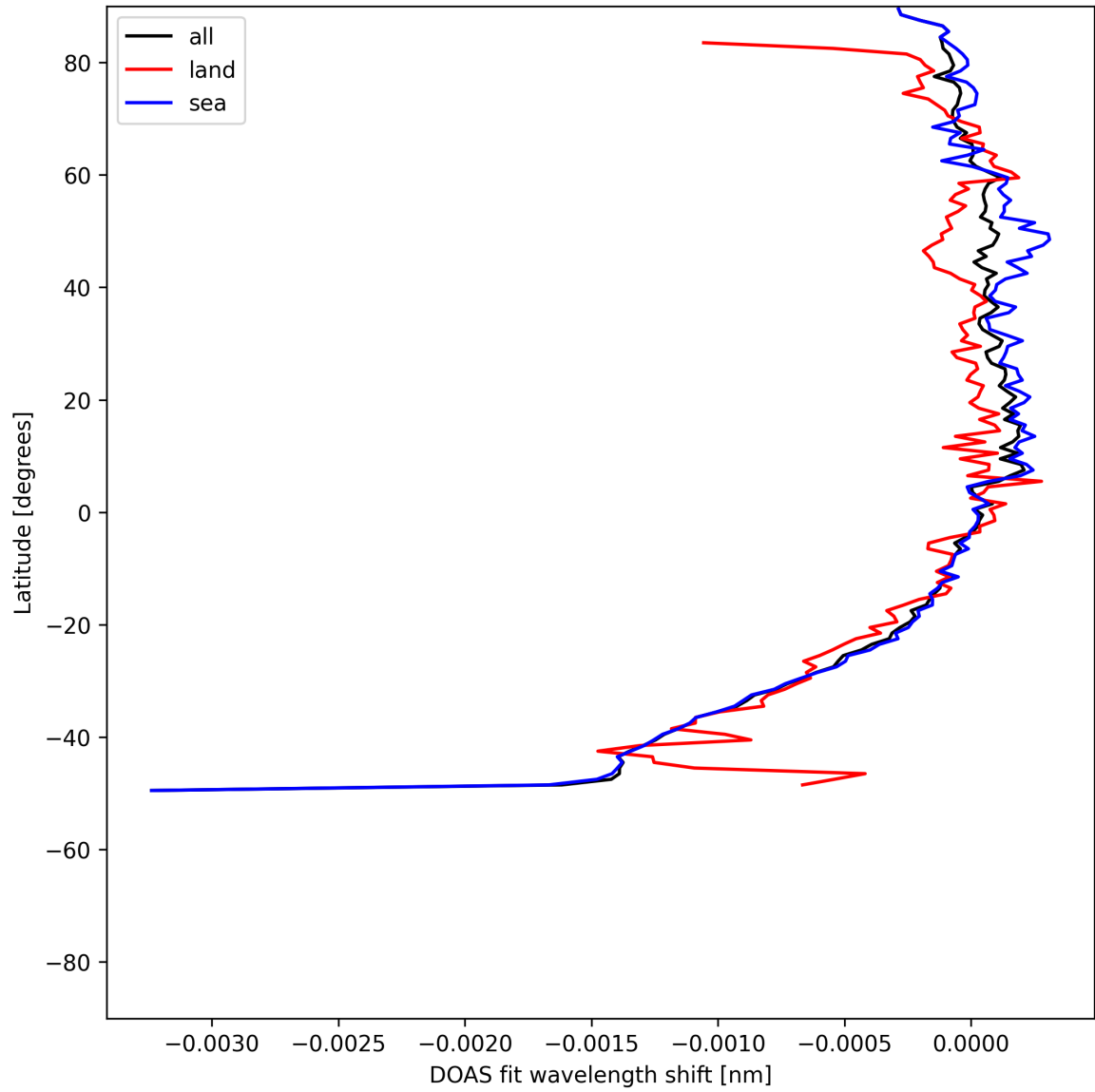
Figure 50: Zonal average of "DOAS fit wavelength shift" for 2025-07-21 to 2025-07-23.
