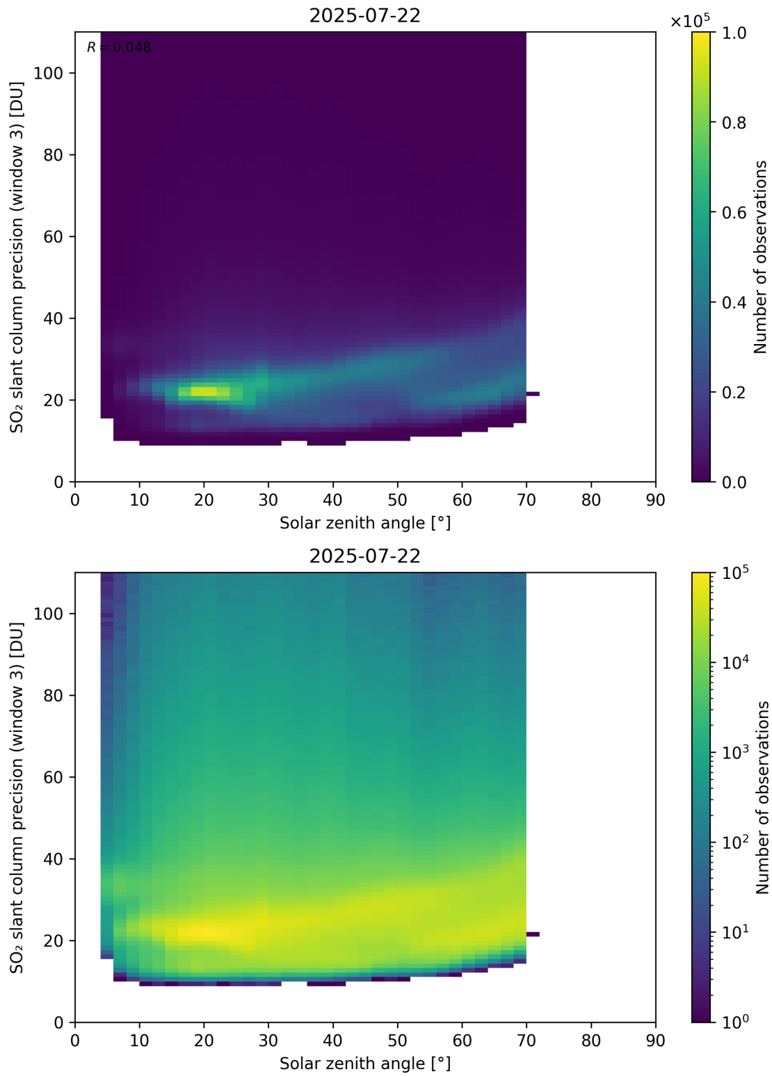
Figure 188: Scatter density plot of “Solar zenith angle” against “SO 2 slant column precision (window 3)” for 2025-07-21 to 2025-07-23.
