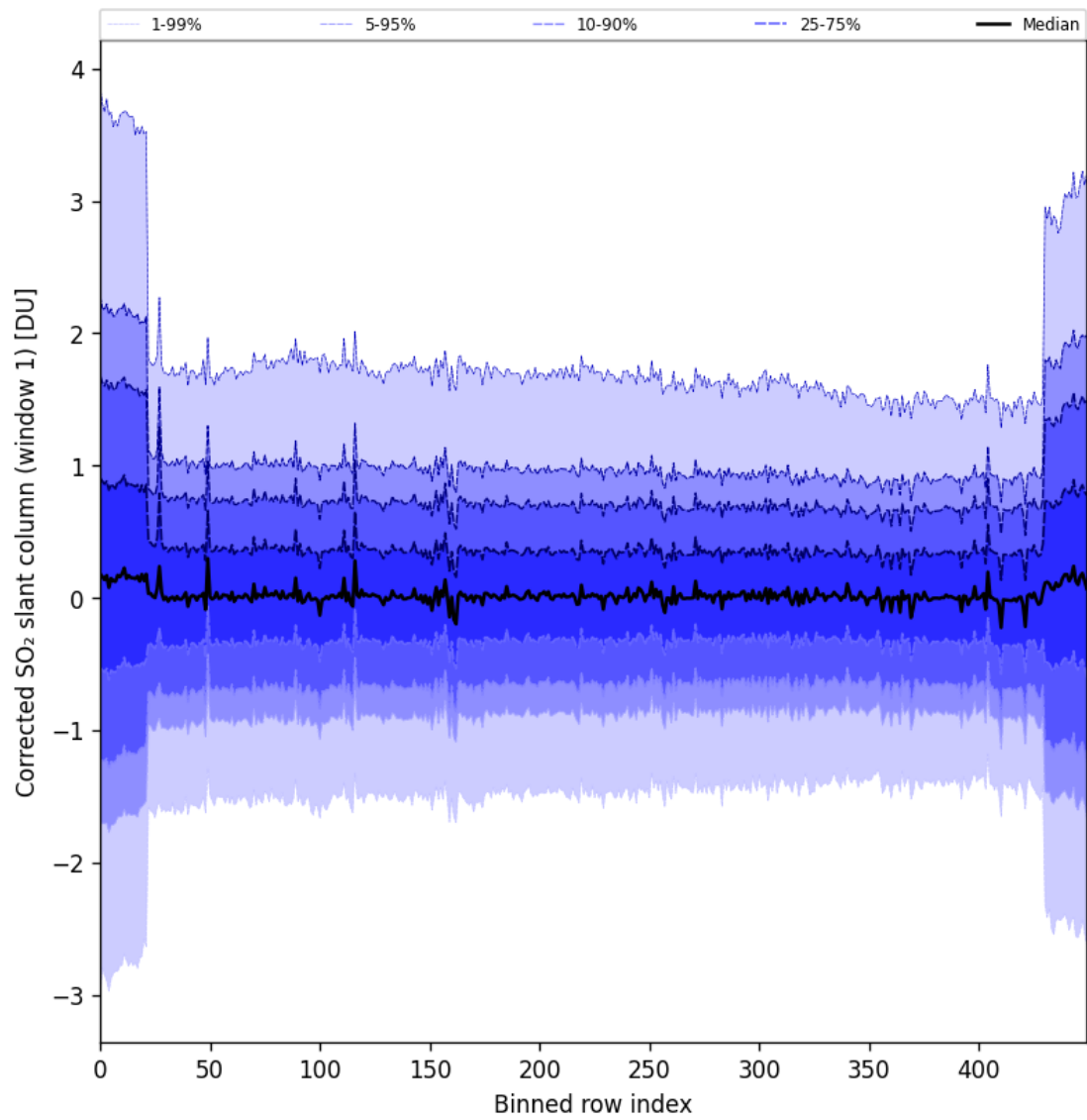
Figure 91: Along track statistics of “Corrected SO 2 slant column (window 1)” for 2025-07-21 to 2025-07-23
