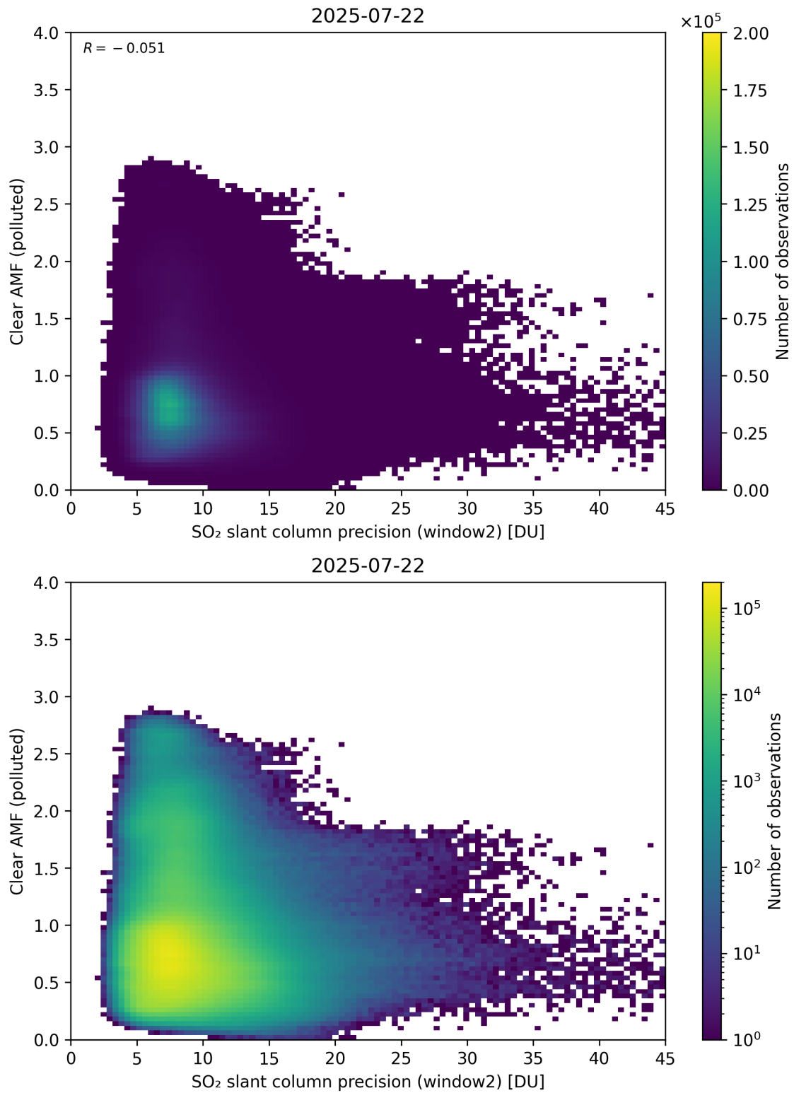
Figure 296: Scatter density plot of “SO 2 slant column precision (window2)” against “Clear AMF (polluted)” for 2025-07-21 to 2025-07-23.
