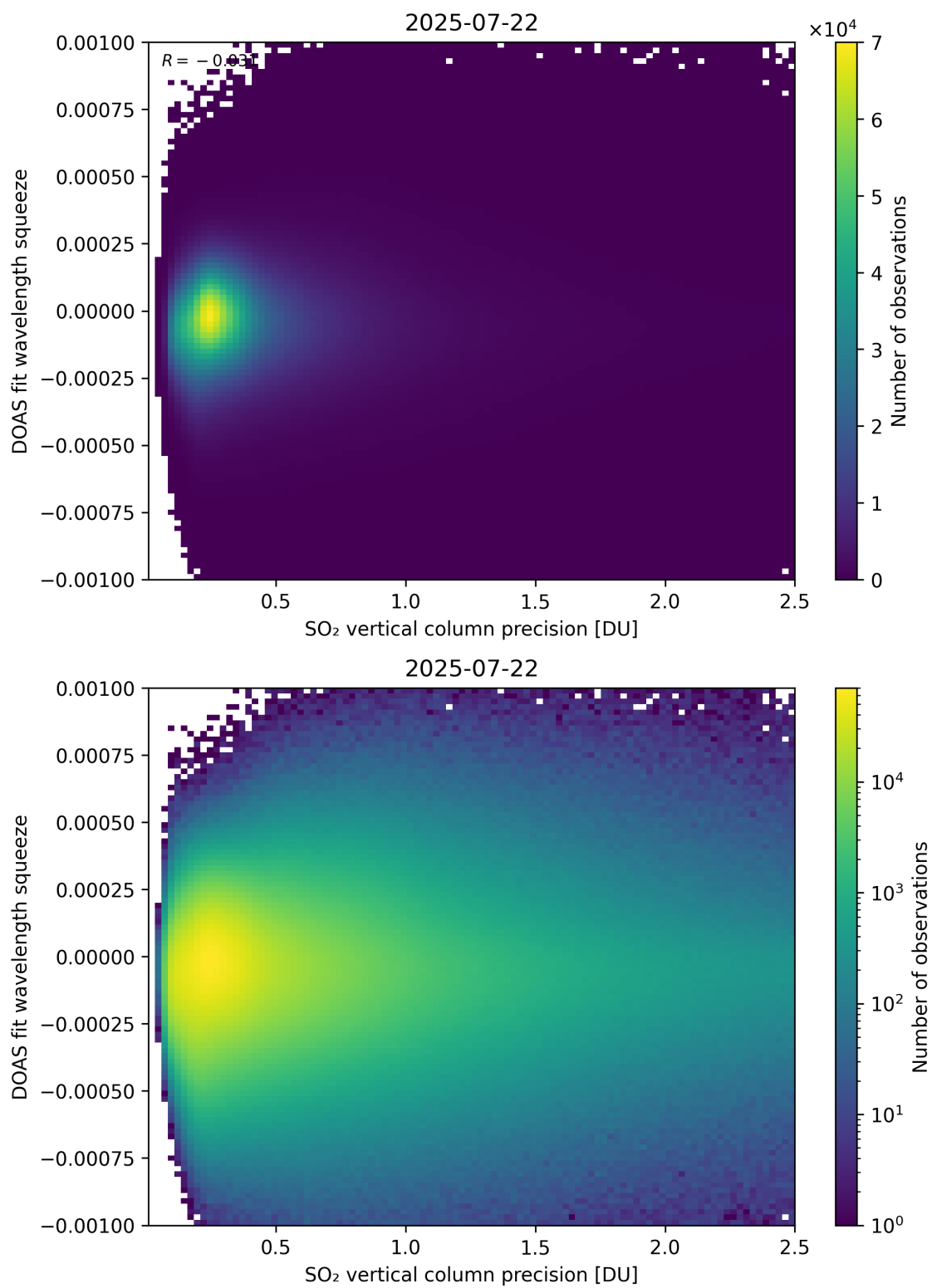
Figure 333: Scatter density plot of “SO 2 vertical column precision” against “DOAS fit wavelength squeeze” for 2025-07-21 to 2025-07-23.
