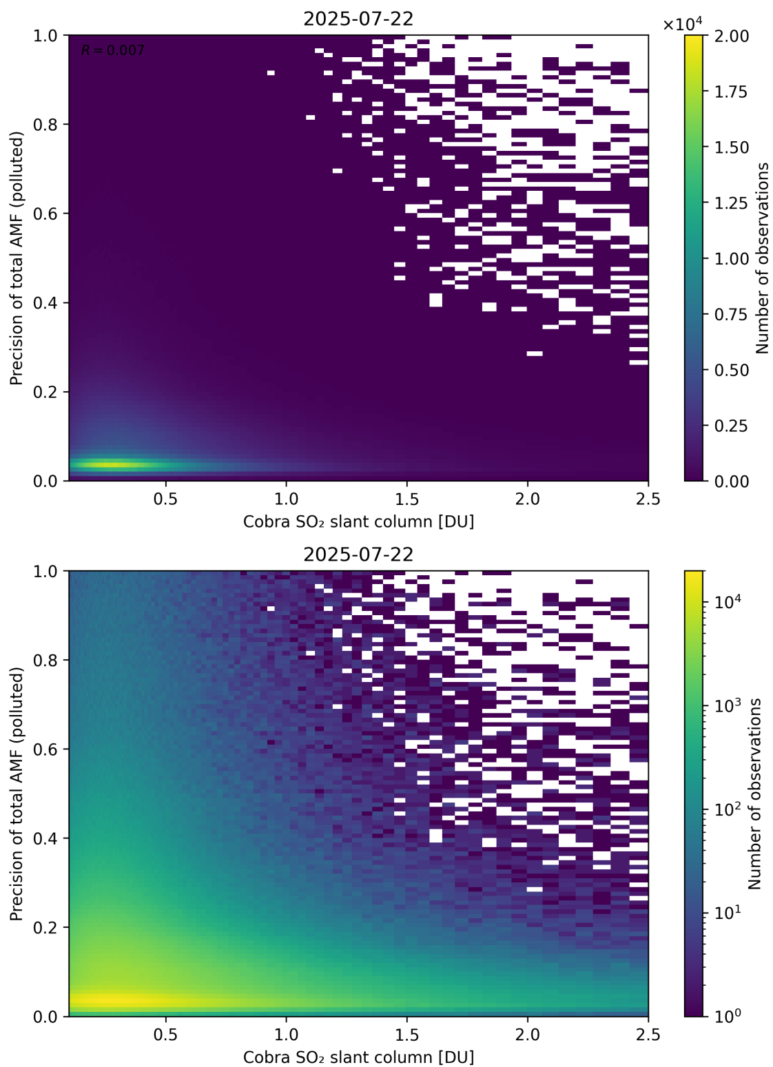
Figure 225: Scatter density plot of “Cobra SO 2 slant column” against “Precision of total AMF (polluted)” for 2025-07-21 to 2025-07-23.
