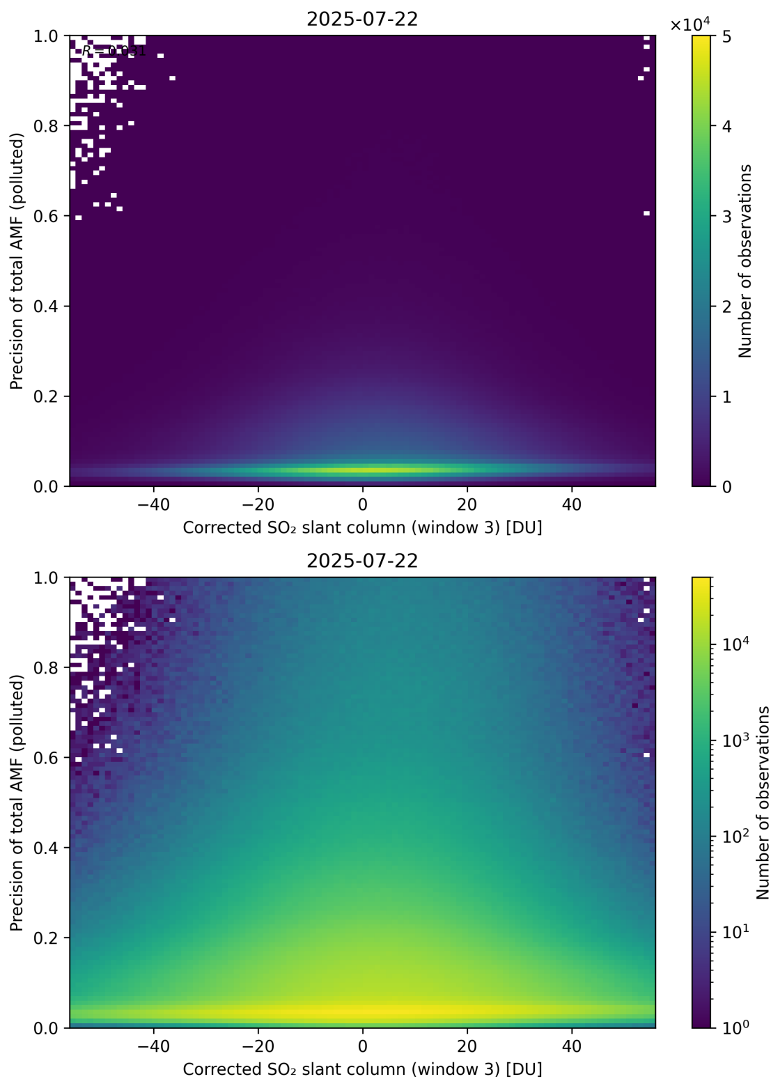
Figure 261: Scatter density plot of “Corrected SO 2 slant column (window 3)” against “Precision of total AMF (polluted)” for 2025-07-21 to 2025-07-23.
