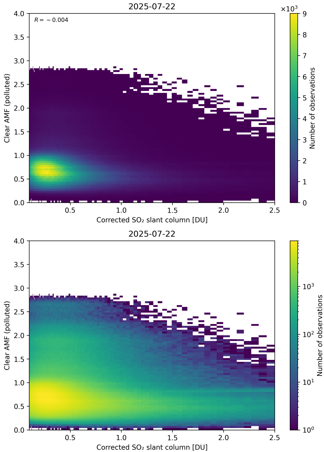
Figure 232: Scatter density plot of “Corrected SO 2 slant column” against “Clear AMF (polluted)” for 2025-07-21 to 2025-07-23.
