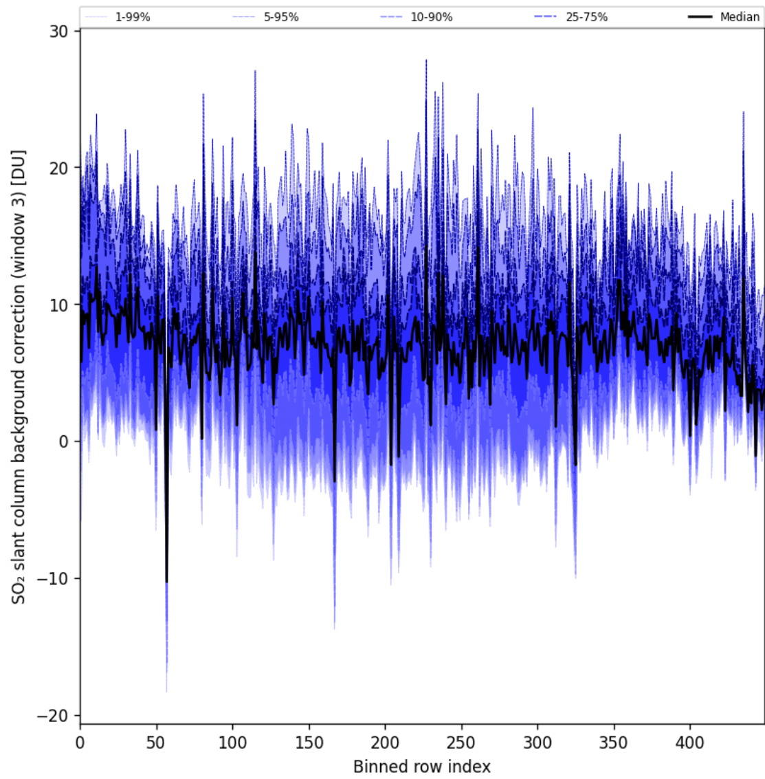
Figure 100: Along track statistics of “SO 2 slant column background correction (window 3)” for 2025-07-21 to 2025-07-23
