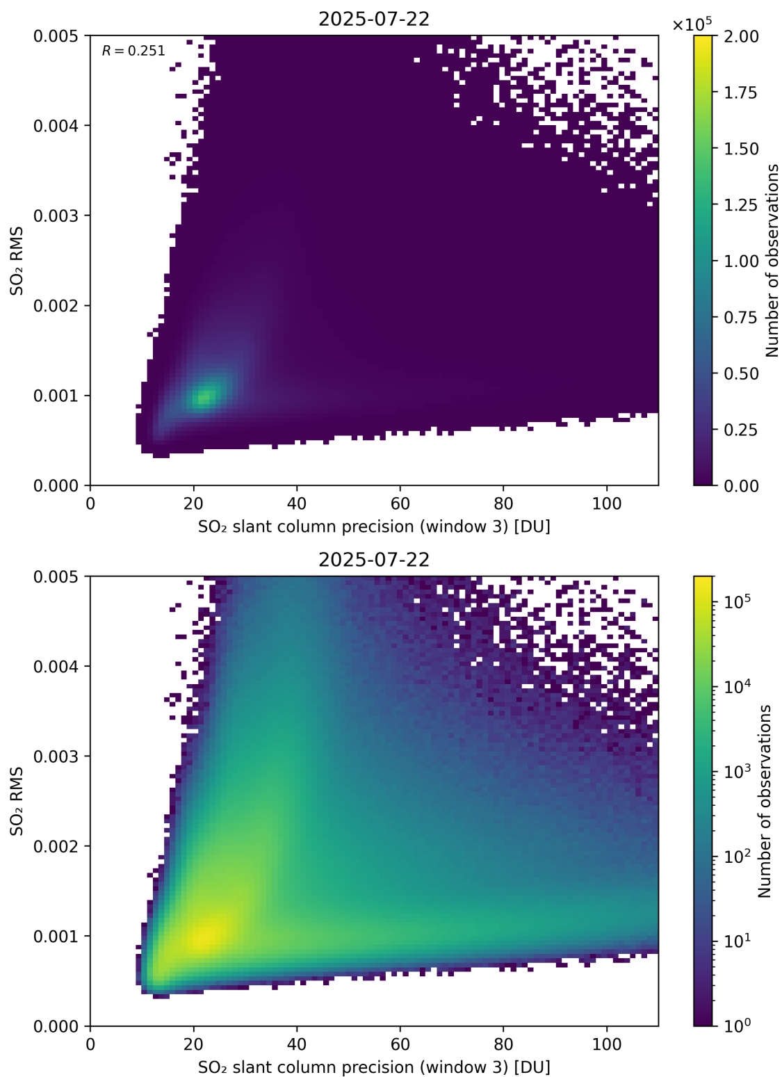
Figure 310: Scatter density plot of “SO 2 slant column precision (window 3)” against “SO 2 RMS” for 2025-07-21 to 2025-07-23.
