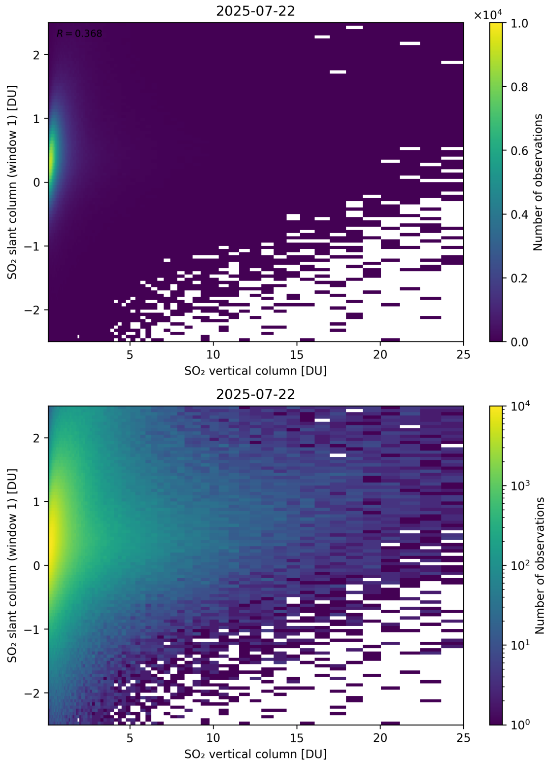
Figure 354: Scatter density plot of “SO 2 vertical column” against “SO 2 slant column (window 1)” for 2025-07-21 to 2025-07-23.
