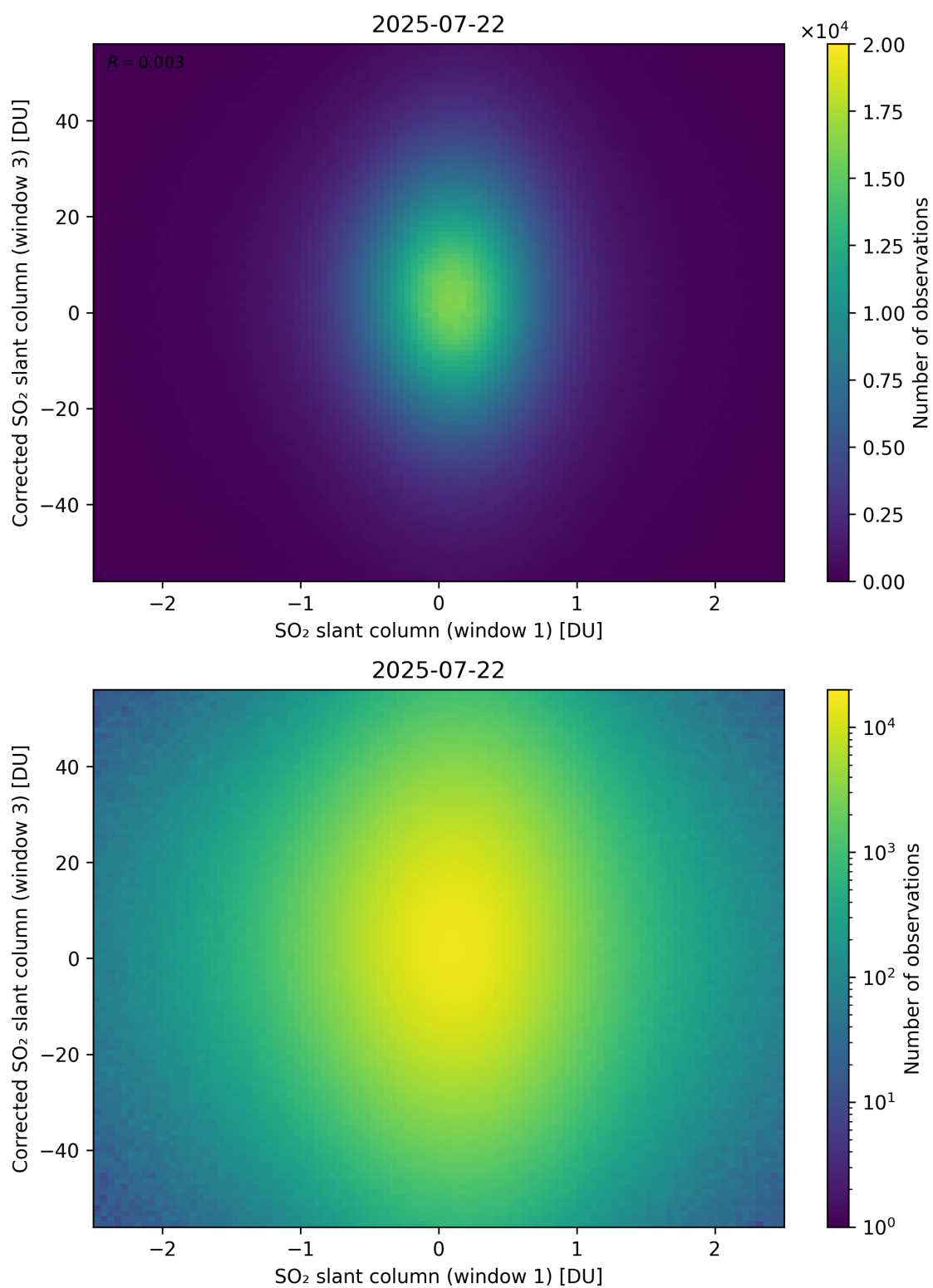
Figure 284: Scatter density plot of “SO 2 slant column (window 1)” against “Corrected SO 2 slant column (window 3)” for 2025-07-21 to 2025-07-23.
