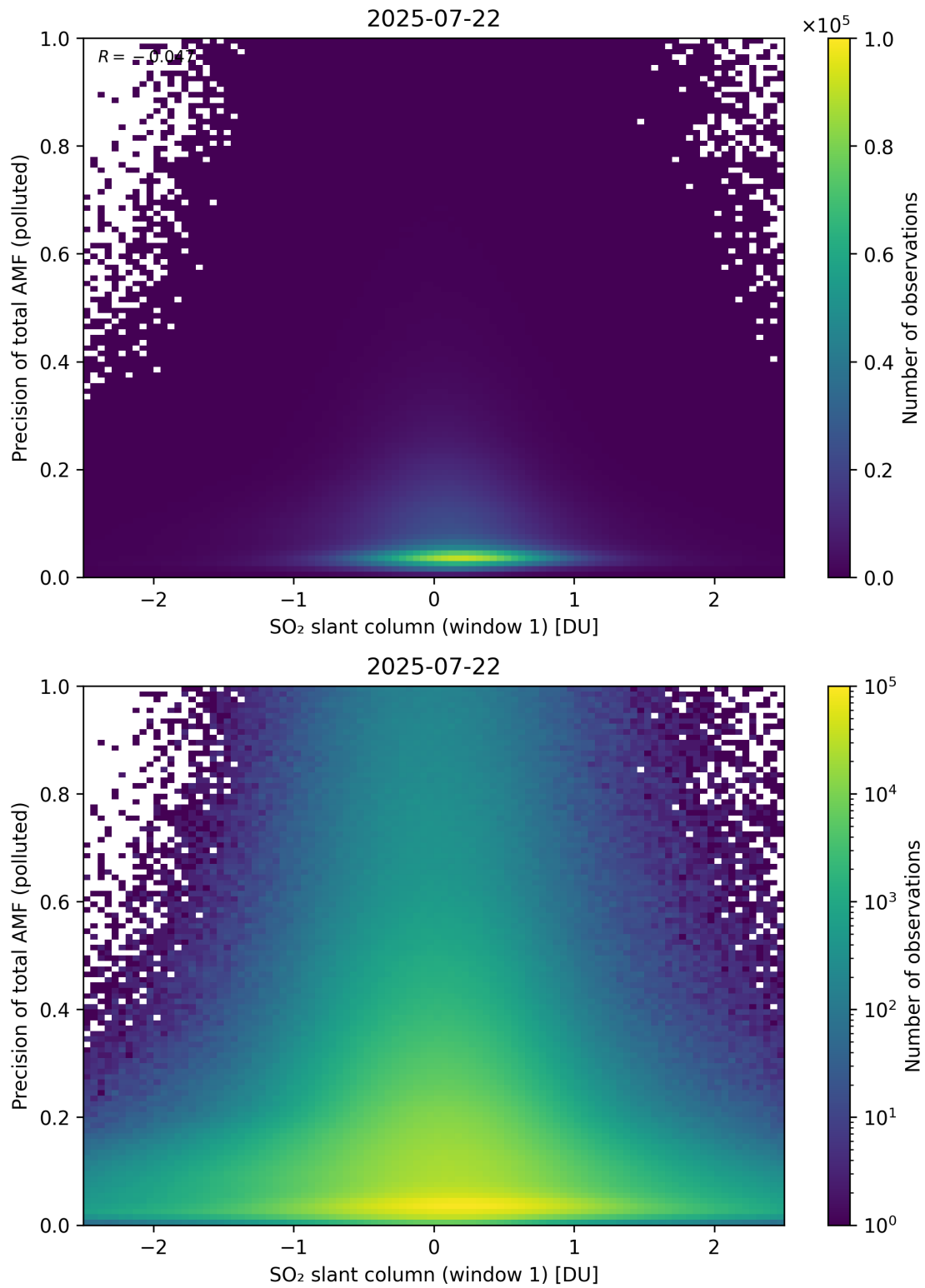
Figure 290: Scatter density plot of “SO 2 slant column (window 1)” against “Precision of total AMF (polluted)” for 2025-07-21 to 2025-07-23.
