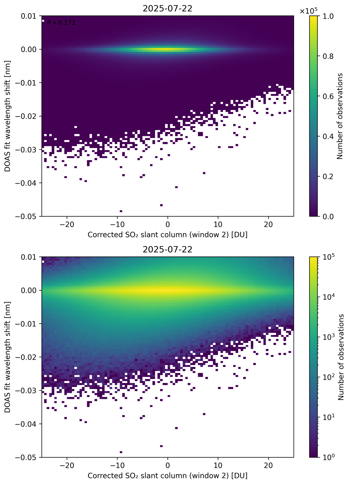
Figure 246: Scatter density plot of “Corrected SO 2 slant column (window 2)” against “DOAS fit wavelength shift” for 2025-07-21 to 2025-07-23.
