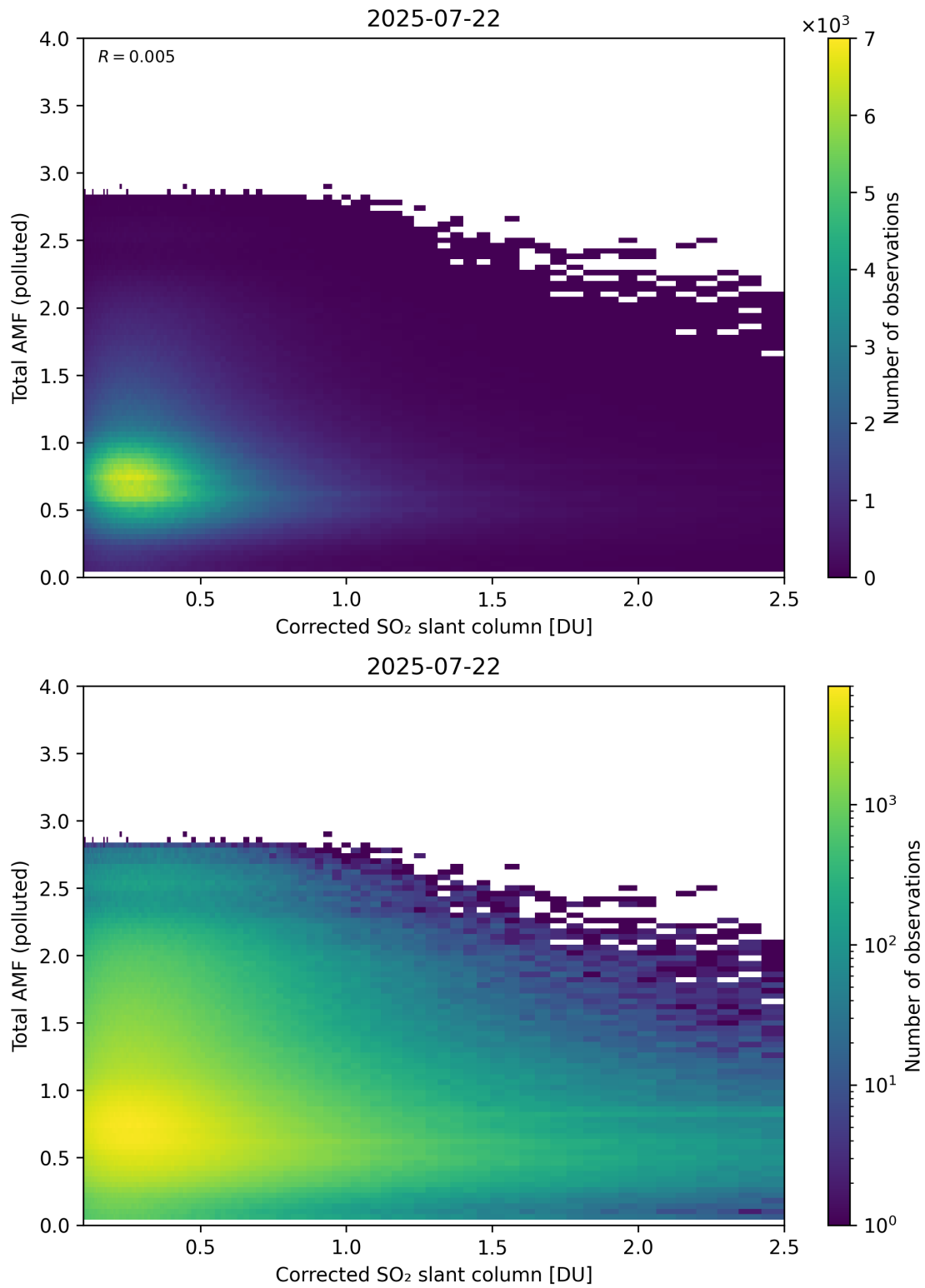
Figure 242: Scatter density plot of “Corrected SO 2 slant column” against “Total AMF (polluted)” for 2025-07-21 to 2025-07-23.
