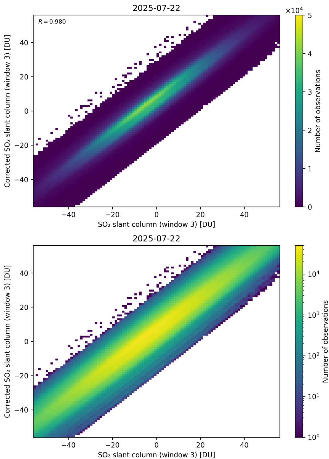
Figure 316: Scatter density plot of “SO 2 slant column (window 3)” against “Corrected SO 2 slant column (window 3)” for 2025-07-21 to 2025-07-23.
