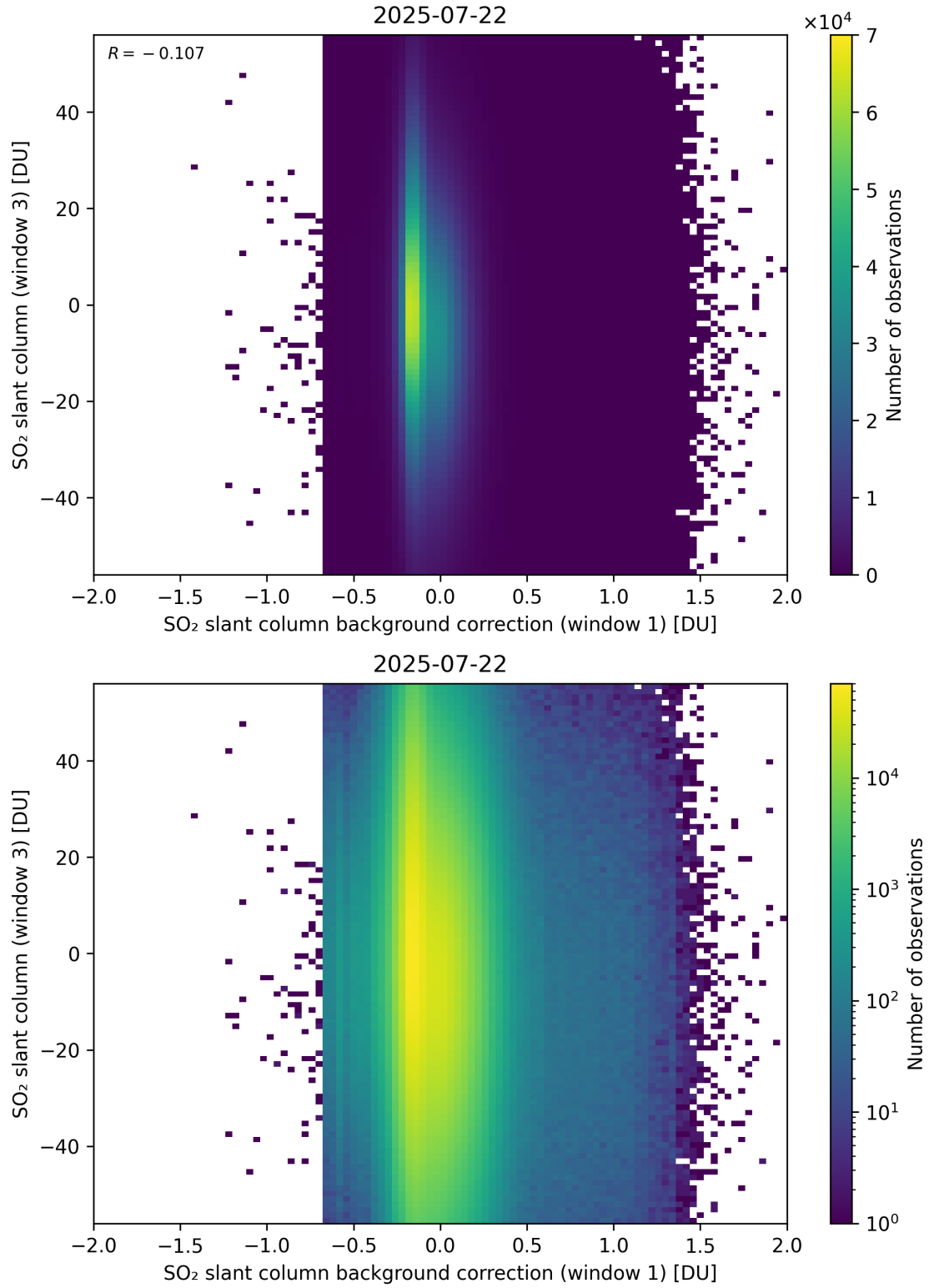
Figure 118: Scatter density plot of “SO 2 slant column background correction (window 1)” against “SO 2 slant column (window 3)” for 2025-07-21 to 2025-07-23.
