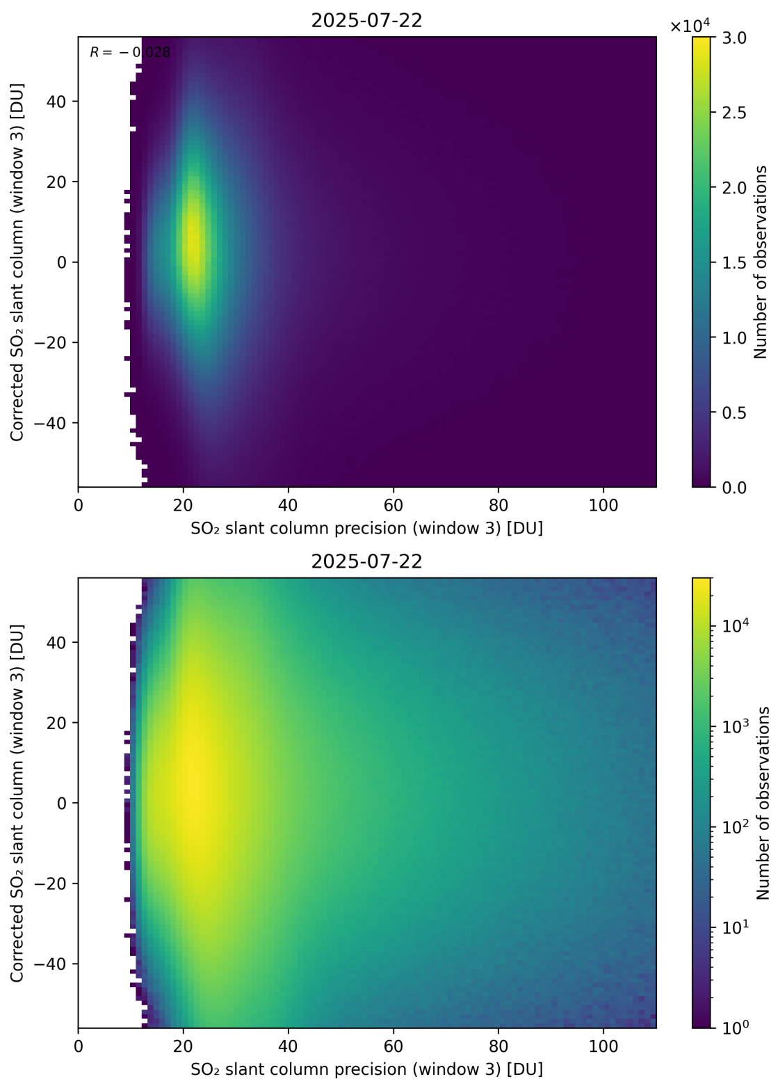
Figure 312: Scatter density plot of “SO 2 slant column precision (window 3)” against “Corrected SO 2 slant column (window 3)” for 2025-07-21 to 2025-07-23.
