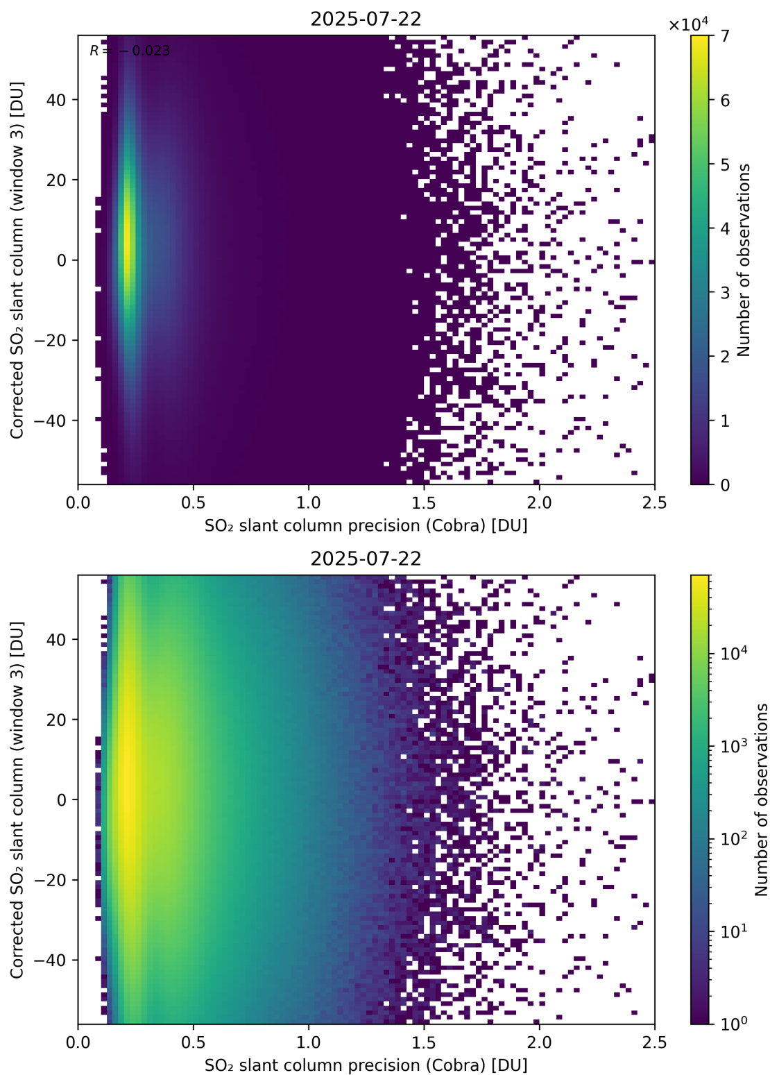
Figure 207: Scatter density plot of “SO 2 slant column precision (Cobra)” against “Corrected SO 2 slant column (window 3)” for 2025-07-21 to 2025-07-23.
