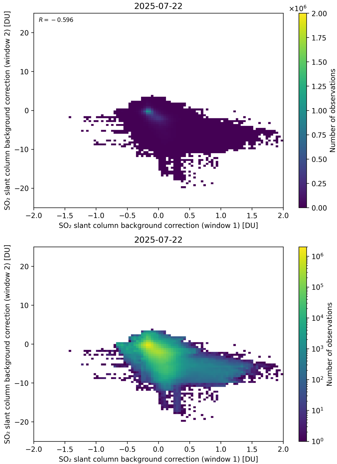
Figure 109: Scatter density plot of “SO 2 slant column background correction (window 1)” against “SO 2 slant column background correction (window 2)” for 2025-07-21 to 2025-07-23.
