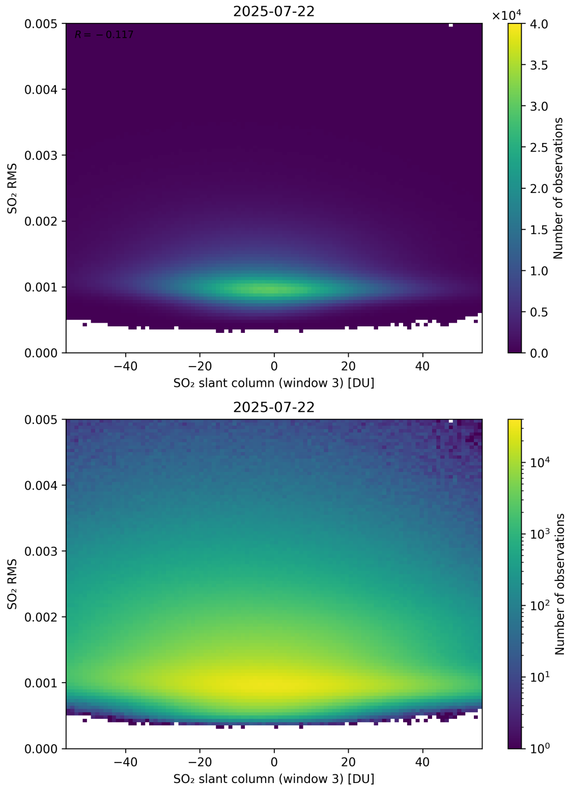
Figure 306: Scatter density plot of “SO 2 slant column (window 3)” against “SO 2 RMS” for 2025-07-21 to 2025-07-23.
