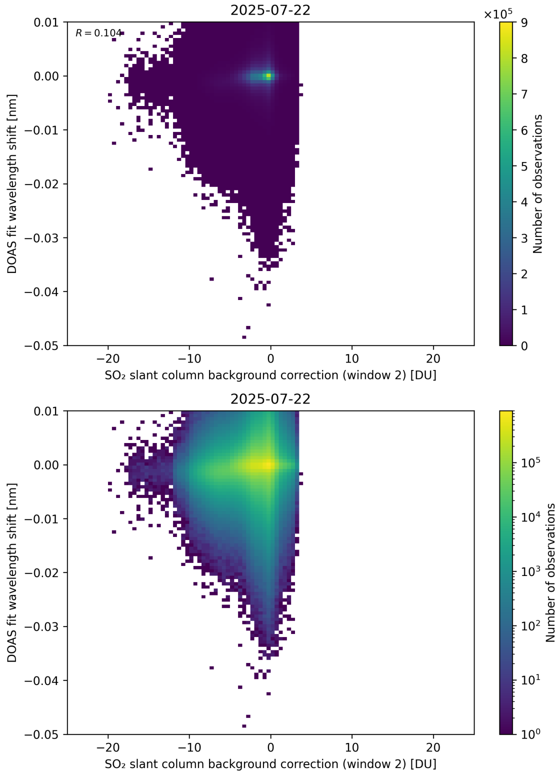
Figure 123: Scatter density plot of “SO 2 slant column background correction (window 2)” against “DOAS fit wavelength shift” for 2025-07-21 to 2025-07-23.
