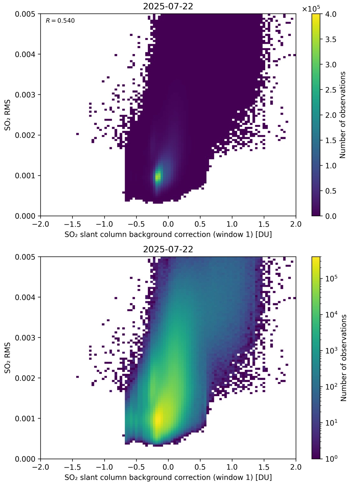
Figure 113: Scatter density plot of “SO 2 slant column background correction (window 1)” against “SO 2 RMS” for 2025-07-21 to 2025-07-23.
