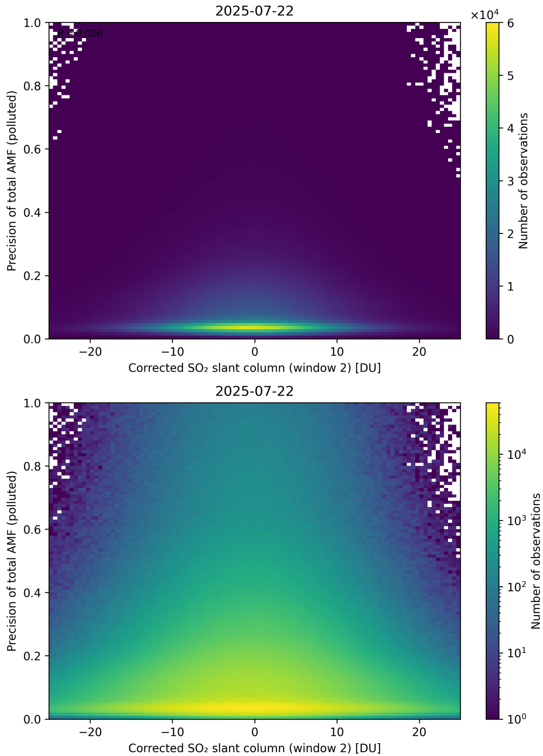
Figure 254: Scatter density plot of “Corrected SO 2 slant column (window 2)” against “Precision of total AMF (polluted)” for 2025-07-21 to 2025-07-23.
