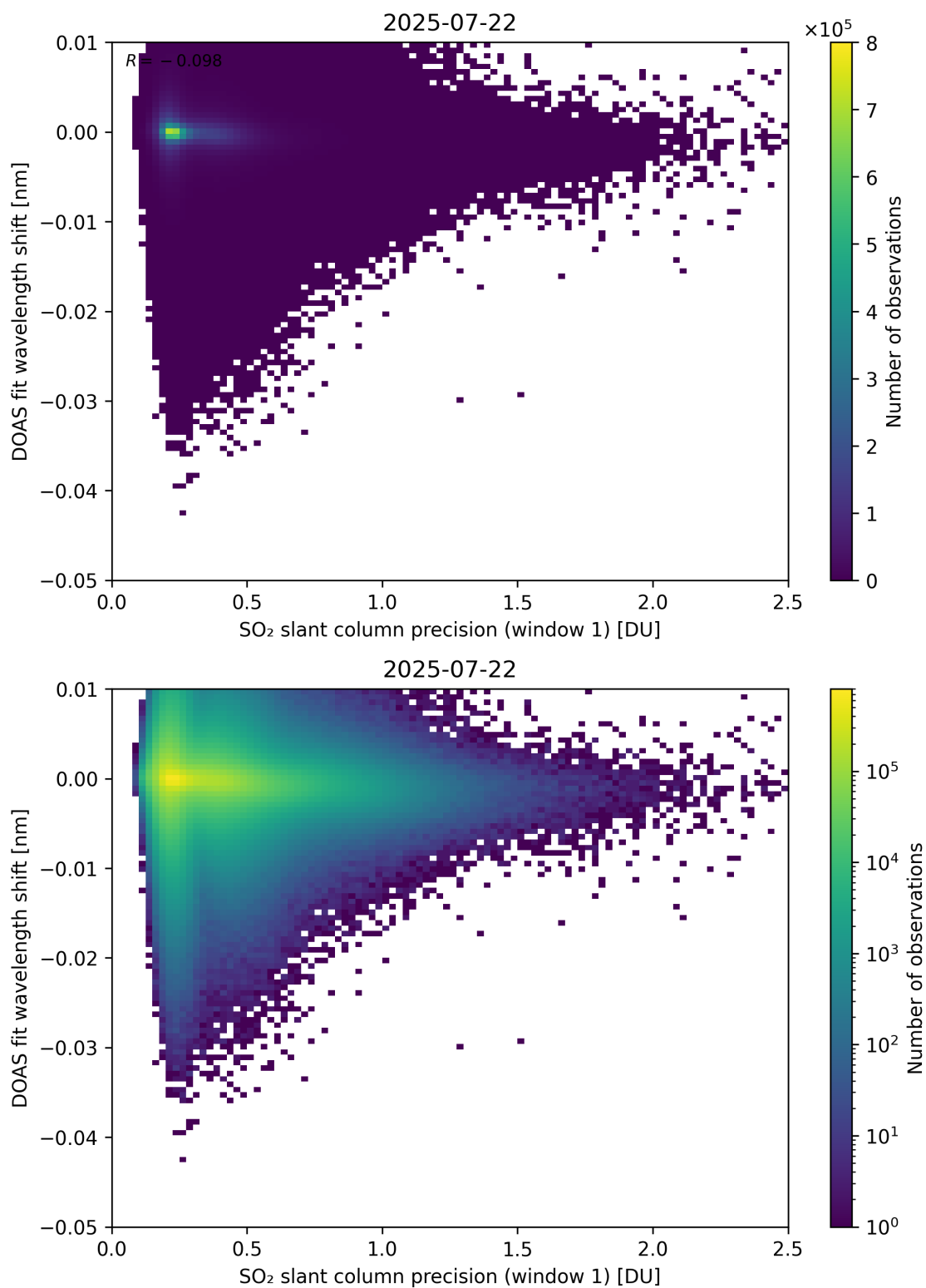
Figure 271: Scatter density plot of “SO 2 slant column precision (window 1)” against “DOAS fit wavelength shift” for 2025-07-21 to 2025-07-23.
