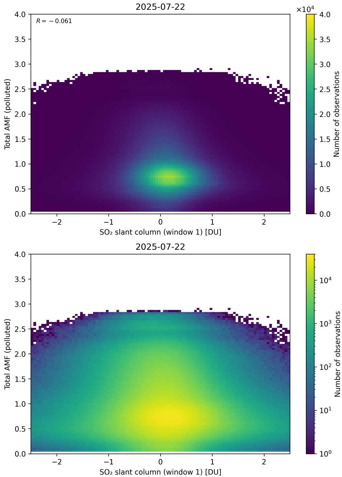
Figure 289: Scatter density plot of “SO 2 slant column (window 1)” against “Total AMF (polluted)” for 2025-07-21 to 2025-07-23.
