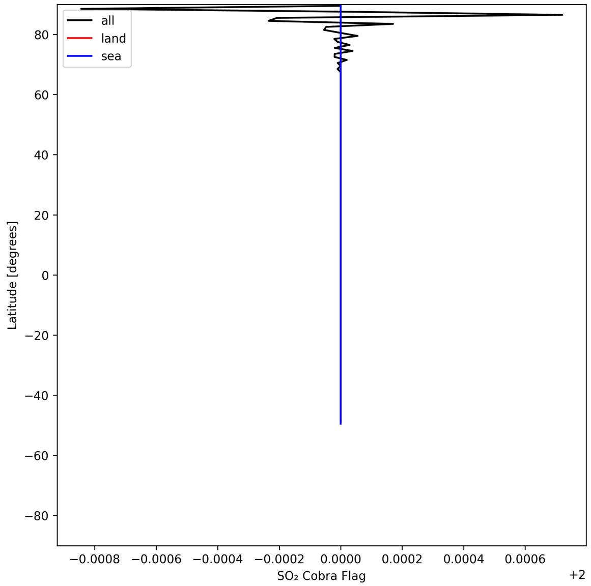
Figure 49: Zonal average of “SO 2 Cobra Flag” for 2025-07-21 to 2025-07-23.
