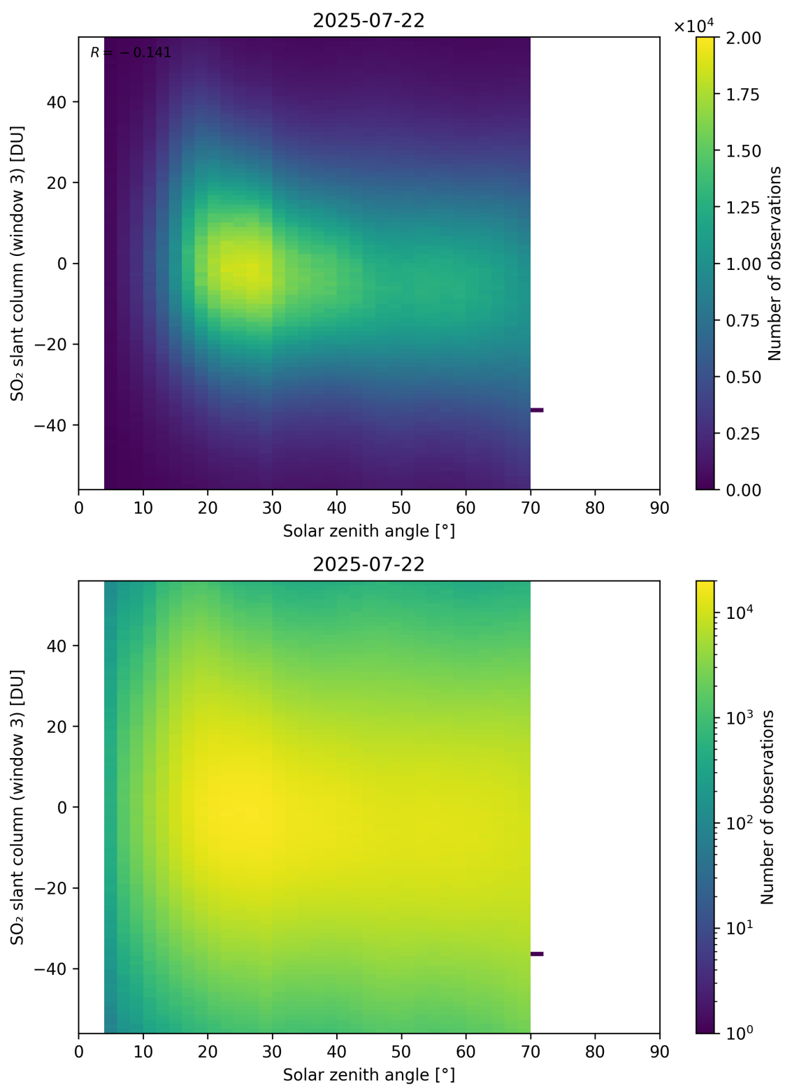
Figure 187: Scatter density plot of “Solar zenith angle” against “SO 2 slant column (window 3)” for 2025-07-21 to 2025-07-23.
