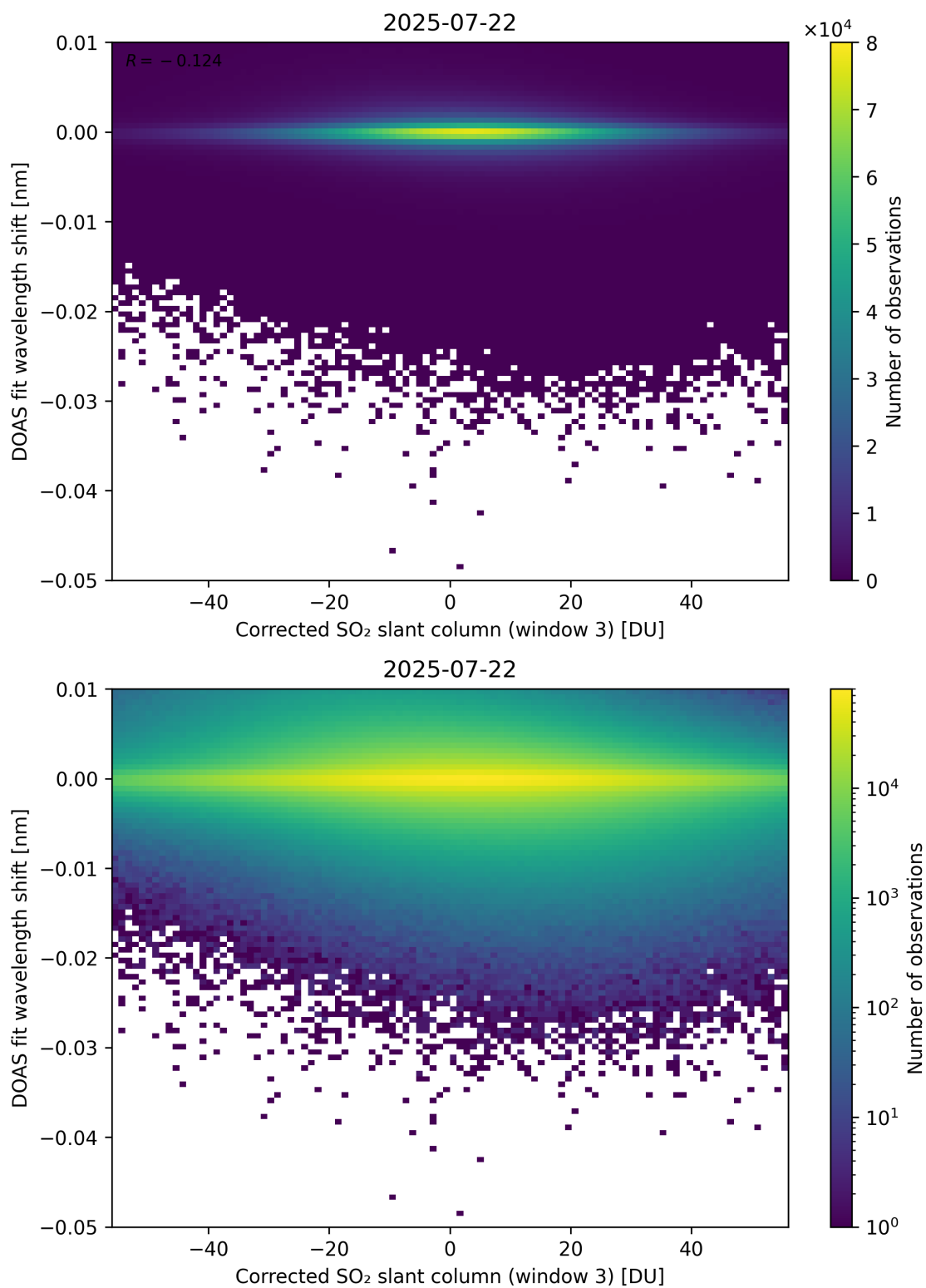
Figure 256: Scatter density plot of “Corrected SO 2 slant column (window 3)” against “DOAS fit wavelength shift” for 2025-07-21 to 2025-07-23.
