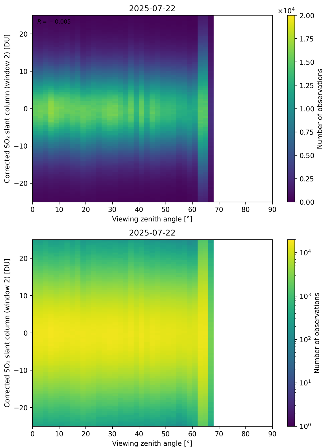
Figure 374: Scatter density plot of “Viewing zenith angle” against “Corrected SO 2 slant column (window 2)” for 2025-07-21 to 2025-07-23.
