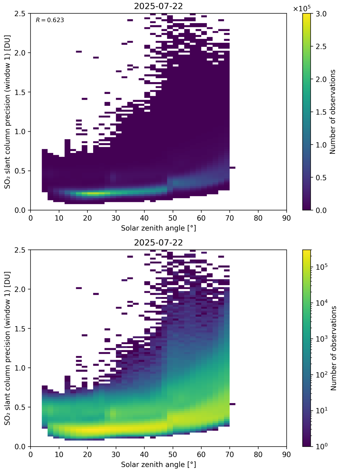
Figure 185: Scatter density plot of “Solar zenith angle” against “SO 2 slant column precision (window 1)” for 2025-07-21 to 2025-07-23.
