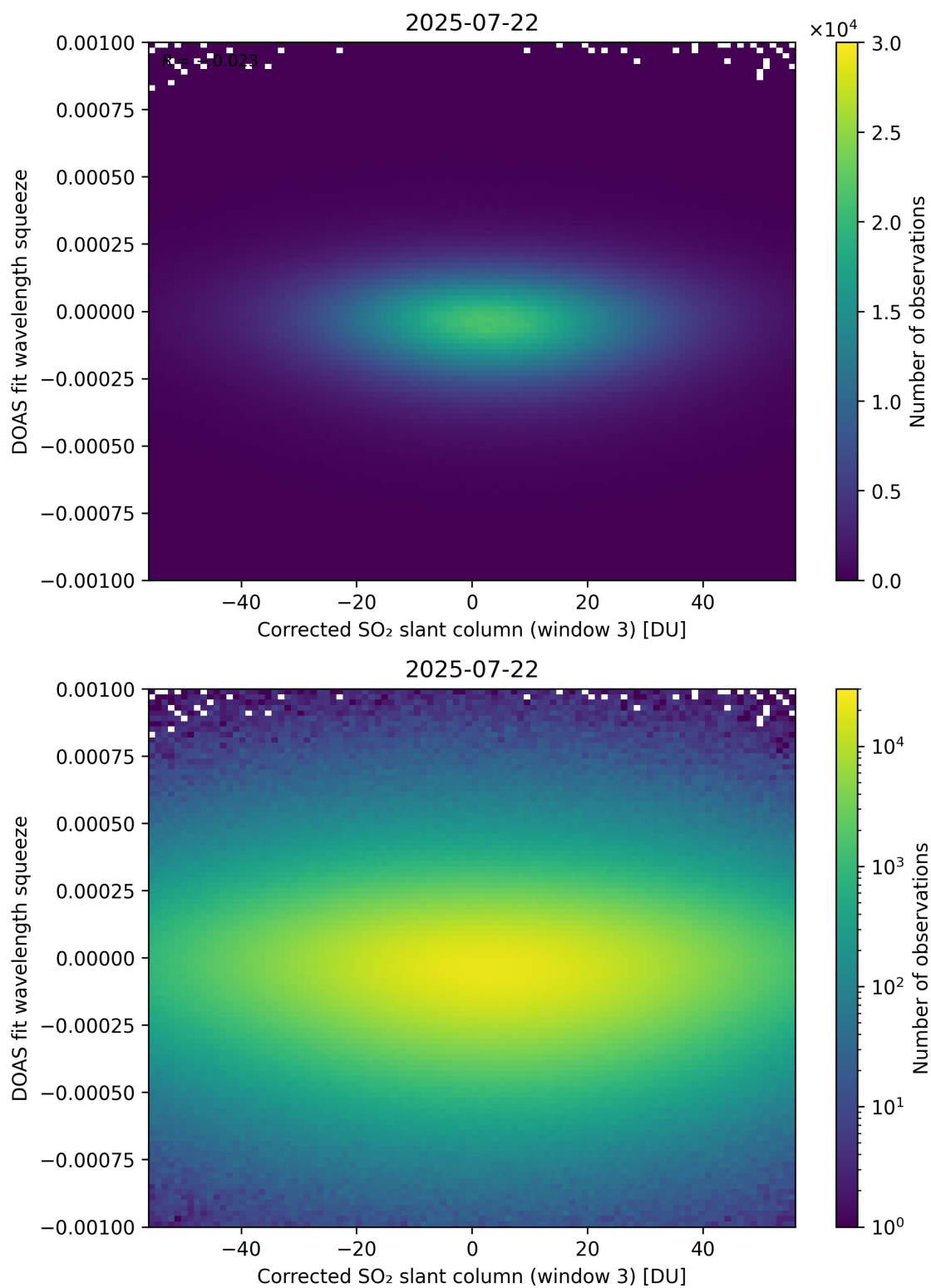
Figure 257: Scatter density plot of “Corrected SO 2 slant column (window 3)” against “DOAS fit wavelength squeeze” for 2025-07-21 to 2025-07-23.
