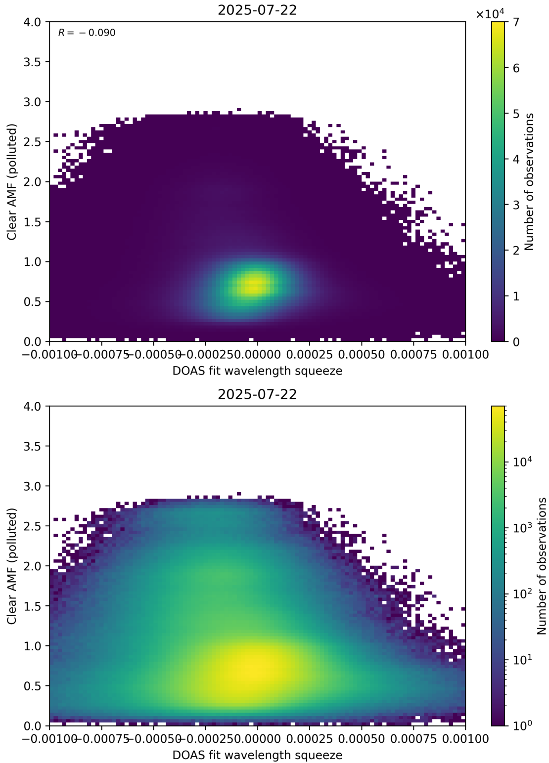
Figure 144: Scatter density plot of “DOAS fit wavelength squeeze” against “Clear AMF (polluted)” for 2025-07-21 to 2025-07-23.
