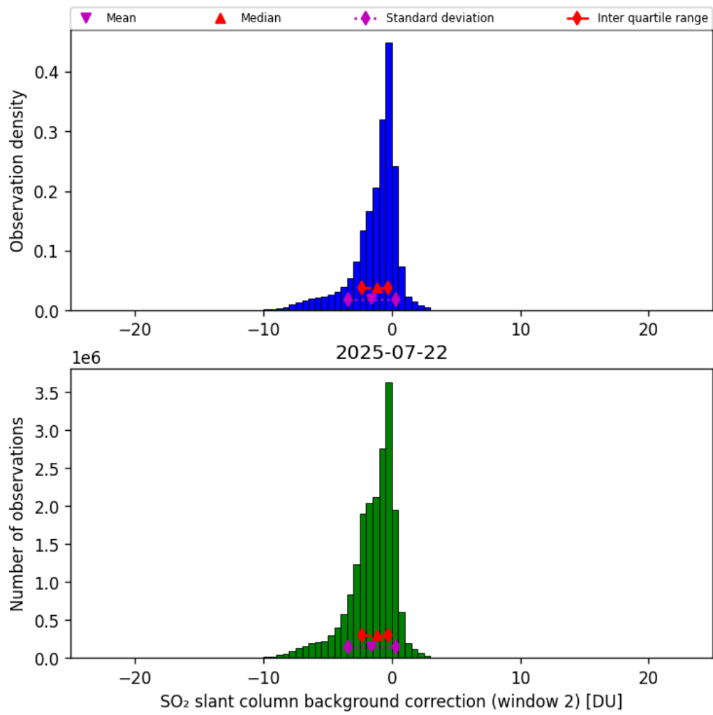
Figure 70: Histogram of “SO 2 slant column background correction (window 2)” for 2025-07-21 to 2025-07-23
