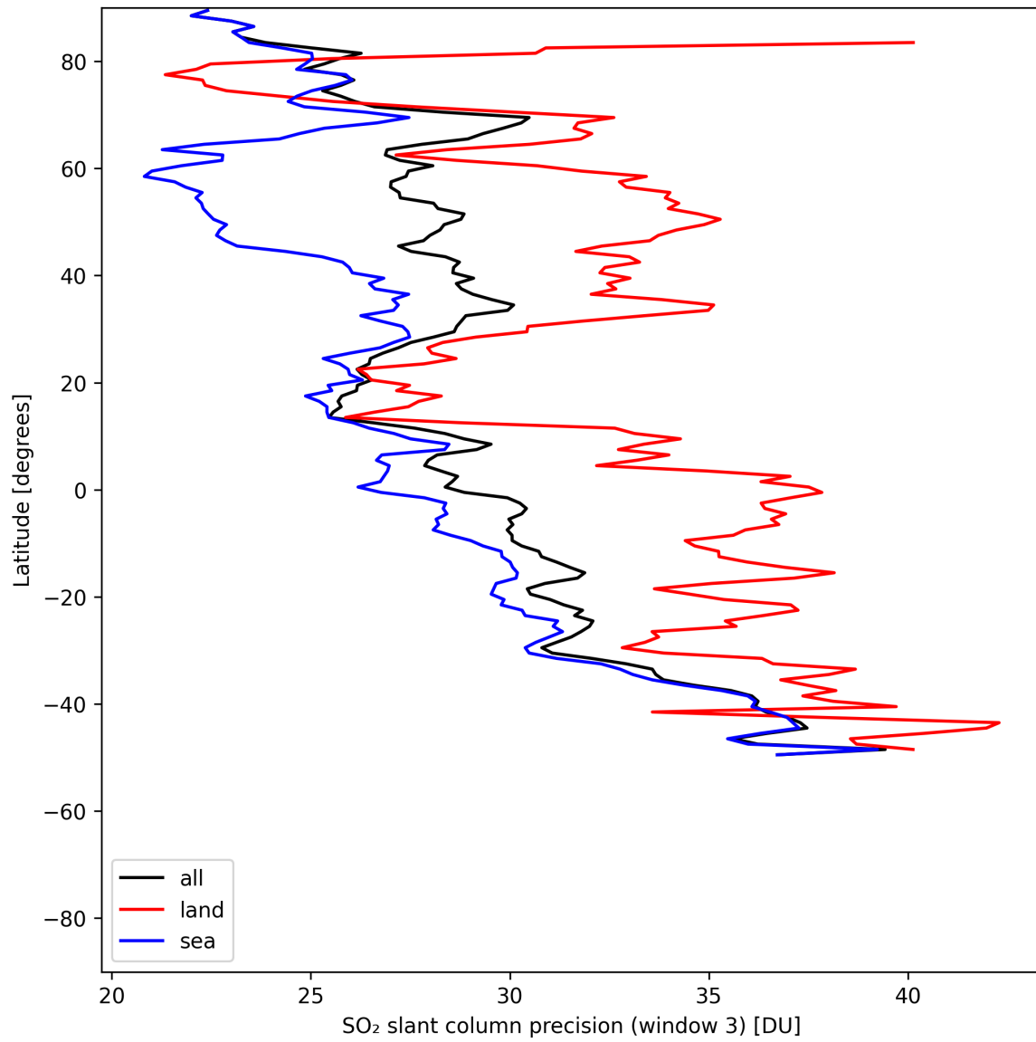
Figure 46: Zonal average of “SO 2 slant column precision (window 3)” for 2025-07-21 to 2025-07-23.
