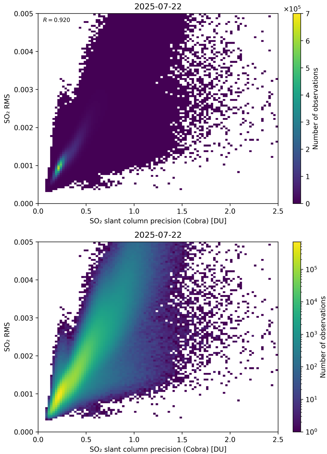
Figure 204: Scatter density plot of “SO 2 slant column precision (Cobra)” against “SO 2 RMS” for 2025-07-21 to 2025-07-23.
