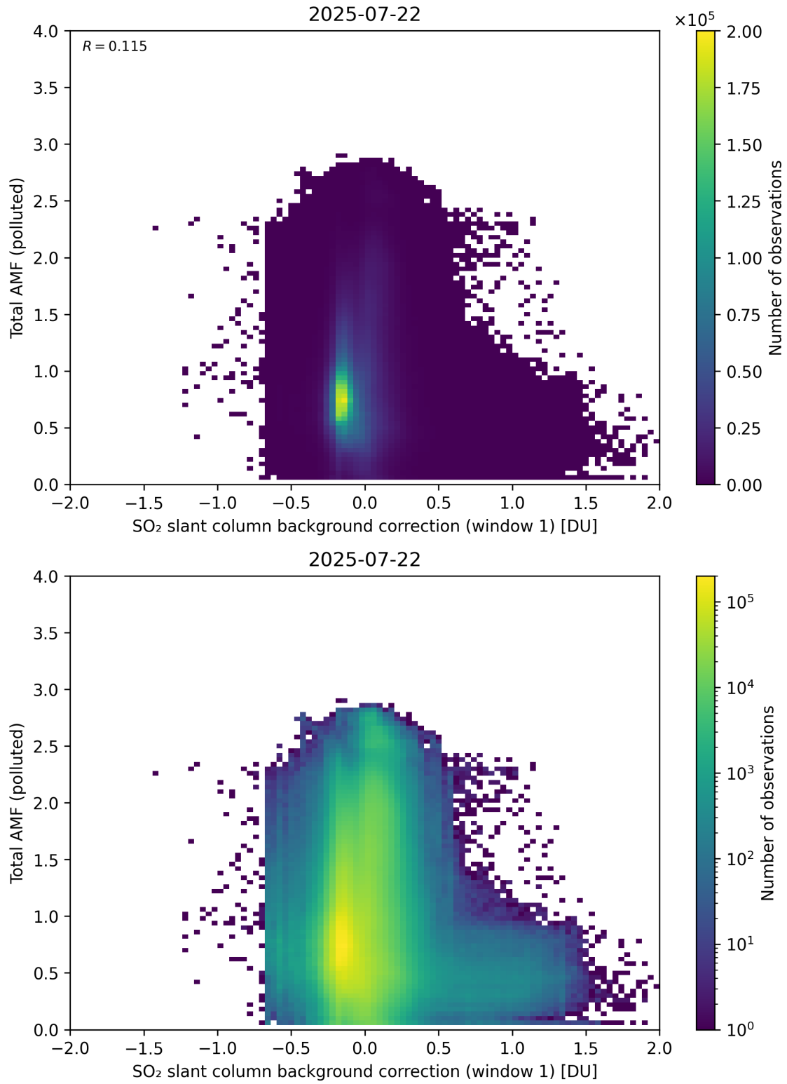
Figure 120: Scatter density plot of “SO 2 slant column background correction (window 1)” against “Total AMF (polluted)” for 2025-07-21 to 2025-07-23.
