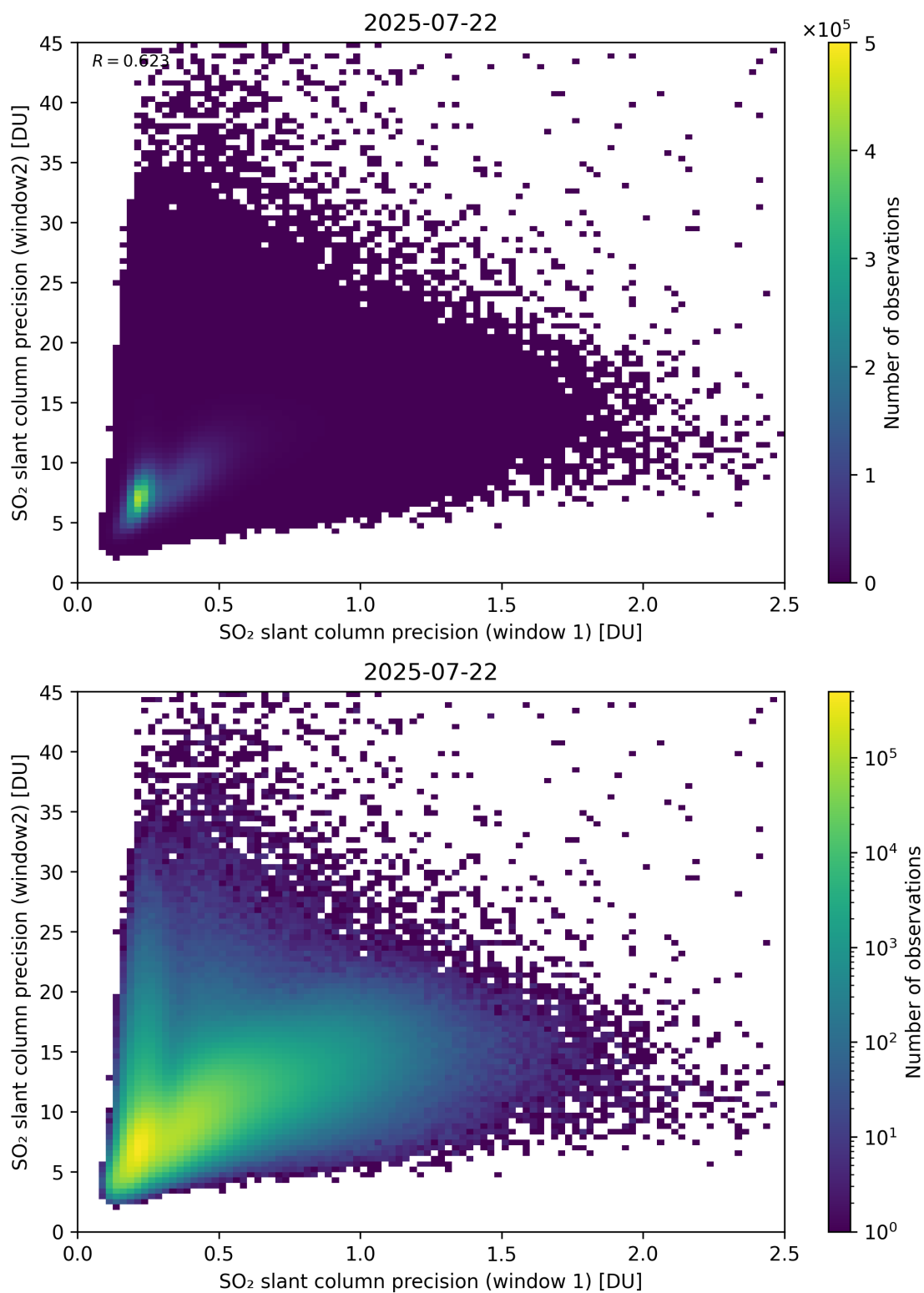
Figure 277: Scatter density plot of “SO 2 slant column precision (window 1)” against “SO 2 slant column precision (window2)” for 2025-07-21 to 2025-07-23.
