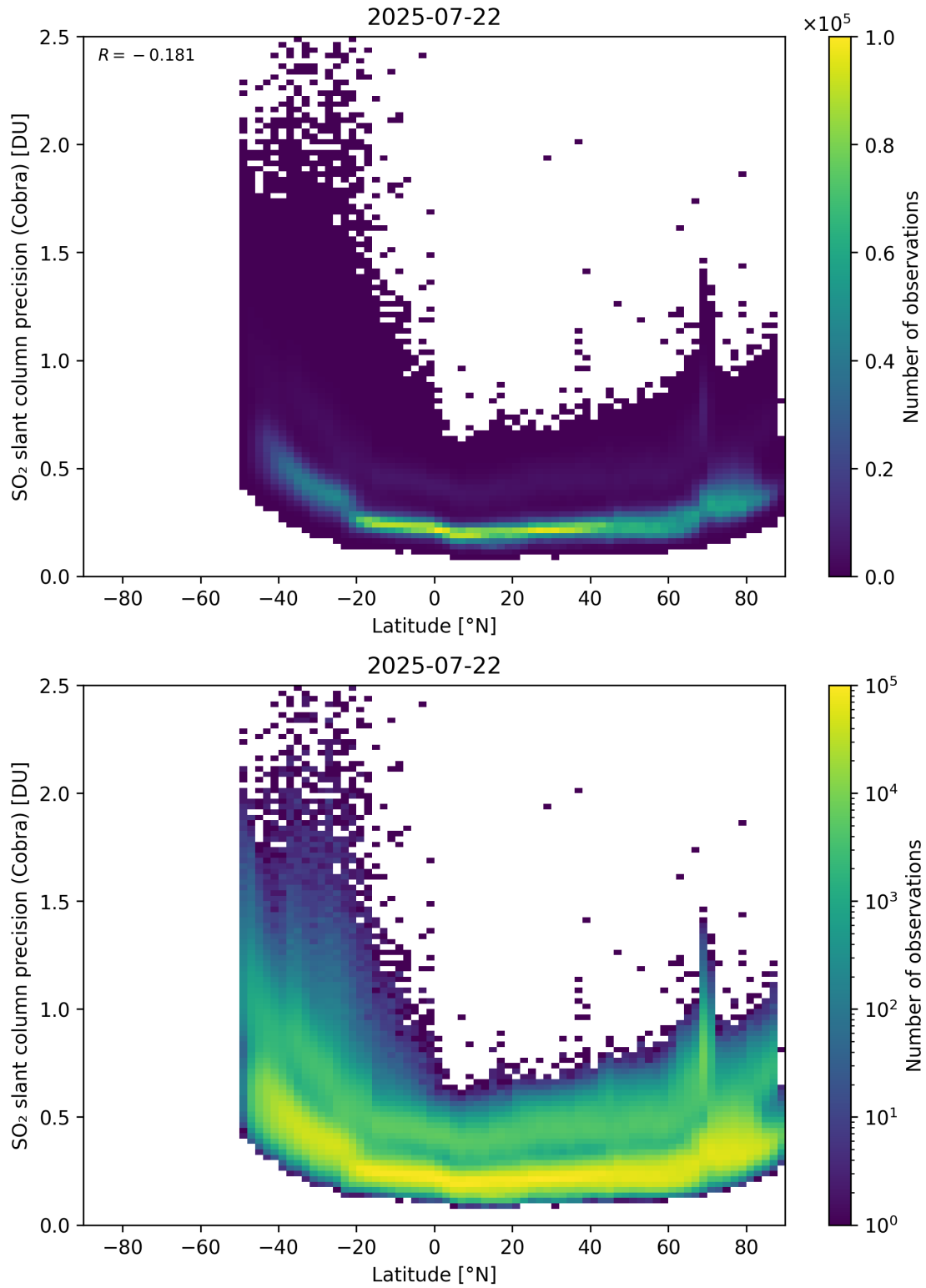
Figure 158: Scatter density plot of “Latitude” against “SO 2 slant column precision (Cobra)” for 2025-07-21 to 2025-07-23.
