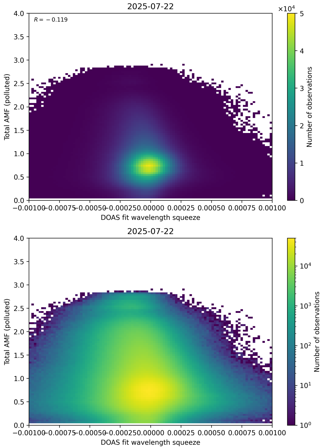
Figure 145: Scatter density plot of “DOAS fit wavelength squeeze” against “Total AMF (polluted)” for 2025-07-21 to 2025-07-23.
