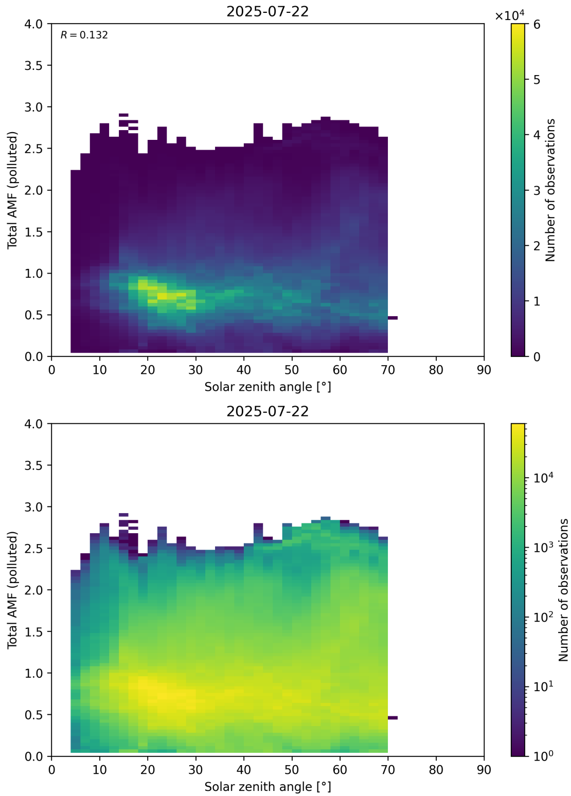
Figure 189: Scatter density plot of “Solar zenith angle” against “Total AMF (polluted)” for 2025-07-21 to 2025-07-23.
