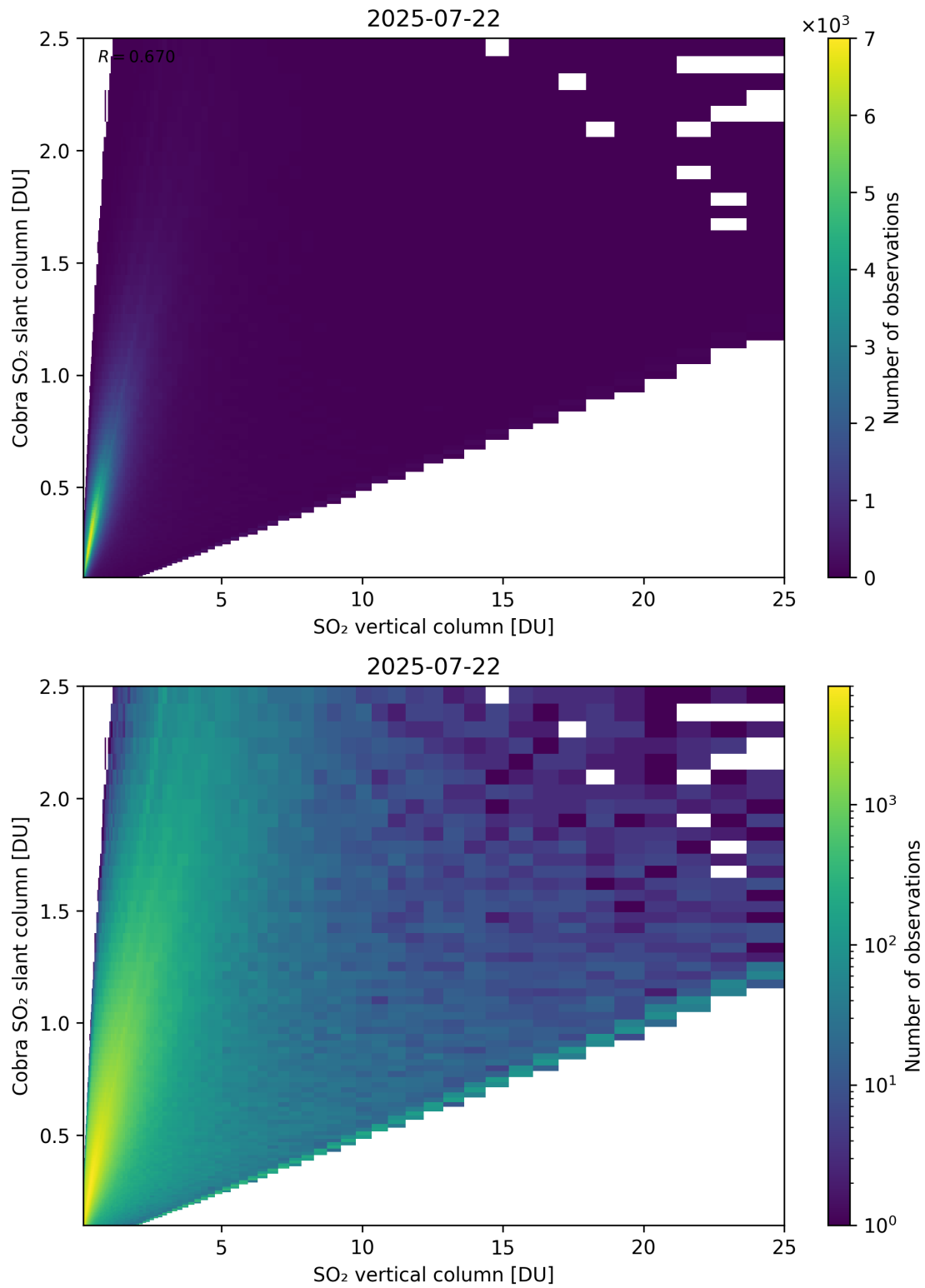
Figure 349: Scatter density plot of “SO 2 vertical column” against “Cobra SO 2 slant column” for 2025-07-21 to 2025-07-23.
