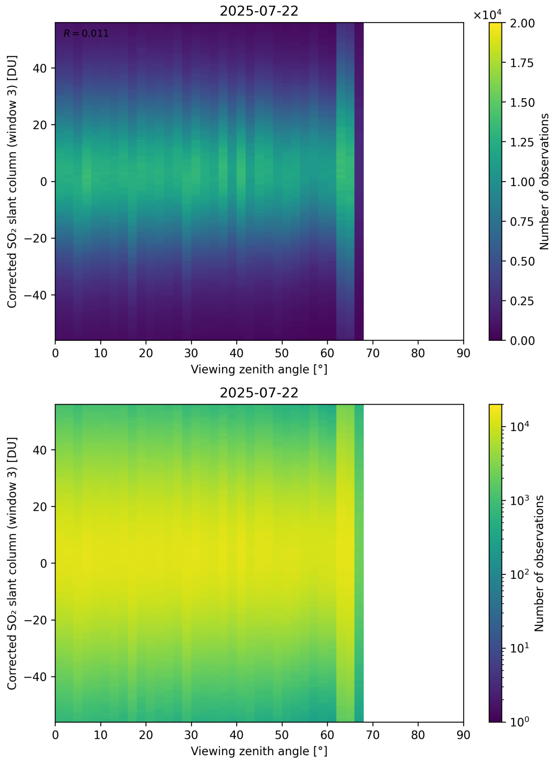
Figure 375: Scatter density plot of “Viewing zenith angle” against “Corrected SO 2 slant column (window 3)” for 2025-07-21 to 2025-07-23.
