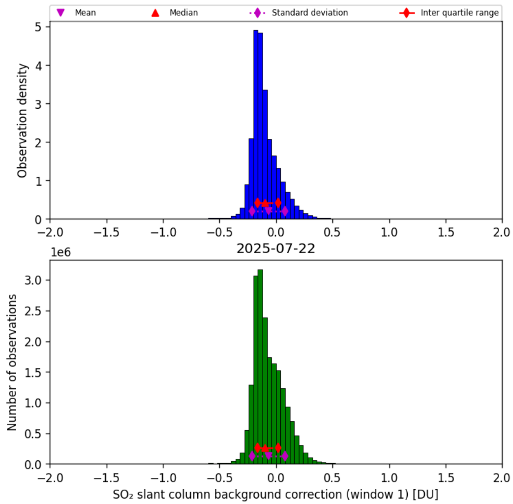
Figure 66: Histogram of “SO 2 slant column background correction (window 1)” for 2025-07-21 to 2025-07-23
