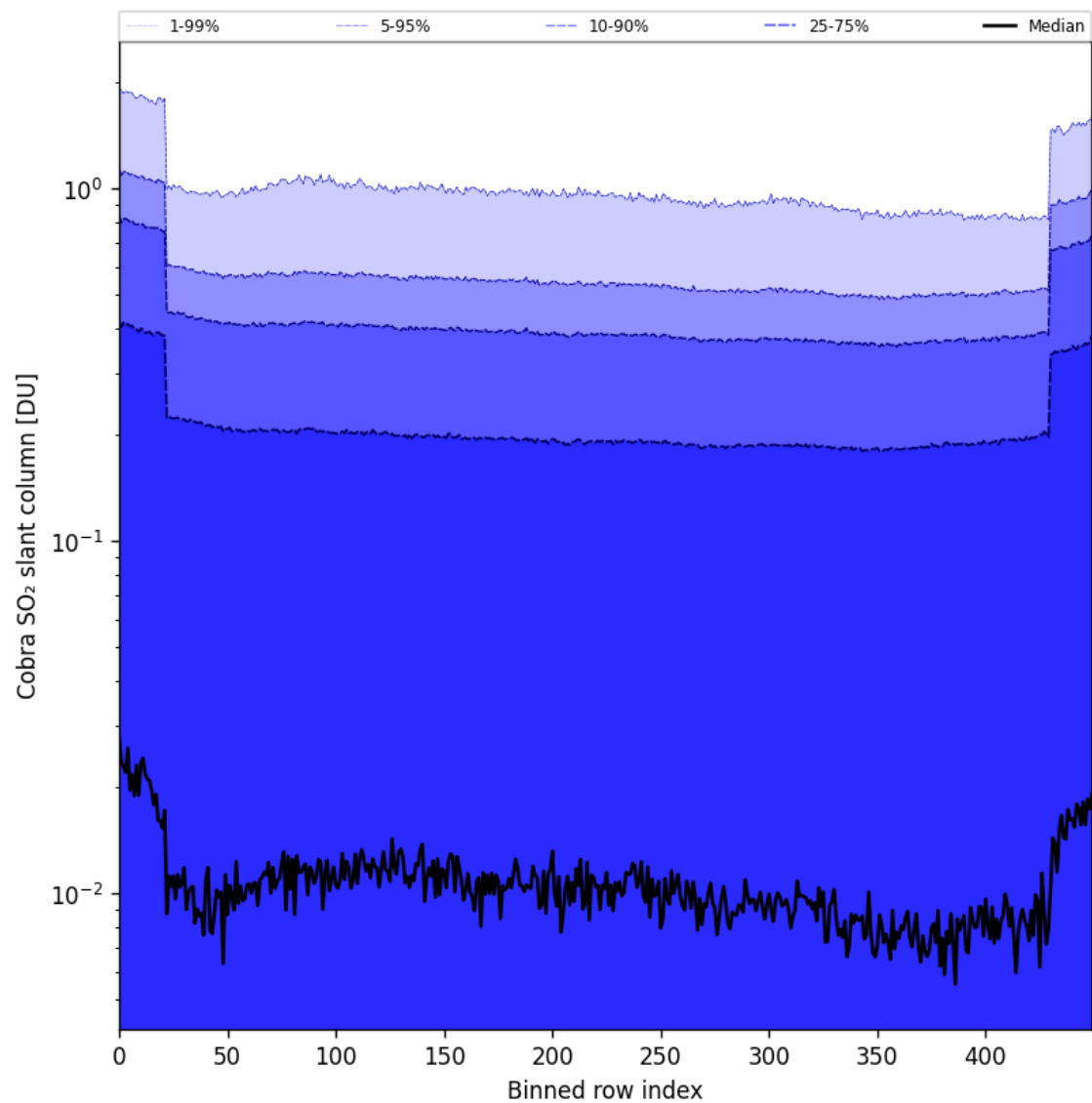
Figure 87: Along track statistics of “Cobra SO 2 slant column” for 2025-07-21 to 2025-07-23
