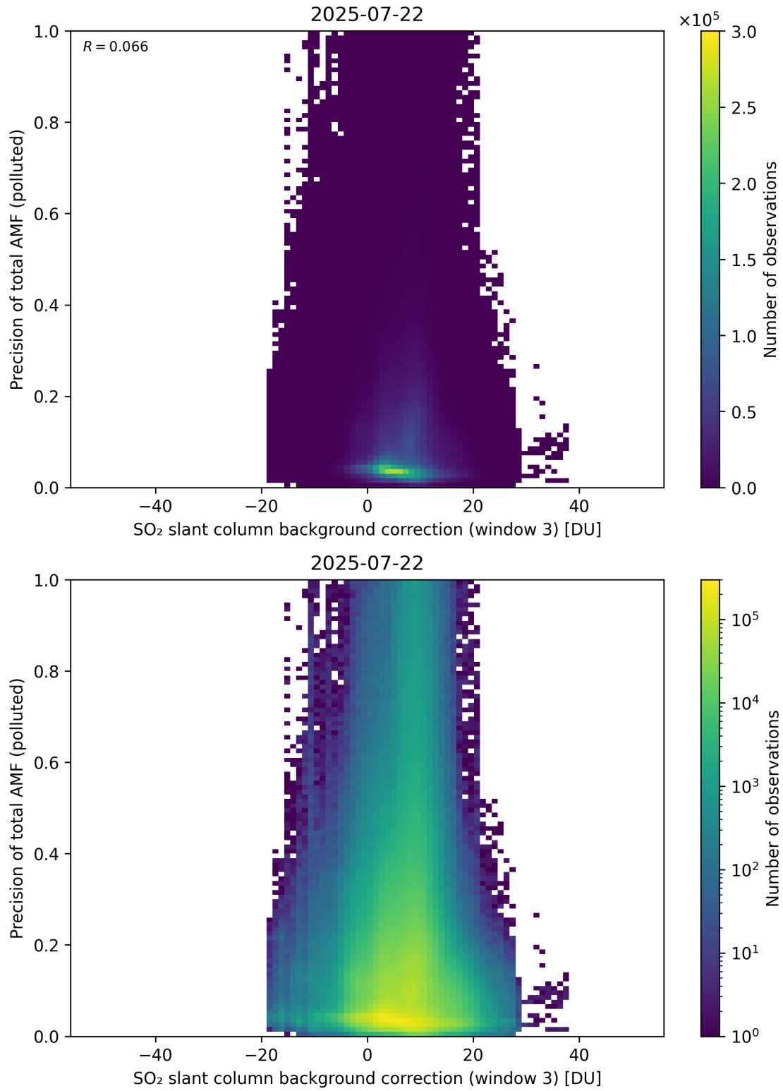
Figure 137: Scatter density plot of “SO 2 slant column background correction (window 3)” against “Precision of total AMF (polluted)” for 2025-07-21 to 2025-07-23.
