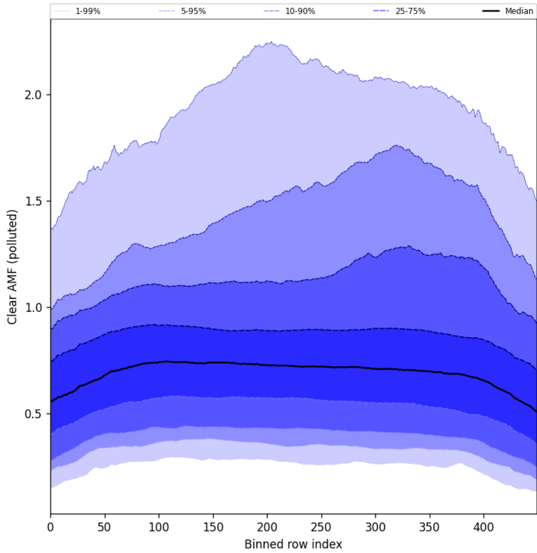
Figure 107: Along track statistics of “Clear AMF (polluted)” for 2025-07-21 to 2025-07-23
