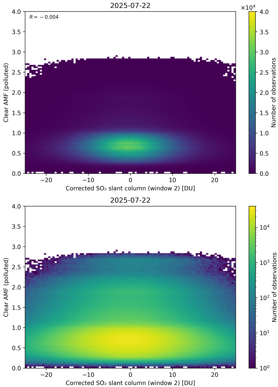
Figure 249: Scatter density plot of “Corrected SO 2 slant column (window 2)” against “Clear AMF (polluted)” for 2025-07-21 to 2025-07-23.
