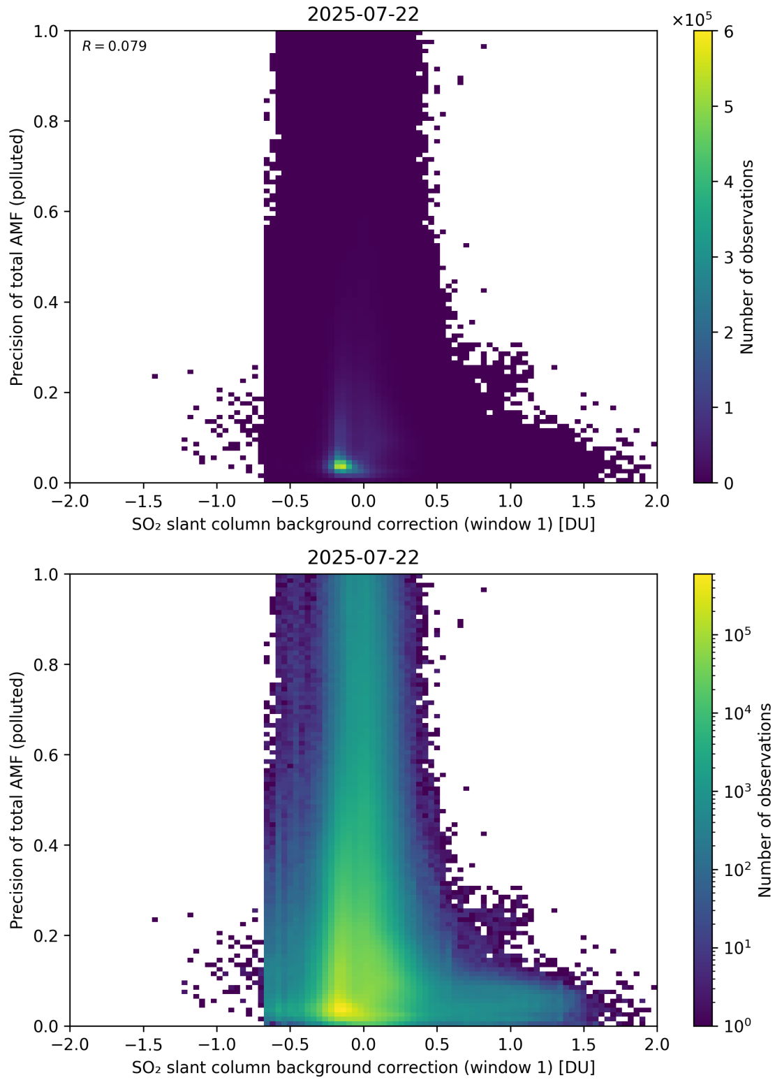
Figure 121: Scatter density plot of “SO 2 slant column background correction (window 1)” against “Precision of total AMF (polluted)” for 2025-07-21 to 2025-07-23.
