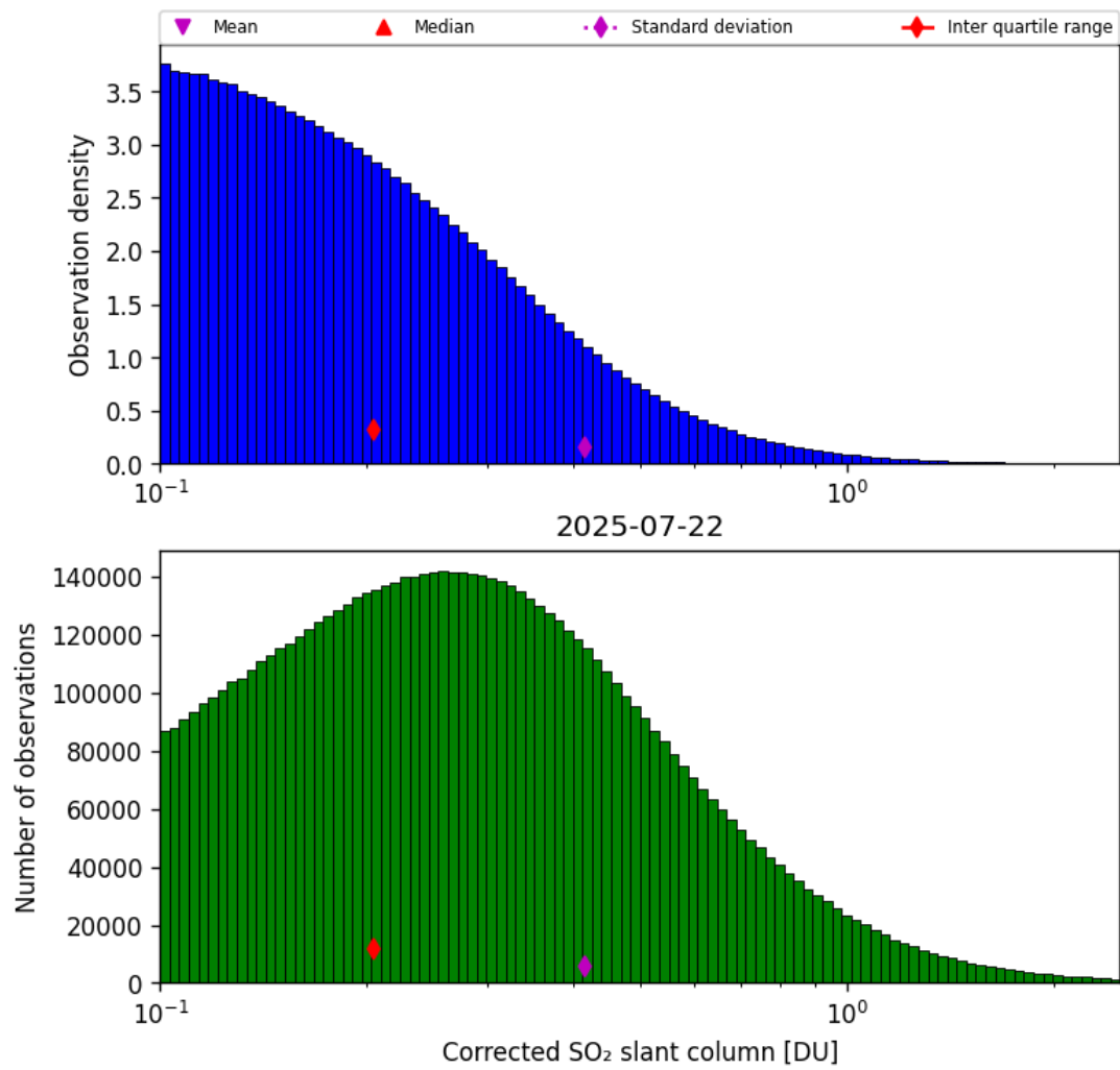
Figure 60: Histogram of “Corrected SO 2 slant column” for 2025-07-21 to 2025-07-23
