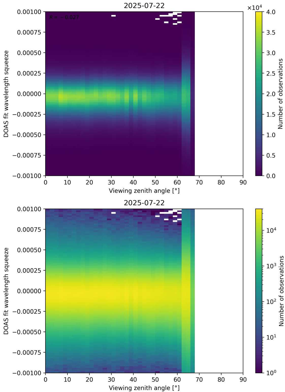
Figure 366: Scatter density plot of “Viewing zenith angle” against “DOAS fit wavelength squeeze” for 2025-07-21 to 2025-07-23.
