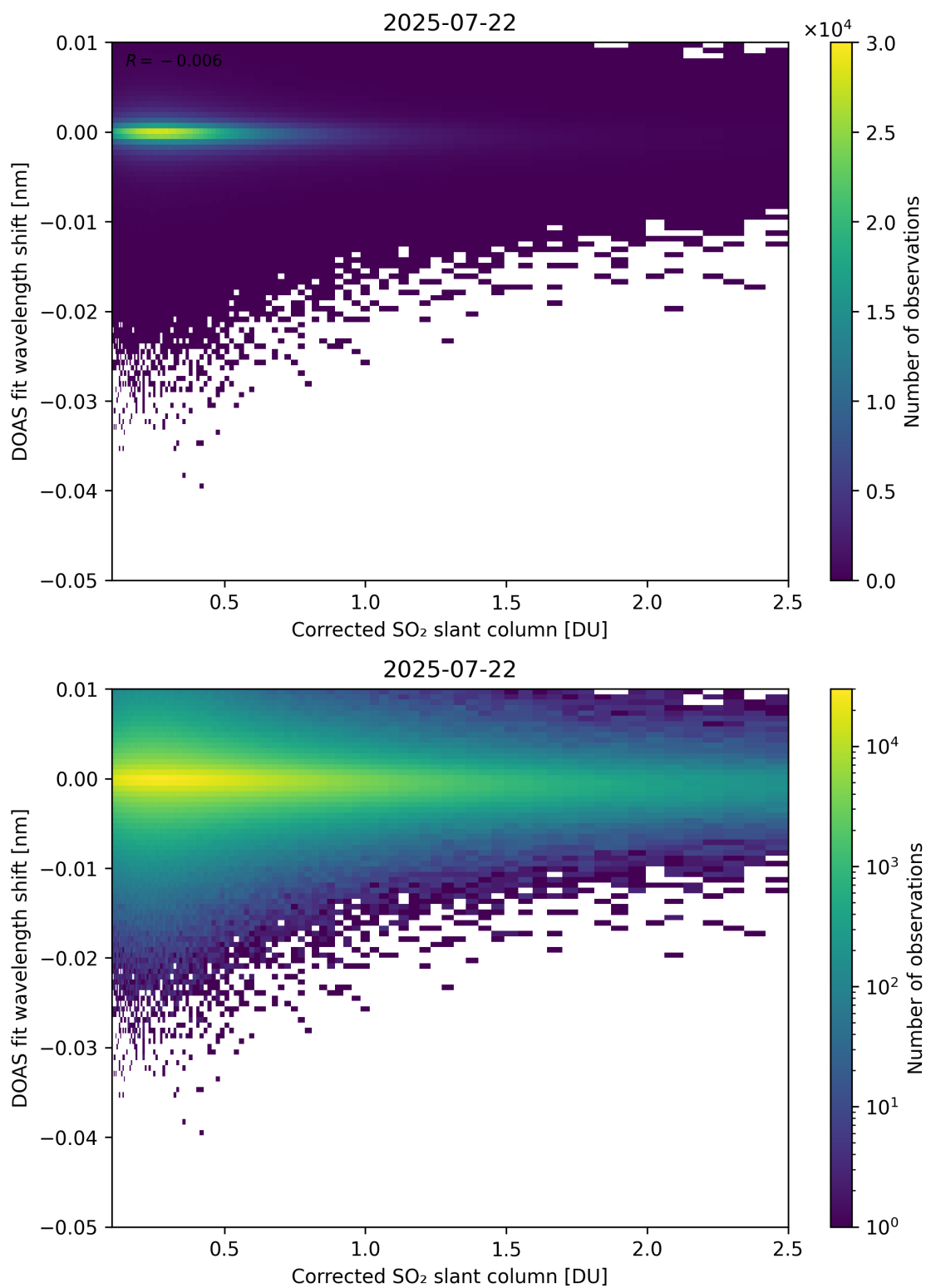
Figure 229: Scatter density plot of “Corrected SO 2 slant column” against “DOAS fit wavelength shift” for 2025-07-21 to 2025-07-23.
