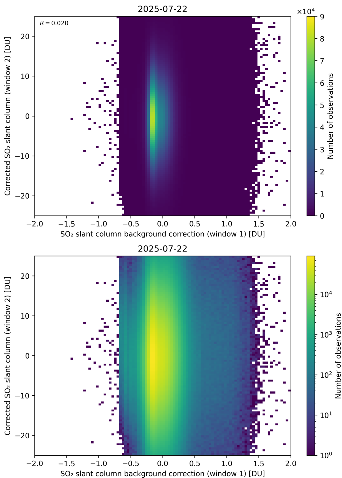
Figure 115: Scatter density plot of “SO 2 slant column background correction (window 1)” against “Corrected SO 2 slant column (window 2)” for 2025-07-21 to 2025-07-23.
