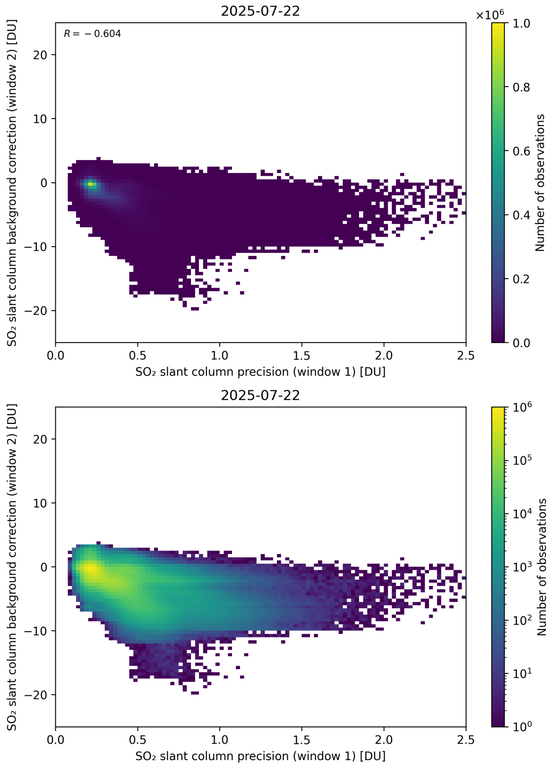
Figure 269: Scatter density plot of “SO 2 slant column precision (window 1)” against “SO 2 slant column background correction (window 2)” for 2025-07-21 to 2025-07-23.
