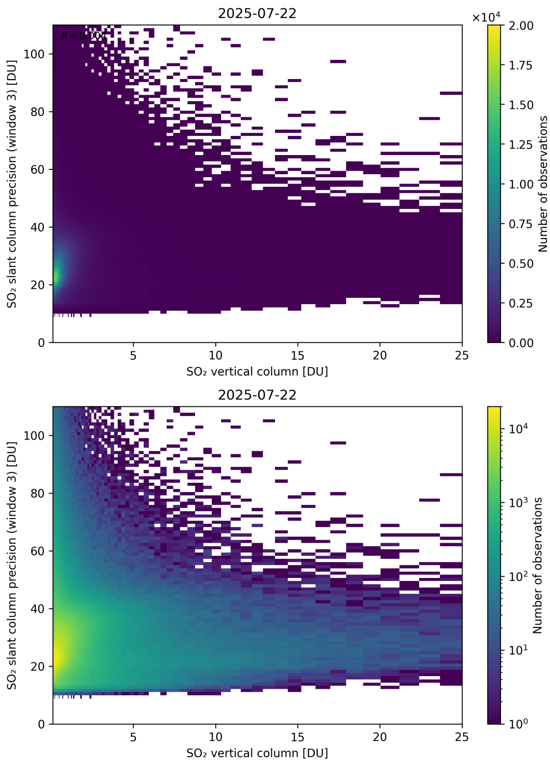
Figure 358: Scatter density plot of “SO 2 vertical column” against “SO 2 slant column precision (window 3)” for 2025-07-21 to 2025-07-23.
