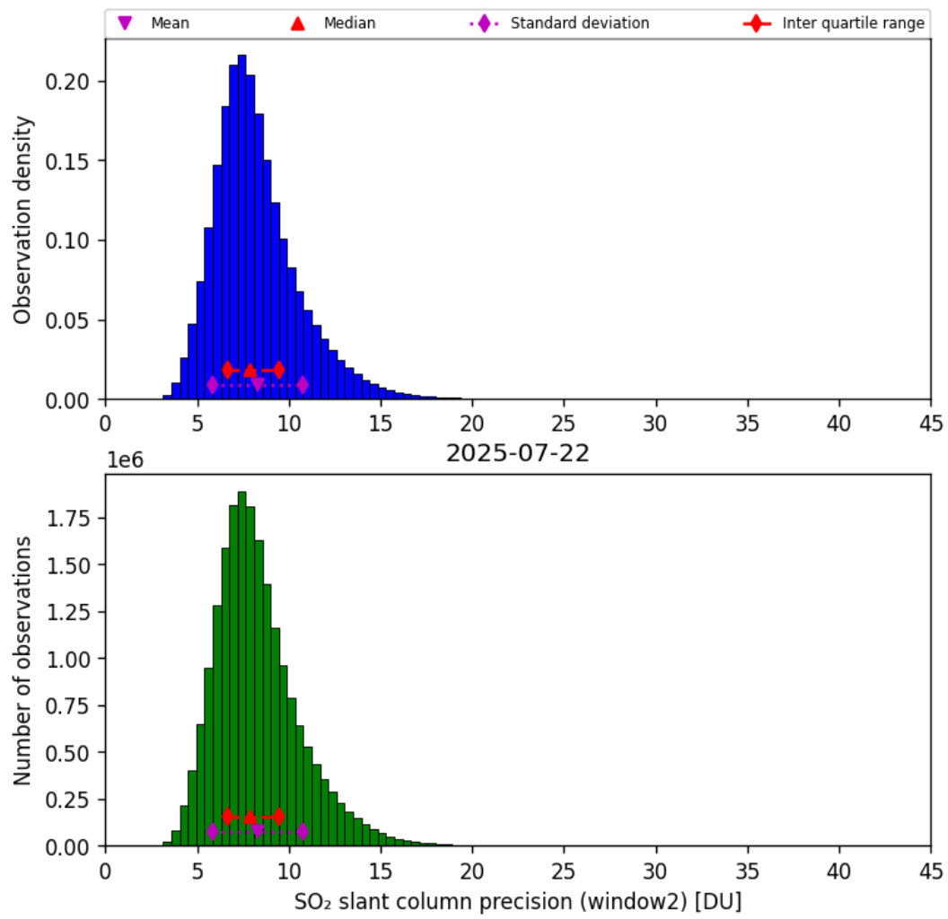
Figure 68: Histogram of “SO 2 slant column precision (window2)” for 2025-07-21 to 2025-07-23
