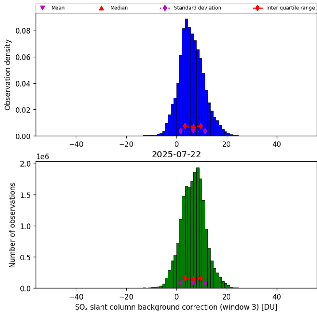
Figure 74: Histogram of “SO 2 slant column background correction (window 3)” for 2025-07-21 to 2025-07-23
