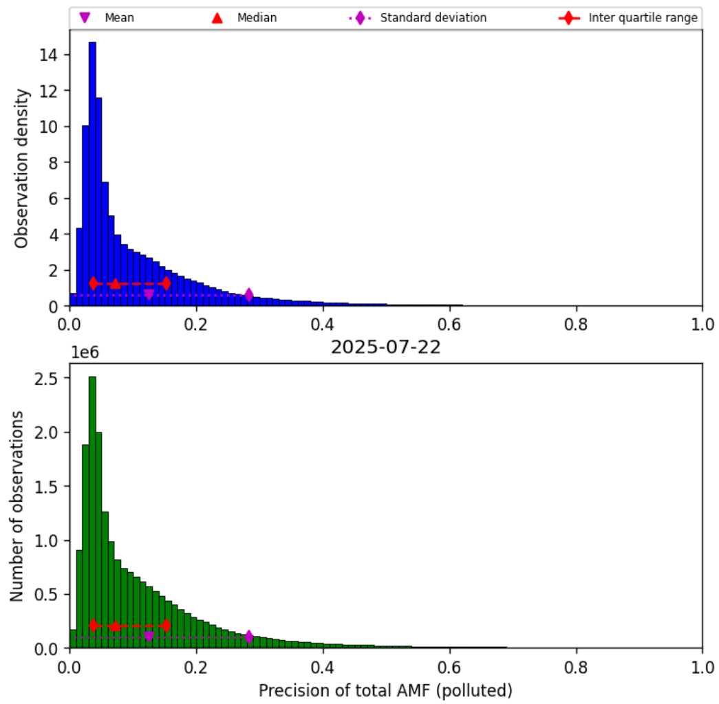
Figure 80: Histogram of “Precision of total AMF (polluted)” for 2025-07-21 to 2025-07-23
