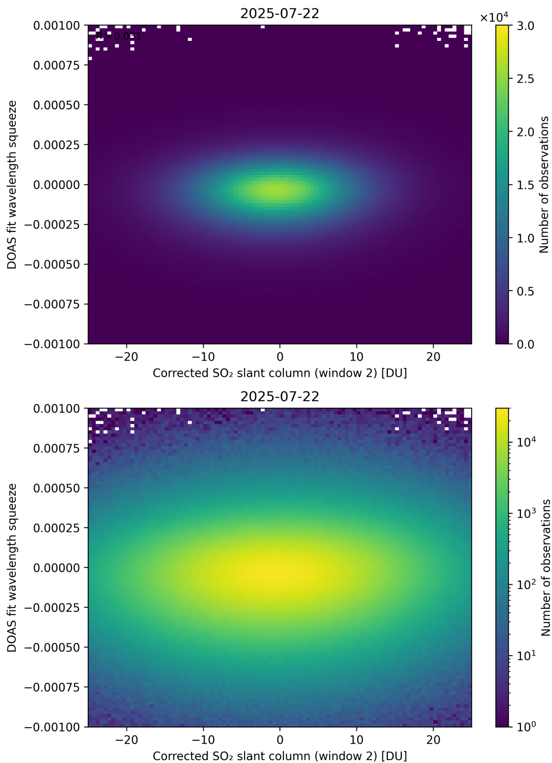
Figure 247: Scatter density plot of “Corrected SO 2 slant column (window 2)” against “DOAS fit wavelength squeeze” for 2025-07-21 to 2025-07-23.
