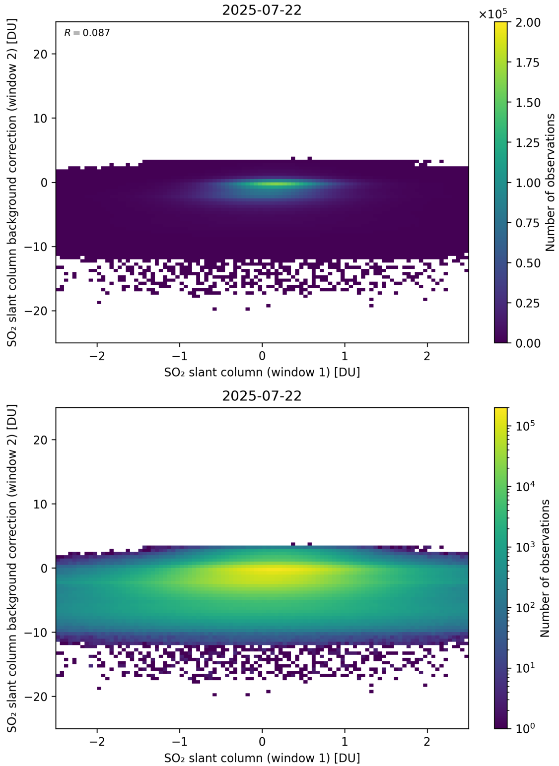
Figure 263: Scatter density plot of “SO 2 slant column (window 1)” against “SO 2 slant column background correction (window 2)” for 2025-07-21 to 2025-07-23.
