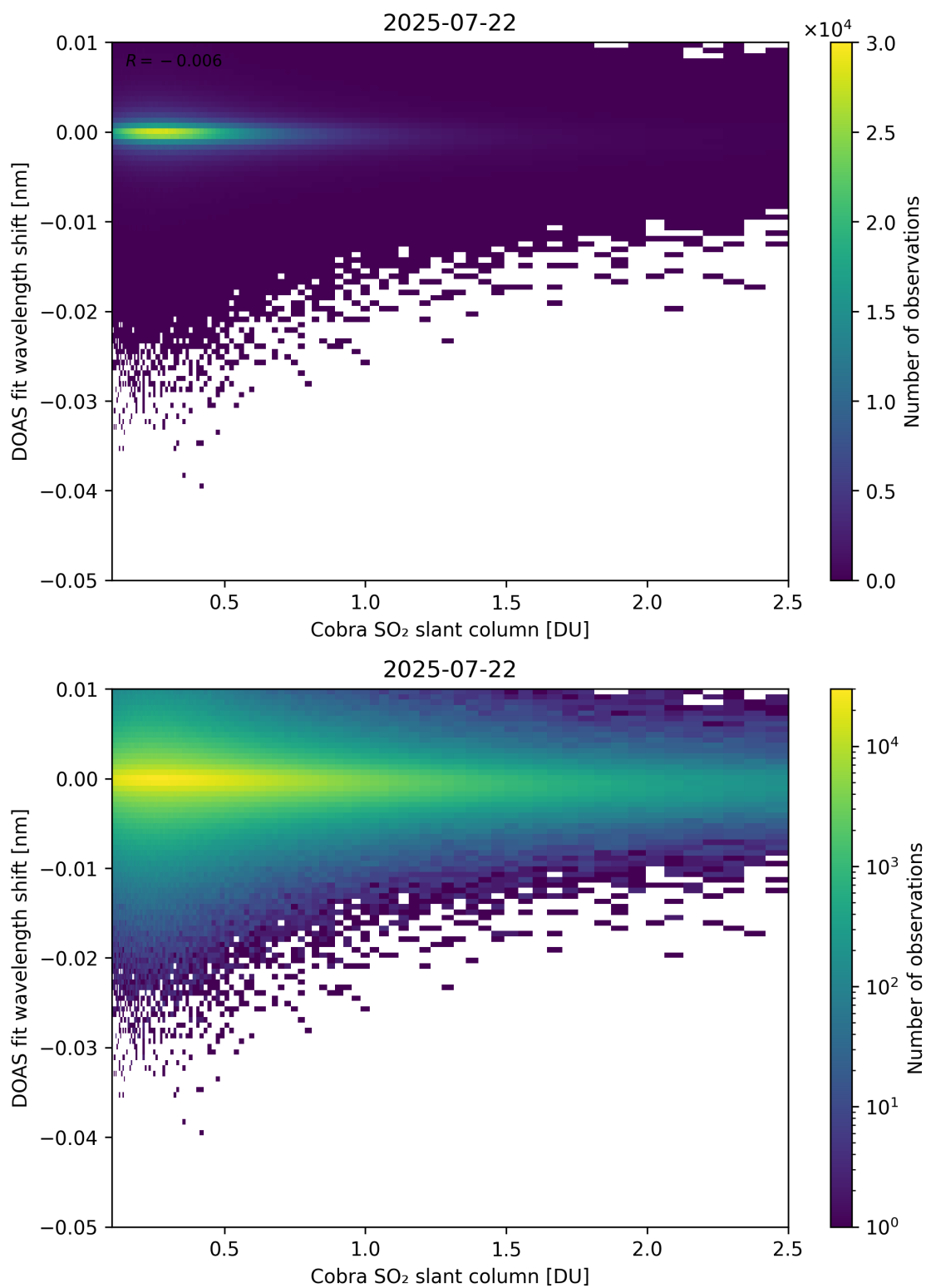
Figure 196: Scatter density plot of “Cobra SO 2 slant column” against “DOAS fit wavelength shift” for 2025-07-21 to 2025-07-23.
