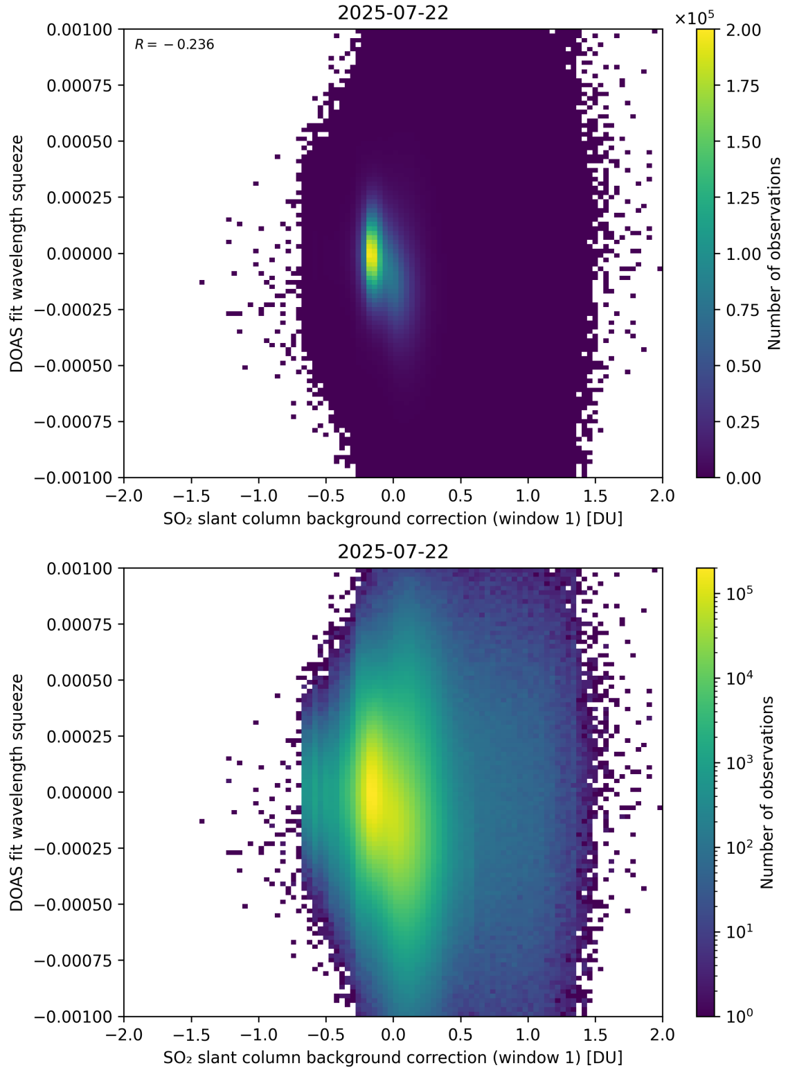
Figure 112: Scatter density plot of “SO 2 slant column background correction (window 1)” against “DOAS fit wavelength squeeze” for 2025-07-21 to 2025-07-23.
