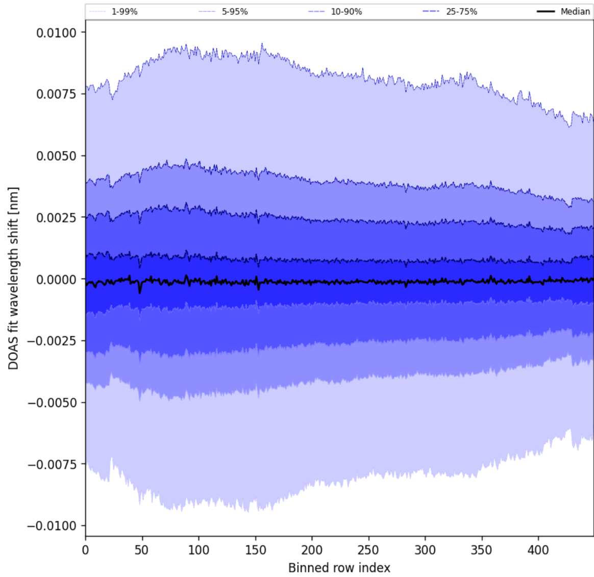
Figure 102: Along track statistics of “DOAS fit wavelength shift” for 2025-07-21 to 2025-07-23
