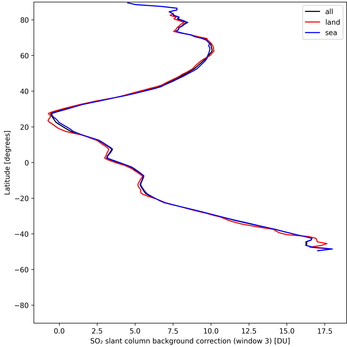
Figure 48: Zonal average of “SO 2 slant column background correction (window 3)” for 2025-07-21 to 2025-07-23.
