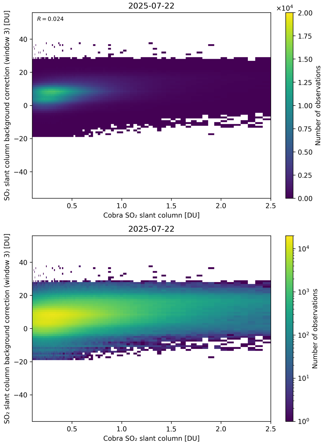
Figure 195: Scatter density plot of “Cobra SO 2 slant column” against “SO 2 slant column background correction (window 3)” for 2025-07-21 to 2025-07-23.
