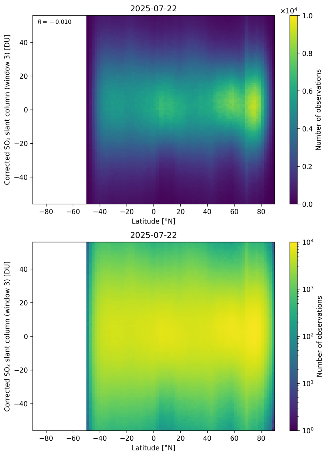
Figure 161: Scatter density plot of “Latitude” against “Corrected SO 2 slant column (window 3)” for 2025-07-21 to 2025-07-23.
