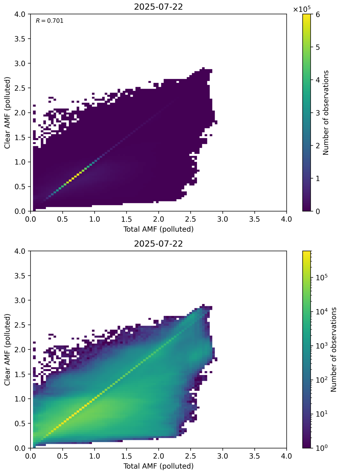
Figure 321: Scatter density plot of “Total AMF (polluted)” against “Clear AMF (polluted)” for 2025-07-21 to 2025-07-23.
