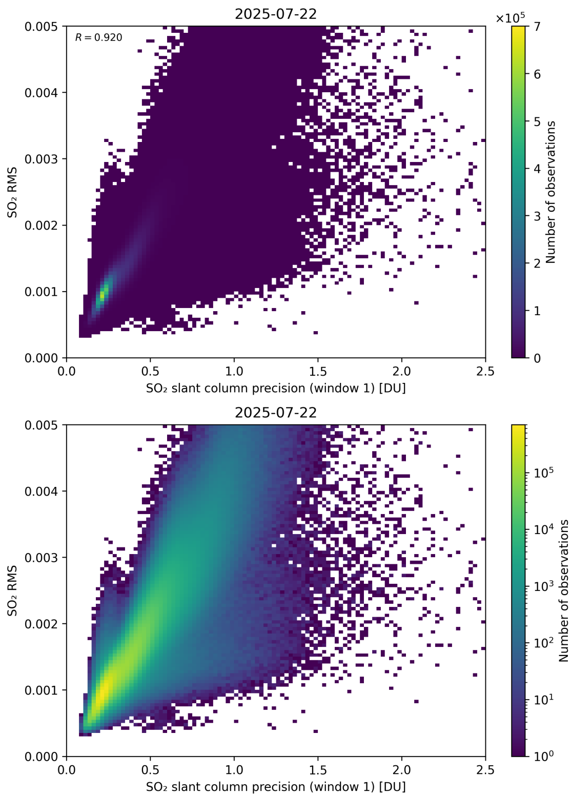
Figure 273: Scatter density plot of “SO 2 slant column precision (window 1)” against “SO 2 RMS” for 2025-07-21 to 2025-07-23.
