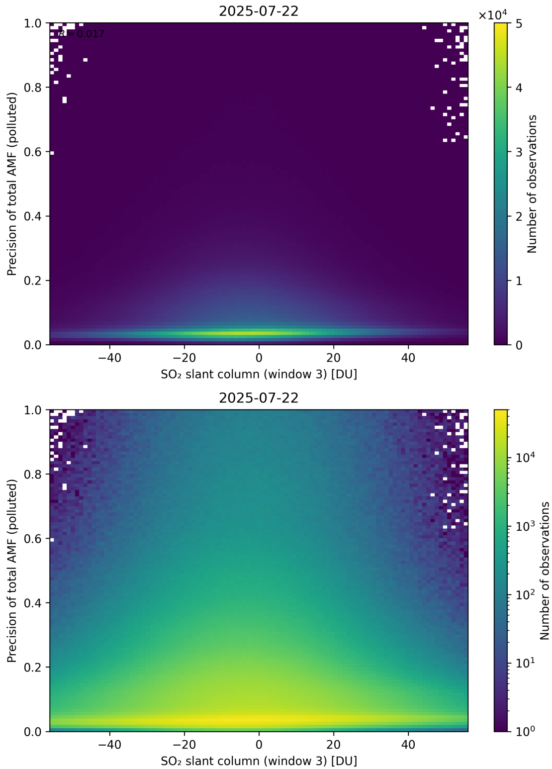
Figure 319: Scatter density plot of “SO 2 slant column (window 3)” against “Precision of total AMF (polluted)” for 2025-07-21 to 2025-07-23.
