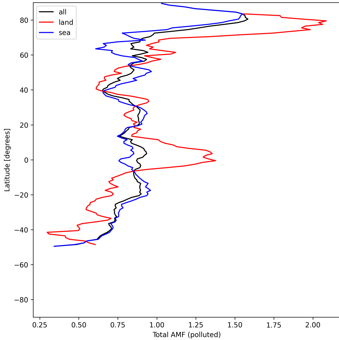
Figure 53: Zonal average of “Total AMF (polluted)” for 2025-07-21 to 2025-07-23.
