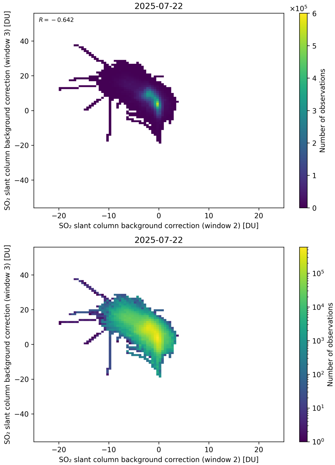
Figure 122: Scatter density plot of “SO 2 slant column background correction (window 2)” against “SO 2 slant column background correction (window 3)” for 2025-07-21 to 2025-07-23.
