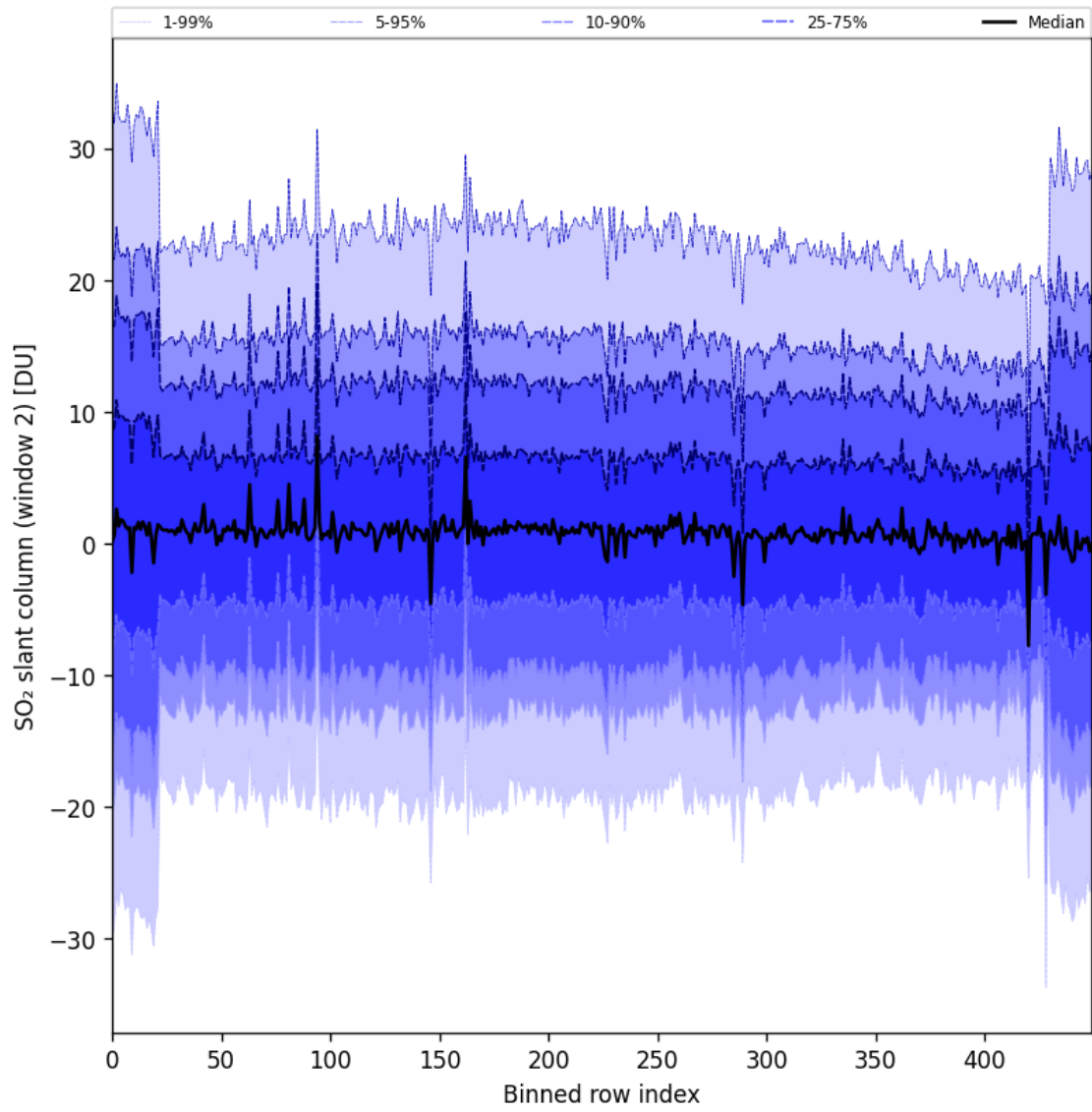
Figure 93: Along track statistics of “SO 2 slant column (window 2)” for 2025-07-21 to 2025-07-23
