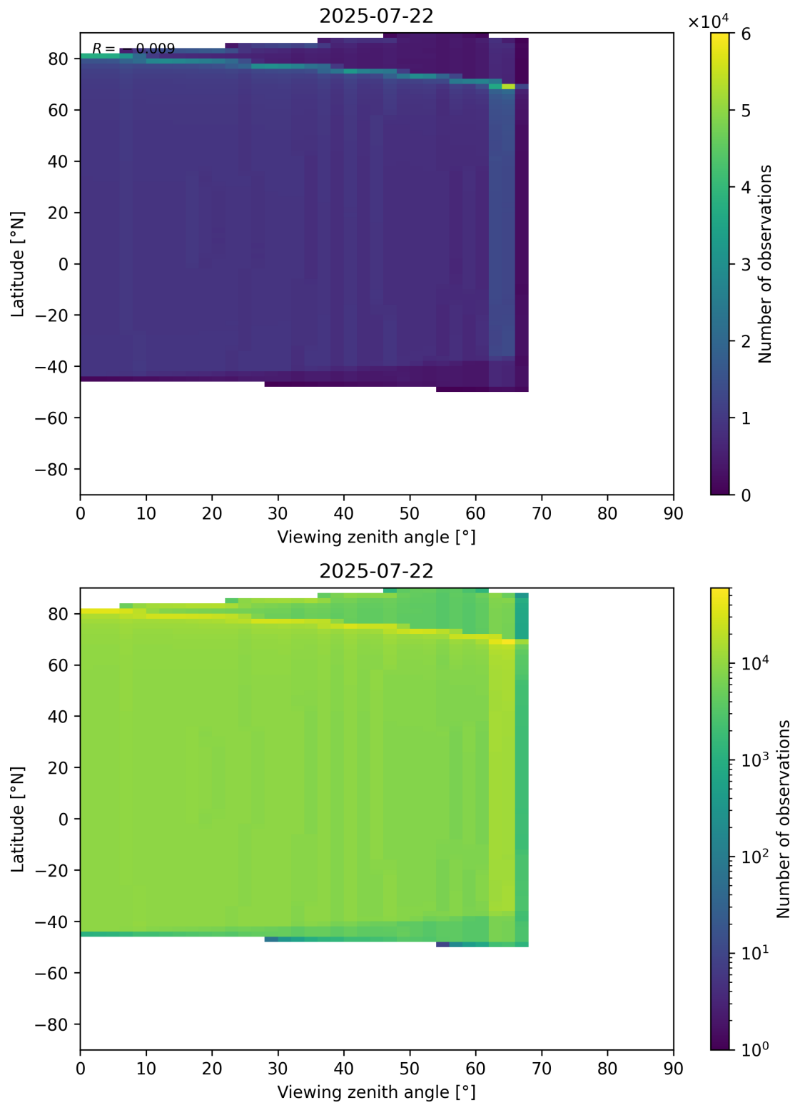
Figure 368: Scatter density plot of “Viewing zenith angle” against “Latitude” for 2025-07-21 to 2025-07-23.
