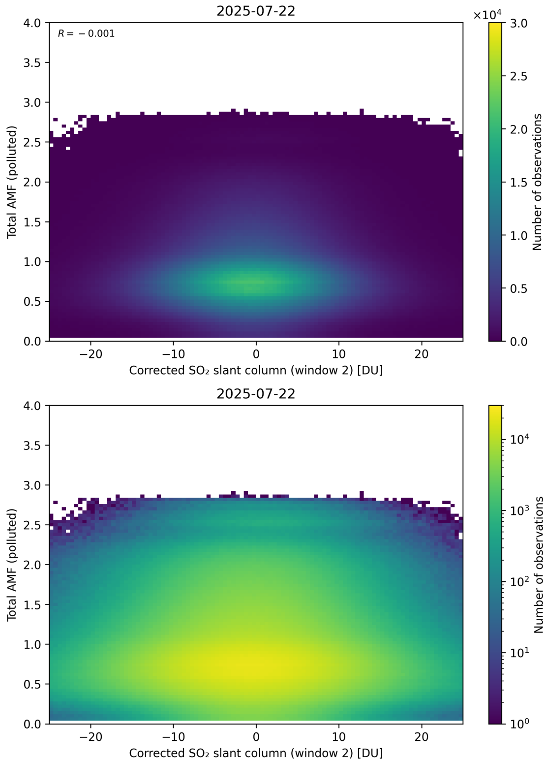
Figure 253: Scatter density plot of “Corrected SO 2 slant column (window 2)” against “Total AMF (polluted)” for 2025-07-21 to 2025-07-23.
