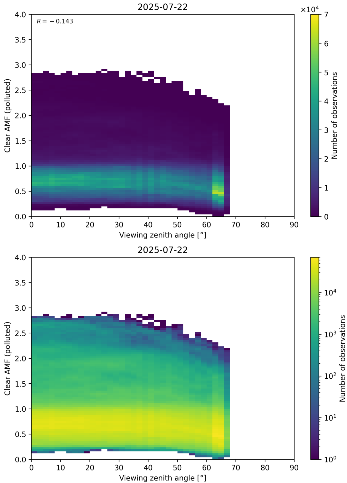
Figure 370: Scatter density plot of “Viewing zenith angle” against “Clear AMF (polluted)” for 2025-07-21 to 2025-07-23.
