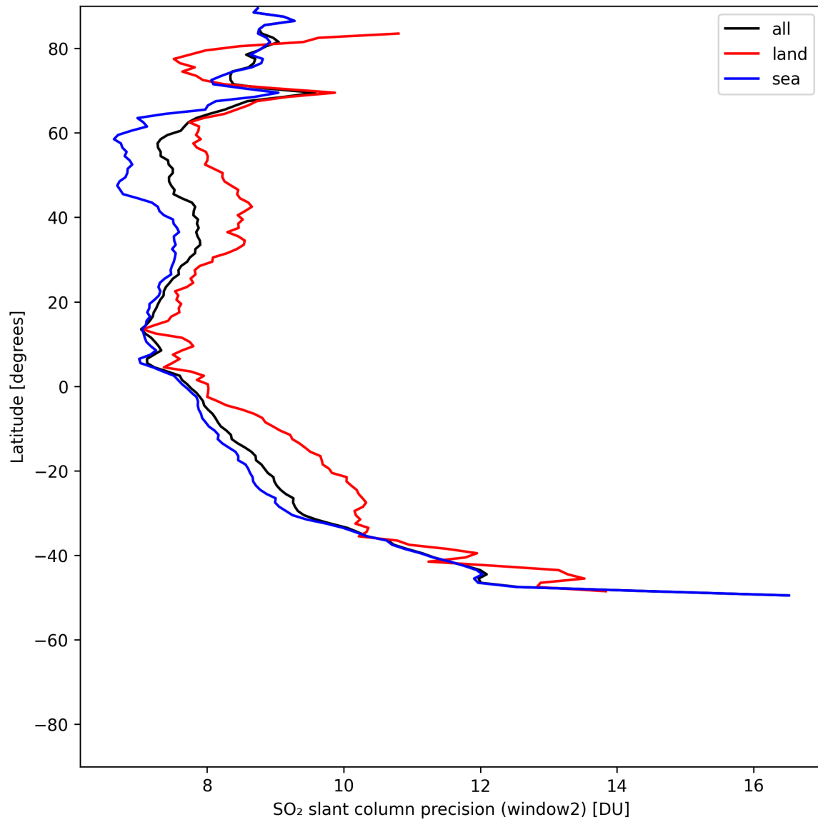
Figure 42: Zonal average of “SO 2 slant column precision (window2)” for 2025-07-21 to 2025-07-23.
