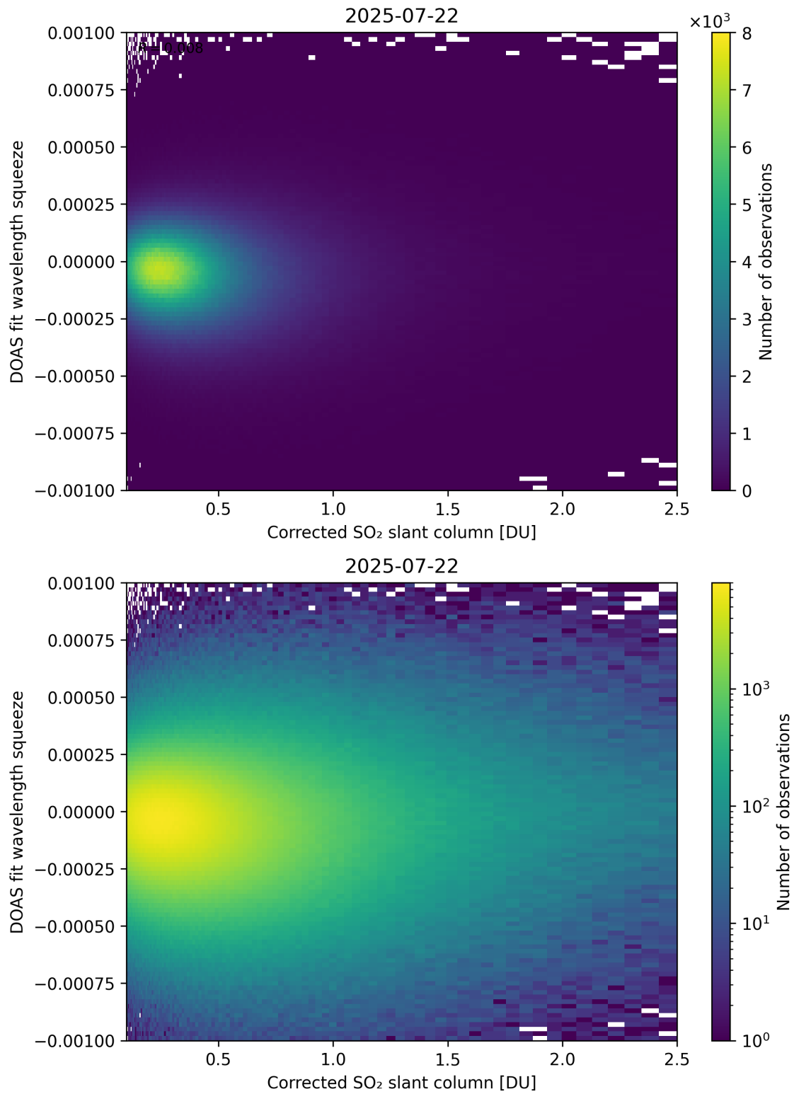
Figure 230: Scatter density plot of “Corrected SO 2 slant column” against “DOAS fit wavelength squeeze” for 2025-07-21 to 2025-07-23.
