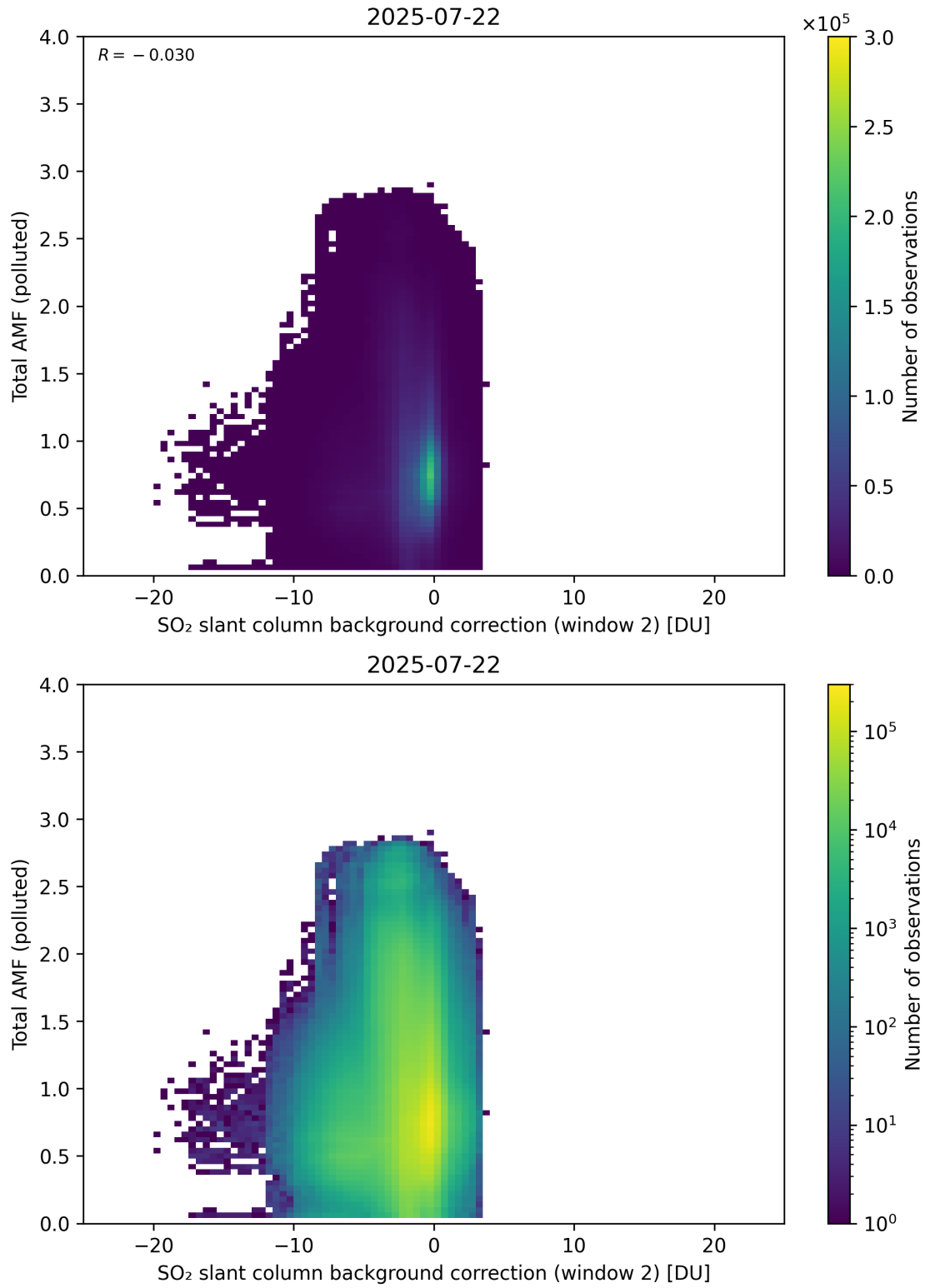
Figure 130: Scatter density plot of “SO 2 slant column background correction (window 2)” against “Total AMF (polluted)” for 2025-07-21 to 2025-07-23.
