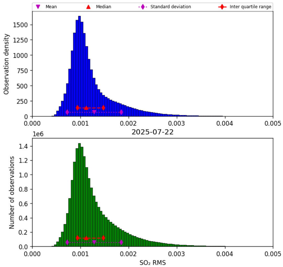
Figure 78: Histogram of “SO 2 RMS” for 2025-07-21 to 2025-07-23
