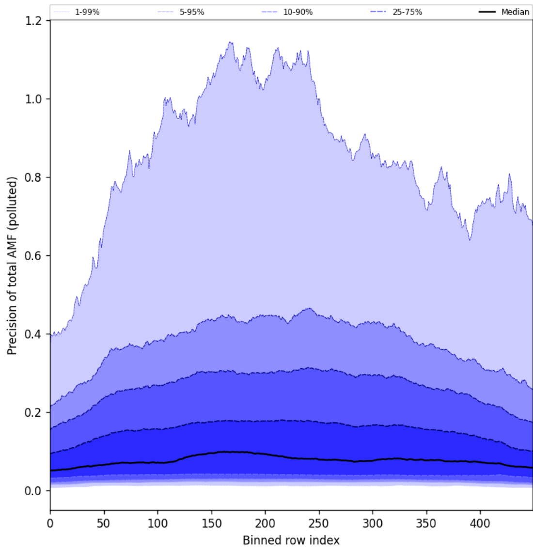
Figure 106: Along track statistics of “Precision of total AMF (polluted)” for 2025-07-21 to 2025-07-23
