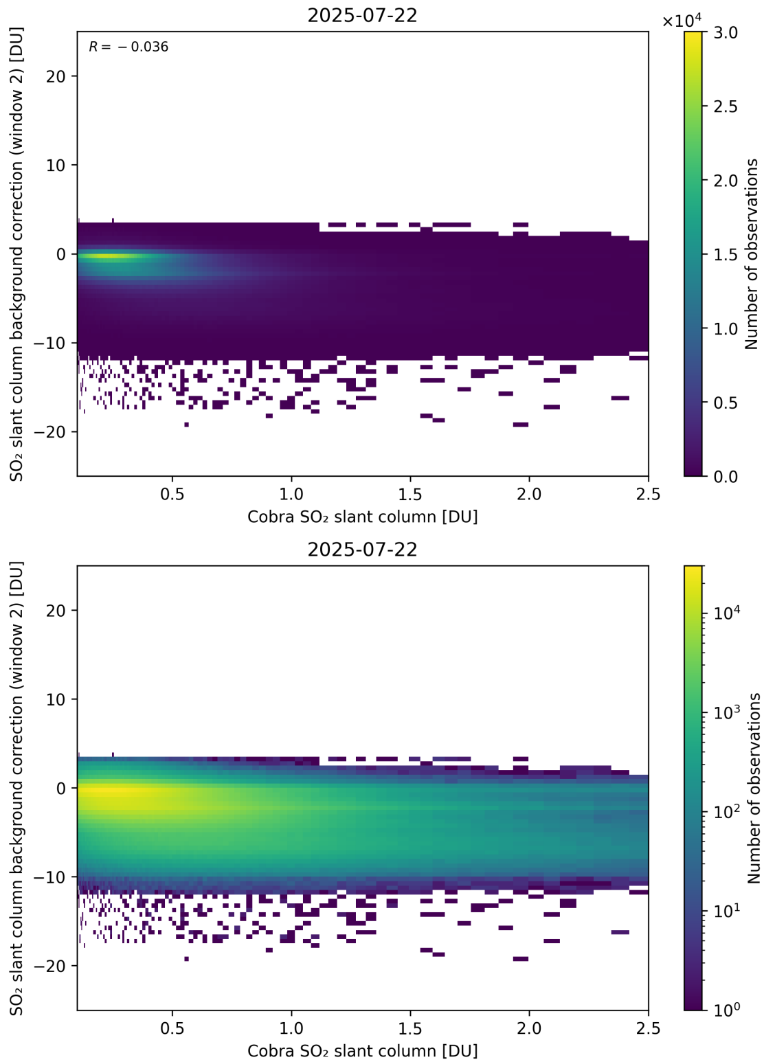
Figure 194: Scatter density plot of “Cobra SO 2 slant column” against “SO 2 slant column background correction (window 2)” for 2025-07-21 to 2025-07-23.
