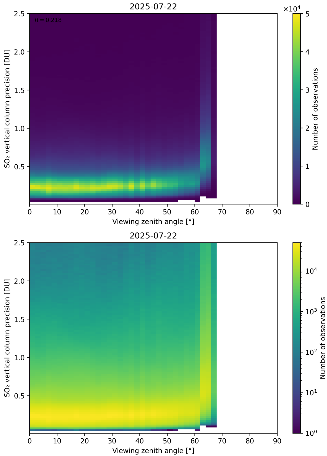
Figure 384: Scatter density plot of “Viewing zenith angle” against “SO 2 vertical column precision” for 2025-07-21 to 2025-07-23.
