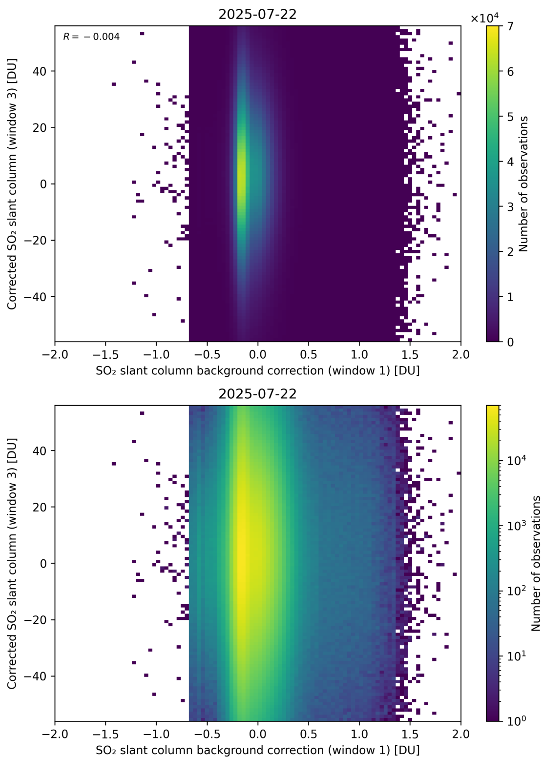
Figure 116: Scatter density plot of “SO 2 slant column background correction (window 1)” against “Corrected SO 2 slant column (window 3)” for 2025-07-21 to 2025-07-23.
