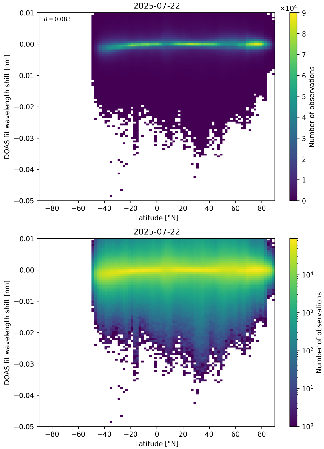
Figure 153: Scatter density plot of “Latitude” against “DOAS fit wavelength shift” for 2025-07-21 to 2025-07-23.
