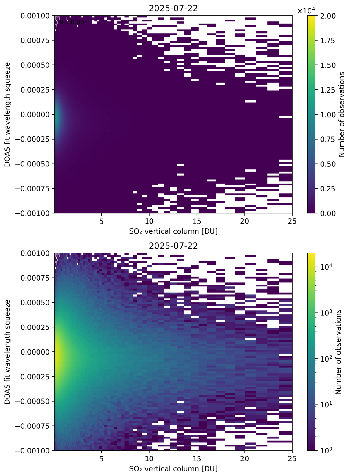
Figure 327: Scatter density plot of “SO 2 vertical column” against “DOAS fit wavelength squeeze” for 2025-07-21 to 2025-07-23.
