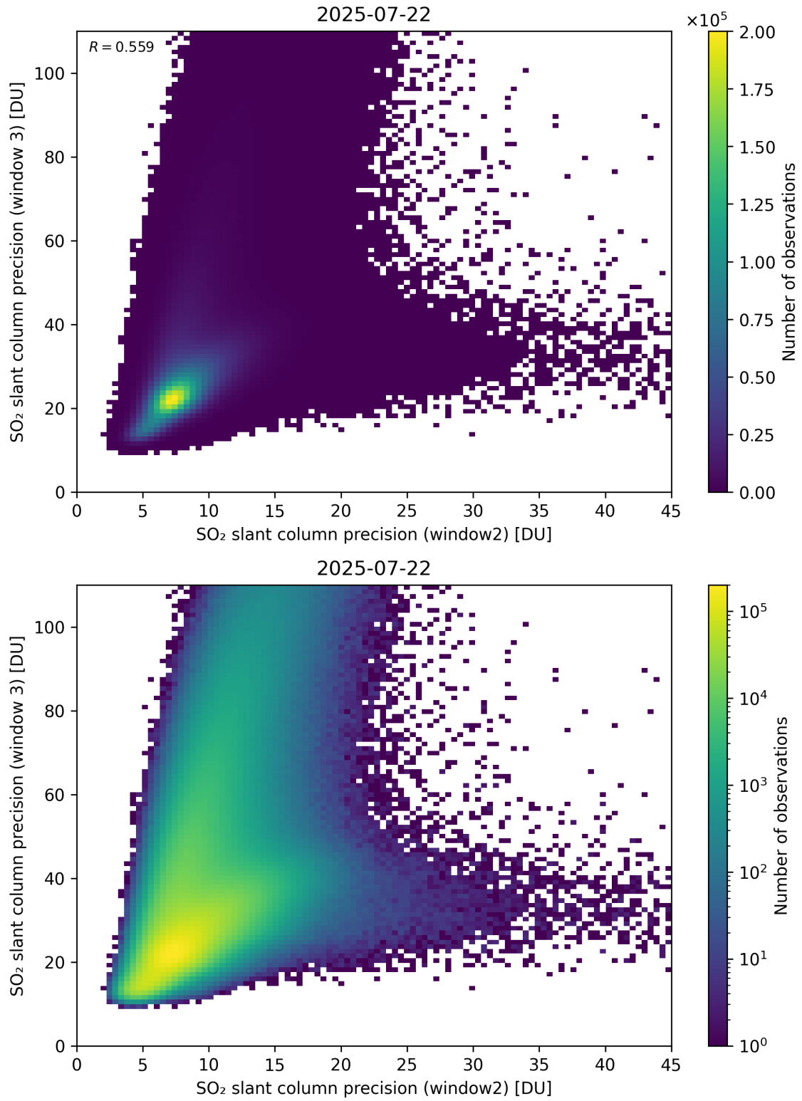
Figure 300: Scatter density plot of “SO 2 slant column precision (window2)” against “SO 2 slant column precision (window 3)” for 2025-07-21 to 2025-07-23.
