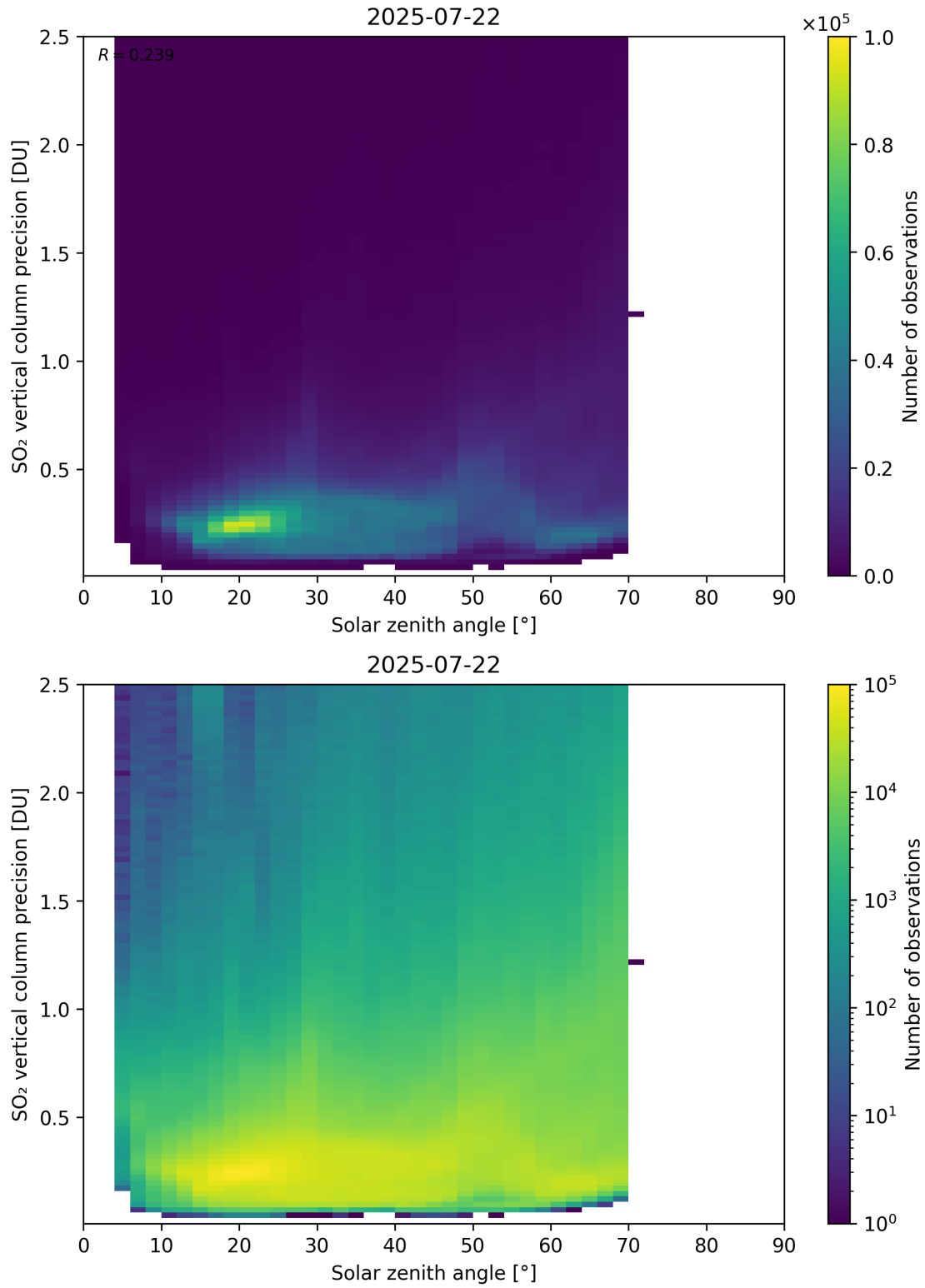
Figure 192: Scatter density plot of “Solar zenith angle” against “SO 2 vertical column precision” for 2025-07-21 to 2025-07-23.
