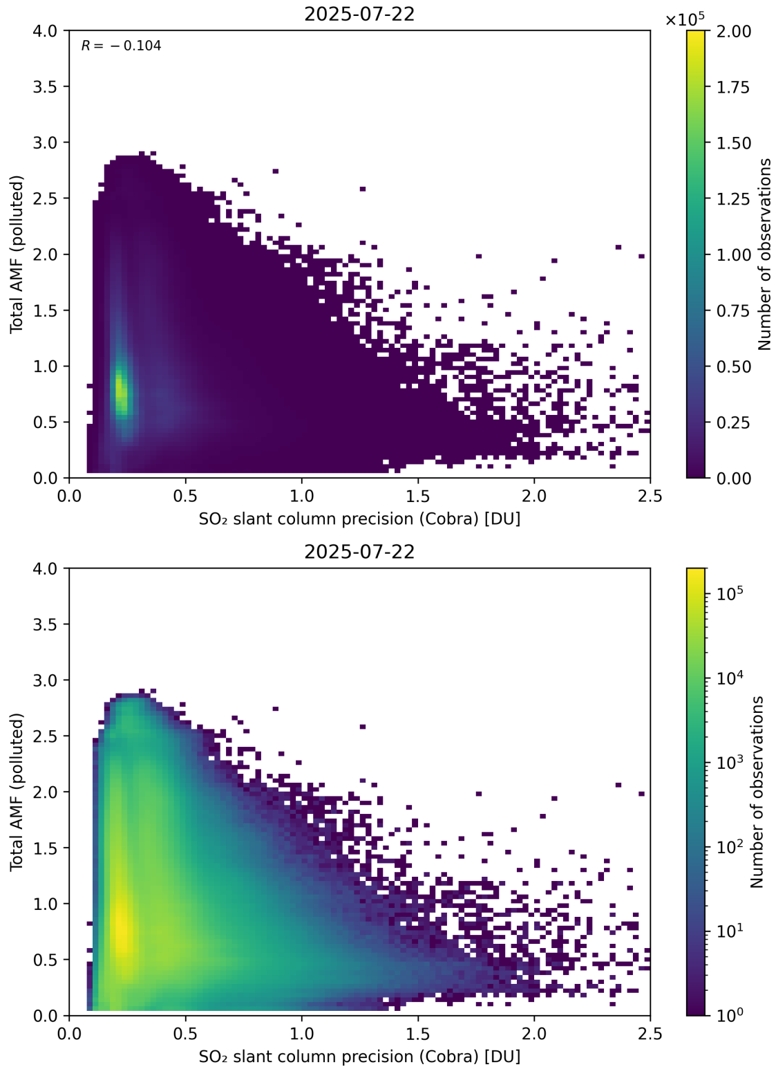
Figure 213: Scatter density plot of “SO 2 slant column precision (Cobra)” against “Total AMF (polluted)” for 2025-07-21 to 2025-07-23.
