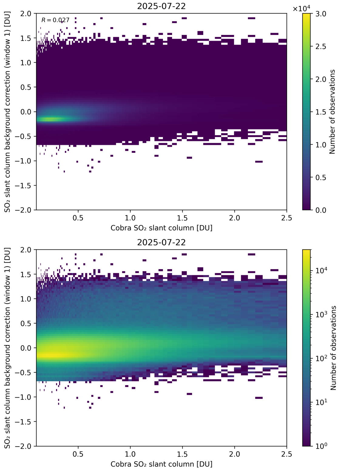
Figure 193: Scatter density plot of “Cobra SO 2 slant column” against “SO 2 slant column background correction (window 1)” for 2025-07-21 to 2025-07-23.
