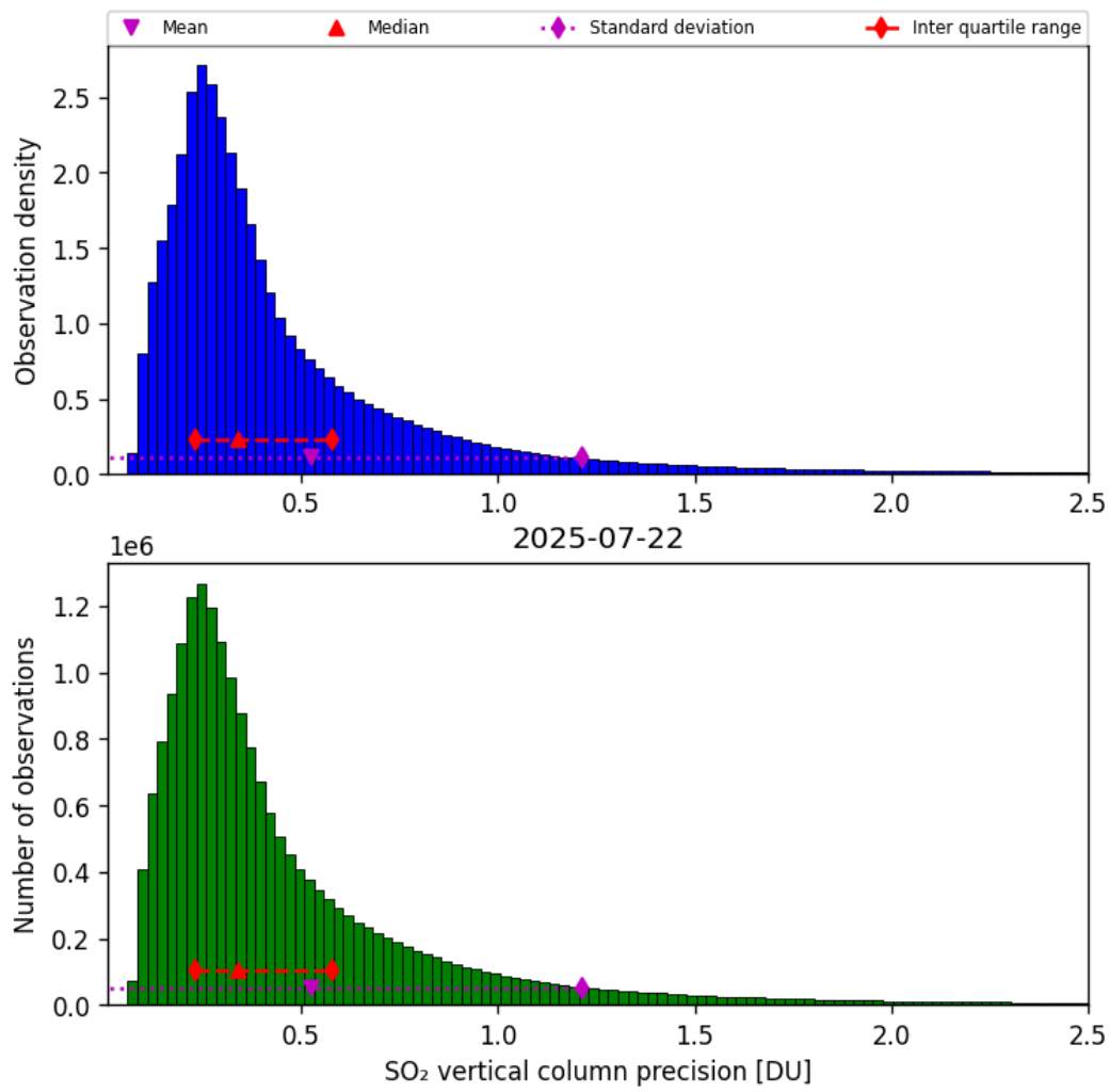
Figure 59: Histogram of “SO 2 vertical column precision” for 2025-07-21 to 2025-07-23
