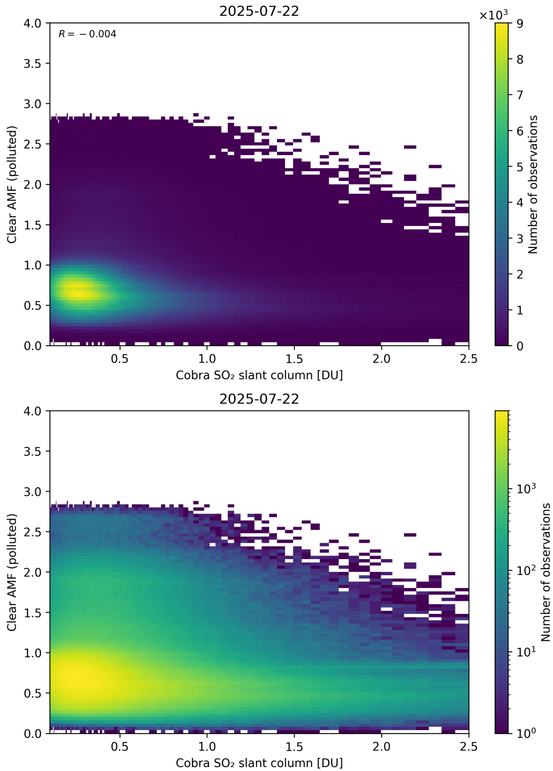
Figure 215: Scatter density plot of “Cobra SO 2 slant column” against “Clear AMF (polluted)” for 2025-07-21 to 2025-07-23.
