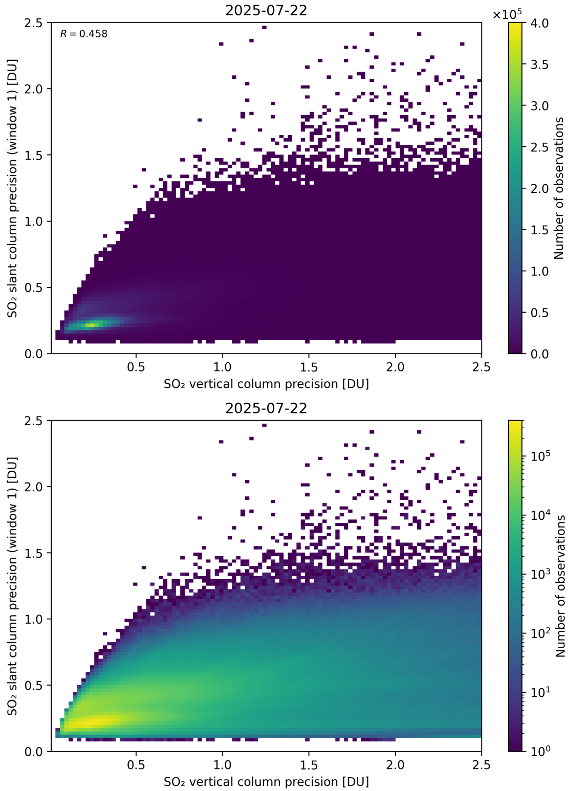
Figure 342: Scatter density plot of “SO 2 vertical column precision” against “SO 2 slant column precision (window 1)” for 2025-07-21 to 2025-07-23.
