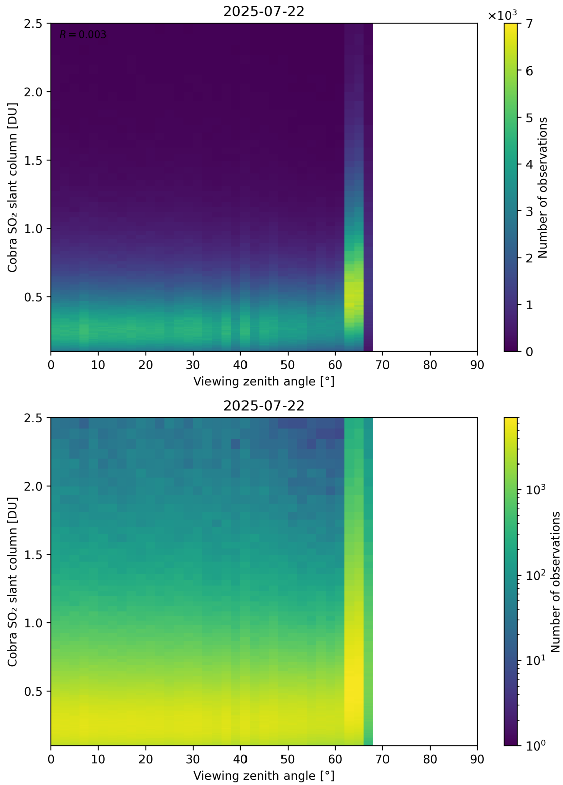
Figure 371: Scatter density plot of “Viewing zenith angle” against “Cobra SO 2 slant column” for 2025-07-21 to 2025-07-23.
