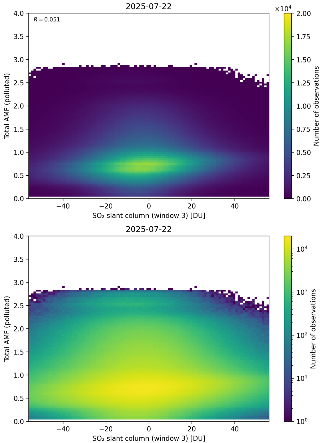
Figure 318: Scatter density plot of “SO 2 slant column (window 3)” against “Total AMF (polluted)” for 2025-07-21 to 2025-07-23.
