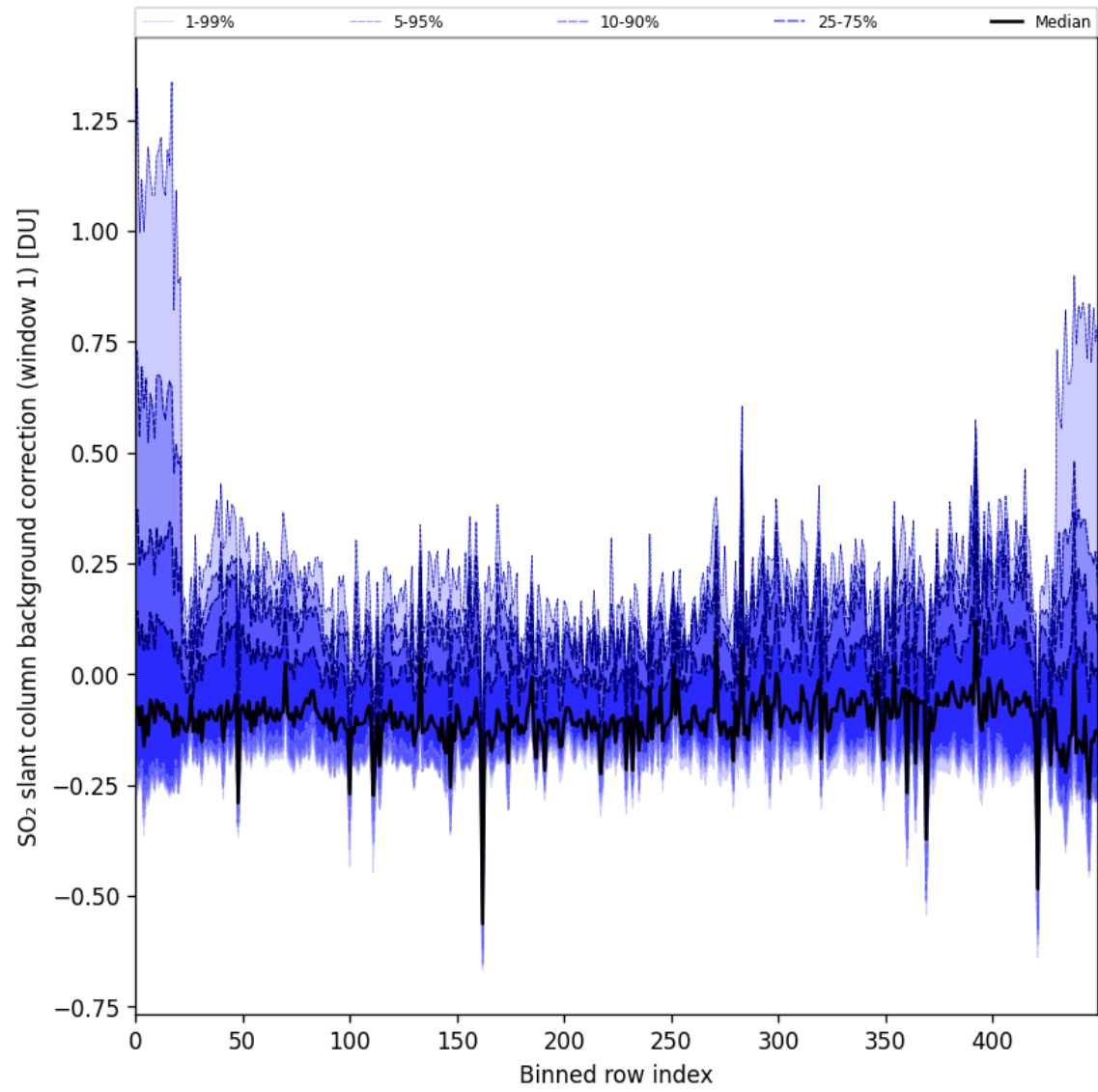
Figure 92: Along track statistics of “SO 2 slant column background correction (window 1)” for 2025-07-21 to 2025-07-23
