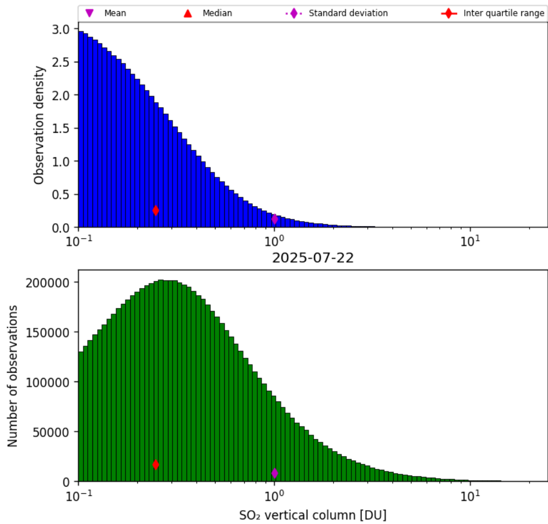
Figure 58: Histogram of “SO 2 vertical column” for 2025-07-21 to 2025-07-23
