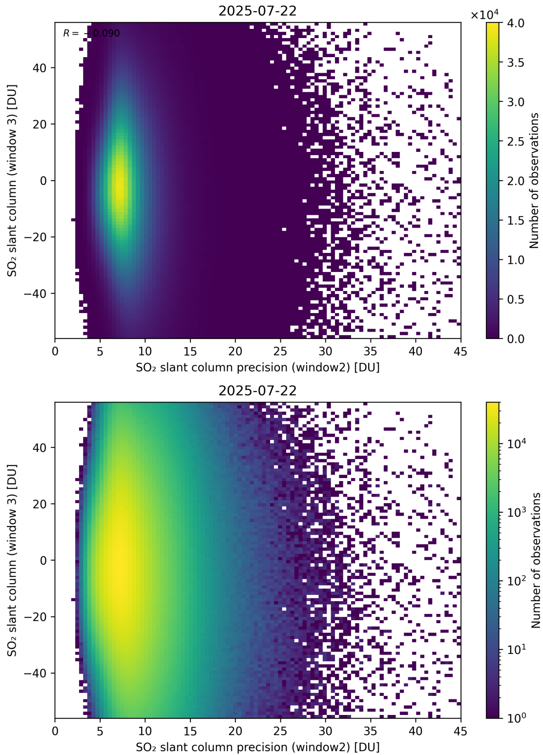
Figure 299: Scatter density plot of “SO 2 slant column precision (window2)” against “SO 2 slant column (window 3)” for 2025-07-21 to 2025-07-23.
