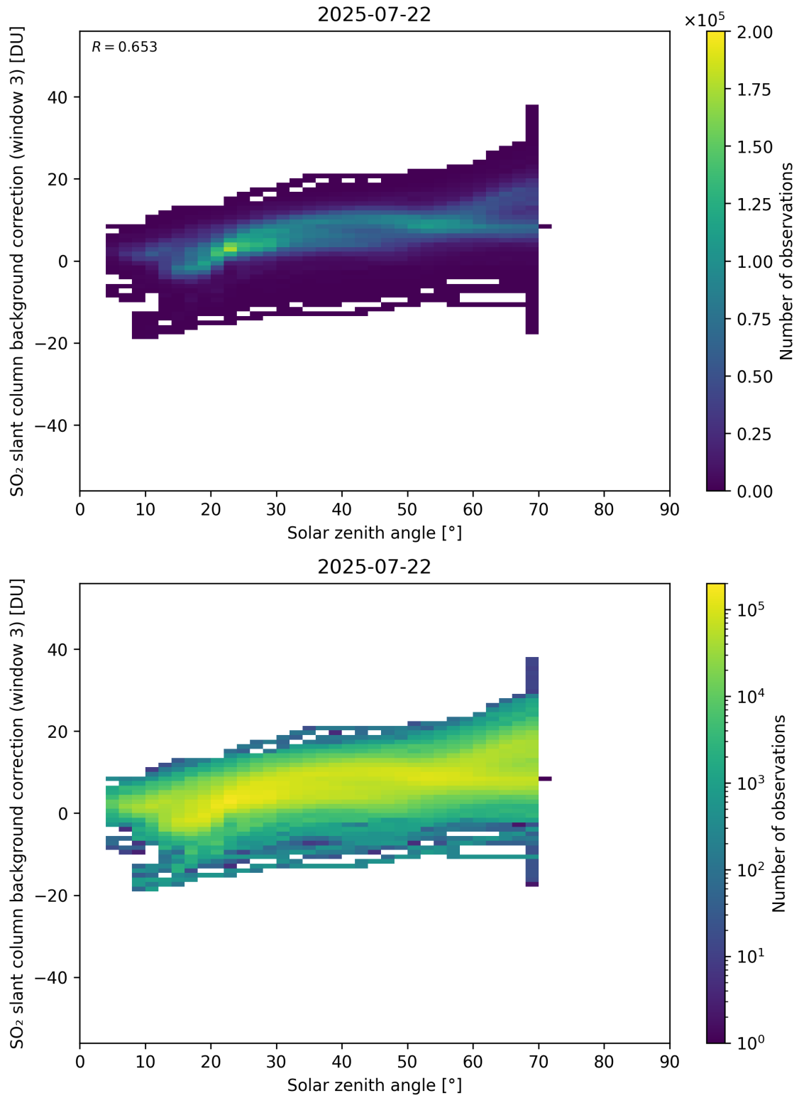
Figure 173: Scatter density plot of “Solar zenith angle” against “SO 2 slant column background correction (window 3)” for 2025-07-21 to 2025-07-23.
