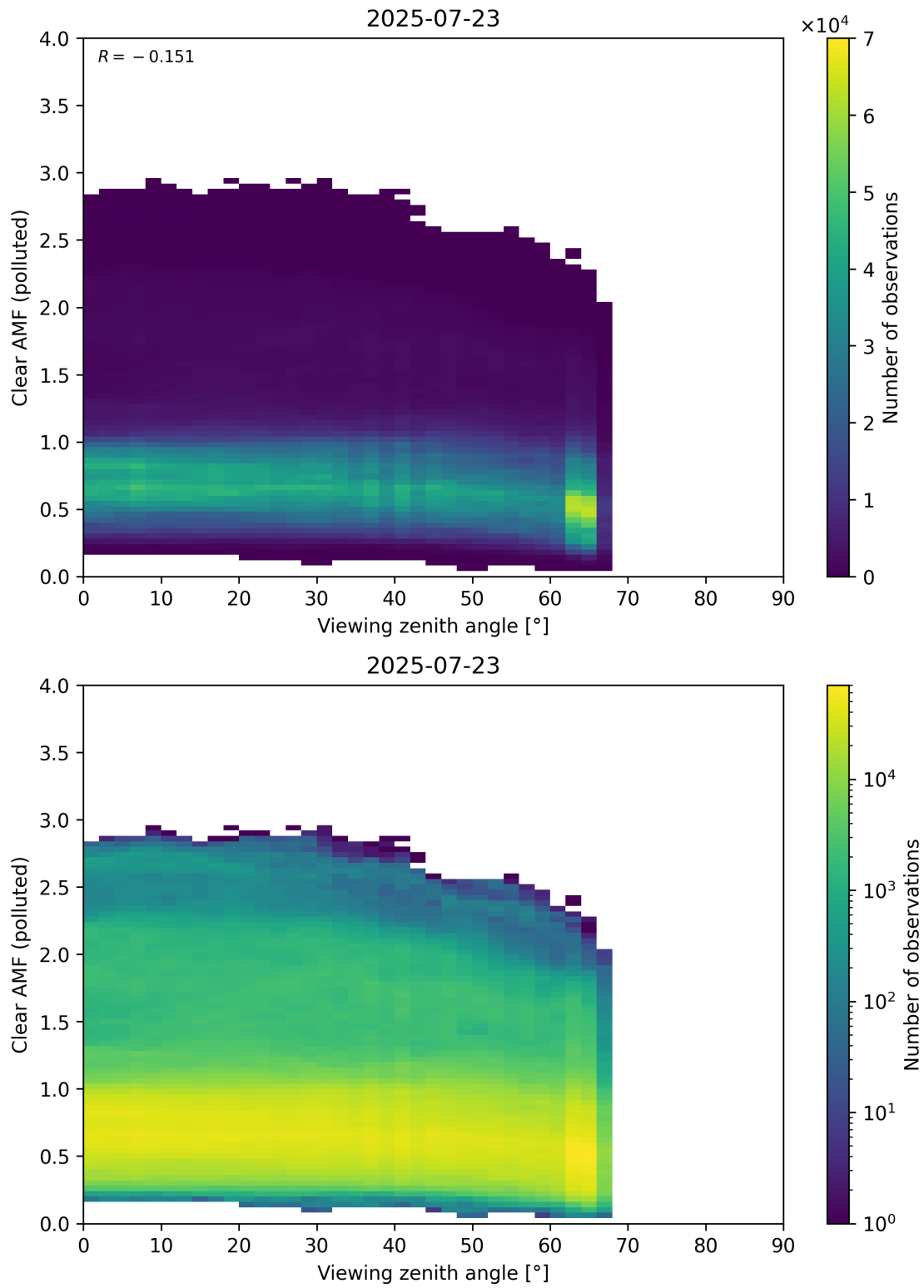
Figure 370: Scatter density plot of “Viewing zenith angle” against “Clear AMF (polluted)” for 2025-07-22 to 2025-07-24.
