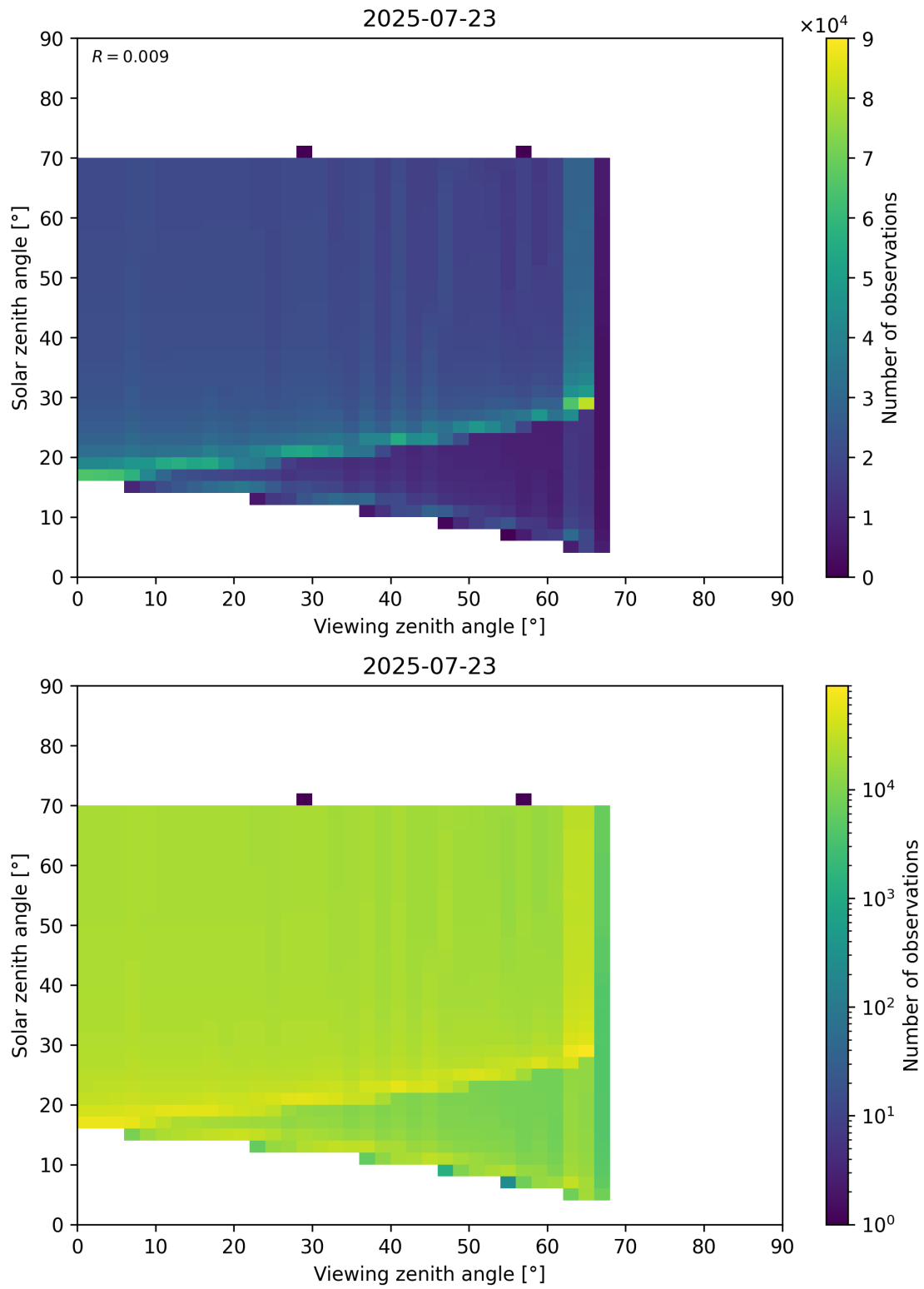
Figure 369: Scatter density plot of “Viewing zenith angle” against “Solar zenith angle” for 2025-07-22 to 2025-07-24.
