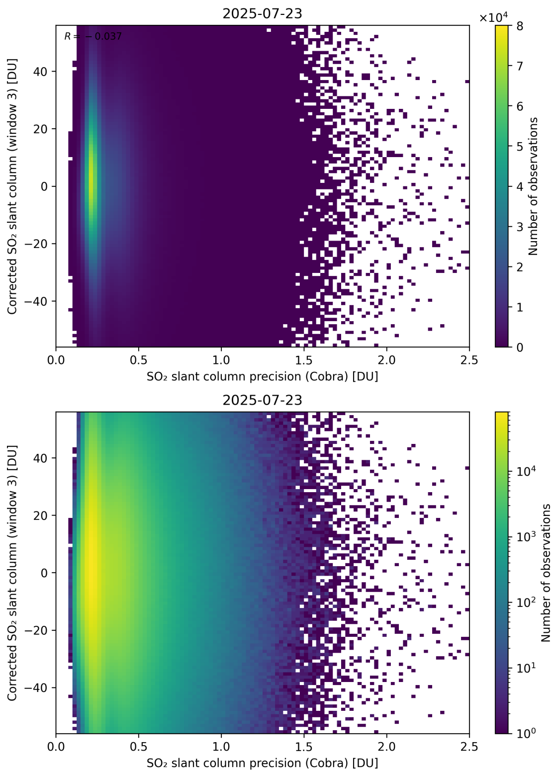
Figure 207: Scatter density plot of “SO 2 slant column precision (Cobra)” against “Corrected SO 2 slant column (window 3)” for 2025-07-22 to 2025-07-24.
