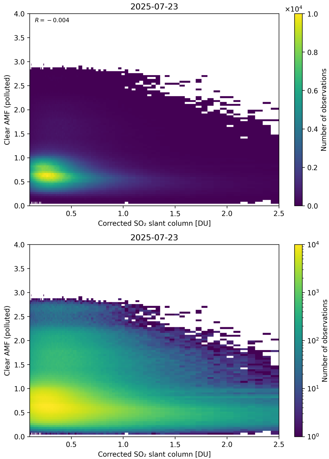
Figure 232: Scatter density plot of “Corrected SO 2 slant column” against “Clear AMF (polluted)” for 2025-07-22 to 2025-07-24.
