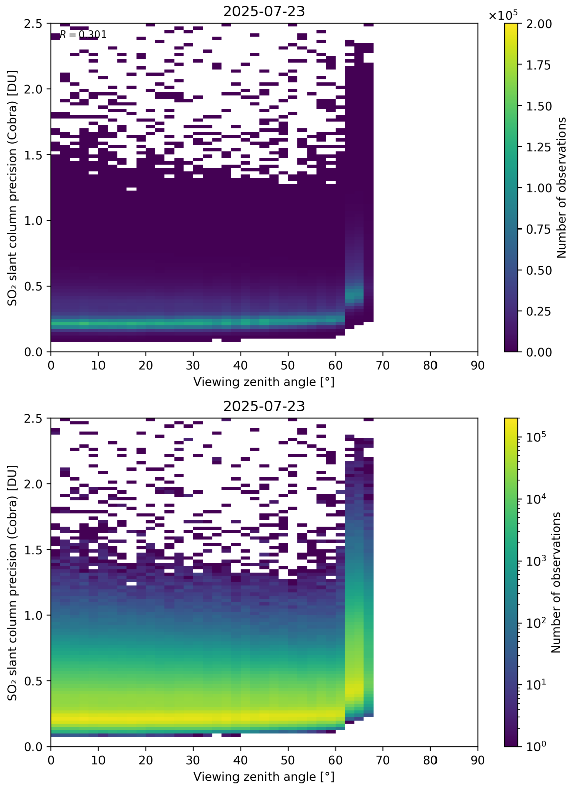
Figure 372: Scatter density plot of “Viewing zenith angle” against “SO 2 slant column precision (Cobra)” for 2025-07-22 to 2025-07-24.
