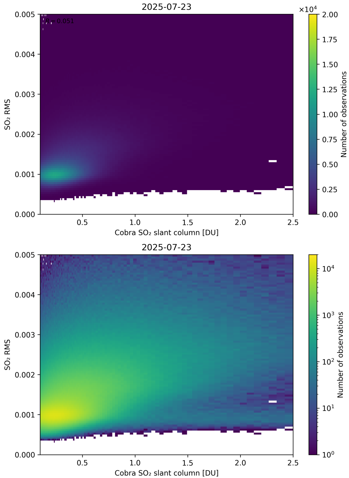
Figure 198: Scatter density plot of “Cobra SO 2 slant column” against “SO 2 RMS” for 2025-07-22 to 2025-07-24.
