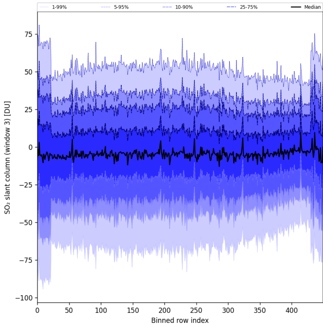
Figure 97: Along track statistics of “SO 2 slant column (window 3)” for 2025-07-22 to 2025-07-24
