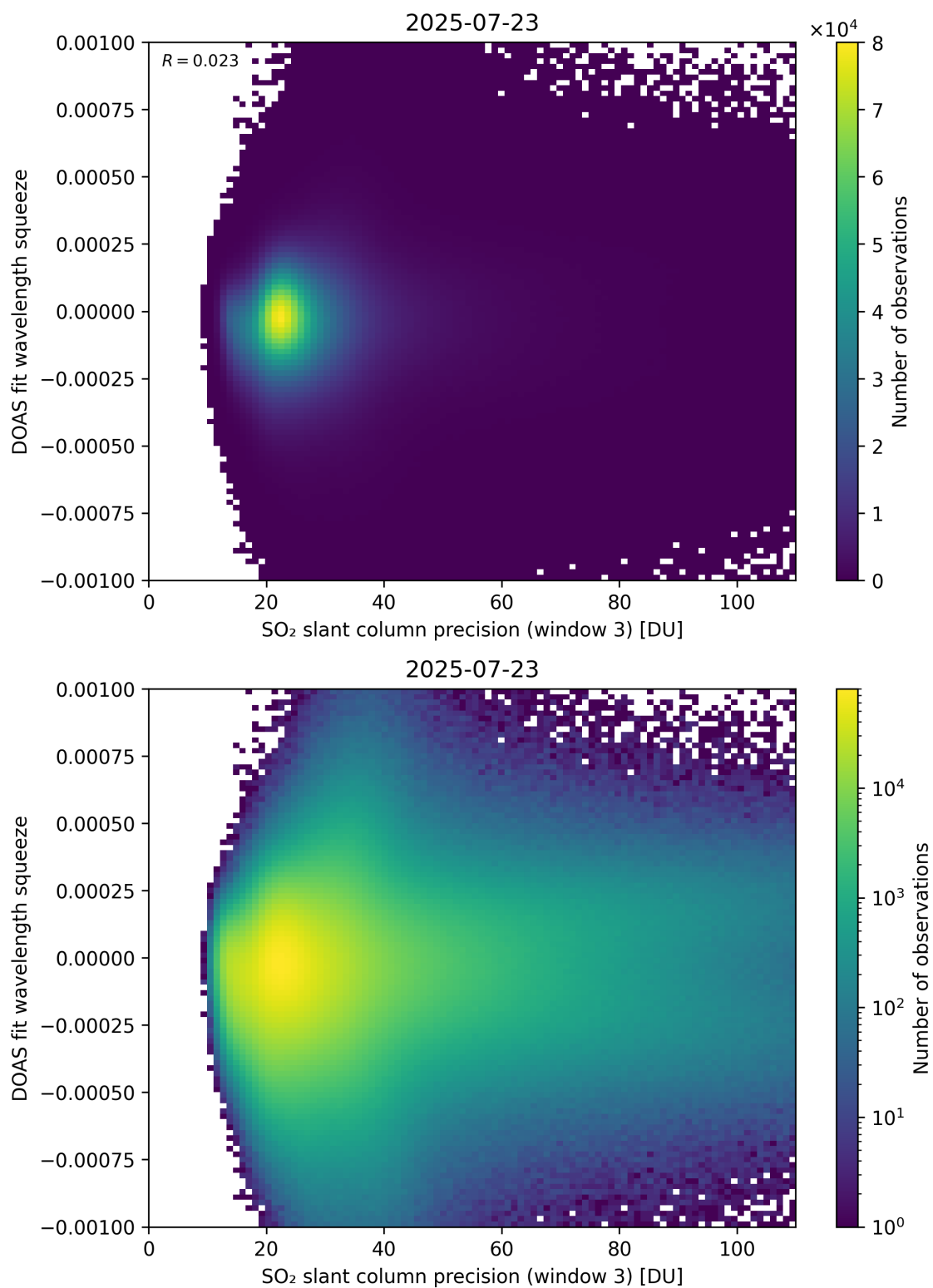
Figure 309: Scatter density plot of “SO 2 slant column precision (window 3)” against “DOAS fit wavelength squeeze” for 2025-07-22 to 2025-07-24.
