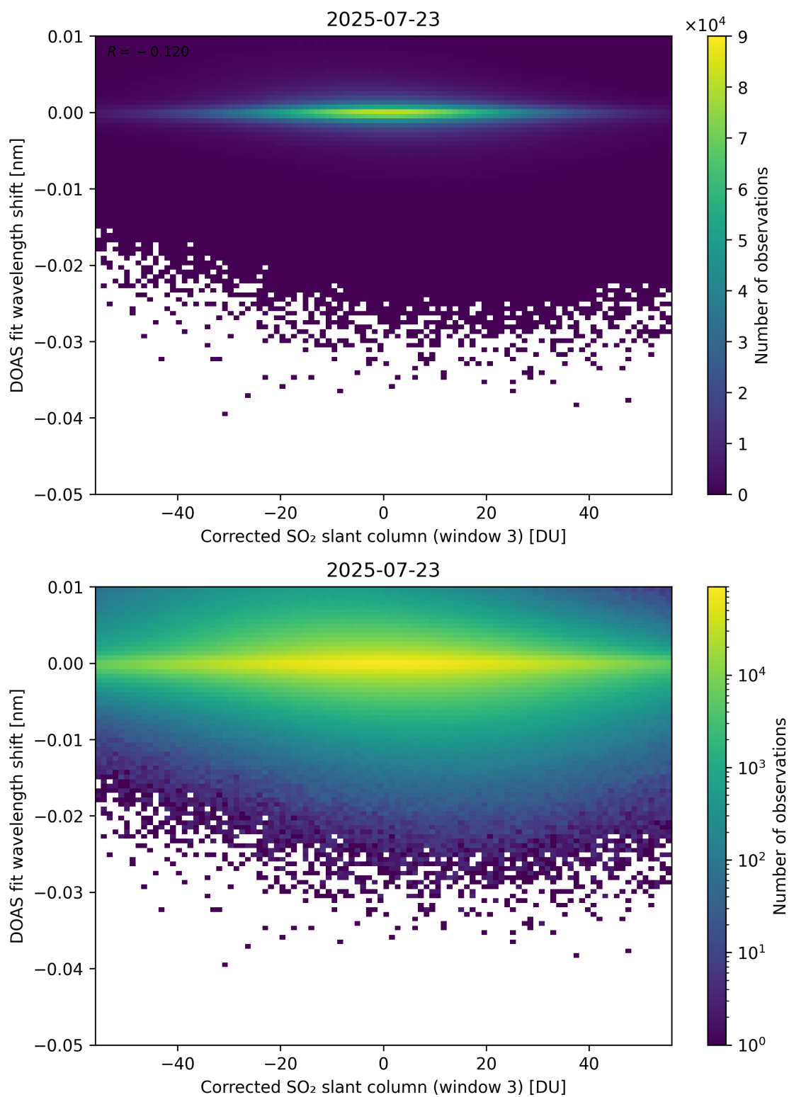
Figure 256: Scatter density plot of “Corrected SO 2 slant column (window 3)” against “DOAS fit wavelength shift” for 2025-07-22 to 2025-07-24.
