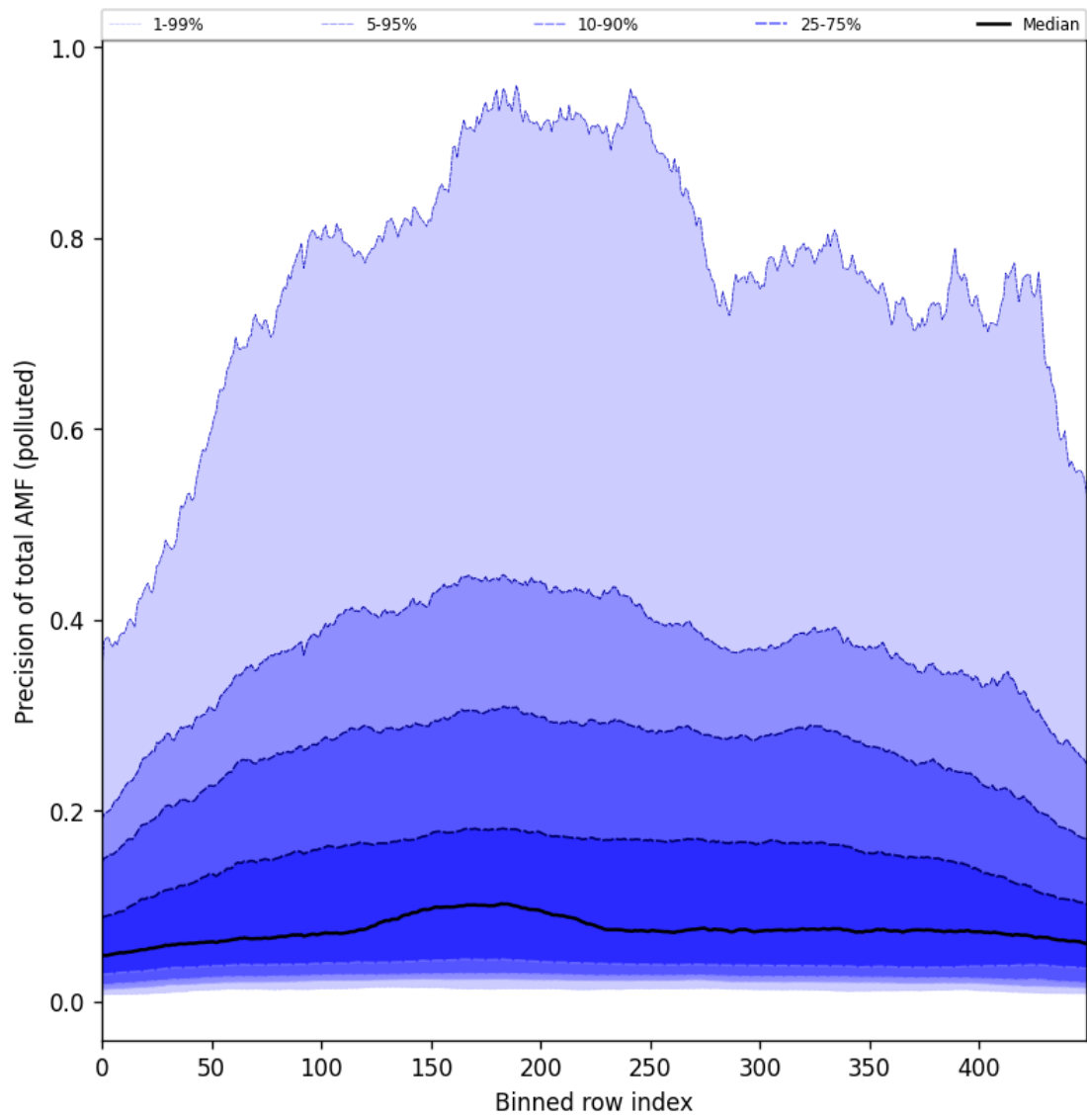
Figure 106: Along track statistics of “Precision of total AMF (polluted)” for 2025-07-22 to 2025-07-24
