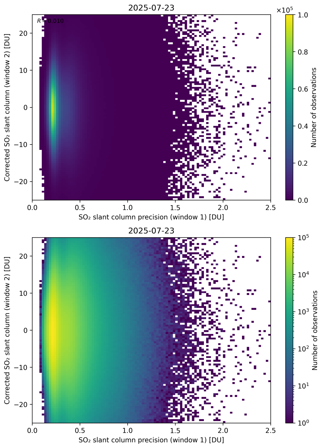
Figure 275: Scatter density plot of “SO 2 slant column precision (window 1)” against “Corrected SO 2 slant column (window 2)” for 2025-07-22 to 2025-07-24.
