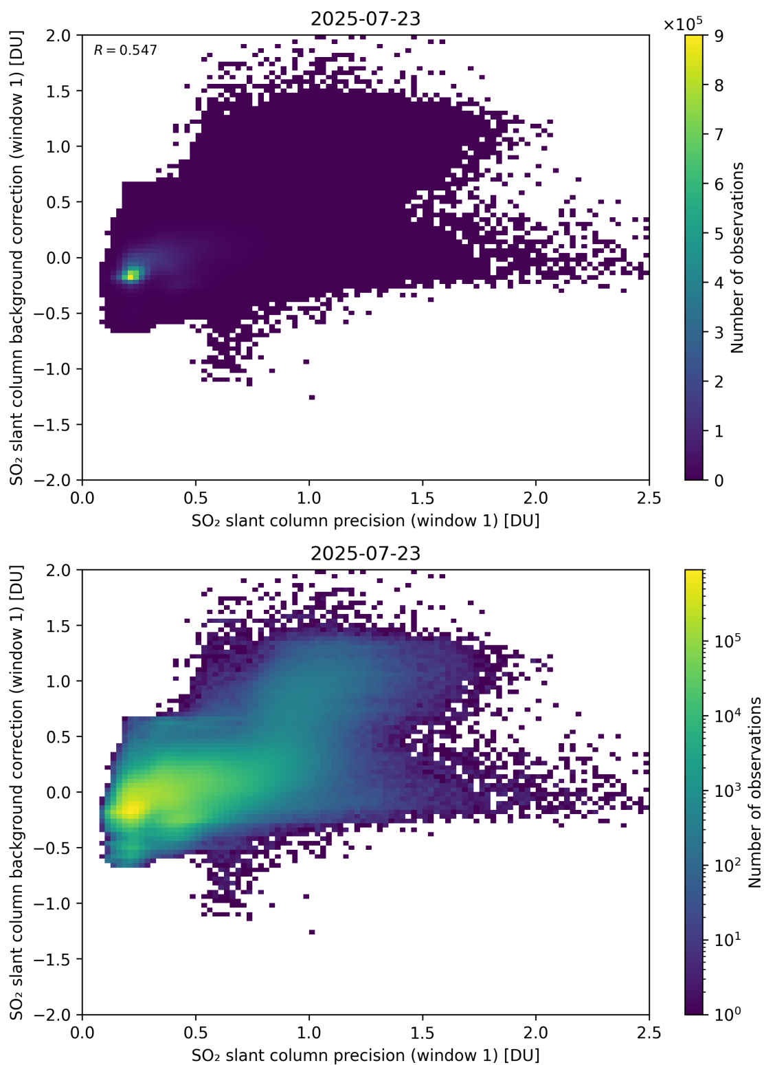
Figure 268: Scatter density plot of “SO 2 slant column precision (window 1)” against “SO 2 slant column background correction (window 1)” for 2025-07-22 to 2025-07-24.
