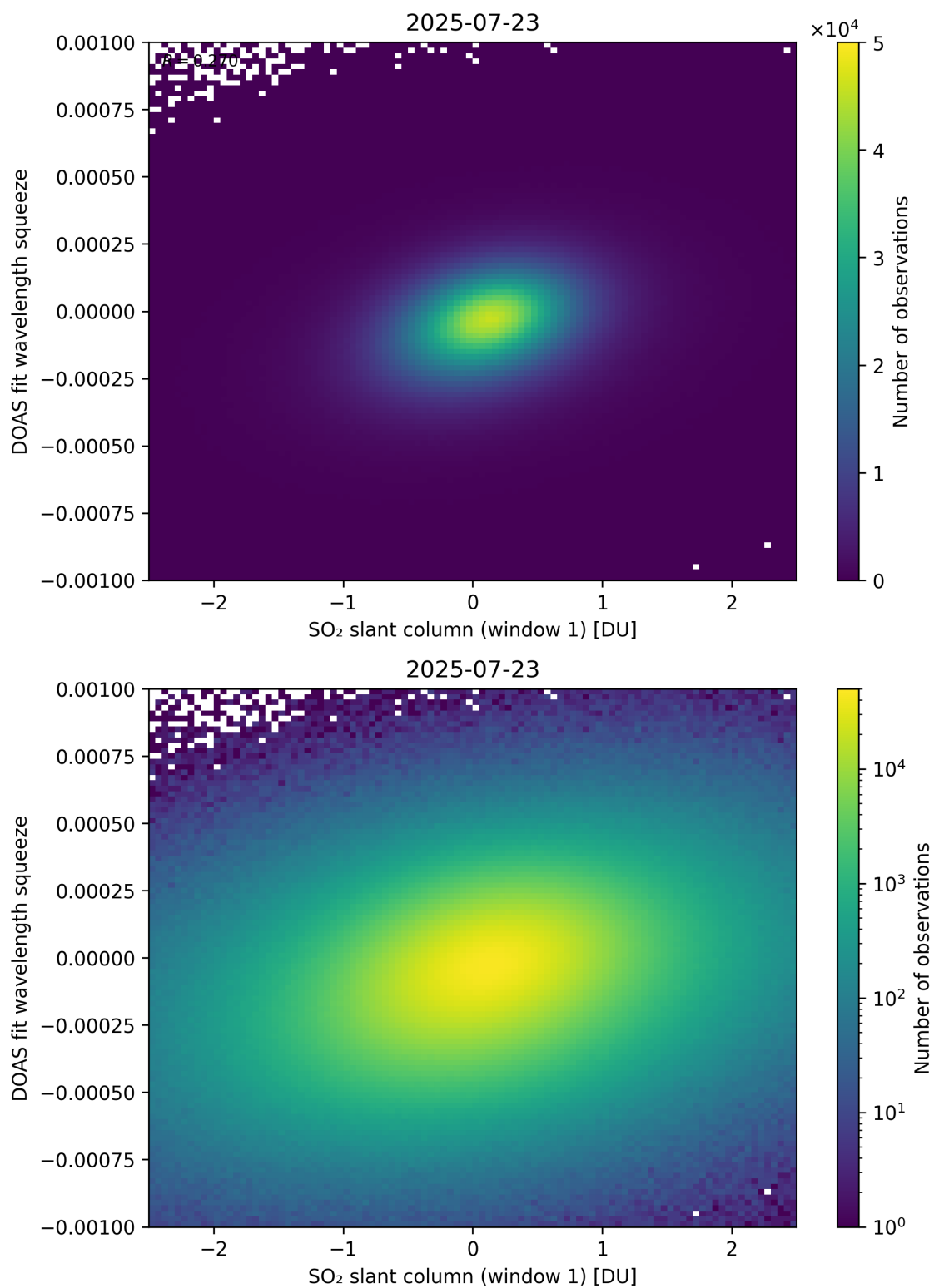
Figure 266: Scatter density plot of “SO 2 slant column (window 1)” against “DOAS fit wavelength squeeze” for 2025-07-22 to 2025-07-24.
