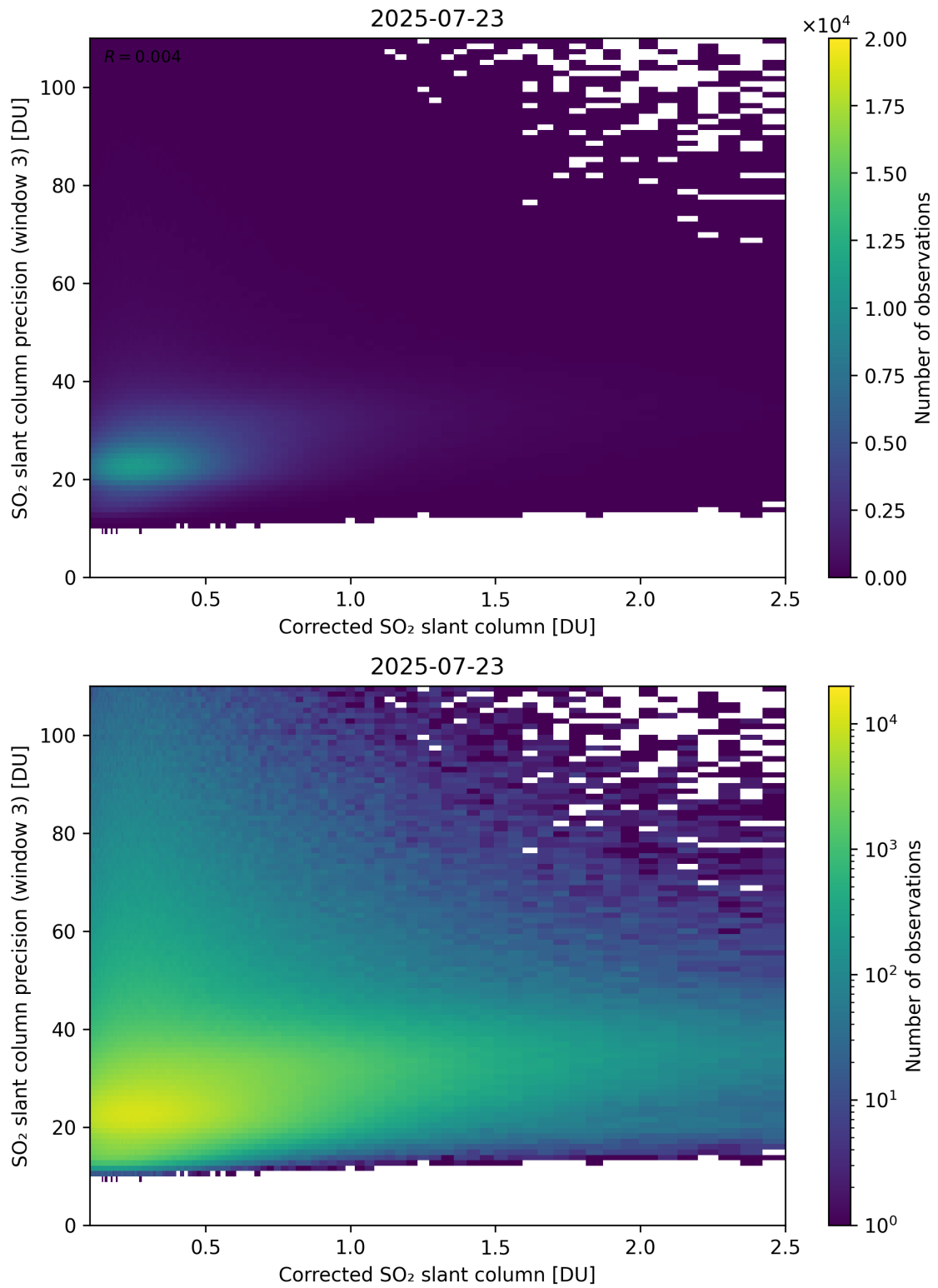
Figure 241: Scatter density plot of “Corrected SO 2 slant column” against “SO 2 slant column precision (window 3)” for 2025-07-22 to 2025-07-24.
