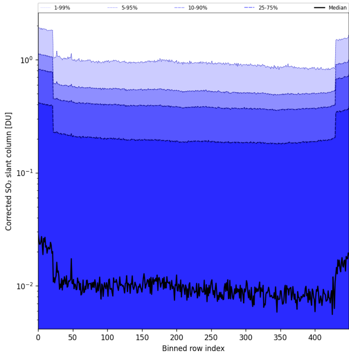
Figure 86: Along track statistics of “Corrected SO 2 slant column” for 2025-07-22 to 2025-07-24
