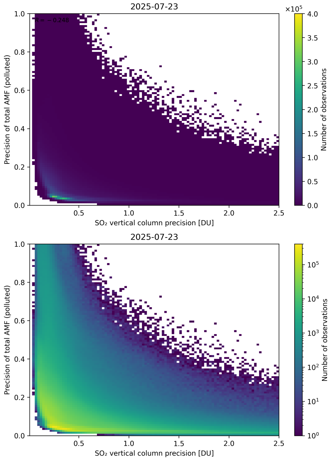
Figure 347: Scatter density plot of “SO 2 vertical column precision” against “Precision of total AMF (polluted)” for 2025-07-22 to 2025-07-24.
