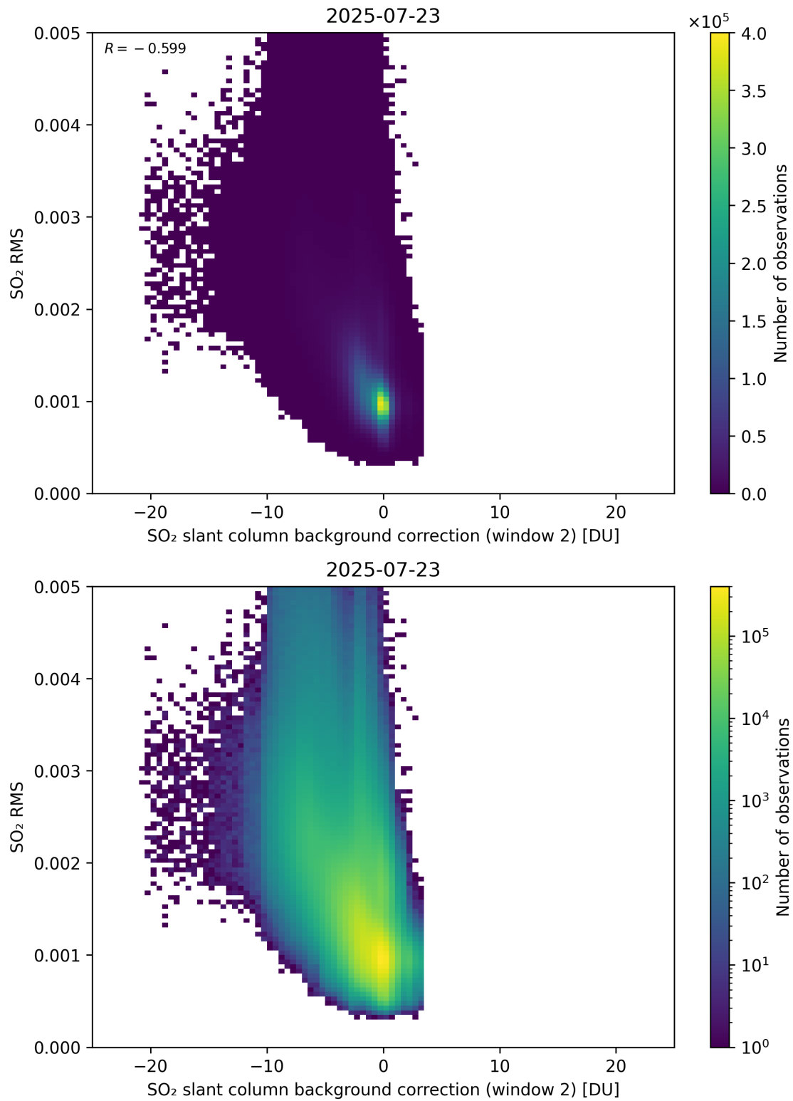
Figure 125: Scatter density plot of “SO 2 slant column background correction (window 2)” against “SO 2 RMS” for 2025-07-22 to 2025-07-24.
