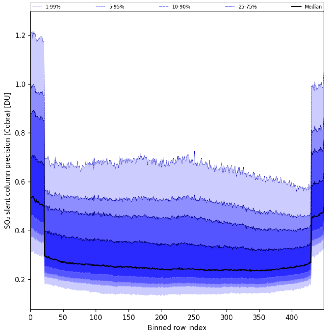
Figure 88: Along track statistics of “SO 2 slant column precision (Cobra)” for 2025-07-22 to 2025-07-24
