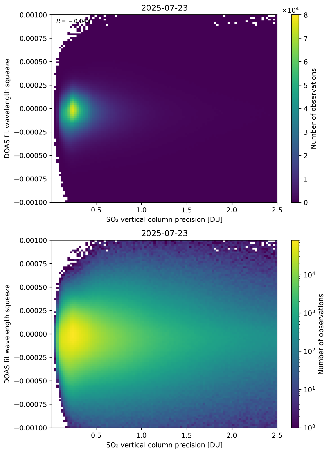
Figure 333: Scatter density plot of “SO 2 vertical column precision” against “DOAS fit wavelength squeeze” for 2025-07-22 to 2025-07-24.
