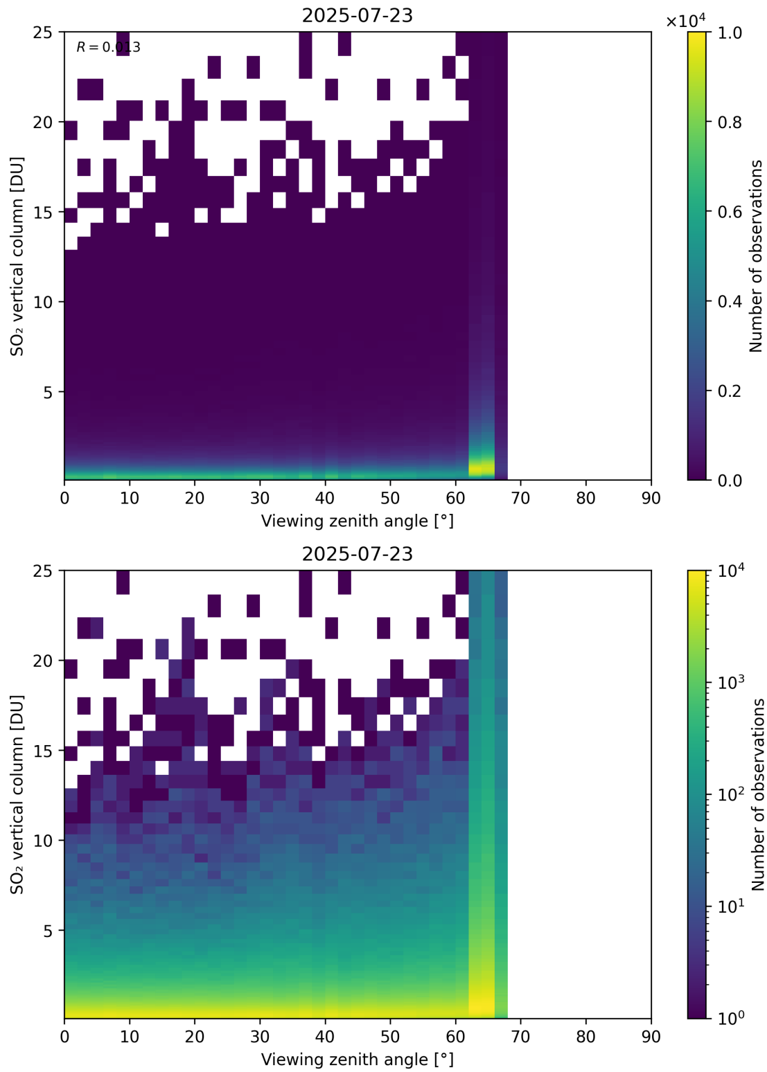
Figure 383: Scatter density plot of “Viewing zenith angle” against “SO 2 vertical column” for 2025-07-22 to 2025-07-24.
