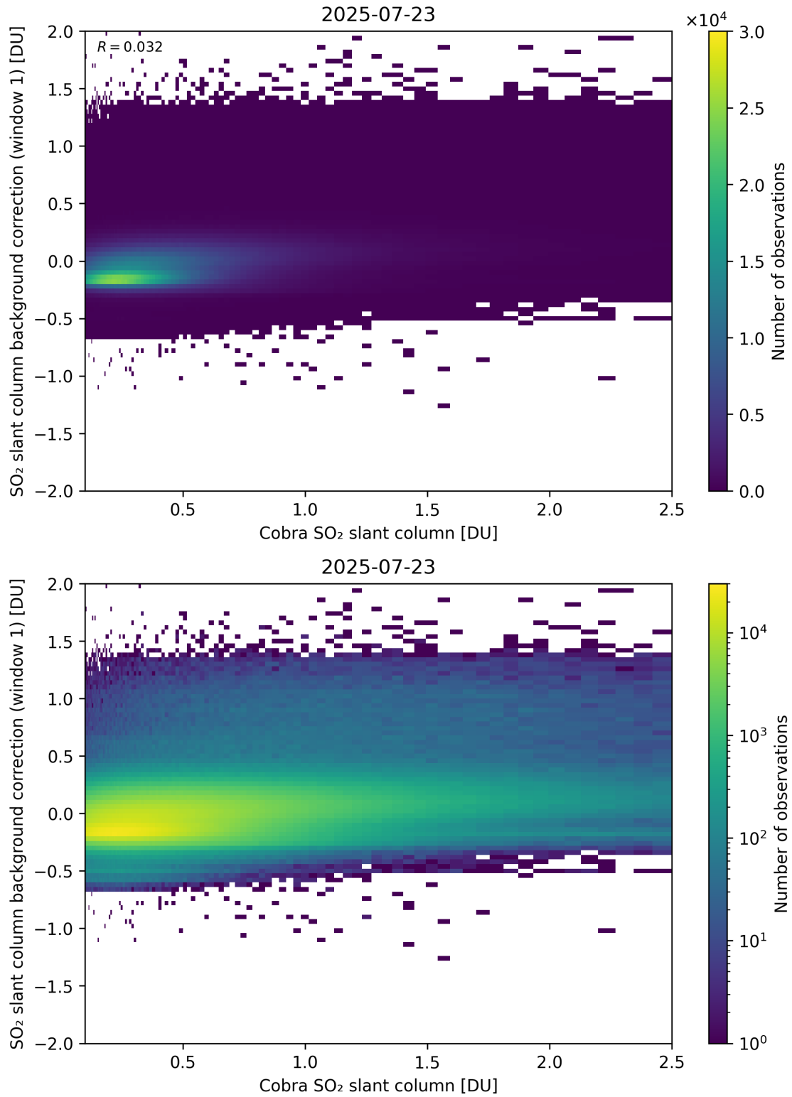
Figure 193: Scatter density plot of “Cobra SO 2 slant column” against “SO 2 slant column background correction (window 1)” for 2025-07-22 to 2025-07-24.
