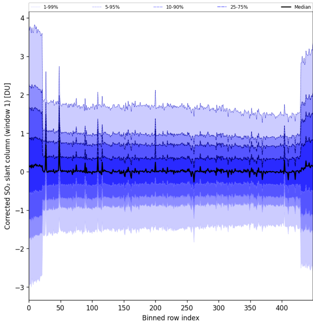
Figure 91: Along track statistics of “Corrected SO 2 slant column (window 1)” for 2025-07-22 to 2025-07-24
