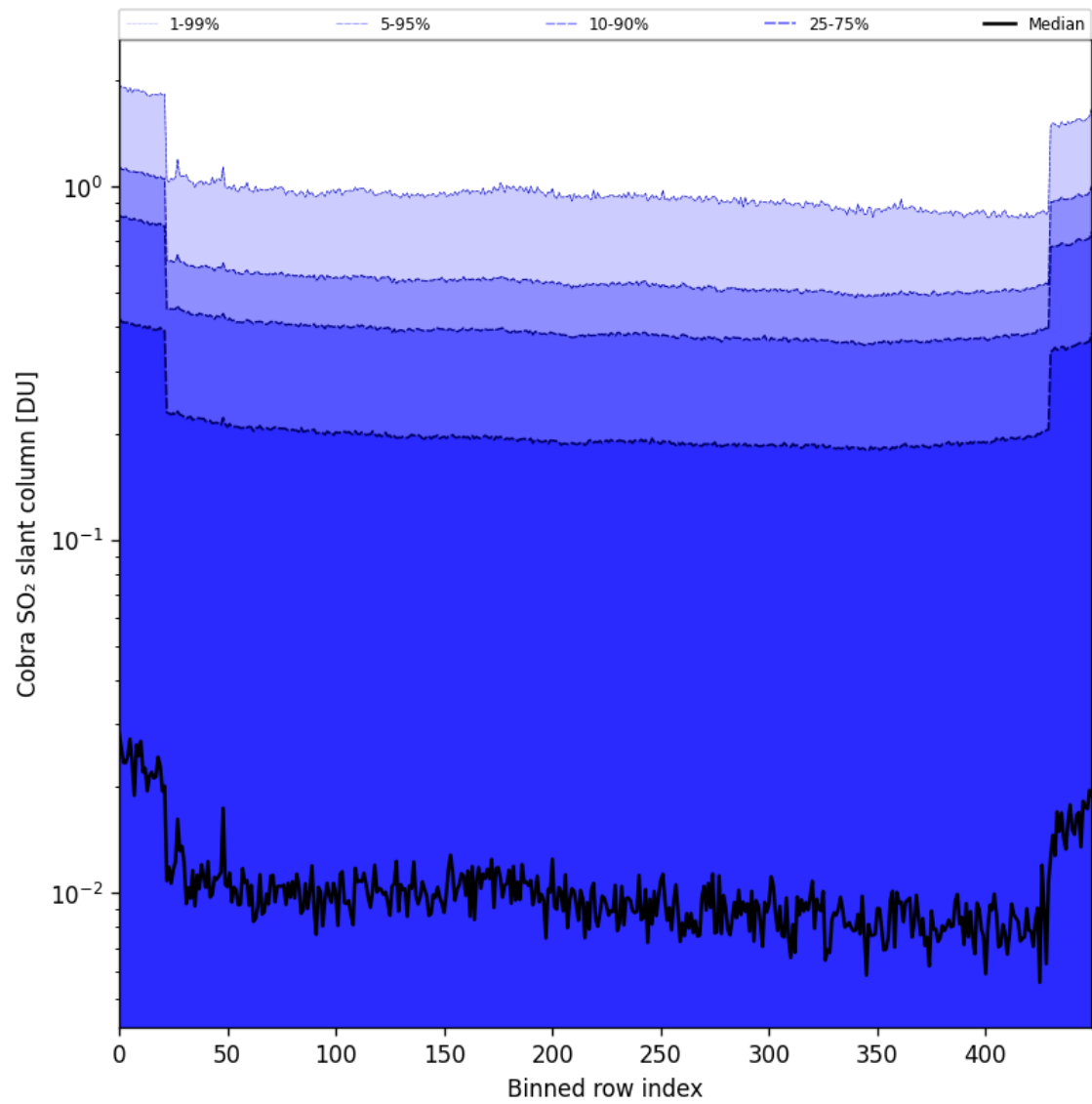
Figure 87: Along track statistics of “Cobra SO 2 slant column” for 2025-07-22 to 2025-07-24
