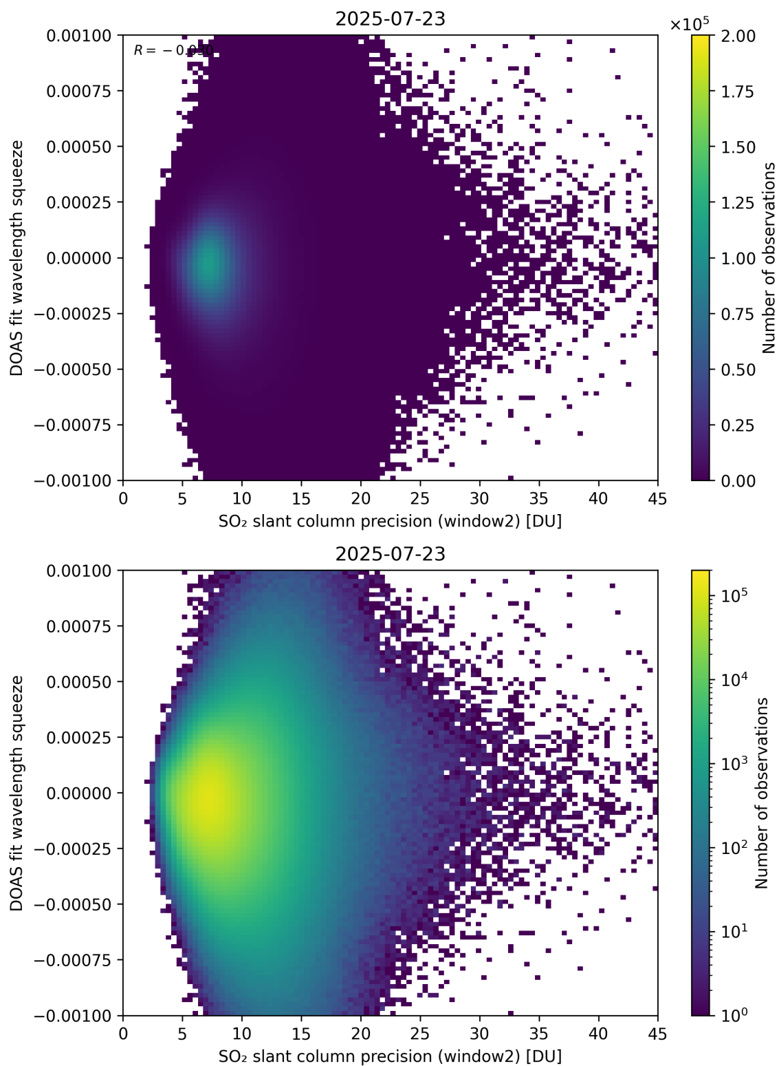
Figure 294: Scatter density plot of “SO 2 slant column precision (window2)” against “DOAS fit wavelength squeeze” for 2025-07-22 to 2025-07-24.
