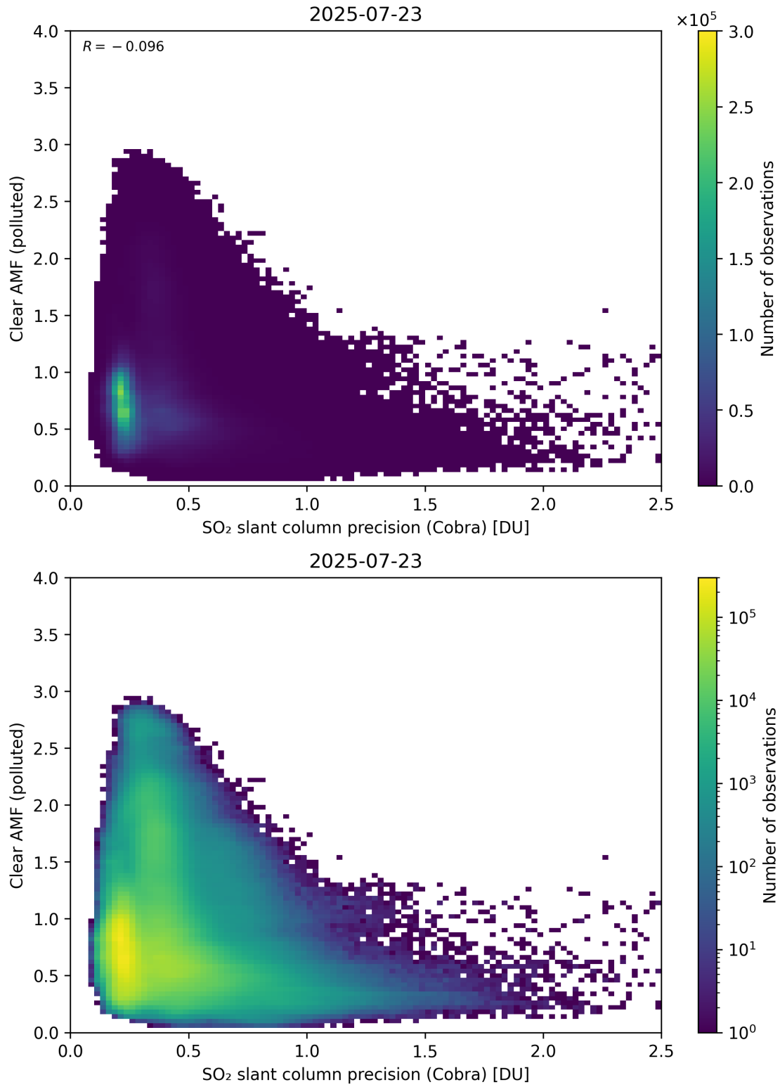
Figure 205: Scatter density plot of “SO 2 slant column precision (Cobra)” against “Clear AMF (polluted)” for 2025-07-22 to 2025-07-24.
