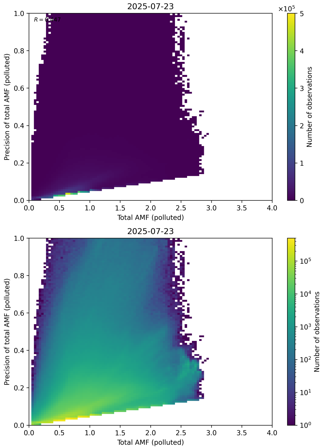
Figure 322: Scatter density plot of “Total AMF (polluted)” against “Precision of total AMF (polluted)” for 2025-07-22 to 2025-07-24.
