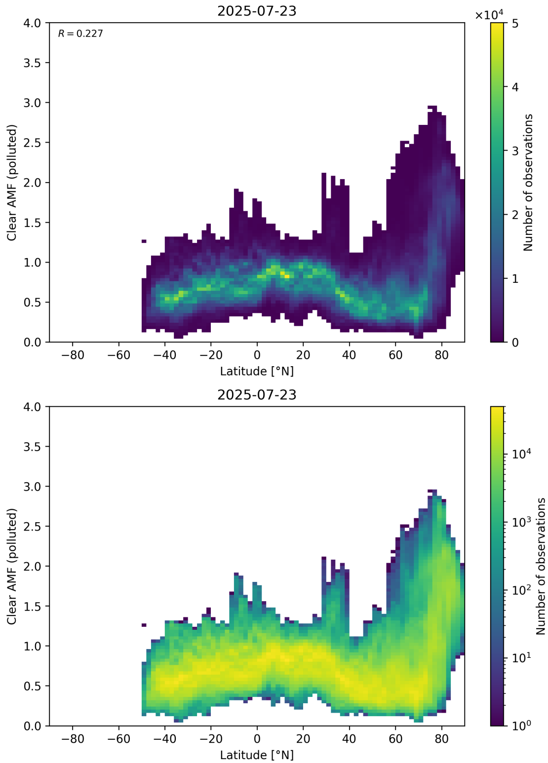
Figure 156: Scatter density plot of “Latitude” against “Clear AMF (polluted)” for 2025-07-22 to 2025-07-24.
