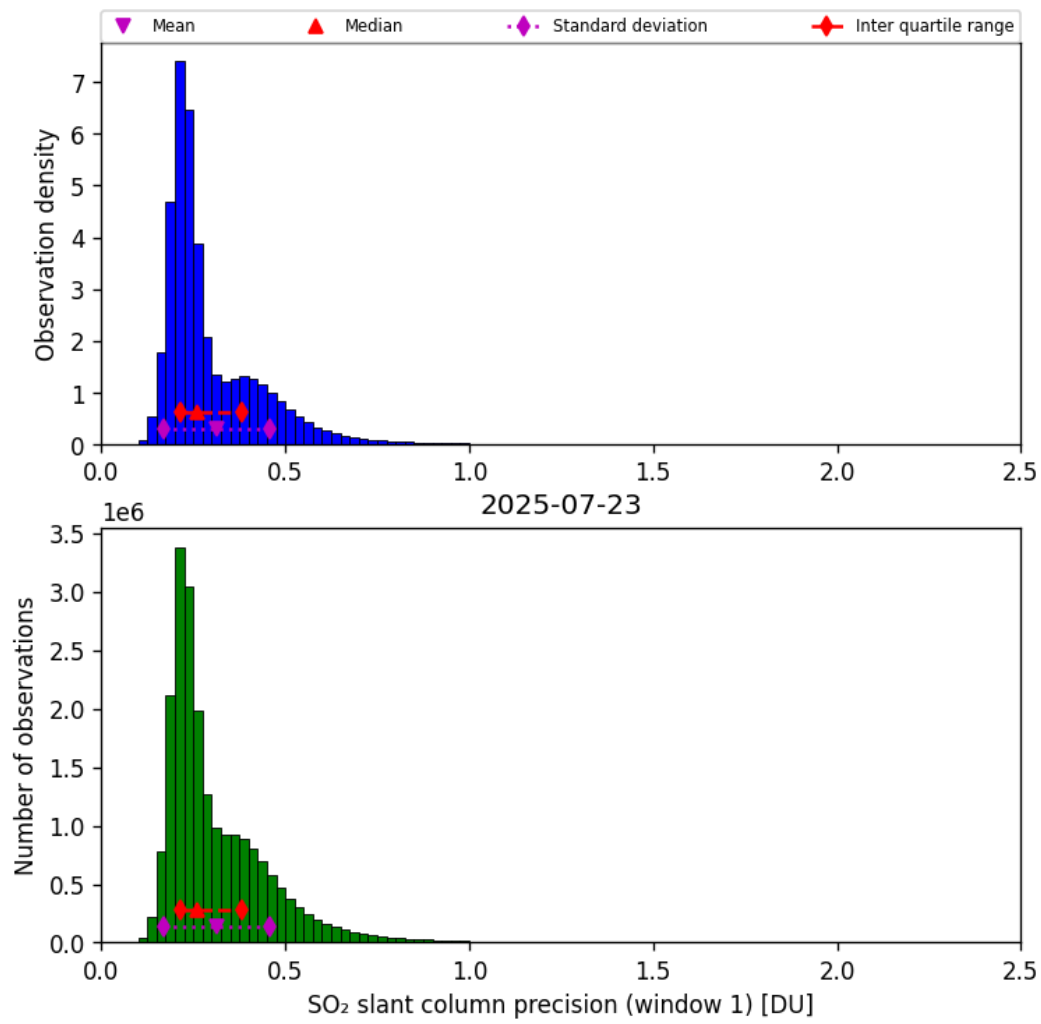
Figure 64: Histogram of “SO 2 slant column precision (window 1)” for 2025-07-22 to 2025-07-24
