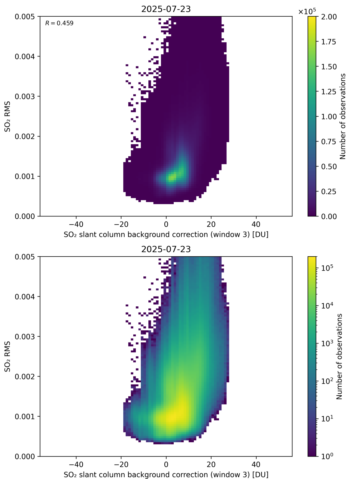
Figure 134: Scatter density plot of “SO 2 slant column background correction (window 3)” against “SO 2 RMS” for 2025-07-22 to 2025-07-24.
