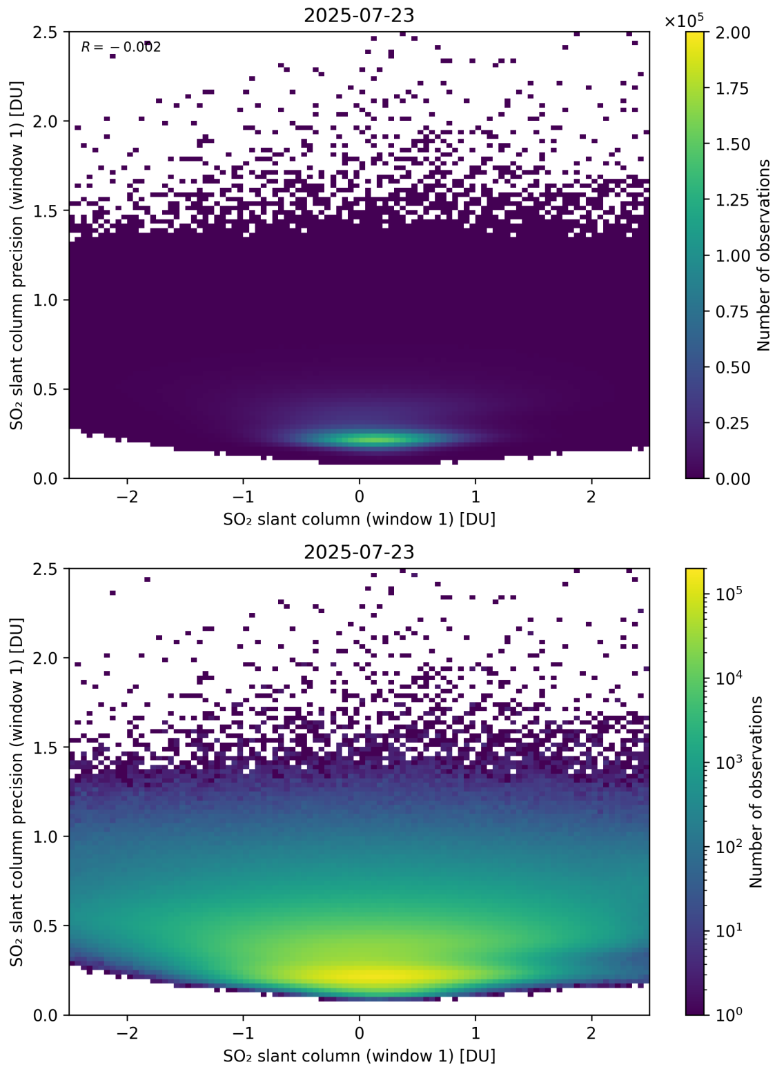
Figure 285: Scatter density plot of “SO 2 slant column (window 1)” against “SO 2 slant column precision (window 1)” for 2025-07-22 to 2025-07-24.
