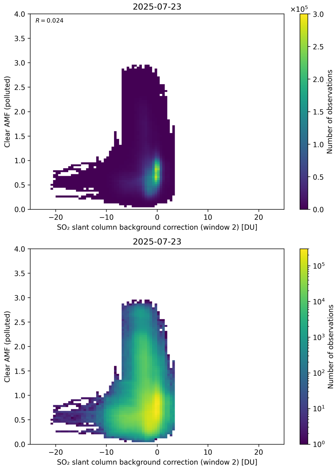
Figure 126: Scatter density plot of “SO 2 slant column background correction (window 2)” against “Clear AMF (polluted)” for 2025-07-22 to 2025-07-24.
