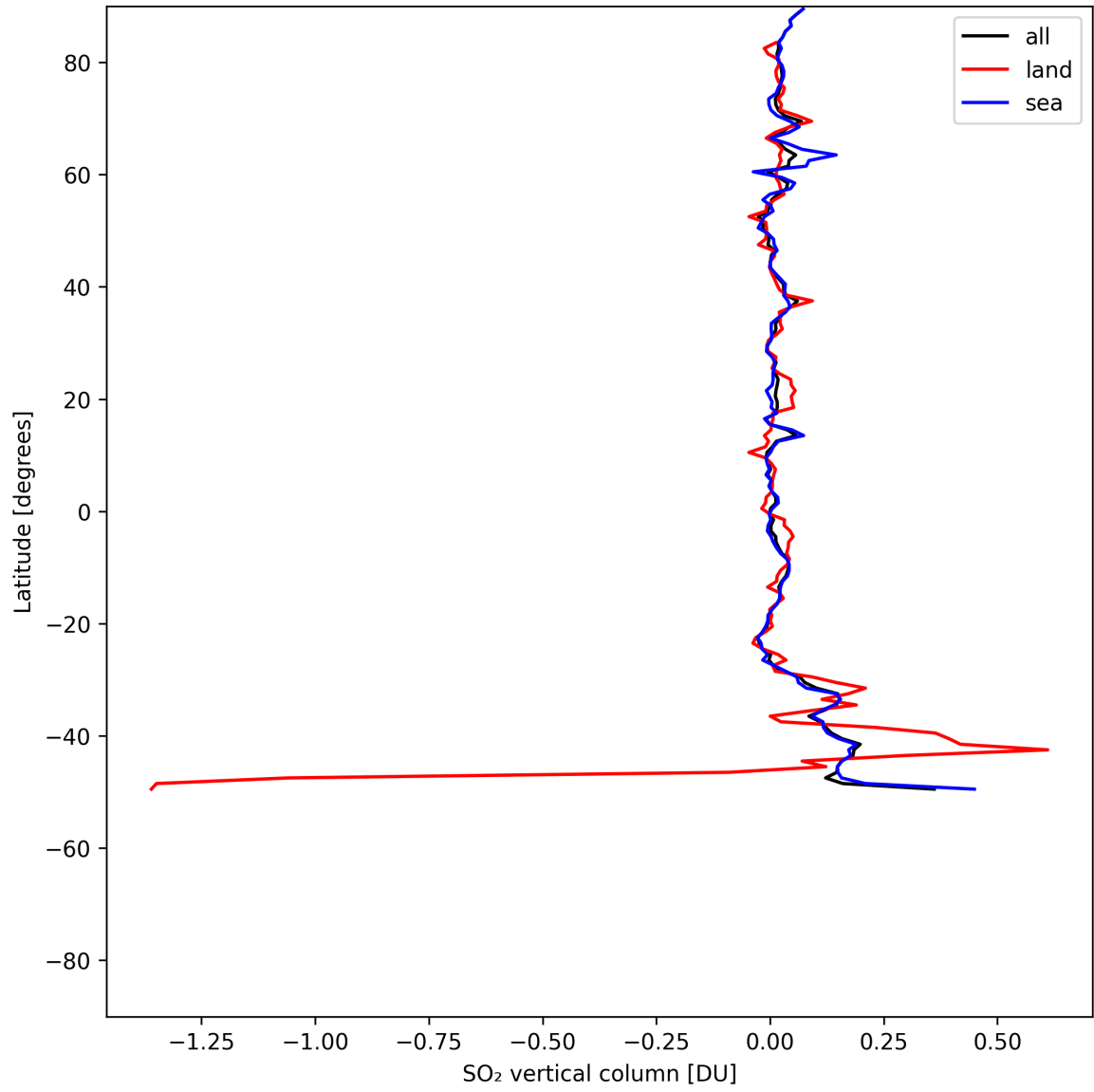
Figure 32: Zonal average of “SO 2 vertical column” for 2025-07-22 to 2025-07-24.
