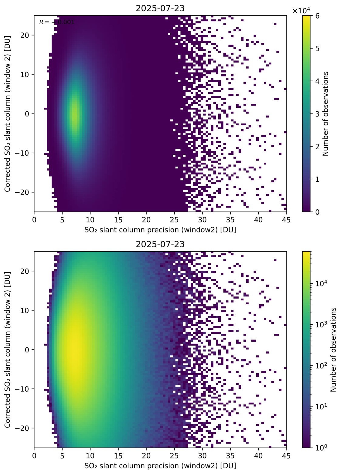
Figure 297: Scatter density plot of “SO 2 slant column precision (window2)” against “Corrected SO 2 slant column (window 2)” for 2025-07-22 to 2025-07-24.
