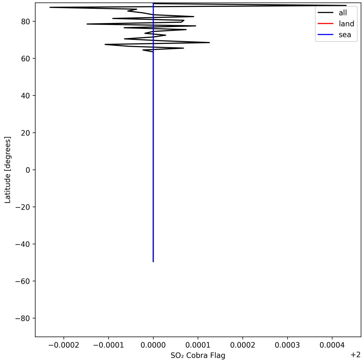
Figure 49: Zonal average of "SO 2 Cobra Flag" for 2025-07-22 to 2025-07-24.
