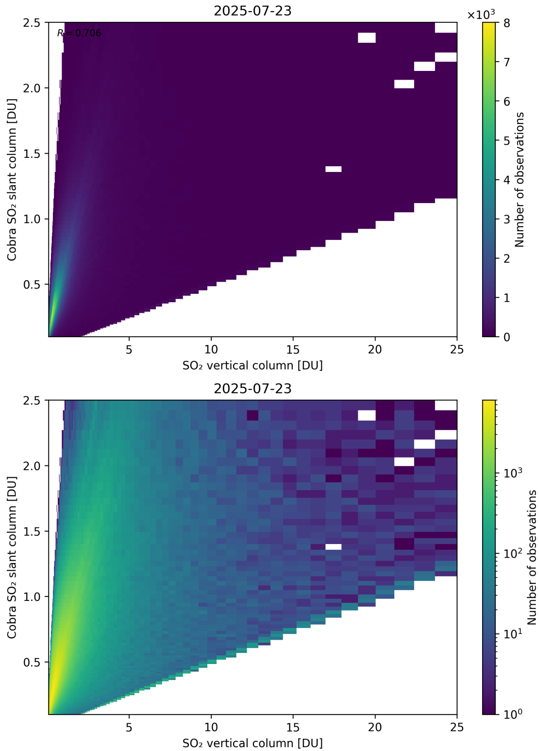
Figure 349: Scatter density plot of “SO 2 vertical column” against “Cobra SO 2 slant column” for 2025-07-22 to 2025-07-24.
