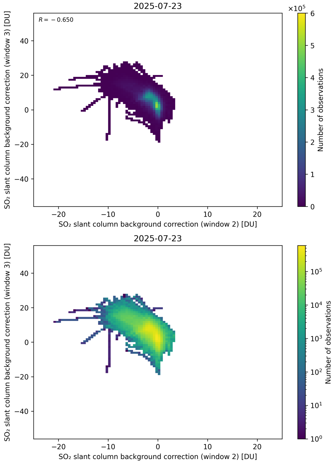
Figure 122: Scatter density plot of “SO 2 slant column background correction (window 2)” against “SO 2 slant column background correction (window 3)” for 2025-07-22 to 2025-07-24.
