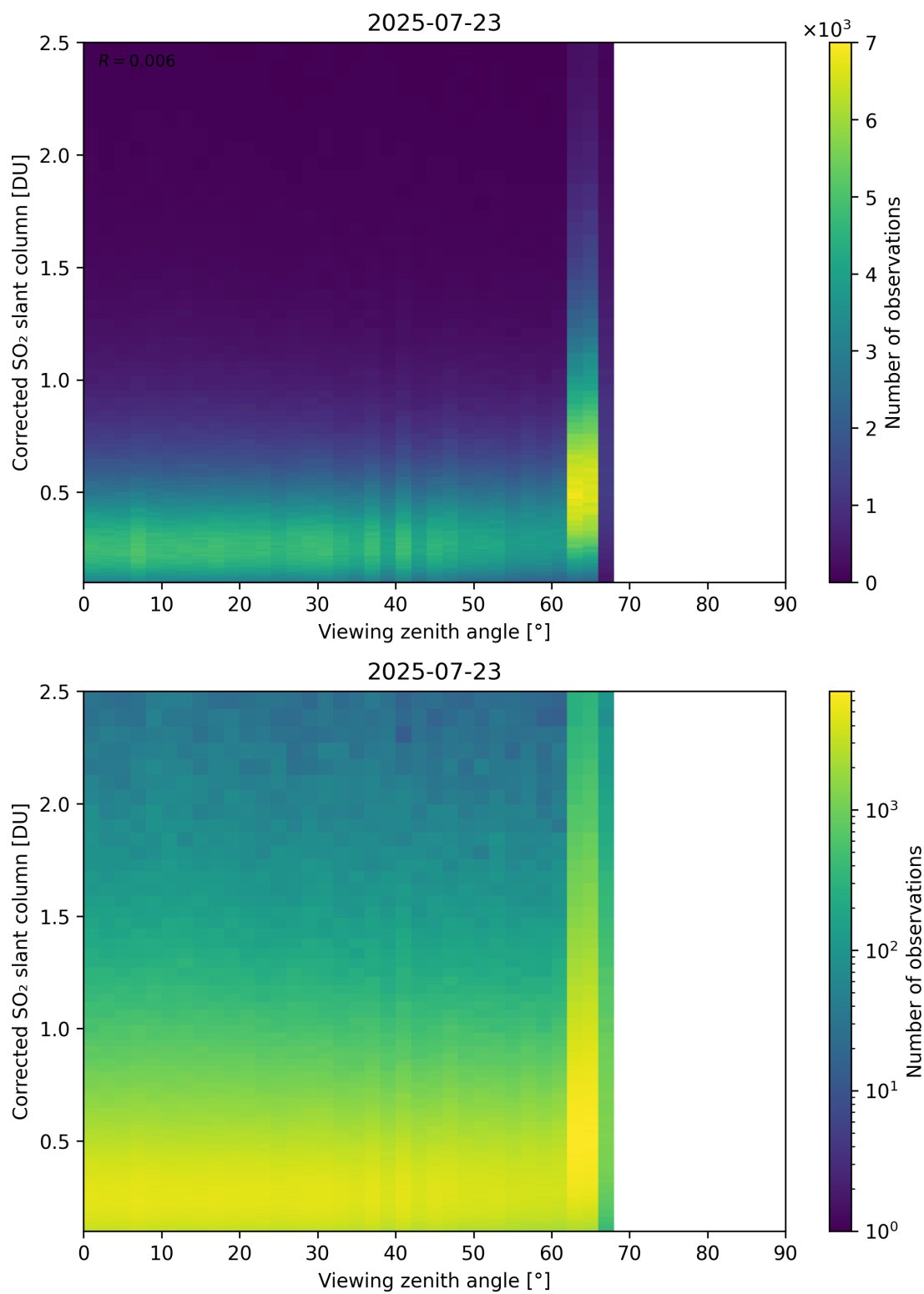
Figure 373: Scatter density plot of “Viewing zenith angle” against “Corrected SO 2 slant column” for 2025-07-22 to 2025-07-24.
