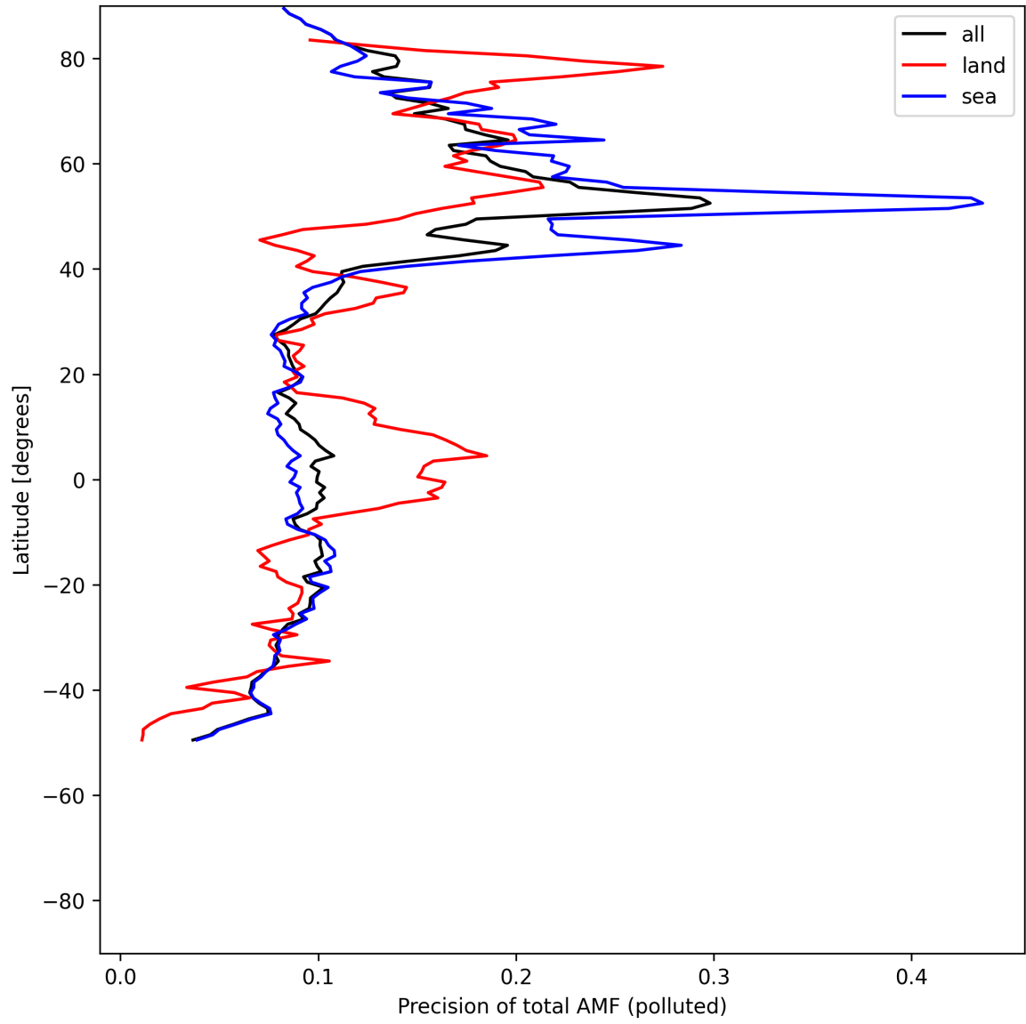
Figure 54: Zonal average of “Precision of total AMF (polluted)” for 2025-07-22 to 2025-07-24.
