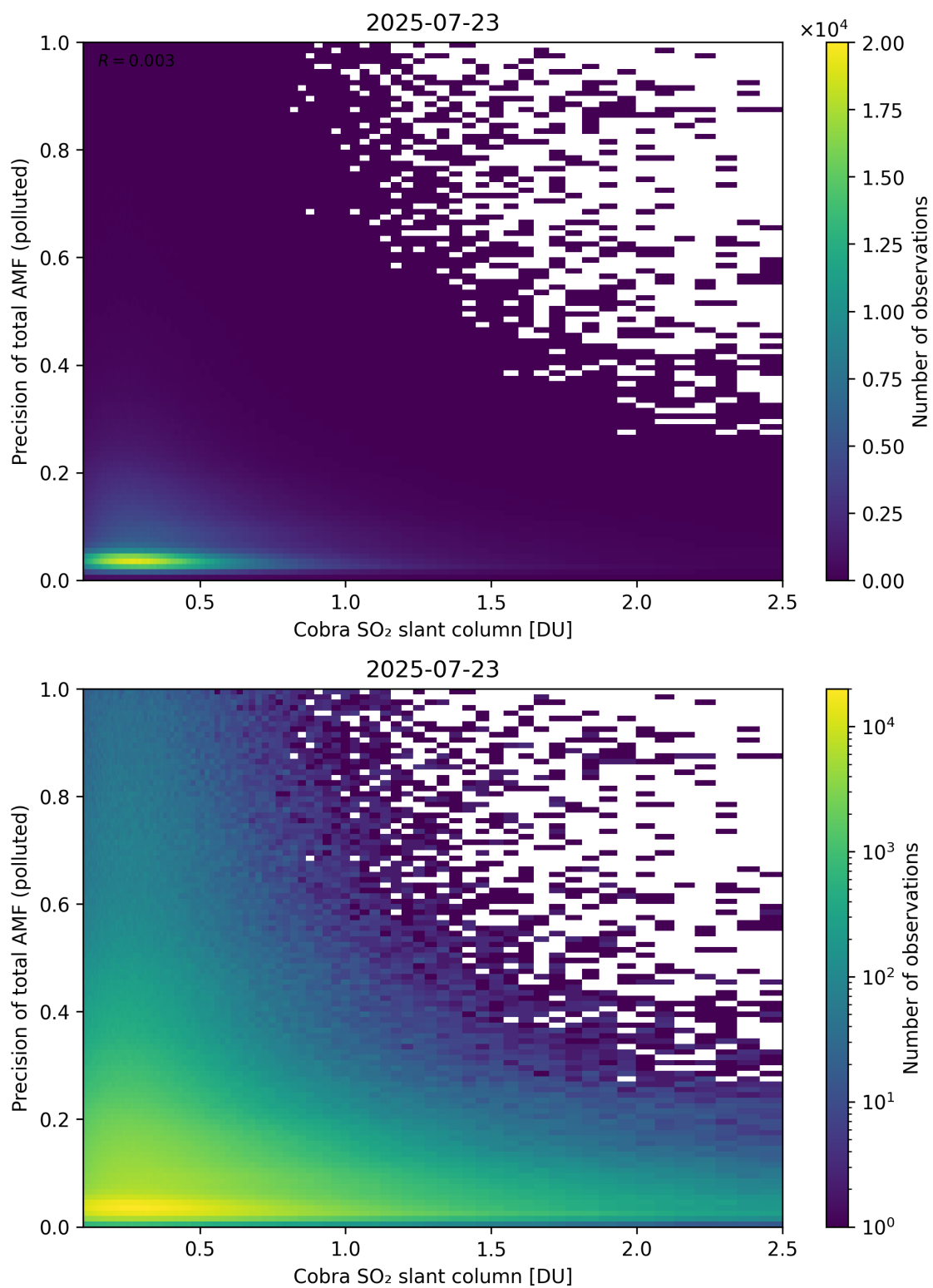
Figure 225: Scatter density plot of “Cobra SO 2 slant column” against “Precision of total AMF (polluted)” for 2025-07-22 to 2025-07-24.
