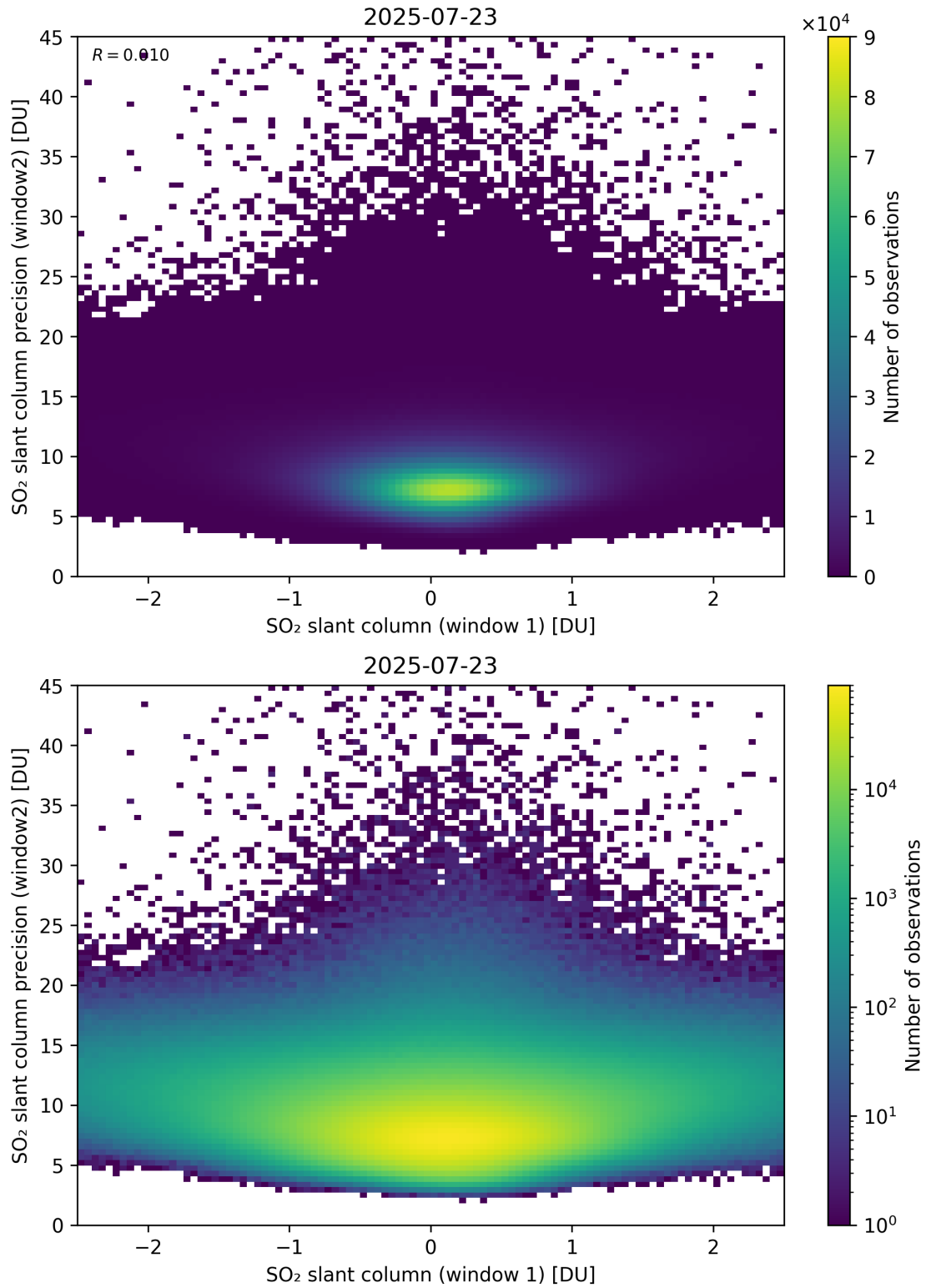
Figure 286: Scatter density plot of “SO 2 slant column (window 1)” against “SO 2 slant column precision (window2)” for 2025-07-22 to 2025-07-24.
