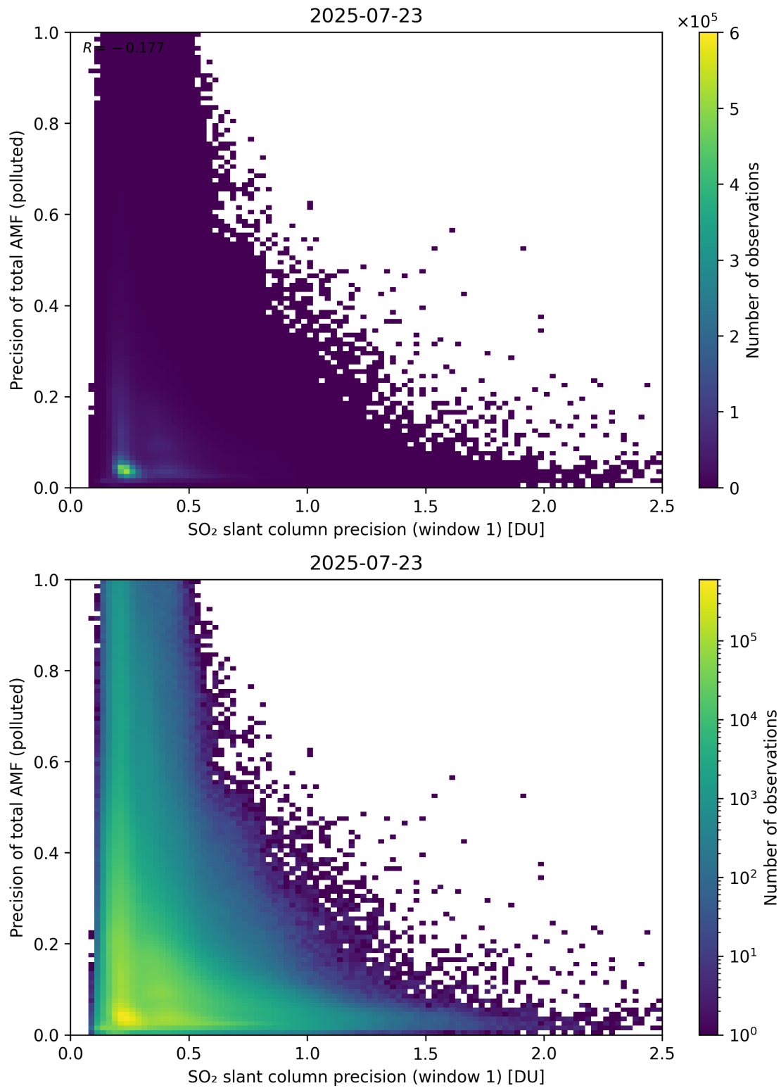
Figure 281: Scatter density plot of “SO 2 slant column precision (window 1)” against “Precision of total AMF (polluted)” for 2025-07-22 to 2025-07-24.
