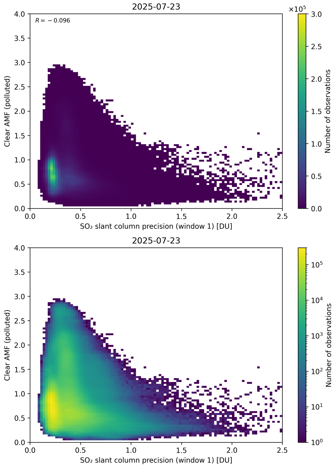
Figure 274: Scatter density plot of “SO 2 slant column precision (window 1)” against “Clear AMF (polluted)” for 2025-07-22 to 2025-07-24.
