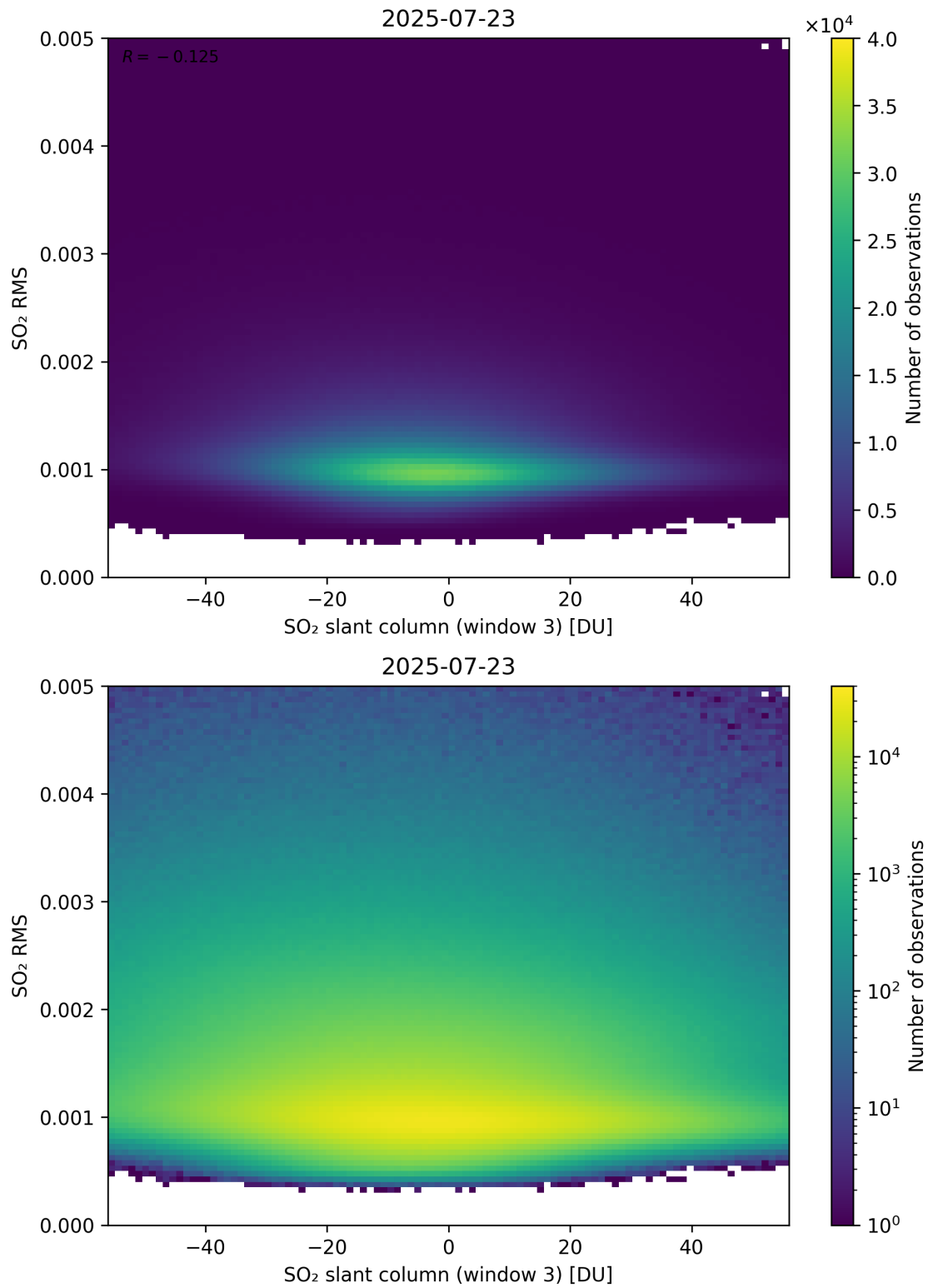
Figure 306: Scatter density plot of “SO 2 slant column (window 3)” against “SO 2 RMS” for 2025-07-22 to 2025-07-24.
