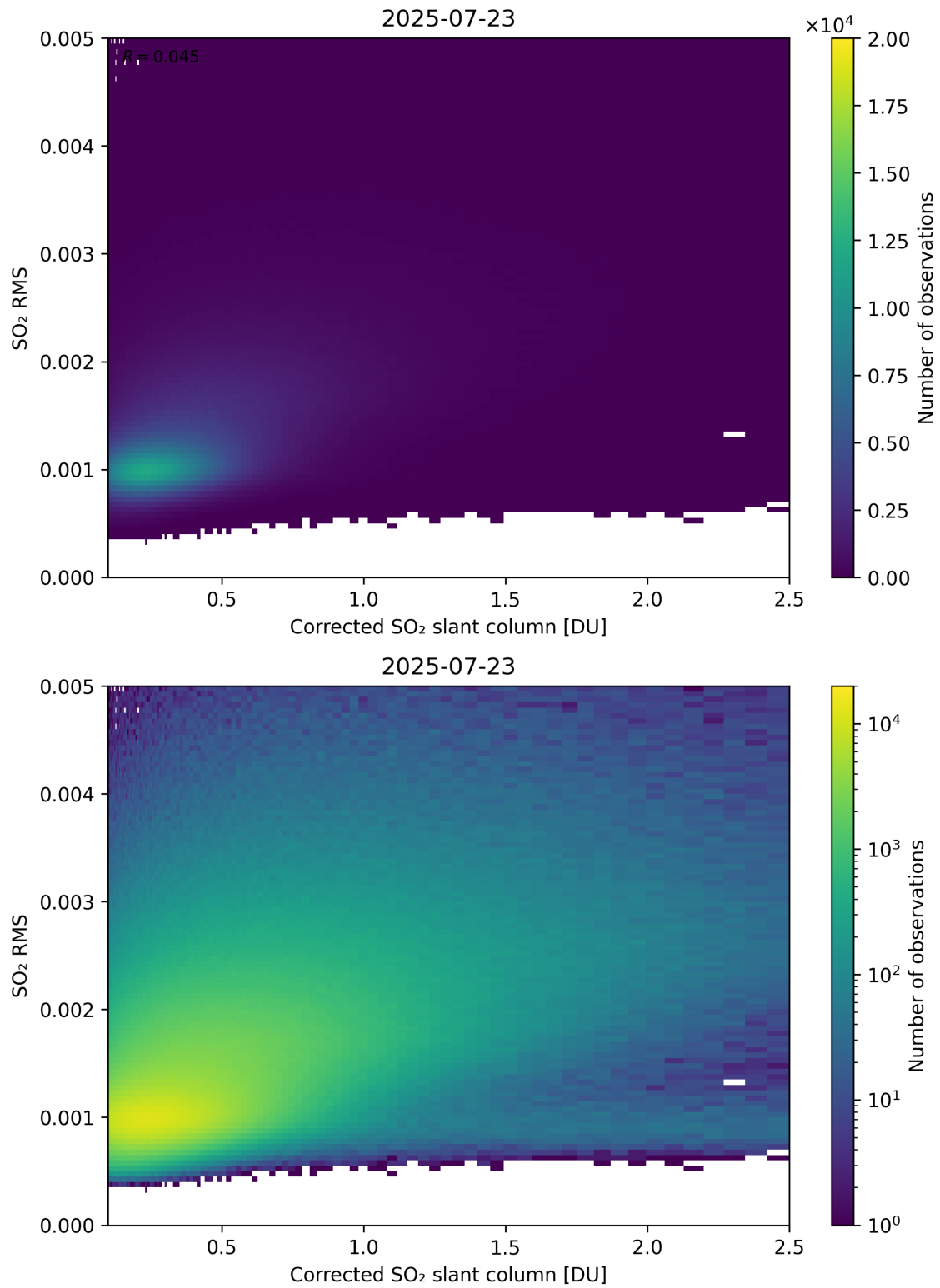
Figure 231: Scatter density plot of “Corrected SO 2 slant column” against “SO 2 RMS” for 2025-07-22 to 2025-07-24.
