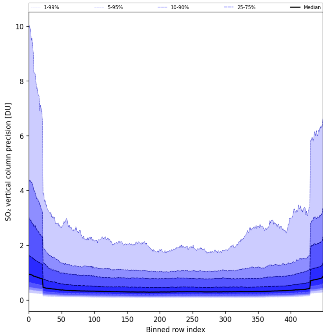
Figure 85: Along track statistics of “SO 2 vertical column precision” for 2025-07-22 to 2025-07-24
