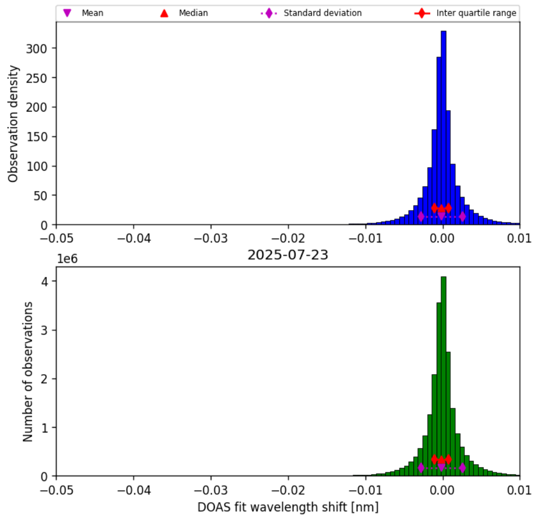
Figure 76: Histogram of “DOAS fit wavelength shift” for 2025-07-22 to 2025-07-24
