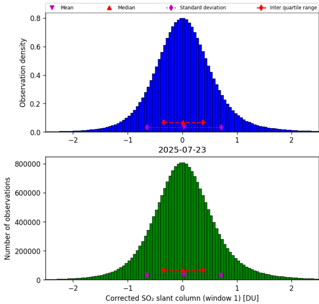
Figure 65: Histogram of “Corrected SO 2 slant column (window 1)” for 2025-07-22 to 2025-07-24
