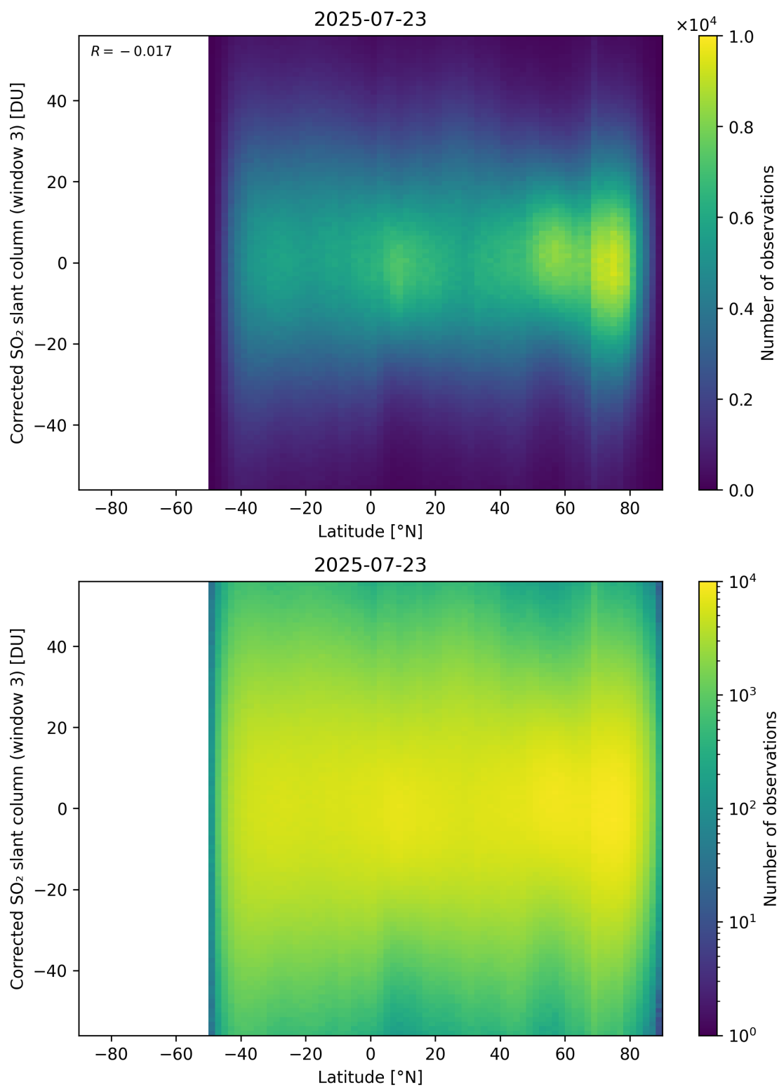
Figure 161: Scatter density plot of “Latitude” against “Corrected SO 2 slant column (window 3)” for 2025-07-22 to 2025-07-24.
