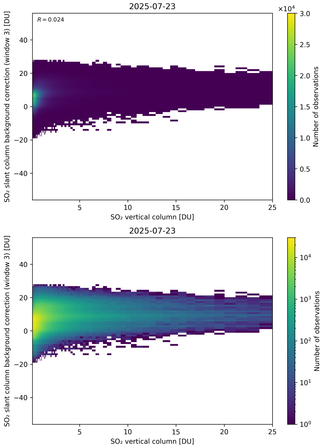
Figure 325: Scatter density plot of “SO 2 vertical column” against “SO 2 slant column background correction (window 3)” for 2025-07-22 to 2025-07-24.
