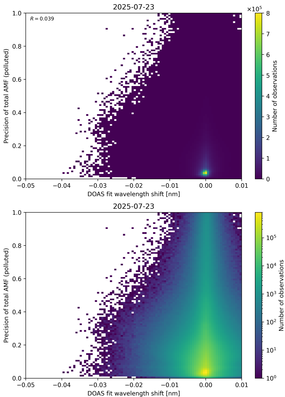
Figure 142: Scatter density plot of “DOAS fit wavelength shift” against “Precision of total AMF (polluted)” for 2025-07-22 to 2025-07-24.
