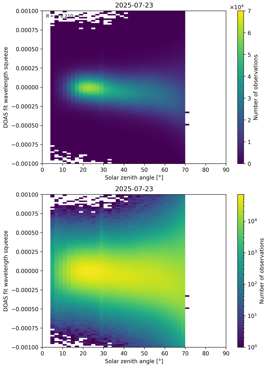
Figure 175: Scatter density plot of “Solar zenith angle” against “DOAS fit wavelength squeeze” for 2025-07-22 to 2025-07-24.
