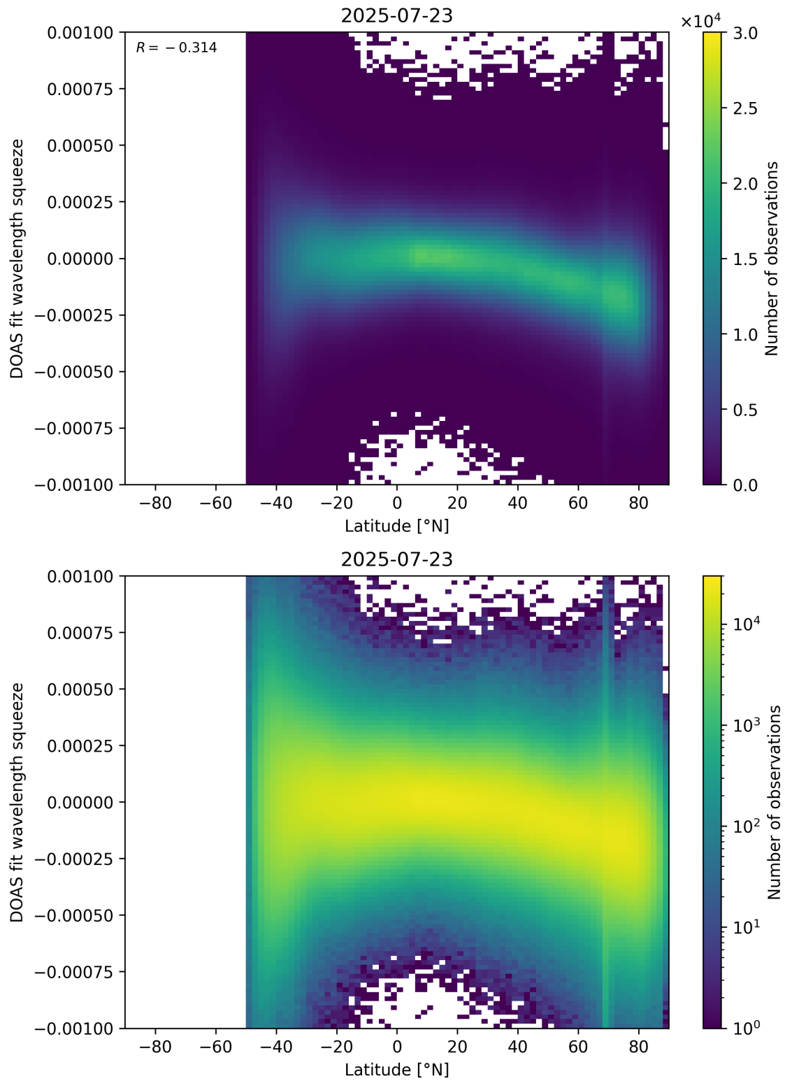
Figure 154: Scatter density plot of “Latitude” against “DOAS fit wavelength squeeze” for 2025-07-22 to 2025-07-24.
