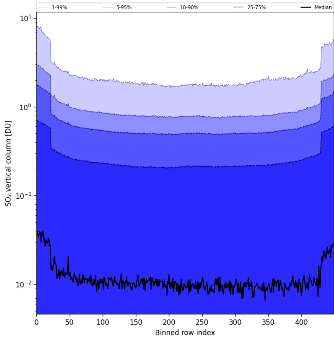
Figure 84: Along track statistics of “SO 2 vertical column” for 2025-07-22 to 2025-07-24
