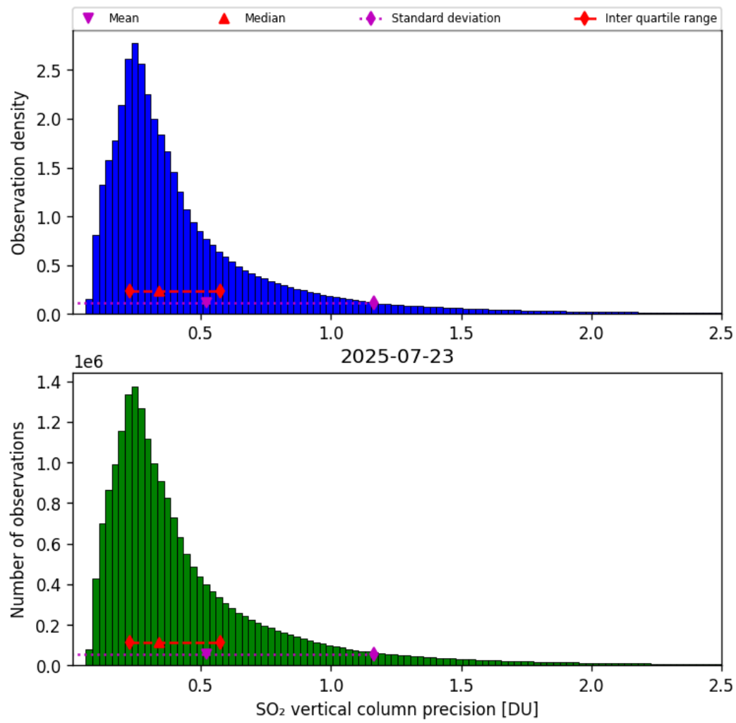
Figure 59: Histogram of “SO 2 vertical column precision” for 2025-07-22 to 2025-07-24
