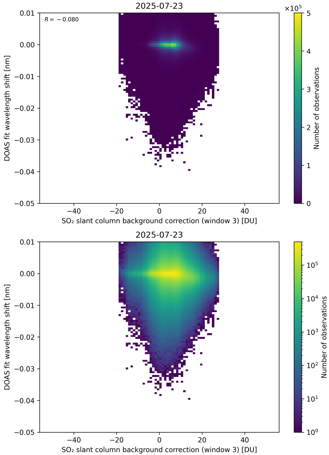
Figure 132: Scatter density plot of “SO 2 slant column background correction (window 3)” against “DOAS fit wavelength shift” for 2025-07-22 to 2025-07-24.
