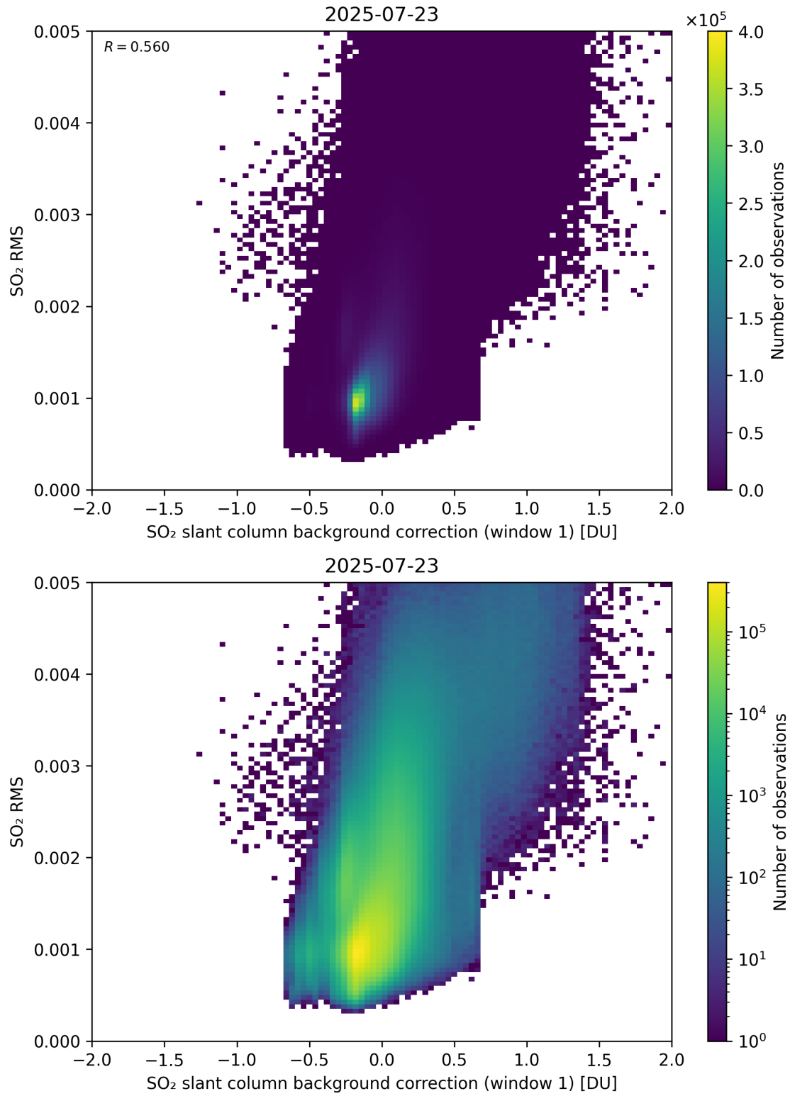
Figure 113: Scatter density plot of “SO 2 slant column background correction (window 1)” against “SO 2 RMS” for 2025-07-22 to 2025-07-24.
