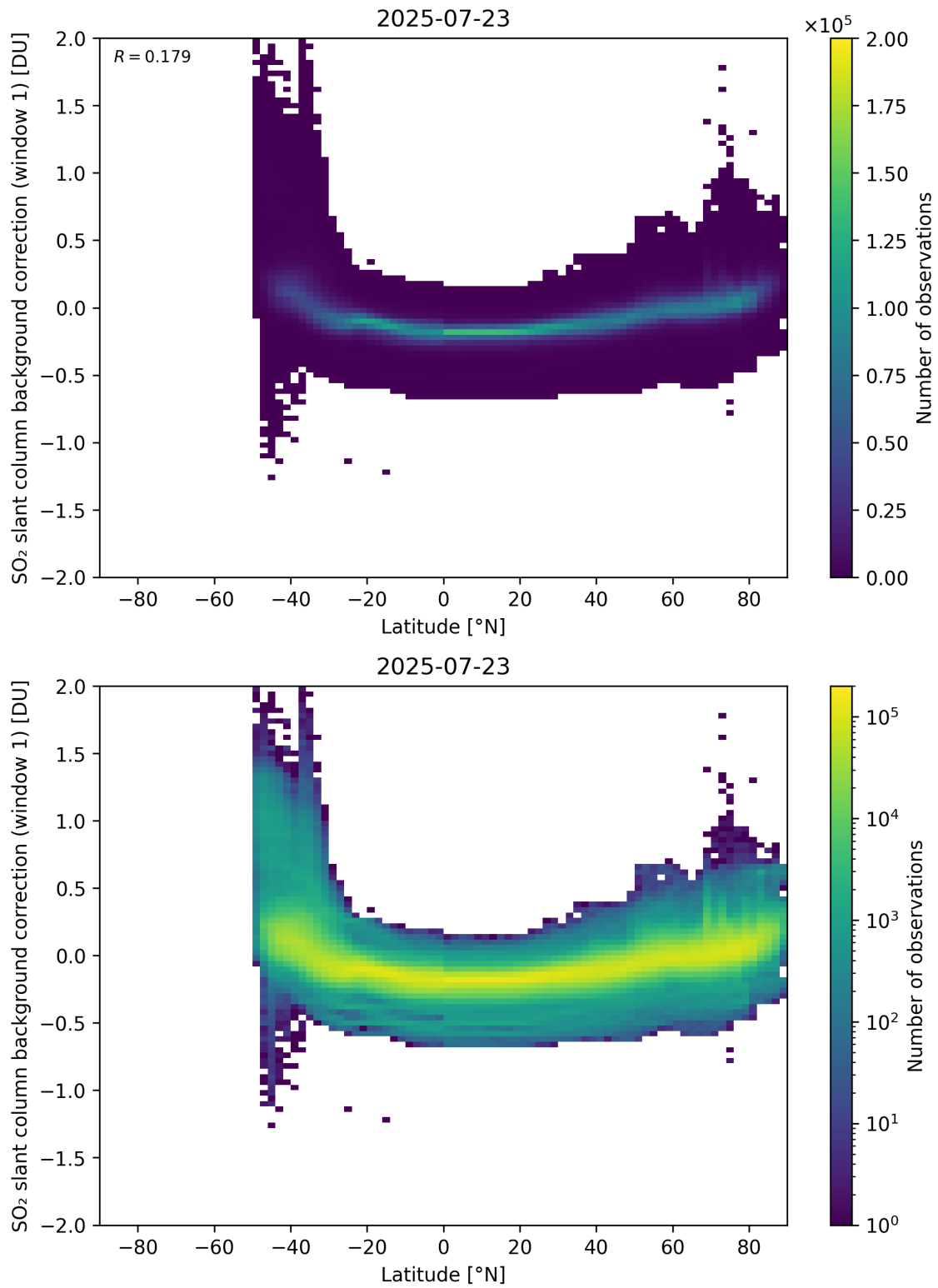
Figure 150: Scatter density plot of “Latitude” against “SO 2 slant column background correction (window 1)” for 2025-07-22 to 2025-07-24.
