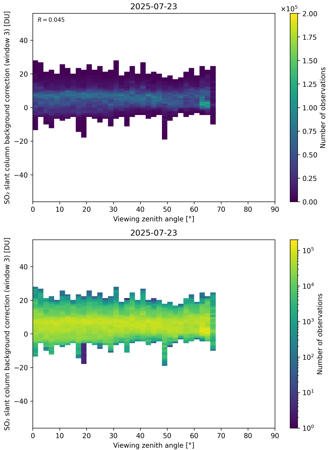
Figure 364: Scatter density plot of “Viewing zenith angle” against “SO 2 slant column background correction (window 3)” for 2025-07-22 to 2025-07-24.
