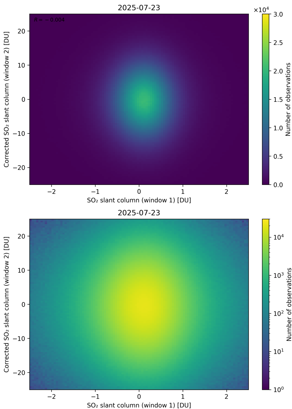
Figure 283: Scatter density plot of “SO 2 slant column (window 1)” against “Corrected SO 2 slant column (window 2)” for 2025-07-22 to 2025-07-24.
