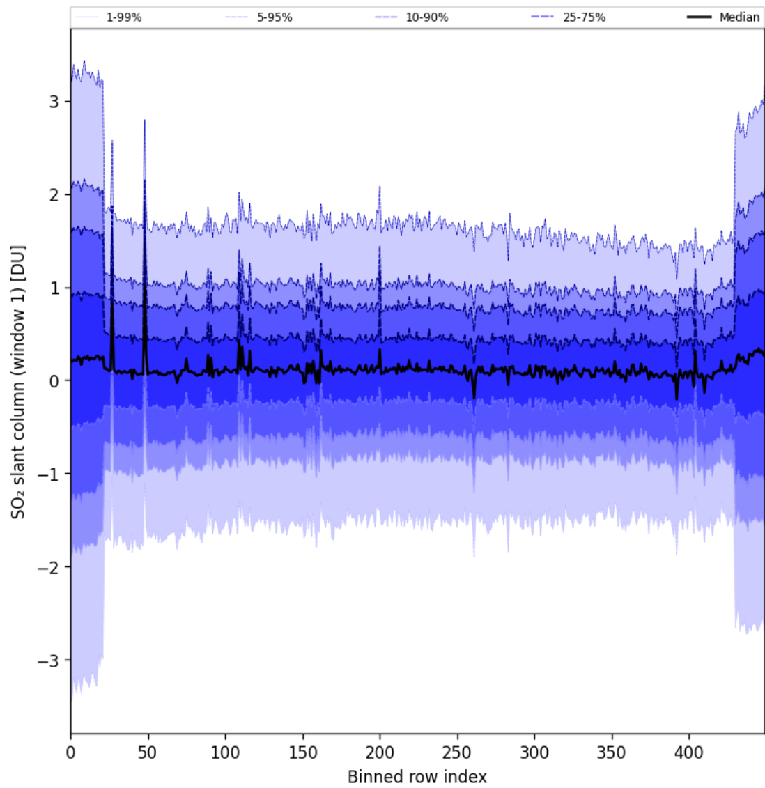
Figure 89: Along track statistics of “SO 2 slant column (window 1)” for 2025-07-22 to 2025-07-24
