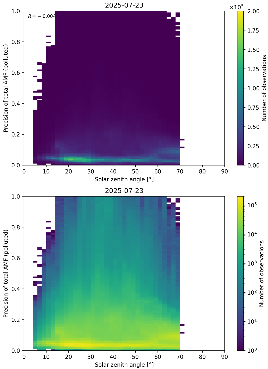
Figure 190: Scatter density plot of “Solar zenith angle” against “Precision of total AMF (polluted)” for 2025-07-22 to 2025-07-24.
