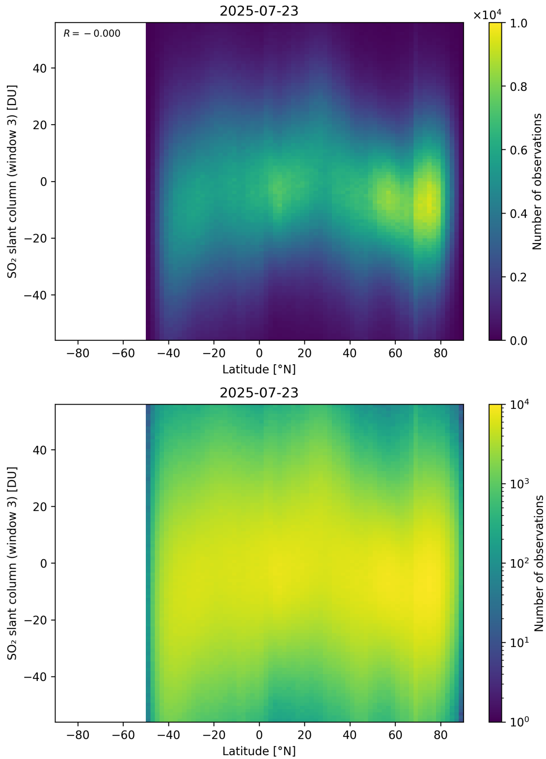
Figure 165: Scatter density plot of “Latitude” against “SO 2 slant column (window 3)” for 2025-07-22 to 2025-07-24.
