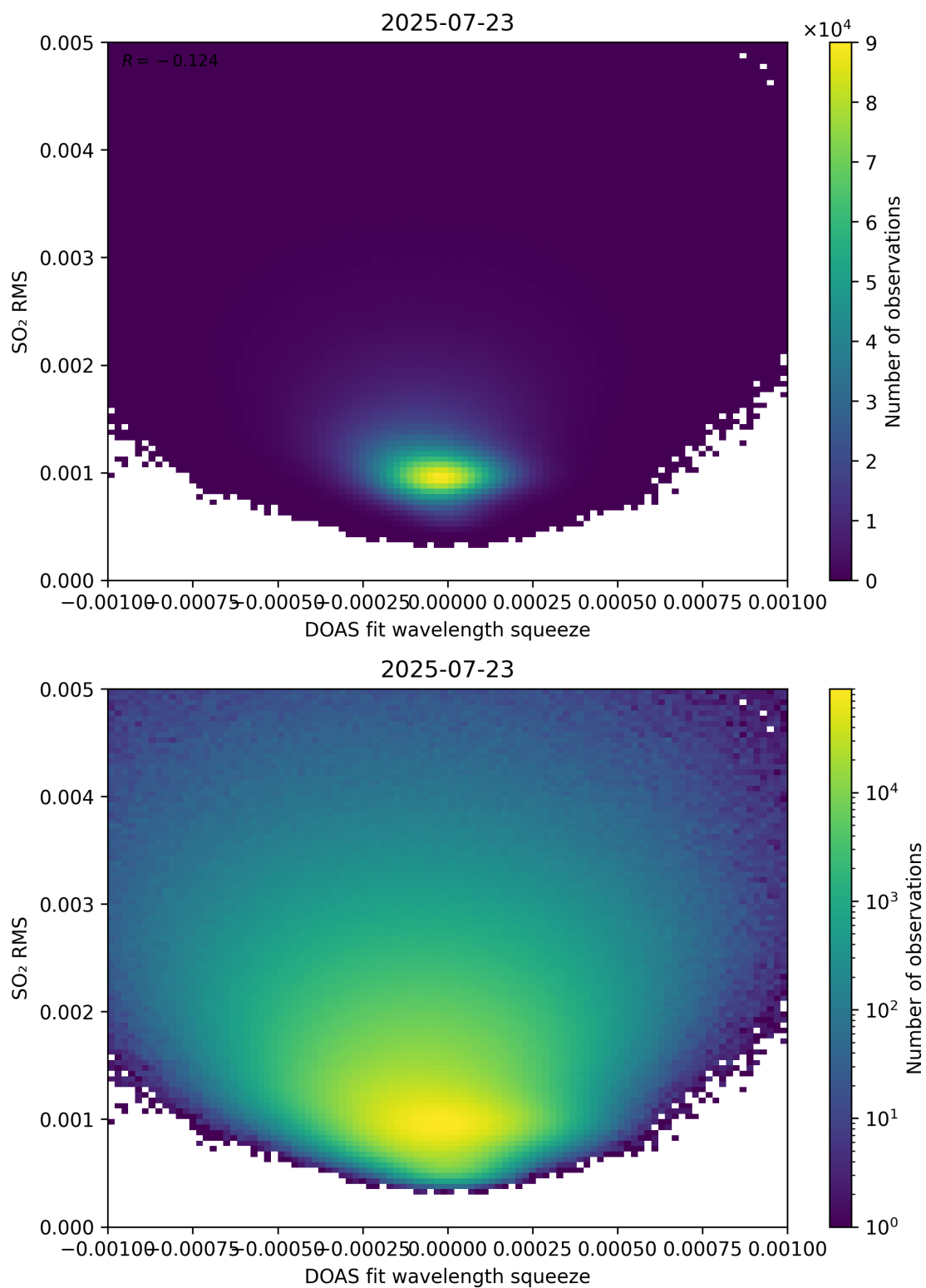
Figure 143: Scatter density plot of “DOAS fit wavelength squeeze” against “SO 2 RMS” for 2025-07-22 to 2025-07-24.
