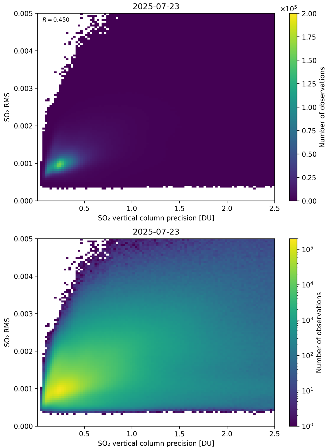
Figure 334: Scatter density plot of “SO 2 vertical column precision” against “SO 2 RMS” for 2025-07-22 to 2025-07-24.
