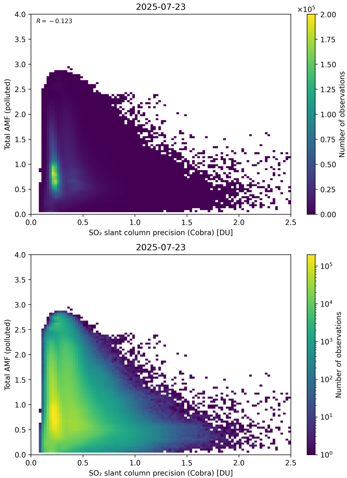
Figure 213: Scatter density plot of “SO 2 slant column precision (Cobra)” against “Total AMF (polluted)” for 2025-07-22 to 2025-07-24.
