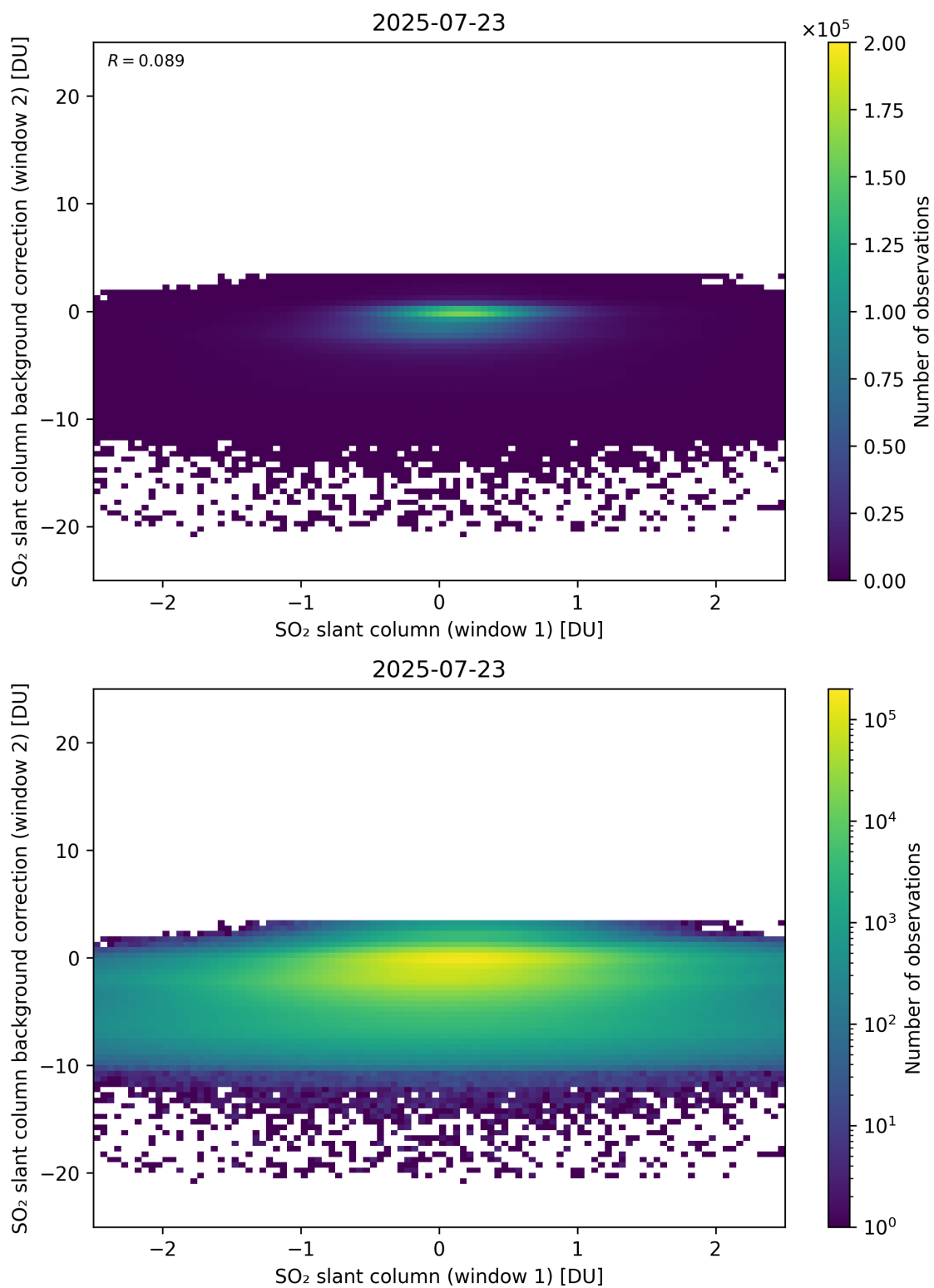
Figure 263: Scatter density plot of “SO 2 slant column (window 1)” against “SO 2 slant column background correction (window 2)” for 2025-07-22 to 2025-07-24.
