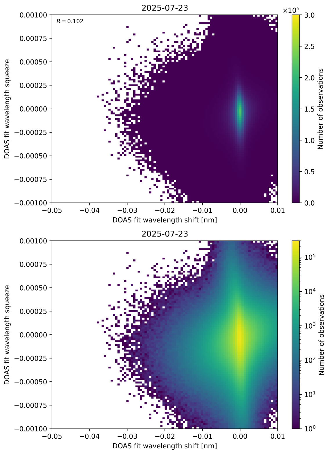
Figure 138: Scatter density plot of “DOAS fit wavelength shift” against “DOAS fit wavelength squeeze” for 2025-07-22 to 2025-07-24.
