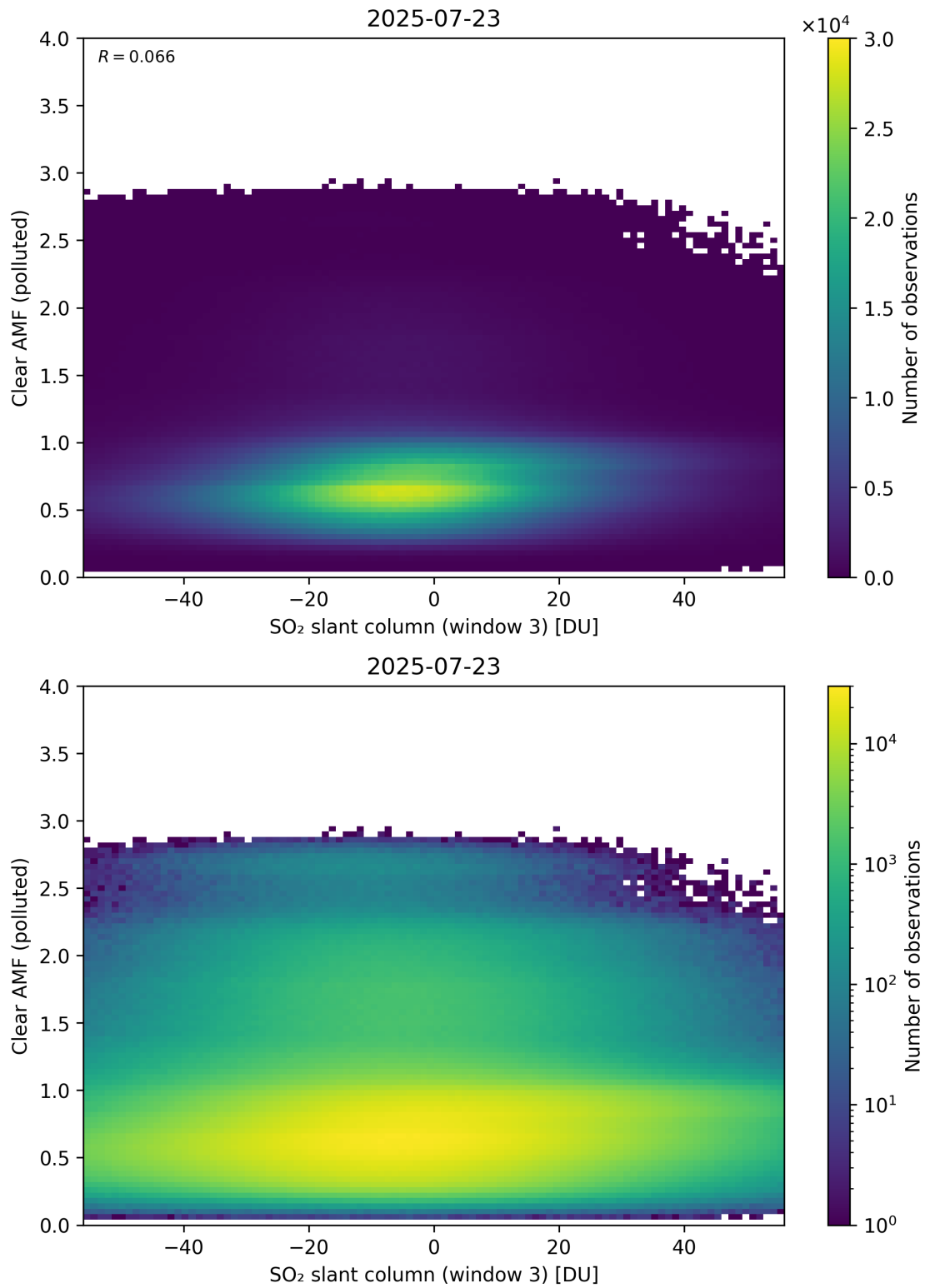
Figure 315: Scatter density plot of “SO 2 slant column (window 3)” against “Clear AMF (polluted)” for 2025-07-22 to 2025-07-24.
