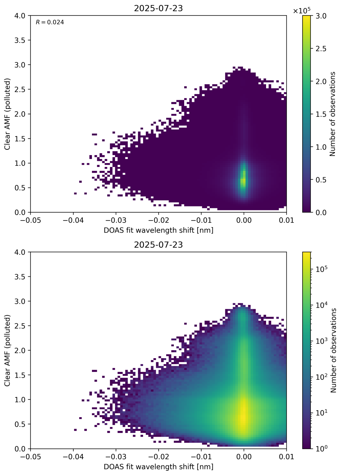
Figure 140: Scatter density plot of “DOAS fit wavelength shift” against “Clear AMF (polluted)” for 2025-07-22 to 2025-07-24.
