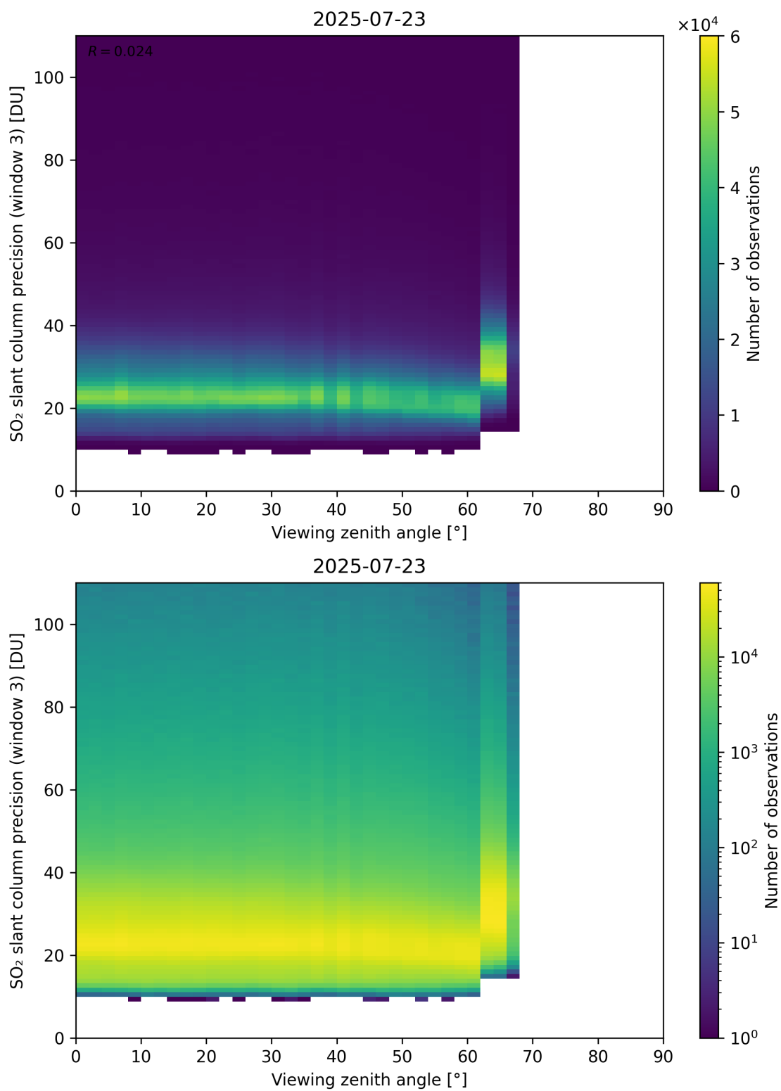
Figure 380: Scatter density plot of “Viewing zenith angle” against “SO 2 slant column precision (window 3)” for 2025-07-22 to 2025-07-24.
