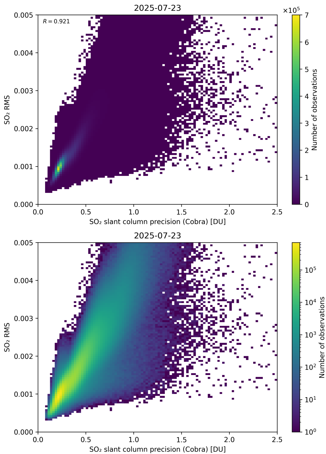
Figure 204: Scatter density plot of “SO 2 slant column precision (Cobra)” against “SO 2 RMS” for 2025-07-22 to 2025-07-24.
