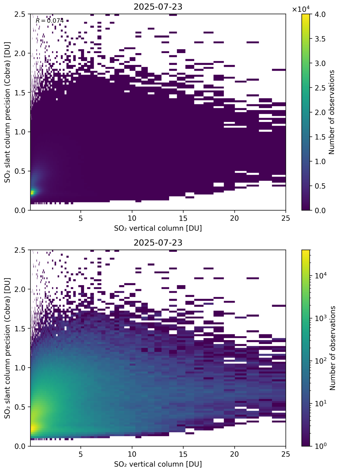
Figure 350: Scatter density plot of “SO 2 vertical column” against “SO 2 slant column precision (Cobra)” for 2025-07-22 to 2025-07-24.
