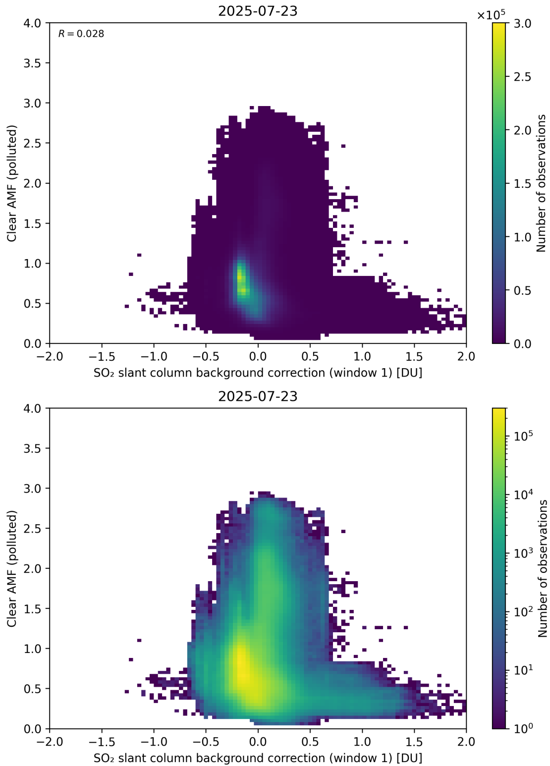
Figure 114: Scatter density plot of “SO 2 slant column background correction (window 1)” against “Clear AMF (polluted)” for 2025-07-22 to 2025-07-24.
