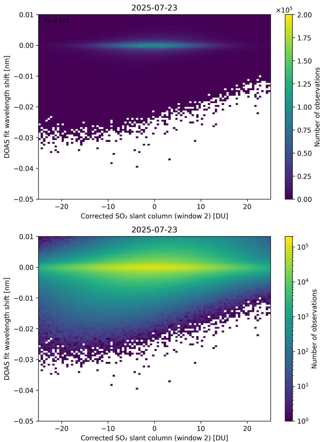
Figure 246: Scatter density plot of “Corrected SO 2 slant column (window 2)” against “DOAS fit wavelength shift” for 2025-07-22 to 2025-07-24.
