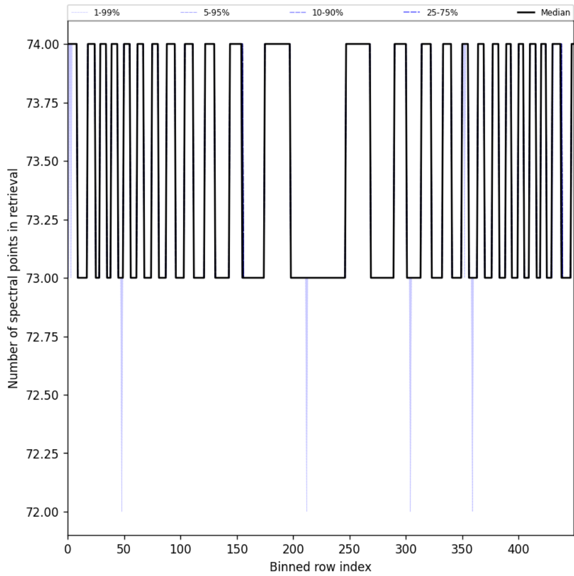
Figure 108: Along track statistics of “Number of spectral points in retrieval” for 2025-07-22 to 2025-07-24
