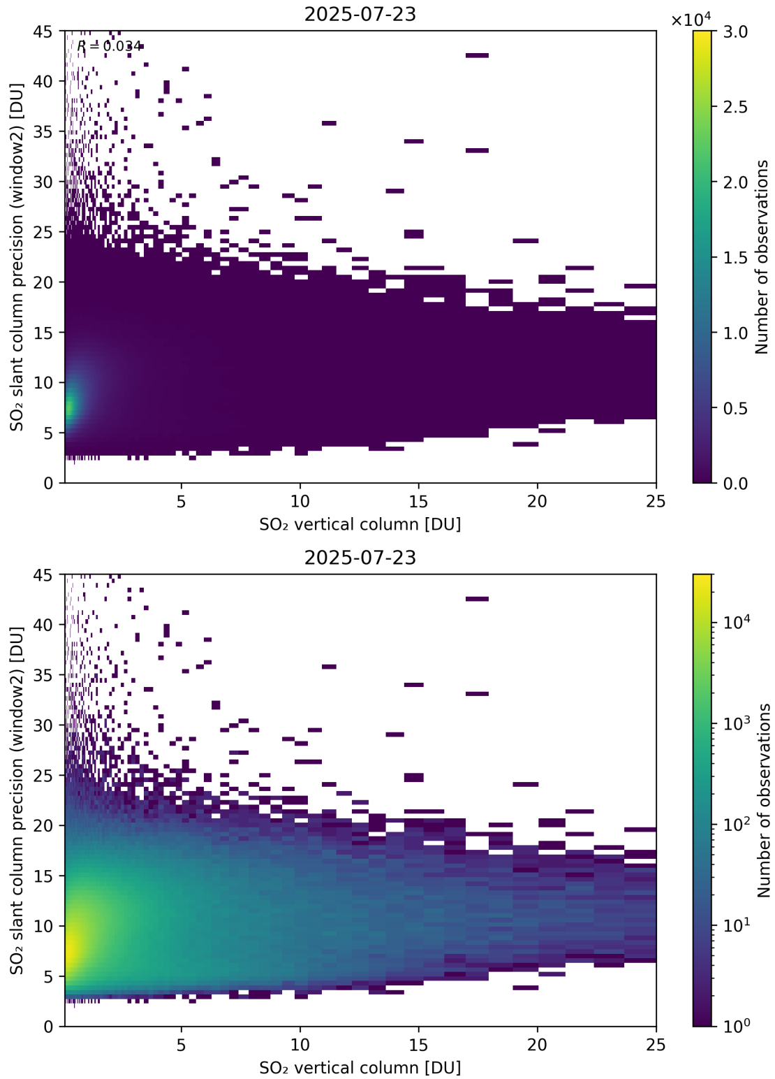
Figure 356: Scatter density plot of “SO 2 vertical column” against “SO 2 slant column precision (window2)” for 2025-07-22 to 2025-07-24.
