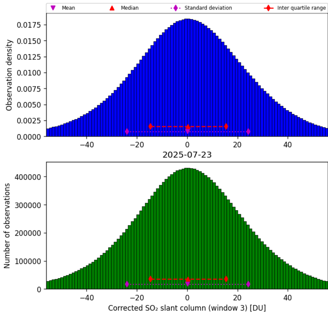
Figure 73: Histogram of “Corrected SO 2 slant column (window 3)” for 2025-07-22 to 2025-07-24
