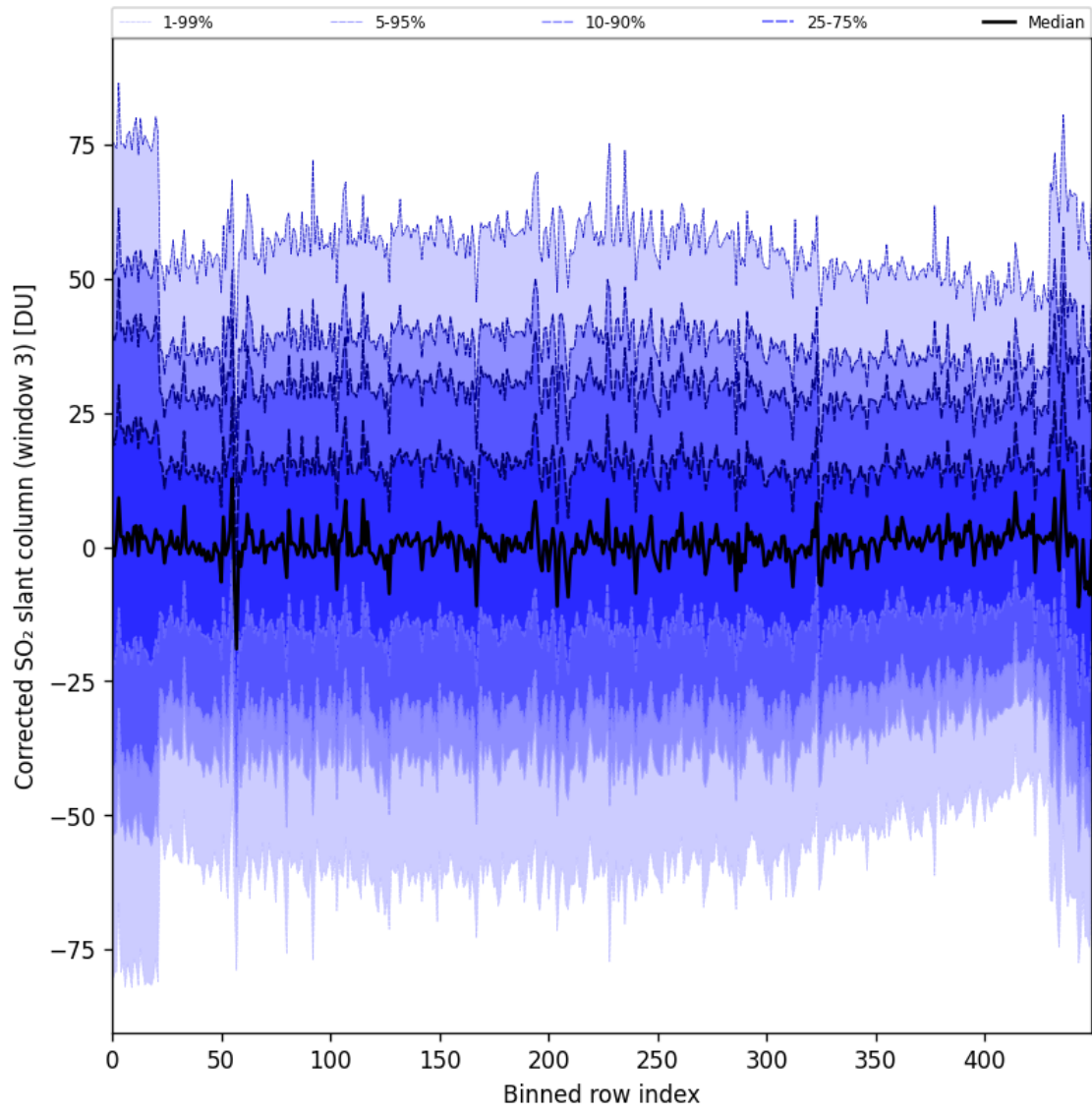
Figure 99: Along track statistics of “Corrected SO 2 slant column (window 3)” for 2025-07-22 to 2025-07-24
