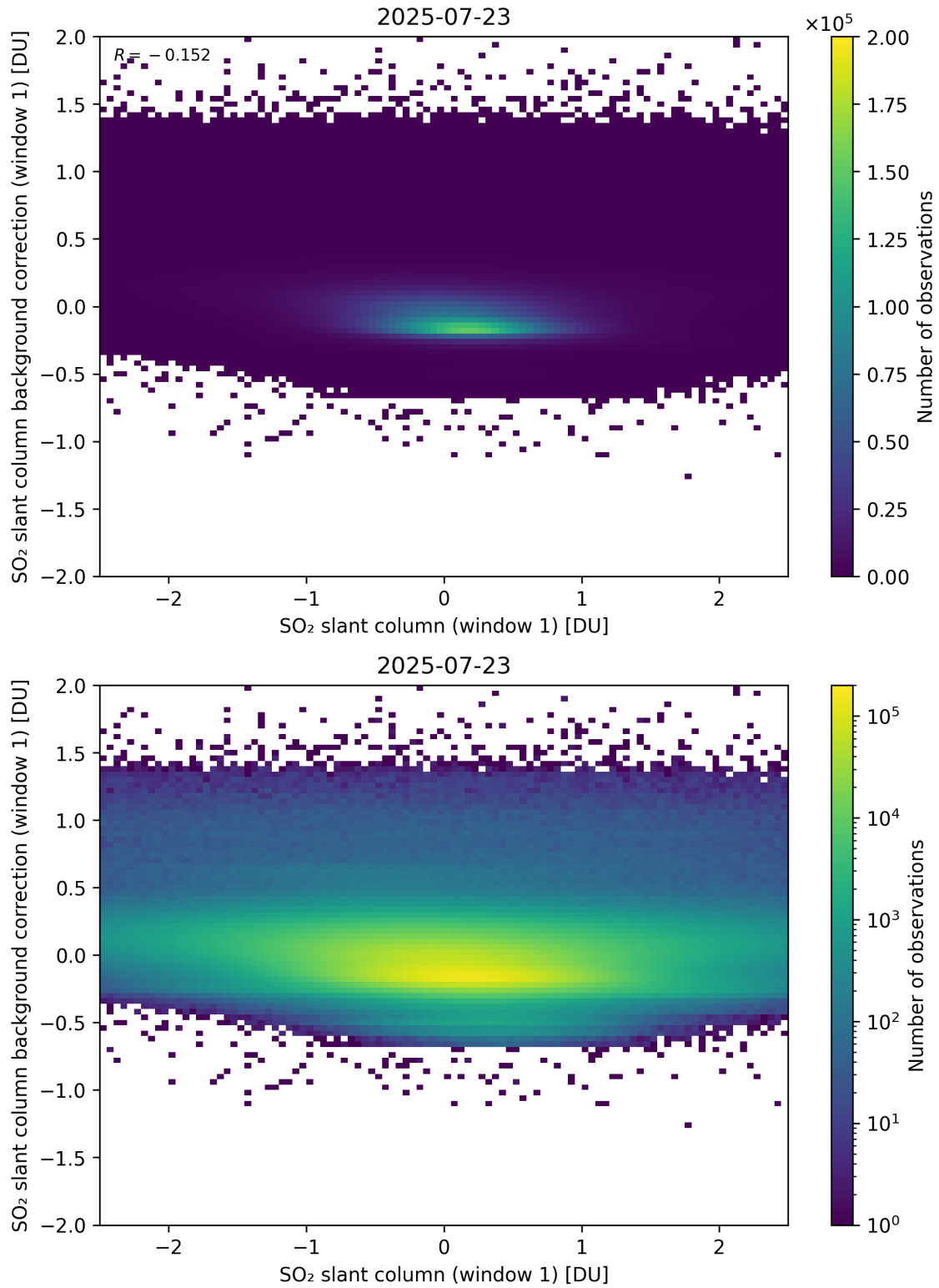
Figure 262: Scatter density plot of “SO 2 slant column (window 1)” against “SO 2 slant column background correction (window 1)” for 2025-07-22 to 2025-07-24.
