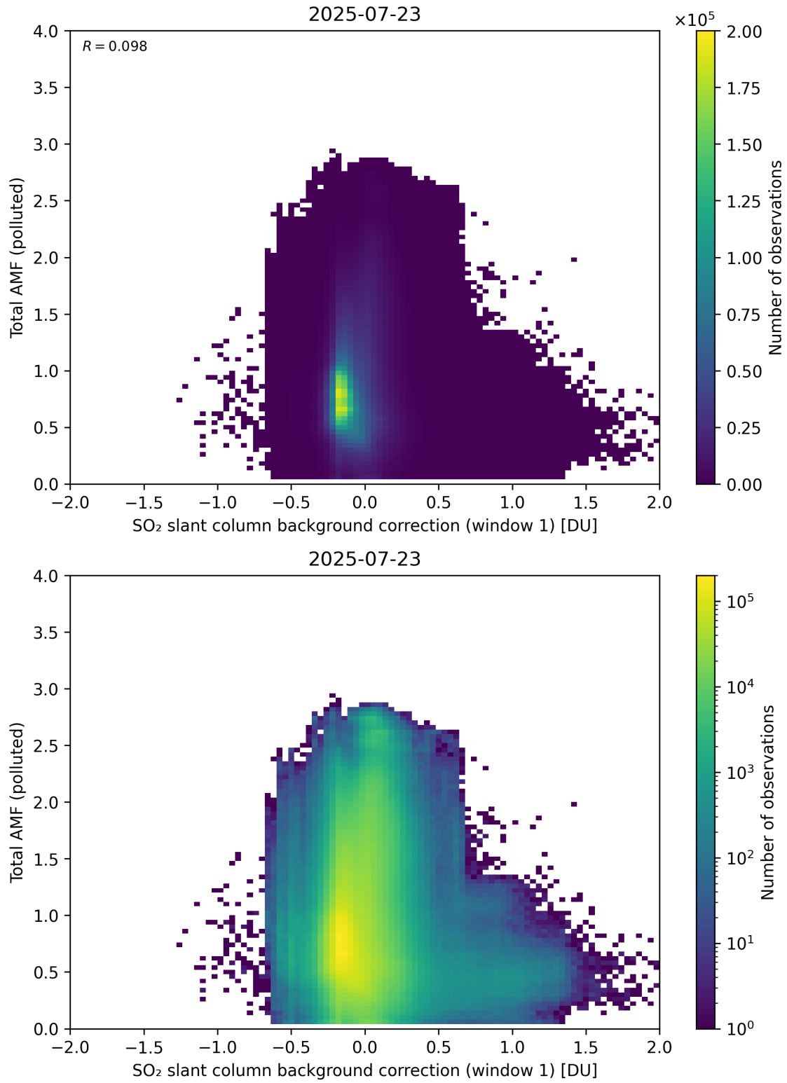
Figure 120: Scatter density plot of “SO 2 slant column background correction (window 1)” against “Total AMF (polluted)” for 2025-07-22 to 2025-07-24.
