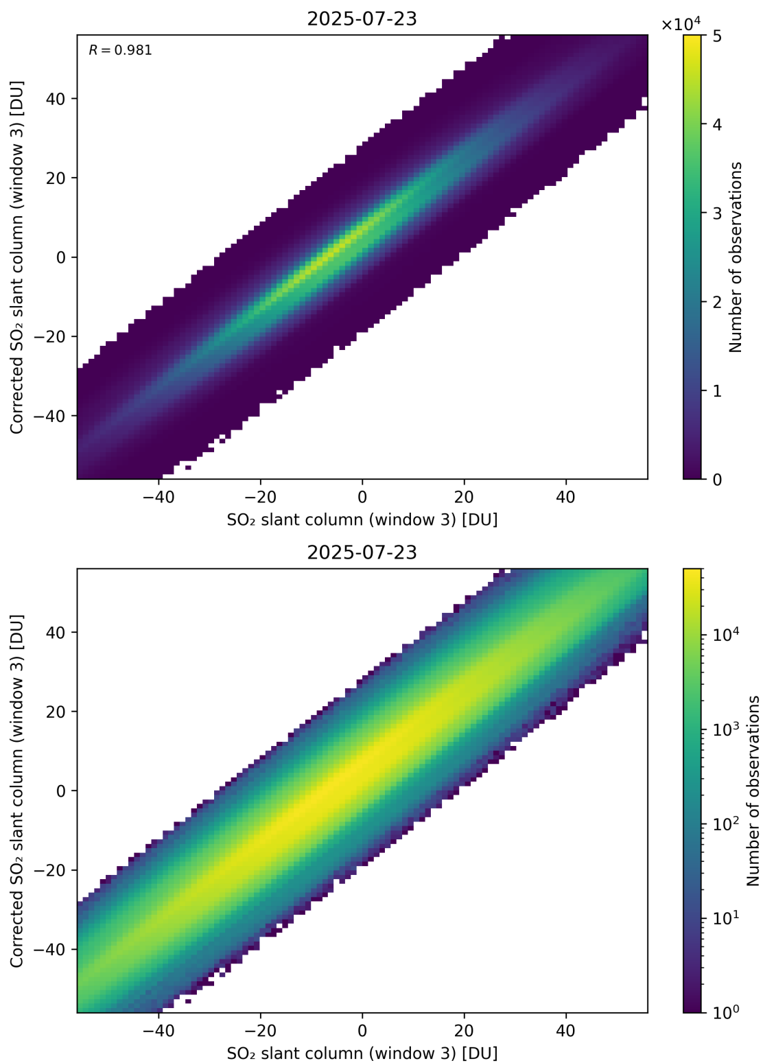
Figure 316: Scatter density plot of “SO 2 slant column (window 3)” against “Corrected SO 2 slant column (window 3)” for 2025-07-22 to 2025-07-24.
