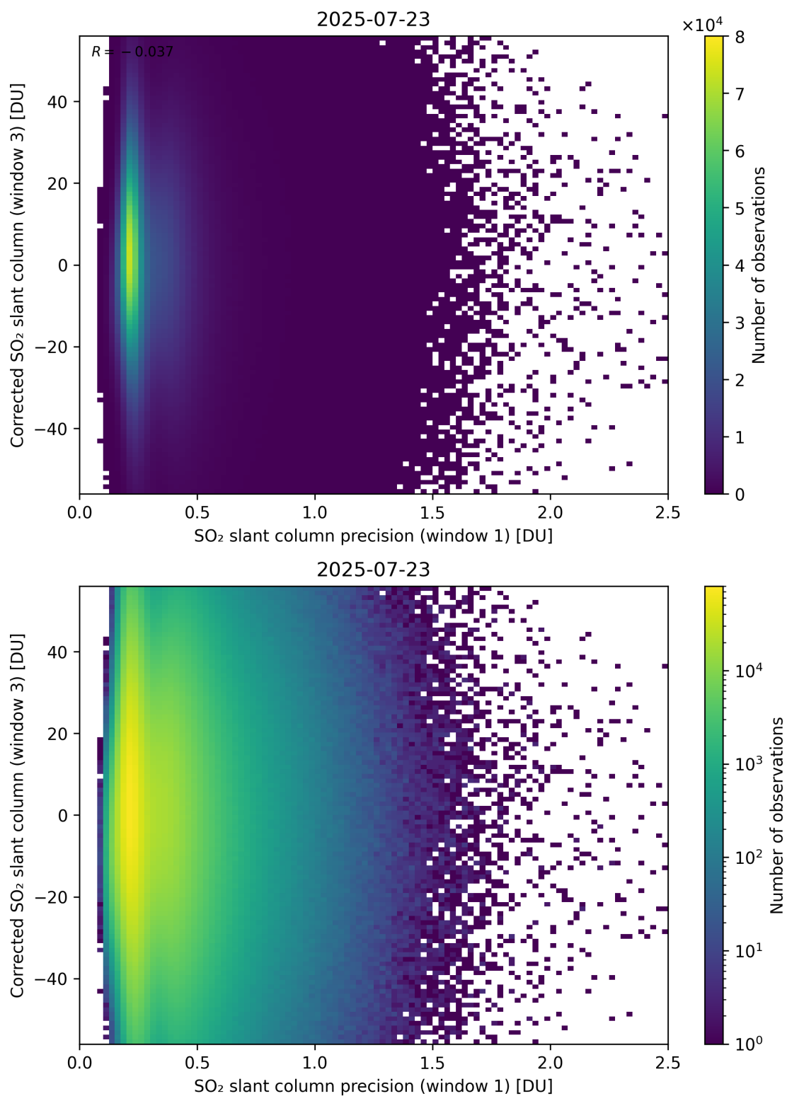
Figure 276: Scatter density plot of “SO 2 slant column precision (window 1)” against “Corrected SO 2 slant column (window 3)” for 2025-07-22 to 2025-07-24.
