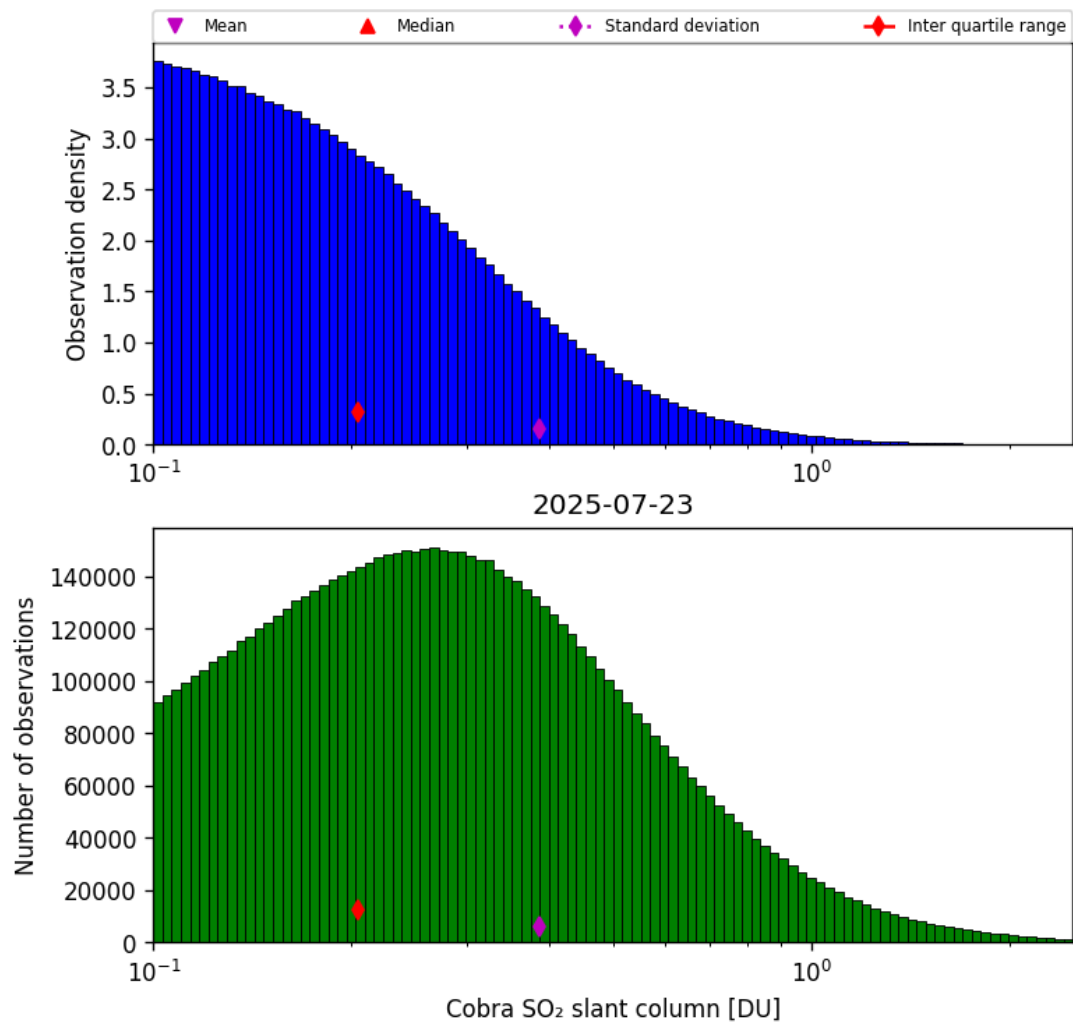
Figure 61: Histogram of “Cobra SO 2 slant column” for 2025-07-22 to 2025-07-24
