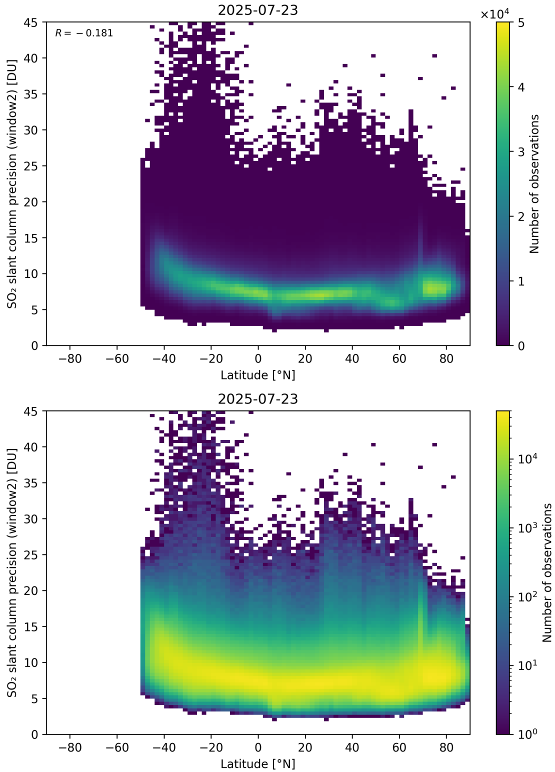
Figure 164: Scatter density plot of “Latitude” against “SO 2 slant column precision (window2)” for 2025-07-22 to 2025-07-24.
