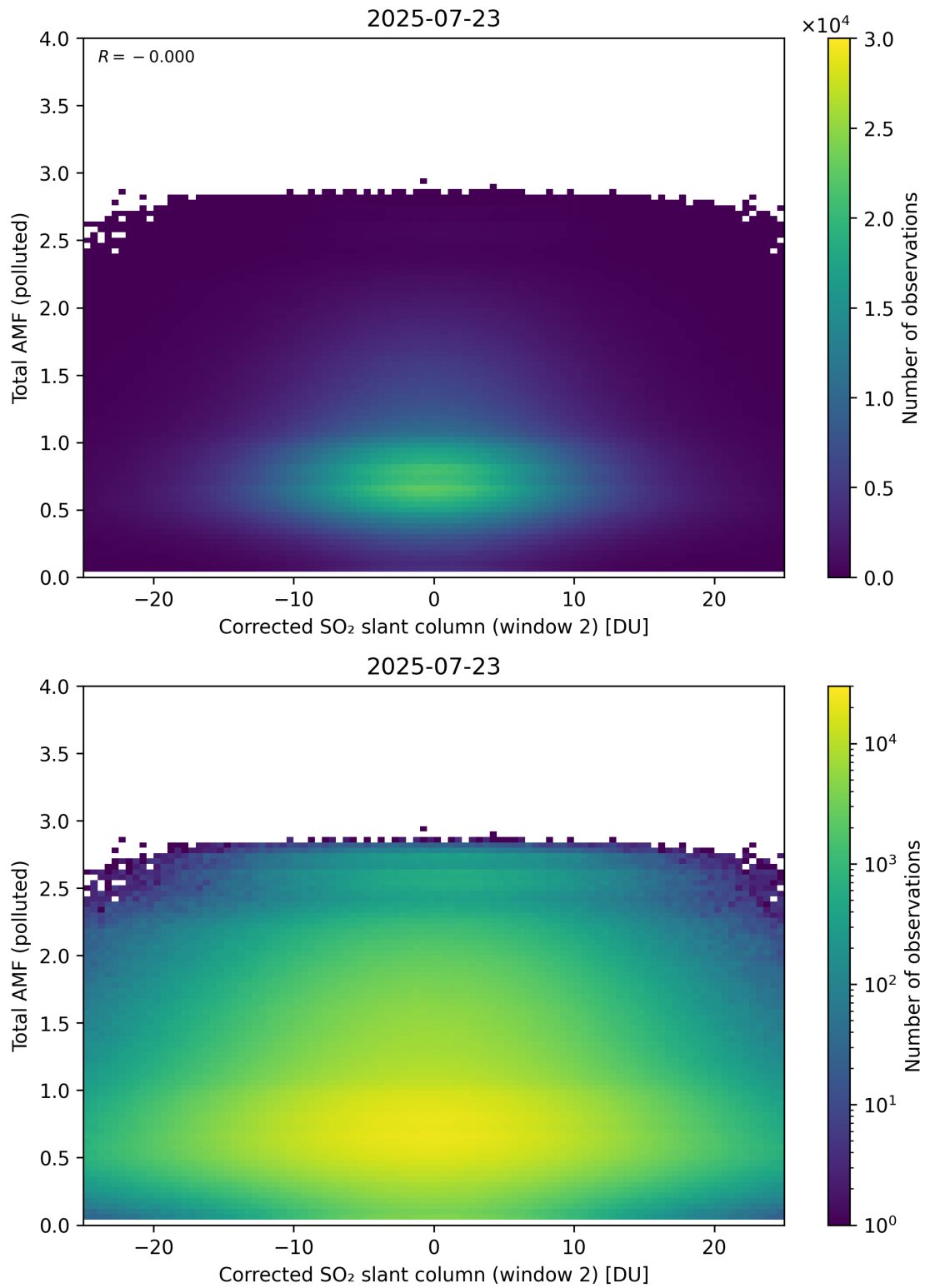
Figure 253: Scatter density plot of “Corrected SO 2 slant column (window 2)” against “Total AMF (polluted)” for 2025-07-22 to 2025-07-24.
