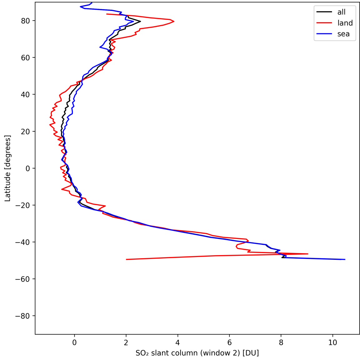
Figure 41: Zonal average of “SO 2 slant column (window 2)” for 2025-07-22 to 2025-07-24.
