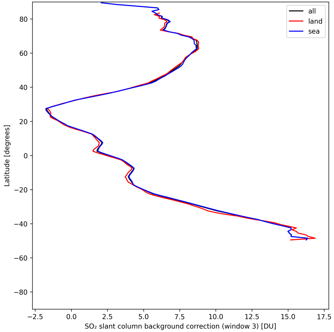
Figure 48: Zonal average of “SO 2 slant column background correction (window 3)” for 2025-07-22 to 2025-07-24.
