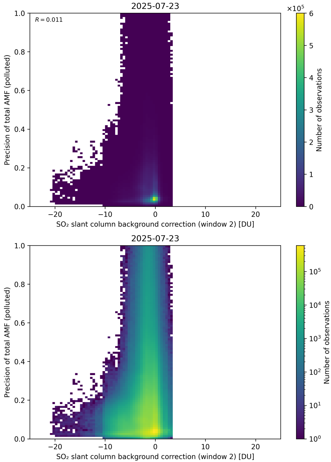
Figure 131: Scatter density plot of “SO 2 slant column background correction (window 2)” against “Precision of total AMF (polluted)” for 2025-07-22 to 2025-07-24.
