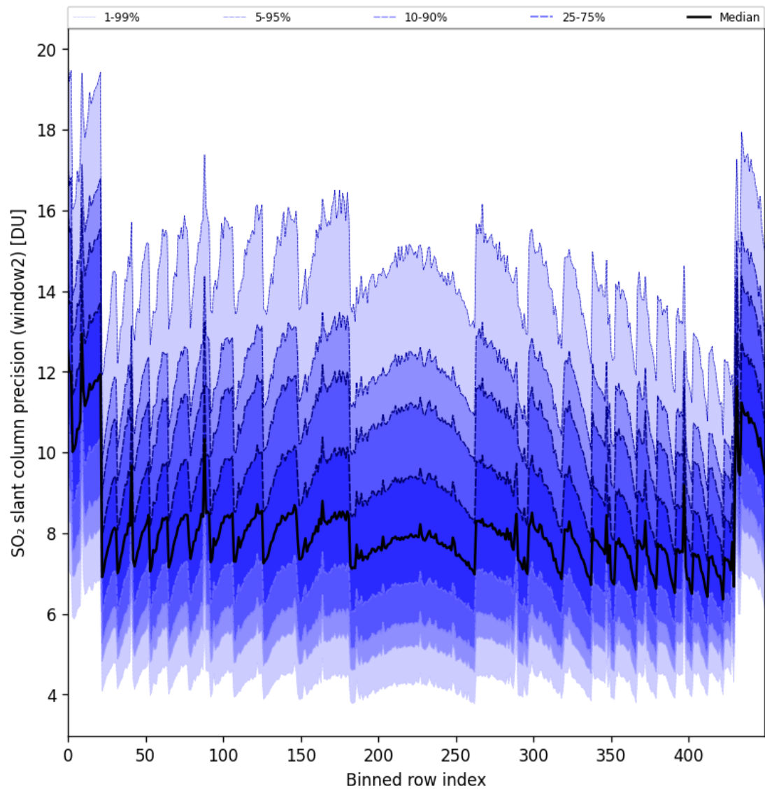
Figure 94: Along track statistics of “SO 2 slant column precision (window2)” for 2025-07-22 to 2025-07-24
