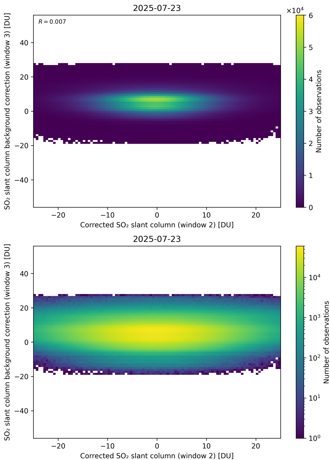
Figure 245: Scatter density plot of “Corrected SO 2 slant column (window 2)” against “SO 2 slant column background correction (window 3)” for 2025-07-22 to 2025-07-24.
