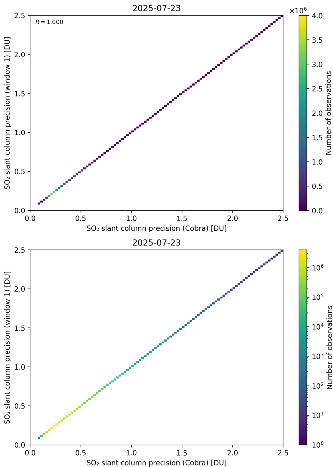
Figure 209: Scatter density plot of “SO 2 slant column precision (Cobra)” against “SO 2 slant column precision (window 1)” for 2025-07-22 to 2025-07-24.
