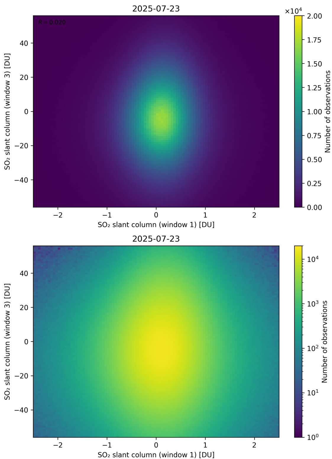
Figure 287: Scatter density plot of “SO 2 slant column (window 1)” against “SO 2 slant column (window 3)” for 2025-07-22 to 2025-07-24.
