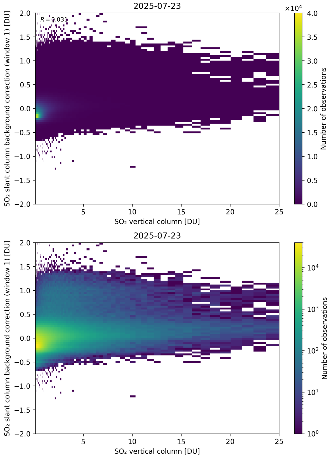
Figure 323: Scatter density plot of “SO 2 vertical column” against “SO 2 slant column background correction (window 1)” for 2025-07-22 to 2025-07-24.
