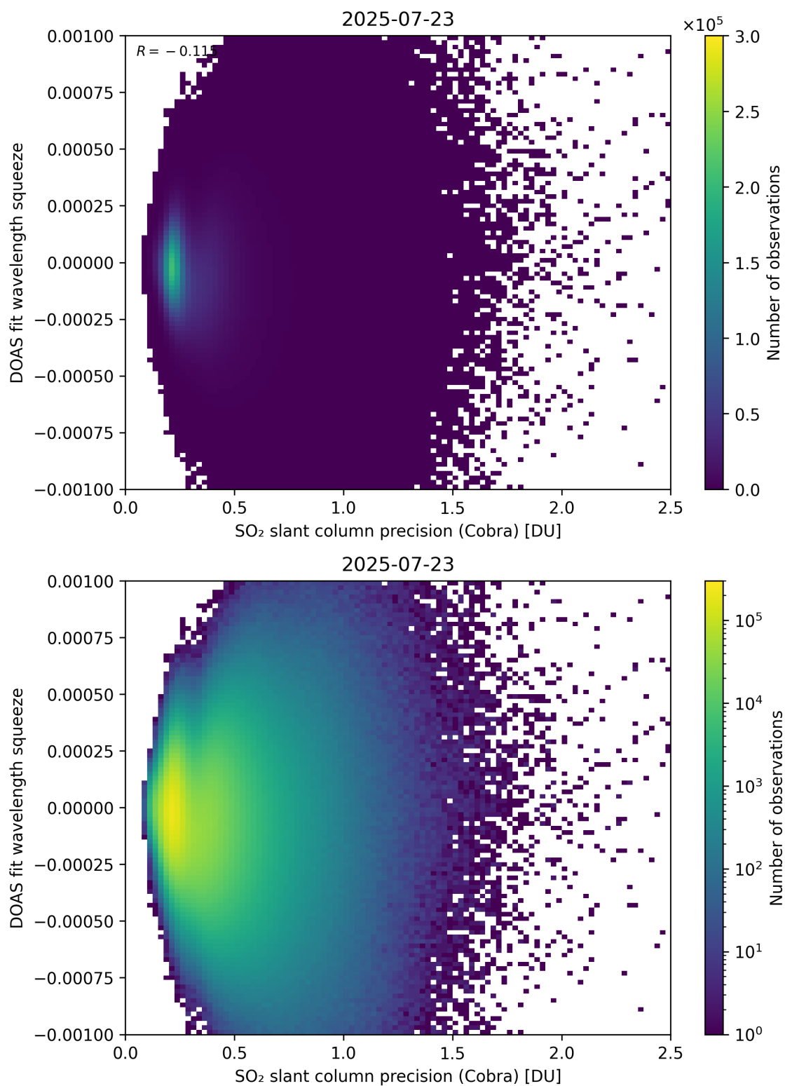
Figure 203: Scatter density plot of “SO 2 slant column precision (Cobra)” against “DOAS fit wavelength squeeze” for 2025-07-22 to 2025-07-24.
