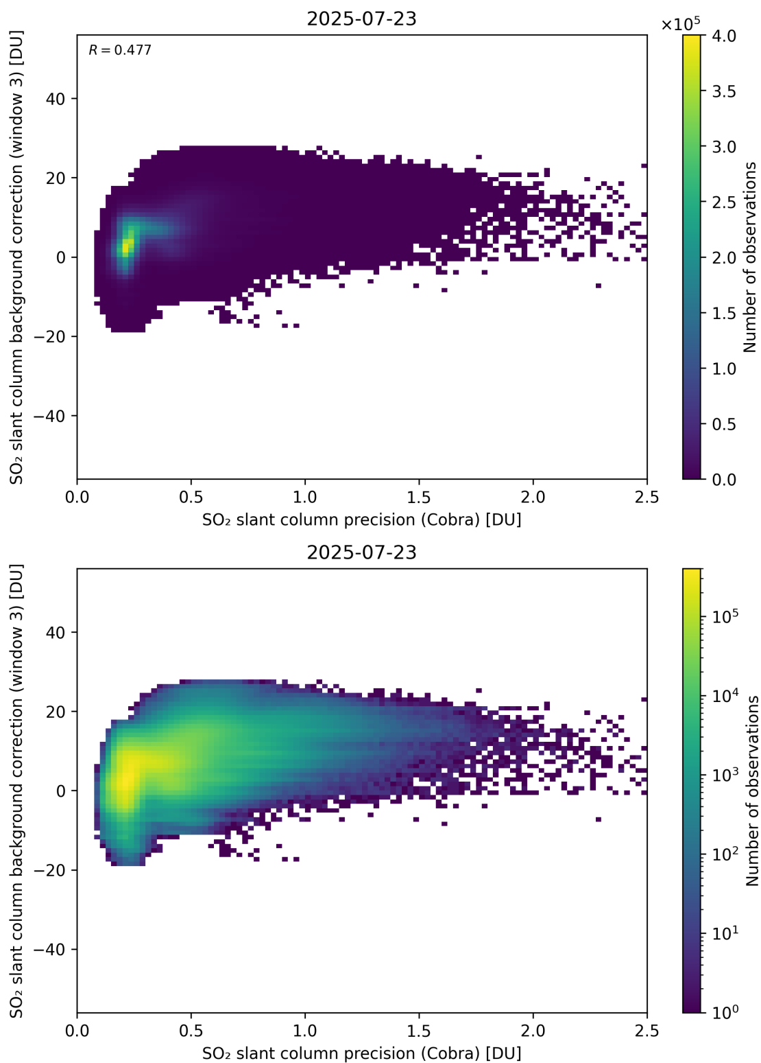
Figure 201: Scatter density plot of “SO 2 slant column precision (Cobra)” against “SO 2 slant column background correction (window 3)” for 2025-07-22 to 2025-07-24.
