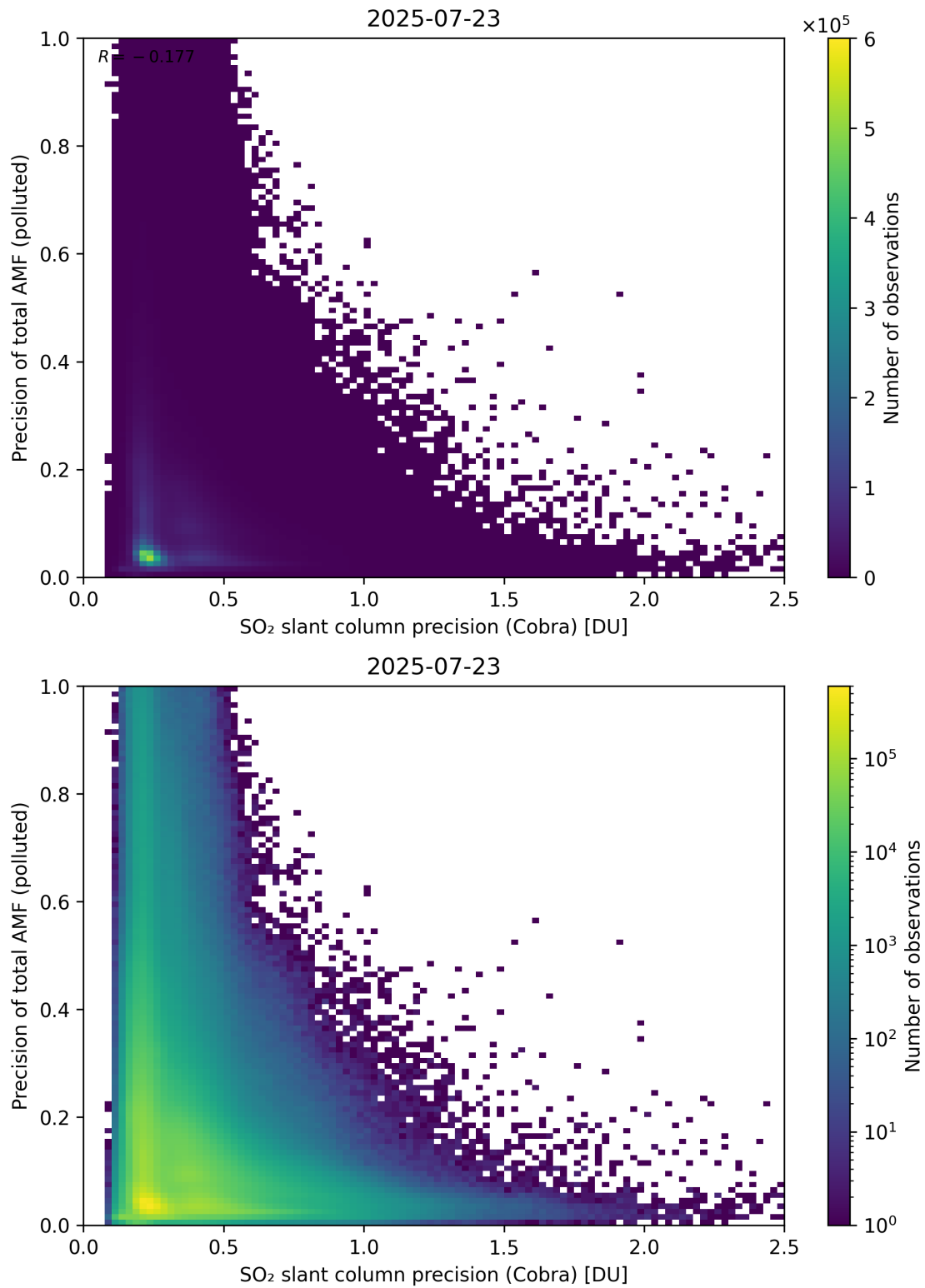
Figure 214: Scatter density plot of “SO 2 slant column precision (Cobra)” against “Precision of total AMF (polluted)” for 2025-07-22 to 2025-07-24.
