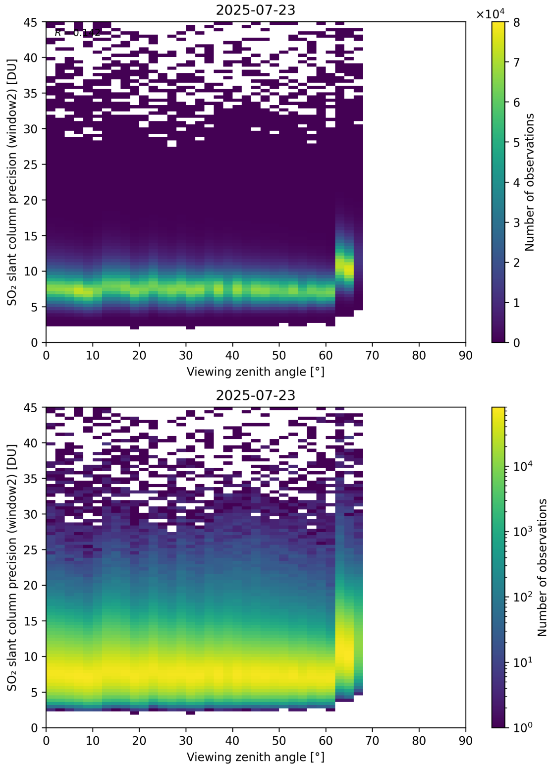
Figure 378: Scatter density plot of “Viewing zenith angle” against “SO 2 slant column precision (window2)” for 2025-07-22 to 2025-07-24.
