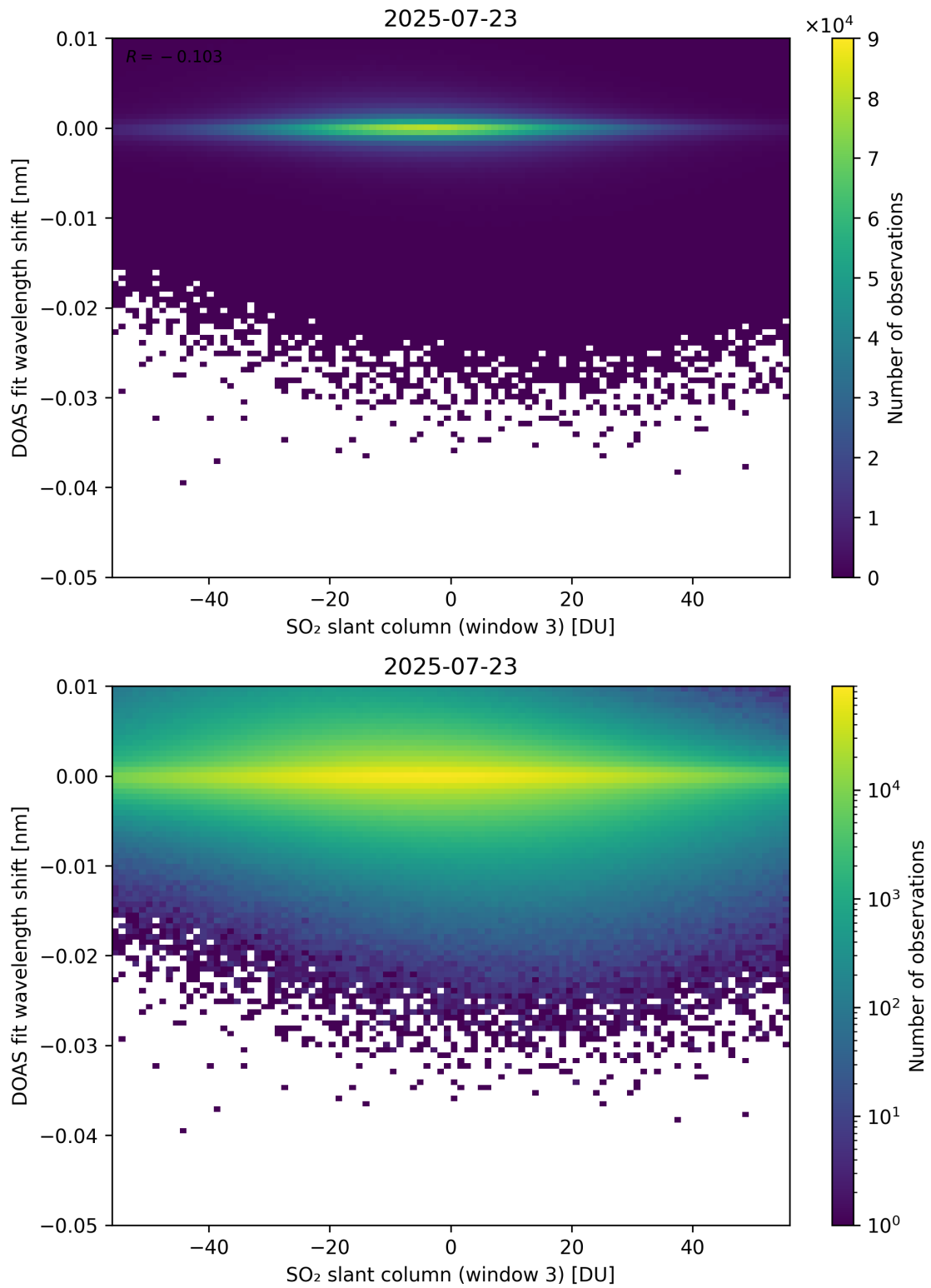
Figure 304: Scatter density plot of “SO 2 slant column (window 3)” against “DOAS fit wavelength shift” for 2025-07-22 to 2025-07-24.
