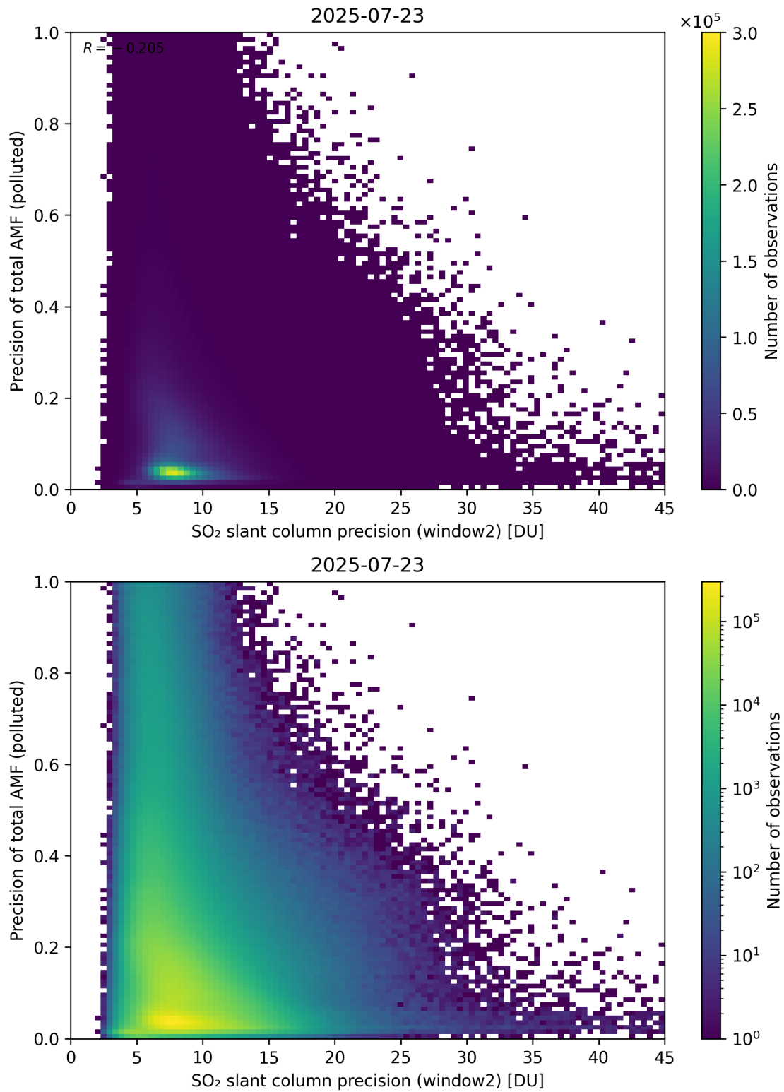
Figure 302: Scatter density plot of “SO 2 slant column precision (window2)” against “Precision of total AMF (polluted)” for 2025-07-22 to 2025-07-24.
