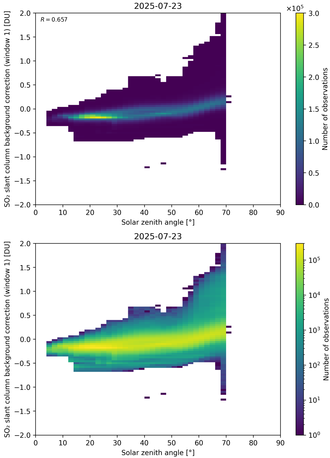
Figure 171: Scatter density plot of “Solar zenith angle” against “SO 2 slant column background correction (window 1)” for 2025-07-22 to 2025-07-24.
