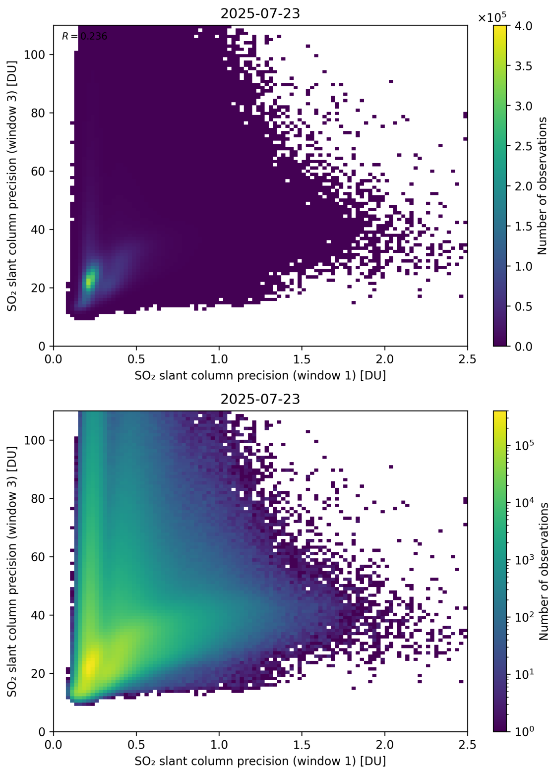
Figure 279: Scatter density plot of “SO 2 slant column precision (window 1)” against “SO 2 slant column precision (window 3)” for 2025-07-22 to 2025-07-24.
