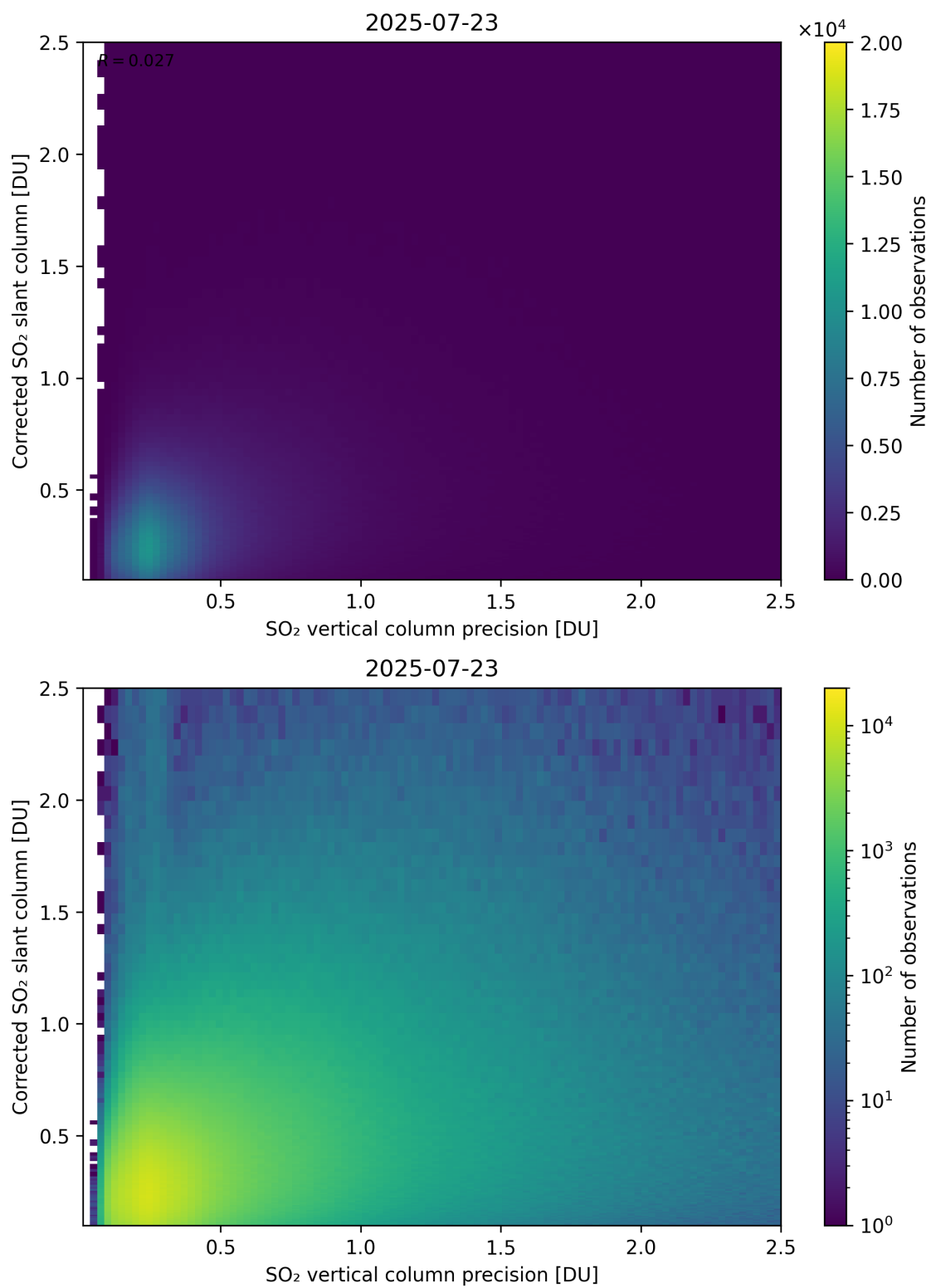
Figure 338: Scatter density plot of “SO 2 vertical column precision” against “Corrected SO 2 slant column” for 2025-07-22 to 2025-07-24.
