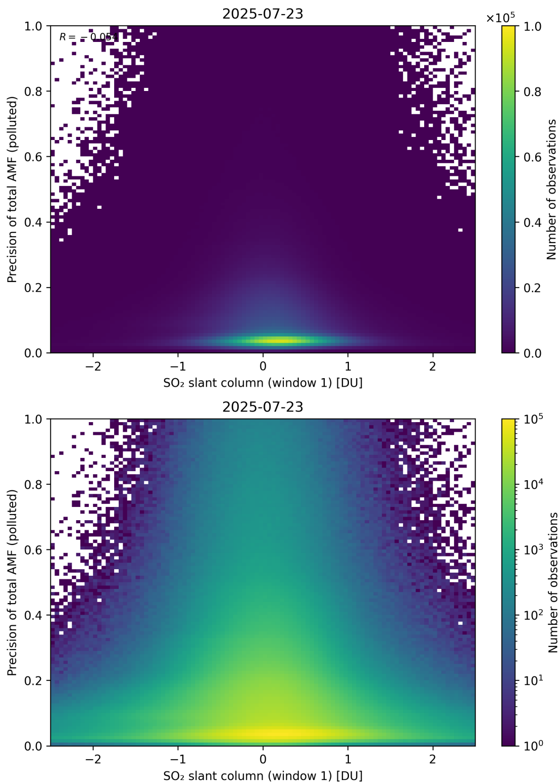
Figure 290: Scatter density plot of “SO 2 slant column (window 1)” against “Precision of total AMF (polluted)” for 2025-07-22 to 2025-07-24.
