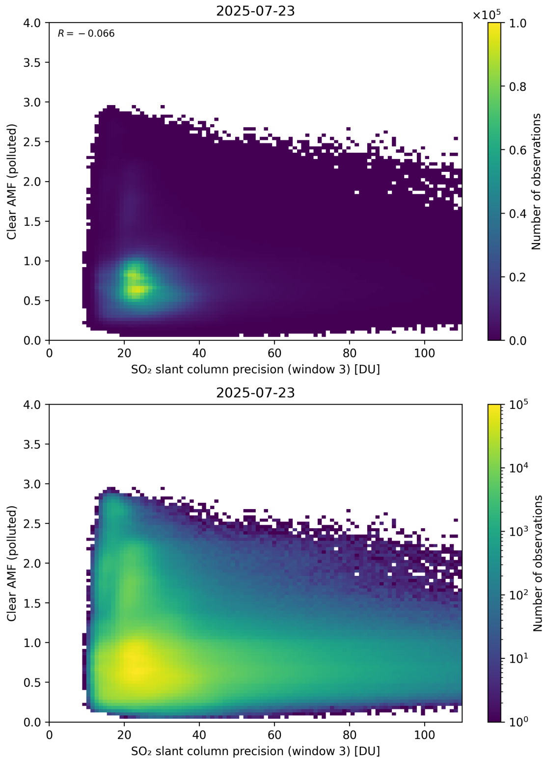
Figure 311: Scatter density plot of “SO 2 slant column precision (window 3)” against “Clear AMF (polluted)” for 2025-07-22 to 2025-07-24.
