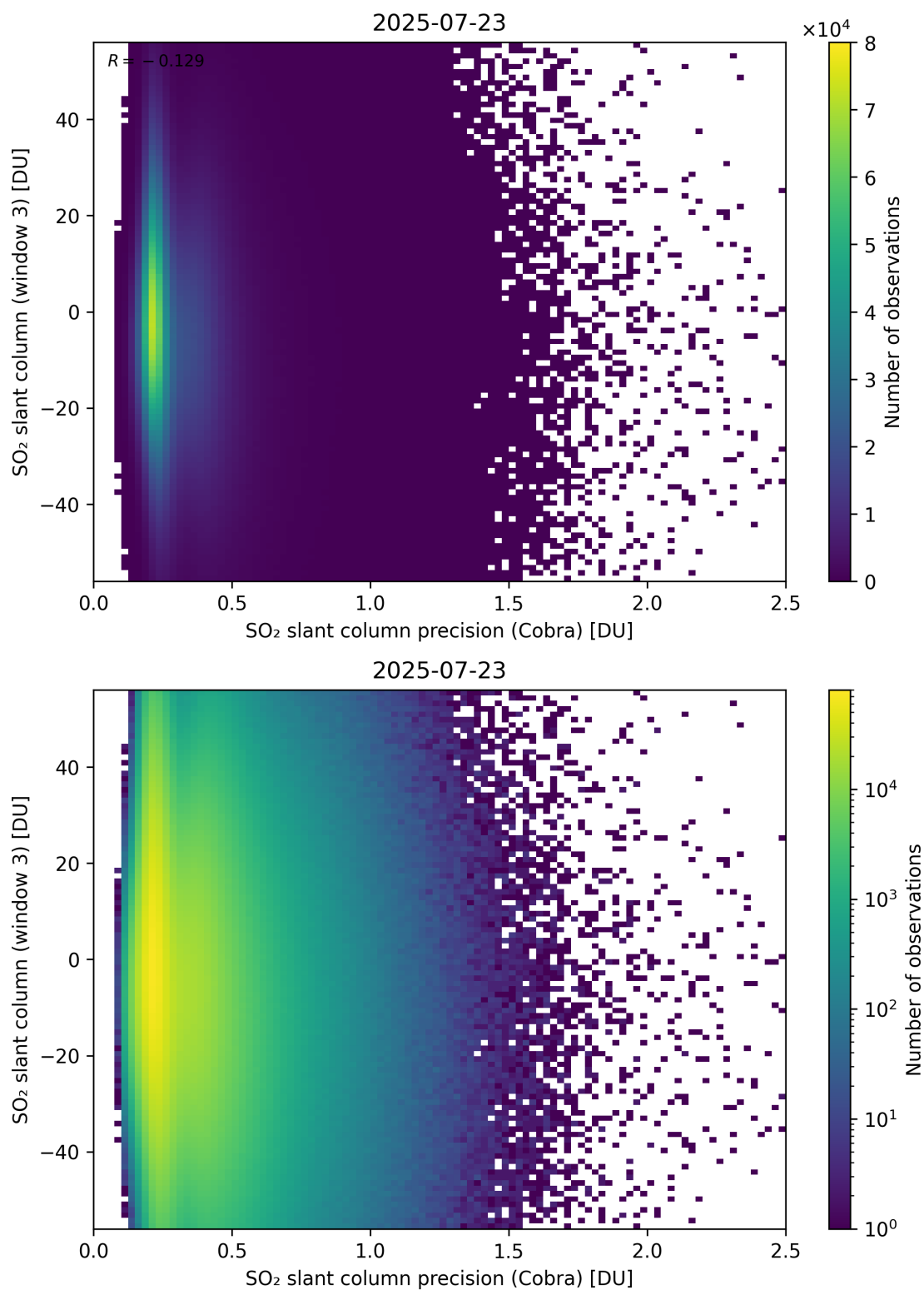
Figure 211: Scatter density plot of “SO 2 slant column precision (Cobra)” against “SO 2 slant column (window 3)” for 2025-07-22 to 2025-07-24.
