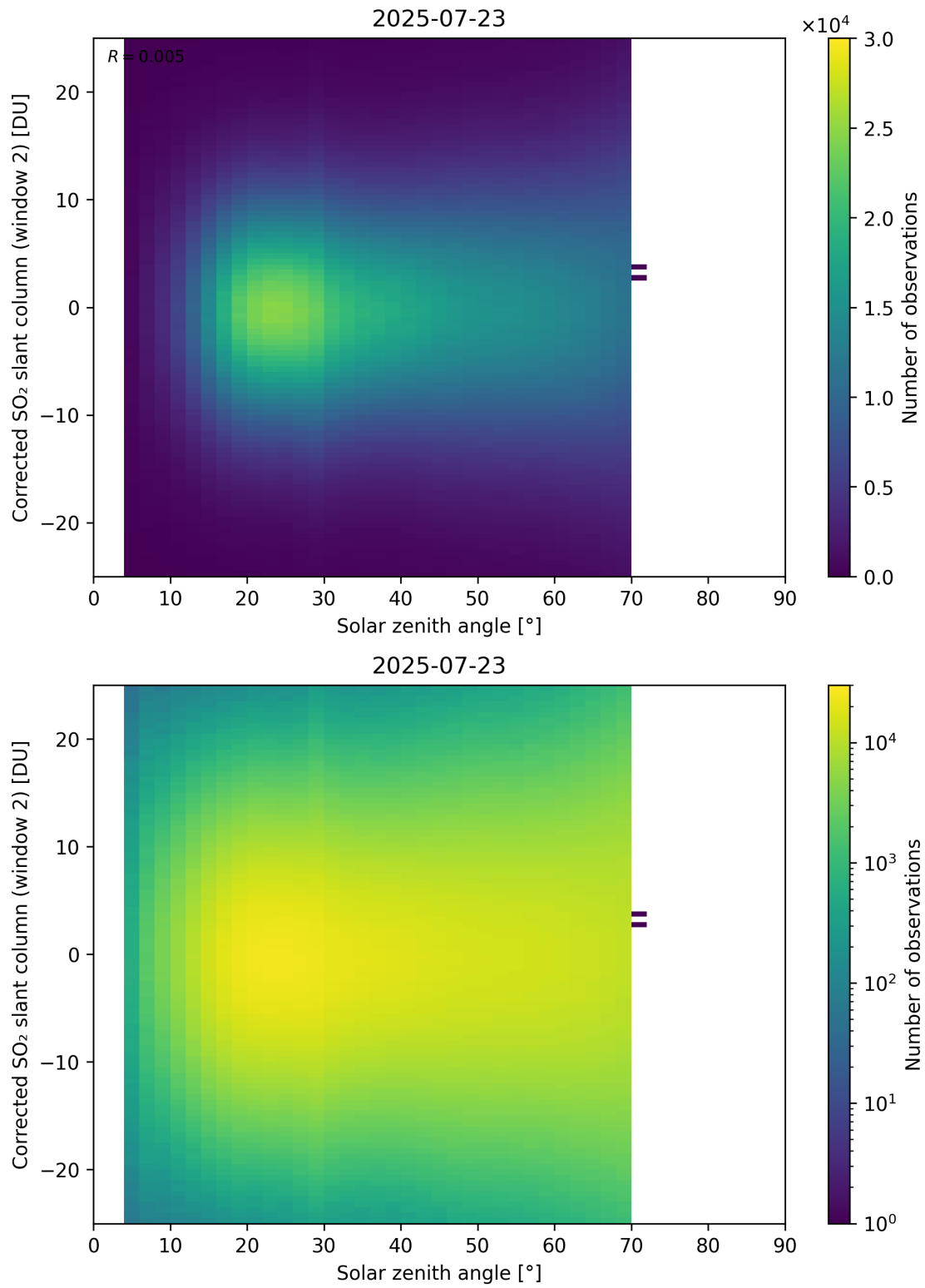
Figure 182: Scatter density plot of “Solar zenith angle” against “Corrected SO 2 slant column (window 2)” for 2025-07-22 to 2025-07-24.
