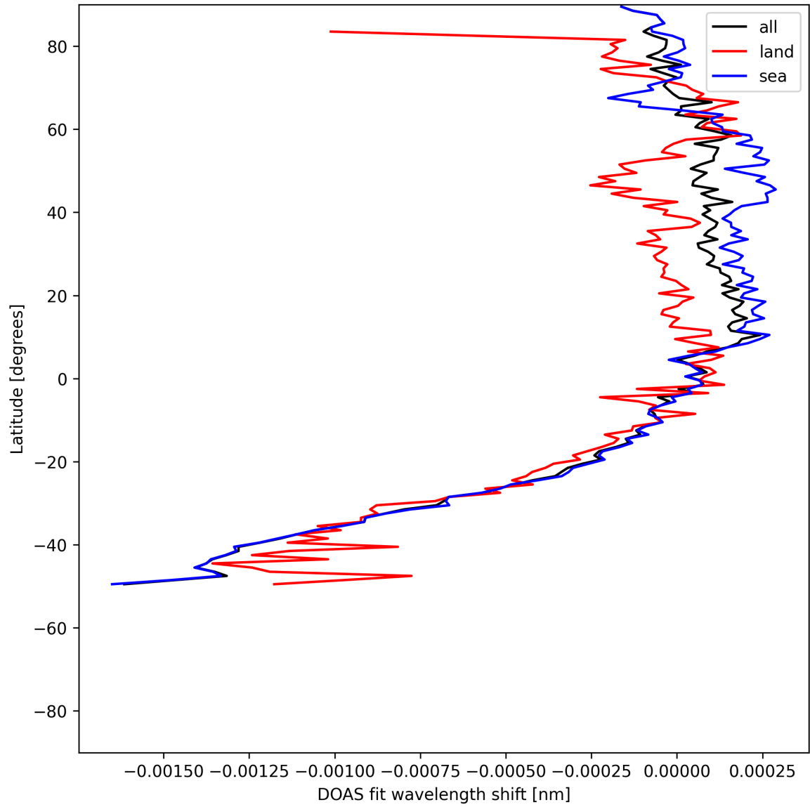
Figure 50: Zonal average of “DOAS fit wavelength shift” for 2025-07-22 to 2025-07-24.
