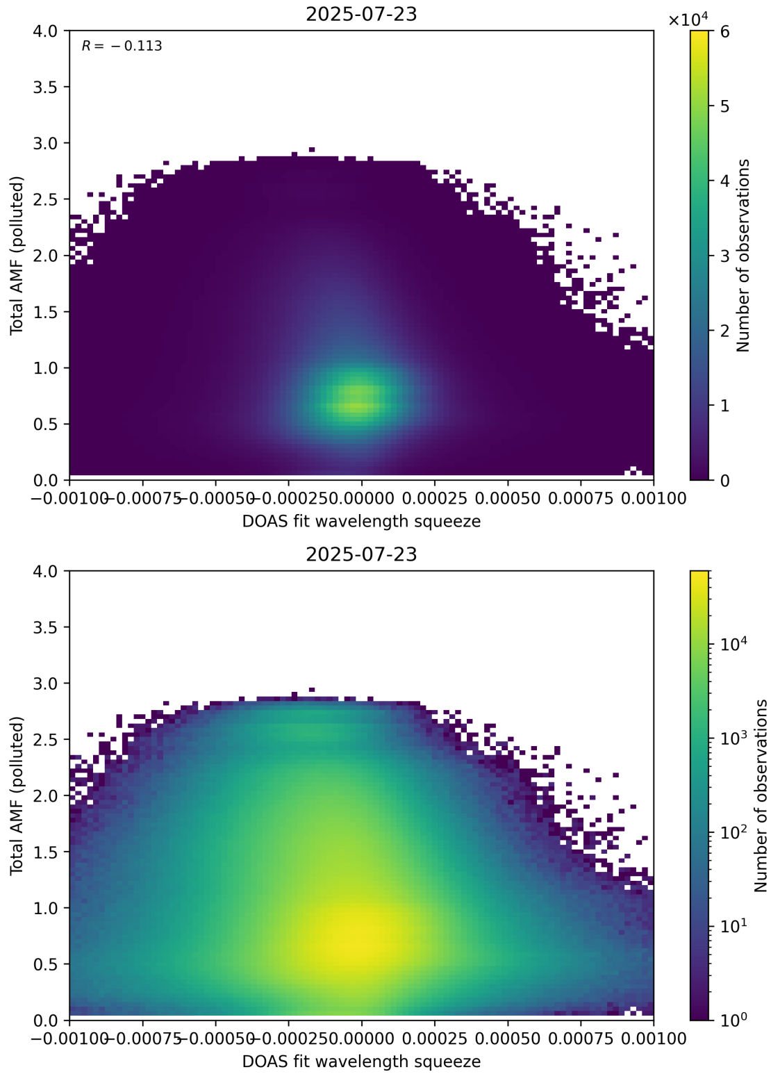
Figure 145: Scatter density plot of “DOAS fit wavelength squeeze” against “Total AMF (polluted)” for 2025-07-22 to 2025-07-24.
