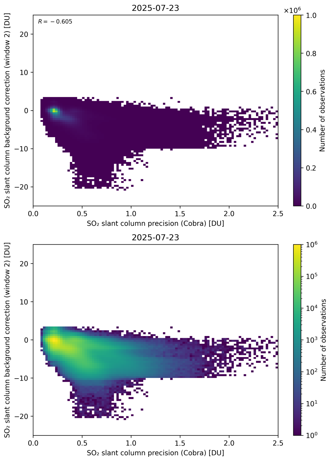
Figure 200: Scatter density plot of “SO 2 slant column precision (Cobra)” against “SO 2 slant column background correction (window 2)” for 2025-07-22 to 2025-07-24.
