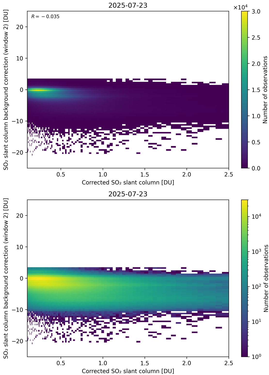
Figure 227: Scatter density plot of “Corrected SO 2 slant column” against “SO 2 slant column background correction (window 2)” for 2025-07-22 to 2025-07-24.
