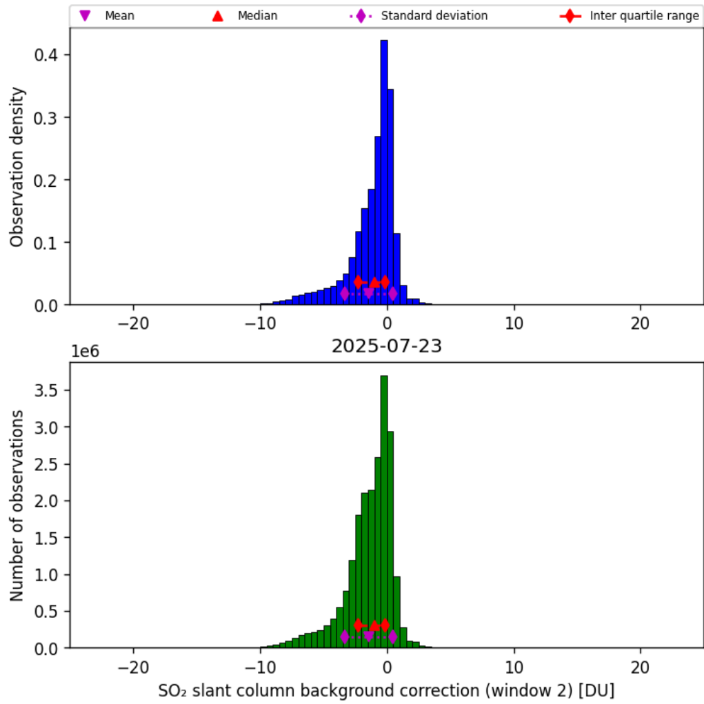
Figure 70: Histogram of “SO 2 slant column background correction (window 2)” for 2025-07-22 to 2025-07-24
