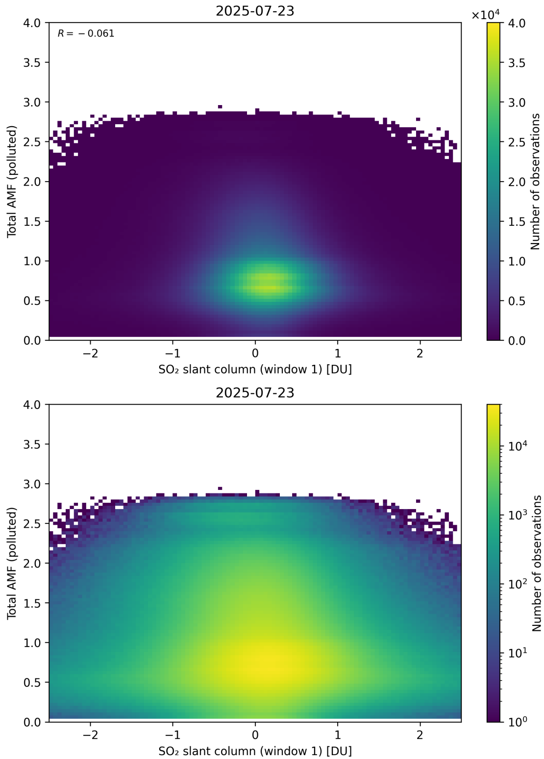
Figure 289: Scatter density plot of “SO 2 slant column (window 1)” against “Total AMF (polluted)” for 2025-07-22 to 2025-07-24.
