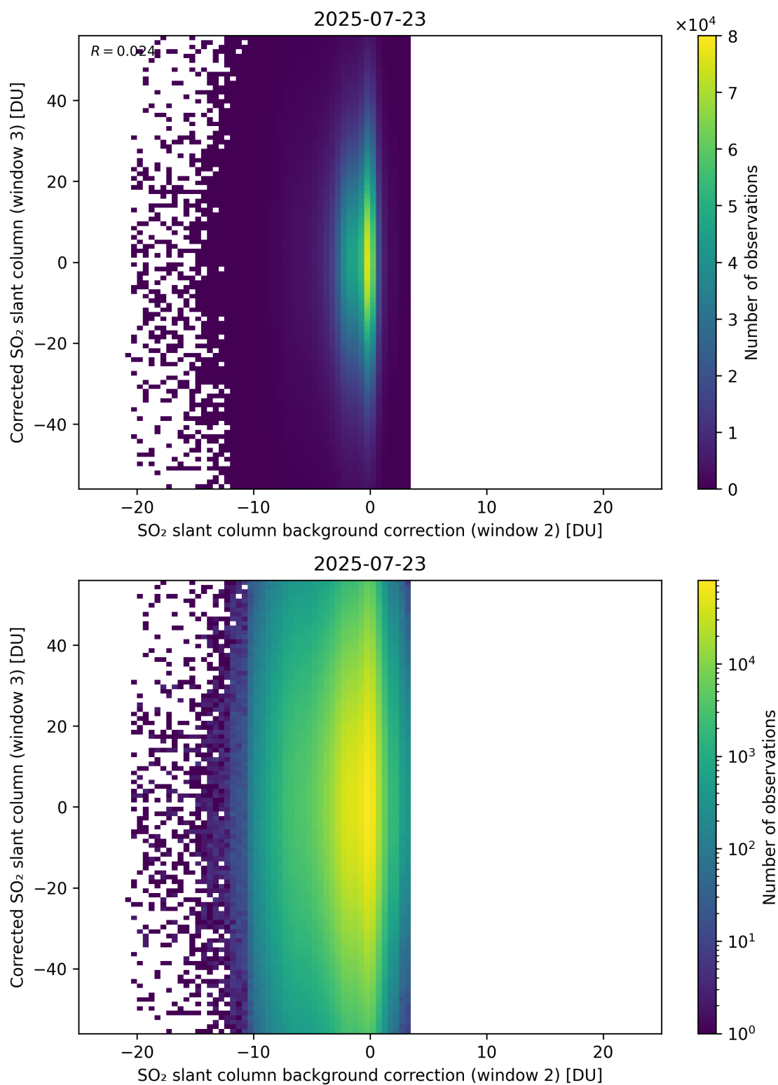
Figure 127: Scatter density plot of “SO 2 slant column background correction (window 2)” against “Corrected SO 2 slant column (window 3)” for 2025-07-22 to 2025-07-24.
