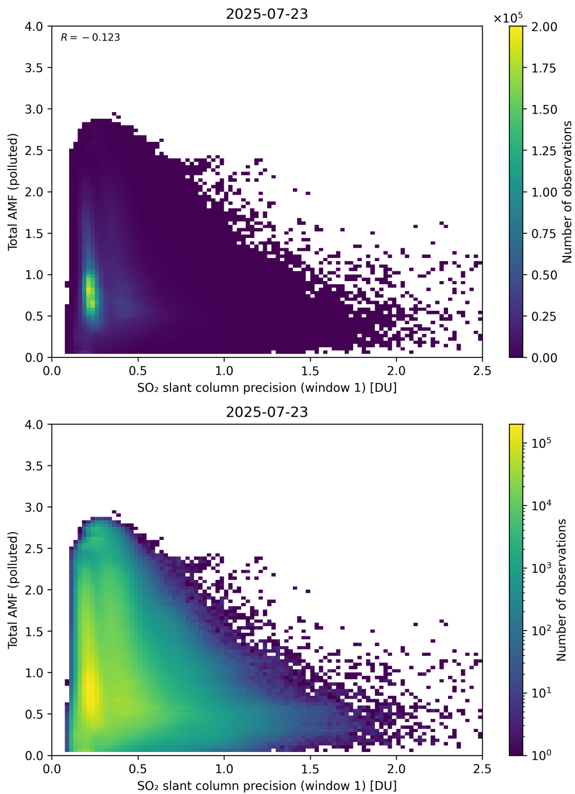
Figure 280: Scatter density plot of “SO 2 slant column precision (window 1)” against “Total AMF (polluted)” for 2025-07-22 to 2025-07-24.
