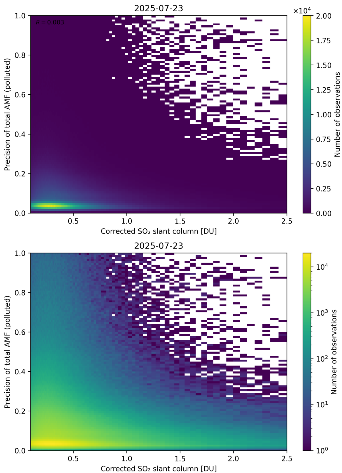
Figure 243: Scatter density plot of “Corrected SO 2 slant column” against “Precision of total AMF (polluted)” for 2025-07-22 to 2025-07-24.
