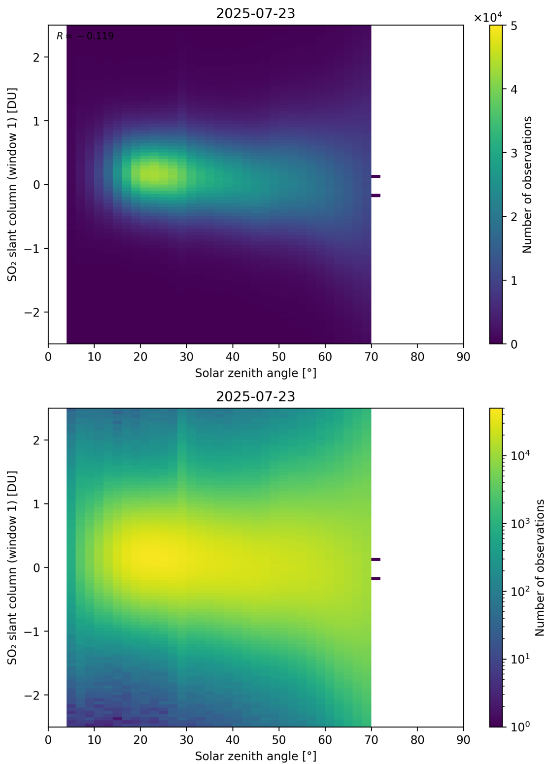
Figure 184: Scatter density plot of “Solar zenith angle” against “SO 2 slant column (window 1)” for 2025-07-22 to 2025-07-24.
