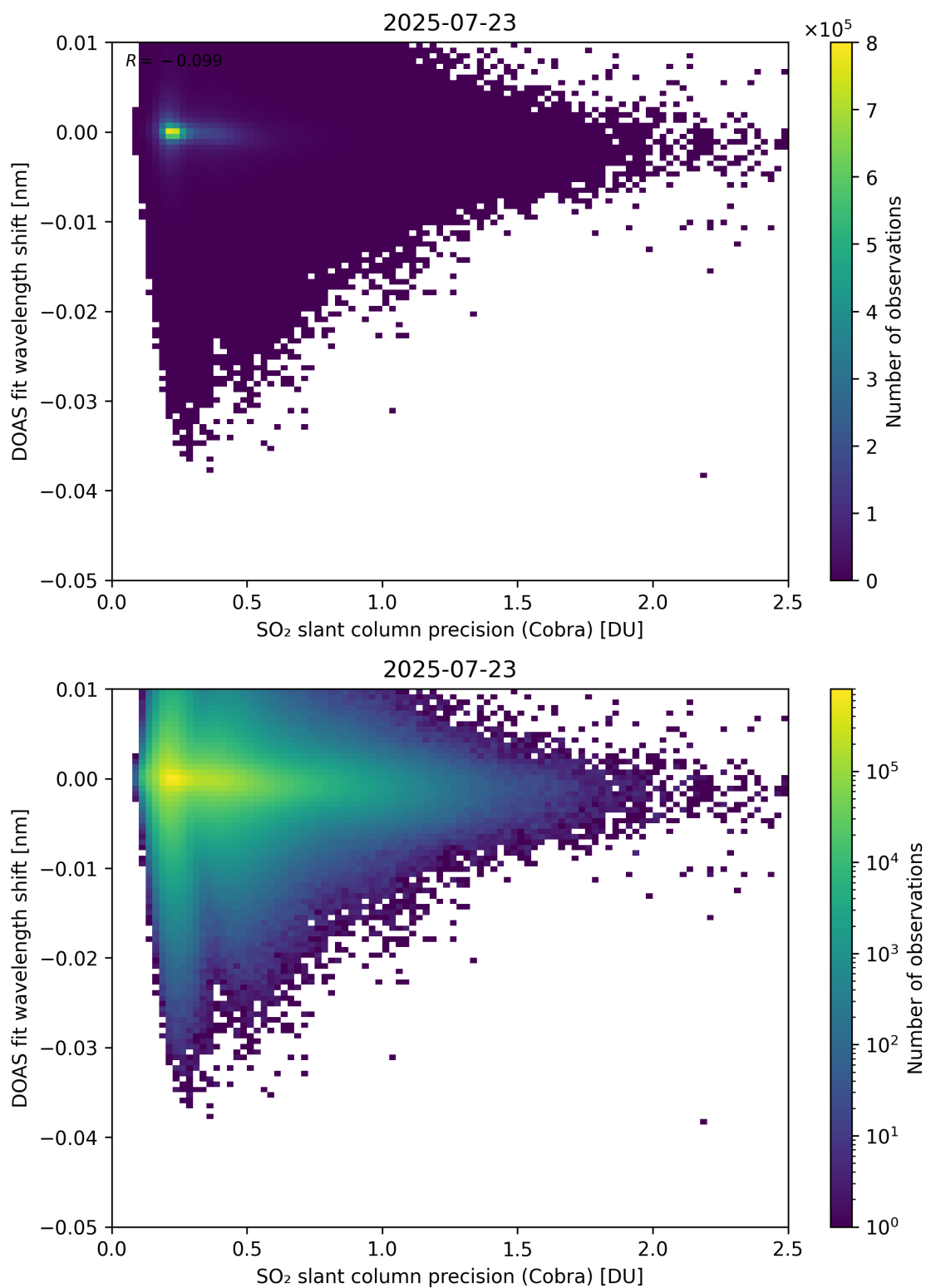
Figure 202: Scatter density plot of “SO 2 slant column precision (Cobra)” against “DOAS fit wavelength shift” for 2025-07-22 to 2025-07-24.
