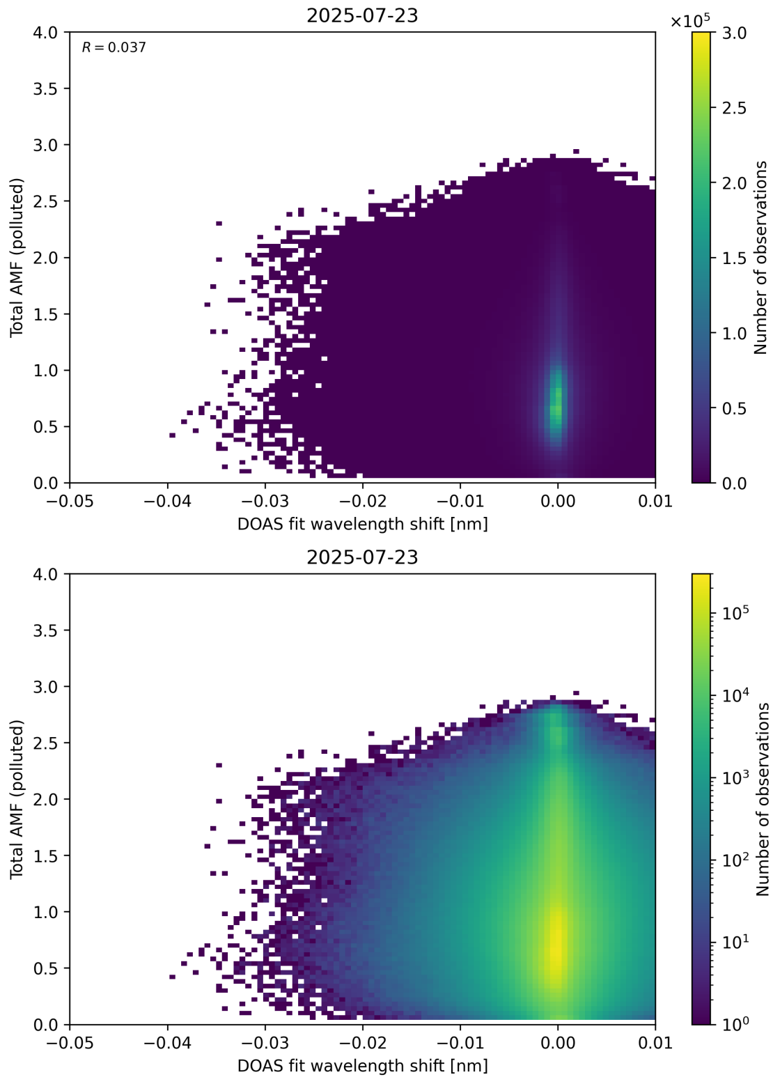
Figure 141: Scatter density plot of “DOAS fit wavelength shift” against “Total AMF (polluted)” for 2025-07-22 to 2025-07-24.
