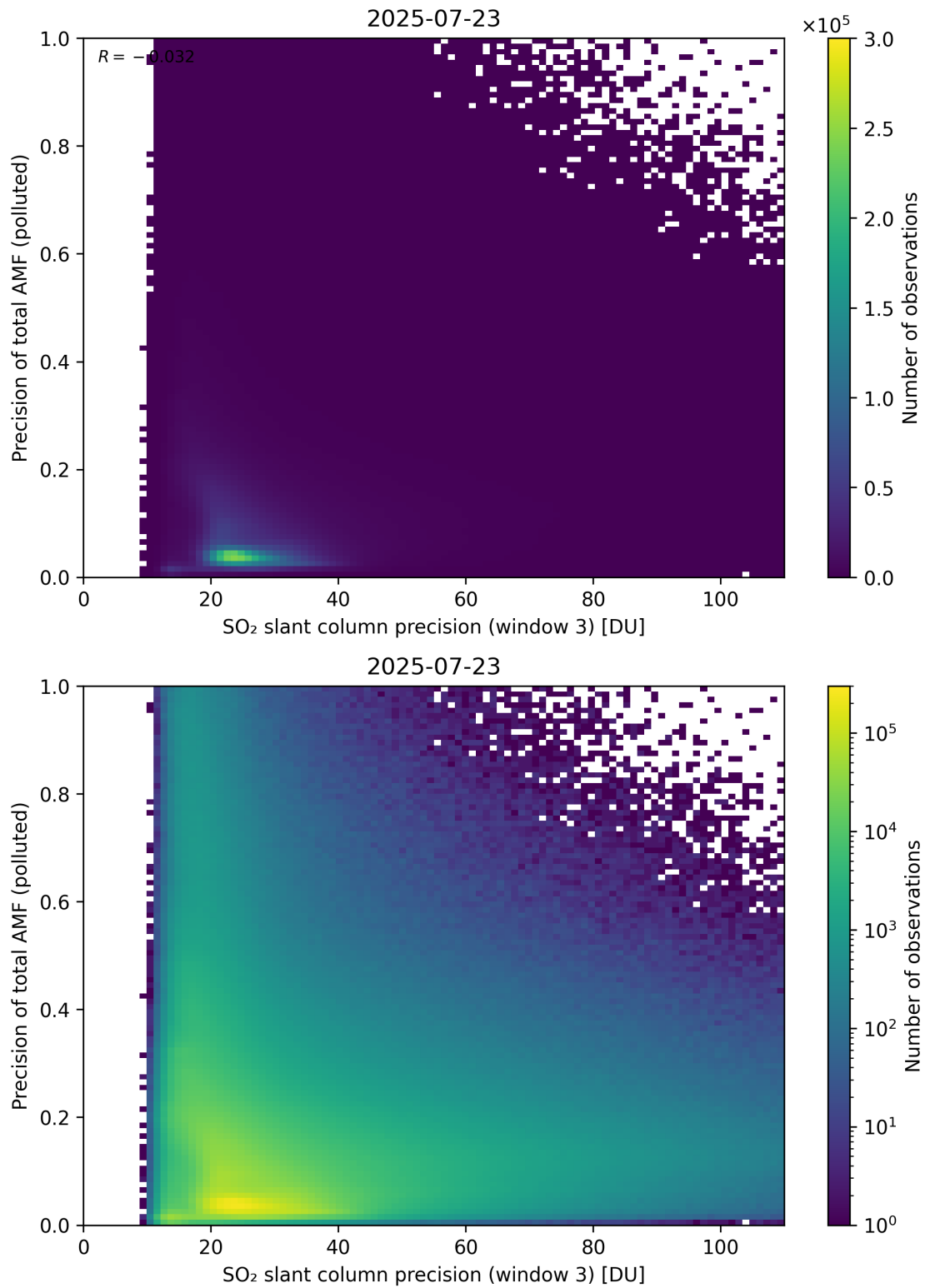
Figure 314: Scatter density plot of “SO 2 slant column precision (window 3)” against “Precision of total AMF (polluted)” for 2025-07-22 to 2025-07-24.
