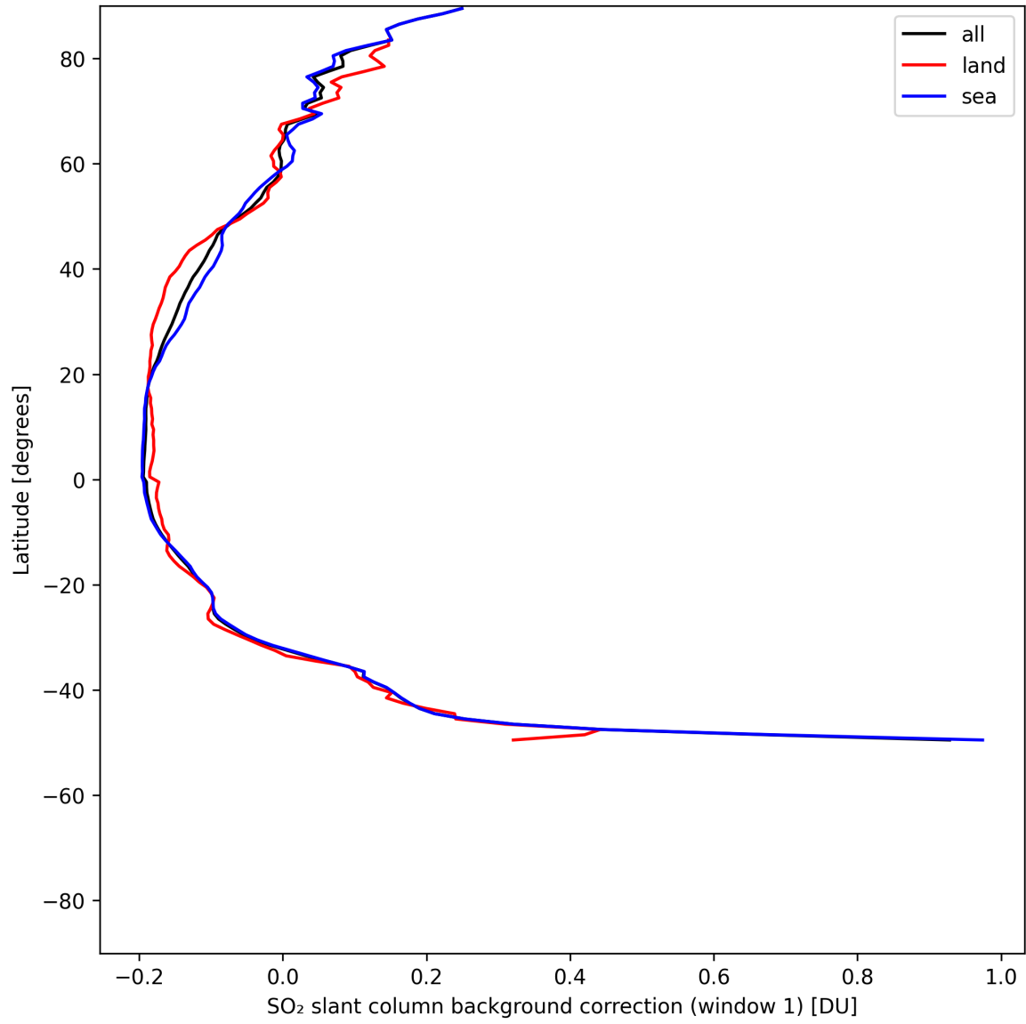
Figure 40: Zonal average of “SO 2 slant column background correction (window 1)” for 2025-07-22 to 2025-07-24.
