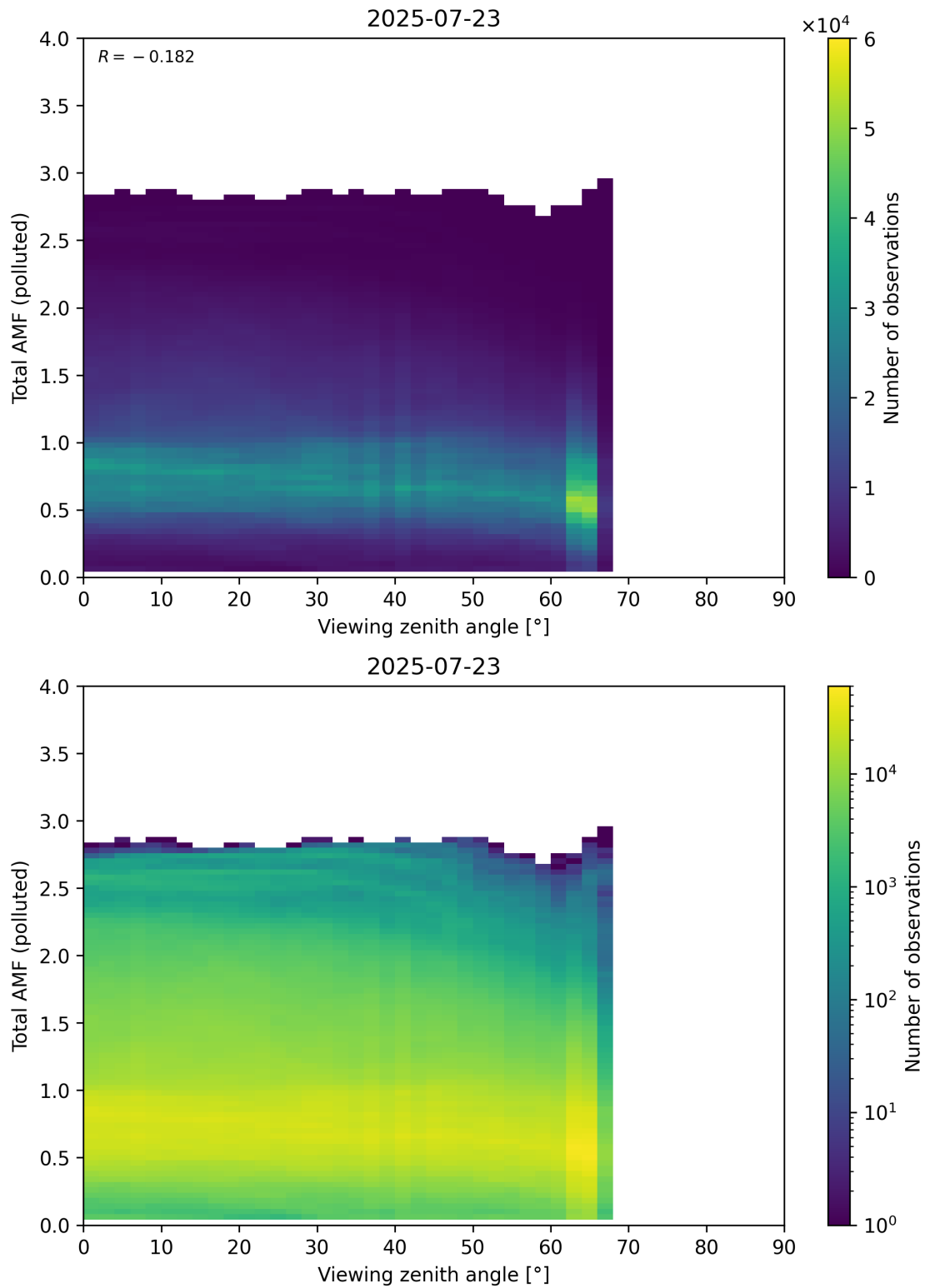
Figure 381: Scatter density plot of “Viewing zenith angle” against “Total AMF (polluted)” for 2025-07-22 to 2025-07-24.
