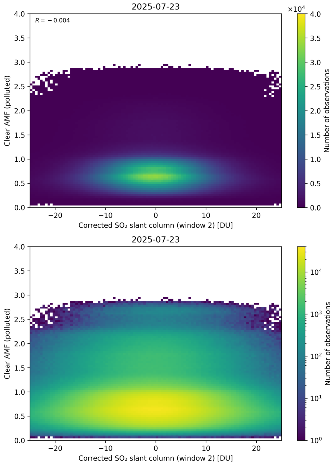
Figure 249: Scatter density plot of “Corrected SO 2 slant column (window 2)” against “Clear AMF (polluted)” for 2025-07-22 to 2025-07-24.
