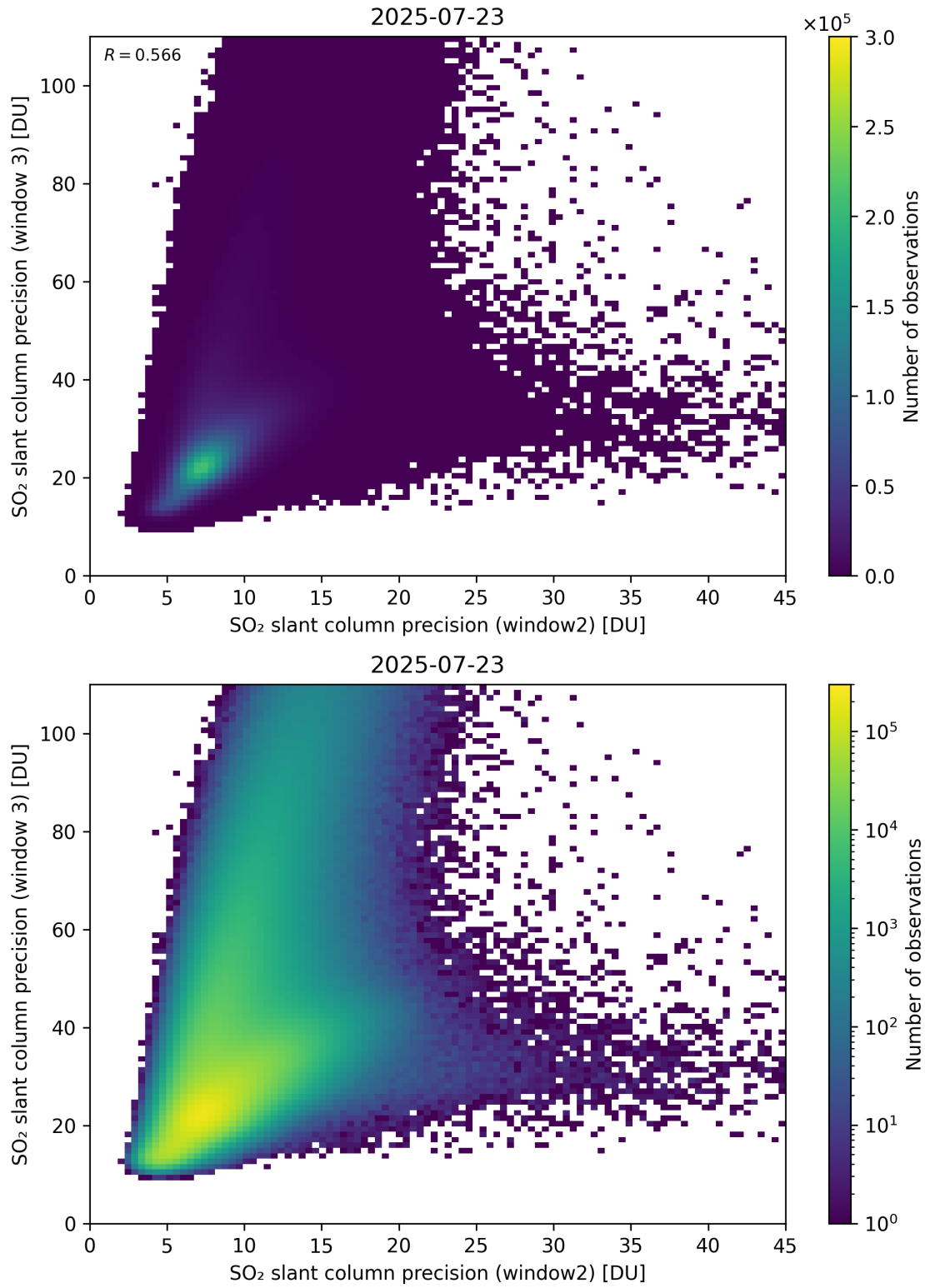
Figure 300: Scatter density plot of “SO 2 slant column precision (window2)” against “SO 2 slant column precision (window 3)” for 2025-07-22 to 2025-07-24.
