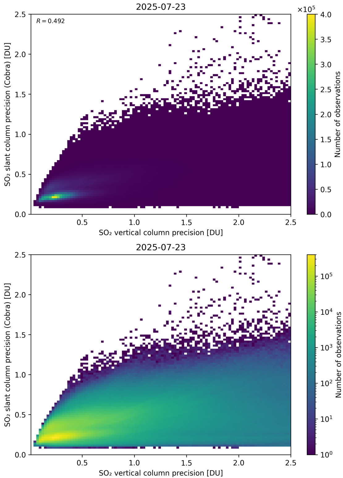
Figure 337: Scatter density plot of “SO 2 vertical column precision” against “SO 2 slant column precision (Cobra)” for 2025-07-22 to 2025-07-24.
