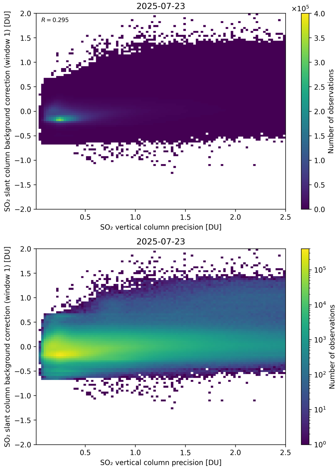
Figure 329: Scatter density plot of “SO 2 vertical column precision” against “SO 2 slant column background correction (window 1)” for 2025-07-22 to 2025-07-24.
