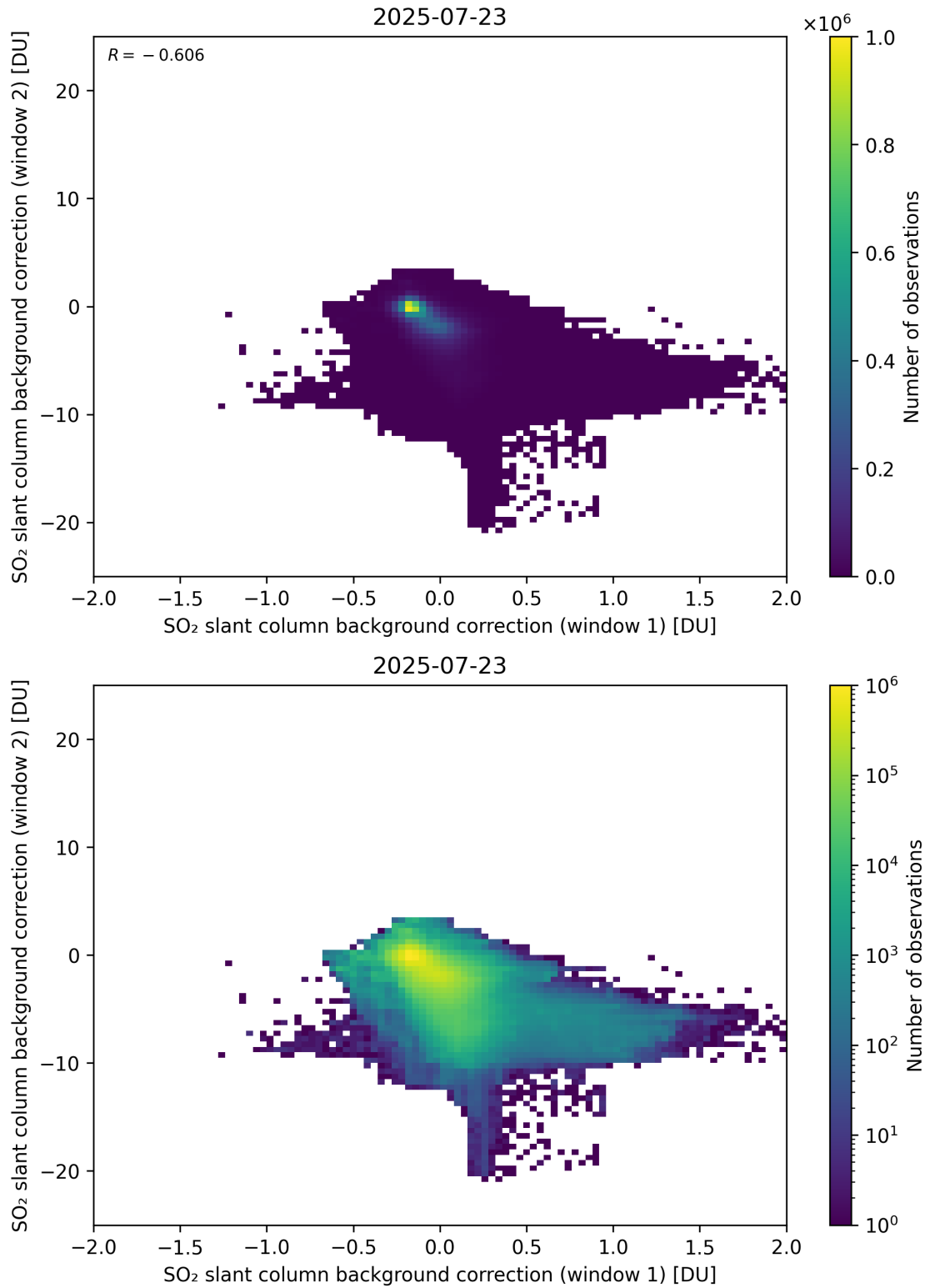
Figure 109: Scatter density plot of “SO 2 slant column background correction (window 1)” against “SO 2 slant column background correction (window 2)” for 2025-07-22 to 2025-07-24.
