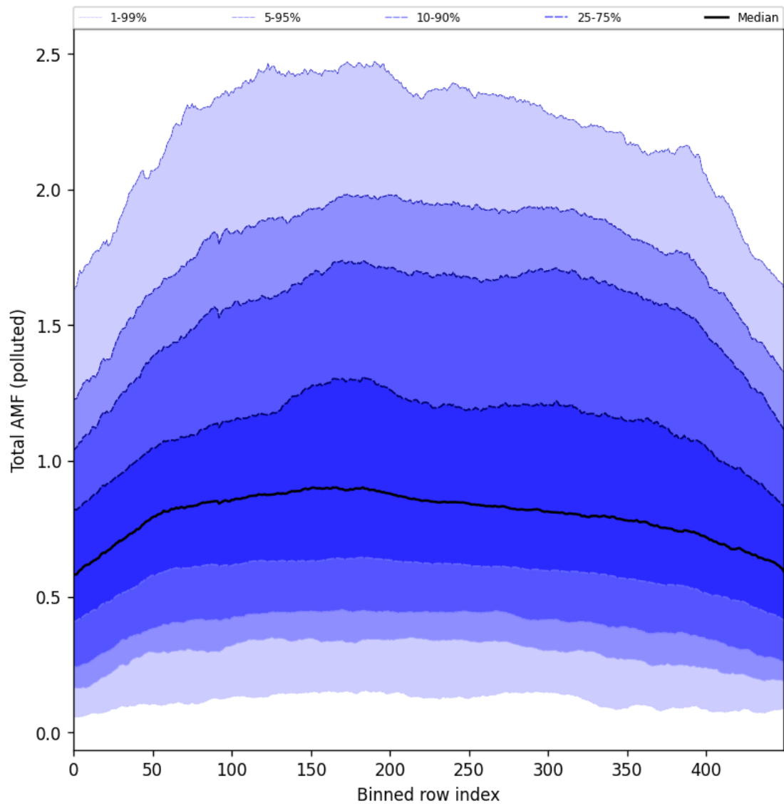
Figure 105: Along track statistics of “Total AMF (polluted)” for 2025-07-22 to 2025-07-24
