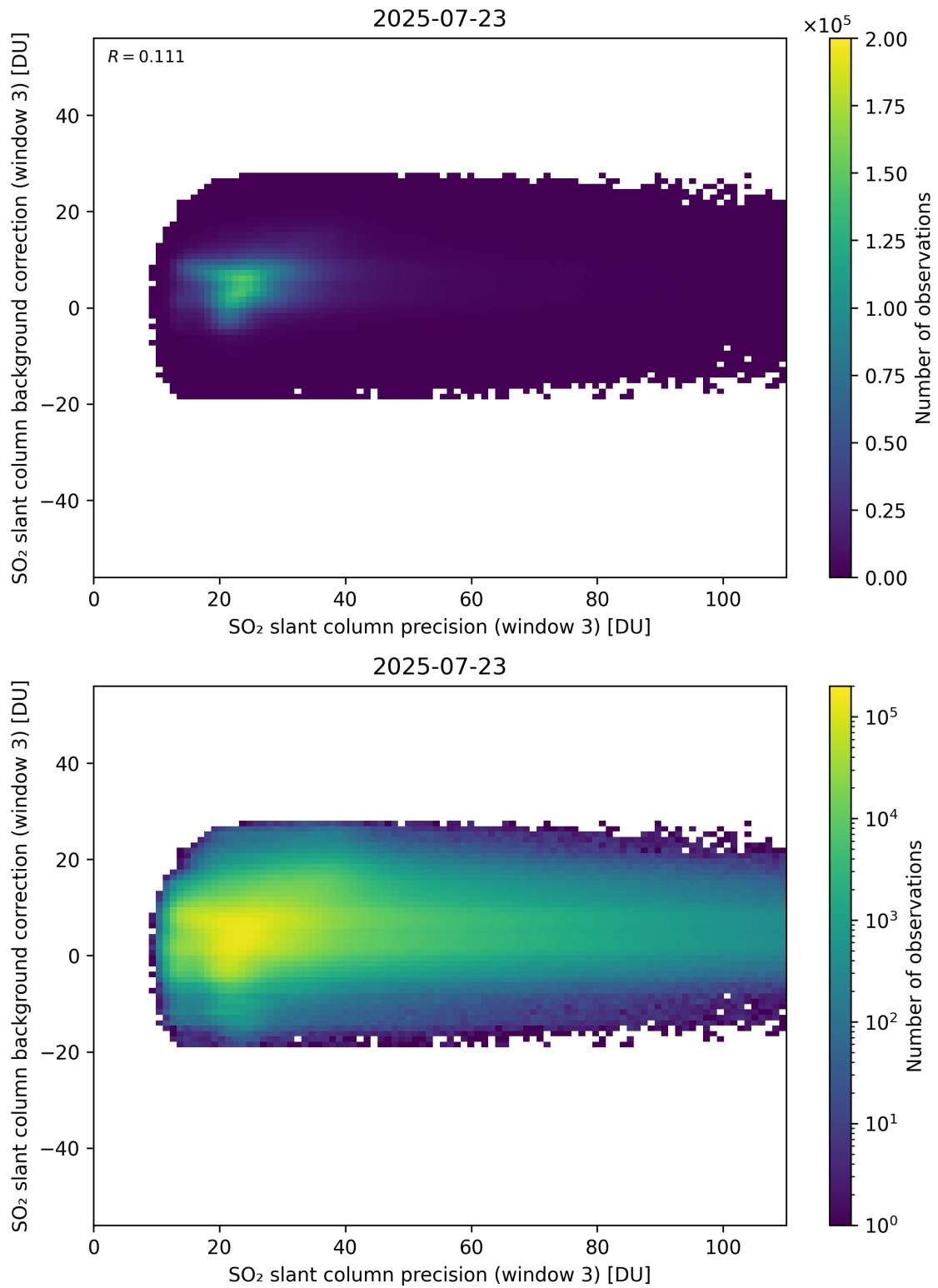
Figure 307: Scatter density plot of “SO 2 slant column precision (window 3)” against “SO 2 slant column background correction (window 3)” for 2025-07-22 to 2025-07-24.
