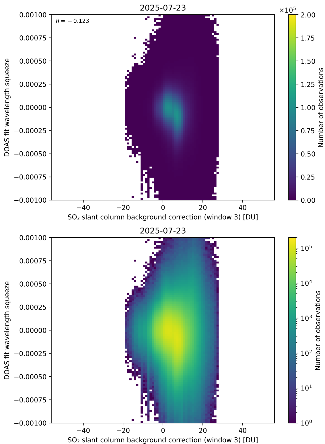
Figure 133: Scatter density plot of “SO 2 slant column background correction (window 3)” against “DOAS fit wavelength squeeze” for 2025-07-22 to 2025-07-24.
