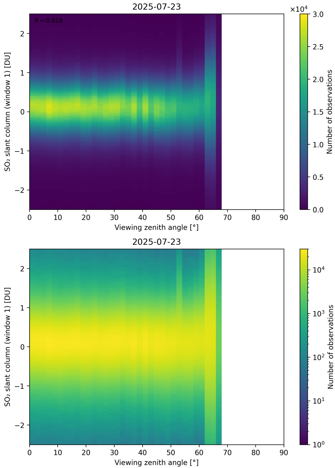
Figure 376: Scatter density plot of “Viewing zenith angle” against “SO 2 slant column (window 1)” for 2025-07-22 to 2025-07-24.
