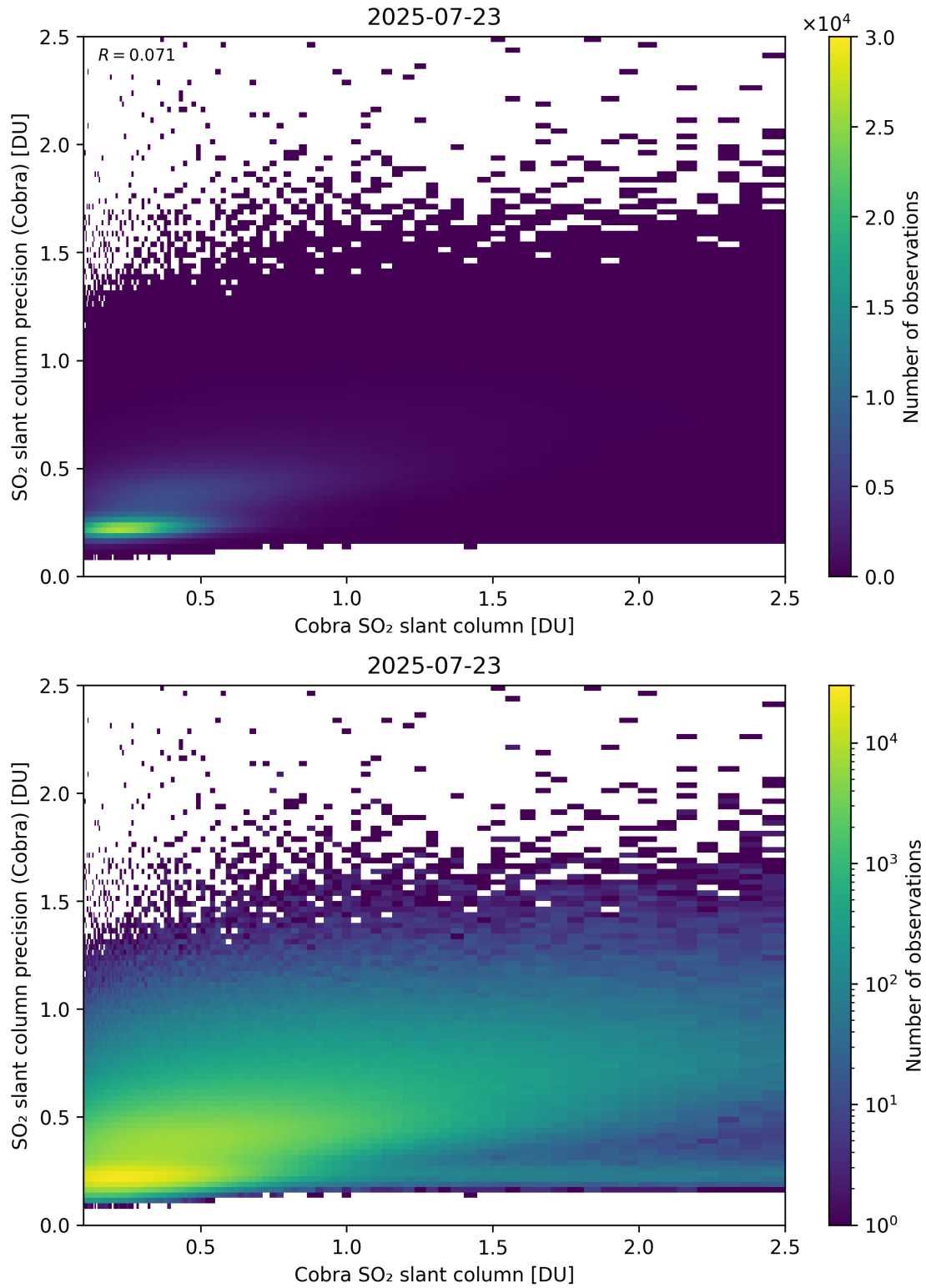
Figure 216: Scatter density plot of “Cobra SO 2 slant column” against “SO 2 slant column precision (Cobra)” for 2025-07-22 to 2025-07-24.
