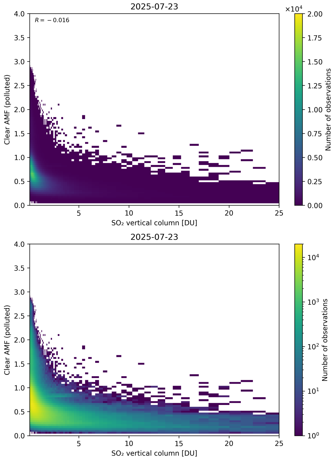
Figure 348: Scatter density plot of “SO 2 vertical column” against “Clear AMF (polluted)” for 2025-07-22 to 2025-07-24.
