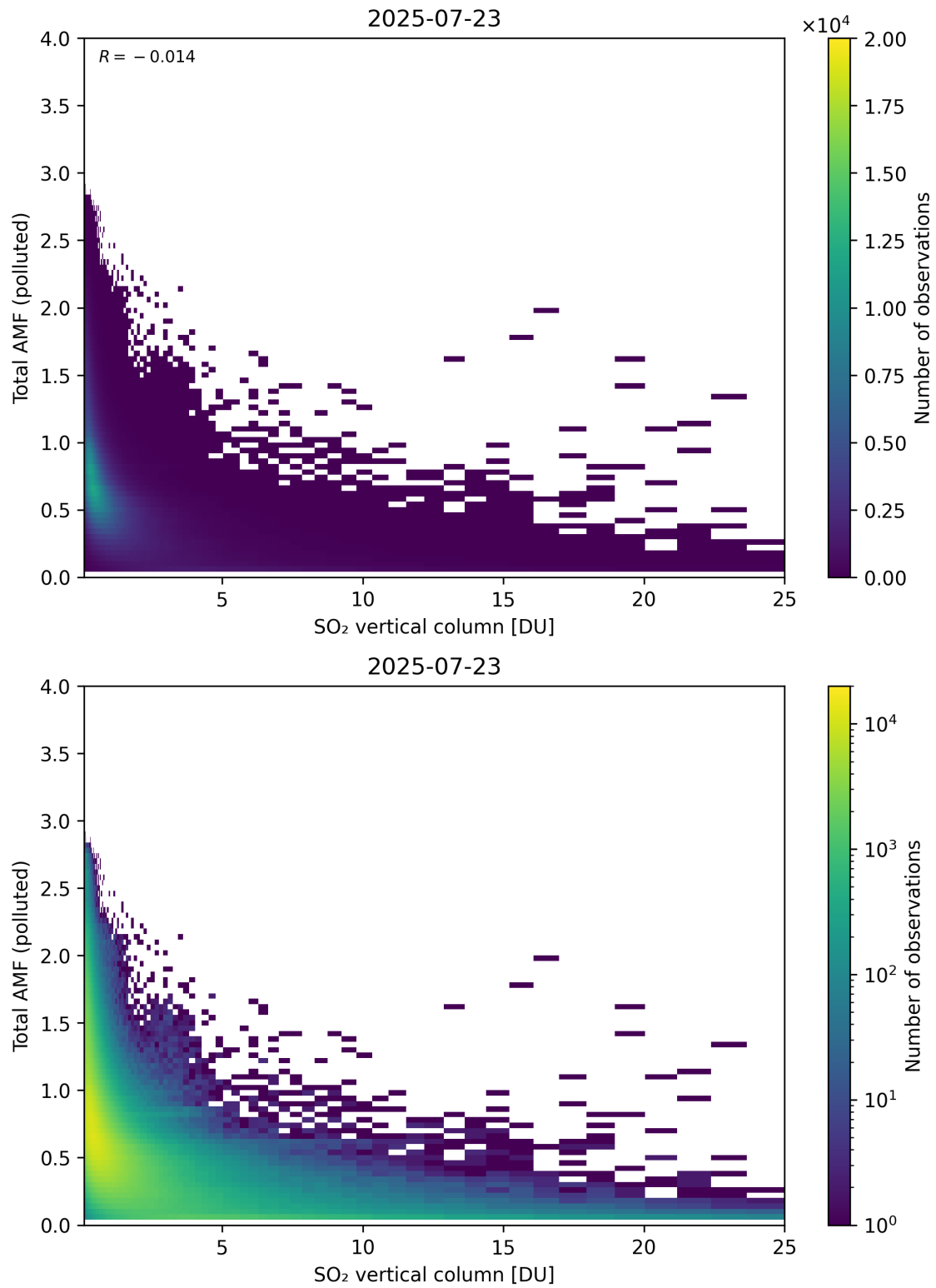
Figure 359: Scatter density plot of “SO 2 vertical column” against “Total AMF (polluted)” for 2025-07-22 to 2025-07-24.
