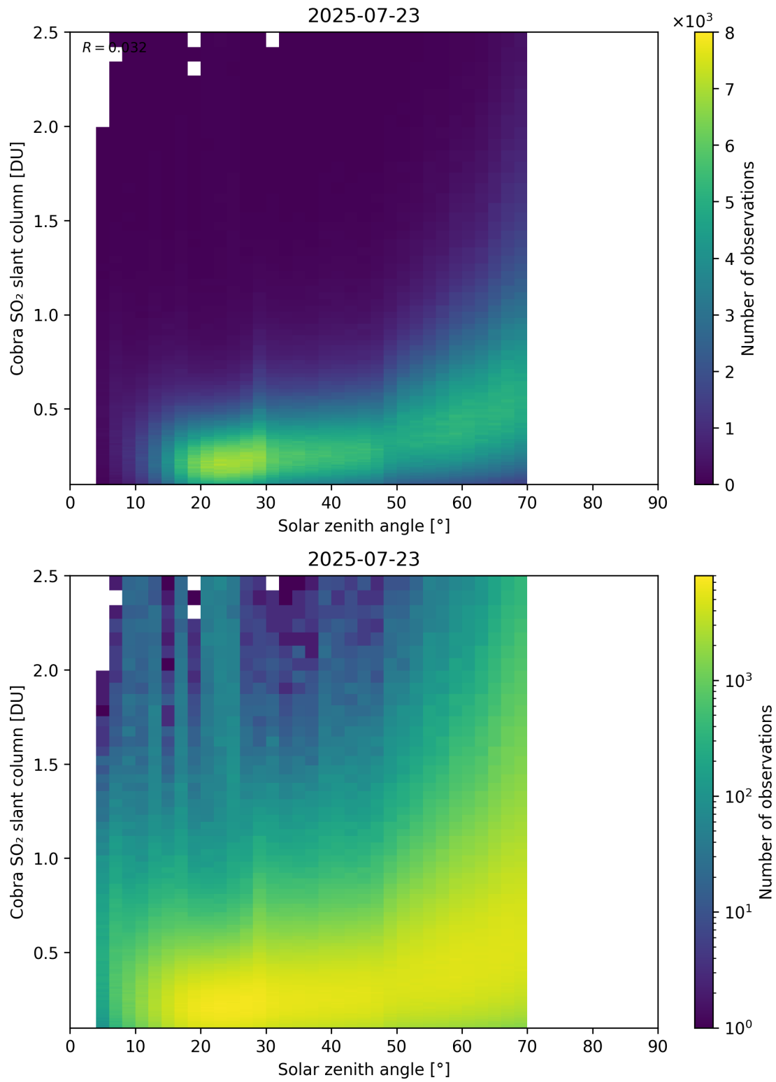
Figure 179: Scatter density plot of “Solar zenith angle” against “Cobra SO 2 slant column” for 2025-07-22 to 2025-07-24.
