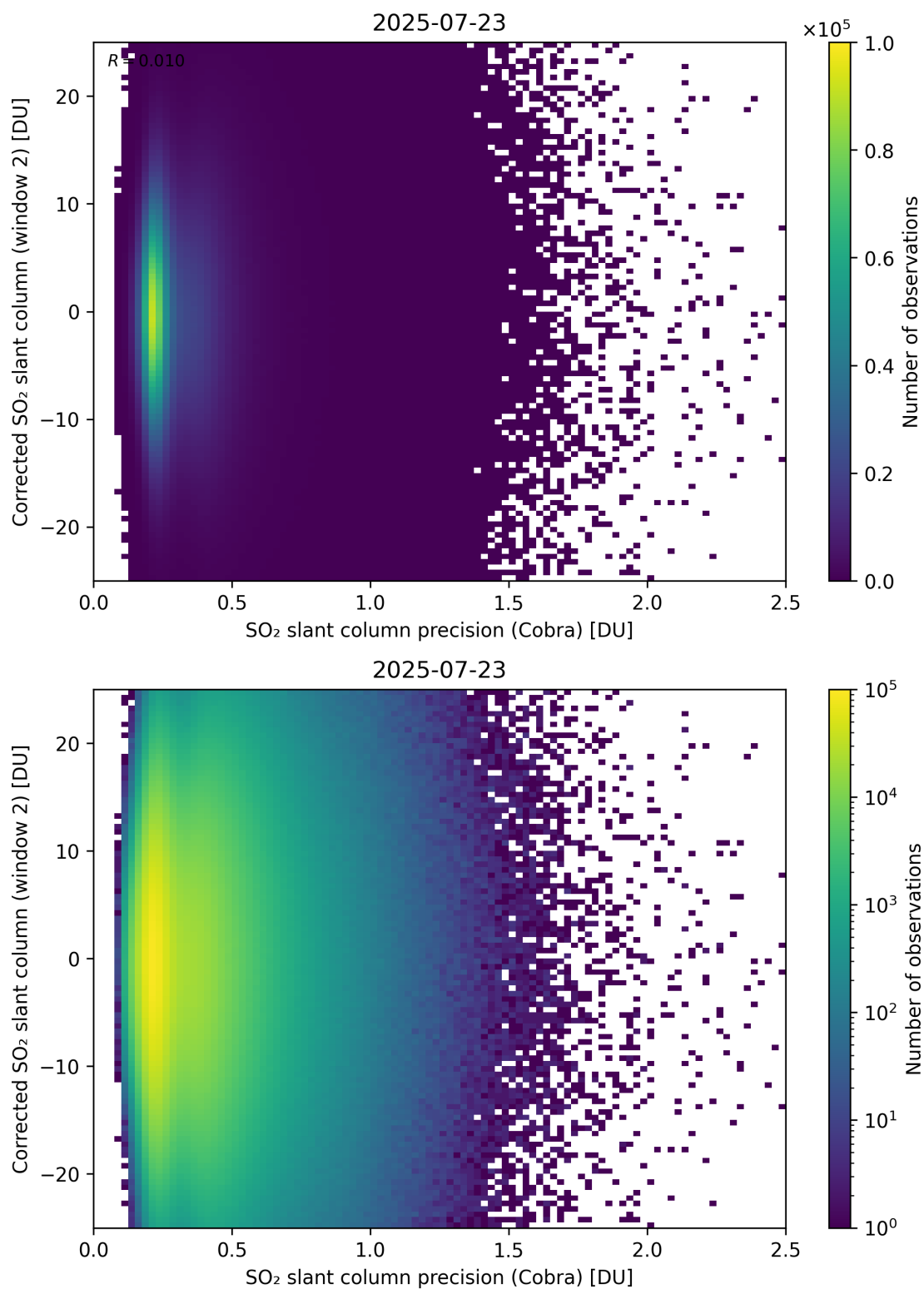
Figure 206: Scatter density plot of “SO 2 slant column precision (Cobra)” against “Corrected SO 2 slant column (window 2)” for 2025-07-22 to 2025-07-24.
