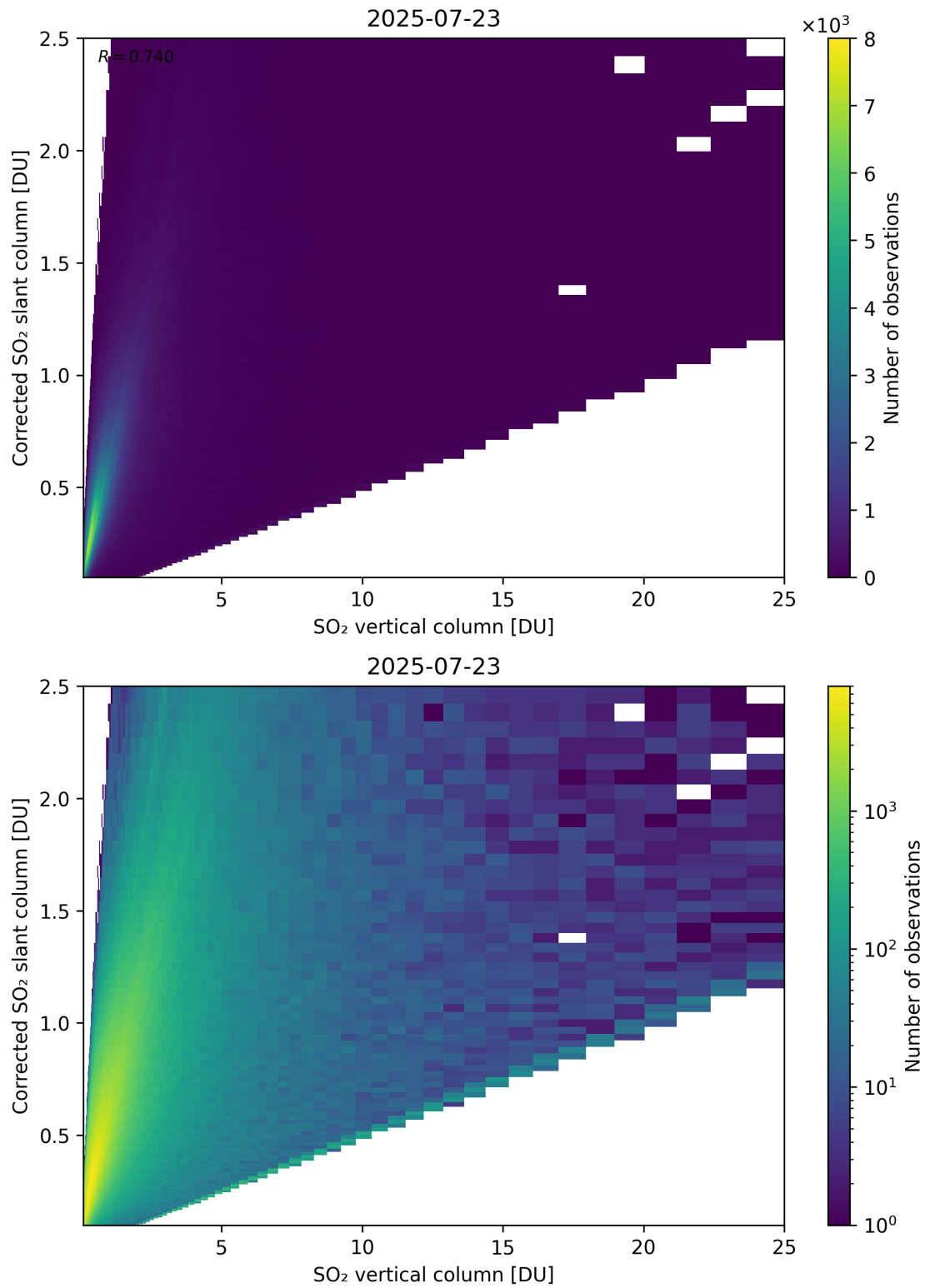
Figure 351: Scatter density plot of “SO 2 vertical column” against “Corrected SO 2 slant column” for 2025-07-22 to 2025-07-24.
