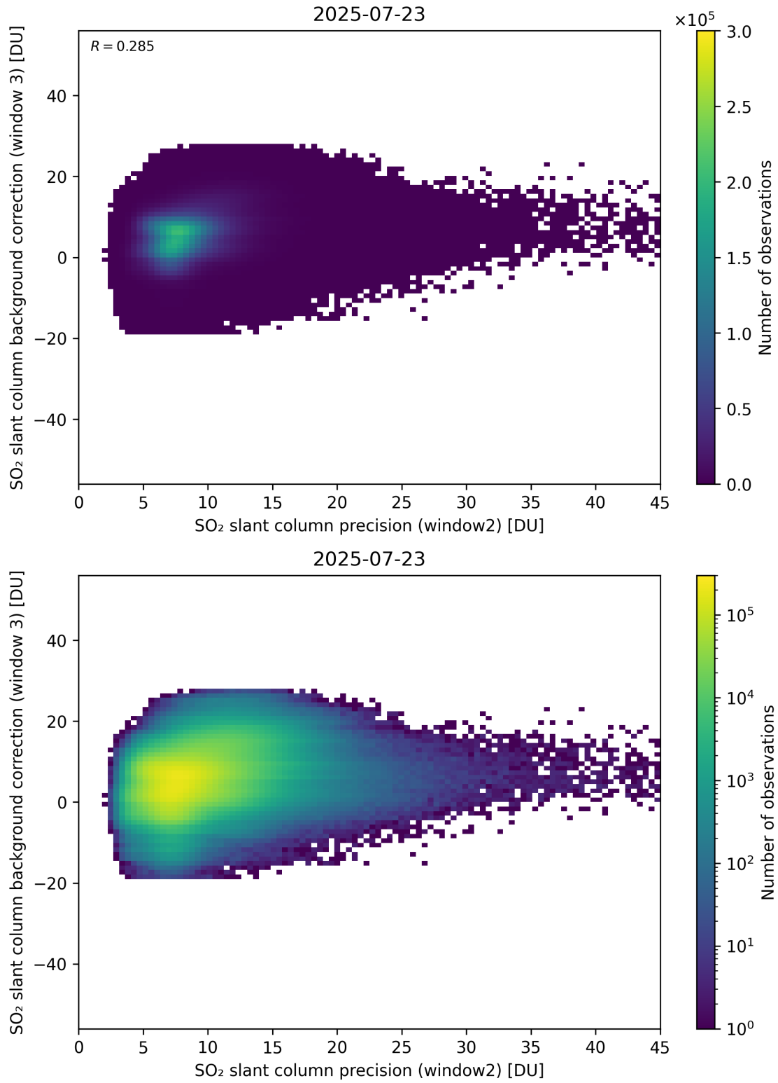
Figure 292: Scatter density plot of “SO 2 slant column precision (window2)” against “SO 2 slant column background correction (window 3)” for 2025-07-22 to 2025-07-24.
