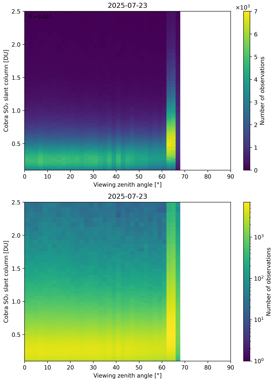
Figure 371: Scatter density plot of “Viewing zenith angle” against “Cobra SO 2 slant column” for 2025-07-22 to 2025-07-24.
