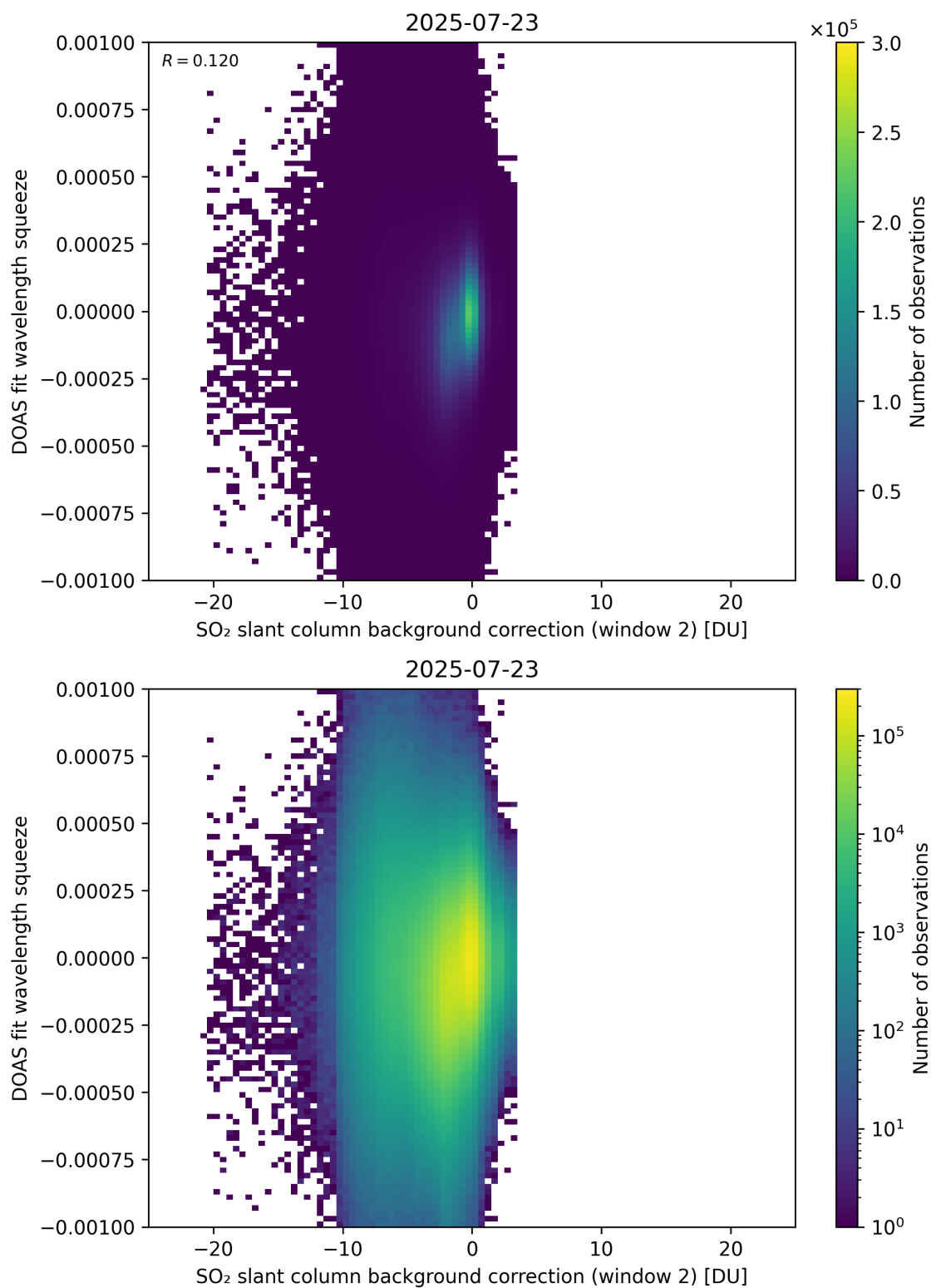
Figure 124: Scatter density plot of “SO 2 slant column background correction (window 2)” against “DOAS fit wavelength squeeze” for 2025-07-22 to 2025-07-24.
