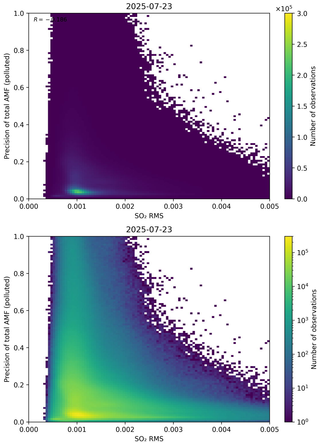
Figure 149: Scatter density plot of “SO 2 RMS” against “Precision of total AMF (polluted)” for 2025-07-22 to 2025-07-24.
