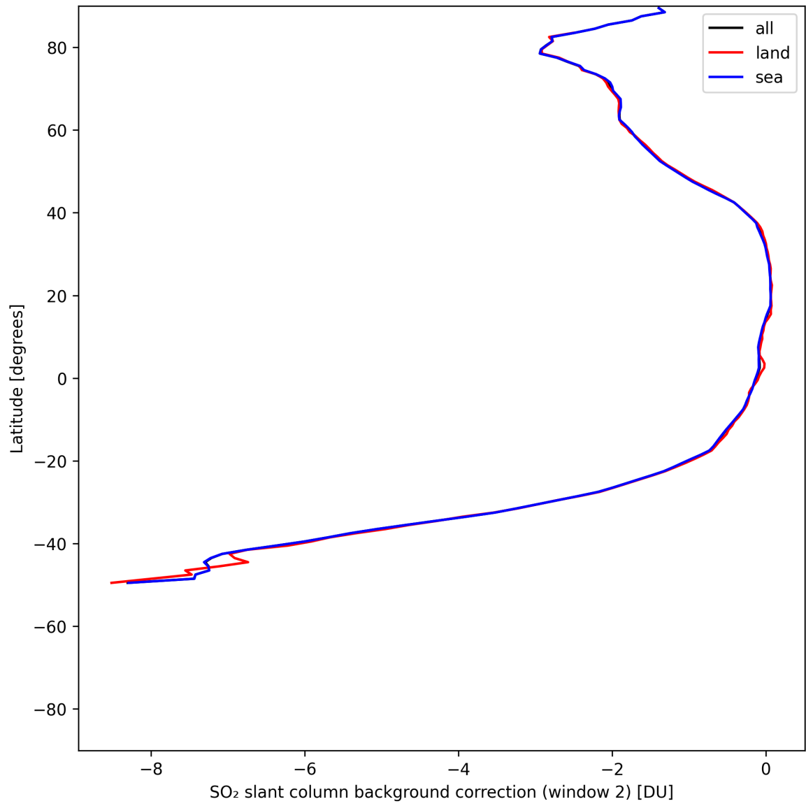
Figure 44: Zonal average of “SO 2 slant column background correction (window 2)” for 2025-07-22 to 2025-07-24.
