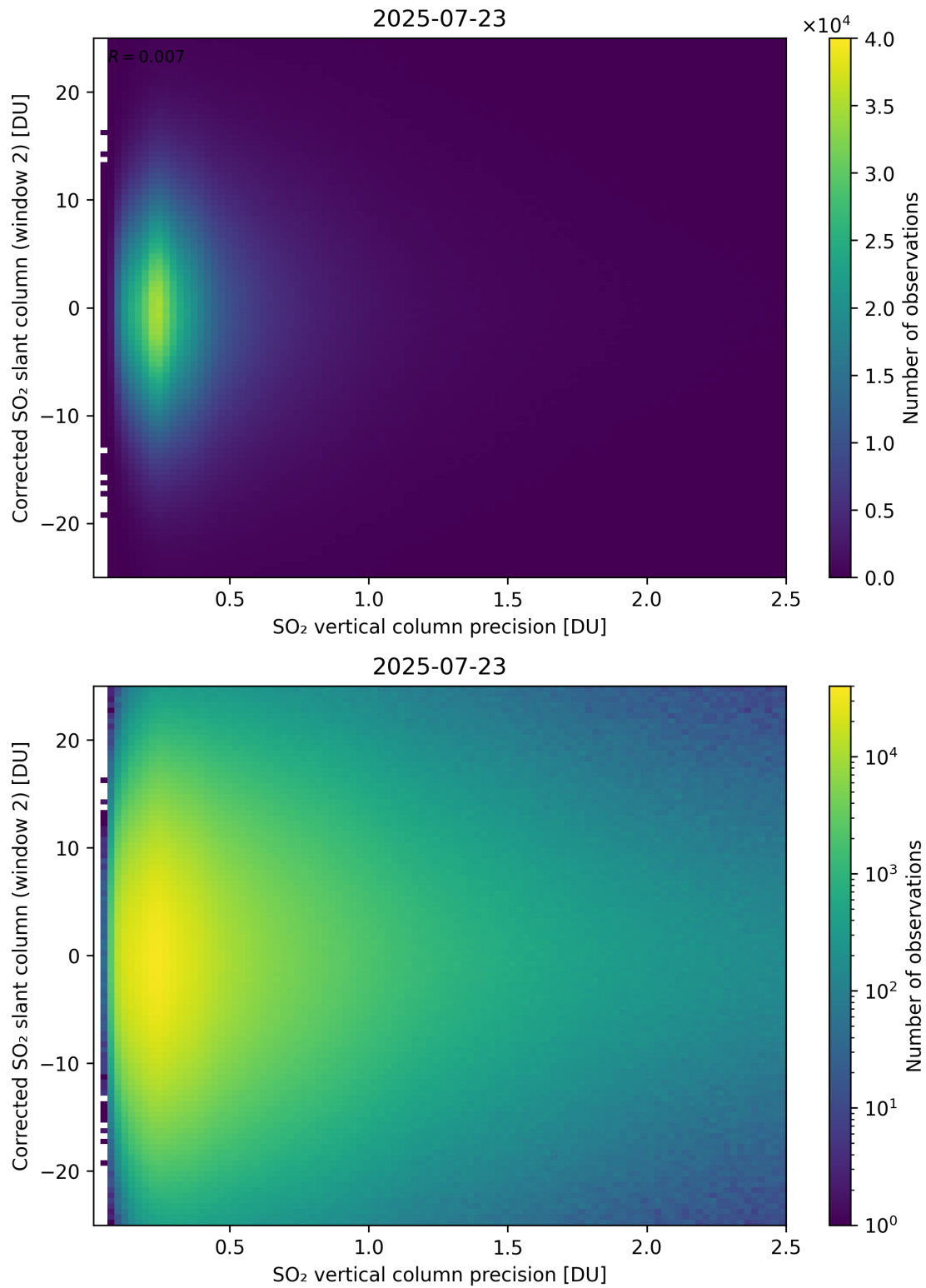
Figure 339: Scatter density plot of “SO 2 vertical column precision” against “Corrected SO 2 slant column (window 2)” for 2025-07-22 to 2025-07-24.
