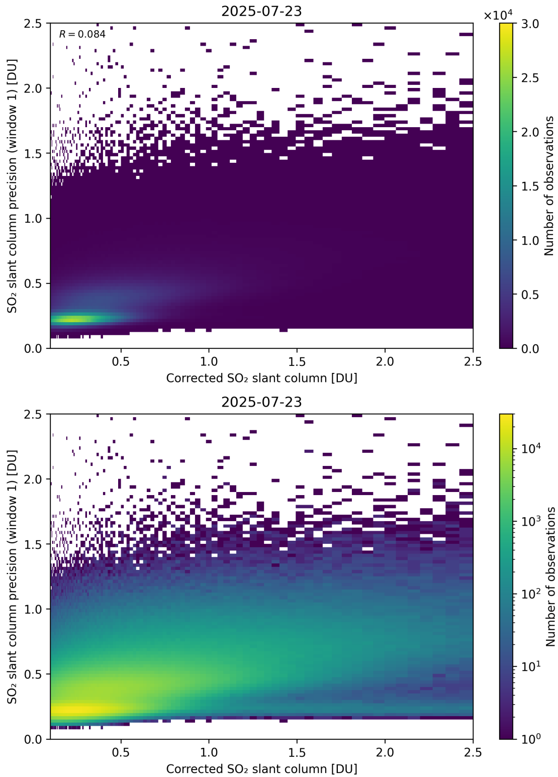
Figure 238: Scatter density plot of “Corrected SO 2 slant column” against “SO 2 slant column precision (window 1)” for 2025-07-22 to 2025-07-24.
