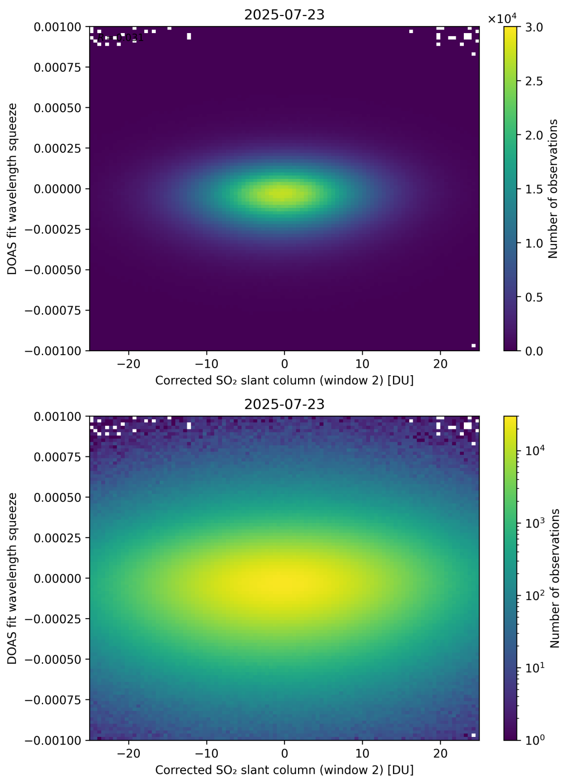
Figure 247: Scatter density plot of “Corrected SO 2 slant column (window 2)” against “DOAS fit wavelength squeeze” for 2025-07-22 to 2025-07-24.
