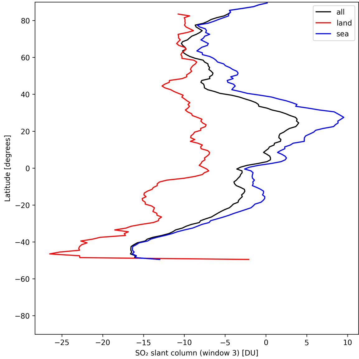
Figure 45: Zonal average of “SO 2 slant column (window 3)” for 2025-07-22 to 2025-07-24.
