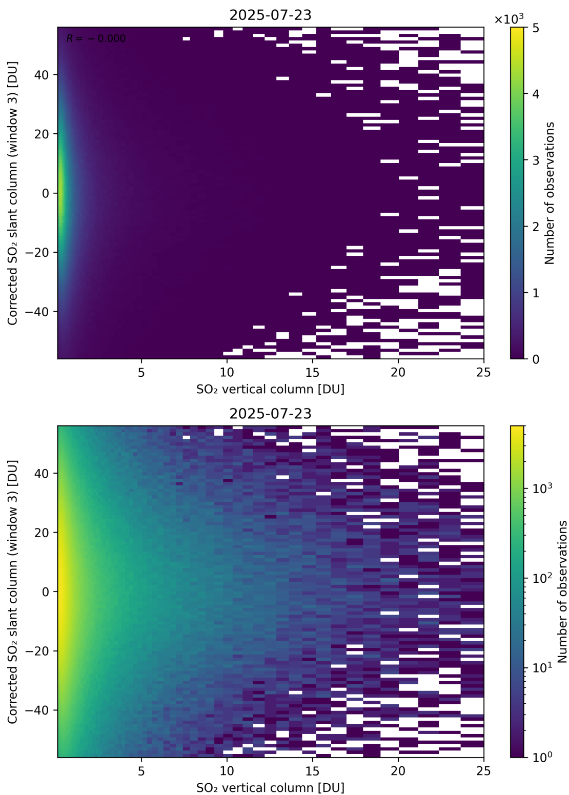
Figure 353: Scatter density plot of “SO 2 vertical column” against “Corrected SO 2 slant column (window 3)” for 2025-07-22 to 2025-07-24.
