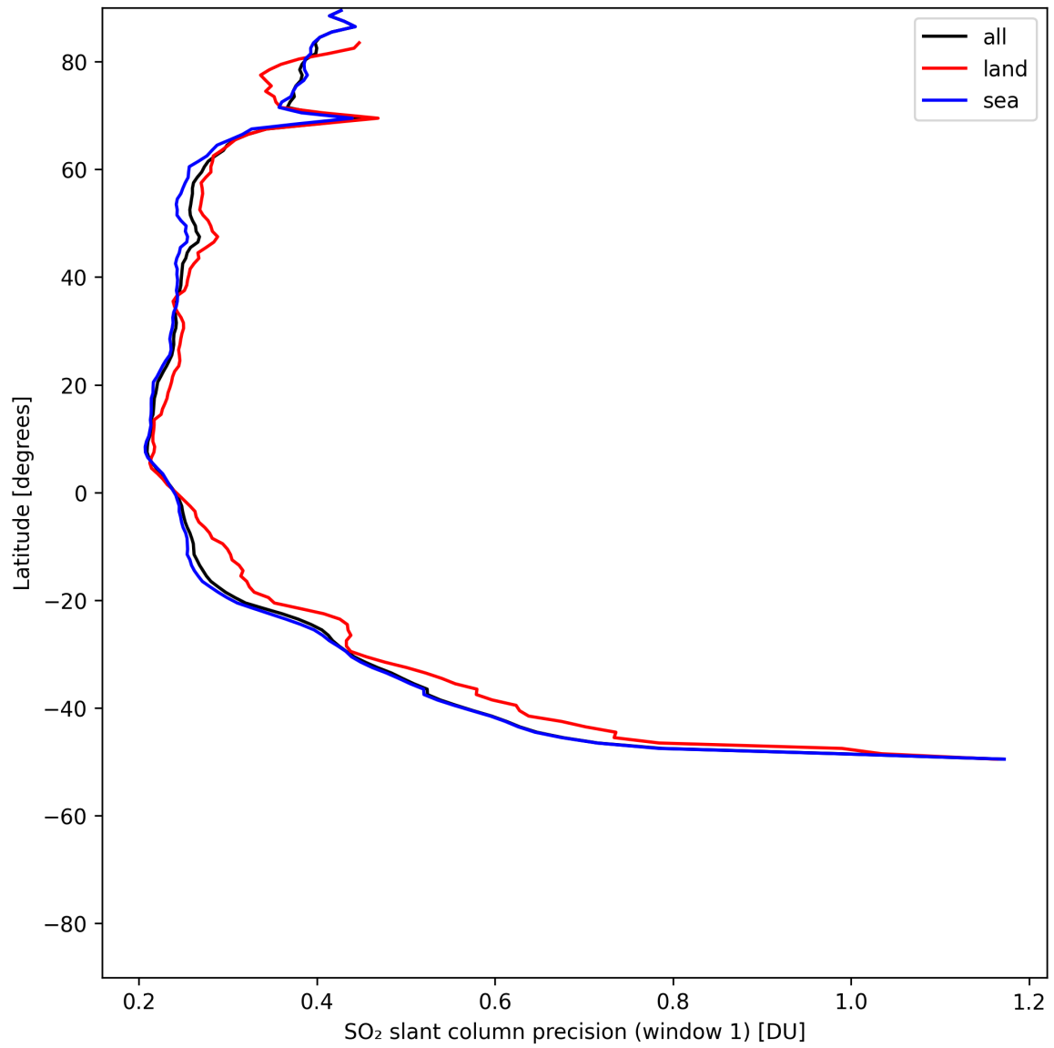
Figure 38: Zonal average of “SO 2 slant column precision (window 1)” for 2025-07-22 to 2025-07-24.
