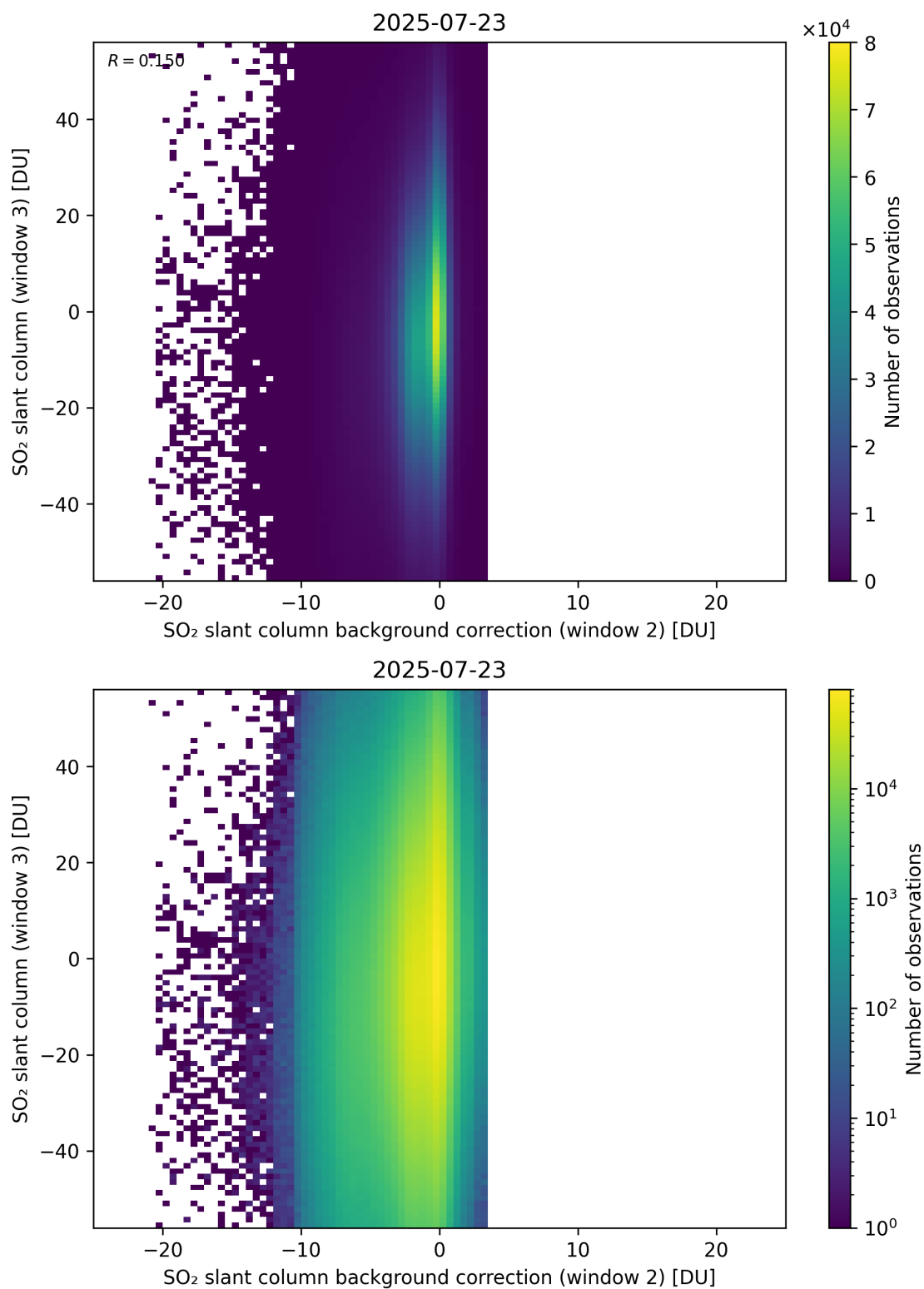
Figure 128: Scatter density plot of “SO 2 slant column background correction (window 2)” against “SO 2 slant column (window 3)” for 2025-07-22 to 2025-07-24.
