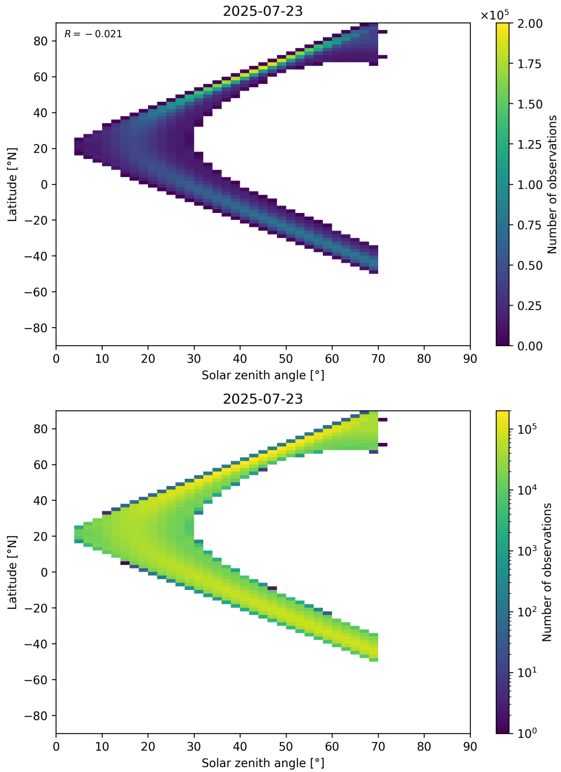
Figure 177: Scatter density plot of “Solar zenith angle” against “Latitude” for 2025-07-22 to 2025-07-24.
