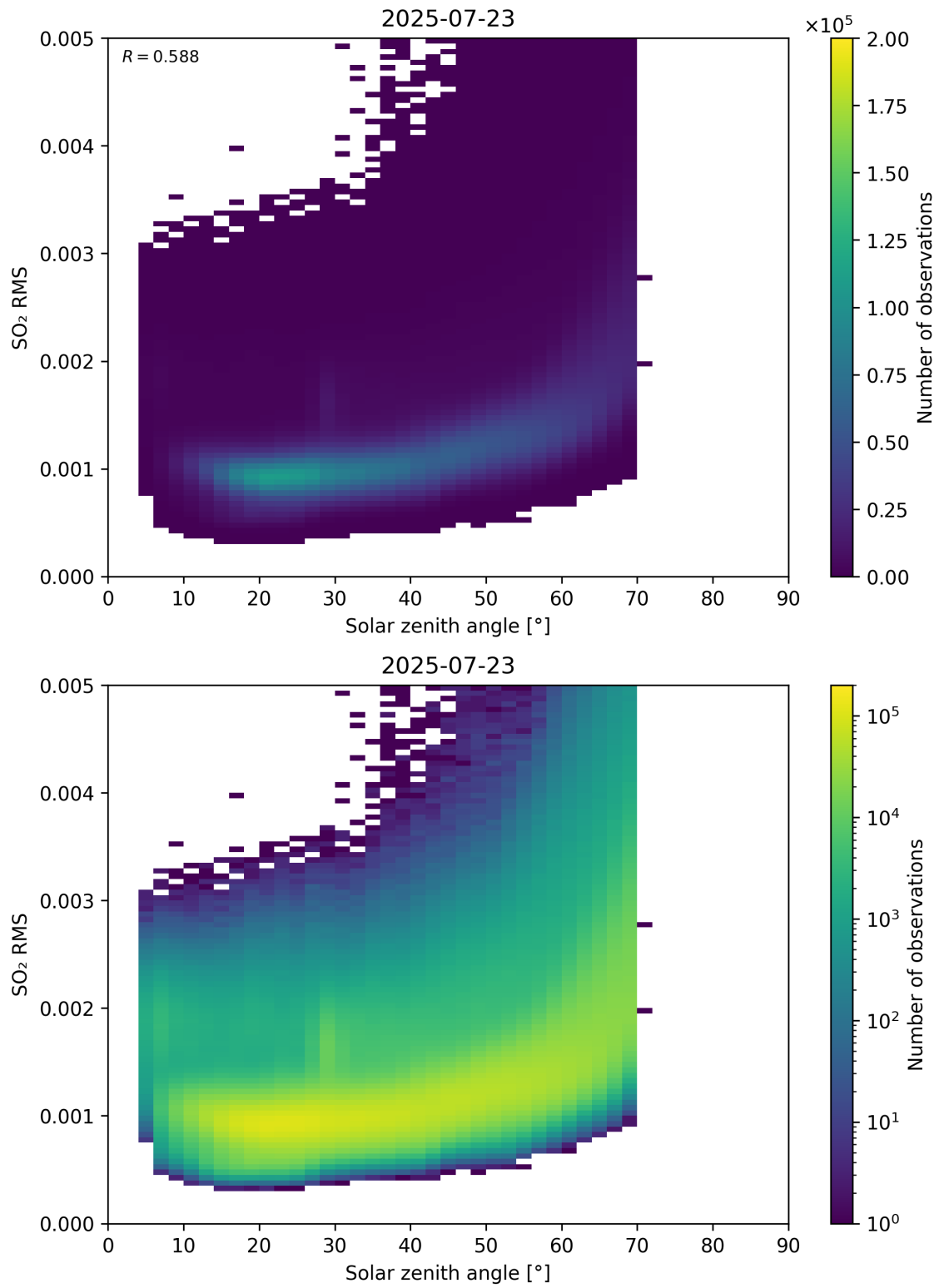
Figure 176: Scatter density plot of “Solar zenith angle” against “SO 2 RMS” for 2025-07-22 to 2025-07-24.
