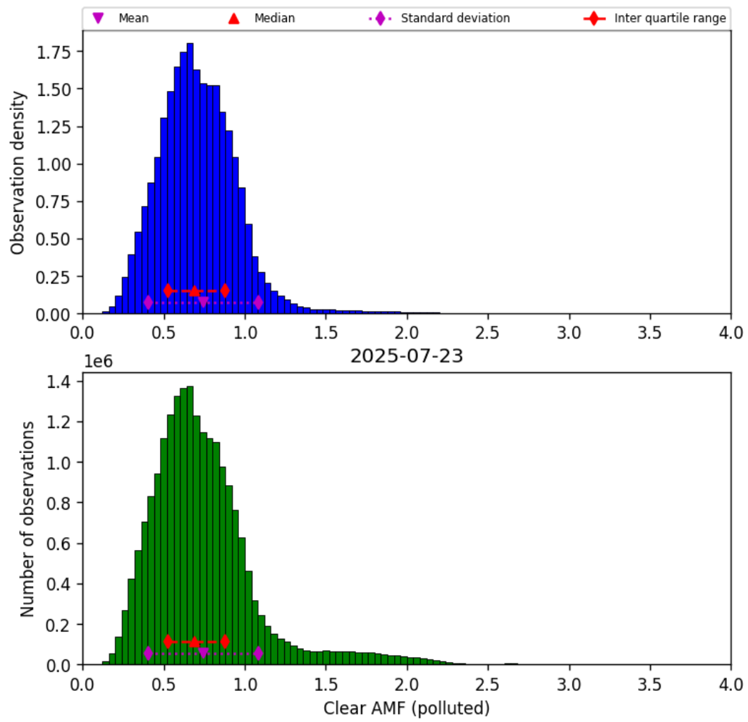
Figure 81: Histogram of “Clear AMF (polluted)” for 2025-07-22 to 2025-07-24
