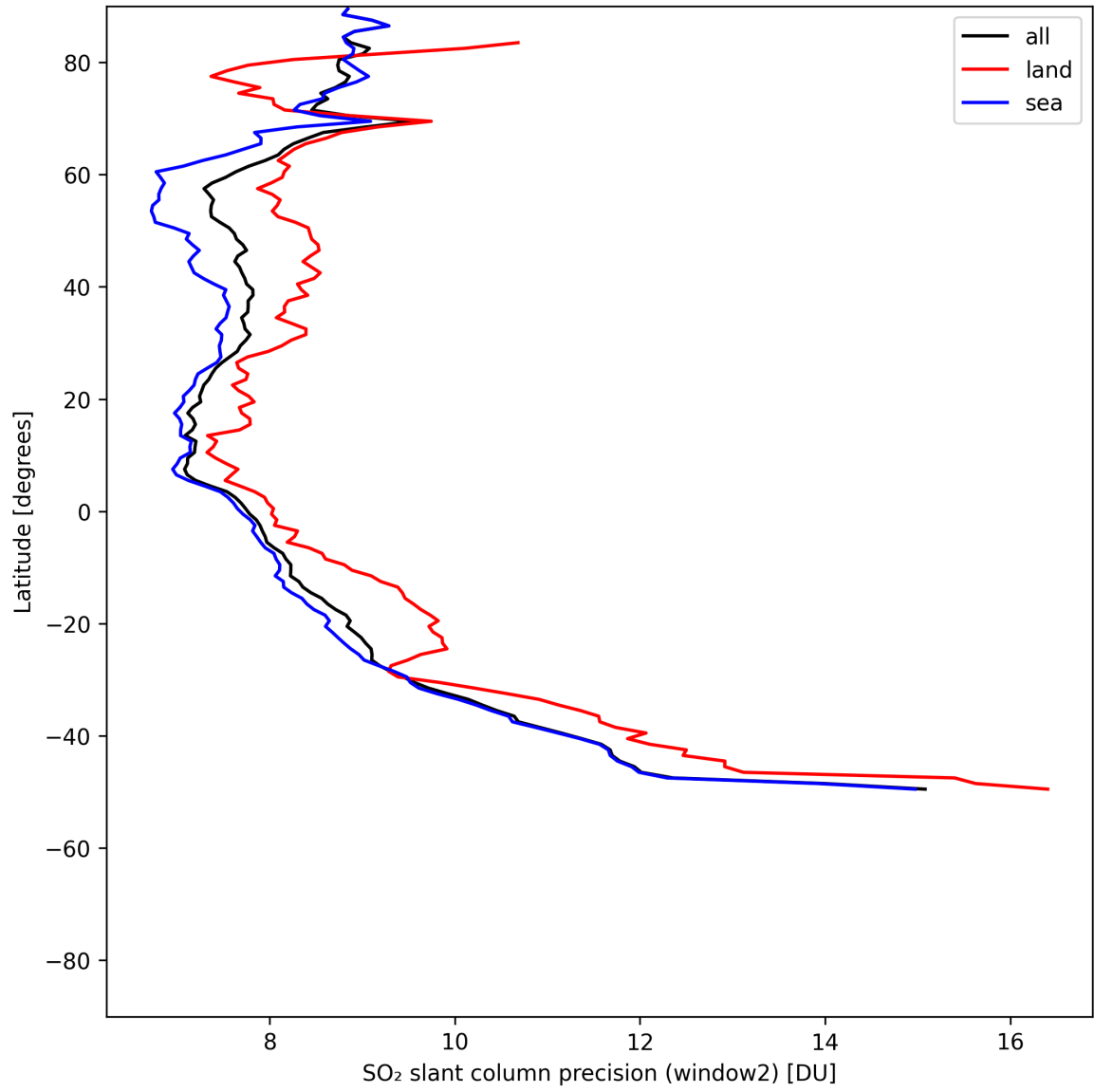
Figure 42: Zonal average of “SO 2 slant column precision (window2)” for 2025-07-22 to 2025-07-24.
