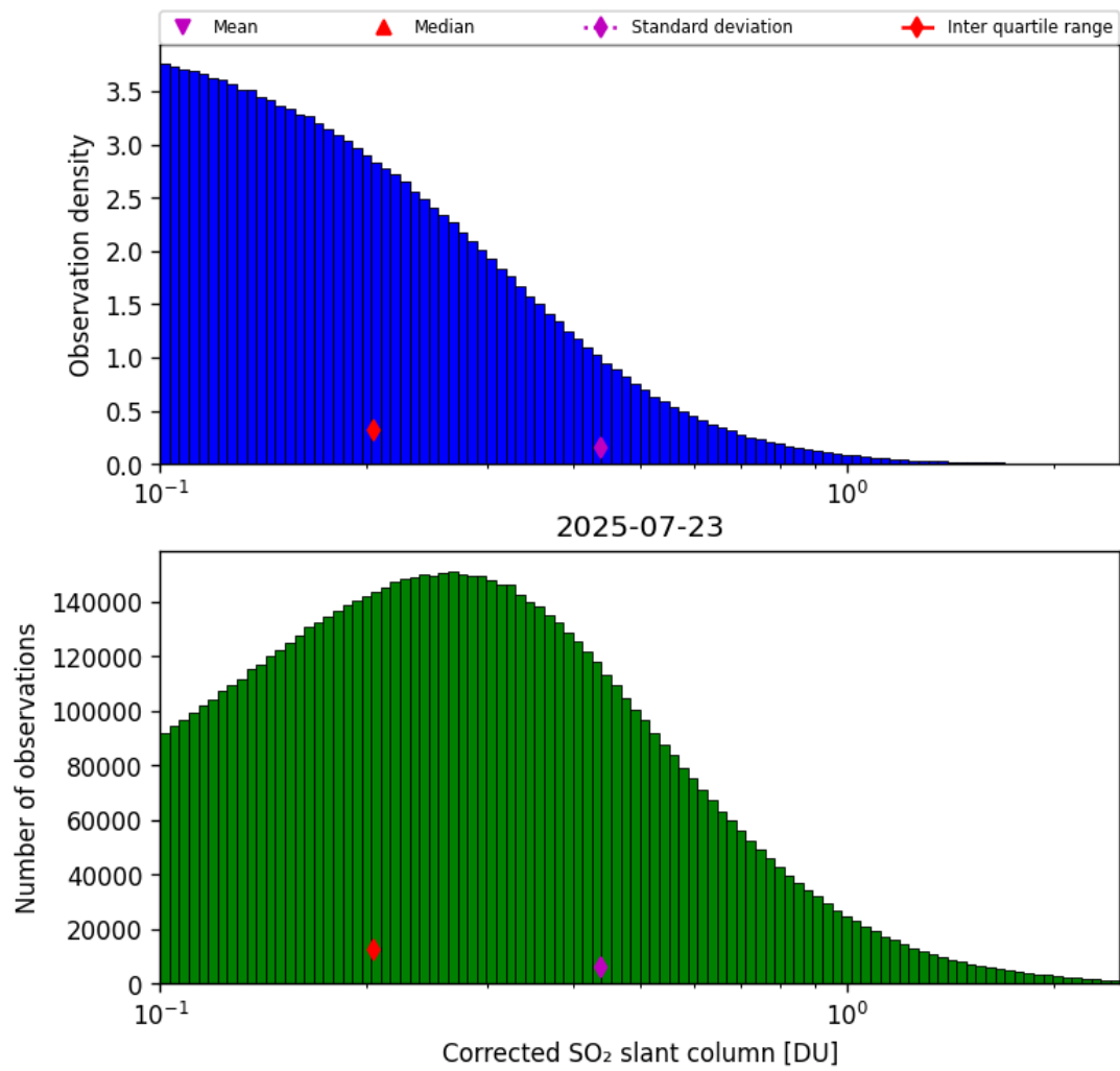
Figure 60: Histogram of “Corrected SO 2 slant column” for 2025-07-22 to 2025-07-24
