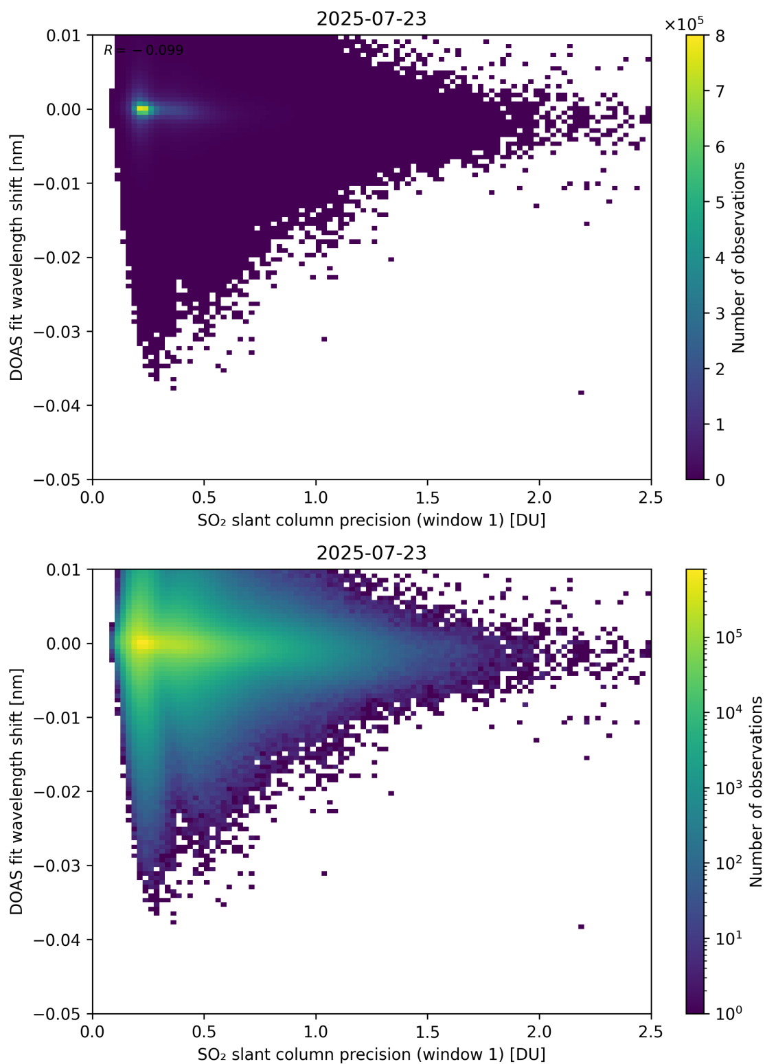
Figure 271: Scatter density plot of “SO 2 slant column precision (window 1)” against “DOAS fit wavelength shift” for 2025-07-22 to 2025-07-24.
