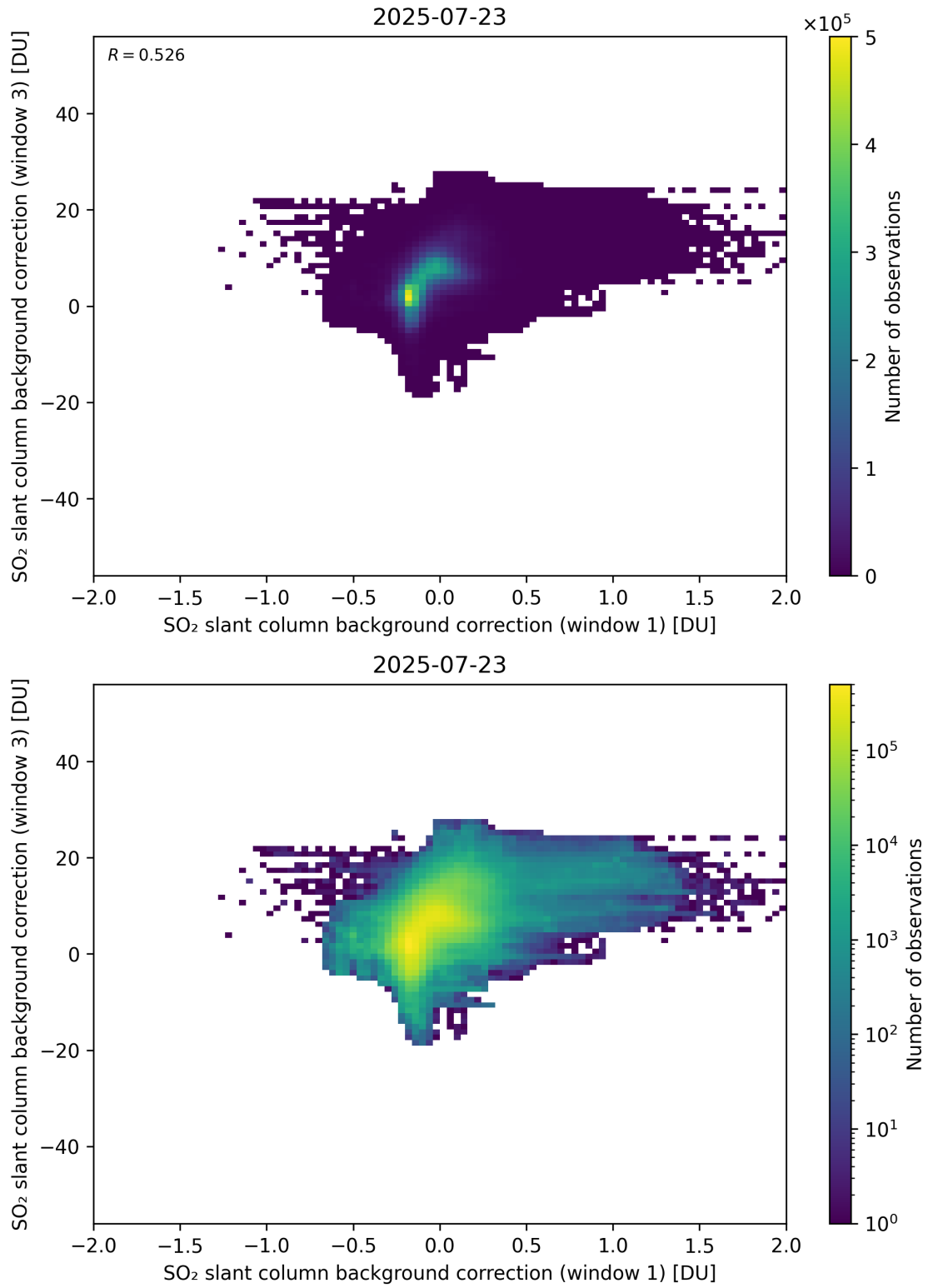
Figure 110: Scatter density plot of “SO 2 slant column background correction (window 1)” against “SO 2 slant column background correction (window 3)” for 2025-07-22 to 2025-07-24.
