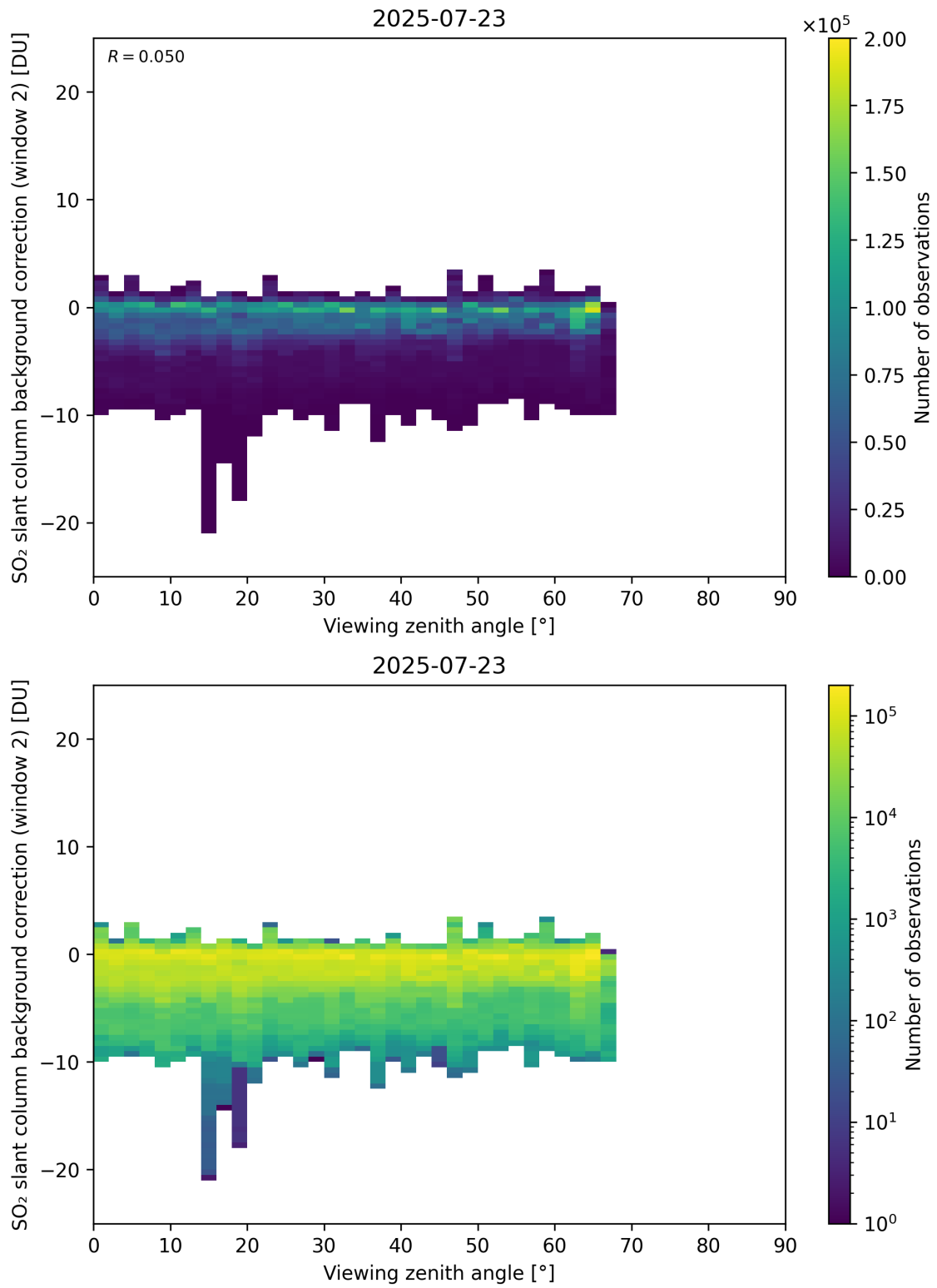
Figure 363: Scatter density plot of “Viewing zenith angle” against “SO 2 slant column background correction (window 2)” for 2025-07-22 to 2025-07-24.
