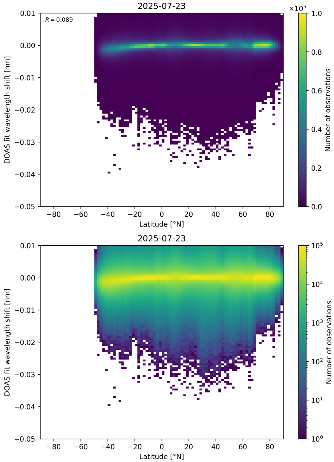
Figure 153: Scatter density plot of “Latitude” against “DOAS fit wavelength shift” for 2025-07-22 to 2025-07-24.
