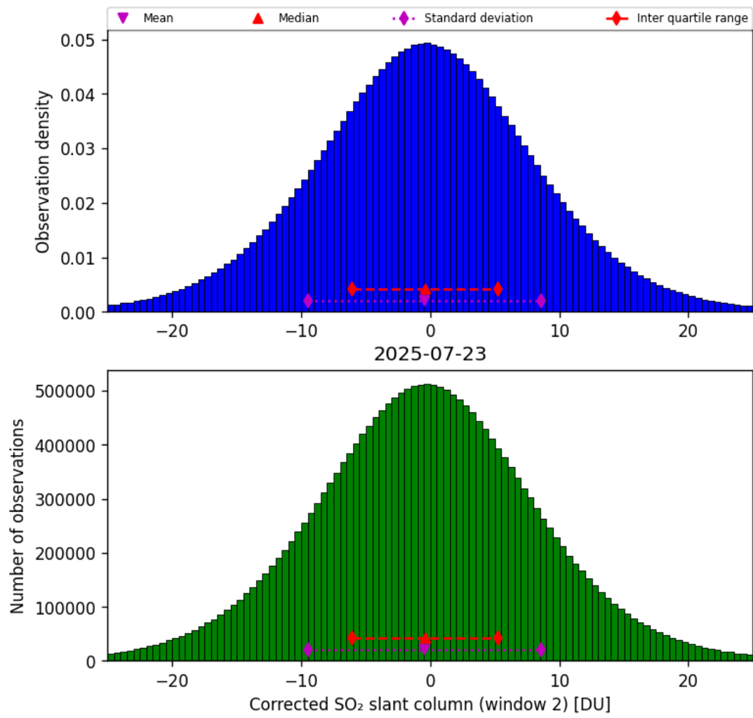
Figure 69: Histogram of “Corrected SO 2 slant column (window 2)” for 2025-07-22 to 2025-07-24
