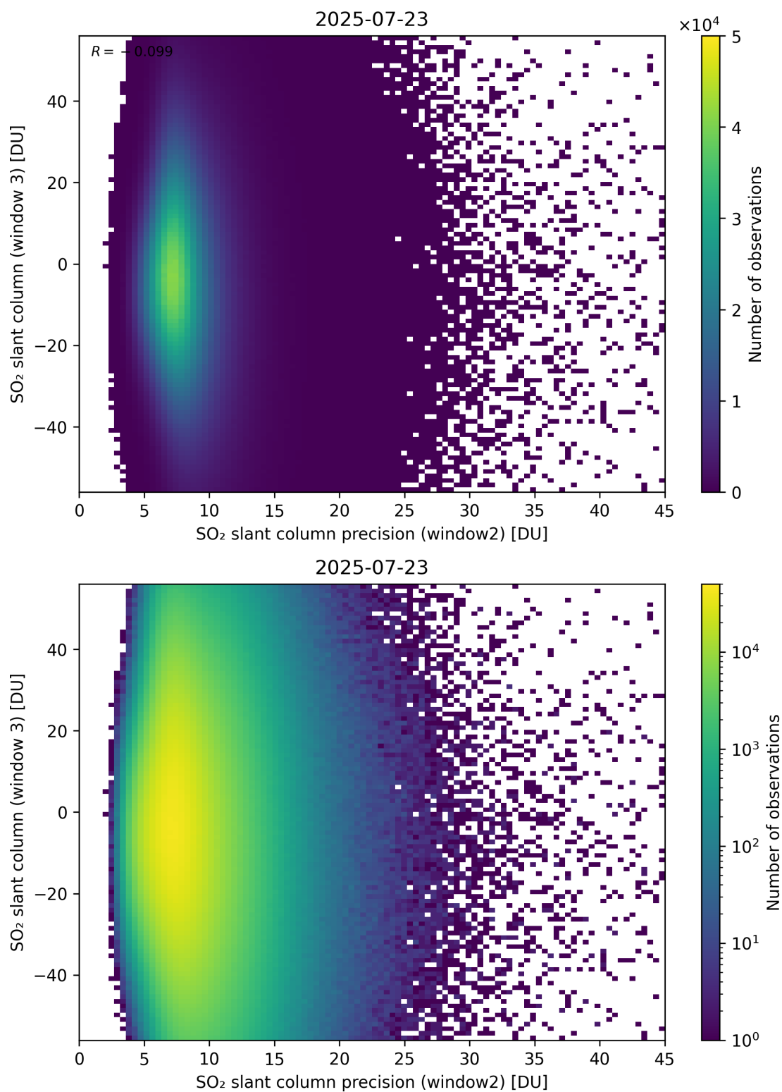
Figure 299: Scatter density plot of “SO 2 slant column precision (window2)” against “SO 2 slant column (window 3)” for 2025-07-22 to 2025-07-24.
