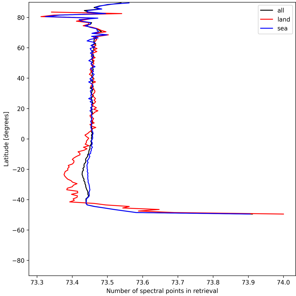
Figure 56: Zonal average of “Number of spectral points in retrieval” for 2025-07-22 to 2025-07-24.
