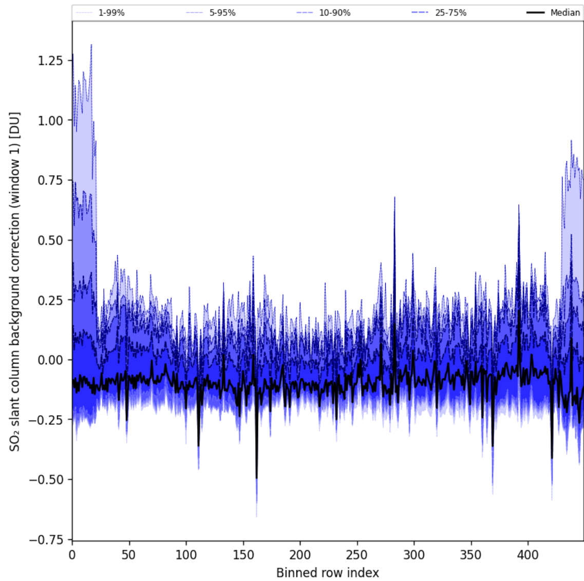
Figure 92: Along track statistics of “SO 2 slant column background correction (window 1)” for 2025-07-22 to 2025-07-24
