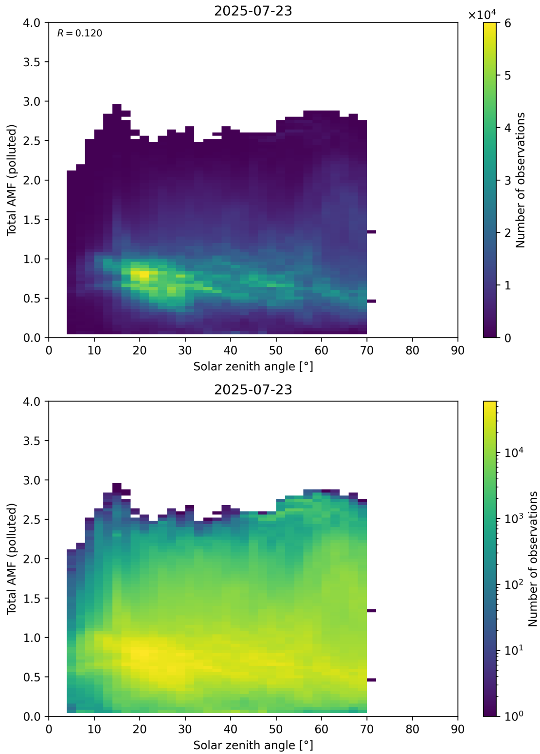
Figure 189: Scatter density plot of “Solar zenith angle” against “Total AMF (polluted)” for 2025-07-22 to 2025-07-24.
