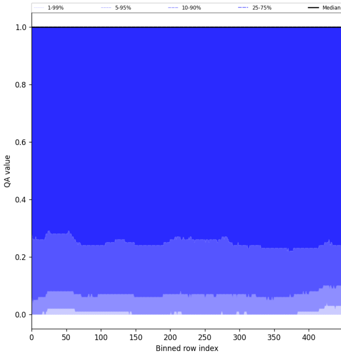
Figure 83: Along track statistics of “QA value” for 2025-07-22 to 2025-07-24
