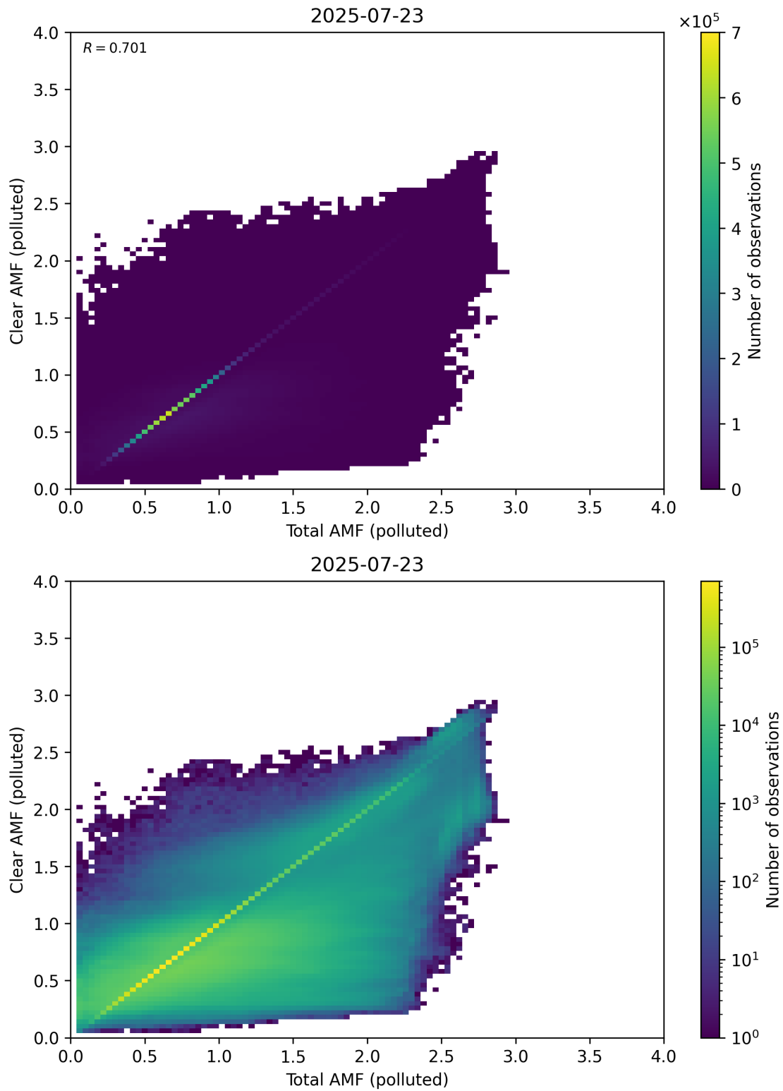
Figure 321: Scatter density plot of “Total AMF (polluted)” against “Clear AMF (polluted)” for 2025-07-22 to 2025-07-24.
