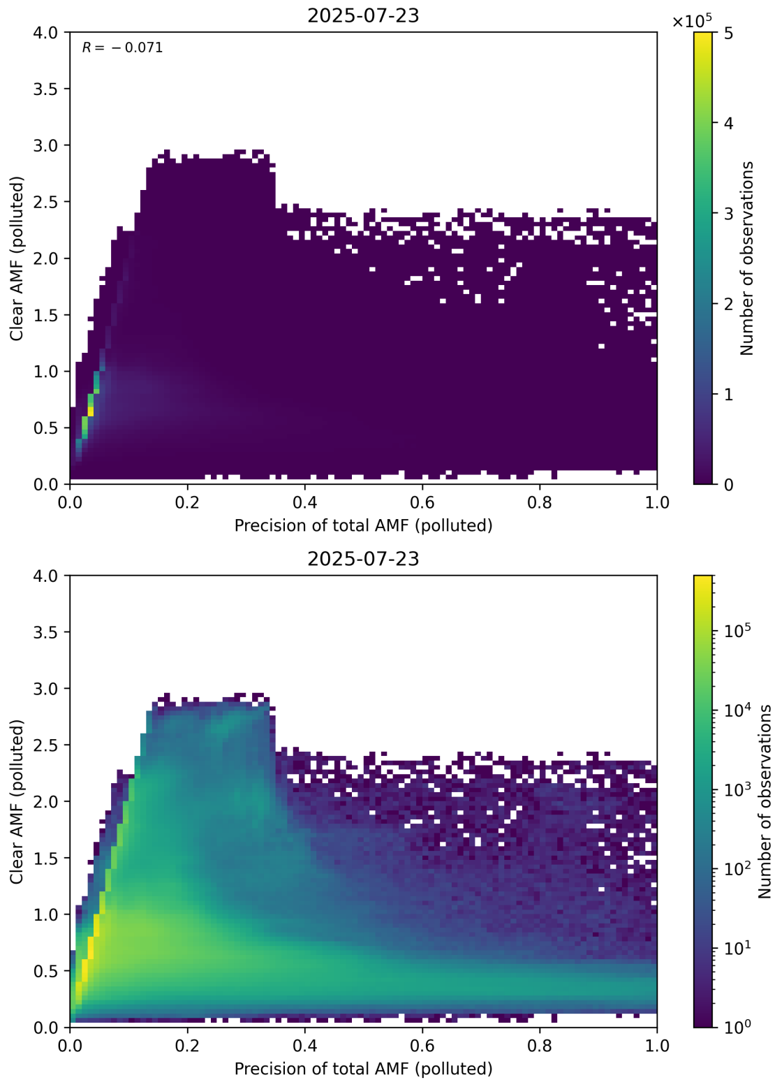
Figure 320: Scatter density plot of “Precision of total AMF (polluted)” against “Clear AMF (polluted)” for 2025-07-22 to 2025-07-24.
