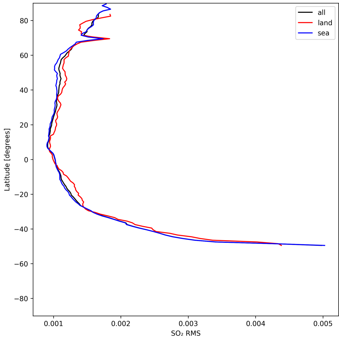
Figure 52: Zonal average of “SO 2 RMS” for 2025-07-22 to 2025-07-24.
