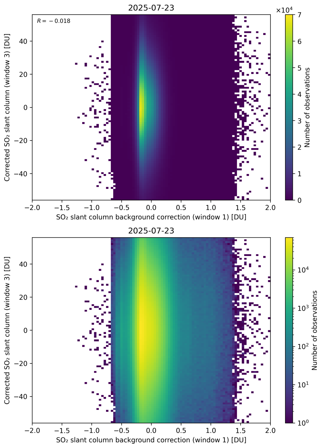
Figure 116: Scatter density plot of “SO 2 slant column background correction (window 1)” against “Corrected SO 2 slant column (window 3)” for 2025-07-22 to 2025-07-24.
