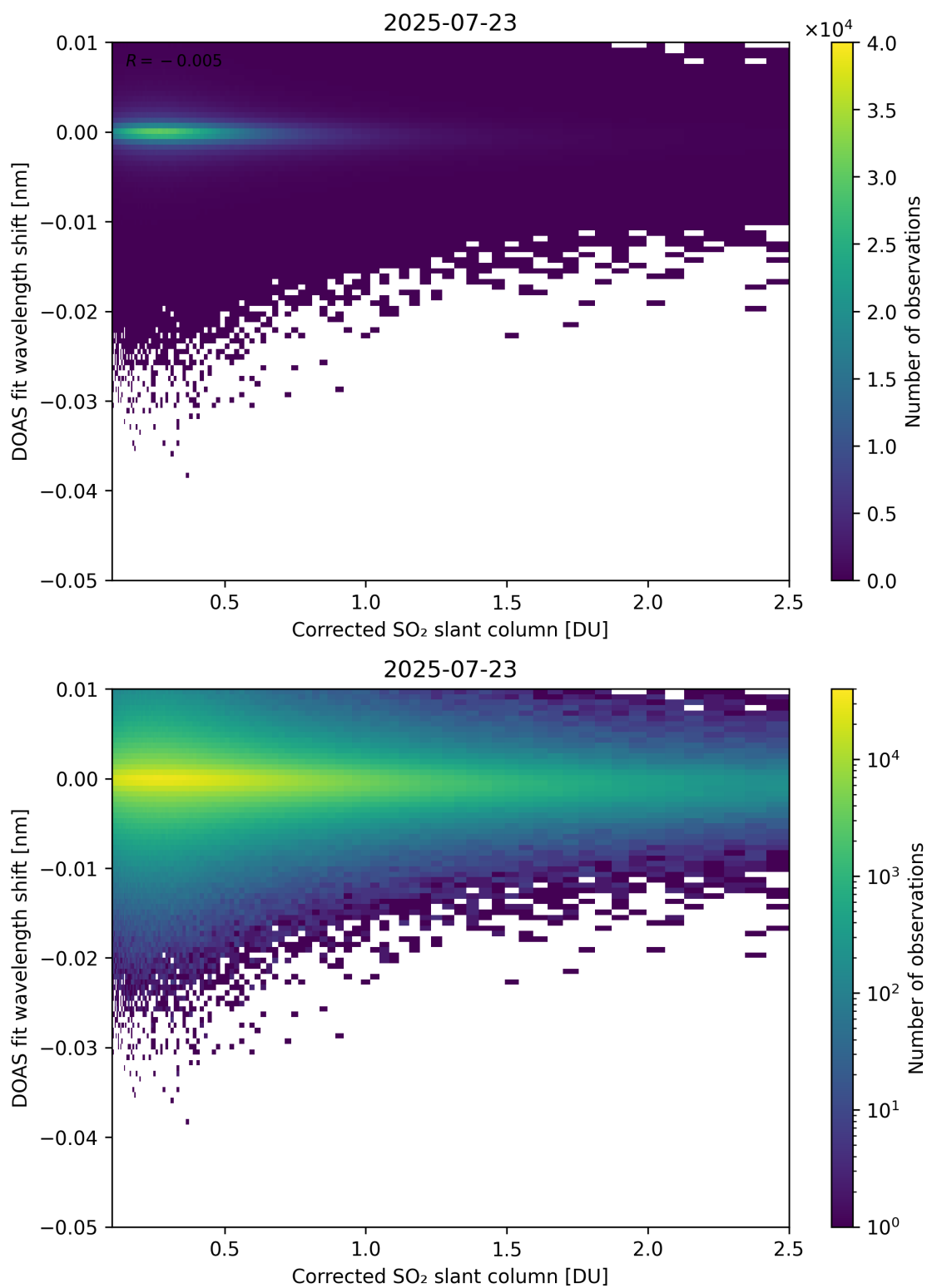
Figure 229: Scatter density plot of “Corrected SO 2 slant column” against “DOAS fit wavelength shift” for 2025-07-22 to 2025-07-24.
