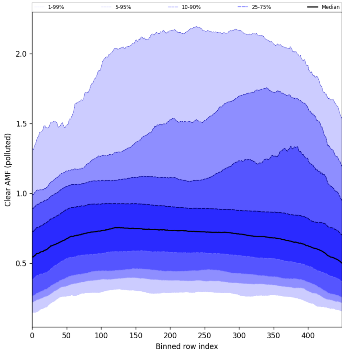
Figure 107: Along track statistics of “Clear AMF (polluted)” for 2025-07-22 to 2025-07-24
