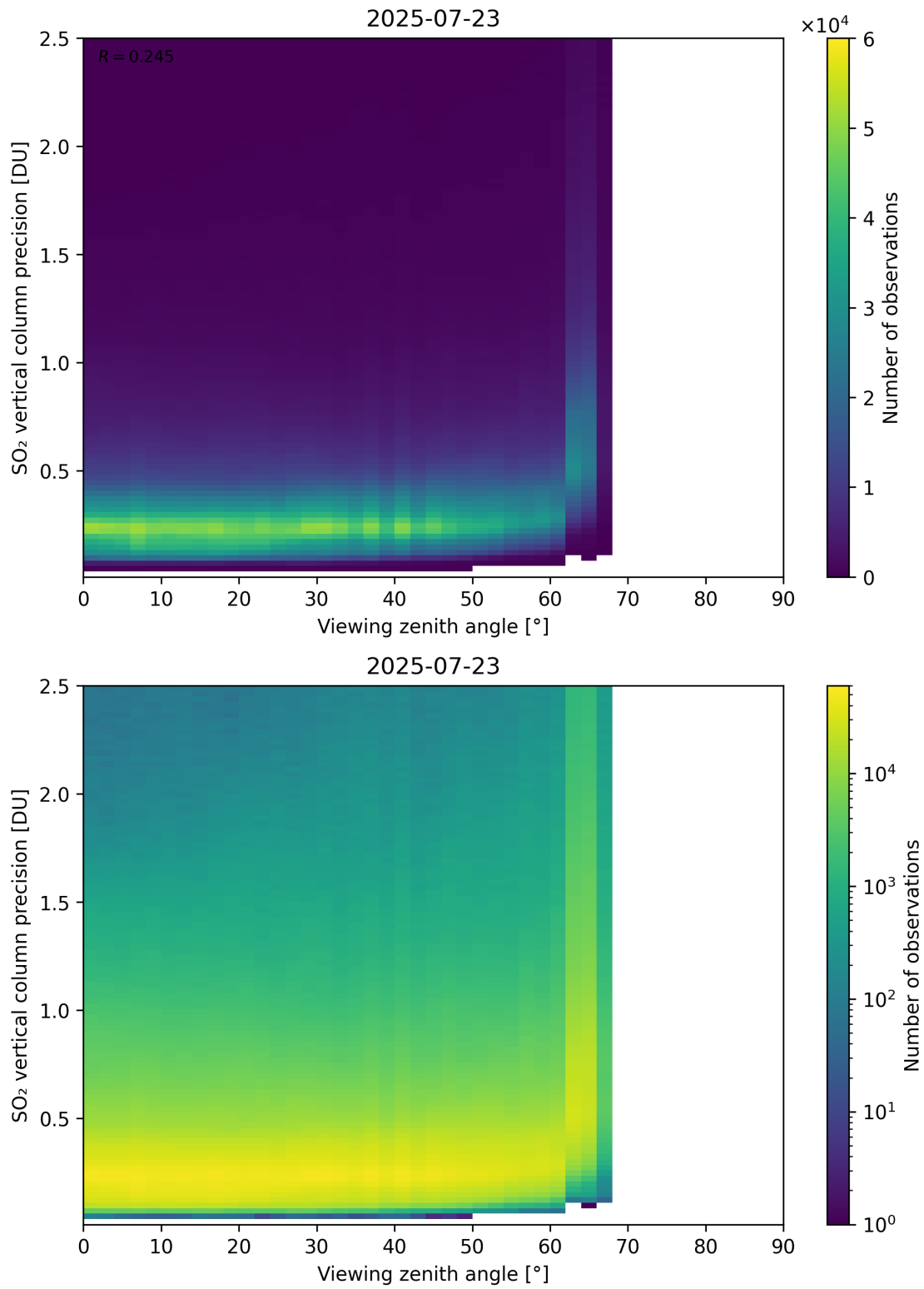
Figure 384: Scatter density plot of “Viewing zenith angle” against “SO 2 vertical column precision” for 2025-07-22 to 2025-07-24.
