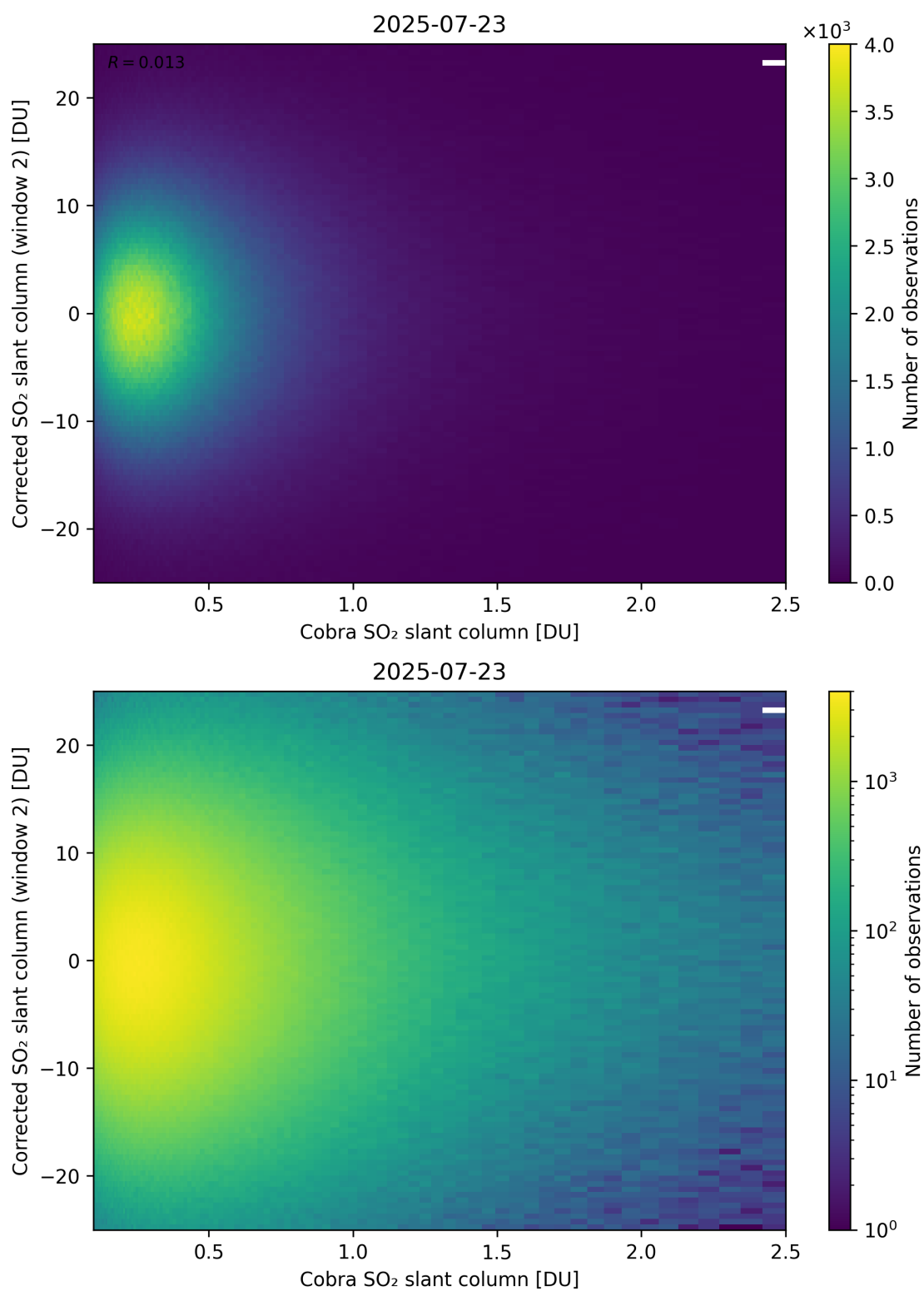
Figure 217: Scatter density plot of “Cobra SO 2 slant column” against “Corrected SO 2 slant column (window 2)” for 2025-07-22 to 2025-07-24.
