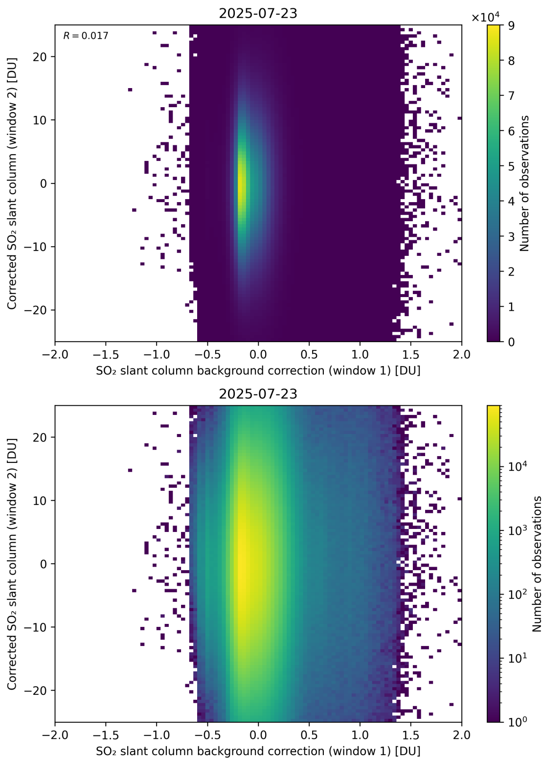
Figure 115: Scatter density plot of “SO 2 slant column background correction (window 1)” against “Corrected SO 2 slant column (window 2)” for 2025-07-22 to 2025-07-24.
