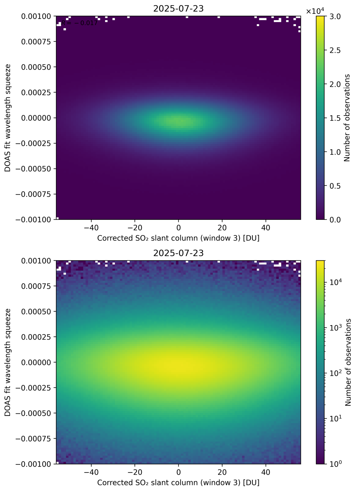
Figure 257: Scatter density plot of “Corrected SO 2 slant column (window 3)” against “DOAS fit wavelength squeeze” for 2025-07-22 to 2025-07-24.
