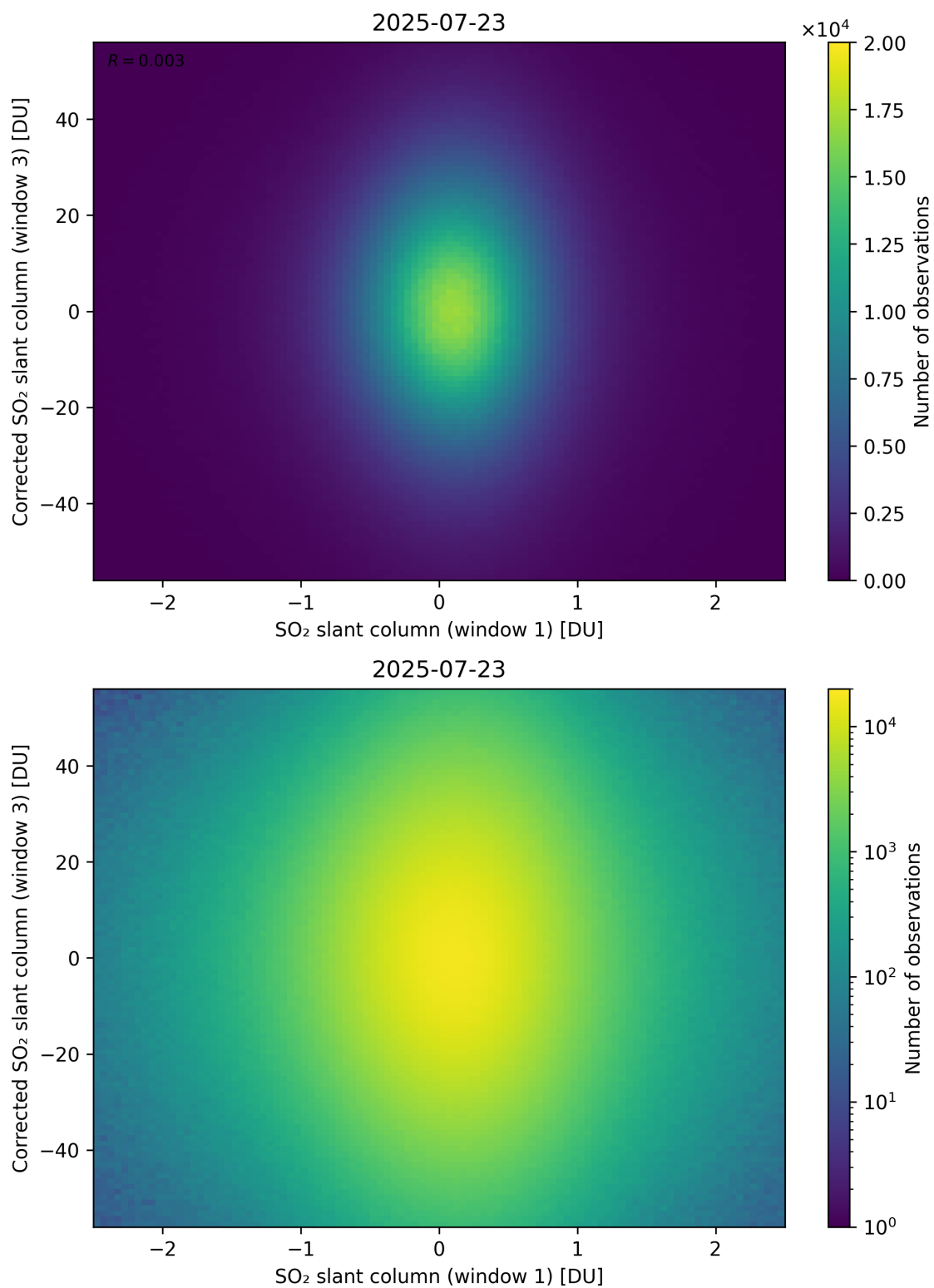
Figure 284: Scatter density plot of “SO 2 slant column (window 1)” against “Corrected SO 2 slant column (window 3)” for 2025-07-22 to 2025-07-24.
