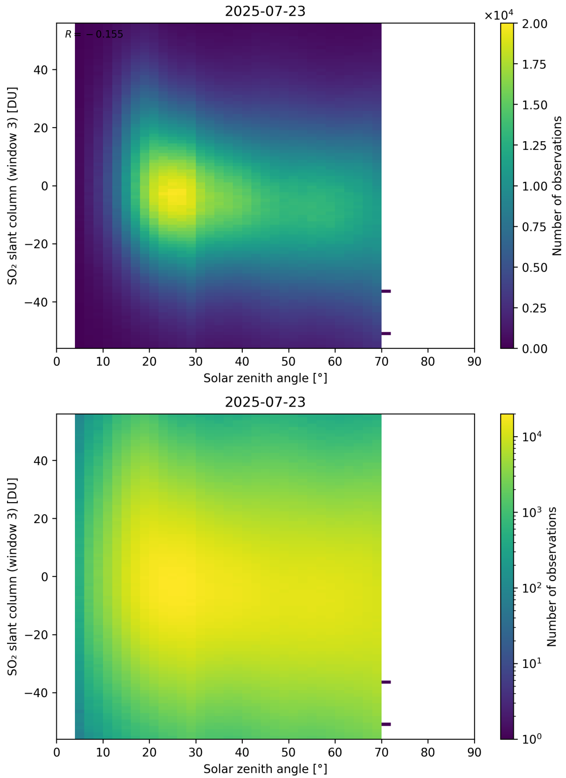
Figure 187: Scatter density plot of “Solar zenith angle” against “SO 2 slant column (window 3)” for 2025-07-22 to 2025-07-24.
