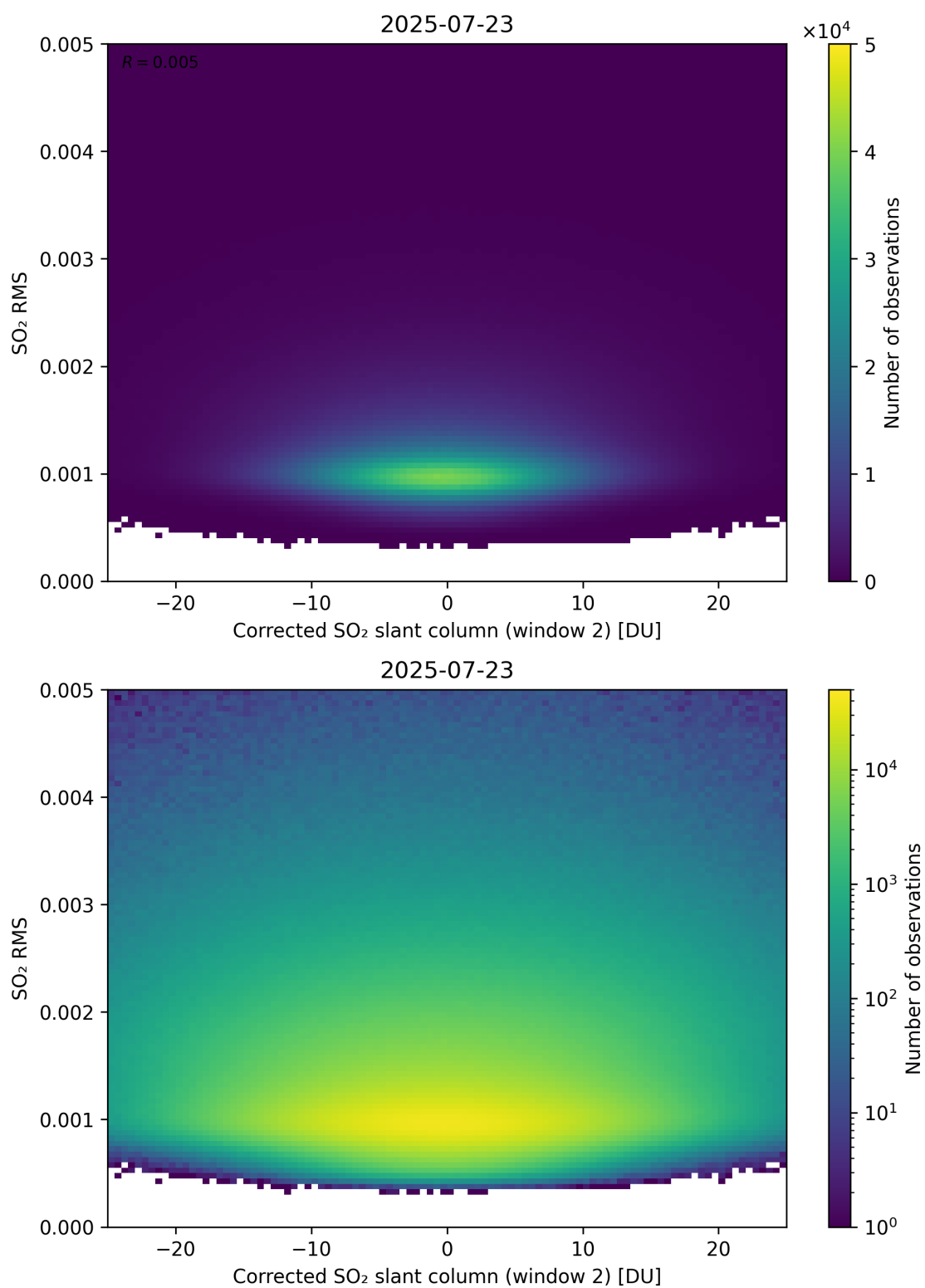
Figure 248: Scatter density plot of “Corrected SO 2 slant column (window 2)” against “SO 2 RMS” for 2025-07-22 to 2025-07-24.
