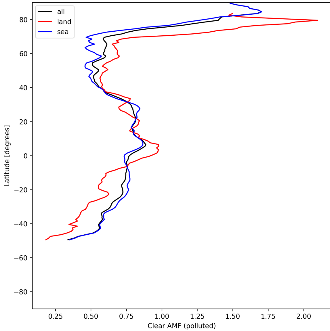
Figure 55: Zonal average of “Clear AMF (polluted)” for 2025-07-22 to 2025-07-24.
