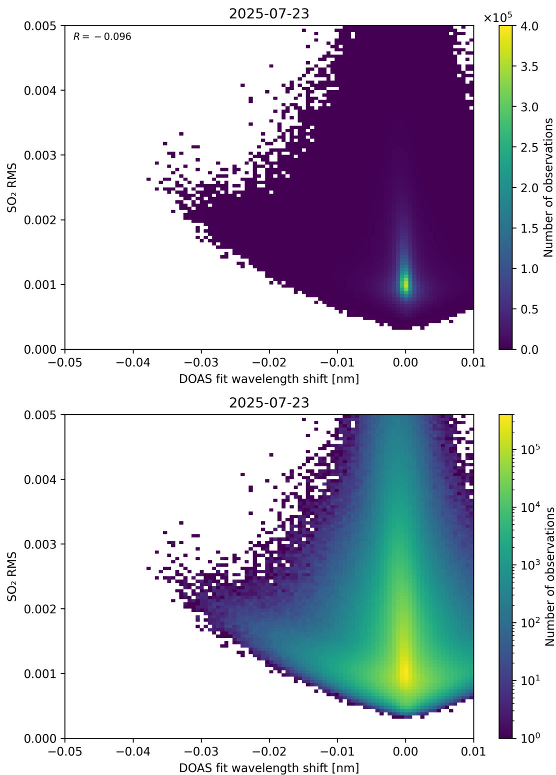
Figure 139: Scatter density plot of “DOAS fit wavelength shift” against “SO 2 RMS” for 2025-07-22 to 2025-07-24.
