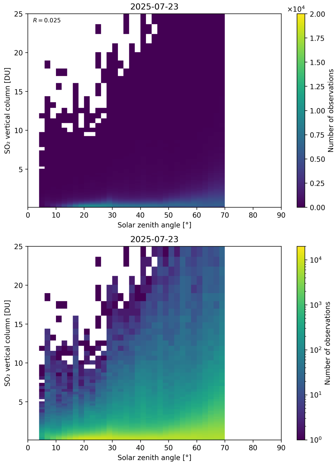
Figure 191: Scatter density plot of “Solar zenith angle” against “SO 2 vertical column” for 2025-07-22 to 2025-07-24.
