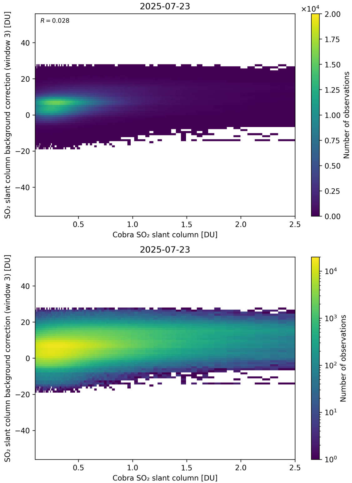
Figure 195: Scatter density plot of “Cobra SO 2 slant column” against “SO 2 slant column background correction (window 3)” for 2025-07-22 to 2025-07-24.
