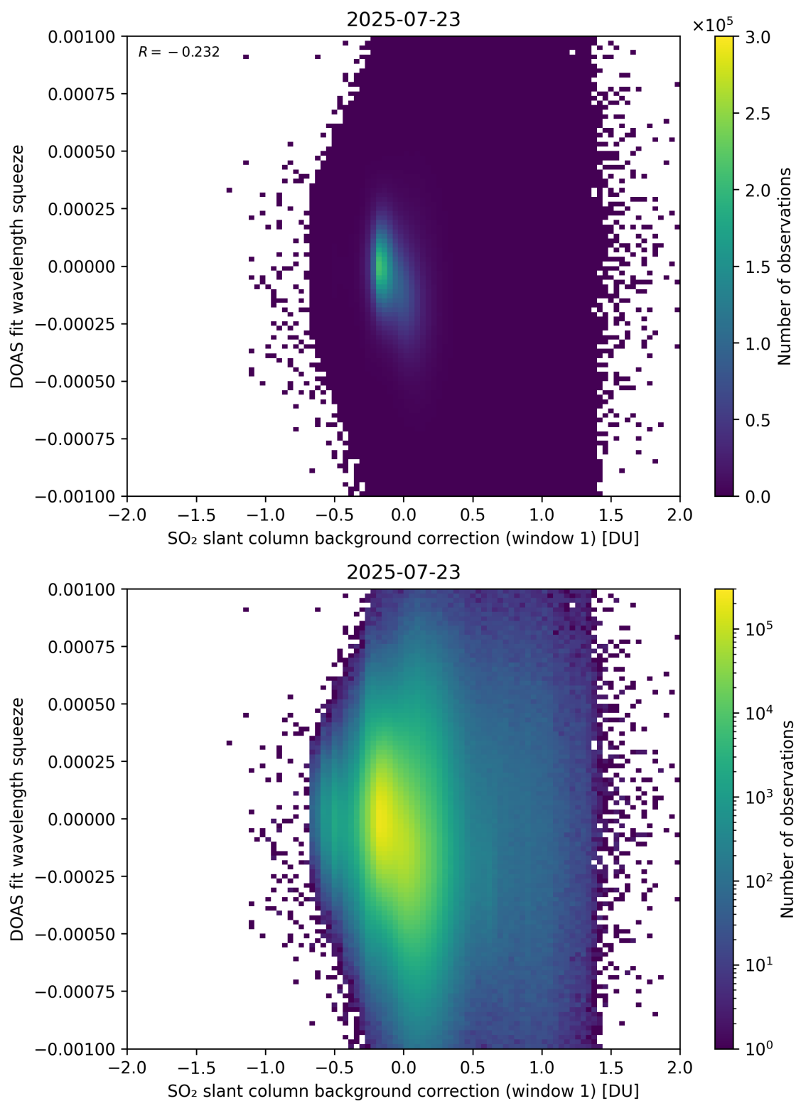
Figure 112: Scatter density plot of “SO 2 slant column background correction (window 1)” against “DOAS fit wavelength squeeze” for 2025-07-22 to 2025-07-24.
