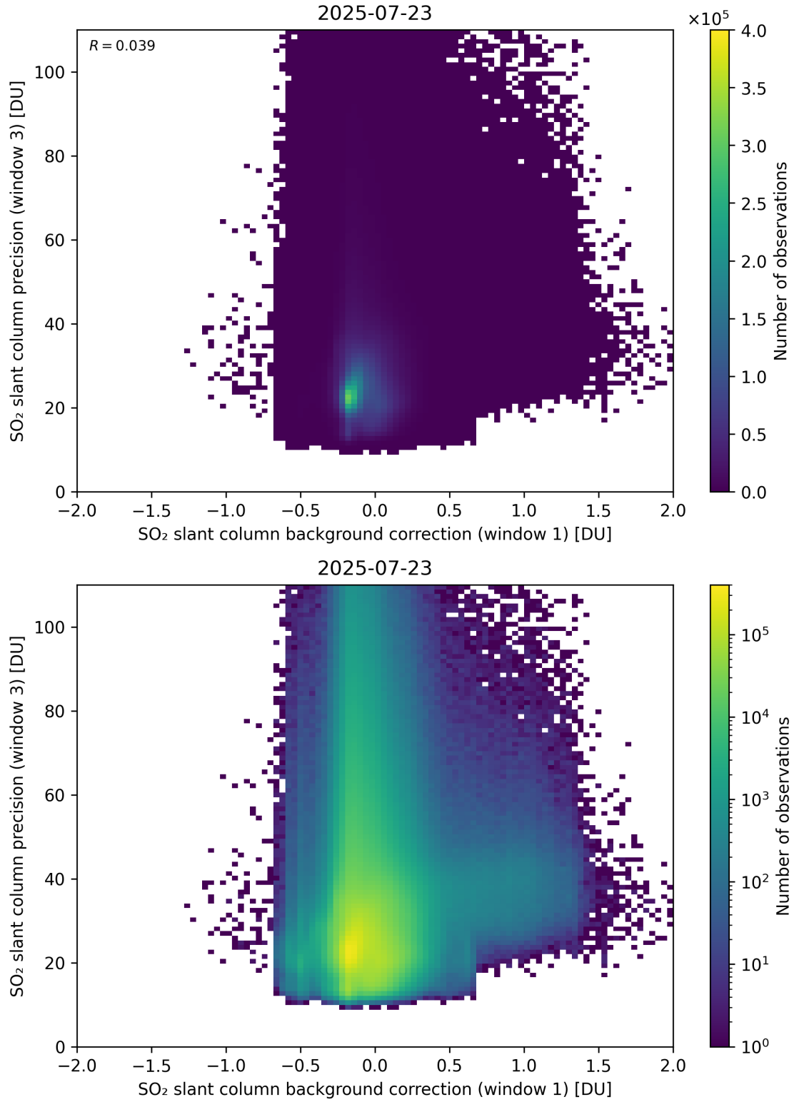
Figure 119: Scatter density plot of “SO 2 slant column background correction (window 1)” against “SO 2 slant column precision (window 3)” for 2025-07-22 to 2025-07-24.
