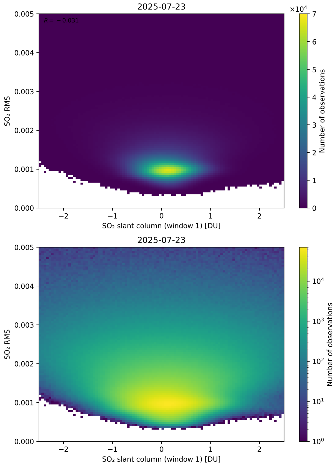
Figure 267: Scatter density plot of “SO 2 slant column (window 1)” against “SO 2 RMS” for 2025-07-22 to 2025-07-24.
