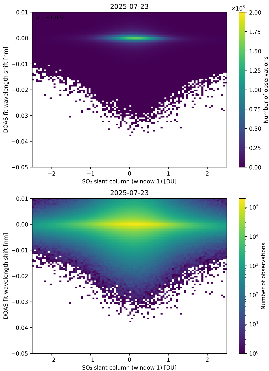
Figure 265: Scatter density plot of “SO 2 slant column (window 1)” against “DOAS fit wavelength shift” for 2025-07-22 to 2025-07-24.
