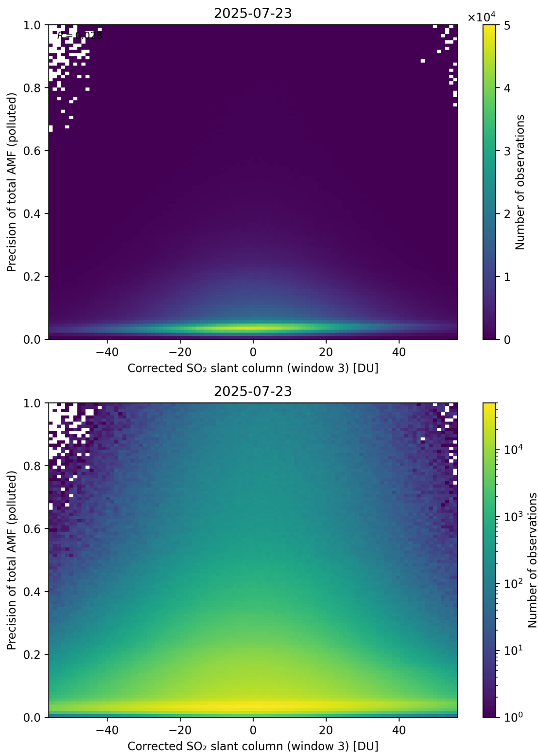
Figure 261: Scatter density plot of “Corrected SO 2 slant column (window 3)” against “Precision of total AMF (polluted)” for 2025-07-22 to 2025-07-24.
