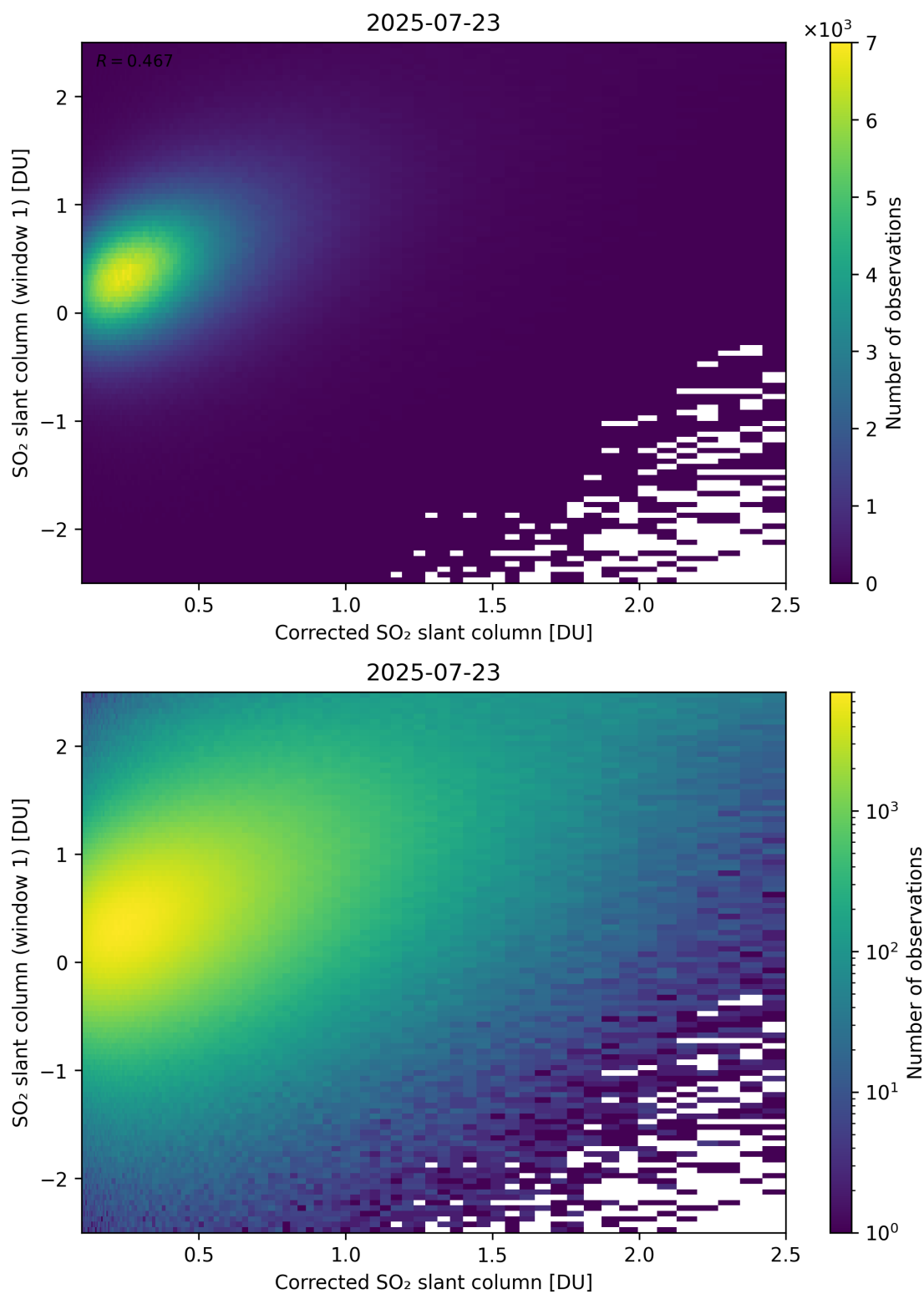
Figure 237: Scatter density plot of “Corrected SO 2 slant column” against “SO 2 slant column (window 1)” for 2025-07-22 to 2025-07-24.
