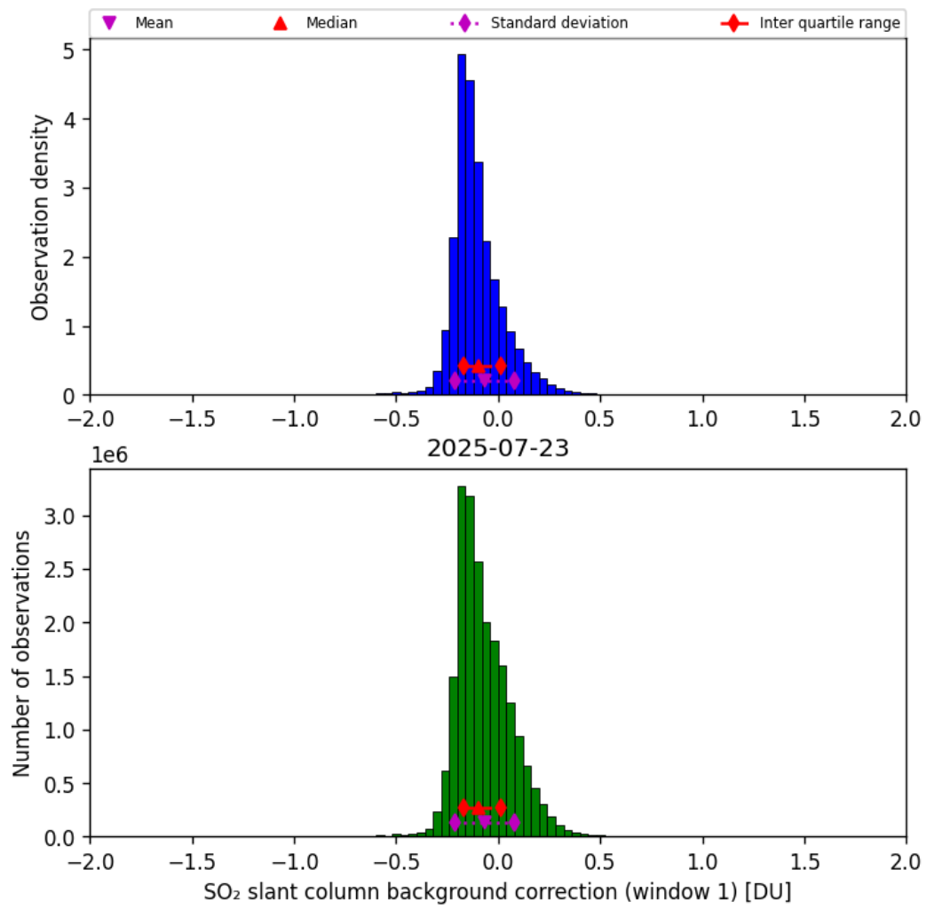
Figure 66: Histogram of “SO 2 slant column background correction (window 1)” for 2025-07-22 to 2025-07-24
