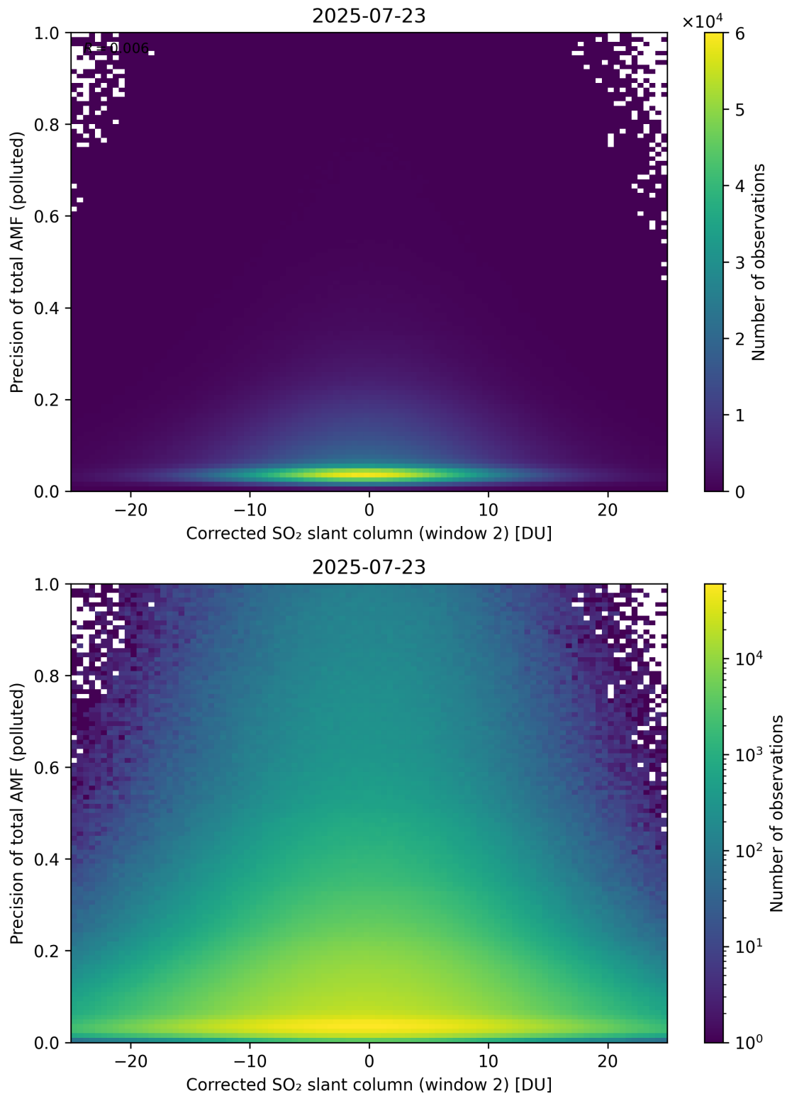
Figure 254: Scatter density plot of “Corrected SO 2 slant column (window 2)” against “Precision of total AMF (polluted)” for 2025-07-22 to 2025-07-24.
