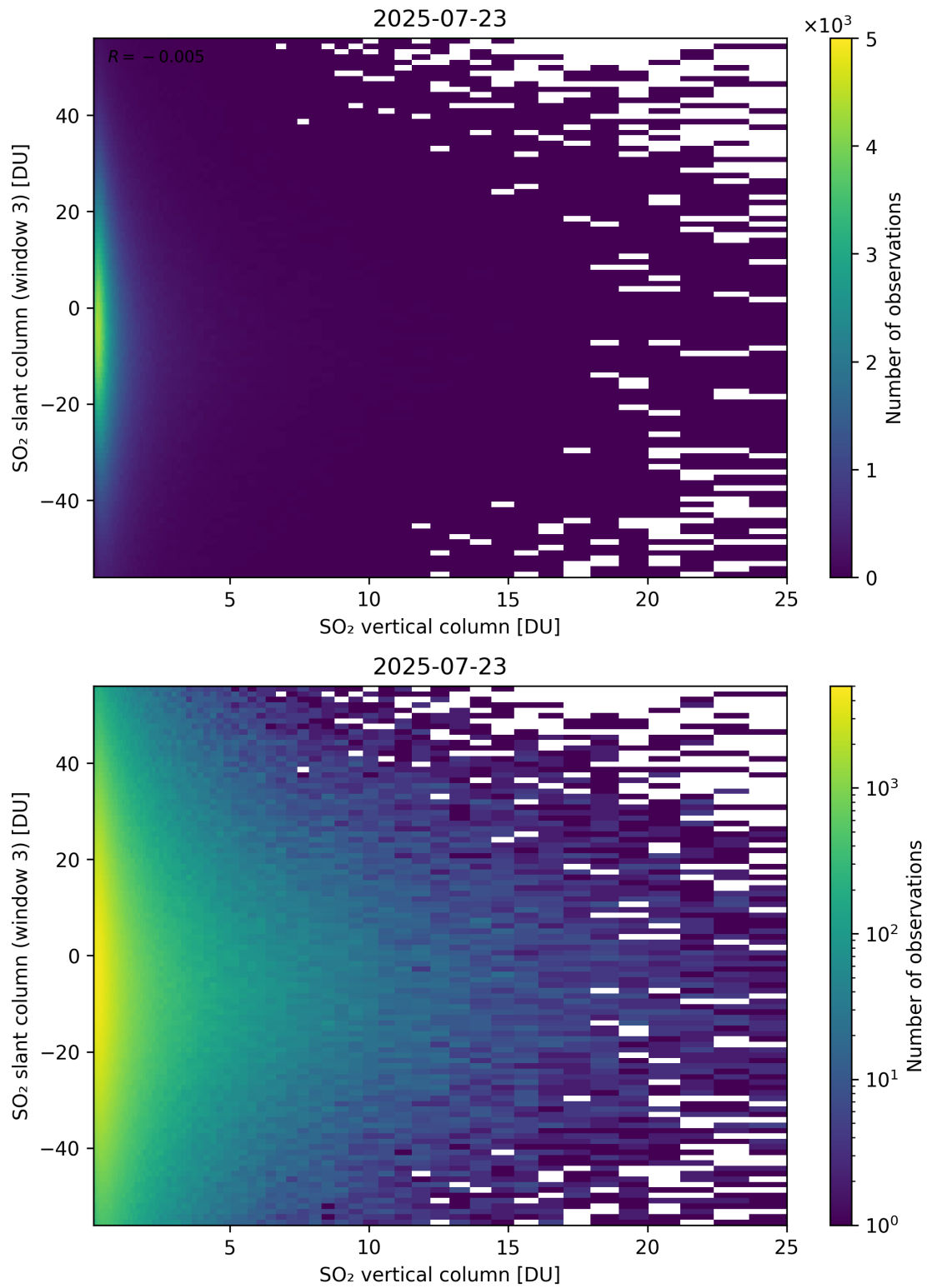
Figure 357: Scatter density plot of “SO 2 vertical column” against “SO 2 slant column (window 3)” for 2025-07-22 to 2025-07-24.
