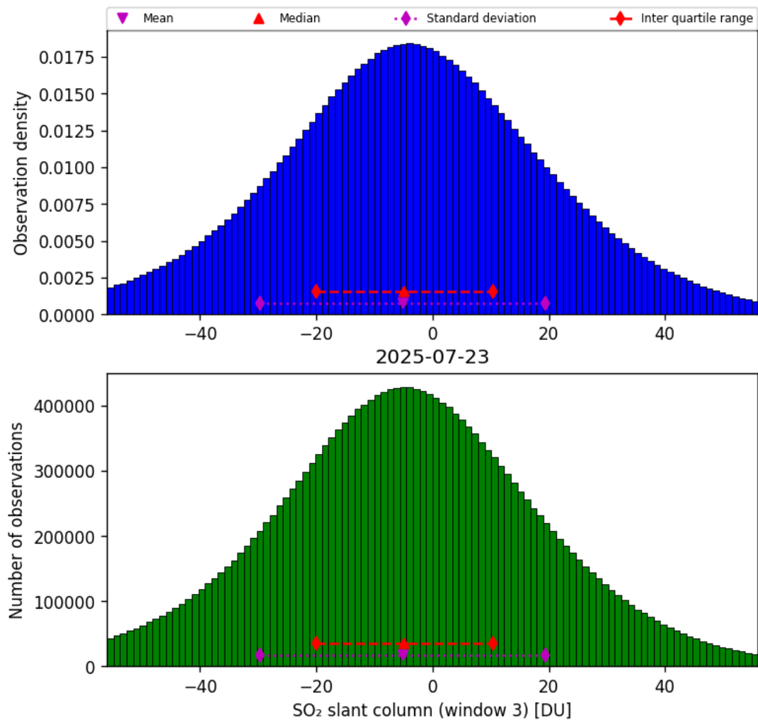
Figure 71: Histogram of “SO 2 slant column (window 3)” for 2025-07-22 to 2025-07-24
