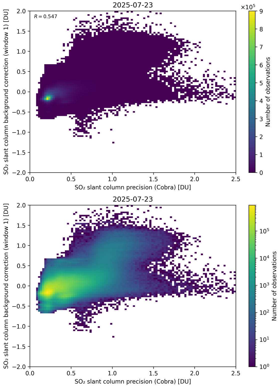
Figure 199: Scatter density plot of “SO 2 slant column precision (Cobra)” against “SO 2 slant column background correction (window 1)” for 2025-07-22 to 2025-07-24.
