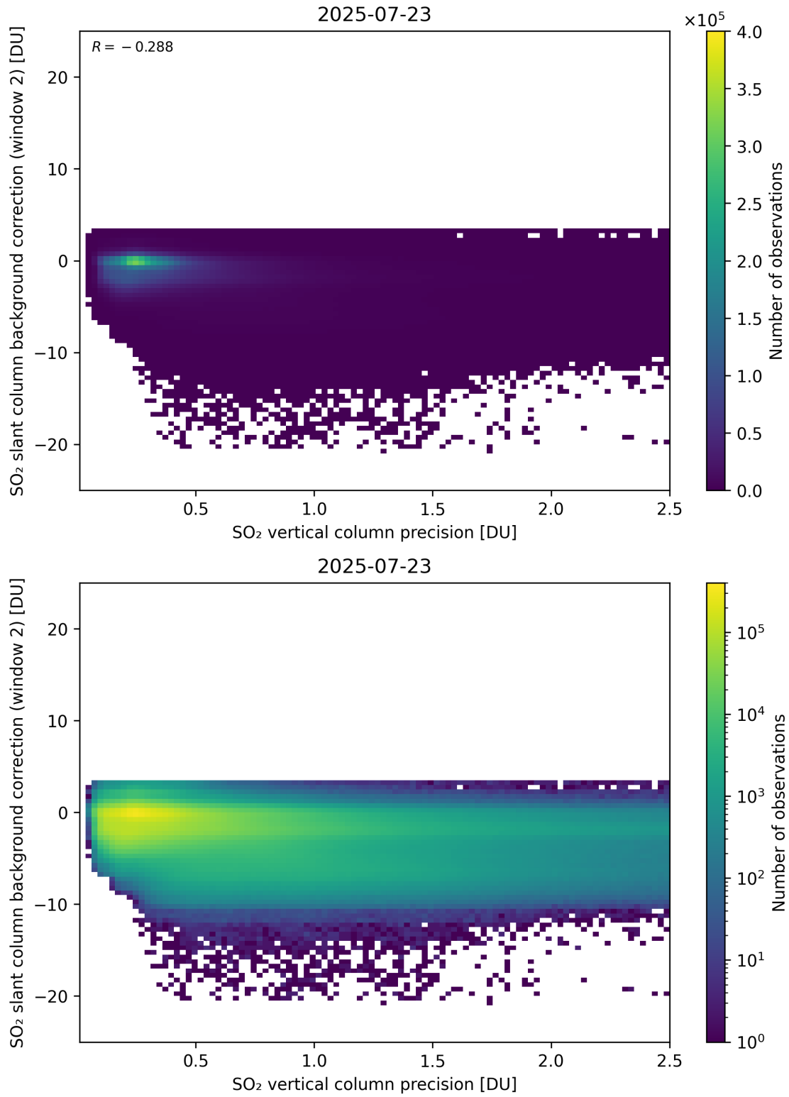
Figure 330: Scatter density plot of “SO 2 vertical column precision” against “SO 2 slant column background correction (window 2)” for 2025-07-22 to 2025-07-24.
