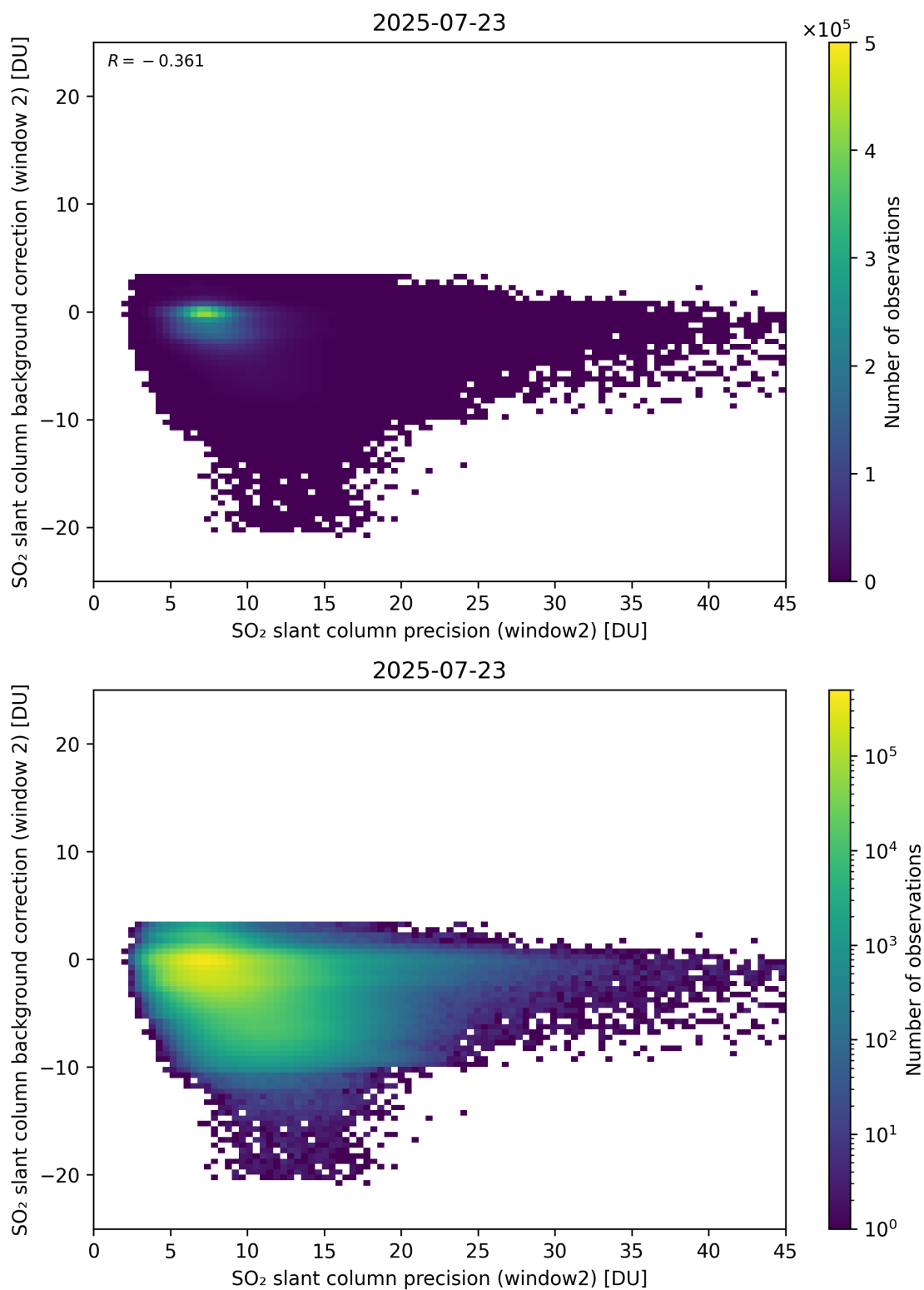
Figure 291: Scatter density plot of “SO 2 slant column precision (window2)” against “SO 2 slant column background correction (window 2)” for 2025-07-22 to 2025-07-24.
