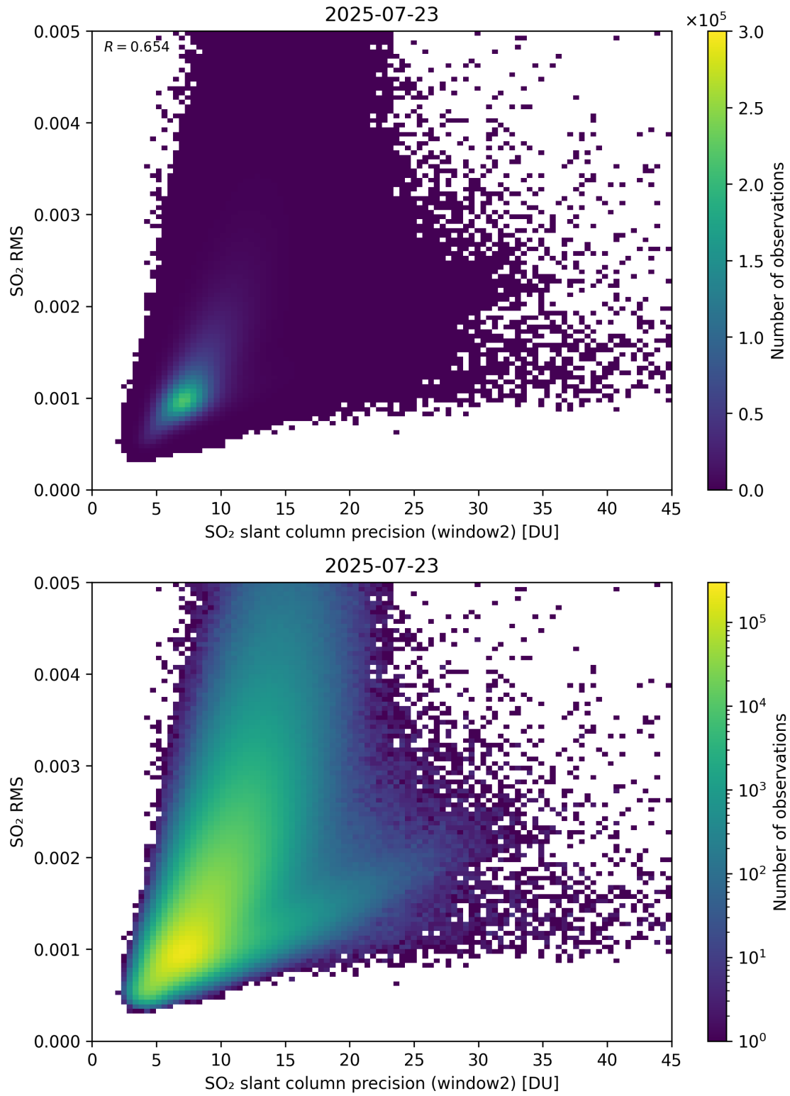
Figure 295: Scatter density plot of “SO 2 slant column precision (window2)” against “SO 2 RMS” for 2025-07-22 to 2025-07-24.
