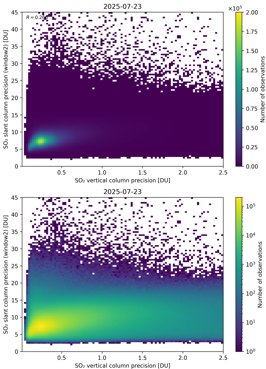
Figure 343: Scatter density plot of “SO 2 vertical column precision” against “SO 2 slant column precision (window2)” for 2025-07-22 to 2025-07-24.
