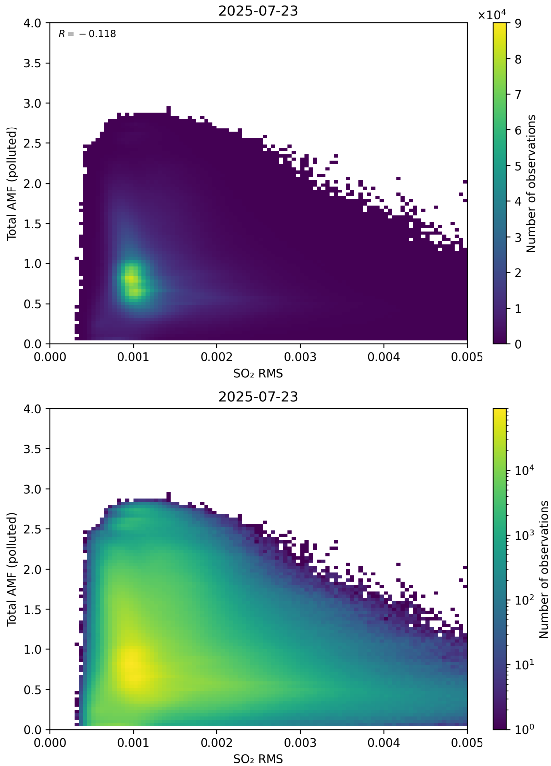
Figure 148: Scatter density plot of “SO 2 RMS” against “Total AMF (polluted)” for 2025-07-22 to 2025-07-24.
