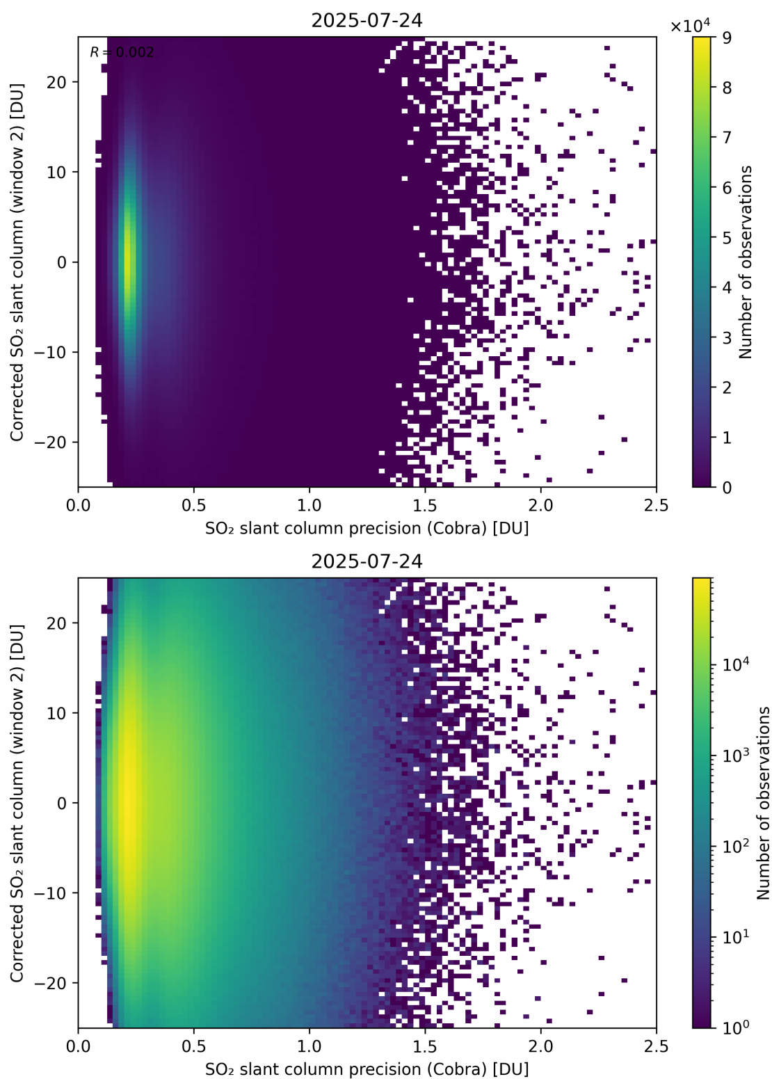
Figure 206: Scatter density plot of “SO 2 slant column precision (Cobra)” against “Corrected SO 2 slant column (window 2)” for 2025-07-24 to 2025-07-25.
