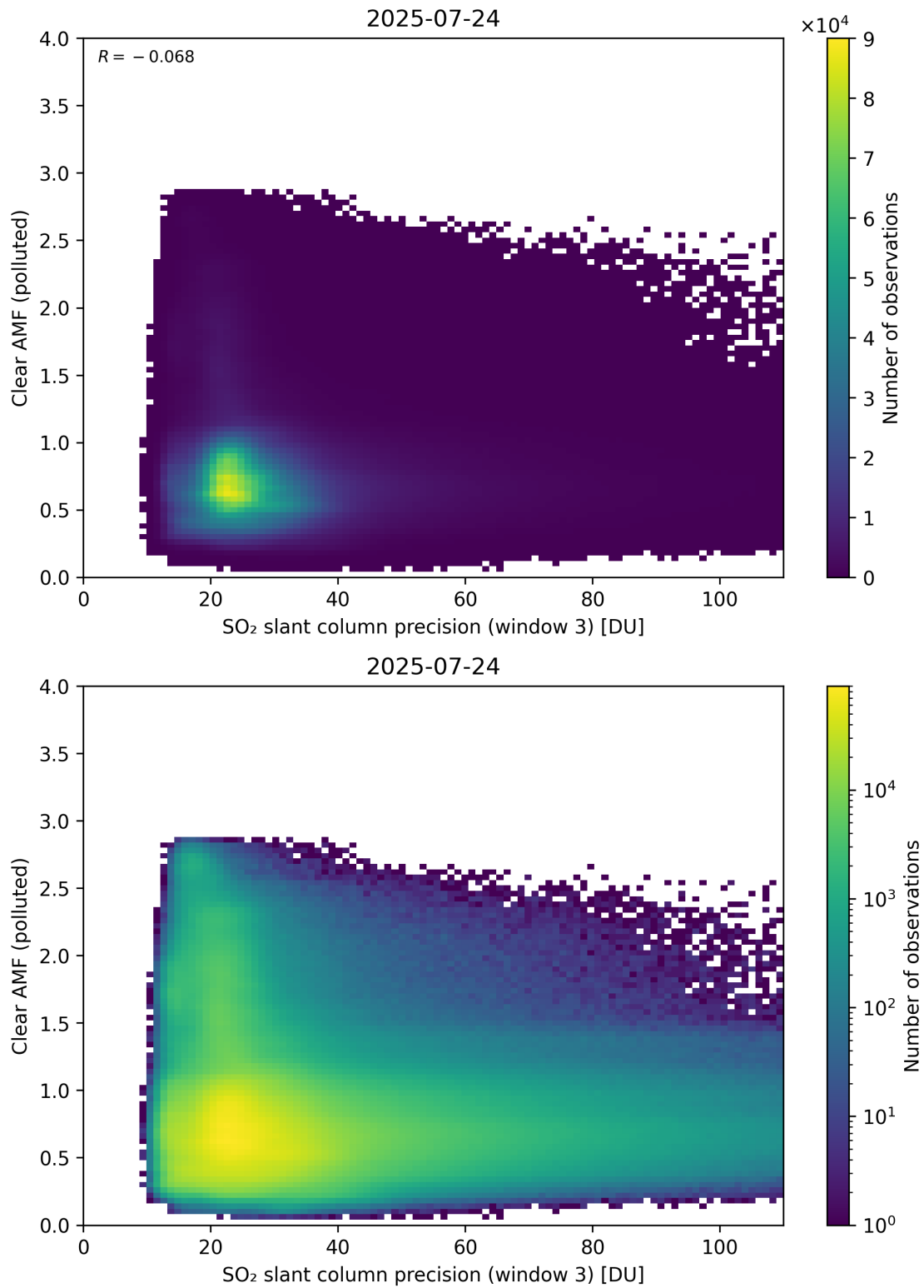
Figure 311: Scatter density plot of “SO 2 slant column precision (window 3)” against “Clear AMF (polluted)” for 2025-07-24 to 2025-07-25.
