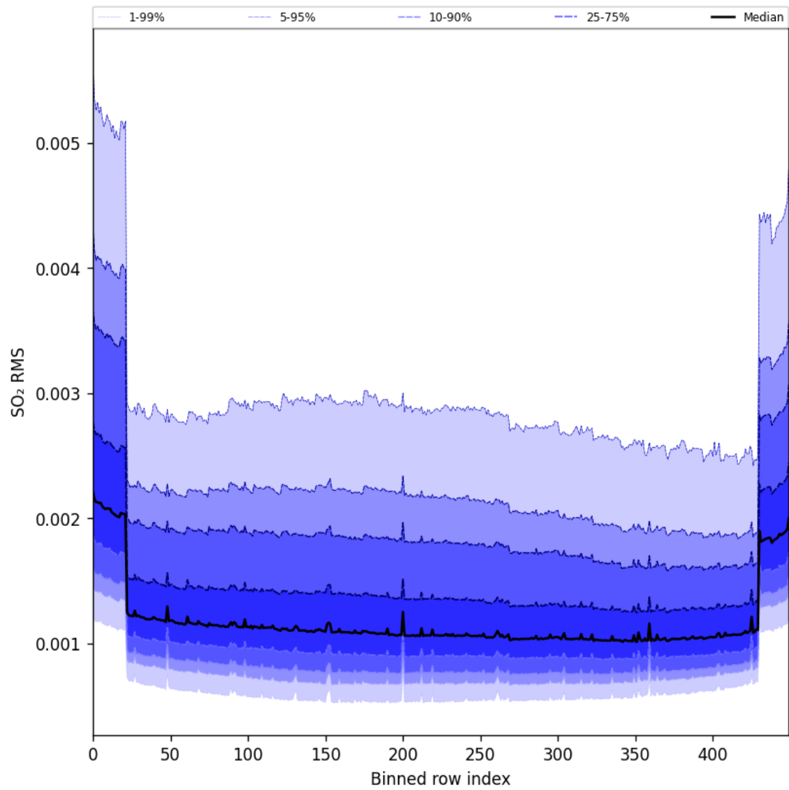
Figure 104: Along track statistics of “SO 2 RMS” for 2025-07-24 to 2025-07-25
