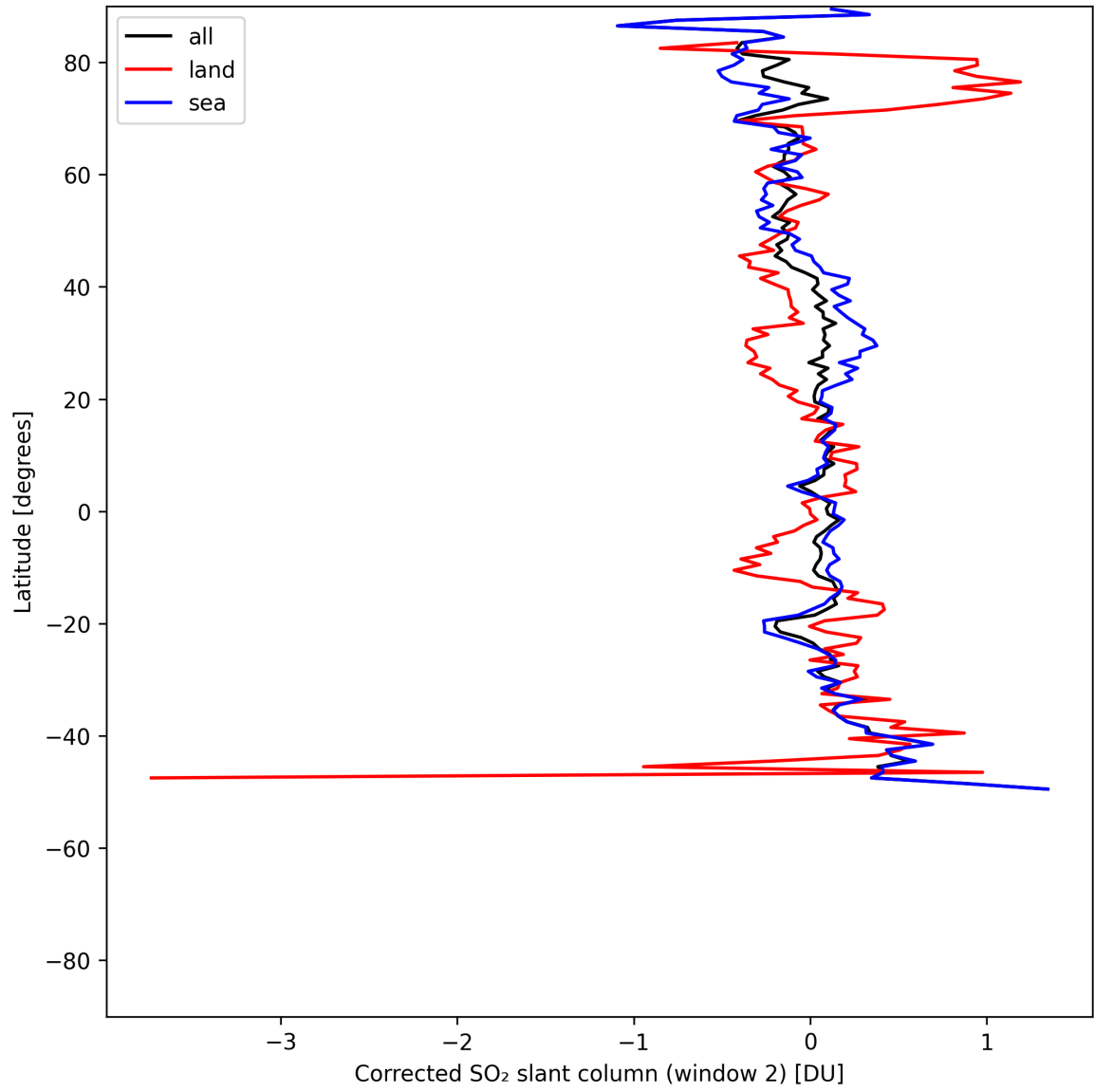
Figure 43: Zonal average of “Corrected SO 2 slant column (window 2)” for 2025-07-24 to 2025-07-25.
