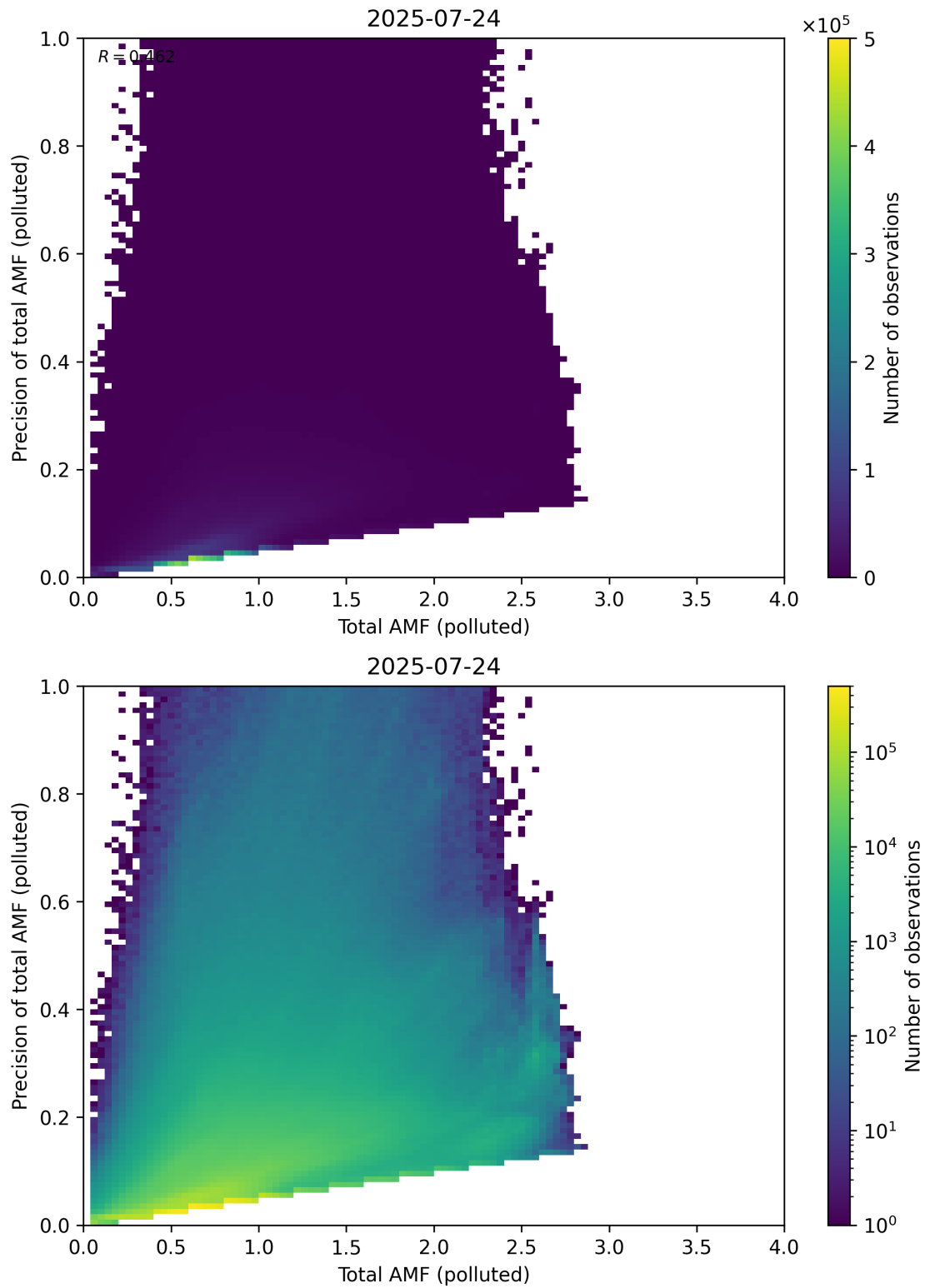
Figure 322: Scatter density plot of “Total AMF (polluted)” against “Precision of total AMF (polluted)” for 2025-07-24 to 2025-07-25.
