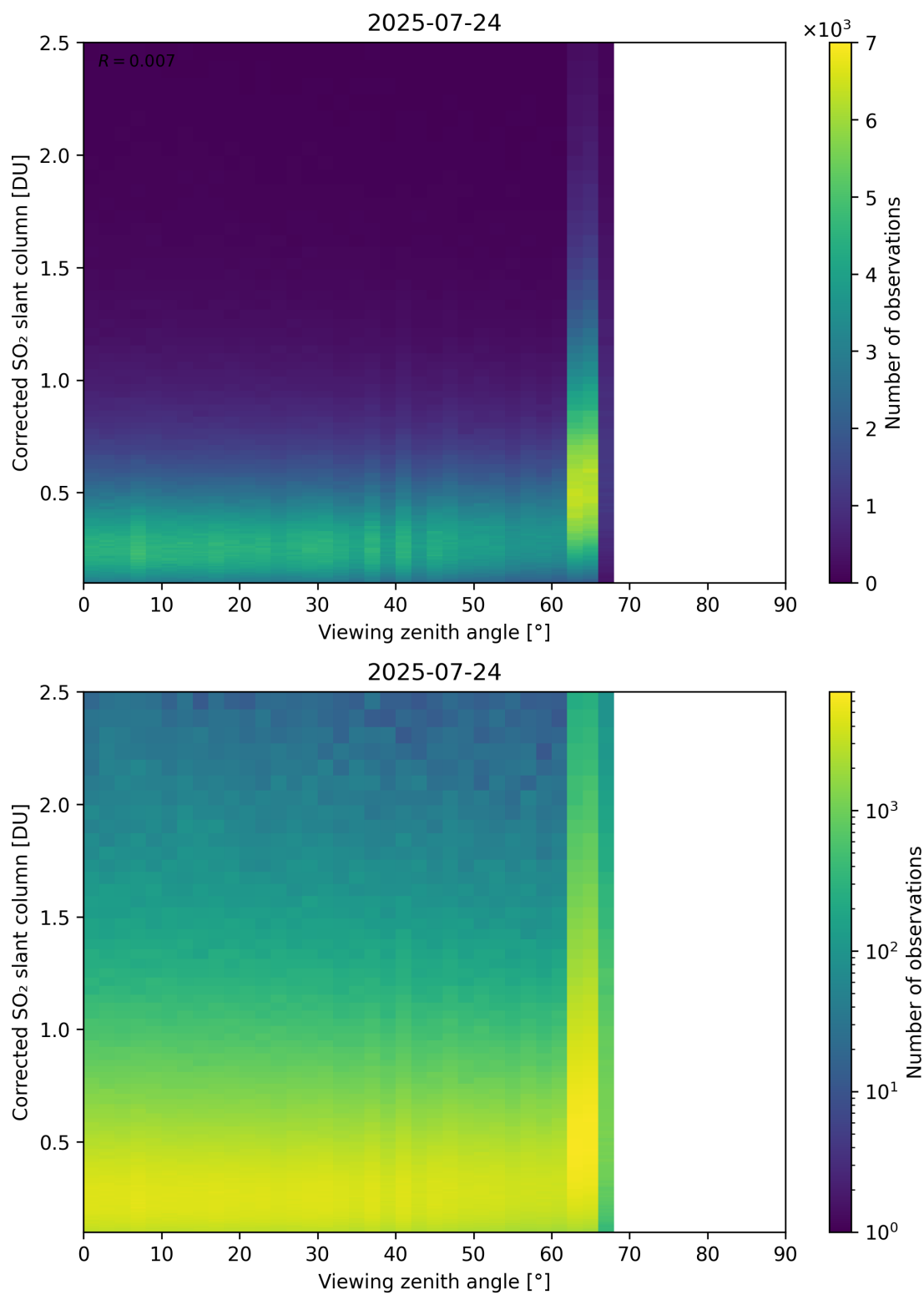
Figure 373: Scatter density plot of “Viewing zenith angle” against “Corrected SO 2 slant column” for 2025-07-24 to 2025-07-25.
