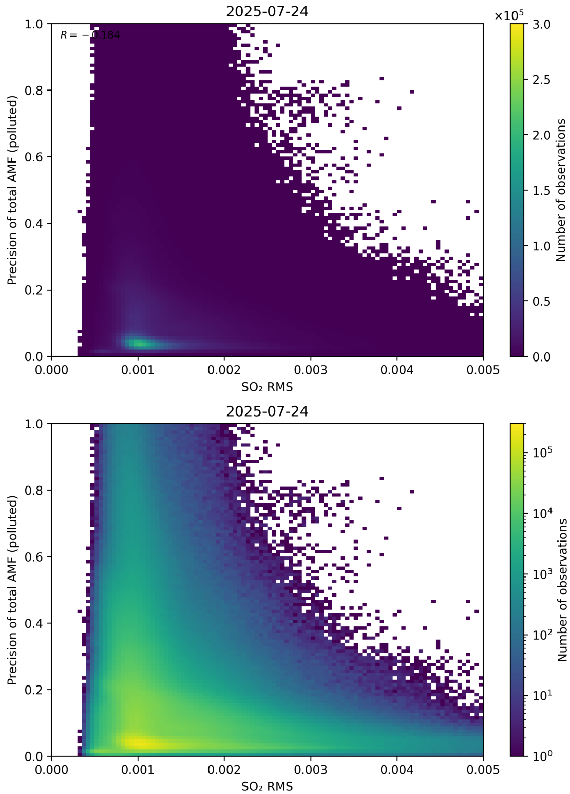
Figure 149: Scatter density plot of “SO 2 RMS” against “Precision of total AMF (polluted)” for 2025-07-24 to 2025-07-25.
