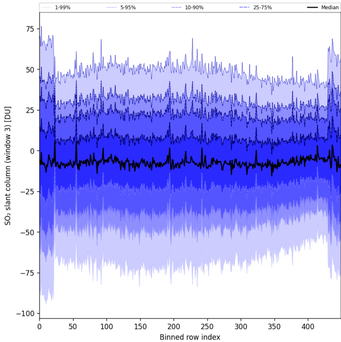
Figure 97: Along track statistics of “SO 2 slant column (window 3)” for 2025-07-24 to 2025-07-25
