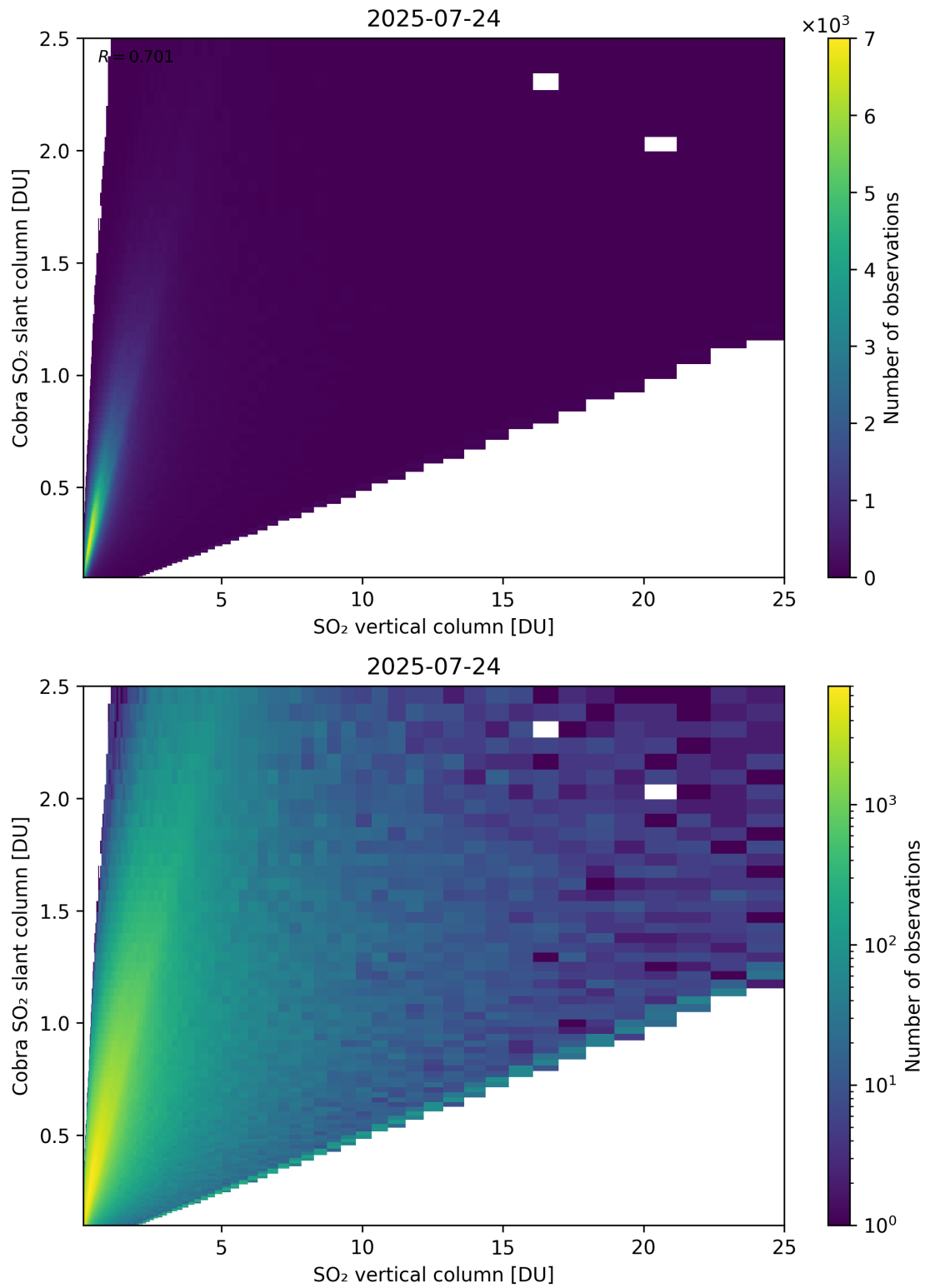
Figure 349: Scatter density plot of “SO 2 vertical column” against “Cobra SO 2 slant column” for 2025-07-24 to 2025-07-25.
