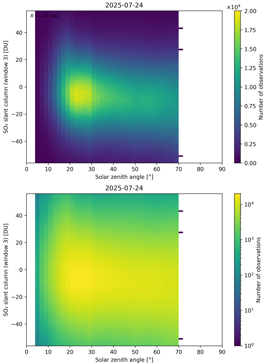
Figure 187: Scatter density plot of “Solar zenith angle” against “SO 2 slant column (window 3)” for 2025-07-24 to 2025-07-25.
