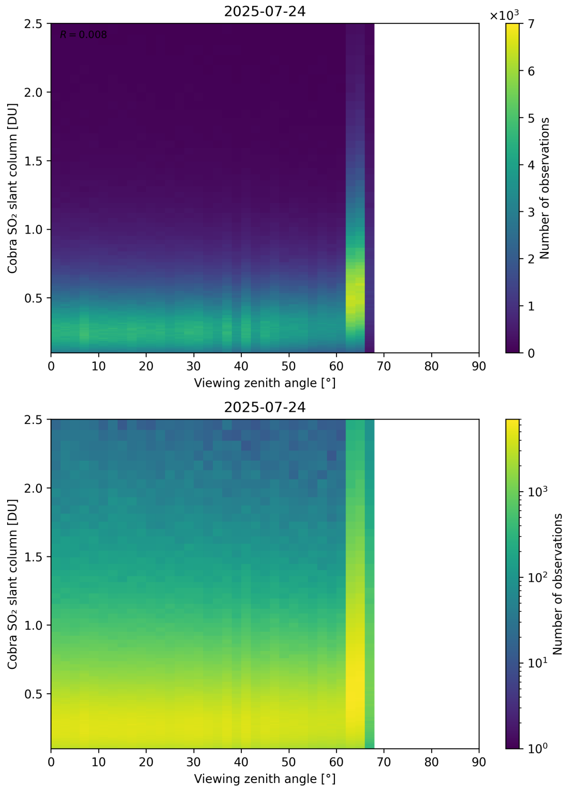
Figure 371: Scatter density plot of “Viewing zenith angle” against “Cobra SO 2 slant column” for 2025-07-24 to 2025-07-25.
