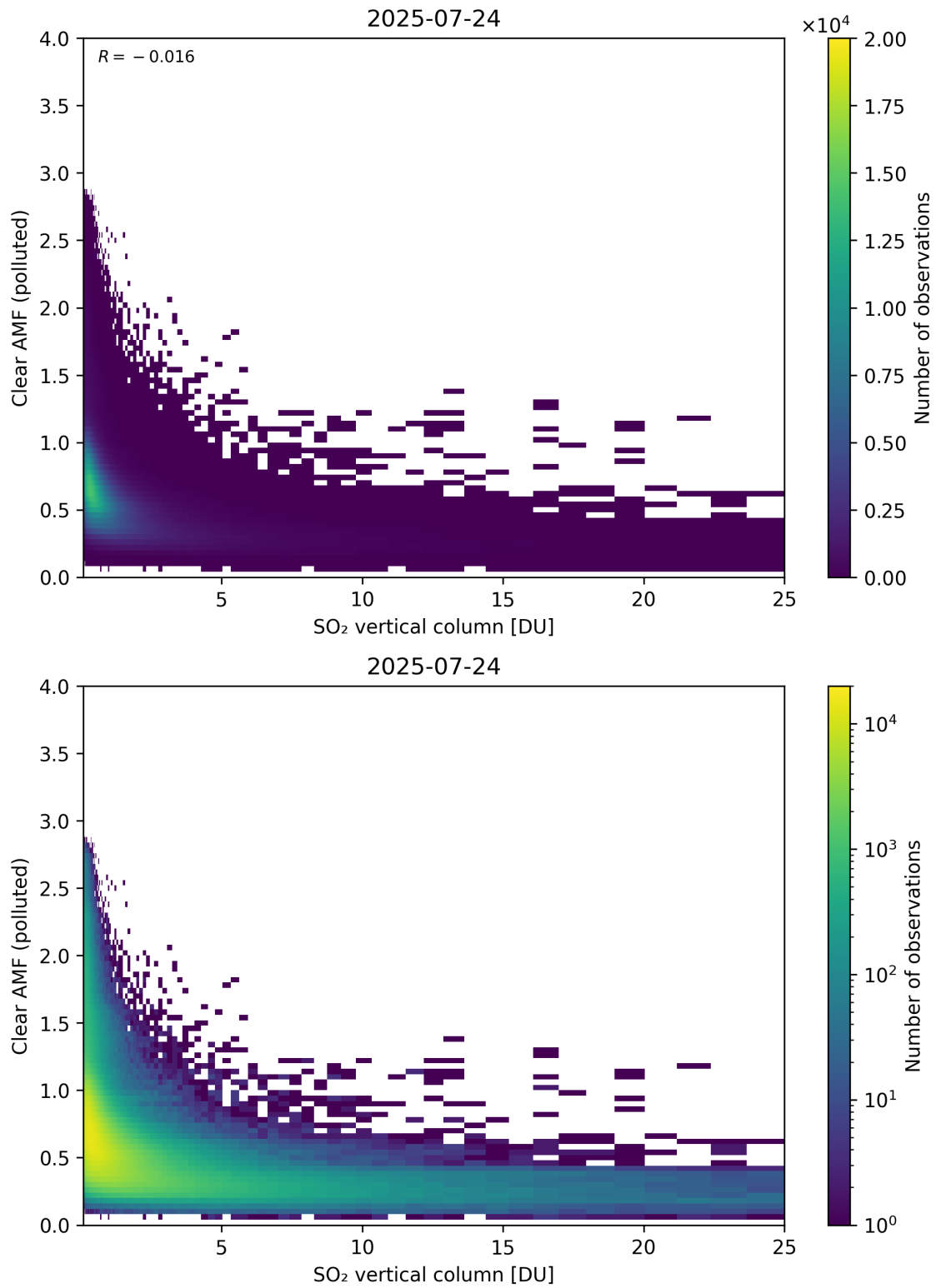
Figure 348: Scatter density plot of “SO 2 vertical column” against “Clear AMF (polluted)” for 2025-07-24 to 2025-07-25.
