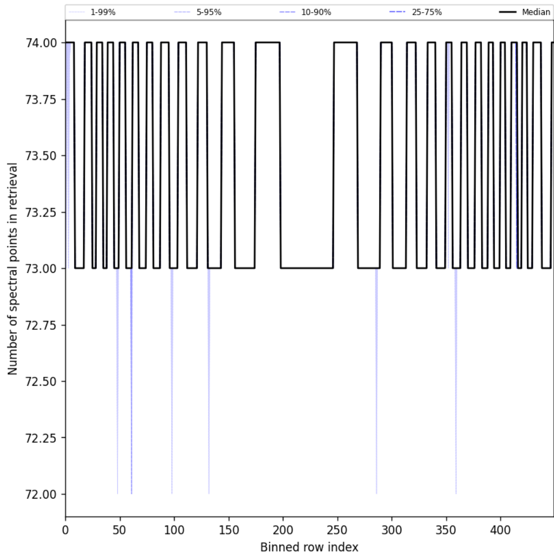
Figure 108: Along track statistics of “Number of spectral points in retrieval” for 2025-07-24 to 2025-07-25
