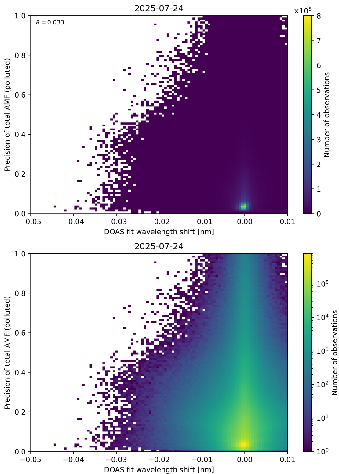
Figure 142: Scatter density plot of “DOAS fit wavelength shift” against “Precision of total AMF (polluted)” for 2025-07-24 to 2025-07-25.
