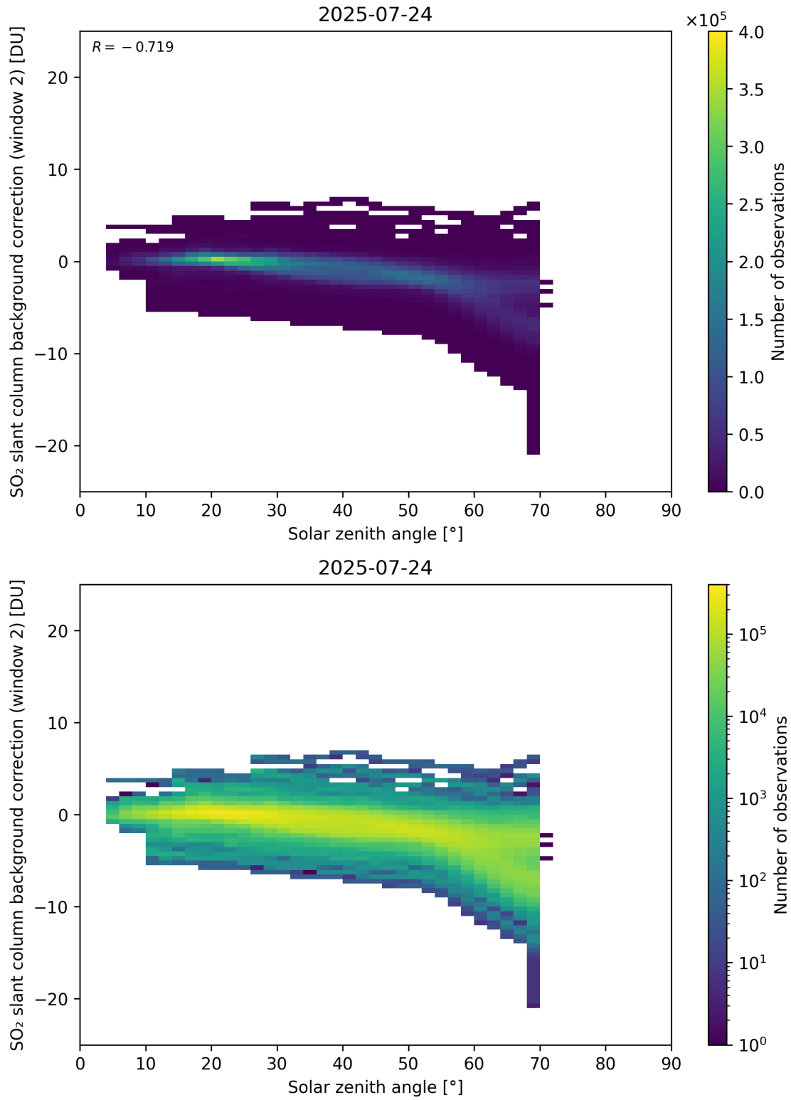
Figure 172: Scatter density plot of “Solar zenith angle” against “SO 2 slant column background correction (window 2)” for 2025-07-24 to 2025-07-25.
