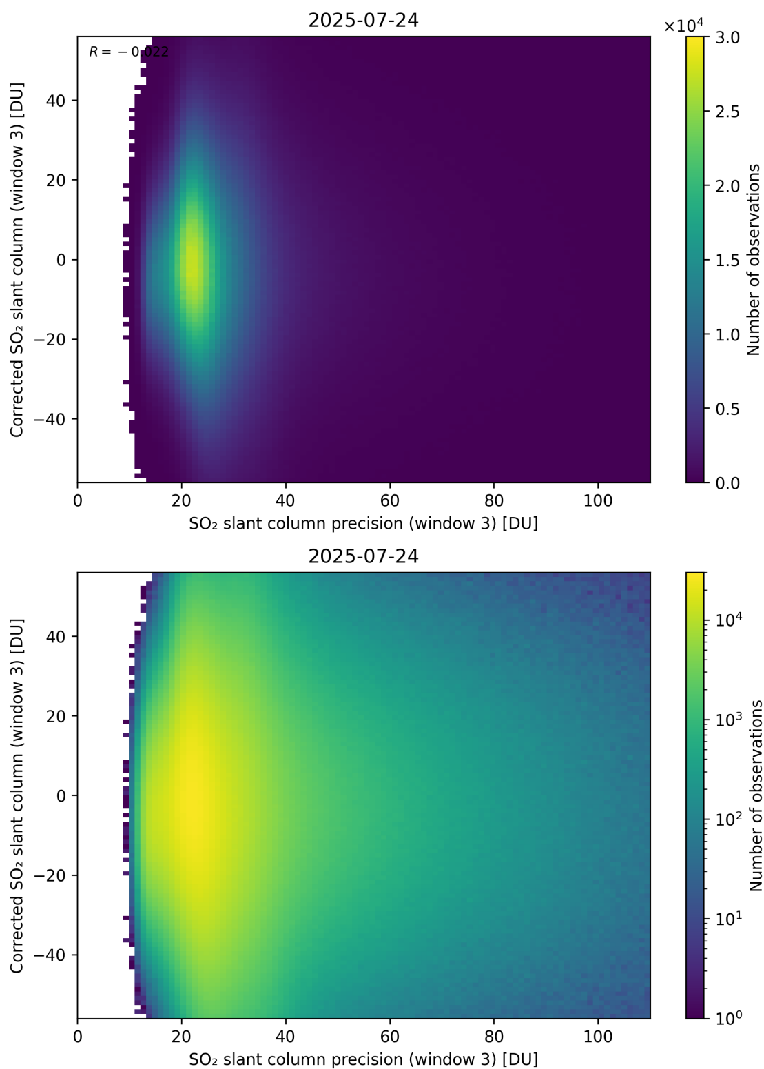
Figure 312: Scatter density plot of “SO 2 slant column precision (window 3)” against “Corrected SO 2 slant column (window 3)” for 2025-07-24 to 2025-07-25.
