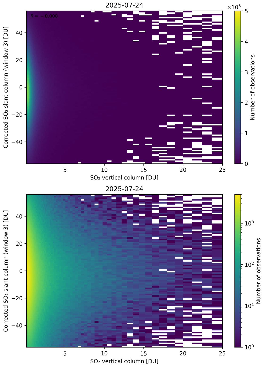
Figure 353: Scatter density plot of “SO 2 vertical column” against “Corrected SO 2 slant column (window 3)” for 2025-07-24 to 2025-07-25.
