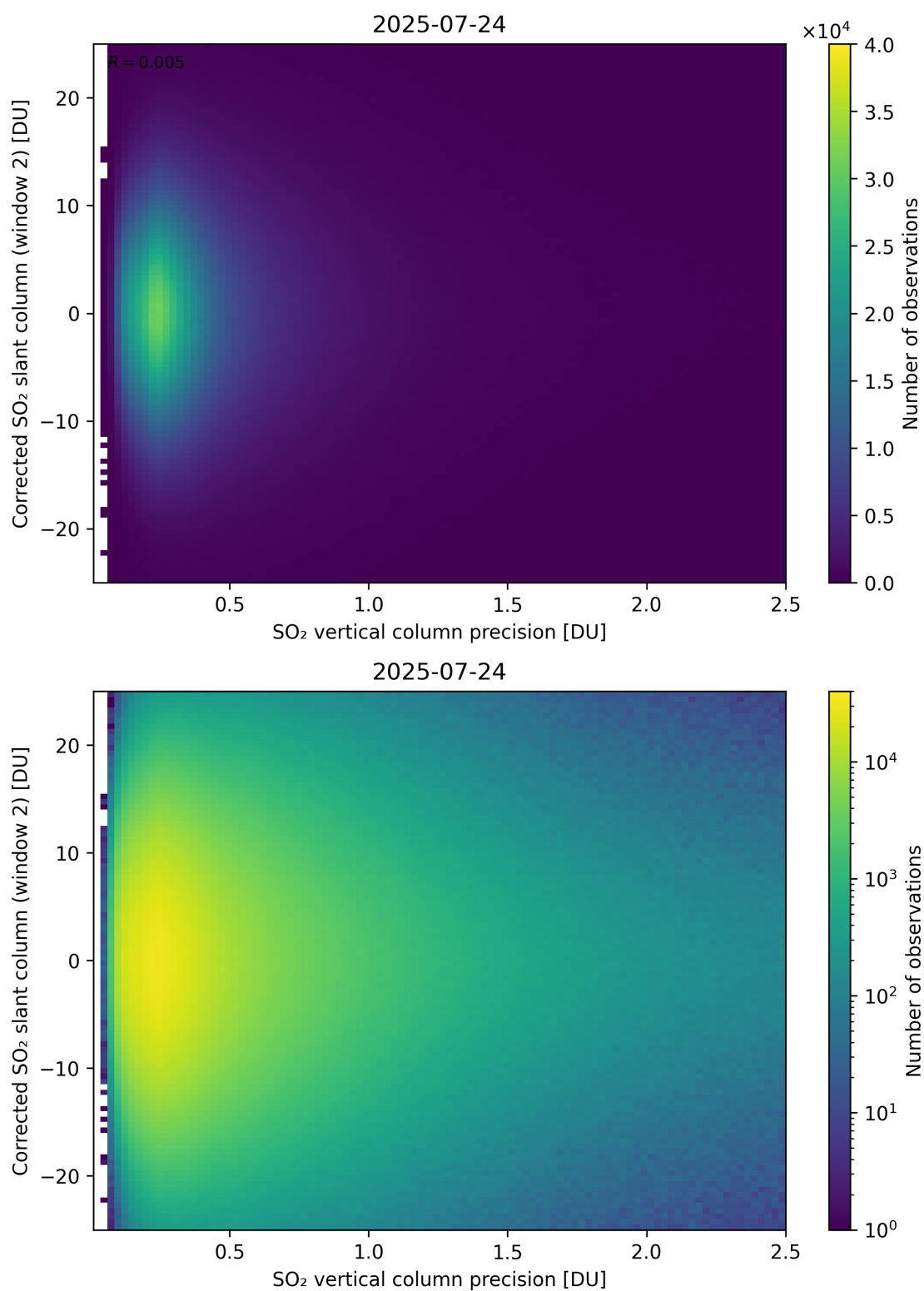
Figure 339: Scatter density plot of “SO 2 vertical column precision” against “Corrected SO 2 slant column (window 2)” for 2025-07-24 to 2025-07-25.
