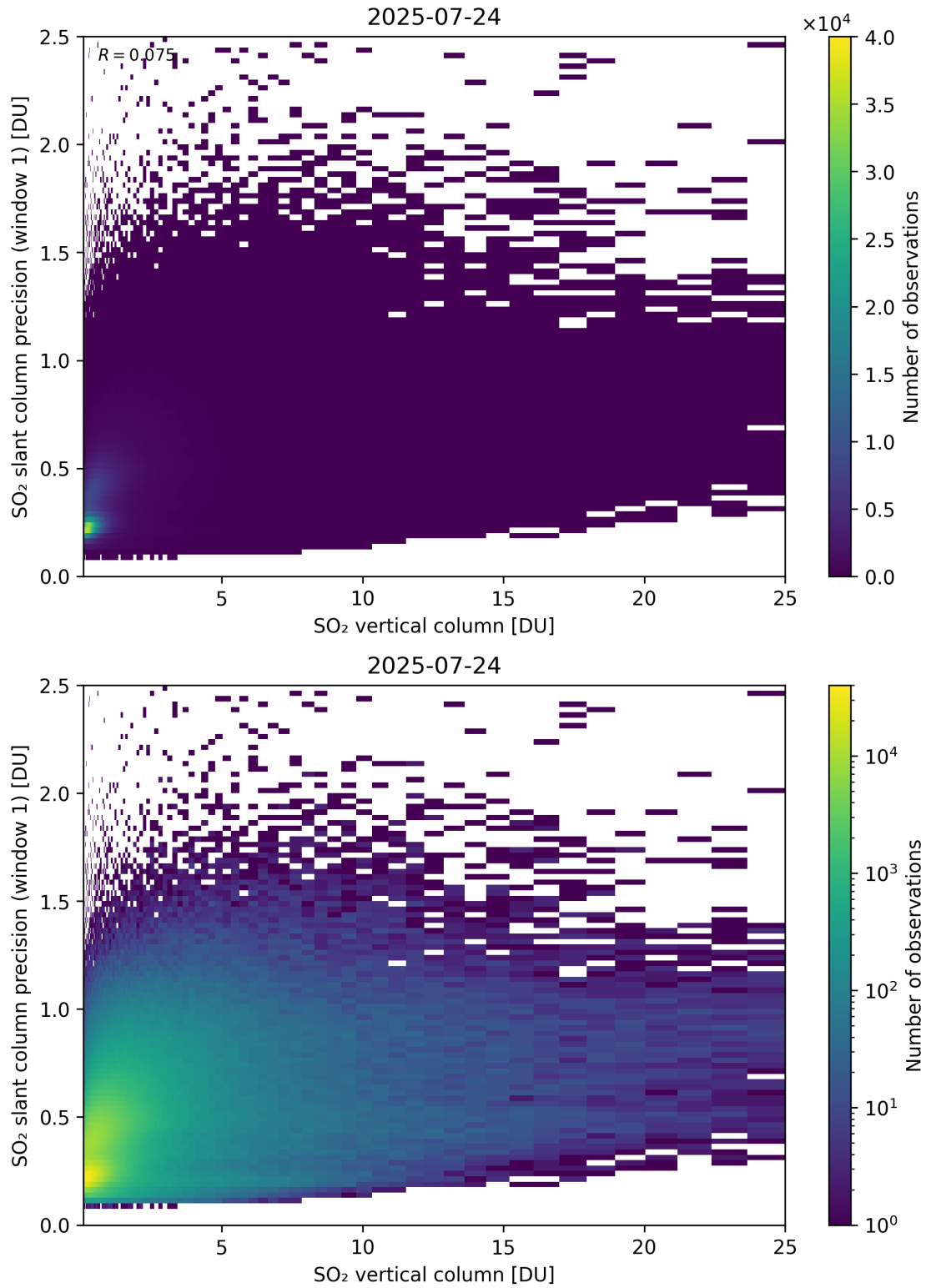
Figure 355: Scatter density plot of “SO 2 vertical column” against “SO 2 slant column precision (window 1)” for 2025-07-24 to 2025-07-25.
