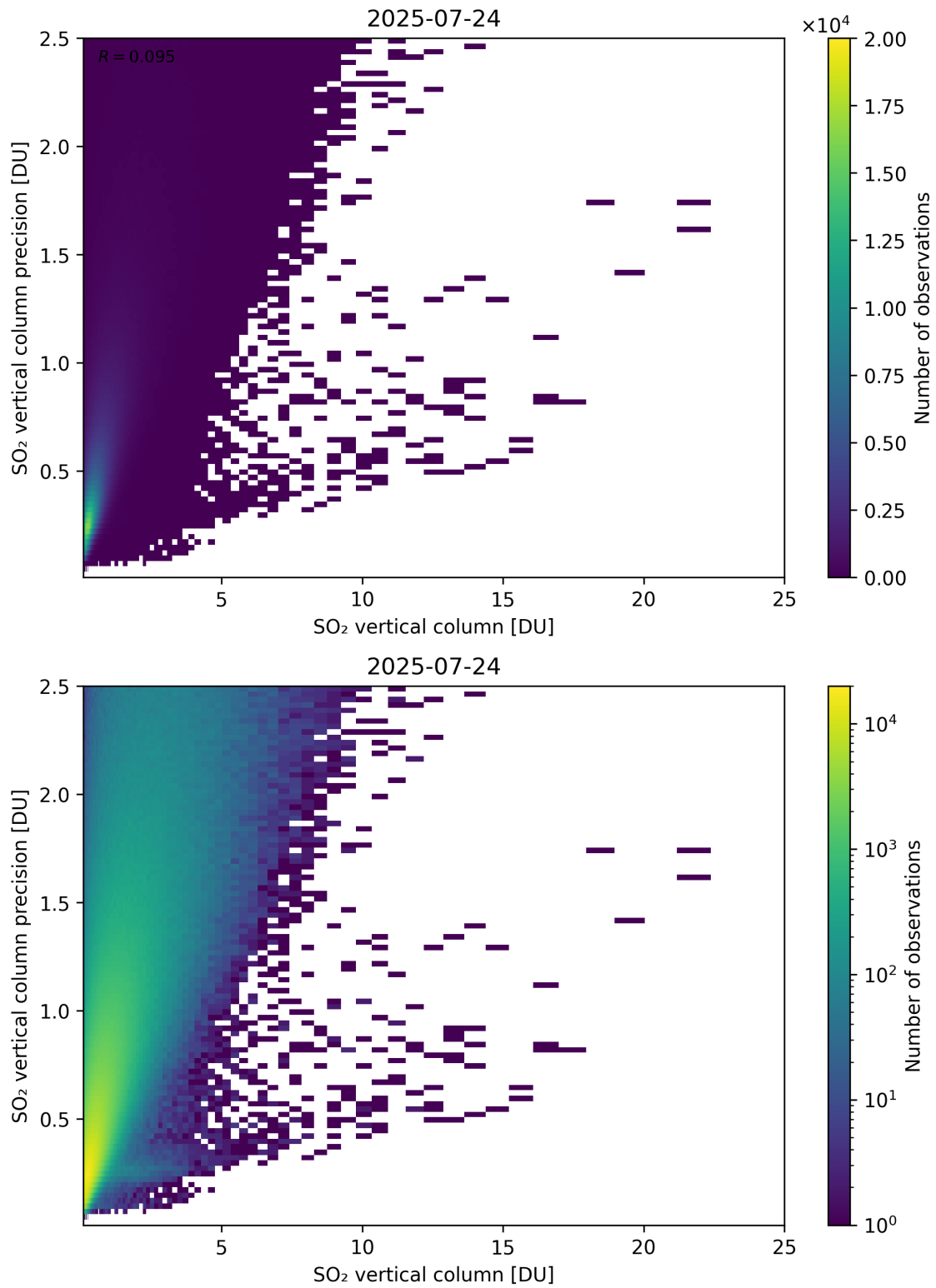
Figure 361: Scatter density plot of “SO 2 vertical column” against “SO 2 vertical column precision” for 2025-07-24 to 2025-07-25.
