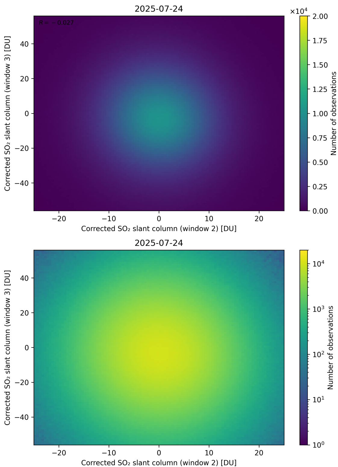
Figure 250: Scatter density plot of “Corrected SO 2 slant column (window 2)” against “Corrected SO 2 slant column (window 3)” for 2025-07-24 to 2025-07-25.
