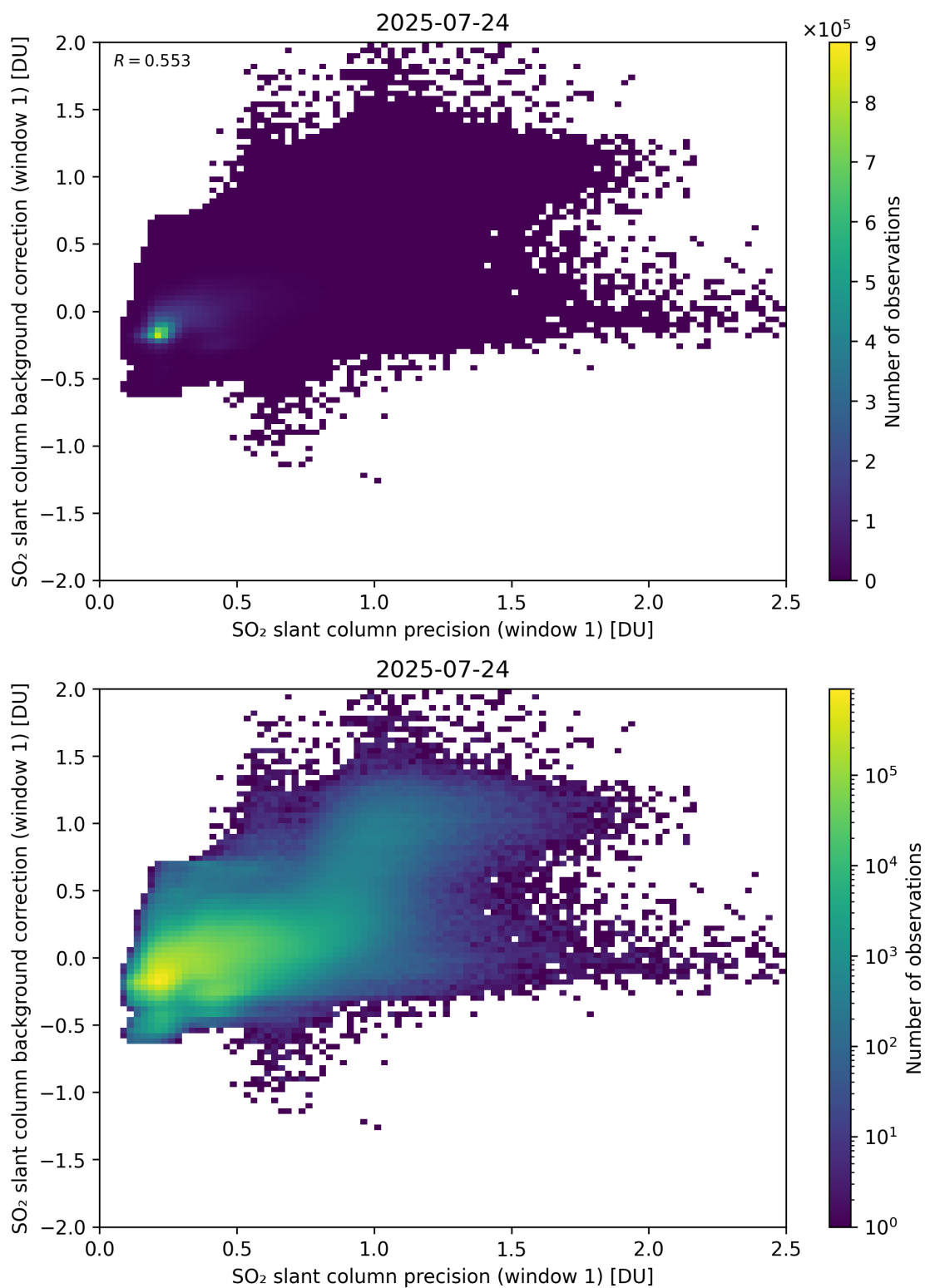
Figure 268: Scatter density plot of “SO 2 slant column precision (window 1)” against “SO 2 slant column background correction (window 1)” for 2025-07-24 to 2025-07-25.
