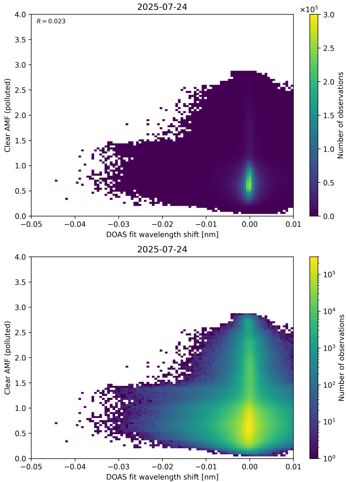
Figure 140: Scatter density plot of “DOAS fit wavelength shift” against “Clear AMF (polluted)” for 2025-07-24 to 2025-07-25.
