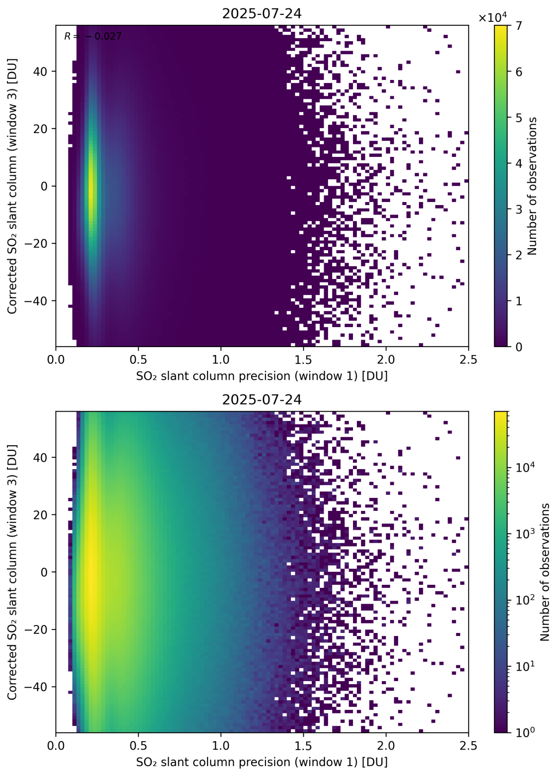
Figure 276: Scatter density plot of “SO 2 slant column precision (window 1)” against “Corrected SO 2 slant column (window 3)” for 2025-07-24 to 2025-07-25.
