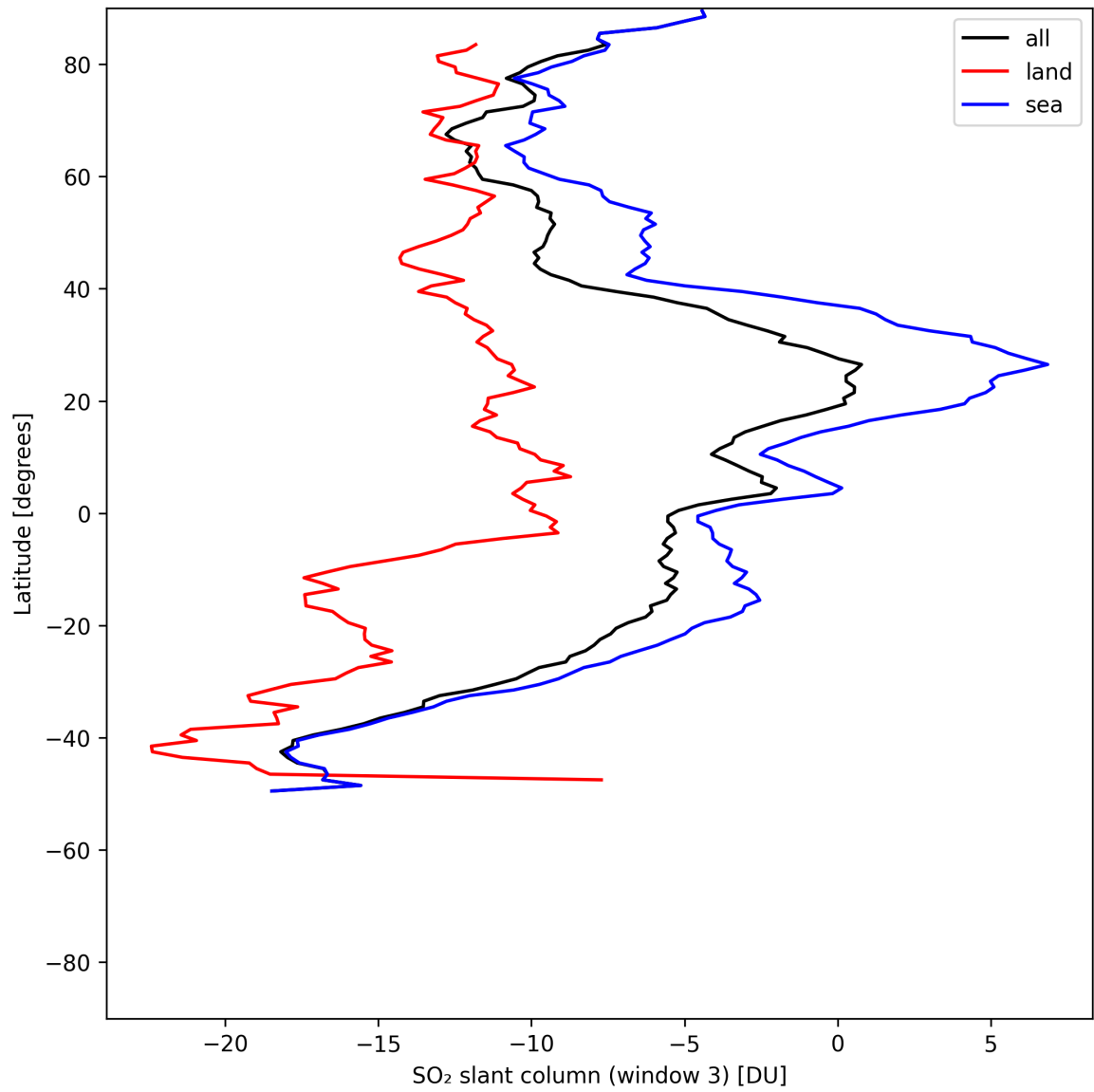
Figure 45: Zonal average of “SO 2 slant column (window 3)” for 2025-07-24 to 2025-07-25.
