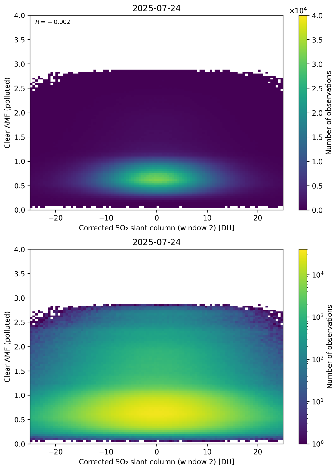
Figure 249: Scatter density plot of “Corrected SO 2 slant column (window 2)” against “Clear AMF (polluted)” for 2025-07-24 to 2025-07-25.
