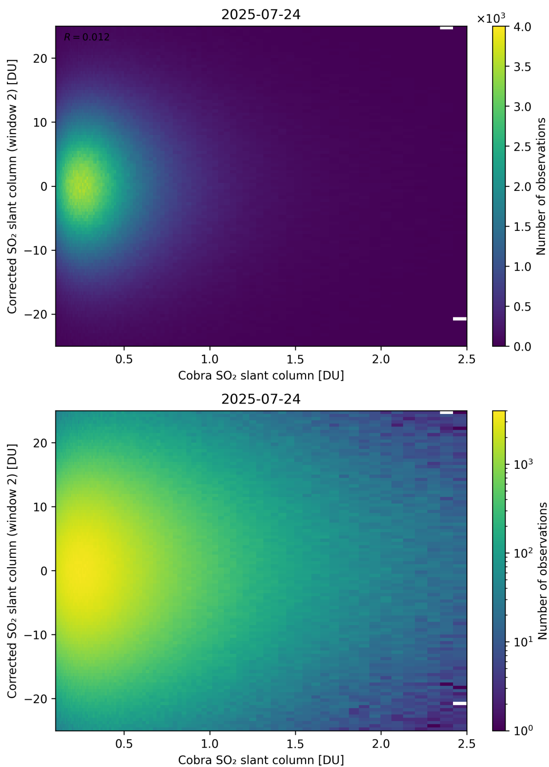
Figure 217: Scatter density plot of “Cobra SO 2 slant column” against “Corrected SO 2 slant column (window 2)” for 2025-07-24 to 2025-07-25.
