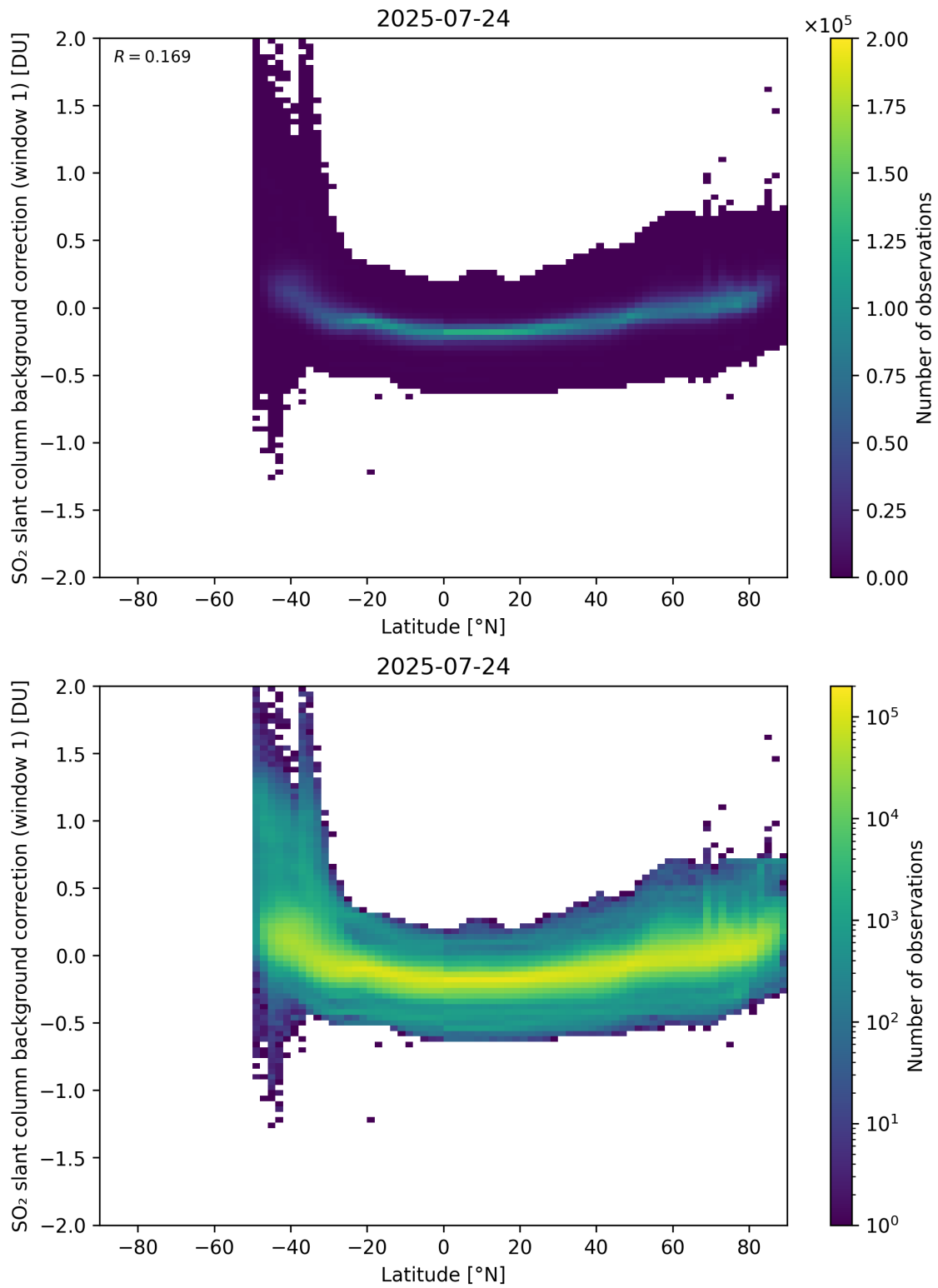
Figure 150: Scatter density plot of “Latitude” against “SO 2 slant column background correction (window 1)” for 2025-07-24 to 2025-07-25.
