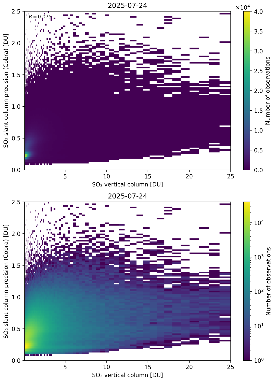
Figure 350: Scatter density plot of “SO 2 vertical column” against “SO 2 slant column precision (Cobra)” for 2025-07-24 to 2025-07-25.
