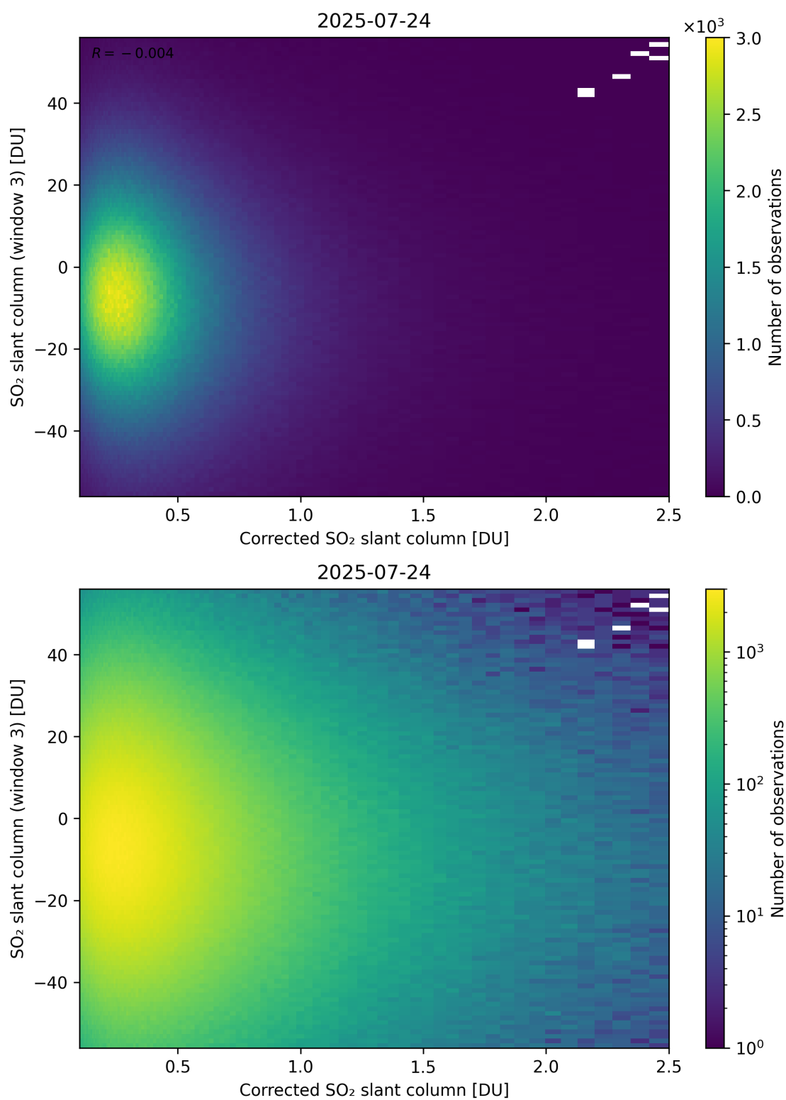
Figure 240: Scatter density plot of “Corrected SO 2 slant column” against “SO 2 slant column (window 3)” for 2025-07-24 to 2025-07-25.
