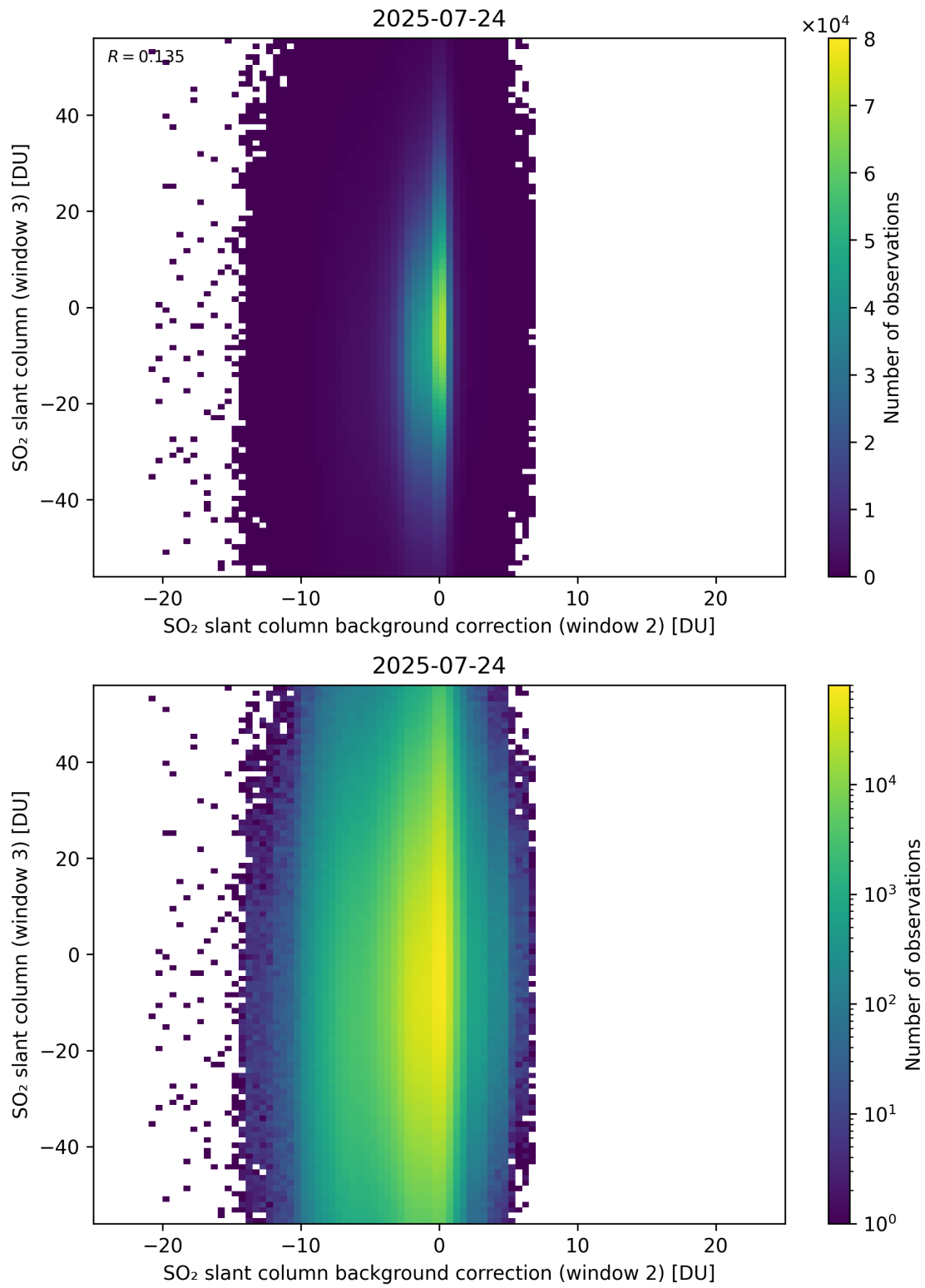
Figure 128: Scatter density plot of “SO 2 slant column background correction (window 2)” against “SO 2 slant column (window 3)” for 2025-07-24 to 2025-07-25.
