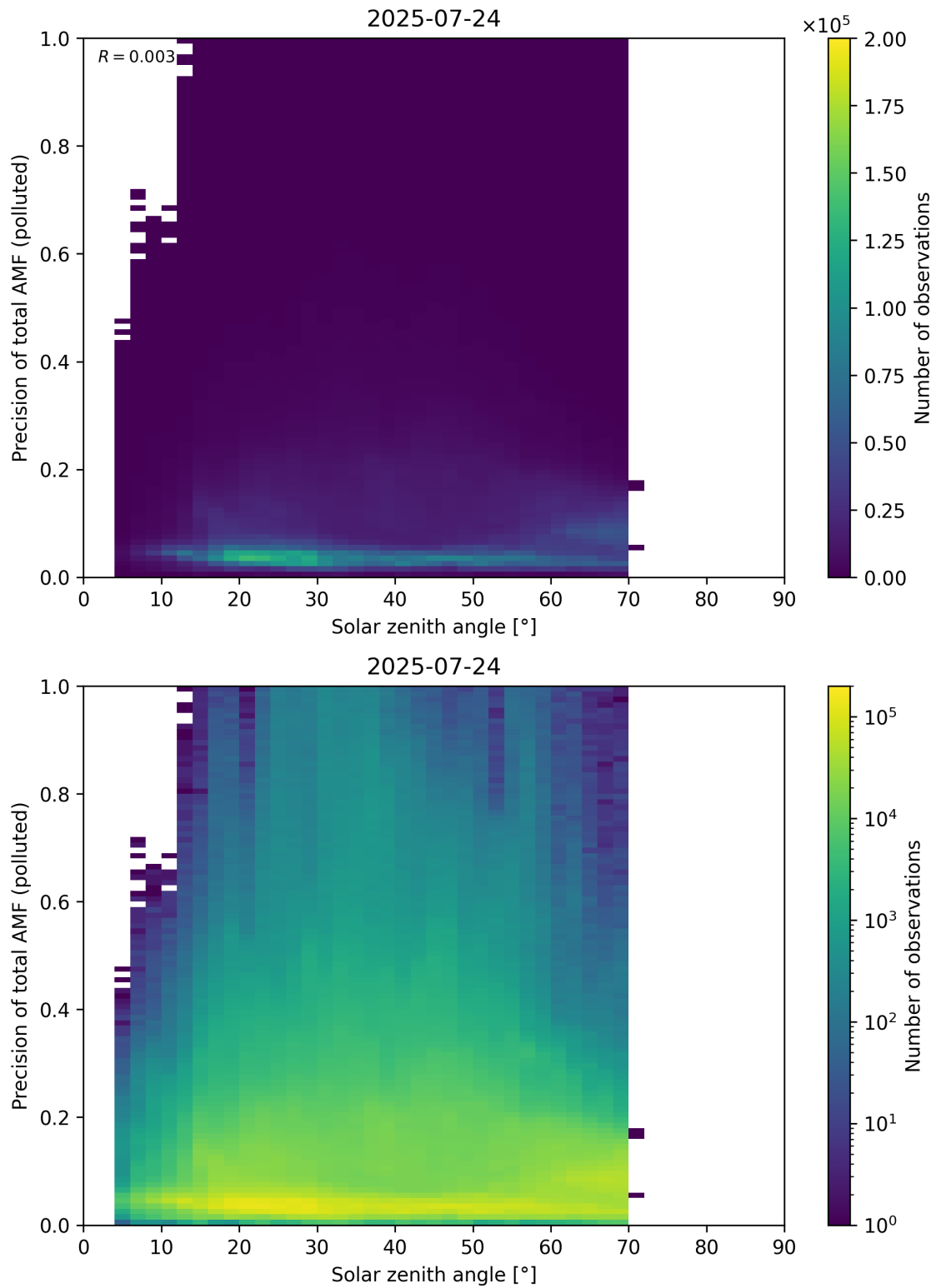
Figure 190: Scatter density plot of “Solar zenith angle” against “Precision of total AMF (polluted)” for 2025-07-24 to 2025-07-25.
