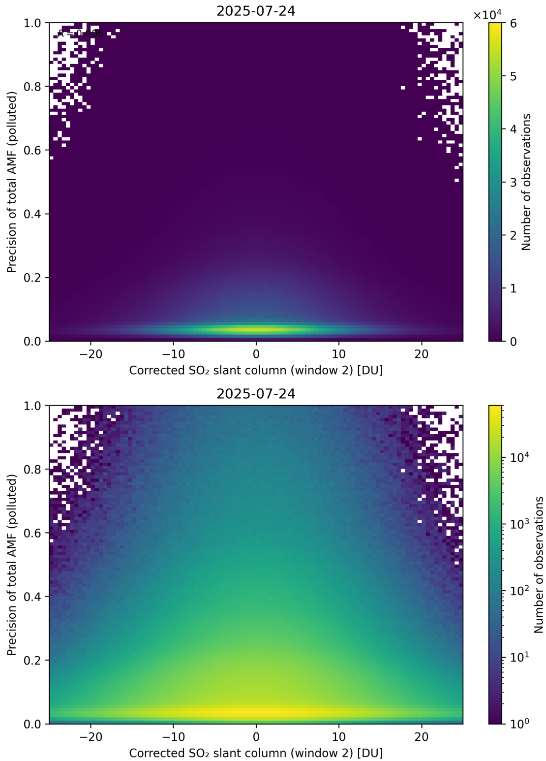
Figure 254: Scatter density plot of “Corrected SO 2 slant column (window 2)” against “Precision of total AMF (polluted)” for 2025-07-24 to 2025-07-25.
