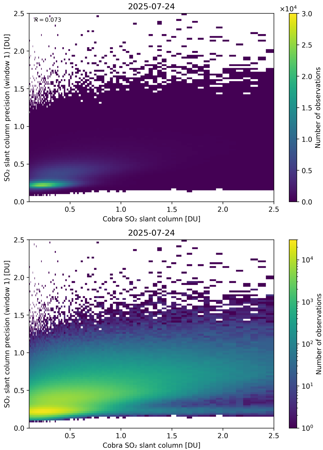
Figure 220: Scatter density plot of “Cobra SO 2 slant column” against “SO 2 slant column precision (window 1)” for 2025-07-24 to 2025-07-25.
