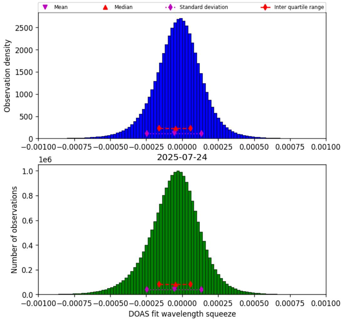
Figure 77: Histogram of “DOAS fit wavelength squeeze” for 2025-07-24 to 2025-07-25
