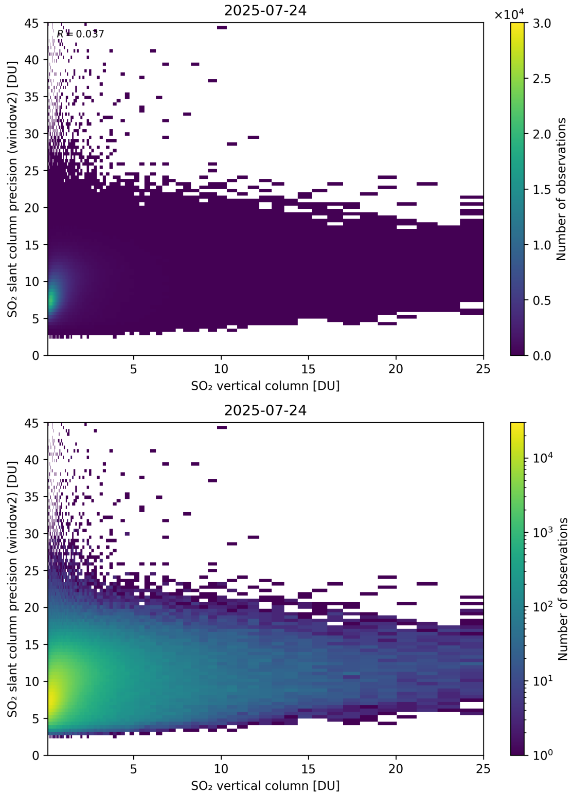
Figure 356: Scatter density plot of “SO 2 vertical column” against “SO 2 slant column precision (window2)” for 2025-07-24 to 2025-07-25.
