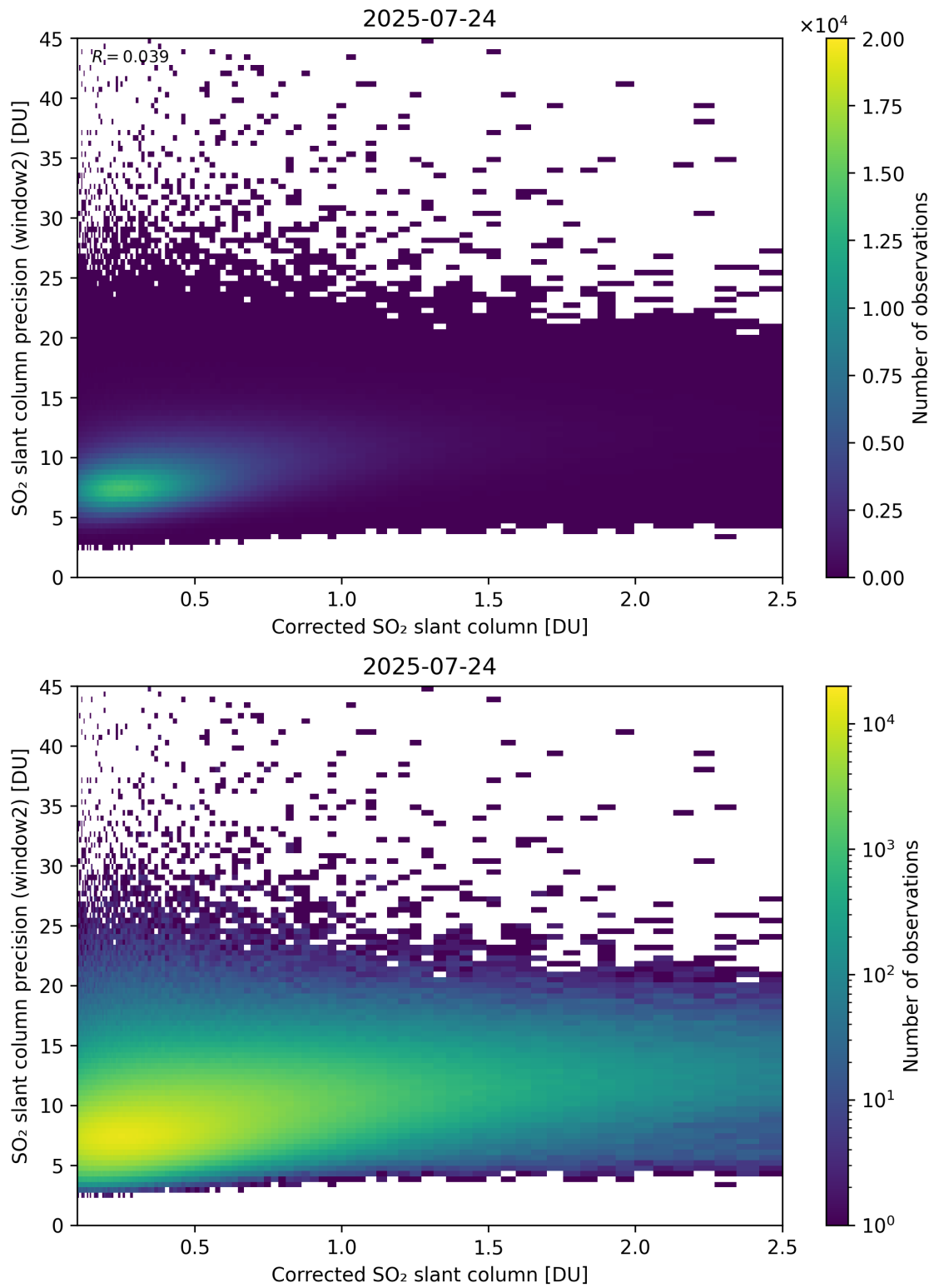
Figure 239: Scatter density plot of “Corrected SO 2 slant column” against “SO 2 slant column precision (window2)” for 2025-07-24 to 2025-07-25.
