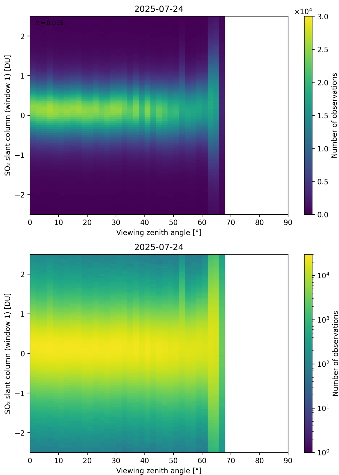
Figure 376: Scatter density plot of “Viewing zenith angle” against “SO 2 slant column (window 1)” for 2025-07-24 to 2025-07-25.
