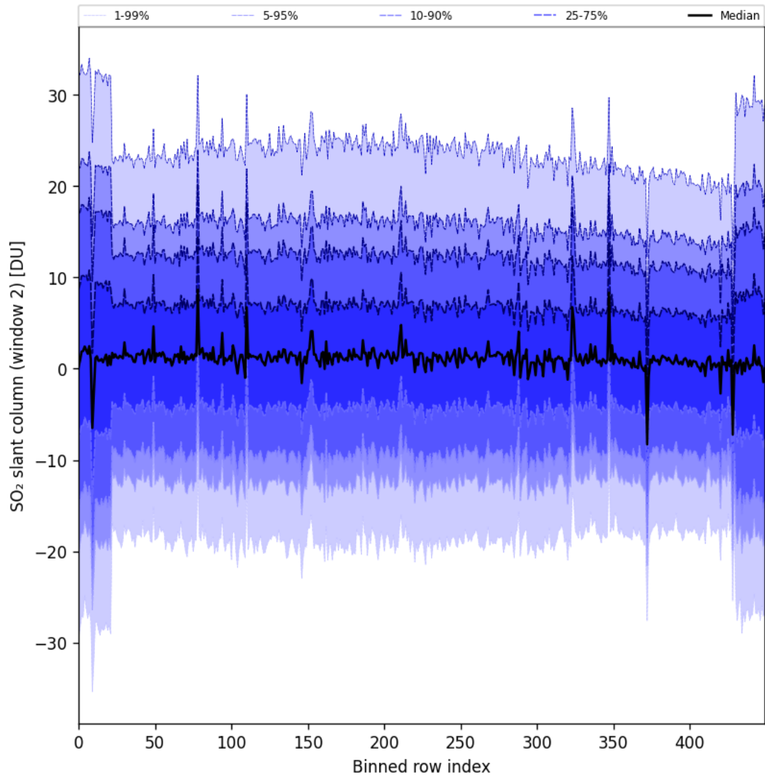
Figure 93: Along track statistics of “SO 2 slant column (window 2)” for 2025-07-24 to 2025-07-25
