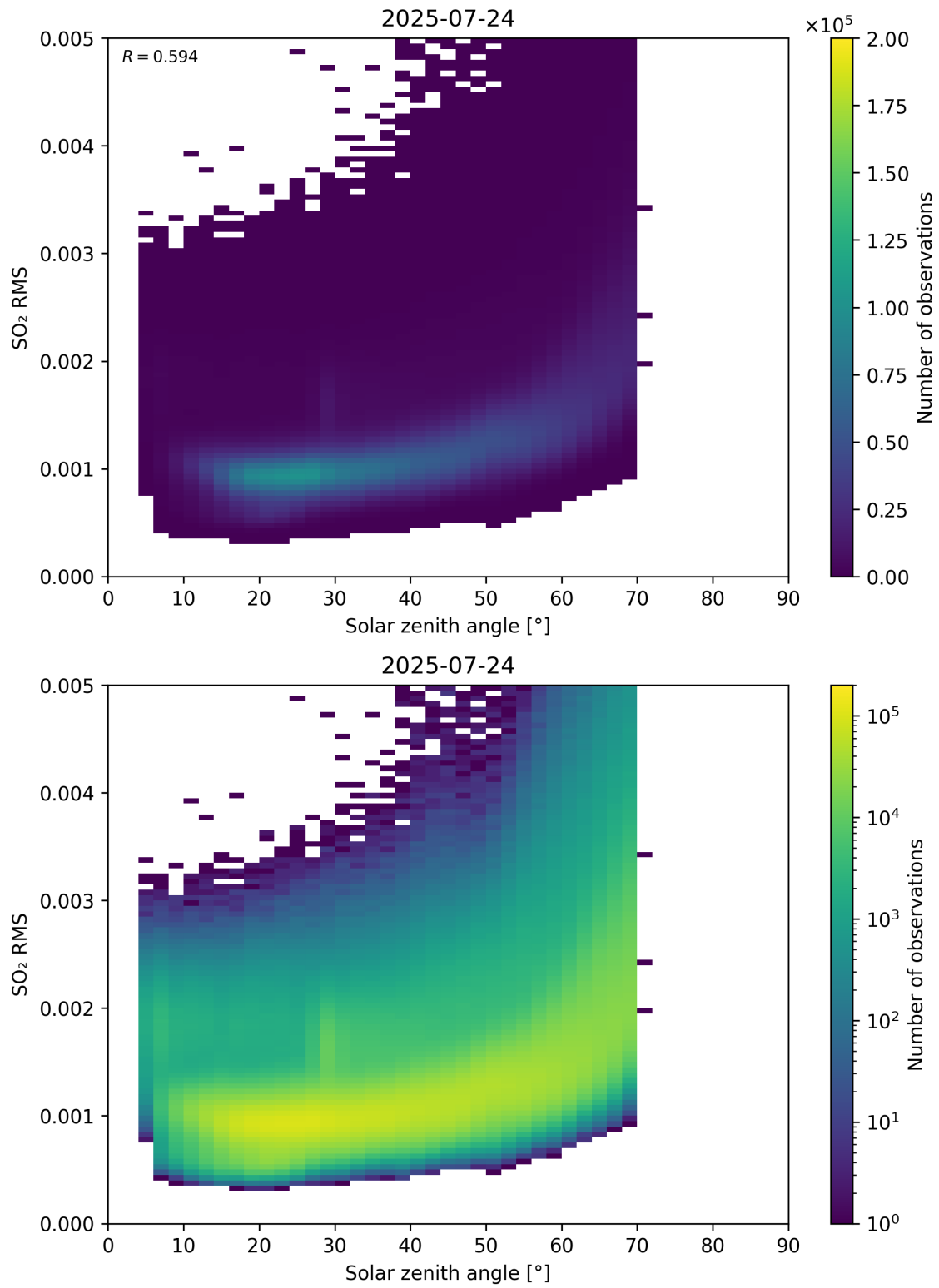
Figure 176: Scatter density plot of “Solar zenith angle” against “SO 2 RMS” for 2025-07-24 to 2025-07-25.
