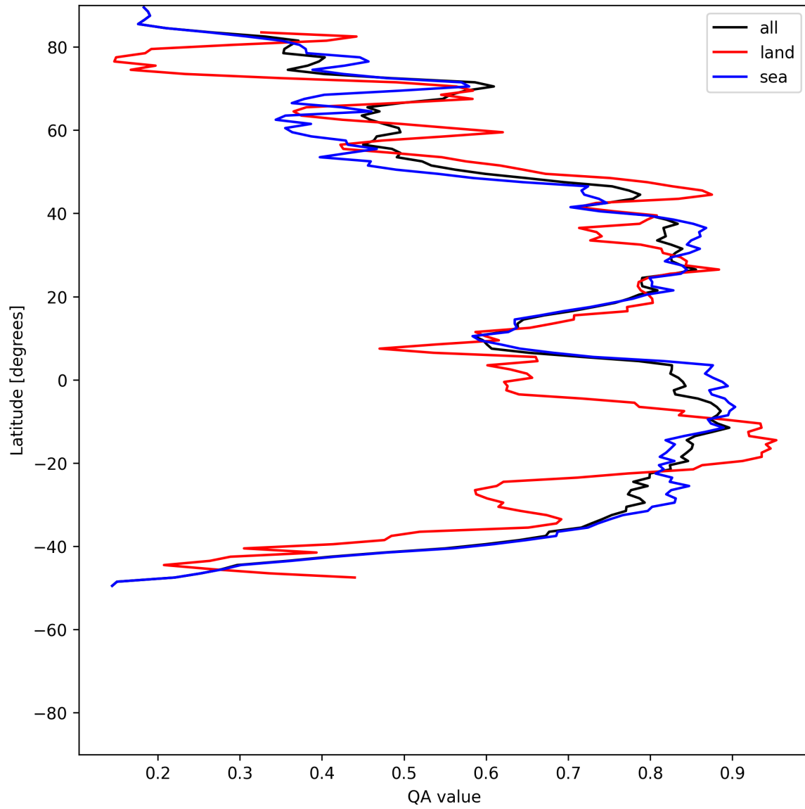
Figure 31: Zonal average of “QA value” for 2025-07-24 to 2025-07-25.
