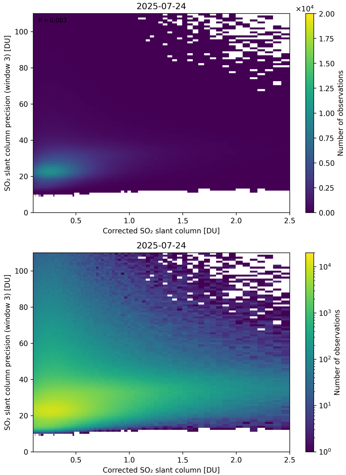
Figure 241: Scatter density plot of “Corrected SO 2 slant column” against “SO 2 slant column precision (window 3)” for 2025-07-24 to 2025-07-25.
