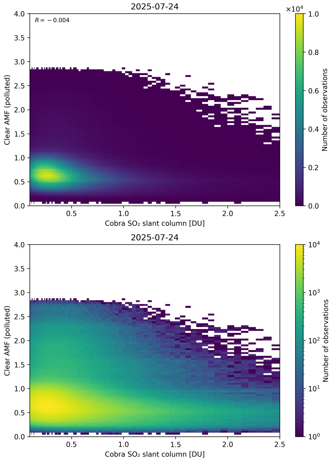
Figure 215: Scatter density plot of “Cobra SO 2 slant column” against “Clear AMF (polluted)” for 2025-07-24 to 2025-07-25.
