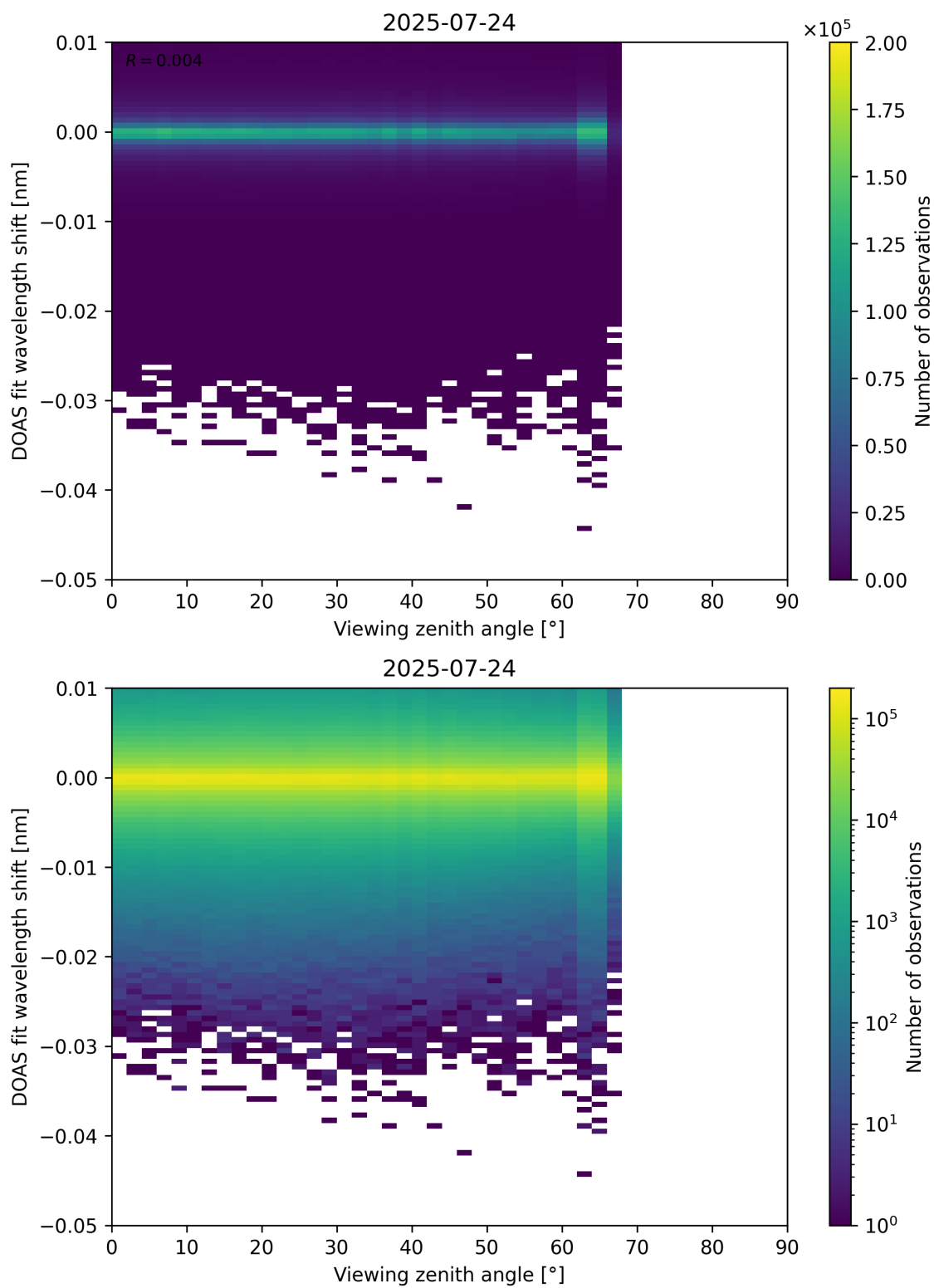
Figure 365: Scatter density plot of “Viewing zenith angle” against “DOAS fit wavelength shift” for 2025-07-24 to 2025-07-25.
