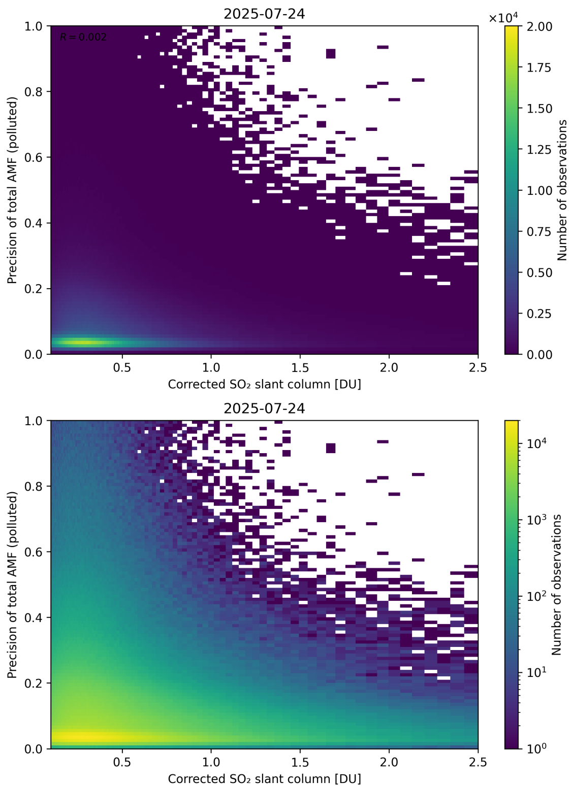
Figure 243: Scatter density plot of “Corrected SO 2 slant column” against “Precision of total AMF (polluted)” for 2025-07-24 to 2025-07-25.
