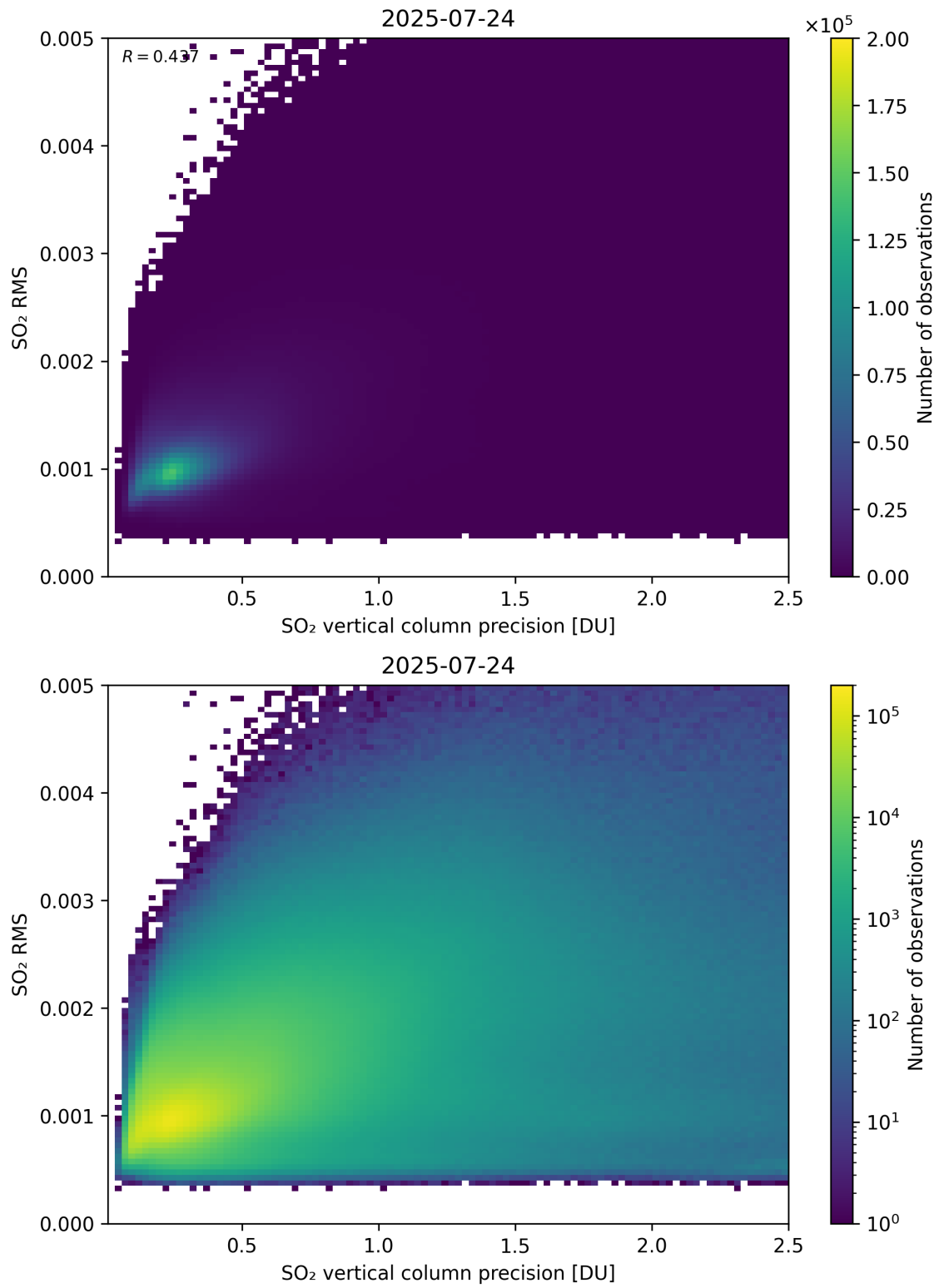
Figure 334: Scatter density plot of “SO 2 vertical column precision” against “SO 2 RMS” for 2025-07-24 to 2025-07-25.
