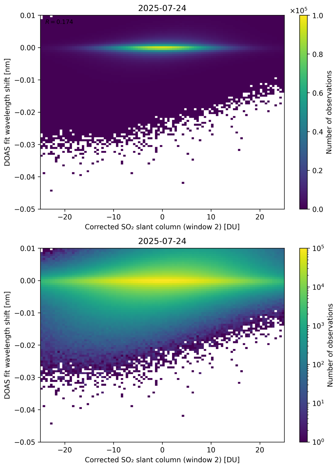
Figure 246: Scatter density plot of “Corrected SO 2 slant column (window 2)” against “DOAS fit wavelength shift” for 2025-07-24 to 2025-07-25.
