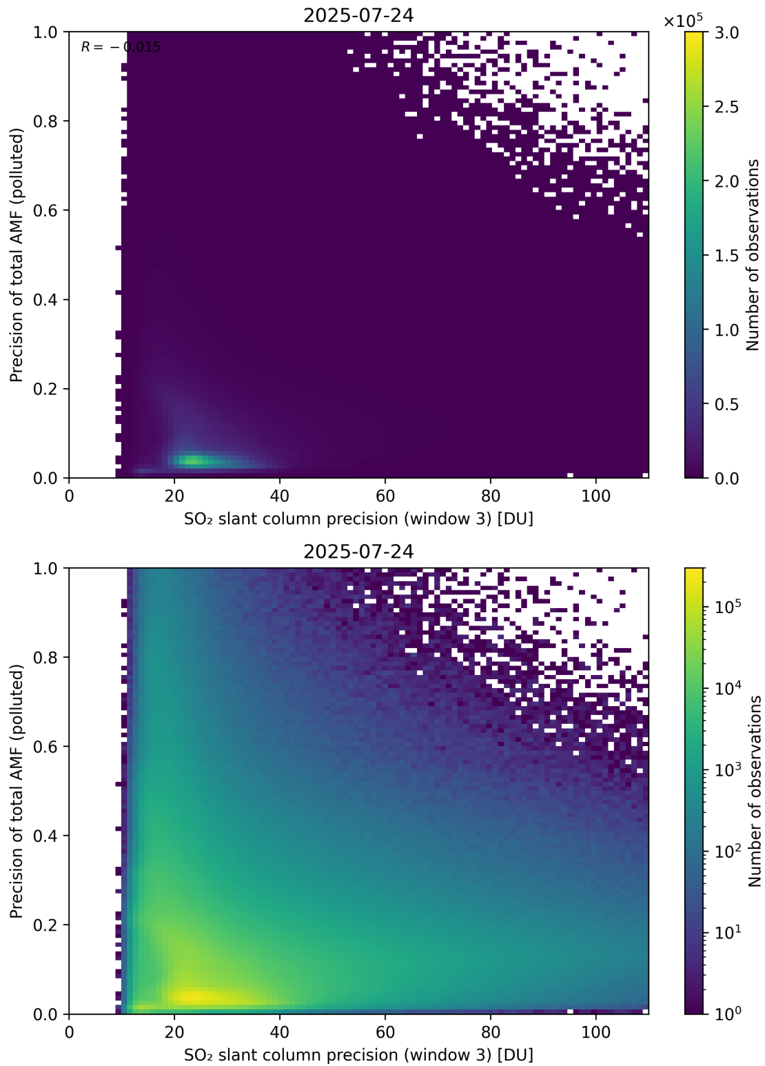
Figure 314: Scatter density plot of “SO 2 slant column precision (window 3)” against “Precision of total AMF (polluted)” for 2025-07-24 to 2025-07-25.
