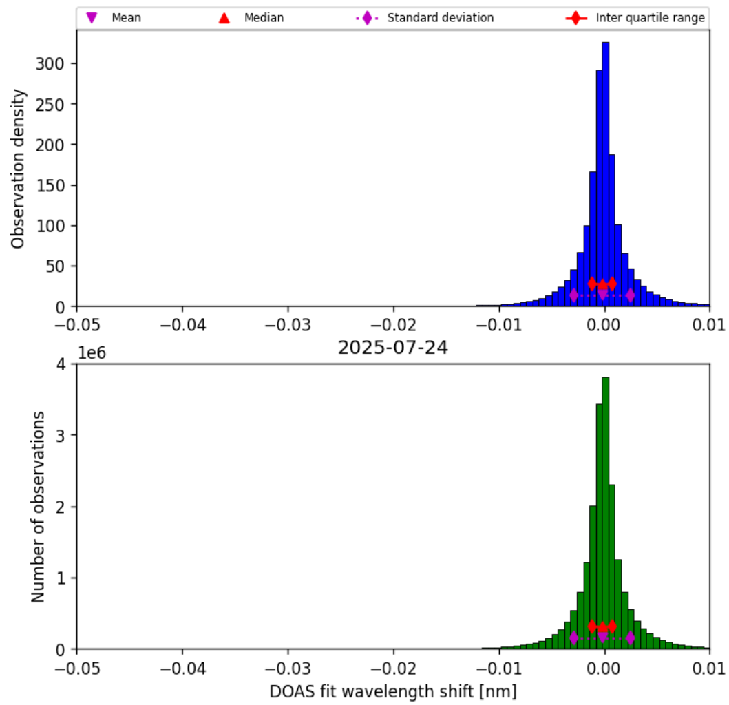
Figure 76: Histogram of “DOAS fit wavelength shift” for 2025-07-24 to 2025-07-25
