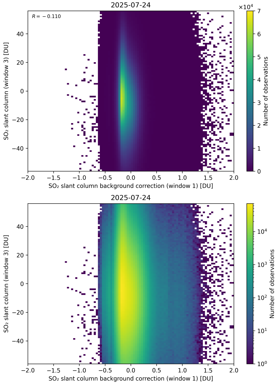
Figure 118: Scatter density plot of “SO 2 slant column background correction (window 1)” against “SO 2 slant column (window 3)” for 2025-07-24 to 2025-07-25.
