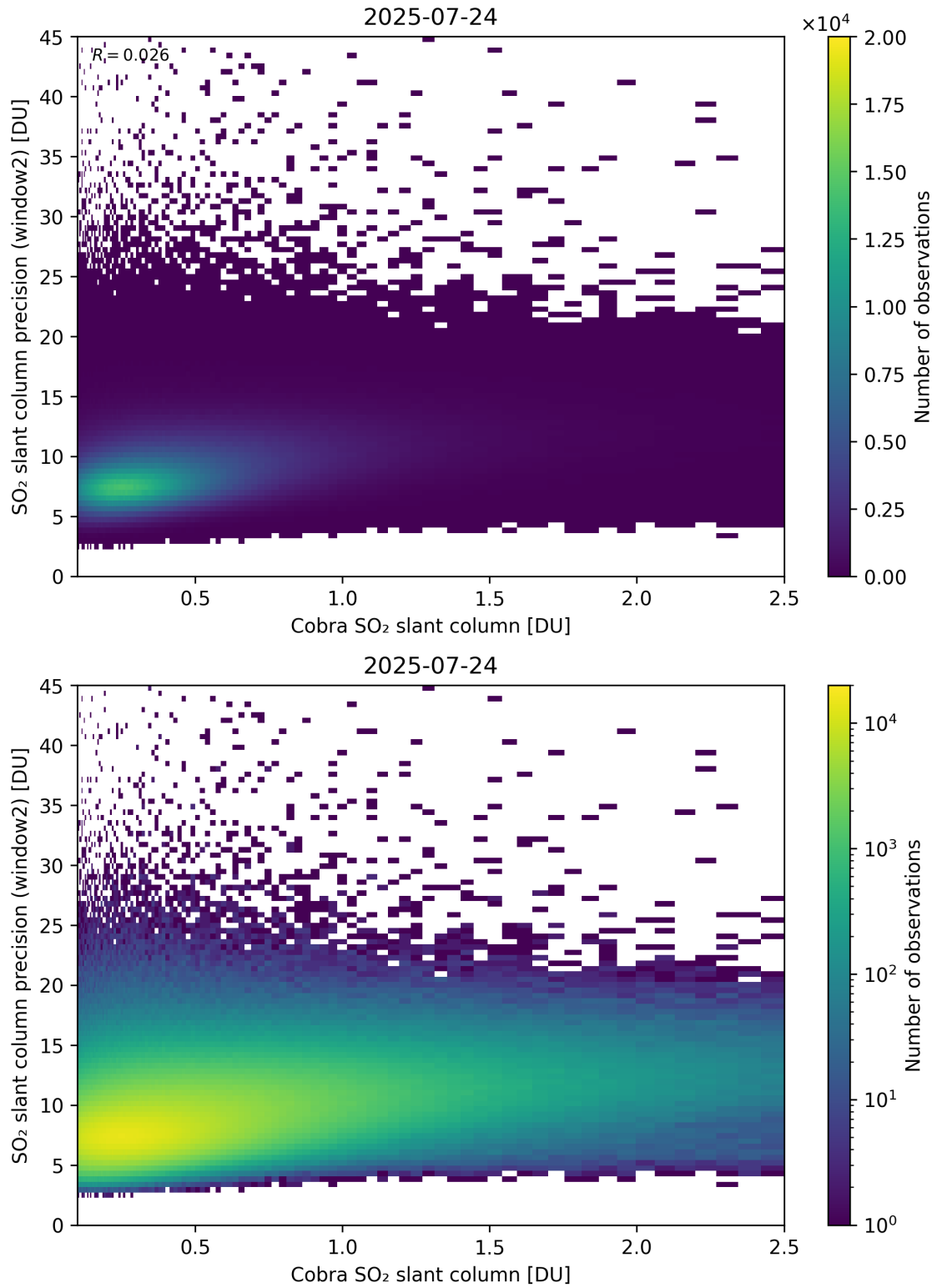
Figure 221: Scatter density plot of “Cobra SO 2 slant column” against “SO 2 slant column precision (window2)” for 2025-07-24 to 2025-07-25.
