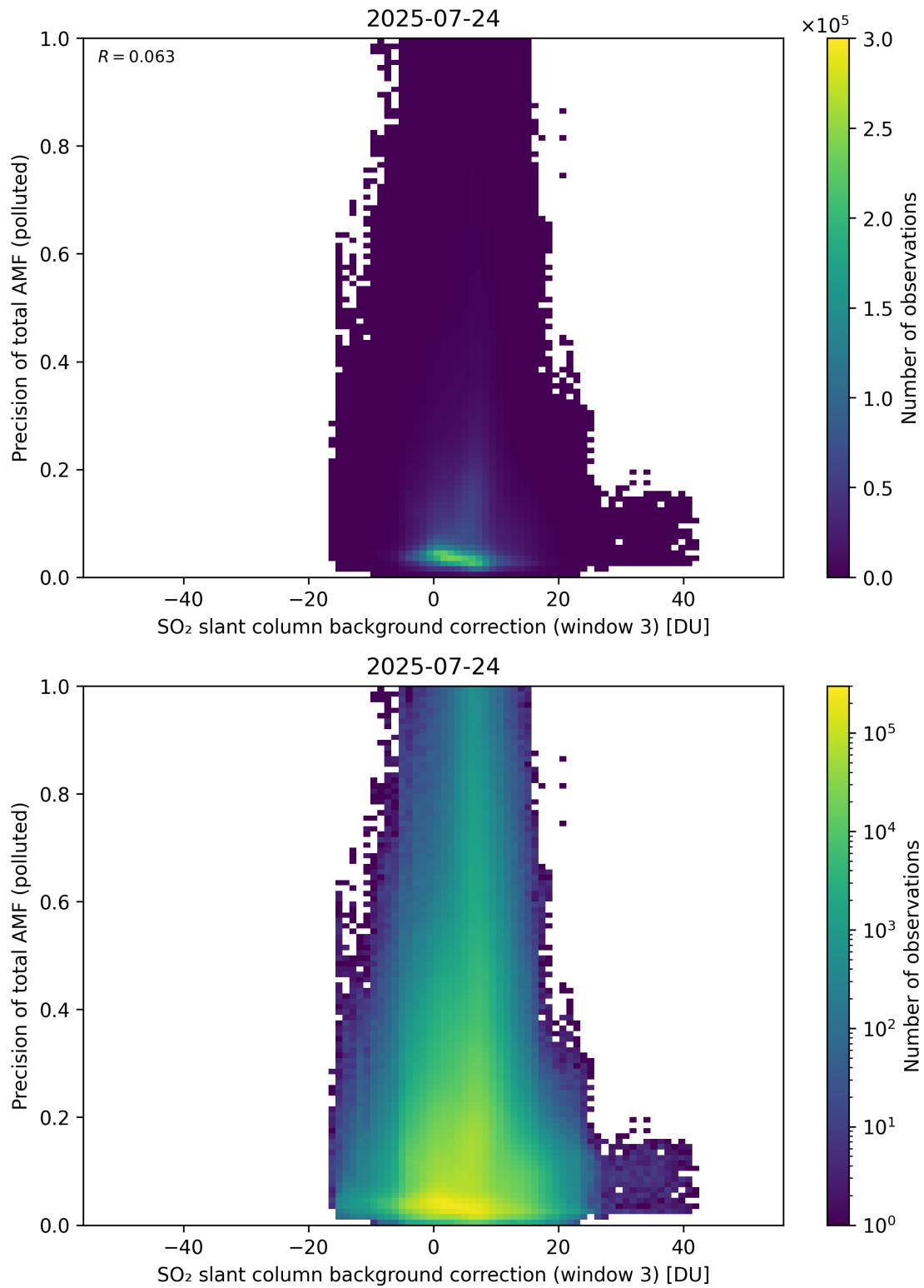
Figure 137: Scatter density plot of “SO 2 slant column background correction (window 3)” against “Precision of total AMF (polluted)” for 2025-07-24 to 2025-07-25.
