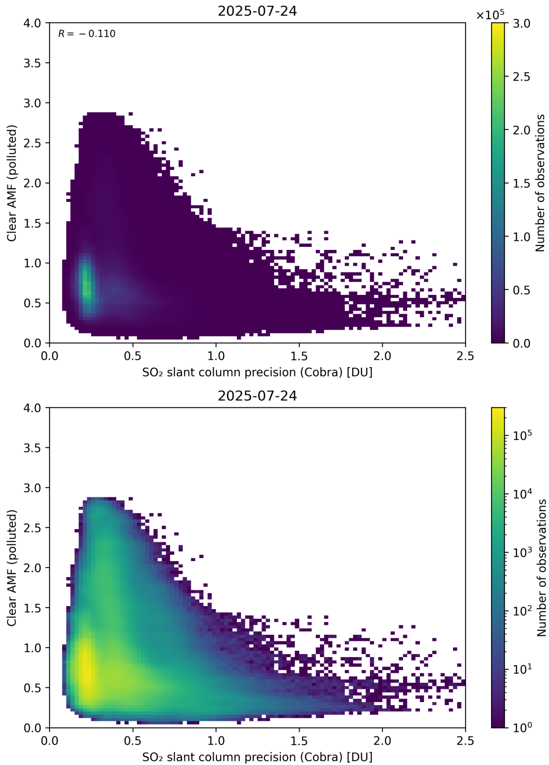
Figure 205: Scatter density plot of “SO 2 slant column precision (Cobra)” against “Clear AMF (polluted)” for 2025-07-24 to 2025-07-25.
