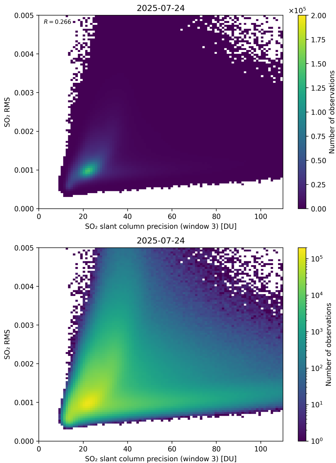
Figure 310: Scatter density plot of “SO 2 slant column precision (window 3)” against “SO 2 RMS” for 2025-07-24 to 2025-07-25.
