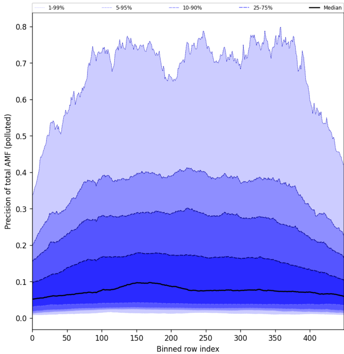
Figure 106: Along track statistics of “Precision of total AMF (polluted)” for 2025-07-24 to 2025-07-25
