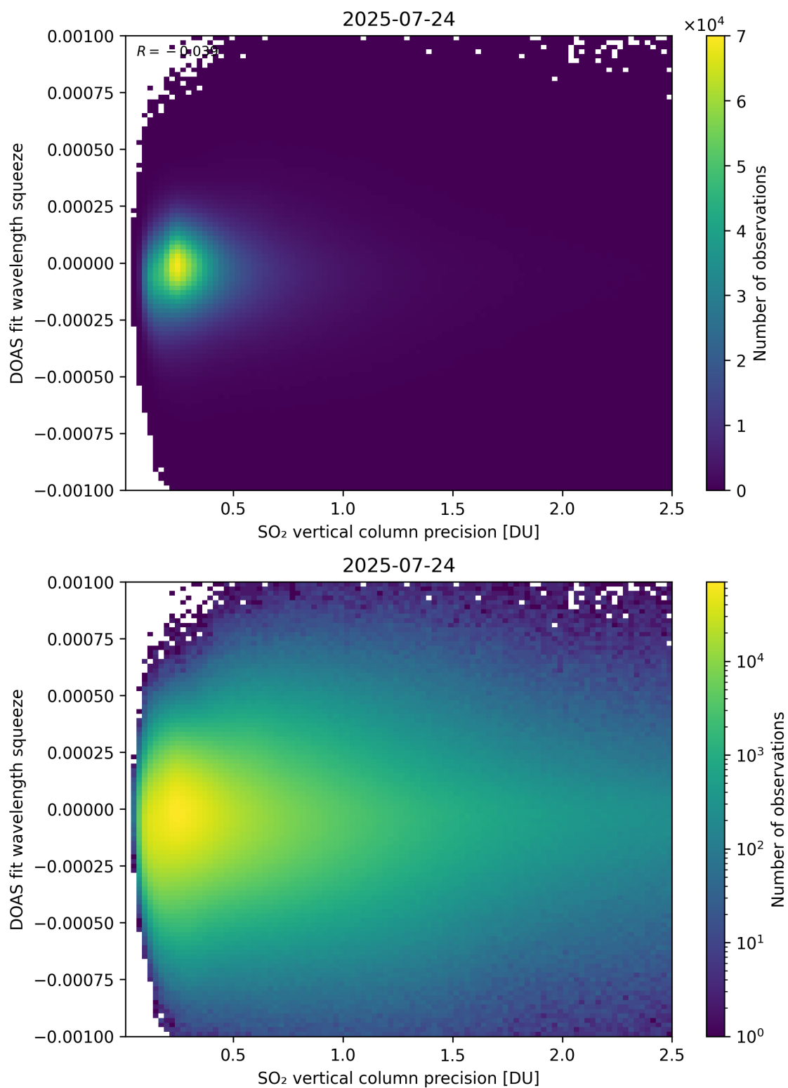
Figure 333: Scatter density plot of “SO 2 vertical column precision” against “DOAS fit wavelength squeeze” for 2025-07-24 to 2025-07-25.
