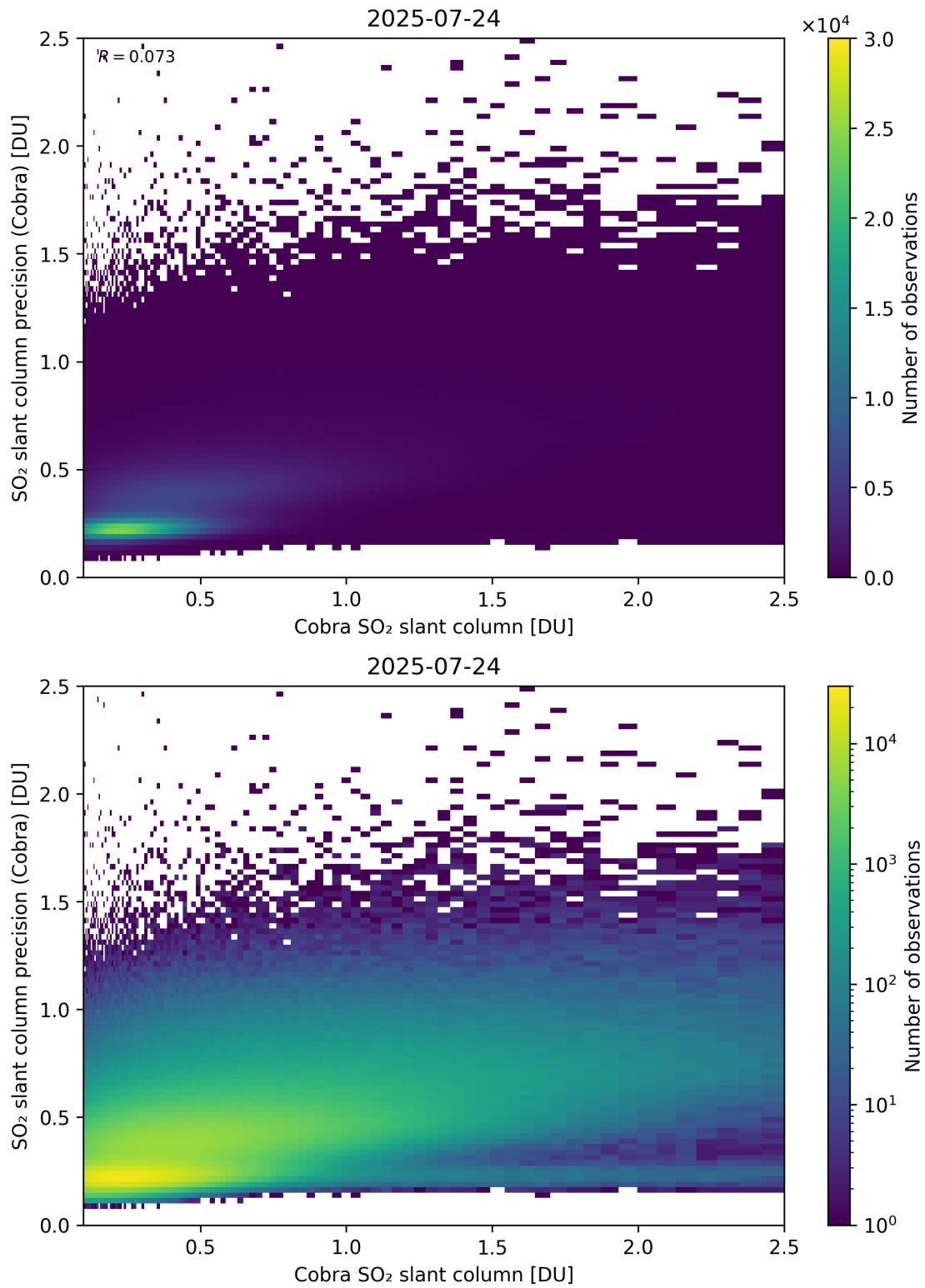
Figure 216: Scatter density plot of “Cobra SO 2 slant column” against “SO 2 slant column precision (Cobra)” for 2025-07-24 to 2025-07-25.
