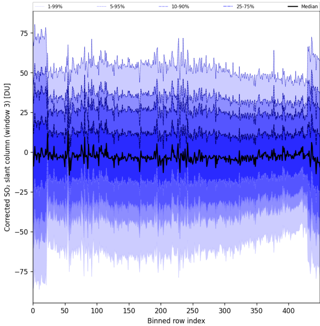
Figure 99: Along track statistics of “Corrected SO 2 slant column (window 3)” for 2025-07-24 to 2025-07-25
