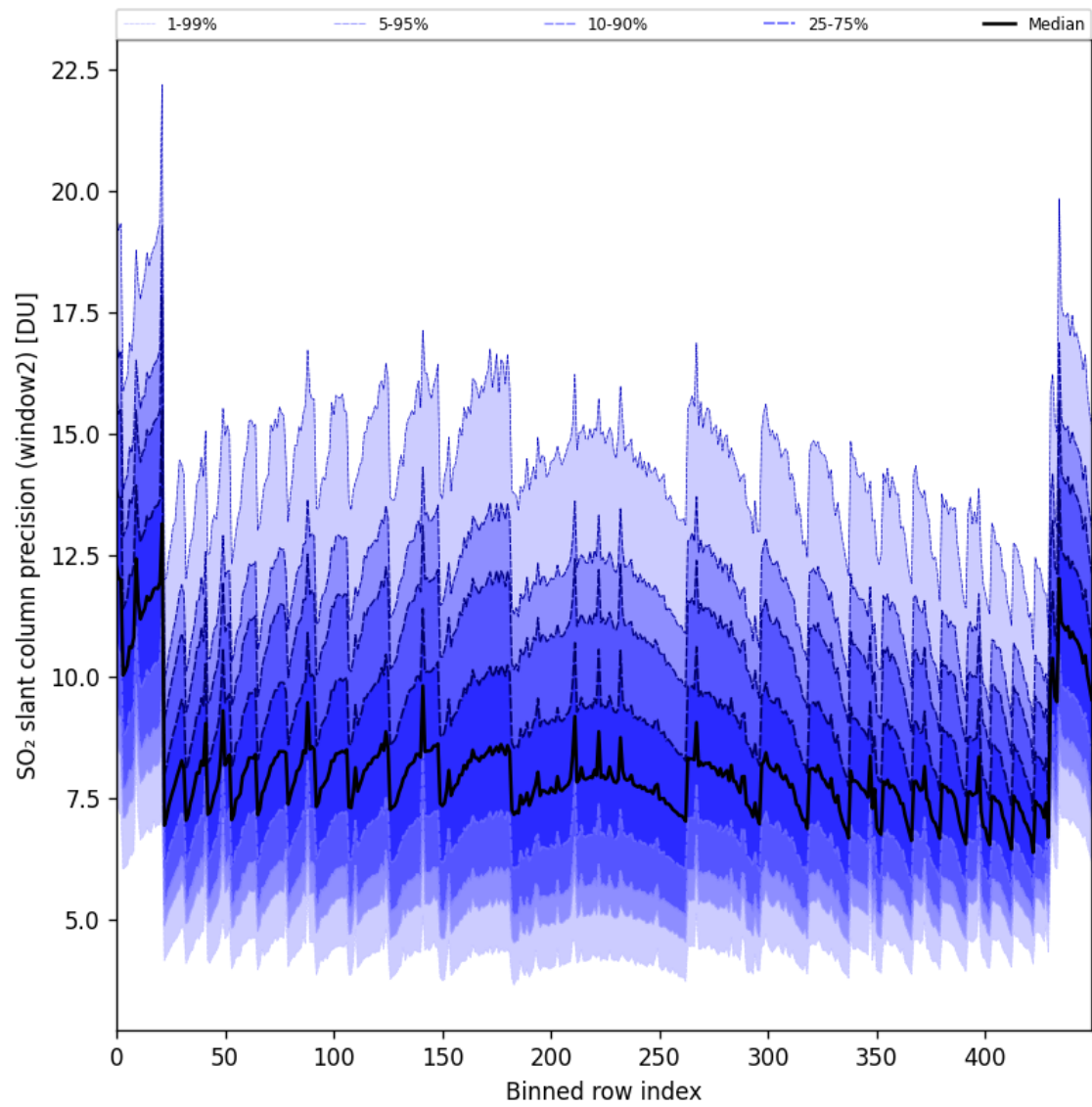
Figure 94: Along track statistics of “SO 2 slant column precision (window2)” for 2025-07-24 to 2025-07-25
