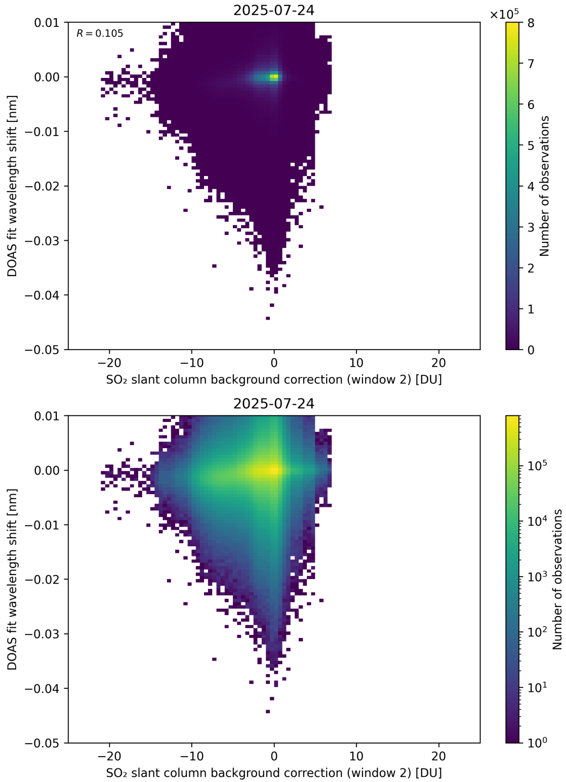
Figure 123: Scatter density plot of “SO 2 slant column background correction (window 2)” against “DOAS fit wavelength shift” for 2025-07-24 to 2025-07-25.
