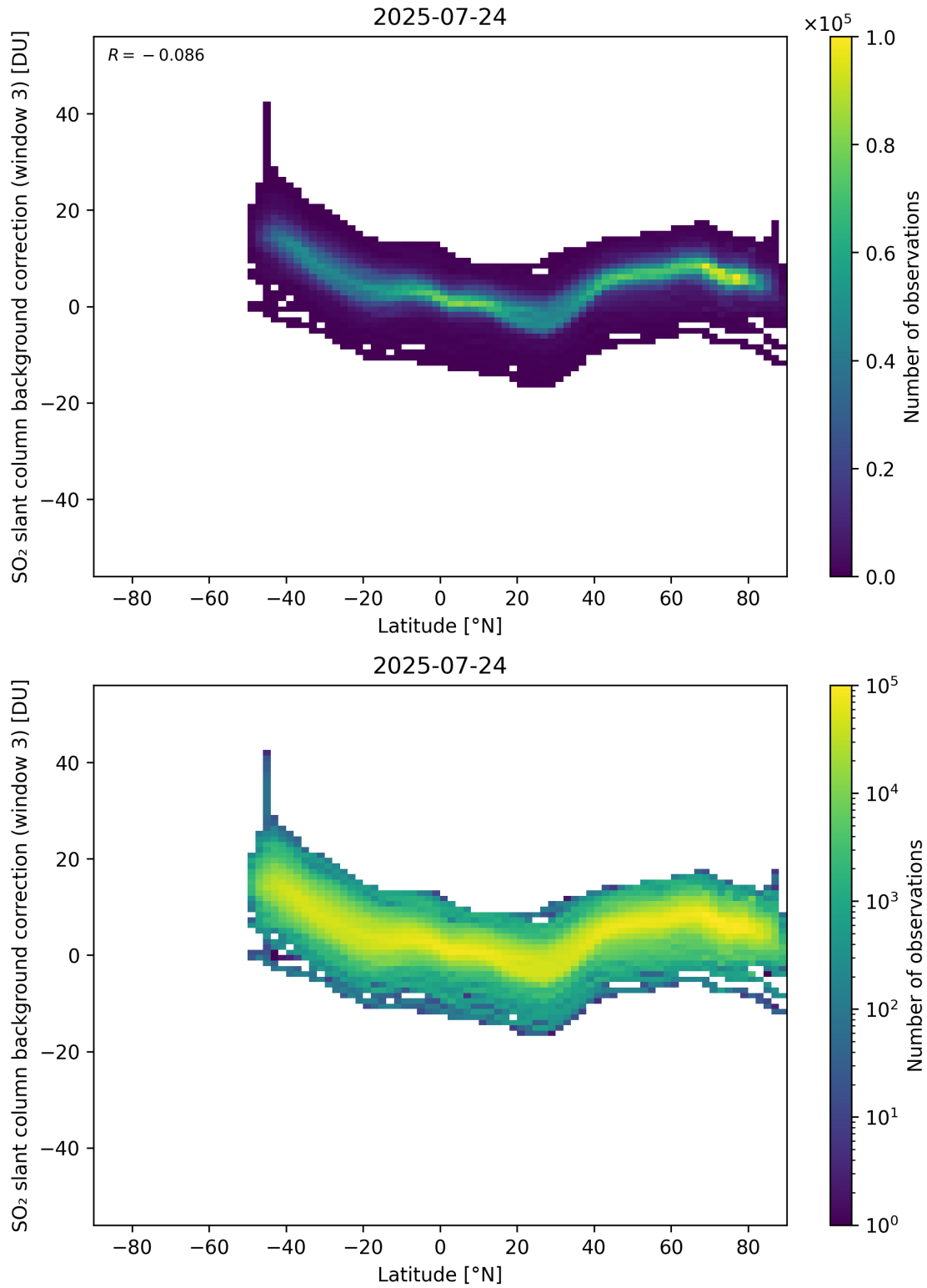
Figure 152: Scatter density plot of “Latitude” against “SO 2 slant column background correction (window 3)” for 2025-07-24 to 2025-07-25.
