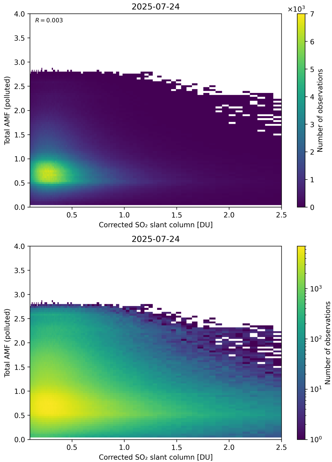
Figure 242: Scatter density plot of “Corrected SO 2 slant column” against “Total AMF (polluted)” for 2025-07-24 to 2025-07-25.
