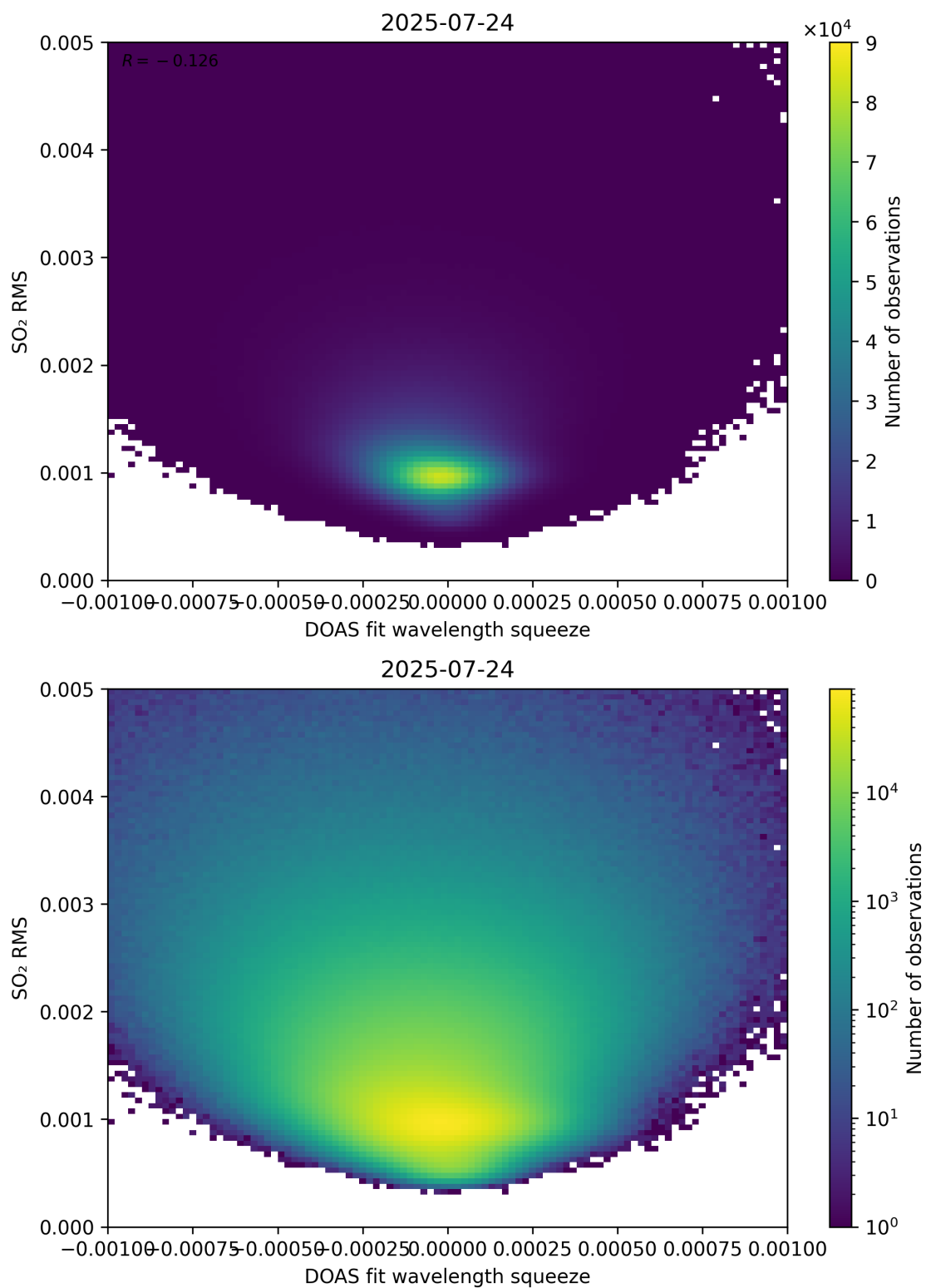
Figure 143: Scatter density plot of “DOAS fit wavelength squeeze” against “SO 2 RMS” for 2025-07-24 to 2025-07-25.
