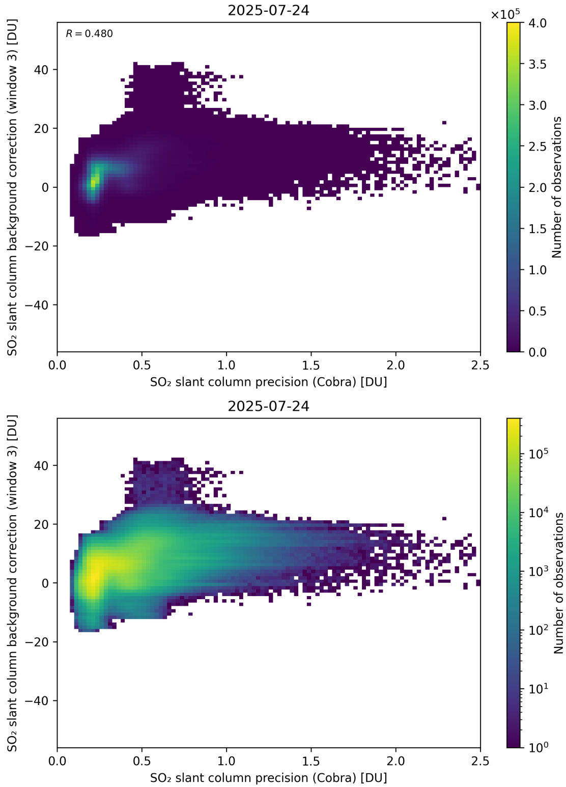
Figure 201: Scatter density plot of “SO 2 slant column precision (Cobra)” against “SO 2 slant column background correction (window 3)” for 2025-07-24 to 2025-07-25.
