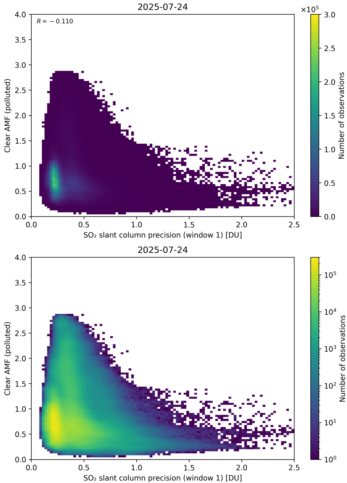
Figure 274: Scatter density plot of “SO 2 slant column precision (window 1)” against “Clear AMF (polluted)” for 2025-07-24 to 2025-07-25.
