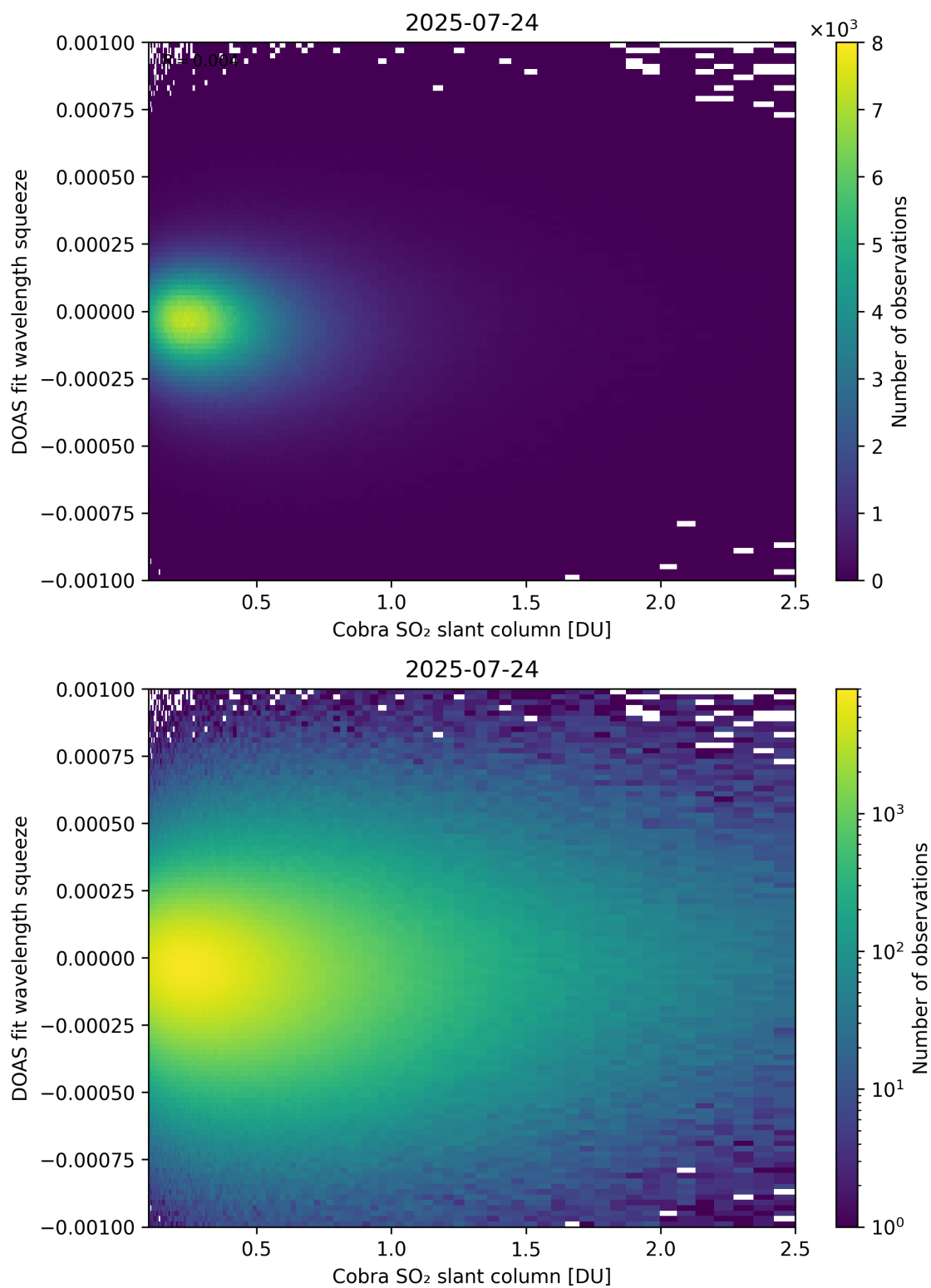
Figure 197: Scatter density plot of “Cobra SO 2 slant column” against “DOAS fit wavelength squeeze” for 2025-07-24 to 2025-07-25.
