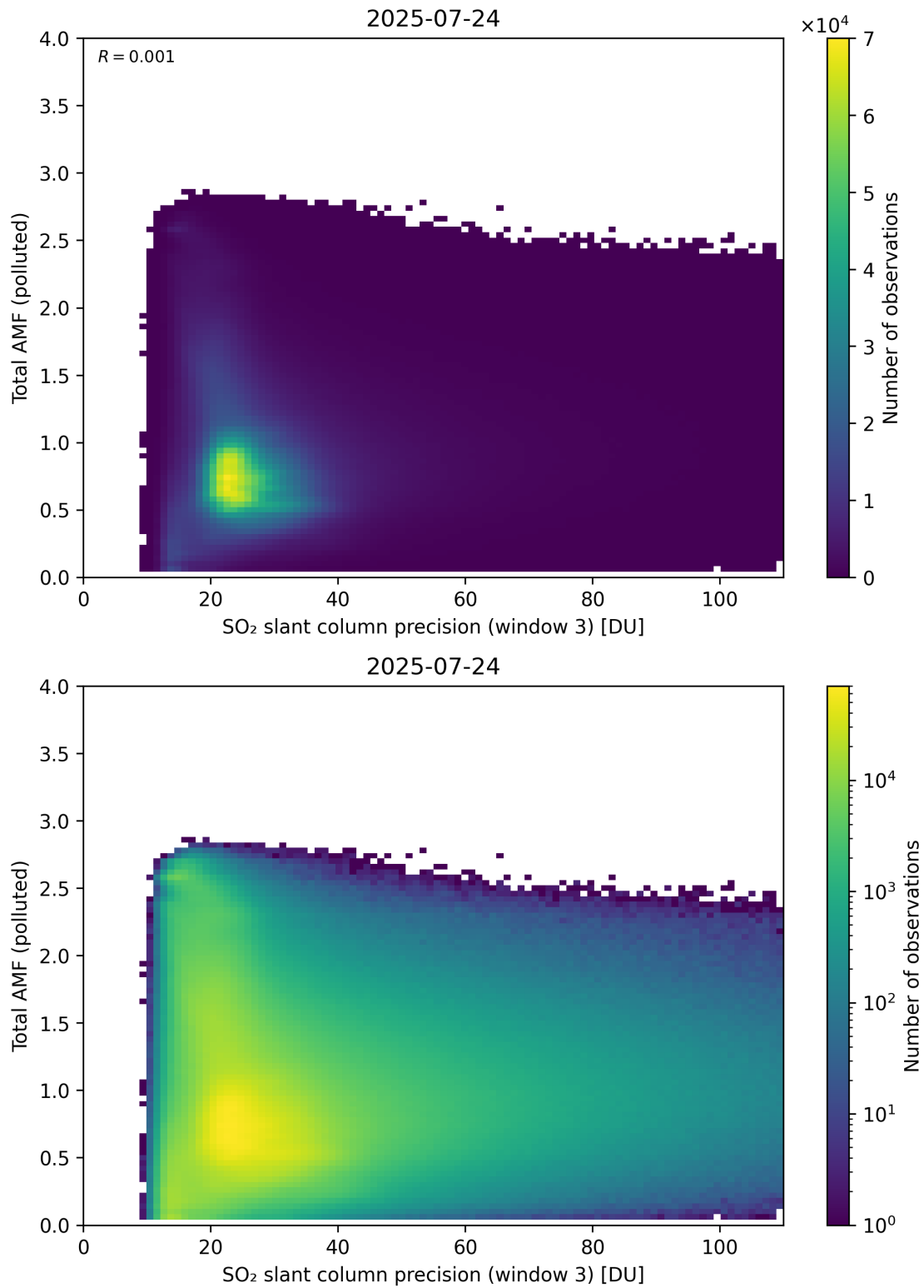
Figure 313: Scatter density plot of “SO 2 slant column precision (window 3)” against “Total AMF (polluted)” for 2025-07-24 to 2025-07-25.
