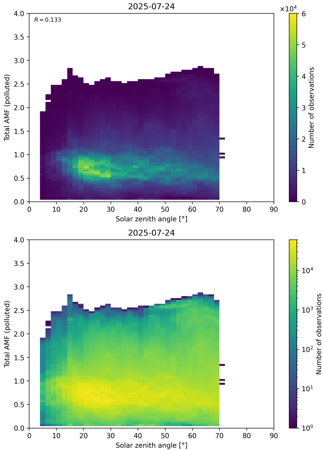
Figure 189: Scatter density plot of “Solar zenith angle” against “Total AMF (polluted)” for 2025-07-24 to 2025-07-25.
