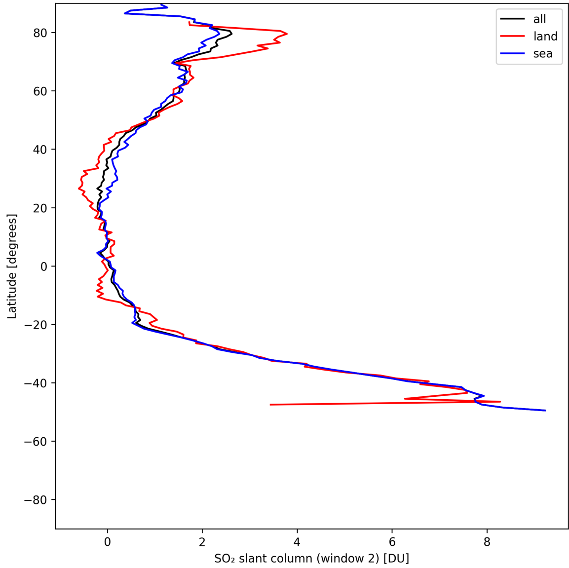
Figure 41: Zonal average of “SO 2 slant column (window 2)” for 2025-07-24 to 2025-07-25.
