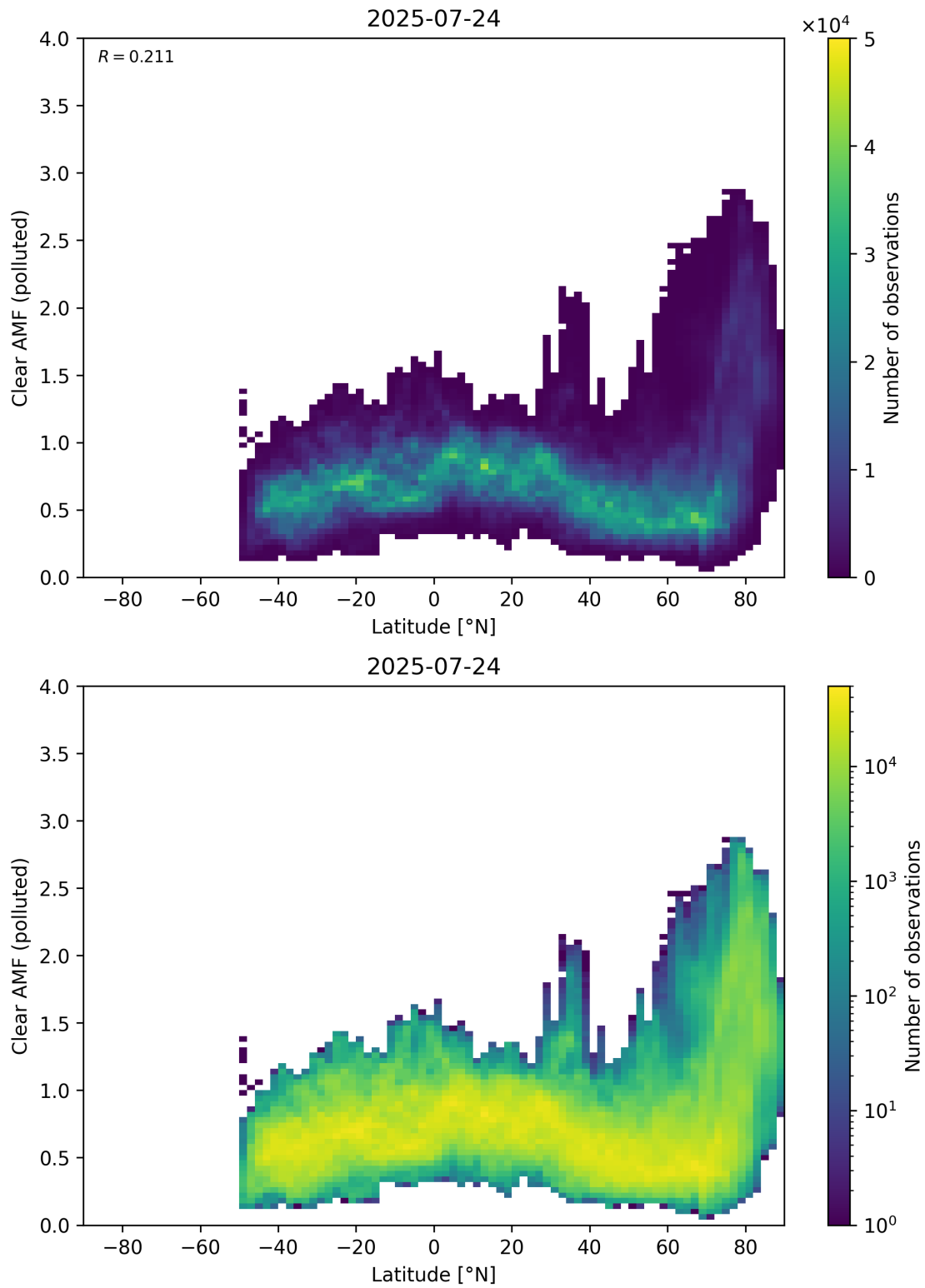
Figure 156: Scatter density plot of “Latitude” against “Clear AMF (polluted)” for 2025-07-24 to 2025-07-25.
