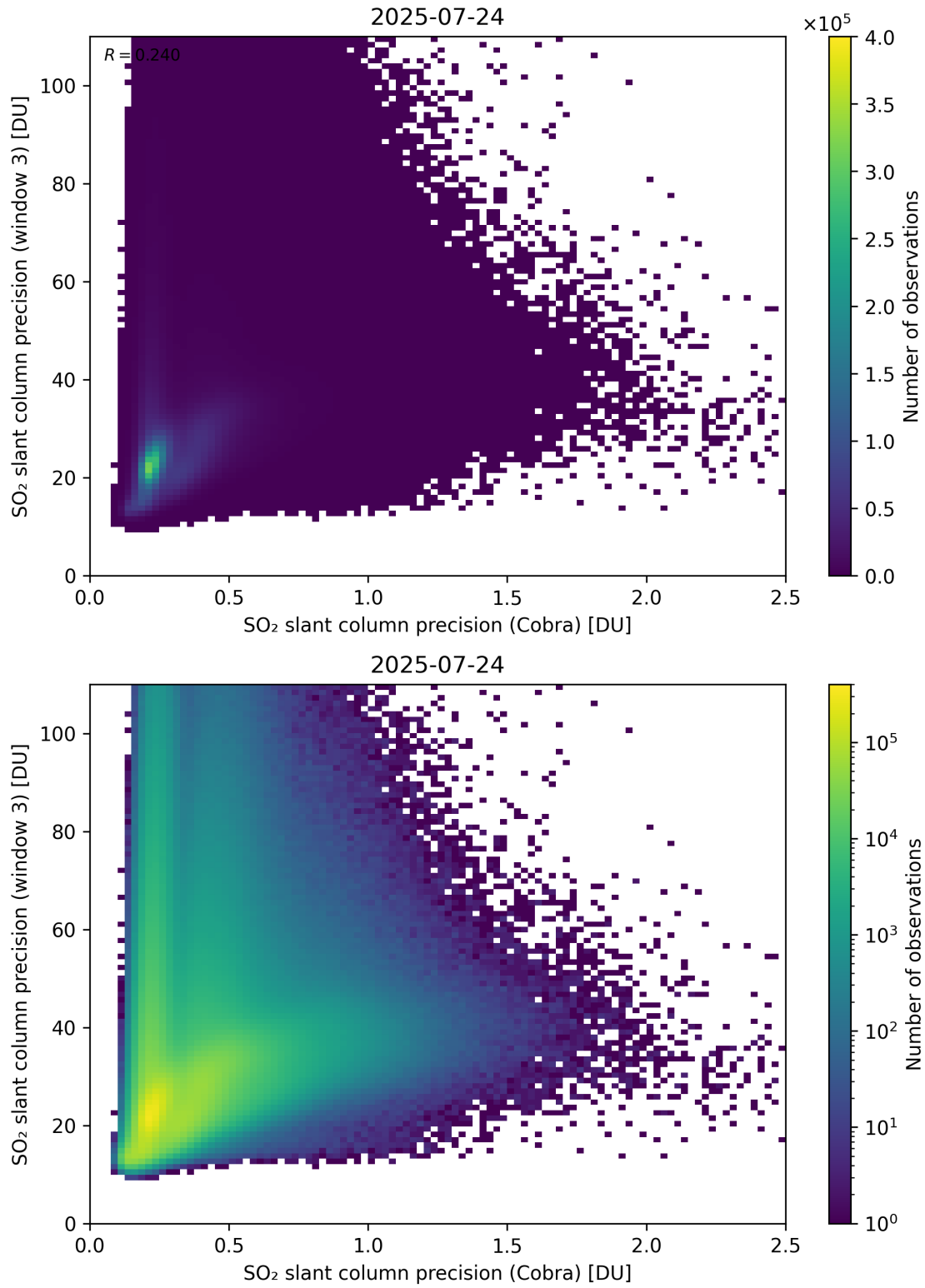
Figure 212: Scatter density plot of “SO 2 slant column precision (Cobra)” against “SO 2 slant column precision (window 3)” for 2025-07-24 to 2025-07-25.
