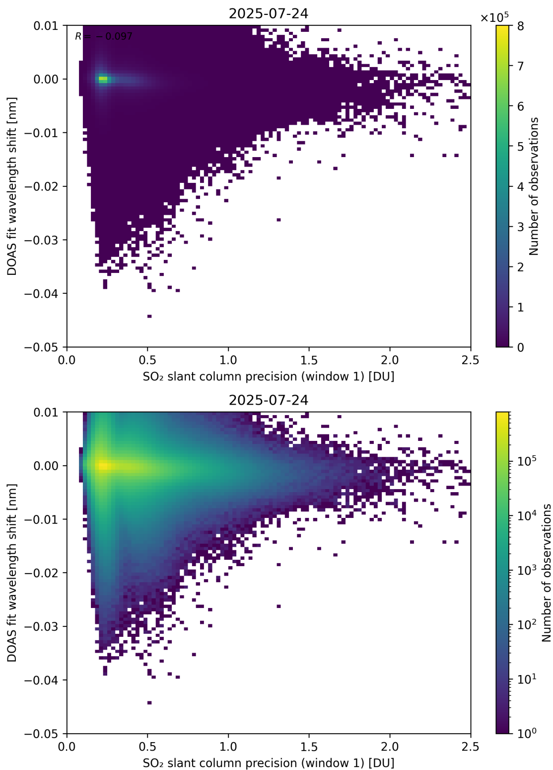
Figure 271: Scatter density plot of “SO 2 slant column precision (window 1)” against “DOAS fit wavelength shift” for 2025-07-24 to 2025-07-25.
