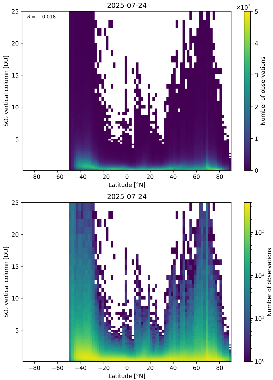
Figure 169: Scatter density plot of “Latitude” against “SO 2 vertical column” for 2025-07-24 to 2025-07-25.
