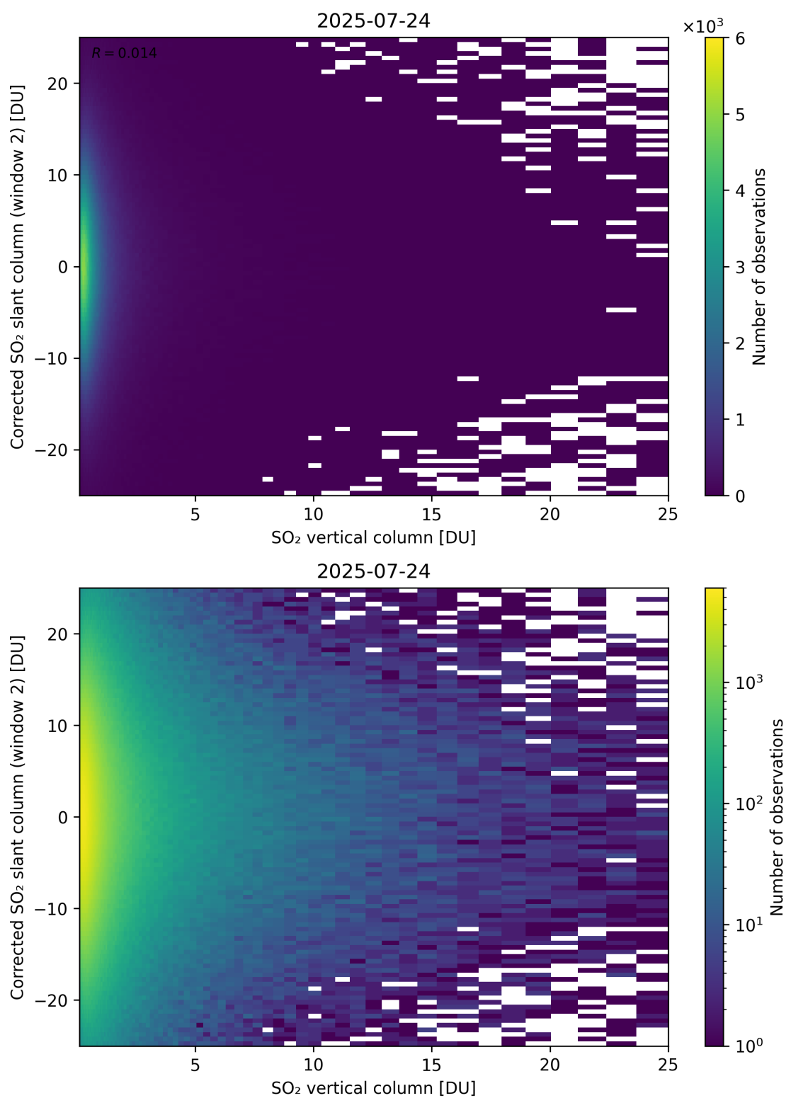
Figure 352: Scatter density plot of “SO 2 vertical column” against “Corrected SO 2 slant column (window 2)” for 2025-07-24 to 2025-07-25.
