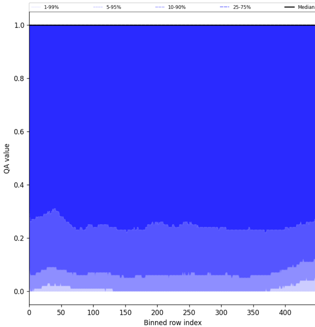
Figure 83: Along track statistics of “QA value” for 2025-07-24 to 2025-07-25
