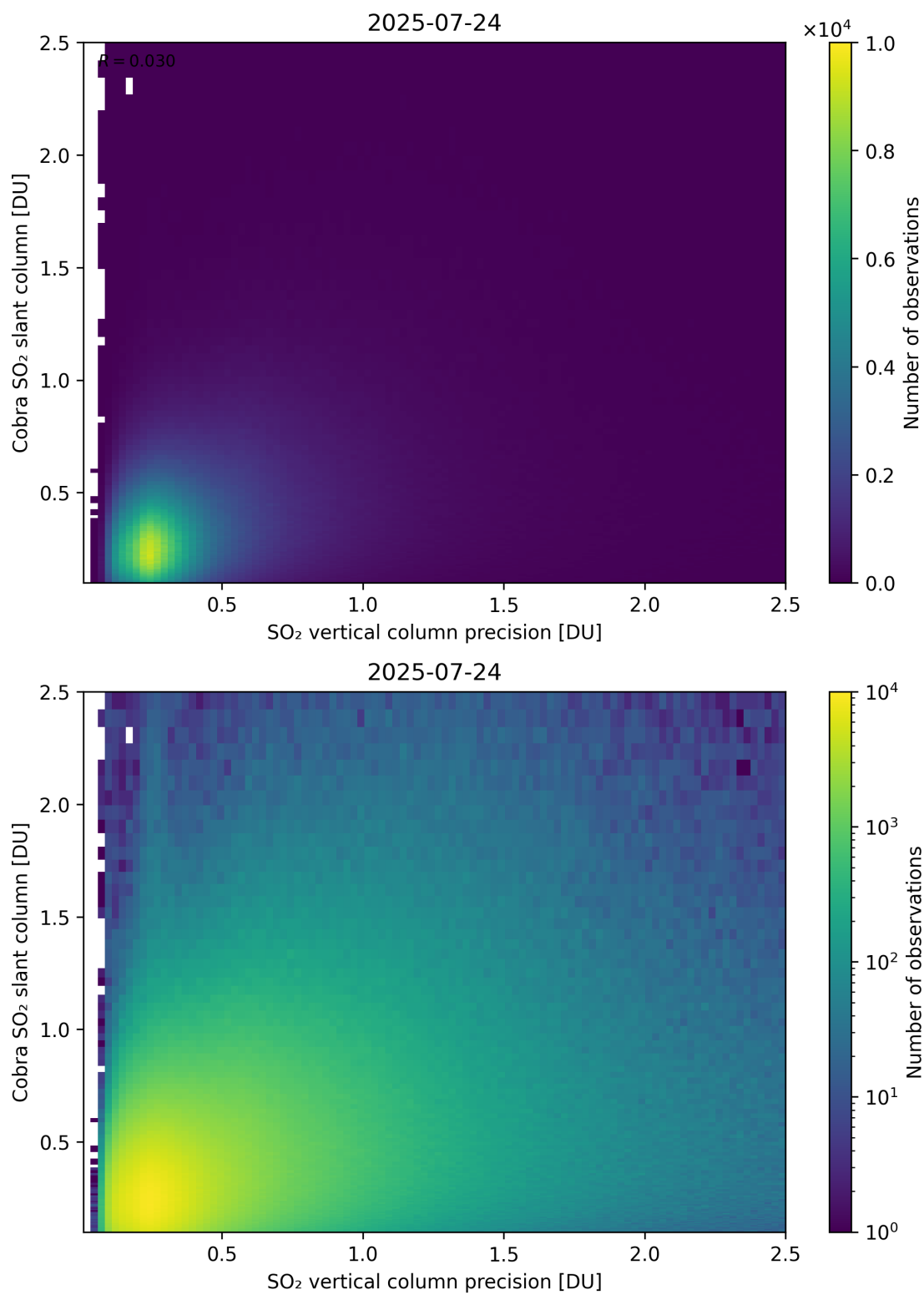
Figure 336: Scatter density plot of “SO 2 vertical column precision” against “Cobra SO 2 slant column” for 2025-07-24 to 2025-07-25.
