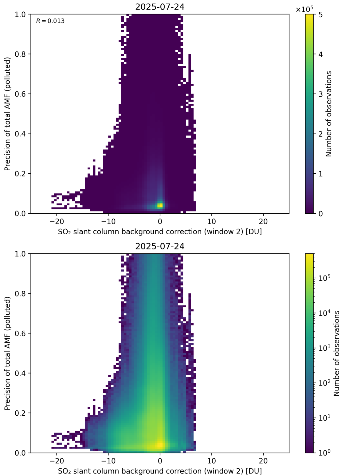
Figure 131: Scatter density plot of “SO 2 slant column background correction (window 2)” against “Precision of total AMF (polluted)” for 2025-07-24 to 2025-07-25.
