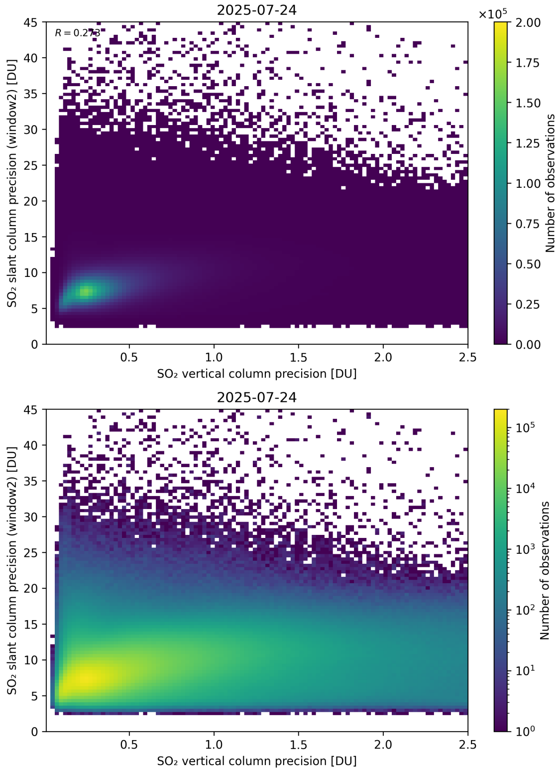
Figure 343: Scatter density plot of “SO 2 vertical column precision” against “SO 2 slant column precision (window2)” for 2025-07-24 to 2025-07-25.
