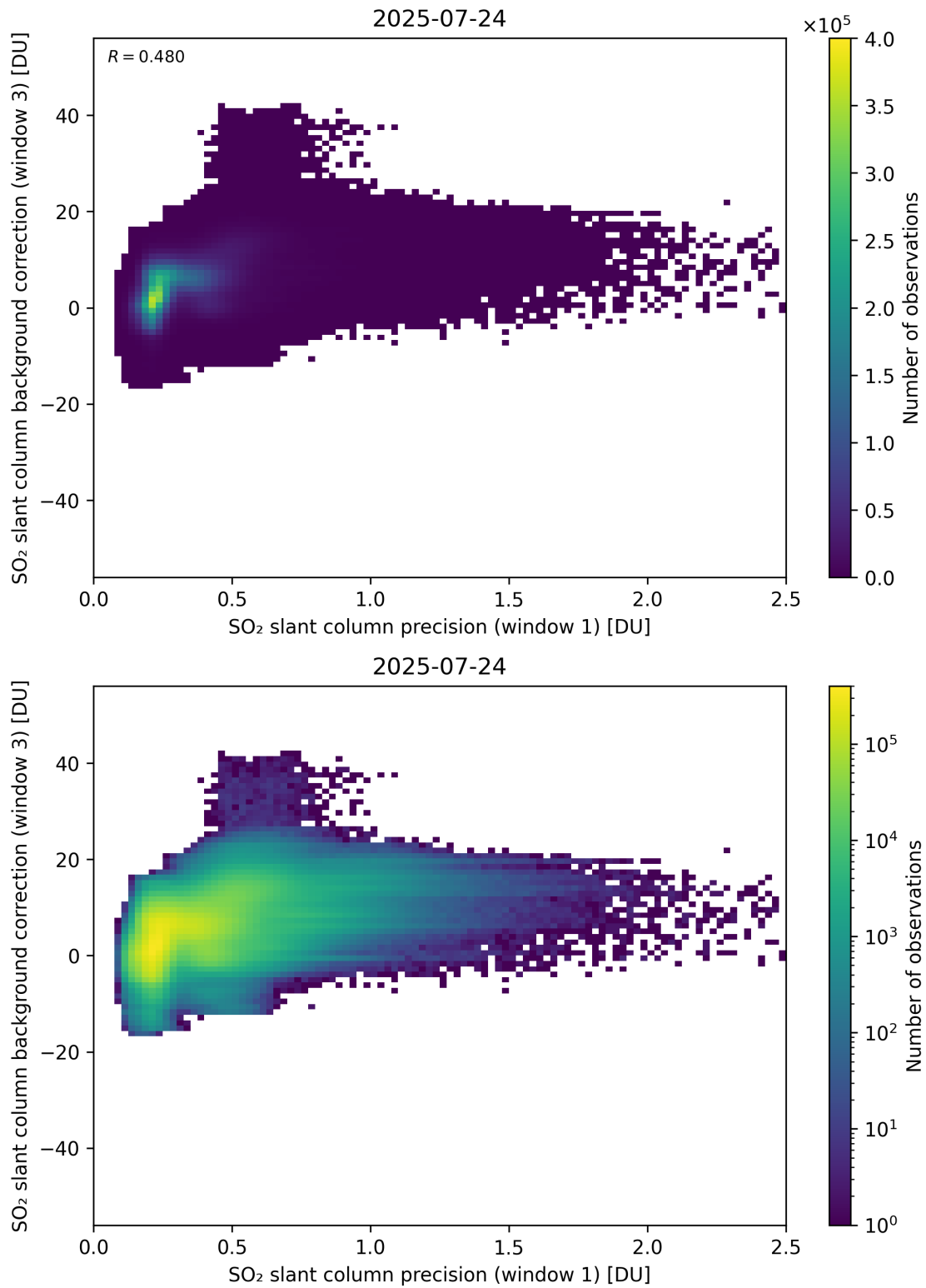
Figure 270: Scatter density plot of “SO 2 slant column precision (window 1)” against “SO 2 slant column background correction (window 3)” for 2025-07-24 to 2025-07-25.
