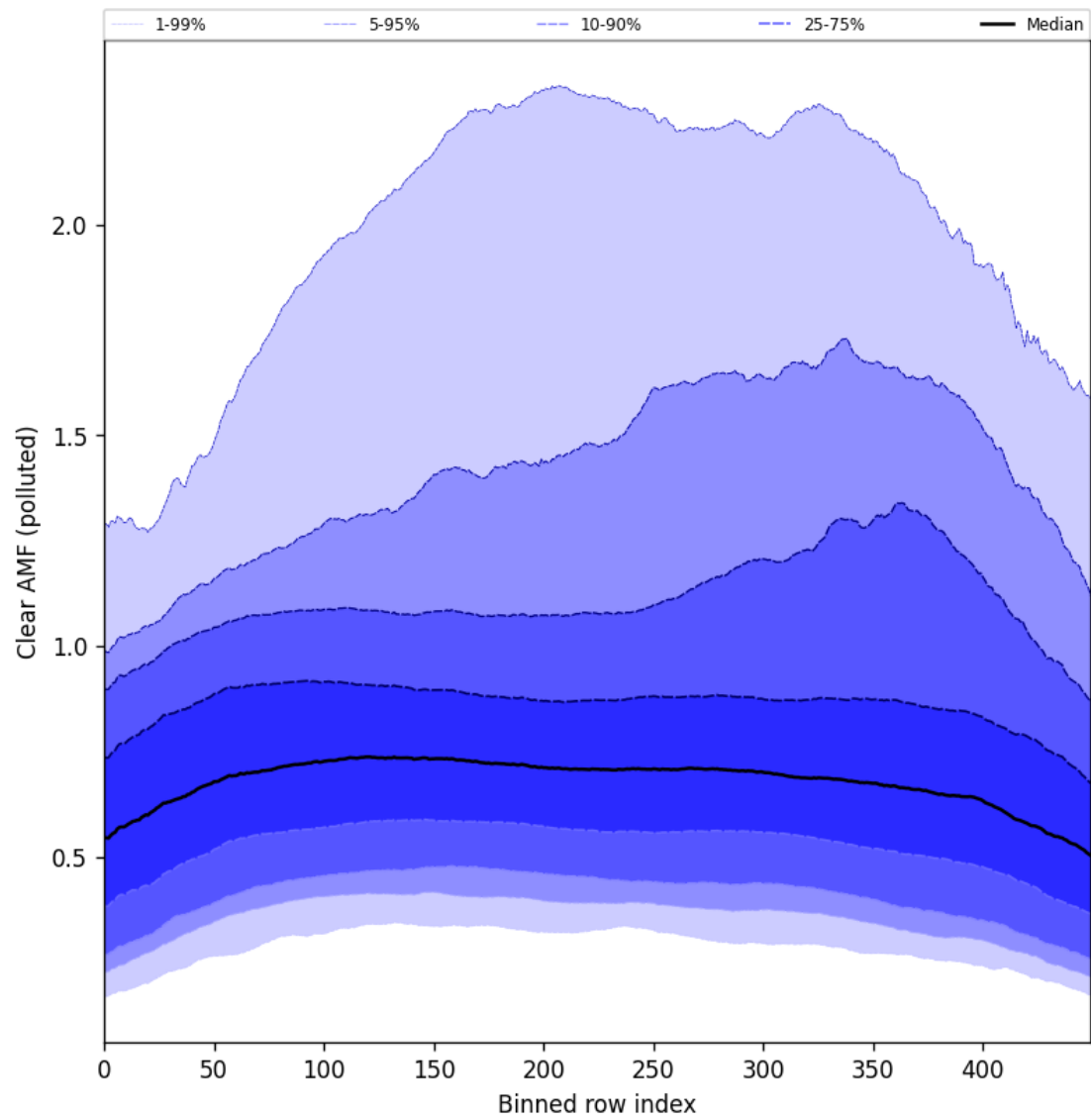
Figure 107: Along track statistics of “Clear AMF (polluted)” for 2025-07-24 to 2025-07-25
