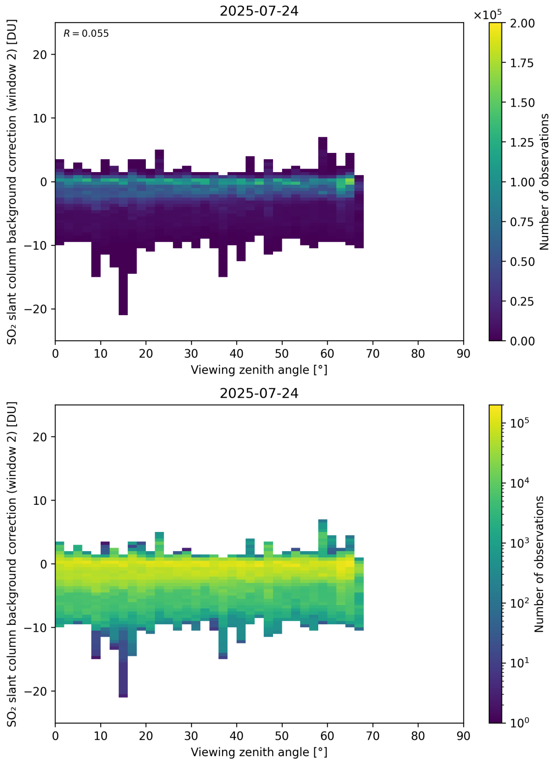
Figure 363: Scatter density plot of “Viewing zenith angle” against “SO 2 slant column background correction (window 2)” for 2025-07-24 to 2025-07-25.
