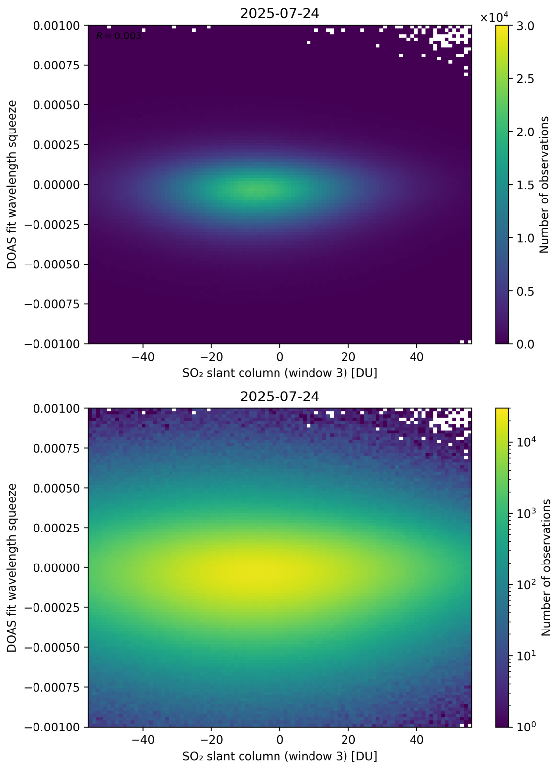
Figure 305: Scatter density plot of “SO 2 slant column (window 3)” against “DOAS fit wavelength squeeze” for 2025-07-24 to 2025-07-25.
