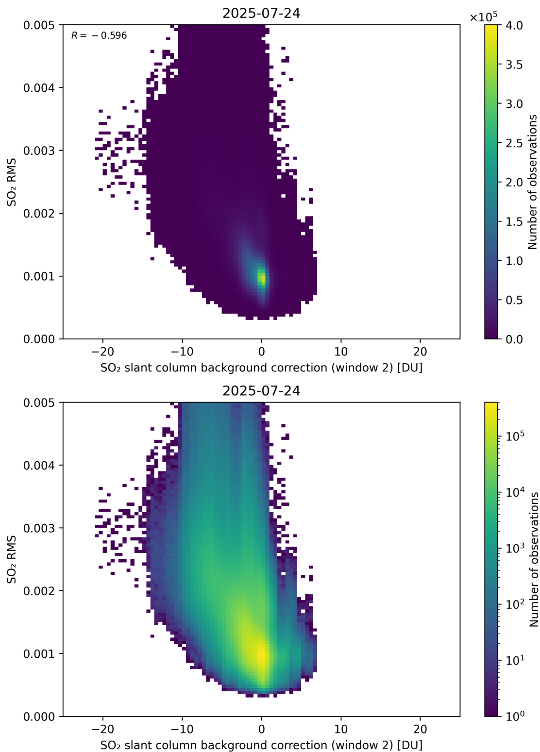
Figure 125: Scatter density plot of “SO 2 slant column background correction (window 2)” against “SO 2 RMS” for 2025-07-24 to 2025-07-25.
