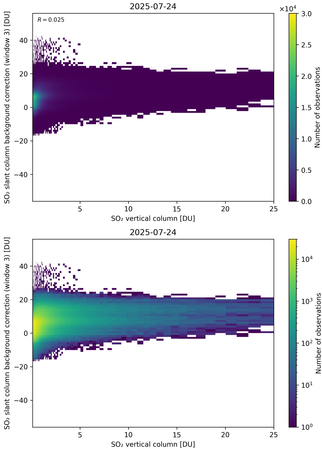
Figure 325: Scatter density plot of “SO 2 vertical column” against “SO 2 slant column background correction (window 3)” for 2025-07-24 to 2025-07-25.
