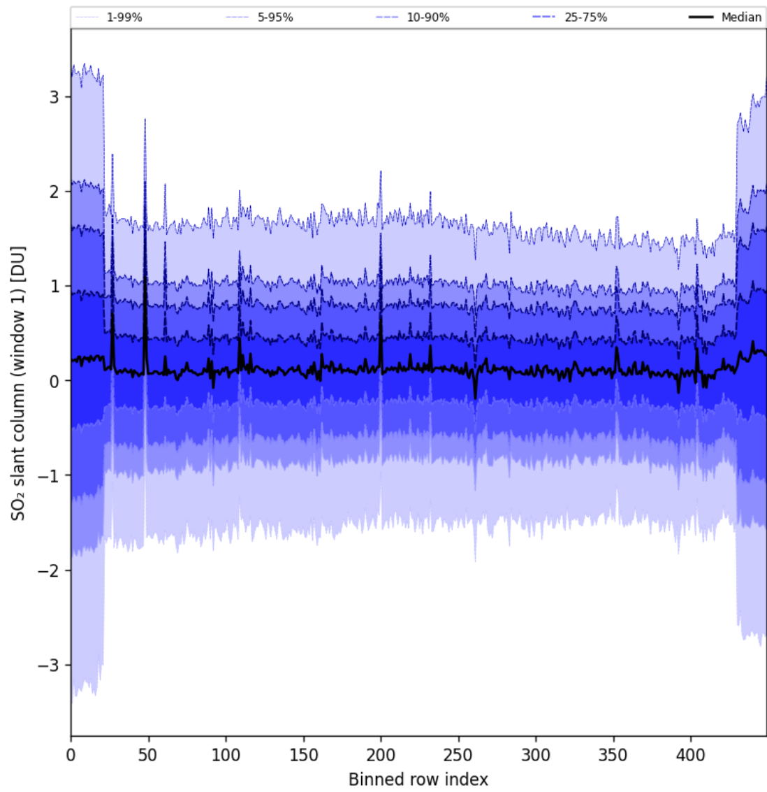
Figure 89: Along track statistics of “SO 2 slant column (window 1)” for 2025-07-24 to 2025-07-25
