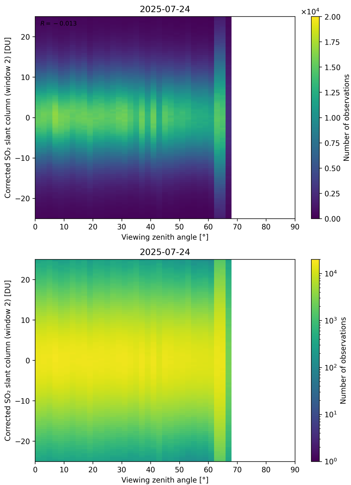
Figure 374: Scatter density plot of “Viewing zenith angle” against “Corrected SO 2 slant column (window 2)” for 2025-07-24 to 2025-07-25.
