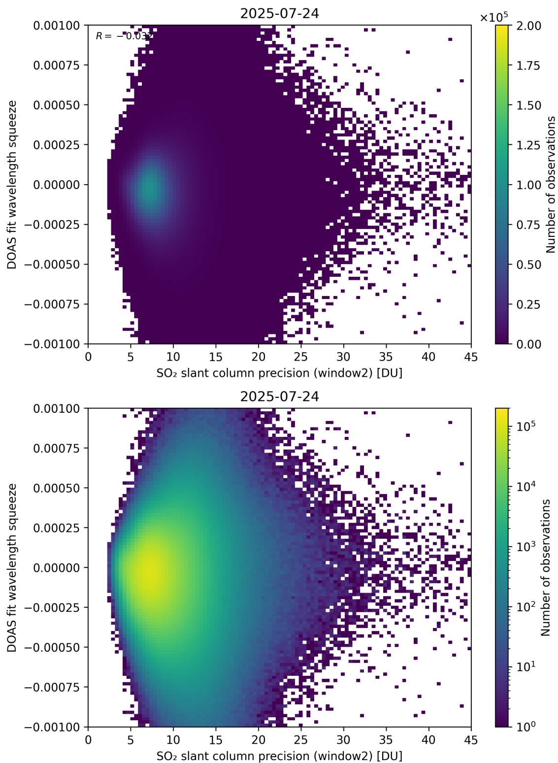
Figure 294: Scatter density plot of “SO 2 slant column precision (window2)” against “DOAS fit wavelength squeeze” for 2025-07-24 to 2025-07-25.
