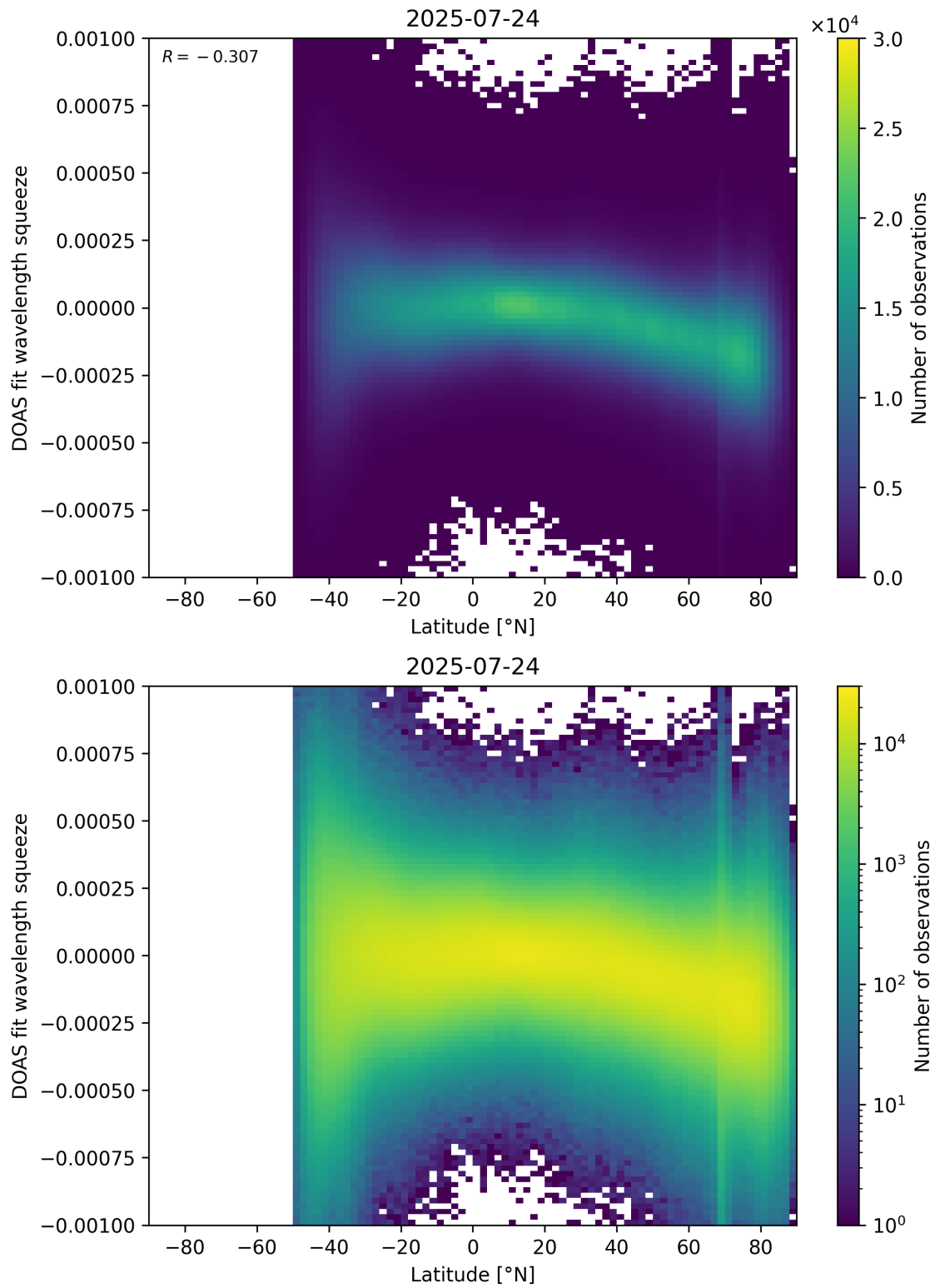
Figure 154: Scatter density plot of “Latitude” against “DOAS fit wavelength squeeze” for 2025-07-24 to 2025-07-25.
