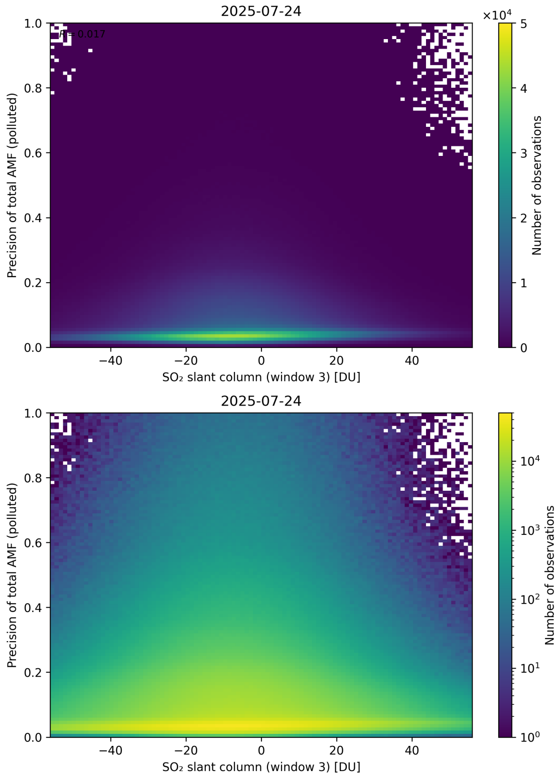
Figure 319: Scatter density plot of “SO 2 slant column (window 3)” against “Precision of total AMF (polluted)” for 2025-07-24 to 2025-07-25.
