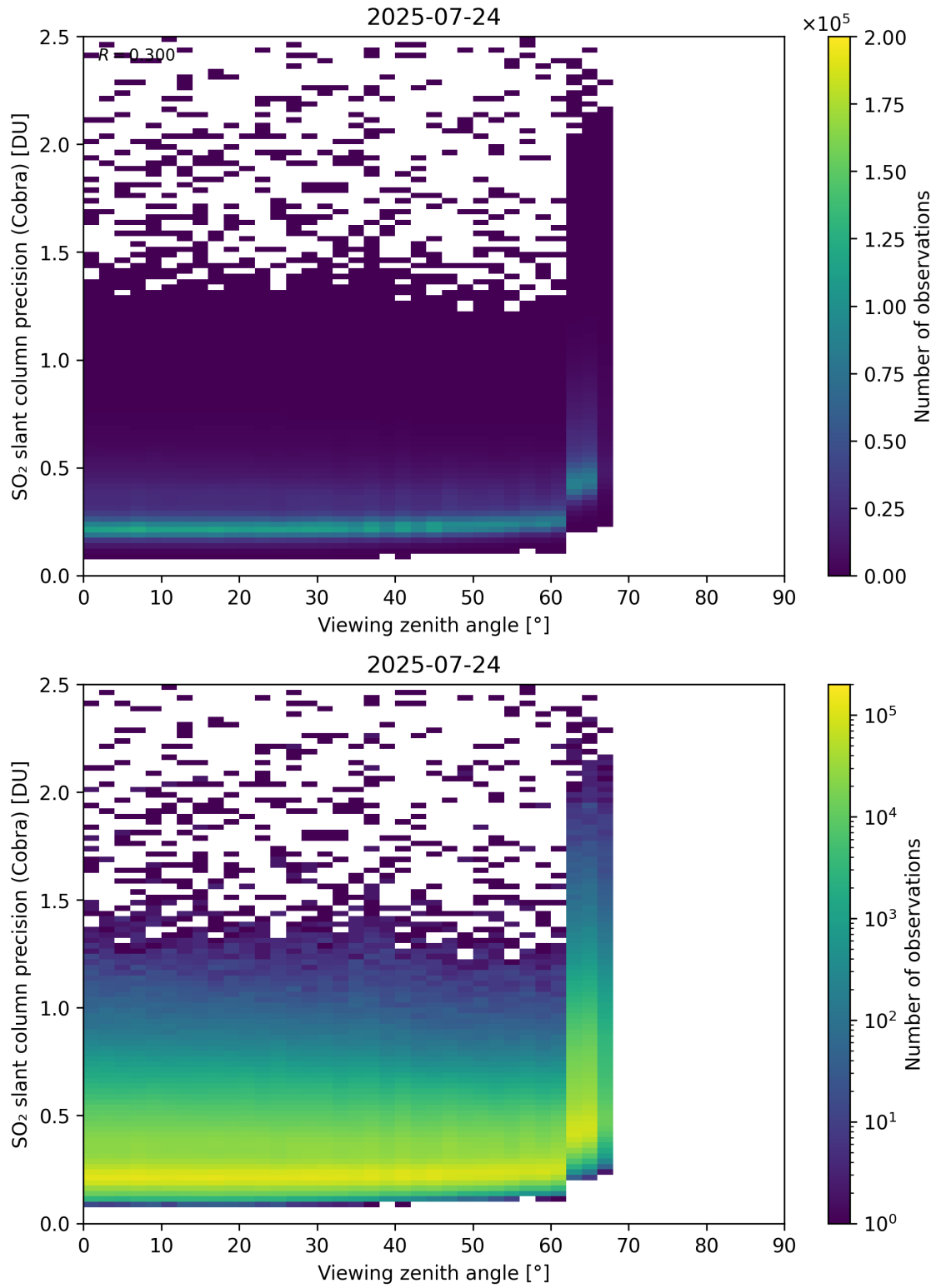
Figure 372: Scatter density plot of “Viewing zenith angle” against “SO 2 slant column precision (Cobra)” for 2025-07-24 to 2025-07-25.
