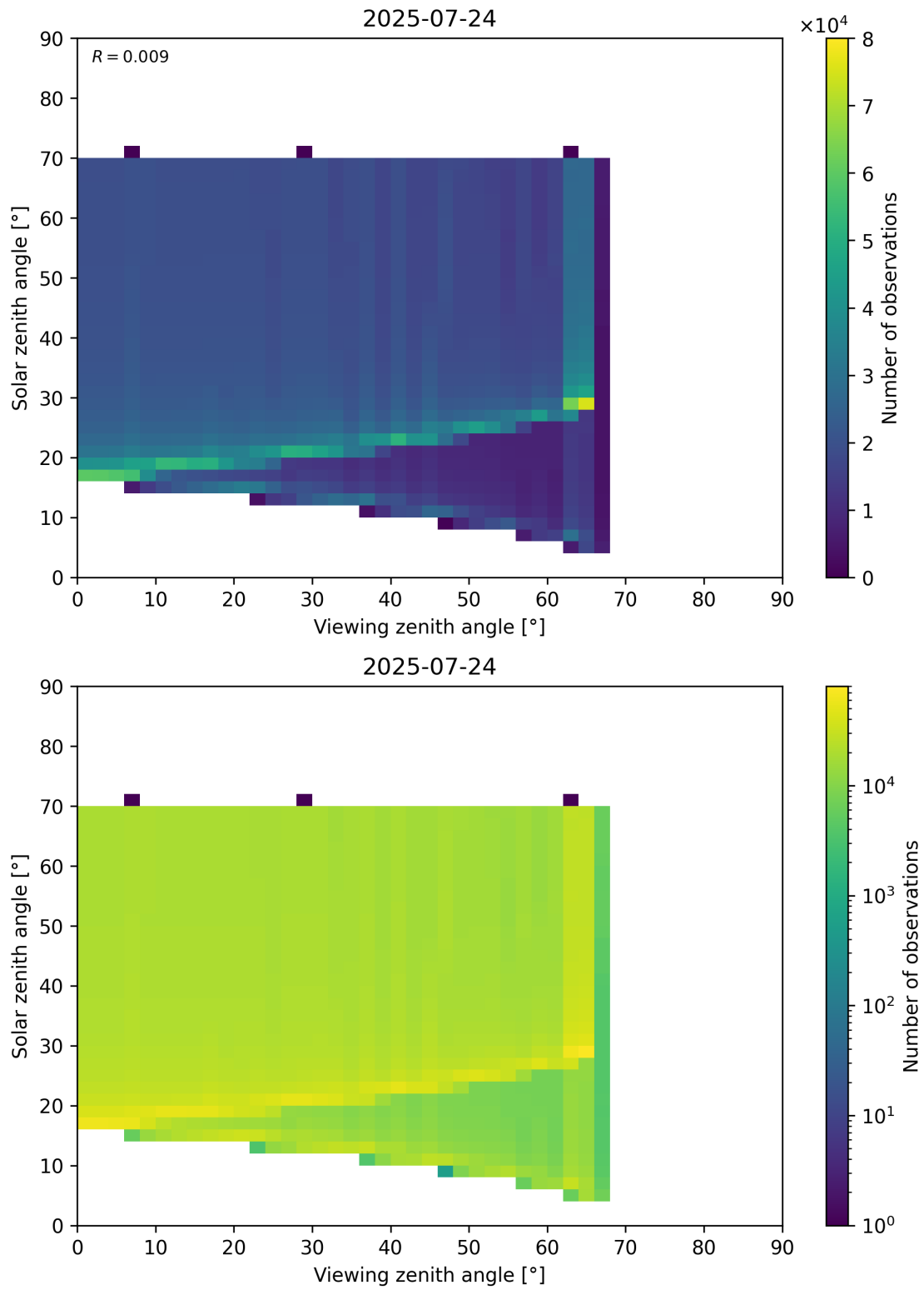
Figure 369: Scatter density plot of “Viewing zenith angle” against “Solar zenith angle” for 2025-07-24 to 2025-07-25.
