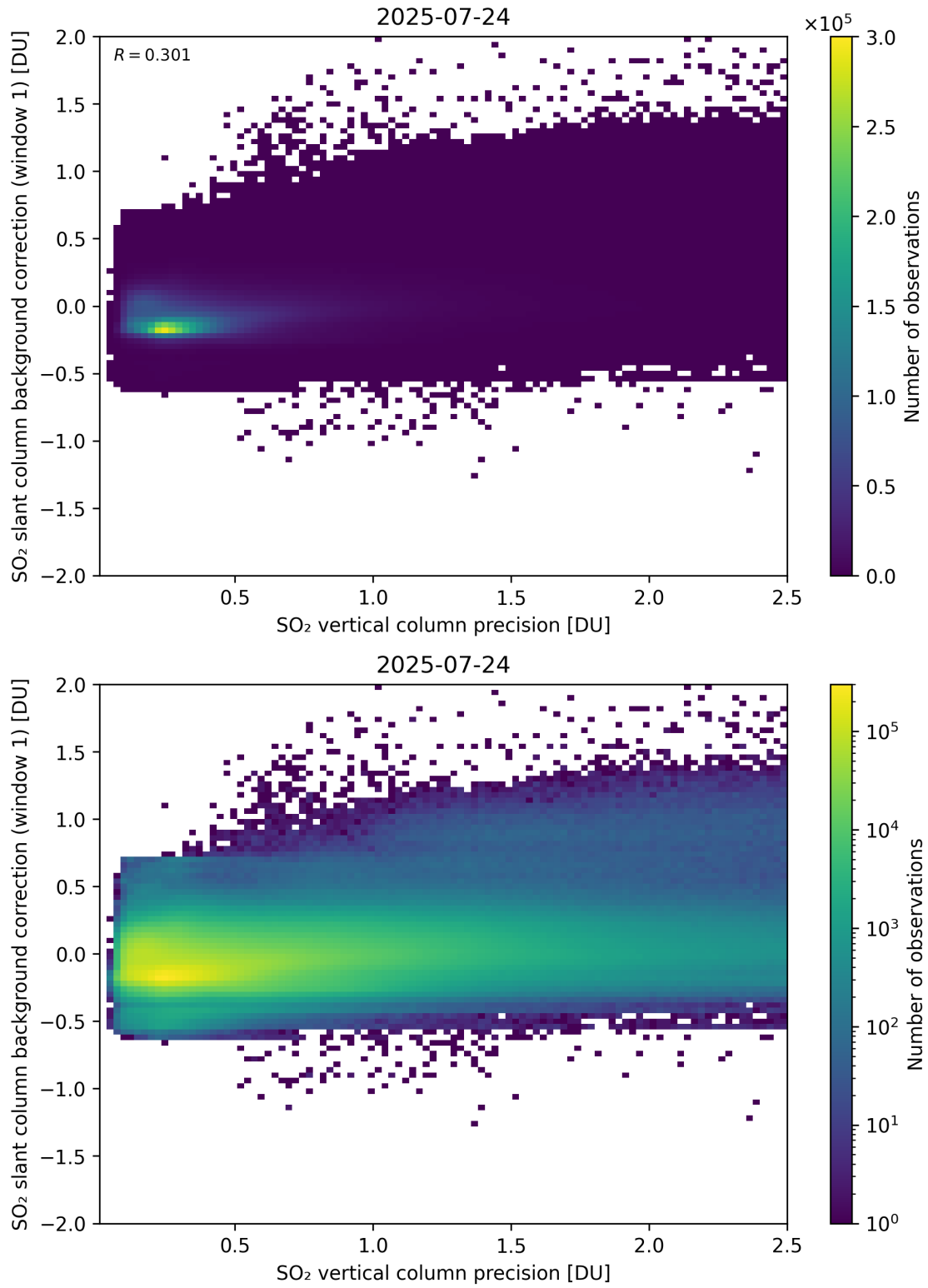
Figure 329: Scatter density plot of “SO 2 vertical column precision” against “SO 2 slant column background correction (window 1)” for 2025-07-24 to 2025-07-25.
