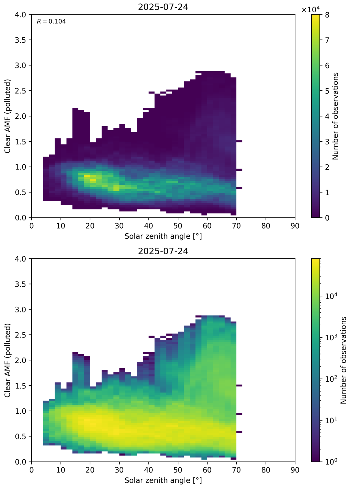
Figure 178: Scatter density plot of “Solar zenith angle” against “Clear AMF (polluted)” for 2025-07-24 to 2025-07-25.
