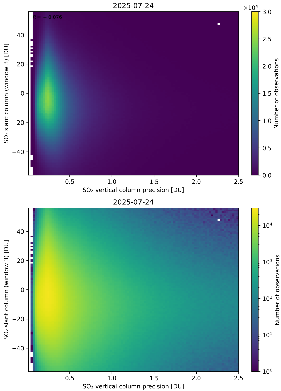
Figure 344: Scatter density plot of “SO 2 vertical column precision” against “SO 2 slant column (window 3)” for 2025-07-24 to 2025-07-25.
