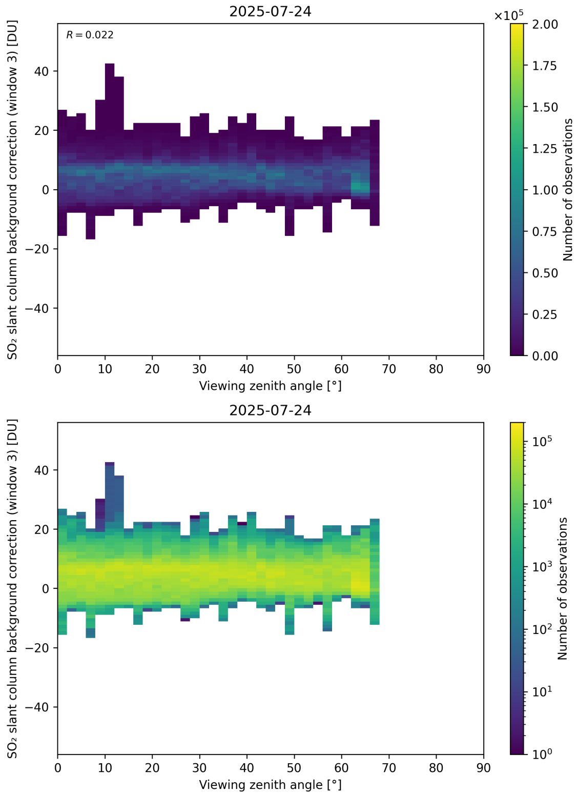
Figure 364: Scatter density plot of “Viewing zenith angle” against “SO 2 slant column background correction (window 3)” for 2025-07-24 to 2025-07-25.
