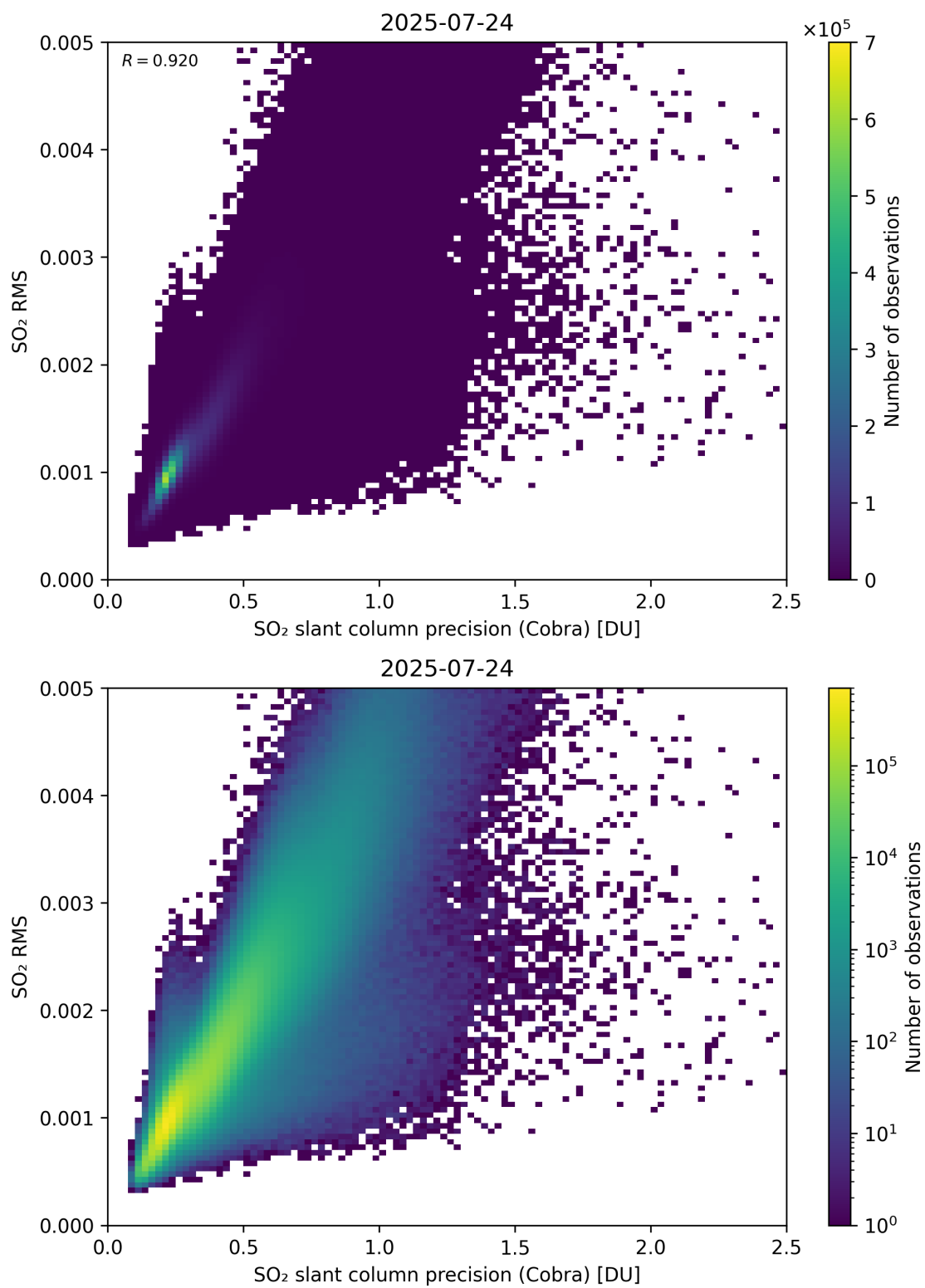
Figure 204: Scatter density plot of “SO 2 slant column precision (Cobra)” against “SO 2 RMS” for 2025-07-24 to 2025-07-25.
