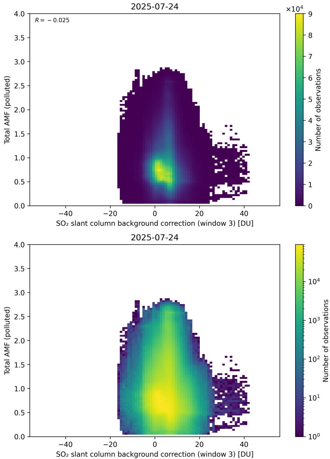
Figure 136: Scatter density plot of “SO 2 slant column background correction (window 3)” against “Total AMF (polluted)” for 2025-07-24 to 2025-07-25.
