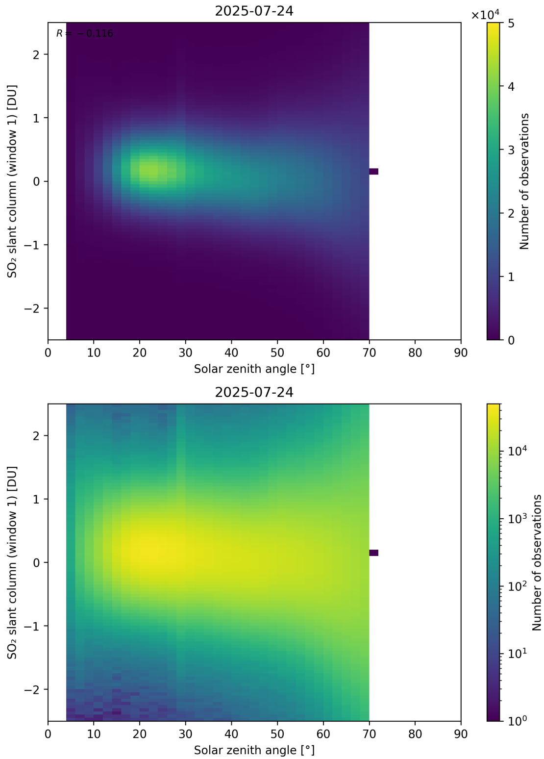
Figure 184: Scatter density plot of “Solar zenith angle” against “SO 2 slant column (window 1)” for 2025-07-24 to 2025-07-25.
