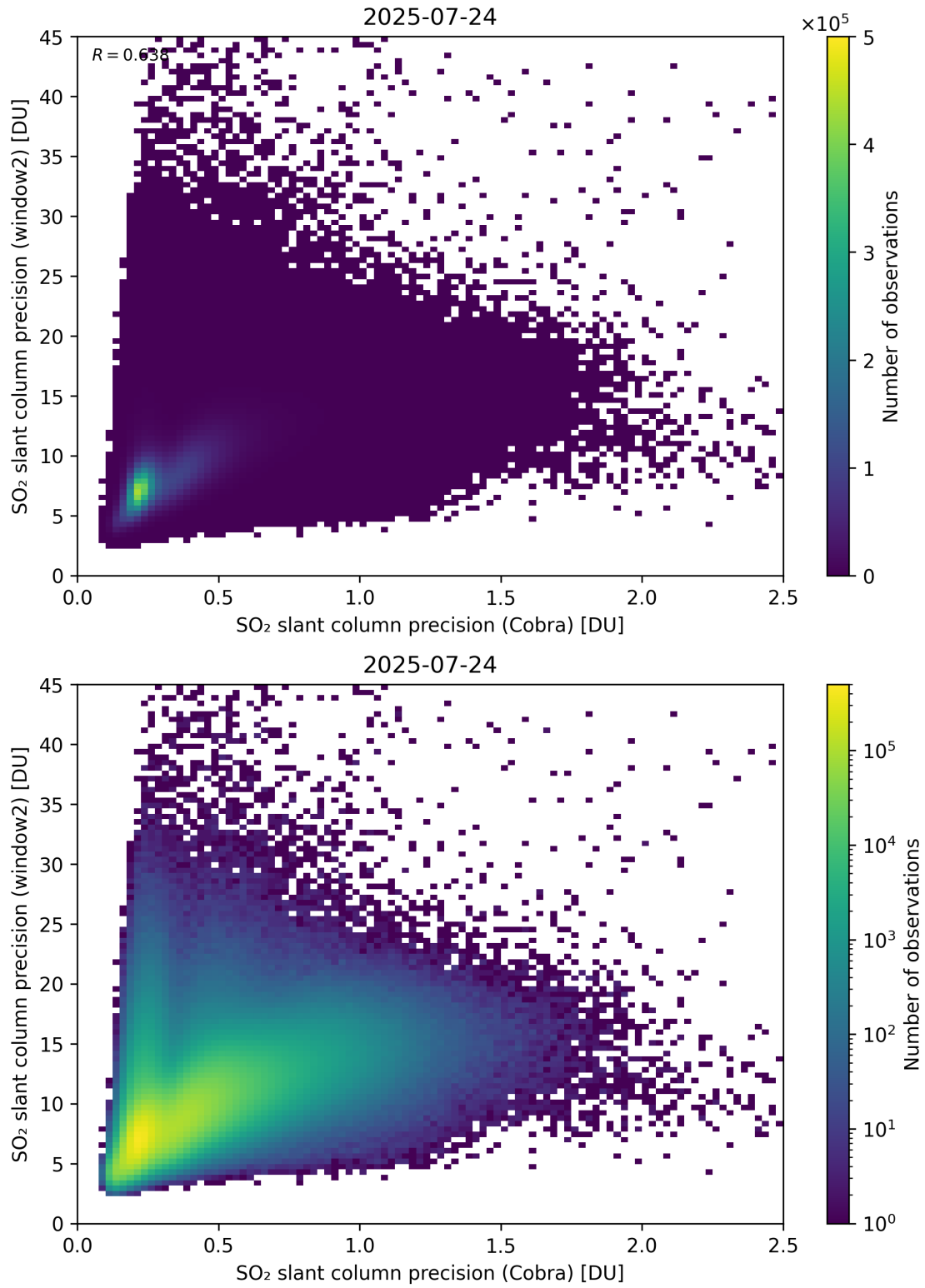
Figure 210: Scatter density plot of “SO 2 slant column precision (Cobra)” against “SO 2 slant column precision (window2)” for 2025-07-24 to 2025-07-25.
