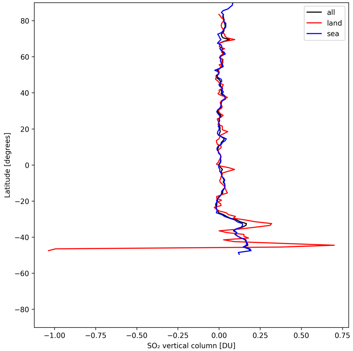
Figure 32: Zonal average of “SO 2 vertical column” for 2025-07-24 to 2025-07-25.
