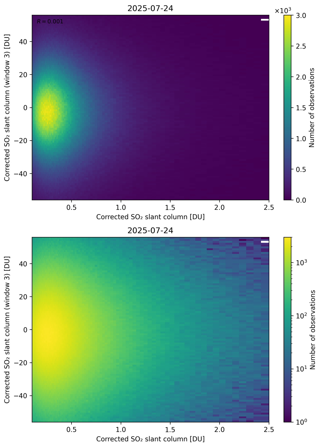
Figure 236: Scatter density plot of “Corrected SO 2 slant column” against “Corrected SO 2 slant column (window 3)” for 2025-07-24 to 2025-07-25.
