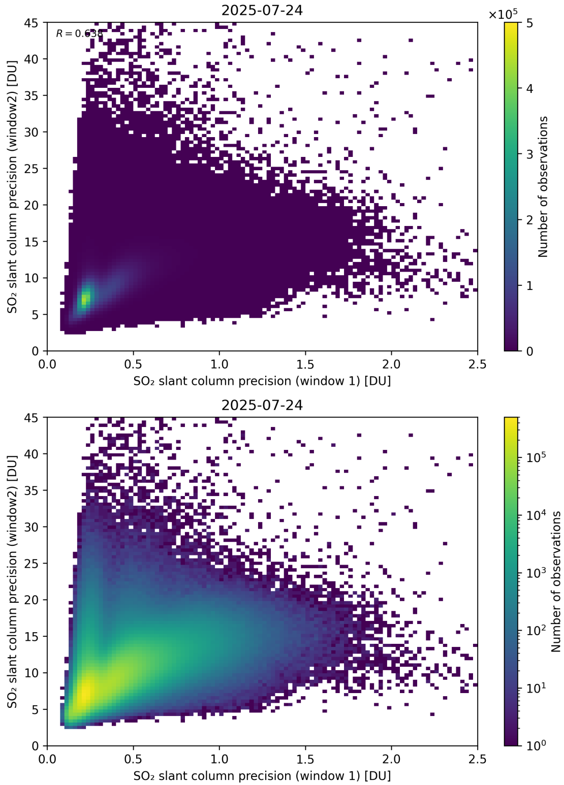
Figure 277: Scatter density plot of “SO 2 slant column precision (window 1)” against “SO 2 slant column precision (window2)” for 2025-07-24 to 2025-07-25.
