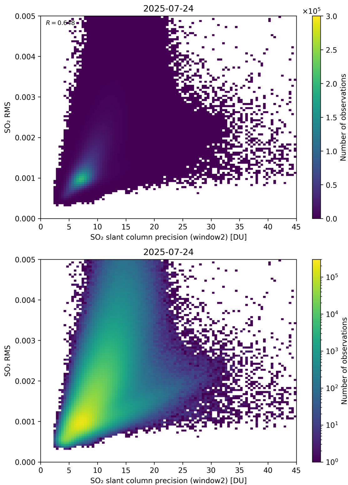
Figure 295: Scatter density plot of “SO 2 slant column precision (window2)” against “SO 2 RMS” for 2025-07-24 to 2025-07-25.
