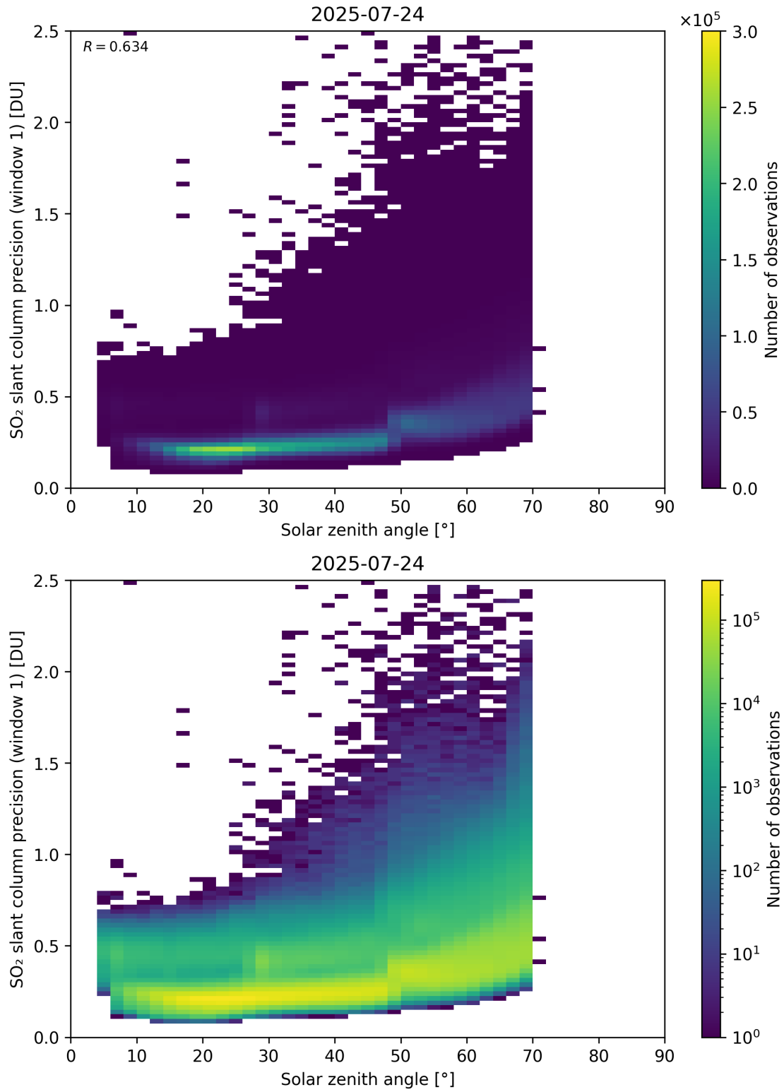
Figure 185: Scatter density plot of “Solar zenith angle” against “SO 2 slant column precision (window 1)” for 2025-07-24 to 2025-07-25.
