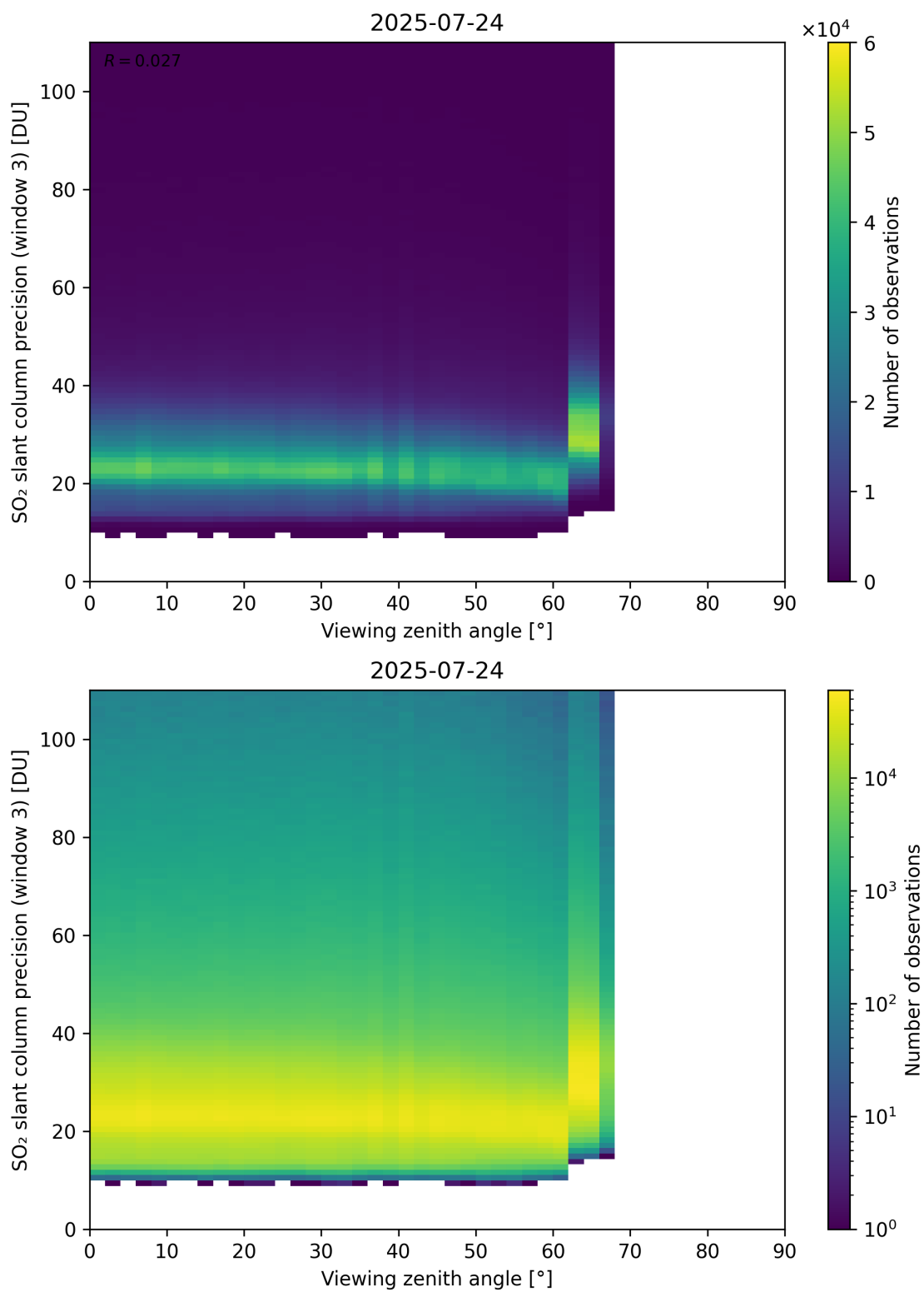
Figure 380: Scatter density plot of “Viewing zenith angle” against “SO 2 slant column precision (window 3)” for 2025-07-24 to 2025-07-25.
