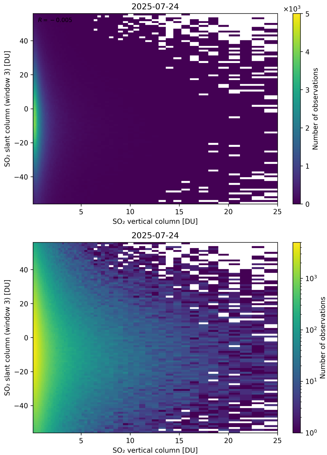
Figure 357: Scatter density plot of “SO 2 vertical column” against “SO 2 slant column (window 3)” for 2025-07-24 to 2025-07-25.
