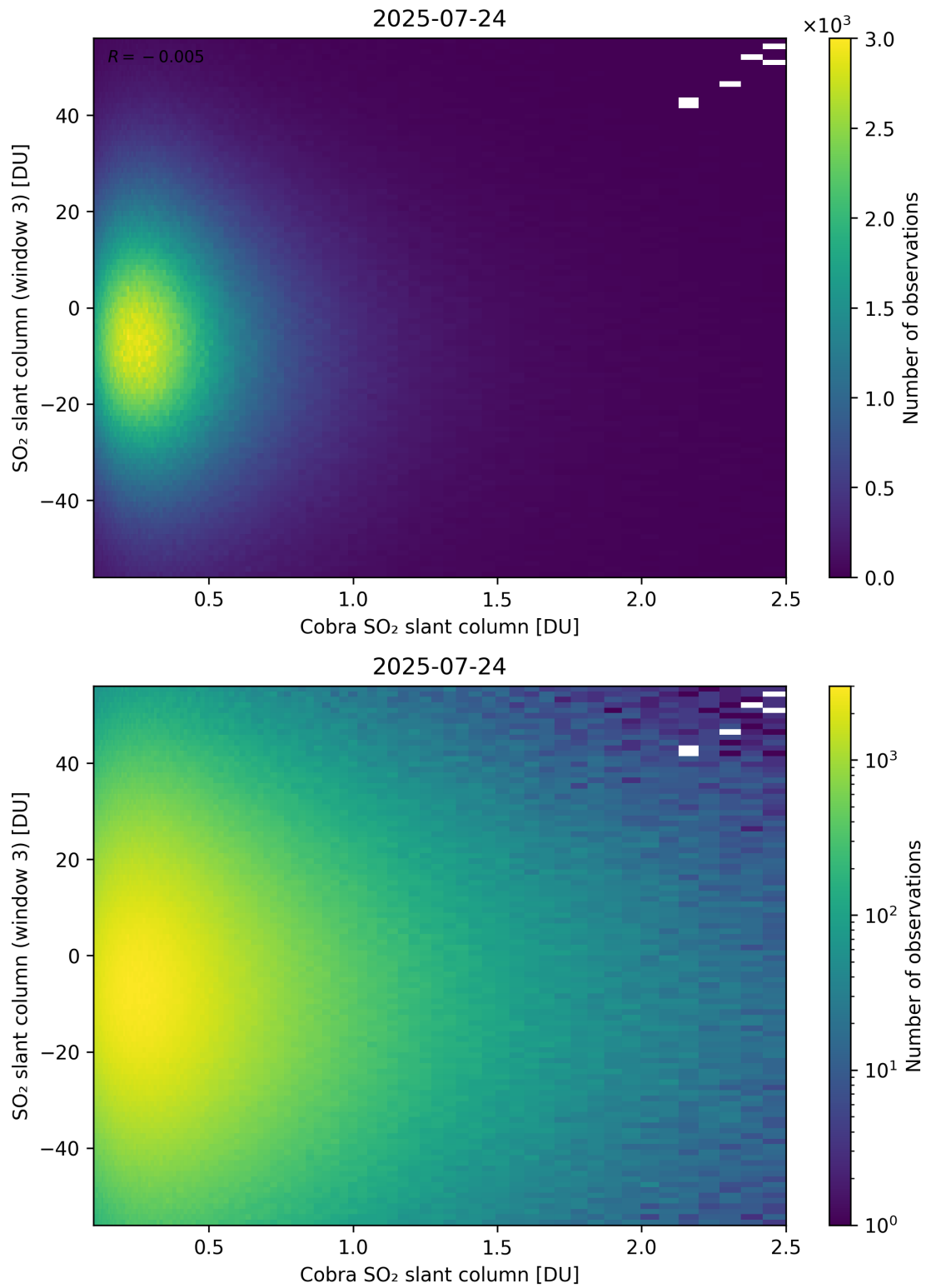
Figure 222: Scatter density plot of “Cobra SO 2 slant column” against “SO 2 slant column (window 3)” for 2025-07-24 to 2025-07-25.
