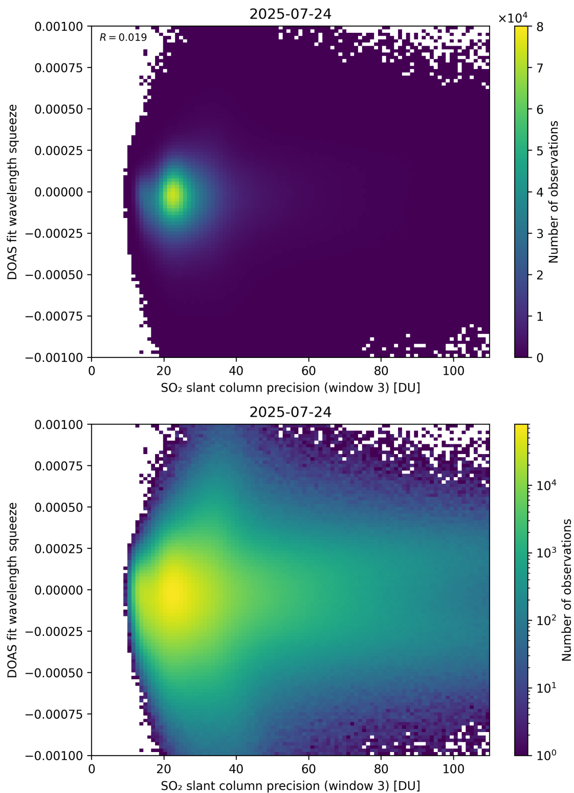
Figure 309: Scatter density plot of “SO 2 slant column precision (window 3)” against “DOAS fit wavelength squeeze” for 2025-07-24 to 2025-07-25.
