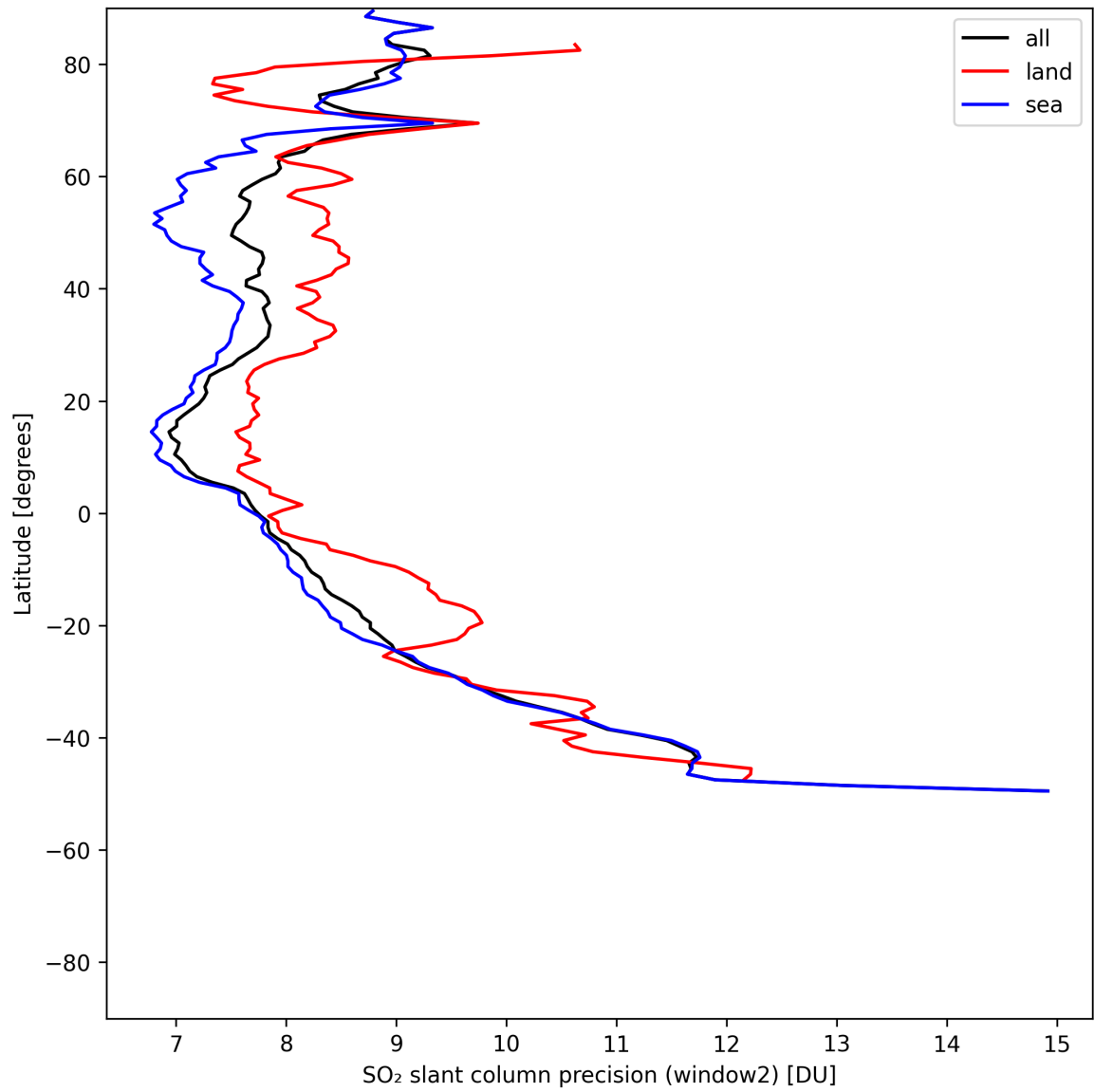
Figure 42: Zonal average of “SO 2 slant column precision (window2)” for 2025-07-24 to 2025-07-25.
