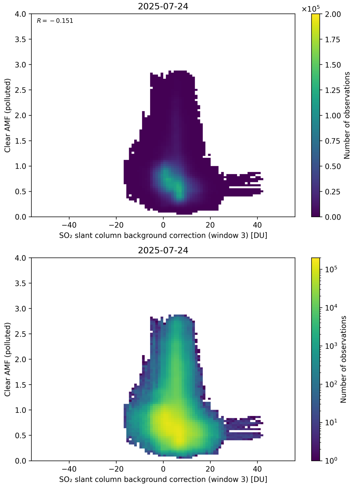
Figure 135: Scatter density plot of “SO 2 slant column background correction (window 3)” against “Clear AMF (polluted)” for 2025-07-24 to 2025-07-25.
