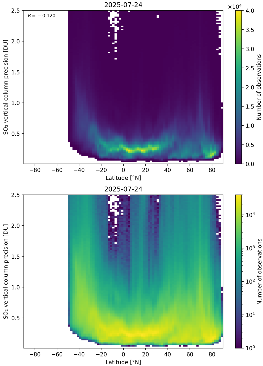
Figure 170: Scatter density plot of “Latitude” against “SO 2 vertical column precision” for 2025-07-24 to 2025-07-25.
