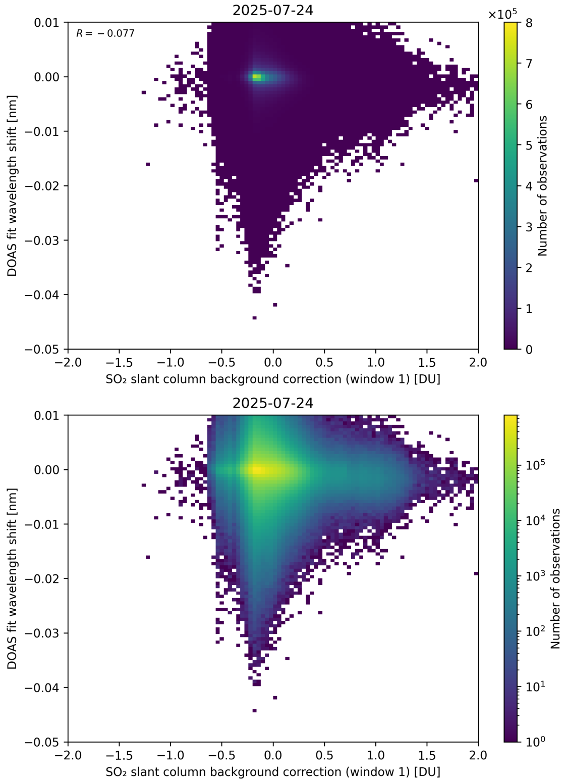
Figure 111: Scatter density plot of “SO 2 slant column background correction (window 1)” against “DOAS fit wavelength shift” for 2025-07-24 to 2025-07-25.
