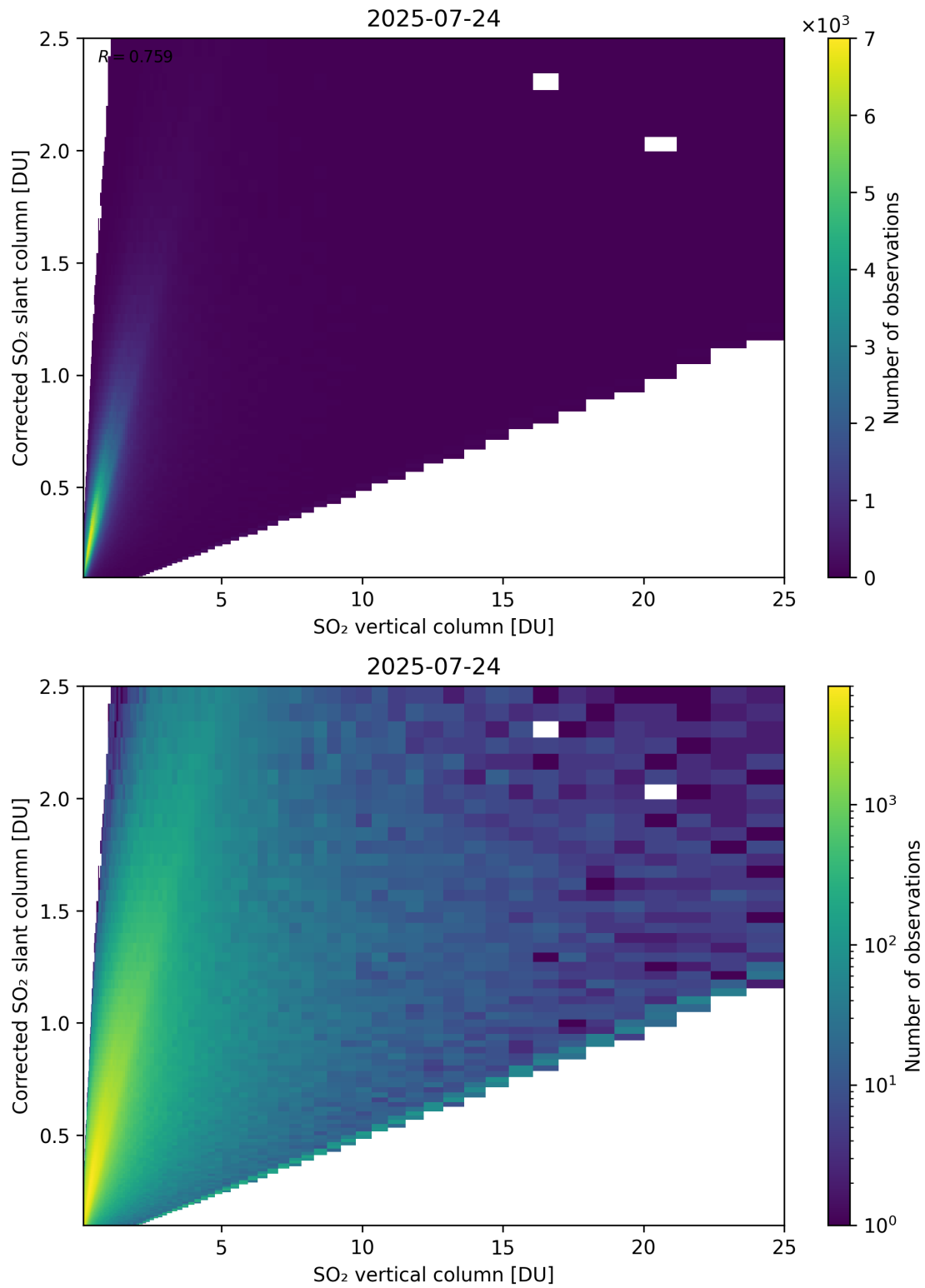
Figure 351: Scatter density plot of “SO 2 vertical column” against “Corrected SO 2 slant column” for 2025-07-24 to 2025-07-25.
