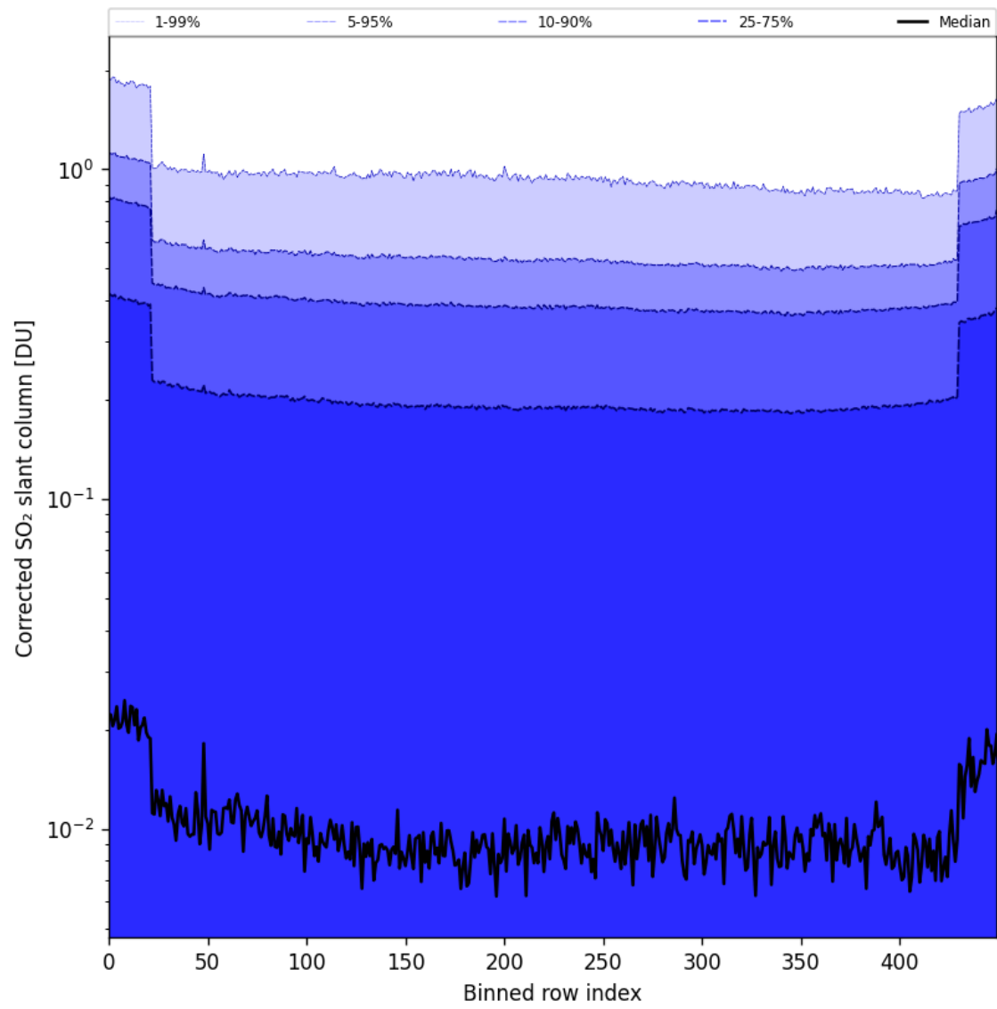
Figure 86: Along track statistics of "Corrected SO 2 slant column" for 2025-07-24 to 2025-07-25
