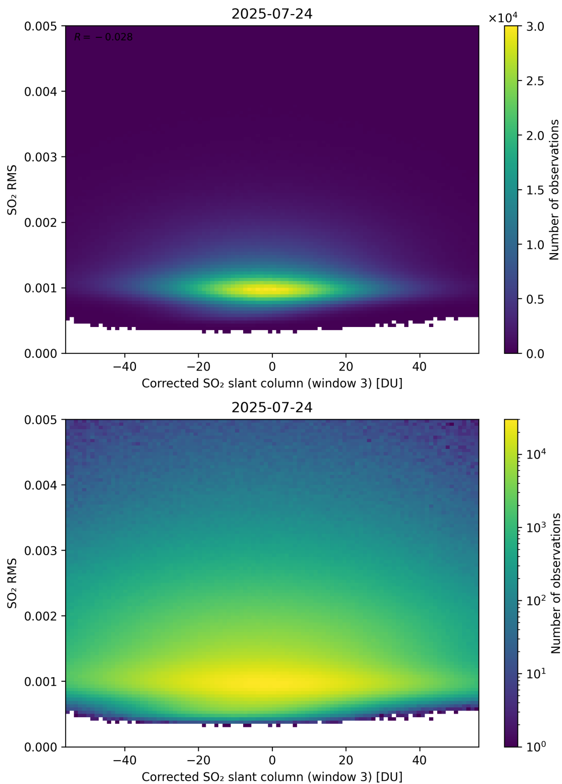
Figure 258: Scatter density plot of “Corrected SO 2 slant column (window 3)” against “SO 2 RMS” for 2025-07-24 to 2025-07-25.
