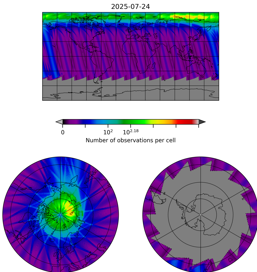
Figure 30: Map of the number of observations for 2025-07-24 to 2025-07-25
