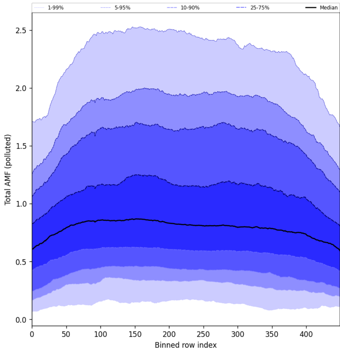
Figure 105: Along track statistics of “Total AMF (polluted)” for 2025-07-24 to 2025-07-25
