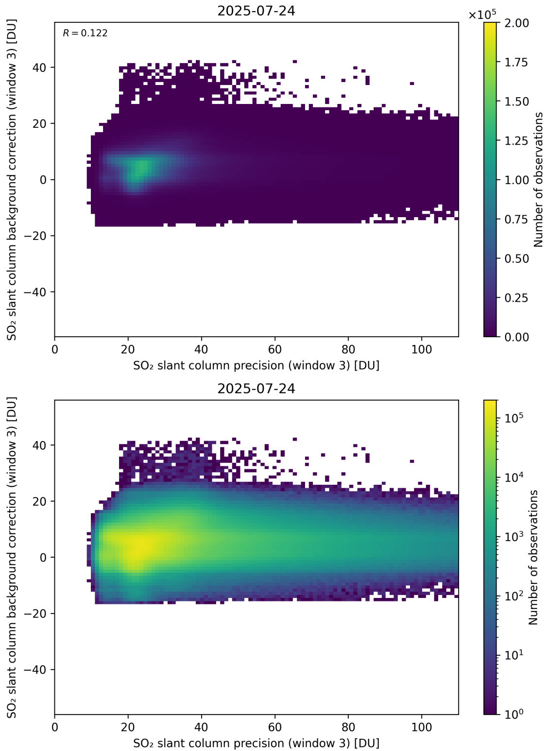
Figure 307: Scatter density plot of “SO 2 slant column precision (window 3)” against “SO 2 slant column background correction (window 3)” for 2025-07-24 to 2025-07-25.
