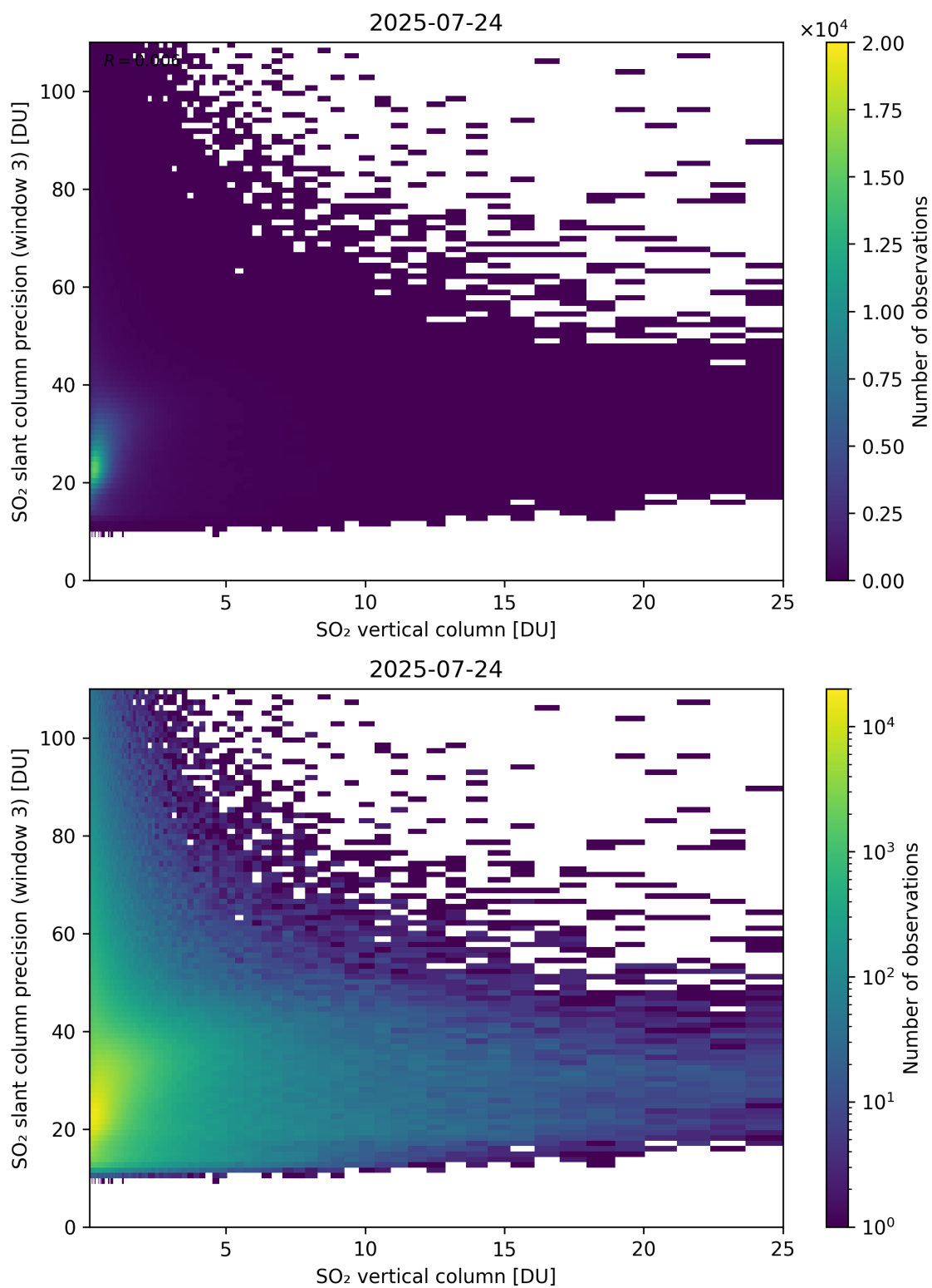
Figure 358: Scatter density plot of “SO 2 vertical column” against “SO 2 slant column precision (window 3)” for 2025-07-24 to 2025-07-25.
