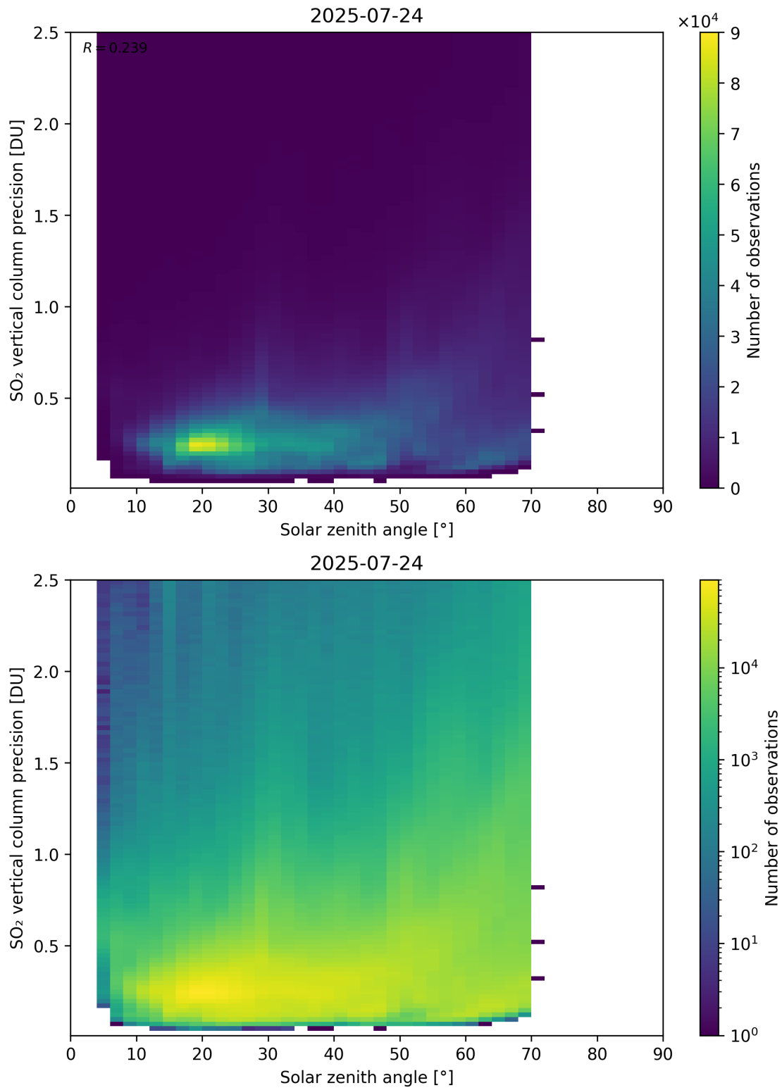
Figure 192: Scatter density plot of “Solar zenith angle” against “SO 2 vertical column precision” for 2025-07-24 to 2025-07-25.
