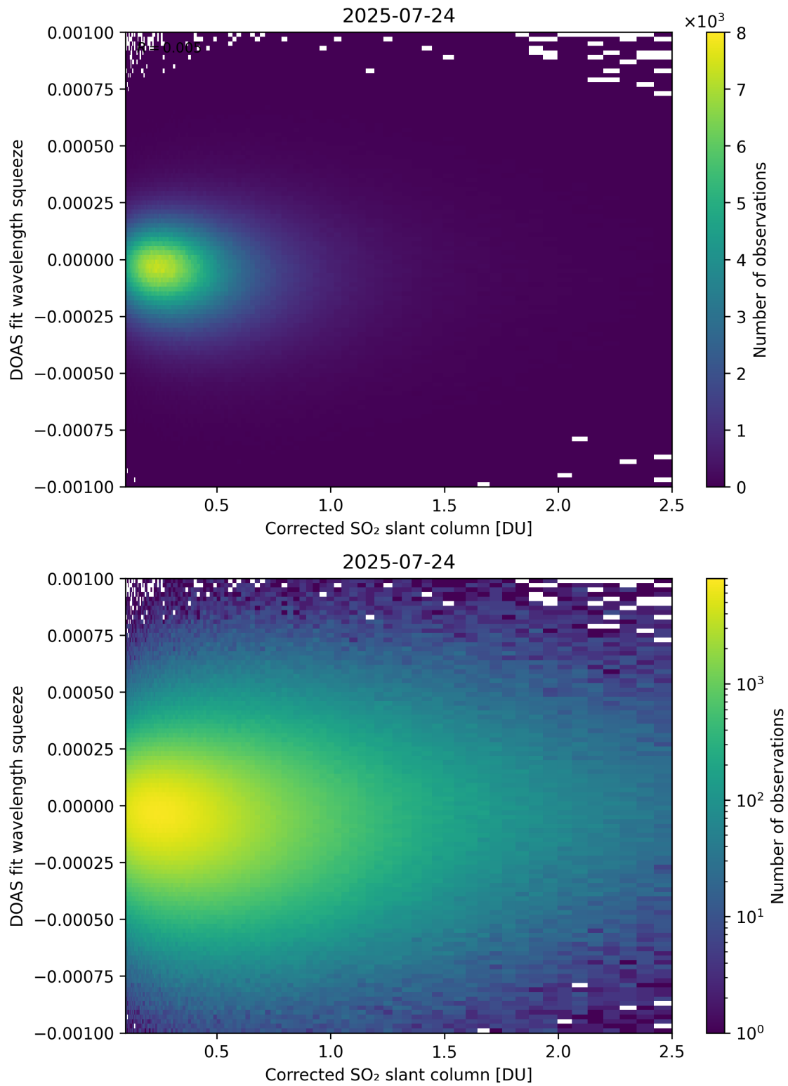
Figure 230: Scatter density plot of “Corrected SO 2 slant column” against “DOAS fit wavelength squeeze” for 2025-07-24 to 2025-07-25.
