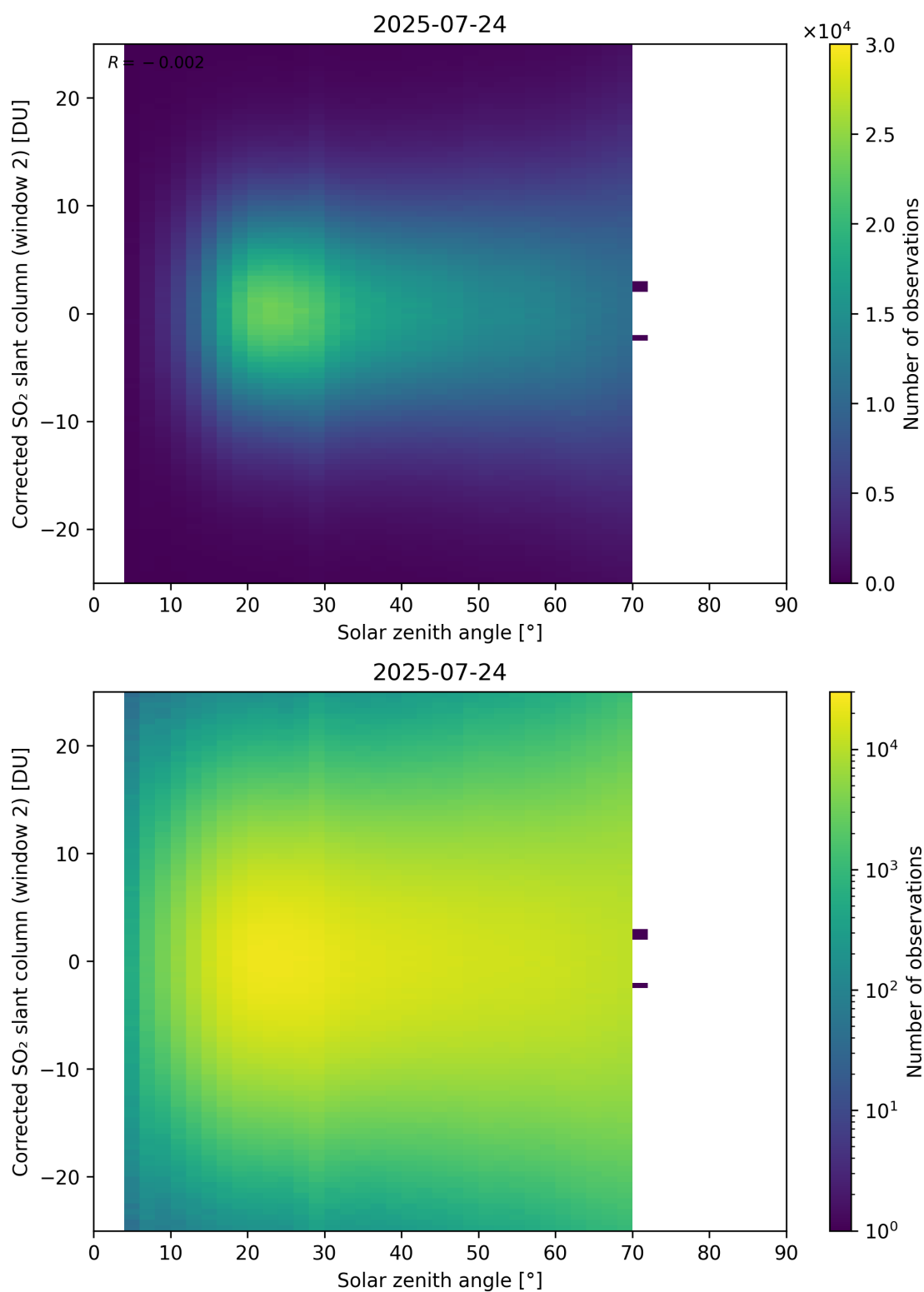
Figure 182: Scatter density plot of “Solar zenith angle” against “Corrected SO 2 slant column (window 2)” for 2025-07-24 to 2025-07-25.
