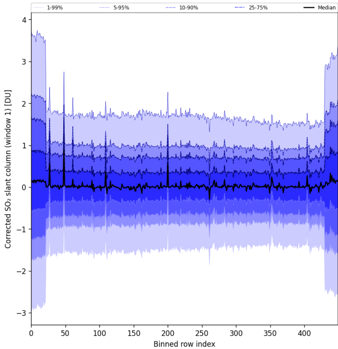
Figure 91: Along track statistics of “Corrected SO 2 slant column (window 1)” for 2025-07-24 to 2025-07-25
