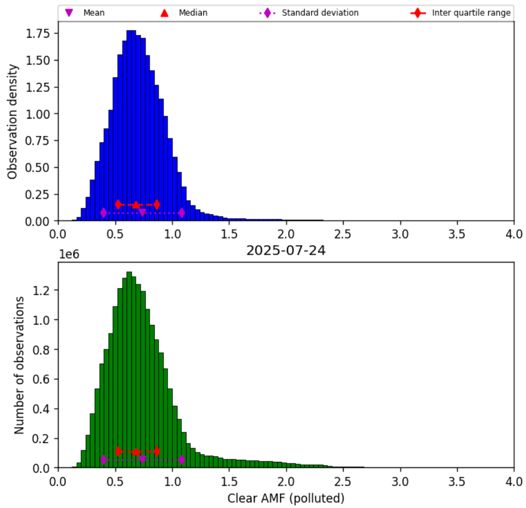
Figure 81: Histogram of “Clear AMF (polluted)” for 2025-07-24 to 2025-07-25
