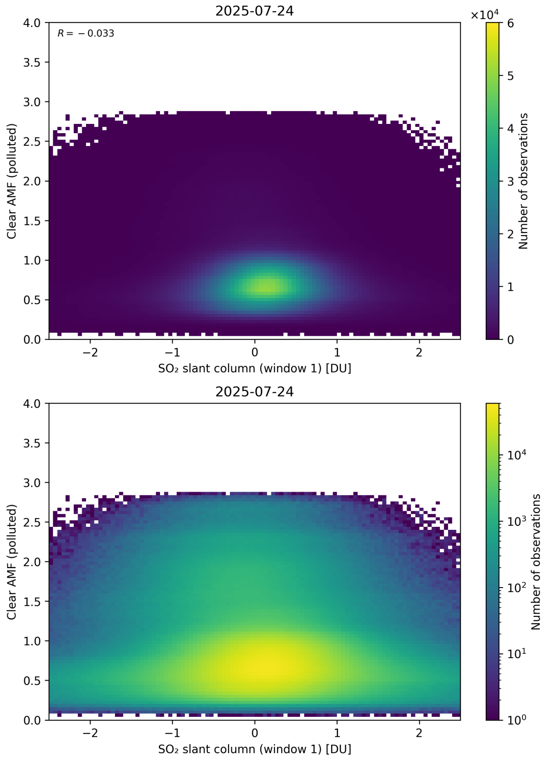
Figure 282: Scatter density plot of “SO 2 slant column (window 1)” against “Clear AMF (polluted)” for 2025-07-24 to 2025-07-25.
