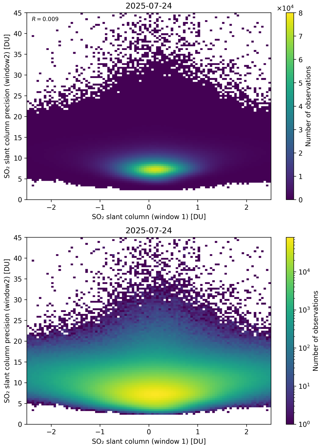
Figure 286: Scatter density plot of “SO 2 slant column (window 1)” against “SO 2 slant column precision (window2)” for 2025-07-24 to 2025-07-25.
