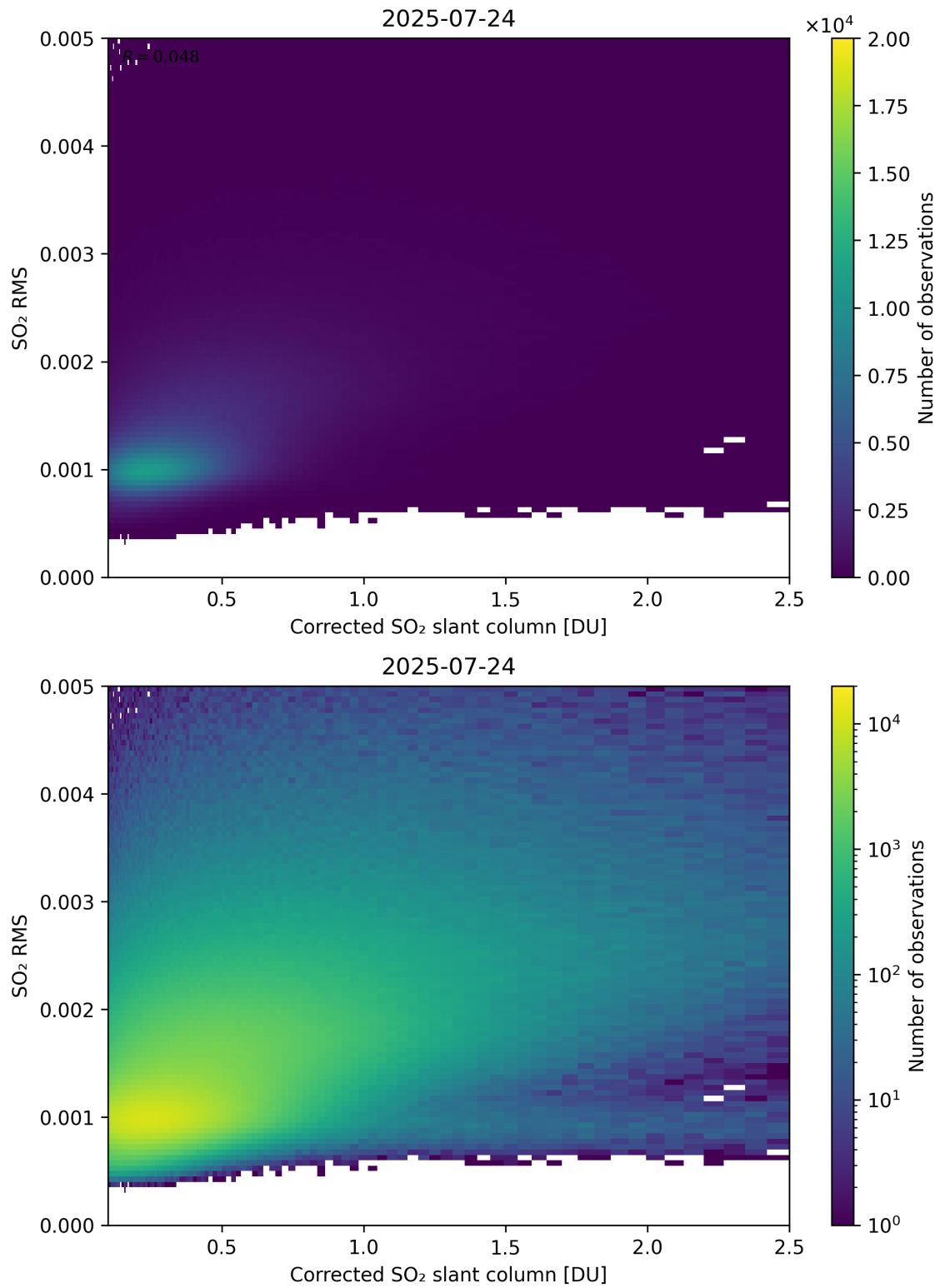
Figure 231: Scatter density plot of “Corrected SO 2 slant column” against “SO 2 RMS” for 2025-07-24 to 2025-07-25.
