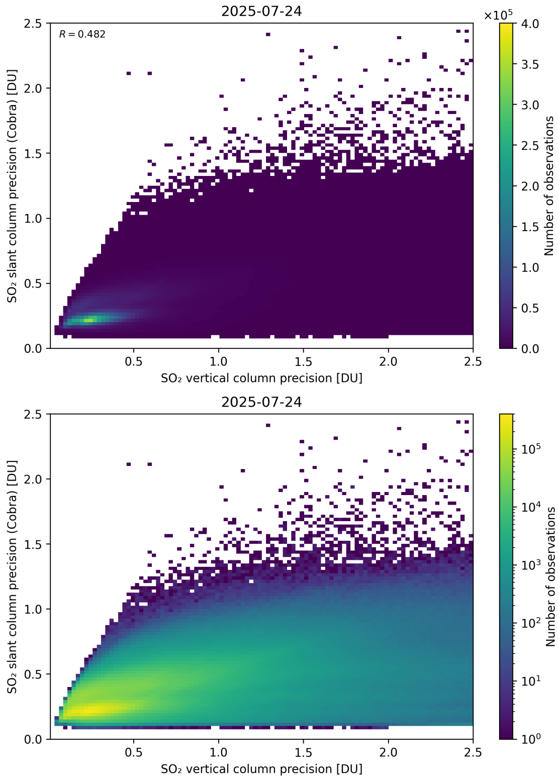
Figure 337: Scatter density plot of “SO 2 vertical column precision” against “SO 2 slant column precision (Cobra)” for 2025-07-24 to 2025-07-25.
