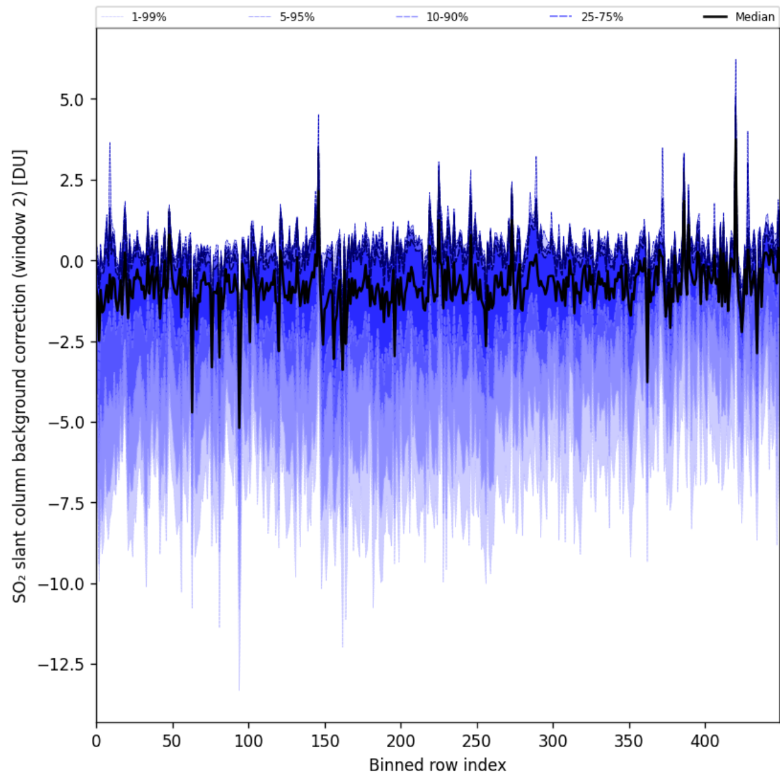
Figure 96: Along track statistics of “SO 2 slant column background correction (window 2)” for 2025-07-24 to 2025-07-25
