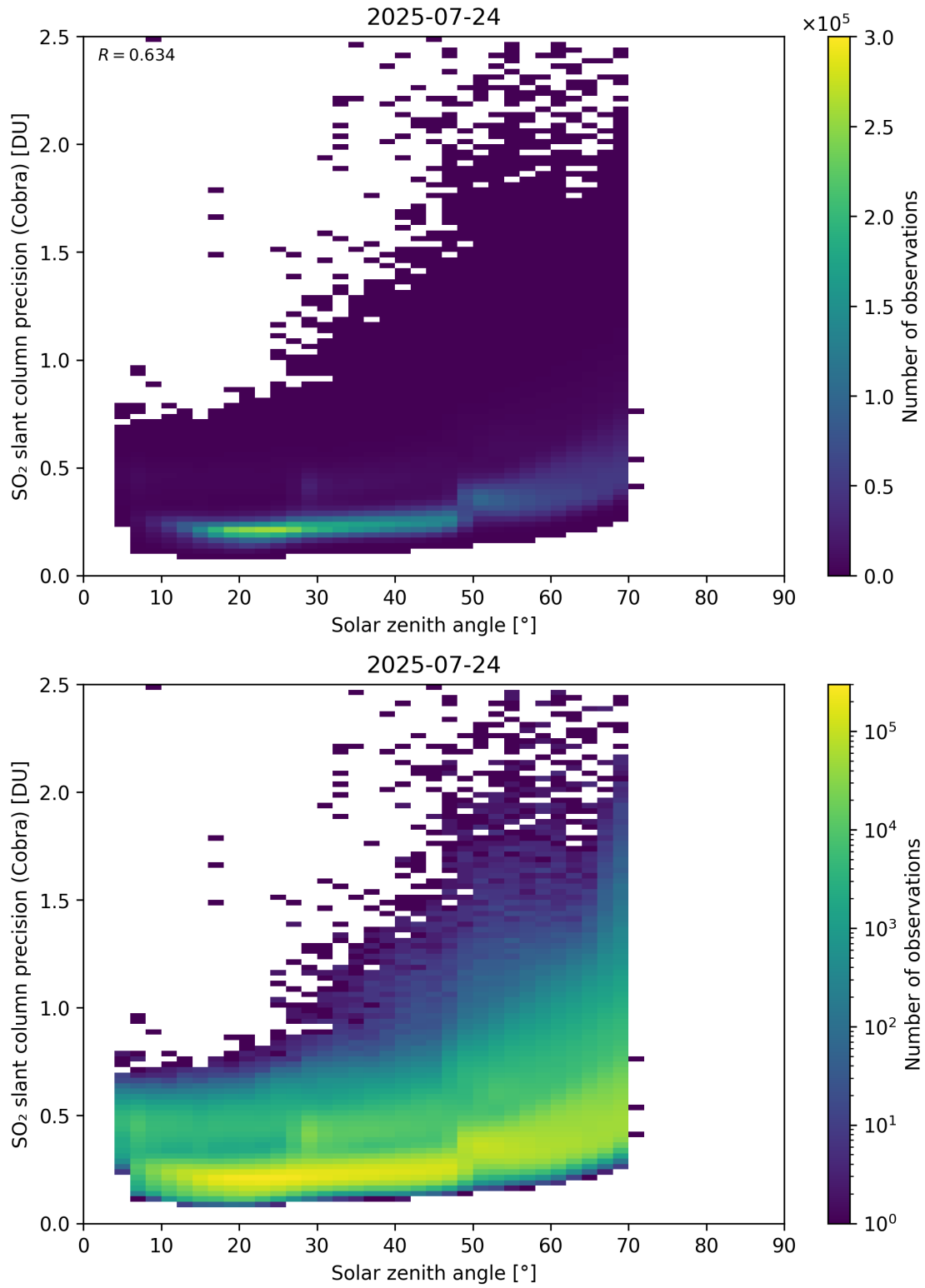
Figure 180: Scatter density plot of “Solar zenith angle” against “SO 2 slant column precision (Cobra)” for 2025-07-24 to 2025-07-25.
