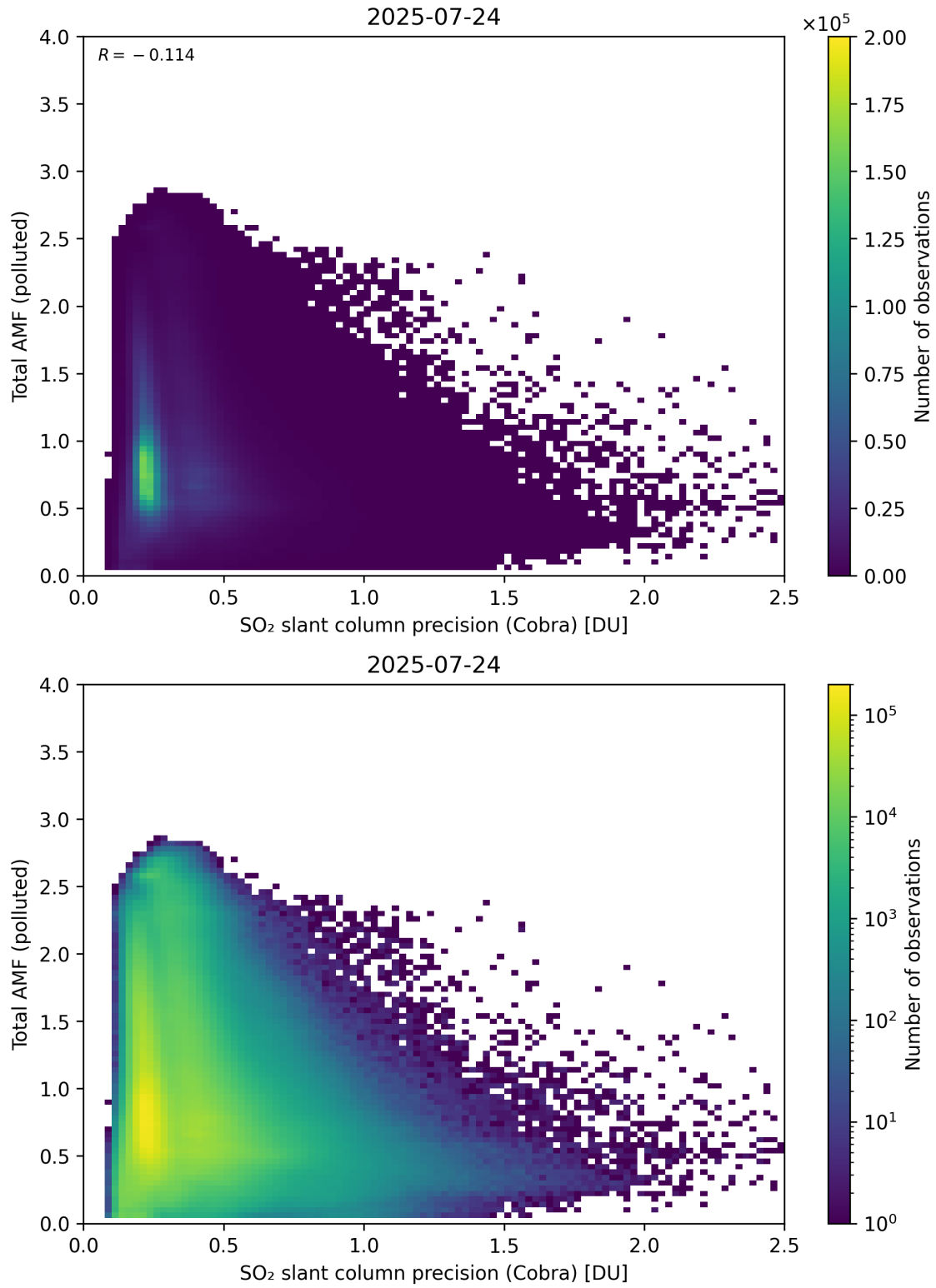
Figure 213: Scatter density plot of “SO 2 slant column precision (Cobra)” against “Total AMF (polluted)” for 2025-07-24 to 2025-07-25.
