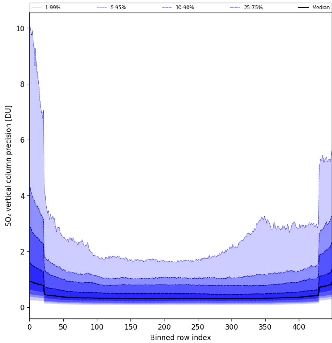
Figure 85: Along track statistics of “SO 2 vertical column precision” for 2025-07-24 to 2025-07-25
