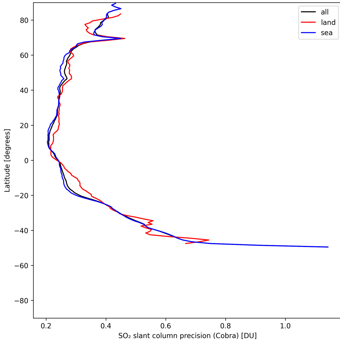
Figure 36: Zonal average of “SO 2 slant column precision (Cobra)” for 2025-07-24 to 2025-07-25.
