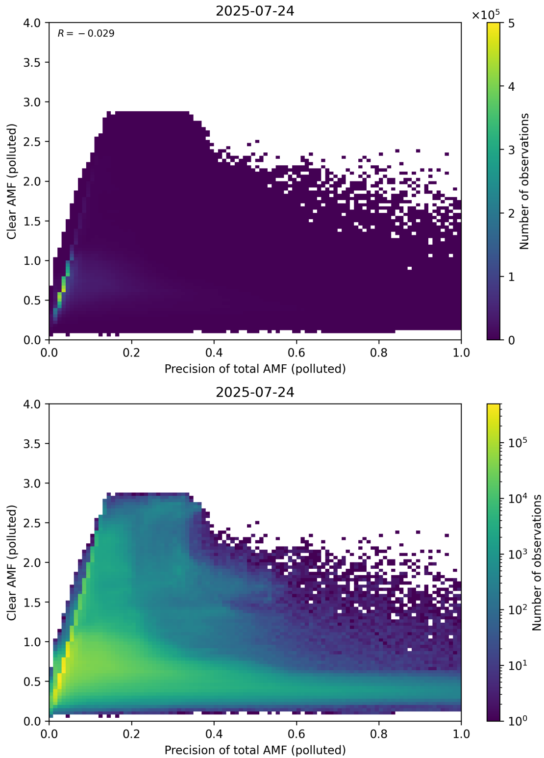
Figure 320: Scatter density plot of “Precision of total AMF (polluted)” against “Clear AMF (polluted)” for 2025-07-24 to 2025-07-25.
