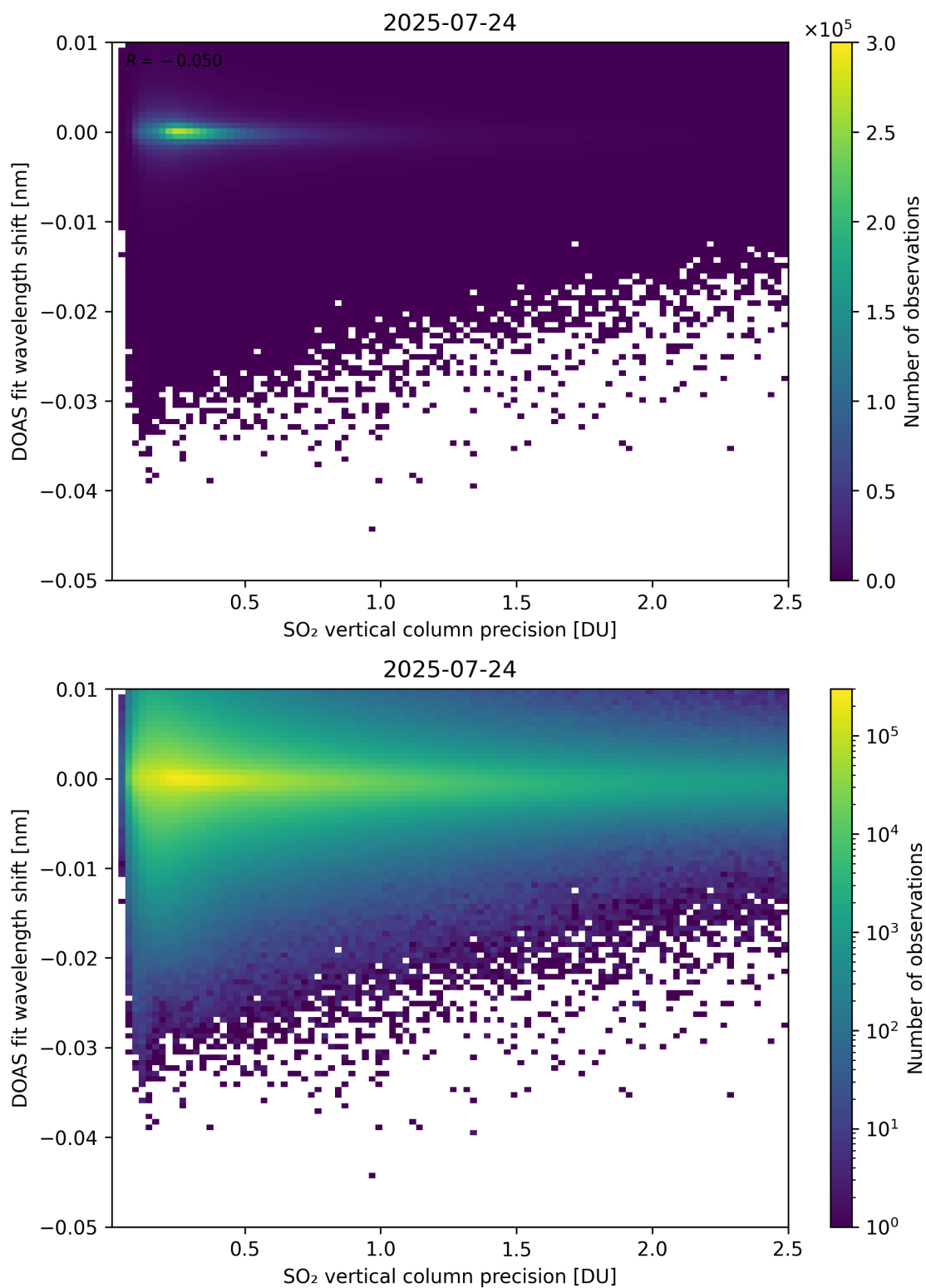
Figure 332: Scatter density plot of “SO 2 vertical column precision” against “DOAS fit wavelength shift” for 2025-07-24 to 2025-07-25.
