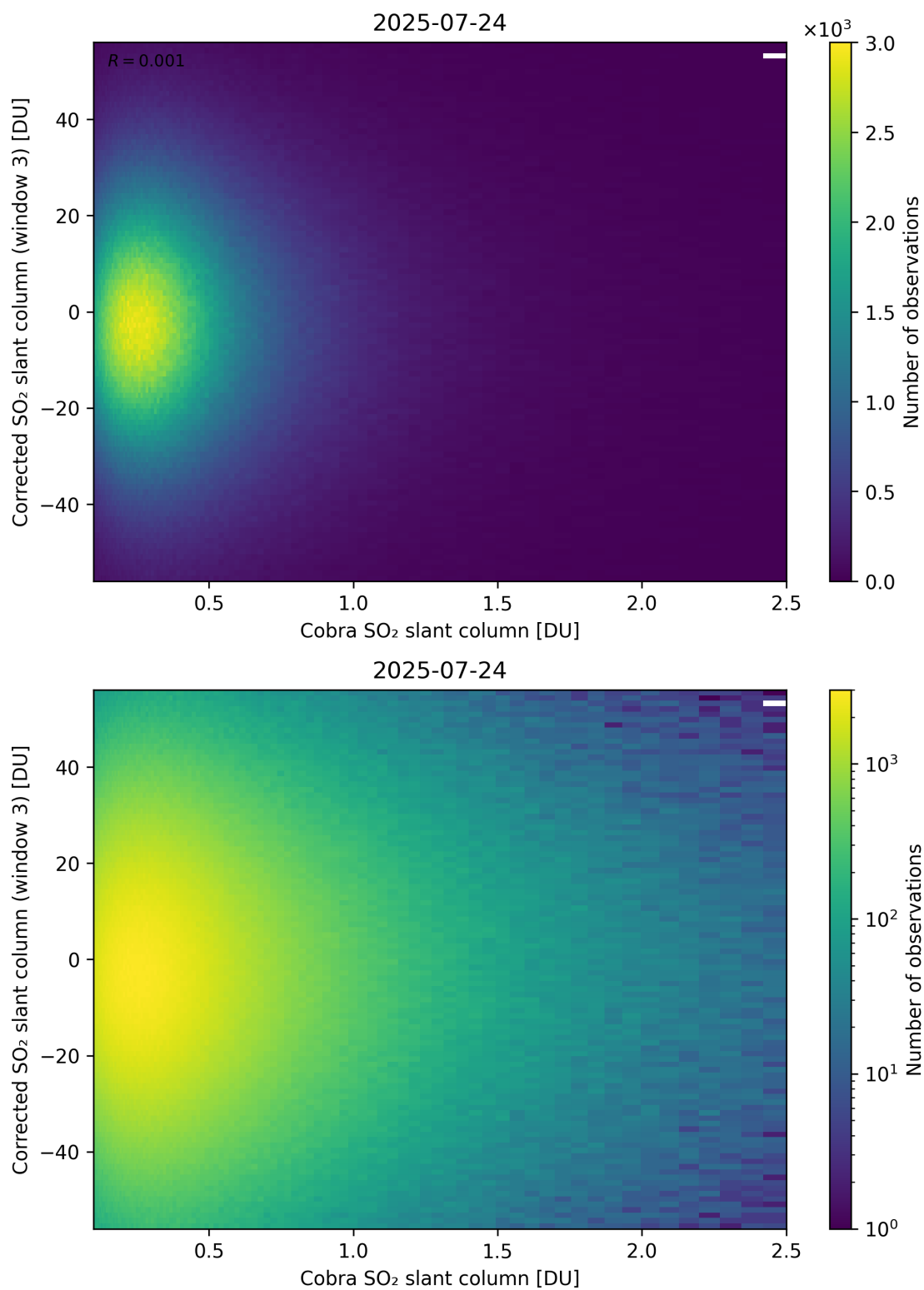
Figure 218: Scatter density plot of “Cobra SO 2 slant column” against “Corrected SO 2 slant column (window 3)” for 2025-07-24 to 2025-07-25.
