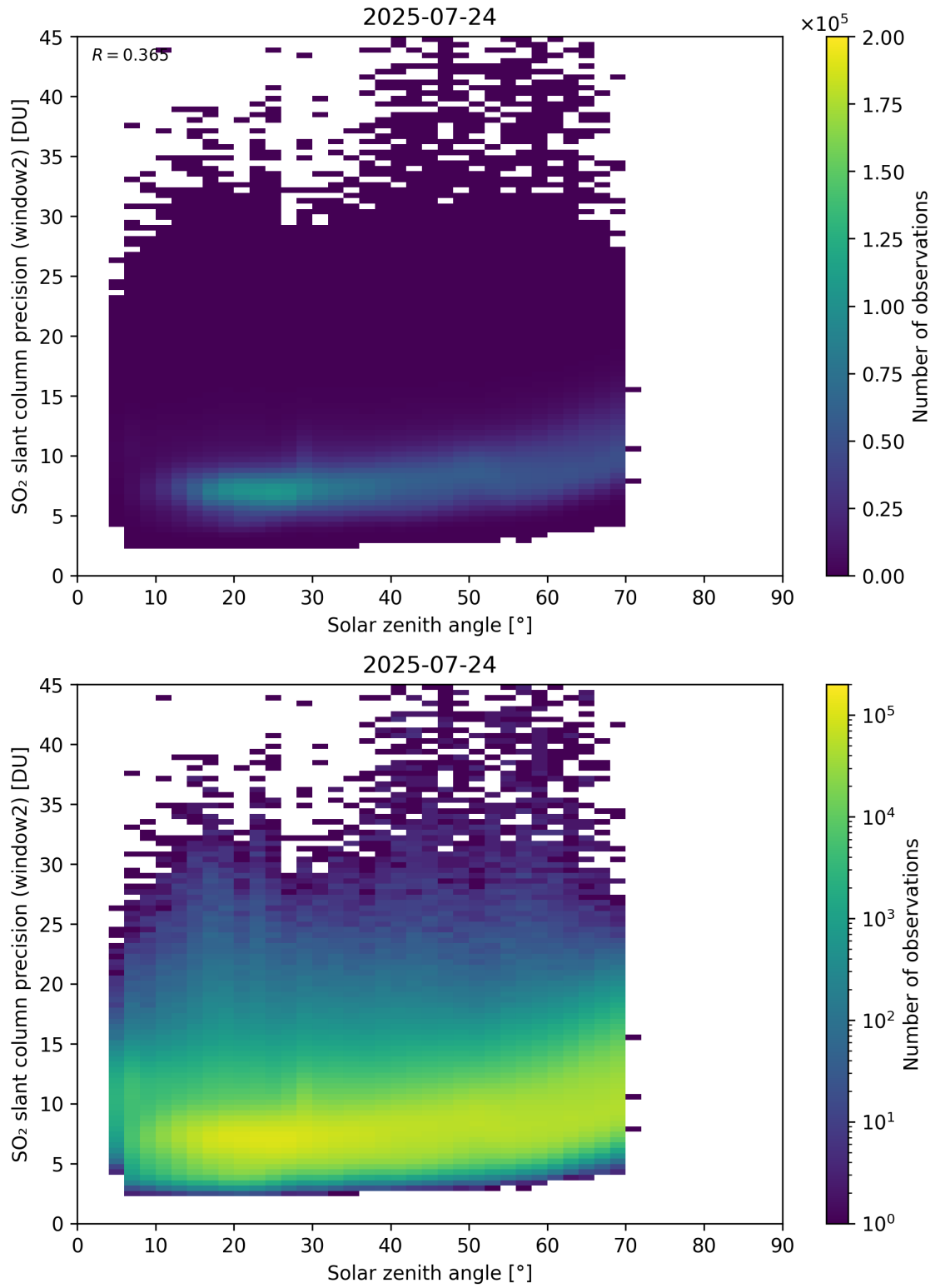
Figure 186: Scatter density plot of “Solar zenith angle” against “SO 2 slant column precision (window2)” for 2025-07-24 to 2025-07-25.
