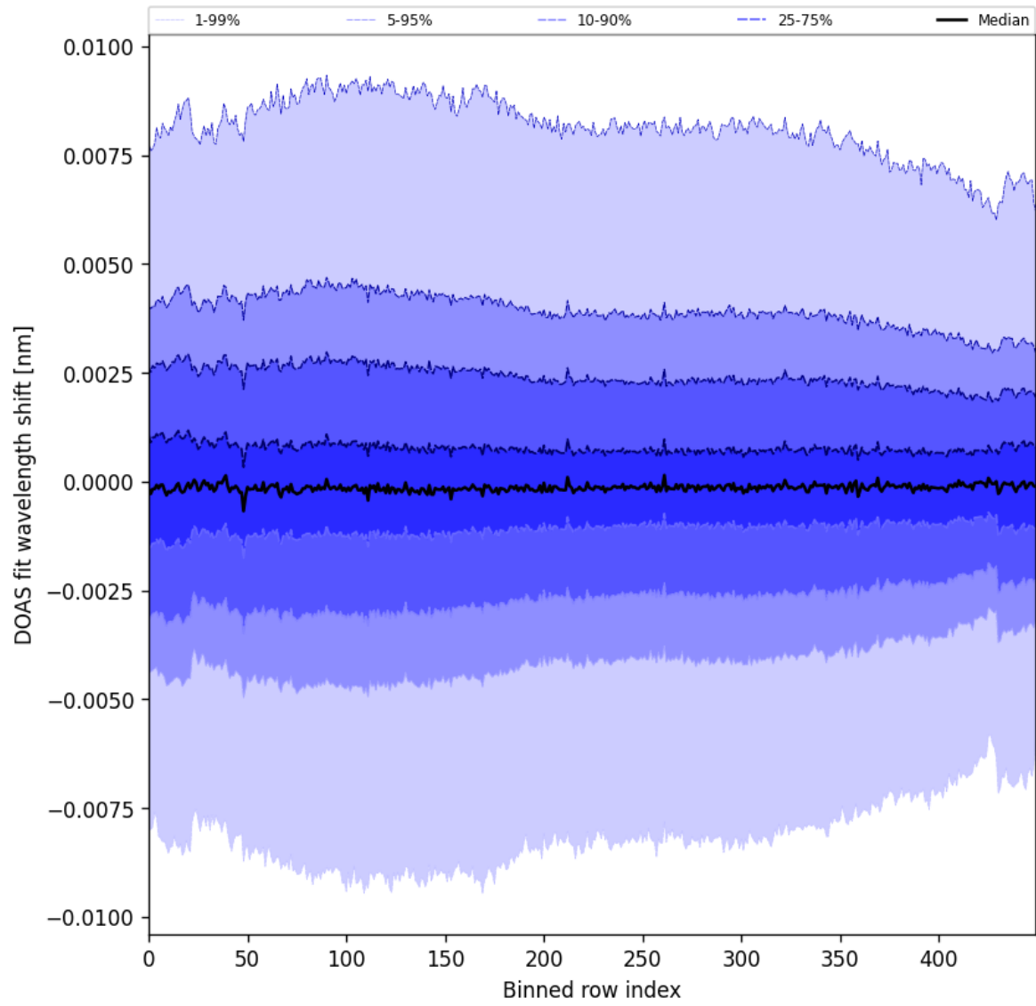
Figure 102: Along track statistics of “DOAS fit wavelength shift” for 2025-07-24 to 2025-07-25
