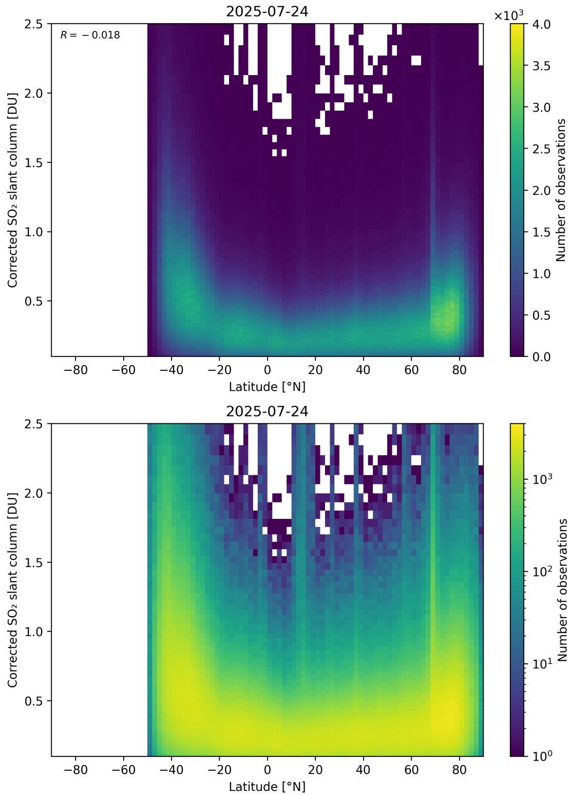
Figure 159: Scatter density plot of “Latitude” against “Corrected SO 2 slant column” for 2025-07-24 to 2025-07-25.
