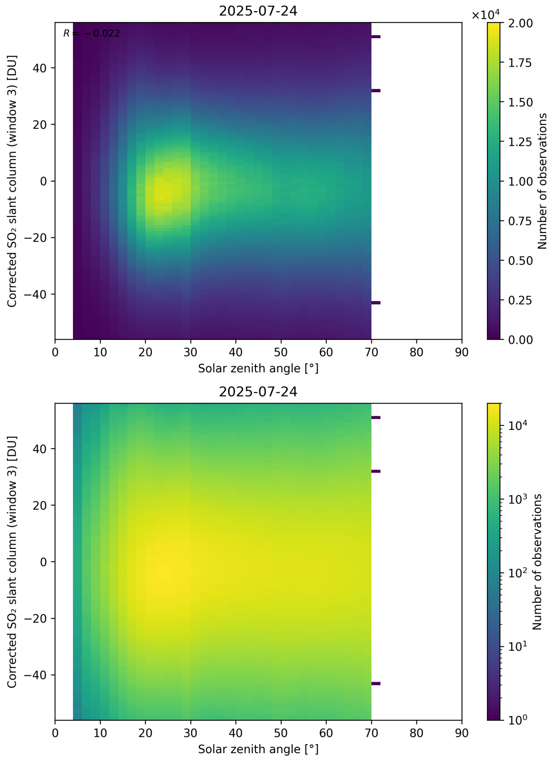
Figure 183: Scatter density plot of “Solar zenith angle” against “Corrected SO 2 slant column (window 3)” for 2025-07-24 to 2025-07-25.
