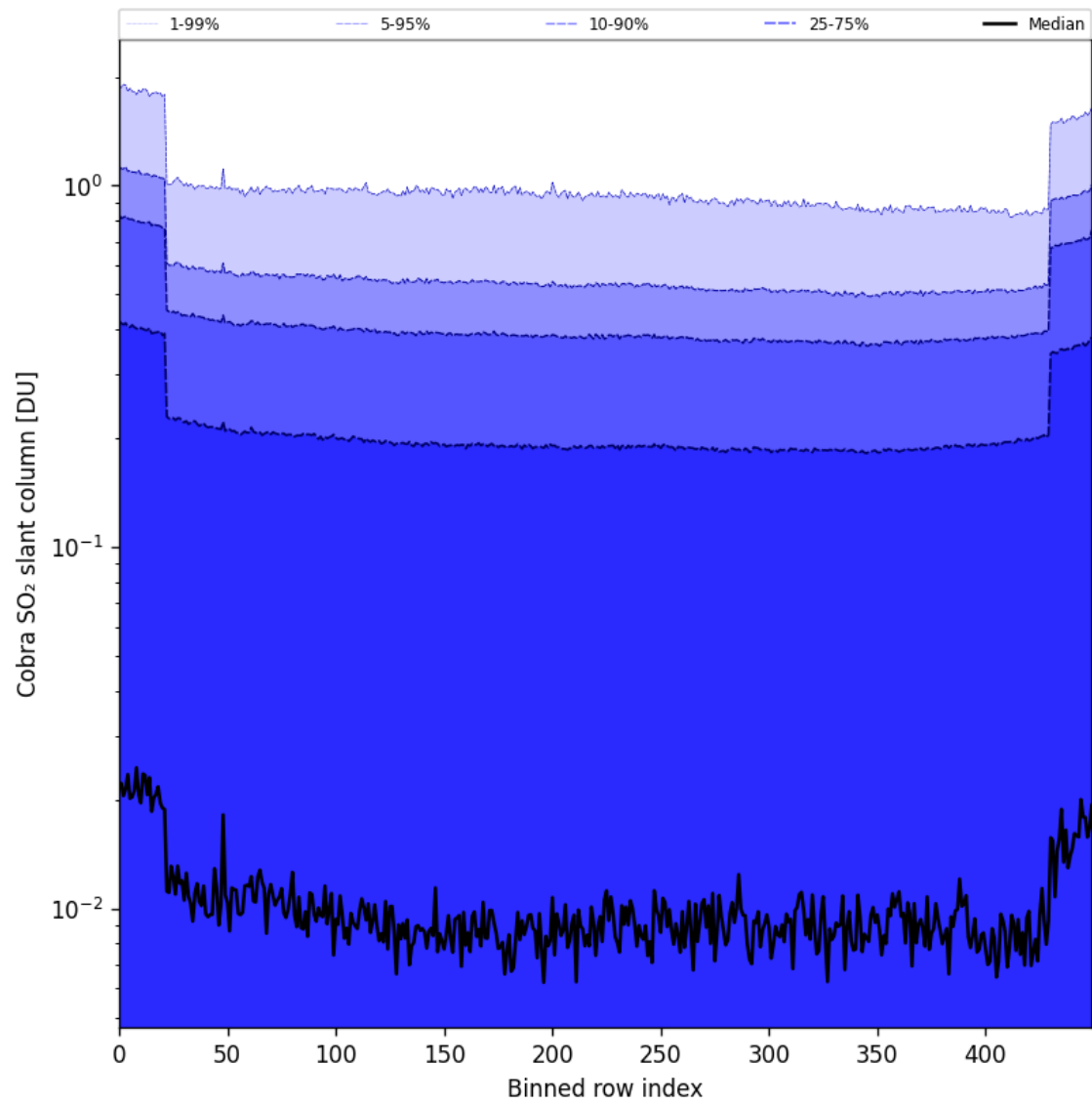
Figure 87: Along track statistics of “Cobra SO 2 slant column” for 2025-07-24 to 2025-07-25
