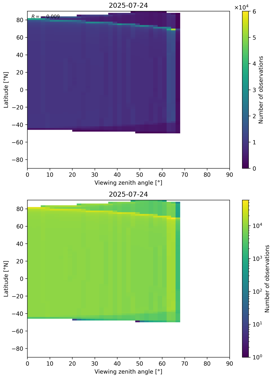
Figure 368: Scatter density plot of “Viewing zenith angle” against “Latitude” for 2025-07-24 to 2025-07-25.
