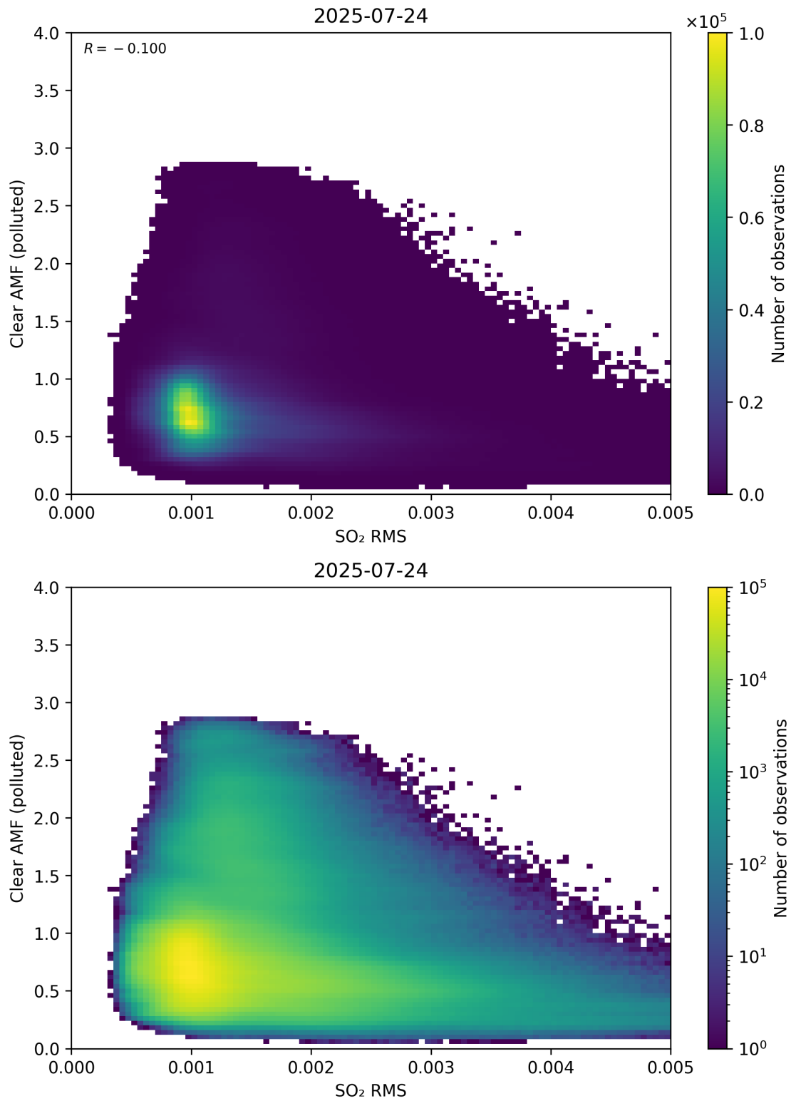
Figure 147: Scatter density plot of “SO 2 RMS” against “Clear AMF (polluted)” for 2025-07-24 to 2025-07-25.
