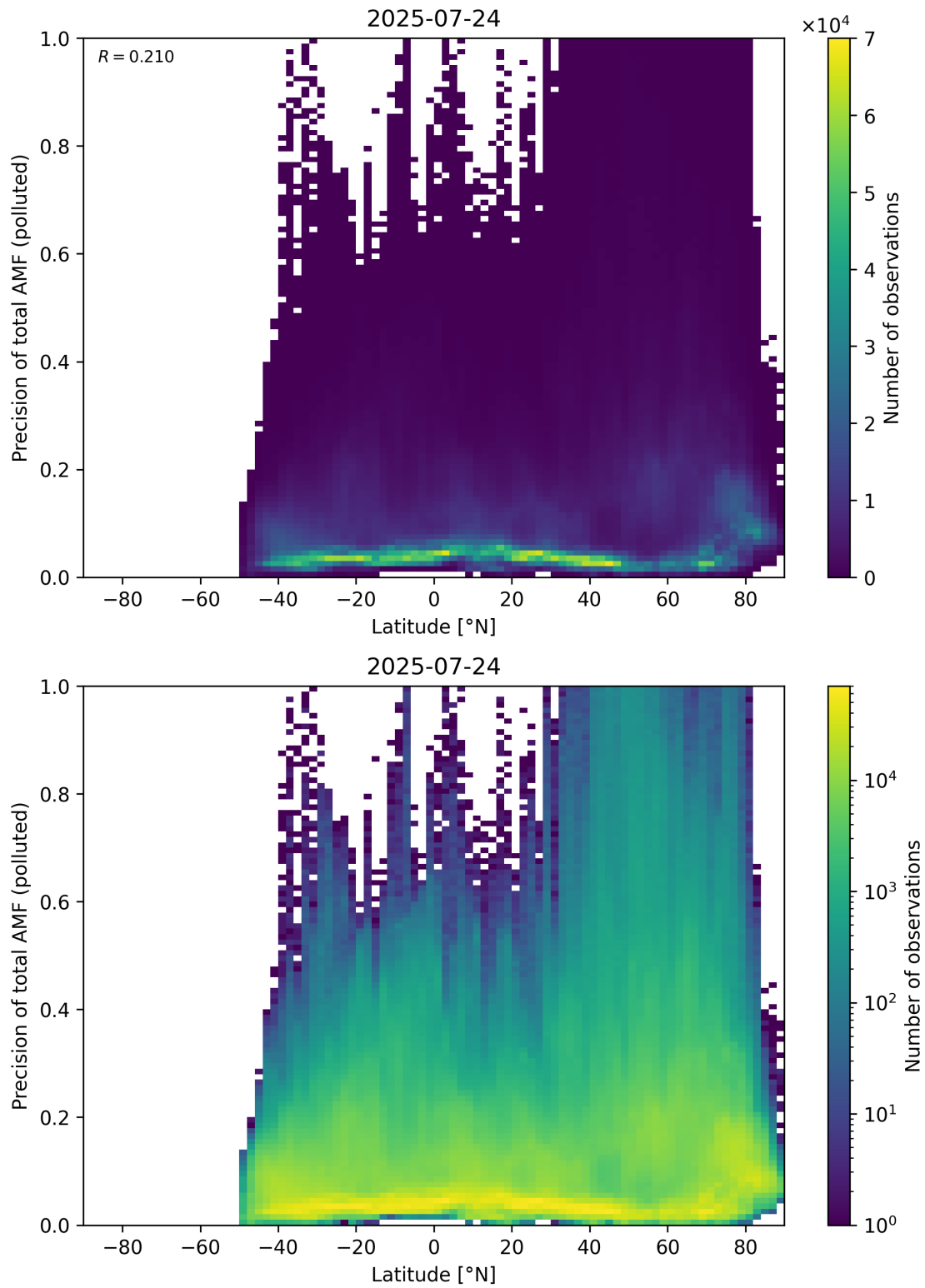
Figure 168: Scatter density plot of “Latitude” against “Precision of total AMF (polluted)” for 2025-07-24 to 2025-07-25.
