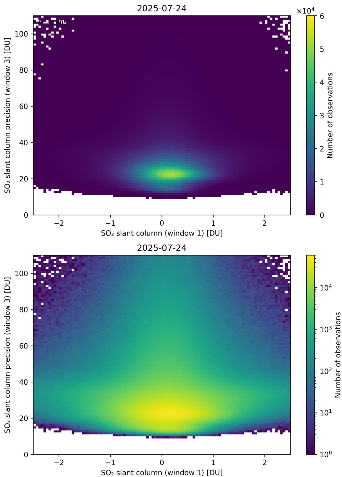
Figure 288: Scatter density plot of “SO 2 slant column (window 1)” against “SO 2 slant column precision (window 3)” for 2025-07-24 to 2025-07-25.
