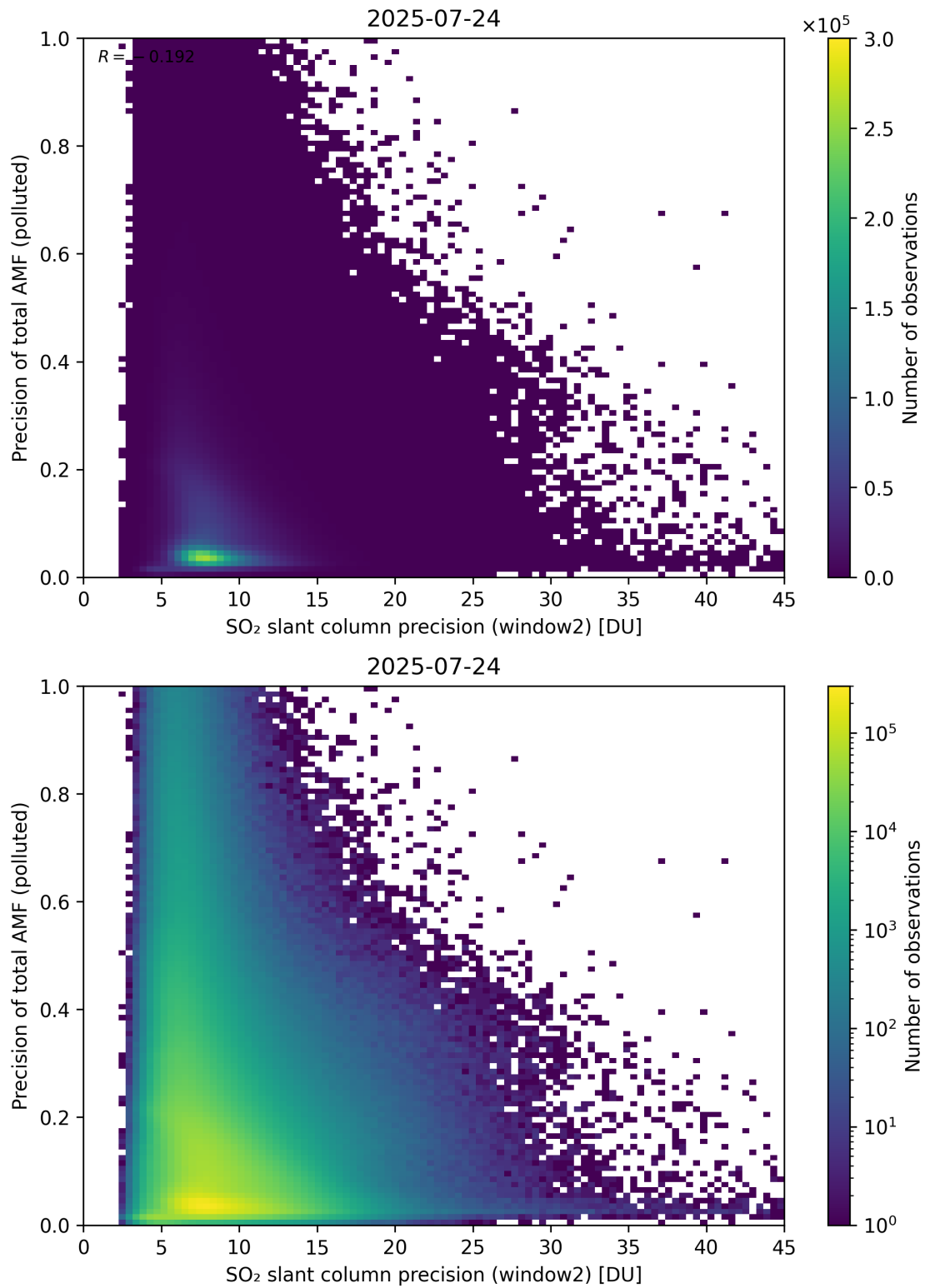
Figure 302: Scatter density plot of “SO 2 slant column precision (window2)” against “Precision of total AMF (polluted)” for 2025-07-24 to 2025-07-25.
