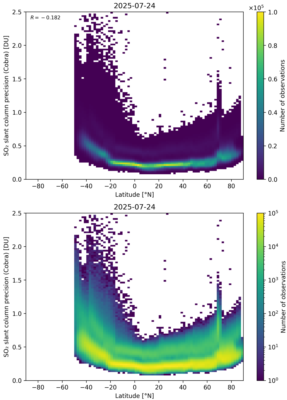
Figure 158: Scatter density plot of “Latitude” against “SO 2 slant column precision (Cobra)” for 2025-07-24 to 2025-07-25.
