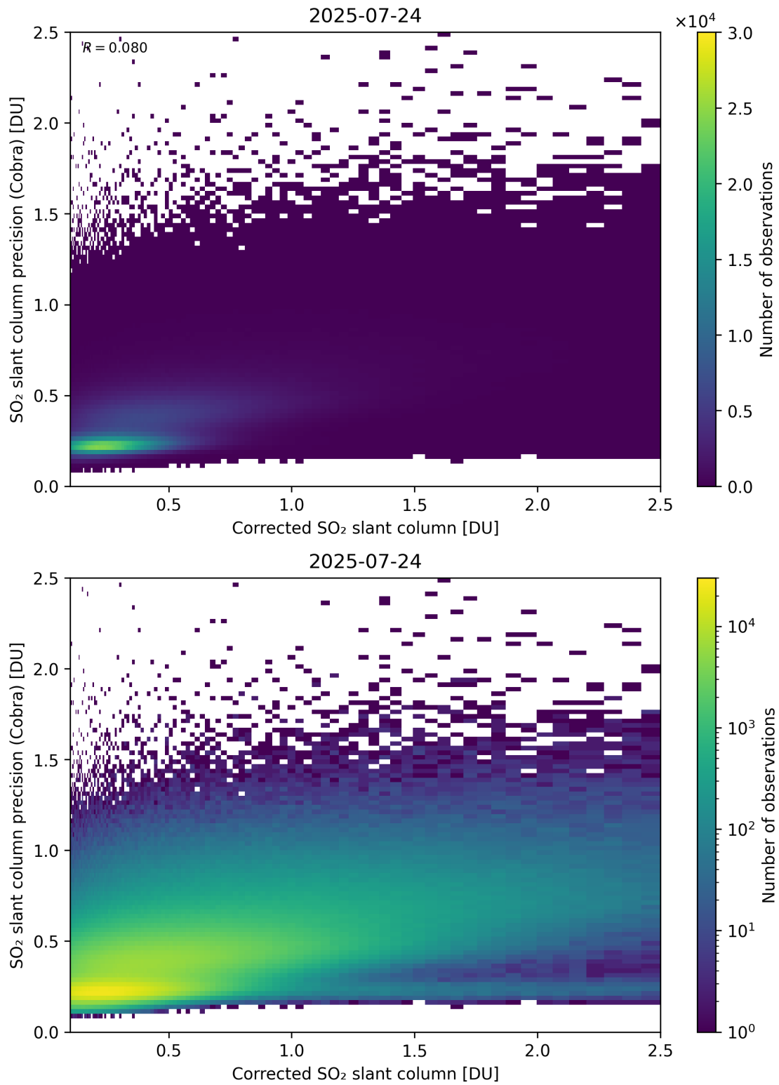
Figure 234: Scatter density plot of “Corrected SO 2 slant column” against “SO 2 slant column precision (Cobra)” for 2025-07-24 to 2025-07-25.
