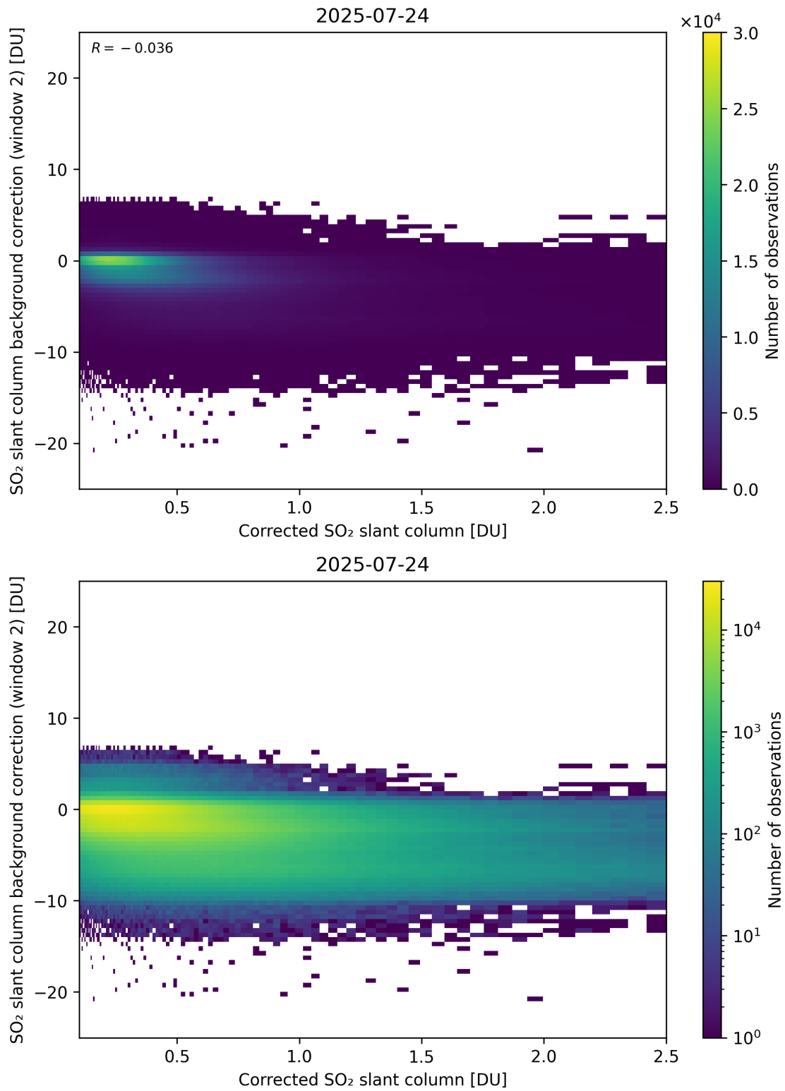
Figure 227: Scatter density plot of “Corrected SO 2 slant column” against “SO 2 slant column background correction (window 2)” for 2025-07-24 to 2025-07-25.
