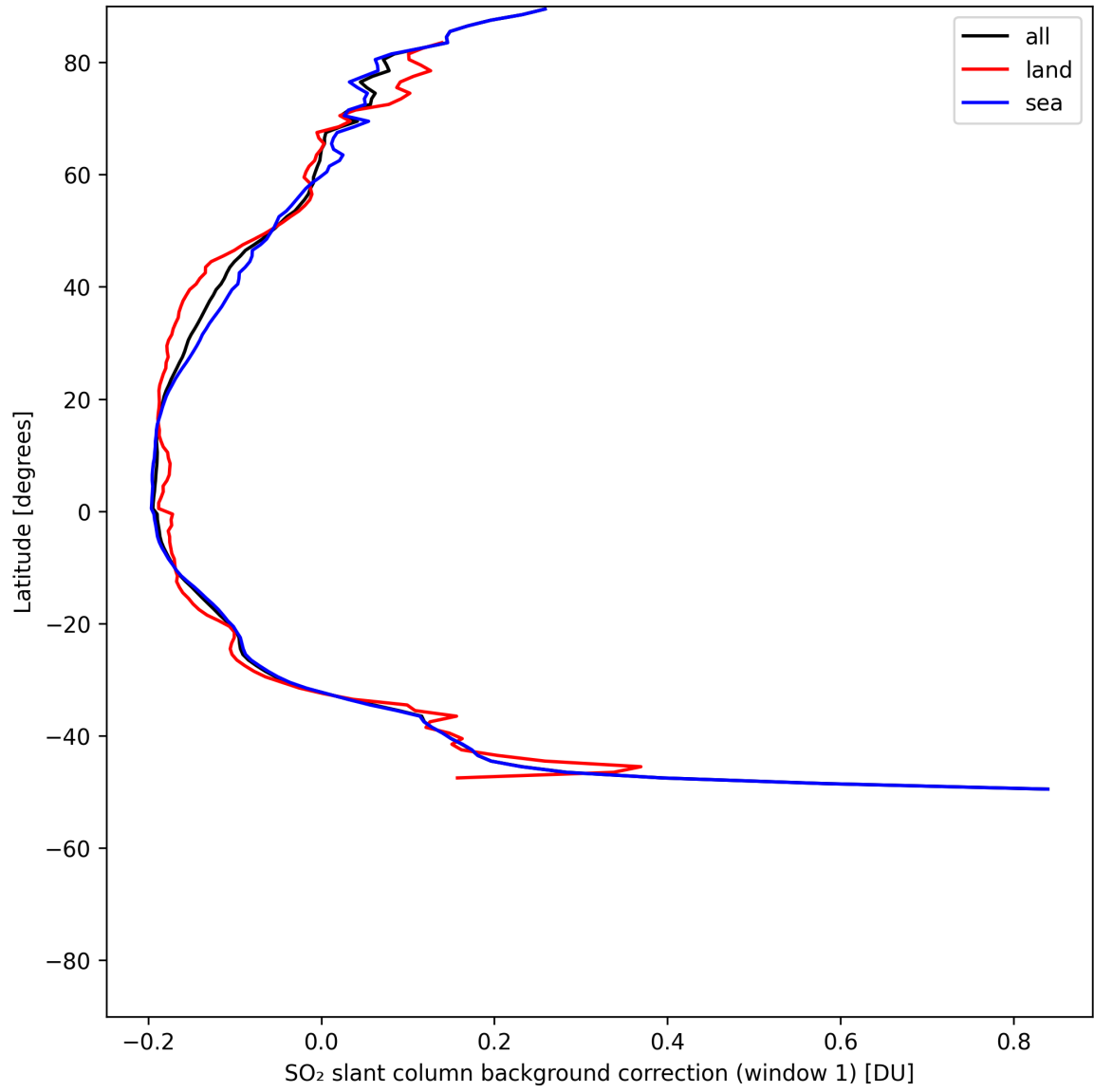
Figure 40: Zonal average of “SO 2 slant column background correction (window 1)” for 2025-07-24 to 2025-07-25.
