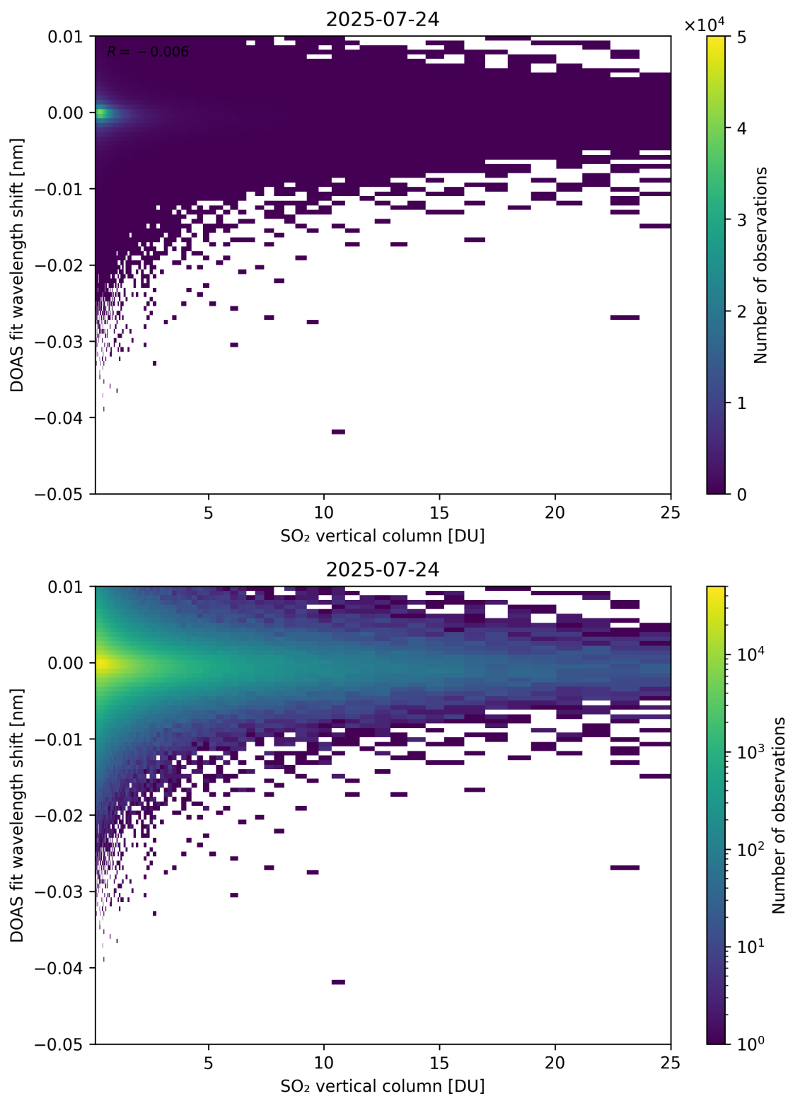
Figure 326: Scatter density plot of “SO 2 vertical column” against “DOAS fit wavelength shift” for 2025-07-24 to 2025-07-25.
