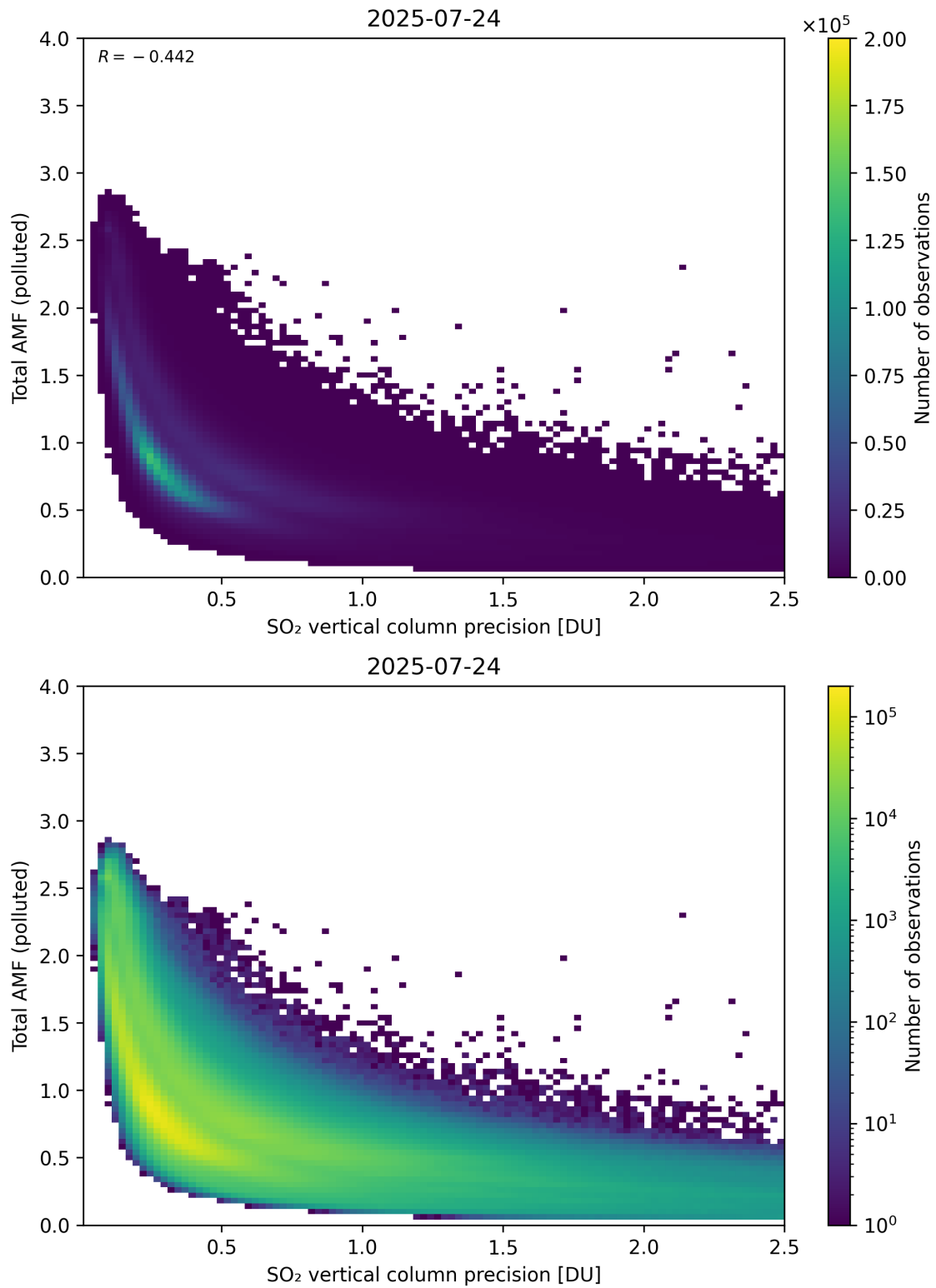
Figure 346: Scatter density plot of “SO 2 vertical column precision” against “Total AMF (polluted)” for 2025-07-24 to 2025-07-25.
