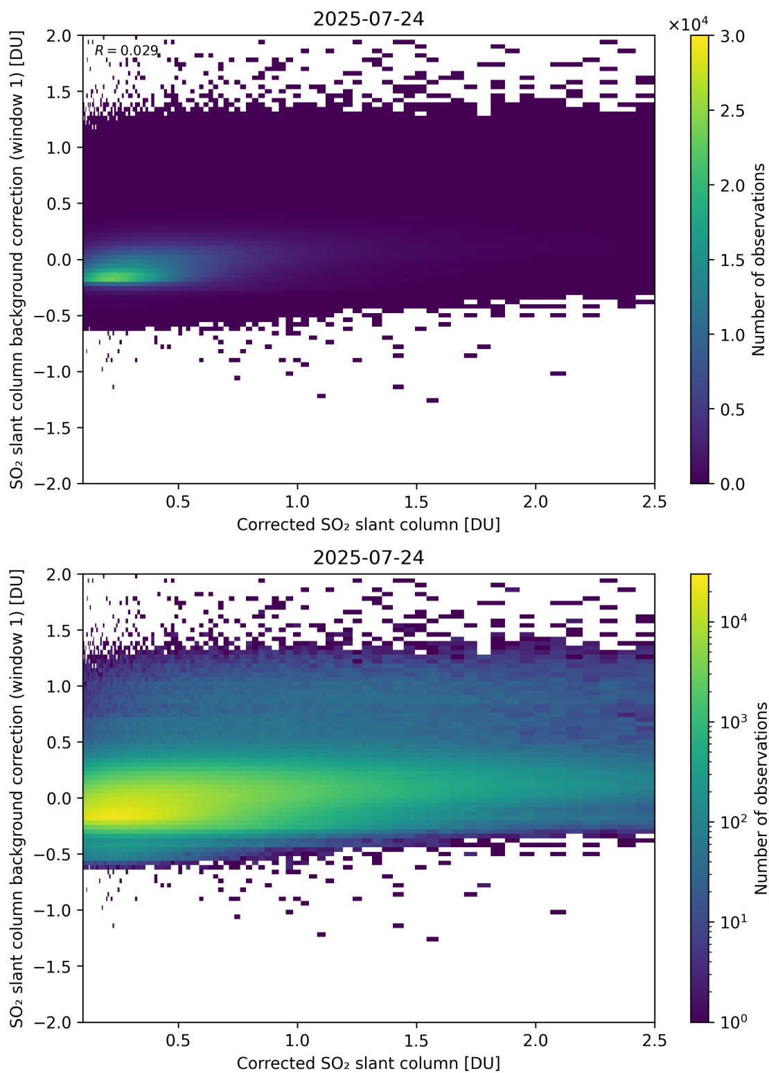
Figure 226: Scatter density plot of “Corrected SO 2 slant column” against “SO 2 slant column background correction (window 1)” for 2025-07-24 to 2025-07-25.
