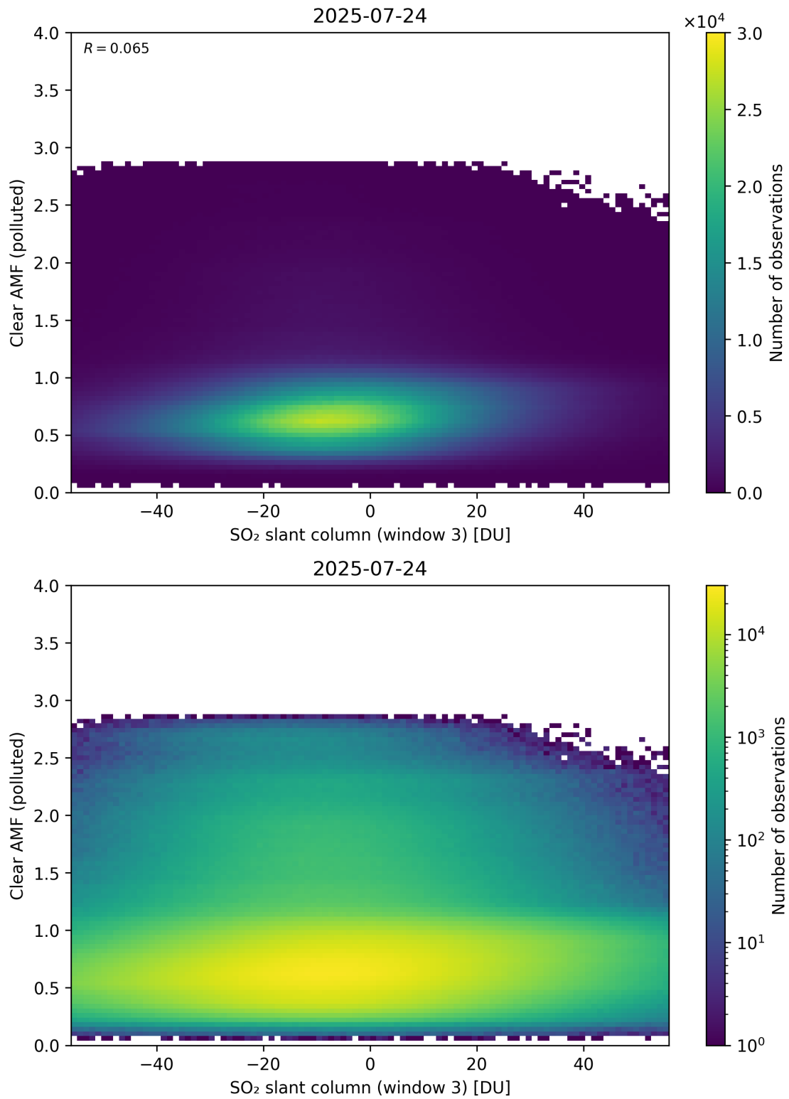
Figure 315: Scatter density plot of “SO 2 slant column (window 3)” against “Clear AMF (polluted)” for 2025-07-24 to 2025-07-25.
