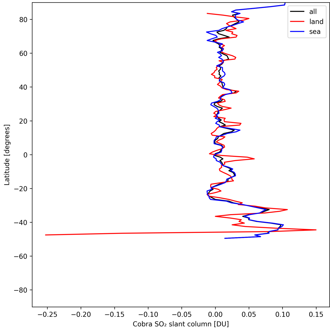
Figure 35: Zonal average of “Cobra SO 2 slant column” for 2025-07-24 to 2025-07-25.
