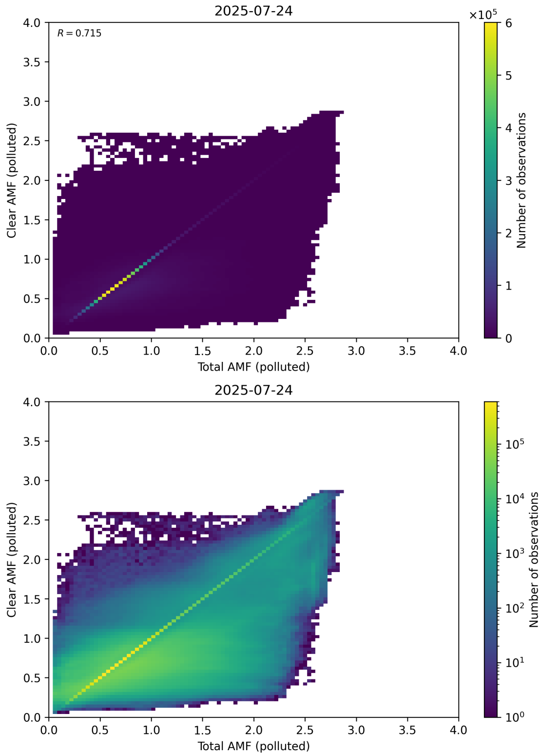
Figure 321: Scatter density plot of “Total AMF (polluted)” against “Clear AMF (polluted)” for 2025-07-24 to 2025-07-25.
