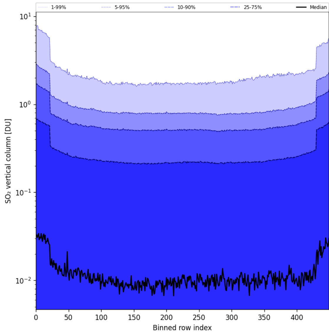
Figure 84: Along track statistics of “SO 2 vertical column” for 2025-07-24 to 2025-07-25
