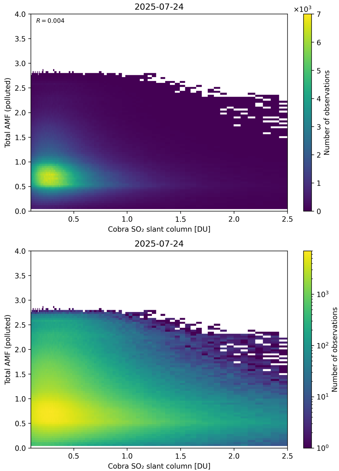
Figure 224: Scatter density plot of “Cobra SO 2 slant column” against “Total AMF (polluted)” for 2025-07-24 to 2025-07-25.
