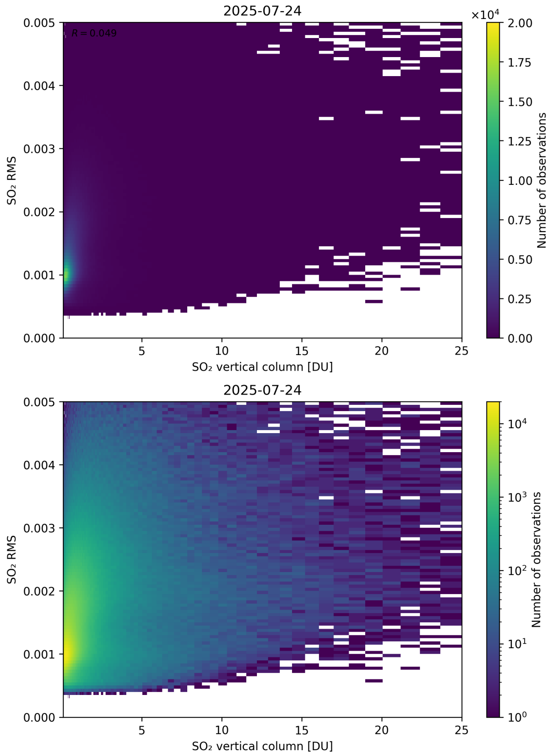
Figure 328: Scatter density plot of “SO 2 vertical column” against “SO 2 RMS” for 2025-07-24 to 2025-07-25.
