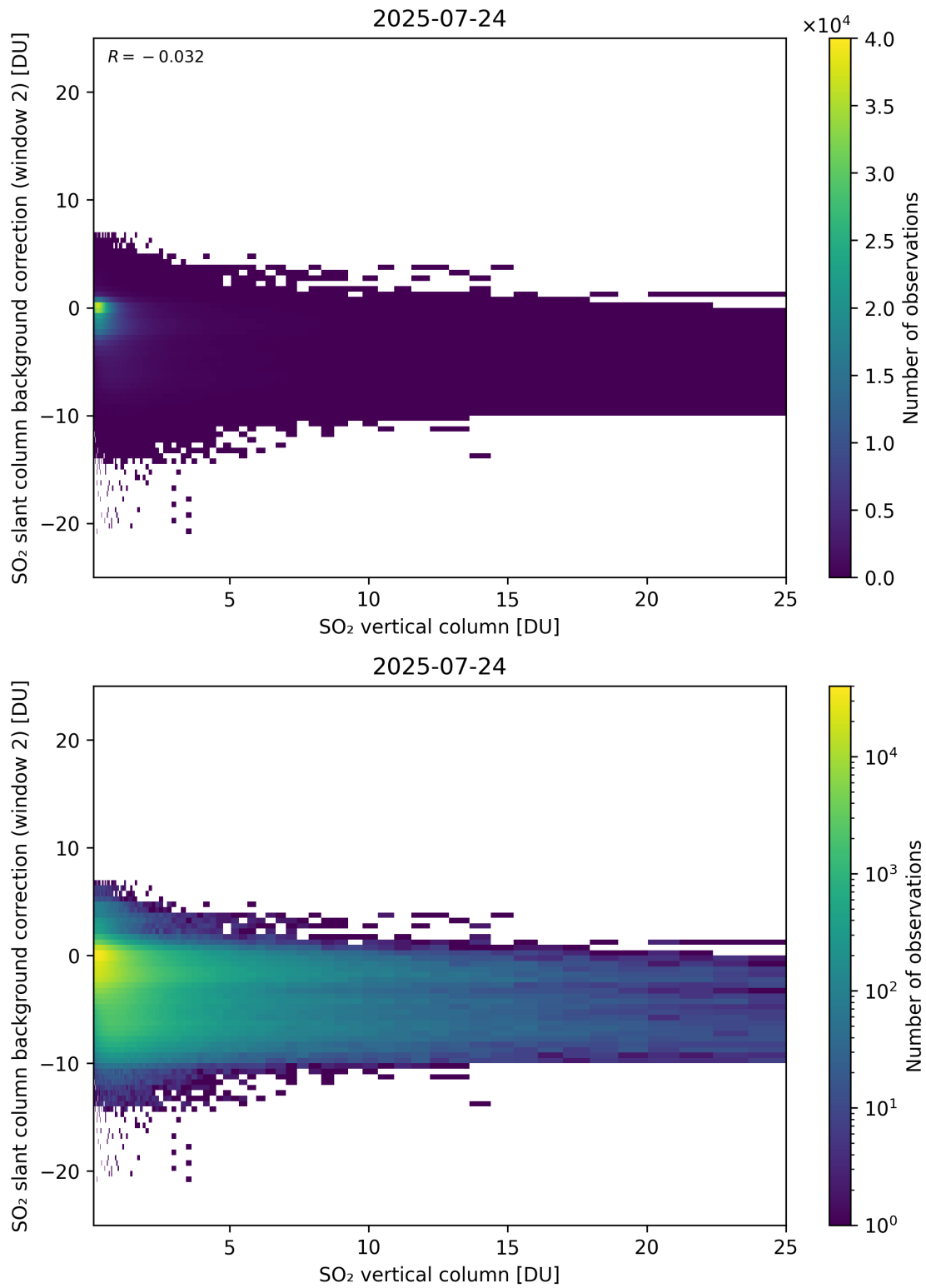
Figure 324: Scatter density plot of “SO 2 vertical column” against “SO 2 slant column background correction (window 2)” for 2025-07-24 to 2025-07-25.
