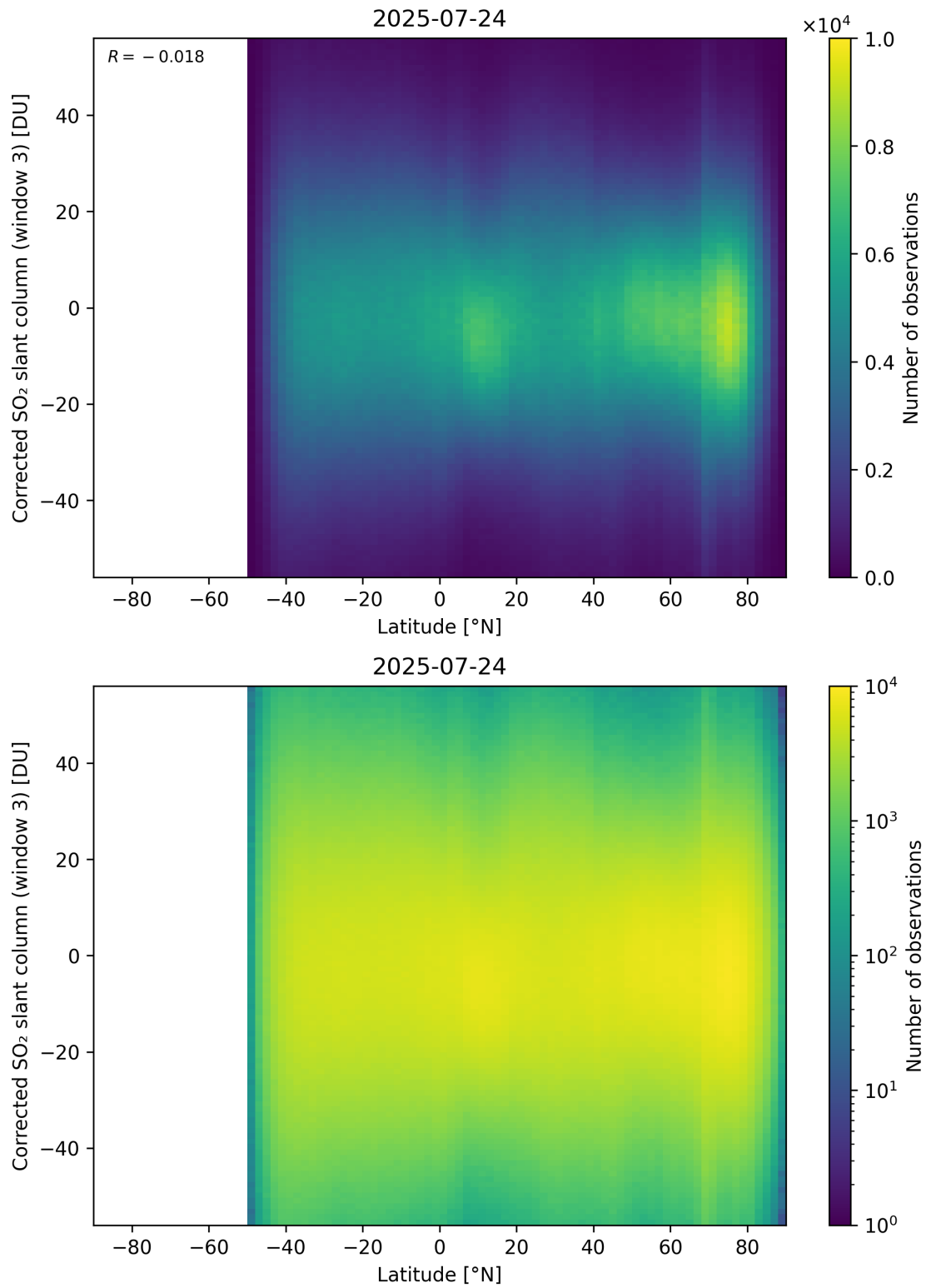
Figure 161: Scatter density plot of “Latitude” against “Corrected SO 2 slant column (window 3)” for 2025-07-24 to 2025-07-25.
