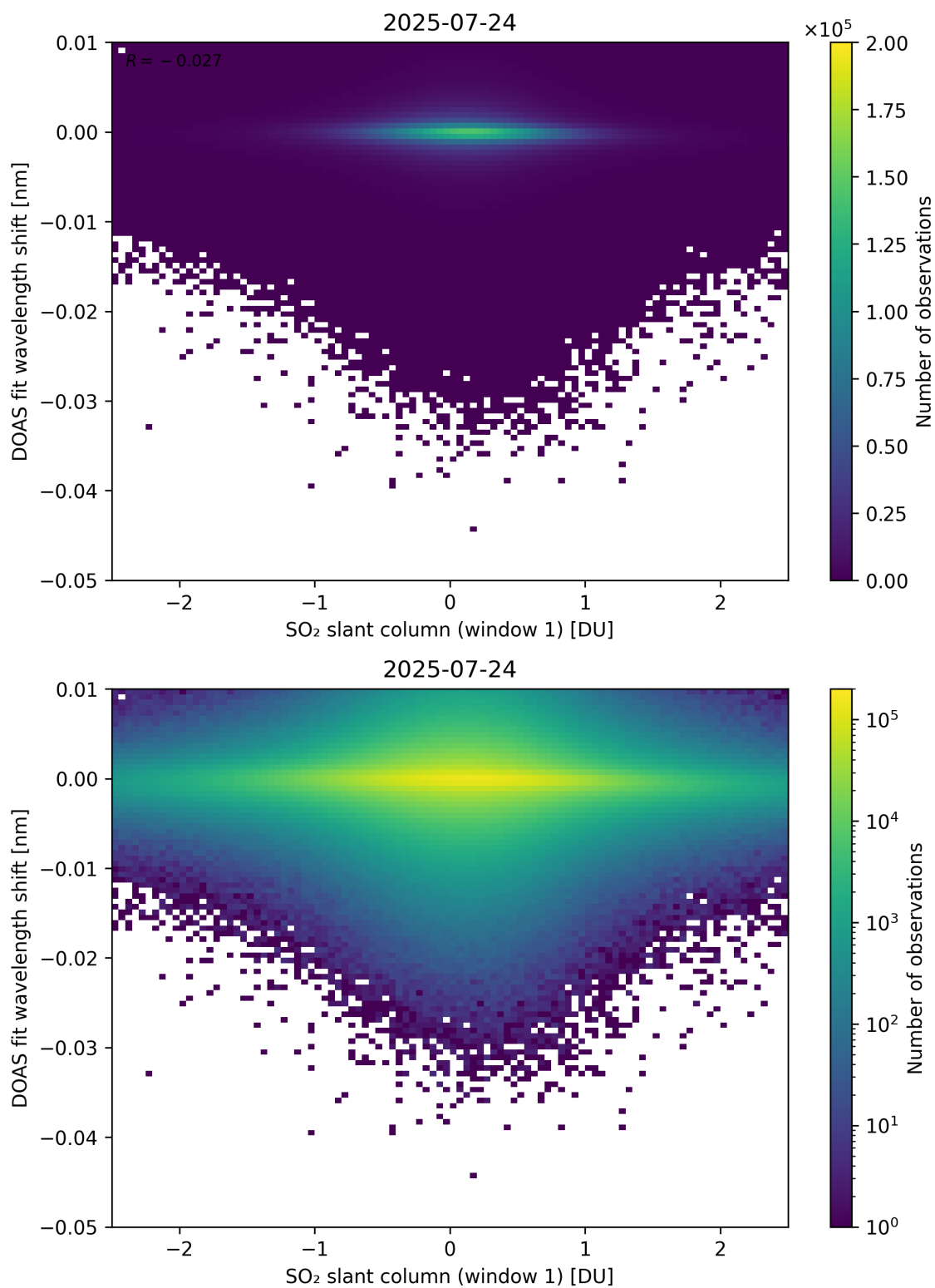
Figure 265: Scatter density plot of “SO 2 slant column (window 1)” against “DOAS fit wavelength shift” for 2025-07-24 to 2025-07-25.
