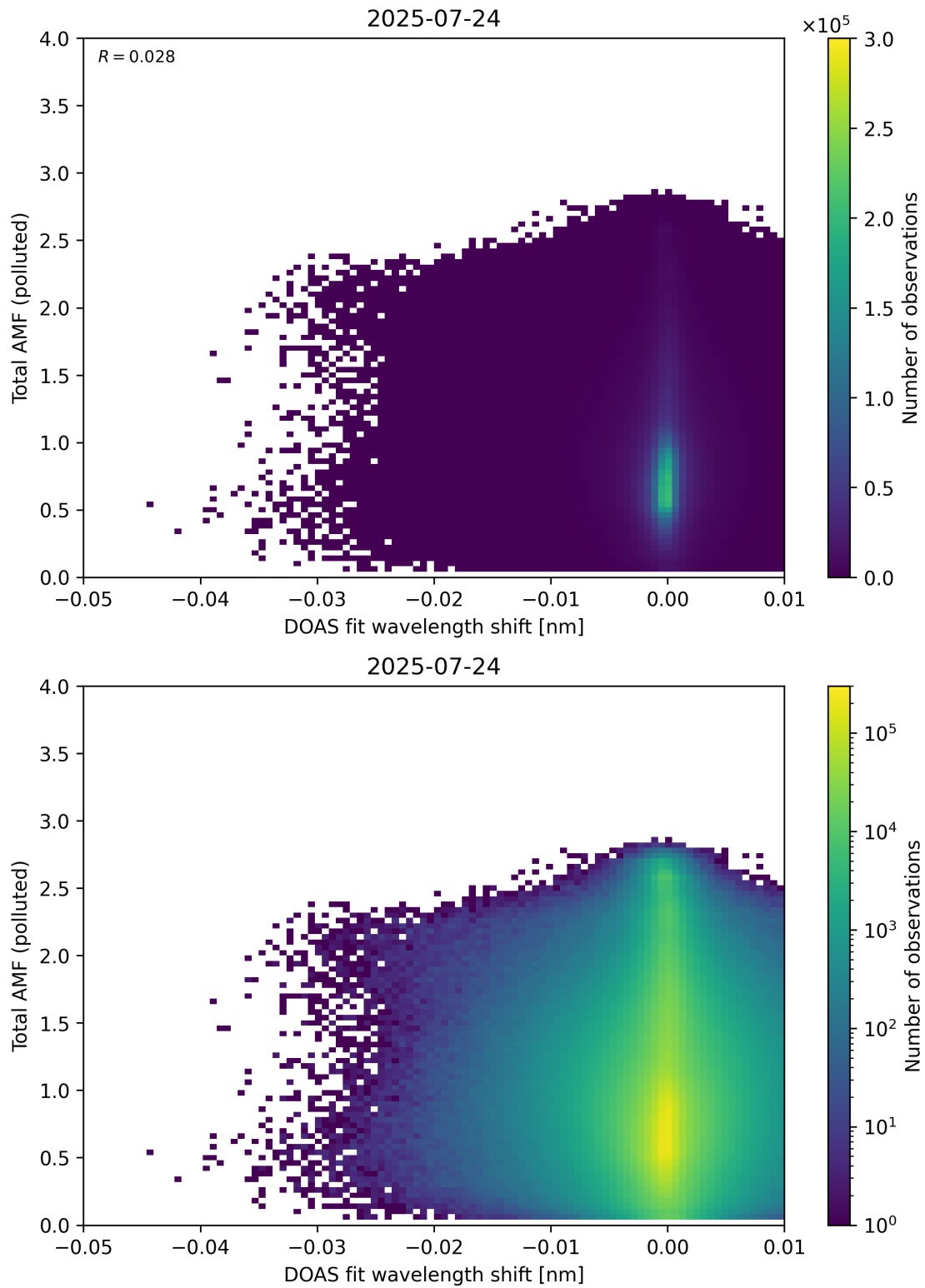
Figure 141: Scatter density plot of “DOAS fit wavelength shift” against “Total AMF (polluted)” for 2025-07-24 to 2025-07-25.
