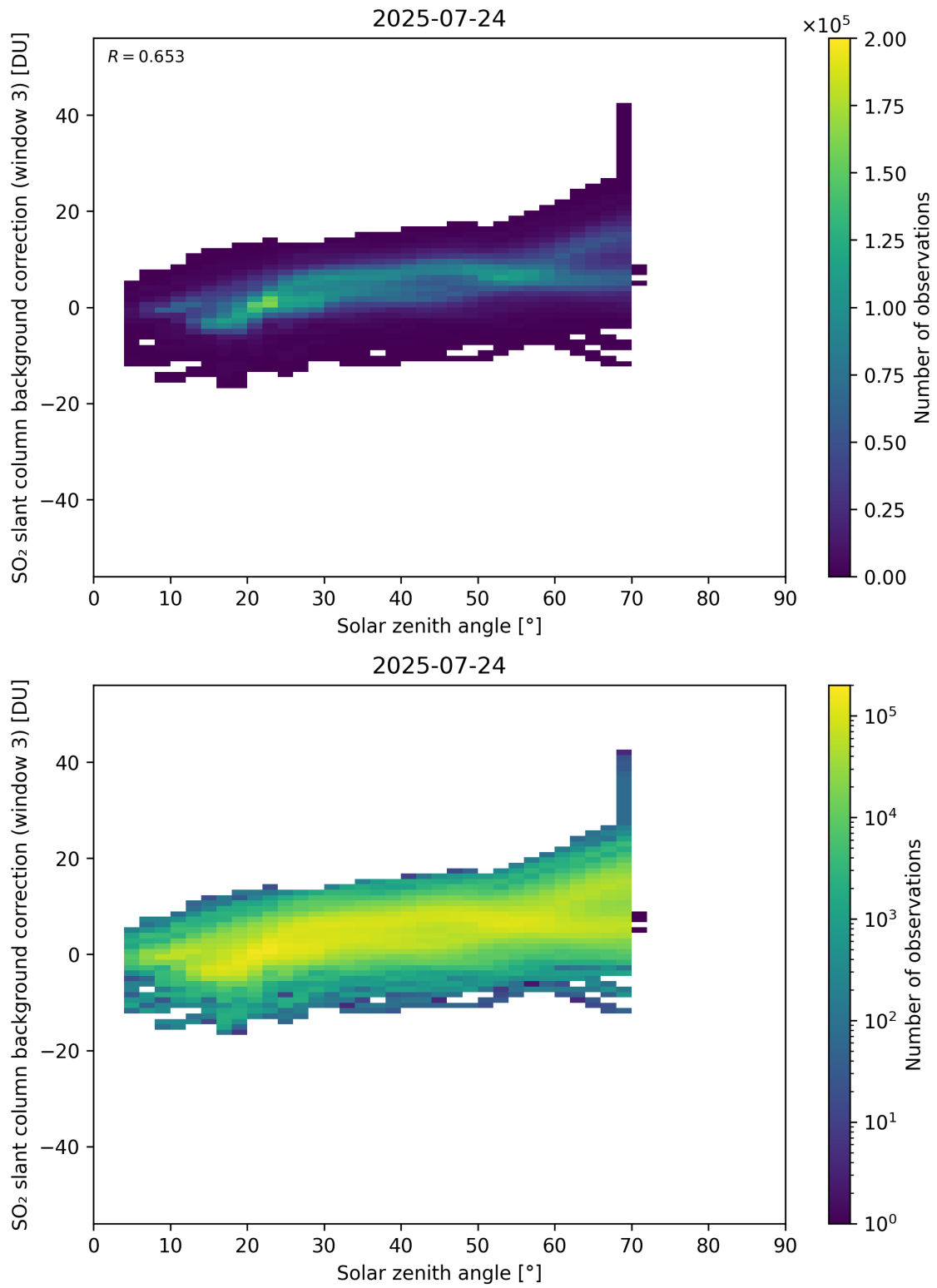
Figure 173: Scatter density plot of “Solar zenith angle” against “SO 2 slant column background correction (window 3)” for 2025-07-24 to 2025-07-25.
