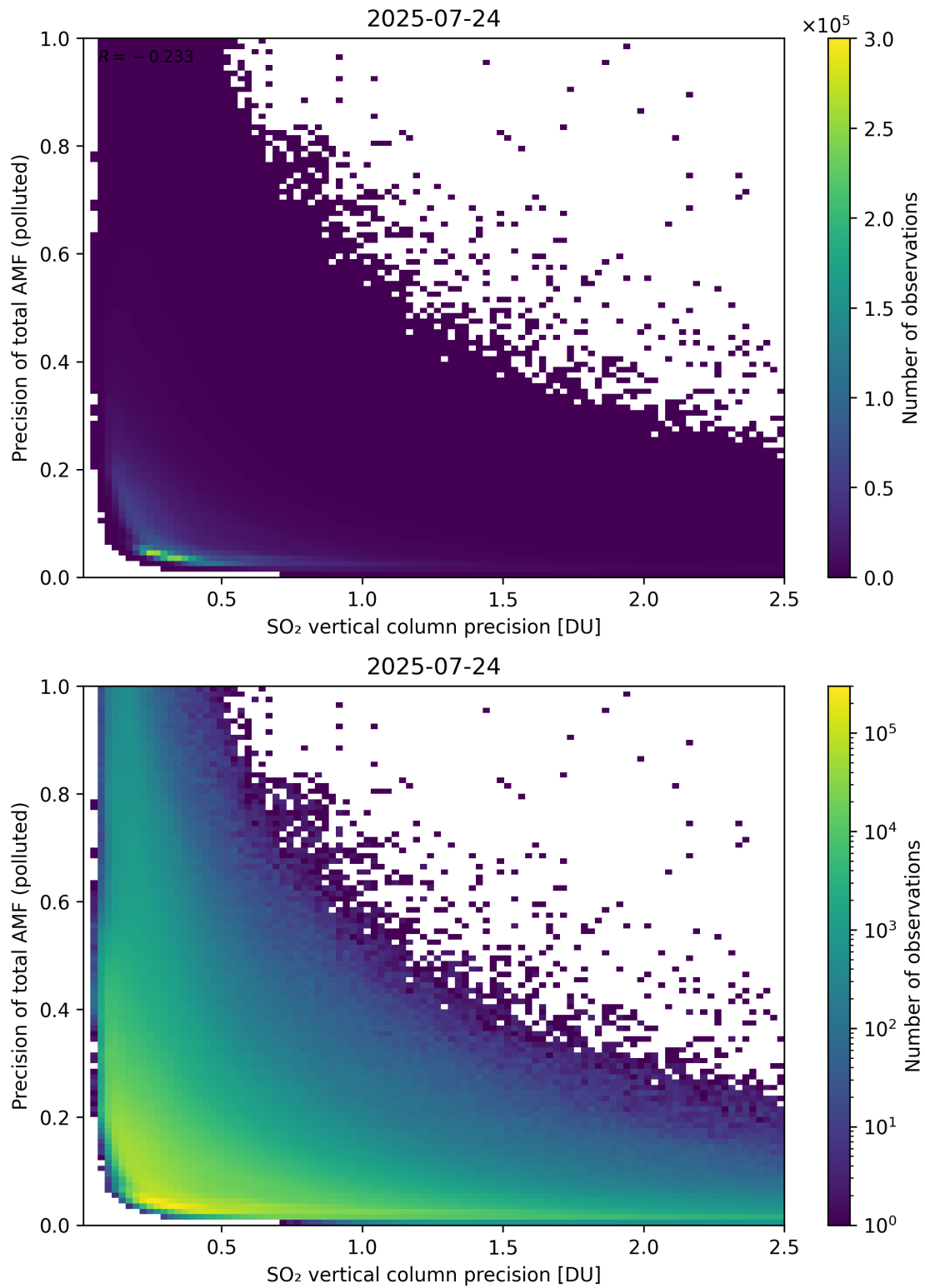
Figure 347: Scatter density plot of “SO 2 vertical column precision” against “Precision of total AMF (polluted)” for 2025-07-24 to 2025-07-25.
