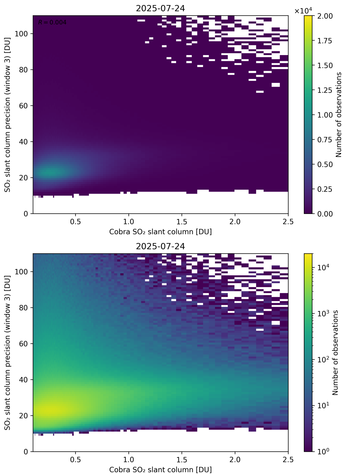
Figure 223: Scatter density plot of “Cobra SO 2 slant column” against “SO 2 slant column precision (window 3)” for 2025-07-24 to 2025-07-25.
