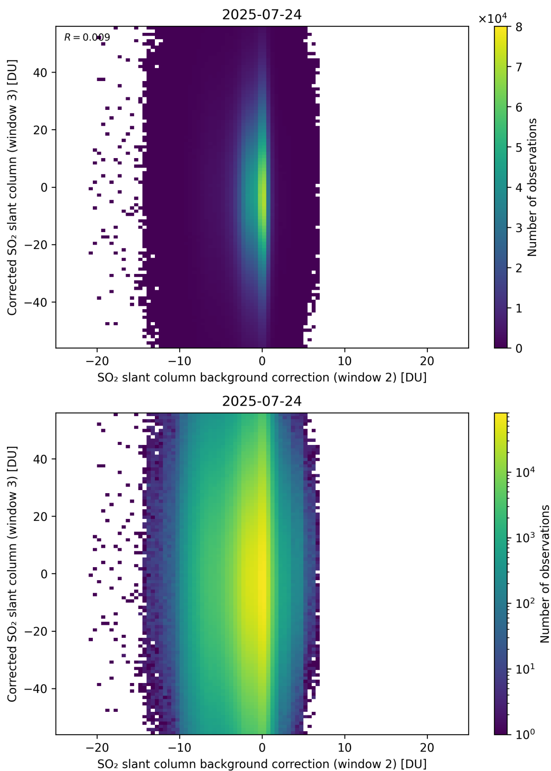
Figure 127: Scatter density plot of “SO 2 slant column background correction (window 2)” against “Corrected SO 2 slant column (window 3)” for 2025-07-24 to 2025-07-25.
