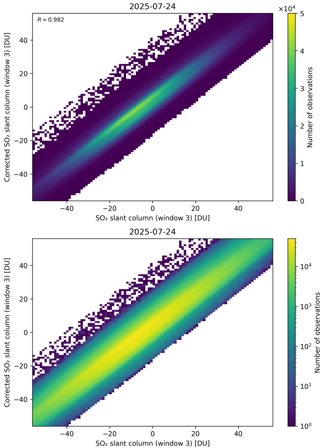
Figure 316: Scatter density plot of “SO 2 slant column (window 3)” against “Corrected SO 2 slant column (window 3)” for 2025-07-24 to 2025-07-25.
