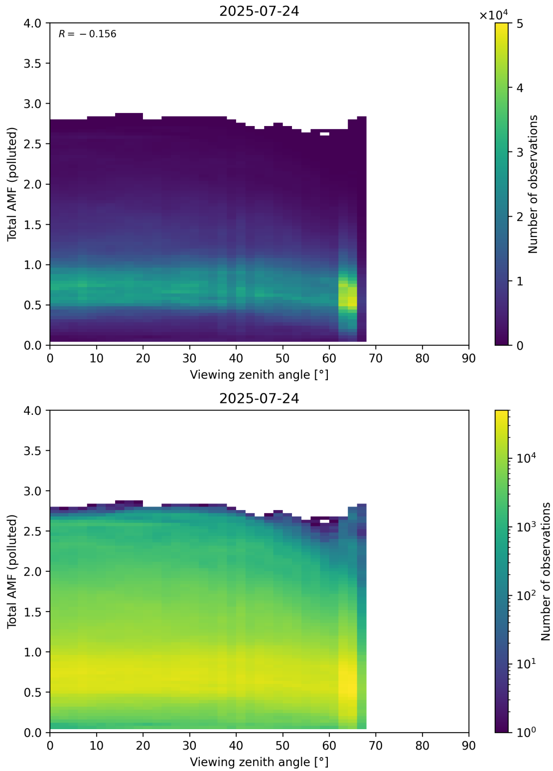
Figure 381: Scatter density plot of “Viewing zenith angle” against “Total AMF (polluted)” for 2025-07-24 to 2025-07-25.
