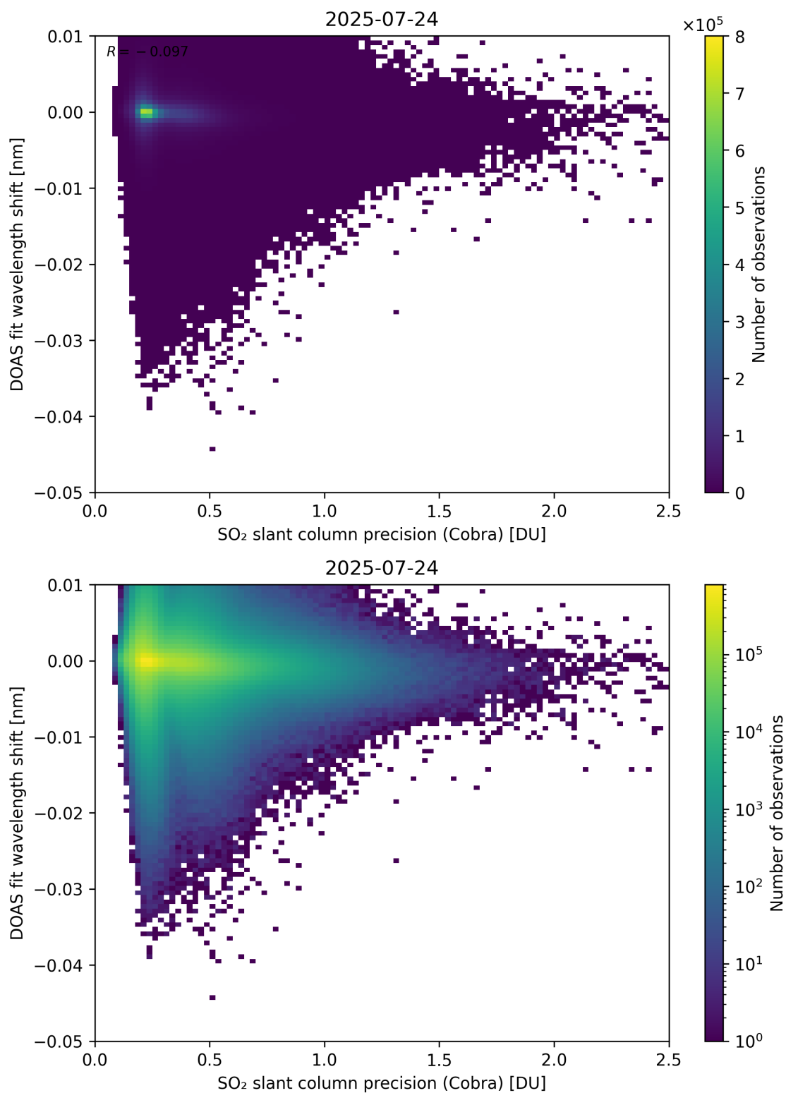
Figure 202: Scatter density plot of “SO 2 slant column precision (Cobra)” against “DOAS fit wavelength shift” for 2025-07-24 to 2025-07-25.
