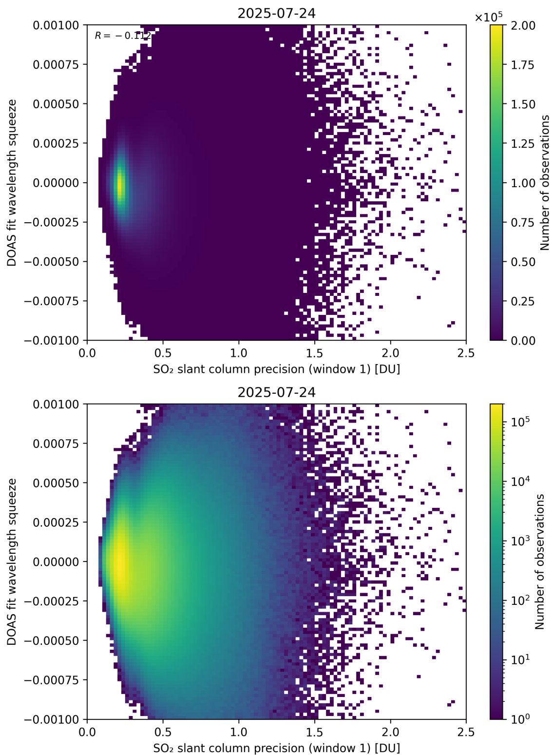
Figure 272: Scatter density plot of “SO 2 slant column precision (window 1)” against “DOAS fit wavelength squeeze” for 2025-07-24 to 2025-07-25.
