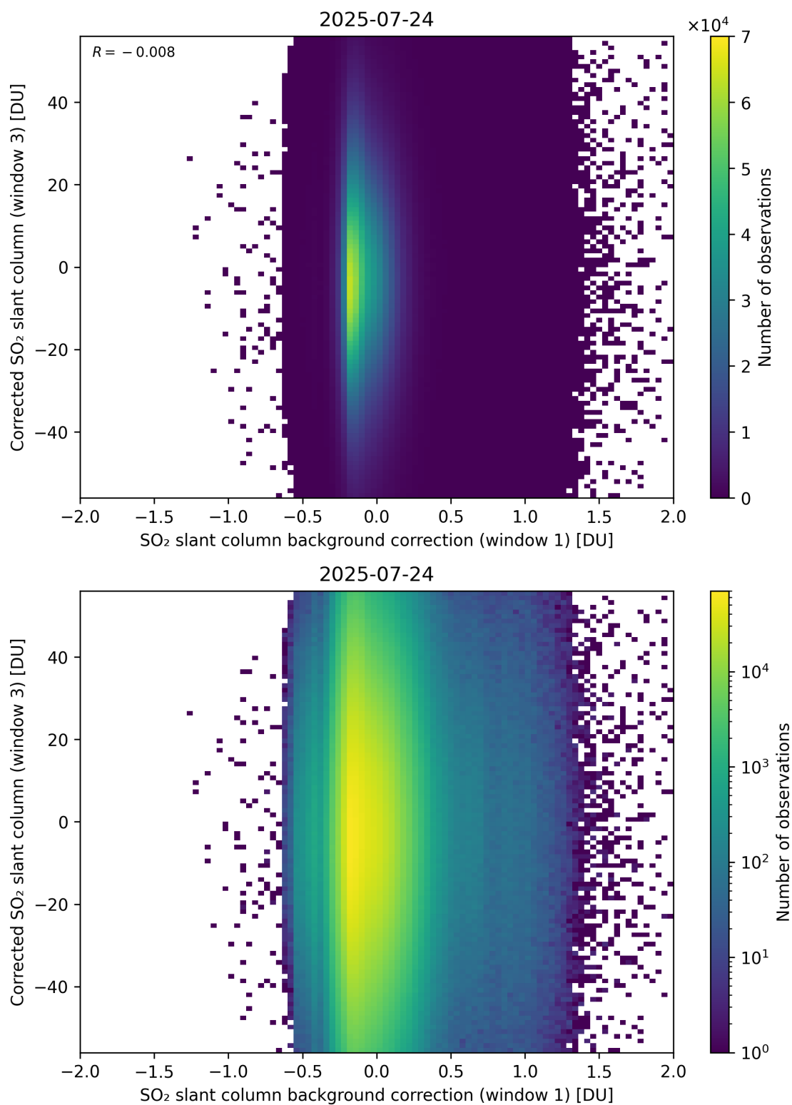
Figure 116: Scatter density plot of “SO 2 slant column background correction (window 1)” against “Corrected SO 2 slant column (window 3)” for 2025-07-24 to 2025-07-25.
