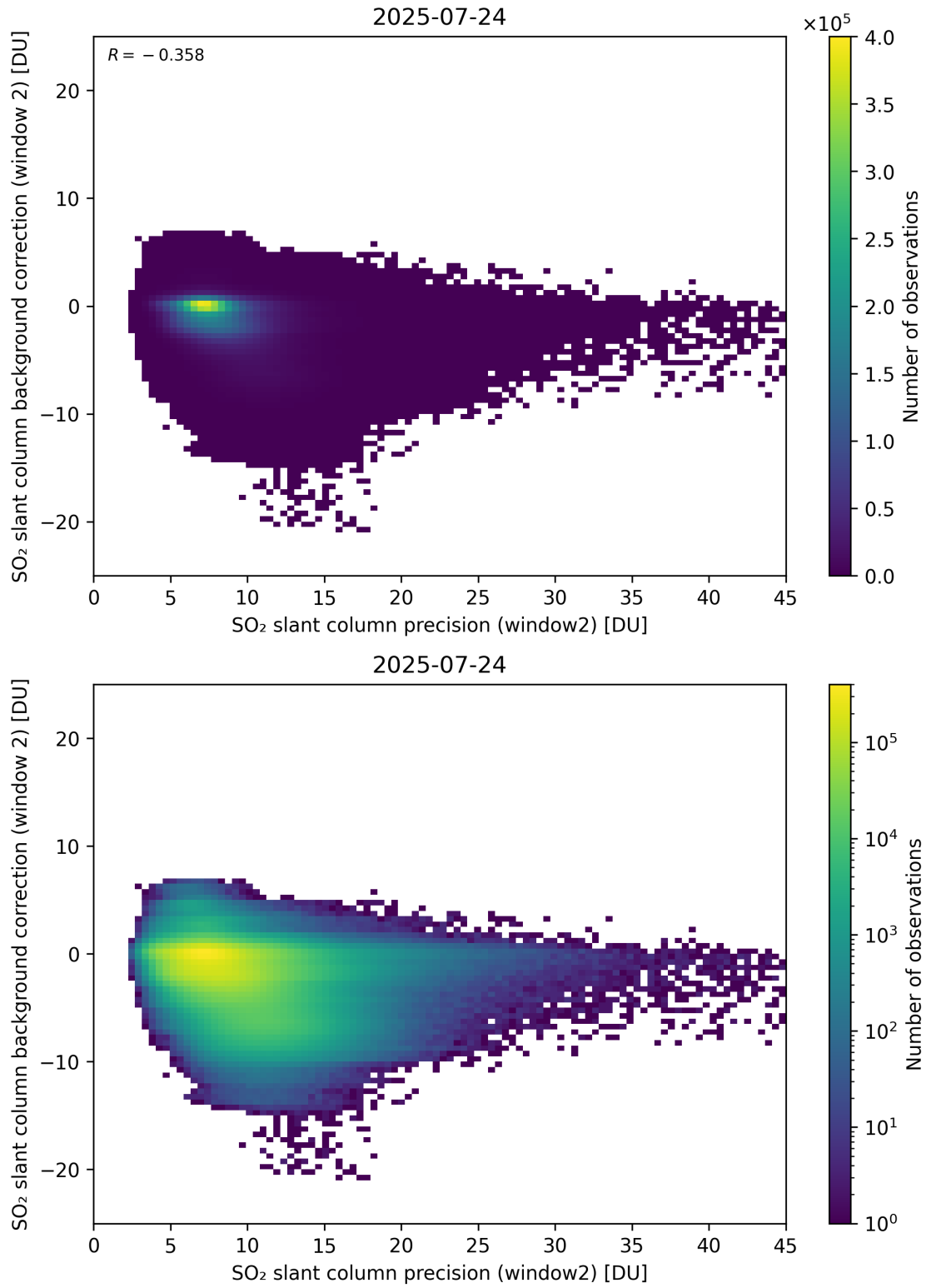
Figure 291: Scatter density plot of “SO 2 slant column precision (window2)” against “SO 2 slant column background correction (window 2)” for 2025-07-24 to 2025-07-25.
