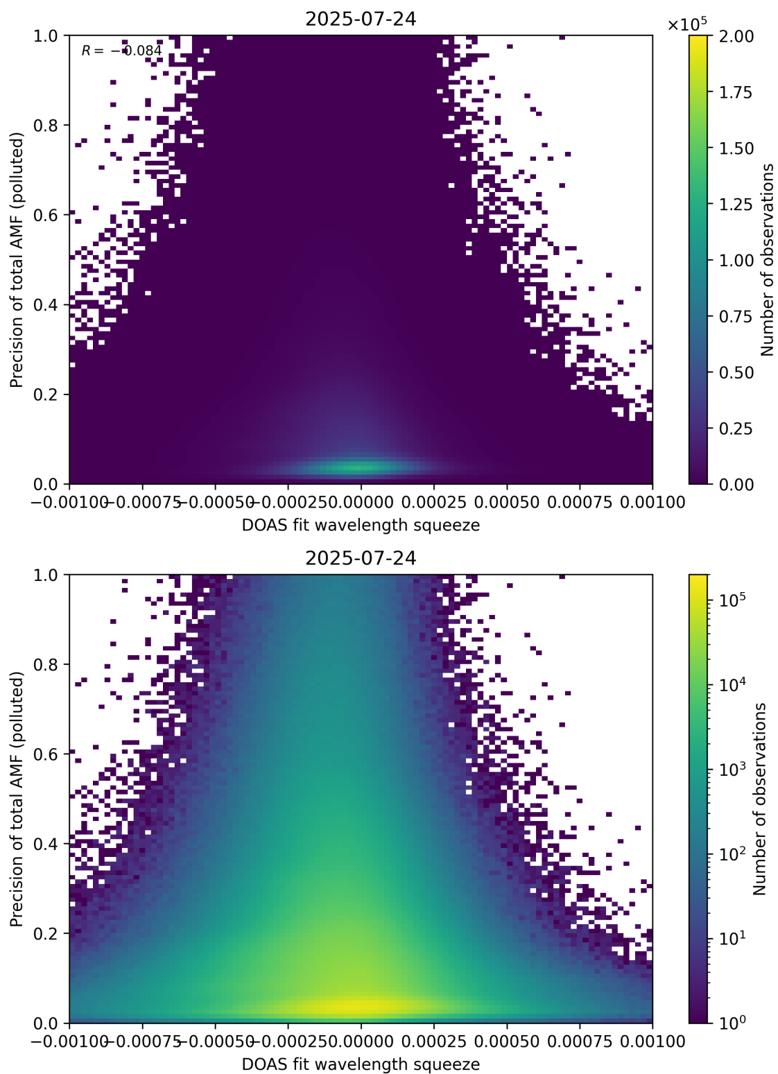
Figure 146: Scatter density plot of “DOAS fit wavelength squeeze” against “Precision of total AMF (polluted)” for 2025-07-24 to 2025-07-25.
