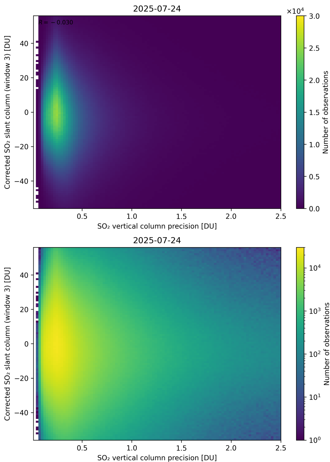
Figure 340: Scatter density plot of “SO 2 vertical column precision” against “Corrected SO 2 slant column (window 3)” for 2025-07-24 to 2025-07-25.
