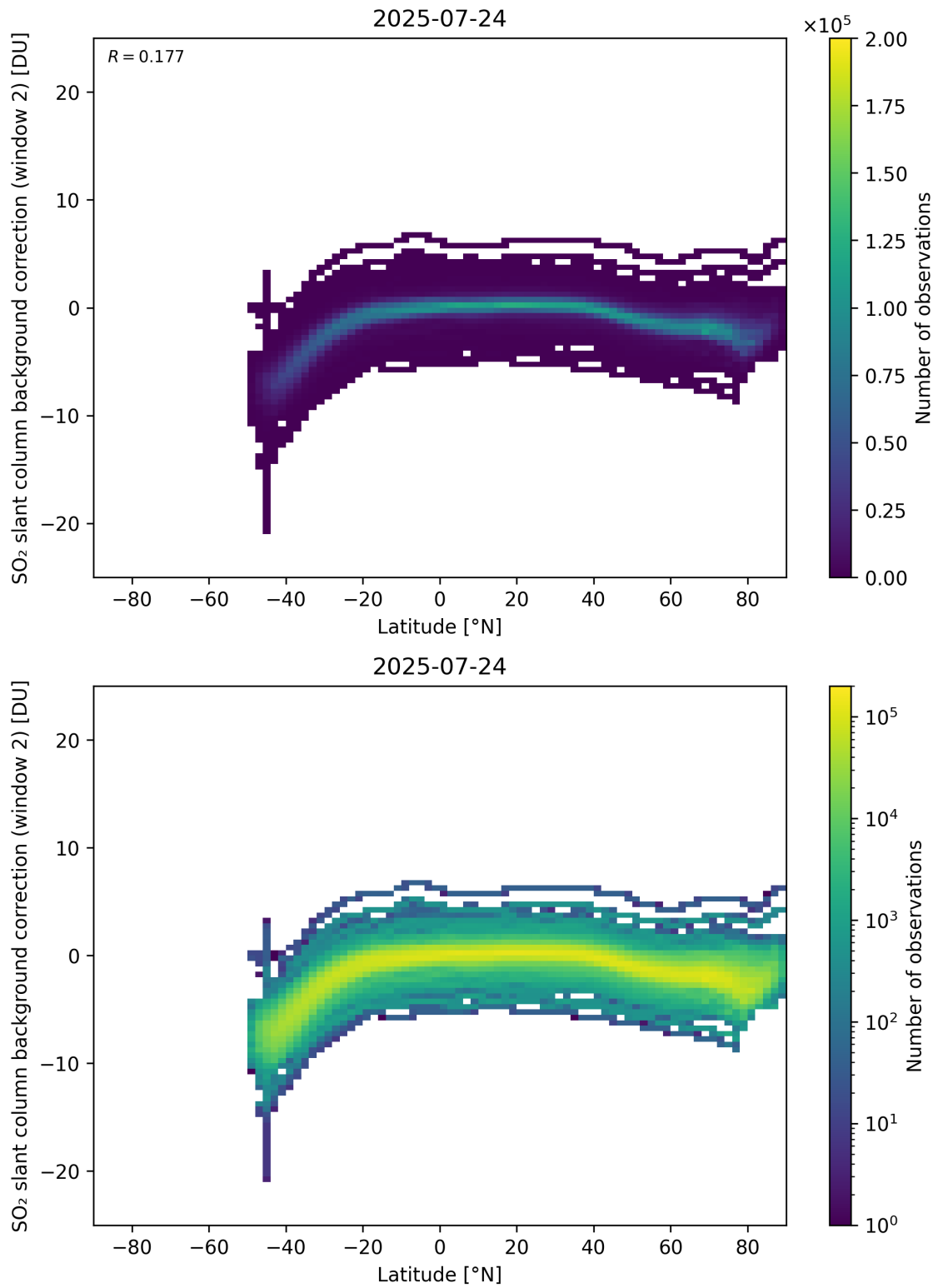
Figure 151: Scatter density plot of “Latitude” against “SO 2 slant column background correction (window 2)” for 2025-07-24 to 2025-07-25.
