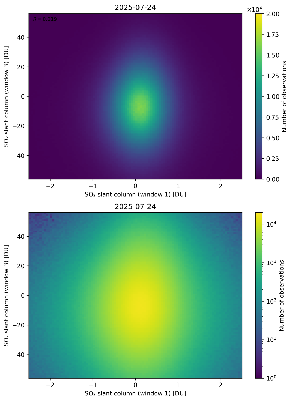
Figure 287: Scatter density plot of “SO 2 slant column (window 1)” against “SO 2 slant column (window 3)” for 2025-07-24 to 2025-07-25.
