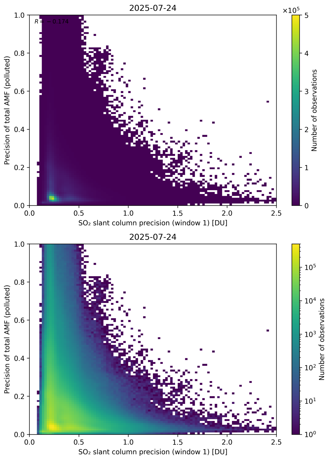
Figure 281: Scatter density plot of “SO 2 slant column precision (window 1)” against “Precision of total AMF (polluted)” for 2025-07-24 to 2025-07-25.
