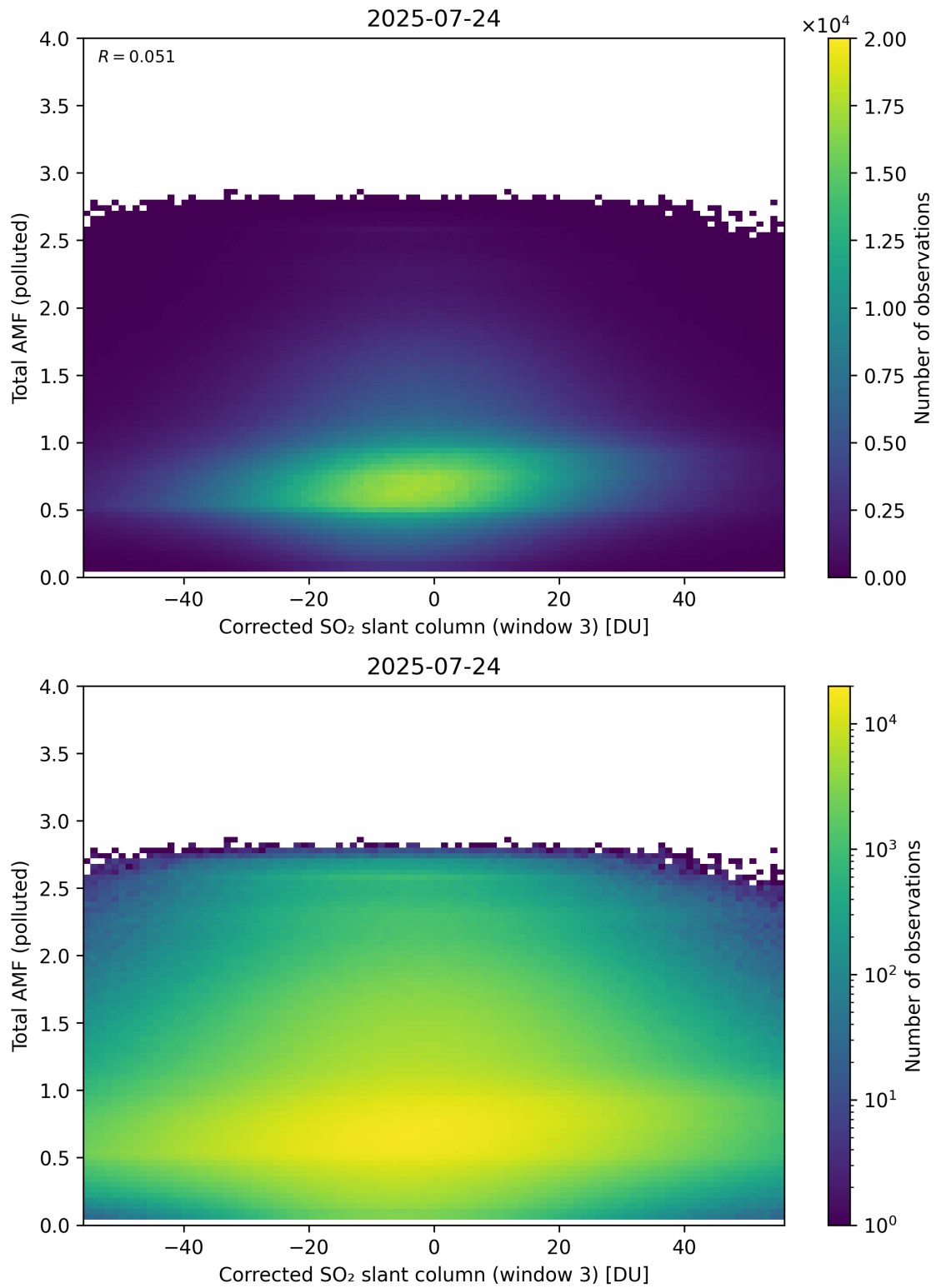
Figure 260: Scatter density plot of “Corrected SO 2 slant column (window 3)” against “Total AMF (polluted)” for 2025-07-24 to 2025-07-25.
