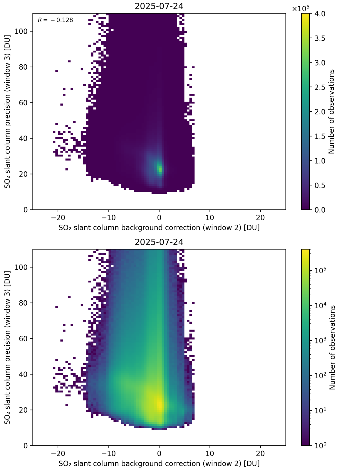
Figure 129: Scatter density plot of “SO 2 slant column background correction (window 2)” against “SO 2 slant column precision (window 3)” for 2025-07-24 to 2025-07-25.
