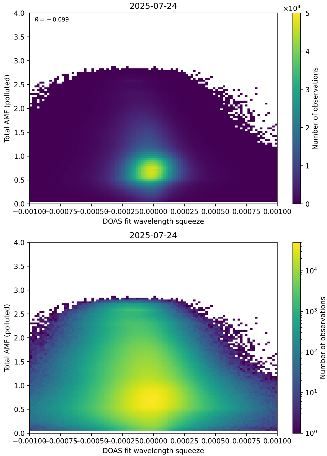
Figure 145: Scatter density plot of “DOAS fit wavelength squeeze” against “Total AMF (polluted)” for 2025-07-24 to 2025-07-25.
