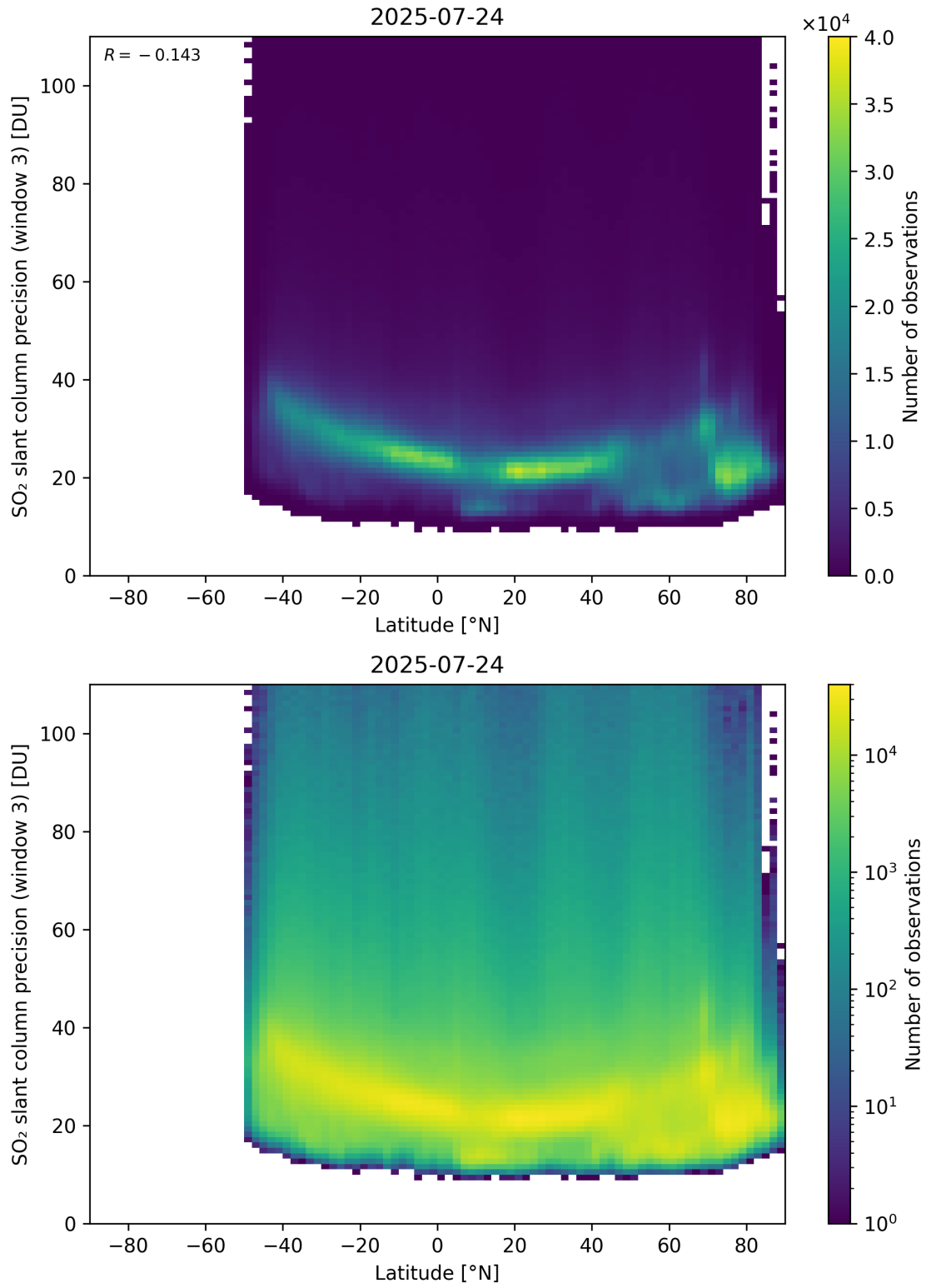
Figure 166: Scatter density plot of “Latitude” against “SO 2 slant column precision (window 3)” for 2025-07-24 to 2025-07-25.
