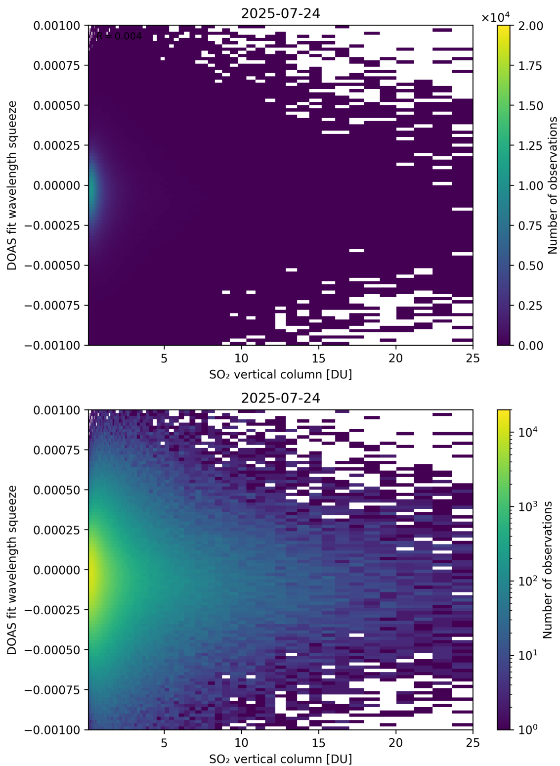
Figure 327: Scatter density plot of “SO 2 vertical column” against “DOAS fit wavelength squeeze” for 2025-07-24 to 2025-07-25.
