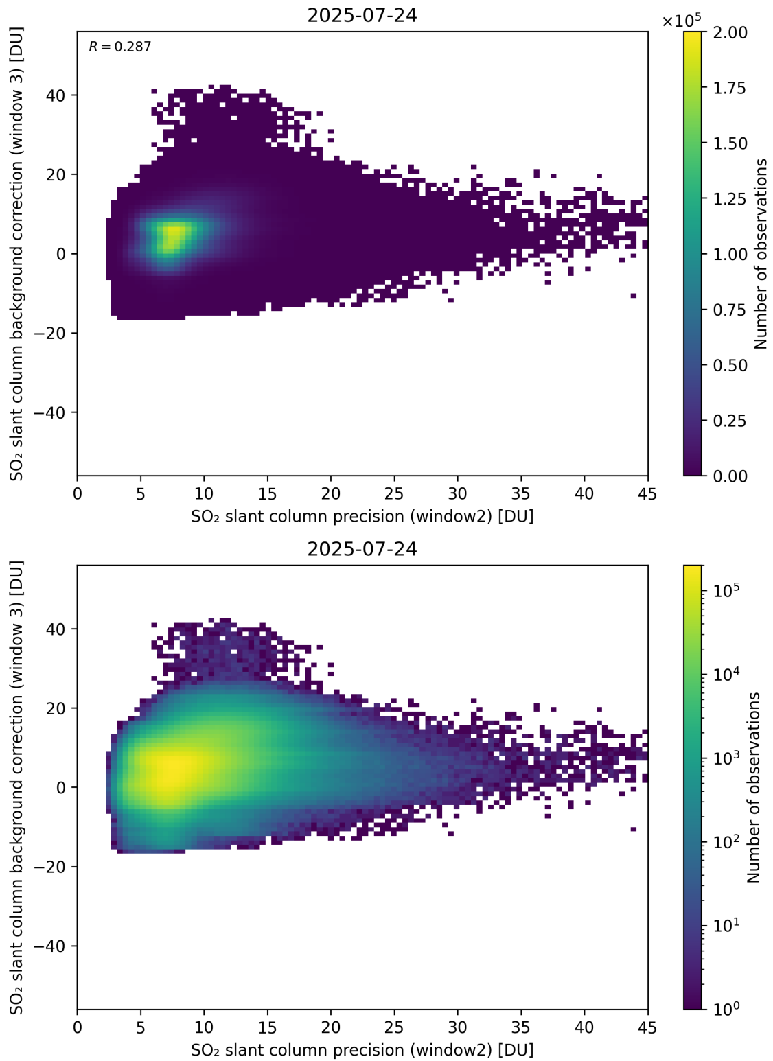
Figure 292: Scatter density plot of “SO 2 slant column precision (window2)” against “SO 2 slant column background correction (window 3)” for 2025-07-24 to 2025-07-25.
