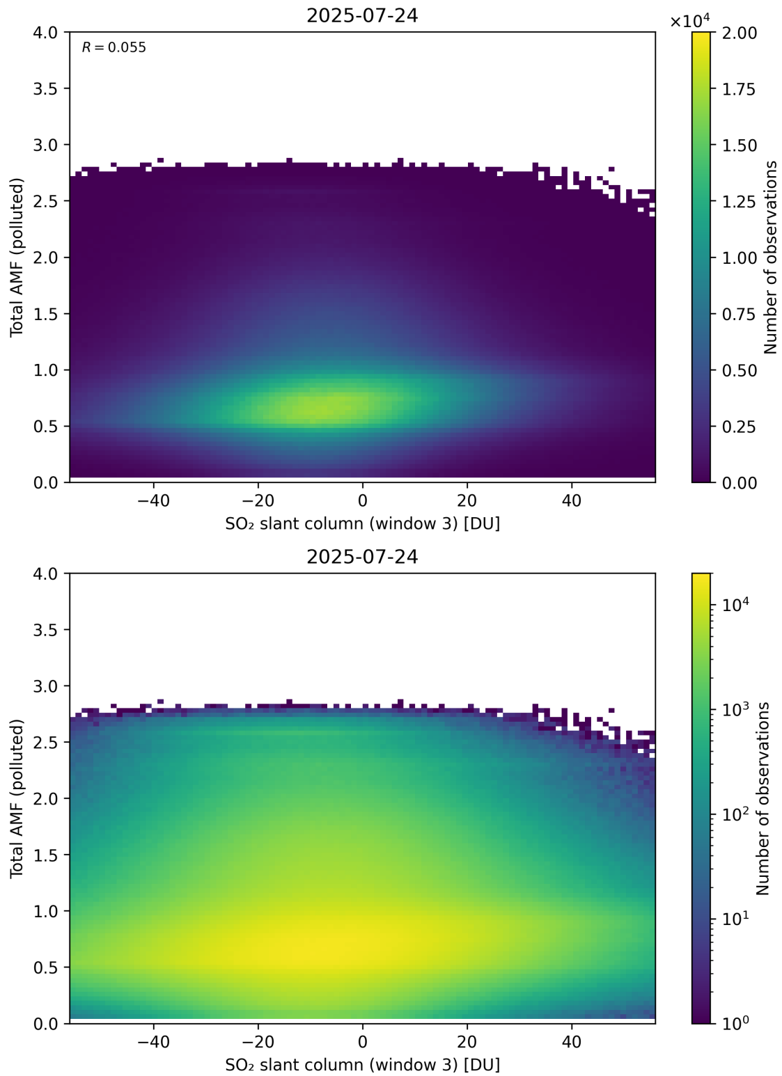
Figure 318: Scatter density plot of “SO 2 slant column (window 3)” against “Total AMF (polluted)” for 2025-07-24 to 2025-07-25.
