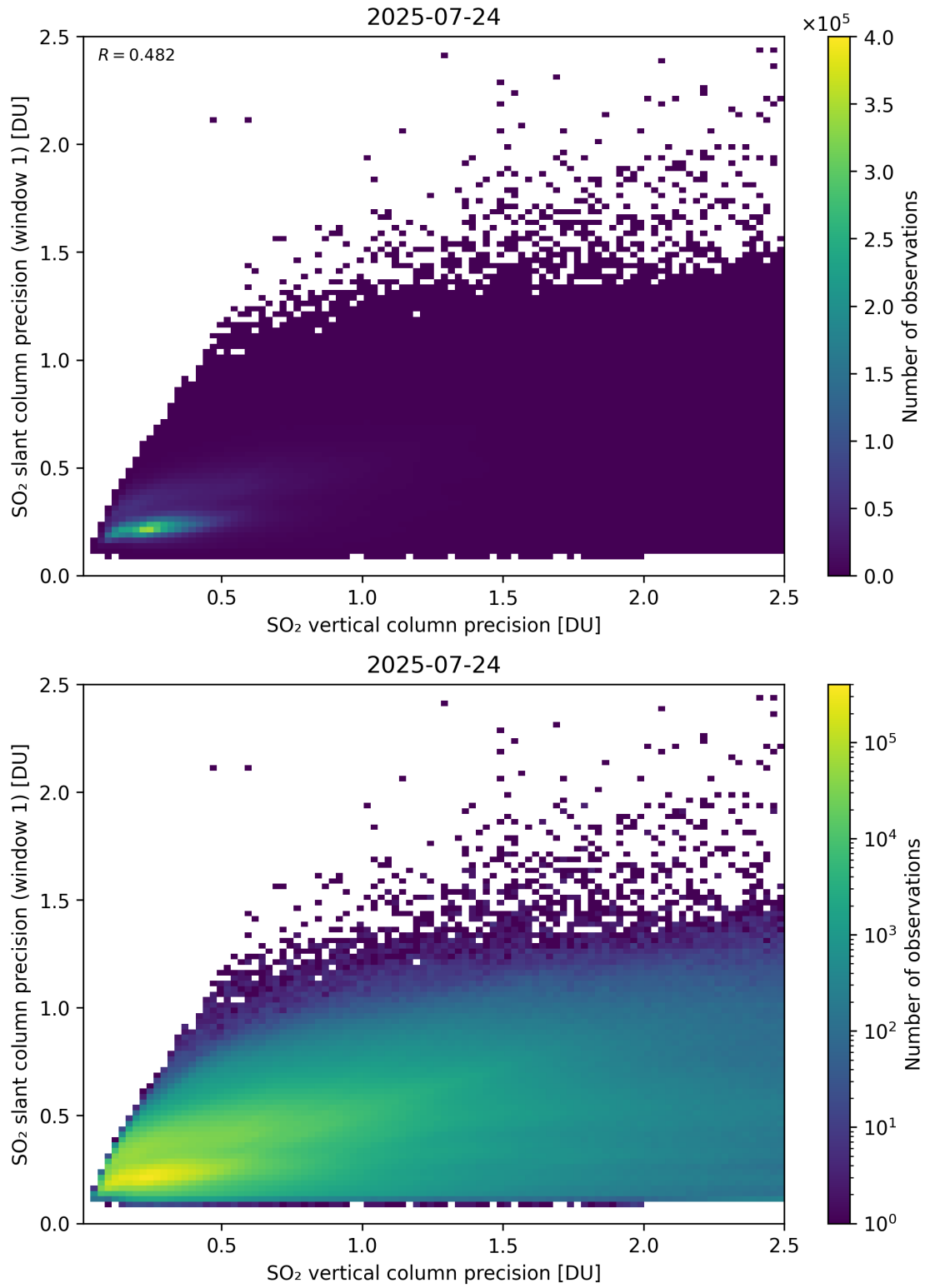
Figure 342: Scatter density plot of “SO 2 vertical column precision” against “SO 2 slant column precision (window 1)” for 2025-07-24 to 2025-07-25.
