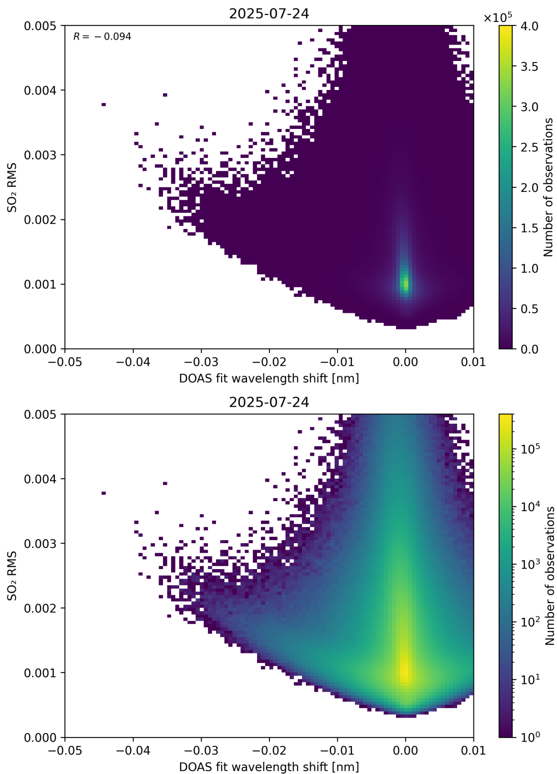
Figure 139: Scatter density plot of “DOAS fit wavelength shift” against “SO 2 RMS” for 2025-07-24 to 2025-07-25.
