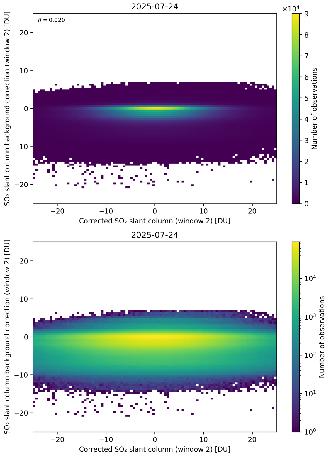
Figure 244: Scatter density plot of “Corrected SO 2 slant column (window 2)” against “SO 2 slant column background correction (window 2)” for 2025-07-24 to 2025-07-25.
