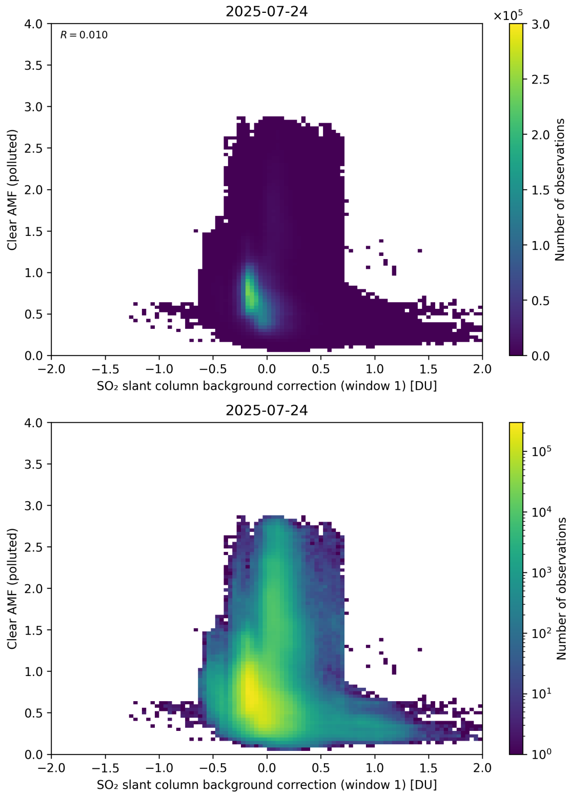
Figure 114: Scatter density plot of “SO 2 slant column background correction (window 1)” against “Clear AMF (polluted)” for 2025-07-24 to 2025-07-25.
