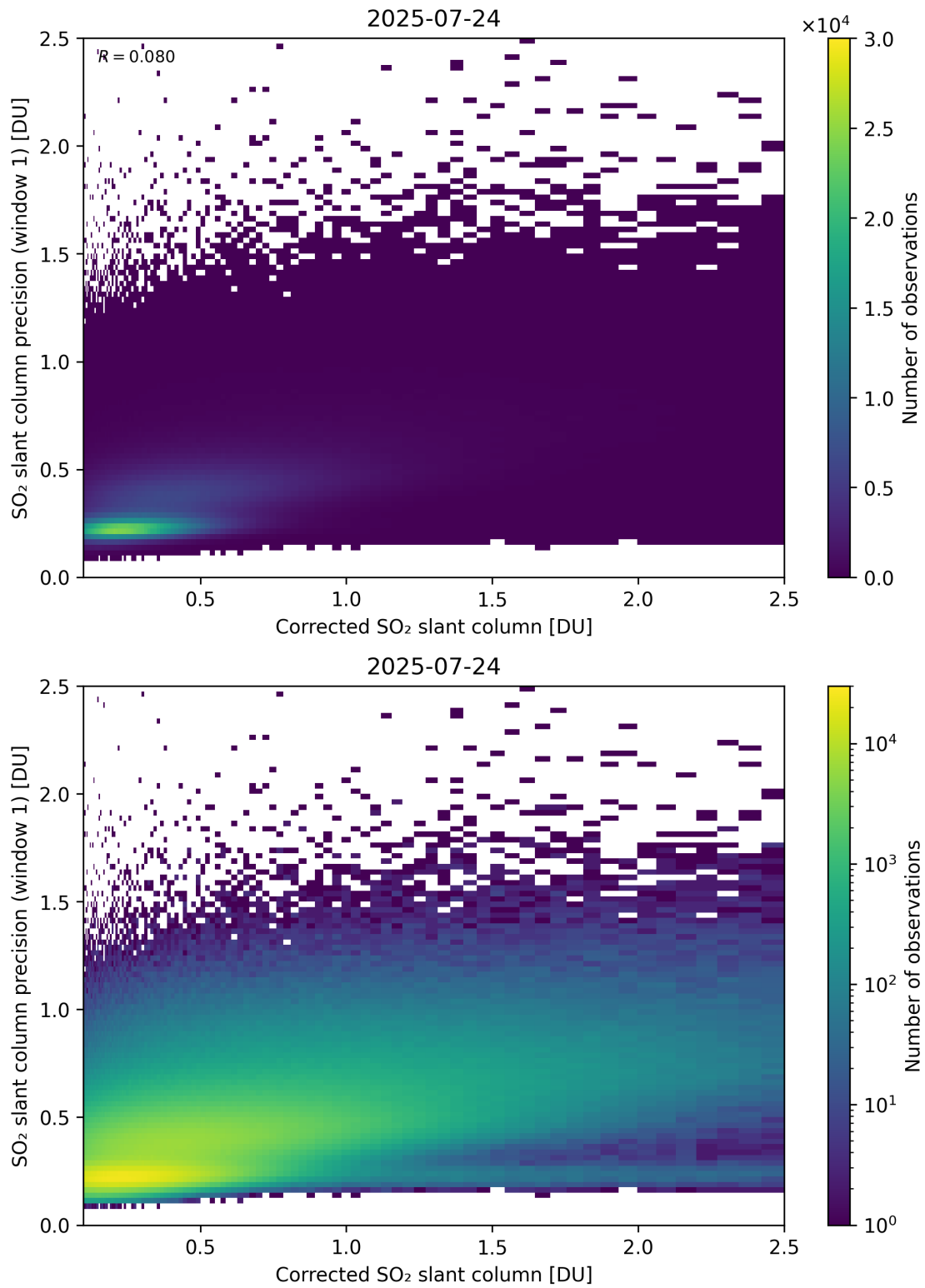
Figure 238: Scatter density plot of “Corrected SO 2 slant column” against “SO 2 slant column precision (window 1)” for 2025-07-24 to 2025-07-25.
