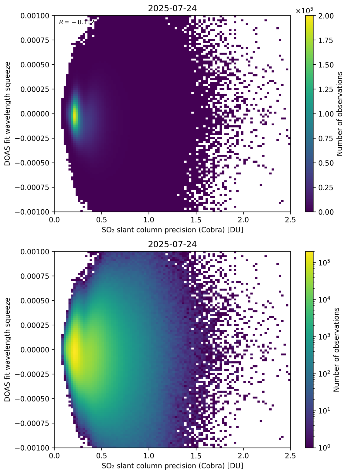
Figure 203: Scatter density plot of “SO 2 slant column precision (Cobra)” against “DOAS fit wavelength squeeze” for 2025-07-24 to 2025-07-25.
