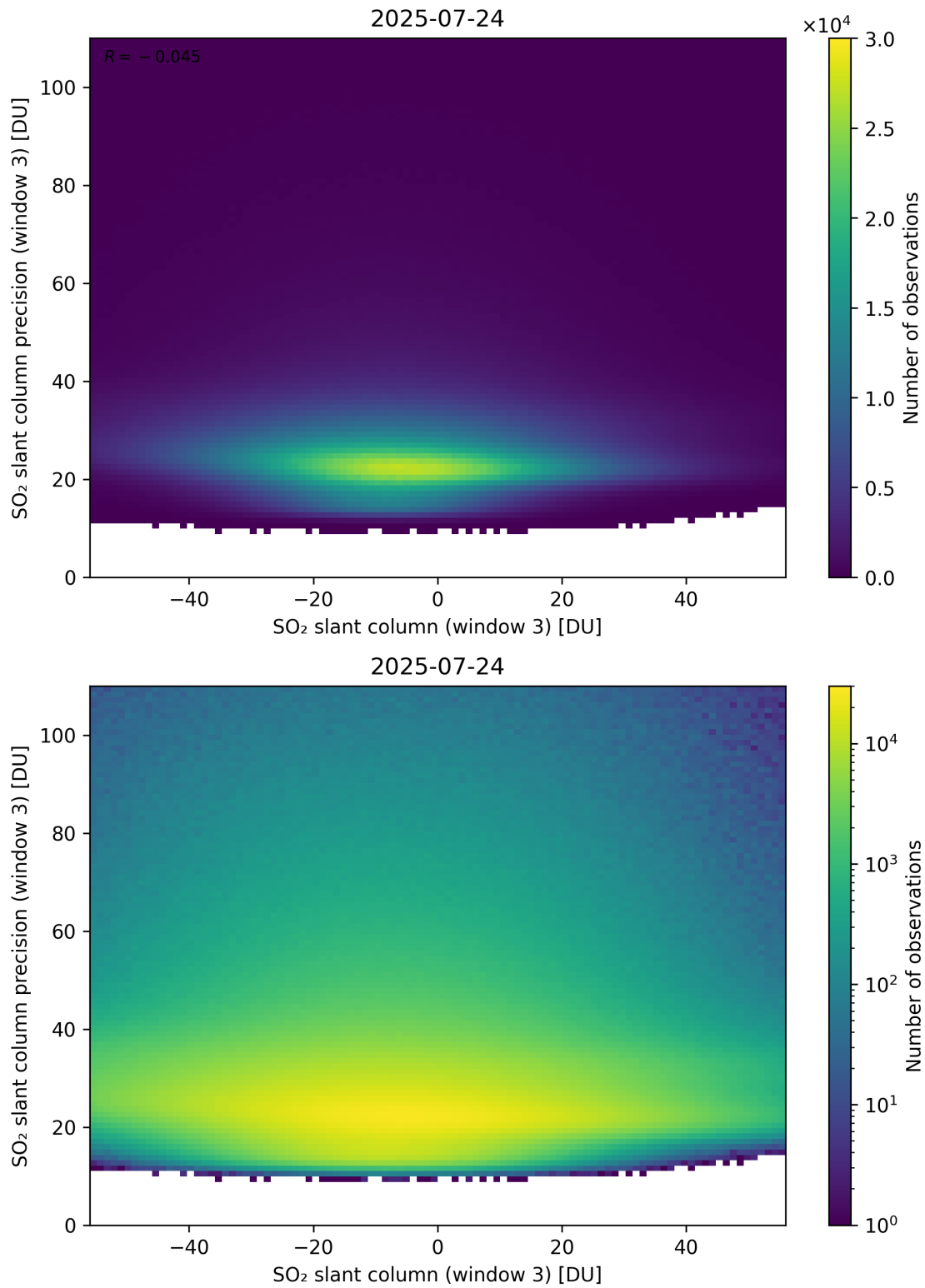
Figure 317: Scatter density plot of “SO 2 slant column (window 3)” against “SO 2 slant column precision (window 3)” for 2025-07-24 to 2025-07-25.
