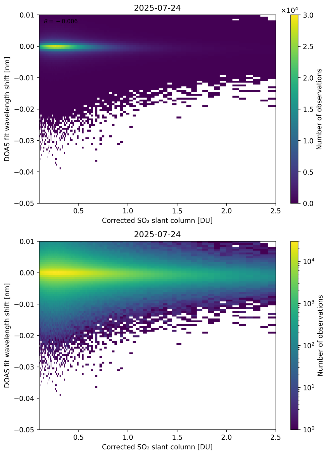
Figure 229: Scatter density plot of “Corrected SO 2 slant column” against “DOAS fit wavelength shift” for 2025-07-24 to 2025-07-25.
