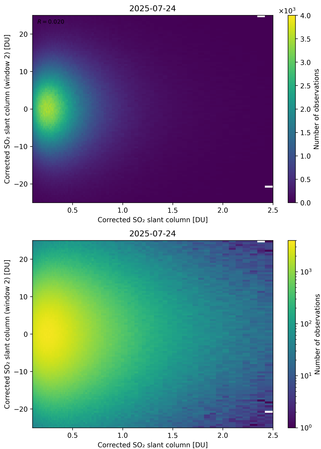
Figure 235: Scatter density plot of “Corrected SO 2 slant column” against “Corrected SO 2 slant column (window 2)” for 2025-07-24 to 2025-07-25.
