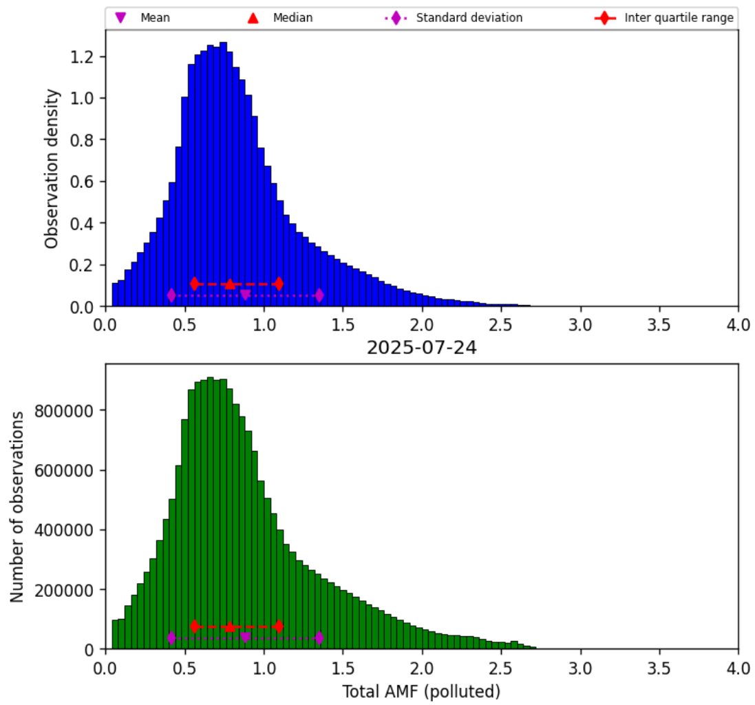
Figure 79: Histogram of “Total AMF (polluted)” for 2025-07-24 to 2025-07-25
