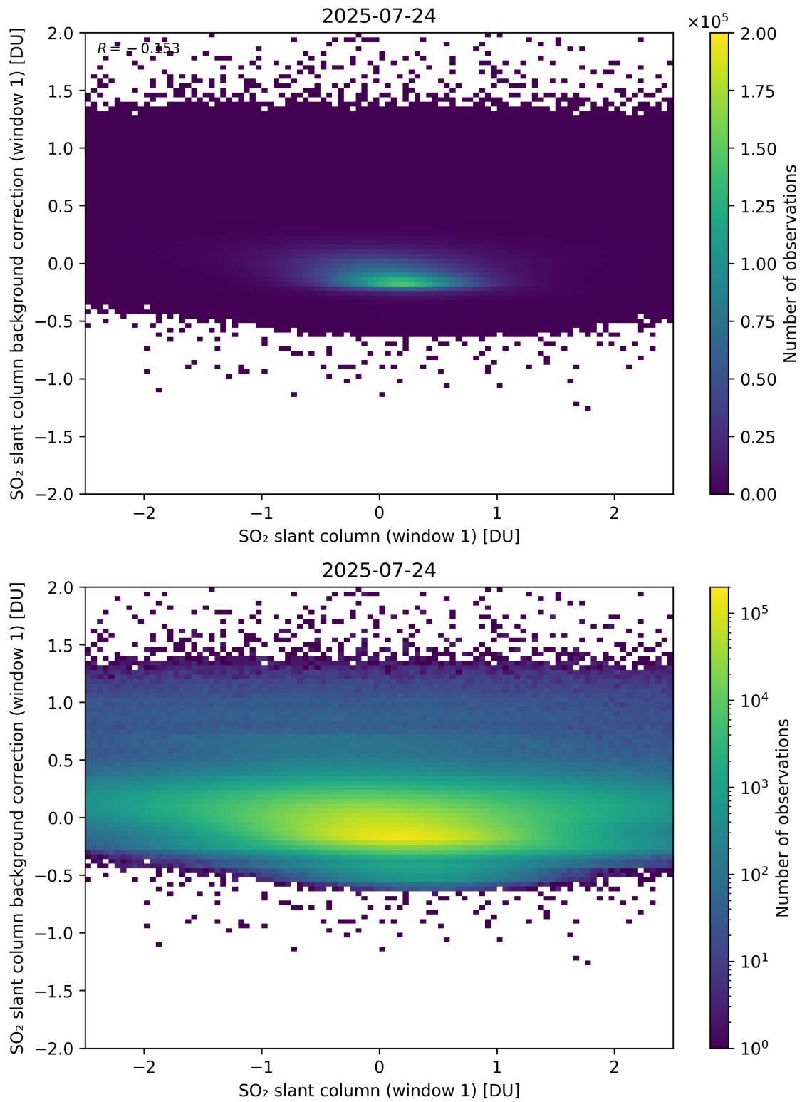
Figure 262: Scatter density plot of “SO 2 slant column (window 1)” against “SO 2 slant column background correction (window 1)” for 2025-07-24 to 2025-07-25.
