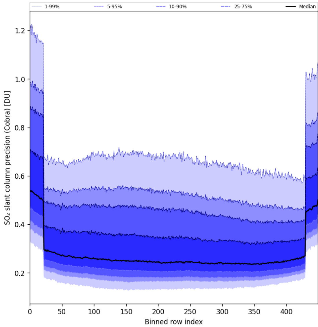
Figure 88: Along track statistics of “SO 2 slant column precision (Cobra)” for 2025-07-24 to 2025-07-25
