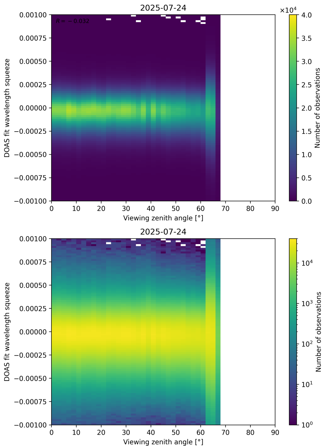
Figure 366: Scatter density plot of “Viewing zenith angle” against “DOAS fit wavelength squeeze” for 2025-07-24 to 2025-07-25.
