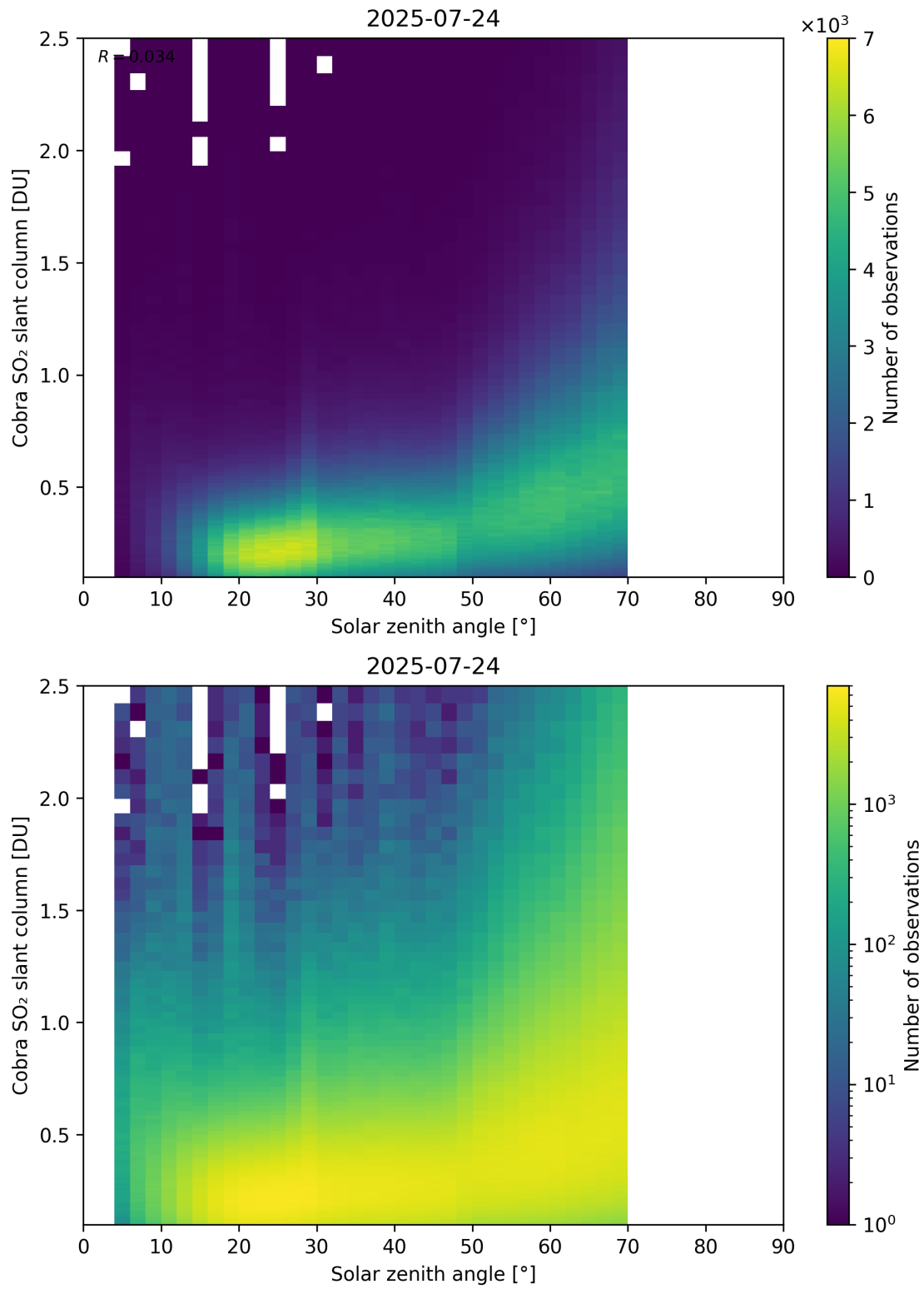
Figure 179: Scatter density plot of “Solar zenith angle” against “Cobra SO 2 slant column” for 2025-07-24 to 2025-07-25.
