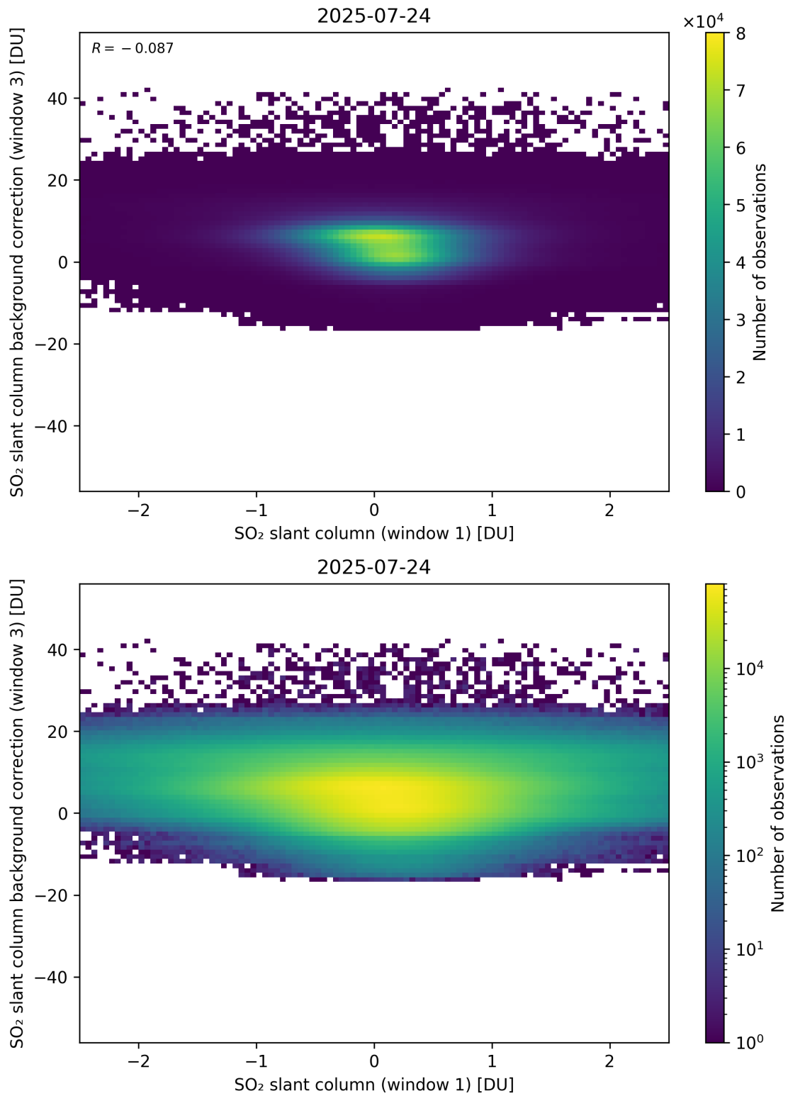
Figure 264: Scatter density plot of “SO 2 slant column (window 1)” against “SO 2 slant column background correction (window 3)” for 2025-07-24 to 2025-07-25.
