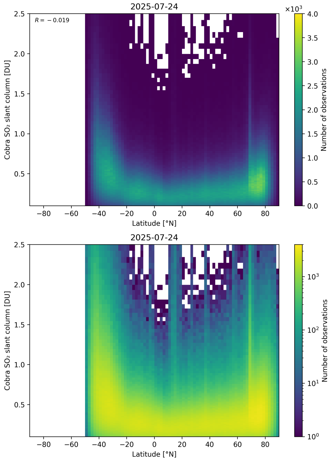
Figure 157: Scatter density plot of “Latitude” against “Cobra SO 2 slant column” for 2025-07-24 to 2025-07-25.
