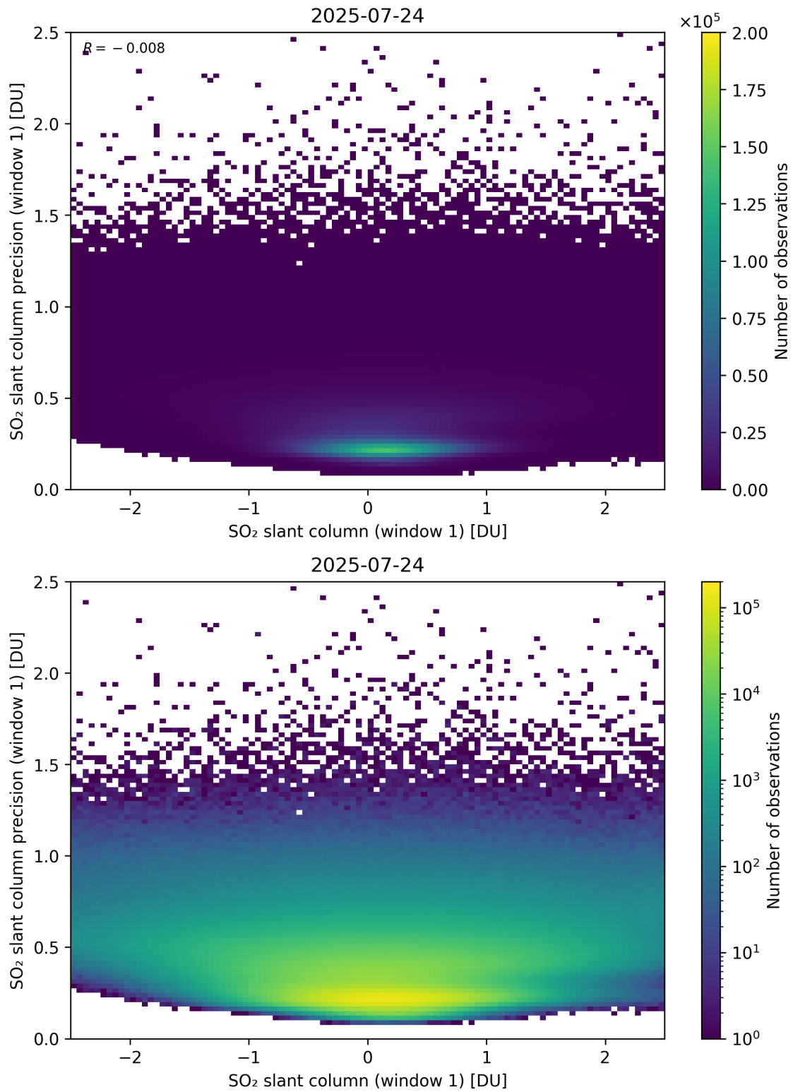
Figure 285: Scatter density plot of “SO 2 slant column (window 1)” against “SO 2 slant column precision (window 1)” for 2025-07-24 to 2025-07-25.
