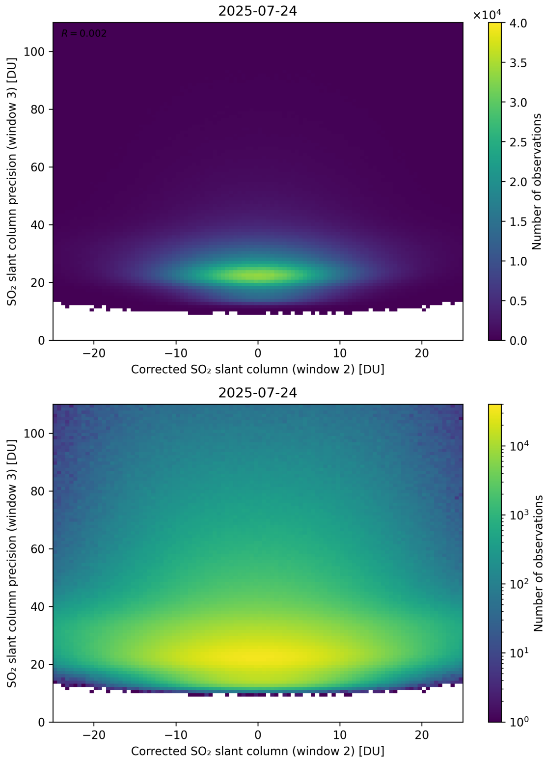
Figure 252: Scatter density plot of “Corrected SO 2 slant column (window 2)” against “SO 2 slant column precision (window 3)” for 2025-07-24 to 2025-07-25.
