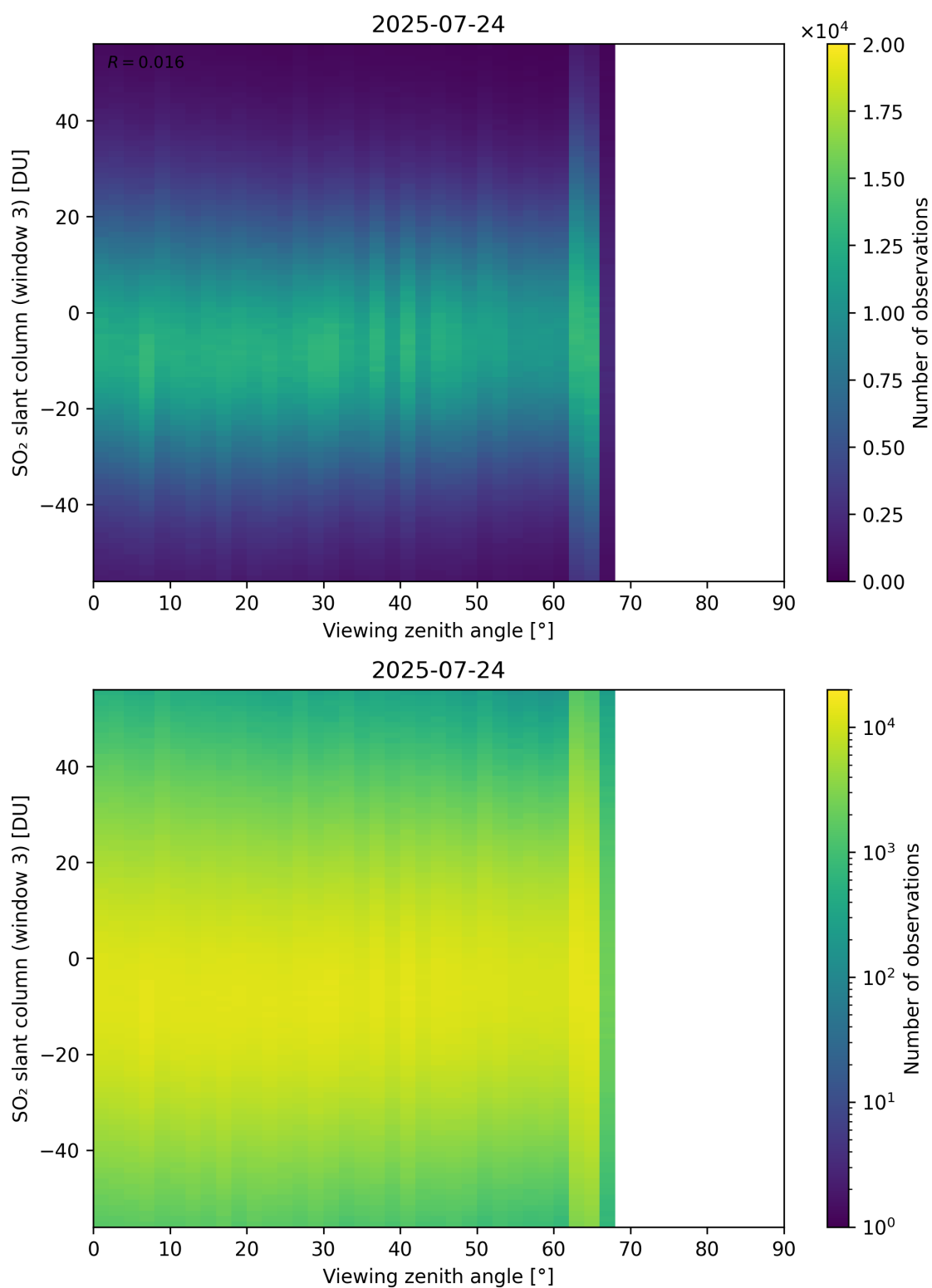
Figure 379: Scatter density plot of “Viewing zenith angle” against “SO 2 slant column (window 3)” for 2025-07-24 to 2025-07-25.
