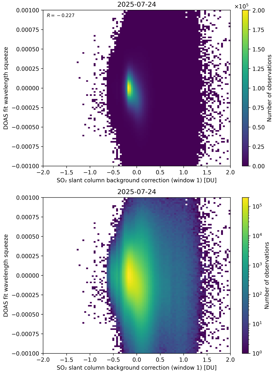
Figure 112: Scatter density plot of “SO 2 slant column background correction (window 1)” against “DOAS fit wavelength squeeze” for 2025-07-24 to 2025-07-25.
