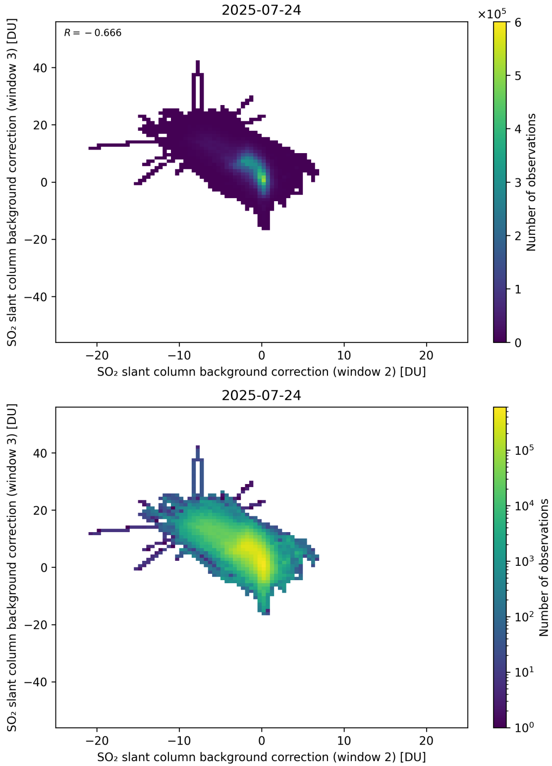
Figure 122: Scatter density plot of “SO 2 slant column background correction (window 2)” against “SO 2 slant column background correction (window 3)” for 2025-07-24 to 2025-07-25.
