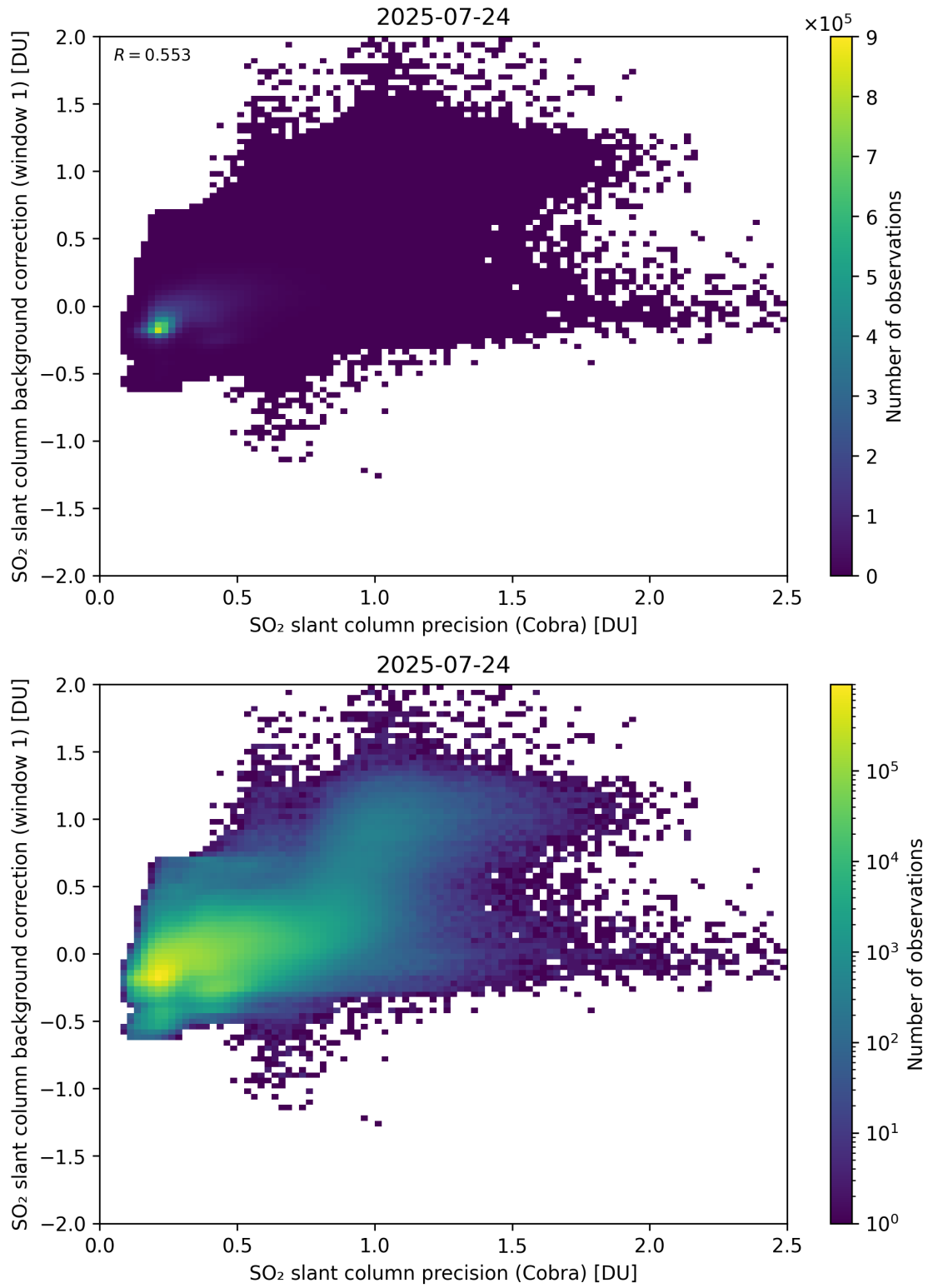
Figure 199: Scatter density plot of “SO 2 slant column precision (Cobra)” against “SO 2 slant column background correction (window 1)” for 2025-07-24 to 2025-07-25.
