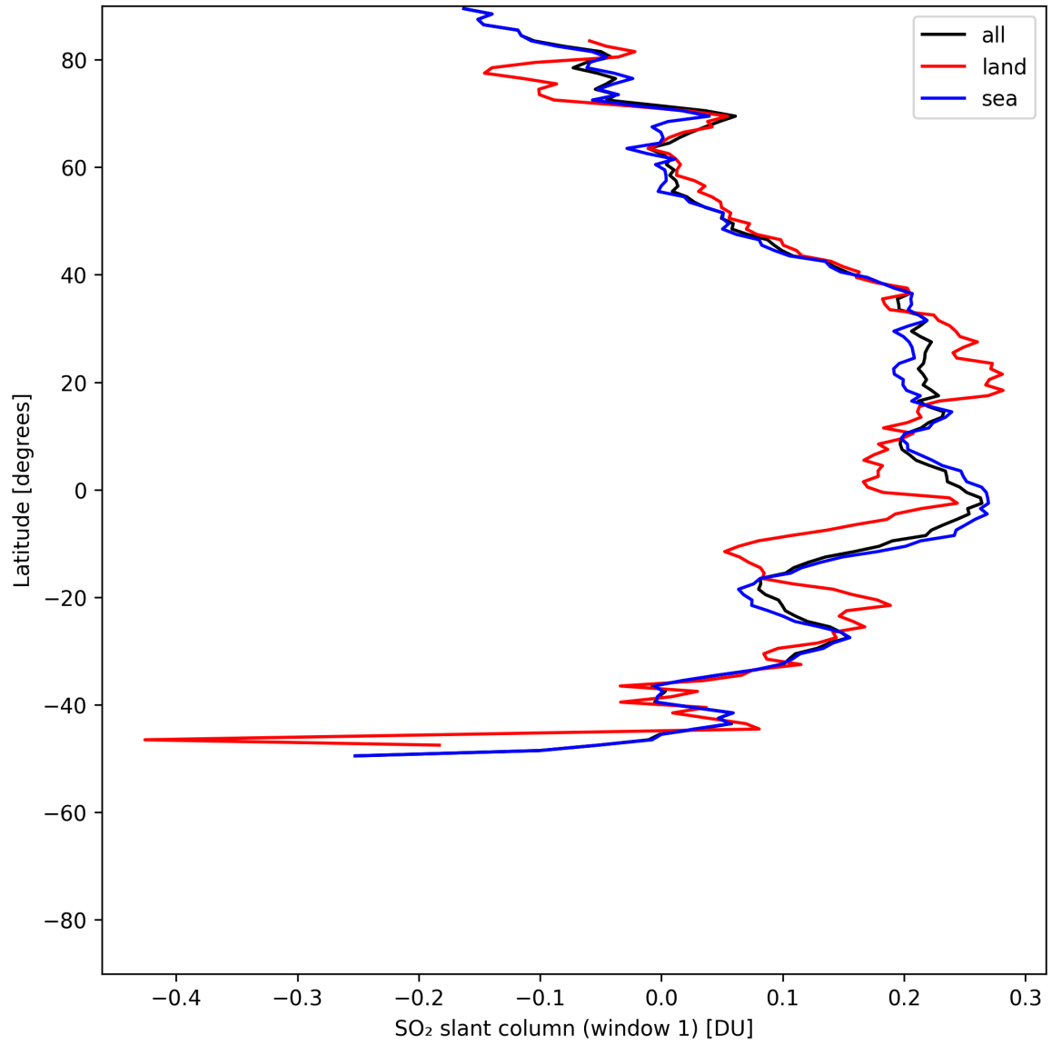
Figure 37: Zonal average of “SO 2 slant column (window 1)” for 2025-07-24 to 2025-07-25.
