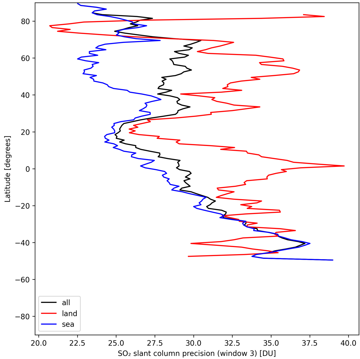
Figure 46: Zonal average of “SO 2 slant column precision (window 3)” for 2025-07-24 to 2025-07-25.
