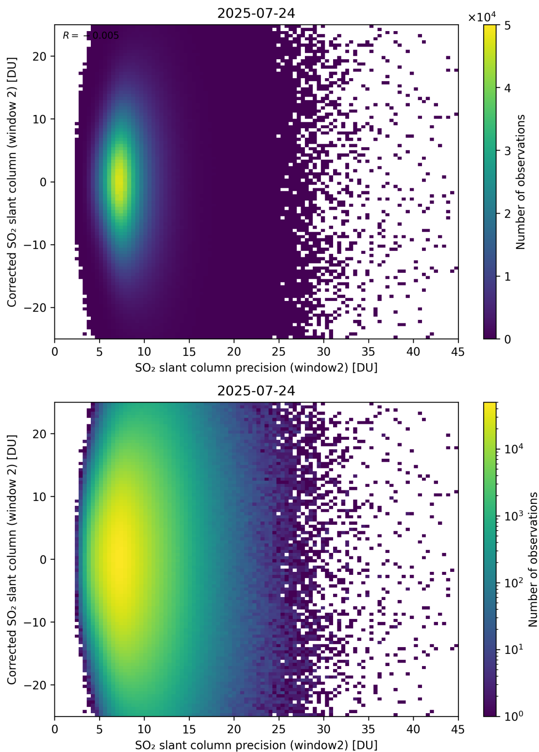
Figure 297: Scatter density plot of “SO 2 slant column precision (window2)” against “Corrected SO 2 slant column (window 2)” for 2025-07-24 to 2025-07-25.
