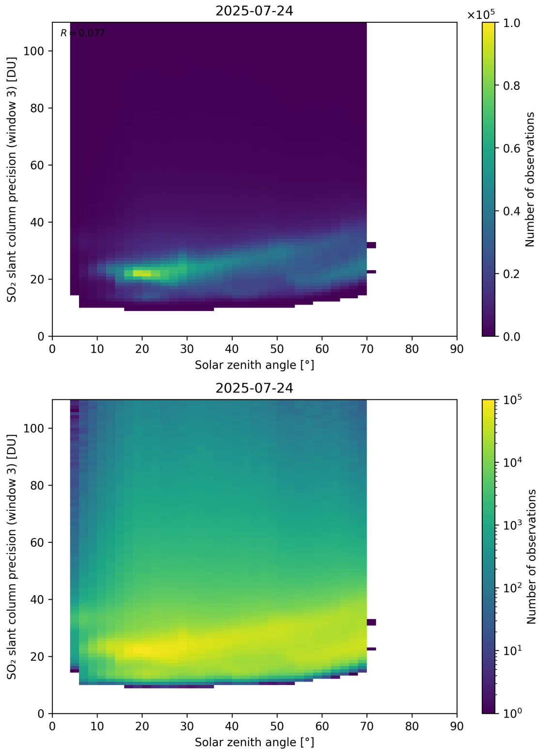
Figure 188: Scatter density plot of “Solar zenith angle” against “SO 2 slant column precision (window 3)” for 2025-07-24 to 2025-07-25.
