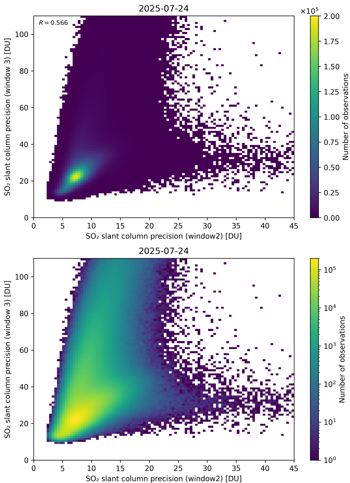
Figure 300: Scatter density plot of “SO 2 slant column precision (window2)” against “SO 2 slant column precision (window 3)” for 2025-07-24 to 2025-07-25.
