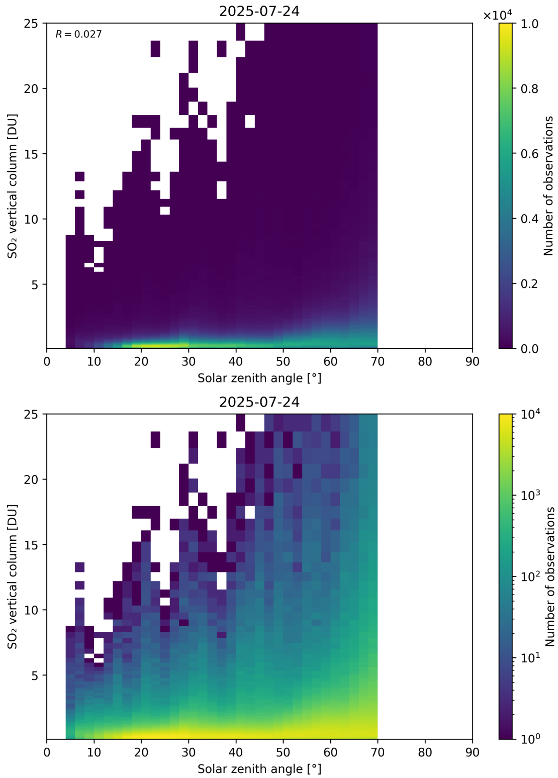
Figure 191: Scatter density plot of “Solar zenith angle” against “SO 2 vertical column” for 2025-07-24 to 2025-07-25.
