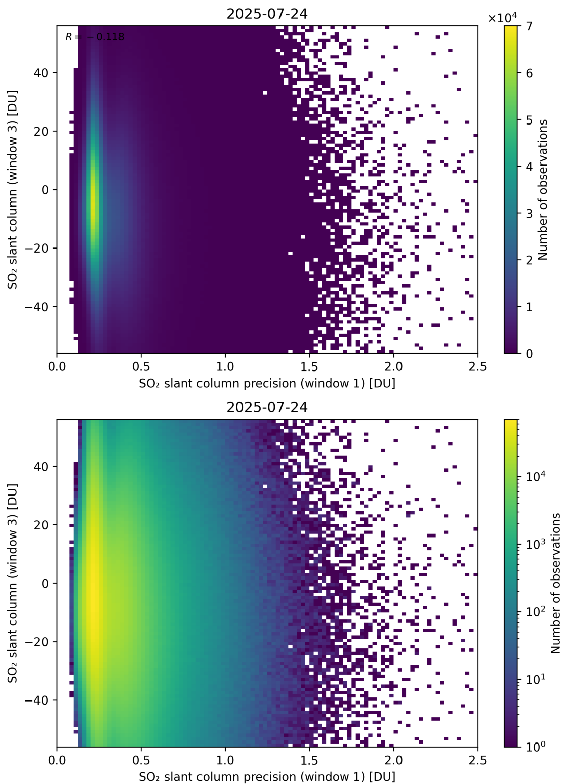
Figure 278: Scatter density plot of “SO 2 slant column precision (window 1)” against “SO 2 slant column (window 3)” for 2025-07-24 to 2025-07-25.
