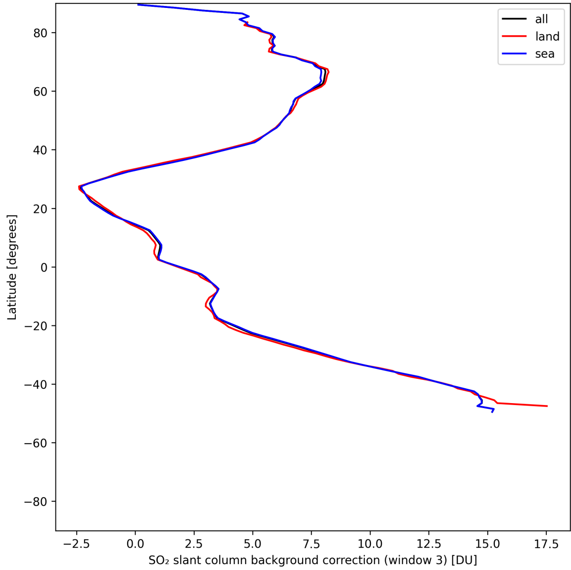
Figure 48: Zonal average of “SO 2 slant column background correction (window 3)” for 2025-07-24 to 2025-07-25.
