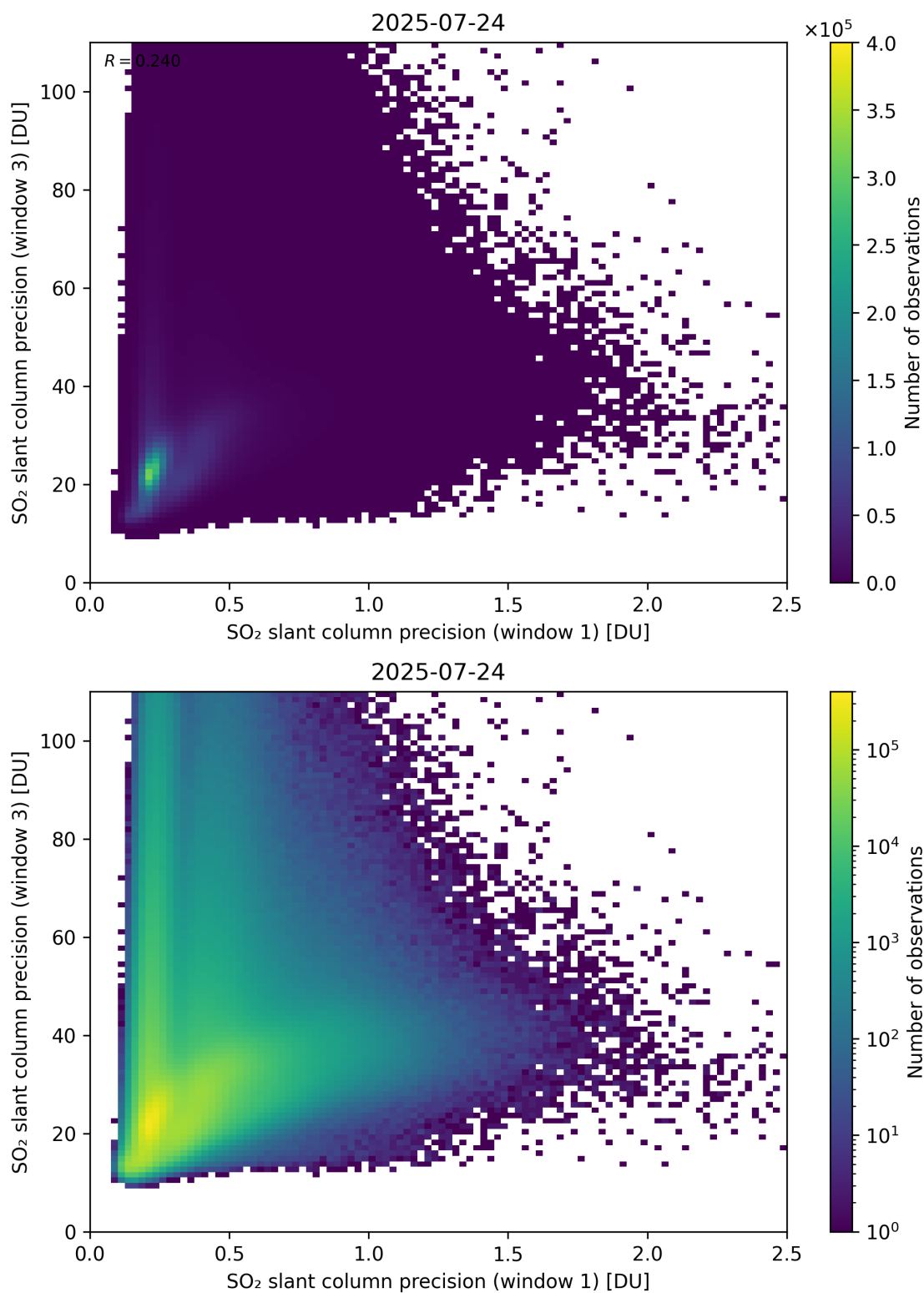
Figure 279: Scatter density plot of “SO 2 slant column precision (window 1)” against “SO 2 slant column precision (window 3)” for 2025-07-24 to 2025-07-25.
