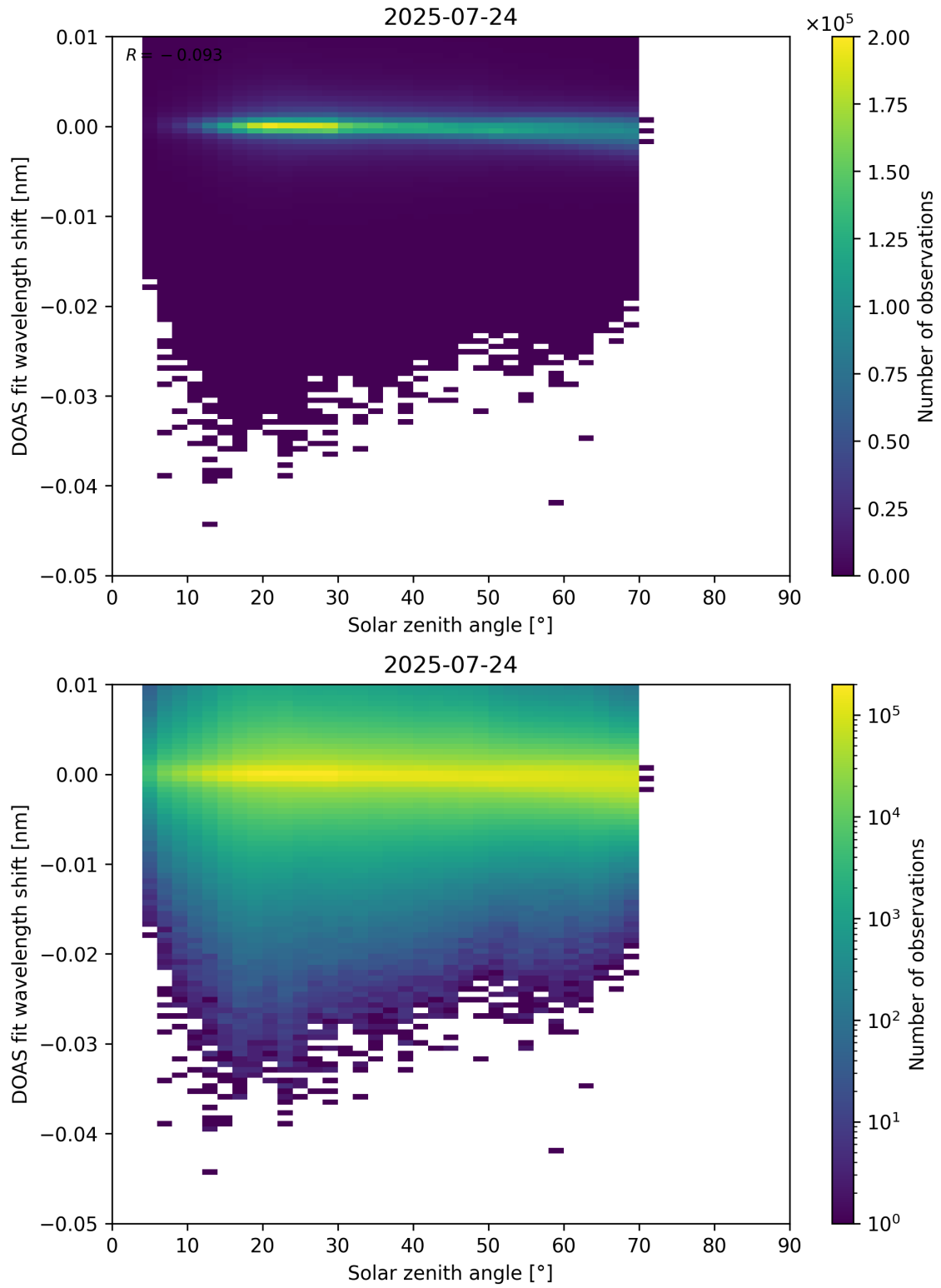
Figure 174: Scatter density plot of “Solar zenith angle” against “DOAS fit wavelength shift” for 2025-07-24 to 2025-07-25.
