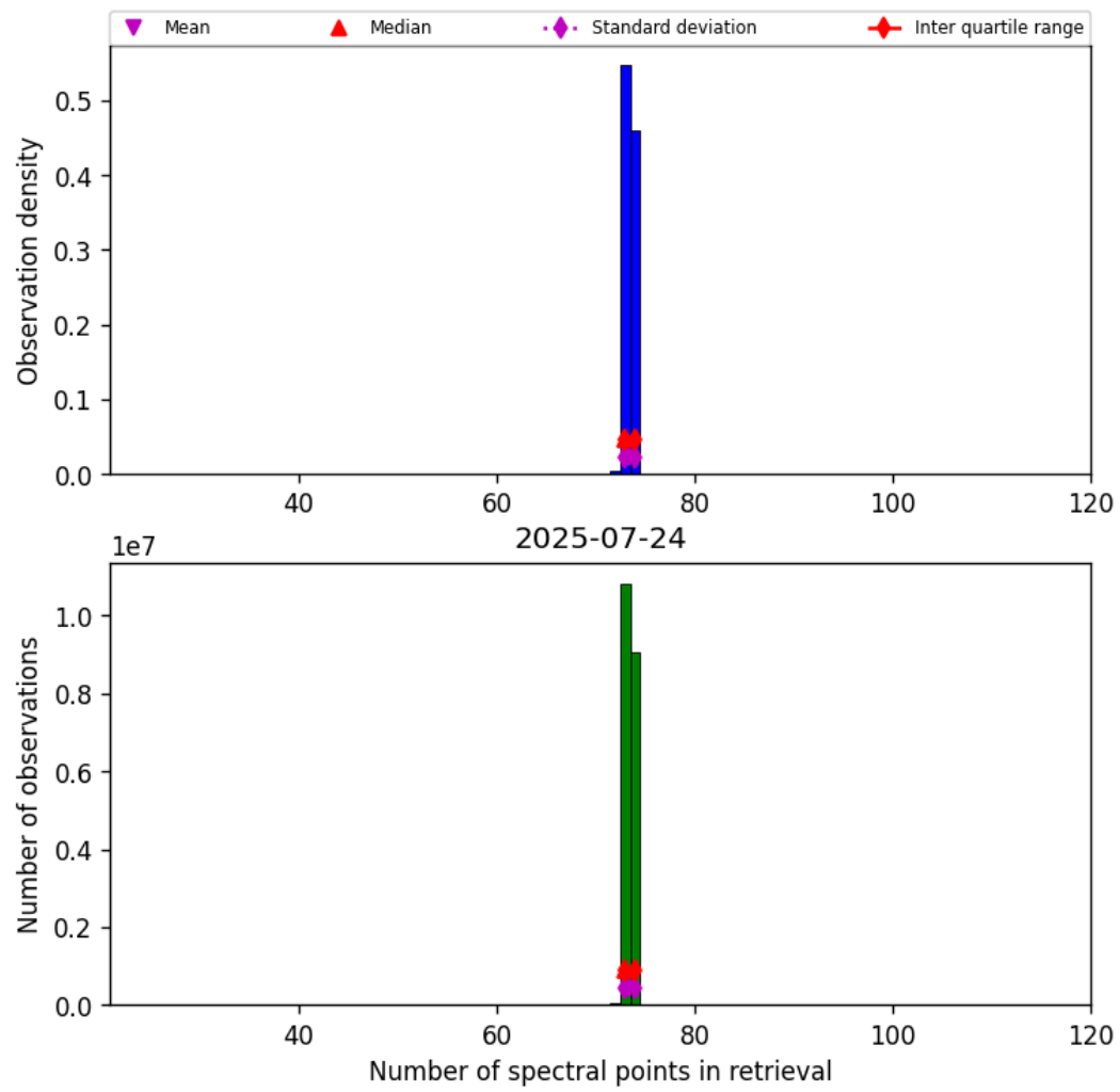
Figure 82: Histogram of “Number of spectral points in retrieval” for 2025-07-24 to 2025-07-25
