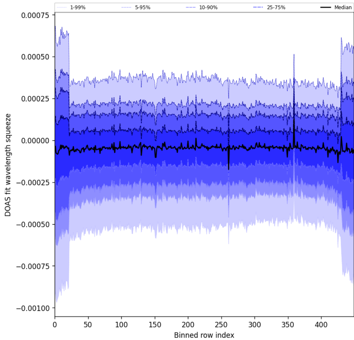
Figure 103: Along track statistics of “DOAS fit wavelength squeeze” for 2025-07-24 to 2025-07-25
