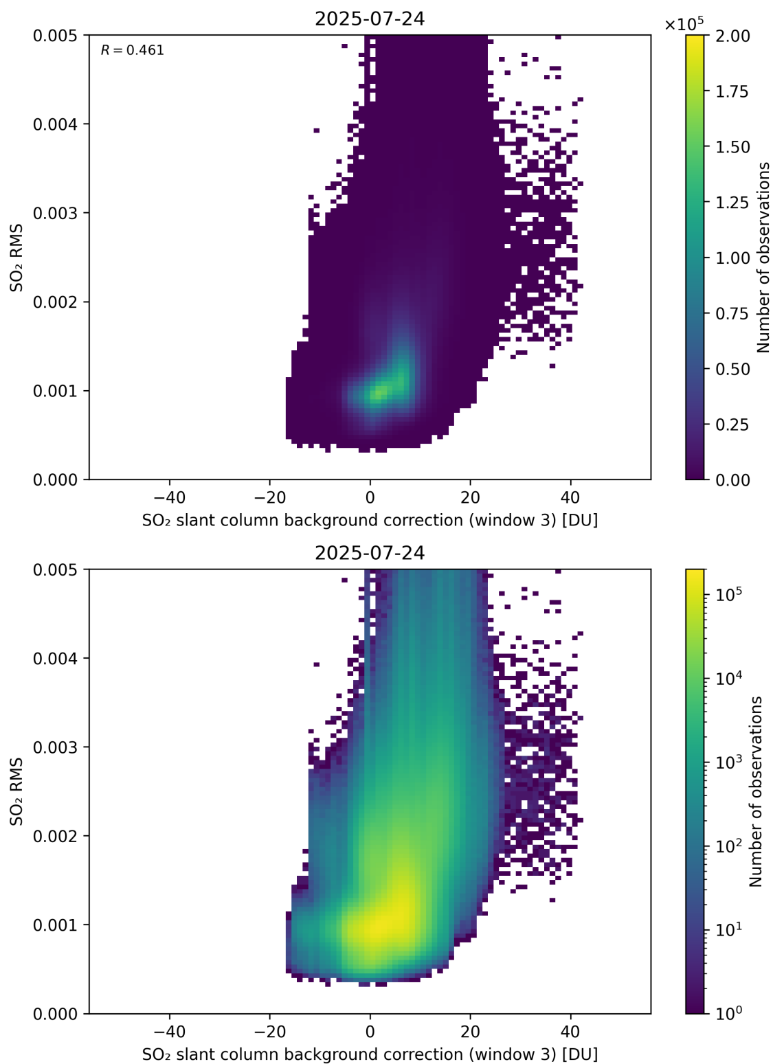
Figure 134: Scatter density plot of “SO 2 slant column background correction (window 3)” against “SO 2 RMS” for 2025-07-24 to 2025-07-25.
