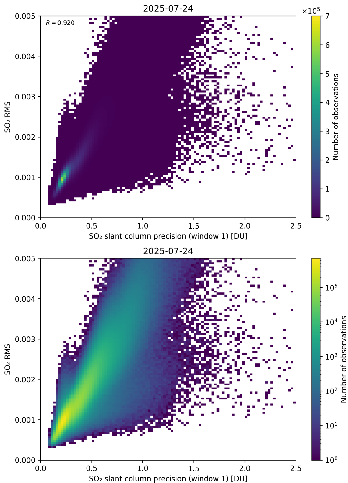
Figure 273: Scatter density plot of “SO 2 slant column precision (window 1)” against “SO 2 RMS” for 2025-07-24 to 2025-07-25.
