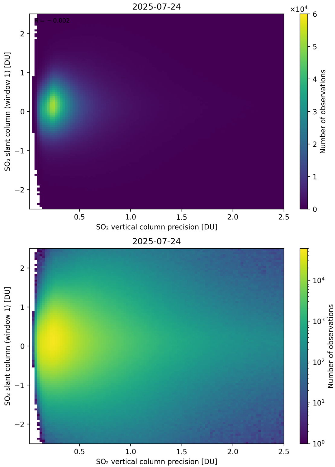
Figure 341: Scatter density plot of “SO 2 vertical column precision” against “SO 2 slant column (window 1)” for 2025-07-24 to 2025-07-25.
