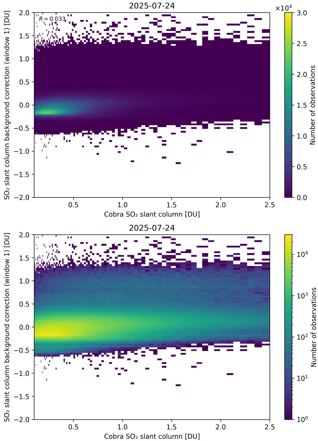
Figure 193: Scatter density plot of “Cobra SO 2 slant column” against “SO 2 slant column background correction (window 1)” for 2025-07-24 to 2025-07-25.
