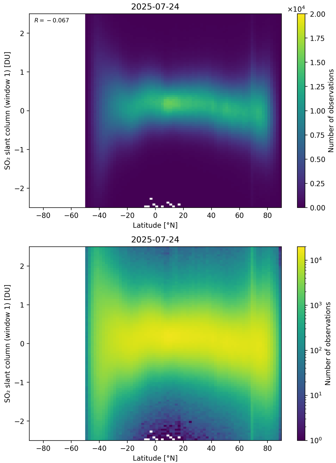
Figure 162: Scatter density plot of “Latitude” against “SO 2 slant column (window 1)” for 2025-07-24 to 2025-07-25.
