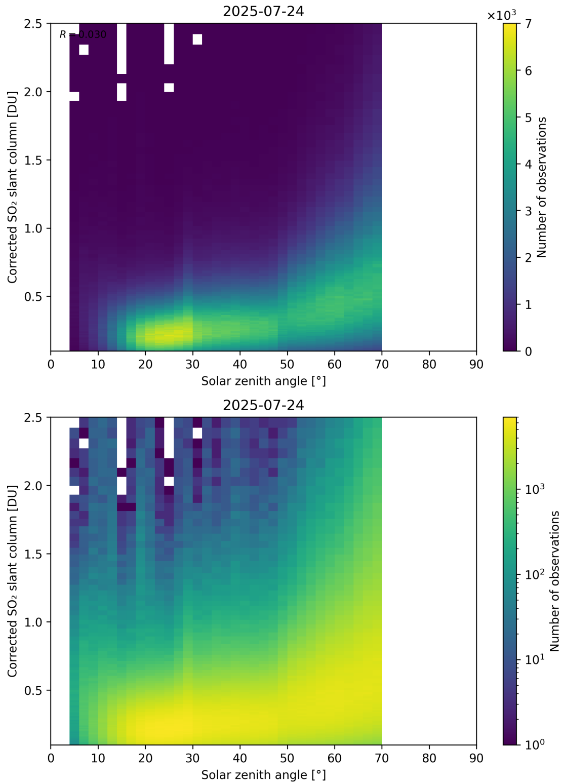
Figure 181: Scatter density plot of “Solar zenith angle” against “Corrected SO 2 slant column” for 2025-07-24 to 2025-07-25.
