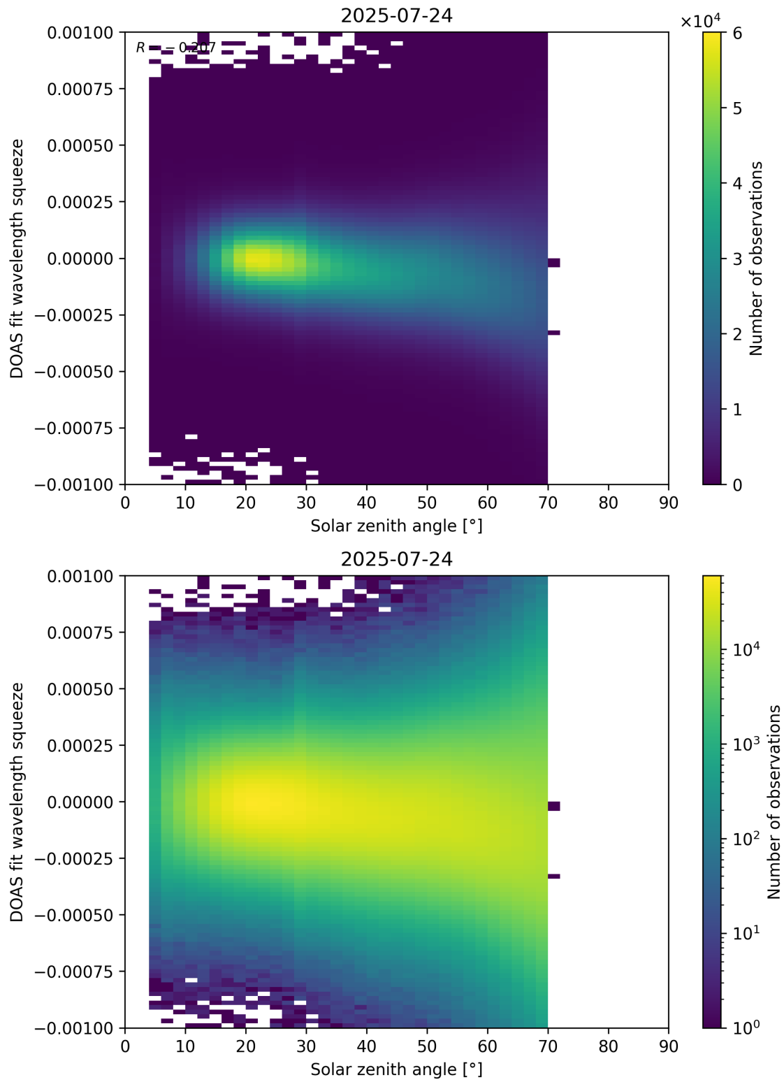
Figure 175: Scatter density plot of “Solar zenith angle” against “DOAS fit wavelength squeeze” for 2025-07-24 to 2025-07-25.
