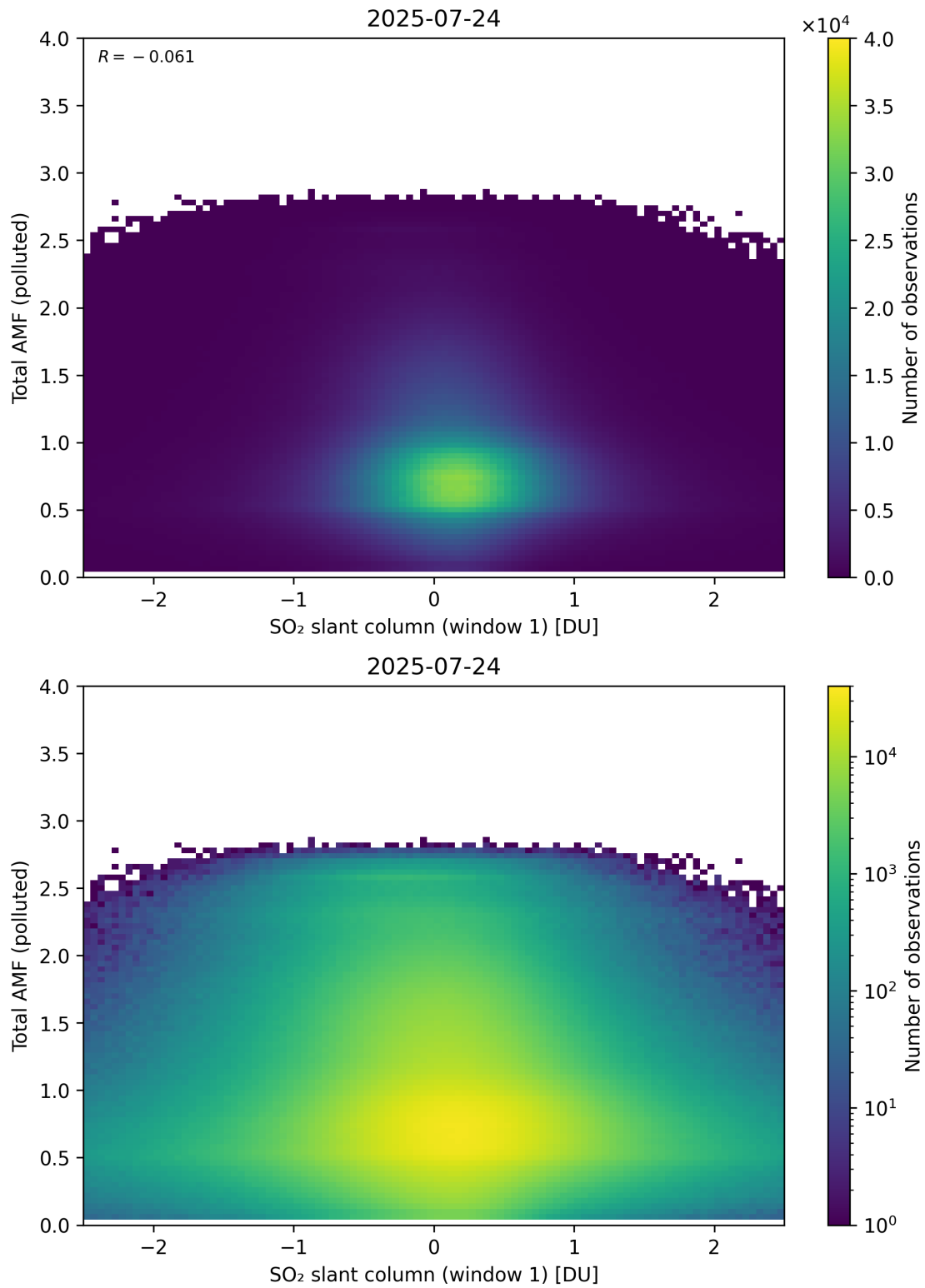
Figure 289: Scatter density plot of “SO 2 slant column (window 1)” against “Total AMF (polluted)” for 2025-07-24 to 2025-07-25.
