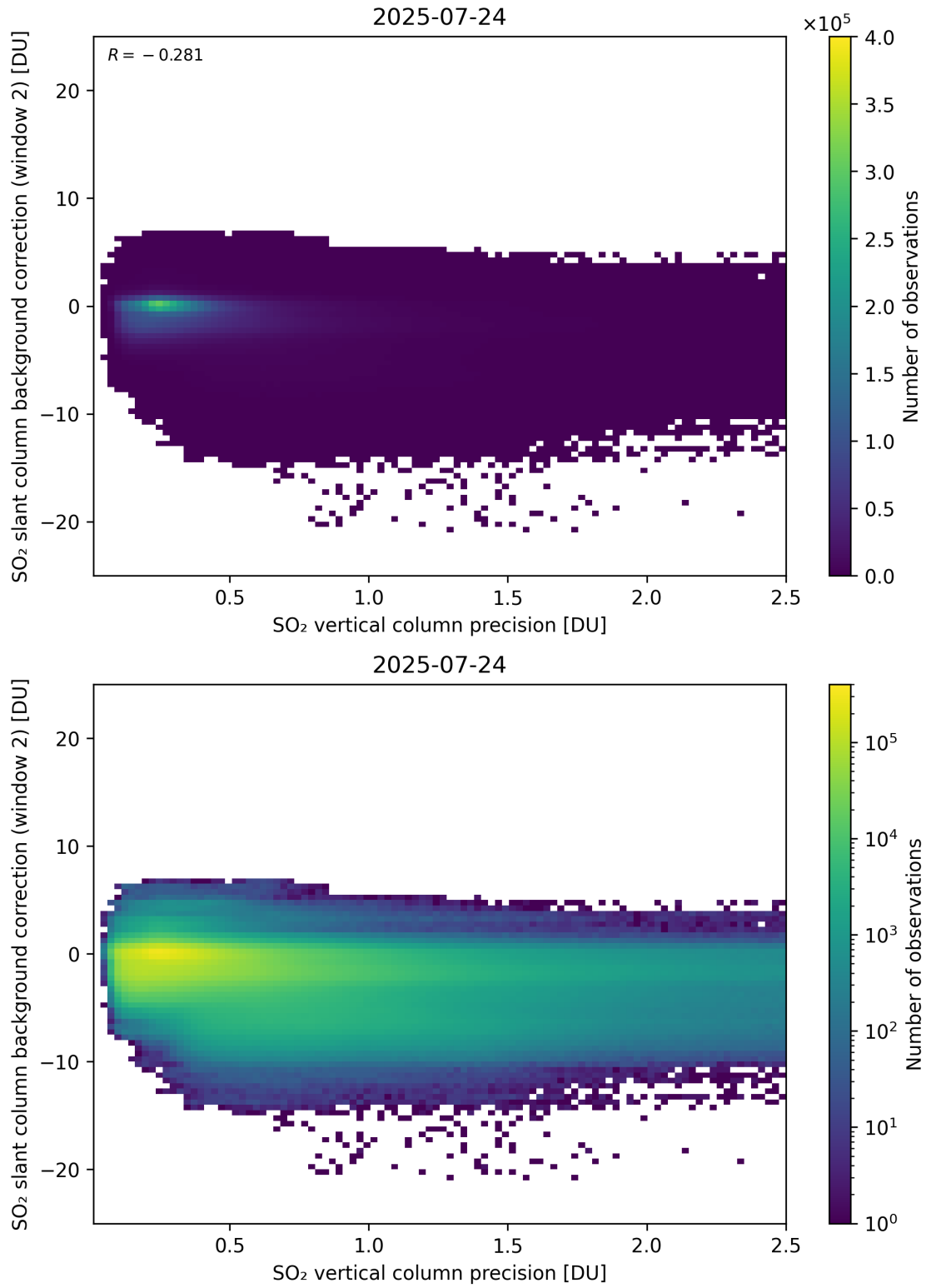
Figure 330: Scatter density plot of “SO 2 vertical column precision” against “SO 2 slant column background correction (window 2)” for 2025-07-24 to 2025-07-25.
