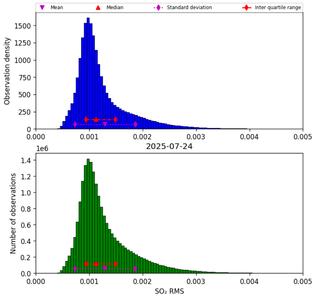
Figure 78: Histogram of “SO 2 RMS” for 2025-07-24 to 2025-07-25
