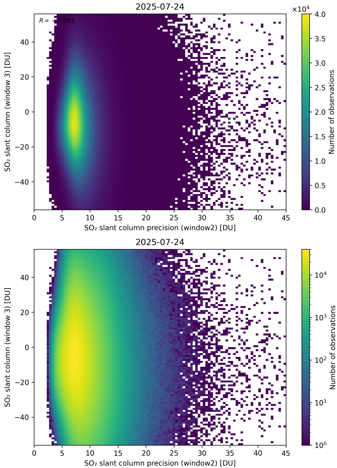
Figure 299: Scatter density plot of “SO 2 slant column precision (window2)” against “SO 2 slant column (window 3)” for 2025-07-24 to 2025-07-25.
