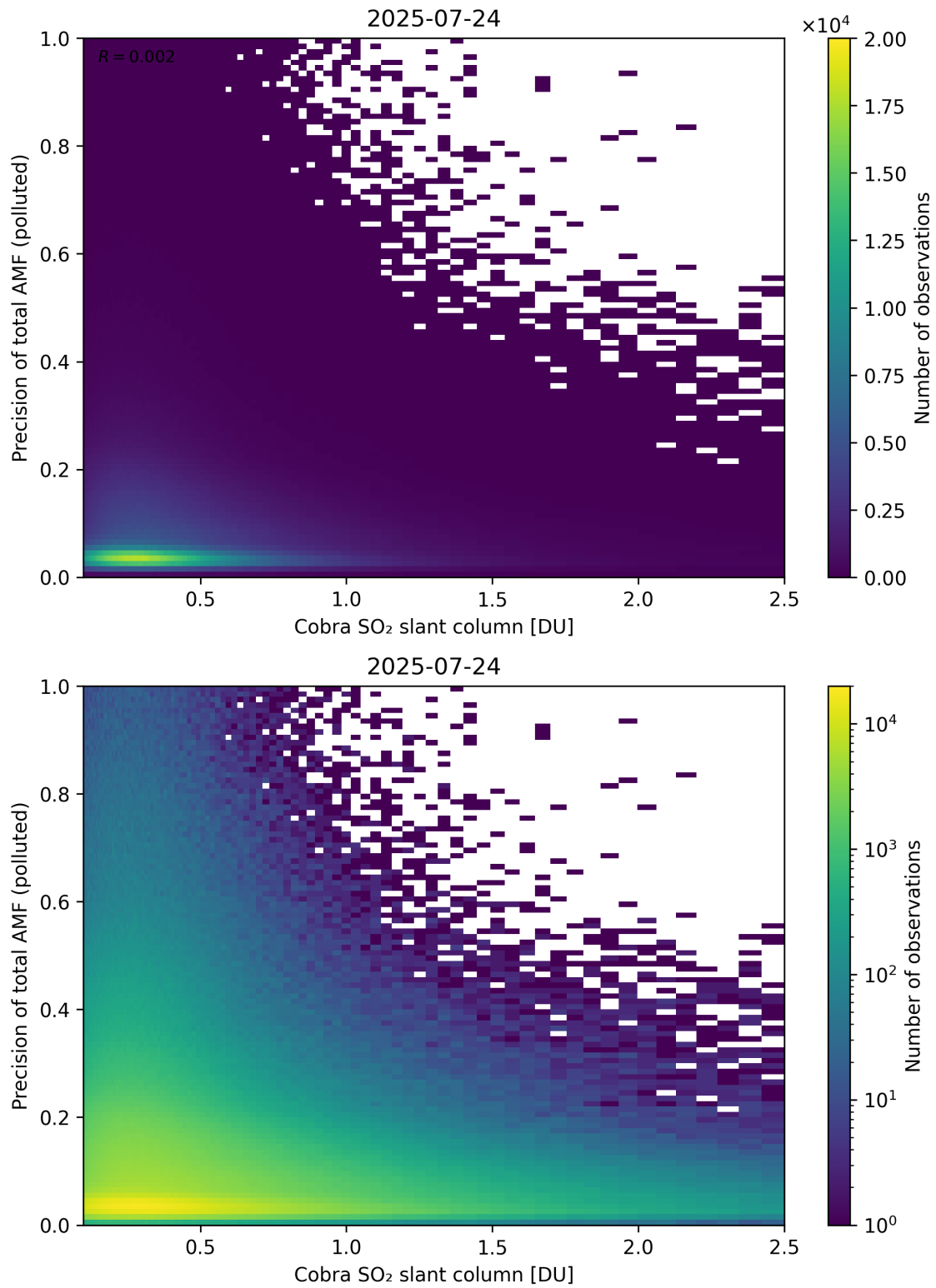
Figure 225: Scatter density plot of “Cobra SO 2 slant column” against “Precision of total AMF (polluted)” for 2025-07-24 to 2025-07-25.
