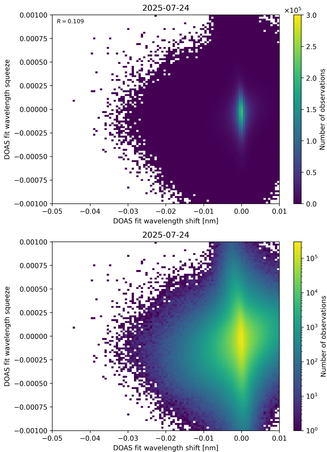
Figure 138: Scatter density plot of “DOAS fit wavelength shift” against “DOAS fit wavelength squeeze” for 2025-07-24 to 2025-07-25.
