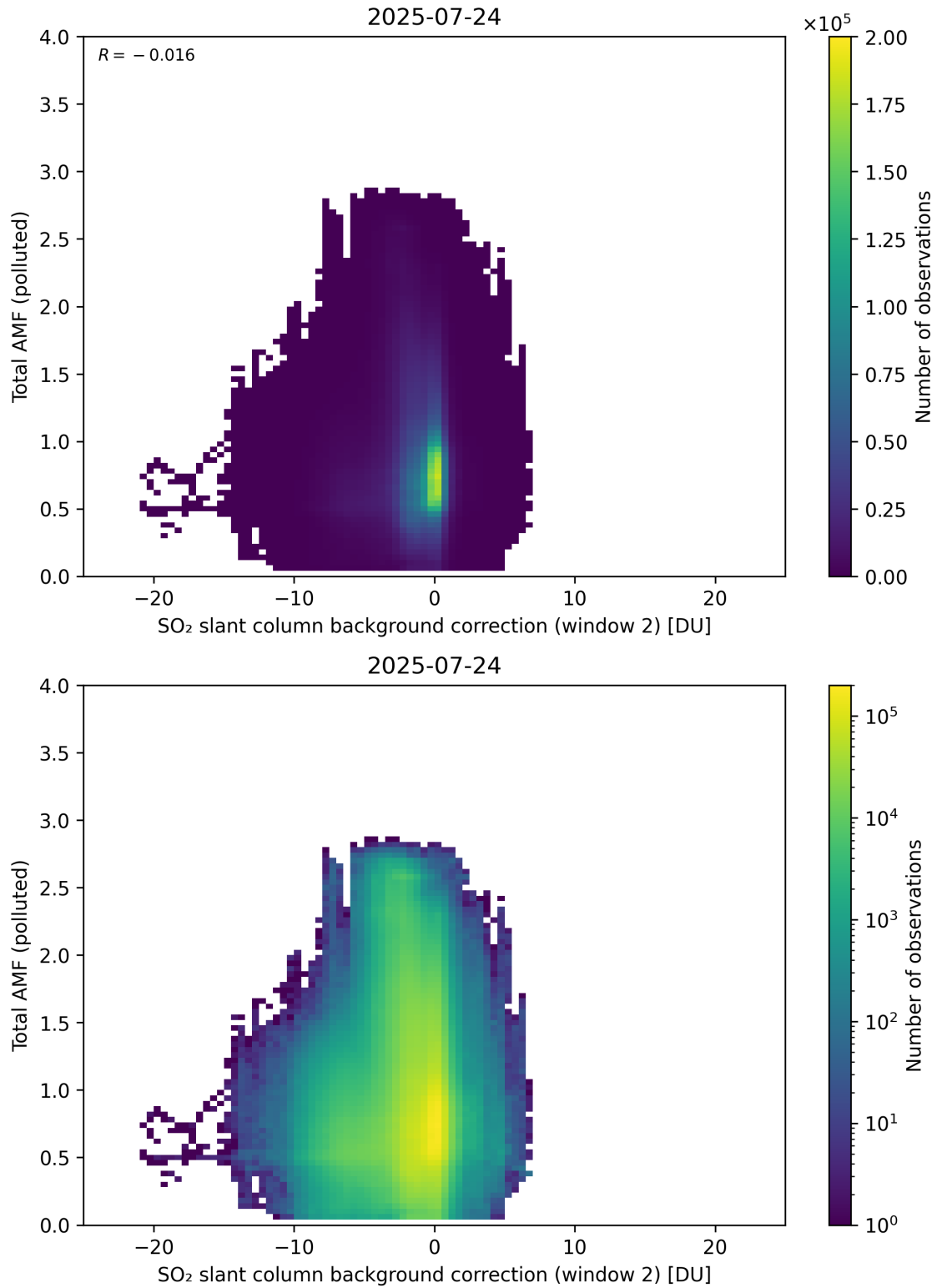
Figure 130: Scatter density plot of “SO 2 slant column background correction (window 2)” against “Total AMF (polluted)” for 2025-07-24 to 2025-07-25.
