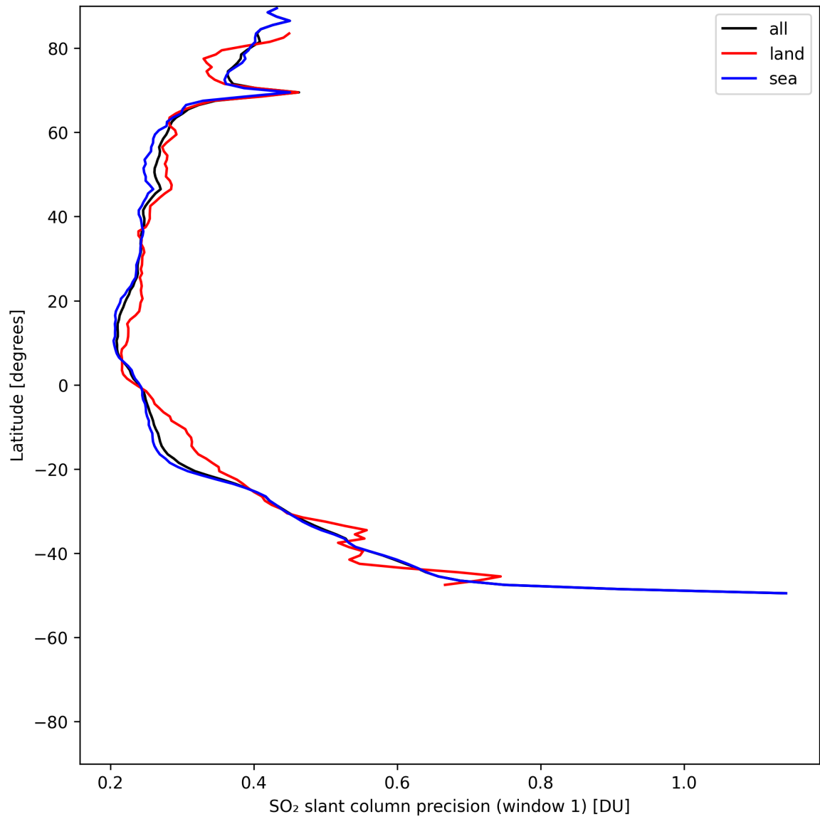
Figure 38: Zonal average of “SO 2 slant column precision (window 1)” for 2025-07-24 to 2025-07-25.
