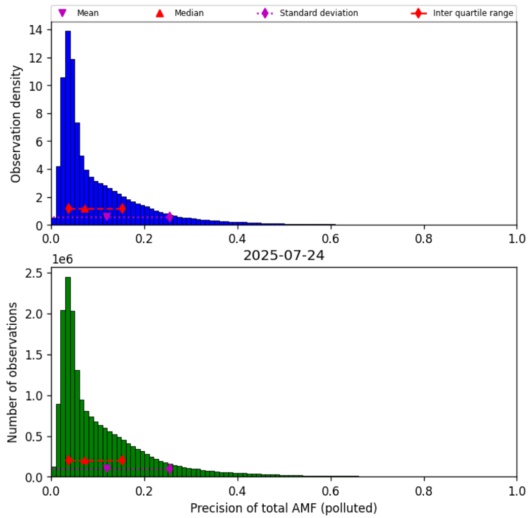
Figure 80: Histogram of “Precision of total AMF (polluted)” for 2025-07-24 to 2025-07-25
