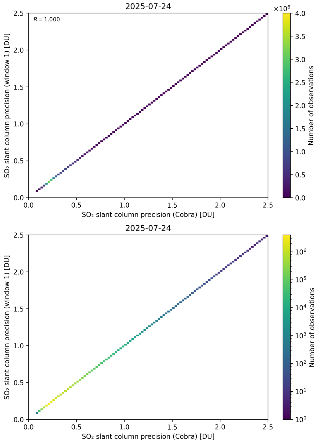
Figure 209: Scatter density plot of “SO 2 slant column precision (Cobra)” against “SO 2 slant column precision (window 1)” for 2025-07-24 to 2025-07-25.
