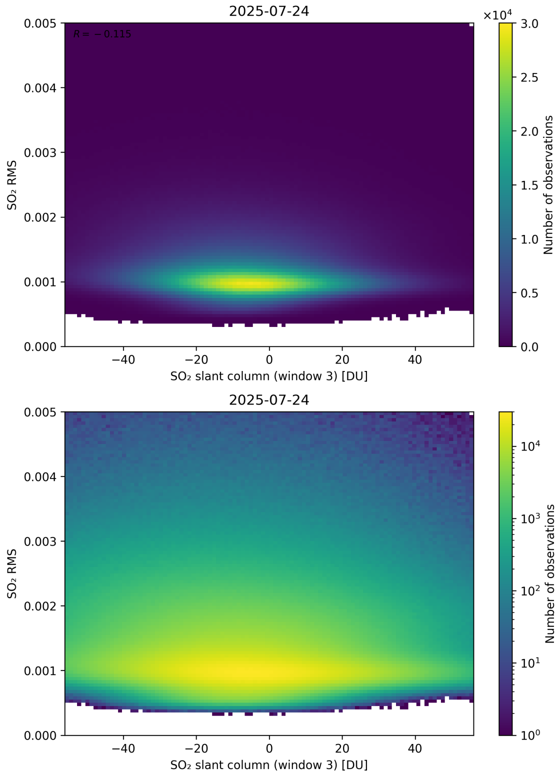
Figure 306: Scatter density plot of “SO 2 slant column (window 3)” against “SO 2 RMS” for 2025-07-24 to 2025-07-25.
