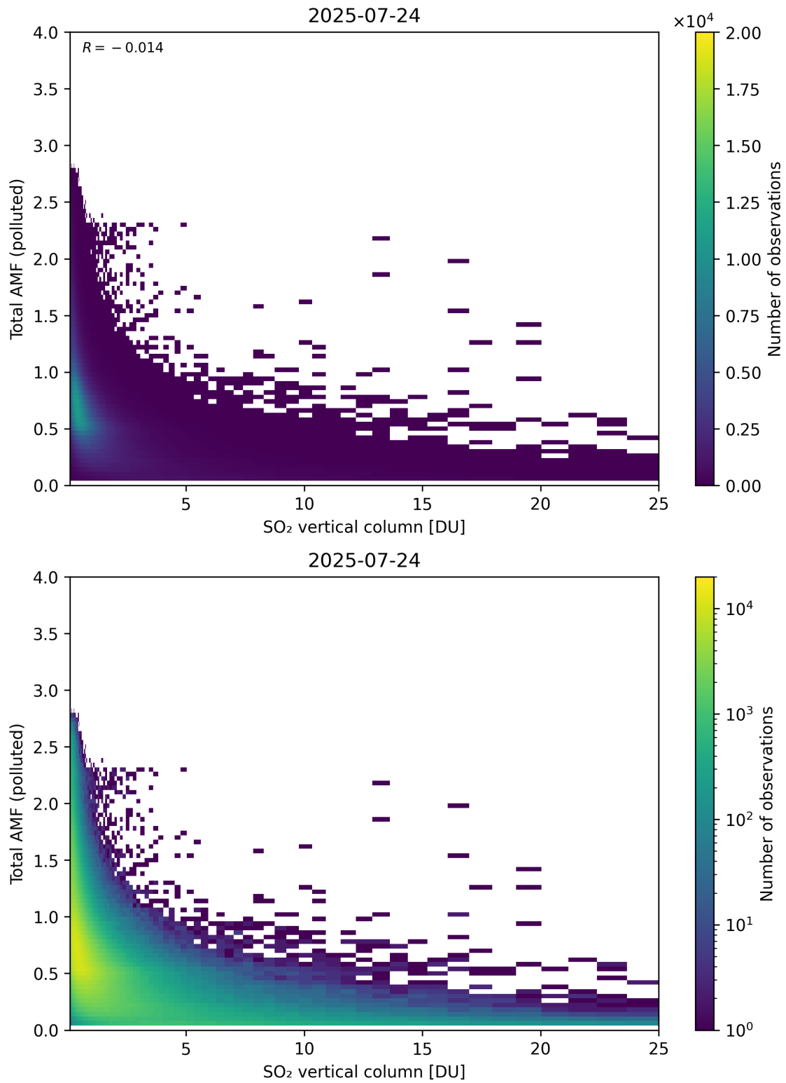
Figure 359: Scatter density plot of “SO 2 vertical column” against “Total AMF (polluted)” for 2025-07-24 to 2025-07-25.
