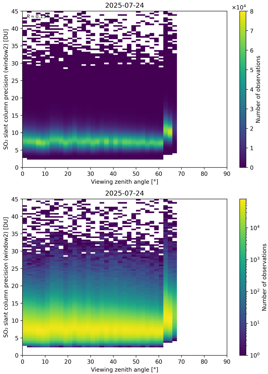
Figure 378: Scatter density plot of “Viewing zenith angle” against “SO 2 slant column precision (window2)” for 2025-07-24 to 2025-07-25.
