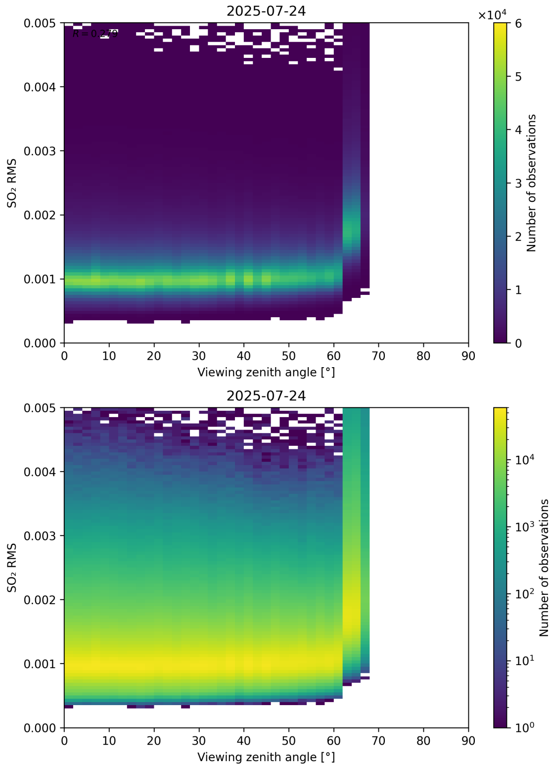
Figure 367: Scatter density plot of “Viewing zenith angle” against “SO 2 RMS” for 2025-07-24 to 2025-07-25.
