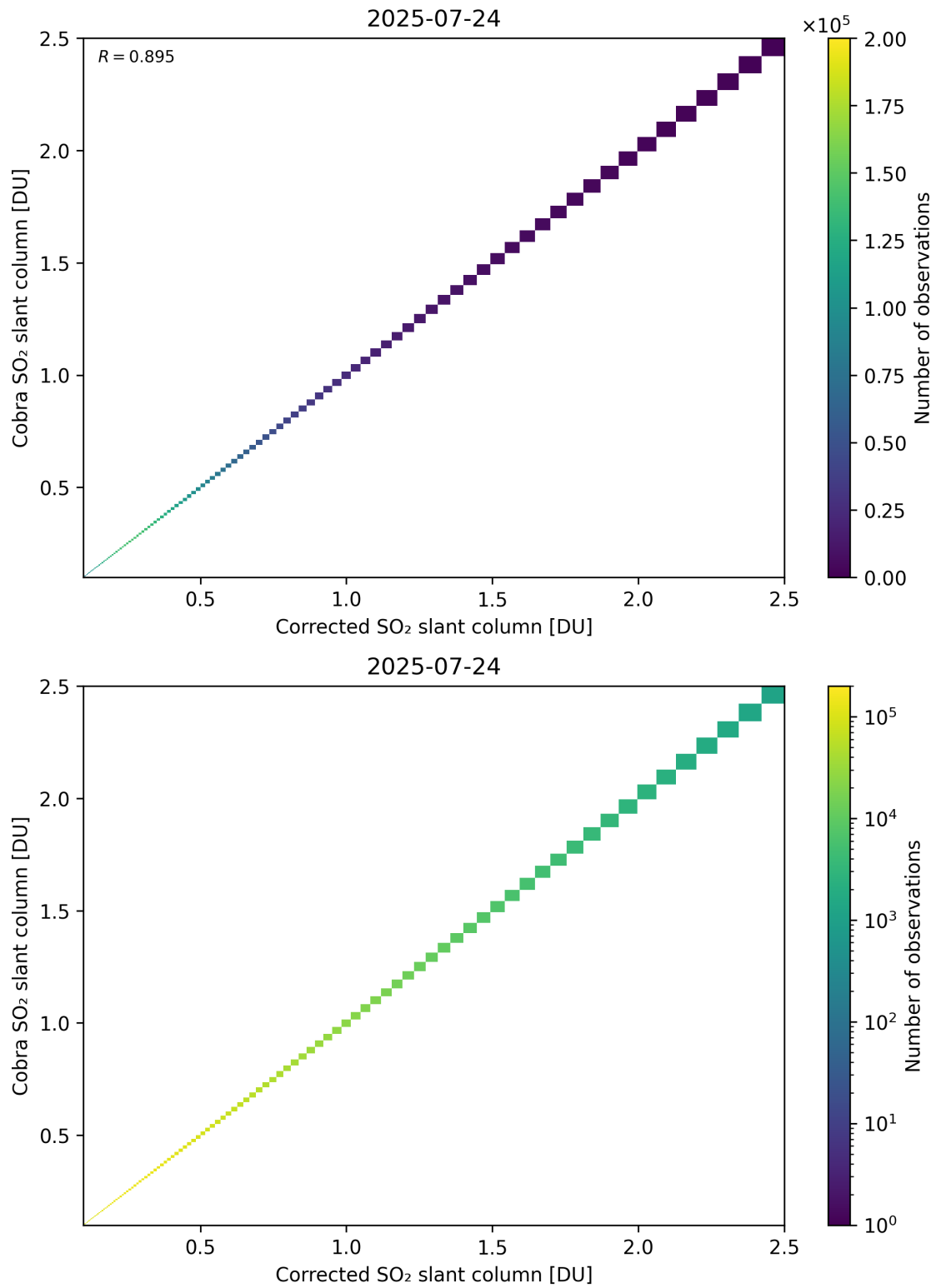
Figure 233: Scatter density plot of “Corrected SO 2 slant column” against “Cobra SO 2 slant column” for 2025-07-24 to 2025-07-25.
