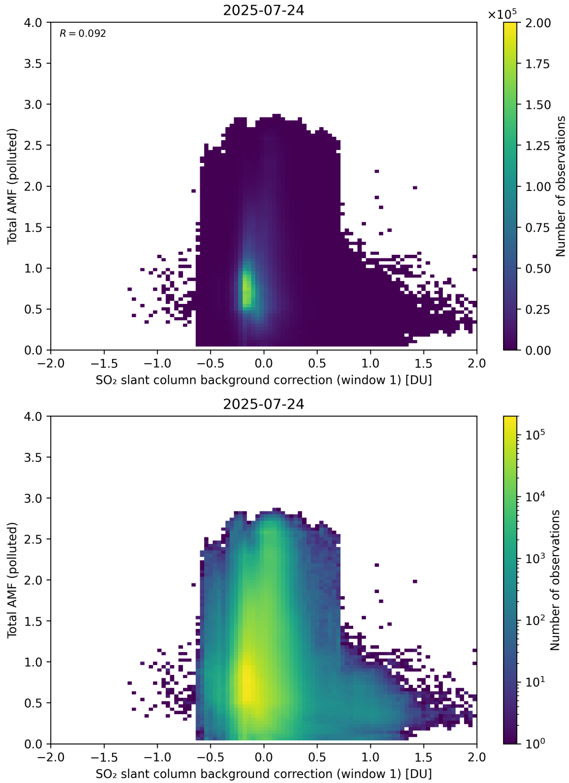
Figure 120: Scatter density plot of “SO 2 slant column background correction (window 1)” against “Total AMF (polluted)” for 2025-07-24 to 2025-07-25.
