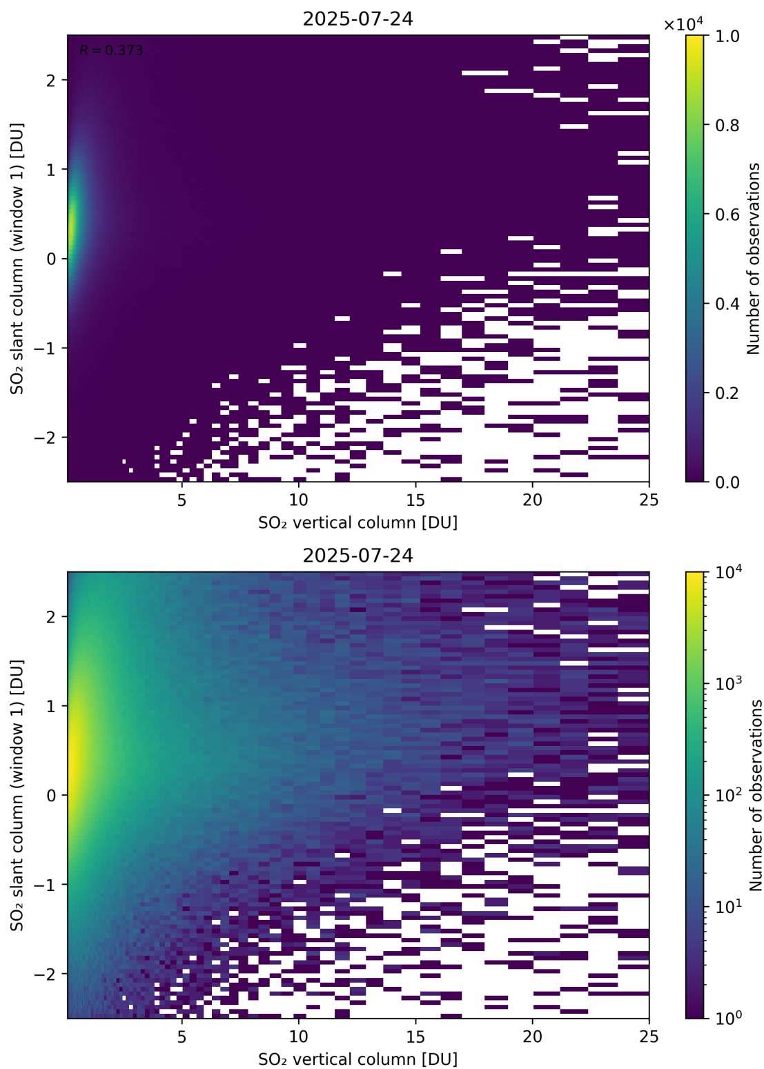
Figure 354: Scatter density plot of “SO 2 vertical column” against “SO 2 slant column (window 1)” for 2025-07-24 to 2025-07-25.
