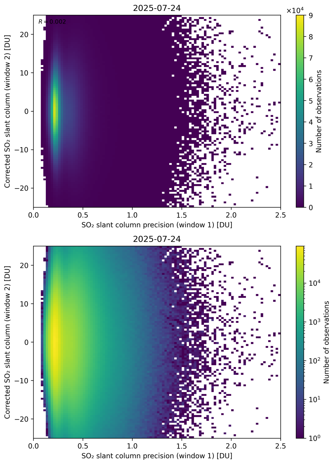
Figure 275: Scatter density plot of “SO 2 slant column precision (window 1)” against “Corrected SO 2 slant column (window 2)” for 2025-07-24 to 2025-07-25.
