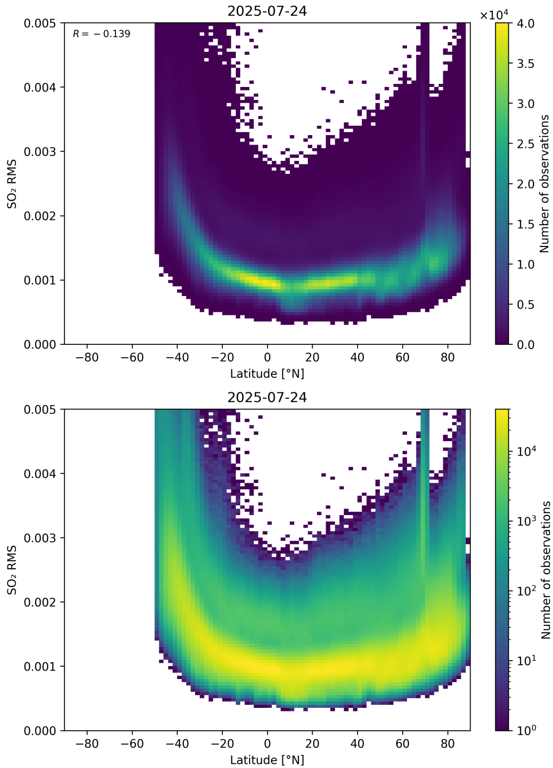
Figure 155: Scatter density plot of “Latitude” against “SO 2 RMS” for 2025-07-24 to 2025-07-25.
