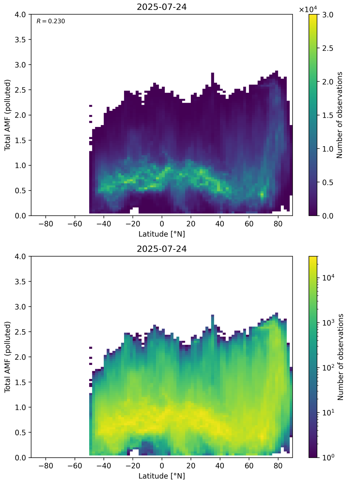
Figure 167: Scatter density plot of “Latitude” against “Total AMF (polluted)” for 2025-07-24 to 2025-07-25.
