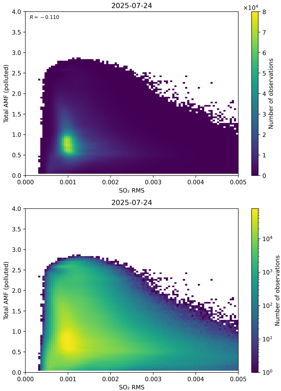
Figure 148: Scatter density plot of “SO 2 RMS” against “Total AMF (polluted)” for 2025-07-24 to 2025-07-25.
