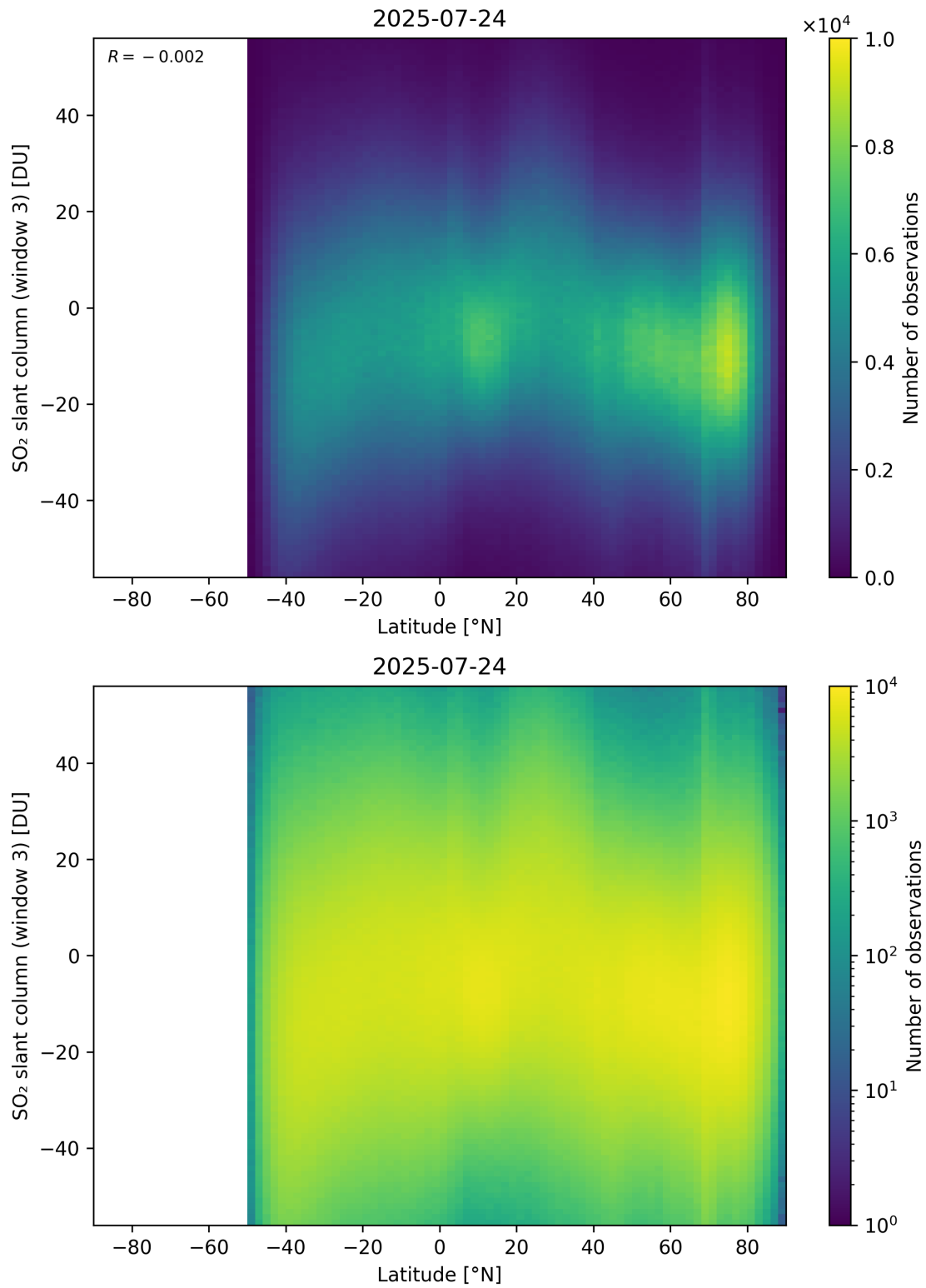
Figure 165: Scatter density plot of “Latitude” against “SO 2 slant column (window 3)” for 2025-07-24 to 2025-07-25.
