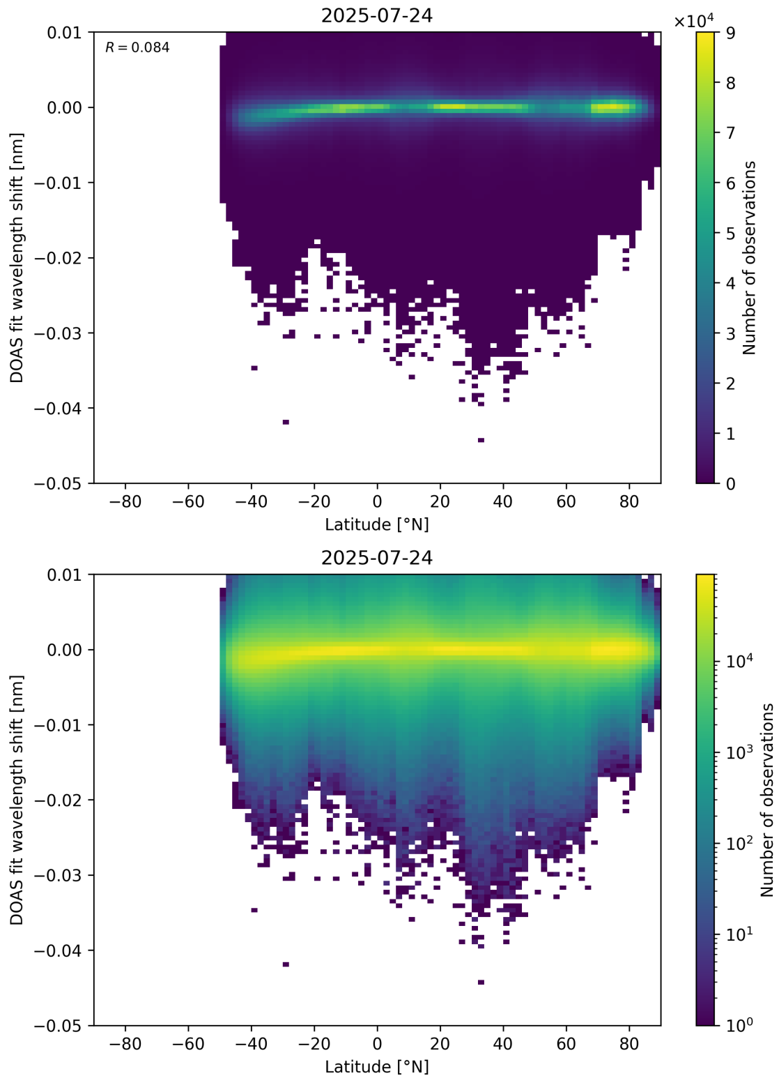
Figure 153: Scatter density plot of “Latitude” against “DOAS fit wavelength shift” for 2025-07-24 to 2025-07-25.
