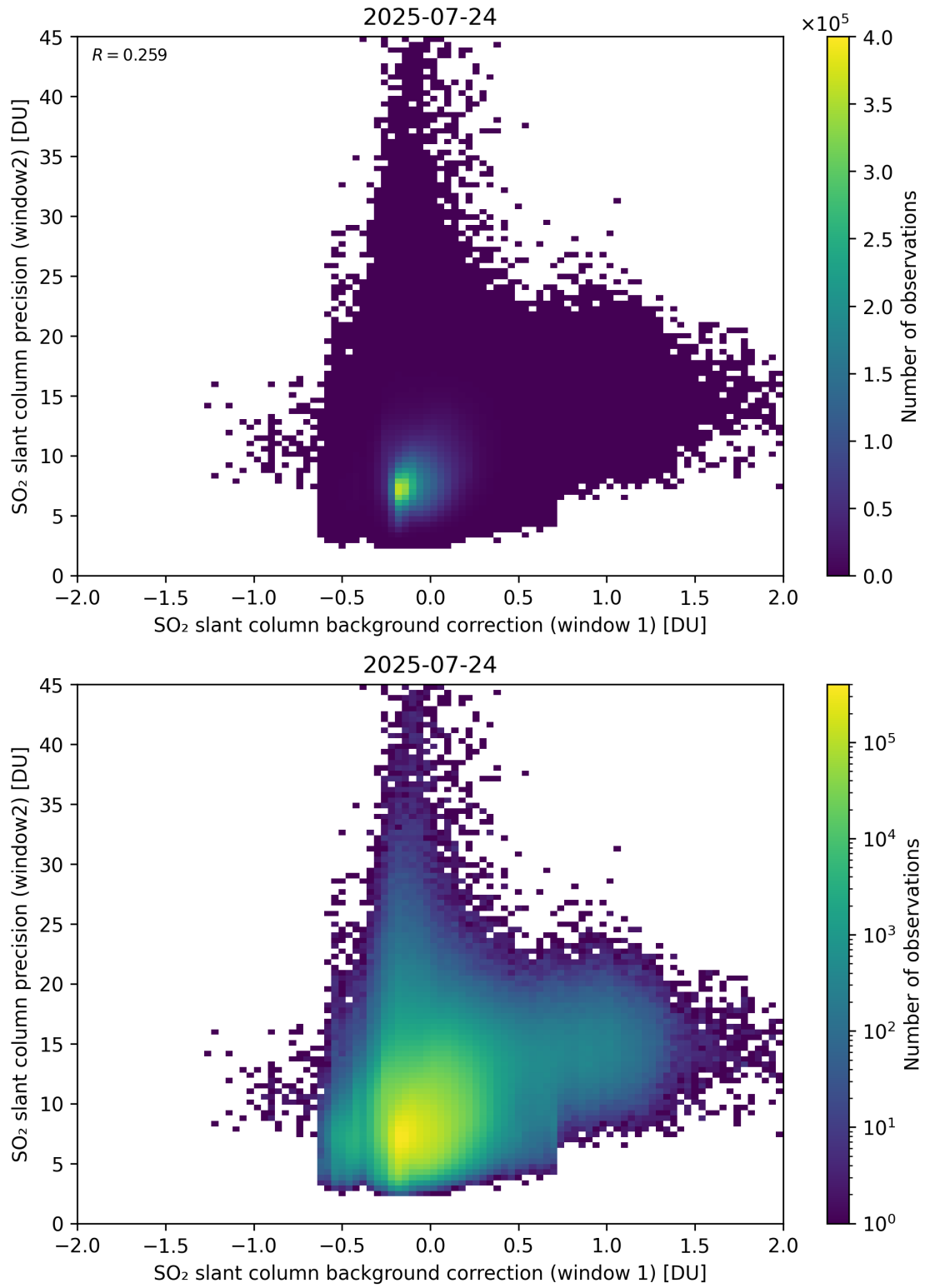
Figure 117: Scatter density plot of “SO 2 slant column background correction (window 1)” against “SO 2 slant column precision (window2)” for 2025-07-24 to 2025-07-25.
