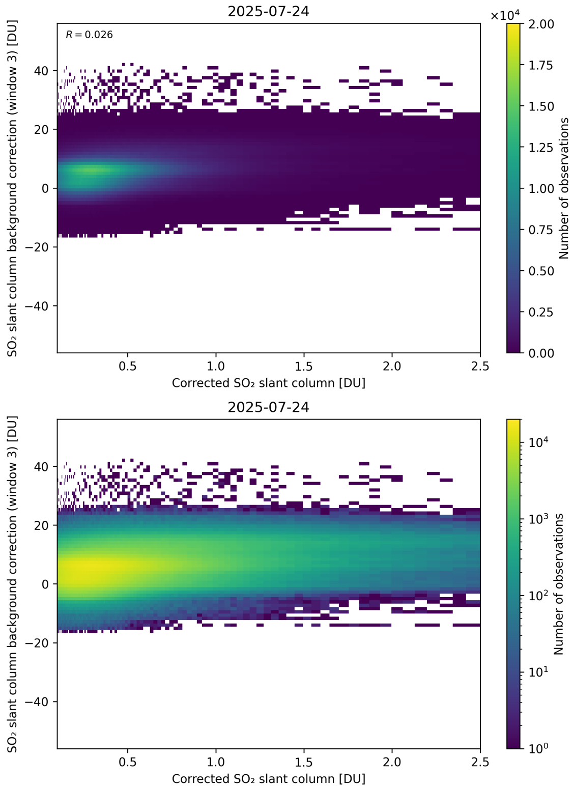
Figure 228: Scatter density plot of “Corrected SO 2 slant column” against “SO 2 slant column background correction (window 3)” for 2025-07-24 to 2025-07-25.
