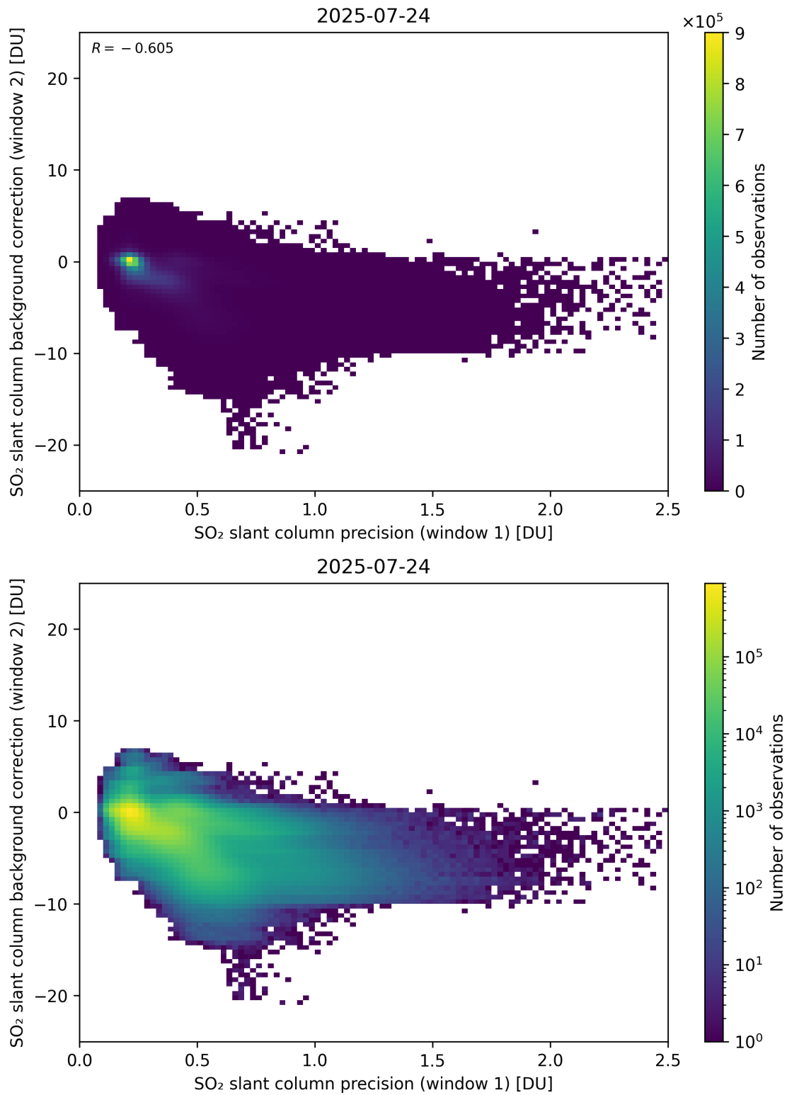
Figure 269: Scatter density plot of “SO 2 slant column precision (window 1)” against “SO 2 slant column background correction (window 2)” for 2025-07-24 to 2025-07-25.
