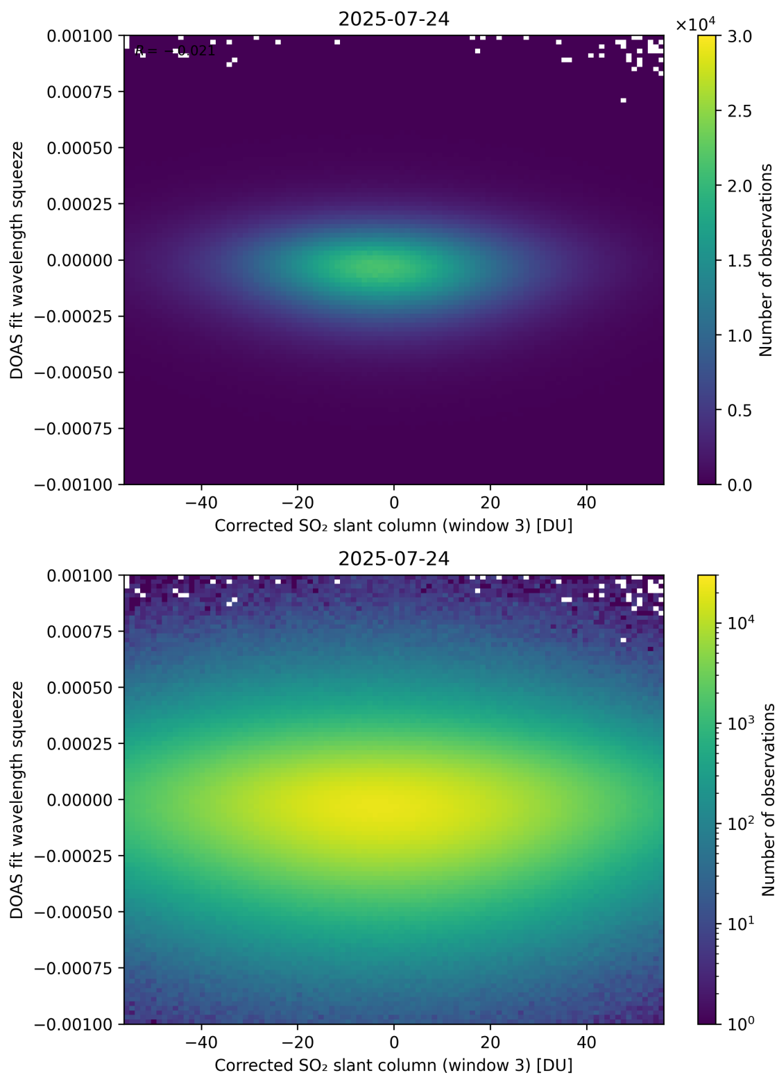
Figure 257: Scatter density plot of “Corrected SO 2 slant column (window 3)” against “DOAS fit wavelength squeeze” for 2025-07-24 to 2025-07-25.
