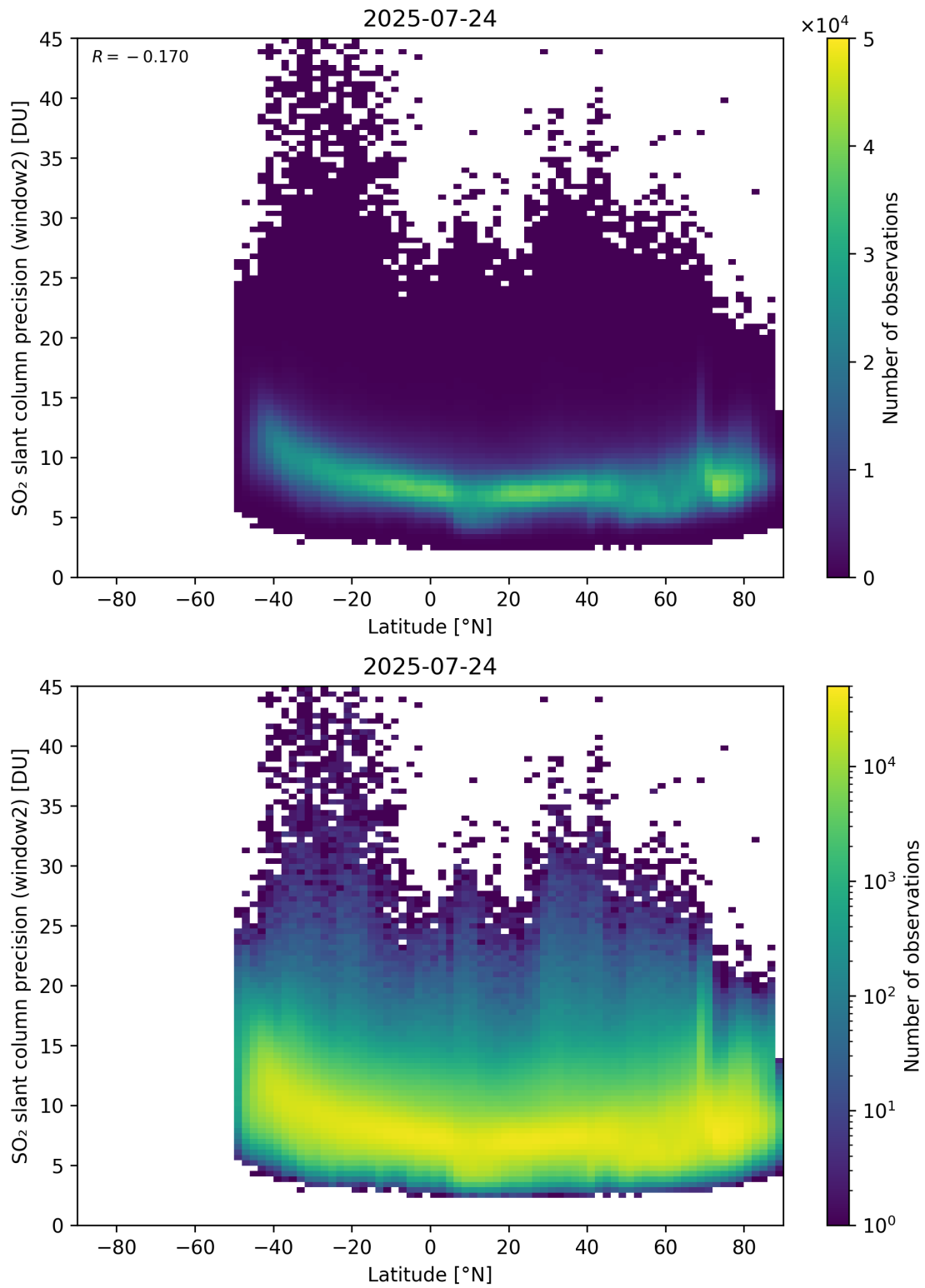
Figure 164: Scatter density plot of “Latitude” against “SO 2 slant column precision (window2)” for 2025-07-24 to 2025-07-25.
