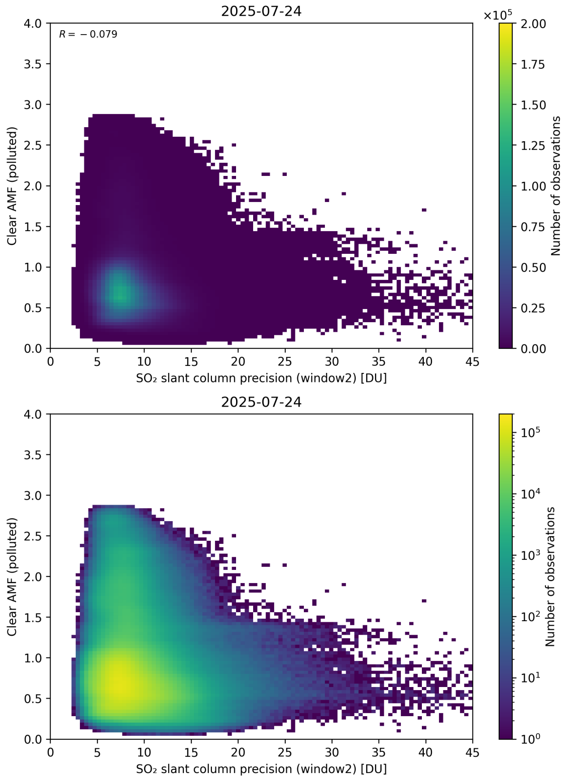
Figure 296: Scatter density plot of “SO 2 slant column precision (window2)” against “Clear AMF (polluted)” for 2025-07-24 to 2025-07-25.
