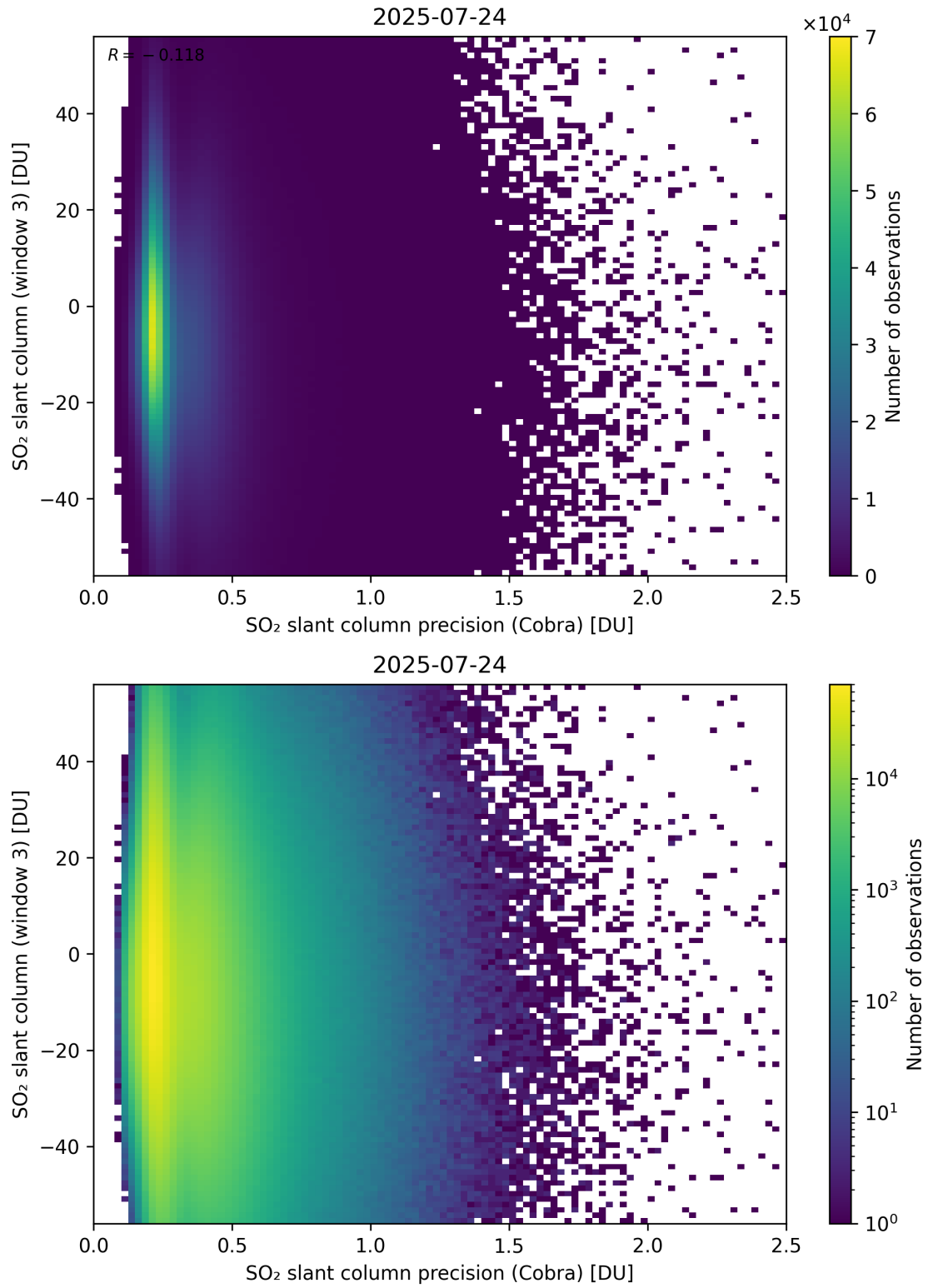
Figure 211: Scatter density plot of “SO 2 slant column precision (Cobra)” against “SO 2 slant column (window 3)” for 2025-07-24 to 2025-07-25.
