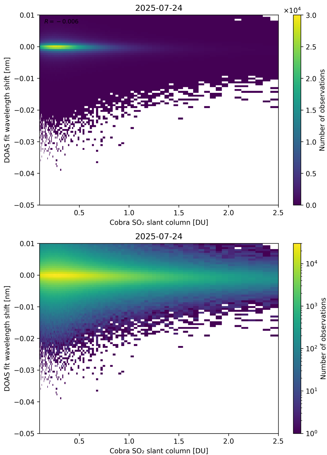
Figure 196: Scatter density plot of “Cobra SO 2 slant column” against “DOAS fit wavelength shift” for 2025-07-24 to 2025-07-25.
