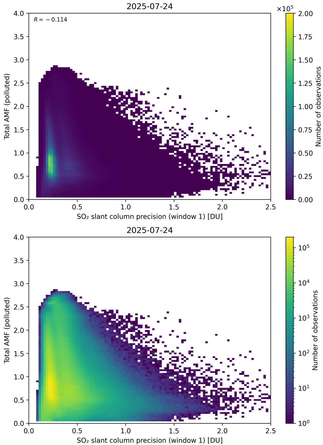
Figure 280: Scatter density plot of “SO 2 slant column precision (window 1)” against “Total AMF (polluted)” for 2025-07-24 to 2025-07-25.
