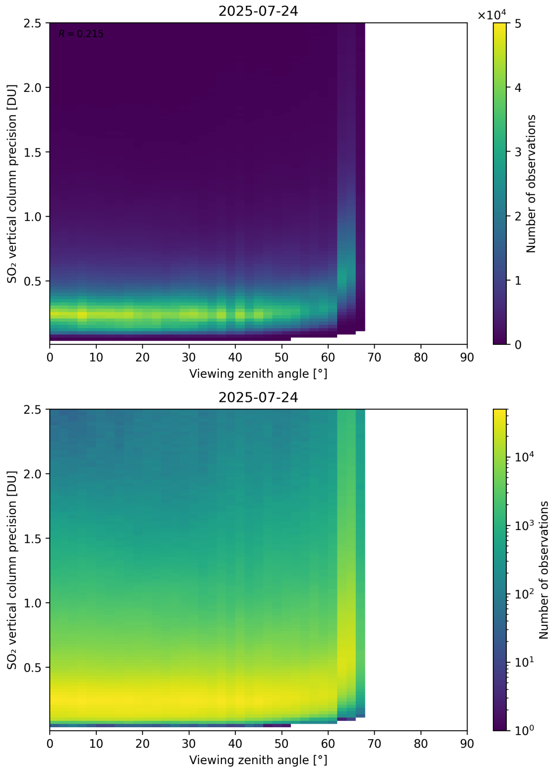
Figure 384: Scatter density plot of “Viewing zenith angle” against “SO 2 vertical column precision” for 2025-07-24 to 2025-07-25.
