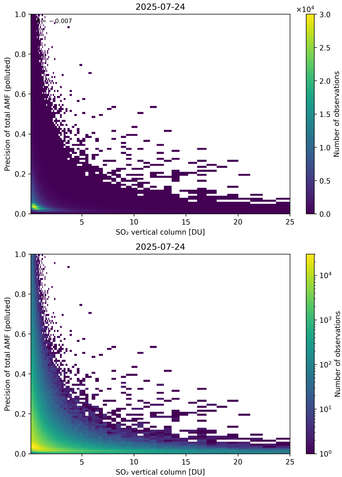
Figure 360: Scatter density plot of “SO 2 vertical column” against “Precision of total AMF (polluted)” for 2025-07-24 to 2025-07-25.
