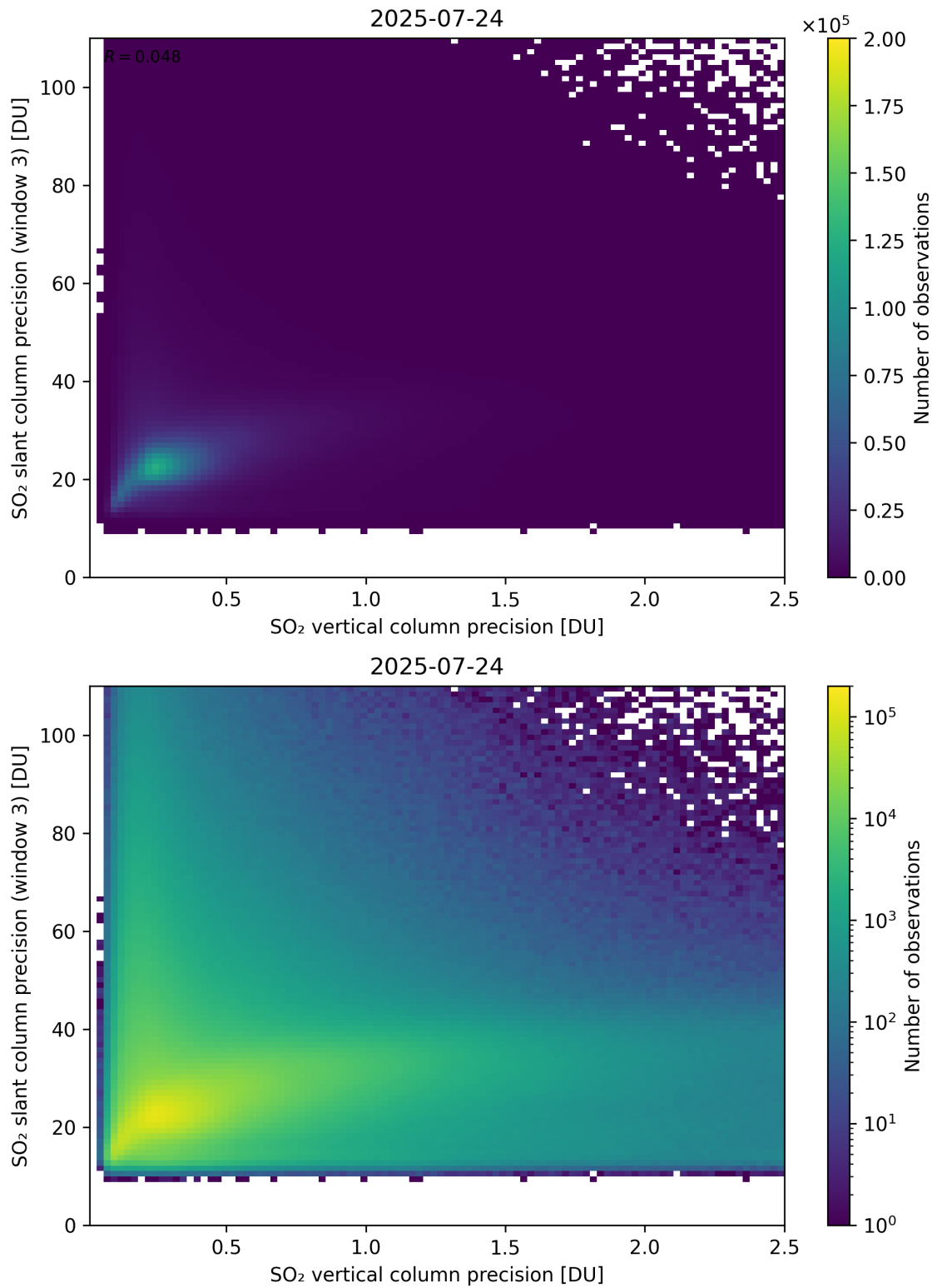
Figure 345: Scatter density plot of “SO 2 vertical column precision” against “SO 2 slant column precision (window 3)” for 2025-07-24 to 2025-07-25.
