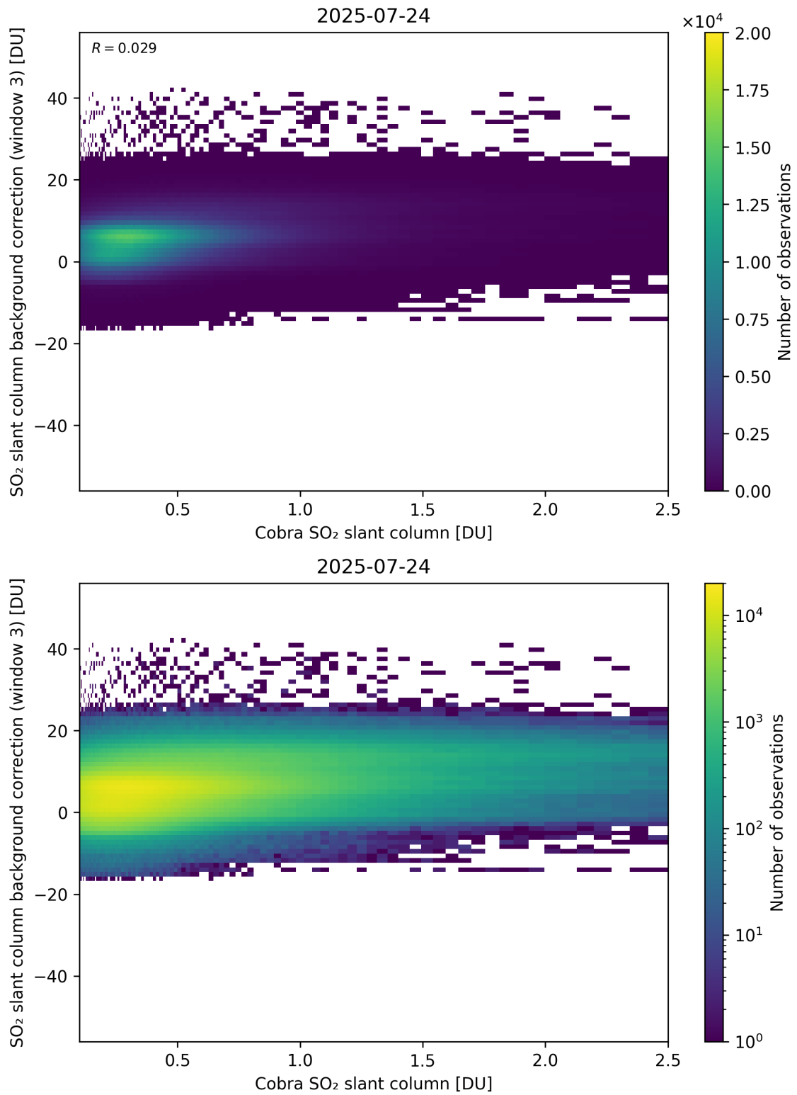
Figure 195: Scatter density plot of “Cobra SO 2 slant column” against “SO 2 slant column background correction (window 3)” for 2025-07-24 to 2025-07-25.
