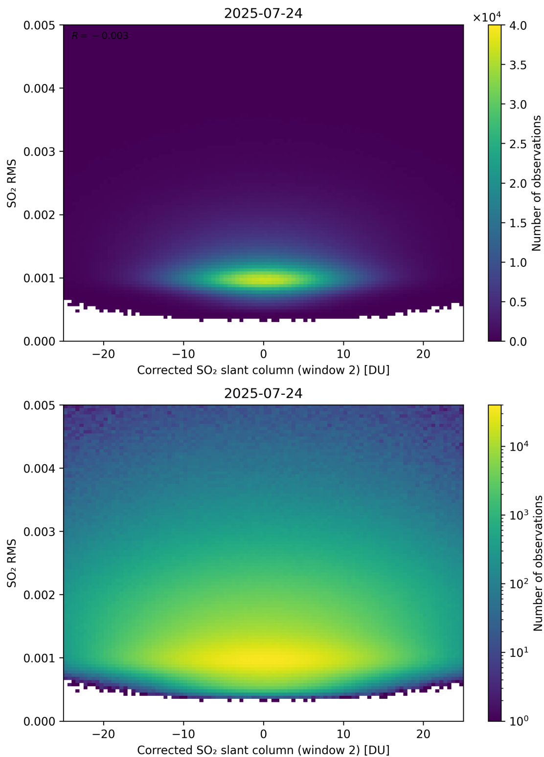
Figure 248: Scatter density plot of “Corrected SO 2 slant column (window 2)” against “SO 2 RMS” for 2025-07-24 to 2025-07-25.
