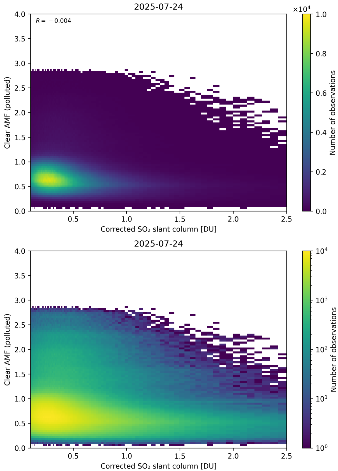
Figure 232: Scatter density plot of “Corrected SO 2 slant column” against “Clear AMF (polluted)” for 2025-07-24 to 2025-07-25.
