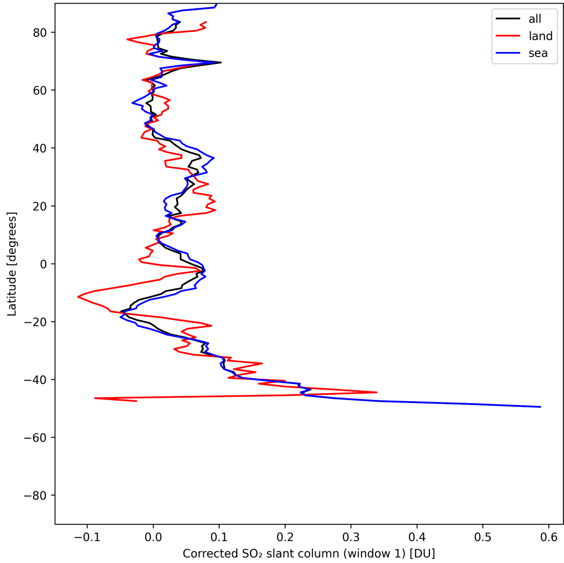
Figure 39: Zonal average of “Corrected SO 2 slant column (window 1)” for 2025-07-24 to 2025-07-25.
