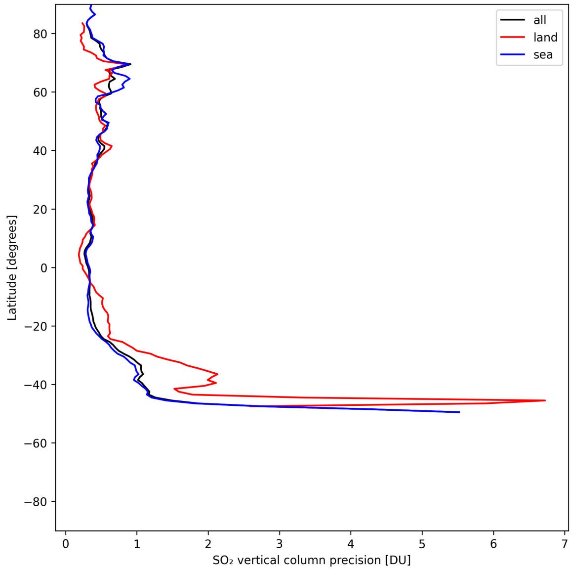
Figure 33: Zonal average of “SO 2 vertical column precision” for 2025-07-24 to 2025-07-25.
