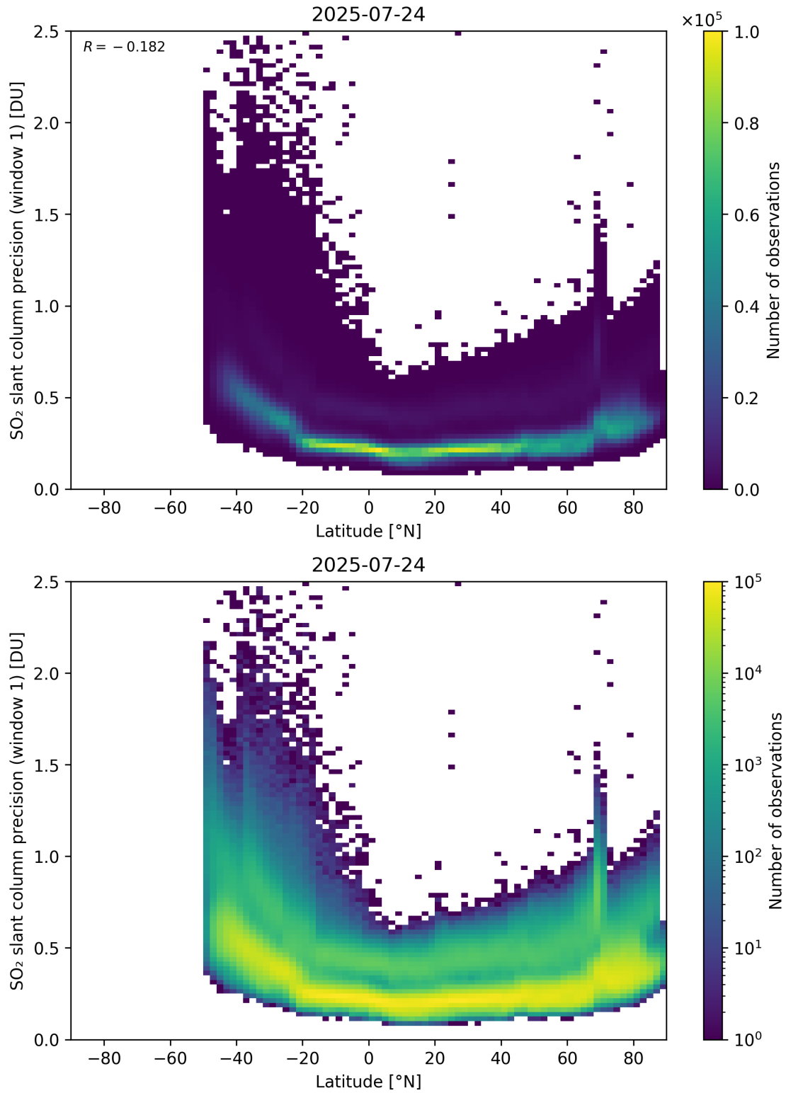
Figure 163: Scatter density plot of “Latitude” against “SO 2 slant column precision (window 1)” for 2025-07-24 to 2025-07-25.
