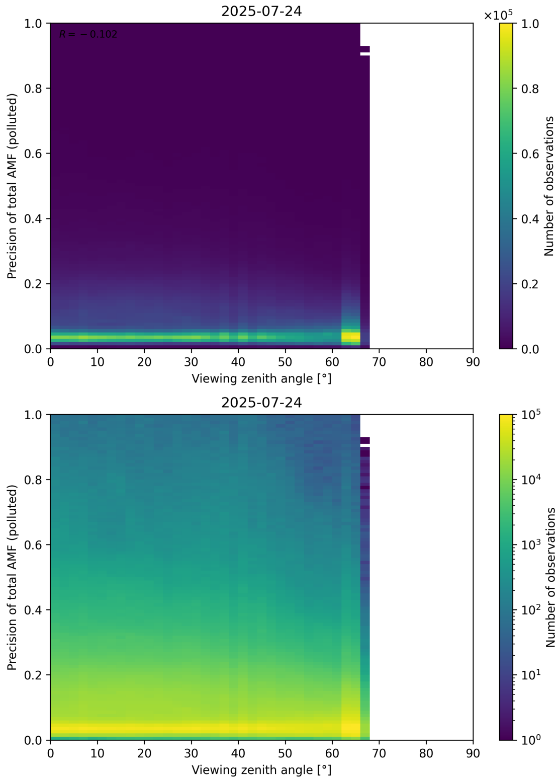
Figure 382: Scatter density plot of “Viewing zenith angle” against “Precision of total AMF (polluted)” for 2025-07-24 to 2025-07-25.
