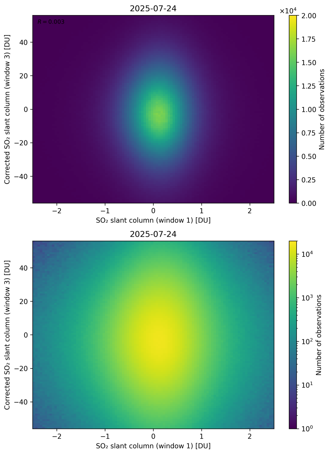
Figure 284: Scatter density plot of “SO 2 slant column (window 1)” against “Corrected SO 2 slant column (window 3)” for 2025-07-24 to 2025-07-25.
