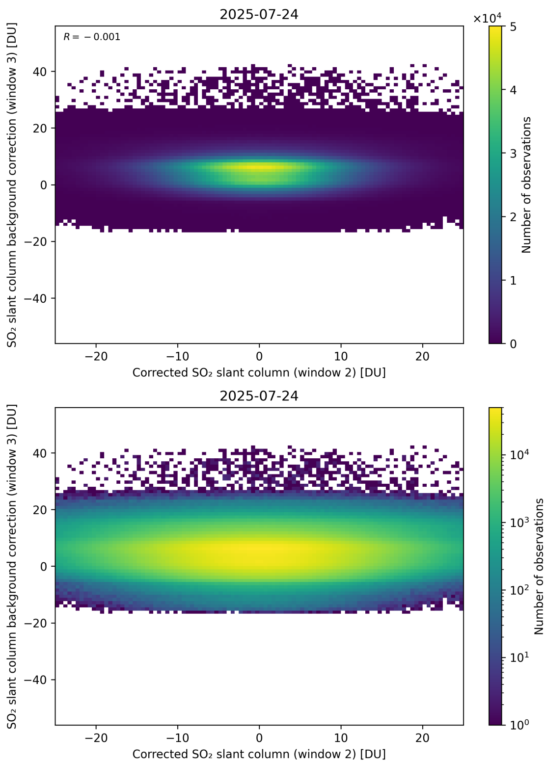
Figure 245: Scatter density plot of “Corrected SO 2 slant column (window 2)” against “SO 2 slant column background correction (window 3)” for 2025-07-24 to 2025-07-25.
