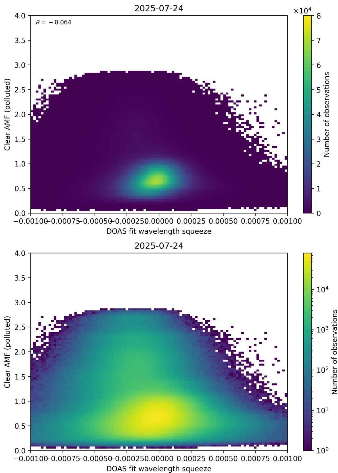
Figure 144: Scatter density plot of “DOAS fit wavelength squeeze” against “Clear AMF (polluted)” for 2025-07-24 to 2025-07-25.
