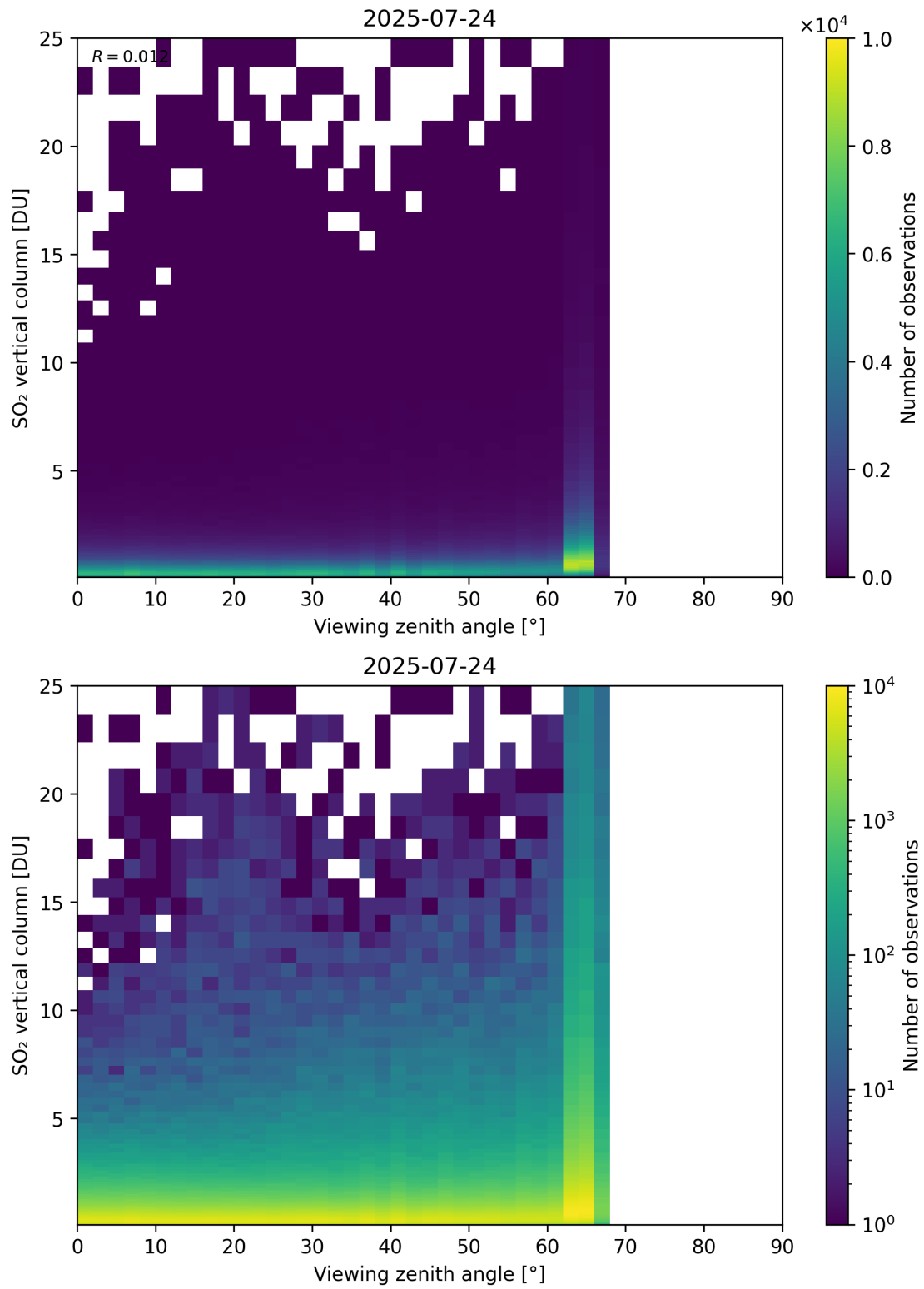
Figure 383: Scatter density plot of “Viewing zenith angle” against “SO 2 vertical column” for 2025-07-24 to 2025-07-25.
