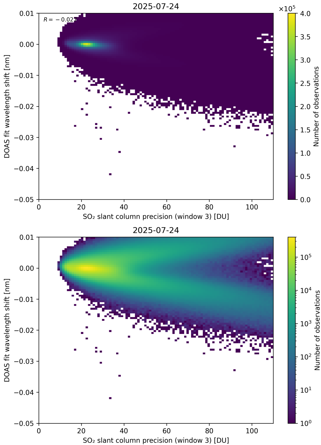
Figure 308: Scatter density plot of “SO 2 slant column precision (window 3)” against “DOAS fit wavelength shift” for 2025-07-24 to 2025-07-25.
