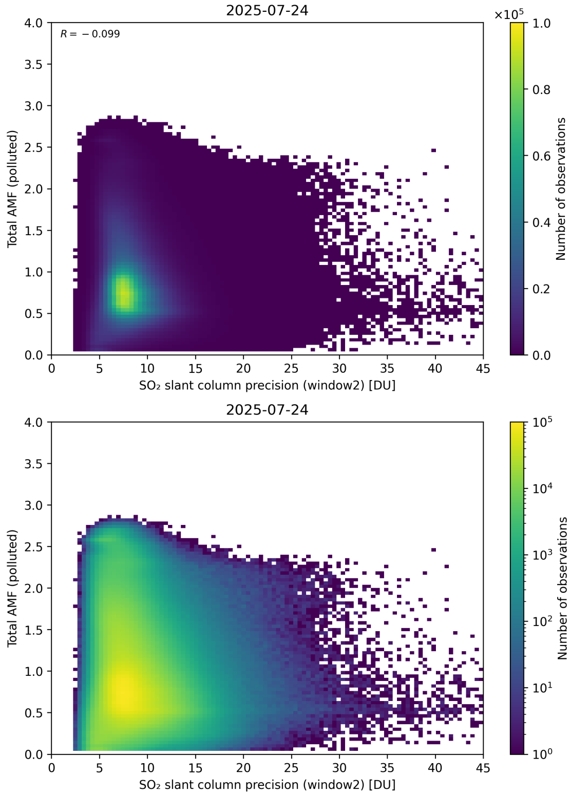
Figure 301: Scatter density plot of “SO 2 slant column precision (window2)” against “Total AMF (polluted)” for 2025-07-24 to 2025-07-25.
