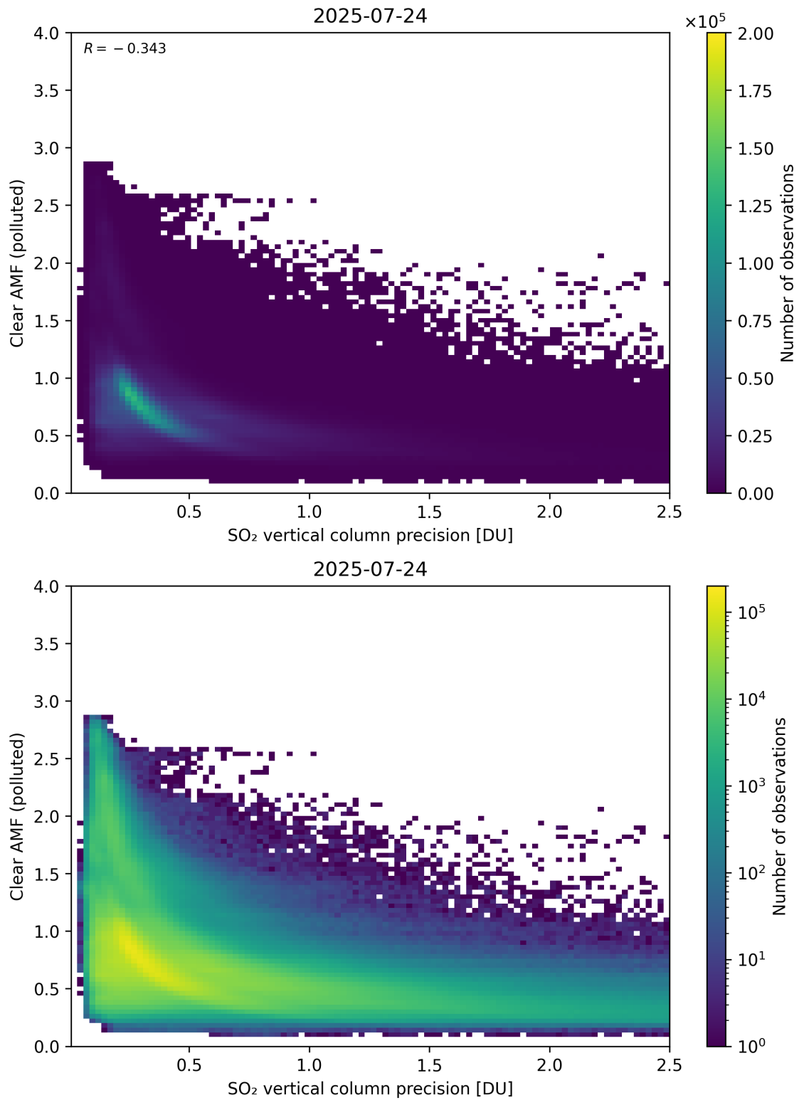
Figure 335: Scatter density plot of “SO 2 vertical column precision” against “Clear AMF (polluted)” for 2025-07-24 to 2025-07-25.
