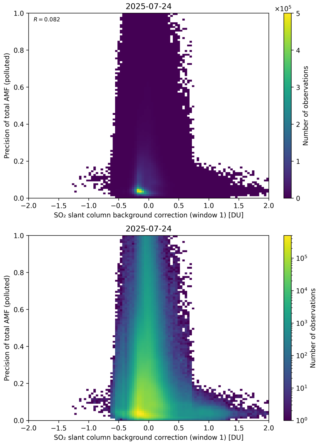
Figure 121: Scatter density plot of “SO 2 slant column background correction (window 1)” against “Precision of total AMF (polluted)” for 2025-07-24 to 2025-07-25.
