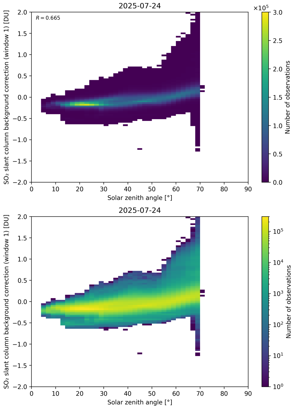
Figure 171: Scatter density plot of “Solar zenith angle” against “SO 2 slant column background correction (window 1)” for 2025-07-24 to 2025-07-25.
