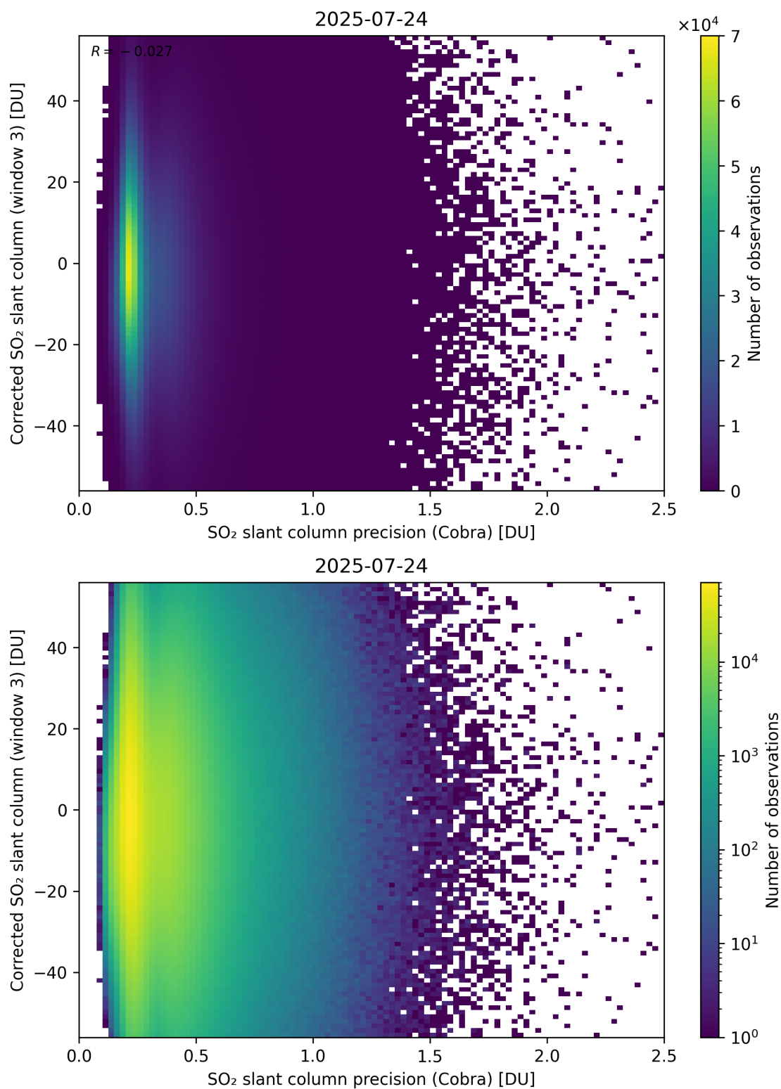
Figure 207: Scatter density plot of “SO 2 slant column precision (Cobra)” against “Corrected SO 2 slant column (window 3)” for 2025-07-24 to 2025-07-25.
