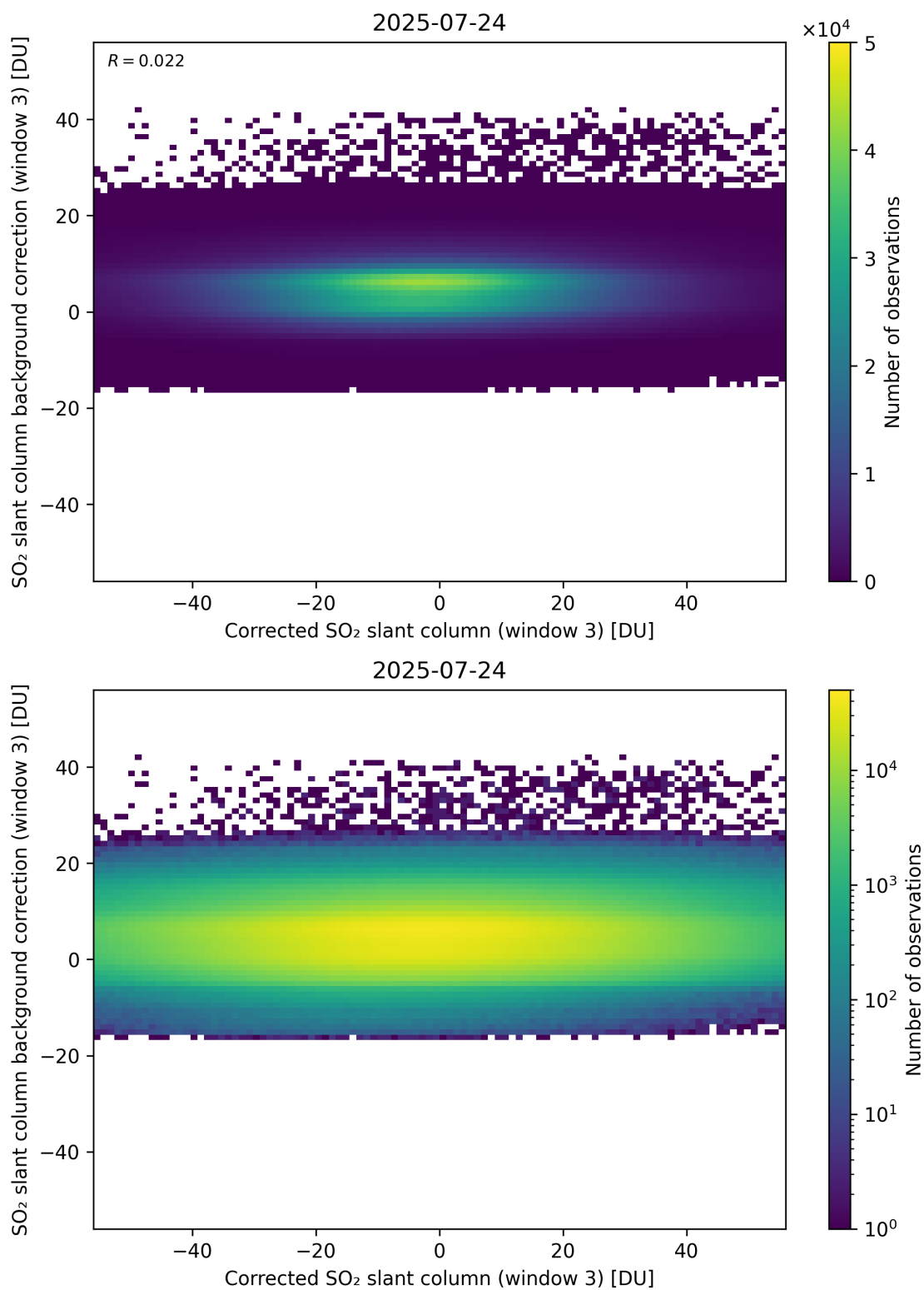
Figure 255: Scatter density plot of “Corrected SO 2 slant column (window 3)” against “SO 2 slant column background correction (window 3)” for 2025-07-24 to 2025-07-25.
