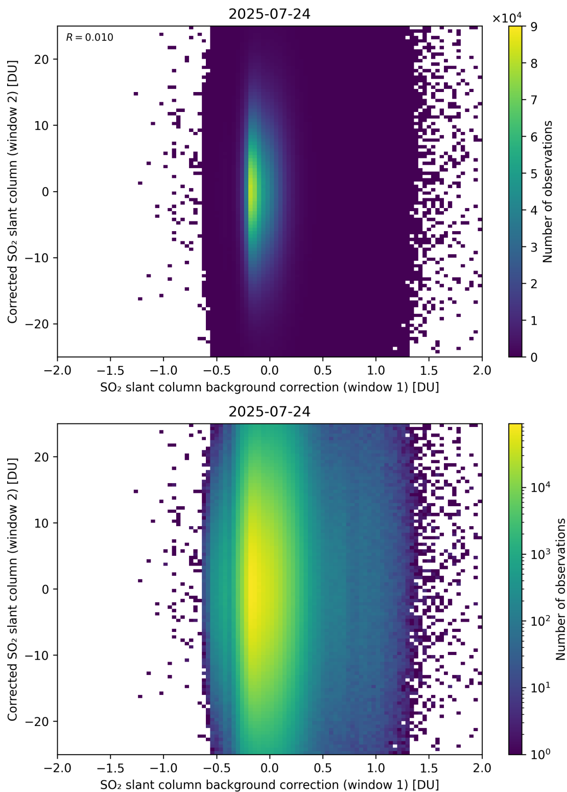
Figure 115: Scatter density plot of “SO 2 slant column background correction (window 1)” against “Corrected SO 2 slant column (window 2)” for 2025-07-24 to 2025-07-25.
