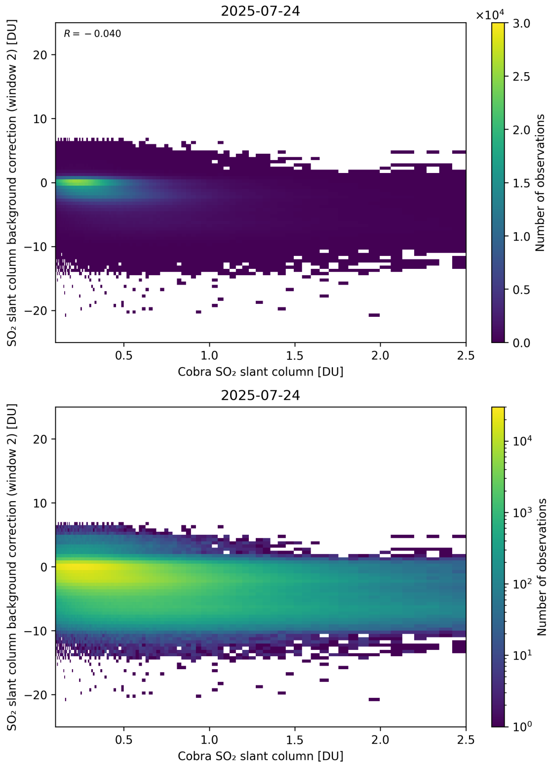
Figure 194: Scatter density plot of “Cobra SO 2 slant column” against “SO 2 slant column background correction (window 2)” for 2025-07-24 to 2025-07-25.
