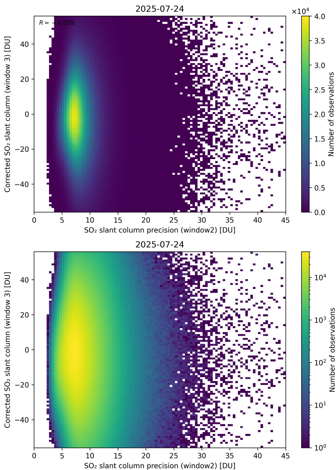
Figure 298: Scatter density plot of “SO 2 slant column precision (window2)” against “Corrected SO 2 slant column (window 3)” for 2025-07-24 to 2025-07-25.
