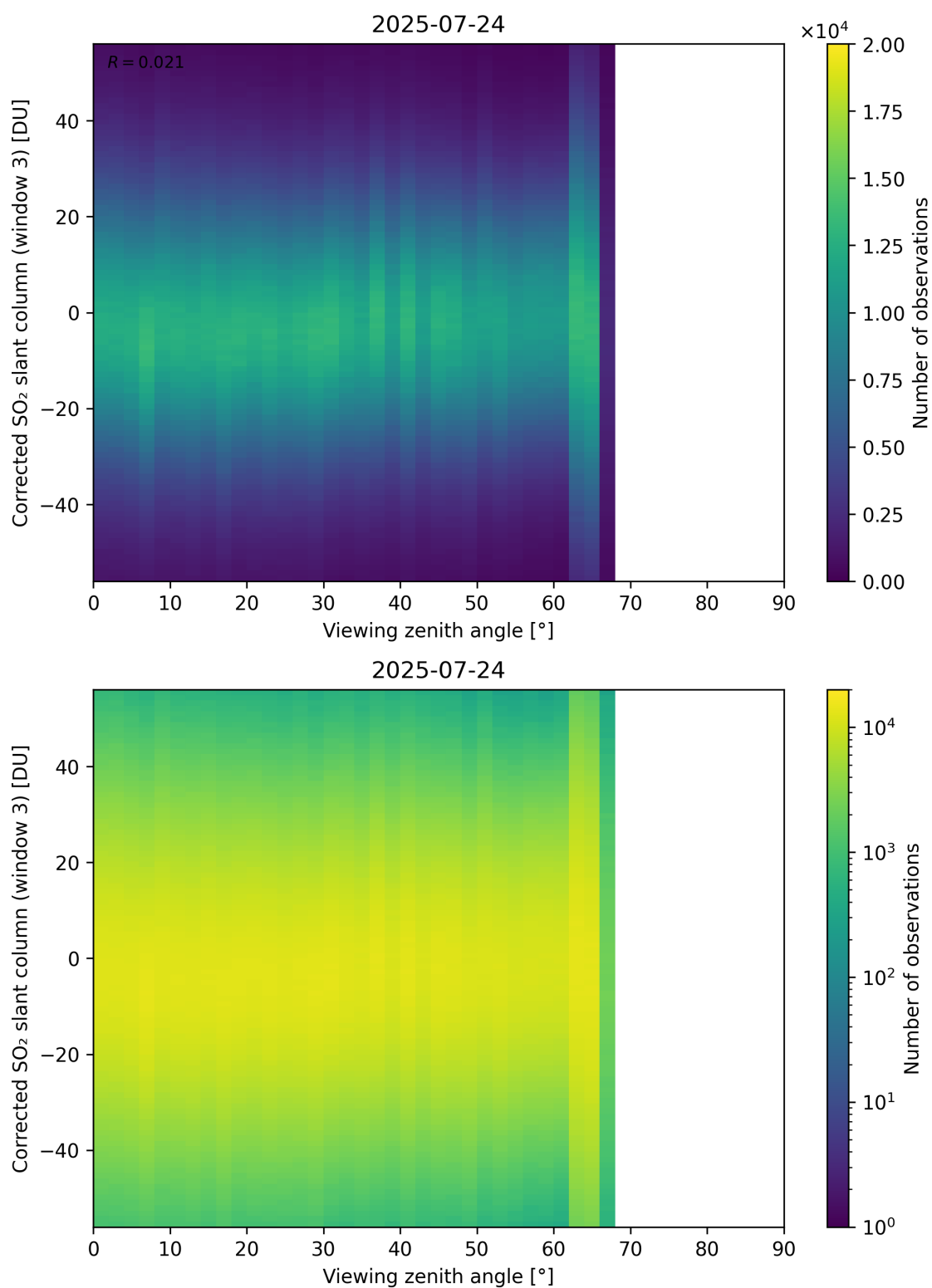
Figure 375: Scatter density plot of “Viewing zenith angle” against “Corrected SO 2 slant column (window 3)” for 2025-07-24 to 2025-07-25.
