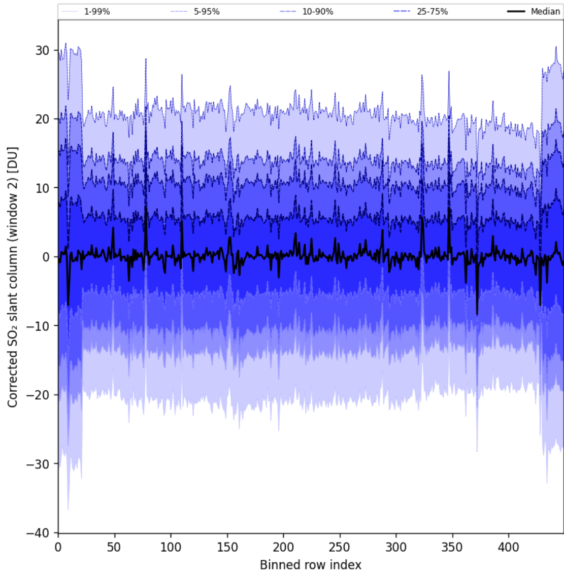
Figure 95: Along track statistics of “Corrected SO 2 slant column (window 2)” for 2025-07-24 to 2025-07-25
