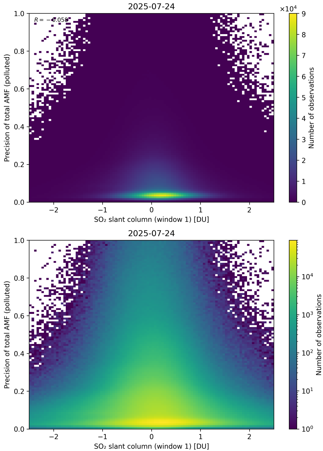
Figure 290: Scatter density plot of “SO 2 slant column (window 1)” against “Precision of total AMF (polluted)” for 2025-07-24 to 2025-07-25.
