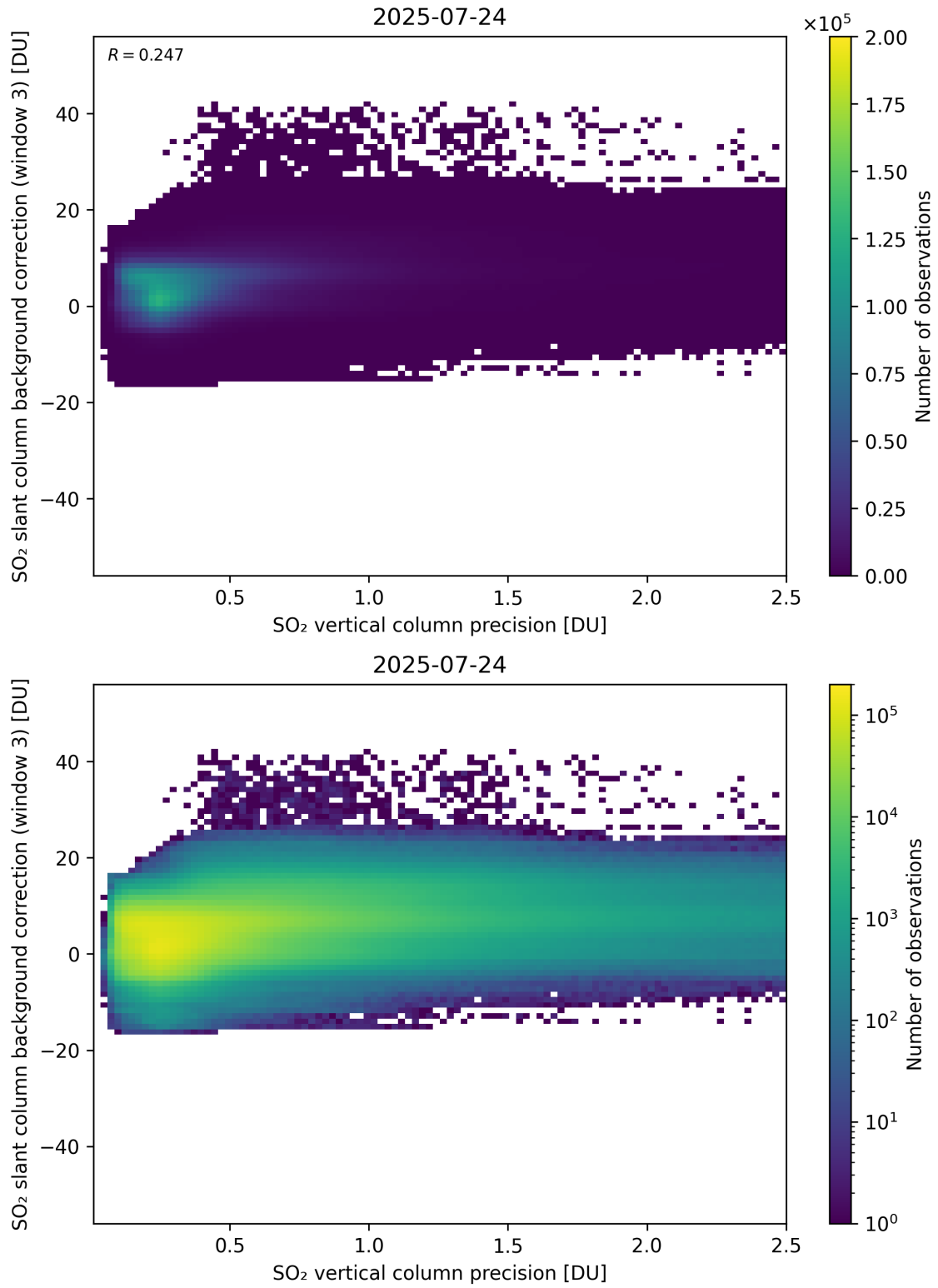
Figure 331: Scatter density plot of “SO 2 vertical column precision” against “SO 2 slant column background correction (window 3)” for 2025-07-24 to 2025-07-25.
