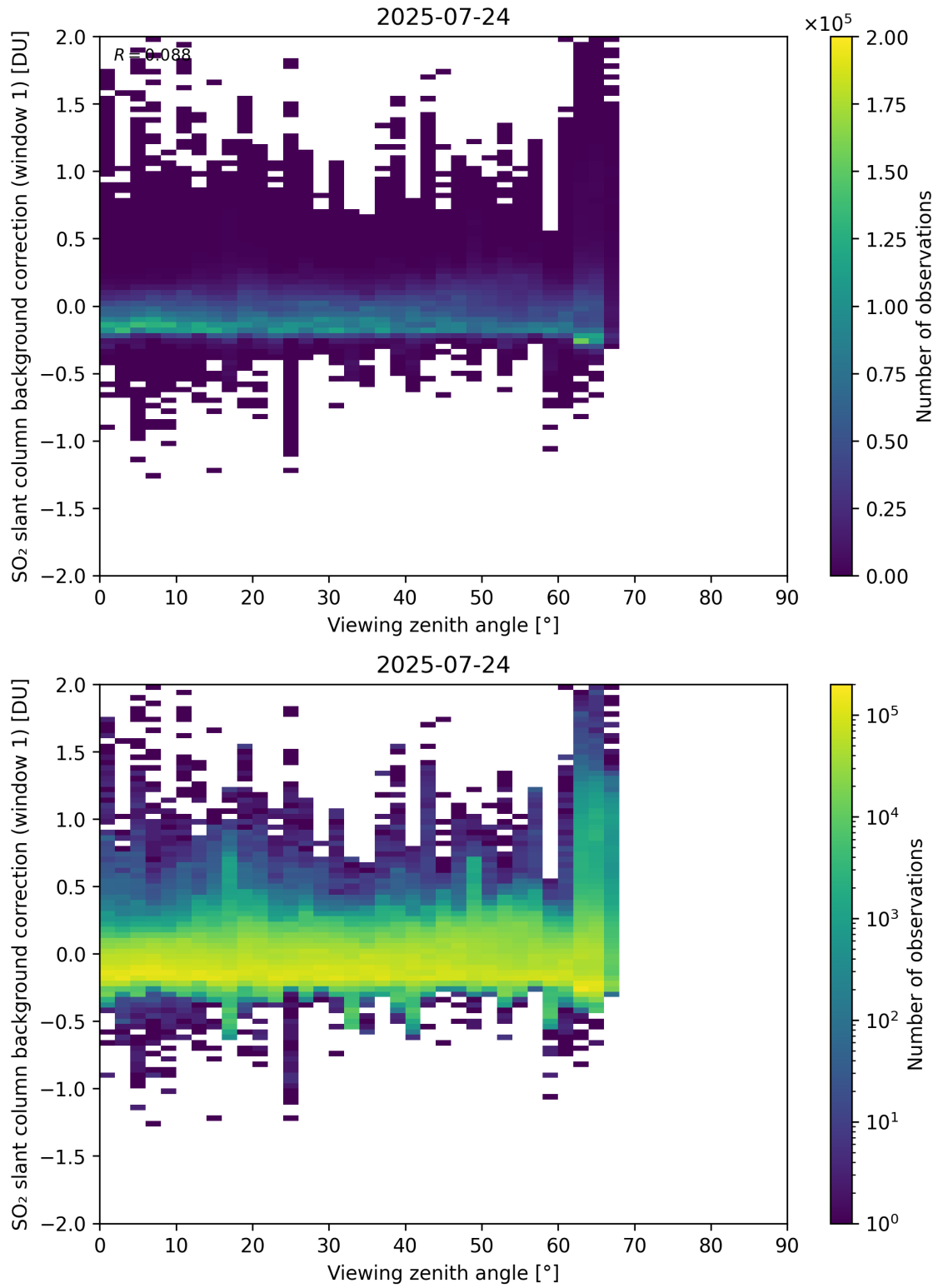
Figure 362: Scatter density plot of “Viewing zenith angle” against “SO 2 slant column background correction (window 1)” for 2025-07-24 to 2025-07-25.
