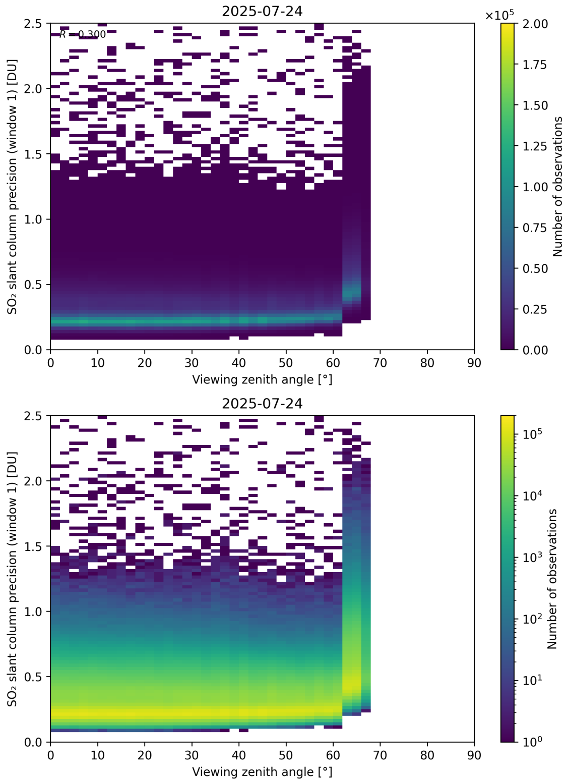
Figure 377: Scatter density plot of “Viewing zenith angle” against “SO 2 slant column precision (window 1)” for 2025-07-24 to 2025-07-25.
