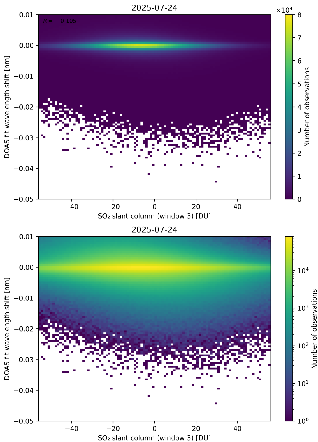
Figure 304: Scatter density plot of “SO 2 slant column (window 3)” against “DOAS fit wavelength shift” for 2025-07-24 to 2025-07-25.
