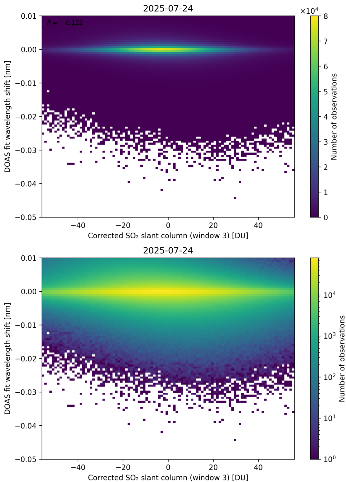
Figure 256: Scatter density plot of “Corrected SO 2 slant column (window 3)” against “DOAS fit wavelength shift” for 2025-07-24 to 2025-07-25.
