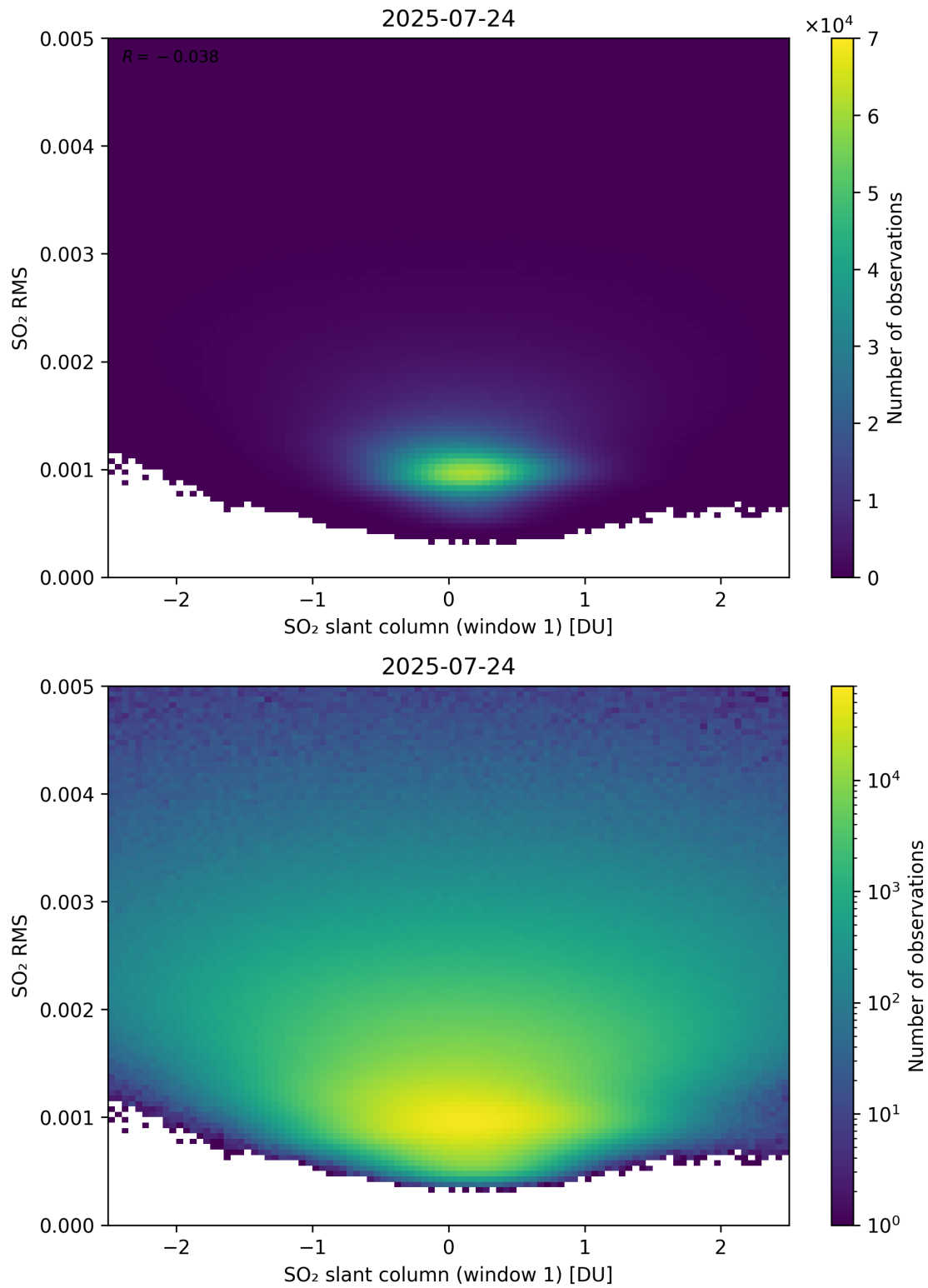
Figure 267: Scatter density plot of “SO 2 slant column (window 1)” against “SO 2 RMS” for 2025-07-24 to 2025-07-25.
