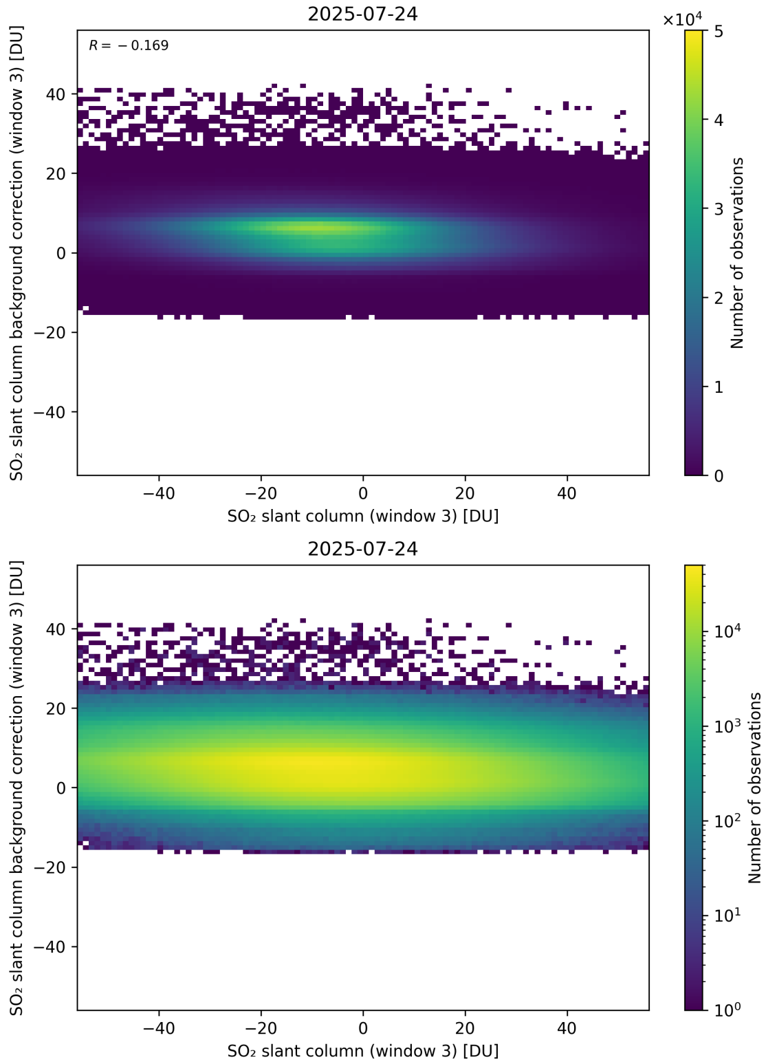
Figure 303: Scatter density plot of “SO 2 slant column (window 3)” against “SO 2 slant column background correction (window 3)” for 2025-07-24 to 2025-07-25.
