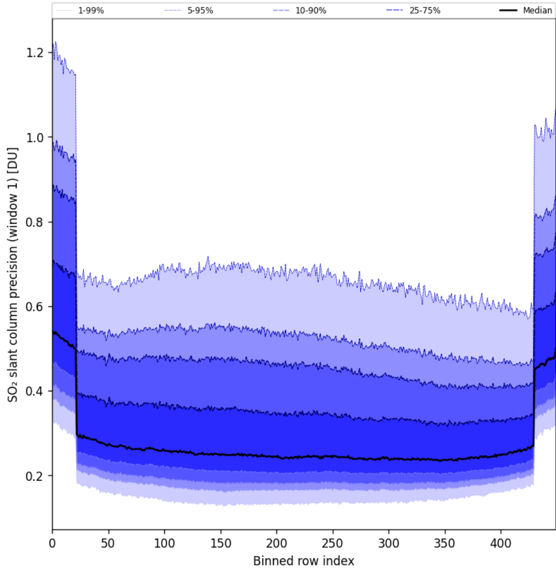
Figure 90: Along track statistics of “SO 2 slant column precision (window 1)” for 2025-07-24 to 2025-07-25
