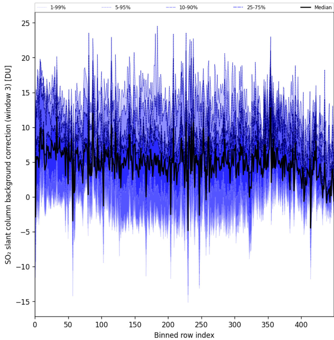
Figure 100: Along track statistics of “SO 2 slant column background correction (window 3)” for 2025-07-24 to 2025-07-25
