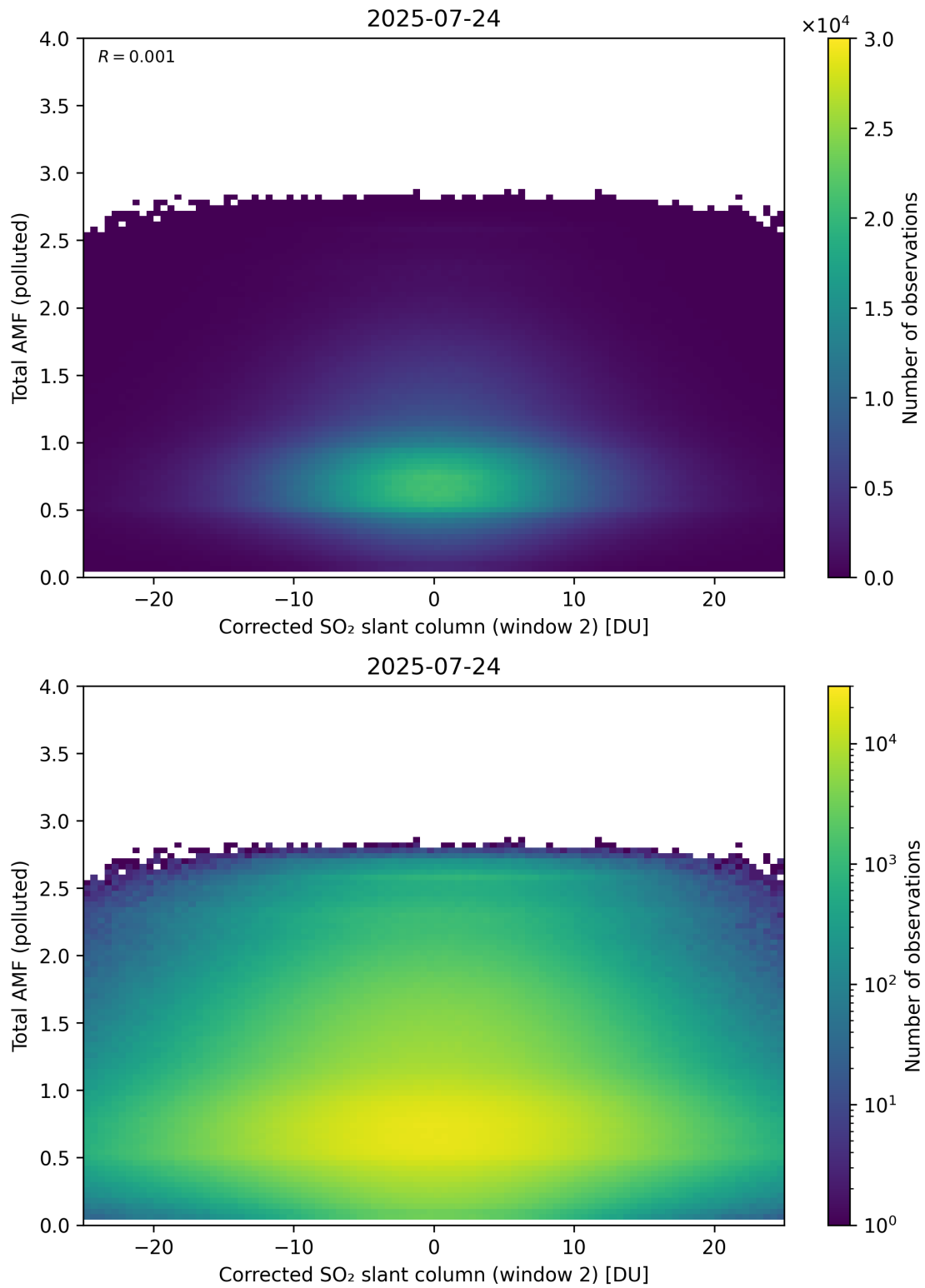
Figure 253: Scatter density plot of “Corrected SO 2 slant column (window 2)” against “Total AMF (polluted)” for 2025-07-24 to 2025-07-25.
