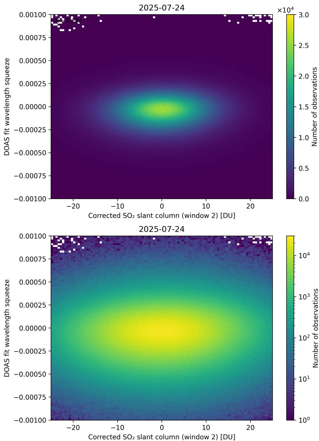
Figure 247: Scatter density plot of “Corrected SO 2 slant column (window 2)” against “DOAS fit wavelength squeeze” for 2025-07-24 to 2025-07-25.
