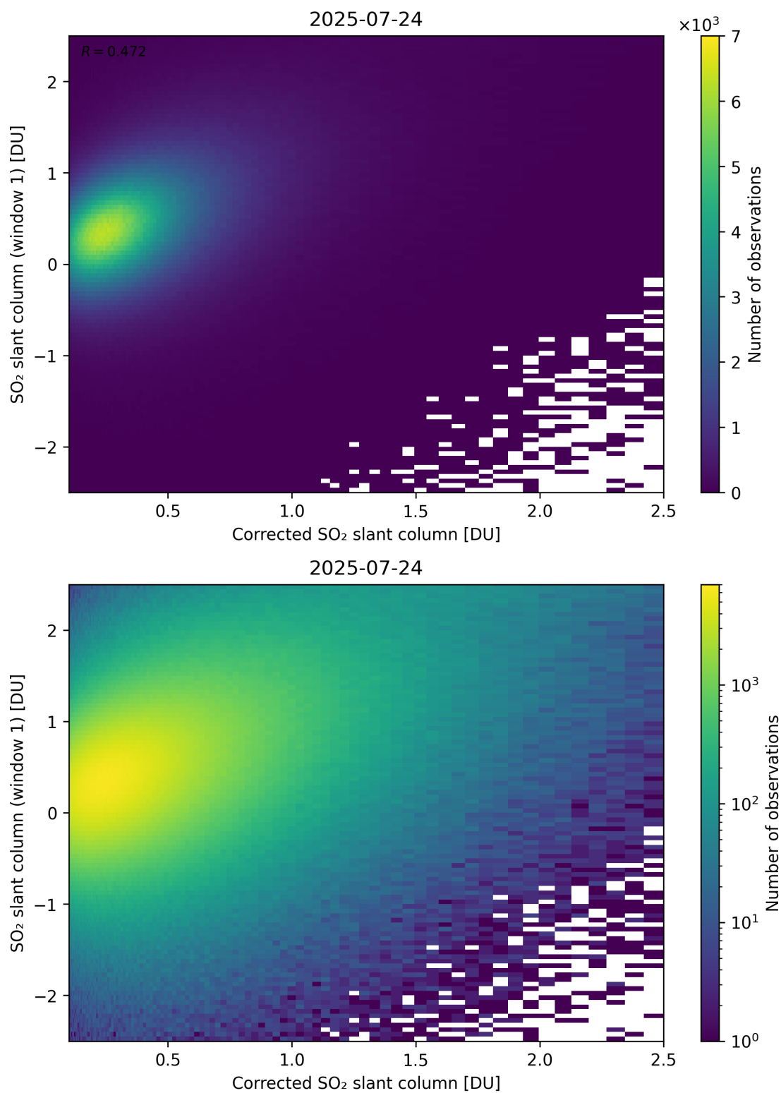
Figure 237: Scatter density plot of “Corrected SO 2 slant column” against “SO 2 slant column (window 1)” for 2025-07-24 to 2025-07-25.
