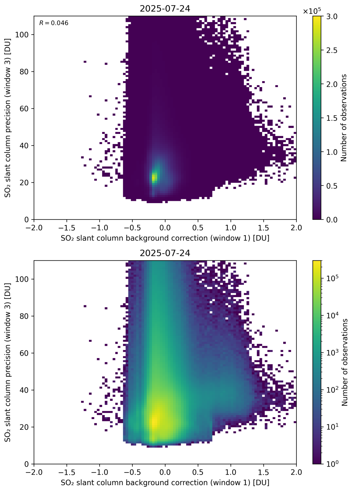
Figure 119: Scatter density plot of “SO 2 slant column background correction (window 1)” against “SO 2 slant column precision (window 3)” for 2025-07-24 to 2025-07-25.
