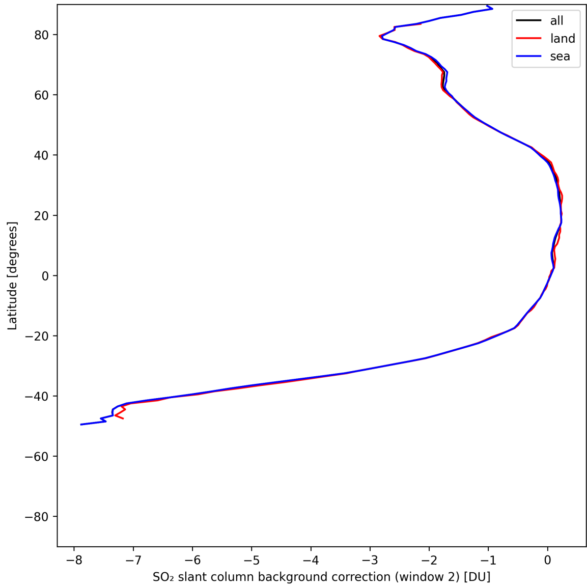
Figure 44: Zonal average of “SO 2 slant column background correction (window 2)” for 2025-07-24 to 2025-07-25.
