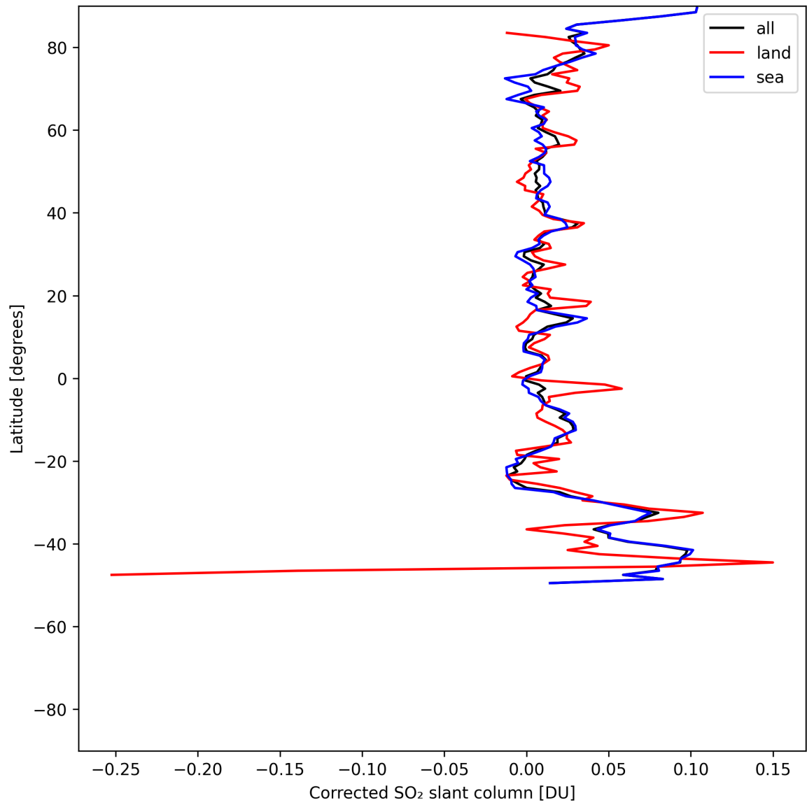
Figure 34: Zonal average of “Corrected SO 2 slant column” for 2025-07-24 to 2025-07-25.
