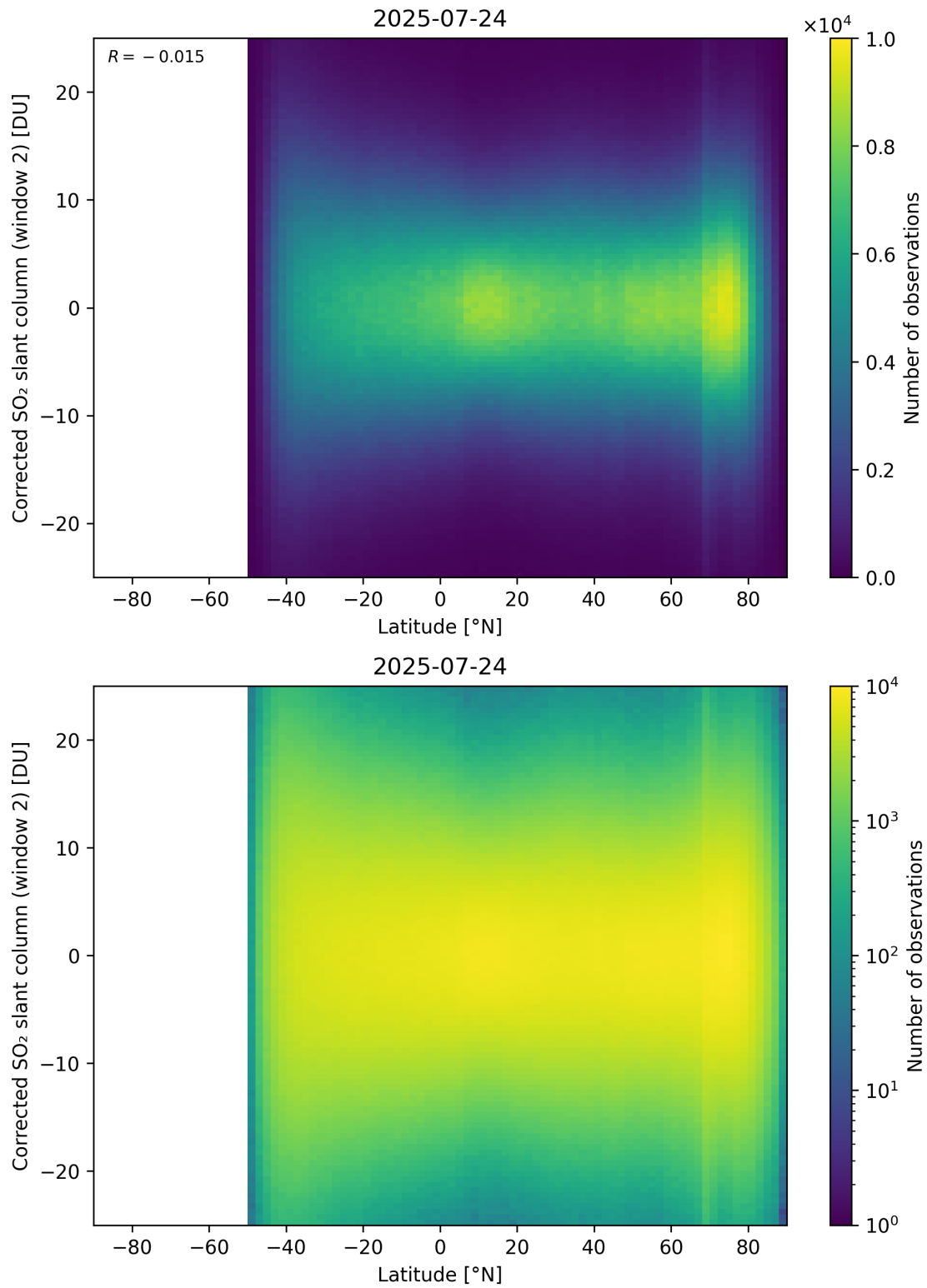
Figure 160: Scatter density plot of “Latitude” against “Corrected SO 2 slant column (window 2)” for 2025-07-24 to 2025-07-25.
