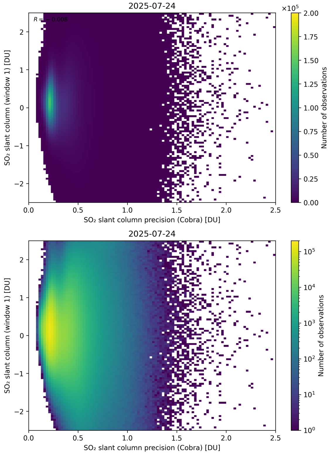
Figure 208: Scatter density plot of “SO 2 slant column precision (Cobra)” against “SO 2 slant column (window 1)” for 2025-07-24 to 2025-07-25.
