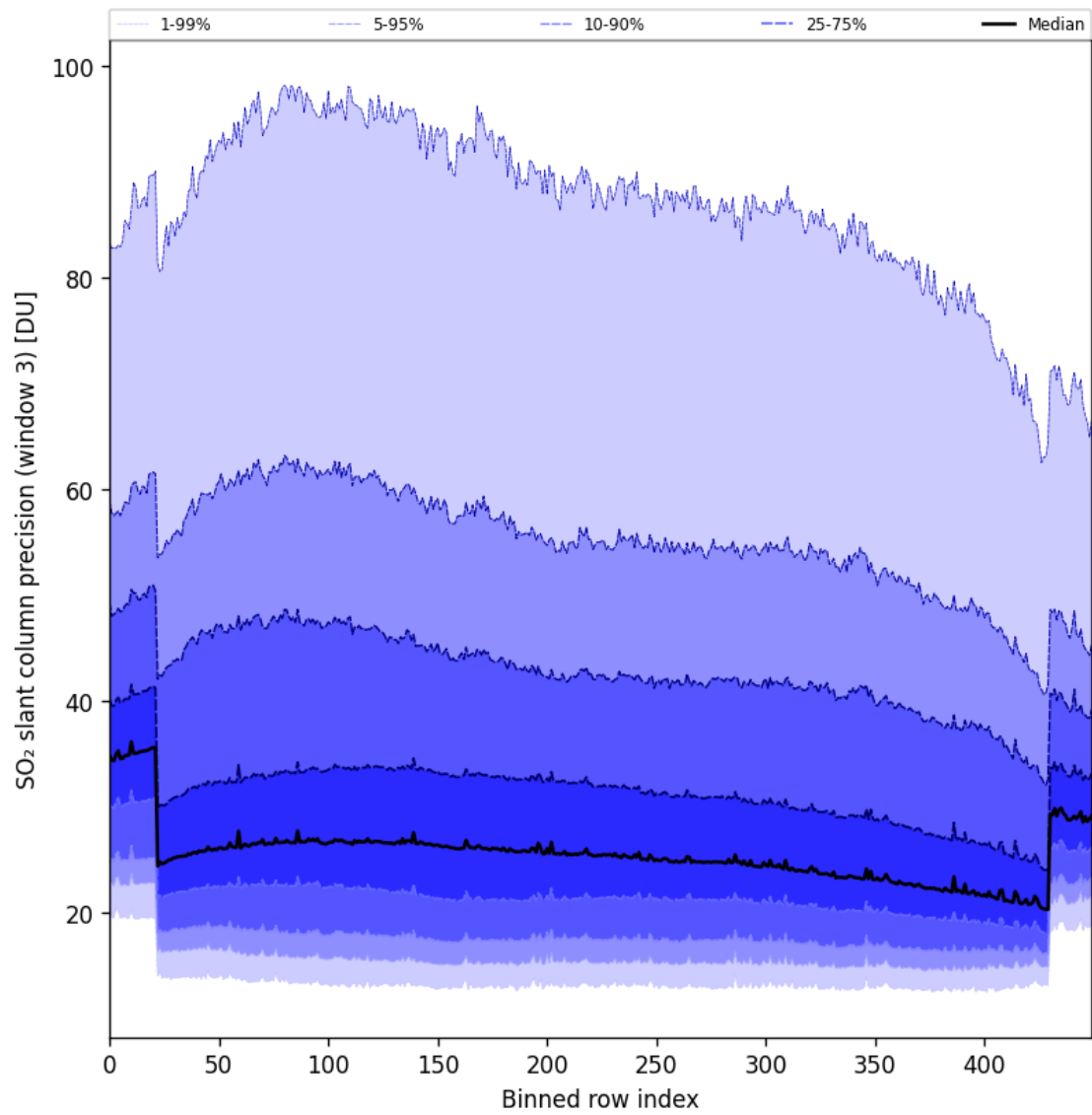
Figure 98: Along track statistics of “SO 2 slant column precision (window 3)” for 2025-07-24 to 2025-07-25
