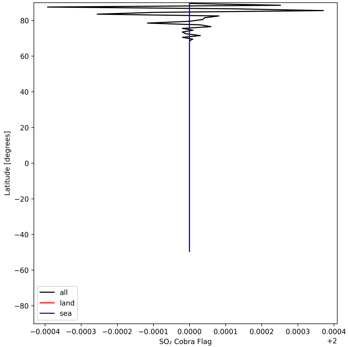
Figure 49: Zonal average of "SO 2 Cobra Flag" for 2025-07-24 to 2025-07-25.
