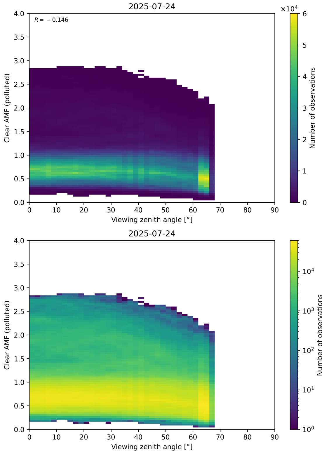
Figure 370: Scatter density plot of “Viewing zenith angle” against “Clear AMF (polluted)” for 2025-07-24 to 2025-07-25.
