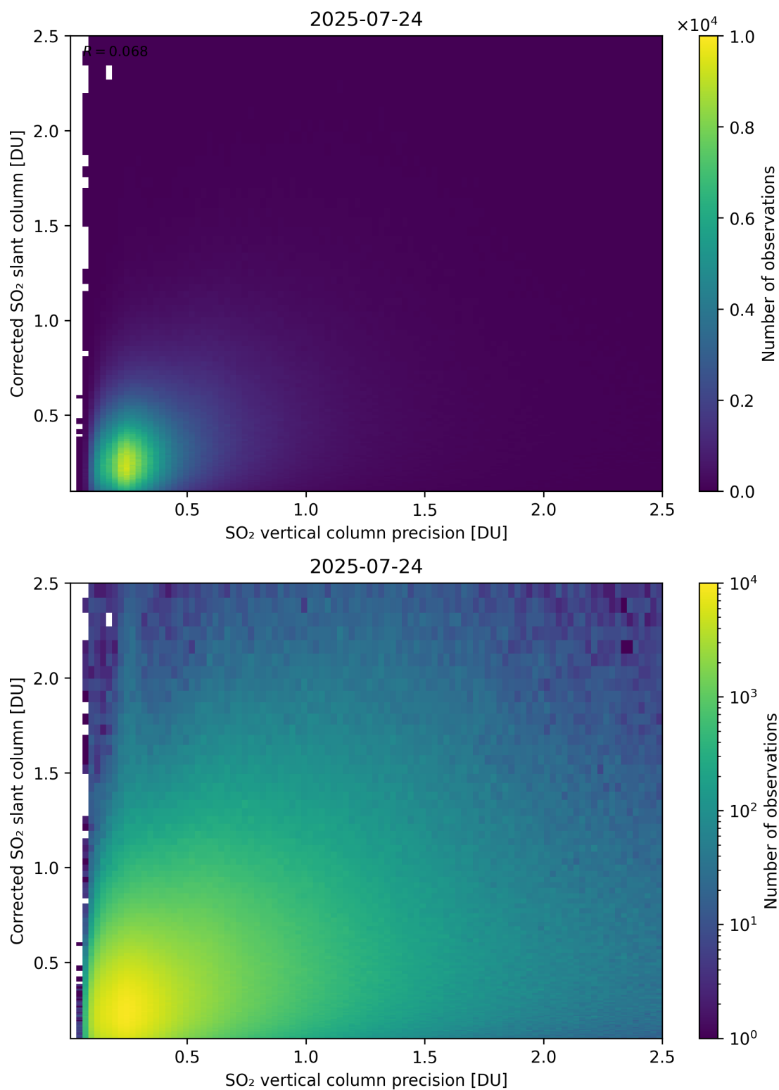
Figure 338: Scatter density plot of “SO 2 vertical column precision” against “Corrected SO 2 slant column” for 2025-07-24 to 2025-07-25.
