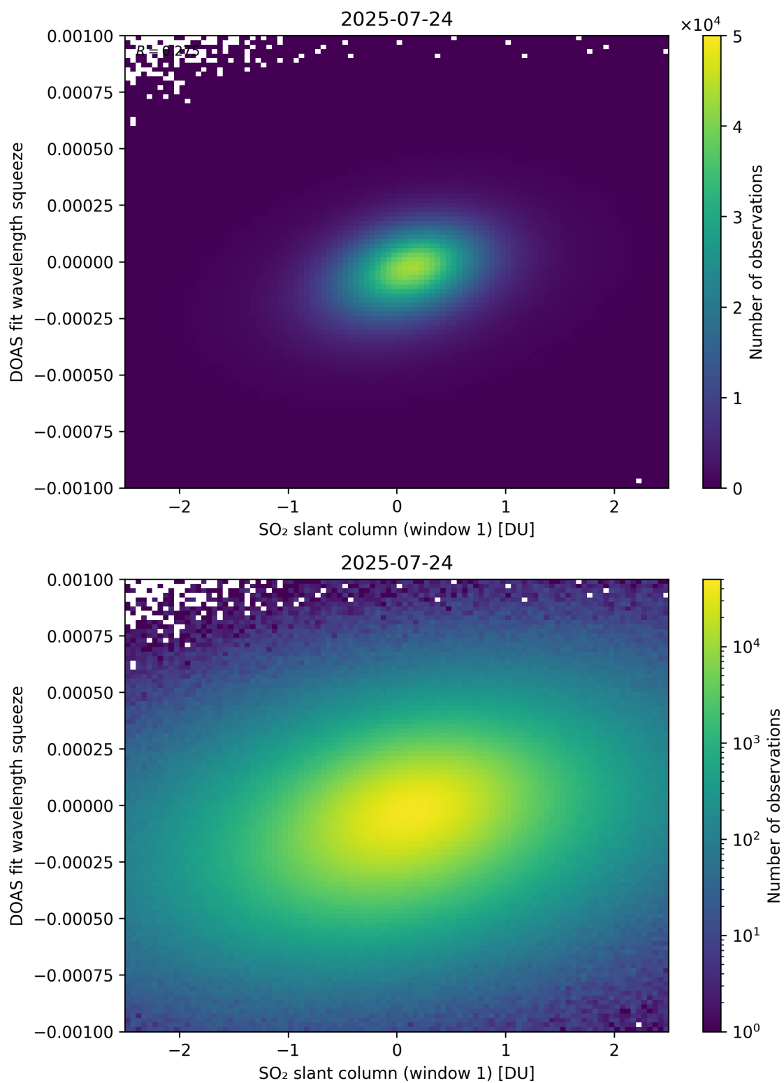
Figure 266: Scatter density plot of “SO 2 slant column (window 1)” against “DOAS fit wavelength squeeze” for 2025-07-24 to 2025-07-25.
