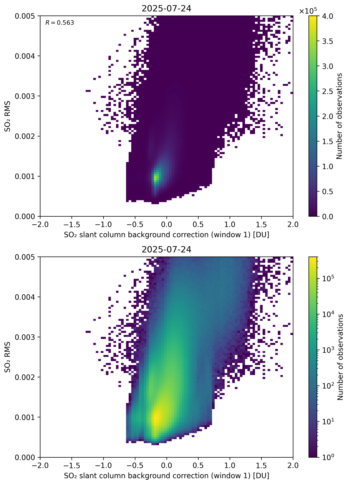
Figure 113: Scatter density plot of “SO 2 slant column background correction (window 1)” against “SO 2 RMS” for 2025-07-24 to 2025-07-25.
