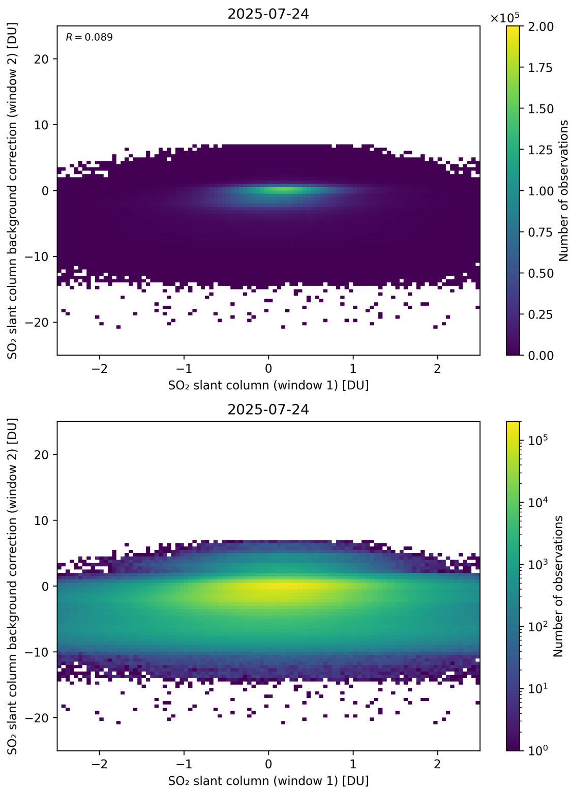
Figure 263: Scatter density plot of “SO 2 slant column (window 1)” against “SO 2 slant column background correction (window 2)” for 2025-07-24 to 2025-07-25.
