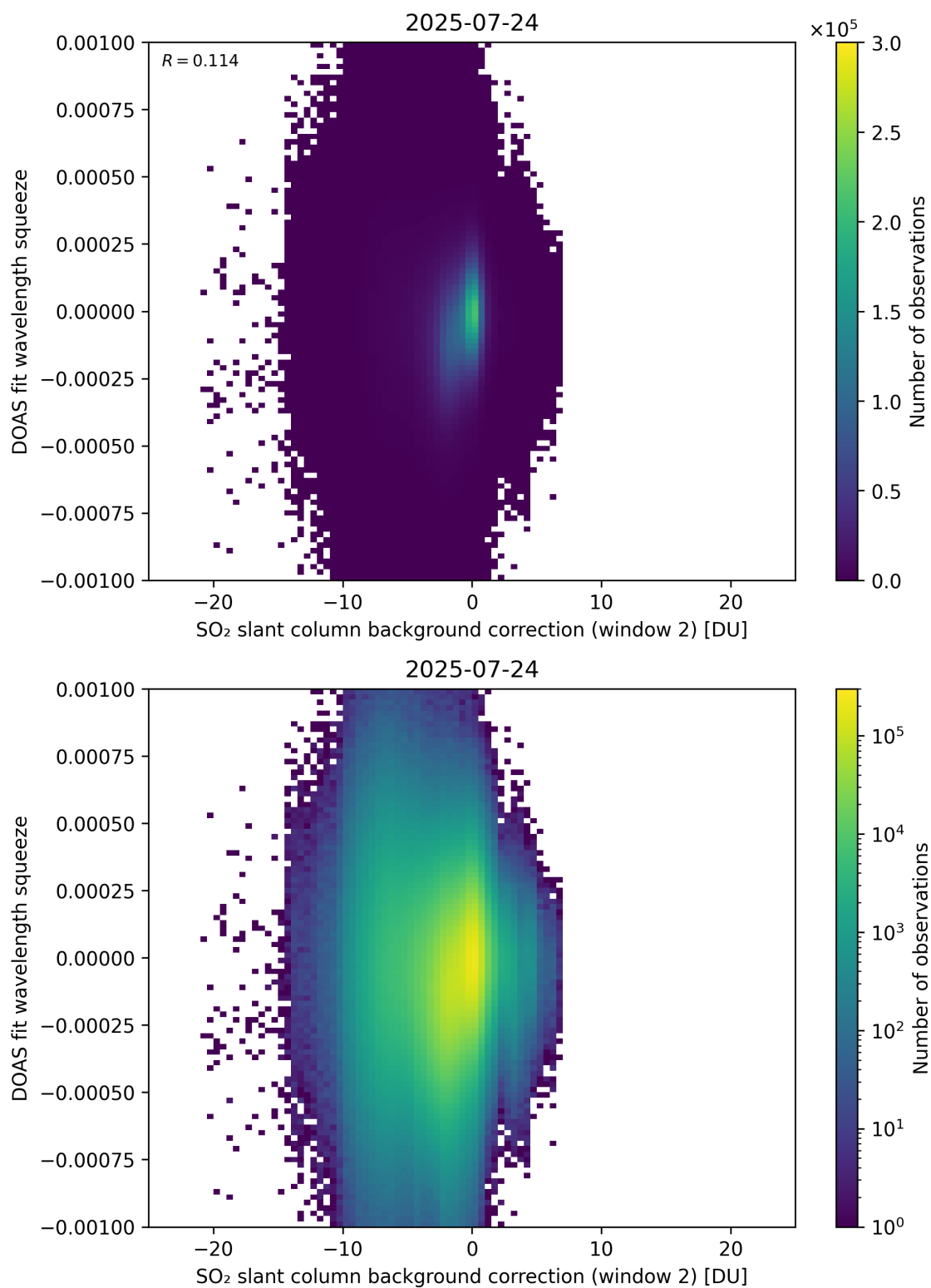
Figure 124: Scatter density plot of “SO 2 slant column background correction (window 2)” against “DOAS fit wavelength squeeze” for 2025-07-24 to 2025-07-25.
