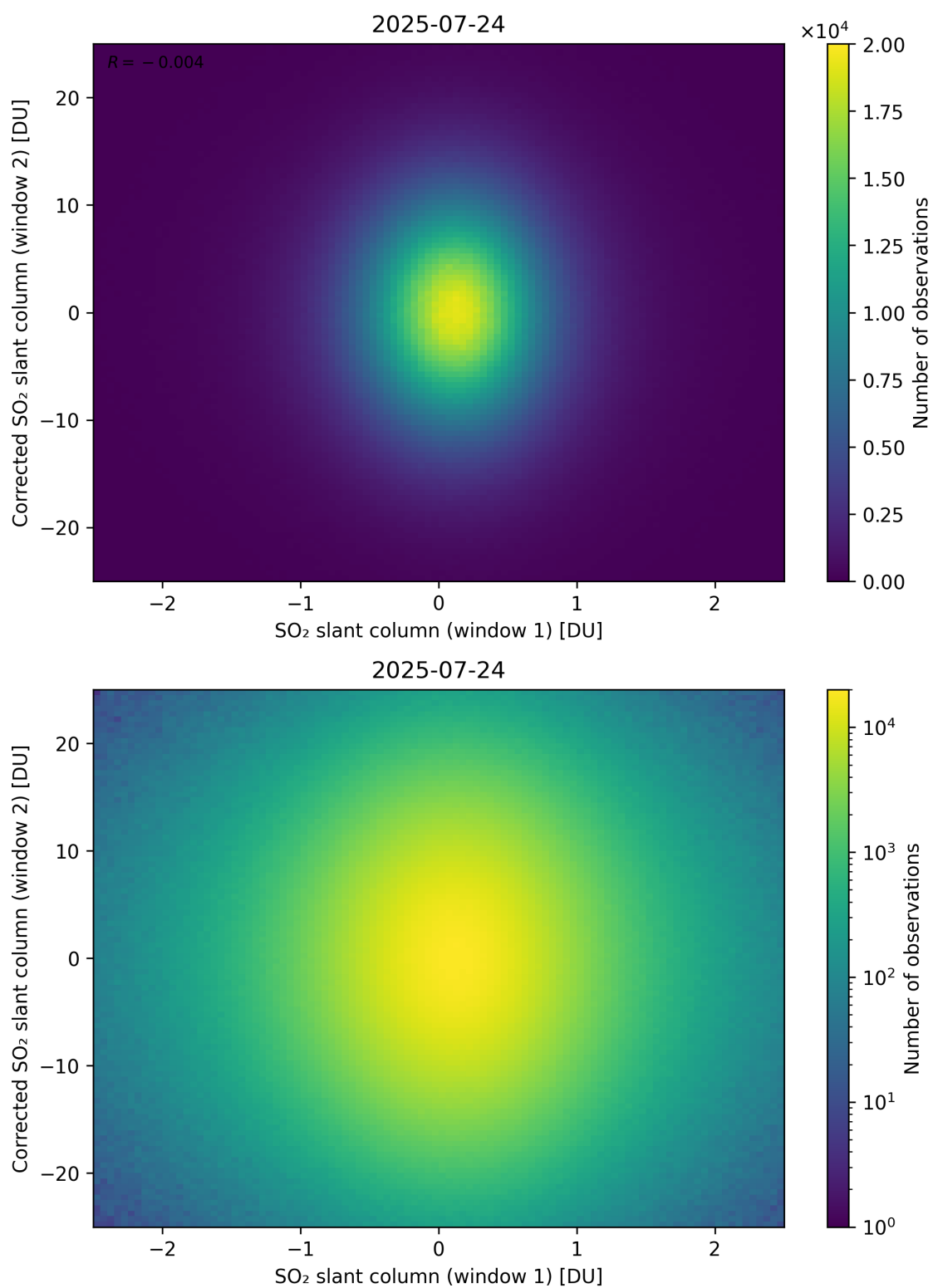
Figure 283: Scatter density plot of “SO 2 slant column (window 1)” against “Corrected SO 2 slant column (window 2)” for 2025-07-24 to 2025-07-25.
