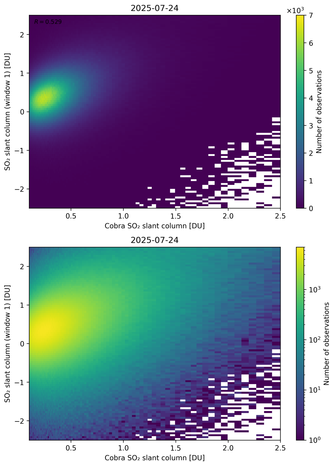
Figure 219: Scatter density plot of “Cobra SO 2 slant column” against “SO 2 slant column (window 1)” for 2025-07-24 to 2025-07-25.
