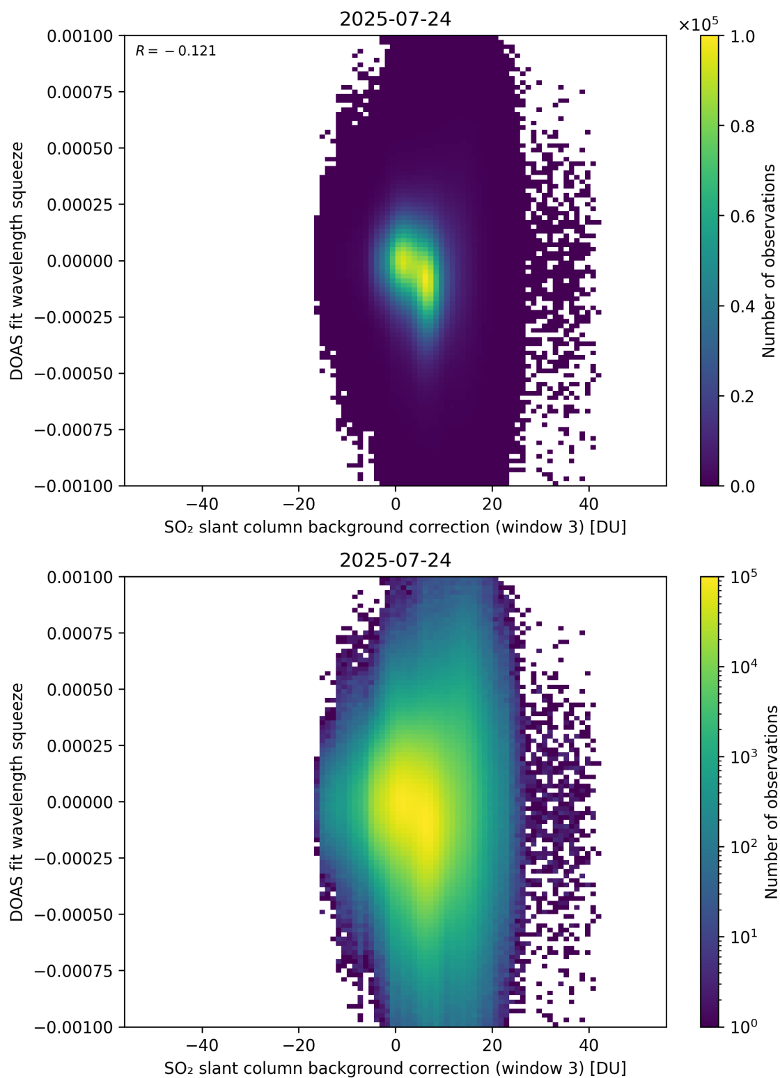
Figure 133: Scatter density plot of “SO 2 slant column background correction (window 3)” against “DOAS fit wavelength squeeze” for 2025-07-24 to 2025-07-25.
