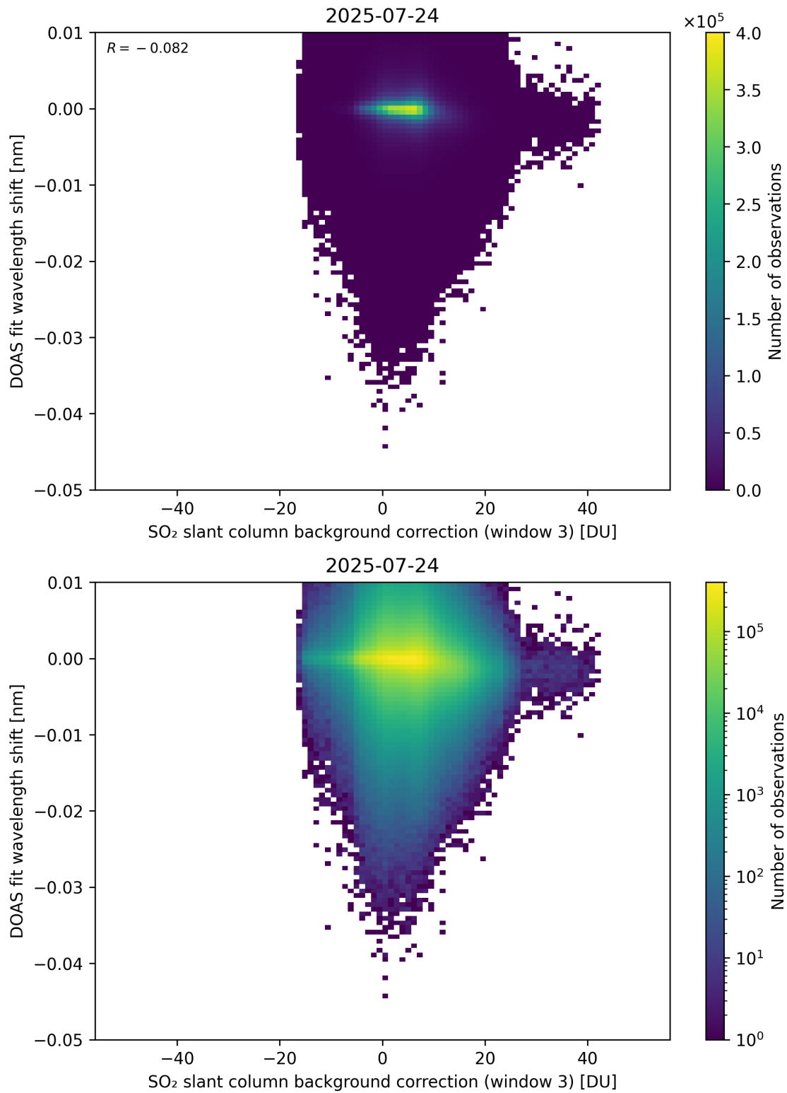
Figure 132: Scatter density plot of “SO 2 slant column background correction (window 3)” against “DOAS fit wavelength shift” for 2025-07-24 to 2025-07-25.
