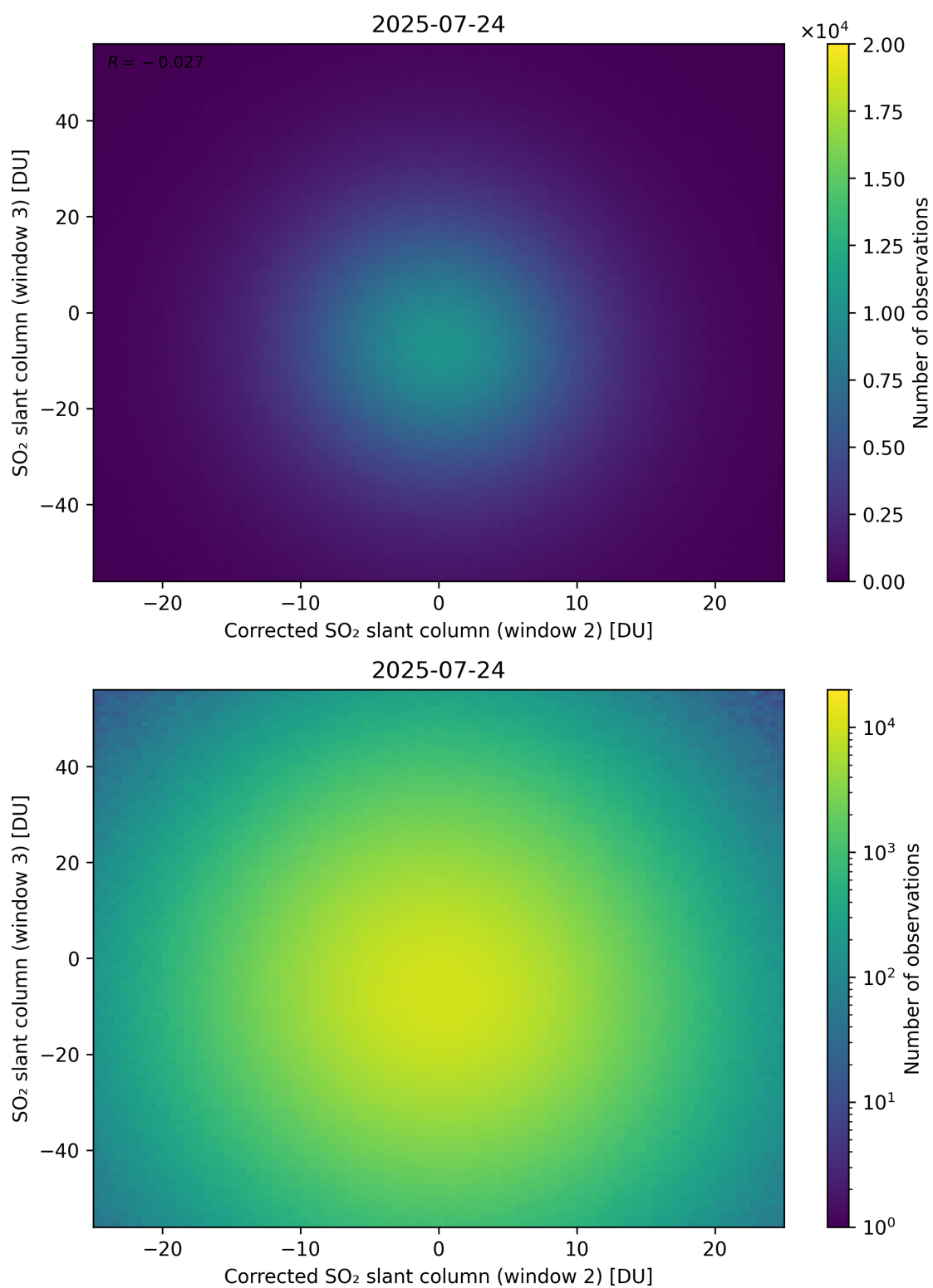
Figure 251: Scatter density plot of “Corrected SO 2 slant column (window 2)” against “SO 2 slant column (window 3)” for 2025-07-24 to 2025-07-25.
