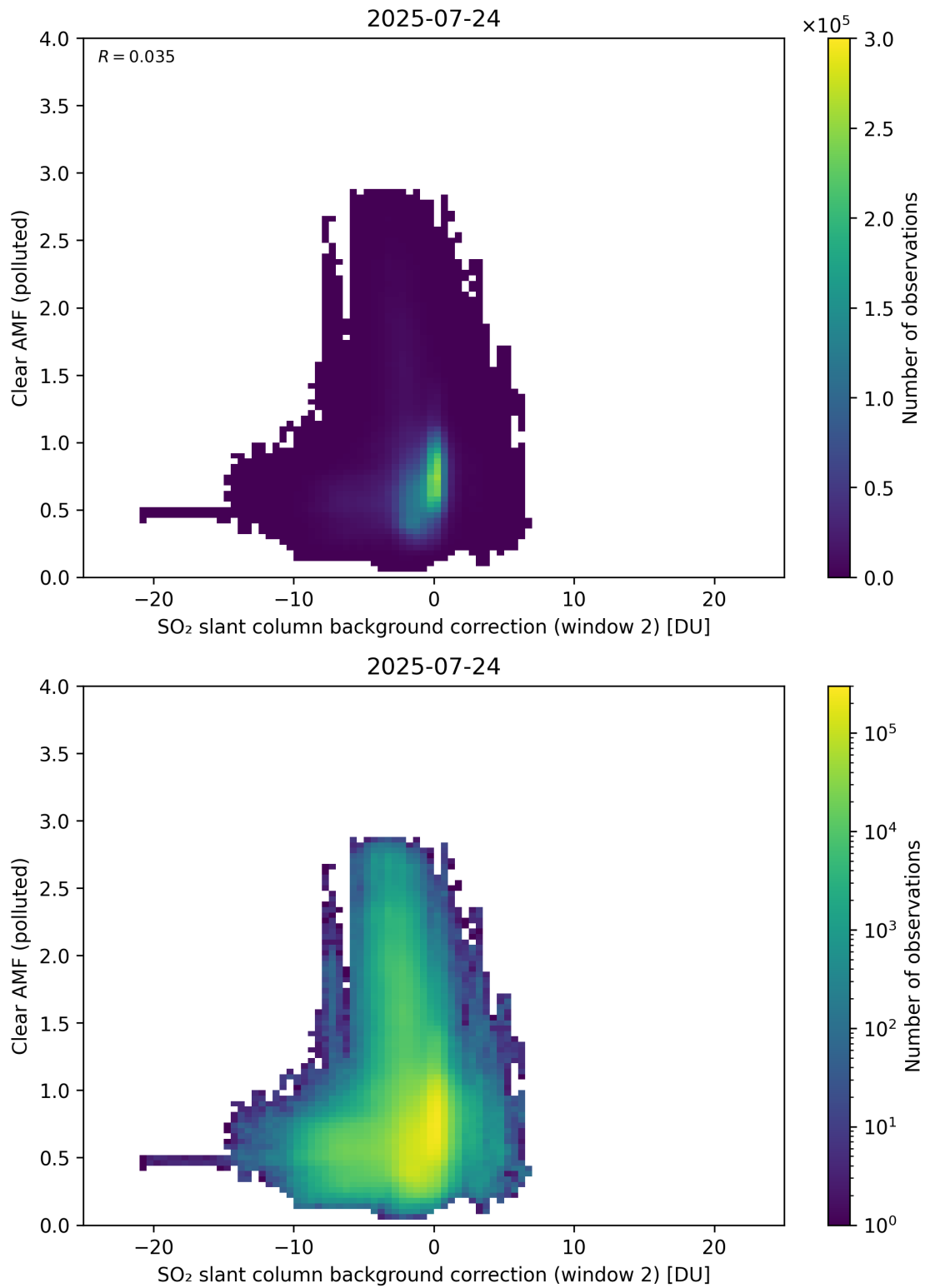
Figure 126: Scatter density plot of “SO 2 slant column background correction (window 2)” against “Clear AMF (polluted)” for 2025-07-24 to 2025-07-25.
