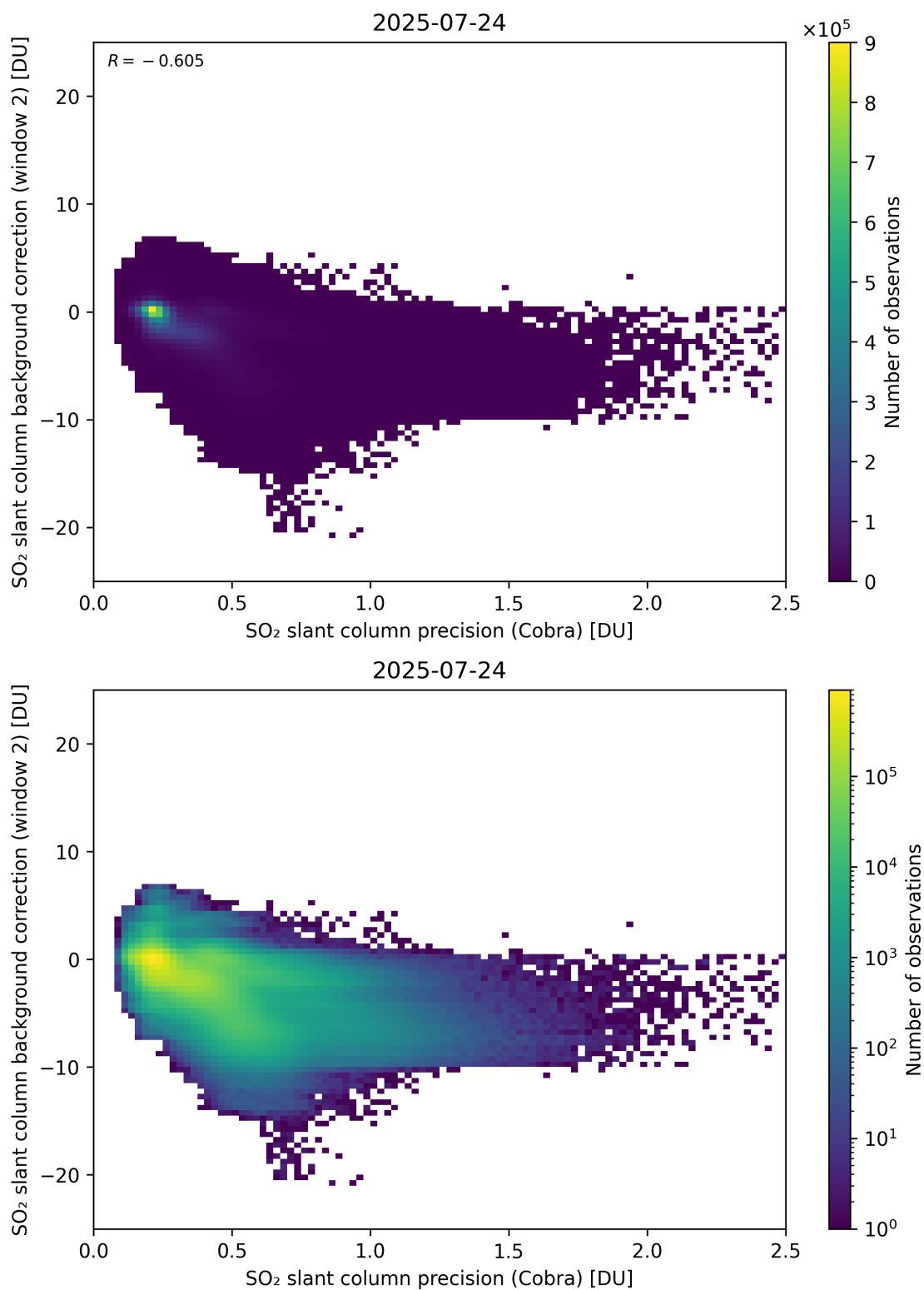
Figure 200: Scatter density plot of “SO 2 slant column precision (Cobra)” against “SO 2 slant column background correction (window 2)” for 2025-07-24 to 2025-07-25.
