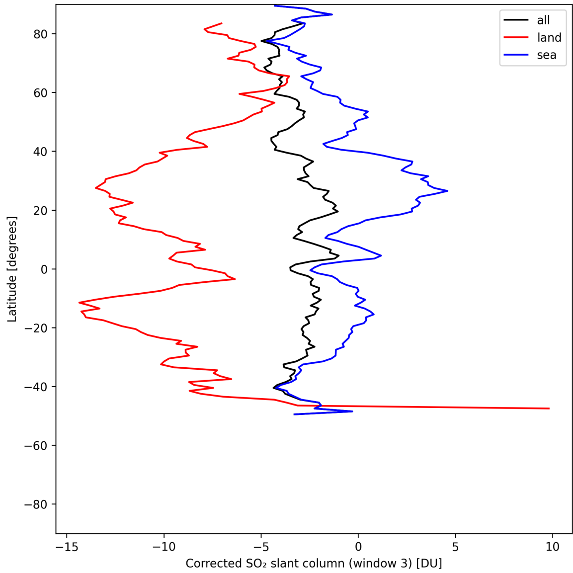
Figure 47: Zonal average of “Corrected SO 2 slant column (window 3)” for 2025-07-24 to 2025-07-25.
