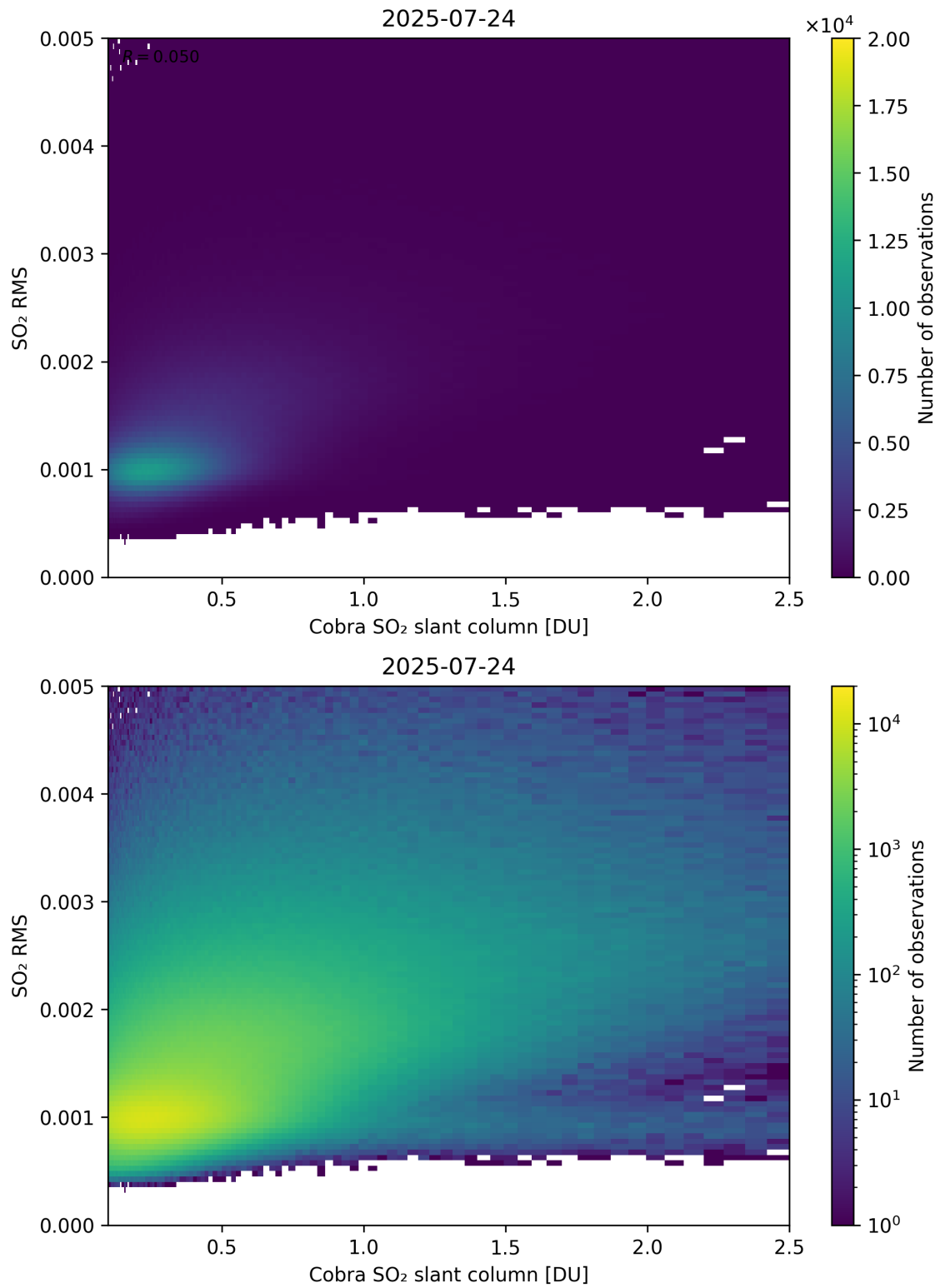
Figure 198: Scatter density plot of “Cobra SO 2 slant column” against “SO 2 RMS” for 2025-07-24 to 2025-07-25.
