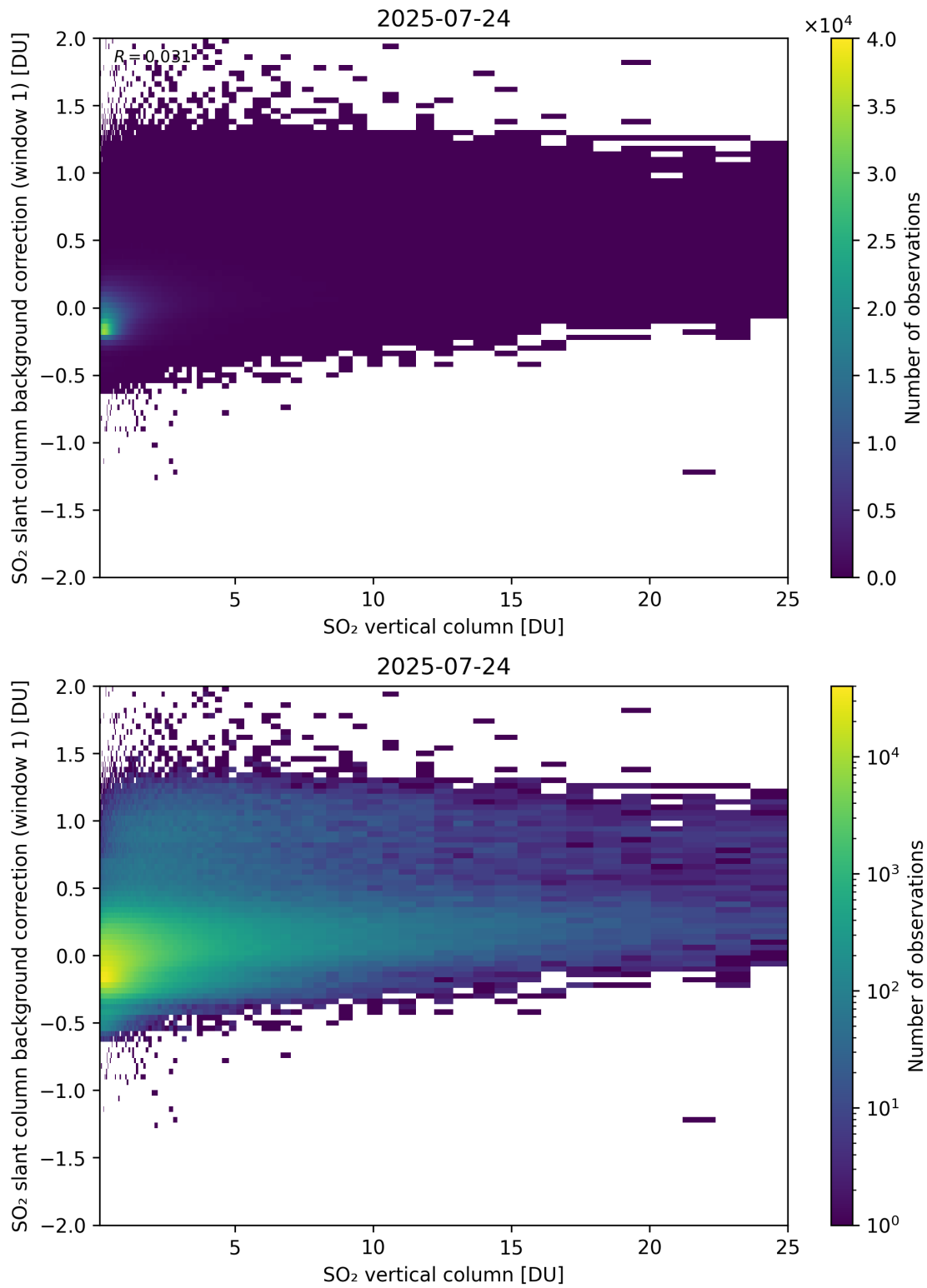
Figure 323: Scatter density plot of “SO 2 vertical column” against “SO 2 slant column background correction (window 1)” for 2025-07-24 to 2025-07-25.
