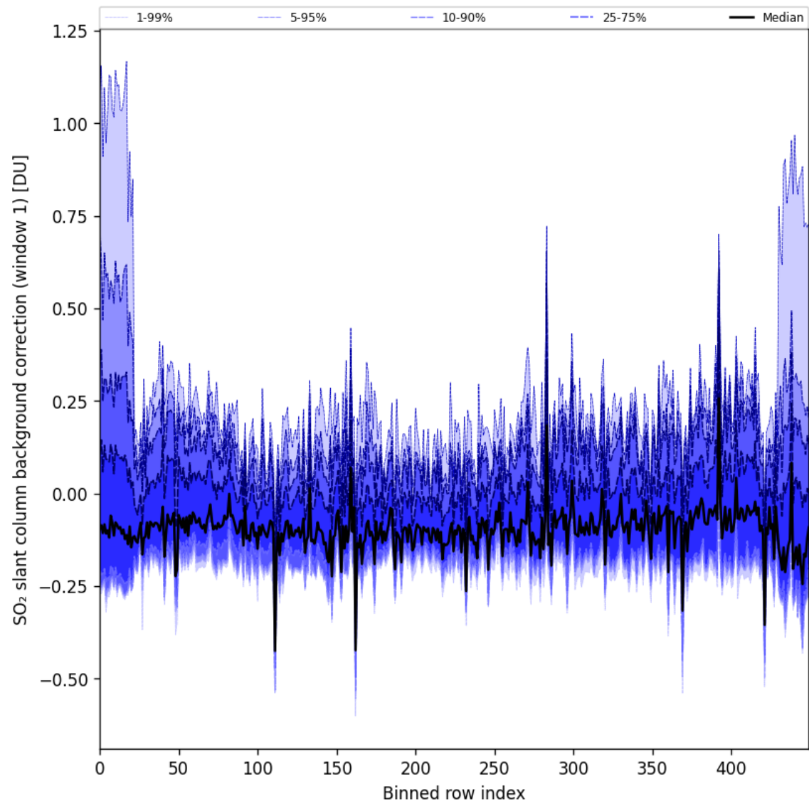
Figure 92: Along track statistics of “SO 2 slant column background correction (window 1)” for 2025-07-24 to 2025-07-25
