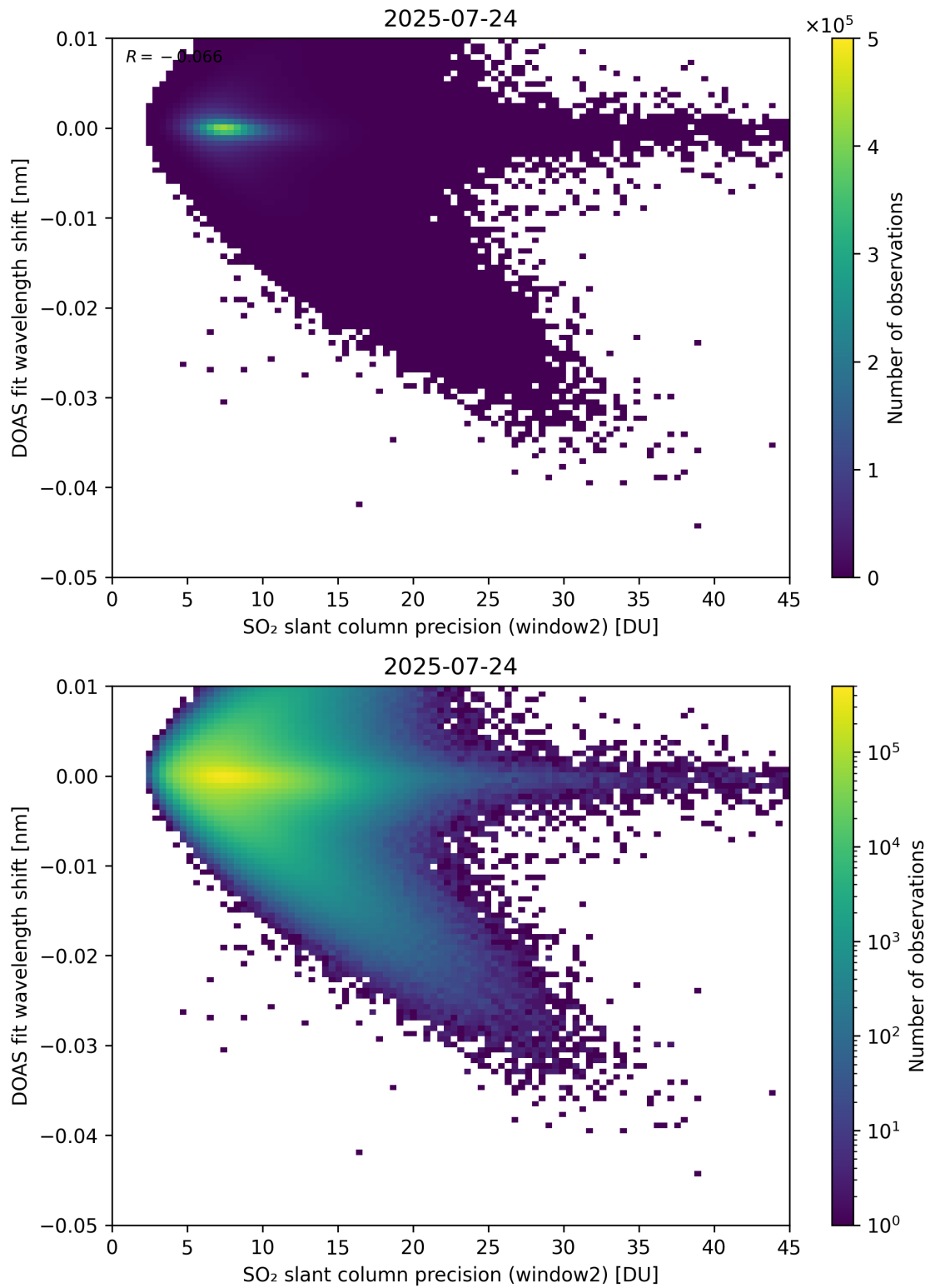
Figure 293: Scatter density plot of “SO 2 slant column precision (window2)” against “DOAS fit wavelength shift” for 2025-07-24 to 2025-07-25.
