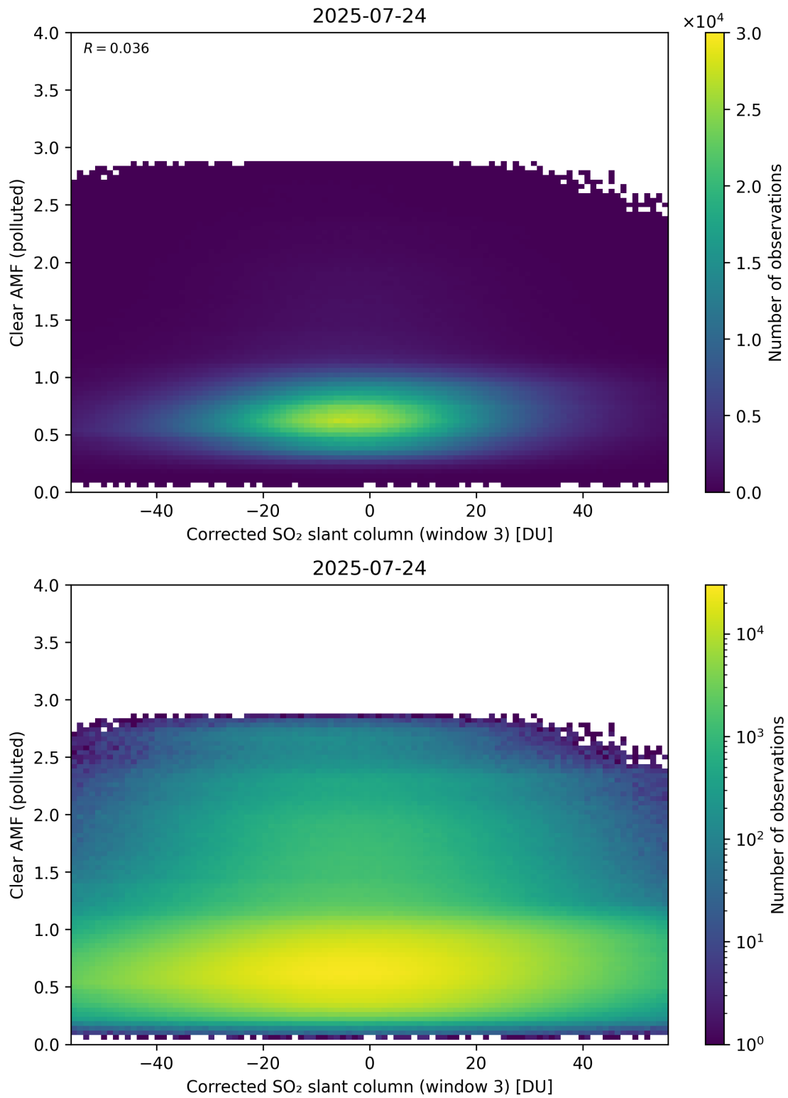
Figure 259: Scatter density plot of “Corrected SO 2 slant column (window 3)” against “Clear AMF (polluted)” for 2025-07-24 to 2025-07-25.
