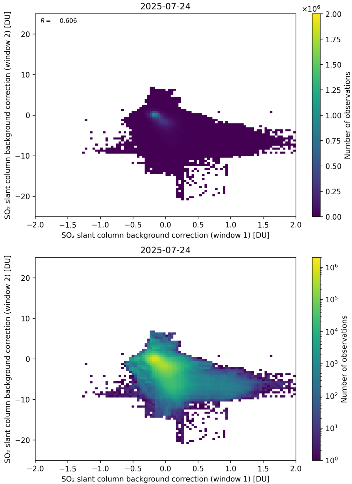
Figure 109: Scatter density plot of “SO 2 slant column background correction (window 1)” against “SO 2 slant column background correction (window 2)” for 2025-07-24 to 2025-07-25.
