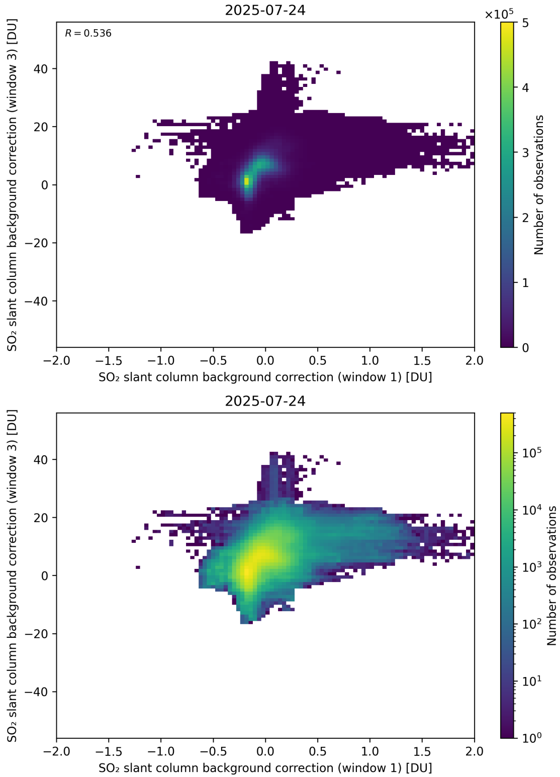
Figure 110: Scatter density plot of “SO 2 slant column background correction (window 1)” against “SO 2 slant column background correction (window 3)” for 2025-07-24 to 2025-07-25.
