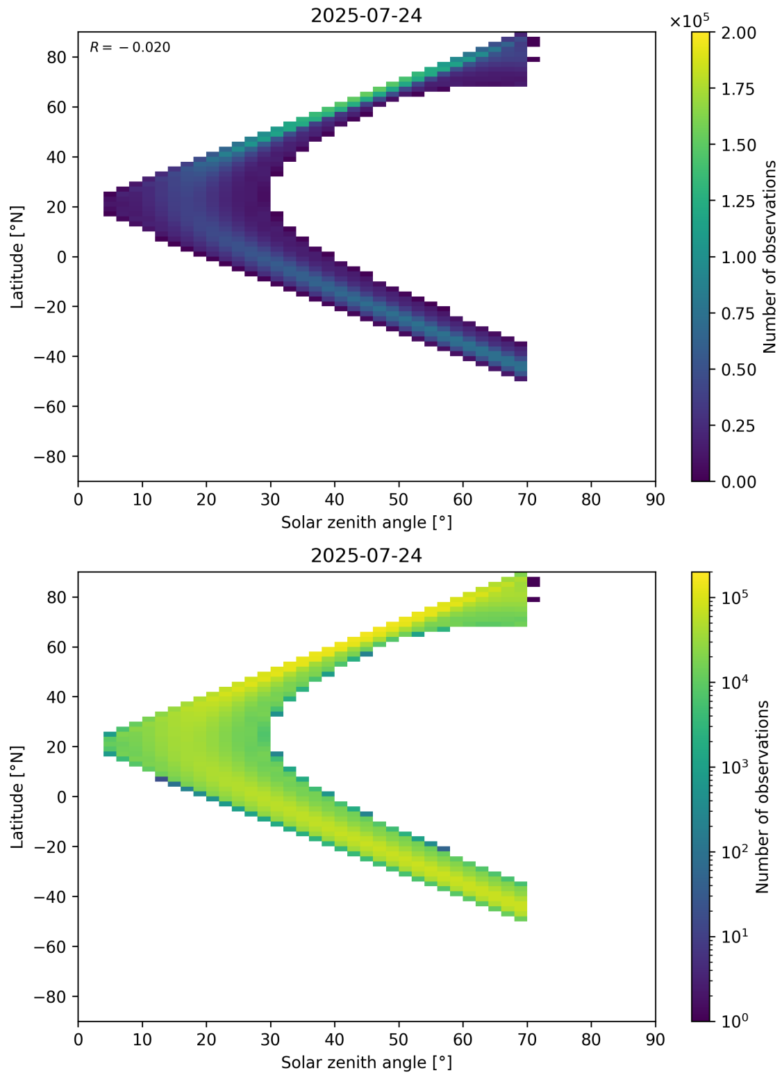
Figure 177: Scatter density plot of “Solar zenith angle” against “Latitude” for 2025-07-24 to 2025-07-25.
