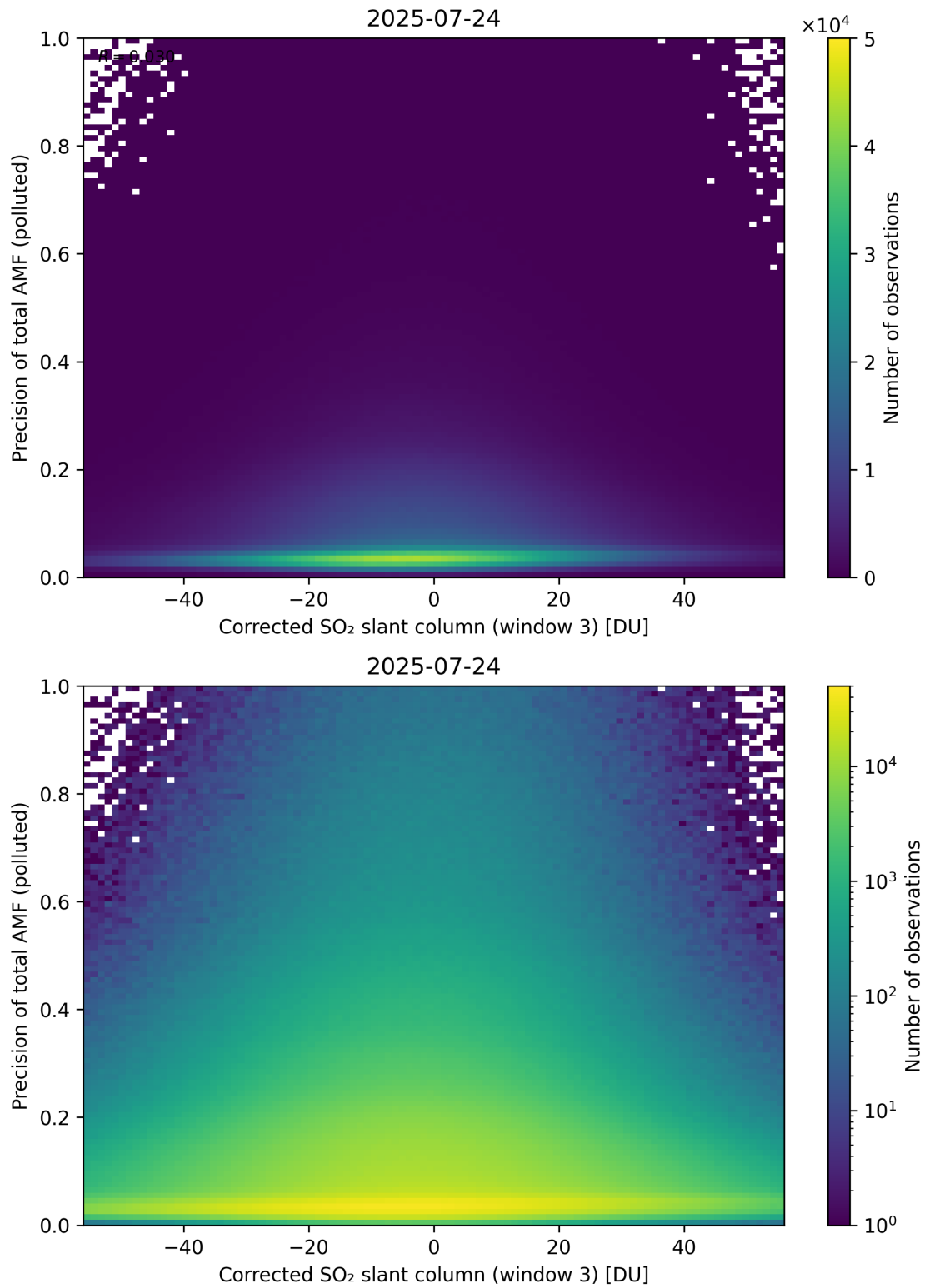
Figure 261: Scatter density plot of “Corrected SO 2 slant column (window 3)” against “Precision of total AMF (polluted)” for 2025-07-24 to 2025-07-25.
