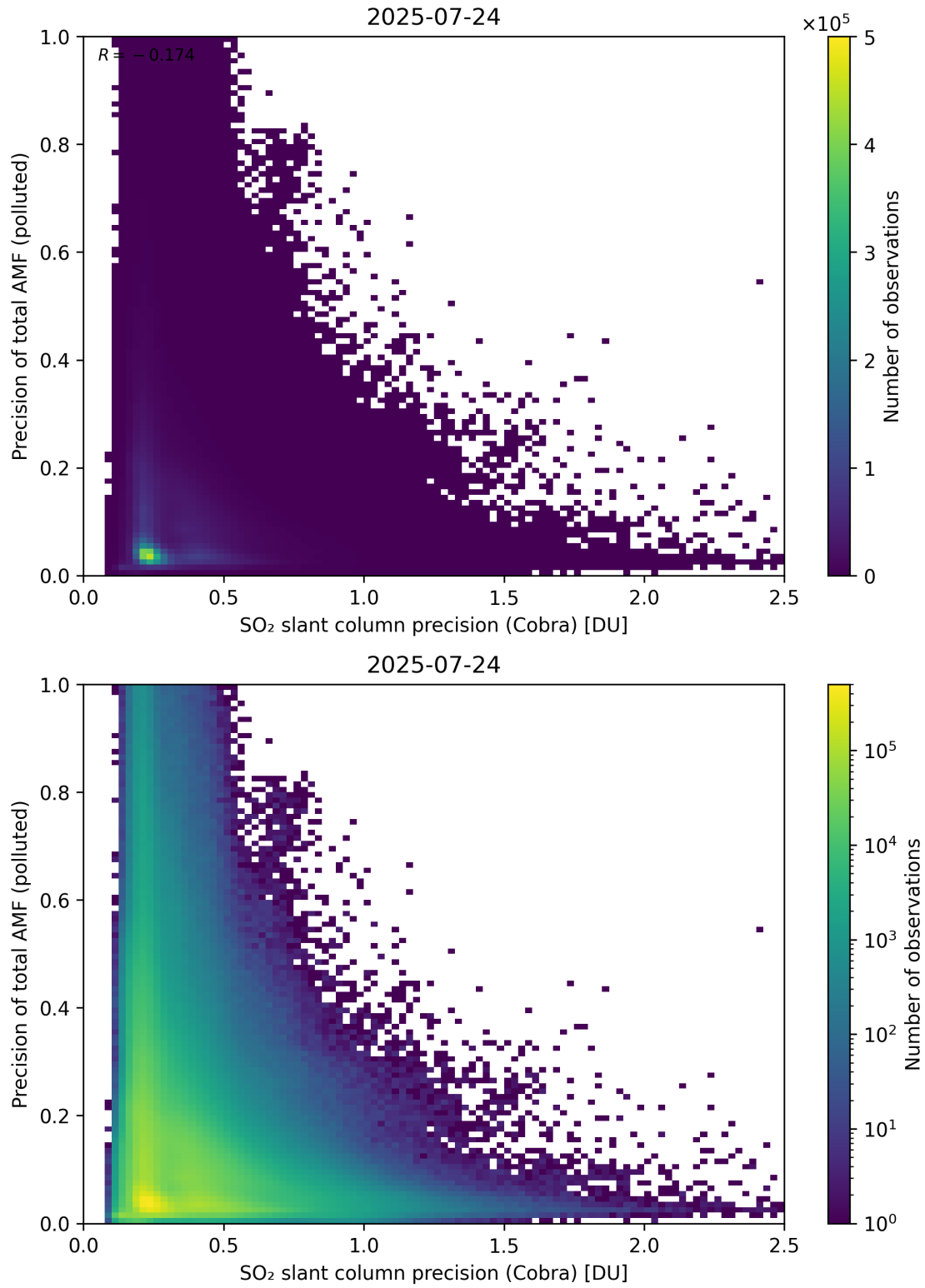
Figure 214: Scatter density plot of “SO 2 slant column precision (Cobra)” against “Precision of total AMF (polluted)” for 2025-07-24 to 2025-07-25.
