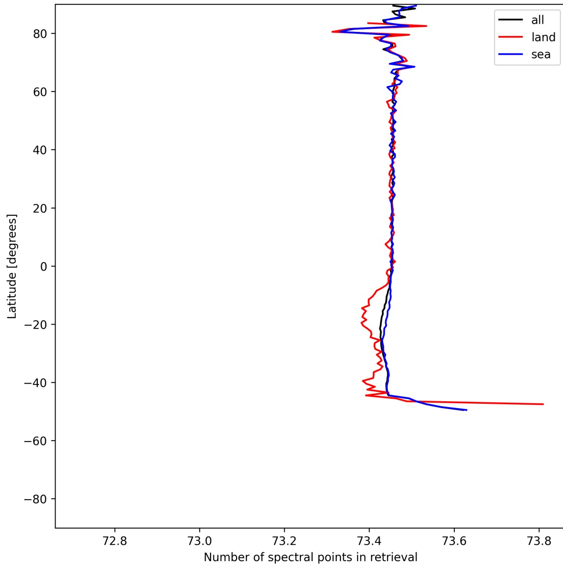
Figure 56: Zonal average of “Number of spectral points in retrieval” for 2025-07-24 to 2025-07-26.
