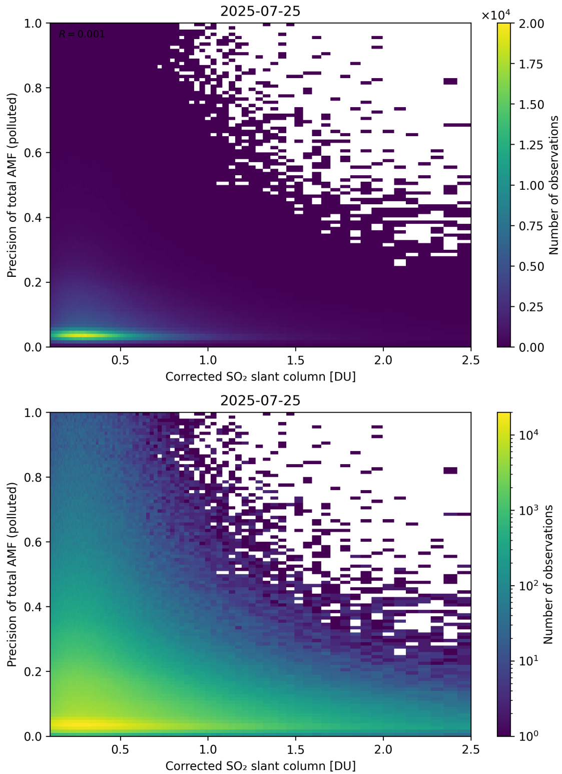
Figure 243: Scatter density plot of “Corrected SO 2 slant column” against “Precision of total AMF (polluted)” for 2025-07-24 to 2025-07-26.
