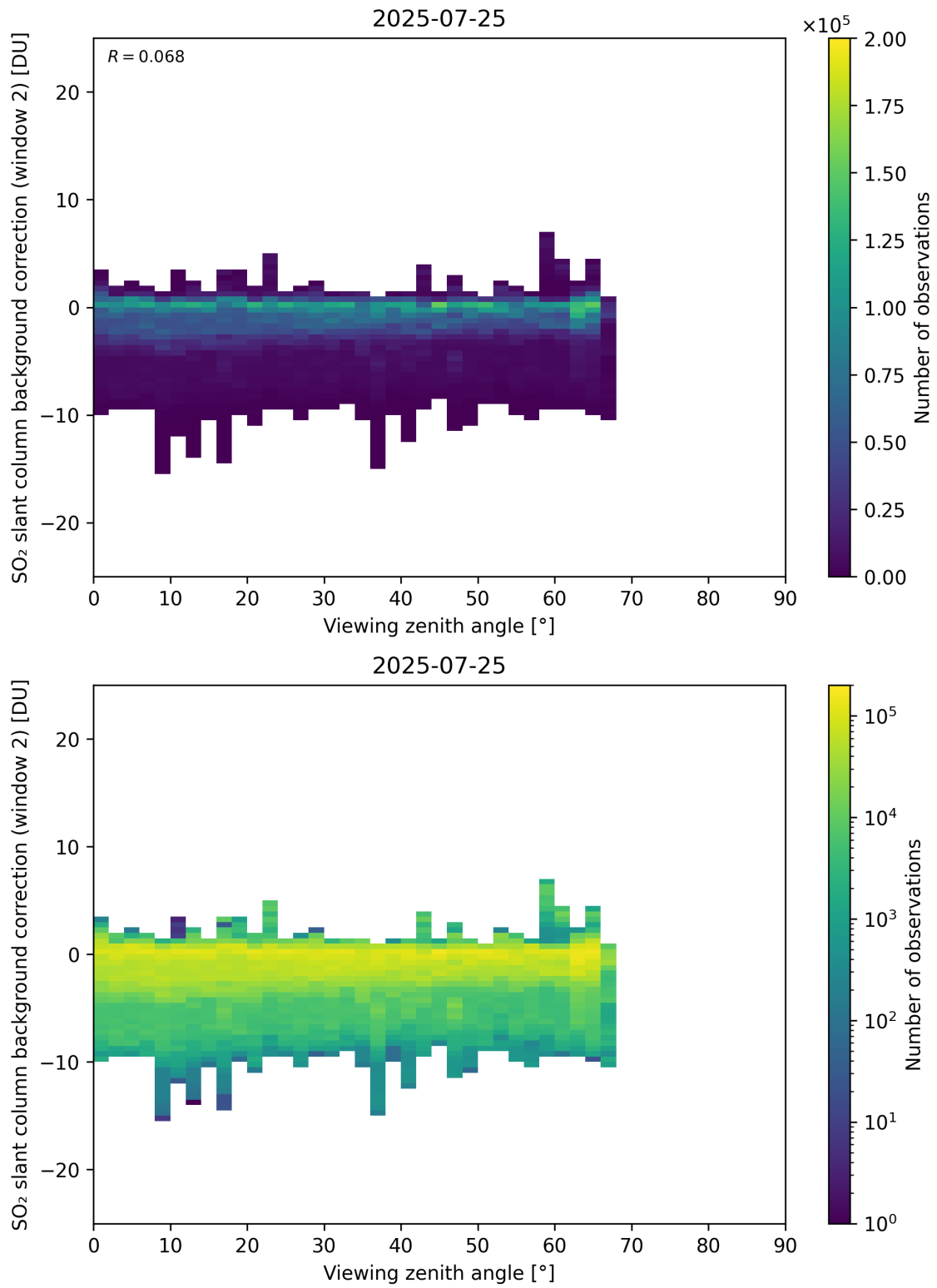
Figure 363: Scatter density plot of “Viewing zenith angle” against “SO 2 slant column background correction (window 2)” for 2025-07-24 to 2025-07-26.
