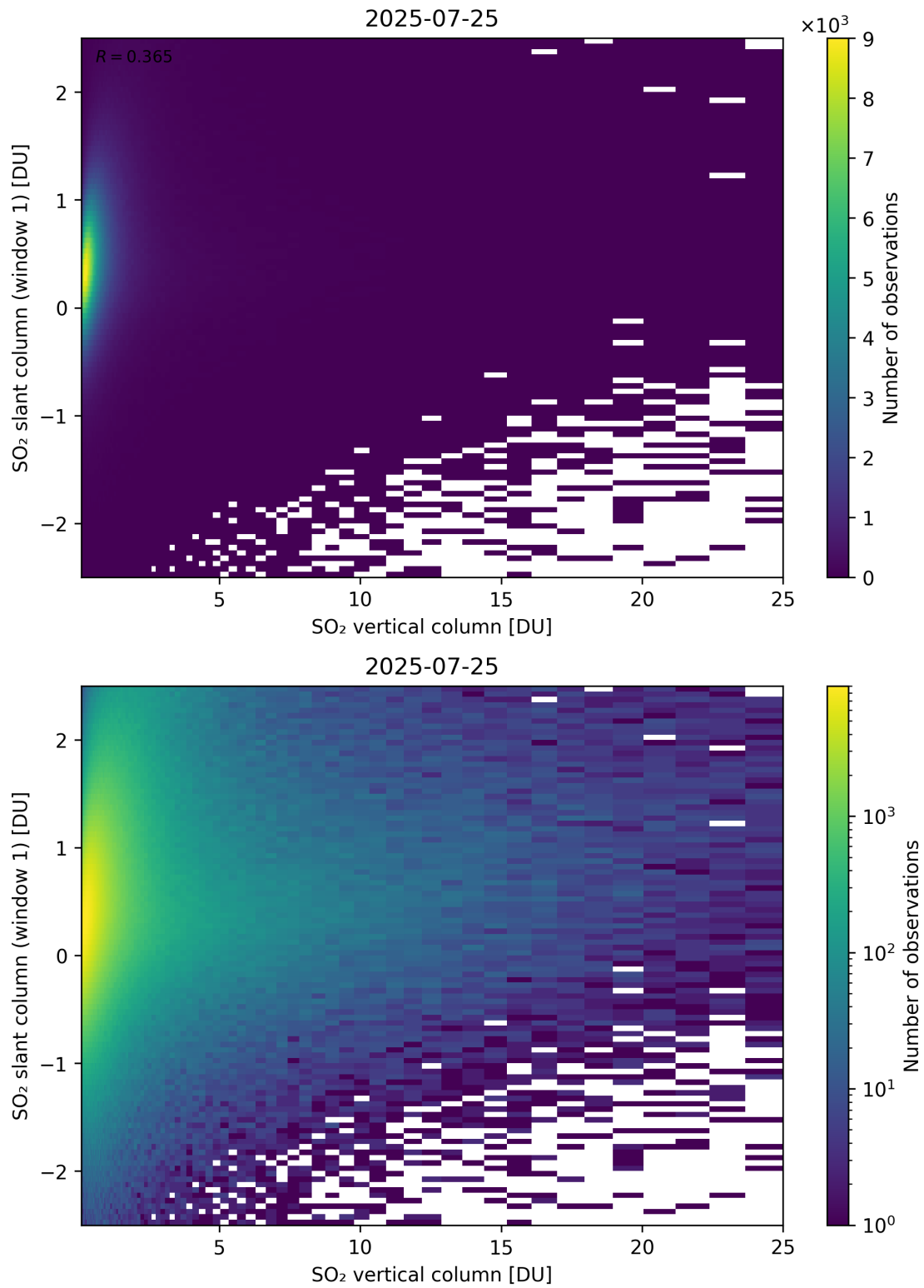
Figure 354: Scatter density plot of “SO 2 vertical column” against “SO 2 slant column (window 1)” for 2025-07-24 to 2025-07-26.
