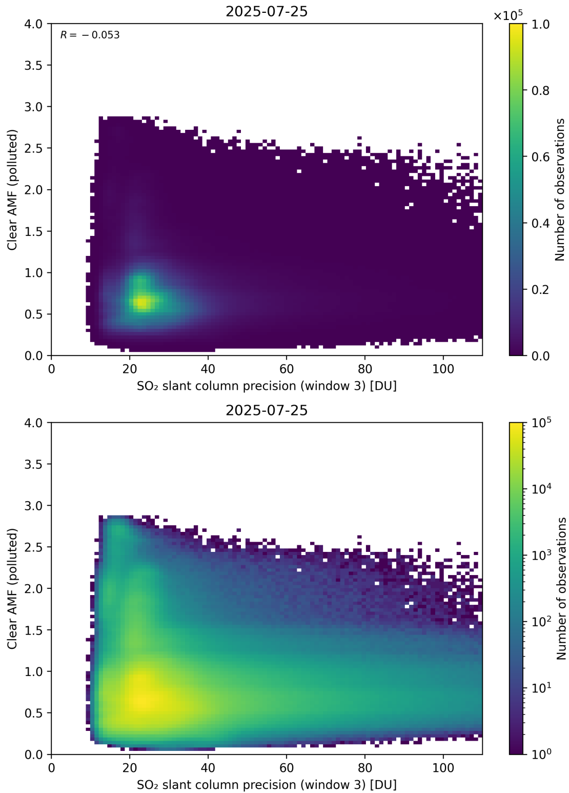
Figure 311: Scatter density plot of “SO 2 slant column precision (window 3)” against “Clear AMF (polluted)” for 2025-07-24 to 2025-07-26.
