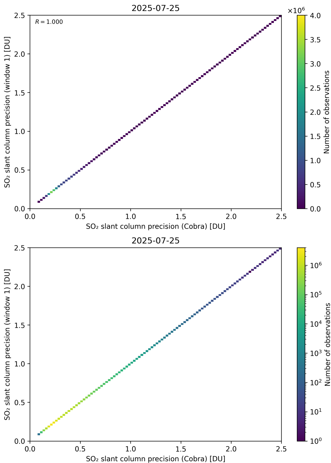
Figure 209: Scatter density plot of “SO 2 slant column precision (Cobra)” against “SO 2 slant column precision (window 1)” for 2025-07-24 to 2025-07-26.
