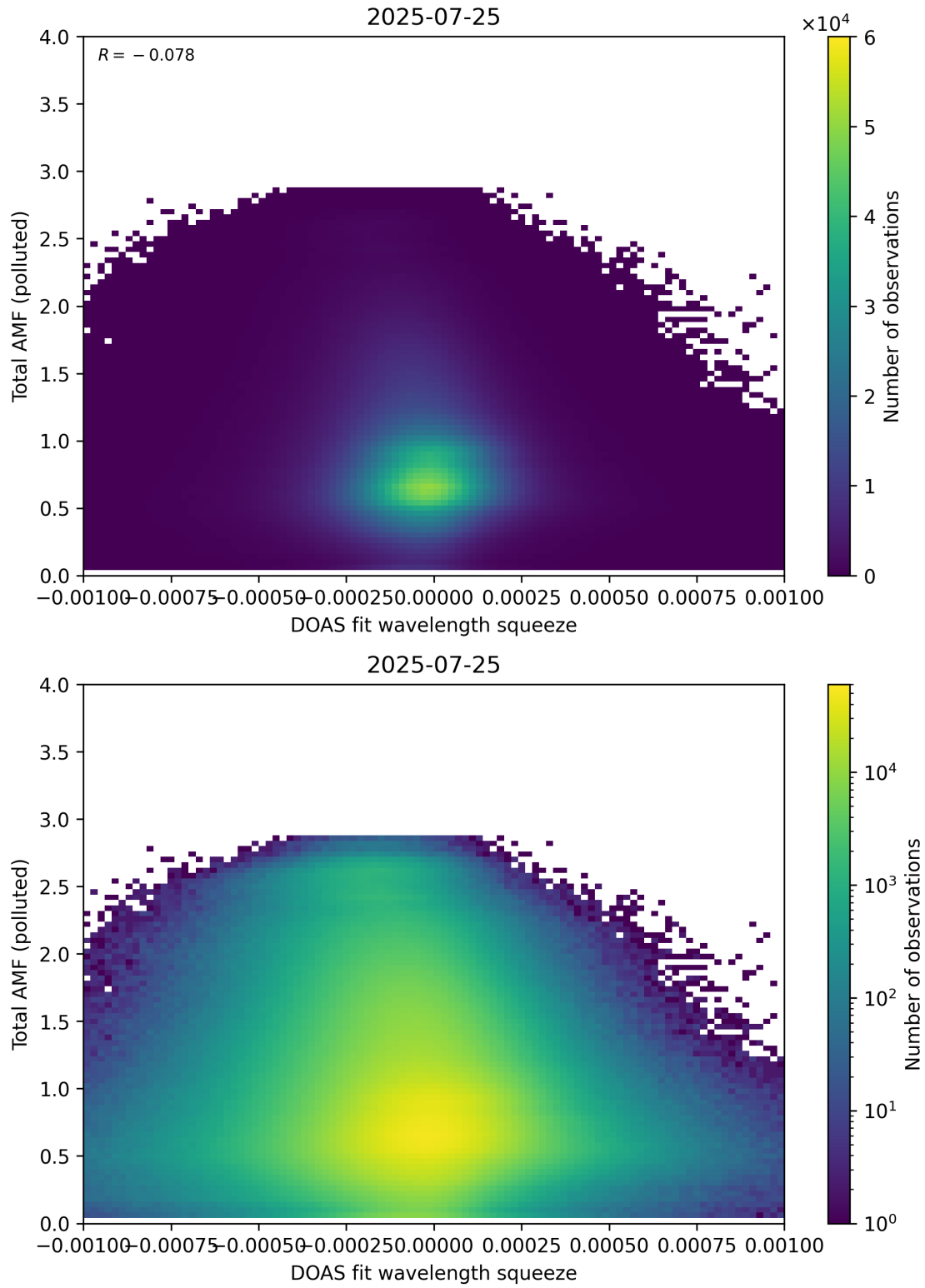
Figure 145: Scatter density plot of “DOAS fit wavelength squeeze” against “Total AMF (polluted)” for 2025-07-24 to 2025-07-26.
