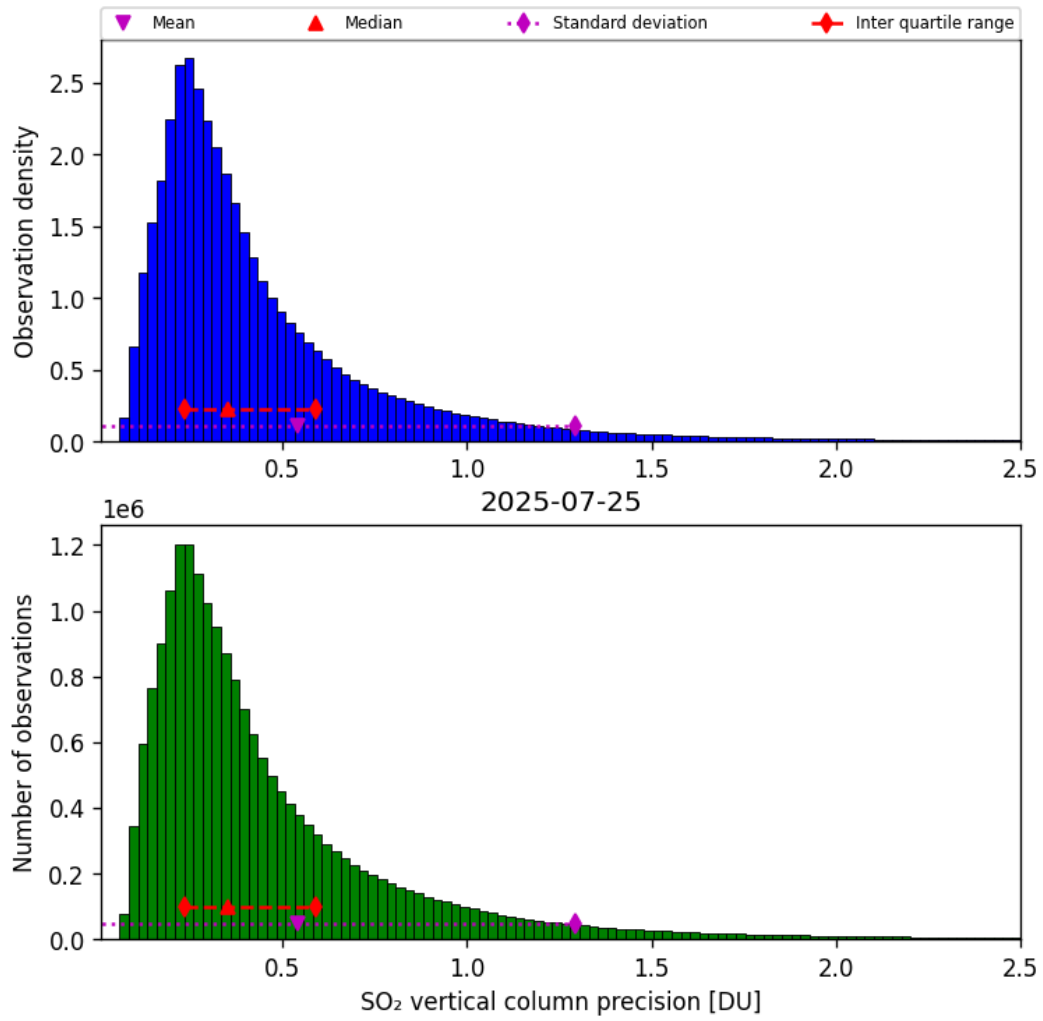
Figure 59: Histogram of “SO 2 vertical column precision” for 2025-07-24 to 2025-07-26
