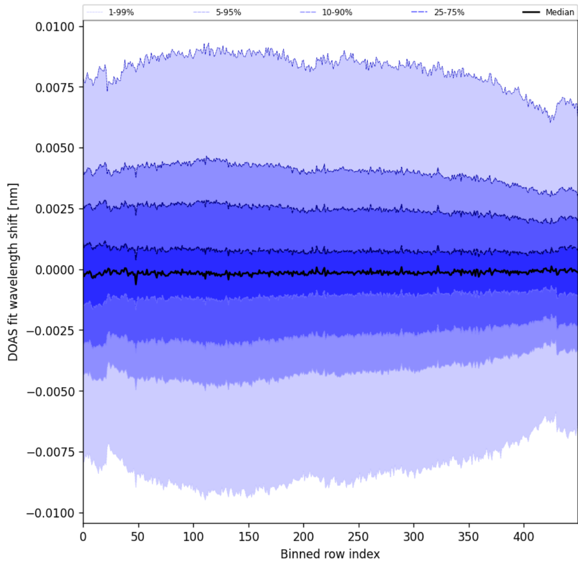
Figure 102: Along track statistics of “DOAS fit wavelength shift” for 2025-07-24 to 2025-07-26
