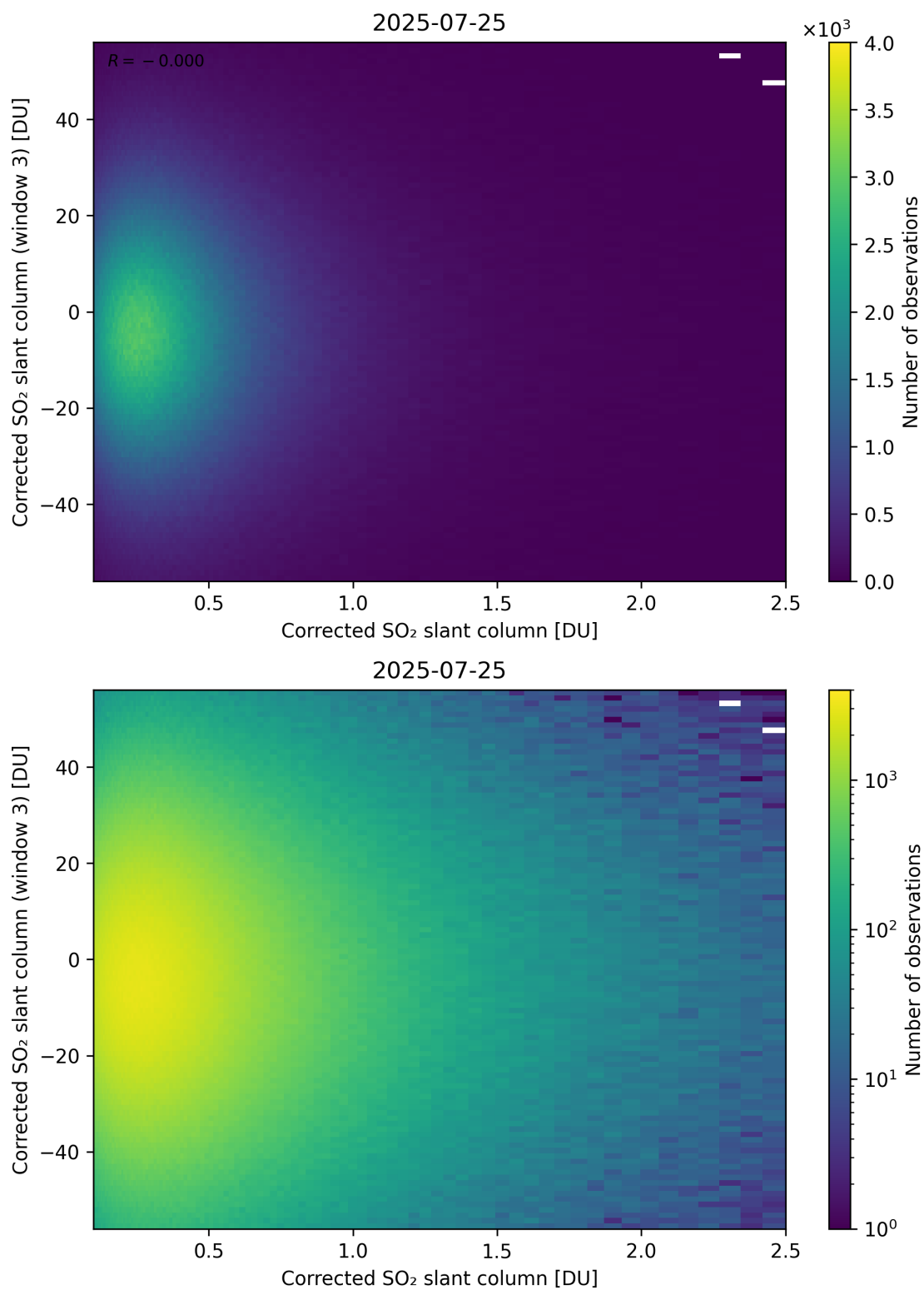
Figure 236: Scatter density plot of “Corrected SO 2 slant column” against “Corrected SO 2 slant column (window 3)” for 2025-07-24 to 2025-07-26.
