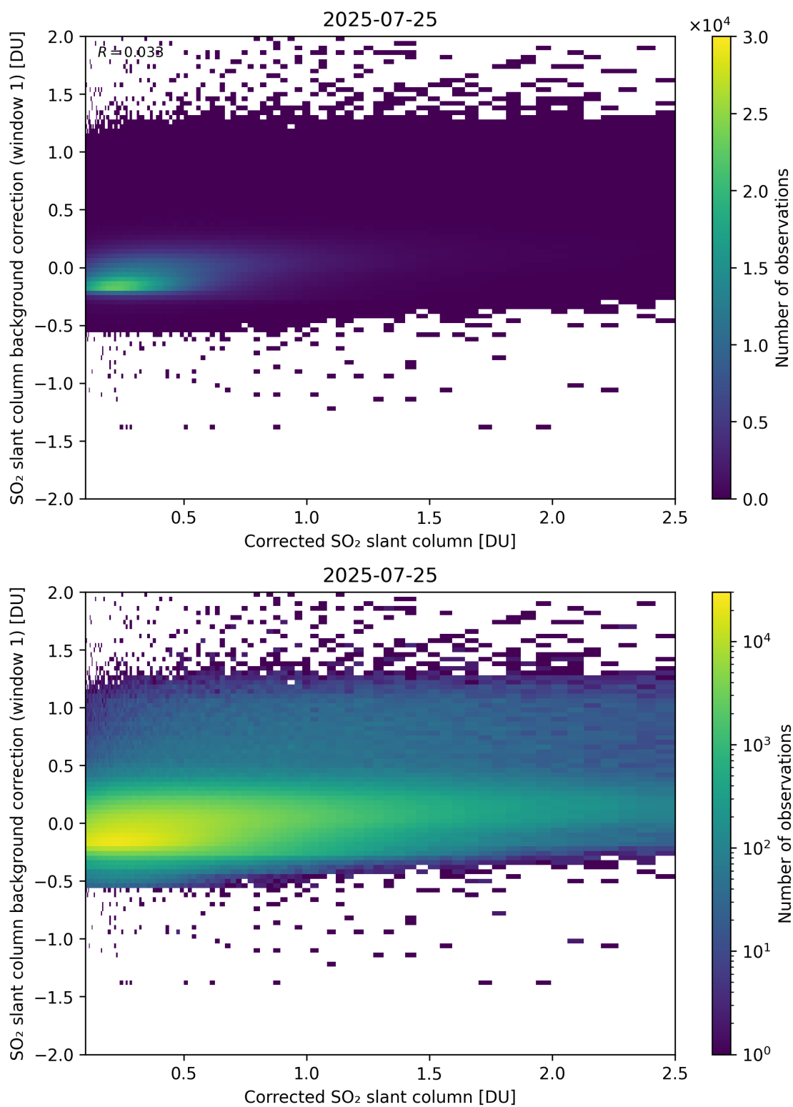
Figure 226: Scatter density plot of “Corrected SO 2 slant column” against “SO 2 slant column background correction (window 1)” for 2025-07-24 to 2025-07-26.
