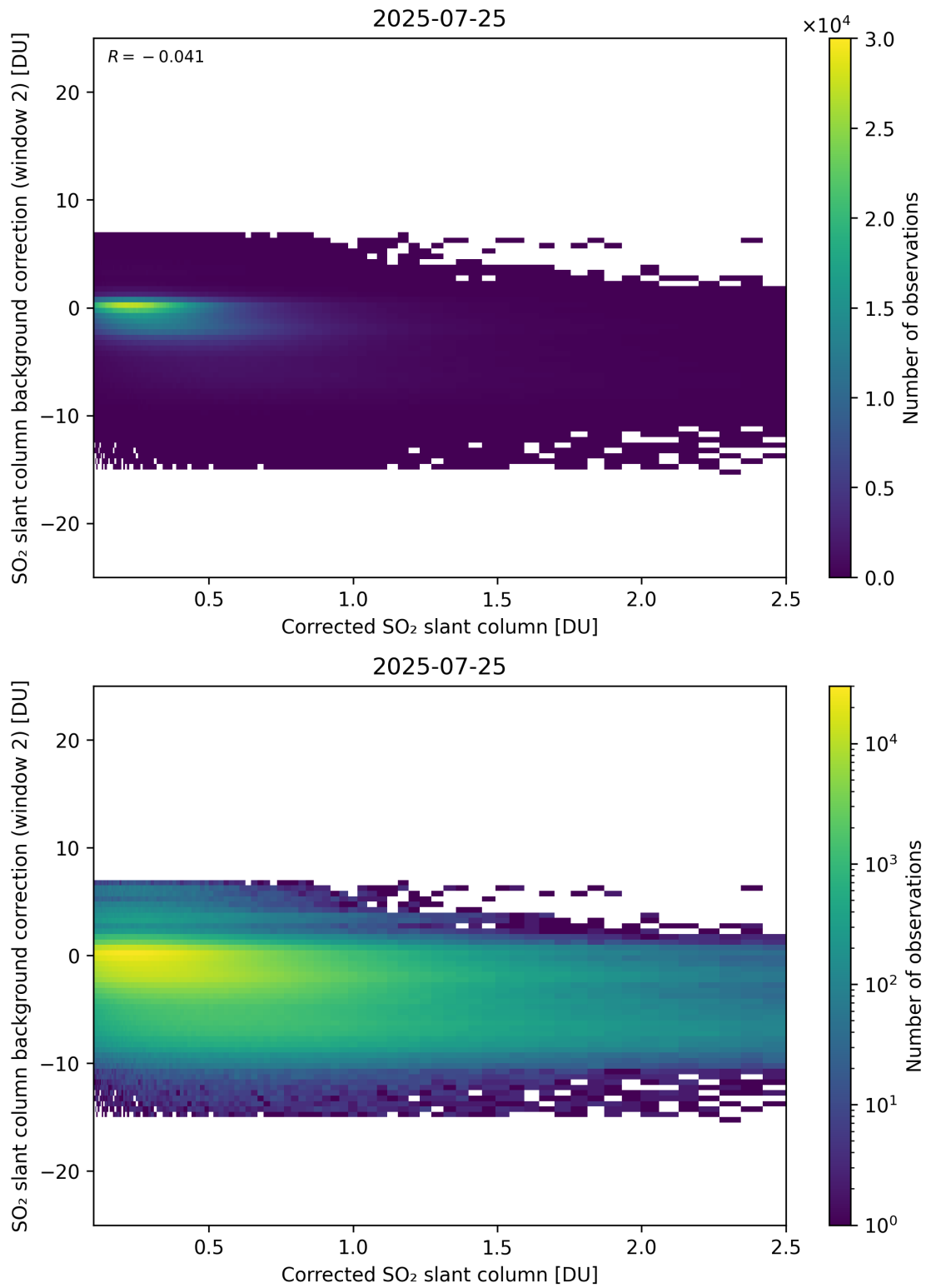
Figure 227: Scatter density plot of “Corrected SO 2 slant column” against “SO 2 slant column background correction (window 2)” for 2025-07-24 to 2025-07-26.
