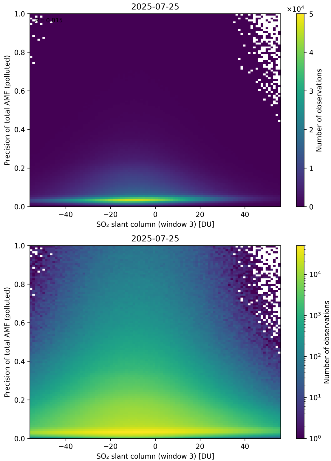
Figure 319: Scatter density plot of “SO 2 slant column (window 3)” against “Precision of total AMF (polluted)” for 2025-07-24 to 2025-07-26.
