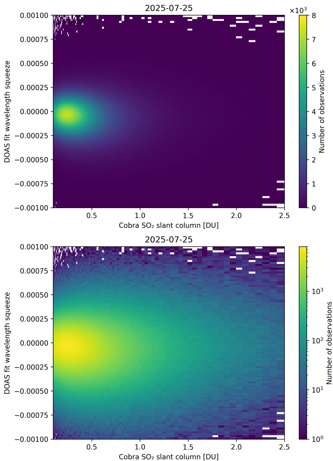
Figure 197: Scatter density plot of “Cobra SO 2 slant column” against “DOAS fit wavelength squeeze” for 2025-07-24 to 2025-07-26.
