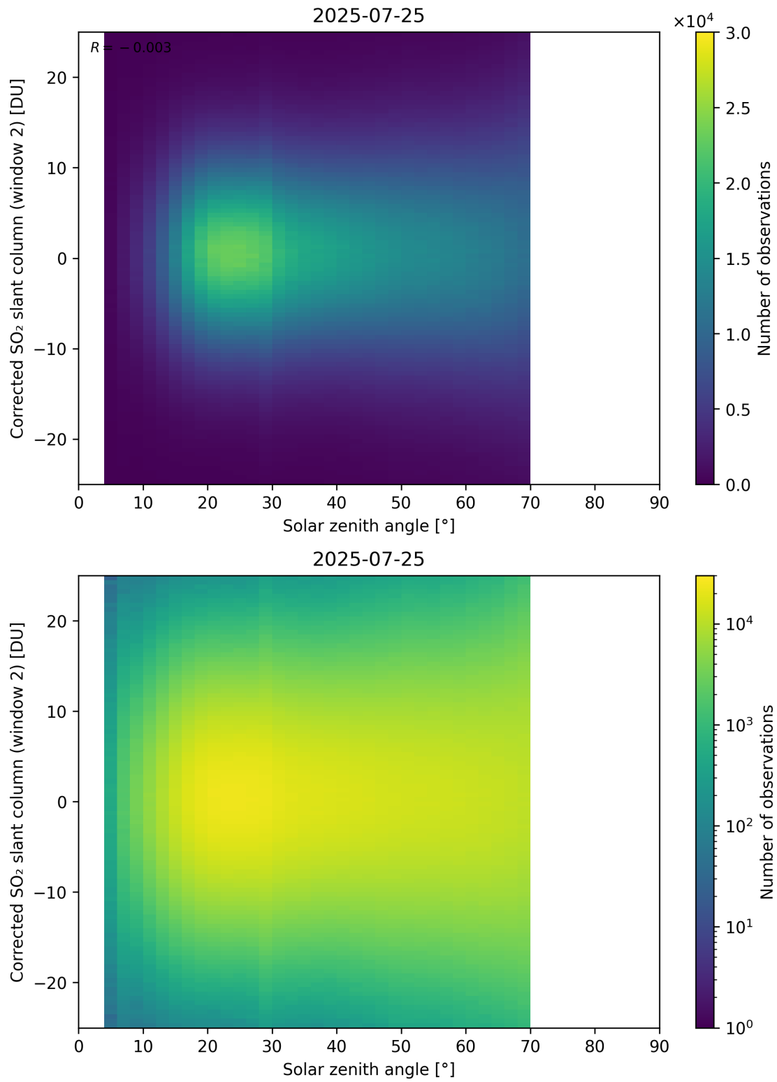
Figure 182: Scatter density plot of “Solar zenith angle” against “Corrected SO 2 slant column (window 2)” for 2025-07-24 to 2025-07-26.
