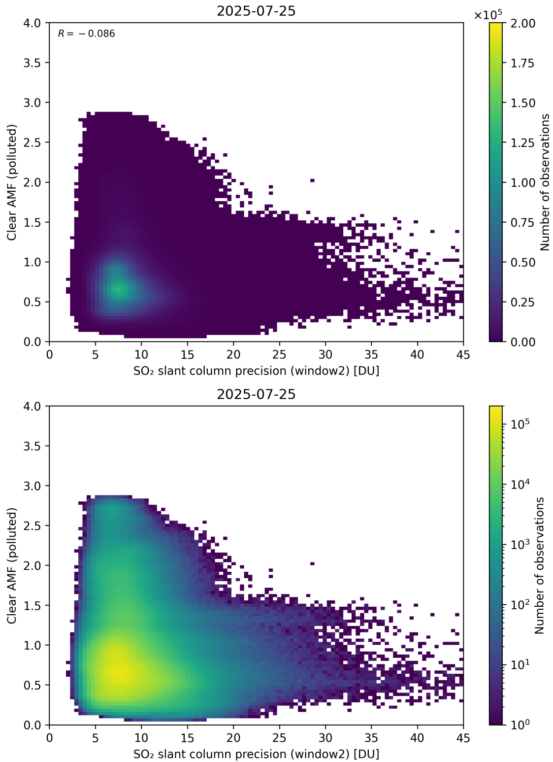
Figure 296: Scatter density plot of “SO 2 slant column precision (window2)” against “Clear AMF (polluted)” for 2025-07-24 to 2025-07-26.
