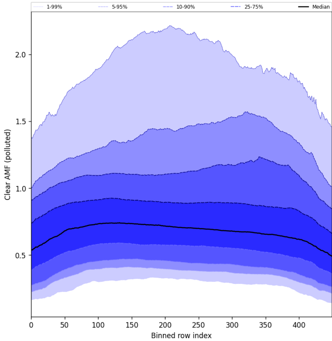
Figure 107: Along track statistics of “Clear AMF (polluted)” for 2025-07-24 to 2025-07-26
