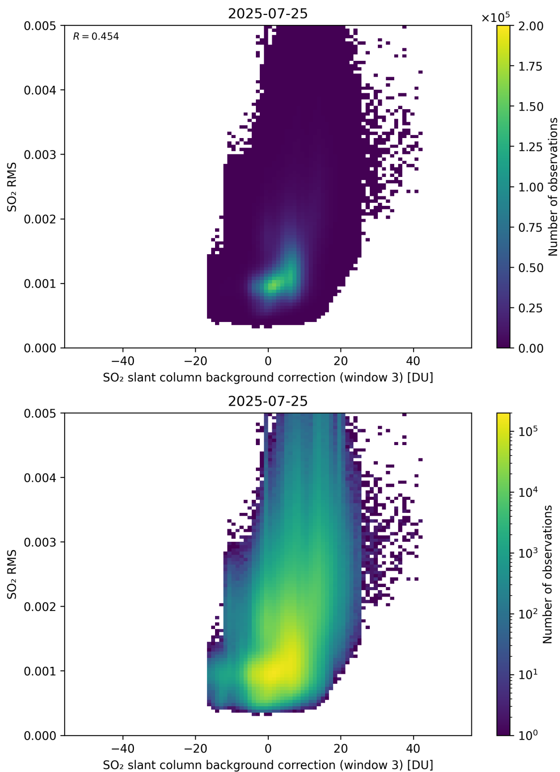
Figure 134: Scatter density plot of “SO 2 slant column background correction (window 3)” against “SO 2 RMS” for 2025-07-24 to 2025-07-26.
