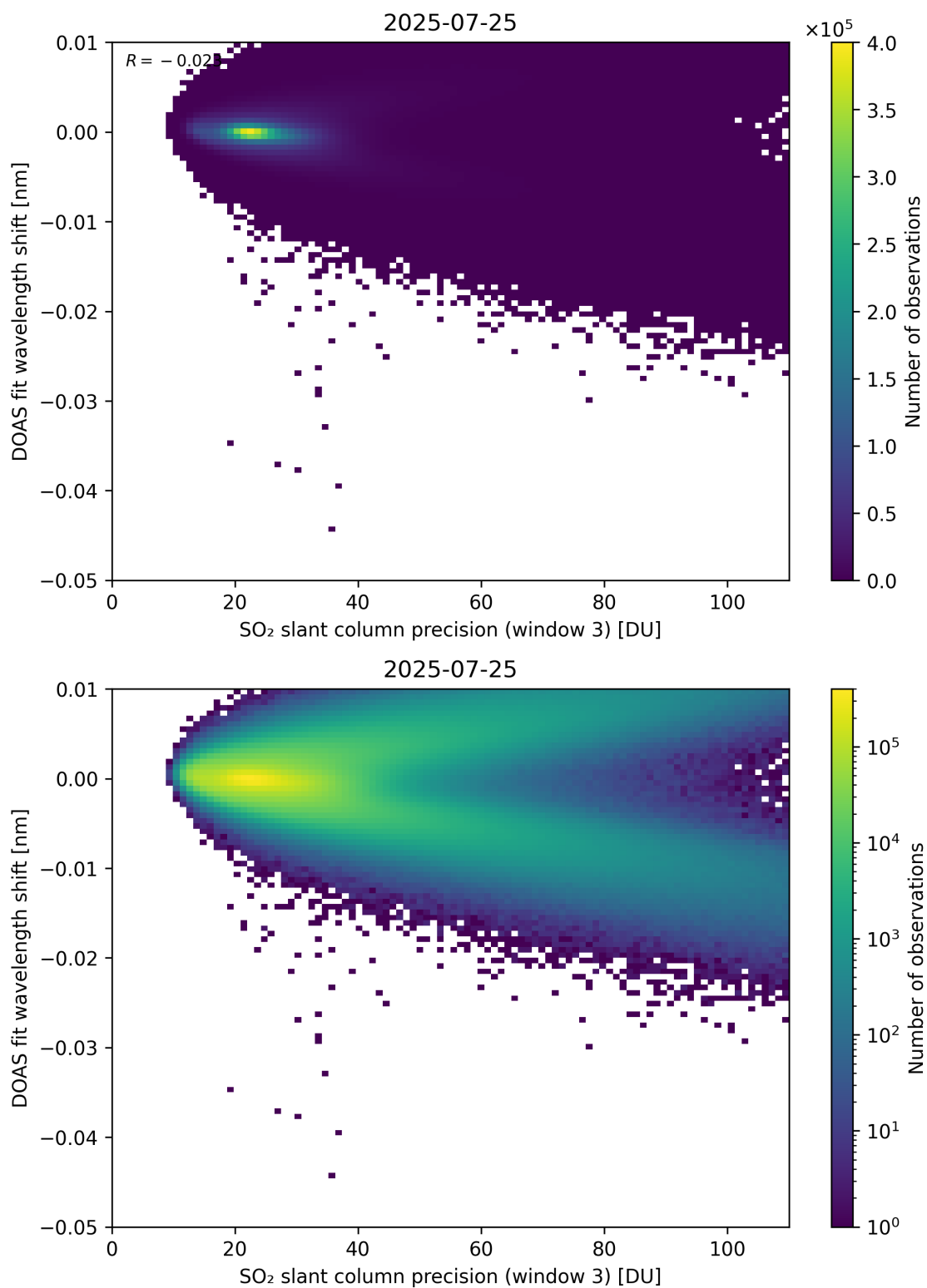
Figure 308: Scatter density plot of “SO 2 slant column precision (window 3)” against “DOAS fit wavelength shift” for 2025-07-24 to 2025-07-26.
