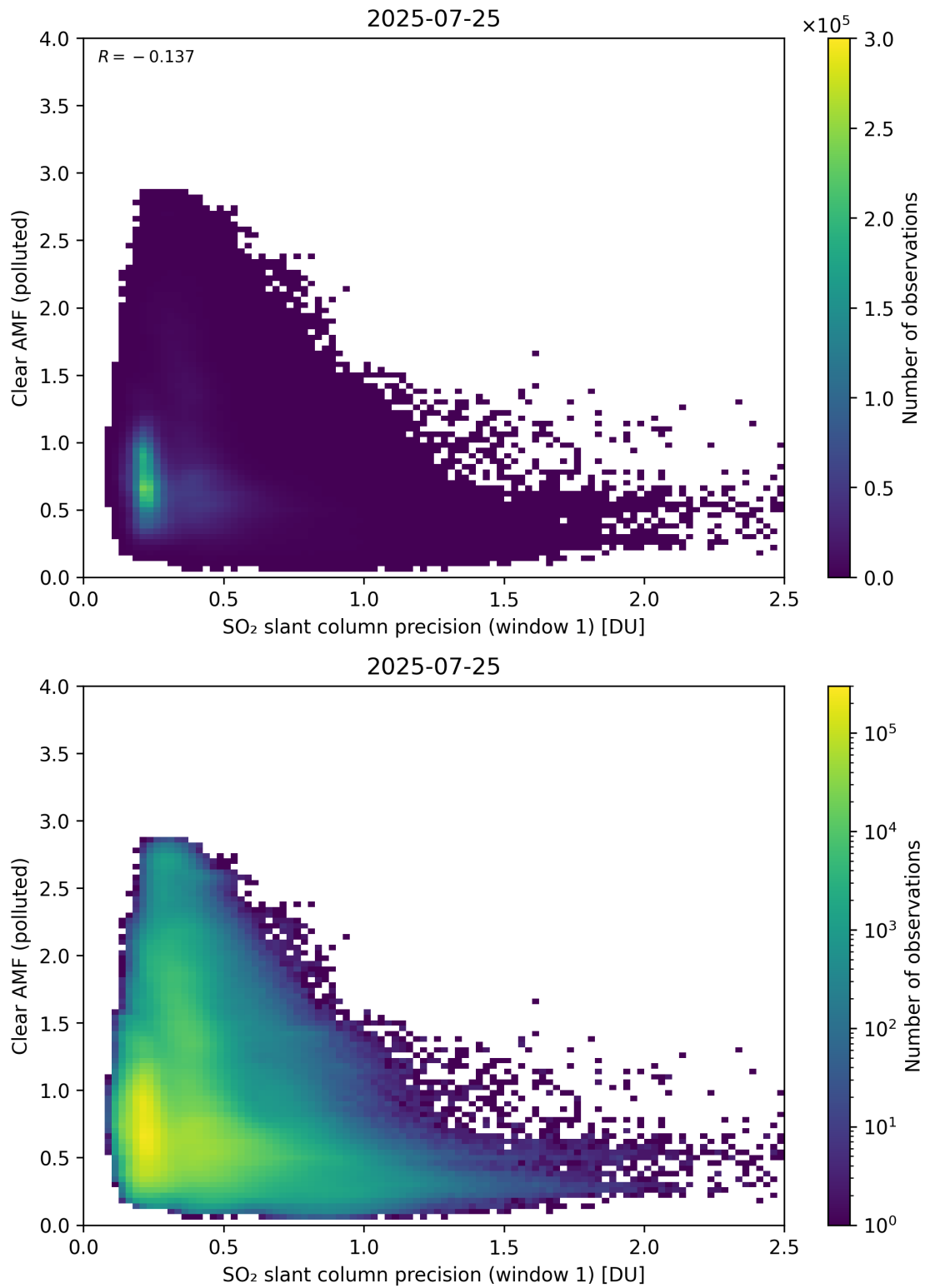
Figure 274: Scatter density plot of “SO 2 slant column precision (window 1)” against “Clear AMF (polluted)” for 2025-07-24 to 2025-07-26.
