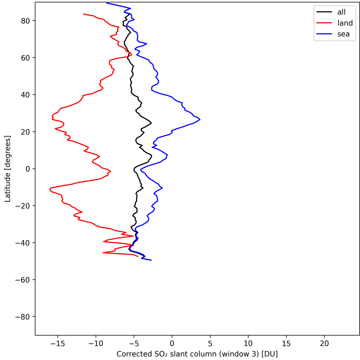
Figure 47: Zonal average of “Corrected SO 2 slant column (window 3)” for 2025-07-24 to 2025-07-26.
