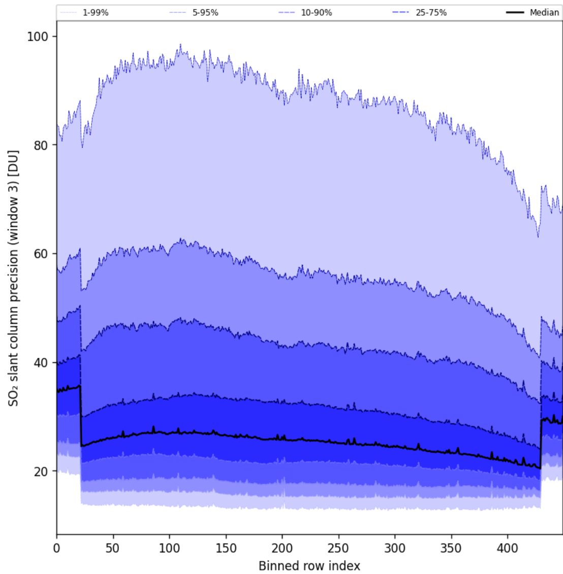
Figure 98: Along track statistics of “SO 2 slant column precision (window 3)” for 2025-07-24 to 2025-07-26
