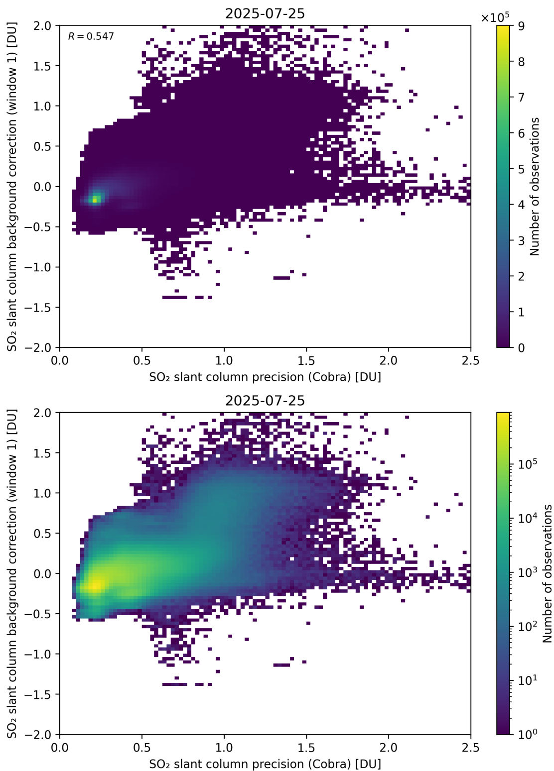
Figure 199: Scatter density plot of “SO 2 slant column precision (Cobra)” against “SO 2 slant column background correction (window 1)” for 2025-07-24 to 2025-07-26.
