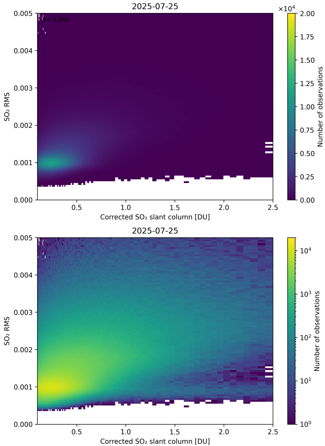
Figure 231: Scatter density plot of “Corrected SO 2 slant column” against “SO 2 RMS” for 2025-07-24 to 2025-07-26.
