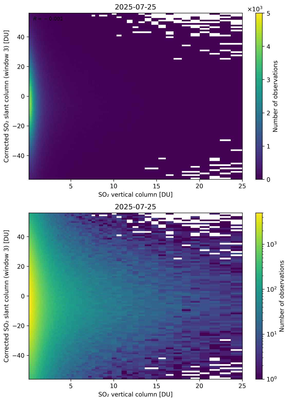
Figure 353: Scatter density plot of “SO 2 vertical column” against “Corrected SO 2 slant column (window 3)” for 2025-07-24 to 2025-07-26.
