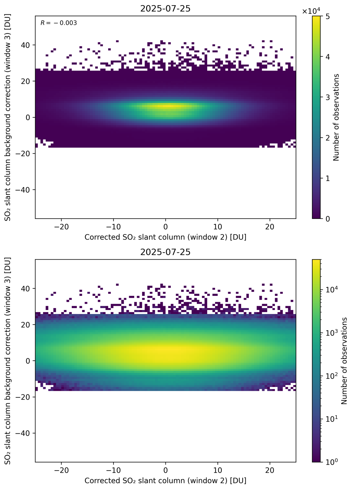
Figure 245: Scatter density plot of “Corrected SO 2 slant column (window 2)” against “SO 2 slant column background correction (window 3)” for 2025-07-24 to 2025-07-26.
