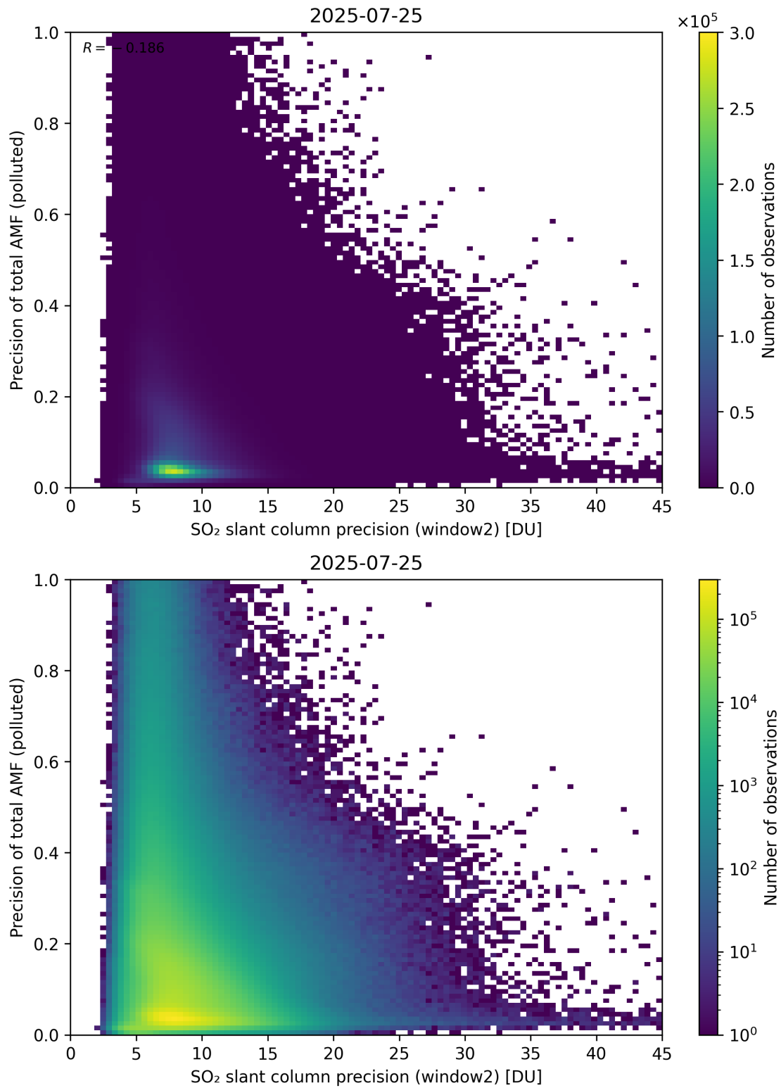
Figure 302: Scatter density plot of “SO 2 slant column precision (window2)” against “Precision of total AMF (polluted)” for 2025-07-24 to 2025-07-26.
