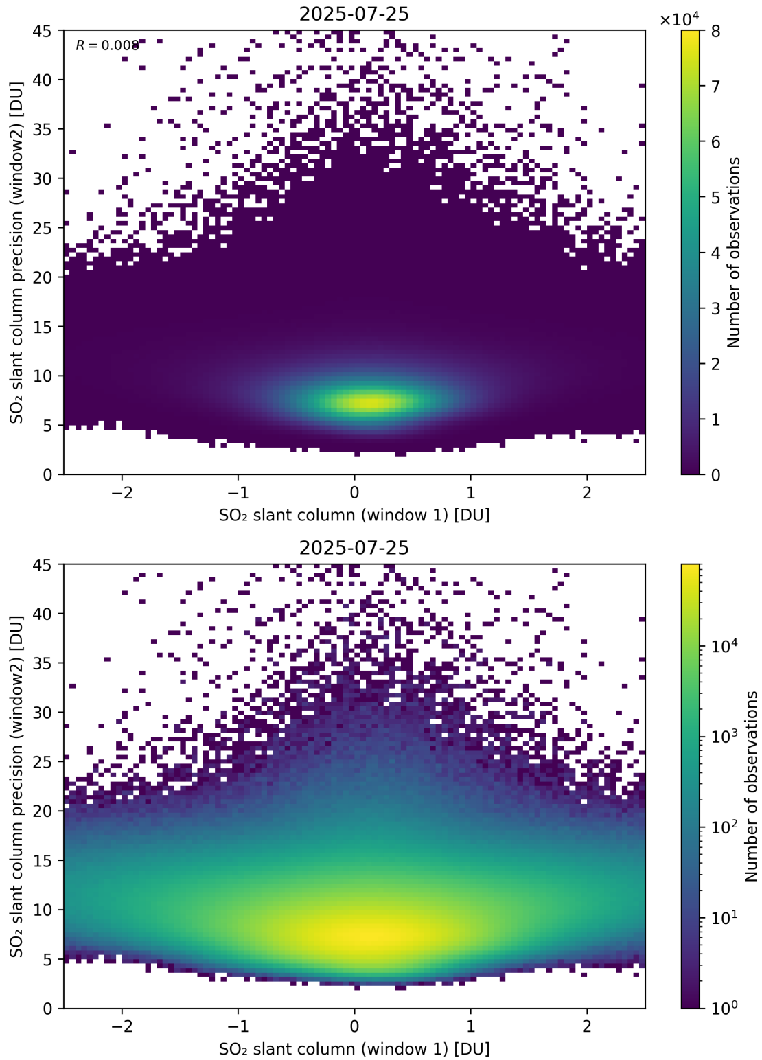
Figure 286: Scatter density plot of “SO 2 slant column (window 1)” against “SO 2 slant column precision (window2)” for 2025-07-24 to 2025-07-26.
