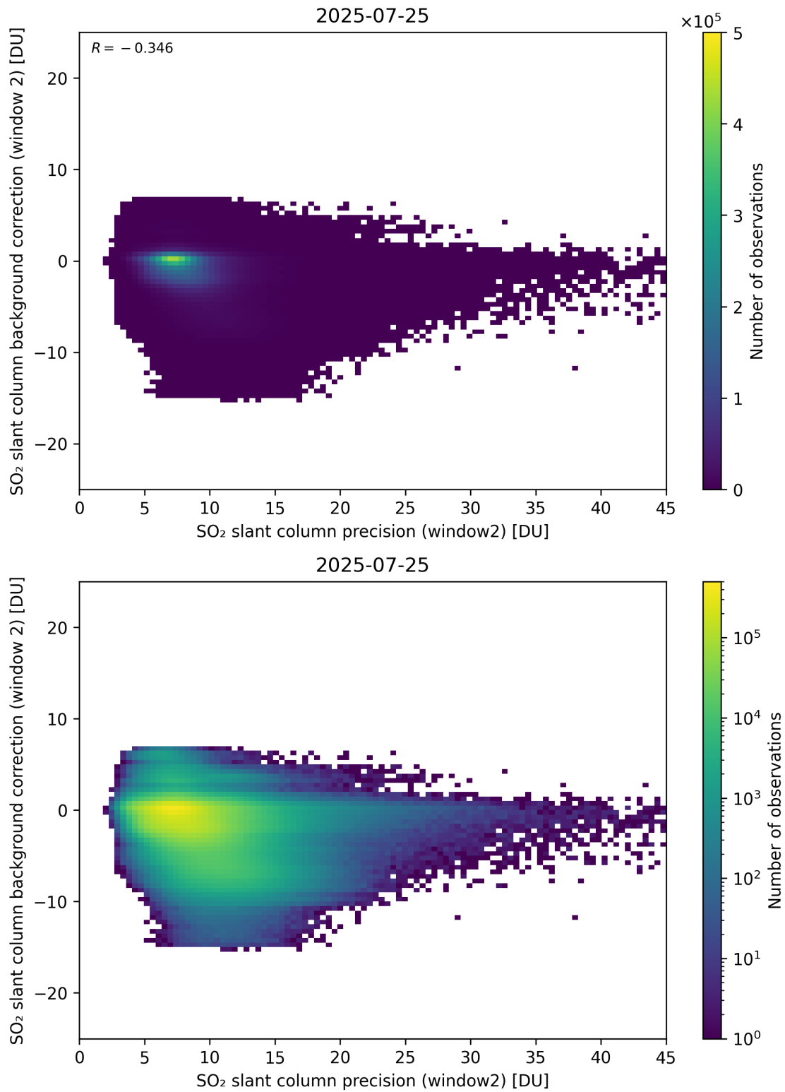
Figure 291: Scatter density plot of “SO 2 slant column precision (window2)” against “SO 2 slant column background correction (window 2)” for 2025-07-24 to 2025-07-26.
