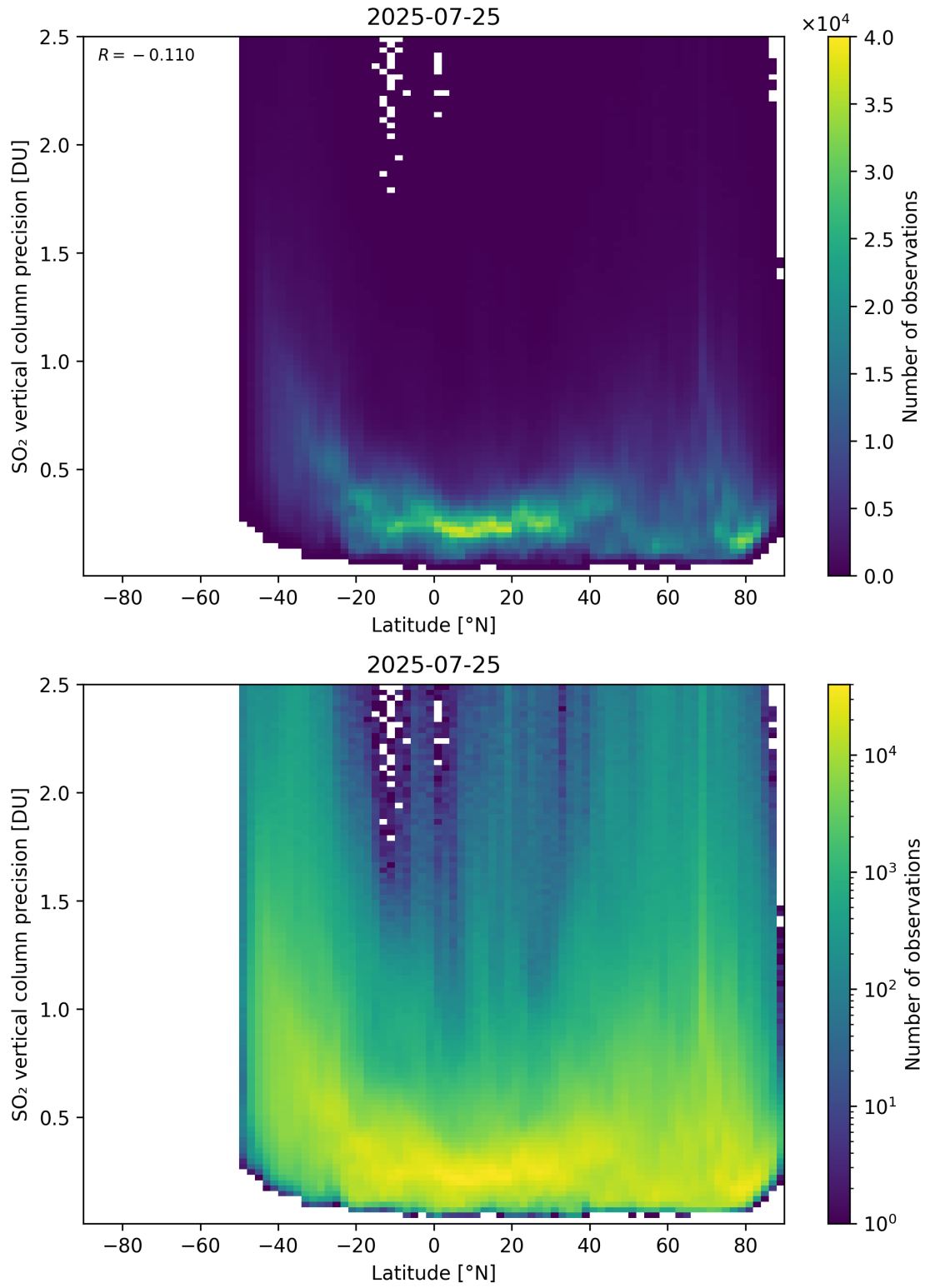
Figure 170: Scatter density plot of “Latitude” against “SO 2 vertical column precision” for 2025-07-24 to 2025-07-26.
