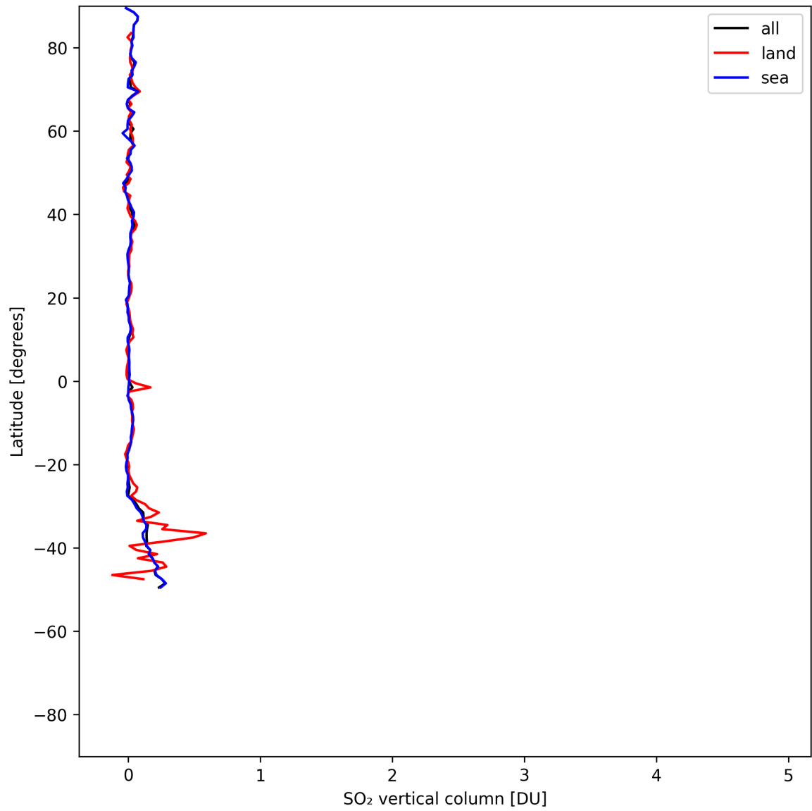
Figure 32: Zonal average of “SO 2 vertical column” for 2025-07-24 to 2025-07-26.
