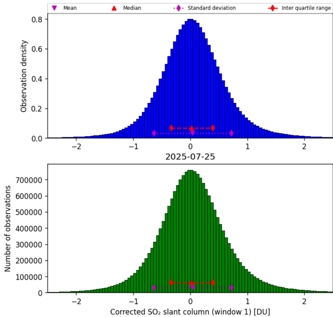
Figure 65: Histogram of “Corrected SO 2 slant column (window 1)” for 2025-07-24 to 2025-07-26
