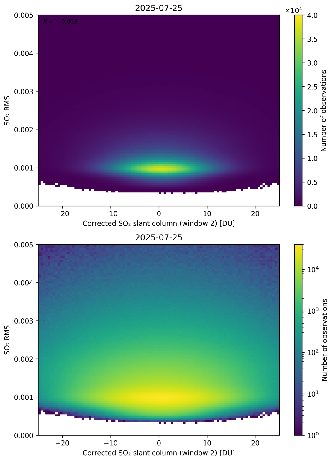
Figure 248: Scatter density plot of “Corrected SO 2 slant column (window 2)” against “SO 2 RMS” for 2025-07-24 to 2025-07-26.
