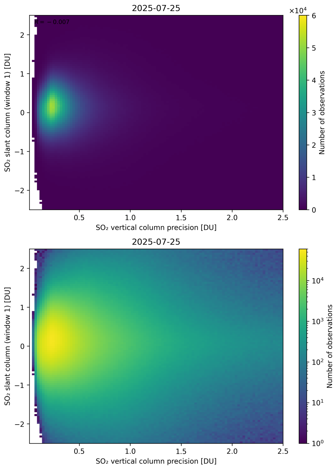
Figure 341: Scatter density plot of “SO 2 vertical column precision” against “SO 2 slant column (window 1)” for 2025-07-24 to 2025-07-26.
