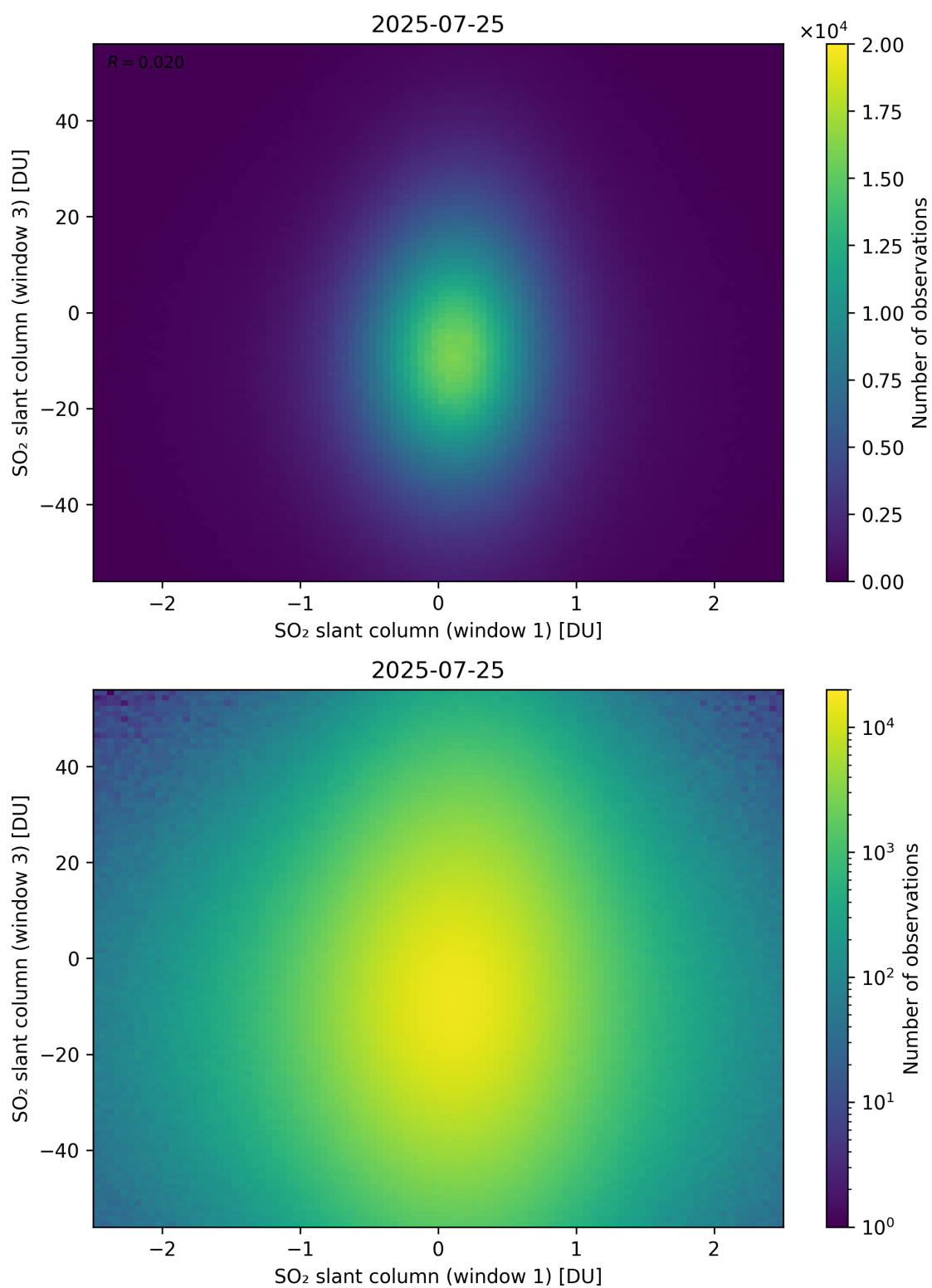
Figure 287: Scatter density plot of “SO 2 slant column (window 1)” against “SO 2 slant column (window 3)” for 2025-07-24 to 2025-07-26.
