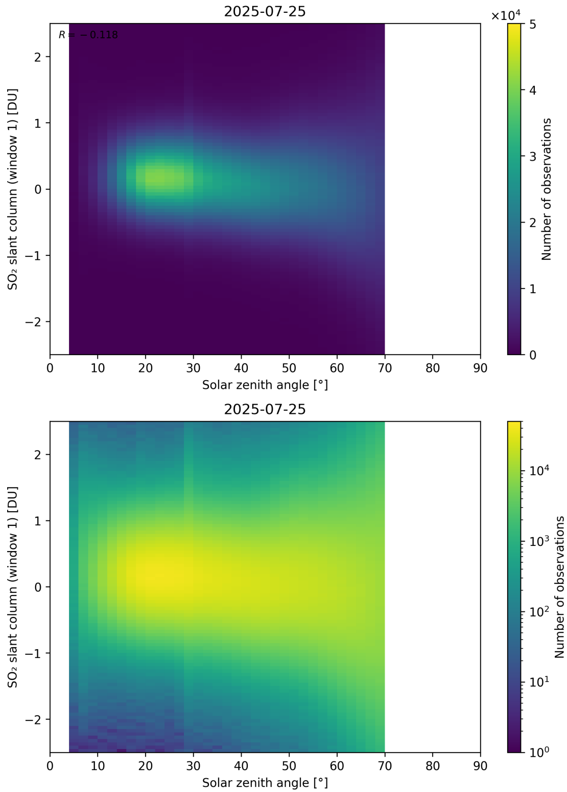
Figure 184: Scatter density plot of “Solar zenith angle” against “SO 2 slant column (window 1)” for 2025-07-24 to 2025-07-26.
