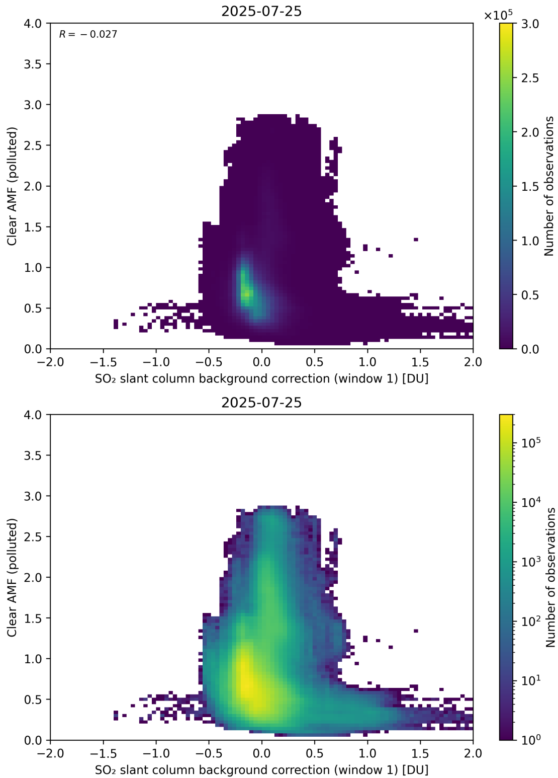
Figure 114: Scatter density plot of “SO 2 slant column background correction (window 1)” against “Clear AMF (polluted)” for 2025-07-24 to 2025-07-26.
