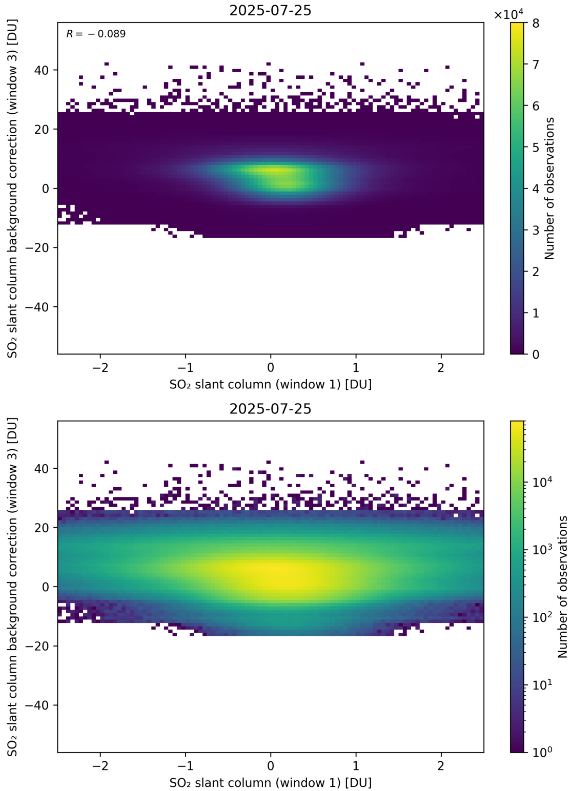
Figure 264: Scatter density plot of “SO 2 slant column (window 1)” against “SO 2 slant column background correction (window 3)” for 2025-07-24 to 2025-07-26.
