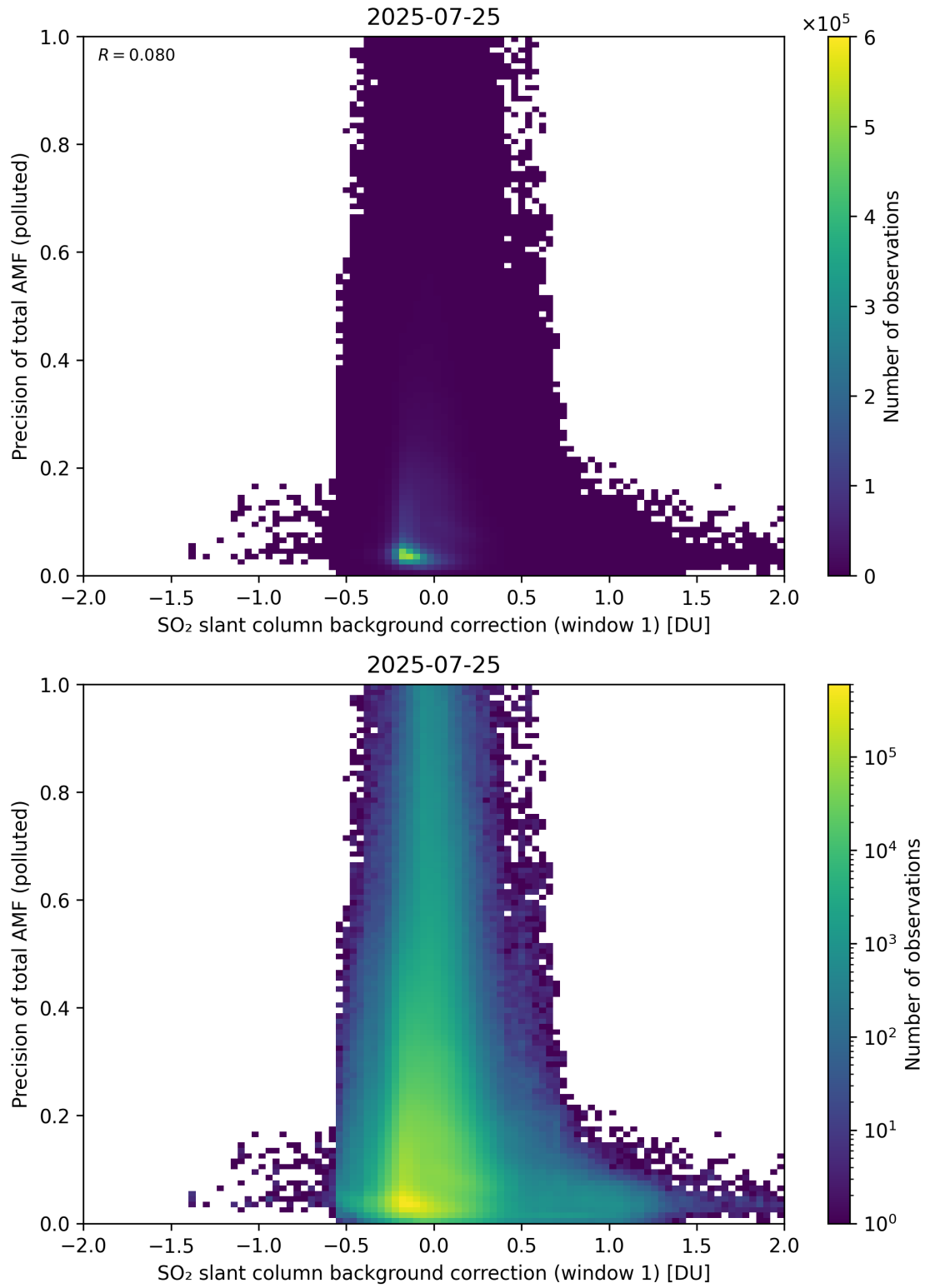
Figure 121: Scatter density plot of “SO 2 slant column background correction (window 1)” against “Precision of total AMF (polluted)” for 2025-07-24 to 2025-07-26.
