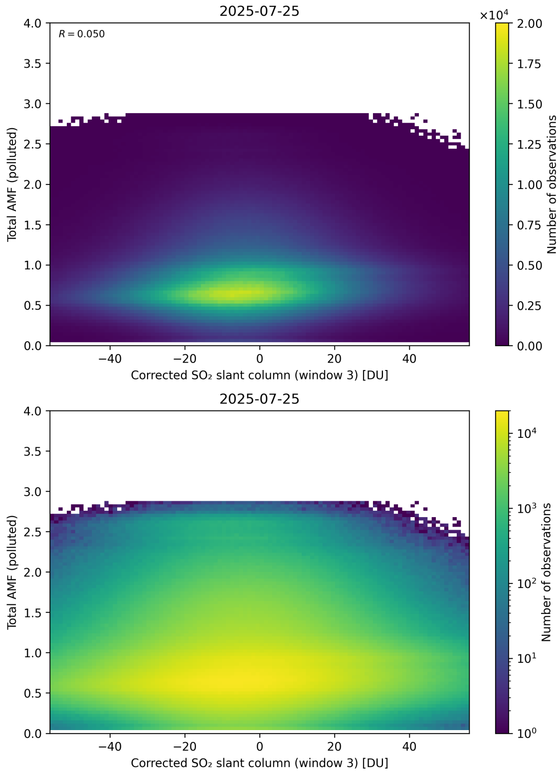
Figure 260: Scatter density plot of “Corrected SO 2 slant column (window 3)” against “Total AMF (polluted)” for 2025-07-24 to 2025-07-26.
