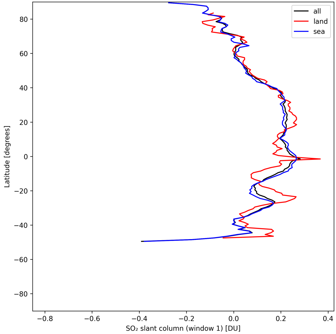
Figure 37: Zonal average of “SO 2 slant column (window 1)” for 2025-07-24 to 2025-07-26.
