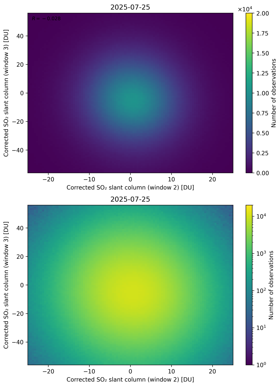
Figure 250: Scatter density plot of “Corrected SO 2 slant column (window 2)” against “Corrected SO 2 slant column (window 3)” for 2025-07-24 to 2025-07-26.
