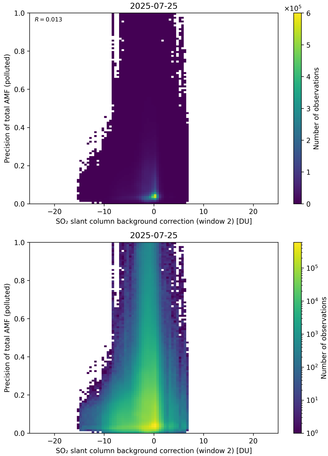
Figure 131: Scatter density plot of “SO 2 slant column background correction (window 2)” against “Precision of total AMF (polluted)” for 2025-07-24 to 2025-07-26.
