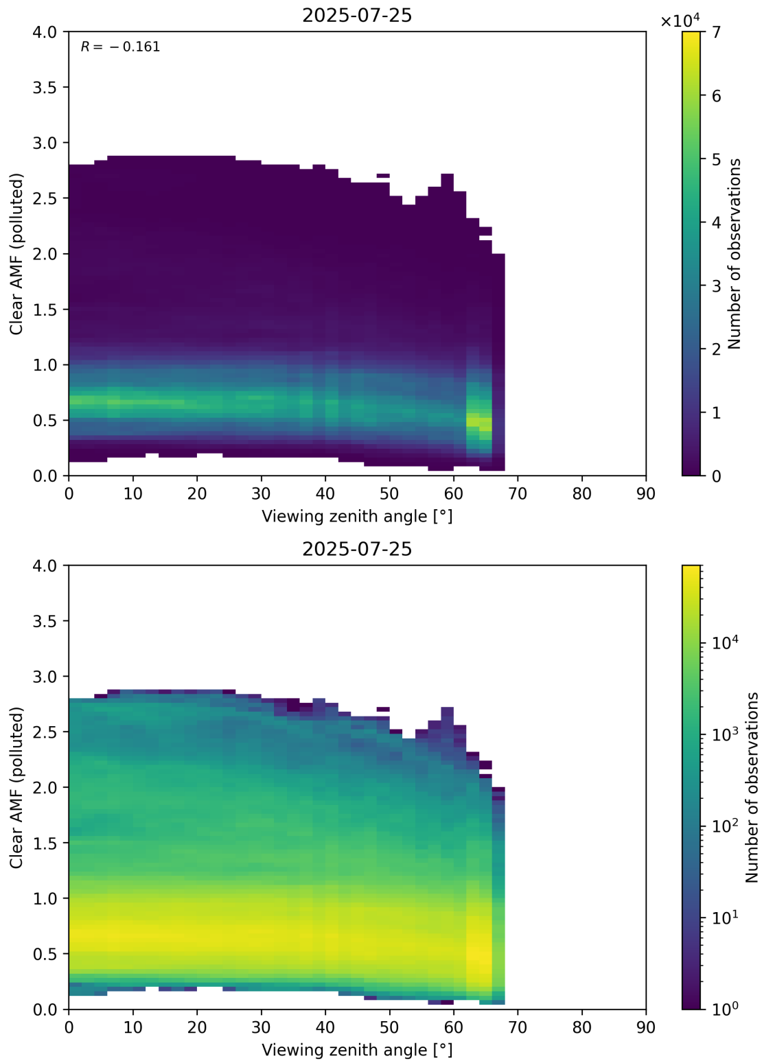
Figure 370: Scatter density plot of “Viewing zenith angle” against “Clear AMF (polluted)” for 2025-07-24 to 2025-07-26.
