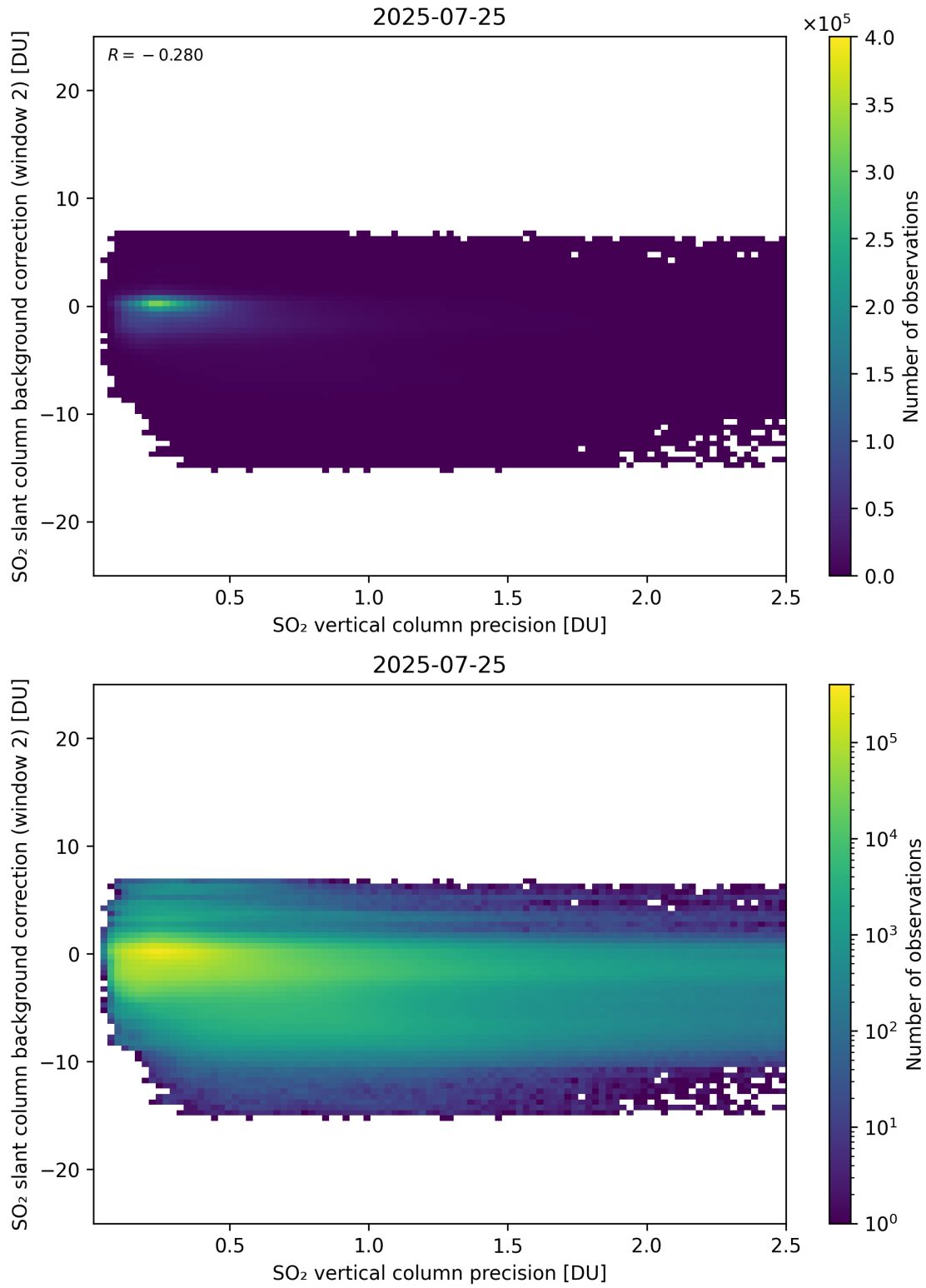
Figure 330: Scatter density plot of “SO 2 vertical column precision” against “SO 2 slant column background correction (window 2)” for 2025-07-24 to 2025-07-26.
