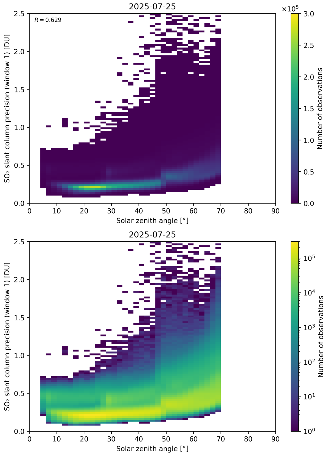
Figure 185: Scatter density plot of “Solar zenith angle” against “SO 2 slant column precision (window 1)” for 2025-07-24 to 2025-07-26.
