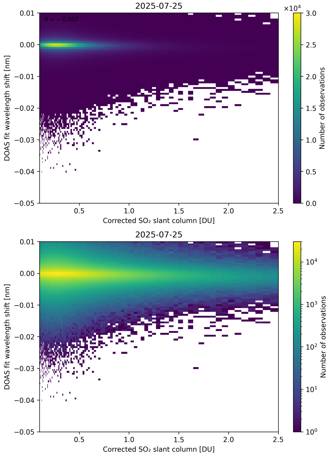
Figure 229: Scatter density plot of “Corrected SO 2 slant column” against “DOAS fit wavelength shift” for 2025-07-24 to 2025-07-26.
