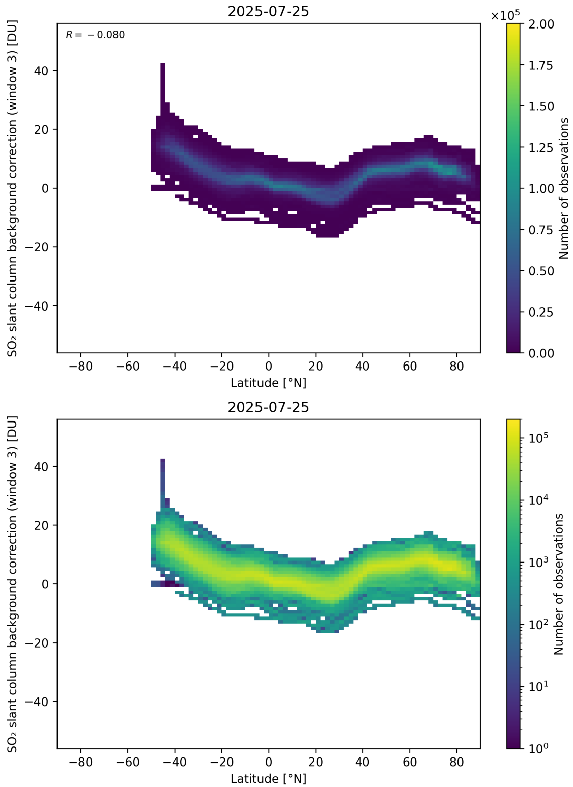
Figure 152: Scatter density plot of “Latitude” against “SO 2 slant column background correction (window 3)” for 2025-07-24 to 2025-07-26.
