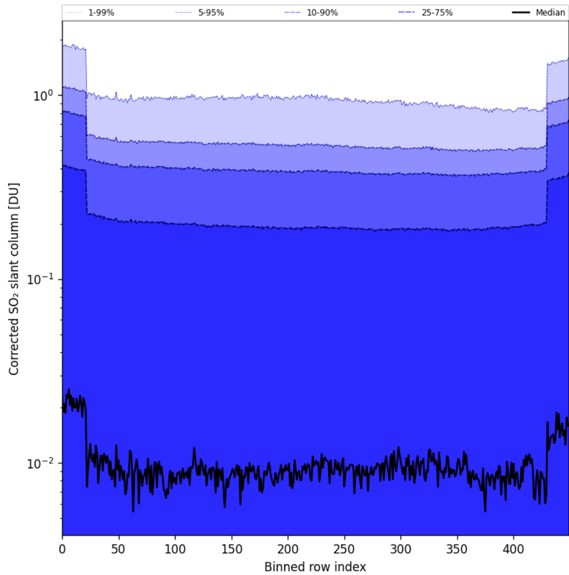
Figure 86: Along track statistics of “Corrected SO 2 slant column” for 2025-07-24 to 2025-07-26
