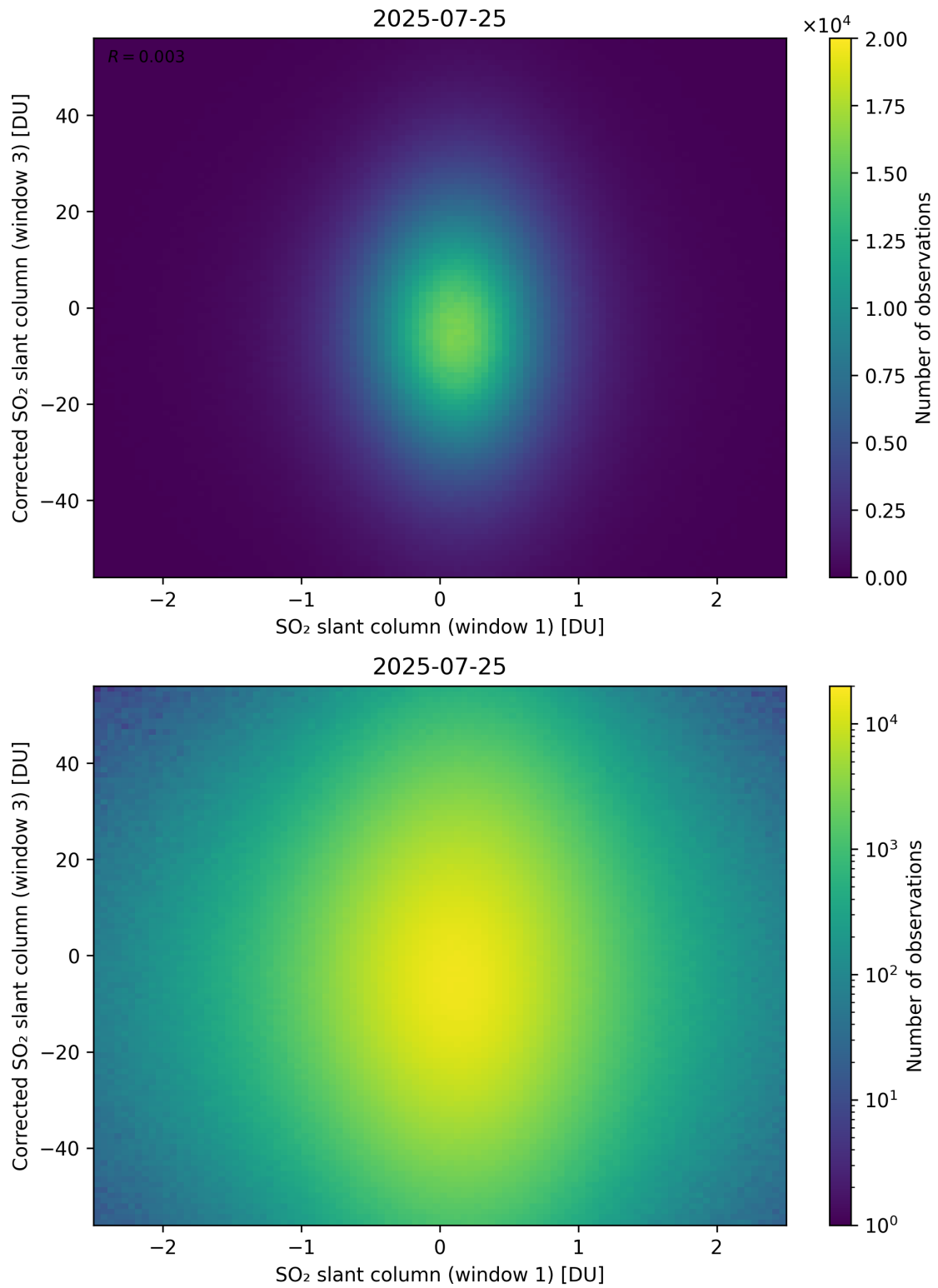
Figure 284: Scatter density plot of “SO 2 slant column (window 1)” against “Corrected SO 2 slant column (window 3)” for 2025-07-24 to 2025-07-26.
