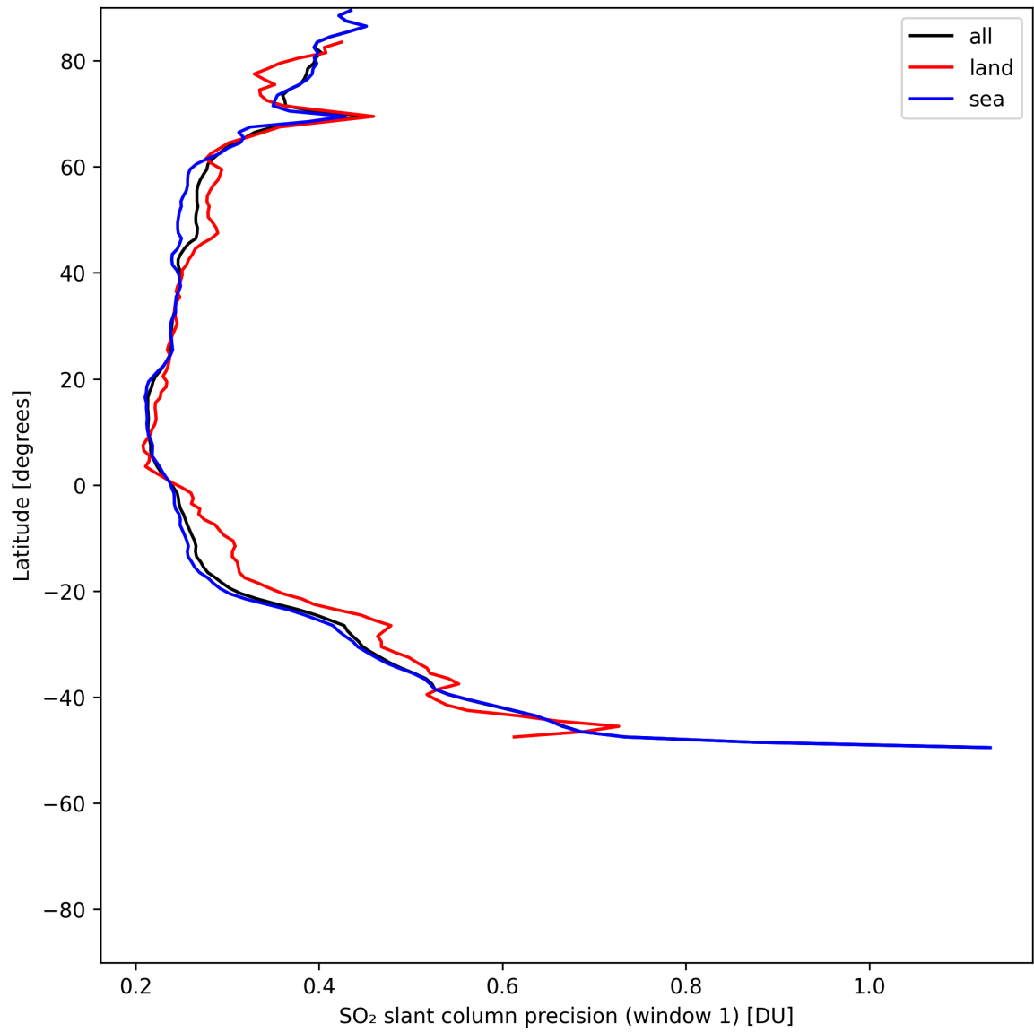
Figure 38: Zonal average of “SO 2 slant column precision (window 1)” for 2025-07-24 to 2025-07-26.
