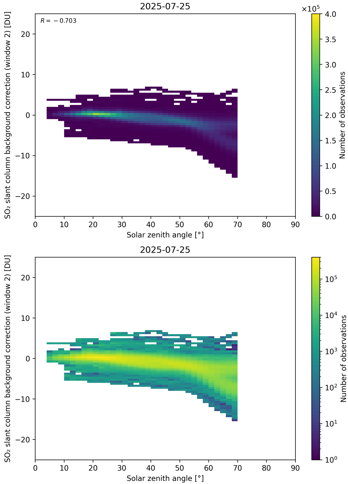
Figure 172: Scatter density plot of “Solar zenith angle” against “SO 2 slant column background correction (window 2)” for 2025-07-24 to 2025-07-26.
