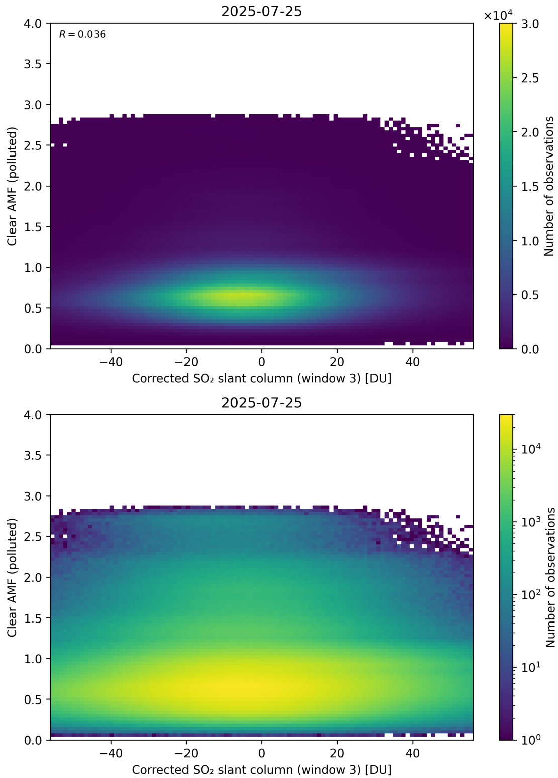
Figure 259: Scatter density plot of “Corrected SO 2 slant column (window 3)” against “Clear AMF (polluted)” for 2025-07-24 to 2025-07-26.
