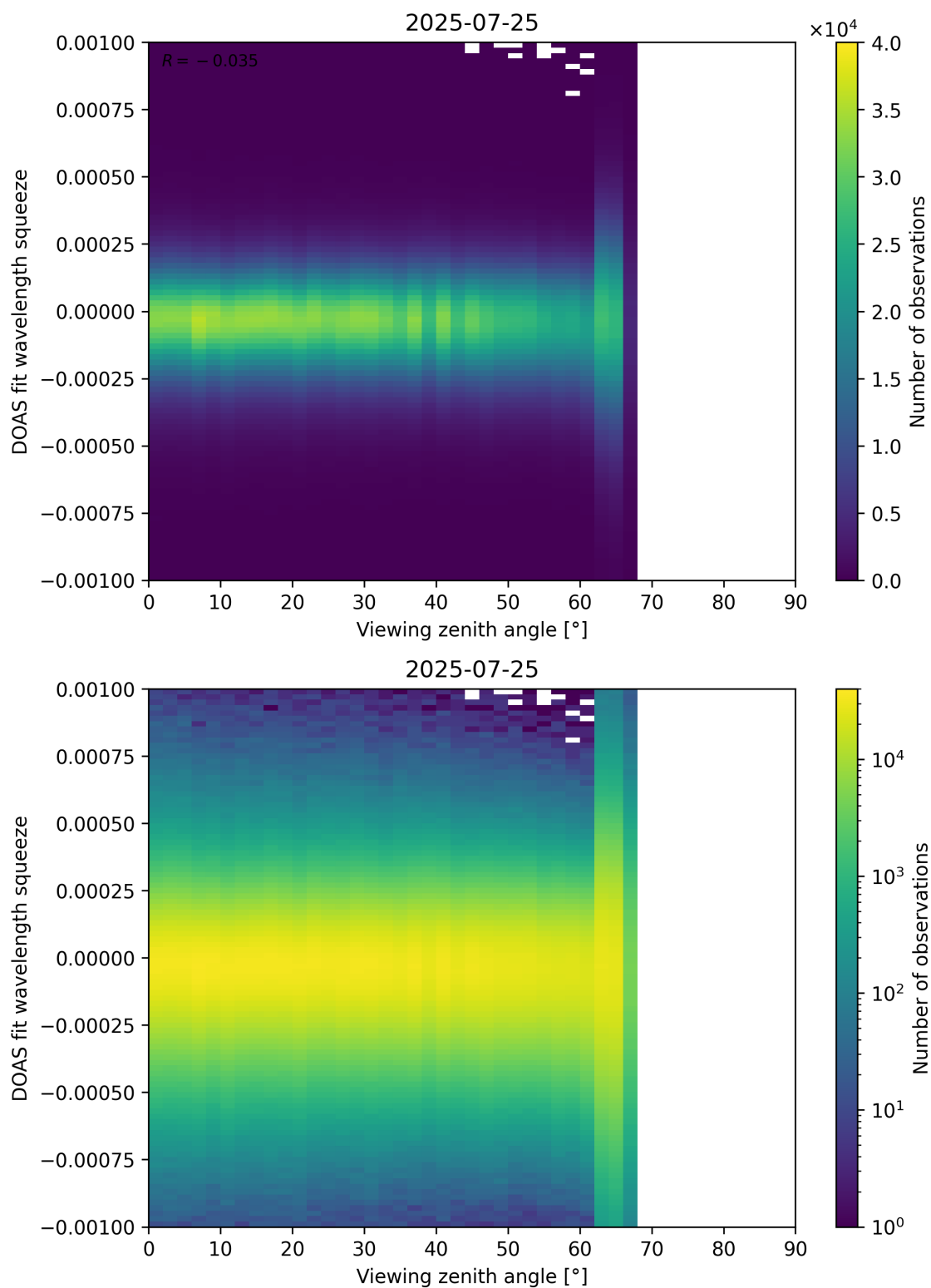
Figure 366: Scatter density plot of “Viewing zenith angle” against “DOAS fit wavelength squeeze” for 2025-07-24 to 2025-07-26.
