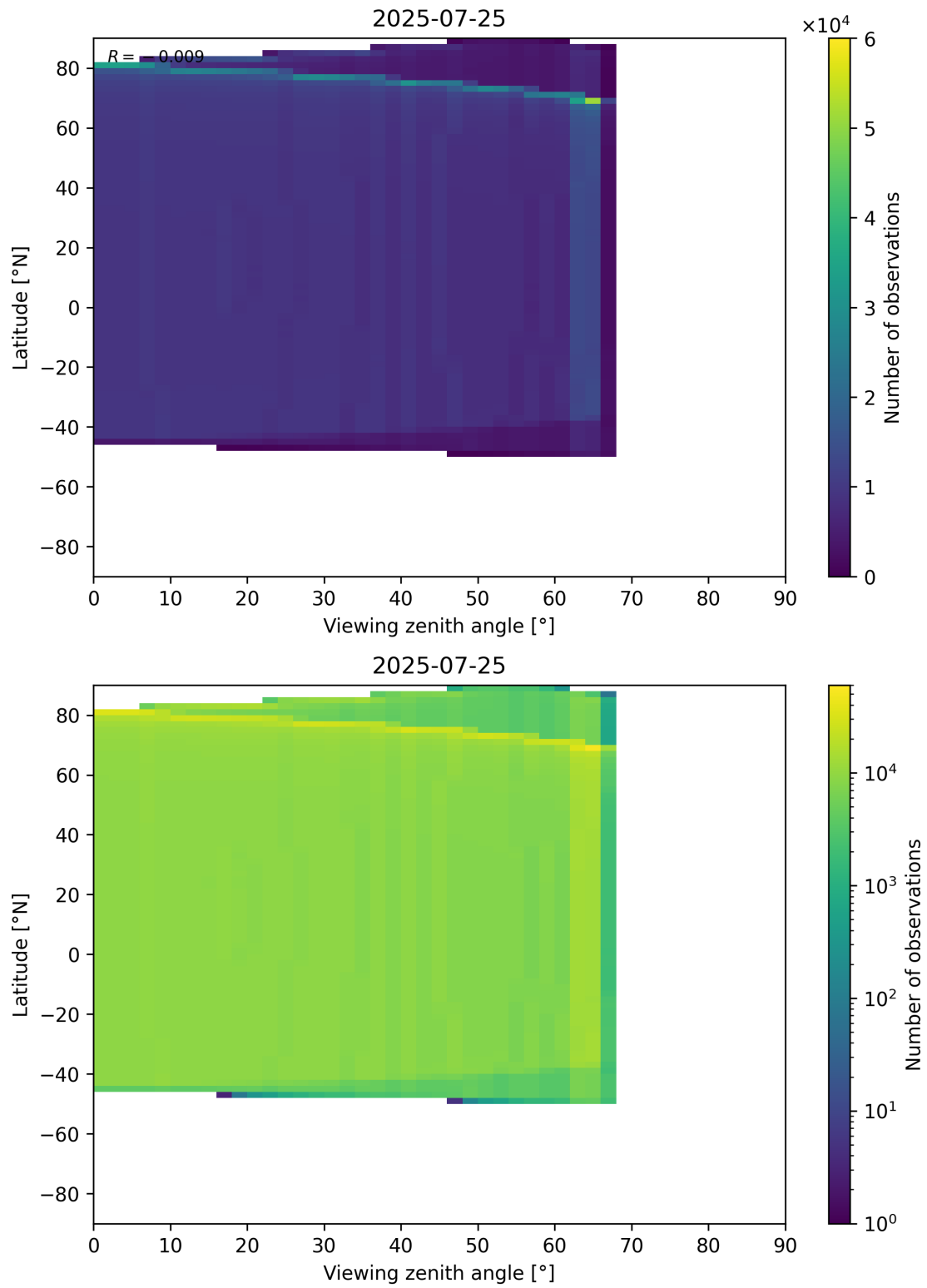
Figure 368: Scatter density plot of “Viewing zenith angle” against “Latitude” for 2025-07-24 to 2025-07-26.
