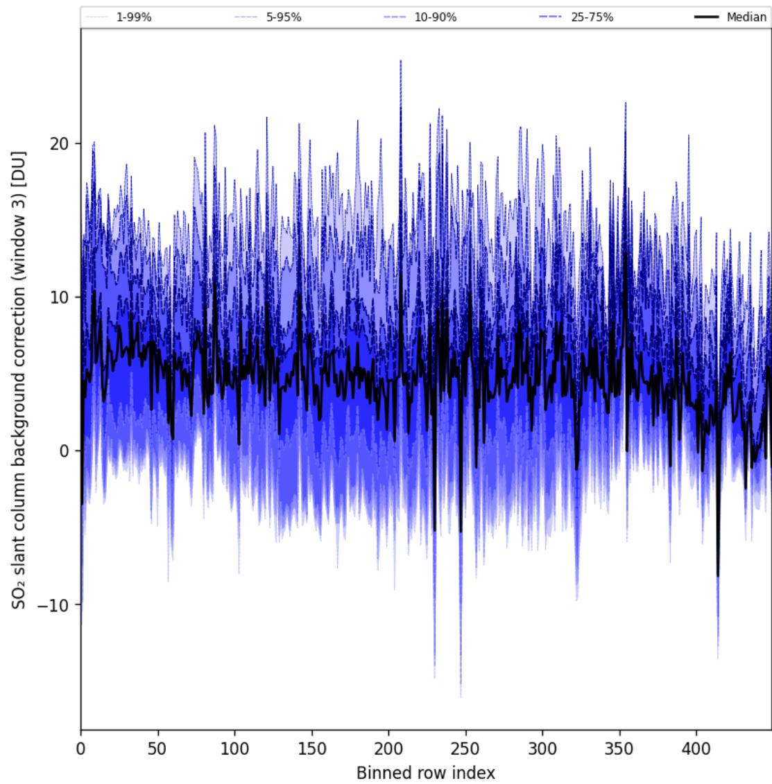
Figure 100: Along track statistics of “SO 2 slant column background correction (window 3)” for 2025-07-24 to 2025-07-26
