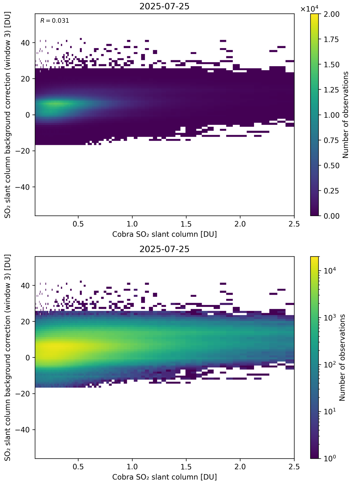
Figure 195: Scatter density plot of “Cobra SO 2 slant column” against “SO 2 slant column background correction (window 3)” for 2025-07-24 to 2025-07-26.
