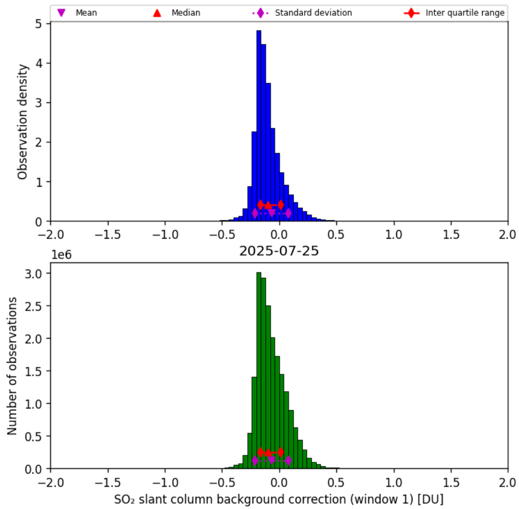
Figure 66: Histogram of “SO 2 slant column background correction (window 1)” for 2025-07-24 to 2025-07-26
