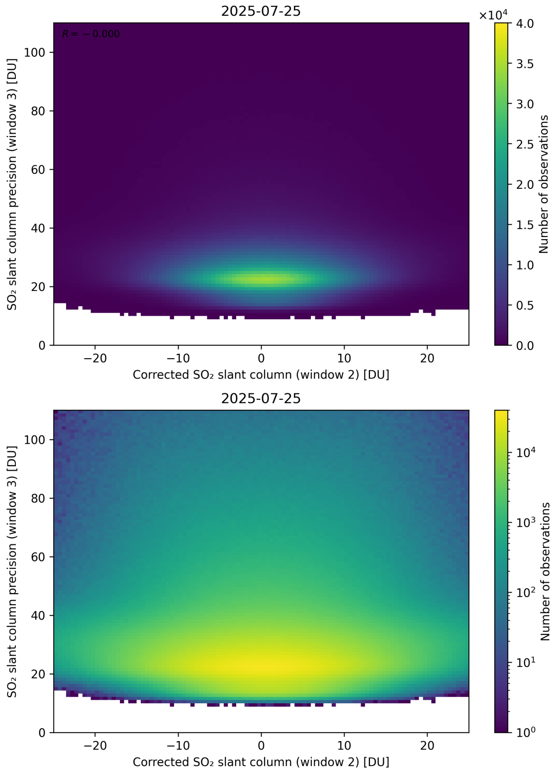
Figure 252: Scatter density plot of “Corrected SO 2 slant column (window 2)” against “SO 2 slant column precision (window 3)” for 2025-07-24 to 2025-07-26.
