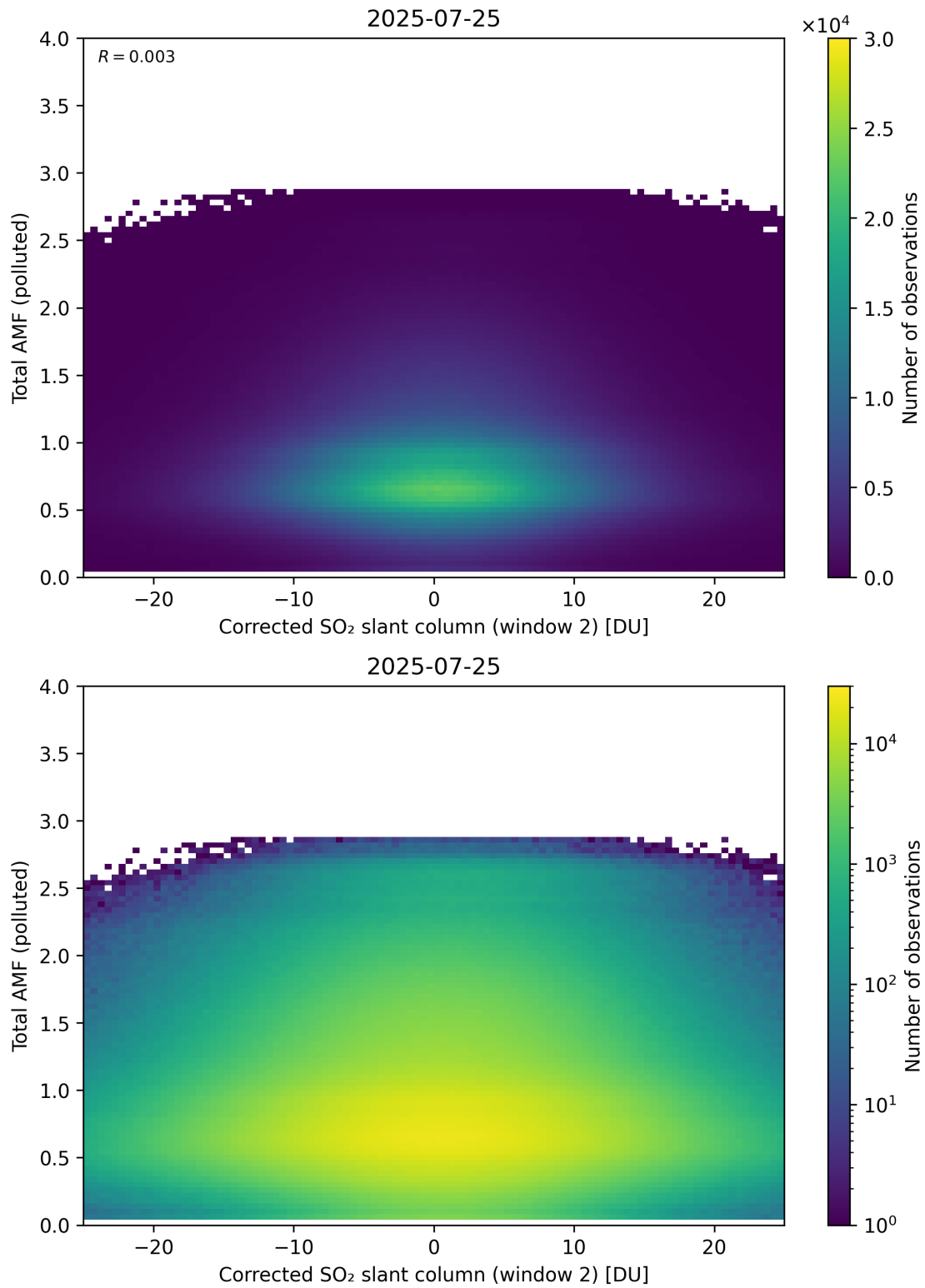
Figure 253: Scatter density plot of “Corrected SO 2 slant column (window 2)” against “Total AMF (polluted)” for 2025-07-24 to 2025-07-26.
