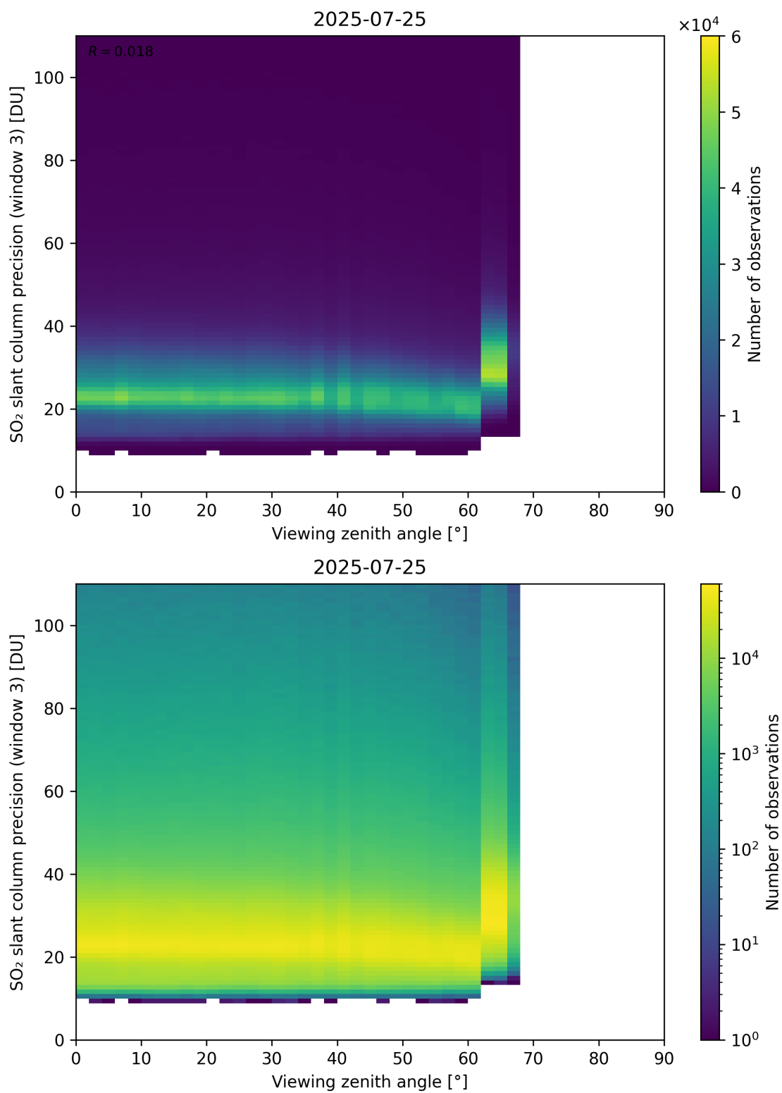
Figure 380: Scatter density plot of “Viewing zenith angle” against “SO 2 slant column precision (window 3)” for 2025-07-24 to 2025-07-26.
