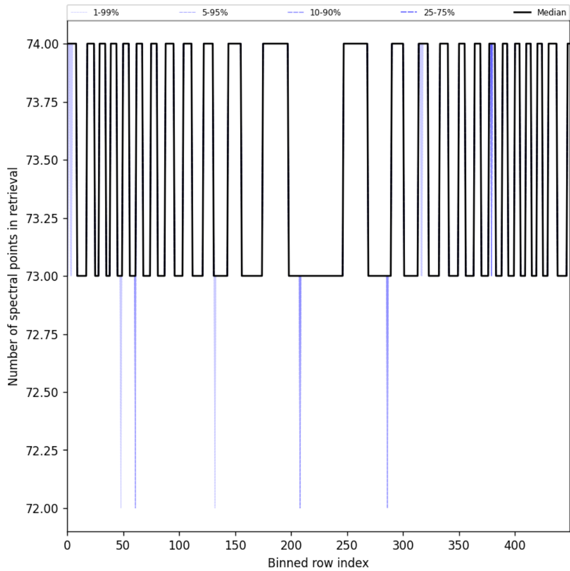
Figure 108: Along track statistics of “Number of spectral points in retrieval” for 2025-07-24 to 2025-07-26
