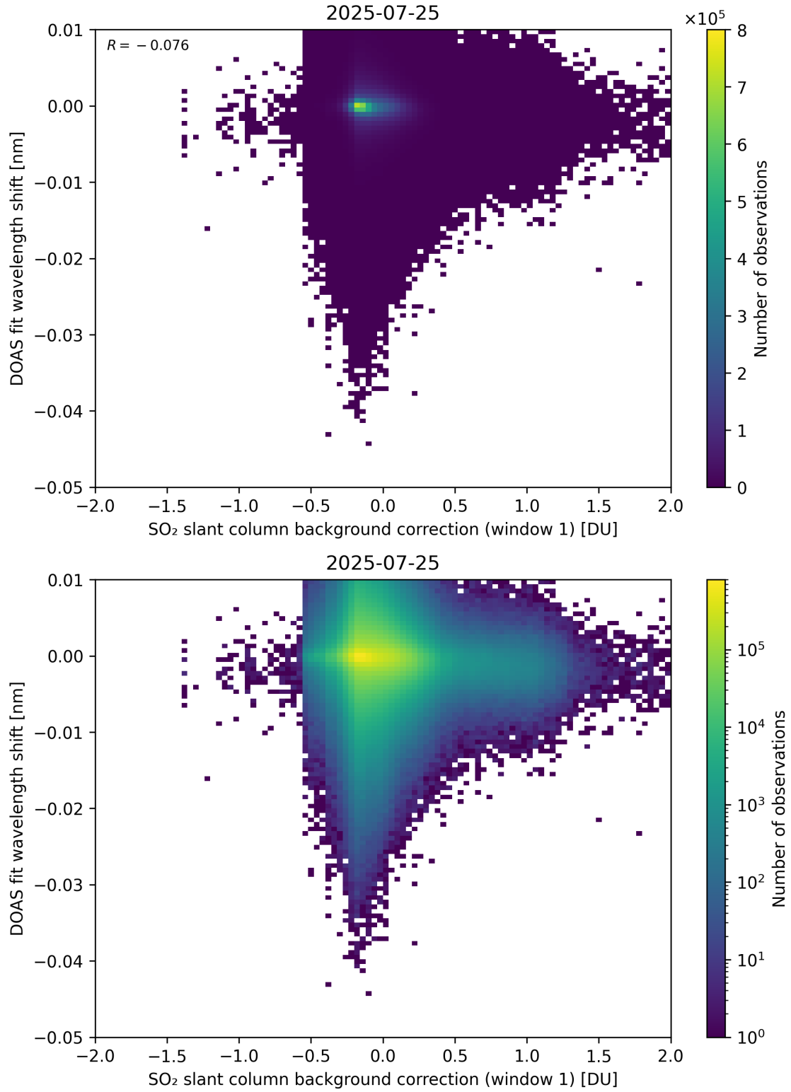
Figure 111: Scatter density plot of “SO 2 slant column background correction (window 1)” against “DOAS fit wavelength shift” for 2025-07-24 to 2025-07-26.
