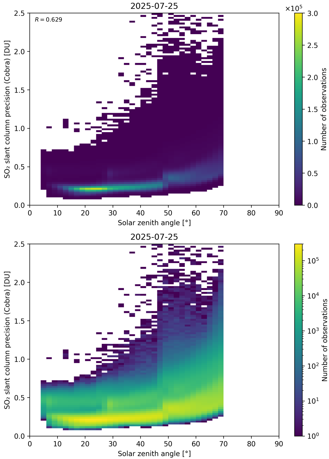
Figure 180: Scatter density plot of “Solar zenith angle” against “SO 2 slant column precision (Cobra)” for 2025-07-24 to 2025-07-26.
