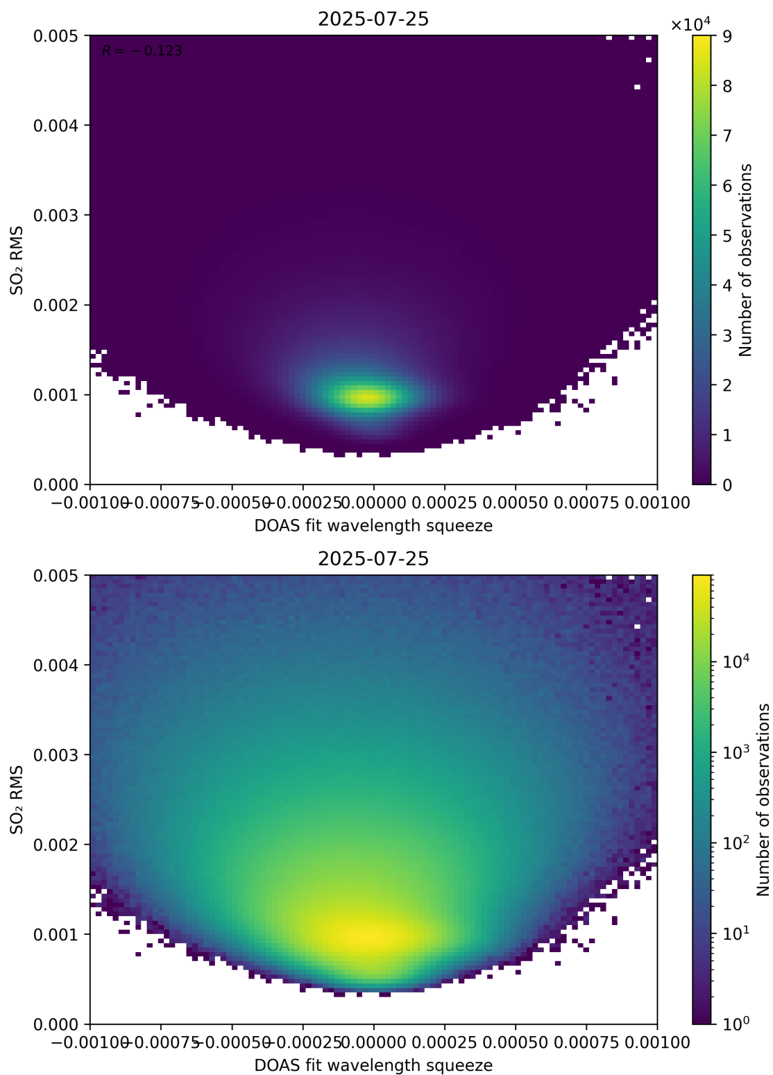
Figure 143: Scatter density plot of “DOAS fit wavelength squeeze” against “SO 2 RMS” for 2025-07-24 to 2025-07-26.
