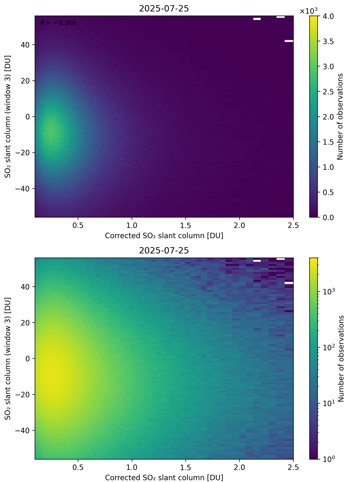
Figure 240: Scatter density plot of “Corrected SO 2 slant column” against “SO 2 slant column (window 3)” for 2025-07-24 to 2025-07-26.
