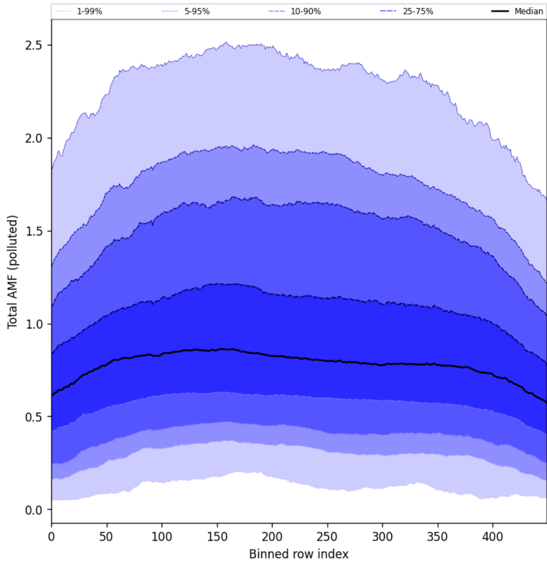
Figure 105: Along track statistics of “Total AMF (polluted)” for 2025-07-24 to 2025-07-26
