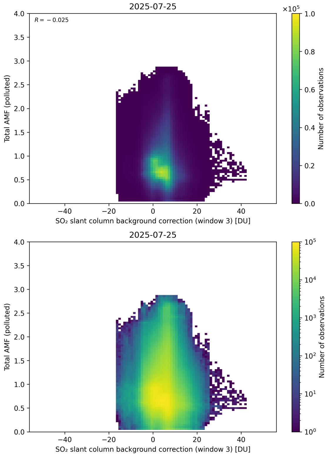
Figure 136: Scatter density plot of “SO 2 slant column background correction (window 3)” against “Total AMF (polluted)” for 2025-07-24 to 2025-07-26.
