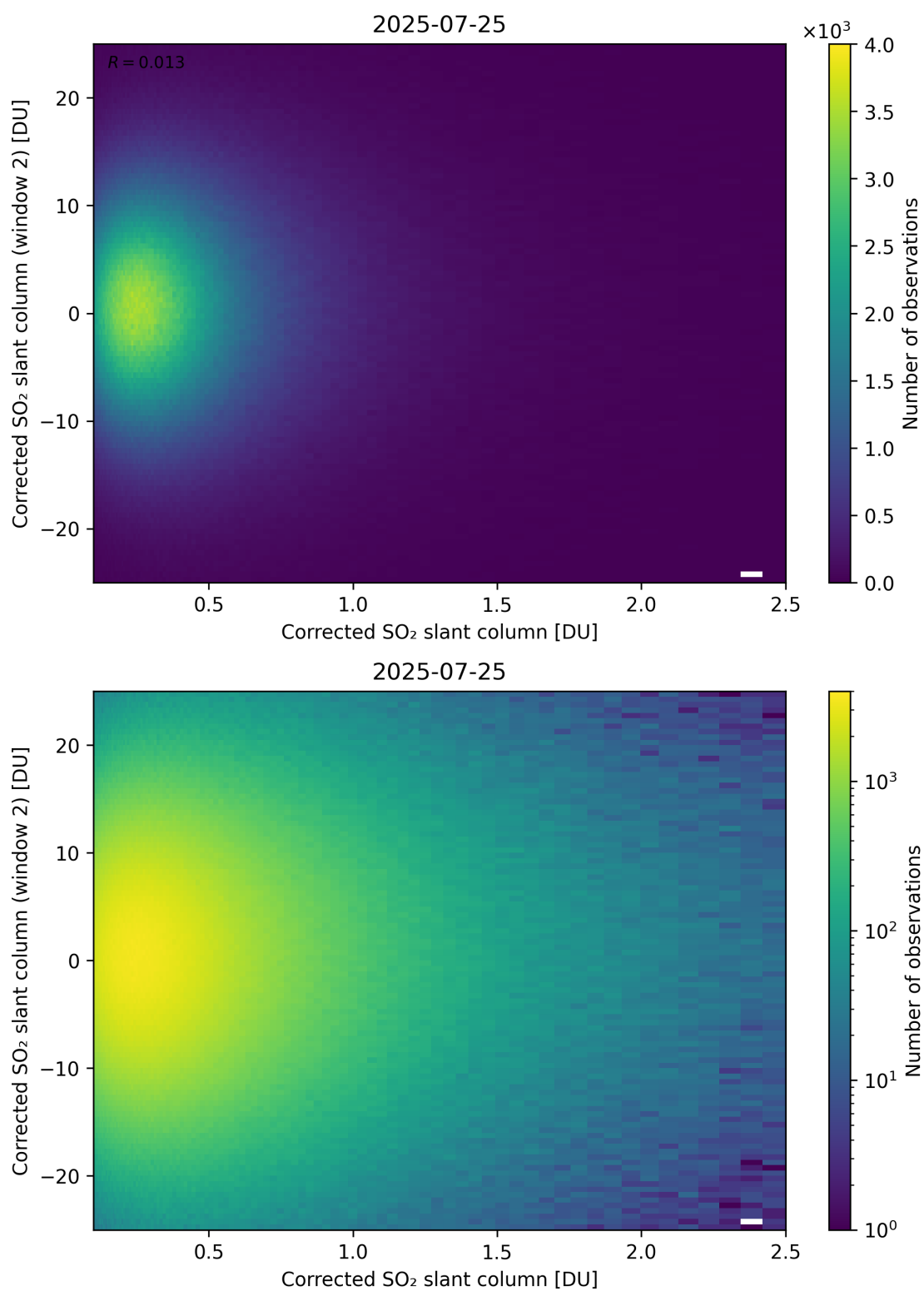
Figure 235: Scatter density plot of “Corrected SO 2 slant column” against “Corrected SO 2 slant column (window 2)” for 2025-07-24 to 2025-07-26.
