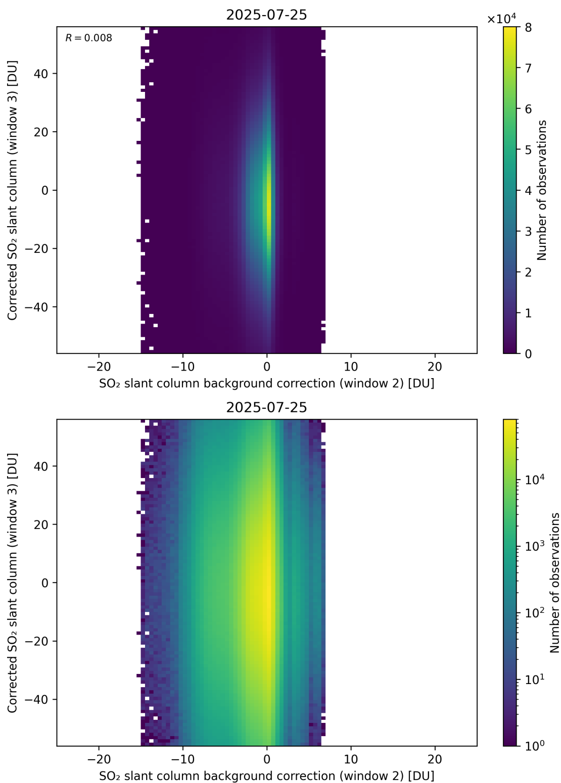
Figure 127: Scatter density plot of “SO 2 slant column background correction (window 2)” against “Corrected SO 2 slant column (window 3)” for 2025-07-24 to 2025-07-26.
