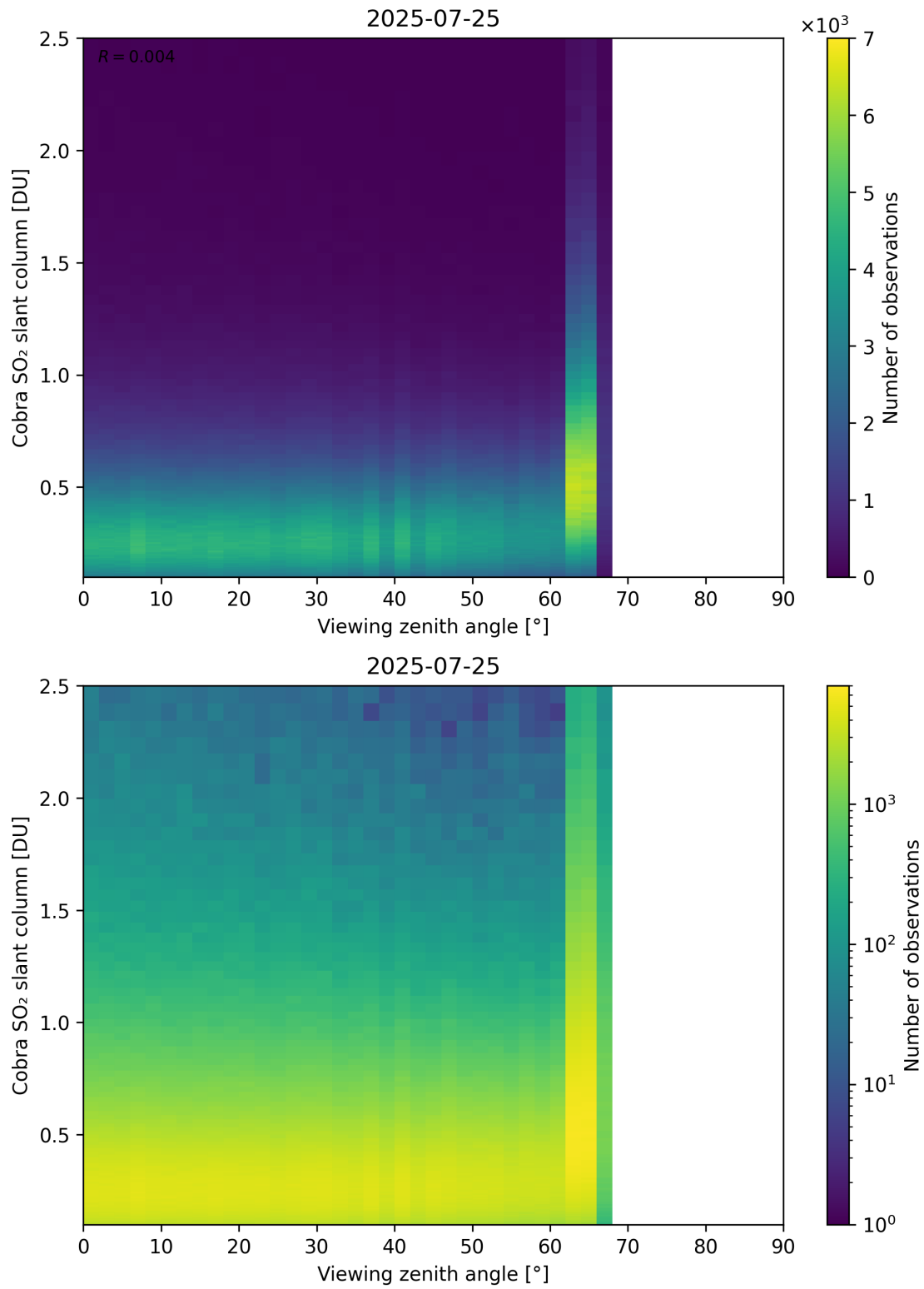
Figure 371: Scatter density plot of “Viewing zenith angle” against “Cobra SO 2 slant column” for 2025-07-24 to 2025-07-26.
