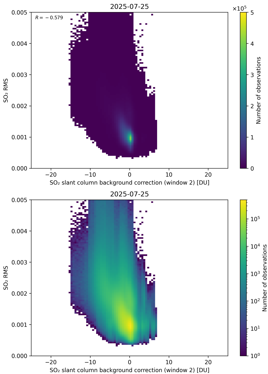
Figure 125: Scatter density plot of “SO 2 slant column background correction (window 2)” against “SO 2 RMS” for 2025-07-24 to 2025-07-26.
