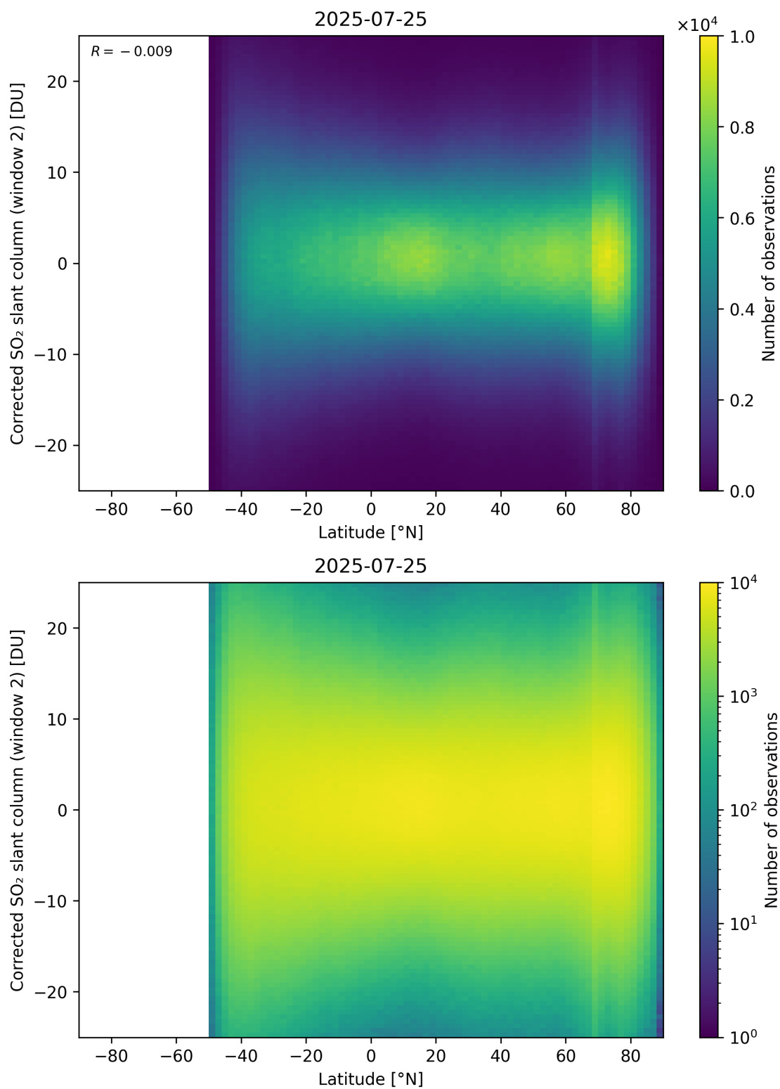
Figure 160: Scatter density plot of “Latitude” against “Corrected SO 2 slant column (window 2)” for 2025-07-24 to 2025-07-26.
