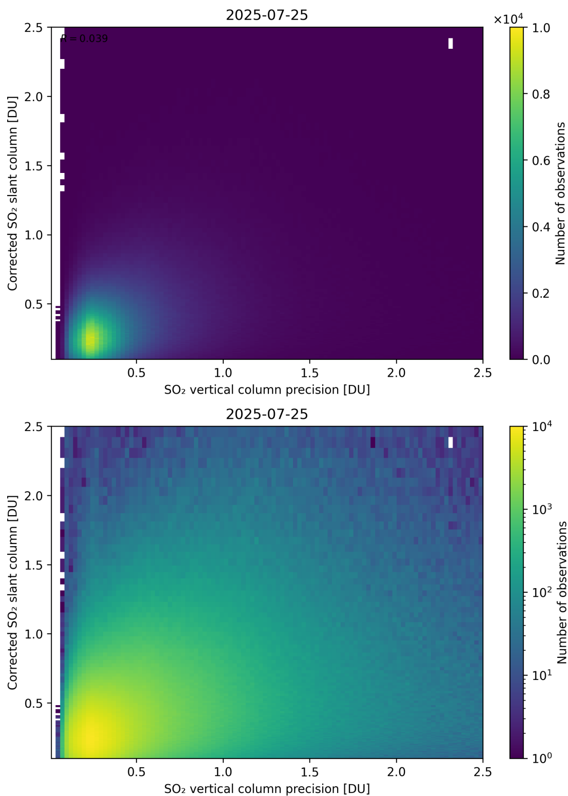
Figure 338: Scatter density plot of “SO 2 vertical column precision” against “Corrected SO 2 slant column” for 2025-07-24 to 2025-07-26.
