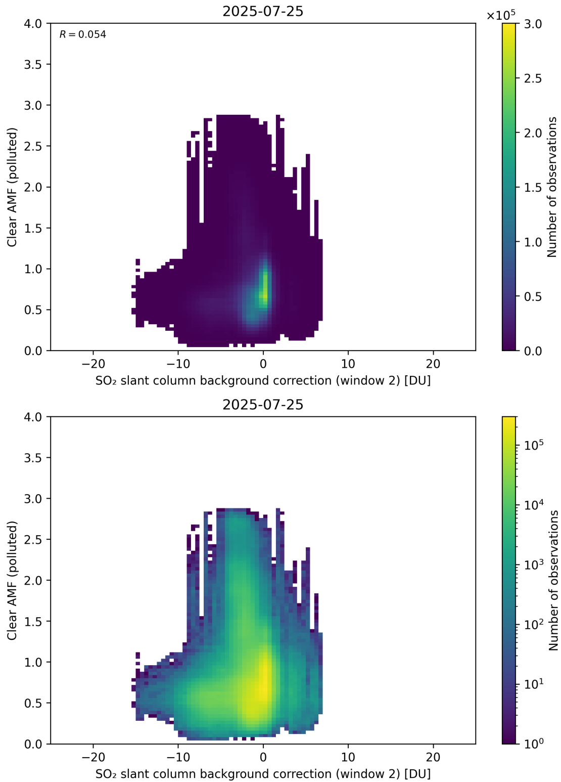
Figure 126: Scatter density plot of “SO 2 slant column background correction (window 2)” against “Clear AMF (polluted)” for 2025-07-24 to 2025-07-26.
