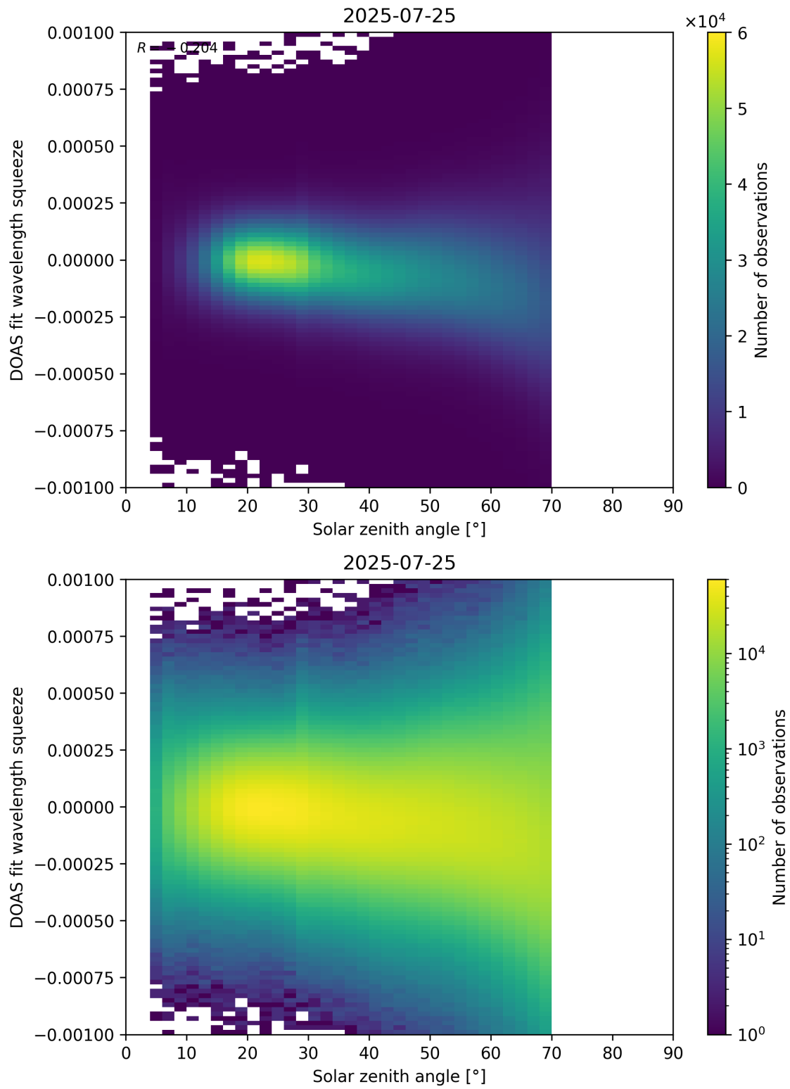
Figure 175: Scatter density plot of “Solar zenith angle” against “DOAS fit wavelength squeeze” for 2025-07-24 to 2025-07-26.
