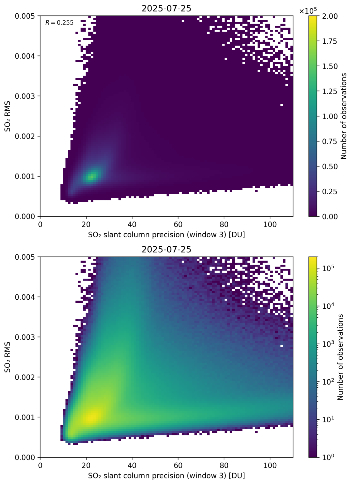
Figure 310: Scatter density plot of “SO 2 slant column precision (window 3)” against “SO 2 RMS” for 2025-07-24 to 2025-07-26.
