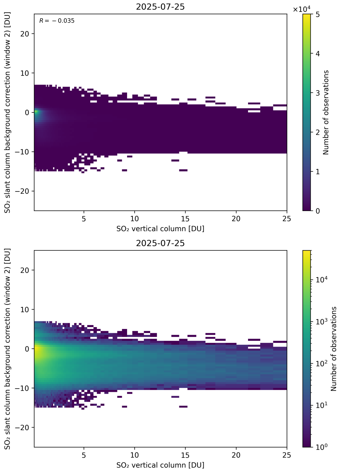
Figure 324: Scatter density plot of “SO 2 vertical column” against “SO 2 slant column background correction (window 2)” for 2025-07-24 to 2025-07-26.
