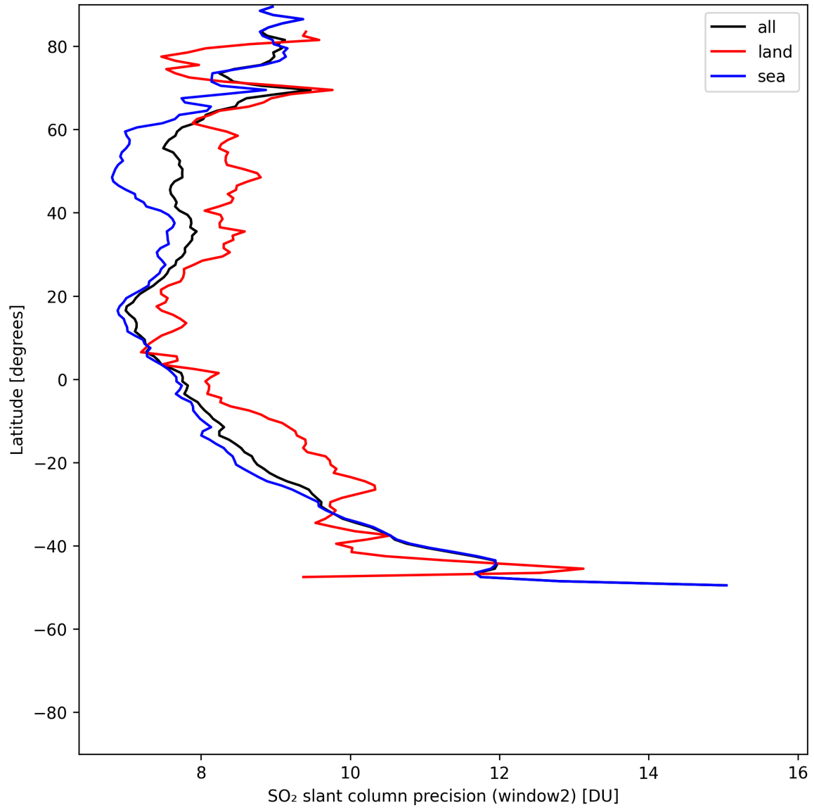
Figure 42: Zonal average of “SO 2 slant column precision (window2)” for 2025-07-24 to 2025-07-26.
