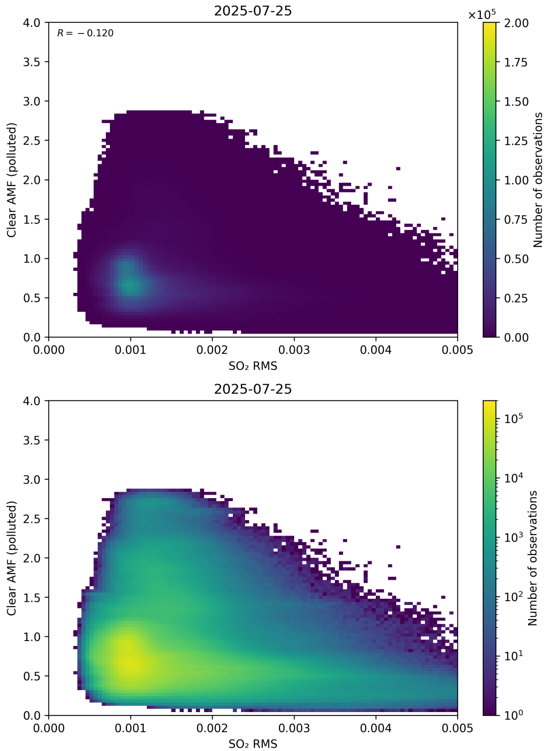
Figure 147: Scatter density plot of “SO 2 RMS” against “Clear AMF (polluted)” for 2025-07-24 to 2025-07-26.
