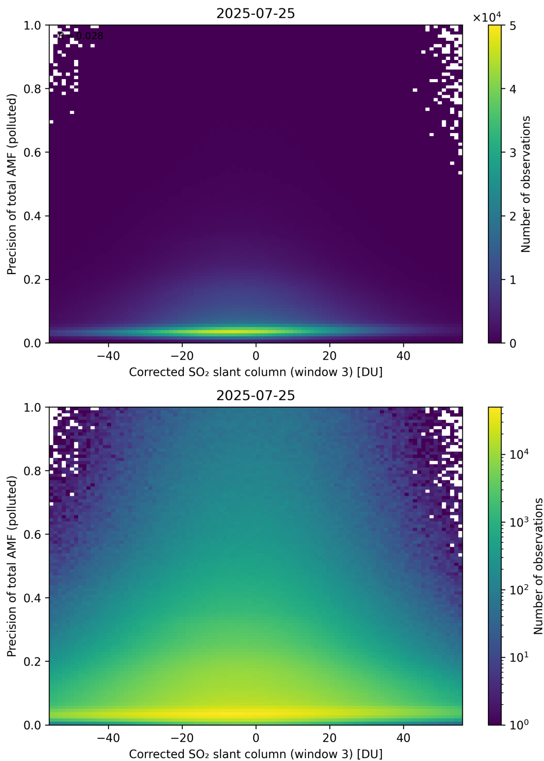
Figure 261: Scatter density plot of “Corrected SO 2 slant column (window 3)” against “Precision of total AMF (polluted)” for 2025-07-24 to 2025-07-26.
