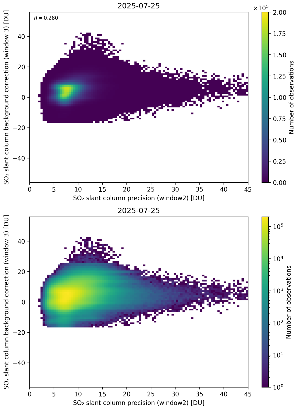
Figure 292: Scatter density plot of “SO 2 slant column precision (window2)” against “SO 2 slant column background correction (window 3)” for 2025-07-24 to 2025-07-26.
