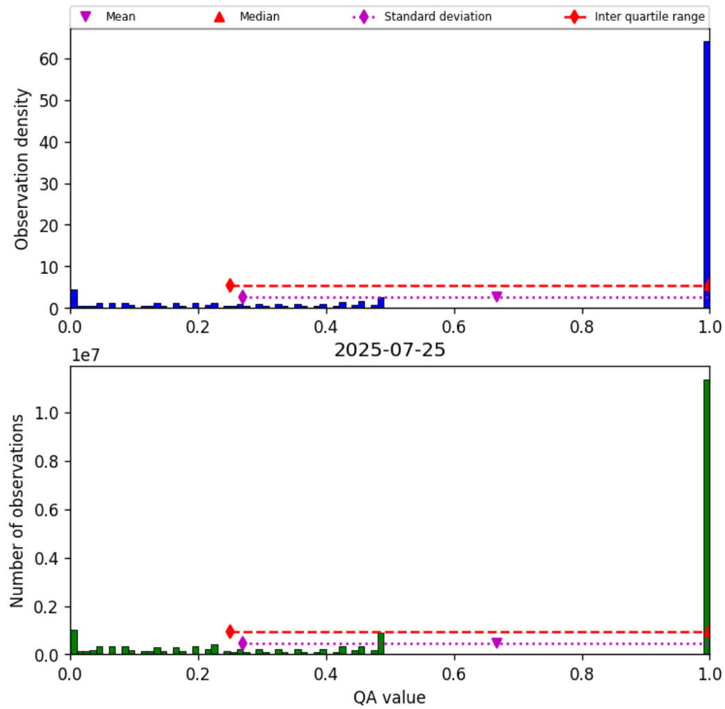
Figure 57: Histogram of “QA value” for 2025-07-24 to 2025-07-26
