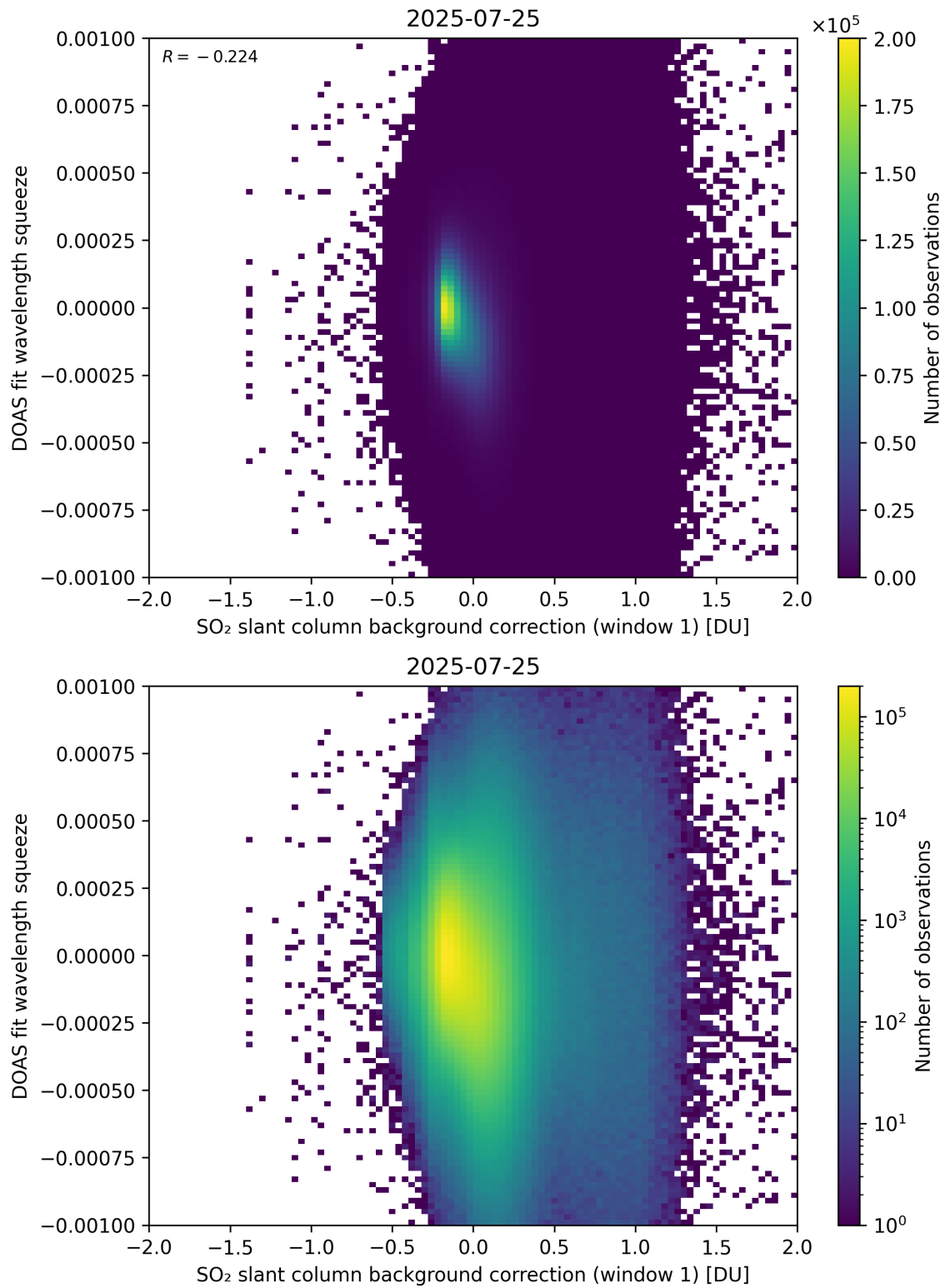
Figure 112: Scatter density plot of “SO 2 slant column background correction (window 1)” against “DOAS fit wavelength squeeze” for 2025-07-24 to 2025-07-26.
