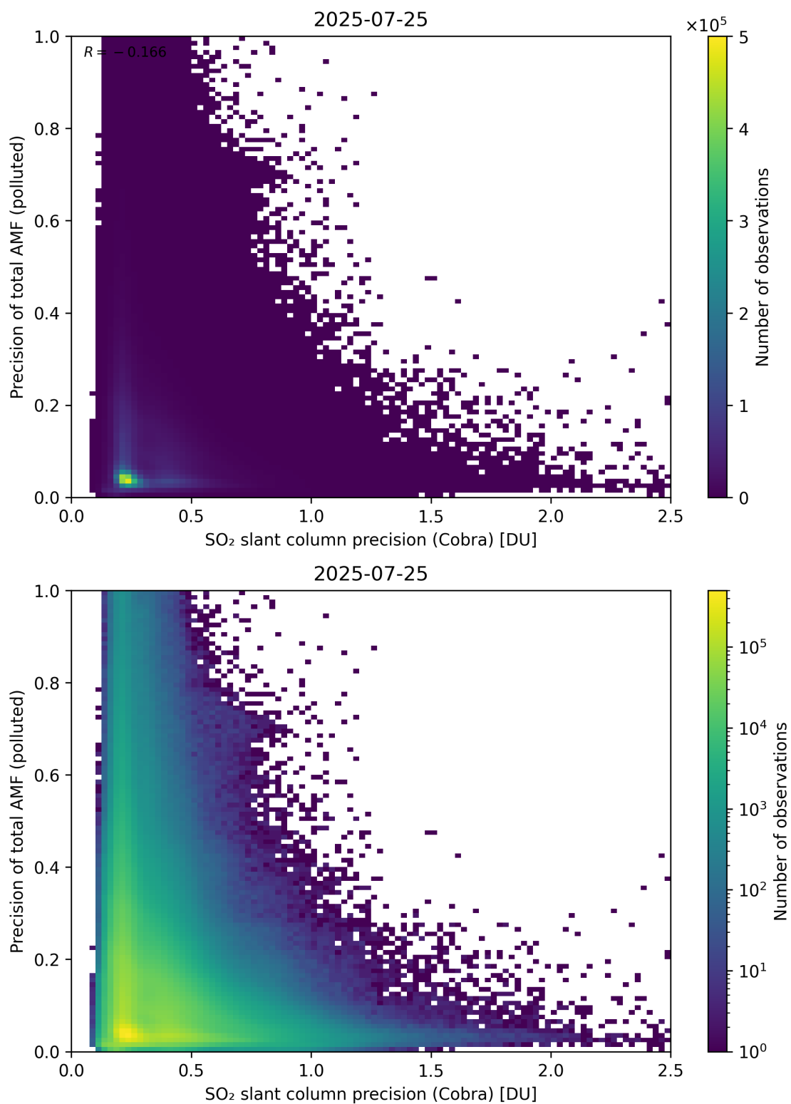
Figure 214: Scatter density plot of “SO 2 slant column precision (Cobra)” against “Precision of total AMF (polluted)” for 2025-07-24 to 2025-07-26.
