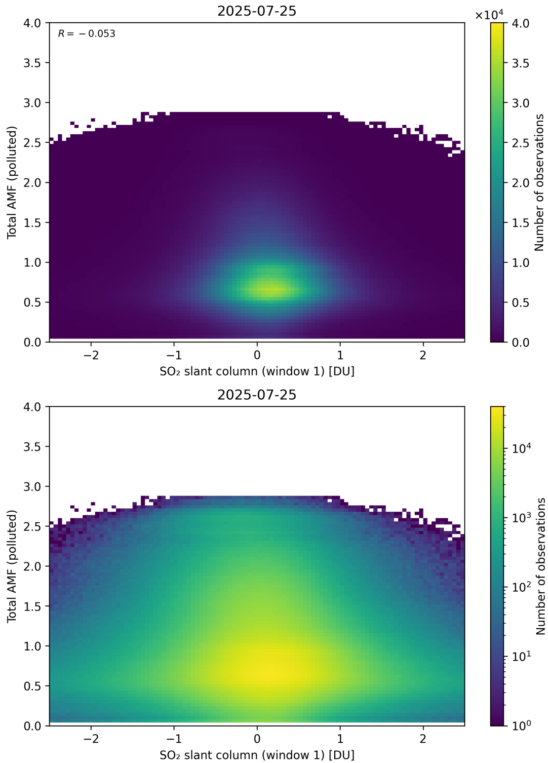
Figure 289: Scatter density plot of “SO 2 slant column (window 1)” against “Total AMF (polluted)” for 2025-07-24 to 2025-07-26.
