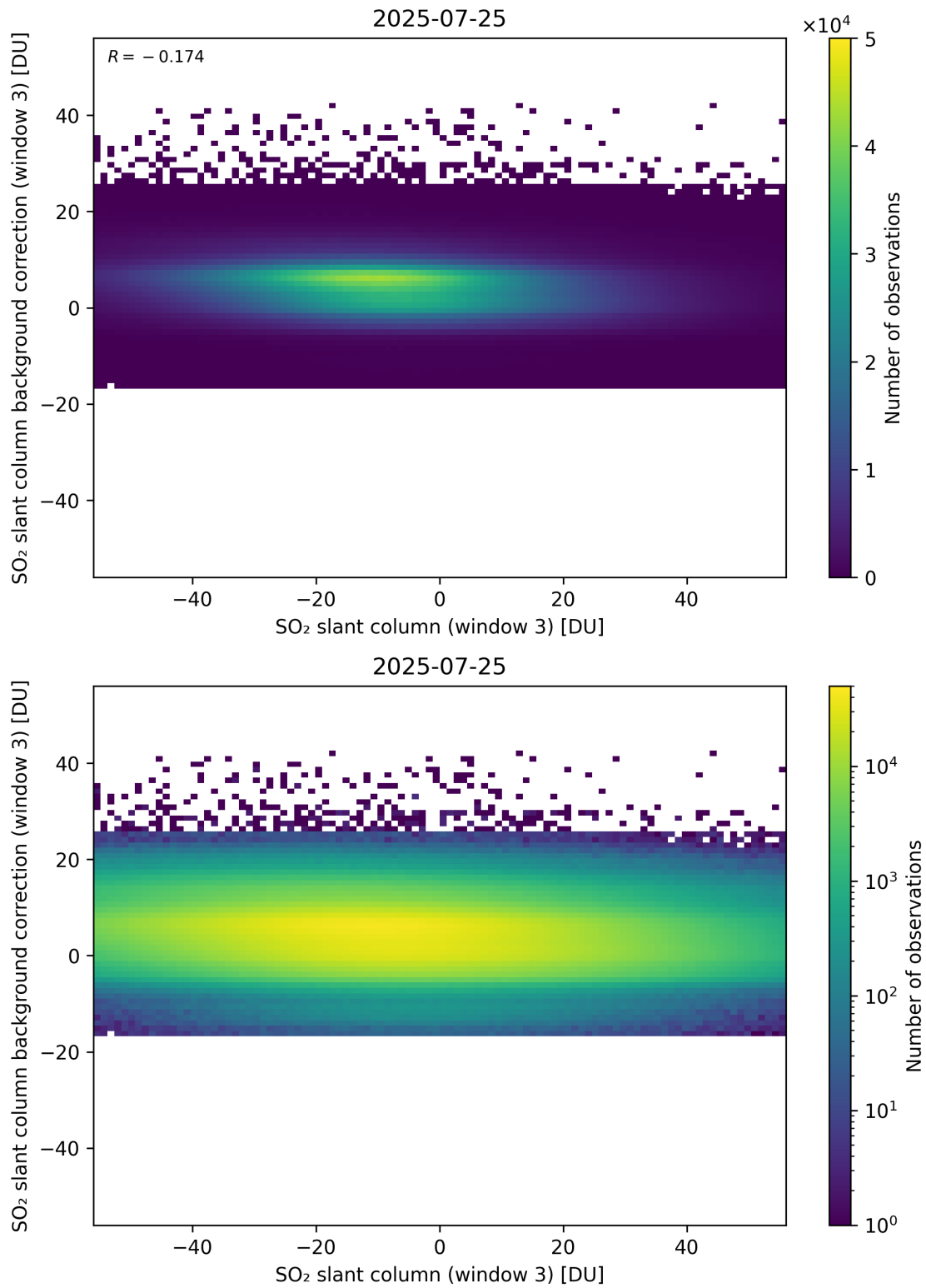
Figure 303: Scatter density plot of “SO 2 slant column (window 3)” against “SO 2 slant column background correction (window 3)” for 2025-07-24 to 2025-07-26.
