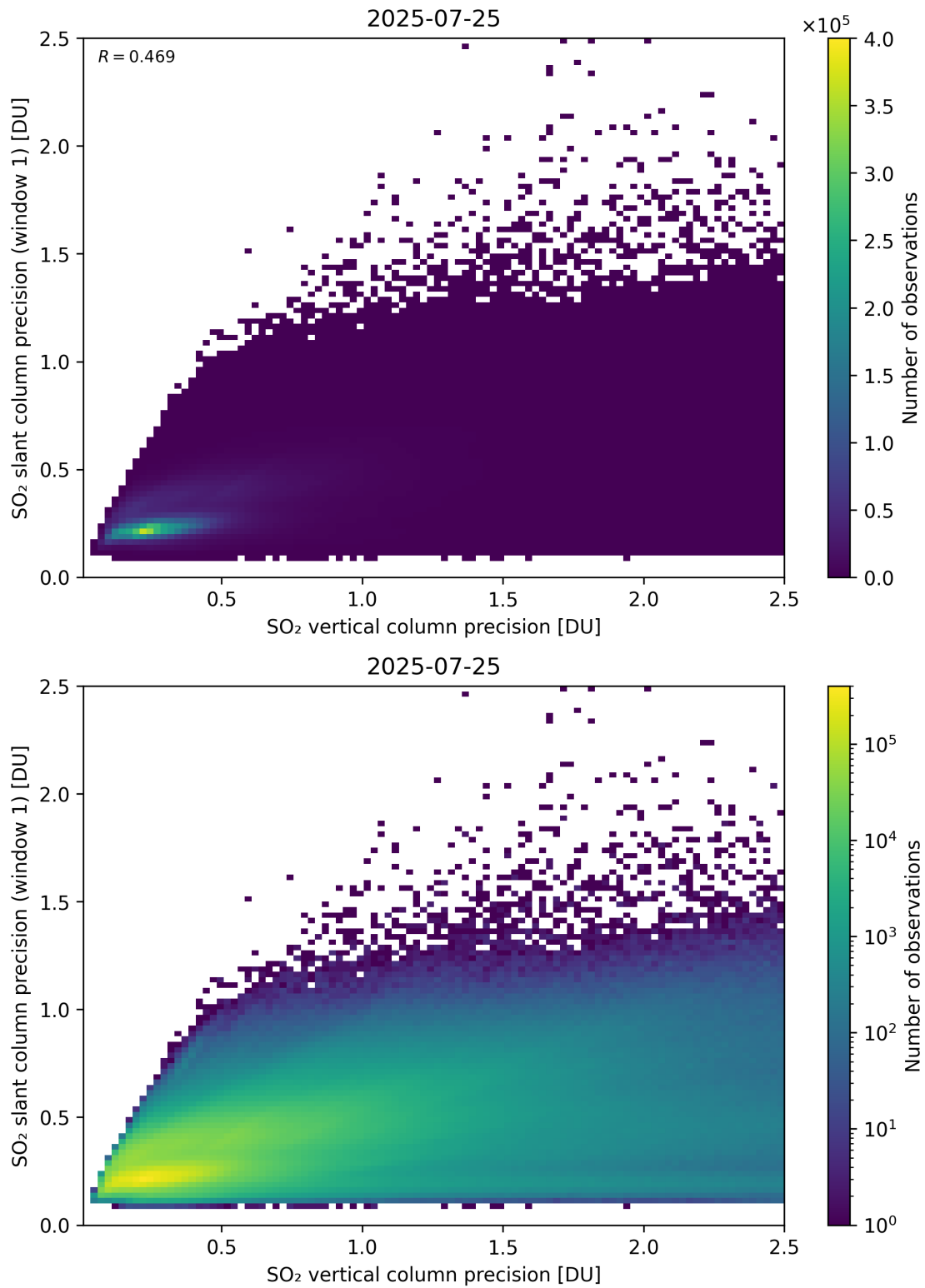
Figure 342: Scatter density plot of “SO 2 vertical column precision” against “SO 2 slant column precision (window 1)” for 2025-07-24 to 2025-07-26.
