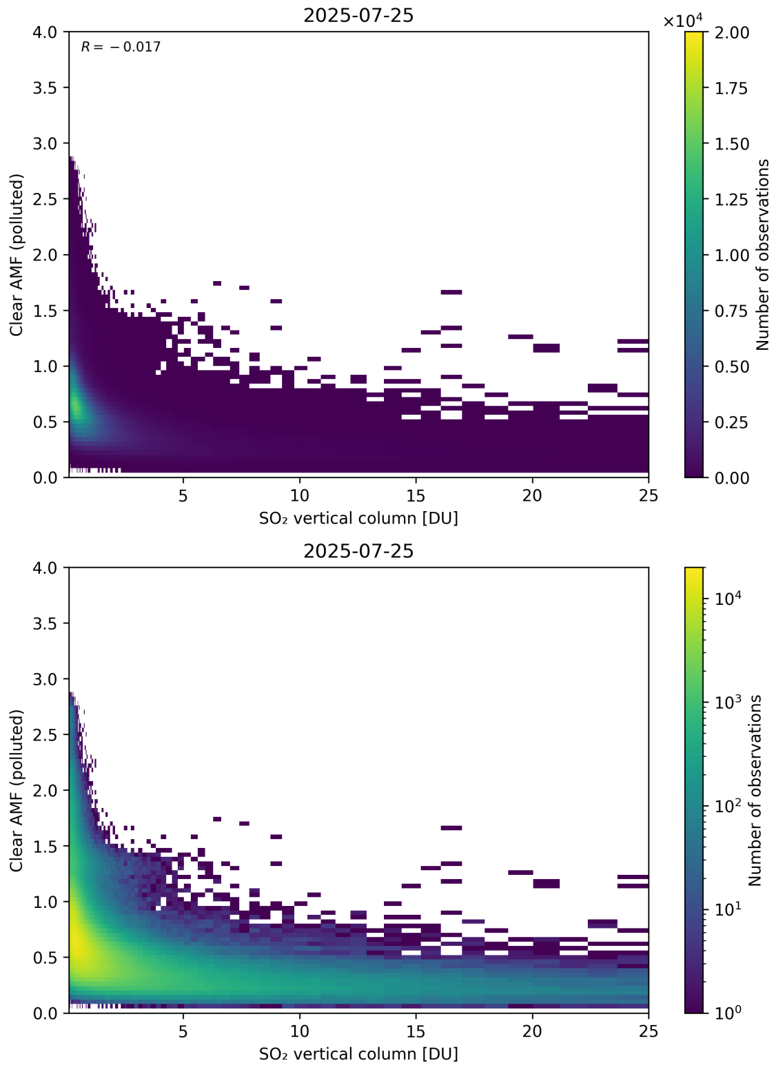
Figure 348: Scatter density plot of “SO 2 vertical column” against “Clear AMF (polluted)” for 2025-07-24 to 2025-07-26.
