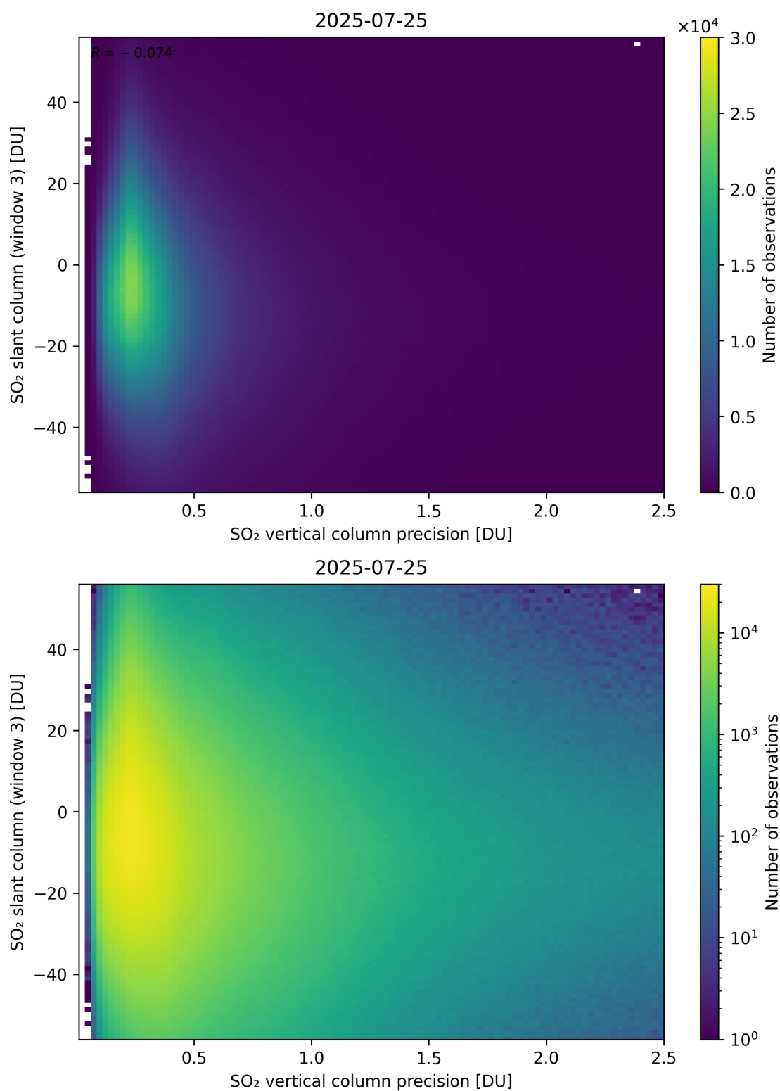
Figure 344: Scatter density plot of “SO 2 vertical column precision” against “SO 2 slant column (window 3)” for 2025-07-24 to 2025-07-26.
