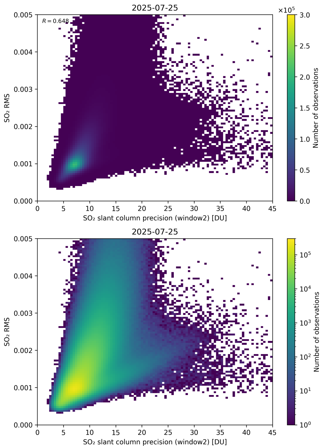
Figure 295: Scatter density plot of “SO 2 slant column precision (window2)” against “SO 2 RMS” for 2025-07-24 to 2025-07-26.
