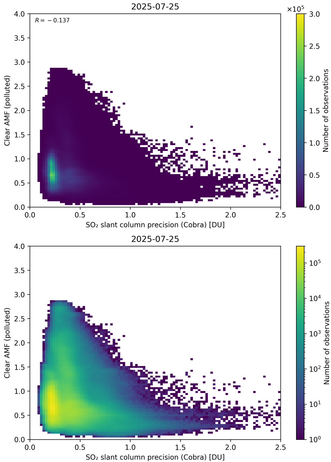
Figure 205: Scatter density plot of “SO 2 slant column precision (Cobra)” against “Clear AMF (polluted)” for 2025-07-24 to 2025-07-26.
