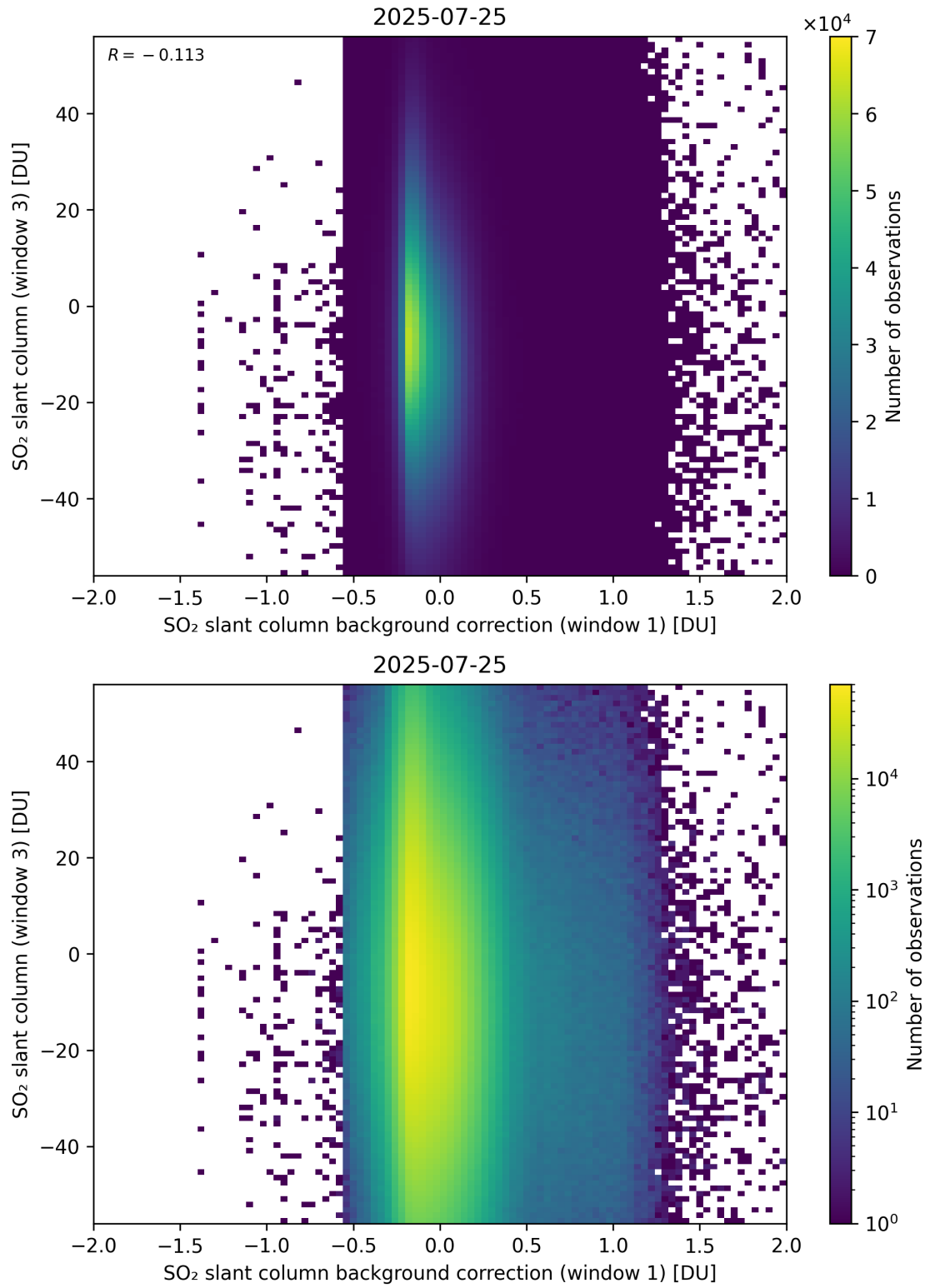
Figure 118: Scatter density plot of “SO 2 slant column background correction (window 1)” against “SO 2 slant column (window 3)” for 2025-07-24 to 2025-07-26.
