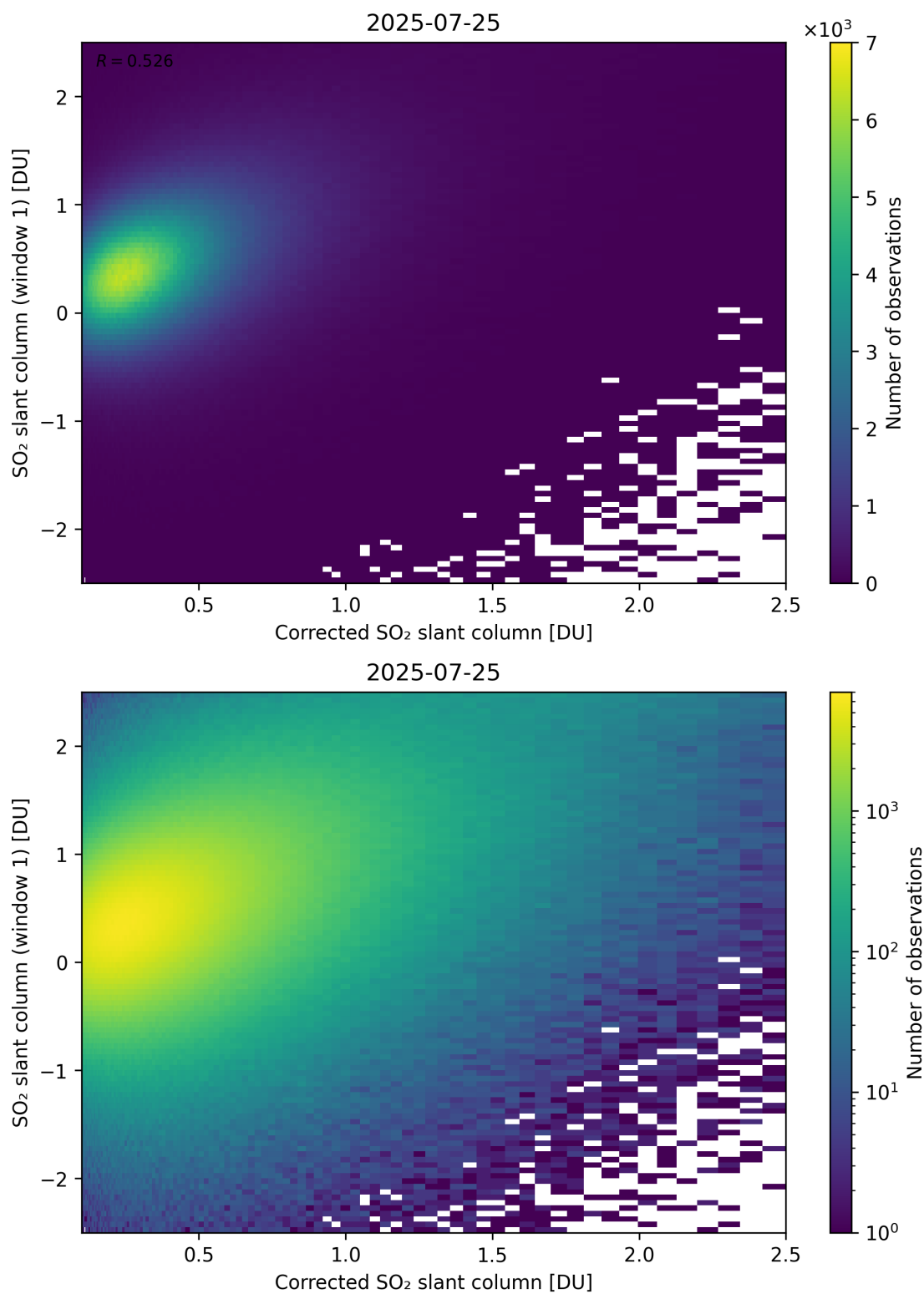
Figure 237: Scatter density plot of “Corrected SO 2 slant column” against “SO 2 slant column (window 1)” for 2025-07-24 to 2025-07-26.
