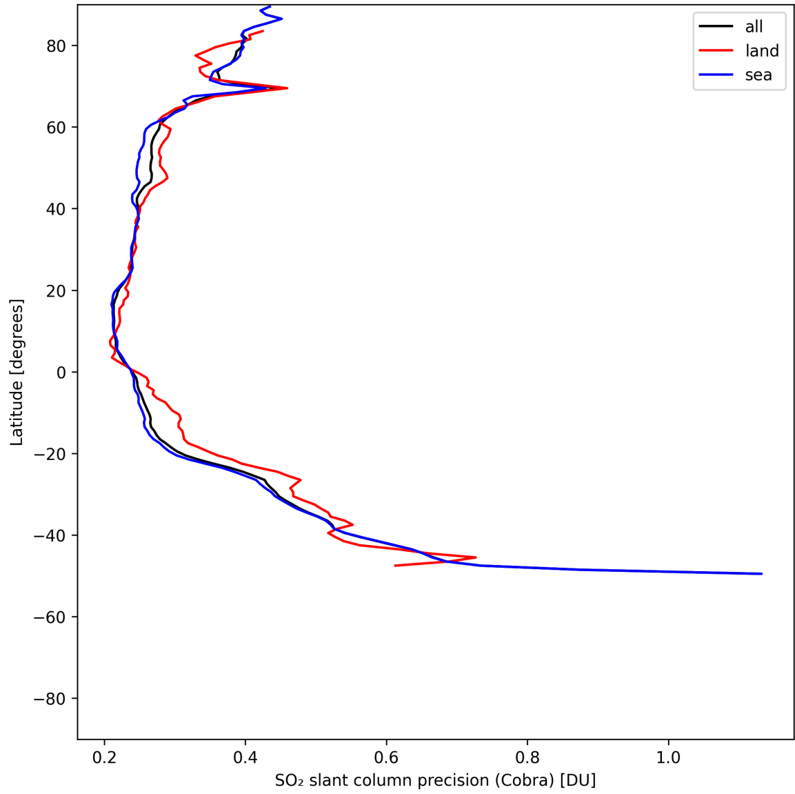
Figure 36: Zonal average of “SO 2 slant column precision (Cobra)” for 2025-07-24 to 2025-07-26.
