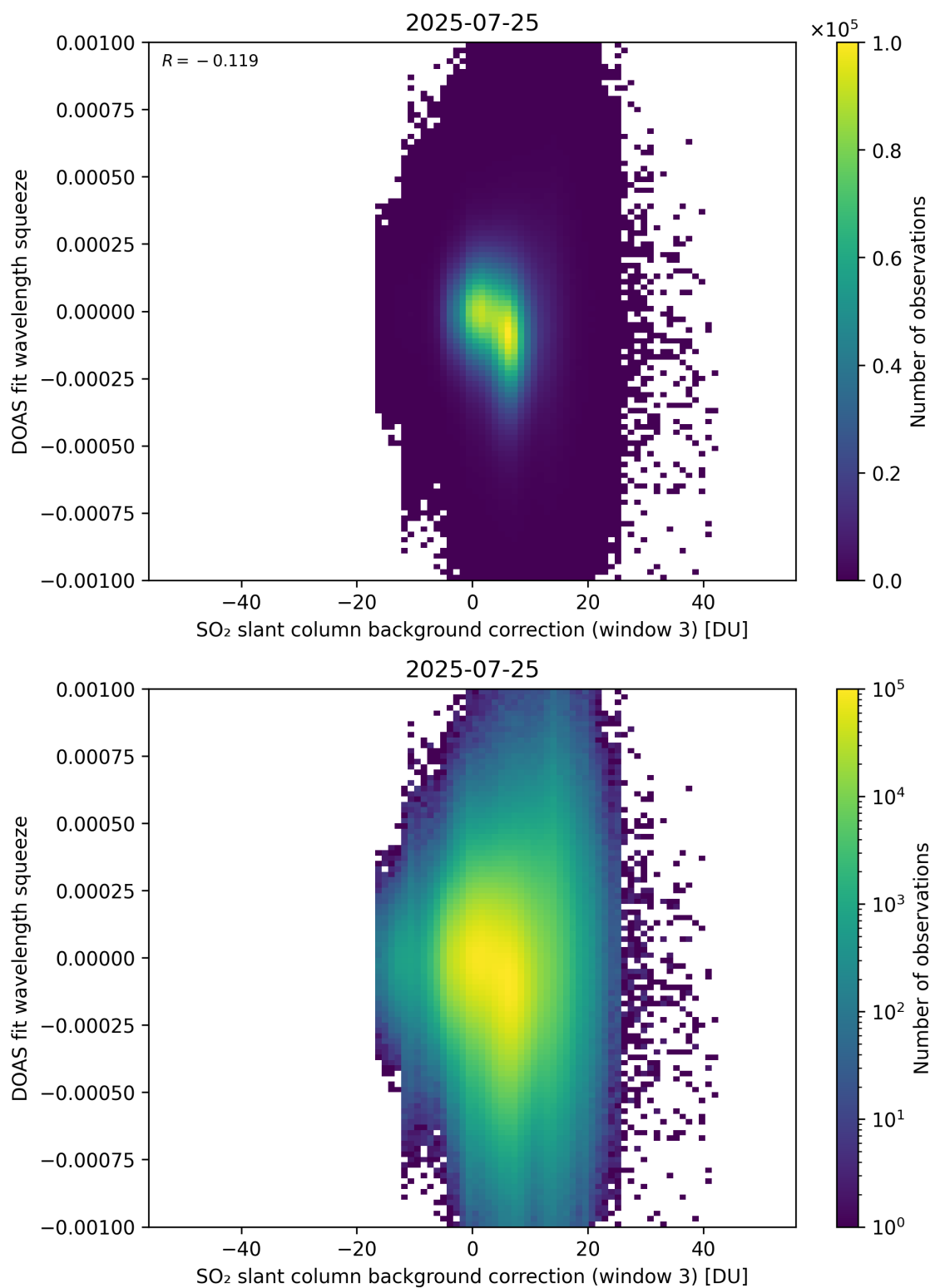
Figure 133: Scatter density plot of “SO 2 slant column background correction (window 3)” against “DOAS fit wavelength squeeze” for 2025-07-24 to 2025-07-26.
