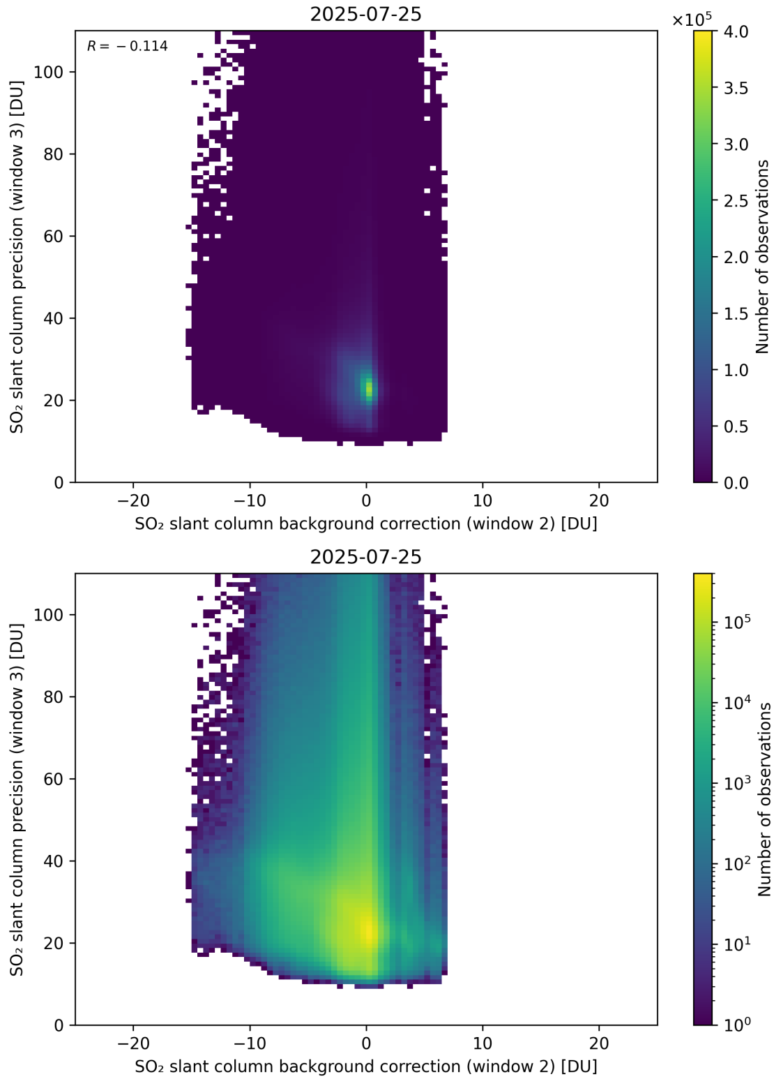
Figure 129: Scatter density plot of “SO 2 slant column background correction (window 2)” against “SO 2 slant column precision (window 3)” for 2025-07-24 to 2025-07-26.
