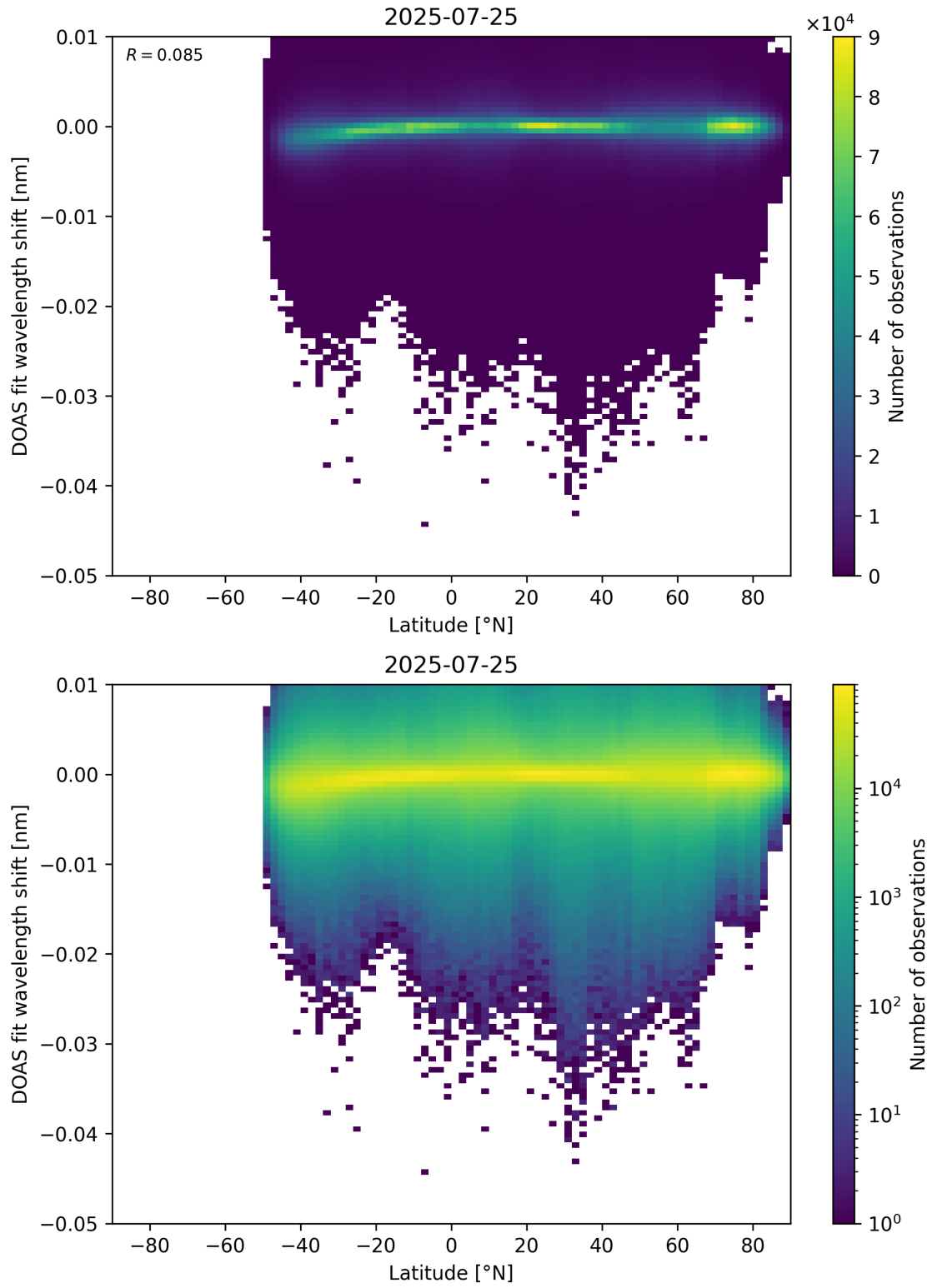
Figure 153: Scatter density plot of “Latitude” against “DOAS fit wavelength shift” for 2025-07-24 to 2025-07-26.
