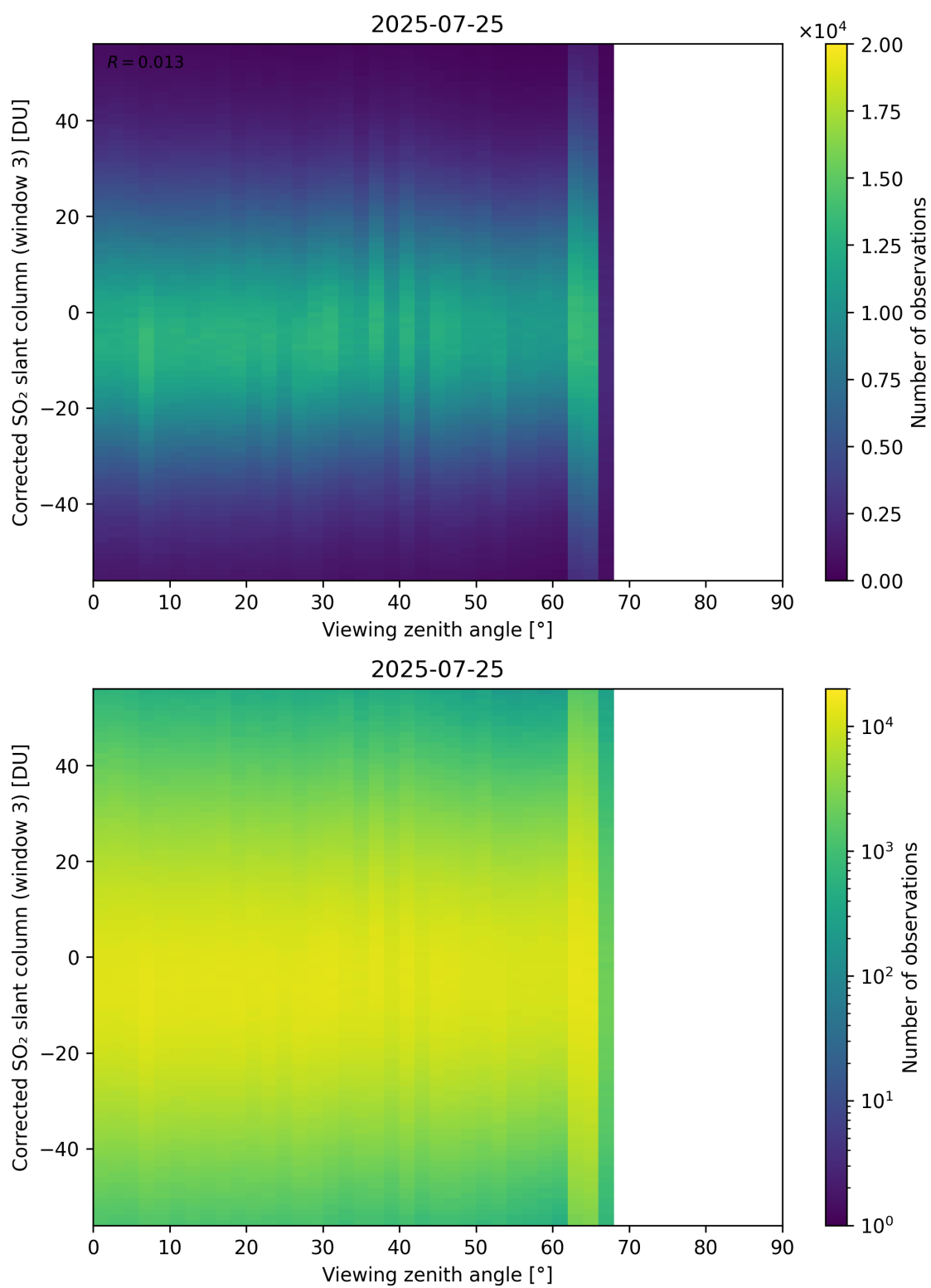
Figure 375: Scatter density plot of “Viewing zenith angle” against “Corrected SO 2 slant column (window 3)” for 2025-07-24 to 2025-07-26.
