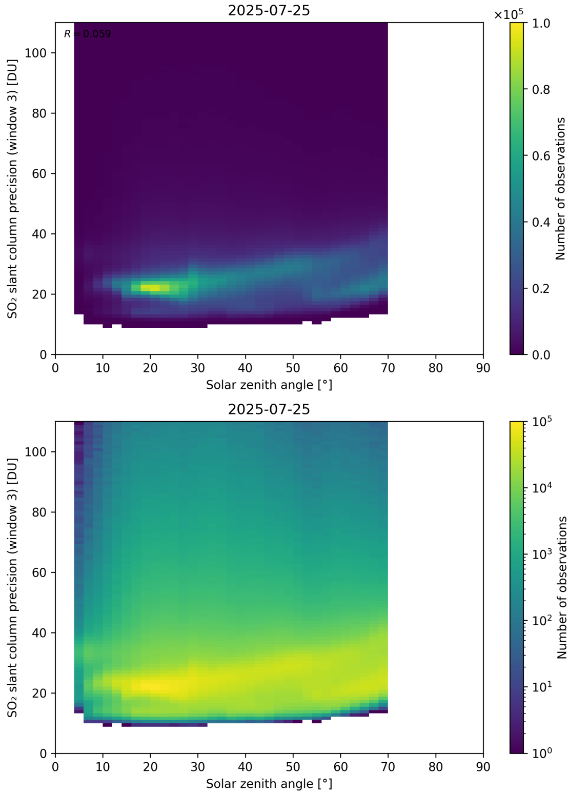
Figure 188: Scatter density plot of “Solar zenith angle” against “SO 2 slant column precision (window 3)” for 2025-07-24 to 2025-07-26.
