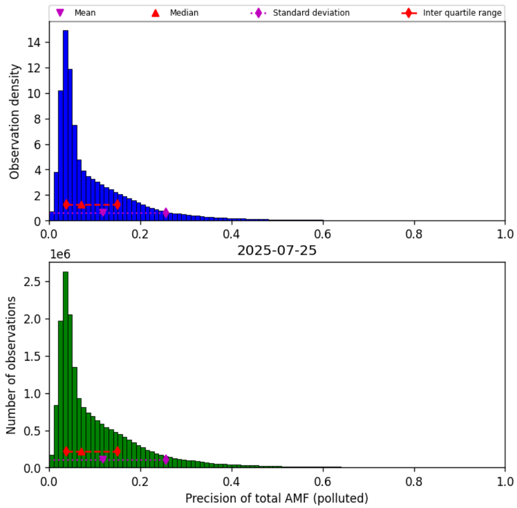
Figure 80: Histogram of “Precision of total AMF (polluted)” for 2025-07-24 to 2025-07-26
