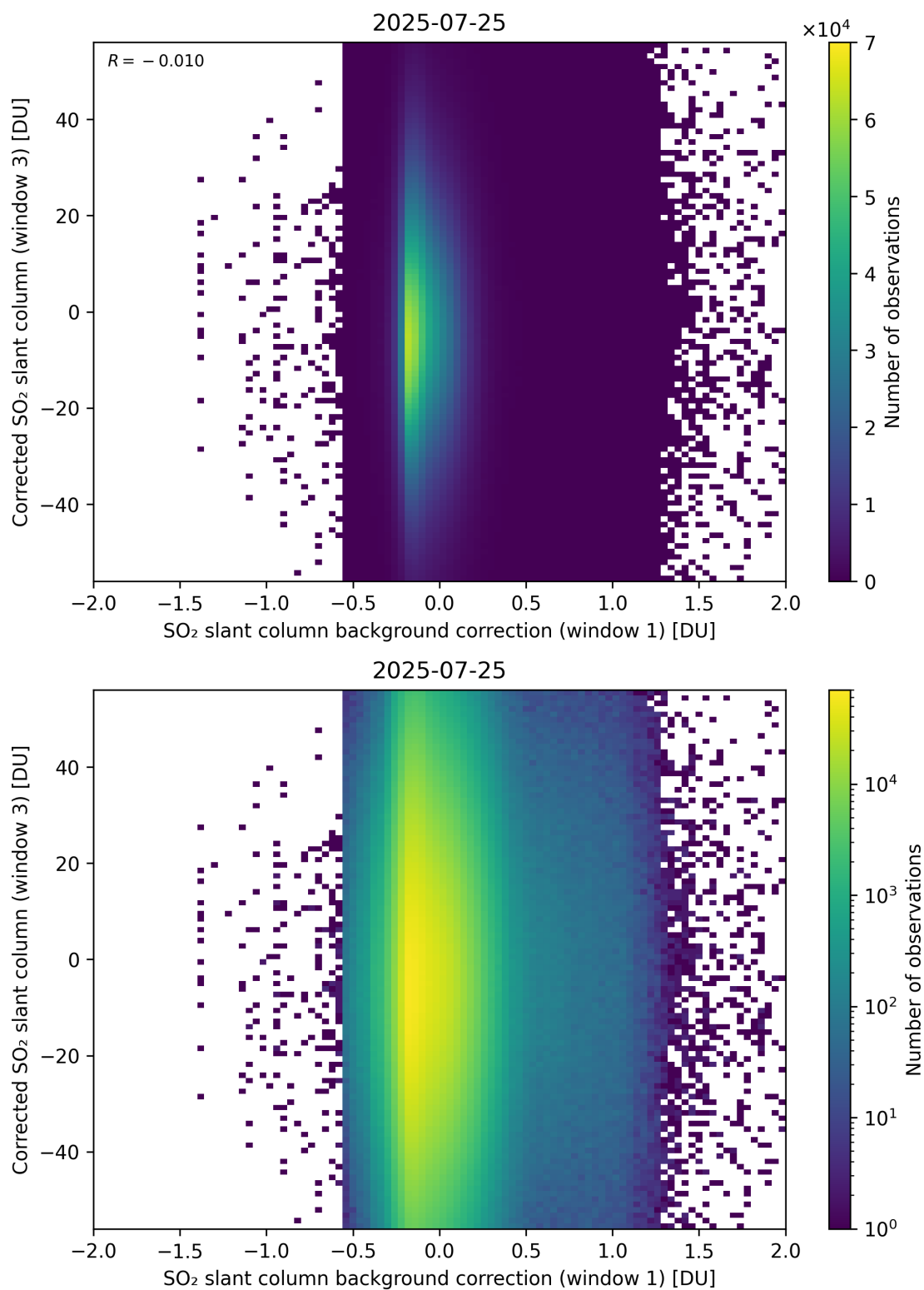
Figure 116: Scatter density plot of “SO 2 slant column background correction (window 1)” against “Corrected SO 2 slant column (window 3)” for 2025-07-24 to 2025-07-26.
