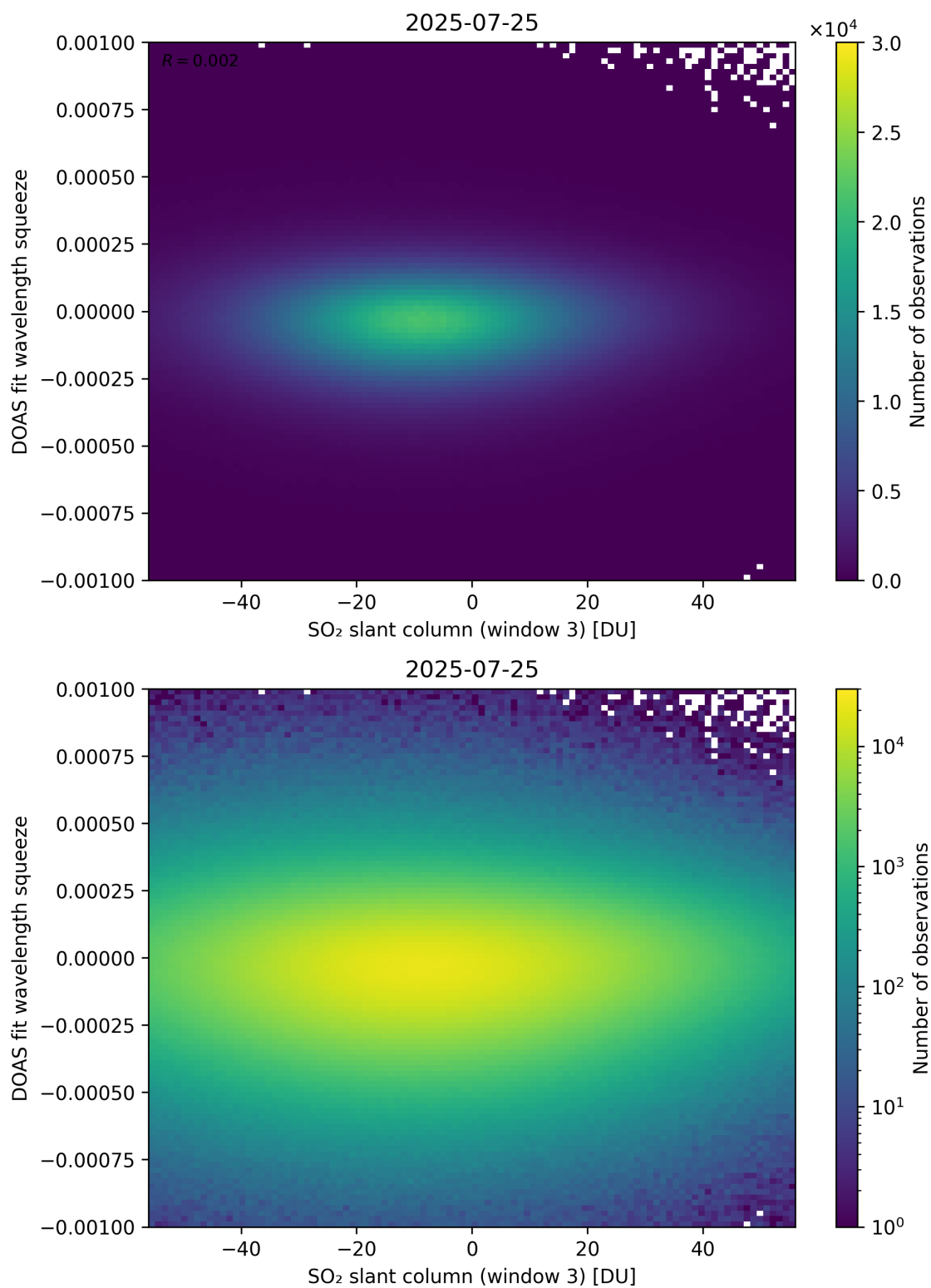
Figure 305: Scatter density plot of “SO 2 slant column (window 3)” against “DOAS fit wavelength squeeze” for 2025-07-24 to 2025-07-26.
