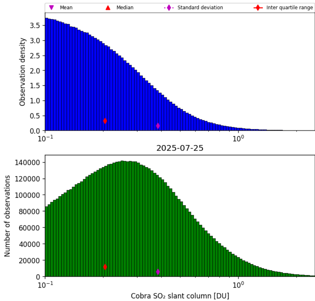
Figure 61: Histogram of “Cobra SO 2 slant column” for 2025-07-24 to 2025-07-26
