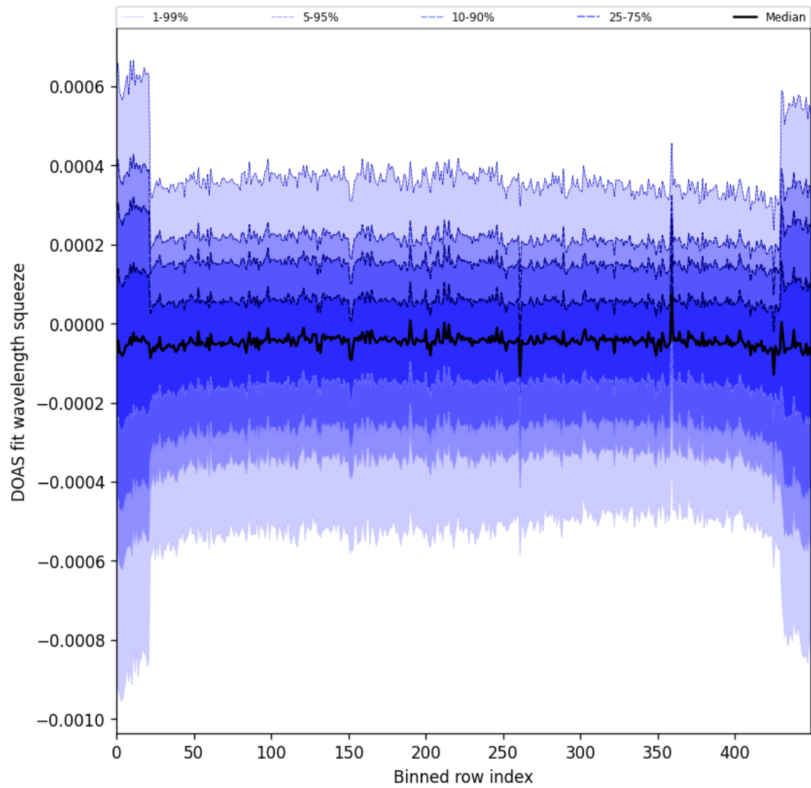
Figure 103: Along track statistics of “DOAS fit wavelength squeeze” for 2025-07-24 to 2025-07-26
