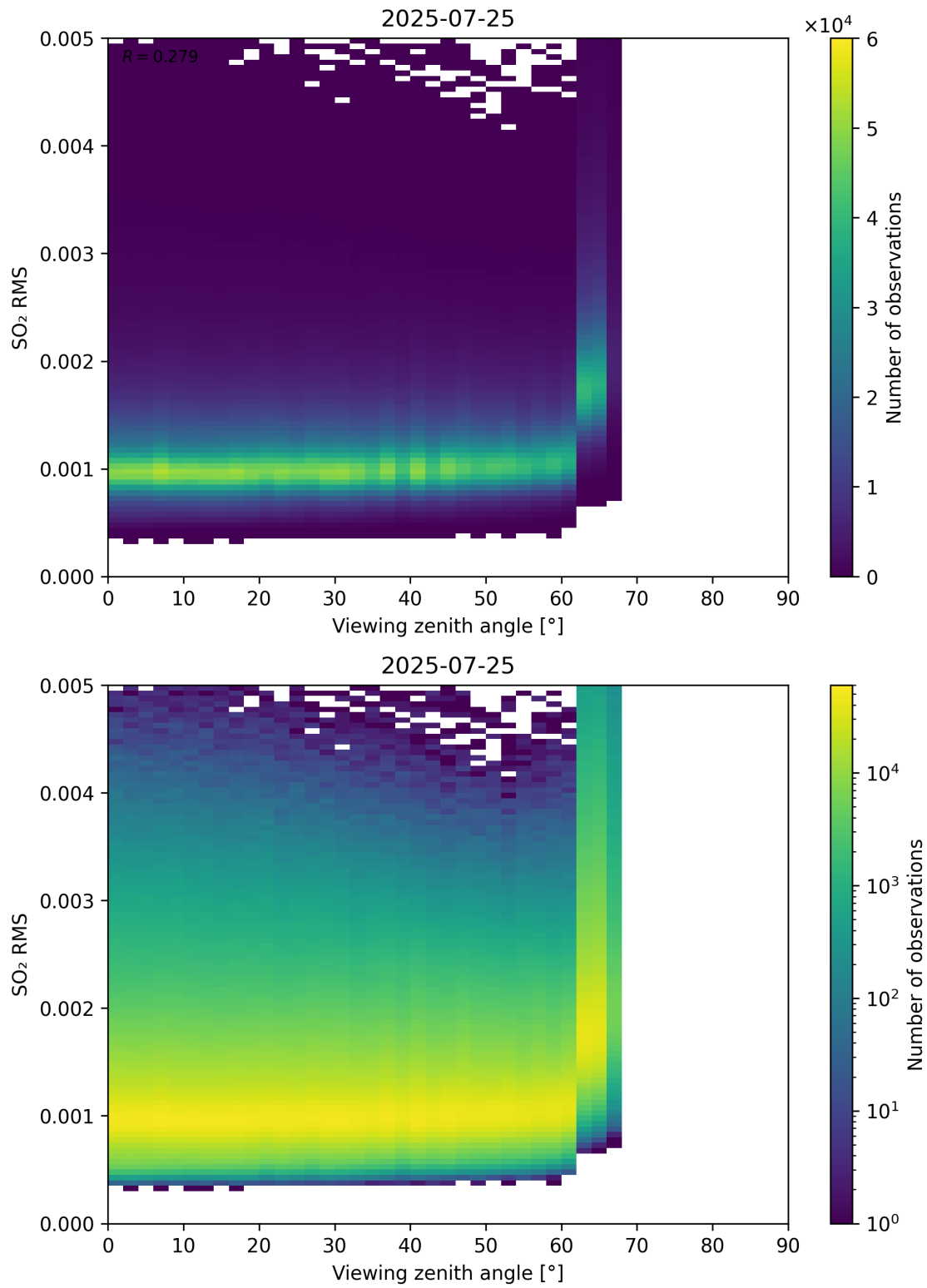
Figure 367: Scatter density plot of “Viewing zenith angle” against “SO 2 RMS” for 2025-07-24 to 2025-07-26.
