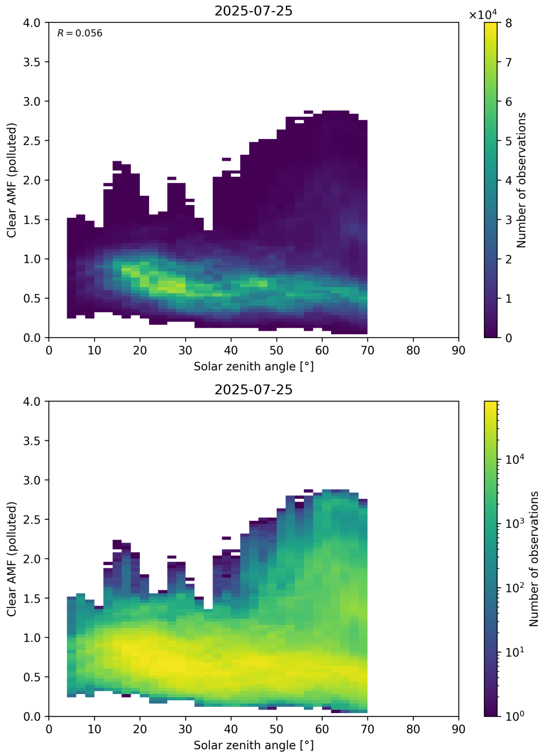
Figure 178: Scatter density plot of “Solar zenith angle” against “Clear AMF (polluted)” for 2025-07-24 to 2025-07-26.
