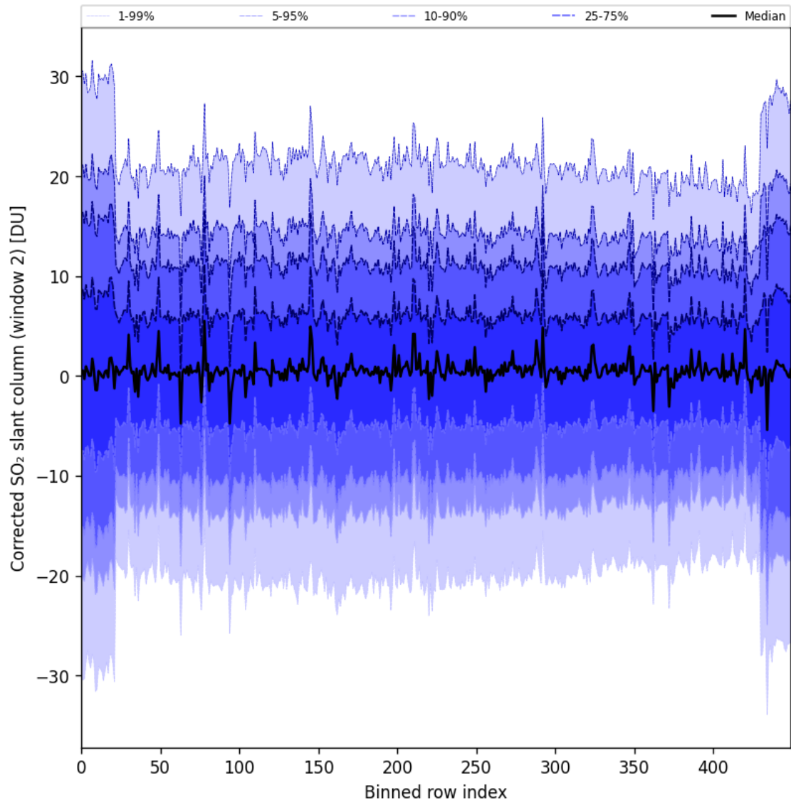
Figure 95: Along track statistics of “Corrected SO 2 slant column (window 2)” for 2025-07-24 to 2025-07-26
