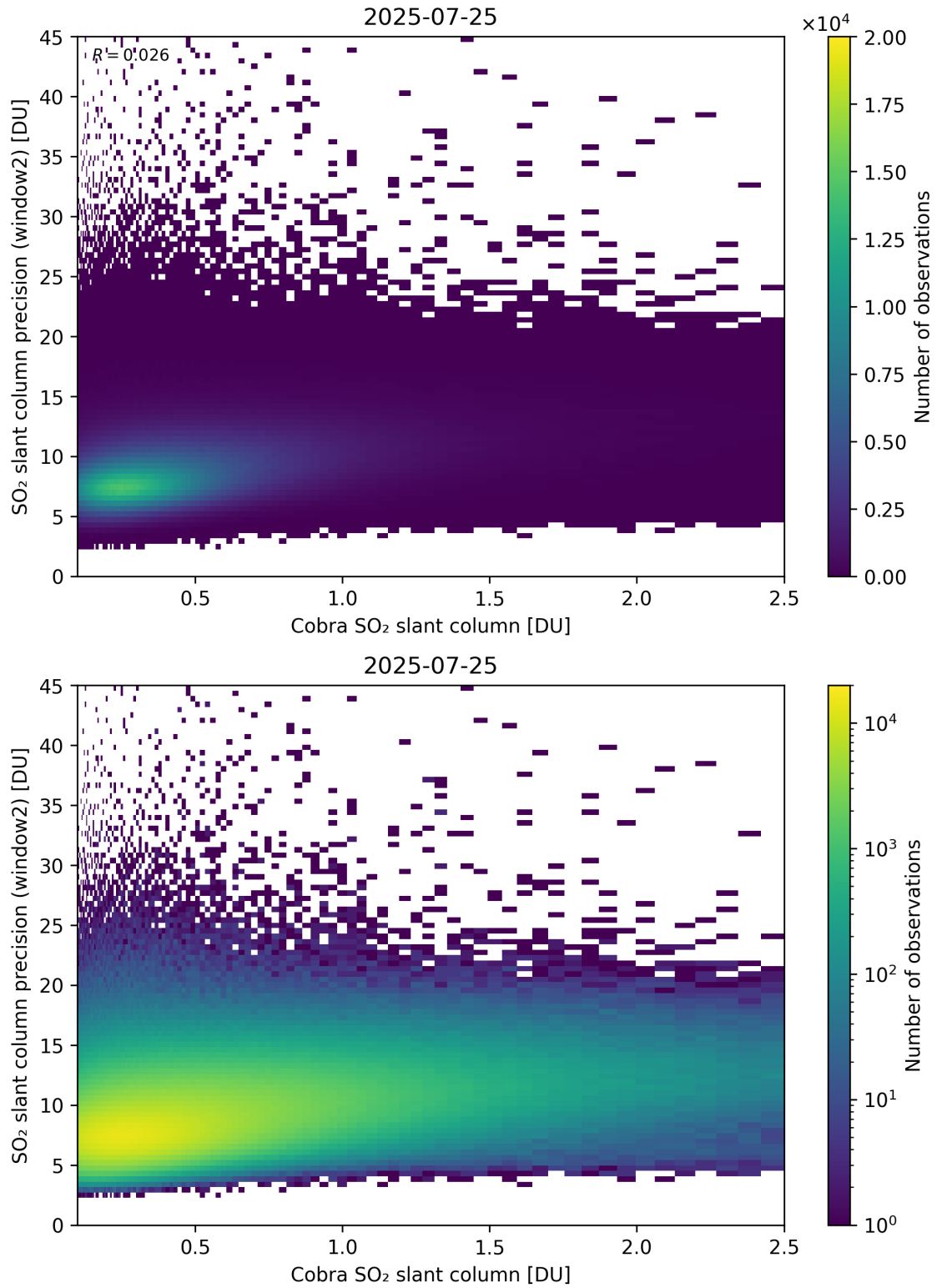
Figure 221: Scatter density plot of “Cobra SO 2 slant column” against “SO 2 slant column precision (window2)” for 2025-07-24 to 2025-07-26.
