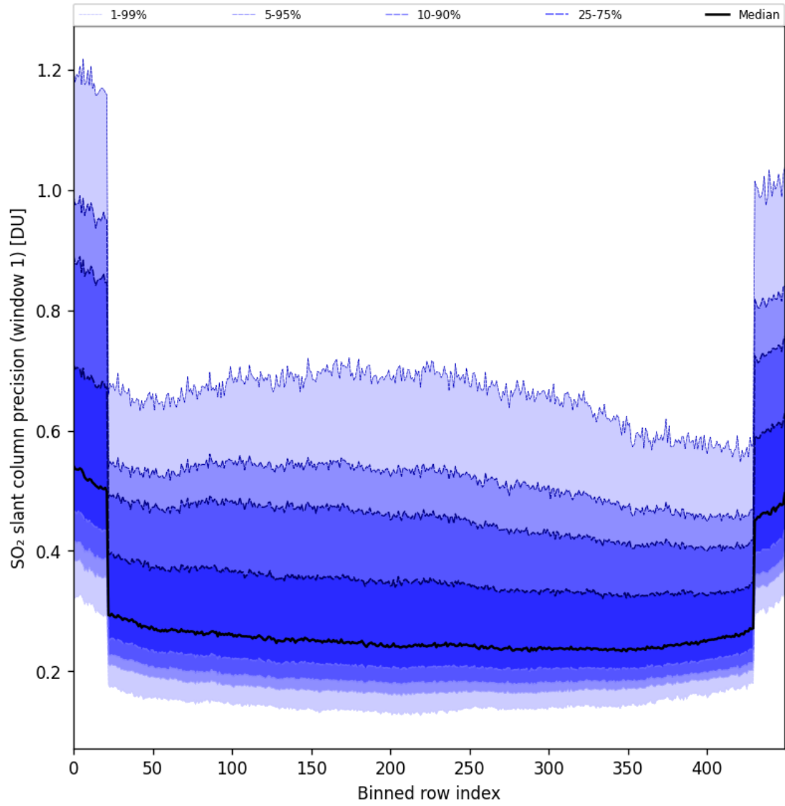
Figure 90: Along track statistics of “SO 2 slant column precision (window 1)” for 2025-07-24 to 2025-07-26
