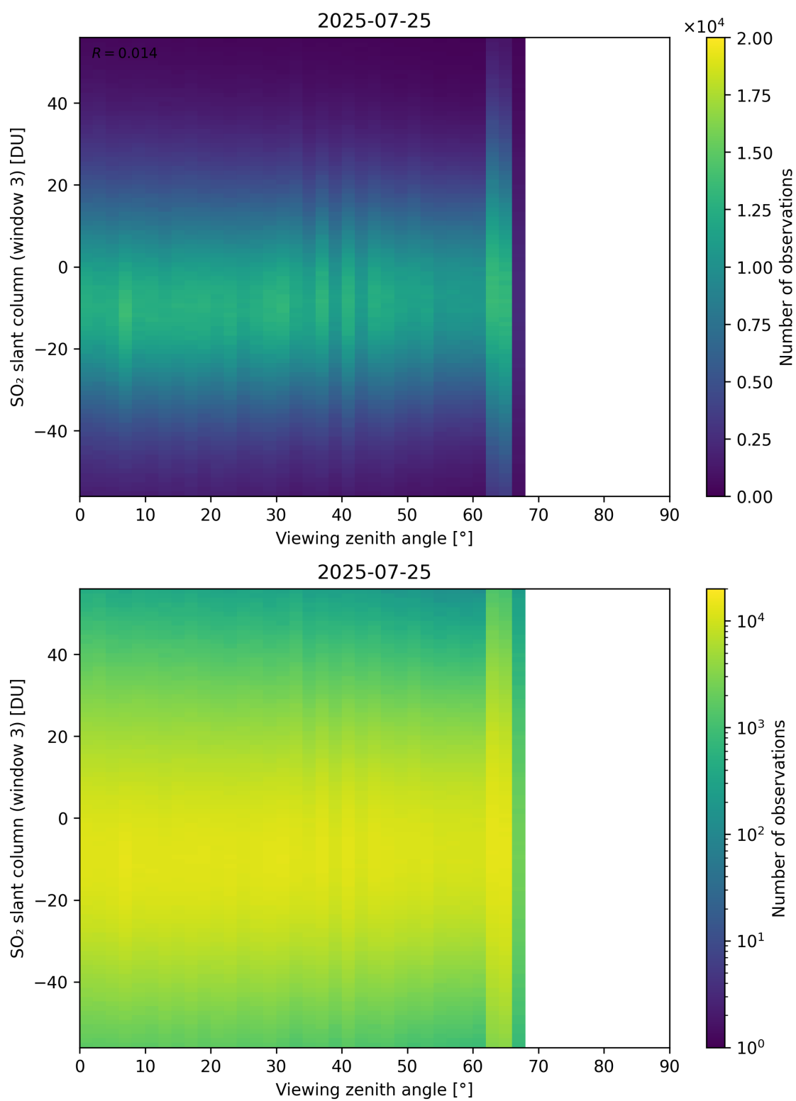
Figure 379: Scatter density plot of “Viewing zenith angle” against “SO 2 slant column (window 3)” for 2025-07-24 to 2025-07-26.
