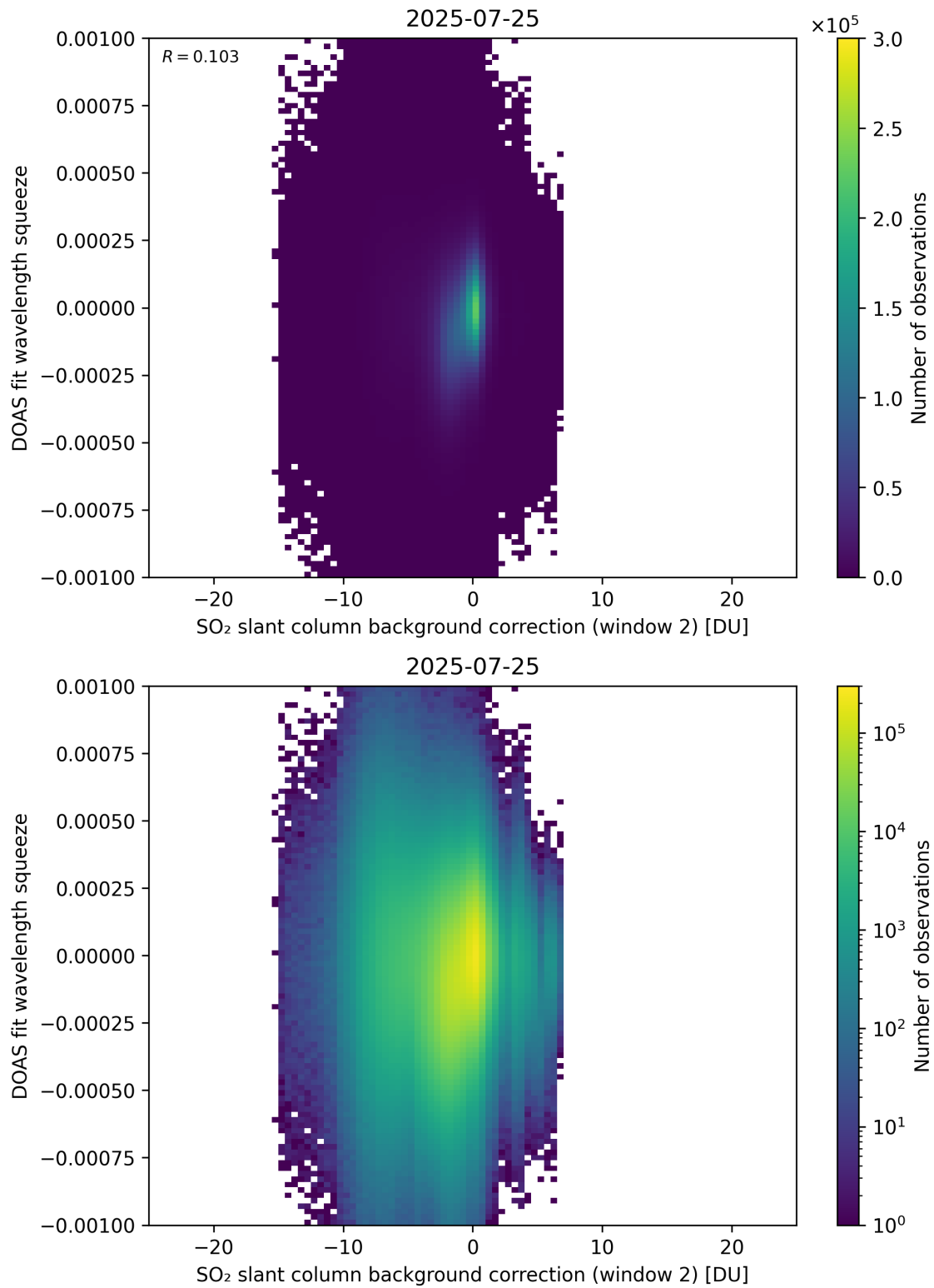
Figure 124: Scatter density plot of “SO 2 slant column background correction (window 2)” against “DOAS fit wavelength squeeze” for 2025-07-24 to 2025-07-26.
