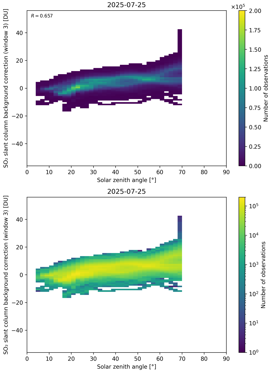
Figure 173: Scatter density plot of “Solar zenith angle” against “SO 2 slant column background correction (window 3)” for 2025-07-24 to 2025-07-26.
