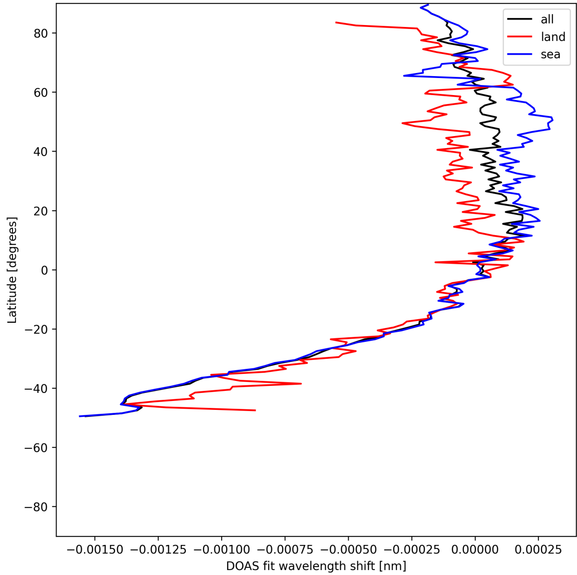
Figure 50: Zonal average of “DOAS fit wavelength shift” for 2025-07-24 to 2025-07-26.
