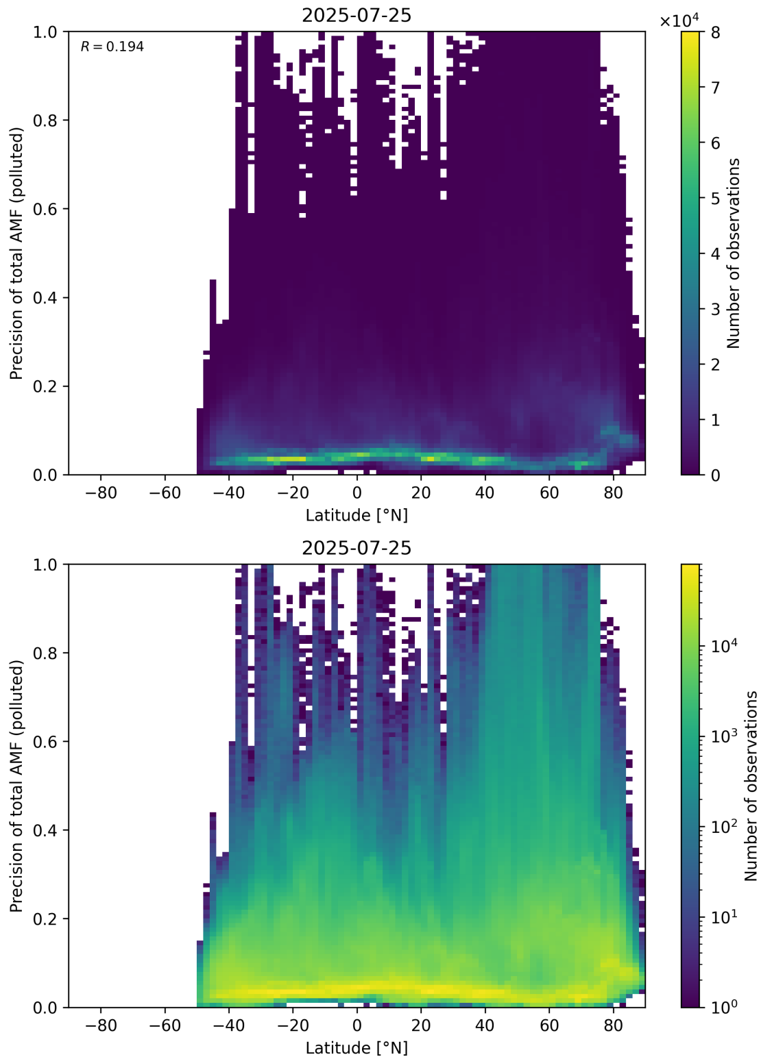
Figure 168: Scatter density plot of “Latitude” against “Precision of total AMF (polluted)” for 2025-07-24 to 2025-07-26.
