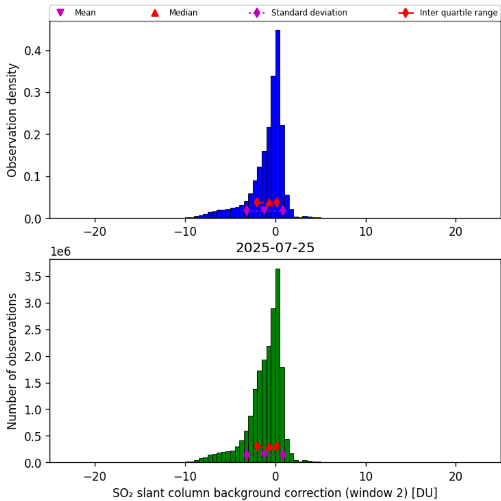
Figure 70: Histogram of “SO 2 slant column background correction (window 2)” for 2025-07-24 to 2025-07-26
