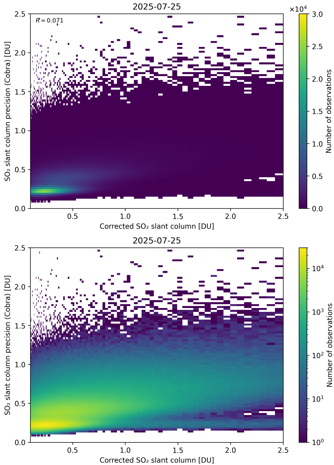
Figure 234: Scatter density plot of “Corrected SO 2 slant column” against “SO 2 slant column precision (Cobra)” for 2025-07-24 to 2025-07-26.
