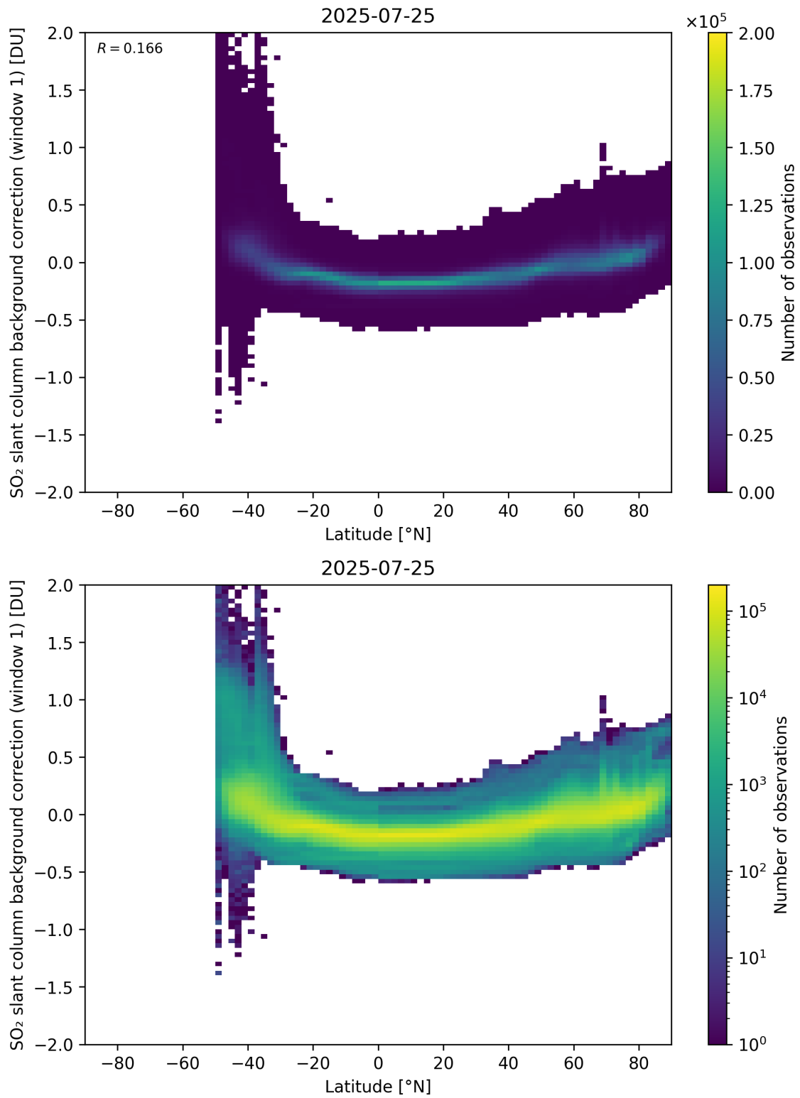
Figure 150: Scatter density plot of “Latitude” against “SO 2 slant column background correction (window 1)” for 2025-07-24 to 2025-07-26.
