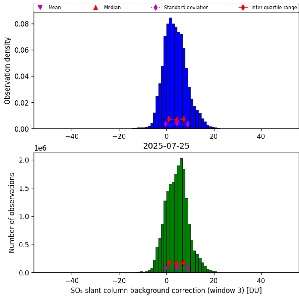
Figure 74: Histogram of “SO 2 slant column background correction (window 3)” for 2025-07-24 to 2025-07-26
