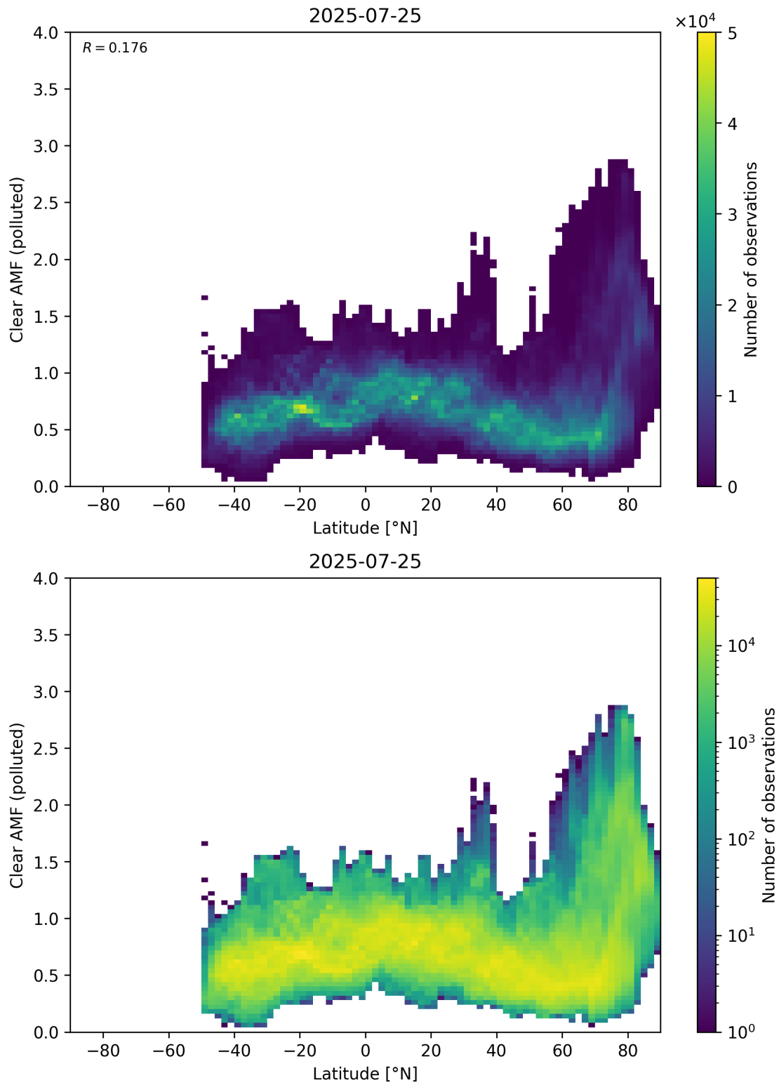
Figure 156: Scatter density plot of “Latitude” against “Clear AMF (polluted)” for 2025-07-24 to 2025-07-26.
