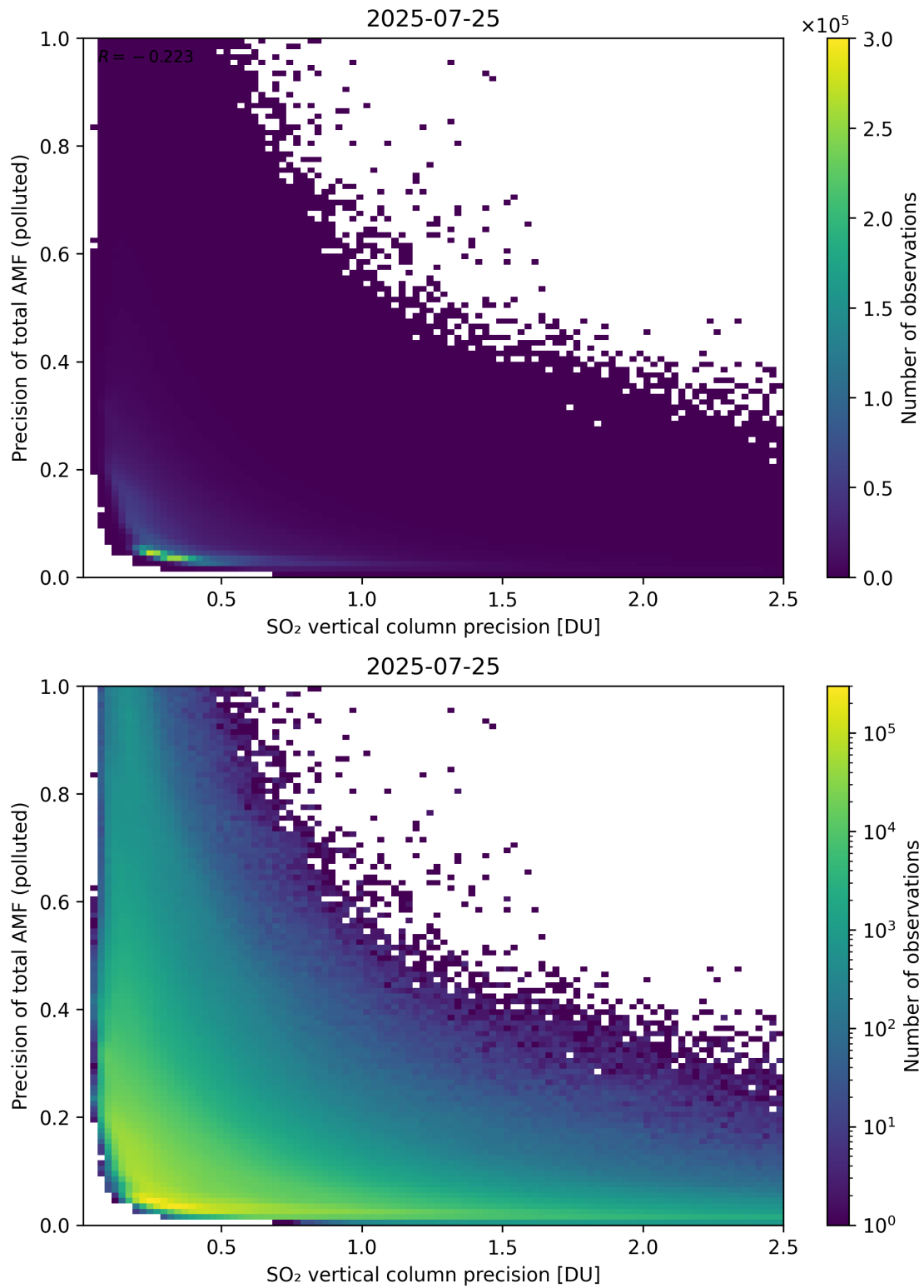
Figure 347: Scatter density plot of “SO 2 vertical column precision” against “Precision of total AMF (polluted)” for 2025-07-24 to 2025-07-26.
