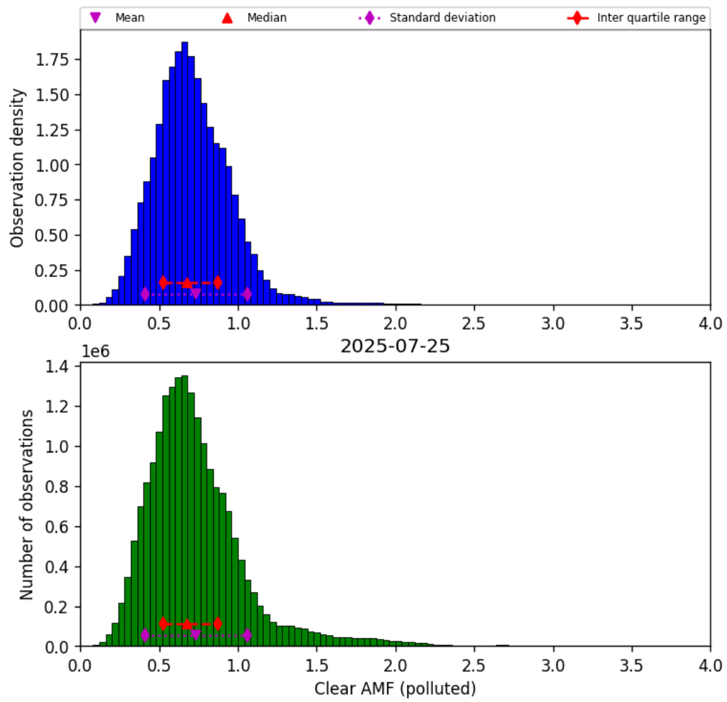
Figure 81: Histogram of “Clear AMF (polluted)” for 2025-07-24 to 2025-07-26
