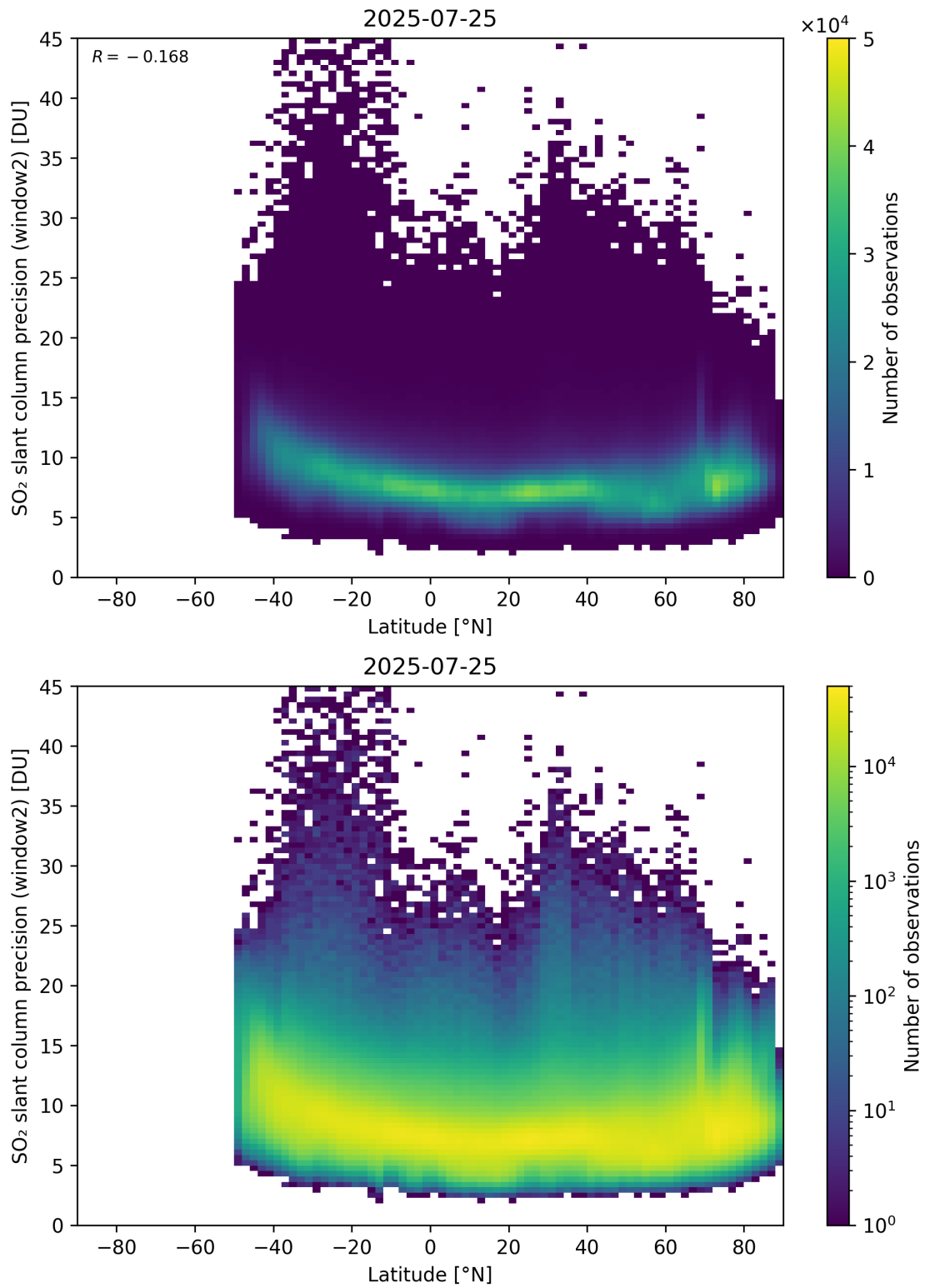
Figure 164: Scatter density plot of “Latitude” against “SO 2 slant column precision (window2)” for 2025-07-24 to 2025-07-26.
