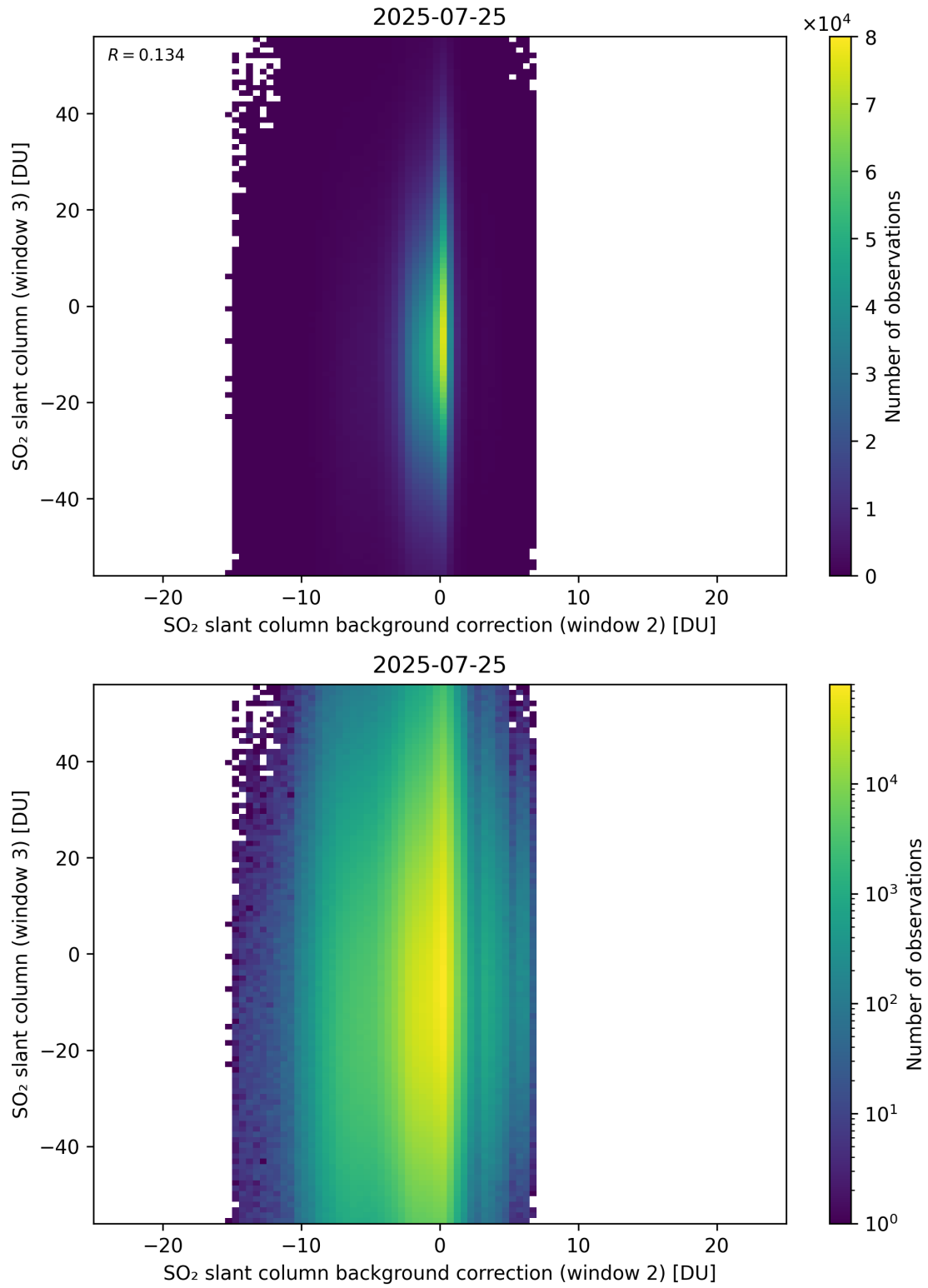
Figure 128: Scatter density plot of “SO 2 slant column background correction (window 2)” against “SO 2 slant column (window 3)” for 2025-07-24 to 2025-07-26.
