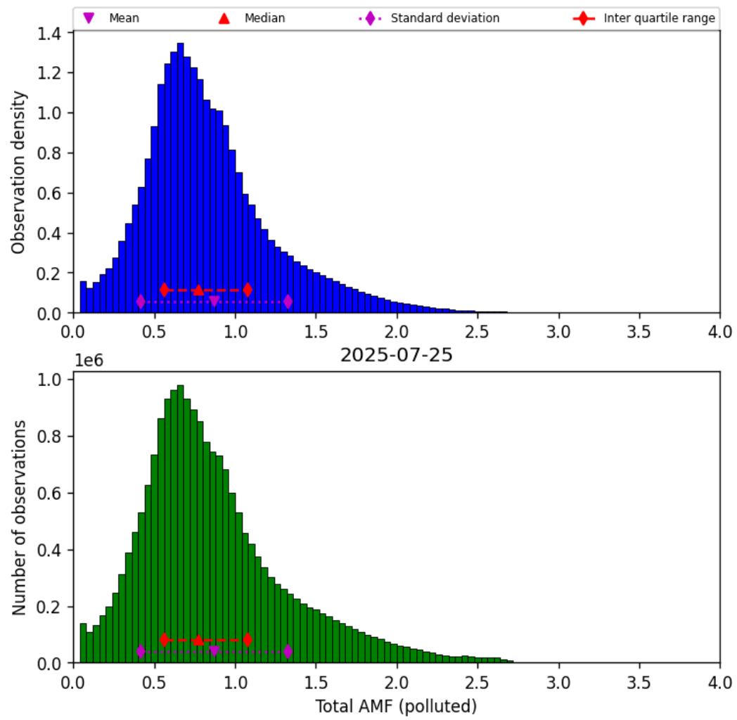
Figure 79: Histogram of “Total AMF (polluted)” for 2025-07-24 to 2025-07-26
