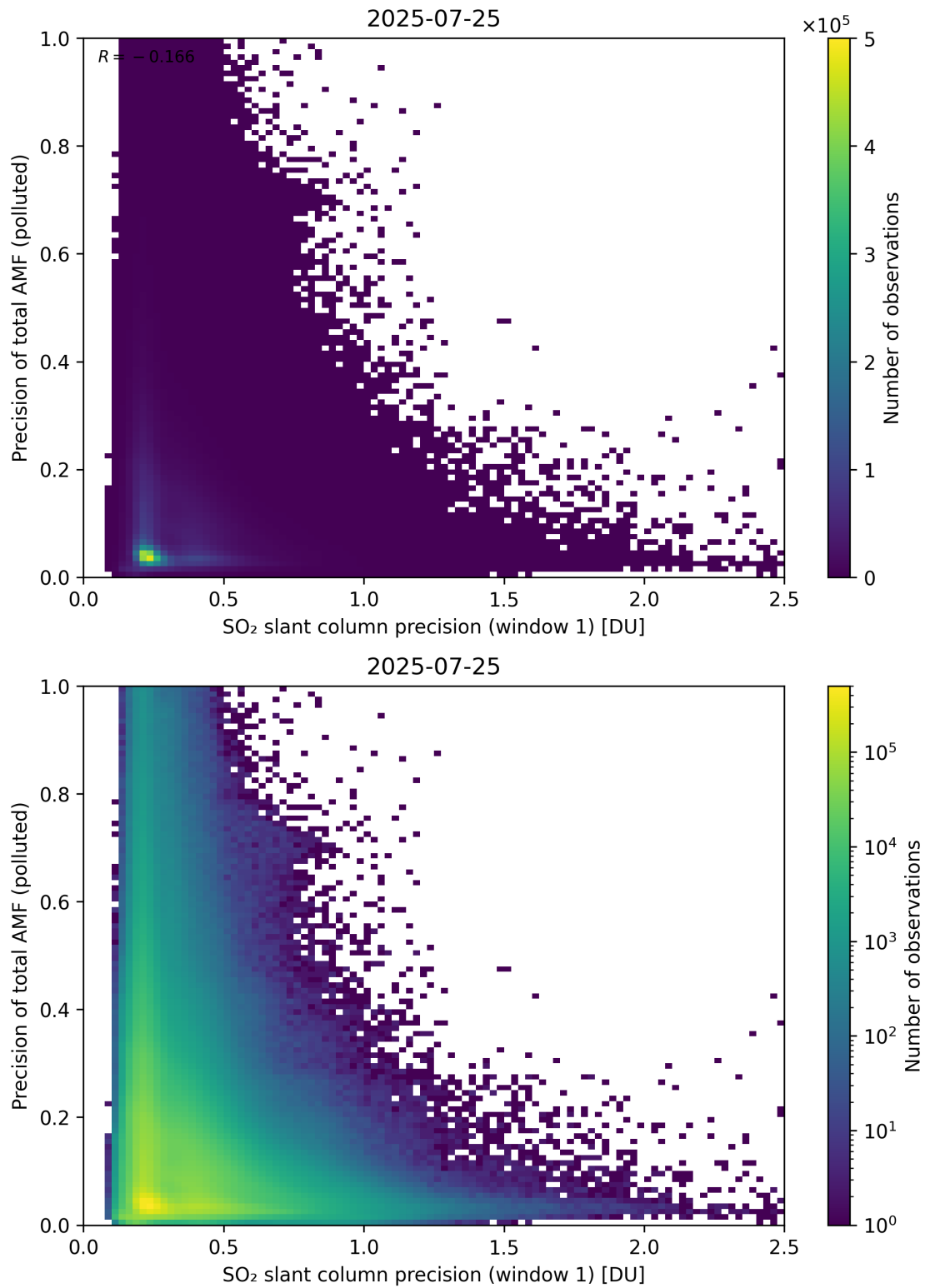
Figure 281: Scatter density plot of “SO 2 slant column precision (window 1)” against “Precision of total AMF (polluted)” for 2025-07-24 to 2025-07-26.
