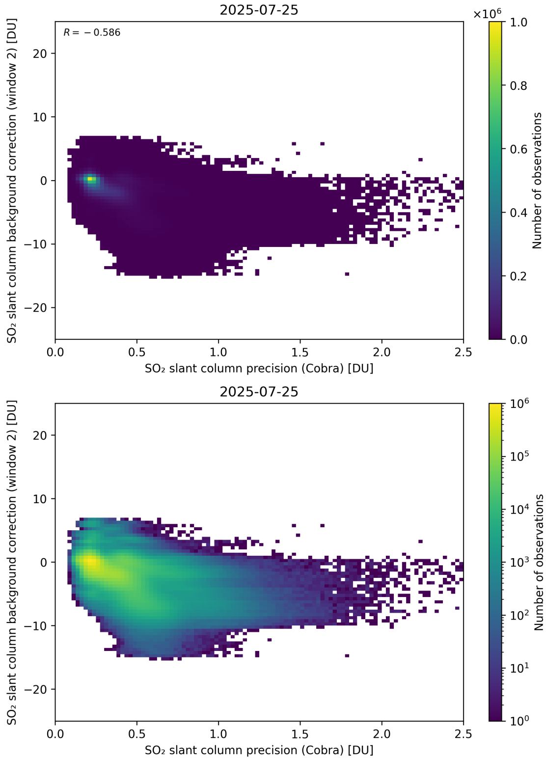
Figure 200: Scatter density plot of “SO 2 slant column precision (Cobra)” against “SO 2 slant column background correction (window 2)” for 2025-07-24 to 2025-07-26.
