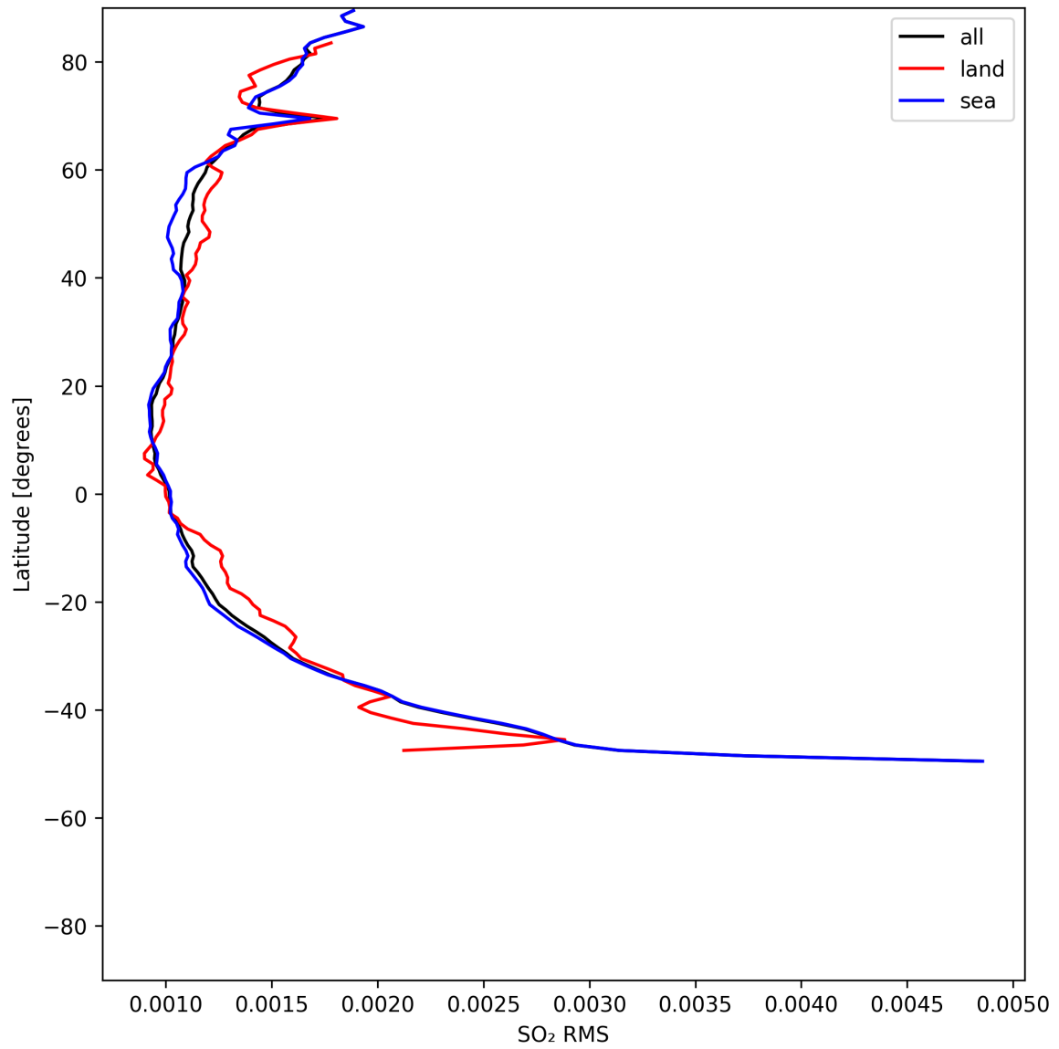
Figure 52: Zonal average of “SO 2 RMS” for 2025-07-24 to 2025-07-26.
