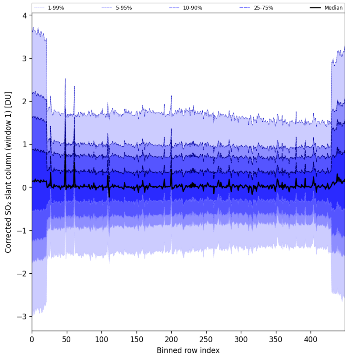
Figure 91: Along track statistics of “Corrected SO 2 slant column (window 1)” for 2025-07-24 to 2025-07-26
