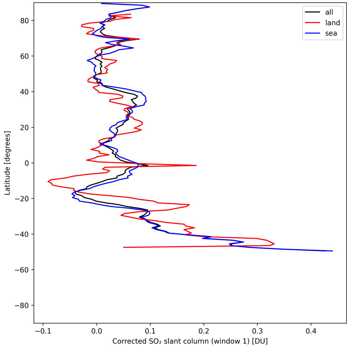
Figure 39: Zonal average of “Corrected SO 2 slant column (window 1)” for 2025-07-24 to 2025-07-26.
