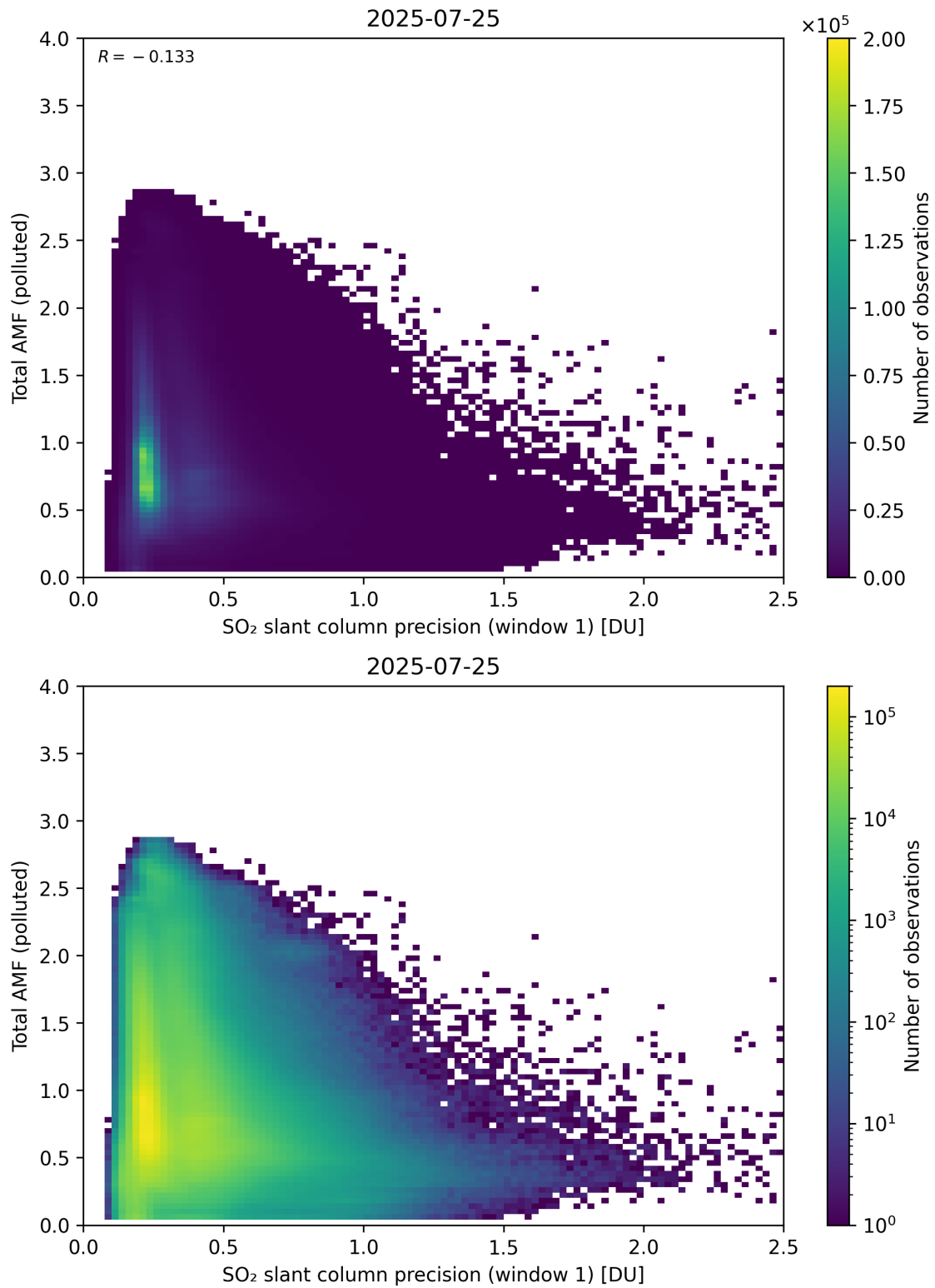
Figure 280: Scatter density plot of “SO 2 slant column precision (window 1)” against “Total AMF (polluted)” for 2025-07-24 to 2025-07-26.
