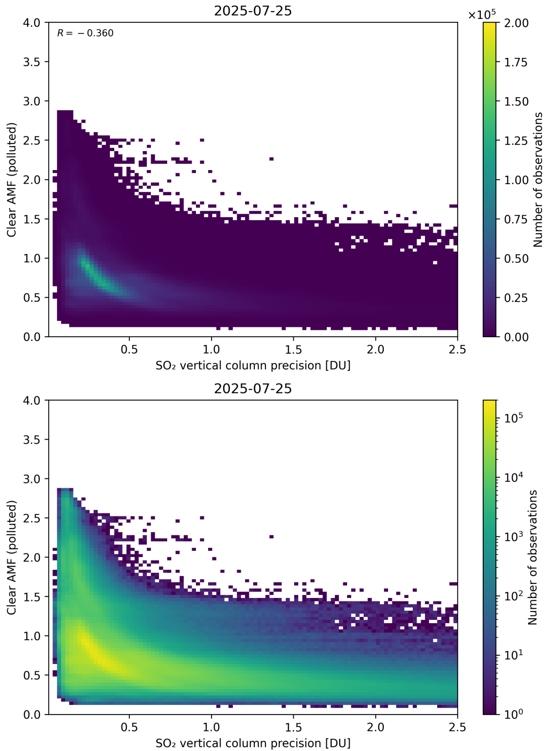
Figure 335: Scatter density plot of “SO 2 vertical column precision” against “Clear AMF (polluted)” for 2025-07-24 to 2025-07-26.
