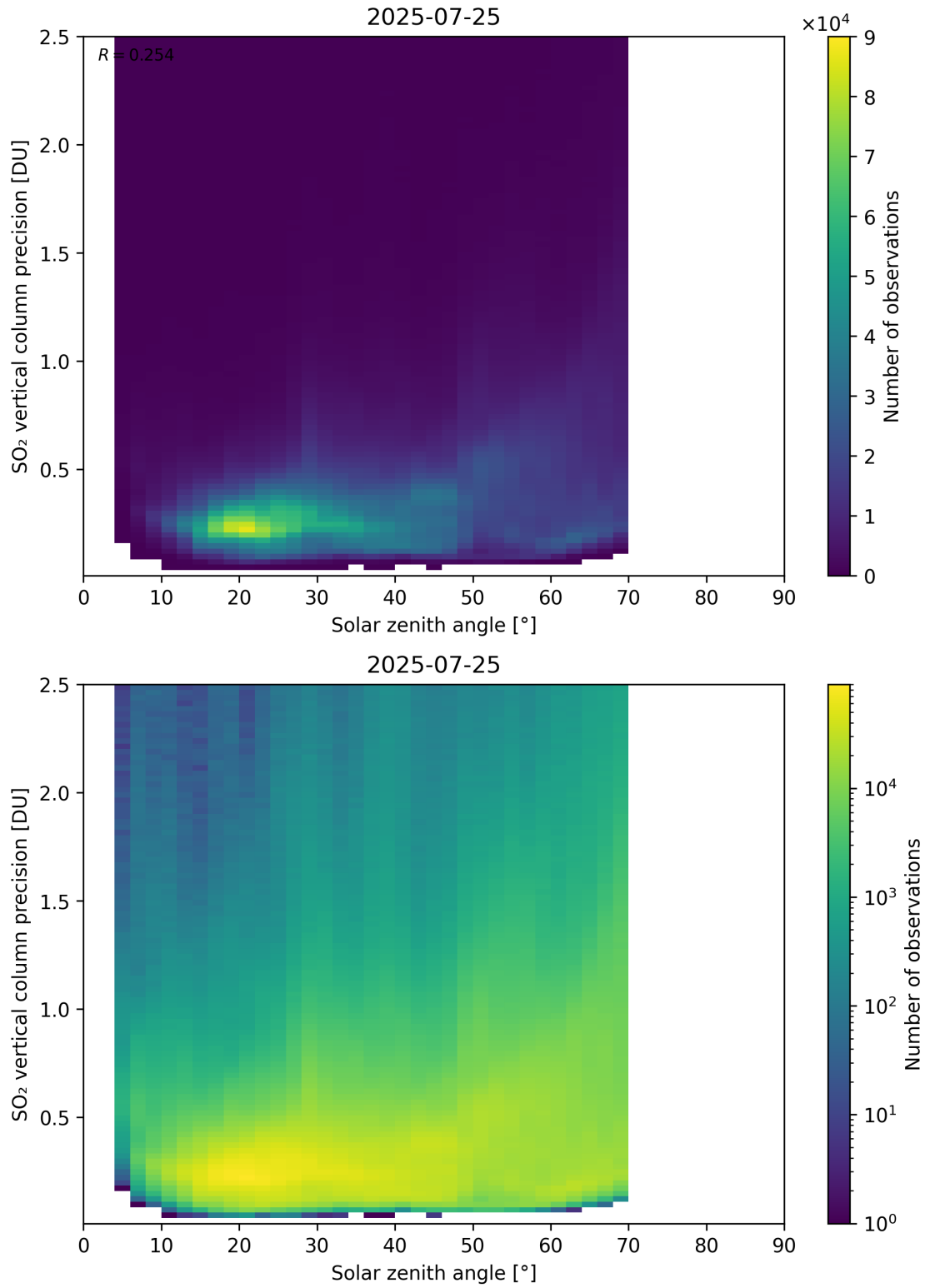
Figure 192: Scatter density plot of “Solar zenith angle” against “SO 2 vertical column precision” for 2025-07-24 to 2025-07-26.
