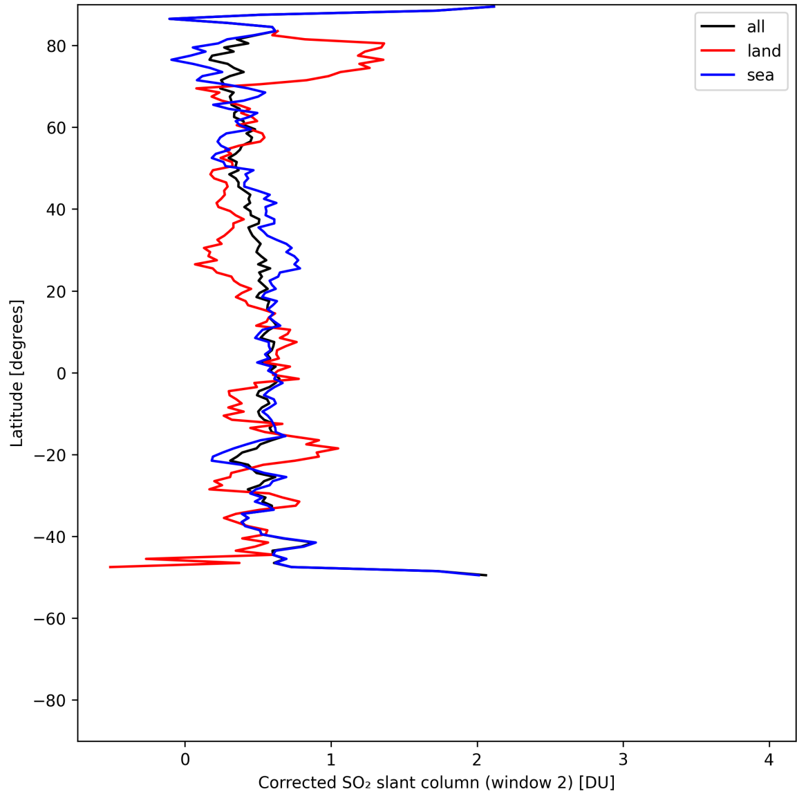
Figure 43: Zonal average of “Corrected SO 2 slant column (window 2)” for 2025-07-24 to 2025-07-26.
