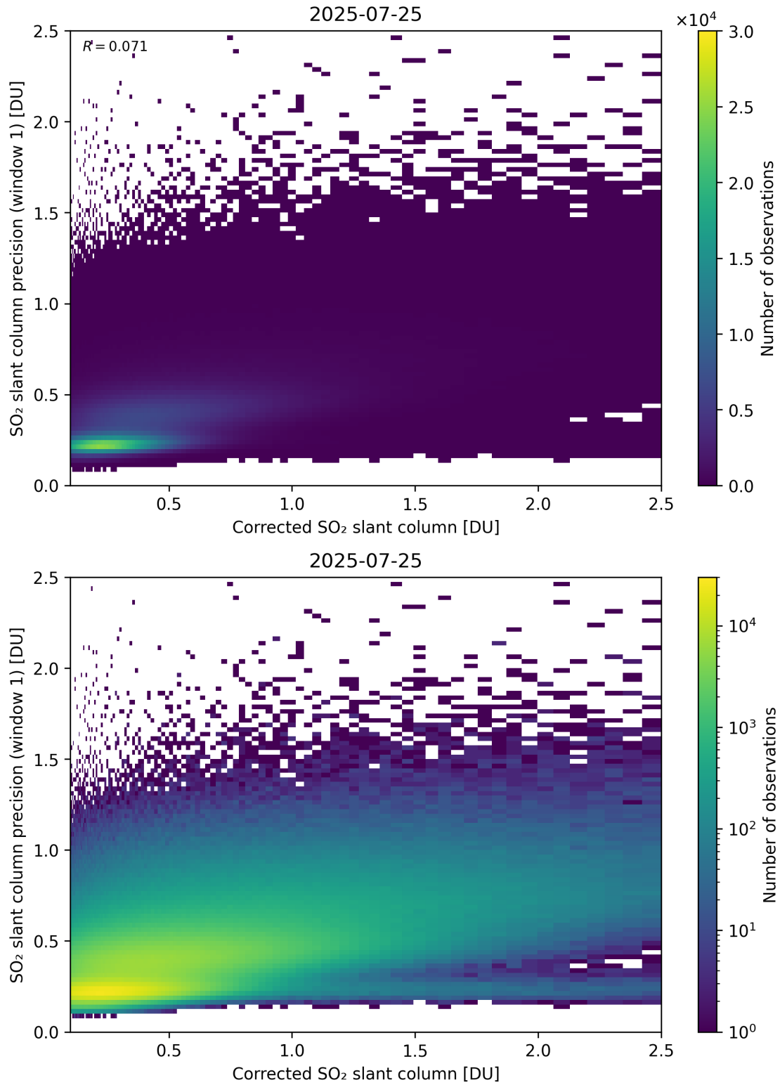
Figure 238: Scatter density plot of “Corrected SO 2 slant column” against “SO 2 slant column precision (window 1)” for 2025-07-24 to 2025-07-26.
