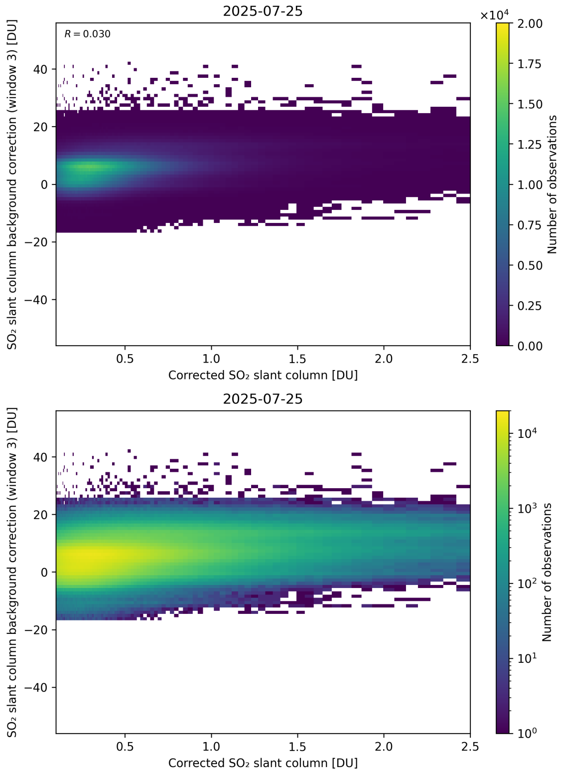
Figure 228: Scatter density plot of “Corrected SO 2 slant column” against “SO 2 slant column background correction (window 3)” for 2025-07-24 to 2025-07-26.
