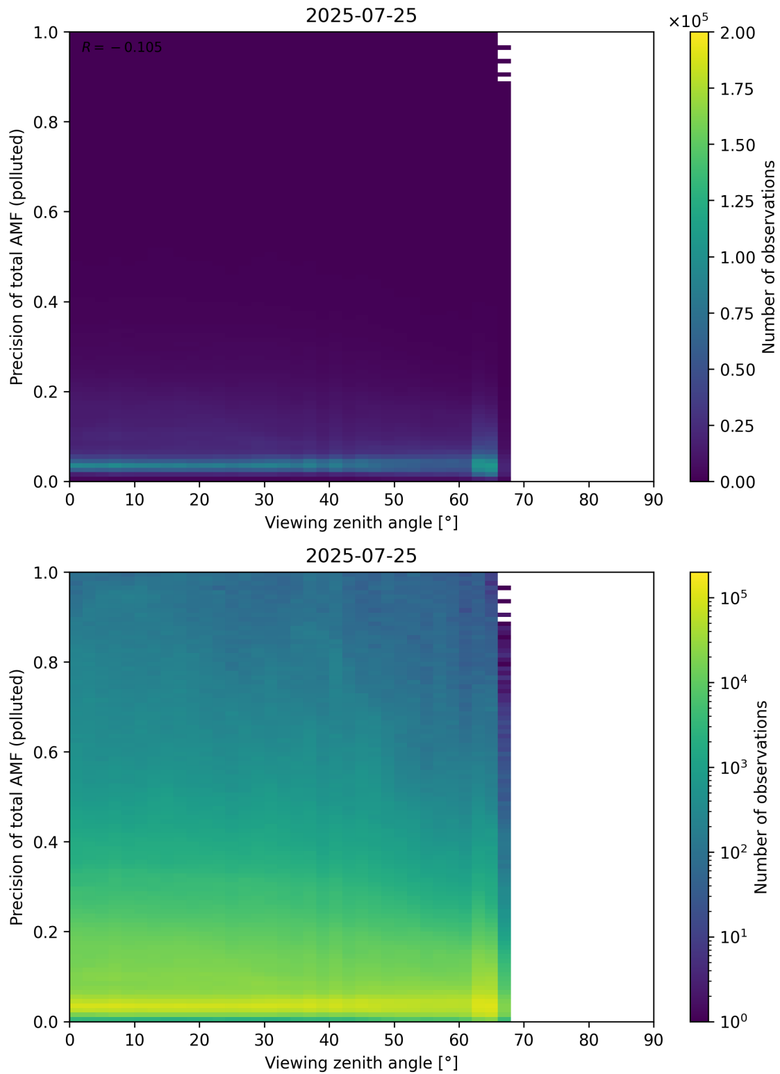
Figure 382: Scatter density plot of “Viewing zenith angle” against “Precision of total AMF (polluted)” for 2025-07-24 to 2025-07-26.
