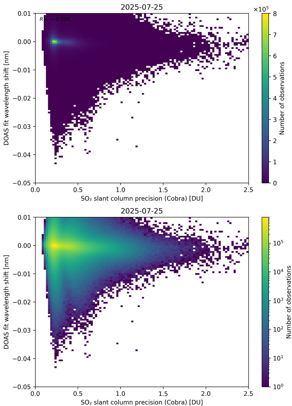
Figure 202: Scatter density plot of “SO 2 slant column precision (Cobra)” against “DOAS fit wavelength shift” for 2025-07-24 to 2025-07-26.
