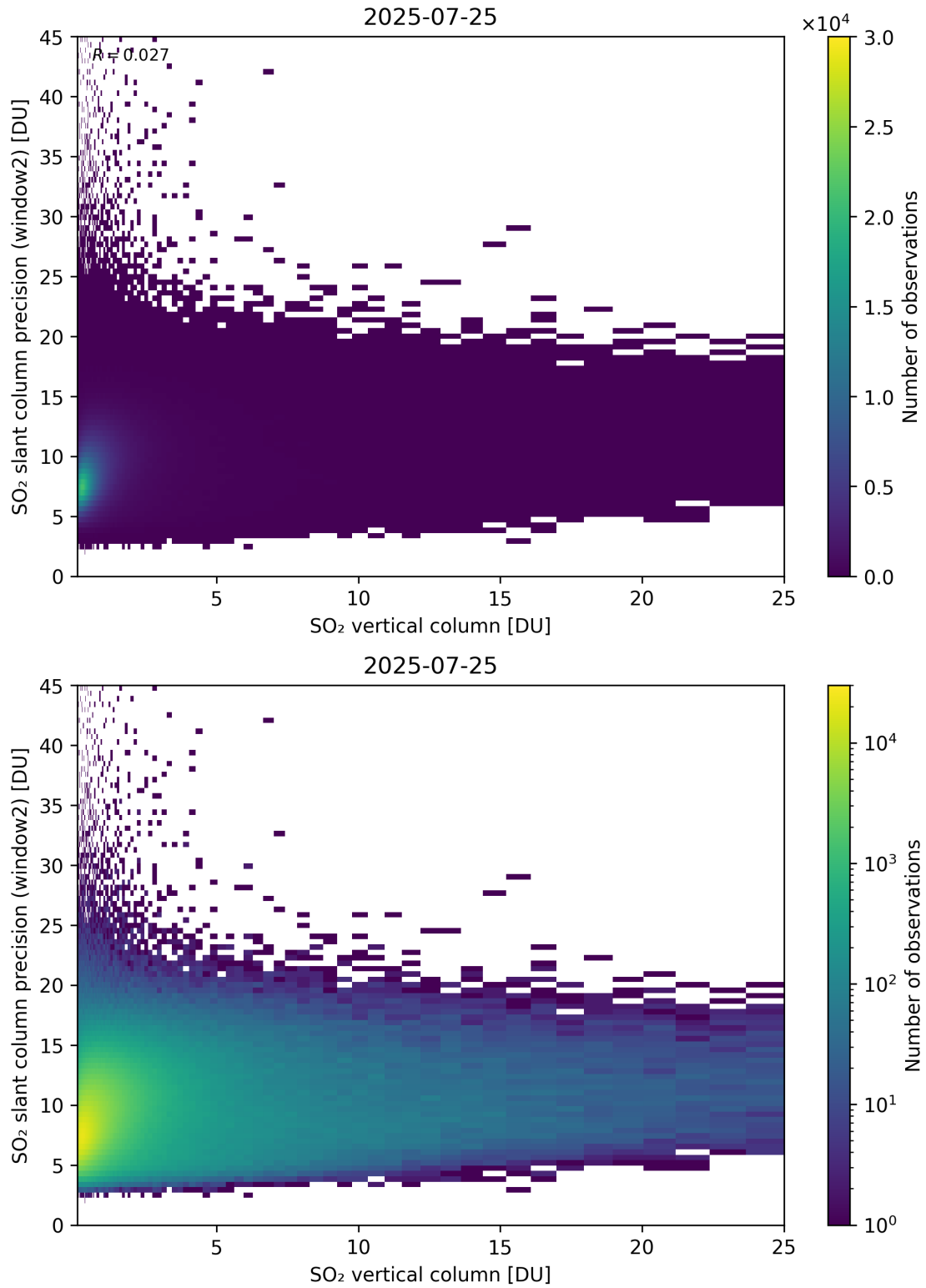
Figure 356: Scatter density plot of “SO 2 vertical column” against “SO 2 slant column precision (window2)” for 2025-07-24 to 2025-07-26.
