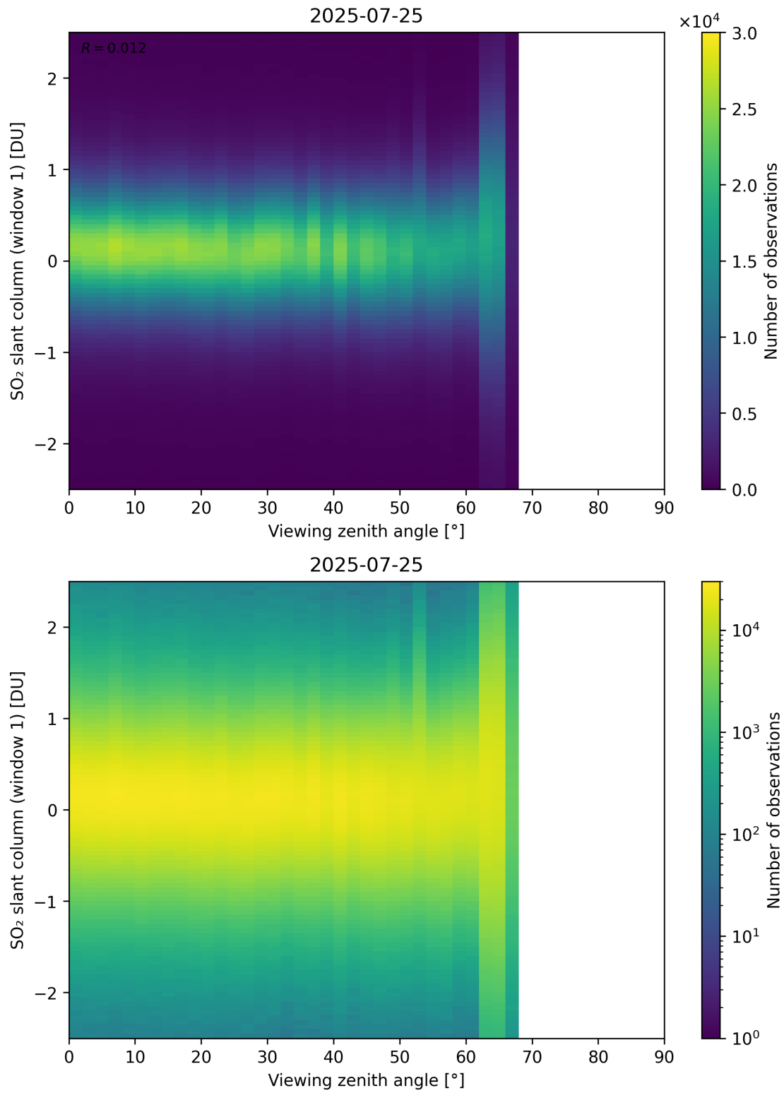
Figure 376: Scatter density plot of “Viewing zenith angle” against “SO 2 slant column (window 1)” for 2025-07-24 to 2025-07-26.
