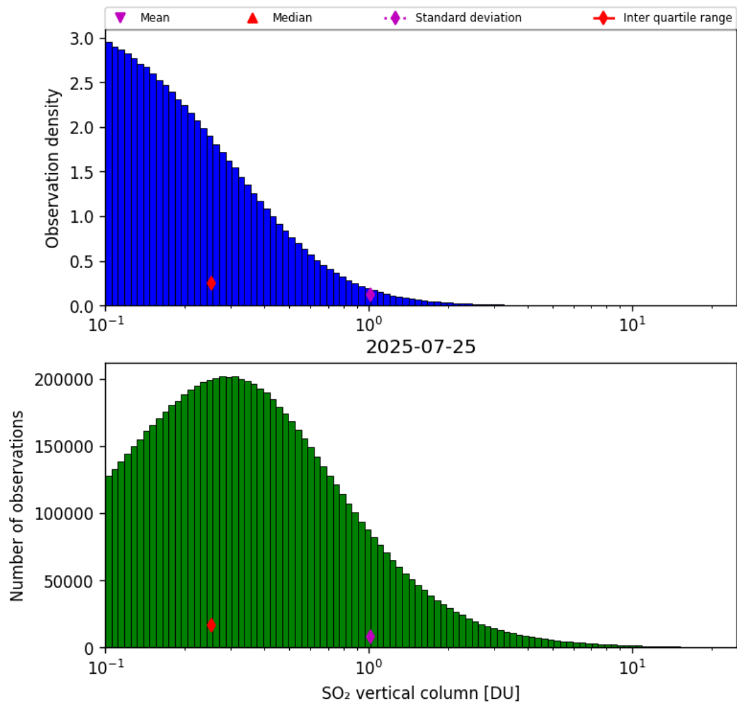
Figure 58: Histogram of “SO 2 vertical column” for 2025-07-24 to 2025-07-26
