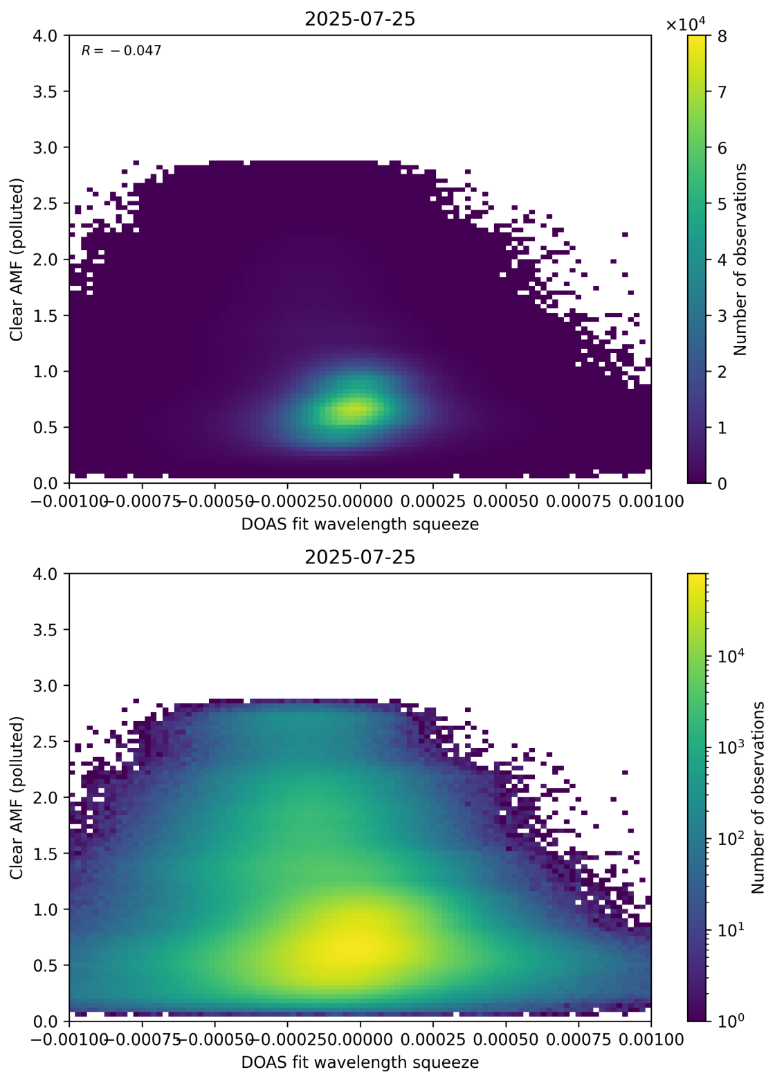
Figure 144: Scatter density plot of “DOAS fit wavelength squeeze” against “Clear AMF (polluted)” for 2025-07-24 to 2025-07-26.
