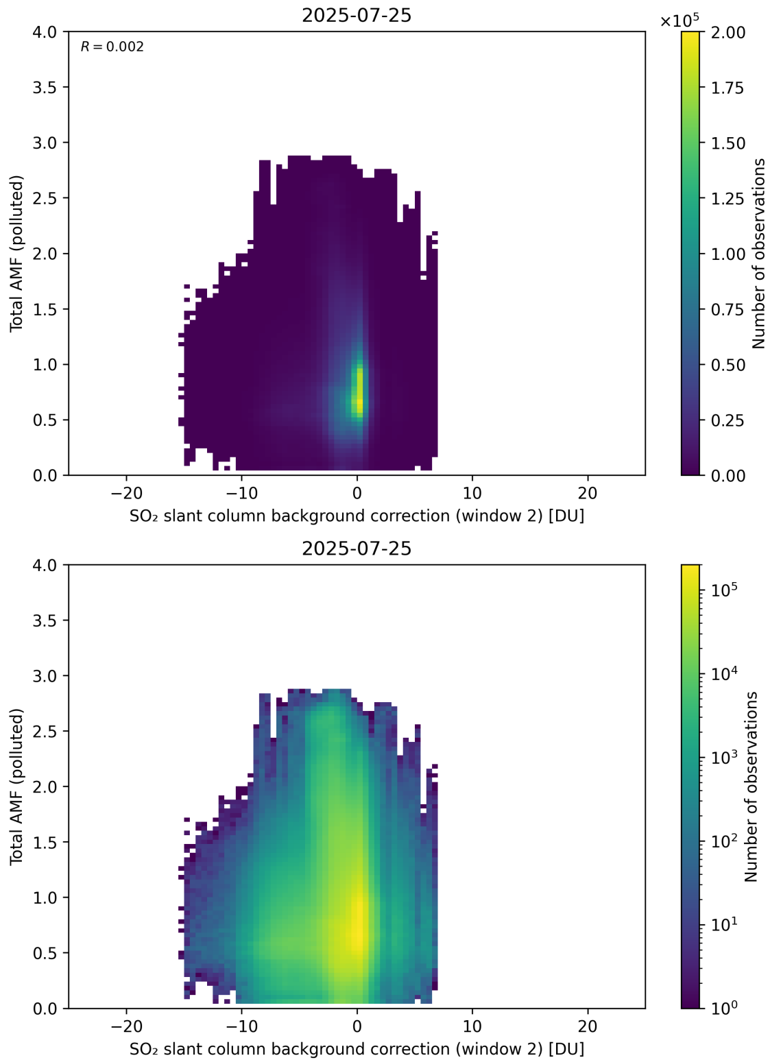
Figure 130: Scatter density plot of “SO 2 slant column background correction (window 2)” against “Total AMF (polluted)” for 2025-07-24 to 2025-07-26.
