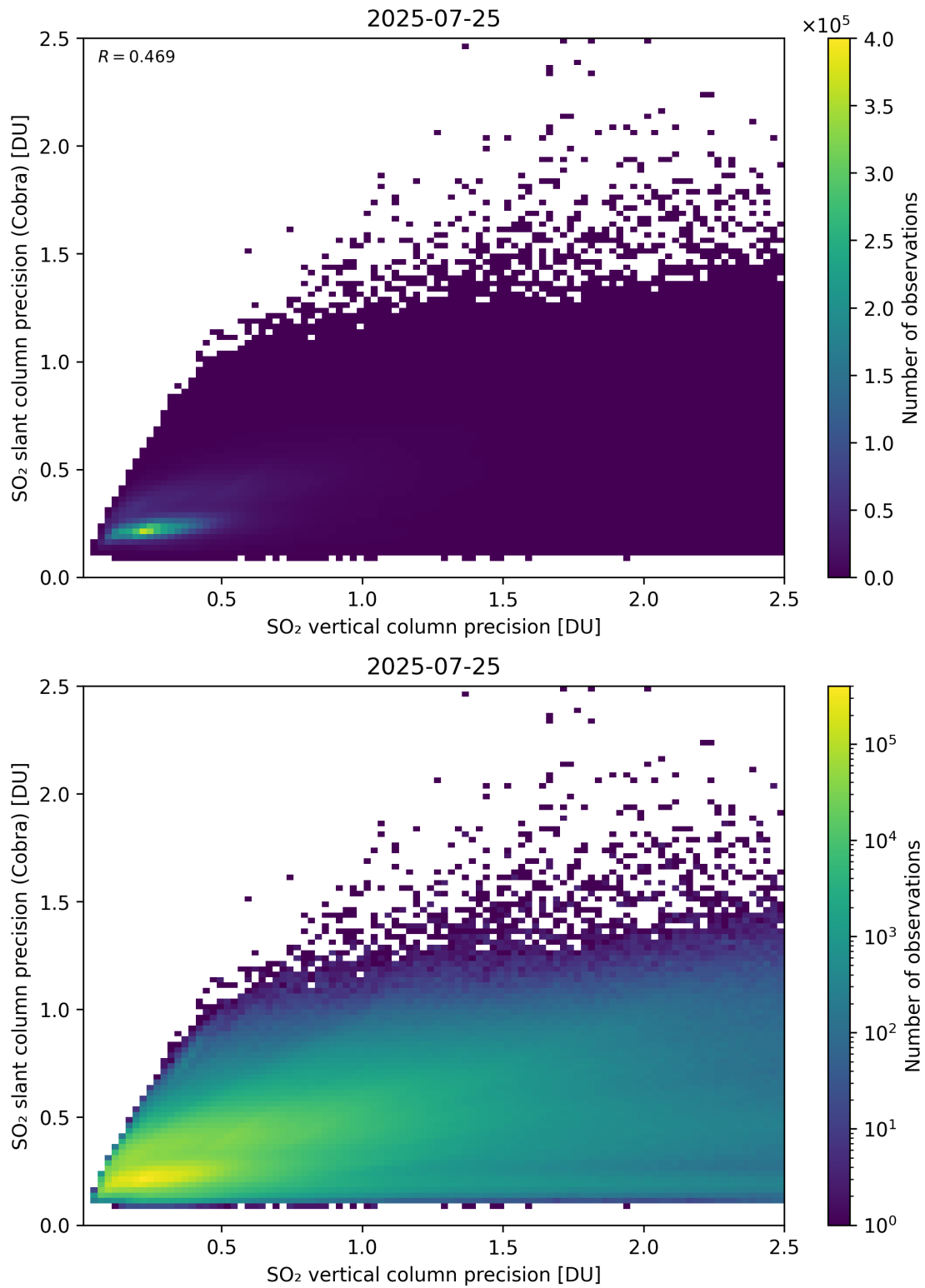
Figure 337: Scatter density plot of “SO 2 vertical column precision” against “SO 2 slant column precision (Cobra)” for 2025-07-24 to 2025-07-26.
