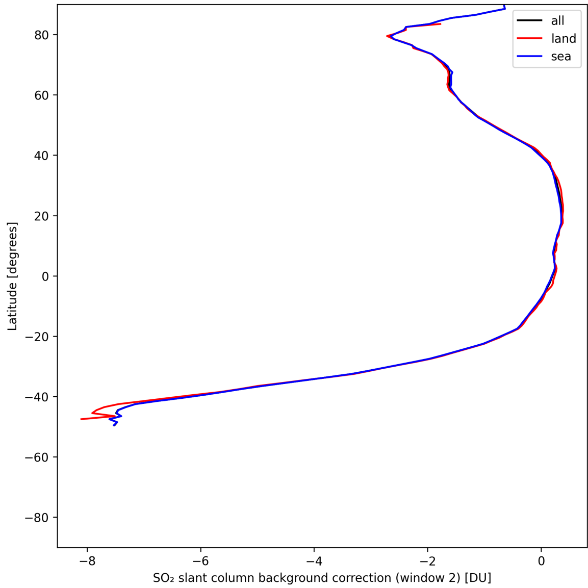
Figure 44: Zonal average of “SO 2 slant column background correction (window 2)” for 2025-07-24 to 2025-07-26.
