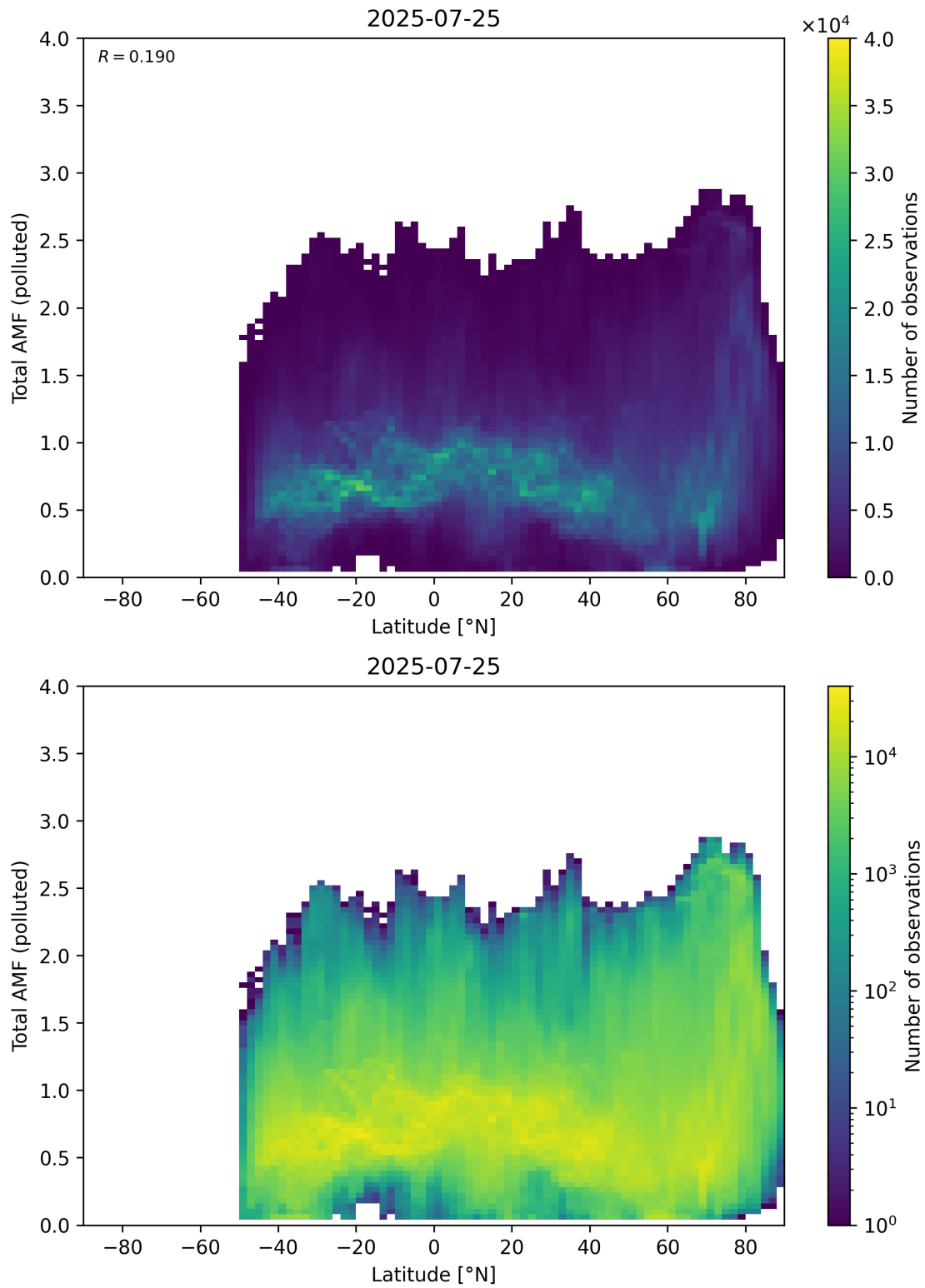
Figure 167: Scatter density plot of “Latitude” against “Total AMF (polluted)” for 2025-07-24 to 2025-07-26.
