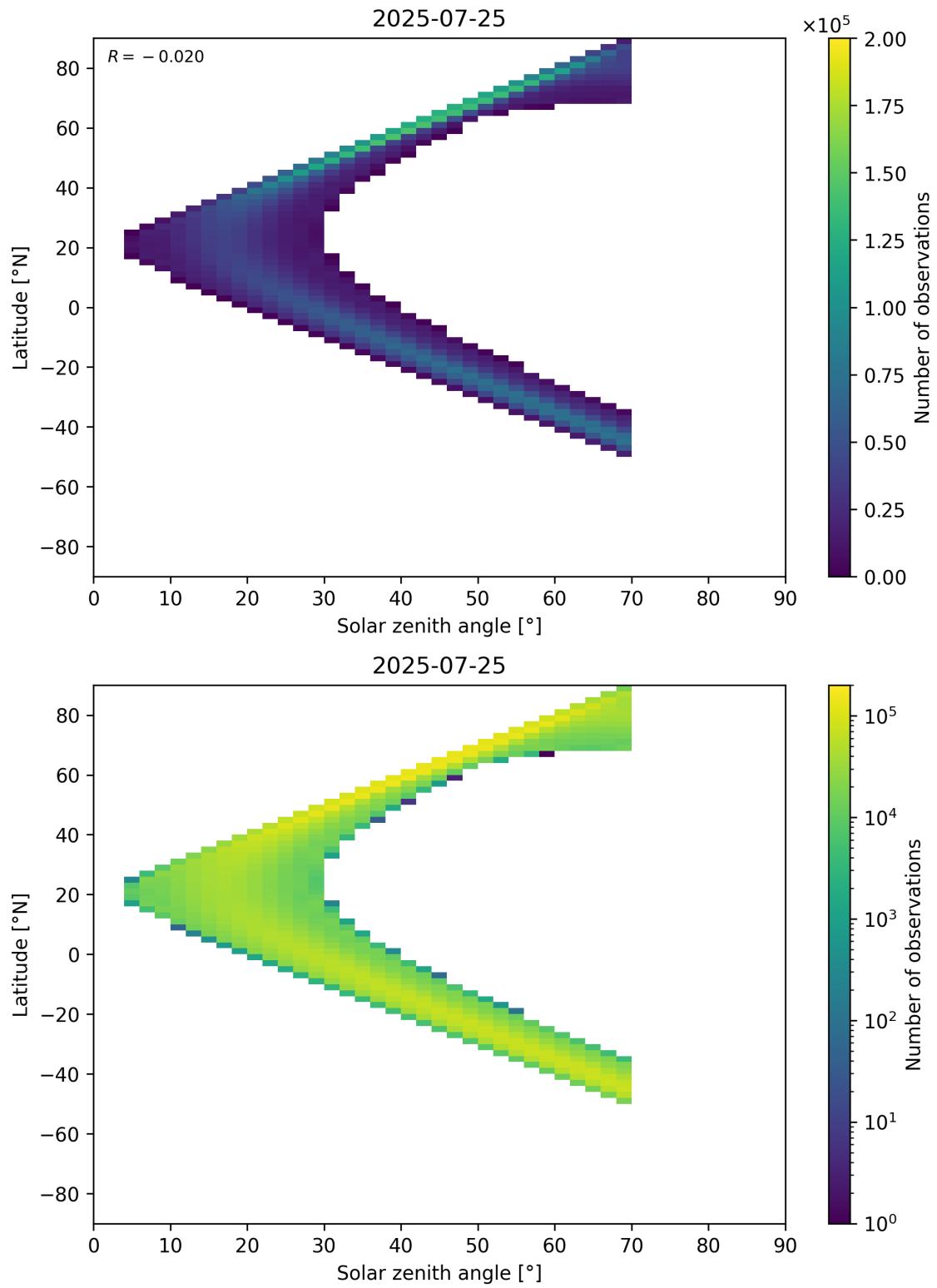
Figure 177: Scatter density plot of “Solar zenith angle” against “Latitude” for 2025-07-24 to 2025-07-26.
