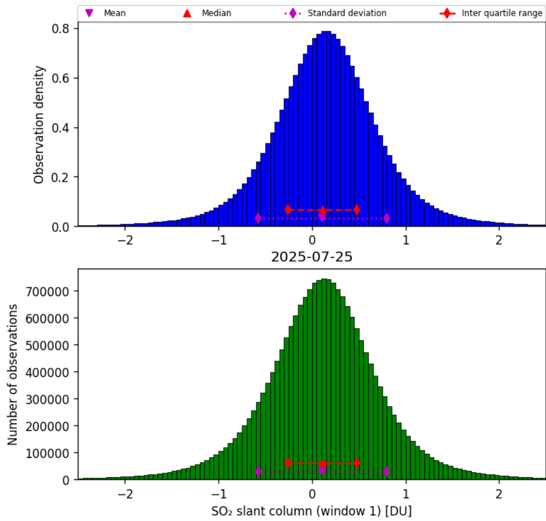
Figure 63: Histogram of “SO 2 slant column (window 1)” for 2025-07-24 to 2025-07-26
