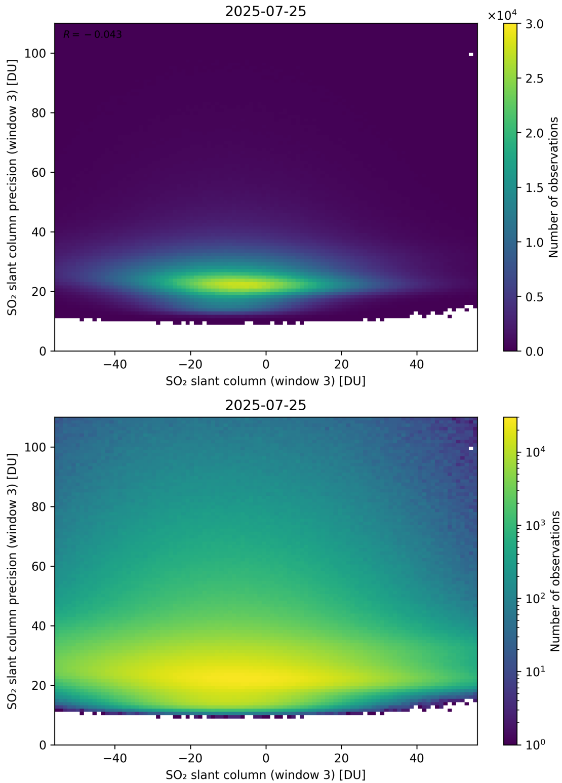
Figure 317: Scatter density plot of “SO 2 slant column (window 3)” against “SO 2 slant column precision (window 3)” for 2025-07-24 to 2025-07-26.
