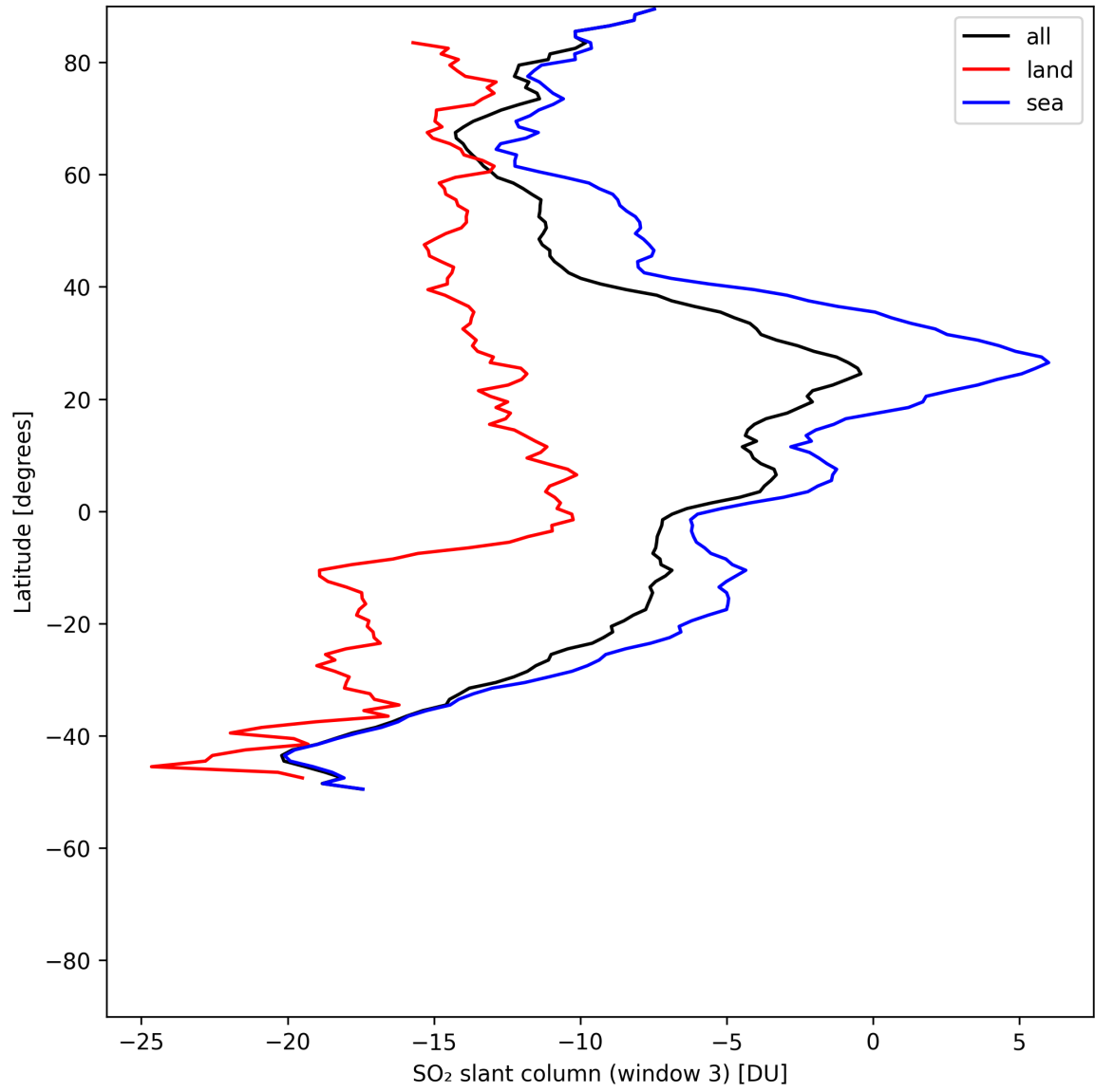
Figure 45: Zonal average of “SO 2 slant column (window 3)” for 2025-07-24 to 2025-07-26.
