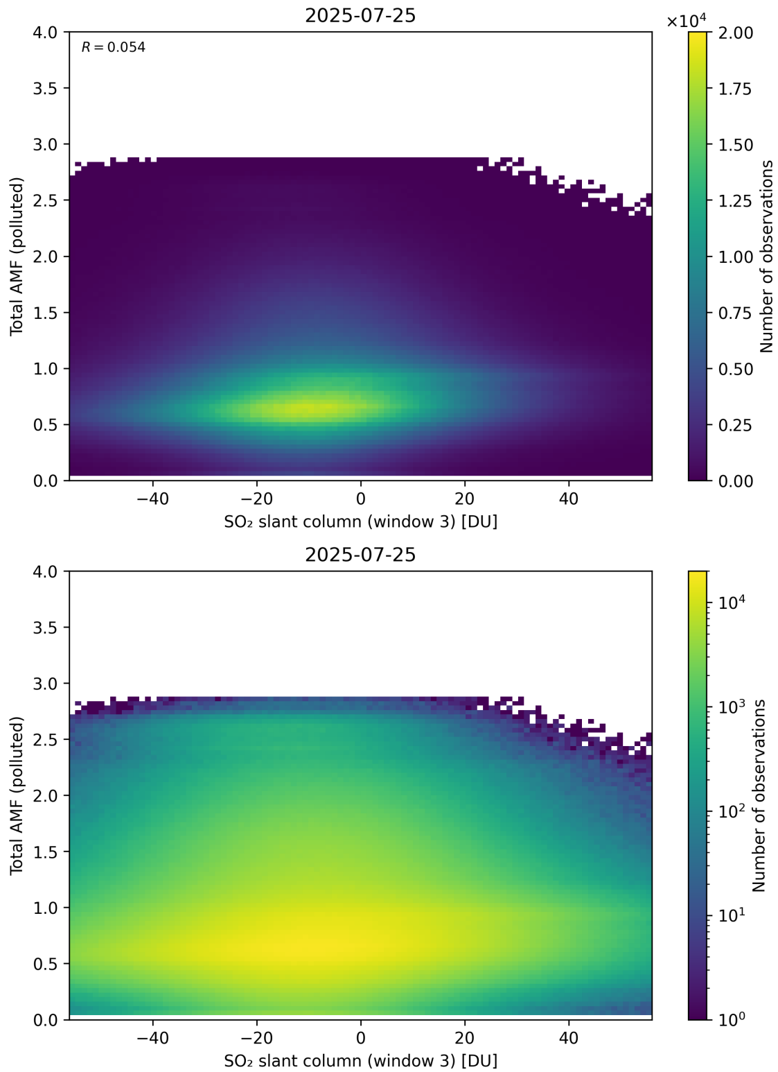
Figure 318: Scatter density plot of “SO 2 slant column (window 3)” against “Total AMF (polluted)” for 2025-07-24 to 2025-07-26.
