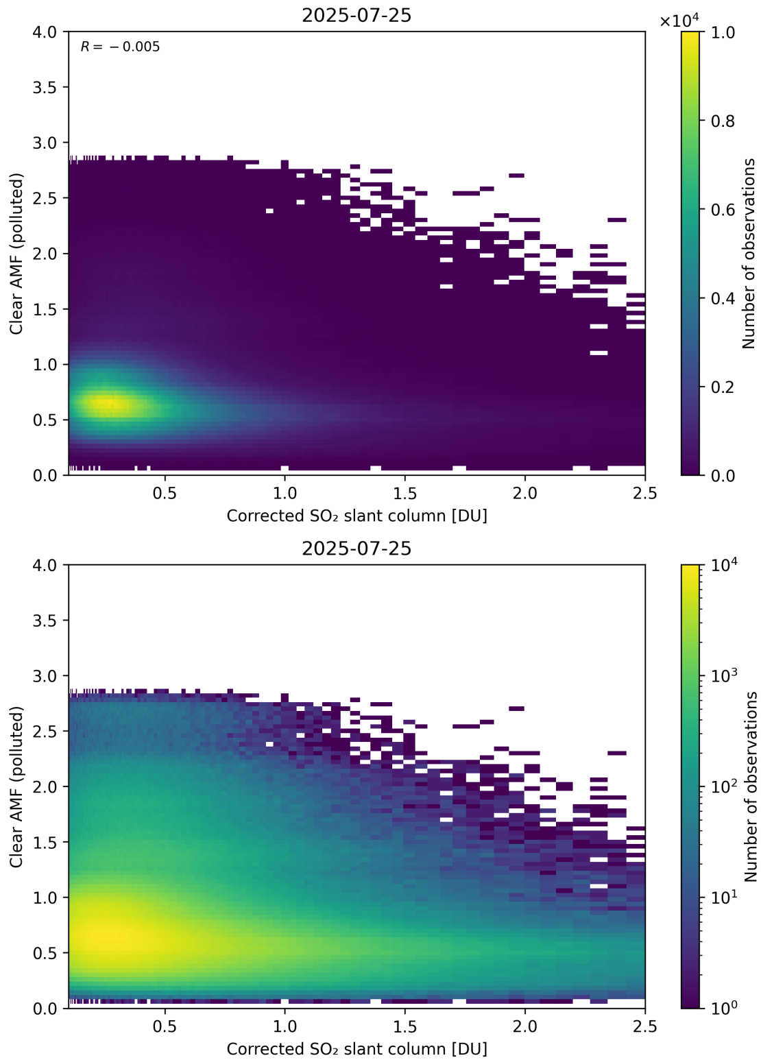
Figure 232: Scatter density plot of “Corrected SO 2 slant column” against “Clear AMF (polluted)” for 2025-07-24 to 2025-07-26.
