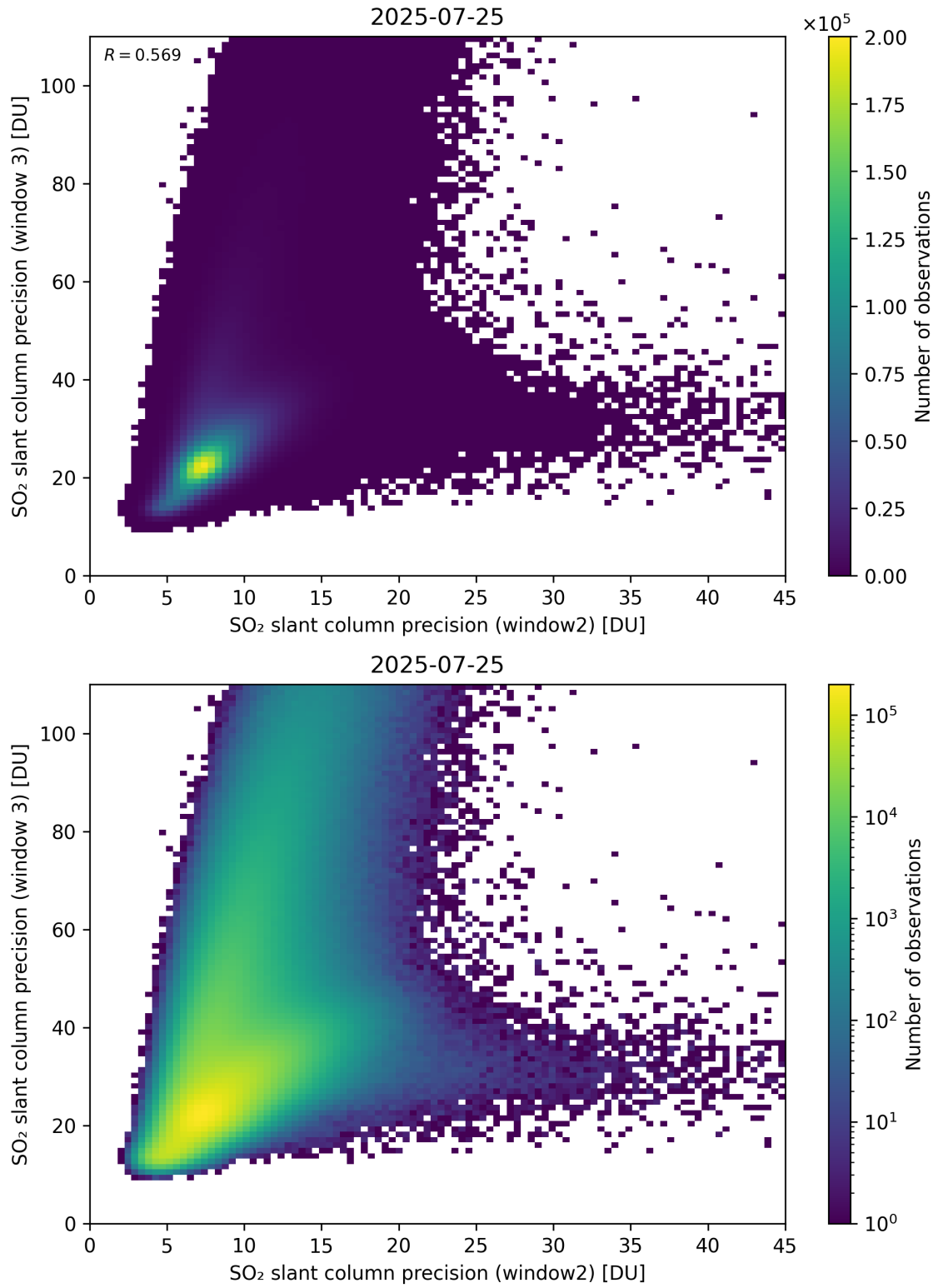
Figure 300: Scatter density plot of “SO 2 slant column precision (window2)” against “SO 2 slant column precision (window 3)” for 2025-07-24 to 2025-07-26.
