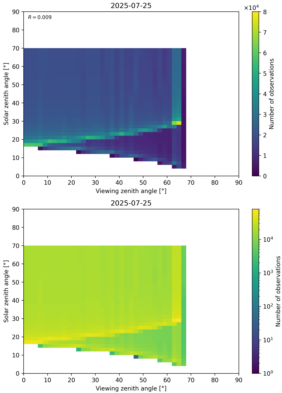
Figure 369: Scatter density plot of “Viewing zenith angle” against “Solar zenith angle” for 2025-07-24 to 2025-07-26.
