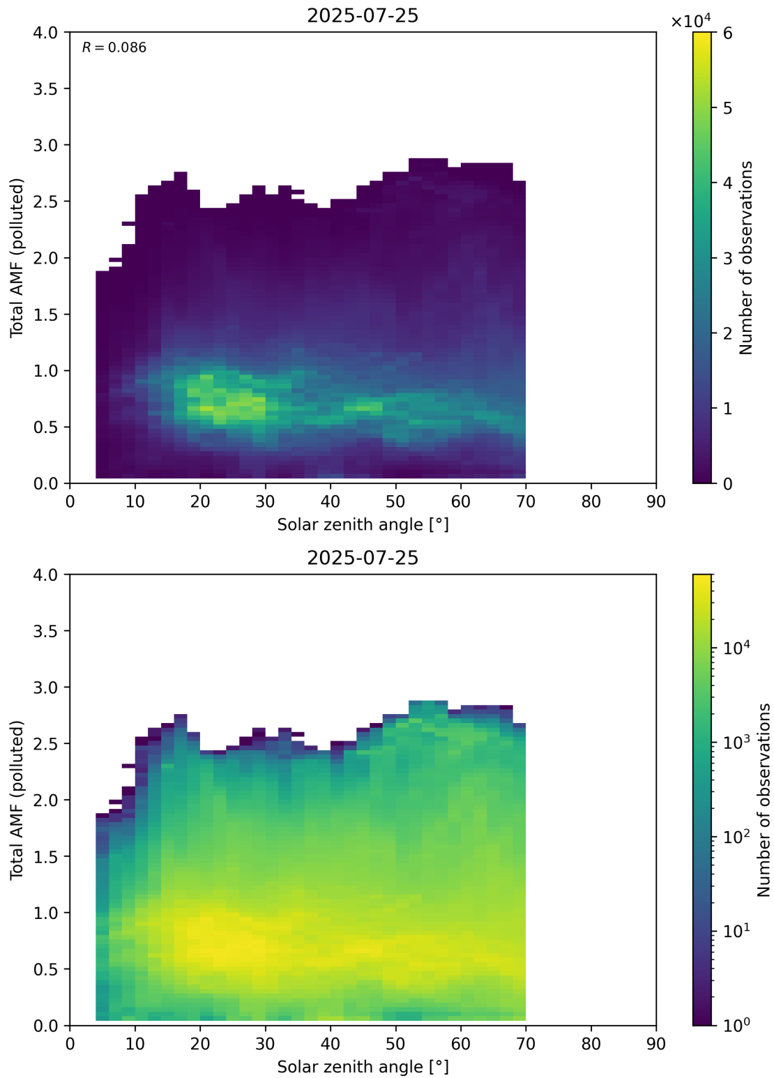
Figure 189: Scatter density plot of “Solar zenith angle” against “Total AMF (polluted)” for 2025-07-24 to 2025-07-26.
