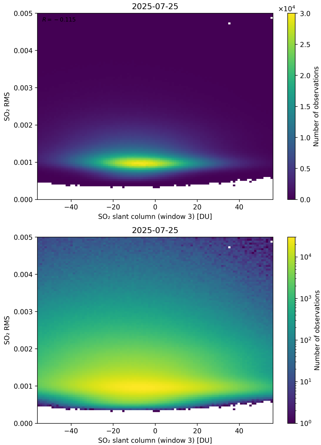
Figure 306: Scatter density plot of “SO 2 slant column (window 3)” against “SO 2 RMS” for 2025-07-24 to 2025-07-26.
