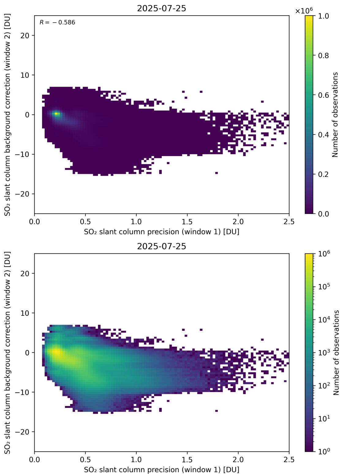
Figure 269: Scatter density plot of “SO 2 slant column precision (window 1)” against “SO 2 slant column background correction (window 2)” for 2025-07-24 to 2025-07-26.
