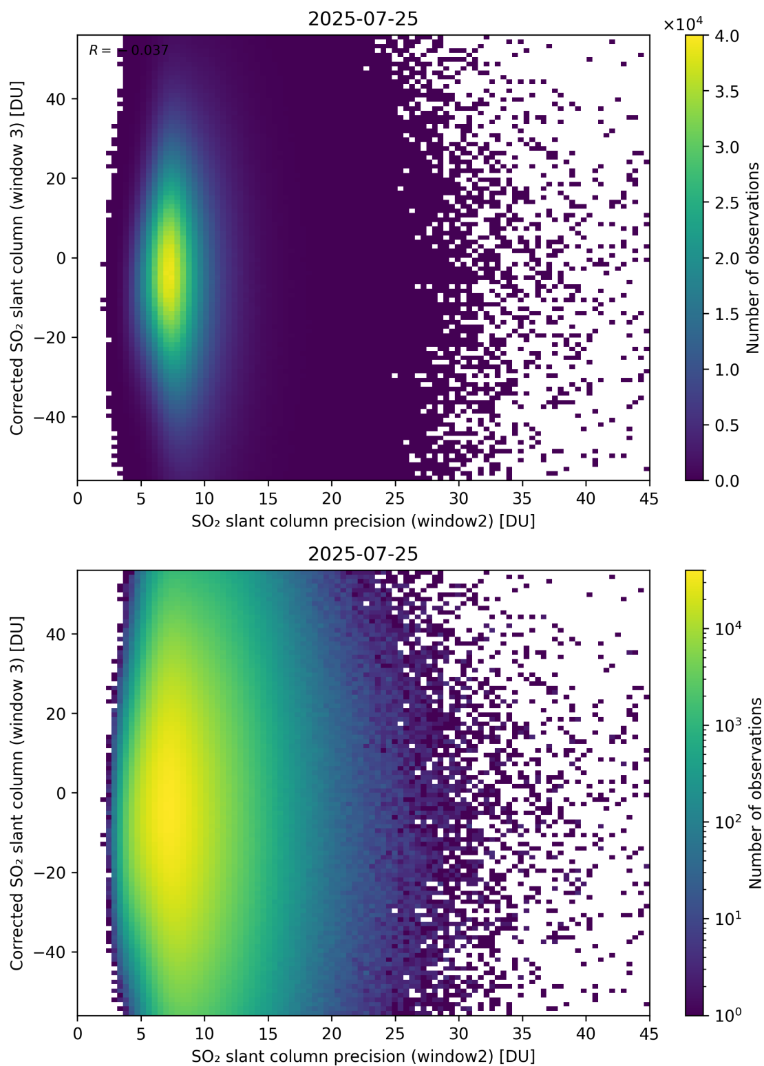
Figure 298: Scatter density plot of “SO 2 slant column precision (window2)” against “Corrected SO 2 slant column (window 3)” for 2025-07-24 to 2025-07-26.
