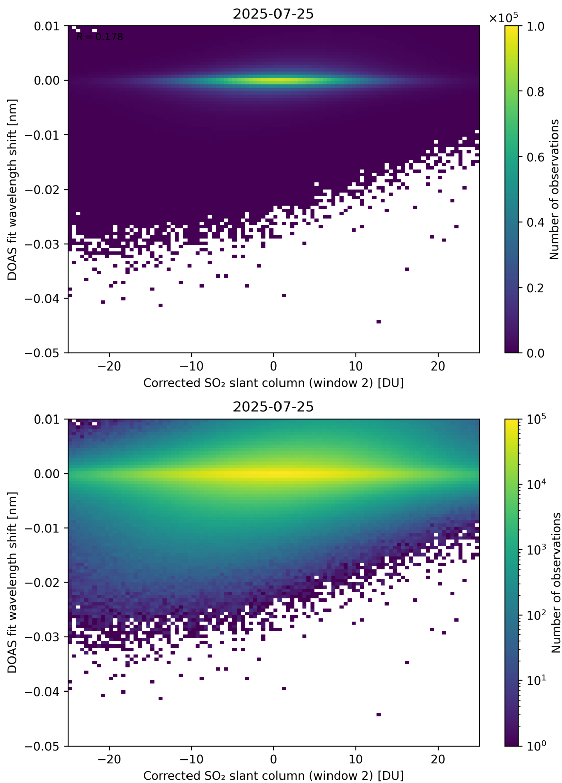
Figure 246: Scatter density plot of “Corrected SO 2 slant column (window 2)” against “DOAS fit wavelength shift” for 2025-07-24 to 2025-07-26.
