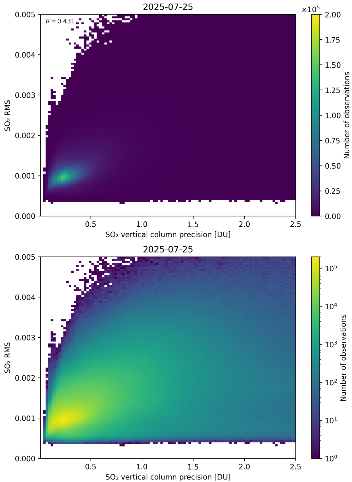
Figure 334: Scatter density plot of “SO 2 vertical column precision” against “SO 2 RMS” for 2025-07-24 to 2025-07-26.
