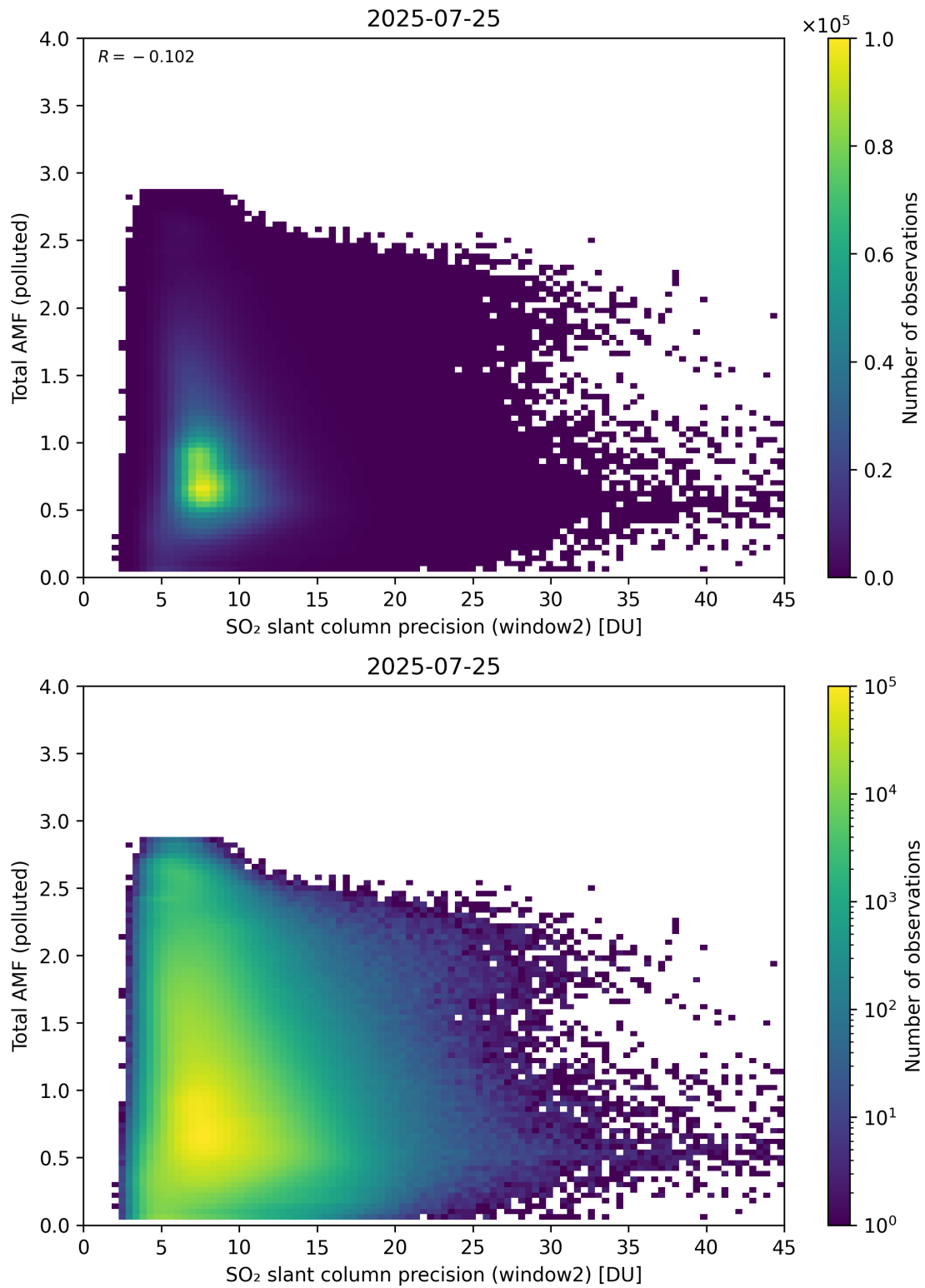
Figure 301: Scatter density plot of “SO 2 slant column precision (window2)” against “Total AMF (polluted)” for 2025-07-24 to 2025-07-26.
