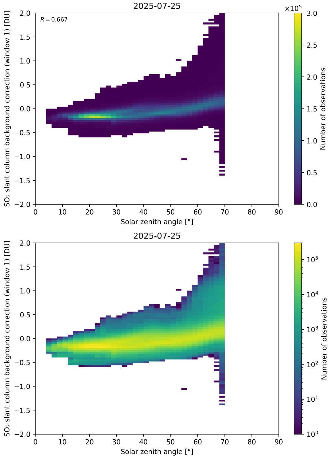
Figure 171: Scatter density plot of “Solar zenith angle” against “SO 2 slant column background correction (window 1)” for 2025-07-24 to 2025-07-26.
