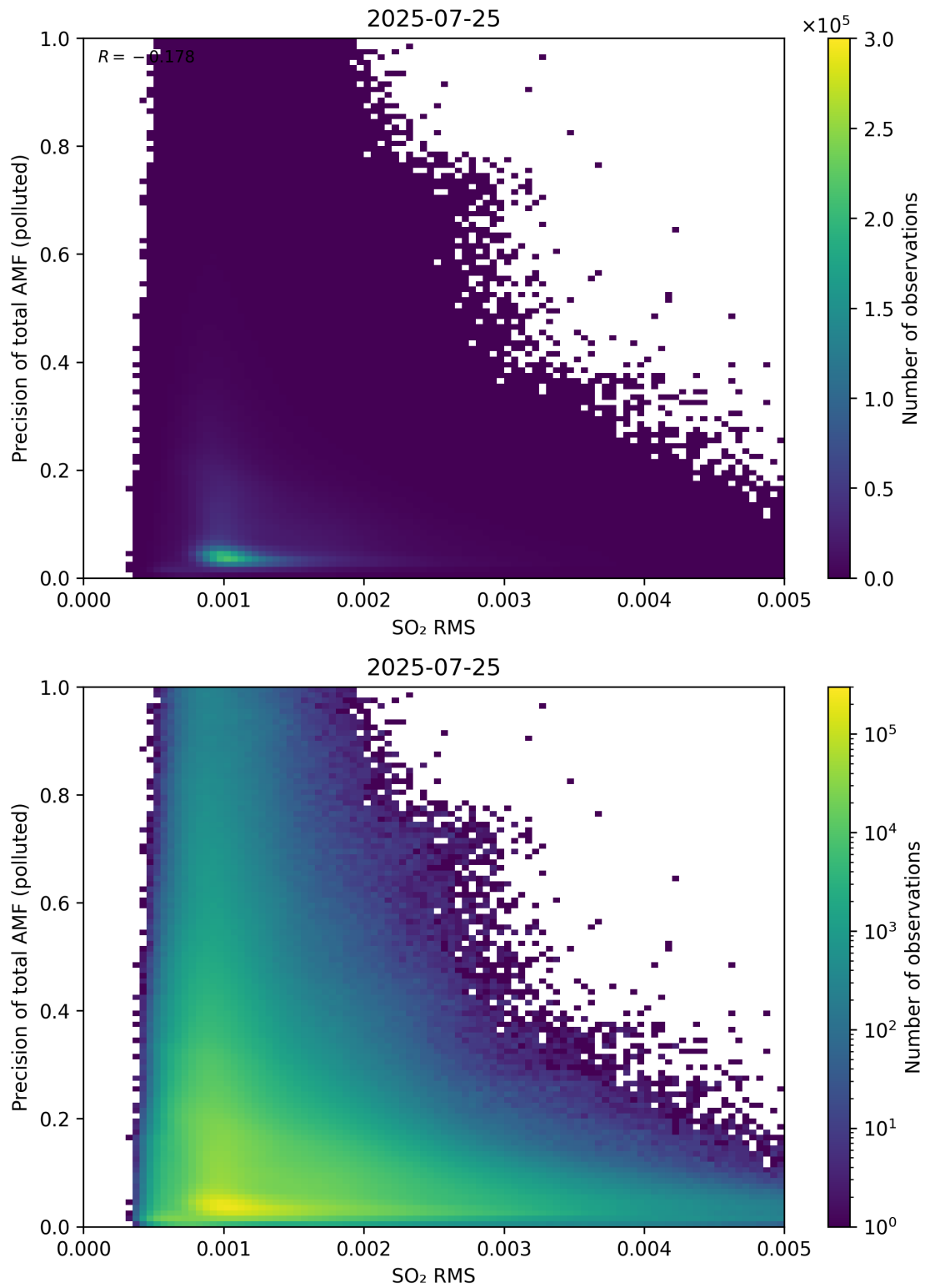
Figure 149: Scatter density plot of “SO 2 RMS” against “Precision of total AMF (polluted)” for 2025-07-24 to 2025-07-26.
