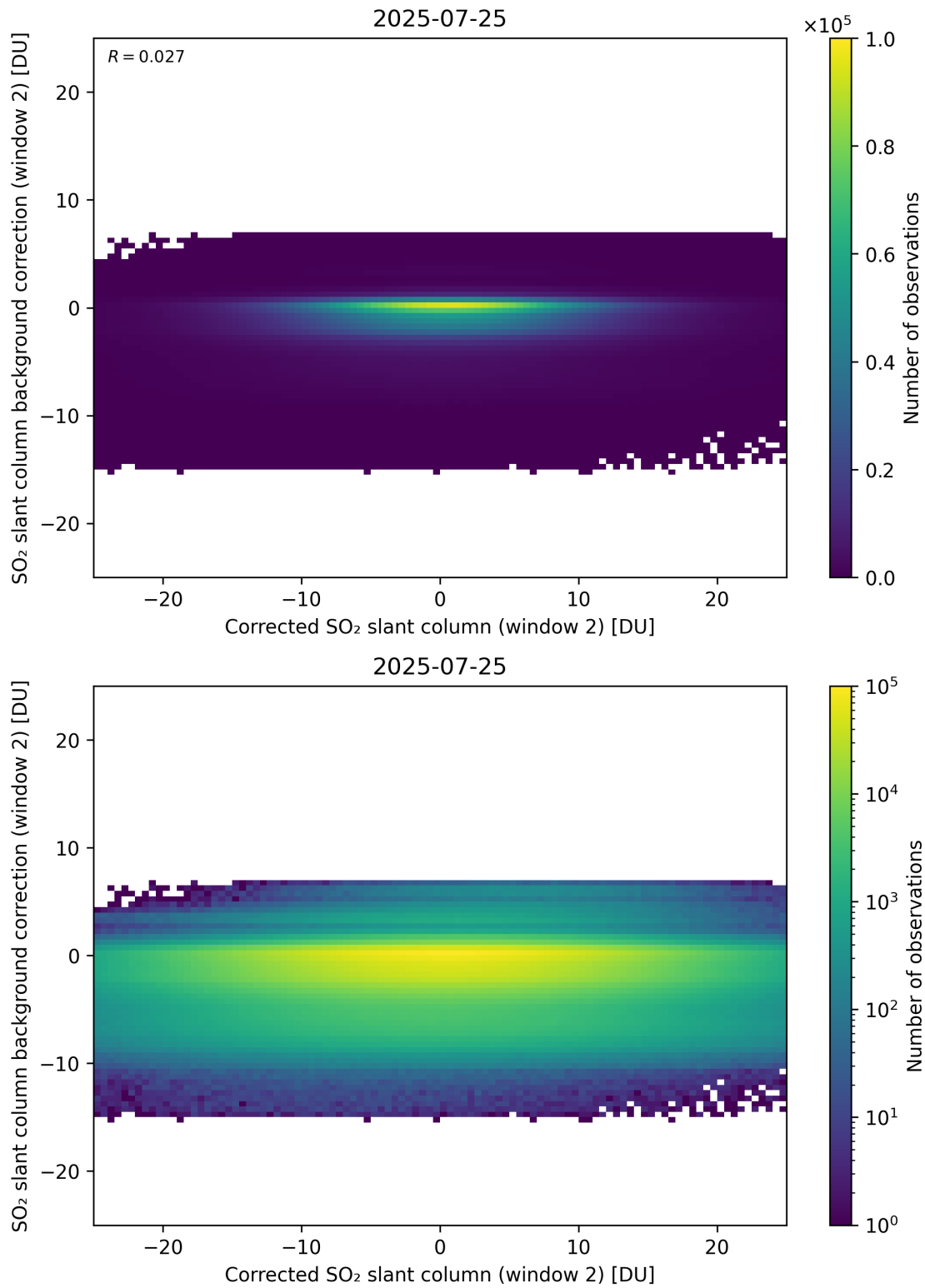
Figure 244: Scatter density plot of “Corrected SO 2 slant column (window 2)” against “SO 2 slant column background correction (window 2)” for 2025-07-24 to 2025-07-26.
