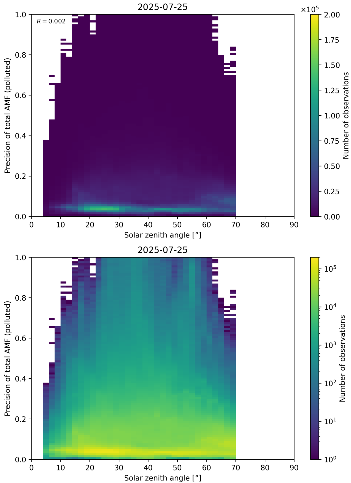
Figure 190: Scatter density plot of “Solar zenith angle” against “Precision of total AMF (polluted)” for 2025-07-24 to 2025-07-26.
