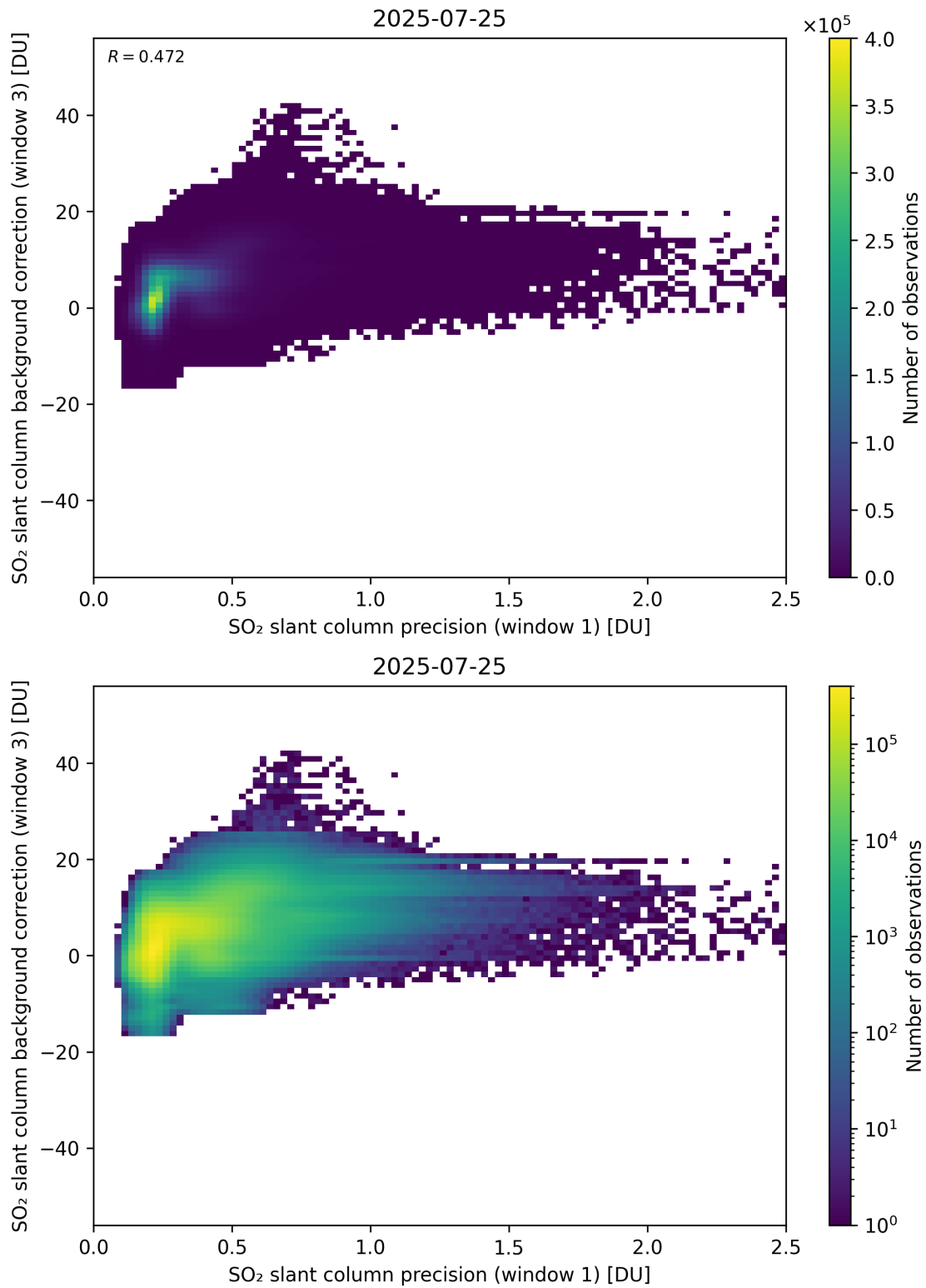
Figure 270: Scatter density plot of “SO 2 slant column precision (window 1)” against “SO 2 slant column background correction (window 3)” for 2025-07-24 to 2025-07-26.
