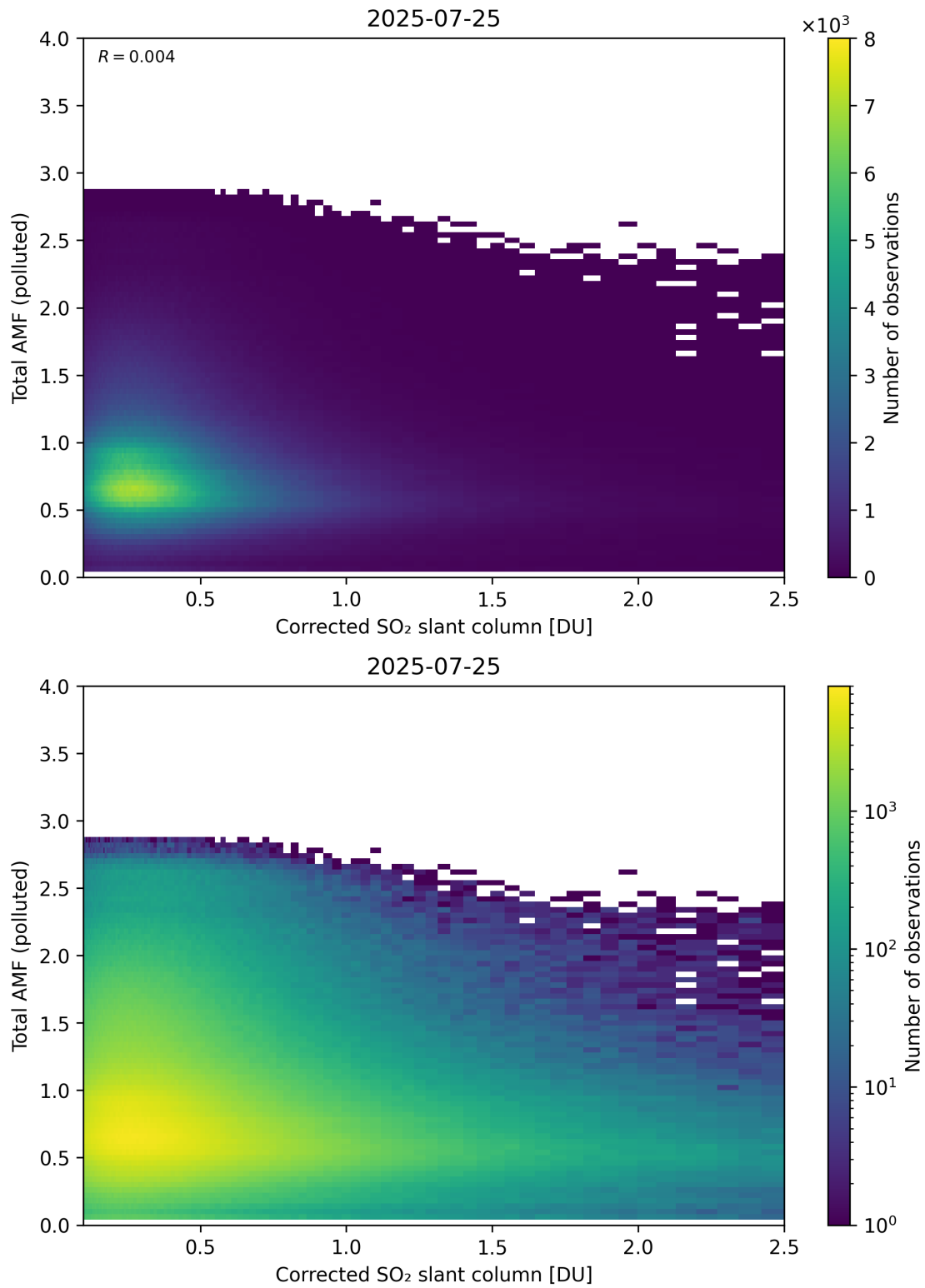
Figure 242: Scatter density plot of “Corrected SO 2 slant column” against “Total AMF (polluted)” for 2025-07-24 to 2025-07-26.
