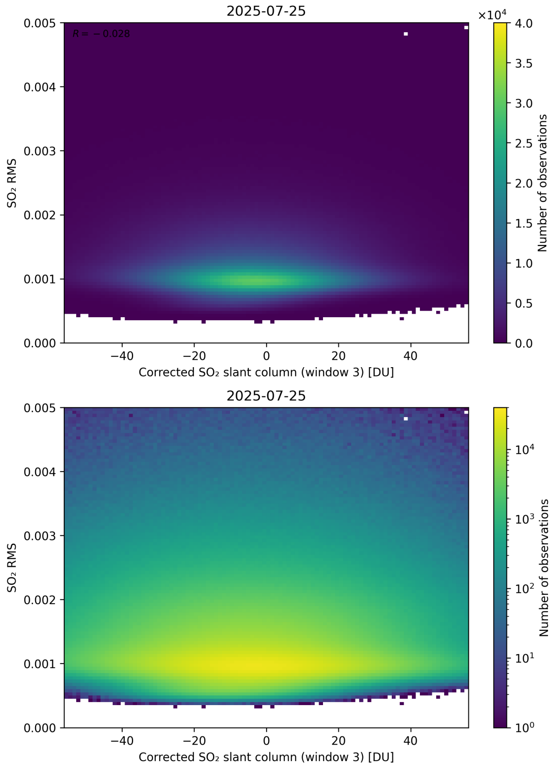
Figure 258: Scatter density plot of “Corrected SO 2 slant column (window 3)” against “SO 2 RMS” for 2025-07-24 to 2025-07-26.
