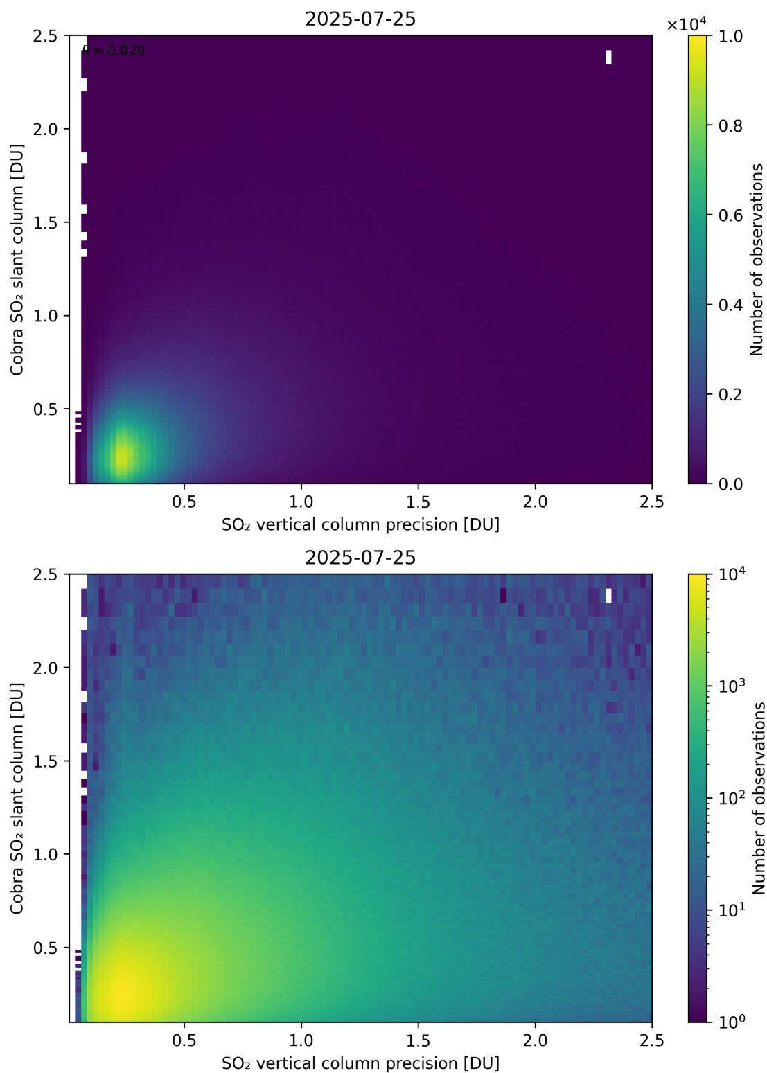
Figure 336: Scatter density plot of “SO 2 vertical column precision” against “Cobra SO 2 slant column” for 2025-07-24 to 2025-07-26.
