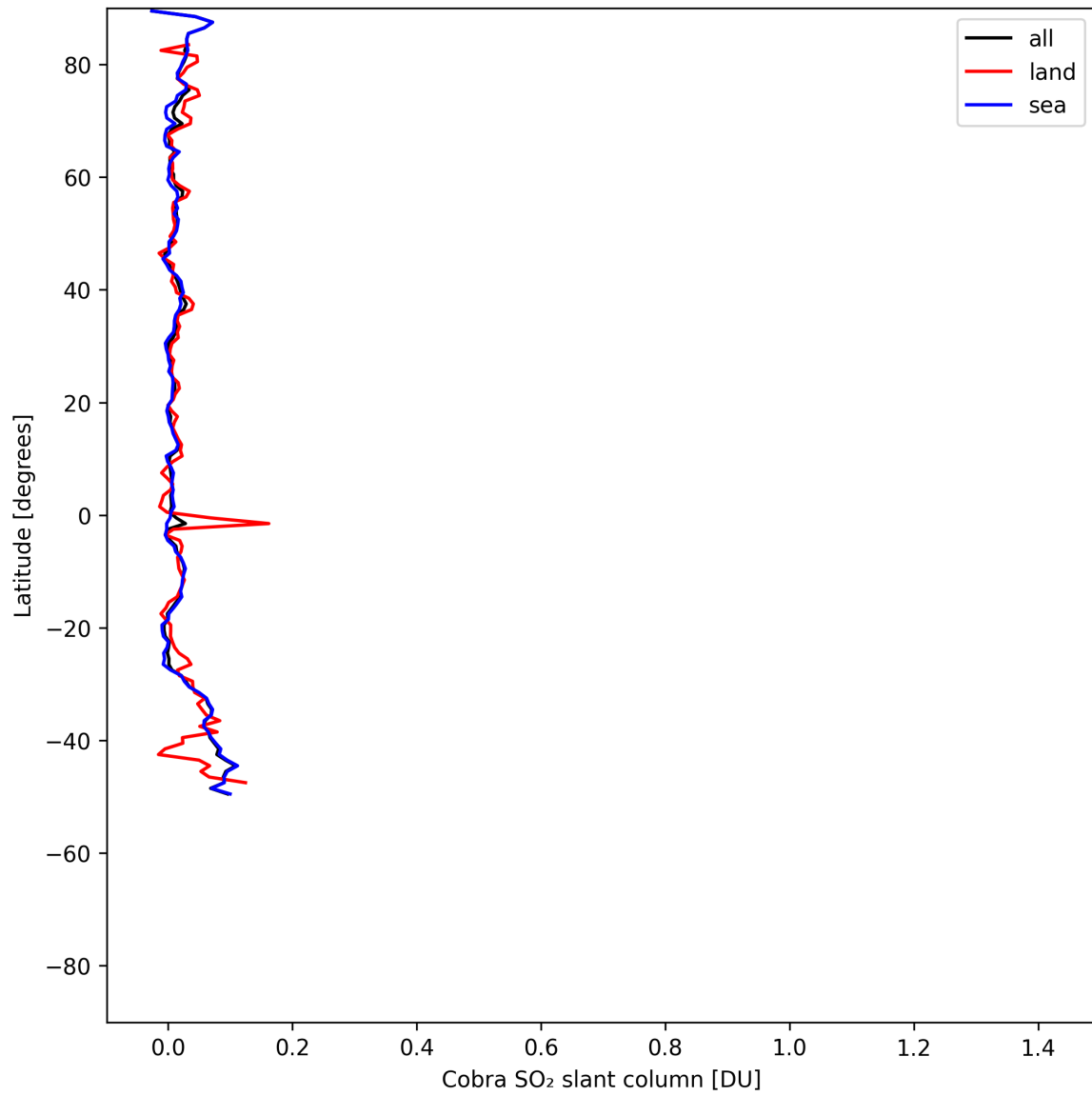
Figure 35: Zonal average of “Cobra SO 2 slant column” for 2025-07-24 to 2025-07-26.
