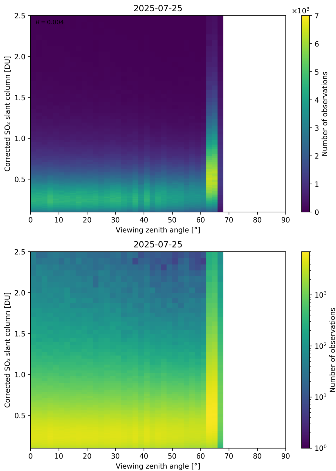
Figure 373: Scatter density plot of “Viewing zenith angle” against “Corrected SO 2 slant column” for 2025-07-24 to 2025-07-26.
