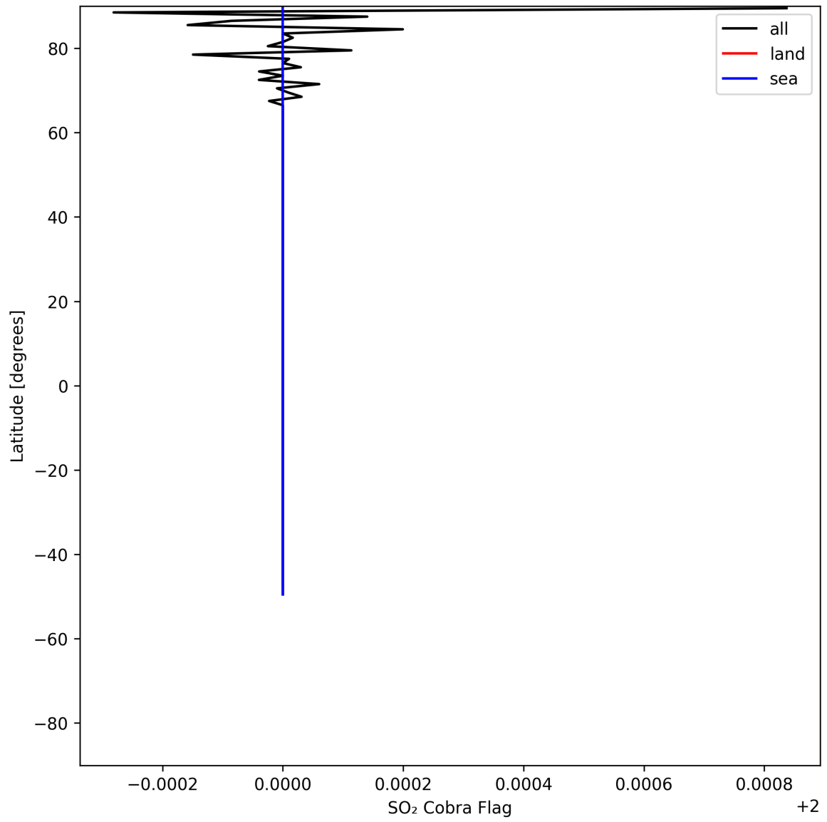
Figure 49: Zonal average of “SO 2 Cobra Flag” for 2025-07-24 to 2025-07-26.
