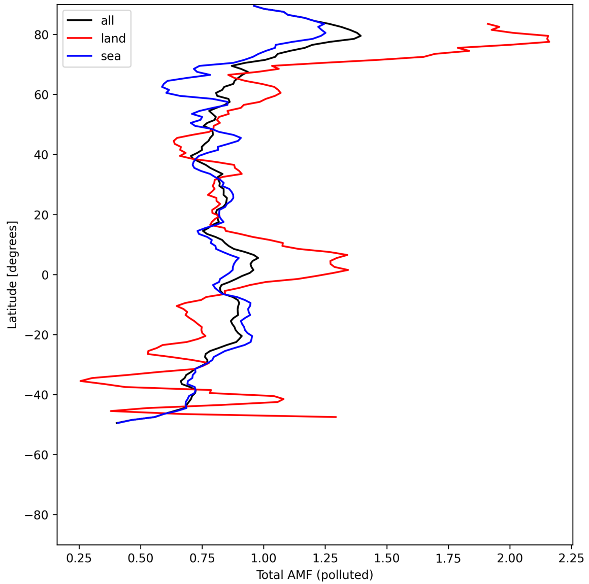
Figure 53: Zonal average of “Total AMF (polluted)” for 2025-07-24 to 2025-07-26.
