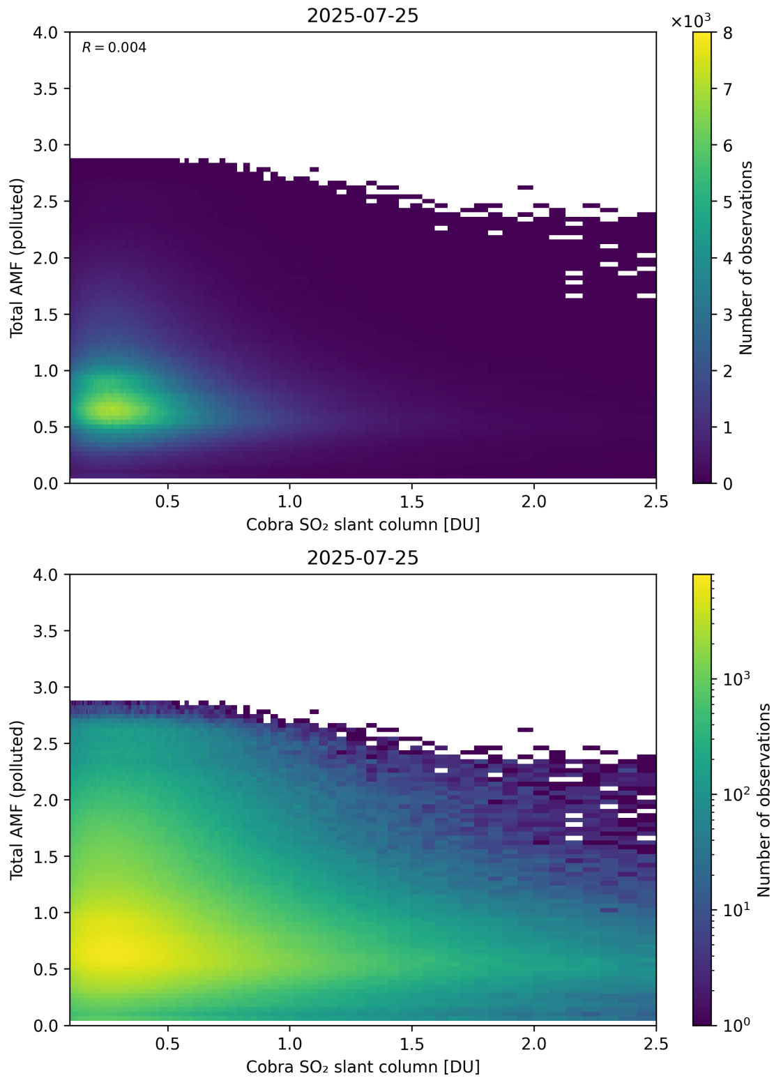
Figure 224: Scatter density plot of “Cobra SO 2 slant column” against “Total AMF (polluted)” for 2025-07-24 to 2025-07-26.
