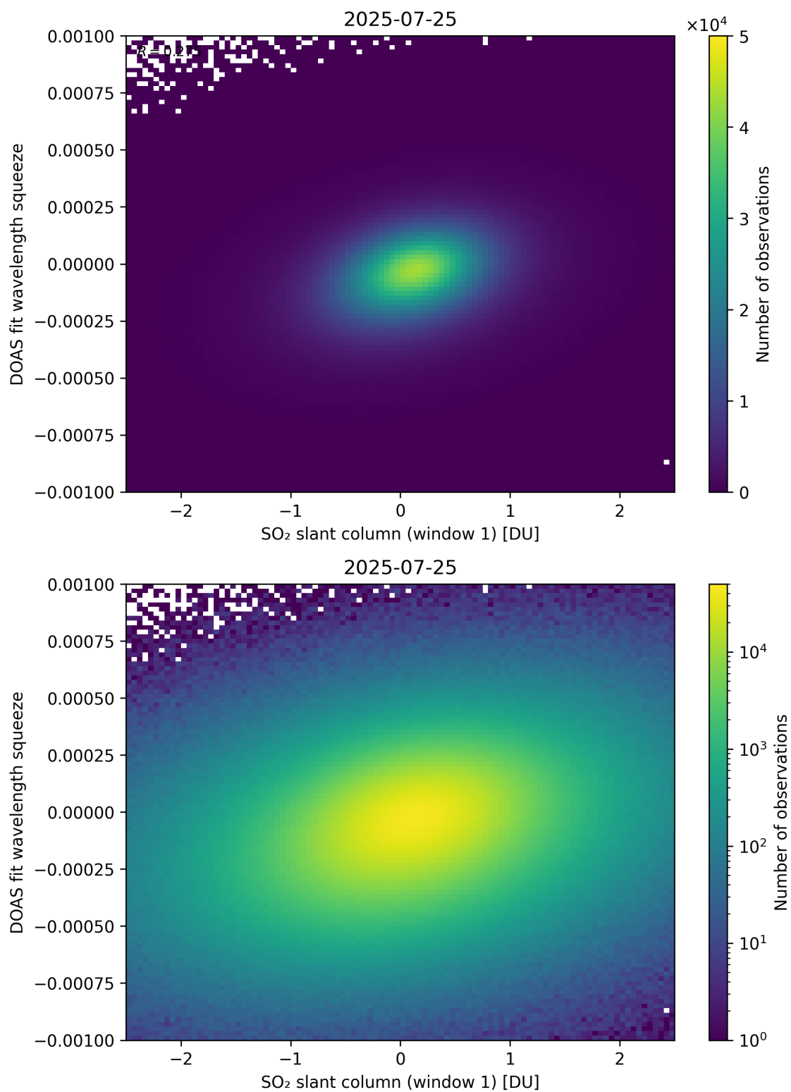
Figure 266: Scatter density plot of “SO 2 slant column (window 1)” against “DOAS fit wavelength squeeze” for 2025-07-24 to 2025-07-26.
