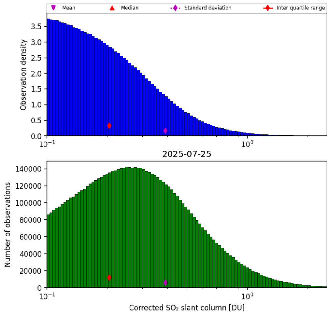
Figure 60: Histogram of “Corrected SO 2 slant column” for 2025-07-24 to 2025-07-26
