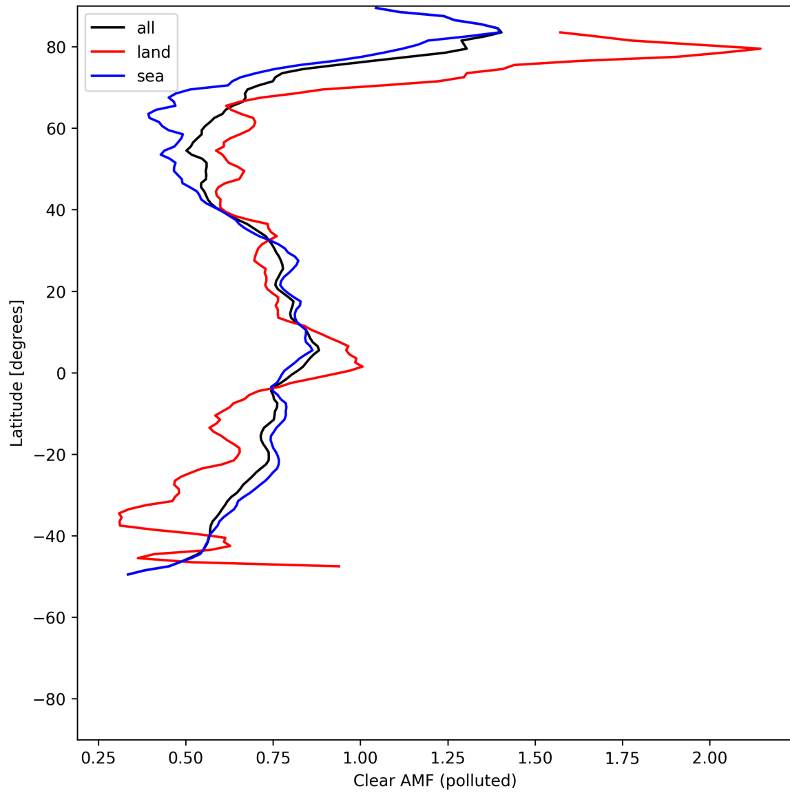
Figure 55: Zonal average of “Clear AMF (polluted)” for 2025-07-24 to 2025-07-26.
