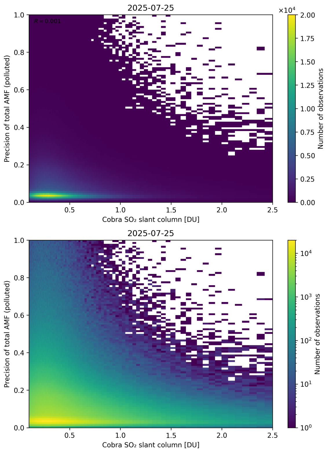
Figure 225: Scatter density plot of “Cobra SO 2 slant column” against “Precision of total AMF (polluted)” for 2025-07-24 to 2025-07-26.
