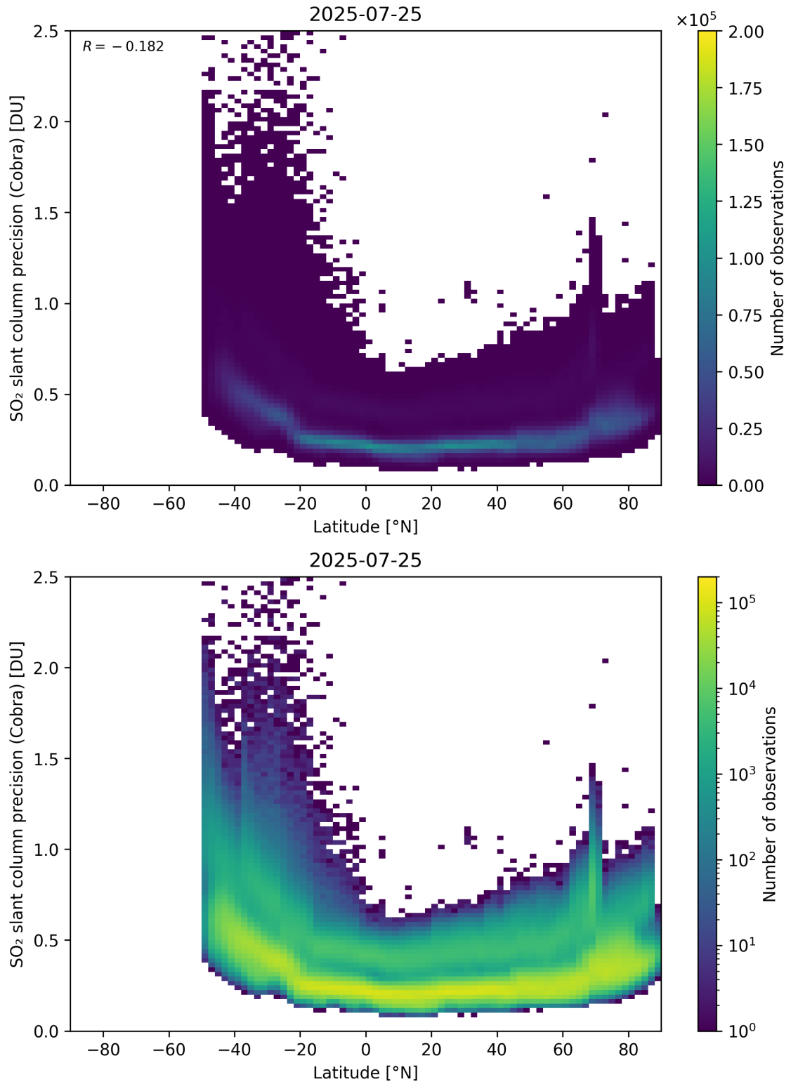
Figure 158: Scatter density plot of “Latitude” against “SO 2 slant column precision (Cobra)” for 2025-07-24 to 2025-07-26.
