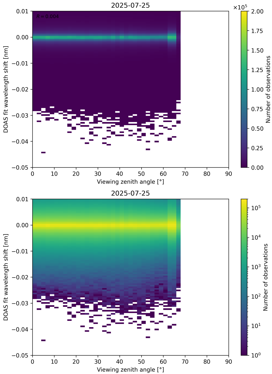
Figure 365: Scatter density plot of “Viewing zenith angle” against “DOAS fit wavelength shift” for 2025-07-24 to 2025-07-26.
