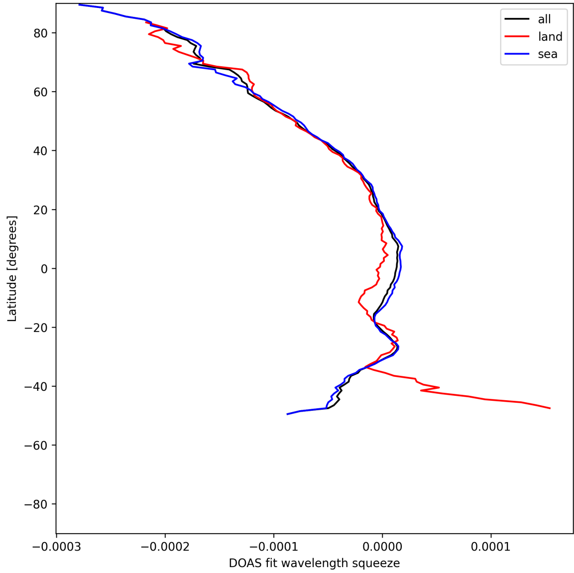
Figure 51: Zonal average of “DOAS fit wavelength squeeze” for 2025-07-24 to 2025-07-26.
