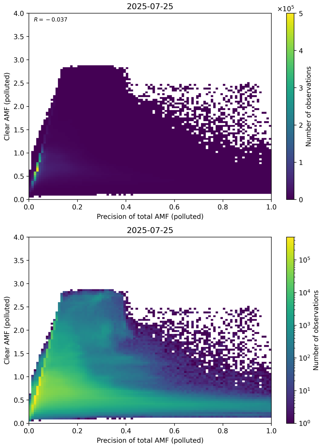
Figure 320: Scatter density plot of “Precision of total AMF (polluted)” against “Clear AMF (polluted)” for 2025-07-24 to 2025-07-26.
