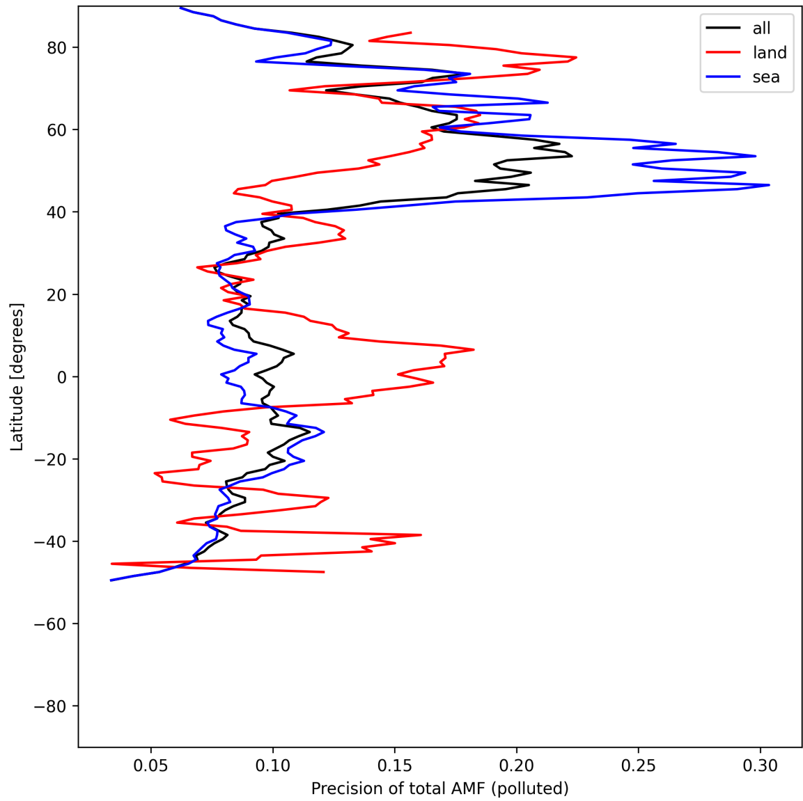
Figure 54: Zonal average of “Precision of total AMF (polluted)” for 2025-07-24 to 2025-07-26.
