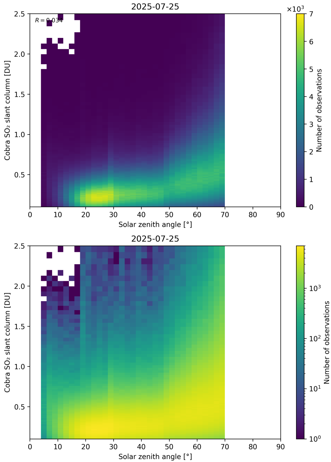
Figure 179: Scatter density plot of “Solar zenith angle” against “Cobra SO 2 slant column” for 2025-07-24 to 2025-07-26.
