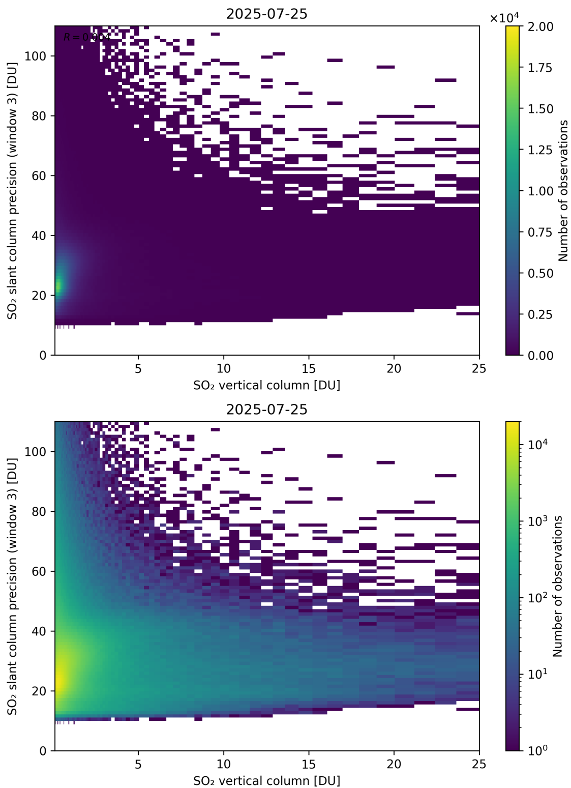
Figure 358: Scatter density plot of “SO 2 vertical column” against “SO 2 slant column precision (window 3)” for 2025-07-24 to 2025-07-26.
