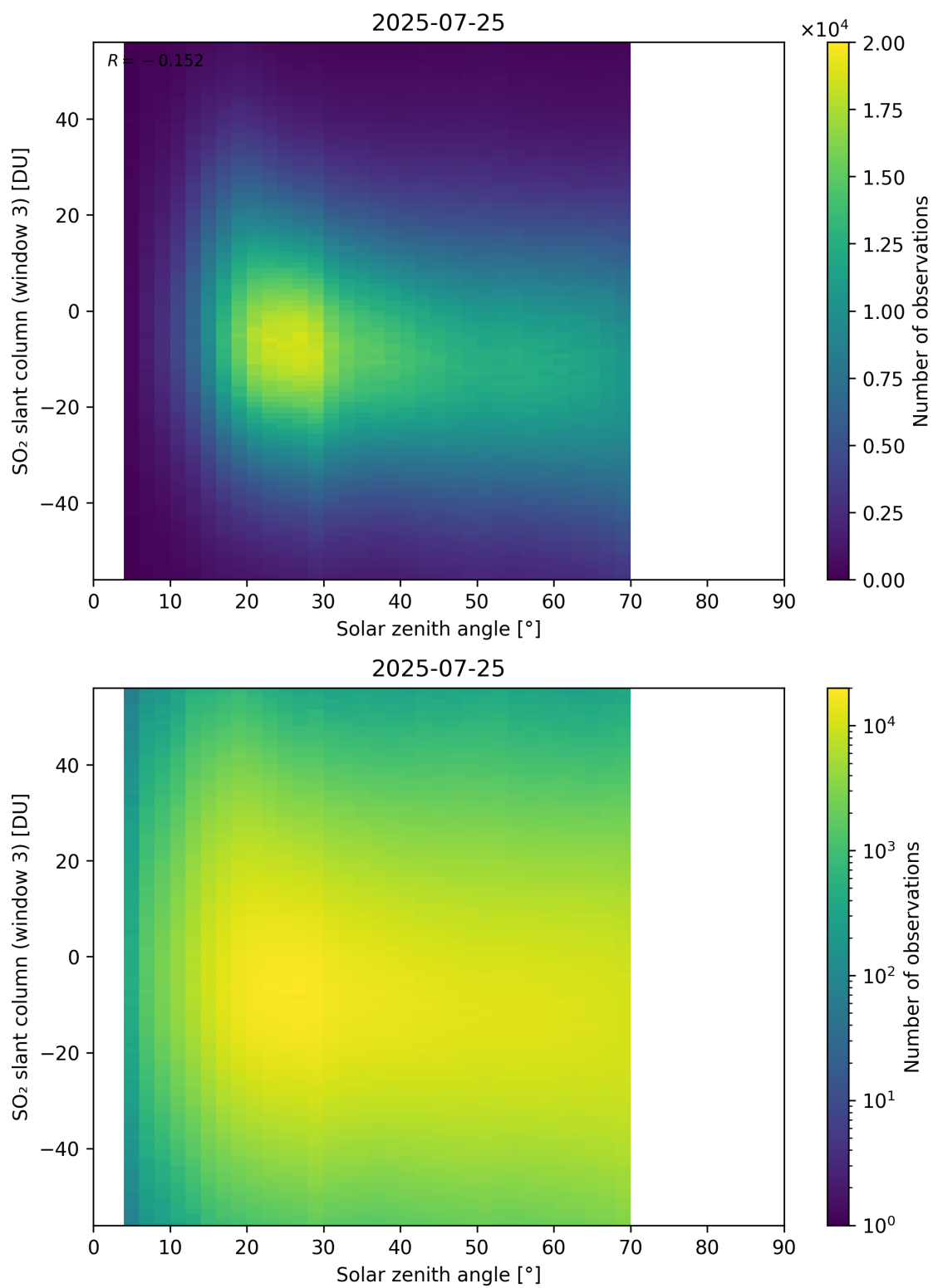
Figure 187: Scatter density plot of “Solar zenith angle” against “SO 2 slant column (window 3)” for 2025-07-24 to 2025-07-26.
