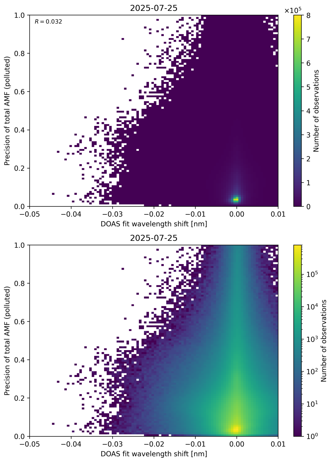
Figure 142: Scatter density plot of “DOAS fit wavelength shift” against “Precision of total AMF (polluted)” for 2025-07-24 to 2025-07-26.
