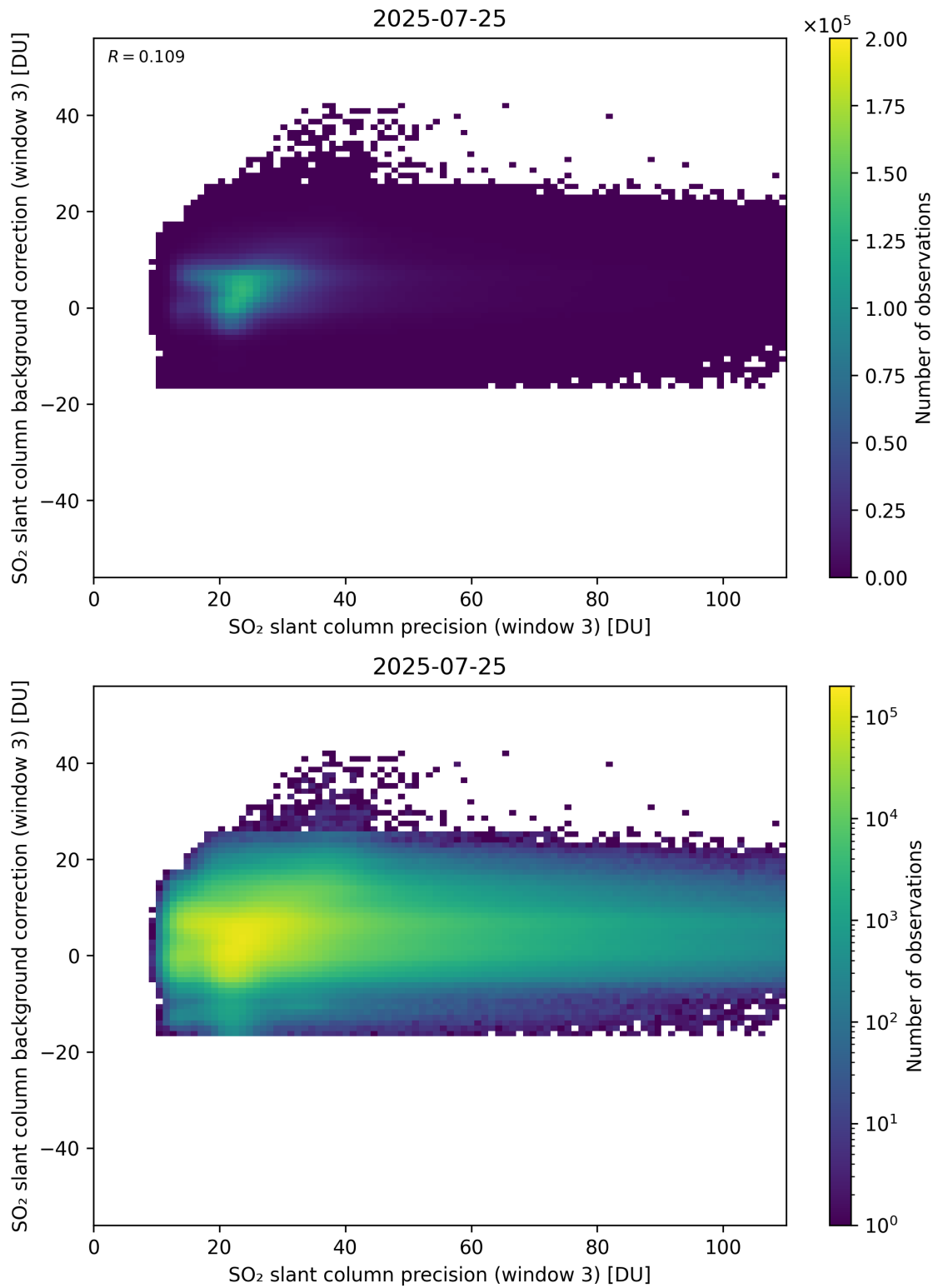
Figure 307: Scatter density plot of “SO 2 slant column precision (window 3)” against “SO 2 slant column background correction (window 3)” for 2025-07-24 to 2025-07-26.
