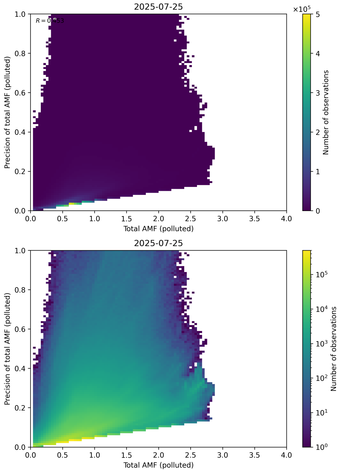
Figure 322: Scatter density plot of “Total AMF (polluted)” against “Precision of total AMF (polluted)” for 2025-07-24 to 2025-07-26.
