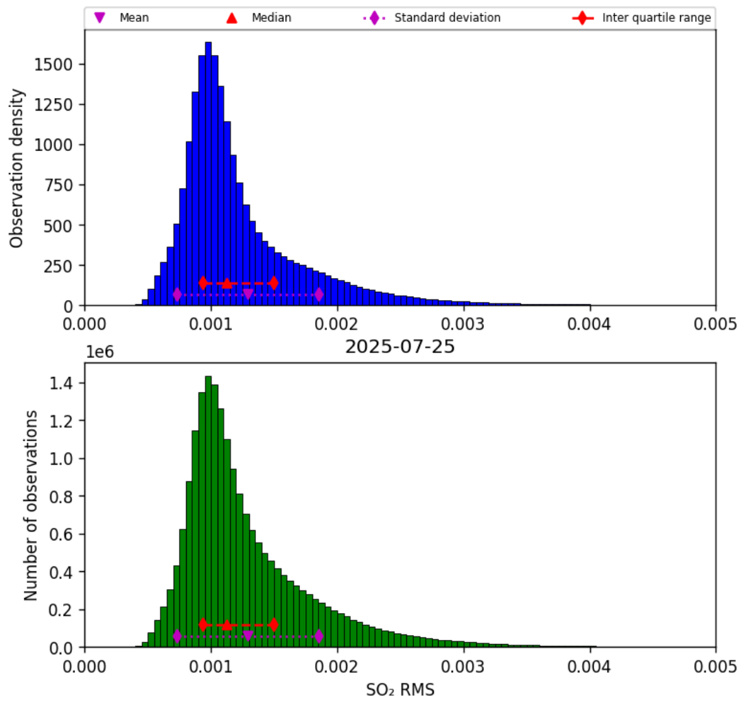
Figure 78: Histogram of “SO 2 RMS” for 2025-07-24 to 2025-07-26
