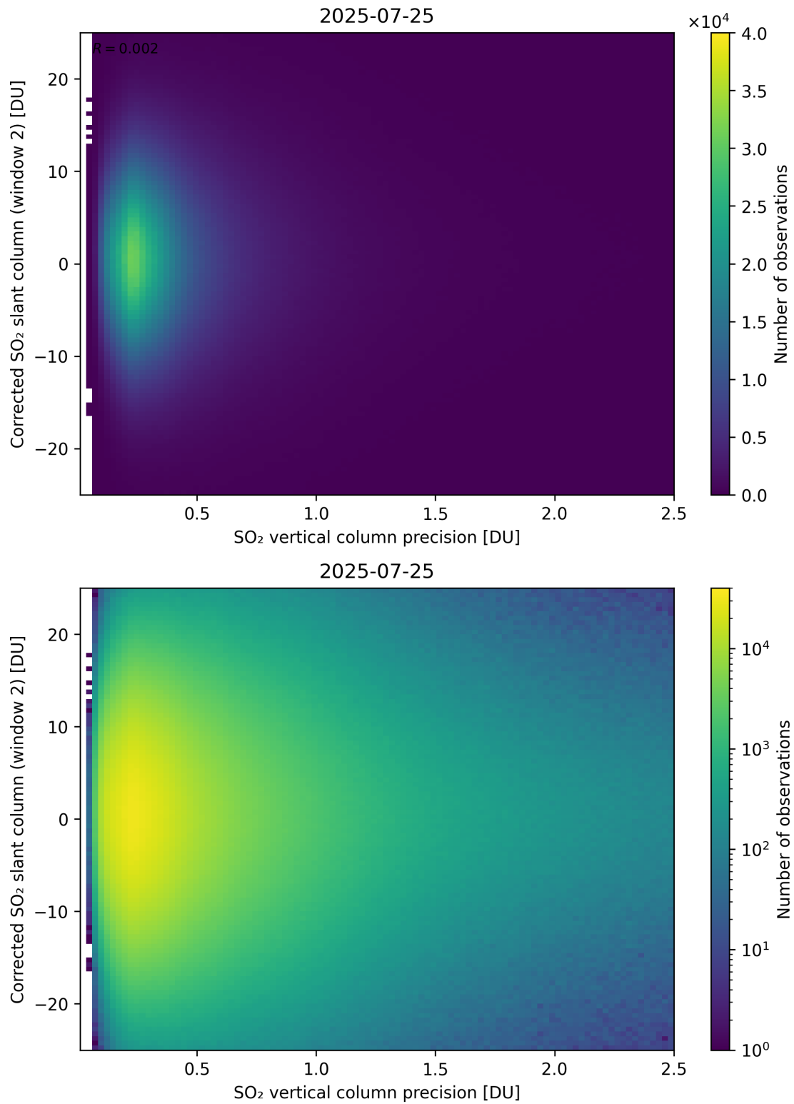
Figure 339: Scatter density plot of “SO 2 vertical column precision” against “Corrected SO 2 slant column (window 2)” for 2025-07-24 to 2025-07-26.
