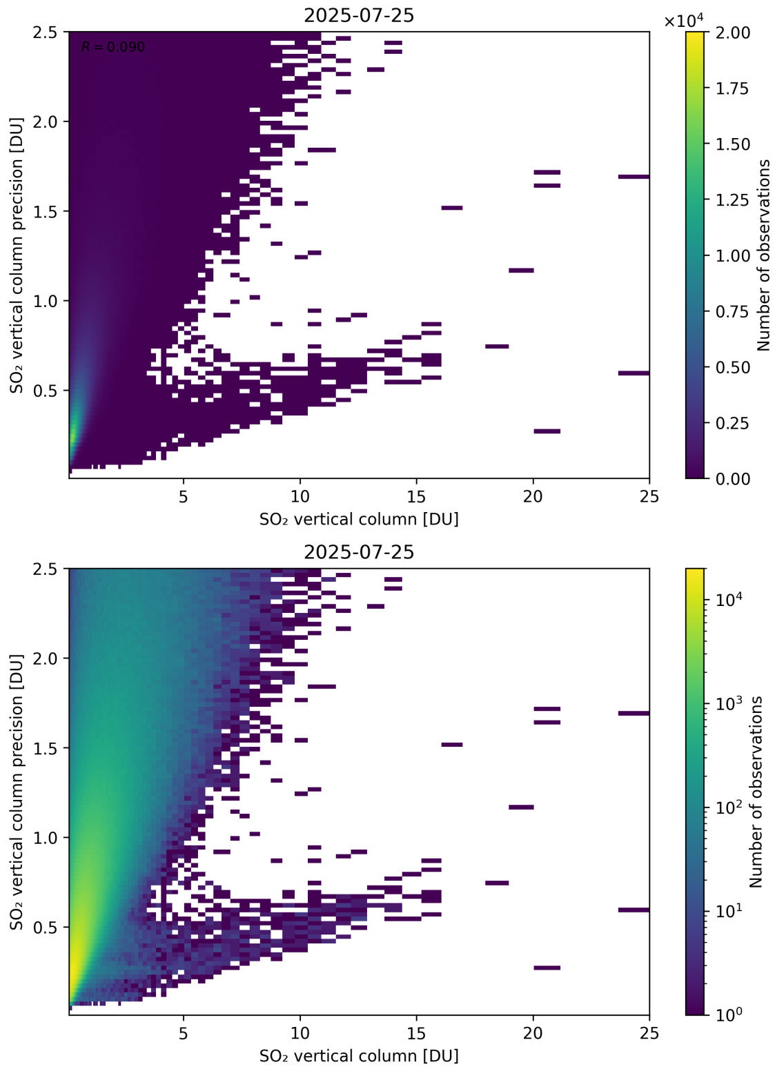
Figure 361: Scatter density plot of “SO 2 vertical column” against “SO 2 vertical column precision” for 2025-07-24 to 2025-07-26.
