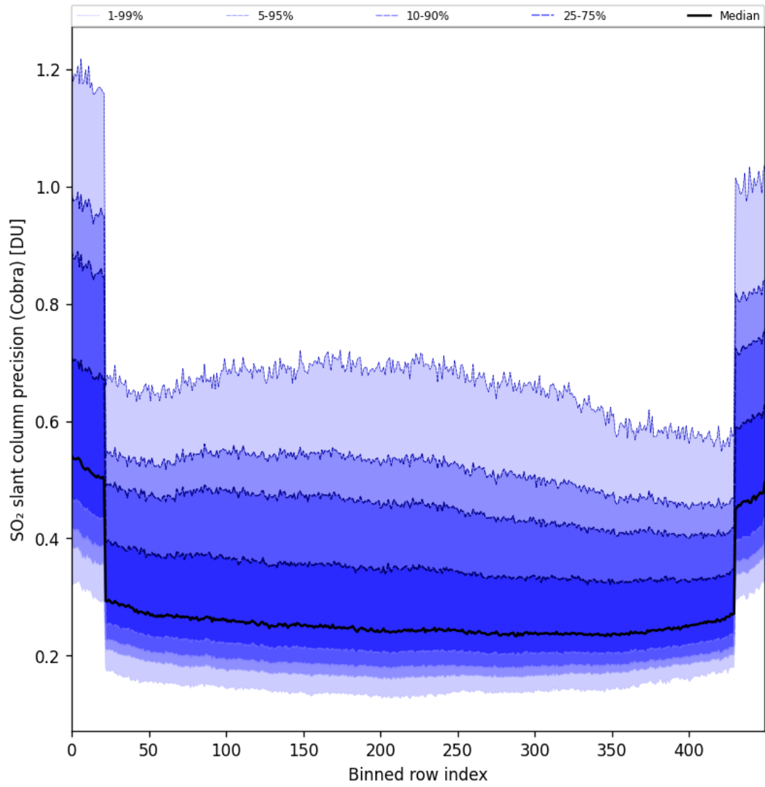
Figure 88: Along track statistics of “SO 2 slant column precision (Cobra)” for 2025-07-24 to 2025-07-26
