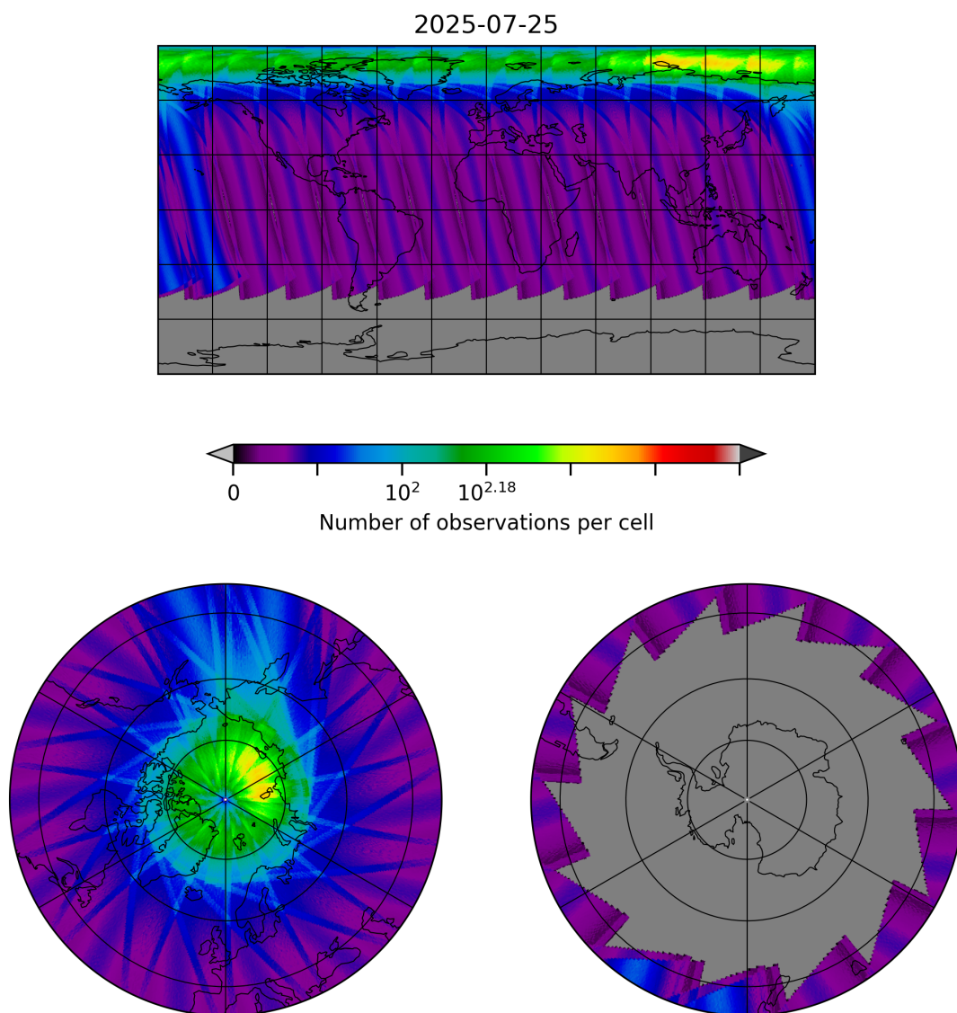
Figure 30: Map of the number of observations for 2025-07-24 to 2025-07-26
