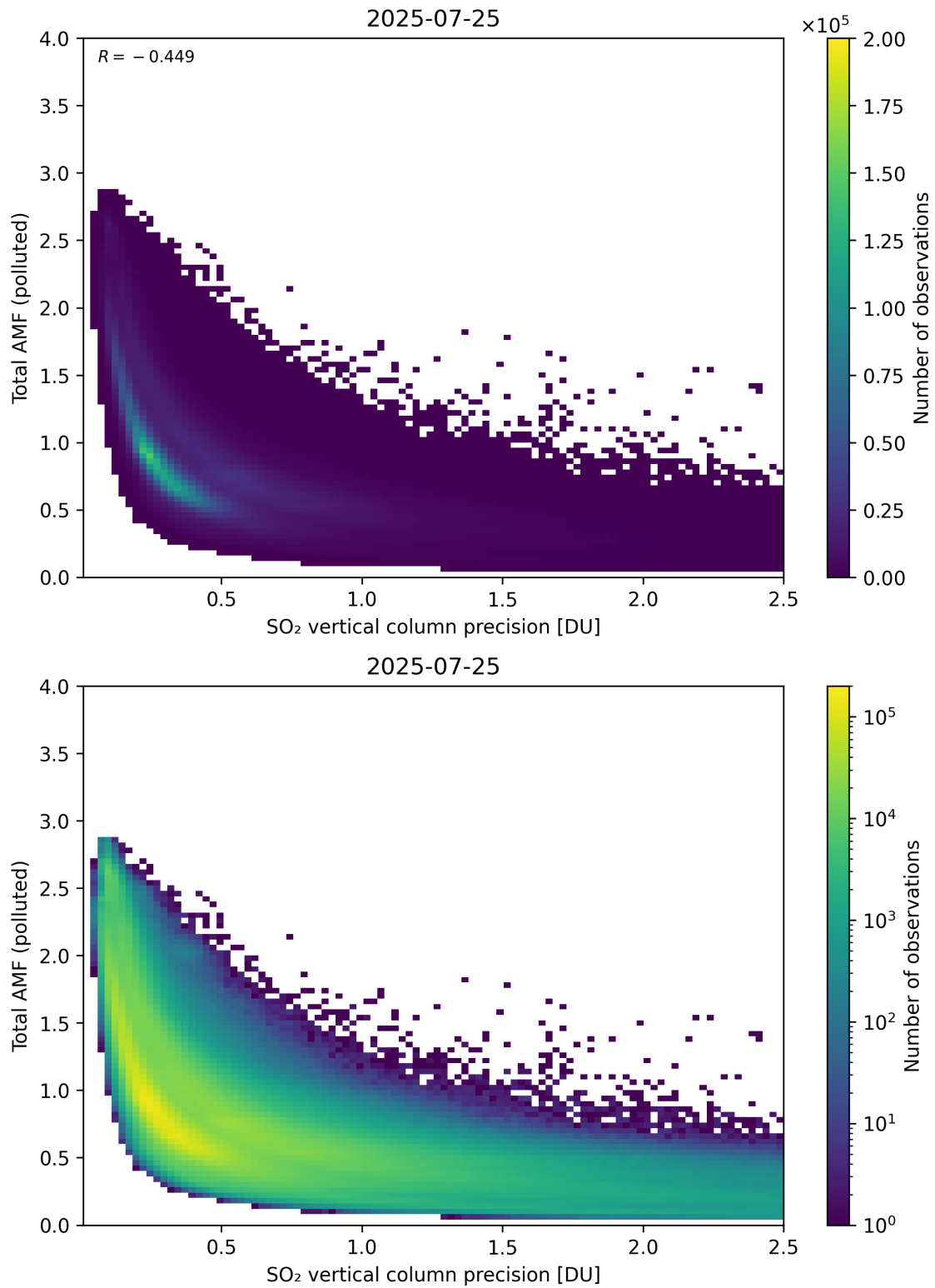
Figure 346: Scatter density plot of “SO 2 vertical column precision” against “Total AMF (polluted)” for 2025-07-24 to 2025-07-26.
