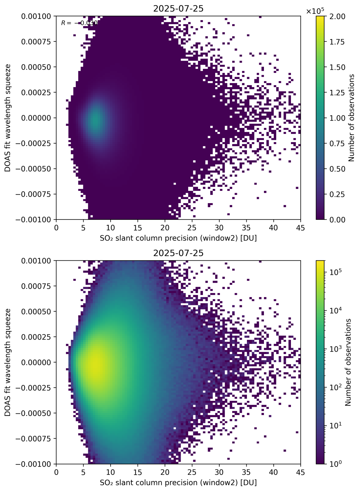
Figure 294: Scatter density plot of “SO 2 slant column precision (window2)” against “DOAS fit wavelength squeeze” for 2025-07-24 to 2025-07-26.
