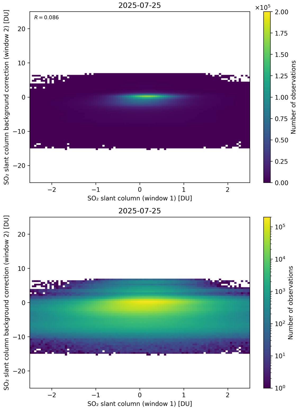
Figure 263: Scatter density plot of “SO 2 slant column (window 1)” against “SO 2 slant column background correction (window 2)” for 2025-07-24 to 2025-07-26.
