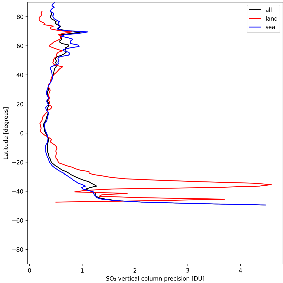
Figure 33: Zonal average of “SO 2 vertical column precision” for 2025-07-24 to 2025-07-26.
