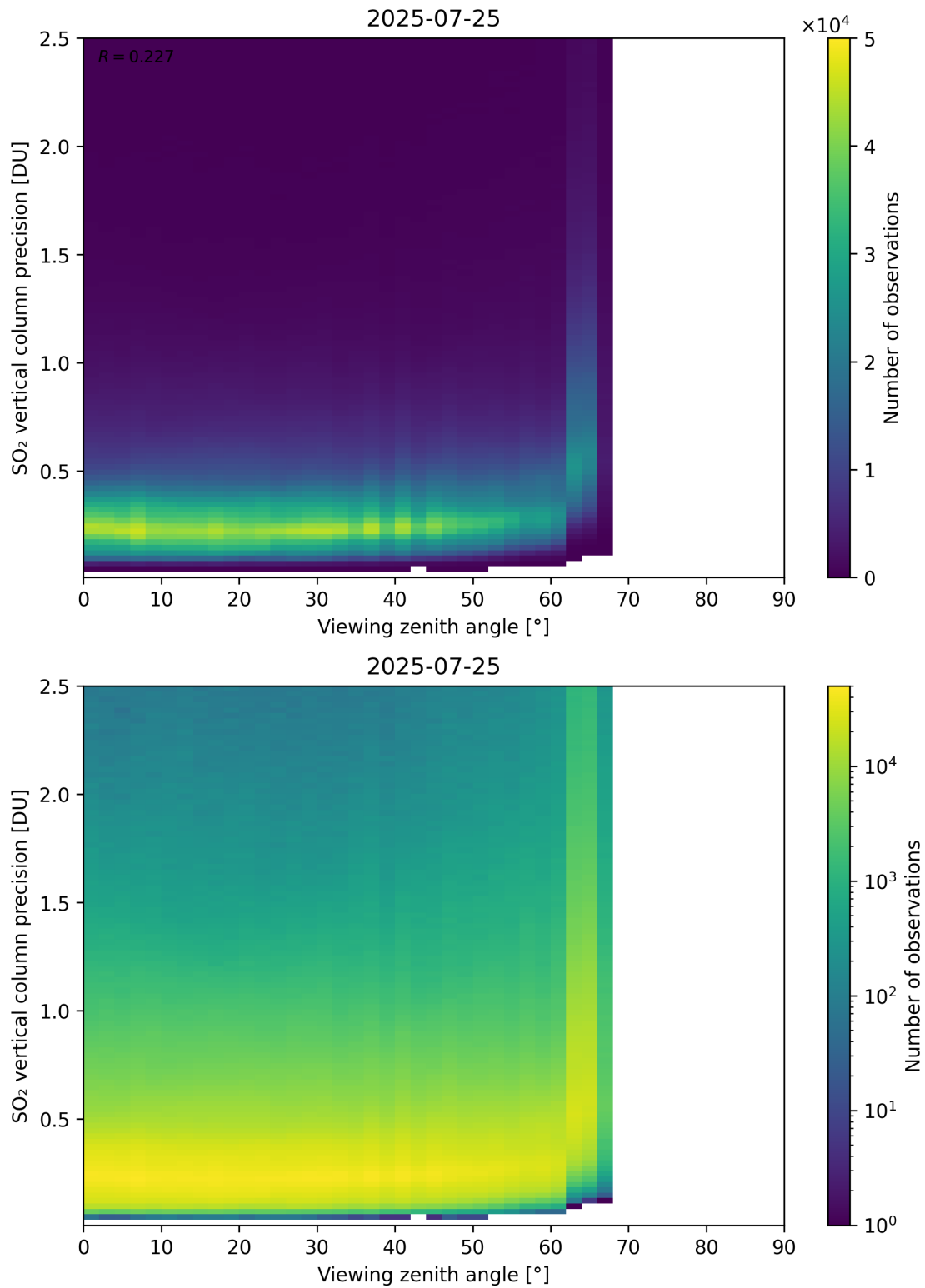
Figure 384: Scatter density plot of “Viewing zenith angle” against “SO 2 vertical column precision” for 2025-07-24 to 2025-07-26.
