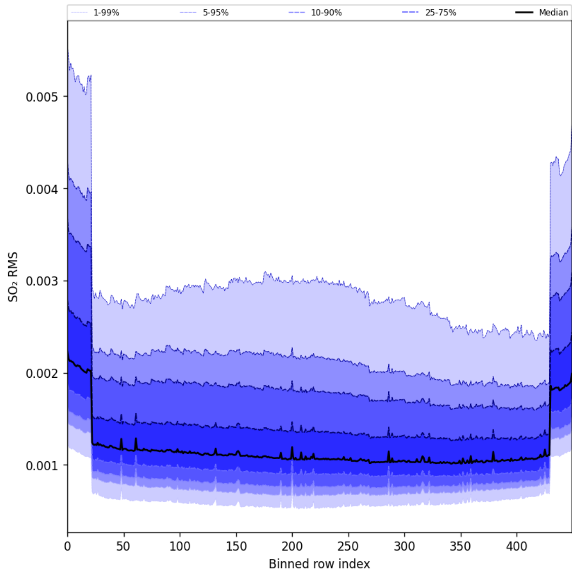
Figure 104: Along track statistics of “SO 2 RMS” for 2025-07-24 to 2025-07-26
