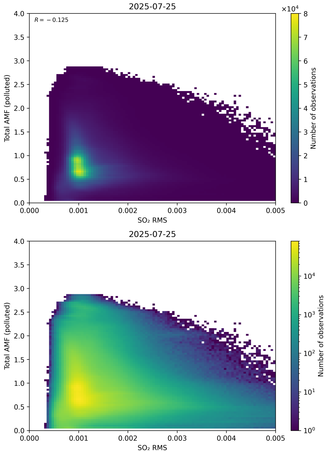
Figure 148: Scatter density plot of “SO 2 RMS” against “Total AMF (polluted)” for 2025-07-24 to 2025-07-26.
