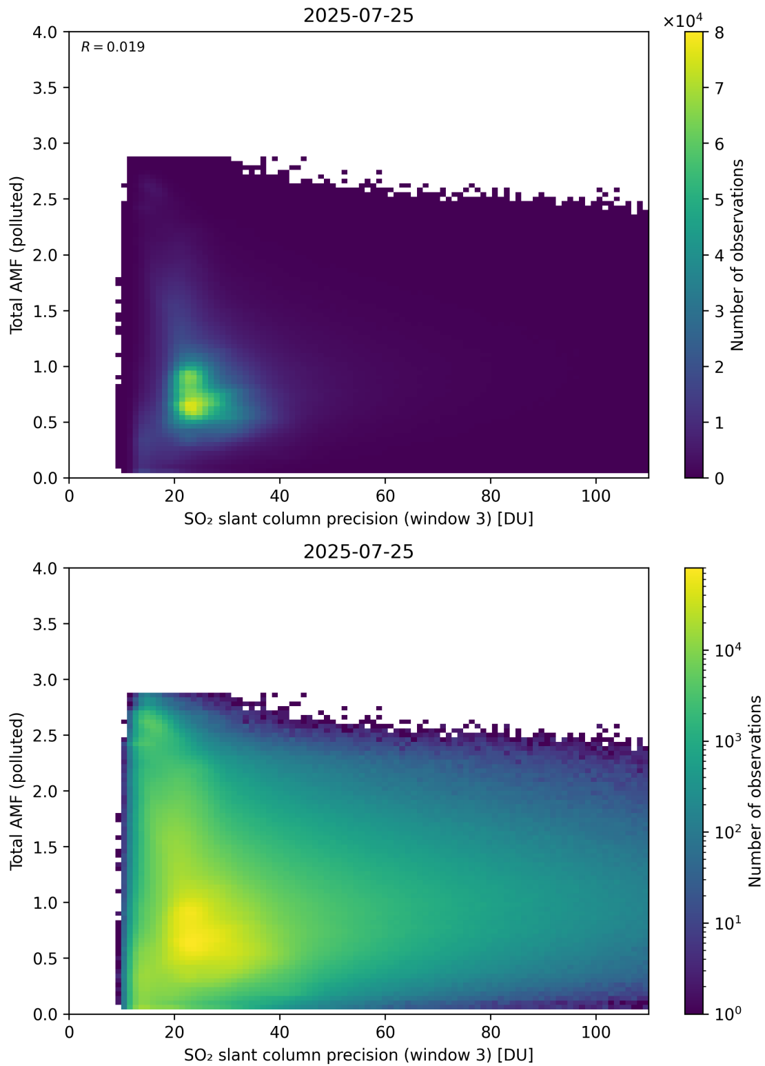
Figure 313: Scatter density plot of “SO 2 slant column precision (window 3)” against “Total AMF (polluted)” for 2025-07-24 to 2025-07-26.
