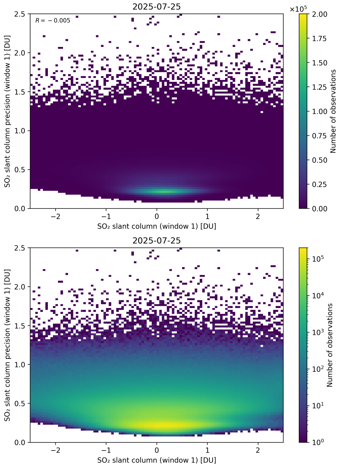
Figure 285: Scatter density plot of “SO 2 slant column (window 1)” against “SO 2 slant column precision (window 1)” for 2025-07-24 to 2025-07-26.
