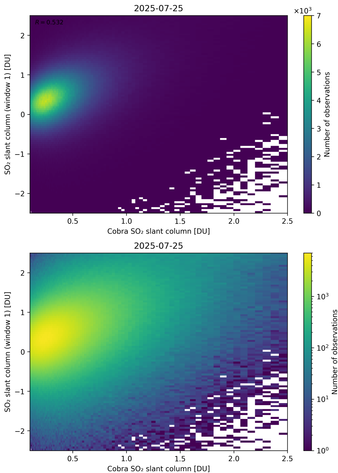
Figure 219: Scatter density plot of “Cobra SO 2 slant column” against “SO 2 slant column (window 1)” for 2025-07-24 to 2025-07-26.
