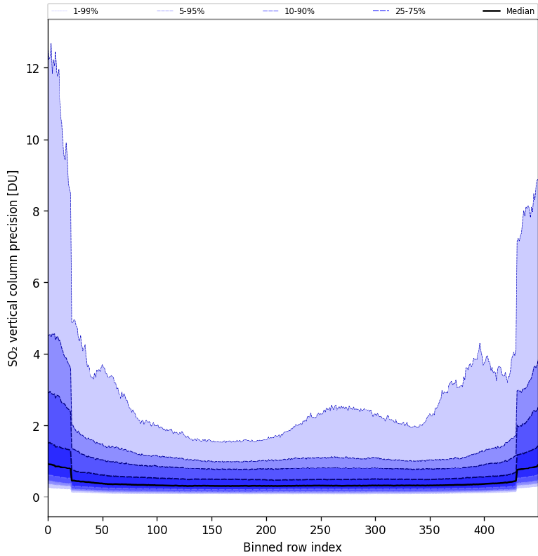
Figure 85: Along track statistics of “SO 2 vertical column precision” for 2025-07-24 to 2025-07-26
