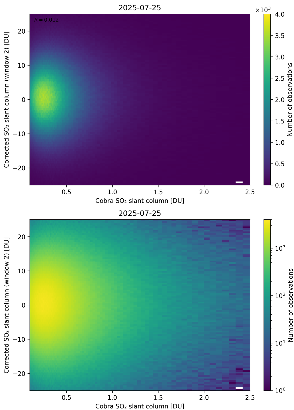
Figure 217: Scatter density plot of “Cobra SO 2 slant column” against “Corrected SO 2 slant column (window 2)” for 2025-07-24 to 2025-07-26.
