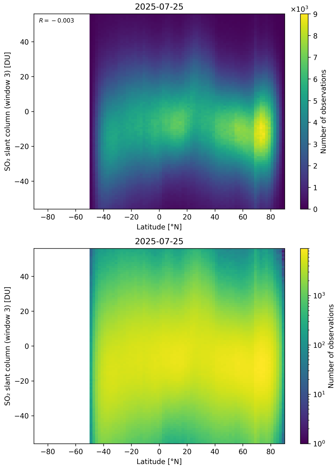
Figure 165: Scatter density plot of “Latitude” against “SO 2 slant column (window 3)” for 2025-07-24 to 2025-07-26.
