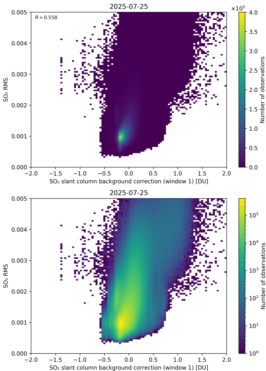
Figure 113: Scatter density plot of “SO 2 slant column background correction (window 1)” against “SO 2 RMS” for 2025-07-24 to 2025-07-26.
