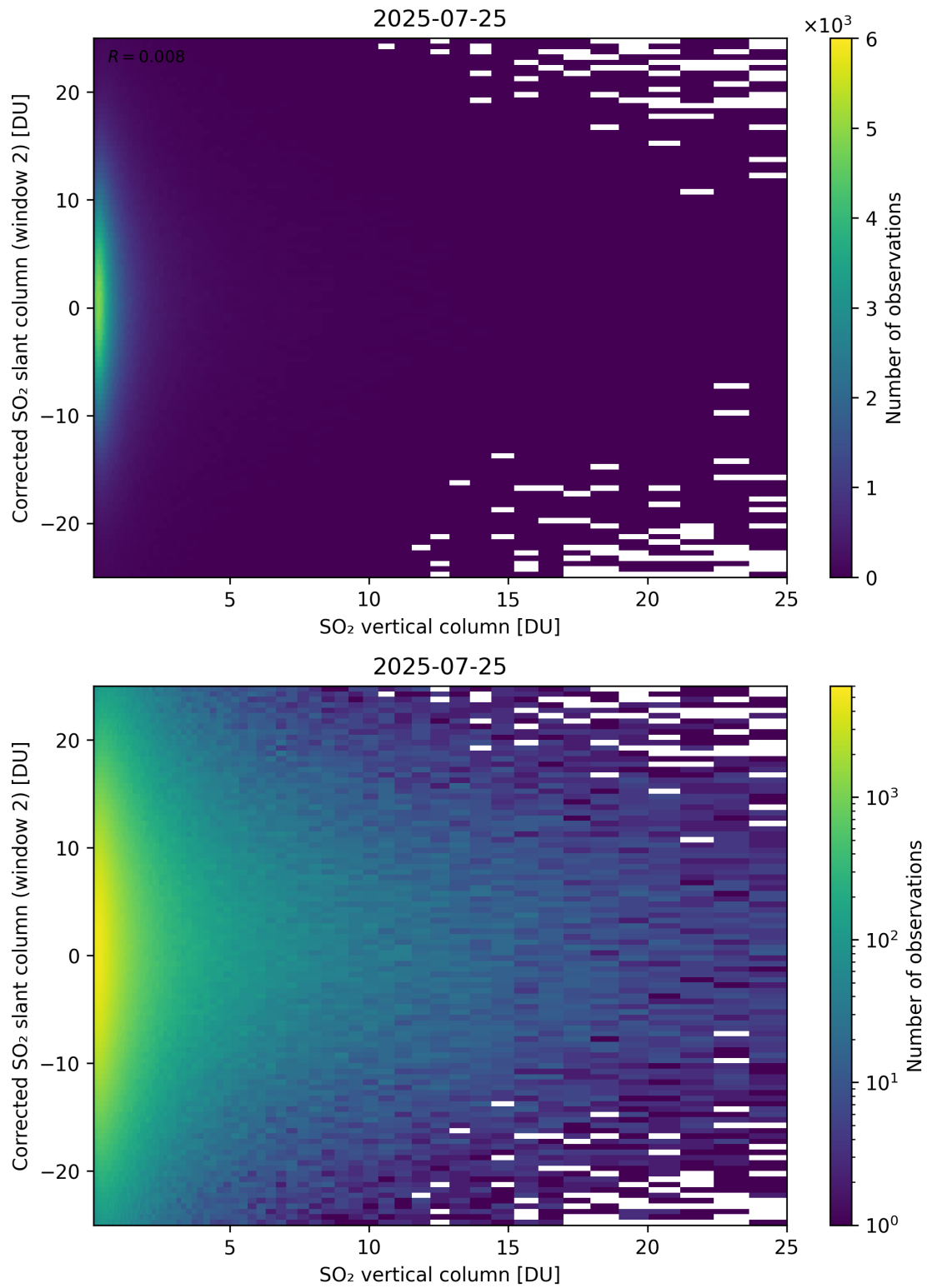
Figure 352: Scatter density plot of “SO 2 vertical column” against “Corrected SO 2 slant column (window 2)” for 2025-07-24 to 2025-07-26.
