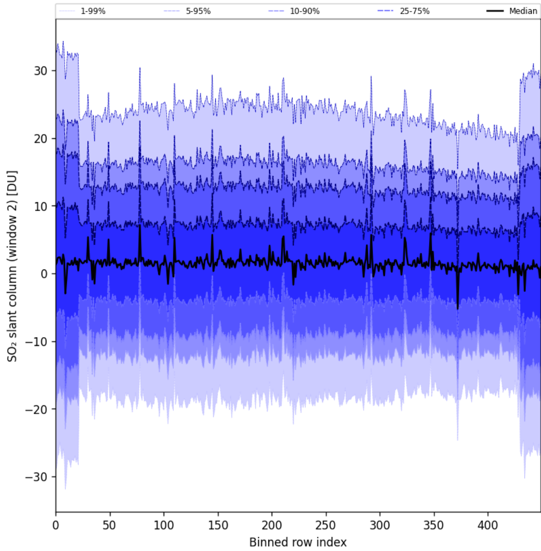
Figure 93: Along track statistics of “SO 2 slant column (window 2)” for 2025-07-24 to 2025-07-26
