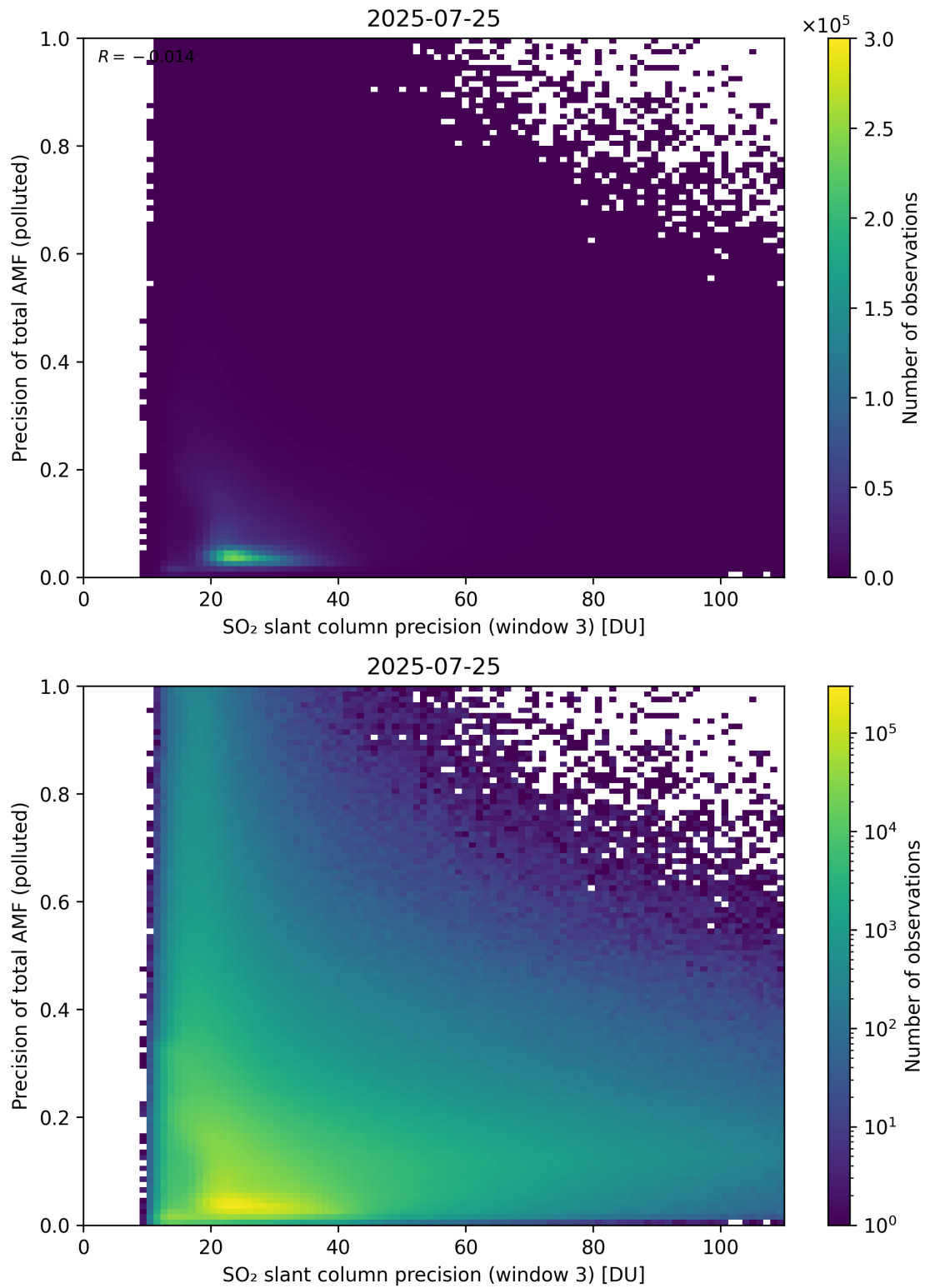
Figure 314: Scatter density plot of “SO 2 slant column precision (window 3)” against “Precision of total AMF (polluted)” for 2025-07-24 to 2025-07-26.
