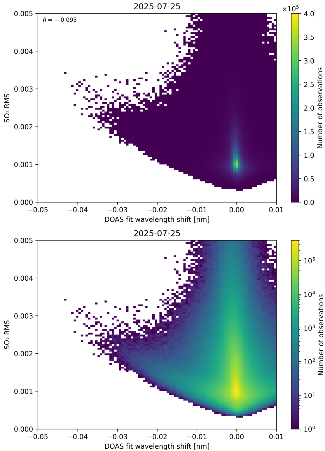
Figure 139: Scatter density plot of “DOAS fit wavelength shift” against “SO 2 RMS” for 2025-07-24 to 2025-07-26.
