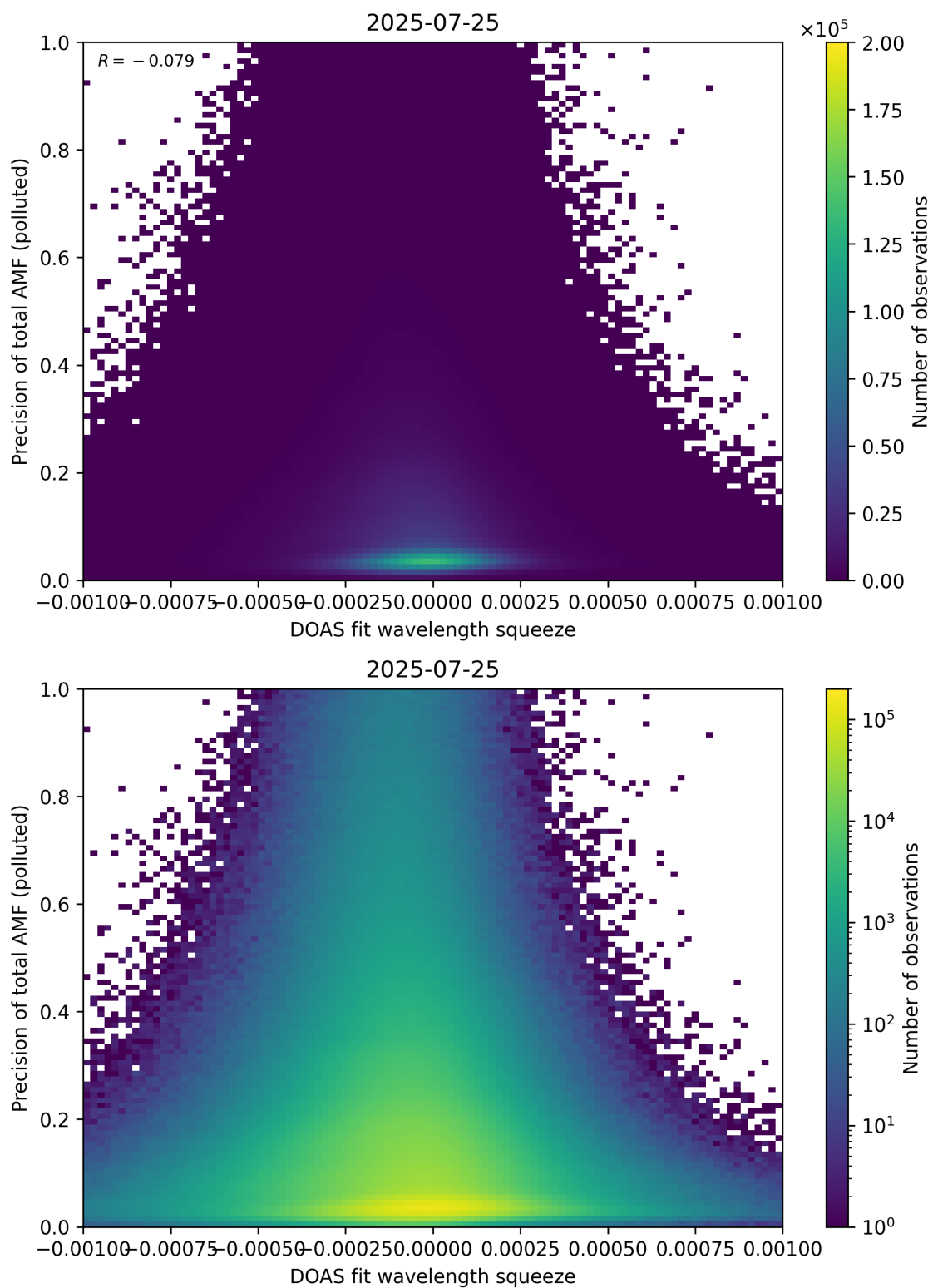
Figure 146: Scatter density plot of “DOAS fit wavelength squeeze” against “Precision of total AMF (polluted)” for 2025-07-24 to 2025-07-26.
