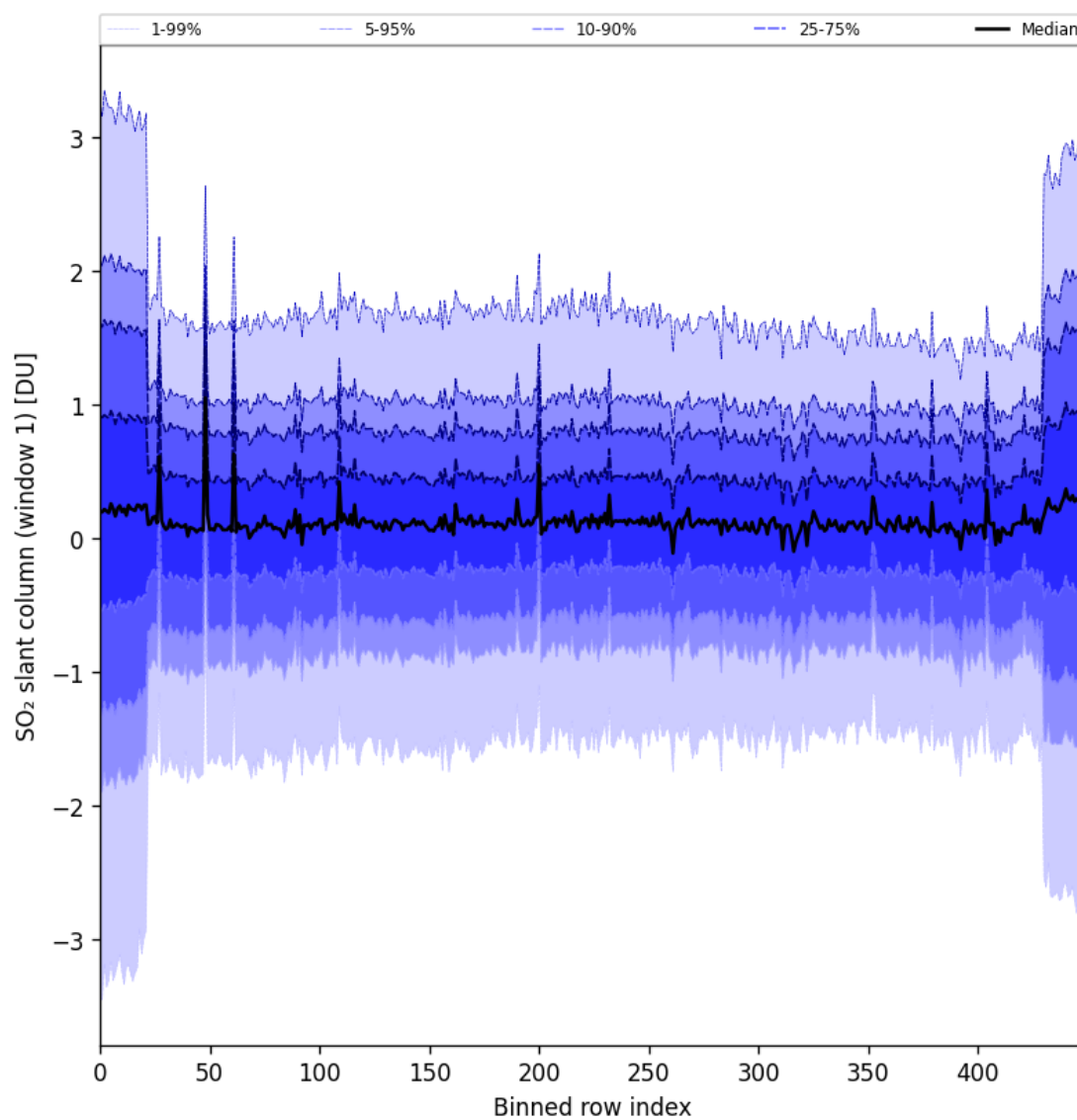
Figure 89: Along track statistics of “SO 2 slant column (window 1)” for 2025-07-24 to 2025-07-26
