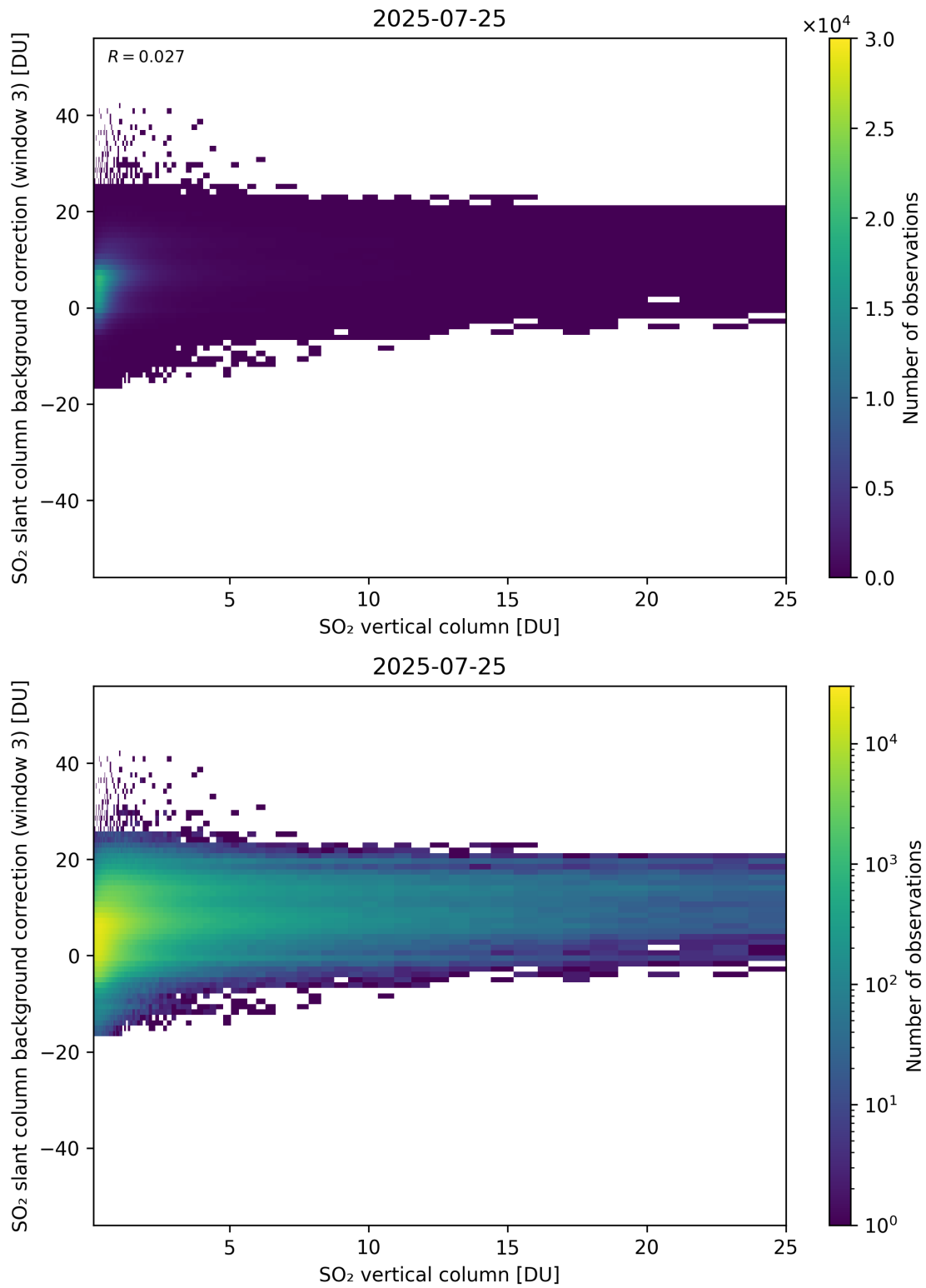
Figure 325: Scatter density plot of “SO 2 vertical column” against “SO 2 slant column background correction (window 3)” for 2025-07-24 to 2025-07-26.
