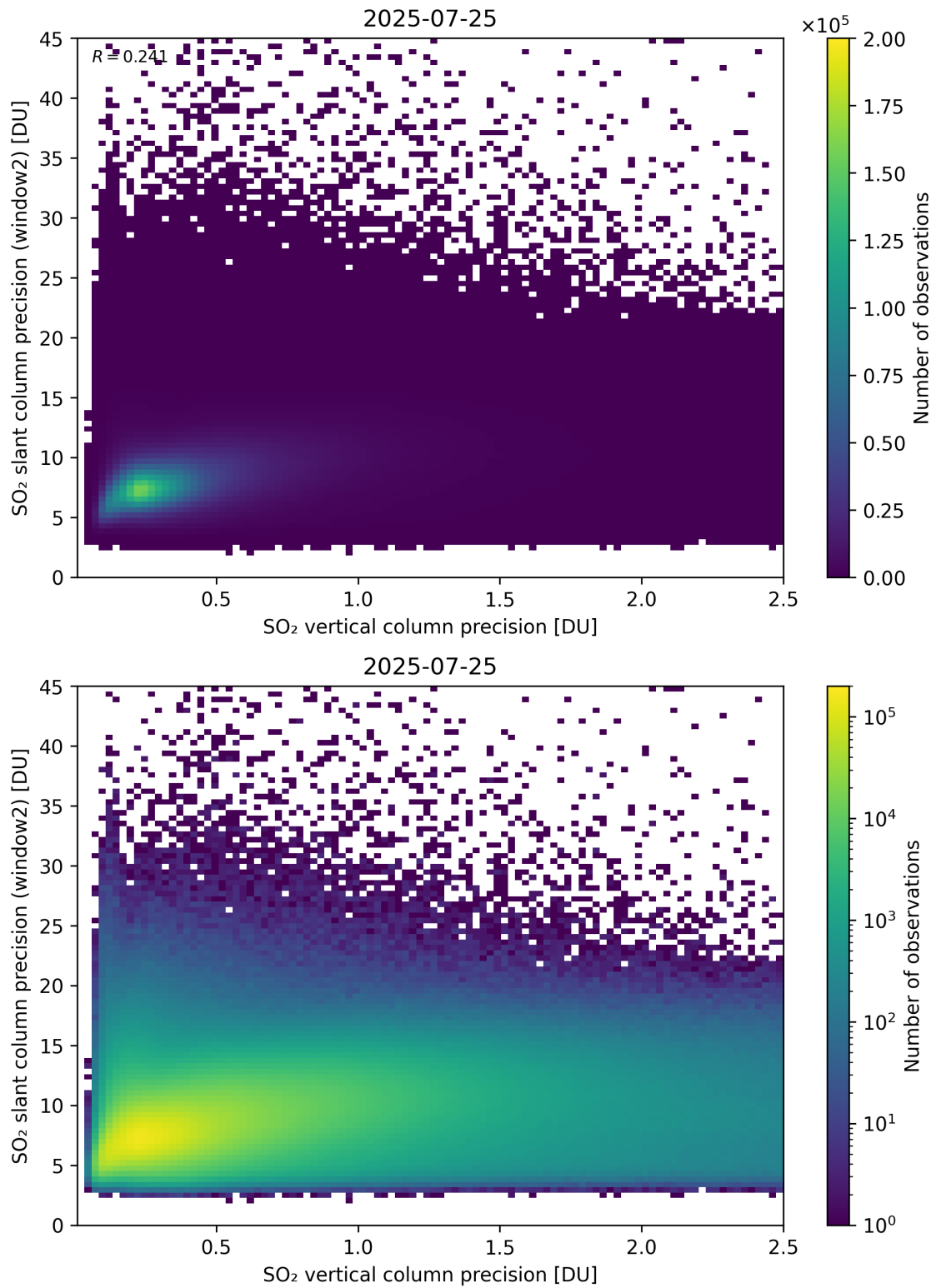
Figure 343: Scatter density plot of “SO 2 vertical column precision” against “SO 2 slant column precision (window2)” for 2025-07-24 to 2025-07-26.
