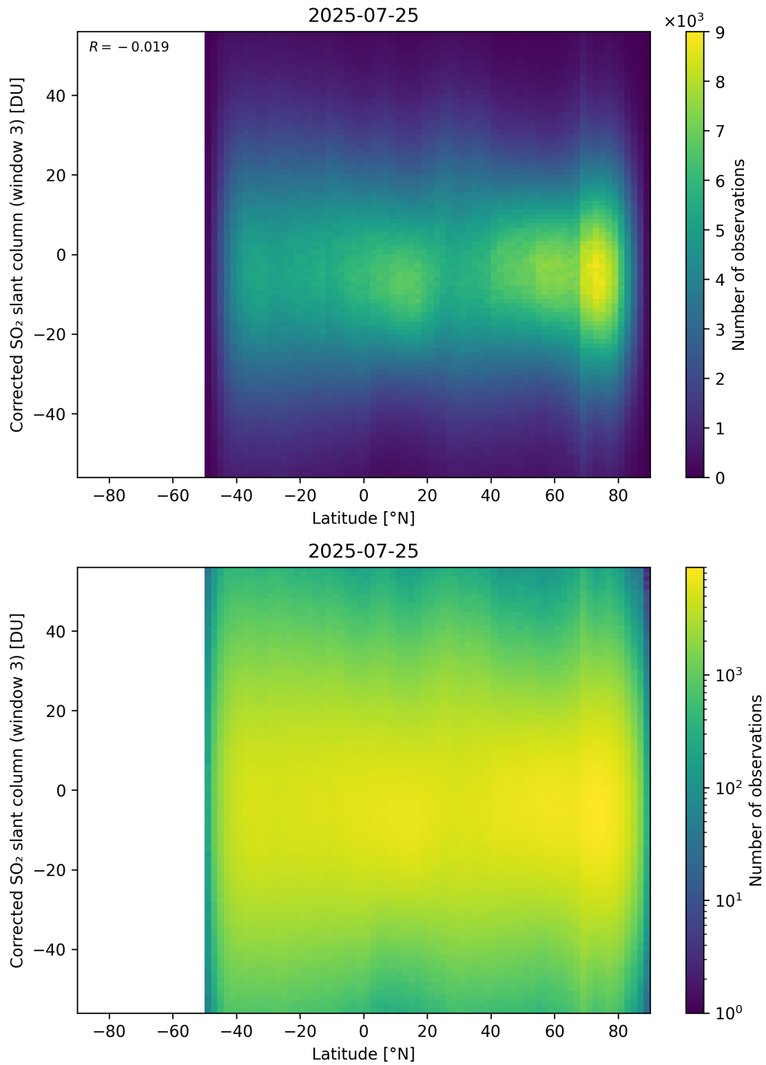
Figure 161: Scatter density plot of “Latitude” against “Corrected SO 2 slant column (window 3)” for 2025-07-24 to 2025-07-26.
