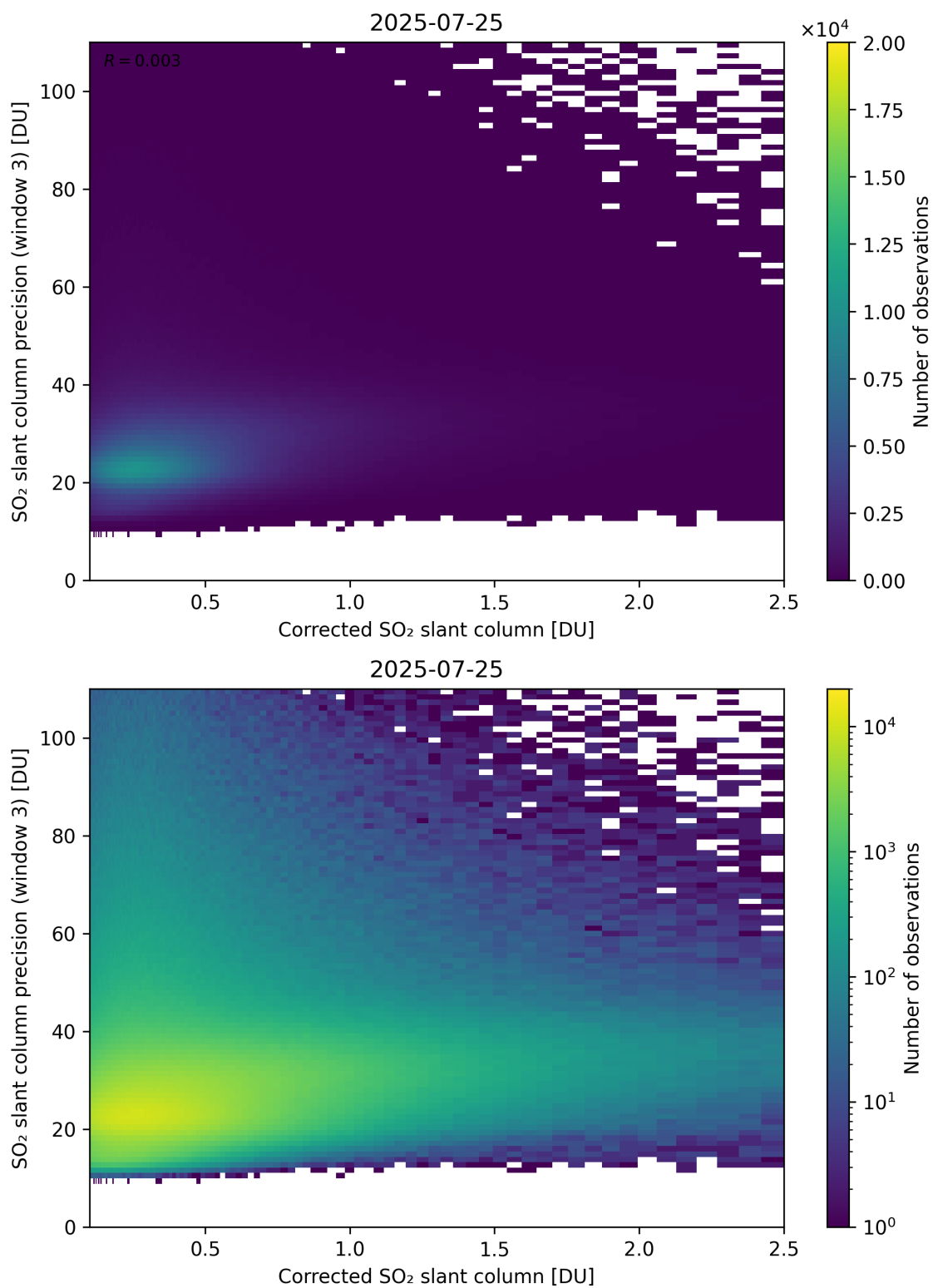
Figure 241: Scatter density plot of “Corrected SO 2 slant column” against “SO 2 slant column precision (window 3)” for 2025-07-24 to 2025-07-26.
