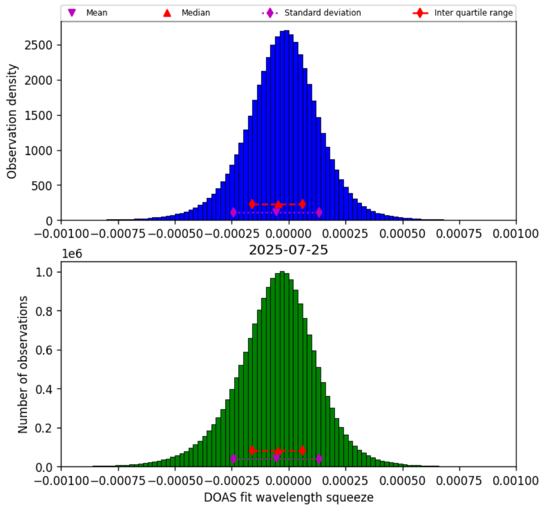
Figure 77: Histogram of “DOAS fit wavelength squeeze” for 2025-07-24 to 2025-07-26
