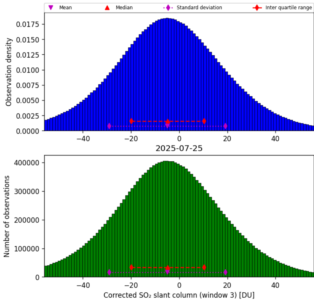
Figure 73: Histogram of “Corrected SO 2 slant column (window 3)” for 2025-07-24 to 2025-07-26
