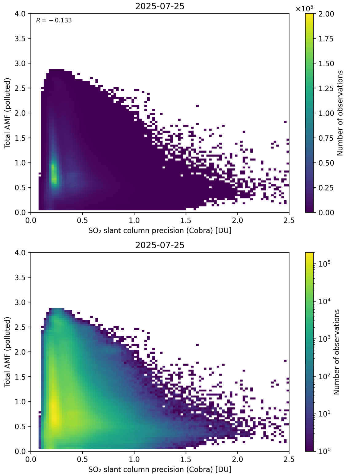
Figure 213: Scatter density plot of “SO 2 slant column precision (Cobra)” against “Total AMF (polluted)” for 2025-07-24 to 2025-07-26.
