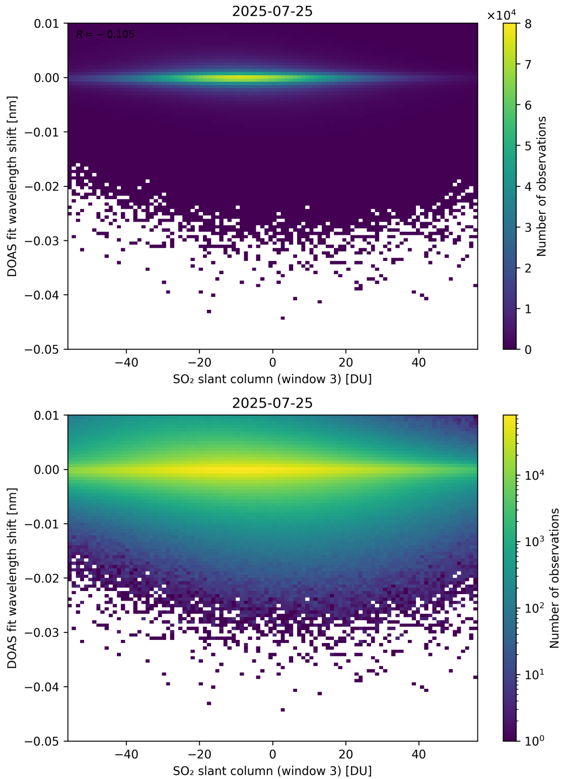
Figure 304: Scatter density plot of “SO 2 slant column (window 3)” against “DOAS fit wavelength shift” for 2025-07-24 to 2025-07-26.
