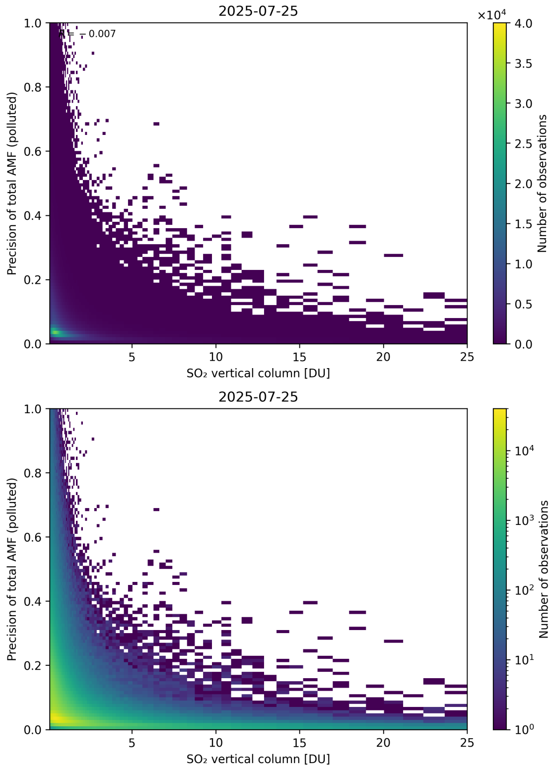
Figure 360: Scatter density plot of “SO 2 vertical column” against “Precision of total AMF (polluted)” for 2025-07-24 to 2025-07-26.
