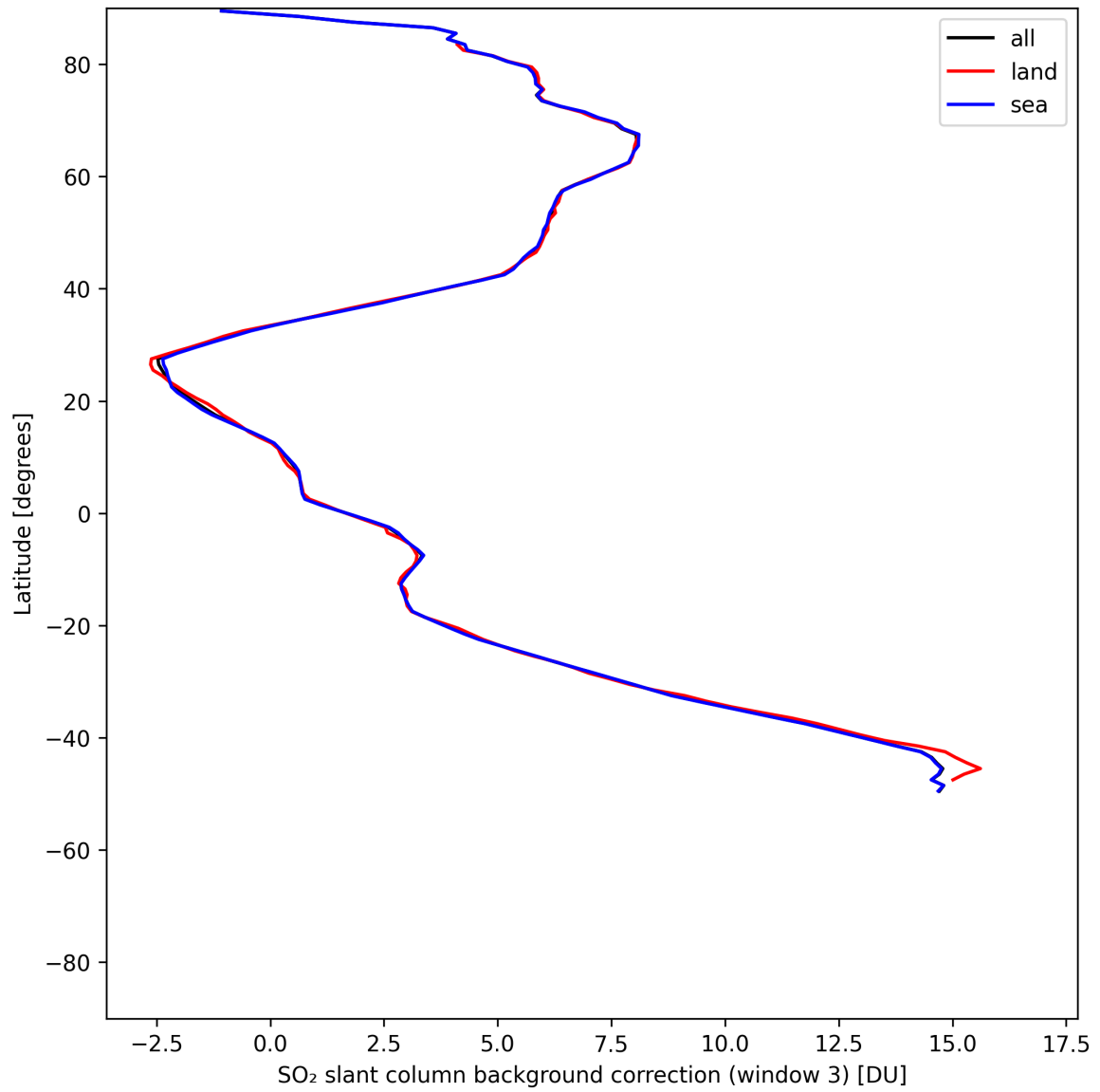
Figure 48: Zonal average of “SO 2 slant column background correction (window 3)” for 2025-07-24 to 2025-07-26.
