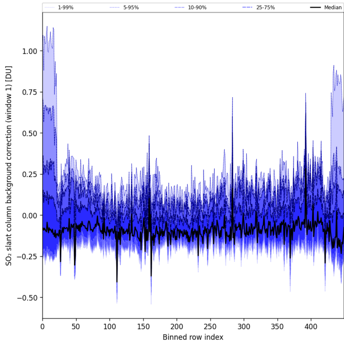
Figure 92: Along track statistics of “SO 2 slant column background correction (window 1)” for 2025-07-24 to 2025-07-26
