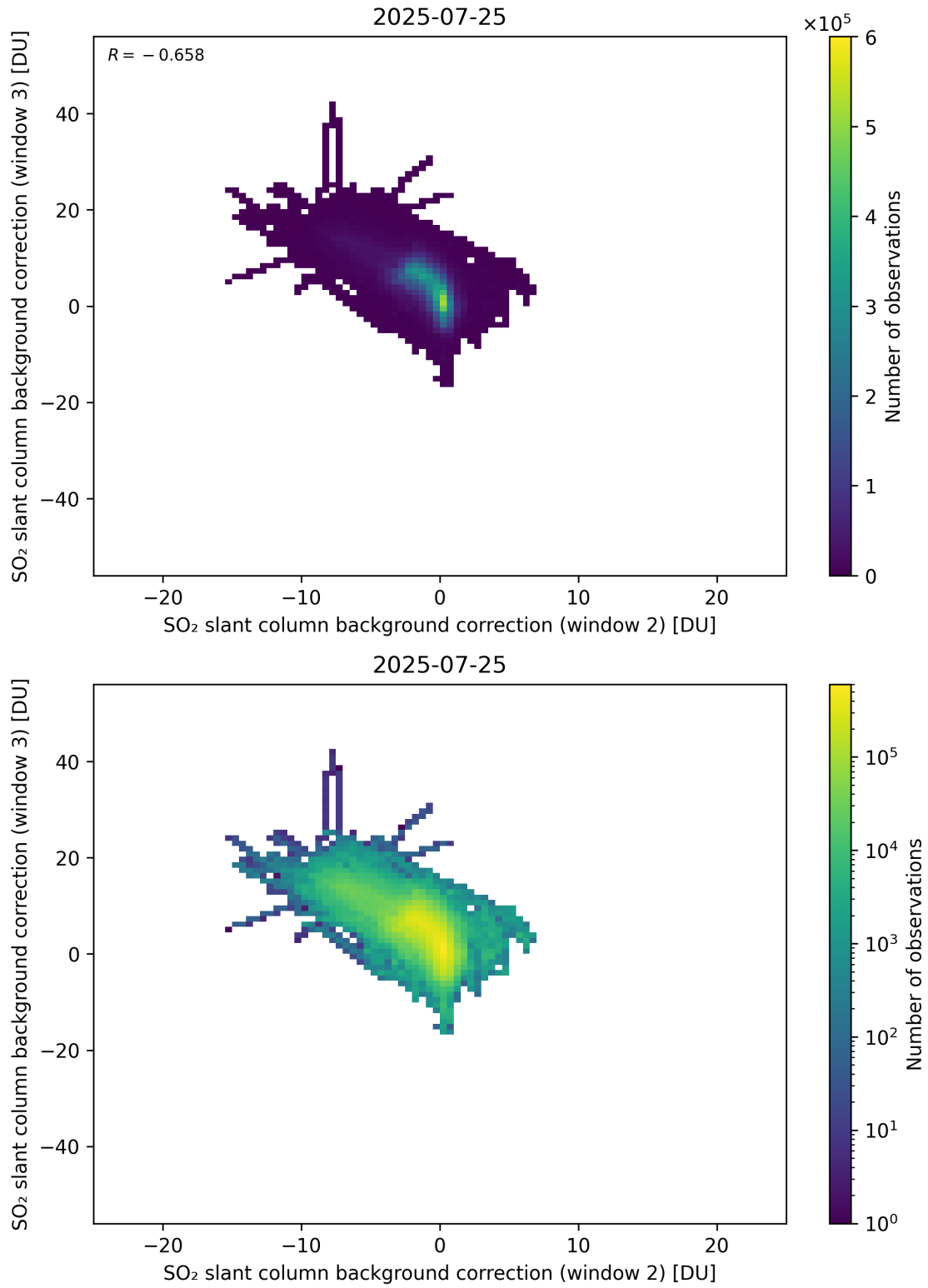
Figure 122: Scatter density plot of “SO 2 slant column background correction (window 2)” against “SO 2 slant column background correction (window 3)” for 2025-07-24 to 2025-07-26.
