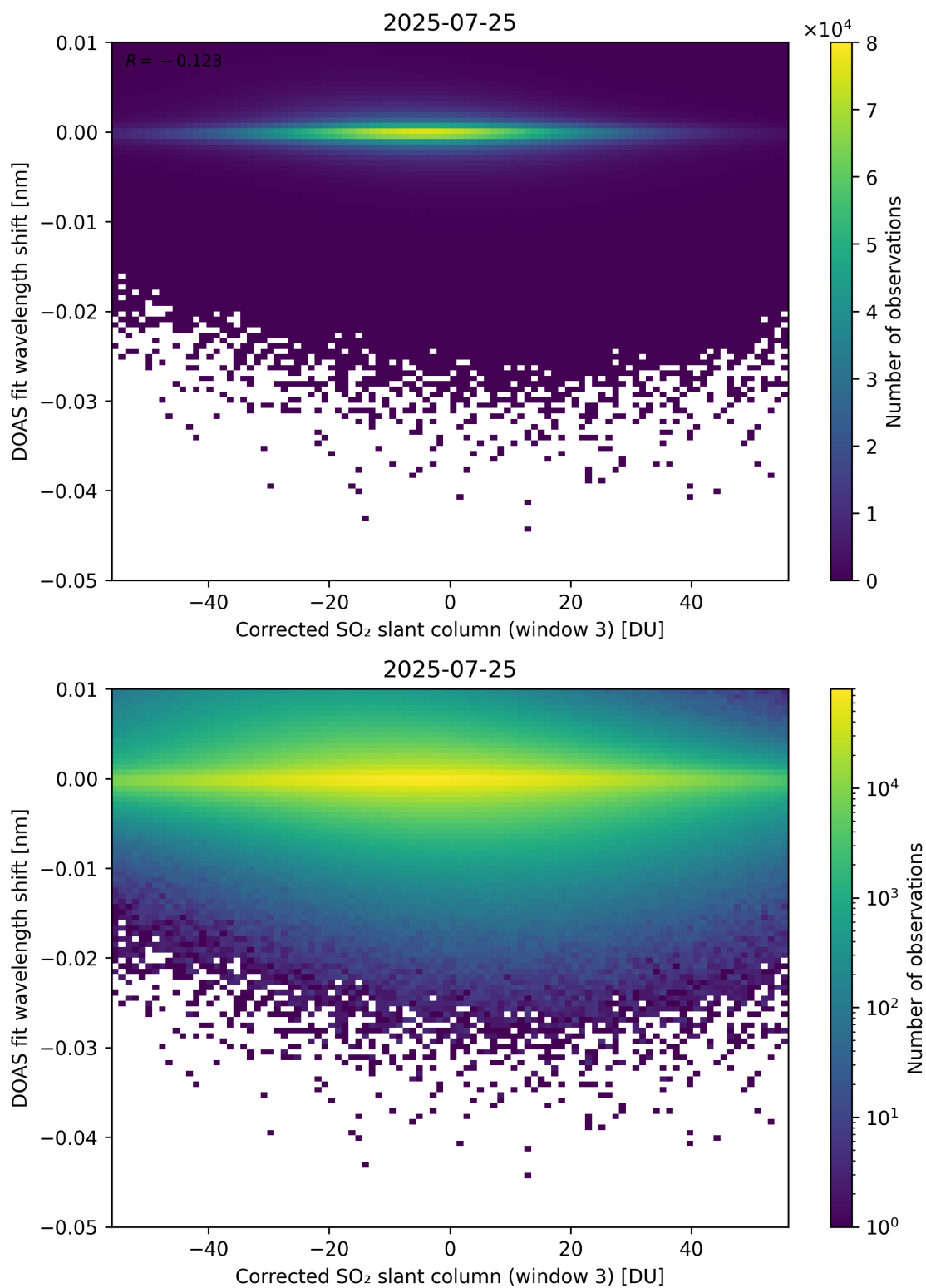
Figure 256: Scatter density plot of “Corrected SO 2 slant column (window 3)” against “DOAS fit wavelength shift” for 2025-07-24 to 2025-07-26.
