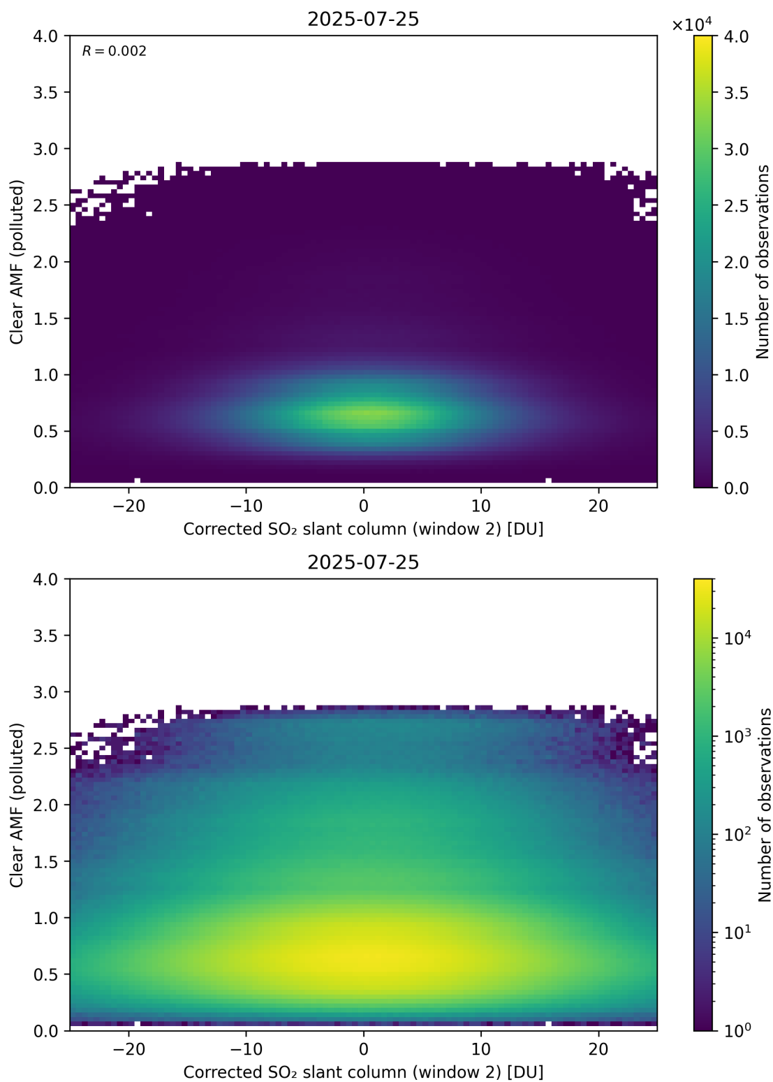
Figure 249: Scatter density plot of “Corrected SO 2 slant column (window 2)” against “Clear AMF (polluted)” for 2025-07-24 to 2025-07-26.
