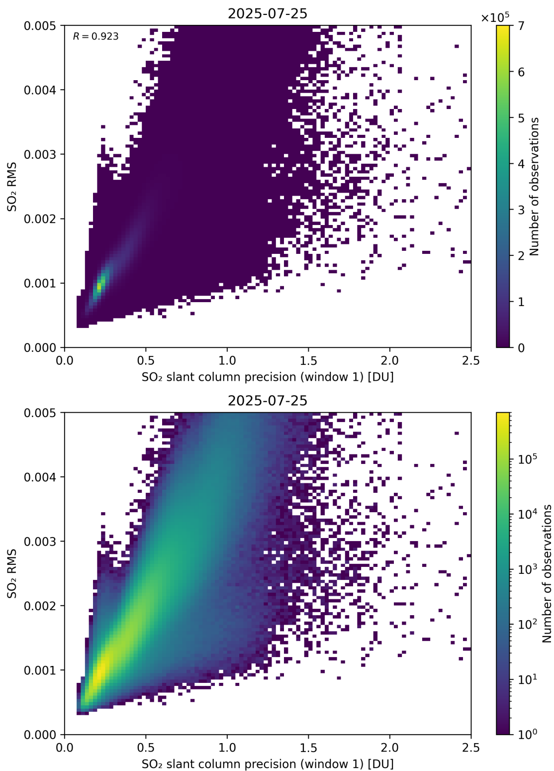
Figure 273: Scatter density plot of “SO 2 slant column precision (window 1)” against “SO 2 RMS” for 2025-07-24 to 2025-07-26.
