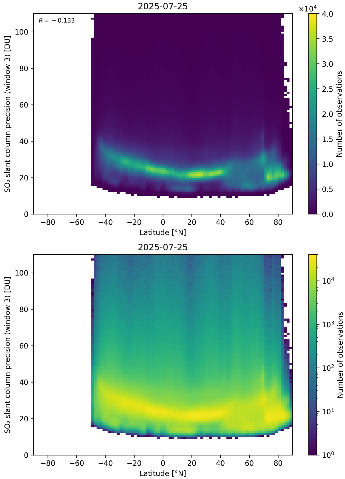
Figure 166: Scatter density plot of “Latitude” against “SO 2 slant column precision (window 3)” for 2025-07-24 to 2025-07-26.
