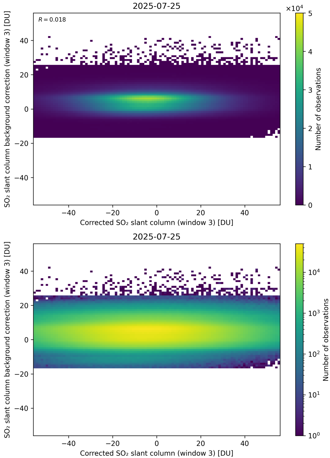
Figure 255: Scatter density plot of “Corrected SO 2 slant column (window 3)” against “SO 2 slant column background correction (window 3)” for 2025-07-24 to 2025-07-26.
