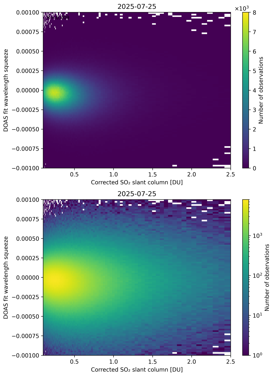
Figure 230: Scatter density plot of “Corrected SO 2 slant column” against “DOAS fit wavelength squeeze” for 2025-07-24 to 2025-07-26.
