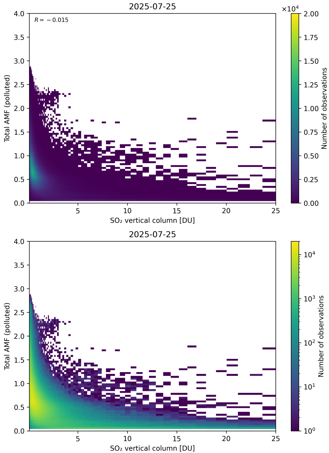
Figure 359: Scatter density plot of “SO 2 vertical column” against “Total AMF (polluted)” for 2025-07-24 to 2025-07-26.
