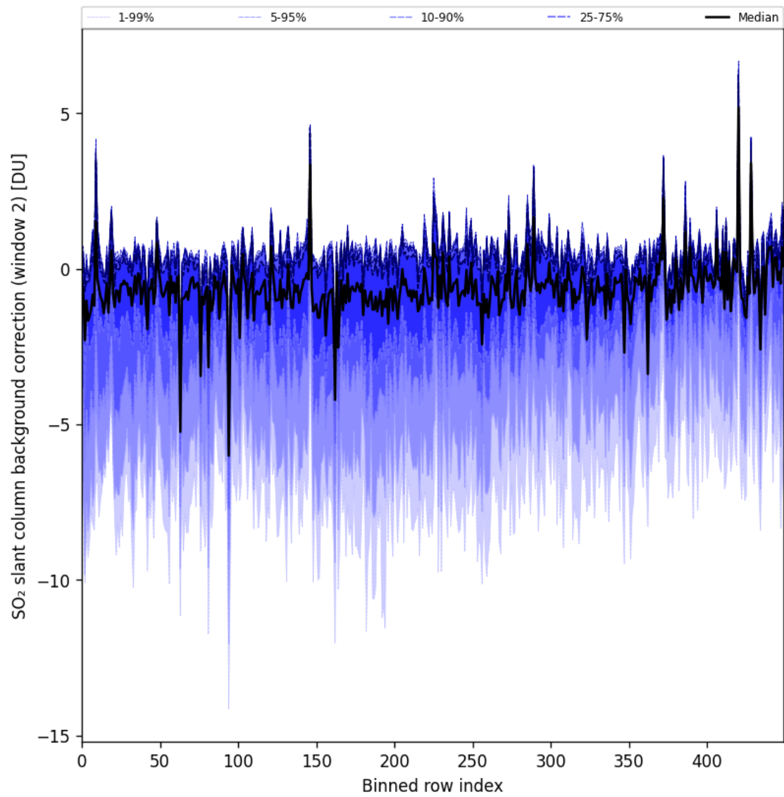
Figure 96: Along track statistics of “SO 2 slant column background correction (window 2)” for 2025-07-24 to 2025-07-26
