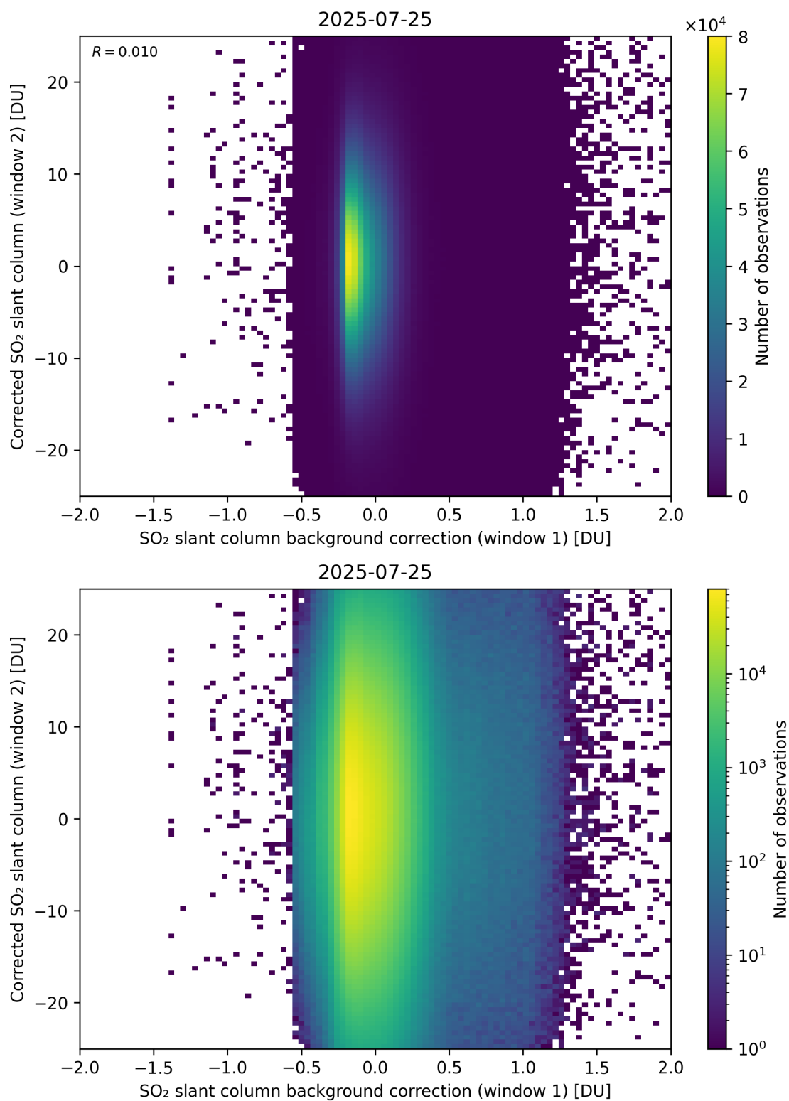
Figure 115: Scatter density plot of “SO 2 slant column background correction (window 1)” against “Corrected SO 2 slant column (window 2)” for 2025-07-24 to 2025-07-26.
