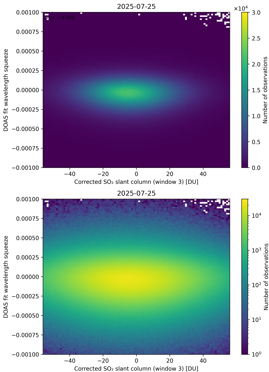
Figure 257: Scatter density plot of “Corrected SO 2 slant column (window 3)” against “DOAS fit wavelength squeeze” for 2025-07-24 to 2025-07-26.
