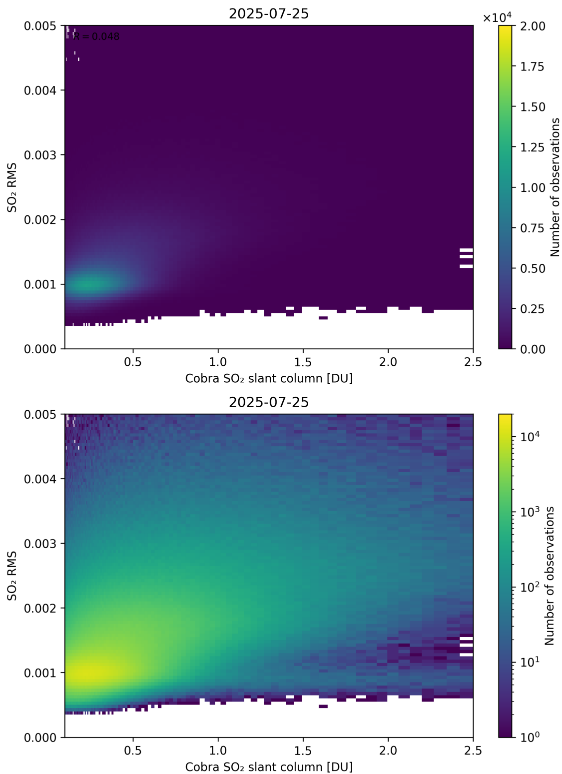
Figure 198: Scatter density plot of “Cobra SO 2 slant column” against “SO 2 RMS” for 2025-07-24 to 2025-07-26.
