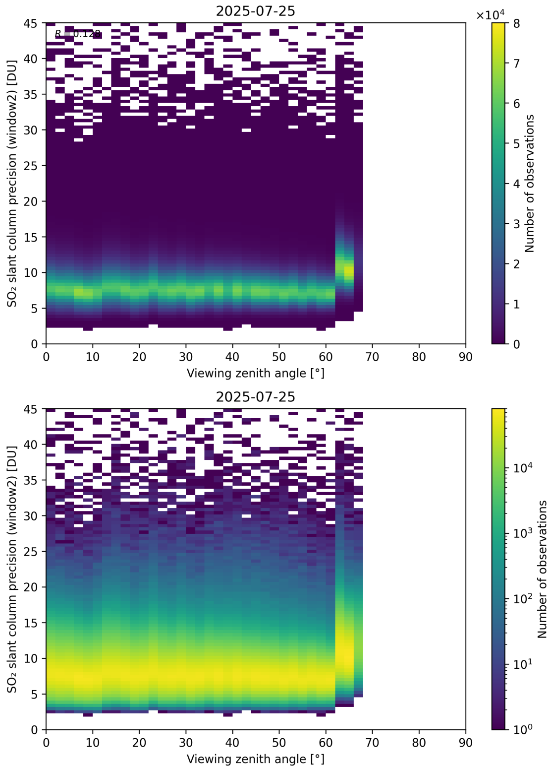
Figure 378: Scatter density plot of “Viewing zenith angle” against “SO 2 slant column precision (window2)” for 2025-07-24 to 2025-07-26.
