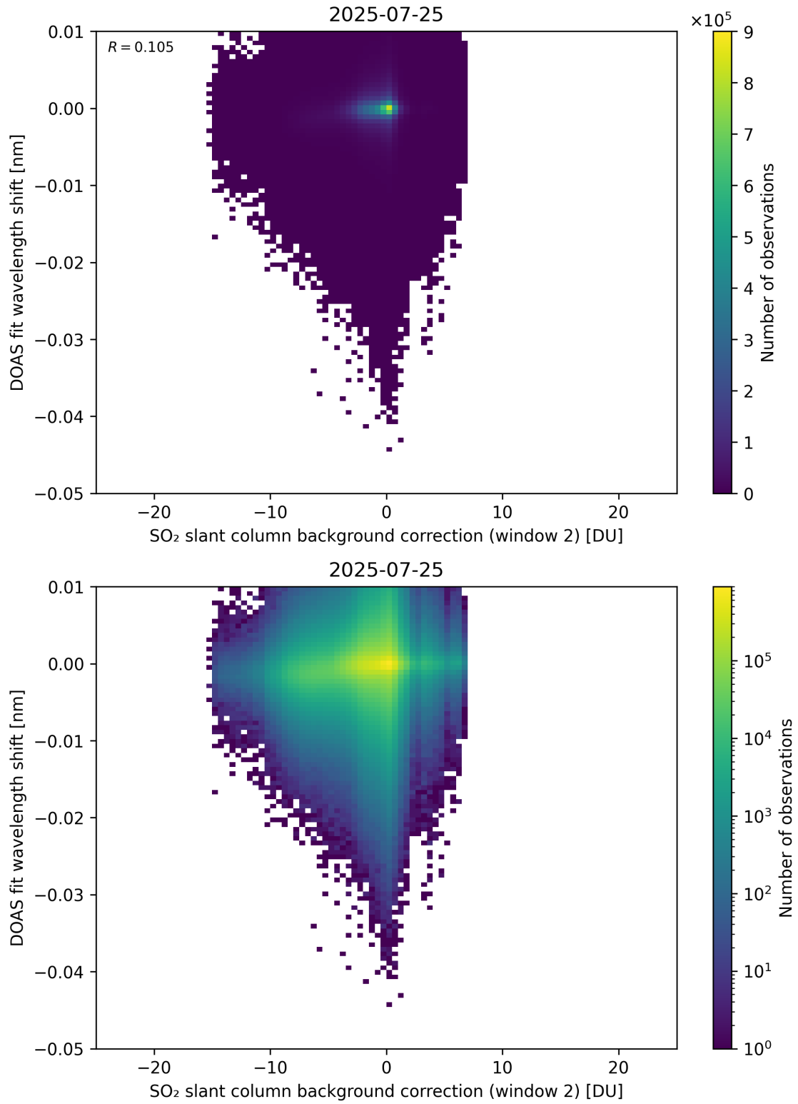
Figure 123: Scatter density plot of “SO 2 slant column background correction (window 2)” against “DOAS fit wavelength shift” for 2025-07-24 to 2025-07-26.
