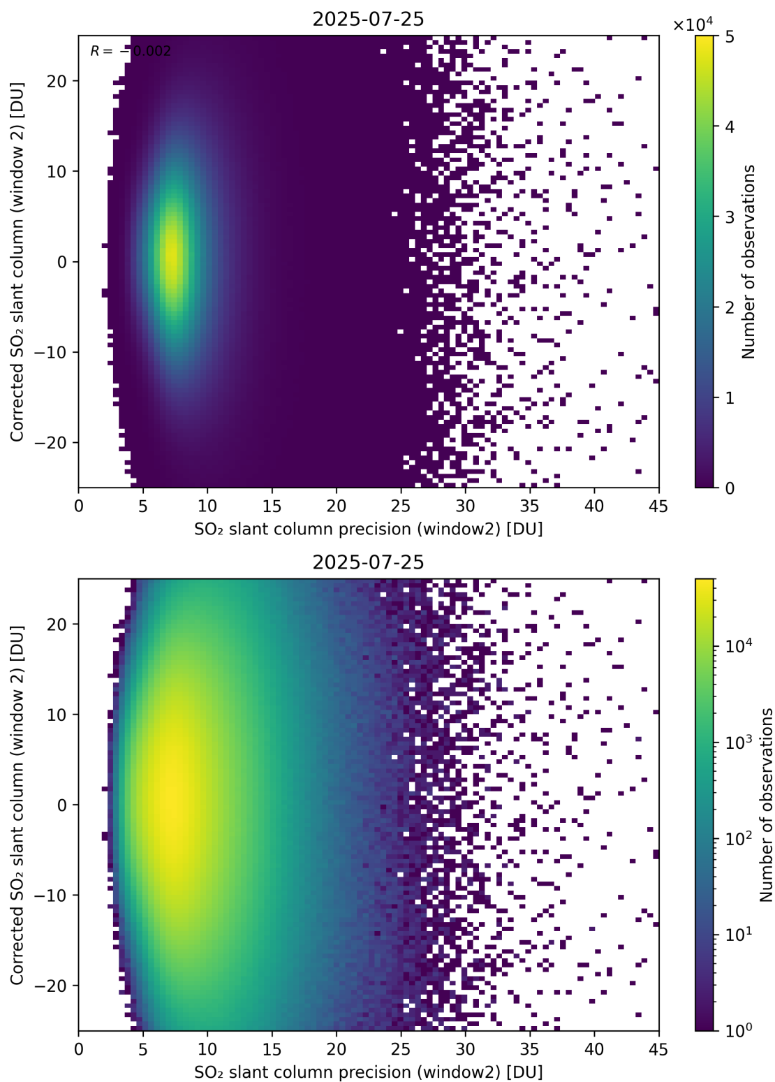
Figure 297: Scatter density plot of “SO 2 slant column precision (window2)” against “Corrected SO 2 slant column (window 2)” for 2025-07-24 to 2025-07-26.
