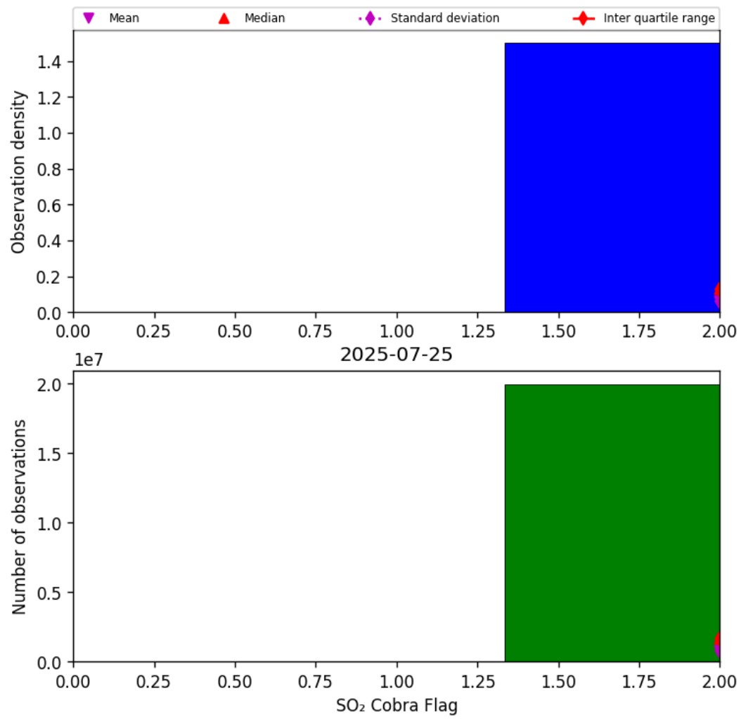
Figure 75: Histogram of “SO 2 Cobra Flag” for 2025-07-24 to 2025-07-26
