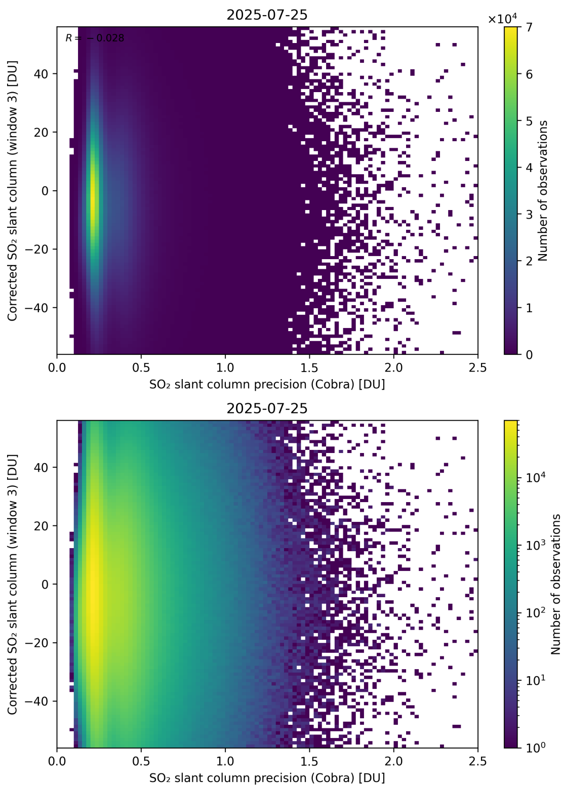
Figure 207: Scatter density plot of “SO 2 slant column precision (Cobra)” against “Corrected SO 2 slant column (window 3)” for 2025-07-24 to 2025-07-26.
