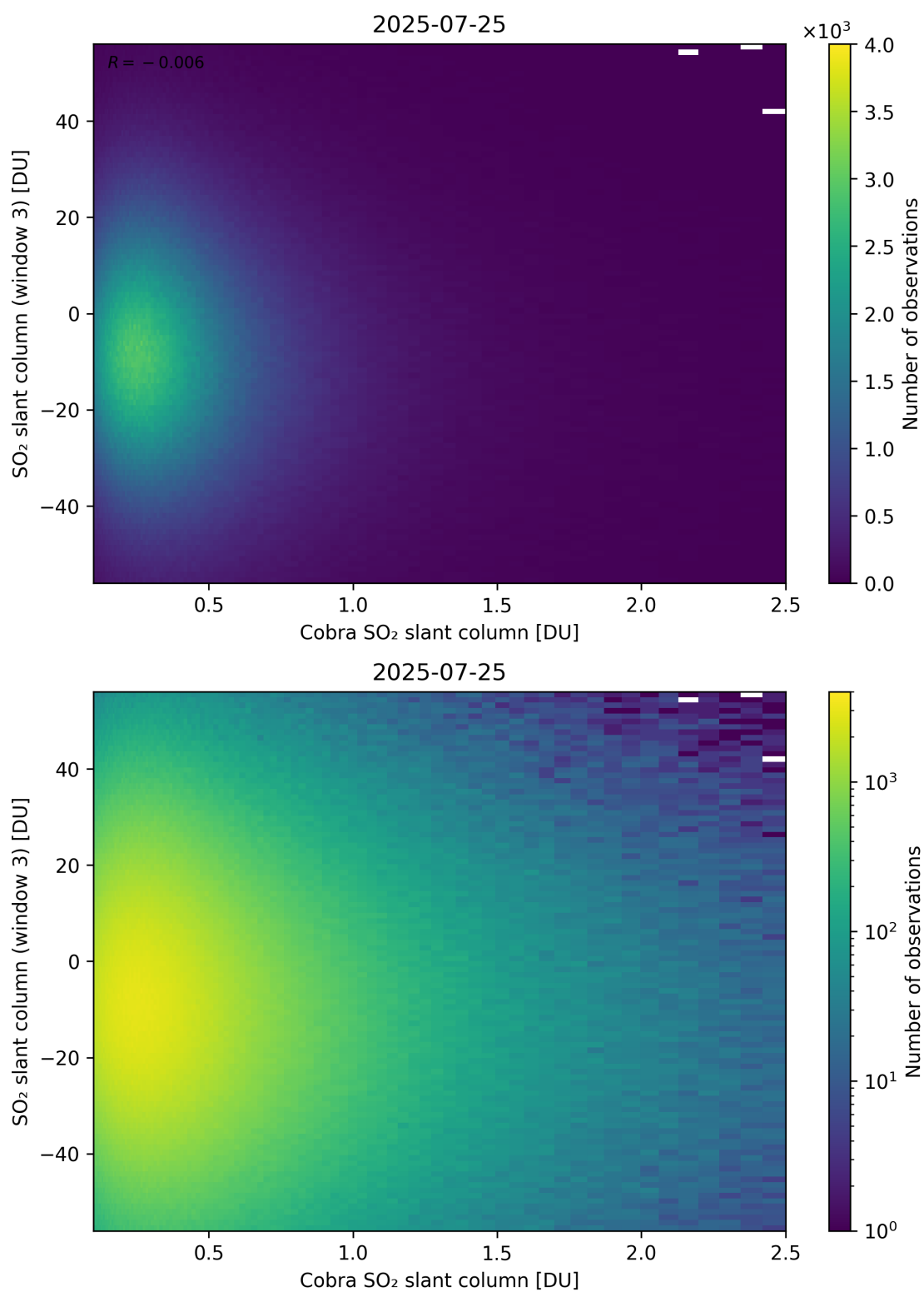
Figure 222: Scatter density plot of “Cobra SO 2 slant column” against “SO 2 slant column (window 3)” for 2025-07-24 to 2025-07-26.
