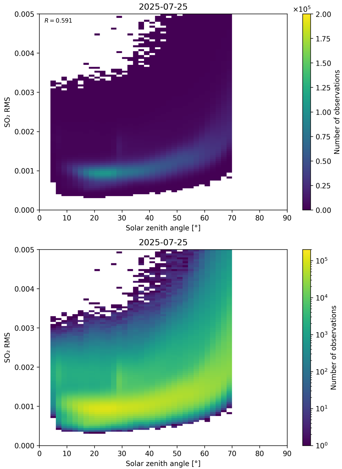
Figure 176: Scatter density plot of “Solar zenith angle” against “SO 2 RMS” for 2025-07-24 to 2025-07-26.
