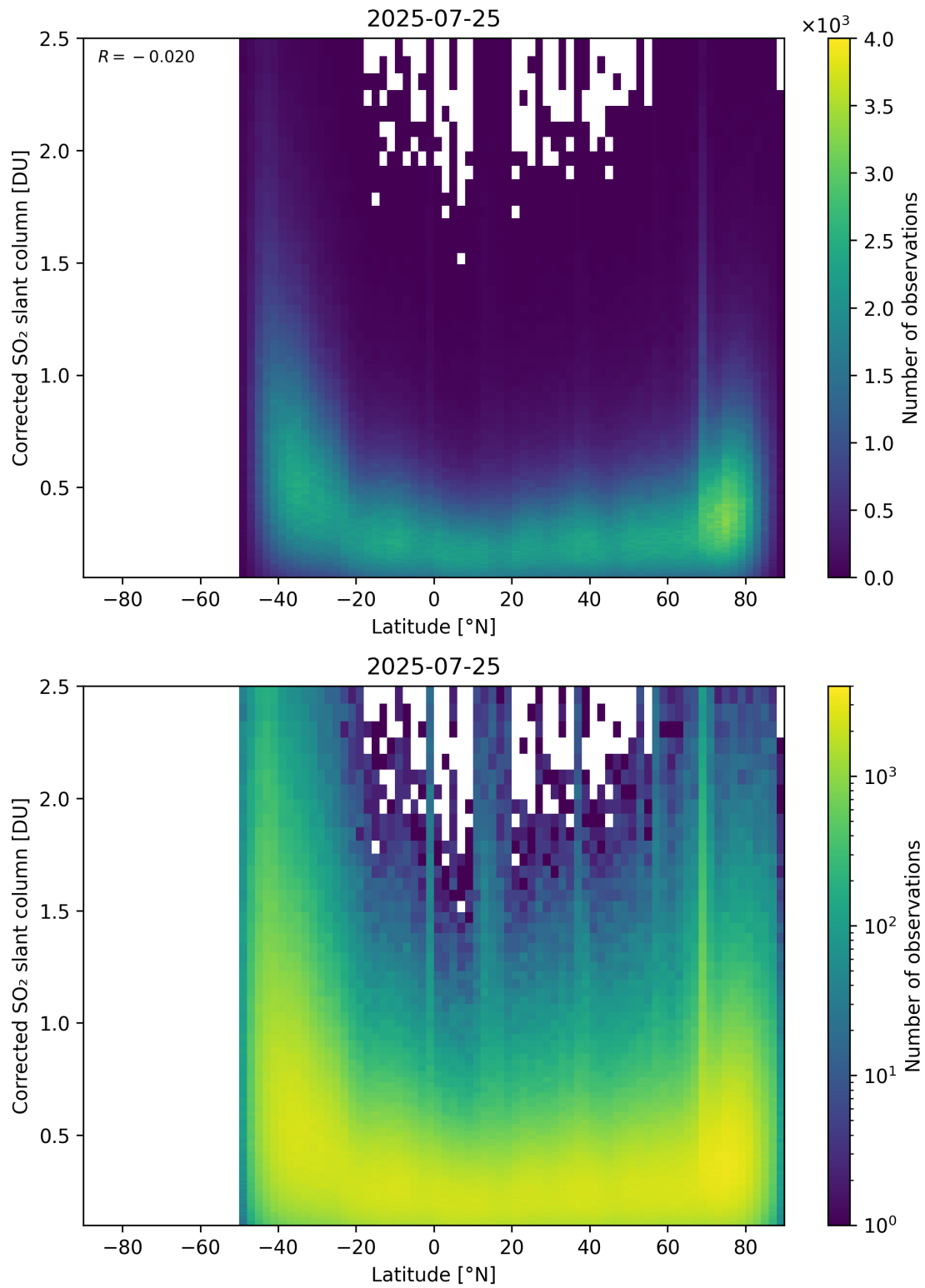
Figure 159: Scatter density plot of “Latitude” against “Corrected SO 2 slant column” for 2025-07-24 to 2025-07-26.
