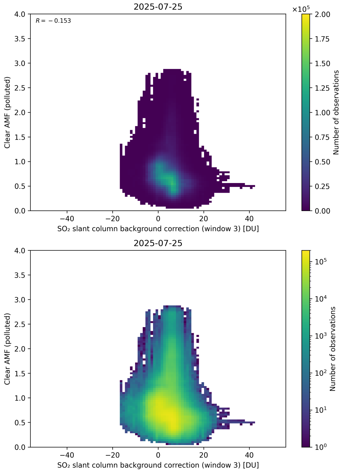
Figure 135: Scatter density plot of “SO 2 slant column background correction (window 3)” against “Clear AMF (polluted)” for 2025-07-24 to 2025-07-26.
