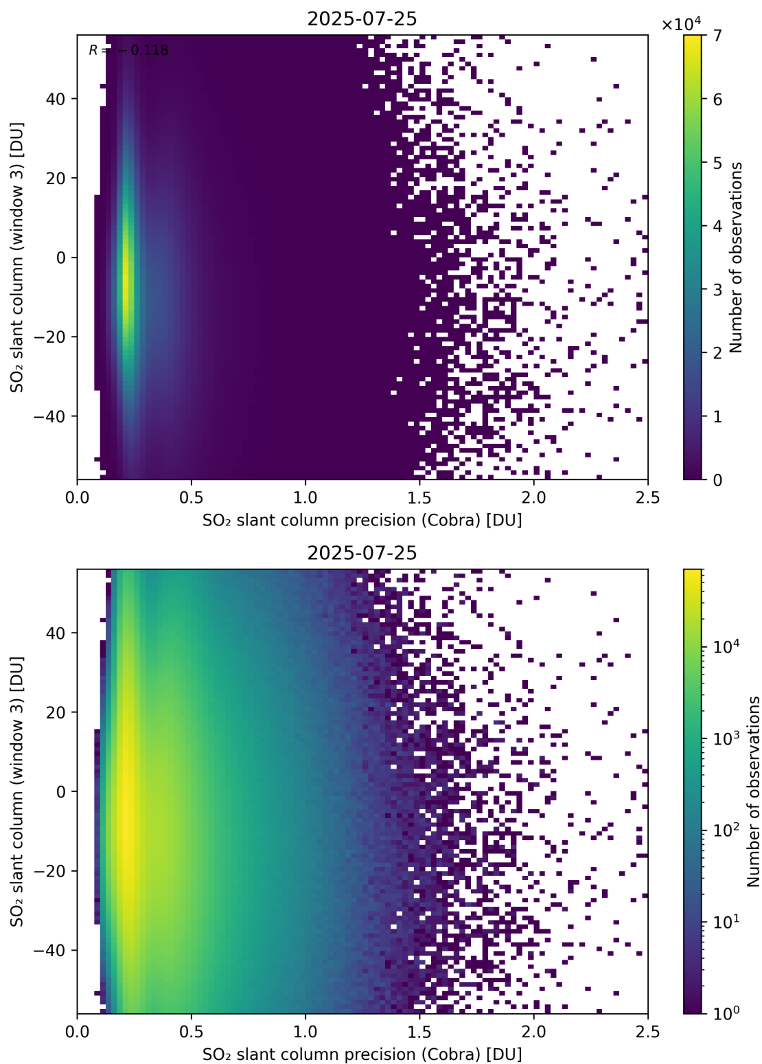
Figure 211: Scatter density plot of “SO 2 slant column precision (Cobra)” against “SO 2 slant column (window 3)” for 2025-07-24 to 2025-07-26.
