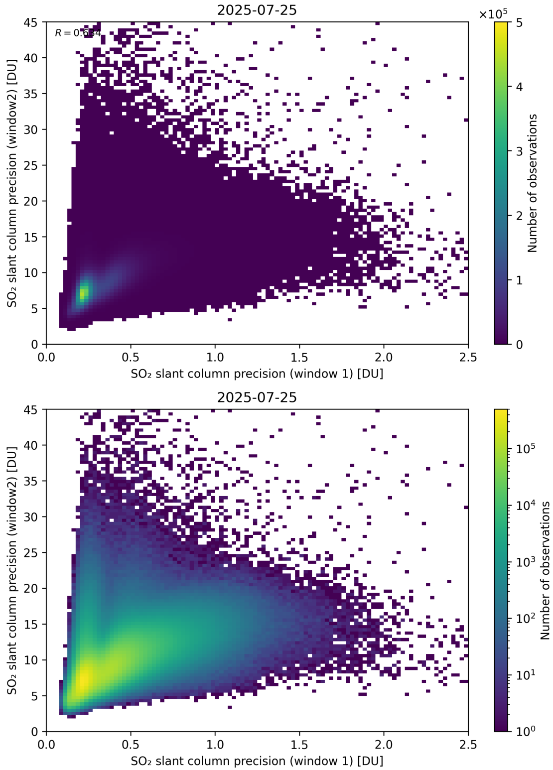
Figure 277: Scatter density plot of “SO 2 slant column precision (window 1)” against “SO 2 slant column precision (window2)” for 2025-07-24 to 2025-07-26.
