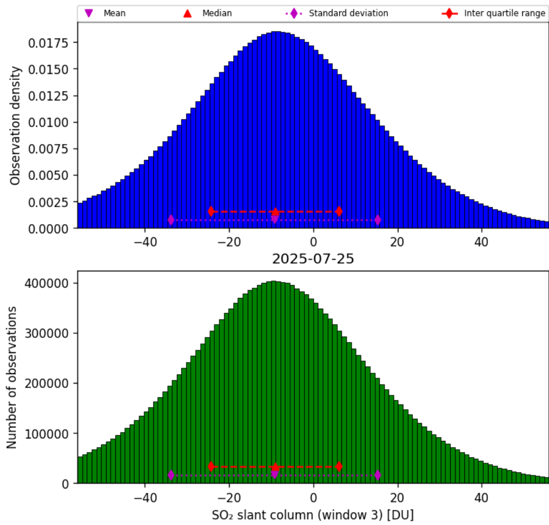
Figure 71: Histogram of “SO 2 slant column (window 3)” for 2025-07-24 to 2025-07-26
