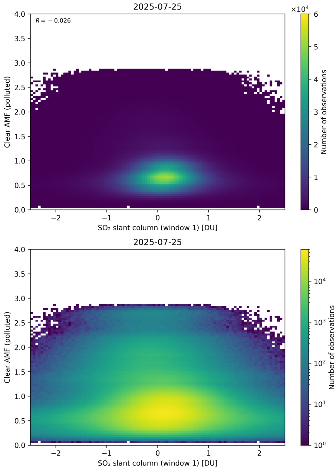
Figure 282: Scatter density plot of “SO 2 slant column (window 1)” against “Clear AMF (polluted)” for 2025-07-24 to 2025-07-26.
