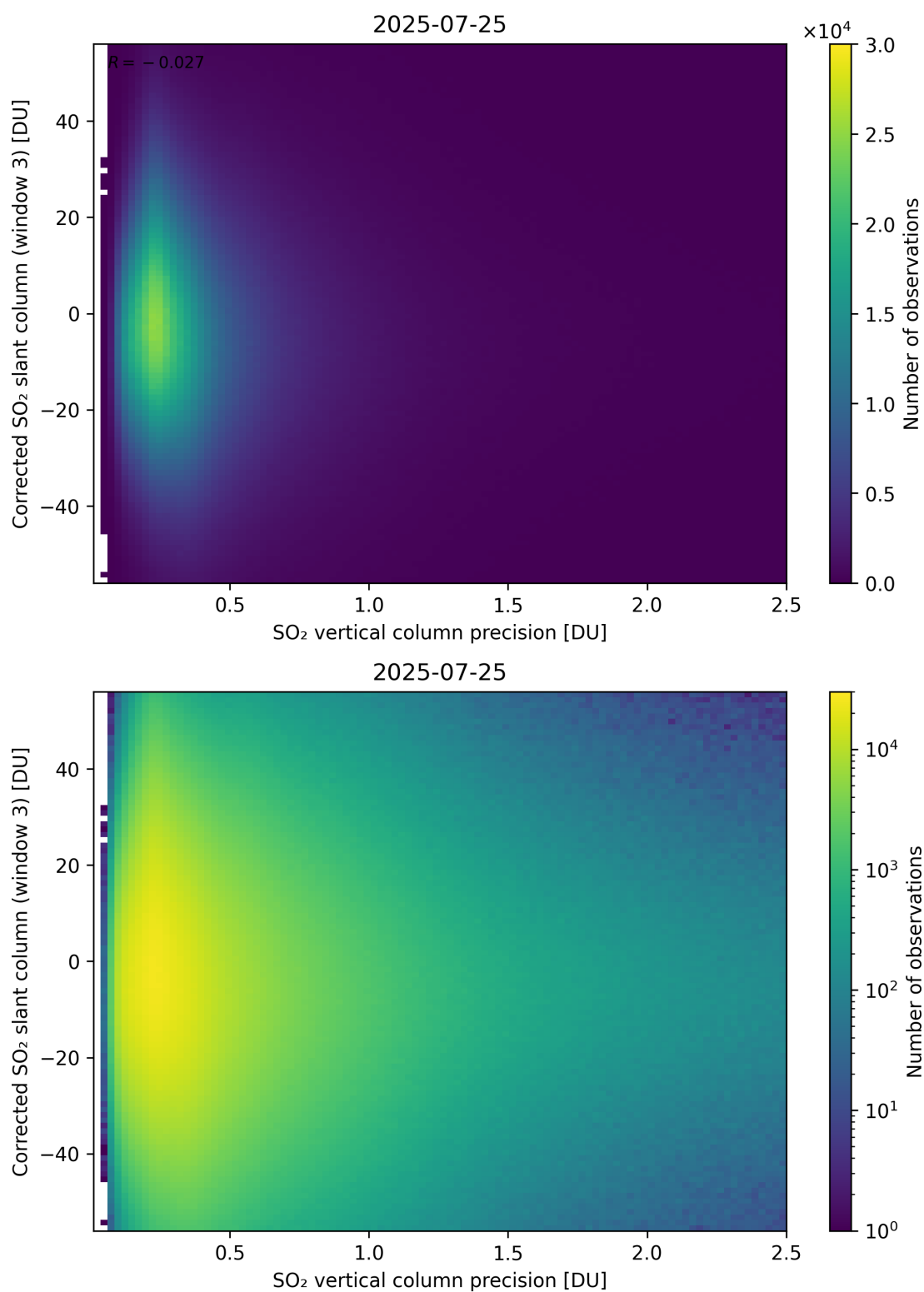
Figure 340: Scatter density plot of “SO 2 vertical column precision” against “Corrected SO 2 slant column (window 3)” for 2025-07-24 to 2025-07-26.
