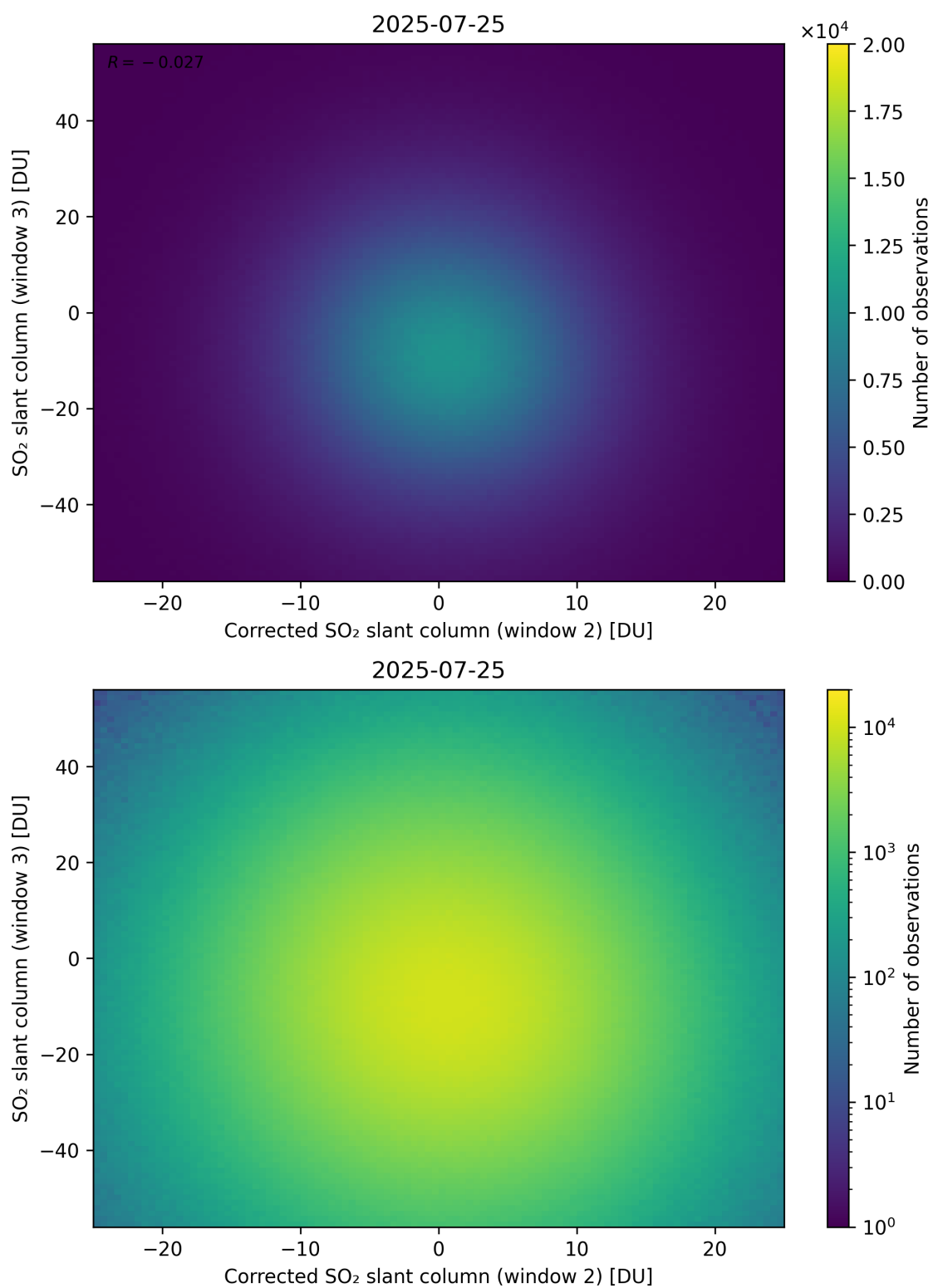
Figure 251: Scatter density plot of “Corrected SO 2 slant column (window 2)” against “SO 2 slant column (window 3)” for 2025-07-24 to 2025-07-26.
