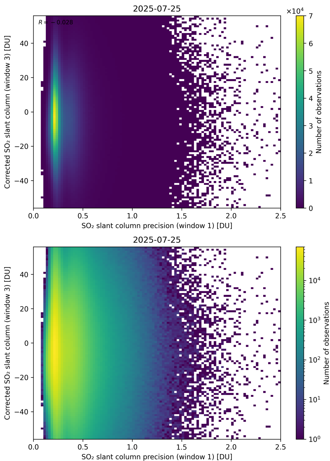
Figure 276: Scatter density plot of “SO 2 slant column precision (window 1)” against “Corrected SO 2 slant column (window 3)” for 2025-07-24 to 2025-07-26.
