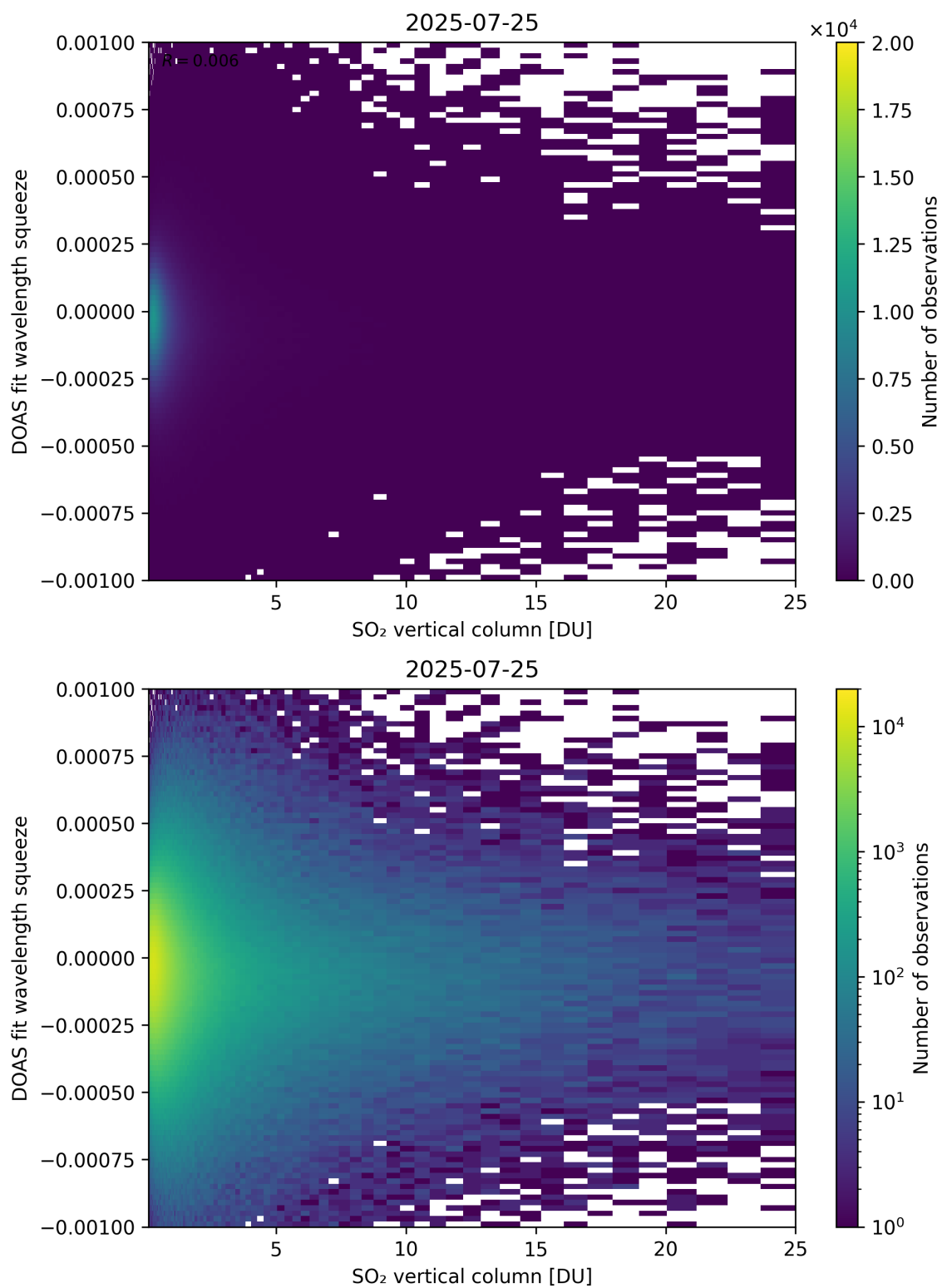
Figure 327: Scatter density plot of “SO 2 vertical column” against “DOAS fit wavelength squeeze” for 2025-07-24 to 2025-07-26.
