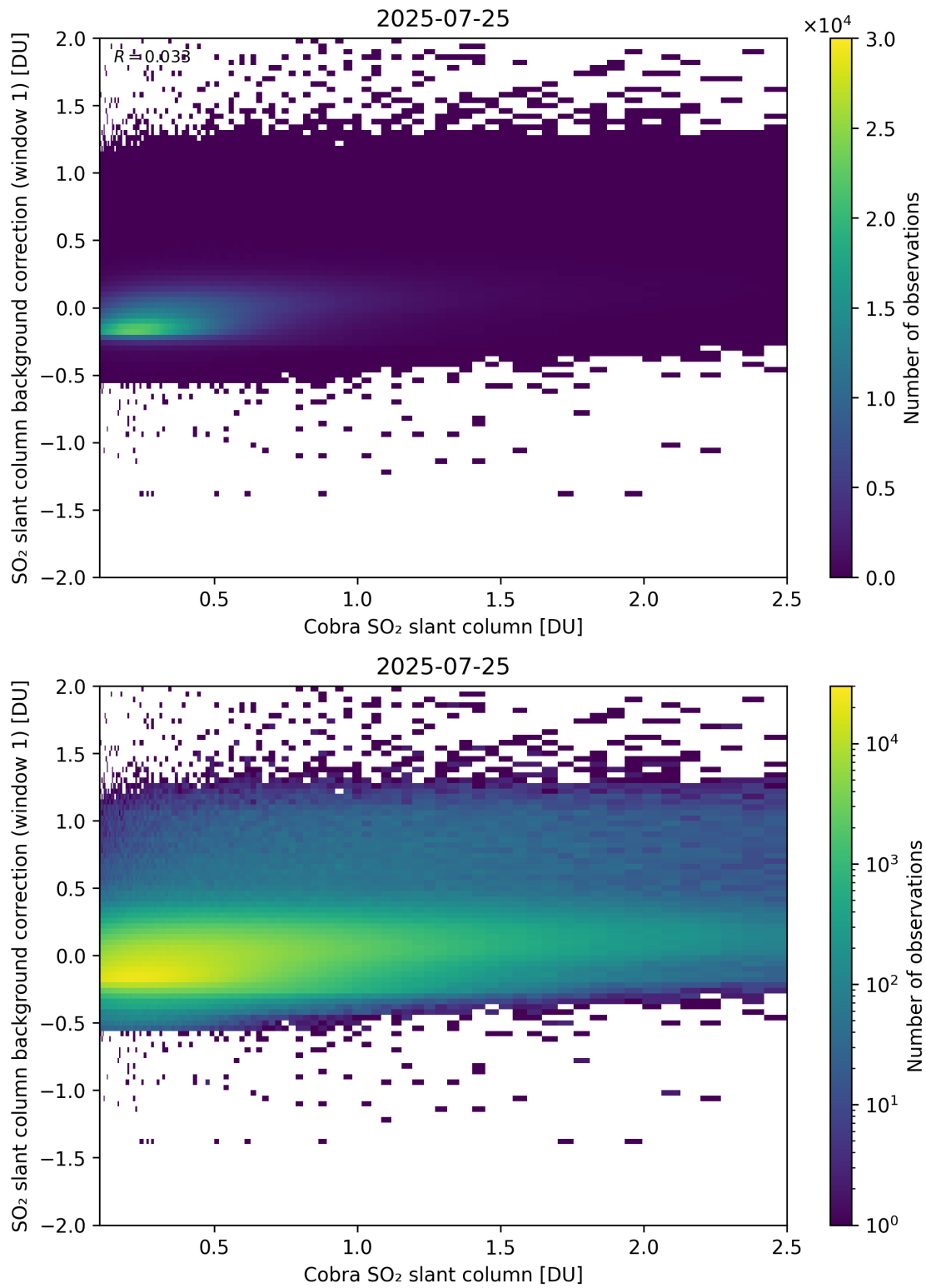
Figure 193: Scatter density plot of “Cobra SO 2 slant column” against “SO 2 slant column background correction (window 1)” for 2025-07-24 to 2025-07-26.
