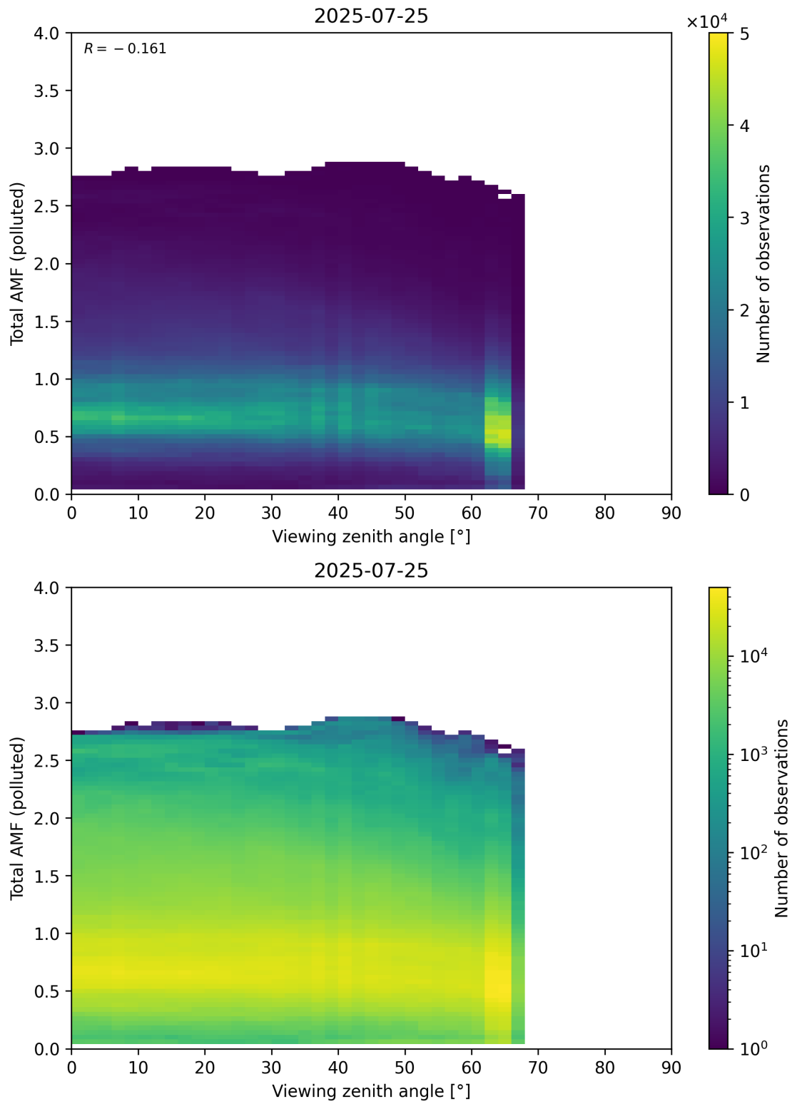
Figure 381: Scatter density plot of “Viewing zenith angle” against “Total AMF (polluted)” for 2025-07-24 to 2025-07-26.
