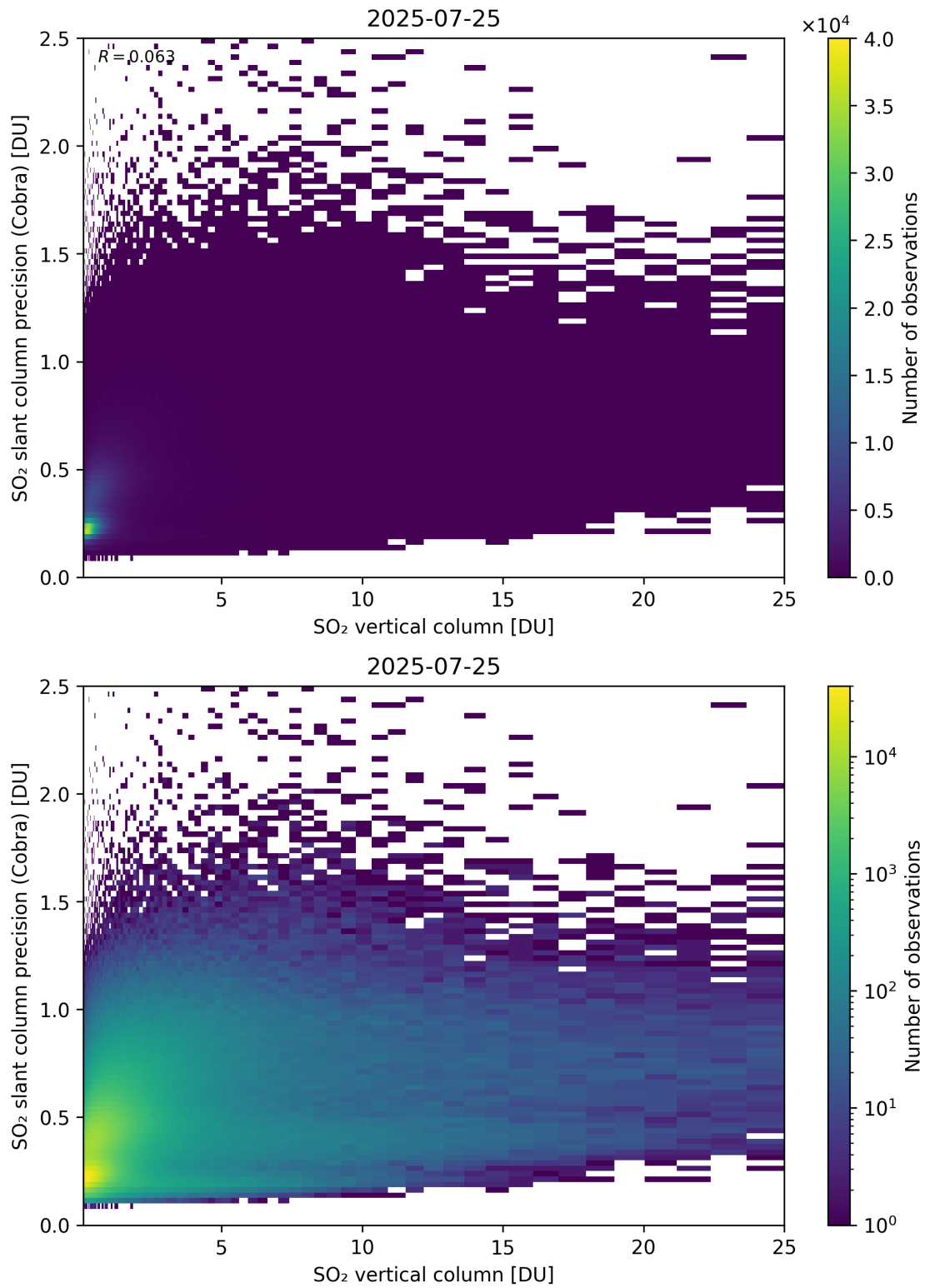
Figure 350: Scatter density plot of “SO 2 vertical column” against “SO 2 slant column precision (Cobra)” for 2025-07-24 to 2025-07-26.
