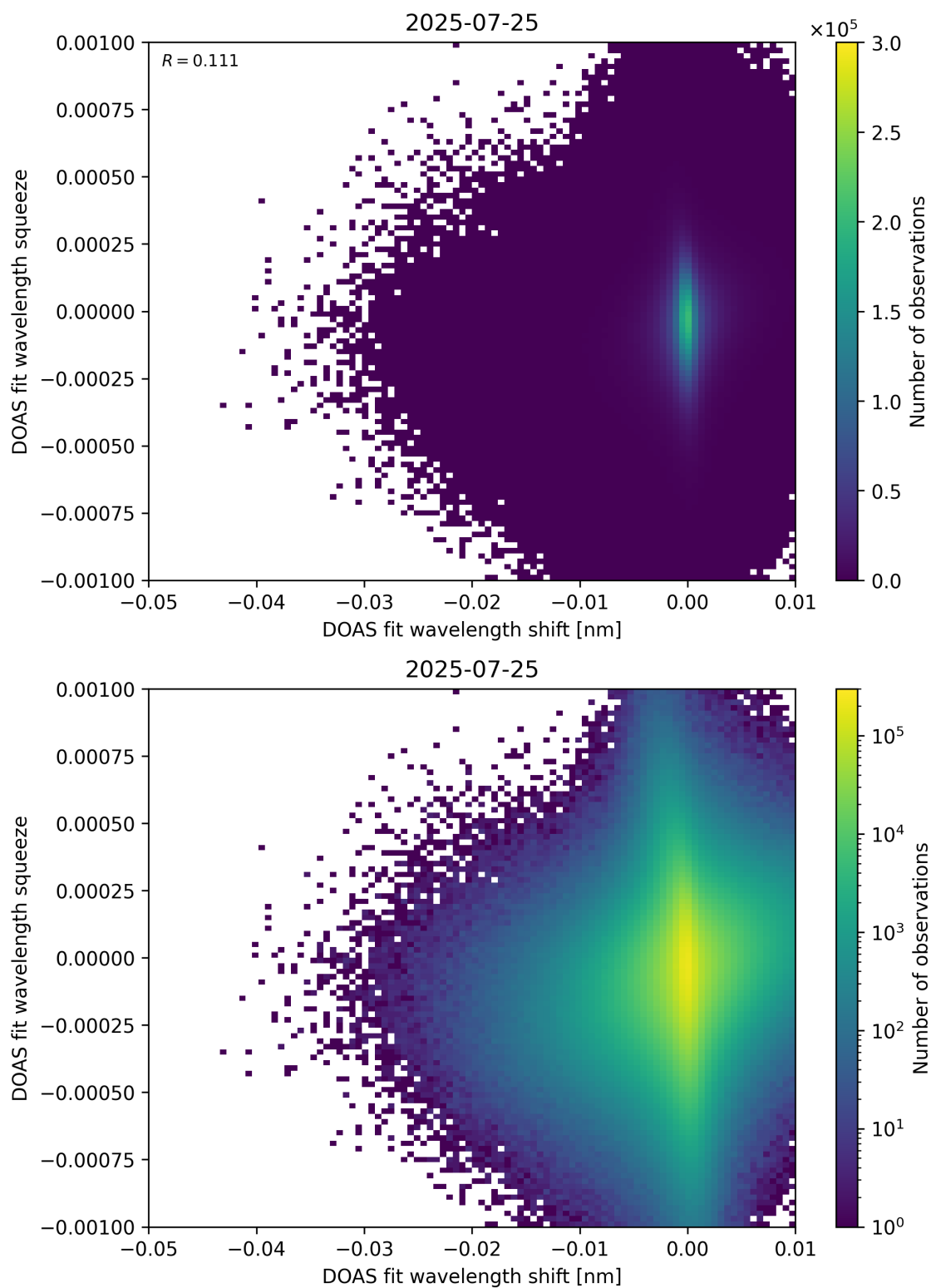
Figure 138: Scatter density plot of “DOAS fit wavelength shift” against “DOAS fit wavelength squeeze” for 2025-07-24 to 2025-07-26.
