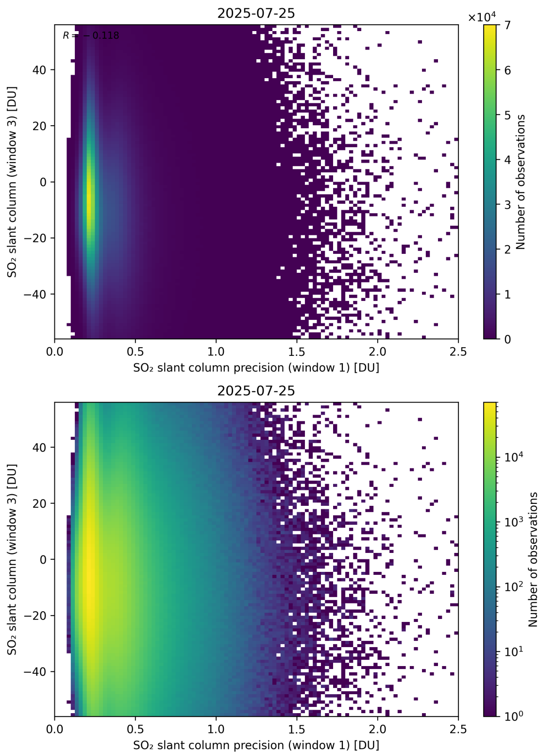
Figure 278: Scatter density plot of “SO 2 slant column precision (window 1)” against “SO 2 slant column (window 3)” for 2025-07-24 to 2025-07-26.
