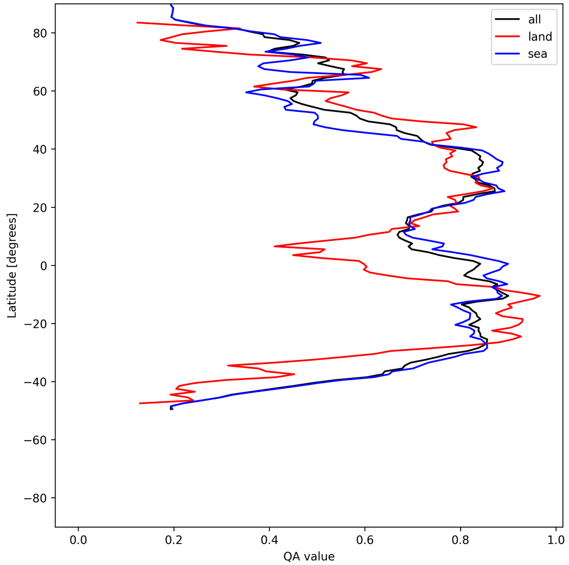
Figure 31: Zonal average of “QA value” for 2025-07-24 to 2025-07-26.
