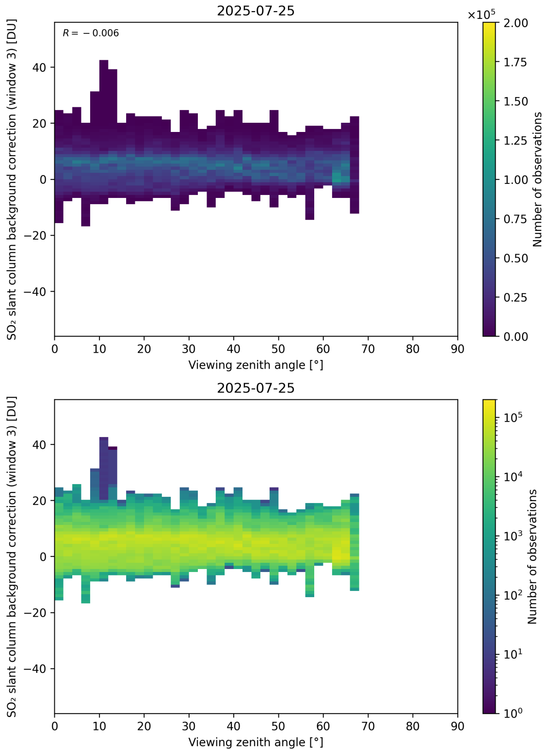
Figure 364: Scatter density plot of “Viewing zenith angle” against “SO 2 slant column background correction (window 3)” for 2025-07-24 to 2025-07-26.
