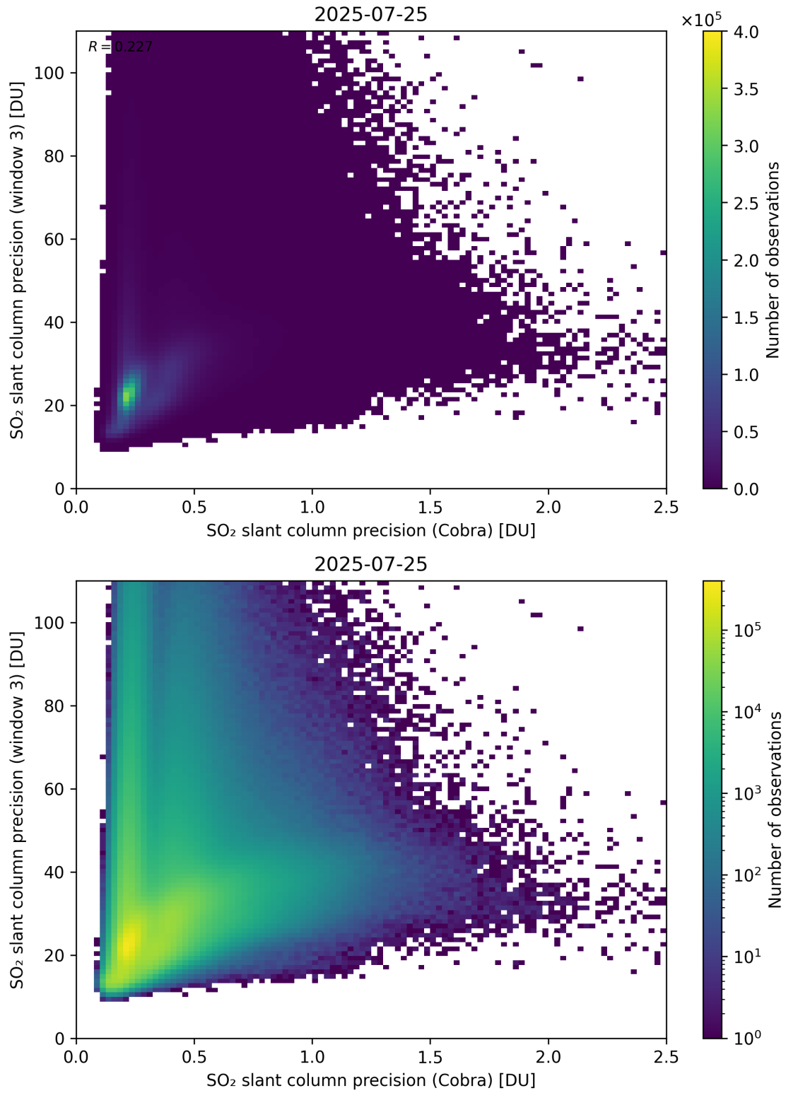
Figure 212: Scatter density plot of “SO 2 slant column precision (Cobra)” against “SO 2 slant column precision (window 3)” for 2025-07-24 to 2025-07-26.
