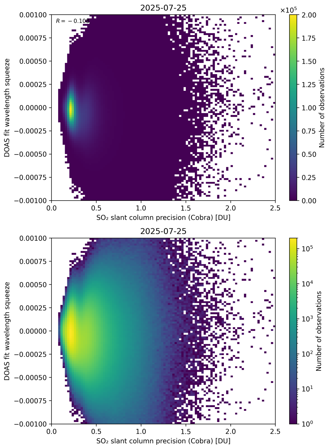
Figure 203: Scatter density plot of “SO 2 slant column precision (Cobra)” against “DOAS fit wavelength squeeze” for 2025-07-24 to 2025-07-26.
