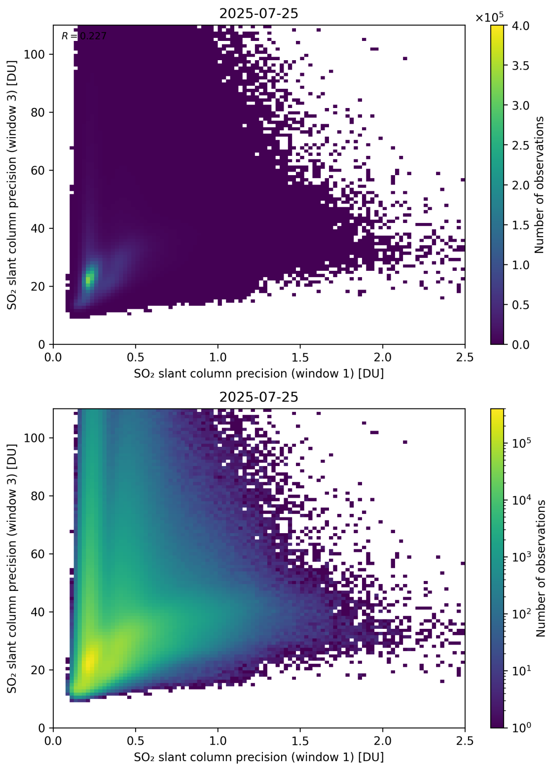
Figure 279: Scatter density plot of “SO 2 slant column precision (window 1)” against “SO 2 slant column precision (window 3)” for 2025-07-24 to 2025-07-26.
