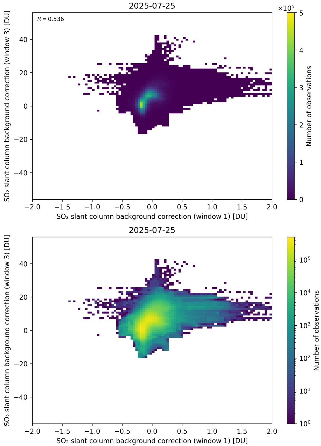
Figure 110: Scatter density plot of “SO 2 slant column background correction (window 1)” against “SO 2 slant column background correction (window 3)” for 2025-07-24 to 2025-07-26.
