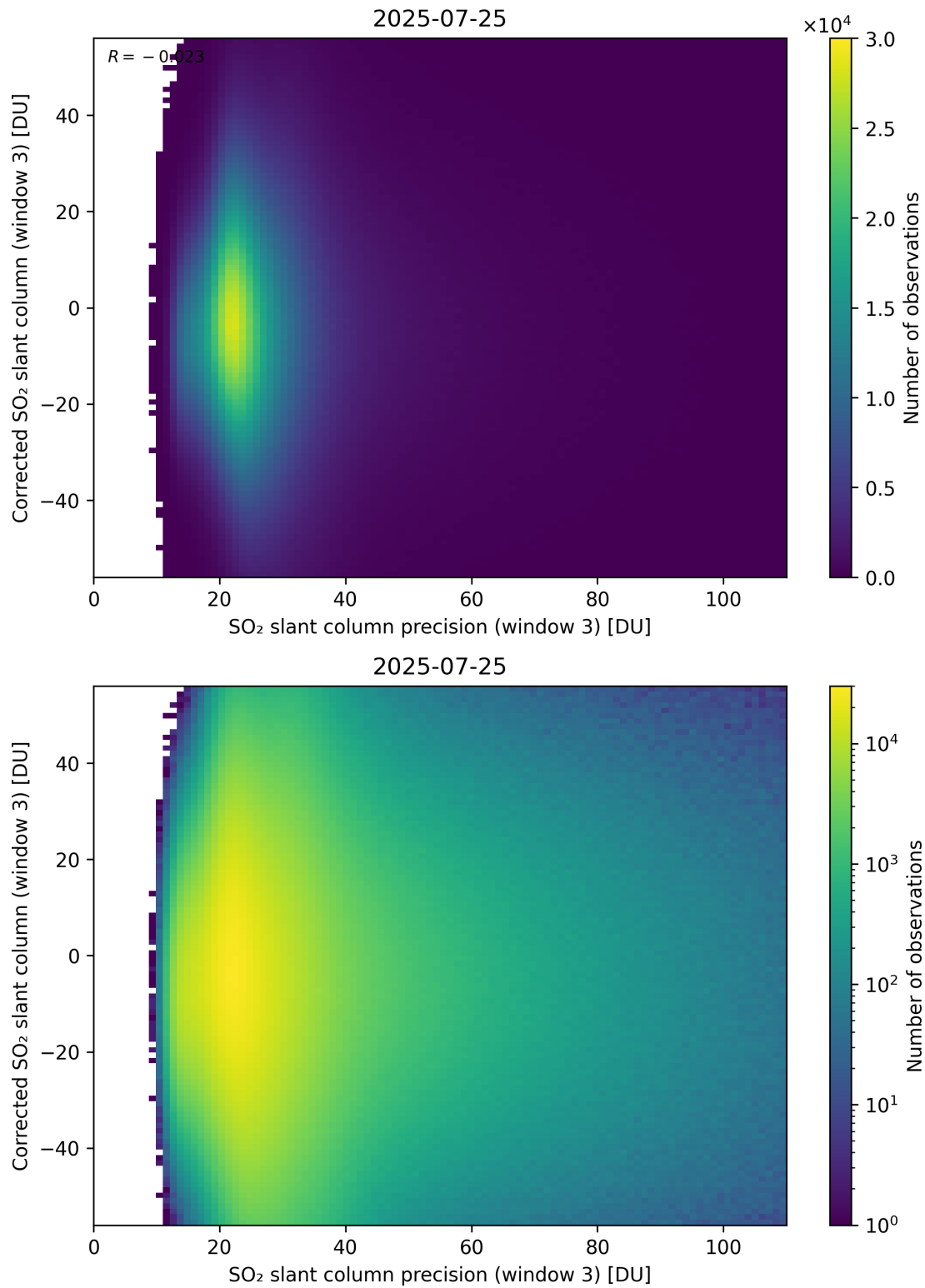
Figure 312: Scatter density plot of “SO 2 slant column precision (window 3)” against “Corrected SO 2 slant column (window 3)” for 2025-07-24 to 2025-07-26.
