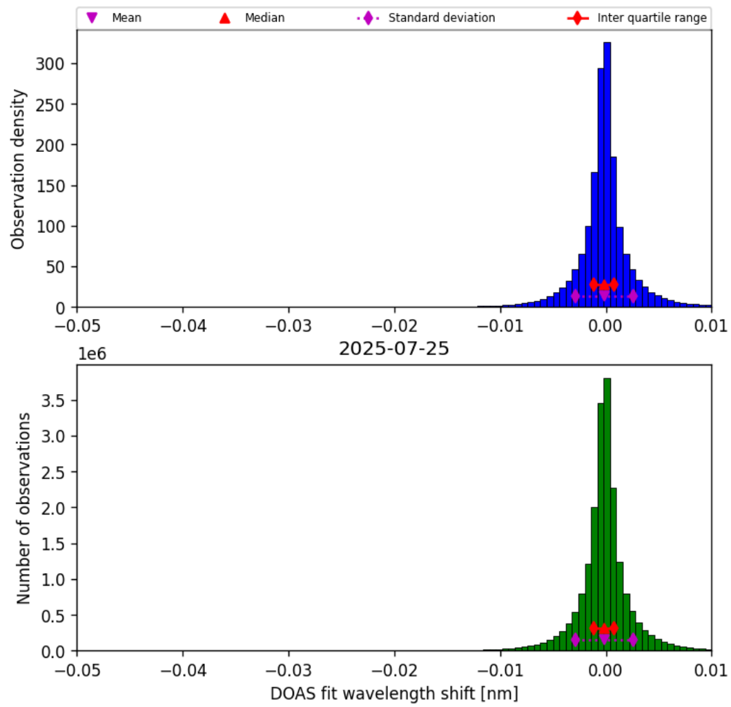
Figure 76: Histogram of “DOAS fit wavelength shift” for 2025-07-24 to 2025-07-26
