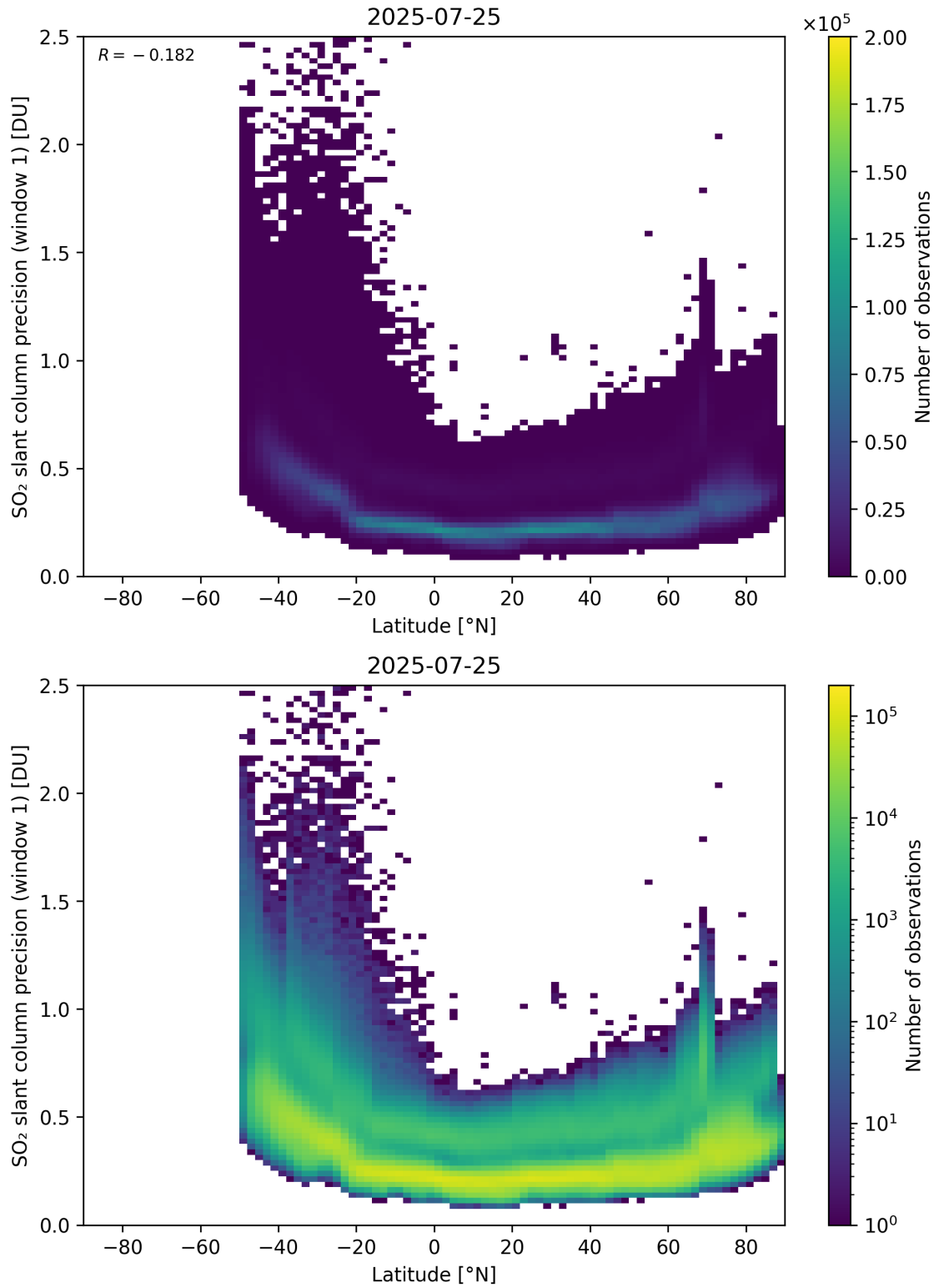
Figure 163: Scatter density plot of “Latitude” against “SO 2 slant column precision (window 1)” for 2025-07-24 to 2025-07-26.
