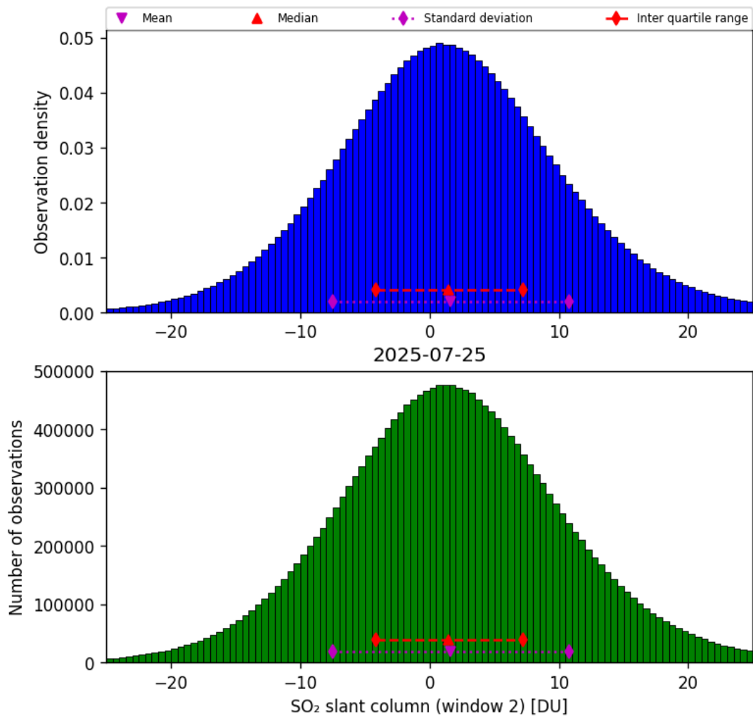
Figure 67: Histogram of “SO 2 slant column (window 2)” for 2025-07-24 to 2025-07-26
