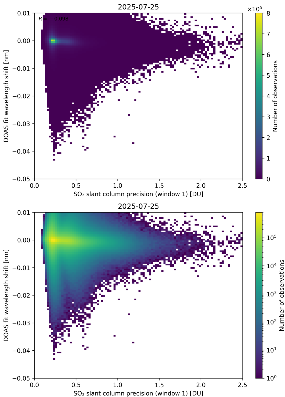
Figure 271: Scatter density plot of “SO 2 slant column precision (window 1)” against “DOAS fit wavelength shift” for 2025-07-24 to 2025-07-26.
