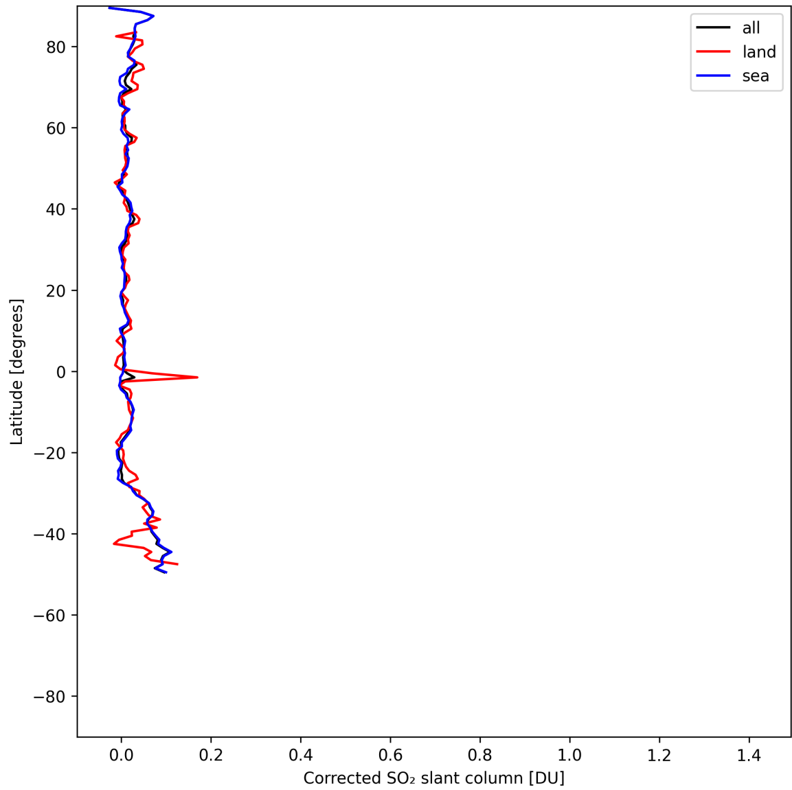
Figure 34: Zonal average of “Corrected SO 2 slant column” for 2025-07-24 to 2025-07-26.
