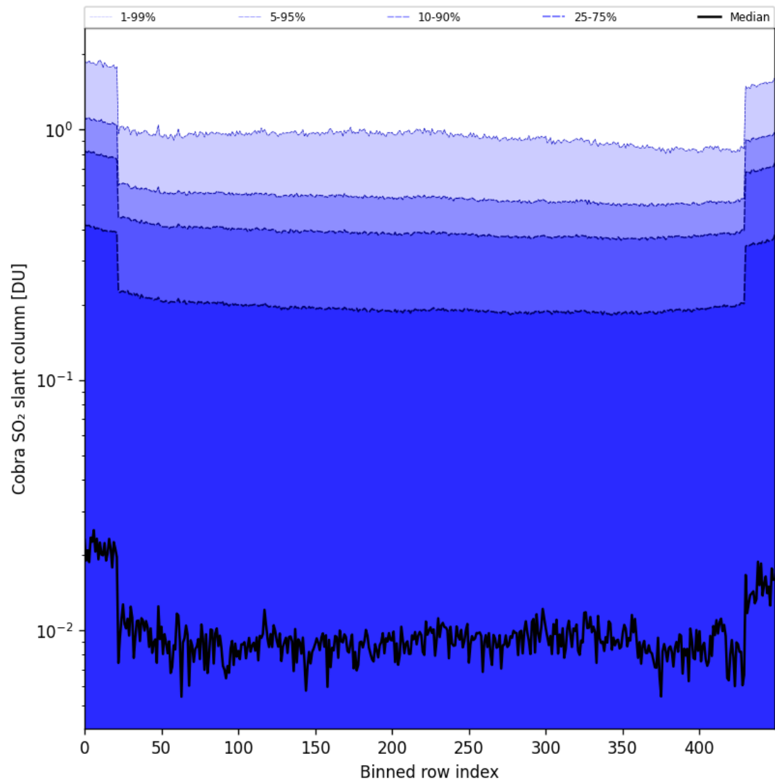
Figure 87: Along track statistics of "Cobra SO 2 slant column" for 2025-07-24 to 2025-07-26
