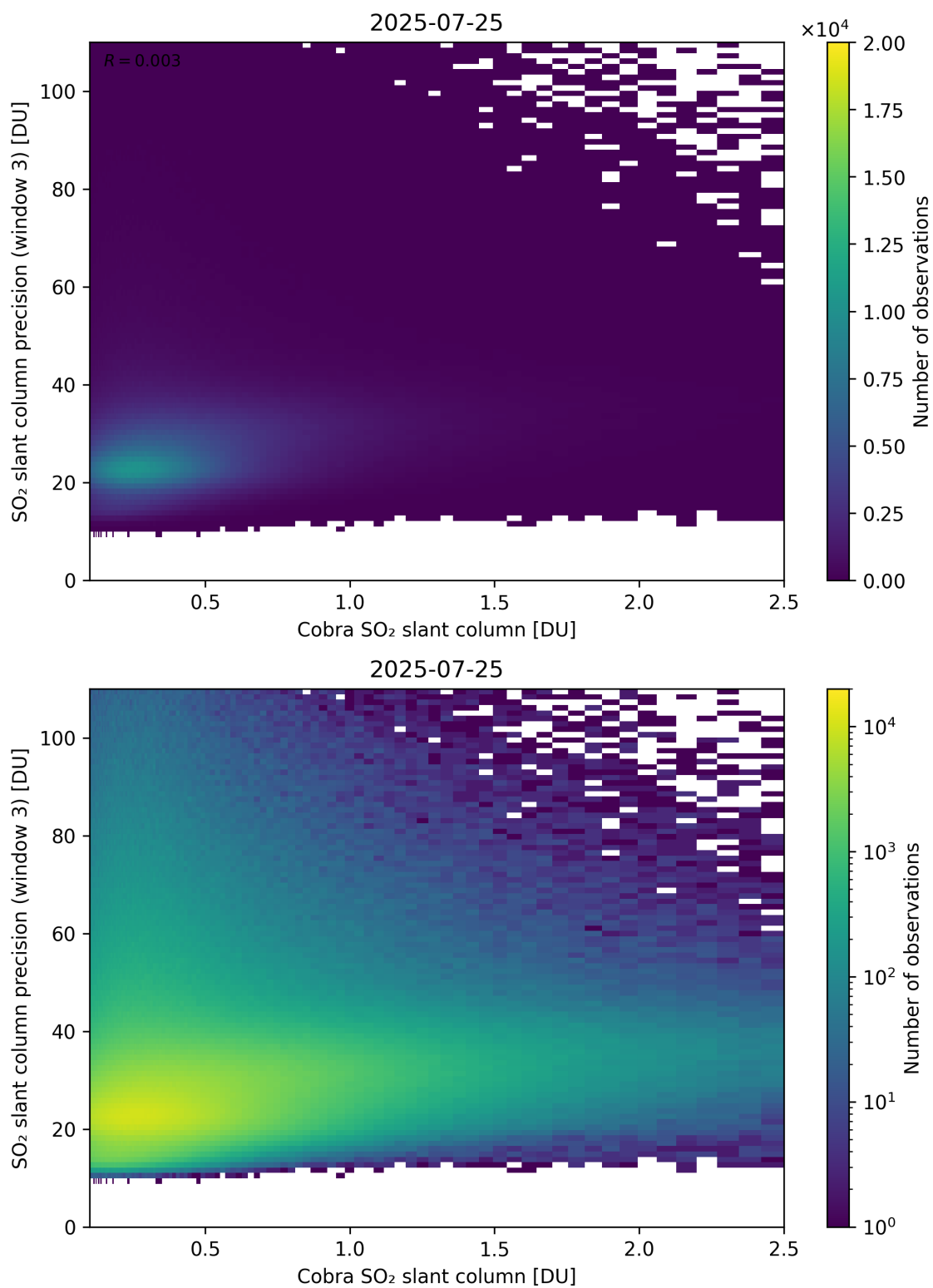
Figure 223: Scatter density plot of “Cobra SO 2 slant column” against “SO 2 slant column precision (window 3)” for 2025-07-24 to 2025-07-26.
