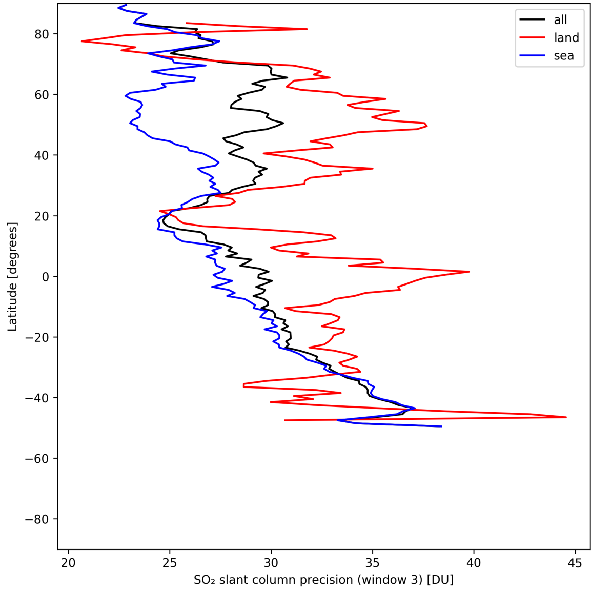
Figure 46: Zonal average of “SO 2 slant column precision (window 3)” for 2025-07-24 to 2025-07-26.
