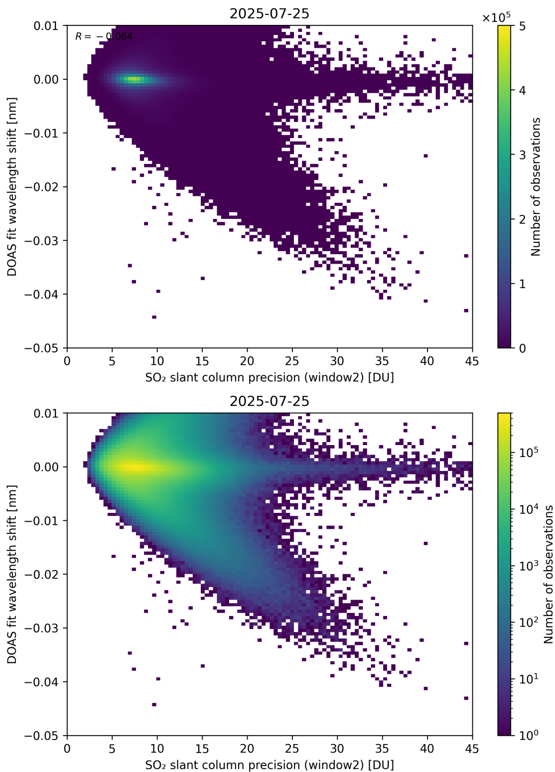
Figure 293: Scatter density plot of “SO 2 slant column precision (window2)” against “DOAS fit wavelength shift” for 2025-07-24 to 2025-07-26.
