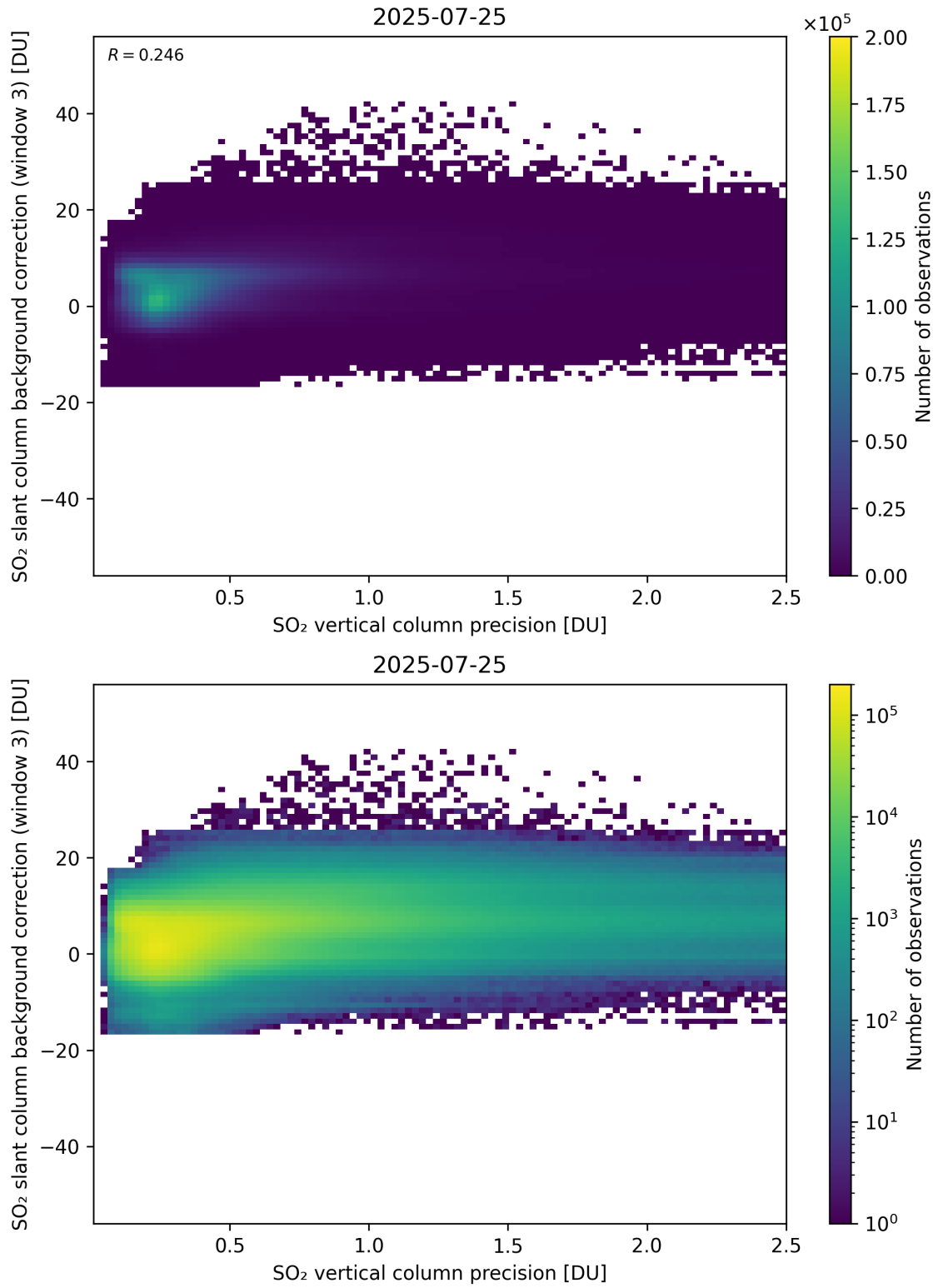
Figure 331: Scatter density plot of “SO 2 vertical column precision” against “SO 2 slant column background correction (window 3)” for 2025-07-24 to 2025-07-26.
