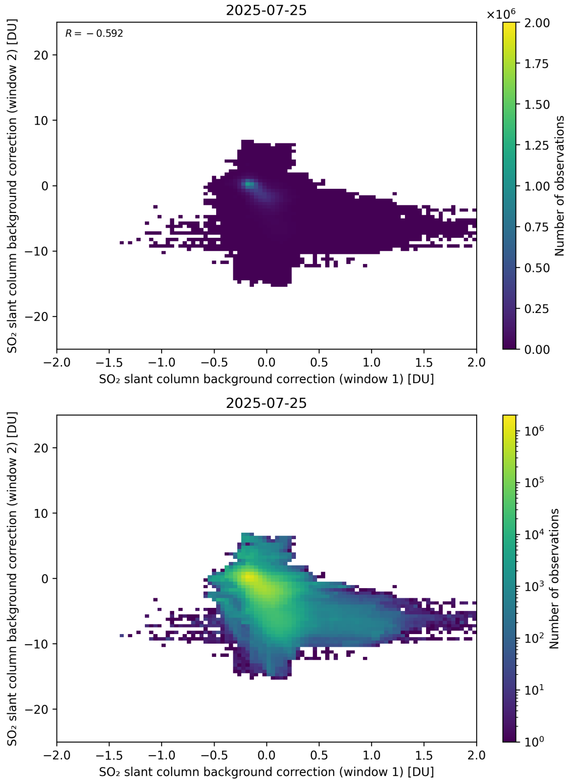
Figure 109: Scatter density plot of “SO 2 slant column background correction (window 1)” against “SO 2 slant column background correction (window 2)” for 2025-07-24 to 2025-07-26.
