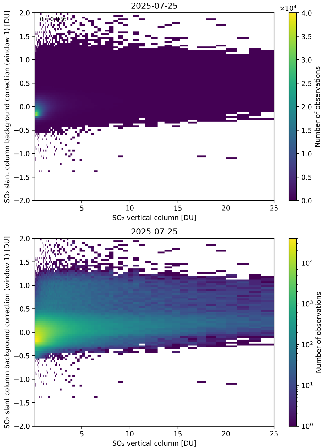
Figure 323: Scatter density plot of “SO 2 vertical column” against “SO 2 slant column background correction (window 1)” for 2025-07-24 to 2025-07-26.
