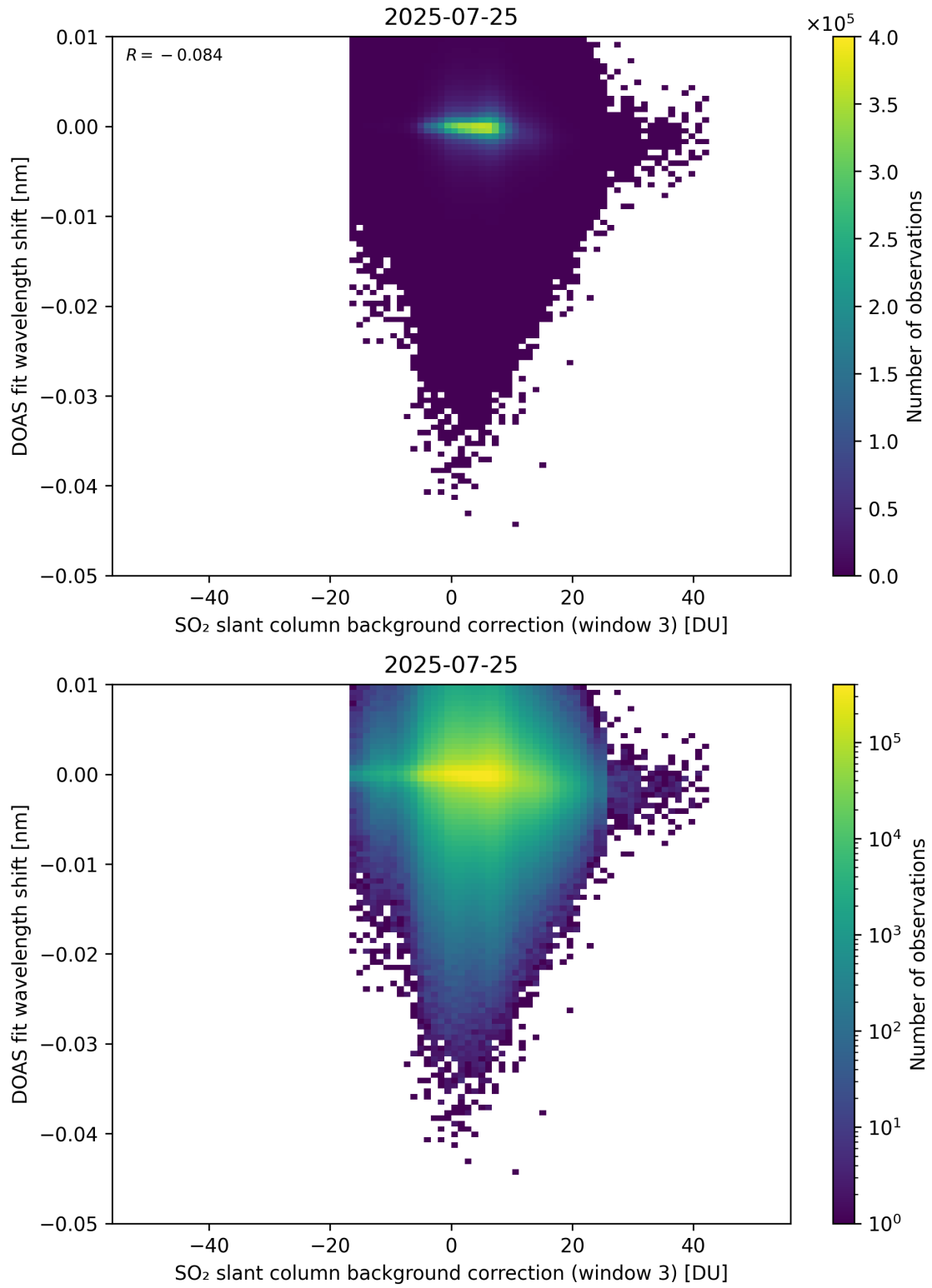
Figure 132: Scatter density plot of “SO 2 slant column background correction (window 3)” against “DOAS fit wavelength shift” for 2025-07-24 to 2025-07-26.
