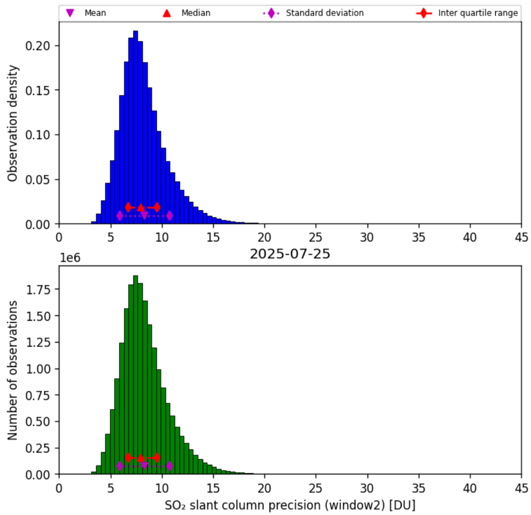
Figure 68: Histogram of “SO 2 slant column precision (window2)” for 2025-07-24 to 2025-07-26
