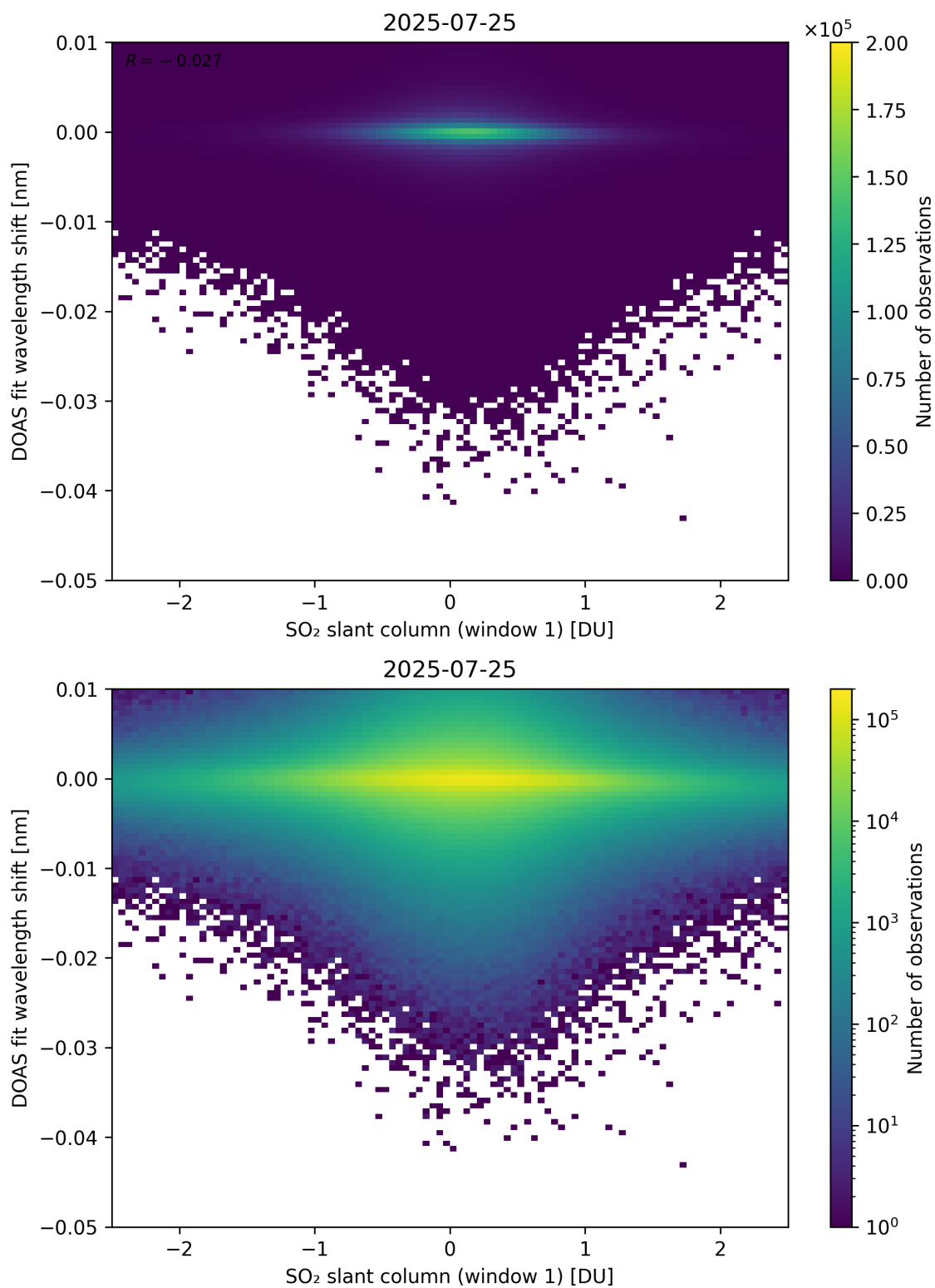
Figure 265: Scatter density plot of “SO 2 slant column (window 1)” against “DOAS fit wavelength shift” for 2025-07-24 to 2025-07-26.
