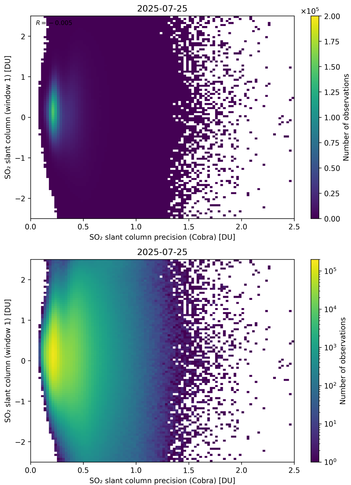
Figure 208: Scatter density plot of “SO 2 slant column precision (Cobra)” against “SO 2 slant column (window 1)” for 2025-07-24 to 2025-07-26.
