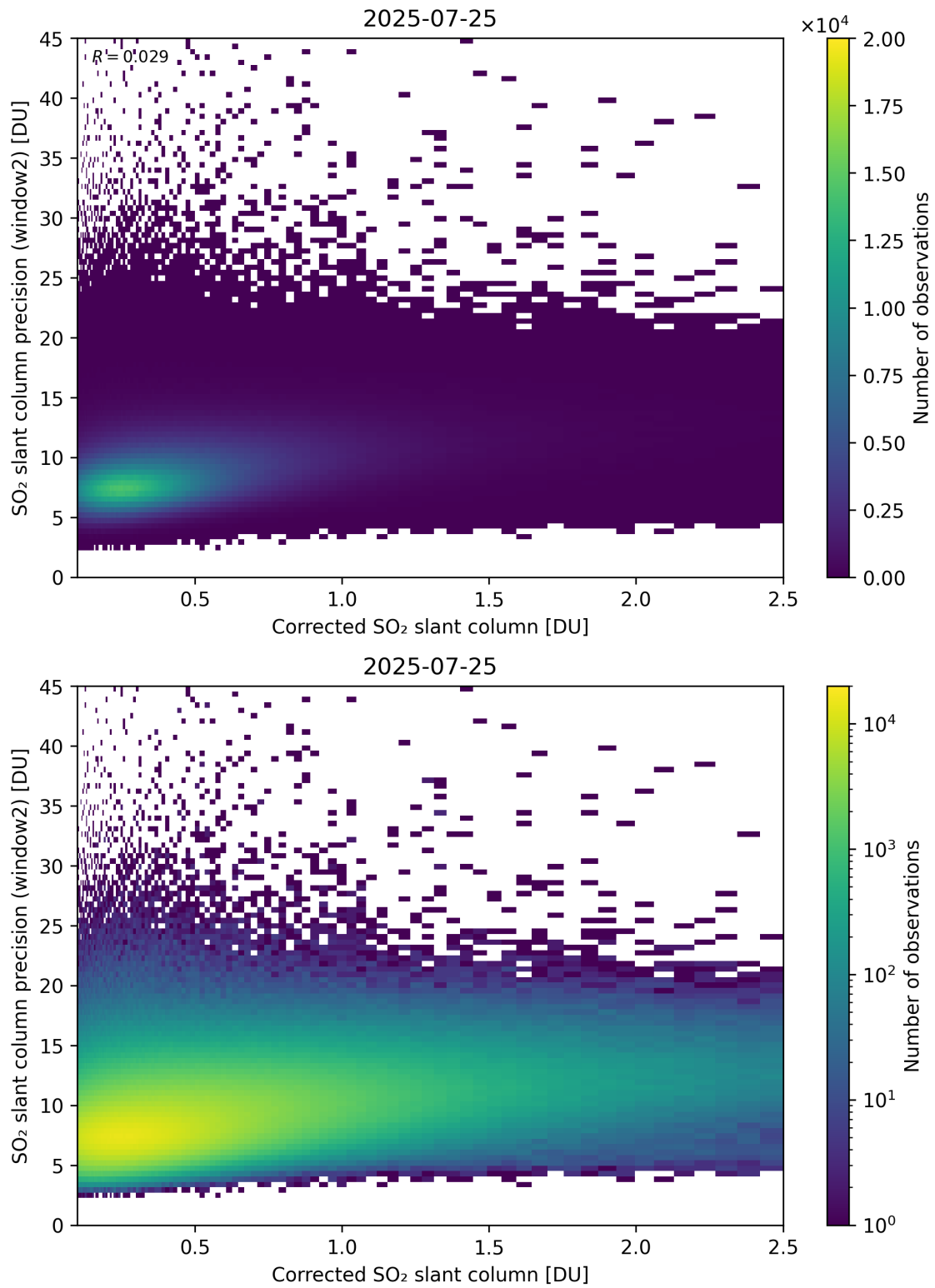
Figure 239: Scatter density plot of “Corrected SO 2 slant column” against “SO 2 slant column precision (window2)” for 2025-07-24 to 2025-07-26.
