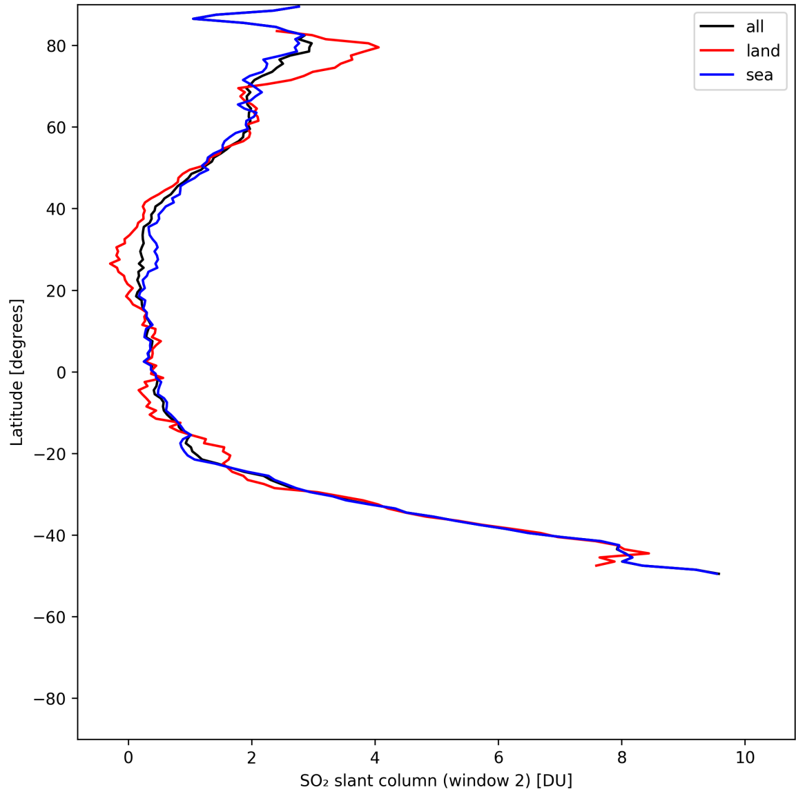
Figure 41: Zonal average of “SO 2 slant column (window 2)” for 2025-07-24 to 2025-07-26.
