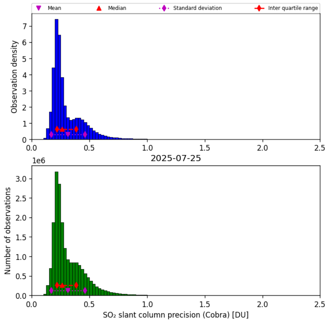
Figure 62: Histogram of “SO 2 slant column precision (Cobra)” for 2025-07-24 to 2025-07-26
