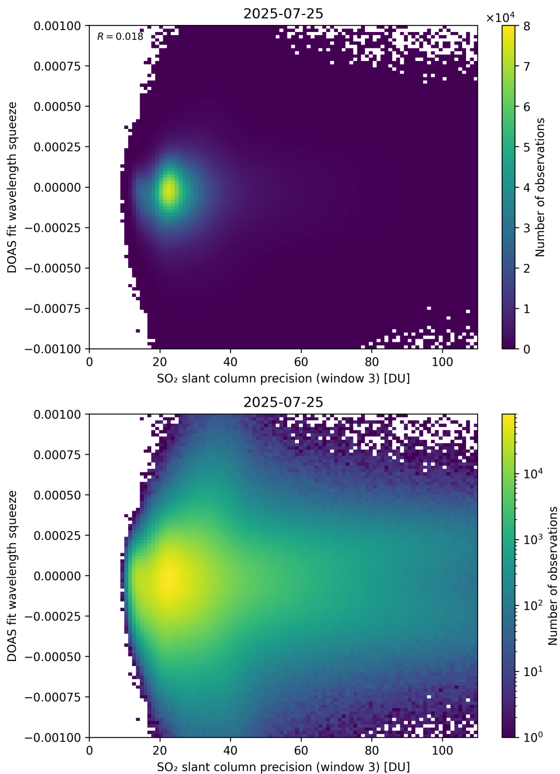
Figure 309: Scatter density plot of “SO 2 slant column precision (window 3)” against “DOAS fit wavelength squeeze” for 2025-07-24 to 2025-07-26.
