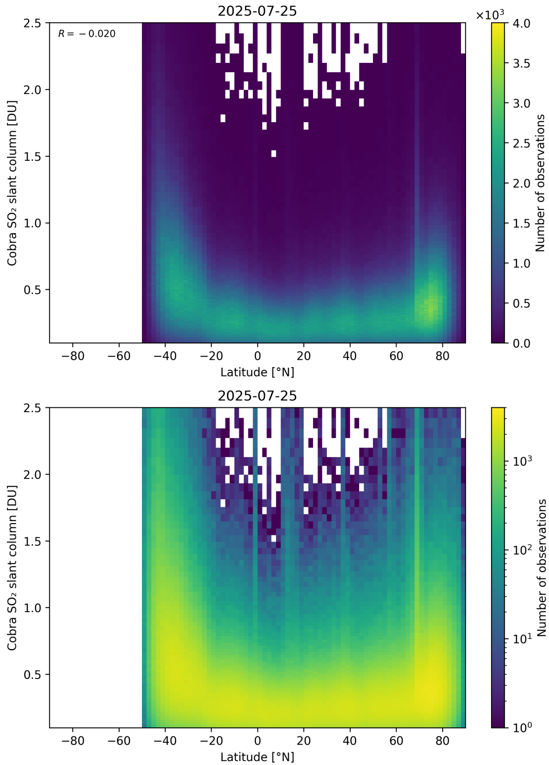
Figure 157: Scatter density plot of “Latitude” against “Cobra SO 2 slant column” for 2025-07-24 to 2025-07-26.
