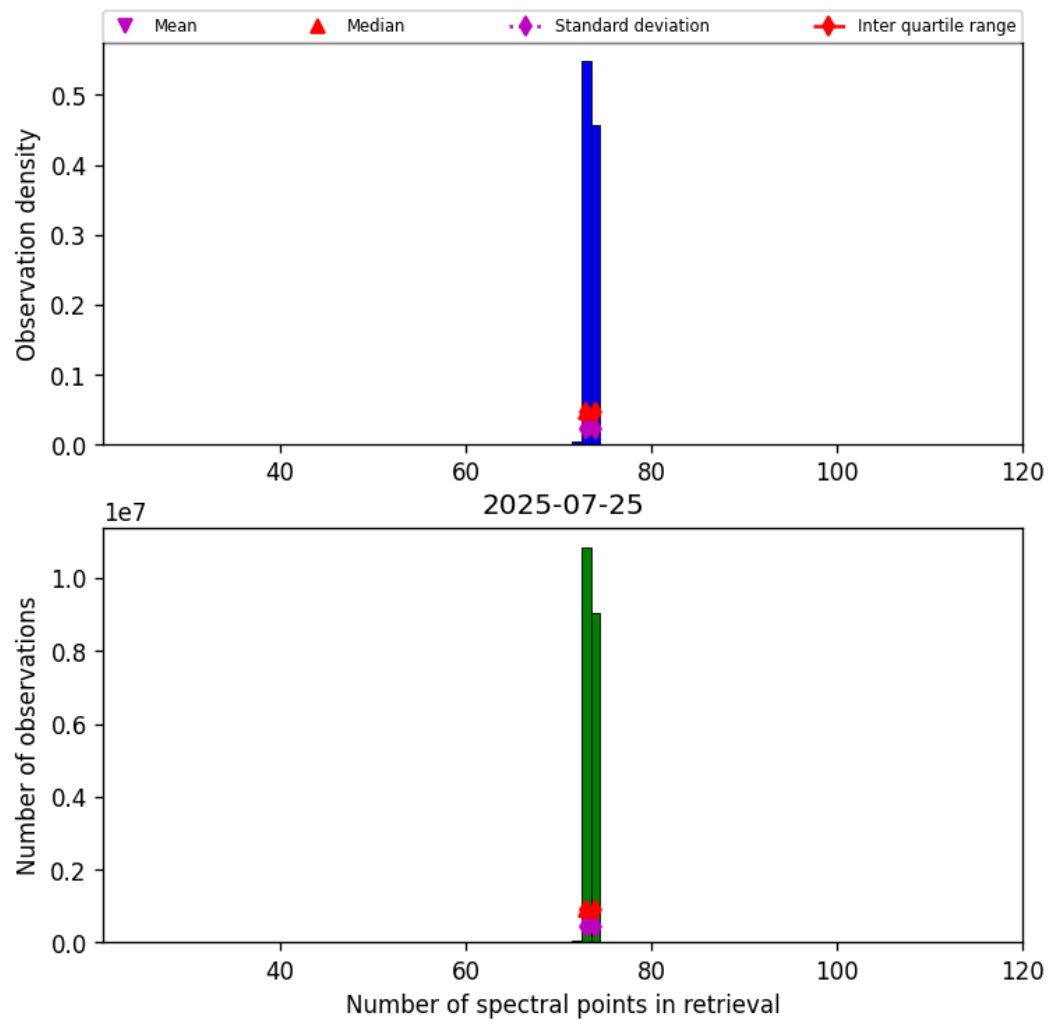
Figure 82: Histogram of “Number of spectral points in retrieval” for 2025-07-24 to 2025-07-26
