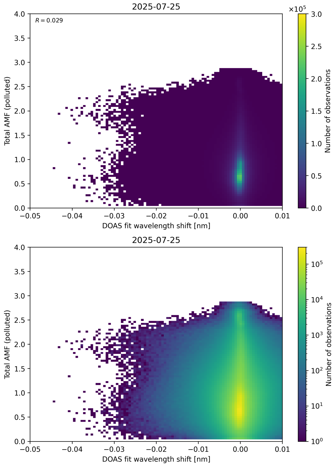
Figure 141: Scatter density plot of “DOAS fit wavelength shift” against “Total AMF (polluted)” for 2025-07-24 to 2025-07-26.
