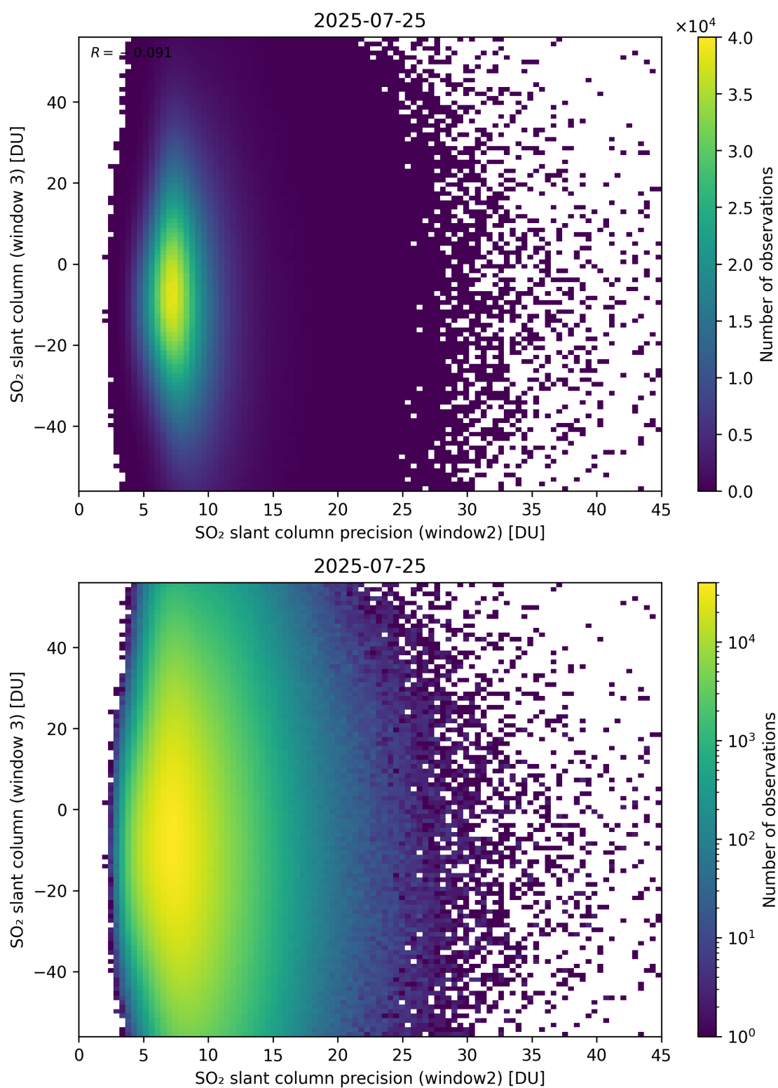
Figure 299: Scatter density plot of “SO 2 slant column precision (window2)” against “SO 2 slant column (window 3)” for 2025-07-24 to 2025-07-26.
