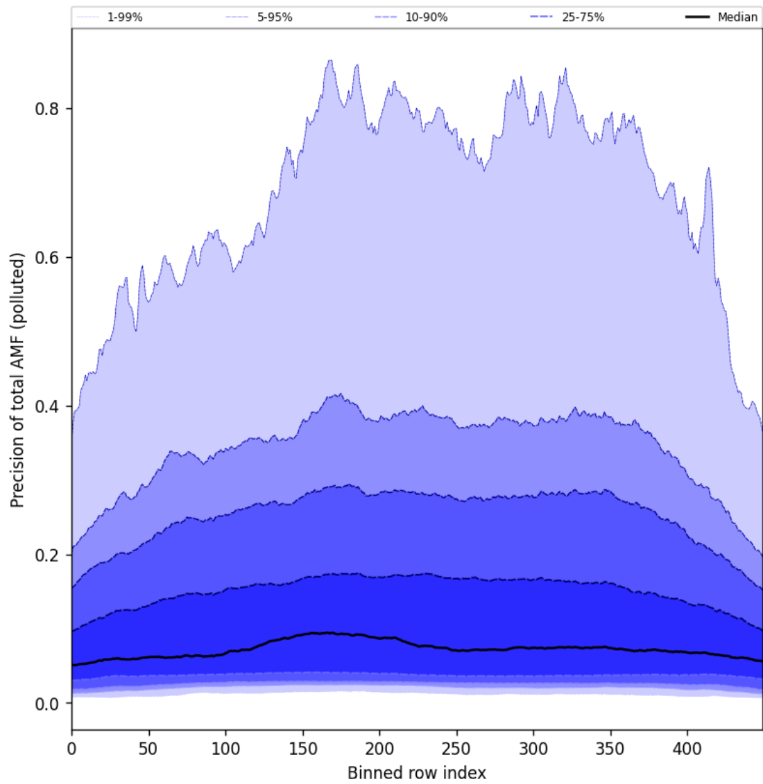
Figure 106: Along track statistics of “Precision of total AMF (polluted)” for 2025-07-24 to 2025-07-26
