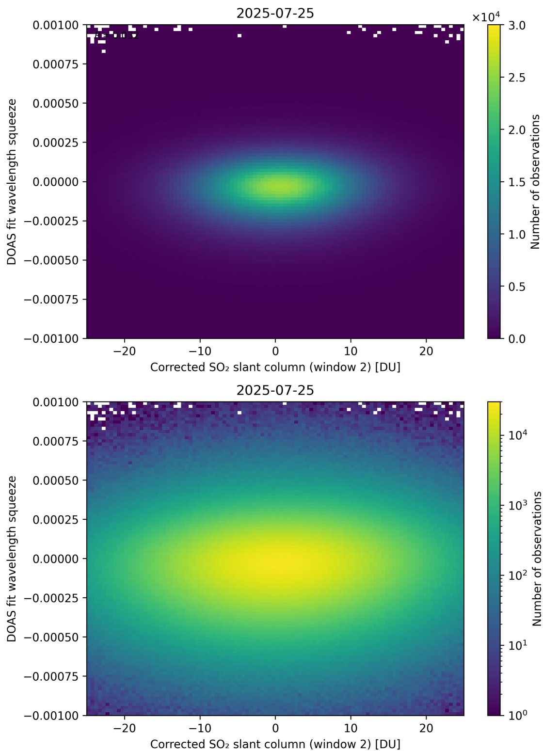
Figure 247: Scatter density plot of “Corrected SO 2 slant column (window 2)” against “DOAS fit wavelength squeeze” for 2025-07-24 to 2025-07-26.
