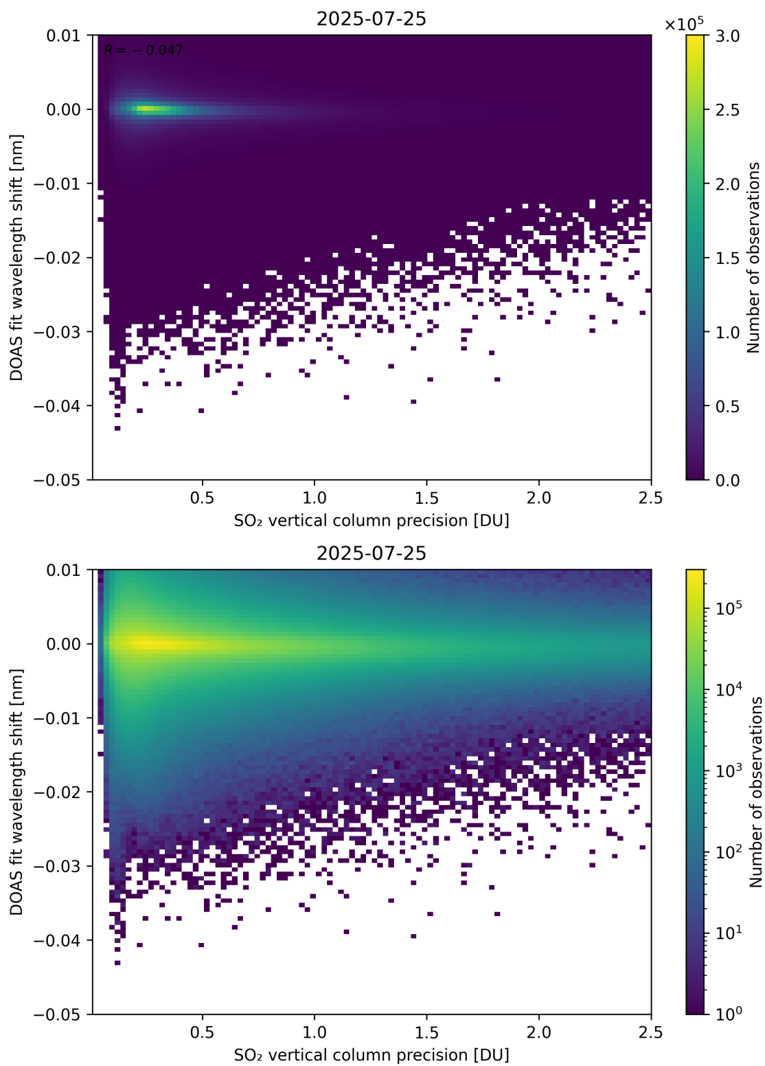
Figure 332: Scatter density plot of “SO 2 vertical column precision” against “DOAS fit wavelength shift” for 2025-07-24 to 2025-07-26.
