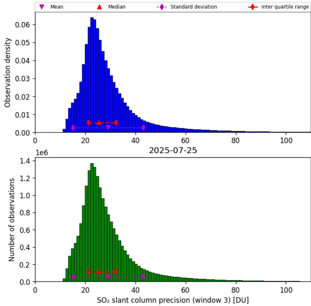
Figure 72: Histogram of “SO 2 slant column precision (window 3)” for 2025-07-24 to 2025-07-26
