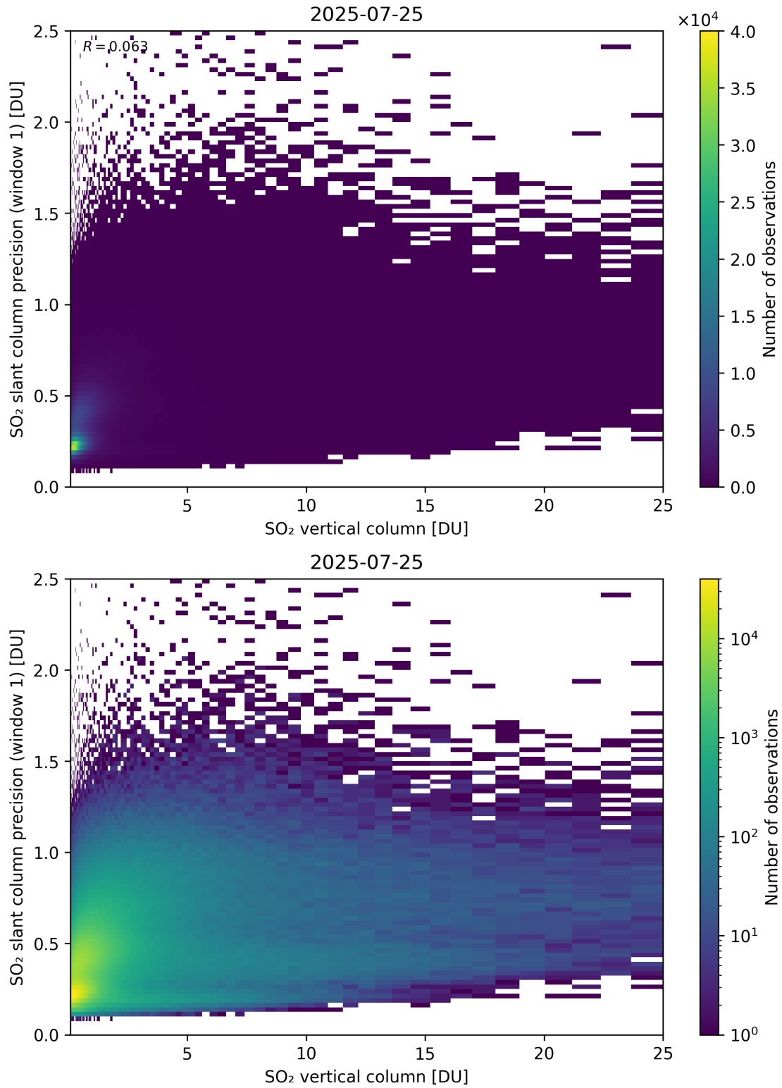
Figure 355: Scatter density plot of “SO 2 vertical column” against “SO 2 slant column precision (window 1)” for 2025-07-24 to 2025-07-26.
