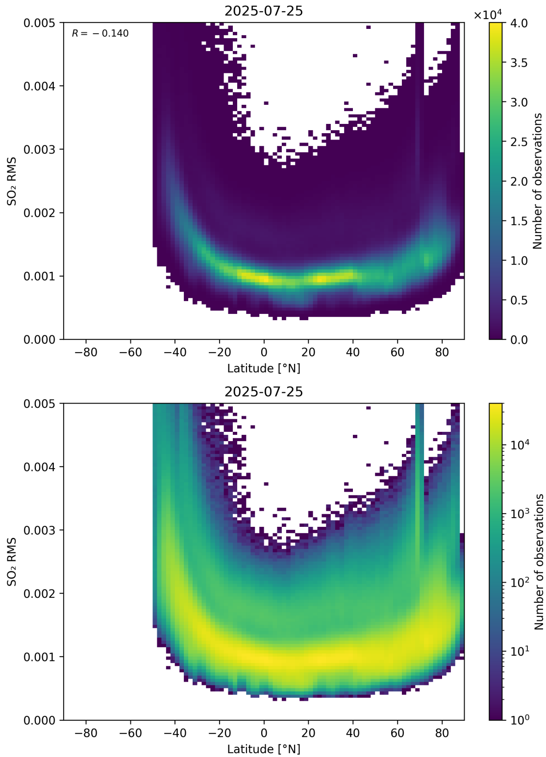
Figure 155: Scatter density plot of “Latitude” against “SO 2 RMS” for 2025-07-24 to 2025-07-26.
