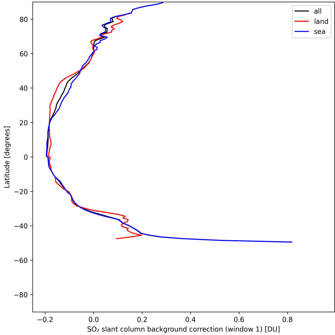
Figure 40: Zonal average of “SO 2 slant column background correction (window 1)” for 2025-07-24 to 2025-07-26.
