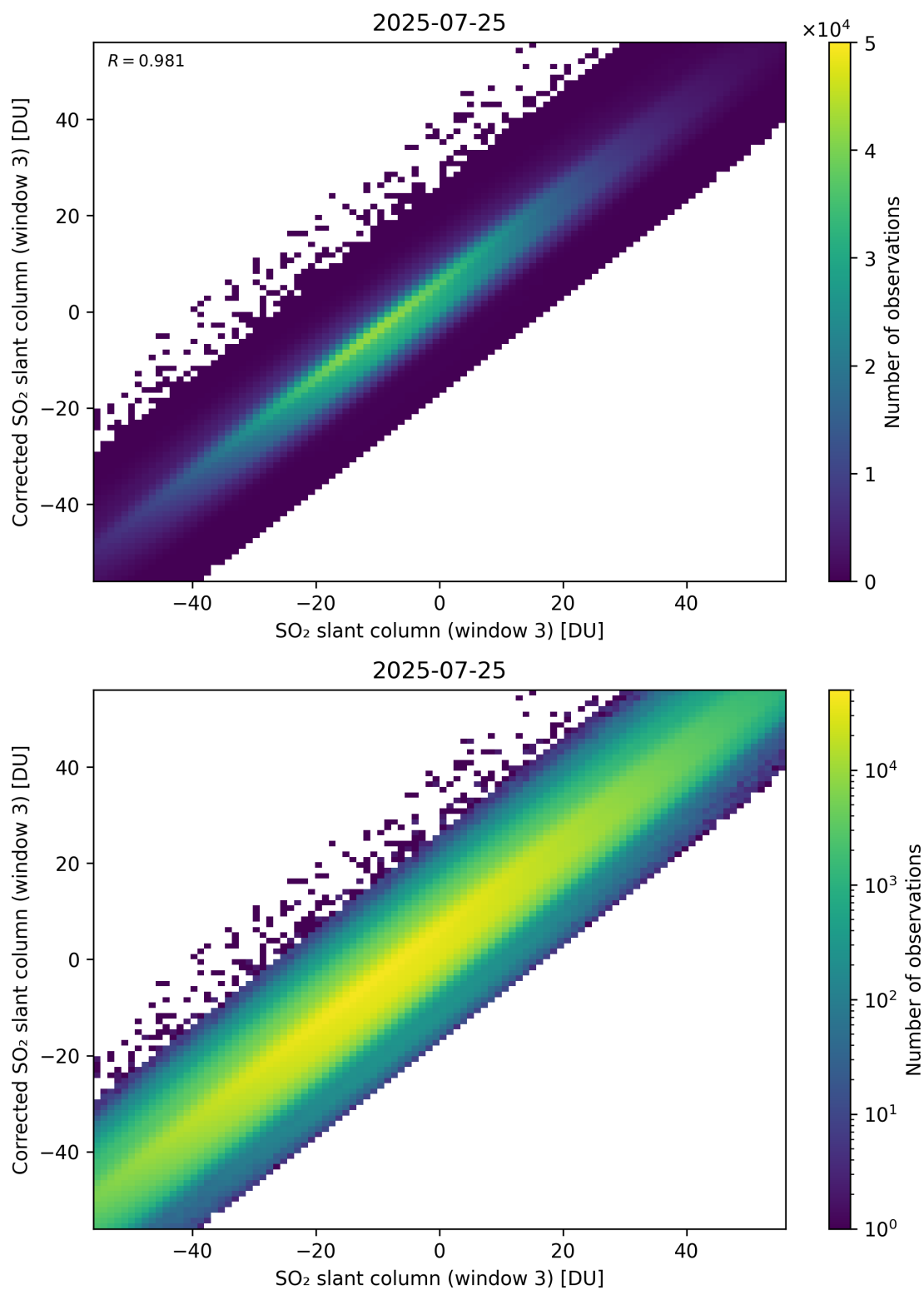
Figure 316: Scatter density plot of “SO 2 slant column (window 3)” against “Corrected SO 2 slant column (window 3)” for 2025-07-24 to 2025-07-26.
