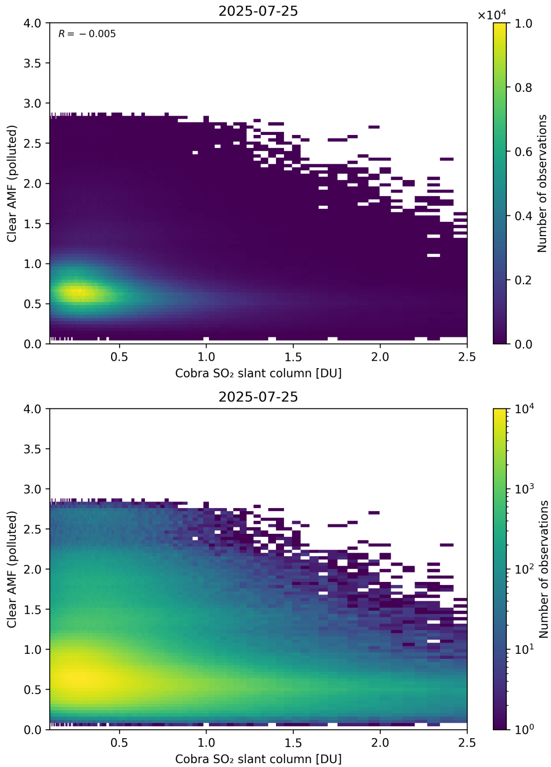
Figure 215: Scatter density plot of “Cobra SO 2 slant column” against “Clear AMF (polluted)” for 2025-07-24 to 2025-07-26.
