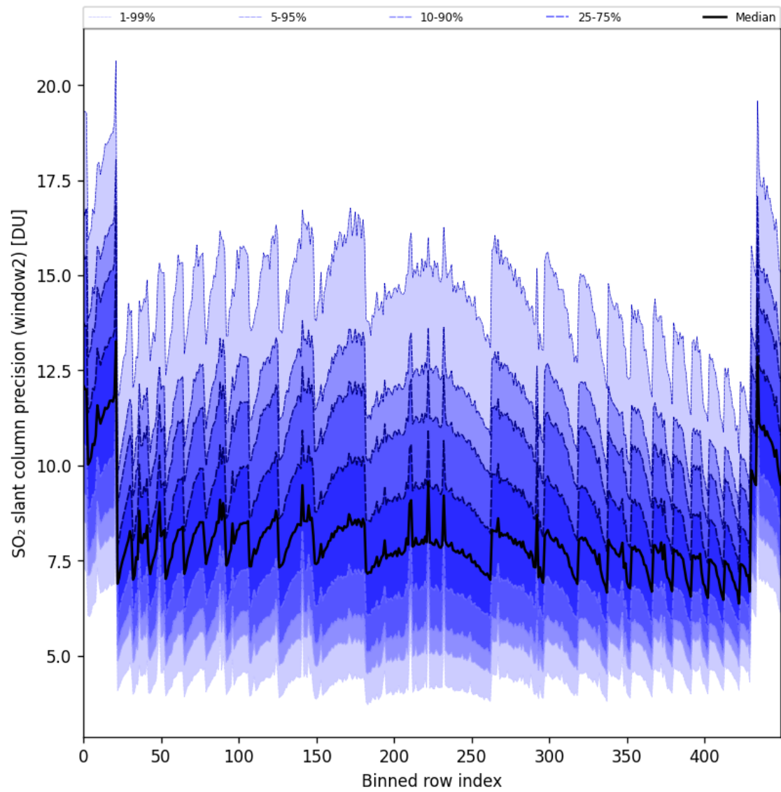
Figure 94: Along track statistics of “SO 2 slant column precision (window2)” for 2025-07-24 to 2025-07-26
