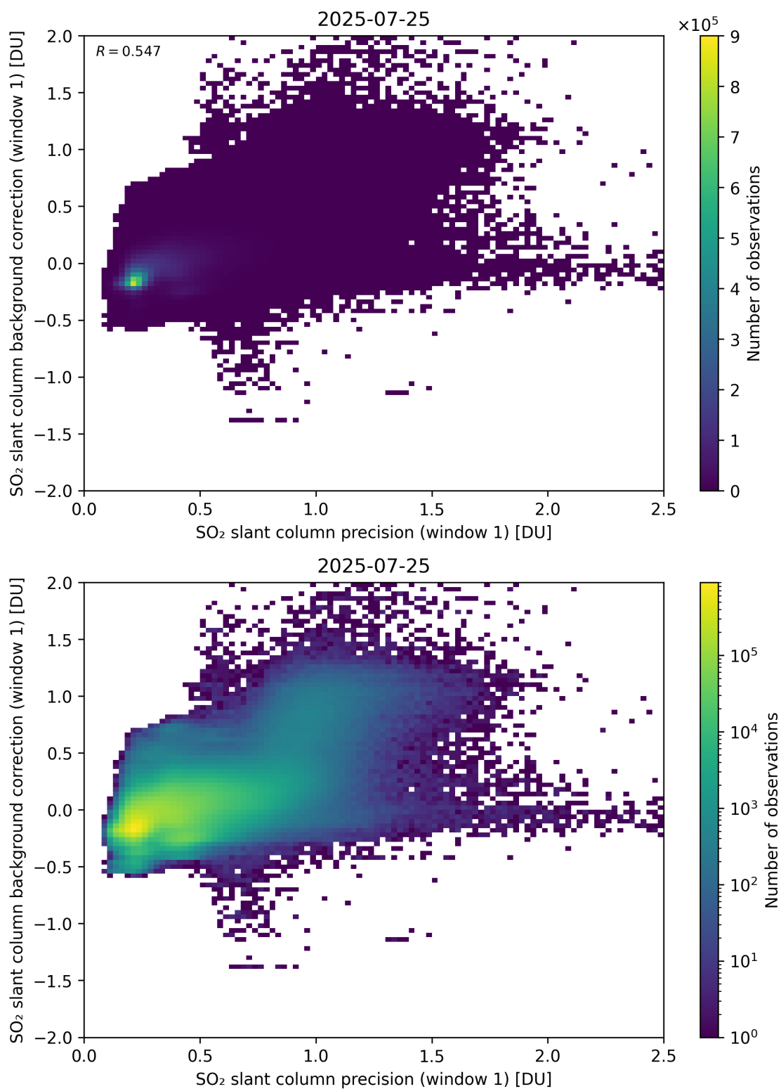
Figure 268: Scatter density plot of “SO 2 slant column precision (window 1)” against “SO 2 slant column background correction (window 1)” for 2025-07-24 to 2025-07-26.
