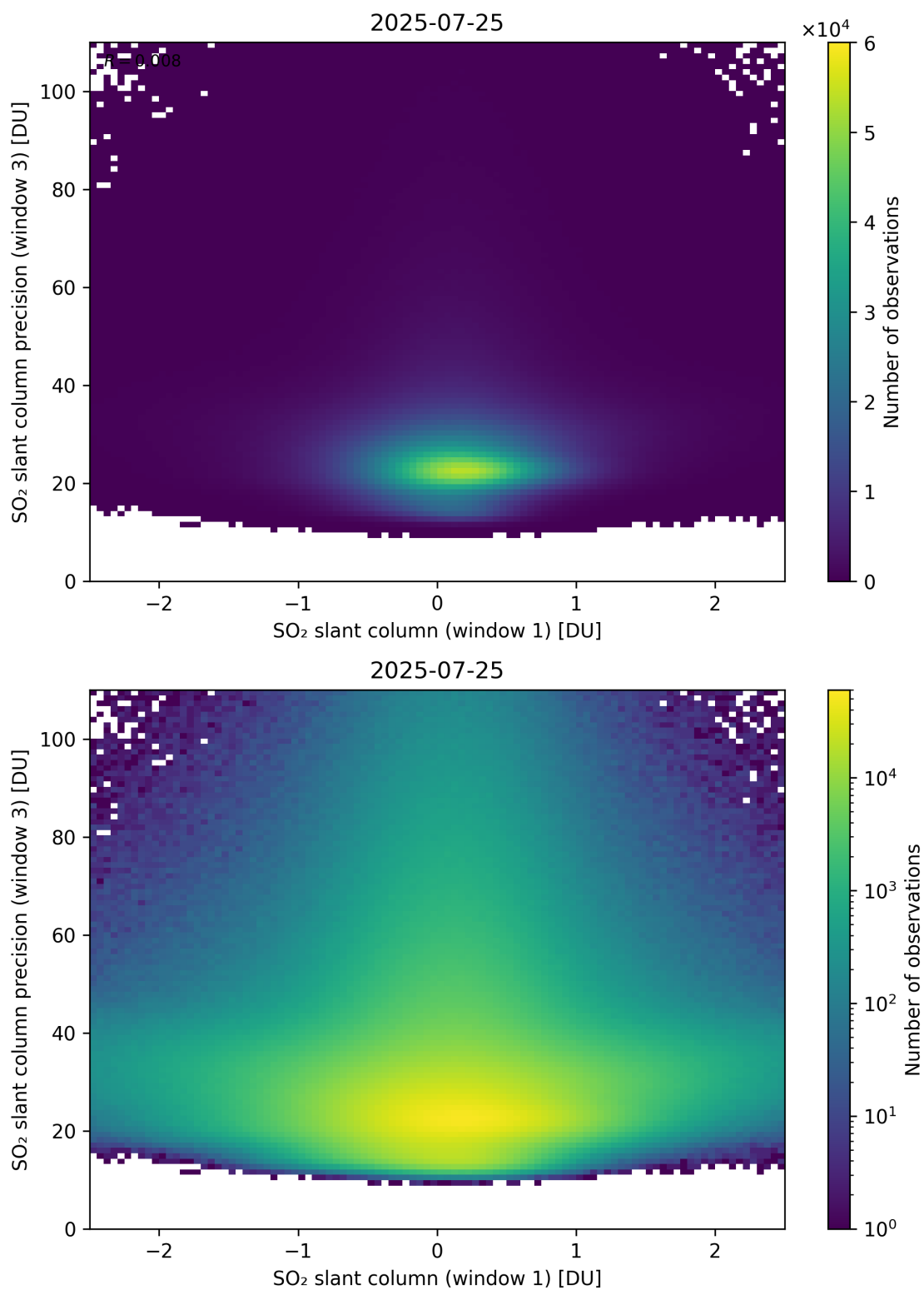
Figure 288: Scatter density plot of “SO 2 slant column (window 1)” against “SO 2 slant column precision (window 3)” for 2025-07-24 to 2025-07-26.
