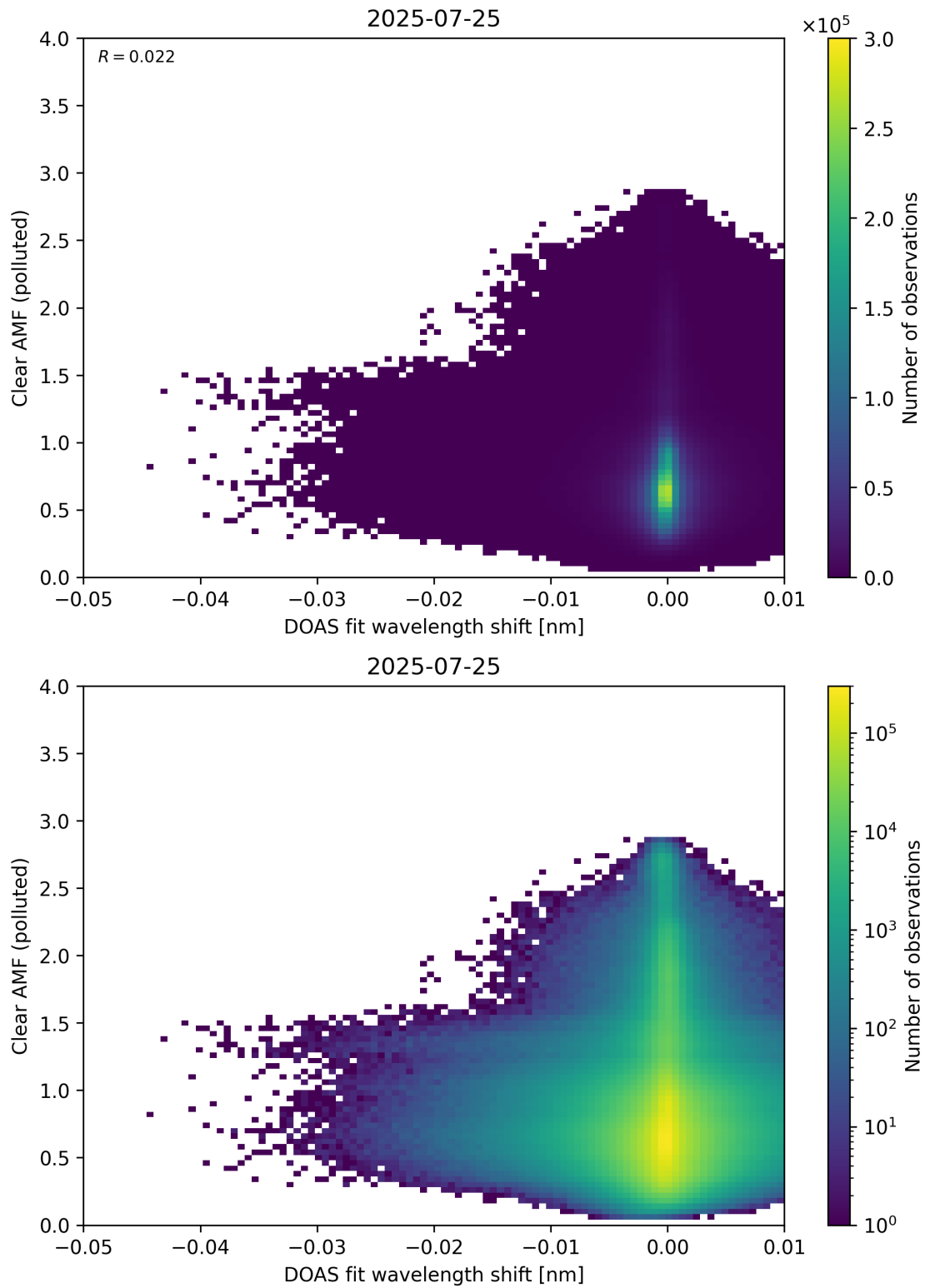
Figure 140: Scatter density plot of “DOAS fit wavelength shift” against “Clear AMF (polluted)” for 2025-07-24 to 2025-07-26.
