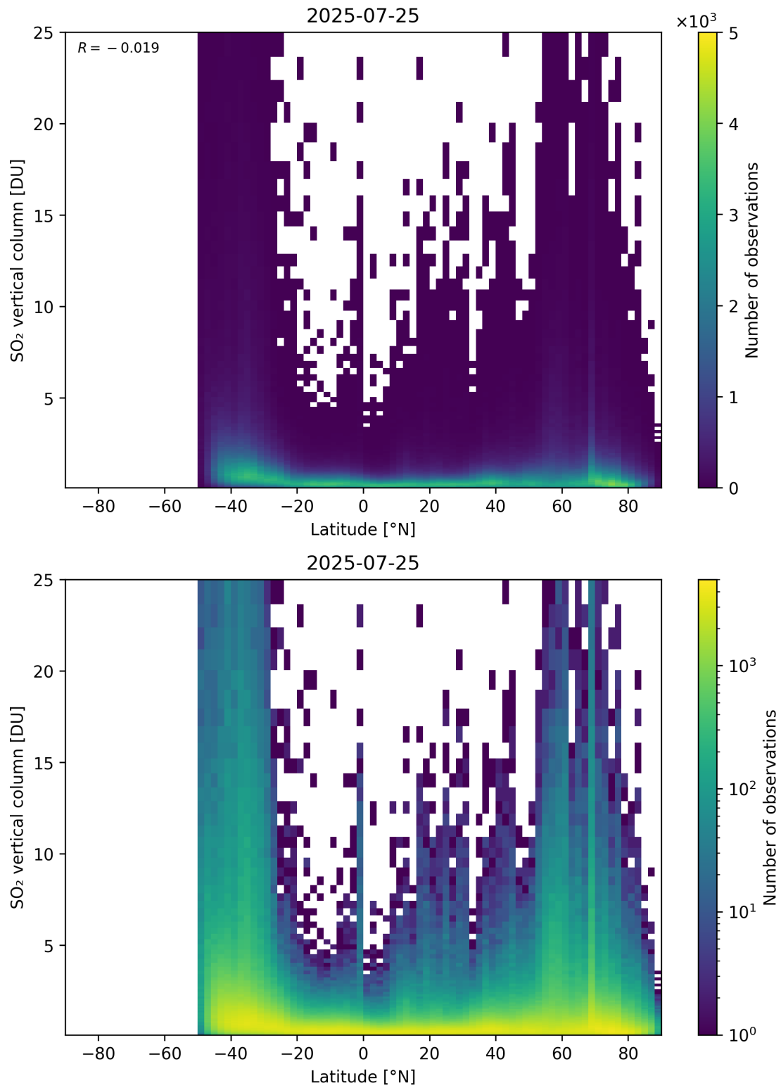
Figure 169: Scatter density plot of “Latitude” against “SO 2 vertical column” for 2025-07-24 to 2025-07-26.
