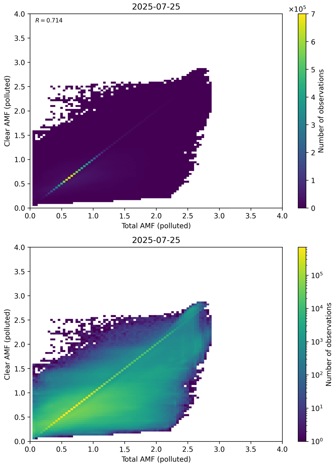
Figure 321: Scatter density plot of “Total AMF (polluted)” against “Clear AMF (polluted)” for 2025-07-24 to 2025-07-26.
