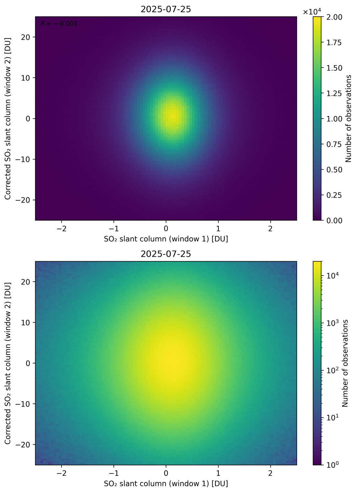
Figure 283: Scatter density plot of “SO 2 slant column (window 1)” against “Corrected SO 2 slant column (window 2)” for 2025-07-24 to 2025-07-26.
