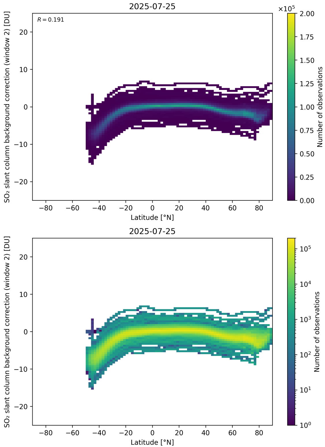
Figure 151: Scatter density plot of “Latitude” against “SO 2 slant column background correction (window 2)” for 2025-07-24 to 2025-07-26.
