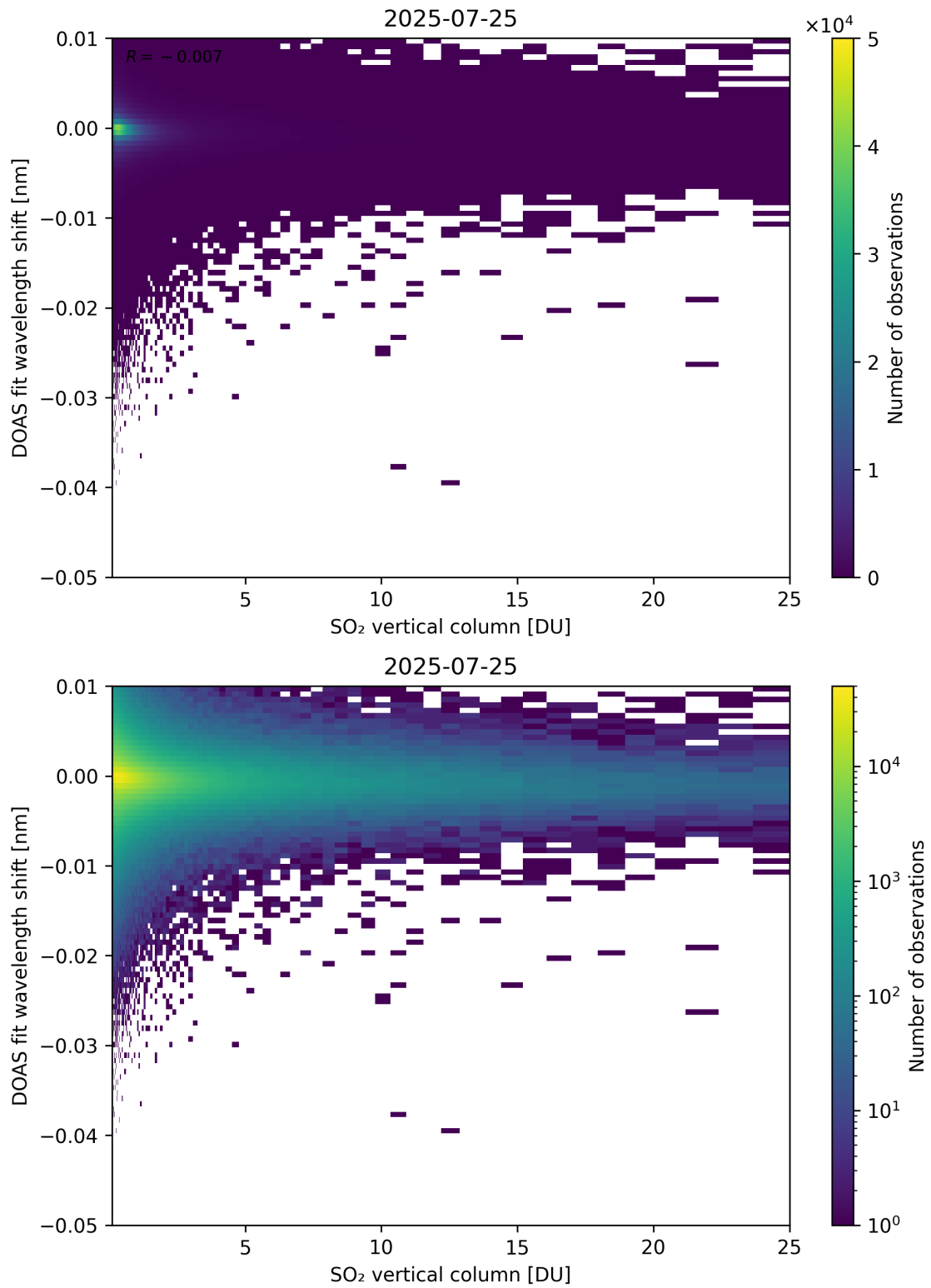
Figure 326: Scatter density plot of “SO 2 vertical column” against “DOAS fit wavelength shift” for 2025-07-24 to 2025-07-26.
