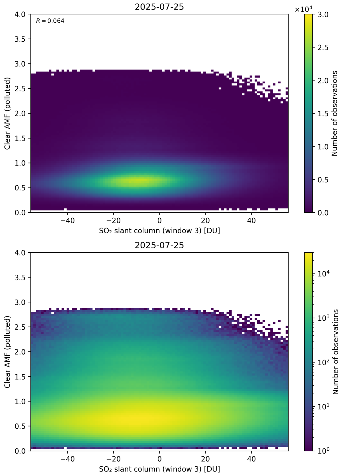
Figure 315: Scatter density plot of “SO 2 slant column (window 3)” against “Clear AMF (polluted)” for 2025-07-24 to 2025-07-26.
