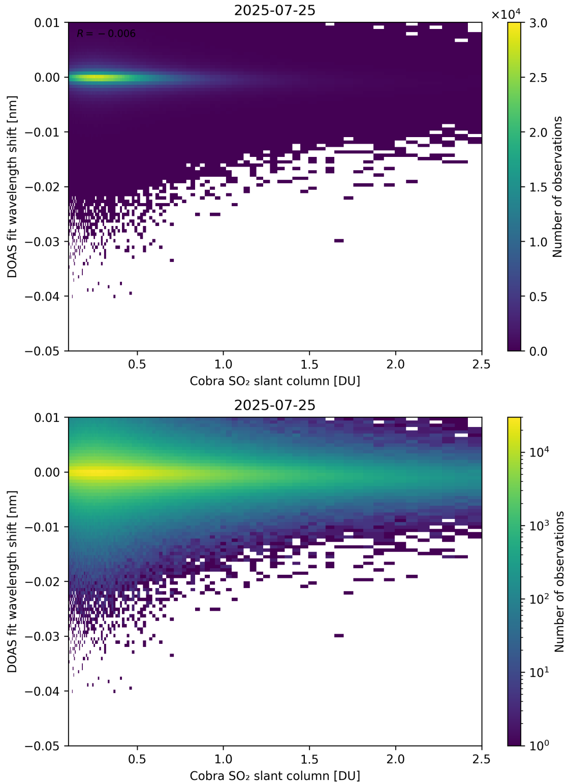
Figure 196: Scatter density plot of “Cobra SO 2 slant column” against “DOAS fit wavelength shift” for 2025-07-24 to 2025-07-26.
