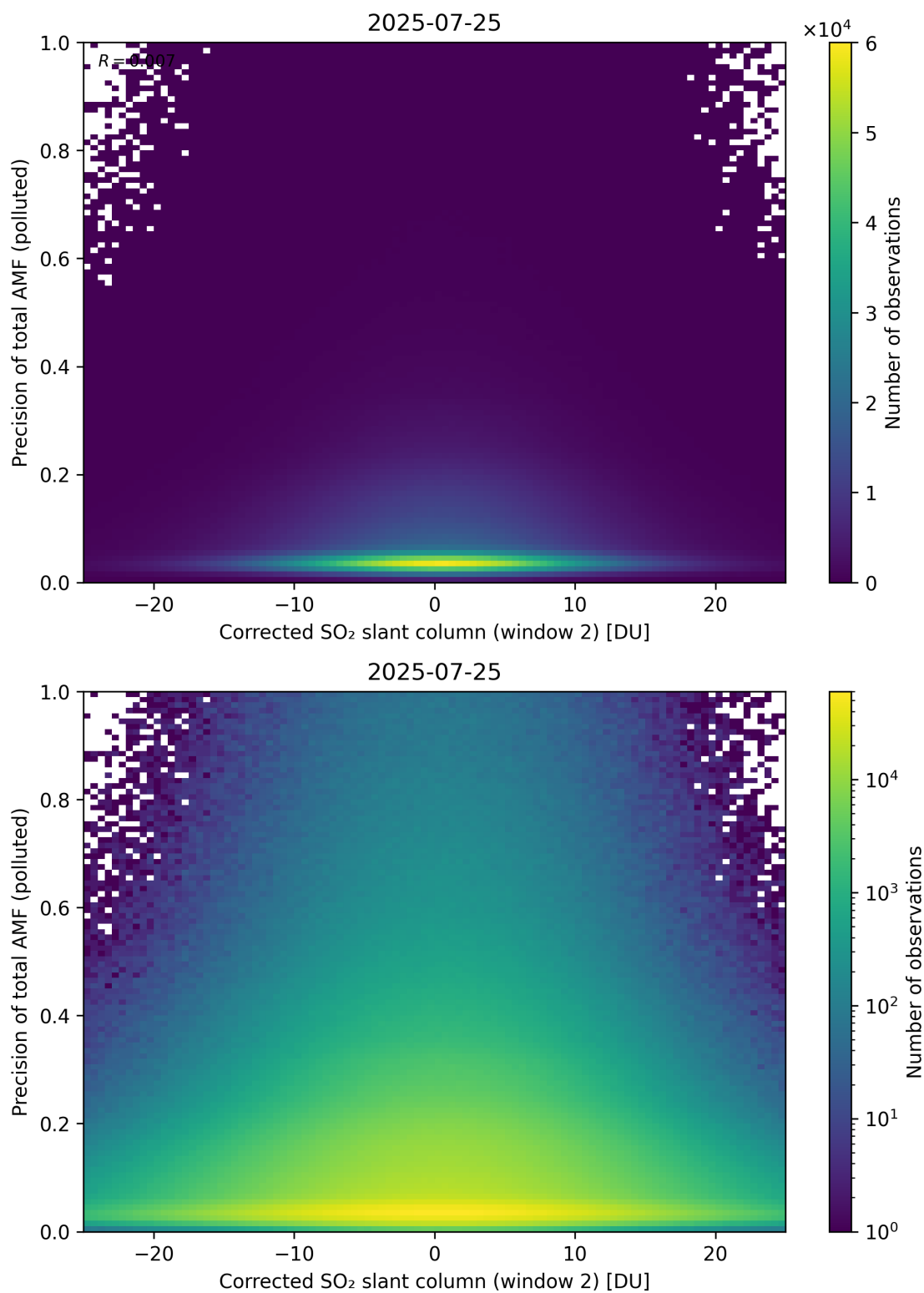
Figure 254: Scatter density plot of “Corrected SO 2 slant column (window 2)” against “Precision of total AMF (polluted)” for 2025-07-24 to 2025-07-26.
