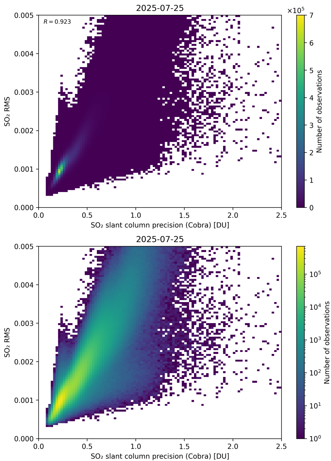
Figure 204: Scatter density plot of “SO 2 slant column precision (Cobra)” against “SO 2 RMS” for 2025-07-24 to 2025-07-26.
