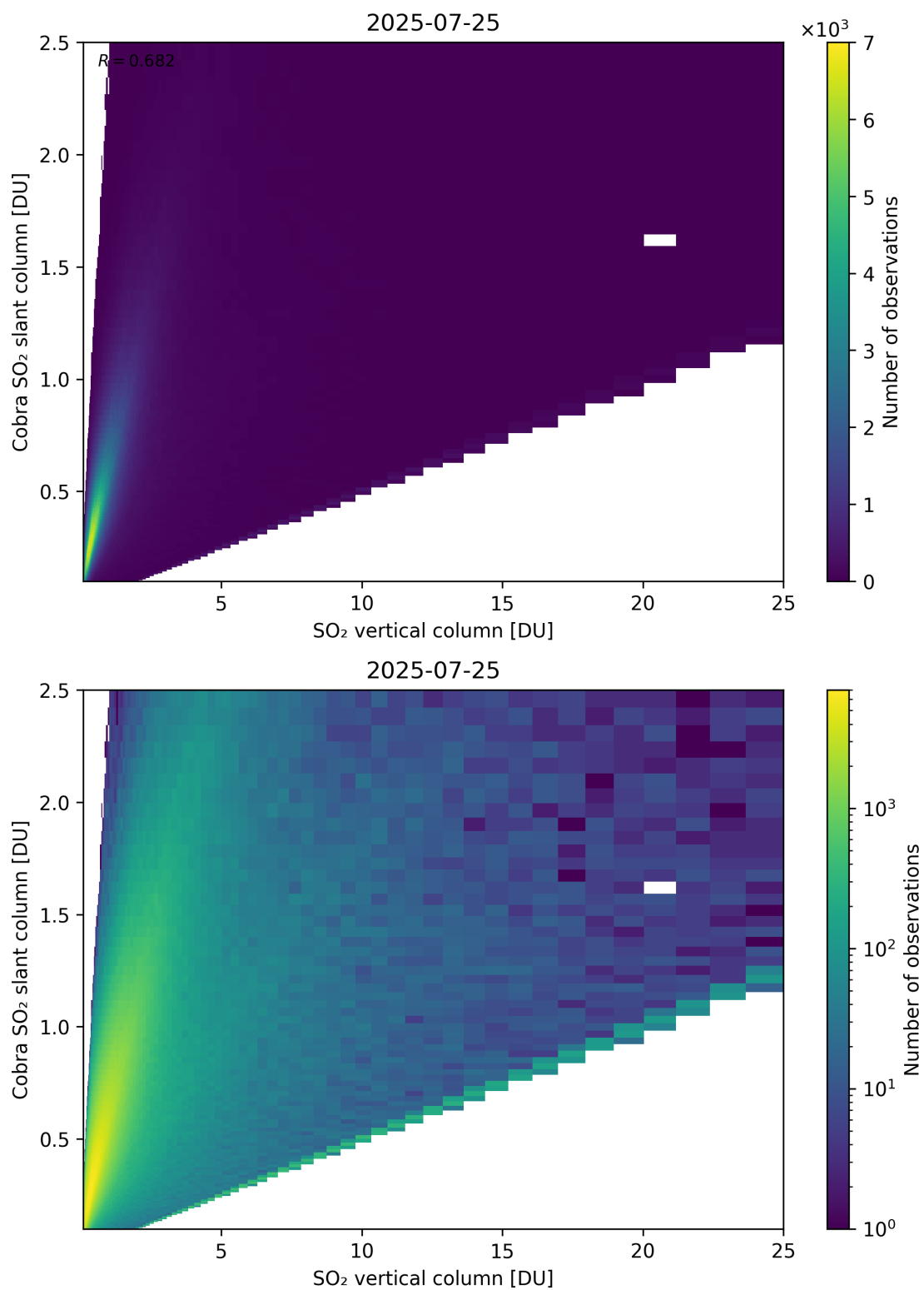
Figure 349: Scatter density plot of “SO 2 vertical column” against “Cobra SO 2 slant column” for 2025-07-24 to 2025-07-26.
