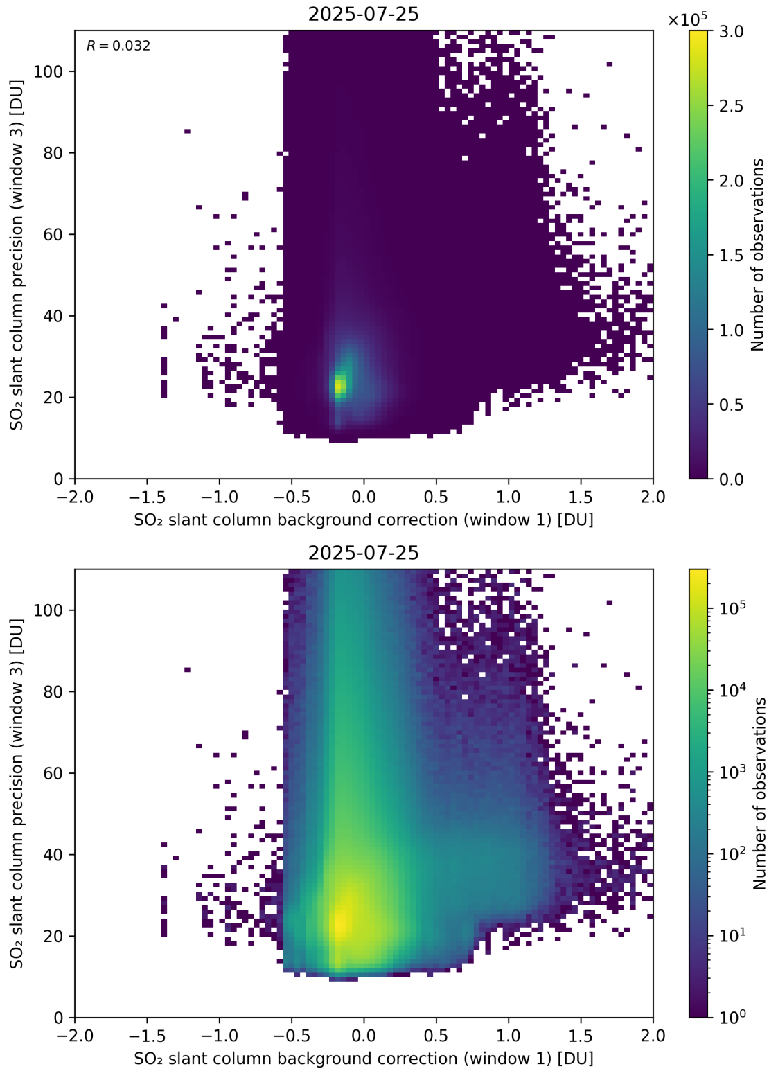
Figure 119: Scatter density plot of “SO 2 slant column background correction (window 1)” against “SO 2 slant column precision (window 3)” for 2025-07-24 to 2025-07-26.
