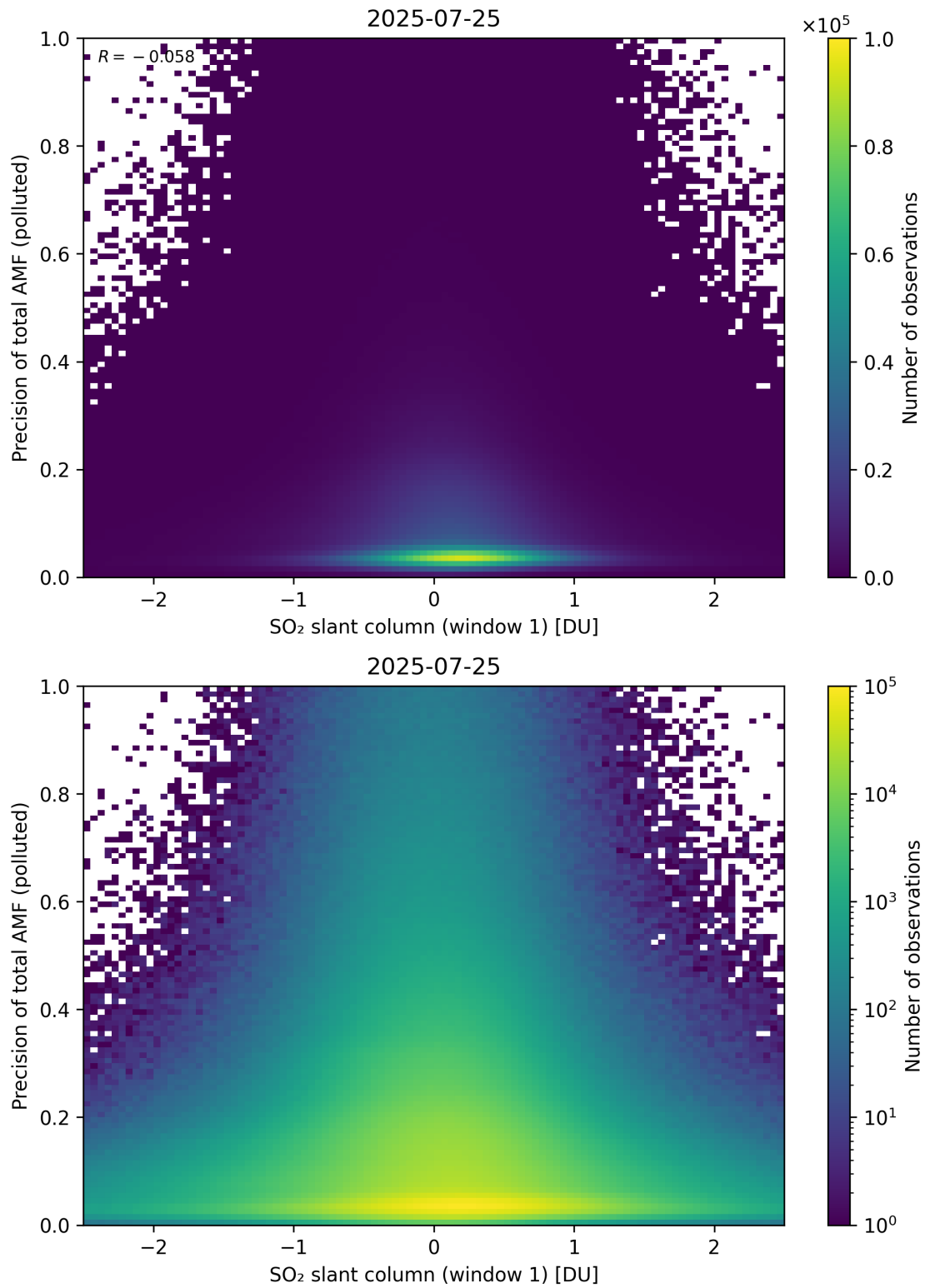
Figure 290: Scatter density plot of “SO 2 slant column (window 1)” against “Precision of total AMF (polluted)” for 2025-07-24 to 2025-07-26.
