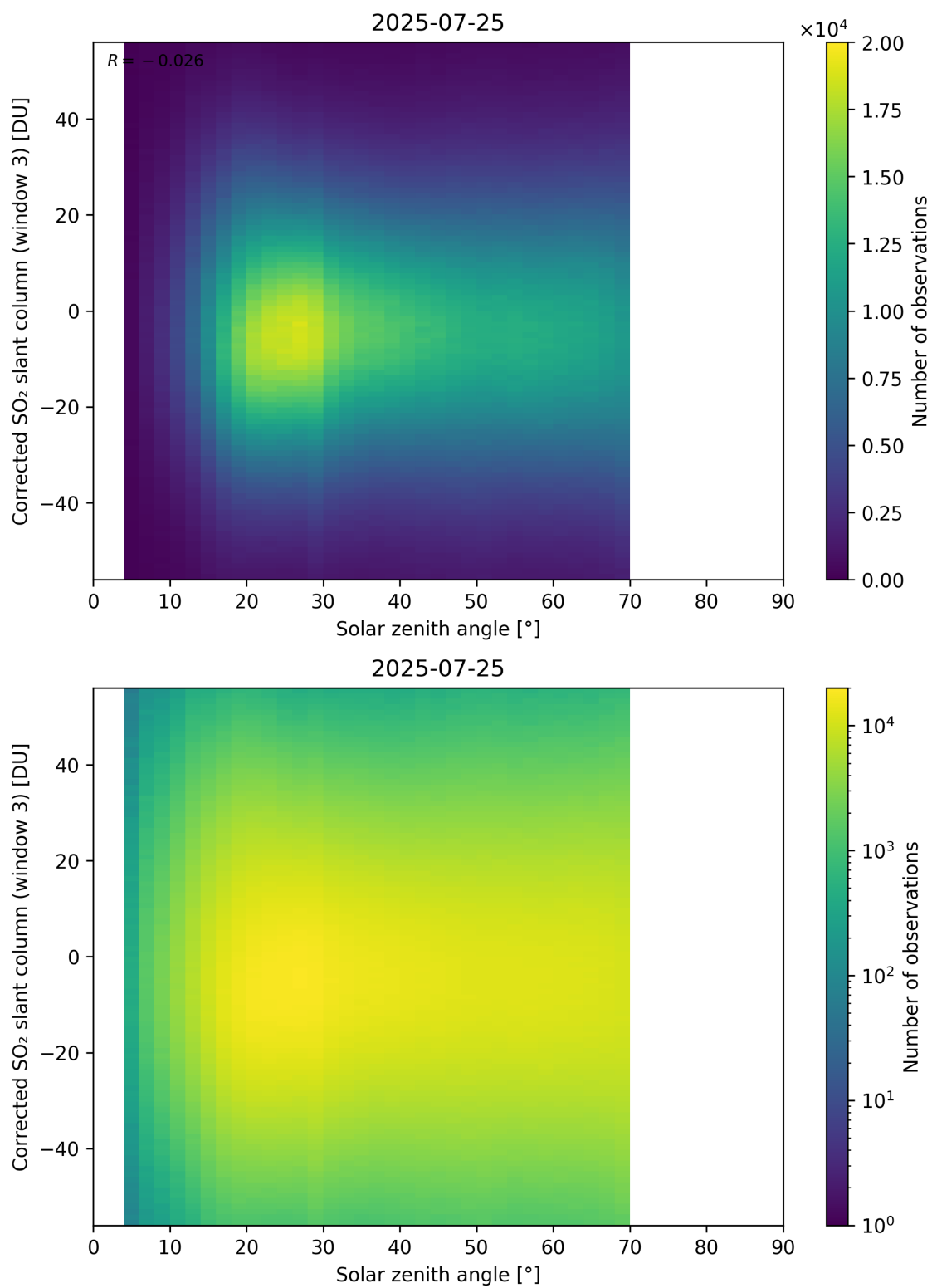
Figure 183: Scatter density plot of “Solar zenith angle” against “Corrected SO 2 slant column (window 3)” for 2025-07-24 to 2025-07-26.
