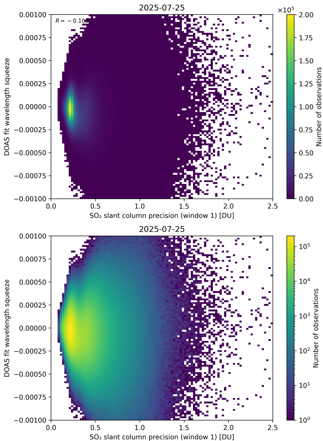
Figure 272: Scatter density plot of “SO 2 slant column precision (window 1)” against “DOAS fit wavelength squeeze” for 2025-07-24 to 2025-07-26.
