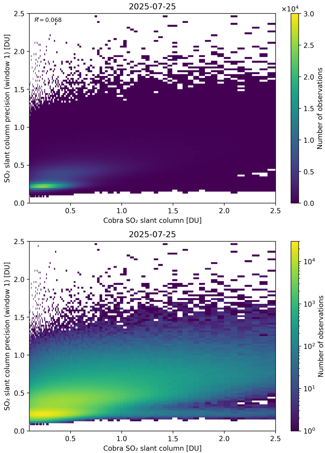
Figure 220: Scatter density plot of “Cobra SO 2 slant column” against “SO 2 slant column precision (window 1)” for 2025-07-24 to 2025-07-26.
