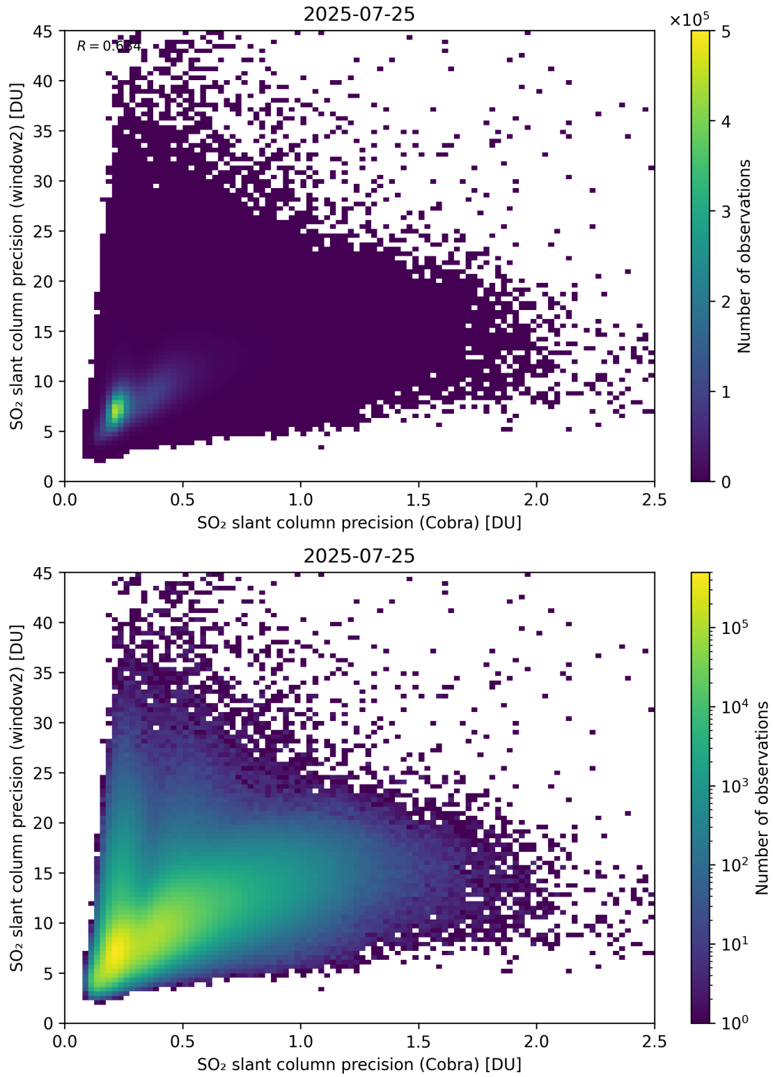
Figure 210: Scatter density plot of “SO 2 slant column precision (Cobra)” against “SO 2 slant column precision (window2)” for 2025-07-24 to 2025-07-26.
