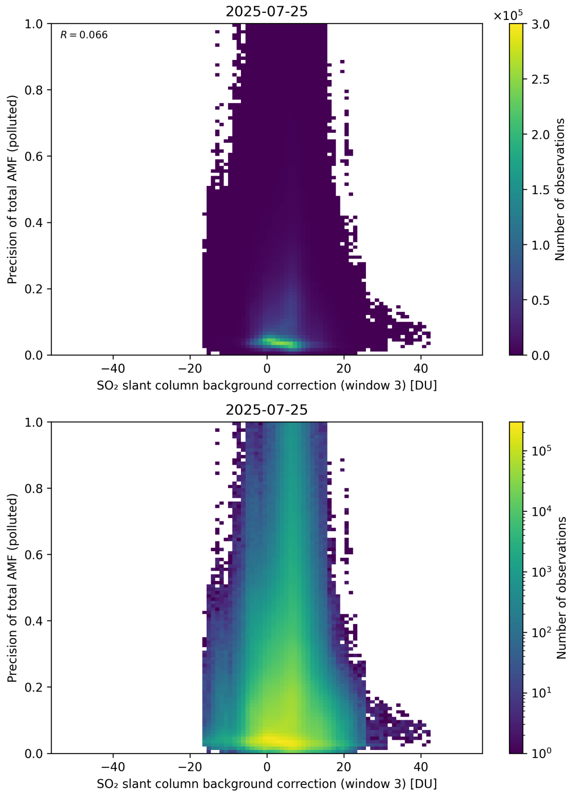
Figure 137: Scatter density plot of “SO 2 slant column background correction (window 3)” against “Precision of total AMF (polluted)” for 2025-07-24 to 2025-07-26.
