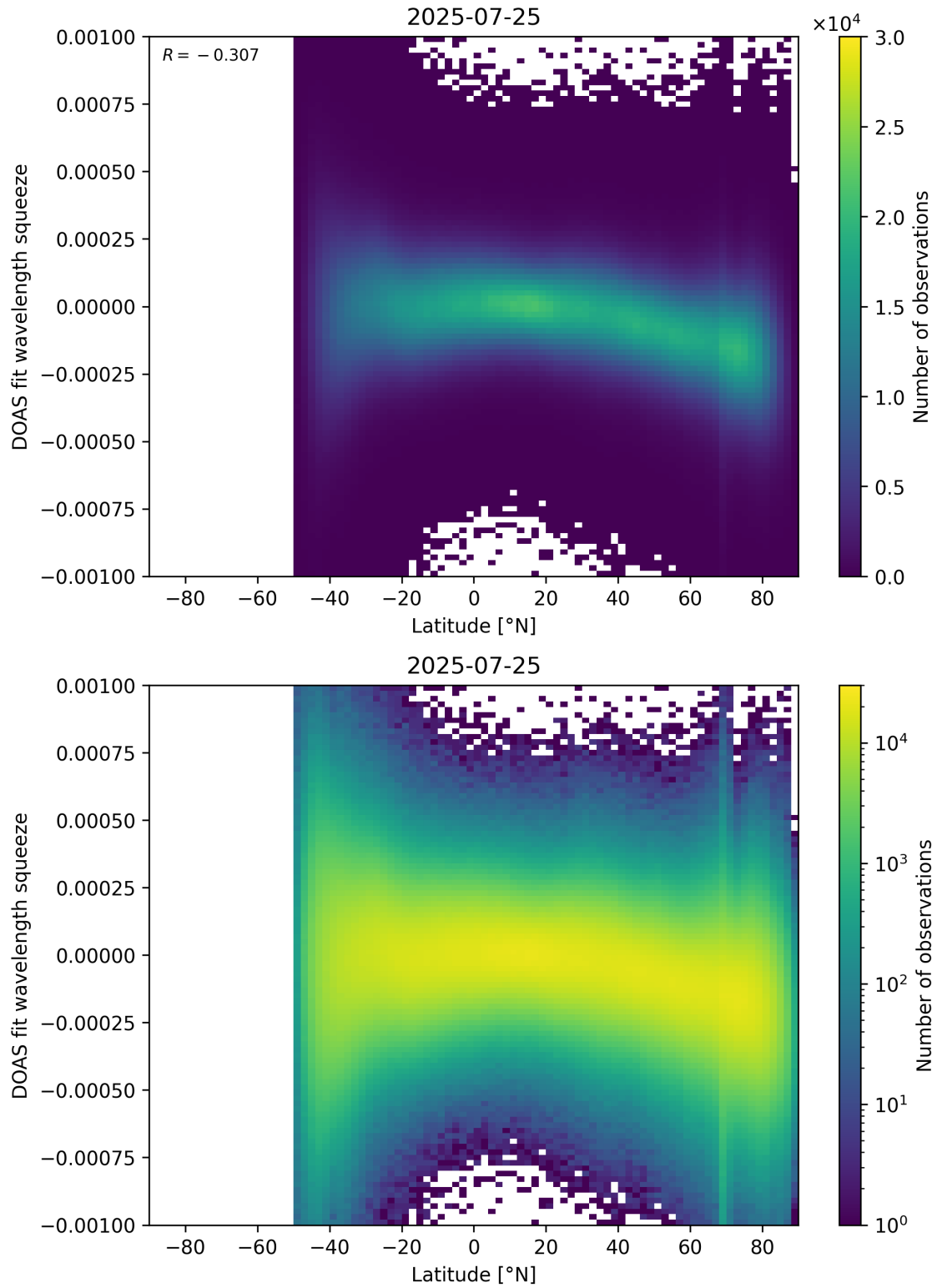
Figure 154: Scatter density plot of “Latitude” against “DOAS fit wavelength squeeze” for 2025-07-24 to 2025-07-26.
