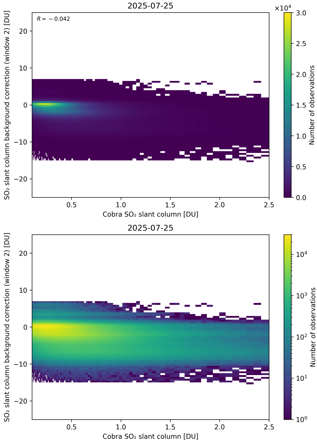
Figure 194: Scatter density plot of “Cobra SO 2 slant column” against “SO 2 slant column background correction (window 2)” for 2025-07-24 to 2025-07-26.
