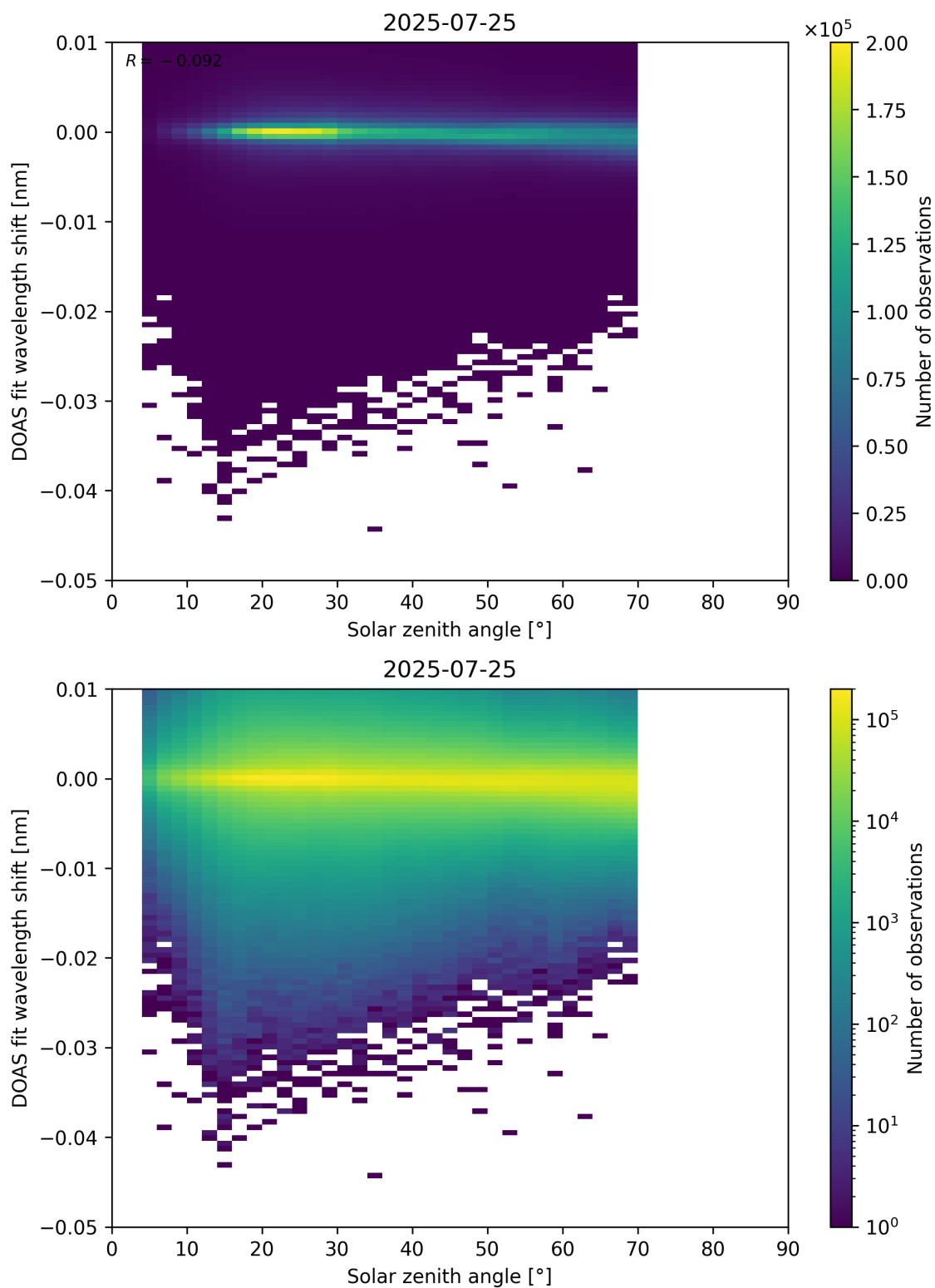
Figure 174: Scatter density plot of “Solar zenith angle” against “DOAS fit wavelength shift” for 2025-07-24 to 2025-07-26.
