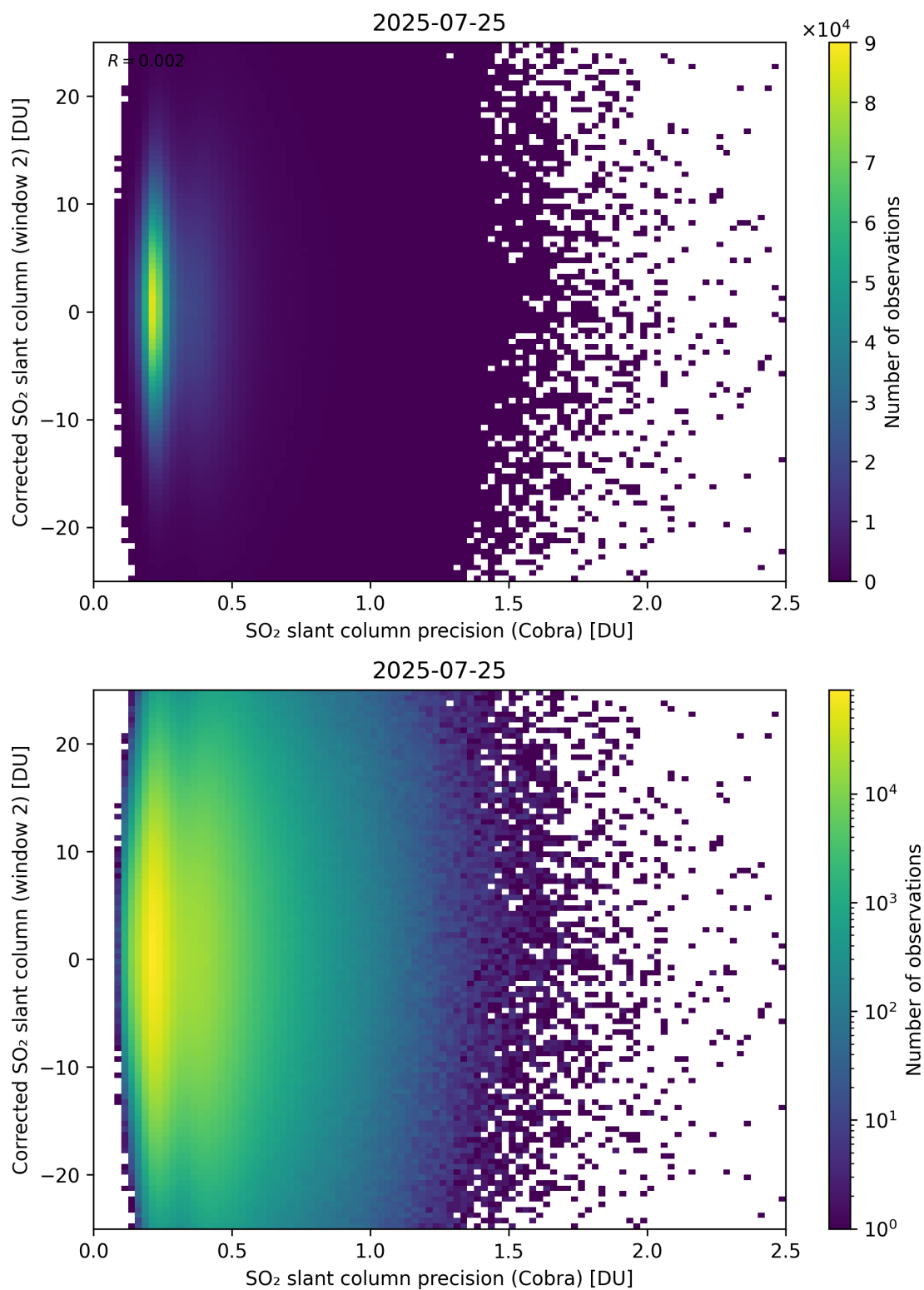
Figure 206: Scatter density plot of “SO 2 slant column precision (Cobra)” against “Corrected SO 2 slant column (window 2)” for 2025-07-24 to 2025-07-26.
