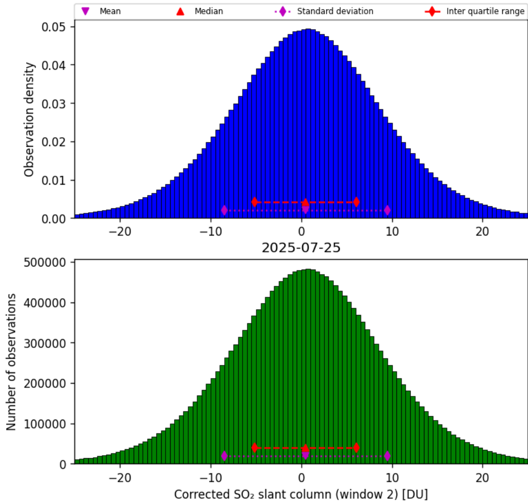
Figure 69: Histogram of “Corrected SO 2 slant column (window 2)” for 2025-07-24 to 2025-07-26
