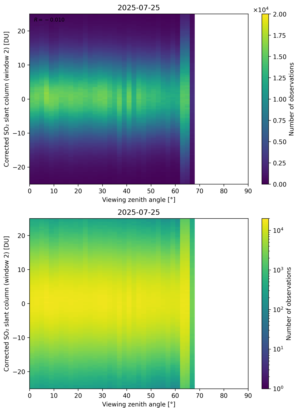
Figure 374: Scatter density plot of “Viewing zenith angle” against “Corrected SO 2 slant column (window 2)” for 2025-07-24 to 2025-07-26.
