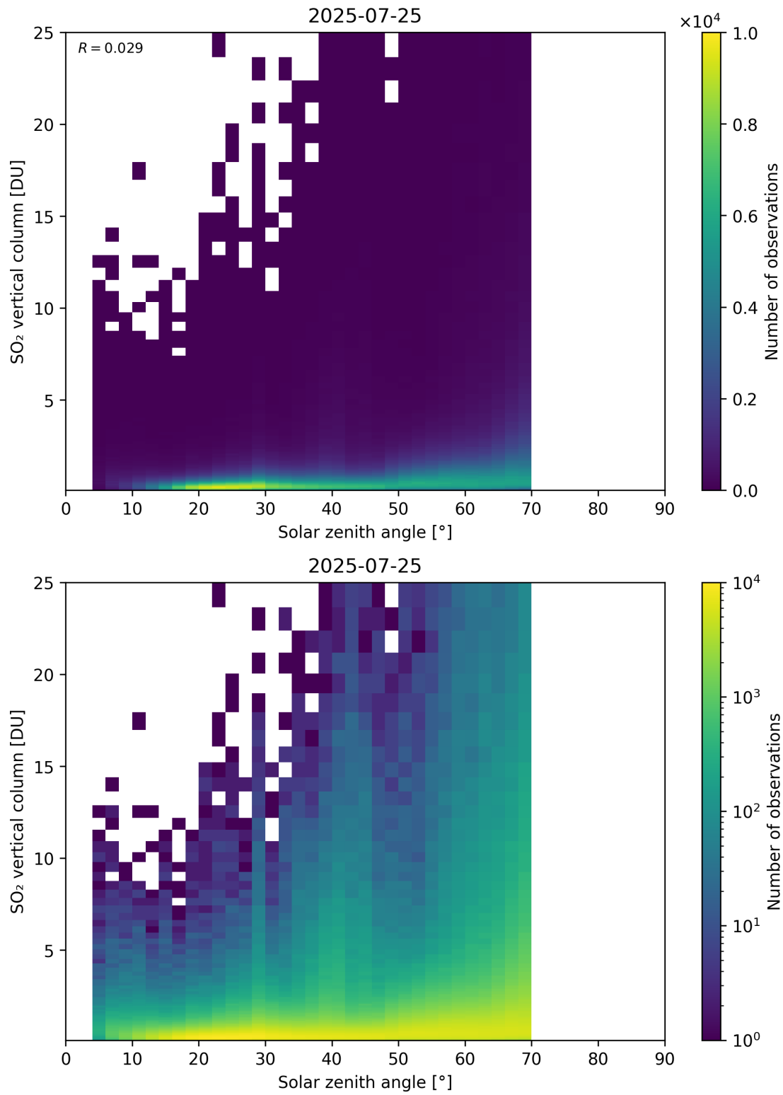
Figure 191: Scatter density plot of “Solar zenith angle” against “SO 2 vertical column” for 2025-07-24 to 2025-07-26.
