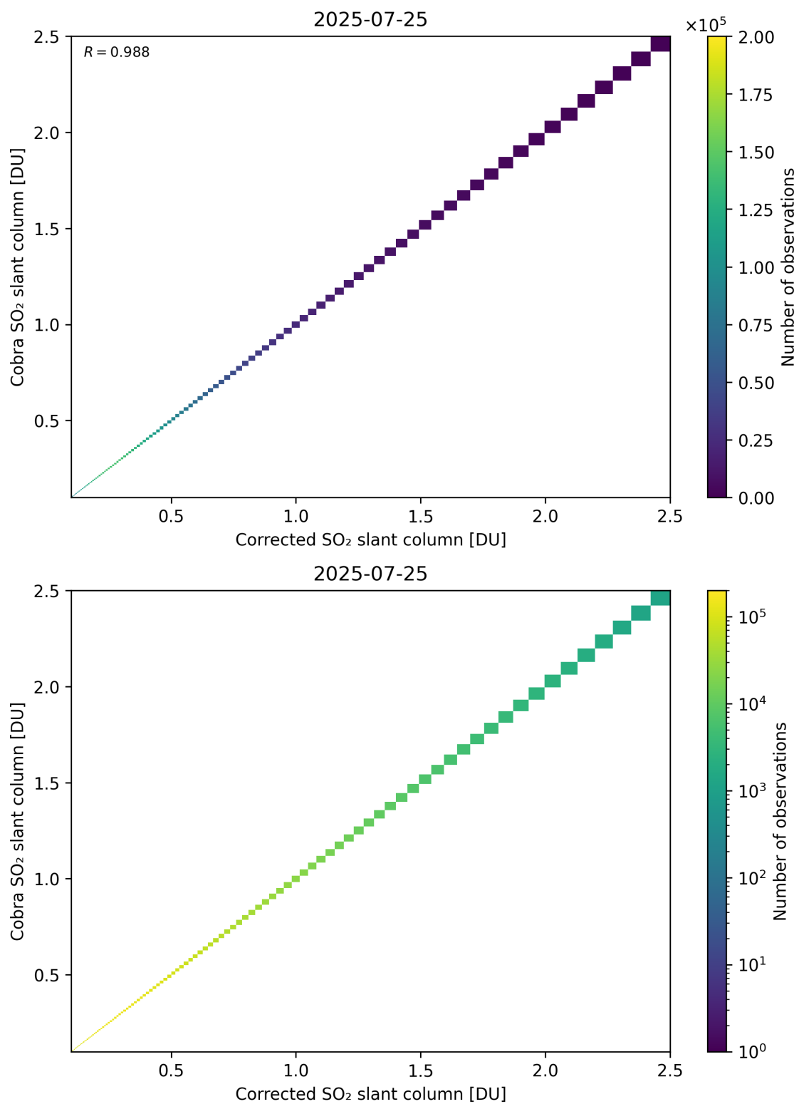
Figure 233: Scatter density plot of “Corrected SO 2 slant column” against “Cobra SO 2 slant column” for 2025-07-24 to 2025-07-26.
