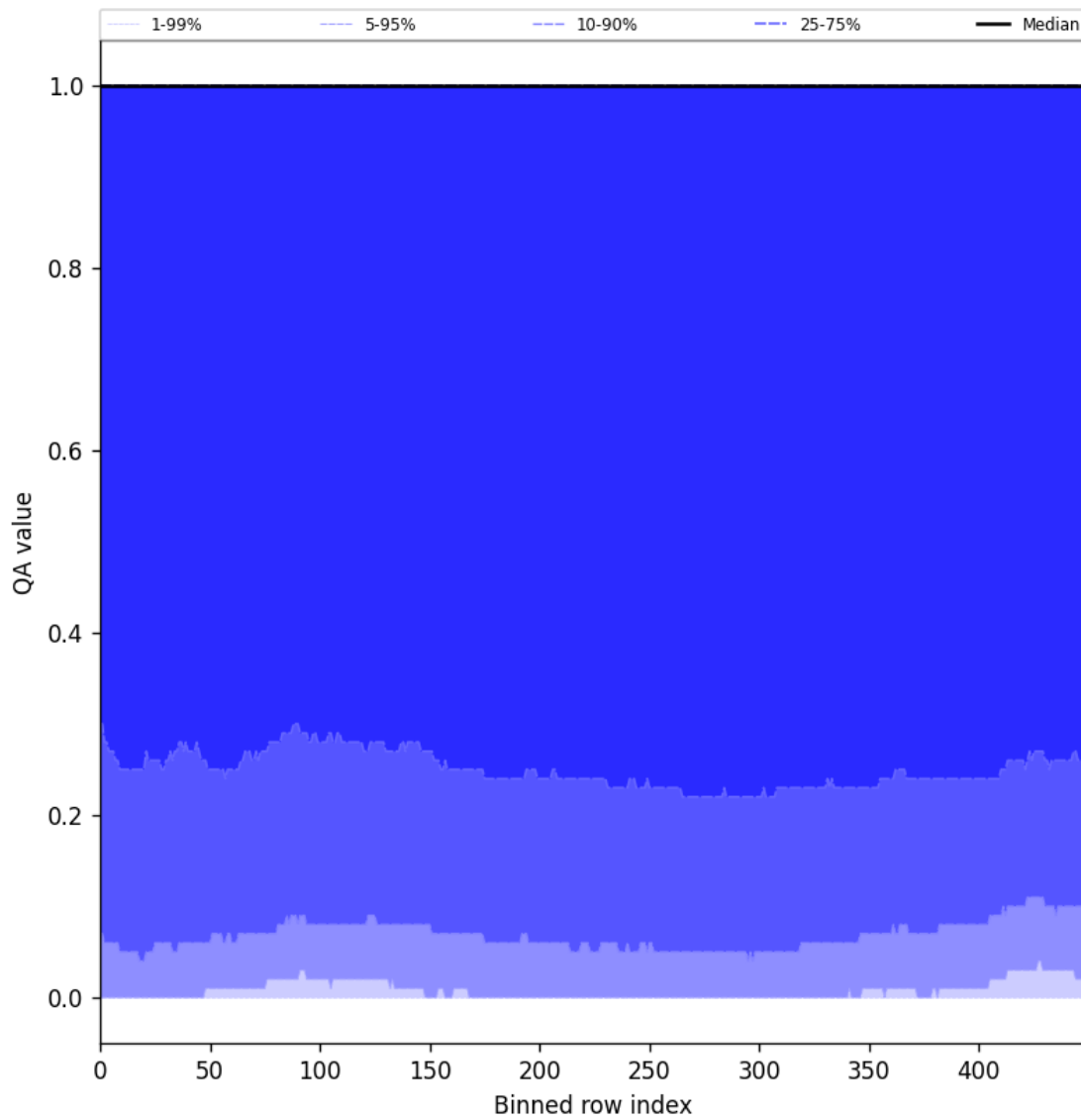
Figure 83: Along track statistics of “QA value” for 2025-07-24 to 2025-07-26
