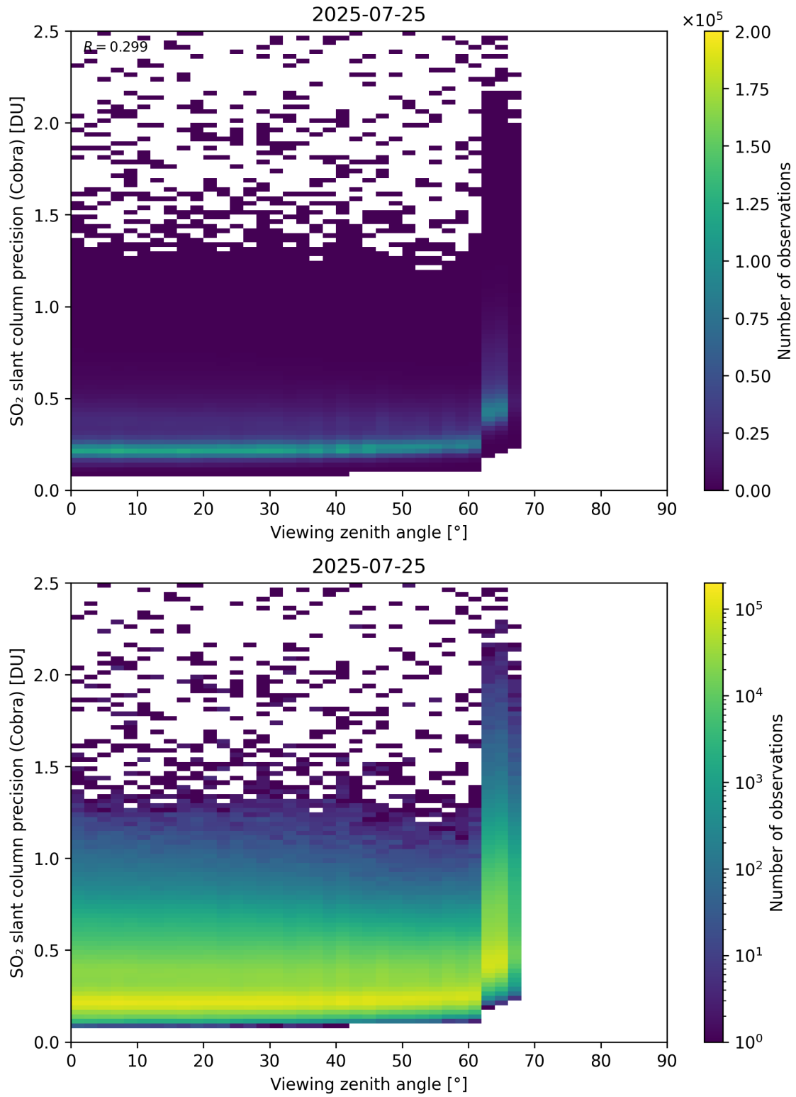
Figure 372: Scatter density plot of “Viewing zenith angle” against “SO 2 slant column precision (Cobra)” for 2025-07-24 to 2025-07-26.
