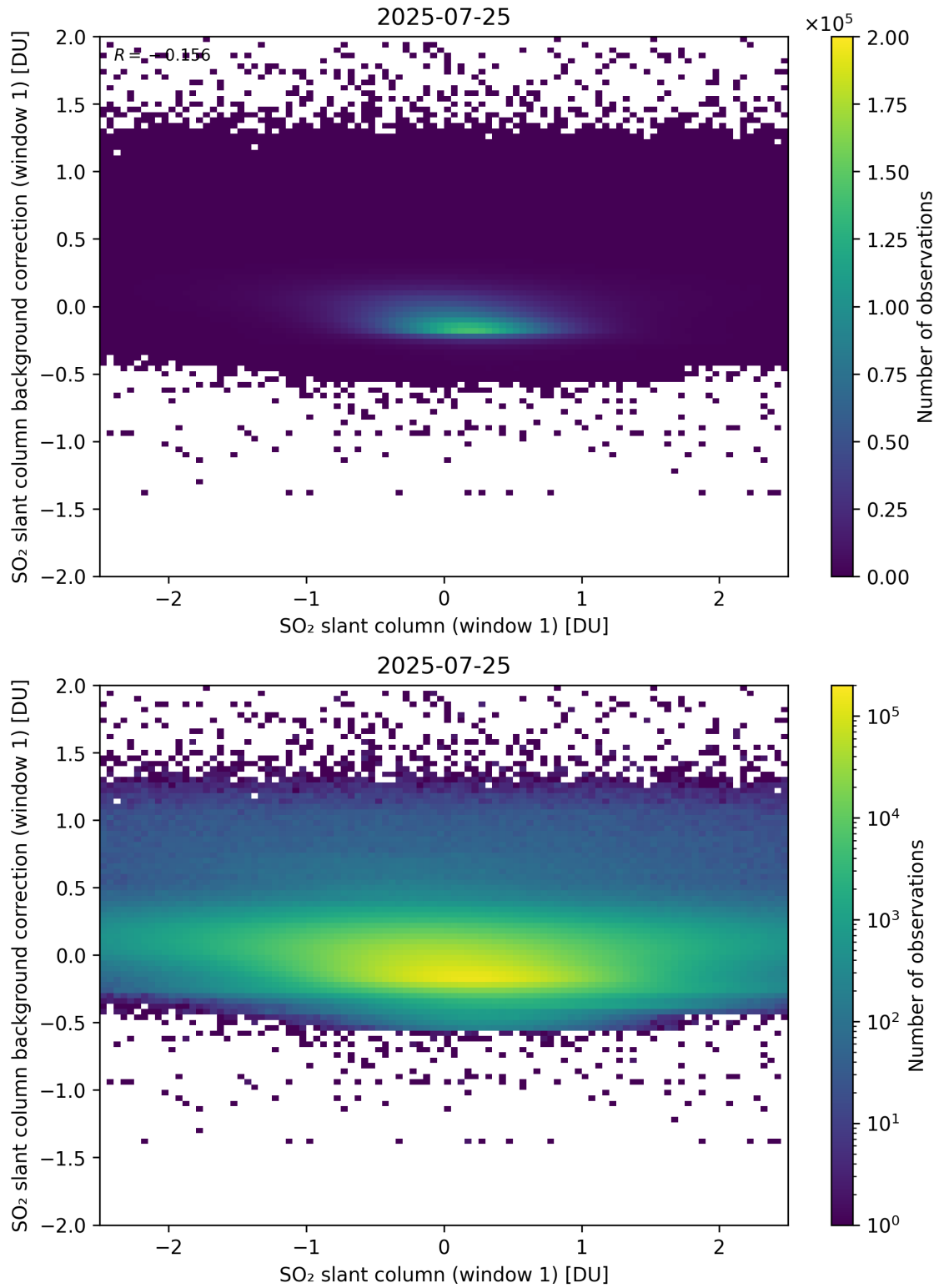
Figure 262: Scatter density plot of “SO 2 slant column (window 1)” against “SO 2 slant column background correction (window 1)” for 2025-07-24 to 2025-07-26.
