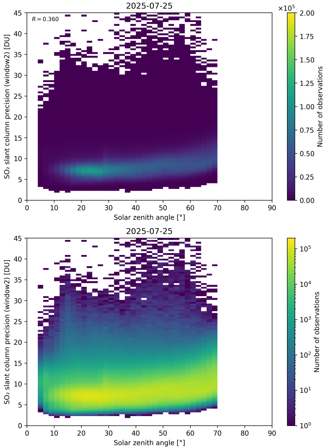
Figure 186: Scatter density plot of “Solar zenith angle” against “SO 2 slant column precision (window2)” for 2025-07-24 to 2025-07-26.
