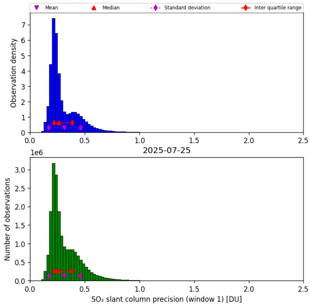
Figure 64: Histogram of “SO 2 slant column precision (window 1)” for 2025-07-24 to 2025-07-26
