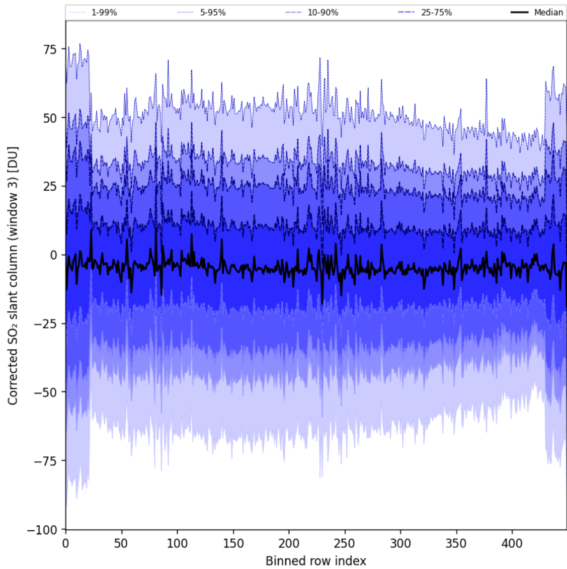
Figure 99: Along track statistics of “Corrected SO 2 slant column (window 3)” for 2025-07-24 to 2025-07-26
