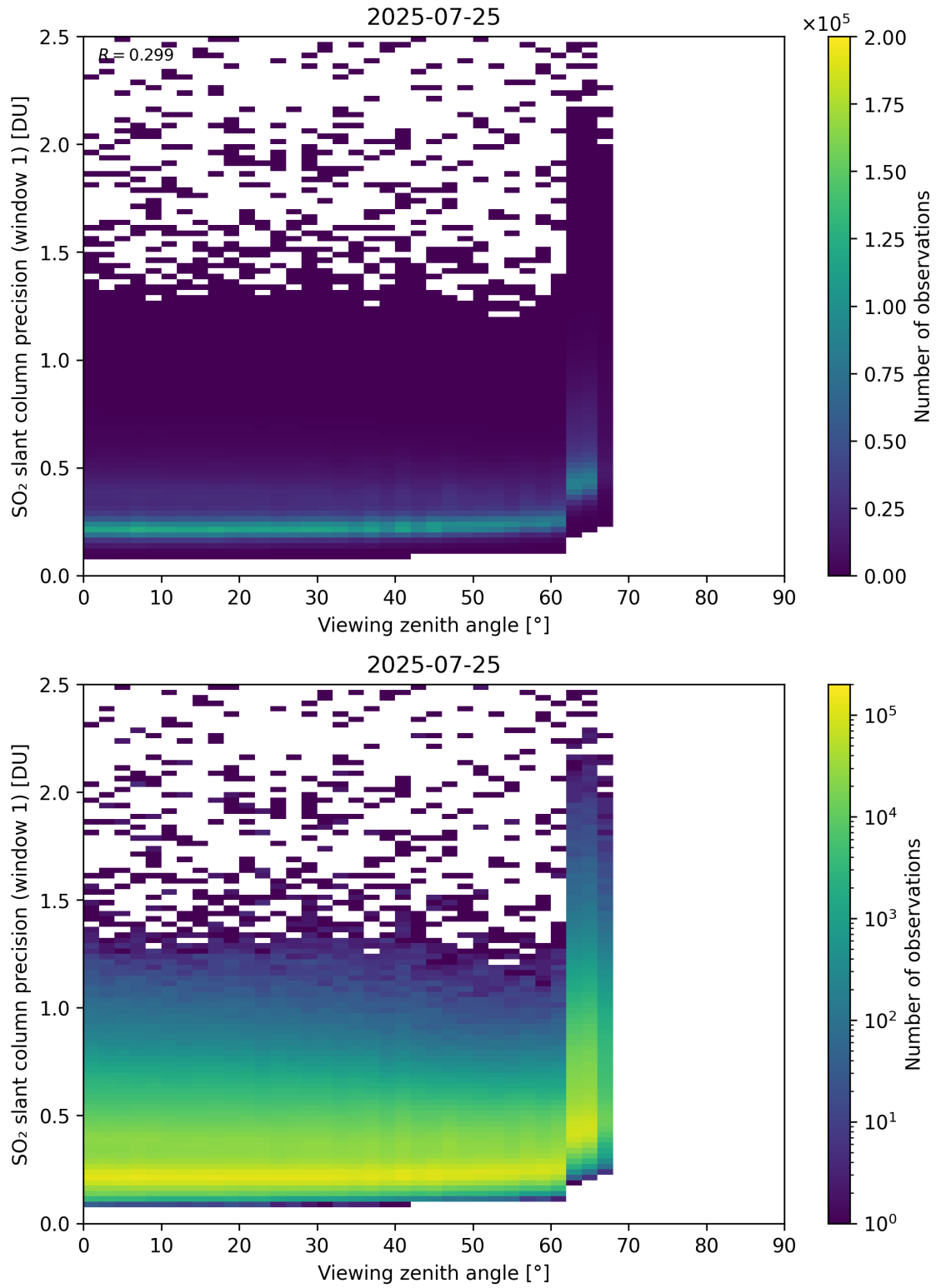
Figure 377: Scatter density plot of “Viewing zenith angle” against “SO 2 slant column precision (window 1)” for 2025-07-24 to 2025-07-26.
