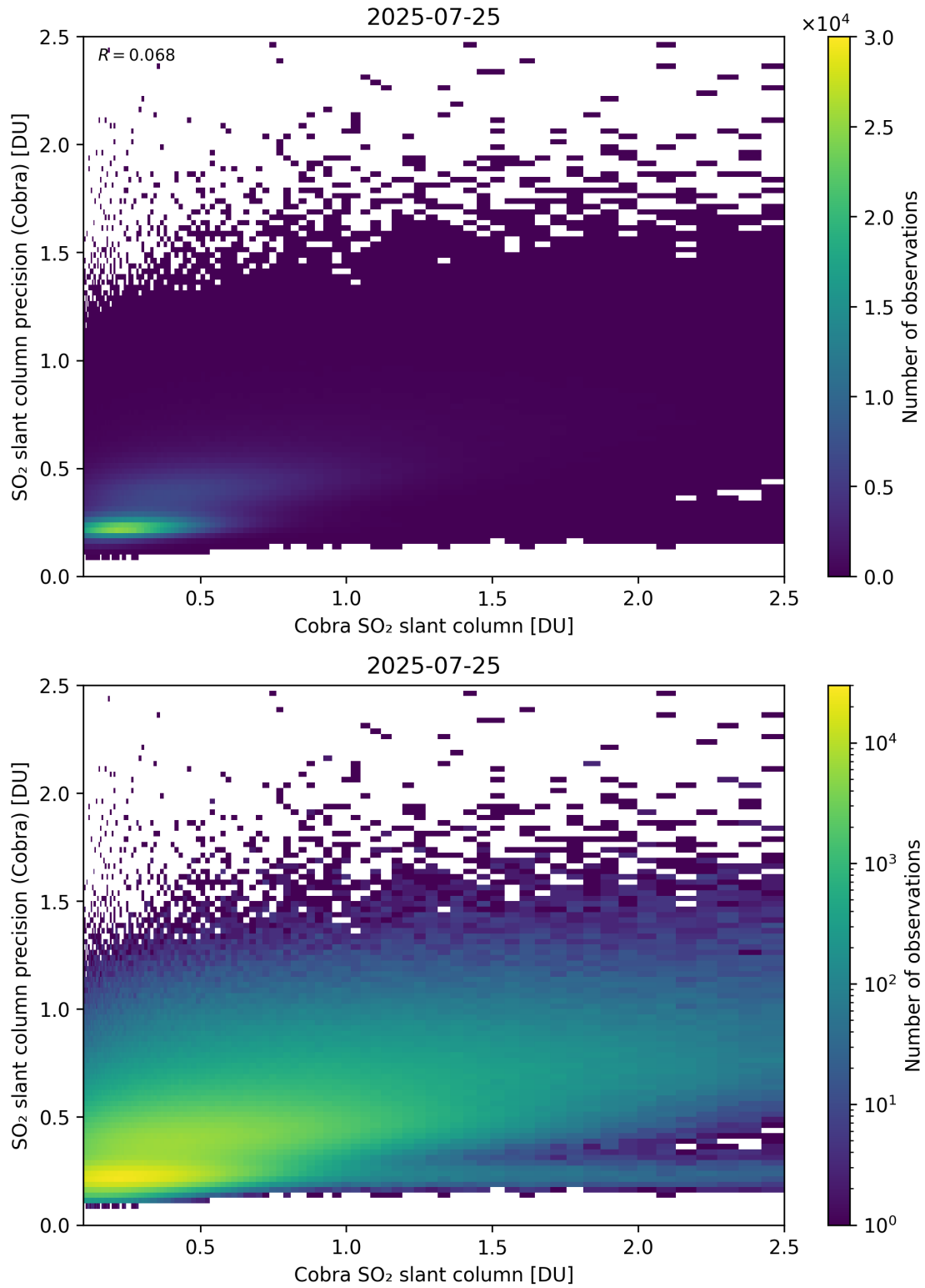
Figure 216: Scatter density plot of “Cobra SO 2 slant column” against “SO 2 slant column precision (Cobra)” for 2025-07-24 to 2025-07-26.
