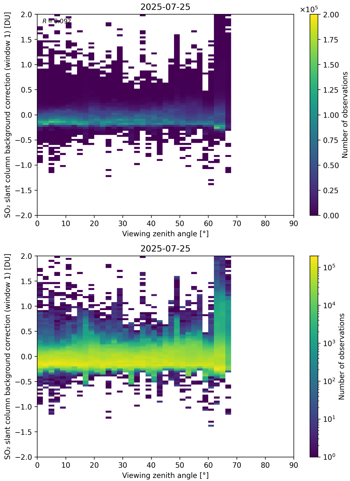
Figure 362: Scatter density plot of “Viewing zenith angle” against “SO 2 slant column background correction (window 1)” for 2025-07-24 to 2025-07-26.
