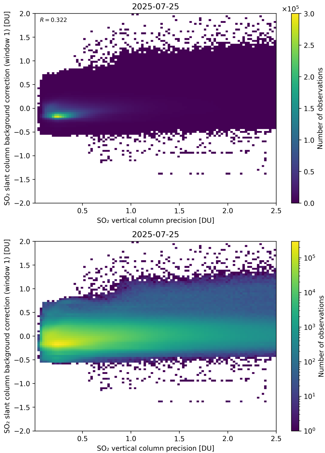
Figure 329: Scatter density plot of “SO 2 vertical column precision” against “SO 2 slant column background correction (window 1)” for 2025-07-24 to 2025-07-26.
