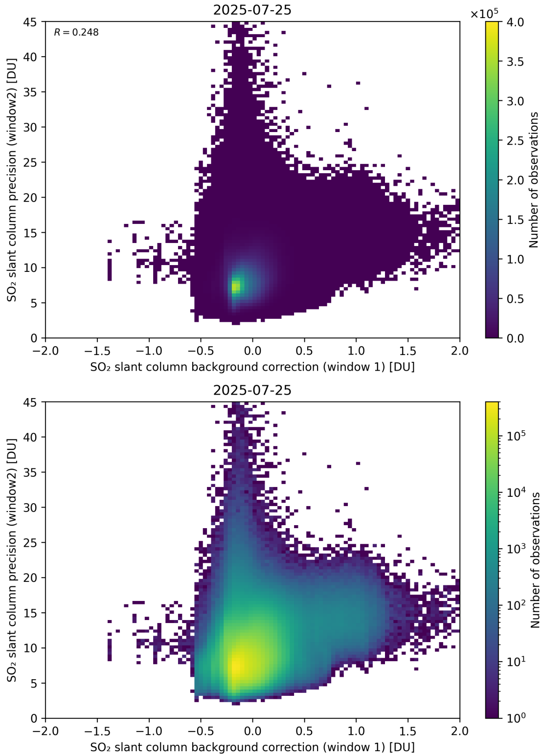
Figure 117: Scatter density plot of “SO 2 slant column background correction (window 1)” against “SO 2 slant column precision (window2)” for 2025-07-24 to 2025-07-26.
