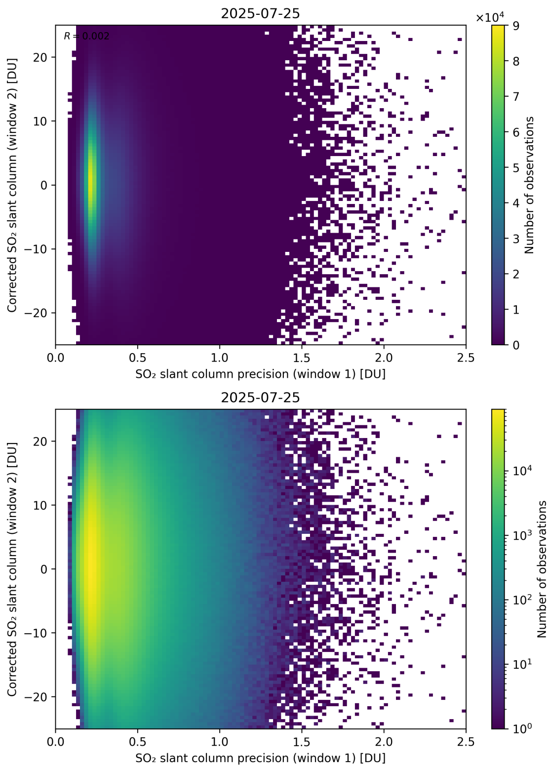
Figure 275: Scatter density plot of “SO 2 slant column precision (window 1)” against “Corrected SO 2 slant column (window 2)” for 2025-07-24 to 2025-07-26.
