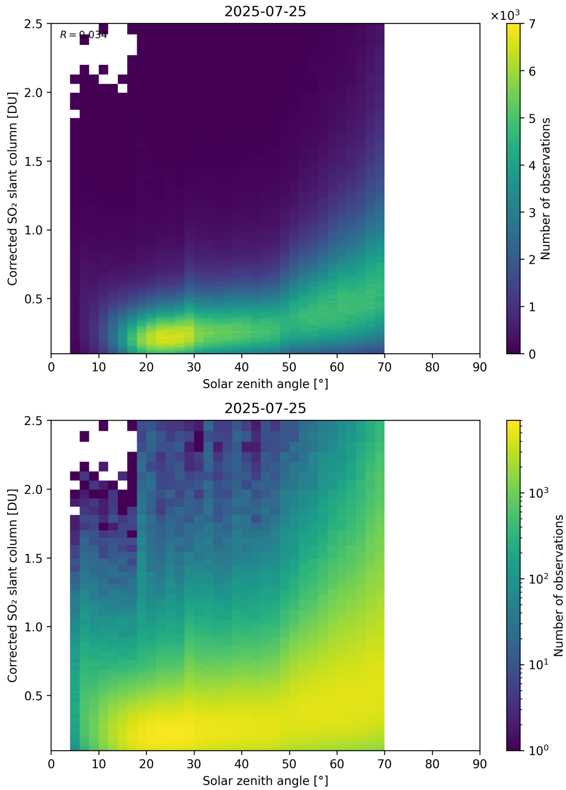
Figure 181: Scatter density plot of “Solar zenith angle” against “Corrected SO 2 slant column” for 2025-07-24 to 2025-07-26.
