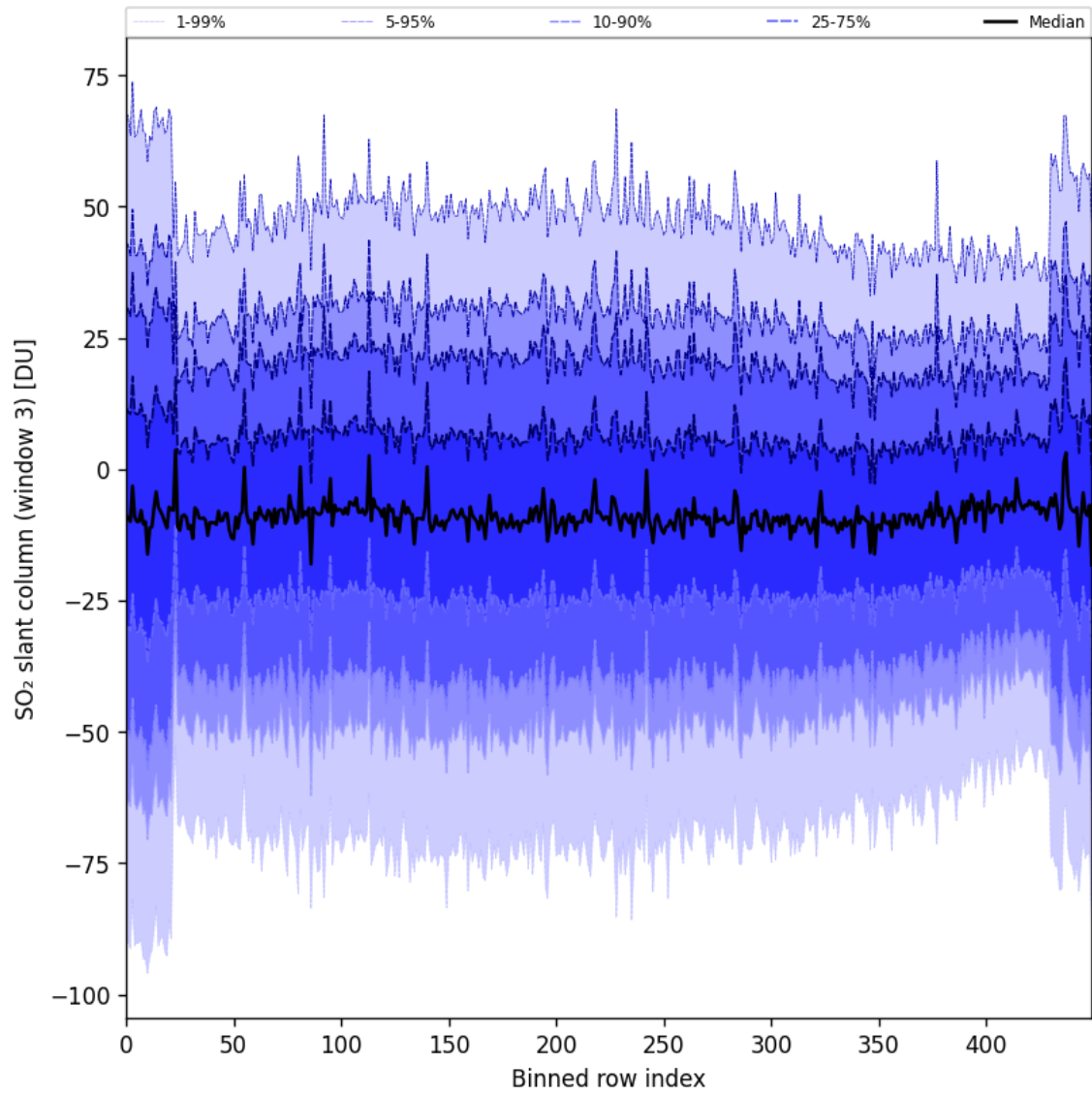
Figure 97: Along track statistics of “SO 2 slant column (window 3)” for 2025-07-24 to 2025-07-26
