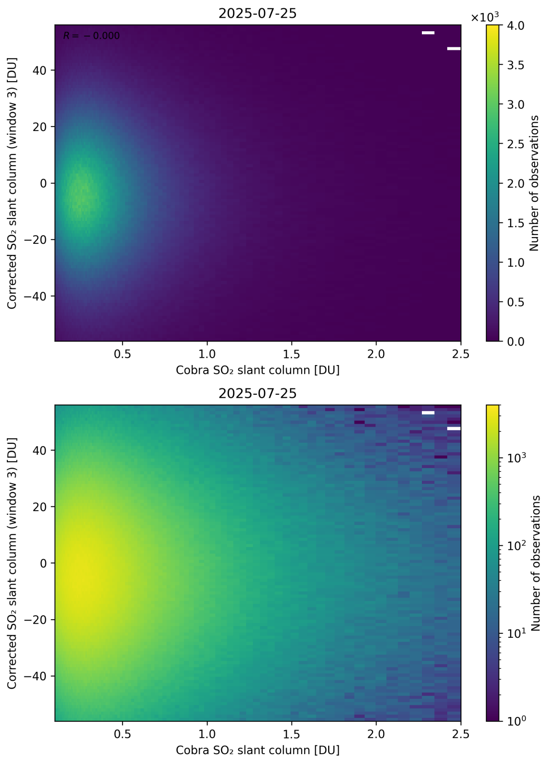
Figure 218: Scatter density plot of “Cobra SO 2 slant column” against “Corrected SO 2 slant column (window 3)” for 2025-07-24 to 2025-07-26.
