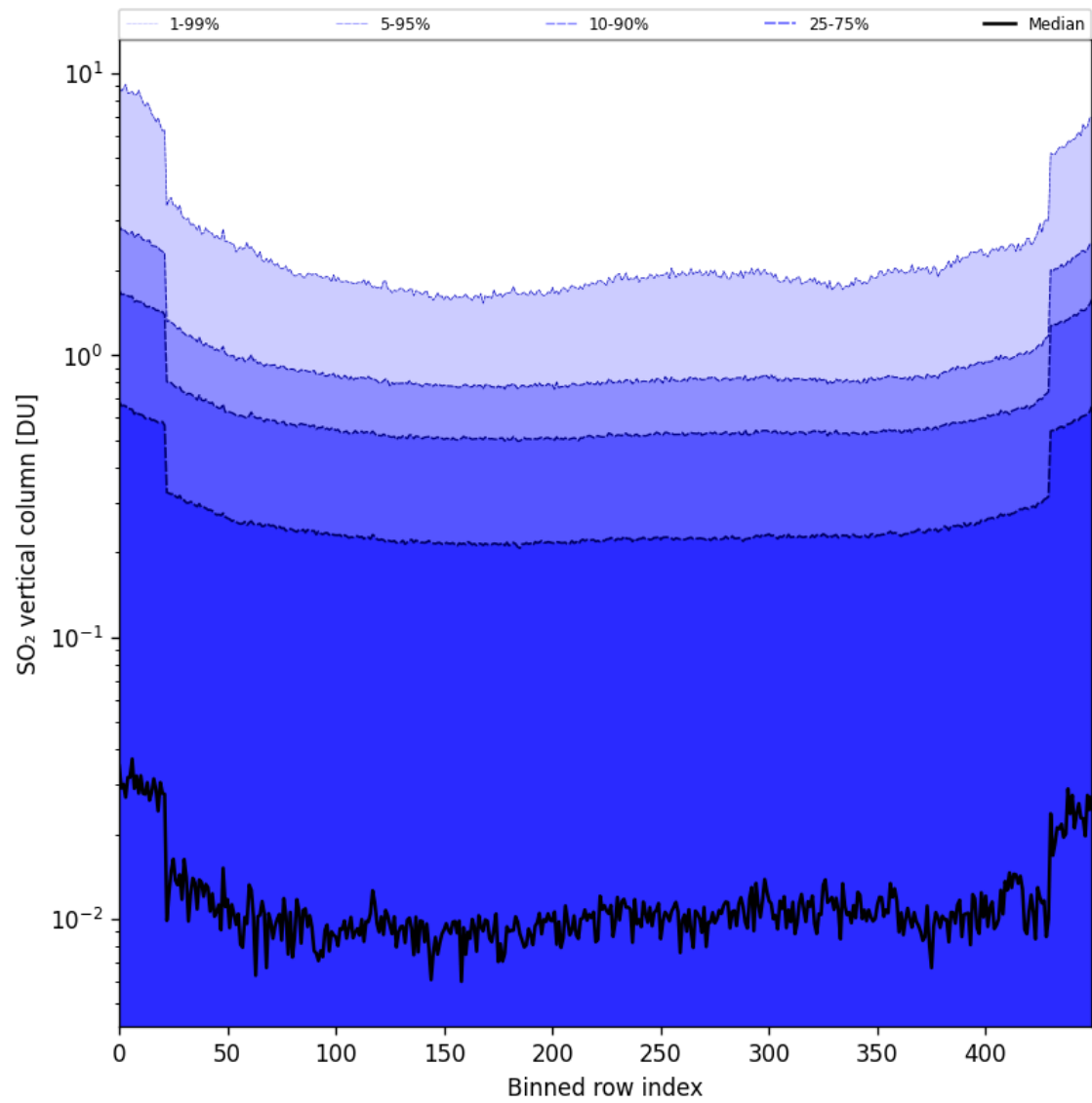
Figure 84: Along track statistics of “SO 2 vertical column” for 2025-07-24 to 2025-07-26
