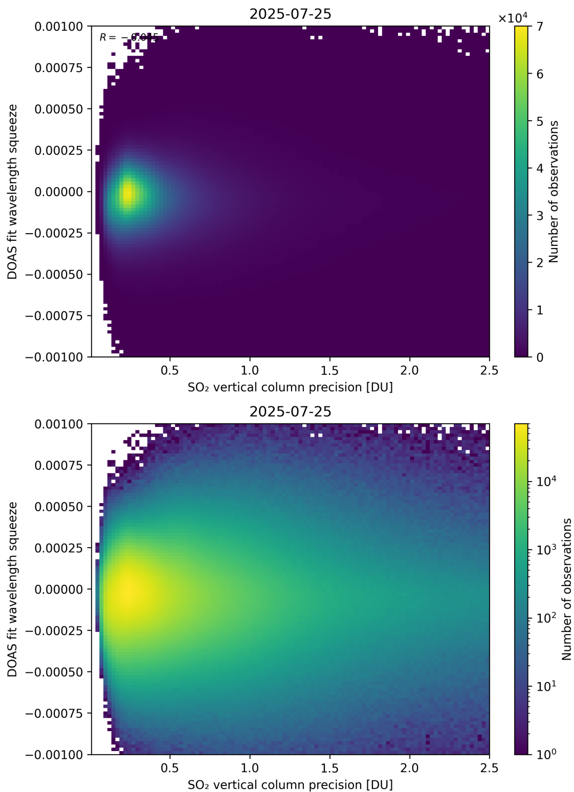
Figure 333: Scatter density plot of “SO 2 vertical column precision” against “DOAS fit wavelength squeeze” for 2025-07-24 to 2025-07-26.
