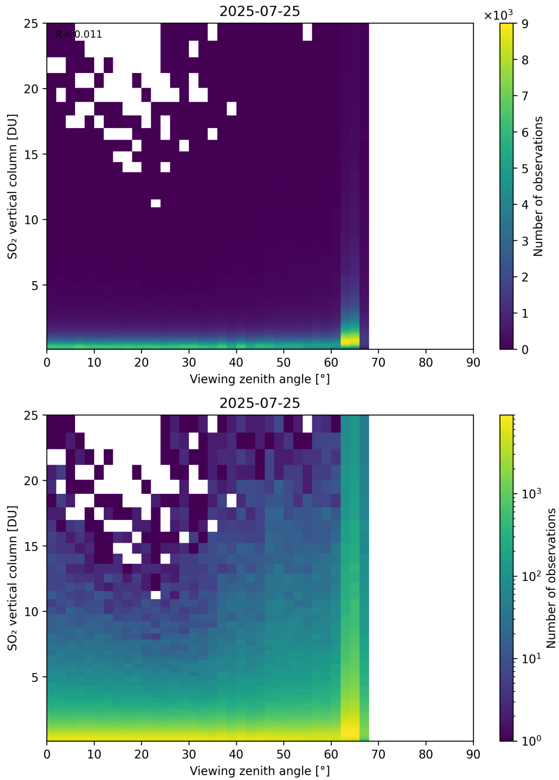
Figure 383: Scatter density plot of “Viewing zenith angle” against “SO 2 vertical column” for 2025-07-24 to 2025-07-26.
