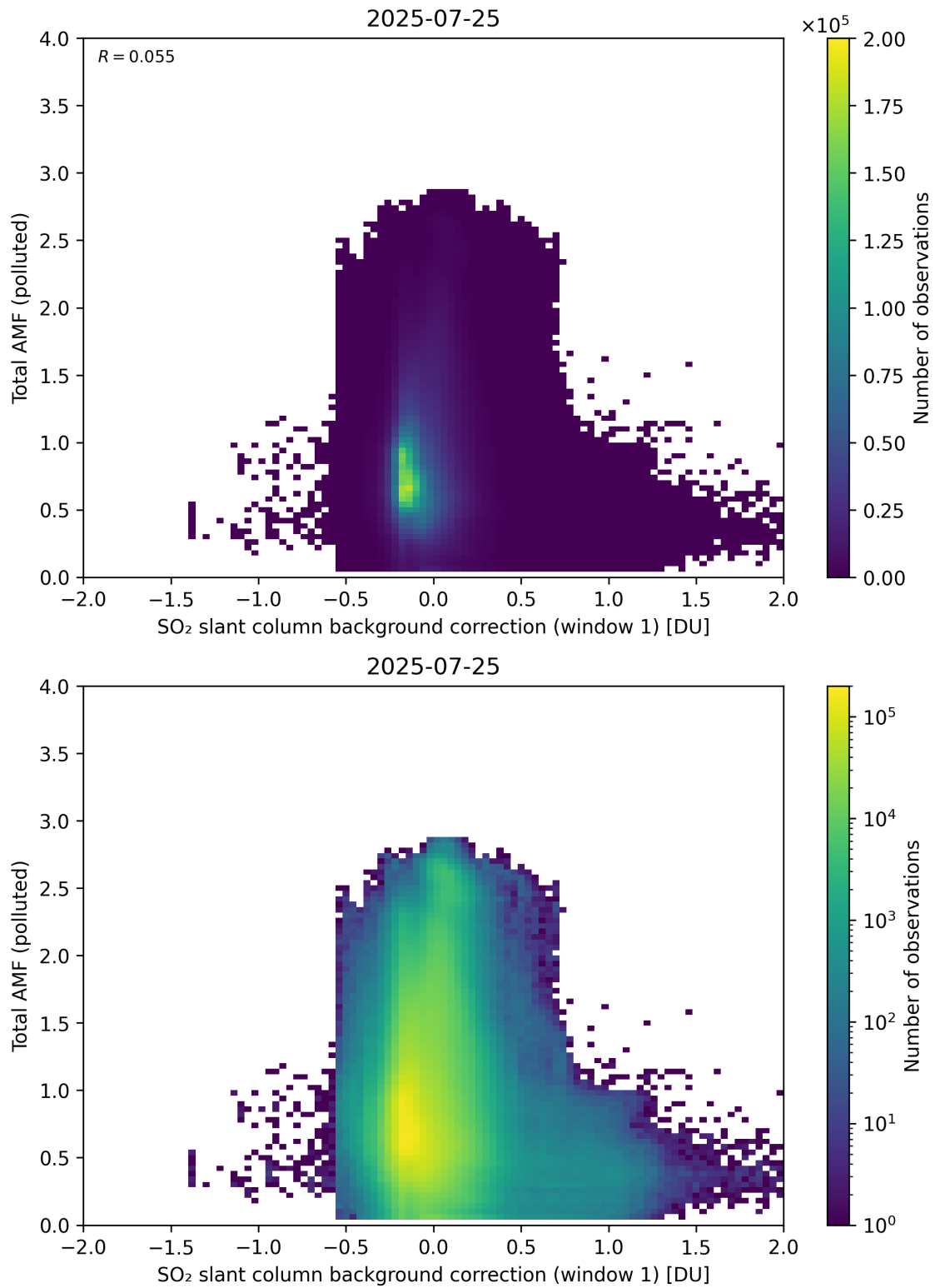
Figure 120: Scatter density plot of “SO 2 slant column background correction (window 1)” against “Total AMF (polluted)” for 2025-07-24 to 2025-07-26.
