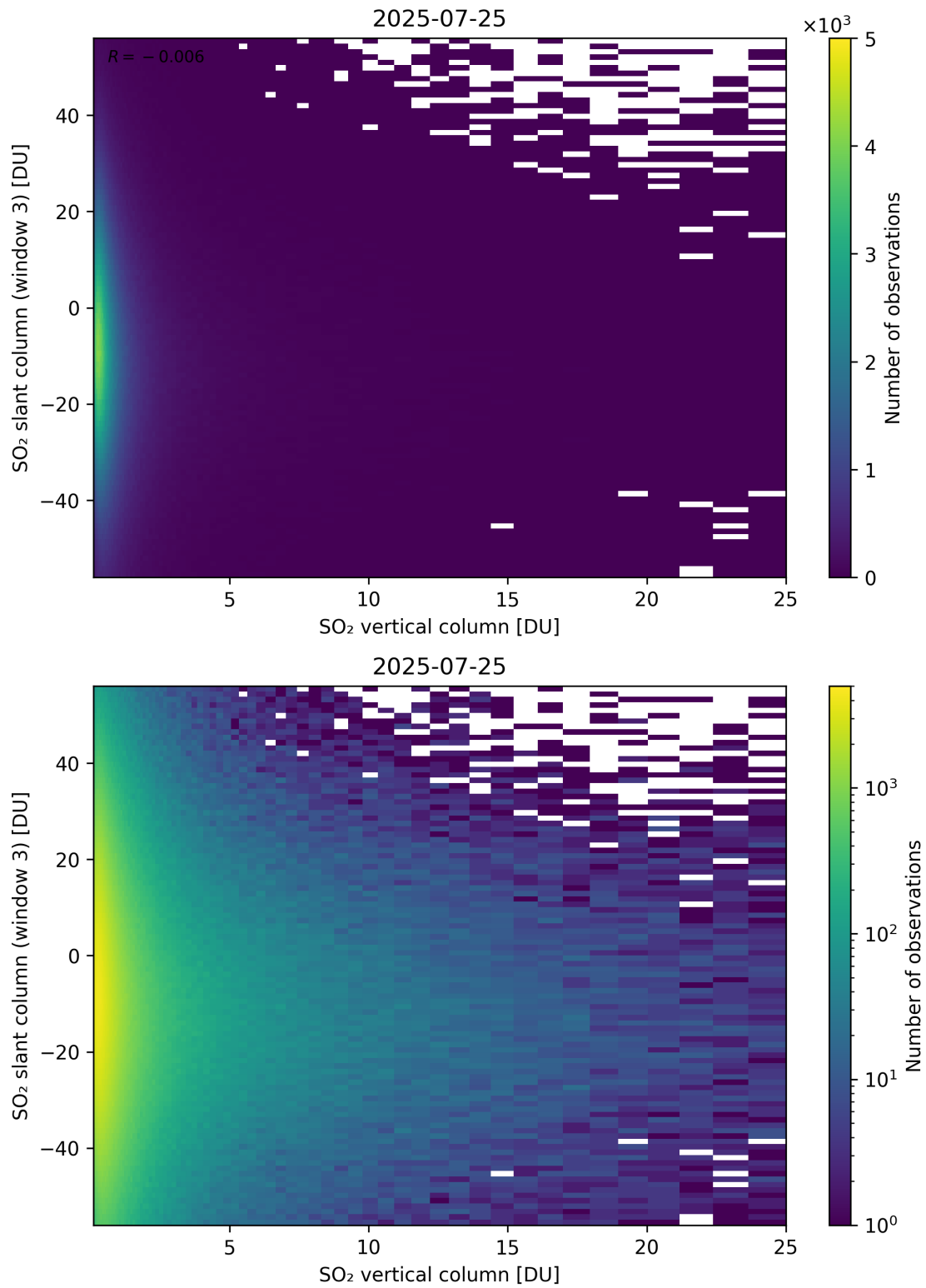
Figure 357: Scatter density plot of “SO 2 vertical column” against “SO 2 slant column (window 3)” for 2025-07-24 to 2025-07-26.
