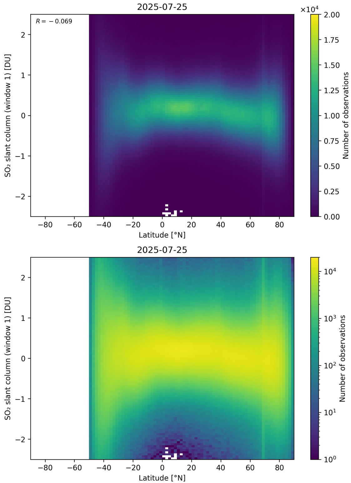
Figure 162: Scatter density plot of “Latitude” against “SO 2 slant column (window 1)” for 2025-07-24 to 2025-07-26.
