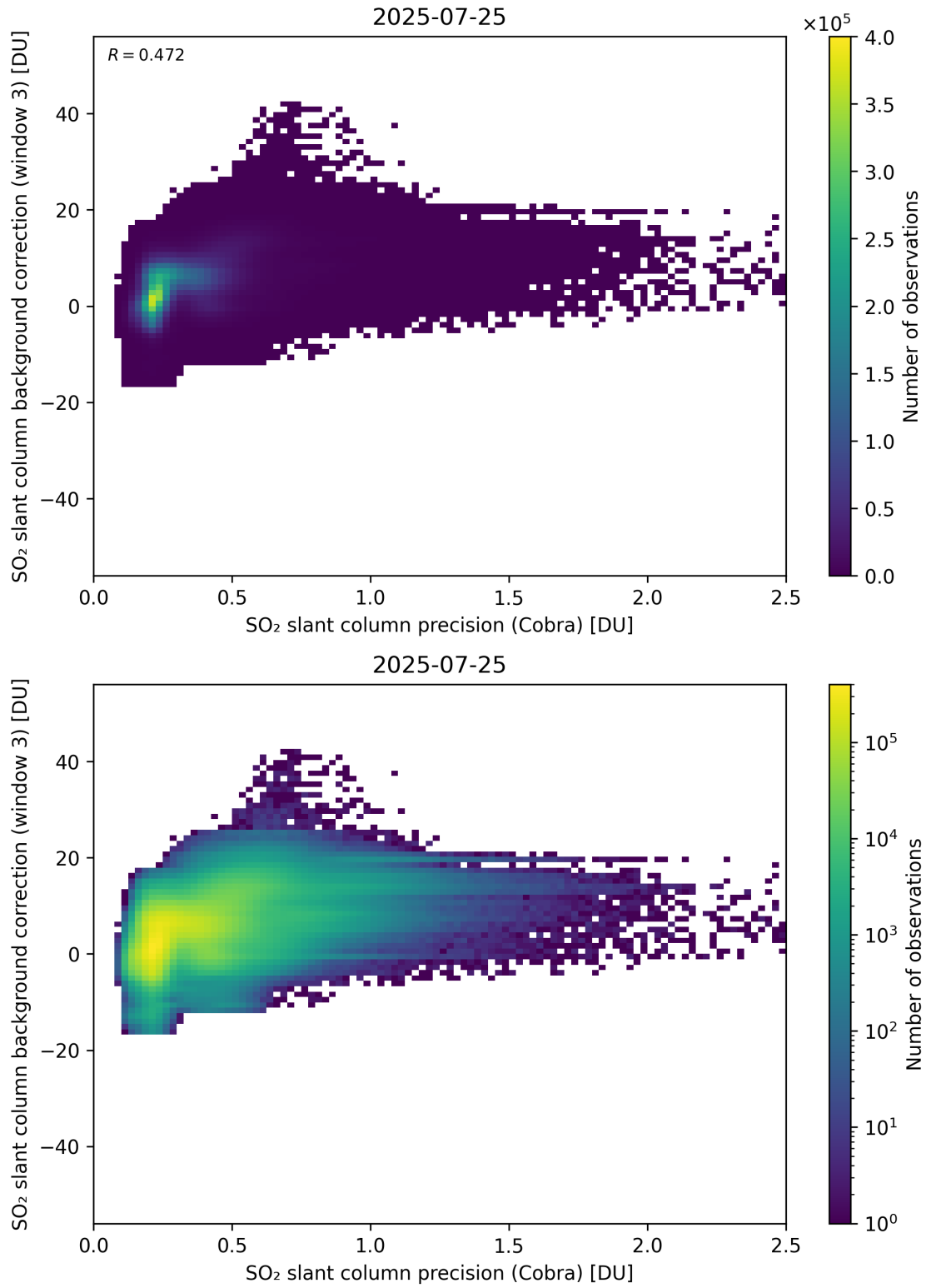
Figure 201: Scatter density plot of “SO 2 slant column precision (Cobra)” against “SO 2 slant column background correction (window 3)” for 2025-07-24 to 2025-07-26.
