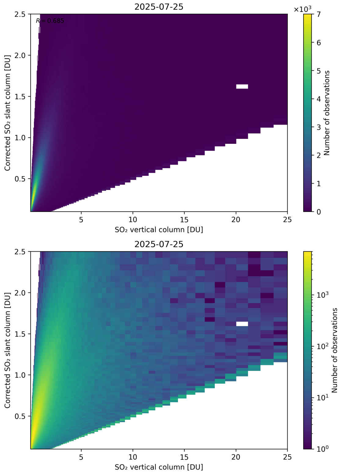
Figure 351: Scatter density plot of “SO 2 vertical column” against “Corrected SO 2 slant column” for 2025-07-24 to 2025-07-26.
