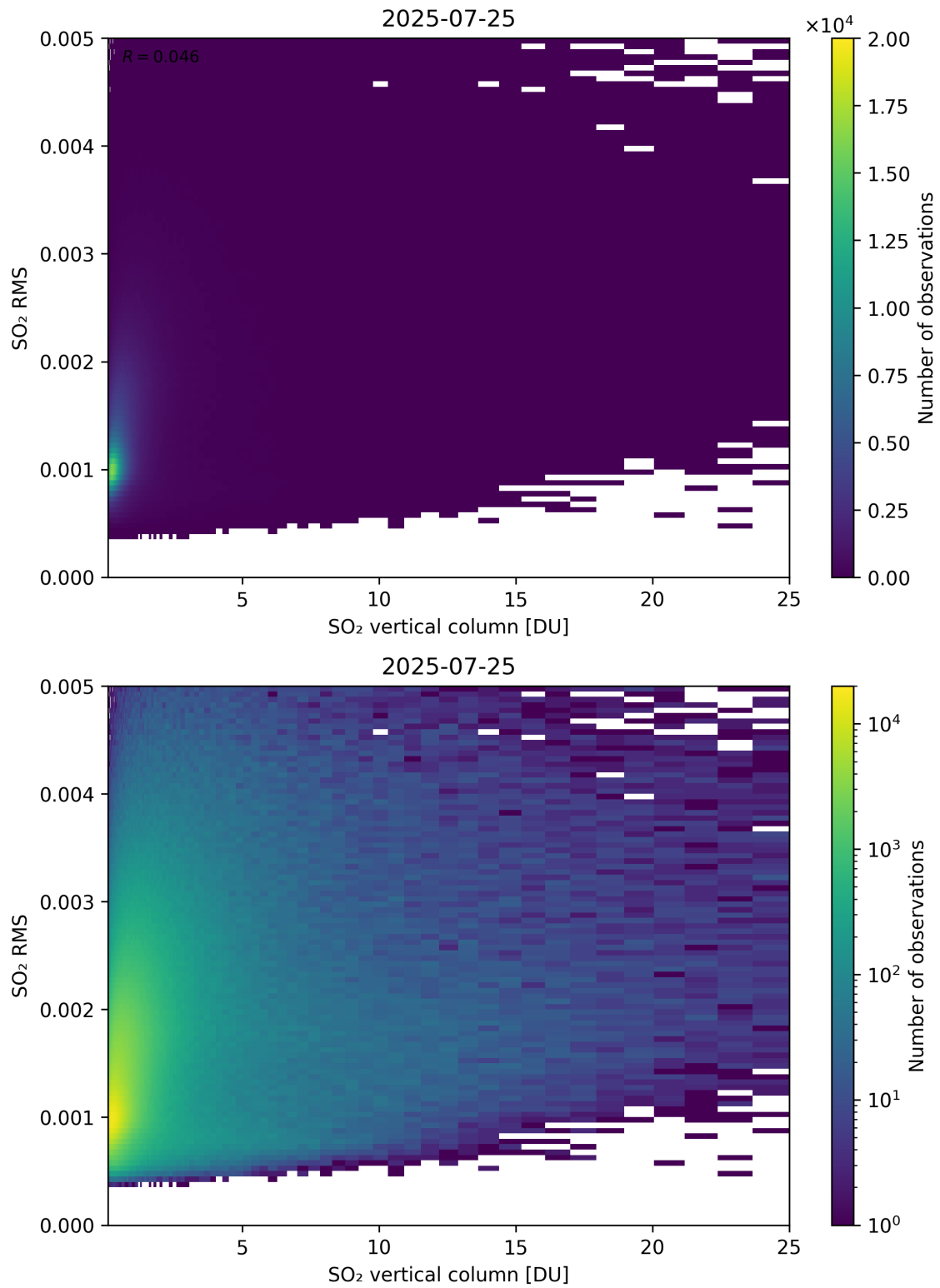
Figure 328: Scatter density plot of “SO 2 vertical column” against “SO 2 RMS” for 2025-07-24 to 2025-07-26.
