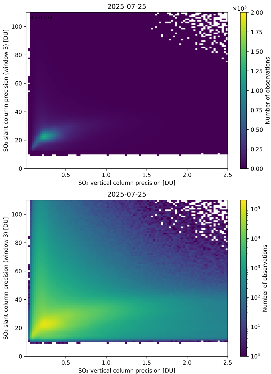
Figure 345: Scatter density plot of “SO 2 vertical column precision” against “SO 2 slant column precision (window 3)” for 2025-07-24 to 2025-07-26.
