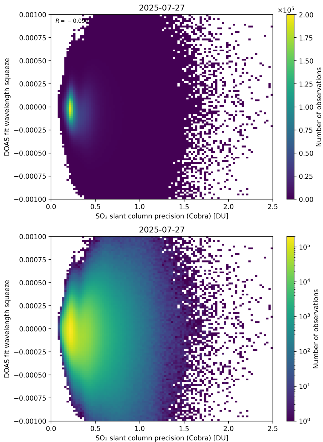
Figure 203: Scatter density plot of “SO 2 slant column precision (Cobra)” against “DOAS fit wavelength squeeze” for 2025-07-26 to 2025-07-28.
