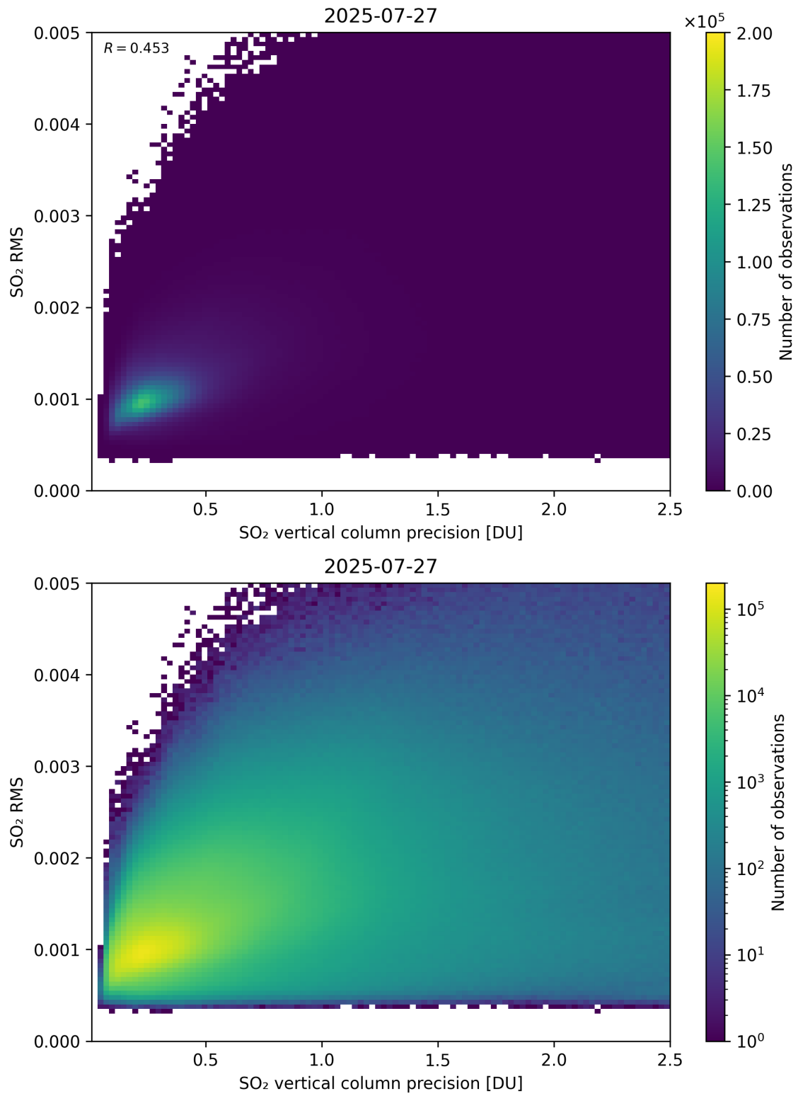
Figure 334: Scatter density plot of “SO 2 vertical column precision” against “SO 2 RMS” for 2025-07-26 to 2025-07-28.
