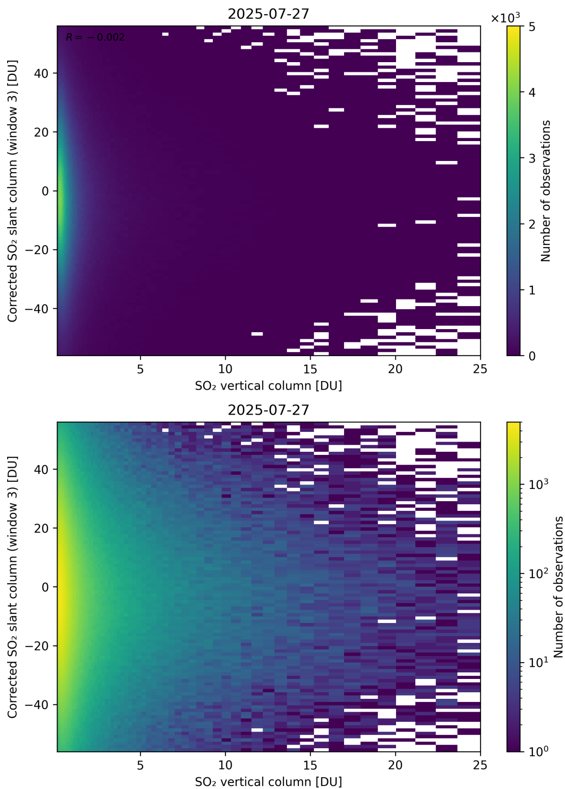
Figure 353: Scatter density plot of “SO 2 vertical column” against “Corrected SO 2 slant column (window 3)” for 2025-07-26 to 2025-07-28.
