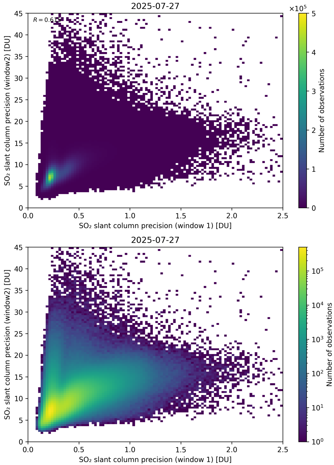
Figure 277: Scatter density plot of “SO 2 slant column precision (window 1)” against “SO 2 slant column precision (window2)” for 2025-07-26 to 2025-07-28.
