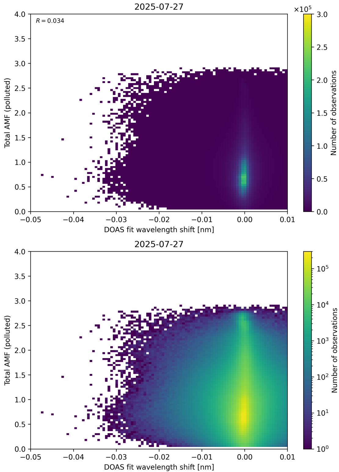
Figure 141: Scatter density plot of “DOAS fit wavelength shift” against “Total AMF (polluted)” for 2025-07-26 to 2025-07-28.
