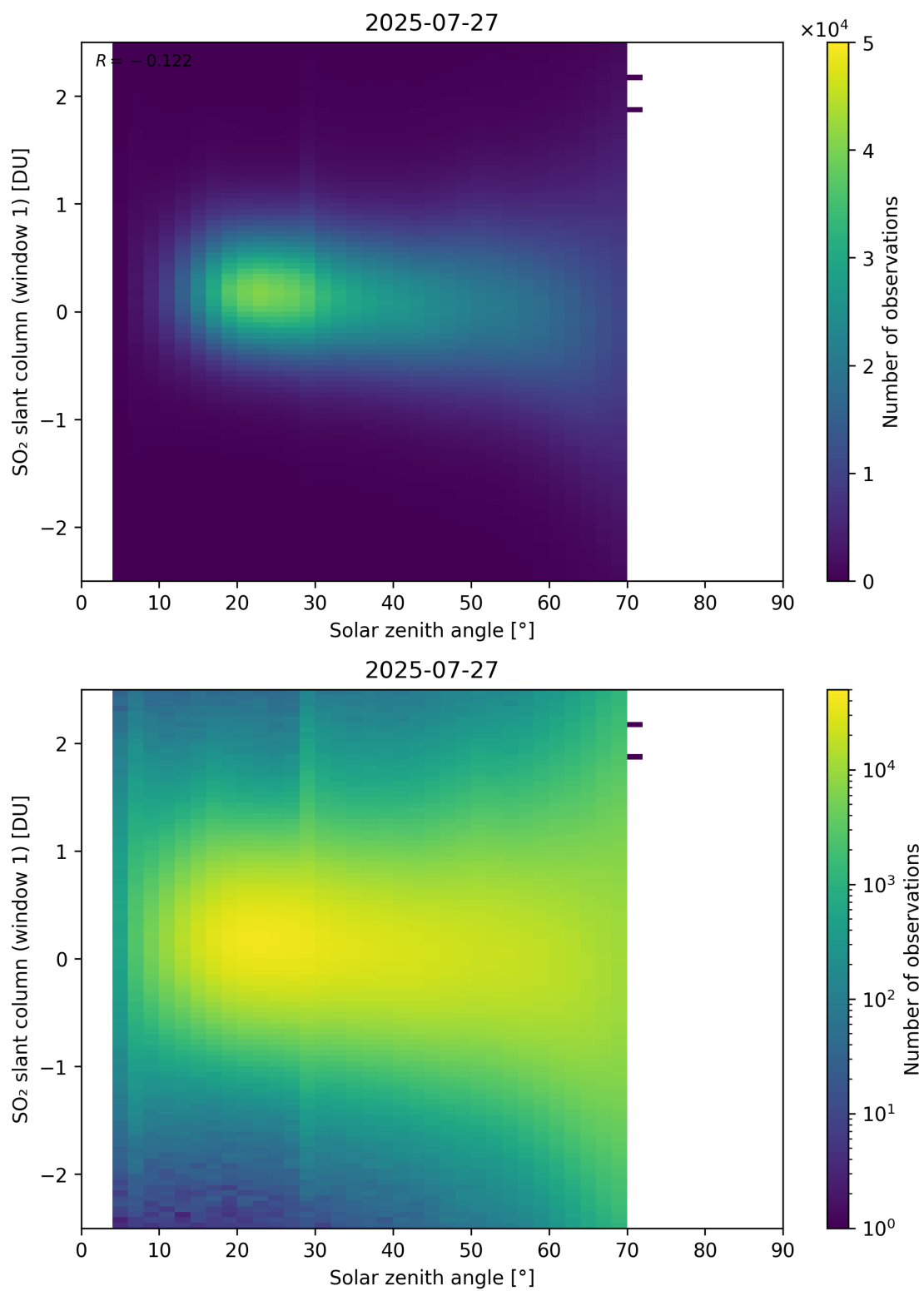
Figure 184: Scatter density plot of “Solar zenith angle” against “SO 2 slant column (window 1)” for 2025-07-26 to 2025-07-28.
