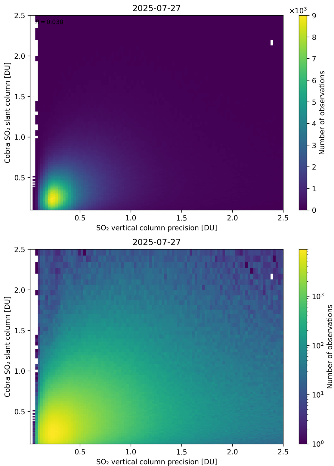
Figure 336: Scatter density plot of “SO 2 vertical column precision” against “Cobra SO 2 slant column” for 2025-07-26 to 2025-07-28.
