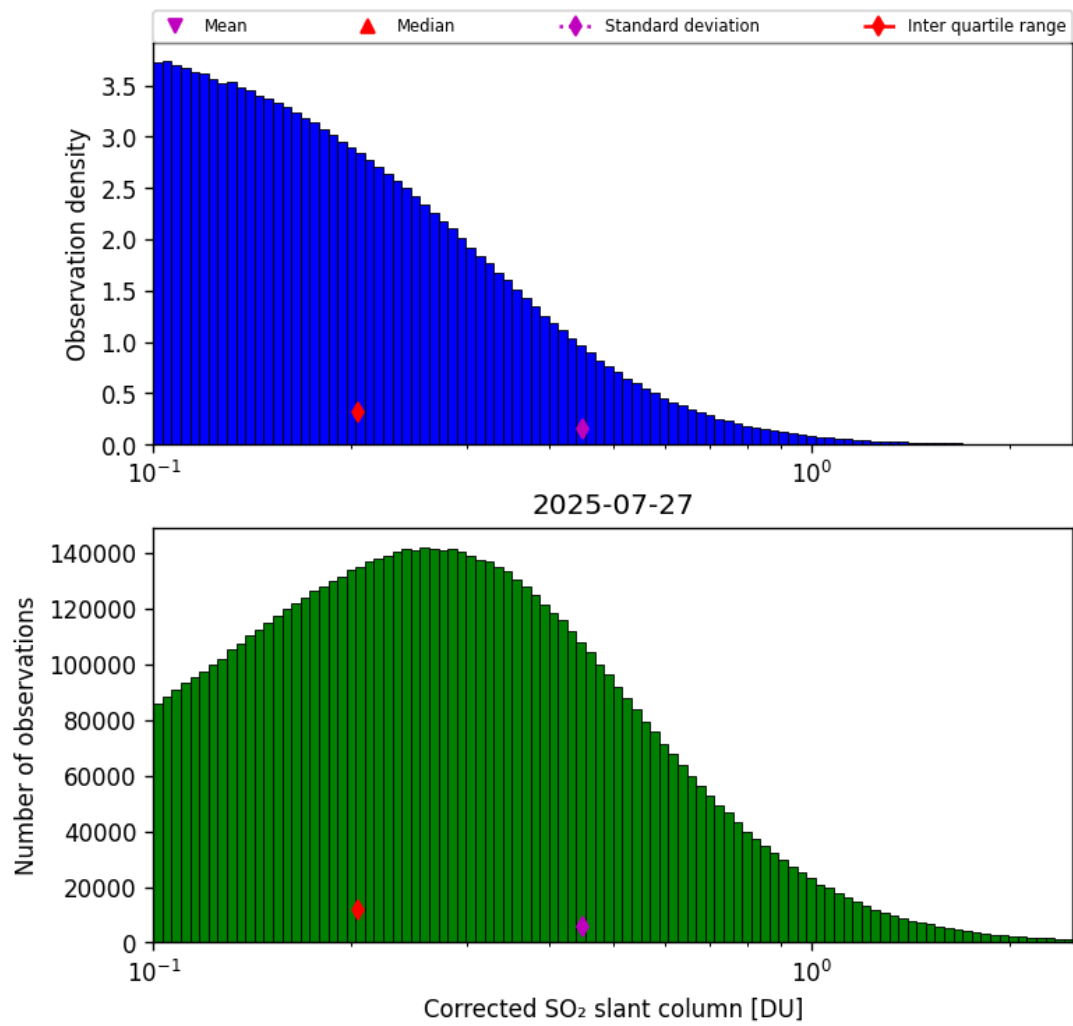
Figure 60: Histogram of “Corrected SO 2 slant column” for 2025-07-26 to 2025-07-28
