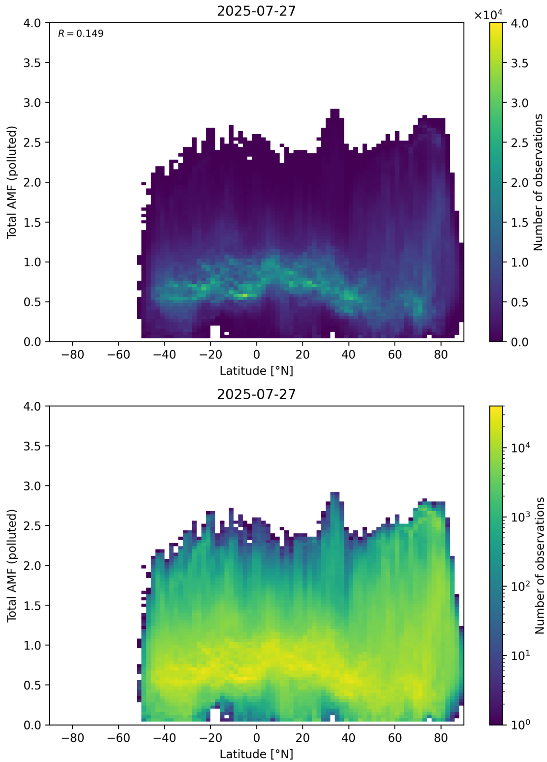
Figure 167: Scatter density plot of “Latitude” against “Total AMF (polluted)” for 2025-07-26 to 2025-07-28.
