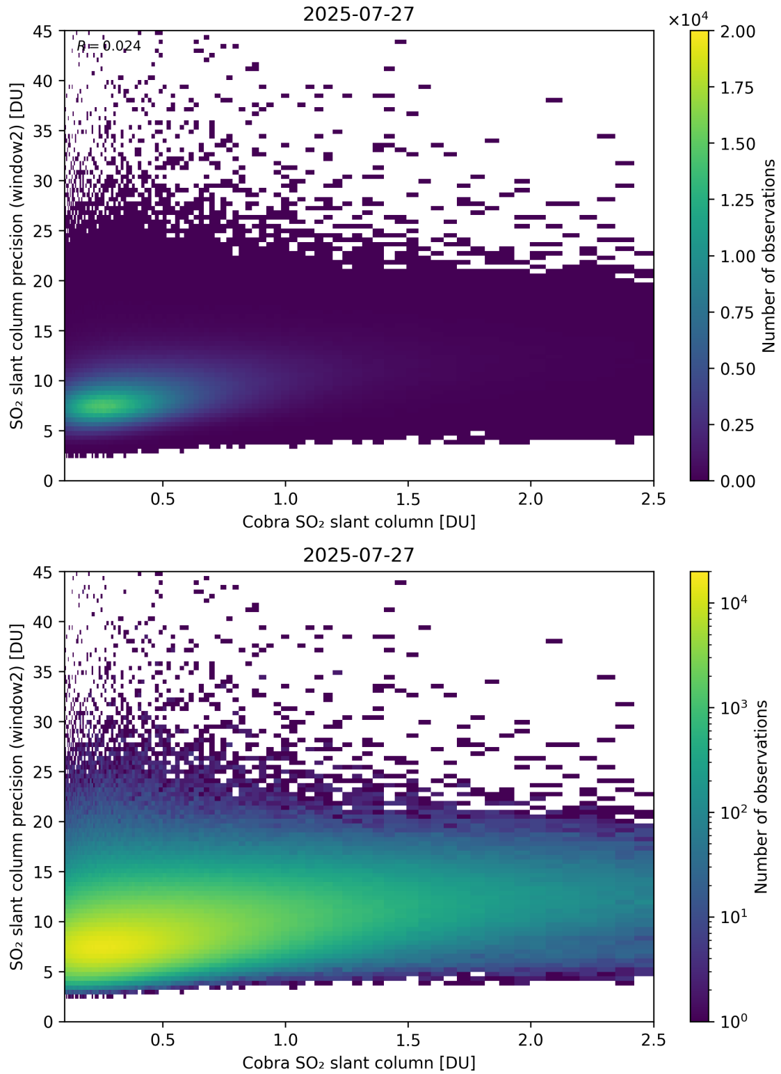
Figure 221: Scatter density plot of “Cobra SO 2 slant column” against “SO 2 slant column precision (window2)” for 2025-07-26 to 2025-07-28.
