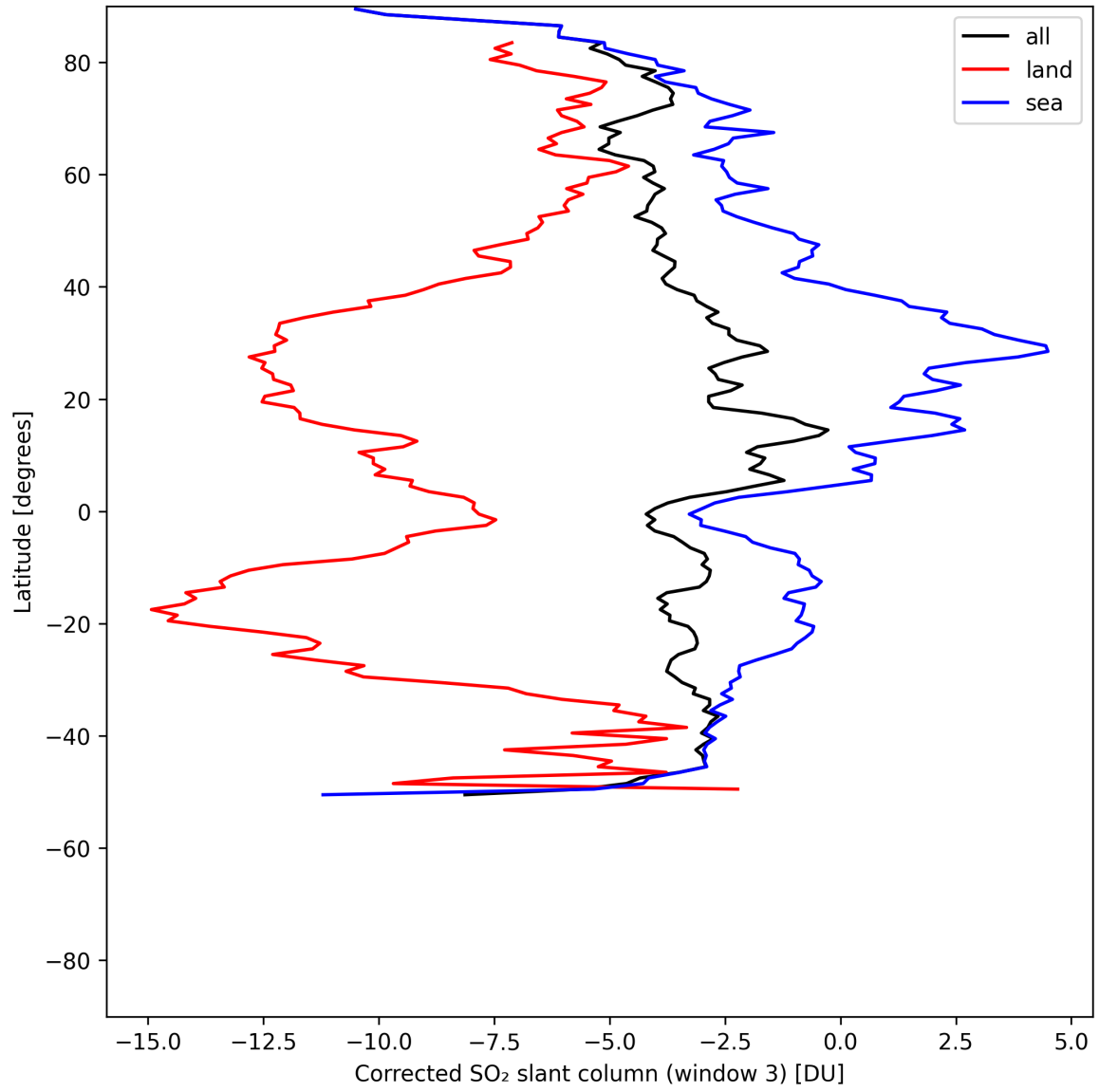
Figure 47: Zonal average of “Corrected SO 2 slant column (window 3)” for 2025-07-26 to 2025-07-28.
