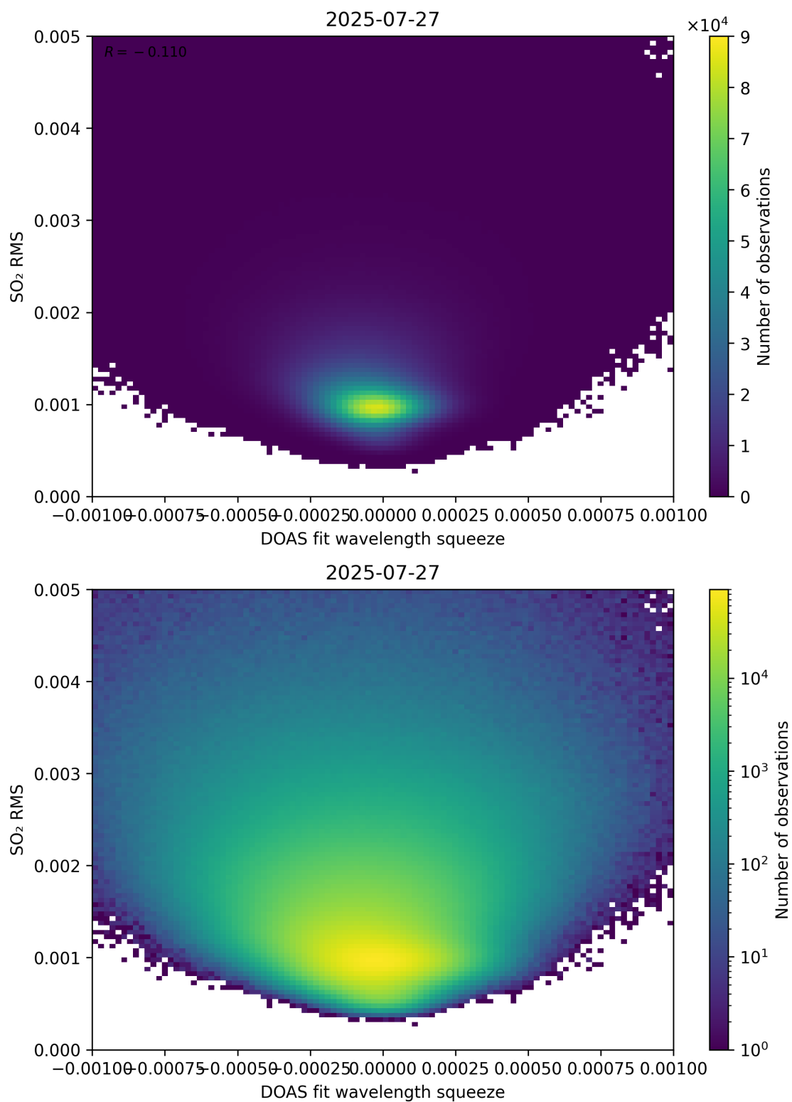
Figure 143: Scatter density plot of “DOAS fit wavelength squeeze” against “SO 2 RMS” for 2025-07-26 to 2025-07-28.
