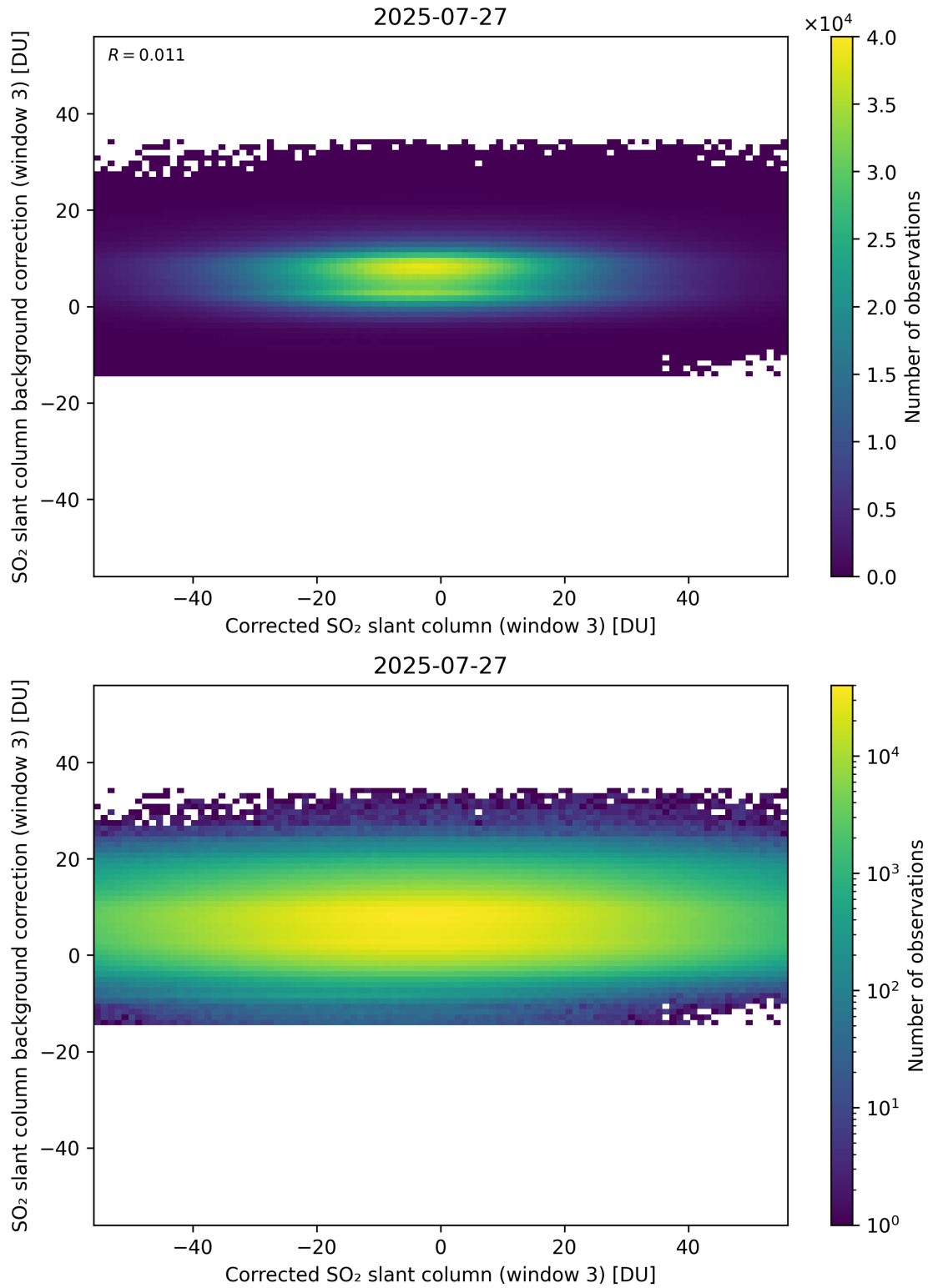
Figure 255: Scatter density plot of “Corrected SO 2 slant column (window 3)” against “SO 2 slant column background correction (window 3)” for 2025-07-26 to 2025-07-28.
