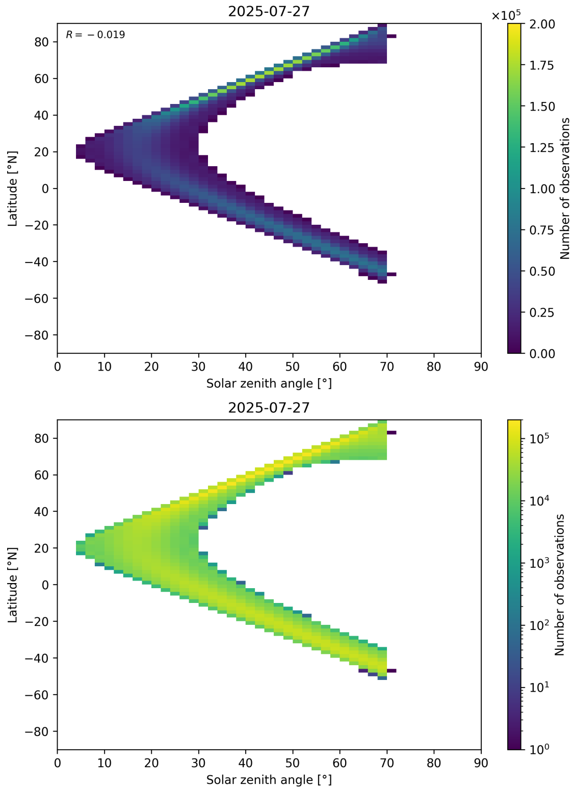
Figure 177: Scatter density plot of “Solar zenith angle” against “Latitude” for 2025-07-26 to 2025-07-28.
