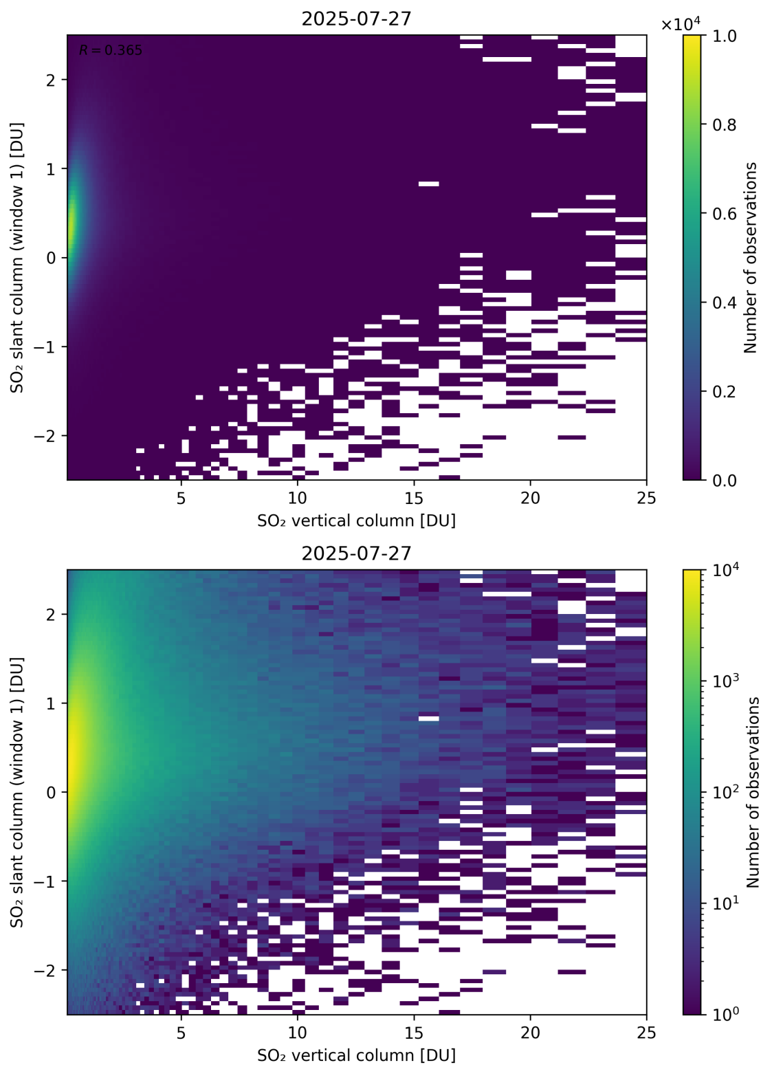
Figure 354: Scatter density plot of “SO 2 vertical column” against “SO 2 slant column (window 1)” for 2025-07-26 to 2025-07-28.
