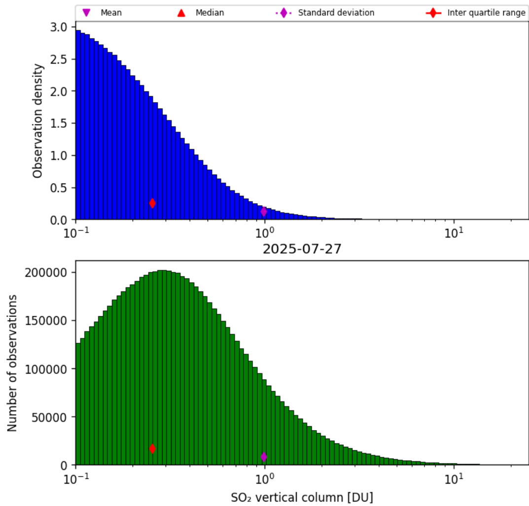
Figure 58: Histogram of “SO 2 vertical column” for 2025-07-26 to 2025-07-28
