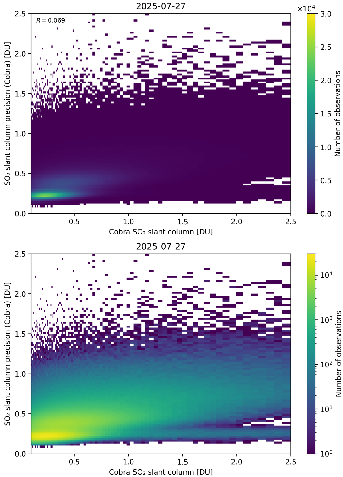
Figure 216: Scatter density plot of “Cobra SO 2 slant column” against “SO 2 slant column precision (Cobra)” for 2025-07-26 to 2025-07-28.
