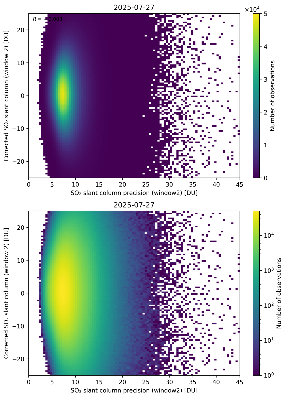
Figure 297: Scatter density plot of “SO 2 slant column precision (window2)” against “Corrected SO 2 slant column (window 2)” for 2025-07-26 to 2025-07-28.
