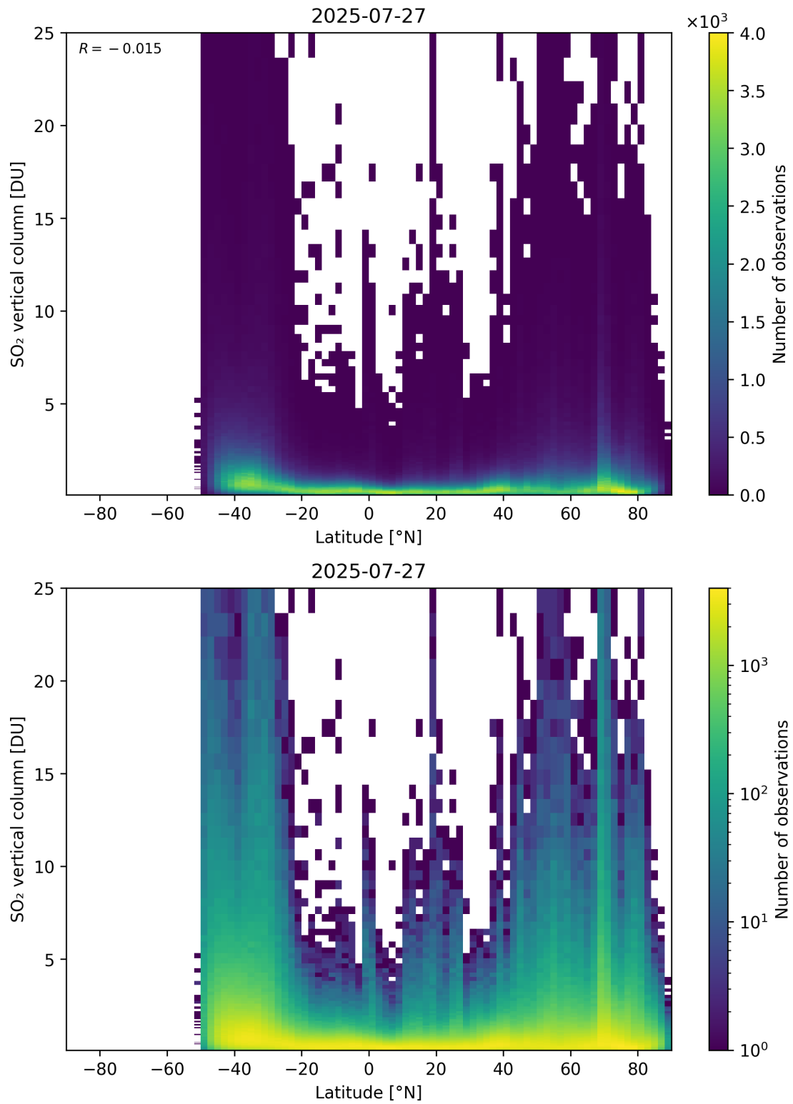
Figure 169: Scatter density plot of “Latitude” against “SO 2 vertical column” for 2025-07-26 to 2025-07-28.
