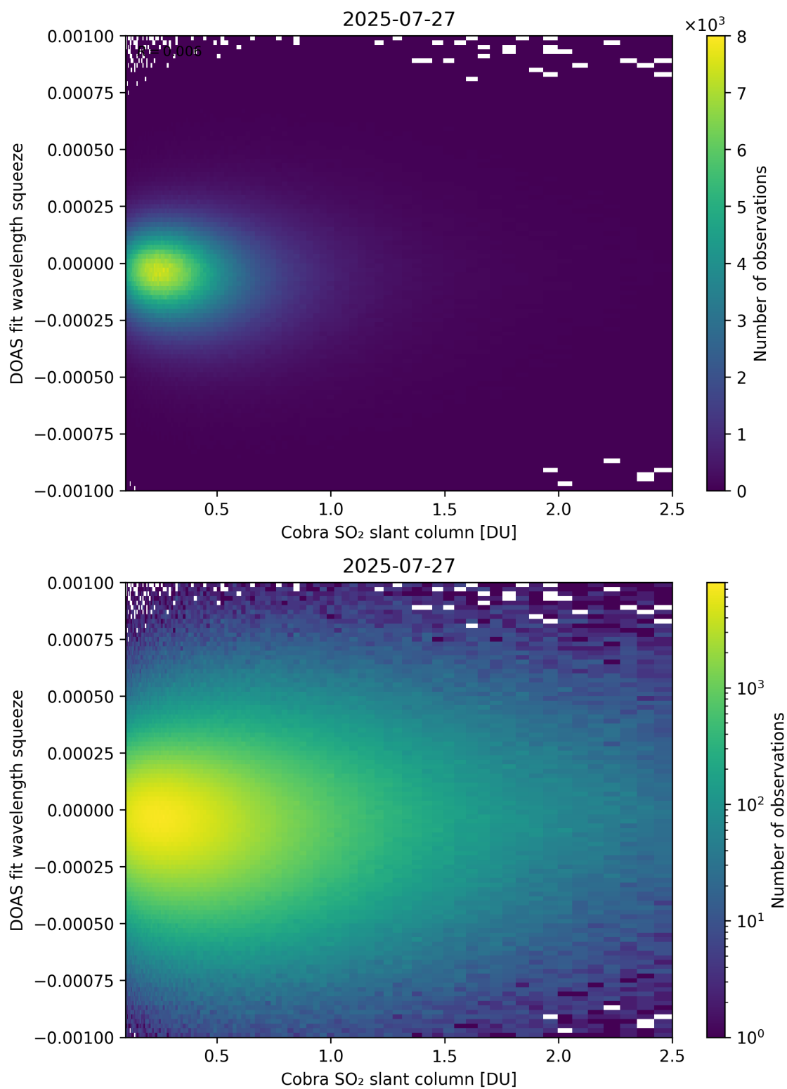
Figure 197: Scatter density plot of “Cobra SO 2 slant column” against “DOAS fit wavelength squeeze” for 2025-07-26 to 2025-07-28.
