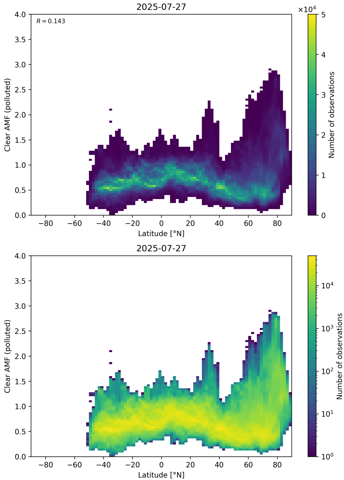
Figure 156: Scatter density plot of “Latitude” against “Clear AMF (polluted)” for 2025-07-26 to 2025-07-28.
