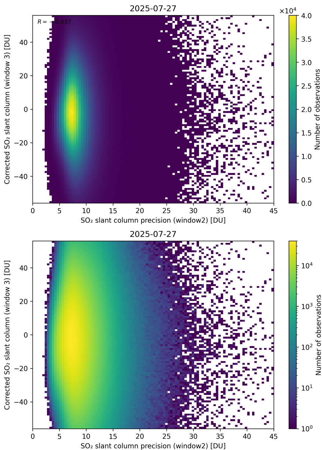
Figure 298: Scatter density plot of “SO 2 slant column precision (window2)” against “Corrected SO 2 slant column (window 3)” for 2025-07-26 to 2025-07-28.
