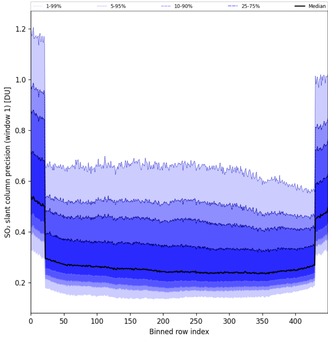
Figure 90: Along track statistics of “SO 2 slant column precision (window 1)” for 2025-07-26 to 2025-07-28
