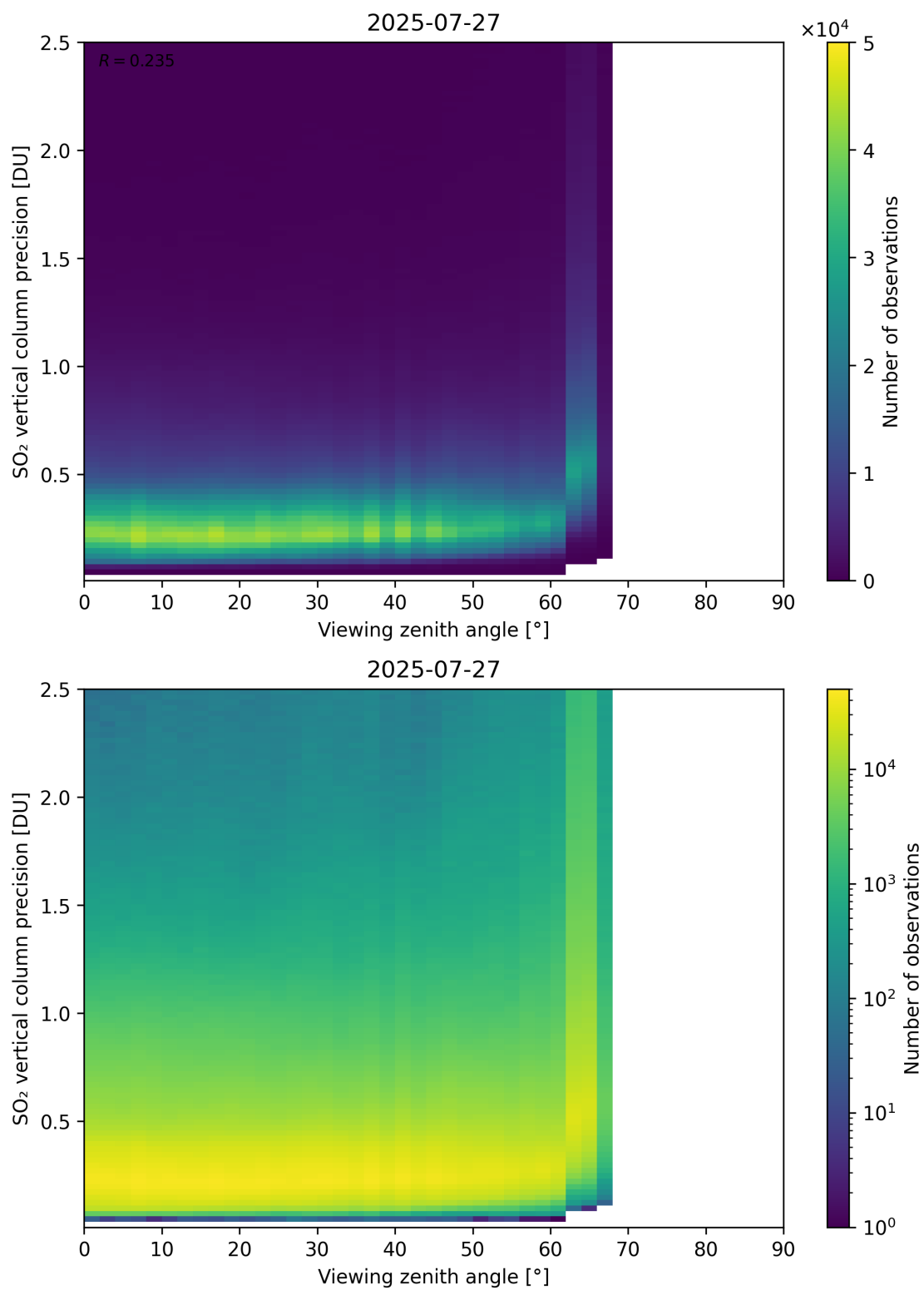
Figure 384: Scatter density plot of “Viewing zenith angle” against “SO 2 vertical column precision” for 2025-07-26 to 2025-07-28.
