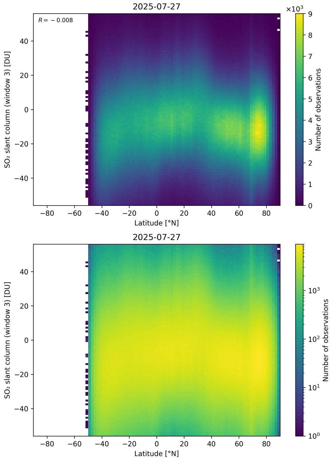
Figure 165: Scatter density plot of “Latitude” against “SO 2 slant column (window 3)” for 2025-07-26 to 2025-07-28.
