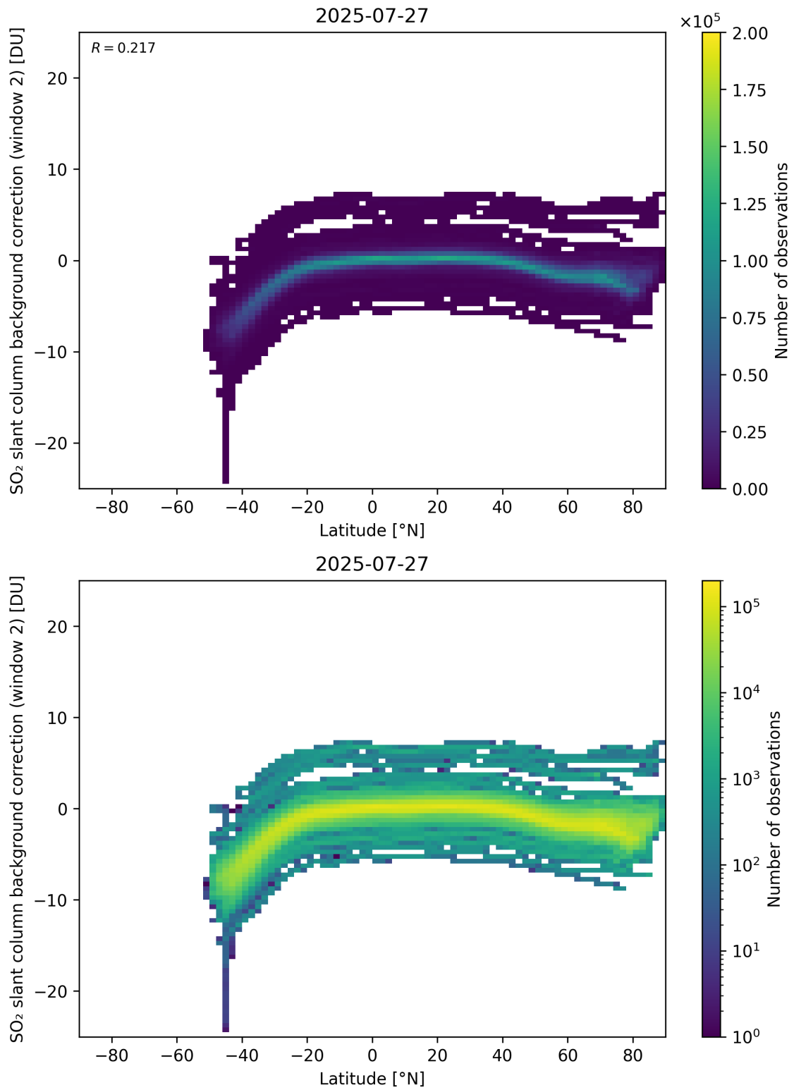
Figure 151: Scatter density plot of “Latitude” against “SO 2 slant column background correction (window 2)” for 2025-07-26 to 2025-07-28.
