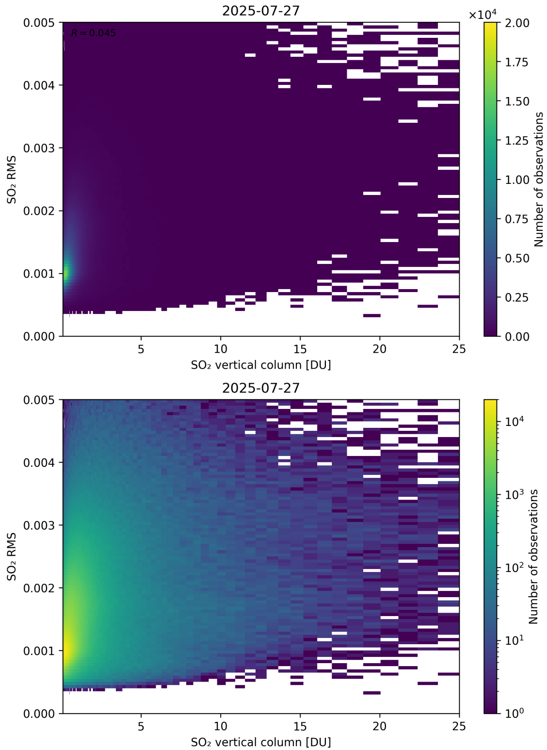
Figure 328: Scatter density plot of “SO 2 vertical column” against “SO 2 RMS” for 2025-07-26 to 2025-07-28.
