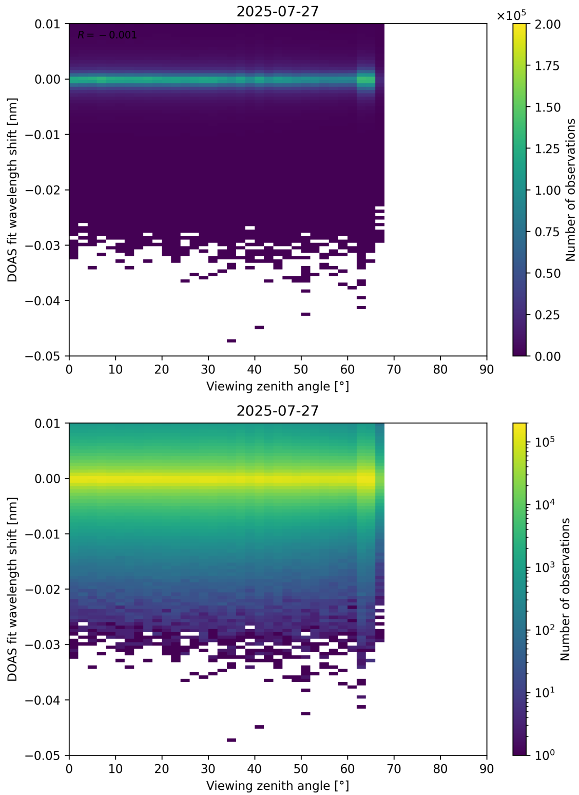
Figure 365: Scatter density plot of “Viewing zenith angle” against “DOAS fit wavelength shift” for 2025-07-26 to 2025-07-28.
