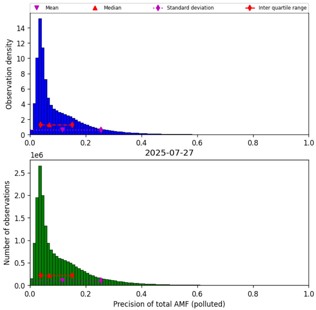
Figure 80: Histogram of “Precision of total AMF (polluted)” for 2025-07-26 to 2025-07-28
