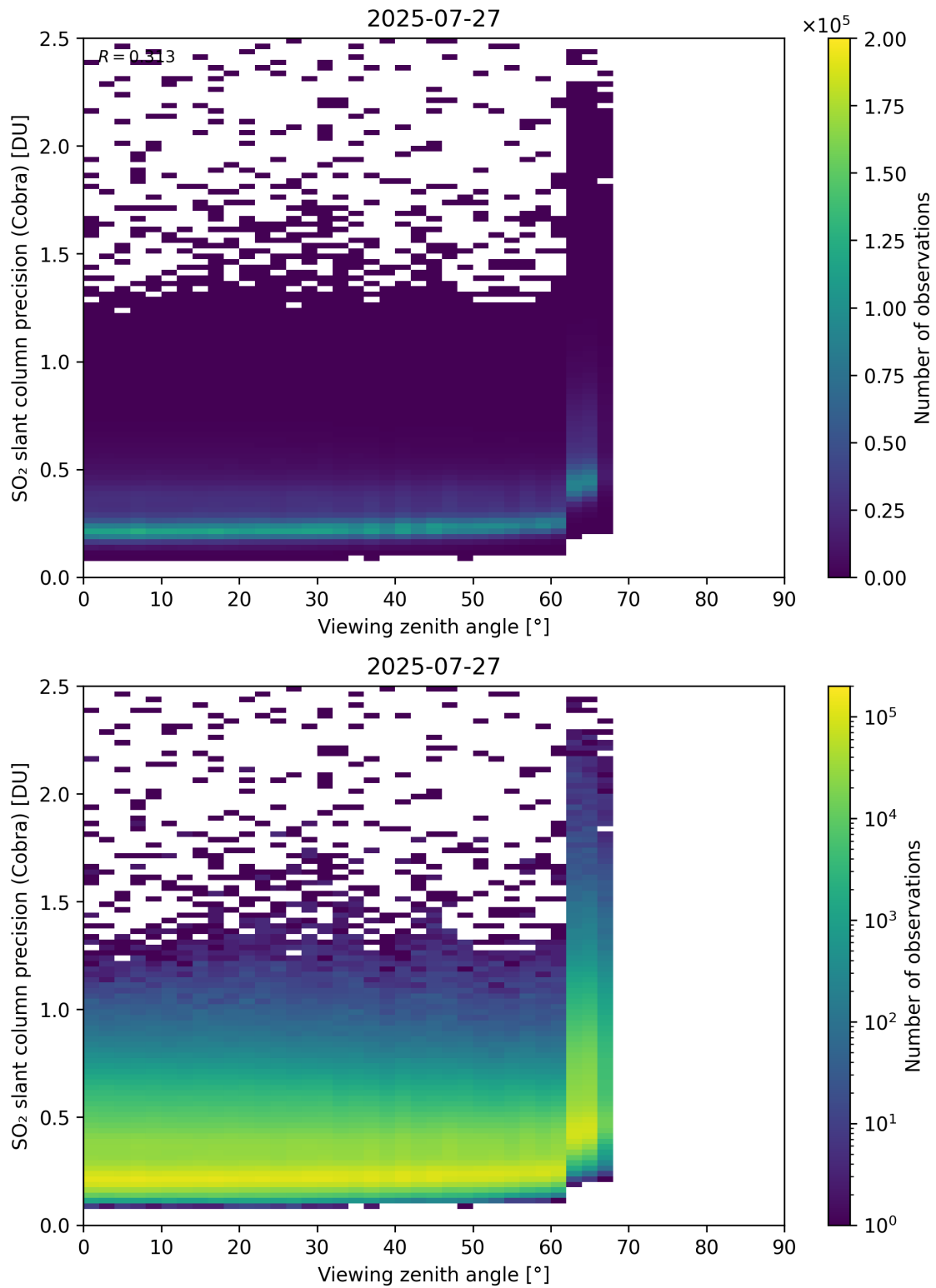
Figure 372: Scatter density plot of “Viewing zenith angle” against “SO 2 slant column precision (Cobra)” for 2025-07-26 to 2025-07-28.
