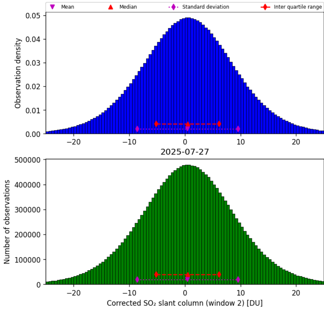
Figure 69: Histogram of “Corrected SO 2 slant column (window 2)” for 2025-07-26 to 2025-07-28
