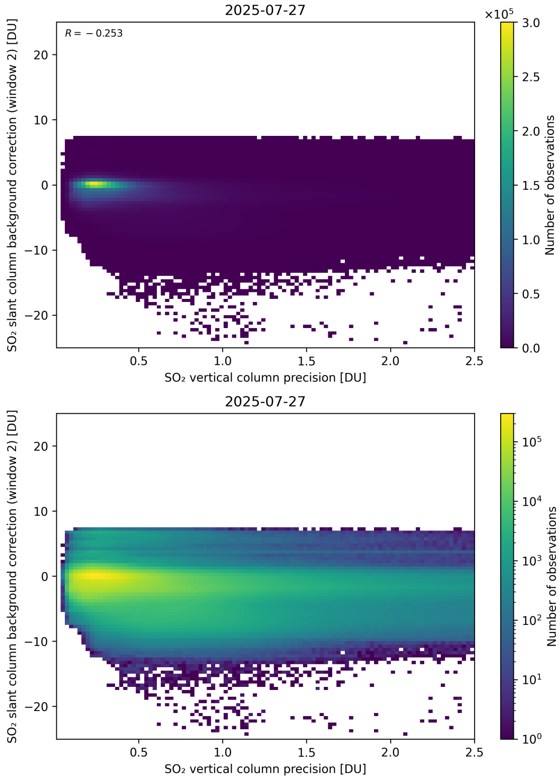
Figure 330: Scatter density plot of “SO 2 vertical column precision” against “SO 2 slant column background correction (window 2)” for 2025-07-26 to 2025-07-28.
