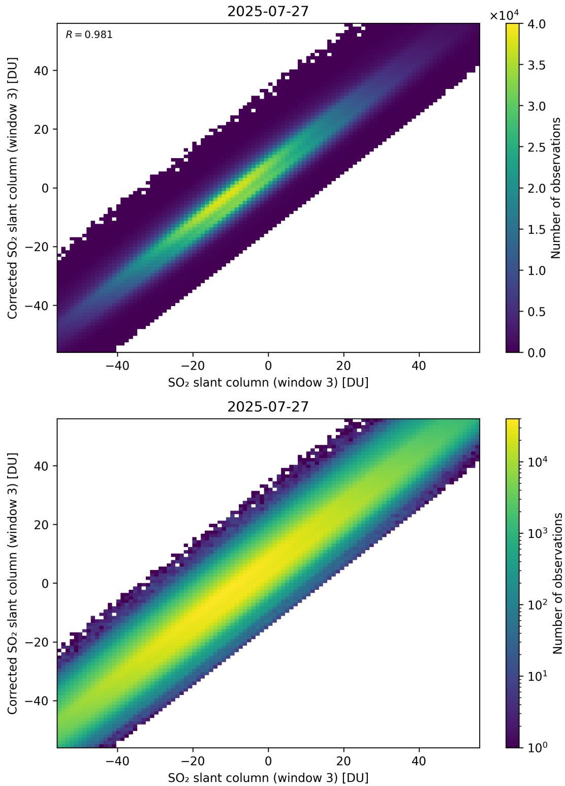
Figure 316: Scatter density plot of “SO 2 slant column (window 3)” against “Corrected SO 2 slant column (window 3)” for 2025-07-26 to 2025-07-28.
