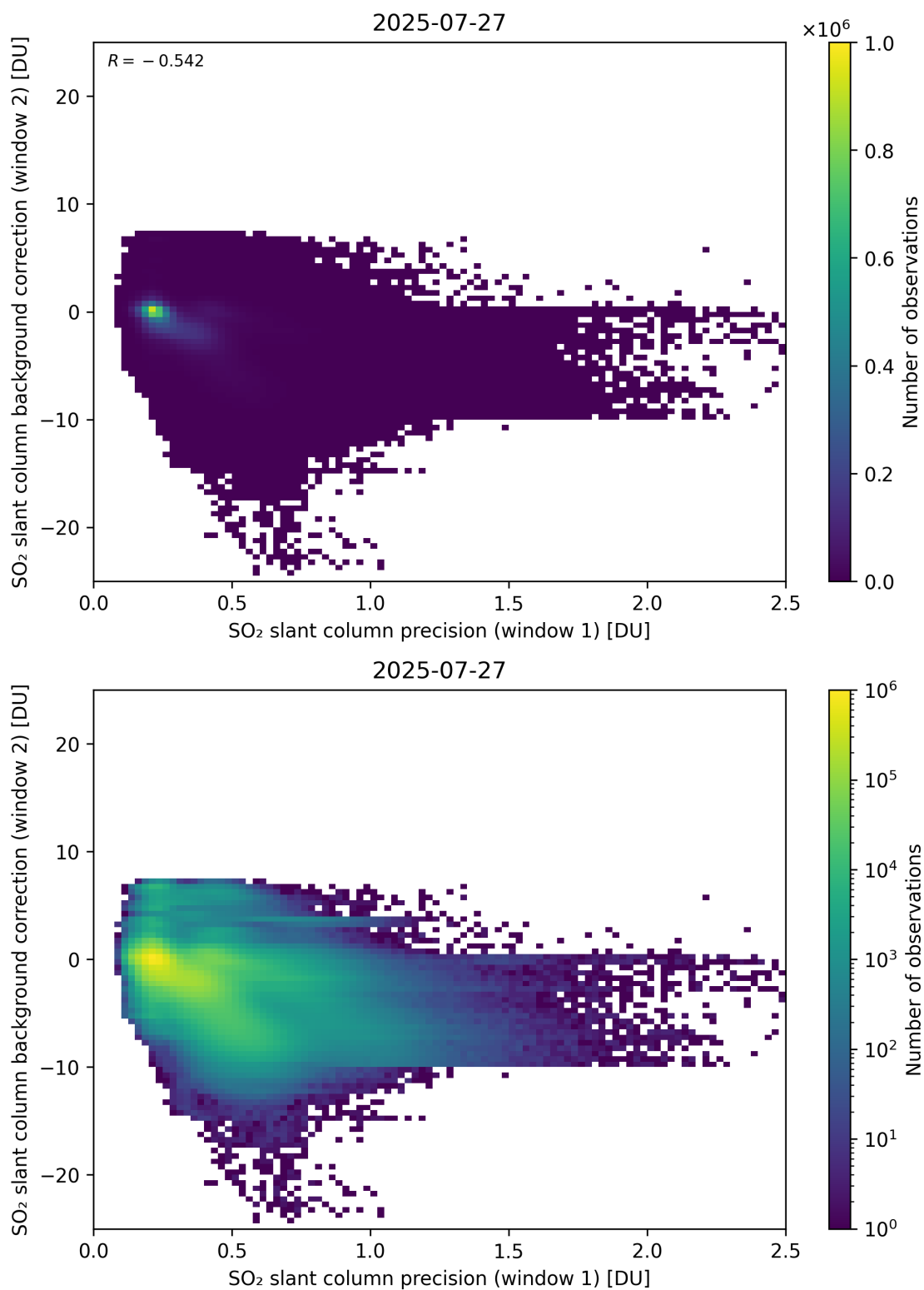
Figure 269: Scatter density plot of “SO 2 slant column precision (window 1)” against “SO 2 slant column background correction (window 2)” for 2025-07-26 to 2025-07-28.
