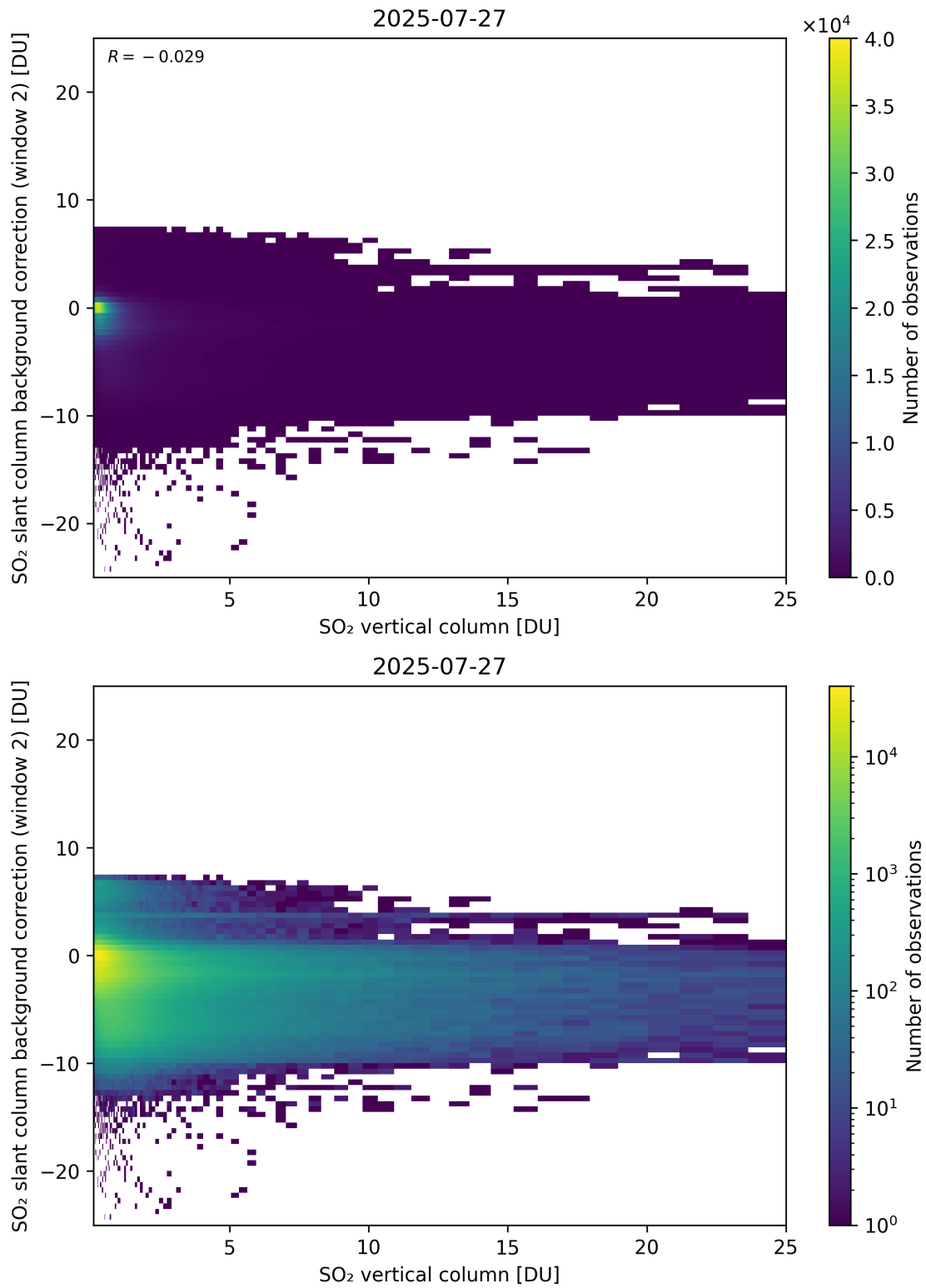
Figure 324: Scatter density plot of “SO 2 vertical column” against “SO 2 slant column background correction (window 2)” for 2025-07-26 to 2025-07-28.
