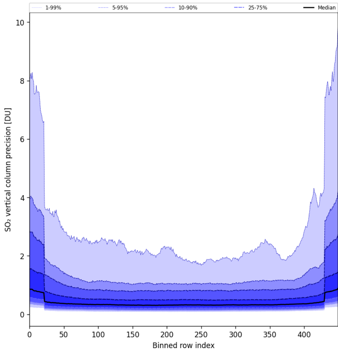
Figure 85: Along track statistics of “SO 2 vertical column precision” for 2025-07-26 to 2025-07-28
