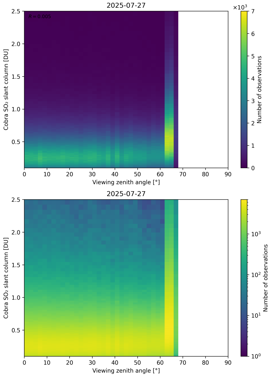
Figure 371: Scatter density plot of “Viewing zenith angle” against “Cobra SO 2 slant column” for 2025-07-26 to 2025-07-28.
