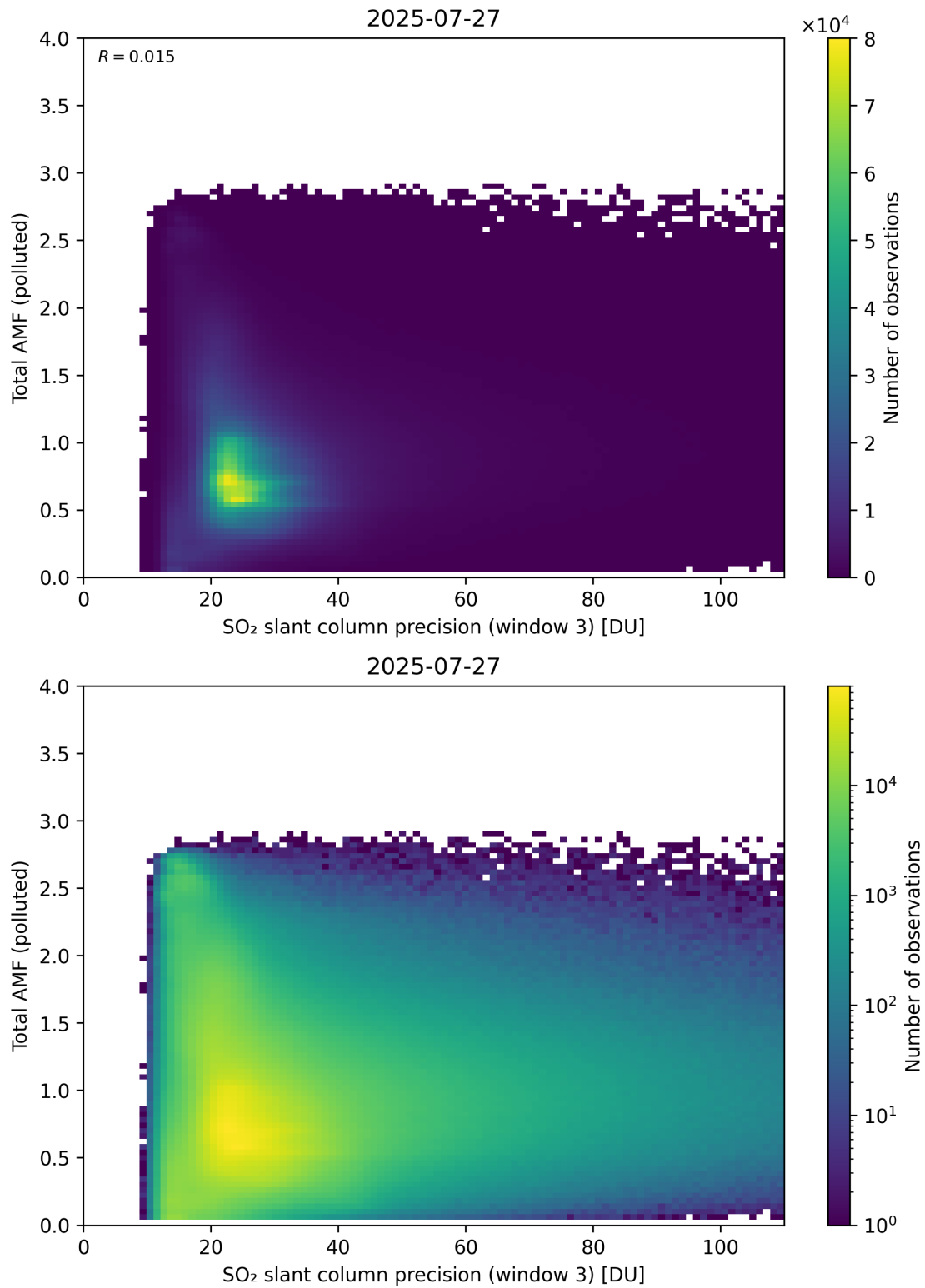
Figure 313: Scatter density plot of “SO 2 slant column precision (window 3)” against “Total AMF (polluted)” for 2025-07-26 to 2025-07-28.
