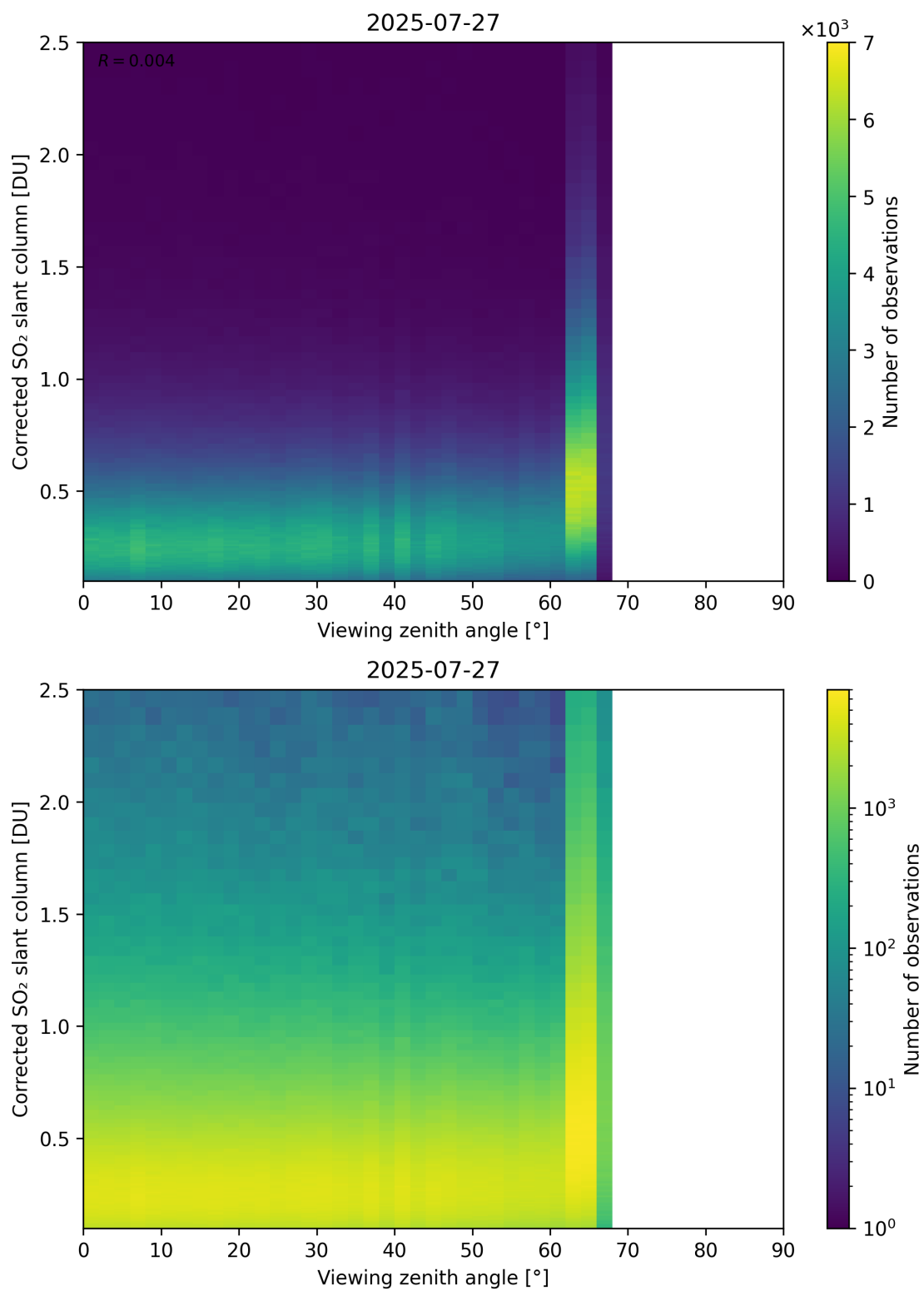
Figure 373: Scatter density plot of “Viewing zenith angle” against “Corrected SO 2 slant column” for 2025-07-26 to 2025-07-28.
