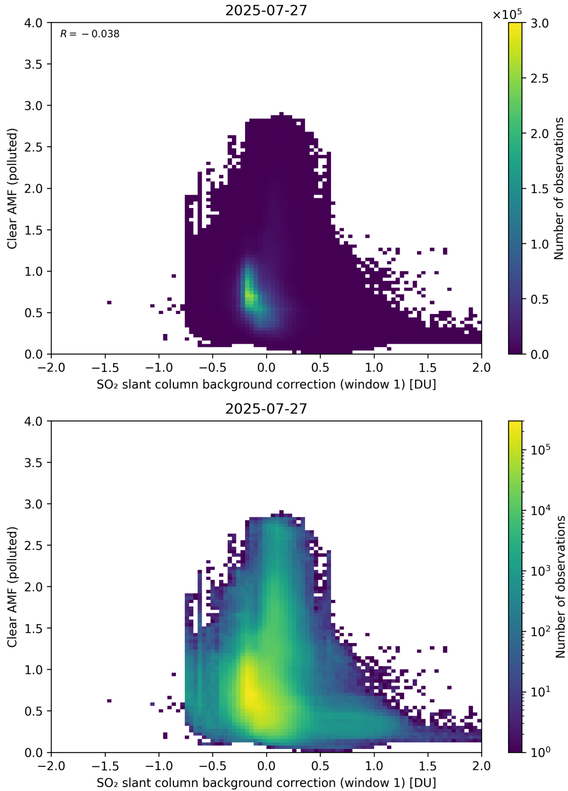
Figure 114: Scatter density plot of “SO 2 slant column background correction (window 1)” against “Clear AMF (polluted)” for 2025-07-26 to 2025-07-28.
