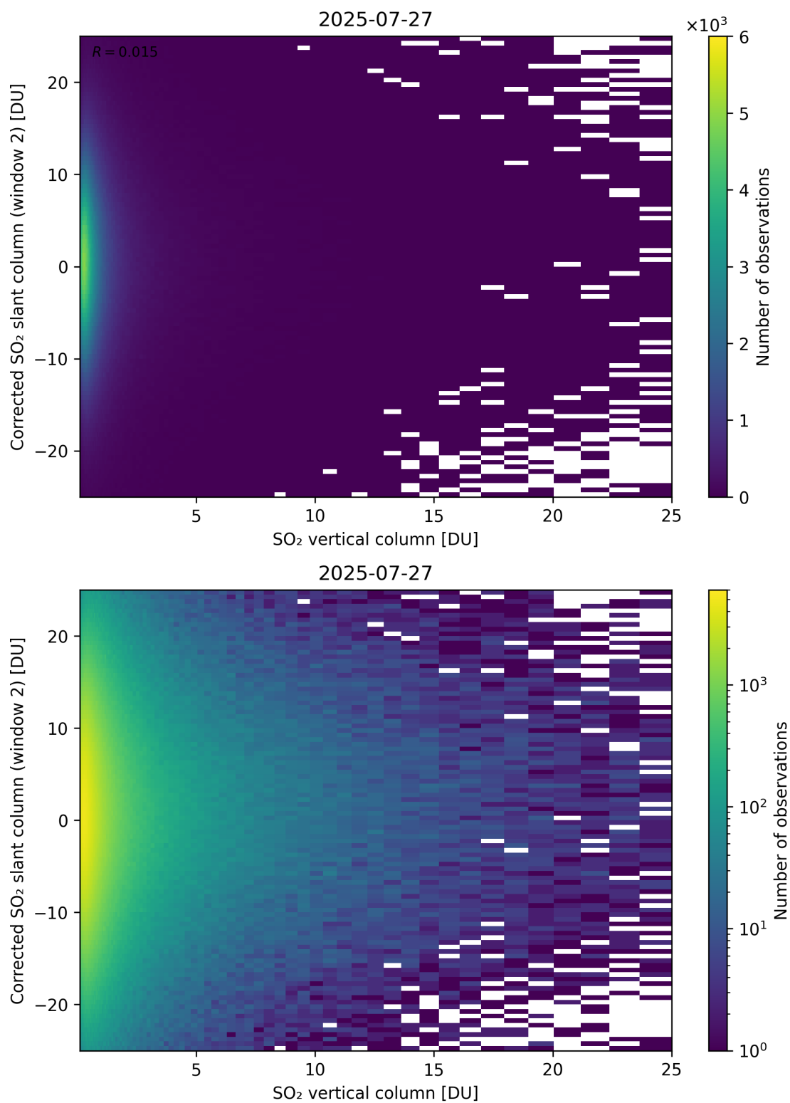
Figure 352: Scatter density plot of “SO 2 vertical column” against “Corrected SO 2 slant column (window 2)” for 2025-07-26 to 2025-07-28.
