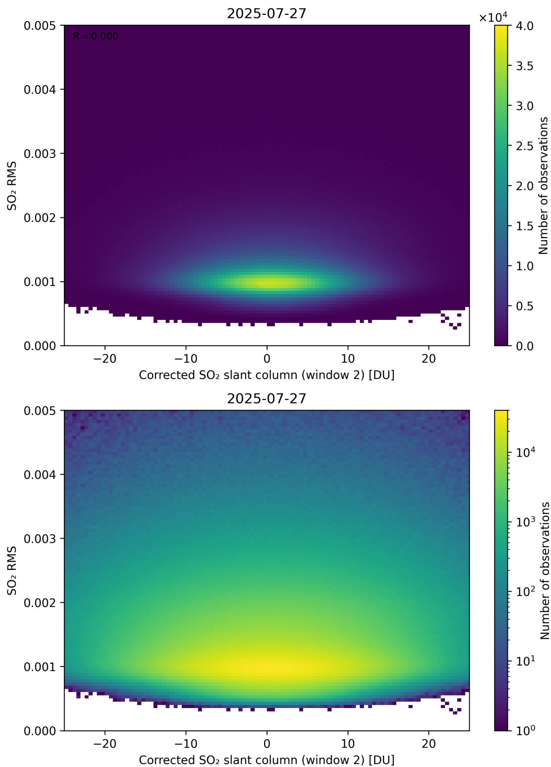
Figure 248: Scatter density plot of “Corrected SO 2 slant column (window 2)” against “SO 2 RMS” for 2025-07-26 to 2025-07-28.
