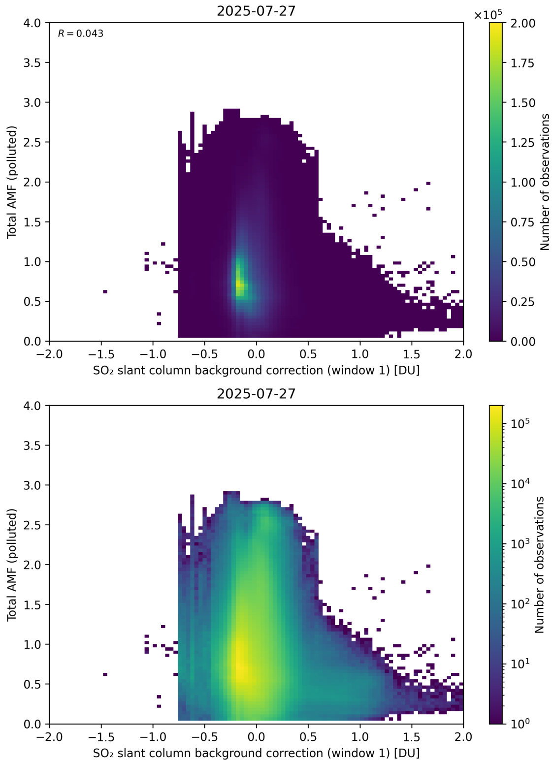
Figure 120: Scatter density plot of “SO 2 slant column background correction (window 1)” against “Total AMF (polluted)” for 2025-07-26 to 2025-07-28.
