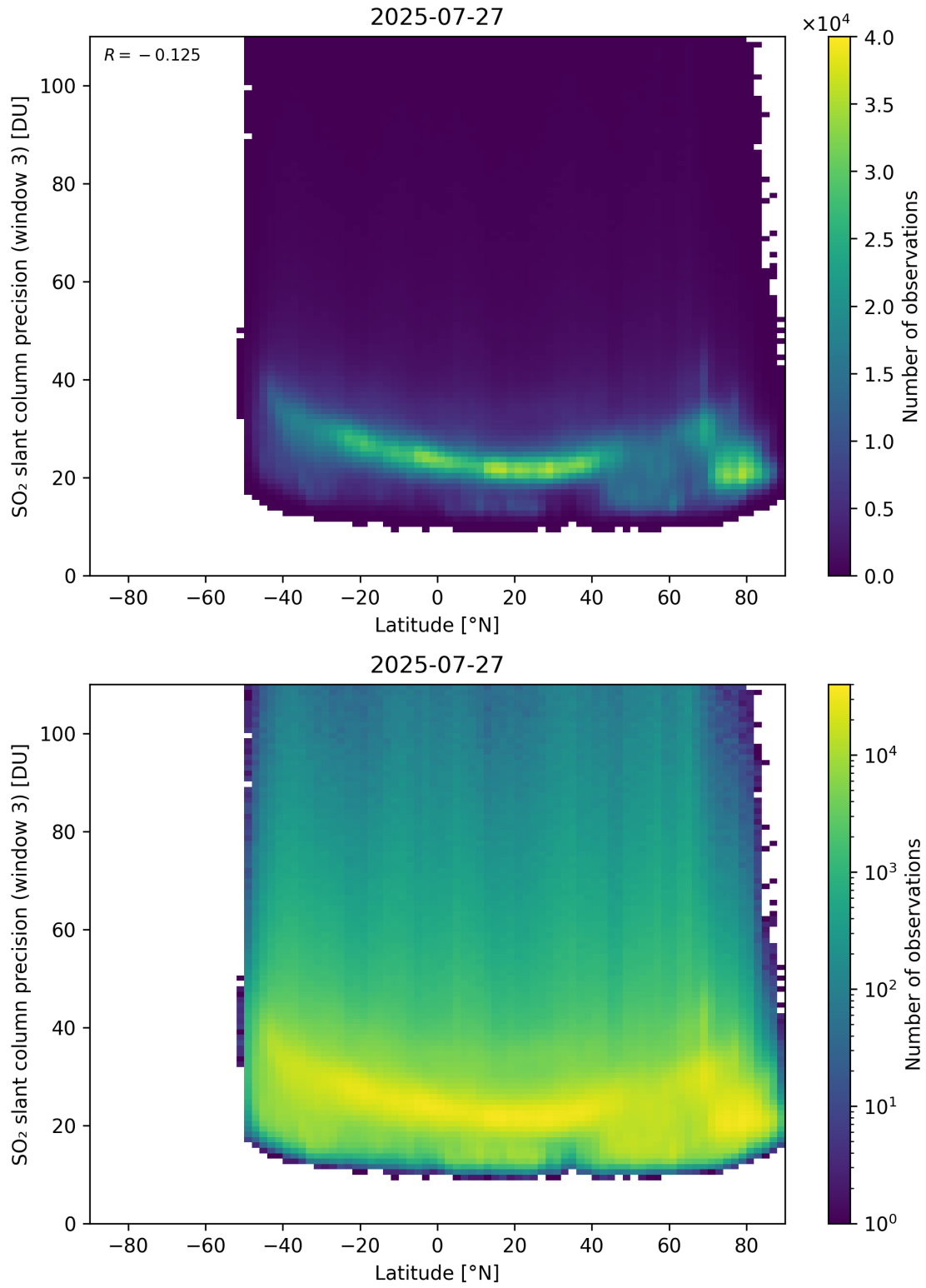
Figure 166: Scatter density plot of “Latitude” against “SO 2 slant column precision (window 3)” for 2025-07-26 to 2025-07-28.
