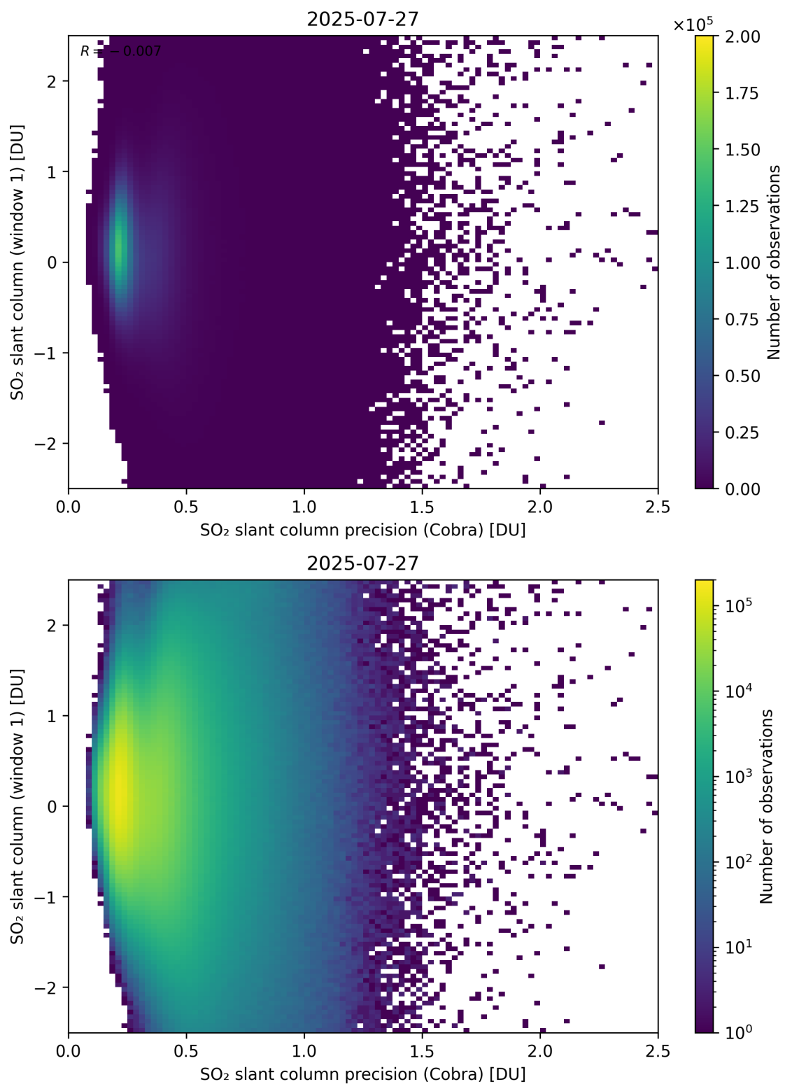
Figure 208: Scatter density plot of “SO 2 slant column precision (Cobra)” against “SO 2 slant column (window 1)” for 2025-07-26 to 2025-07-28.
