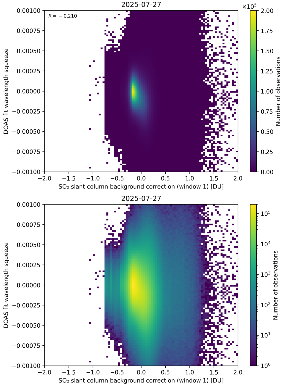
Figure 112: Scatter density plot of “SO 2 slant column background correction (window 1)” against “DOAS fit wavelength squeeze” for 2025-07-26 to 2025-07-28.
