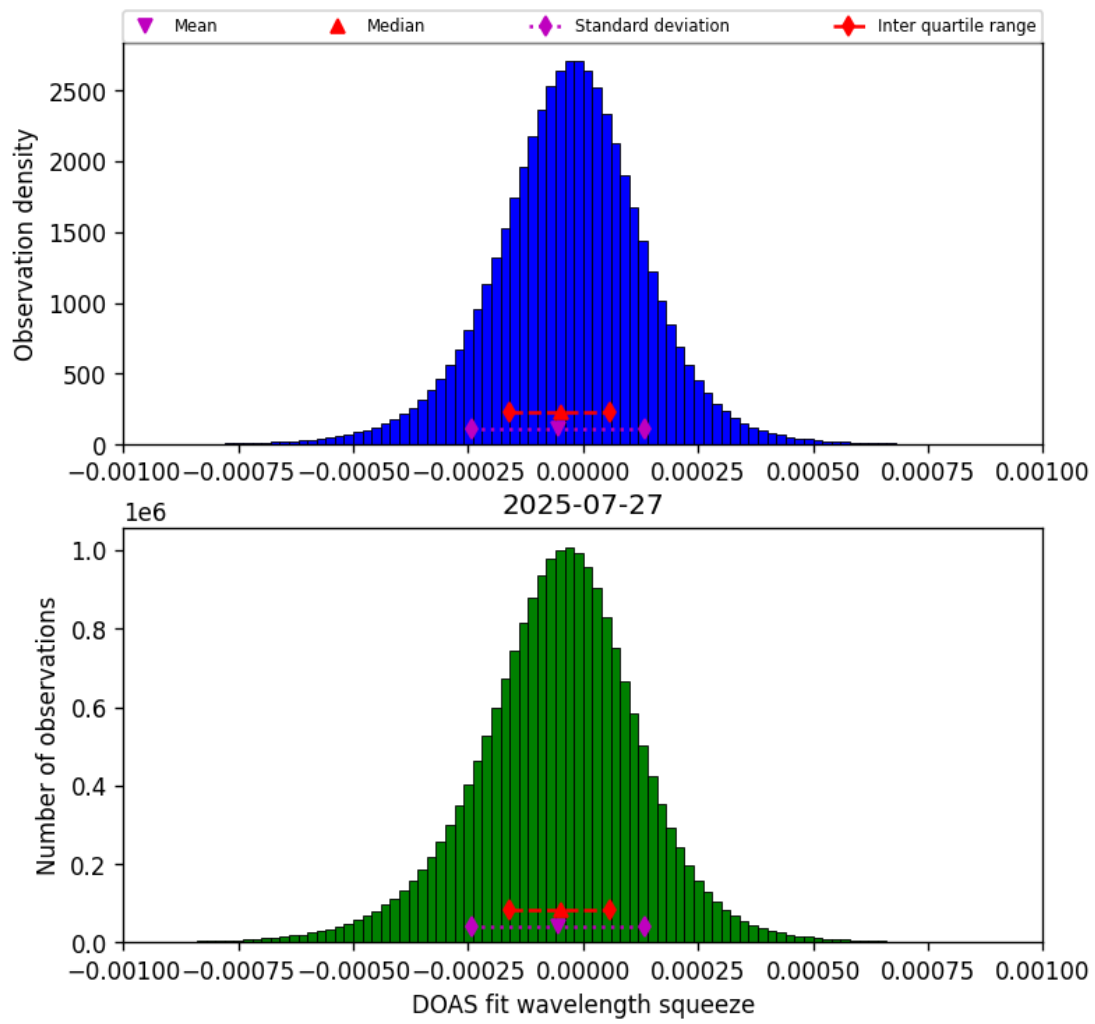
Figure 77: Histogram of “DOAS fit wavelength squeeze” for 2025-07-26 to 2025-07-28
