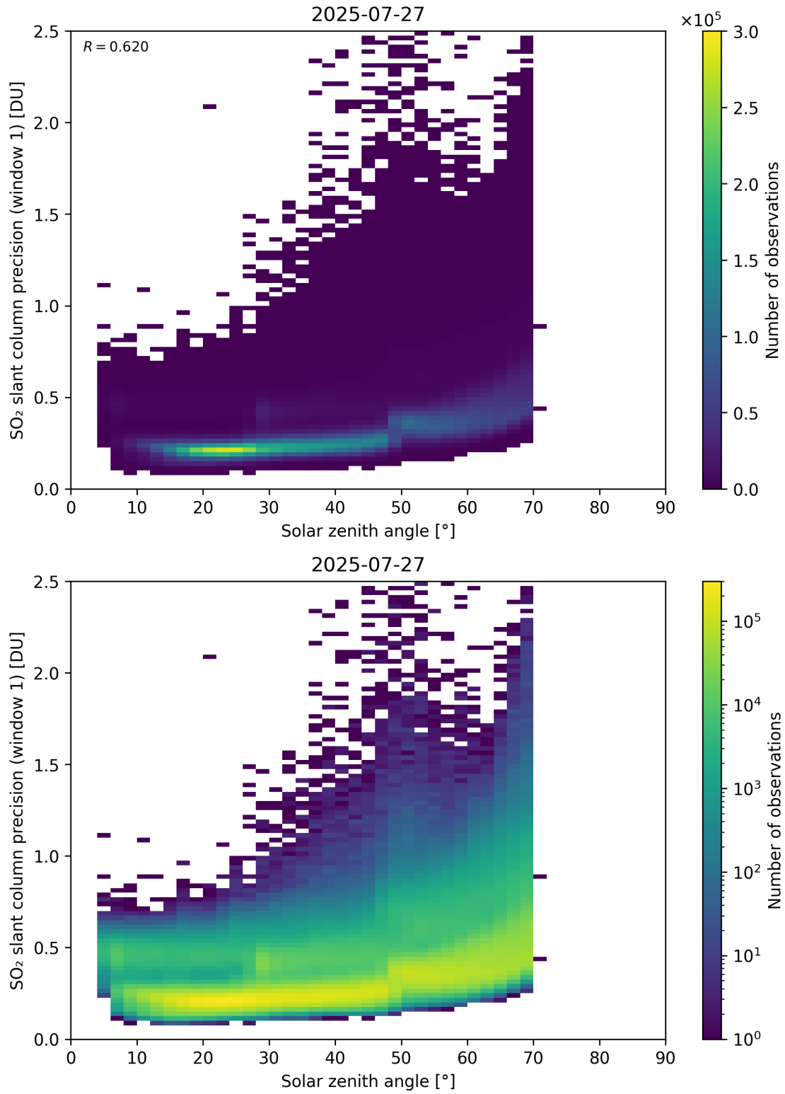
Figure 185: Scatter density plot of “Solar zenith angle” against “SO 2 slant column precision (window 1)” for 2025-07-26 to 2025-07-28.
