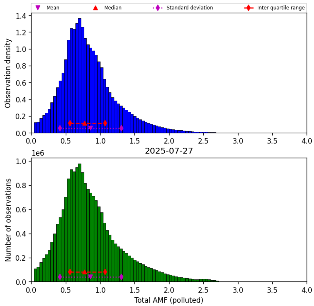
Figure 79: Histogram of “Total AMF (polluted)” for 2025-07-26 to 2025-07-28
