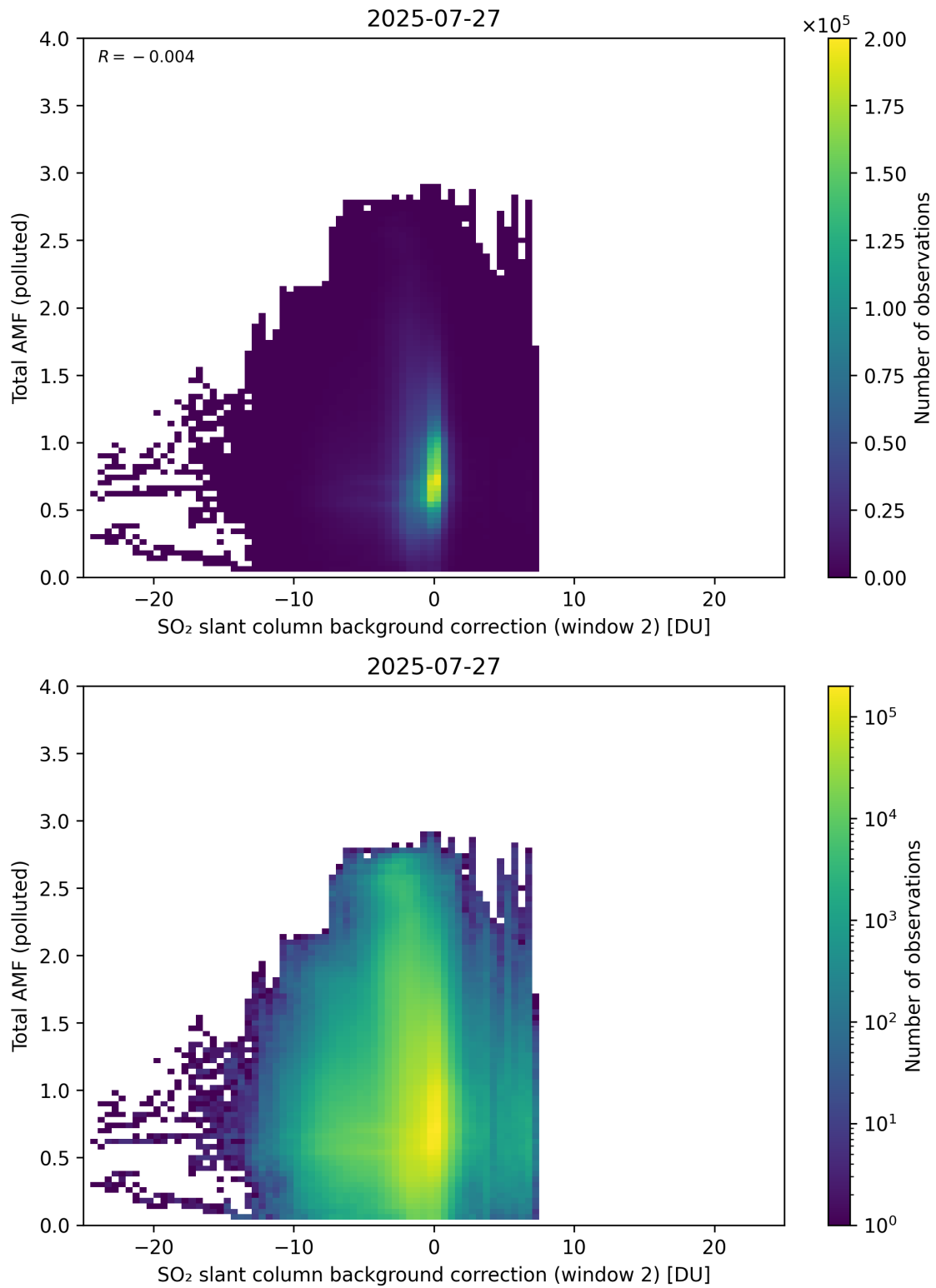
Figure 130: Scatter density plot of “SO 2 slant column background correction (window 2)” against “Total AMF (polluted)” for 2025-07-26 to 2025-07-28.
