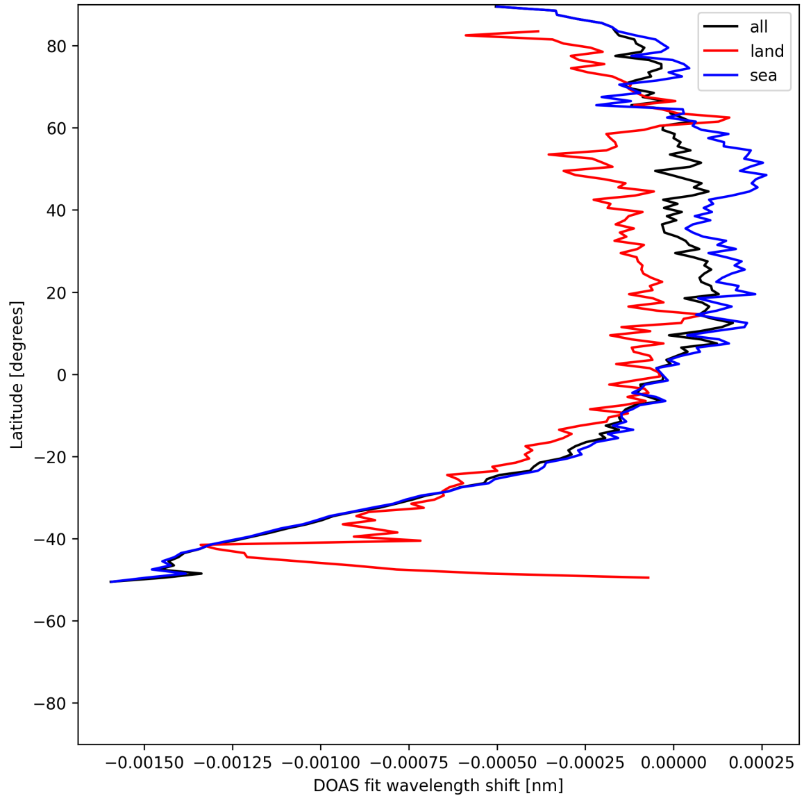
Figure 50: Zonal average of “DOAS fit wavelength shift” for 2025-07-26 to 2025-07-28.
