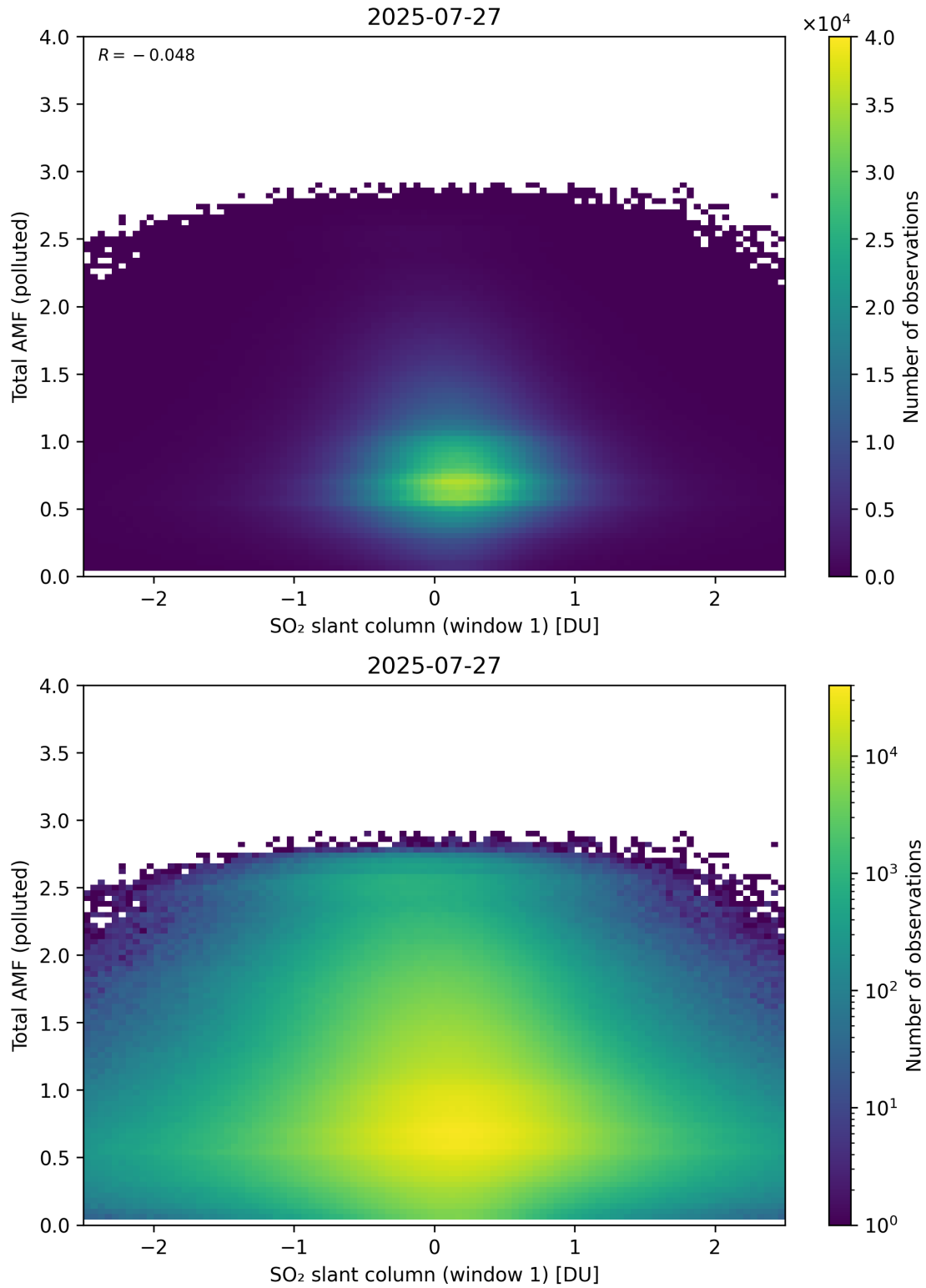
Figure 289: Scatter density plot of “SO 2 slant column (window 1)” against “Total AMF (polluted)” for 2025-07-26 to 2025-07-28.
