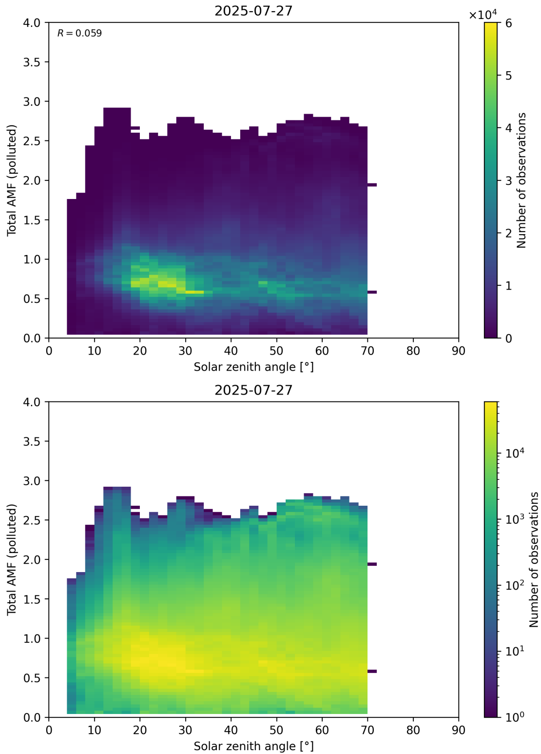
Figure 189: Scatter density plot of “Solar zenith angle” against “Total AMF (polluted)” for 2025-07-26 to 2025-07-28.
