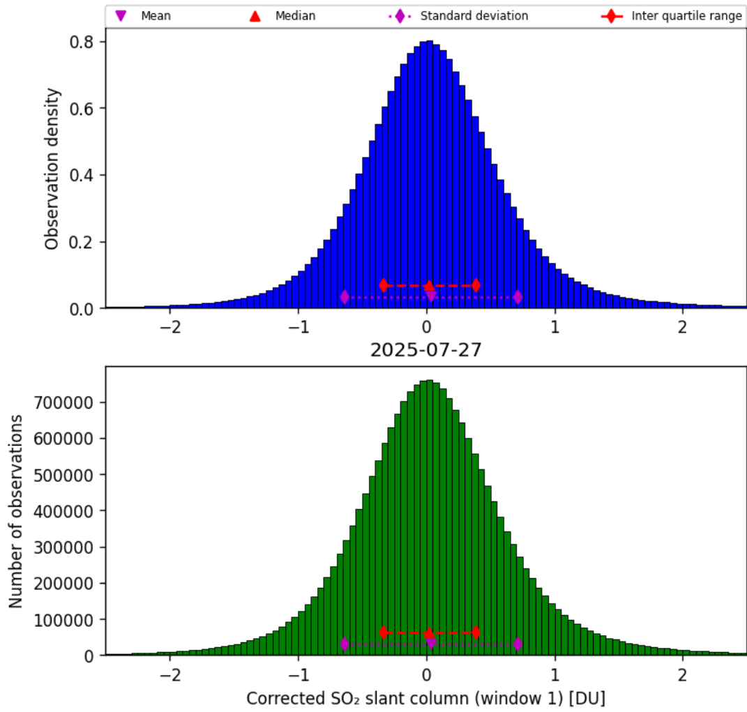
Figure 65: Histogram of “Corrected SO 2 slant column (window 1)” for 2025-07-26 to 2025-07-28
