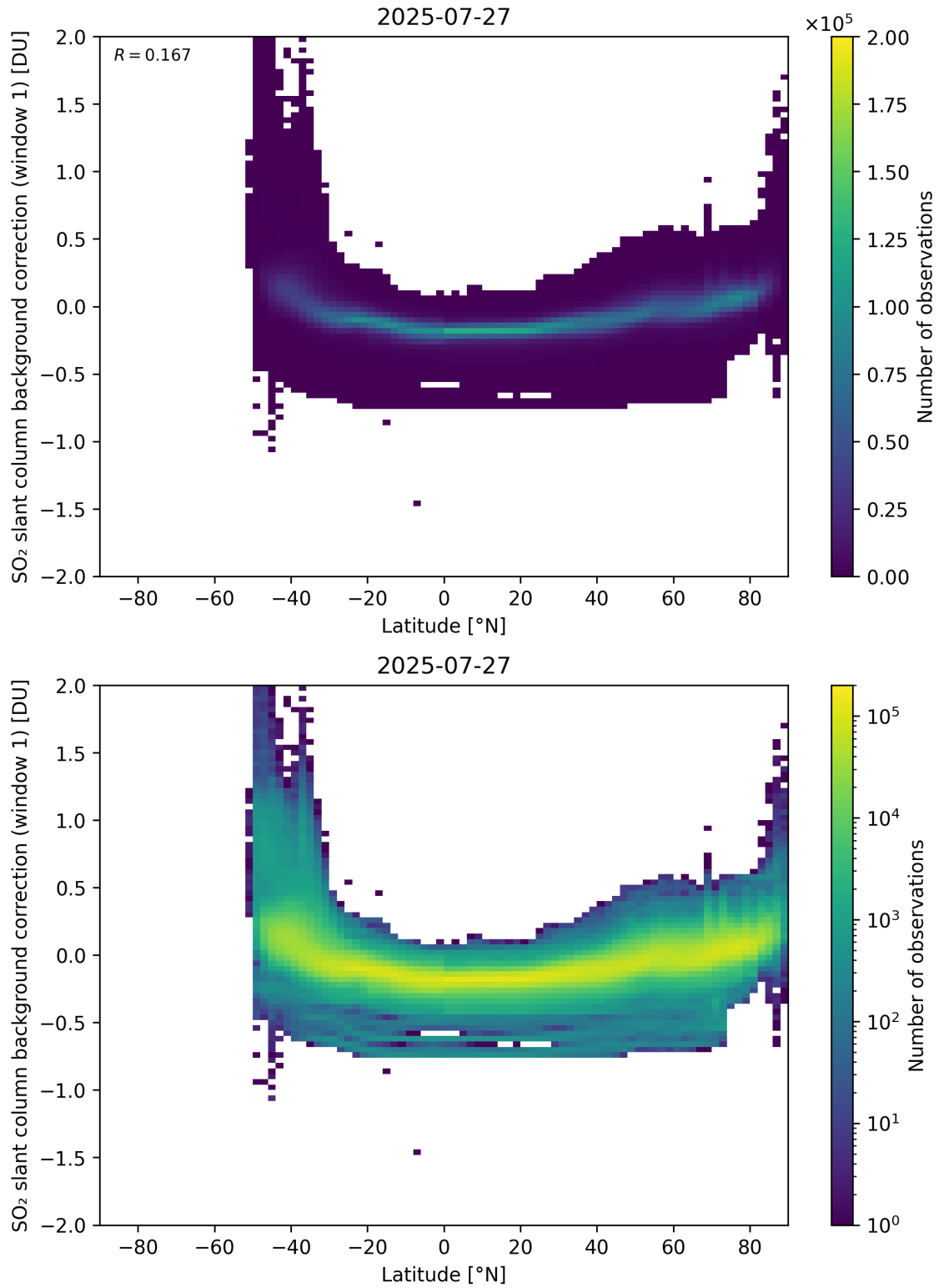
Figure 150: Scatter density plot of “Latitude” against “SO 2 slant column background correction (window 1)” for 2025-07-26 to 2025-07-28.
