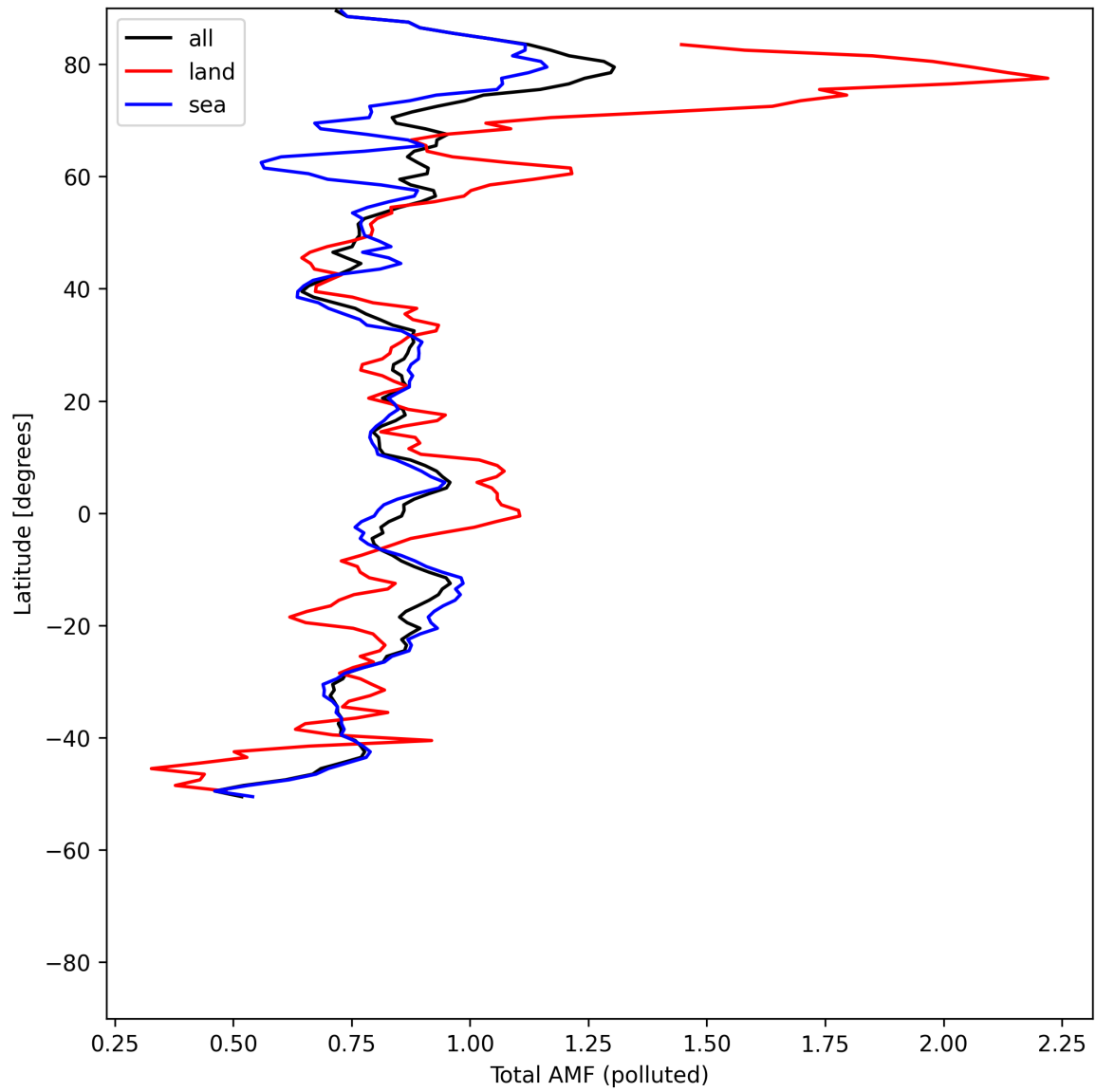
Figure 53: Zonal average of “Total AMF (polluted)” for 2025-07-26 to 2025-07-28.
