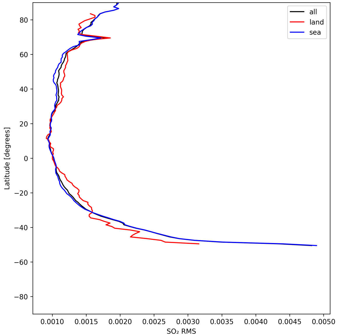
Figure 52: Zonal average of “SO 2 RMS” for 2025-07-26 to 2025-07-28.
