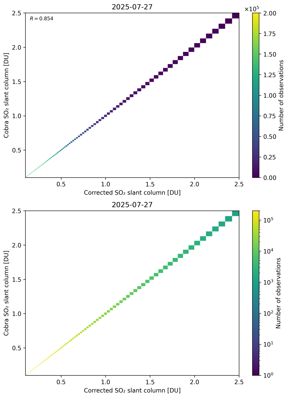
Figure 233: Scatter density plot of “Corrected SO 2 slant column” against “Cobra SO 2 slant column” for 2025-07-26 to 2025-07-28.
