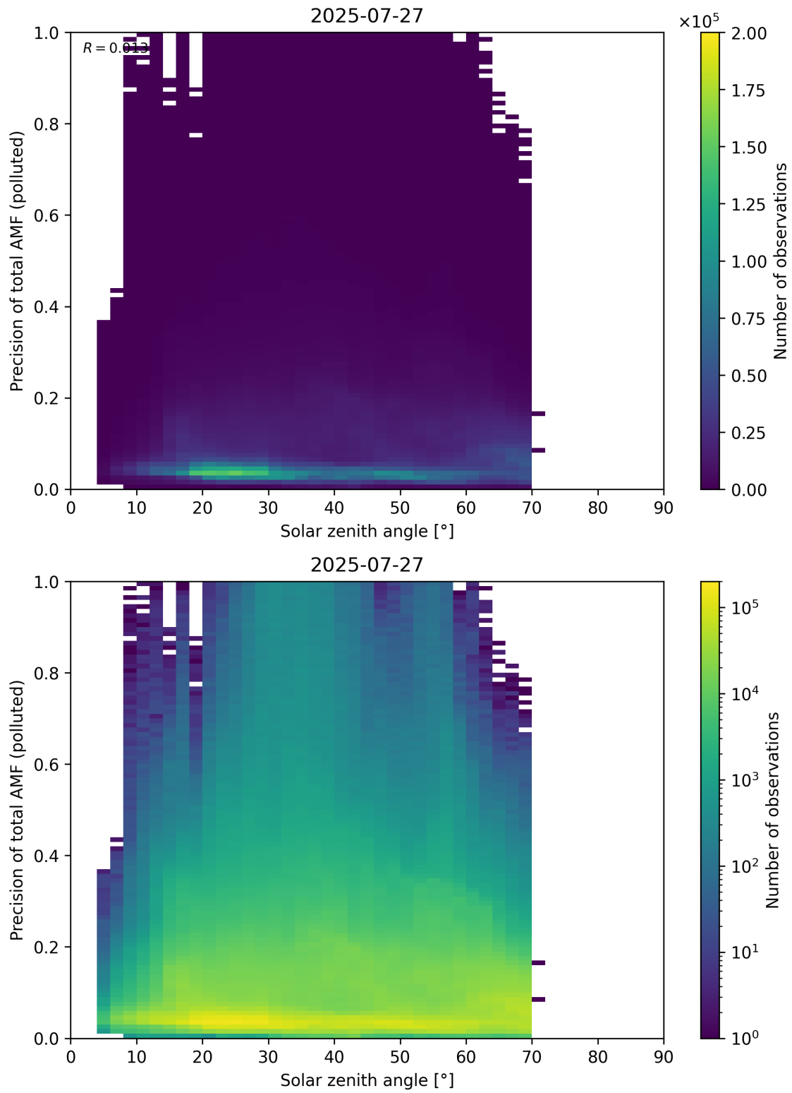
Figure 190: Scatter density plot of “Solar zenith angle” against “Precision of total AMF (polluted)” for 2025-07-26 to 2025-07-28.
