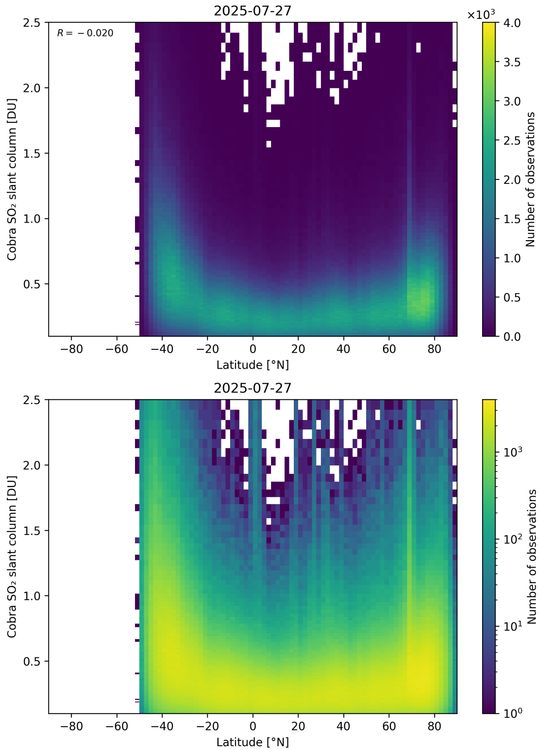
Figure 157: Scatter density plot of “Latitude” against “Cobra SO 2 slant column” for 2025-07-26 to 2025-07-28.
