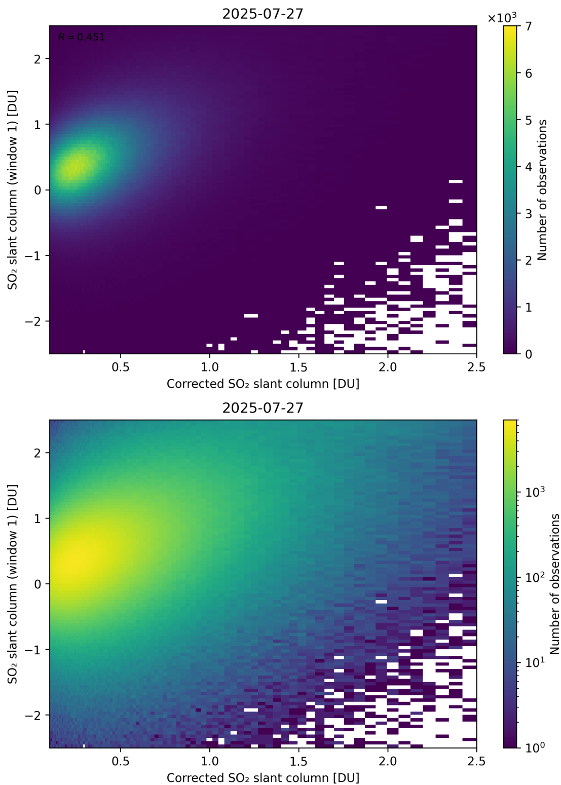
Figure 237: Scatter density plot of “Corrected SO 2 slant column” against “SO 2 slant column (window 1)” for 2025-07-26 to 2025-07-28.
