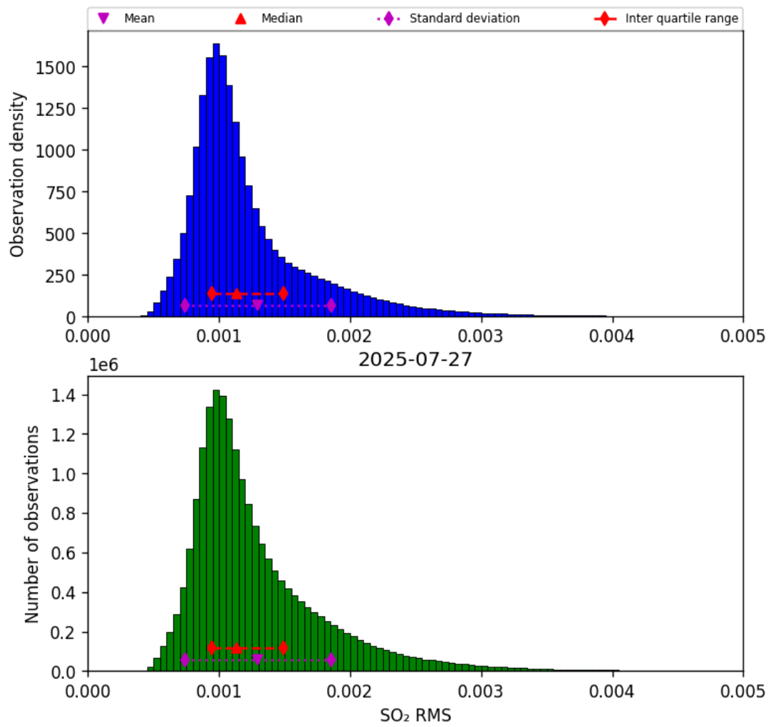
Figure 78: Histogram of “SO 2 RMS” for 2025-07-26 to 2025-07-28
