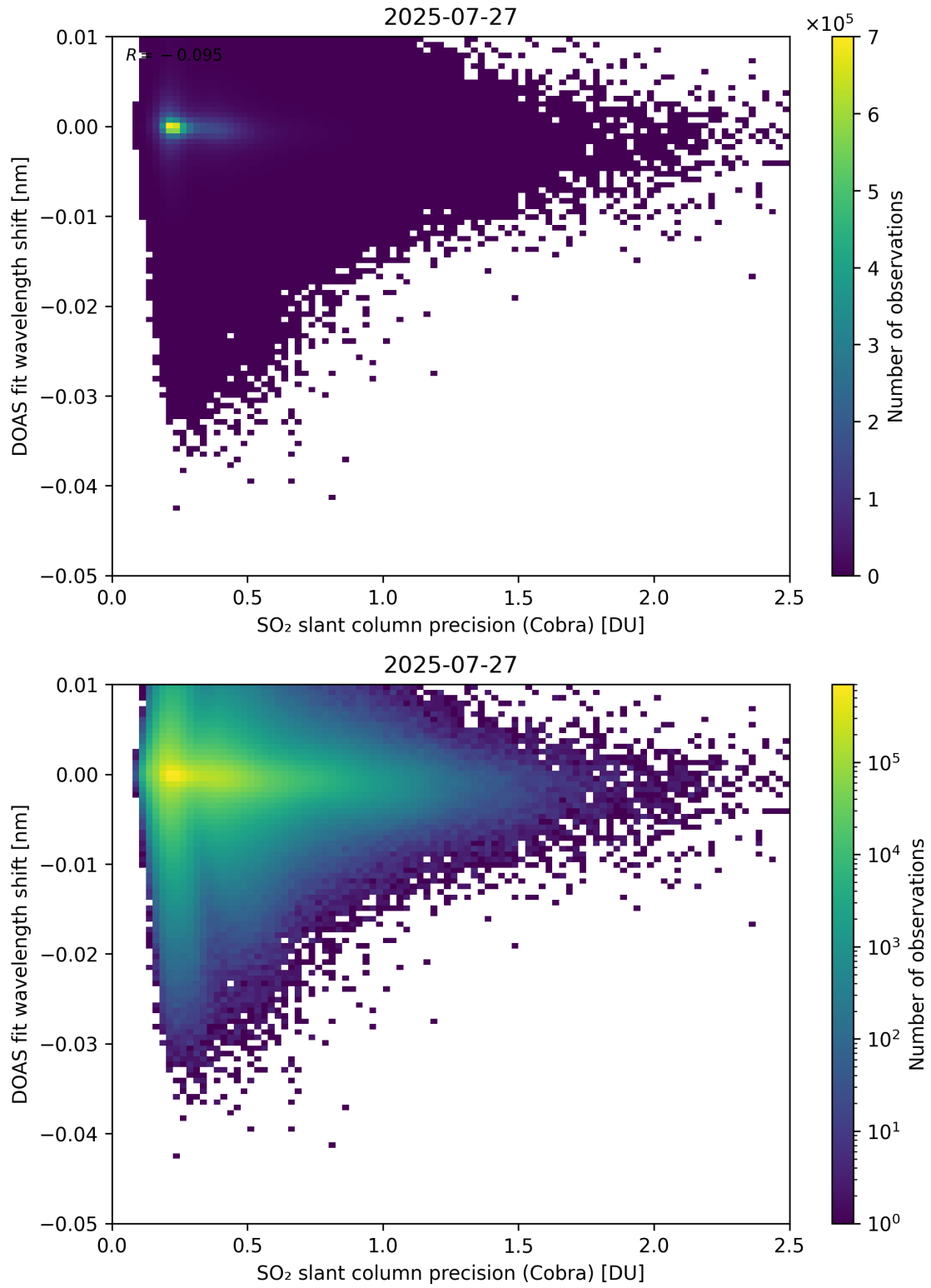
Figure 202: Scatter density plot of “SO 2 slant column precision (Cobra)” against “DOAS fit wavelength shift” for 2025-07-26 to 2025-07-28.
