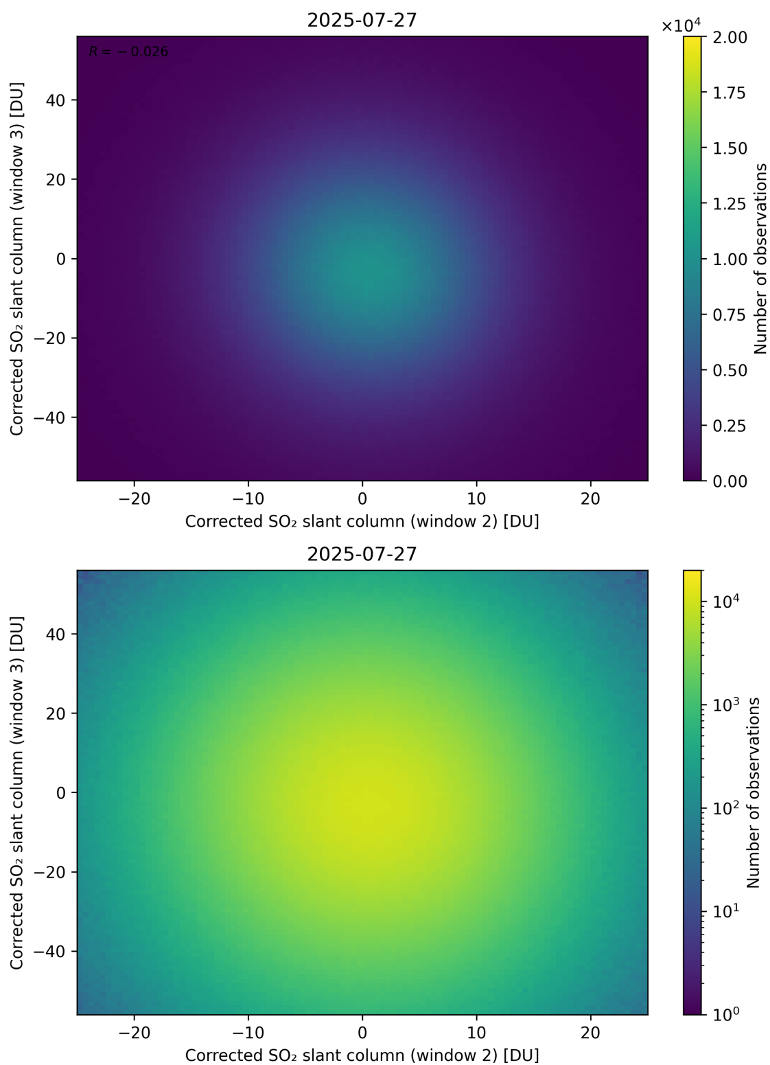
Figure 250: Scatter density plot of “Corrected SO 2 slant column (window 2)” against “Corrected SO 2 slant column (window 3)” for 2025-07-26 to 2025-07-28.
