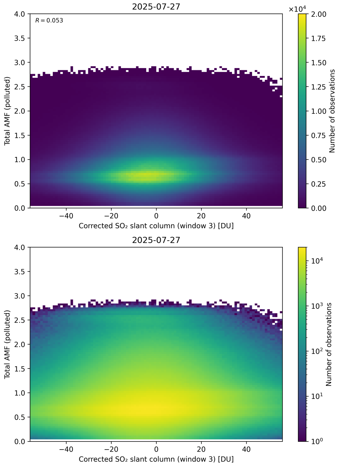
Figure 260: Scatter density plot of “Corrected SO 2 slant column (window 3)” against “Total AMF (polluted)” for 2025-07-26 to 2025-07-28.
