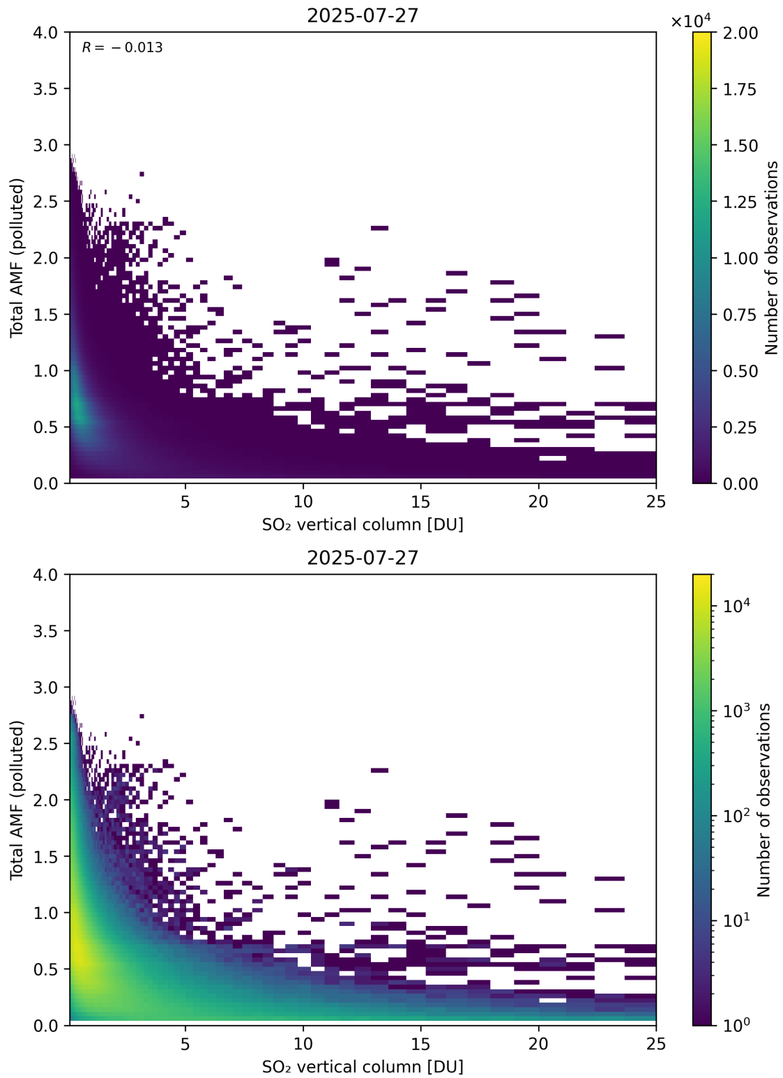
Figure 359: Scatter density plot of “SO 2 vertical column” against “Total AMF (polluted)” for 2025-07-26 to 2025-07-28.
