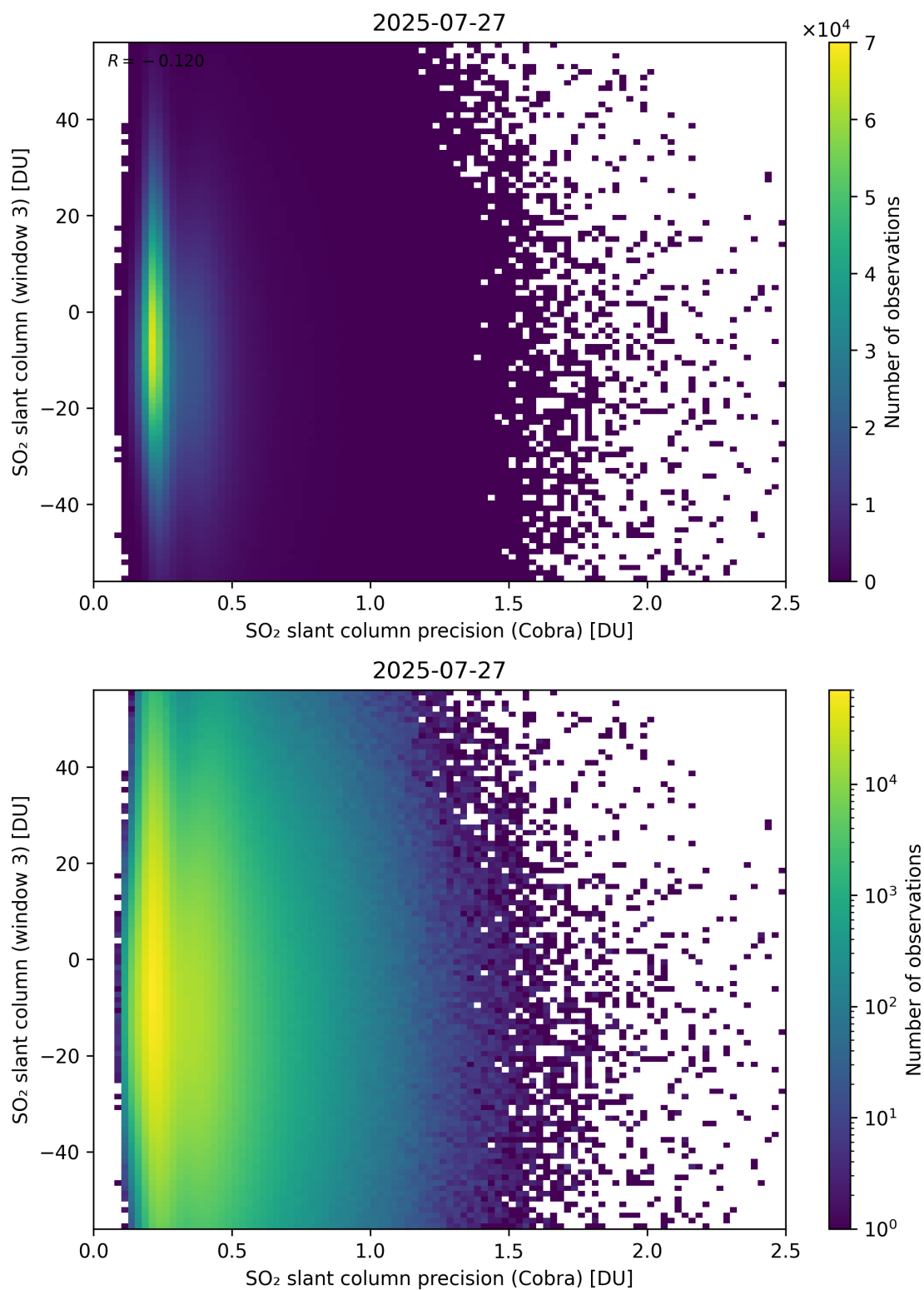
Figure 211: Scatter density plot of “SO 2 slant column precision (Cobra)” against “SO 2 slant column (window 3)” for 2025-07-26 to 2025-07-28.
