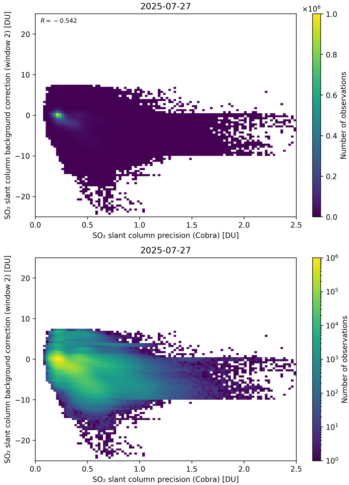
Figure 200: Scatter density plot of “SO 2 slant column precision (Cobra)” against “SO 2 slant column background correction (window 2)” for 2025-07-26 to 2025-07-28.
