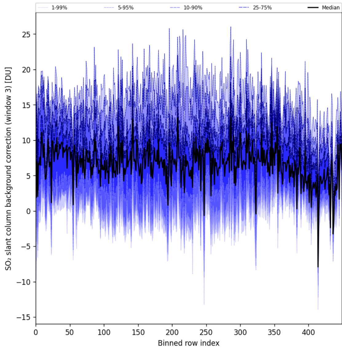
Figure 100: Along track statistics of “SO 2 slant column background correction (window 3)” for 2025-07-26 to 2025-07-28
