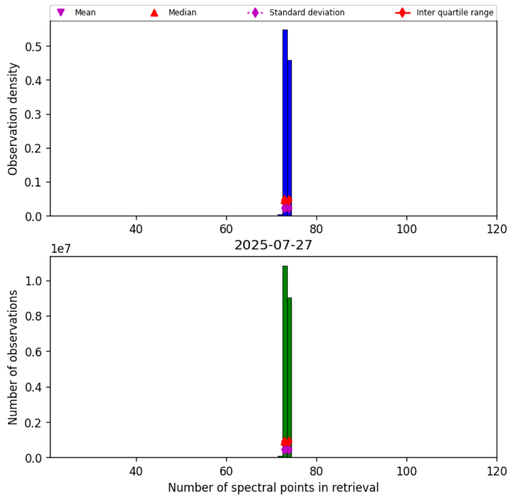
Figure 82: Histogram of “Number of spectral points in retrieval” for 2025-07-26 to 2025-07-28
