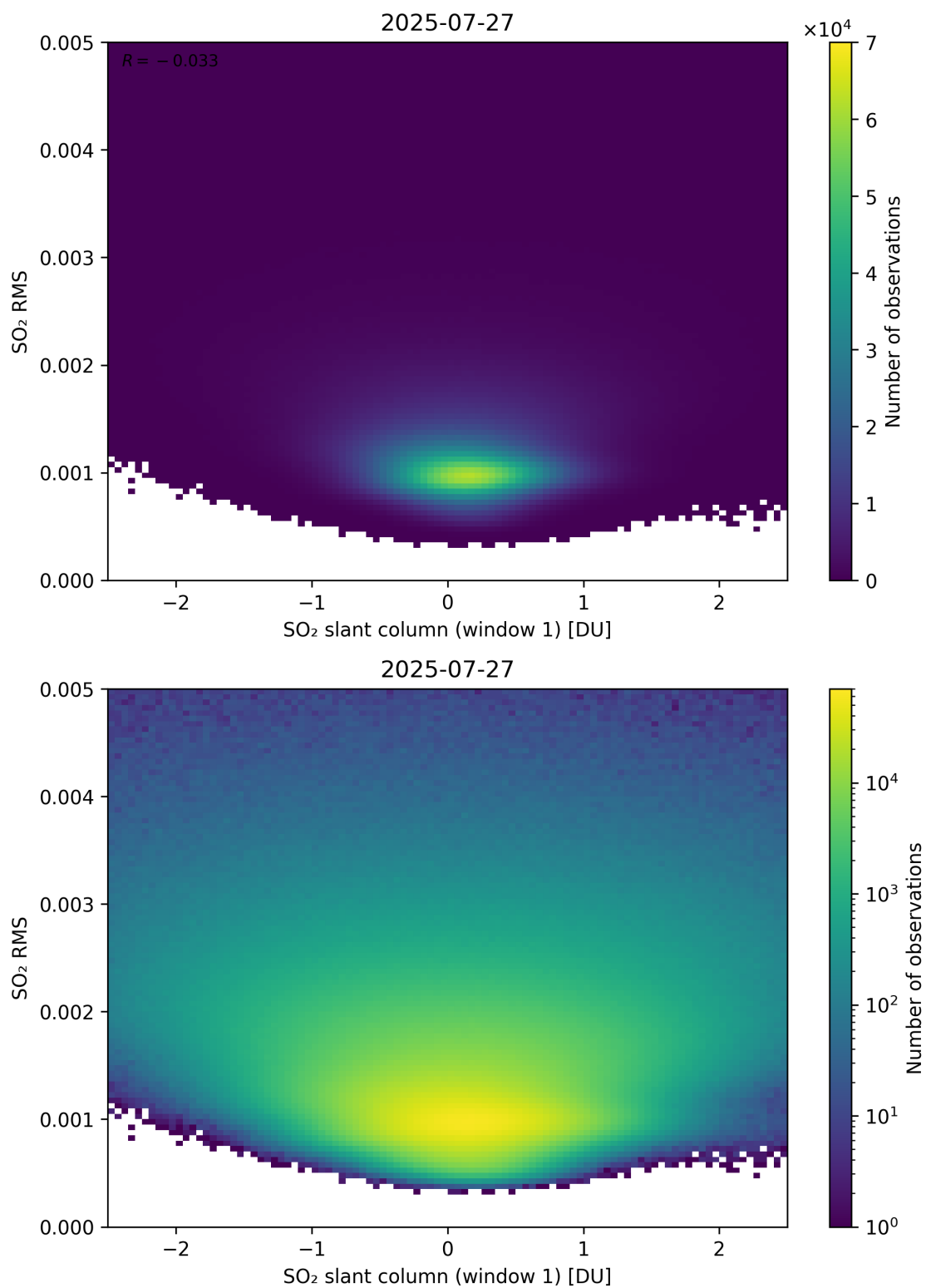
Figure 267: Scatter density plot of “SO 2 slant column (window 1)” against “SO 2 RMS” for 2025-07-26 to 2025-07-28.
