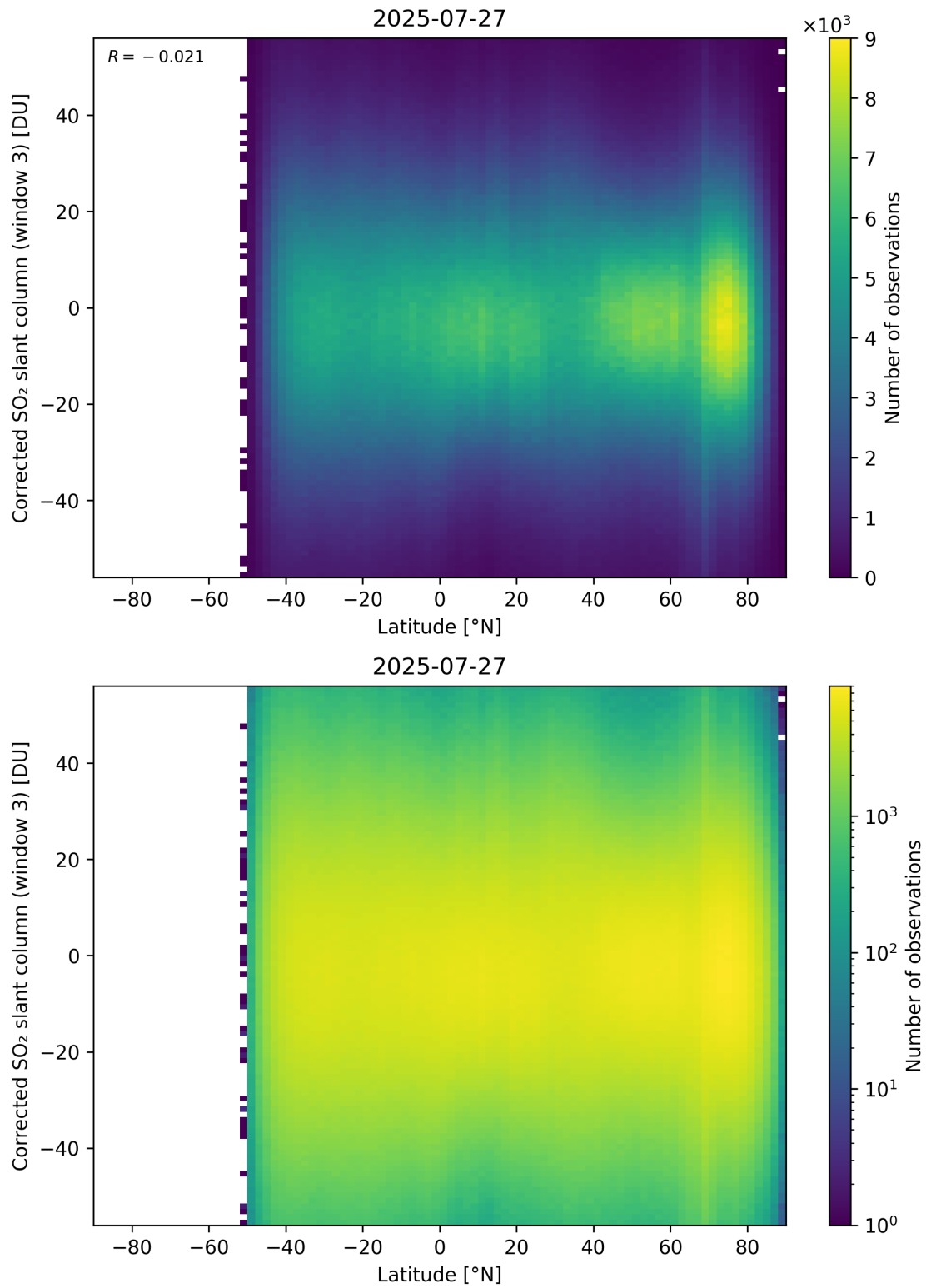
Figure 161: Scatter density plot of “Latitude” against “Corrected SO 2 slant column (window 3)” for 2025-07-26 to 2025-07-28.
