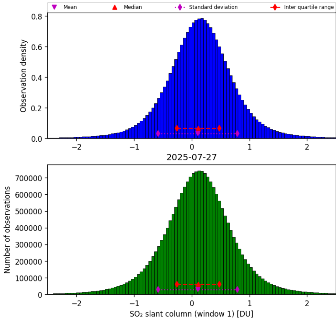
Figure 63: Histogram of “SO 2 slant column (window 1)” for 2025-07-26 to 2025-07-28
