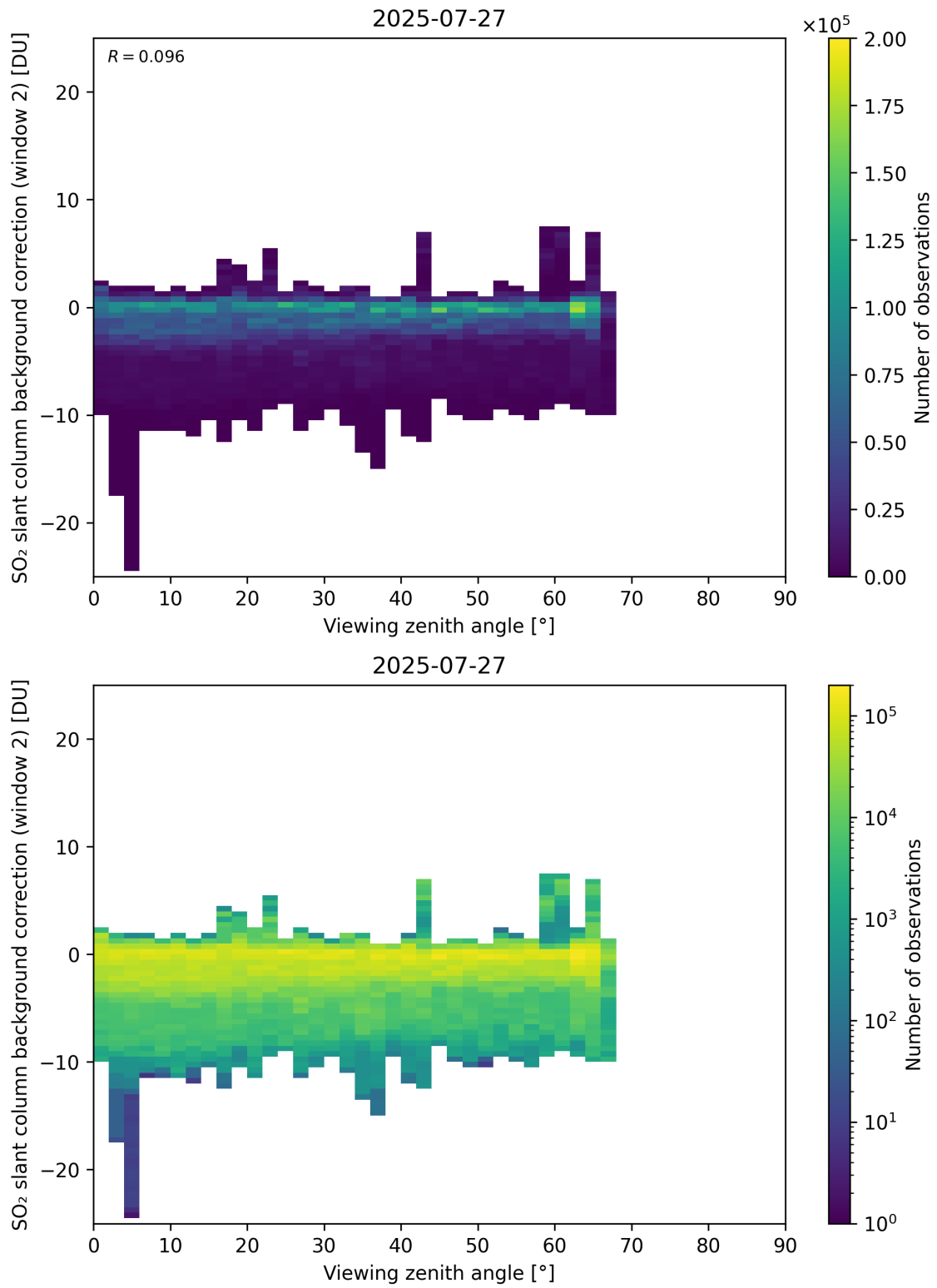
Figure 363: Scatter density plot of “Viewing zenith angle” against “SO 2 slant column background correction (window 2)” for 2025-07-26 to 2025-07-28.
