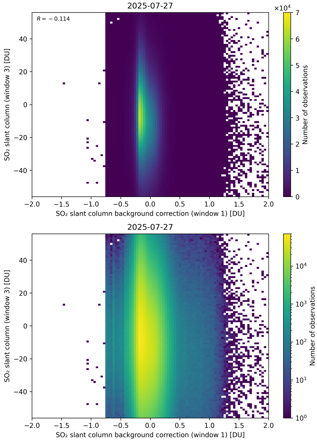
Figure 118: Scatter density plot of “SO 2 slant column background correction (window 1)” against “SO 2 slant column (window 3)” for 2025-07-26 to 2025-07-28.
