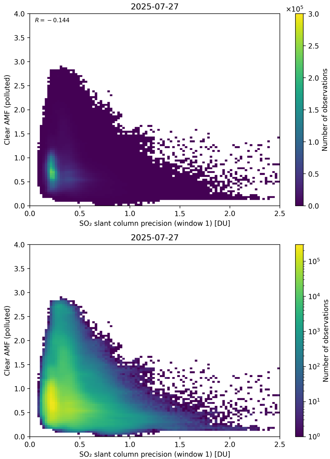
Figure 274: Scatter density plot of “SO 2 slant column precision (window 1)” against “Clear AMF (polluted)” for 2025-07-26 to 2025-07-28.
