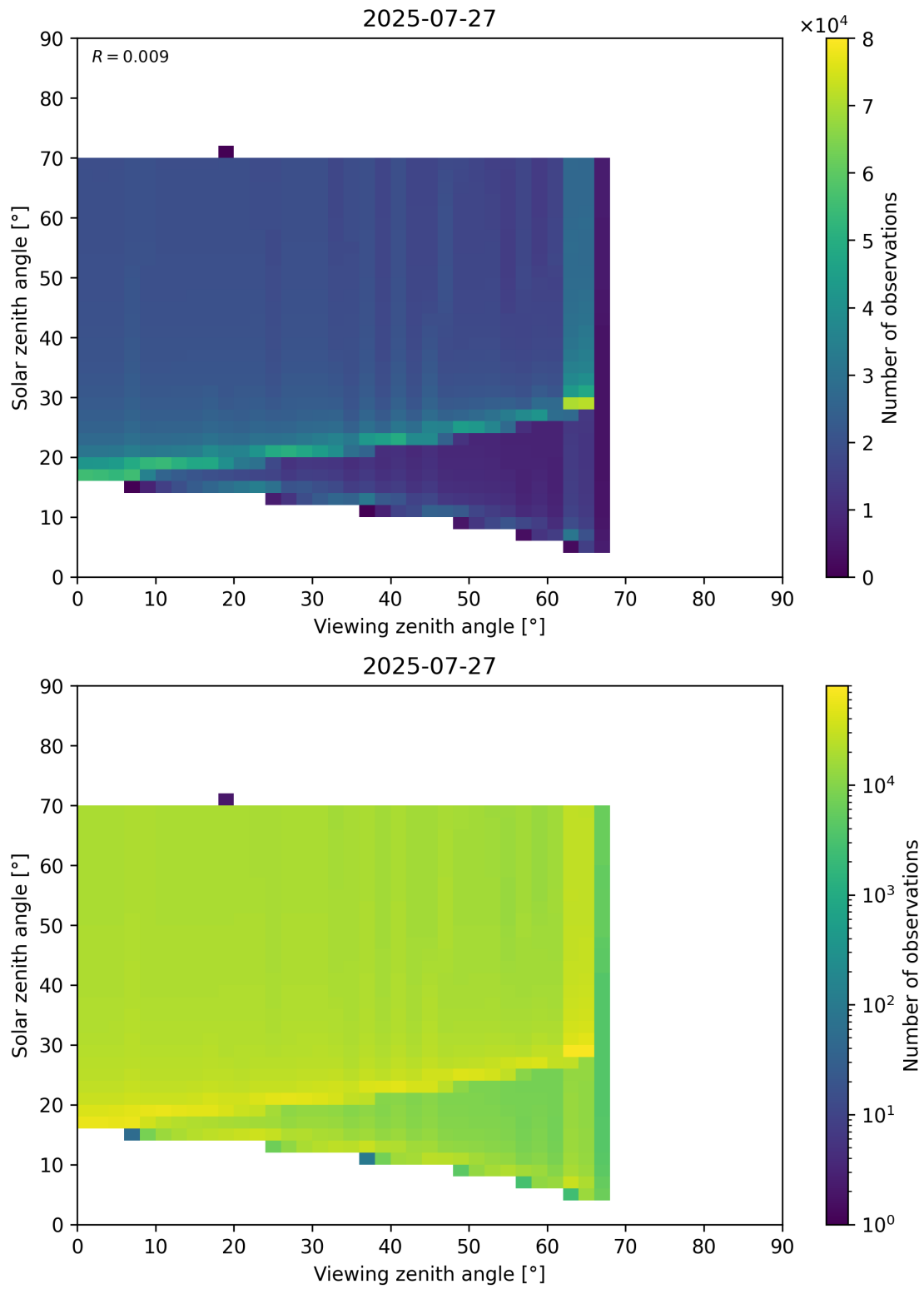
Figure 369: Scatter density plot of “Viewing zenith angle” against “Solar zenith angle” for 2025-07-26 to 2025-07-28.
