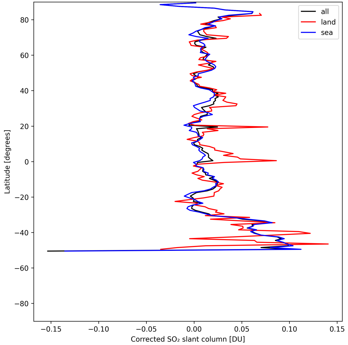
Figure 34: Zonal average of “Corrected SO 2 slant column” for 2025-07-26 to 2025-07-28.
