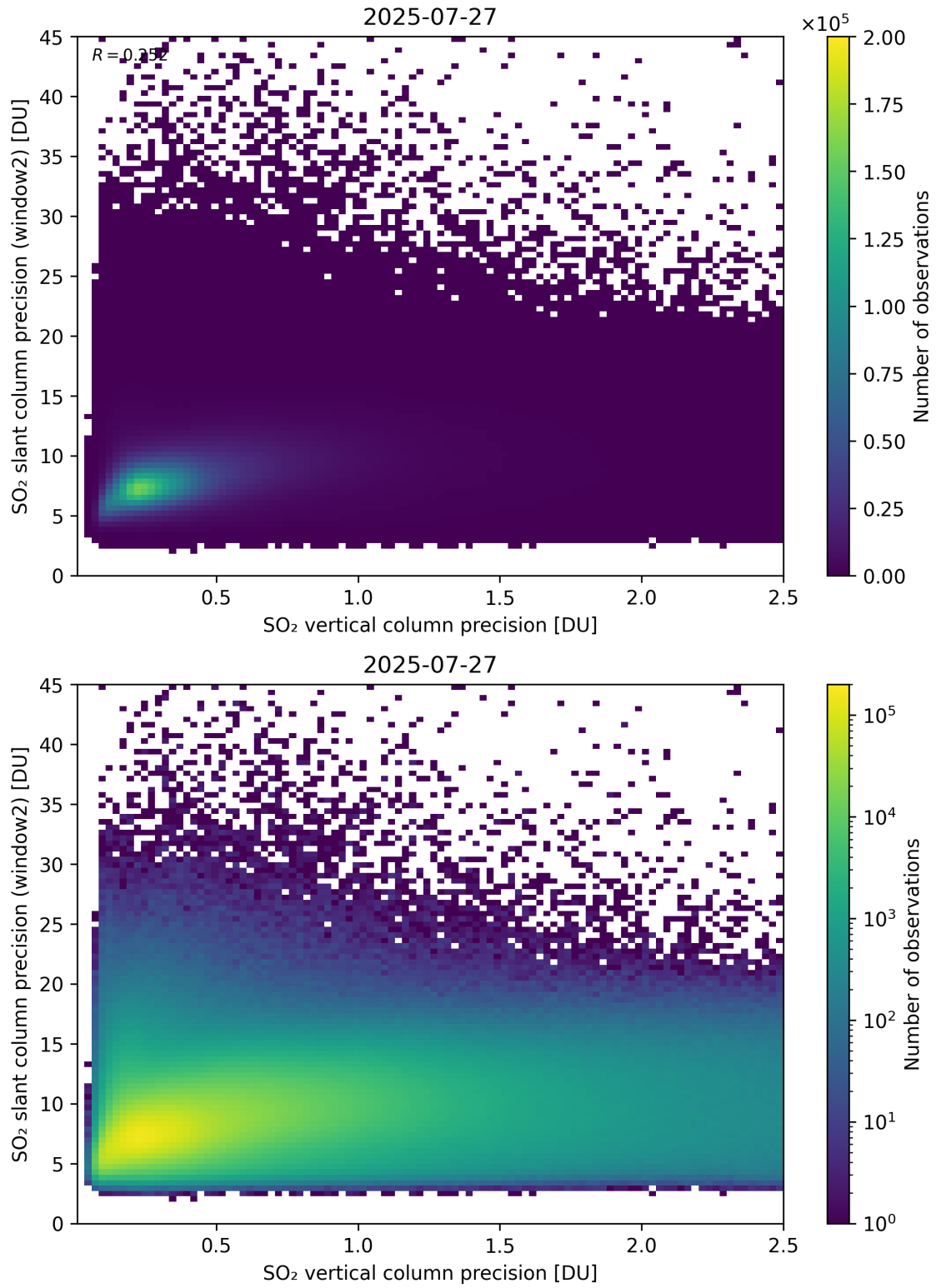
Figure 343: Scatter density plot of “SO 2 vertical column precision” against “SO 2 slant column precision (window2)” for 2025-07-26 to 2025-07-28.
