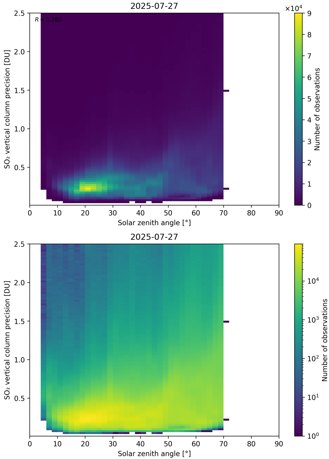
Figure 192: Scatter density plot of “Solar zenith angle” against “SO 2 vertical column precision” for 2025-07-26 to 2025-07-28.
