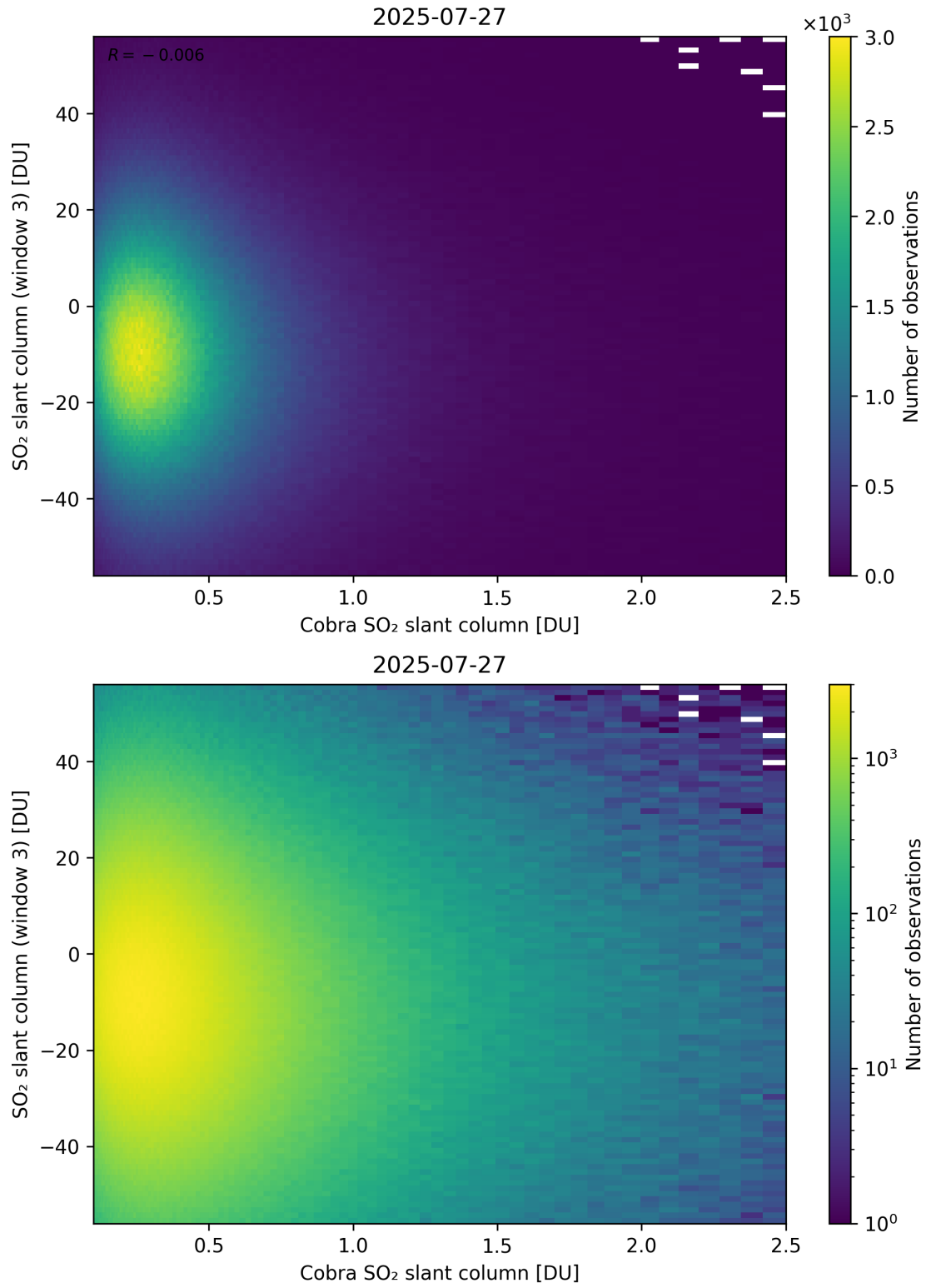
Figure 222: Scatter density plot of “Cobra SO 2 slant column” against “SO 2 slant column (window 3)” for 2025-07-26 to 2025-07-28.
