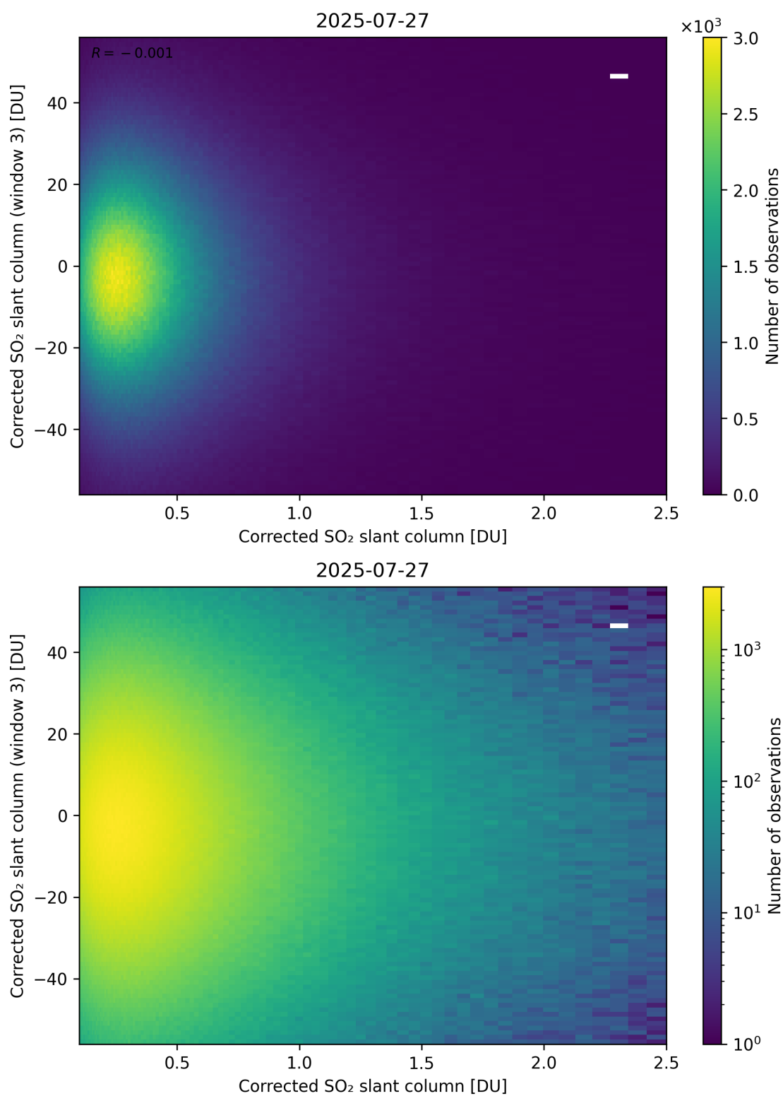
Figure 236: Scatter density plot of “Corrected SO 2 slant column” against “Corrected SO 2 slant column (window 3)” for 2025-07-26 to 2025-07-28.
