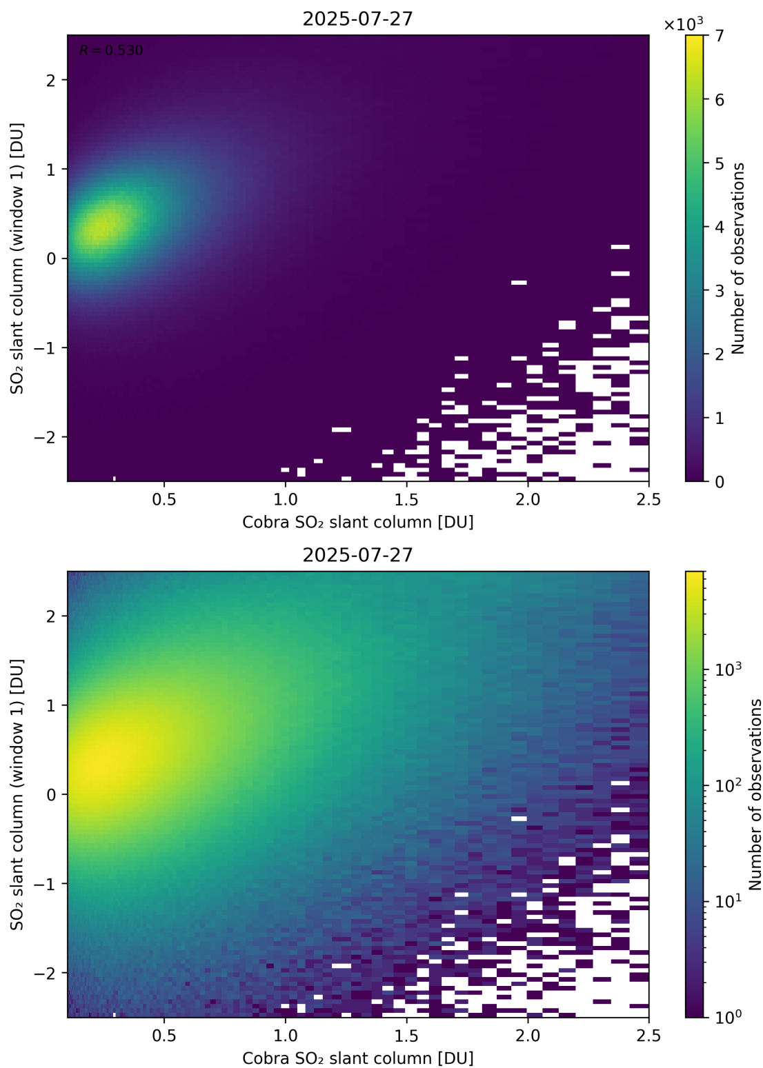
Figure 219: Scatter density plot of “Cobra SO 2 slant column” against “SO 2 slant column (window 1)” for 2025-07-26 to 2025-07-28.
