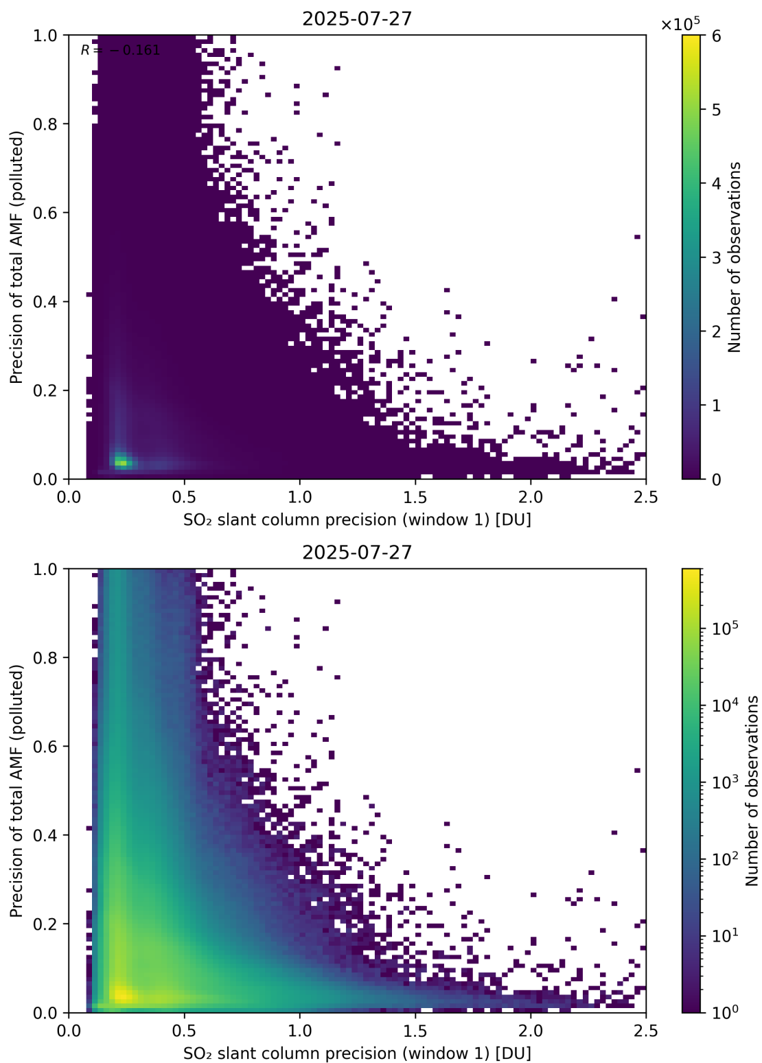
Figure 281: Scatter density plot of “SO 2 slant column precision (window 1)” against “Precision of total AMF (polluted)” for 2025-07-26 to 2025-07-28.
