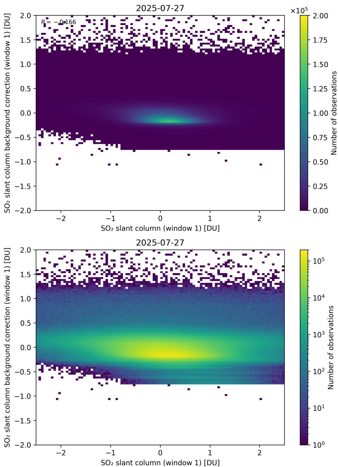
Figure 262: Scatter density plot of “SO 2 slant column (window 1)” against “SO 2 slant column background correction (window 1)” for 2025-07-26 to 2025-07-28.
