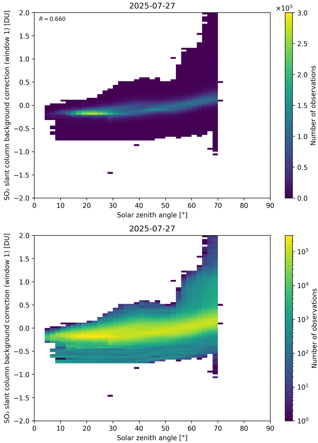
Figure 171: Scatter density plot of “Solar zenith angle” against “SO 2 slant column background correction (window 1)” for 2025-07-26 to 2025-07-28.
