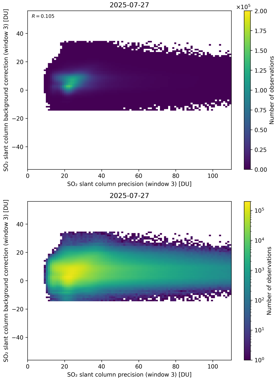
Figure 307: Scatter density plot of “SO 2 slant column precision (window 3)” against “SO 2 slant column background correction (window 3)” for 2025-07-26 to 2025-07-28.
