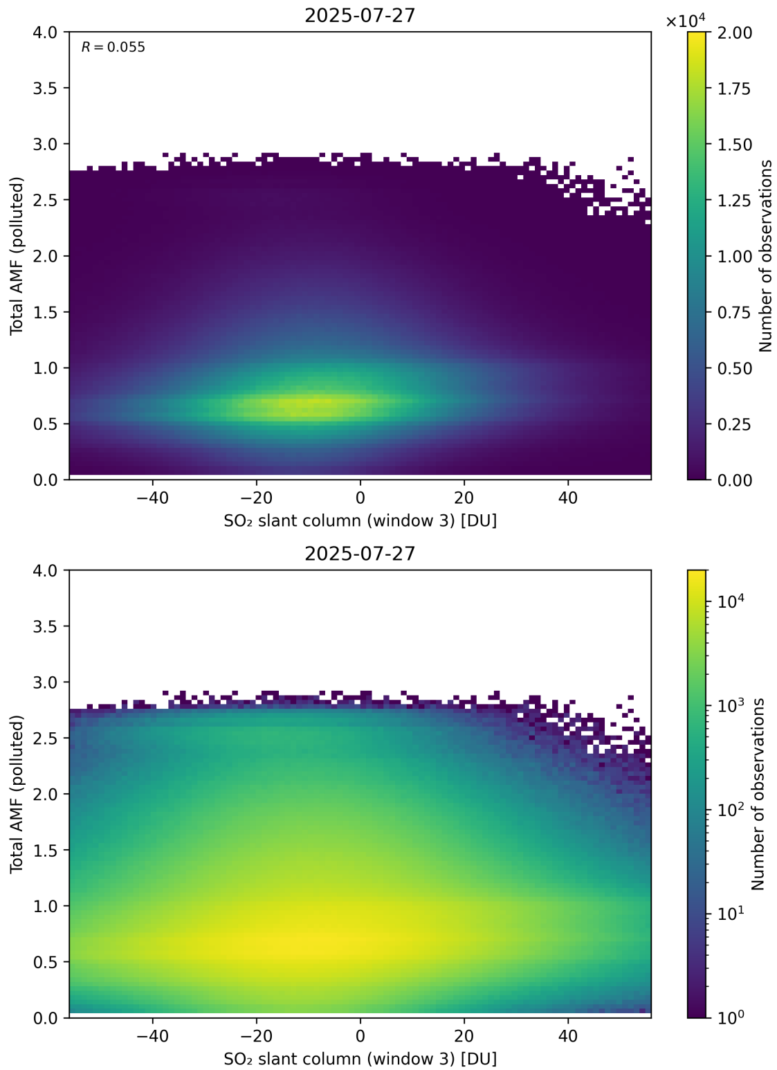
Figure 318: Scatter density plot of “SO 2 slant column (window 3)” against “Total AMF (polluted)” for 2025-07-26 to 2025-07-28.
