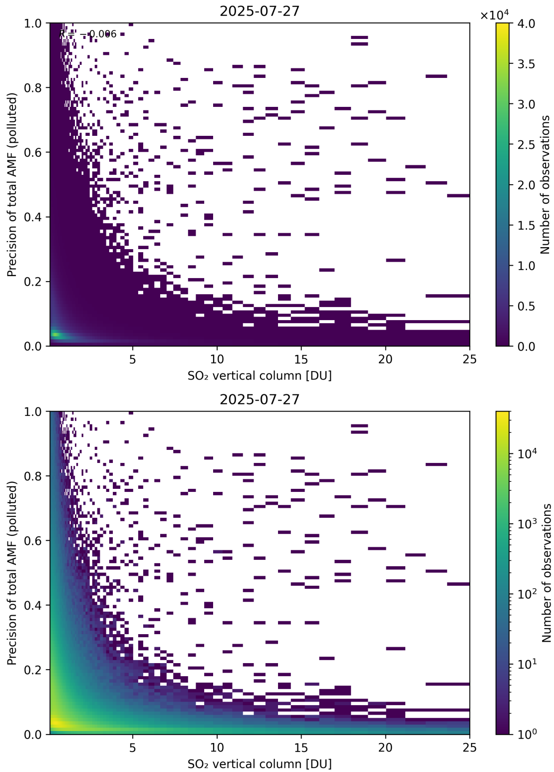
Figure 360: Scatter density plot of “SO 2 vertical column” against “Precision of total AMF (polluted)” for 2025-07-26 to 2025-07-28.
