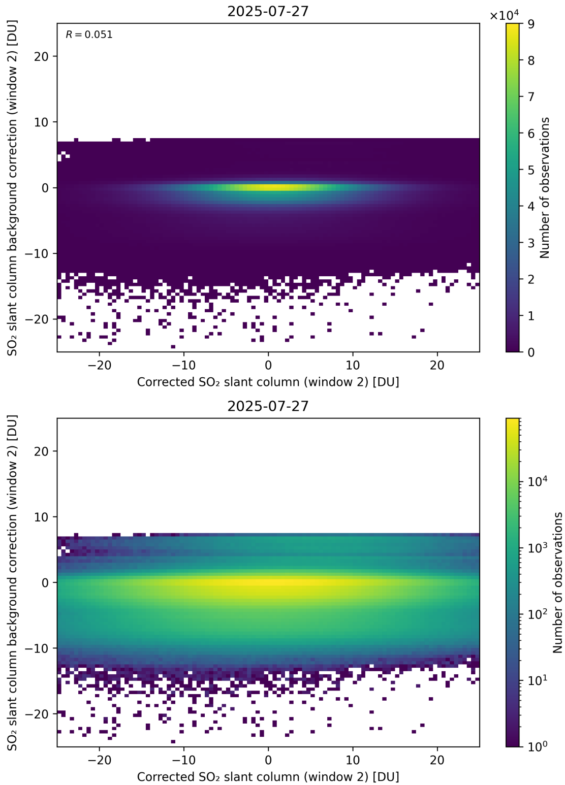
Figure 244: Scatter density plot of “Corrected SO 2 slant column (window 2)” against “SO 2 slant column background correction (window 2)” for 2025-07-26 to 2025-07-28.
