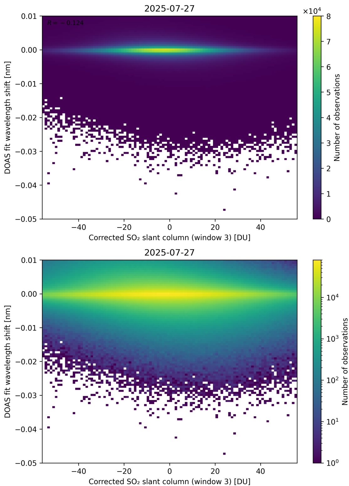
Figure 256: Scatter density plot of “Corrected SO 2 slant column (window 3)” against “DOAS fit wavelength shift” for 2025-07-26 to 2025-07-28.
