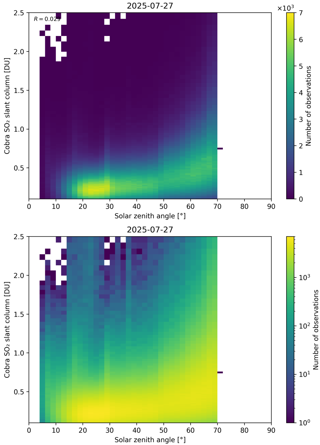
Figure 179: Scatter density plot of “Solar zenith angle” against “Cobra SO 2 slant column” for 2025-07-26 to 2025-07-28.
