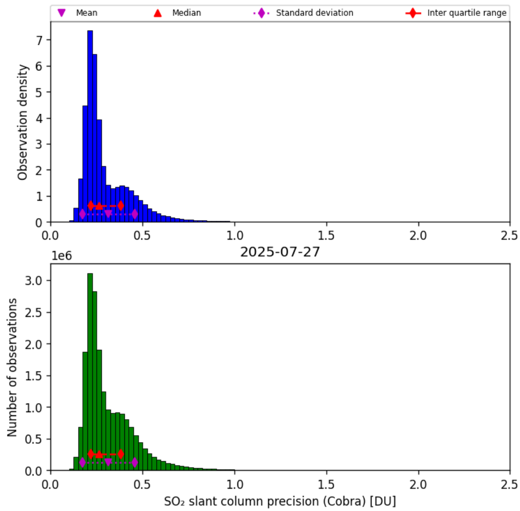
Figure 62: Histogram of “SO 2 slant column precision (Cobra)” for 2025-07-26 to 2025-07-28
