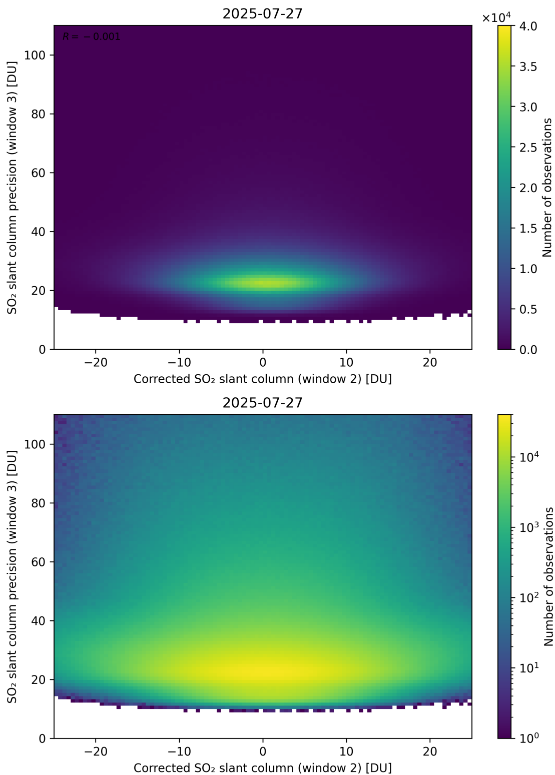
Figure 252: Scatter density plot of “Corrected SO 2 slant column (window 2)” against “SO 2 slant column precision (window 3)” for 2025-07-26 to 2025-07-28.
