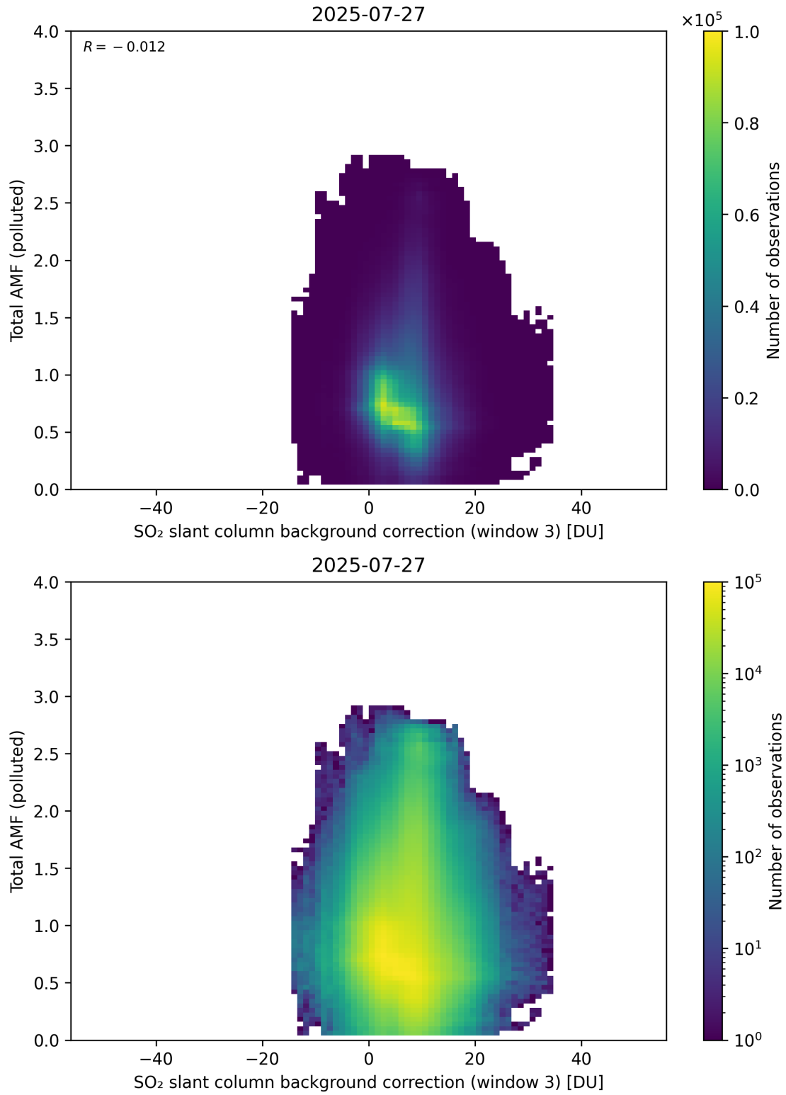
Figure 136: Scatter density plot of “SO 2 slant column background correction (window 3)” against “Total AMF (polluted)” for 2025-07-26 to 2025-07-28.
