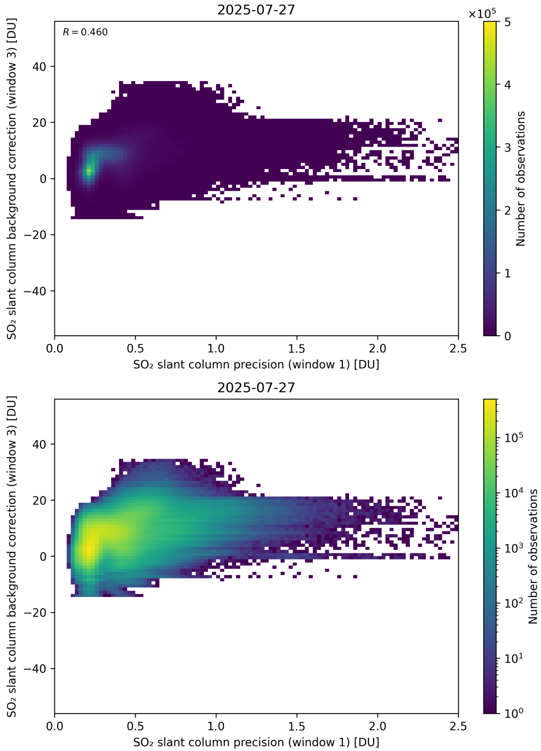
Figure 270: Scatter density plot of “SO 2 slant column precision (window 1)” against “SO 2 slant column background correction (window 3)” for 2025-07-26 to 2025-07-28.
