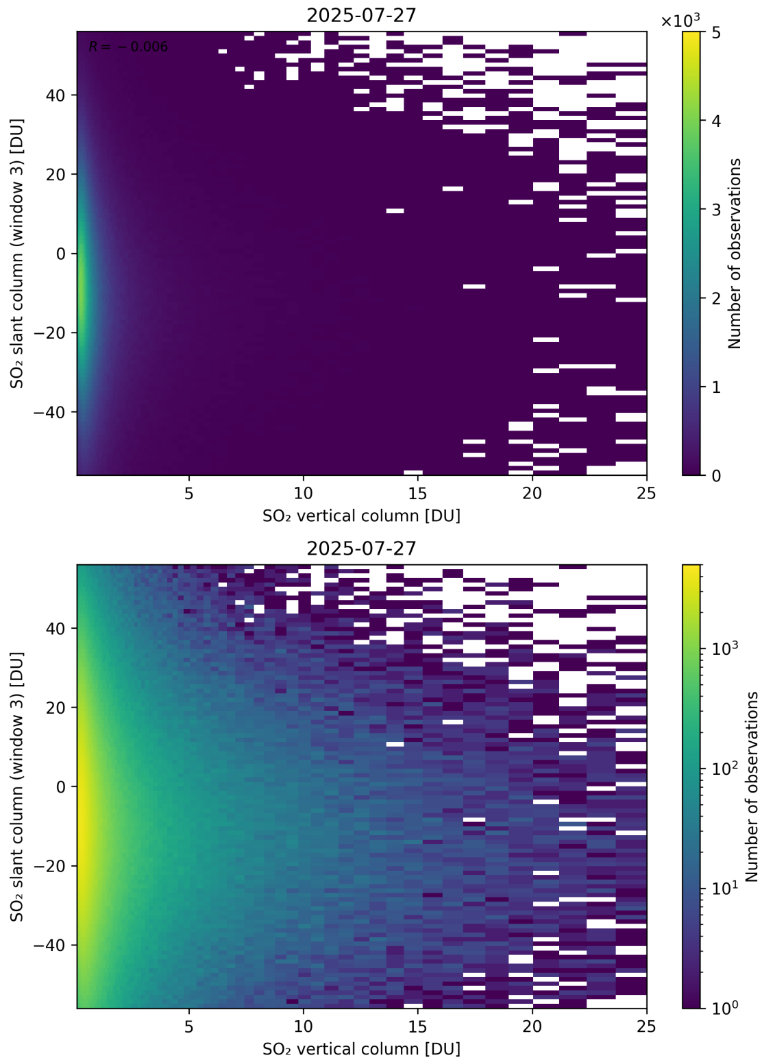
Figure 357: Scatter density plot of “SO 2 vertical column” against “SO 2 slant column (window 3)” for 2025-07-26 to 2025-07-28.
