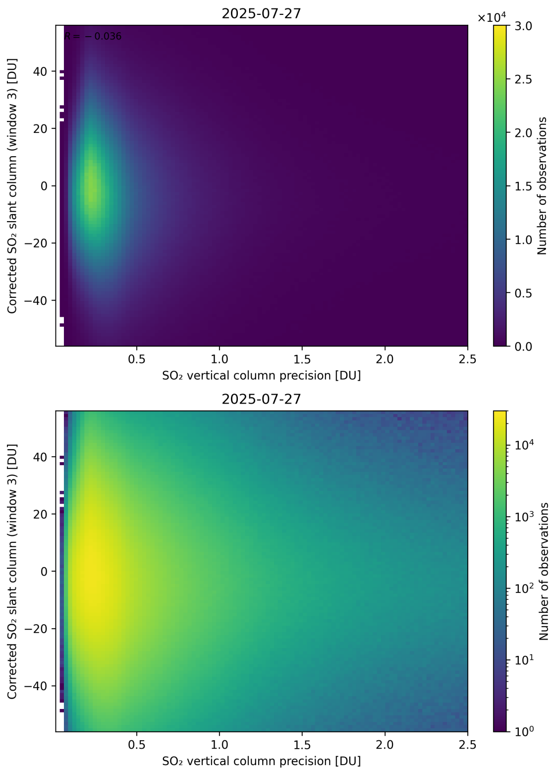
Figure 340: Scatter density plot of “SO 2 vertical column precision” against “Corrected SO 2 slant column (window 3)” for 2025-07-26 to 2025-07-28.
