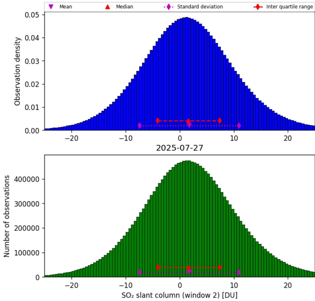
Figure 67: Histogram of “SO 2 slant column (window 2)” for 2025-07-26 to 2025-07-28
