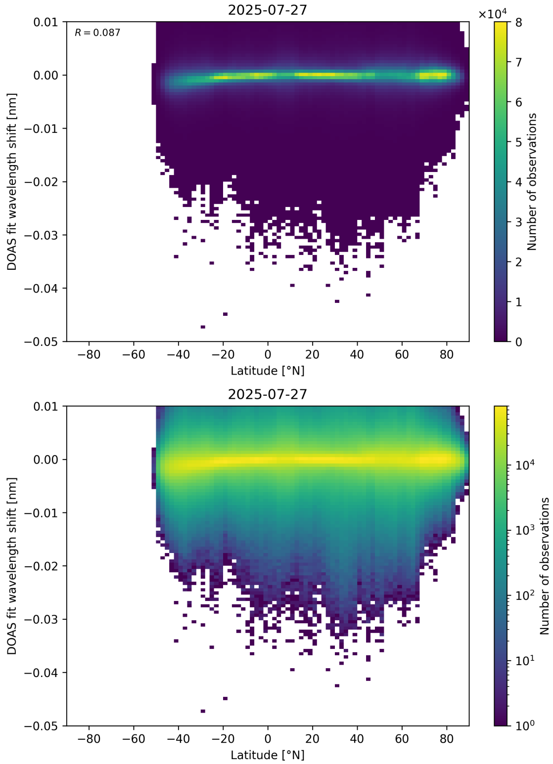
Figure 153: Scatter density plot of “Latitude” against “DOAS fit wavelength shift” for 2025-07-26 to 2025-07-28.
