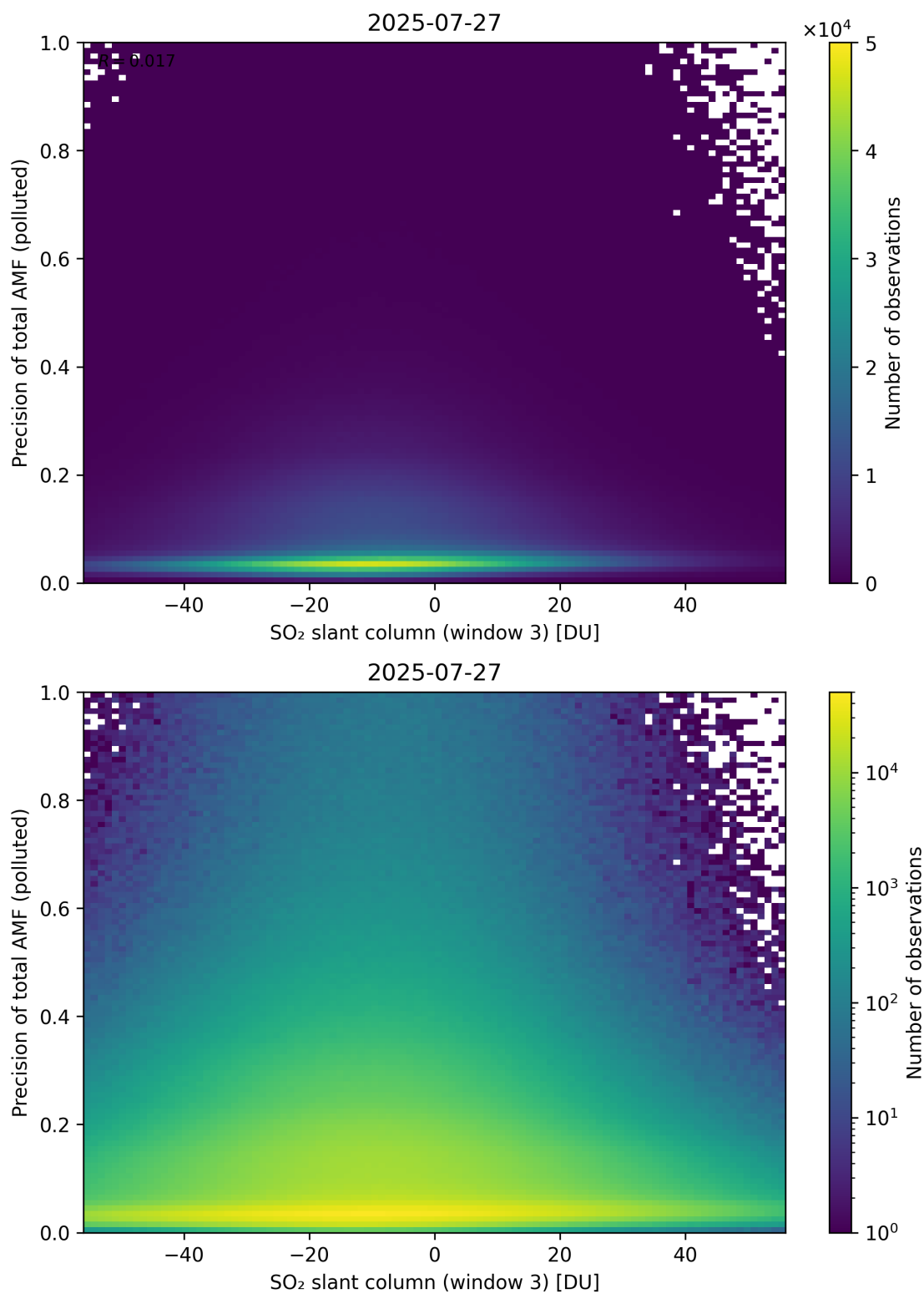
Figure 319: Scatter density plot of “SO 2 slant column (window 3)” against “Precision of total AMF (polluted)” for 2025-07-26 to 2025-07-28.
