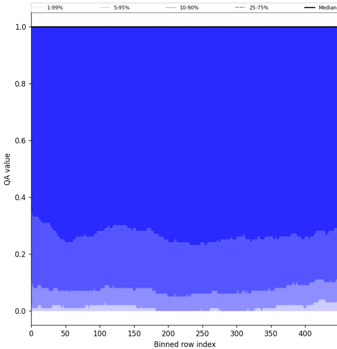
Figure 83: Along track statistics of “QA value” for 2025-07-26 to 2025-07-28
