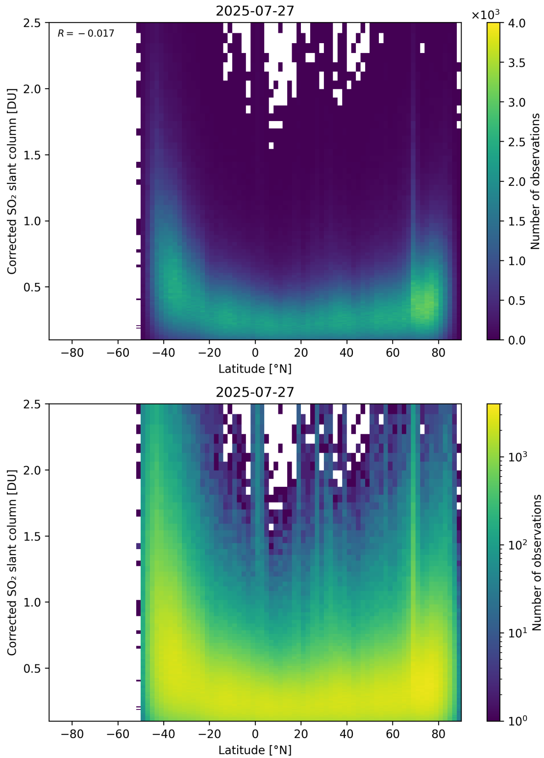
Figure 159: Scatter density plot of “Latitude” against “Corrected SO 2 slant column” for 2025-07-26 to 2025-07-28.
