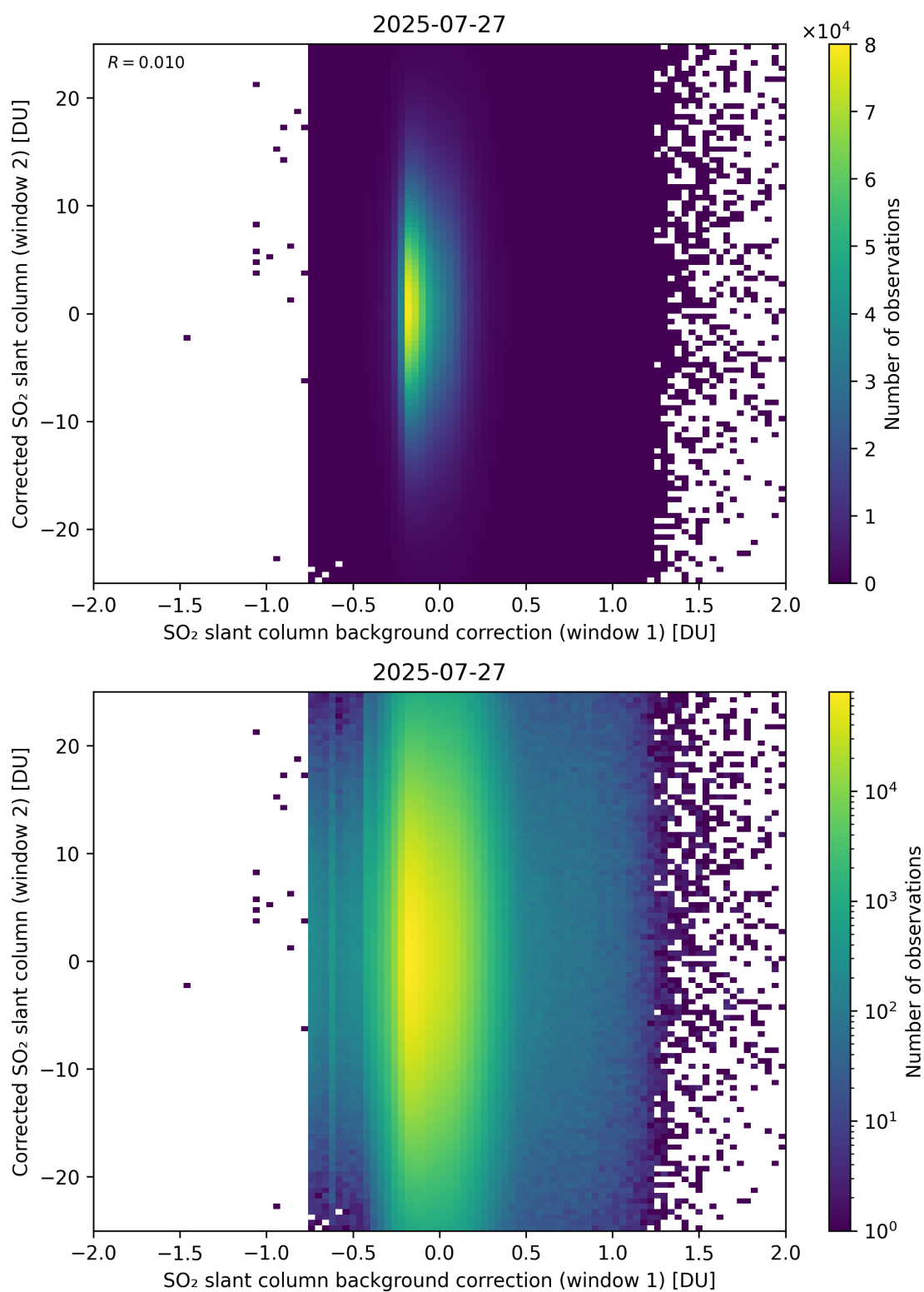
Figure 115: Scatter density plot of “SO 2 slant column background correction (window 1)” against “Corrected SO 2 slant column (window 2)” for 2025-07-26 to 2025-07-28.
