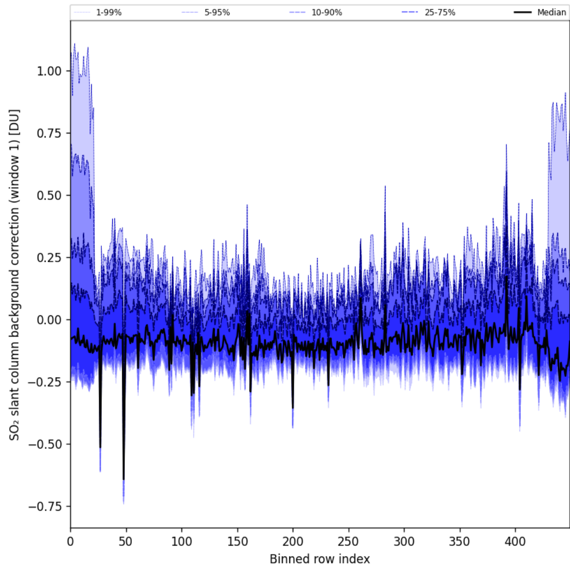
Figure 92: Along track statistics of “SO 2 slant column background correction (window 1)” for 2025-07-26 to 2025-07-28
