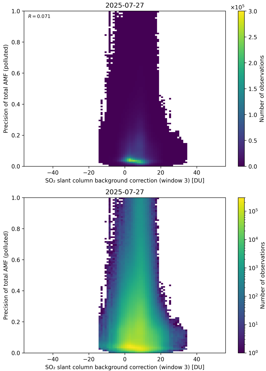
Figure 137: Scatter density plot of “SO 2 slant column background correction (window 3)” against “Precision of total AMF (polluted)” for 2025-07-26 to 2025-07-28.
