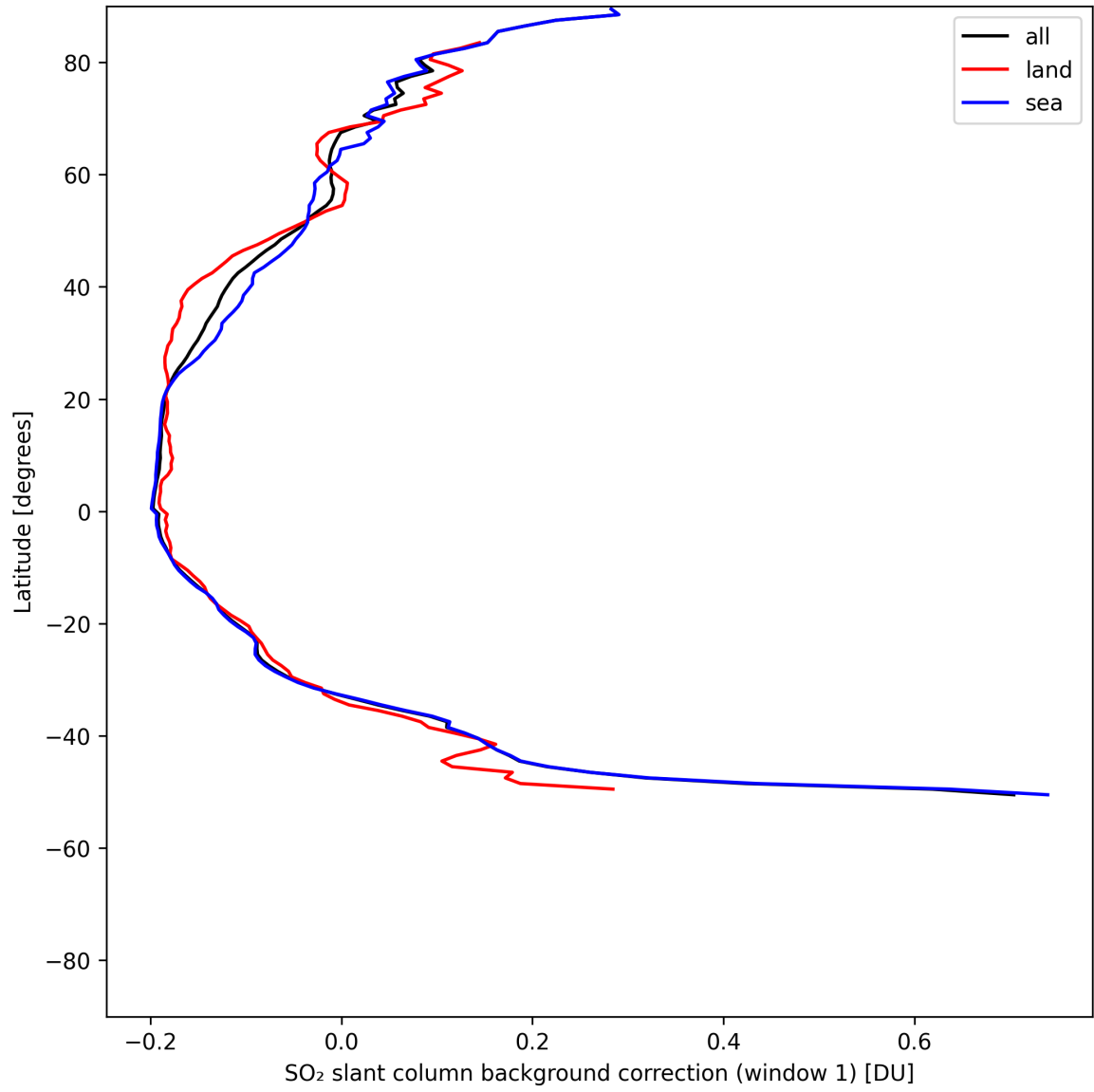
Figure 40: Zonal average of "SO 2 slant column background correction (window 1)" for 2025-07-26 to 2025-07-28.
