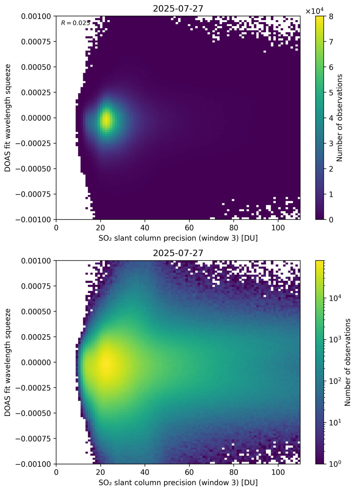
Figure 309: Scatter density plot of “SO 2 slant column precision (window 3)” against “DOAS fit wavelength squeeze” for 2025-07-26 to 2025-07-28.
