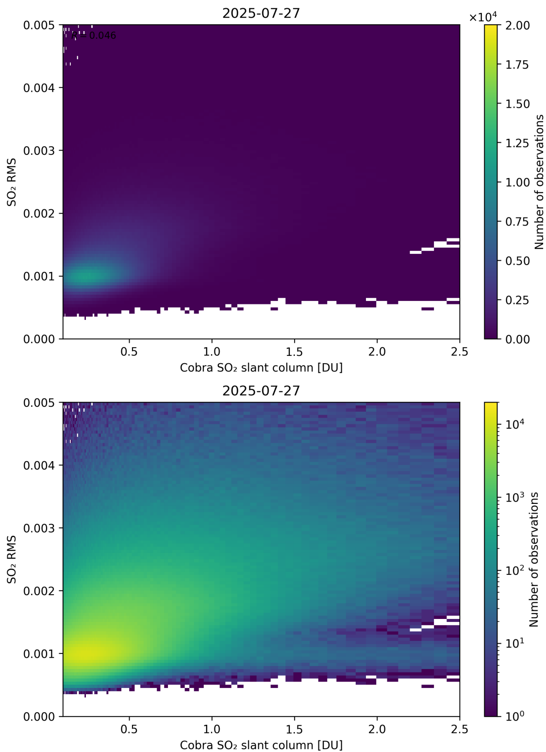
Figure 198: Scatter density plot of “Cobra SO 2 slant column” against “SO 2 RMS” for 2025-07-26 to 2025-07-28.
