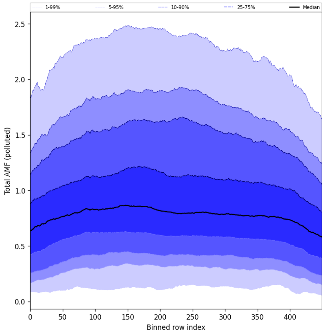
Figure 105: Along track statistics of “Total AMF (polluted)” for 2025-07-26 to 2025-07-28
