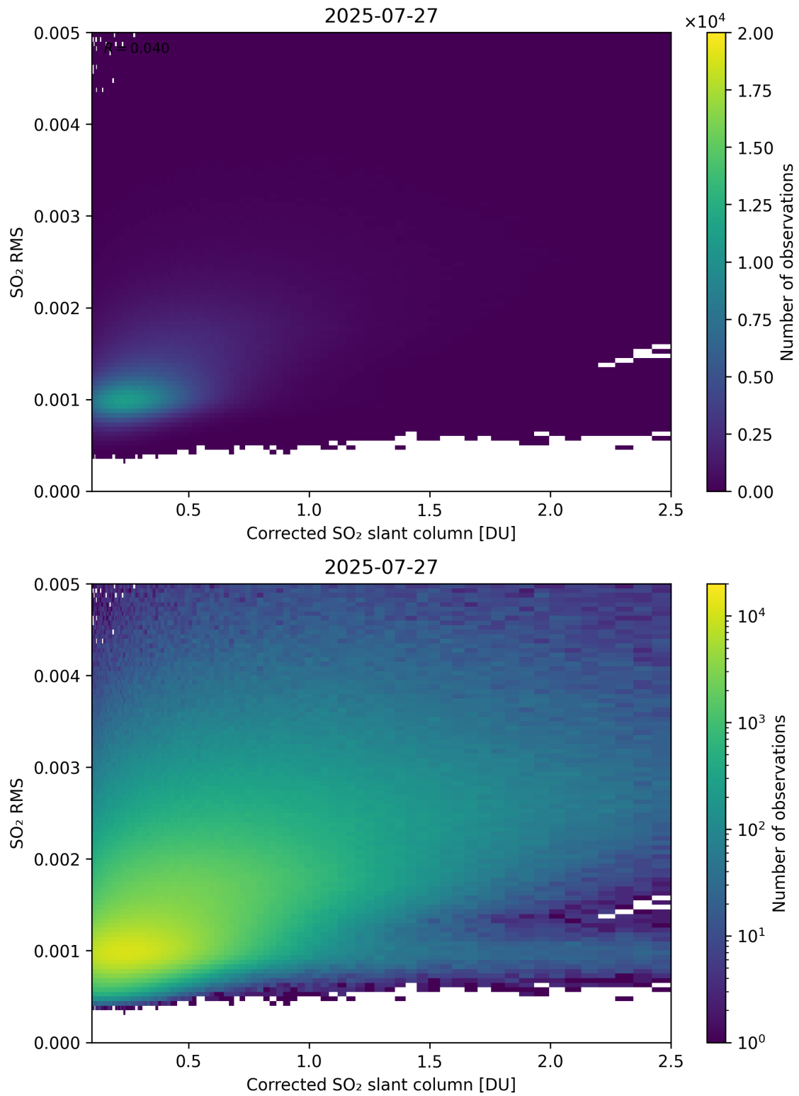
Figure 231: Scatter density plot of “Corrected SO 2 slant column” against “SO 2 RMS” for 2025-07-26 to 2025-07-28.
