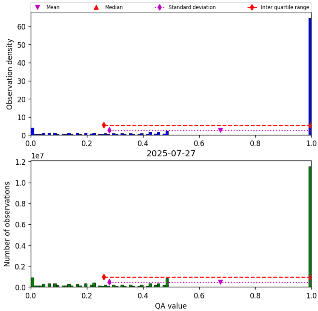
Figure 57: Histogram of “QA value” for 2025-07-26 to 2025-07-28
