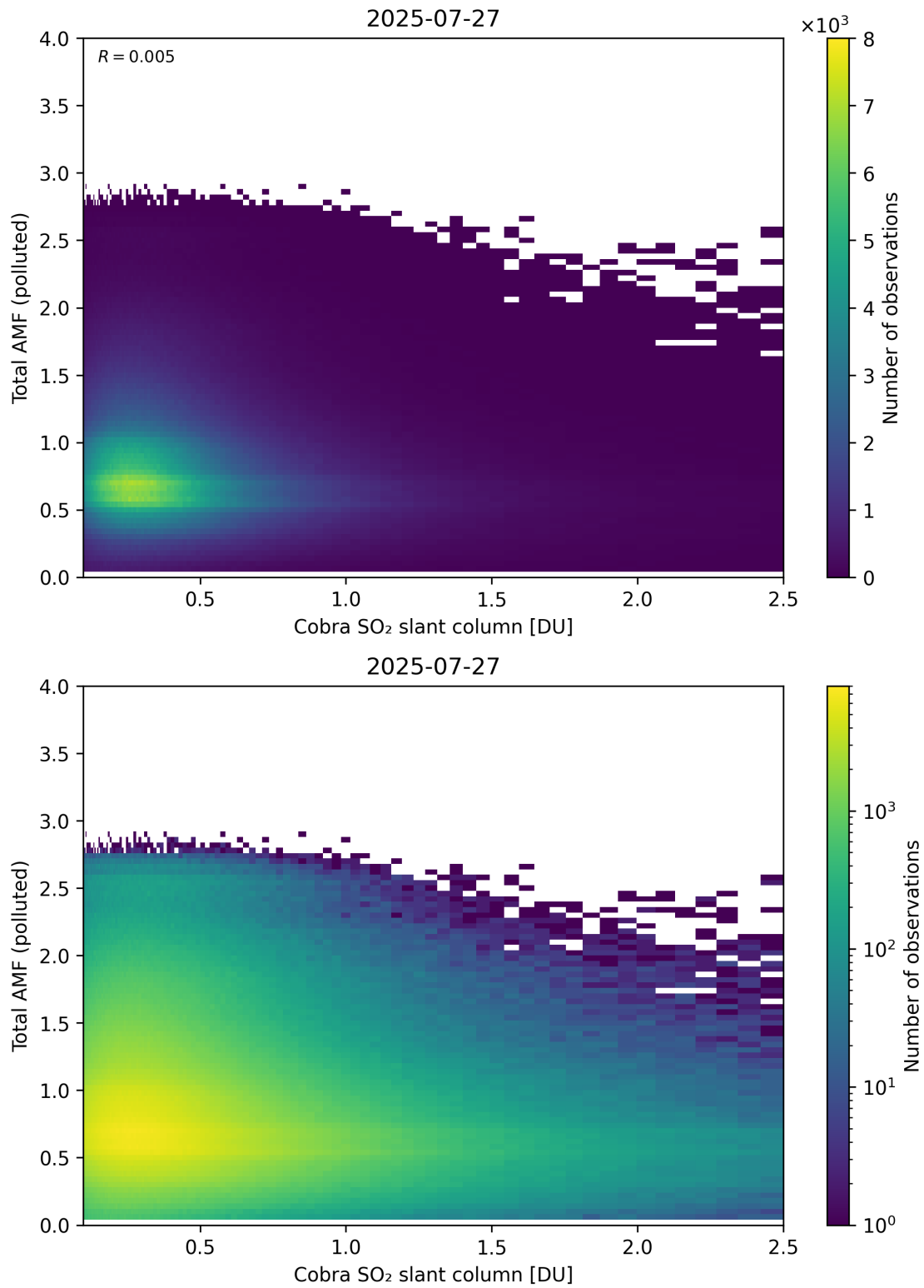
Figure 224: Scatter density plot of “Cobra SO 2 slant column” against “Total AMF (polluted)” for 2025-07-26 to 2025-07-28.
