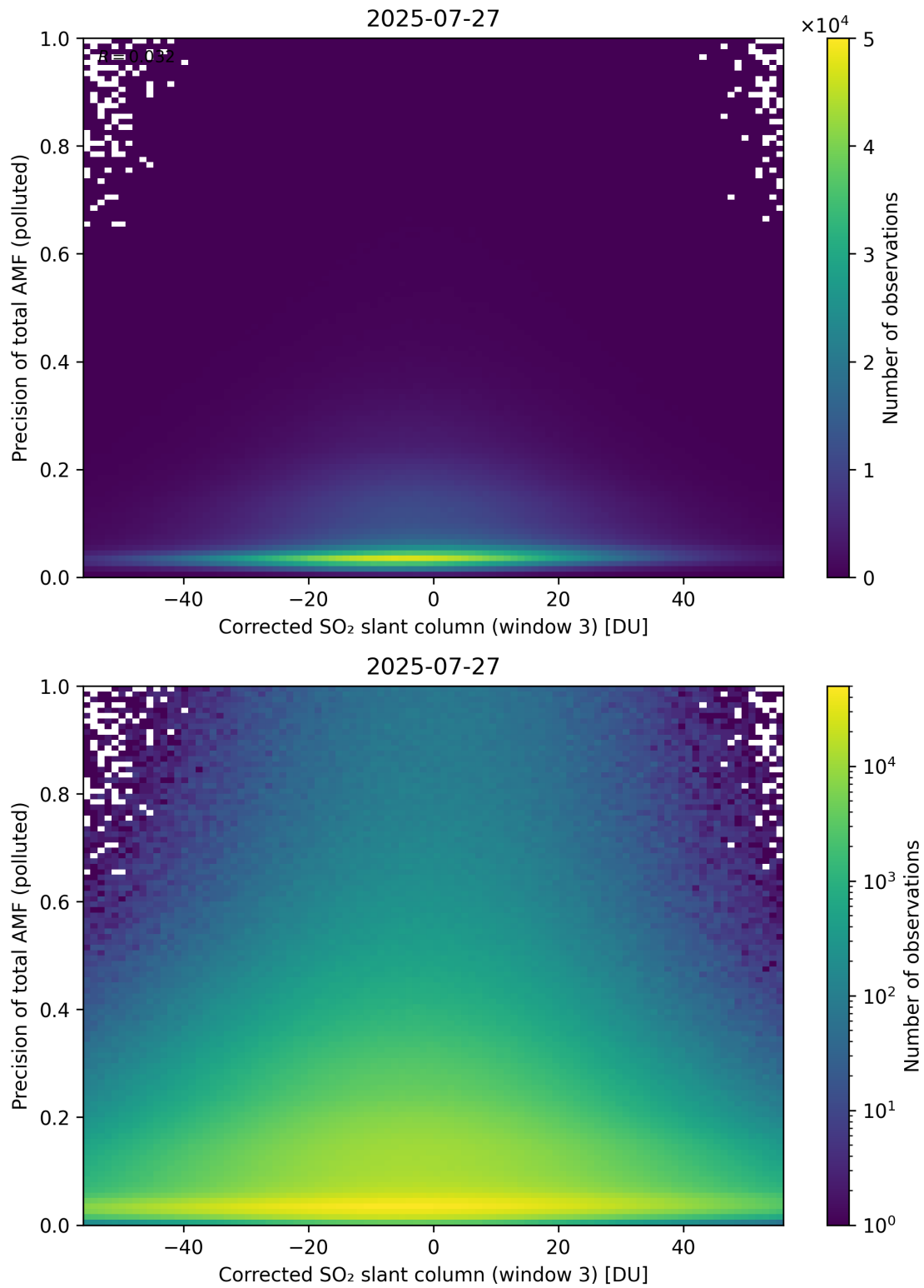
Figure 261: Scatter density plot of “Corrected SO 2 slant column (window 3)” against “Precision of total AMF (polluted)” for 2025-07-26 to 2025-07-28.
