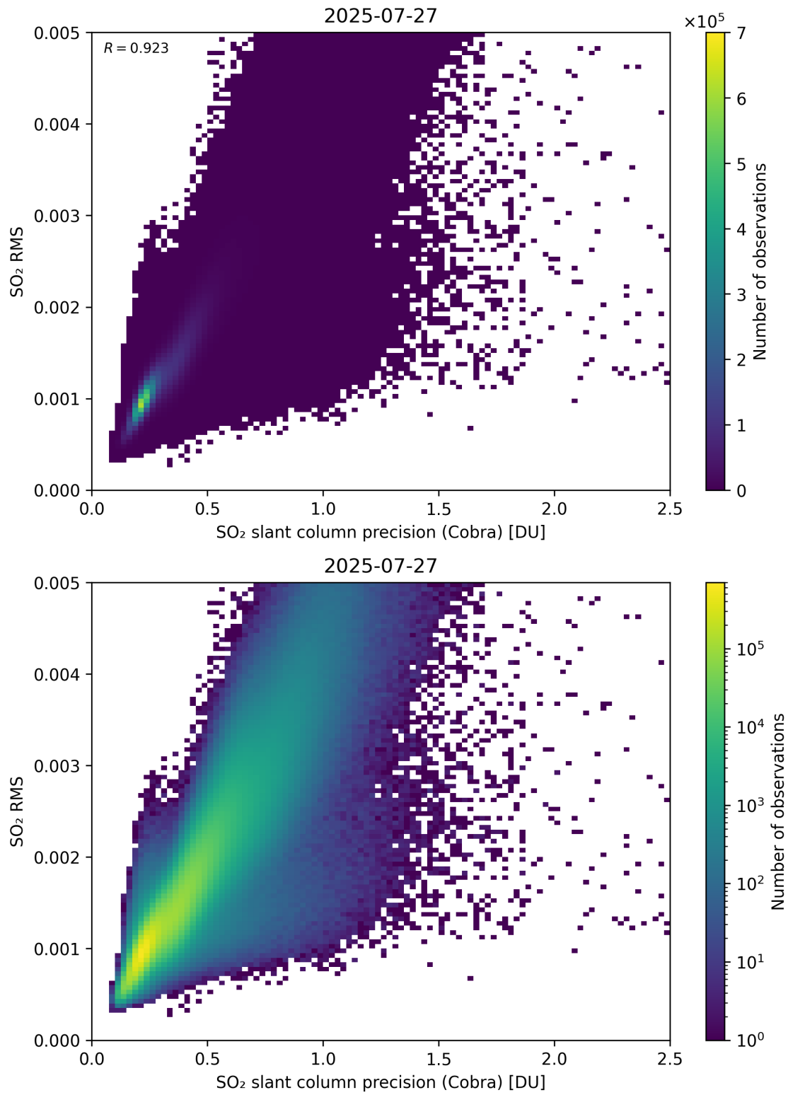
Figure 204: Scatter density plot of “SO 2 slant column precision (Cobra)” against “SO 2 RMS” for 2025-07-26 to 2025-07-28.
