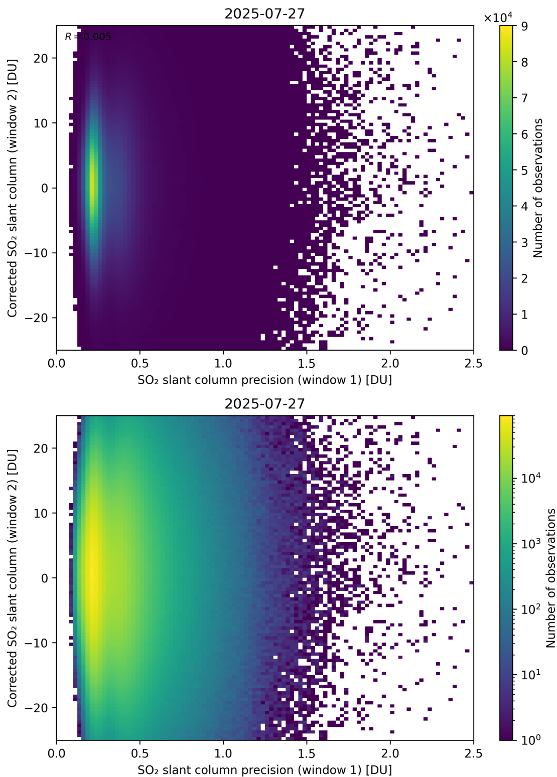
Figure 275: Scatter density plot of “SO 2 slant column precision (window 1)” against “Corrected SO 2 slant column (window 2)” for 2025-07-26 to 2025-07-28.
