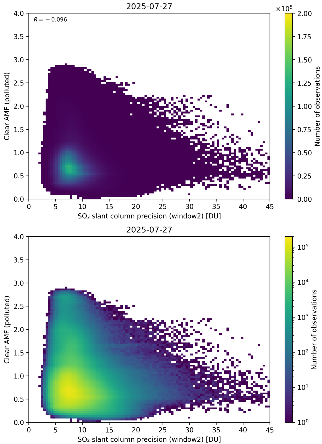
Figure 296: Scatter density plot of “SO 2 slant column precision (window2)” against “Clear AMF (polluted)” for 2025-07-26 to 2025-07-28.
