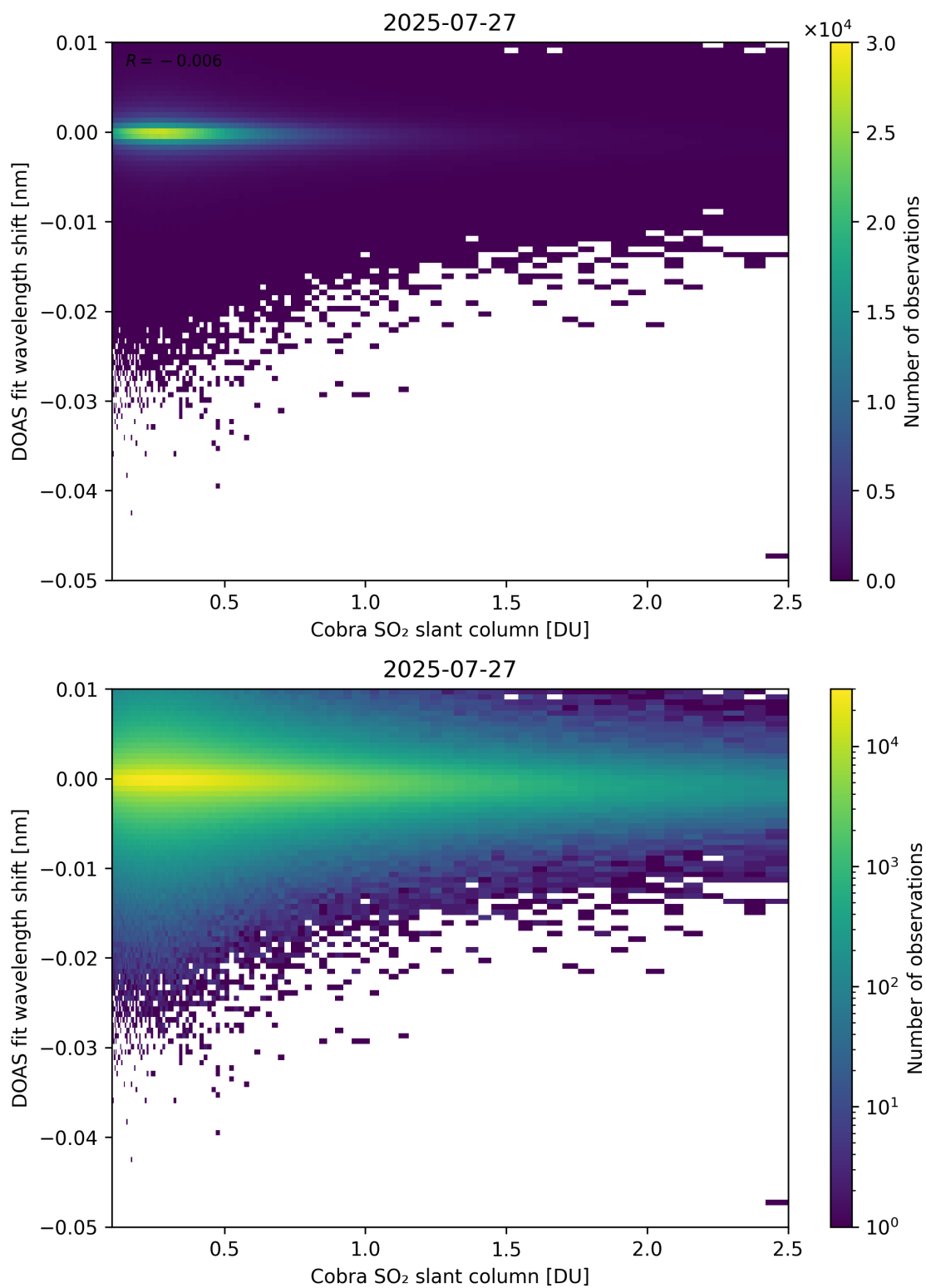
Figure 196: Scatter density plot of “Cobra SO 2 slant column” against “DOAS fit wavelength shift” for 2025-07-26 to 2025-07-28.
