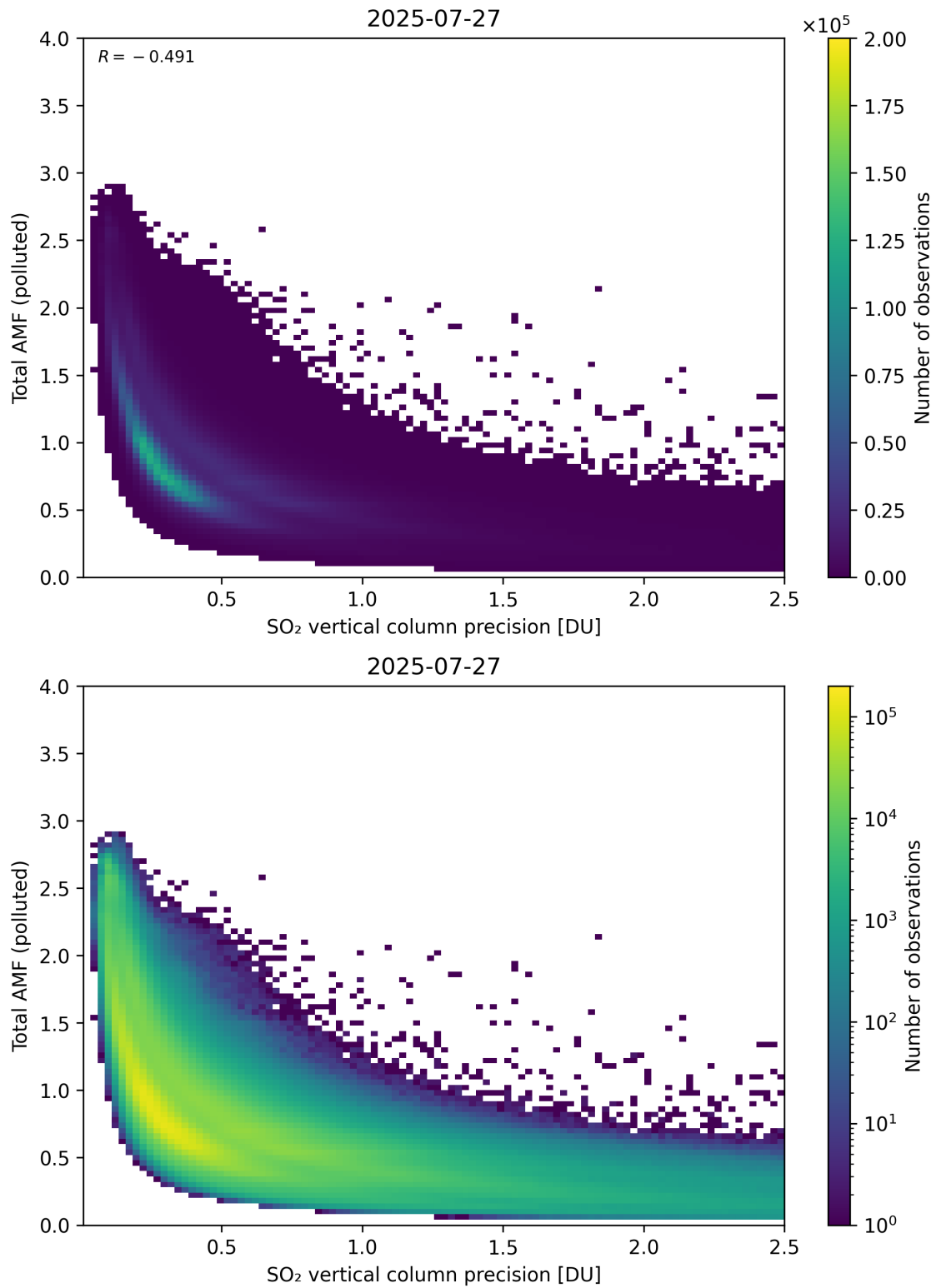
Figure 346: Scatter density plot of “SO 2 vertical column precision” against “Total AMF (polluted)” for 2025-07-26 to 2025-07-28.
