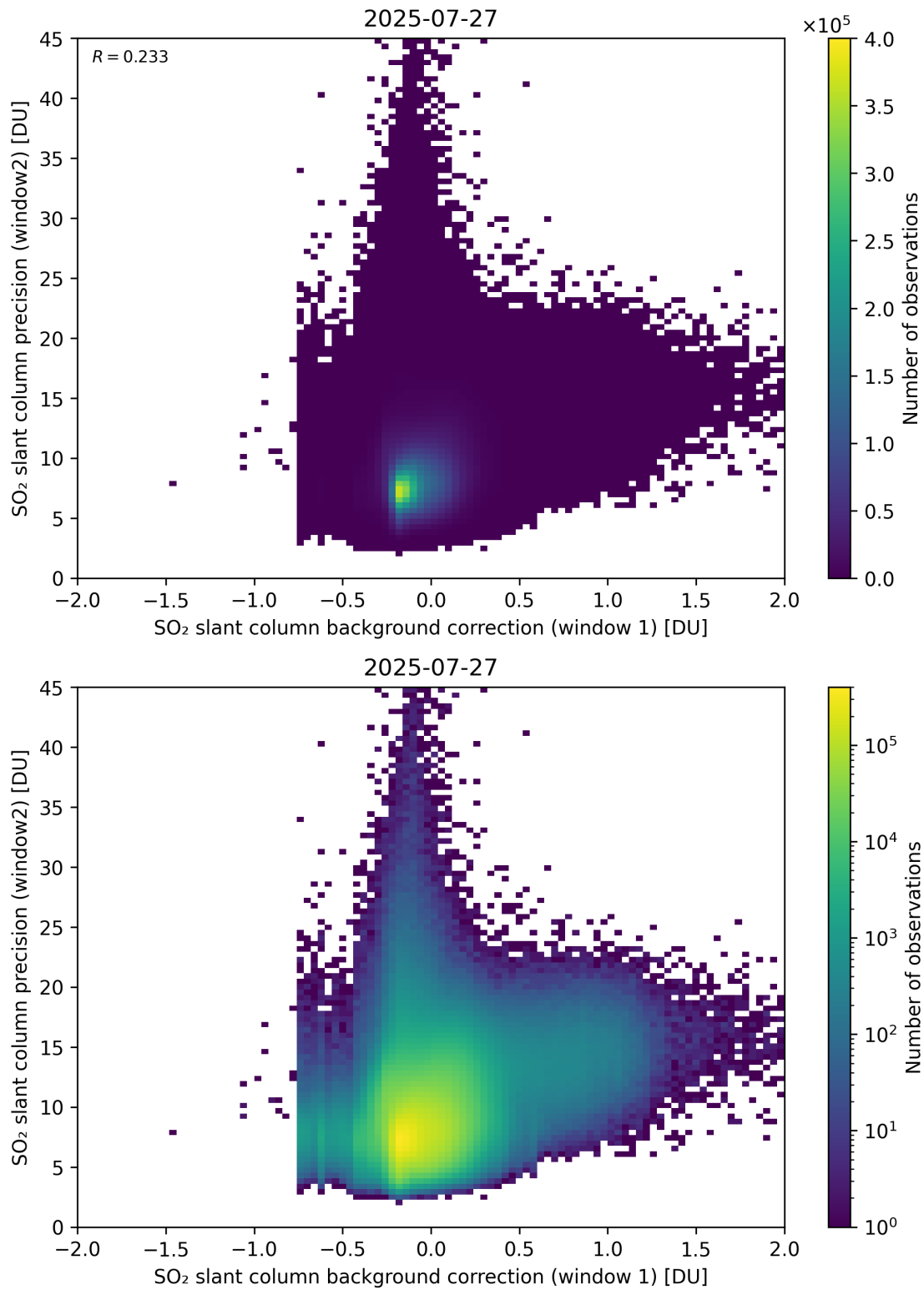
Figure 117: Scatter density plot of “SO 2 slant column background correction (window 1)” against “SO 2 slant column precision (window2)” for 2025-07-26 to 2025-07-28.
