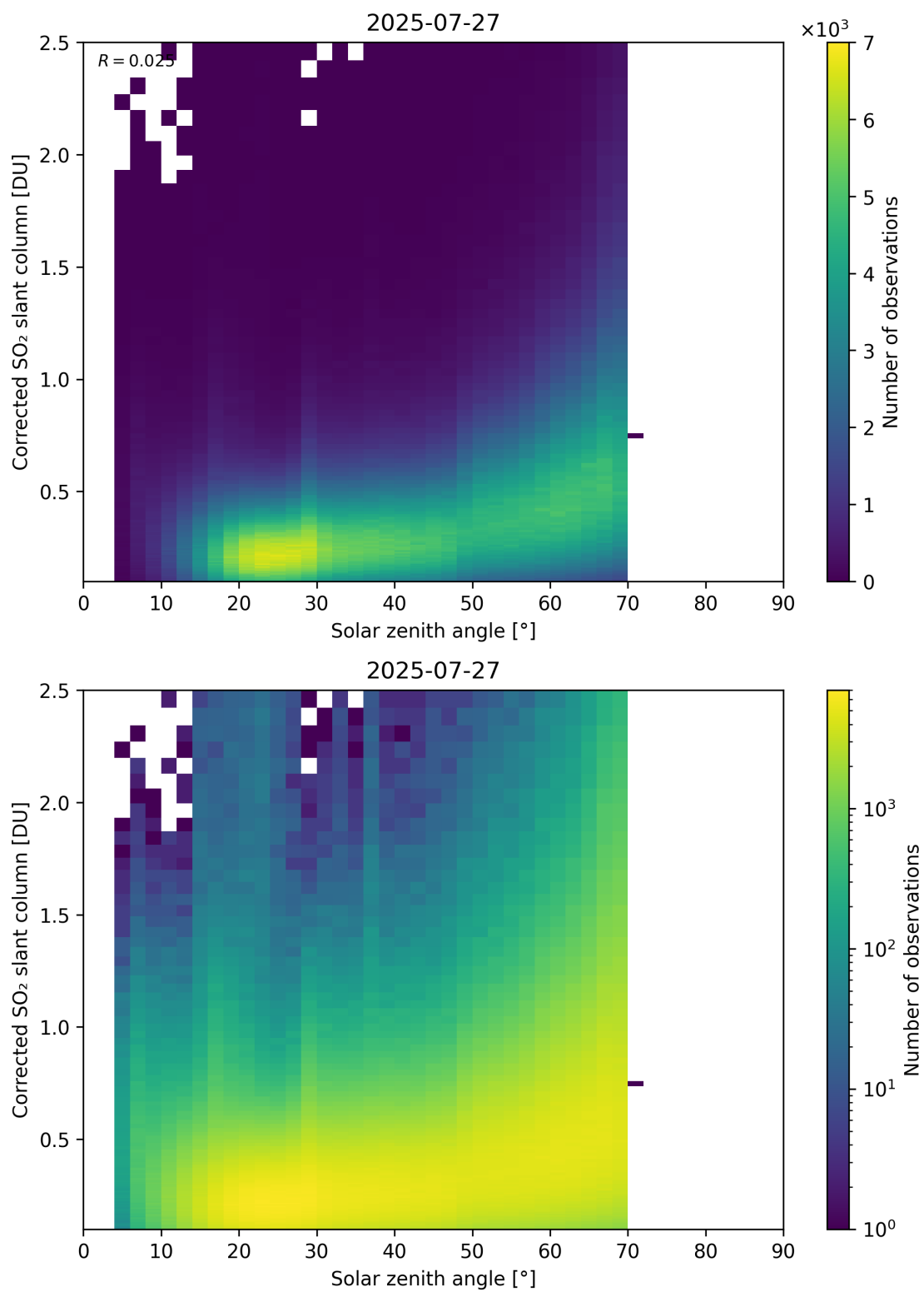
Figure 181: Scatter density plot of “Solar zenith angle” against “Corrected SO 2 slant column” for 2025-07-26 to 2025-07-28.
