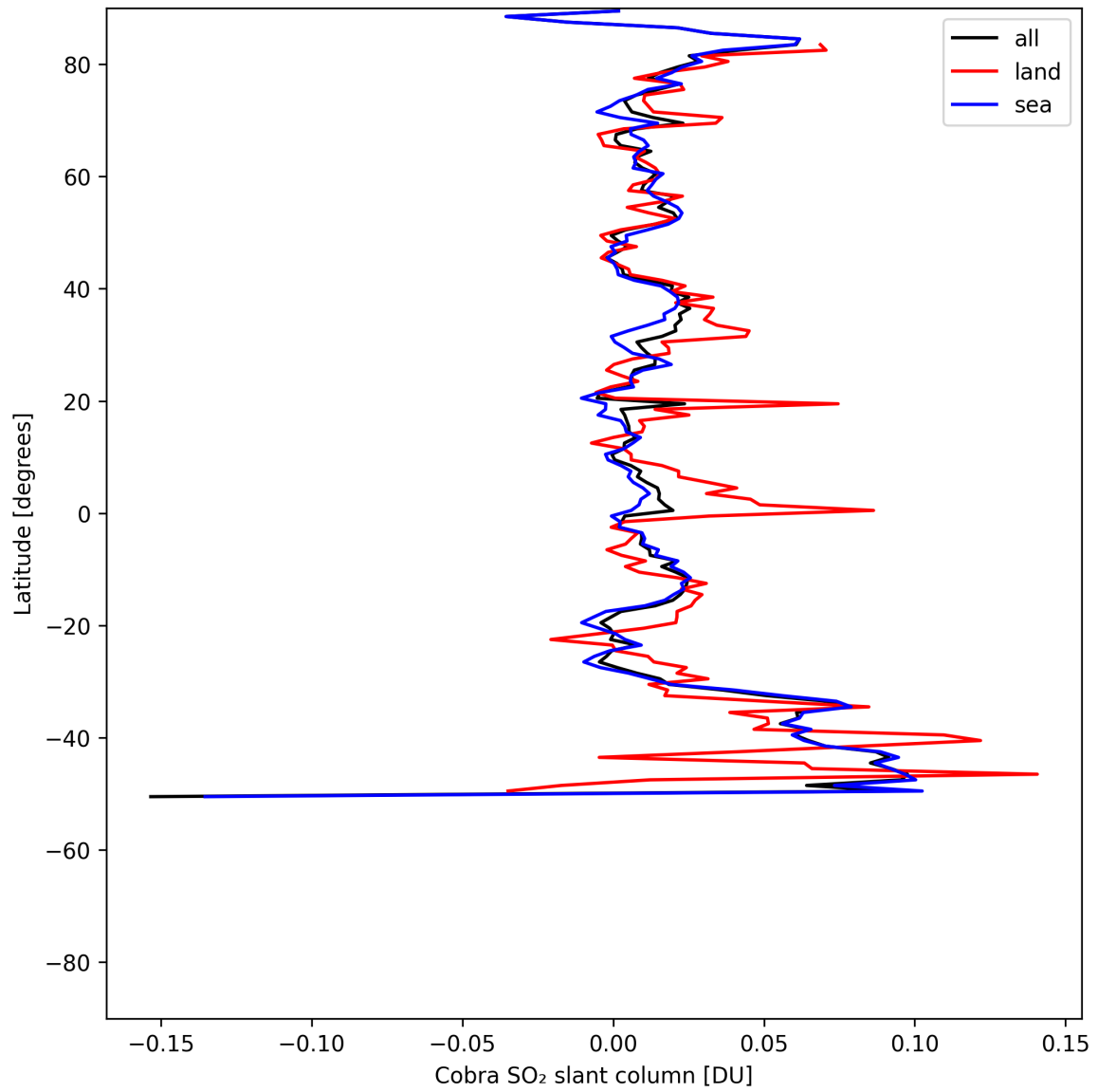
Figure 35: Zonal average of “Cobra SO 2 slant column” for 2025-07-26 to 2025-07-28.
