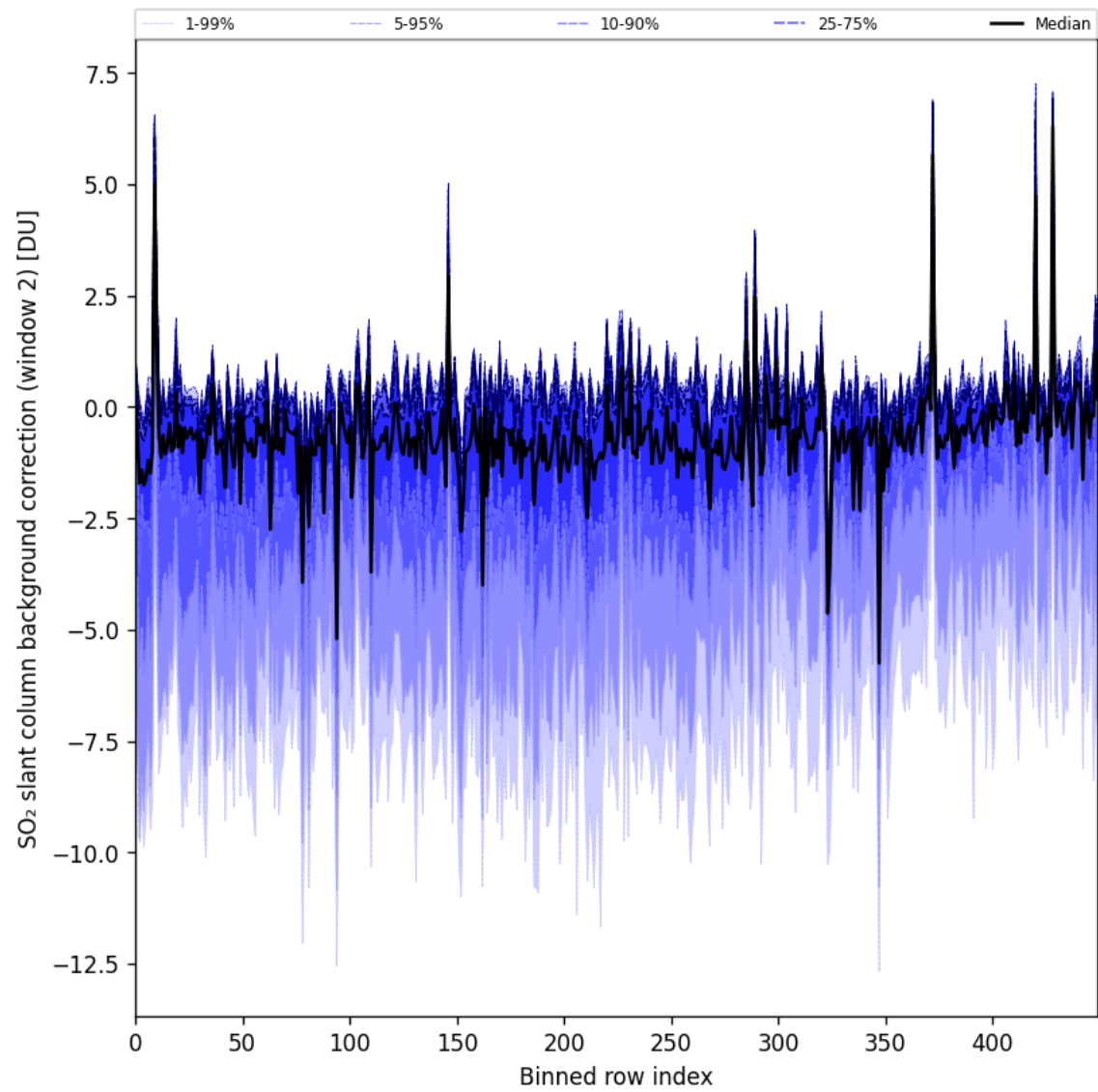
Figure 96: Along track statistics of “SO 2 slant column background correction (window 2)” for 2025-07-26 to 2025-07-28
