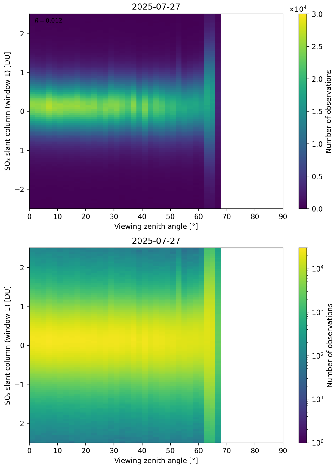
Figure 376: Scatter density plot of “Viewing zenith angle” against “SO 2 slant column (window 1)” for 2025-07-26 to 2025-07-28.
