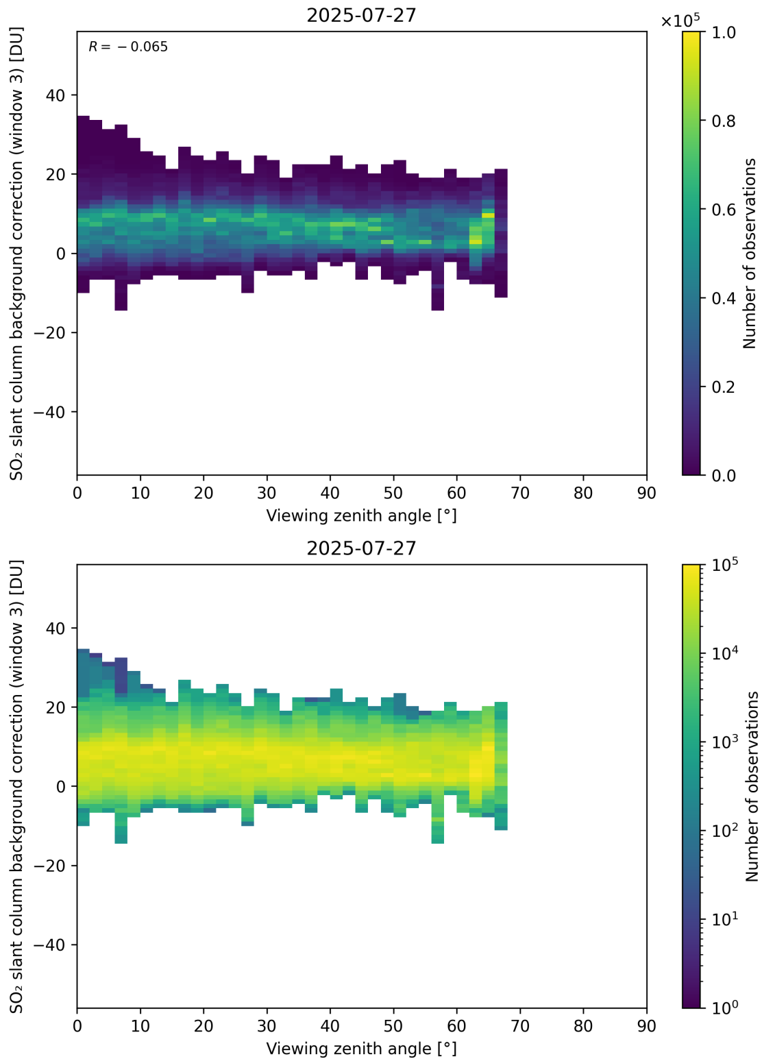
Figure 364: Scatter density plot of “Viewing zenith angle” against “SO 2 slant column background correction (window 3)” for 2025-07-26 to 2025-07-28.
