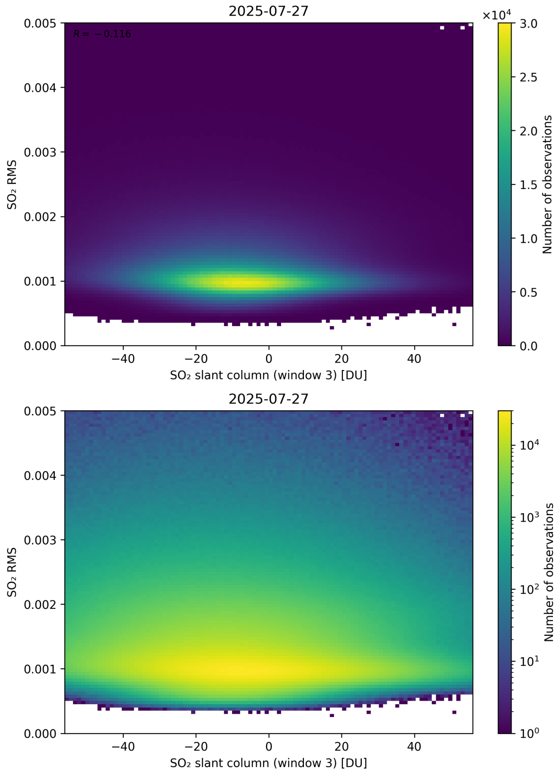
Figure 306: Scatter density plot of “SO 2 slant column (window 3)” against “SO 2 RMS” for 2025-07-26 to 2025-07-28.
