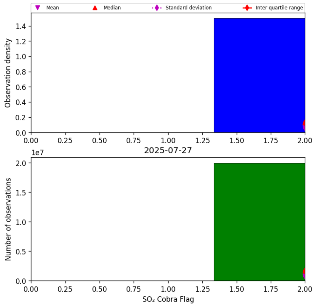
Figure 75: Histogram of “SO 2 Cobra Flag” for 2025-07-26 to 2025-07-28
