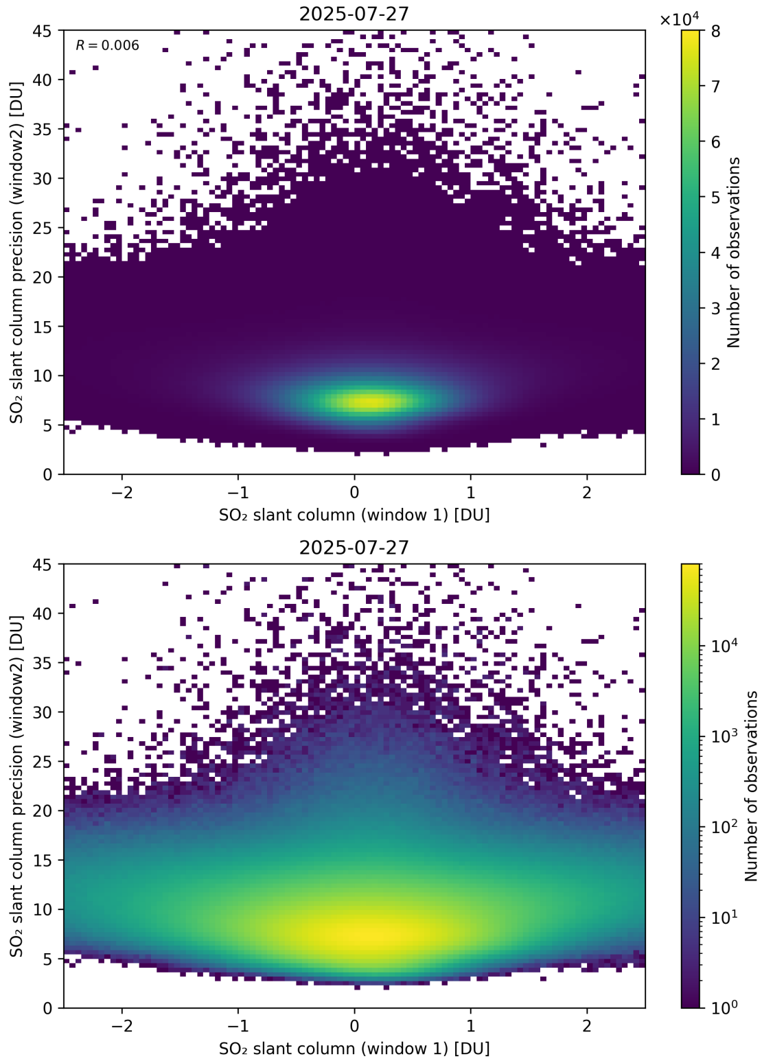
Figure 286: Scatter density plot of “SO 2 slant column (window 1)” against “SO 2 slant column precision (window2)” for 2025-07-26 to 2025-07-28.
