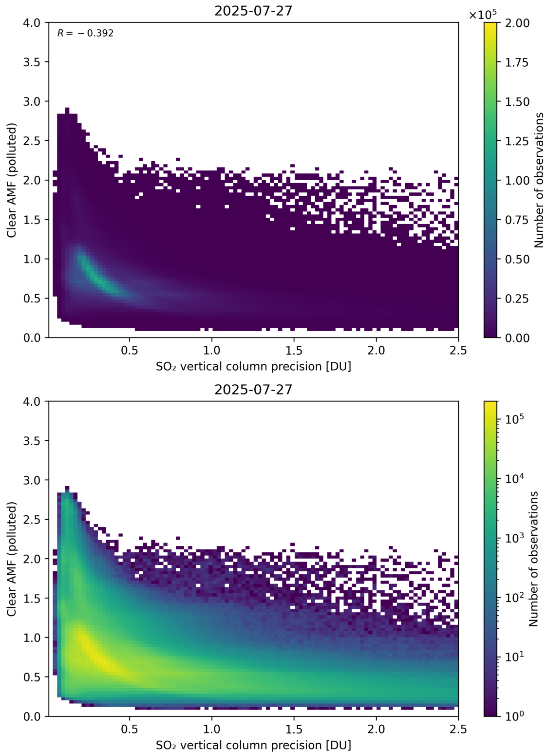
Figure 335: Scatter density plot of “SO 2 vertical column precision” against “Clear AMF (polluted)” for 2025-07-26 to 2025-07-28.
