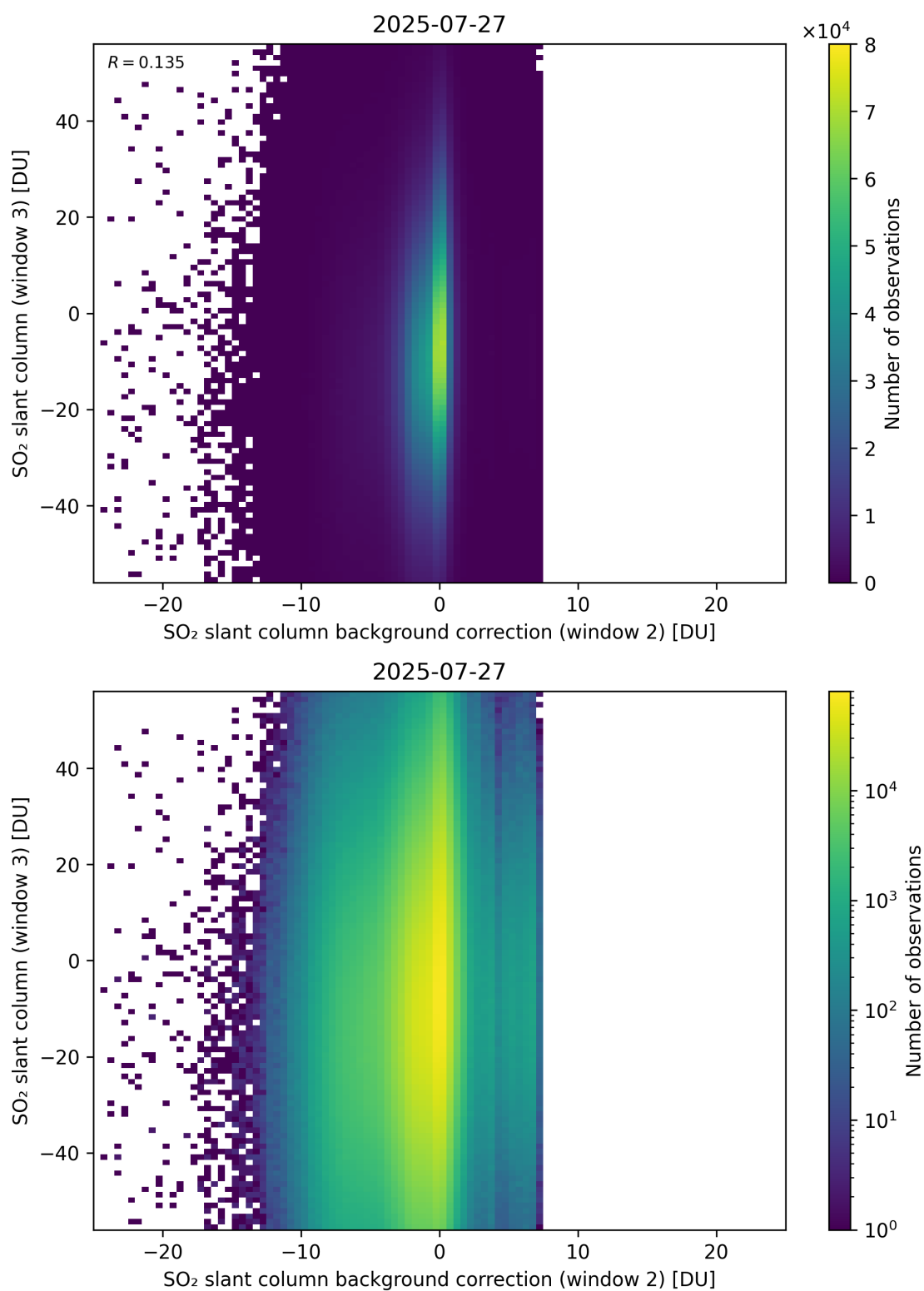
Figure 128: Scatter density plot of “SO 2 slant column background correction (window 2)” against “SO 2 slant column (window 3)” for 2025-07-26 to 2025-07-28.
