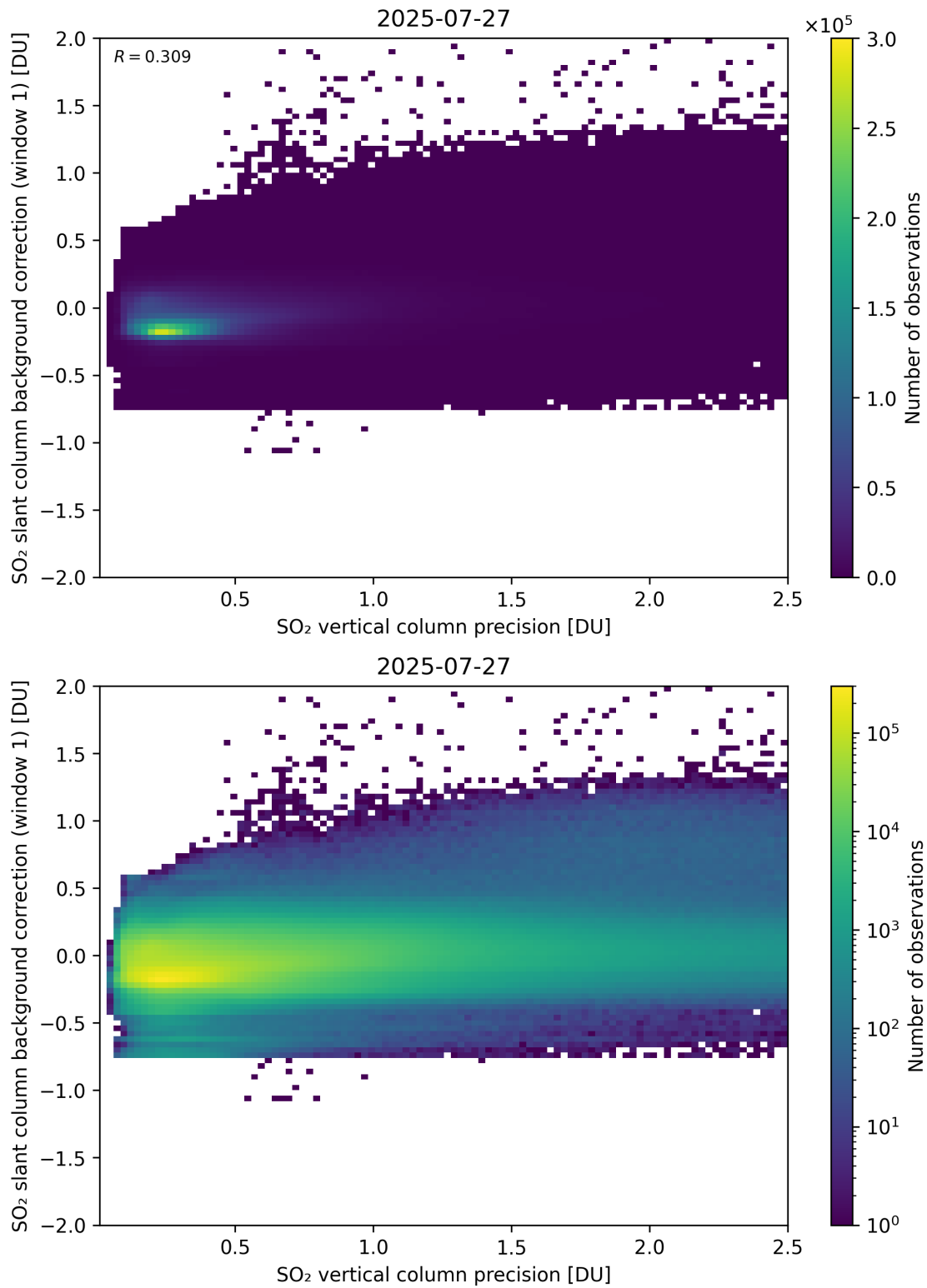
Figure 329: Scatter density plot of “SO 2 vertical column precision” against “SO 2 slant column background correction (window 1)” for 2025-07-26 to 2025-07-28.
