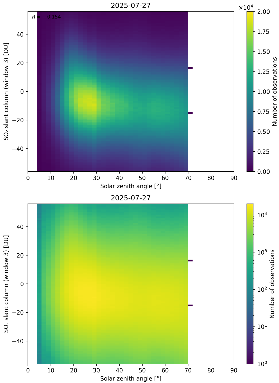
Figure 187: Scatter density plot of “Solar zenith angle” against “SO 2 slant column (window 3)” for 2025-07-26 to 2025-07-28.
