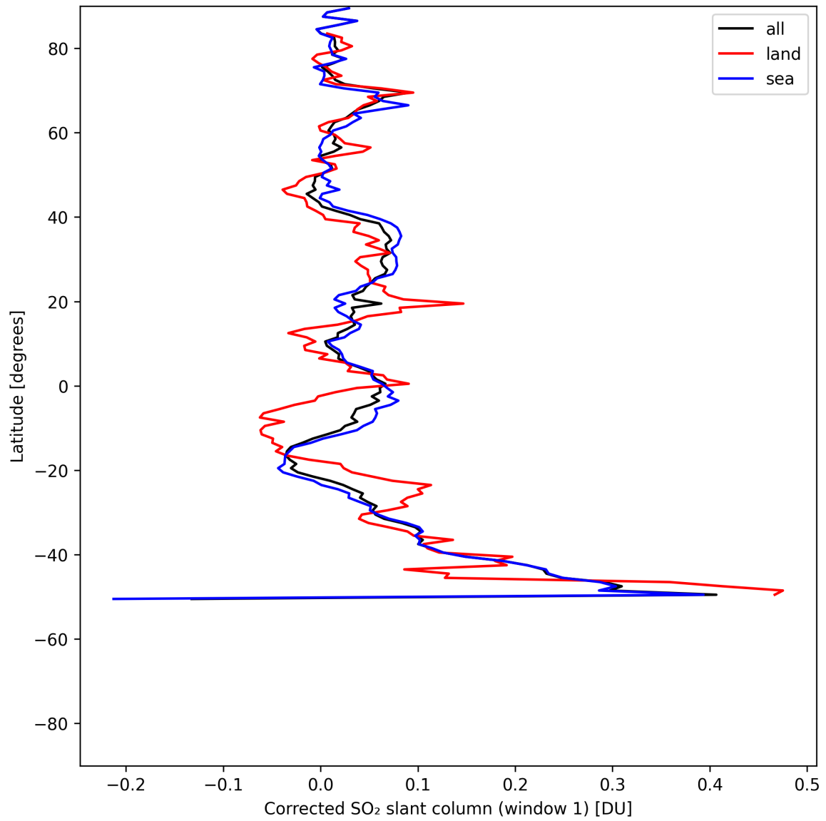
Figure 39: Zonal average of “Corrected SO 2 slant column (window 1)” for 2025-07-26 to 2025-07-28.
