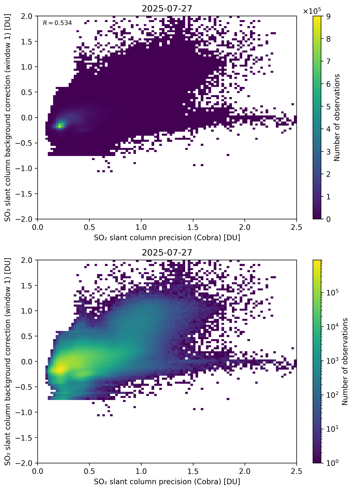
Figure 199: Scatter density plot of “SO 2 slant column precision (Cobra)” against “SO 2 slant column background correction (window 1)” for 2025-07-26 to 2025-07-28.
