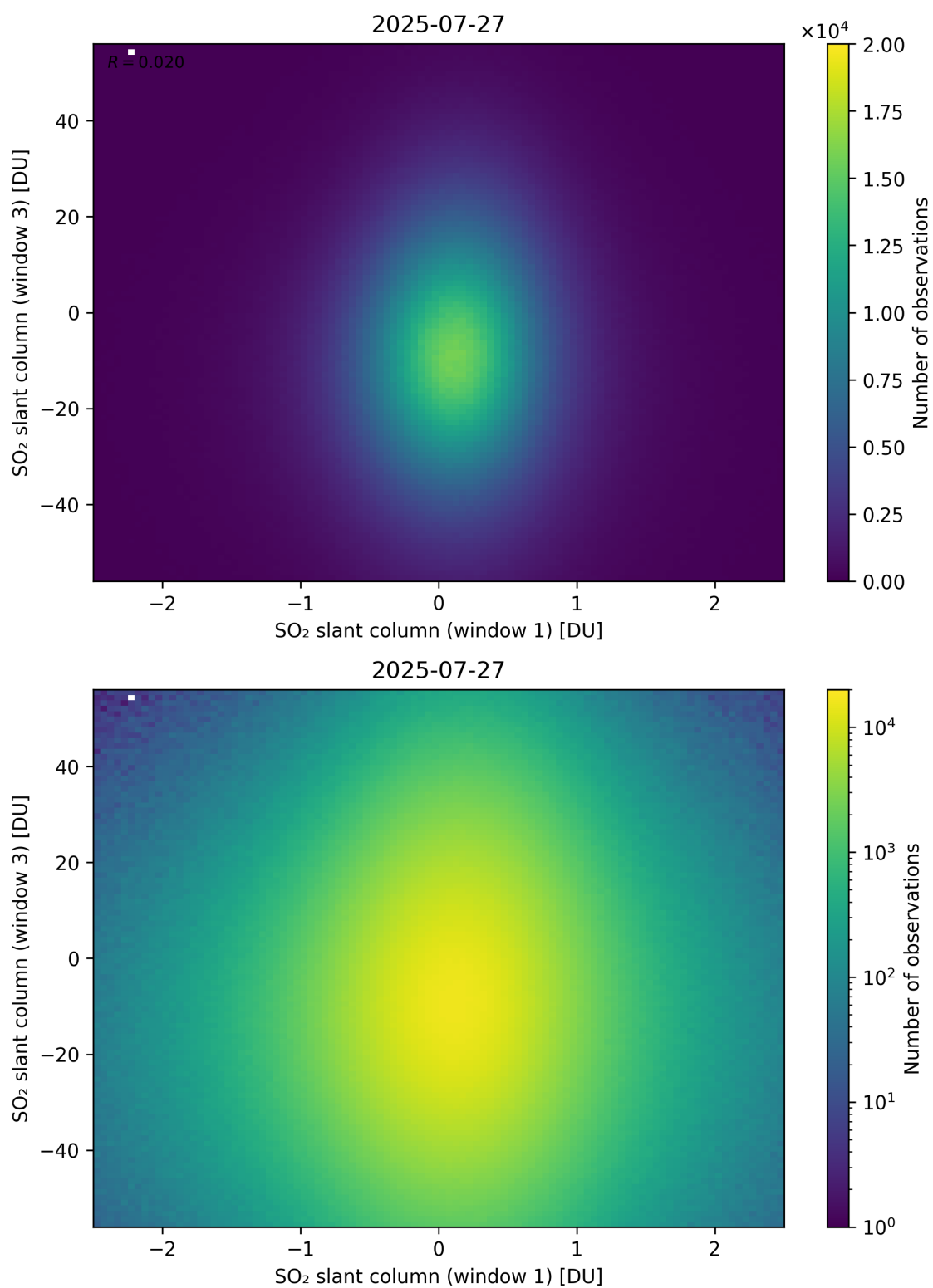
Figure 287: Scatter density plot of “SO 2 slant column (window 1)” against “SO 2 slant column (window 3)” for 2025-07-26 to 2025-07-28.
