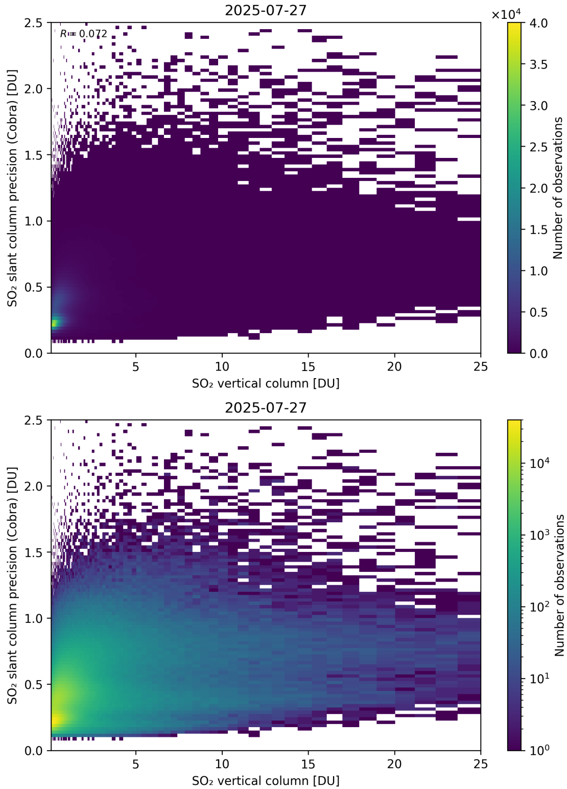
Figure 350: Scatter density plot of “SO 2 vertical column” against “SO 2 slant column precision (Cobra)” for 2025-07-26 to 2025-07-28.
