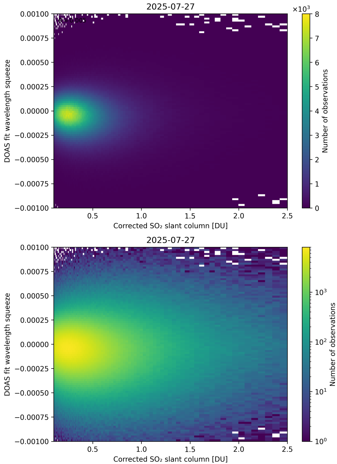
Figure 230: Scatter density plot of "Corrected SO 2 slant column" against "DOAS fit wavelength squeeze" for 2025-07-26 to 2025-07-28.
