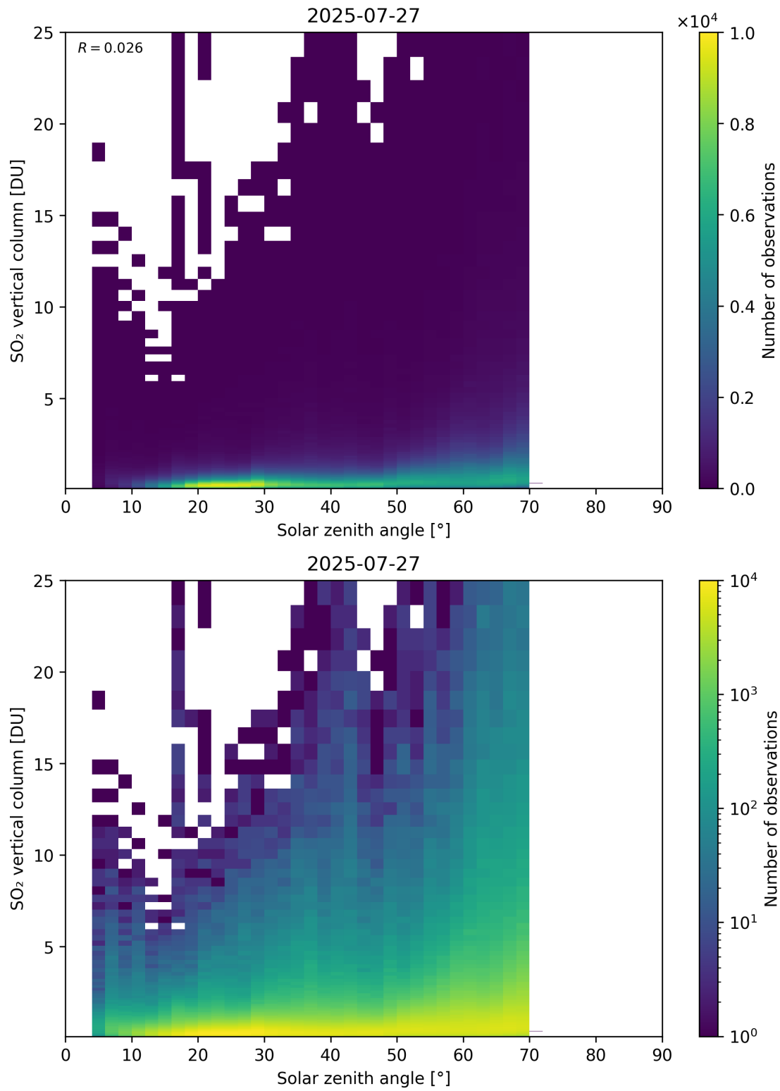
Figure 191: Scatter density plot of “Solar zenith angle” against “SO 2 vertical column” for 2025-07-26 to 2025-07-28.
