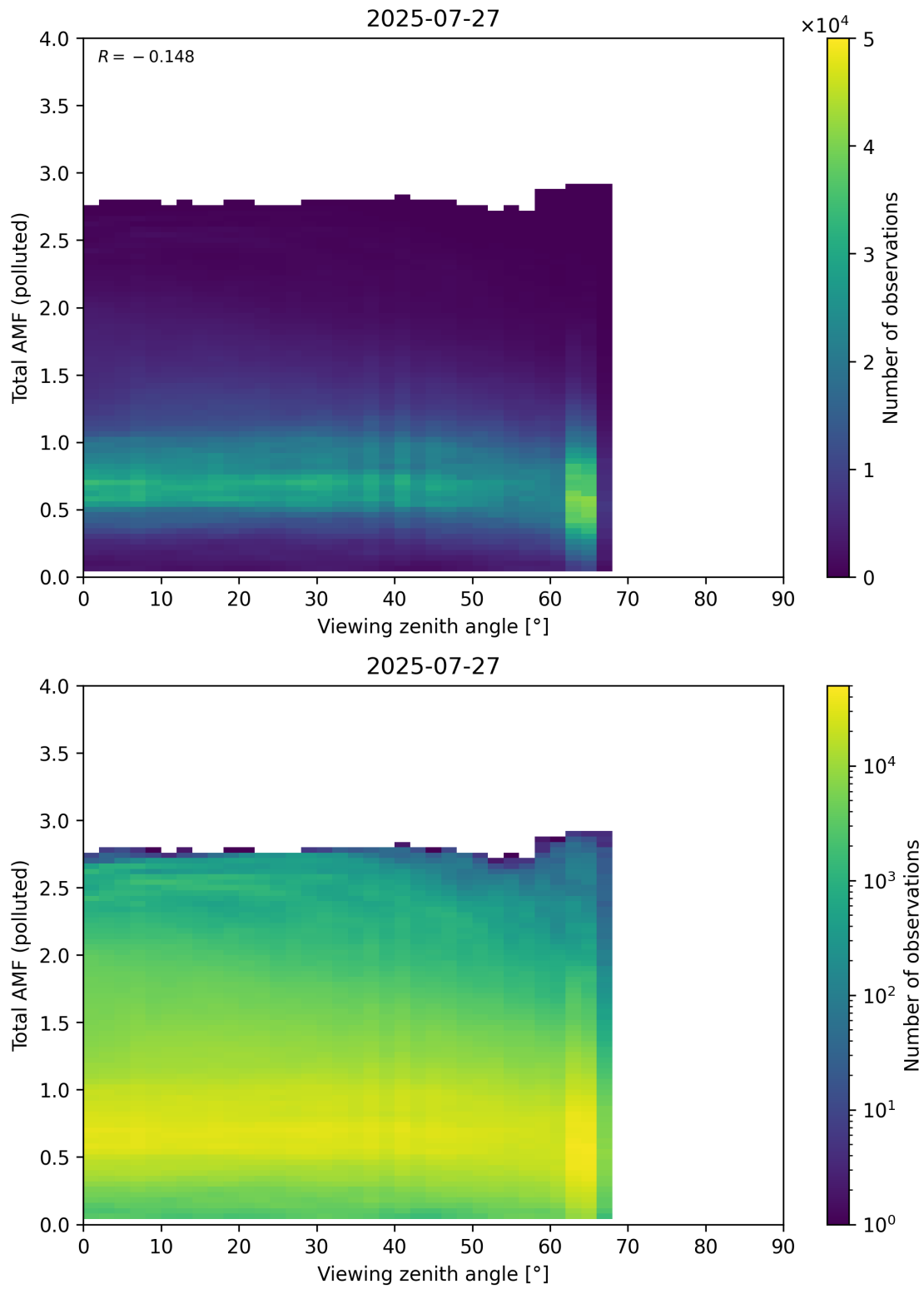
Figure 381: Scatter density plot of “Viewing zenith angle” against “Total AMF (polluted)” for 2025-07-26 to 2025-07-28.
