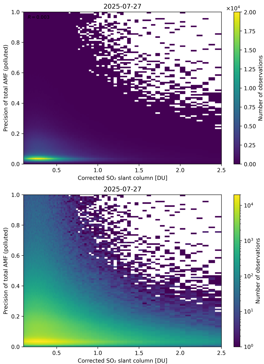
Figure 243: Scatter density plot of “Corrected SO 2 slant column” against “Precision of total AMF (polluted)” for 2025-07-26 to 2025-07-28.
