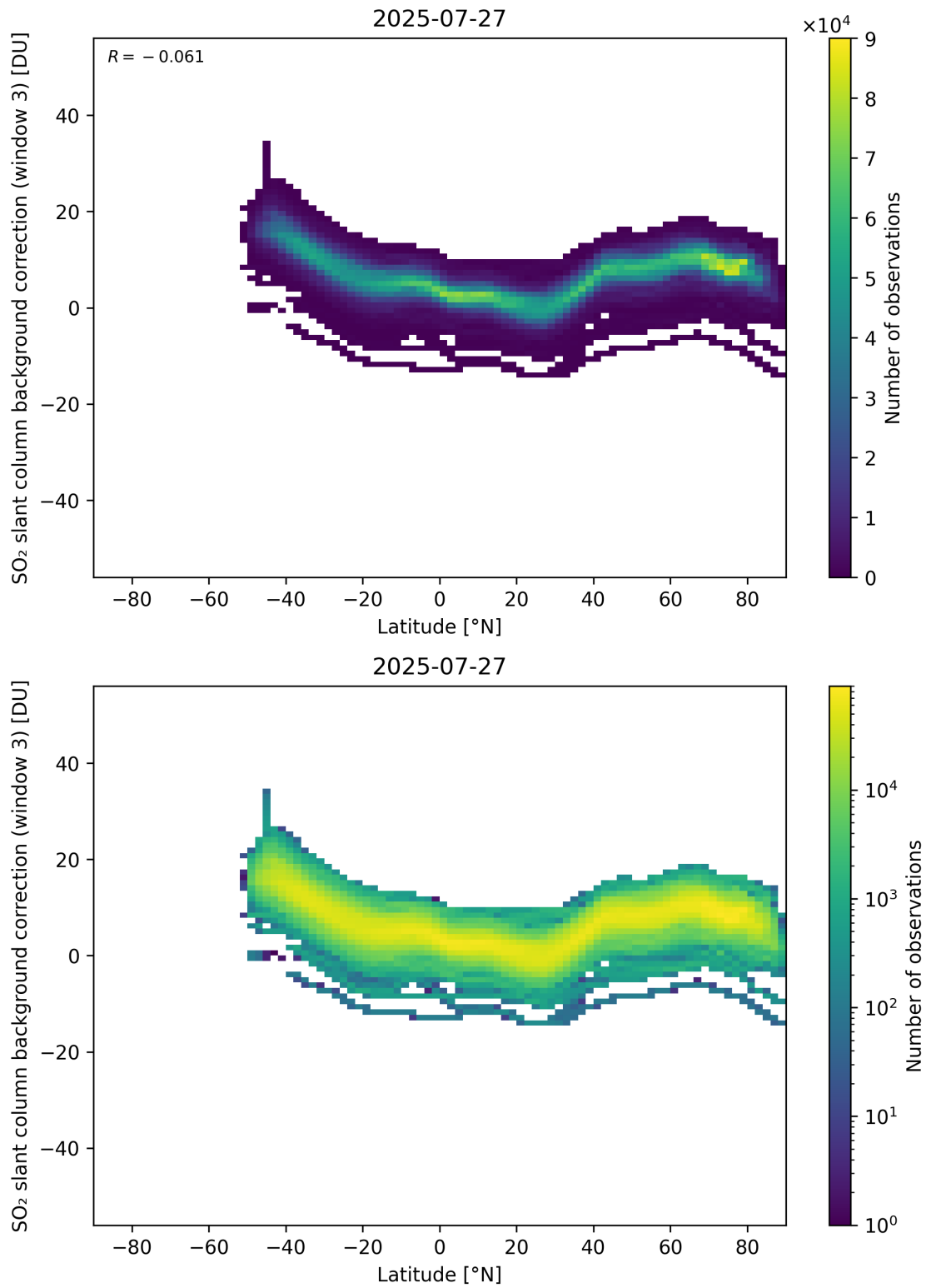
Figure 152: Scatter density plot of “Latitude” against “SO 2 slant column background correction (window 3)” for 2025-07-26 to 2025-07-28.
