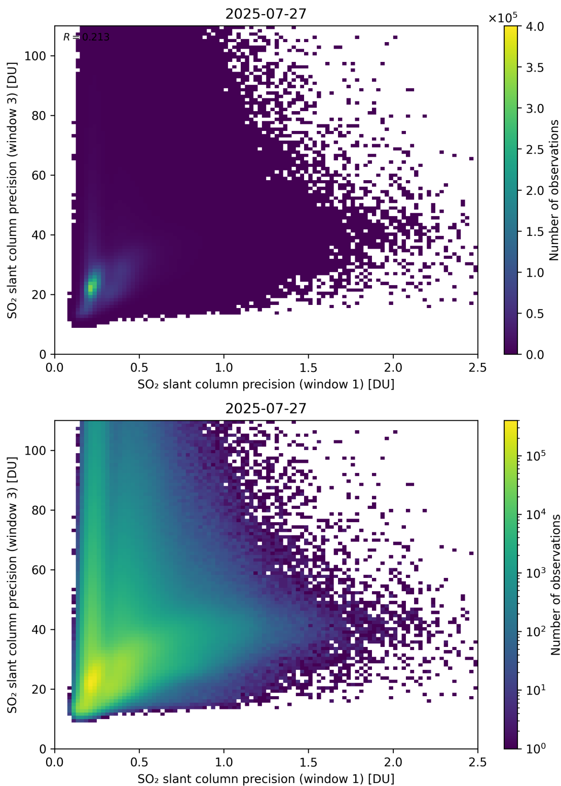
Figure 279: Scatter density plot of “SO 2 slant column precision (window 1)” against “SO 2 slant column precision (window 3)” for 2025-07-26 to 2025-07-28.
