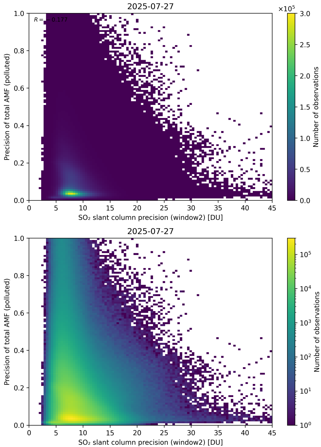
Figure 302: Scatter density plot of “SO 2 slant column precision (window2)” against “Precision of total AMF (polluted)” for 2025-07-26 to 2025-07-28.
