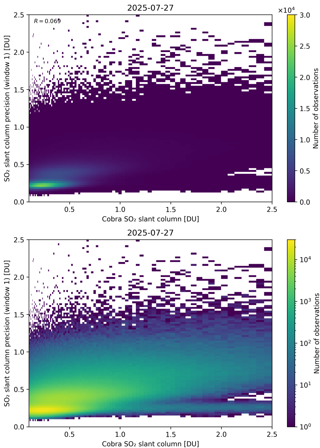
Figure 220: Scatter density plot of “Cobra SO 2 slant column” against “SO 2 slant column precision (window 1)” for 2025-07-26 to 2025-07-28.
