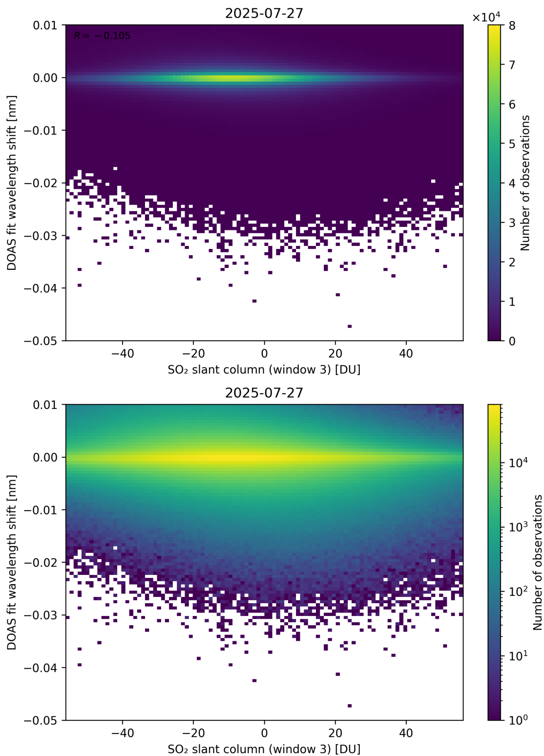
Figure 304: Scatter density plot of “SO 2 slant column (window 3)” against “DOAS fit wavelength shift” for 2025-07-26 to 2025-07-28.
