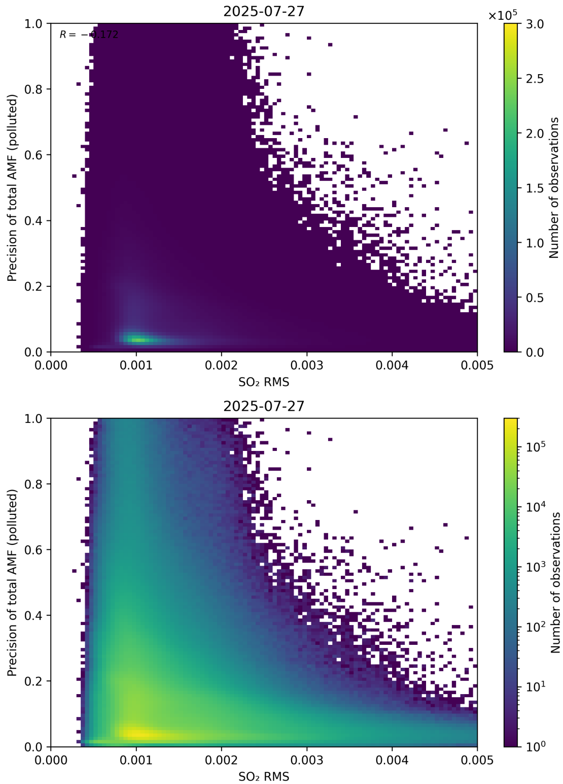
Figure 149: Scatter density plot of “SO 2 RMS” against “Precision of total AMF (polluted)” for 2025-07-26 to 2025-07-28.
