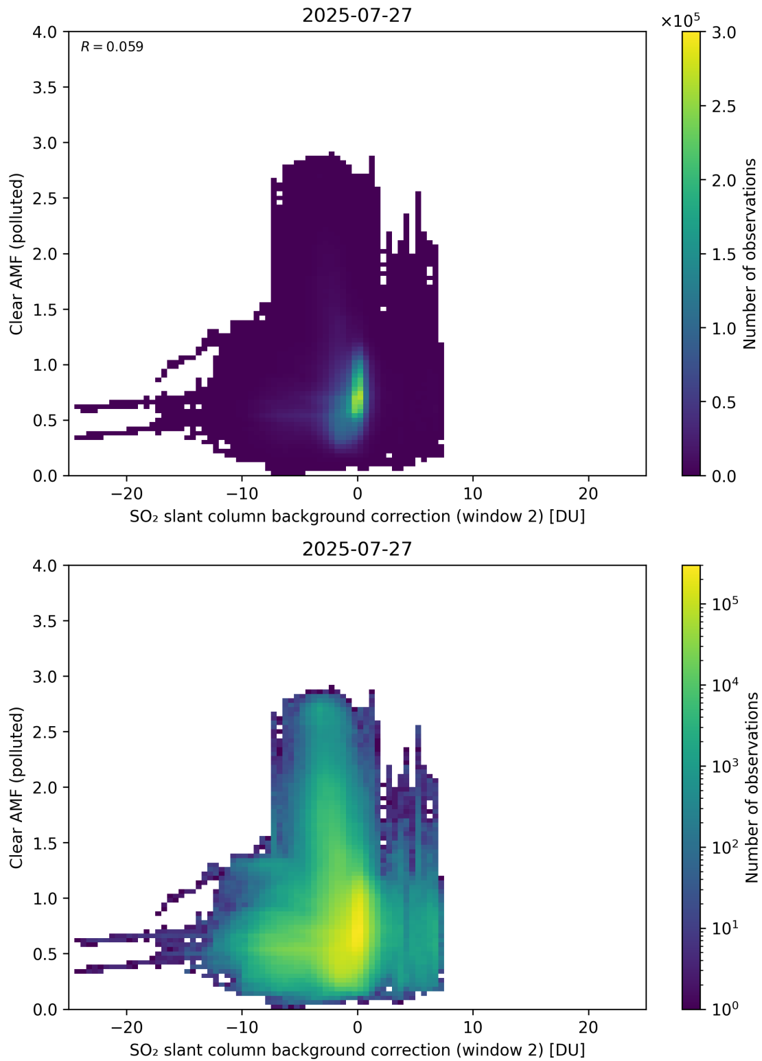
Figure 126: Scatter density plot of “SO 2 slant column background correction (window 2)” against “Clear AMF (polluted)” for 2025-07-26 to 2025-07-28.
