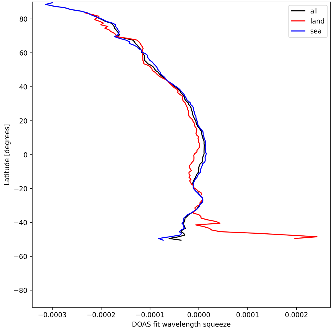
Figure 51: Zonal average of “DOAS fit wavelength squeeze” for 2025-07-26 to 2025-07-28.
