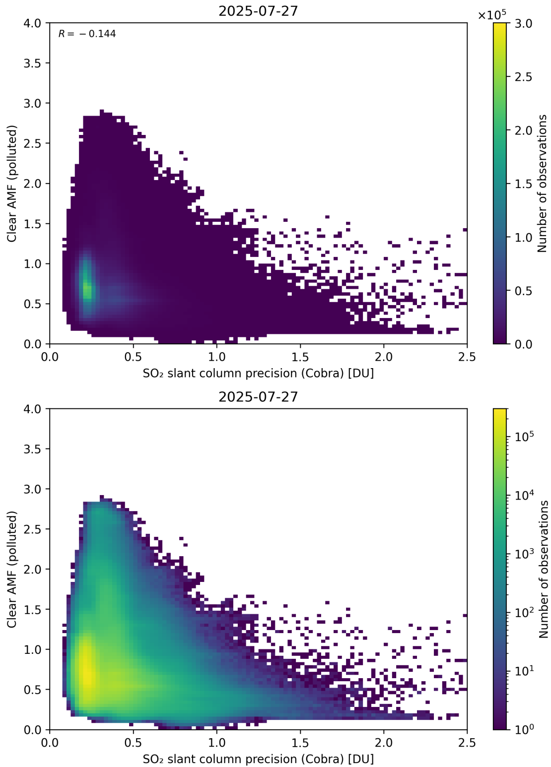
Figure 205: Scatter density plot of “SO 2 slant column precision (Cobra)” against “Clear AMF (polluted)” for 2025-07-26 to 2025-07-28.
