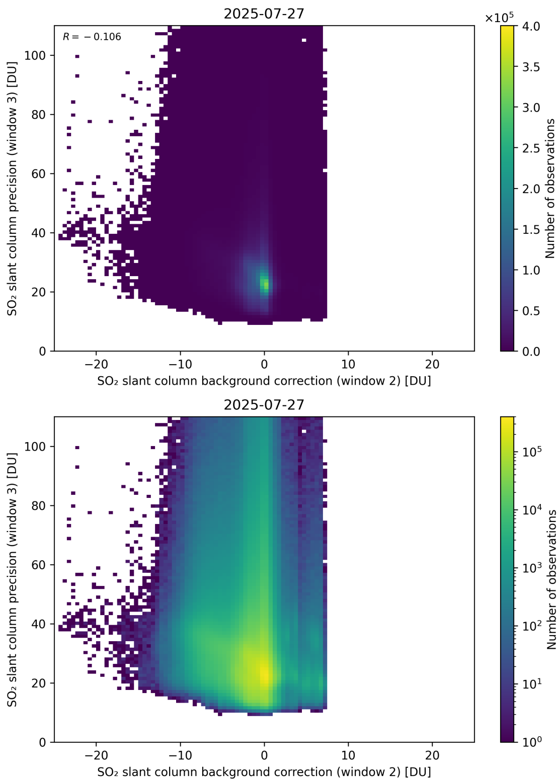
Figure 129: Scatter density plot of “SO 2 slant column background correction (window 2)” against “SO 2 slant column precision (window 3)” for 2025-07-26 to 2025-07-28.
