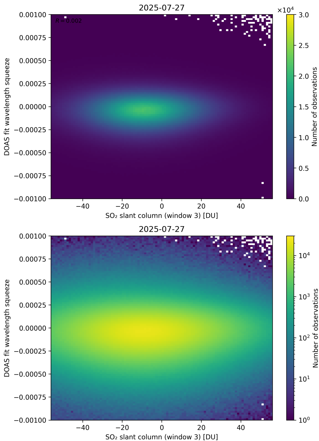
Figure 305: Scatter density plot of “SO 2 slant column (window 3)” against “DOAS fit wavelength squeeze” for 2025-07-26 to 2025-07-28.
