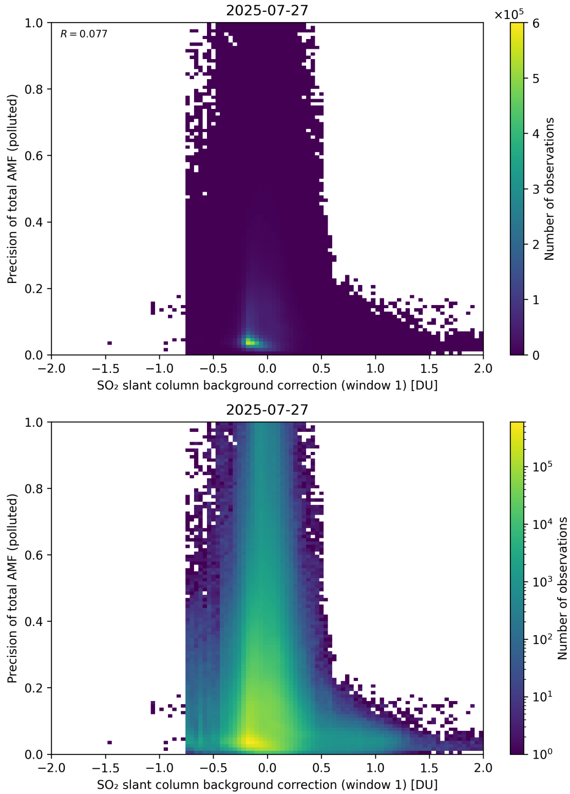
Figure 121: Scatter density plot of “SO 2 slant column background correction (window 1)” against “Precision of total AMF (polluted)” for 2025-07-26 to 2025-07-28.
