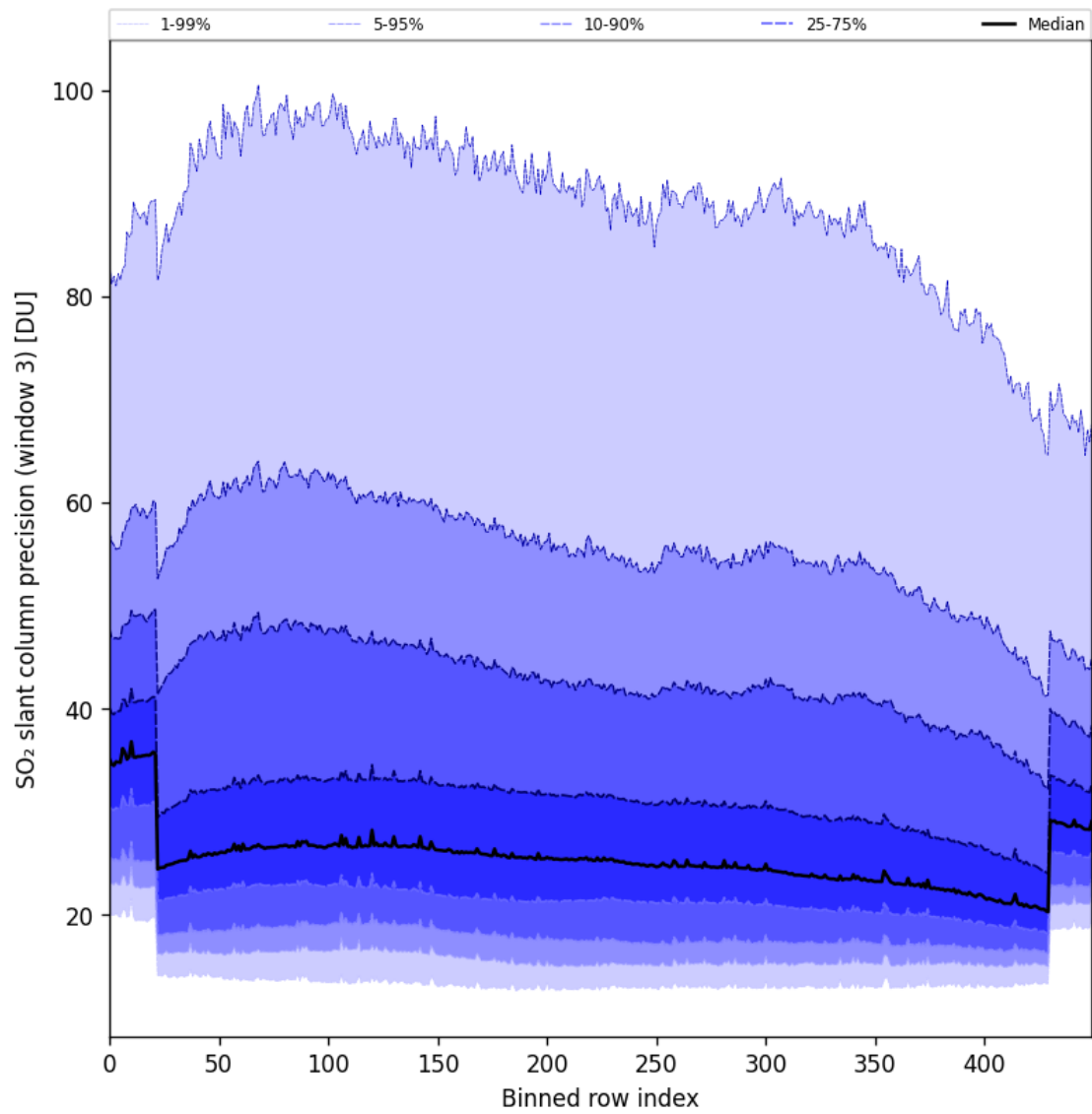
Figure 98: Along track statistics of “SO 2 slant column precision (window 3)” for 2025-07-26 to 2025-07-28
