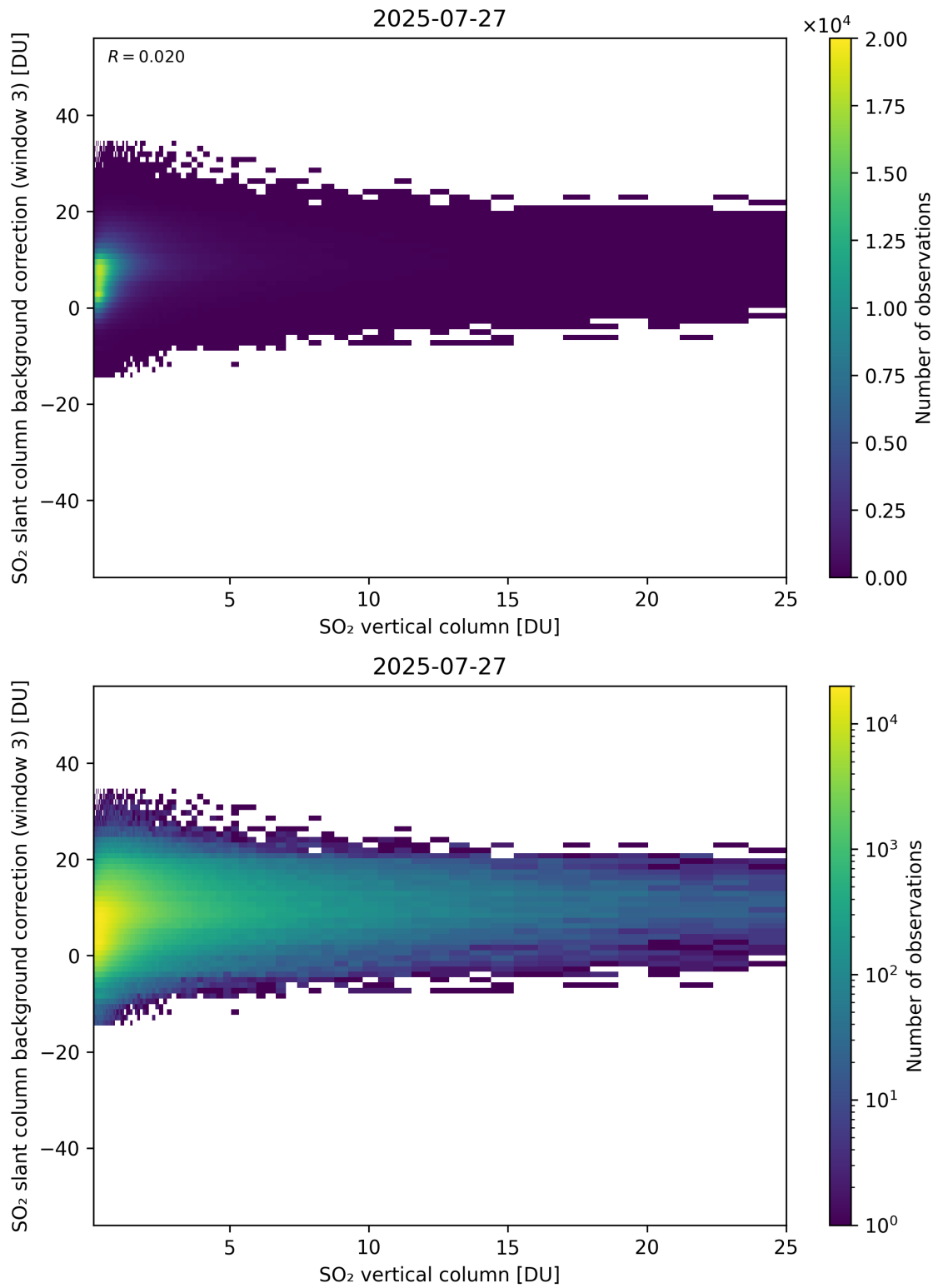
Figure 325: Scatter density plot of “SO 2 vertical column” against “SO 2 slant column background correction (window 3)” for 2025-07-26 to 2025-07-28.
