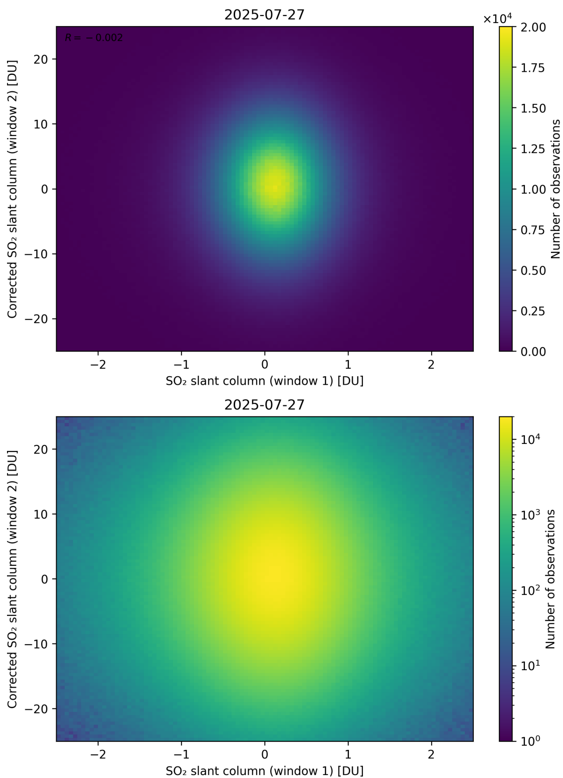
Figure 283: Scatter density plot of “SO 2 slant column (window 1)” against “Corrected SO 2 slant column (window 2)” for 2025-07-26 to 2025-07-28.
