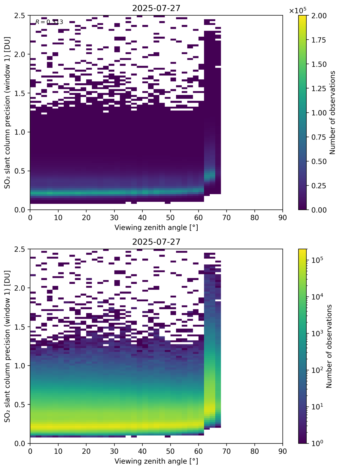
Figure 377: Scatter density plot of “Viewing zenith angle” against “SO 2 slant column precision (window 1)” for 2025-07-26 to 2025-07-28.
