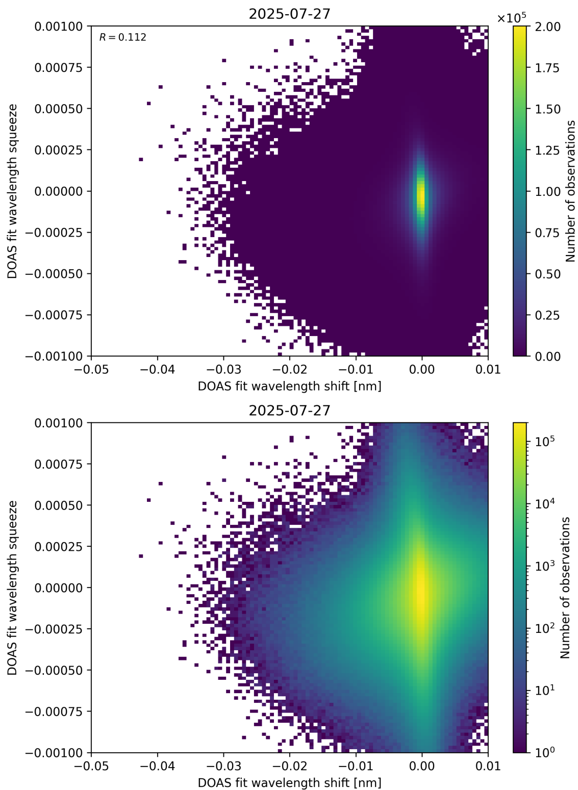
Figure 138: Scatter density plot of “DOAS fit wavelength shift” against “DOAS fit wavelength squeeze” for 2025-07-26 to 2025-07-28.
