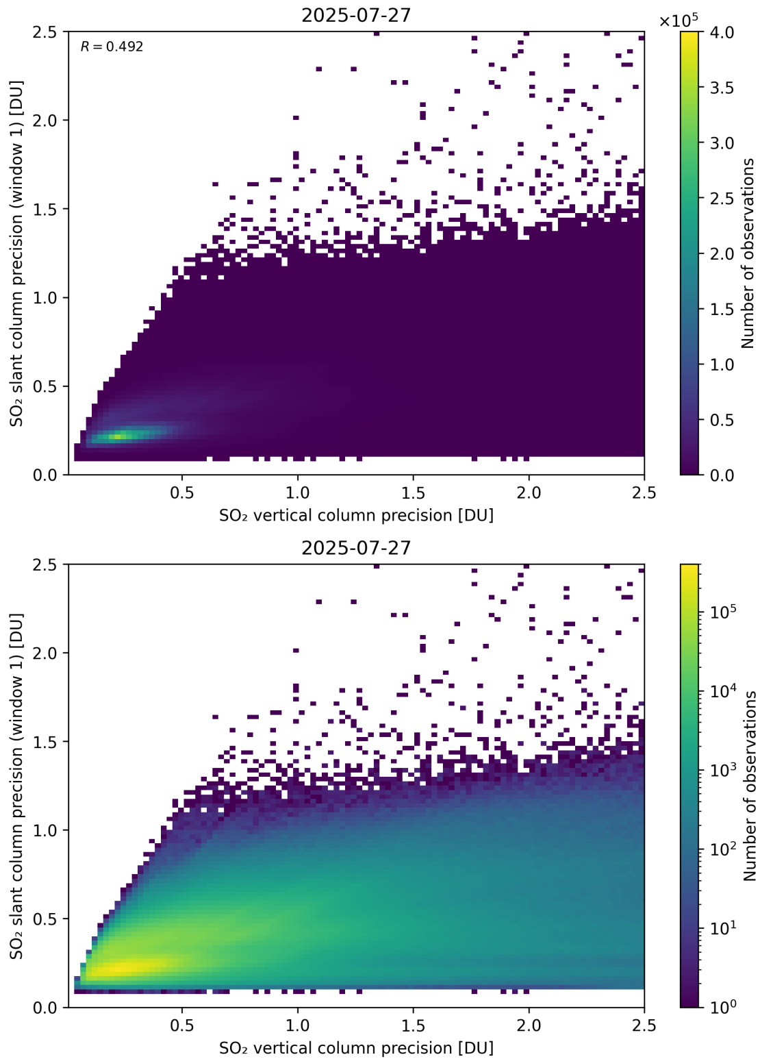
Figure 342: Scatter density plot of “SO 2 vertical column precision” against “SO 2 slant column precision (window 1)” for 2025-07-26 to 2025-07-28.
