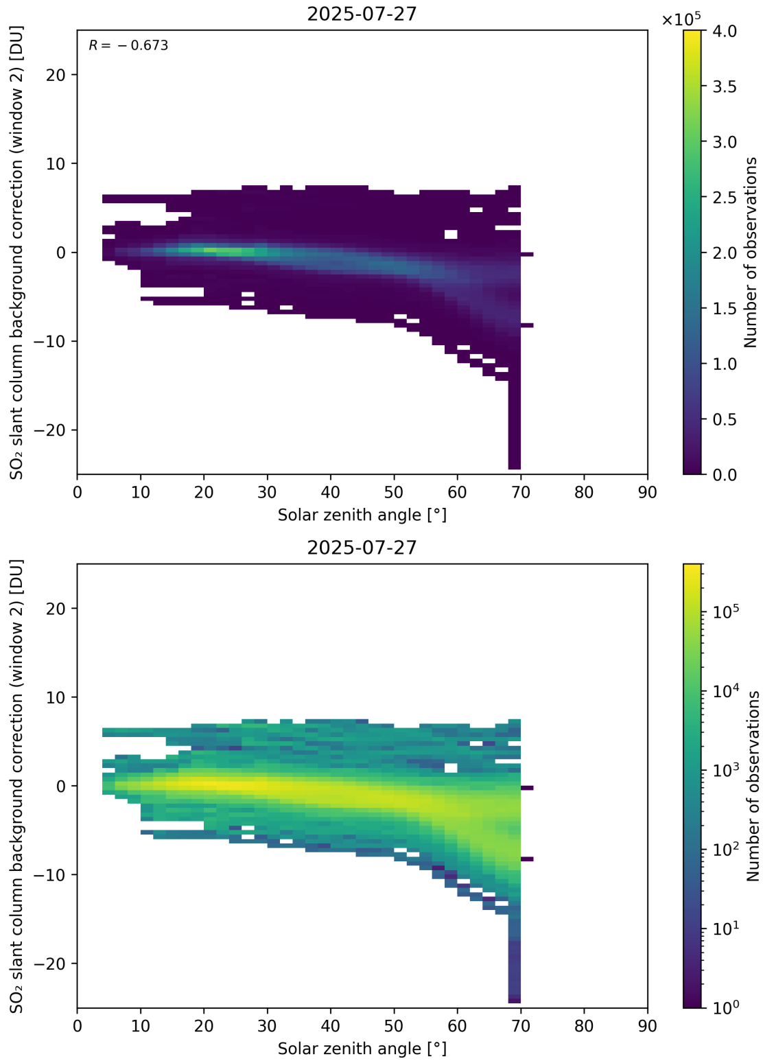
Figure 172: Scatter density plot of “Solar zenith angle” against “SO 2 slant column background correction (window 2)” for 2025-07-26 to 2025-07-28.
