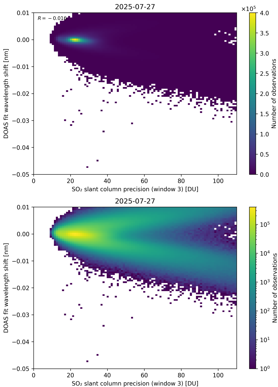
Figure 308: Scatter density plot of “SO 2 slant column precision (window 3)” against “DOAS fit wavelength shift” for 2025-07-26 to 2025-07-28.
