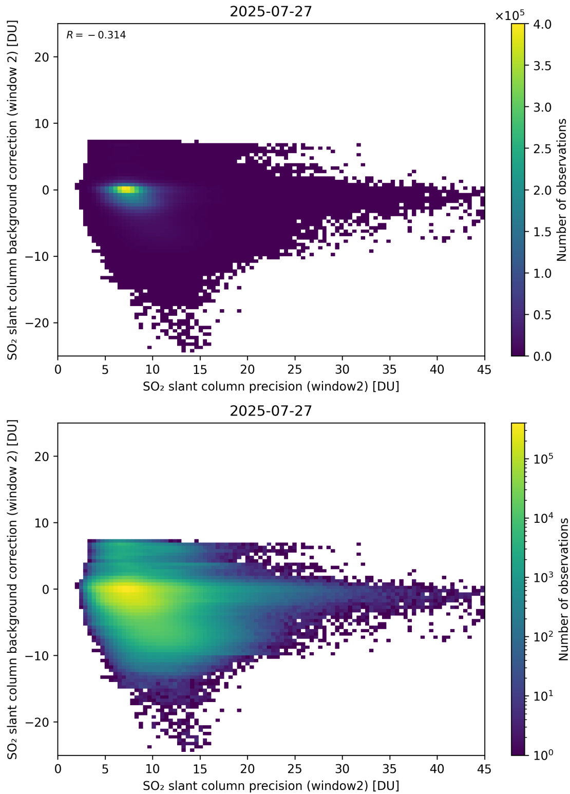
Figure 291: Scatter density plot of “SO 2 slant column precision (window2)” against “SO 2 slant column background correction (window 2)” for 2025-07-26 to 2025-07-28.
