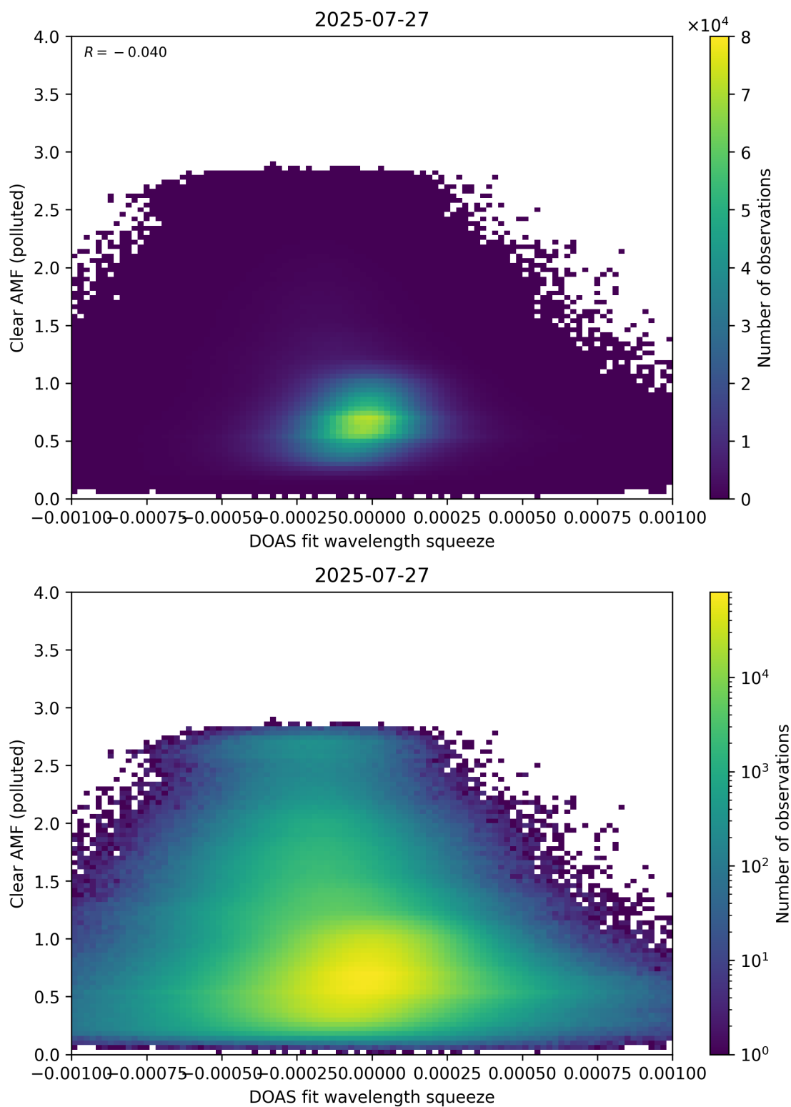
Figure 144: Scatter density plot of “DOAS fit wavelength squeeze” against “Clear AMF (polluted)” for 2025-07-26 to 2025-07-28.
