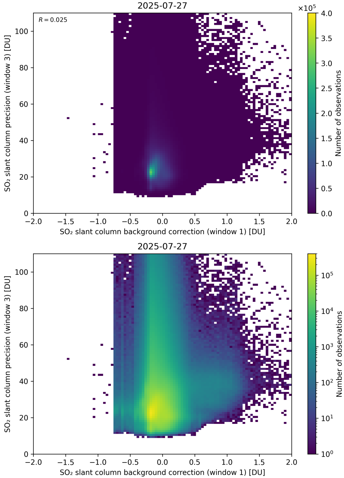
Figure 119: Scatter density plot of “SO 2 slant column background correction (window 1)” against “SO 2 slant column precision (window 3)” for 2025-07-26 to 2025-07-28.
