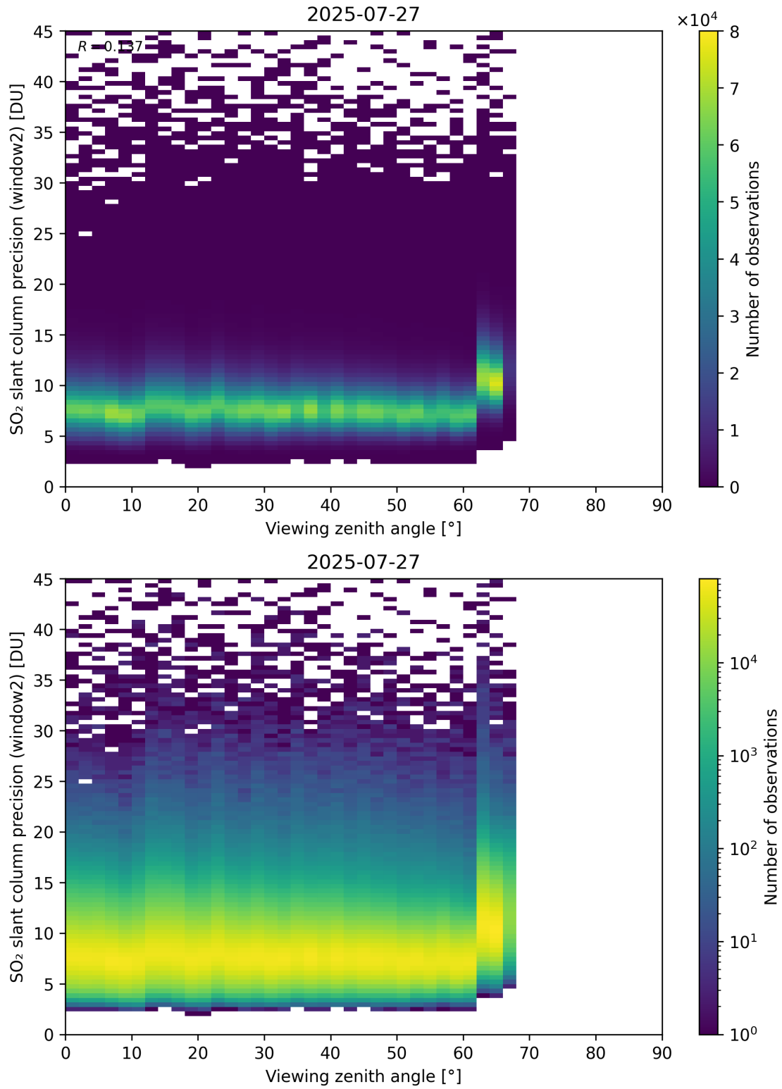
Figure 378: Scatter density plot of “Viewing zenith angle” against “SO 2 slant column precision (window2)” for 2025-07-26 to 2025-07-28.
