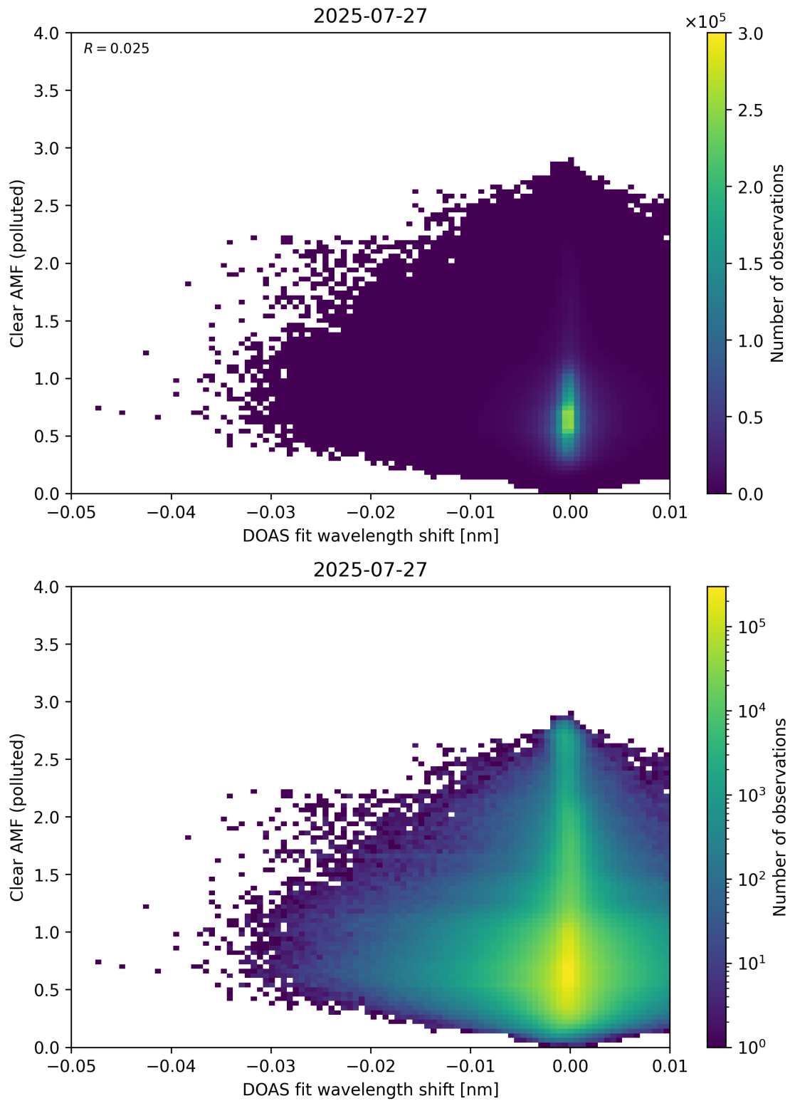
Figure 140: Scatter density plot of “DOAS fit wavelength shift” against “Clear AMF (polluted)” for 2025-07-26 to 2025-07-28.
