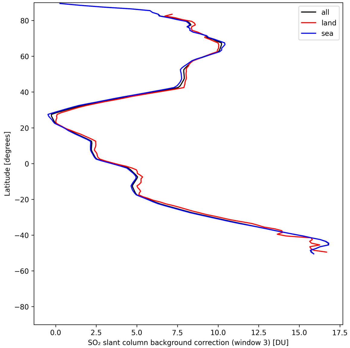
Figure 48: Zonal average of “SO 2 slant column background correction (window 3)” for 2025-07-26 to 2025-07-28.
