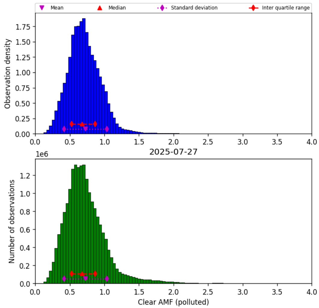
Figure 81: Histogram of “Clear AMF (polluted)” for 2025-07-26 to 2025-07-28
