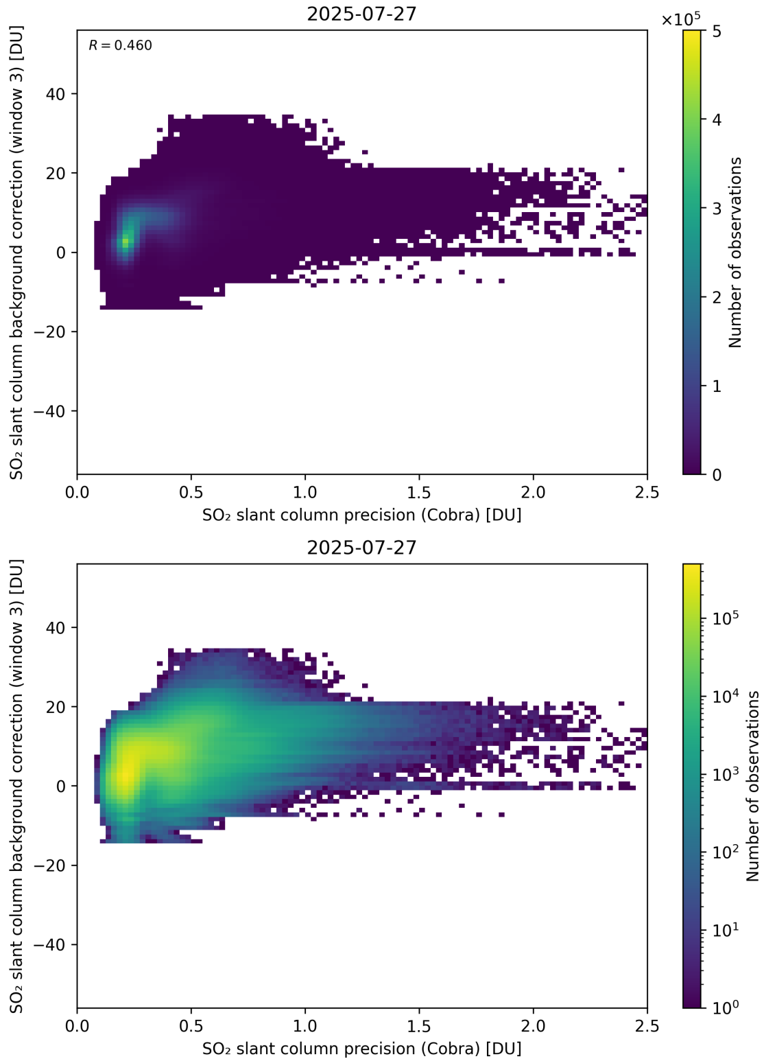
Figure 201: Scatter density plot of “SO 2 slant column precision (Cobra)” against “SO 2 slant column background correction (window 3)” for 2025-07-26 to 2025-07-28.
