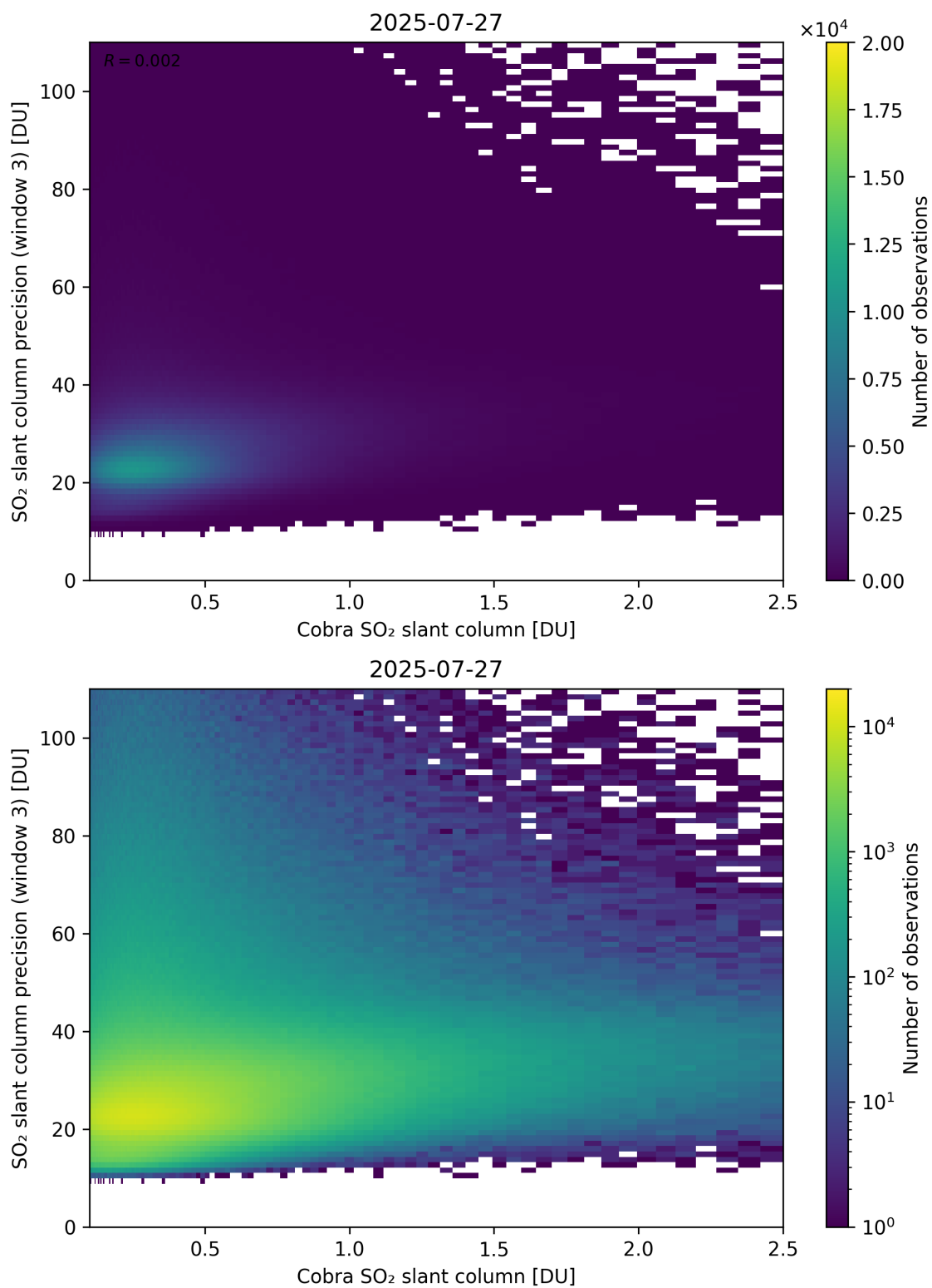
Figure 223: Scatter density plot of “Cobra SO 2 slant column” against “SO 2 slant column precision (window 3)” for 2025-07-26 to 2025-07-28.
