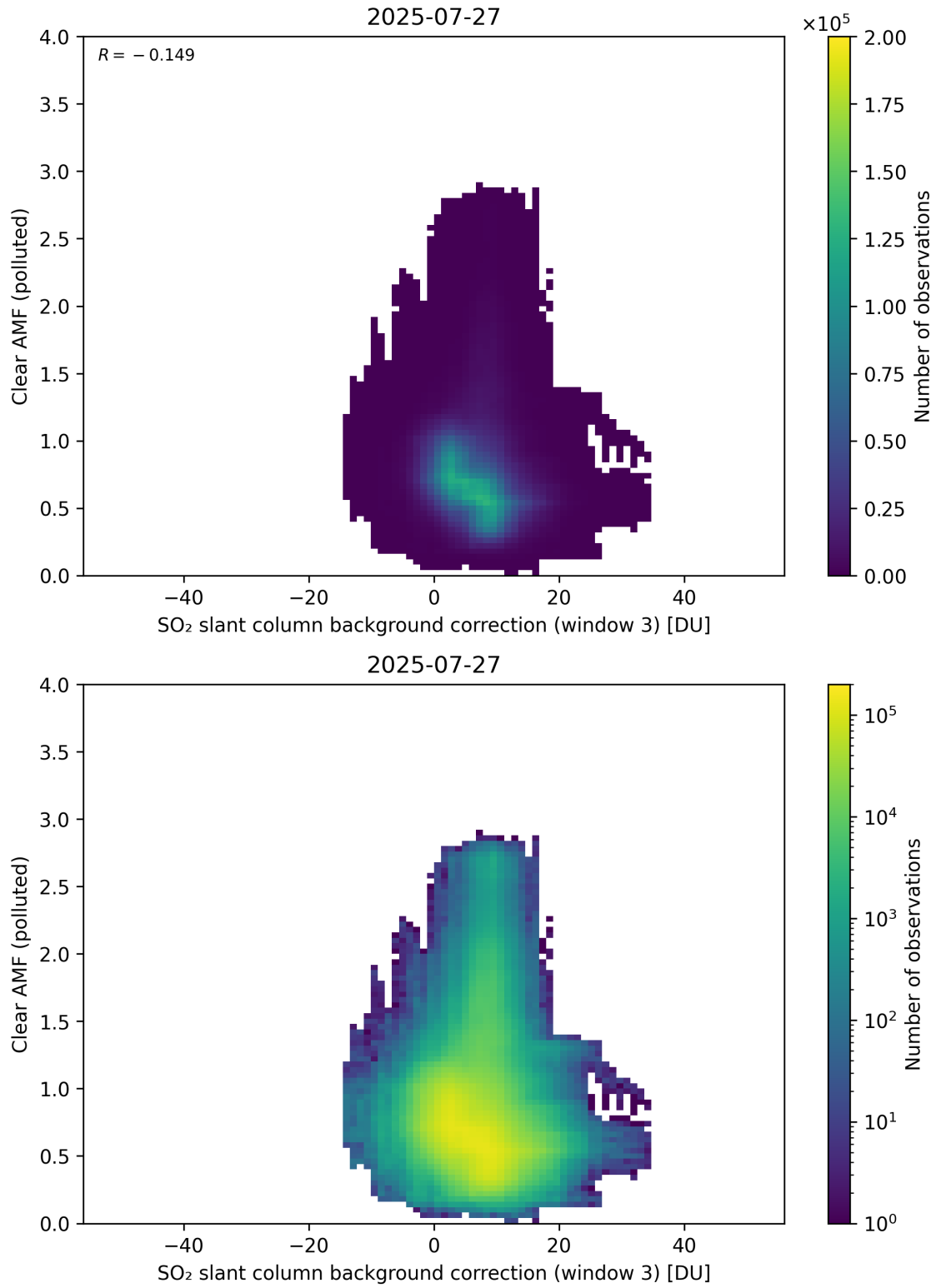
Figure 135: Scatter density plot of “SO 2 slant column background correction (window 3)” against “Clear AMF (polluted)” for 2025-07-26 to 2025-07-28.
