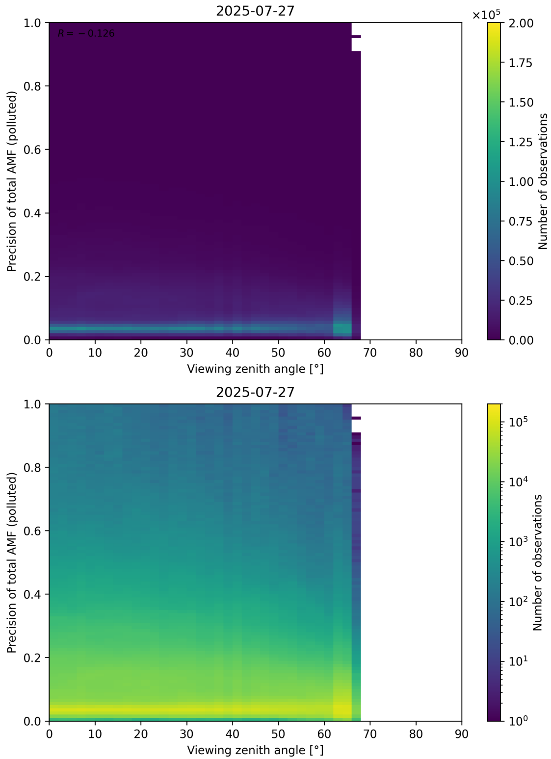
Figure 382: Scatter density plot of “Viewing zenith angle” against “Precision of total AMF (polluted)” for 2025-07-26 to 2025-07-28.
