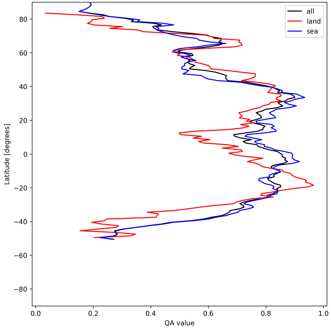
Figure 31: Zonal average of “QA value” for 2025-07-26 to 2025-07-28.
