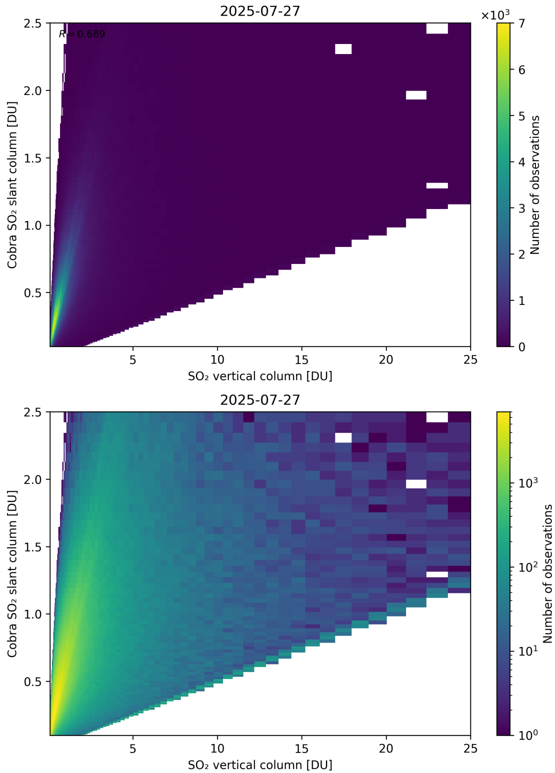
Figure 349: Scatter density plot of “SO 2 vertical column” against “Cobra SO 2 slant column” for 2025-07-26 to 2025-07-28.
