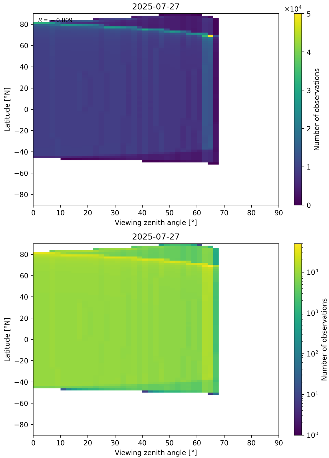
Figure 368: Scatter density plot of “Viewing zenith angle” against “Latitude” for 2025-07-26 to 2025-07-28.
