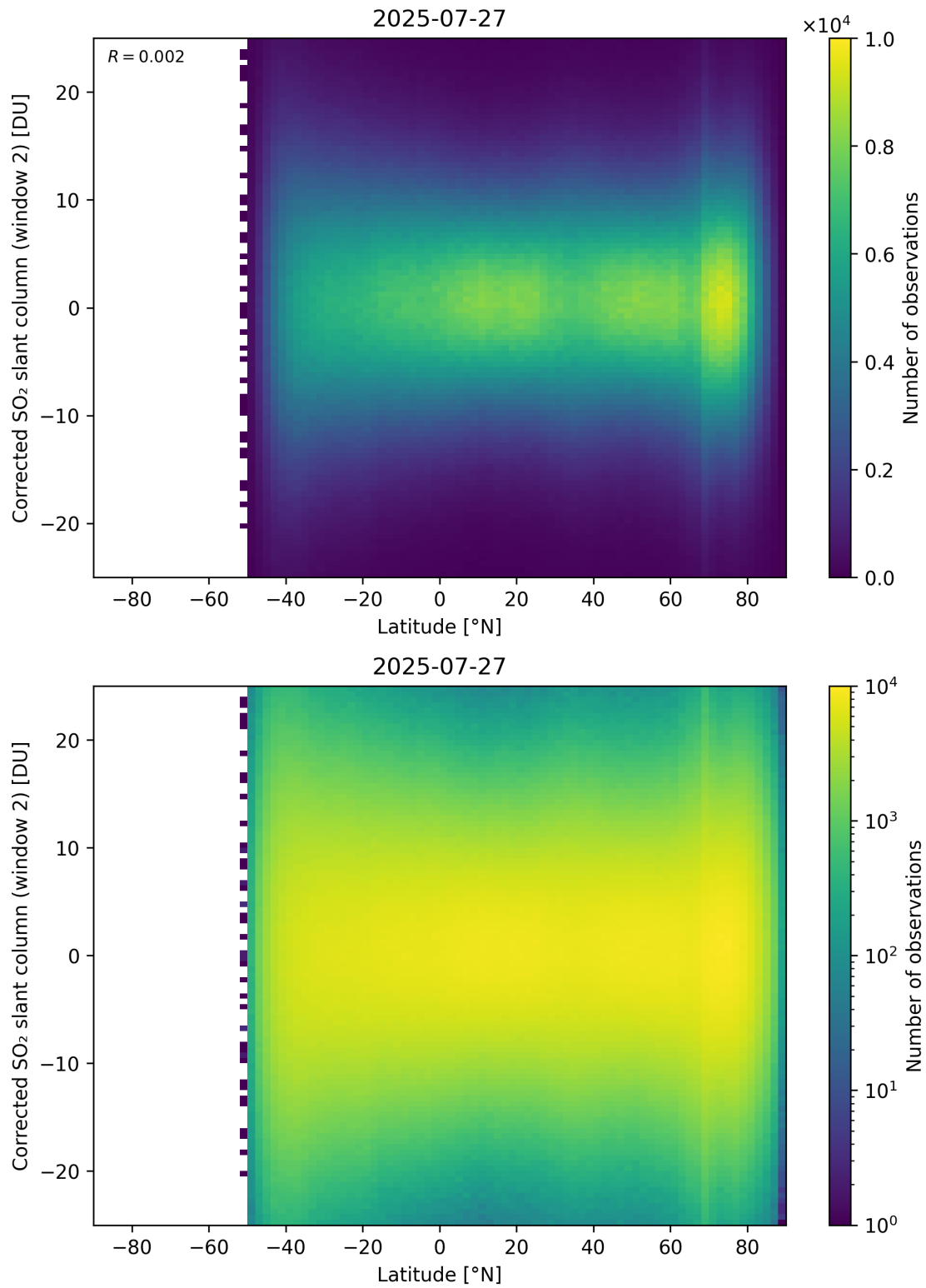
Figure 160: Scatter density plot of “Latitude” against “Corrected SO 2 slant column (window 2)” for 2025-07-26 to 2025-07-28.
