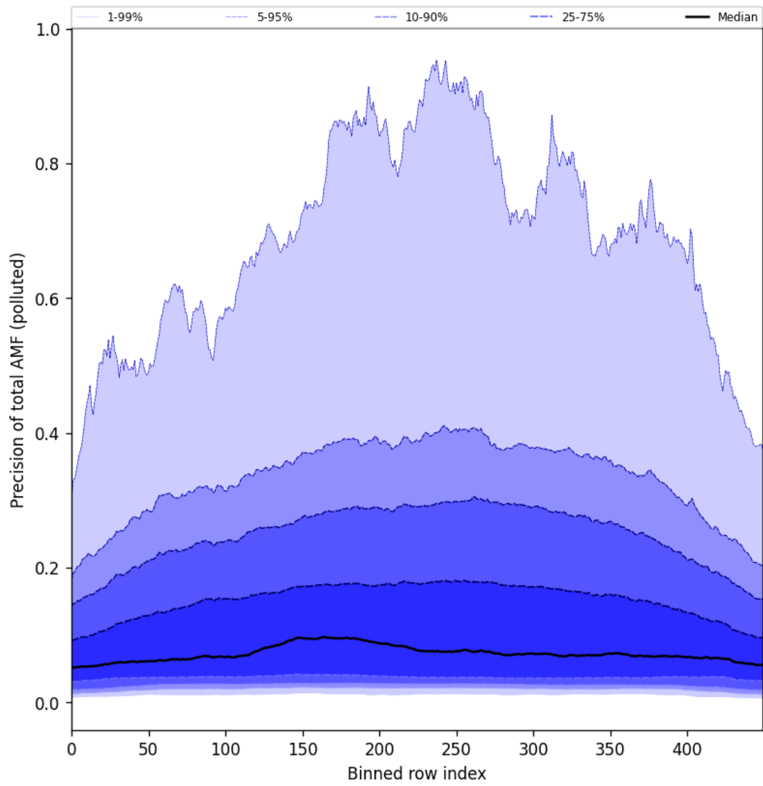
Figure 106: Along track statistics of “Precision of total AMF (polluted)” for 2025-07-26 to 2025-07-28
