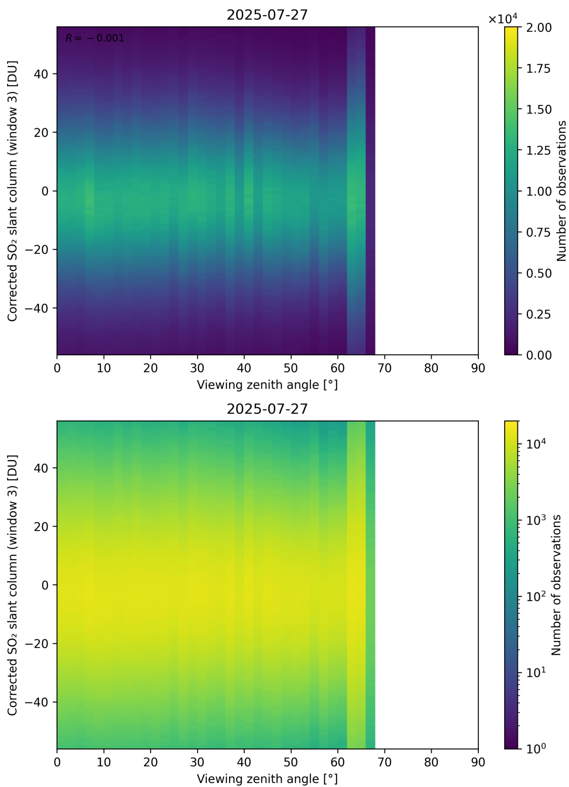
Figure 375: Scatter density plot of “Viewing zenith angle” against “Corrected SO 2 slant column (window 3)” for 2025-07-26 to 2025-07-28.
