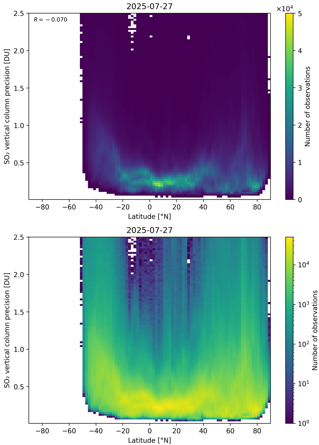
Figure 170: Scatter density plot of “Latitude” against “SO 2 vertical column precision” for 2025-07-26 to 2025-07-28.
