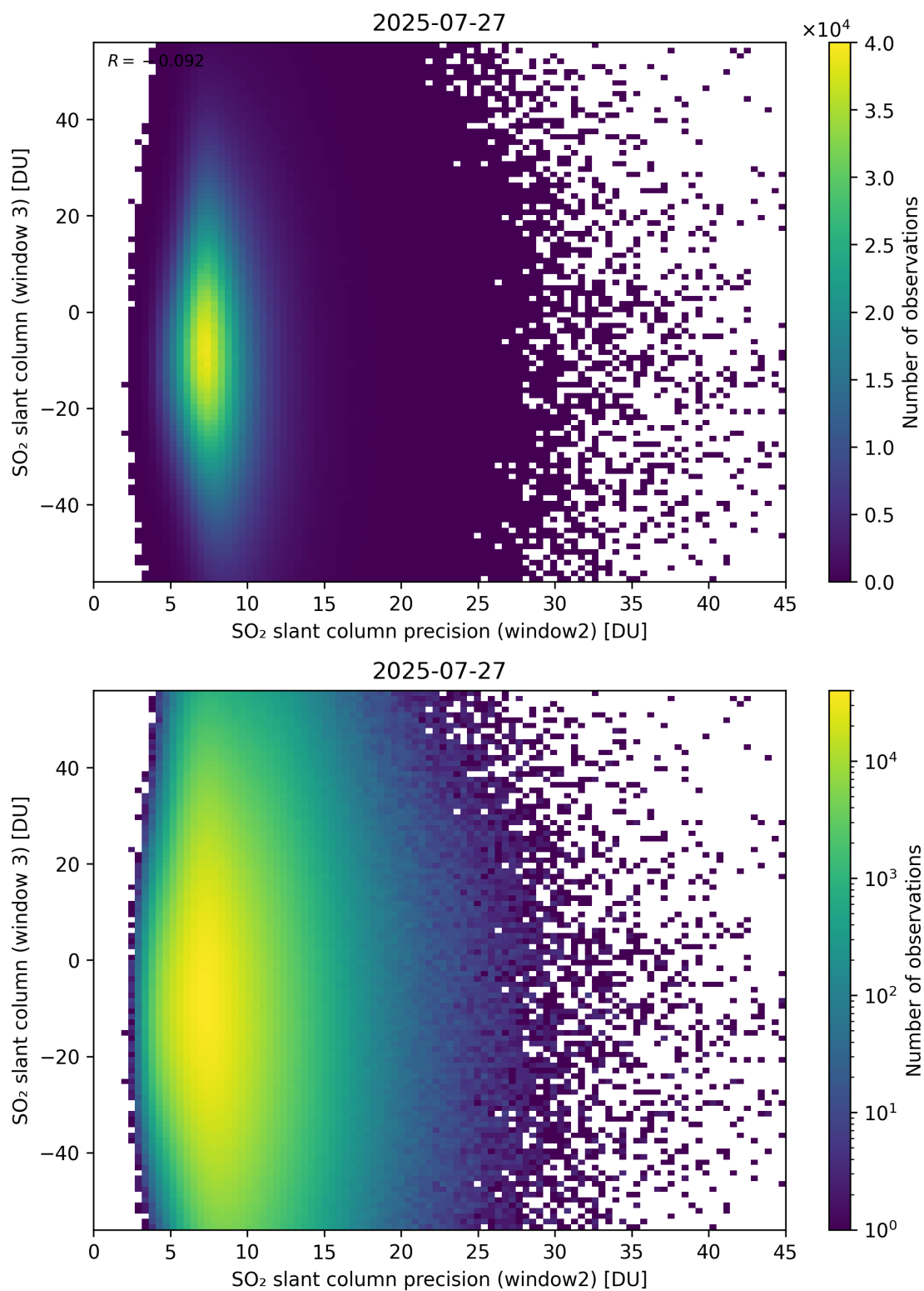
Figure 299: Scatter density plot of “SO 2 slant column precision (window2)” against “SO 2 slant column (window 3)” for 2025-07-26 to 2025-07-28.
