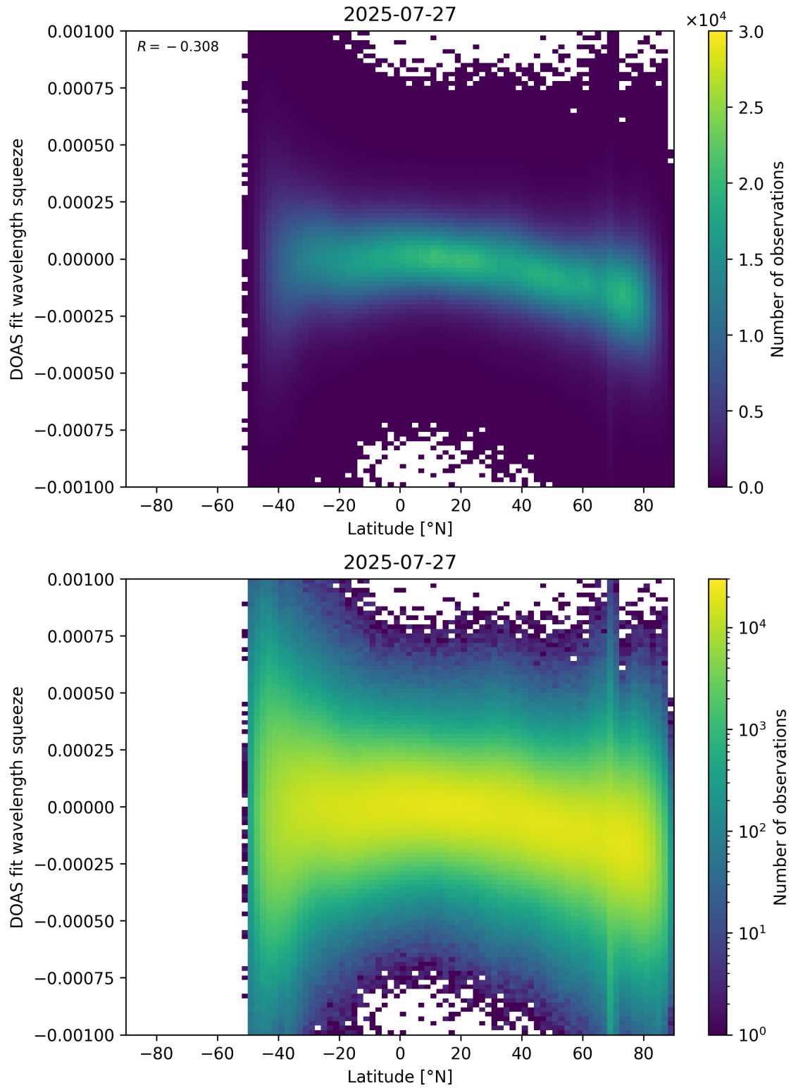
Figure 154: Scatter density plot of “Latitude” against “DOAS fit wavelength squeeze” for 2025-07-26 to 2025-07-28.
