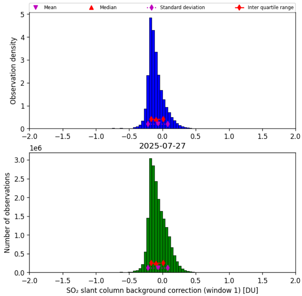
Figure 66: Histogram of “SO 2 slant column background correction (window 1)” for 2025-07-26 to 2025-07-28
