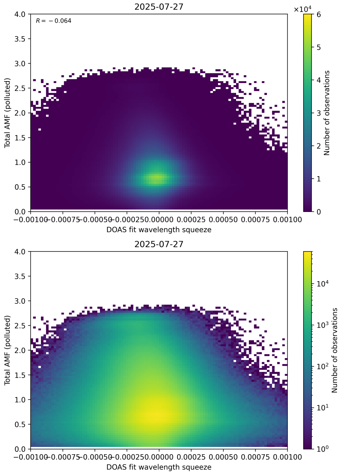
Figure 145: Scatter density plot of “DOAS fit wavelength squeeze” against “Total AMF (polluted)” for 2025-07-26 to 2025-07-28.
