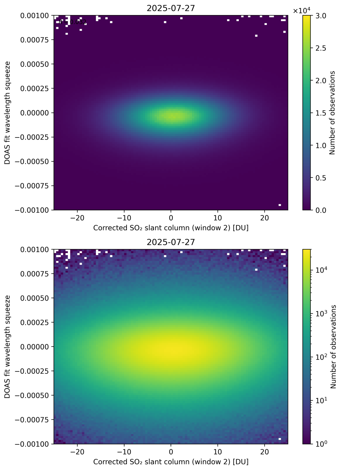
Figure 247: Scatter density plot of “Corrected SO 2 slant column (window 2)” against “DOAS fit wavelength squeeze” for 2025-07-26 to 2025-07-28.
