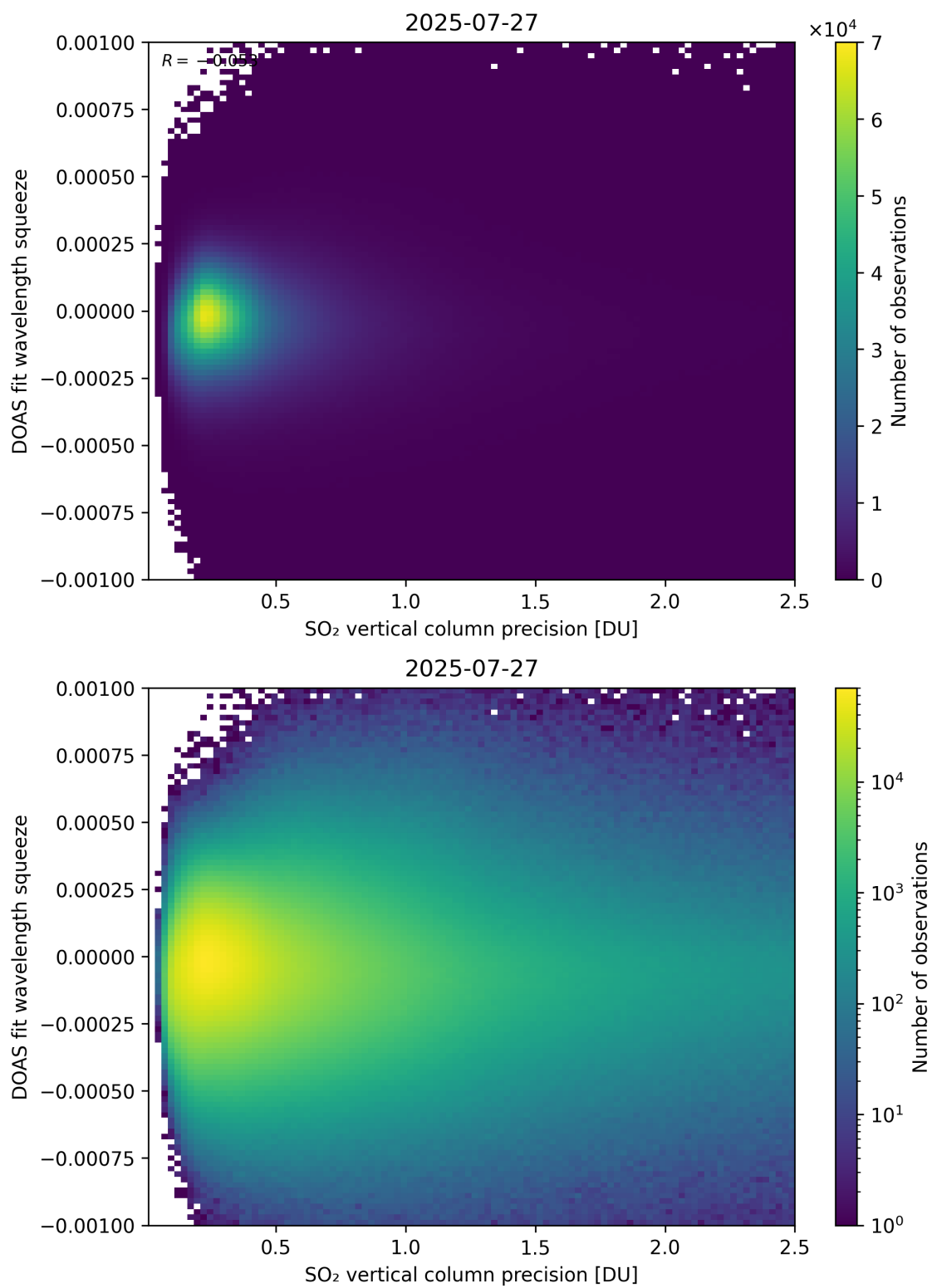
Figure 333: Scatter density plot of “SO 2 vertical column precision” against “DOAS fit wavelength squeeze” for 2025-07-26 to 2025-07-28.
