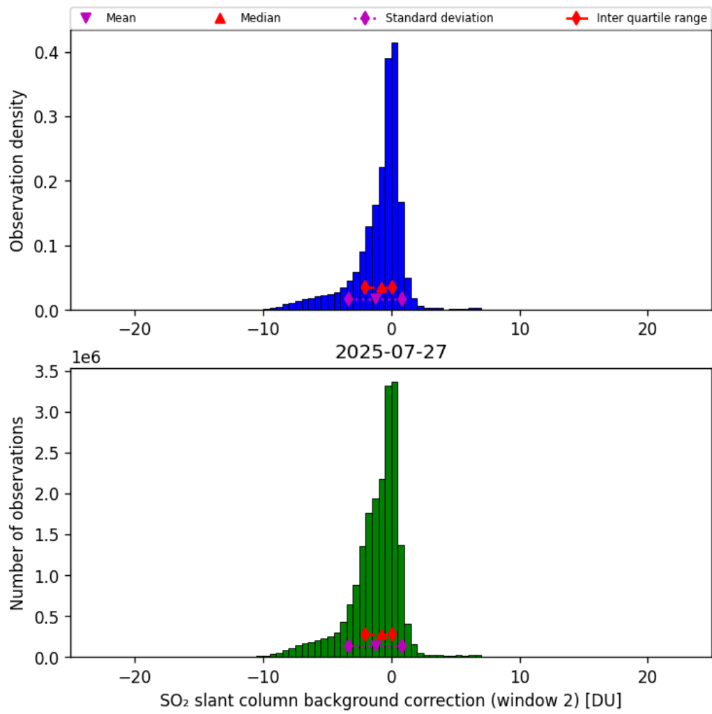
Figure 70: Histogram of “SO 2 slant column background correction (window 2)” for 2025-07-26 to 2025-07-28
