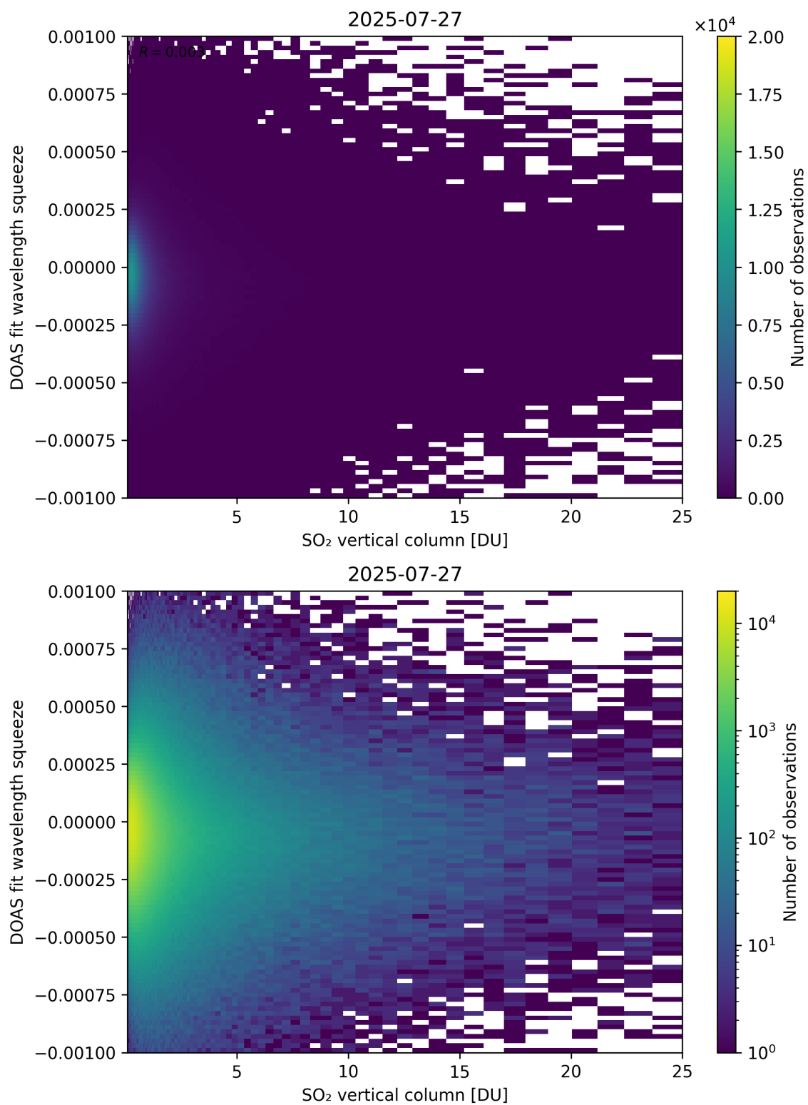
Figure 327: Scatter density plot of “SO 2 vertical column” against “DOAS fit wavelength squeeze” for 2025-07-26 to 2025-07-28.
