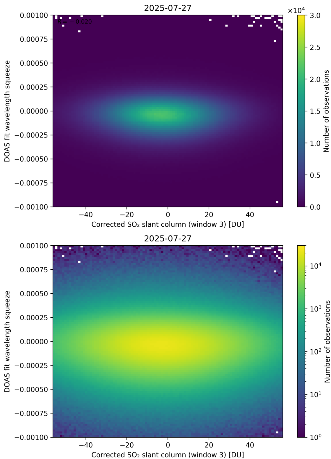
Figure 257: Scatter density plot of “Corrected SO 2 slant column (window 3)” against “DOAS fit wavelength squeeze” for 2025-07-26 to 2025-07-28.
