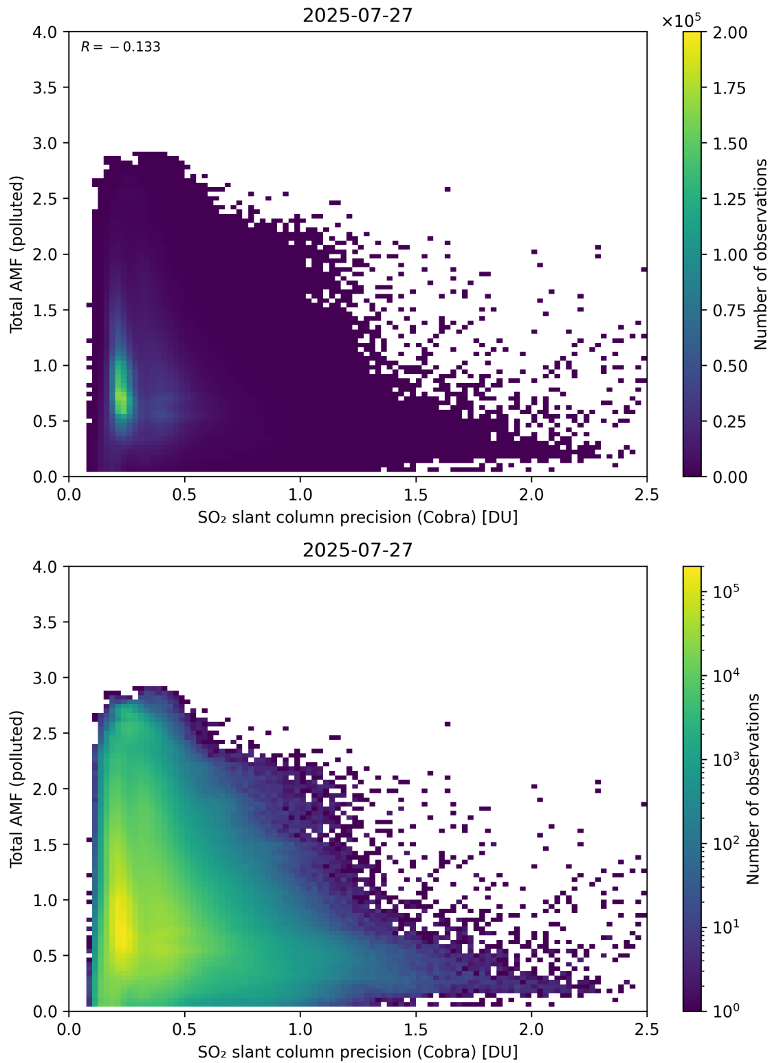
Figure 213: Scatter density plot of “SO 2 slant column precision (Cobra)” against “Total AMF (polluted)” for 2025-07-26 to 2025-07-28.
