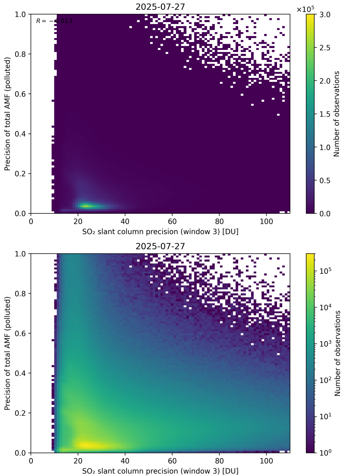
Figure 314: Scatter density plot of “SO 2 slant column precision (window 3)” against “Precision of total AMF (polluted)” for 2025-07-26 to 2025-07-28.
