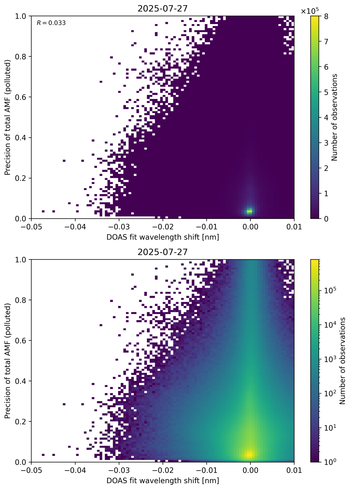
Figure 142: Scatter density plot of “DOAS fit wavelength shift” against “Precision of total AMF (polluted)” for 2025-07-26 to 2025-07-28.
