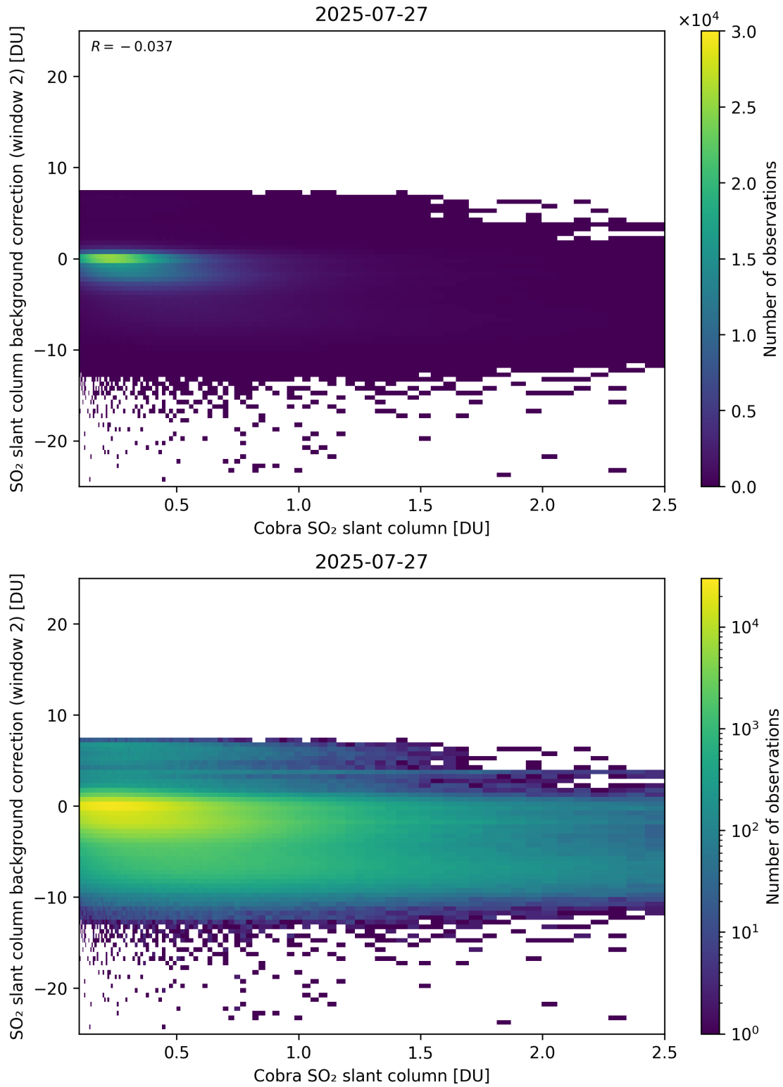
Figure 194: Scatter density plot of “Cobra SO 2 slant column” against “SO 2 slant column background correction (window 2)” for 2025-07-26 to 2025-07-28.
