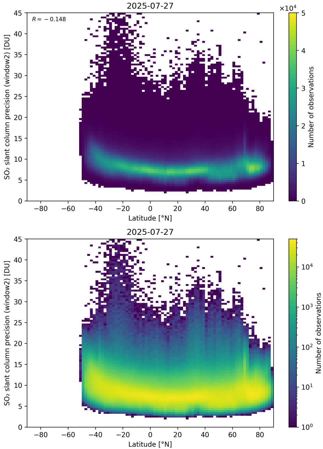
Figure 164: Scatter density plot of “Latitude” against “SO 2 slant column precision (window2)” for 2025-07-26 to 2025-07-28.
