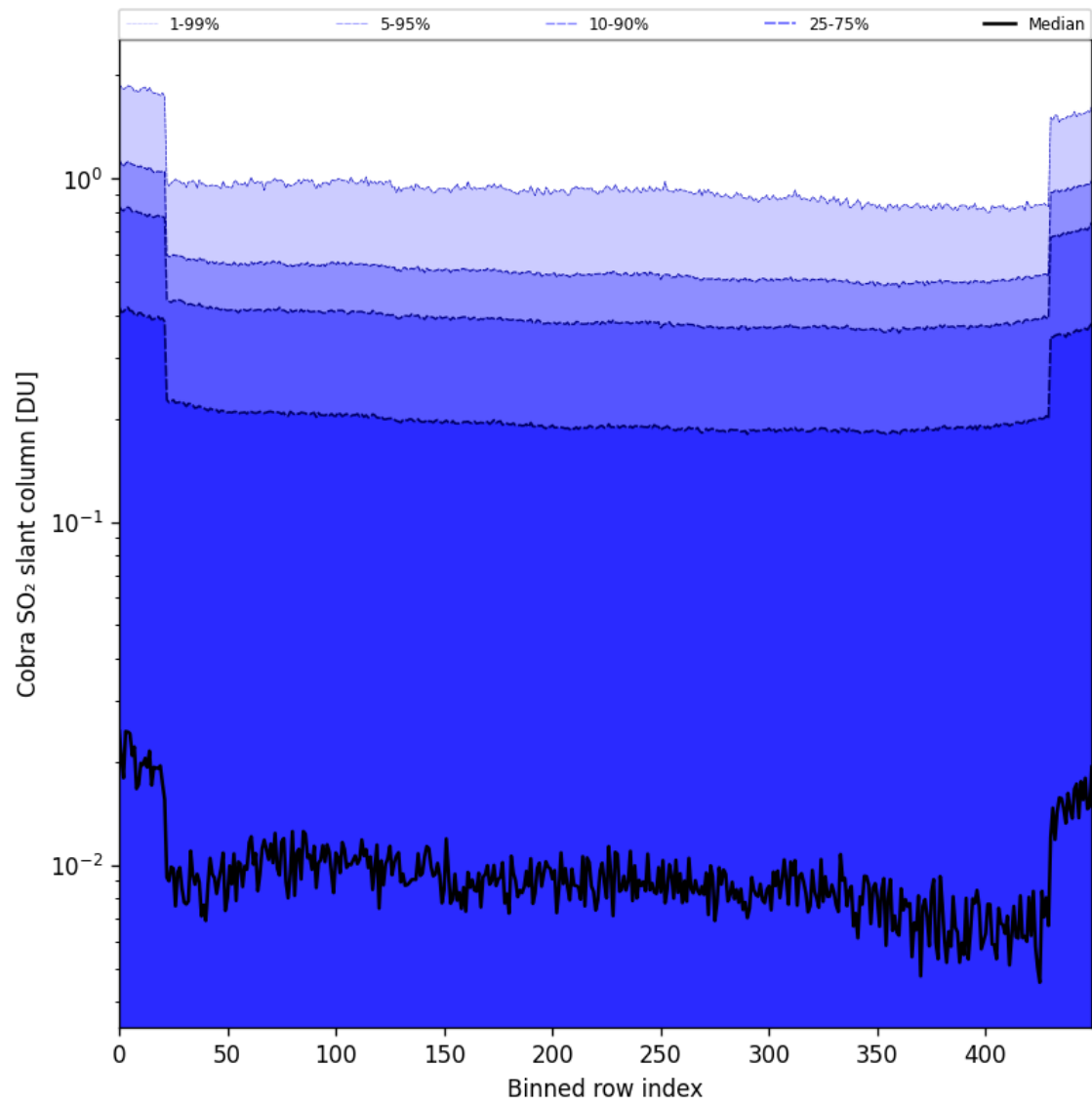
Figure 87: Along track statistics of “Cobra SO 2 slant column” for 2025-07-26 to 2025-07-28
