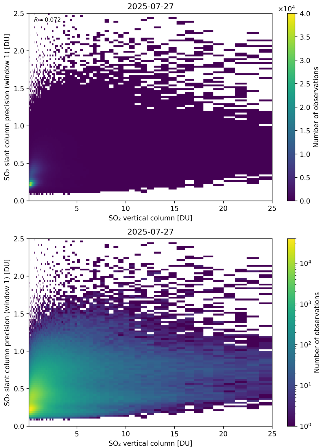
Figure 355: Scatter density plot of “SO 2 vertical column” against “SO 2 slant column precision (window 1)” for 2025-07-26 to 2025-07-28.
