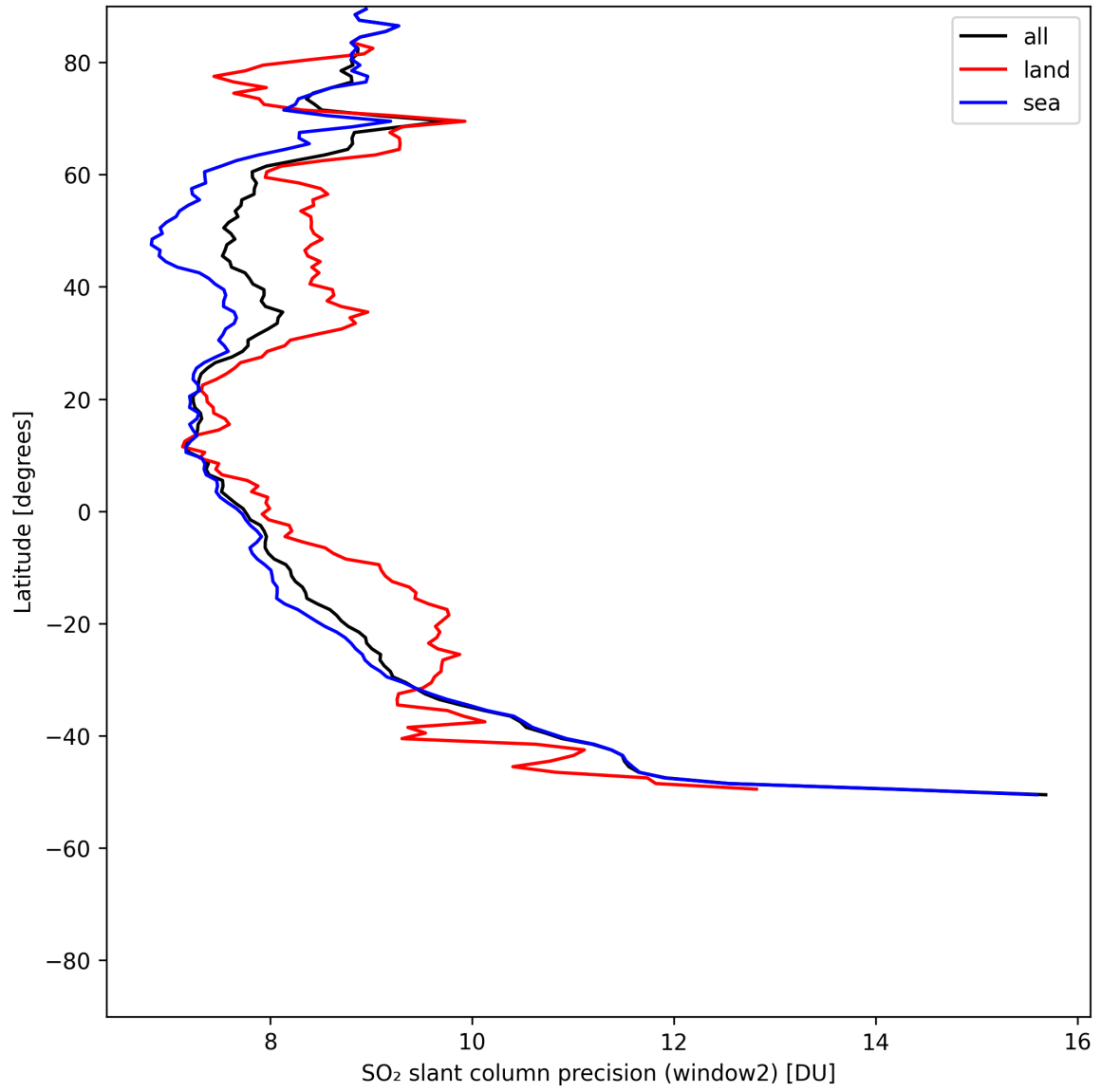
Figure 42: Zonal average of “SO 2 slant column precision (window2)” for 2025-07-26 to 2025-07-28.
