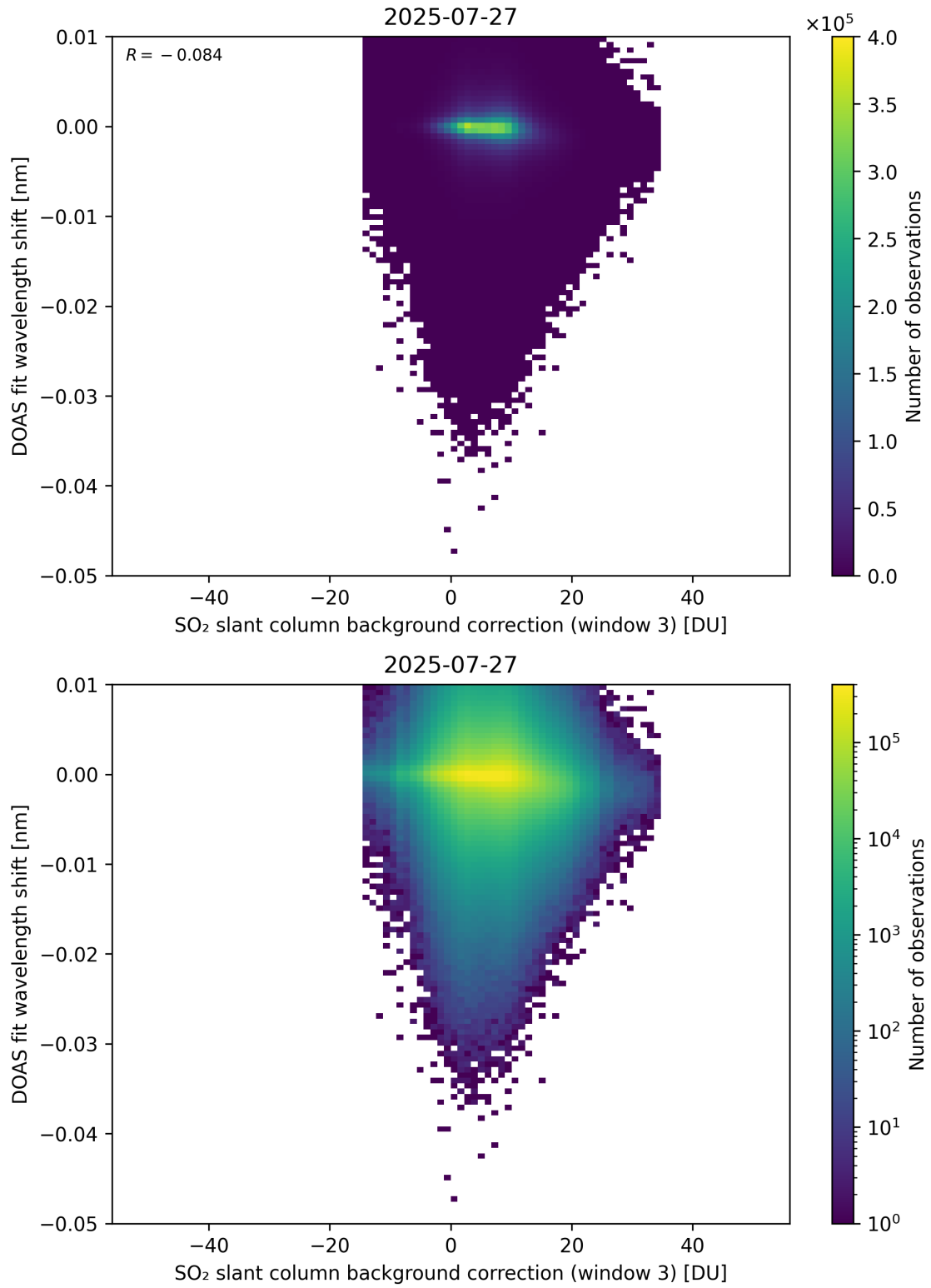
Figure 132: Scatter density plot of “SO 2 slant column background correction (window 3)” against “DOAS fit wavelength shift” for 2025-07-26 to 2025-07-28.
