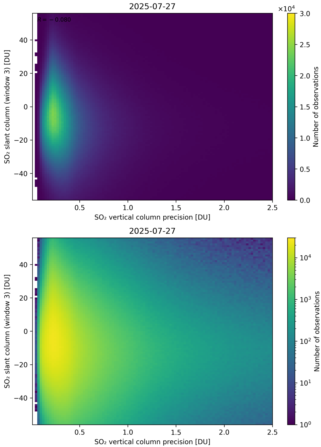
Figure 344: Scatter density plot of “SO 2 vertical column precision” against “SO 2 slant column (window 3)” for 2025-07-26 to 2025-07-28.
