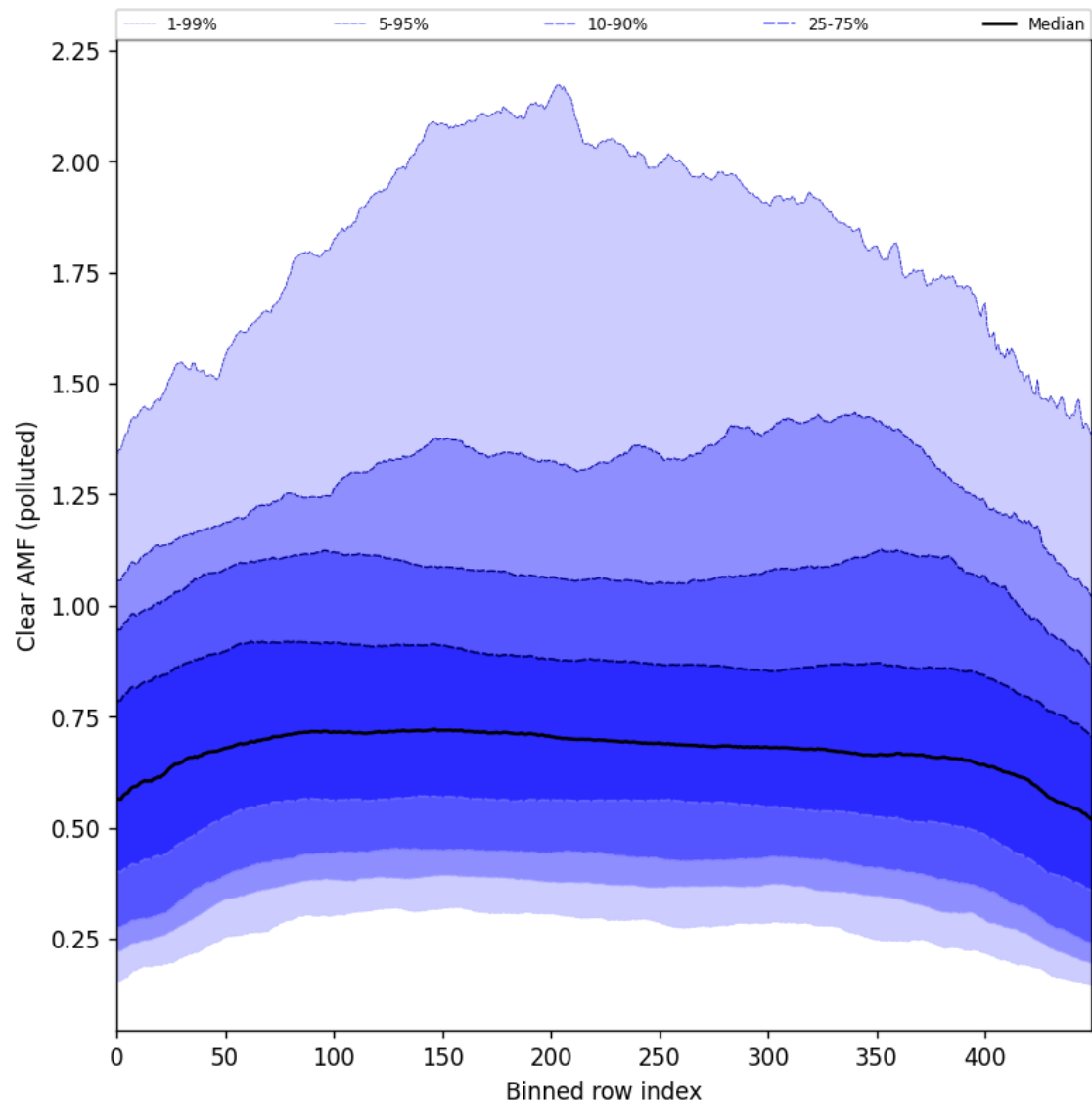
Figure 107: Along track statistics of “Clear AMF (polluted)” for 2025-07-26 to 2025-07-28
