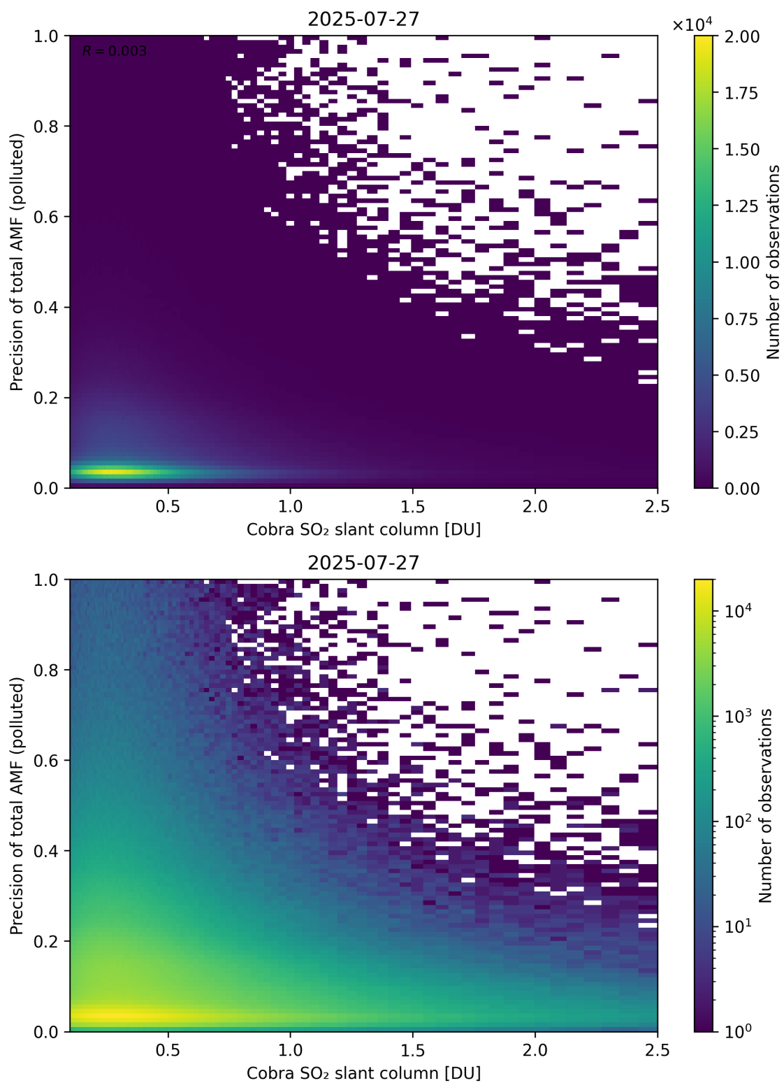
Figure 225: Scatter density plot of “Cobra SO 2 slant column” against “Precision of total AMF (polluted)” for 2025-07-26 to 2025-07-28.
