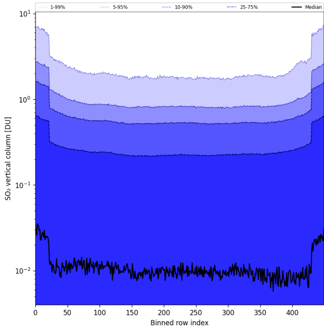
Figure 84: Along track statistics of “SO 2 vertical column” for 2025-07-26 to 2025-07-28
