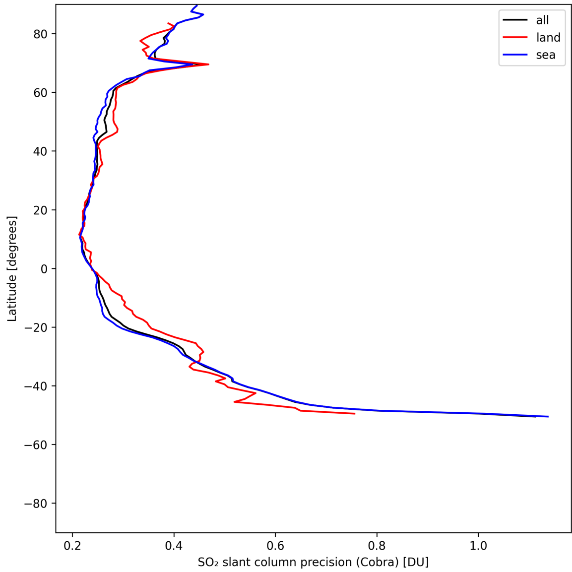
Figure 36: Zonal average of “SO 2 slant column precision (Cobra)” for 2025-07-26 to 2025-07-28.
