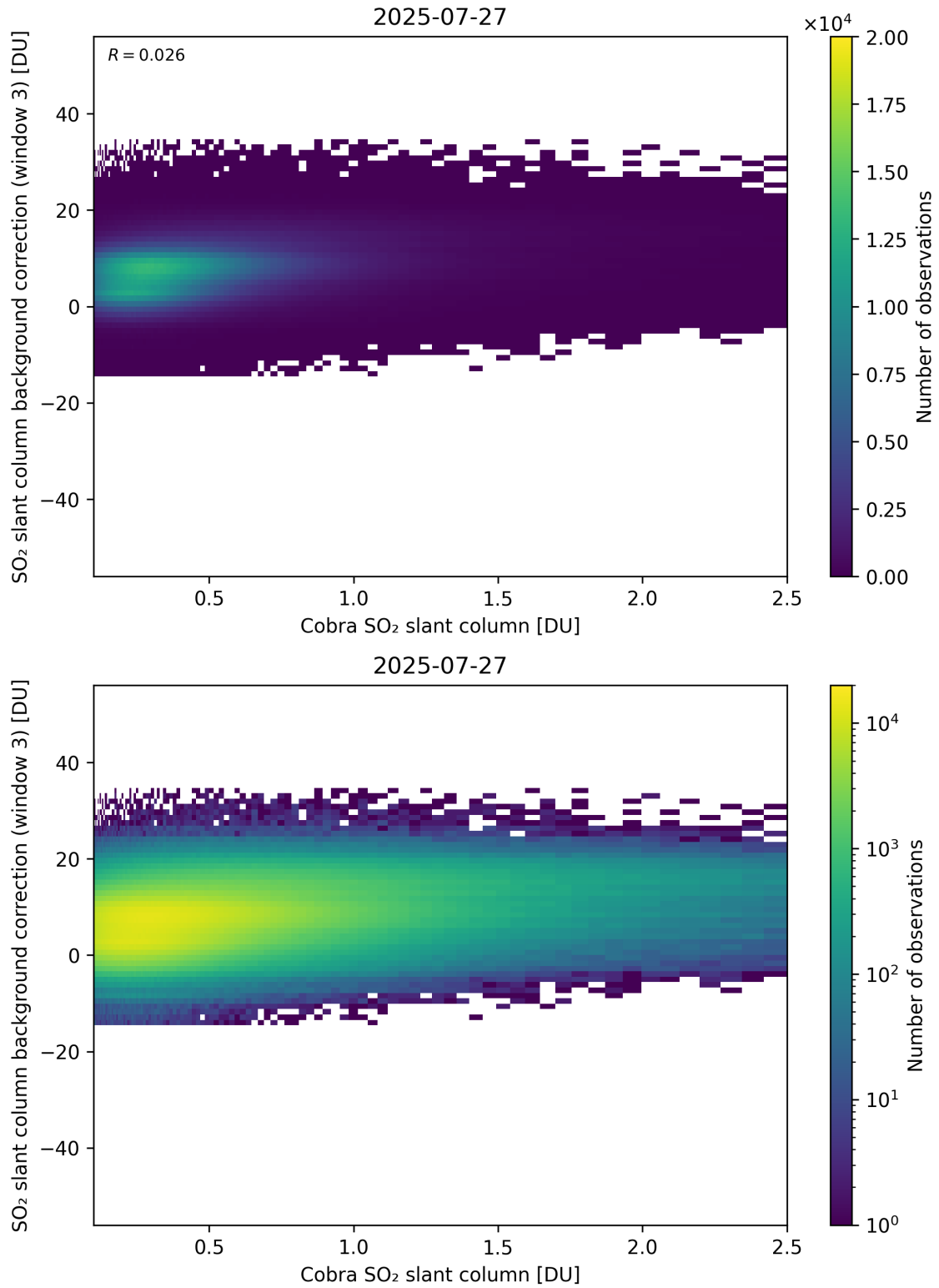
Figure 195: Scatter density plot of “Cobra SO 2 slant column” against “SO 2 slant column background correction (window 3)” for 2025-07-26 to 2025-07-28.
