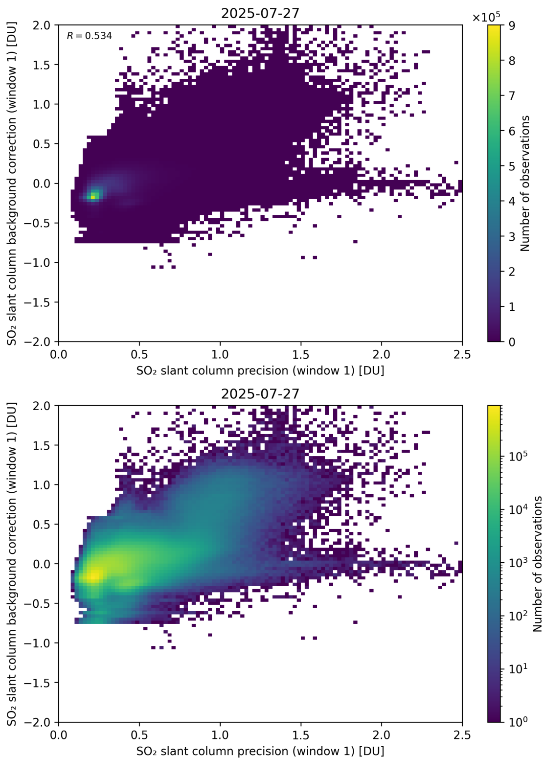
Figure 268: Scatter density plot of “SO 2 slant column precision (window 1)” against “SO 2 slant column background correction (window 1)” for 2025-07-26 to 2025-07-28.
