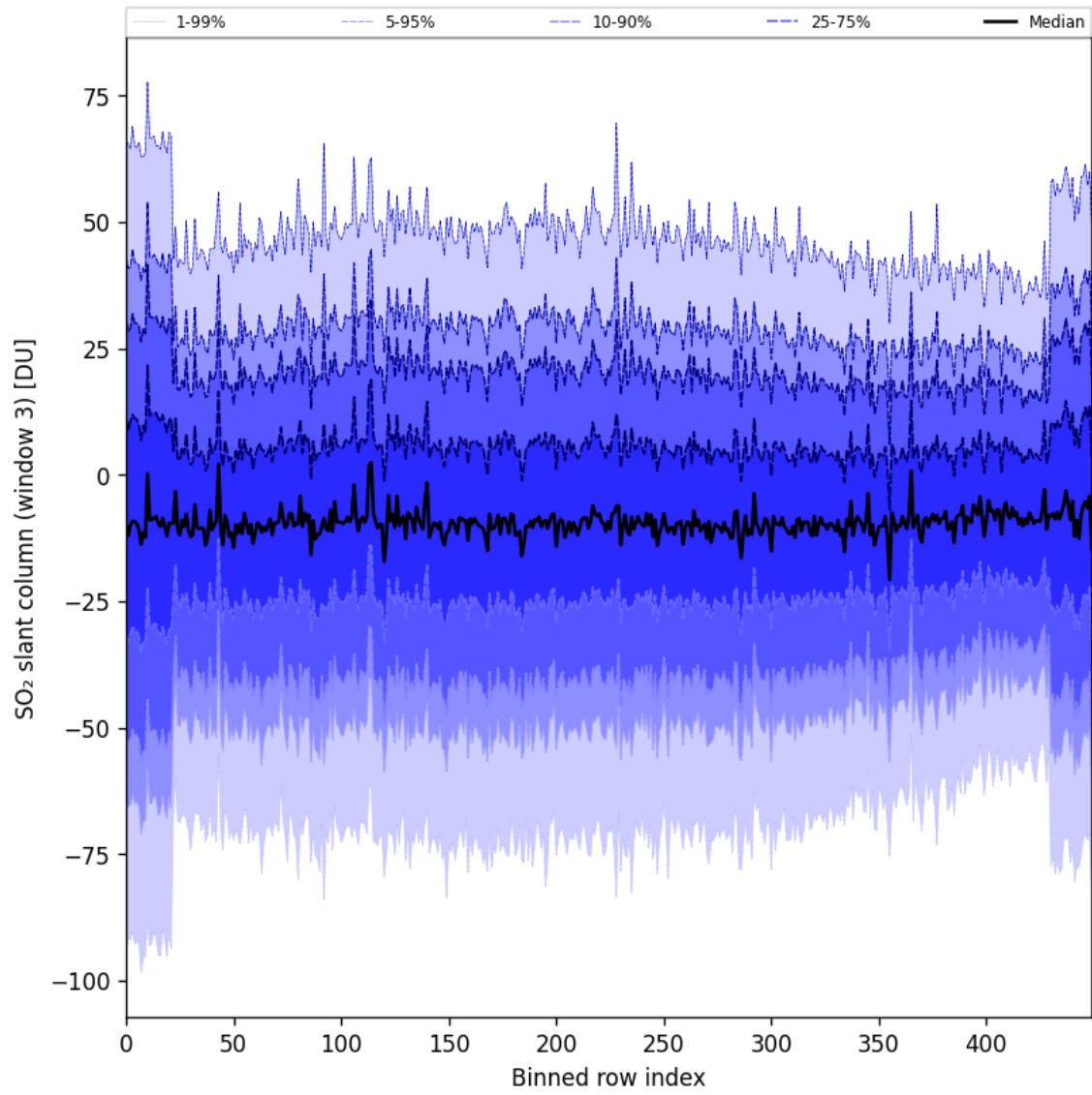
Figure 97: Along track statistics of “SO 2 slant column (window 3)” for 2025-07-26 to 2025-07-28
