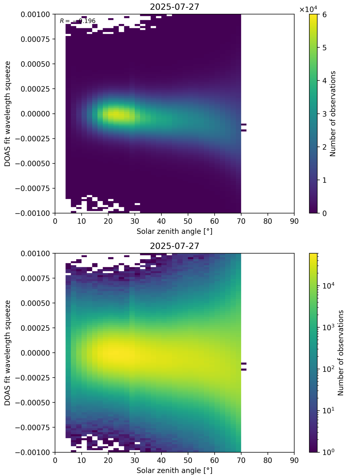
Figure 175: Scatter density plot of “Solar zenith angle” against “DOAS fit wavelength squeeze” for 2025-07-26 to 2025-07-28.
