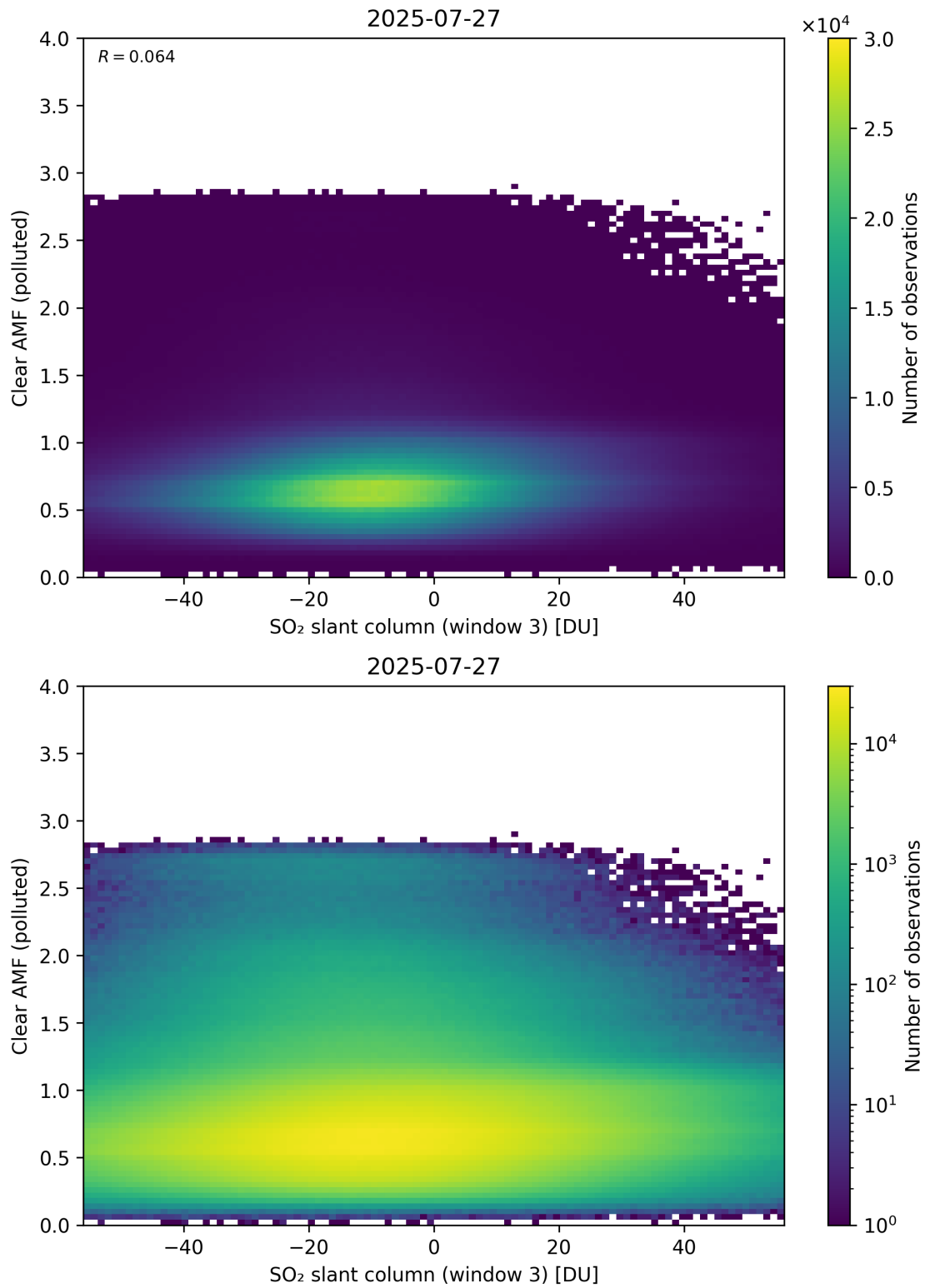
Figure 315: Scatter density plot of “SO 2 slant column (window 3)” against “Clear AMF (polluted)” for 2025-07-26 to 2025-07-28.
