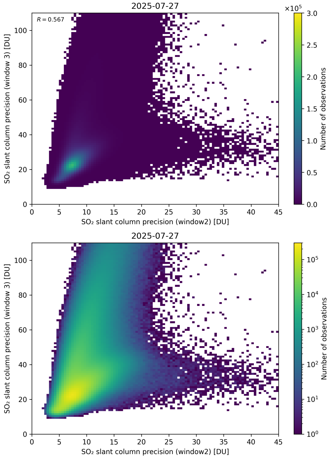
Figure 300: Scatter density plot of “SO 2 slant column precision (window2)” against “SO 2 slant column precision (window 3)” for 2025-07-26 to 2025-07-28.
