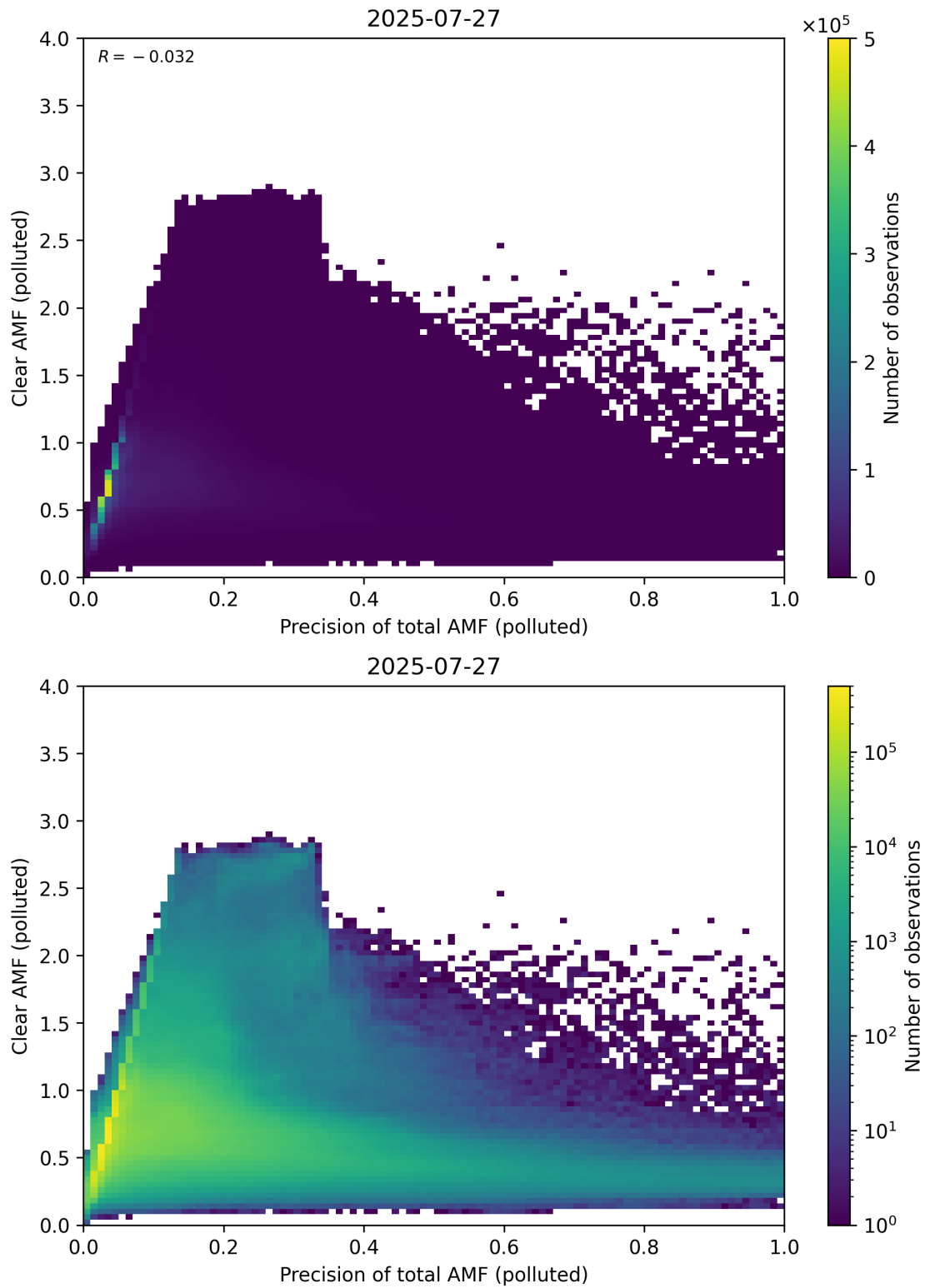
Figure 320: Scatter density plot of “Precision of total AMF (polluted)” against “Clear AMF (polluted)” for 2025-07-26 to 2025-07-28.
