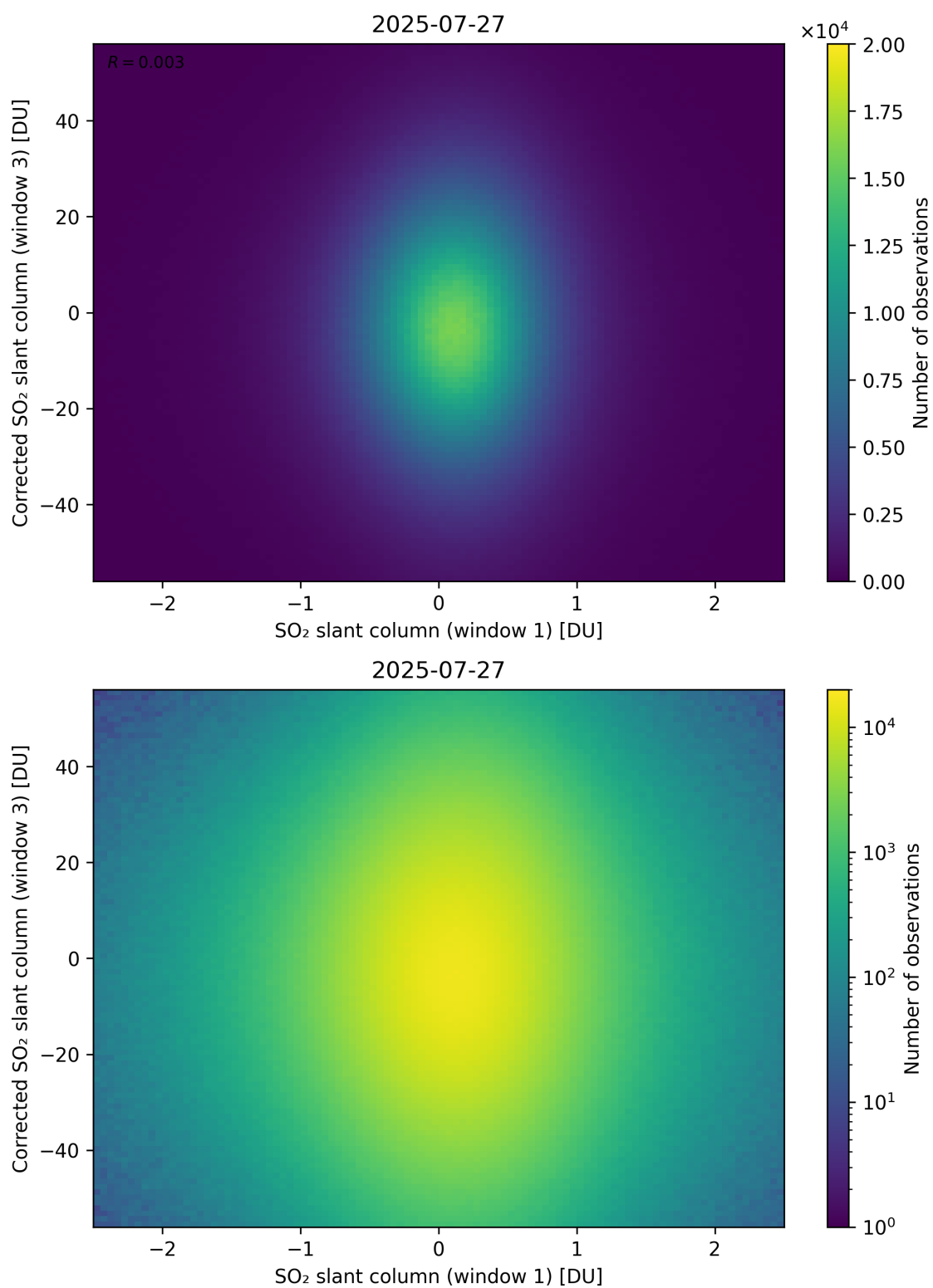
Figure 284: Scatter density plot of “SO 2 slant column (window 1)” against “Corrected SO 2 slant column (window 3)” for 2025-07-26 to 2025-07-28.
