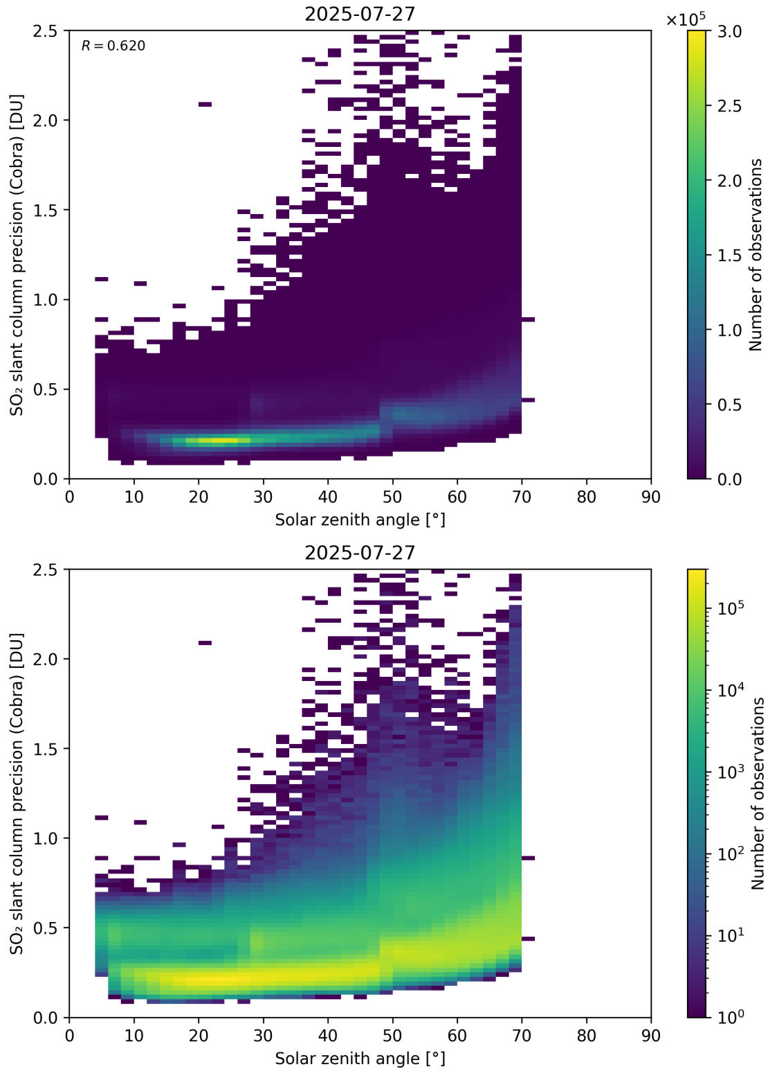
Figure 180: Scatter density plot of “Solar zenith angle” against “SO 2 slant column precision (Cobra)” for 2025-07-26 to 2025-07-28.
