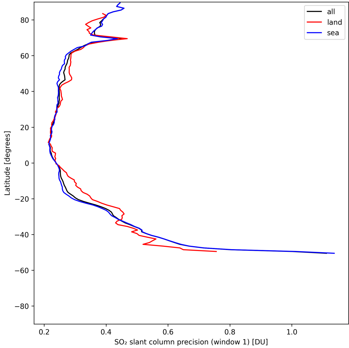
Figure 38: Zonal average of “SO 2 slant column precision (window 1)” for 2025-07-26 to 2025-07-28.
