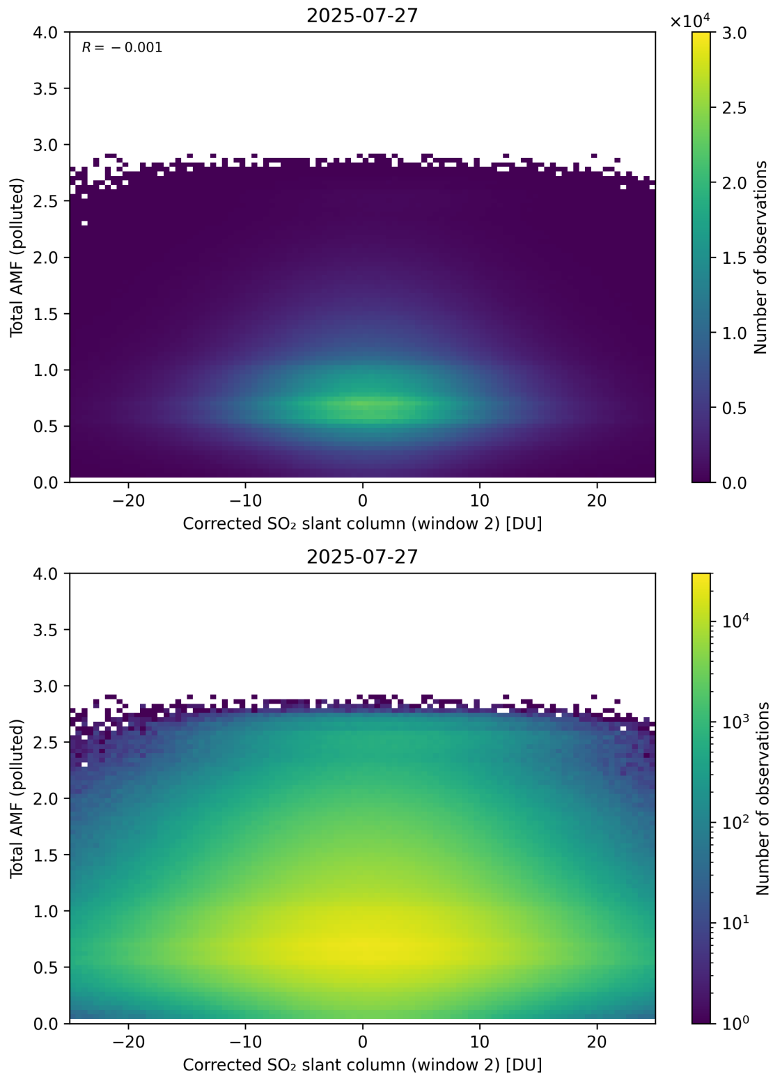
Figure 253: Scatter density plot of “Corrected SO 2 slant column (window 2)” against “Total AMF (polluted)” for 2025-07-26 to 2025-07-28.
