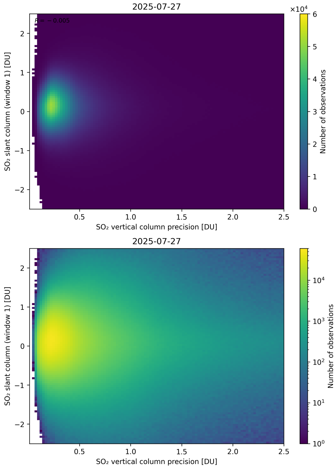
Figure 341: Scatter density plot of “SO 2 vertical column precision” against “SO 2 slant column (window 1)” for 2025-07-26 to 2025-07-28.
