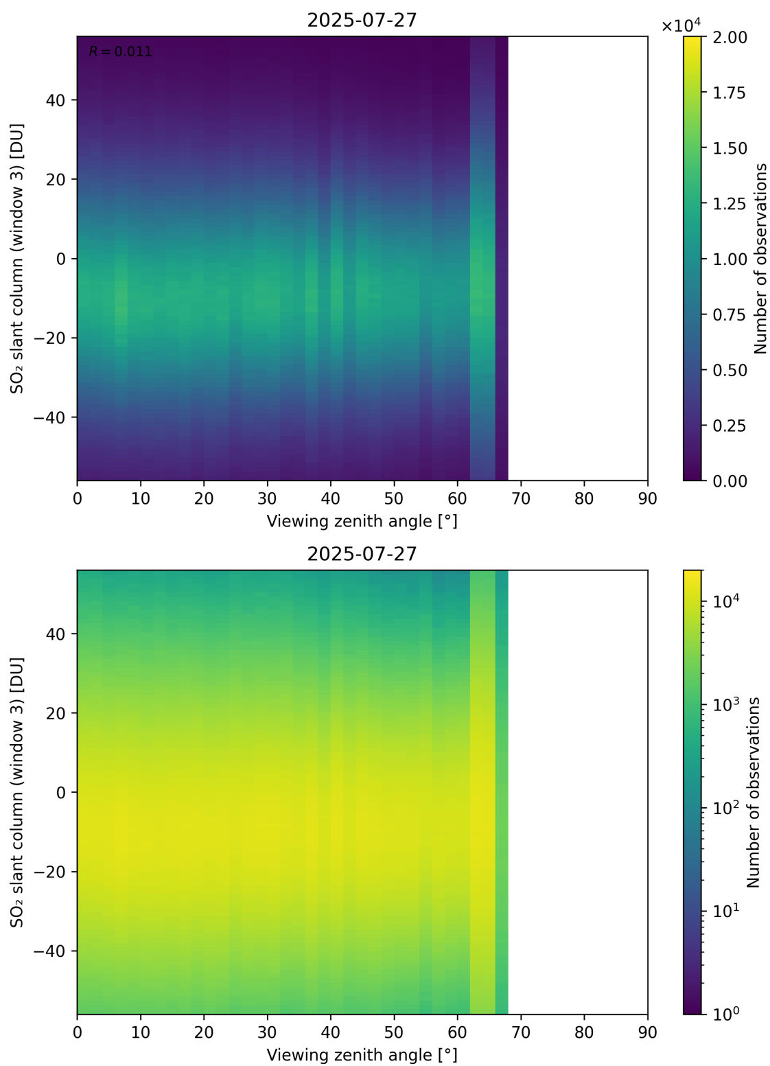
Figure 379: Scatter density plot of “Viewing zenith angle” against “SO 2 slant column (window 3)” for 2025-07-26 to 2025-07-28.
