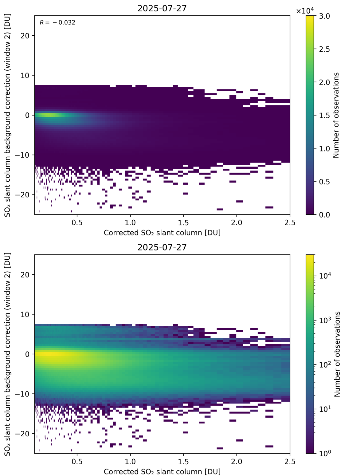
Figure 227: Scatter density plot of “Corrected SO 2 slant column” against “SO 2 slant column background correction (window 2)” for 2025-07-26 to 2025-07-28.
