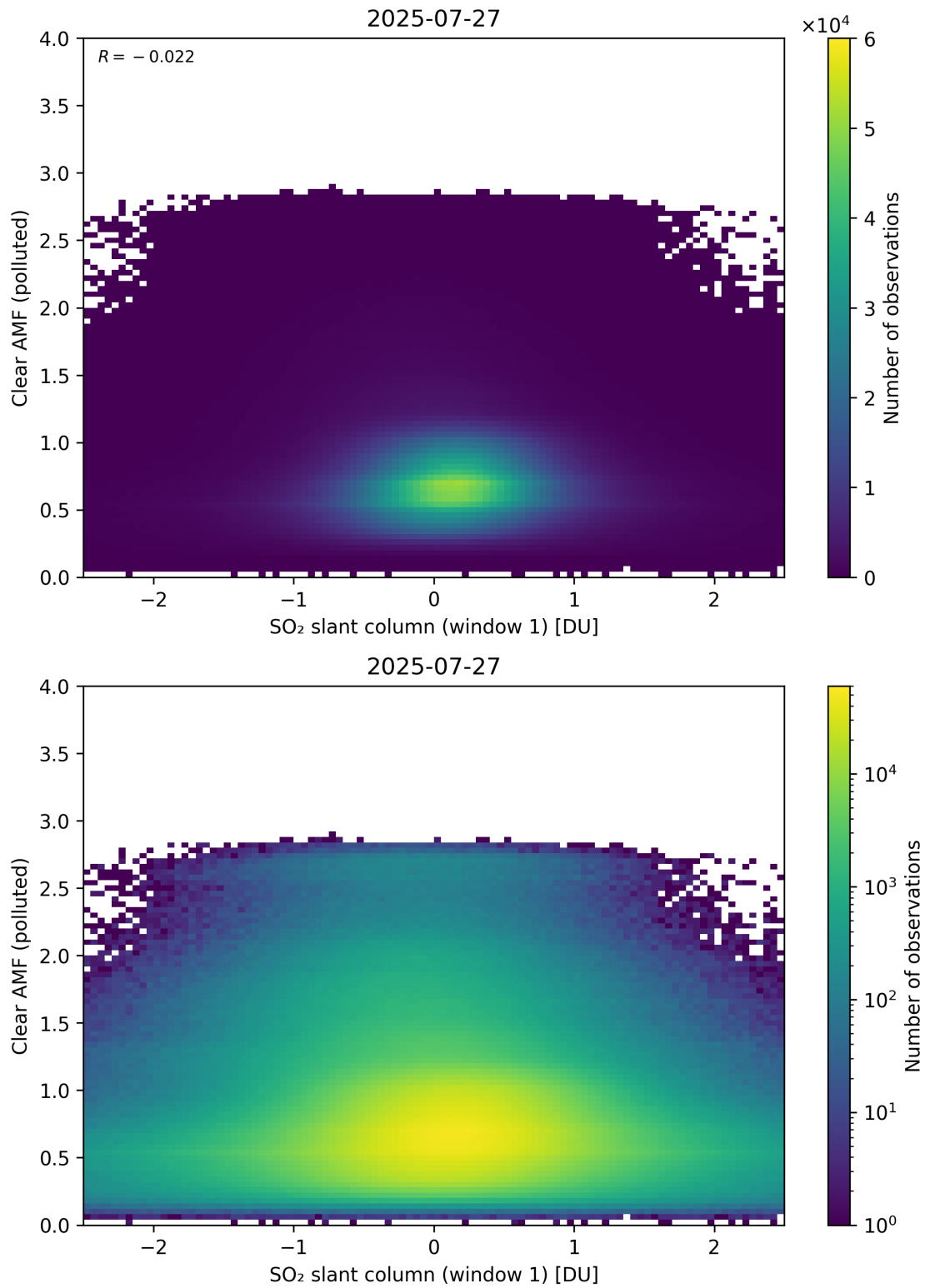
Figure 282: Scatter density plot of “SO 2 slant column (window 1)” against “Clear AMF (polluted)” for 2025-07-26 to 2025-07-28.
