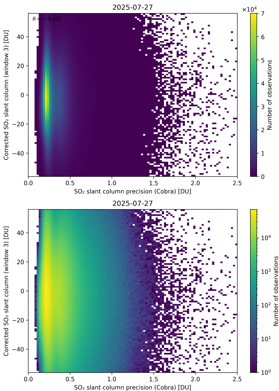
Figure 207: Scatter density plot of “SO 2 slant column precision (Cobra)” against “Corrected SO 2 slant column (window 3)” for 2025-07-26 to 2025-07-28.
