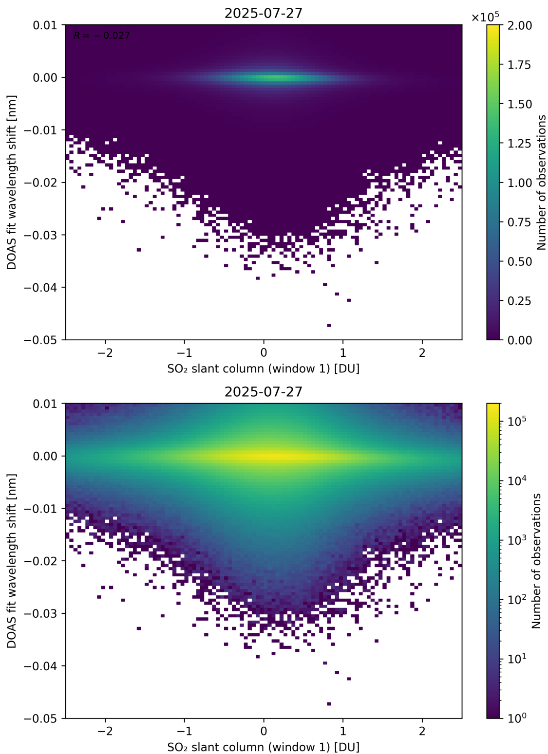
Figure 265: Scatter density plot of “SO 2 slant column (window 1)” against “DOAS fit wavelength shift” for 2025-07-26 to 2025-07-28.
