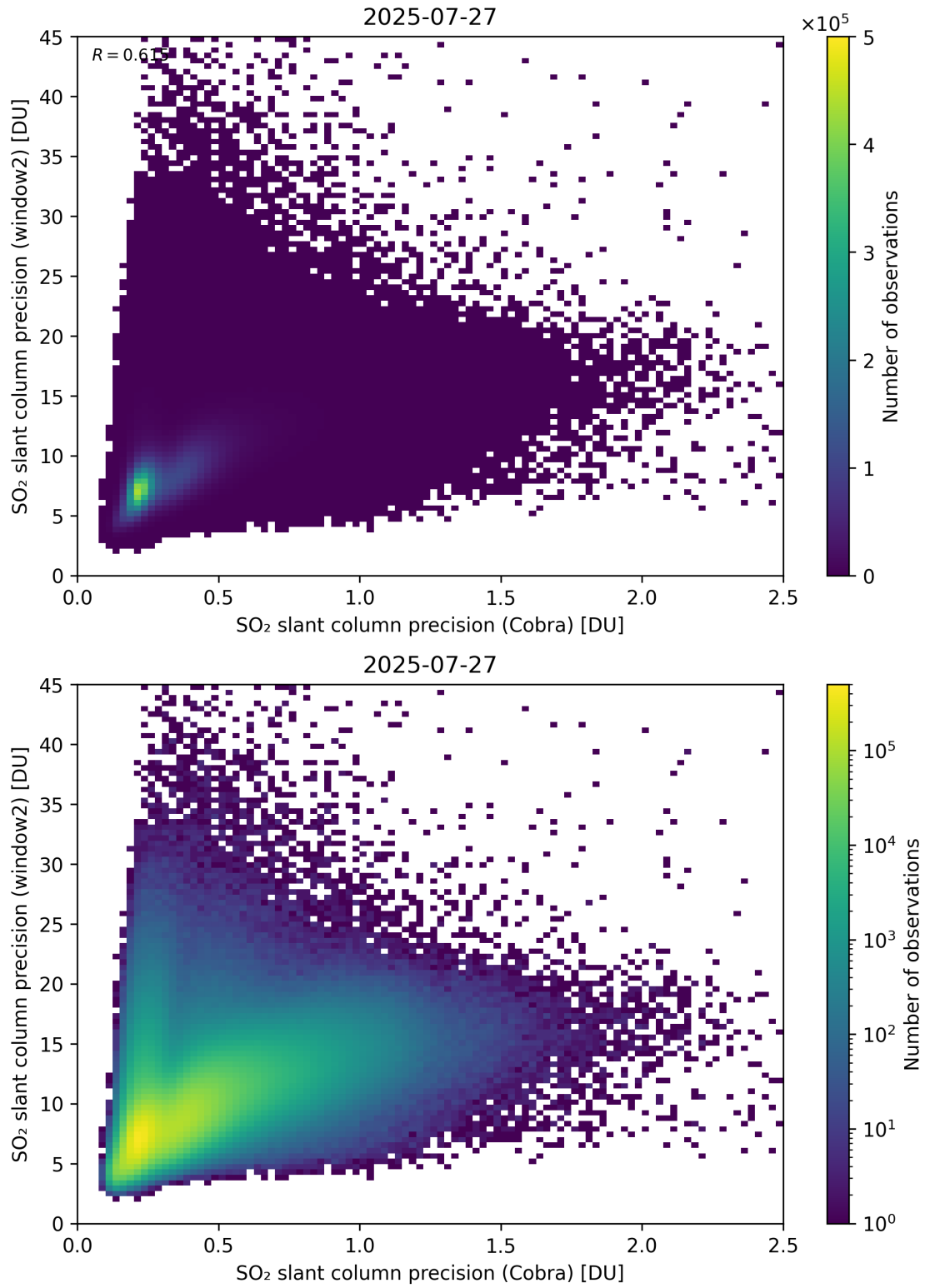
Figure 210: Scatter density plot of “SO 2 slant column precision (Cobra)” against “SO 2 slant column precision (window2)” for 2025-07-26 to 2025-07-28.
