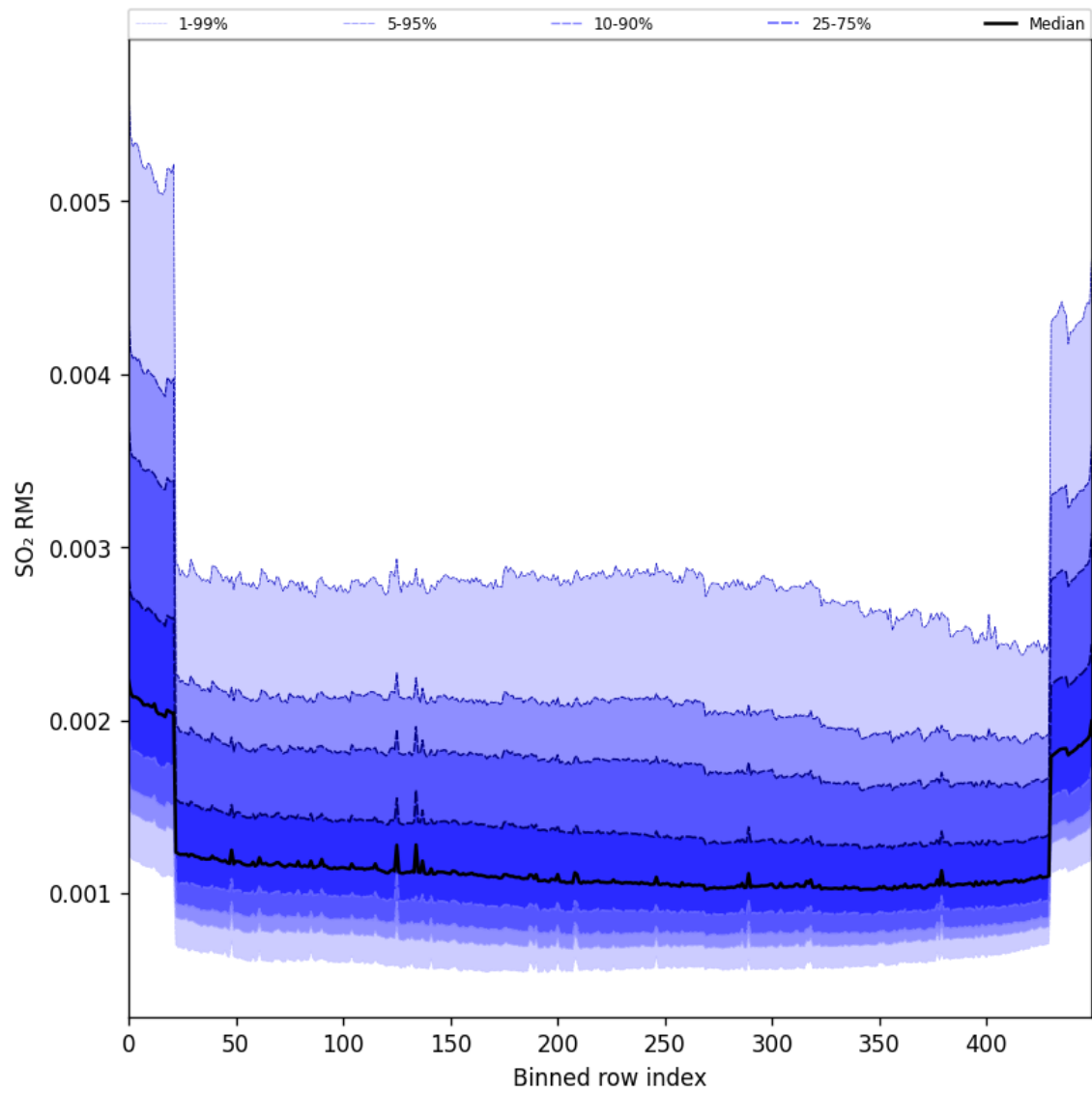
Figure 104: Along track statistics of “SO 2 RMS” for 2025-07-26 to 2025-07-28
