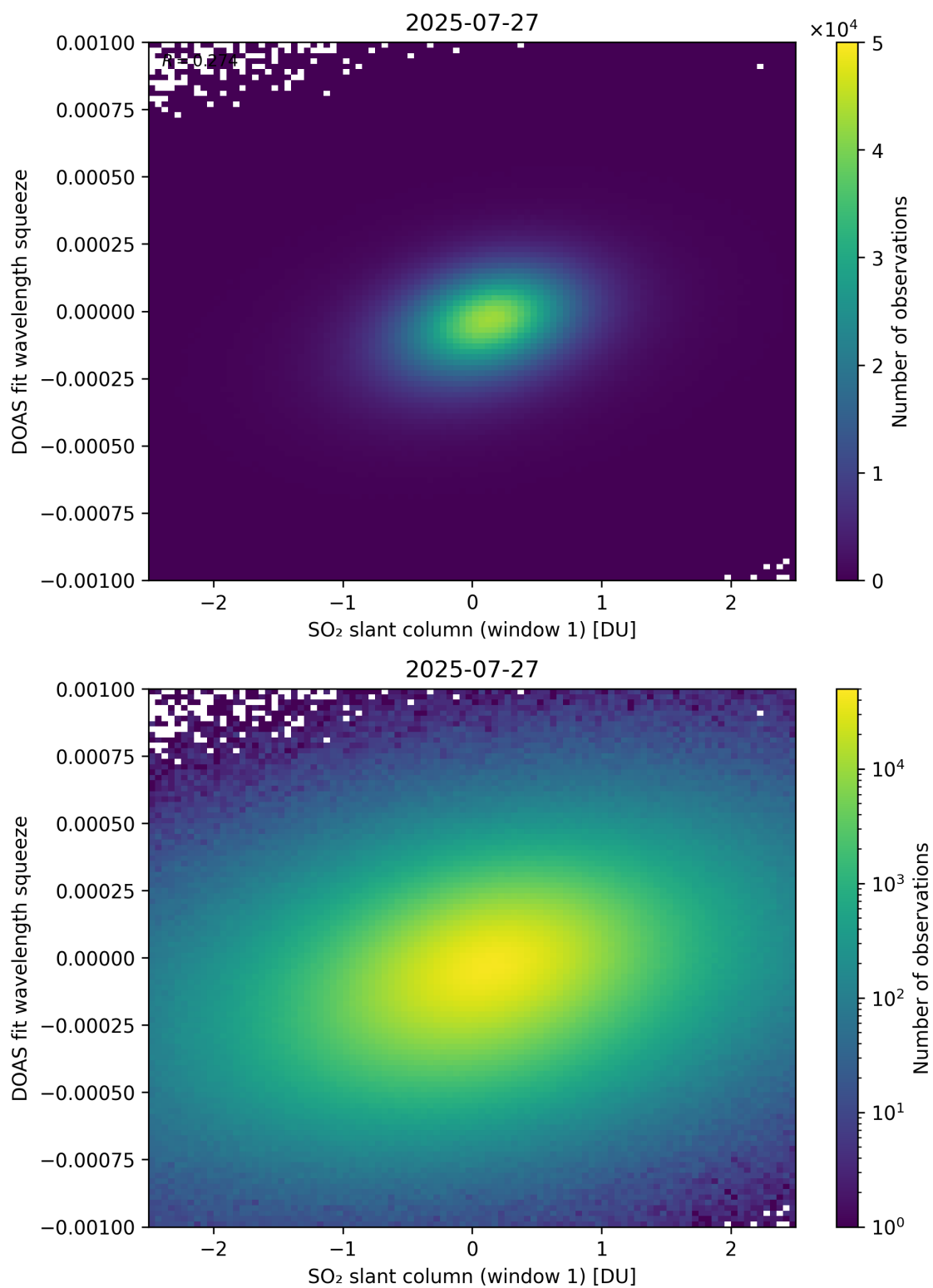
Figure 266: Scatter density plot of “SO 2 slant column (window 1)” against “DOAS fit wavelength squeeze” for 2025-07-26 to 2025-07-28.
