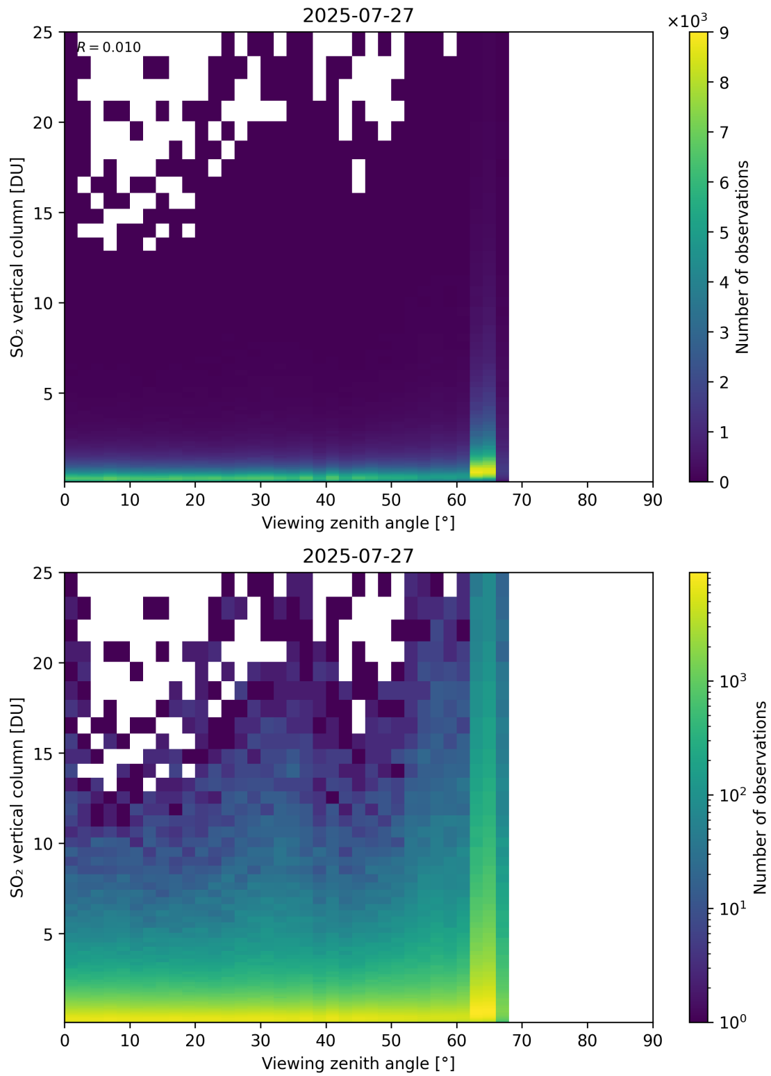
Figure 383: Scatter density plot of “Viewing zenith angle” against “SO 2 vertical column” for 2025-07-26 to 2025-07-28.
