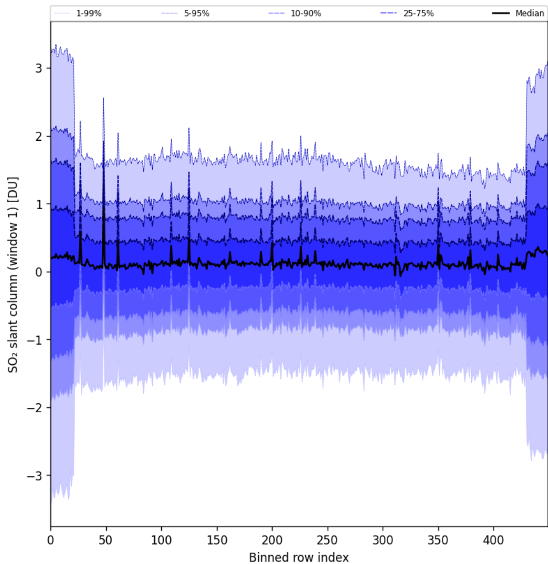
Figure 89: Along track statistics of “SO 2 slant column (window 1)” for 2025-07-26 to 2025-07-28
