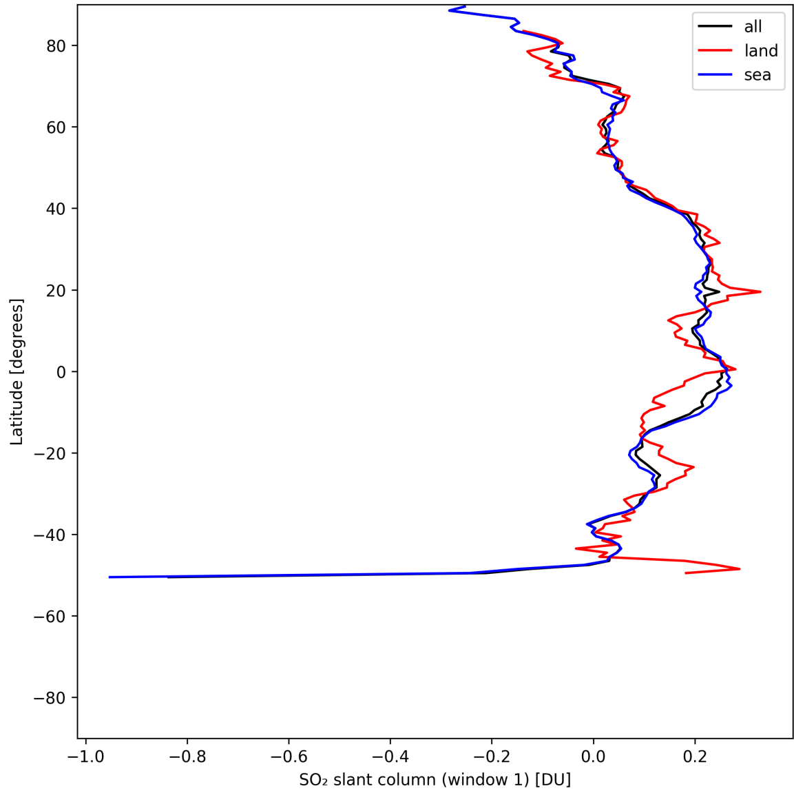
Figure 37: Zonal average of “SO 2 slant column (window 1)” for 2025-07-26 to 2025-07-28.
