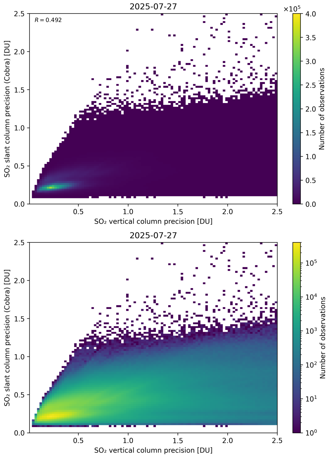
Figure 337: Scatter density plot of “SO 2 vertical column precision” against “SO 2 slant column precision (Cobra)” for 2025-07-26 to 2025-07-28.
