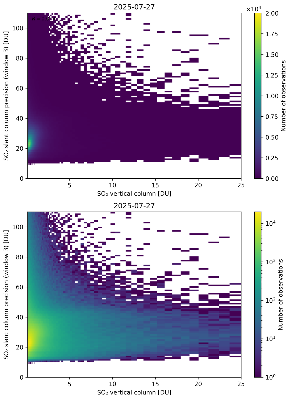
Figure 358: Scatter density plot of “SO 2 vertical column” against “SO 2 slant column precision (window 3)” for 2025-07-26 to 2025-07-28.
