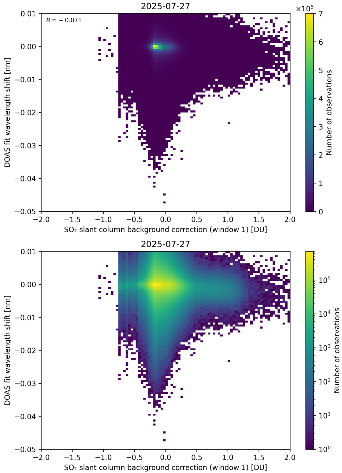
Figure 111: Scatter density plot of “SO 2 slant column background correction (window 1)” against “DOAS fit wavelength shift” for 2025-07-26 to 2025-07-28.
