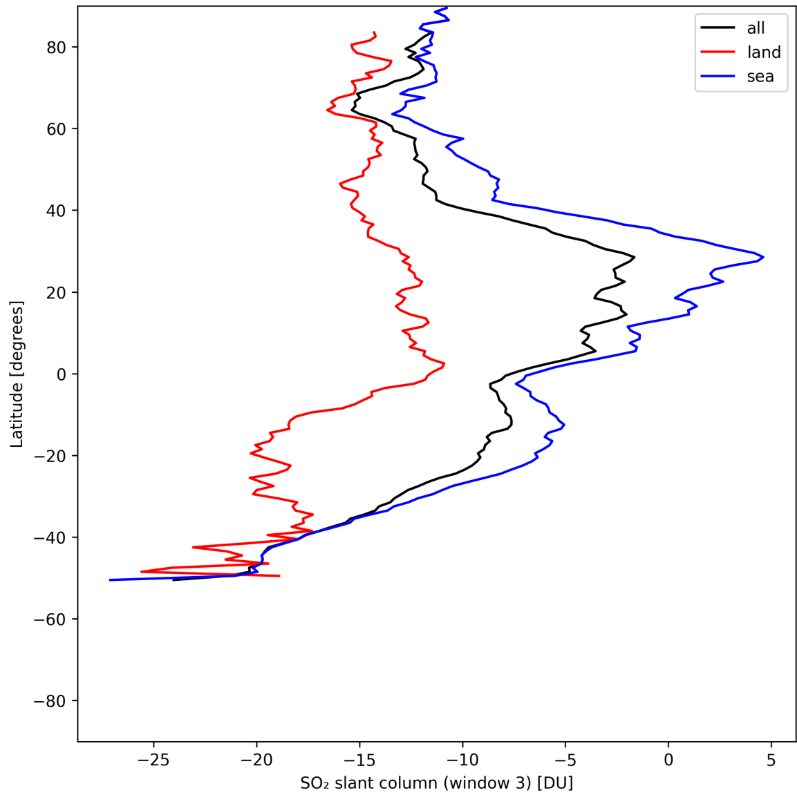
Figure 45: Zonal average of “SO 2 slant column (window 3)” for 2025-07-26 to 2025-07-28.
