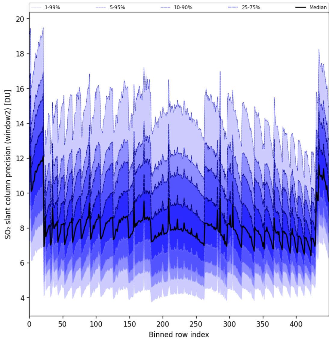
Figure 94: Along track statistics of “SO 2 slant column precision (window2)” for 2025-07-26 to 2025-07-28
