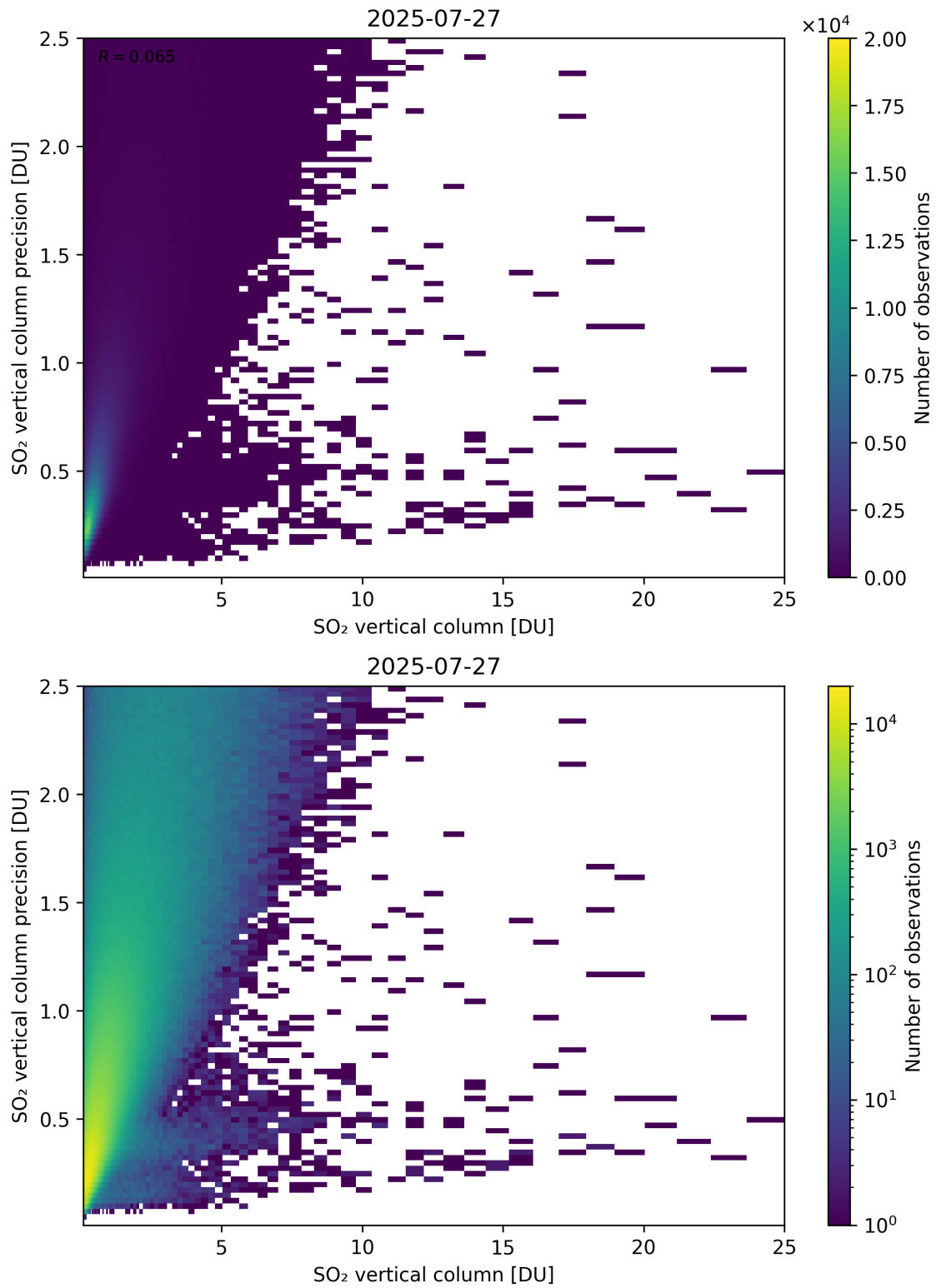
Figure 361: Scatter density plot of “SO 2 vertical column” against “SO 2 vertical column precision” for 2025-07-26 to 2025-07-28.
