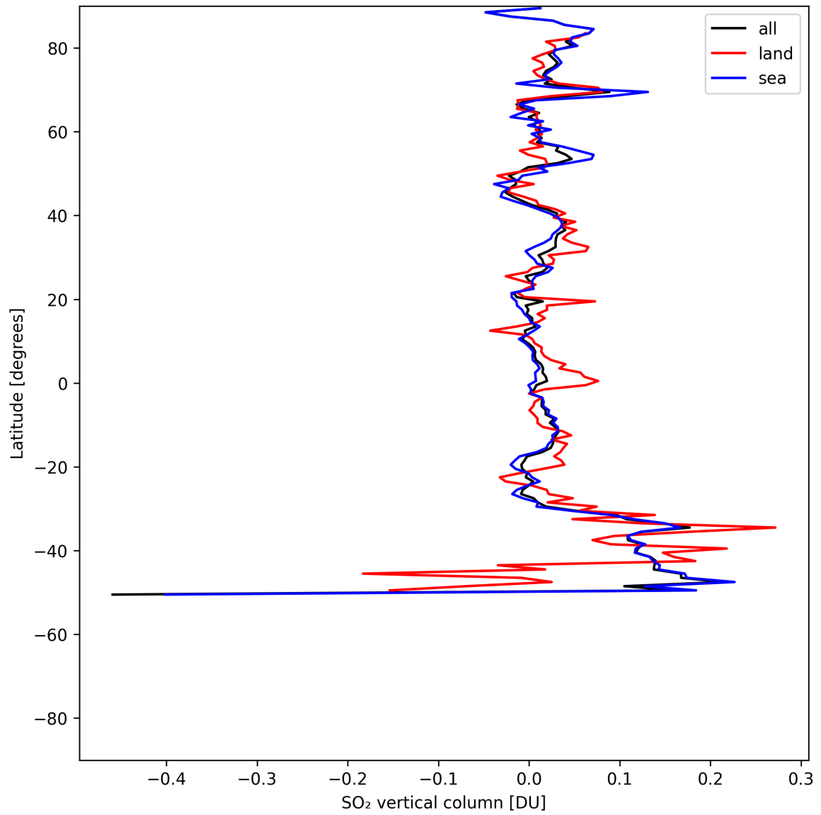
Figure 32: Zonal average of “SO 2 vertical column” for 2025-07-26 to 2025-07-28.
