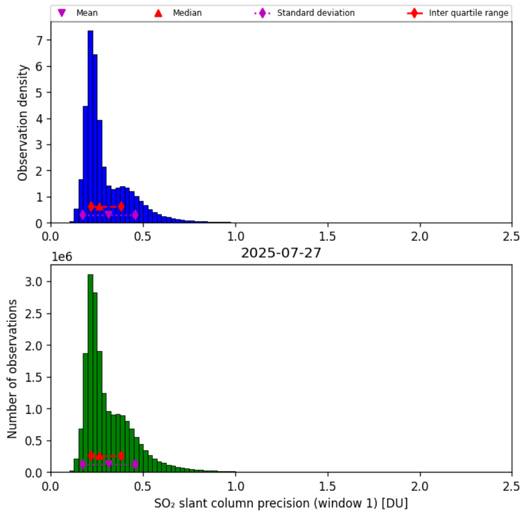
Figure 64: Histogram of “SO 2 slant column precision (window 1)” for 2025-07-26 to 2025-07-28
