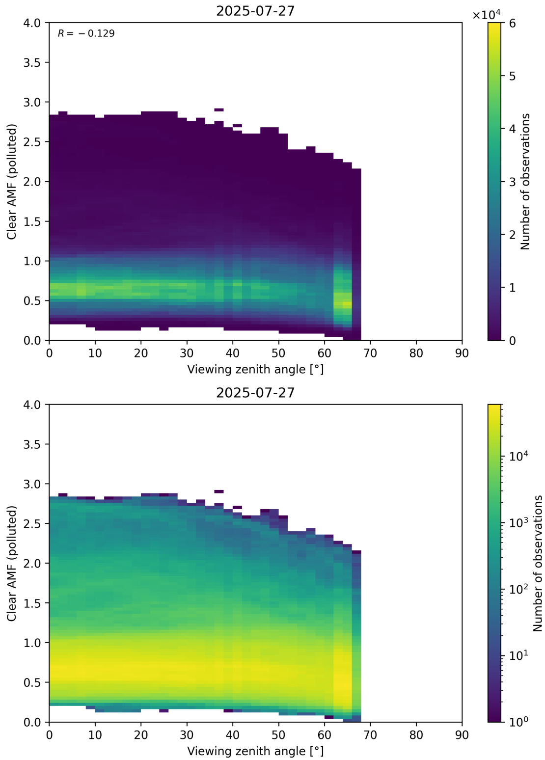
Figure 370: Scatter density plot of “Viewing zenith angle” against “Clear AMF (polluted)” for 2025-07-26 to 2025-07-28.
