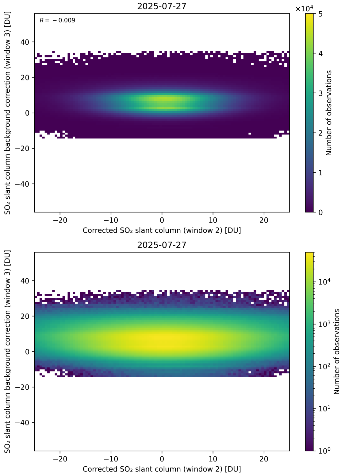
Figure 245: Scatter density plot of “Corrected SO 2 slant column (window 2)” against “SO 2 slant column background correction (window 3)” for 2025-07-26 to 2025-07-28.
