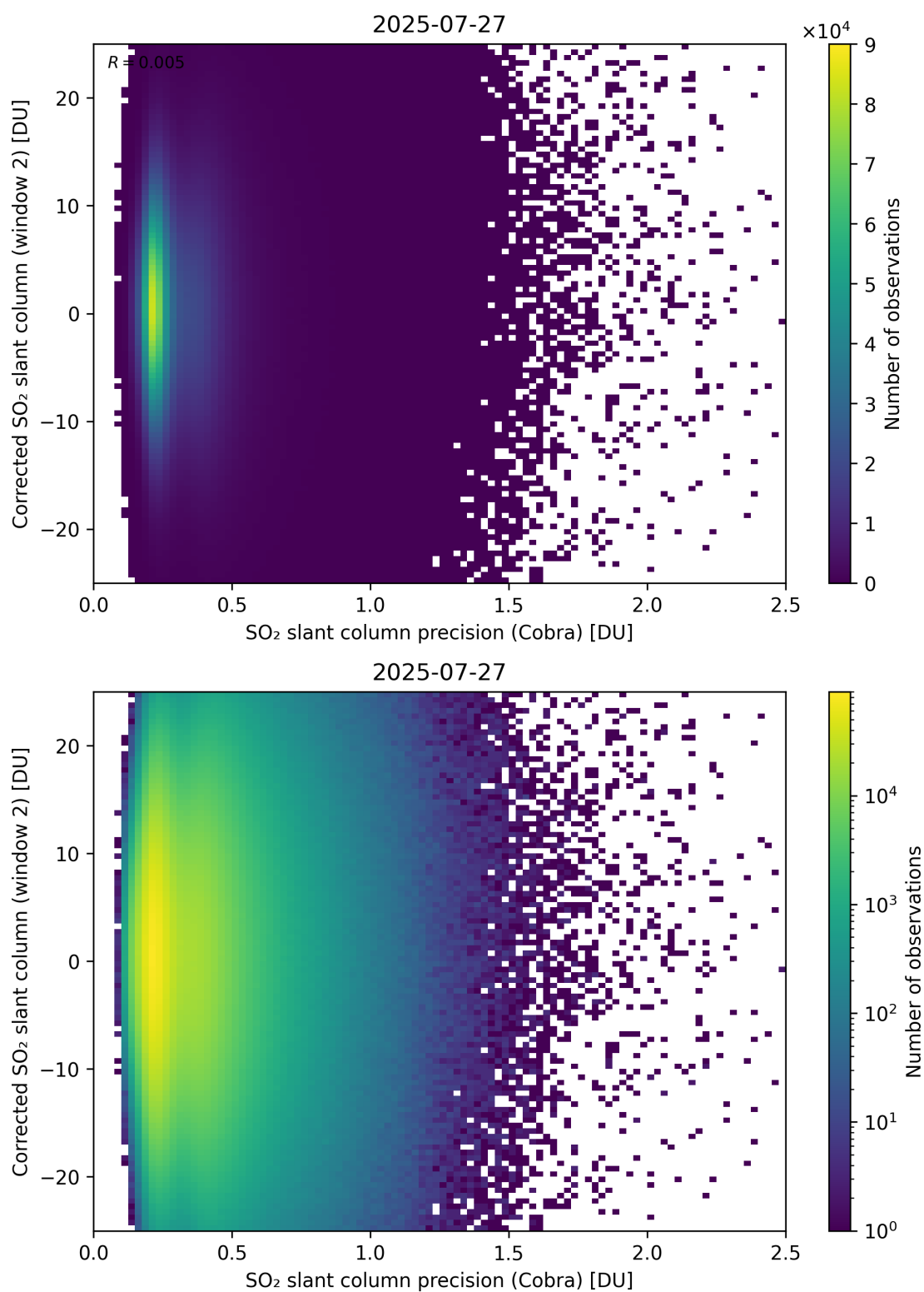
Figure 206: Scatter density plot of “SO 2 slant column precision (Cobra)” against “Corrected SO 2 slant column (window 2)” for 2025-07-26 to 2025-07-28.
