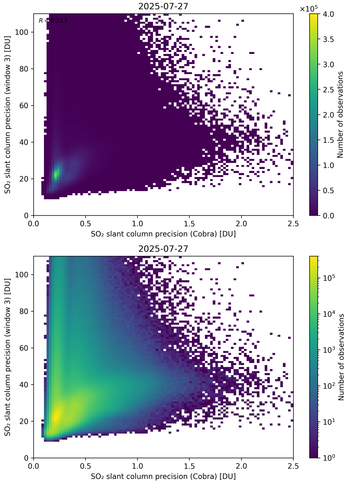
Figure 212: Scatter density plot of “SO 2 slant column precision (Cobra)” against “SO 2 slant column precision (window 3)” for 2025-07-26 to 2025-07-28.
