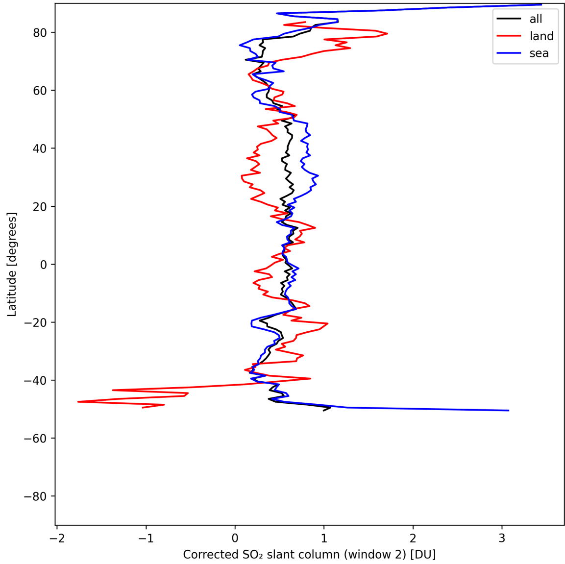
Figure 43: Zonal average of “Corrected SO 2 slant column (window 2)” for 2025-07-26 to 2025-07-28.
