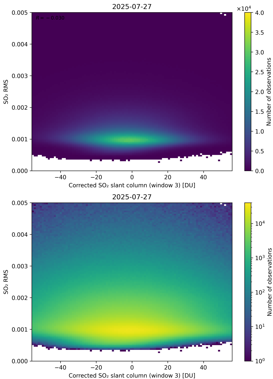
Figure 258: Scatter density plot of “Corrected SO 2 slant column (window 3)” against “SO 2 RMS” for 2025-07-26 to 2025-07-28.
