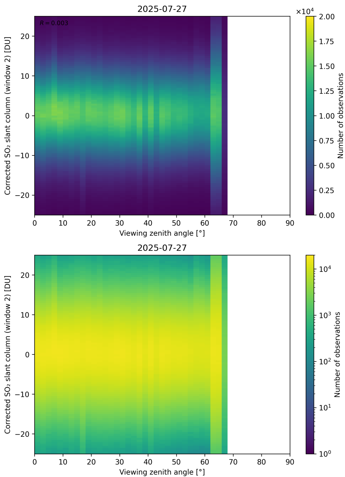
Figure 374: Scatter density plot of “Viewing zenith angle” against “Corrected SO 2 slant column (window 2)” for 2025-07-26 to 2025-07-28.
