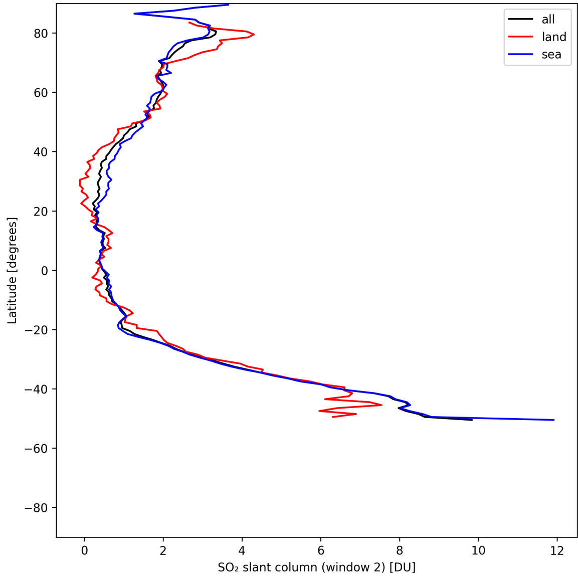
Figure 41: Zonal average of “SO 2 slant column (window 2)” for 2025-07-26 to 2025-07-28.
