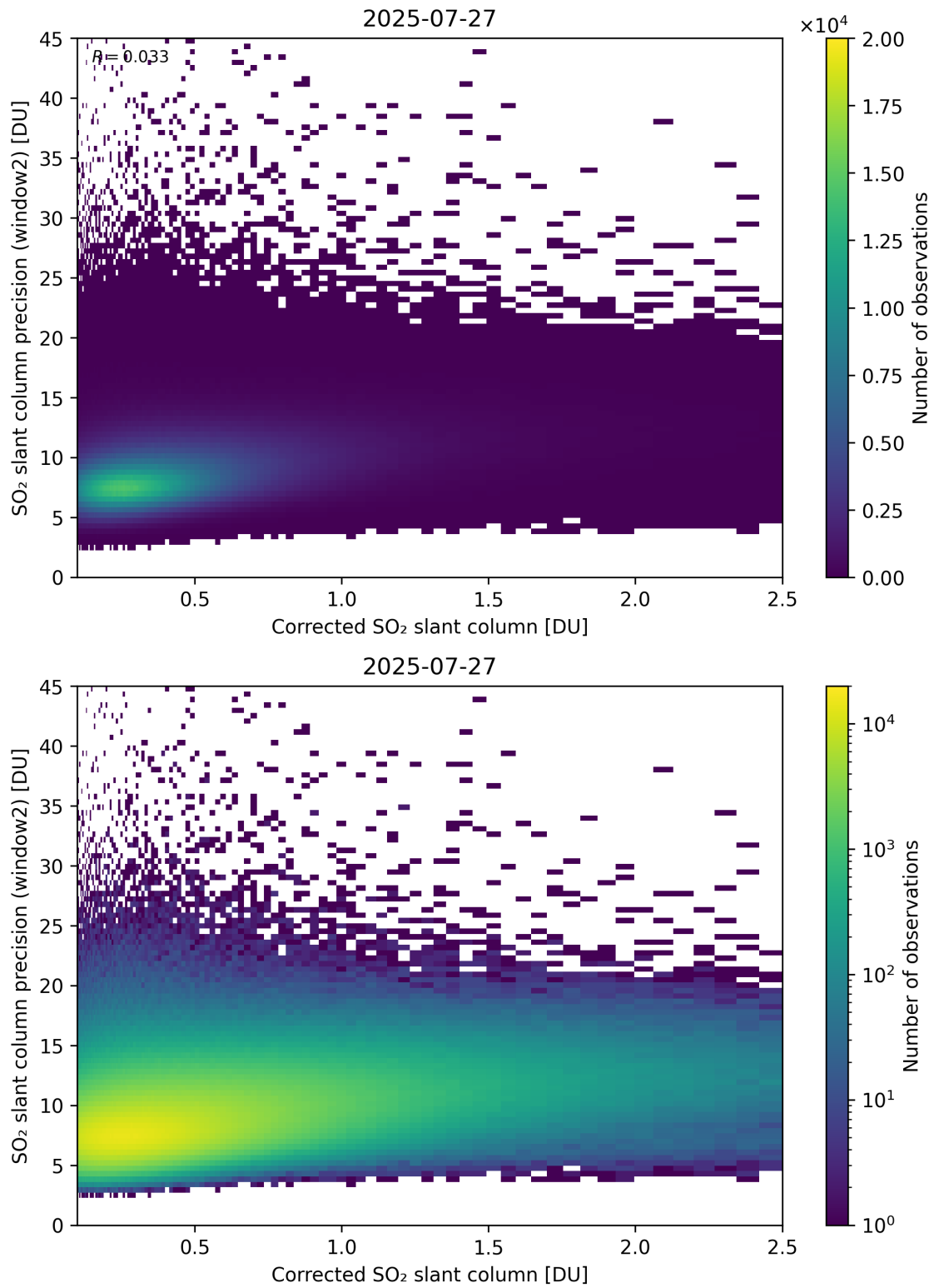
Figure 239: Scatter density plot of “Corrected SO 2 slant column” against “SO 2 slant column precision (window2)” for 2025-07-26 to 2025-07-28.
