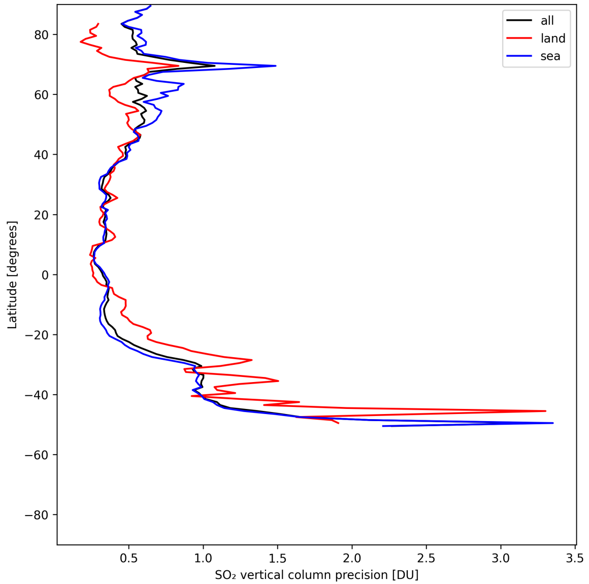
Figure 33: Zonal average of “SO 2 vertical column precision” for 2025-07-26 to 2025-07-28.
