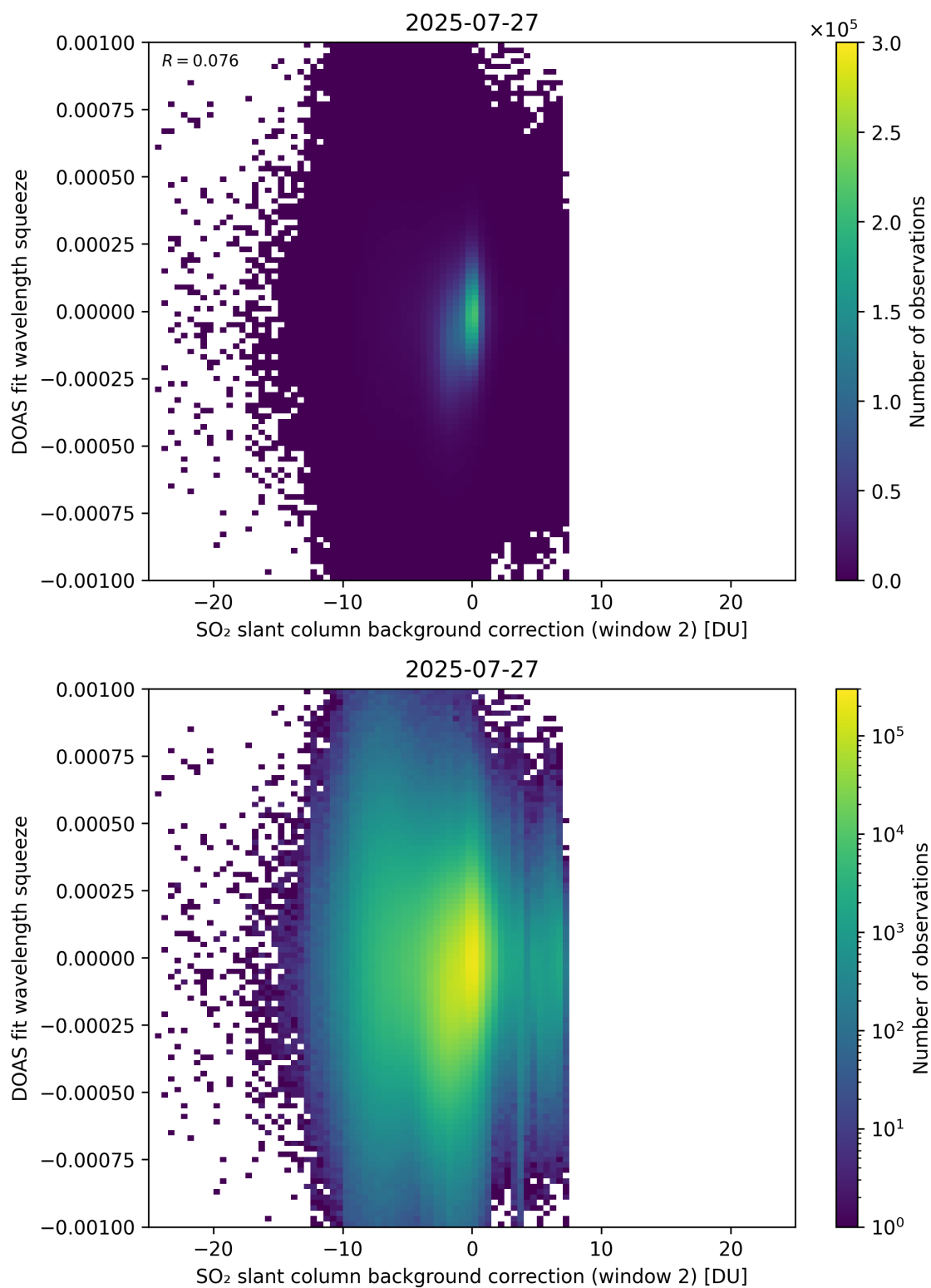
Figure 124: Scatter density plot of “SO 2 slant column background correction (window 2)” against “DOAS fit wavelength squeeze” for 2025-07-26 to 2025-07-28.
