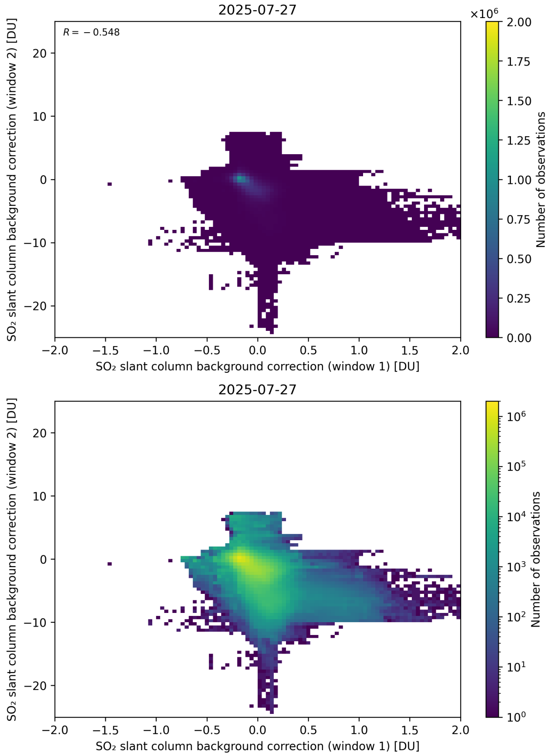
Figure 109: Scatter density plot of “SO 2 slant column background correction (window 1)” against “SO 2 slant column background correction (window 2)” for 2025-07-26 to 2025-07-28.
