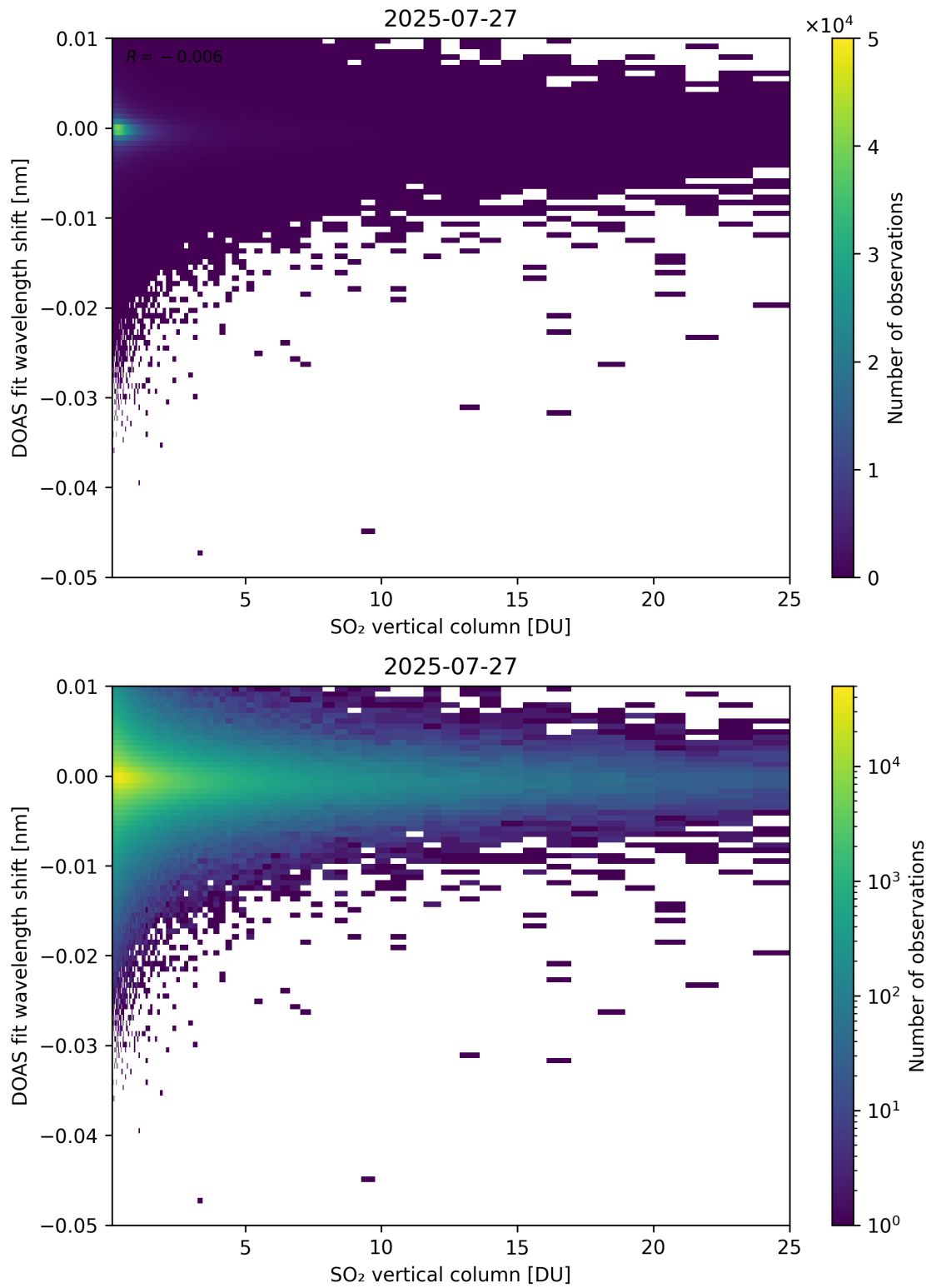
Figure 326: Scatter density plot of “SO 2 vertical column” against “DOAS fit wavelength shift” for 2025-07-26 to 2025-07-28.
