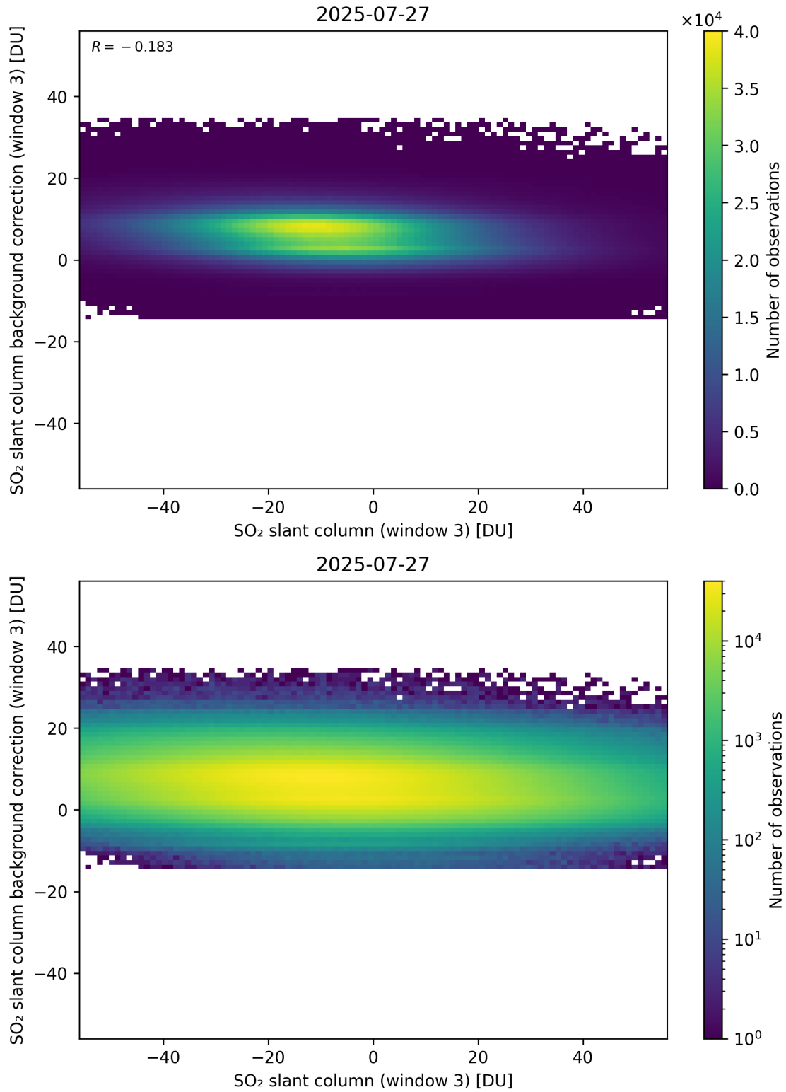
Figure 303: Scatter density plot of “SO 2 slant column (window 3)” against “SO 2 slant column background correction (window 3)” for 2025-07-26 to 2025-07-28.
