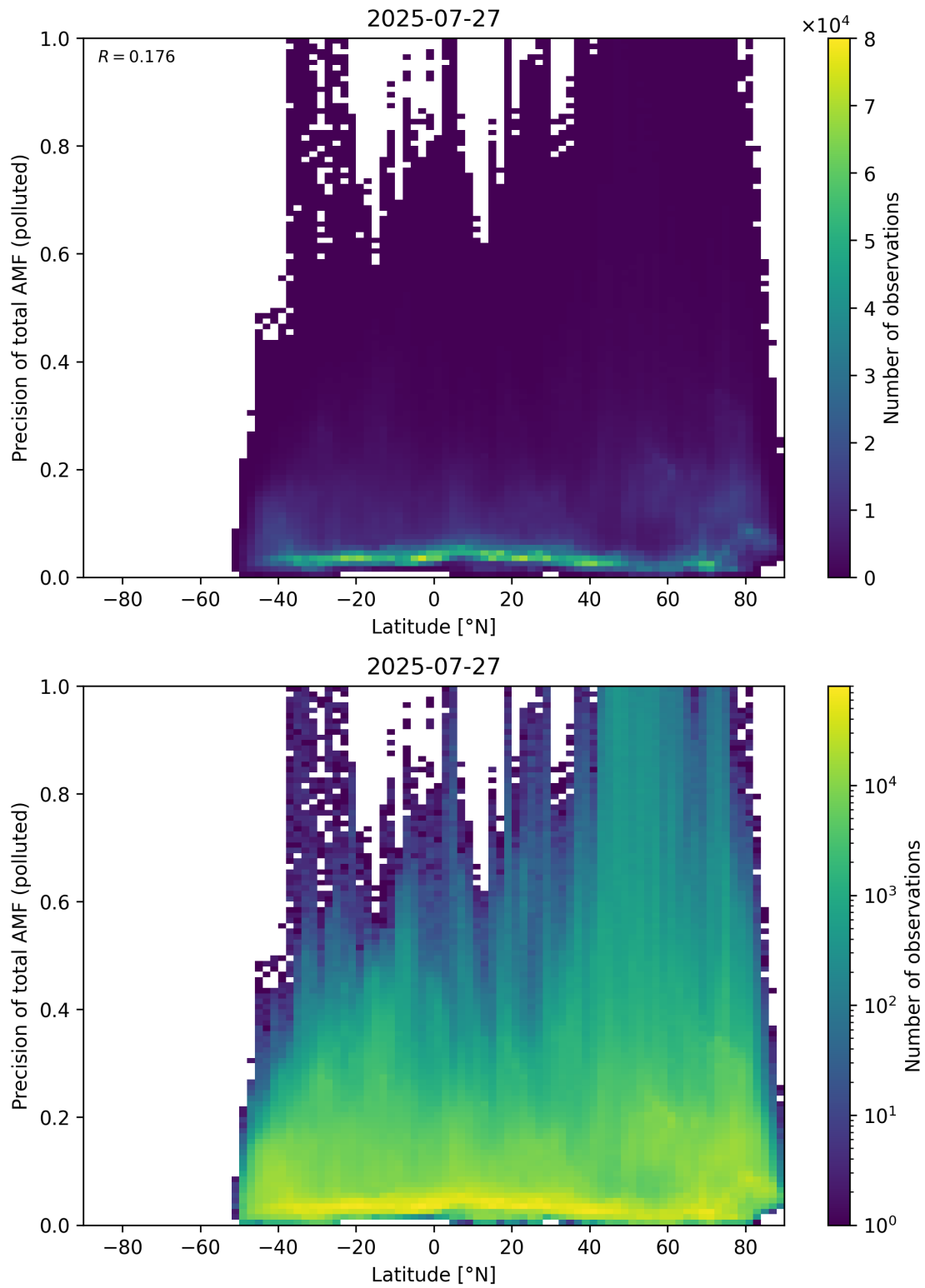
Figure 168: Scatter density plot of “Latitude” against “Precision of total AMF (polluted)” for 2025-07-26 to 2025-07-28.
