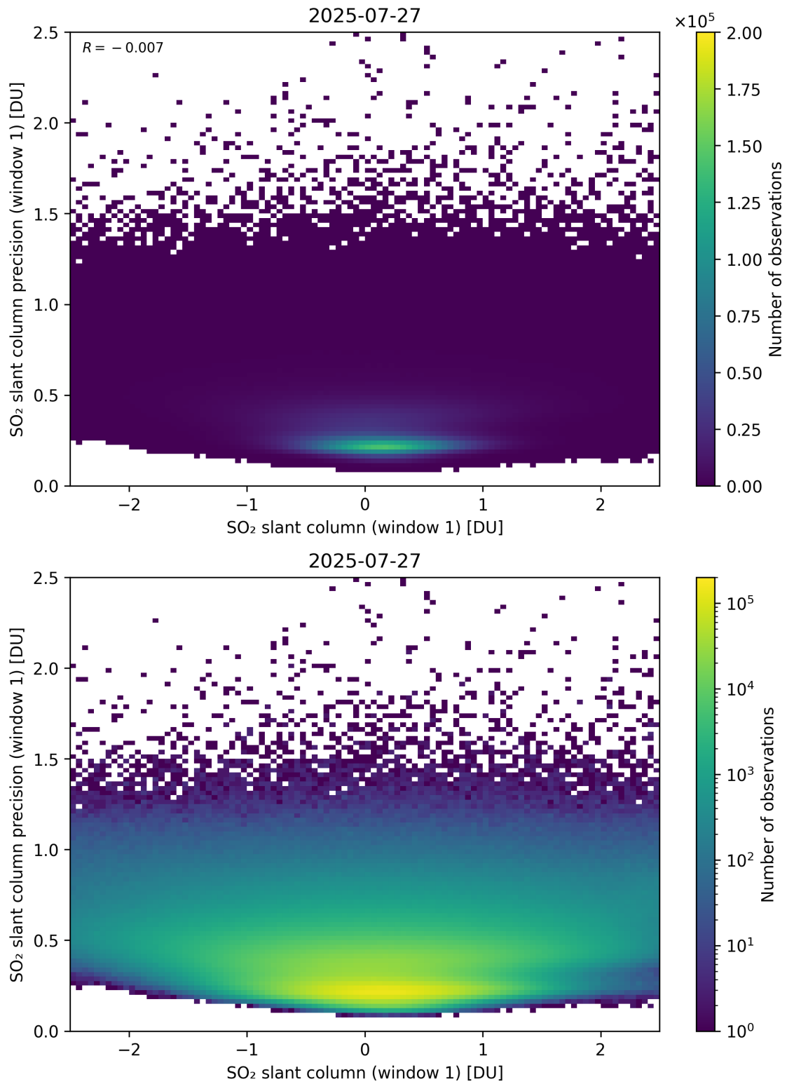
Figure 285: Scatter density plot of “SO 2 slant column (window 1)” against “SO 2 slant column precision (window 1)” for 2025-07-26 to 2025-07-28.
