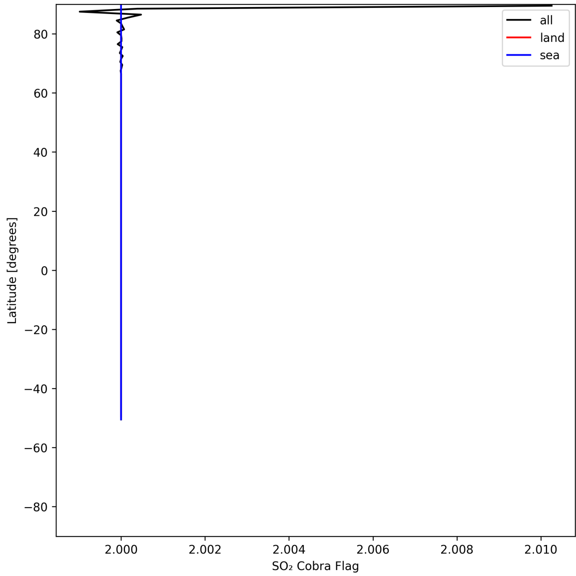
Figure 49: Zonal average of “SO 2 Cobra Flag” for 2025-07-26 to 2025-07-28.
