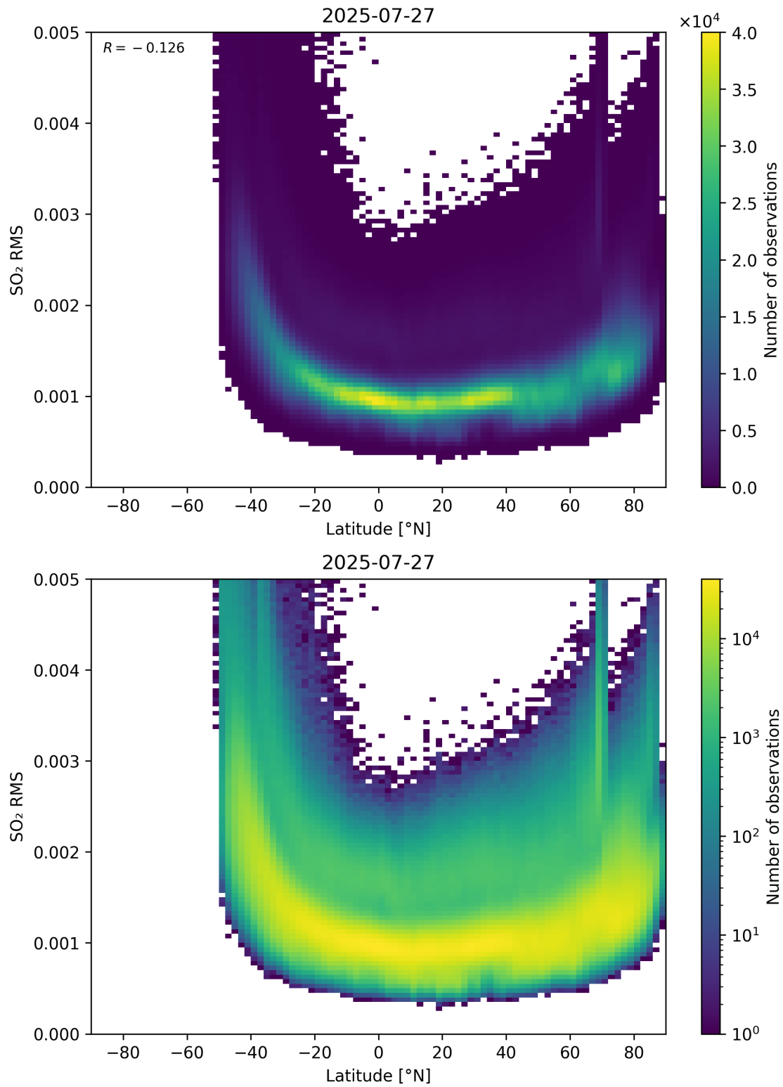
Figure 155: Scatter density plot of “Latitude” against “SO 2 RMS” for 2025-07-26 to 2025-07-28.
