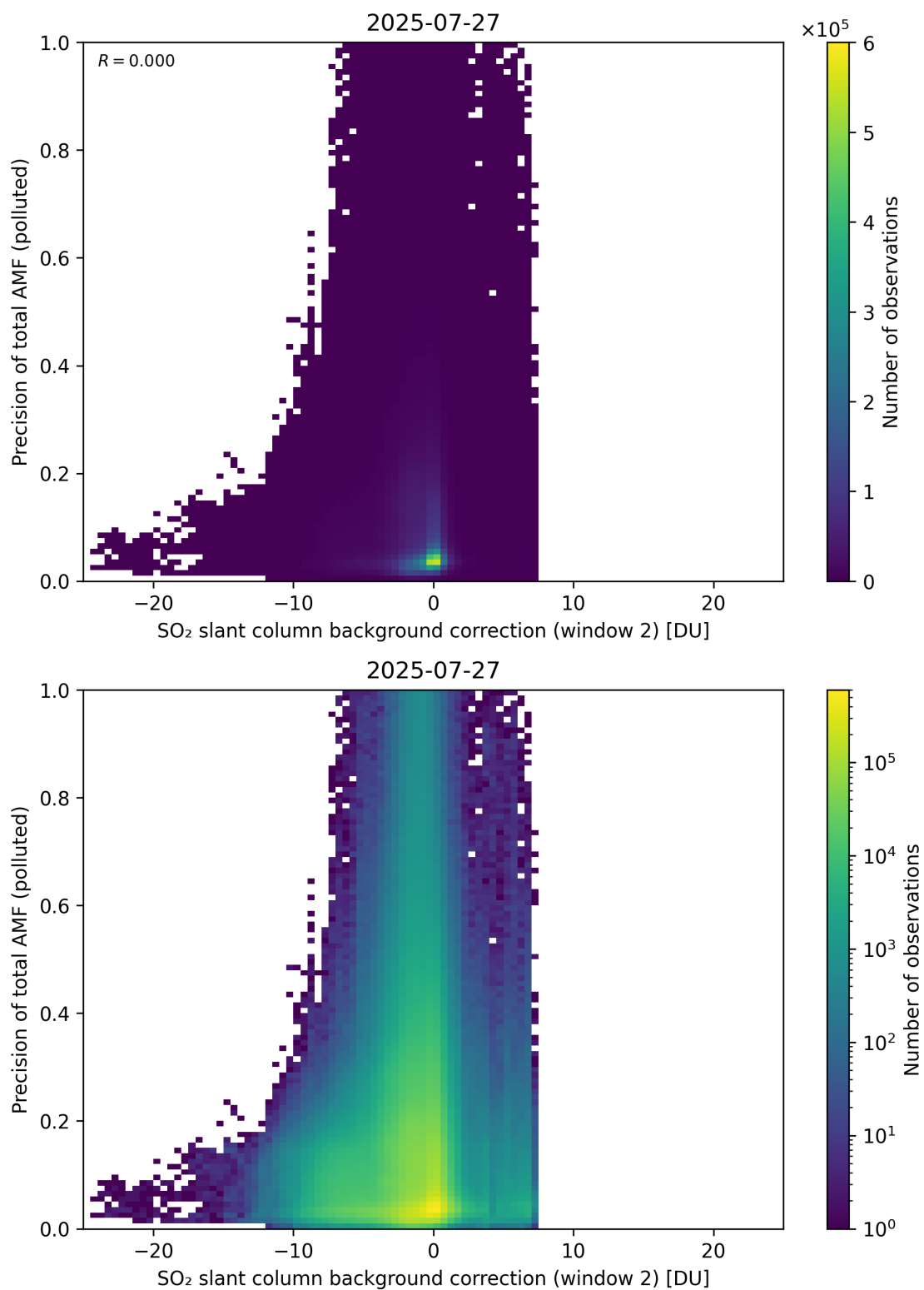
Figure 131: Scatter density plot of “SO 2 slant column background correction (window 2)” against “Precision of total AMF (polluted)” for 2025-07-26 to 2025-07-28.
