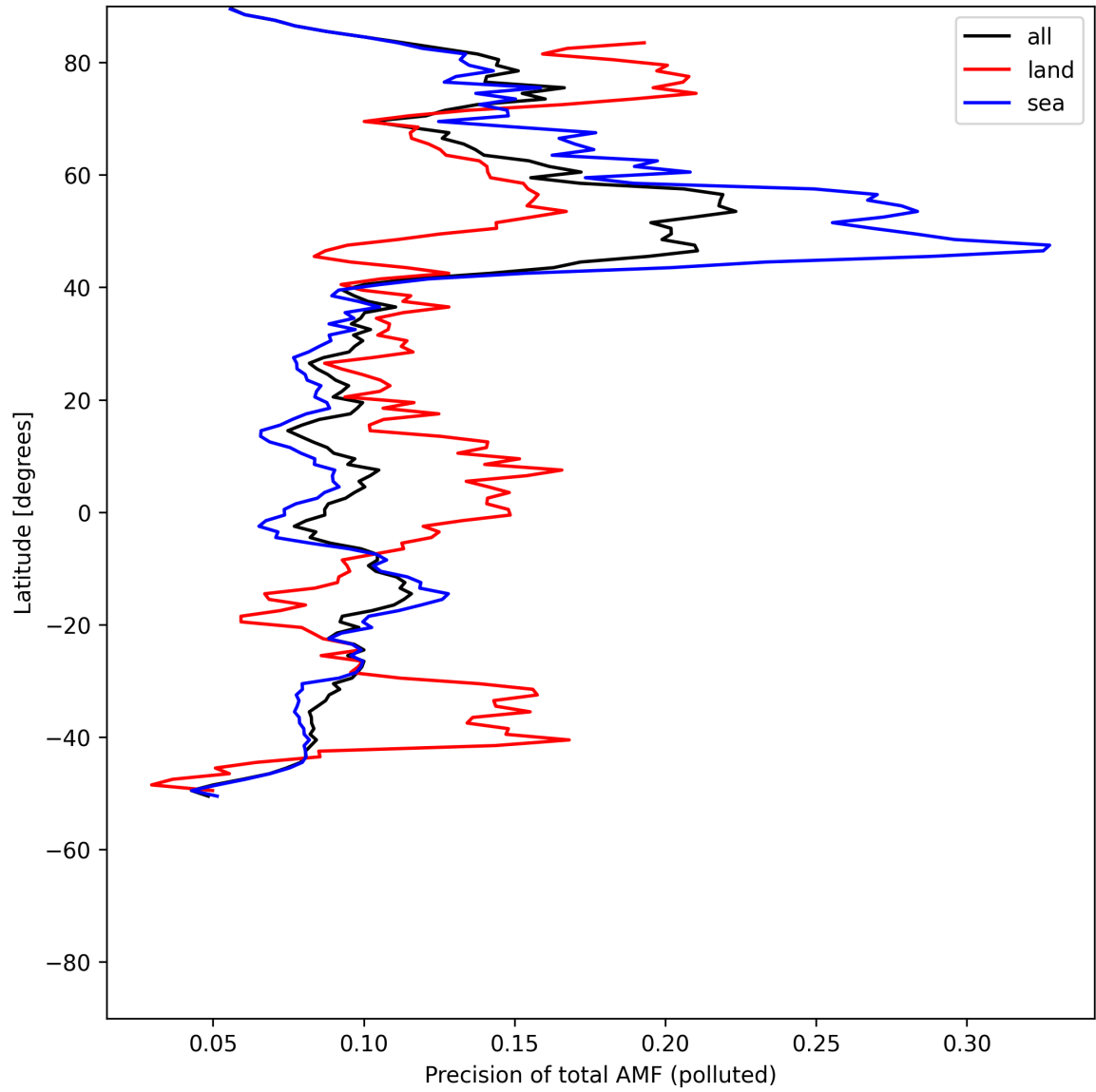
Figure 54: Zonal average of “Precision of total AMF (polluted)” for 2025-07-26 to 2025-07-28.
