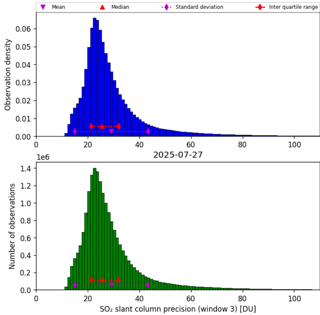
Figure 72: Histogram of “SO 2 slant column precision (window 3)” for 2025-07-26 to 2025-07-28
