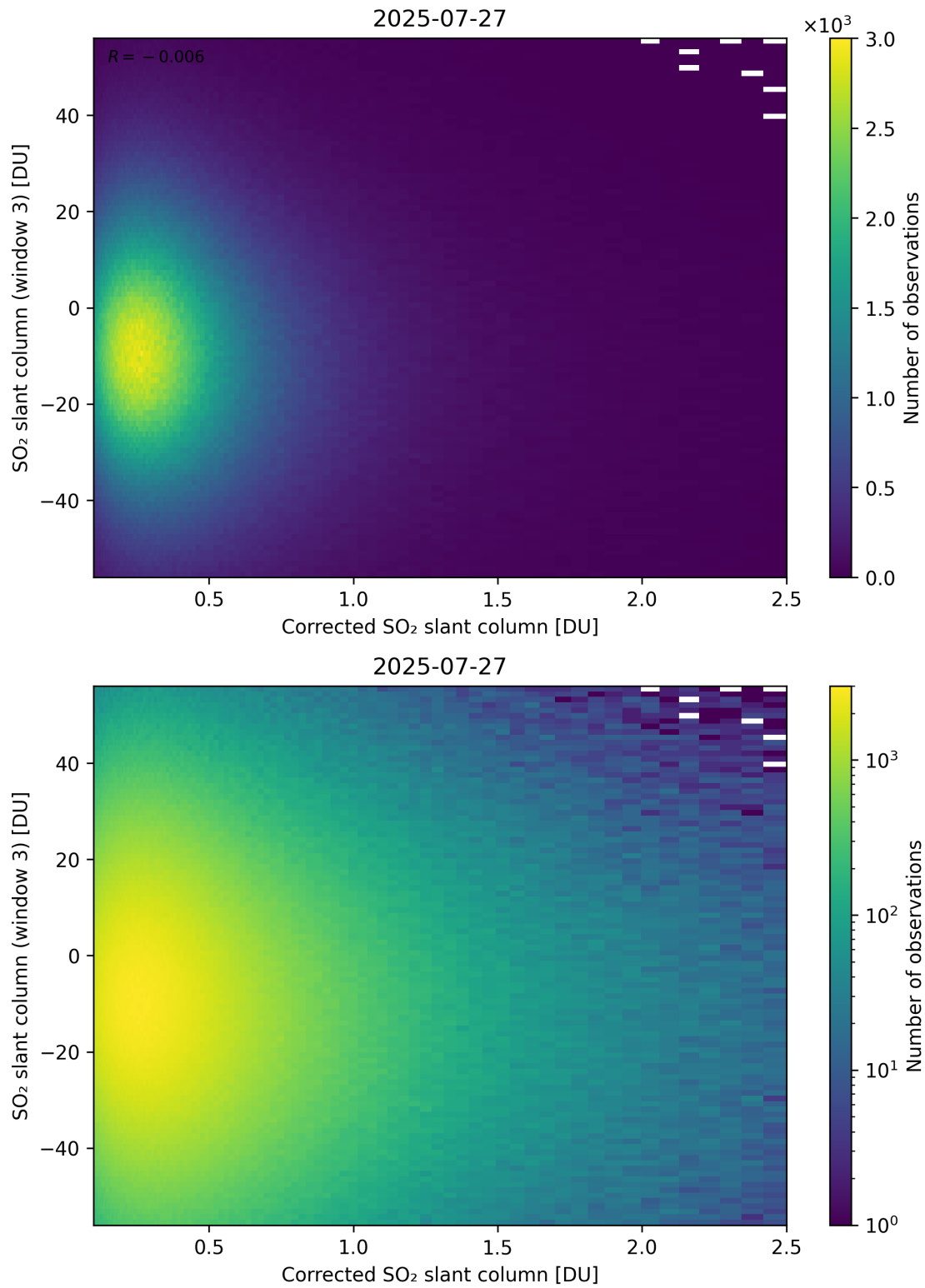
Figure 240: Scatter density plot of “Corrected SO 2 slant column” against “SO 2 slant column (window 3)” for 2025-07-26 to 2025-07-28.
