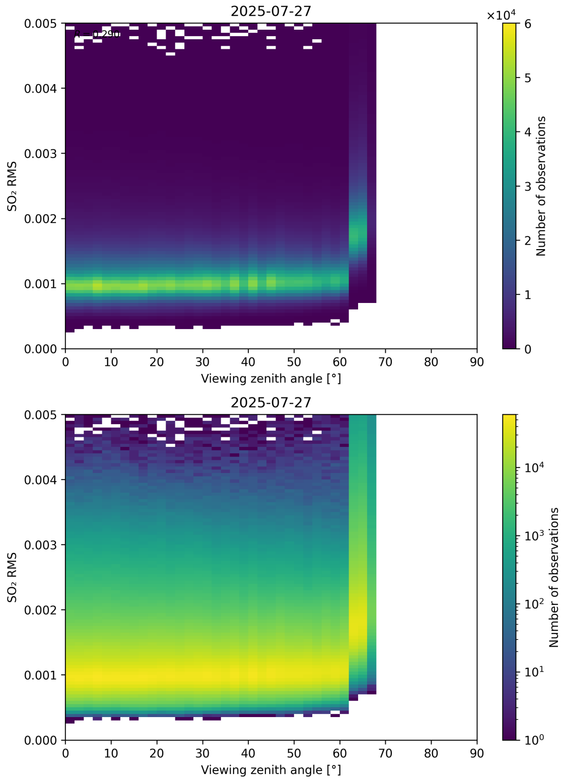
Figure 367: Scatter density plot of “Viewing zenith angle” against “SO 2 RMS” for 2025-07-26 to 2025-07-28.
