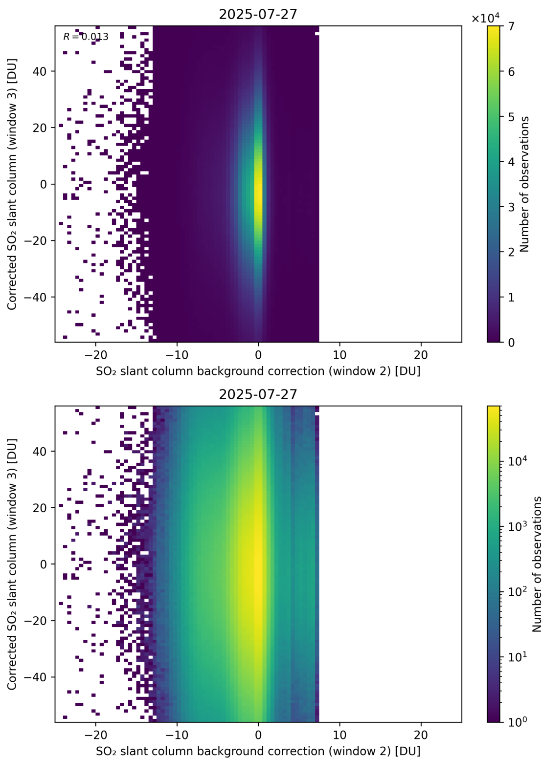
Figure 127: Scatter density plot of “SO 2 slant column background correction (window 2)” against “Corrected SO 2 slant column (window 3)” for 2025-07-26 to 2025-07-28.
