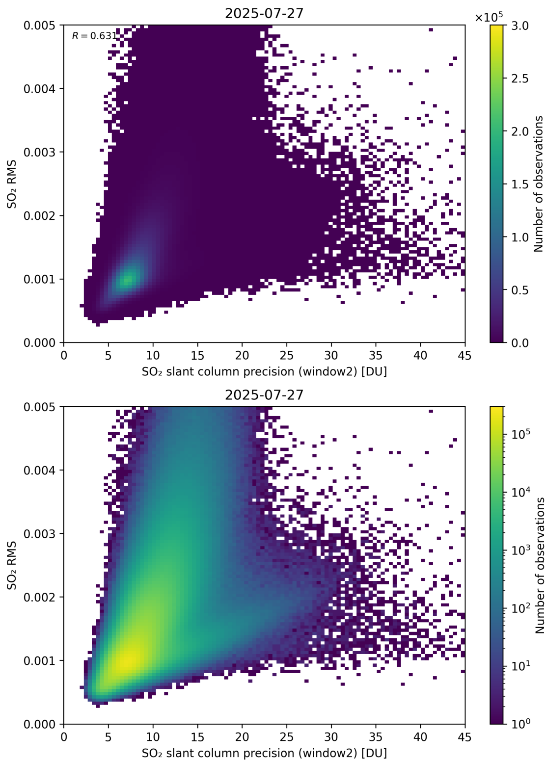
Figure 295: Scatter density plot of “SO 2 slant column precision (window2)” against “SO 2 RMS” for 2025-07-26 to 2025-07-28.
