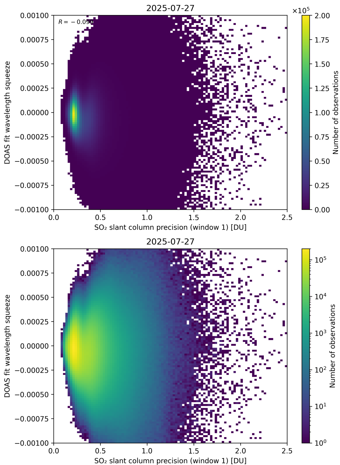
Figure 272: Scatter density plot of “SO 2 slant column precision (window 1)” against “DOAS fit wavelength squeeze” for 2025-07-26 to 2025-07-28.
