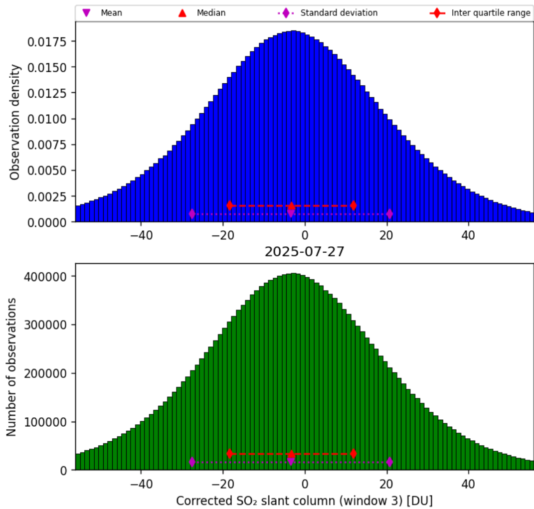
Figure 73: Histogram of “Corrected SO 2 slant column (window 3)” for 2025-07-26 to 2025-07-28
