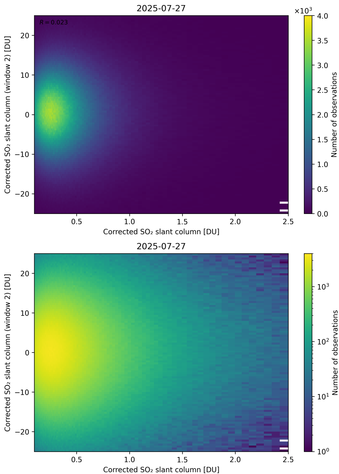
Figure 235: Scatter density plot of “Corrected SO 2 slant column” against “Corrected SO 2 slant column (window 2)” for 2025-07-26 to 2025-07-28.
