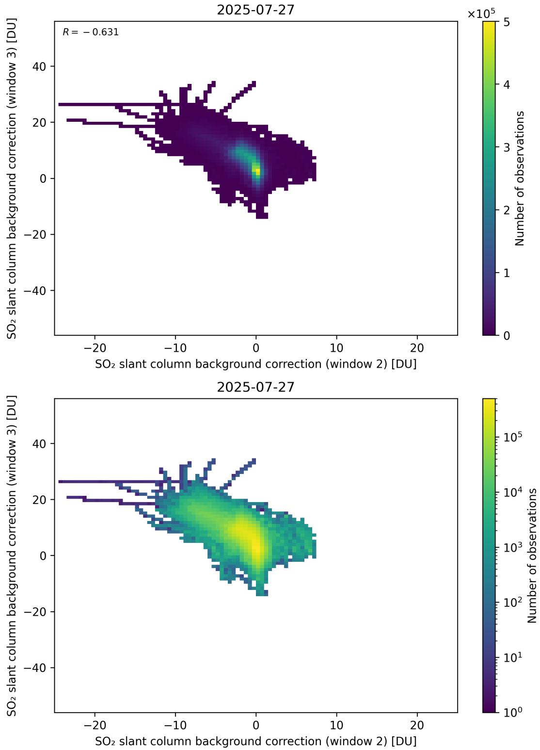
Figure 122: Scatter density plot of “SO 2 slant column background correction (window 2)” against “SO 2 slant column background correction (window 3)” for 2025-07-26 to 2025-07-28.
