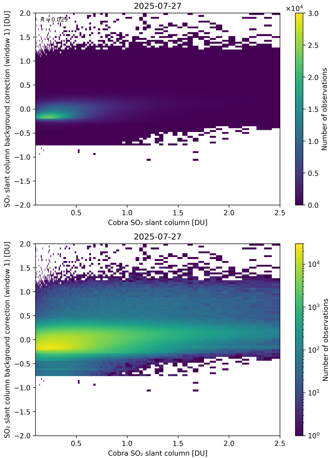
Figure 193: Scatter density plot of “Cobra SO 2 slant column” against “SO 2 slant column background correction (window 1)” for 2025-07-26 to 2025-07-28.
