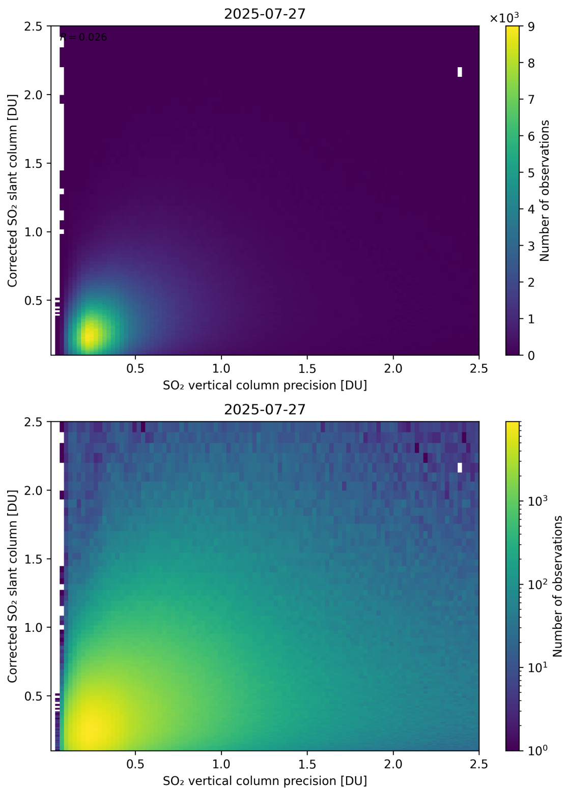
Figure 338: Scatter density plot of “SO 2 vertical column precision” against “Corrected SO 2 slant column” for 2025-07-26 to 2025-07-28.
