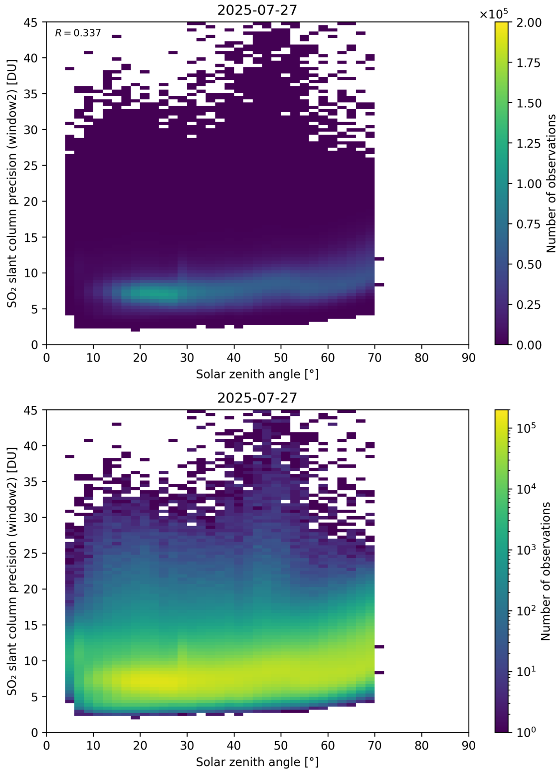
Figure 186: Scatter density plot of “Solar zenith angle” against “SO 2 slant column precision (window2)” for 2025-07-26 to 2025-07-28.
