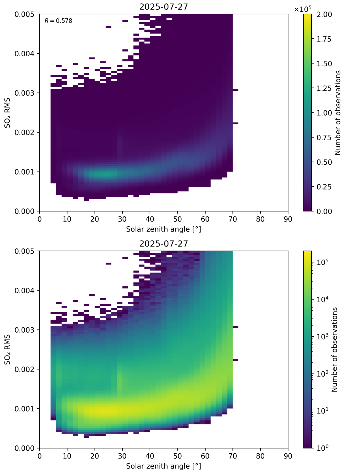
Figure 176: Scatter density plot of “Solar zenith angle” against “SO 2 RMS” for 2025-07-26 to 2025-07-28.
