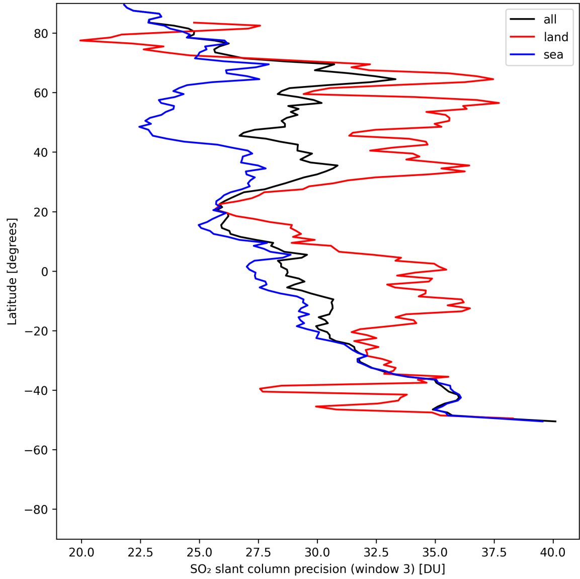
Figure 46: Zonal average of “SO 2 slant column precision (window 3)” for 2025-07-26 to 2025-07-28.
