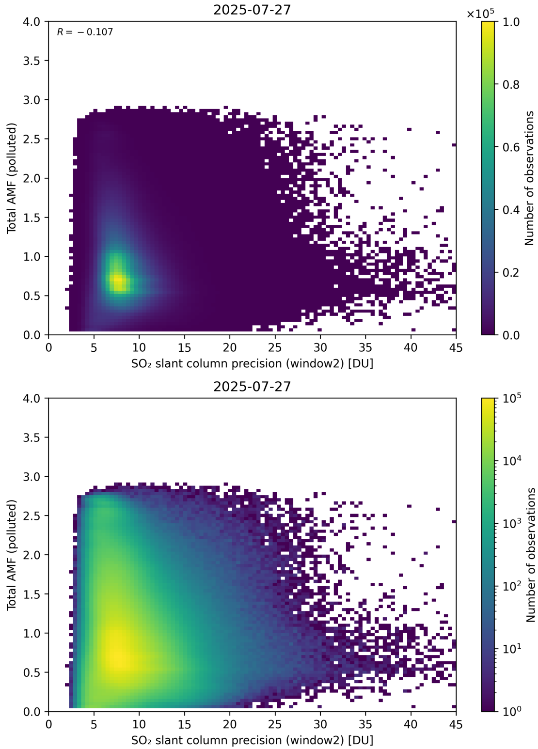
Figure 301: Scatter density plot of “SO 2 slant column precision (window2)” against “Total AMF (polluted)” for 2025-07-26 to 2025-07-28.
