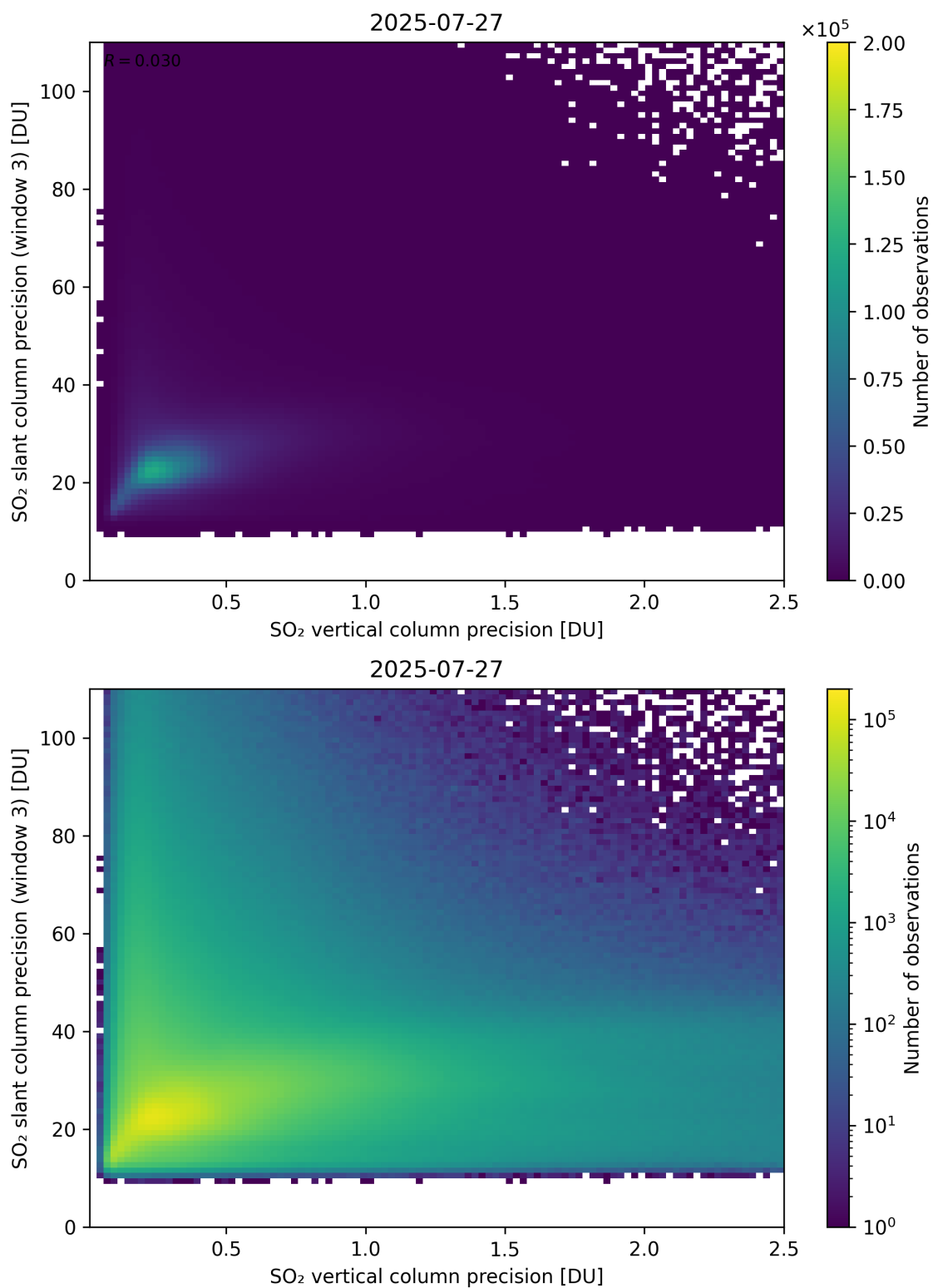
Figure 345: Scatter density plot of “SO 2 vertical column precision” against “SO 2 slant column precision (window 3)” for 2025-07-26 to 2025-07-28.
