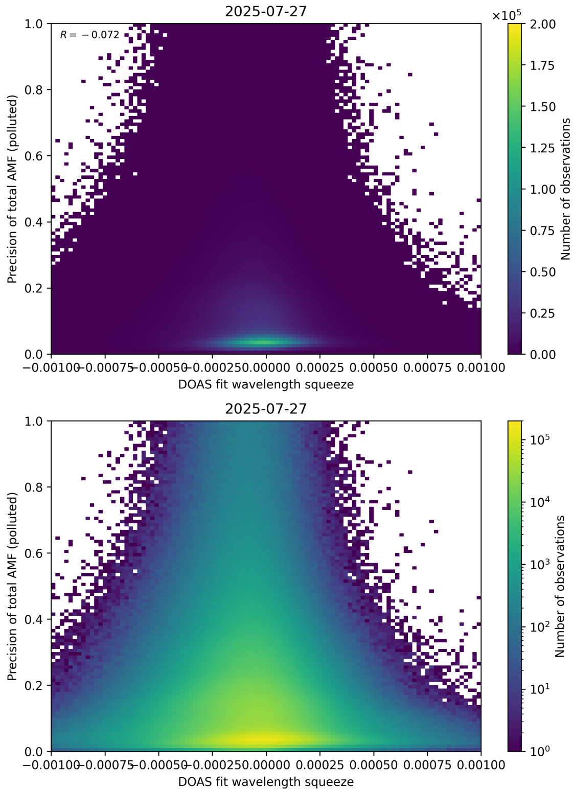
Figure 146: Scatter density plot of “DOAS fit wavelength squeeze” against “Precision of total AMF (polluted)” for 2025-07-26 to 2025-07-28.
