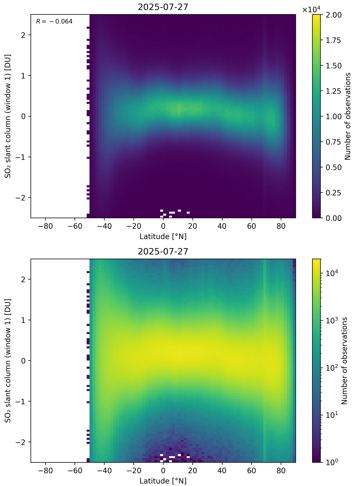
Figure 162: Scatter density plot of “Latitude” against “SO 2 slant column (window 1)” for 2025-07-26 to 2025-07-28.
