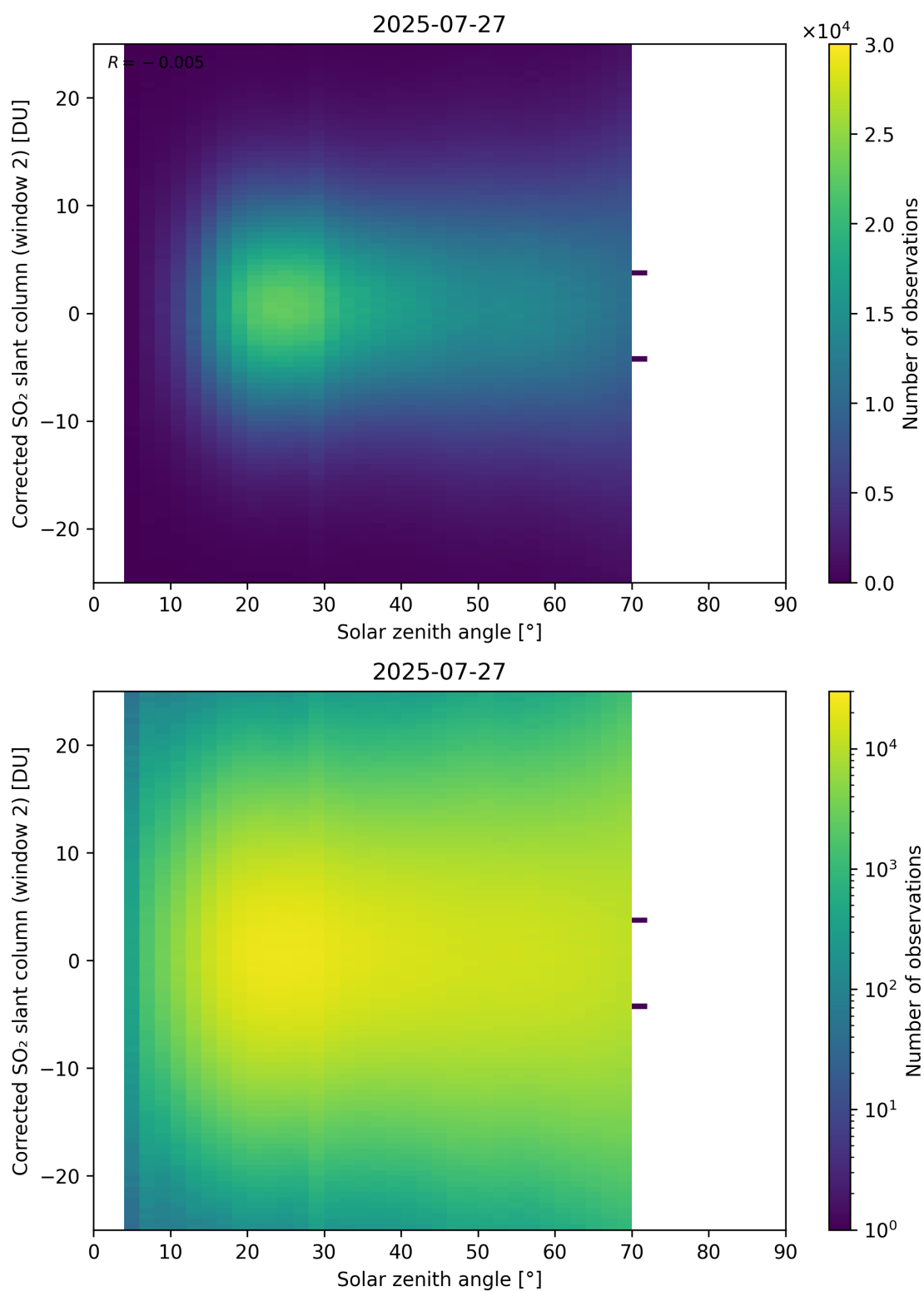
Figure 182: Scatter density plot of “Solar zenith angle” against “Corrected SO 2 slant column (window 2)” for 2025-07-26 to 2025-07-28.
