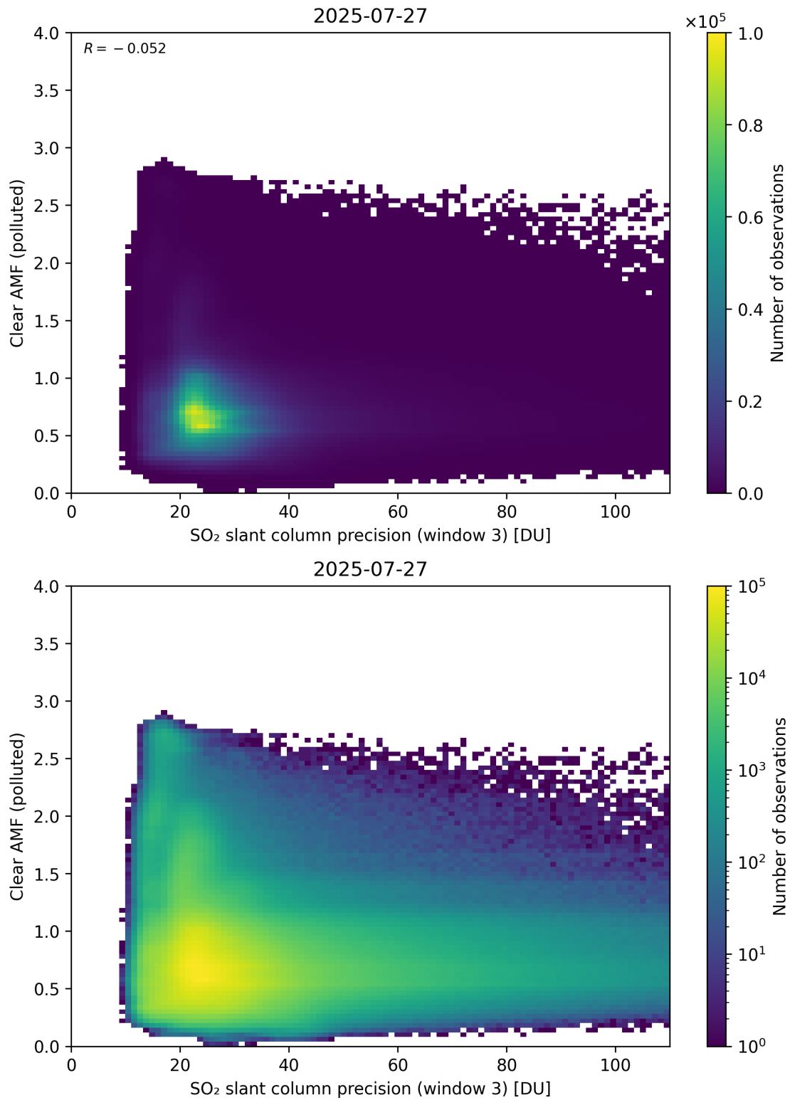
Figure 311: Scatter density plot of “SO 2 slant column precision (window 3)” against “Clear AMF (polluted)” for 2025-07-26 to 2025-07-28.
