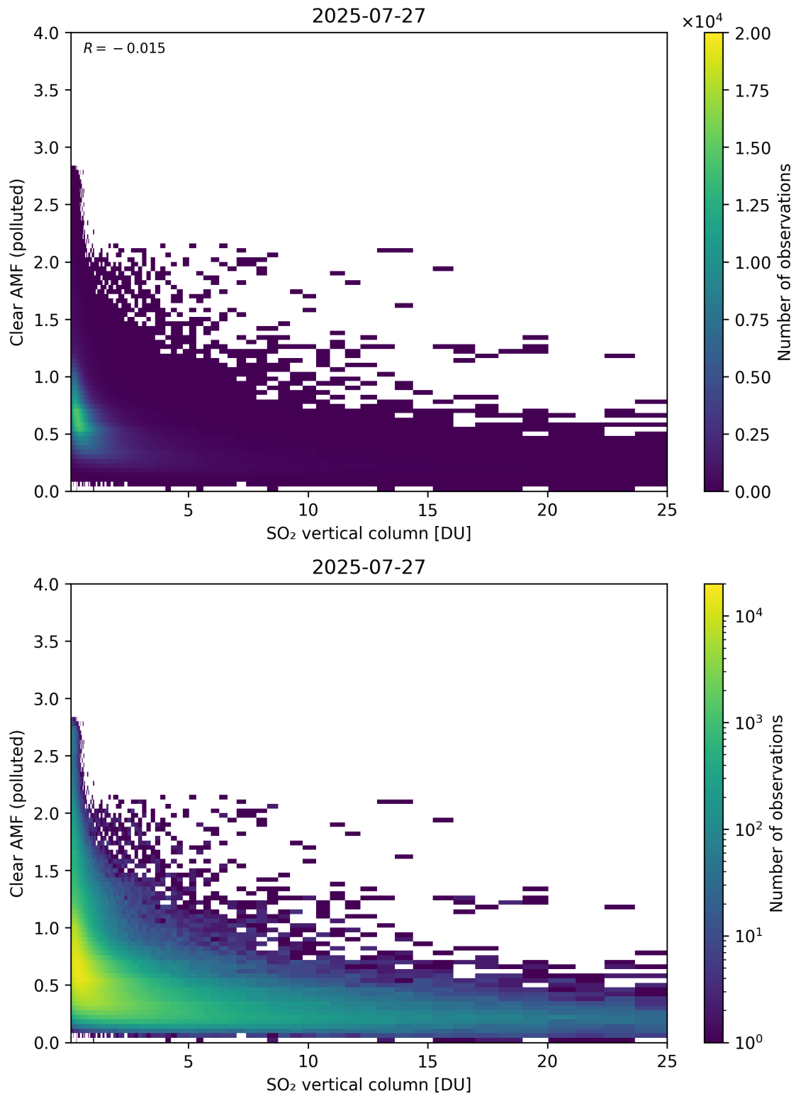
Figure 348: Scatter density plot of “SO 2 vertical column” against “Clear AMF (polluted)” for 2025-07-26 to 2025-07-28.
