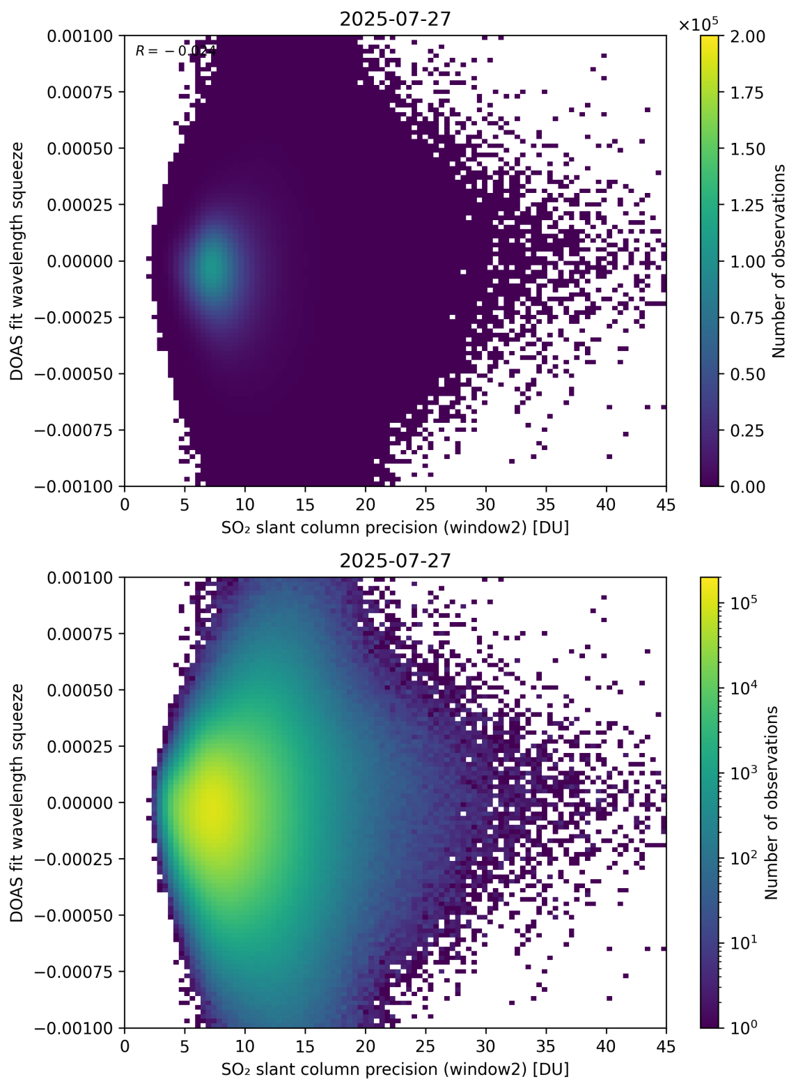
Figure 294: Scatter density plot of “SO 2 slant column precision (window2)” against “DOAS fit wavelength squeeze” for 2025-07-26 to 2025-07-28.
