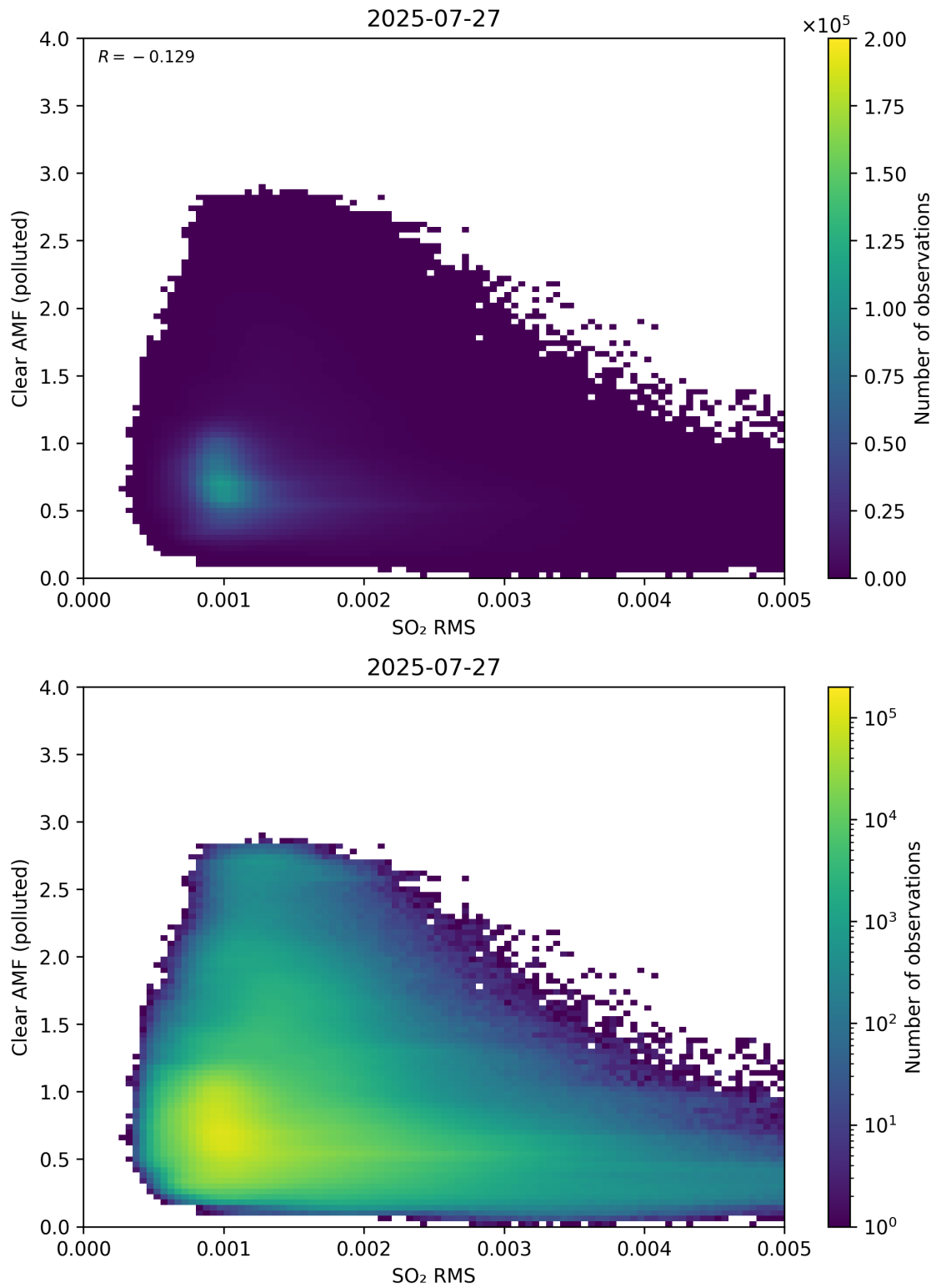
Figure 147: Scatter density plot of “SO 2 RMS” against “Clear AMF (polluted)” for 2025-07-26 to 2025-07-28.
