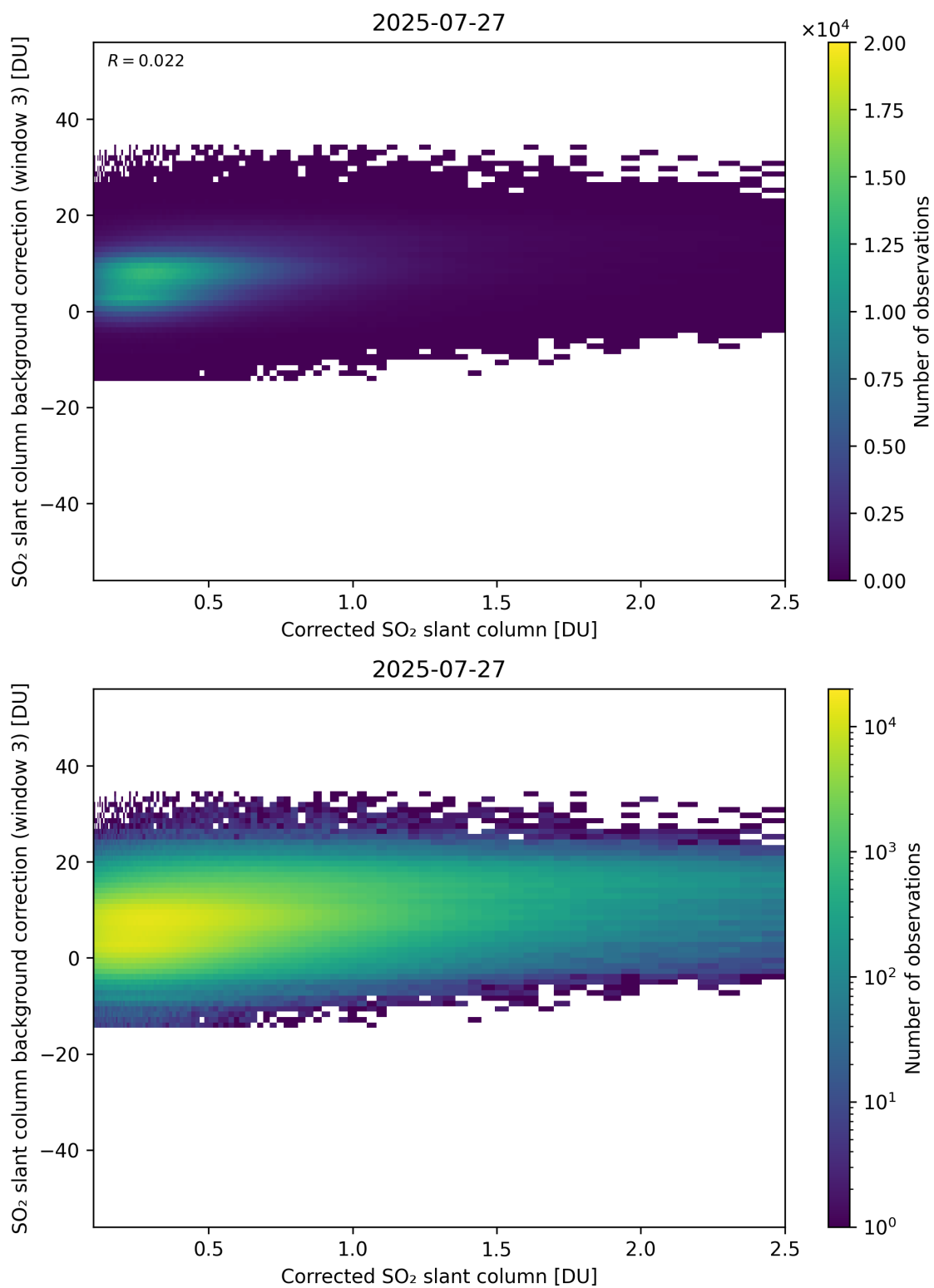
Figure 228: Scatter density plot of “Corrected SO 2 slant column” against “SO 2 slant column background correction (window 3)” for 2025-07-26 to 2025-07-28.
