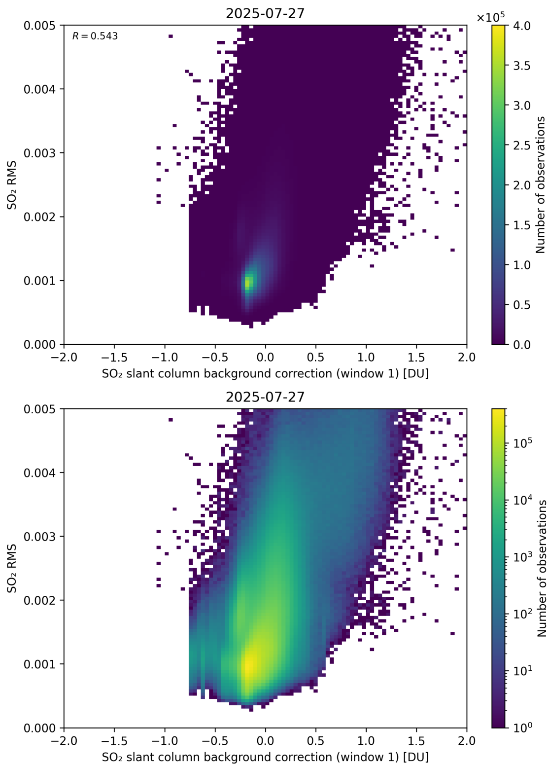
Figure 113: Scatter density plot of “SO 2 slant column background correction (window 1)” against “SO 2 RMS” for 2025-07-26 to 2025-07-28.
