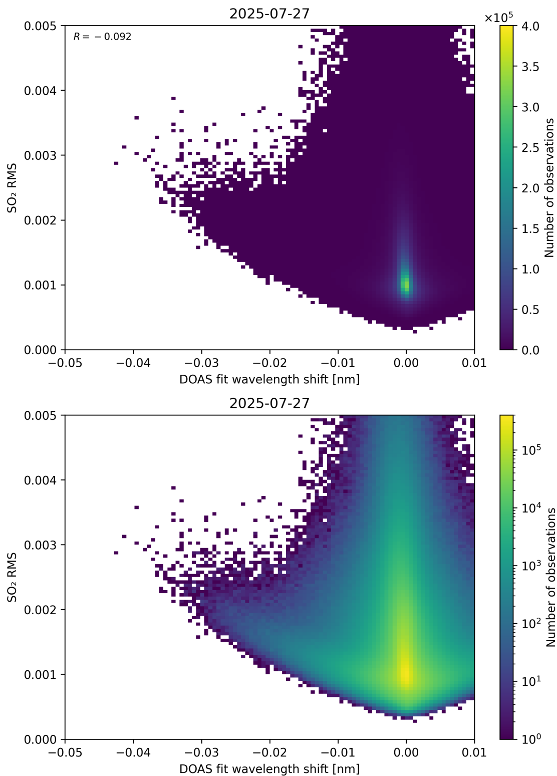
Figure 139: Scatter density plot of “DOAS fit wavelength shift” against “SO 2 RMS” for 2025-07-26 to 2025-07-28.
