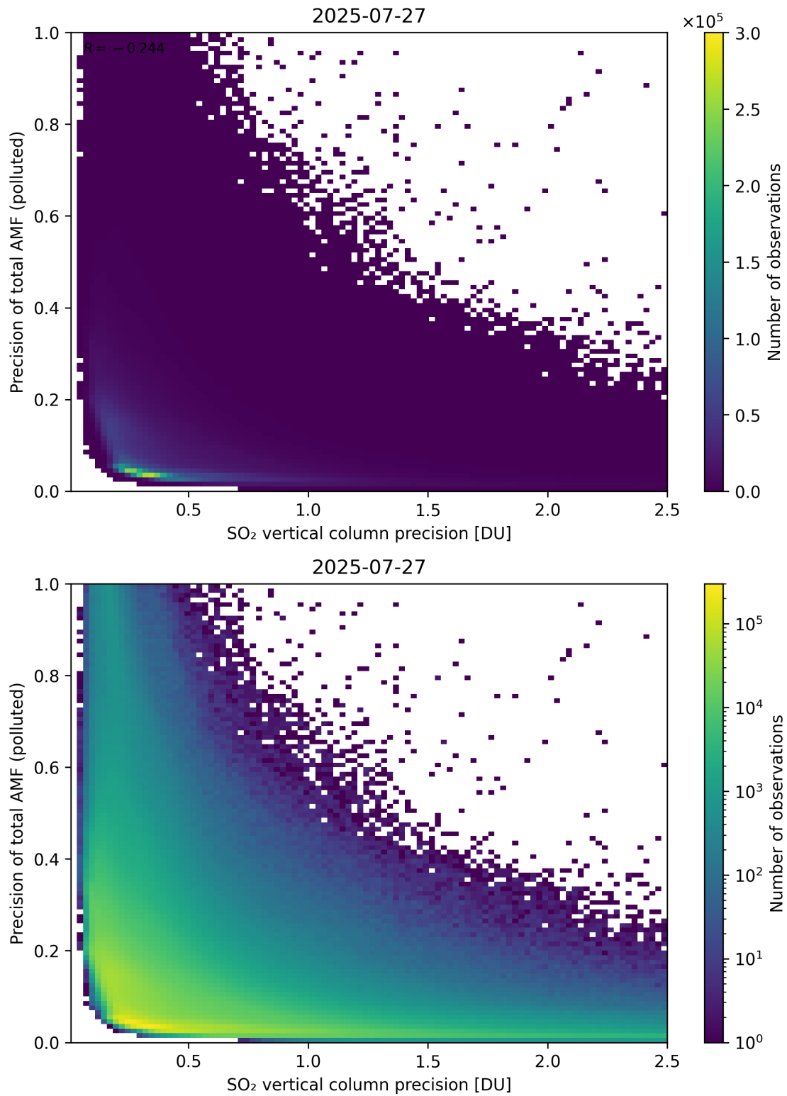
Figure 347: Scatter density plot of “SO 2 vertical column precision” against “Precision of total AMF (polluted)” for 2025-07-26 to 2025-07-28.
