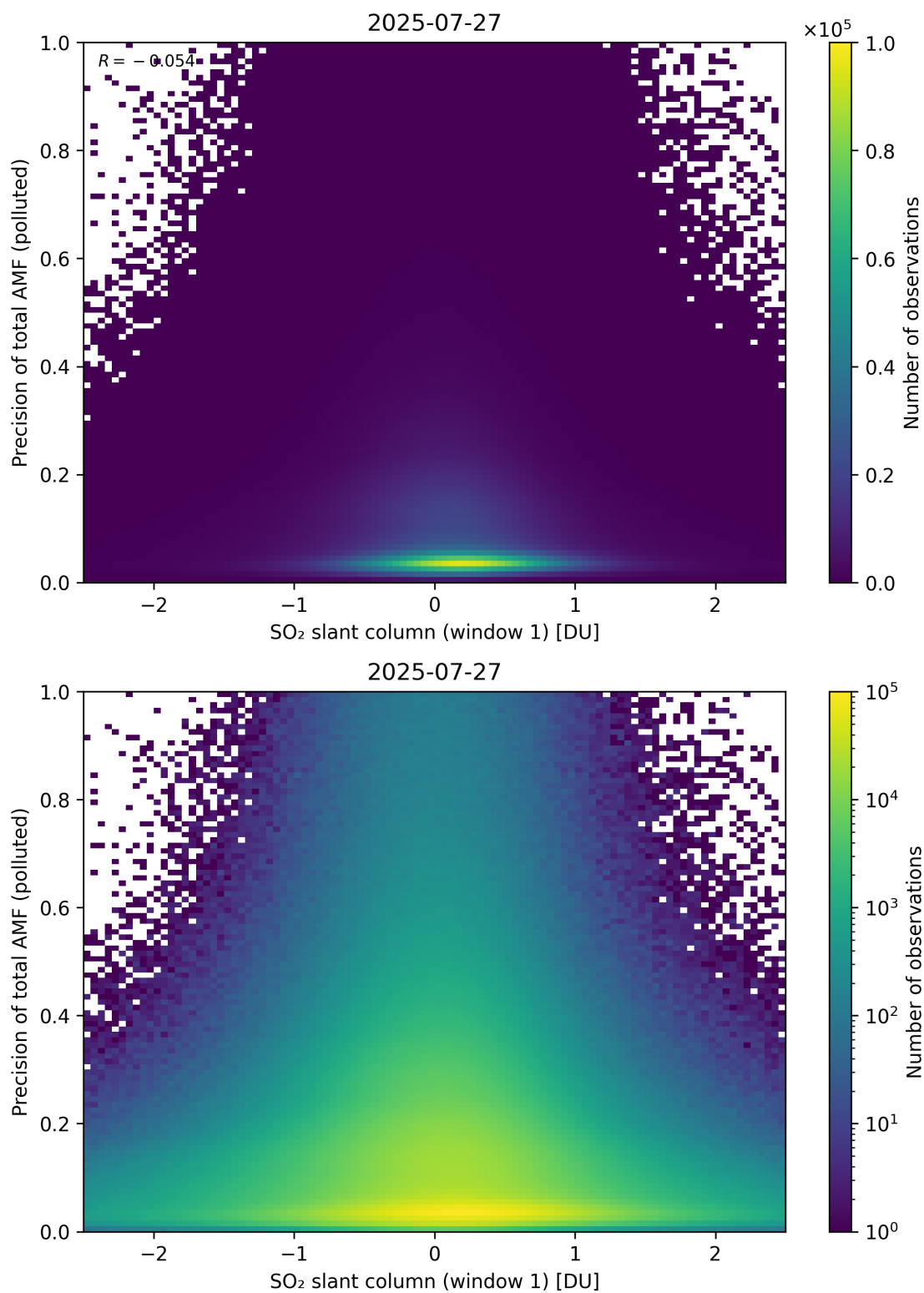
Figure 290: Scatter density plot of “SO 2 slant column (window 1)” against “Precision of total AMF (polluted)” for 2025-07-26 to 2025-07-28.
