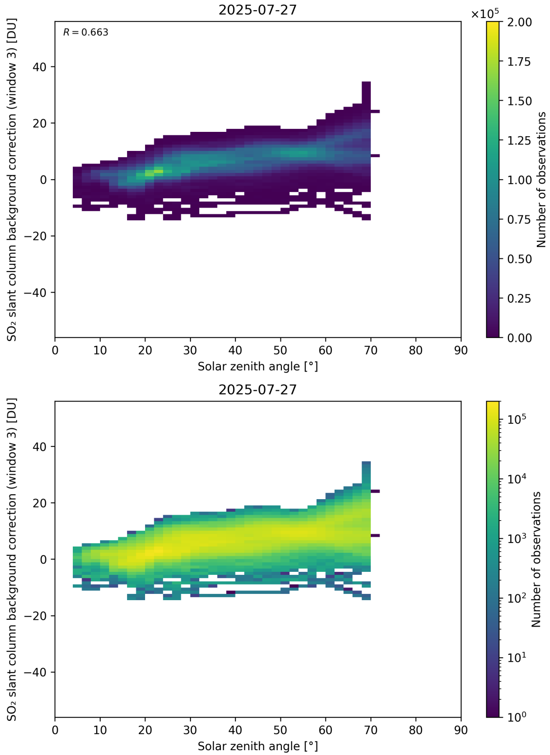
Figure 173: Scatter density plot of “Solar zenith angle” against “SO 2 slant column background correction (window 3)” for 2025-07-26 to 2025-07-28.
