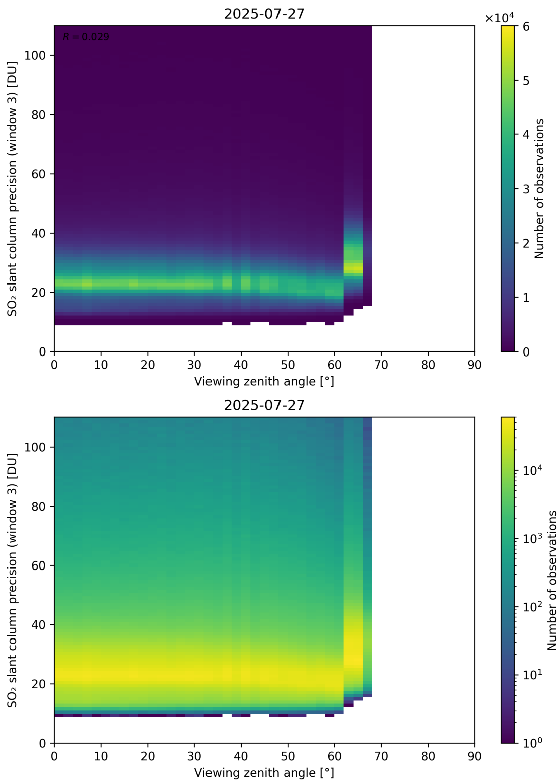
Figure 380: Scatter density plot of “Viewing zenith angle” against “SO 2 slant column precision (window 3)” for 2025-07-26 to 2025-07-28.
