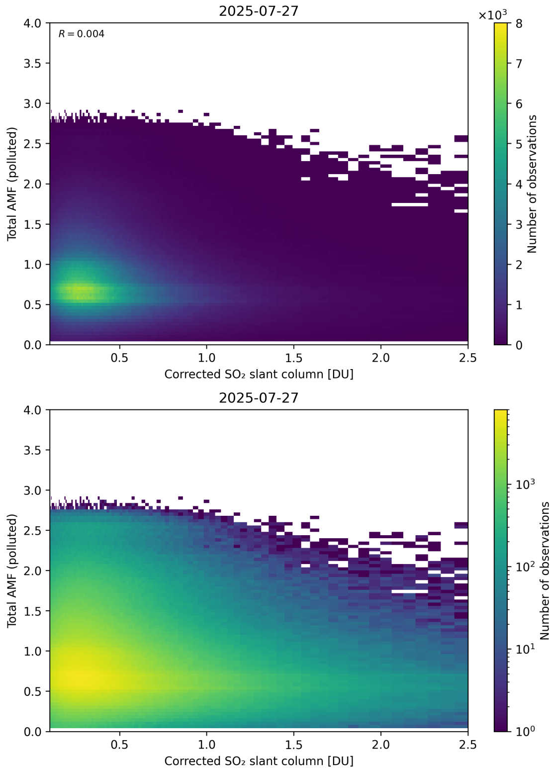
Figure 242: Scatter density plot of “Corrected SO 2 slant column” against “Total AMF (polluted)” for 2025-07-26 to 2025-07-28.
