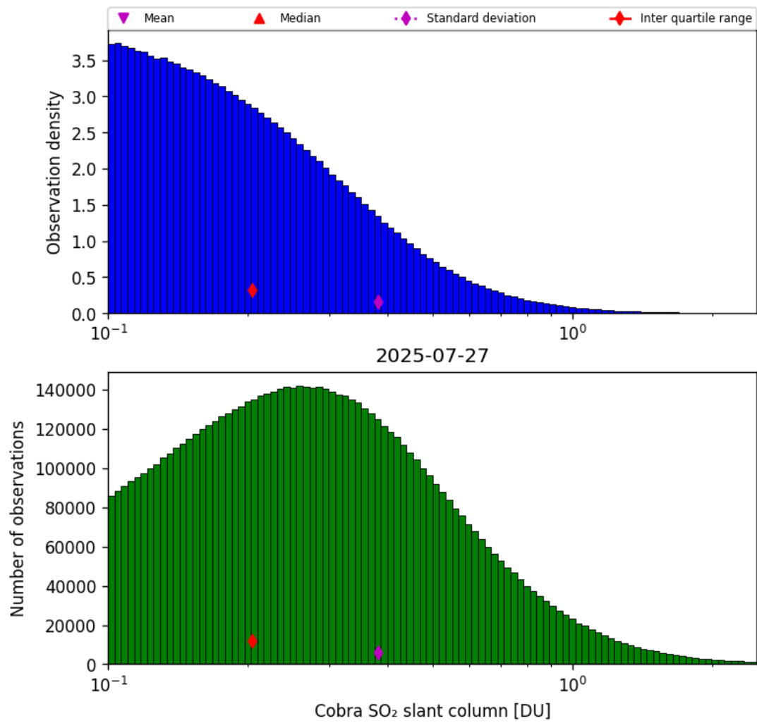
Figure 61: Histogram of “Cobra SO 2 slant column” for 2025-07-26 to 2025-07-28
