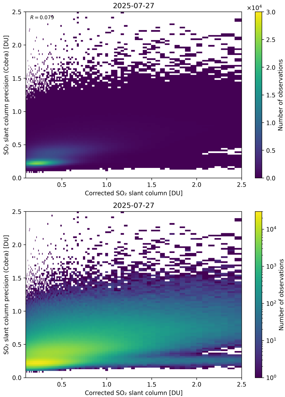
Figure 234: Scatter density plot of “Corrected SO 2 slant column” against “SO 2 slant column precision (Cobra)” for 2025-07-26 to 2025-07-28.
