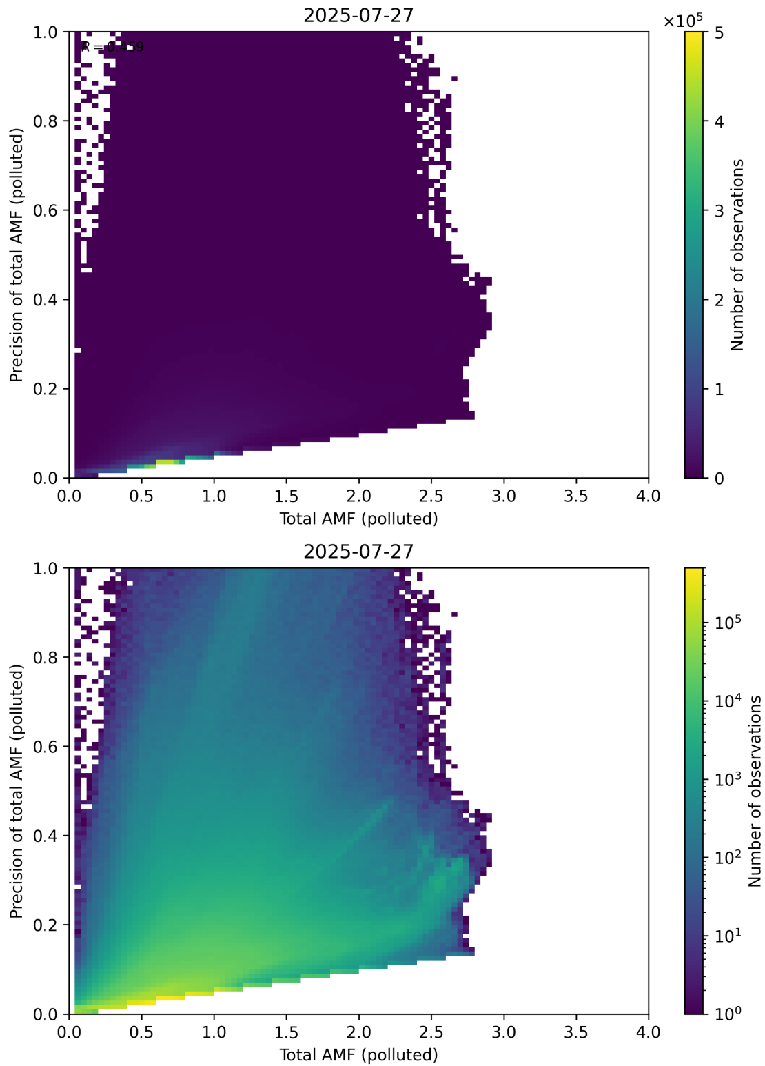
Figure 322: Scatter density plot of “Total AMF (polluted)” against “Precision of total AMF (polluted)” for 2025-07-26 to 2025-07-28.
