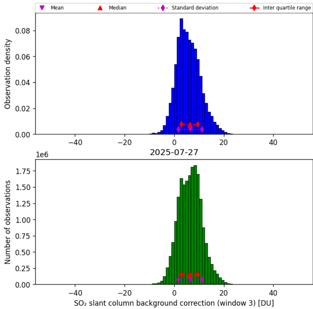
Figure 74: Histogram of “SO 2 slant column background correction (window 3)” for 2025-07-26 to 2025-07-28
