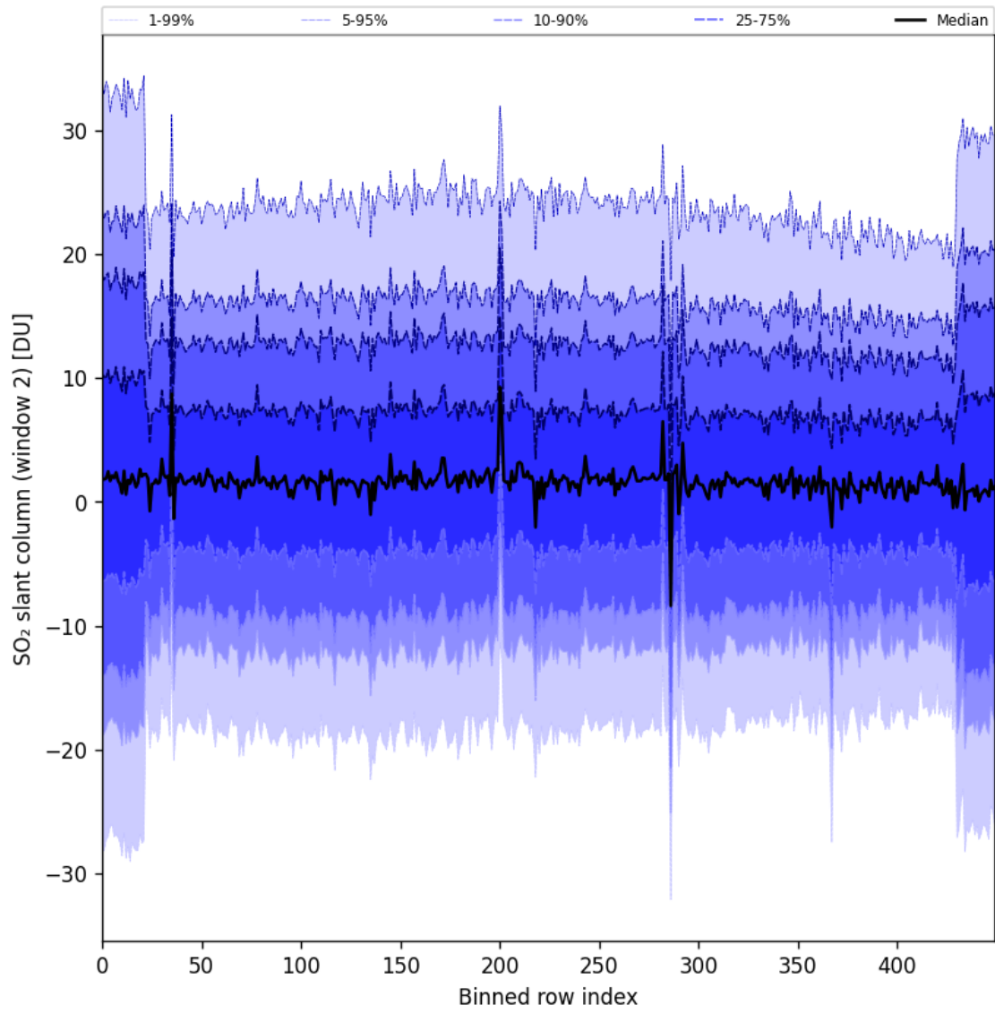
Figure 93: Along track statistics of “SO 2 slant column (window 2)” for 2025-07-26 to 2025-07-28
