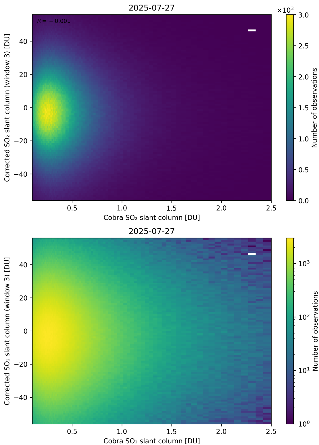
Figure 218: Scatter density plot of “Cobra SO 2 slant column” against “Corrected SO 2 slant column (window 3)” for 2025-07-26 to 2025-07-28.
