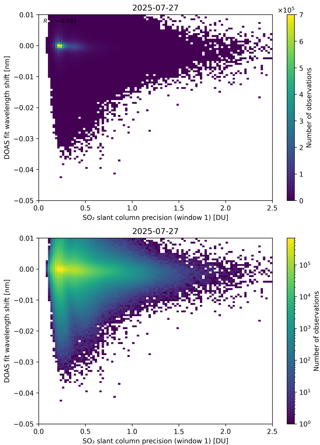
Figure 271: Scatter density plot of “SO 2 slant column precision (window 1)” against “DOAS fit wavelength shift” for 2025-07-26 to 2025-07-28.
