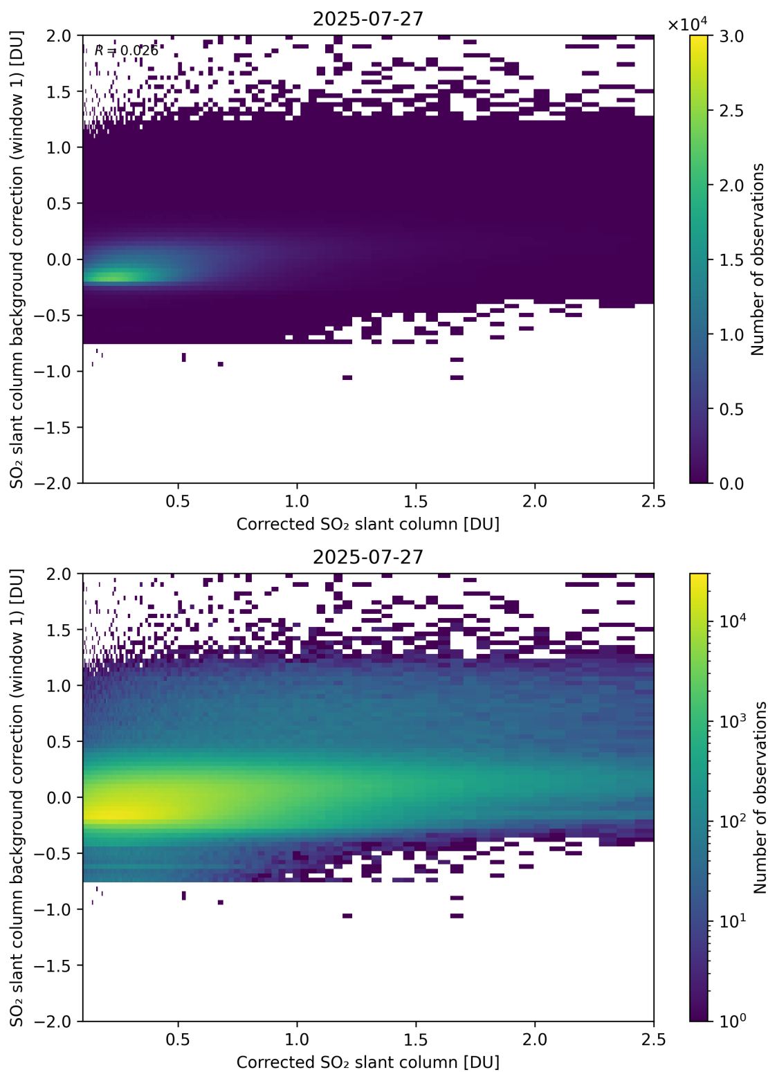
Figure 226: Scatter density plot of “Corrected SO 2 slant column” against “SO 2 slant column background correction (window 1)” for 2025-07-26 to 2025-07-28.
