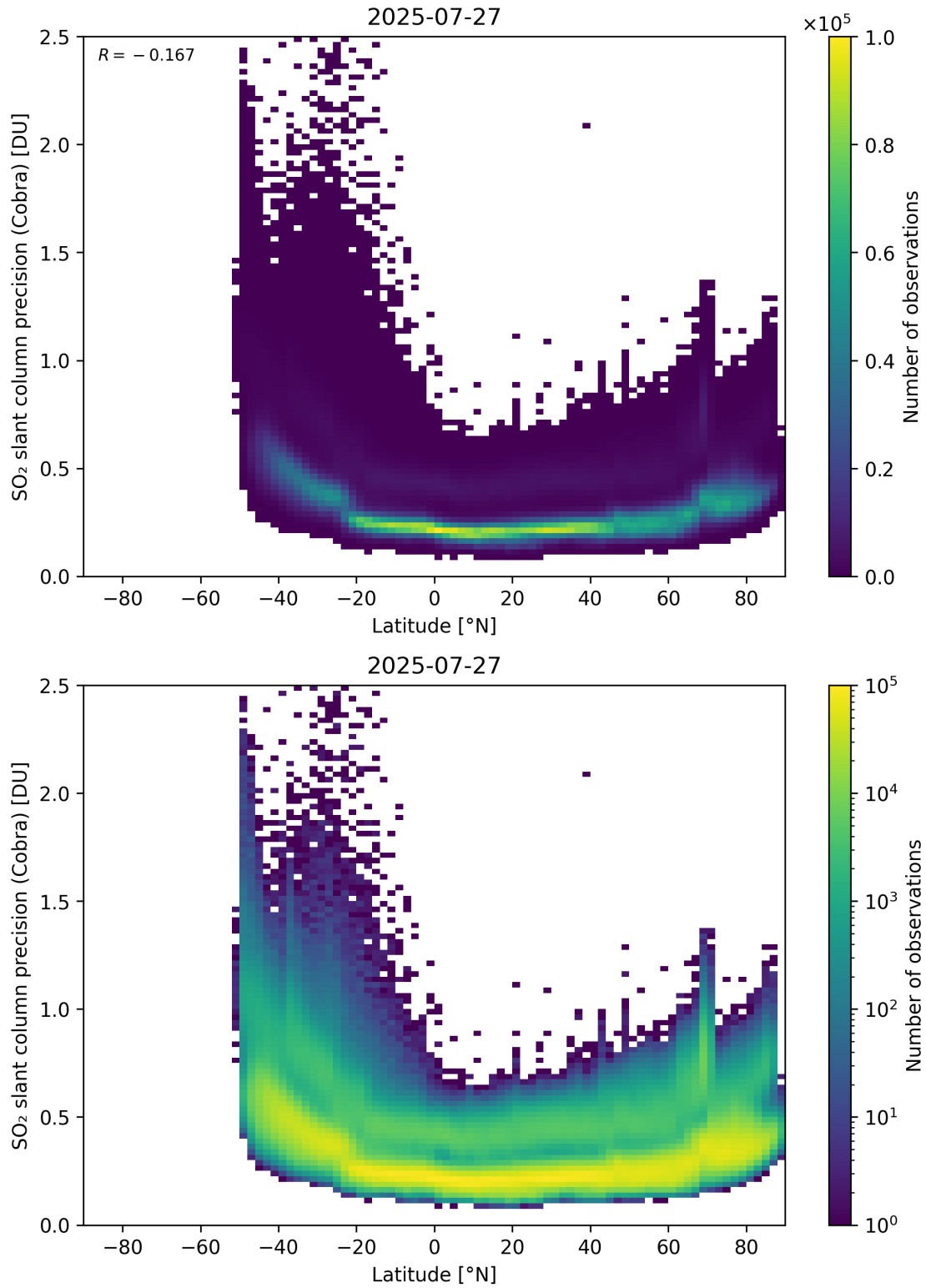
Figure 158: Scatter density plot of “Latitude” against “SO 2 slant column precision (Cobra)” for 2025-07-26 to 2025-07-28.
