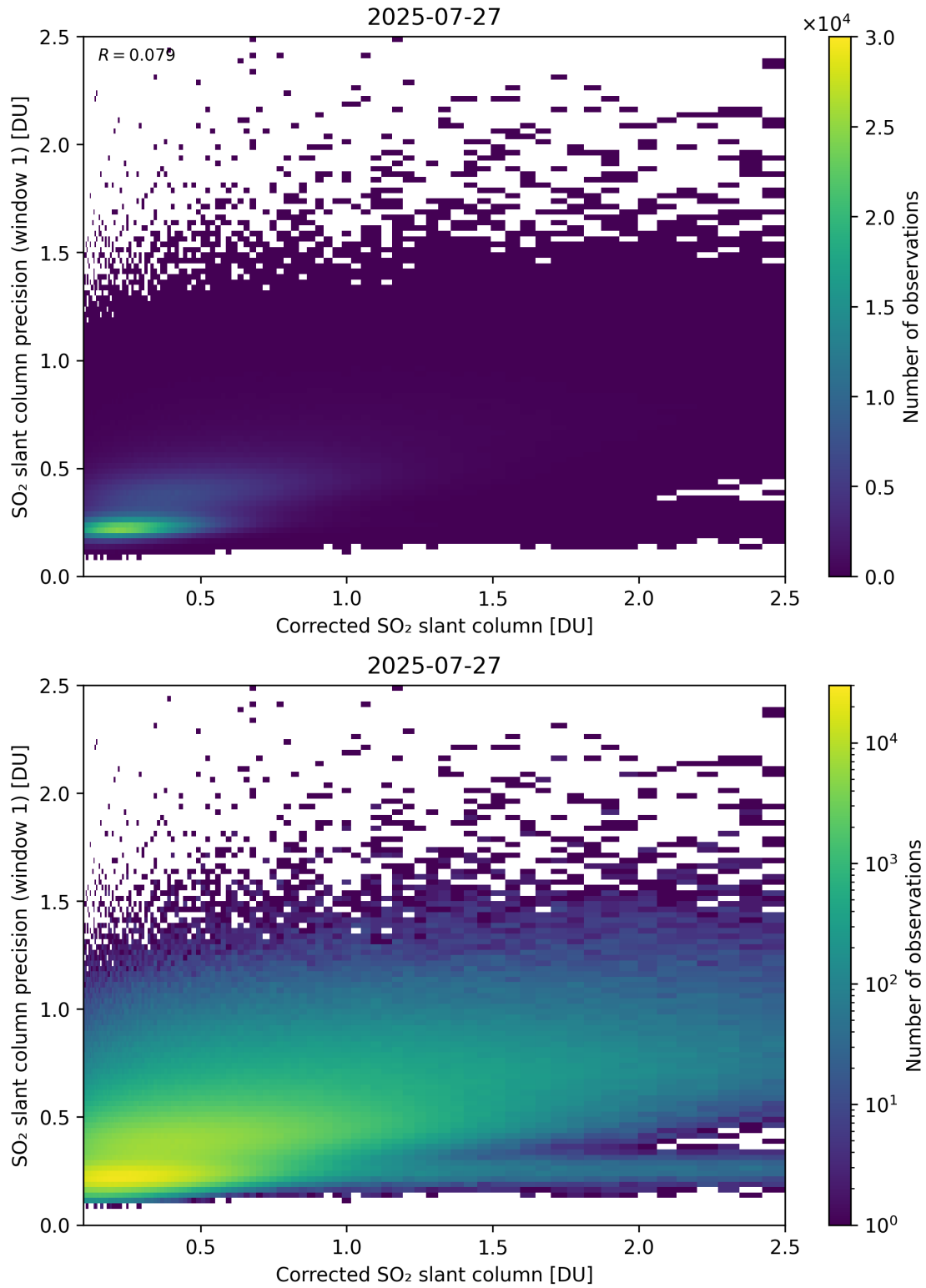
Figure 238: Scatter density plot of “Corrected SO 2 slant column” against “SO 2 slant column precision (window 1)” for 2025-07-26 to 2025-07-28.
