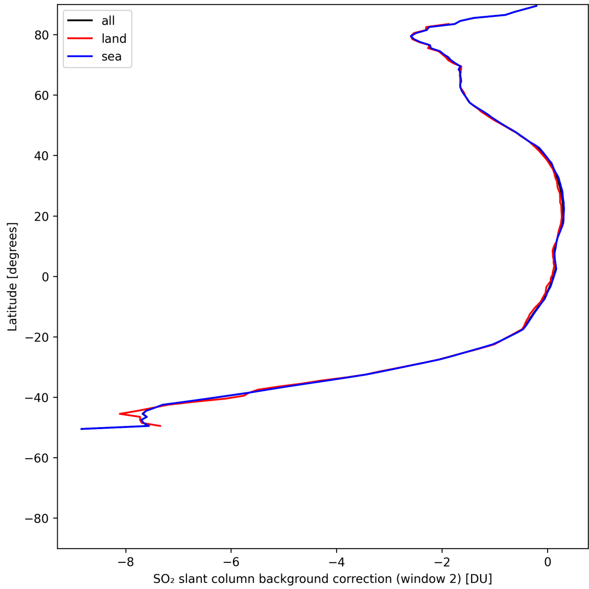
Figure 44: Zonal average of “SO 2 slant column background correction (window 2)” for 2025-07-26 to 2025-07-28.
