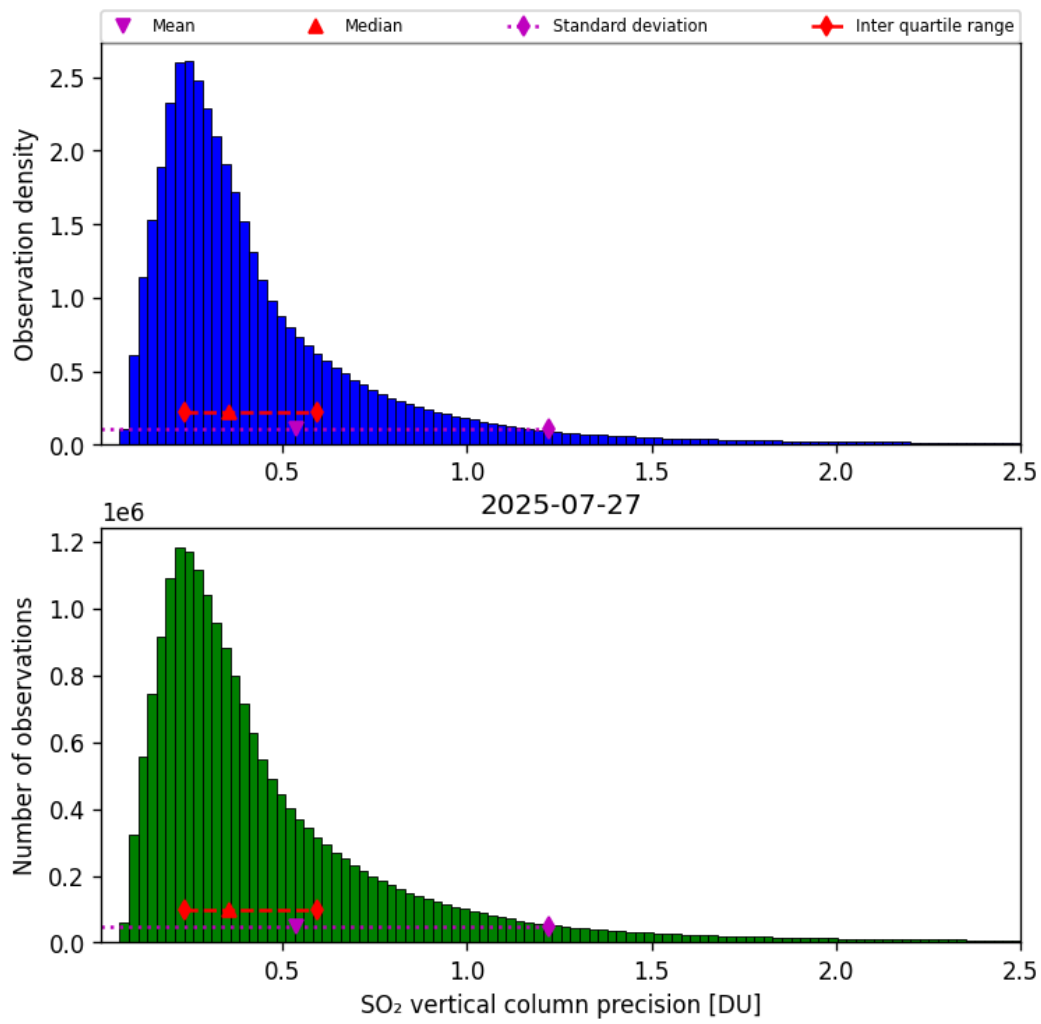
Figure 59: Histogram of “SO 2 vertical column precision” for 2025-07-26 to 2025-07-28
