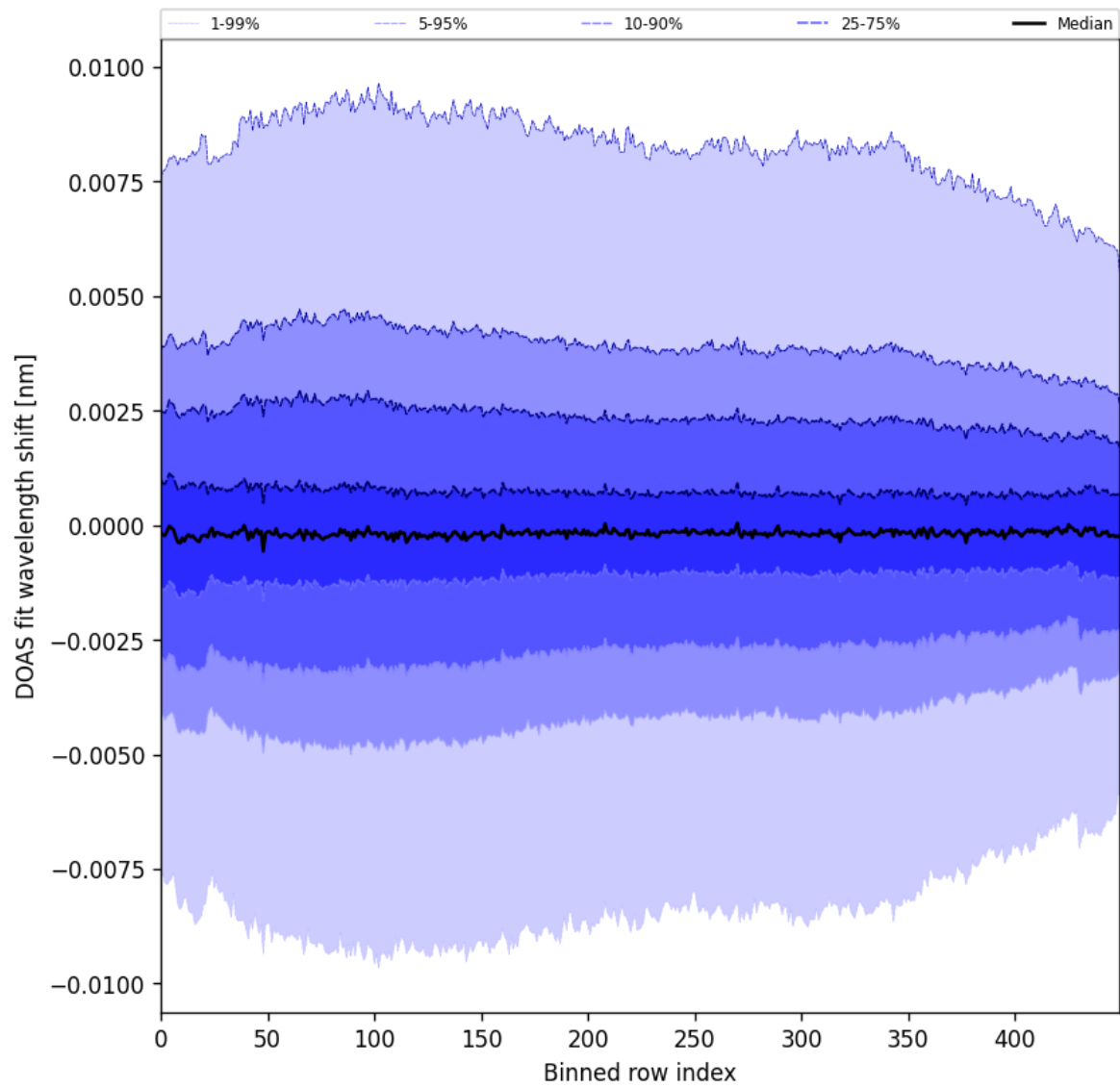
Figure 102: Along track statistics of “DOAS fit wavelength shift” for 2025-07-26 to 2025-07-28
