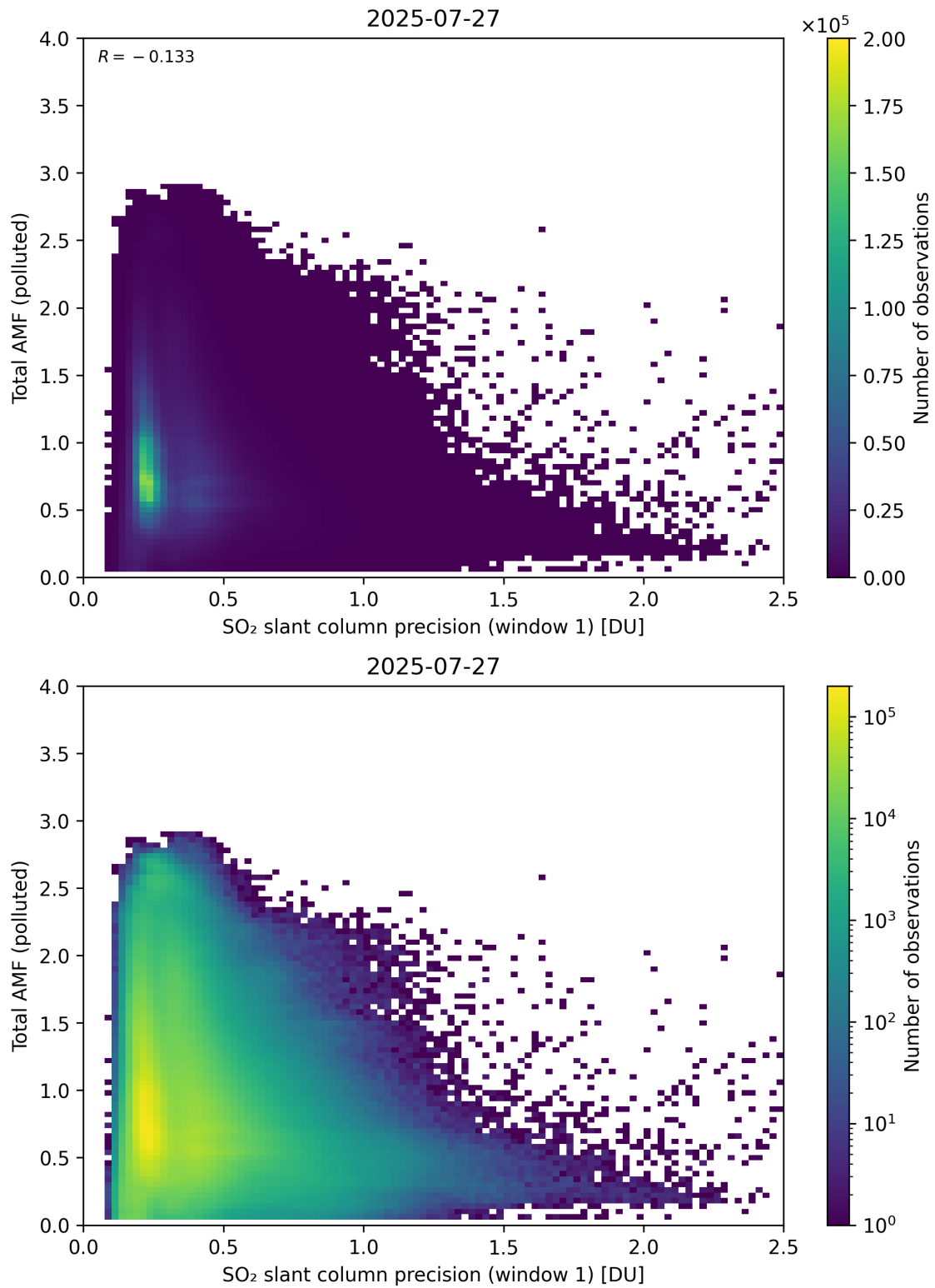
Figure 280: Scatter density plot of “SO 2 slant column precision (window 1)” against “Total AMF (polluted)” for 2025-07-26 to 2025-07-28.
