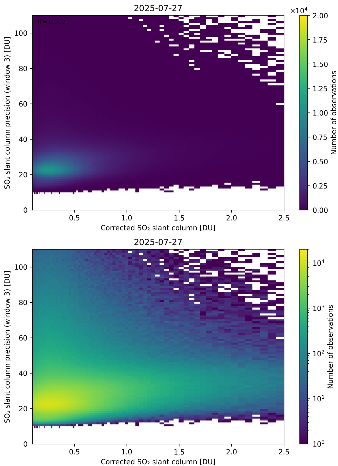
Figure 241: Scatter density plot of “Corrected SO 2 slant column” against “SO 2 slant column precision (window 3)” for 2025-07-26 to 2025-07-28.
