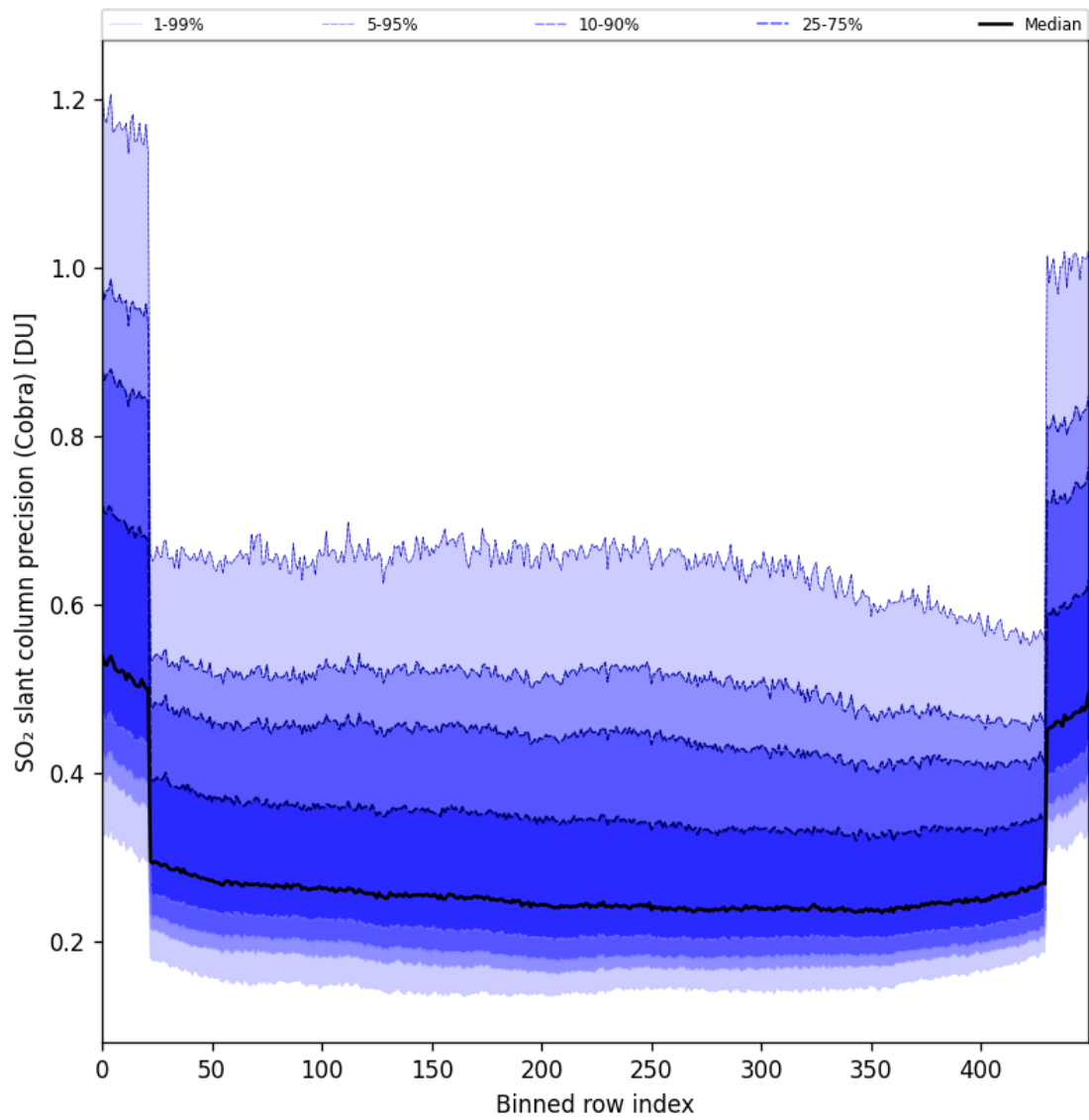
Figure 88: Along track statistics of “SO 2 slant column precision (Cobra)” for 2025-07-26 to 2025-07-28
