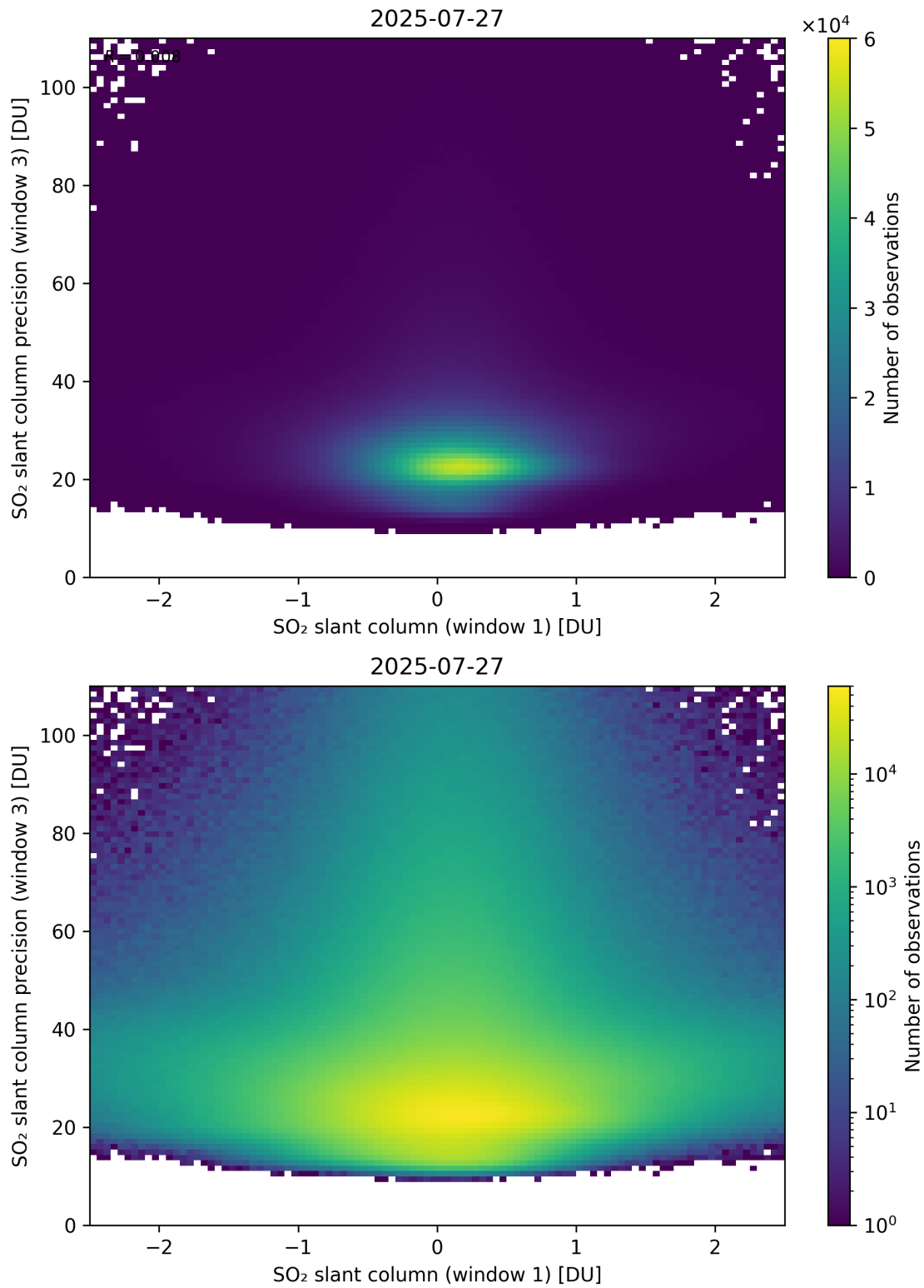
Figure 288: Scatter density plot of “SO 2 slant column (window 1)” against “SO 2 slant column precision (window 3)” for 2025-07-26 to 2025-07-28.
