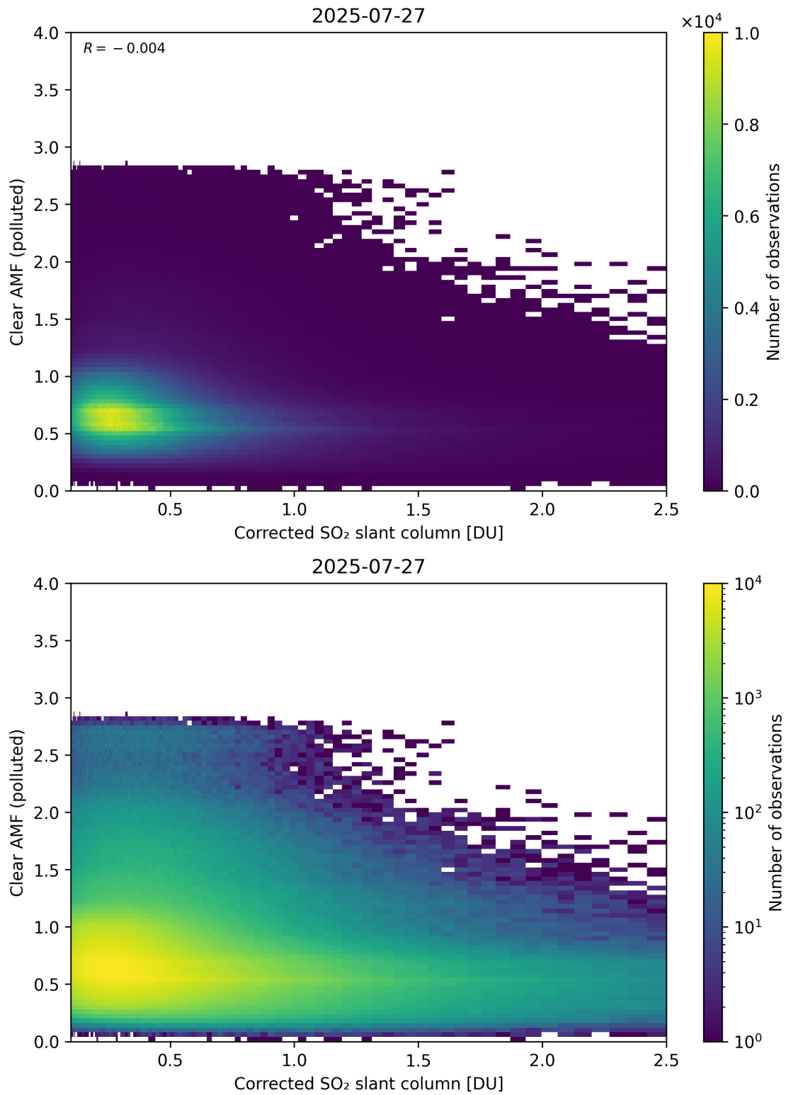
Figure 232: Scatter density plot of “Corrected SO 2 slant column” against “Clear AMF (polluted)” for 2025-07-26 to 2025-07-28.
