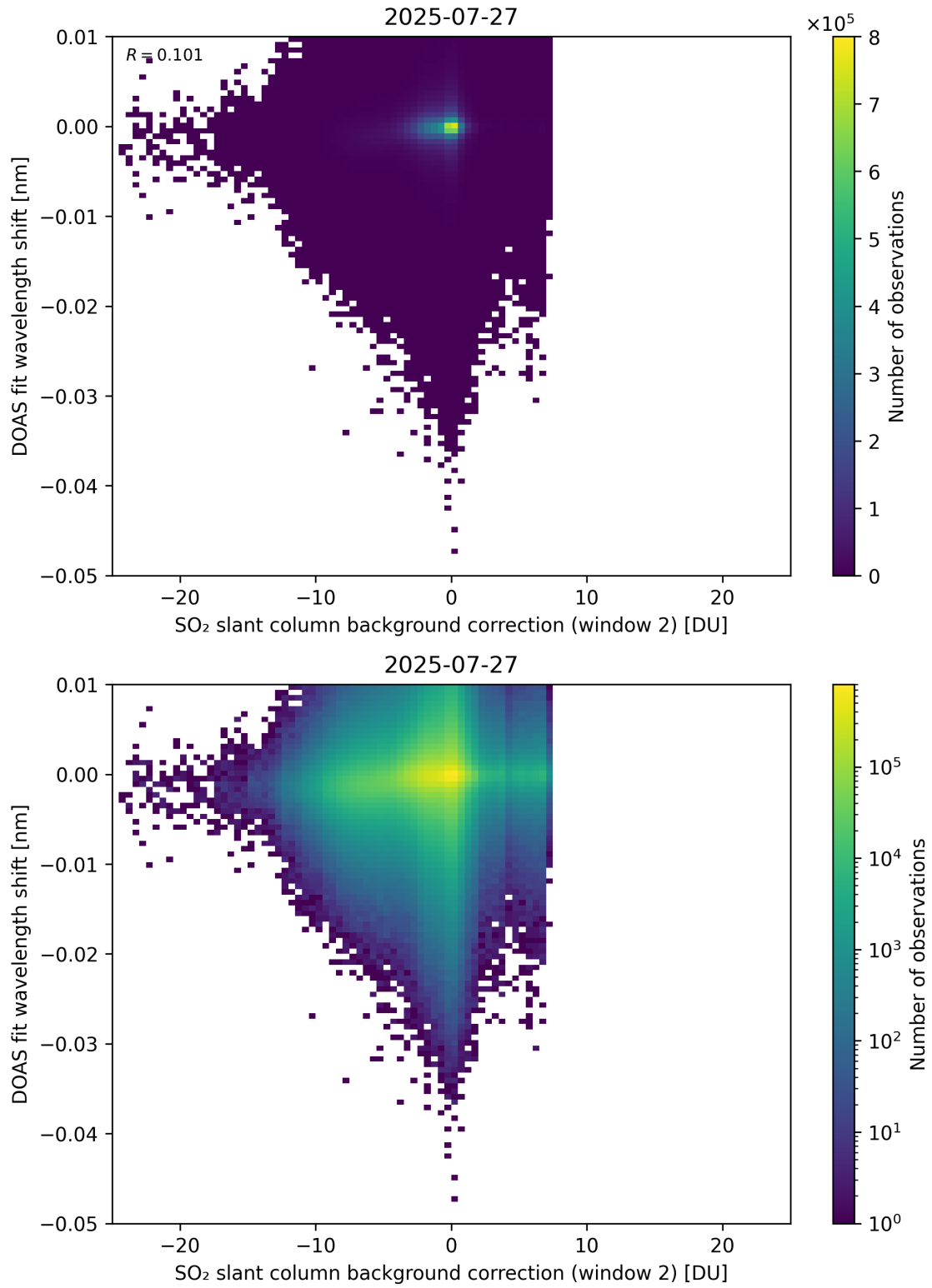
Figure 123: Scatter density plot of “SO 2 slant column background correction (window 2)” against “DOAS fit wavelength shift” for 2025-07-26 to 2025-07-28.
