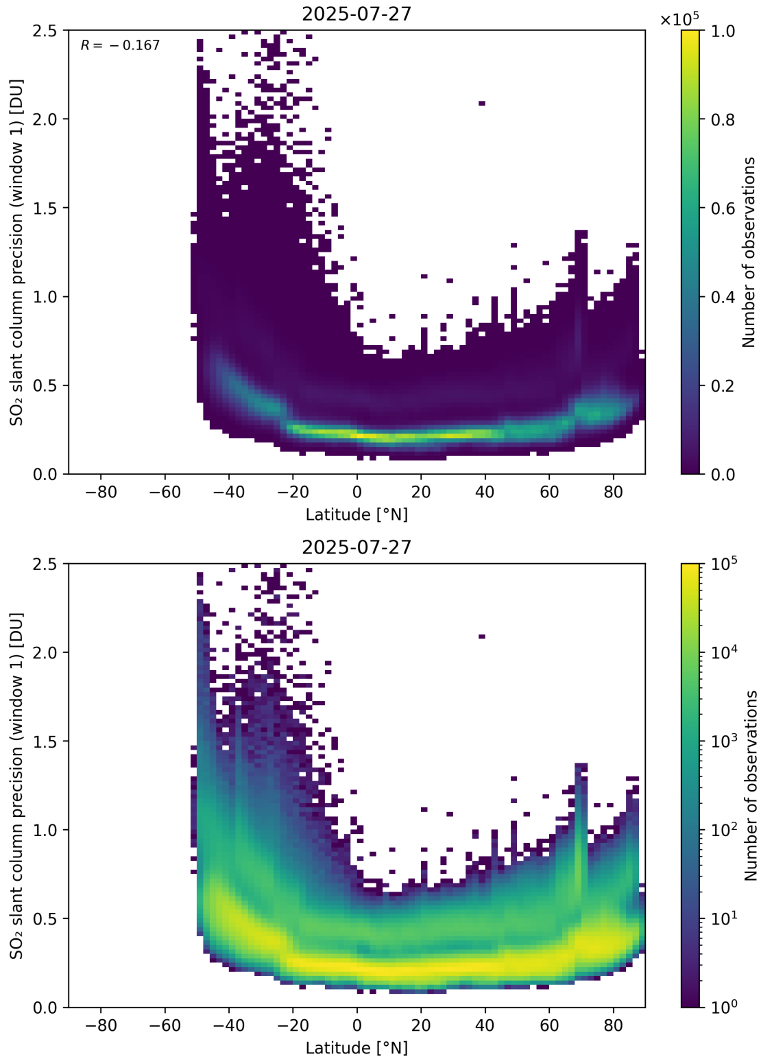
Figure 163: Scatter density plot of “Latitude” against “SO 2 slant column precision (window 1)” for 2025-07-26 to 2025-07-28.
