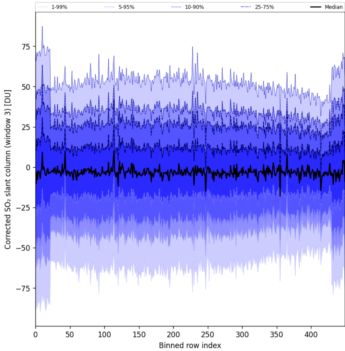
Figure 99: Along track statistics of “Corrected SO 2 slant column (window 3)” for 2025-07-26 to 2025-07-28
