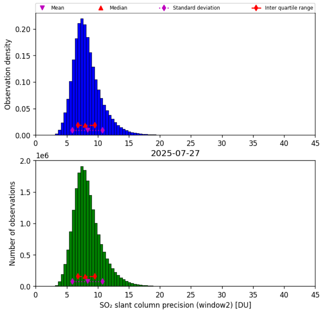
Figure 68: Histogram of “SO 2 slant column precision (window2)” for 2025-07-26 to 2025-07-28
