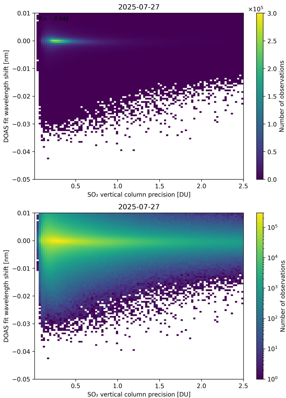
Figure 332: Scatter density plot of “SO 2 vertical column precision” against “DOAS fit wavelength shift” for 2025-07-26 to 2025-07-28.
