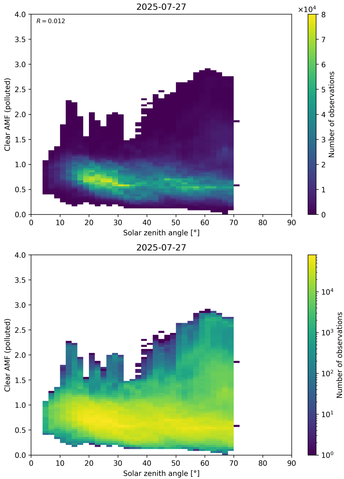
Figure 178: Scatter density plot of “Solar zenith angle” against “Clear AMF (polluted)” for 2025-07-26 to 2025-07-28.
