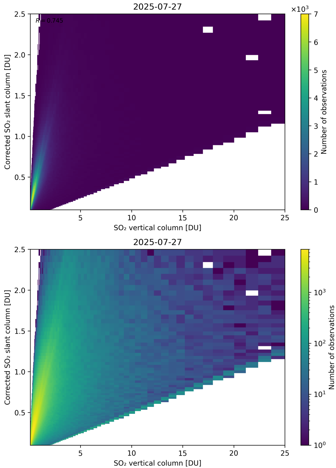
Figure 351: Scatter density plot of “SO 2 vertical column” against “Corrected SO 2 slant column” for 2025-07-26 to 2025-07-28.
