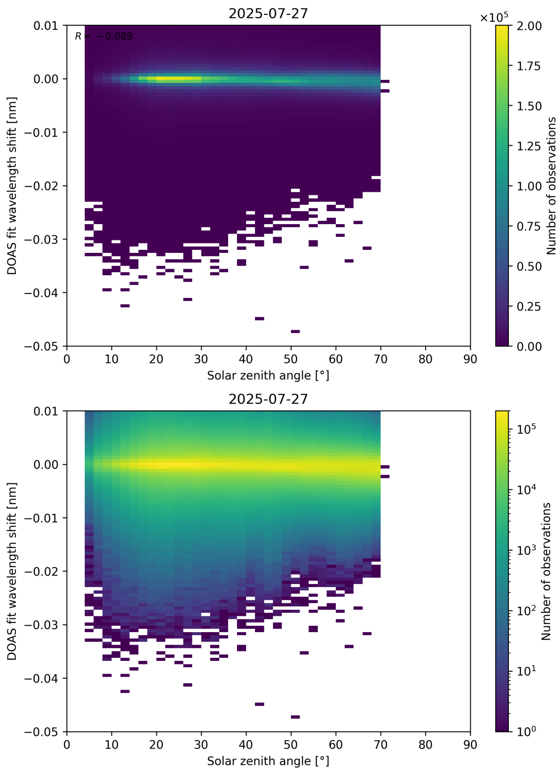
Figure 174: Scatter density plot of “Solar zenith angle” against “DOAS fit wavelength shift” for 2025-07-26 to 2025-07-28.
