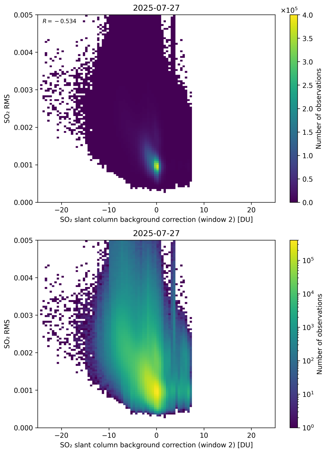
Figure 125: Scatter density plot of “SO 2 slant column background correction (window 2)” against “SO 2 RMS” for 2025-07-26 to 2025-07-28.
