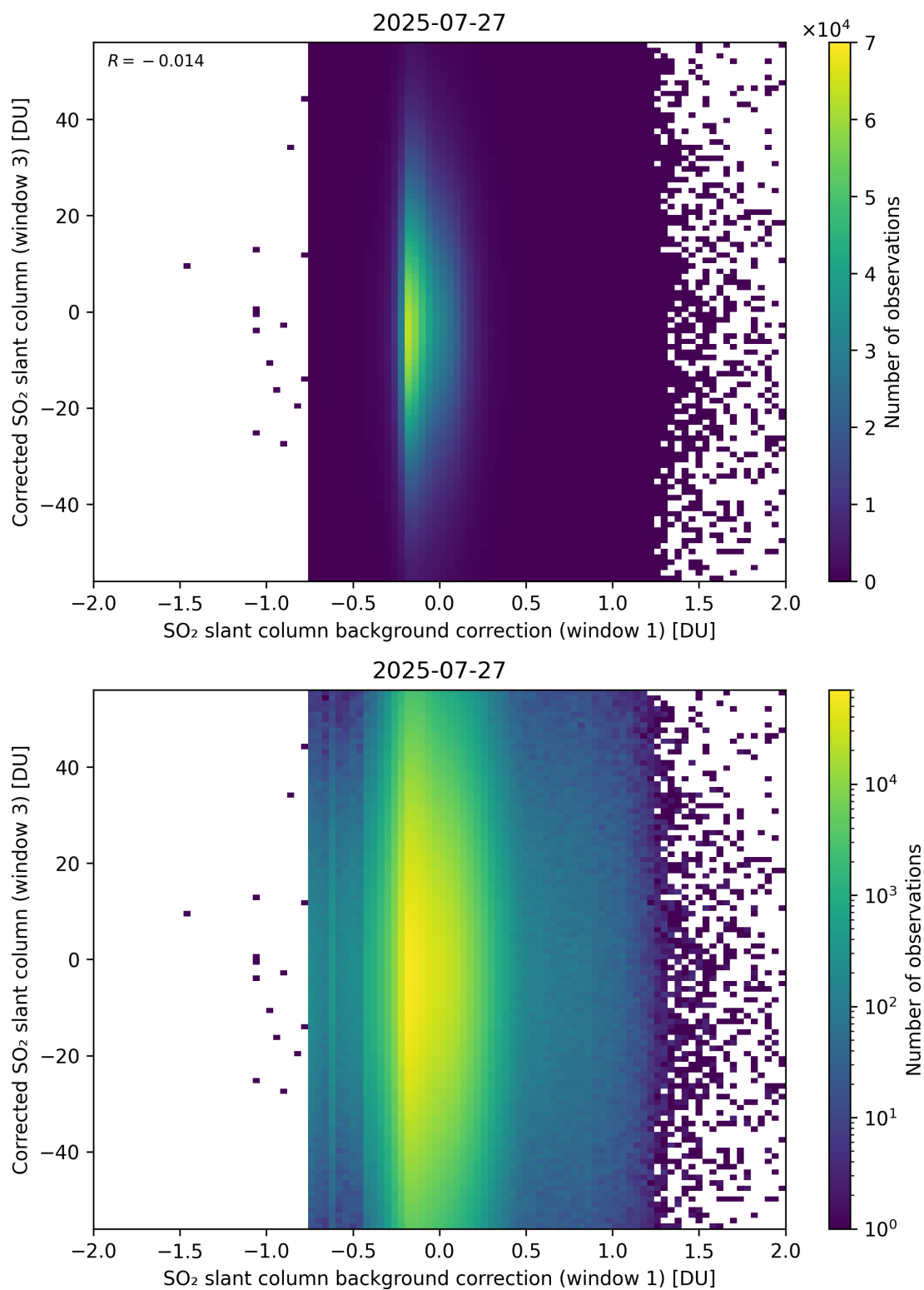
Figure 116: Scatter density plot of “SO 2 slant column background correction (window 1)” against “Corrected SO 2 slant column (window 3)” for 2025-07-26 to 2025-07-28.
