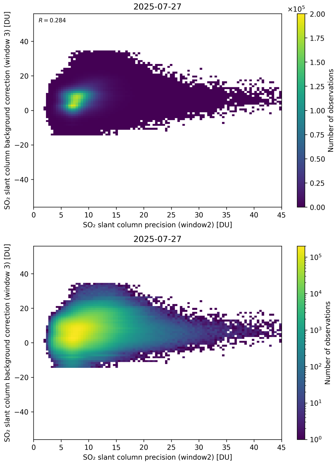
Figure 292: Scatter density plot of “SO 2 slant column precision (window2)” against “SO 2 slant column background correction (window 3)” for 2025-07-26 to 2025-07-28.
