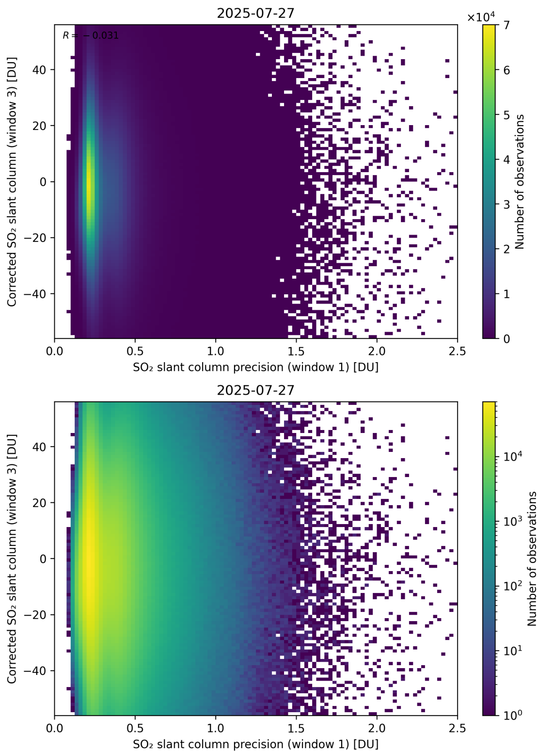
Figure 276: Scatter density plot of “SO 2 slant column precision (window 1)” against “Corrected SO 2 slant column (window 3)” for 2025-07-26 to 2025-07-28.
