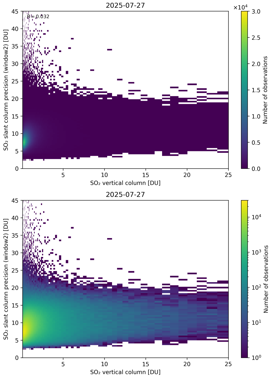
Figure 356: Scatter density plot of “SO 2 vertical column” against “SO 2 slant column precision (window2)” for 2025-07-26 to 2025-07-28.
