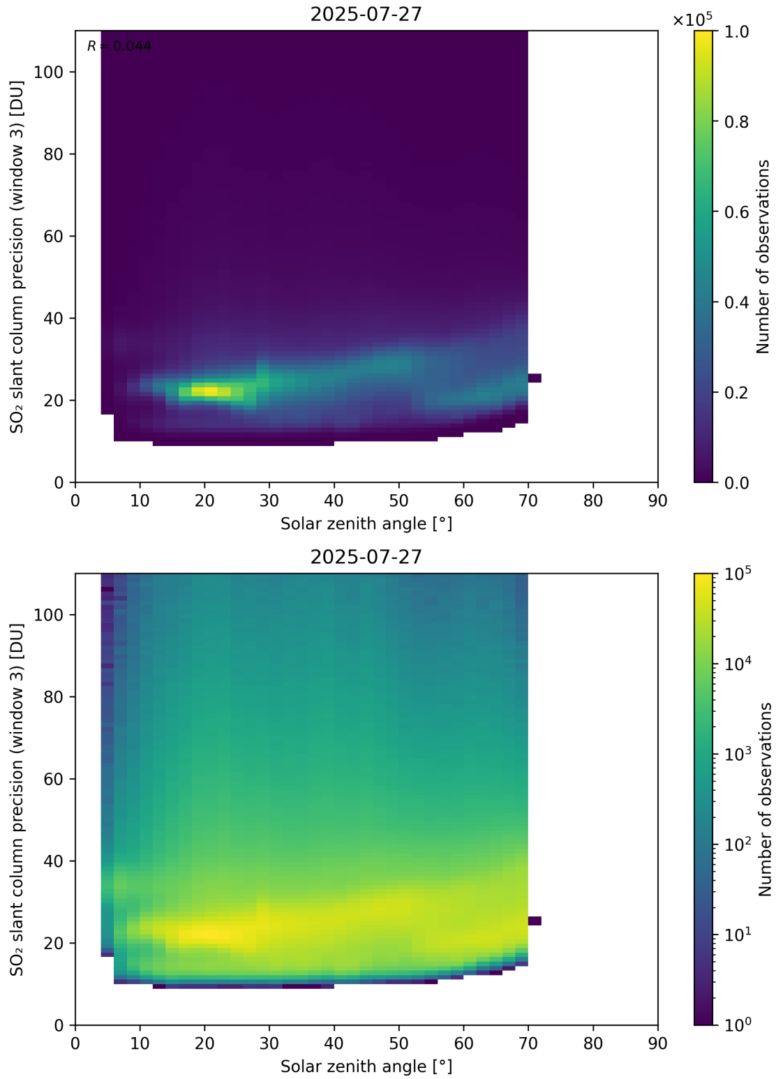
Figure 188: Scatter density plot of “Solar zenith angle” against “SO 2 slant column precision (window 3)” for 2025-07-26 to 2025-07-28.
