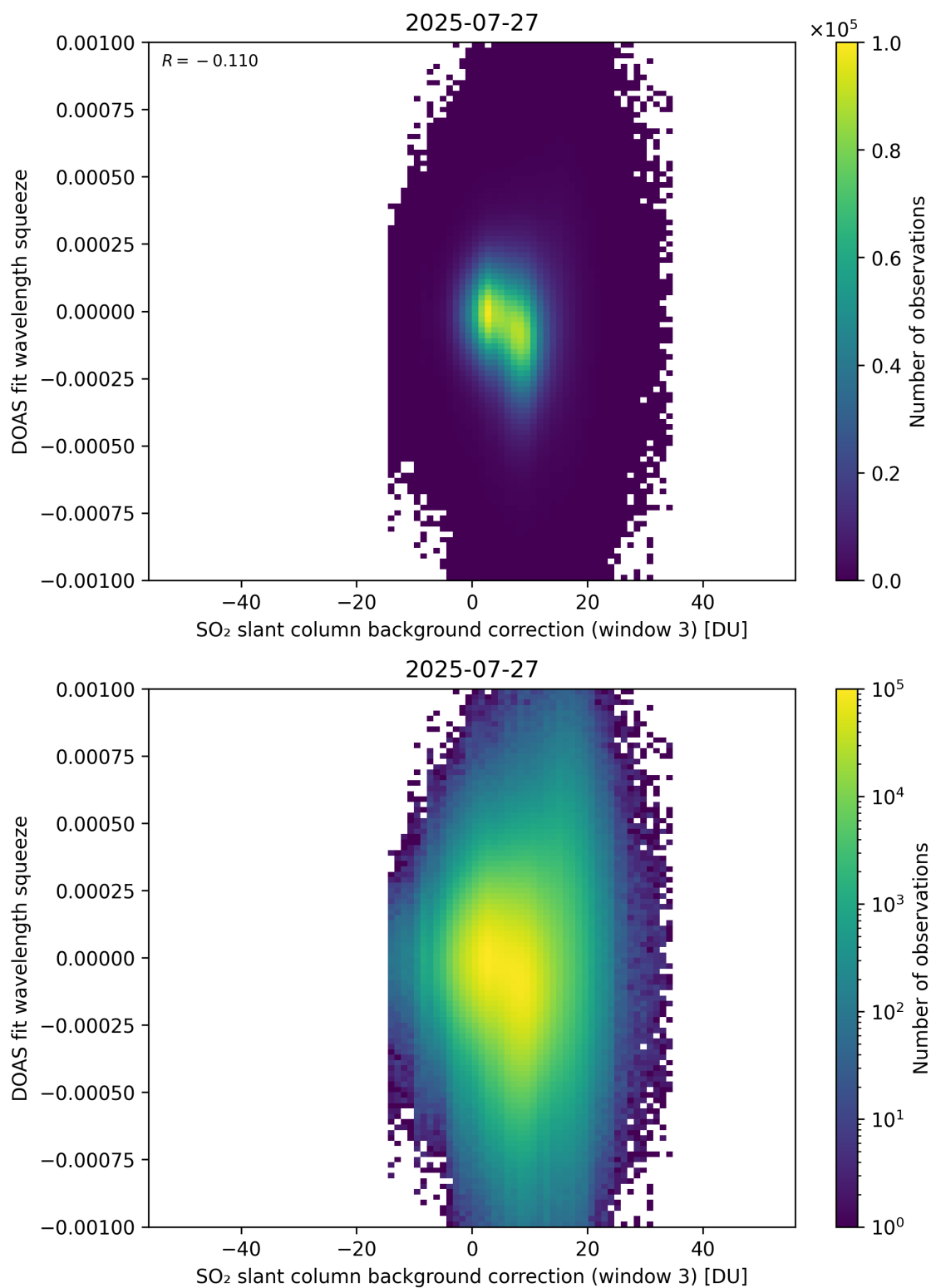
Figure 133: Scatter density plot of “SO 2 slant column background correction (window 3)” against “DOAS fit wavelength squeeze” for 2025-07-26 to 2025-07-28.
