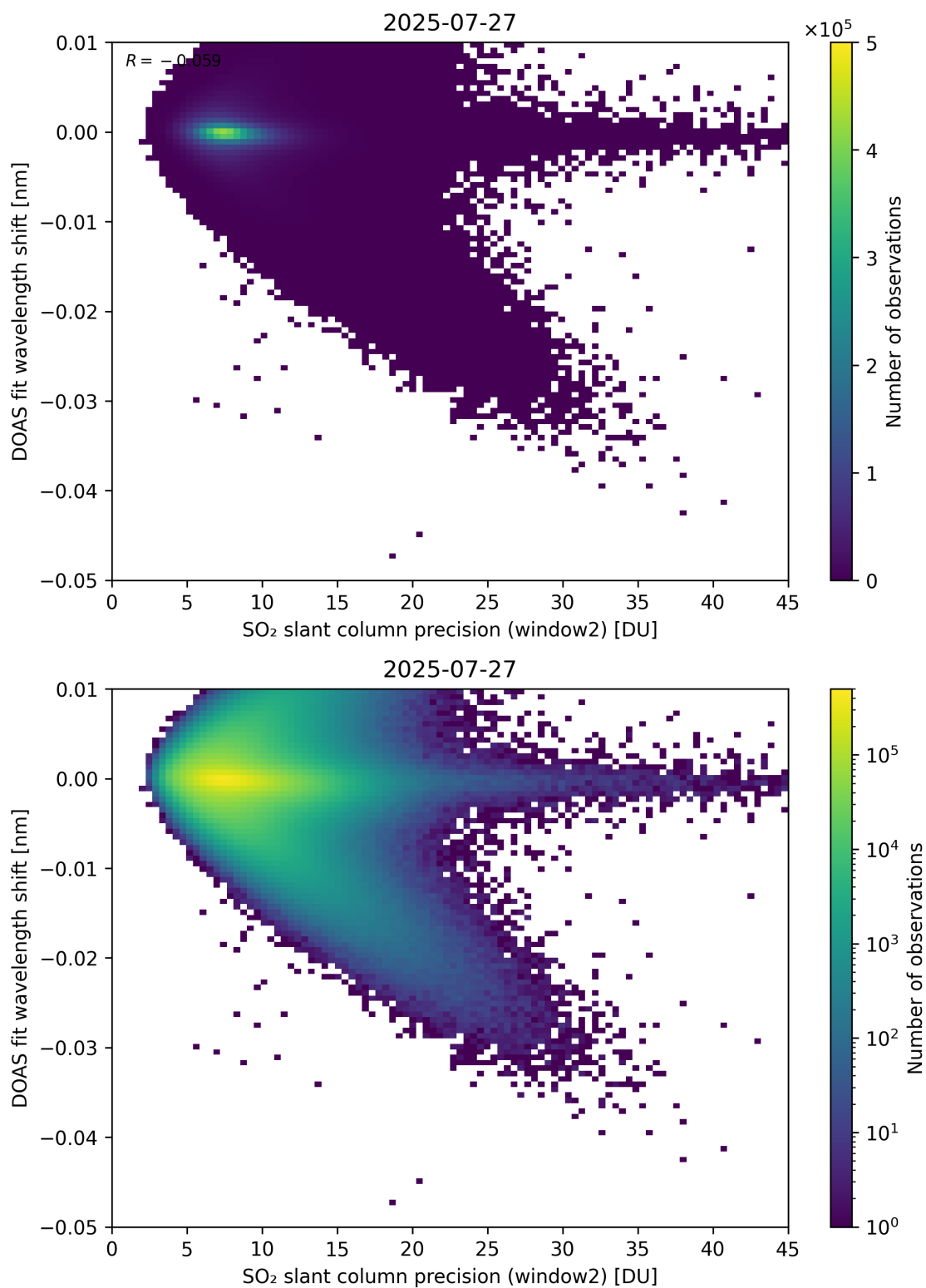
Figure 293: Scatter density plot of “SO 2 slant column precision (window2)” against “DOAS fit wavelength shift” for 2025-07-26 to 2025-07-28.
