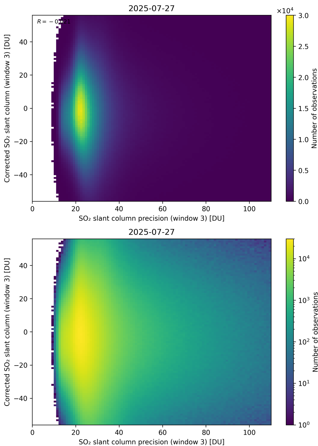
Figure 312: Scatter density plot of “SO 2 slant column precision (window 3)” against “Corrected SO 2 slant column (window 3)” for 2025-07-26 to 2025-07-28.
