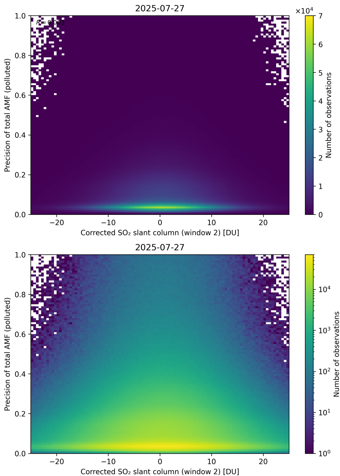
Figure 254: Scatter density plot of “Corrected SO 2 slant column (window 2)” against “Precision of total AMF (polluted)” for 2025-07-26 to 2025-07-28.
