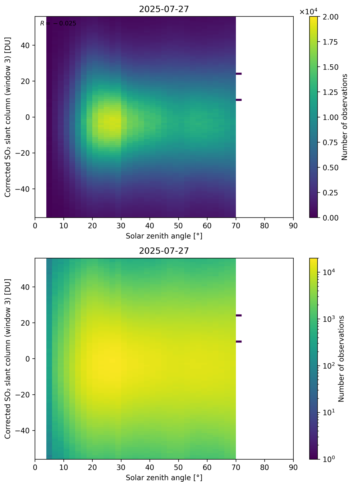
Figure 183: Scatter density plot of “Solar zenith angle” against “Corrected SO 2 slant column (window 3)” for 2025-07-26 to 2025-07-28.
