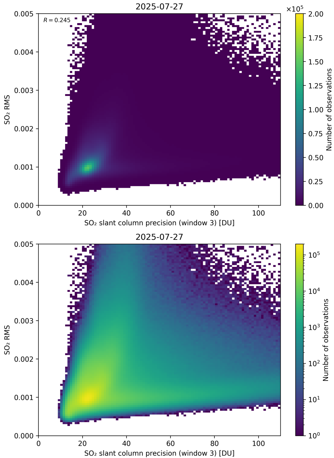
Figure 310: Scatter density plot of “SO 2 slant column precision (window 3)” against “SO 2 RMS” for 2025-07-26 to 2025-07-28.
