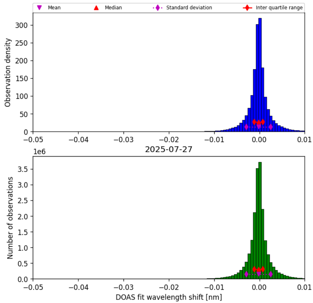
Figure 76: Histogram of “DOAS fit wavelength shift” for 2025-07-26 to 2025-07-28
