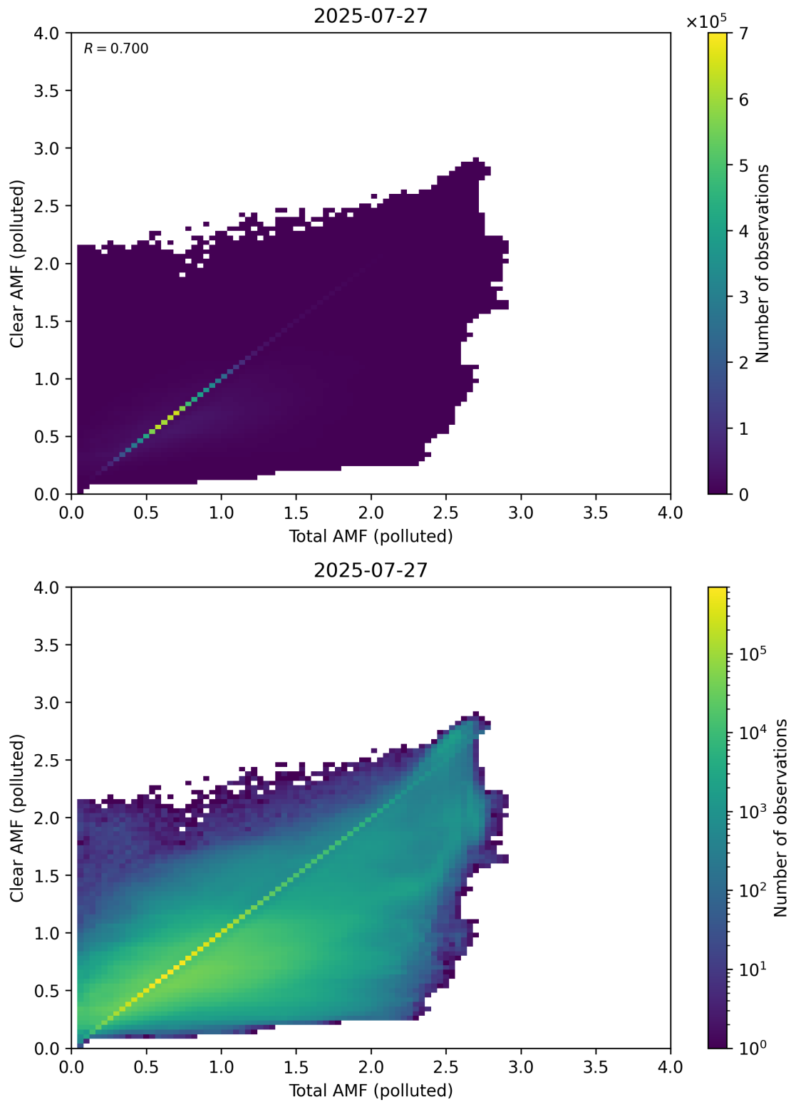
Figure 321: Scatter density plot of “Total AMF (polluted)” against “Clear AMF (polluted)” for 2025-07-26 to 2025-07-28.
