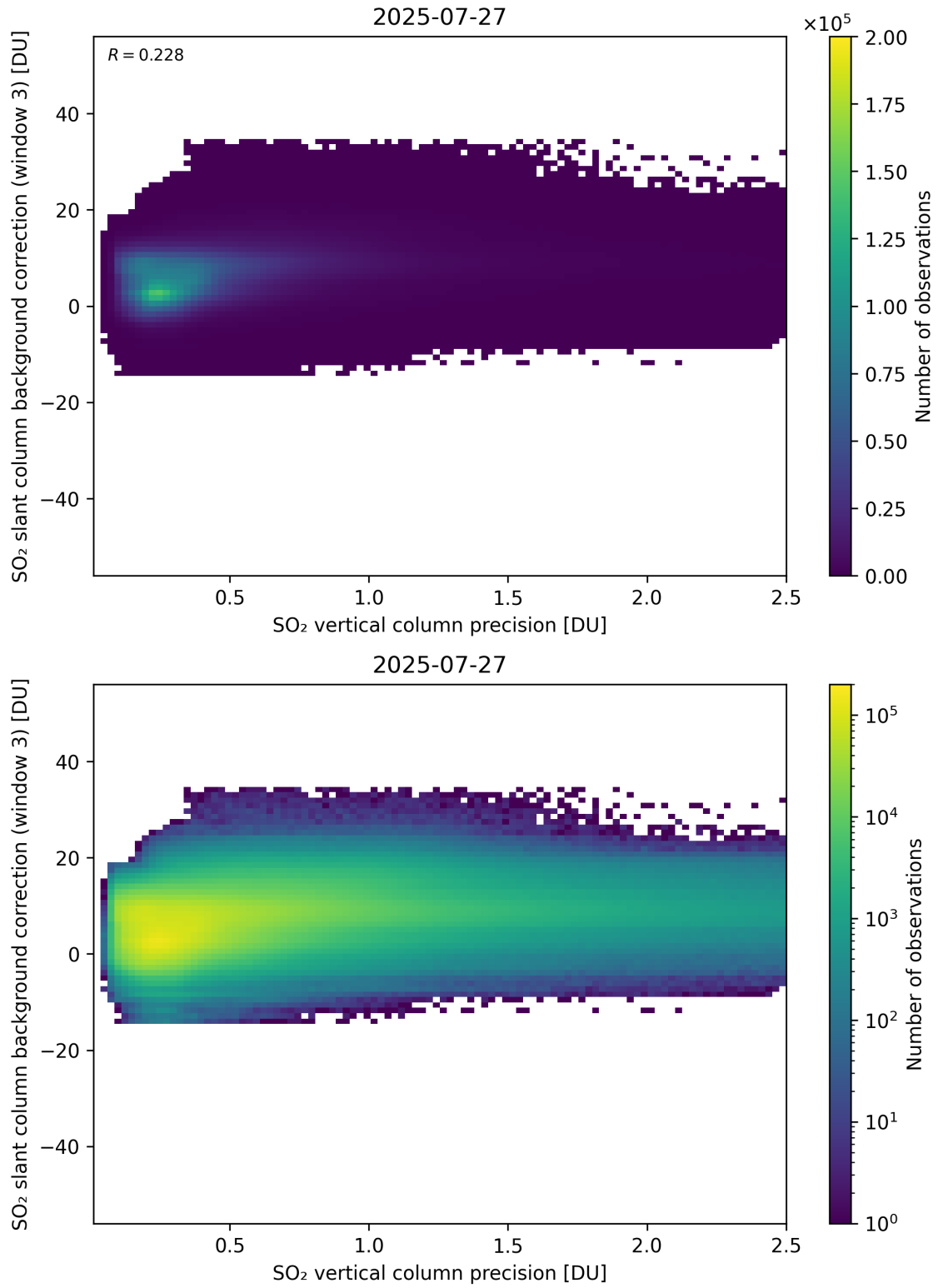
Figure 331: Scatter density plot of “SO 2 vertical column precision” against “SO 2 slant column background correction (window 3)” for 2025-07-26 to 2025-07-28.
