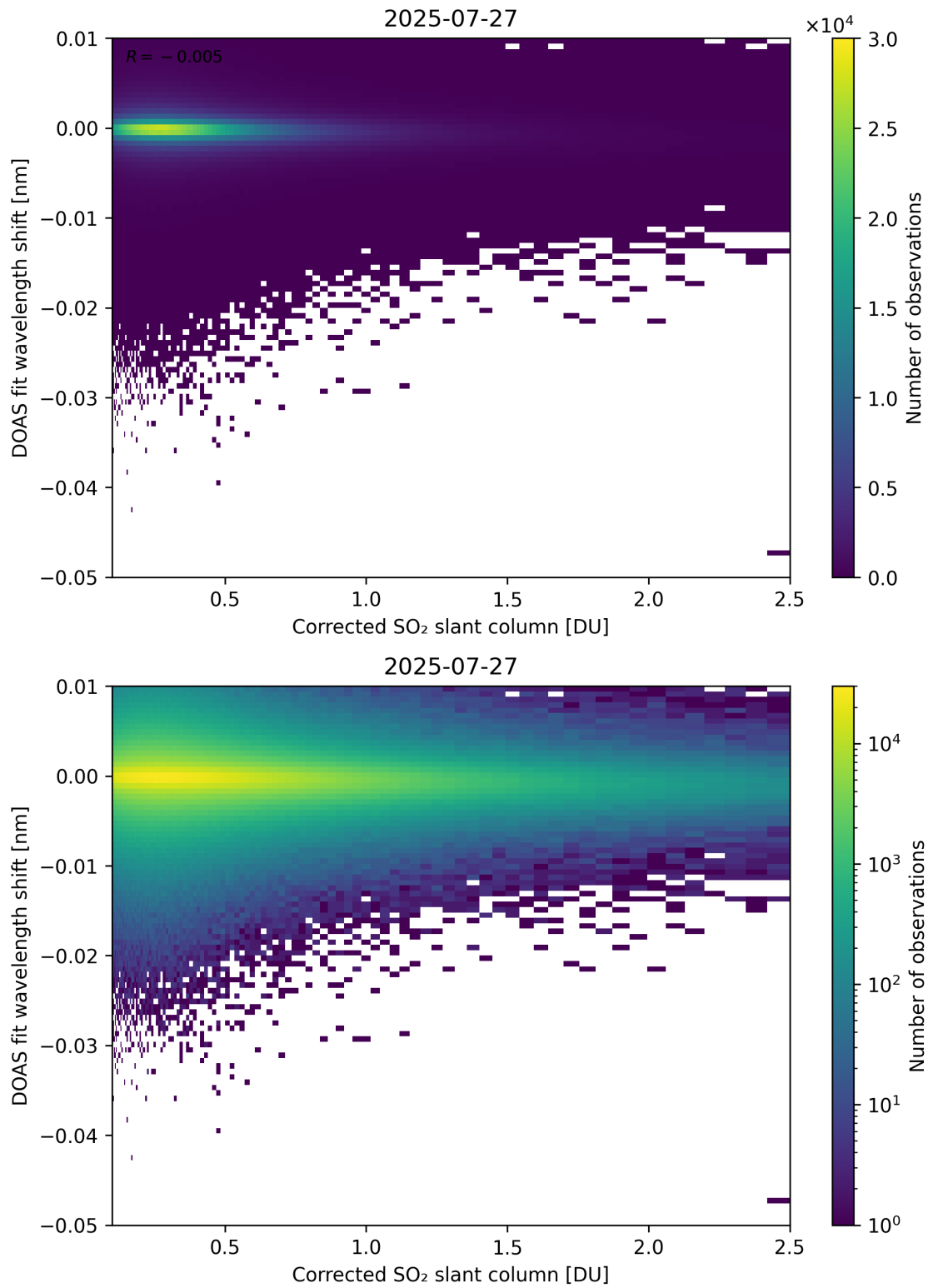
Figure 229: Scatter density plot of “Corrected SO 2 slant column” against “DOAS fit wavelength shift” for 2025-07-26 to 2025-07-28.
