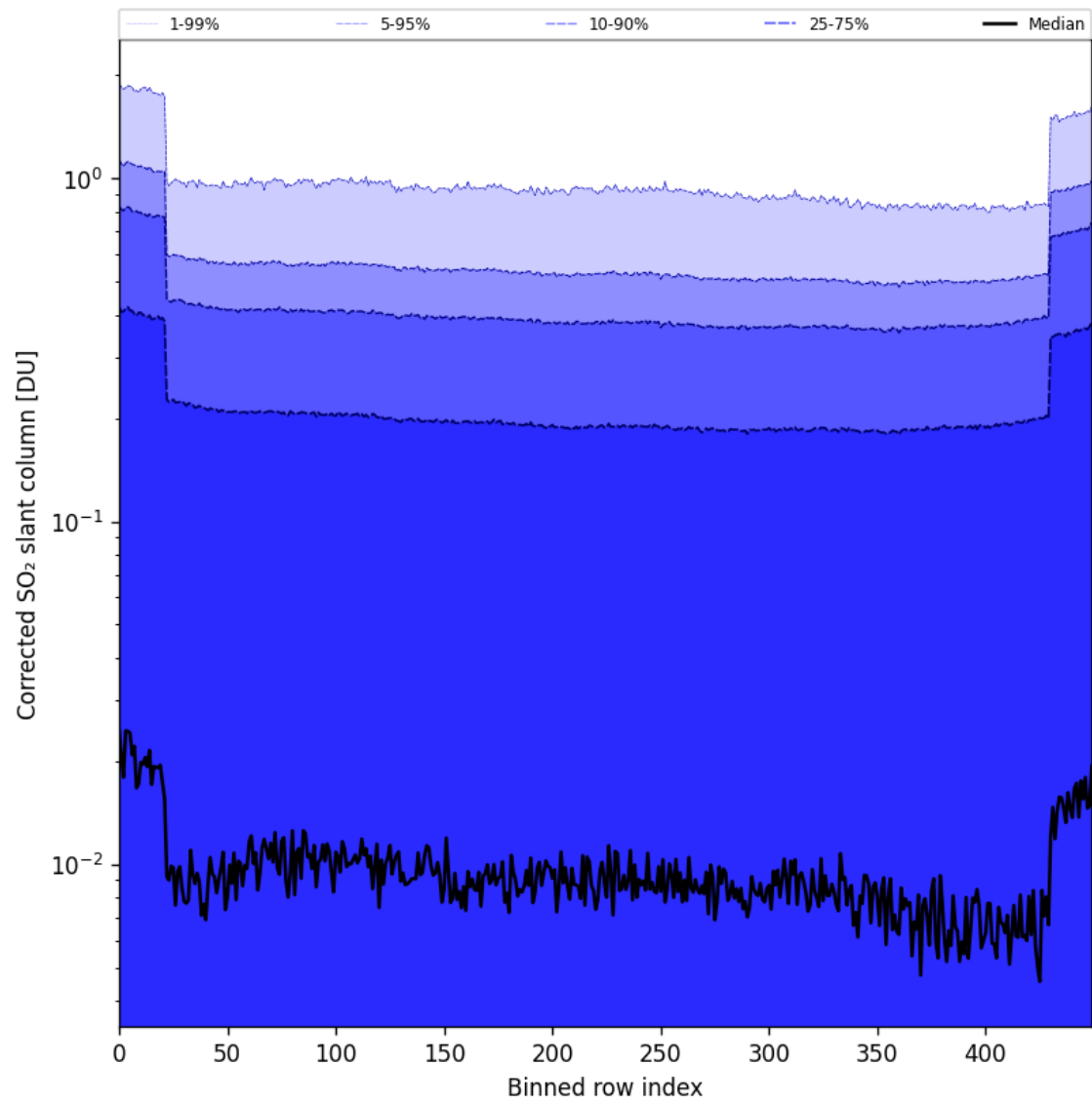
Figure 86: Along track statistics of “Corrected SO 2 slant column” for 2025-07-26 to 2025-07-28
