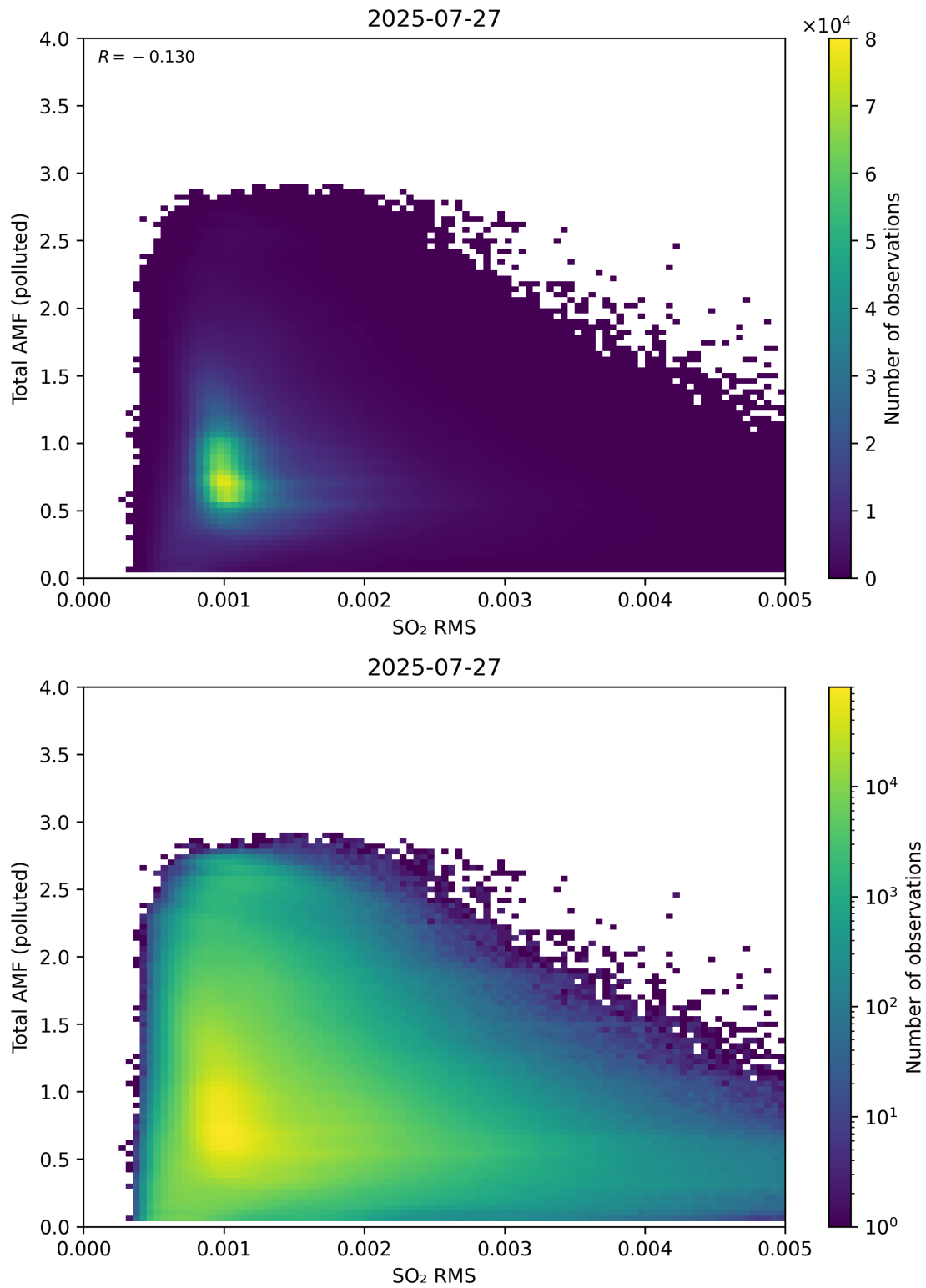
Figure 148: Scatter density plot of “SO 2 RMS” against “Total AMF (polluted)” for 2025-07-26 to 2025-07-28.
