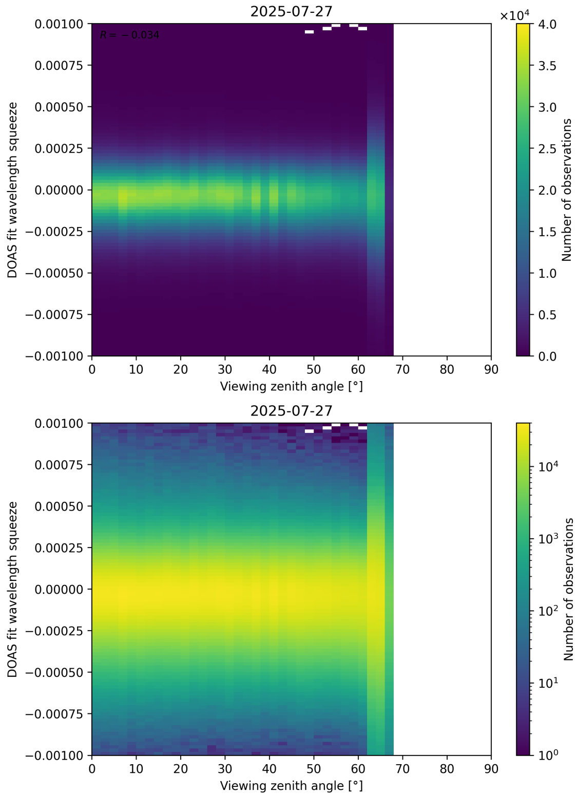
Figure 366: Scatter density plot of “Viewing zenith angle” against “DOAS fit wavelength squeeze” for 2025-07-26 to 2025-07-28.
