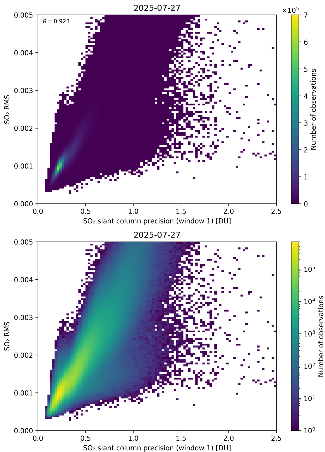
Figure 273: Scatter density plot of “SO 2 slant column precision (window 1)” against “SO 2 RMS” for 2025-07-26 to 2025-07-28.
