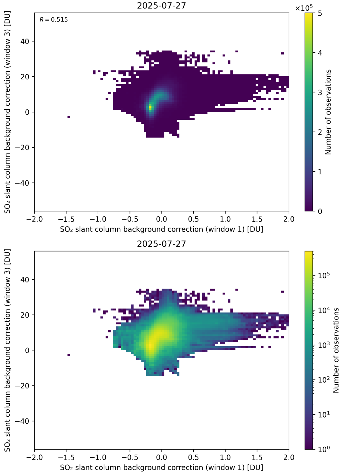
Figure 110: Scatter density plot of “SO 2 slant column background correction (window 1)” against “SO 2 slant column background correction (window 3)” for 2025-07-26 to 2025-07-28.
