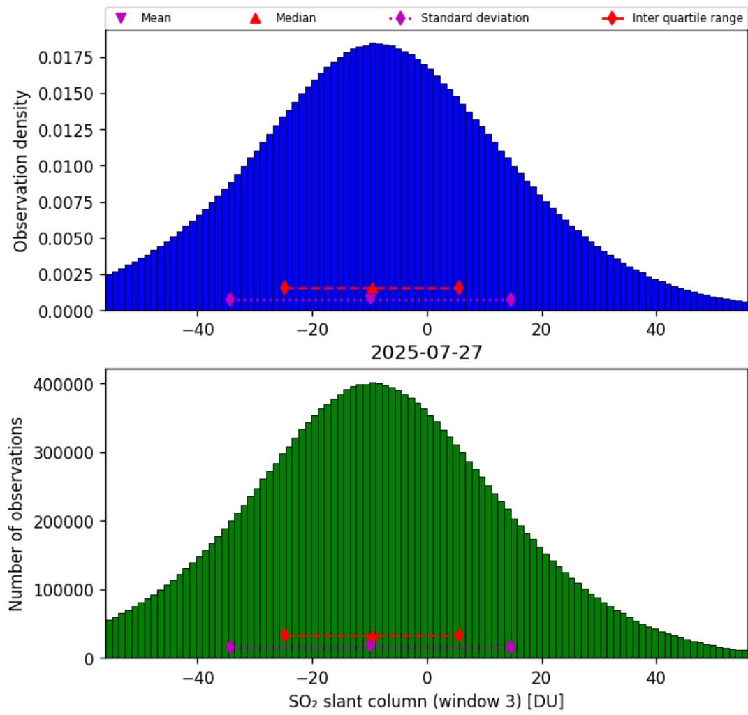
Figure 71: Histogram of “SO 2 slant column (window 3)” for 2025-07-26 to 2025-07-28
