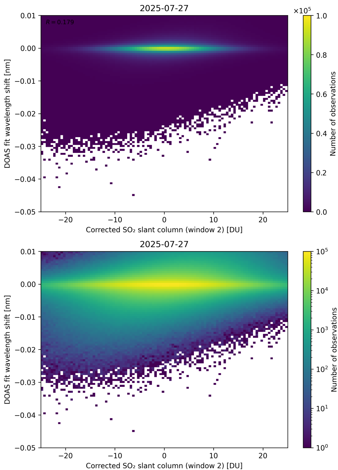
Figure 246: Scatter density plot of “Corrected SO 2 slant column (window 2)” against “DOAS fit wavelength shift” for 2025-07-26 to 2025-07-28.
