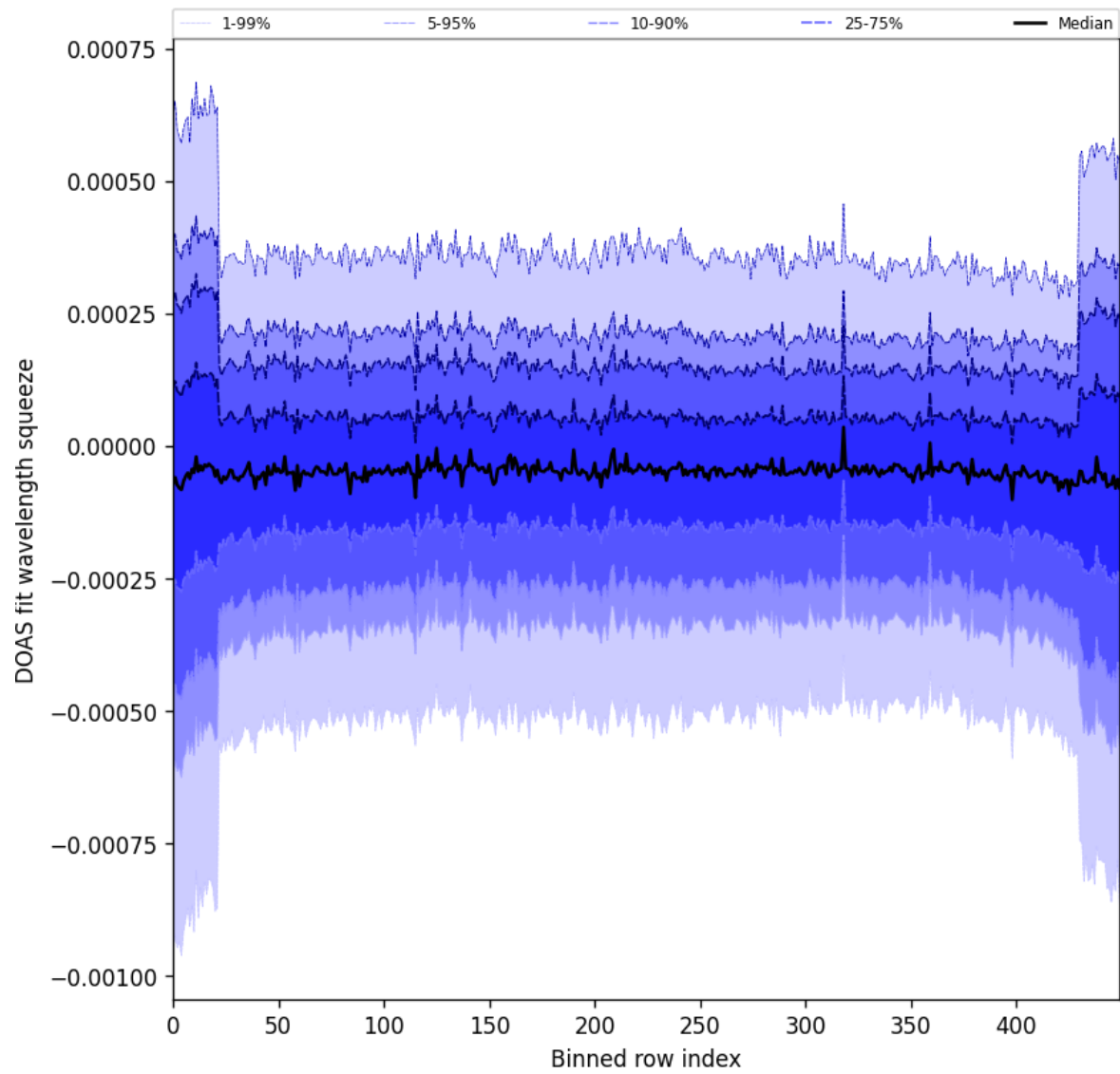
Figure 103: Along track statistics of “DOAS fit wavelength squeeze” for 2025-07-26 to 2025-07-28
