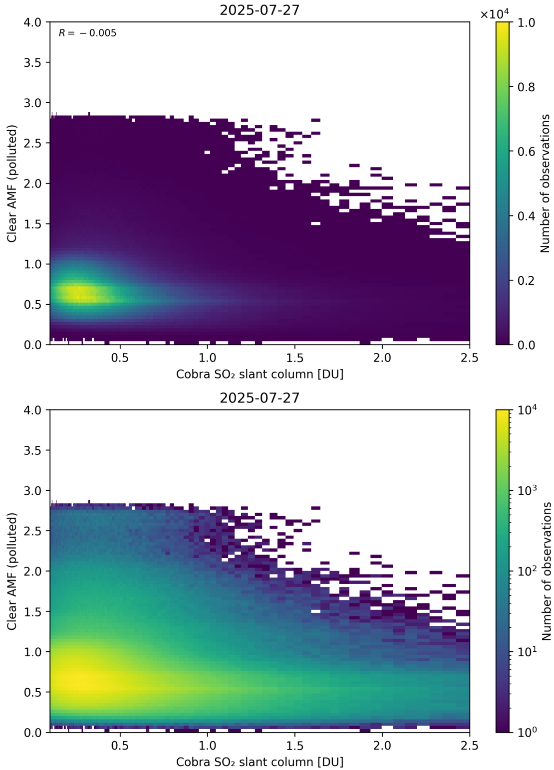
Figure 215: Scatter density plot of “Cobra SO 2 slant column” against “Clear AMF (polluted)” for 2025-07-26 to 2025-07-28.
