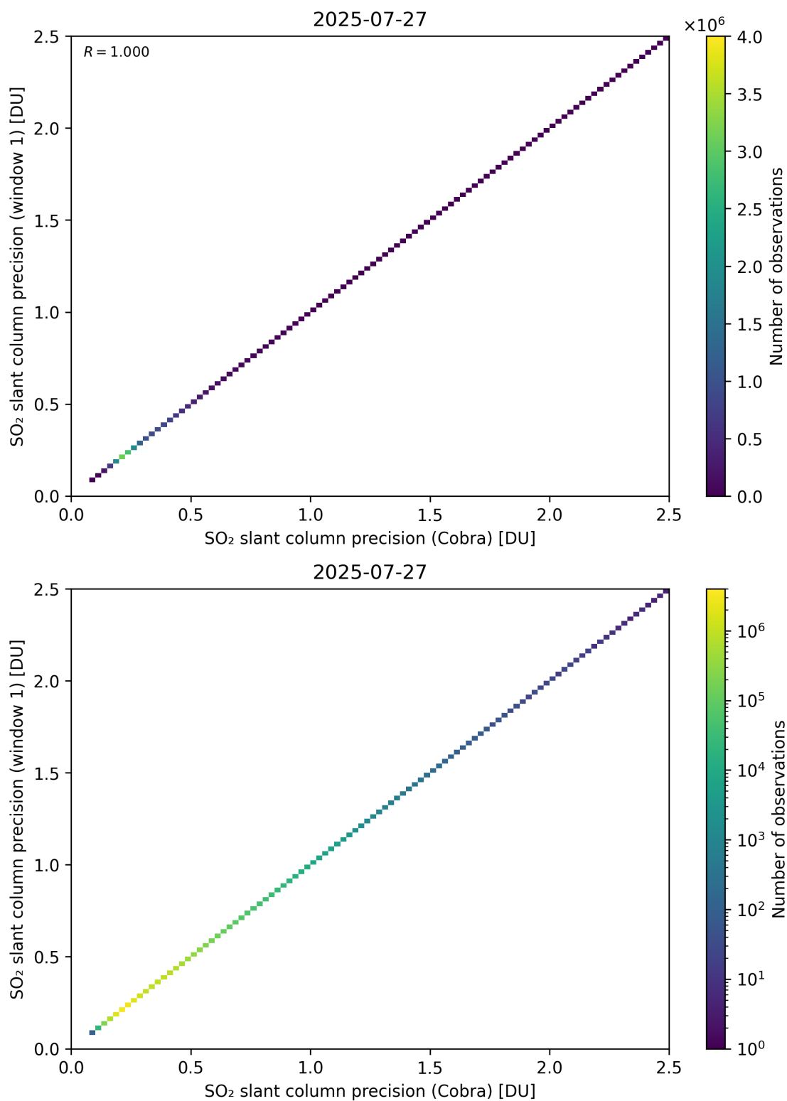
Figure 209: Scatter density plot of “SO 2 slant column precision (Cobra)” against “SO 2 slant column precision (window 1)” for 2025-07-26 to 2025-07-28.
