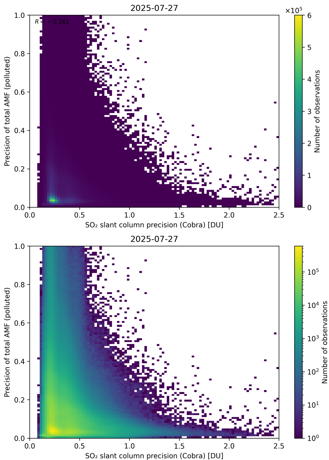
Figure 214: Scatter density plot of “SO 2 slant column precision (Cobra)” against “Precision of total AMF (polluted)” for 2025-07-26 to 2025-07-28.
