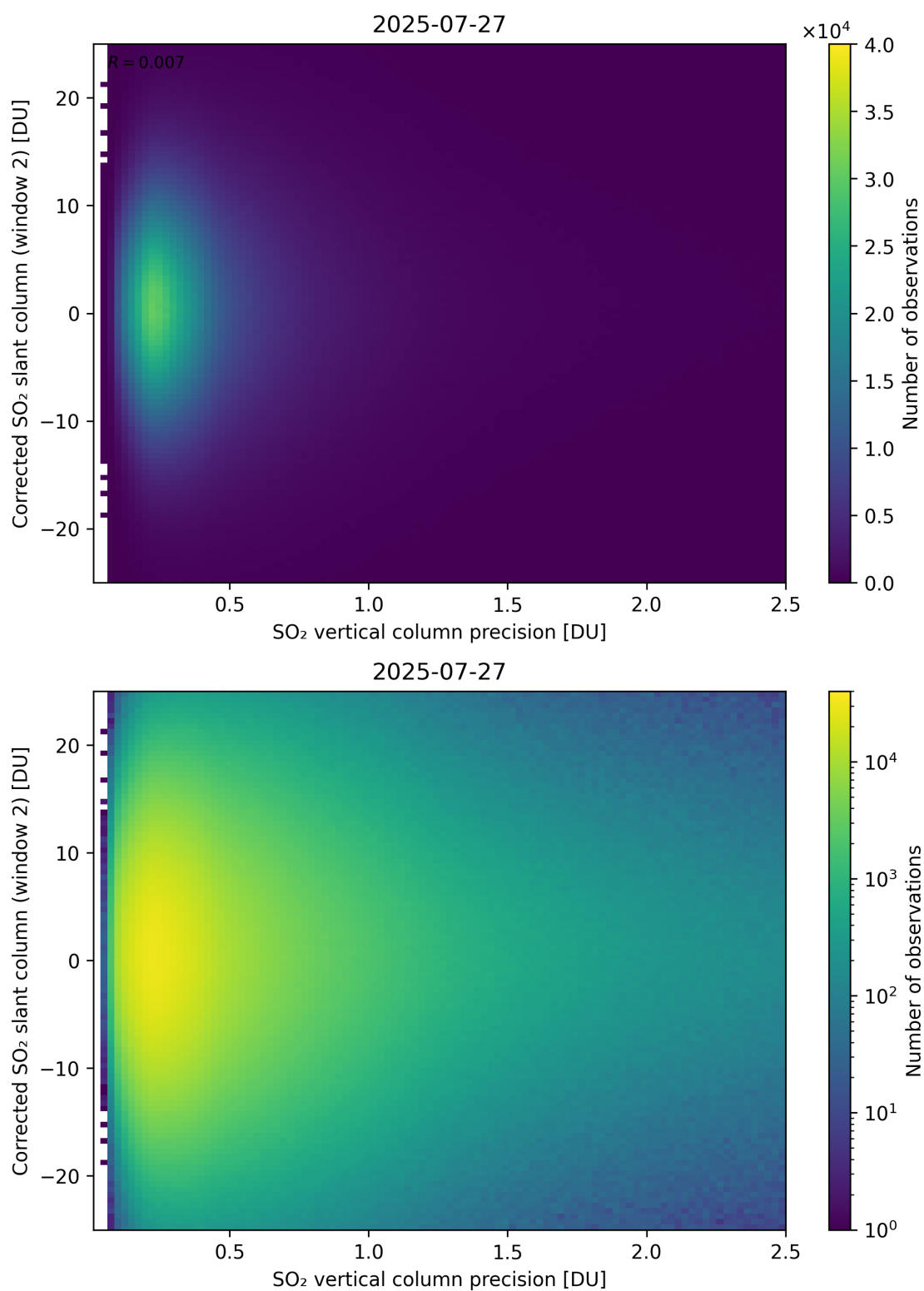
Figure 339: Scatter density plot of “SO 2 vertical column precision” against “Corrected SO 2 slant column (window 2)” for 2025-07-26 to 2025-07-28.
