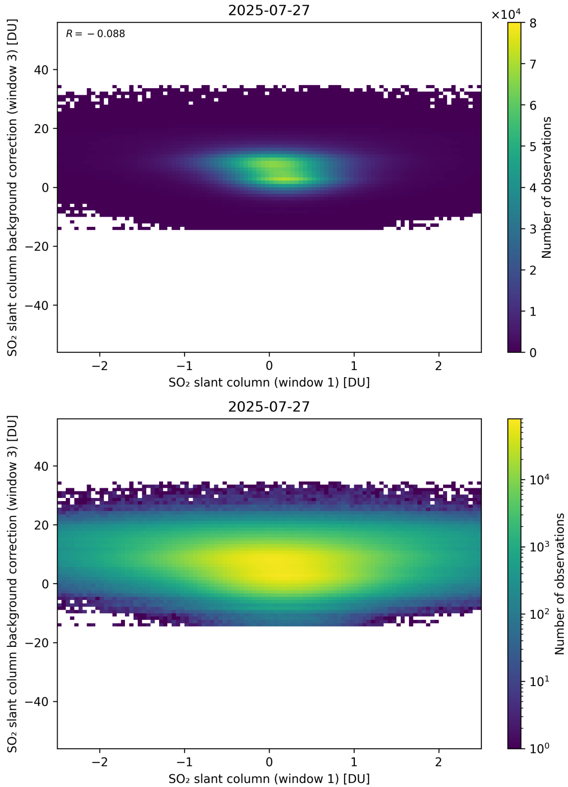
Figure 264: Scatter density plot of “SO 2 slant column (window 1)” against “SO 2 slant column background correction (window 3)” for 2025-07-26 to 2025-07-28.
