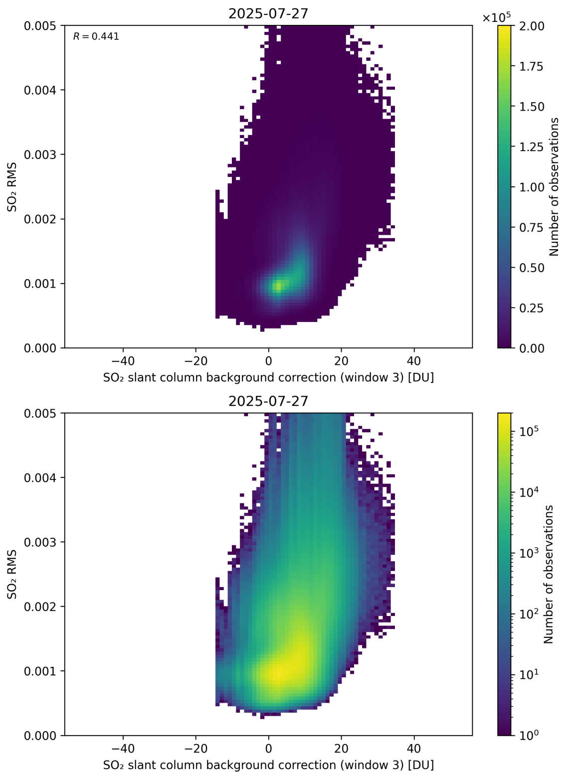
Figure 134: Scatter density plot of “SO 2 slant column background correction (window 3)” against “SO 2 RMS” for 2025-07-26 to 2025-07-28.
