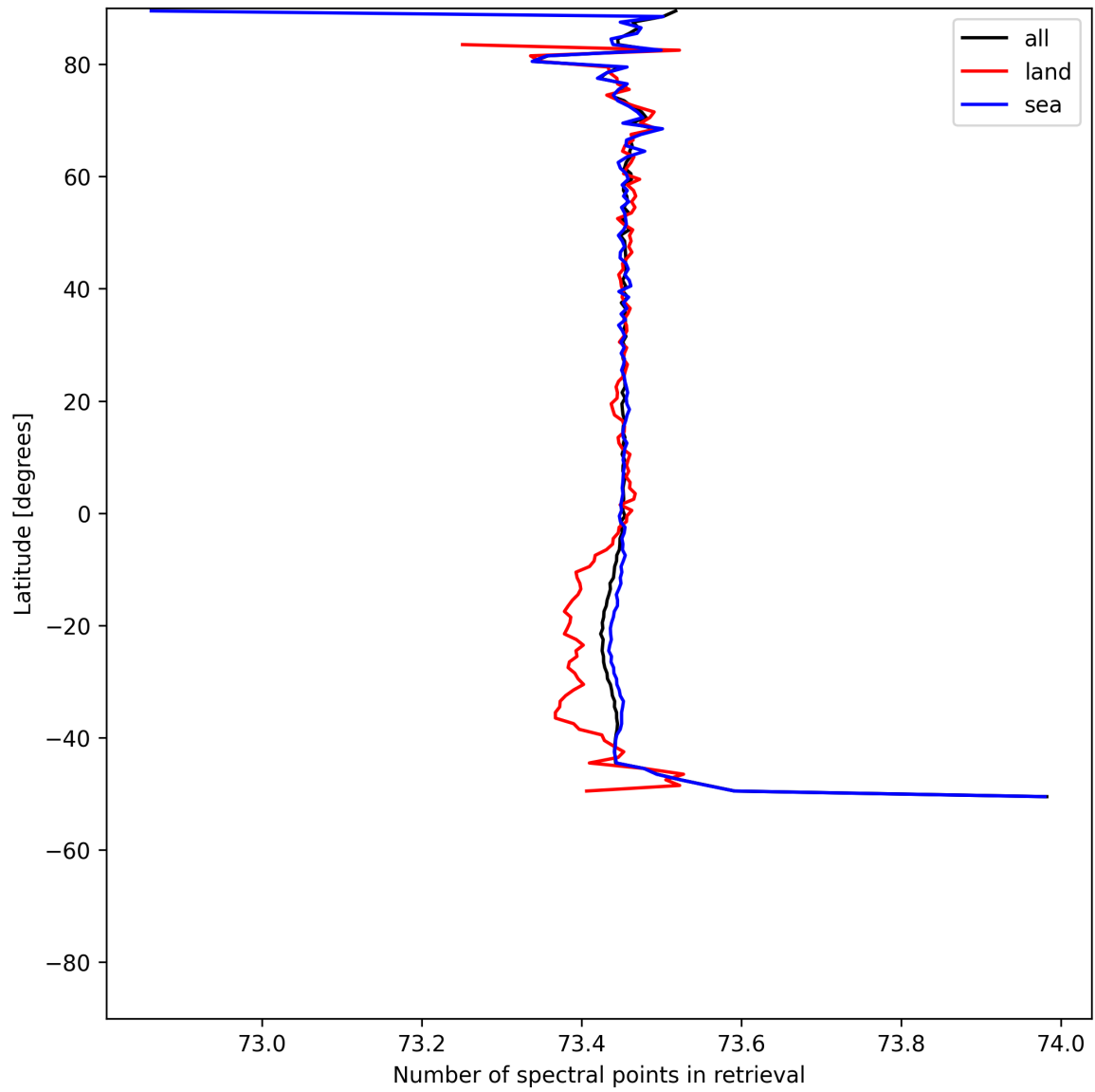
Figure 56: Zonal average of “Number of spectral points in retrieval” for 2025-07-26 to 2025-07-28.
