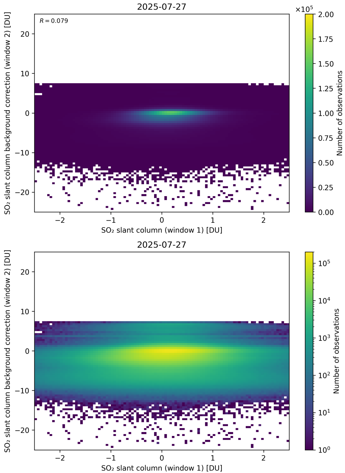
Figure 263: Scatter density plot of “SO 2 slant column (window 1)” against “SO 2 slant column background correction (window 2)” for 2025-07-26 to 2025-07-28.
