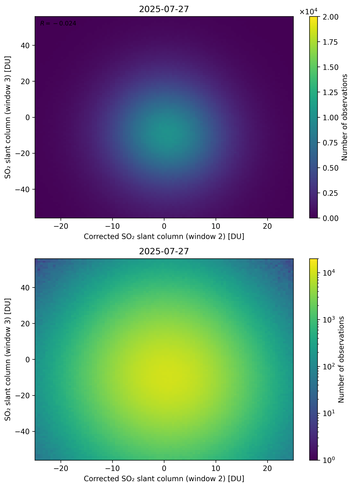
Figure 251: Scatter density plot of “Corrected SO 2 slant column (window 2)” against “SO 2 slant column (window 3)” for 2025-07-26 to 2025-07-28.
