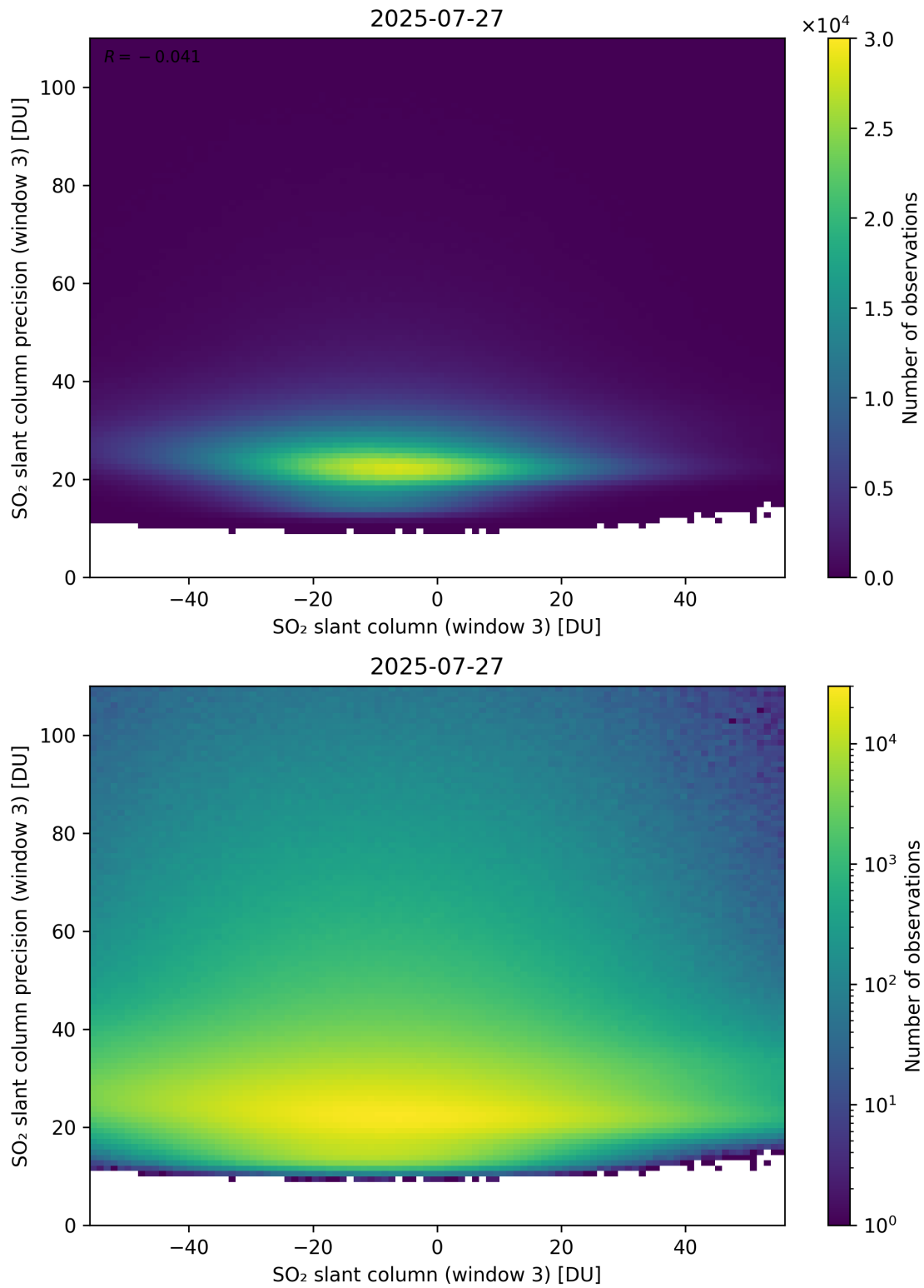
Figure 317: Scatter density plot of “SO 2 slant column (window 3)” against “SO 2 slant column precision (window 3)” for 2025-07-26 to 2025-07-28.
