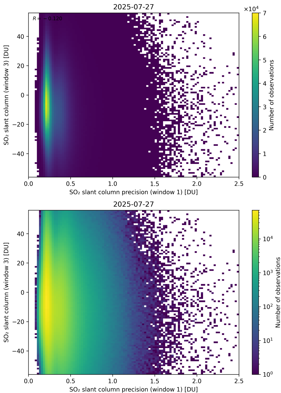
Figure 278: Scatter density plot of “SO 2 slant column precision (window 1)” against “SO 2 slant column (window 3)” for 2025-07-26 to 2025-07-28.
