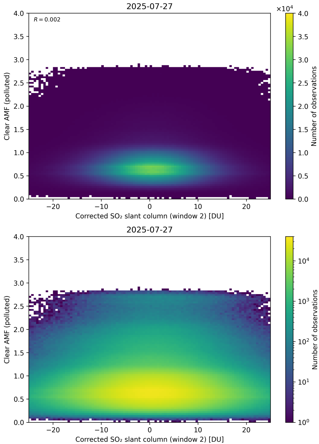
Figure 249: Scatter density plot of “Corrected SO 2 slant column (window 2)” against “Clear AMF (polluted)” for 2025-07-26 to 2025-07-28.
