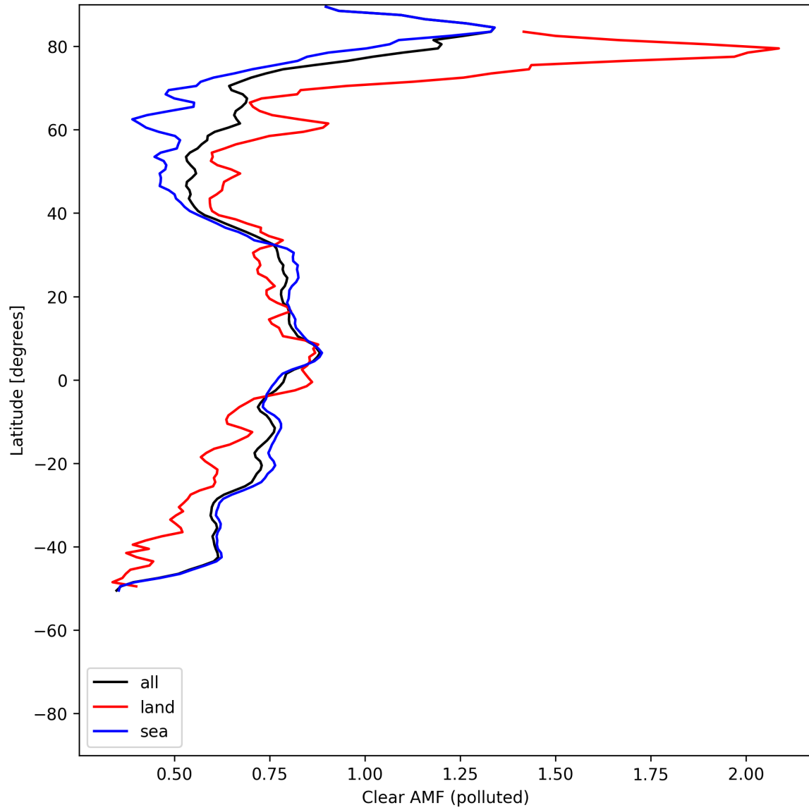
Figure 55: Zonal average of “Clear AMF (polluted)” for 2025-07-26 to 2025-07-28.
