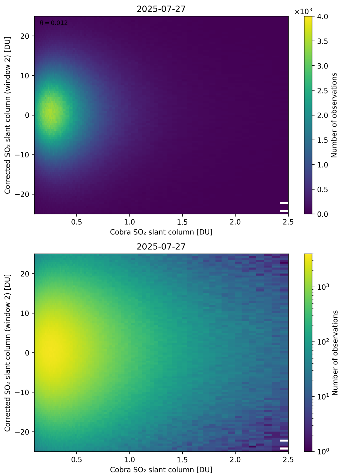
Figure 217: Scatter density plot of “Cobra SO 2 slant column” against “Corrected SO 2 slant column (window 2)” for 2025-07-26 to 2025-07-28.
