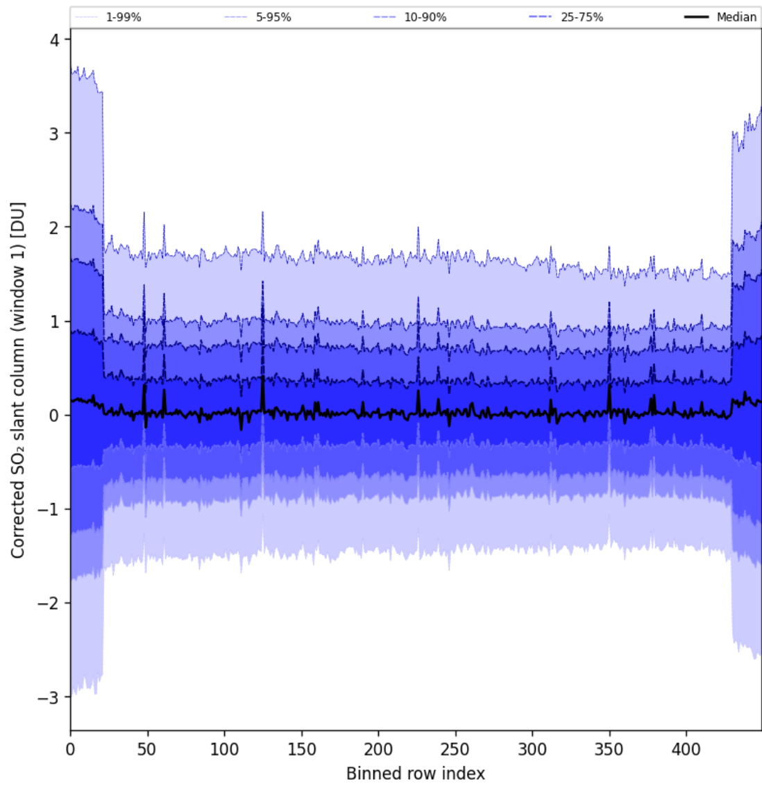
Figure 91: Along track statistics of "Corrected SO 2 slant column (window 1)" for 2025-07-26 to 2025-07-28
