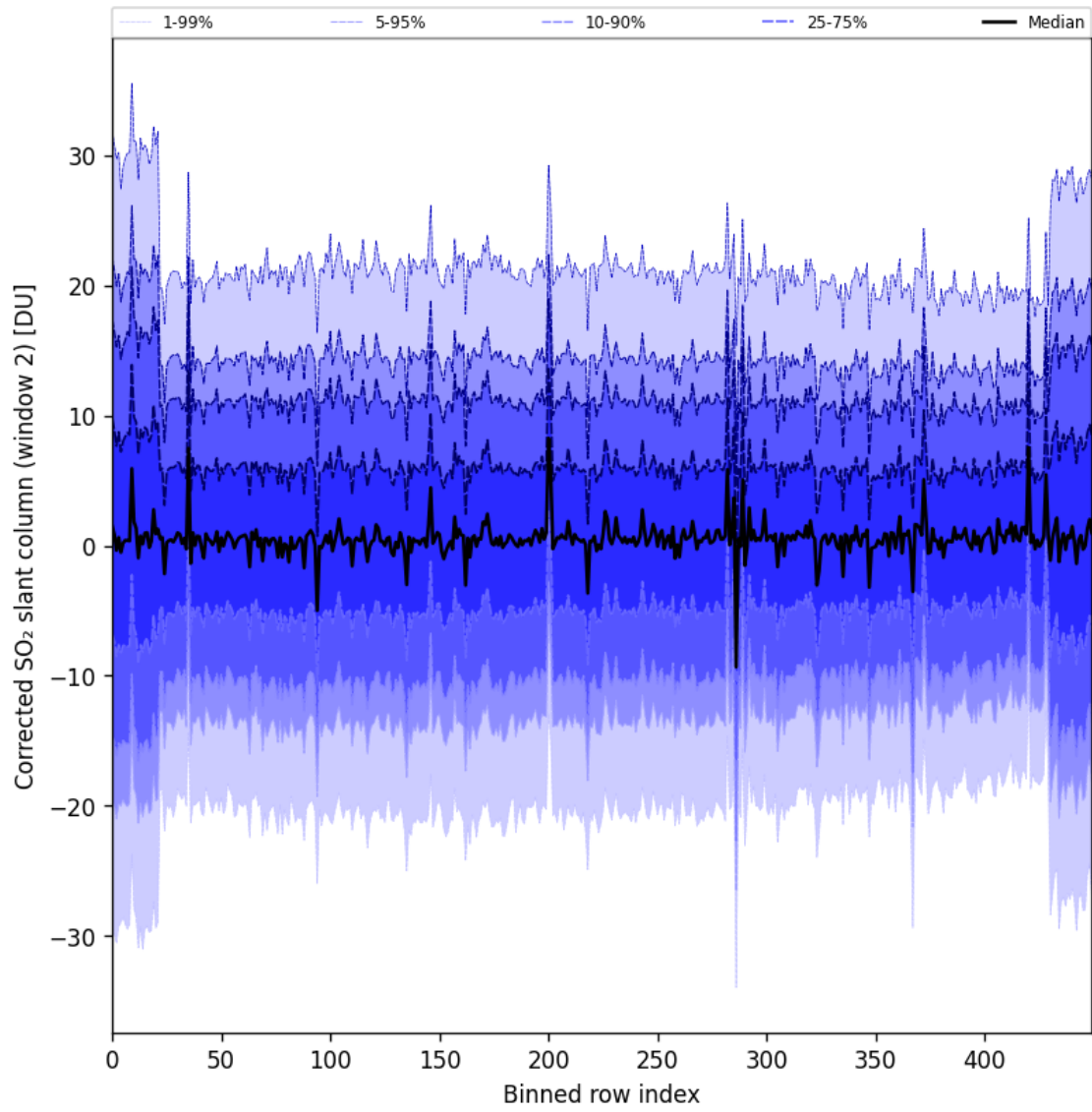
Figure 95: Along track statistics of “Corrected SO 2 slant column (window 2)” for 2025-07-26 to 2025-07-28
