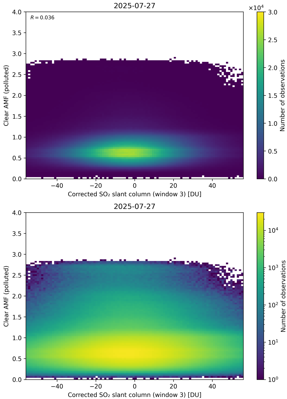
Figure 259: Scatter density plot of “Corrected SO 2 slant column (window 3)” against “Clear AMF (polluted)” for 2025-07-26 to 2025-07-28.
