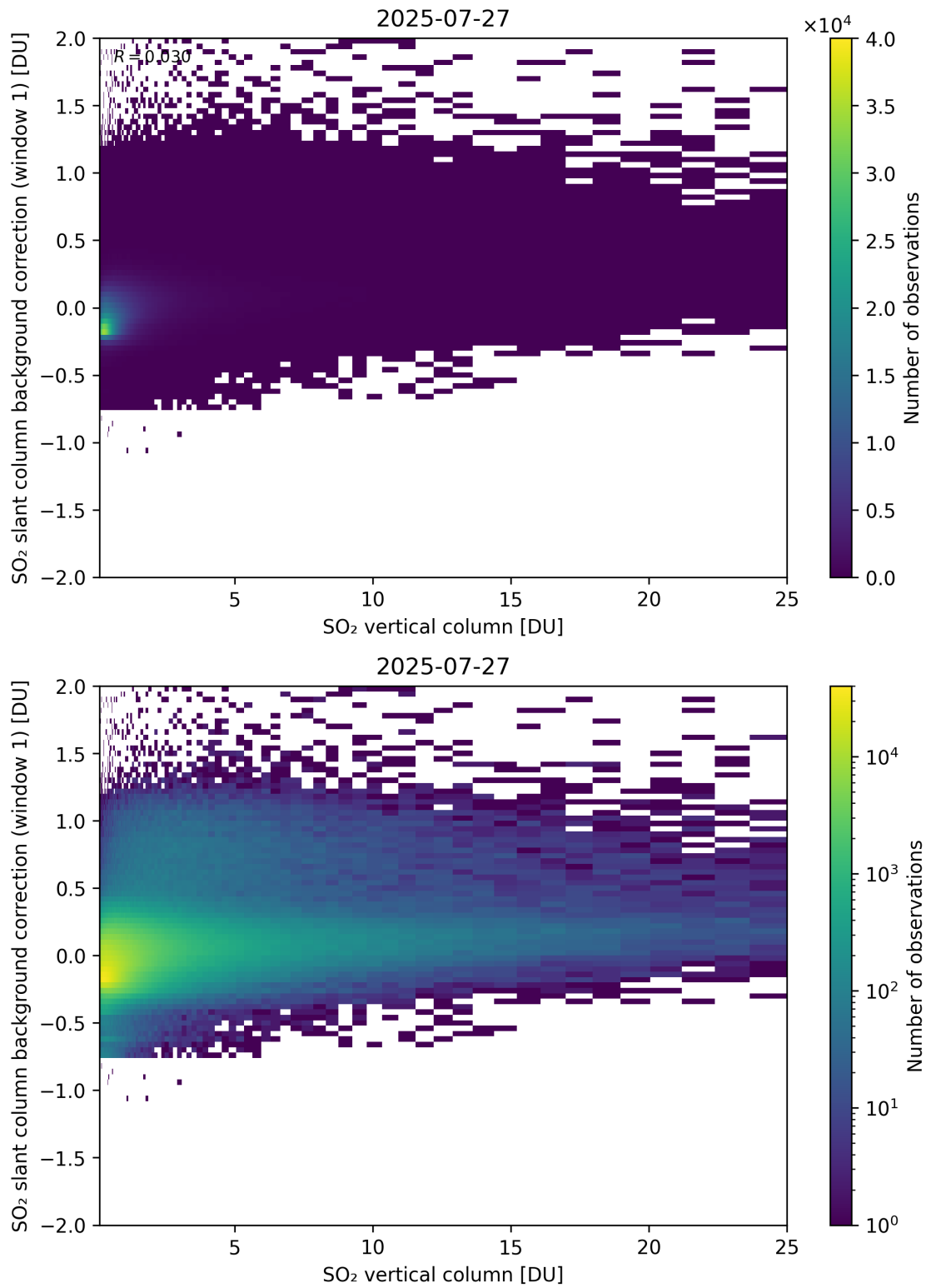
Figure 323: Scatter density plot of “SO 2 vertical column” against “SO 2 slant column background correction (window 1)” for 2025-07-26 to 2025-07-28.
