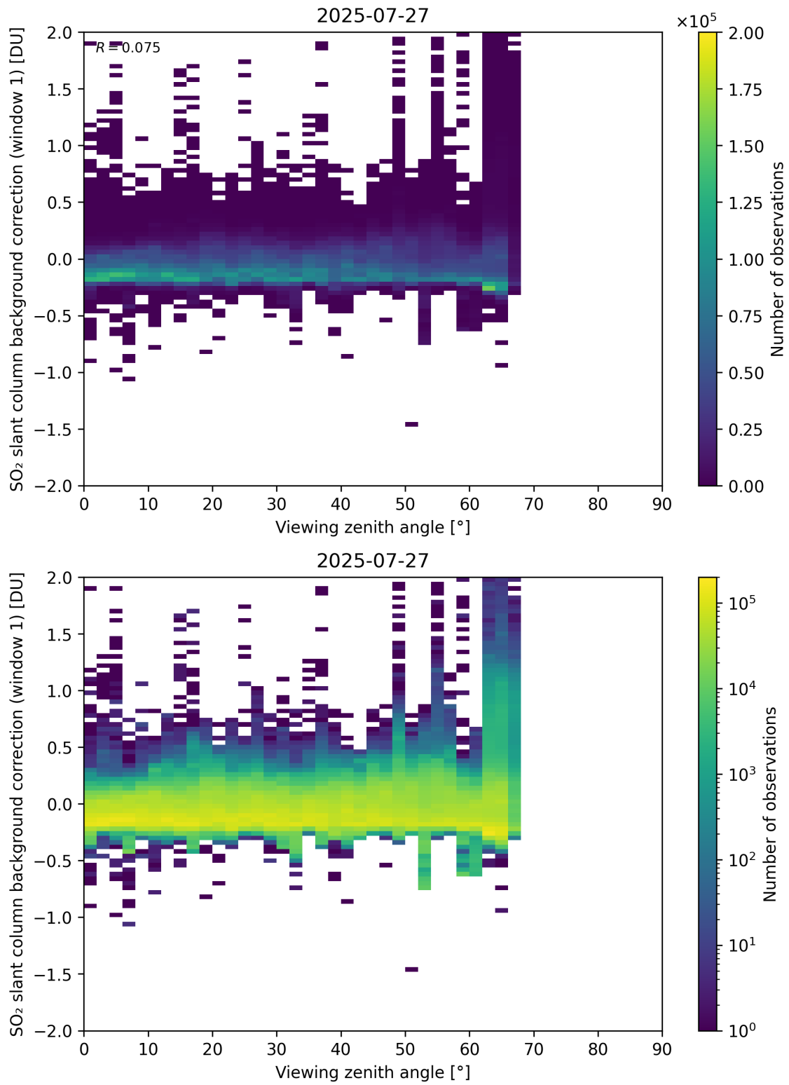
Figure 362: Scatter density plot of “Viewing zenith angle” against “SO 2 slant column background correction (window 1)” for 2025-07-26 to 2025-07-28.
