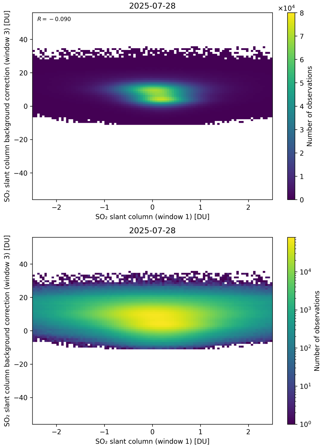
Figure 264: Scatter density plot of “SO 2 slant column (window 1)” against “SO 2 slant column background correction (window 3)” for 2025-07-27 to 2025-07-29.
