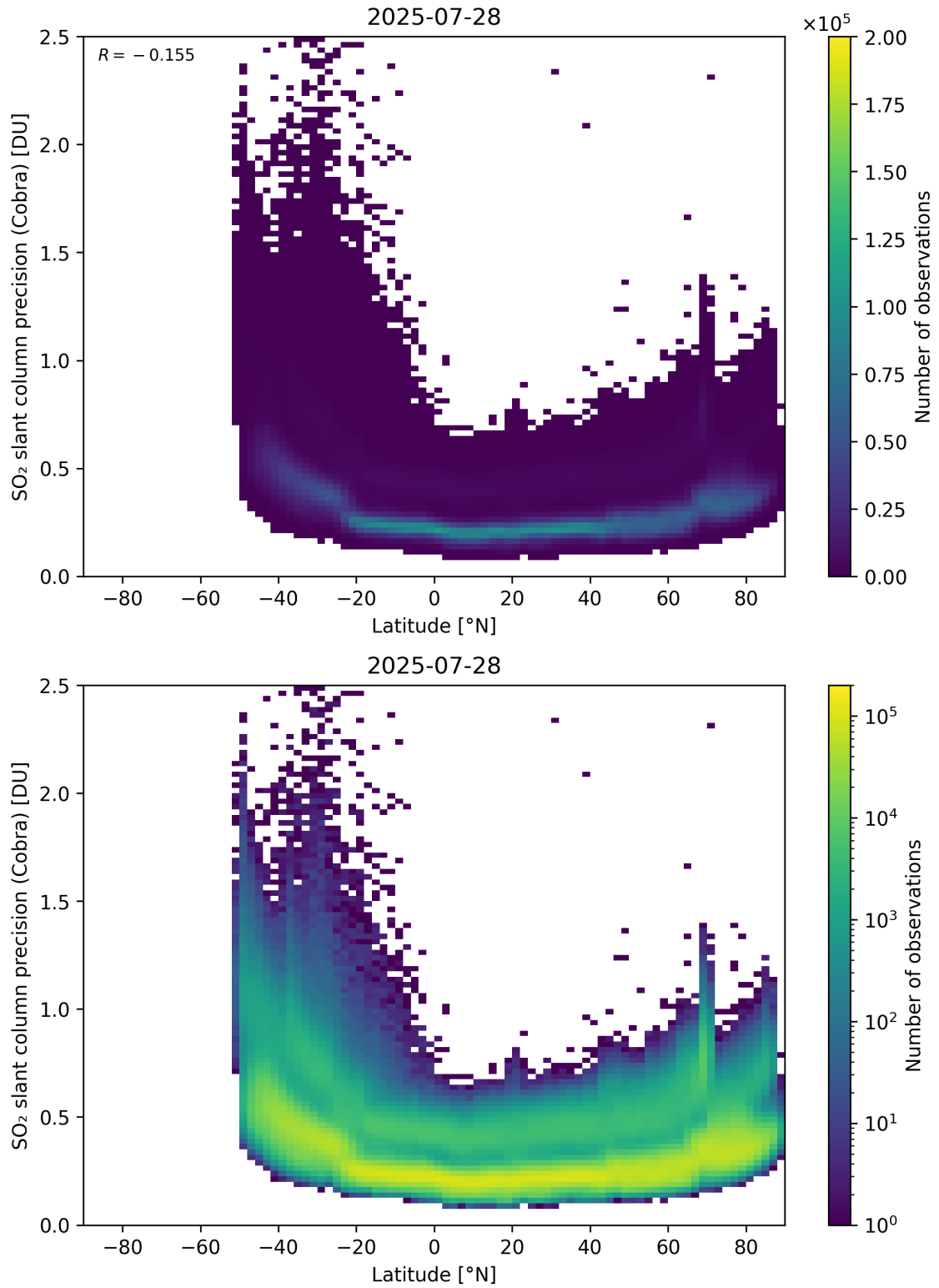
Figure 158: Scatter density plot of “Latitude” against “SO 2 slant column precision (Cobra)” for 2025-07-27 to 2025-07-29.
