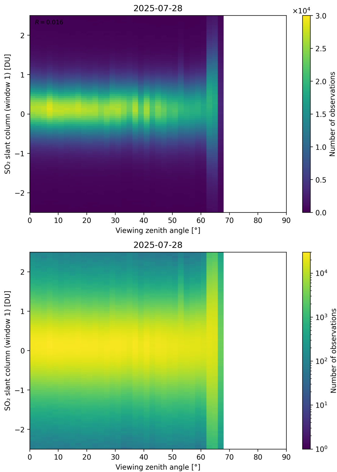
Figure 376: Scatter density plot of “Viewing zenith angle” against “SO 2 slant column (window 1)” for 2025-07-27 to 2025-07-29.
