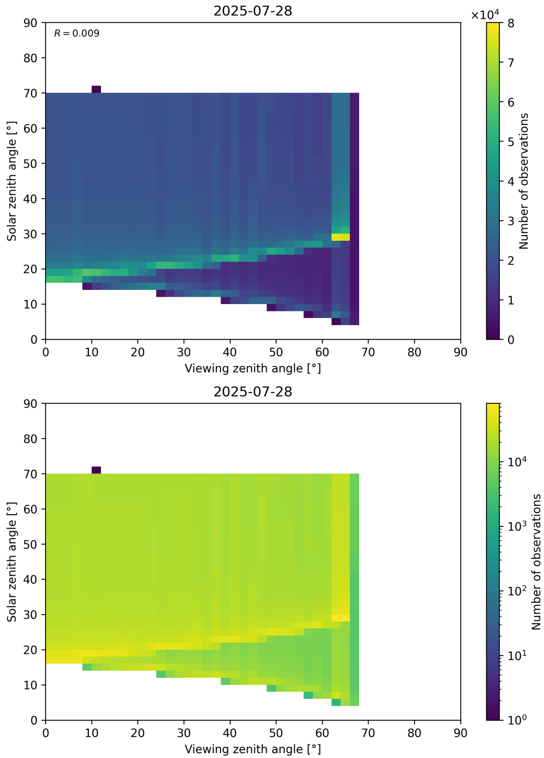
Figure 369: Scatter density plot of “Viewing zenith angle” against “Solar zenith angle” for 2025-07-27 to 2025-07-29.
