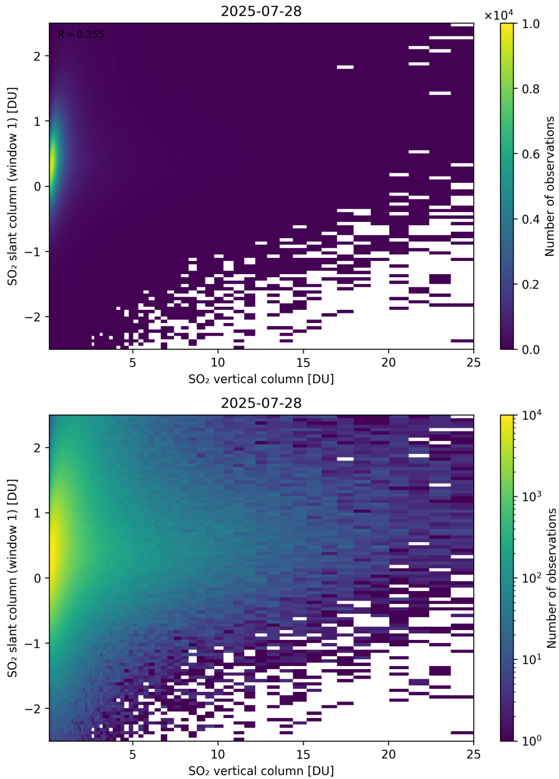
Figure 354: Scatter density plot of “SO 2 vertical column” against “SO 2 slant column (window 1)” for 2025-07-27 to 2025-07-29.
