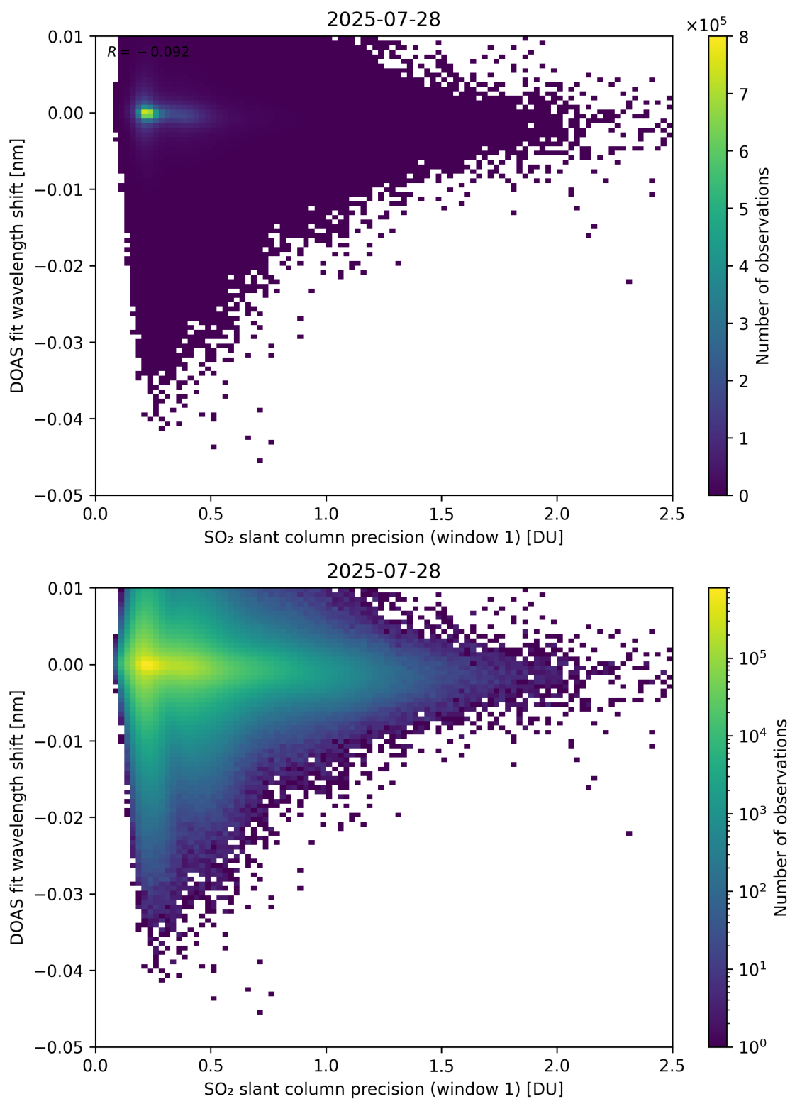
Figure 271: Scatter density plot of “SO 2 slant column precision (window 1)” against “DOAS fit wavelength shift” for 2025-07-27 to 2025-07-29.
