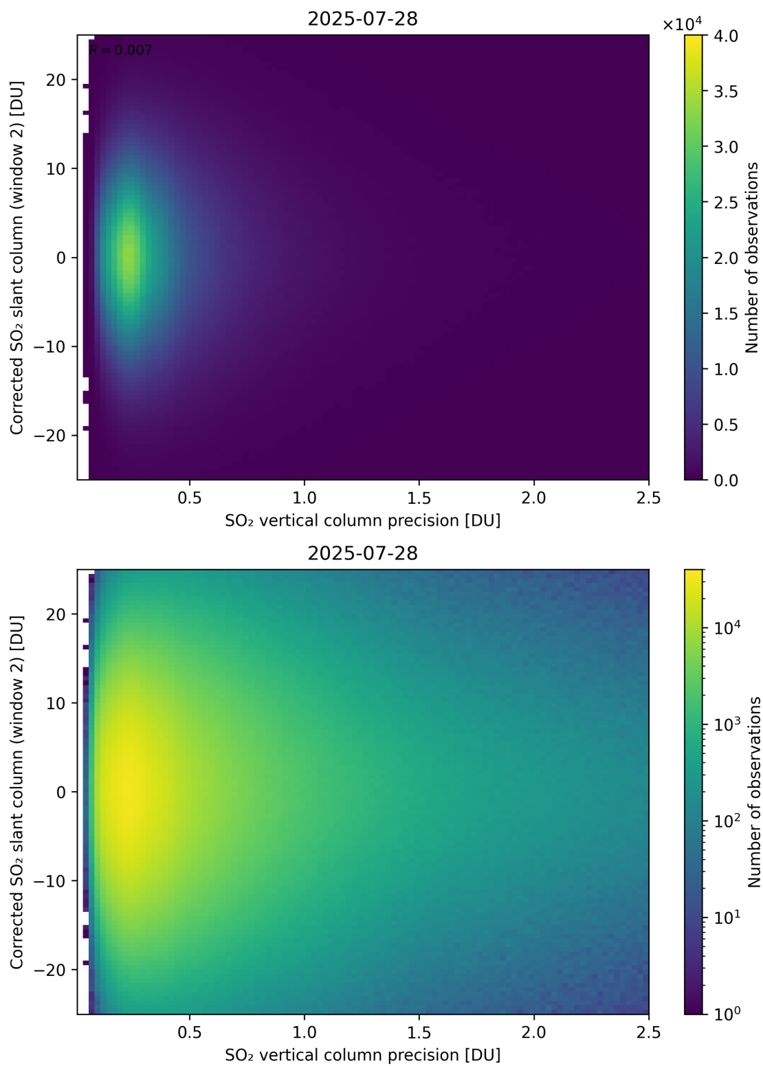
Figure 339: Scatter density plot of “SO 2 vertical column precision” against “Corrected SO 2 slant column (window 2)” for 2025-07-27 to 2025-07-29.
