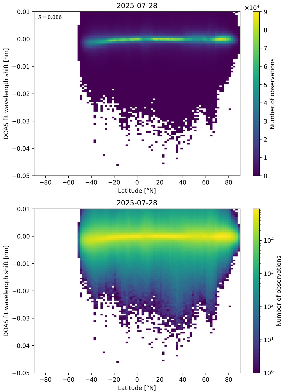
Figure 153: Scatter density plot of “Latitude” against “DOAS fit wavelength shift” for 2025-07-27 to 2025-07-29.
