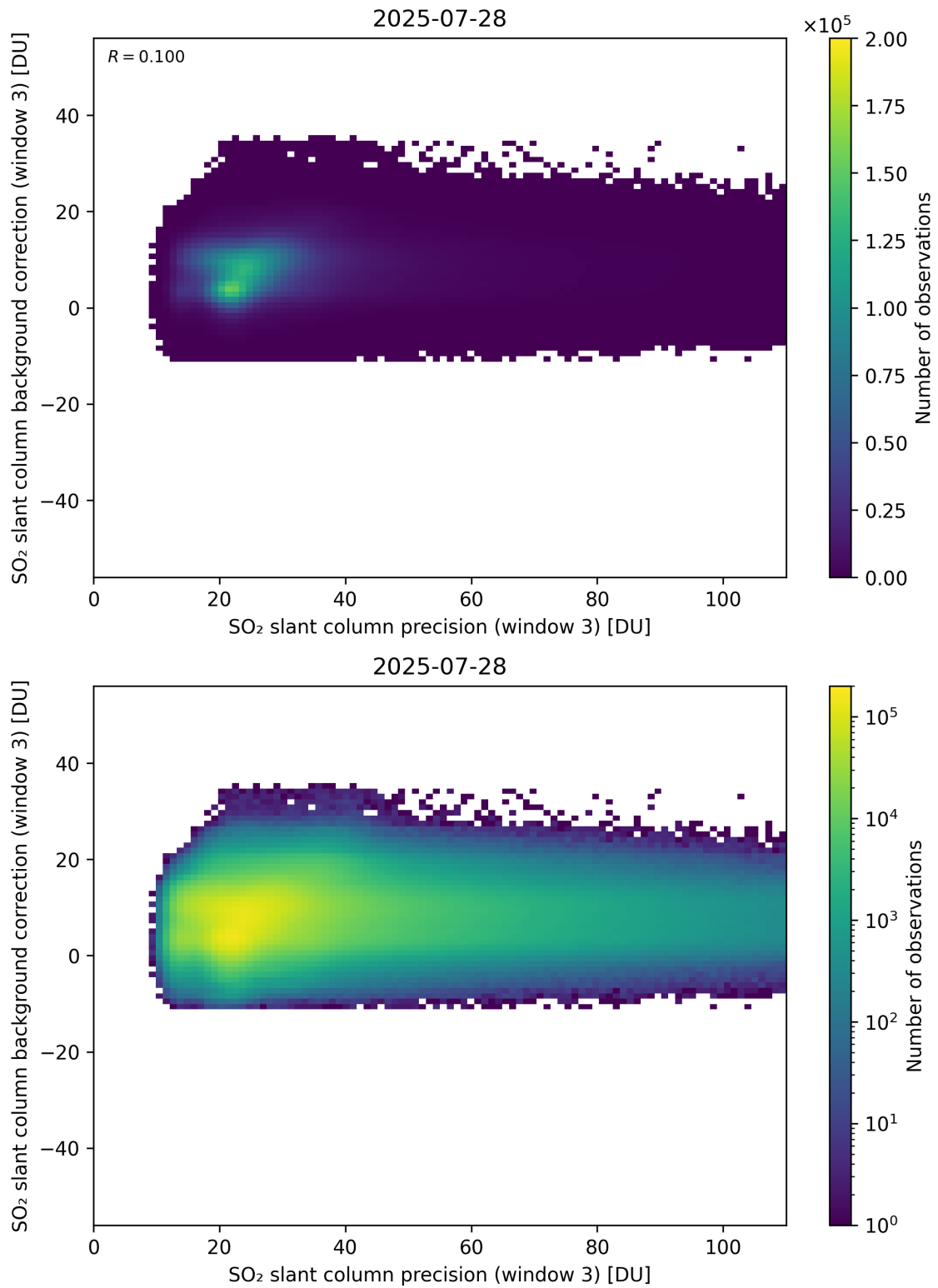
Figure 307: Scatter density plot of “SO 2 slant column precision (window 3)” against “SO 2 slant column background correction (window 3)” for 2025-07-27 to 2025-07-29.
