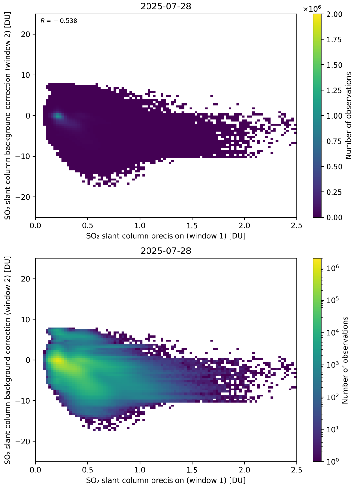
Figure 269: Scatter density plot of “SO 2 slant column precision (window 1)” against “SO 2 slant column background correction (window 2)” for 2025-07-27 to 2025-07-29.
