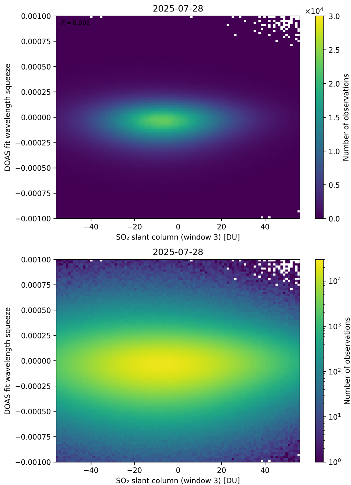
Figure 305: Scatter density plot of “SO 2 slant column (window 3)” against “DOAS fit wavelength squeeze” for 2025-07-27 to 2025-07-29.
