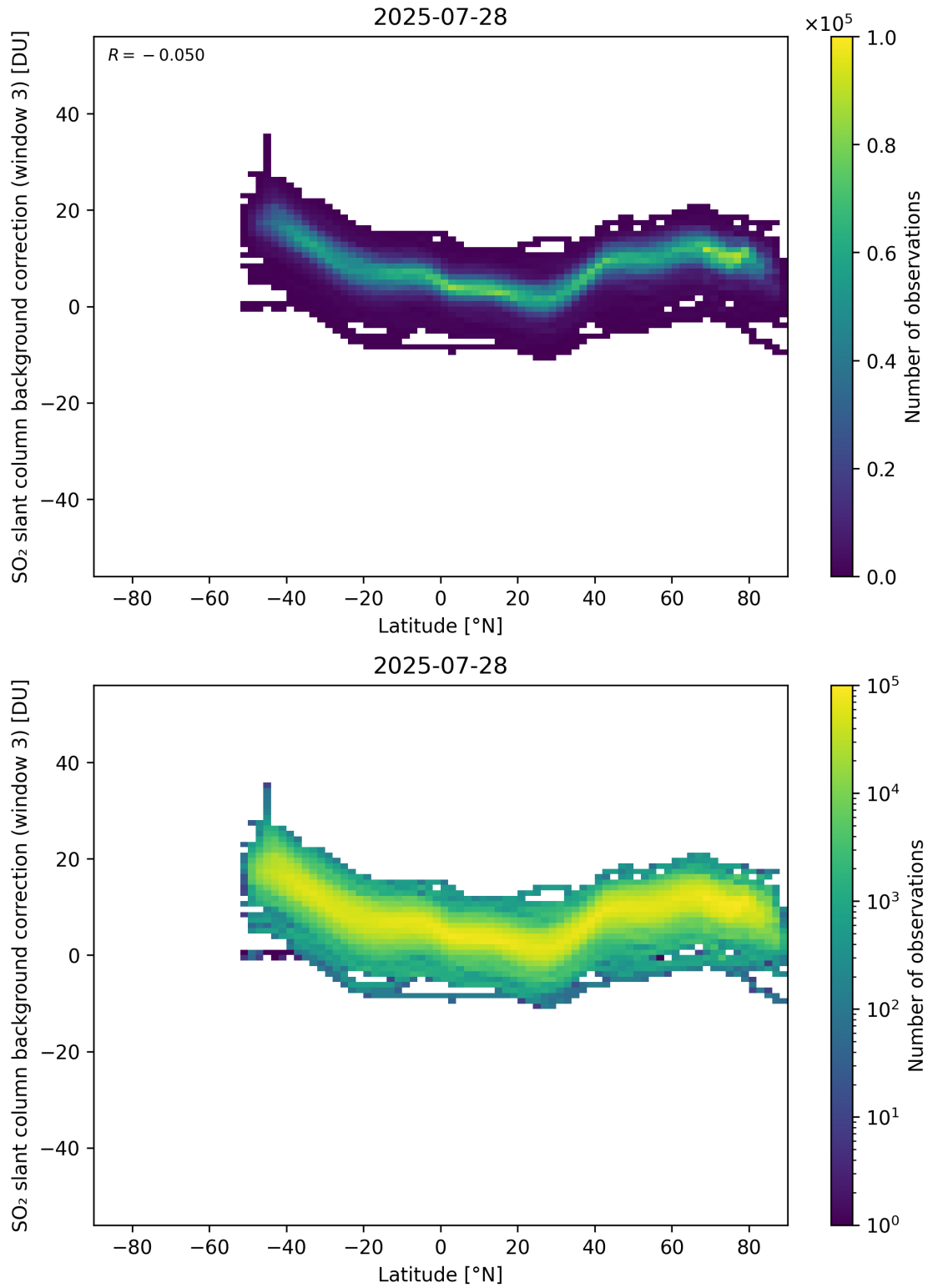
Figure 152: Scatter density plot of “Latitude” against “SO 2 slant column background correction (window 3)” for 2025-07-27 to 2025-07-29.
