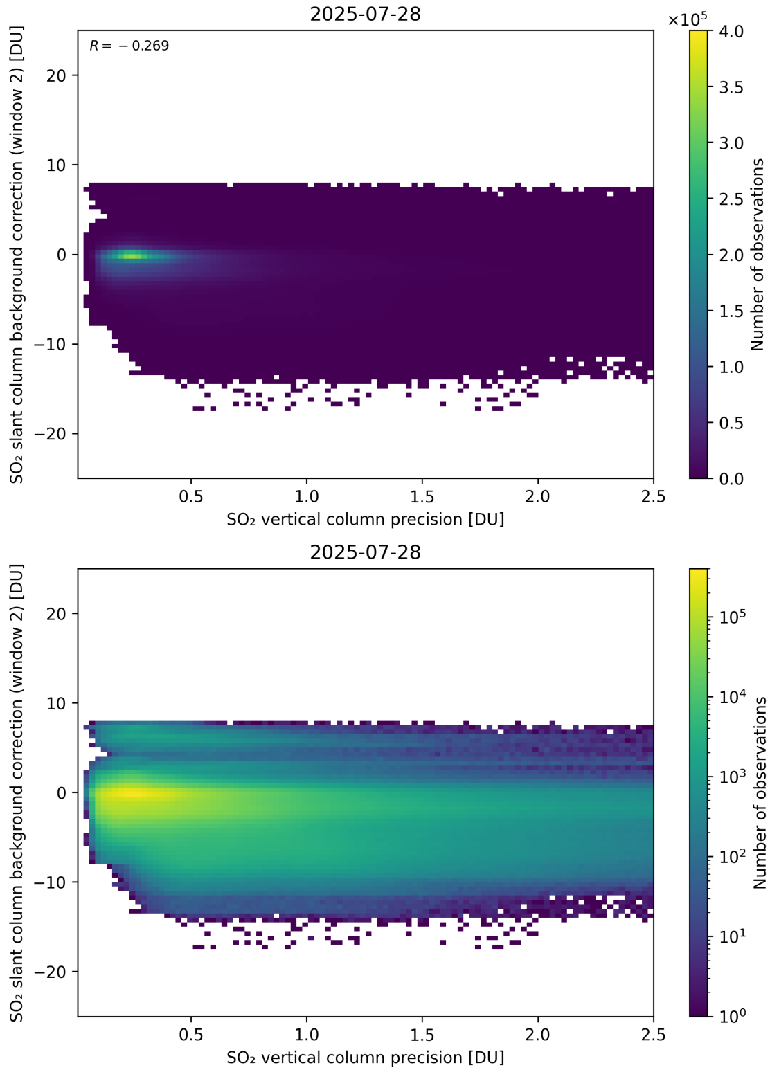
Figure 330: Scatter density plot of “SO 2 vertical column precision” against “SO 2 slant column background correction (window 2)” for 2025-07-27 to 2025-07-29.
