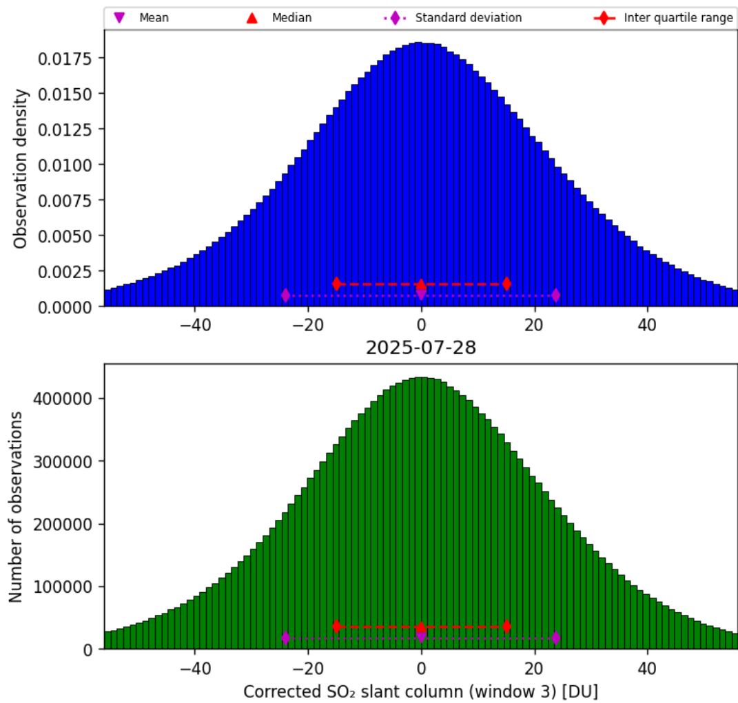
Figure 73: Histogram of “Corrected SO 2 slant column (window 3)” for 2025-07-27 to 2025-07-29
