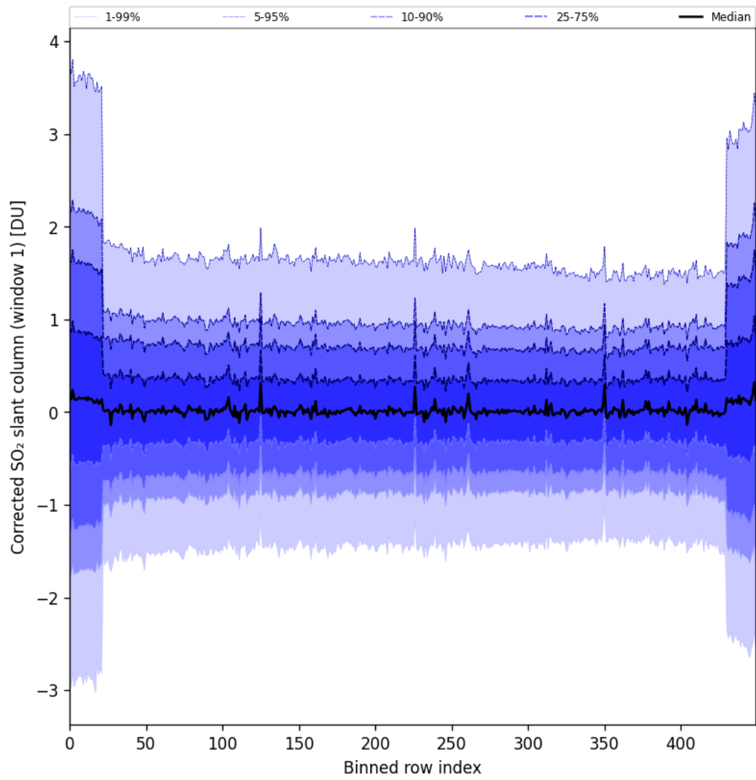
Figure 91: Along track statistics of “Corrected SO 2 slant column (window 1)” for 2025-07-27 to 2025-07-29
