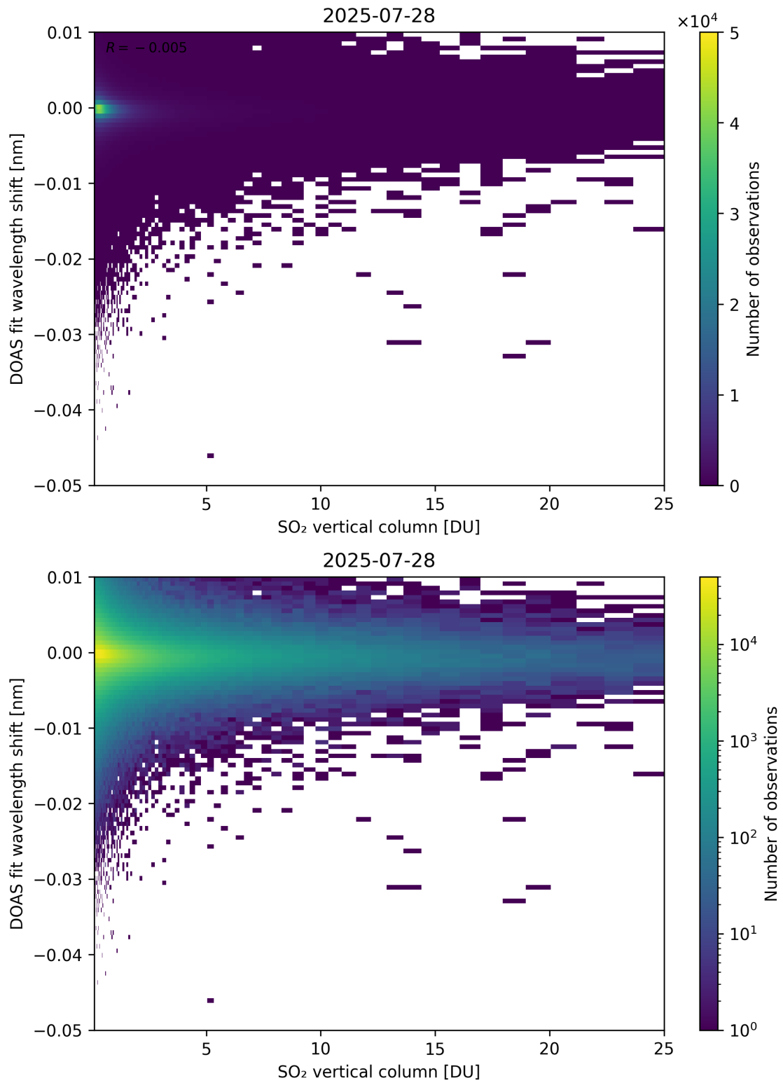
Figure 326: Scatter density plot of “SO 2 vertical column” against “DOAS fit wavelength shift” for 2025-07-27 to 2025-07-29.
