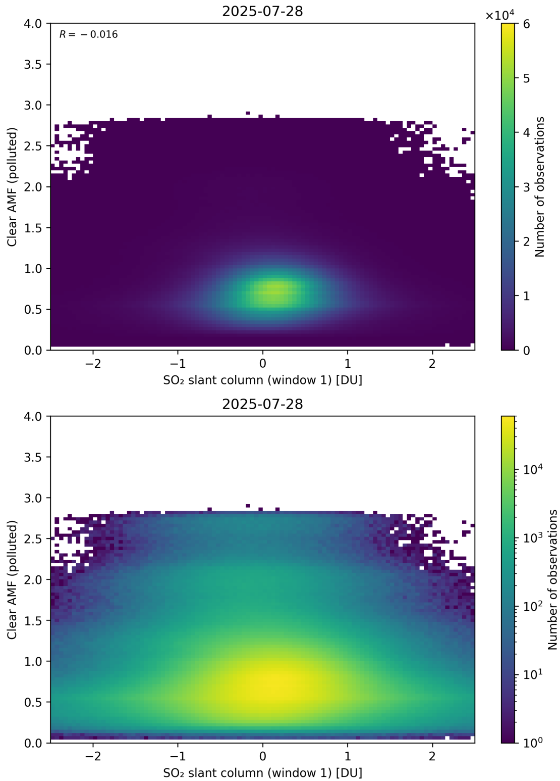
Figure 282: Scatter density plot of “SO 2 slant column (window 1)” against “Clear AMF (polluted)” for 2025-07-27 to 2025-07-29.
