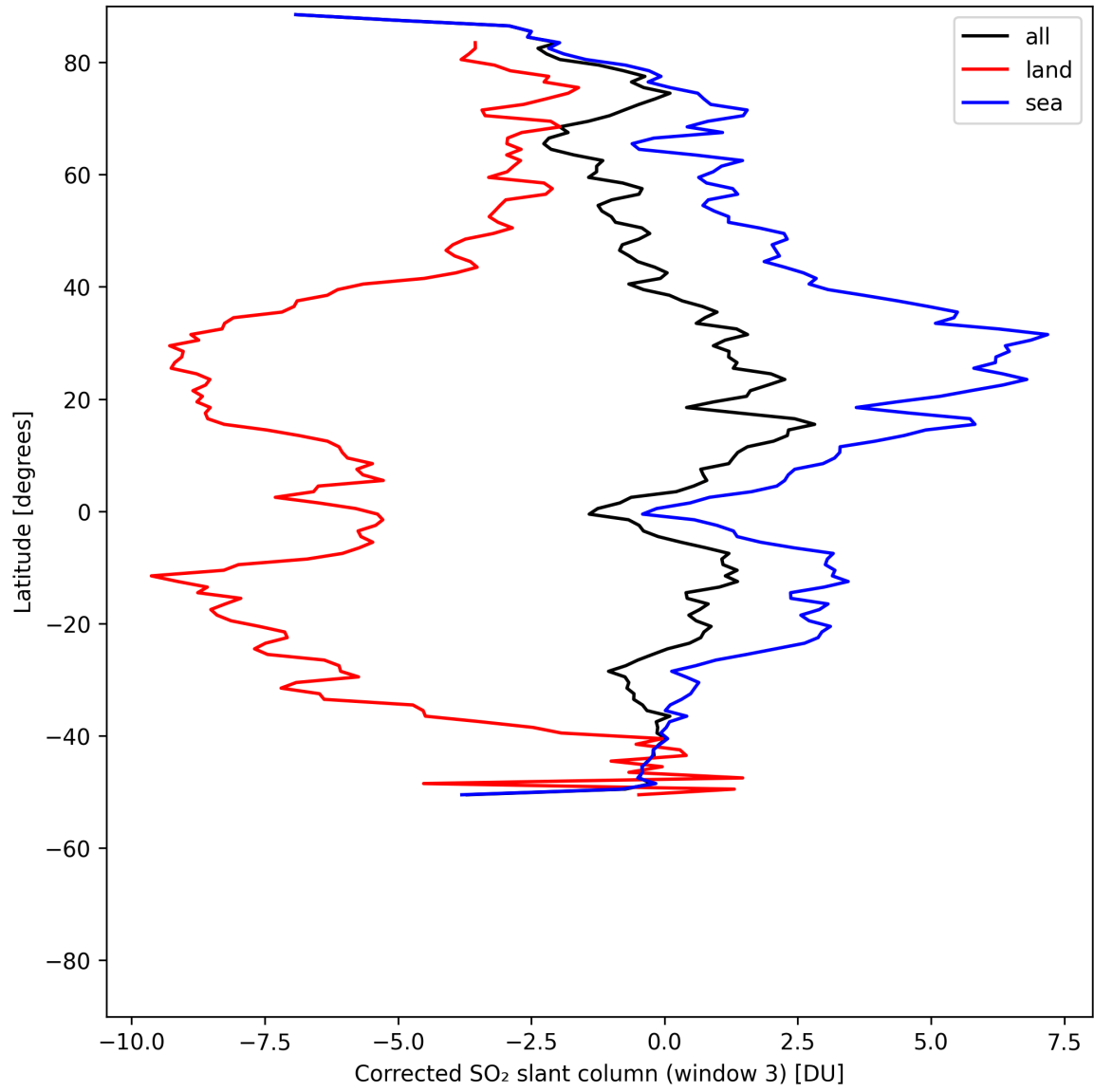
Figure 47: Zonal average of “Corrected SO 2 slant column (window 3)” for 2025-07-27 to 2025-07-29.
