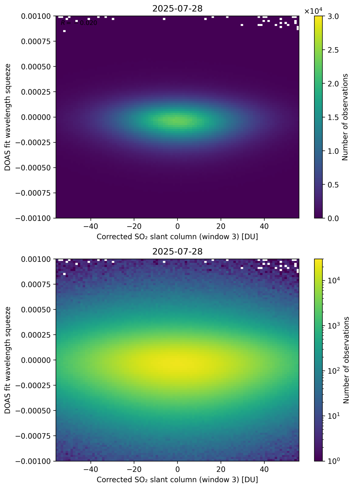
Figure 257: Scatter density plot of “Corrected SO 2 slant column (window 3)” against “DOAS fit wavelength squeeze” for 2025-07-27 to 2025-07-29.
