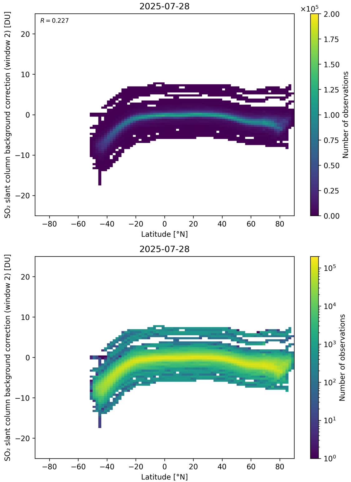
Figure 151: Scatter density plot of “Latitude” against “SO 2 slant column background correction (window 2)” for 2025-07-27 to 2025-07-29.
