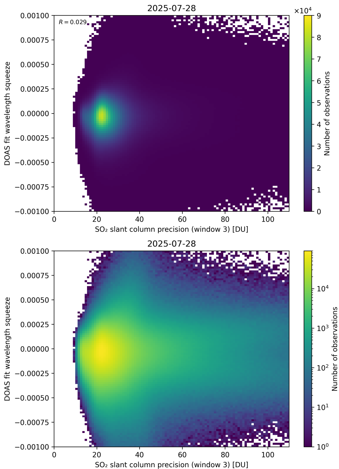
Figure 309: Scatter density plot of “SO 2 slant column precision (window 3)” against “DOAS fit wavelength squeeze” for 2025-07-27 to 2025-07-29.
