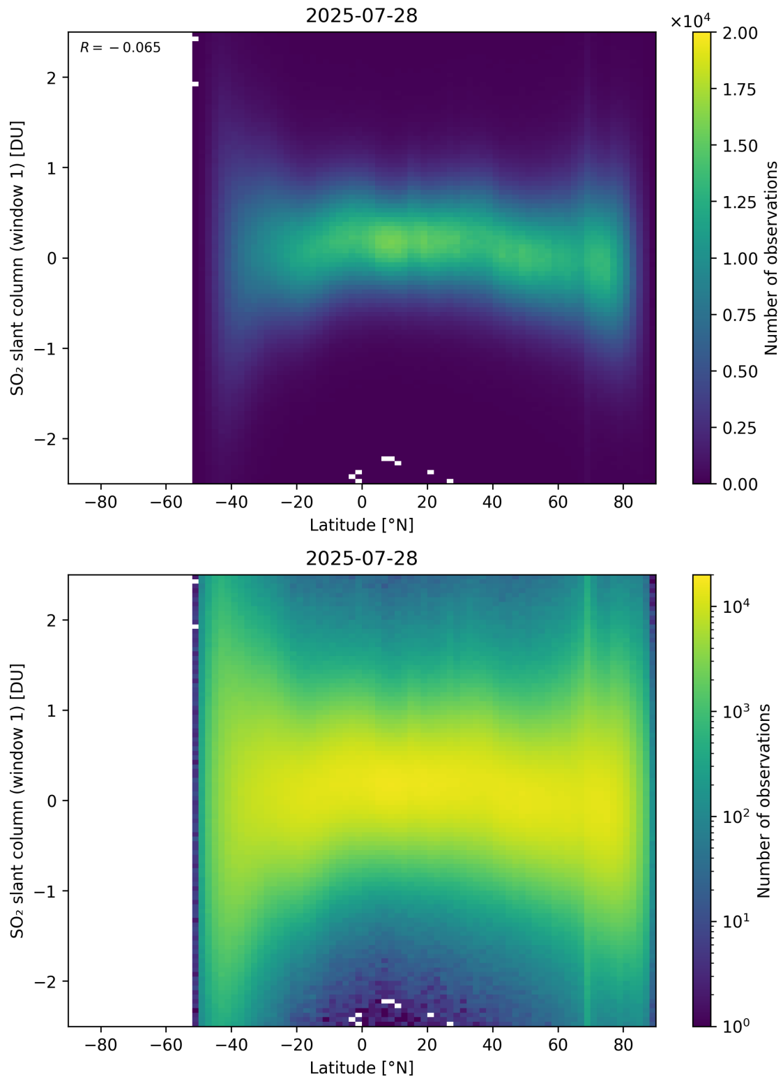
Figure 162: Scatter density plot of “Latitude” against “SO 2 slant column (window 1)” for 2025-07-27 to 2025-07-29.
