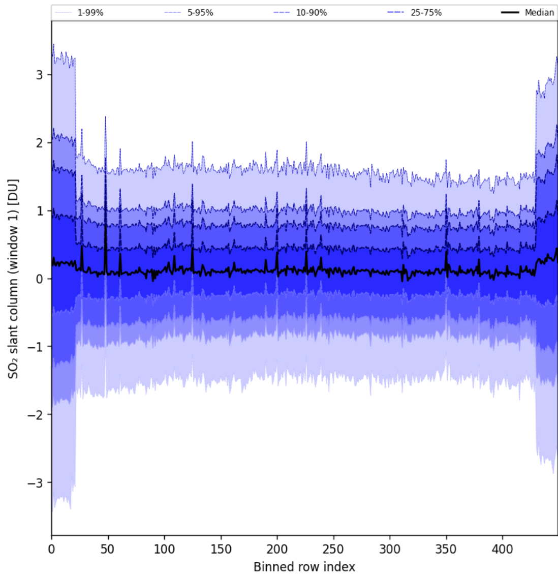
Figure 89: Along track statistics of “SO 2 slant column (window 1)” for 2025-07-27 to 2025-07-29
