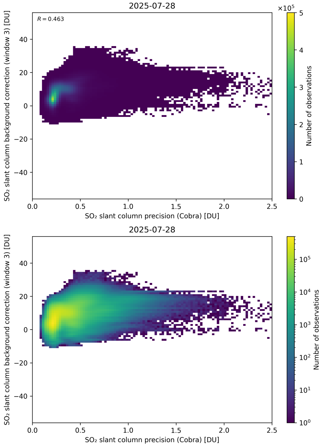
Figure 201: Scatter density plot of “SO 2 slant column precision (Cobra)” against “SO 2 slant column background correction (window 3)” for 2025-07-27 to 2025-07-29.
