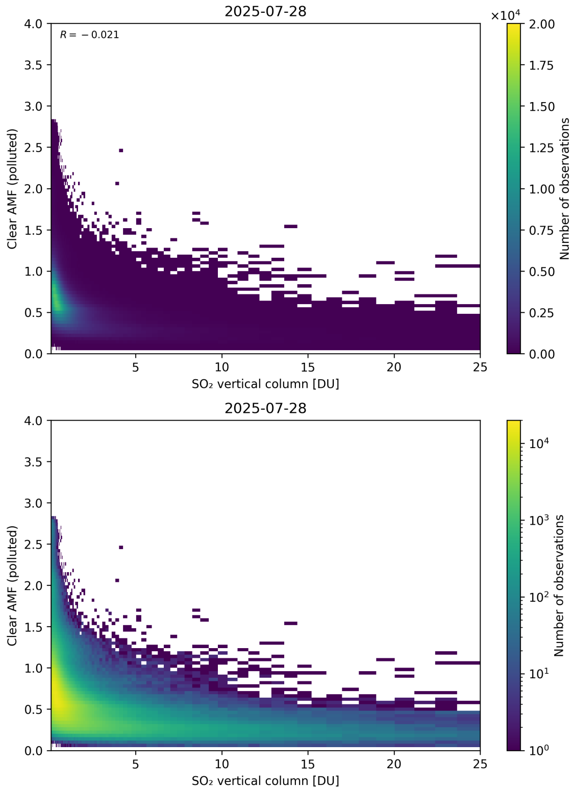
Figure 348: Scatter density plot of “SO 2 vertical column” against “Clear AMF (polluted)” for 2025-07-27 to 2025-07-29.
