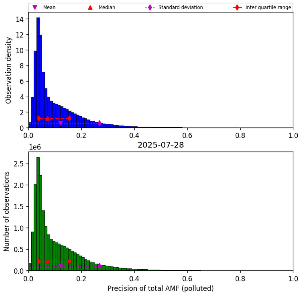
Figure 80: Histogram of “Precision of total AMF (polluted)” for 2025-07-27 to 2025-07-29
