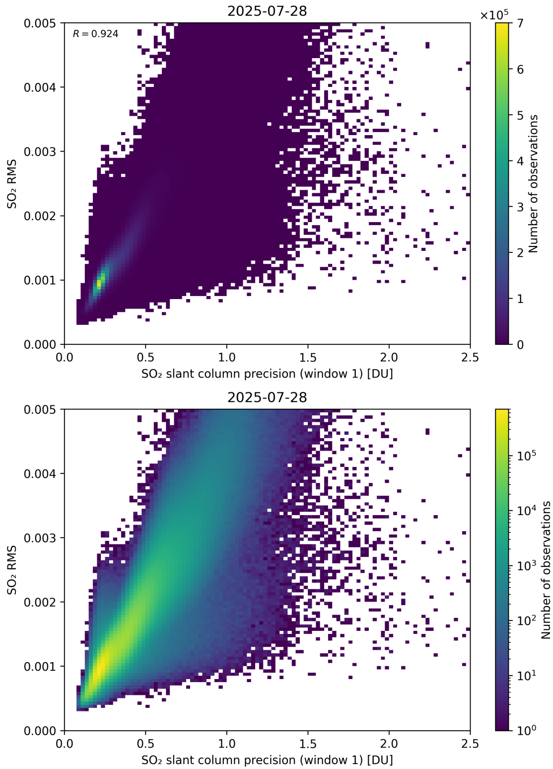
Figure 273: Scatter density plot of “SO 2 slant column precision (window 1)” against “SO 2 RMS” for 2025-07-27 to 2025-07-29.
