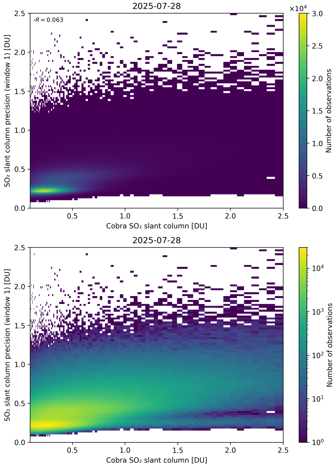
Figure 220: Scatter density plot of “Cobra SO 2 slant column” against “SO 2 slant column precision (window 1)” for 2025-07-27 to 2025-07-29.
