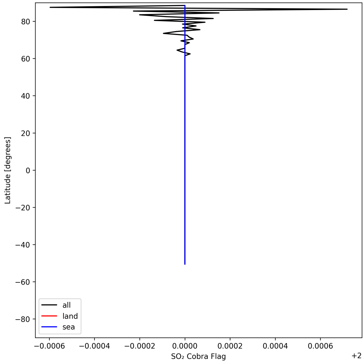
Figure 49: Zonal average of "SO 2 Cobra Flag" for 2025-07-27 to 2025-07-29.
