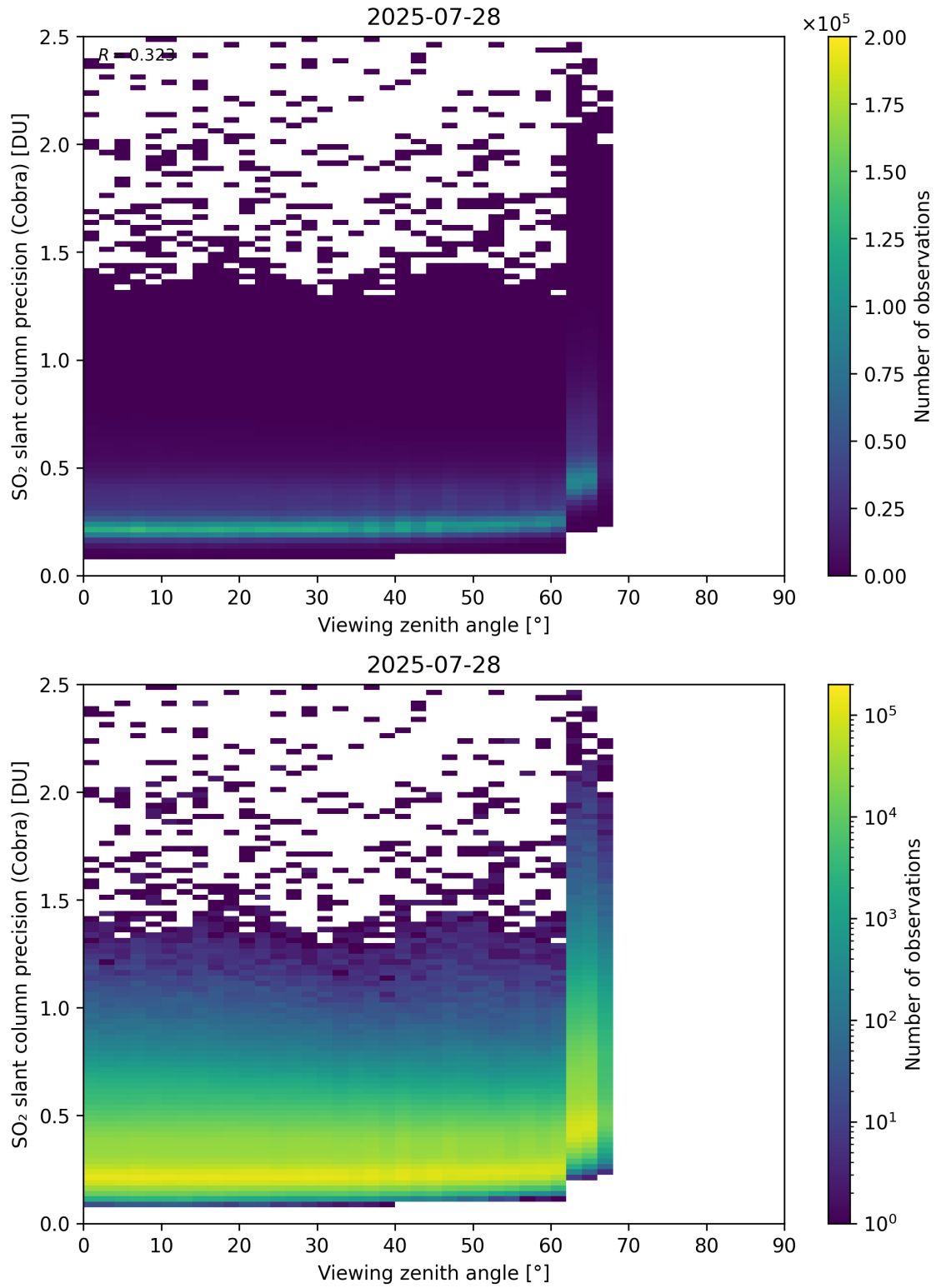
Figure 372: Scatter density plot of “Viewing zenith angle” against “SO 2 slant column precision (Cobra)” for 2025-07-27 to 2025-07-29.
