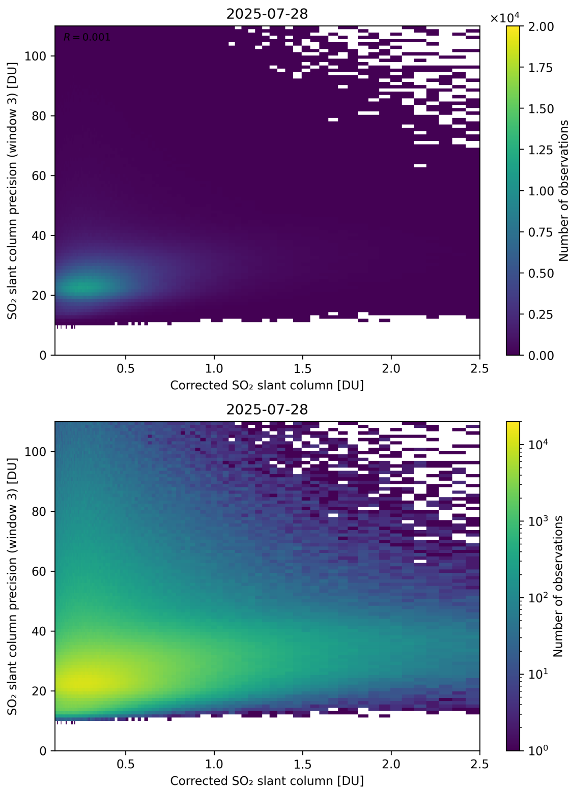
Figure 241: Scatter density plot of “Corrected SO 2 slant column” against “SO 2 slant column precision (window 3)” for 2025-07-27 to 2025-07-29.
