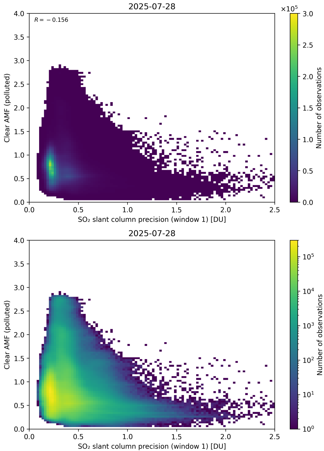
Figure 274: Scatter density plot of “SO 2 slant column precision (window 1)” against “Clear AMF (polluted)” for 2025-07-27 to 2025-07-29.
