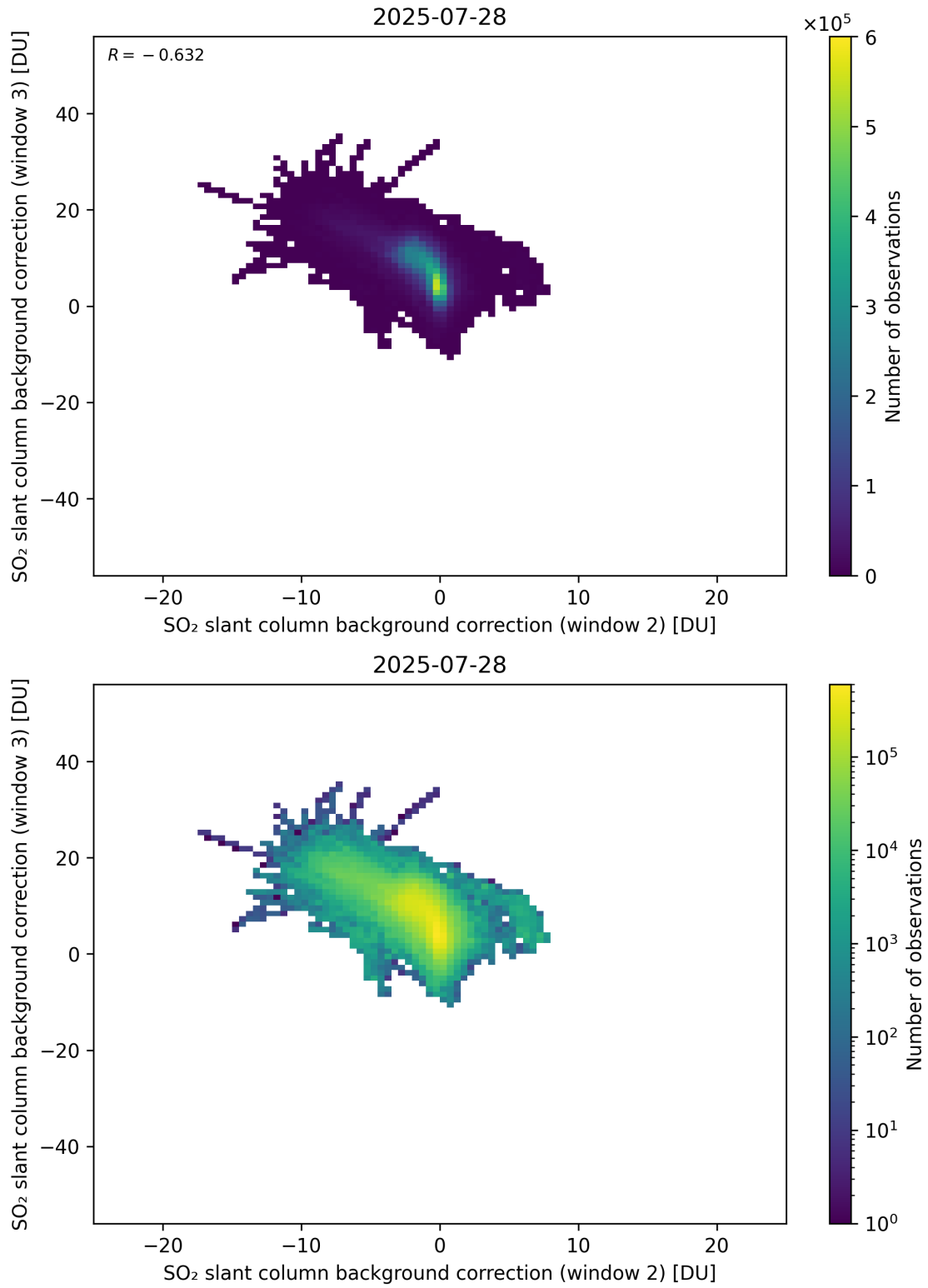
Figure 122: Scatter density plot of “SO 2 slant column background correction (window 2)” against “SO 2 slant column background correction (window 3)” for 2025-07-27 to 2025-07-29.
