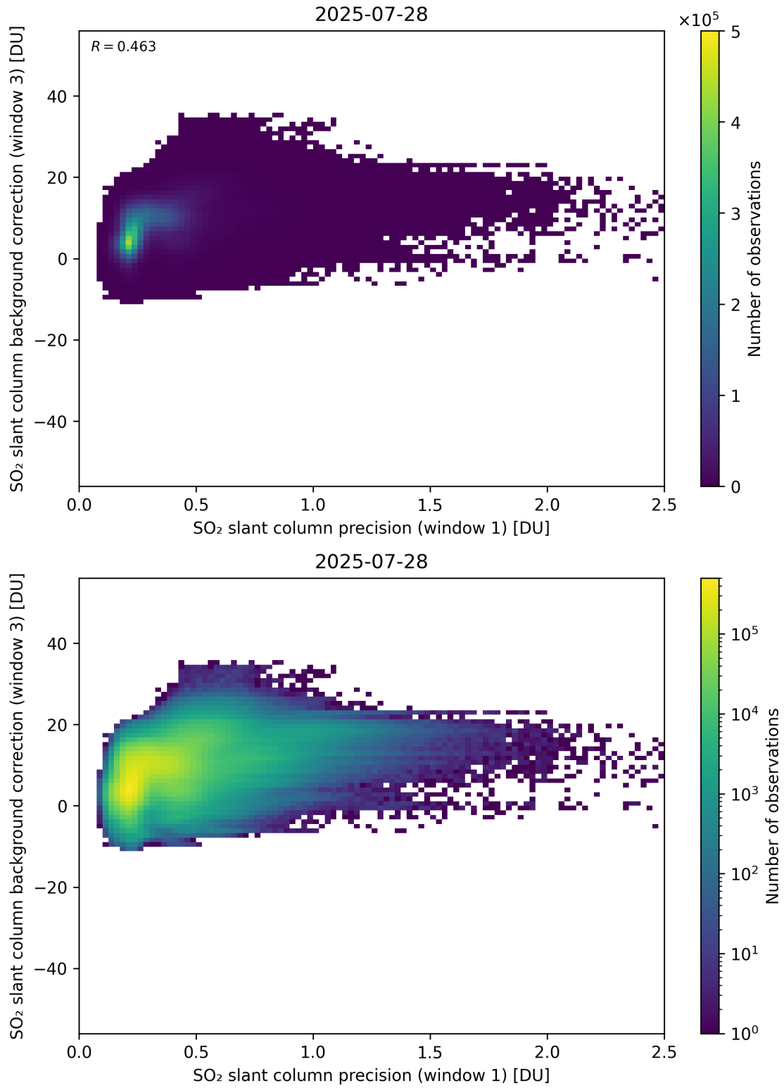
Figure 270: Scatter density plot of “SO 2 slant column precision (window 1)” against “SO 2 slant column background correction (window 3)” for 2025-07-27 to 2025-07-29.
