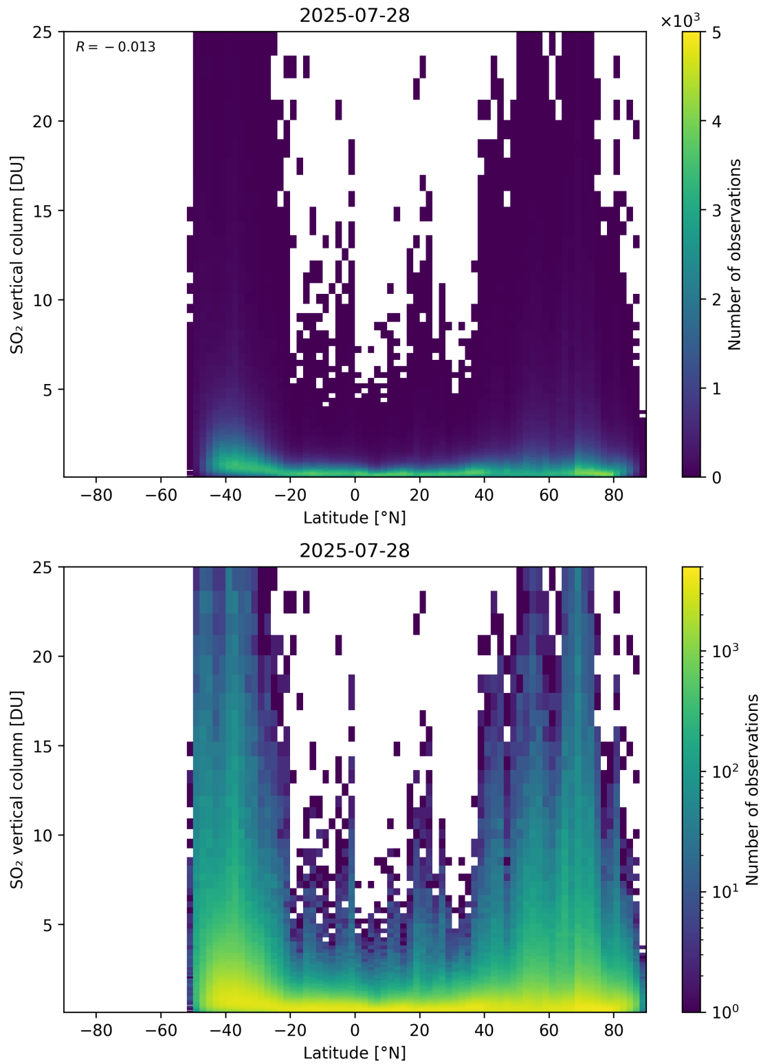
Figure 169: Scatter density plot of “Latitude” against “SO 2 vertical column” for 2025-07-27 to 2025-07-29.
