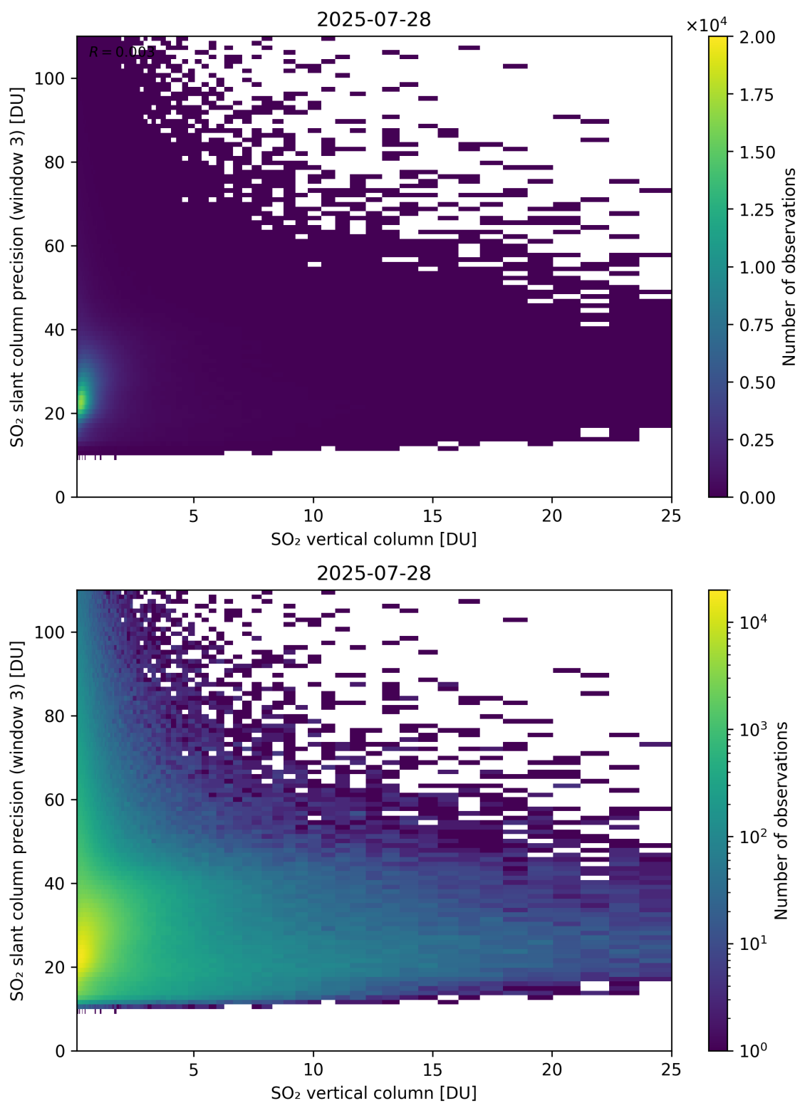
Figure 358: Scatter density plot of “SO 2 vertical column” against “SO 2 slant column precision (window 3)” for 2025-07-27 to 2025-07-29.
