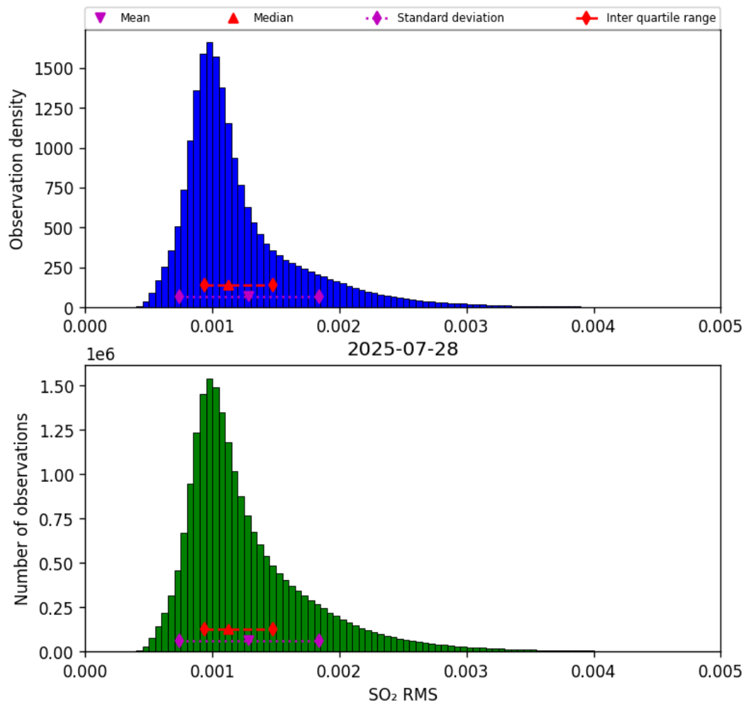
Figure 78: Histogram of “SO 2 RMS” for 2025-07-27 to 2025-07-29
