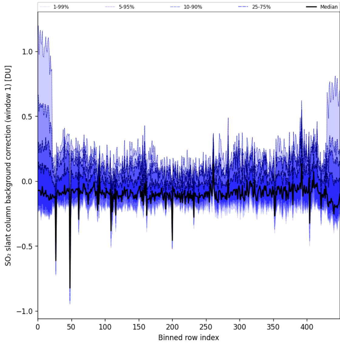
Figure 92: Along track statistics of “SO 2 slant column background correction (window 1)” for 2025-07-27 to 2025-07-29
