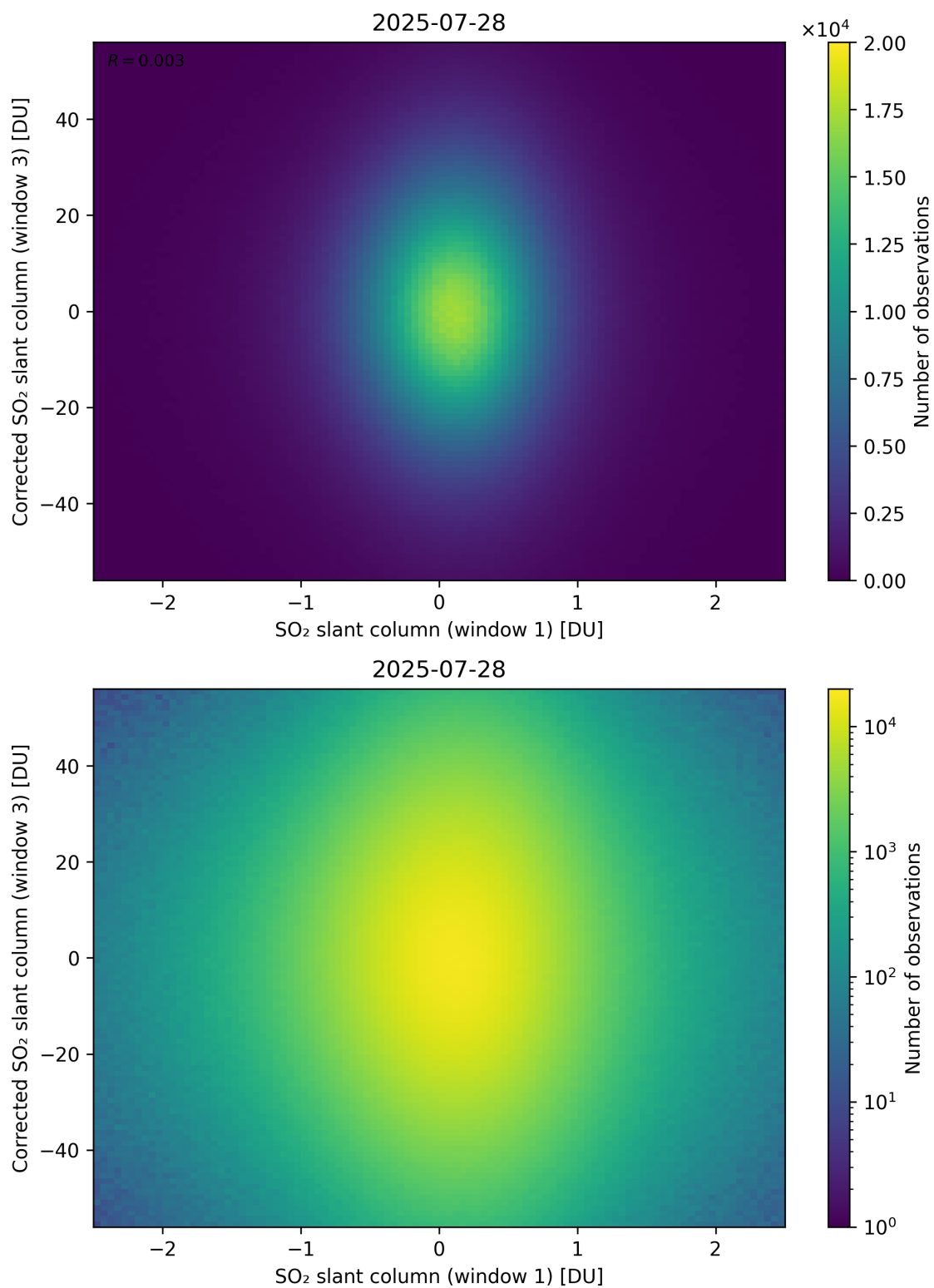
Figure 284: Scatter density plot of “SO 2 slant column (window 1)” against “Corrected SO 2 slant column (window 3)” for 2025-07-27 to 2025-07-29.
