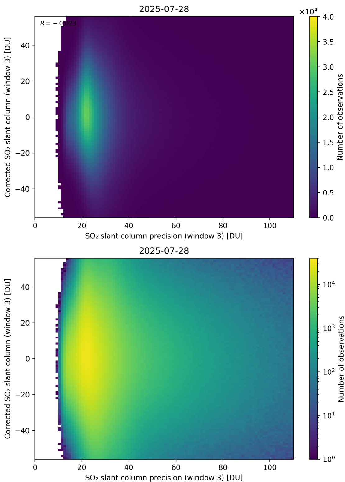
Figure 312: Scatter density plot of “SO 2 slant column precision (window 3)” against “Corrected SO 2 slant column (window 3)” for 2025-07-27 to 2025-07-29.
