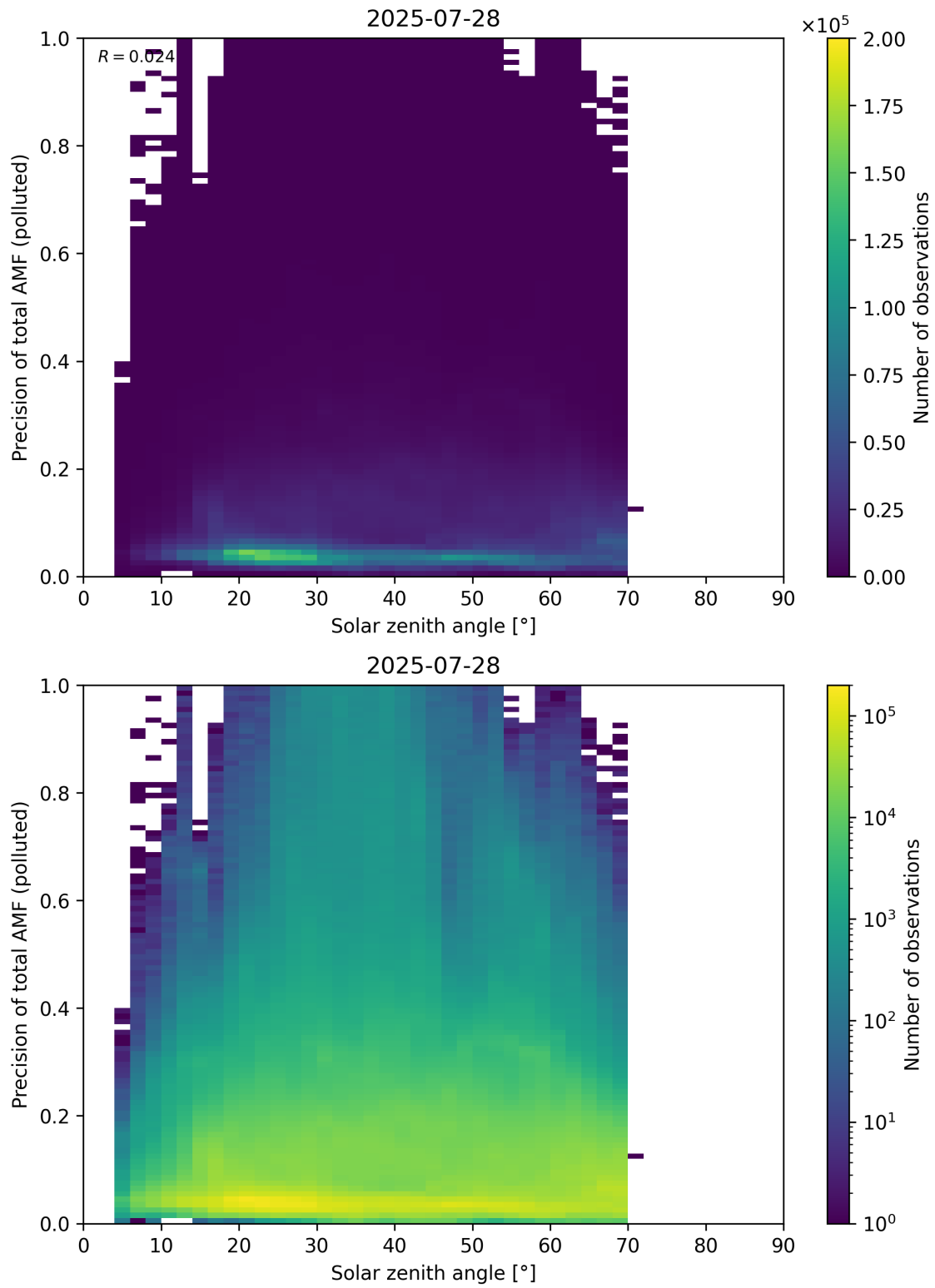
Figure 190: Scatter density plot of “Solar zenith angle” against “Precision of total AMF (polluted)” for 2025-07-27 to 2025-07-29.
