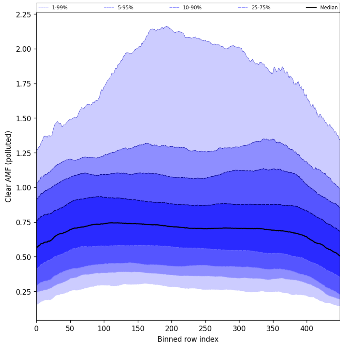
Figure 107: Along track statistics of “Clear AMF (polluted)” for 2025-07-27 to 2025-07-29
