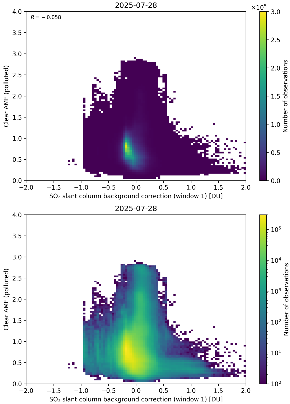
Figure 114: Scatter density plot of “SO 2 slant column background correction (window 1)” against “Clear AMF (polluted)” for 2025-07-27 to 2025-07-29.
