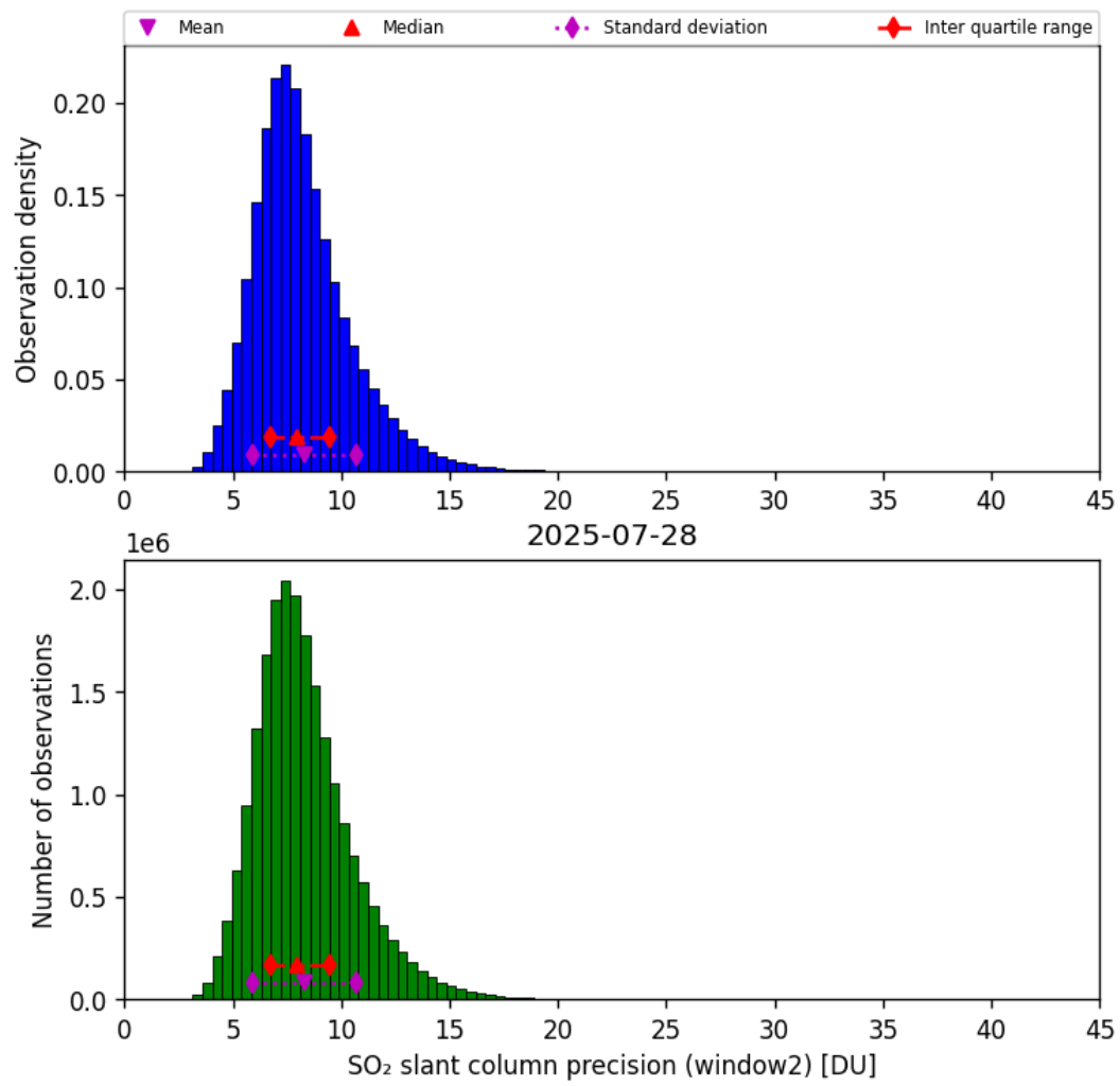
Figure 68: Histogram of “SO 2 slant column precision (window2)” for 2025-07-27 to 2025-07-29
