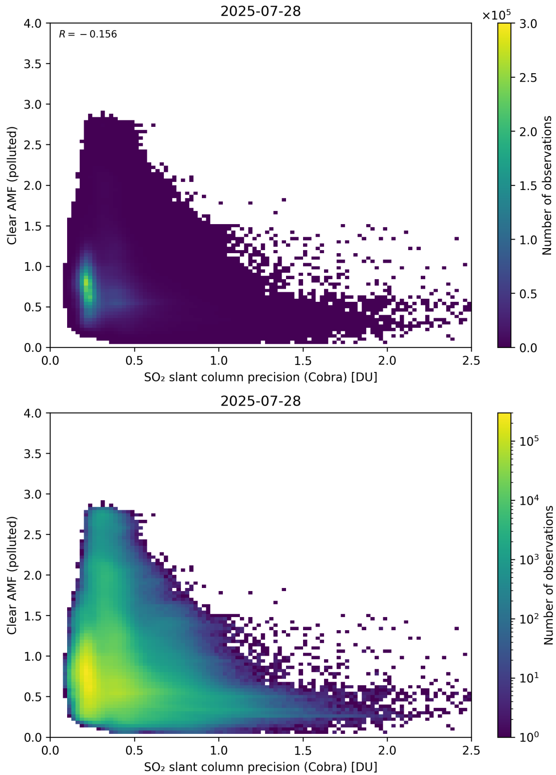
Figure 205: Scatter density plot of “SO 2 slant column precision (Cobra)” against “Clear AMF (polluted)” for 2025-07-27 to 2025-07-29.
