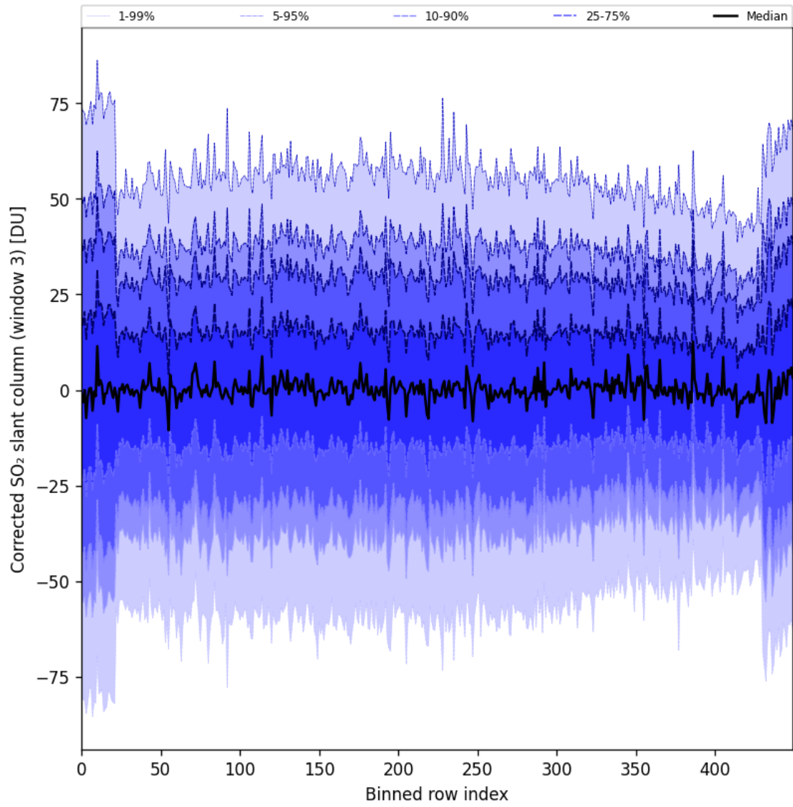
Figure 99: Along track statistics of “Corrected SO 2 slant column (window 3)” for 2025-07-27 to 2025-07-29
