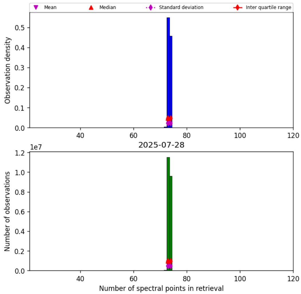
Figure 82: Histogram of “Number of spectral points in retrieval” for 2025-07-27 to 2025-07-29
