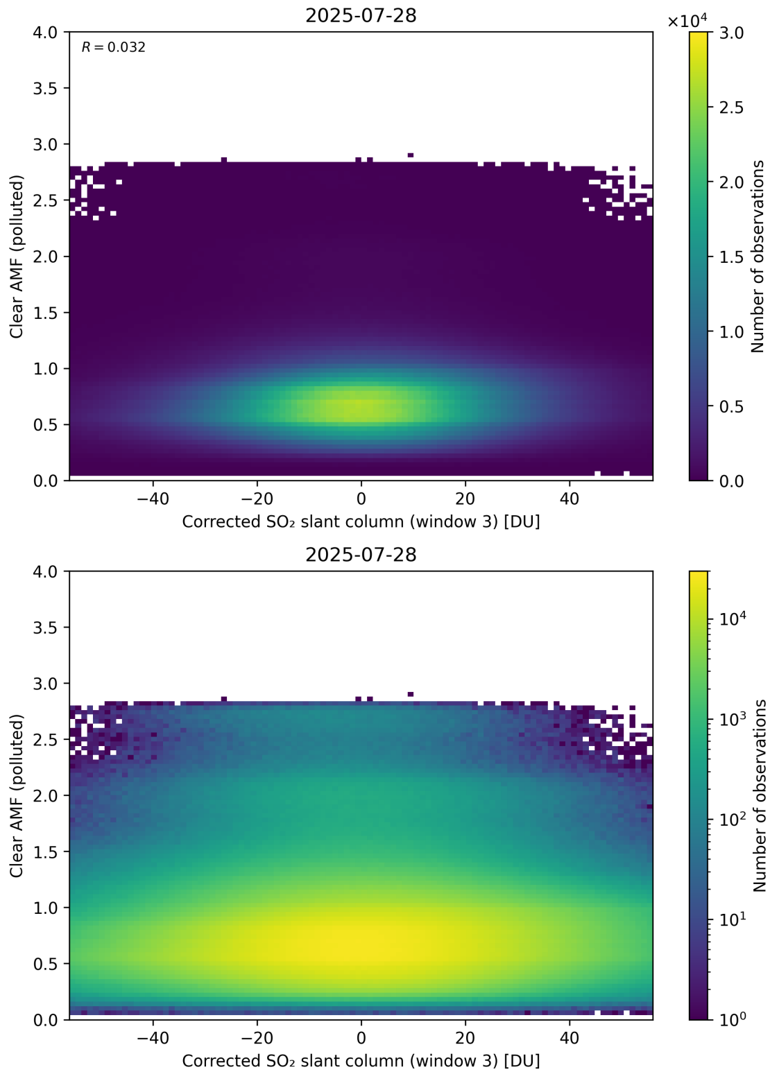
Figure 259: Scatter density plot of “Corrected SO 2 slant column (window 3)” against “Clear AMF (polluted)” for 2025-07-27 to 2025-07-29.
