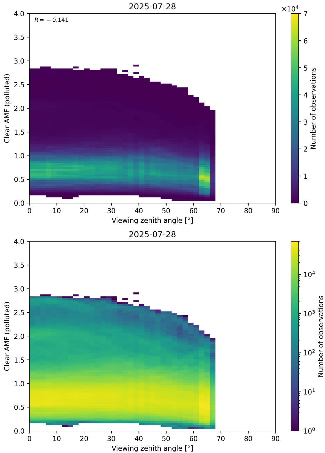
Figure 370: Scatter density plot of “Viewing zenith angle” against “Clear AMF (polluted)” for 2025-07-27 to 2025-07-29.
