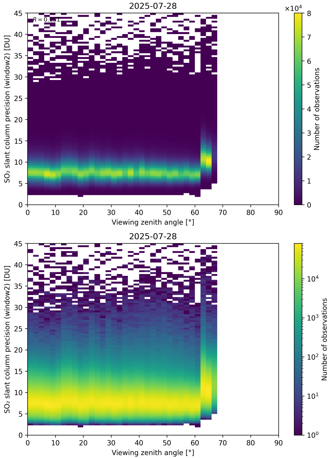
Figure 378: Scatter density plot of “Viewing zenith angle” against “SO 2 slant column precision (window2)” for 2025-07-27 to 2025-07-29.
