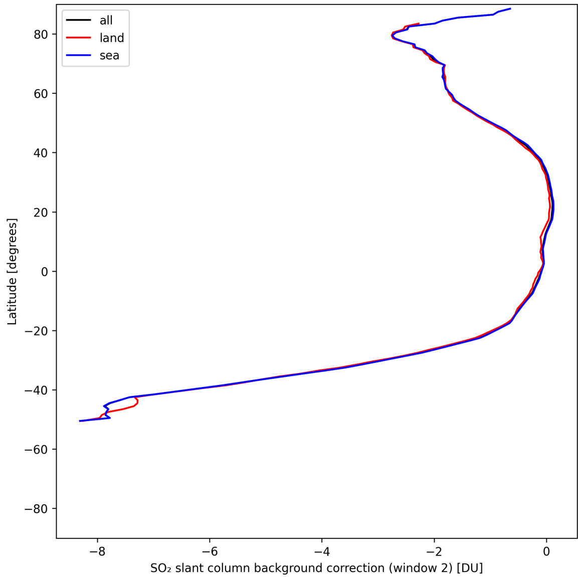
Figure 44: Zonal average of “SO 2 slant column background correction (window 2)” for 2025-07-27 to 2025-07-29.
