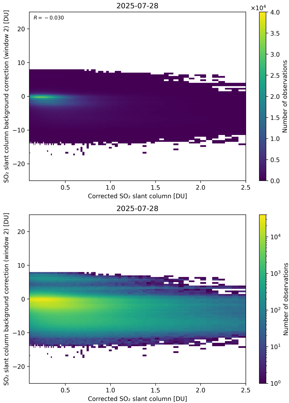
Figure 227: Scatter density plot of “Corrected SO 2 slant column” against “SO 2 slant column background correction (window 2)” for 2025-07-27 to 2025-07-29.
