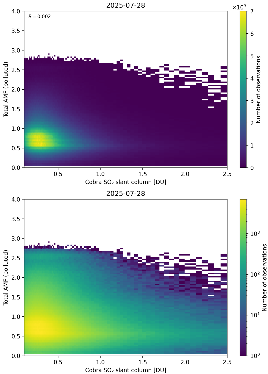
Figure 224: Scatter density plot of “Cobra SO 2 slant column” against “Total AMF (polluted)” for 2025-07-27 to 2025-07-29.
