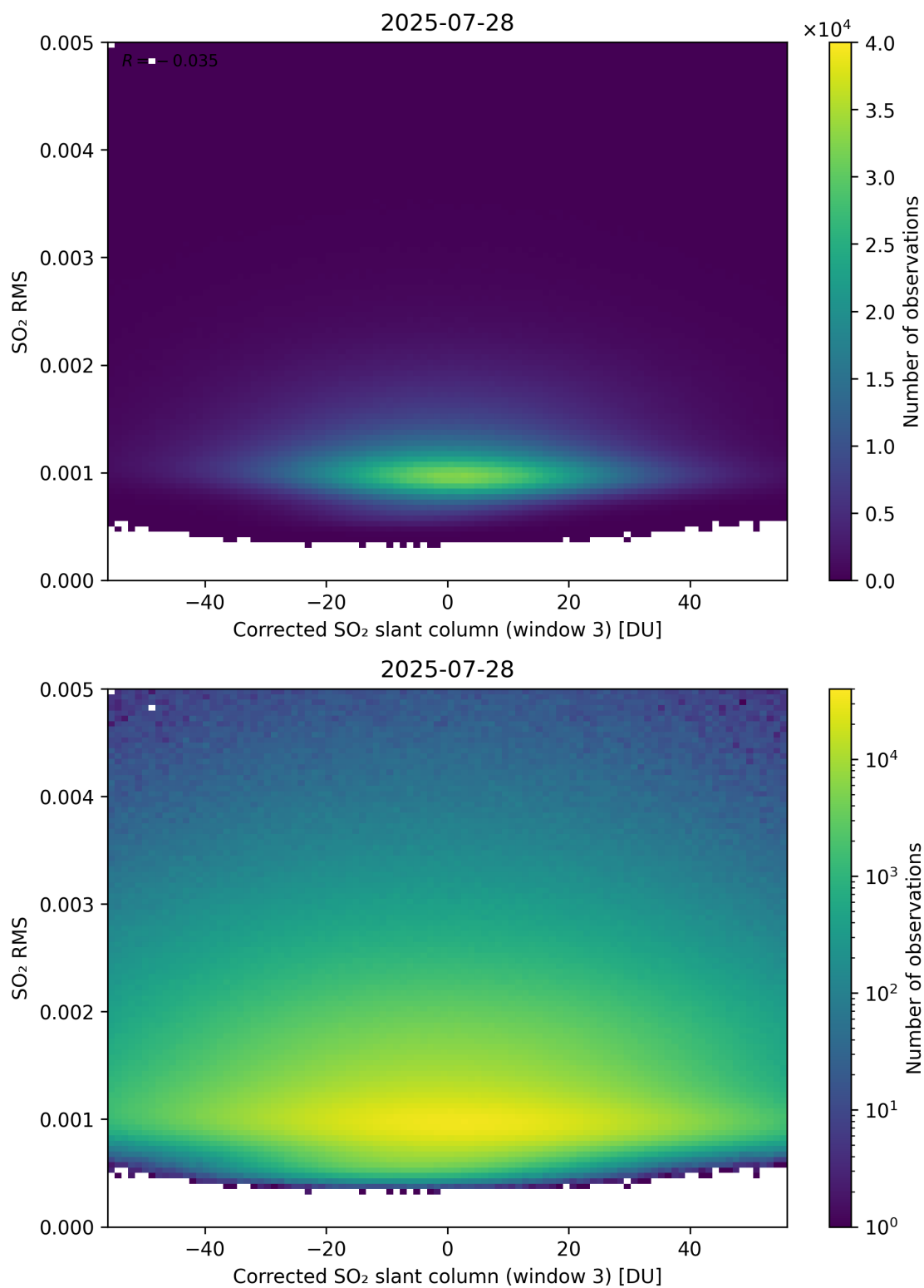
Figure 258: Scatter density plot of “Corrected SO 2 slant column (window 3)” against “SO 2 RMS” for 2025-07-27 to 2025-07-29.
