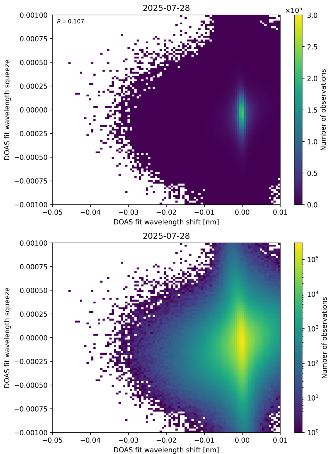
Figure 138: Scatter density plot of “DOAS fit wavelength shift” against “DOAS fit wavelength squeeze” for 2025-07-27 to 2025-07-29.
