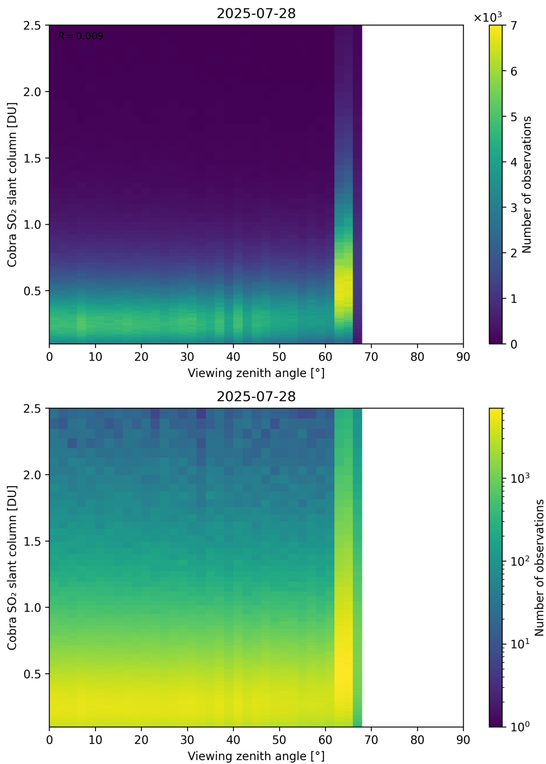
Figure 371: Scatter density plot of “Viewing zenith angle” against “Cobra SO 2 slant column” for 2025-07-27 to 2025-07-29.
