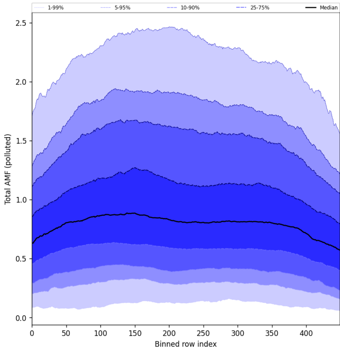
Figure 105: Along track statistics of “Total AMF (polluted)” for 2025-07-27 to 2025-07-29
