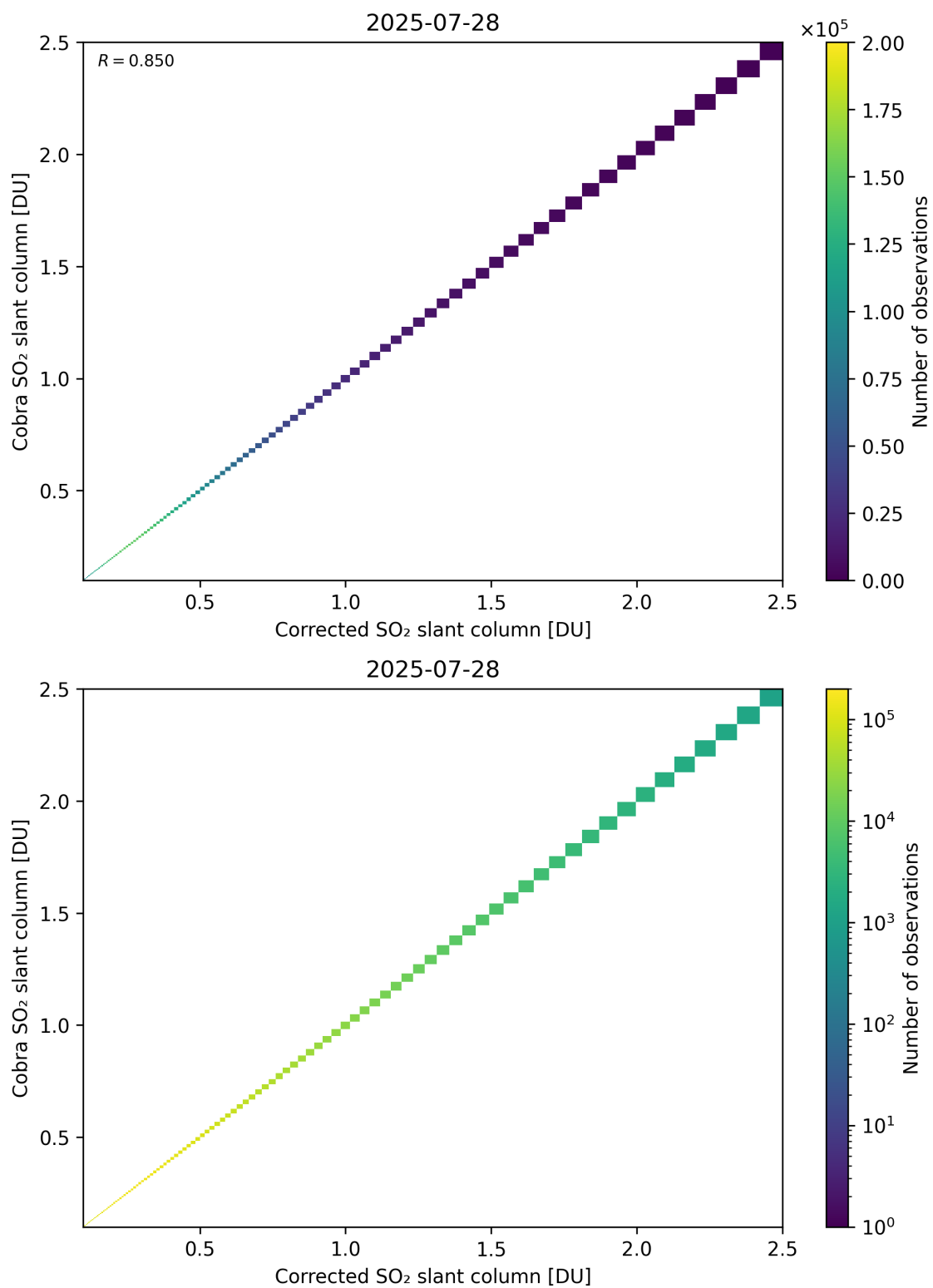
Figure 233: Scatter density plot of “Corrected SO 2 slant column” against “Cobra SO 2 slant column” for 2025-07-27 to 2025-07-29.
