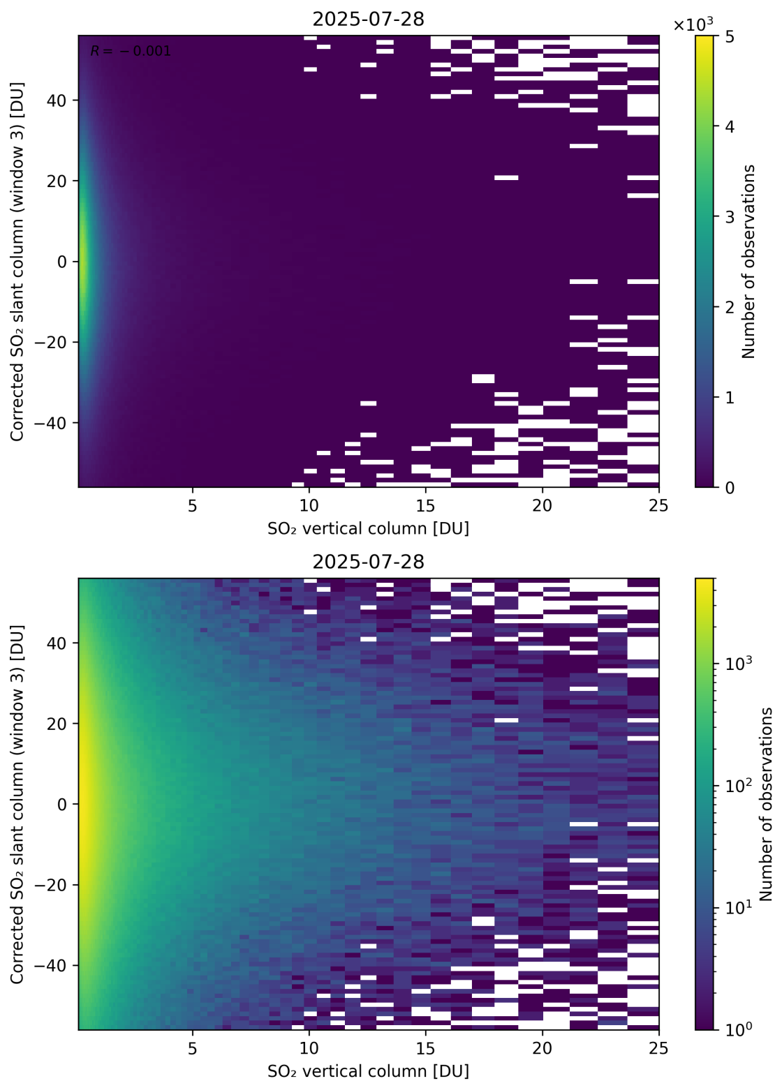
Figure 353: Scatter density plot of “SO 2 vertical column” against “Corrected SO 2 slant column (window 3)” for 2025-07-27 to 2025-07-29.
