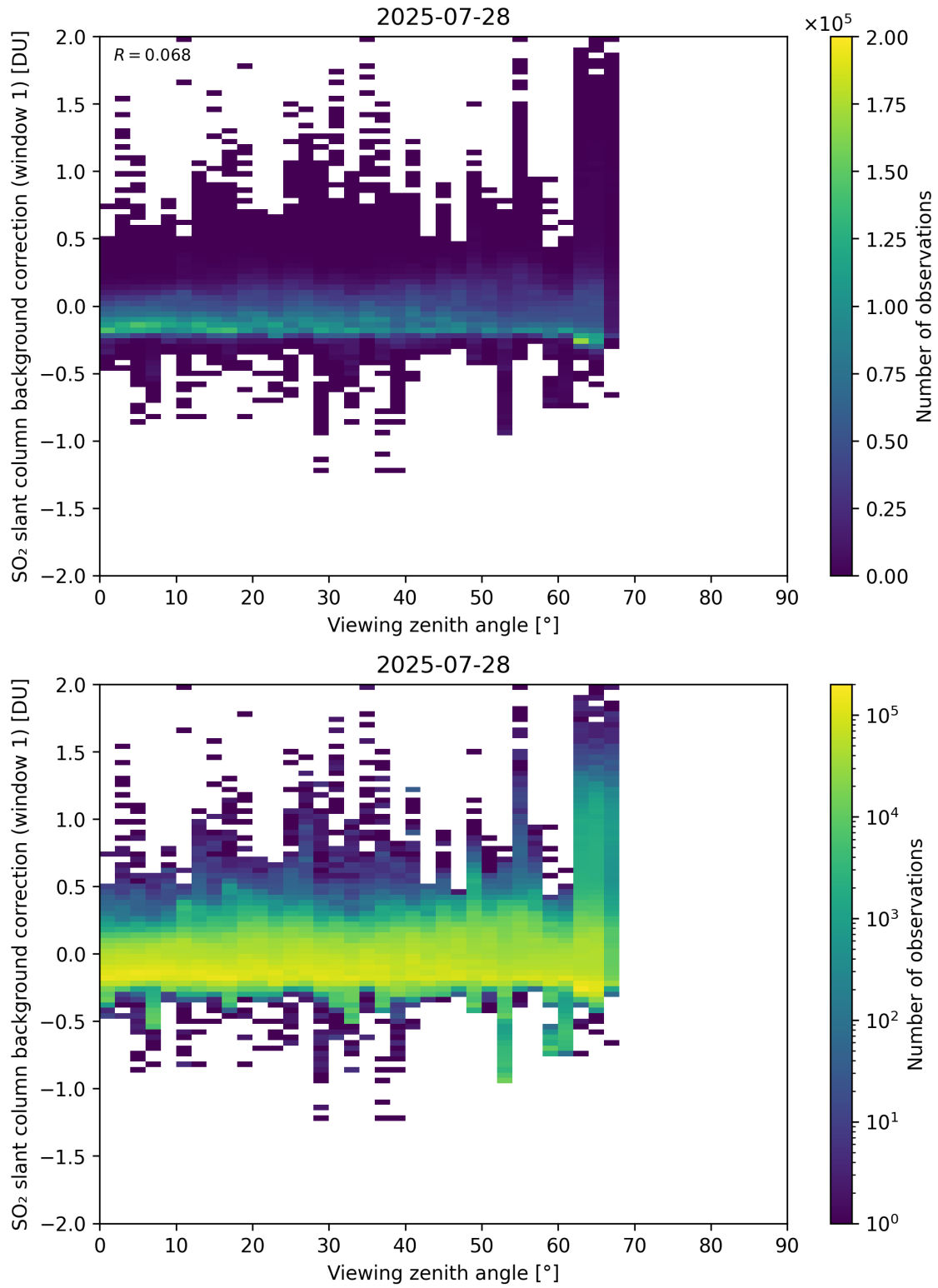
Figure 362: Scatter density plot of “Viewing zenith angle” against “SO 2 slant column background correction (window 1)” for 2025-07-27 to 2025-07-29.
