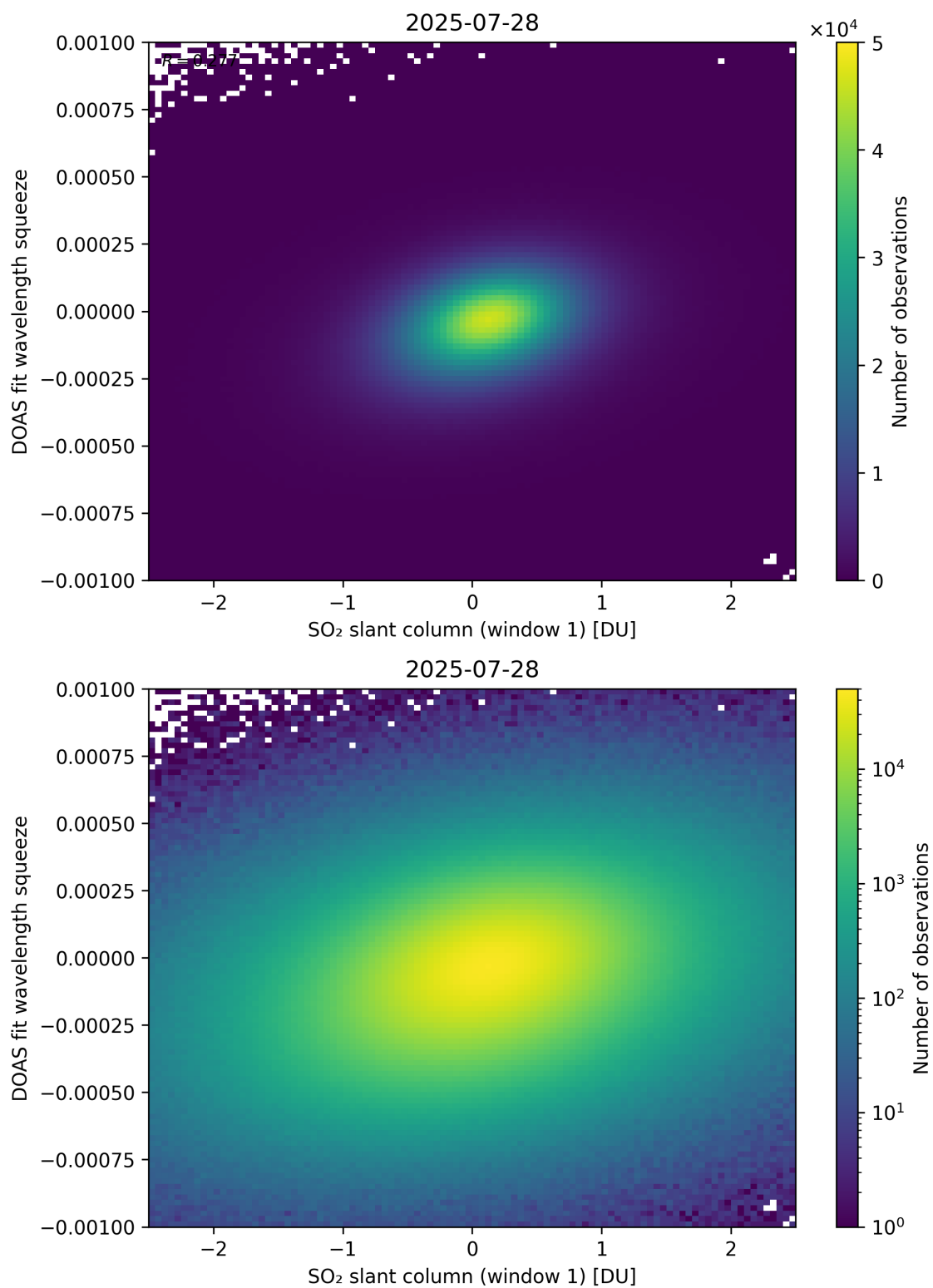
Figure 266: Scatter density plot of “SO 2 slant column (window 1)” against “DOAS fit wavelength squeeze” for 2025-07-27 to 2025-07-29.
