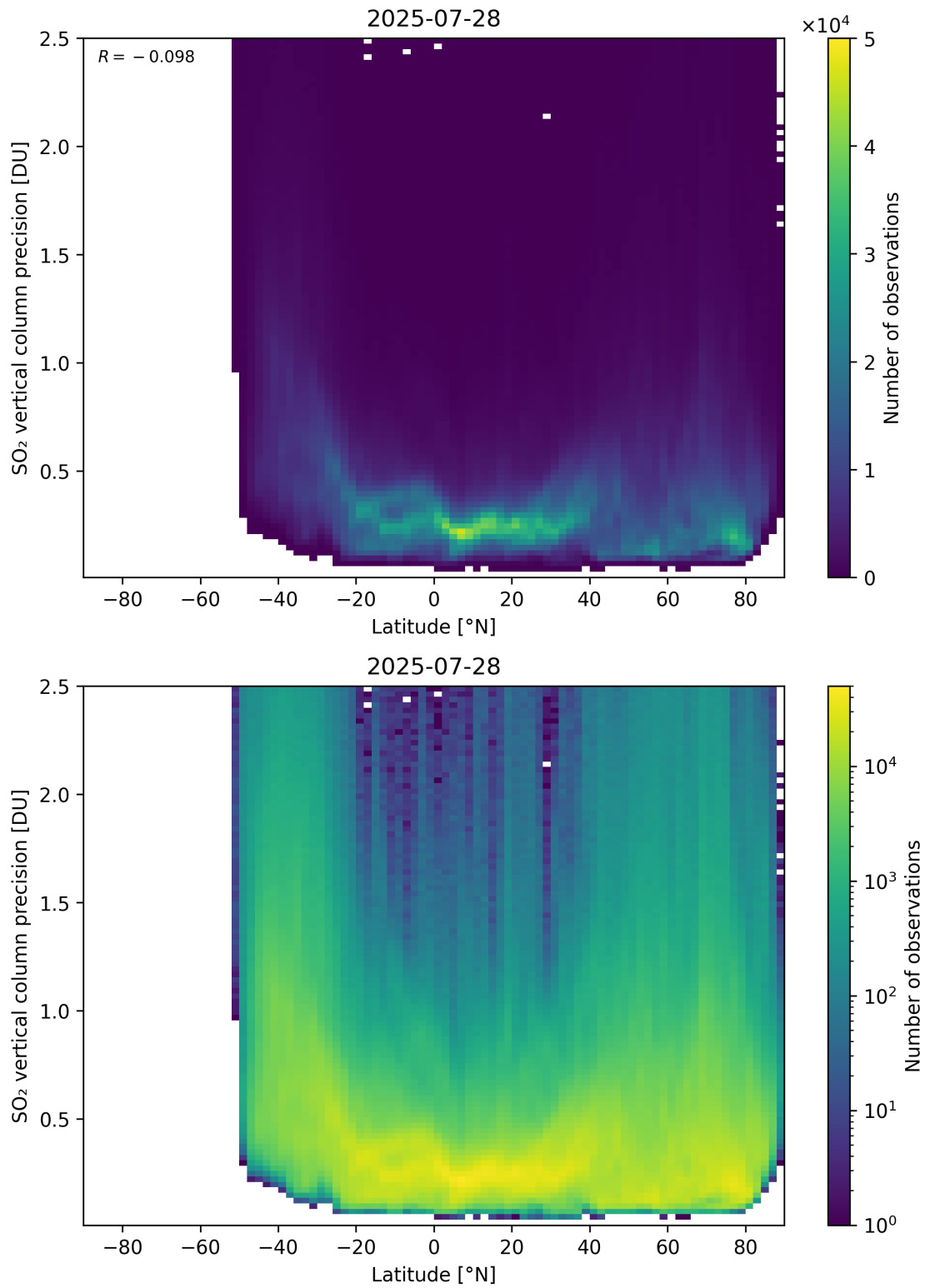
Figure 170: Scatter density plot of “Latitude” against “SO 2 vertical column precision” for 2025-07-27 to 2025-07-29.
