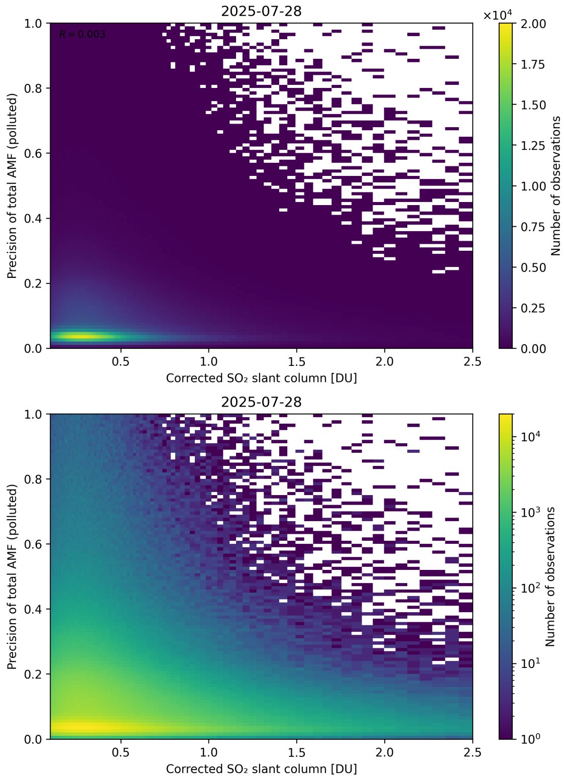
Figure 243: Scatter density plot of “Corrected SO 2 slant column” against “Precision of total AMF (polluted)” for 2025-07-27 to 2025-07-29.
