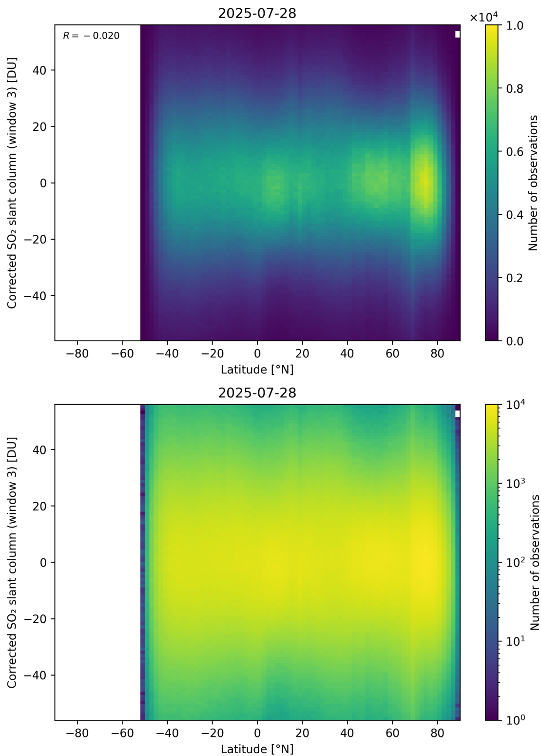
Figure 161: Scatter density plot of “Latitude” against “Corrected SO 2 slant column (window 3)” for 2025-07-27 to 2025-07-29.
