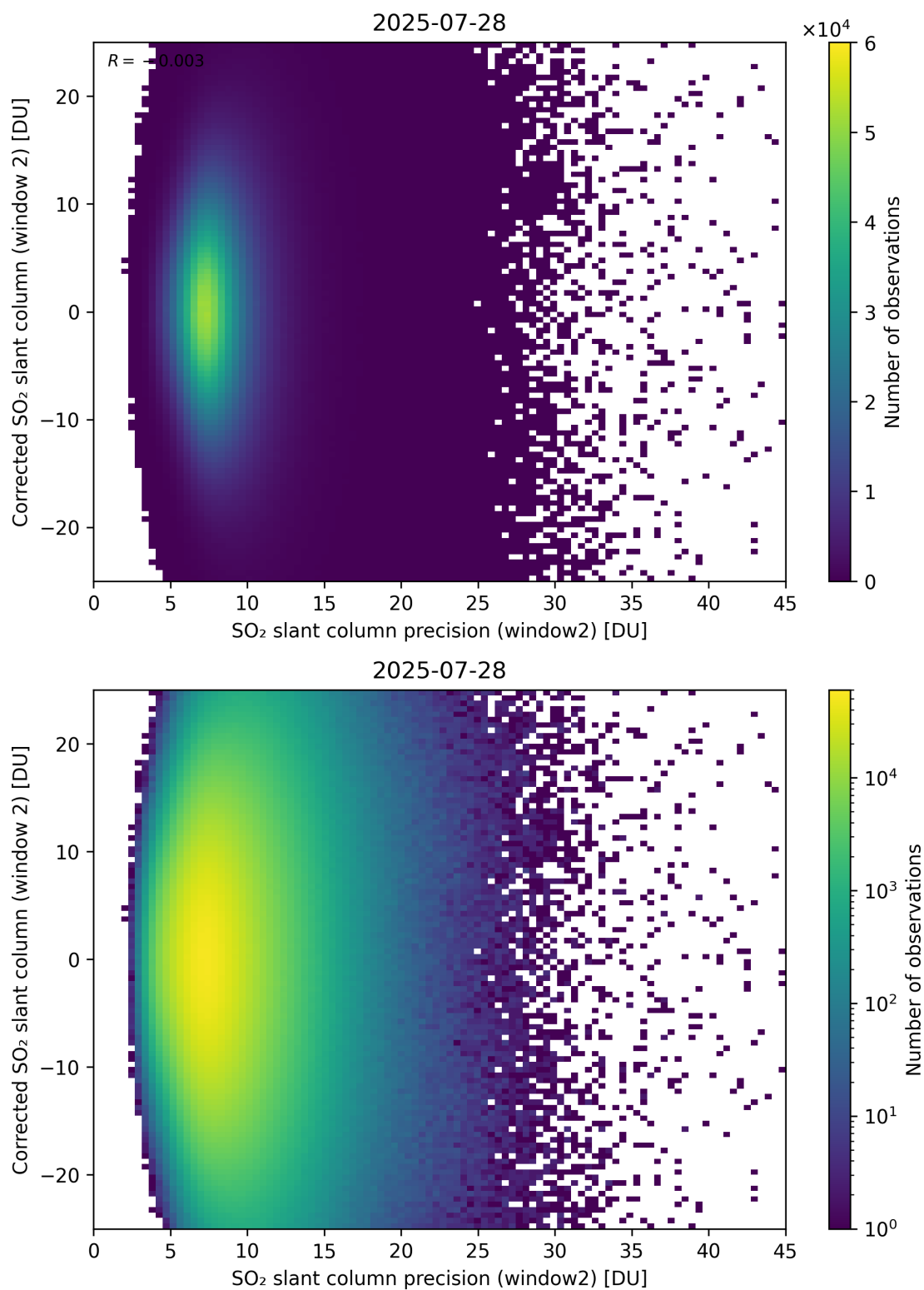
Figure 297: Scatter density plot of “SO 2 slant column precision (window2)” against “Corrected SO 2 slant column (window 2)” for 2025-07-27 to 2025-07-29.
