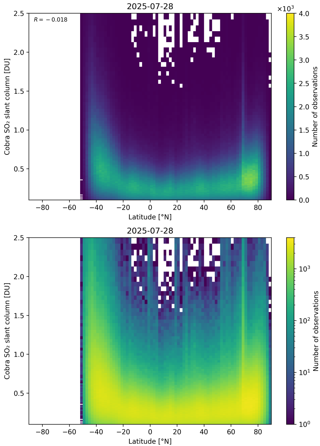
Figure 157: Scatter density plot of “Latitude” against “Cobra SO 2 slant column” for 2025-07-27 to 2025-07-29.
