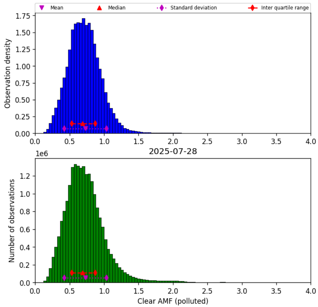
Figure 81: Histogram of “Clear AMF (polluted)” for 2025-07-27 to 2025-07-29
