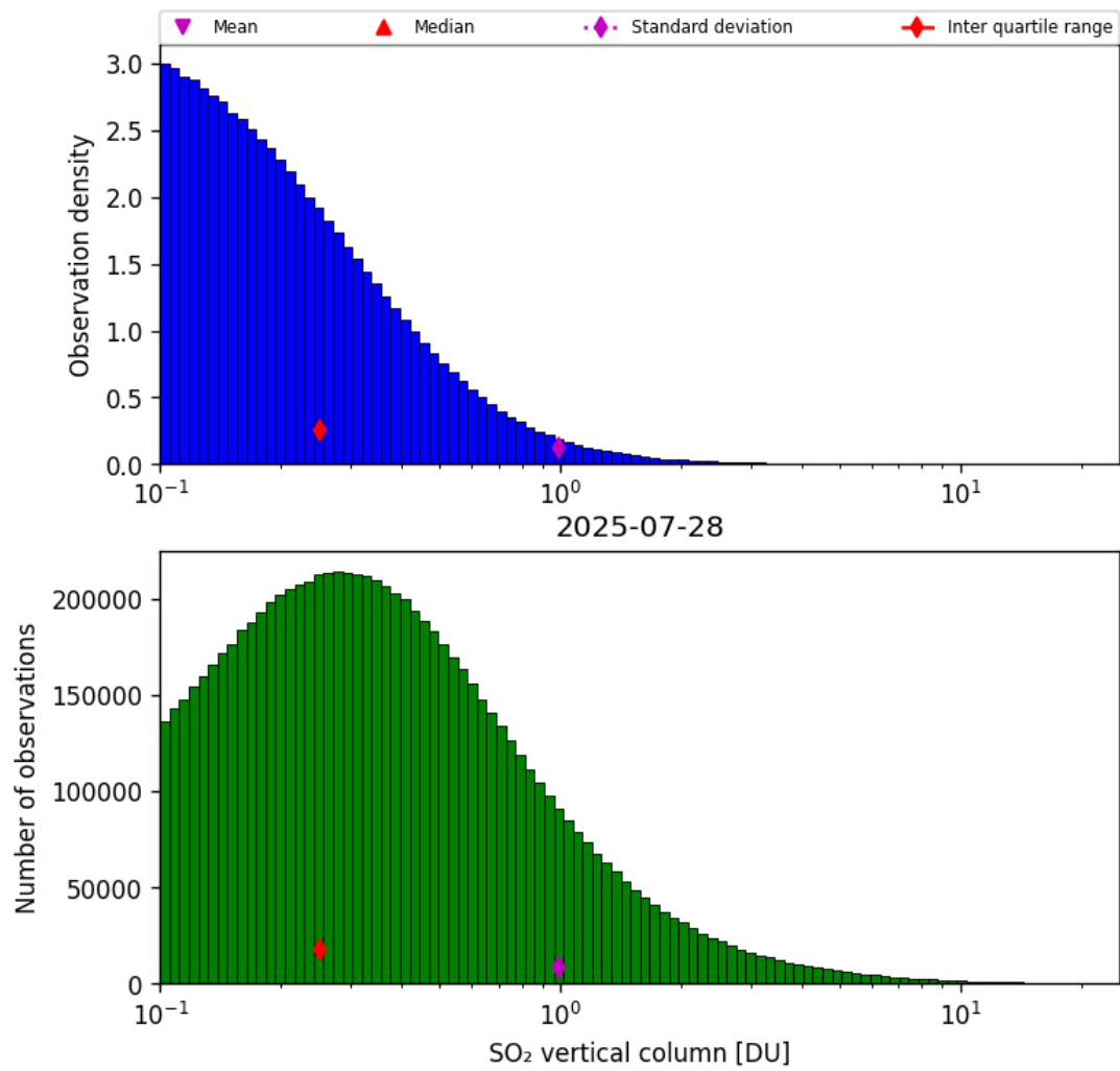
Figure 58: Histogram of “SO 2 vertical column” for 2025-07-27 to 2025-07-29
