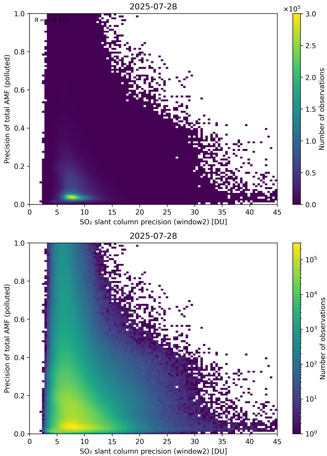
Figure 302: Scatter density plot of “SO 2 slant column precision (window2)” against “Precision of total AMF (polluted)” for 2025-07-27 to 2025-07-29.
