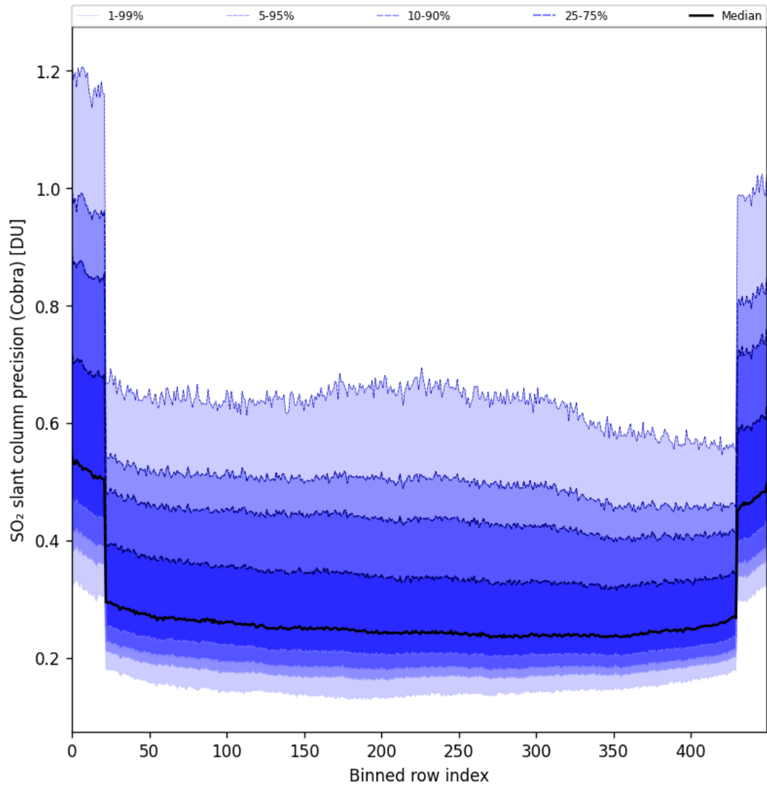
Figure 88: Along track statistics of “SO 2 slant column precision (Cobra)” for 2025-07-27 to 2025-07-29
