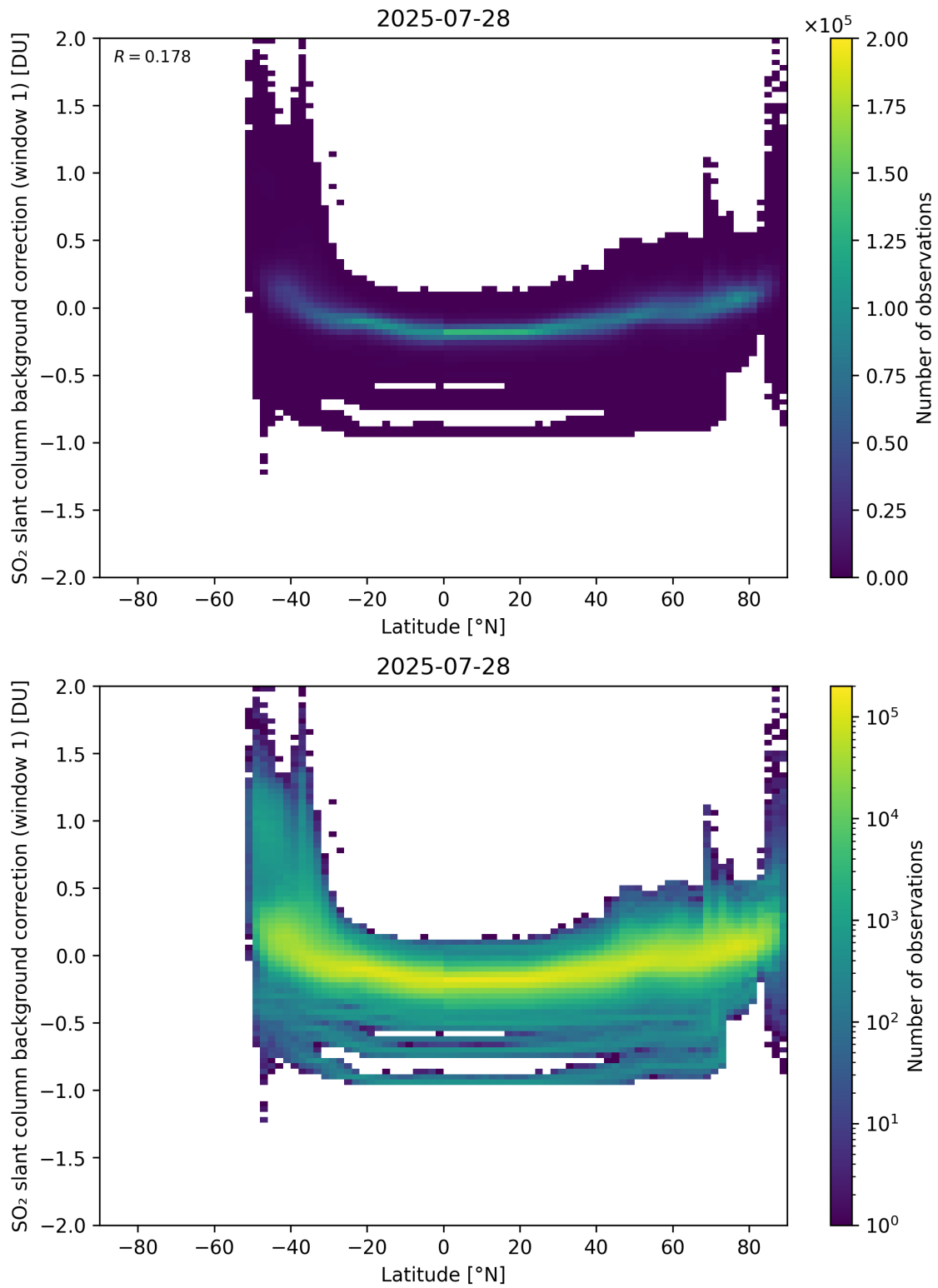
Figure 150: Scatter density plot of “Latitude” against “SO 2 slant column background correction (window 1)” for 2025-07-27 to 2025-07-29.
