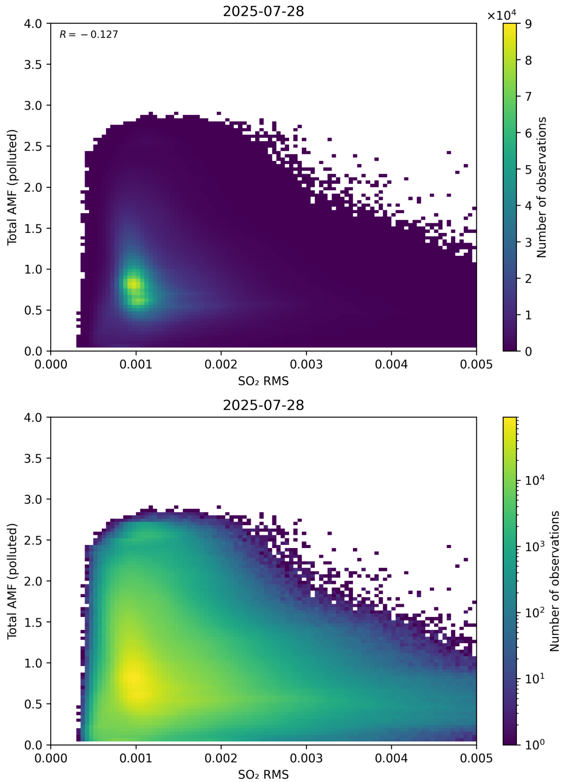
Figure 148: Scatter density plot of “SO 2 RMS” against “Total AMF (polluted)” for 2025-07-27 to 2025-07-29.
