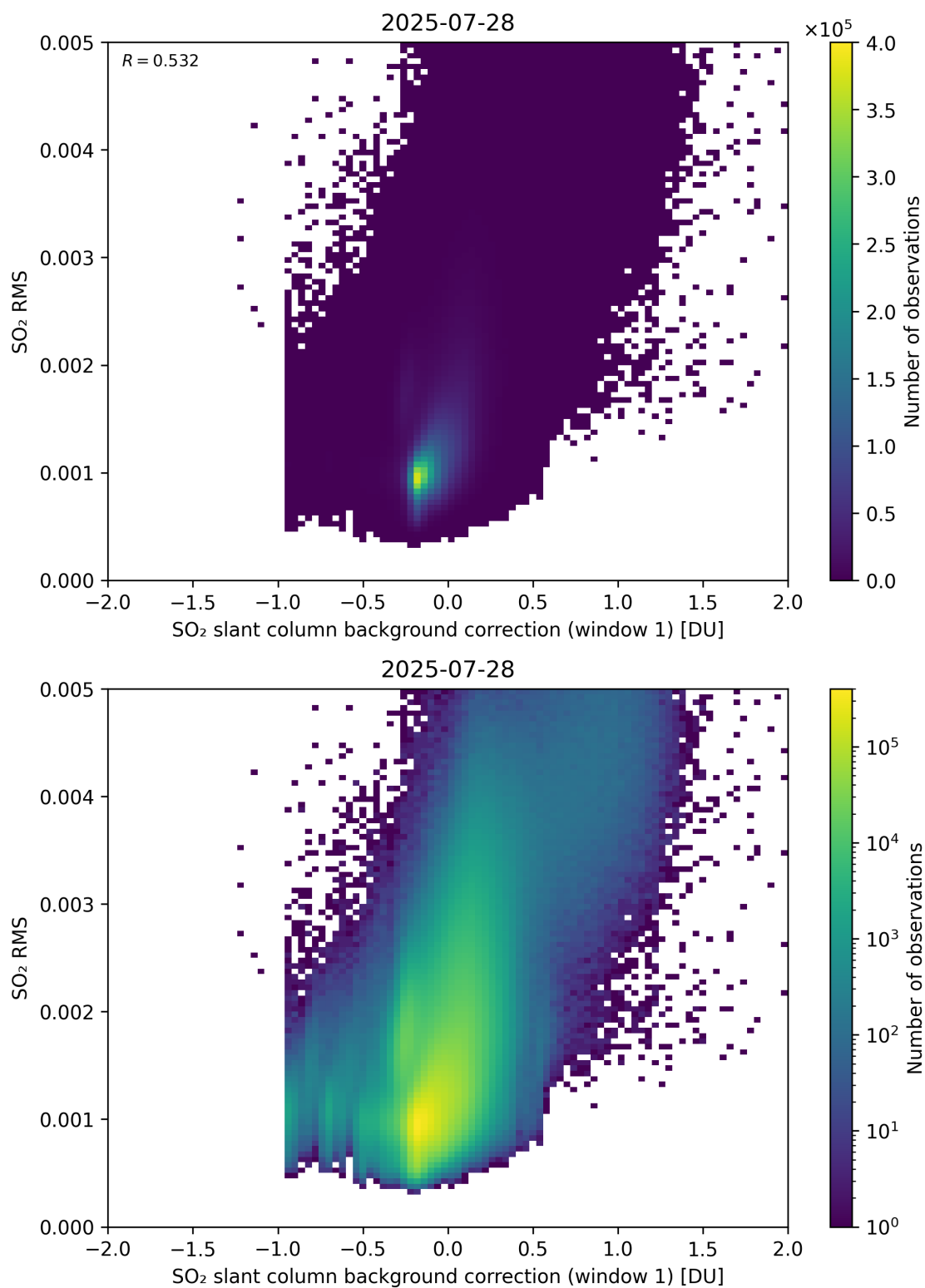
Figure 113: Scatter density plot of “SO 2 slant column background correction (window 1)” against “SO 2 RMS” for 2025-07-27 to 2025-07-29.
