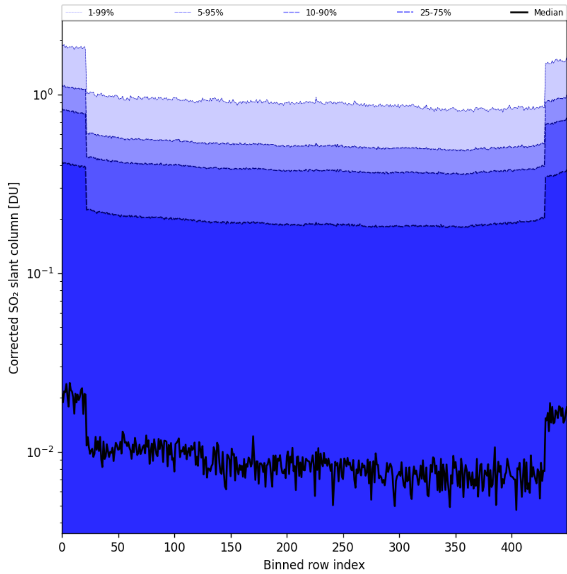
Figure 86: Along track statistics of "Corrected SO 2 slant column" for 2025-07-27 to 2025-07-29
