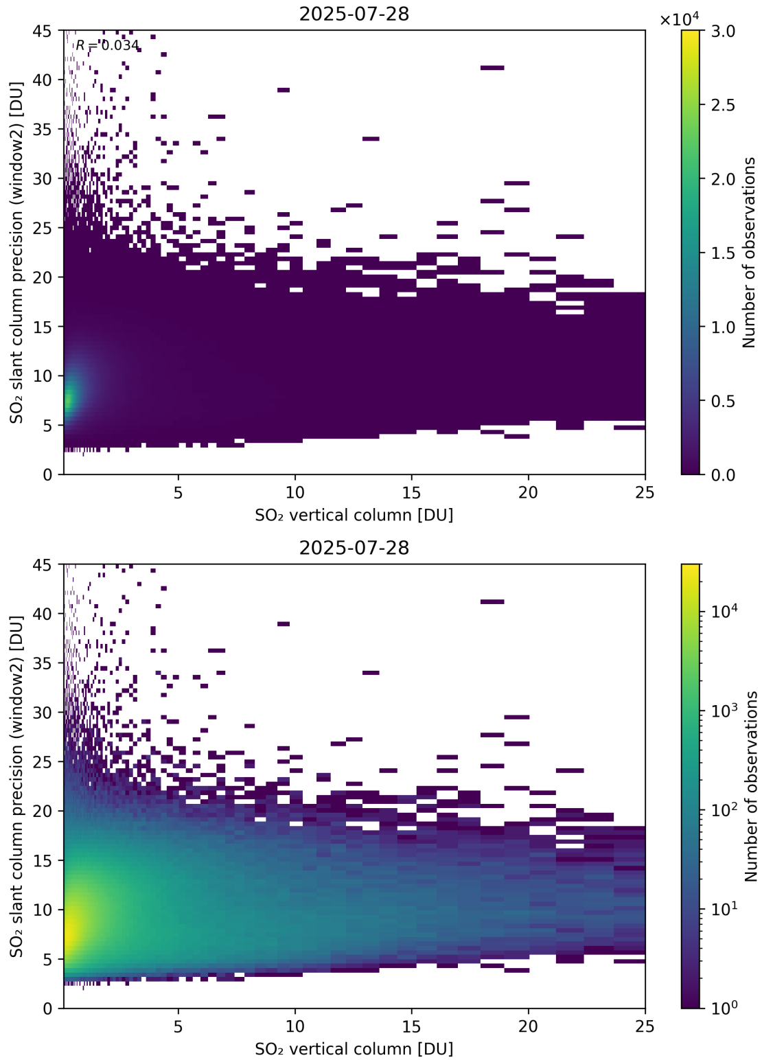
Figure 356: Scatter density plot of “SO 2 vertical column” against “SO 2 slant column precision (window2)” for 2025-07-27 to 2025-07-29.
