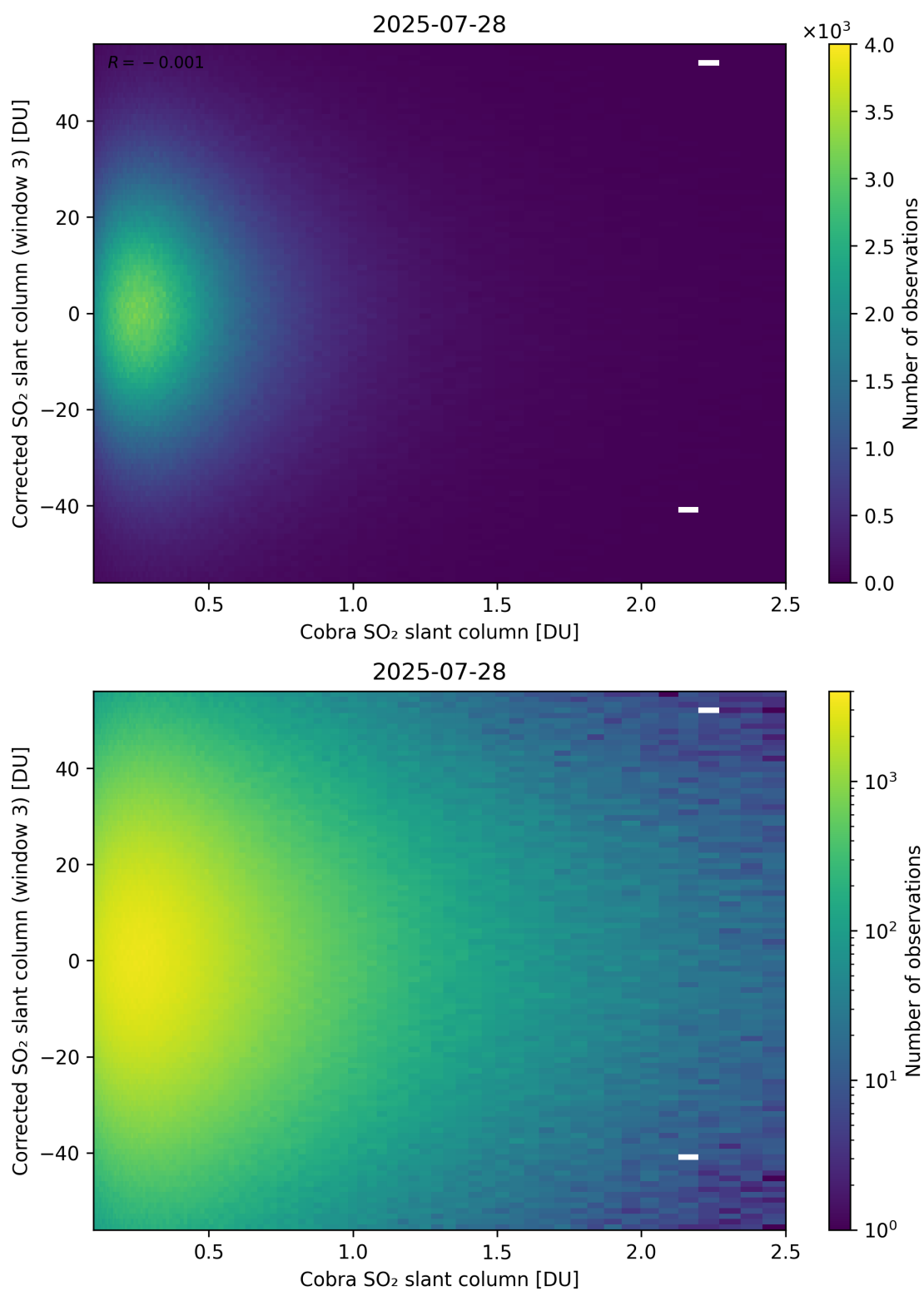
Figure 218: Scatter density plot of “Cobra SO 2 slant column” against “Corrected SO 2 slant column (window 3)” for 2025-07-27 to 2025-07-29.
