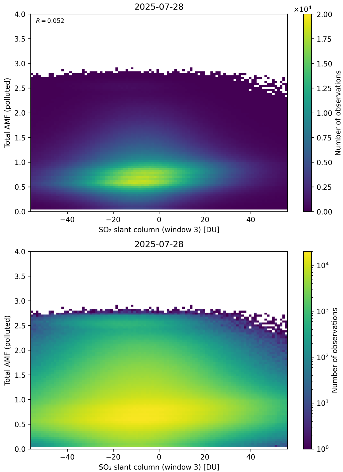
Figure 318: Scatter density plot of “SO 2 slant column (window 3)” against “Total AMF (polluted)” for 2025-07-27 to 2025-07-29.
