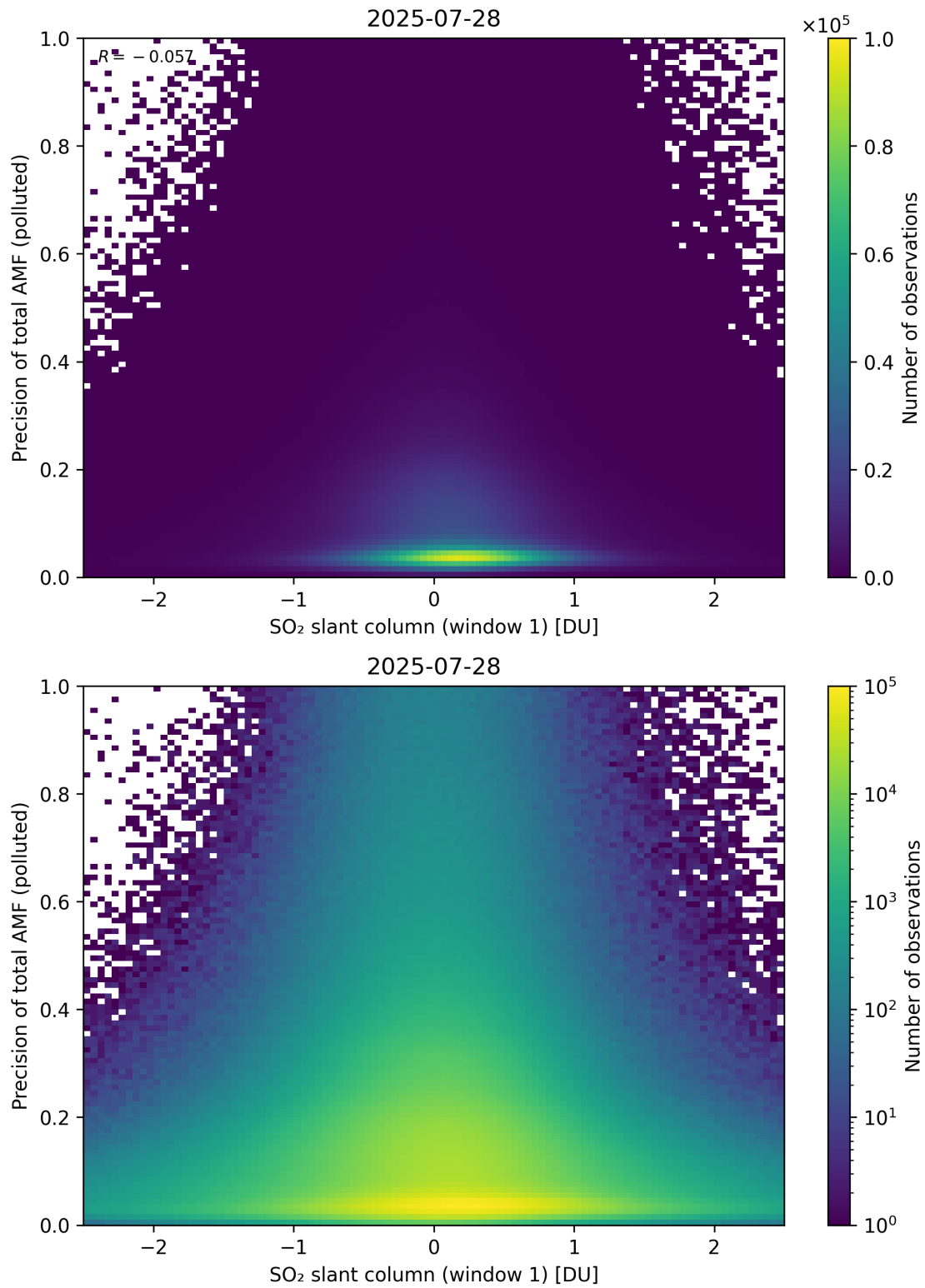
Figure 290: Scatter density plot of “SO 2 slant column (window 1)” against “Precision of total AMF (polluted)” for 2025-07-27 to 2025-07-29.
