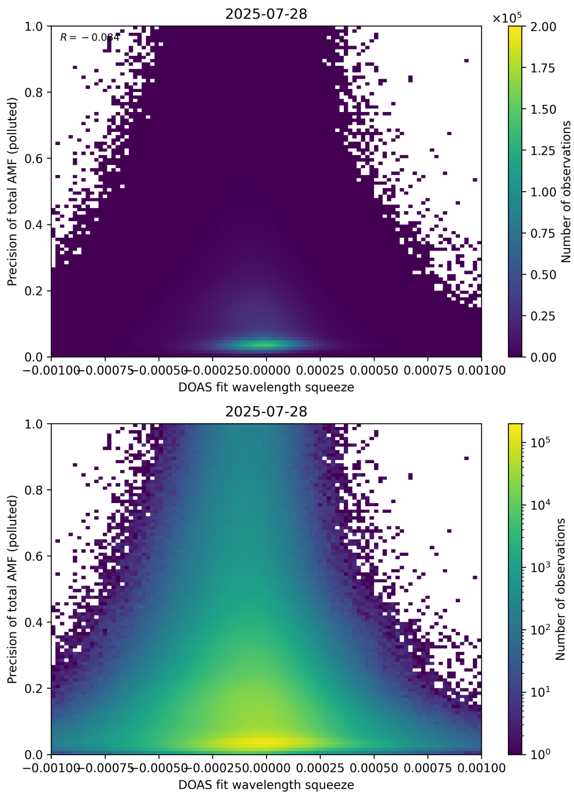
Figure 146: Scatter density plot of “DOAS fit wavelength squeeze” against “Precision of total AMF (polluted)” for 2025-07-27 to 2025-07-29.
