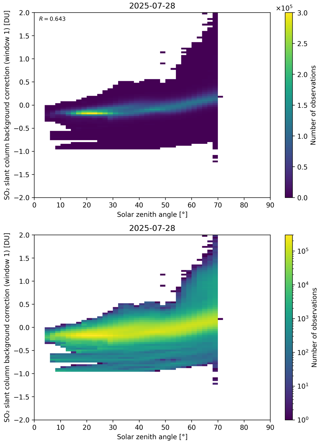
Figure 171: Scatter density plot of “Solar zenith angle” against “SO 2 slant column background correction (window 1)” for 2025-07-27 to 2025-07-29.
