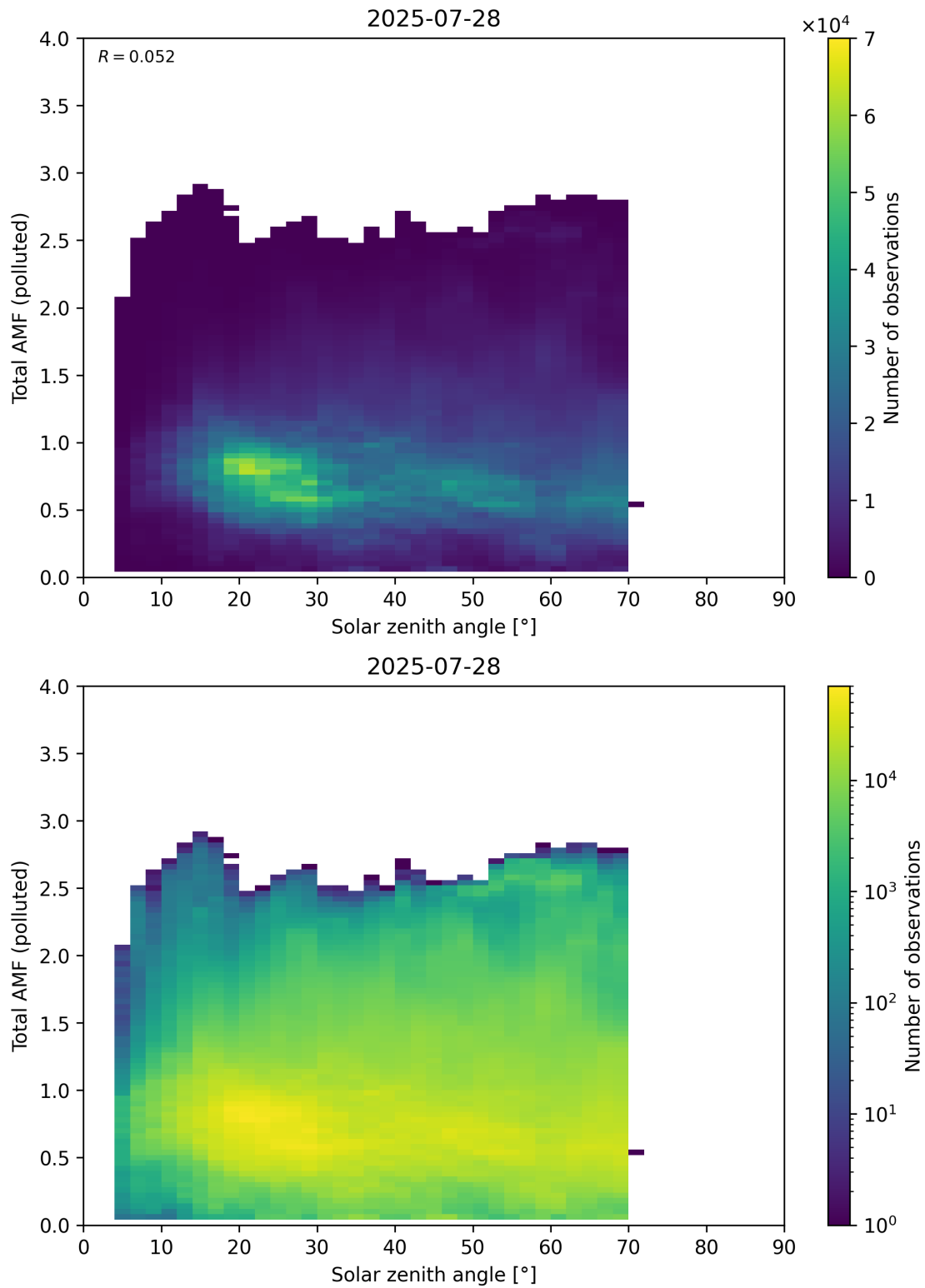
Figure 189: Scatter density plot of “Solar zenith angle” against “Total AMF (polluted)” for 2025-07-27 to 2025-07-29.
