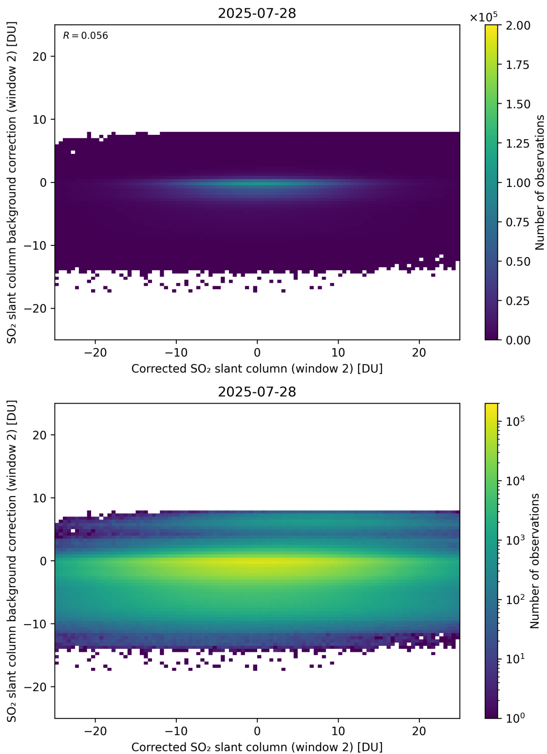
Figure 244: Scatter density plot of “Corrected SO 2 slant column (window 2)” against “SO 2 slant column background correction (window 2)” for 2025-07-27 to 2025-07-29.
