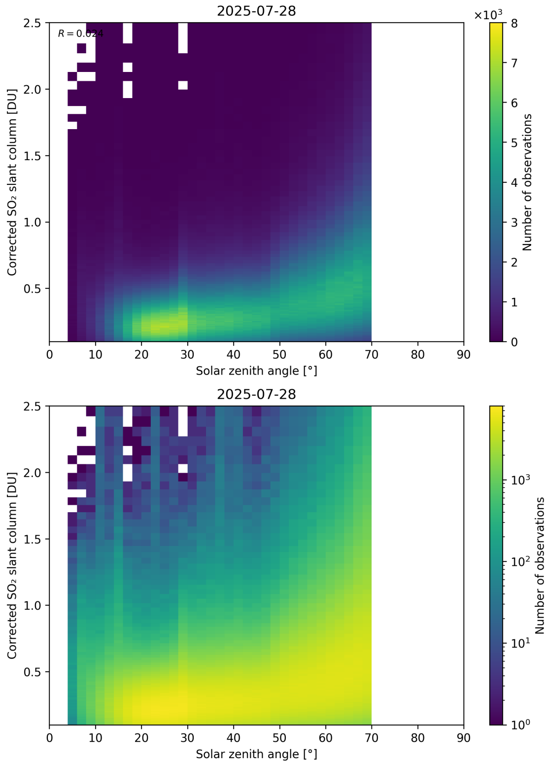
Figure 181: Scatter density plot of “Solar zenith angle” against “Corrected SO 2 slant column” for 2025-07-27 to 2025-07-29.
