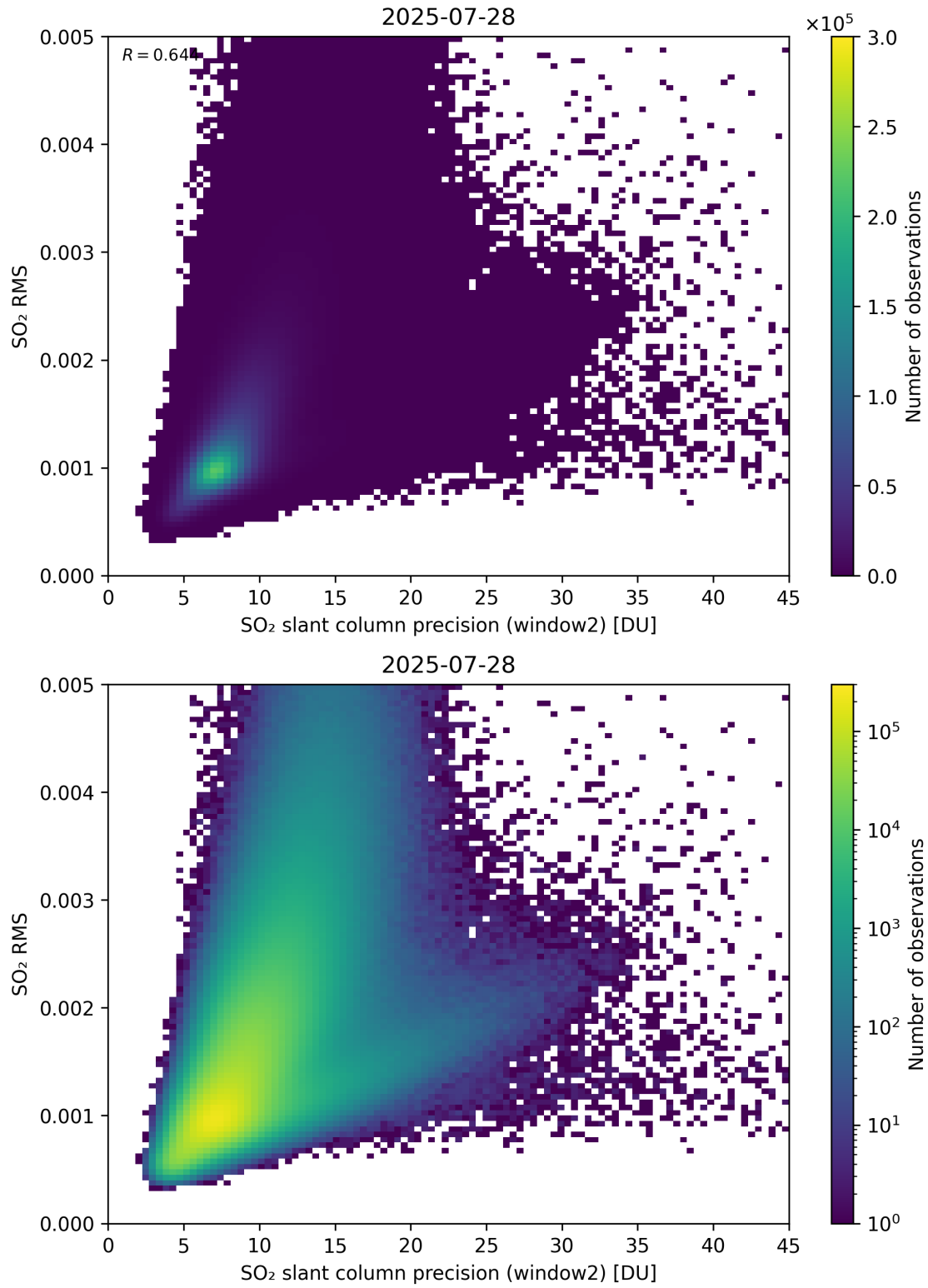
Figure 295: Scatter density plot of “SO 2 slant column precision (window2)” against “SO 2 RMS” for 2025-07-27 to 2025-07-29.
