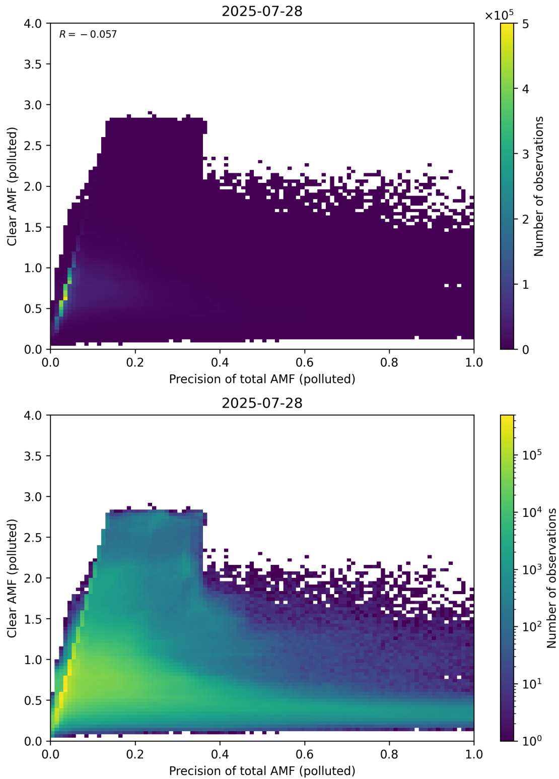
Figure 320: Scatter density plot of “Precision of total AMF (polluted)” against “Clear AMF (polluted)” for 2025-07-27 to 2025-07-29.
