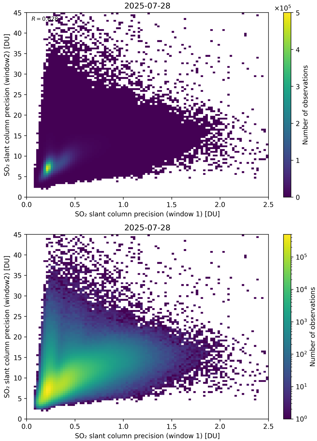
Figure 277: Scatter density plot of “SO 2 slant column precision (window 1)” against “SO 2 slant column precision (window2)” for 2025-07-27 to 2025-07-29.
