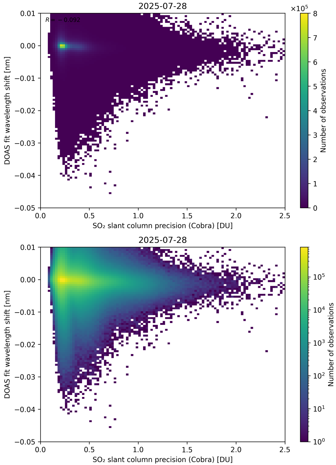
Figure 202: Scatter density plot of “SO 2 slant column precision (Cobra)” against “DOAS fit wavelength shift” for 2025-07-27 to 2025-07-29.
