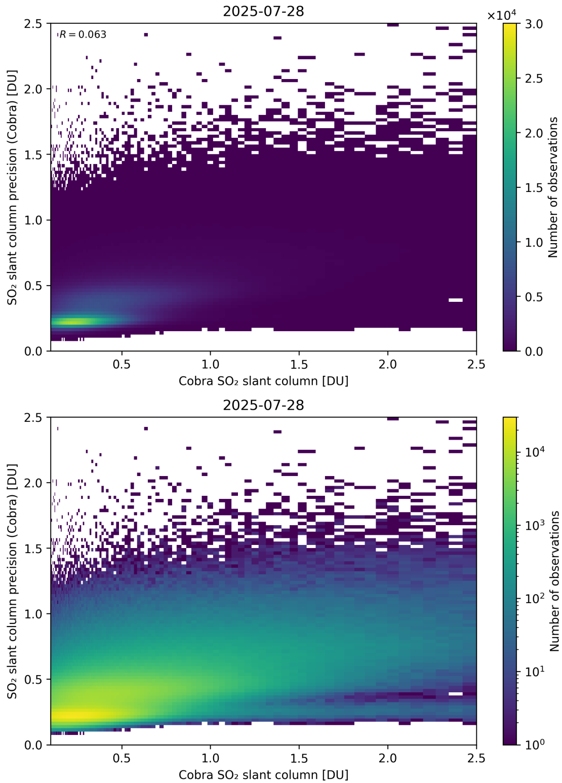
Figure 216: Scatter density plot of “Cobra SO 2 slant column” against “SO 2 slant column precision (Cobra)” for 2025-07-27 to 2025-07-29.
