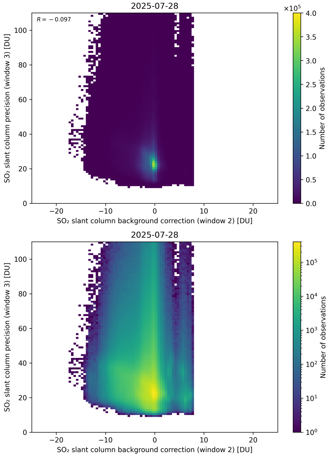
Figure 129: Scatter density plot of “SO 2 slant column background correction (window 2)” against “SO 2 slant column precision (window 3)” for 2025-07-27 to 2025-07-29.
