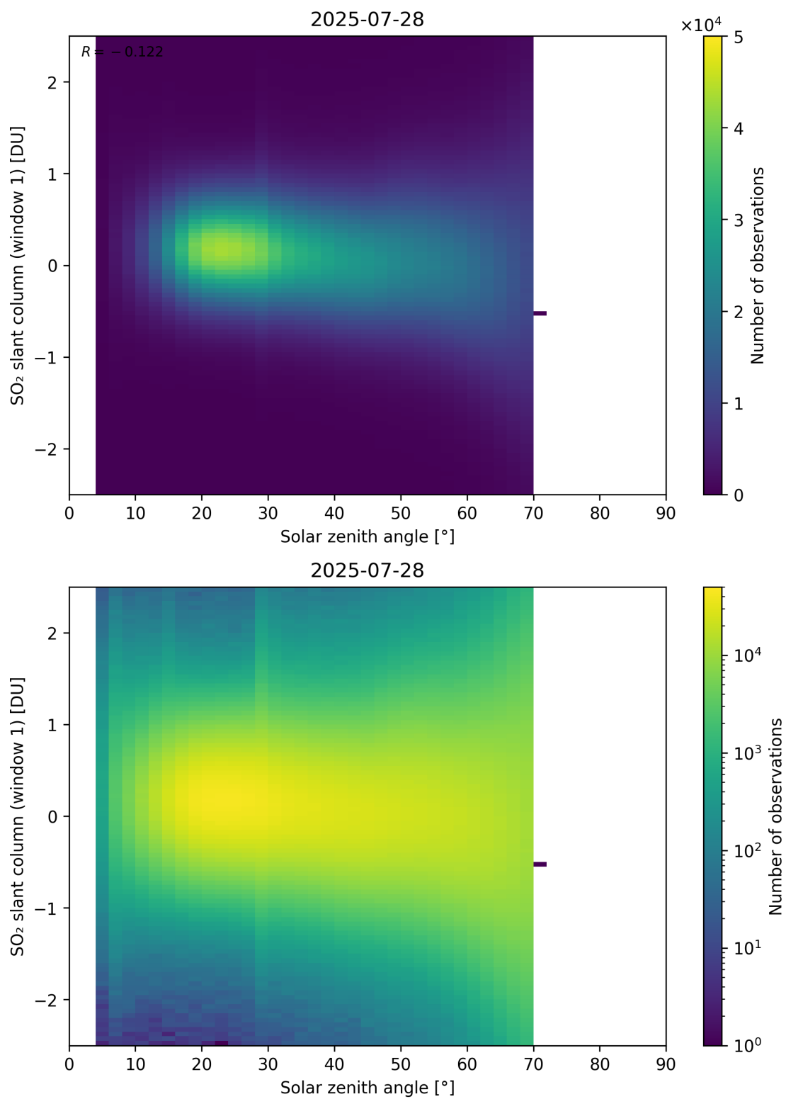
Figure 184: Scatter density plot of “Solar zenith angle” against “SO 2 slant column (window 1)” for 2025-07-27 to 2025-07-29.
