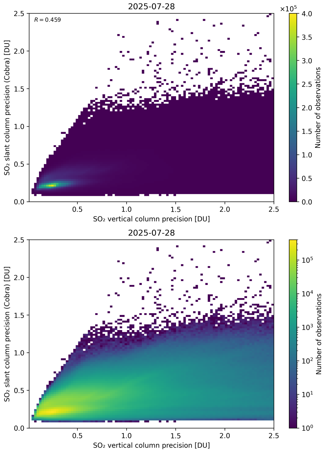
Figure 337: Scatter density plot of “SO 2 vertical column precision” against “SO 2 slant column precision (Cobra)” for 2025-07-27 to 2025-07-29.
