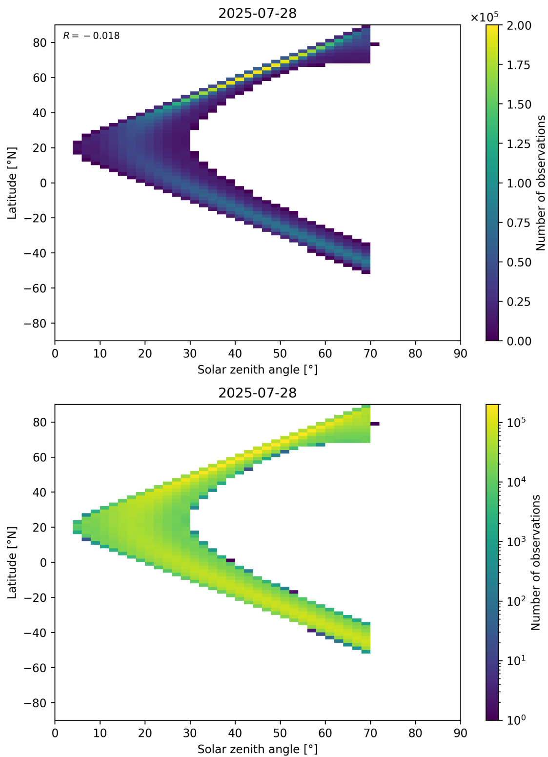
Figure 177: Scatter density plot of “Solar zenith angle” against “Latitude” for 2025-07-27 to 2025-07-29.
