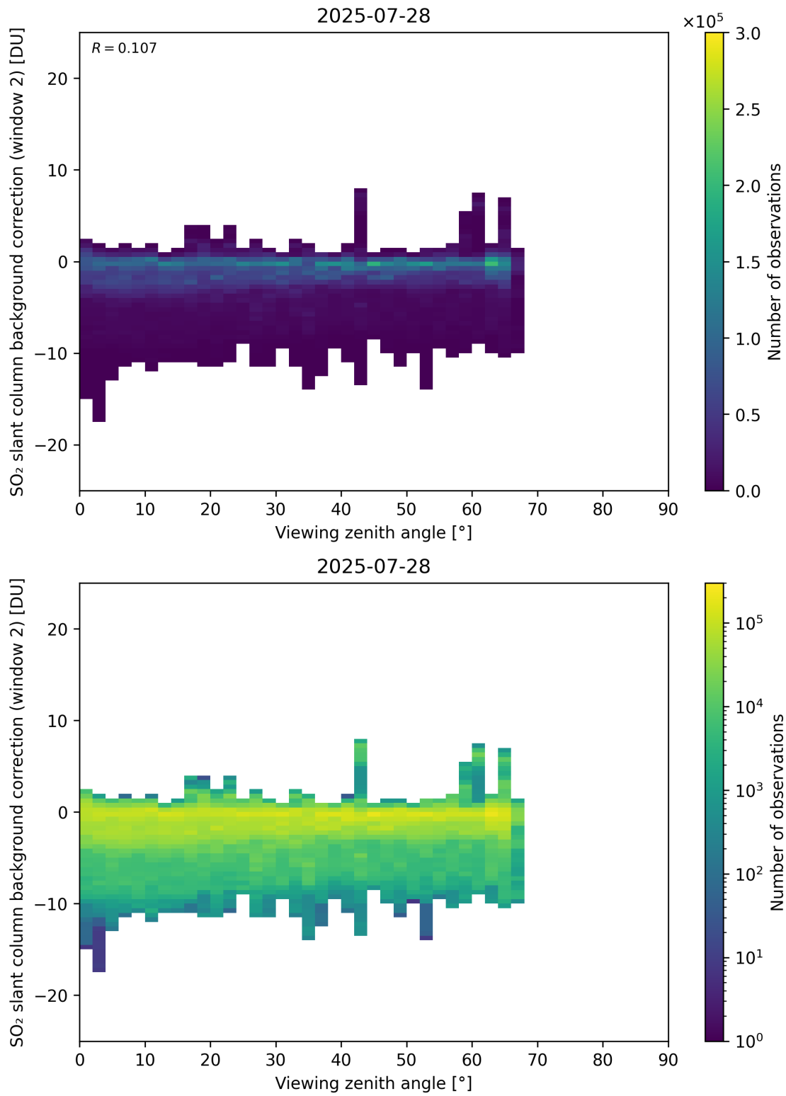
Figure 363: Scatter density plot of “Viewing zenith angle” against “SO 2 slant column background correction (window 2)” for 2025-07-27 to 2025-07-29.
