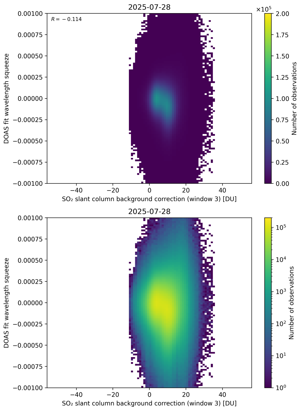
Figure 133: Scatter density plot of “SO 2 slant column background correction (window 3)” against “DOAS fit wavelength squeeze” for 2025-07-27 to 2025-07-29.
