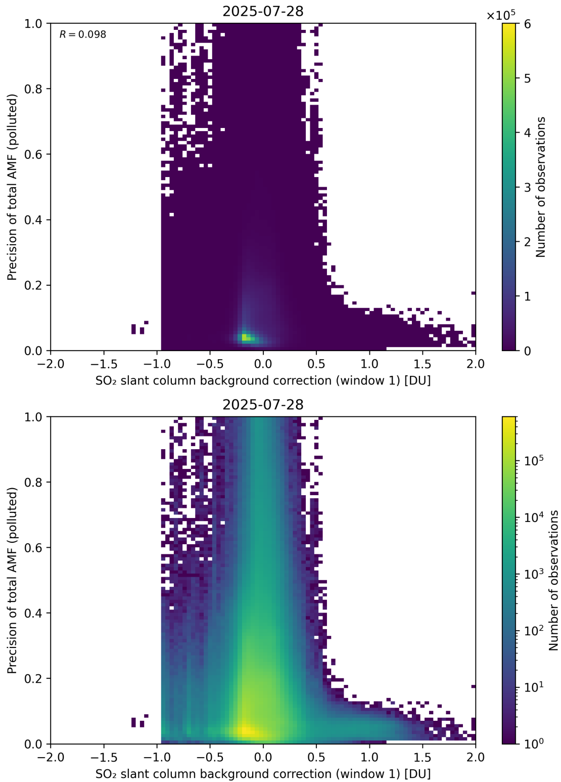
Figure 121: Scatter density plot of “SO 2 slant column background correction (window 1)” against “Precision of total AMF (polluted)” for 2025-07-27 to 2025-07-29.
