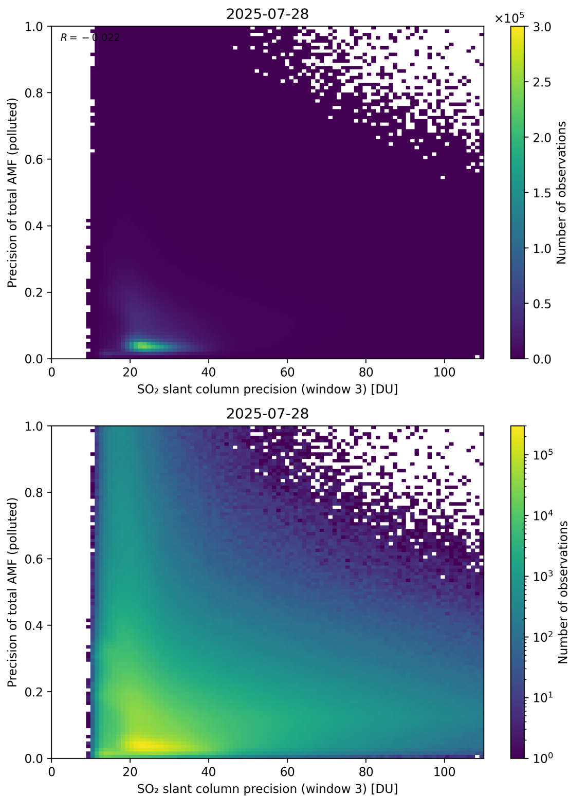
Figure 314: Scatter density plot of “SO 2 slant column precision (window 3)” against “Precision of total AMF (polluted)” for 2025-07-27 to 2025-07-29.
