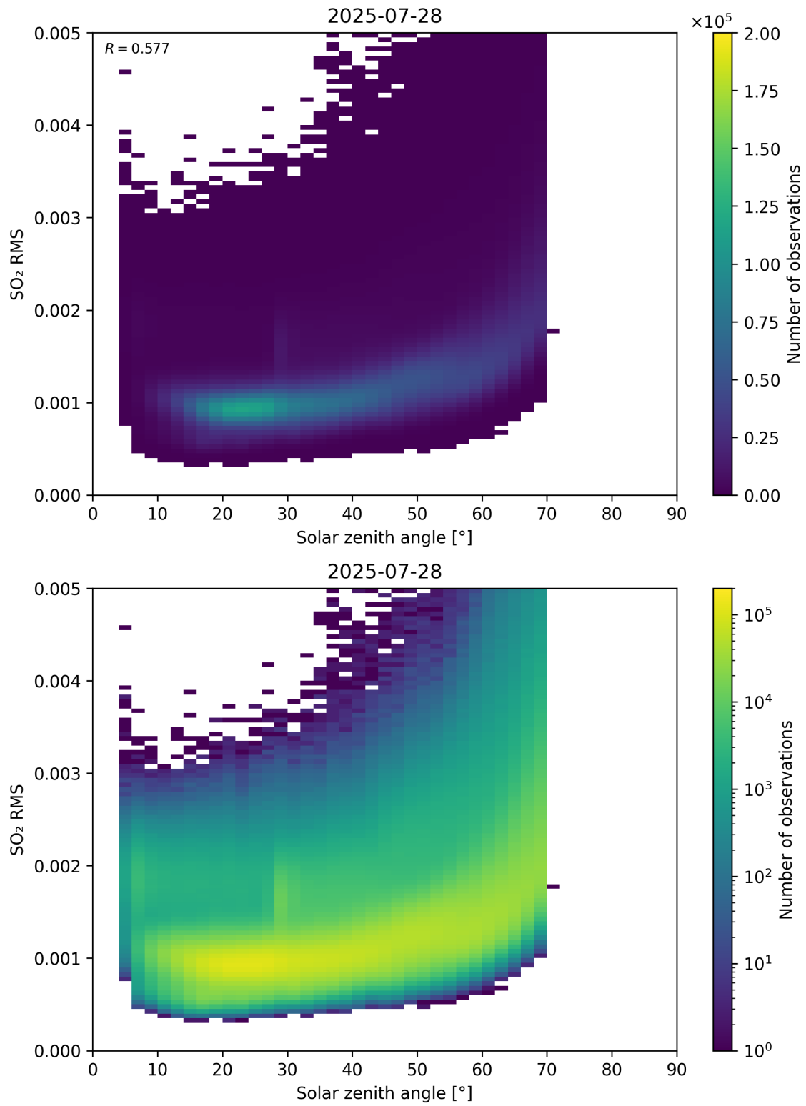
Figure 176: Scatter density plot of “Solar zenith angle” against “SO 2 RMS” for 2025-07-27 to 2025-07-29.
