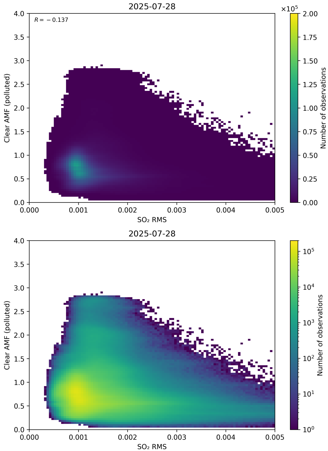
Figure 147: Scatter density plot of “SO 2 RMS” against “Clear AMF (polluted)” for 2025-07-27 to 2025-07-29.
