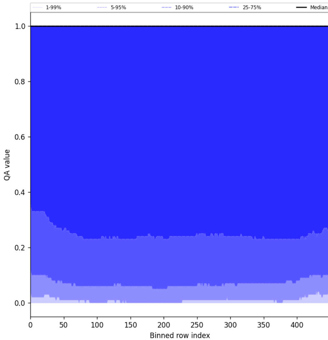
Figure 83: Along track statistics of “QA value” for 2025-07-27 to 2025-07-29
