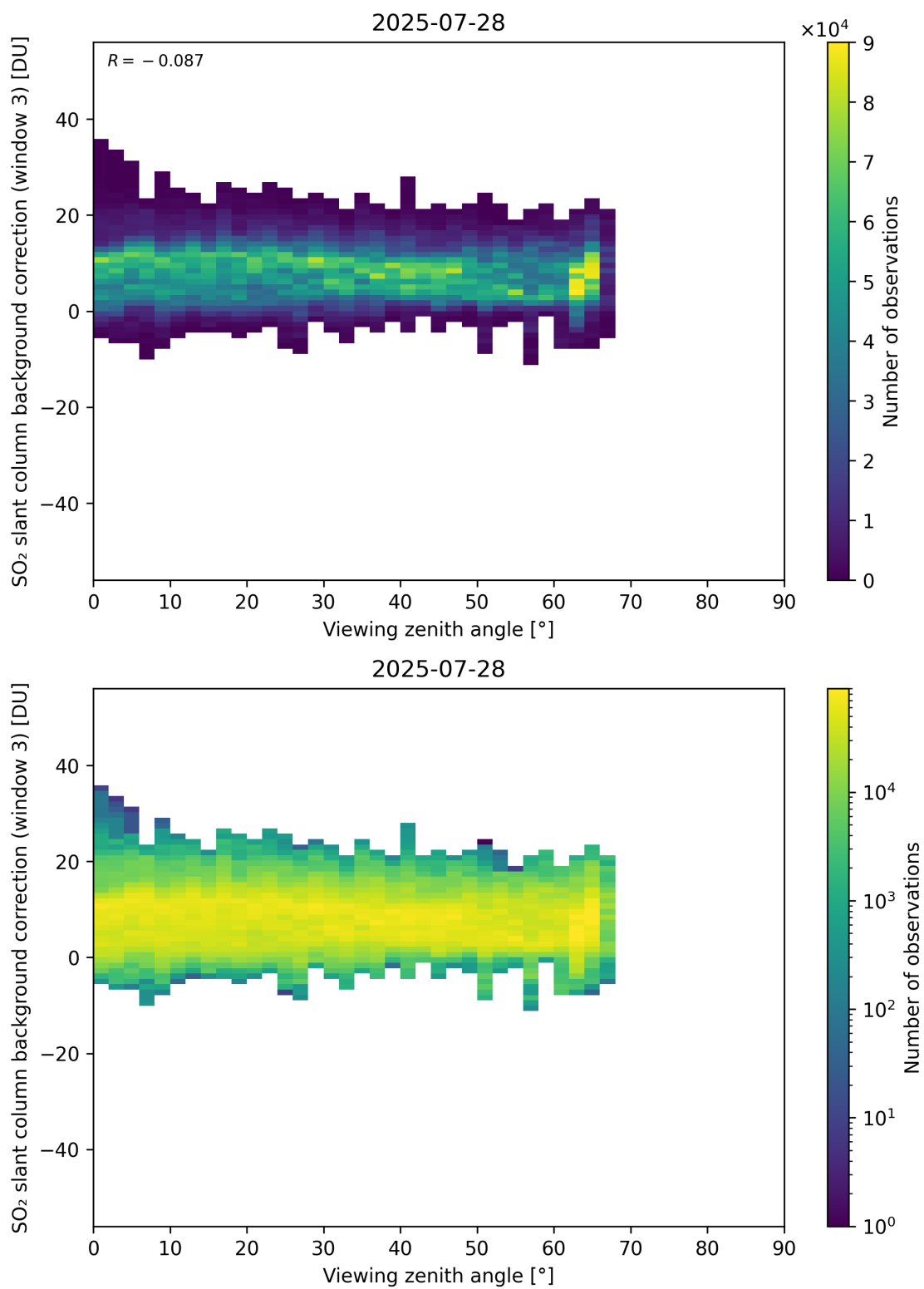
Figure 364: Scatter density plot of “Viewing zenith angle” against “SO 2 slant column background correction (window 3)” for 2025-07-27 to 2025-07-29.
