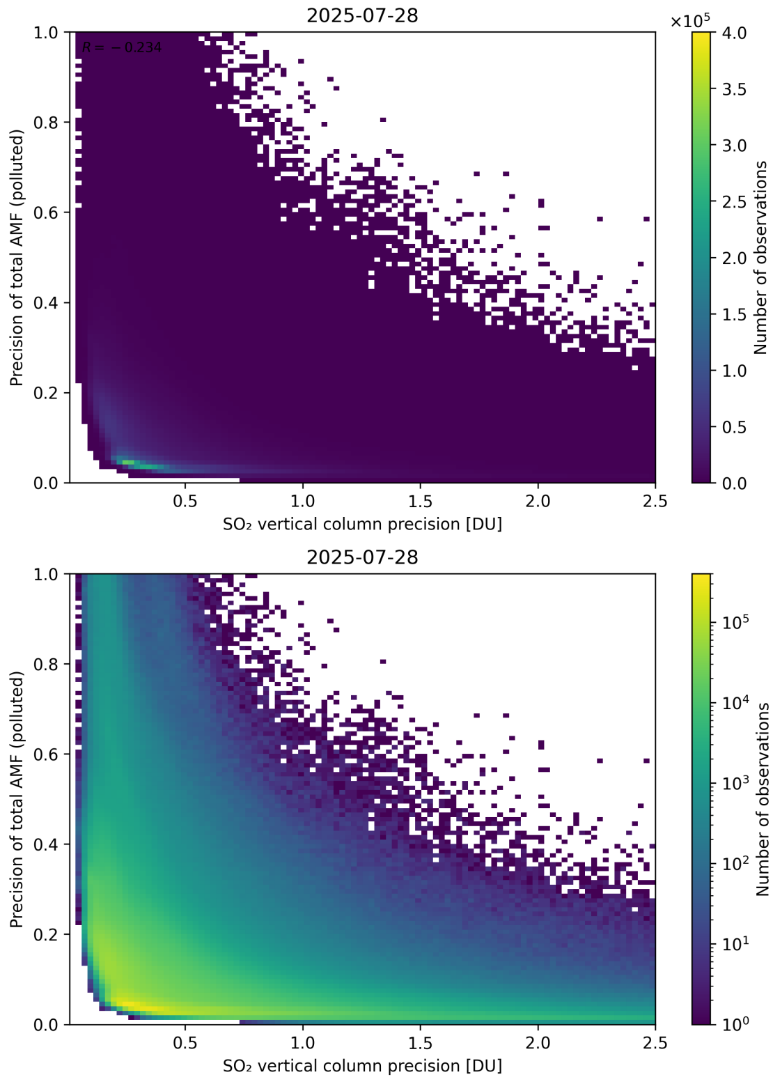
Figure 347: Scatter density plot of “SO 2 vertical column precision” against “Precision of total AMF (polluted)” for 2025-07-27 to 2025-07-29.
