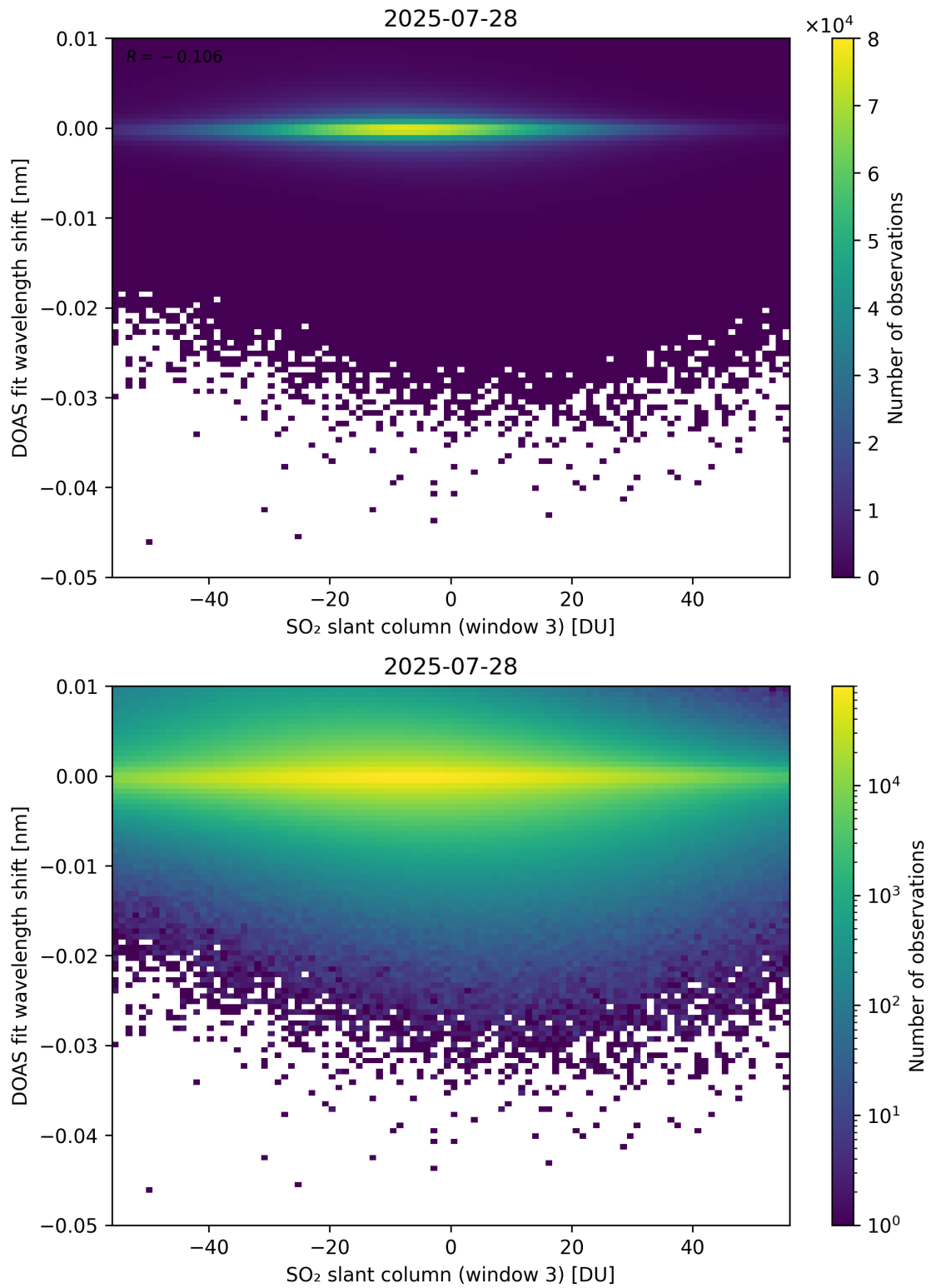
Figure 304: Scatter density plot of “SO 2 slant column (window 3)” against “DOAS fit wavelength shift” for 2025-07-27 to 2025-07-29.
