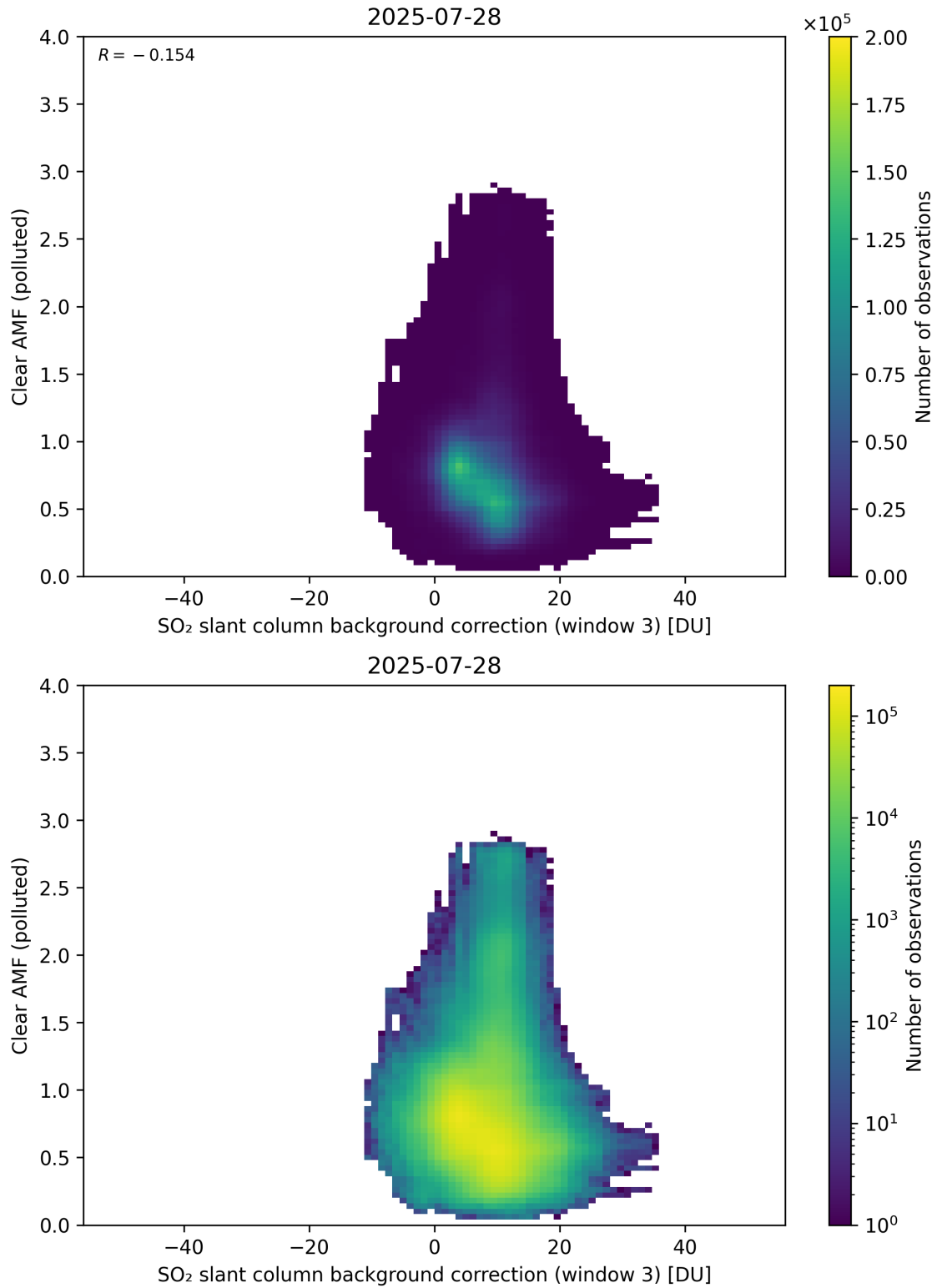
Figure 135: Scatter density plot of “SO 2 slant column background correction (window 3)” against “Clear AMF (polluted)” for 2025-07-27 to 2025-07-29.
