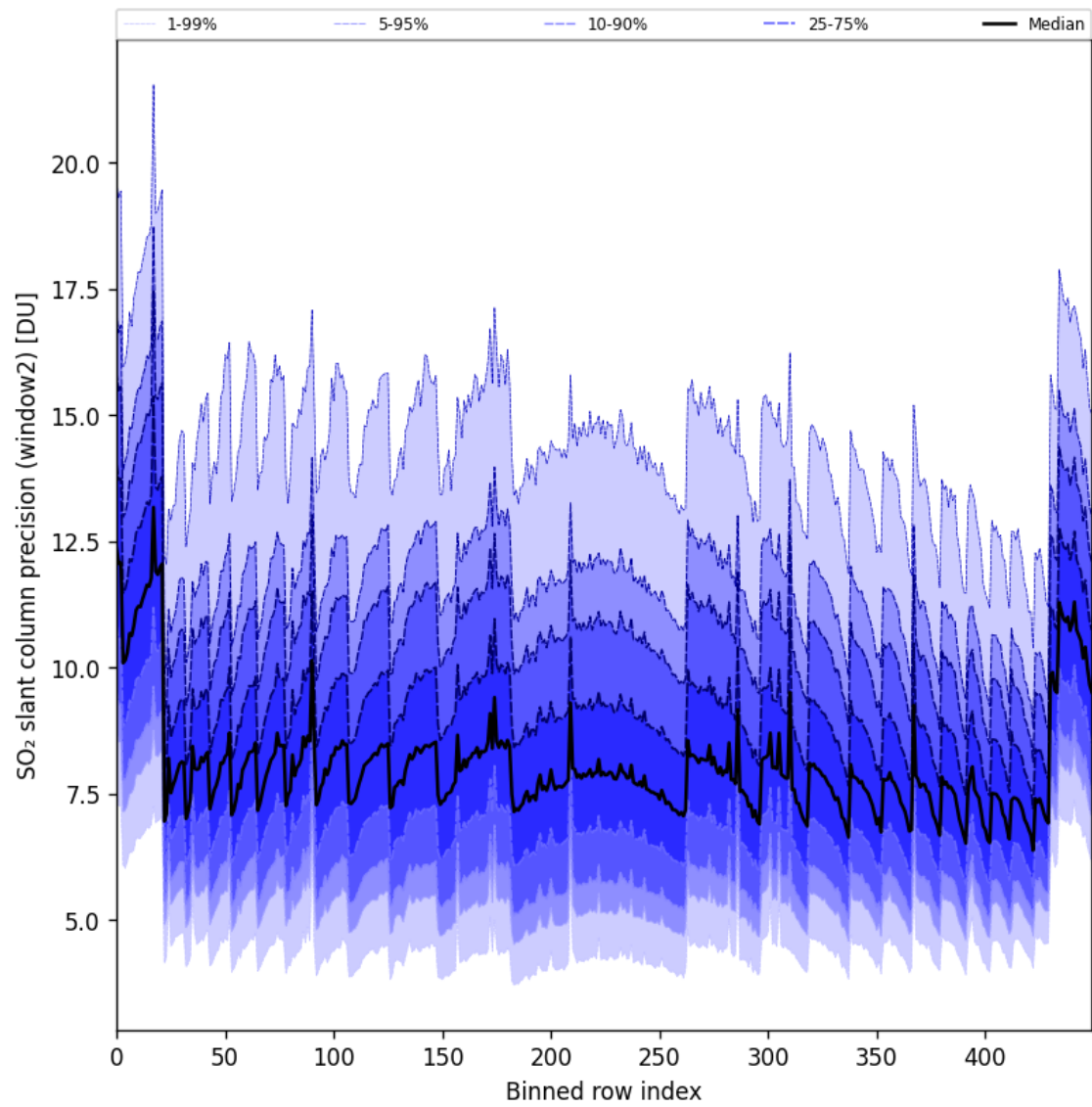
Figure 94: Along track statistics of “SO 2 slant column precision (window2)” for 2025-07-27 to 2025-07-29
