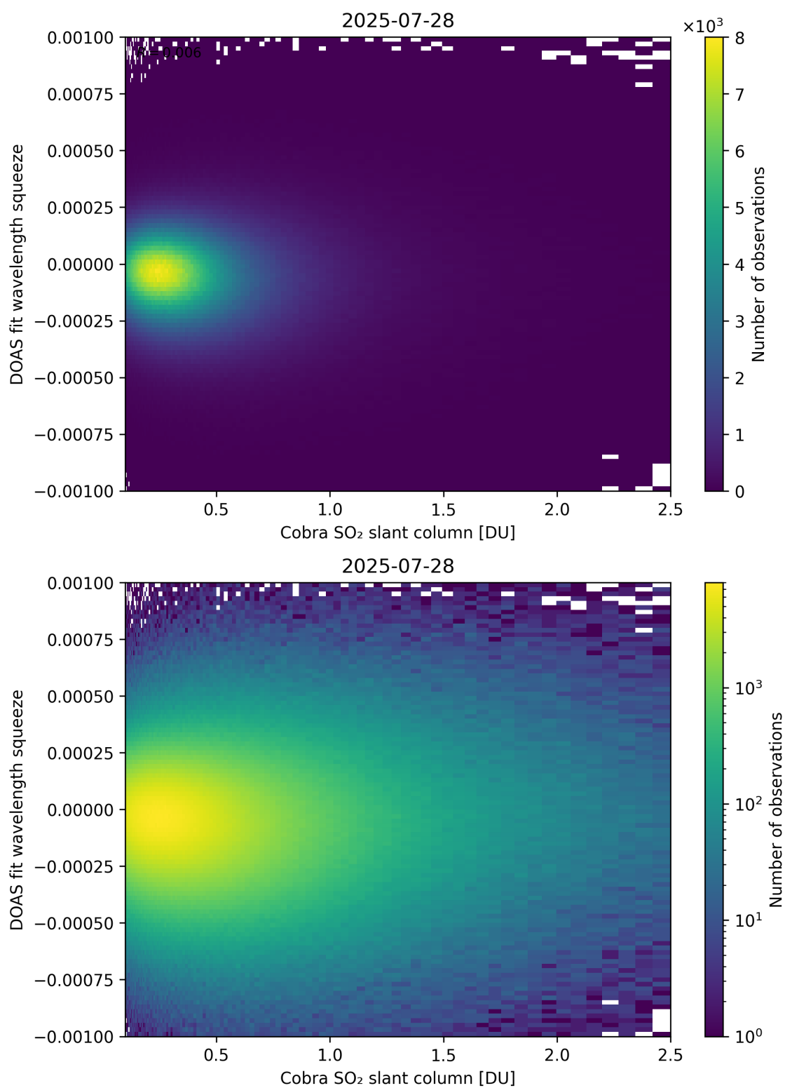
Figure 197: Scatter density plot of “Cobra SO 2 slant column” against “DOAS fit wavelength squeeze” for 2025-07-27 to 2025-07-29.
