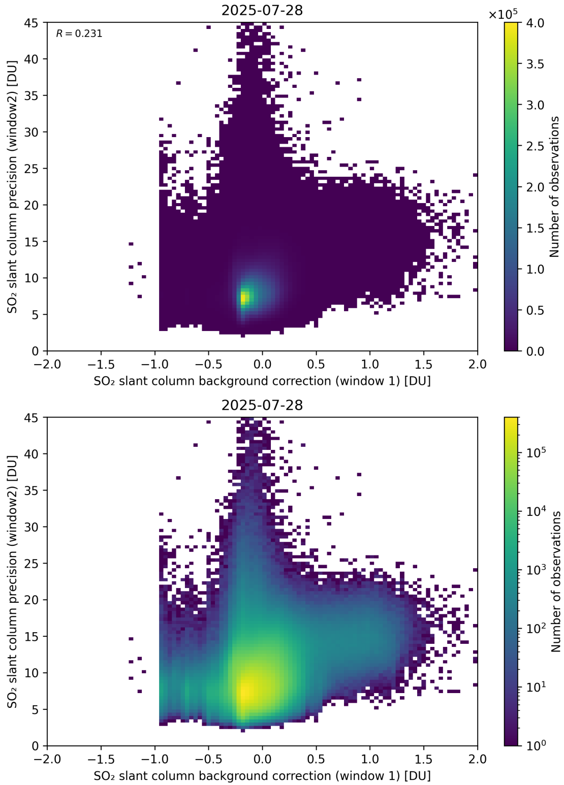
Figure 117: Scatter density plot of “SO 2 slant column background correction (window 1)” against “SO 2 slant column precision (window2)” for 2025-07-27 to 2025-07-29.
