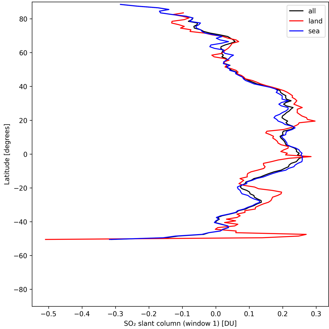
Figure 37: Zonal average of “SO 2 slant column (window 1)” for 2025-07-27 to 2025-07-29.
