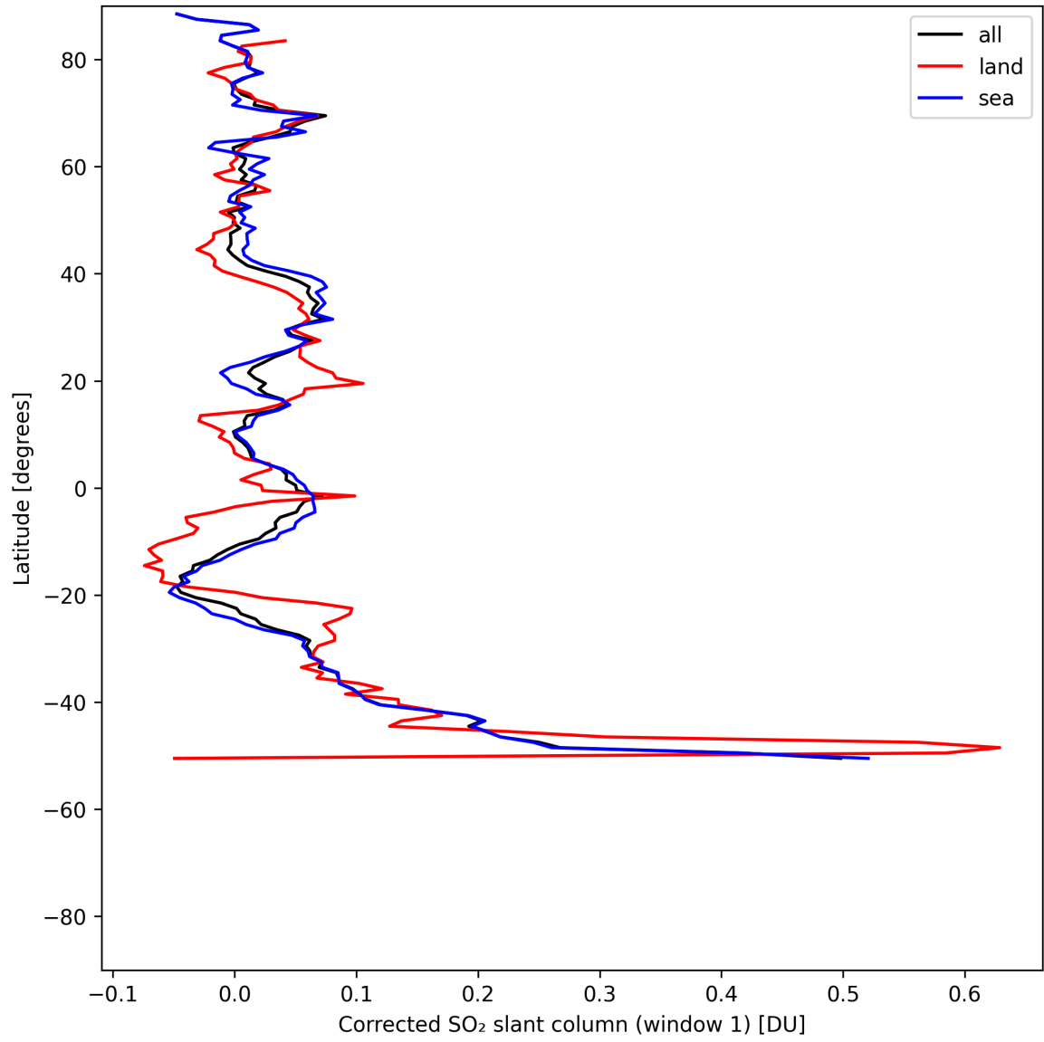
Figure 39: Zonal average of “Corrected SO 2 slant column (window 1)” for 2025-07-27 to 2025-07-29.
