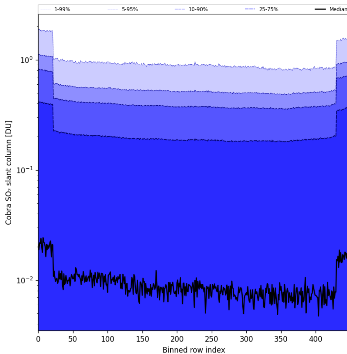
Figure 87: Along track statistics of "Cobra SO 2 slant column" for 2025-07-27 to 2025-07-29
