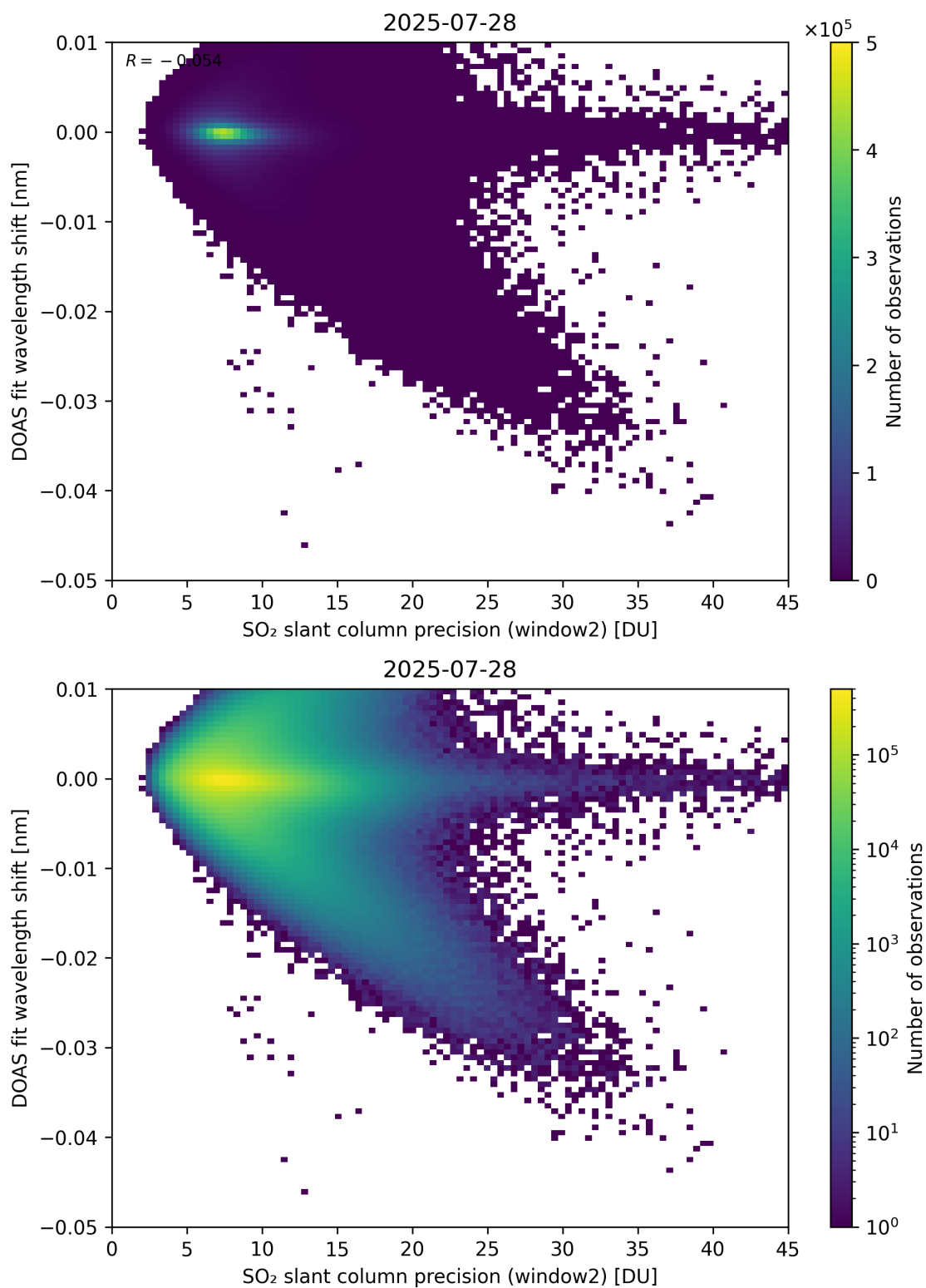
Figure 293: Scatter density plot of “SO 2 slant column precision (window2)” against “DOAS fit wavelength shift” for 2025-07-27 to 2025-07-29.
