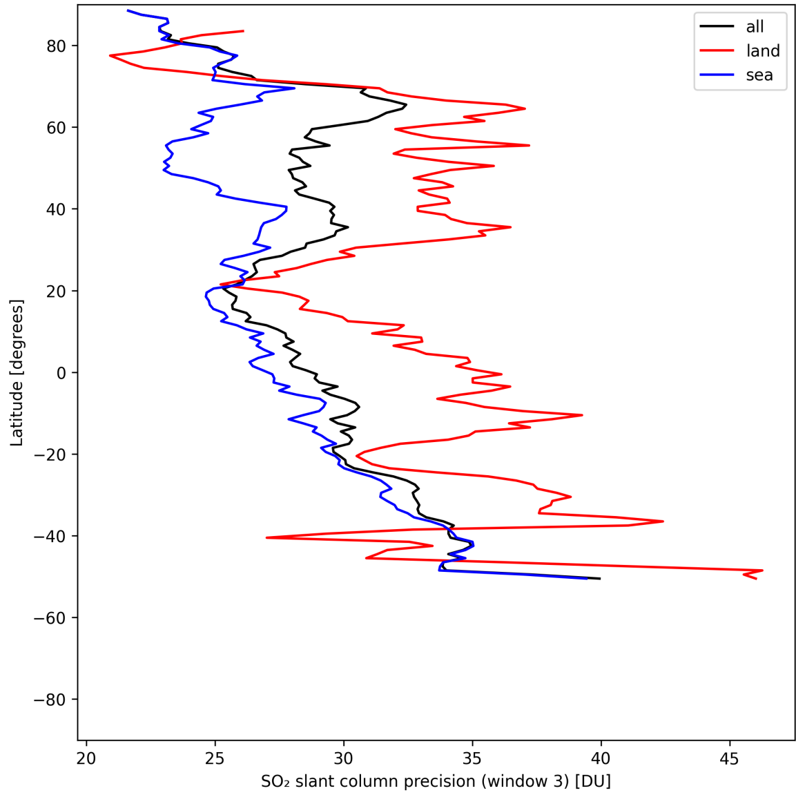
Figure 46: Zonal average of “SO 2 slant column precision (window 3)” for 2025-07-27 to 2025-07-29.
