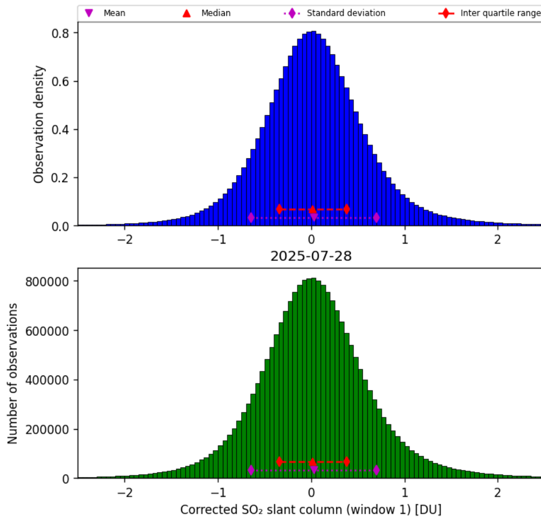
Figure 65: Histogram of “Corrected SO 2 slant column (window 1)” for 2025-07-27 to 2025-07-29
