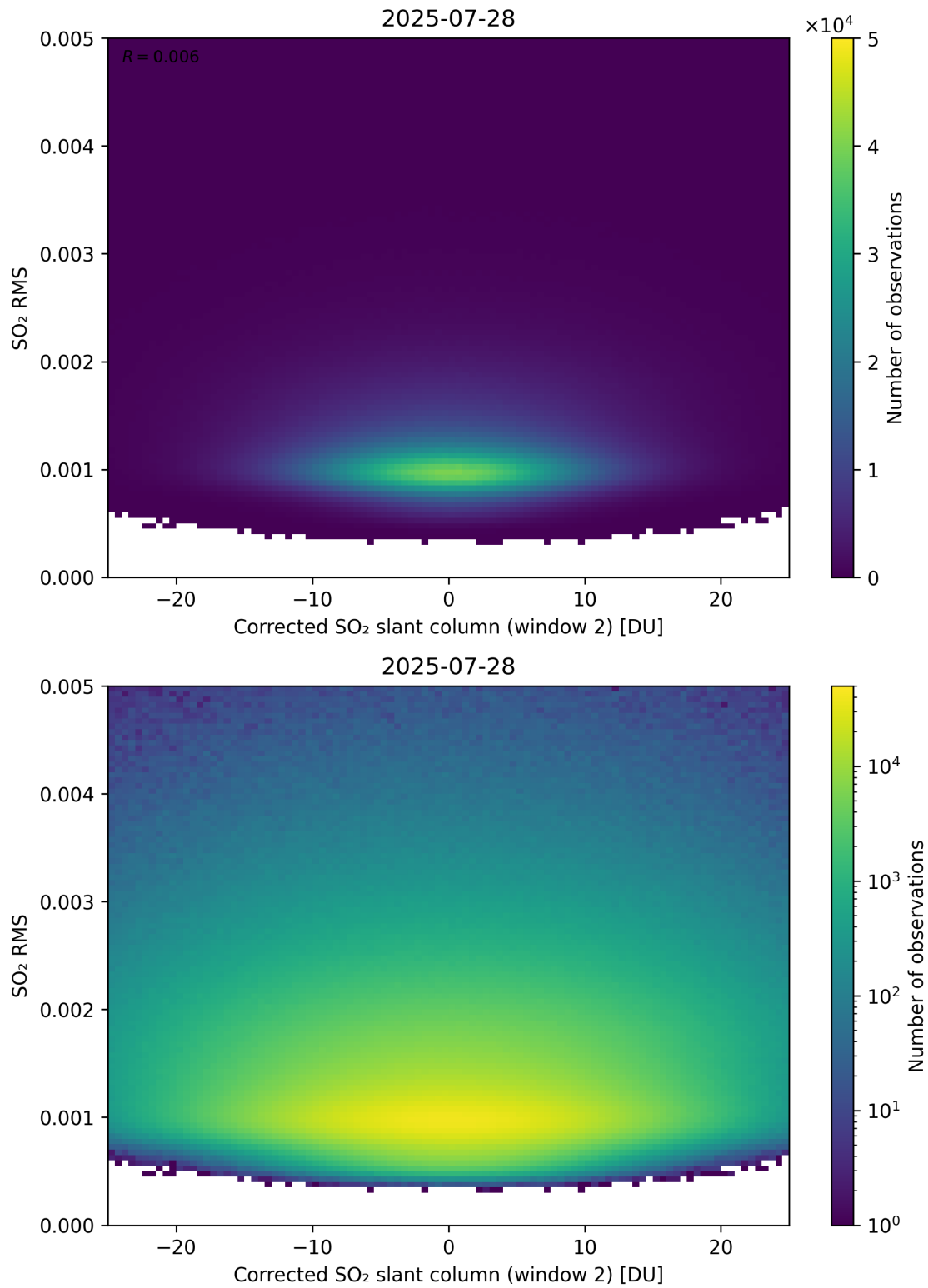
Figure 248: Scatter density plot of “Corrected SO 2 slant column (window 2)” against “SO 2 RMS” for 2025-07-27 to 2025-07-29.
