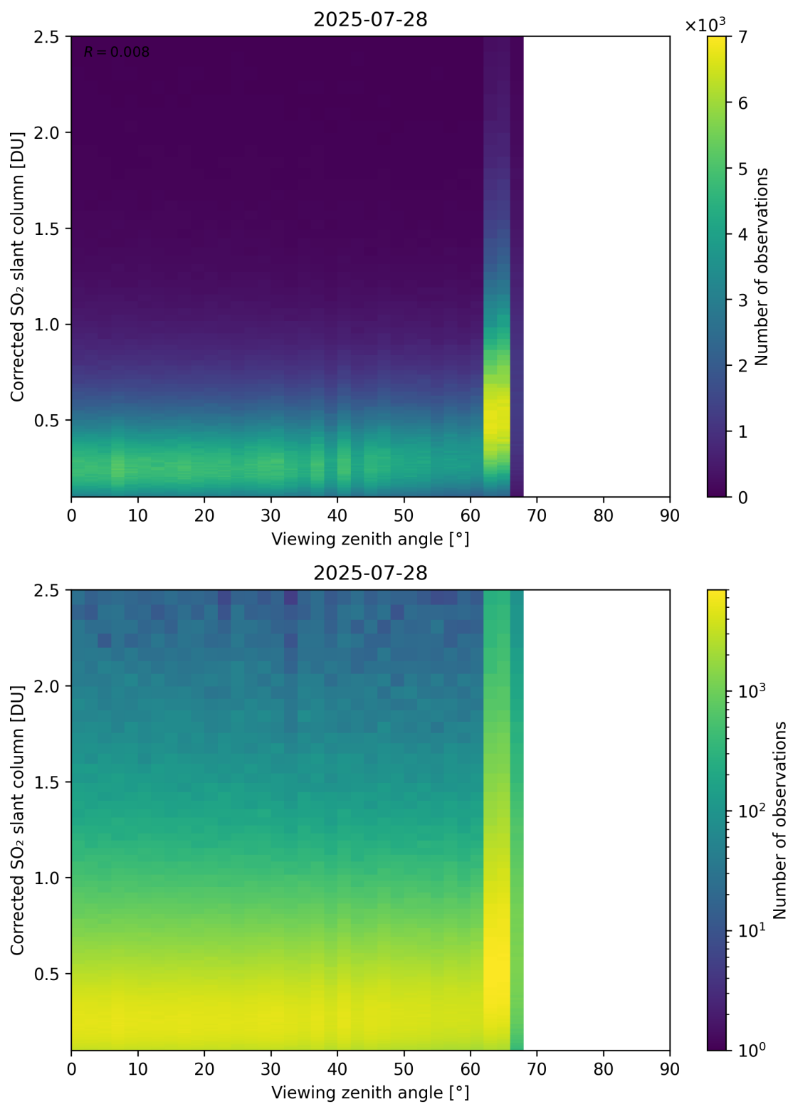
Figure 373: Scatter density plot of “Viewing zenith angle” against “Corrected SO 2 slant column” for 2025-07-27 to 2025-07-29.
