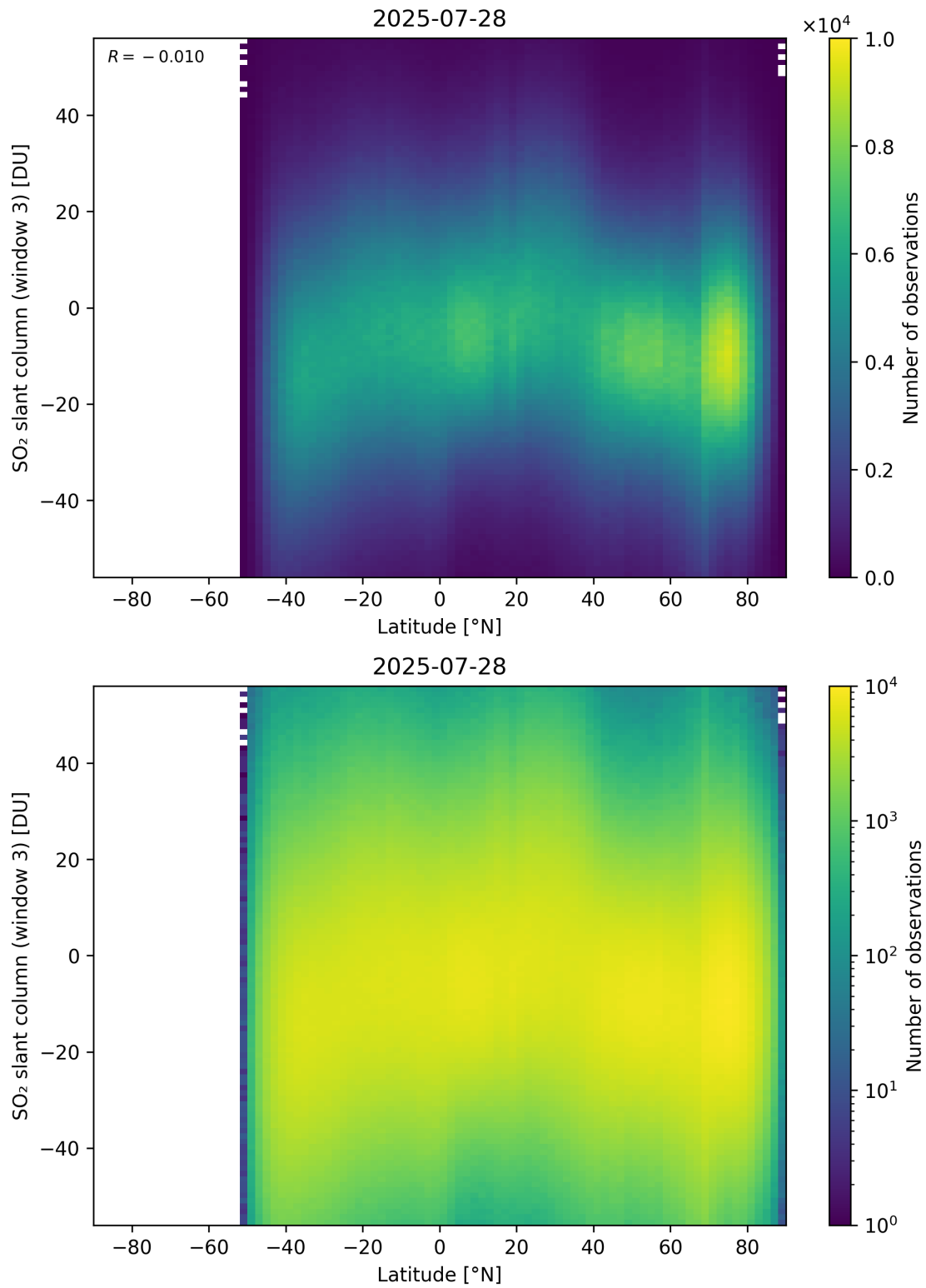
Figure 165: Scatter density plot of “Latitude” against “SO 2 slant column (window 3)” for 2025-07-27 to 2025-07-29.
