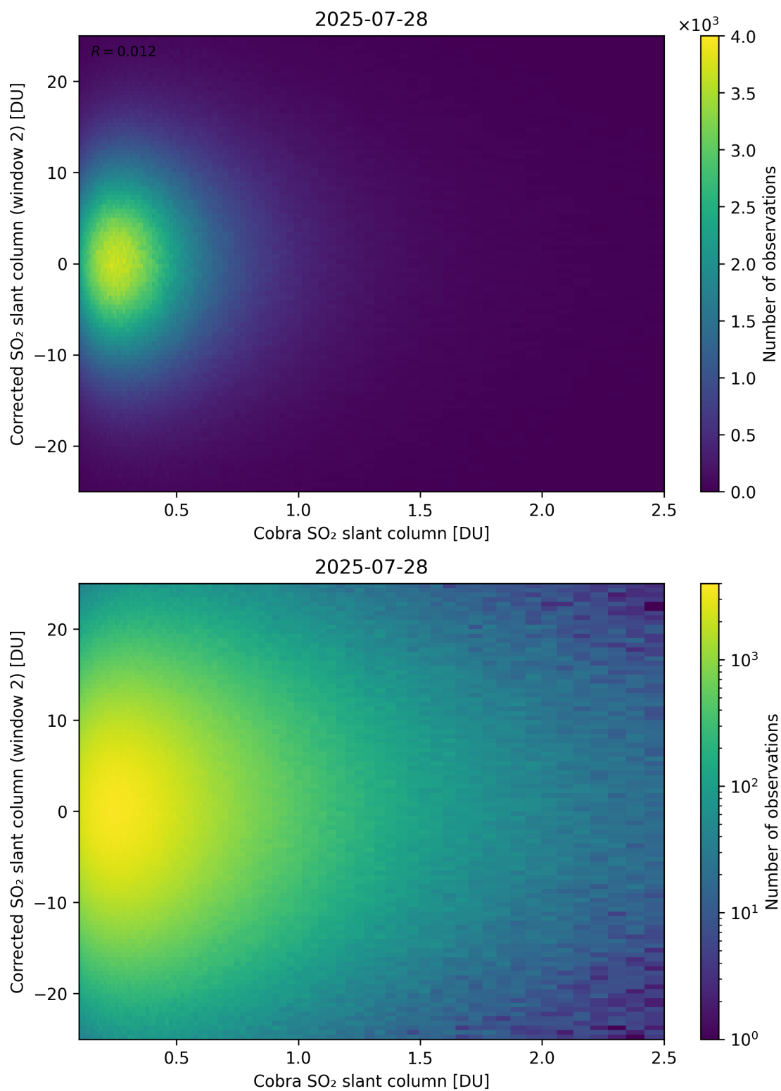
Figure 217: Scatter density plot of “Cobra SO 2 slant column” against “Corrected SO 2 slant column (window 2)” for 2025-07-27 to 2025-07-29.
