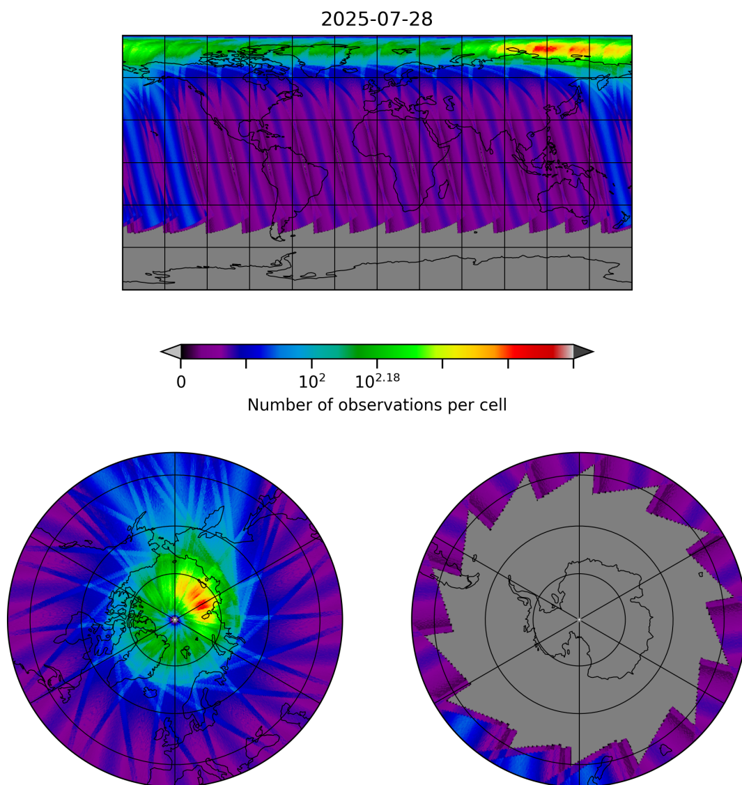
Figure 30: Map of the number of observations for 2025-07-27 to 2025-07-29
