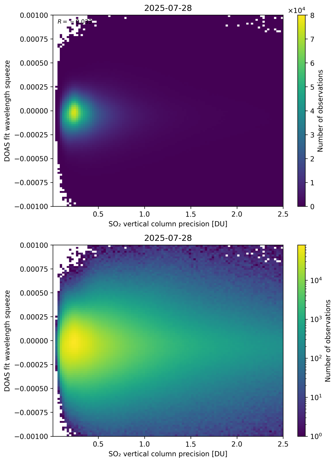
Figure 333: Scatter density plot of “SO 2 vertical column precision” against “DOAS fit wavelength squeeze” for 2025-07-27 to 2025-07-29.
