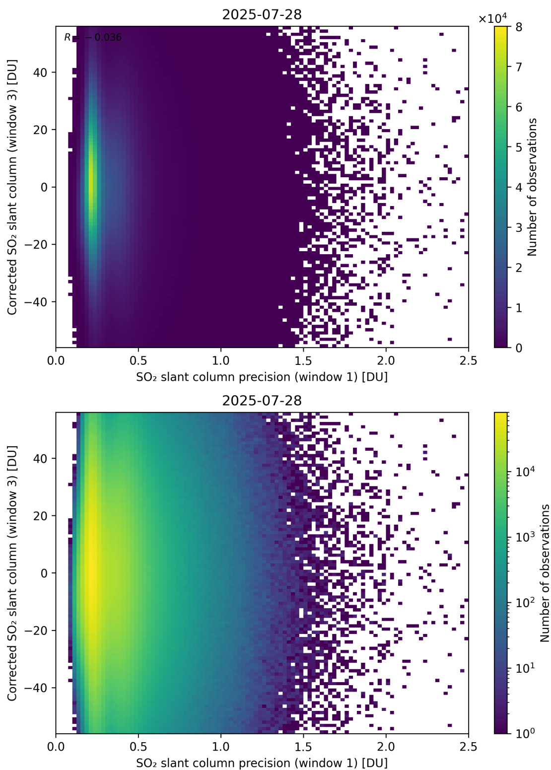
Figure 276: Scatter density plot of “SO 2 slant column precision (window 1)” against “Corrected SO 2 slant column (window 3)” for 2025-07-27 to 2025-07-29.
