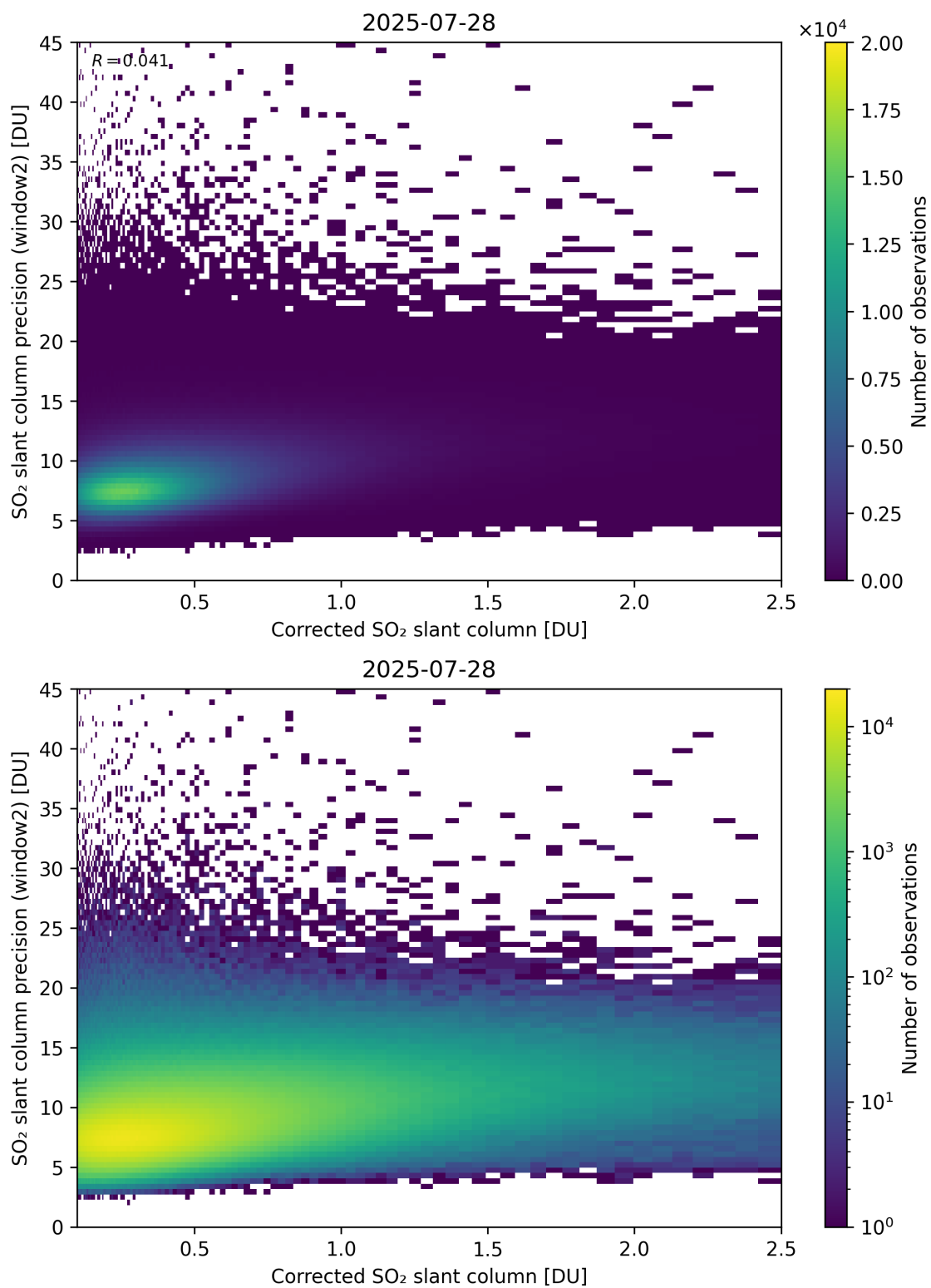
Figure 239: Scatter density plot of “Corrected SO 2 slant column” against “SO 2 slant column precision (window2)” for 2025-07-27 to 2025-07-29.
