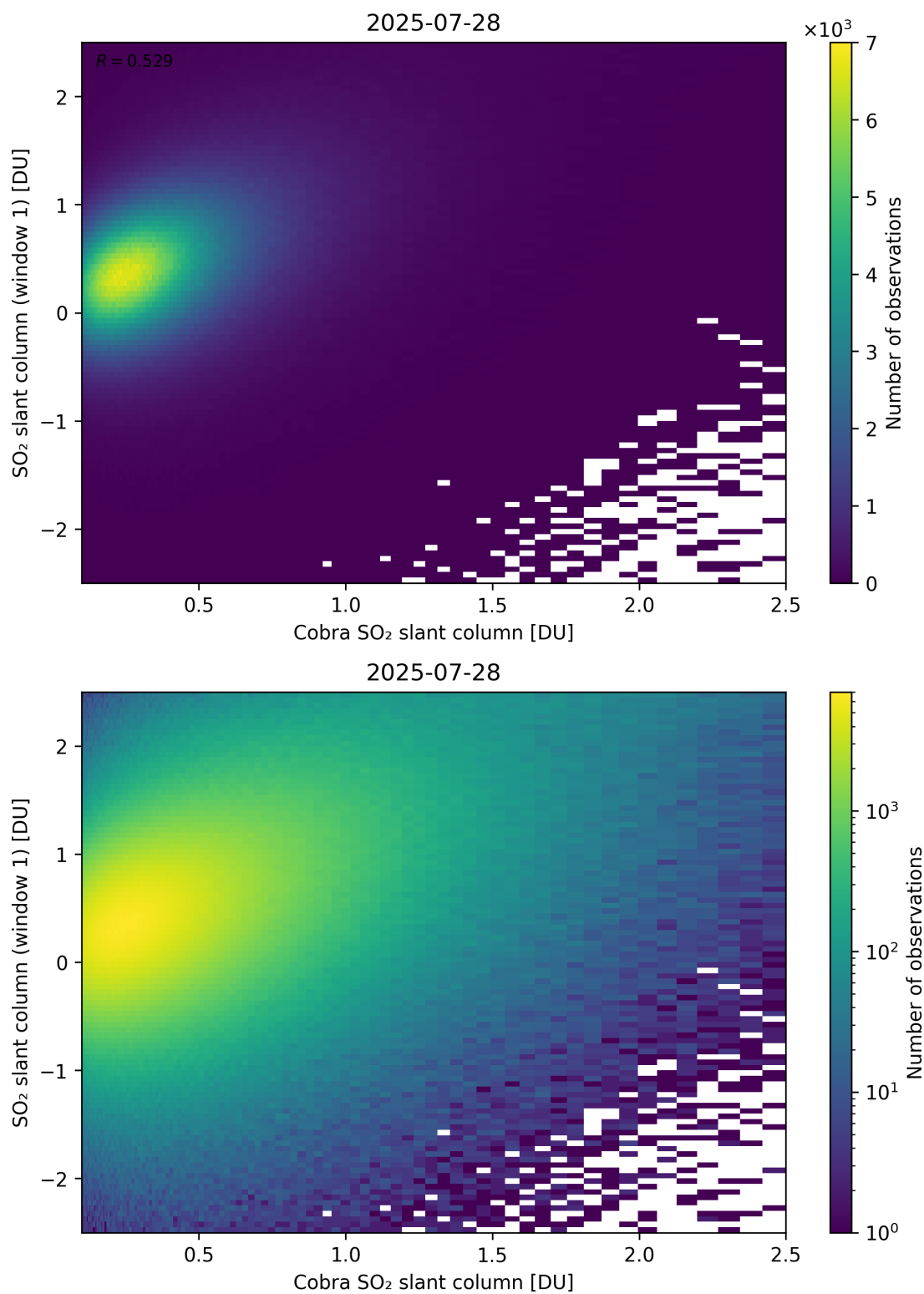
Figure 219: Scatter density plot of “Cobra SO 2 slant column” against “SO 2 slant column (window 1)” for 2025-07-27 to 2025-07-29.
