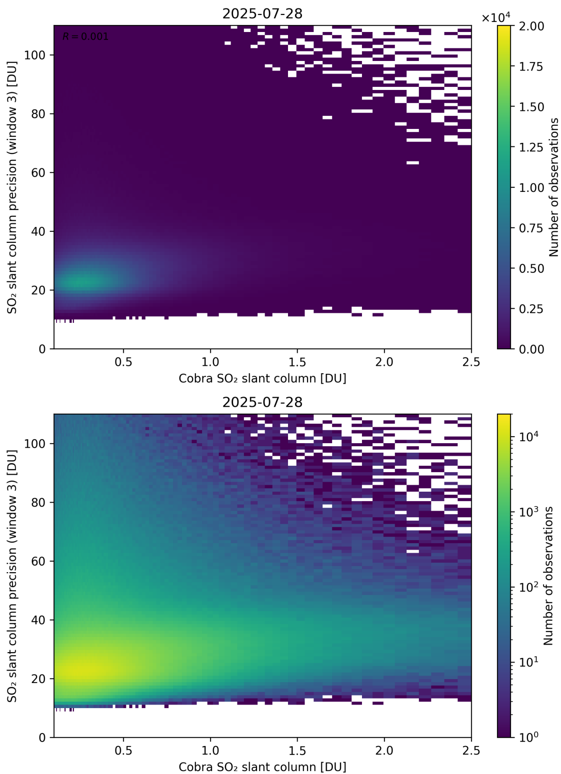
Figure 223: Scatter density plot of “Cobra SO 2 slant column” against “SO 2 slant column precision (window 3)” for 2025-07-27 to 2025-07-29.
