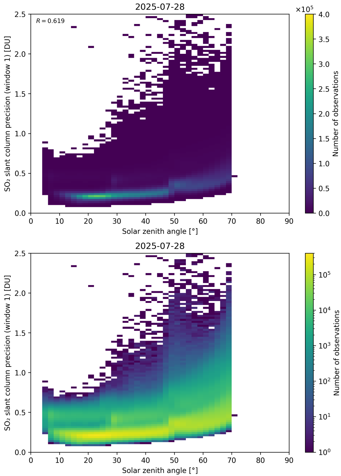
Figure 185: Scatter density plot of “Solar zenith angle” against “SO 2 slant column precision (window 1)” for 2025-07-27 to 2025-07-29.
