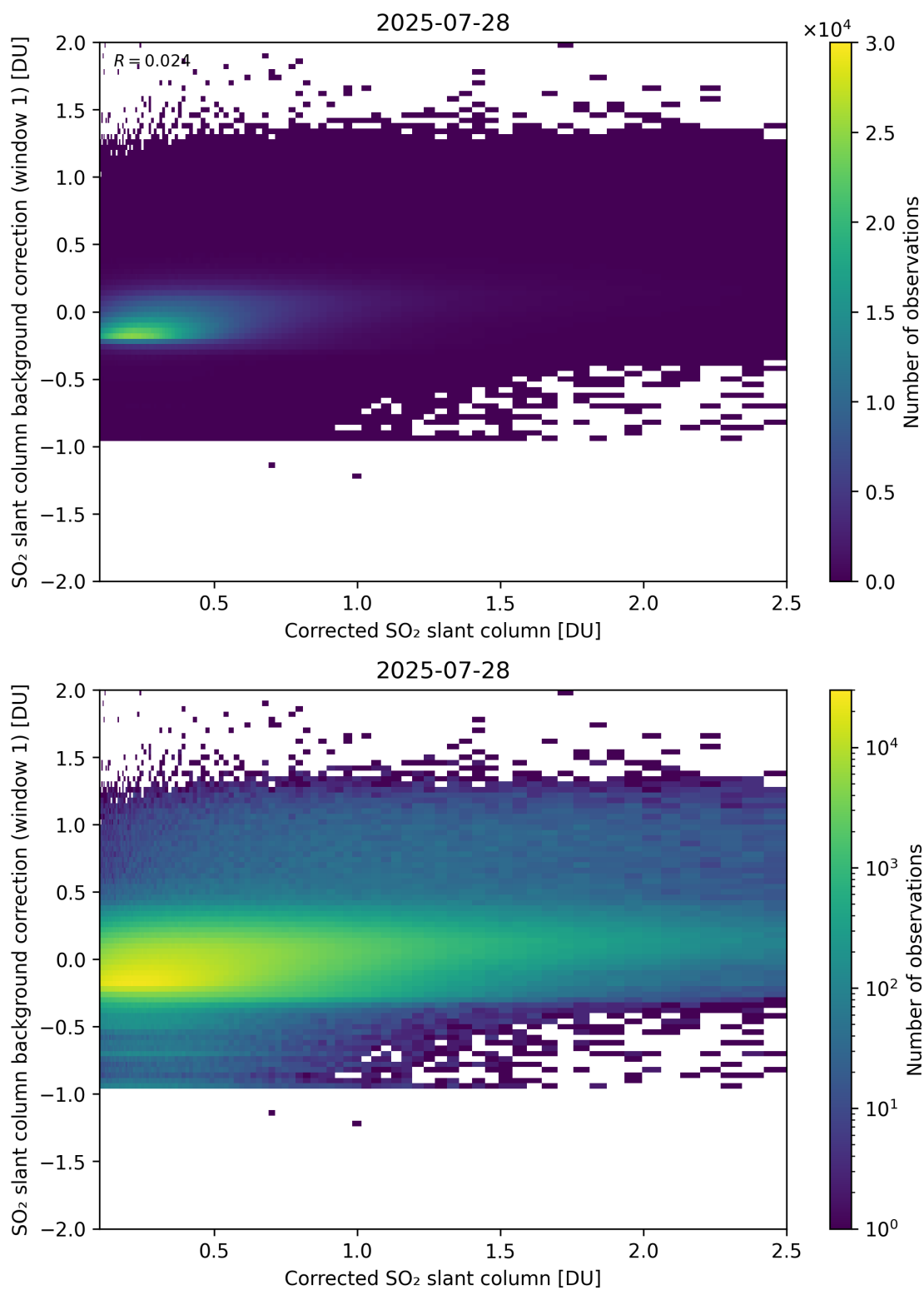
Figure 226: Scatter density plot of “Corrected SO 2 slant column” against “SO 2 slant column background correction (window 1)” for 2025-07-27 to 2025-07-29.
