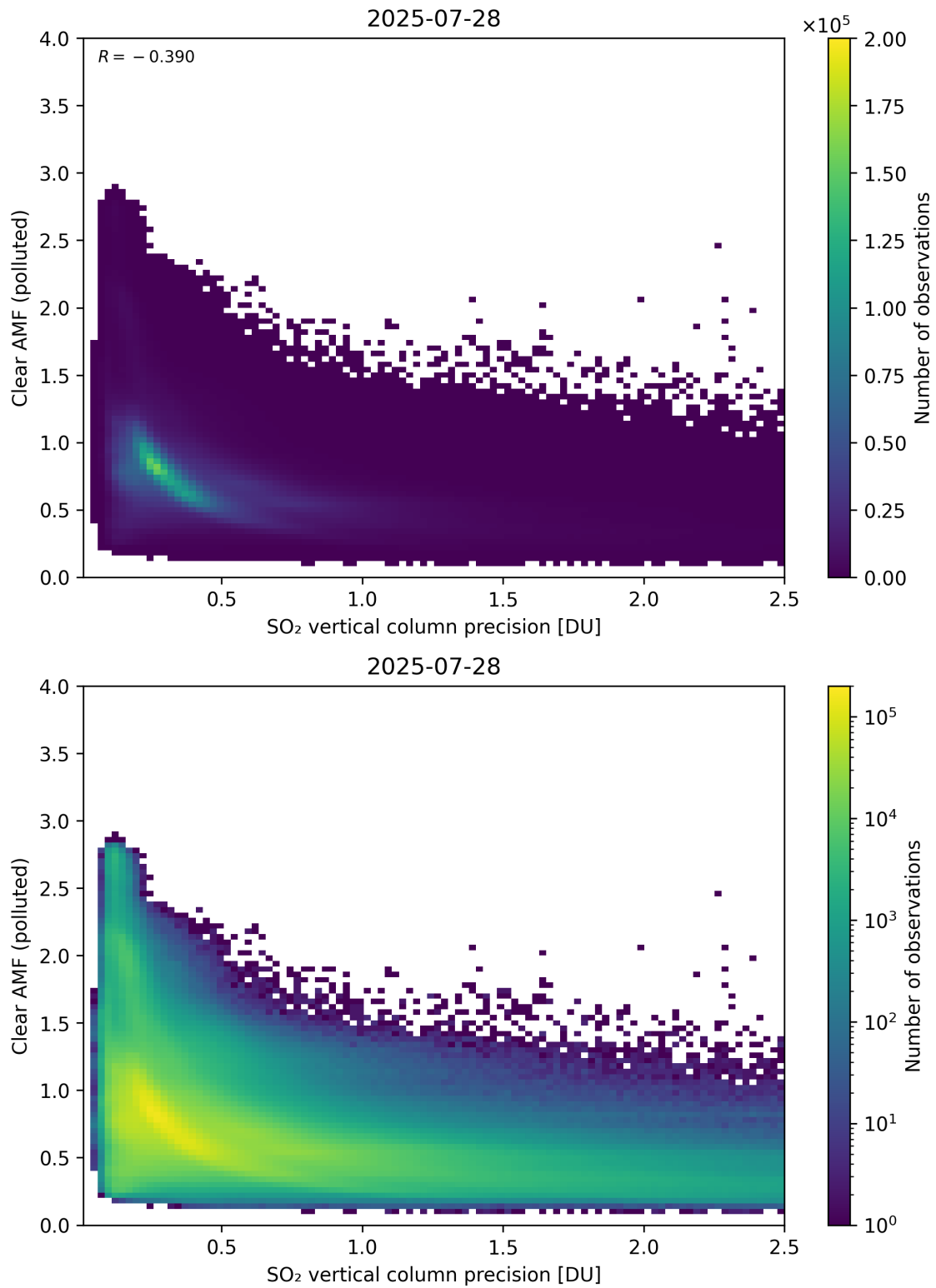
Figure 335: Scatter density plot of “SO 2 vertical column precision” against “Clear AMF (polluted)” for 2025-07-27 to 2025-07-29.
