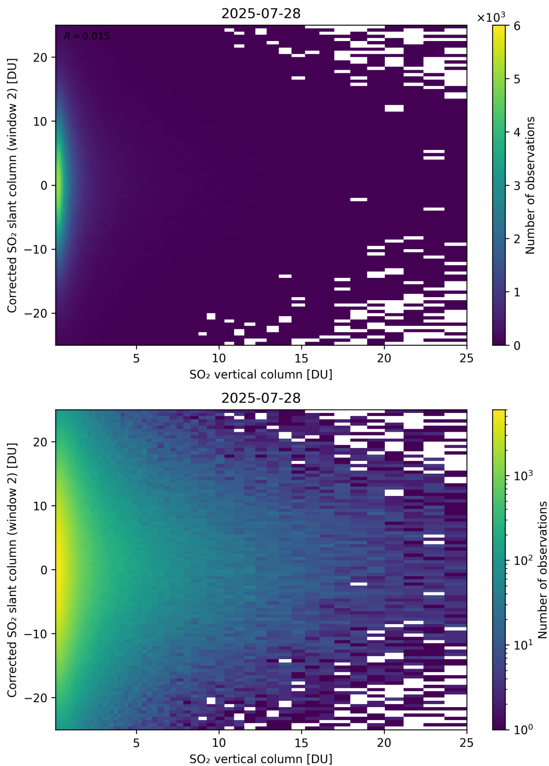
Figure 352: Scatter density plot of “SO 2 vertical column” against “Corrected SO 2 slant column (window 2)” for 2025-07-27 to 2025-07-29.
