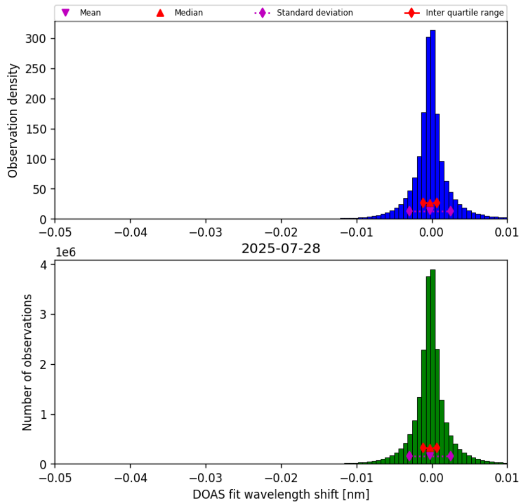
Figure 76: Histogram of “DOAS fit wavelength shift” for 2025-07-27 to 2025-07-29
