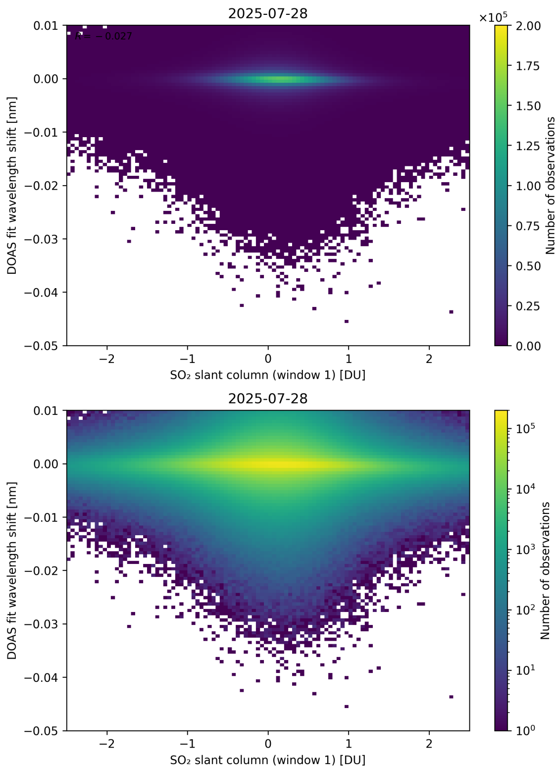
Figure 265: Scatter density plot of “SO 2 slant column (window 1)” against “DOAS fit wavelength shift” for 2025-07-27 to 2025-07-29.
