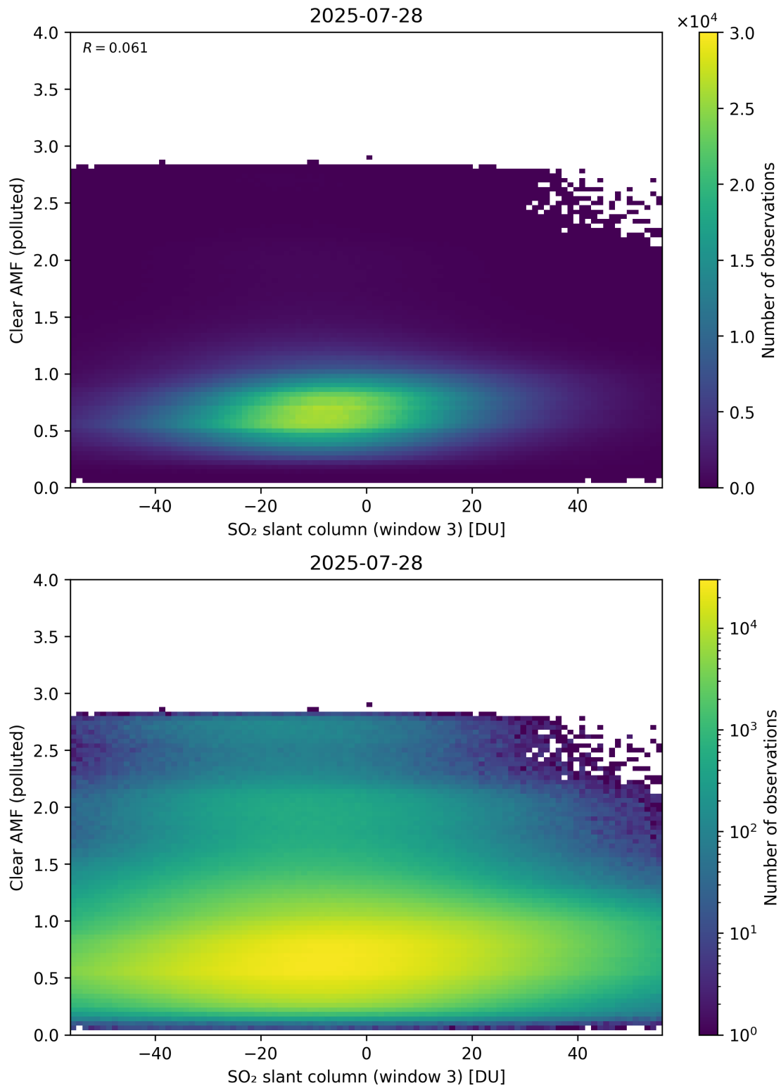
Figure 315: Scatter density plot of “SO 2 slant column (window 3)” against “Clear AMF (polluted)” for 2025-07-27 to 2025-07-29.
