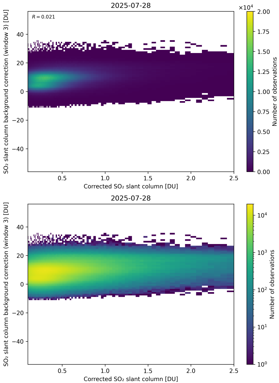
Figure 228: Scatter density plot of “Corrected SO 2 slant column” against “SO 2 slant column background correction (window 3)” for 2025-07-27 to 2025-07-29.
