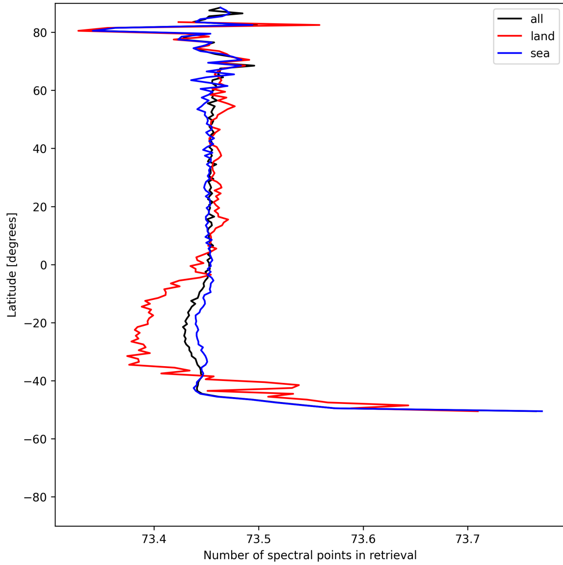
Figure 56: Zonal average of “Number of spectral points in retrieval” for 2025-07-27 to 2025-07-29.
