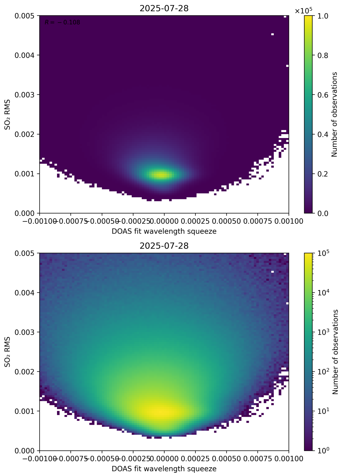
Figure 143: Scatter density plot of “DOAS fit wavelength squeeze” against “SO 2 RMS” for 2025-07-27 to 2025-07-29.
