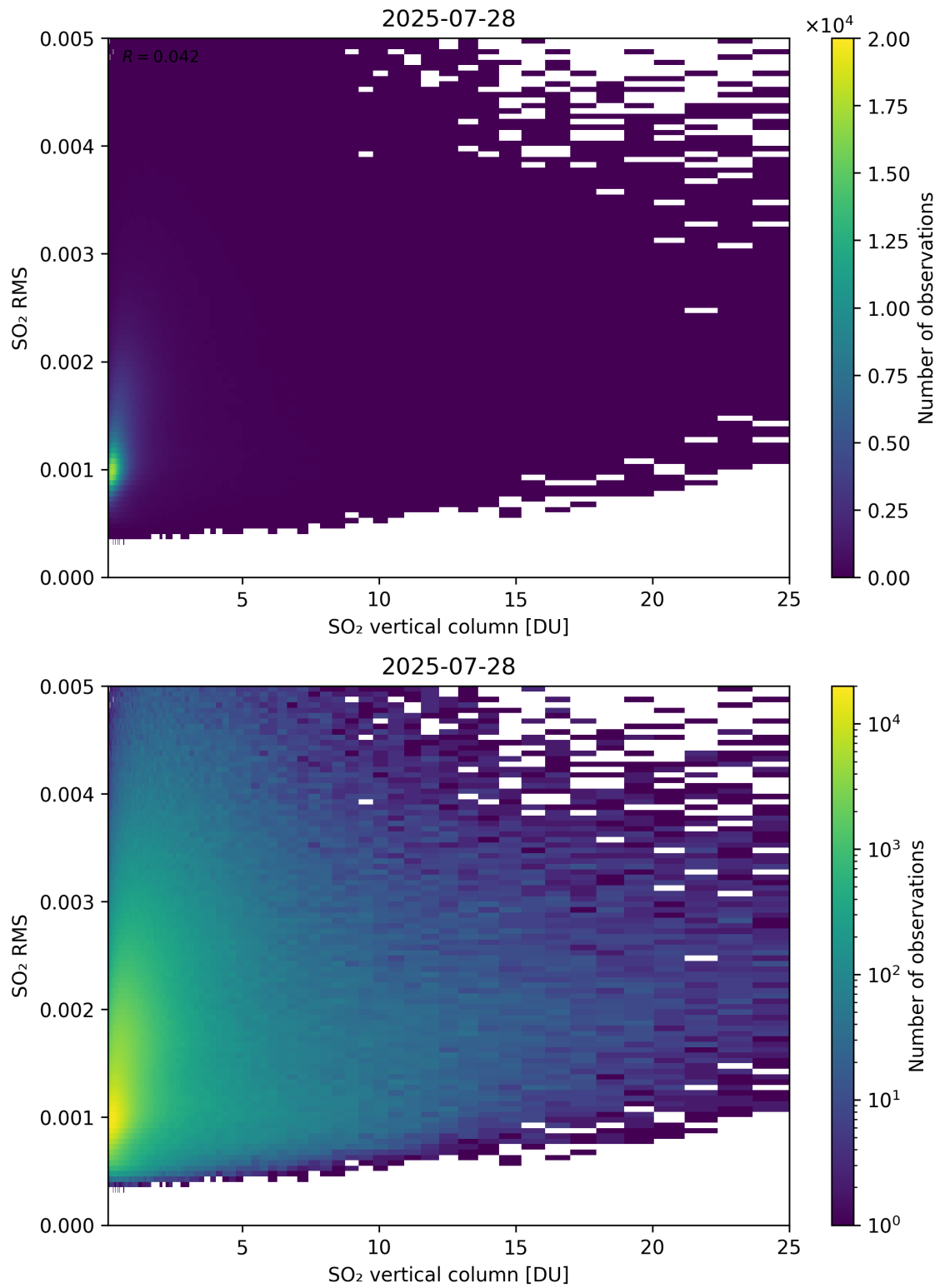
Figure 328: Scatter density plot of “SO 2 vertical column” against “SO 2 RMS” for 2025-07-27 to 2025-07-29.
