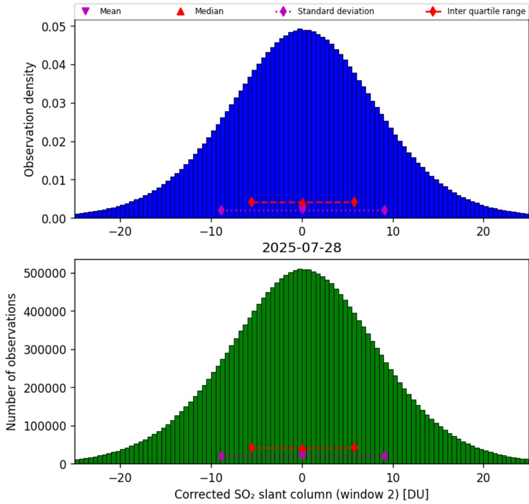
Figure 69: Histogram of “Corrected SO 2 slant column (window 2)” for 2025-07-27 to 2025-07-29
