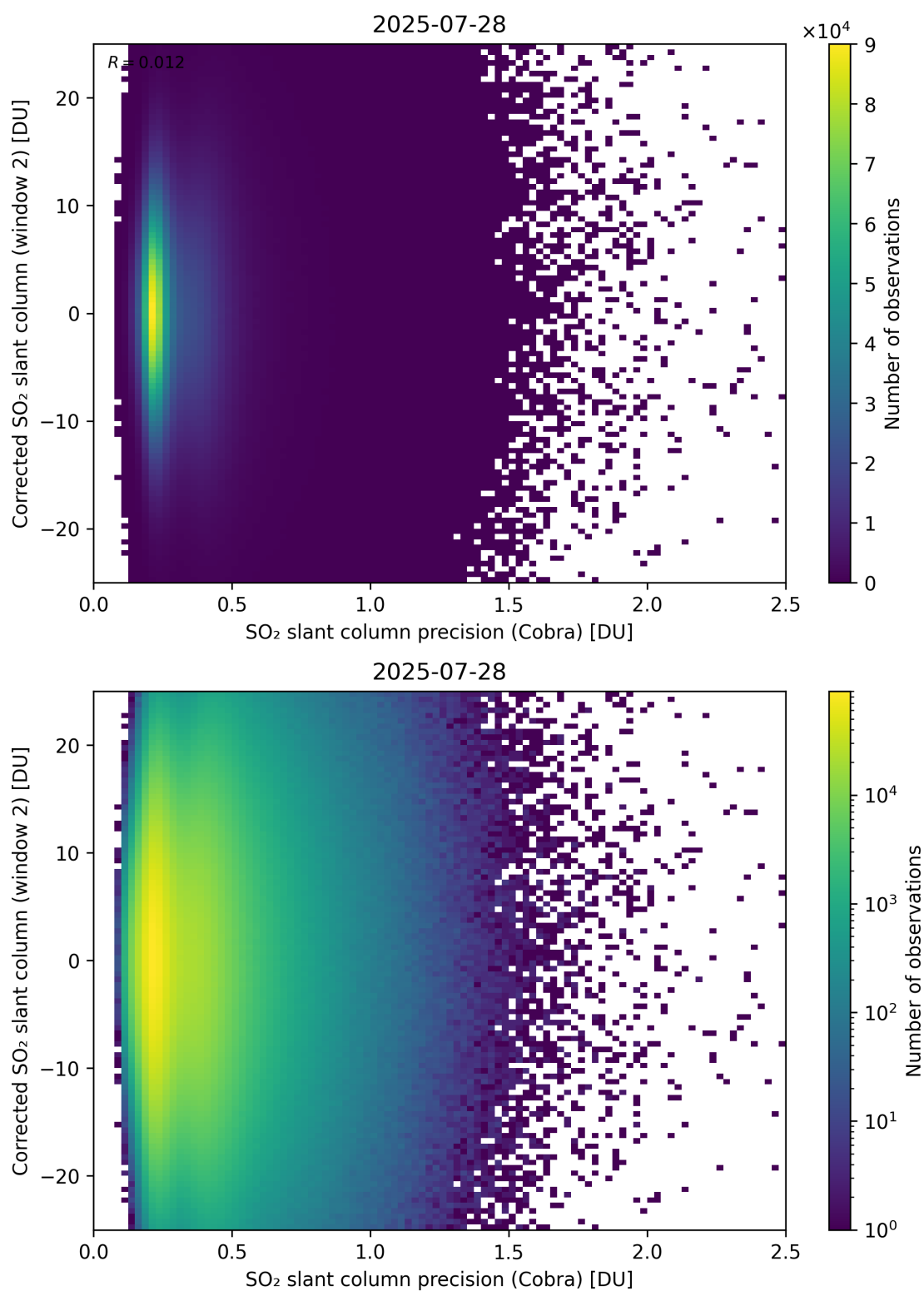
Figure 206: Scatter density plot of “SO 2 slant column precision (Cobra)” against “Corrected SO 2 slant column (window 2)” for 2025-07-27 to 2025-07-29.
