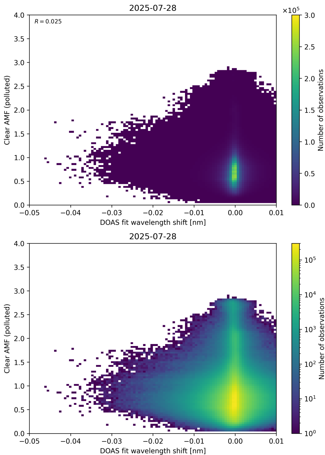
Figure 140: Scatter density plot of “DOAS fit wavelength shift” against “Clear AMF (polluted)” for 2025-07-27 to 2025-07-29.
