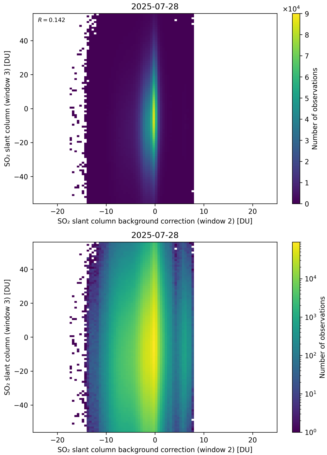
Figure 128: Scatter density plot of “SO 2 slant column background correction (window 2)” against “SO 2 slant column (window 3)” for 2025-07-27 to 2025-07-29.
