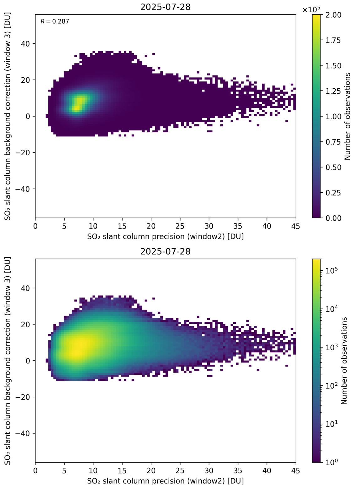
Figure 292: Scatter density plot of “SO 2 slant column precision (window2)” against “SO 2 slant column background correction (window 3)” for 2025-07-27 to 2025-07-29.
