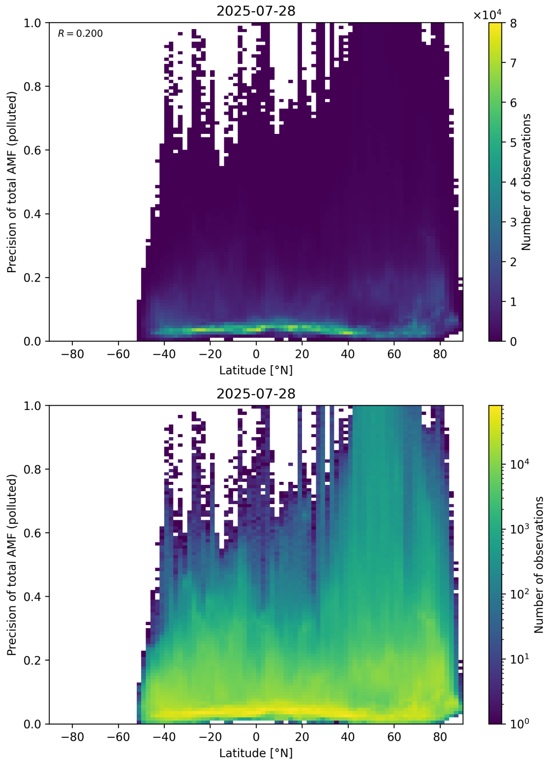
Figure 168: Scatter density plot of “Latitude” against “Precision of total AMF (polluted)” for 2025-07-27 to 2025-07-29.
