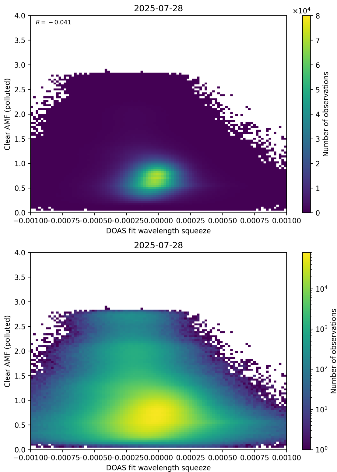
Figure 144: Scatter density plot of “DOAS fit wavelength squeeze” against “Clear AMF (polluted)” for 2025-07-27 to 2025-07-29.
