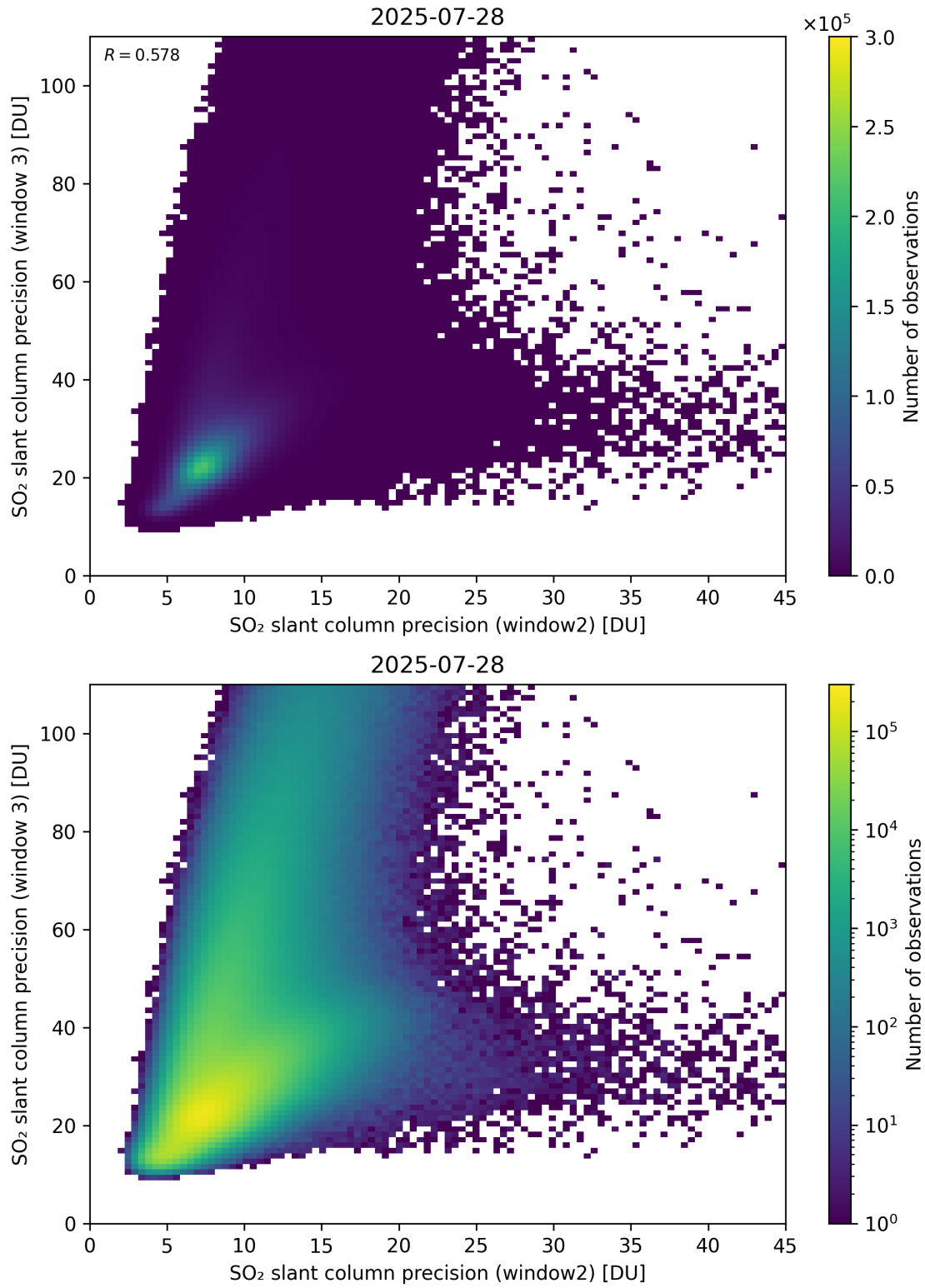
Figure 300: Scatter density plot of “SO 2 slant column precision (window2)” against “SO 2 slant column precision (window 3)” for 2025-07-27 to 2025-07-29.
