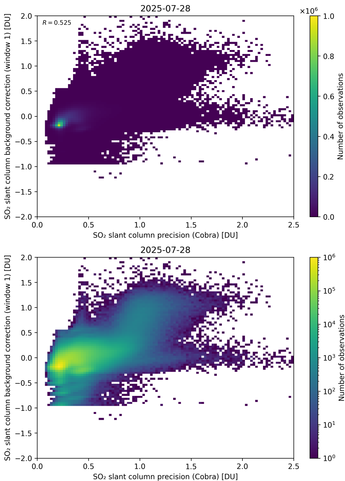
Figure 199: Scatter density plot of “SO 2 slant column precision (Cobra)” against “SO 2 slant column background correction (window 1)” for 2025-07-27 to 2025-07-29.
