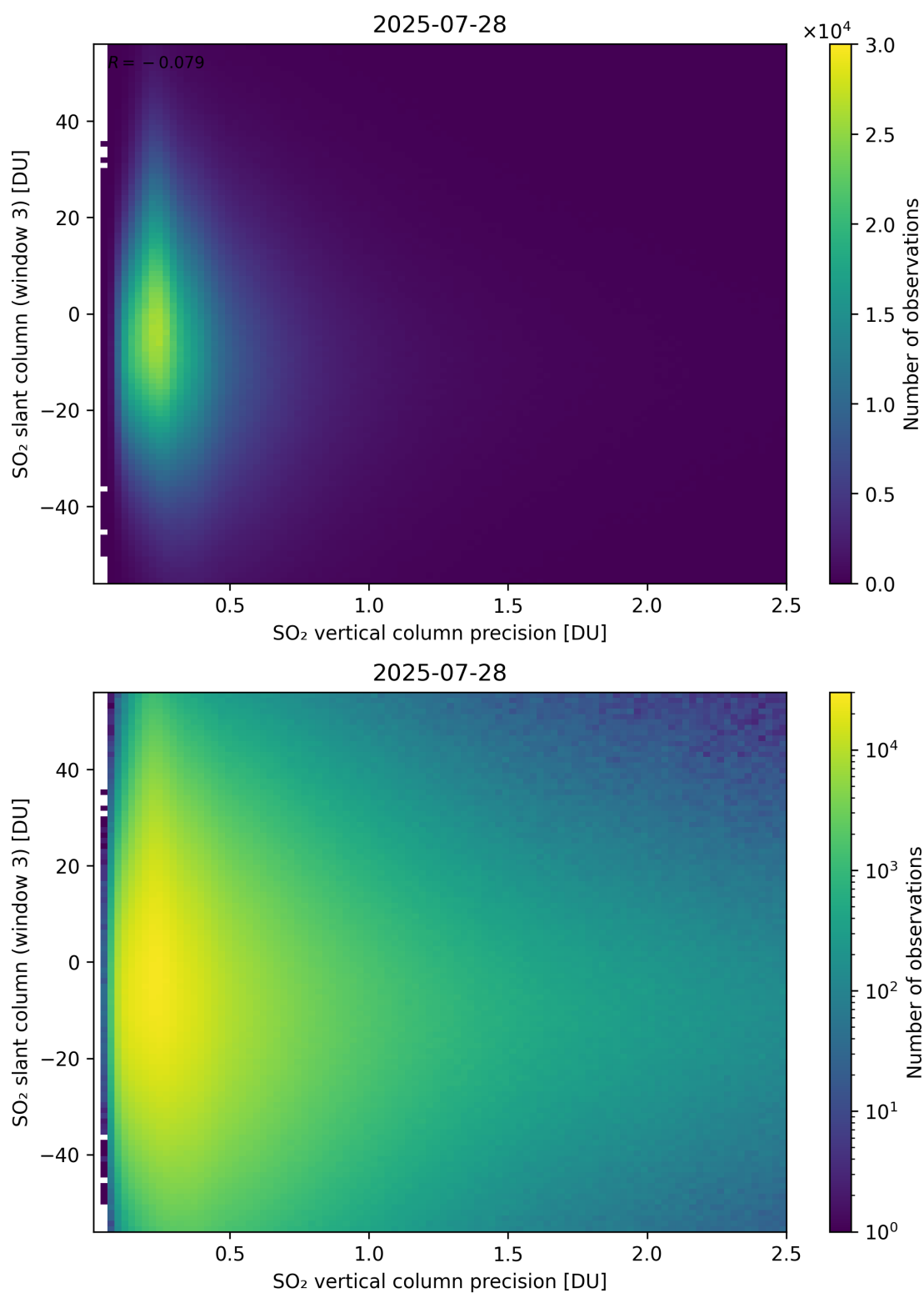
Figure 344: Scatter density plot of “SO 2 vertical column precision” against “SO 2 slant column (window 3)” for 2025-07-27 to 2025-07-29.
