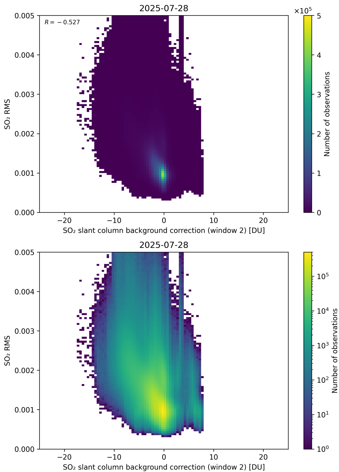
Figure 125: Scatter density plot of “SO 2 slant column background correction (window 2)” against “SO 2 RMS” for 2025-07-27 to 2025-07-29.
