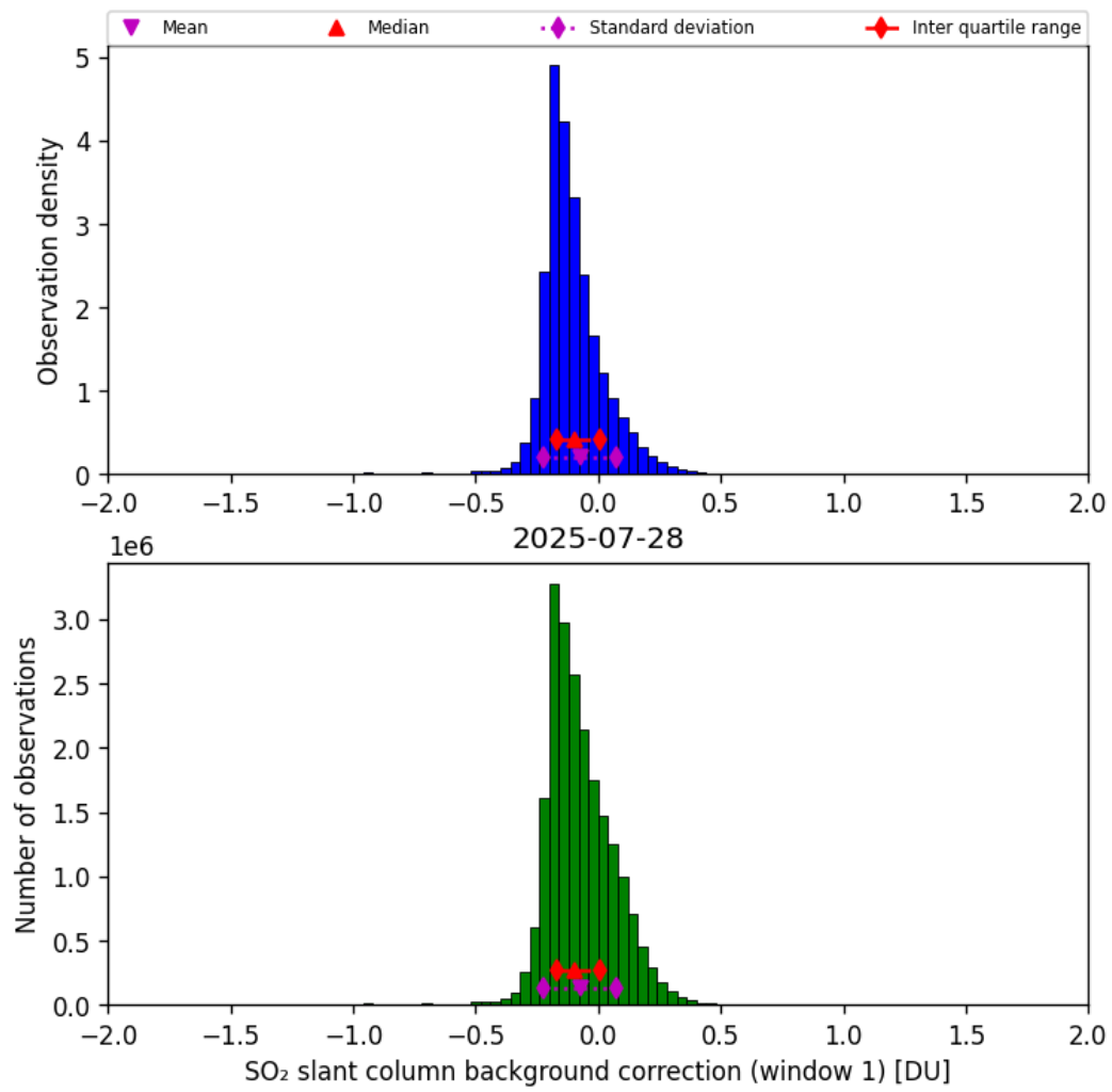
Figure 66: Histogram of “SO 2 slant column background correction (window 1)” for 2025-07-27 to 2025-07-29
