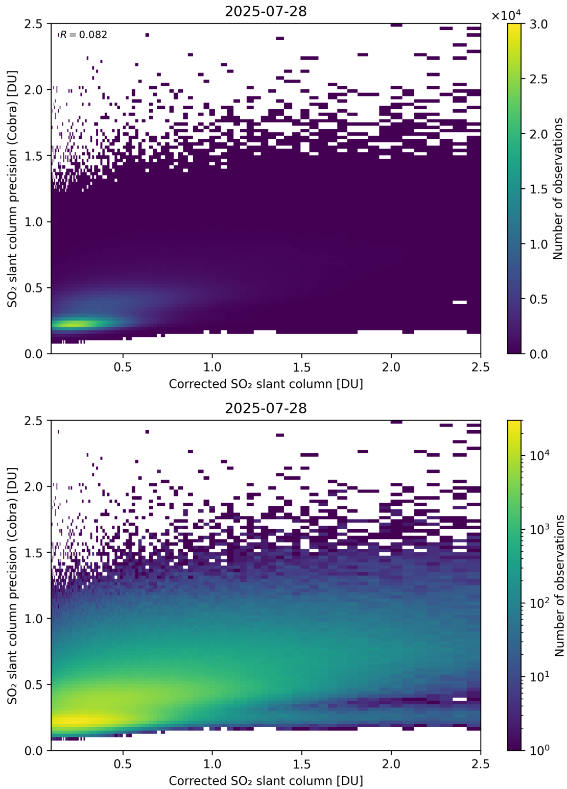
Figure 234: Scatter density plot of “Corrected SO 2 slant column” against “SO 2 slant column precision (Cobra)” for 2025-07-27 to 2025-07-29.
