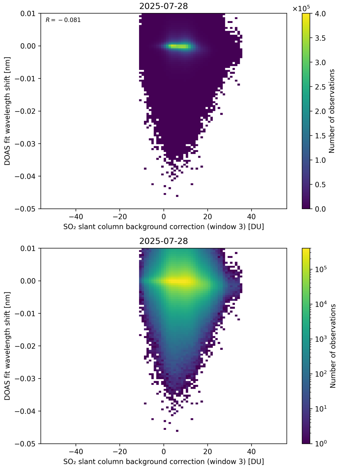
Figure 132: Scatter density plot of “SO 2 slant column background correction (window 3)” against “DOAS fit wavelength shift” for 2025-07-27 to 2025-07-29.
