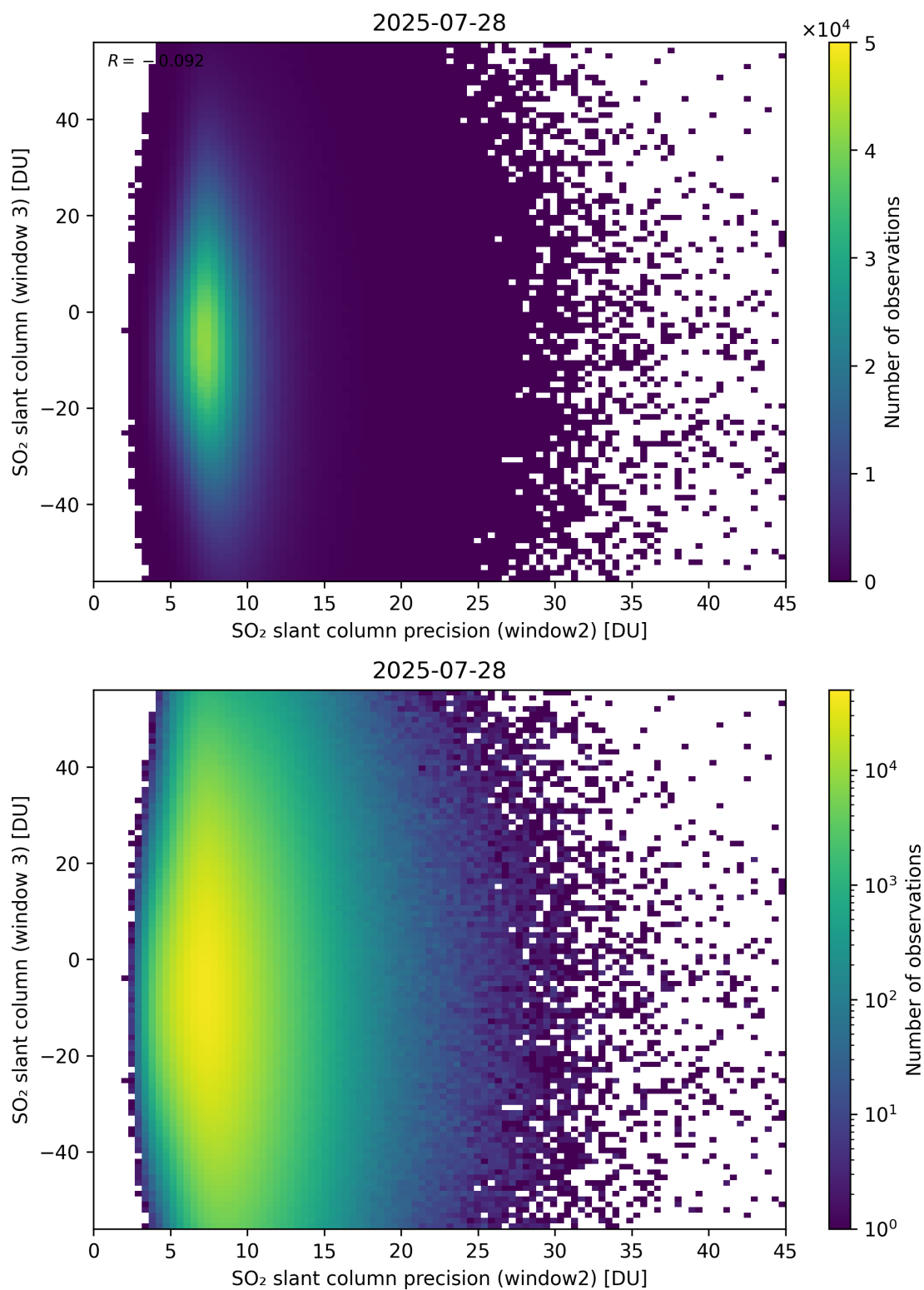
Figure 299: Scatter density plot of “SO 2 slant column precision (window2)” against “SO 2 slant column (window 3)” for 2025-07-27 to 2025-07-29.
