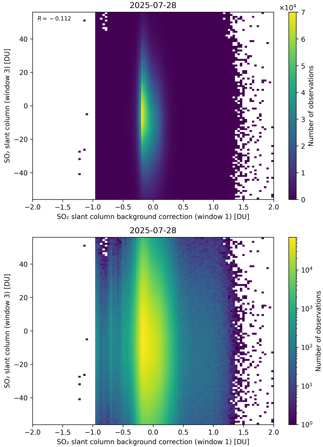
Figure 118: Scatter density plot of “SO 2 slant column background correction (window 1)” against “SO 2 slant column (window 3)” for 2025-07-27 to 2025-07-29.
