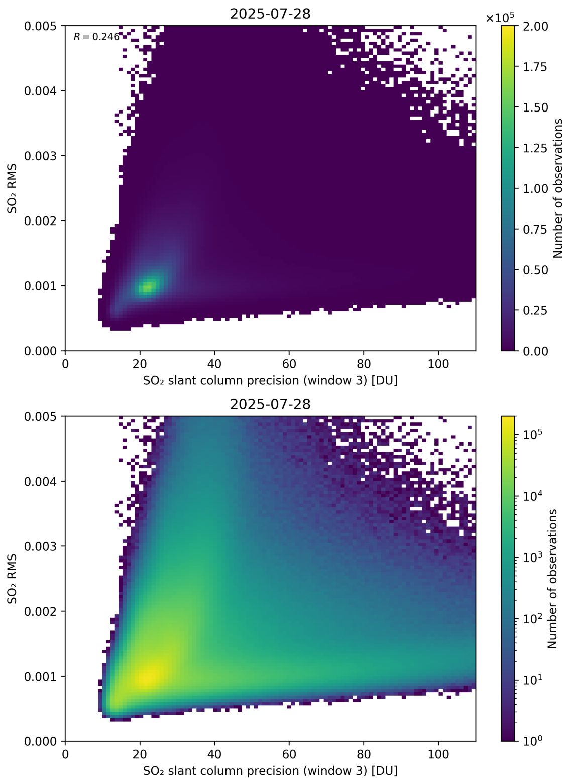
Figure 310: Scatter density plot of “SO 2 slant column precision (window 3)” against “SO 2 RMS” for 2025-07-27 to 2025-07-29.
