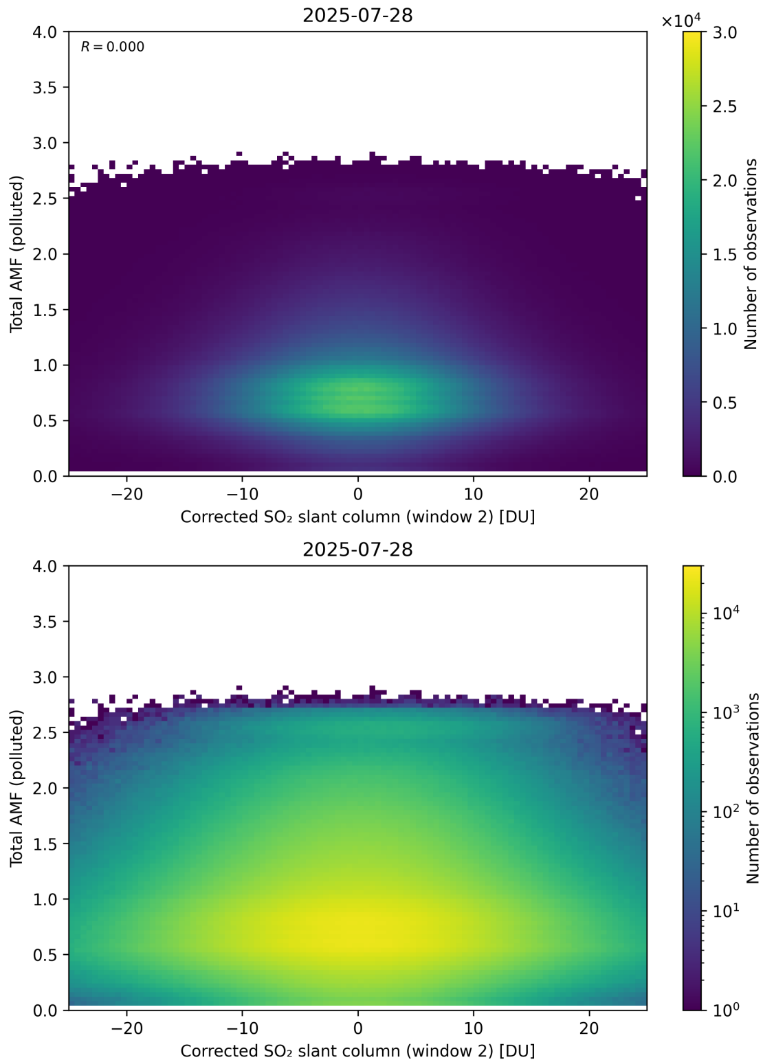
Figure 253: Scatter density plot of “Corrected SO 2 slant column (window 2)” against “Total AMF (polluted)” for 2025-07-27 to 2025-07-29.
