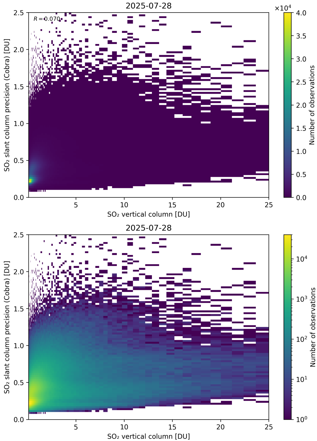
Figure 350: Scatter density plot of “SO 2 vertical column” against “SO 2 slant column precision (Cobra)” for 2025-07-27 to 2025-07-29.
