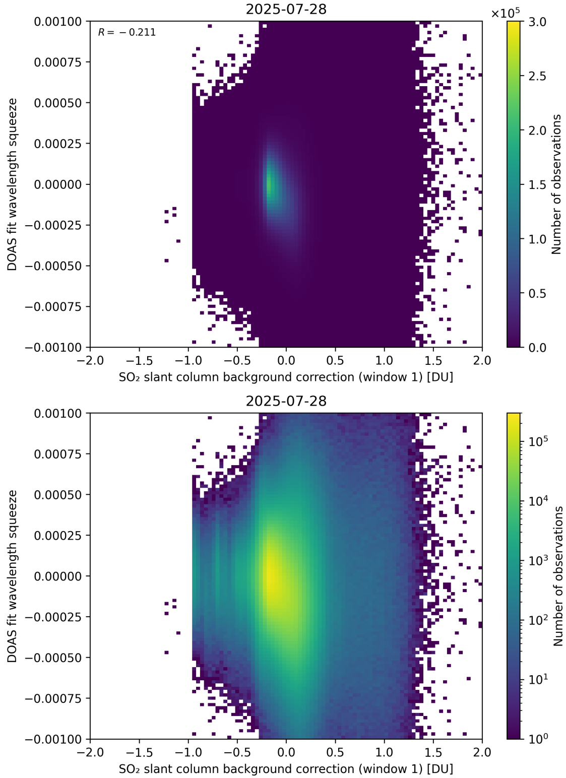
Figure 112: Scatter density plot of “SO 2 slant column background correction (window 1)” against “DOAS fit wavelength squeeze” for 2025-07-27 to 2025-07-29.
