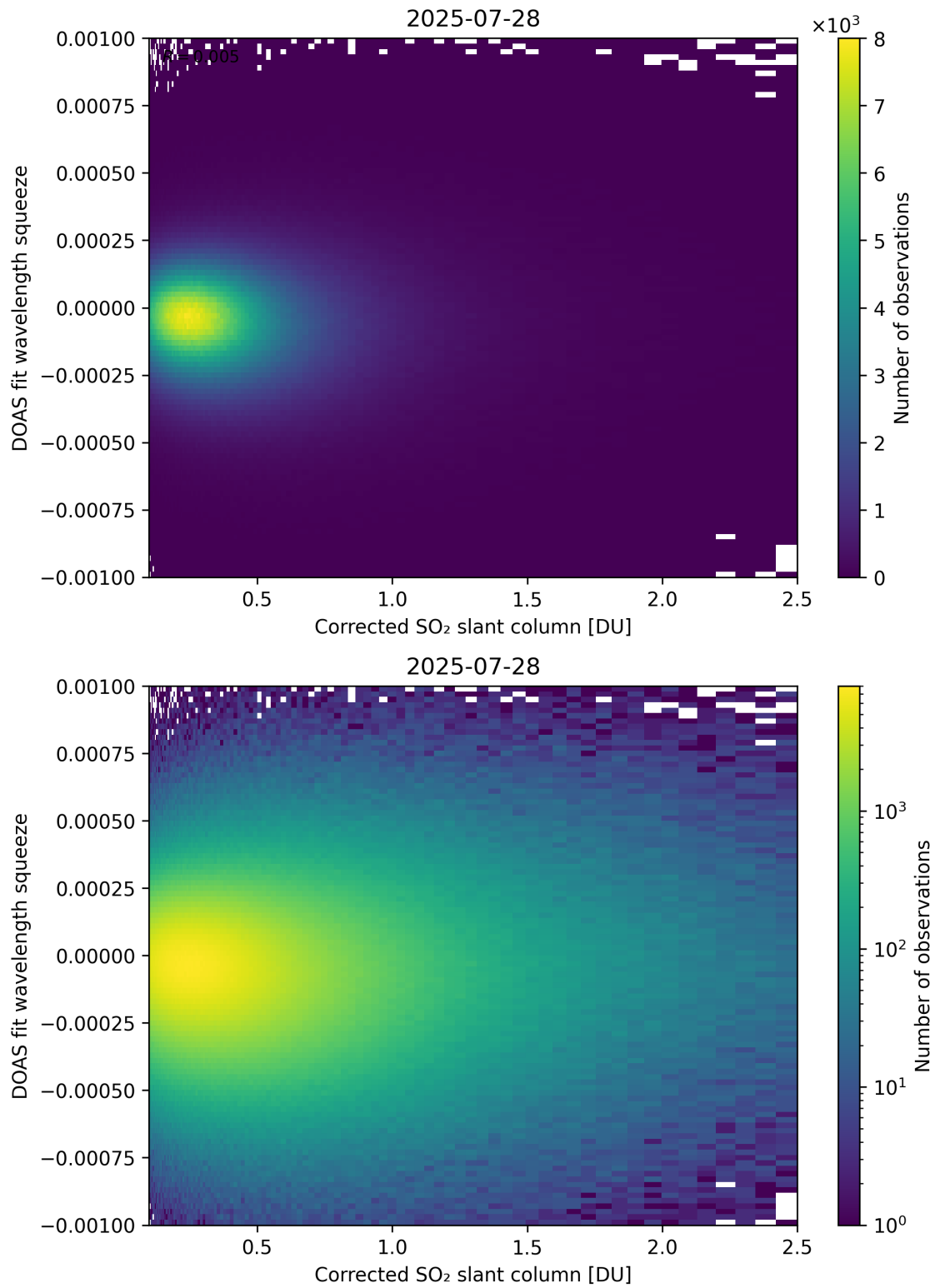
Figure 230: Scatter density plot of “Corrected SO 2 slant column” against “DOAS fit wavelength squeeze” for 2025-07-27 to 2025-07-29.
