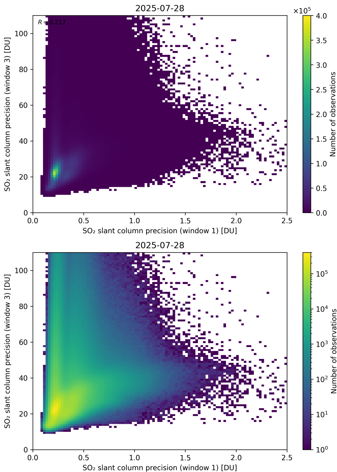
Figure 279: Scatter density plot of “SO 2 slant column precision (window 1)” against “SO 2 slant column precision (window 3)” for 2025-07-27 to 2025-07-29.
