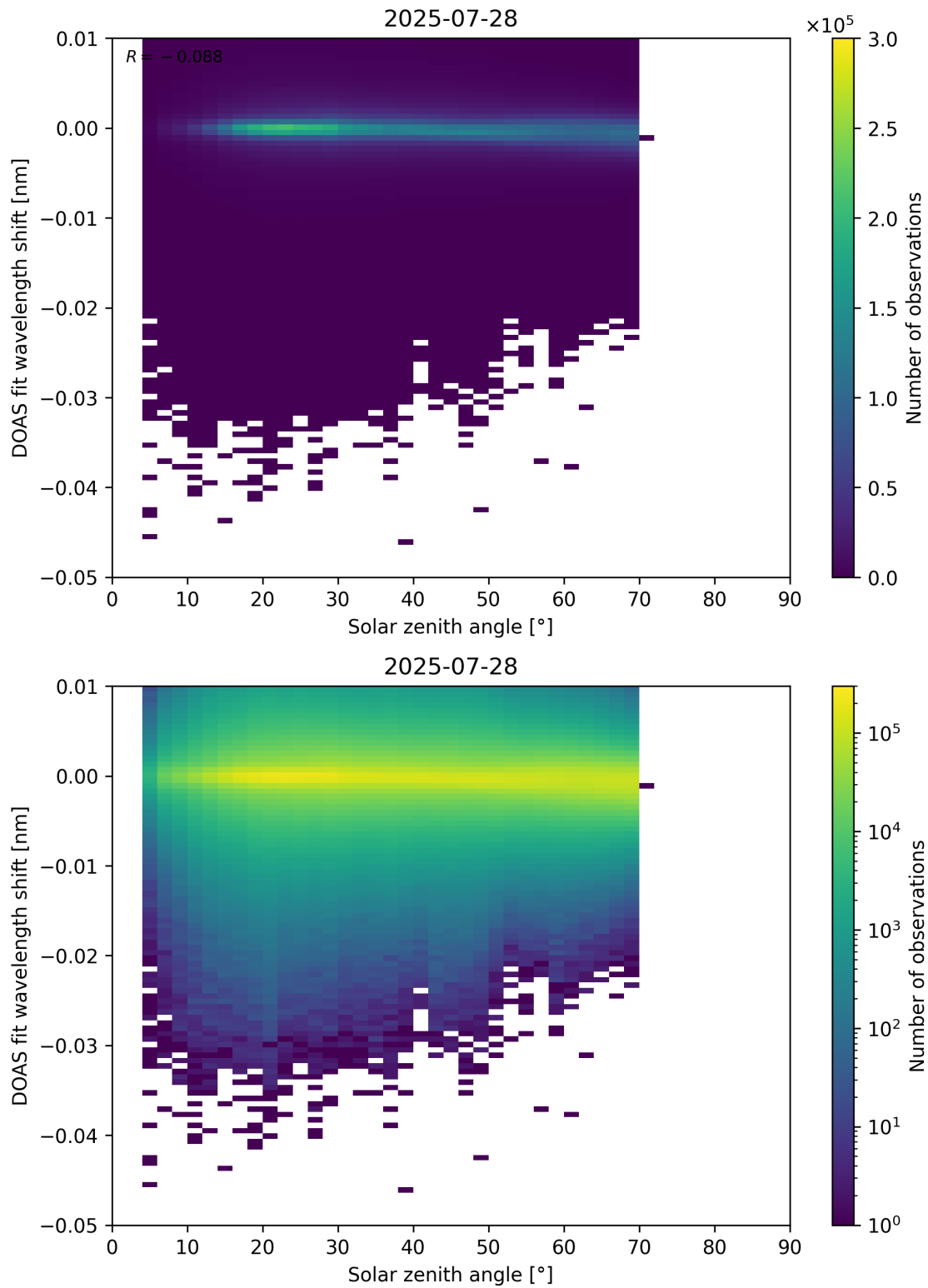
Figure 174: Scatter density plot of “Solar zenith angle” against “DOAS fit wavelength shift” for 2025-07-27 to 2025-07-29.
