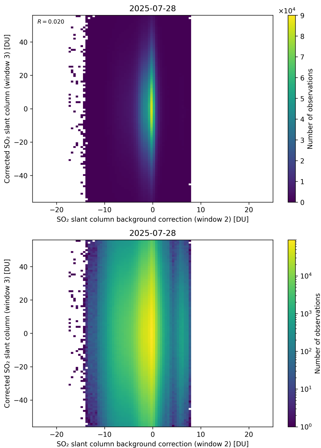
Figure 127: Scatter density plot of “SO 2 slant column background correction (window 2)” against “Corrected SO 2 slant column (window 3)” for 2025-07-27 to 2025-07-29.
