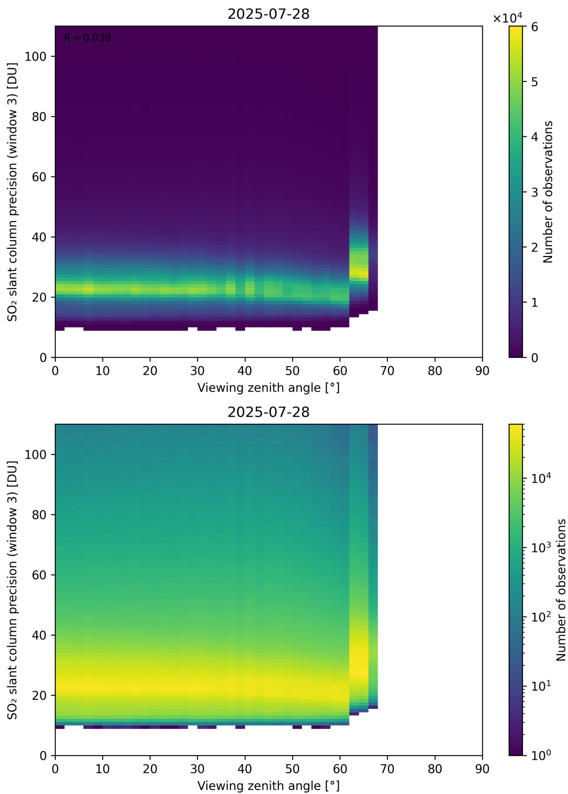
Figure 380: Scatter density plot of “Viewing zenith angle” against “SO 2 slant column precision (window 3)” for 2025-07-27 to 2025-07-29.
