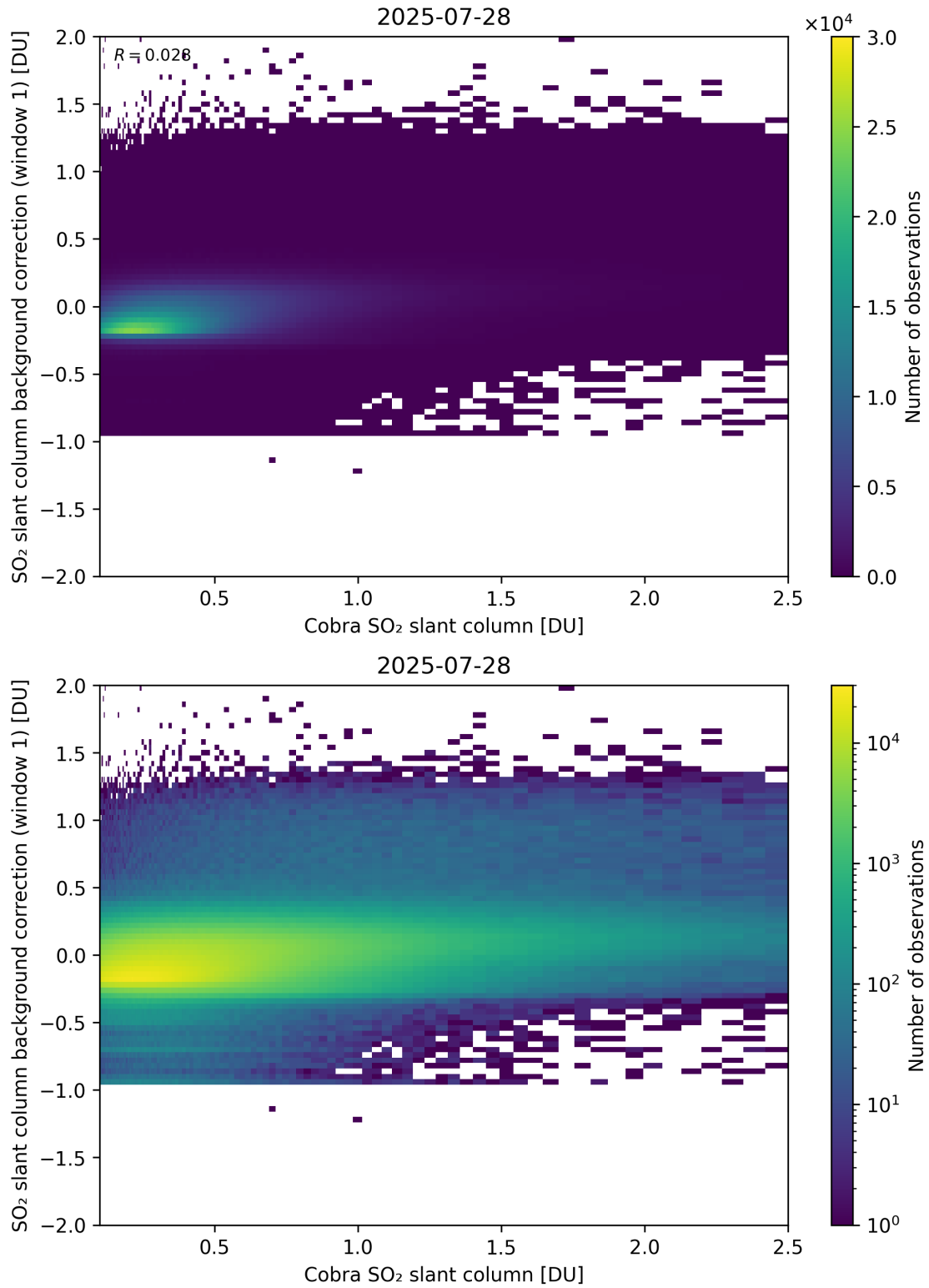
Figure 193: Scatter density plot of “Cobra SO 2 slant column” against “SO 2 slant column background correction (window 1)” for 2025-07-27 to 2025-07-29.
