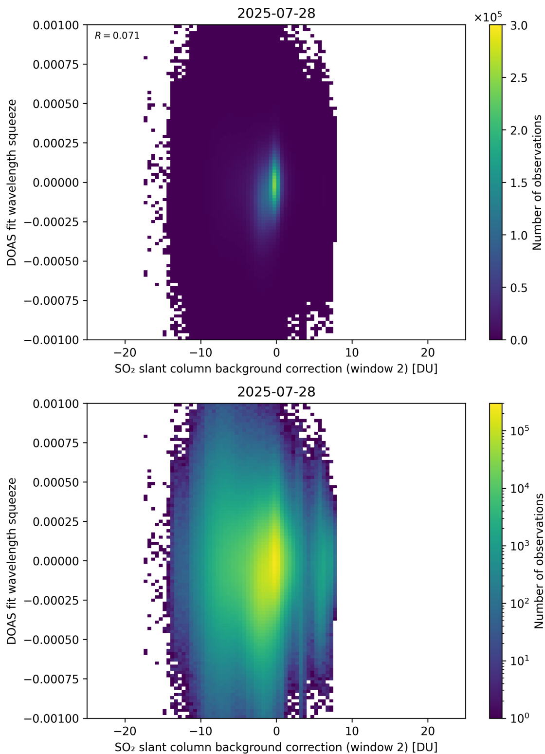
Figure 124: Scatter density plot of “SO 2 slant column background correction (window 2)” against “DOAS fit wavelength squeeze” for 2025-07-27 to 2025-07-29.
