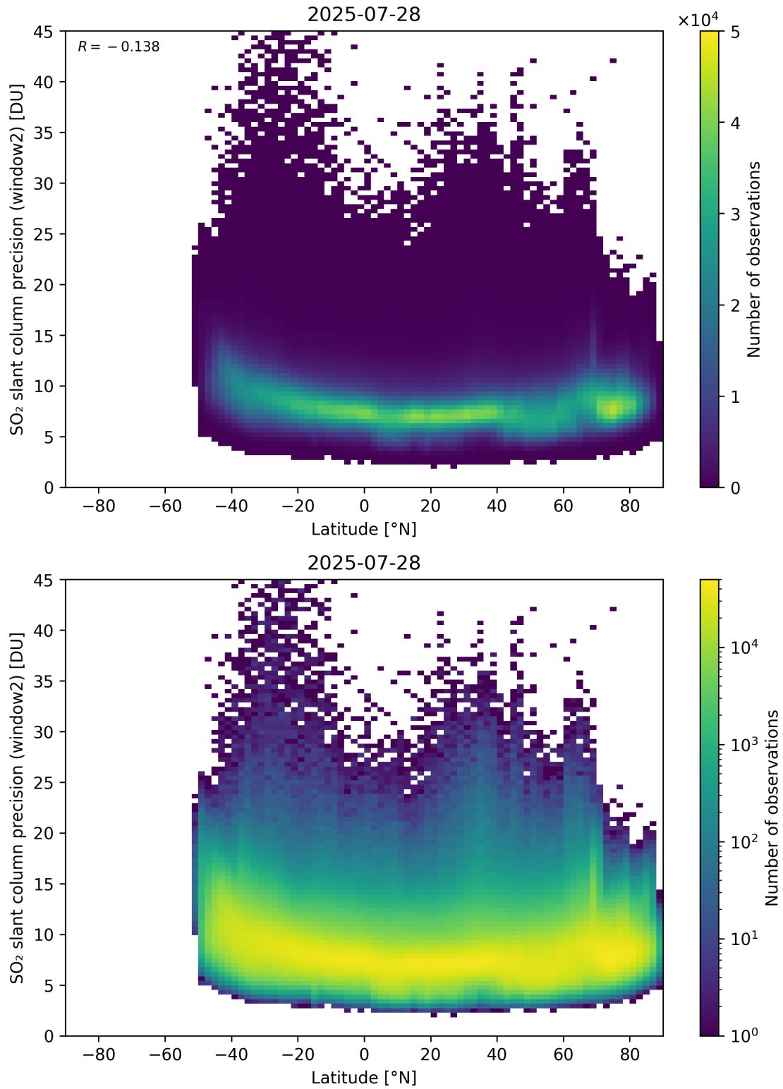
Figure 164: Scatter density plot of “Latitude” against “SO 2 slant column precision (window2)” for 2025-07-27 to 2025-07-29.
