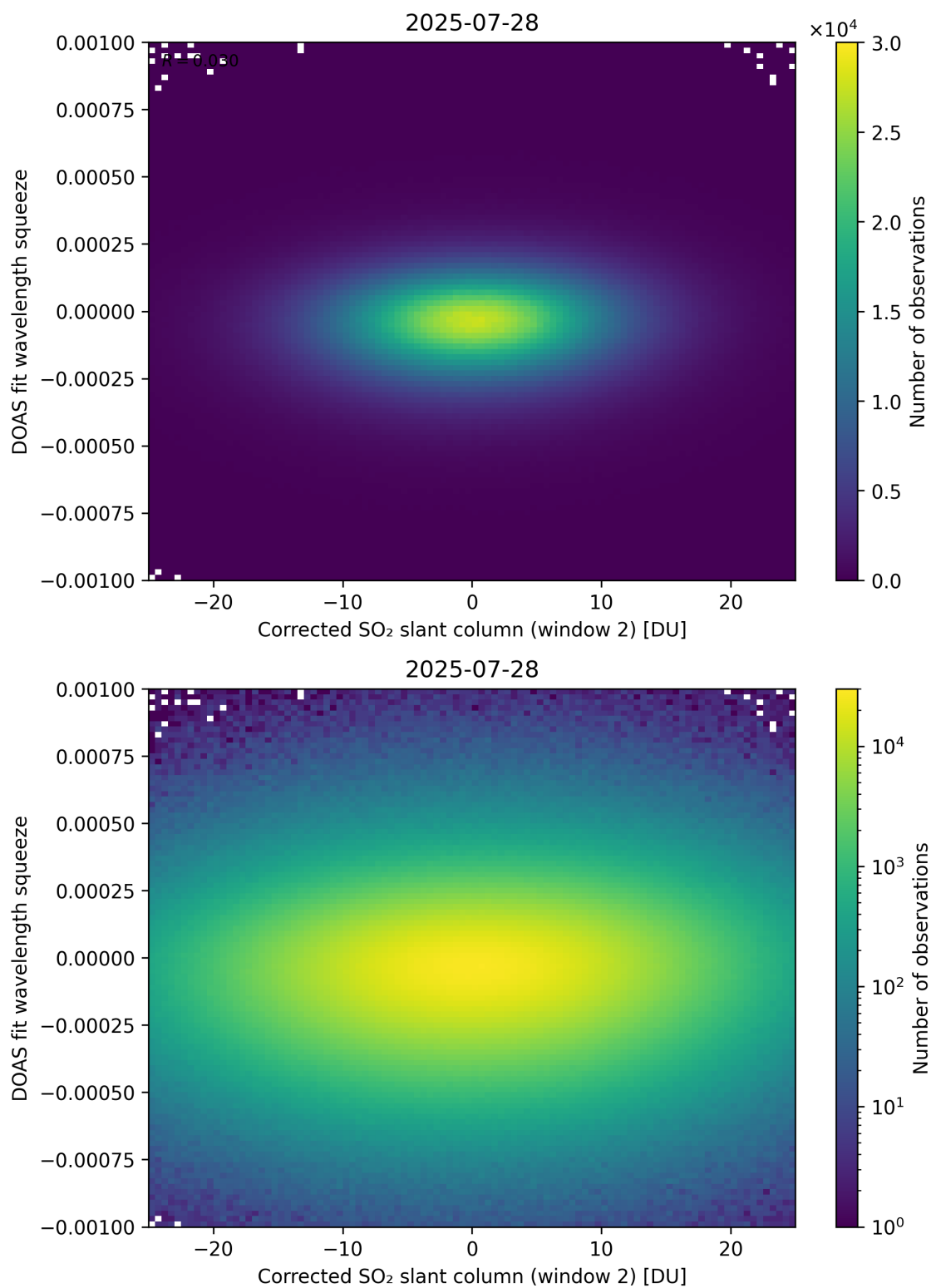
Figure 247: Scatter density plot of “Corrected SO 2 slant column (window 2)” against “DOAS fit wavelength squeeze” for 2025-07-27 to 2025-07-29.
