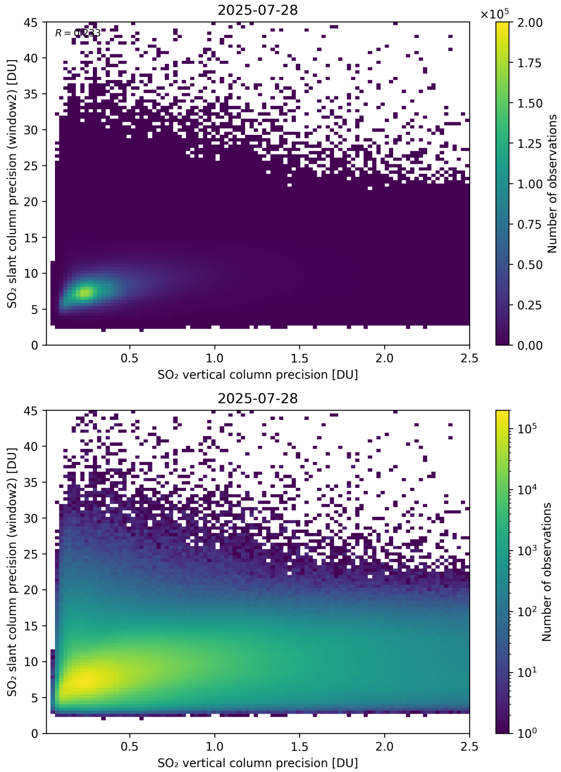
Figure 343: Scatter density plot of “SO 2 vertical column precision” against “SO 2 slant column precision (window2)” for 2025-07-27 to 2025-07-29.
