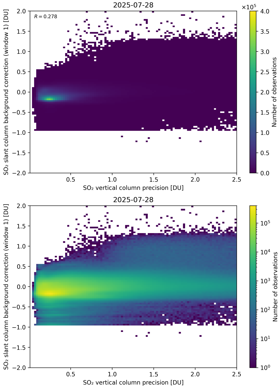
Figure 329: Scatter density plot of “SO 2 vertical column precision” against “SO 2 slant column background correction (window 1)” for 2025-07-27 to 2025-07-29.
