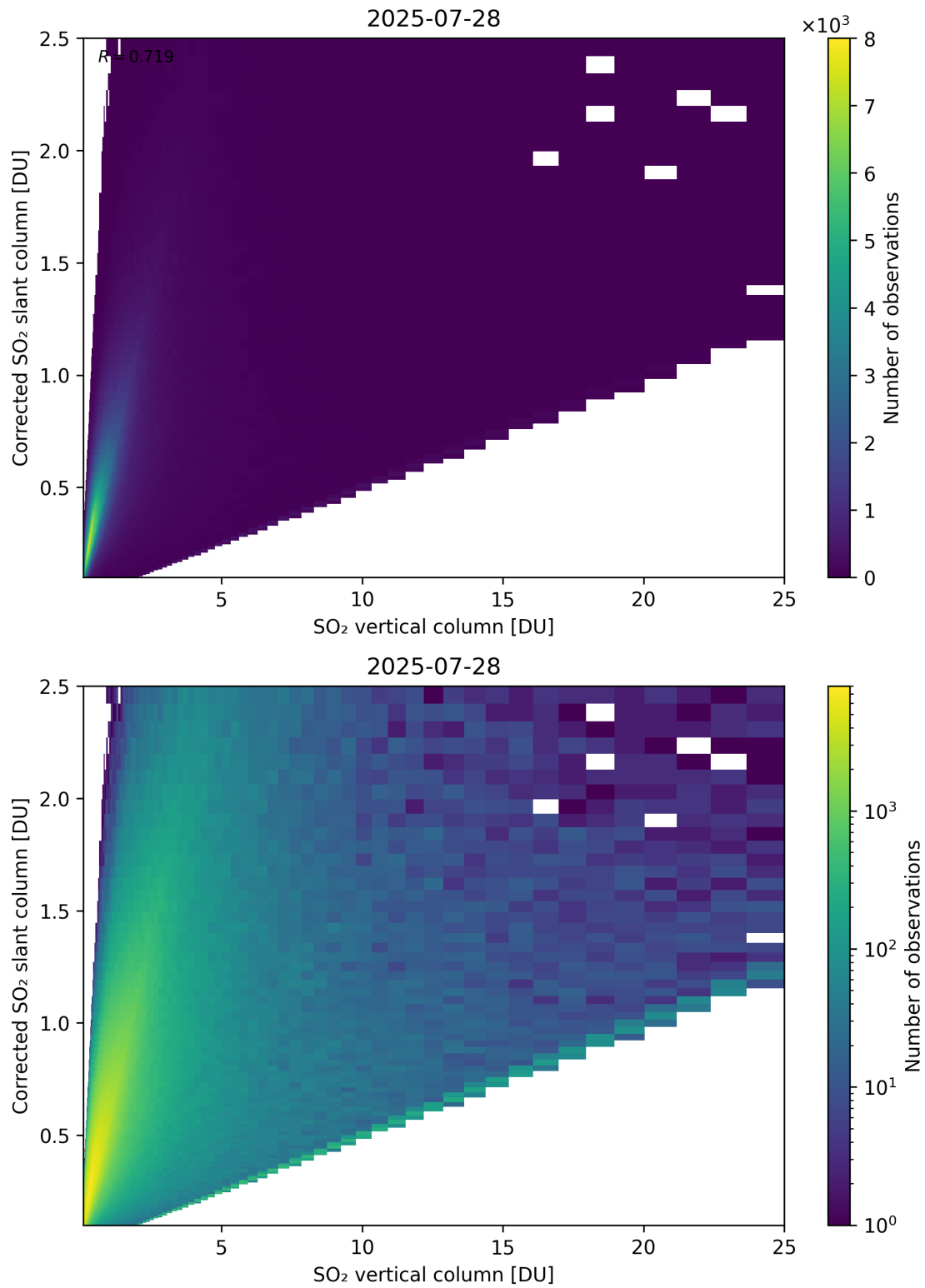
Figure 351: Scatter density plot of “SO 2 vertical column” against “Corrected SO 2 slant column” for 2025-07-27 to 2025-07-29.
