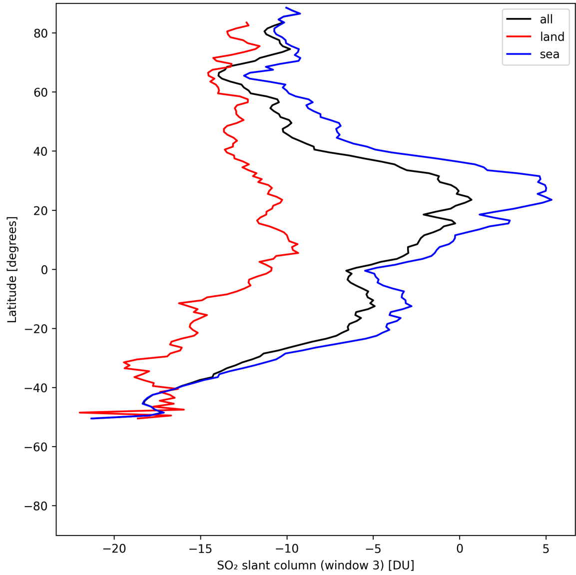
Figure 45: Zonal average of “SO 2 slant column (window 3)” for 2025-07-27 to 2025-07-29.
