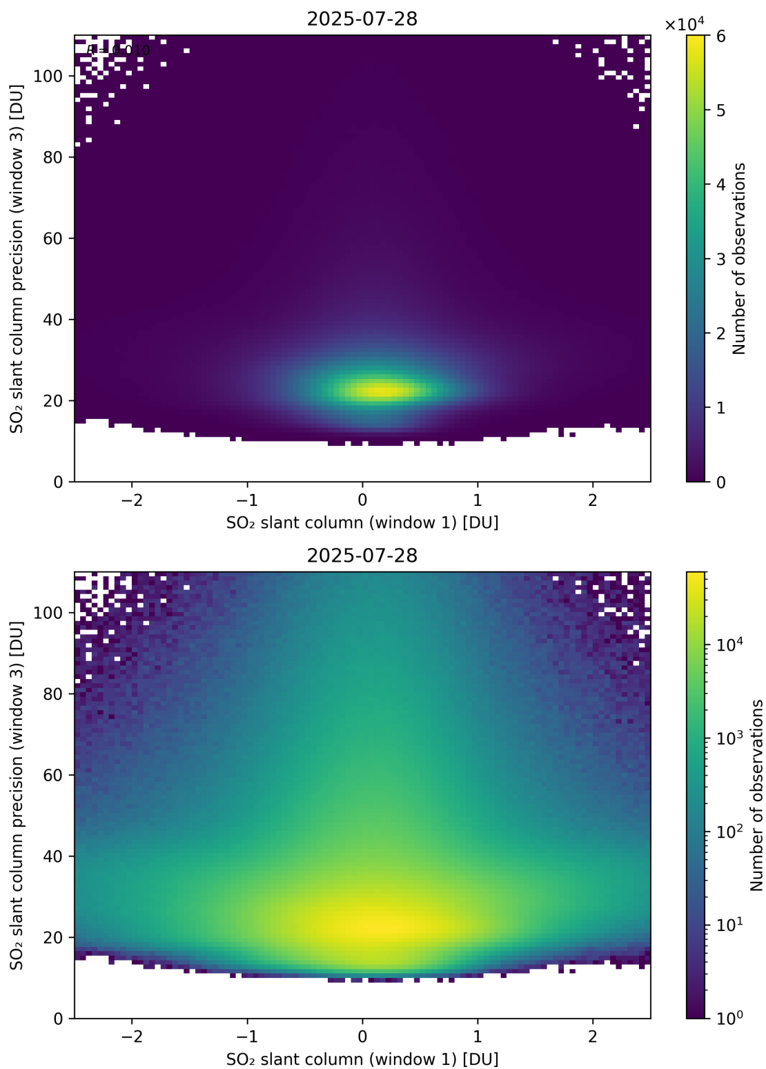
Figure 288: Scatter density plot of “SO 2 slant column (window 1)” against “SO 2 slant column precision (window 3)” for 2025-07-27 to 2025-07-29.
