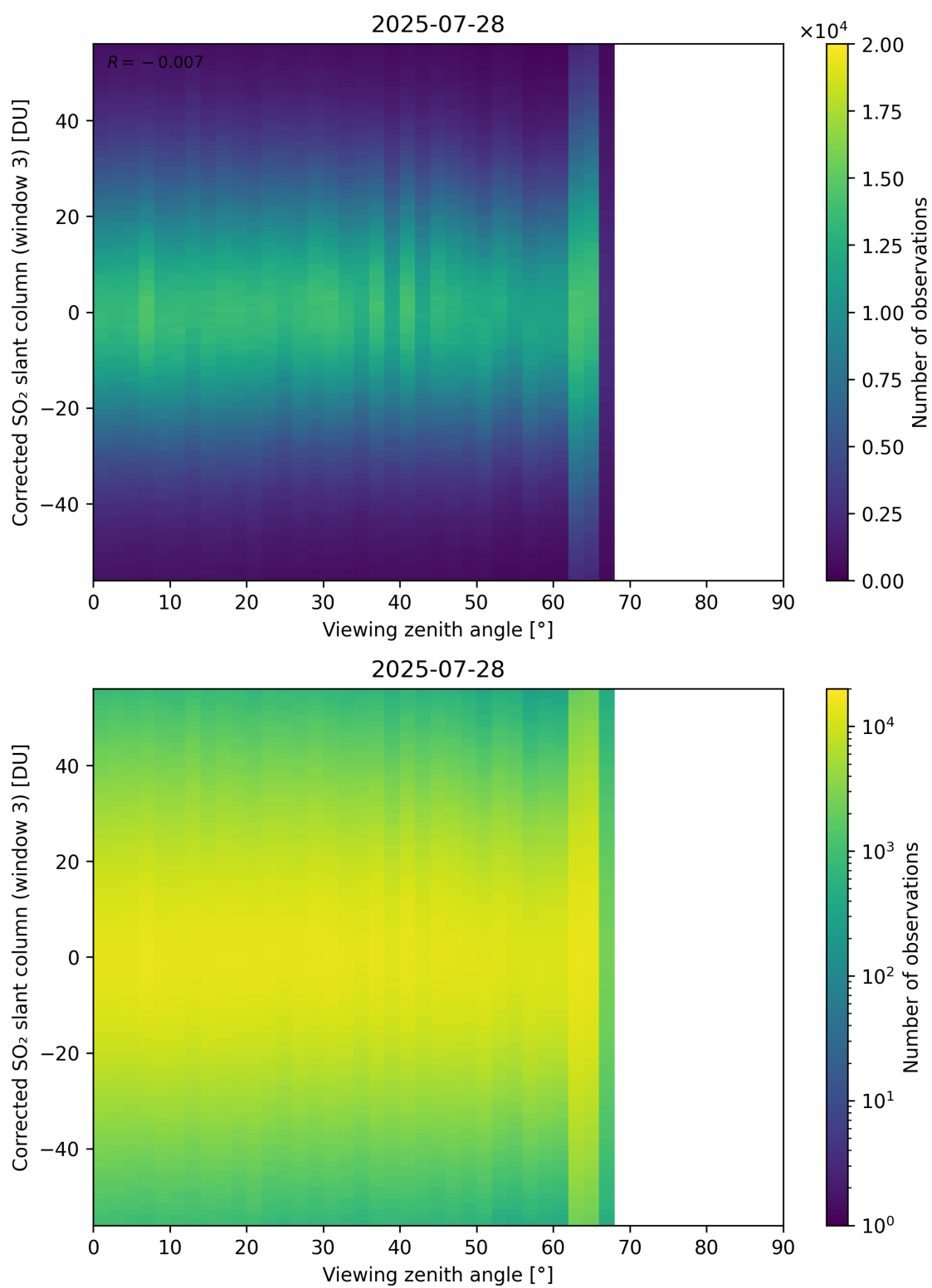
Figure 375: Scatter density plot of “Viewing zenith angle” against “Corrected SO 2 slant column (window 3)” for 2025-07-27 to 2025-07-29.
