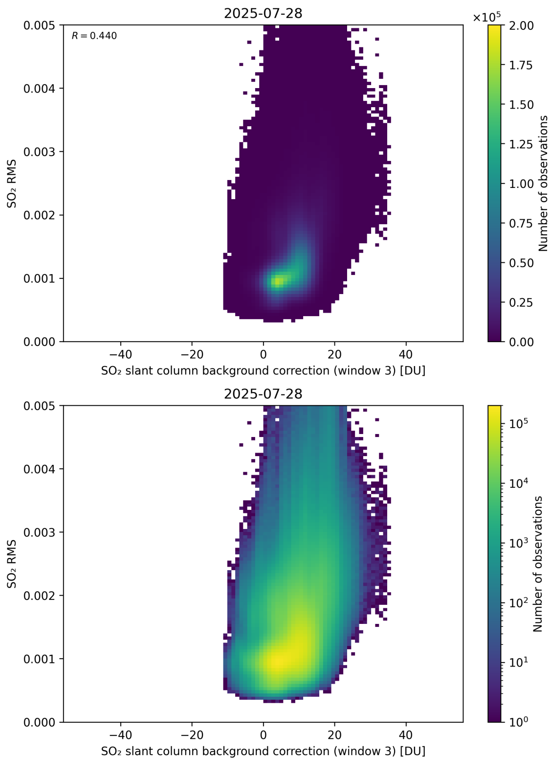
Figure 134: Scatter density plot of “SO 2 slant column background correction (window 3)” against “SO 2 RMS” for 2025-07-27 to 2025-07-29.
