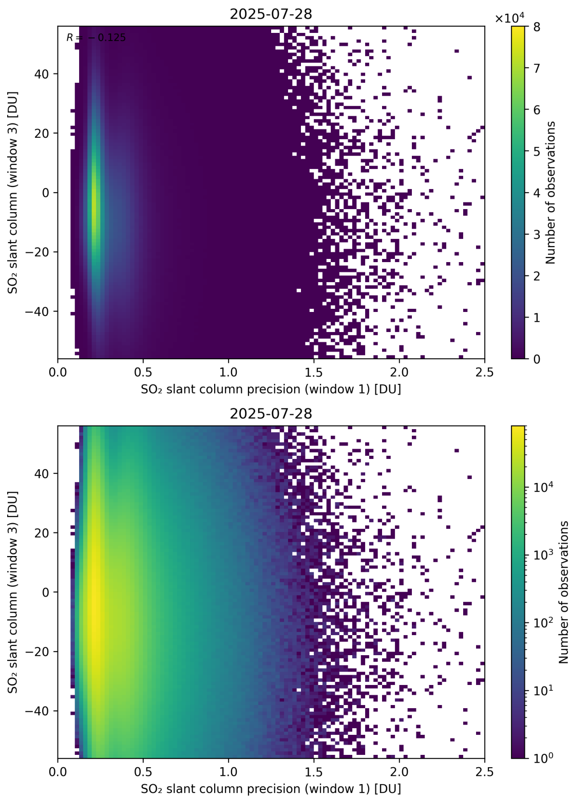
Figure 278: Scatter density plot of “SO 2 slant column precision (window 1)” against “SO 2 slant column (window 3)” for 2025-07-27 to 2025-07-29.
