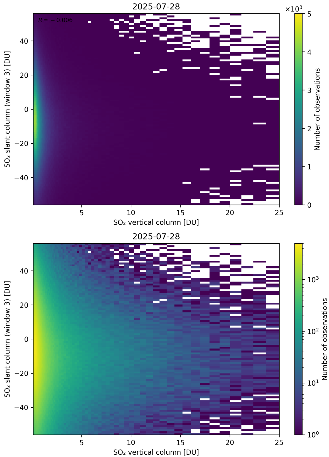
Figure 357: Scatter density plot of “SO 2 vertical column” against “SO 2 slant column (window 3)” for 2025-07-27 to 2025-07-29.
