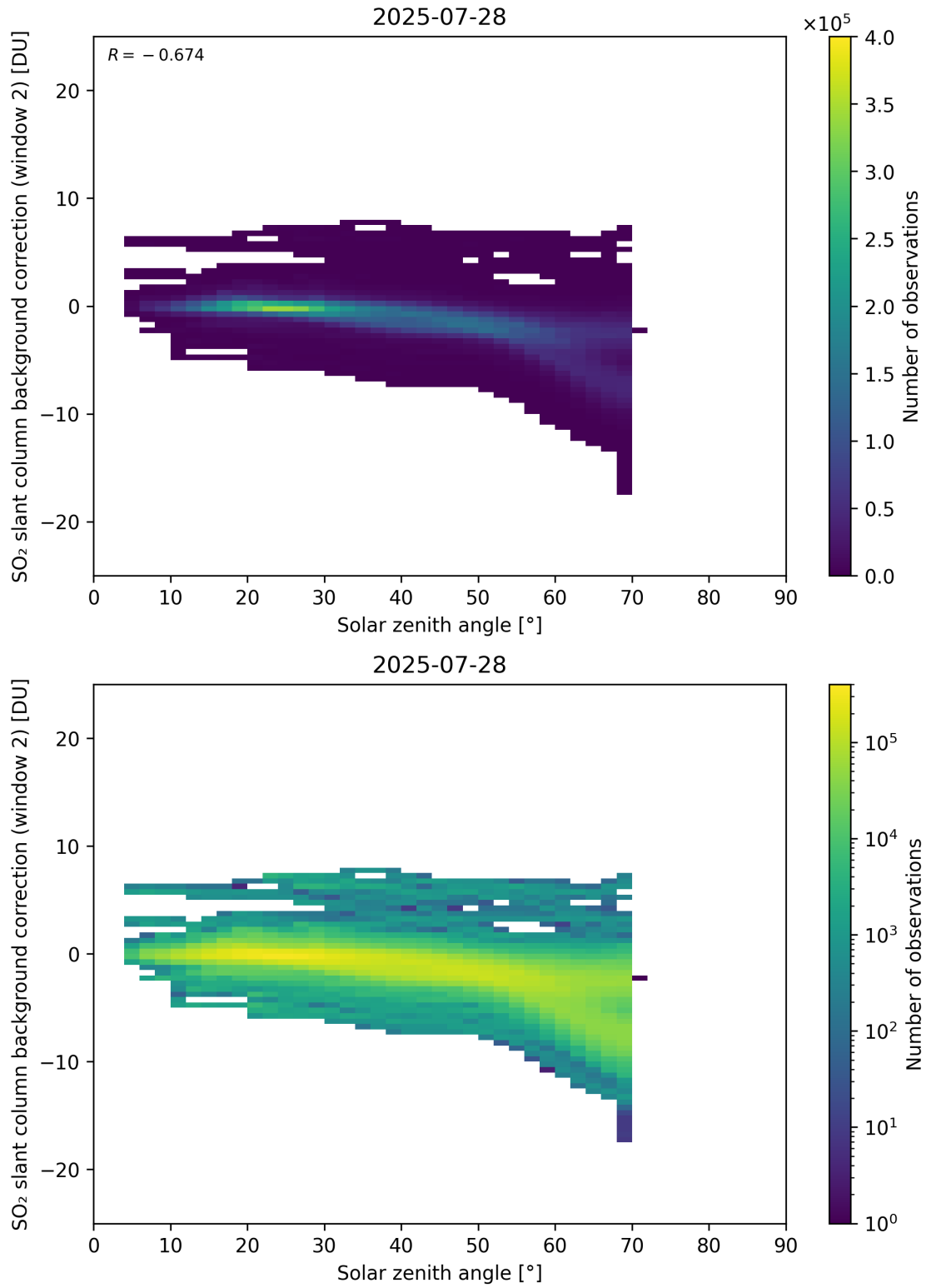
Figure 172: Scatter density plot of “Solar zenith angle” against “SO 2 slant column background correction (window 2)” for 2025-07-27 to 2025-07-29.
