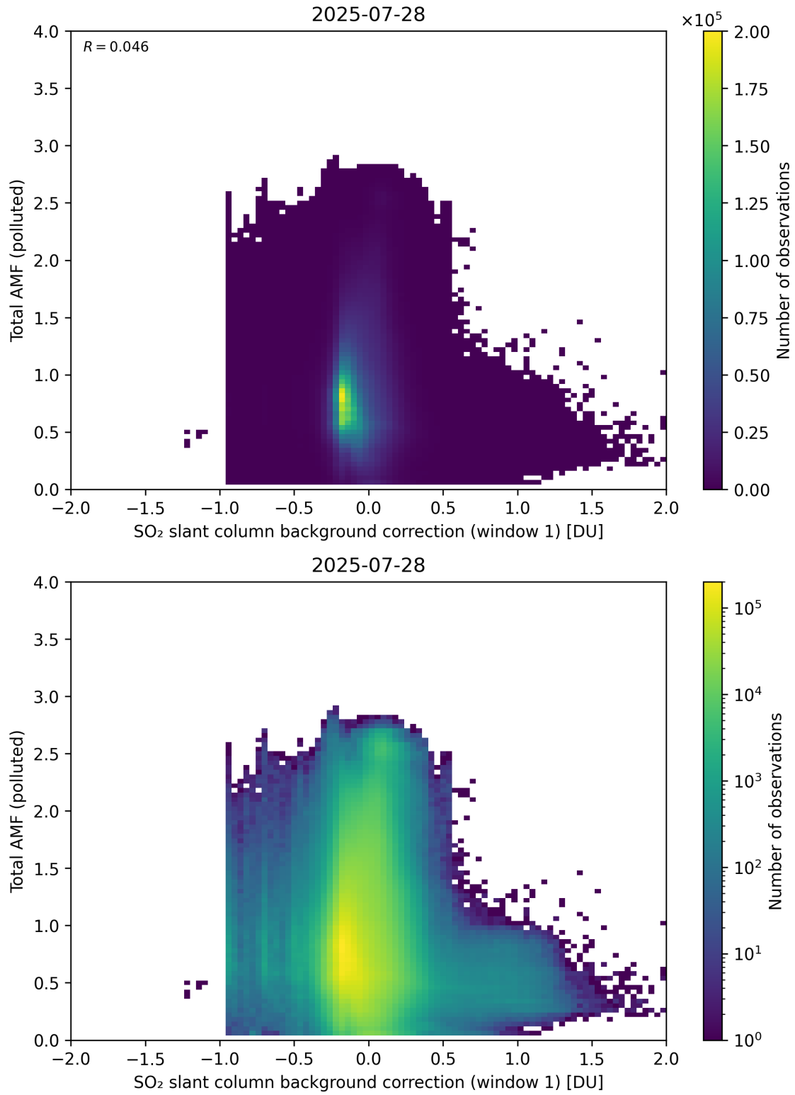
Figure 120: Scatter density plot of “SO 2 slant column background correction (window 1)” against “Total AMF (polluted)” for 2025-07-27 to 2025-07-29.
