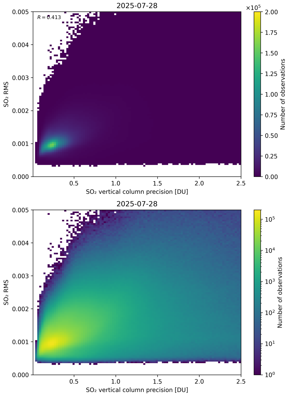
Figure 334: Scatter density plot of “SO 2 vertical column precision” against “SO 2 RMS” for 2025-07-27 to 2025-07-29.
