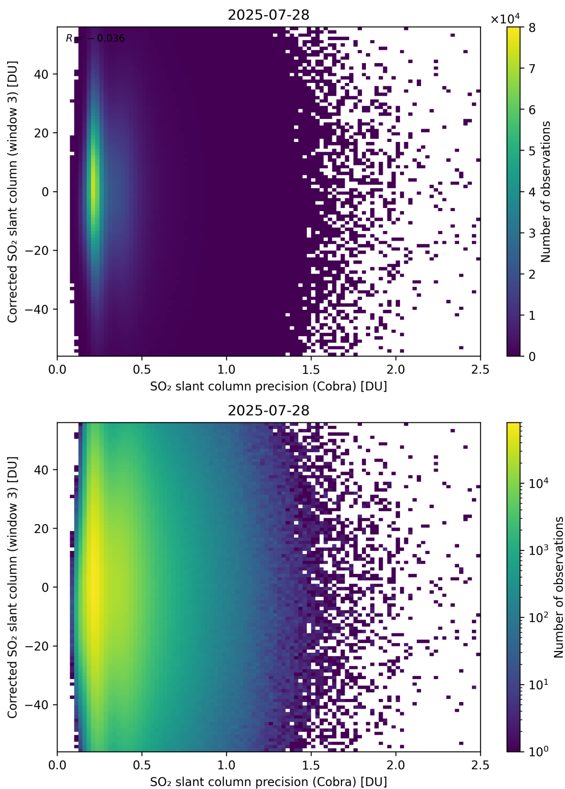
Figure 207: Scatter density plot of “SO 2 slant column precision (Cobra)” against “Corrected SO 2 slant column (window 3)” for 2025-07-27 to 2025-07-29.
