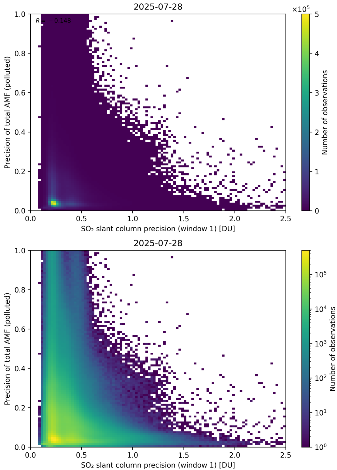
Figure 281: Scatter density plot of “SO 2 slant column precision (window 1)” against “Precision of total AMF (polluted)” for 2025-07-27 to 2025-07-29.
