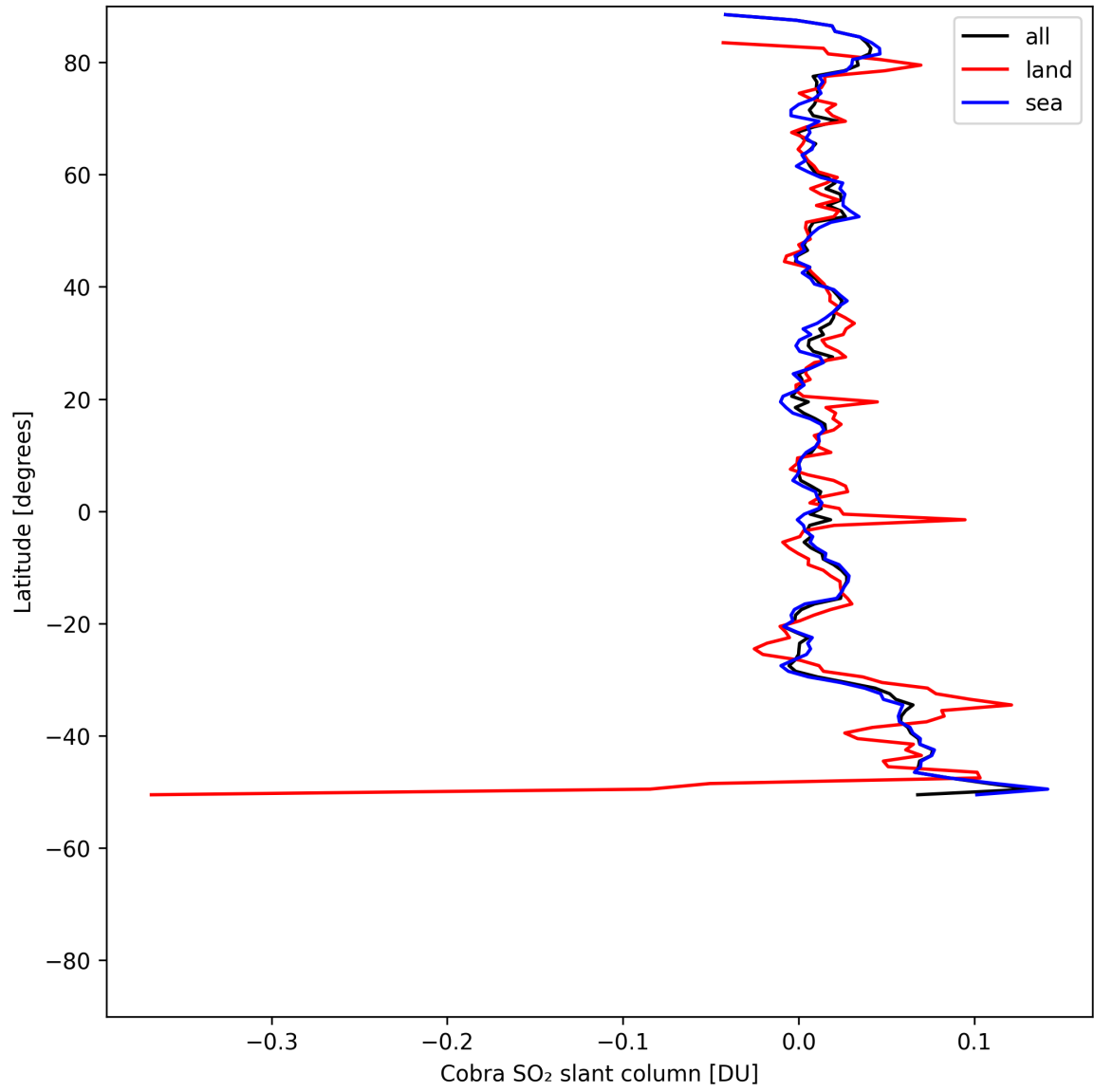
Figure 35: Zonal average of “Cobra SO 2 slant column” for 2025-07-27 to 2025-07-29.
