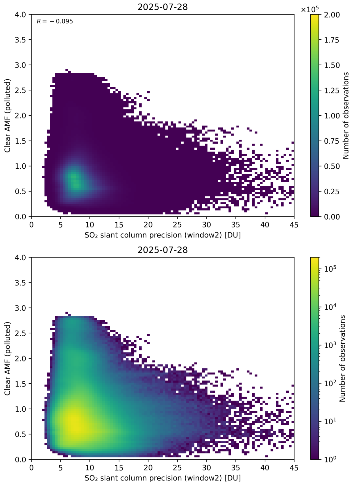
Figure 296: Scatter density plot of “SO 2 slant column precision (window2)” against “Clear AMF (polluted)” for 2025-07-27 to 2025-07-29.
