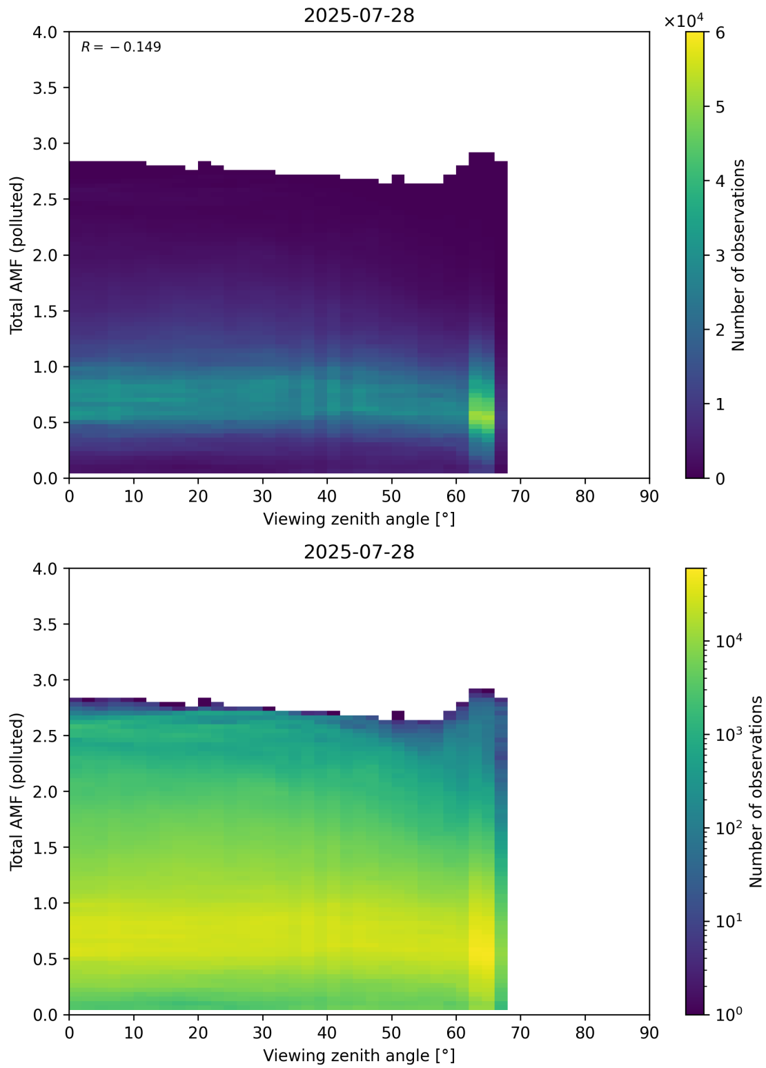
Figure 381: Scatter density plot of “Viewing zenith angle” against “Total AMF (polluted)” for 2025-07-27 to 2025-07-29.
