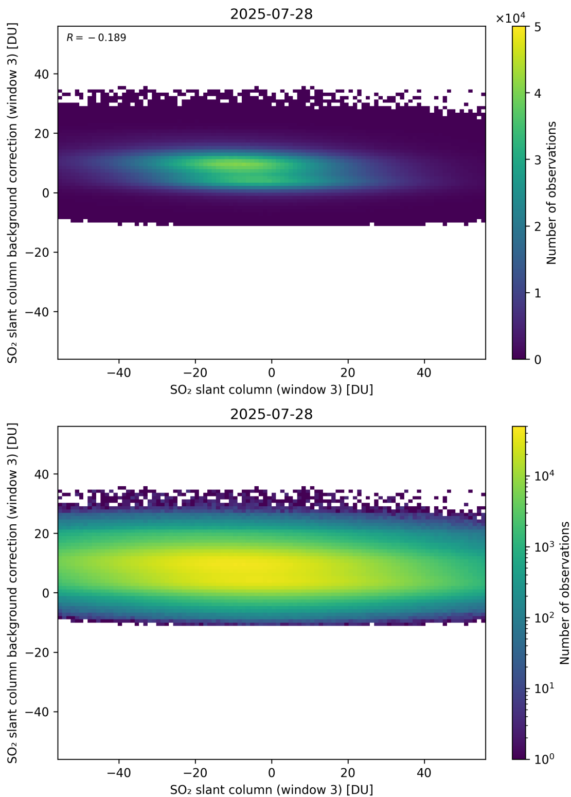
Figure 303: Scatter density plot of “SO 2 slant column (window 3)” against “SO 2 slant column background correction (window 3)” for 2025-07-27 to 2025-07-29.
