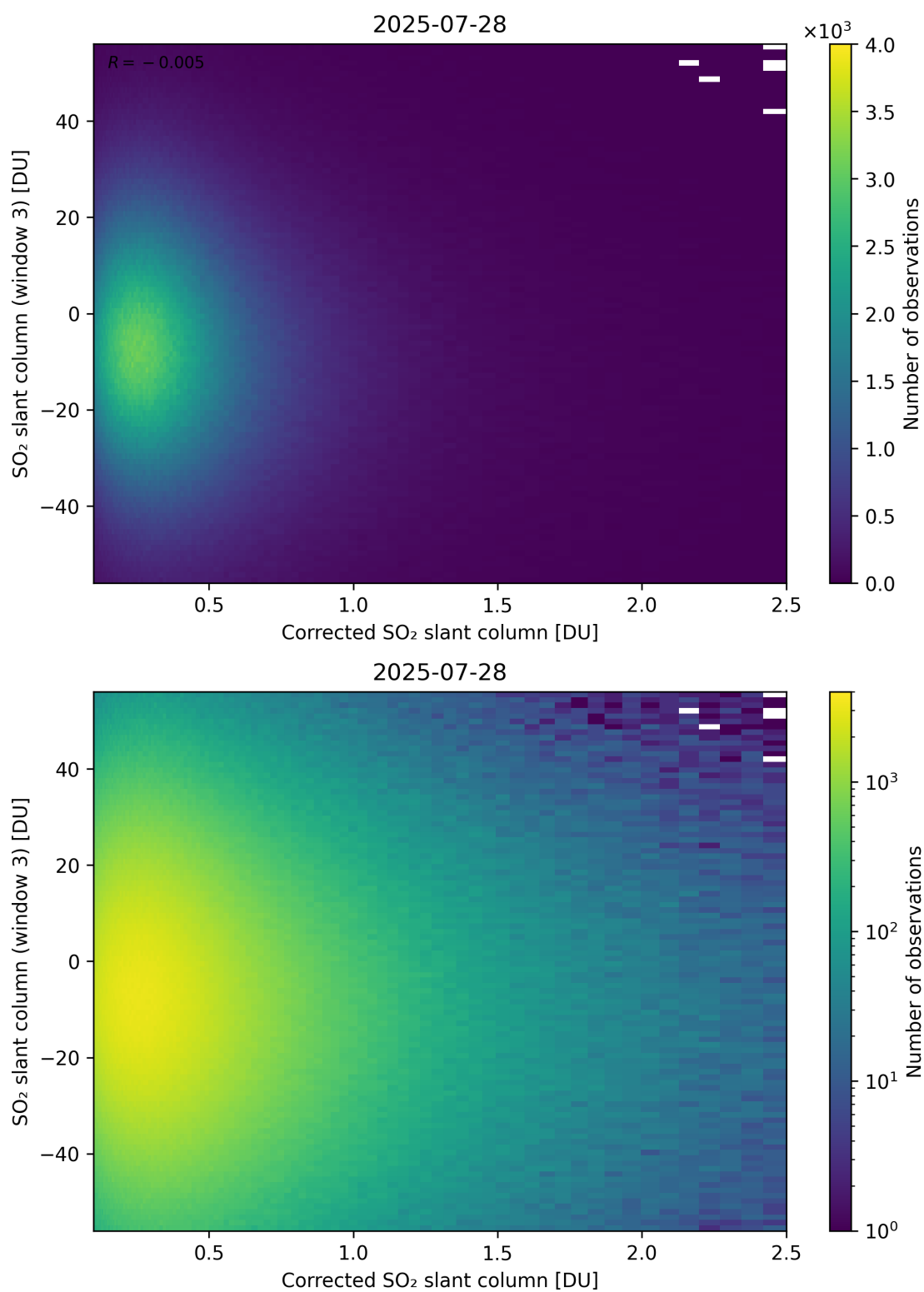
Figure 240: Scatter density plot of “Corrected SO 2 slant column” against “SO 2 slant column (window 3)” for 2025-07-27 to 2025-07-29.
