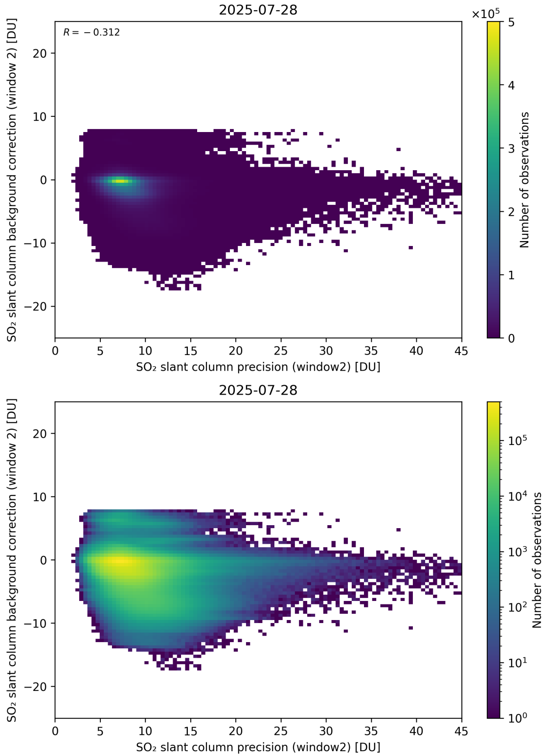
Figure 291: Scatter density plot of “SO 2 slant column precision (window2)” against “SO 2 slant column background correction (window 2)” for 2025-07-27 to 2025-07-29.
