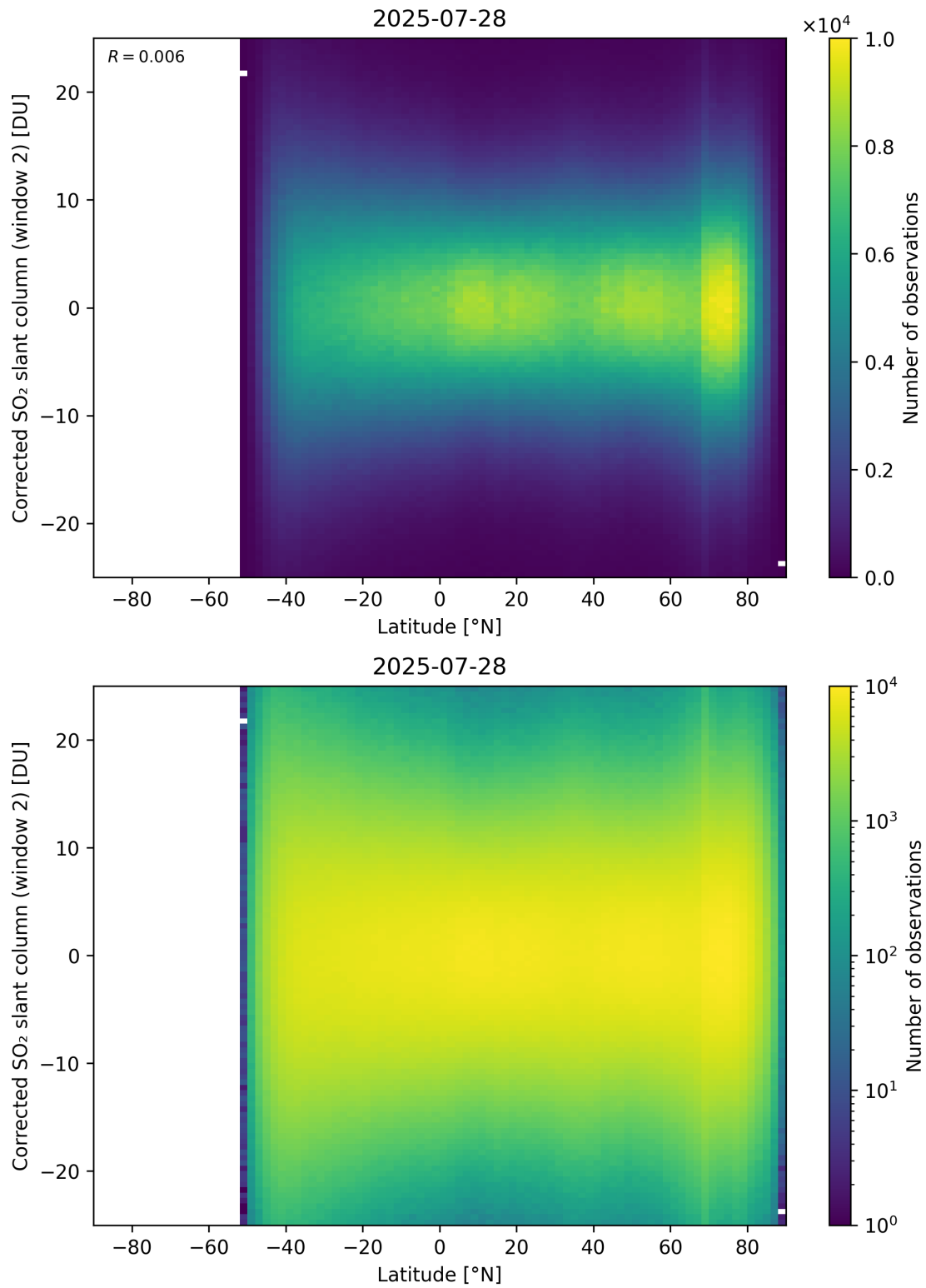
Figure 160: Scatter density plot of “Latitude” against “Corrected SO 2 slant column (window 2)” for 2025-07-27 to 2025-07-29.
