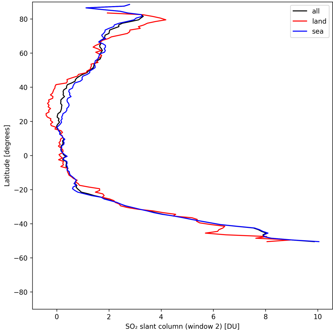
Figure 41: Zonal average of “SO 2 slant column (window 2)” for 2025-07-27 to 2025-07-29.
