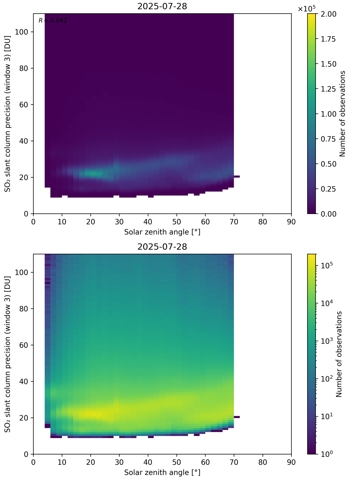
Figure 188: Scatter density plot of “Solar zenith angle” against “SO 2 slant column precision (window 3)” for 2025-07-27 to 2025-07-29.
