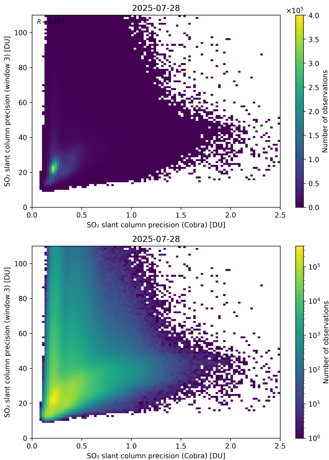
Figure 212: Scatter density plot of “SO 2 slant column precision (Cobra)” against “SO 2 slant column precision (window 3)” for 2025-07-27 to 2025-07-29.
