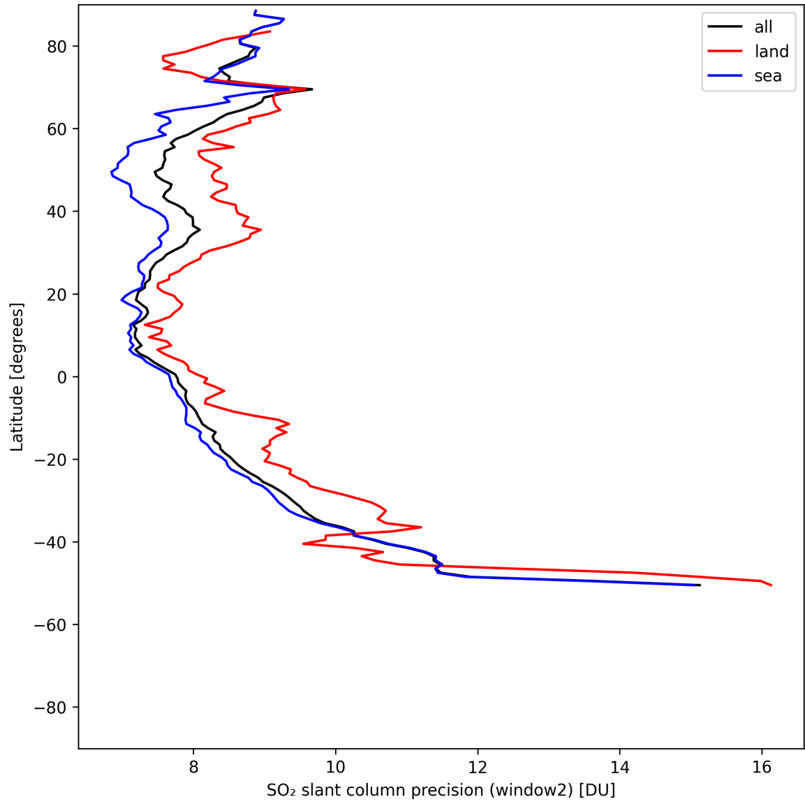
Figure 42: Zonal average of “SO 2 slant column precision (window2)” for 2025-07-27 to 2025-07-29.
