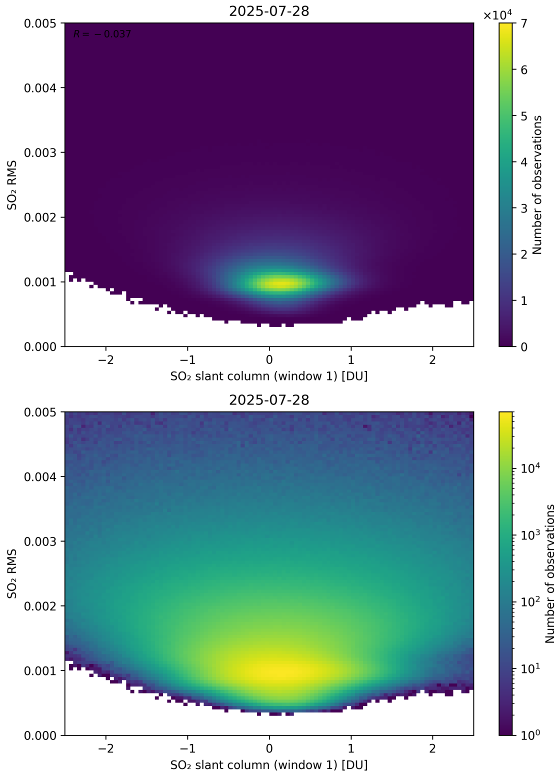
Figure 267: Scatter density plot of “SO 2 slant column (window 1)” against “SO 2 RMS” for 2025-07-27 to 2025-07-29.
