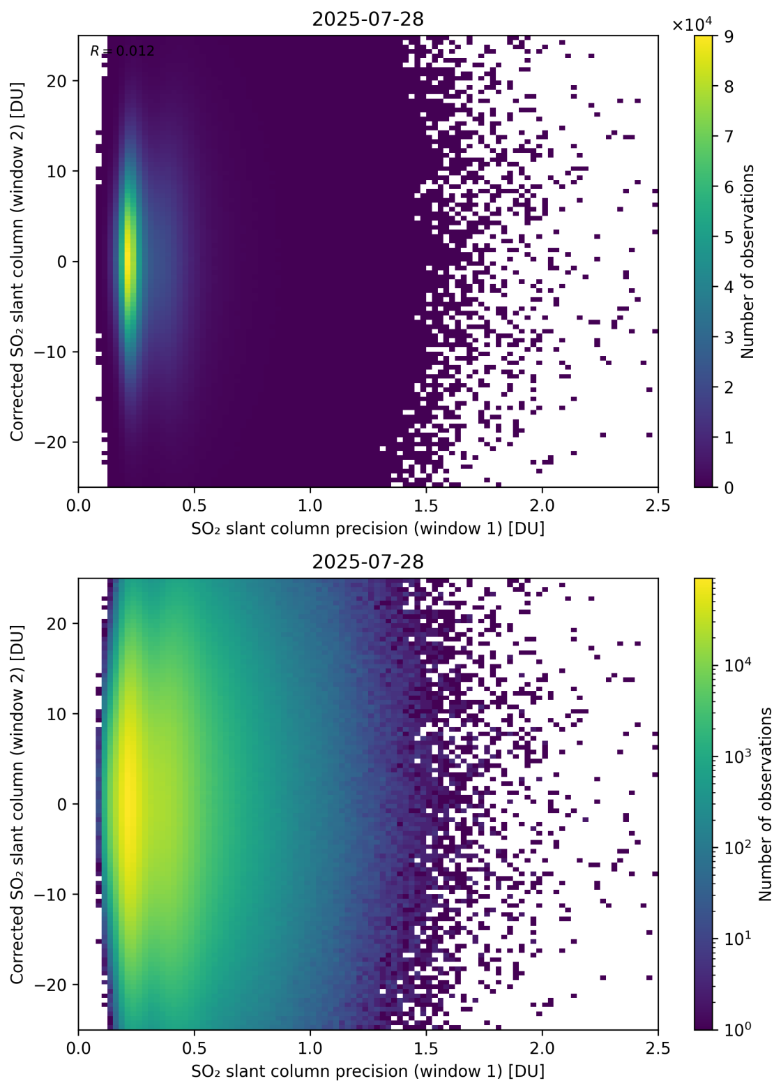
Figure 275: Scatter density plot of “SO 2 slant column precision (window 1)” against “Corrected SO 2 slant column (window 2)” for 2025-07-27 to 2025-07-29.
