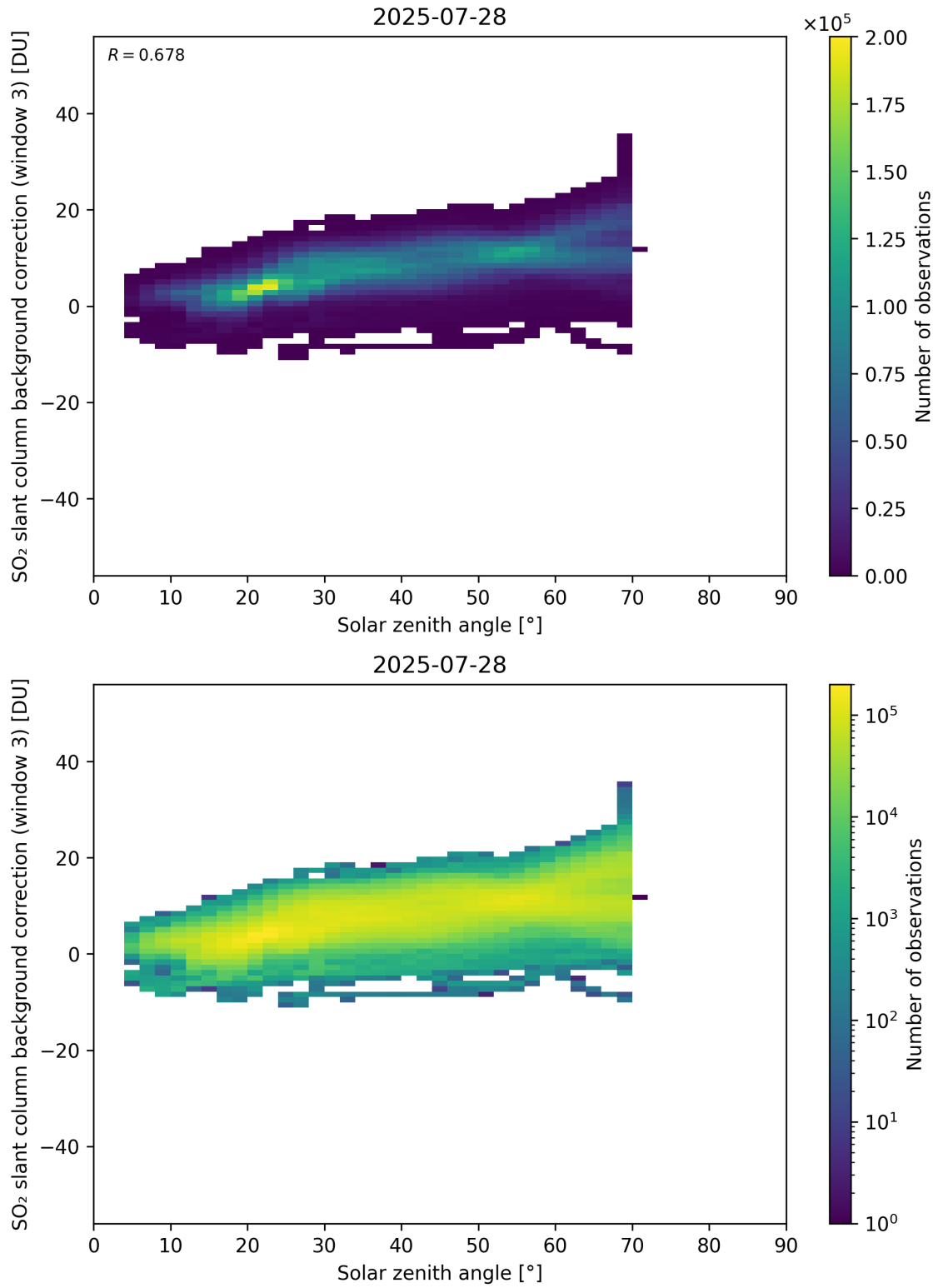
Figure 173: Scatter density plot of “Solar zenith angle” against “SO 2 slant column background correction (window 3)” for 2025-07-27 to 2025-07-29.
