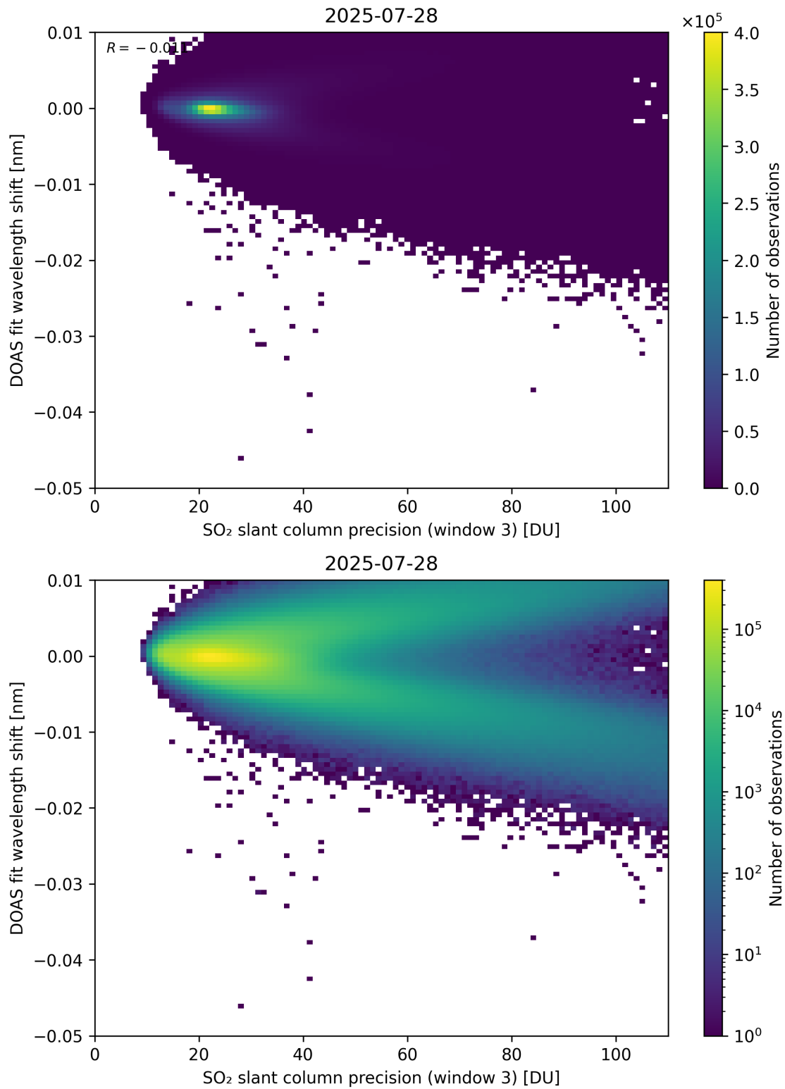
Figure 308: Scatter density plot of “SO 2 slant column precision (window 3)” against “DOAS fit wavelength shift” for 2025-07-27 to 2025-07-29.
