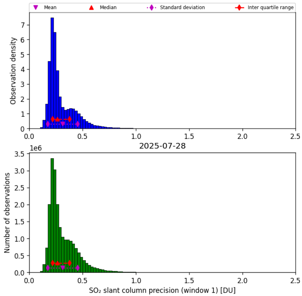
Figure 64: Histogram of “SO 2 slant column precision (window 1)” for 2025-07-27 to 2025-07-29
