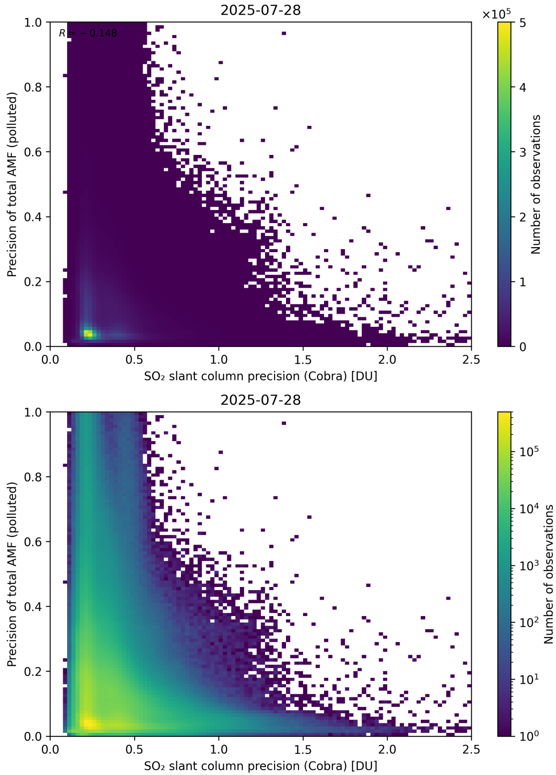
Figure 214: Scatter density plot of “SO 2 slant column precision (Cobra)” against “Precision of total AMF (polluted)” for 2025-07-27 to 2025-07-29.
