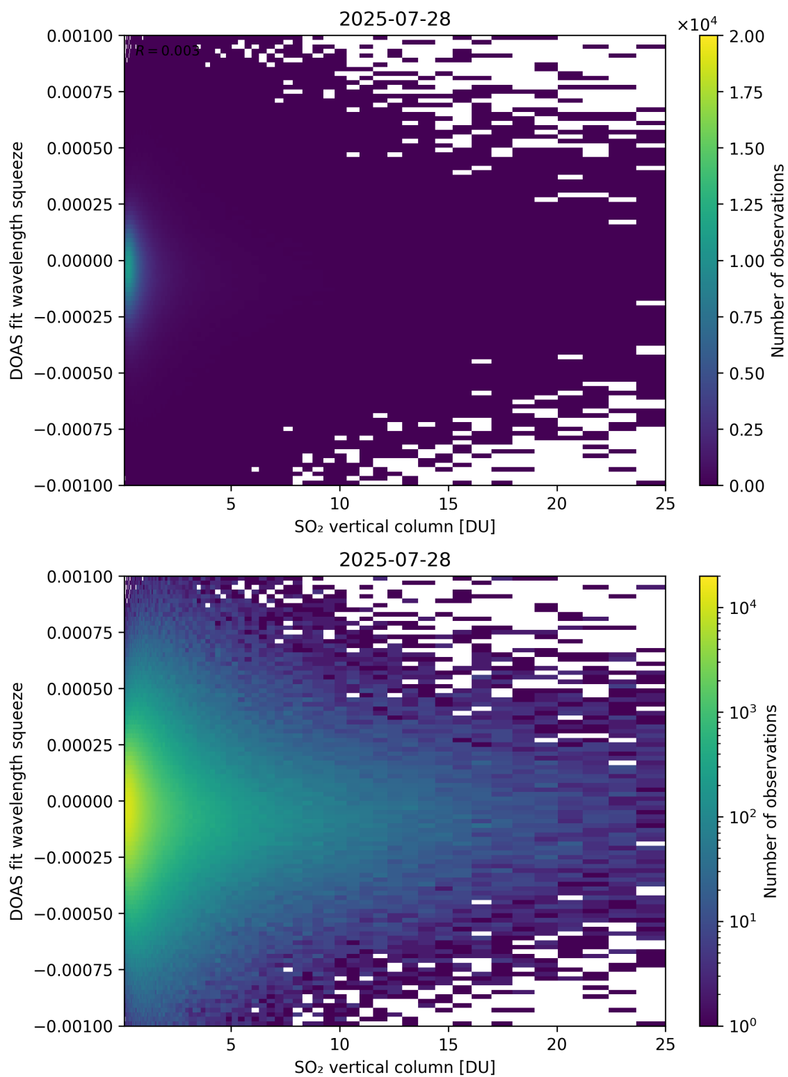
Figure 327: Scatter density plot of “SO 2 vertical column” against “DOAS fit wavelength squeeze” for 2025-07-27 to 2025-07-29.
