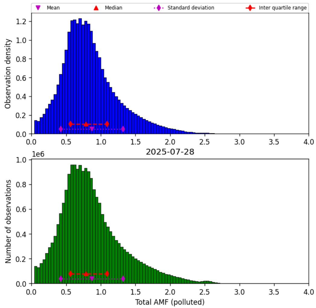
Figure 79: Histogram of “Total AMF (polluted)” for 2025-07-27 to 2025-07-29
