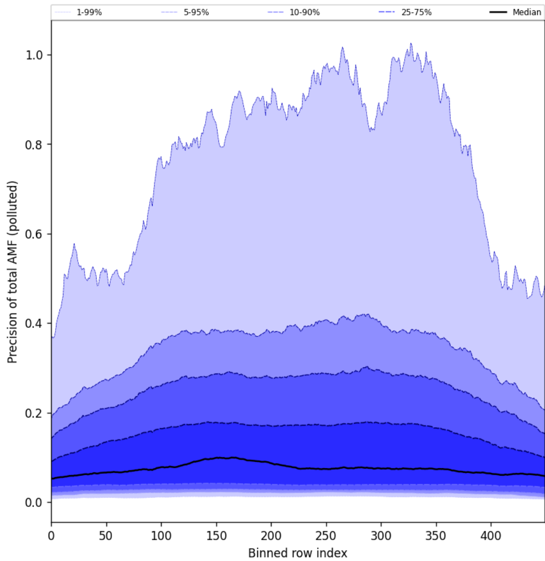
Figure 106: Along track statistics of “Precision of total AMF (polluted)” for 2025-07-27 to 2025-07-29
