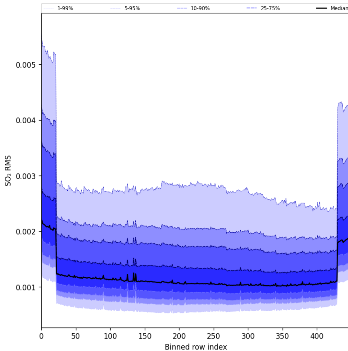
Figure 104: Along track statistics of “SO 2 RMS” for 2025-07-27 to 2025-07-29
