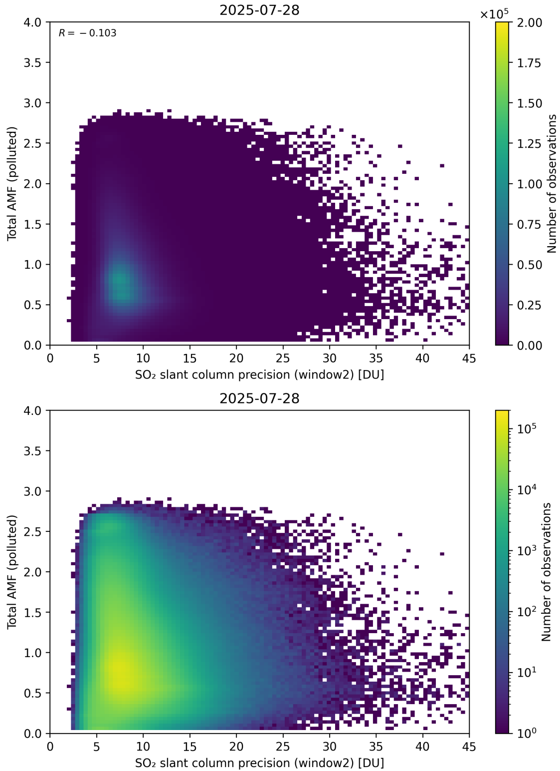
Figure 301: Scatter density plot of “SO 2 slant column precision (window2)” against “Total AMF (polluted)” for 2025-07-27 to 2025-07-29.
