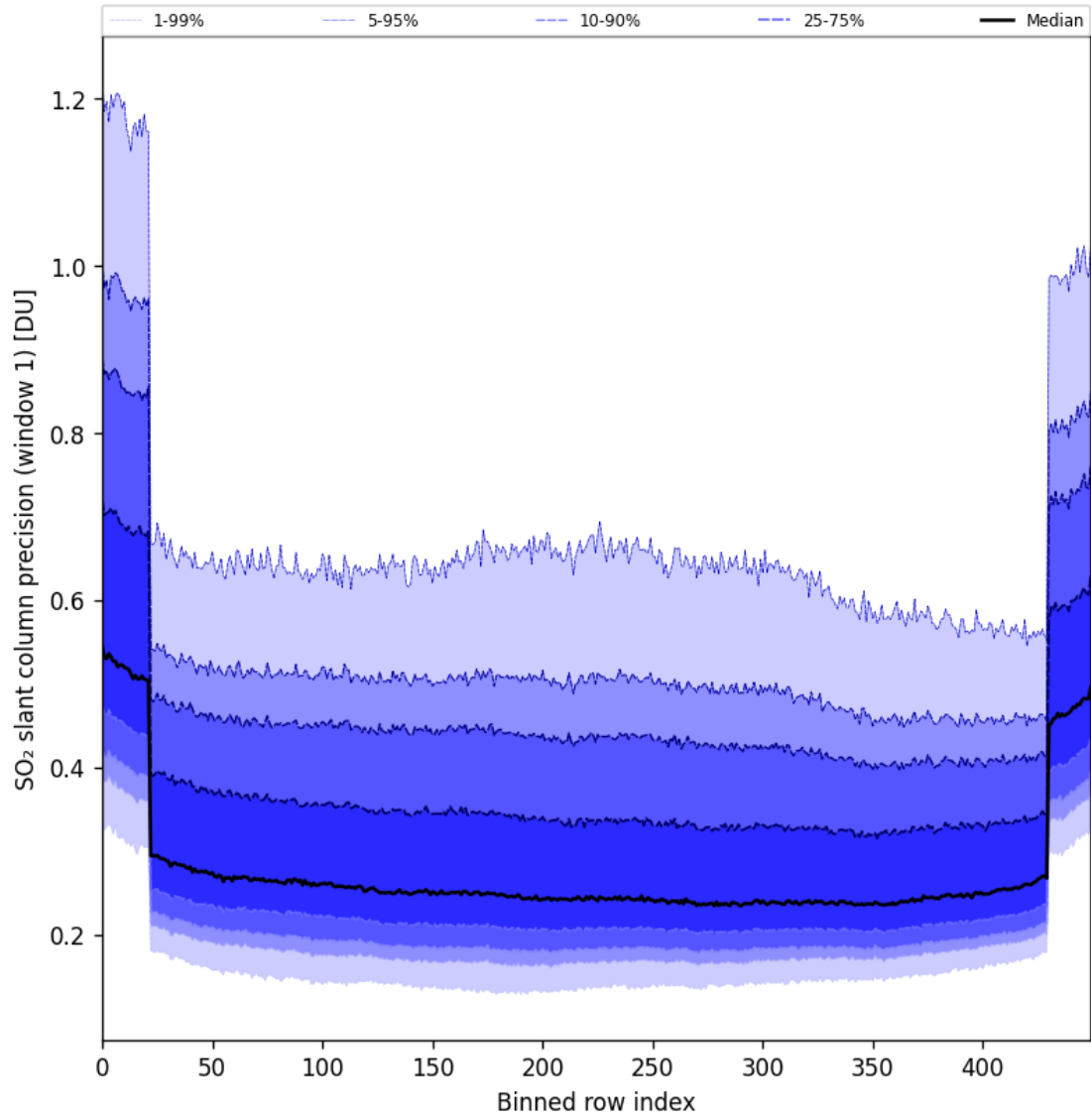
Figure 90: Along track statistics of “SO 2 slant column precision (window 1)” for 2025-07-27 to 2025-07-29
