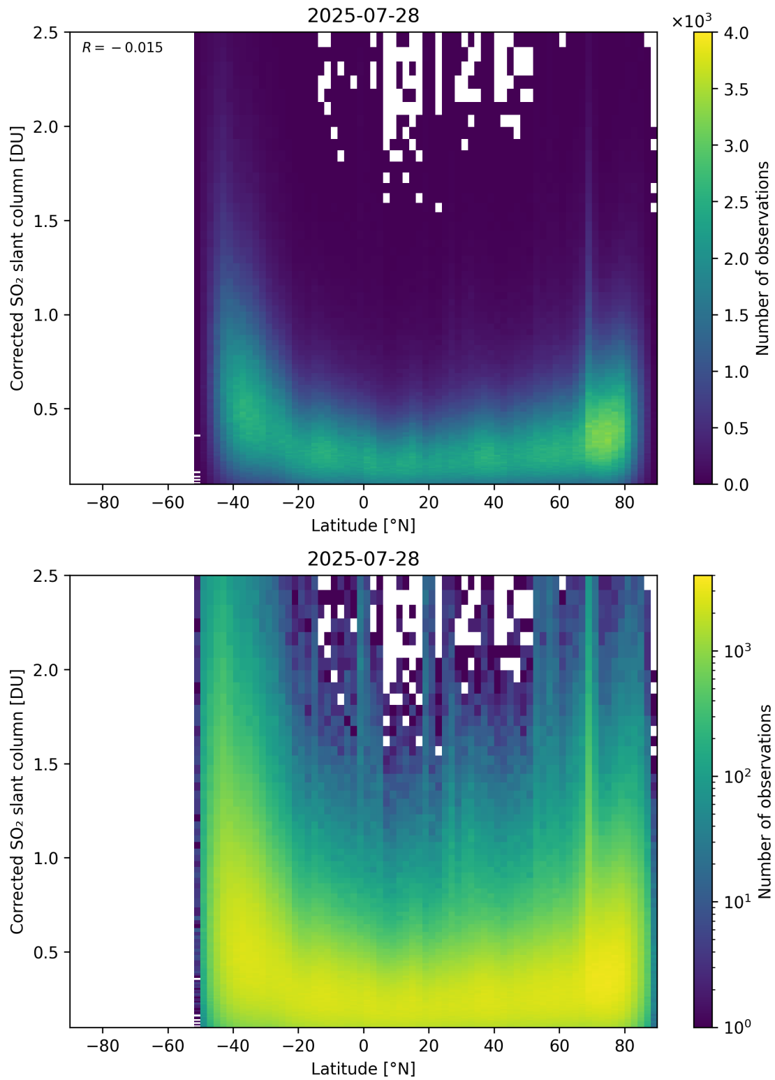
Figure 159: Scatter density plot of “Latitude” against “Corrected SO 2 slant column” for 2025-07-27 to 2025-07-29.
