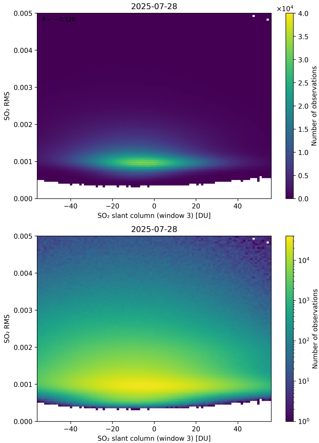
Figure 306: Scatter density plot of “SO 2 slant column (window 3)” against “SO 2 RMS” for 2025-07-27 to 2025-07-29.
