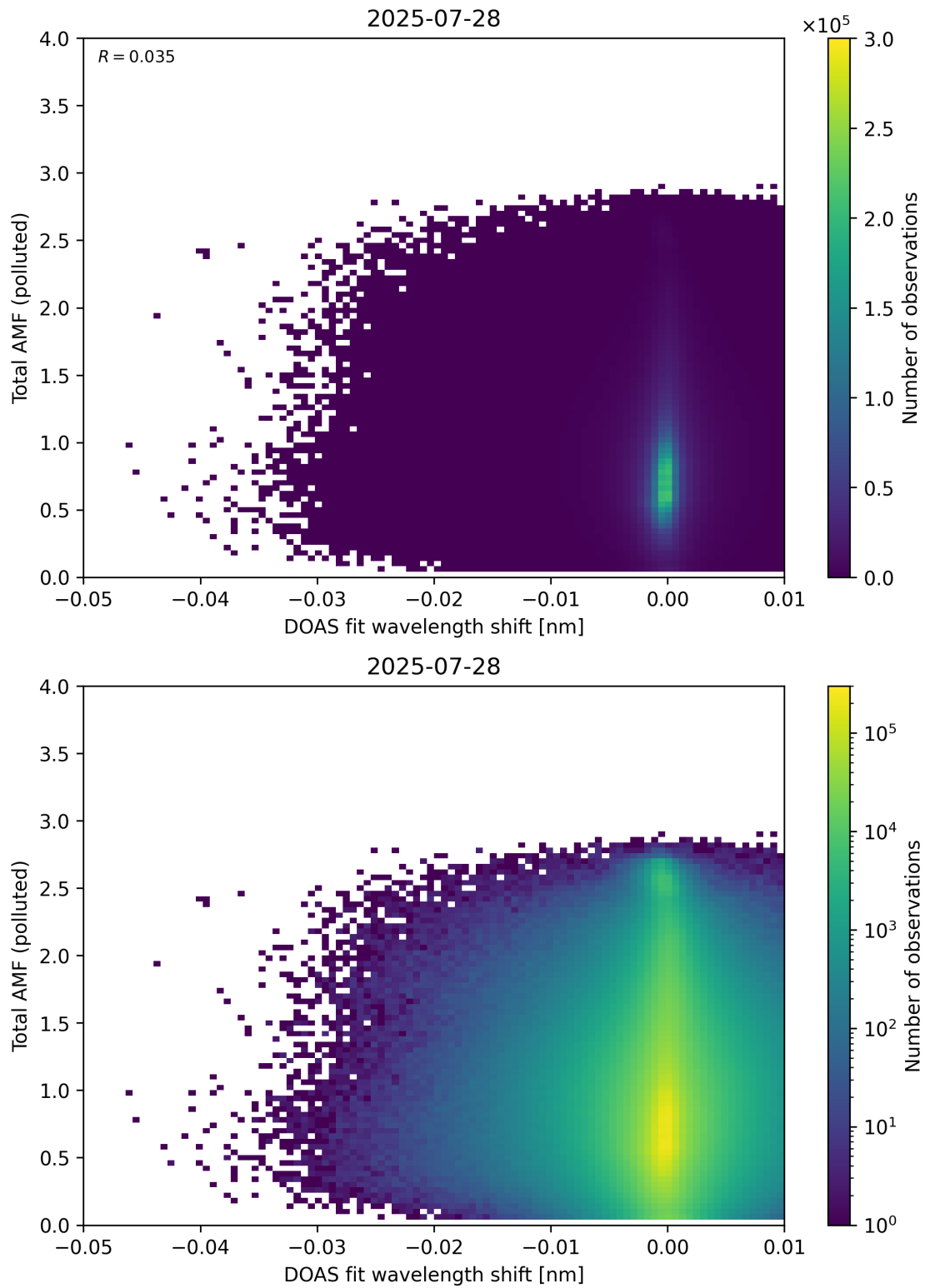
Figure 141: Scatter density plot of “DOAS fit wavelength shift” against “Total AMF (polluted)” for 2025-07-27 to 2025-07-29.
