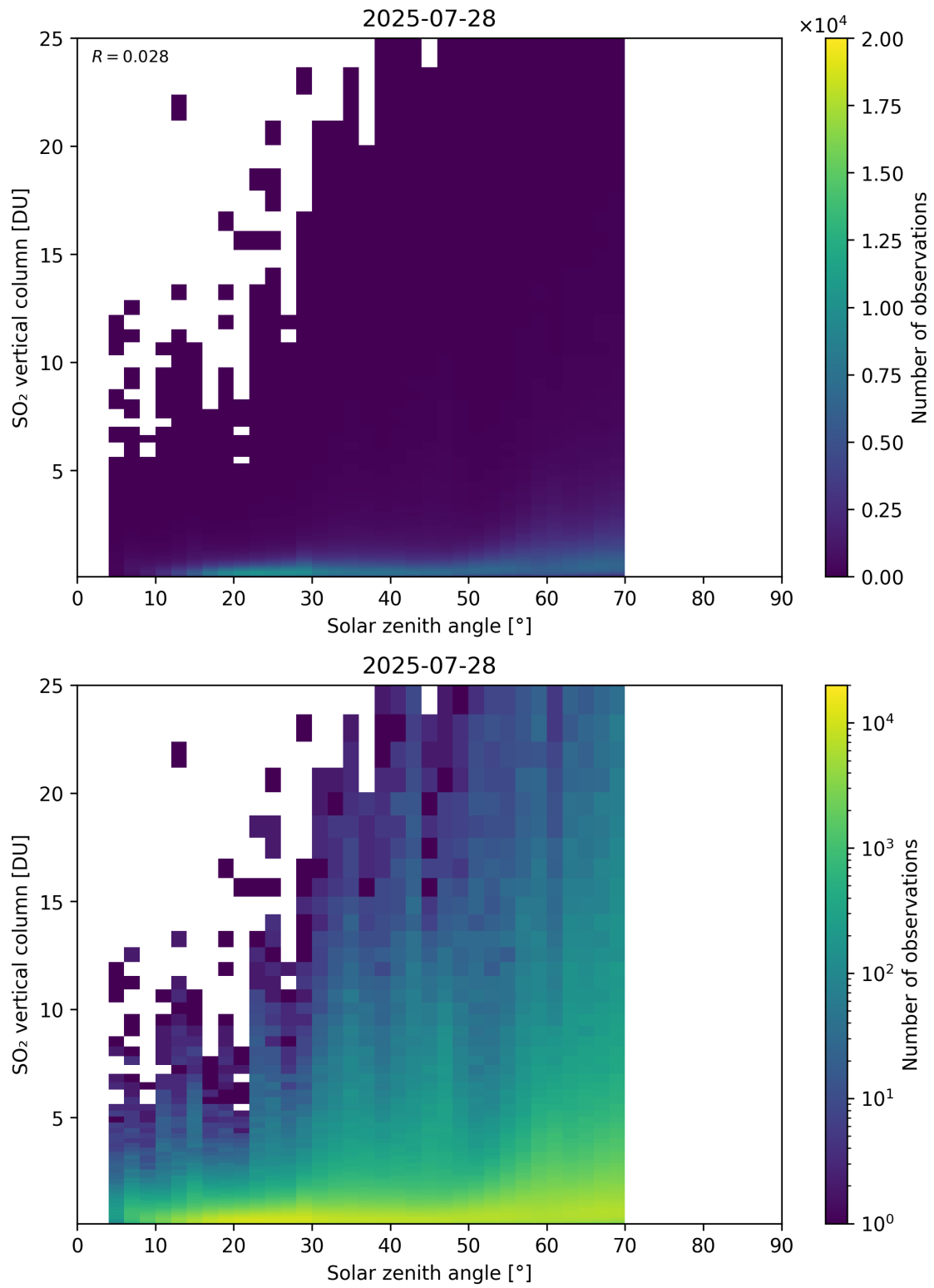
Figure 191: Scatter density plot of “Solar zenith angle” against “SO 2 vertical column” for 2025-07-27 to 2025-07-29.
