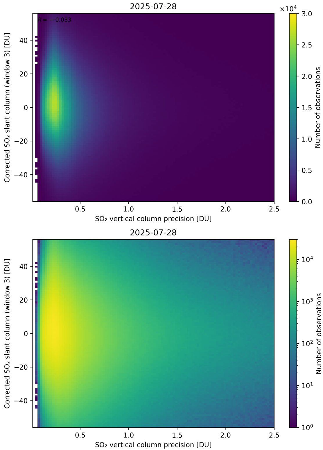
Figure 340: Scatter density plot of “SO 2 vertical column precision” against “Corrected SO 2 slant column (window 3)” for 2025-07-27 to 2025-07-29.
