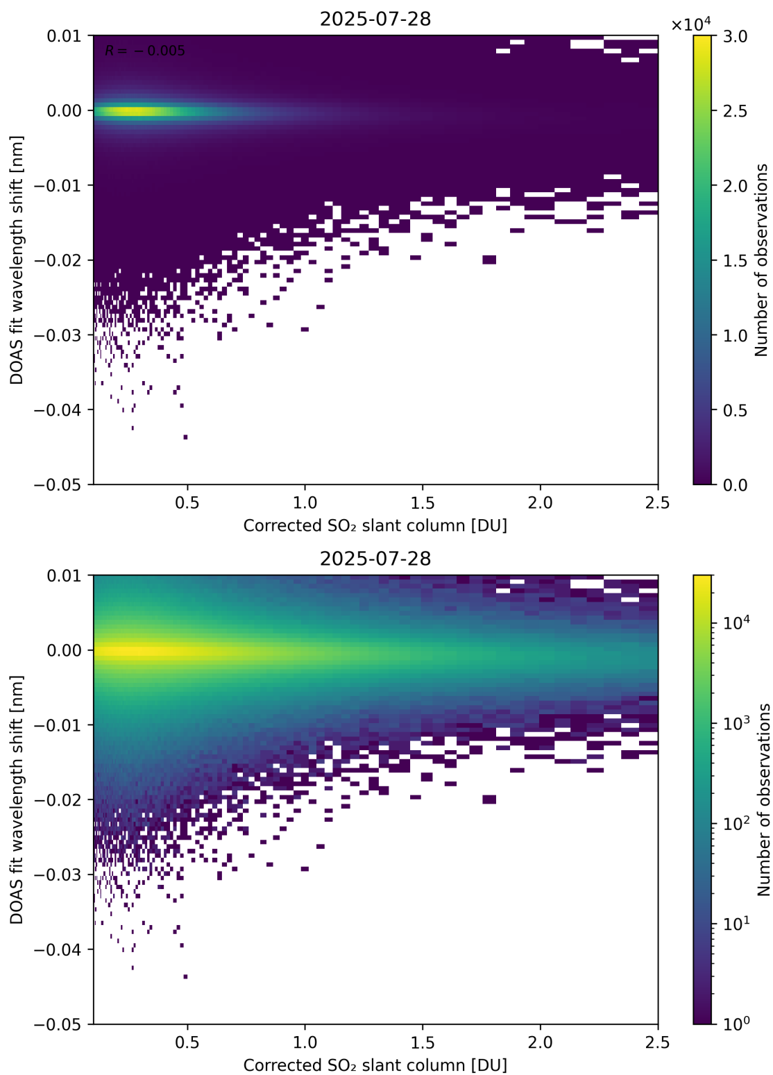
Figure 229: Scatter density plot of “Corrected SO 2 slant column” against “DOAS fit wavelength shift” for 2025-07-27 to 2025-07-29.
