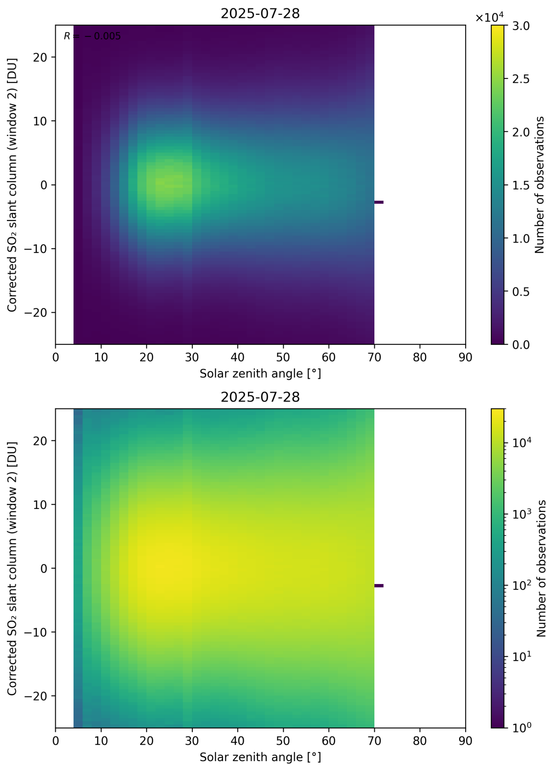
Figure 182: Scatter density plot of “Solar zenith angle” against “Corrected SO 2 slant column (window 2)” for 2025-07-27 to 2025-07-29.
