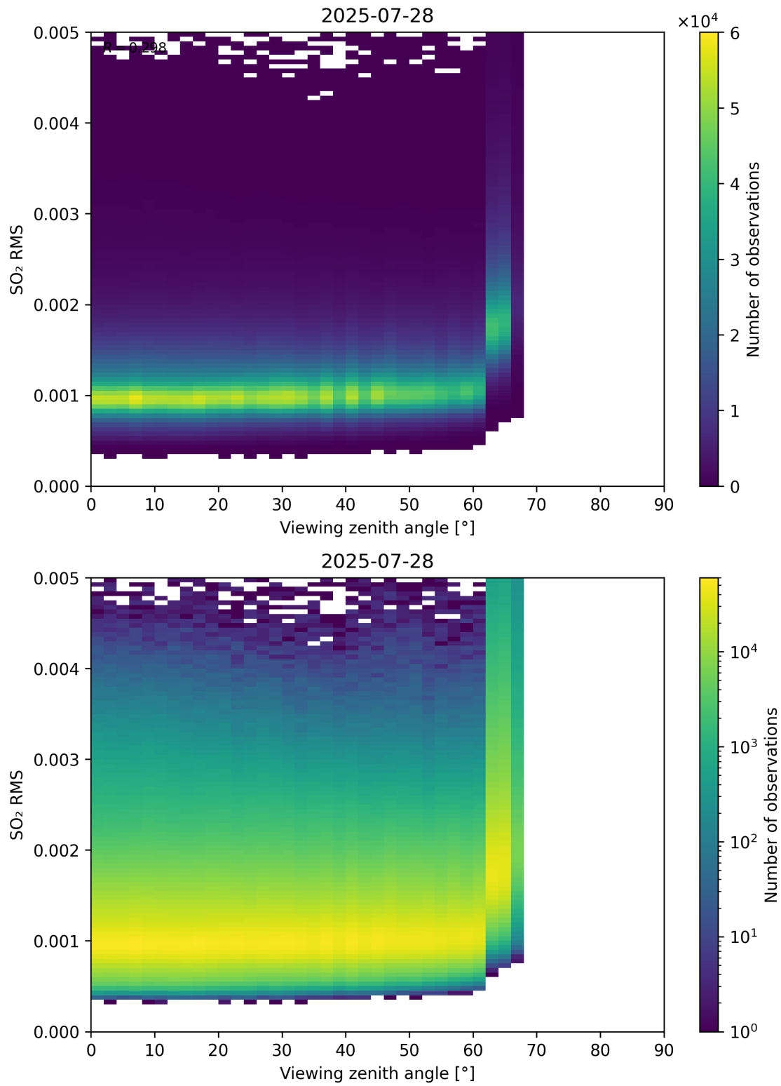
Figure 367: Scatter density plot of “Viewing zenith angle” against “SO 2 RMS” for 2025-07-27 to 2025-07-29.
