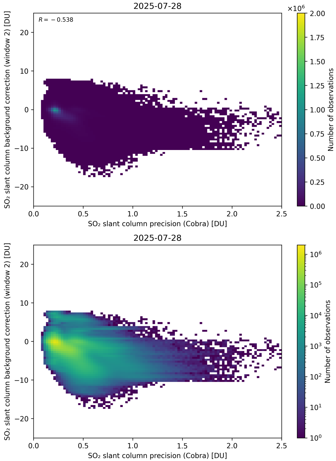
Figure 200: Scatter density plot of “SO 2 slant column precision (Cobra)” against “SO 2 slant column background correction (window 2)” for 2025-07-27 to 2025-07-29.
