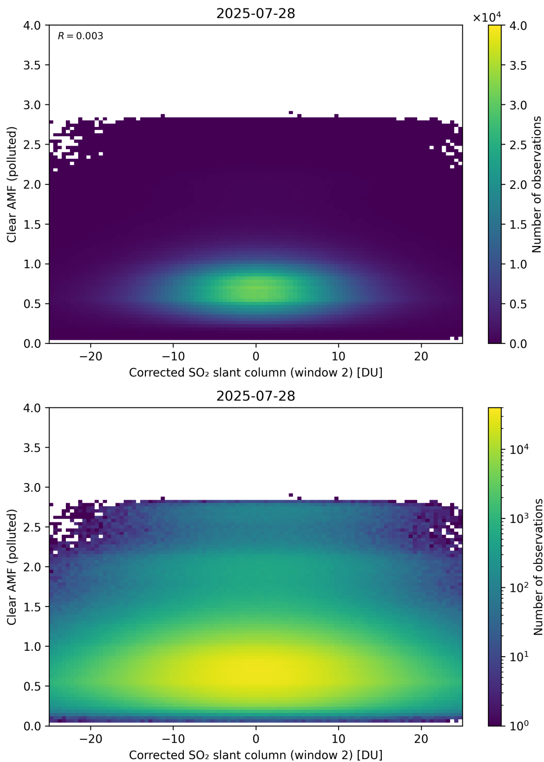
Figure 249: Scatter density plot of “Corrected SO 2 slant column (window 2)” against “Clear AMF (polluted)” for 2025-07-27 to 2025-07-29.
