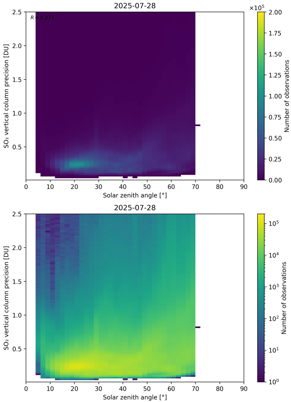
Figure 192: Scatter density plot of “Solar zenith angle” against “SO 2 vertical column precision” for 2025-07-27 to 2025-07-29.
