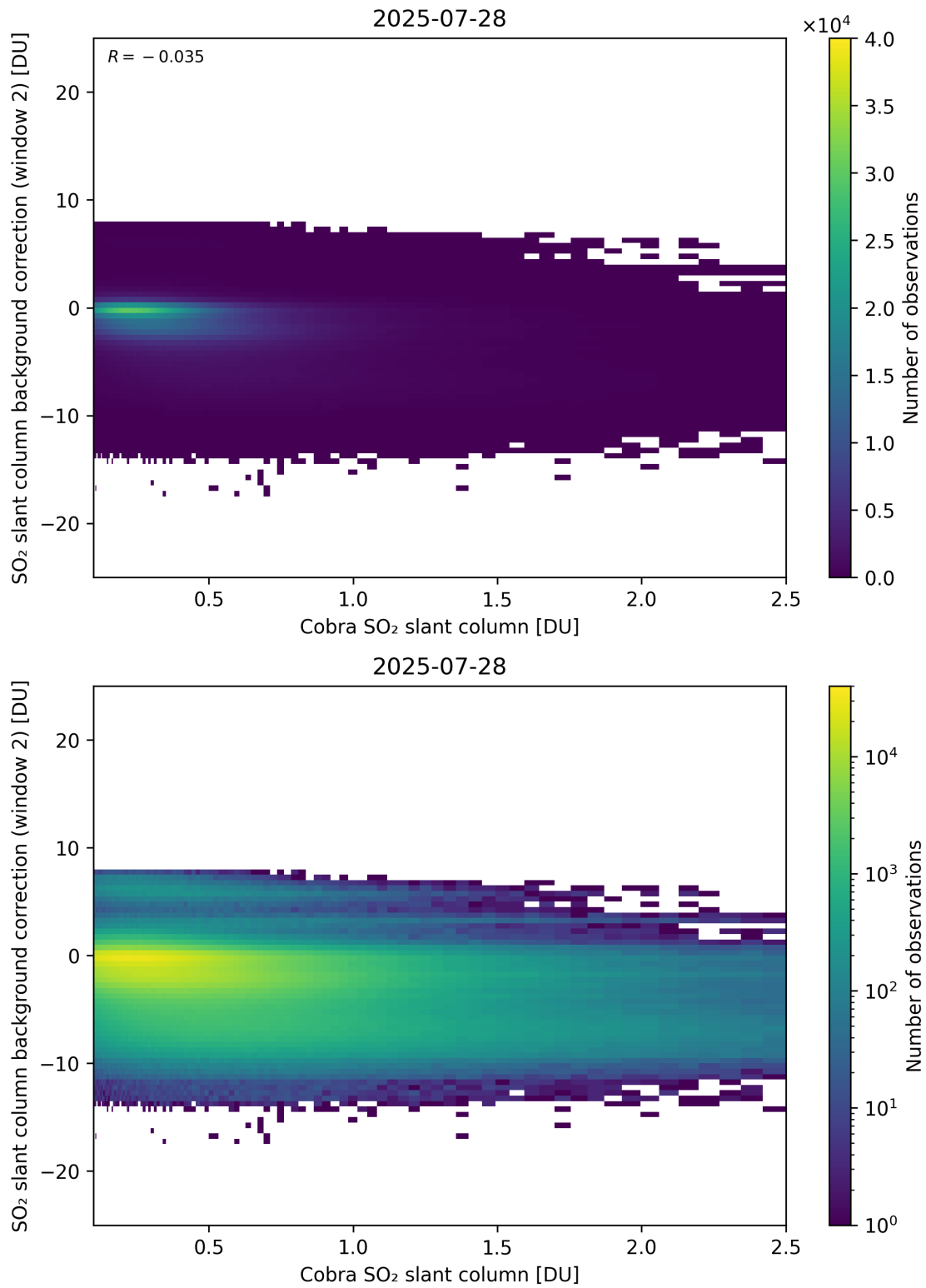
Figure 194: Scatter density plot of “Cobra SO 2 slant column” against “SO 2 slant column background correction (window 2)” for 2025-07-27 to 2025-07-29.
