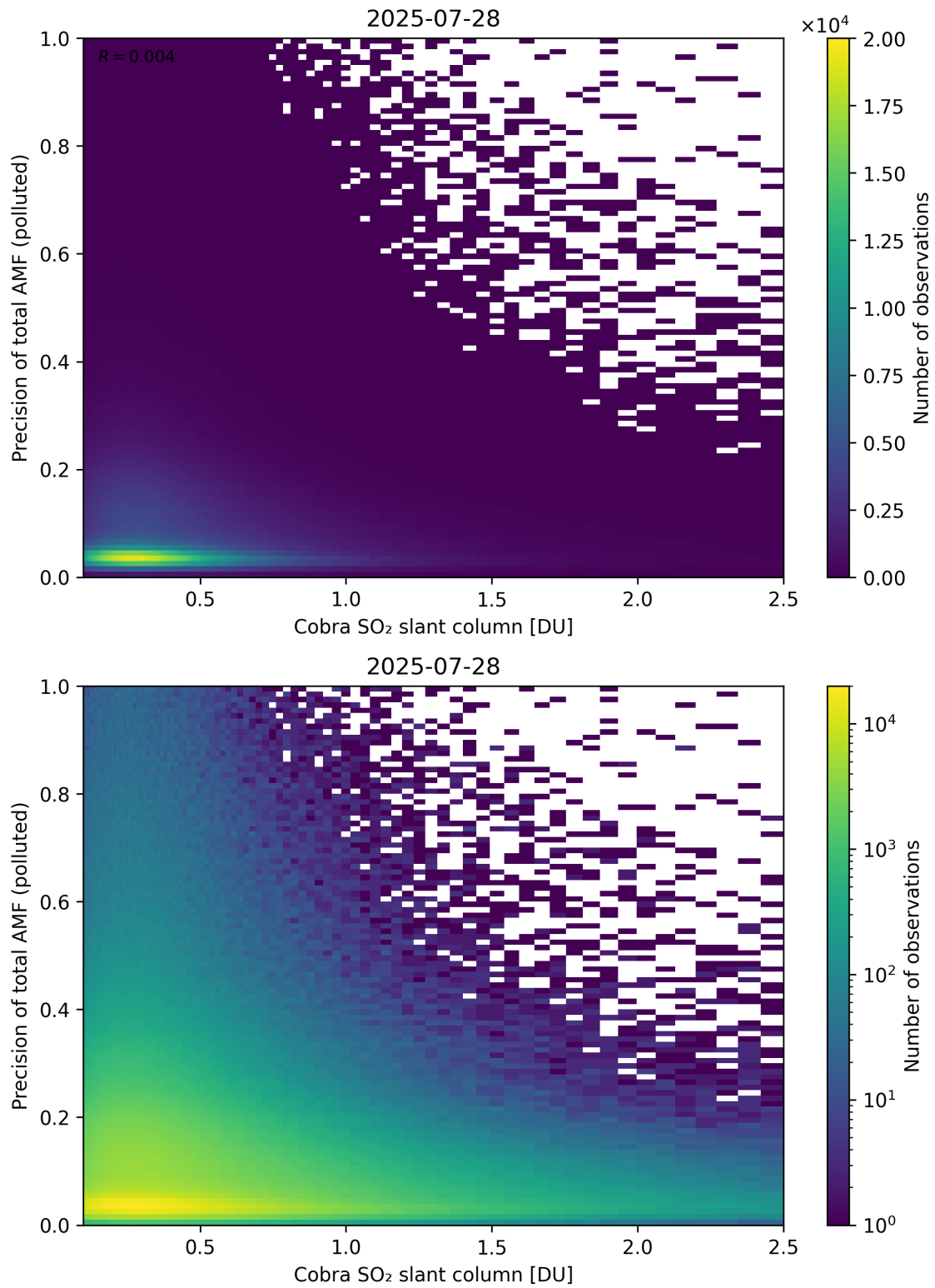
Figure 225: Scatter density plot of “Cobra SO 2 slant column” against “Precision of total AMF (polluted)” for 2025-07-27 to 2025-07-29.
