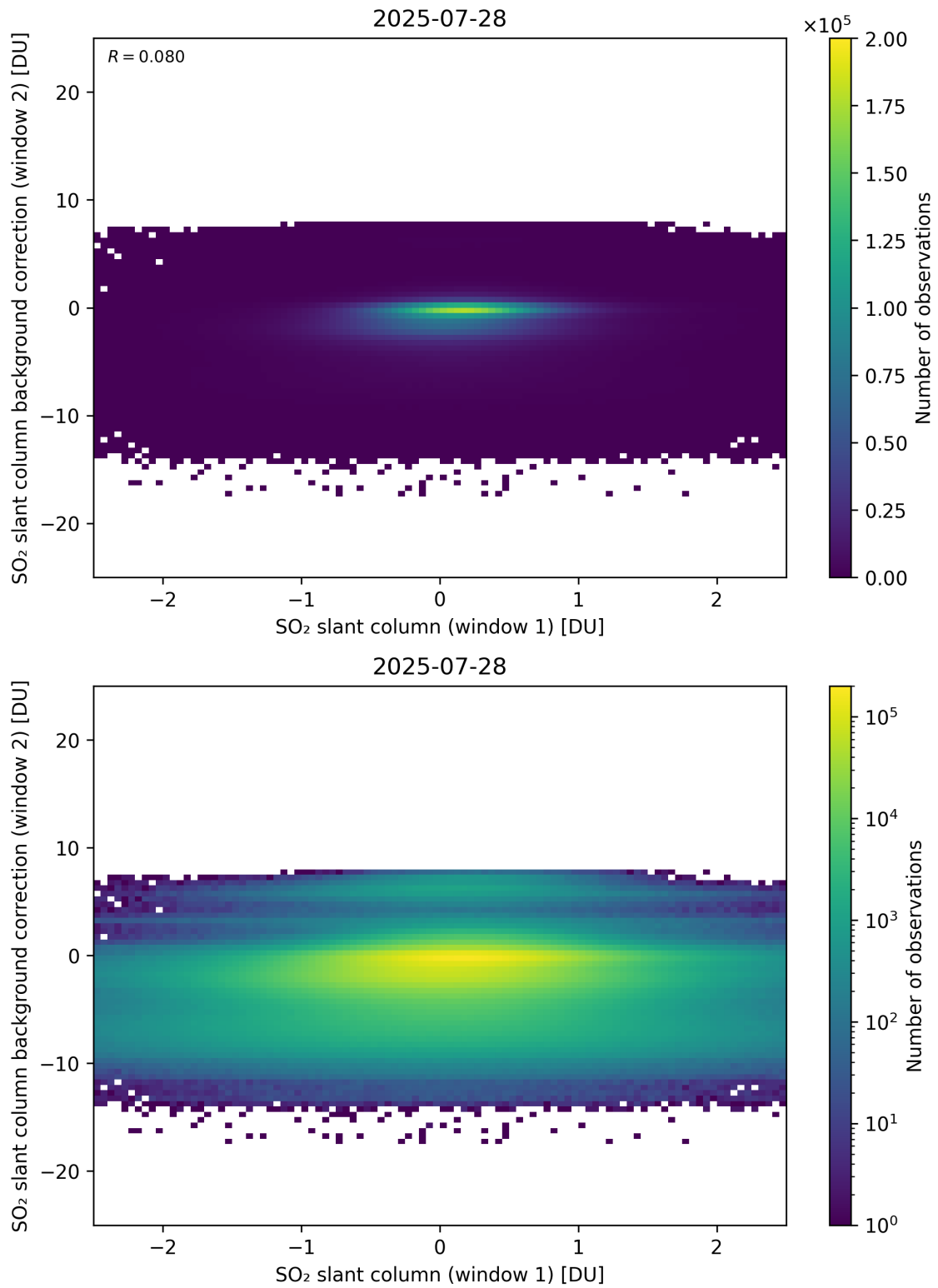
Figure 263: Scatter density plot of “SO 2 slant column (window 1)” against “SO 2 slant column background correction (window 2)” for 2025-07-27 to 2025-07-29.
