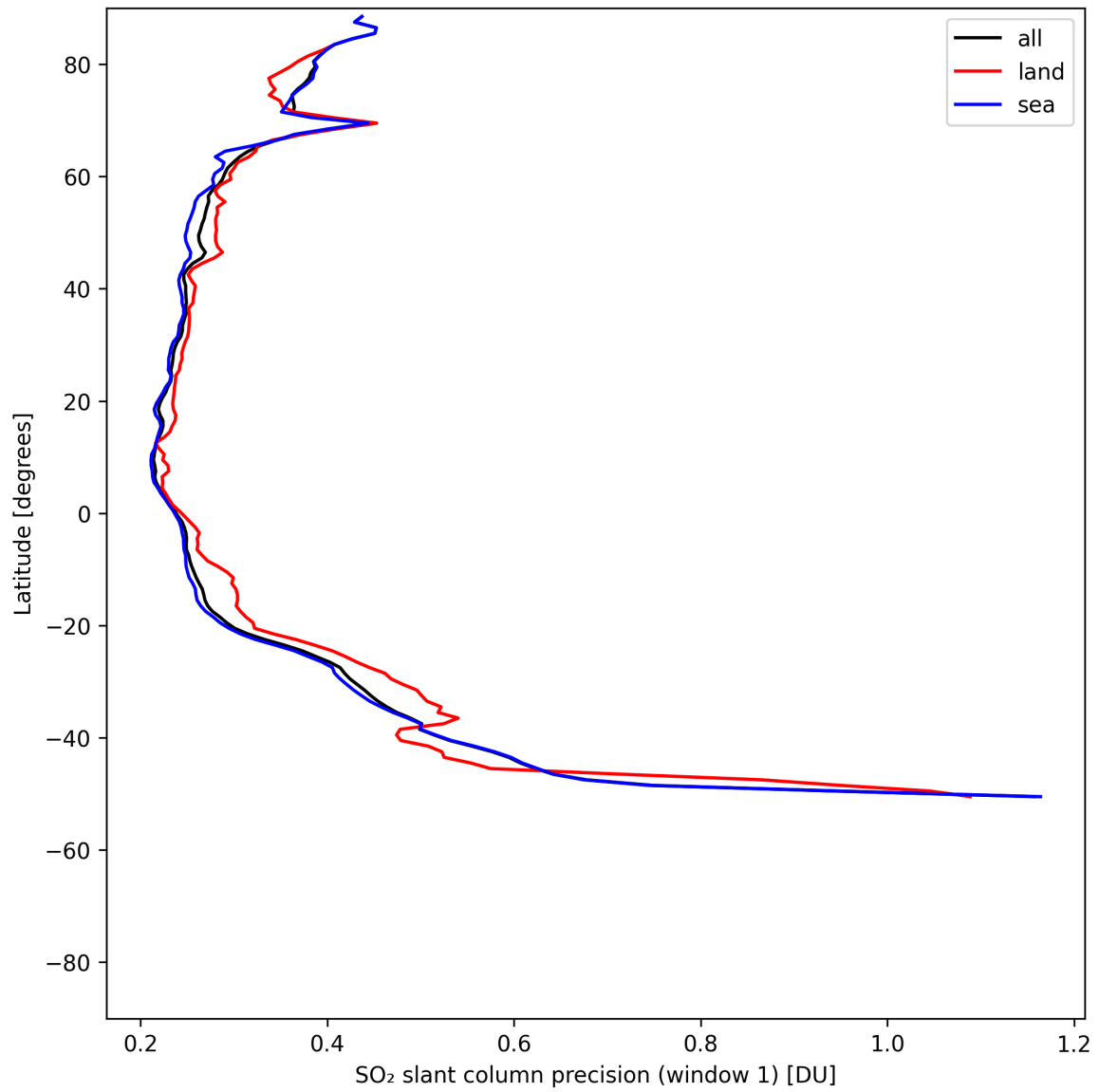
Figure 38: Zonal average of “SO 2 slant column precision (window 1)” for 2025-07-27 to 2025-07-29.
