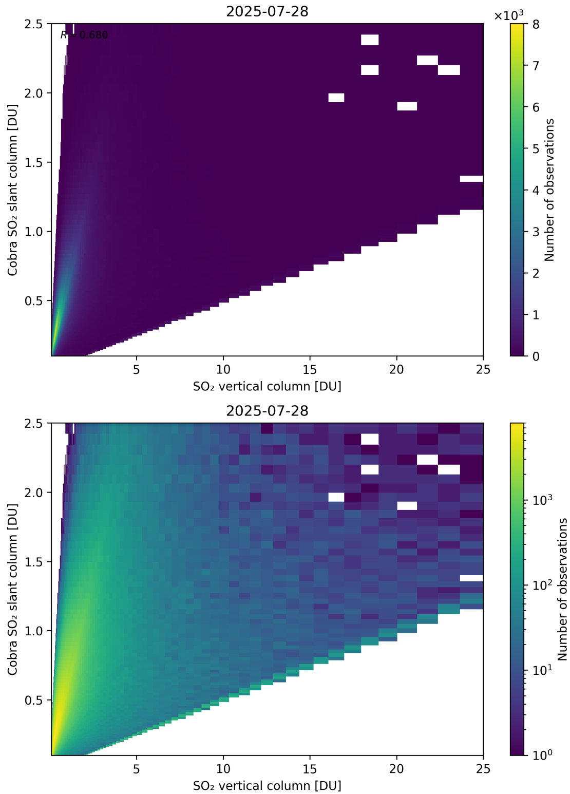
Figure 349: Scatter density plot of “SO 2 vertical column” against “Cobra SO 2 slant column” for 2025-07-27 to 2025-07-29.
