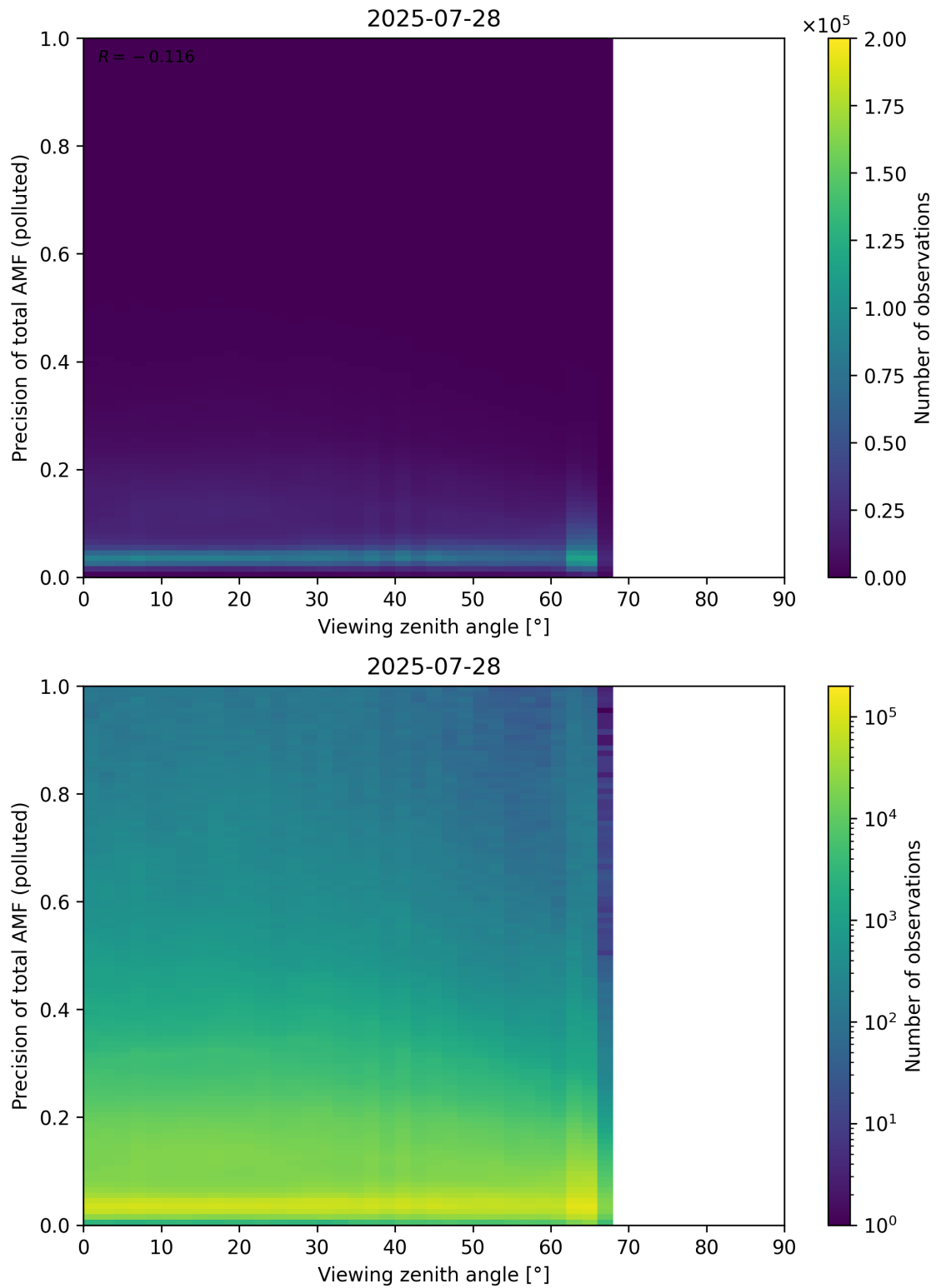
Figure 382: Scatter density plot of “Viewing zenith angle” against “Precision of total AMF (polluted)” for 2025-07-27 to 2025-07-29.
