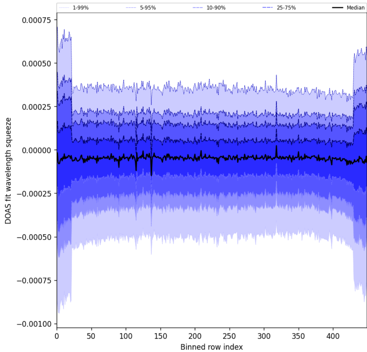
Figure 103: Along track statistics of “DOAS fit wavelength squeeze” for 2025-07-27 to 2025-07-29
