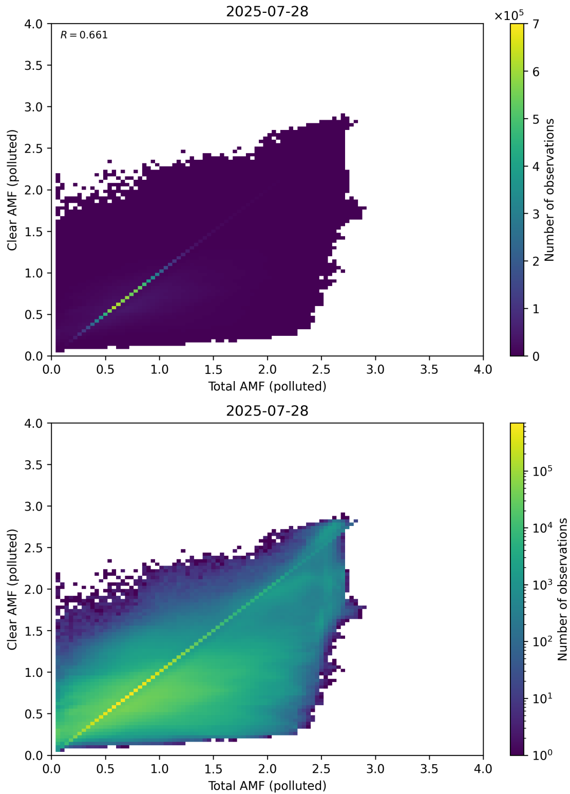
Figure 321: Scatter density plot of “Total AMF (polluted)” against “Clear AMF (polluted)” for 2025-07-27 to 2025-07-29.
