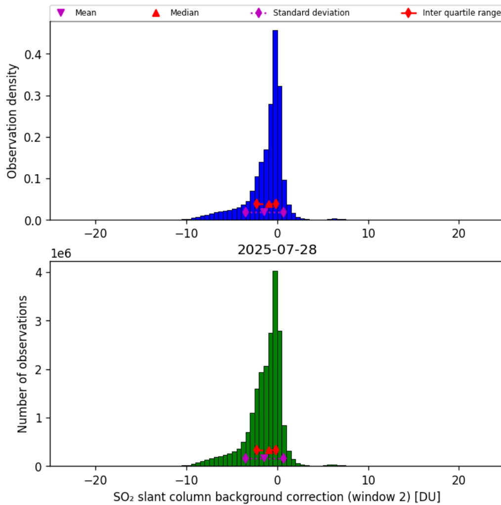
Figure 70: Histogram of “SO 2 slant column background correction (window 2)” for 2025-07-27 to 2025-07-29
