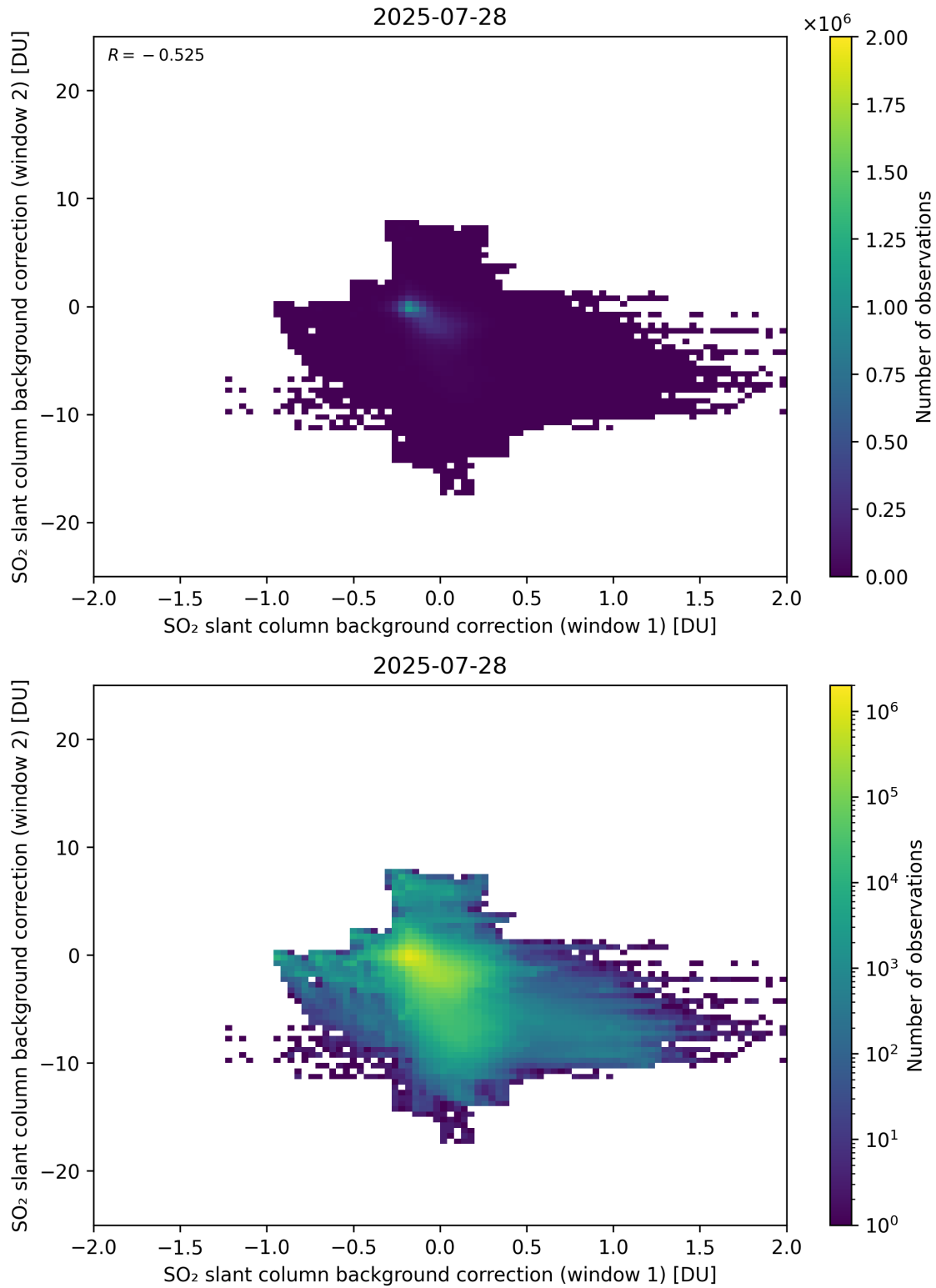
Figure 109: Scatter density plot of “SO 2 slant column background correction (window 1)” against “SO 2 slant column background correction (window 2)” for 2025-07-27 to 2025-07-29.
