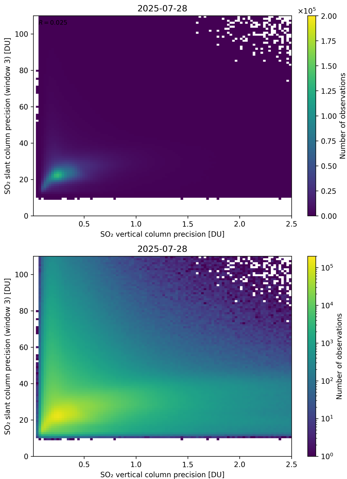
Figure 345: Scatter density plot of “SO 2 vertical column precision” against “SO 2 slant column precision (window 3)” for 2025-07-27 to 2025-07-29.
