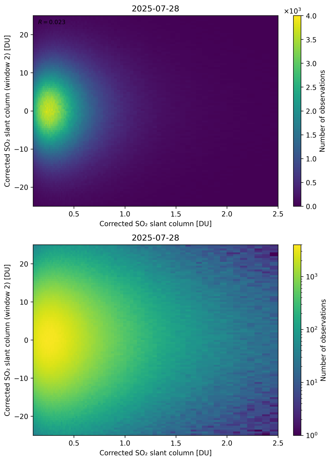
Figure 235: Scatter density plot of “Corrected SO 2 slant column” against “Corrected SO 2 slant column (window 2)” for 2025-07-27 to 2025-07-29.
