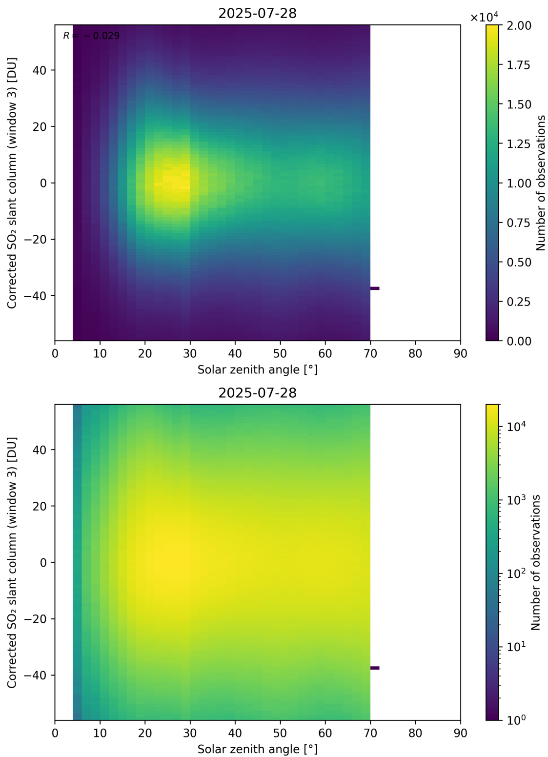
Figure 183: Scatter density plot of “Solar zenith angle” against “Corrected SO 2 slant column (window 3)” for 2025-07-27 to 2025-07-29.
