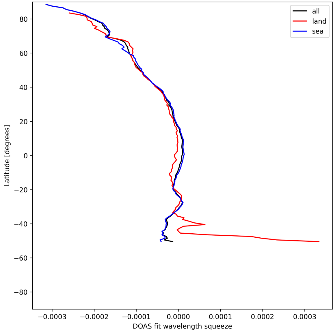
Figure 51: Zonal average of “DOAS fit wavelength squeeze” for 2025-07-27 to 2025-07-29.
