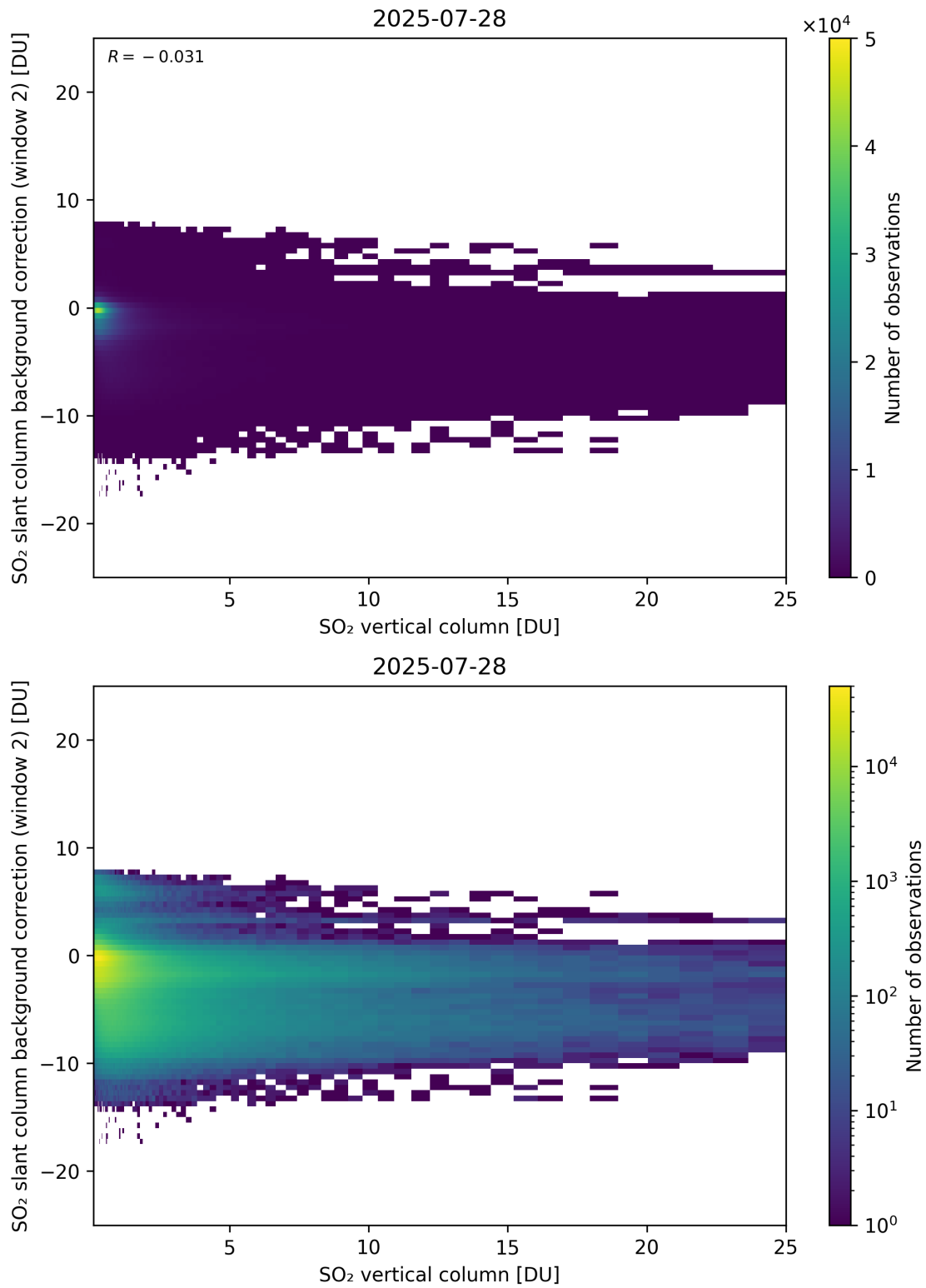
Figure 324: Scatter density plot of “SO 2 vertical column” against “SO 2 slant column background correction (window 2)” for 2025-07-27 to 2025-07-29.
