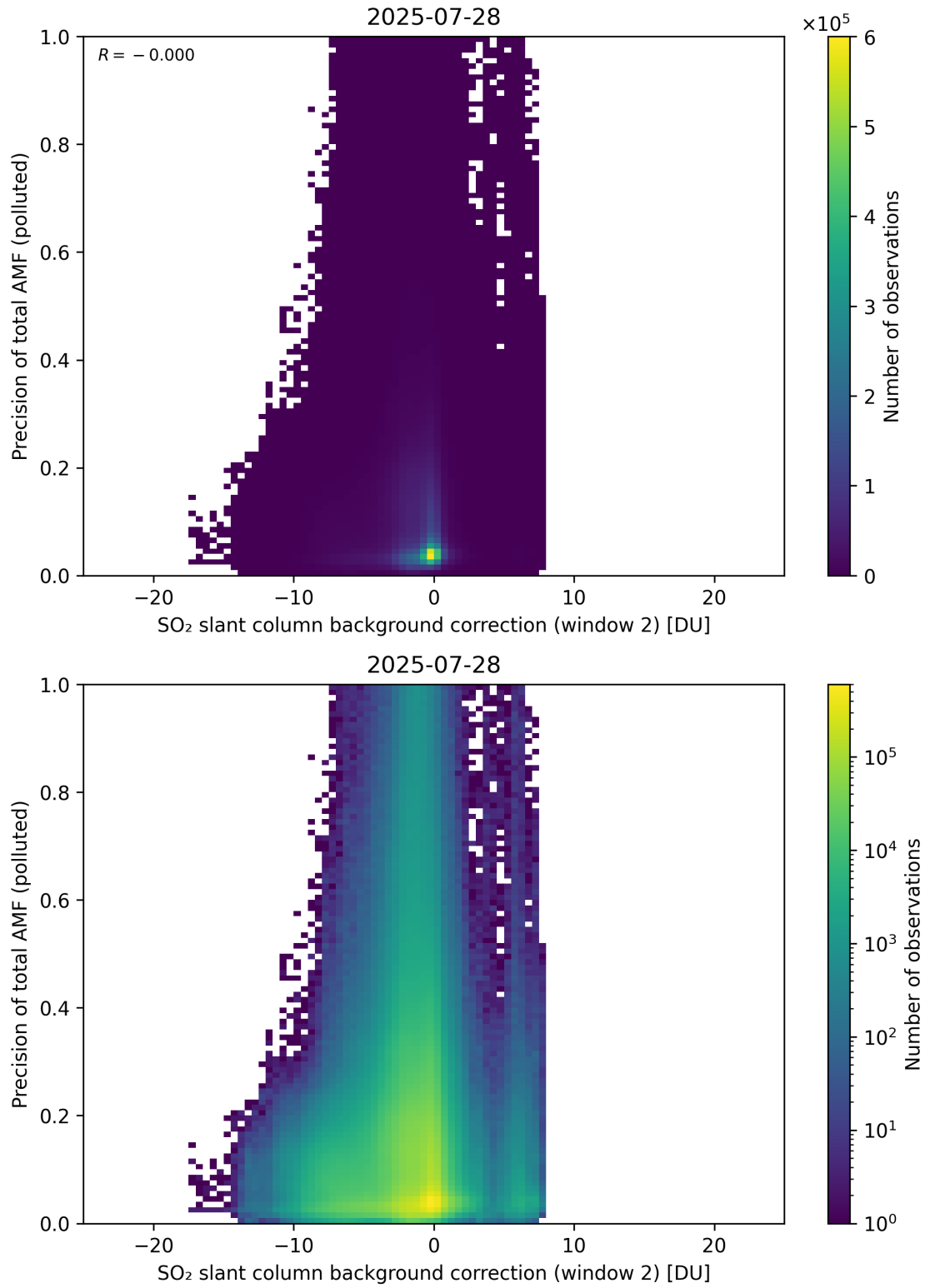
Figure 131: Scatter density plot of “SO 2 slant column background correction (window 2)” against “Precision of total AMF (polluted)” for 2025-07-27 to 2025-07-29.
