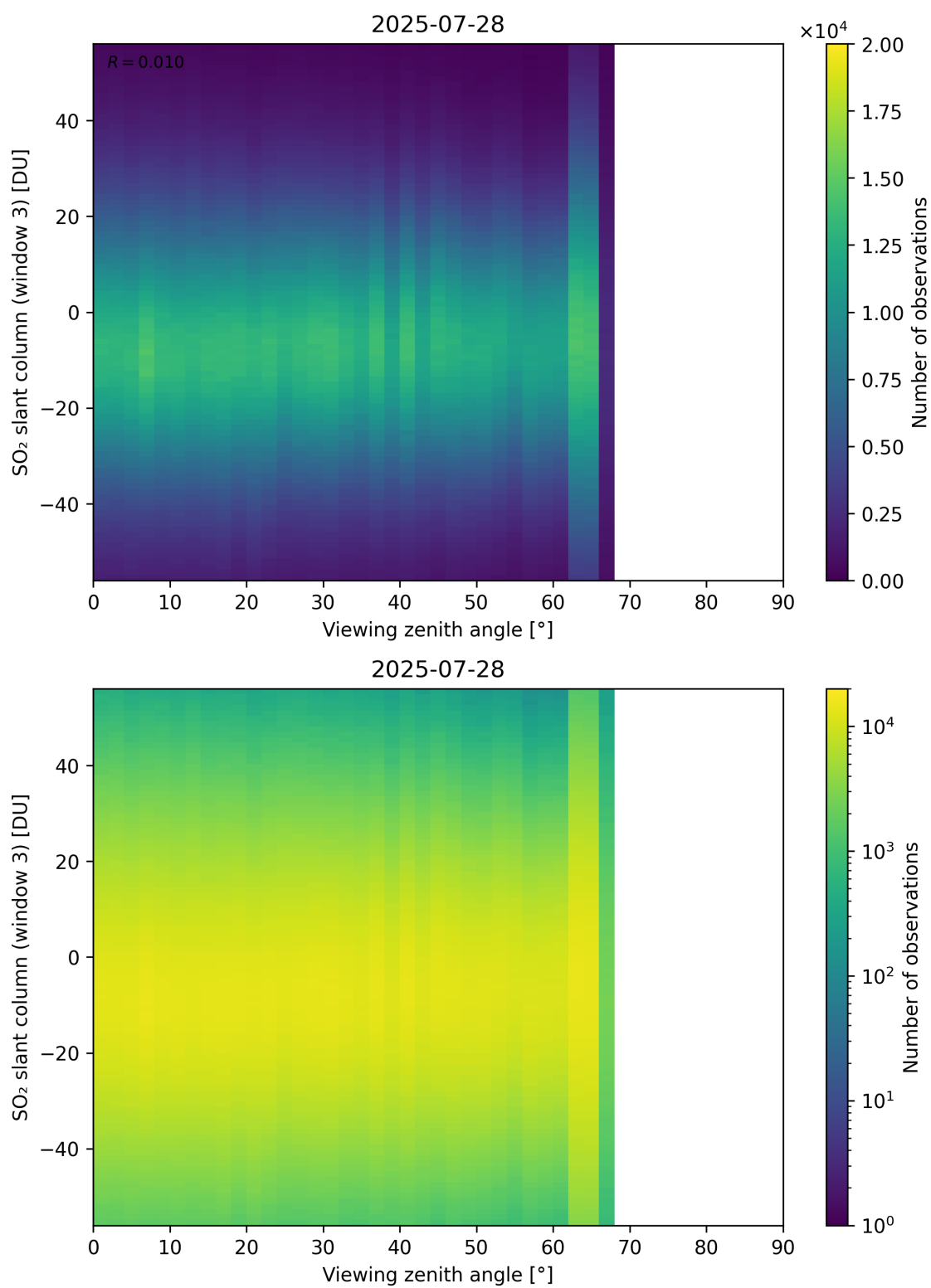
Figure 379: Scatter density plot of “Viewing zenith angle” against “SO 2 slant column (window 3)” for 2025-07-27 to 2025-07-29.
