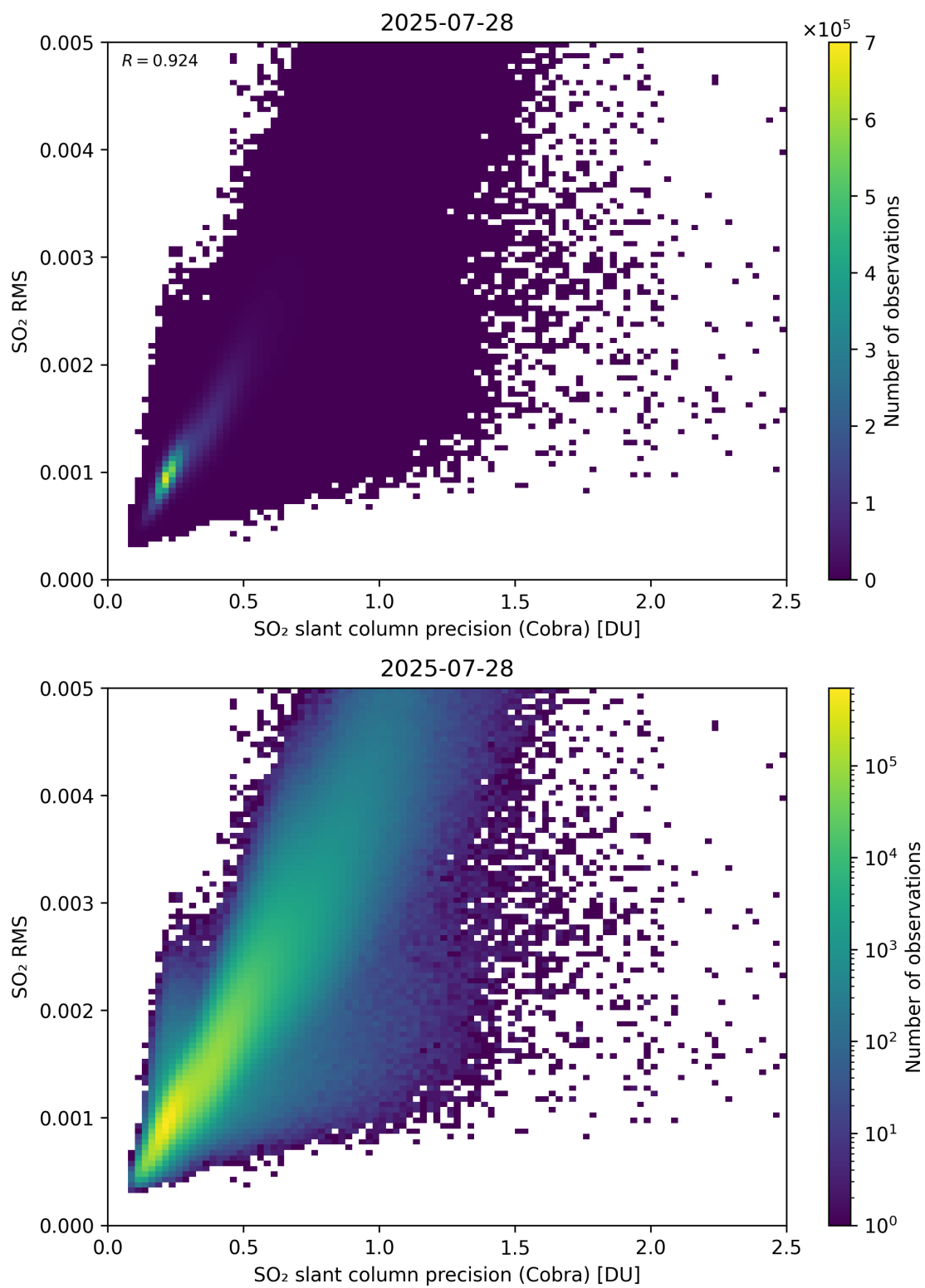
Figure 204: Scatter density plot of “SO 2 slant column precision (Cobra)” against “SO 2 RMS” for 2025-07-27 to 2025-07-29.
