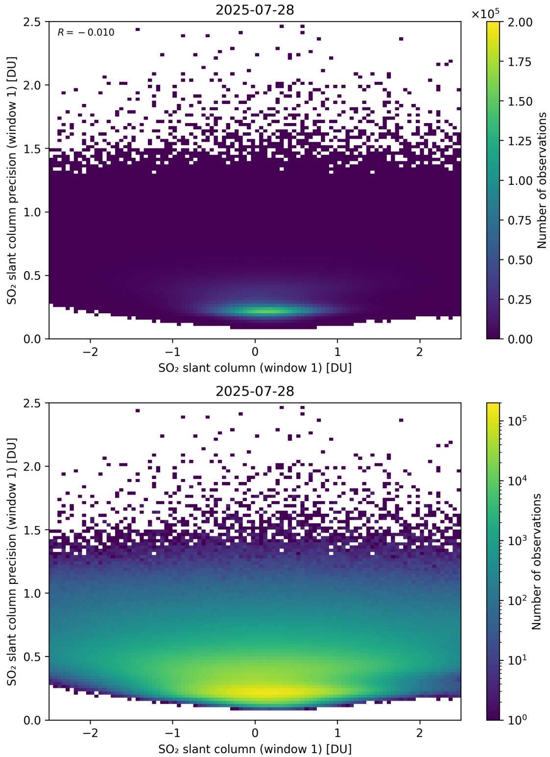
Figure 285: Scatter density plot of “SO 2 slant column (window 1)” against “SO 2 slant column precision (window 1)” for 2025-07-27 to 2025-07-29.
