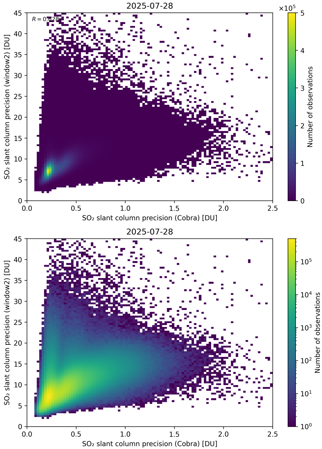
Figure 210: Scatter density plot of “SO 2 slant column precision (Cobra)” against “SO 2 slant column precision (window2)” for 2025-07-27 to 2025-07-29.
