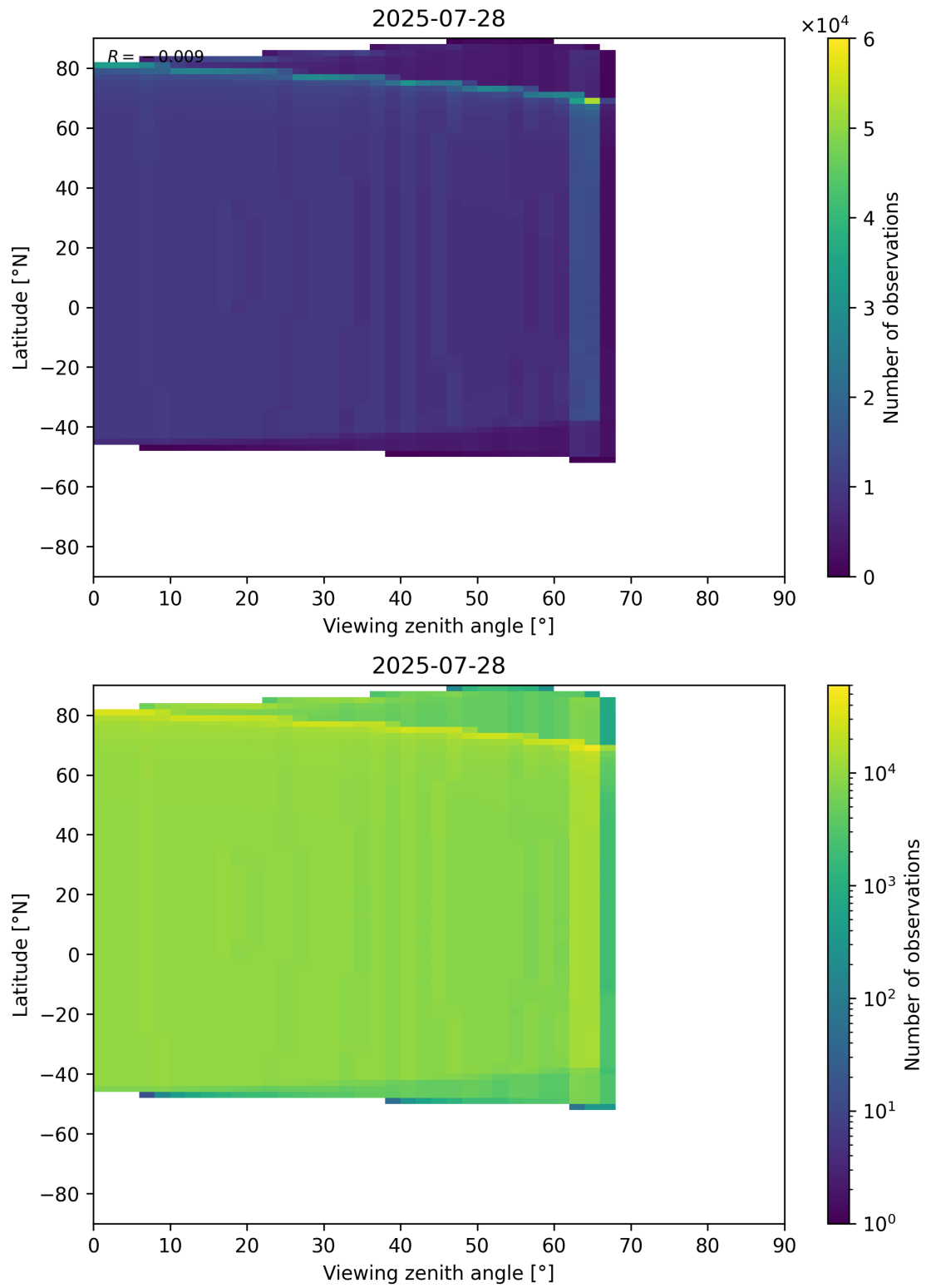
Figure 368: Scatter density plot of “Viewing zenith angle” against “Latitude” for 2025-07-27 to 2025-07-29.
