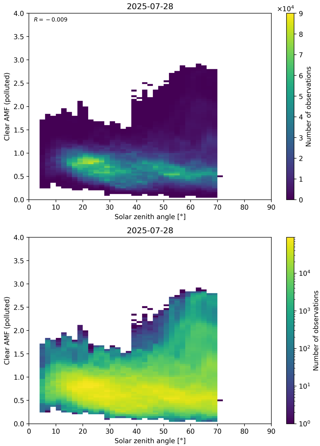
Figure 178: Scatter density plot of “Solar zenith angle” against “Clear AMF (polluted)” for 2025-07-27 to 2025-07-29.
