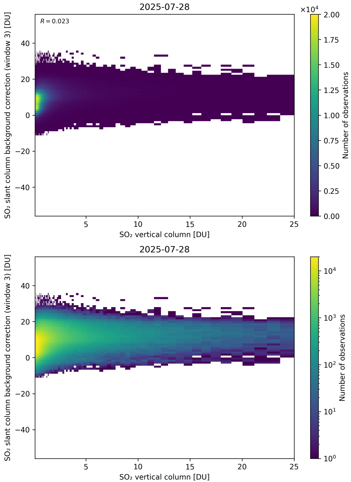
Figure 325: Scatter density plot of “SO 2 vertical column” against “SO 2 slant column background correction (window 3)” for 2025-07-27 to 2025-07-29.
