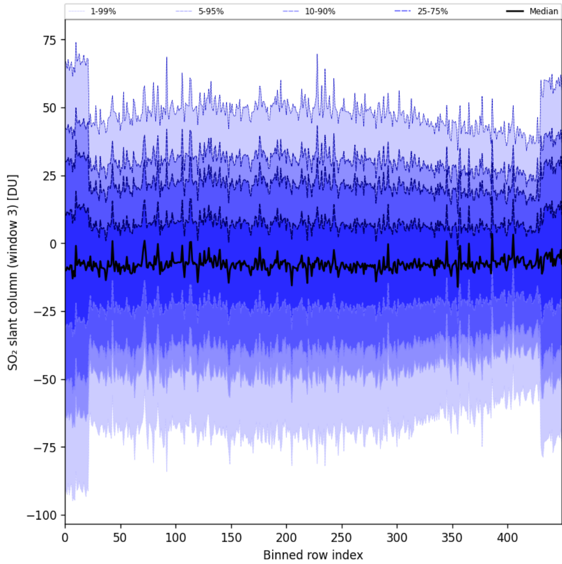
Figure 97: Along track statistics of “SO 2 slant column (window 3)” for 2025-07-27 to 2025-07-29
