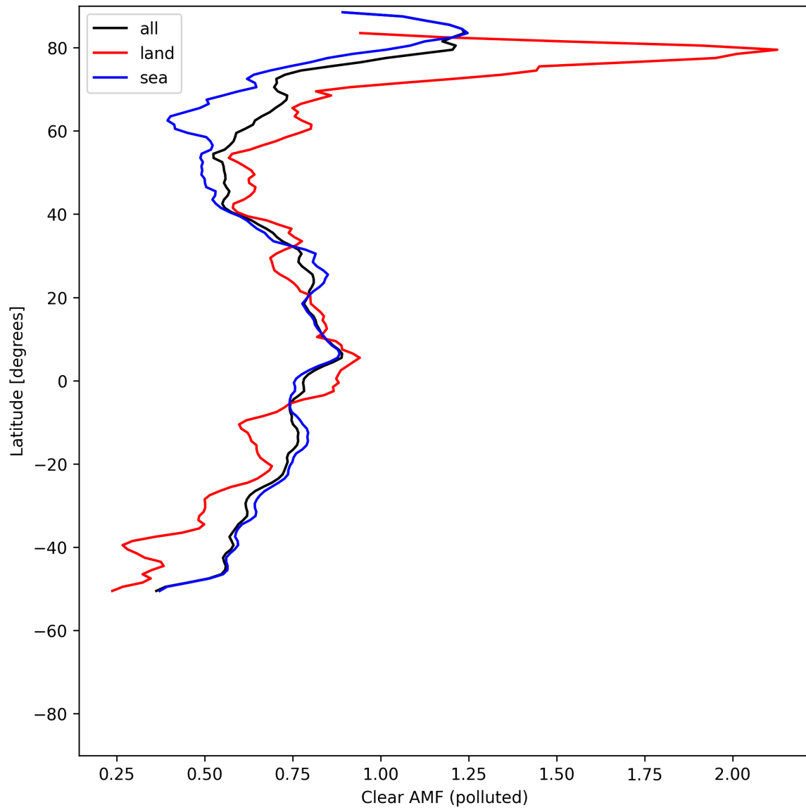
Figure 55: Zonal average of “Clear AMF (polluted)” for 2025-07-27 to 2025-07-29.
