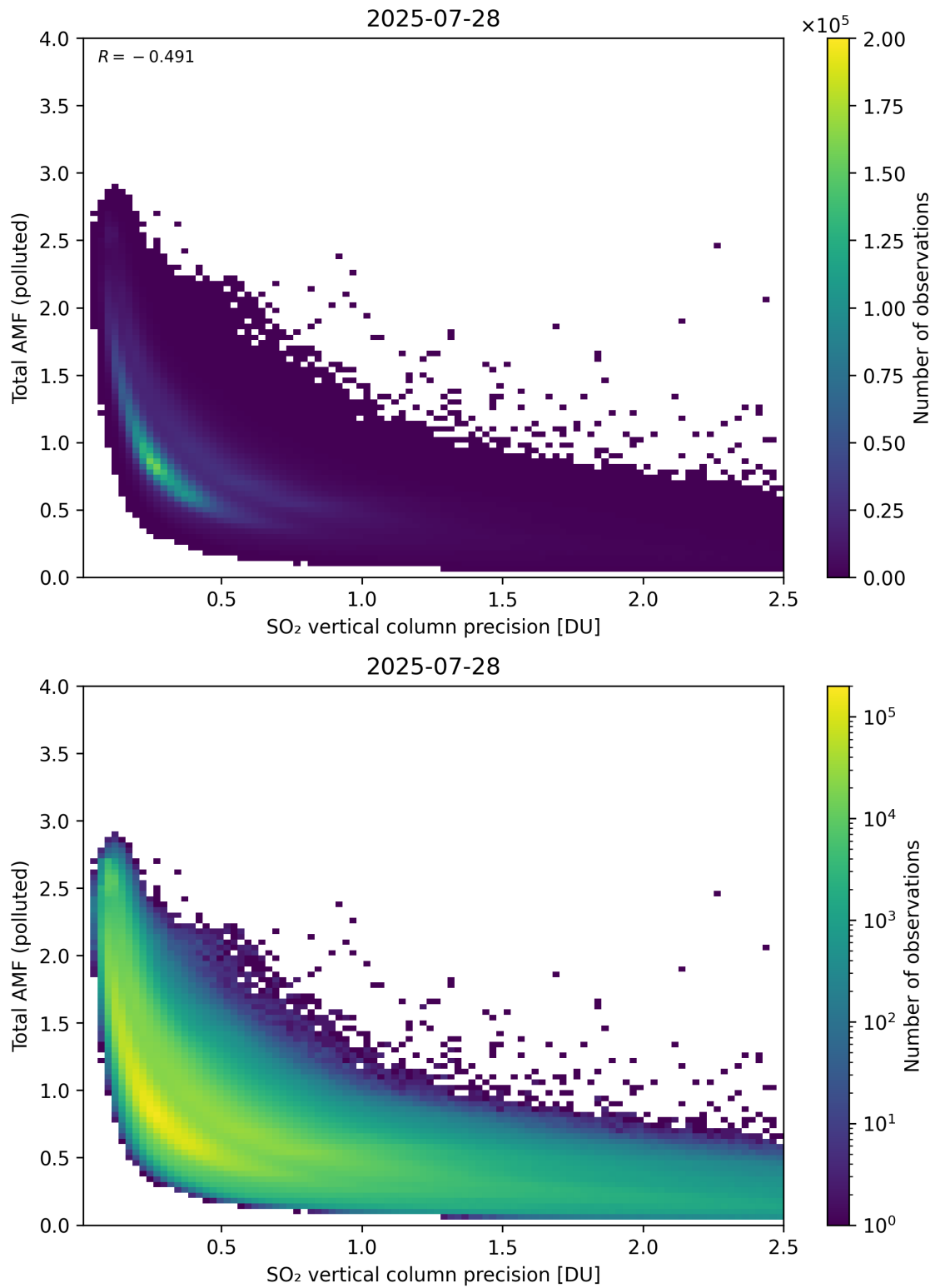
Figure 346: Scatter density plot of “SO 2 vertical column precision” against “Total AMF (polluted)” for 2025-07-27 to 2025-07-29.
