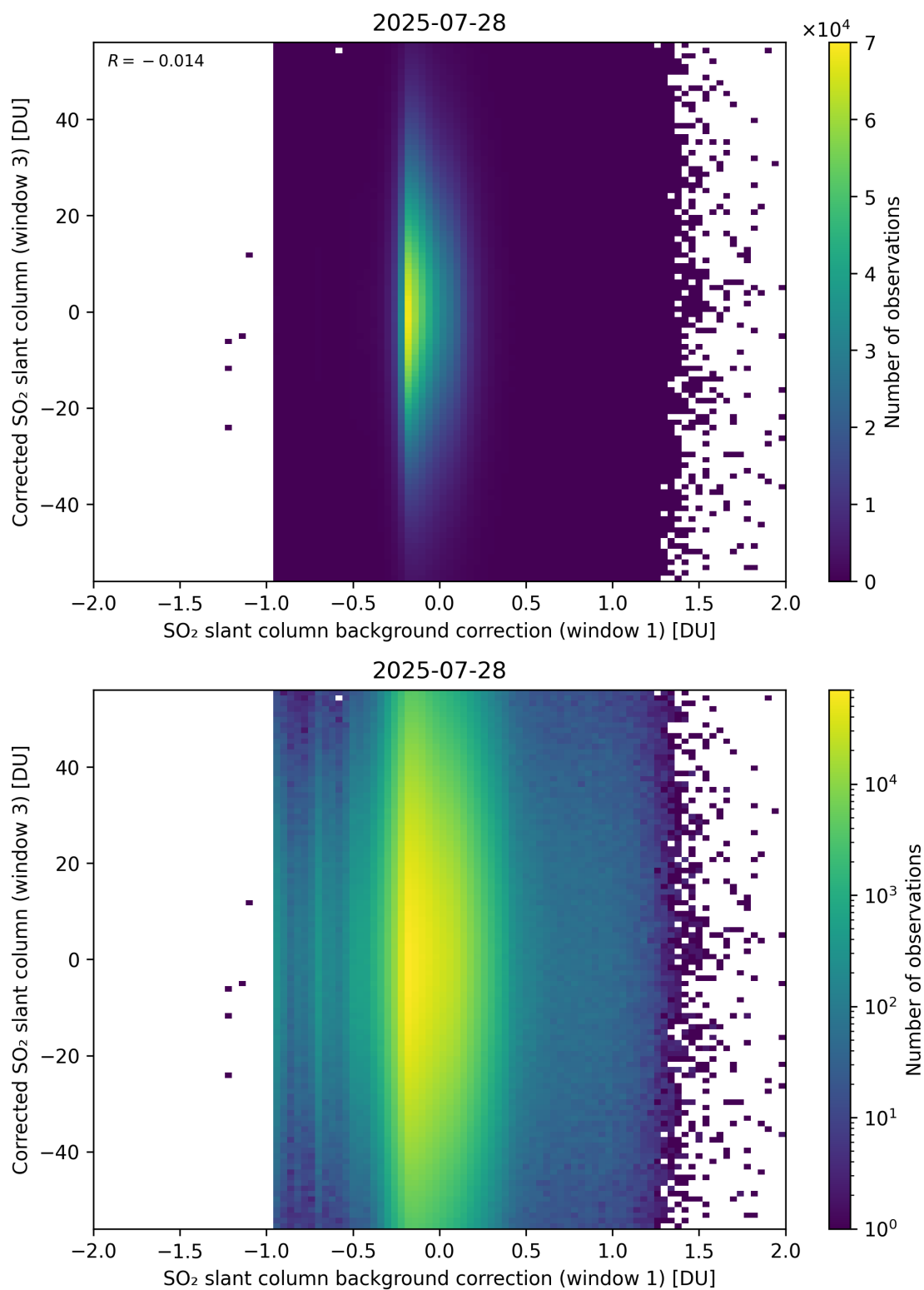
Figure 116: Scatter density plot of “SO 2 slant column background correction (window 1)” against “Corrected SO 2 slant column (window 3)” for 2025-07-27 to 2025-07-29.
