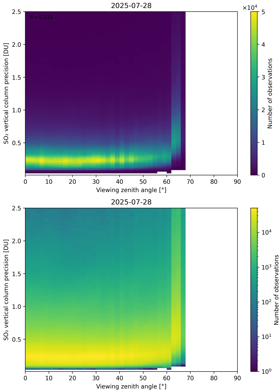
Figure 384: Scatter density plot of “Viewing zenith angle” against “SO 2 vertical column precision” for 2025-07-27 to 2025-07-29.
