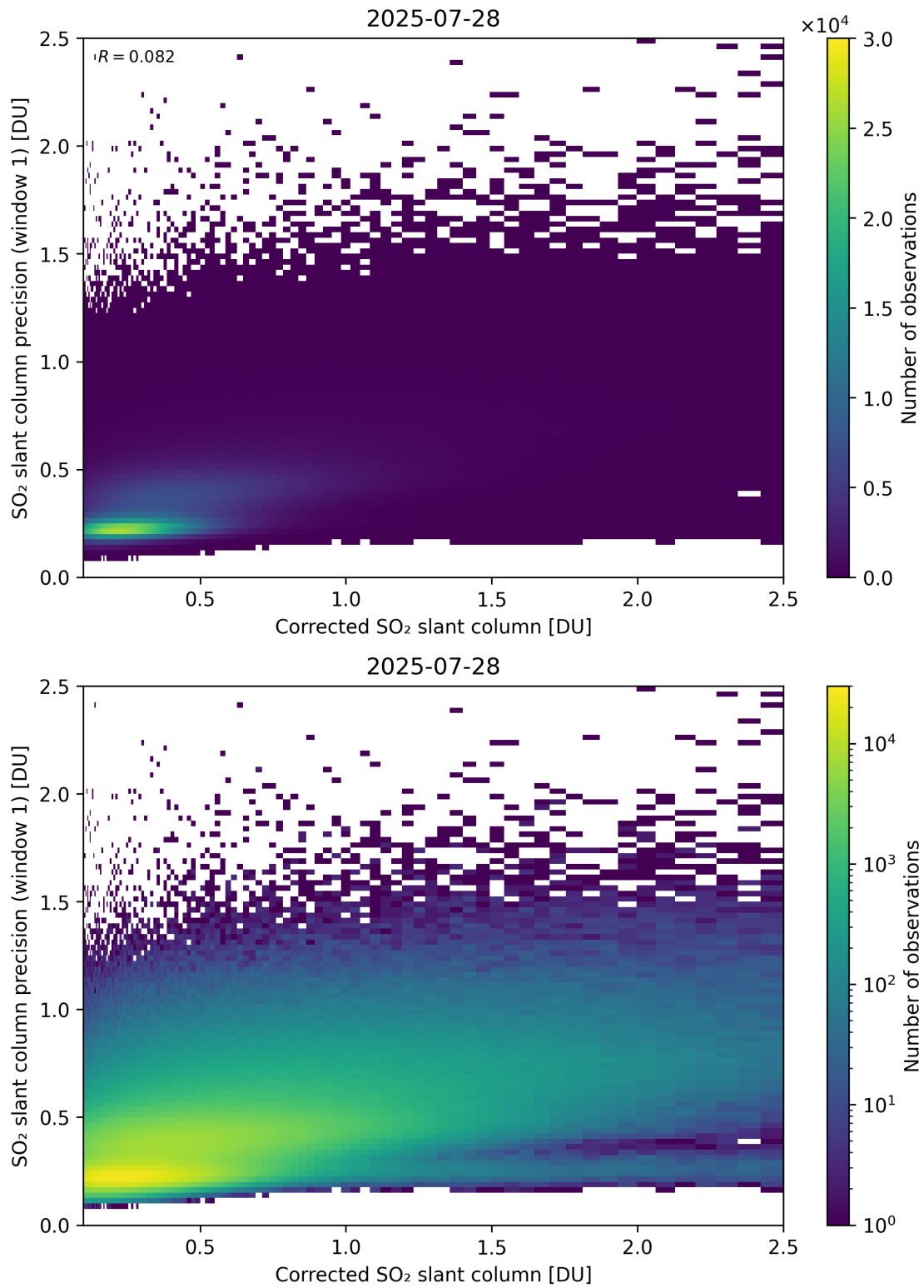
Figure 238: Scatter density plot of “Corrected SO 2 slant column” against “SO 2 slant column precision (window 1)” for 2025-07-27 to 2025-07-29.
