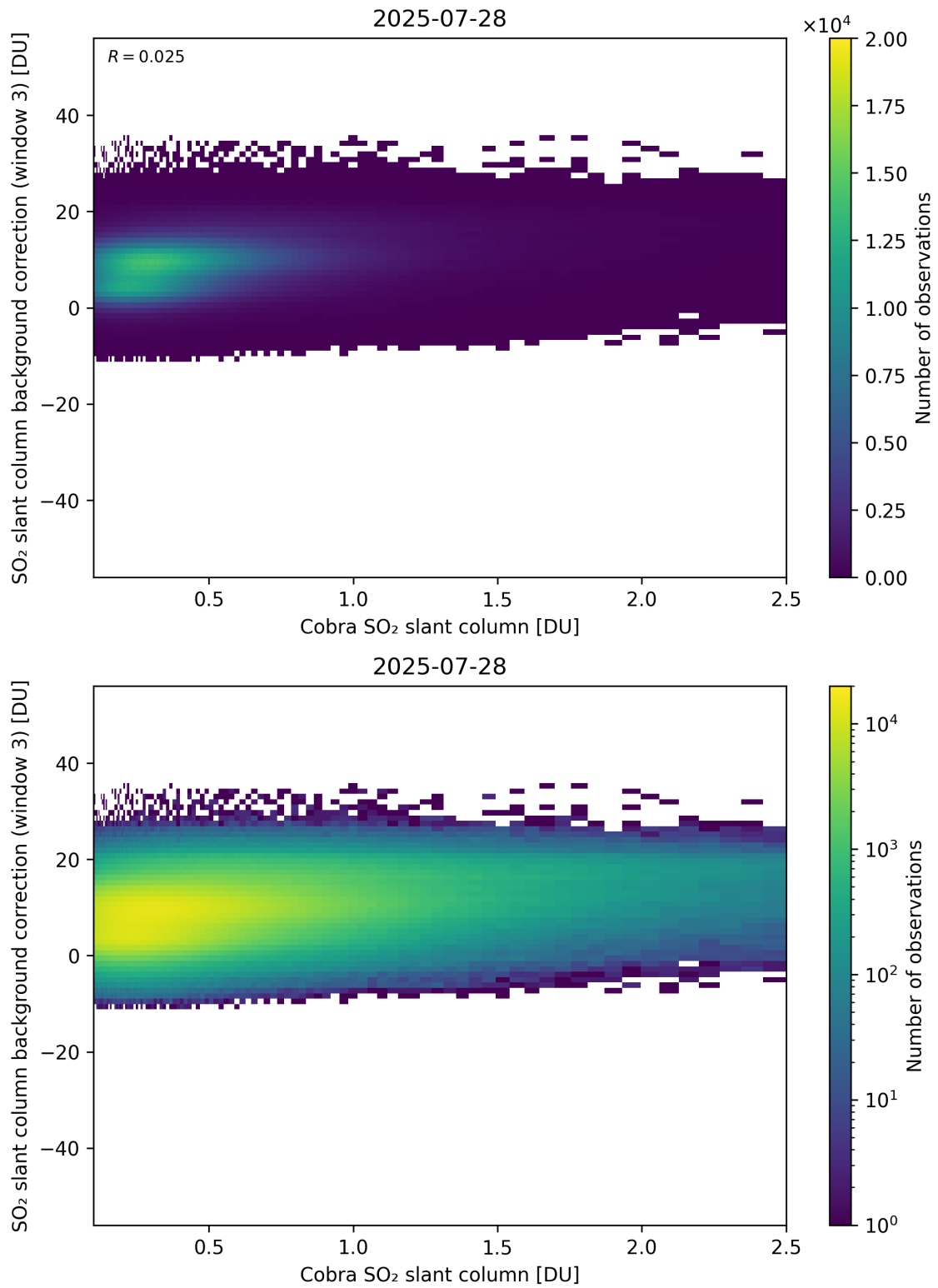
Figure 195: Scatter density plot of “Cobra SO 2 slant column” against “SO 2 slant column background correction (window 3)” for 2025-07-27 to 2025-07-29.
