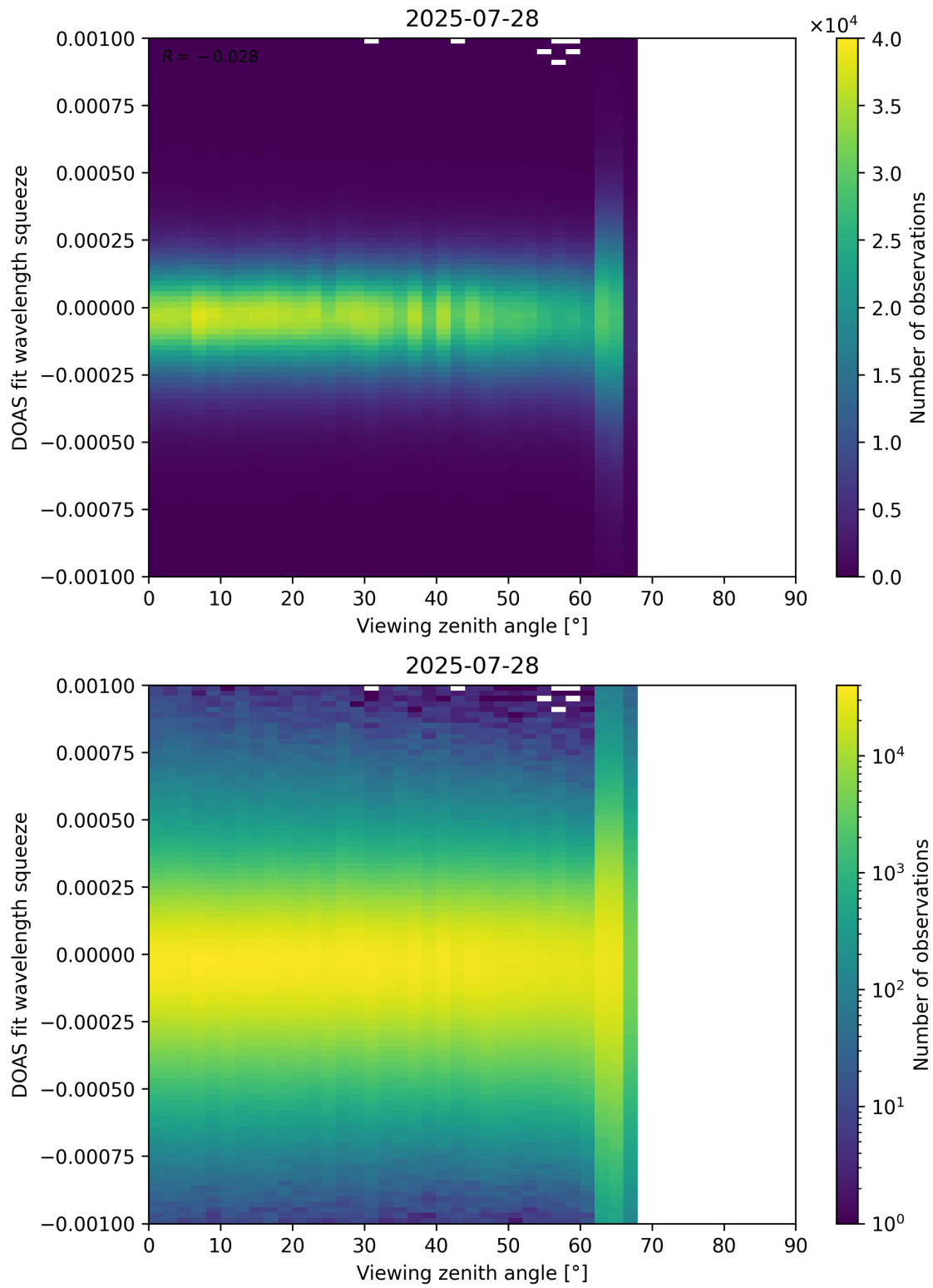
Figure 366: Scatter density plot of “Viewing zenith angle” against “DOAS fit wavelength squeeze” for 2025-07-27 to 2025-07-29.
