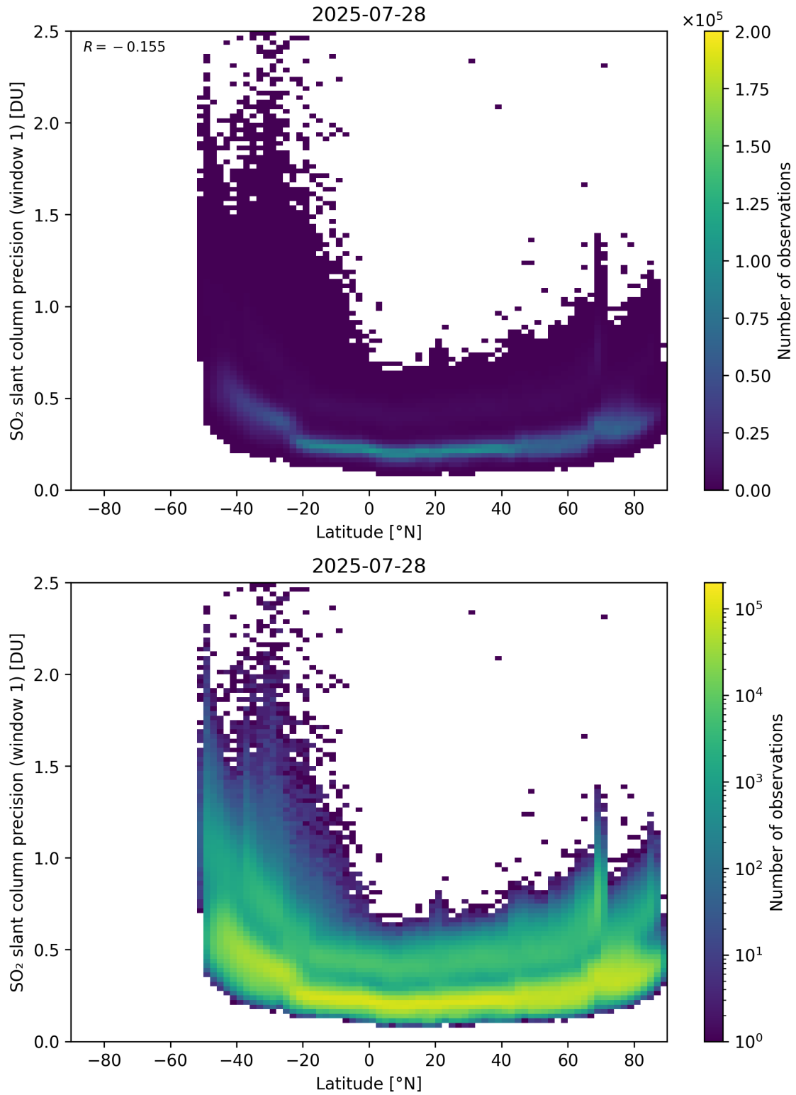
Figure 163: Scatter density plot of “Latitude” against “SO 2 slant column precision (window 1)” for 2025-07-27 to 2025-07-29.
