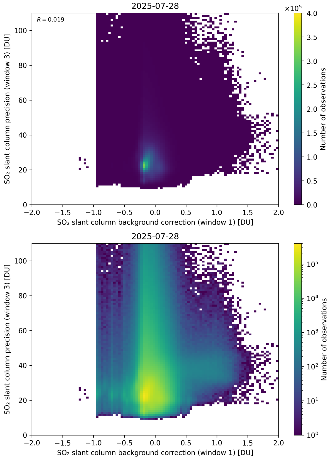
Figure 119: Scatter density plot of “SO 2 slant column background correction (window 1)” against “SO 2 slant column precision (window 3)” for 2025-07-27 to 2025-07-29.
