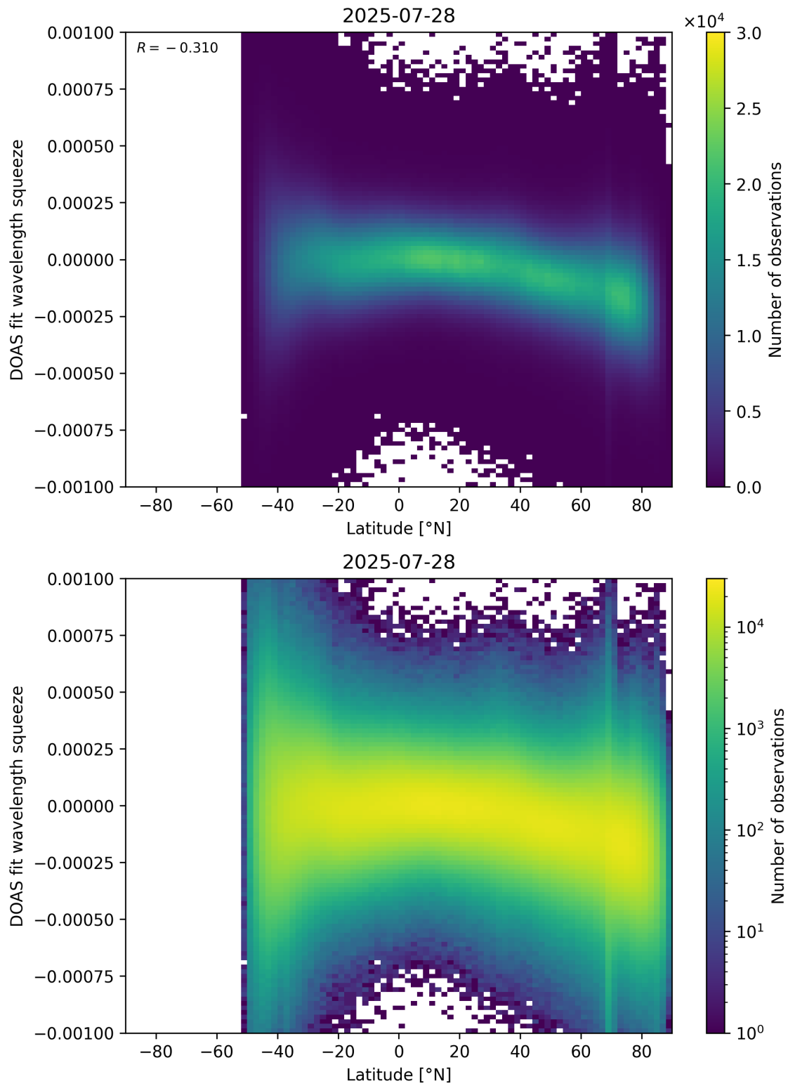
Figure 154: Scatter density plot of “Latitude” against “DOAS fit wavelength squeeze” for 2025-07-27 to 2025-07-29.
