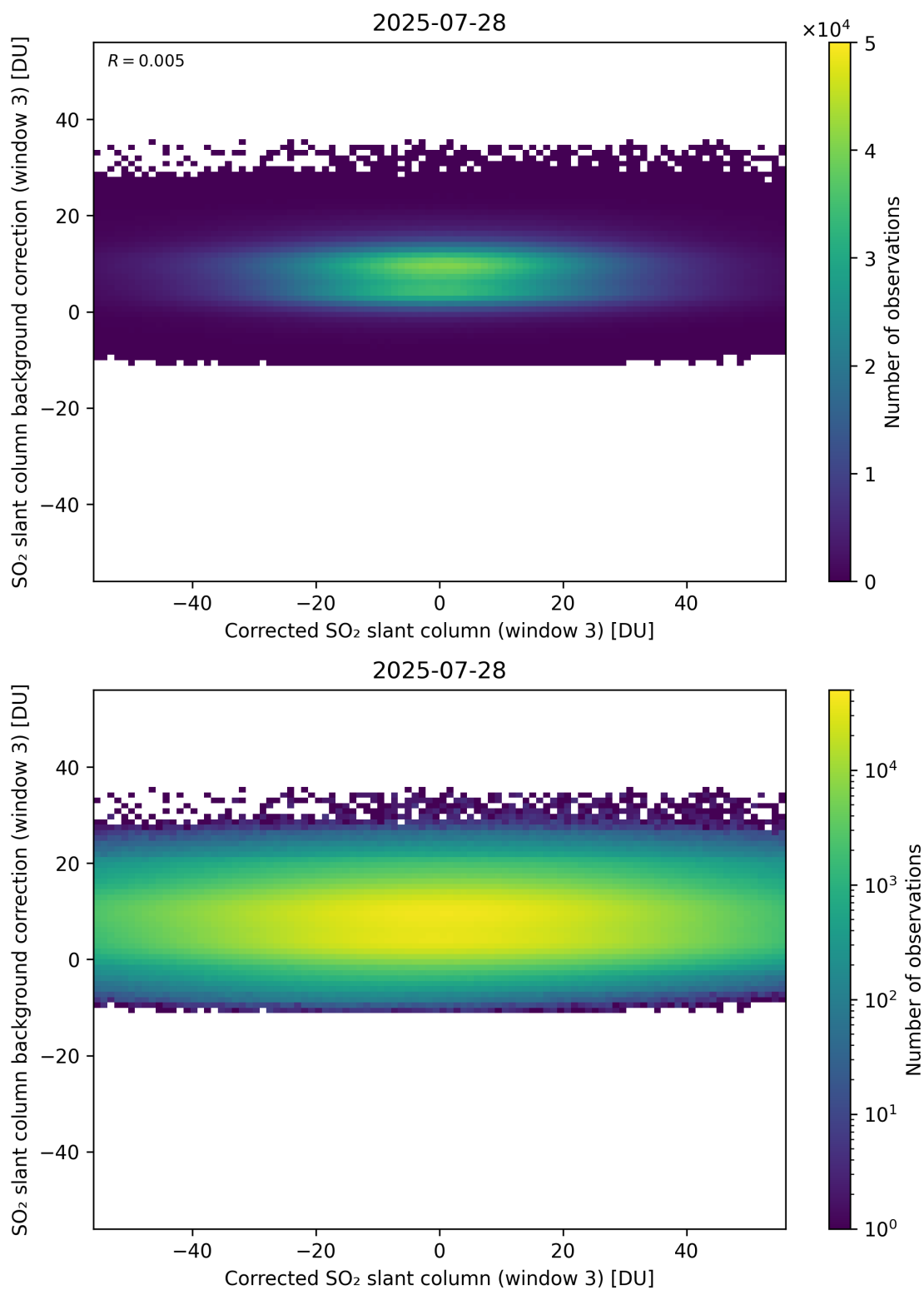
Figure 255: Scatter density plot of “Corrected SO 2 slant column (window 3)” against “SO 2 slant column background correction (window 3)” for 2025-07-27 to 2025-07-29.
