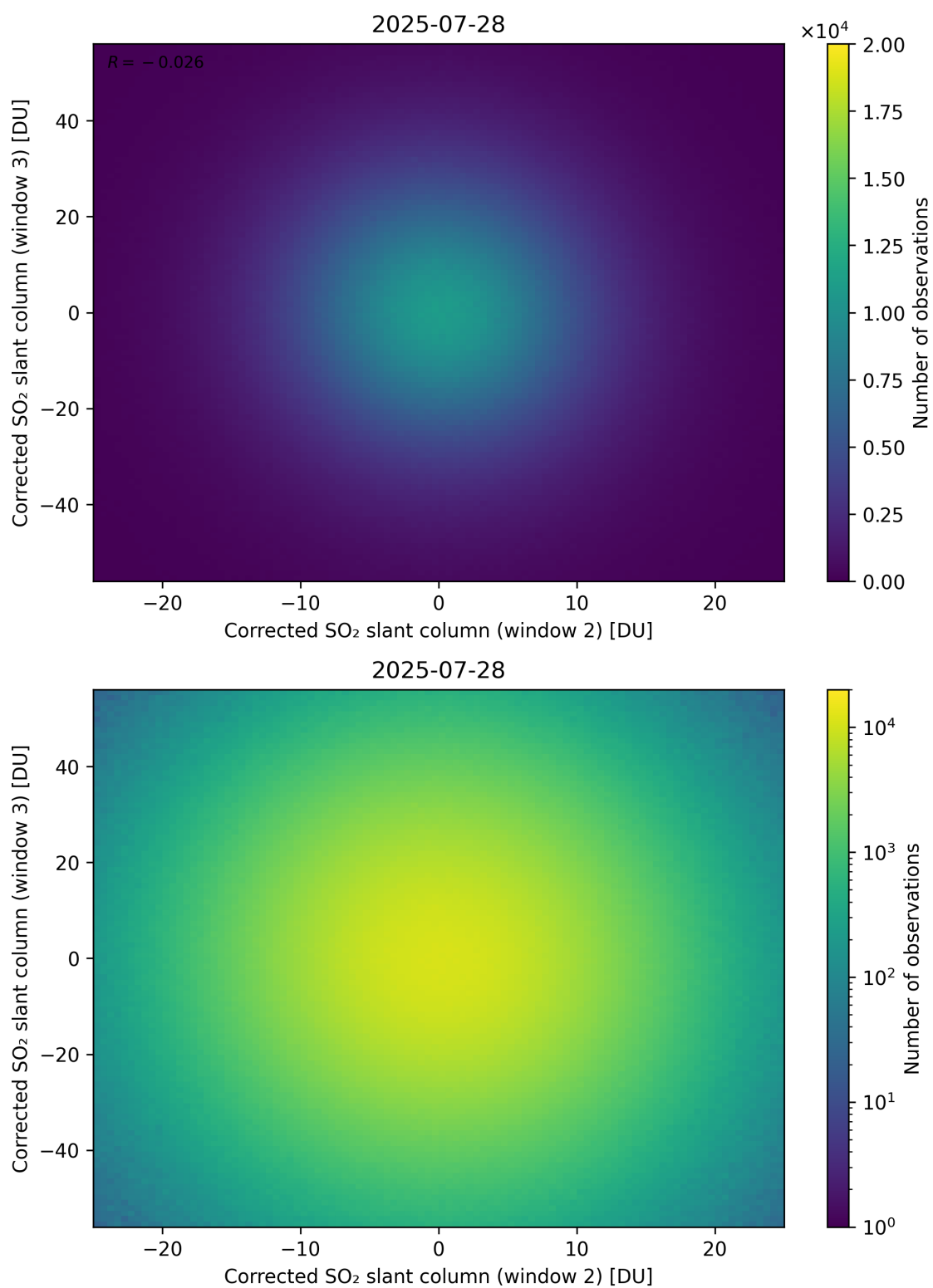
Figure 250: Scatter density plot of “Corrected SO 2 slant column (window 2)” against “Corrected SO 2 slant column (window 3)” for 2025-07-27 to 2025-07-29.
