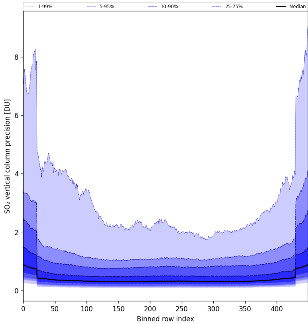
Figure 85: Along track statistics of “SO 2 vertical column precision” for 2025-07-27 to 2025-07-29
