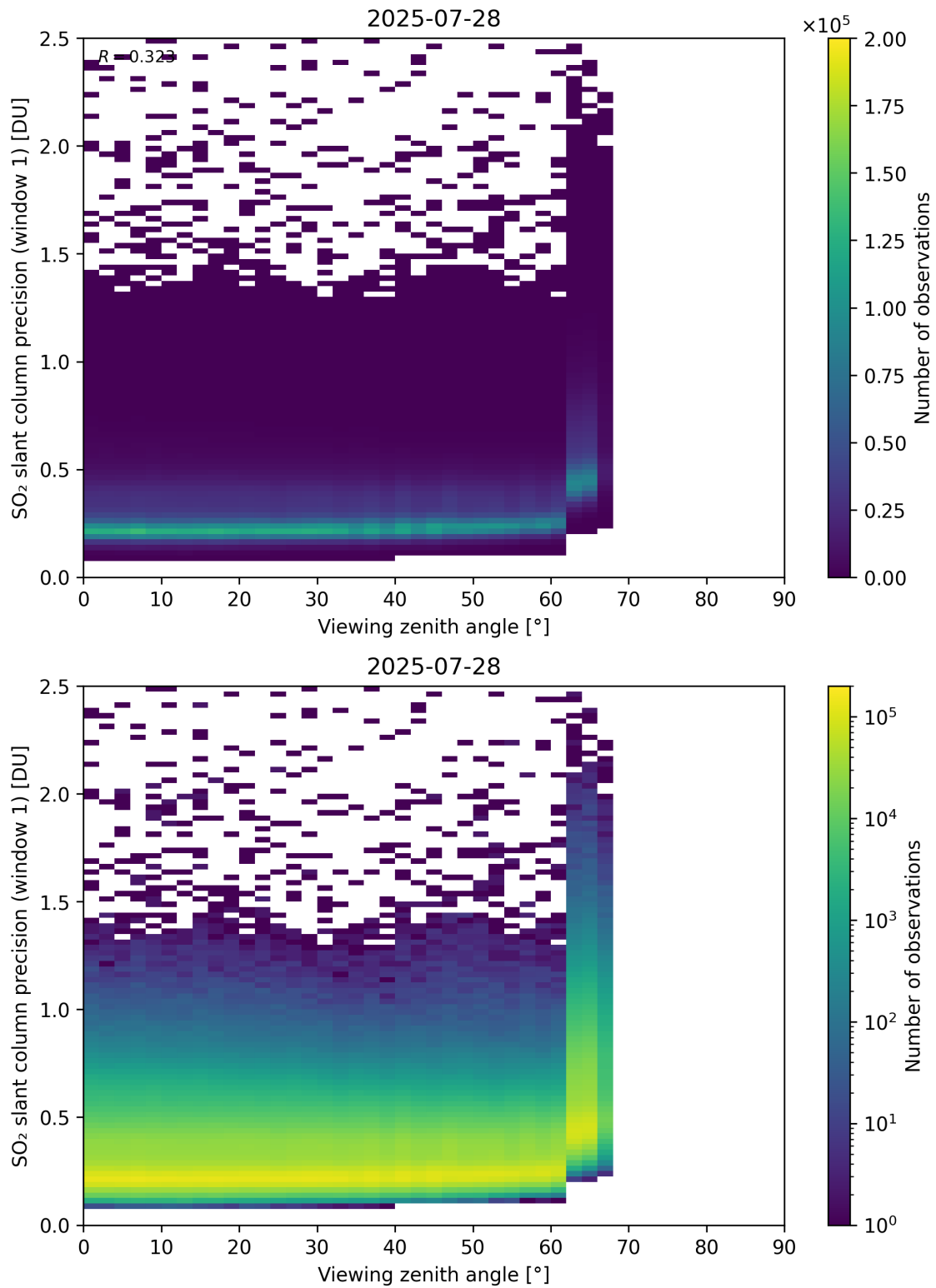
Figure 377: Scatter density plot of “Viewing zenith angle” against “SO 2 slant column precision (window 1)” for 2025-07-27 to 2025-07-29.
