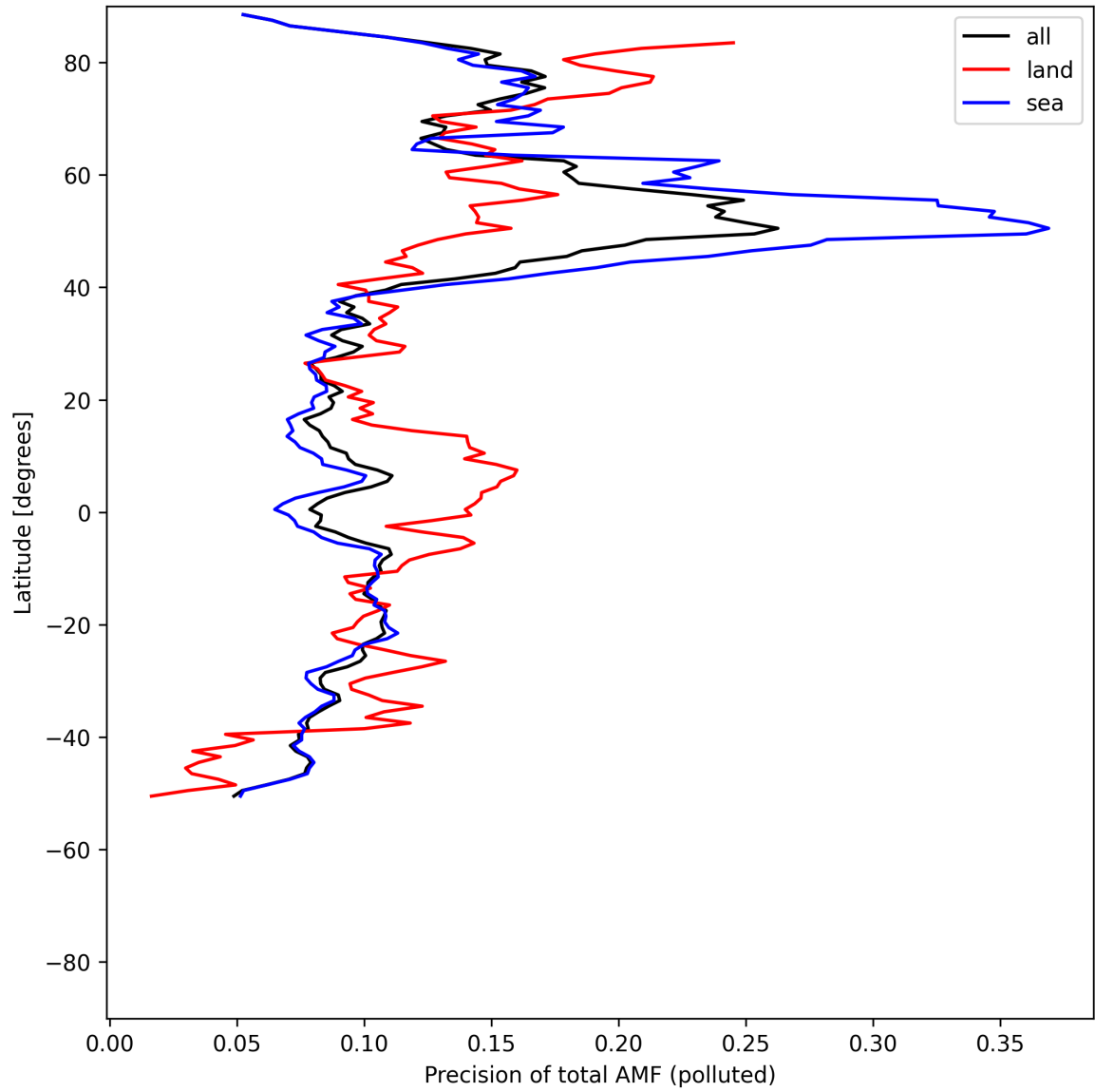
Figure 54: Zonal average of “Precision of total AMF (polluted)” for 2025-07-27 to 2025-07-29.
