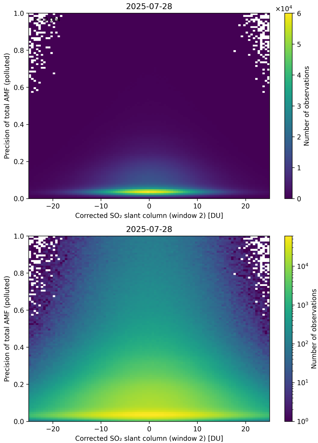
Figure 254: Scatter density plot of “Corrected SO 2 slant column (window 2)” against “Precision of total AMF (polluted)” for 2025-07-27 to 2025-07-29.
