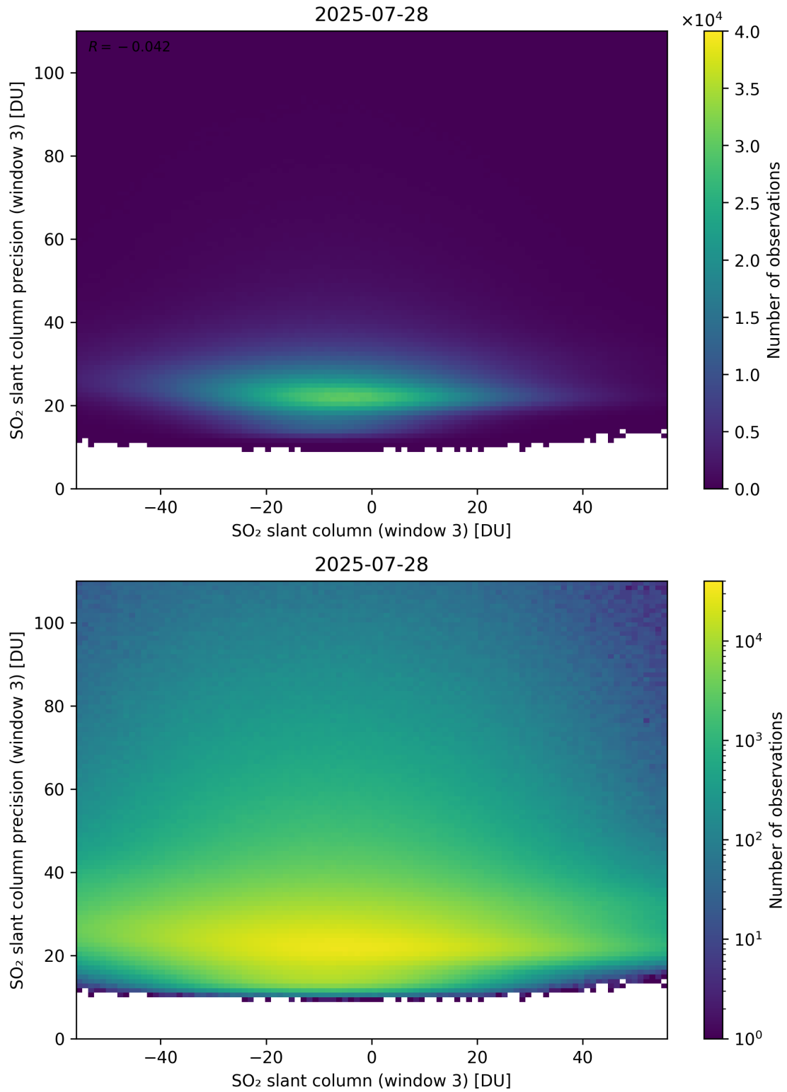
Figure 317: Scatter density plot of “SO 2 slant column (window 3)” against “SO 2 slant column precision (window 3)” for 2025-07-27 to 2025-07-29.
