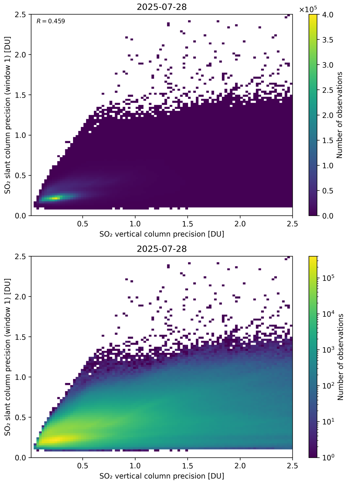
Figure 342: Scatter density plot of “SO 2 vertical column precision” against “SO 2 slant column precision (window 1)” for 2025-07-27 to 2025-07-29.
