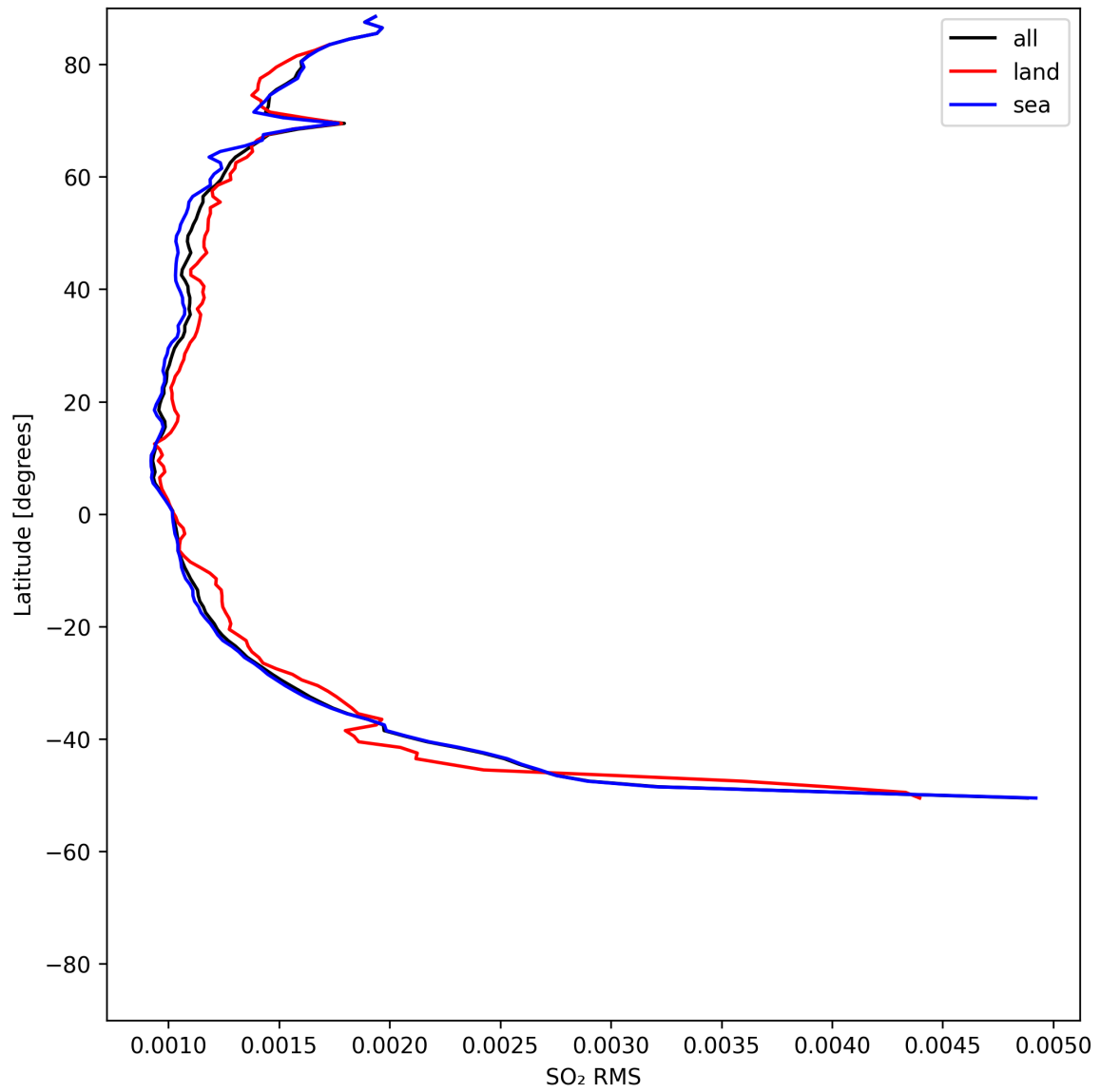
Figure 52: Zonal average of “SO 2 RMS” for 2025-07-27 to 2025-07-29.
