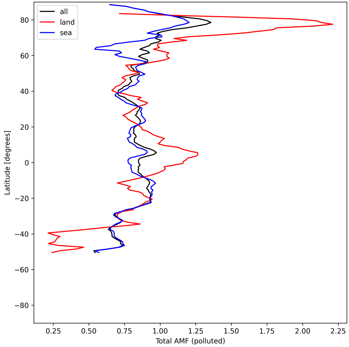
Figure 53: Zonal average of “Total AMF (polluted)” for 2025-07-27 to 2025-07-29.
