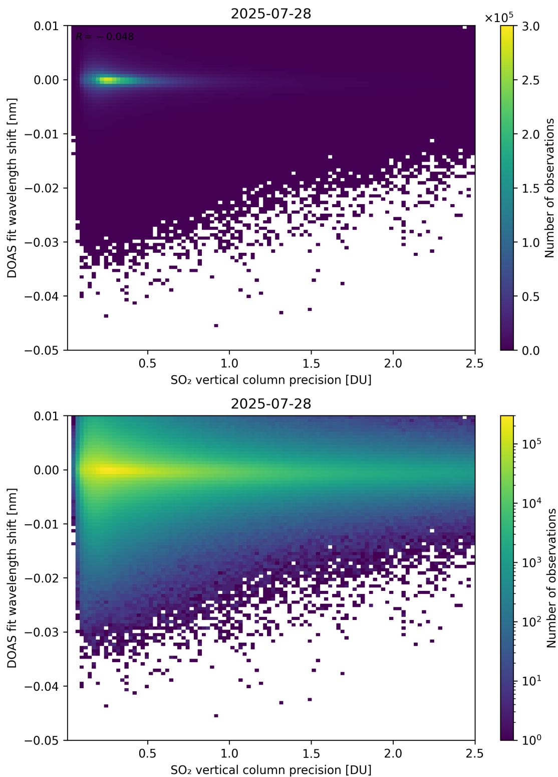
Figure 332: Scatter density plot of “SO 2 vertical column precision” against “DOAS fit wavelength shift” for 2025-07-27 to 2025-07-29.
