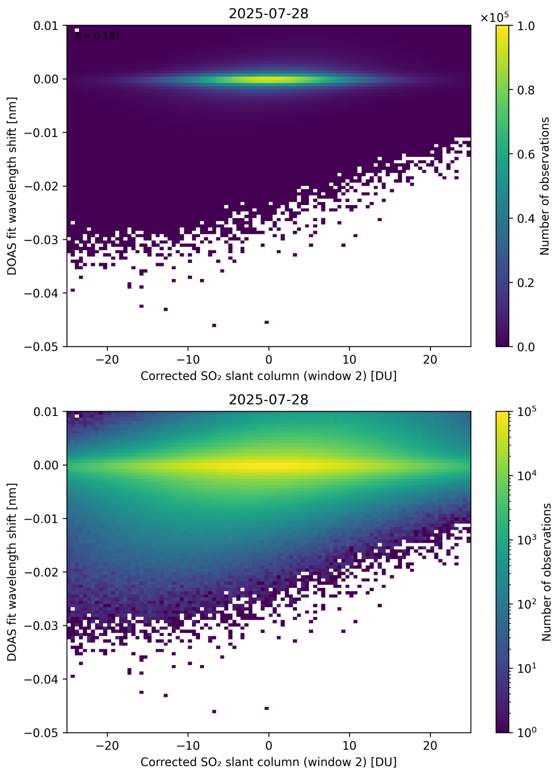
Figure 246: Scatter density plot of “Corrected SO 2 slant column (window 2)” against “DOAS fit wavelength shift” for 2025-07-27 to 2025-07-29.
