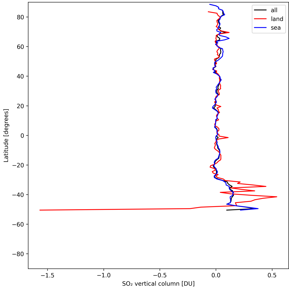
Figure 32: Zonal average of “SO 2 vertical column” for 2025-07-27 to 2025-07-29.
