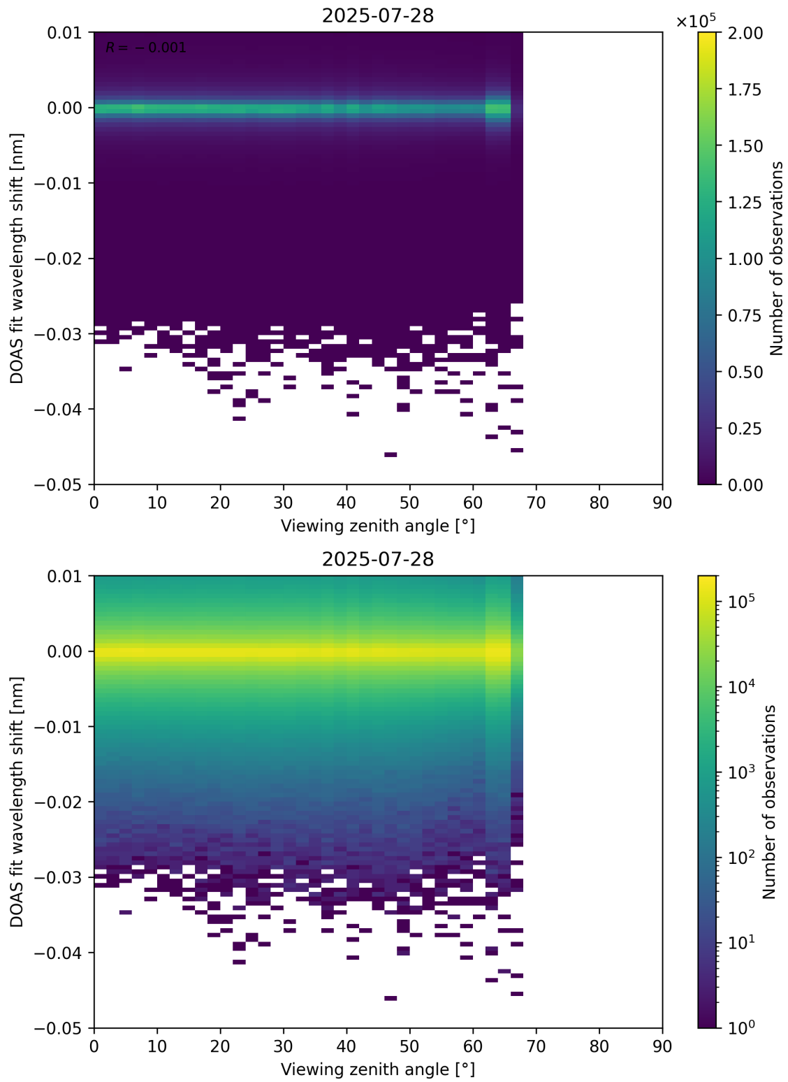
Figure 365: Scatter density plot of “Viewing zenith angle” against “DOAS fit wavelength shift” for 2025-07-27 to 2025-07-29.
