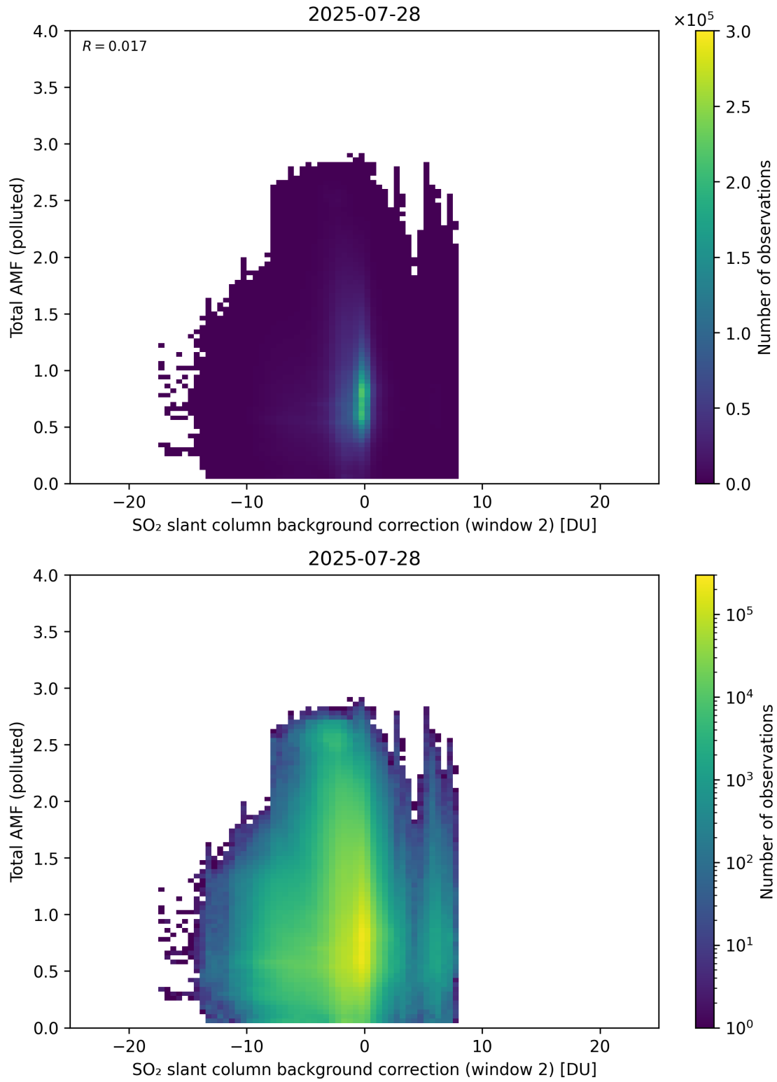
Figure 130: Scatter density plot of “SO 2 slant column background correction (window 2)” against “Total AMF (polluted)” for 2025-07-27 to 2025-07-29.
