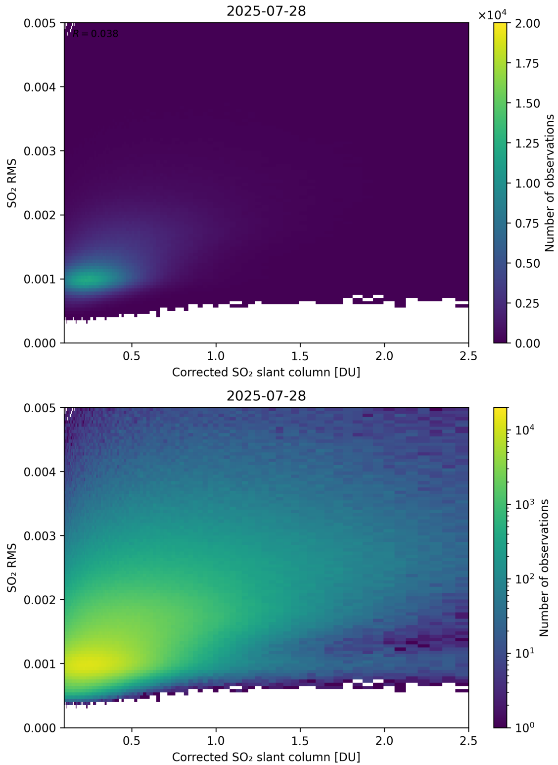
Figure 231: Scatter density plot of “Corrected SO 2 slant column” against “SO 2 RMS” for 2025-07-27 to 2025-07-29.
