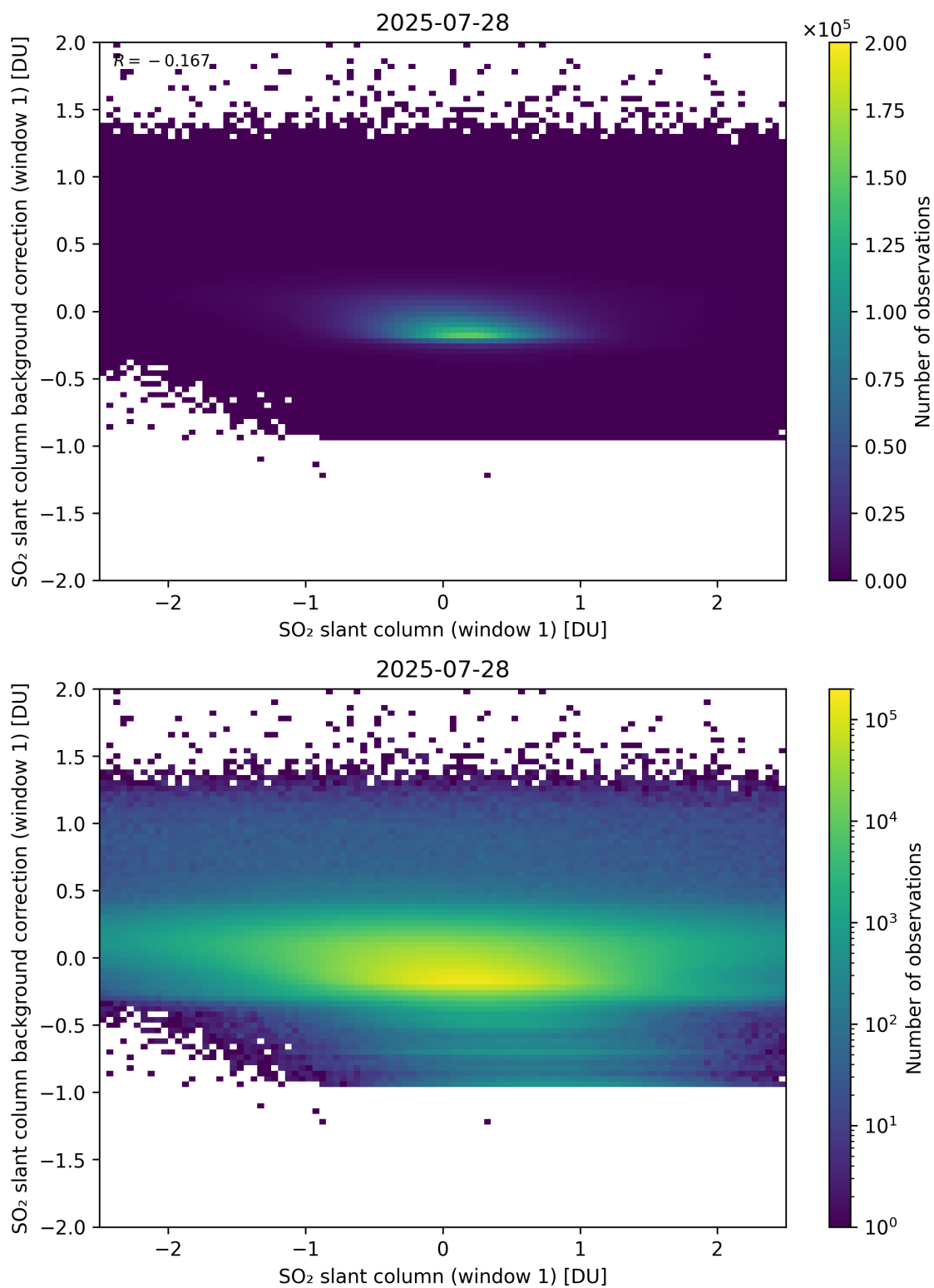
Figure 262: Scatter density plot of “SO 2 slant column (window 1)” against “SO 2 slant column background correction (window 1)” for 2025-07-27 to 2025-07-29.
