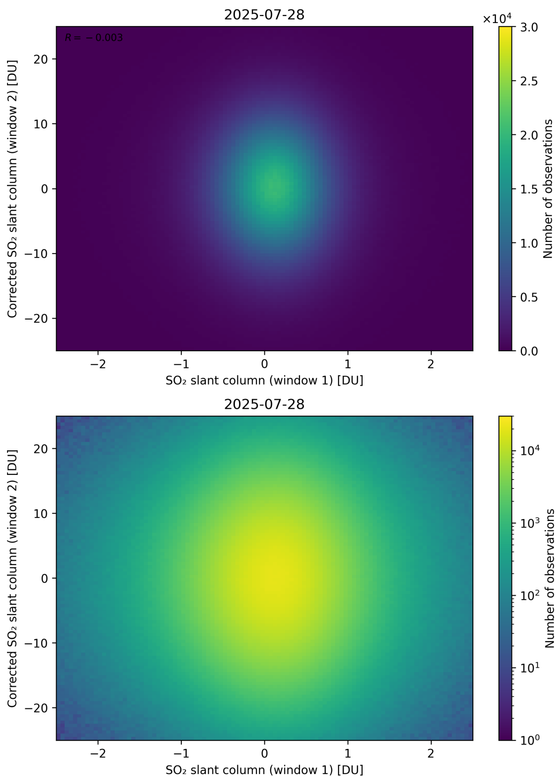
Figure 283: Scatter density plot of “SO 2 slant column (window 1)” against “Corrected SO 2 slant column (window 2)” for 2025-07-27 to 2025-07-29.
