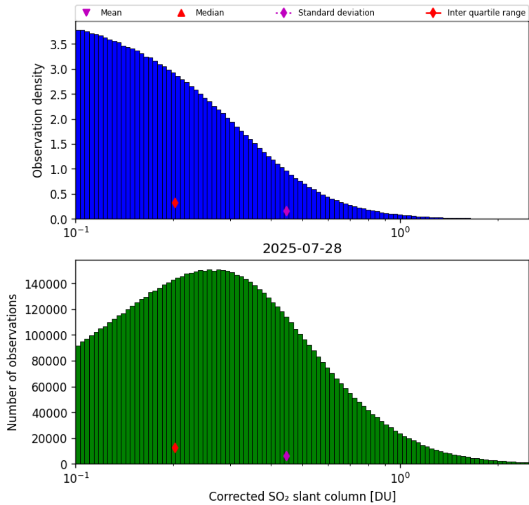
Figure 60: Histogram of “Corrected SO 2 slant column” for 2025-07-27 to 2025-07-29
