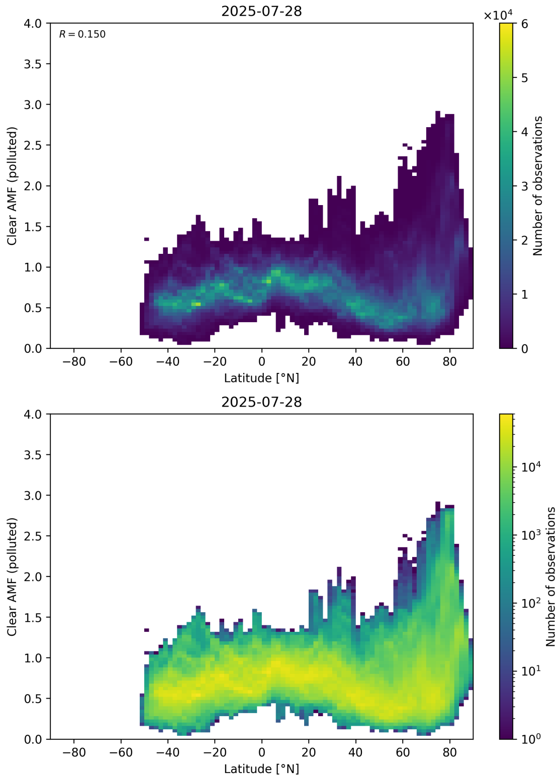
Figure 156: Scatter density plot of “Latitude” against “Clear AMF (polluted)” for 2025-07-27 to 2025-07-29.
