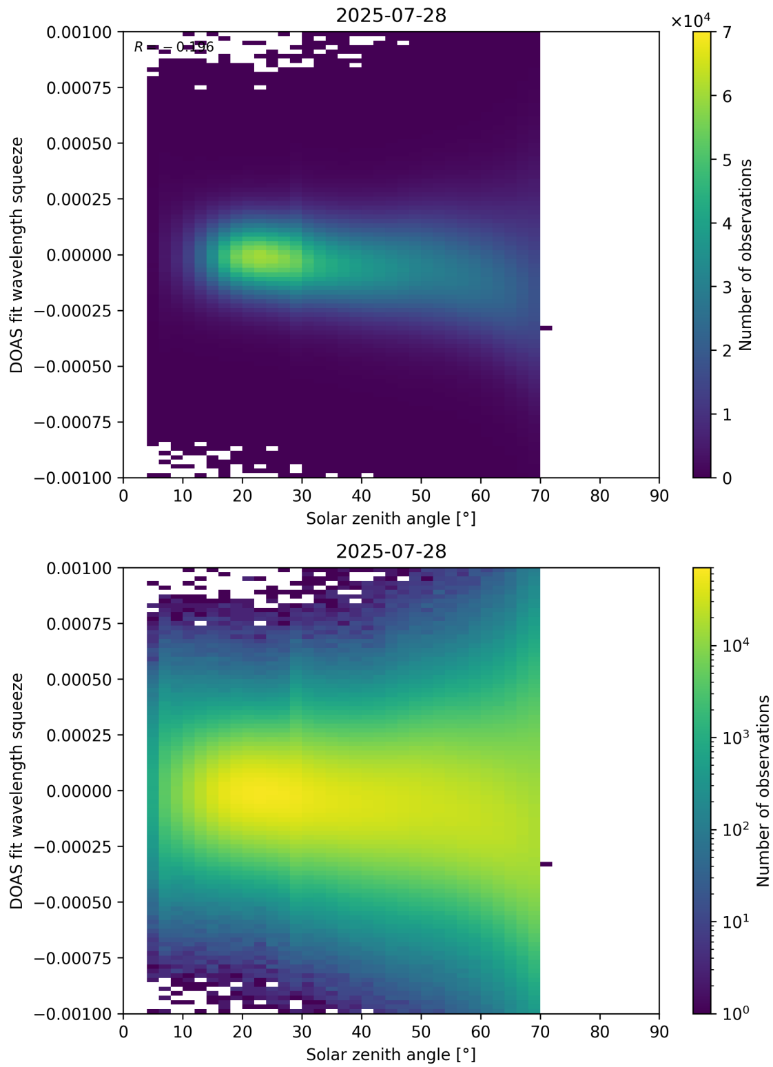
Figure 175: Scatter density plot of “Solar zenith angle” against “DOAS fit wavelength squeeze” for 2025-07-27 to 2025-07-29.
