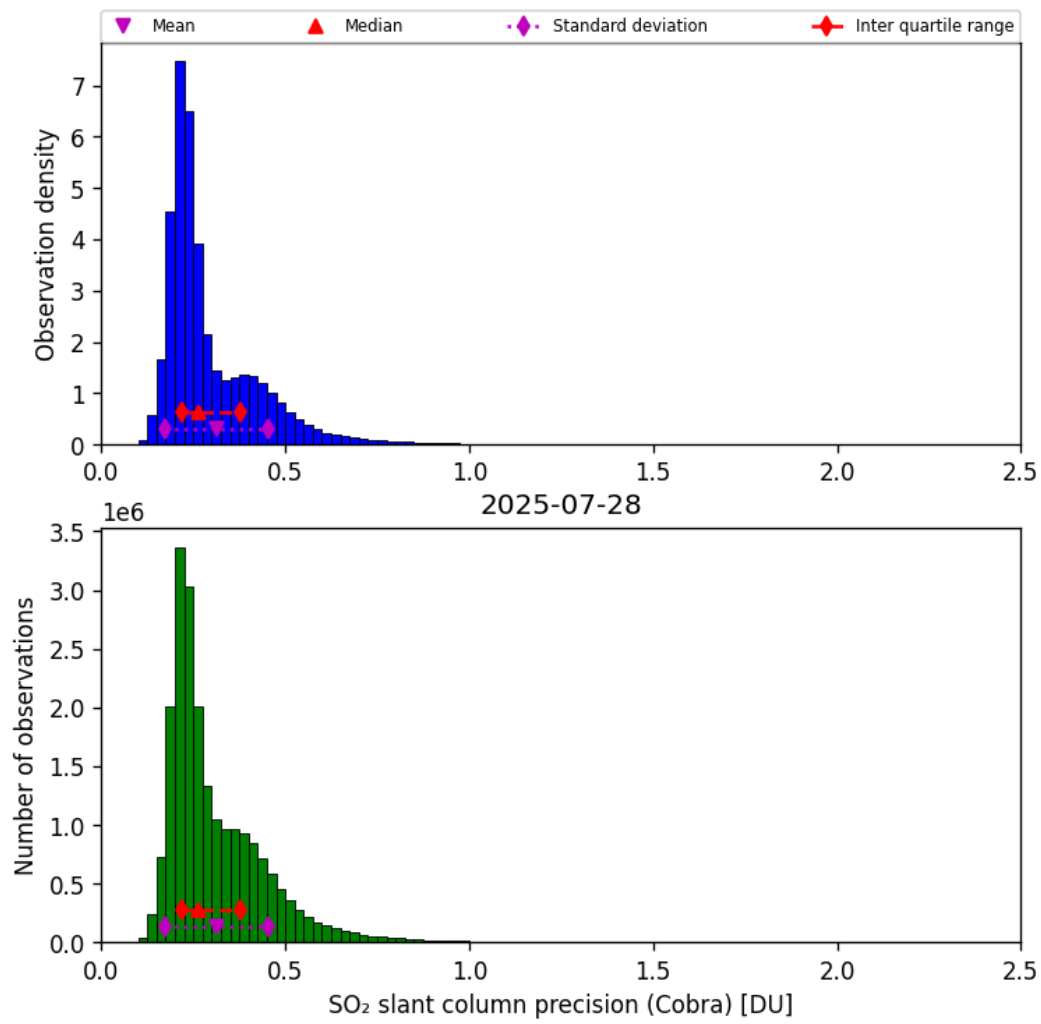
Figure 62: Histogram of “SO 2 slant column precision (Cobra)” for 2025-07-27 to 2025-07-29
