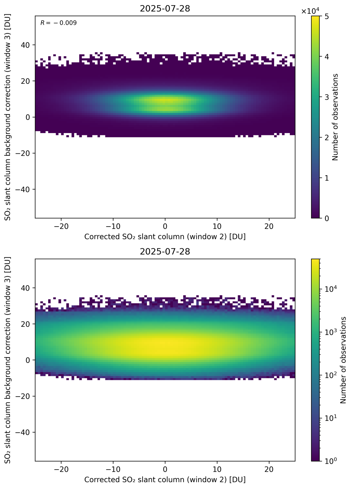
Figure 245: Scatter density plot of “Corrected SO 2 slant column (window 2)” against “SO 2 slant column background correction (window 3)” for 2025-07-27 to 2025-07-29.
