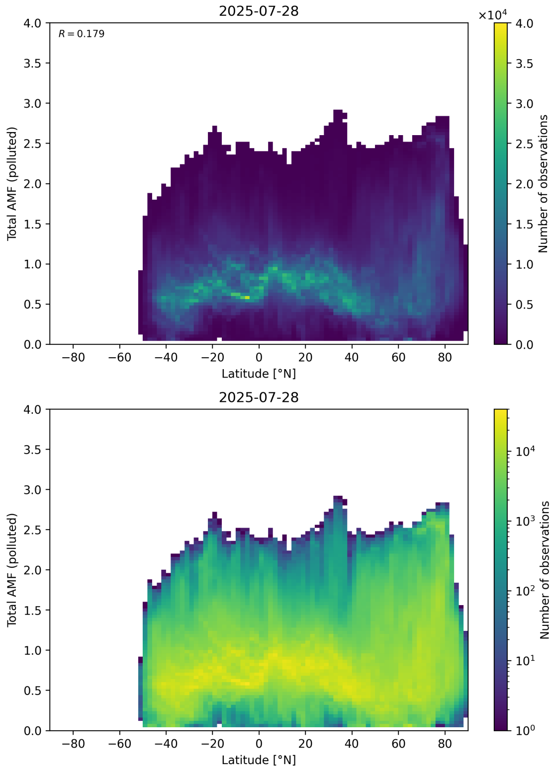
Figure 167: Scatter density plot of “Latitude” against “Total AMF (polluted)” for 2025-07-27 to 2025-07-29.
