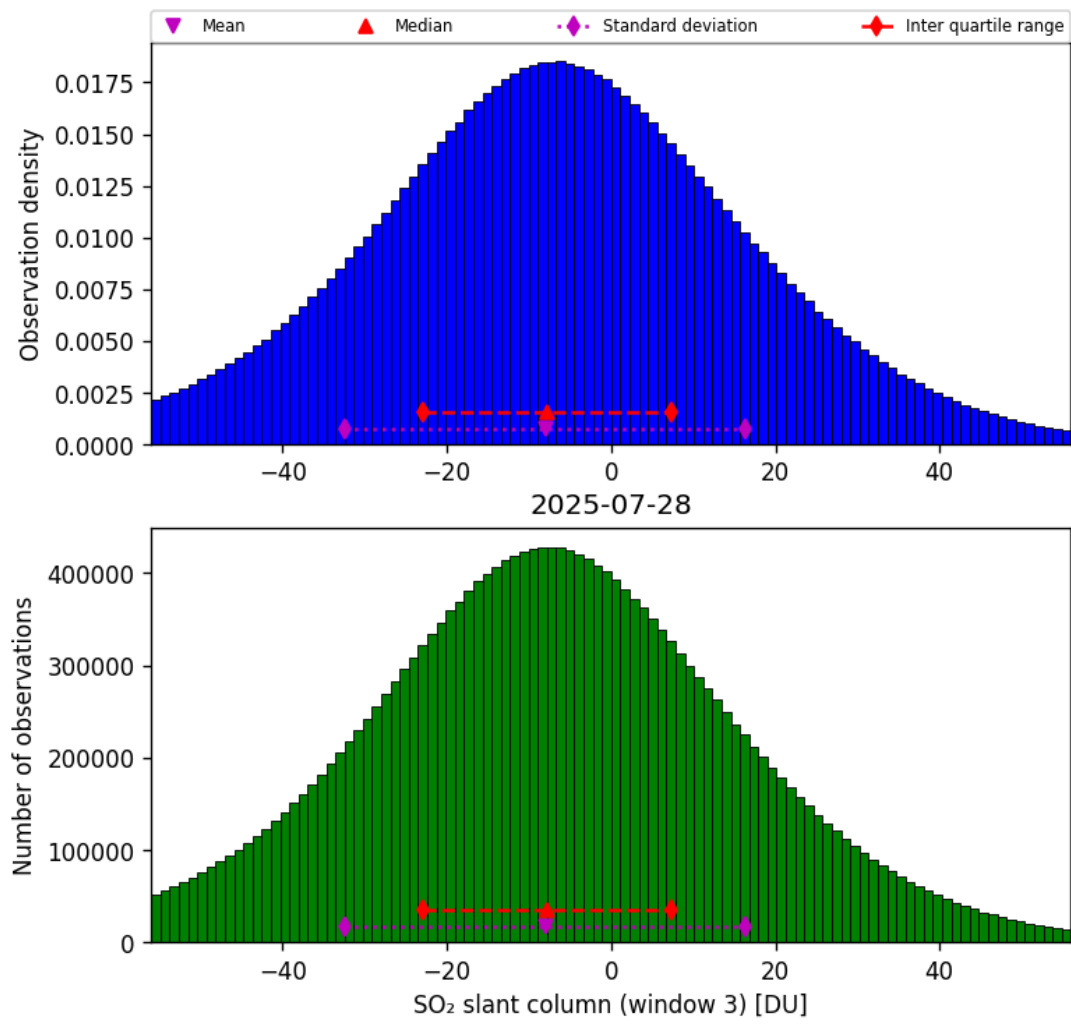
Figure 71: Histogram of “SO 2 slant column (window 3)” for 2025-07-27 to 2025-07-29
