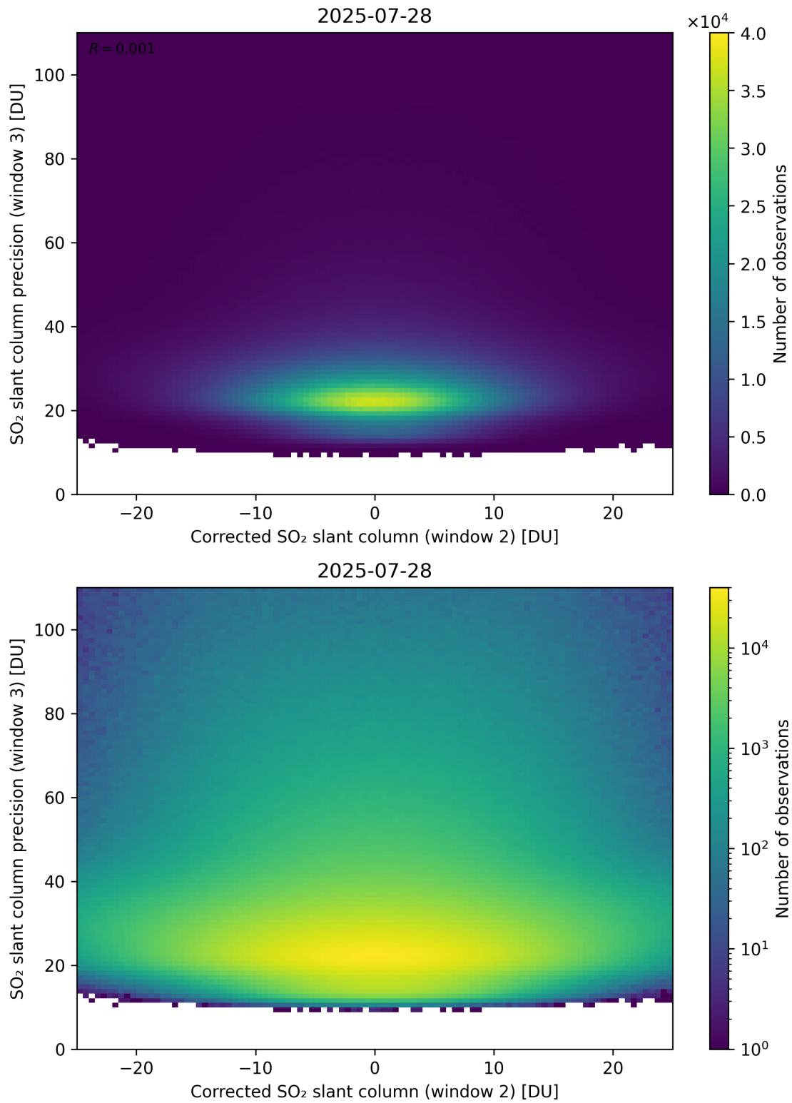
Figure 252: Scatter density plot of “Corrected SO 2 slant column (window 2)” against “SO 2 slant column precision (window 3)” for 2025-07-27 to 2025-07-29.
