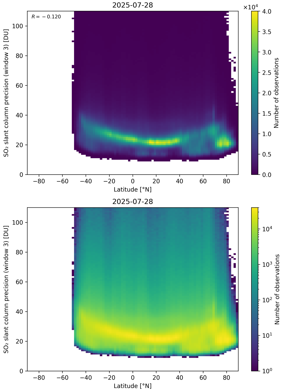
Figure 166: Scatter density plot of “Latitude” against “SO 2 slant column precision (window 3)” for 2025-07-27 to 2025-07-29.
