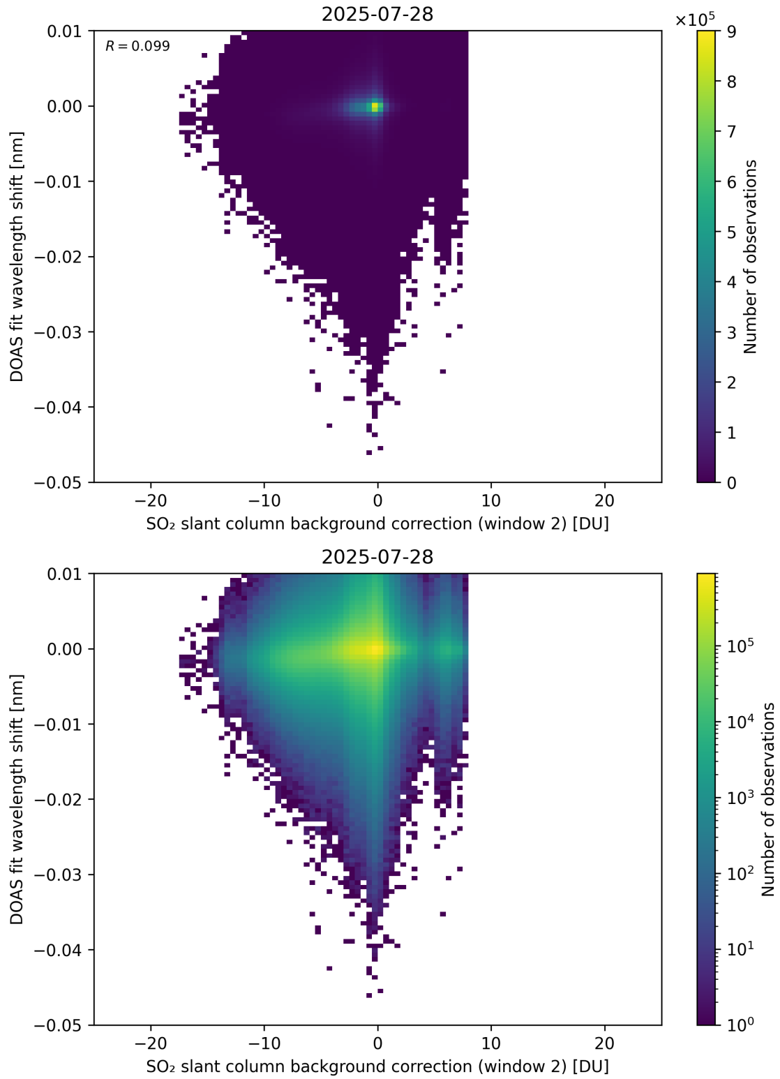
Figure 123: Scatter density plot of “SO 2 slant column background correction (window 2)” against “DOAS fit wavelength shift” for 2025-07-27 to 2025-07-29.
