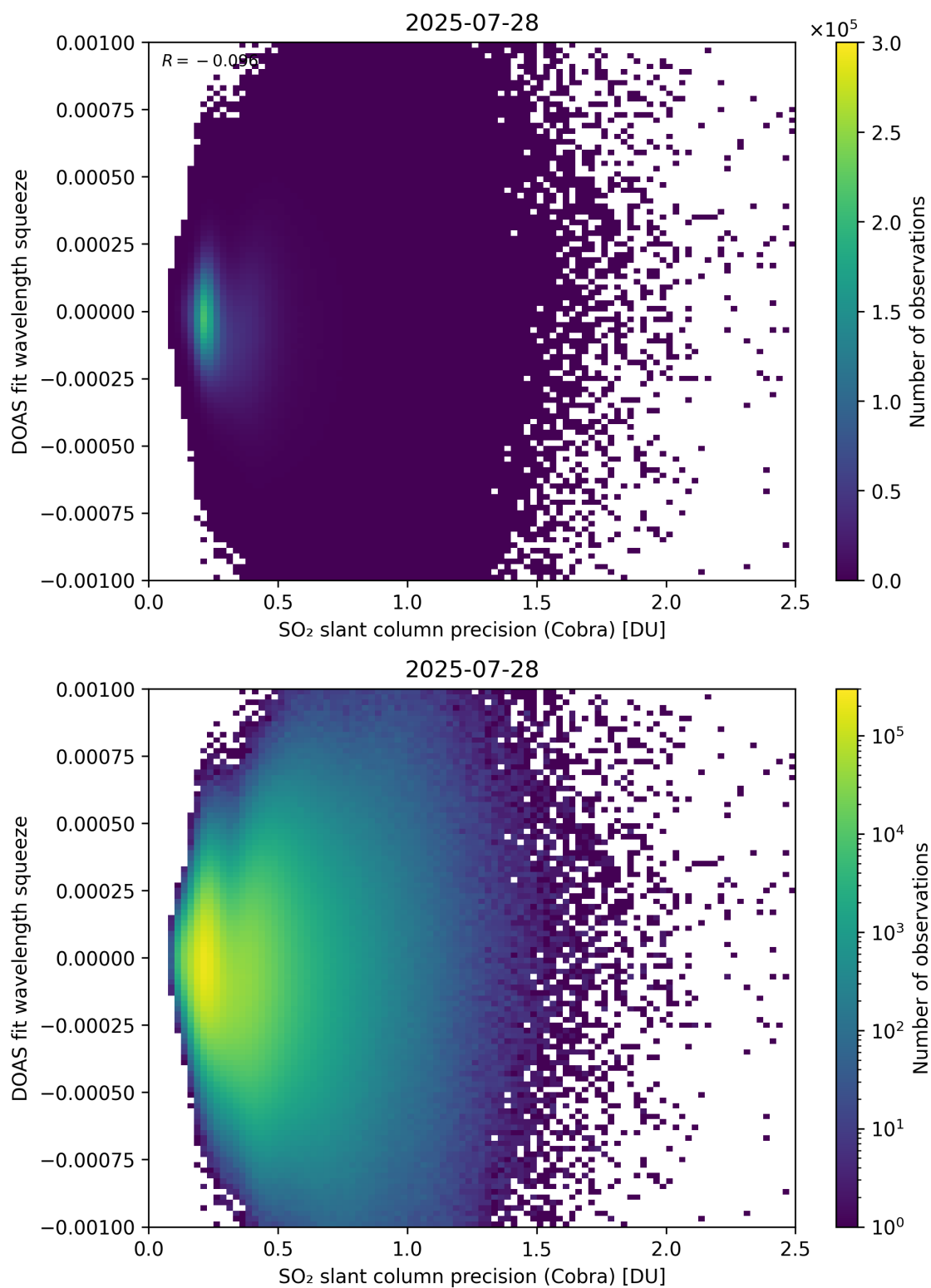
Figure 203: Scatter density plot of “SO 2 slant column precision (Cobra)” against “DOAS fit wavelength squeeze” for 2025-07-27 to 2025-07-29.
