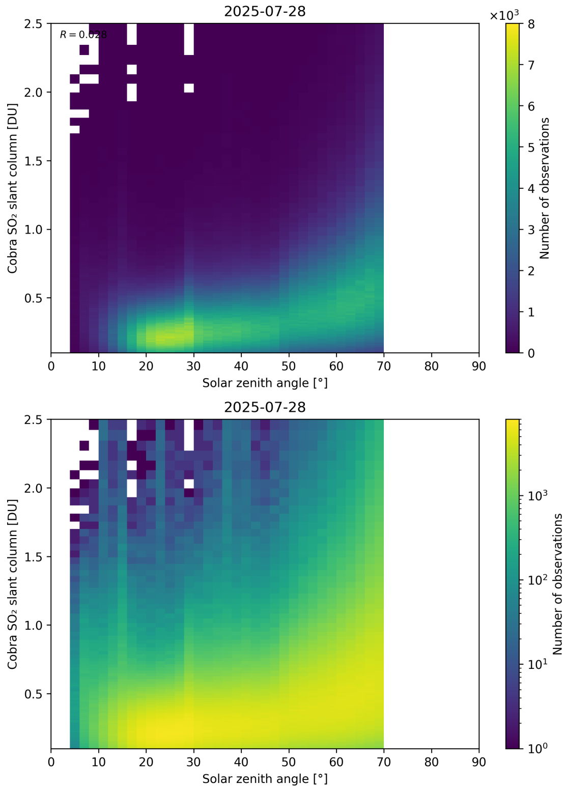
Figure 179: Scatter density plot of “Solar zenith angle” against “Cobra SO 2 slant column” for 2025-07-27 to 2025-07-29.
