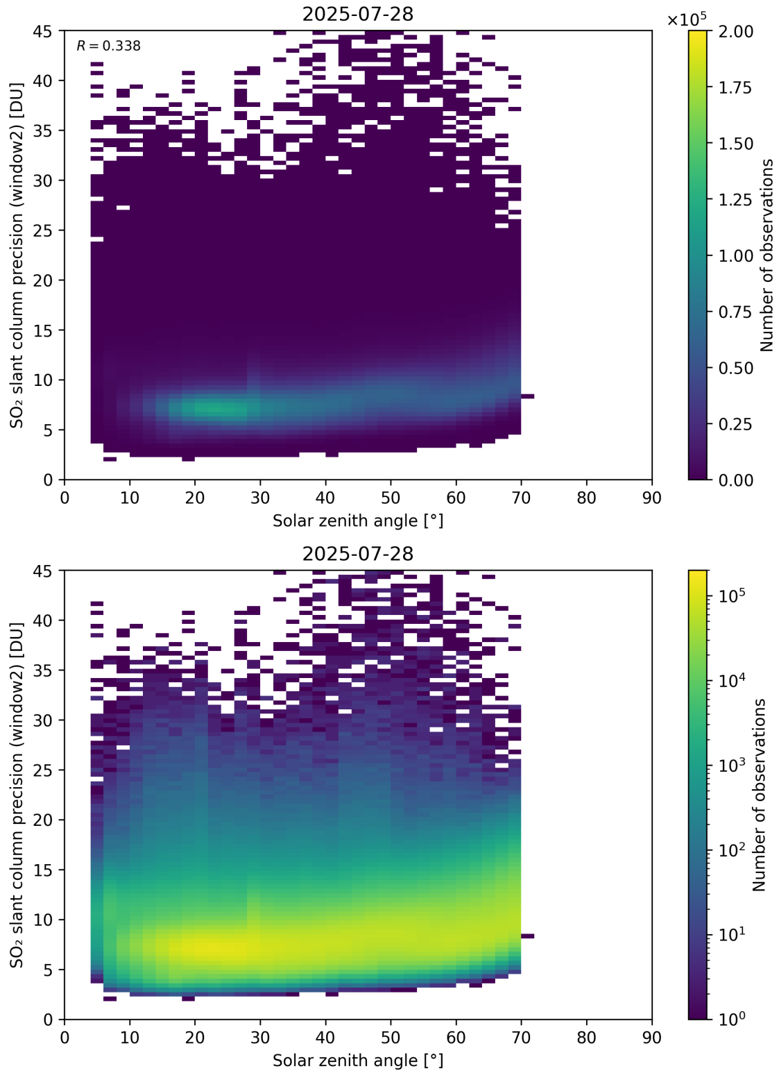
Figure 186: Scatter density plot of “Solar zenith angle” against “SO 2 slant column precision (window2)” for 2025-07-27 to 2025-07-29.
