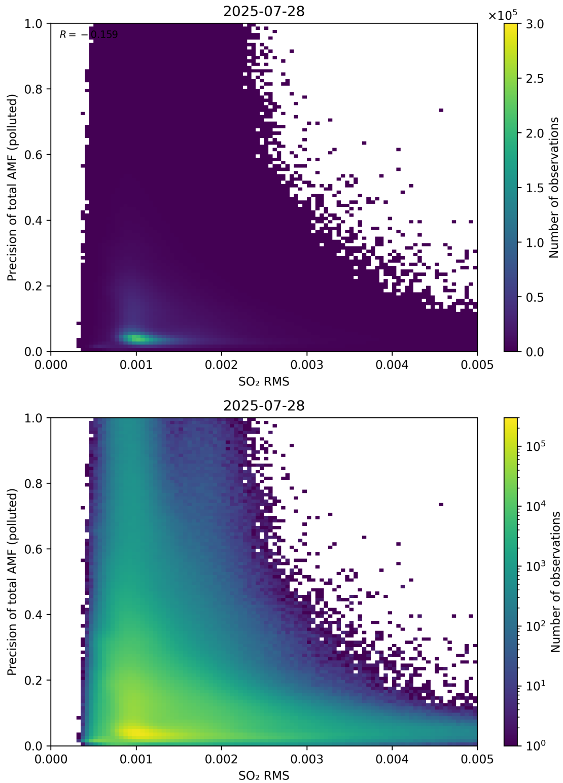
Figure 149: Scatter density plot of “SO 2 RMS” against “Precision of total AMF (polluted)” for 2025-07-27 to 2025-07-29.
