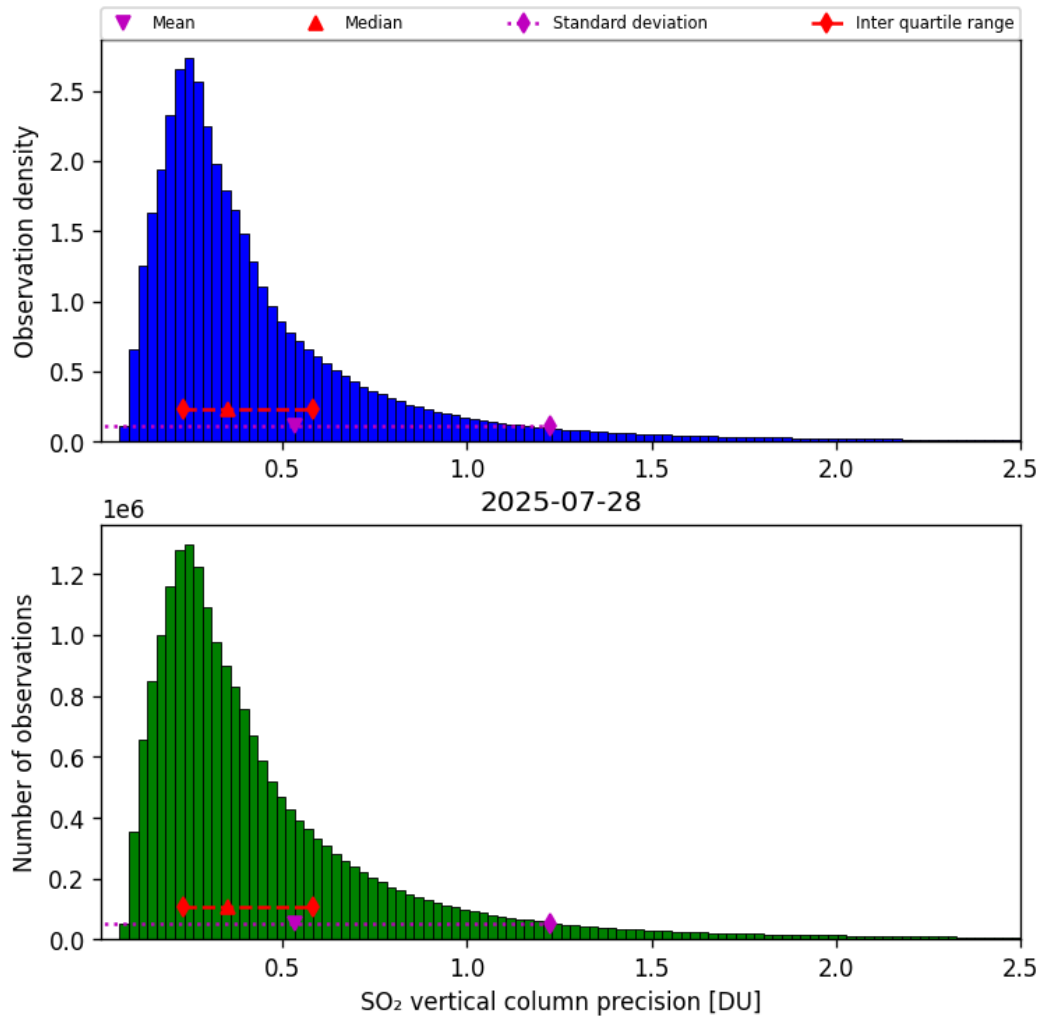
Figure 59: Histogram of “SO 2 vertical column precision” for 2025-07-27 to 2025-07-29
