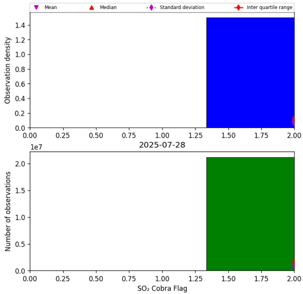
Figure 75: Histogram of “SO 2 Cobra Flag” for 2025-07-27 to 2025-07-29
