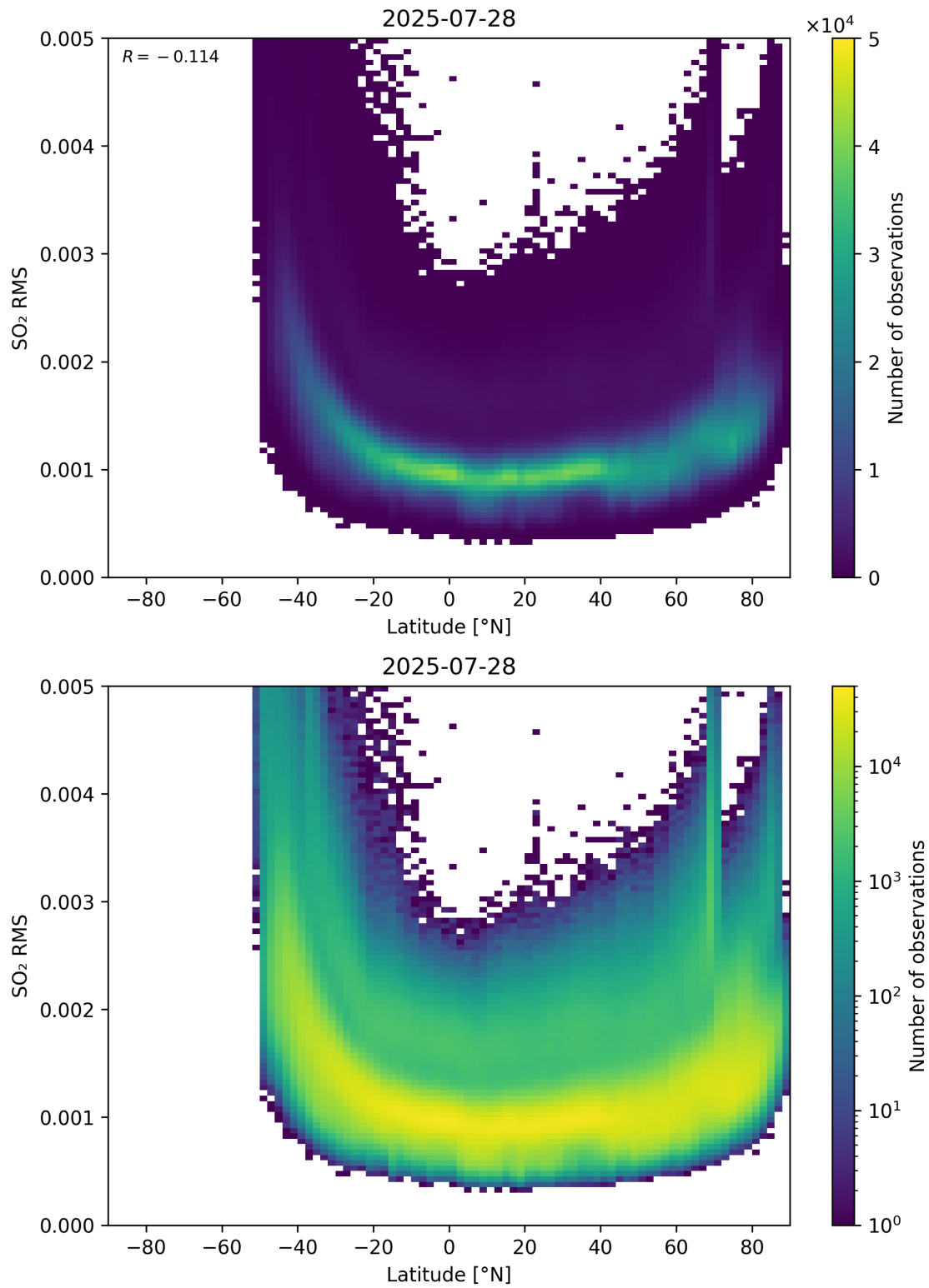
Figure 155: Scatter density plot of “Latitude” against “SO 2 RMS” for 2025-07-27 to 2025-07-29.
