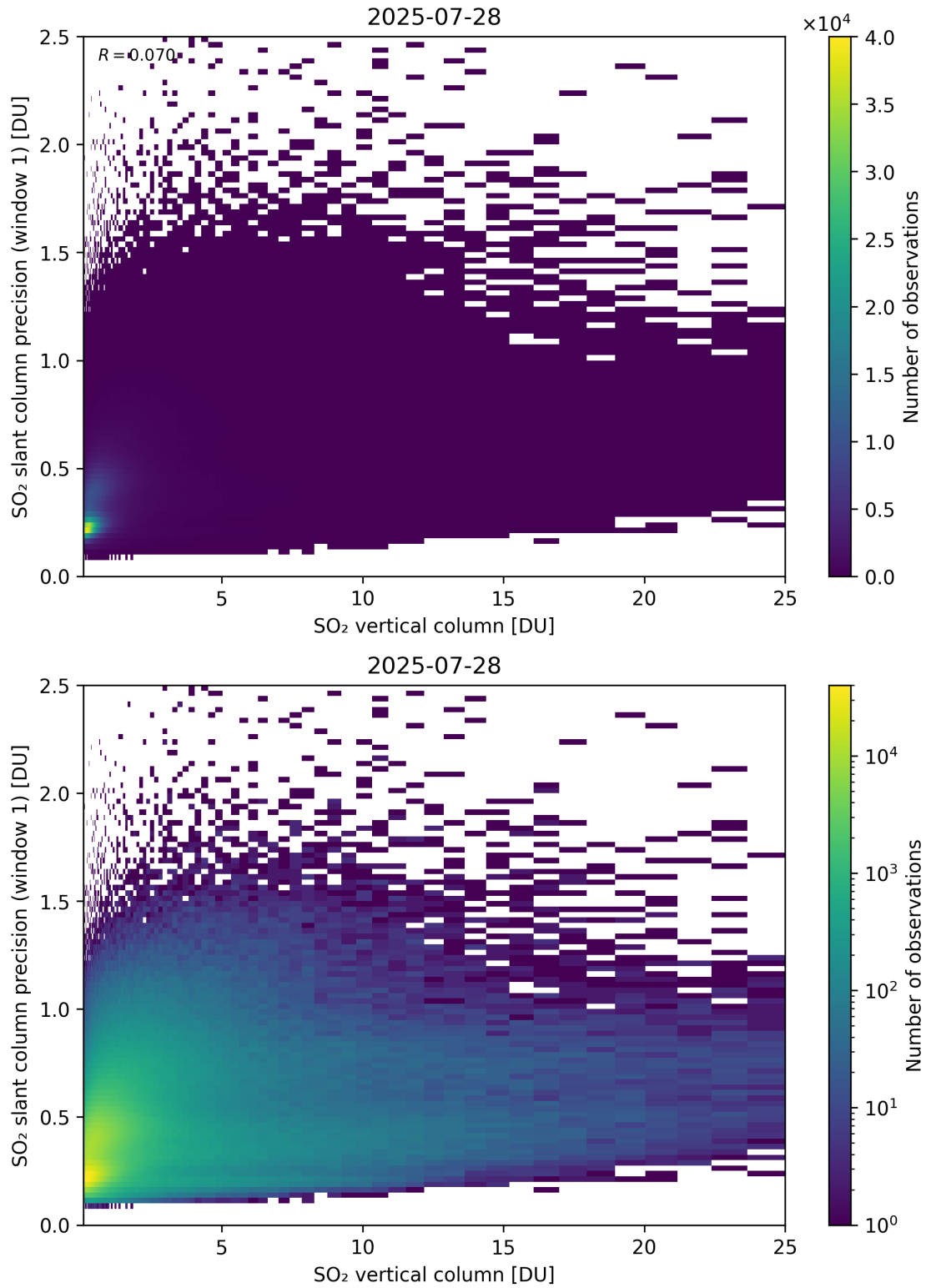
Figure 355: Scatter density plot of “SO 2 vertical column” against “SO 2 slant column precision (window 1)” for 2025-07-27 to 2025-07-29.
