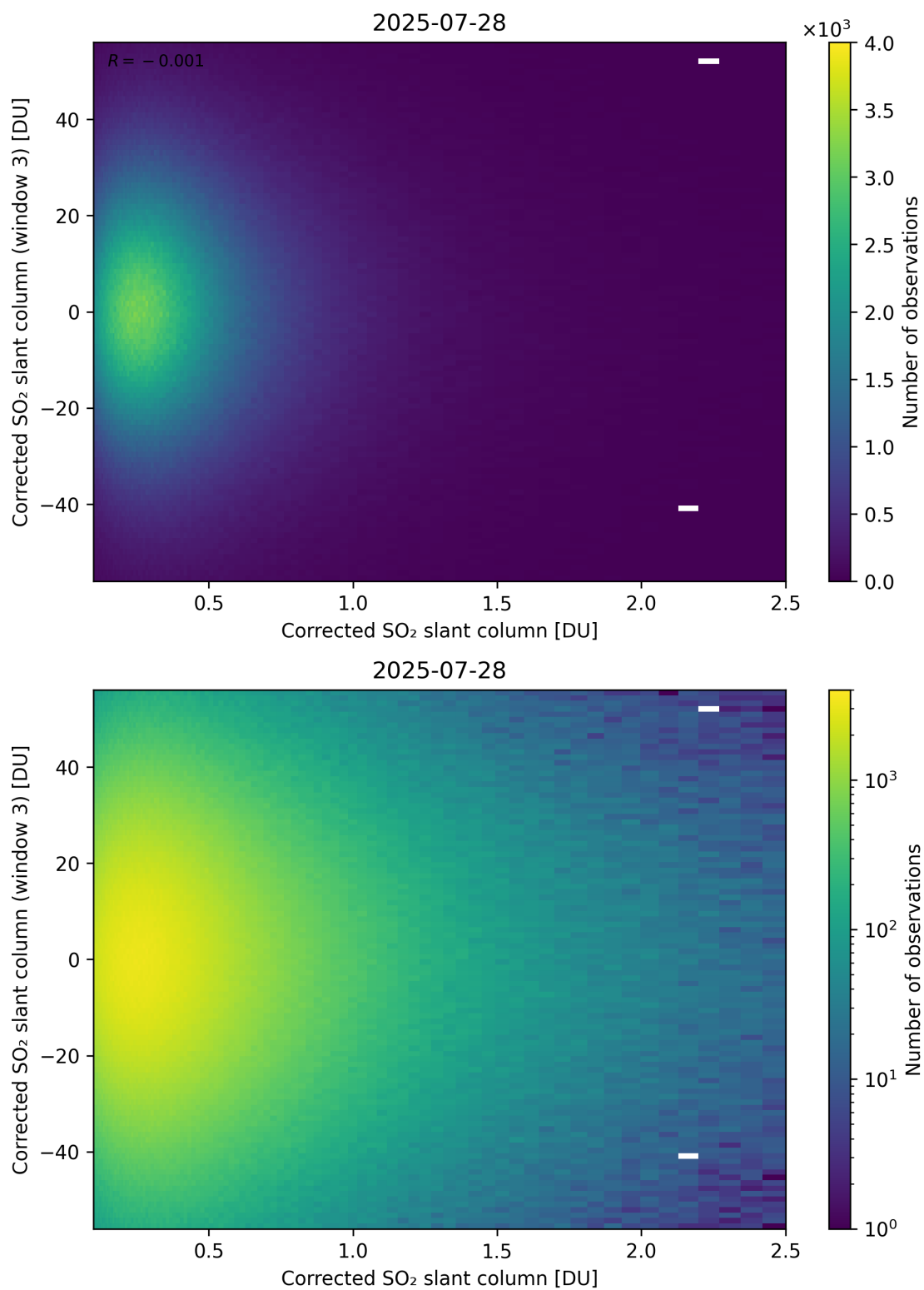
Figure 236: Scatter density plot of “Corrected SO 2 slant column” against “Corrected SO 2 slant column (window 3)” for 2025-07-27 to 2025-07-29.
