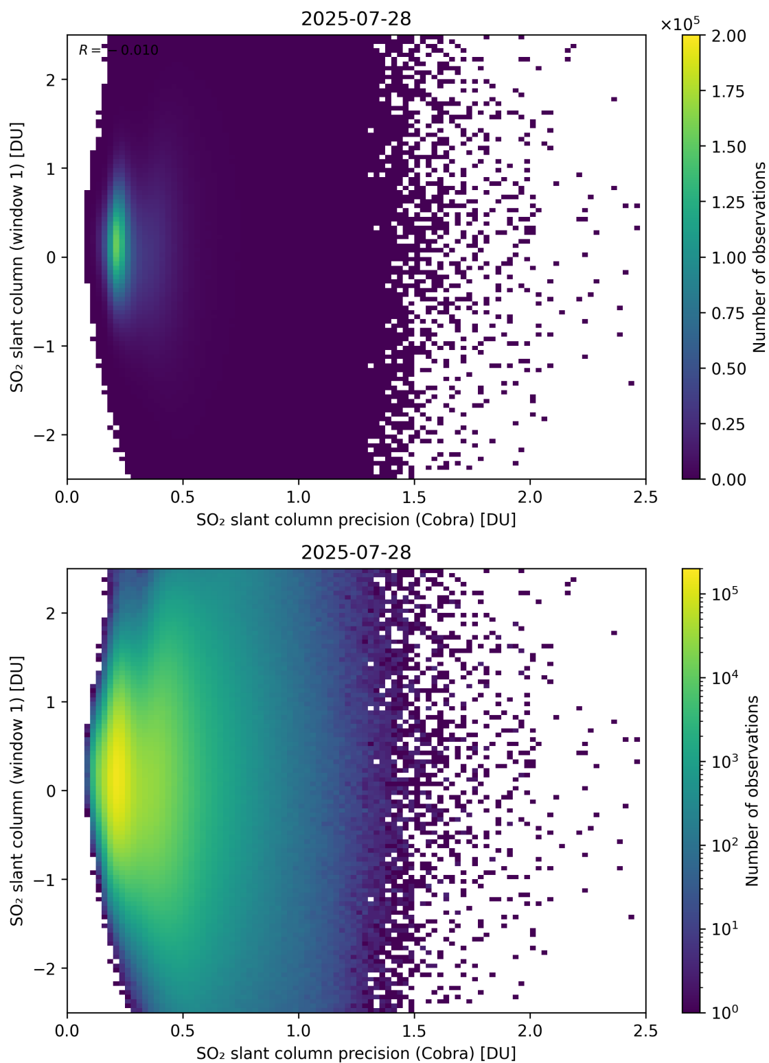
Figure 208: Scatter density plot of “SO 2 slant column precision (Cobra)” against “SO 2 slant column (window 1)” for 2025-07-27 to 2025-07-29.
