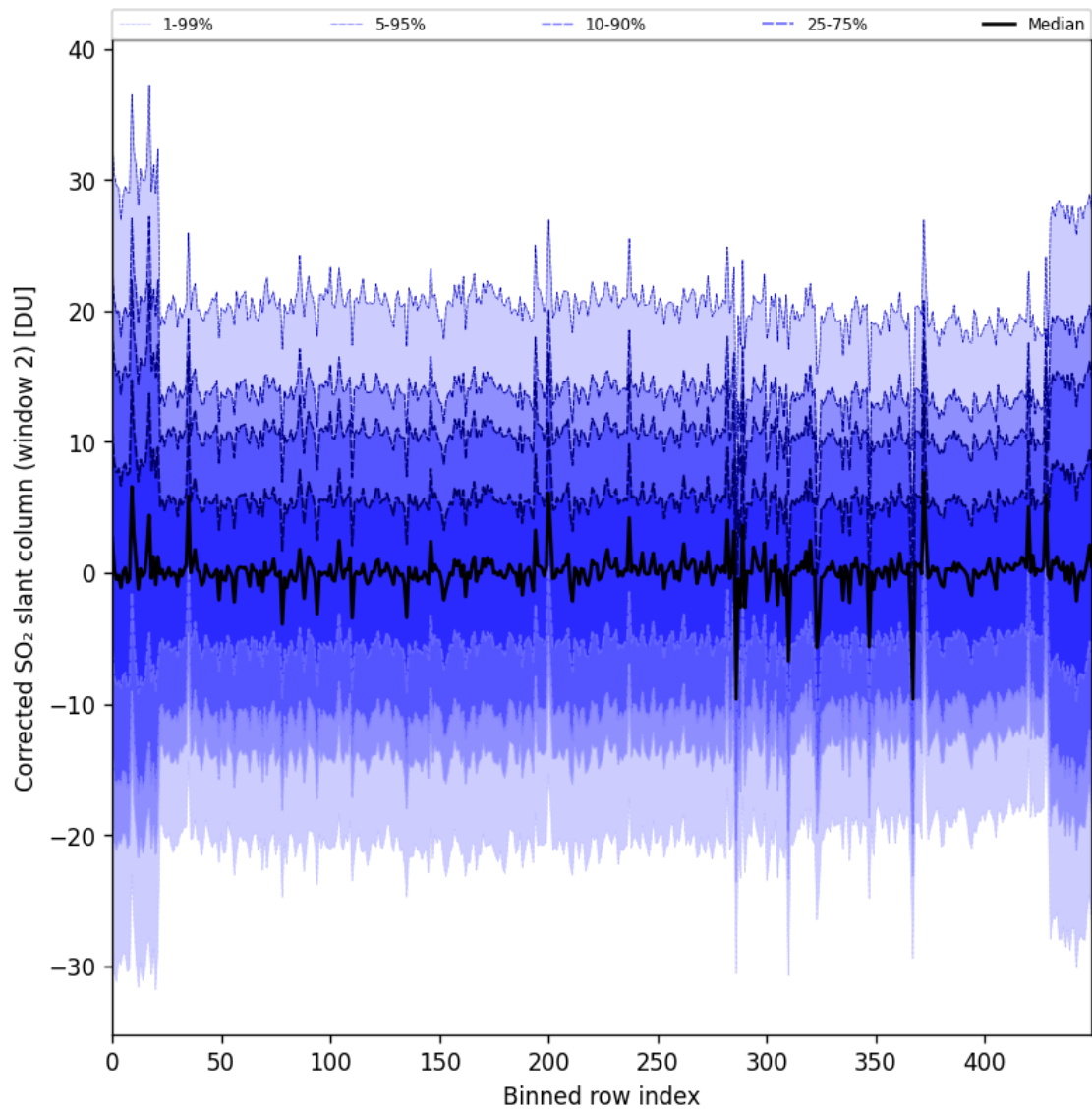
Figure 95: Along track statistics of “Corrected SO 2 slant column (window 2)” for 2025-07-27 to 2025-07-29
