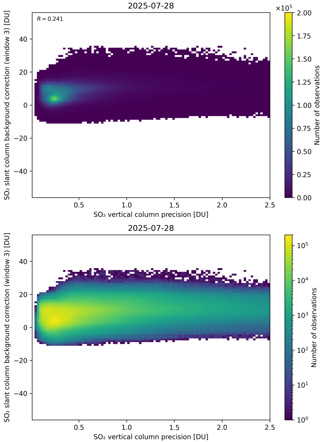
Figure 331: Scatter density plot of “SO 2 vertical column precision” against “SO 2 slant column background correction (window 3)” for 2025-07-27 to 2025-07-29.
