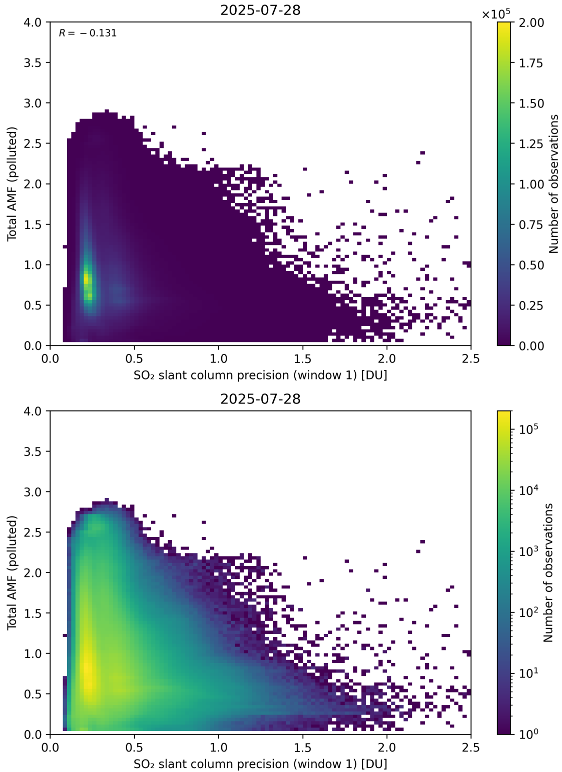
Figure 280: Scatter density plot of “SO 2 slant column precision (window 1)” against “Total AMF (polluted)” for 2025-07-27 to 2025-07-29.
