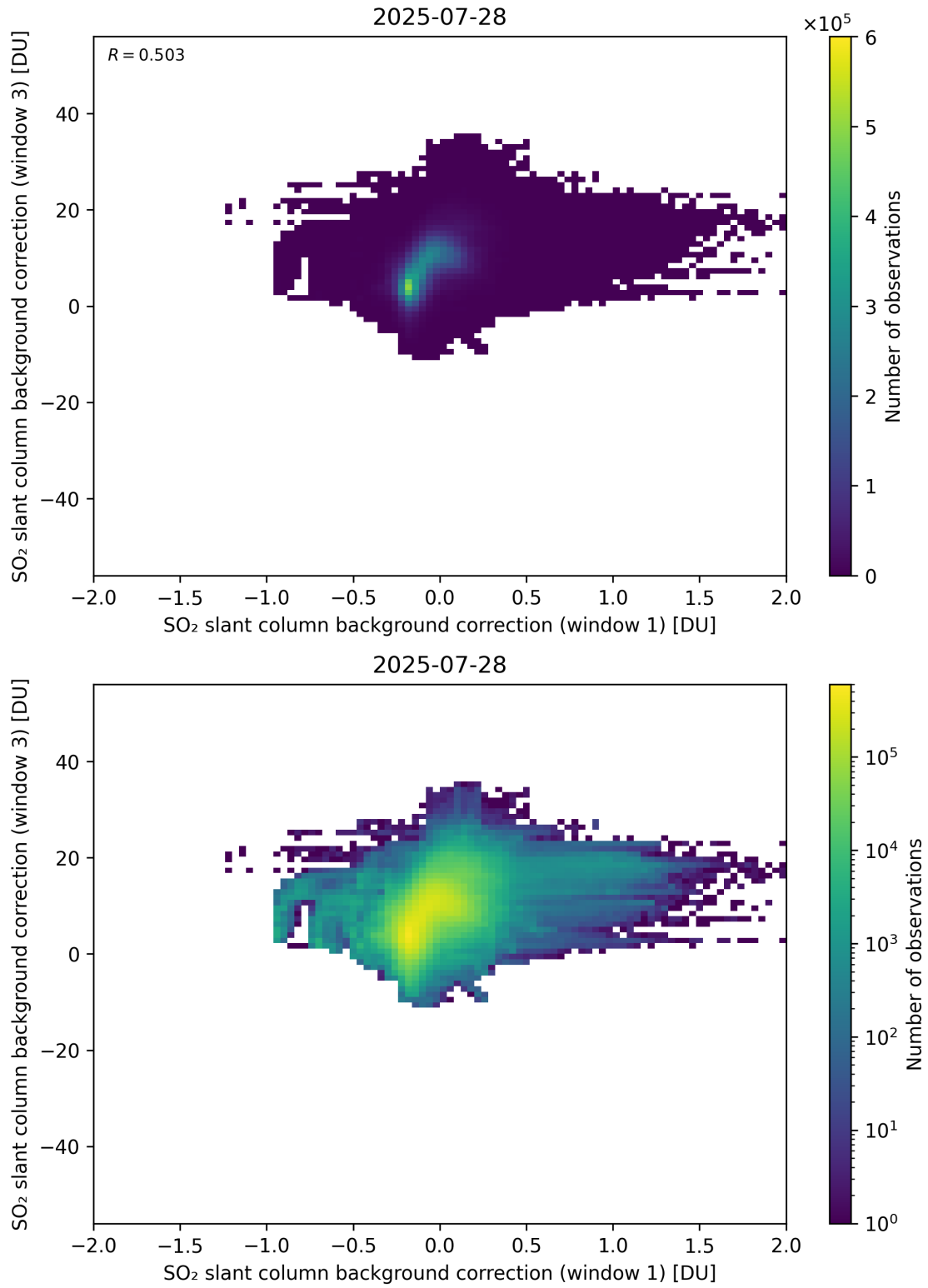
Figure 110: Scatter density plot of “SO 2 slant column background correction (window 1)” against “SO 2 slant column background correction (window 3)” for 2025-07-27 to 2025-07-29.
