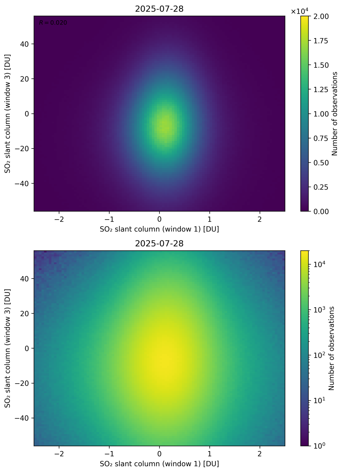
Figure 287: Scatter density plot of “SO 2 slant column (window 1)” against “SO 2 slant column (window 3)” for 2025-07-27 to 2025-07-29.
