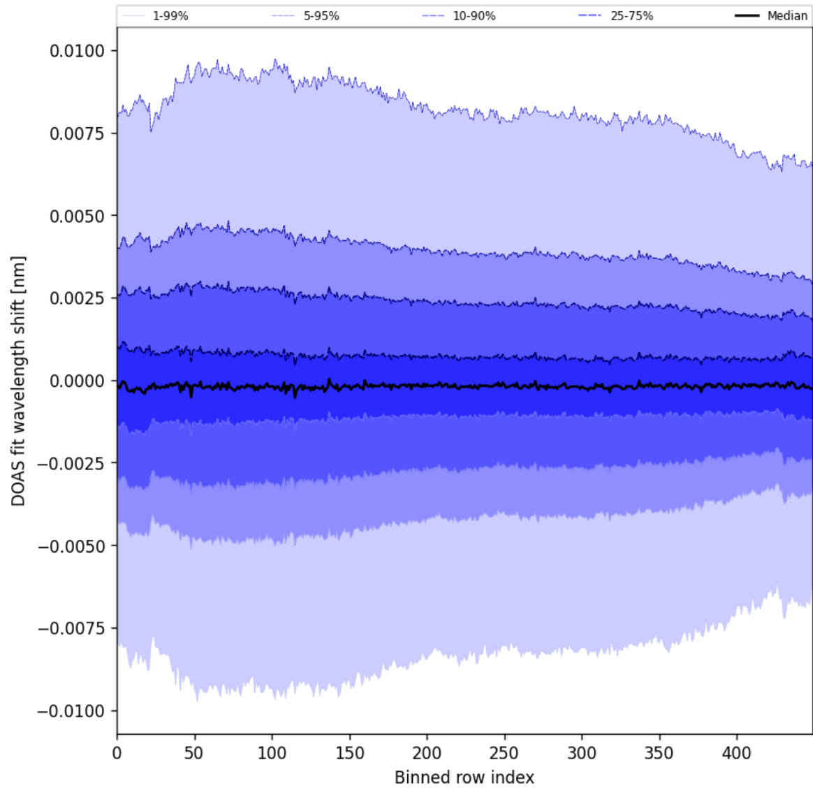
Figure 102: Along track statistics of “DOAS fit wavelength shift” for 2025-07-27 to 2025-07-29
