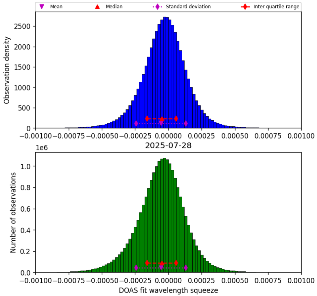
Figure 77: Histogram of “DOAS fit wavelength squeeze” for 2025-07-27 to 2025-07-29
