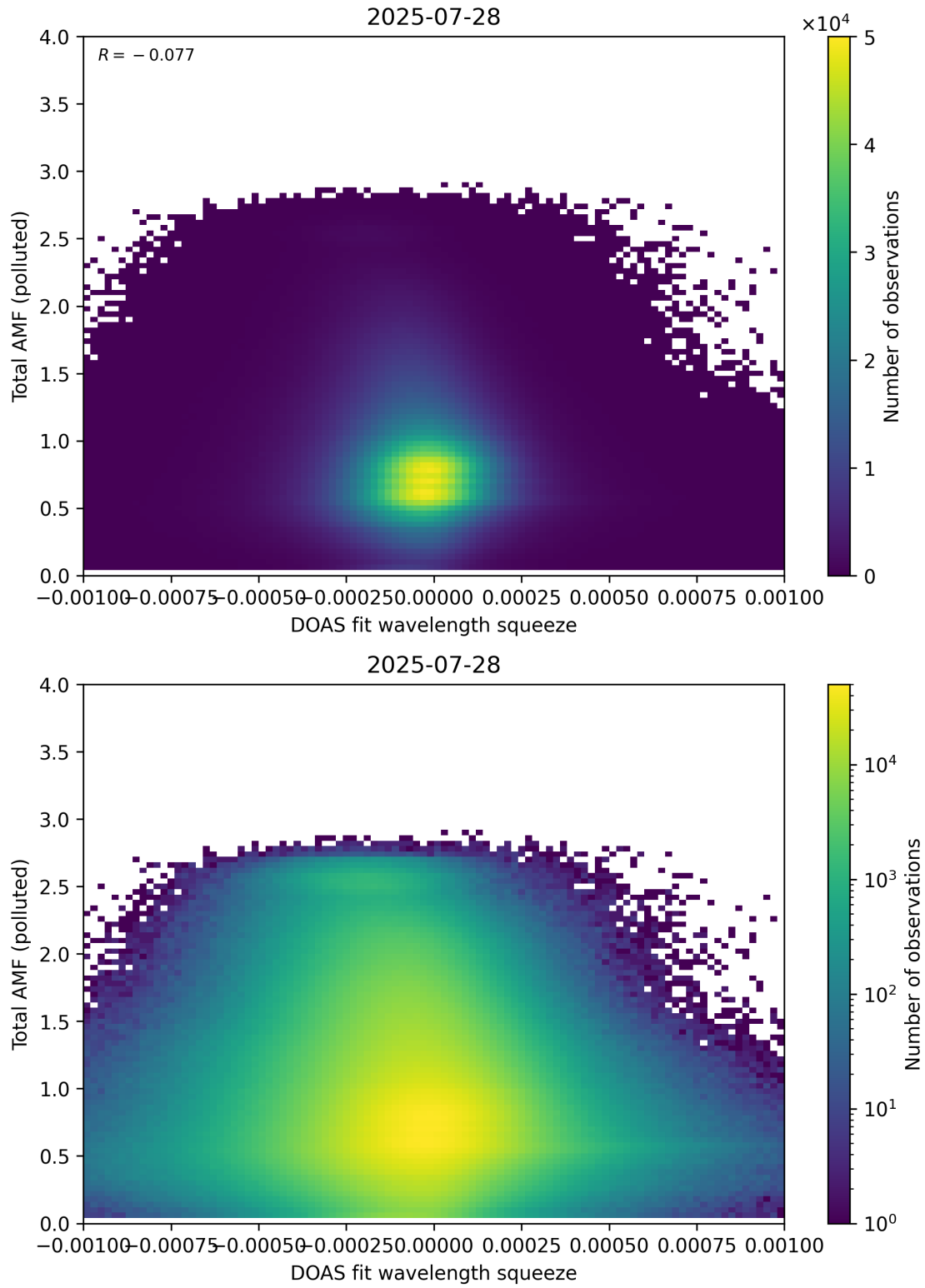
Figure 145: Scatter density plot of “DOAS fit wavelength squeeze” against “Total AMF (polluted)” for 2025-07-27 to 2025-07-29.
