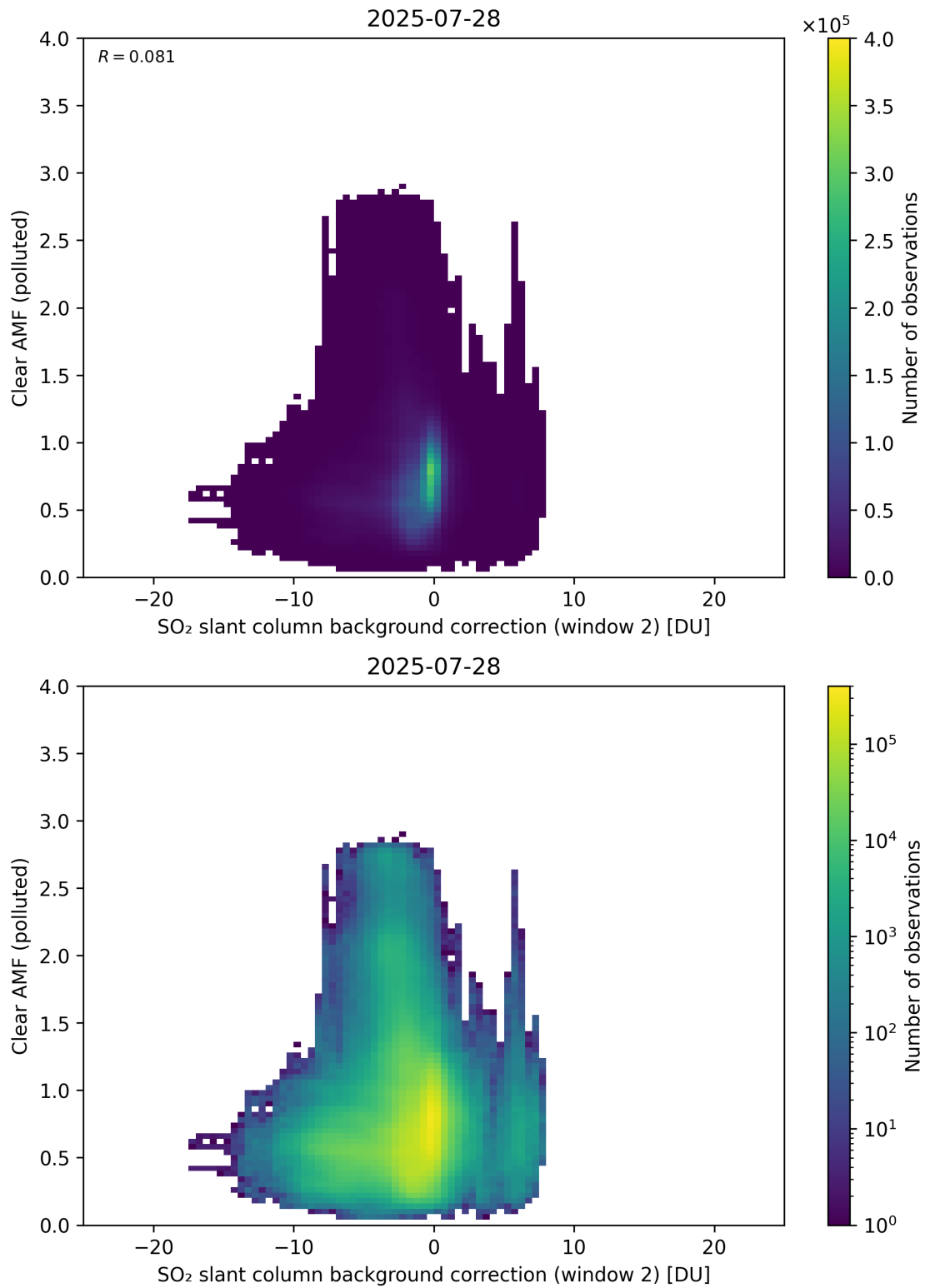
Figure 126: Scatter density plot of “SO 2 slant column background correction (window 2)” against “Clear AMF (polluted)” for 2025-07-27 to 2025-07-29.
