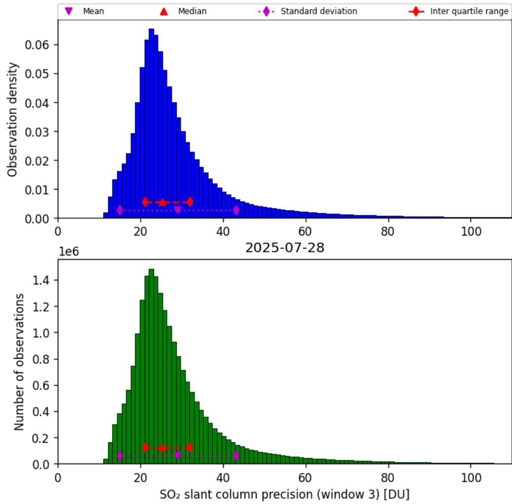
Figure 72: Histogram of “SO 2 slant column precision (window 3)” for 2025-07-27 to 2025-07-29
