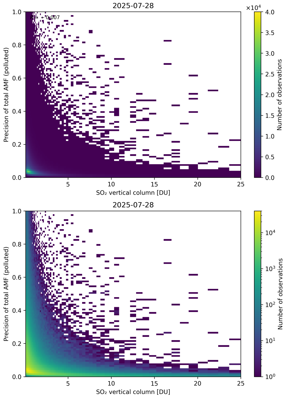
Figure 360: Scatter density plot of “SO 2 vertical column” against “Precision of total AMF (polluted)” for 2025-07-27 to 2025-07-29.
