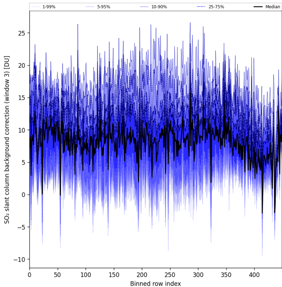
Figure 100: Along track statistics of “SO 2 slant column background correction (window 3)” for 2025-07-27 to 2025-07-29
