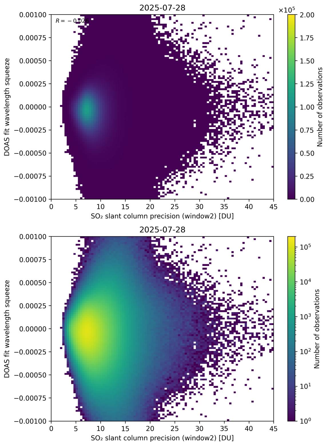
Figure 294: Scatter density plot of “SO 2 slant column precision (window2)” against “DOAS fit wavelength squeeze” for 2025-07-27 to 2025-07-29.
