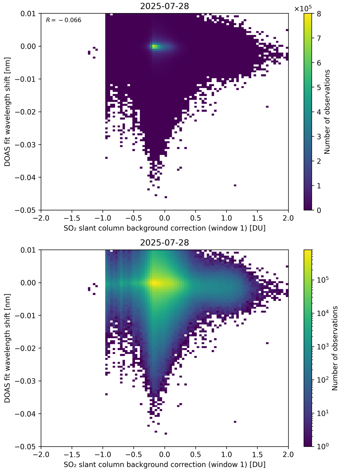
Figure 111: Scatter density plot of “SO 2 slant column background correction (window 1)” against “DOAS fit wavelength shift” for 2025-07-27 to 2025-07-29.
