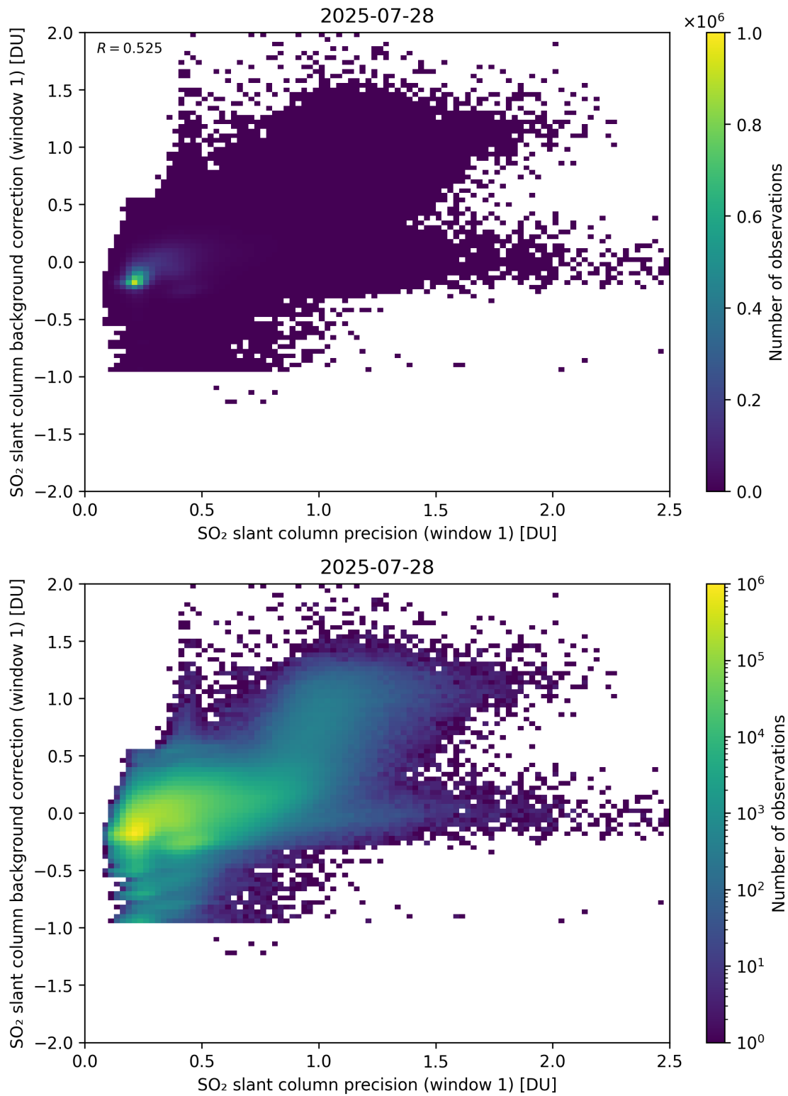
Figure 268: Scatter density plot of “SO 2 slant column precision (window 1)” against “SO 2 slant column background correction (window 1)” for 2025-07-27 to 2025-07-29.
