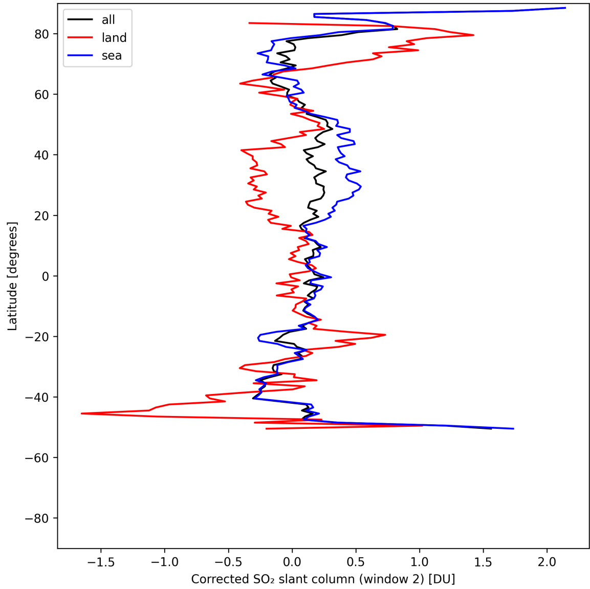
Figure 43: Zonal average of “Corrected SO 2 slant column (window 2)” for 2025-07-27 to 2025-07-29.
