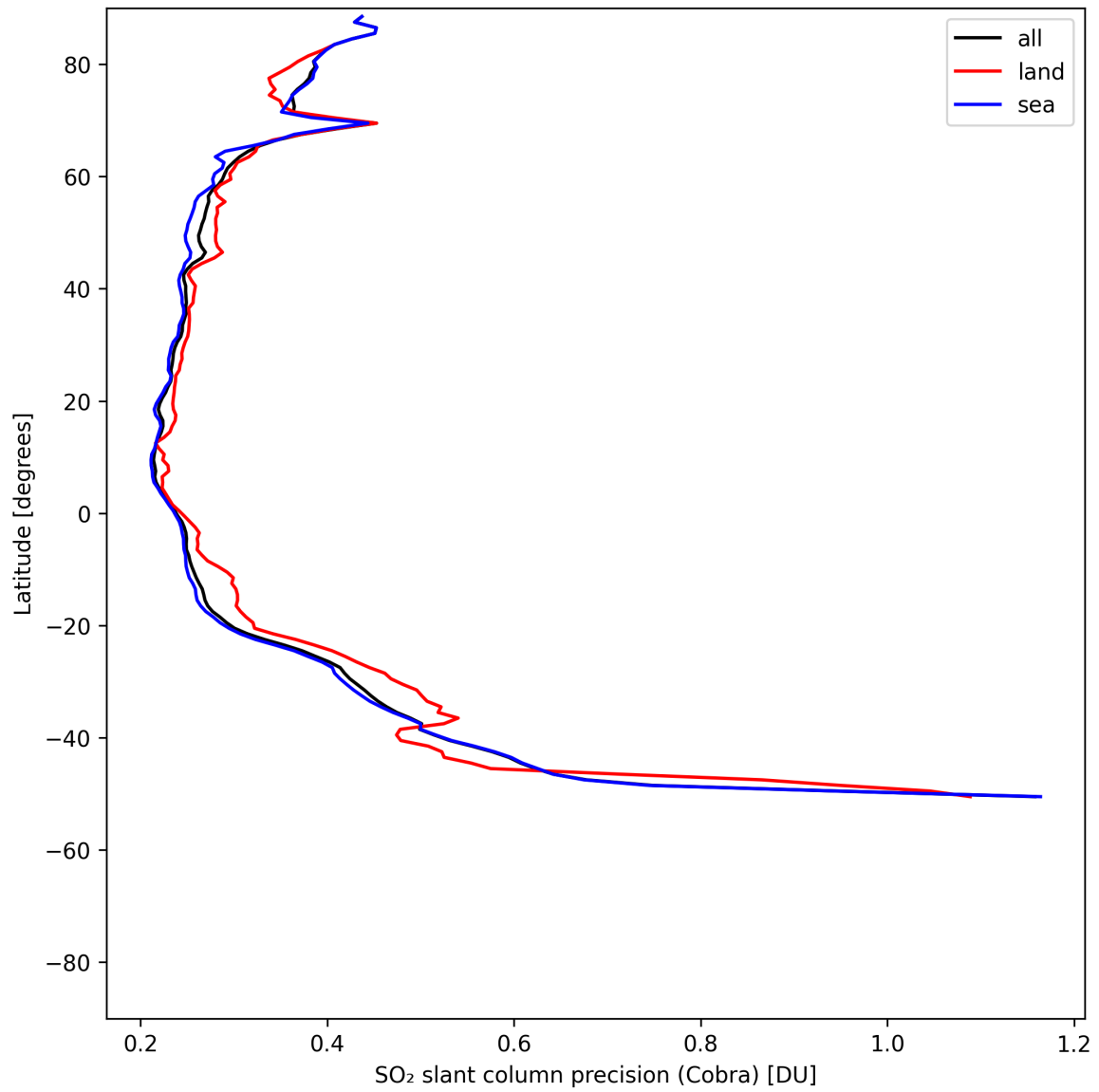
Figure 36: Zonal average of “SO 2 slant column precision (Cobra)” for 2025-07-27 to 2025-07-29.
