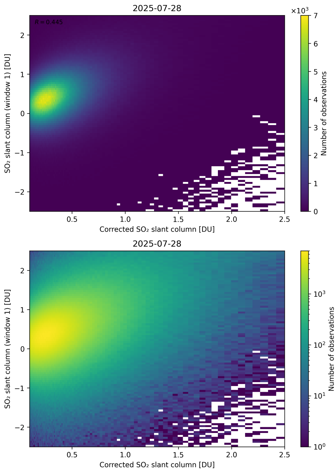
Figure 237: Scatter density plot of “Corrected SO 2 slant column” against “SO 2 slant column (window 1)” for 2025-07-27 to 2025-07-29.
