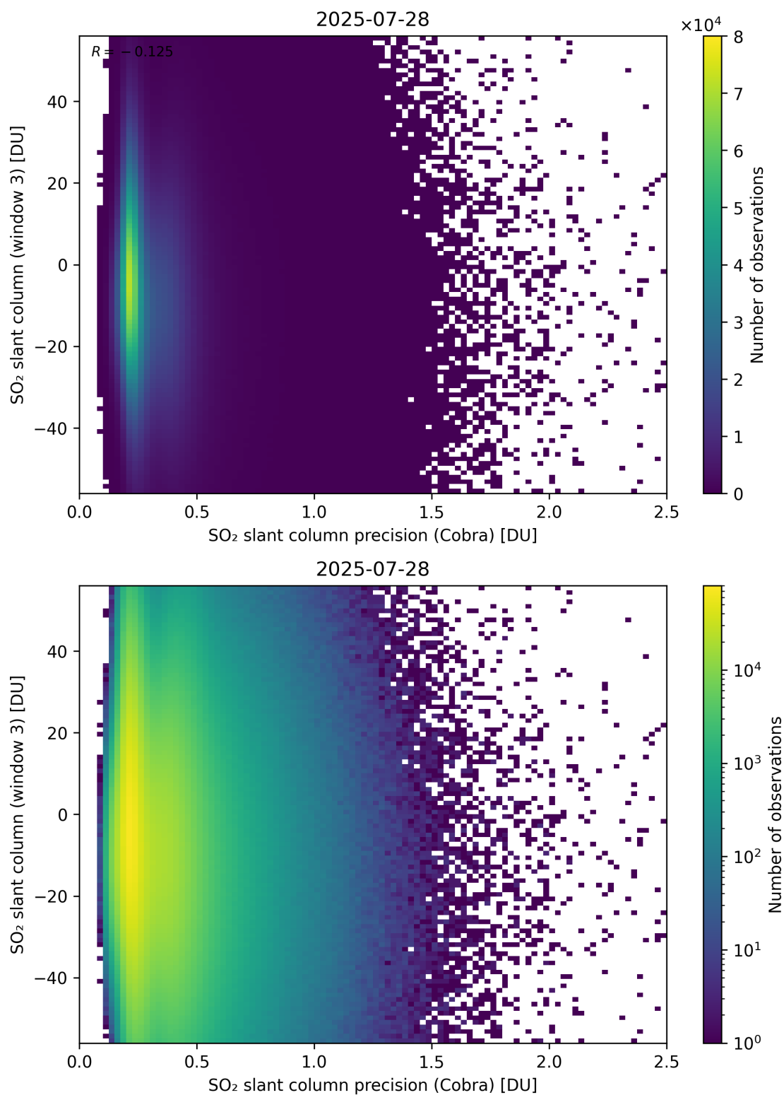
Figure 211: Scatter density plot of “SO 2 slant column precision (Cobra)” against “SO 2 slant column (window 3)” for 2025-07-27 to 2025-07-29.
