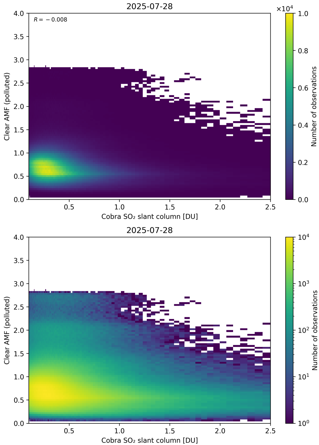
Figure 215: Scatter density plot of “Cobra SO 2 slant column” against “Clear AMF (polluted)” for 2025-07-27 to 2025-07-29.
