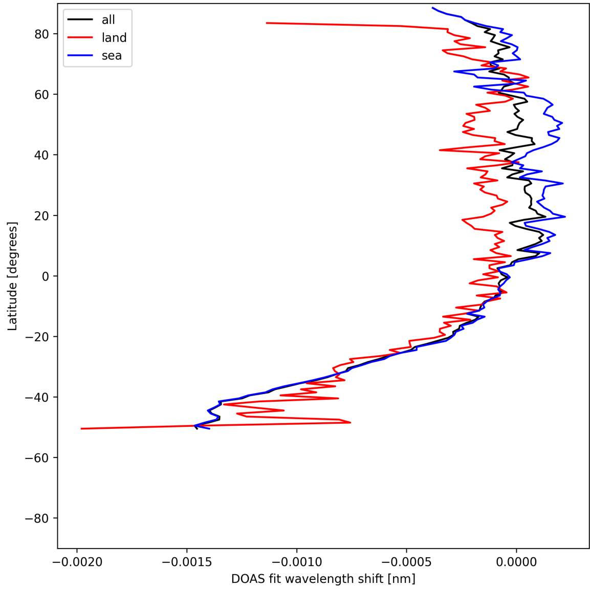
Figure 50: Zonal average of “DOAS fit wavelength shift” for 2025-07-27 to 2025-07-29.
