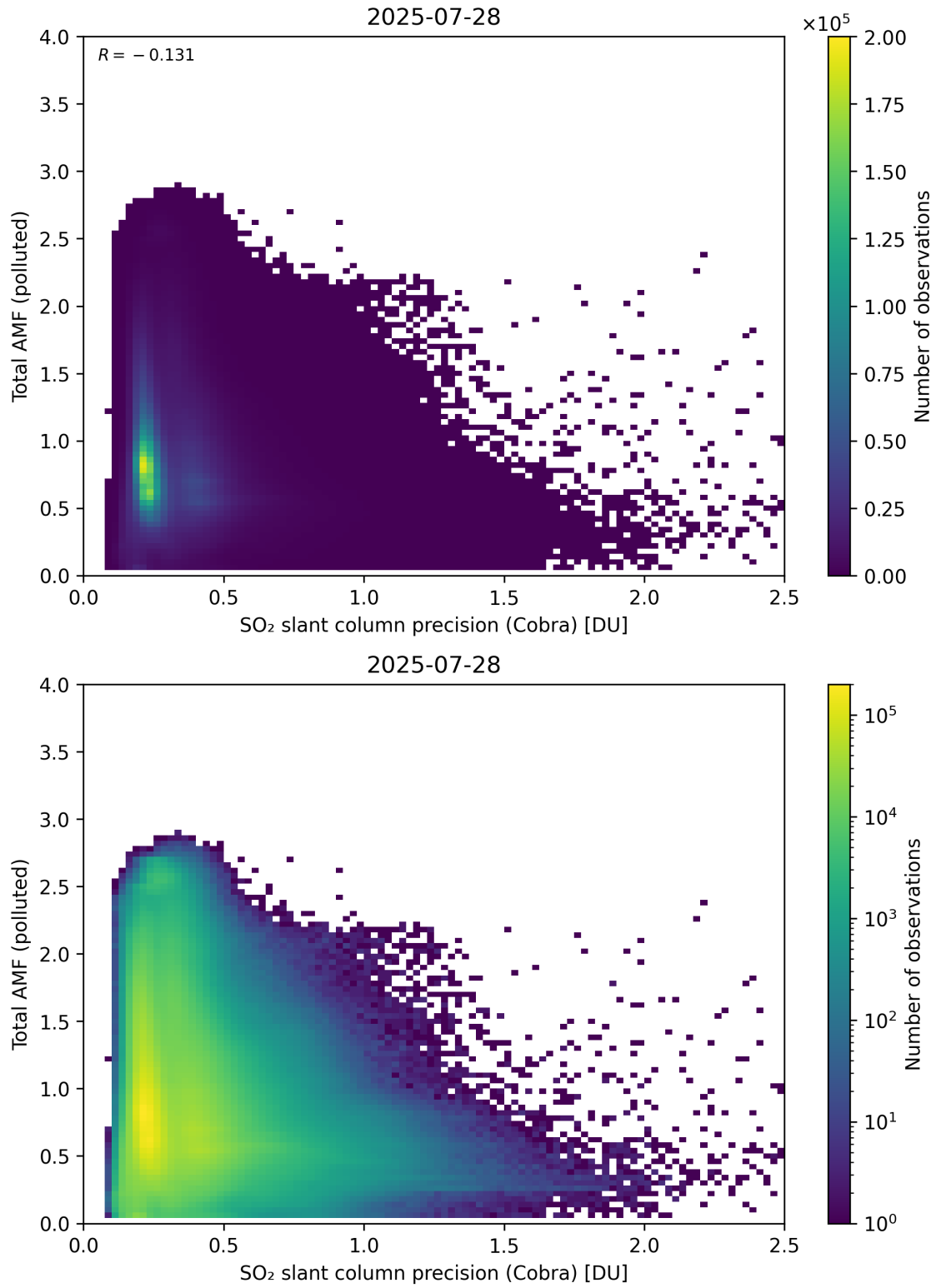
Figure 213: Scatter density plot of “SO 2 slant column precision (Cobra)” against “Total AMF (polluted)” for 2025-07-27 to 2025-07-29.
