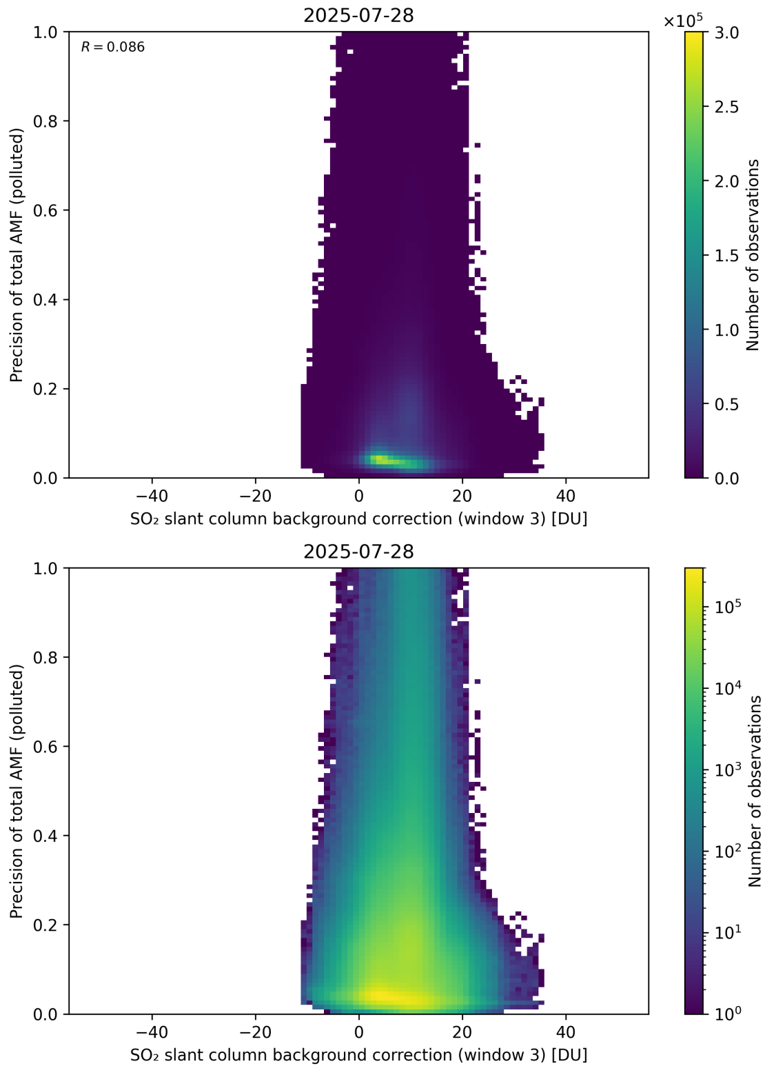
Figure 137: Scatter density plot of “SO 2 slant column background correction (window 3)” against “Precision of total AMF (polluted)” for 2025-07-27 to 2025-07-29.
