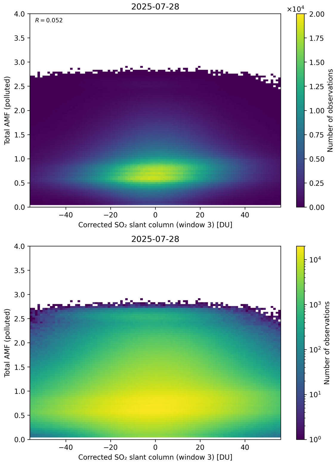
Figure 260: Scatter density plot of “Corrected SO 2 slant column (window 3)” against “Total AMF (polluted)” for 2025-07-27 to 2025-07-29.
