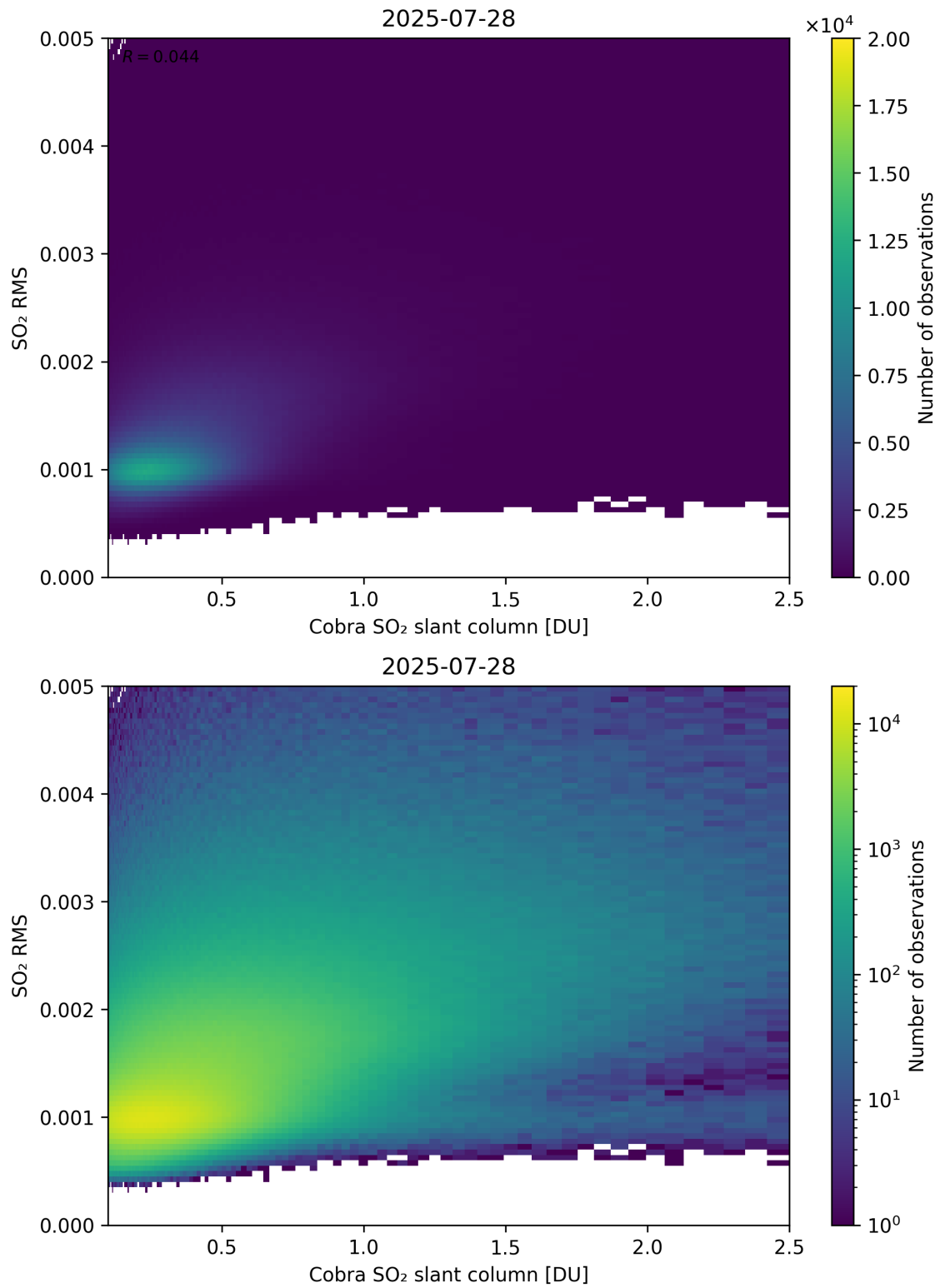
Figure 198: Scatter density plot of “Cobra SO 2 slant column” against “SO 2 RMS” for 2025-07-27 to 2025-07-29.
