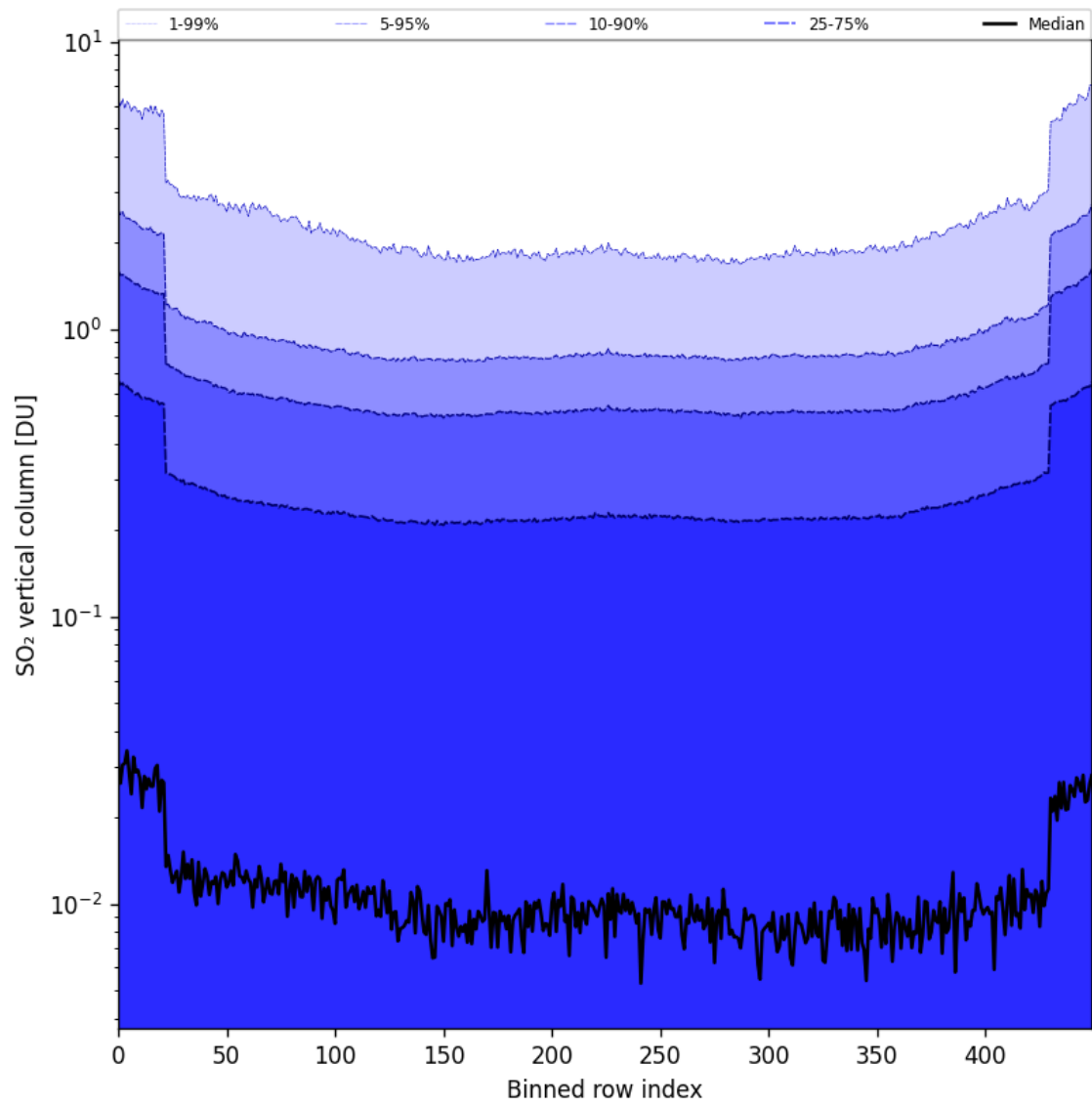
Figure 84: Along track statistics of “SO 2 vertical column” for 2025-07-27 to 2025-07-29
