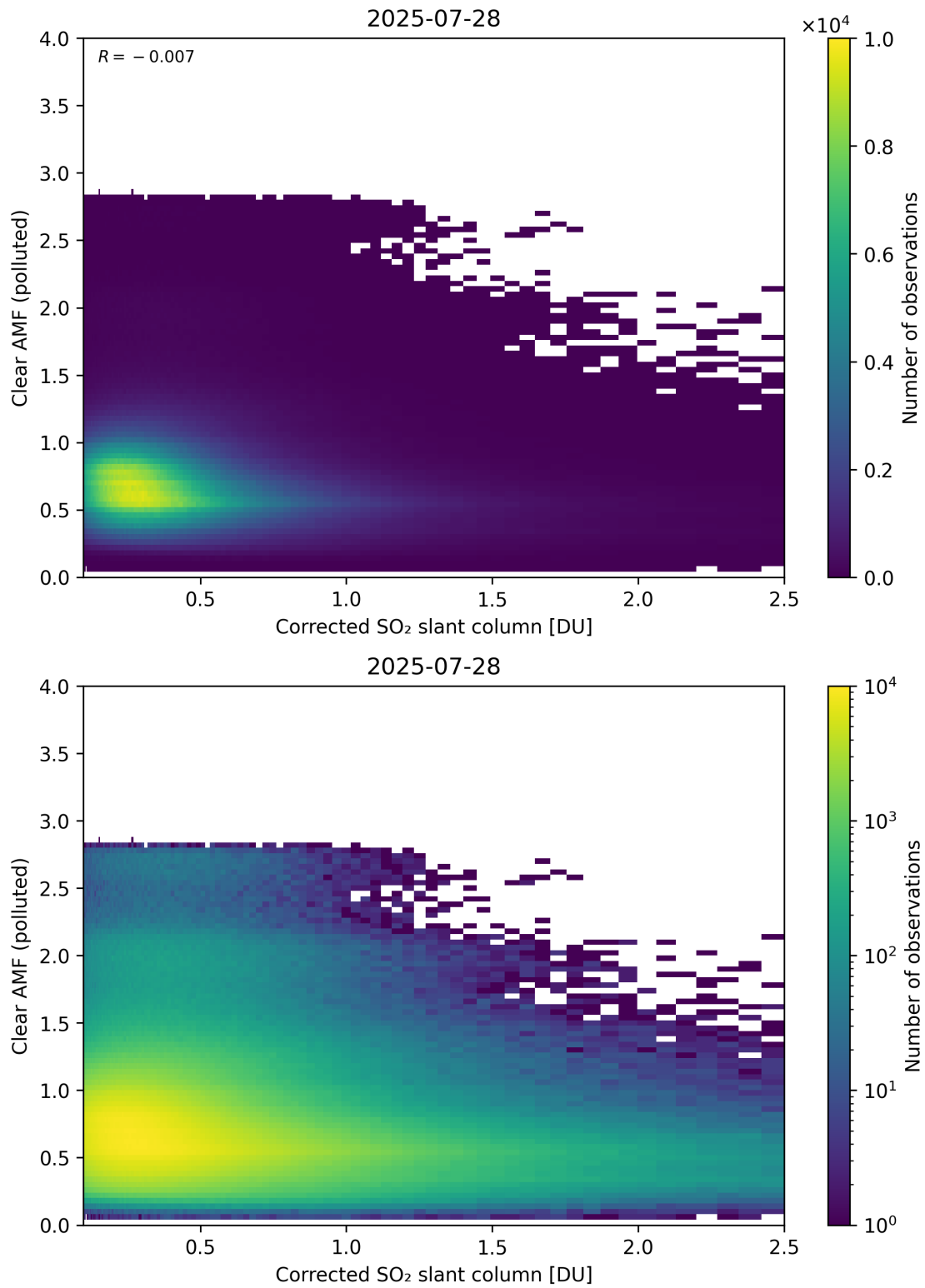
Figure 232: Scatter density plot of “Corrected SO 2 slant column” against “Clear AMF (polluted)” for 2025-07-27 to 2025-07-29.
