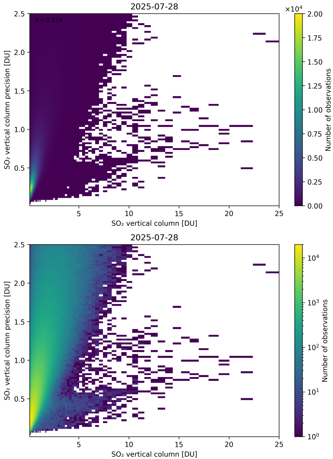
Figure 361: Scatter density plot of “SO 2 vertical column” against “SO 2 vertical column precision” for 2025-07-27 to 2025-07-29.
