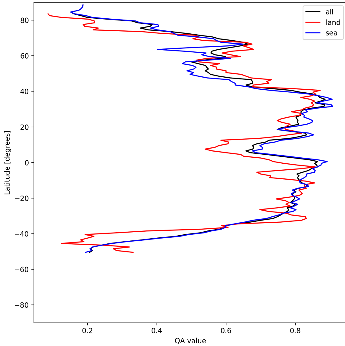
Figure 31: Zonal average of “QA value” for 2025-07-27 to 2025-07-29.
