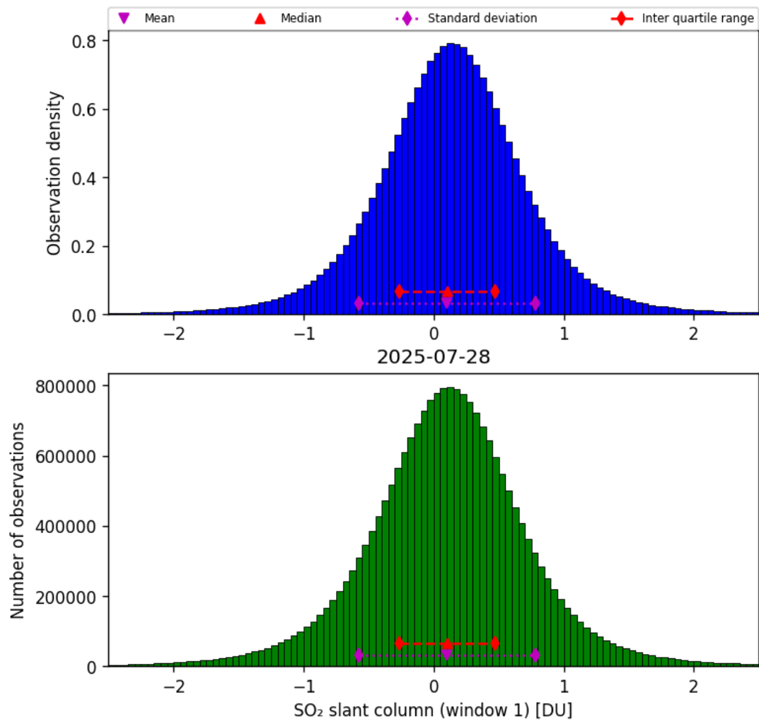
Figure 63: Histogram of “SO 2 slant column (window 1)” for 2025-07-27 to 2025-07-29
