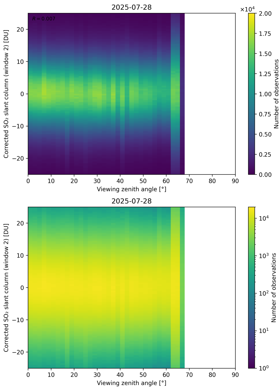
Figure 374: Scatter density plot of “Viewing zenith angle” against “Corrected SO 2 slant column (window 2)” for 2025-07-27 to 2025-07-29.
