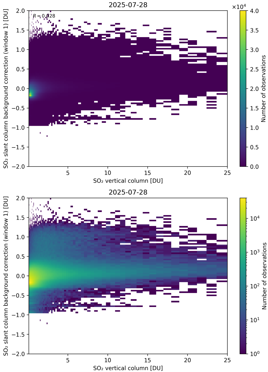
Figure 323: Scatter density plot of “SO 2 vertical column” against “SO 2 slant column background correction (window 1)” for 2025-07-27 to 2025-07-29.
