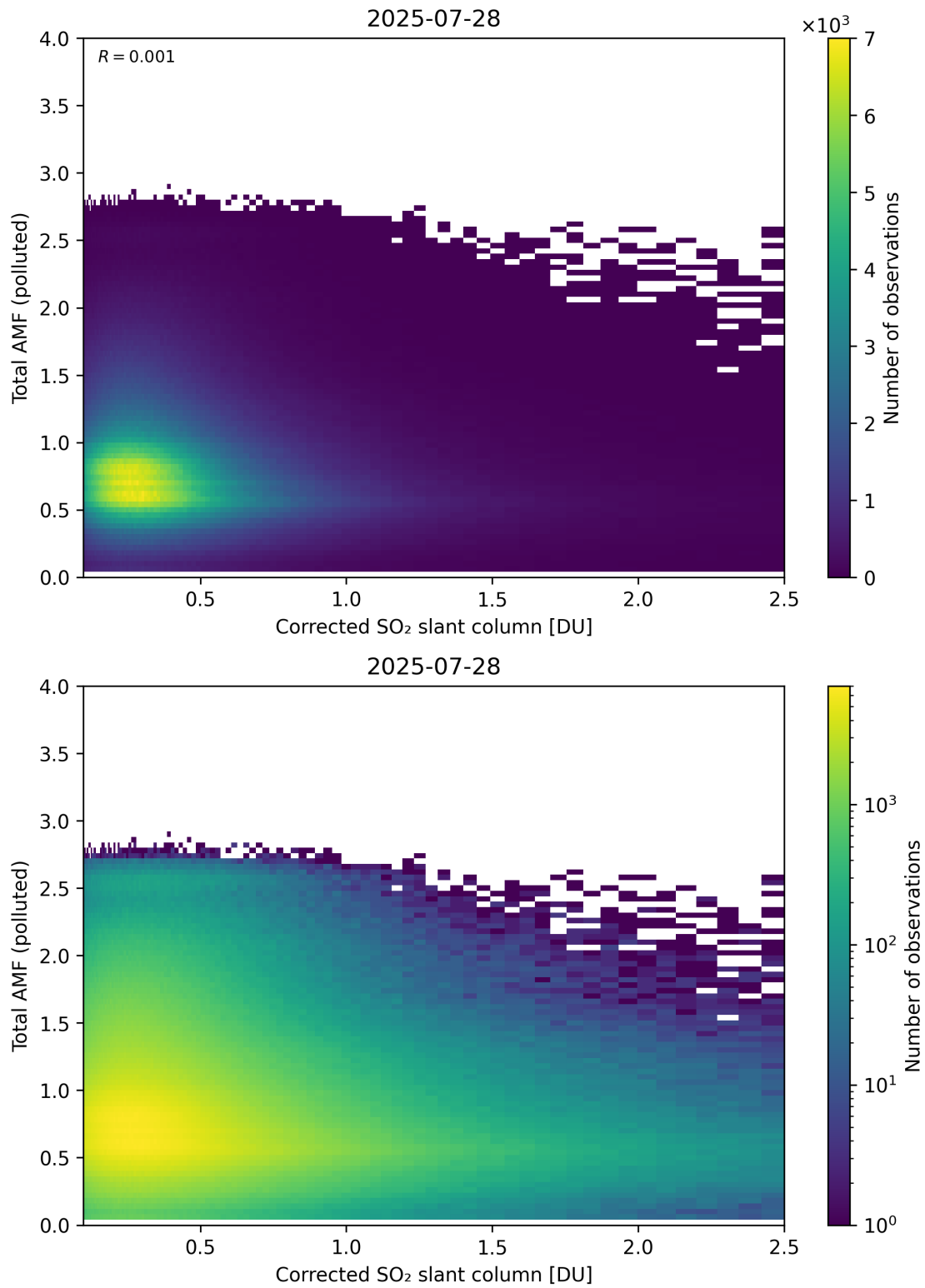
Figure 242: Scatter density plot of “Corrected SO 2 slant column” against “Total AMF (polluted)” for 2025-07-27 to 2025-07-29.
