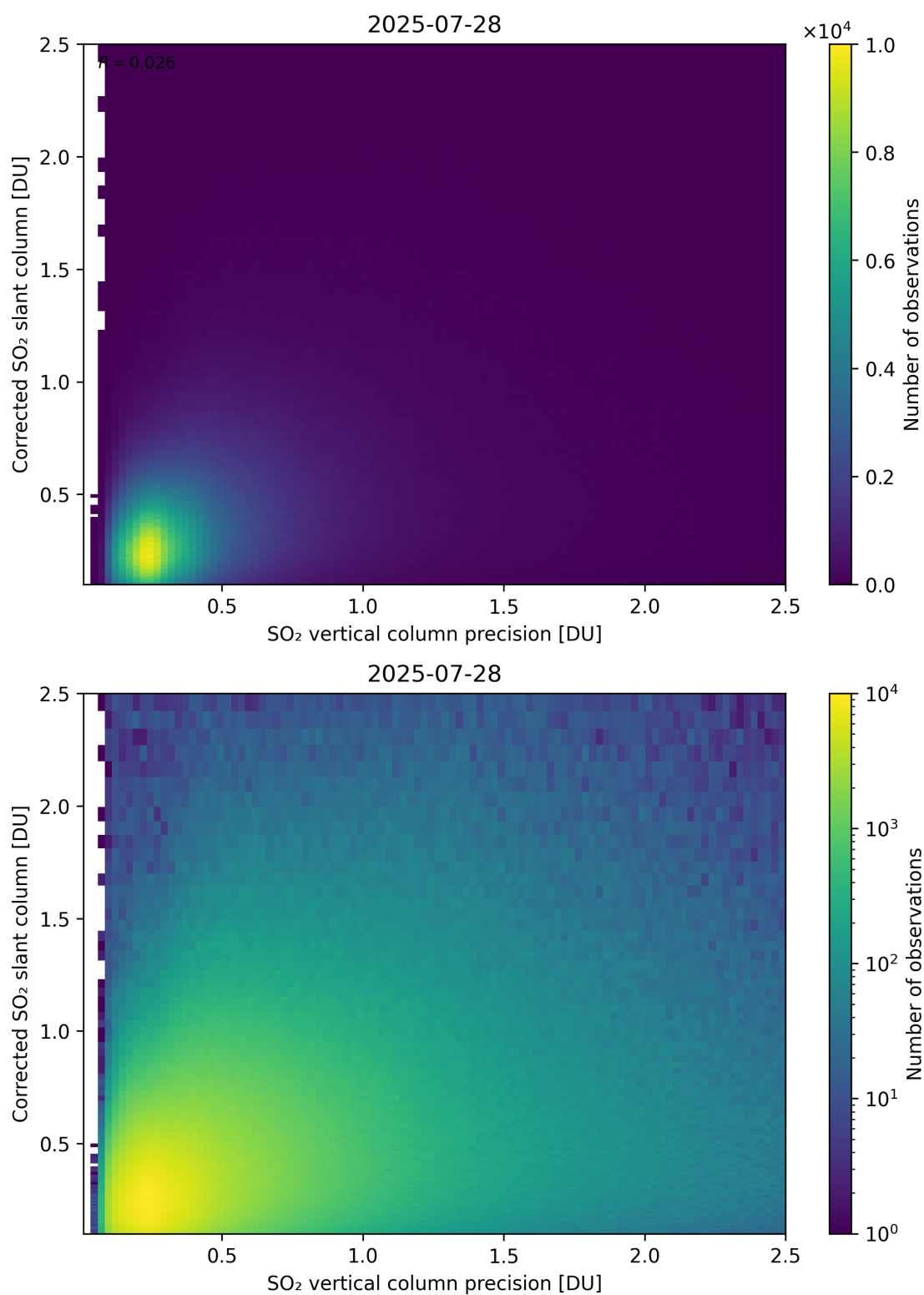
Figure 338: Scatter density plot of “SO 2 vertical column precision” against “Corrected SO 2 slant column” for 2025-07-27 to 2025-07-29.
