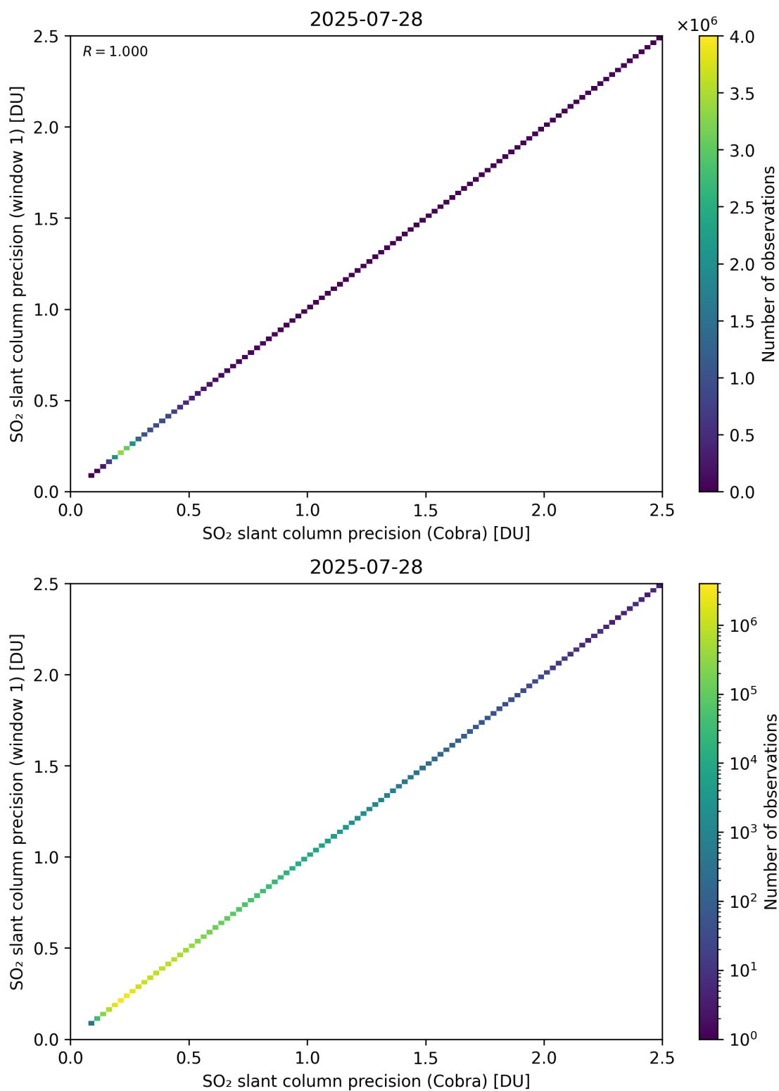
Figure 209: Scatter density plot of “SO 2 slant column precision (Cobra)” against “SO 2 slant column precision (window 1)” for 2025-07-27 to 2025-07-29.
