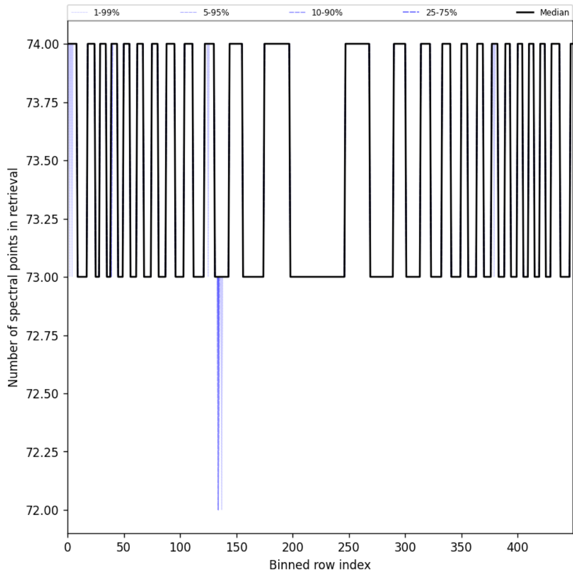
Figure 108: Along track statistics of “Number of spectral points in retrieval” for 2025-07-27 to 2025-07-29
