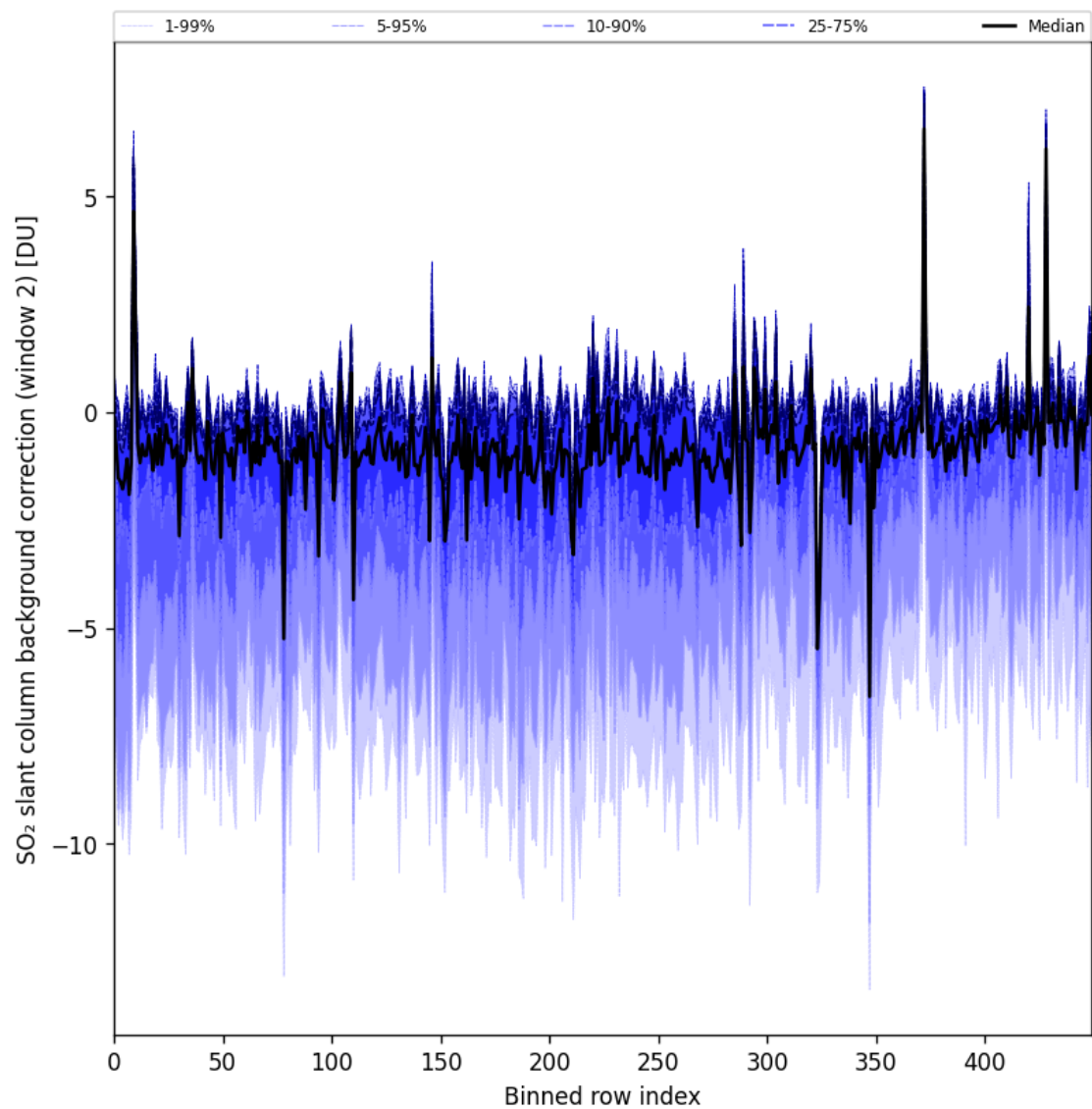
Figure 96: Along track statistics of “SO 2 slant column background correction (window 2)” for 2025-07-27 to 2025-07-29
