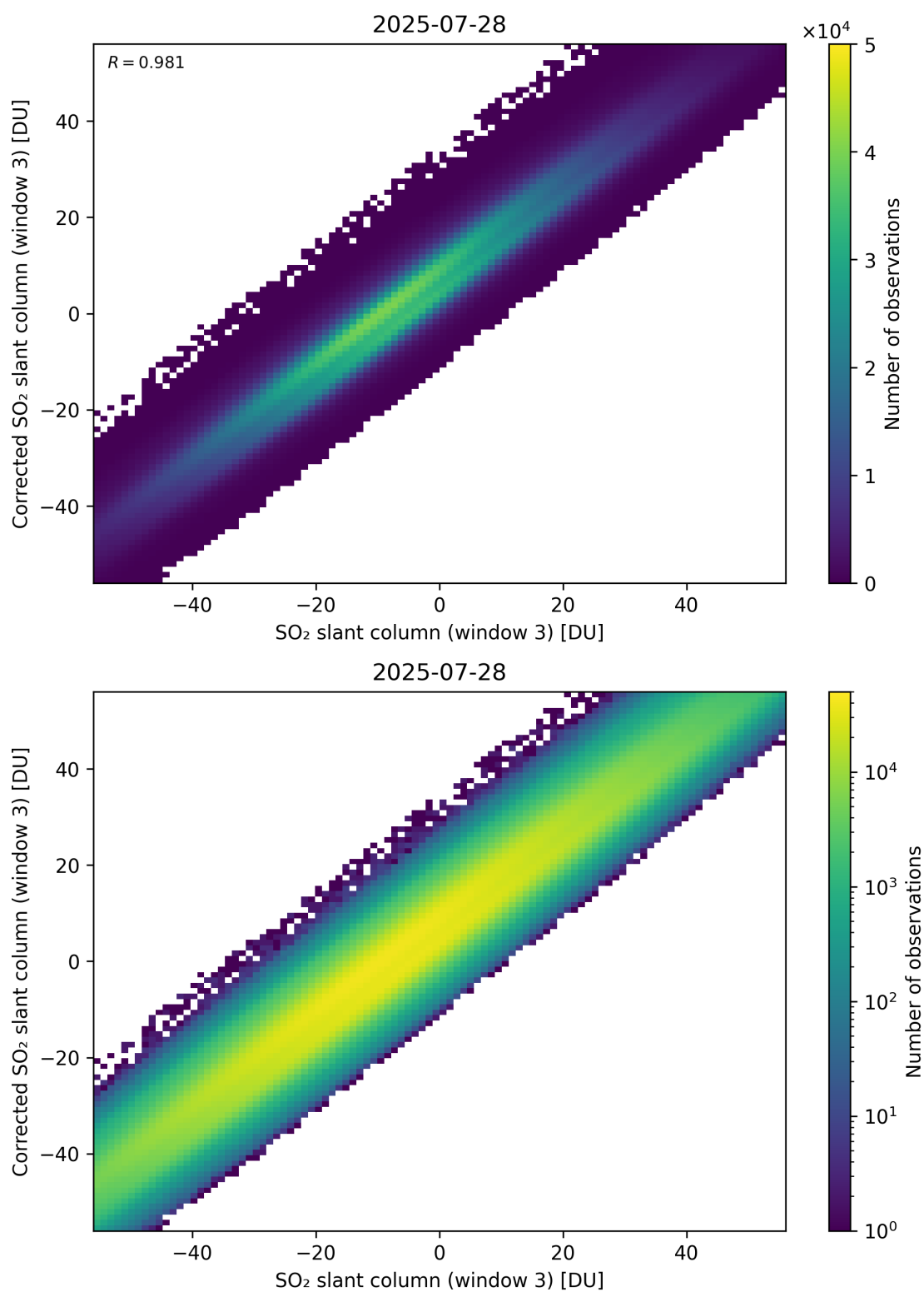
Figure 316: Scatter density plot of “SO 2 slant column (window 3)” against “Corrected SO 2 slant column (window 3)” for 2025-07-27 to 2025-07-29.
