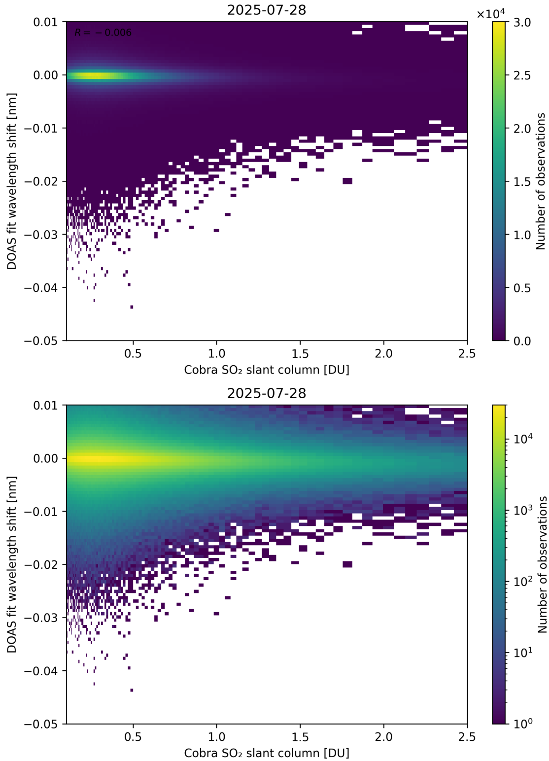
Figure 196: Scatter density plot of “Cobra SO 2 slant column” against “DOAS fit wavelength shift” for 2025-07-27 to 2025-07-29.
