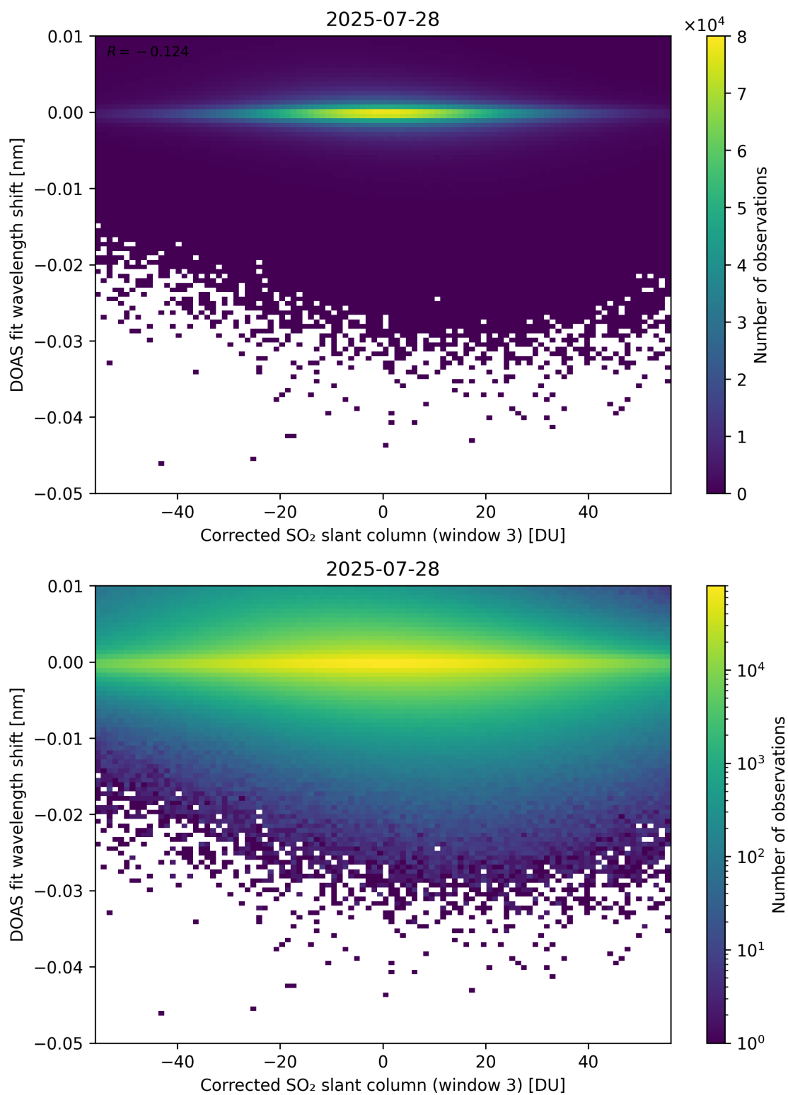
Figure 256: Scatter density plot of “Corrected SO 2 slant column (window 3)” against “DOAS fit wavelength shift” for 2025-07-27 to 2025-07-29.
