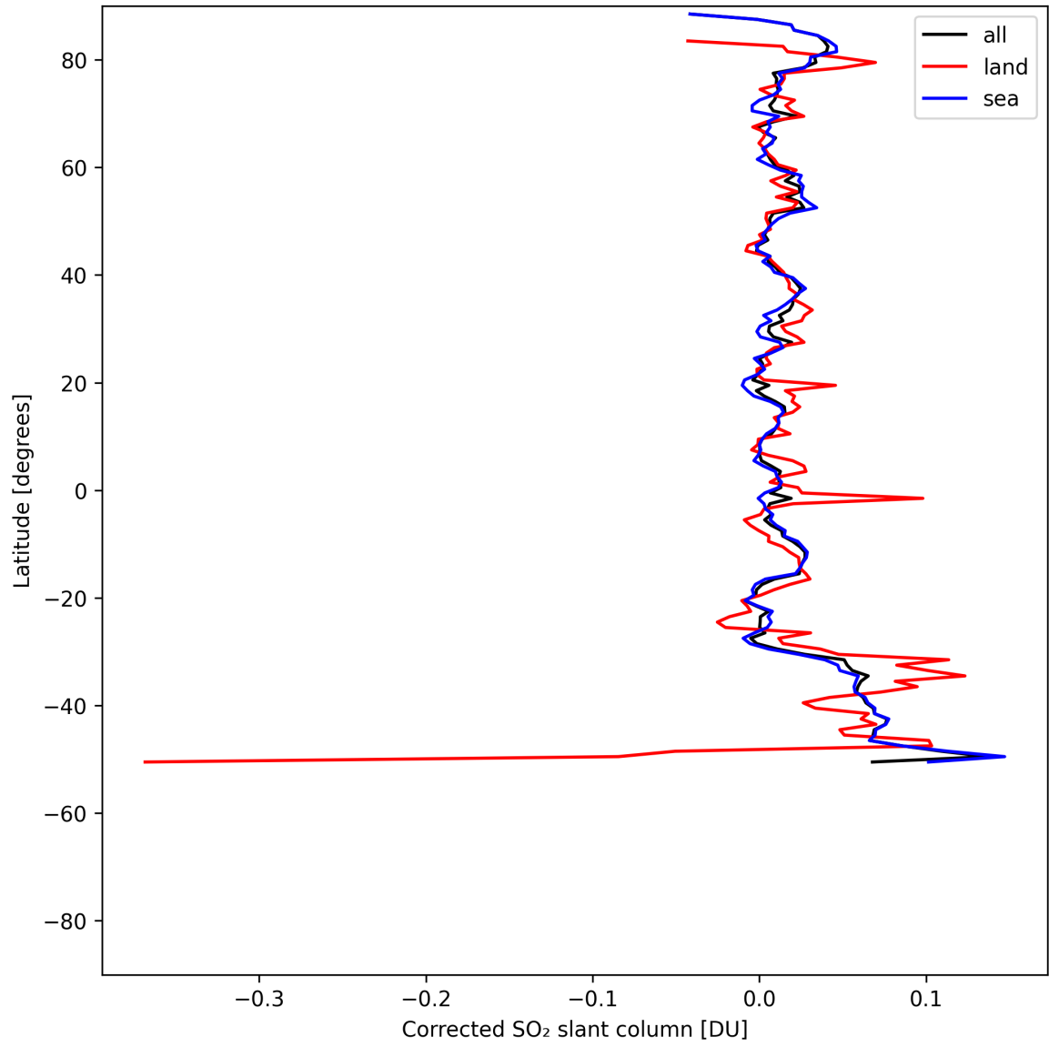
Figure 34: Zonal average of “Corrected SO 2 slant column” for 2025-07-27 to 2025-07-29.
