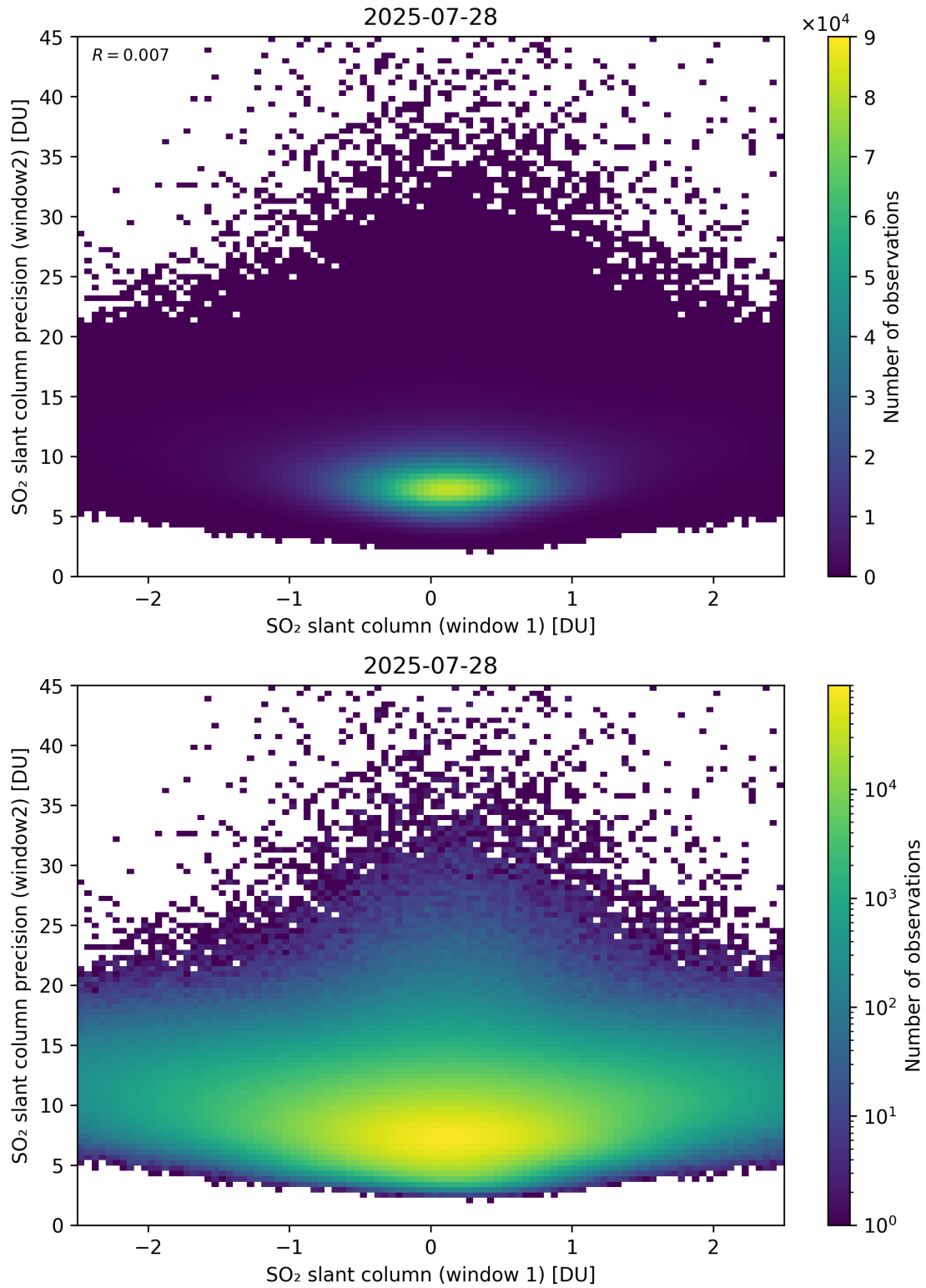
Figure 286: Scatter density plot of “SO 2 slant column (window 1)” against “SO 2 slant column precision (window2)” for 2025-07-27 to 2025-07-29.
