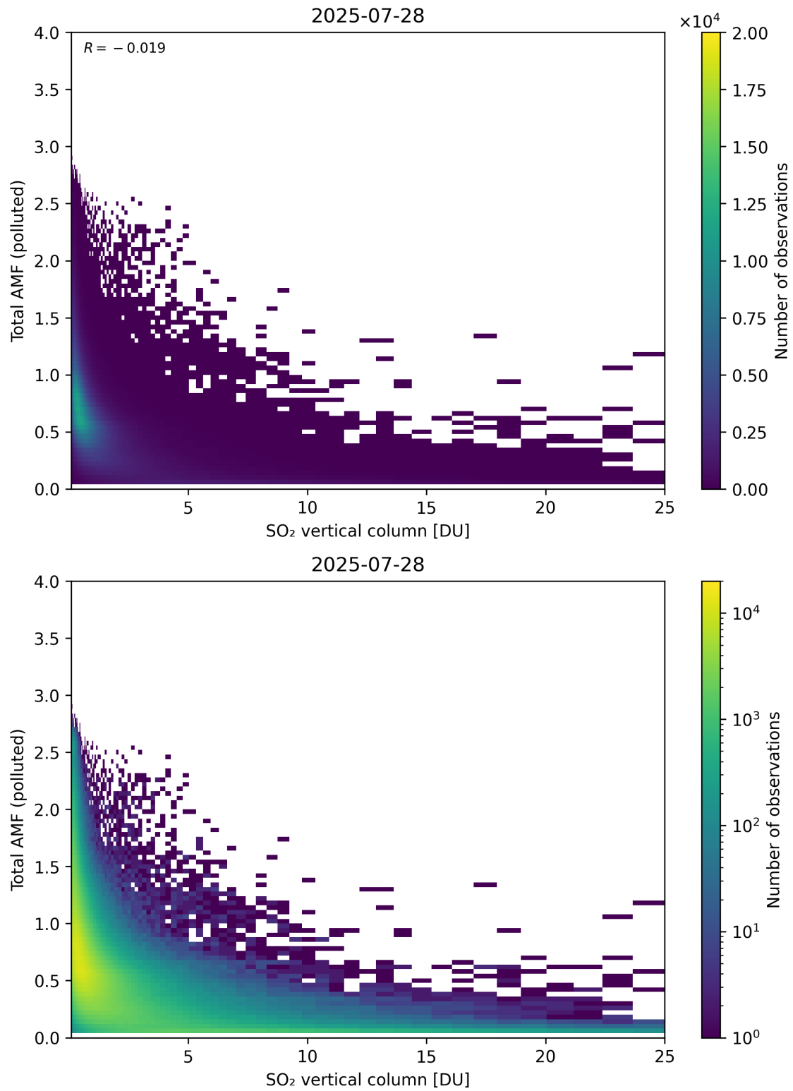
Figure 359: Scatter density plot of “SO 2 vertical column” against “Total AMF (polluted)” for 2025-07-27 to 2025-07-29.
