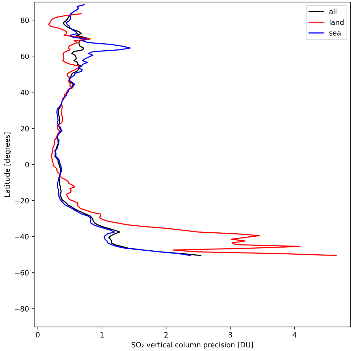
Figure 33: Zonal average of “SO 2 vertical column precision” for 2025-07-27 to 2025-07-29.
