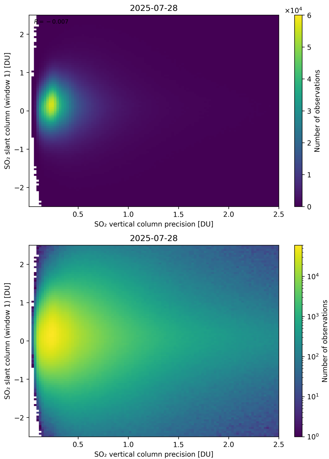
Figure 341: Scatter density plot of “SO 2 vertical column precision” against “SO 2 slant column (window 1)” for 2025-07-27 to 2025-07-29.
