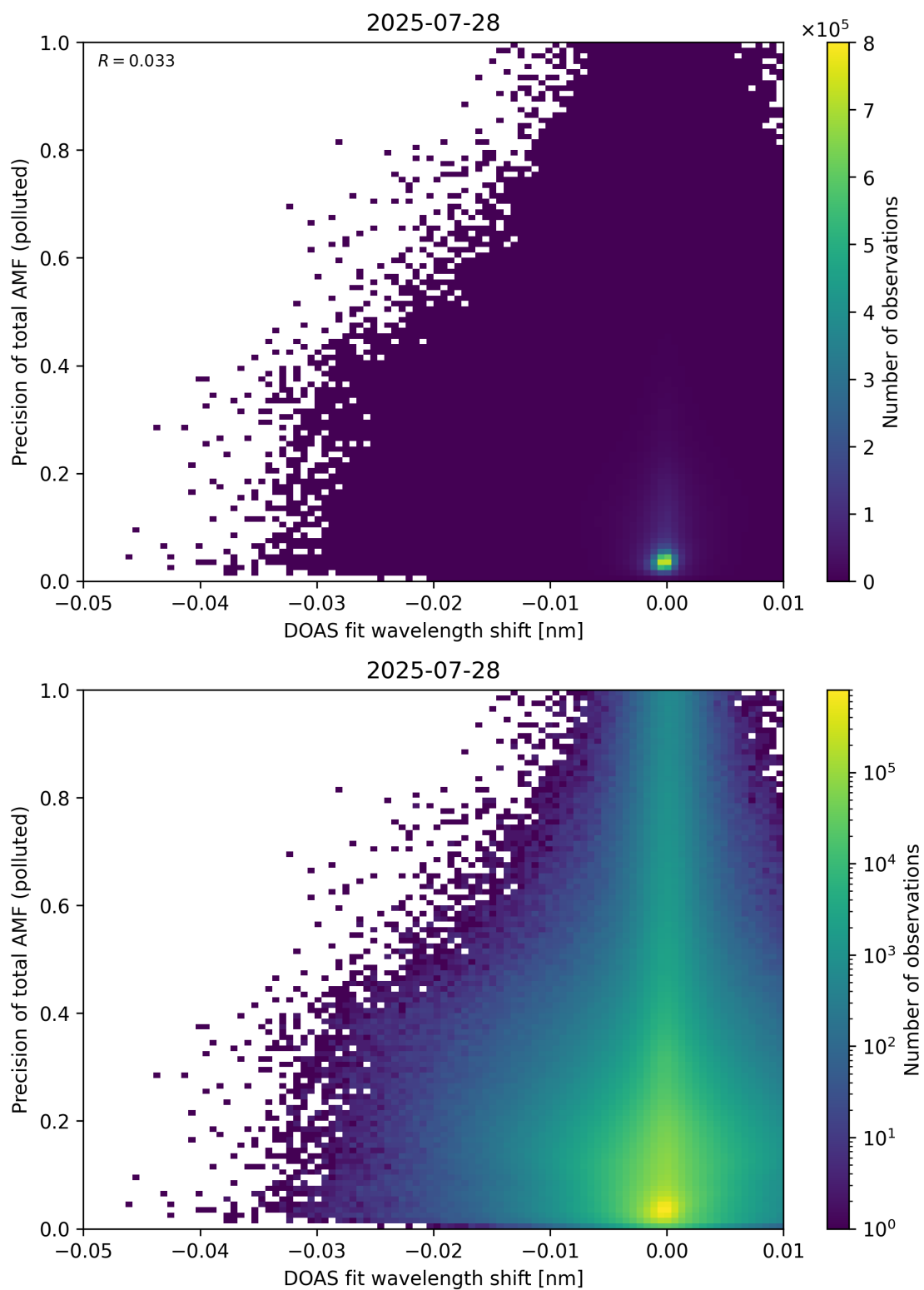
Figure 142: Scatter density plot of “DOAS fit wavelength shift” against “Precision of total AMF (polluted)” for 2025-07-27 to 2025-07-29.
