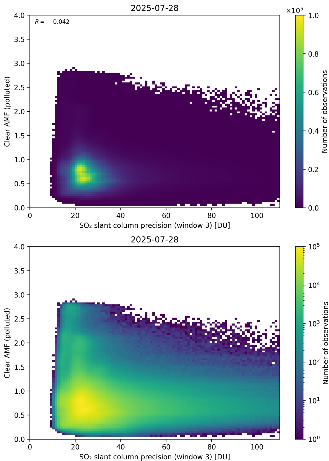
Figure 311: Scatter density plot of “SO 2 slant column precision (window 3)” against “Clear AMF (polluted)” for 2025-07-27 to 2025-07-29.
