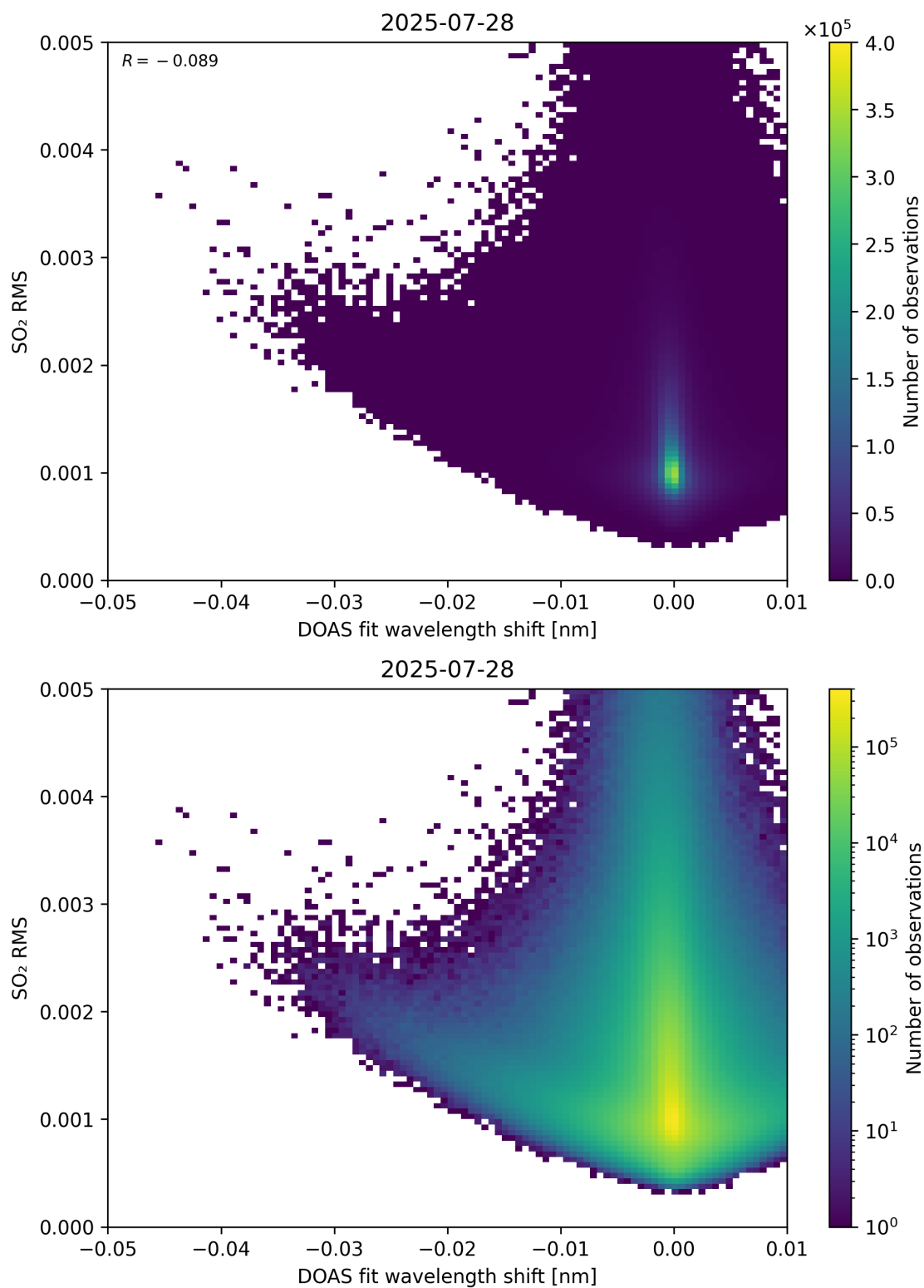
Figure 139: Scatter density plot of “DOAS fit wavelength shift” against “SO 2 RMS” for 2025-07-27 to 2025-07-29.
