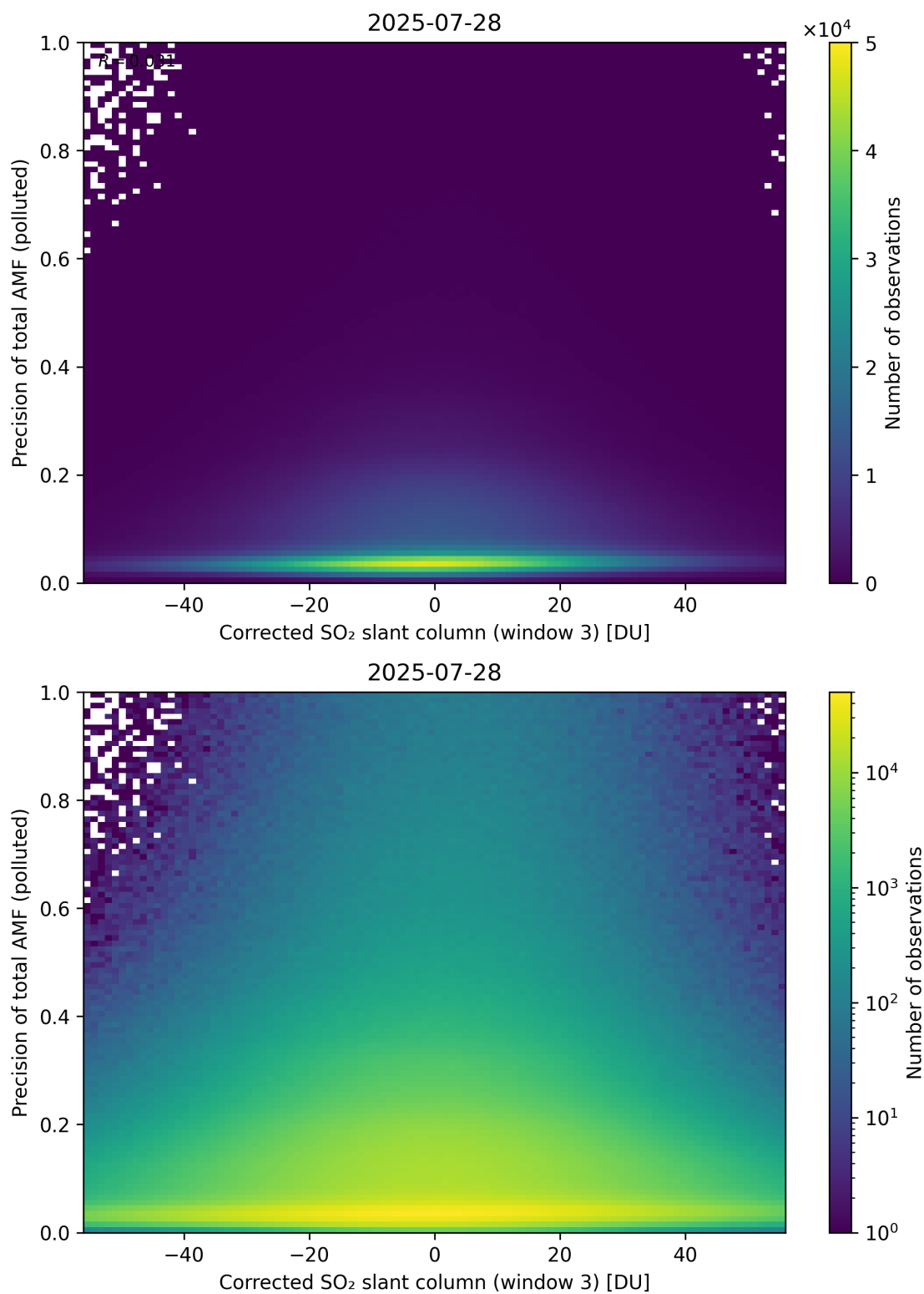
Figure 261: Scatter density plot of “Corrected SO 2 slant column (window 3)” against “Precision of total AMF (polluted)” for 2025-07-27 to 2025-07-29.
