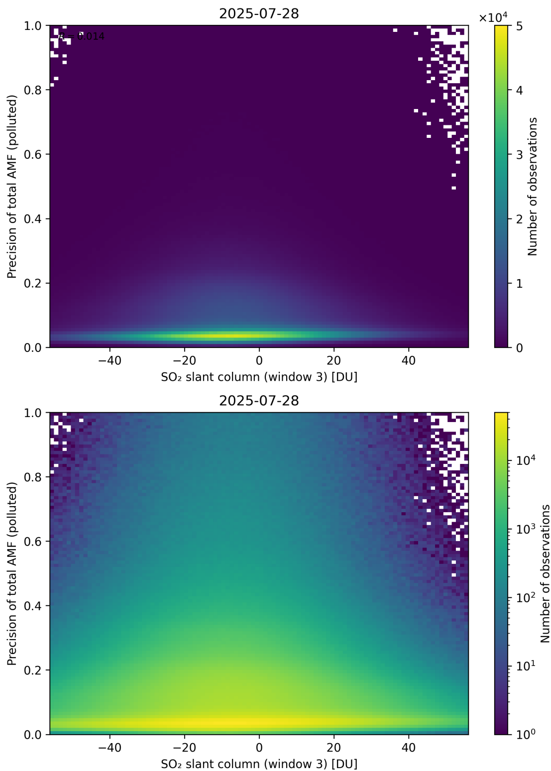
Figure 319: Scatter density plot of “SO 2 slant column (window 3)” against “Precision of total AMF (polluted)” for 2025-07-27 to 2025-07-29.
