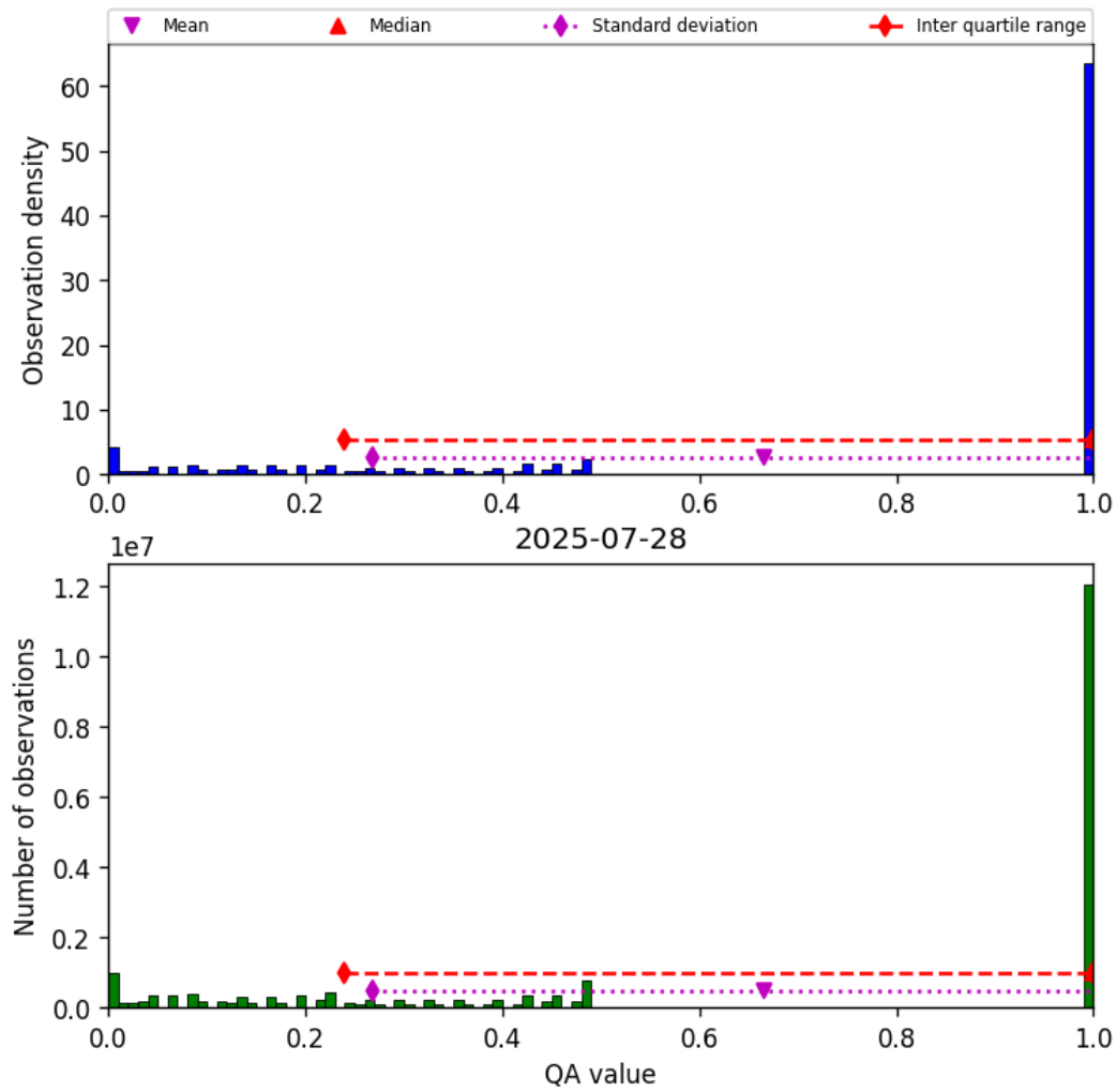
Figure 57: Histogram of “QA value” for 2025-07-27 to 2025-07-29
