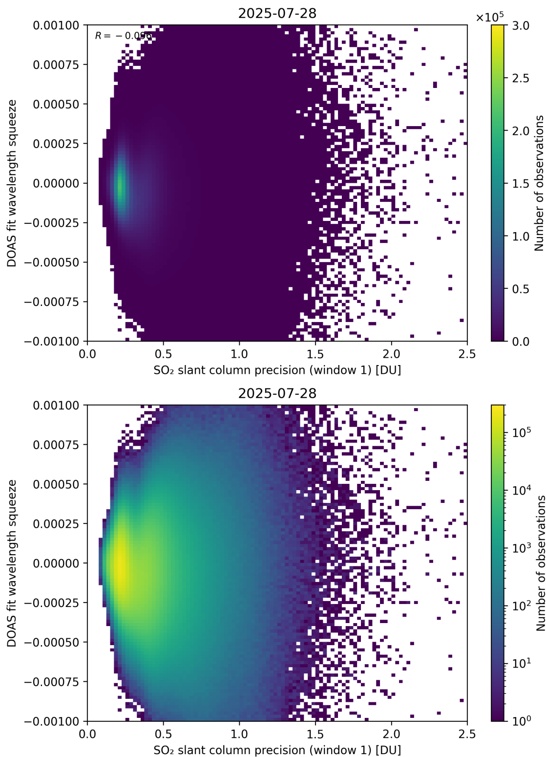
Figure 272: Scatter density plot of “SO 2 slant column precision (window 1)” against “DOAS fit wavelength squeeze” for 2025-07-27 to 2025-07-29.
