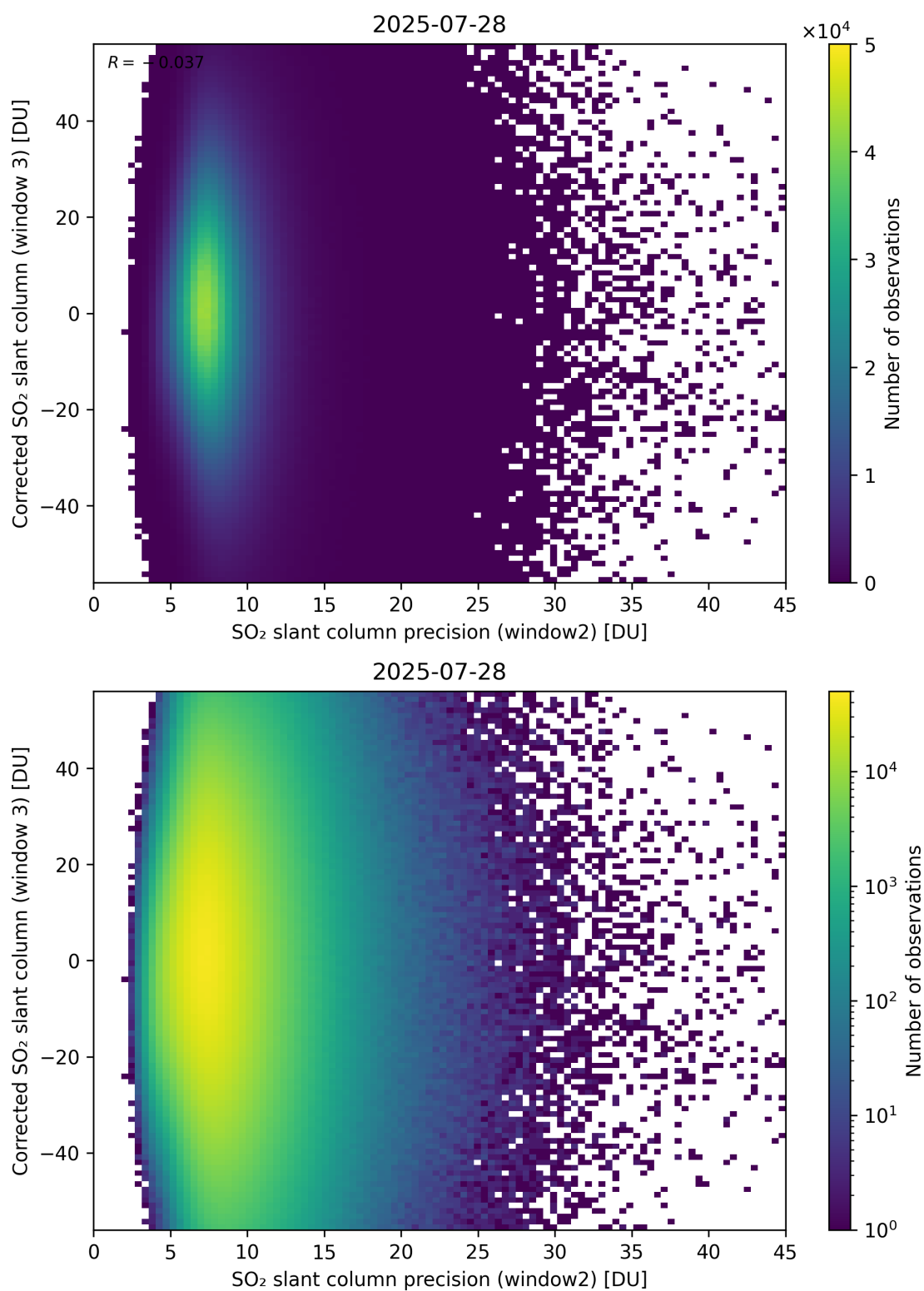
Figure 298: Scatter density plot of “SO 2 slant column precision (window2)” against “Corrected SO 2 slant column (window 3)” for 2025-07-27 to 2025-07-29.
