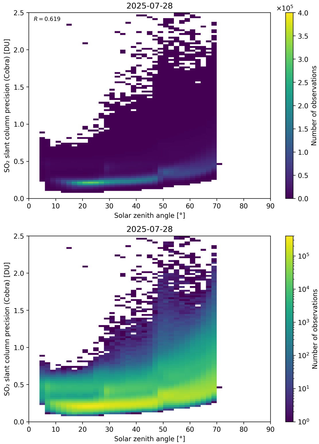
Figure 180: Scatter density plot of “Solar zenith angle” against “SO 2 slant column precision (Cobra)” for 2025-07-27 to 2025-07-29.
