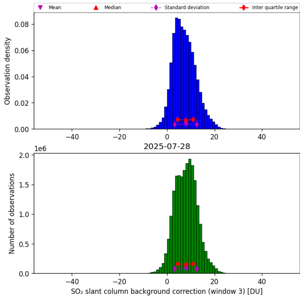
Figure 74: Histogram of “SO 2 slant column background correction (window 3)” for 2025-07-27 to 2025-07-29
