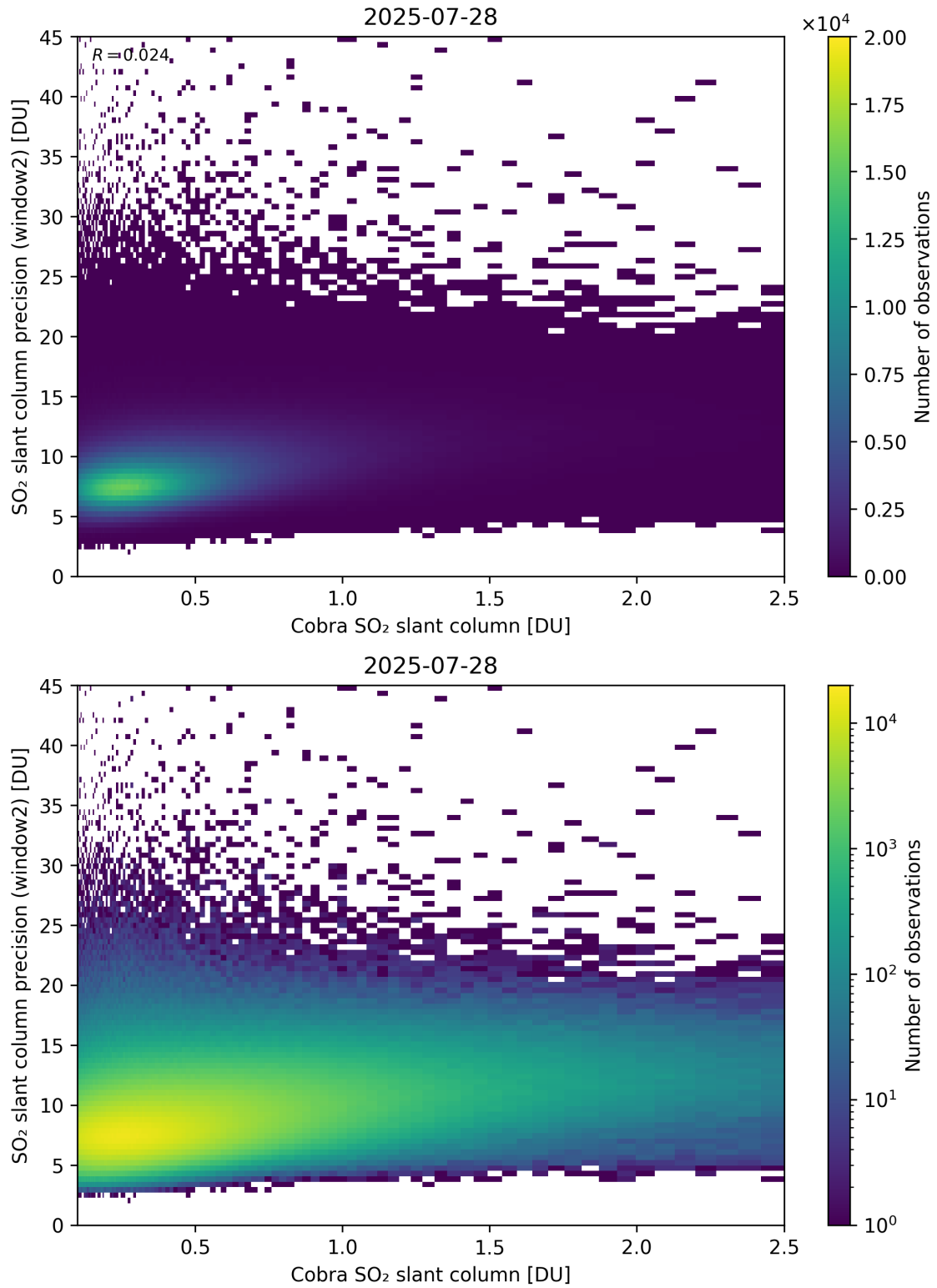
Figure 221: Scatter density plot of “Cobra SO 2 slant column” against “SO 2 slant column precision (window2)” for 2025-07-27 to 2025-07-29.
