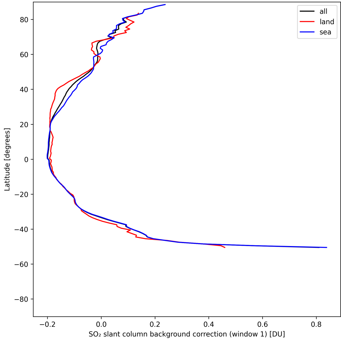
Figure 40: Zonal average of “SO 2 slant column background correction (window 1)” for 2025-07-27 to 2025-07-29.
