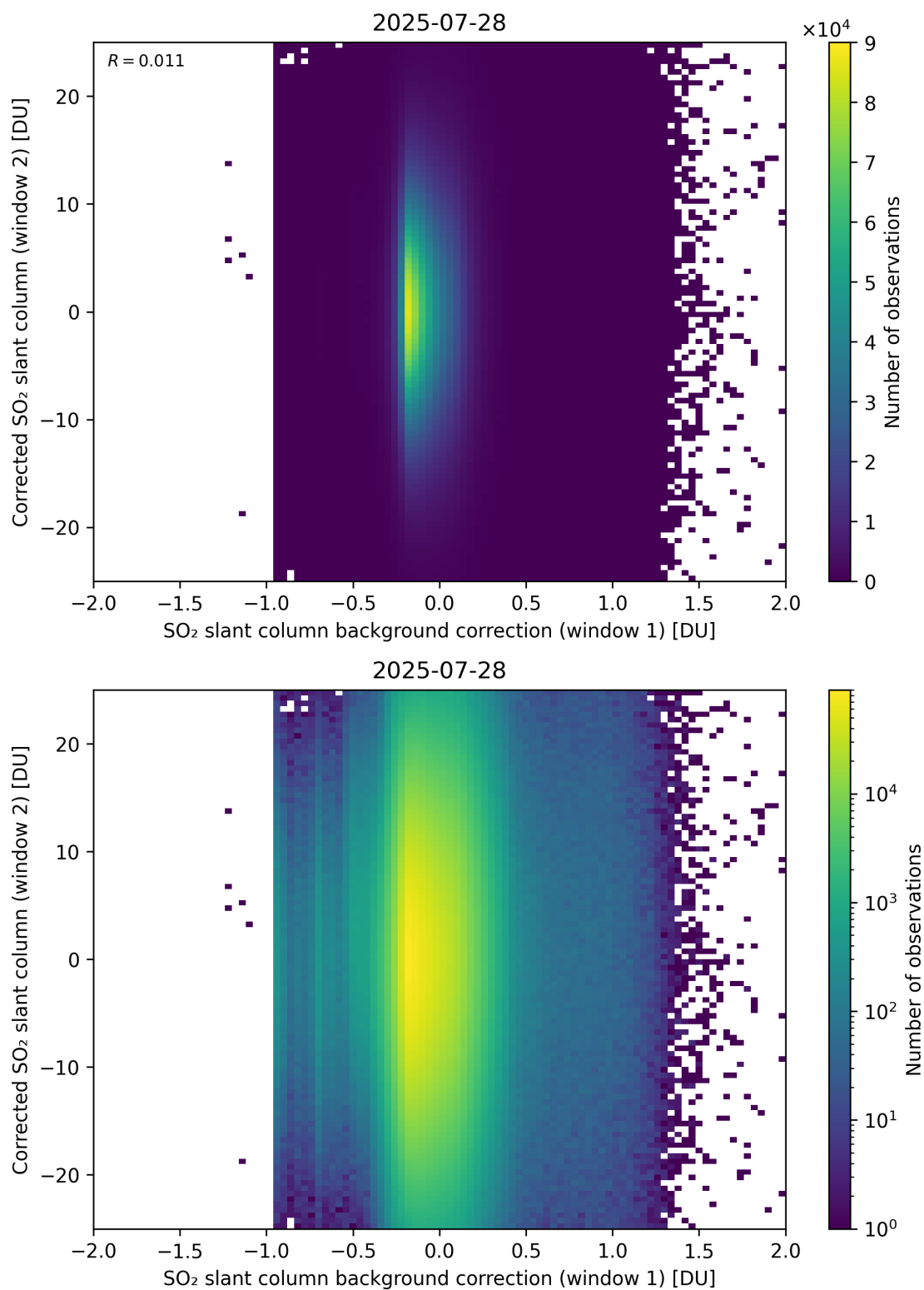
Figure 115: Scatter density plot of “SO 2 slant column background correction (window 1)” against “Corrected SO 2 slant column (window 2)” for 2025-07-27 to 2025-07-29.
