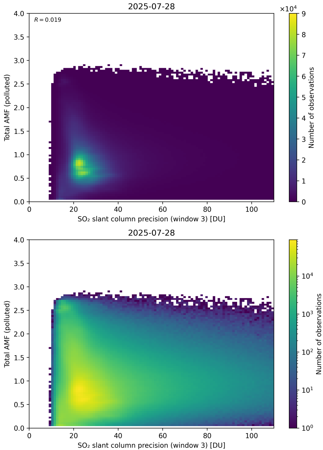
Figure 313: Scatter density plot of “SO 2 slant column precision (window 3)” against “Total AMF (polluted)” for 2025-07-27 to 2025-07-29.
