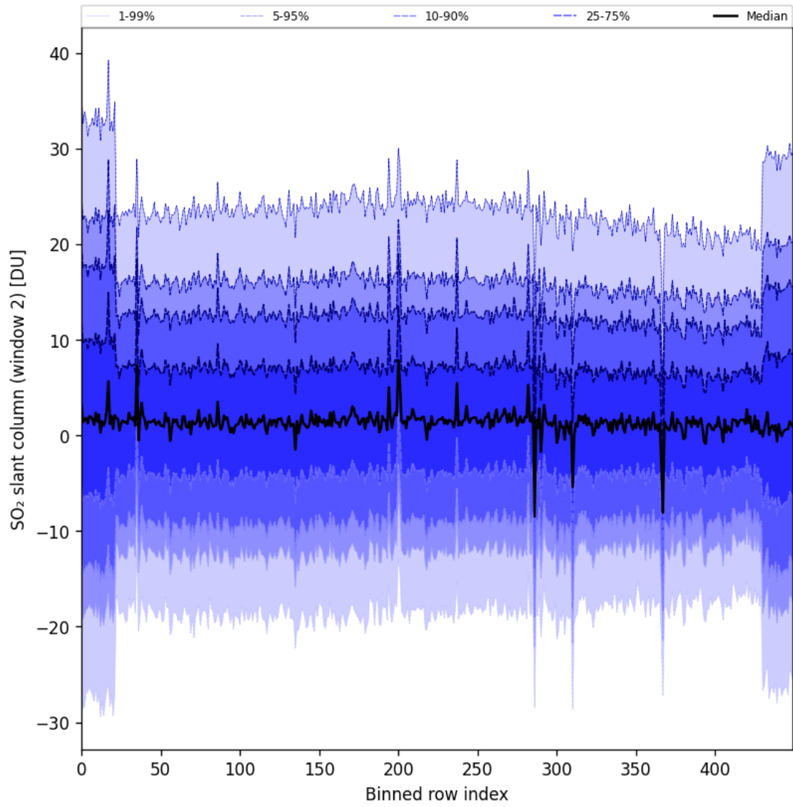
Figure 93: Along track statistics of “SO 2 slant column (window 2)” for 2025-07-27 to 2025-07-29
