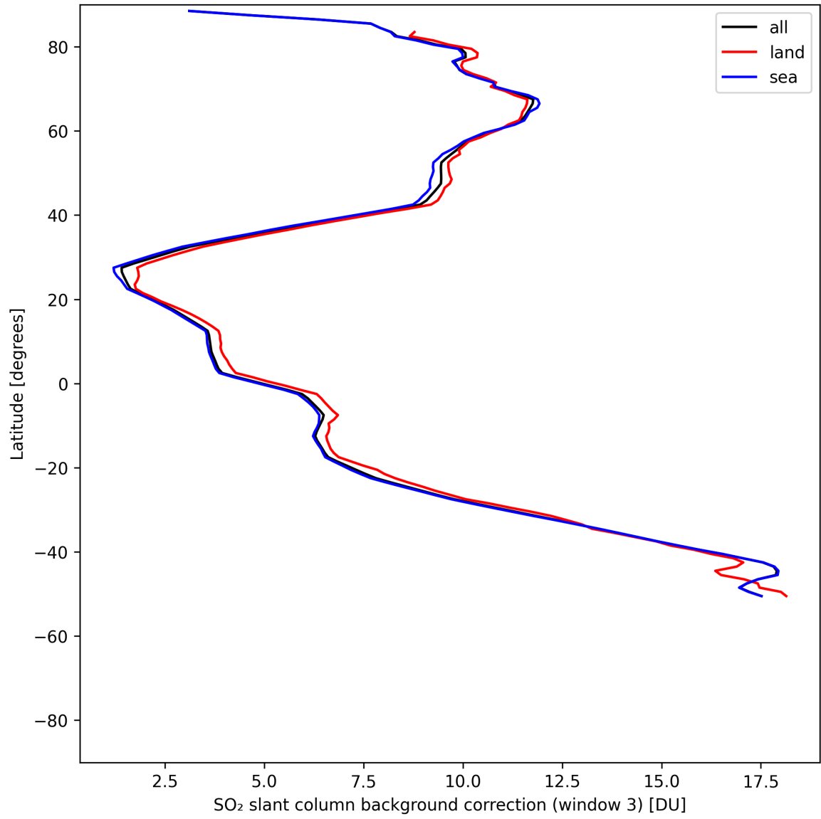
Figure 48: Zonal average of “SO 2 slant column background correction (window 3)” for 2025-07-27 to 2025-07-29.
