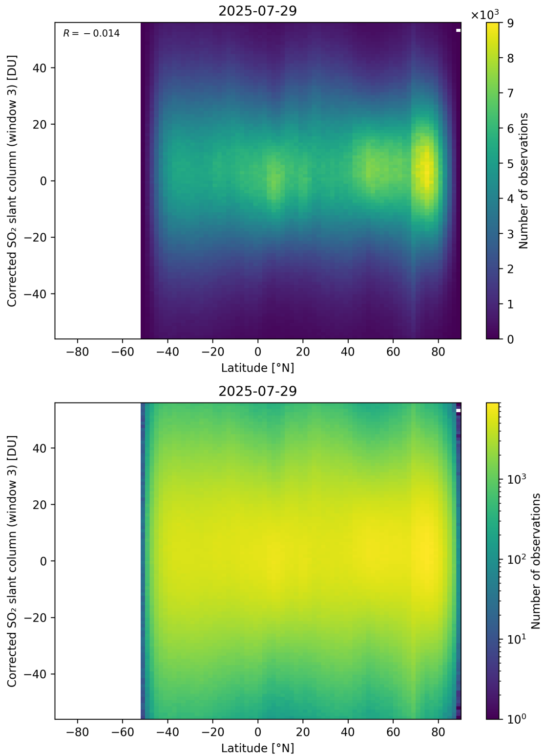
Figure 161: Scatter density plot of “Latitude” against “Corrected SO 2 slant column (window 3)” for 2025-07-29 to 2025-07-30.
