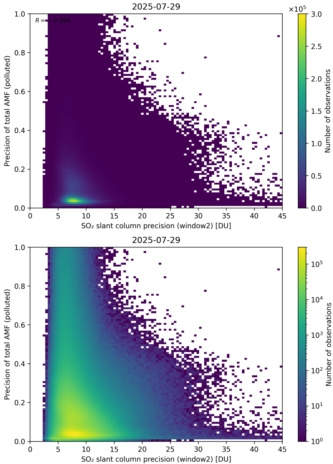
Figure 302: Scatter density plot of “SO 2 slant column precision (window2)” against “Precision of total AMF (polluted)” for 2025-07-29 to 2025-07-30.
