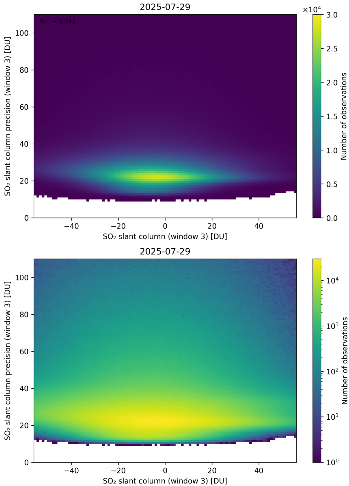
Figure 317: Scatter density plot of “SO 2 slant column (window 3)” against “SO 2 slant column precision (window 3)” for 2025-07-29 to 2025-07-30.
