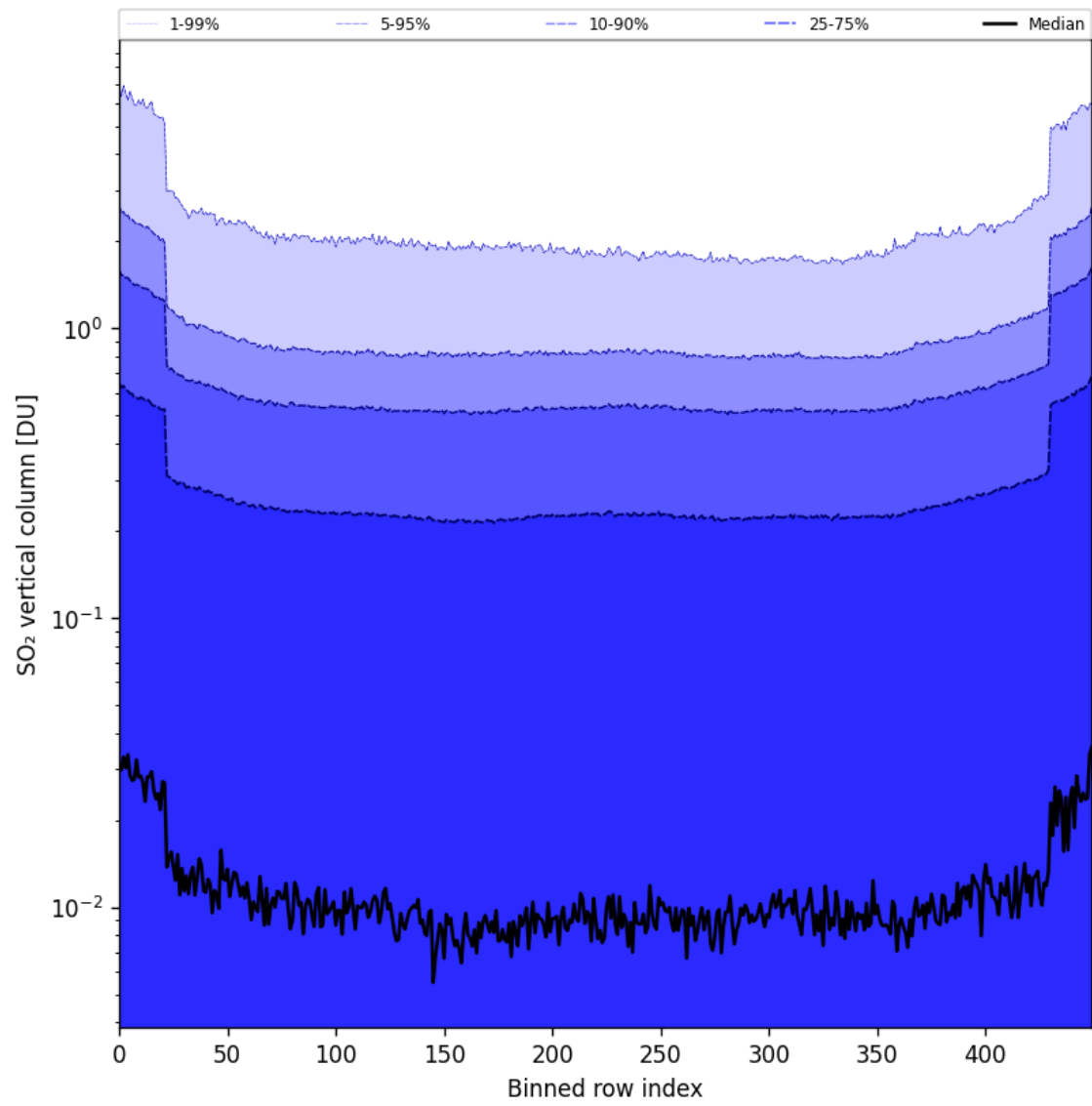
Figure 84: Along track statistics of “SO 2 vertical column” for 2025-07-29 to 2025-07-30
