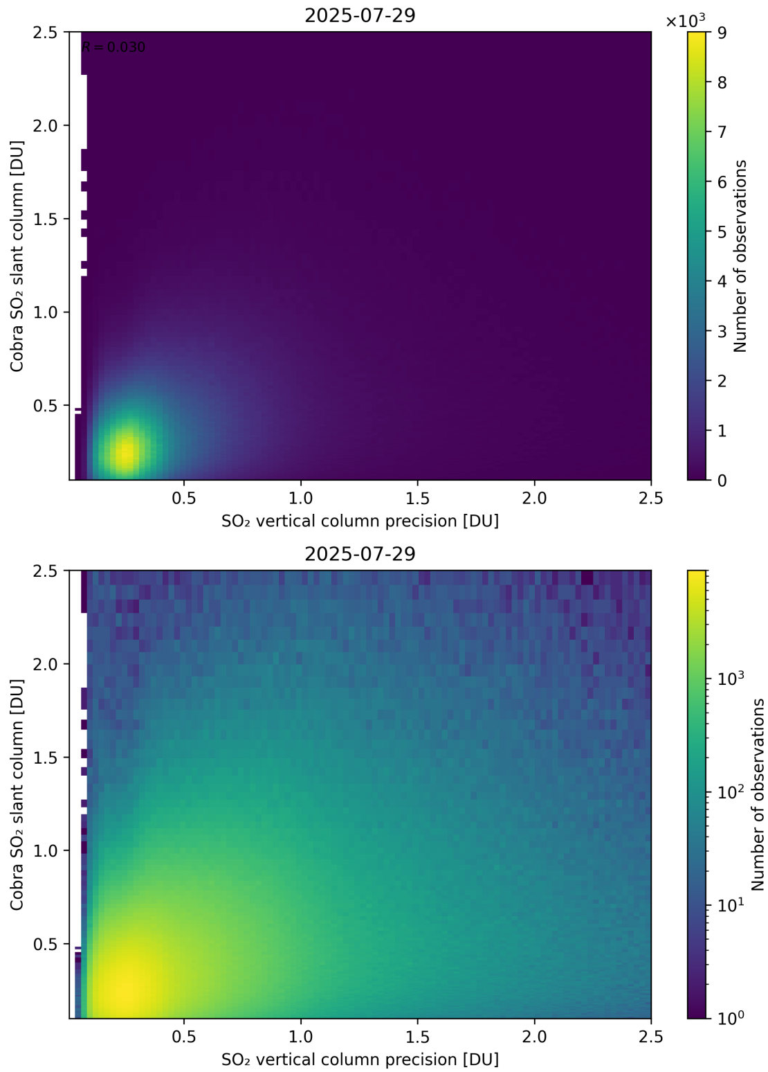
Figure 336: Scatter density plot of “SO 2 vertical column precision” against “Cobra SO 2 slant column” for 2025-07-29 to 2025-07-30.
