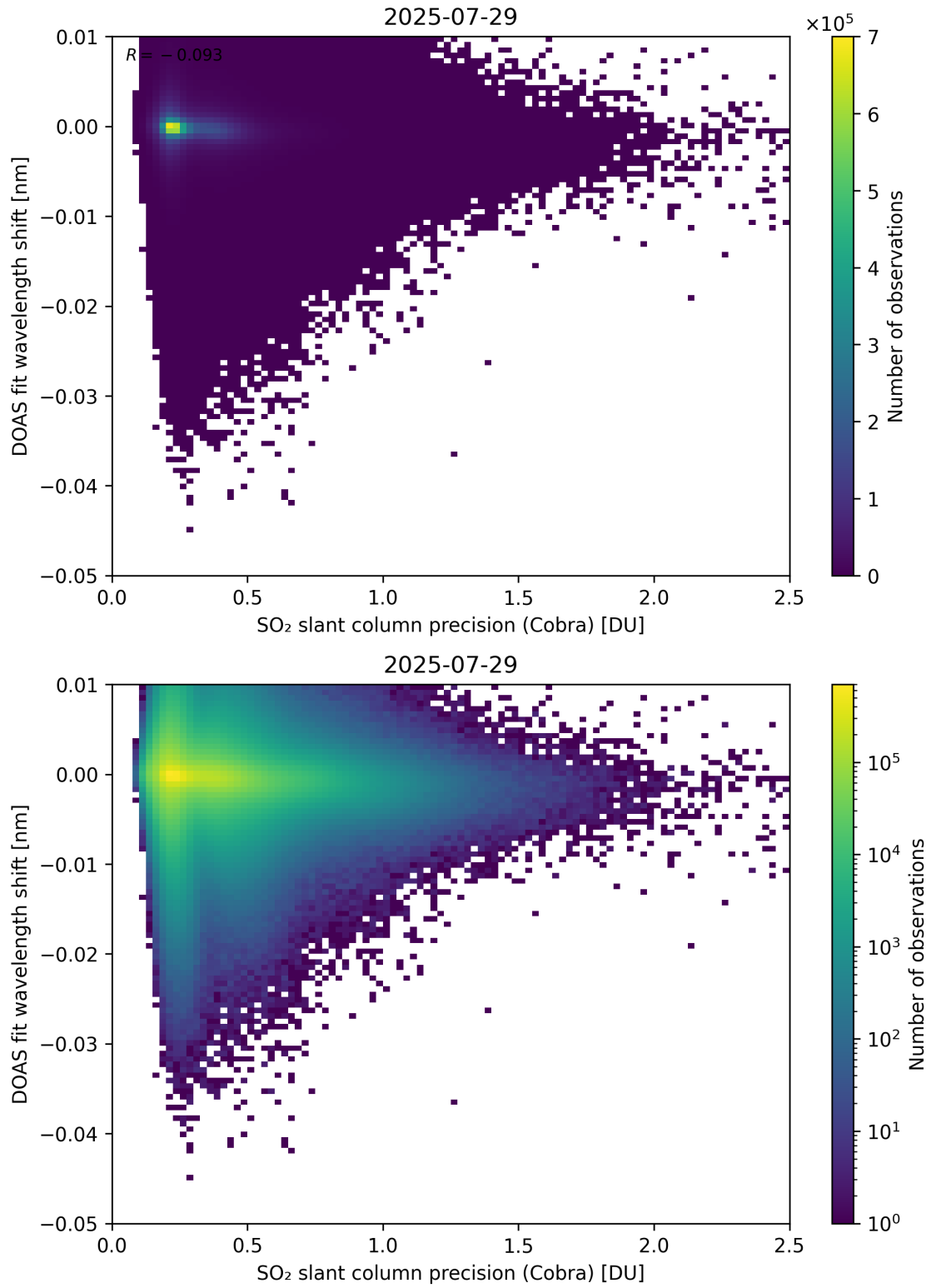
Figure 202: Scatter density plot of “SO 2 slant column precision (Cobra)” against “DOAS fit wavelength shift” for 2025-07-29 to 2025-07-30.
