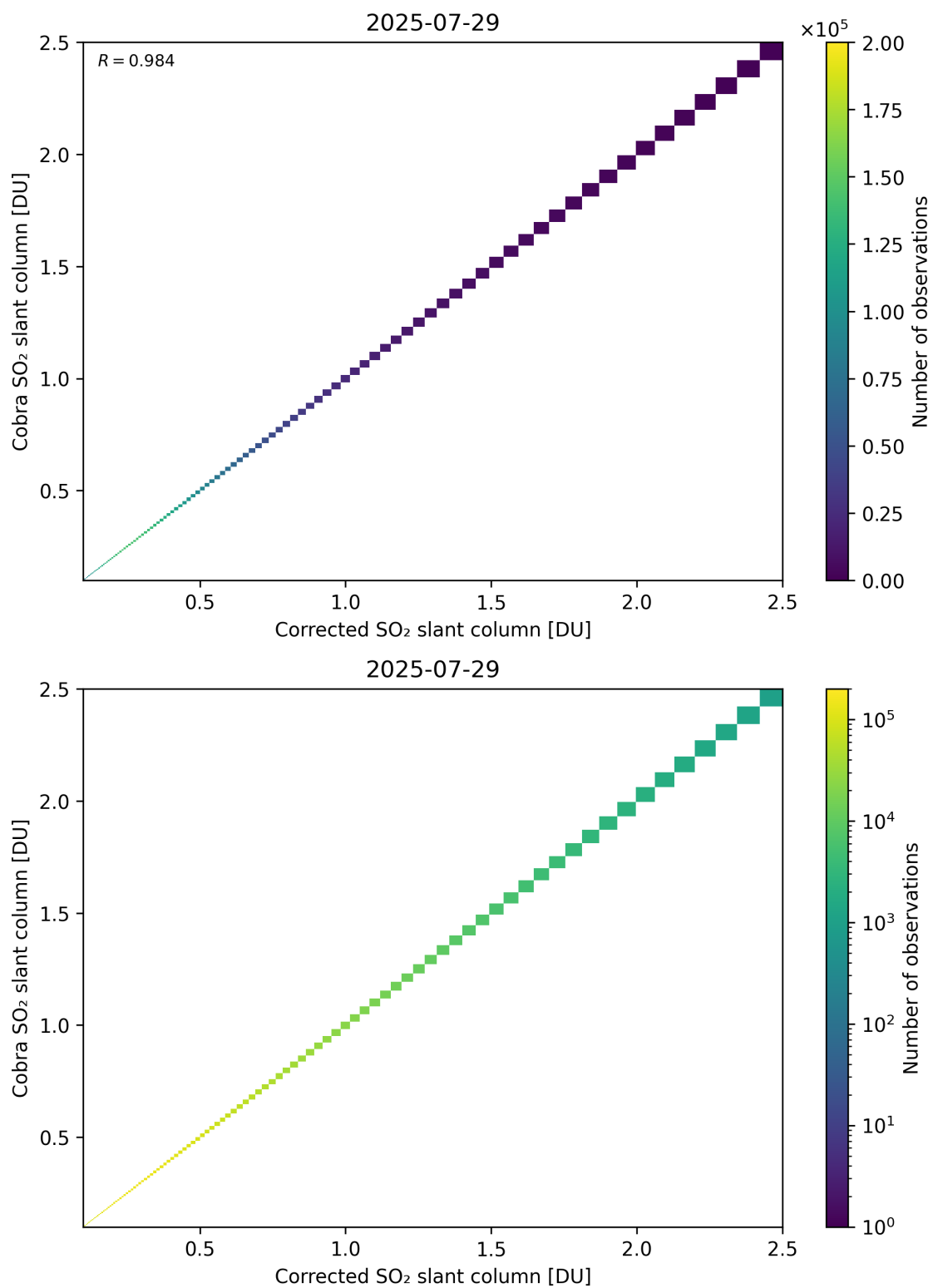
Figure 233: Scatter density plot of “Corrected SO 2 slant column” against “Cobra SO 2 slant column” for 2025-07-29 to 2025-07-30.
