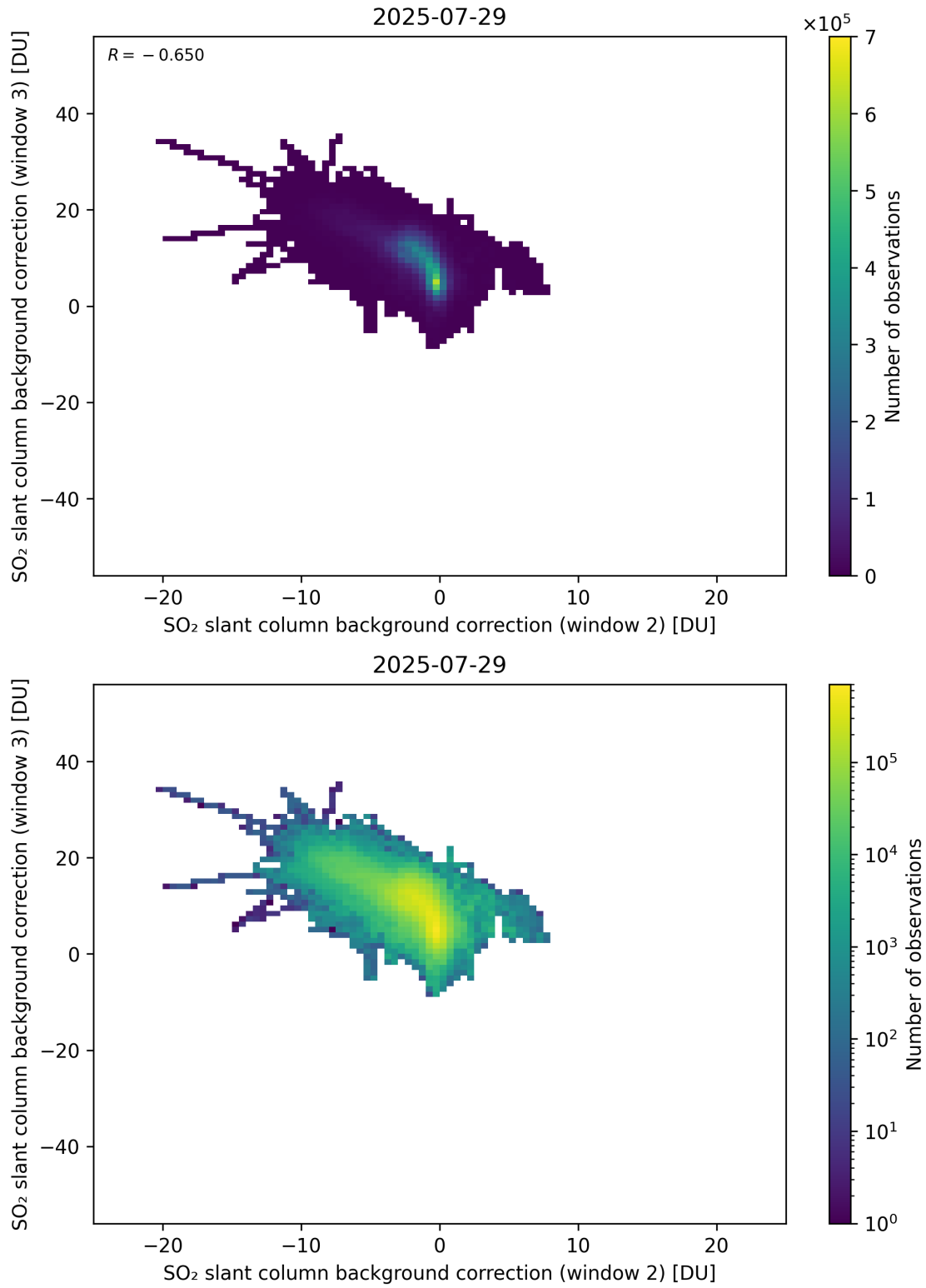
Figure 122: Scatter density plot of “SO 2 slant column background correction (window 2)” against “SO 2 slant column background correction (window 3)” for 2025-07-29 to 2025-07-30.
