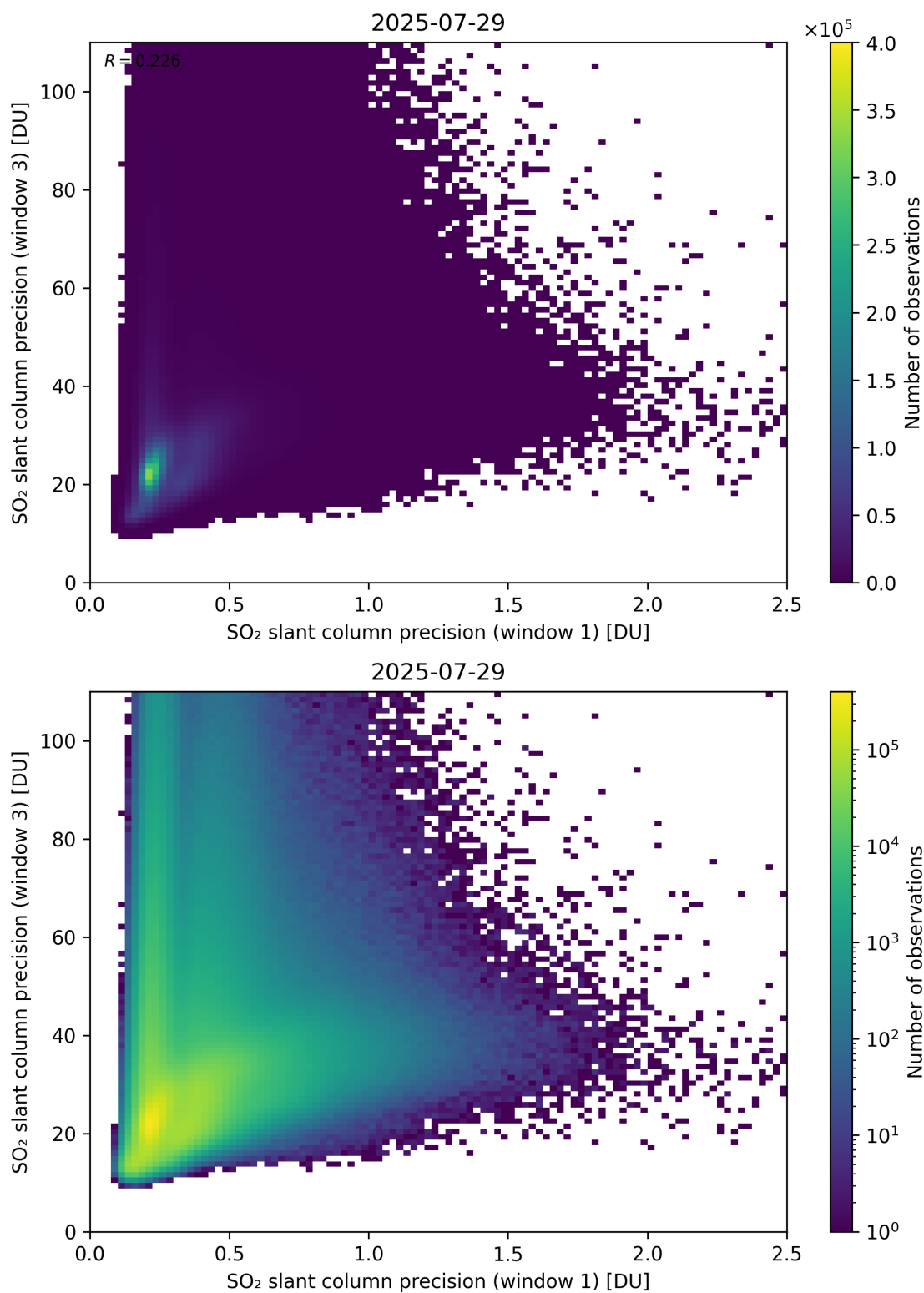
Figure 279: Scatter density plot of “SO 2 slant column precision (window 1)” against “SO 2 slant column precision (window 3)” for 2025-07-29 to 2025-07-30.
