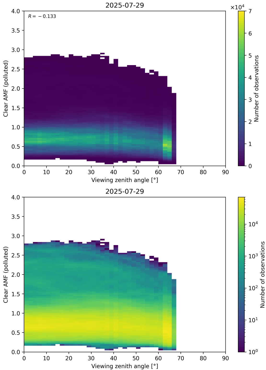
Figure 370: Scatter density plot of “Viewing zenith angle” against “Clear AMF (polluted)” for 2025-07-29 to 2025-07-30.
