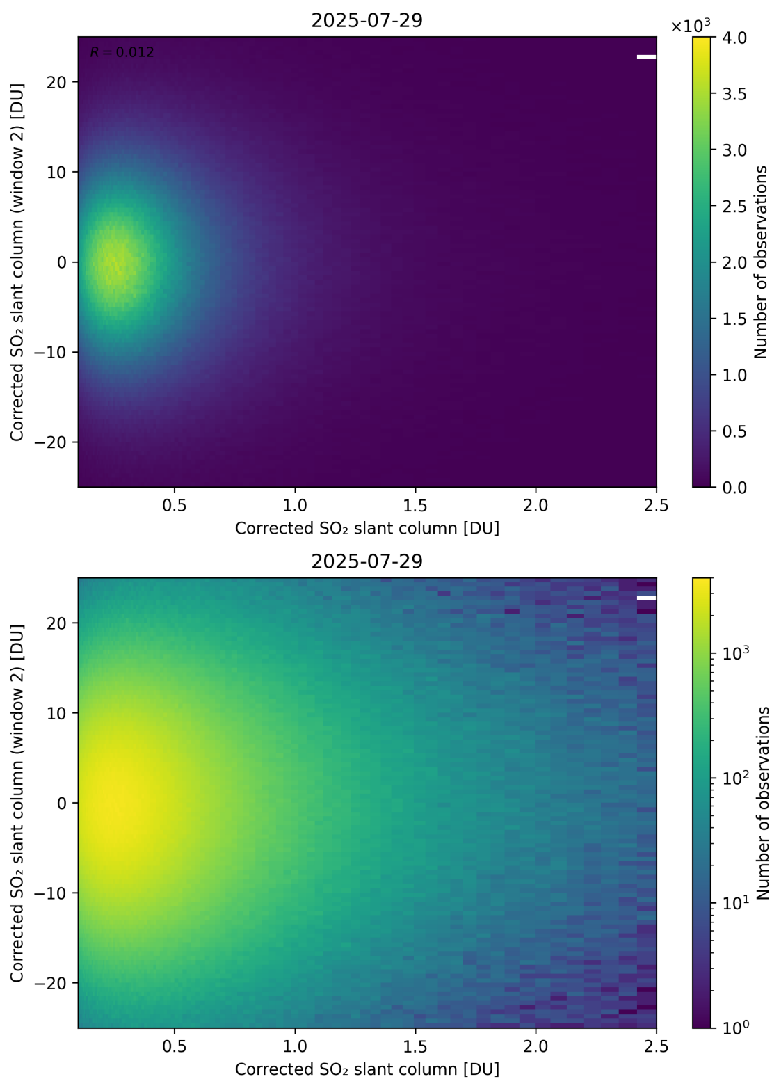
Figure 235: Scatter density plot of “Corrected SO 2 slant column” against “Corrected SO 2 slant column (window 2)” for 2025-07-29 to 2025-07-30.
