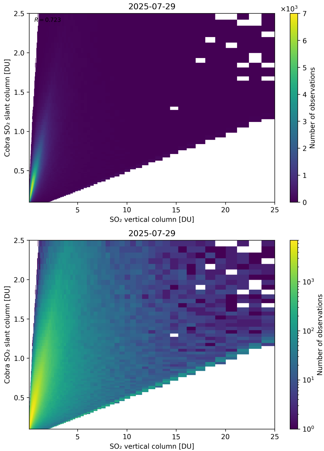
Figure 349: Scatter density plot of “SO 2 vertical column” against “Cobra SO 2 slant column” for 2025-07-29 to 2025-07-30.
