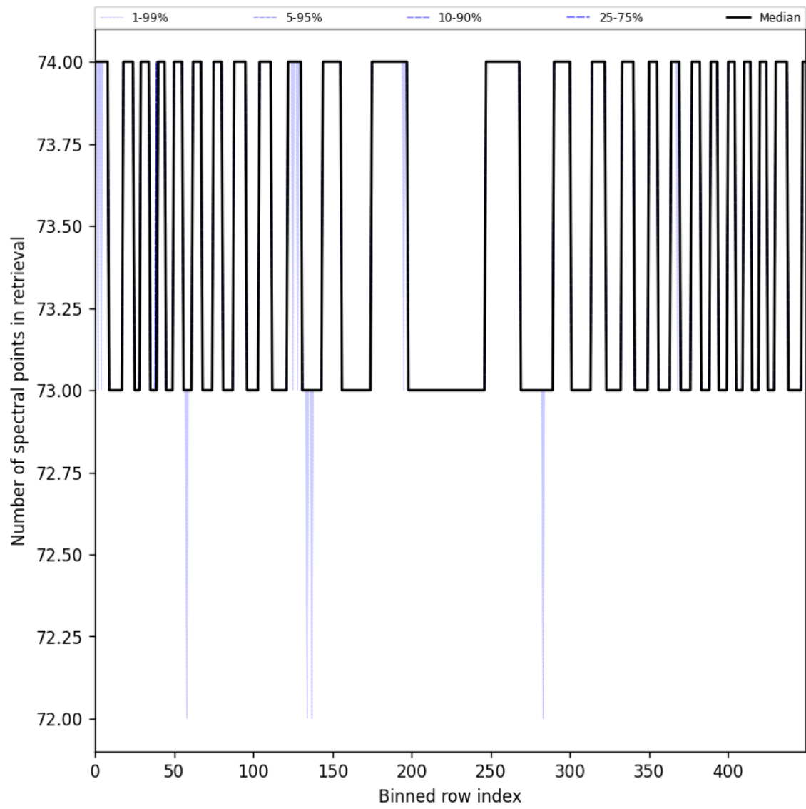
Figure 108: Along track statistics of “Number of spectral points in retrieval” for 2025-07-29 to 2025-07-30
