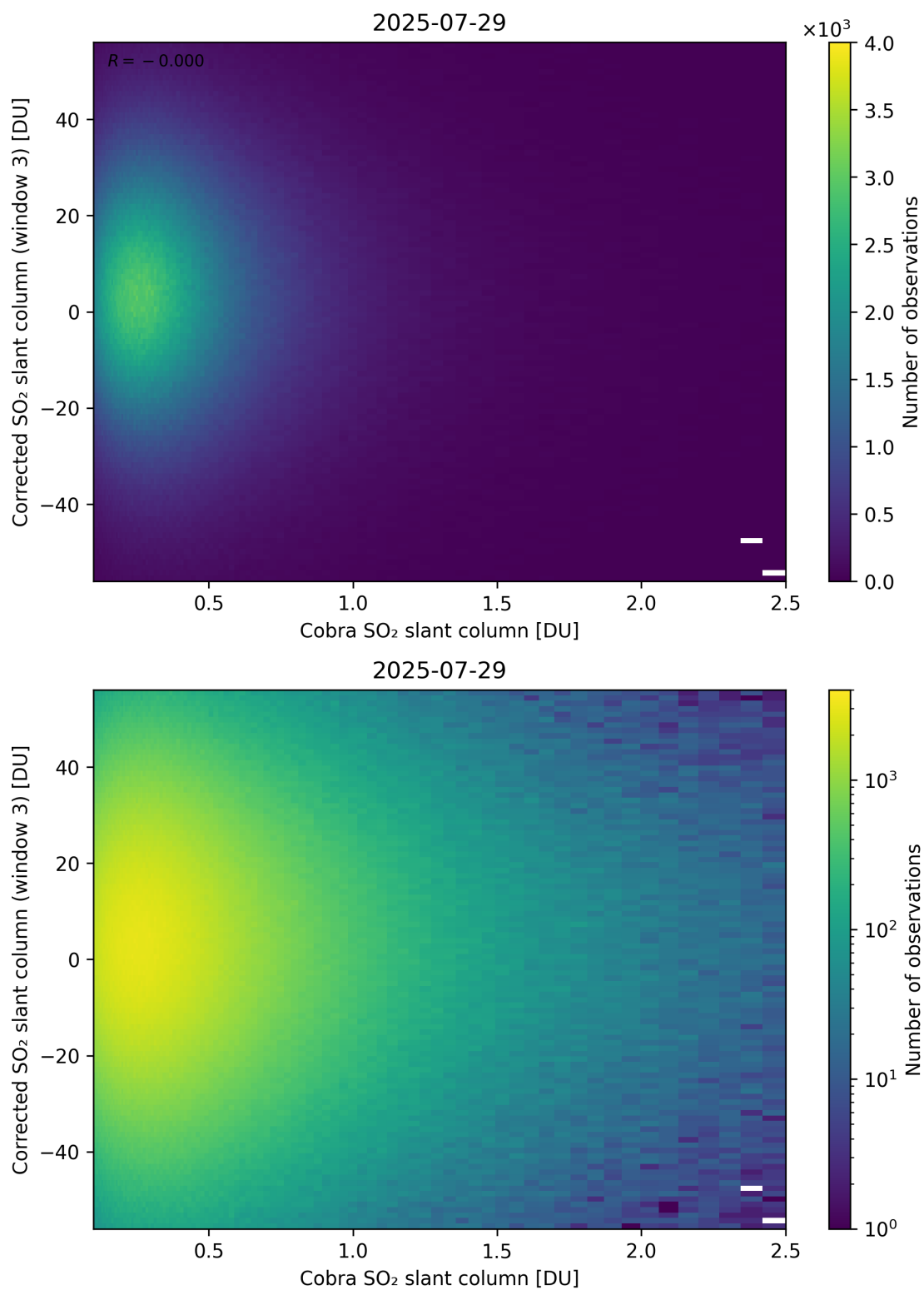
Figure 218: Scatter density plot of “Cobra SO 2 slant column” against “Corrected SO 2 slant column (window 3)” for 2025-07-29 to 2025-07-30.
