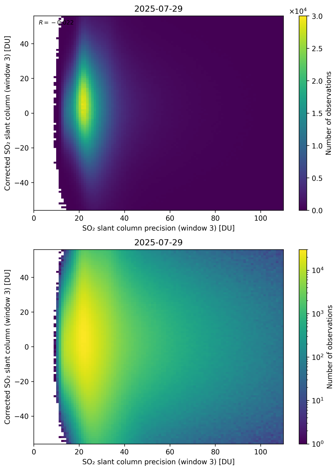
Figure 312: Scatter density plot of “SO 2 slant column precision (window 3)” against “Corrected SO 2 slant column (window 3)” for 2025-07-29 to 2025-07-30.
