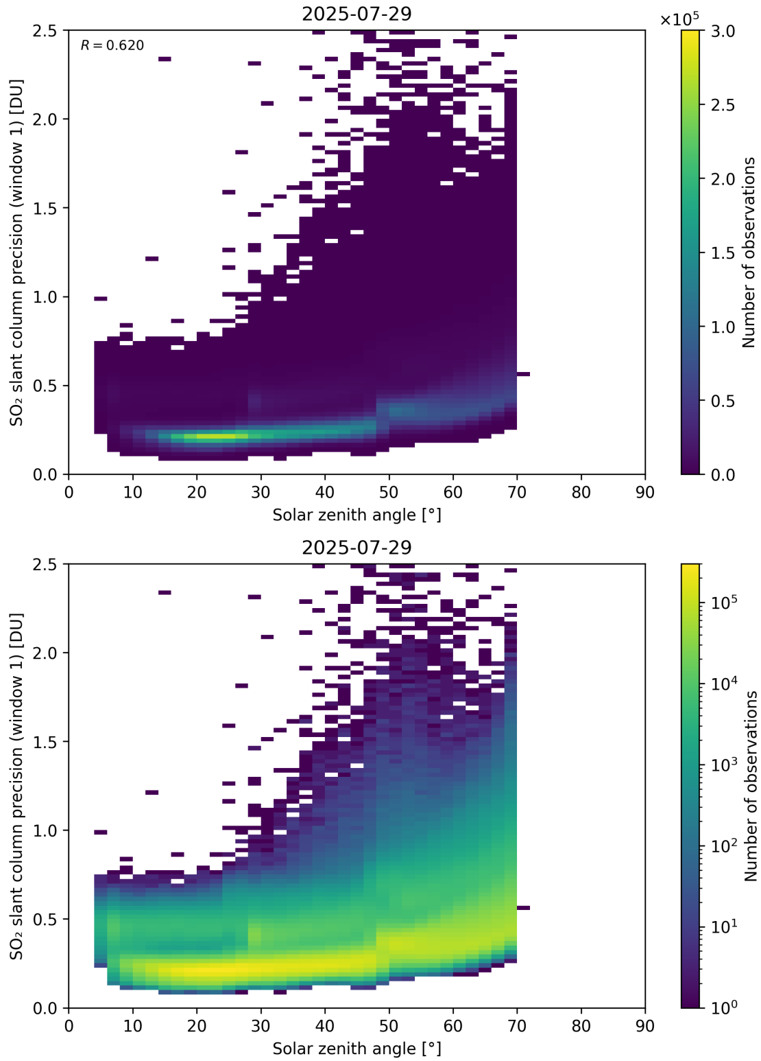
Figure 185: Scatter density plot of “Solar zenith angle” against “SO 2 slant column precision (window 1)” for 2025-07-29 to 2025-07-30.
