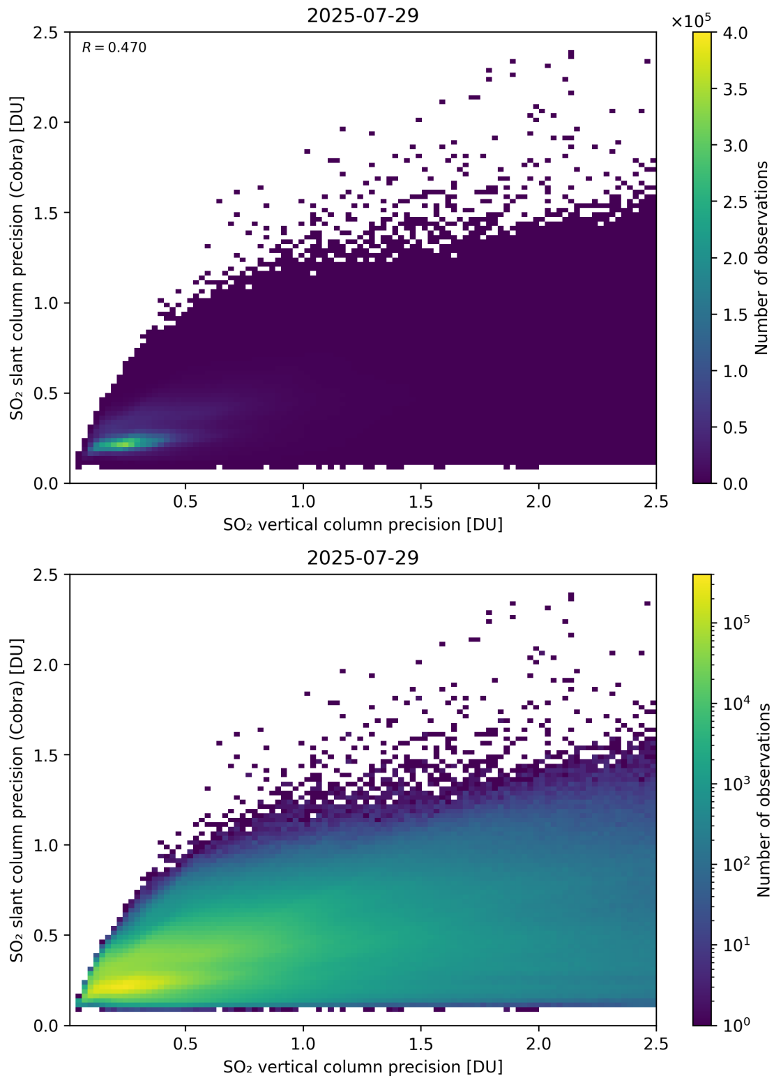
Figure 337: Scatter density plot of “SO 2 vertical column precision” against “SO 2 slant column precision (Cobra)” for 2025-07-29 to 2025-07-30.
