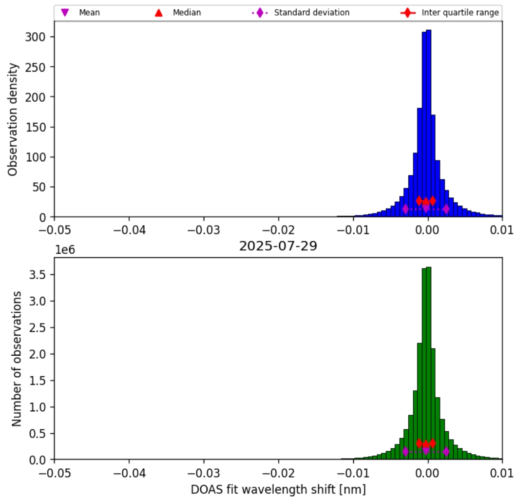
Figure 76: Histogram of “DOAS fit wavelength shift” for 2025-07-29 to 2025-07-30
