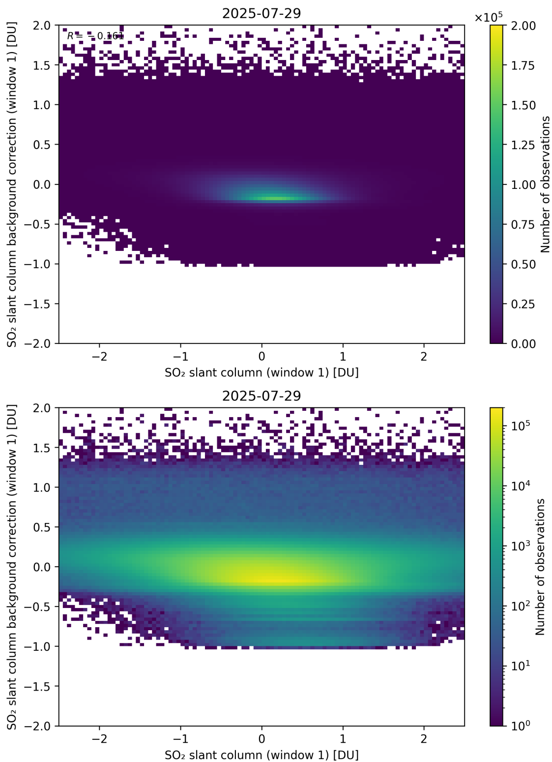
Figure 262: Scatter density plot of “SO 2 slant column (window 1)” against “SO 2 slant column background correction (window 1)” for 2025-07-29 to 2025-07-30.
