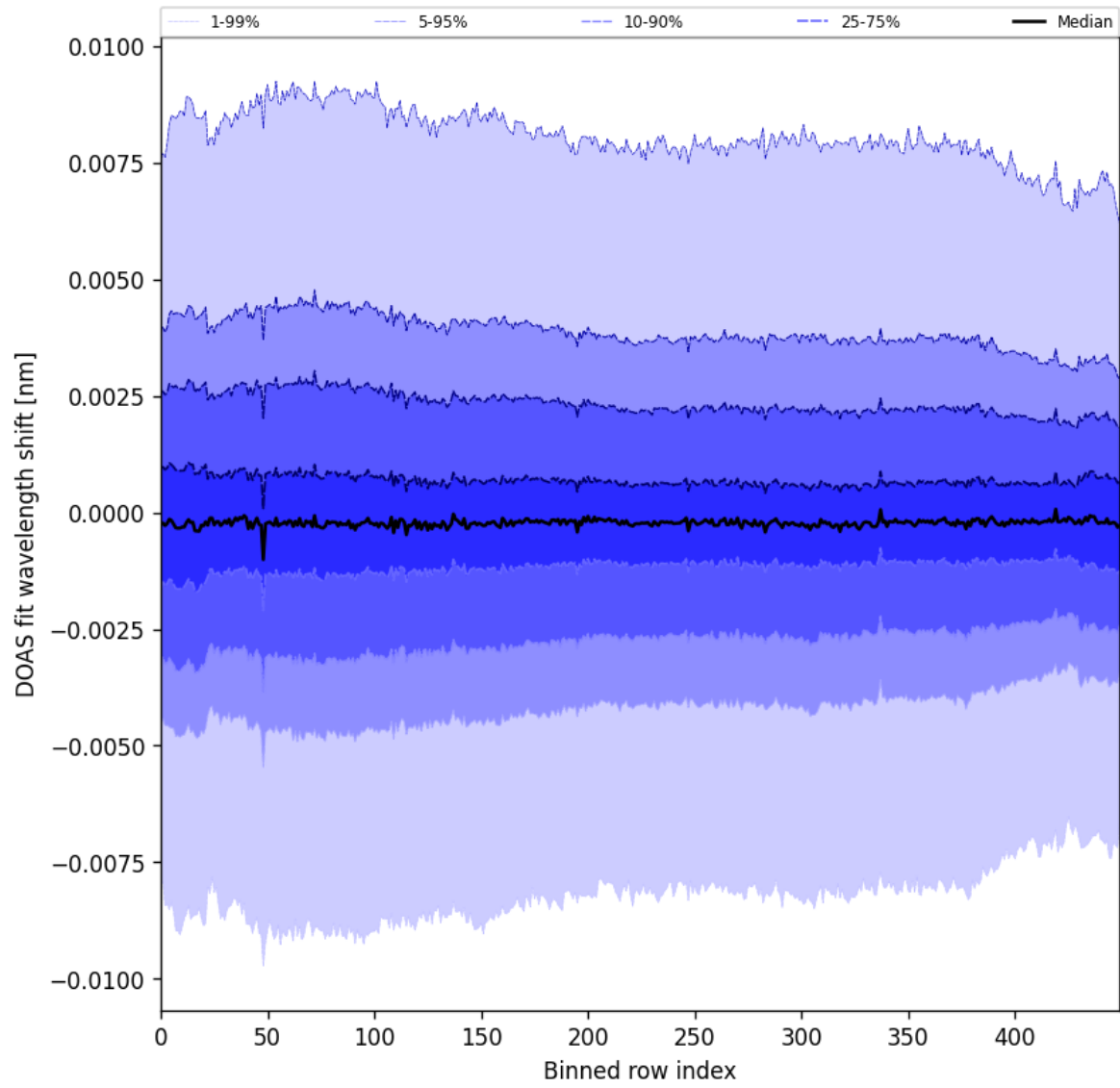
Figure 102: Along track statistics of “DOAS fit wavelength shift” for 2025-07-29 to 2025-07-30
