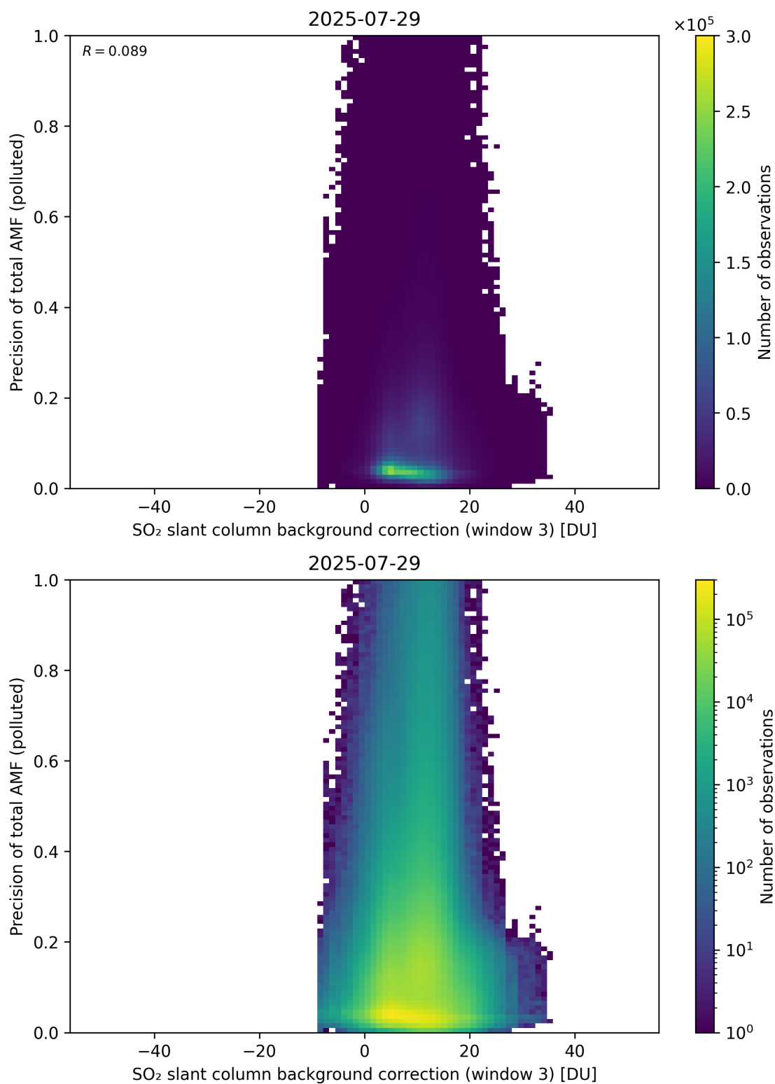
Figure 137: Scatter density plot of “SO 2 slant column background correction (window 3)” against “Precision of total AMF (polluted)” for 2025-07-29 to 2025-07-30.
