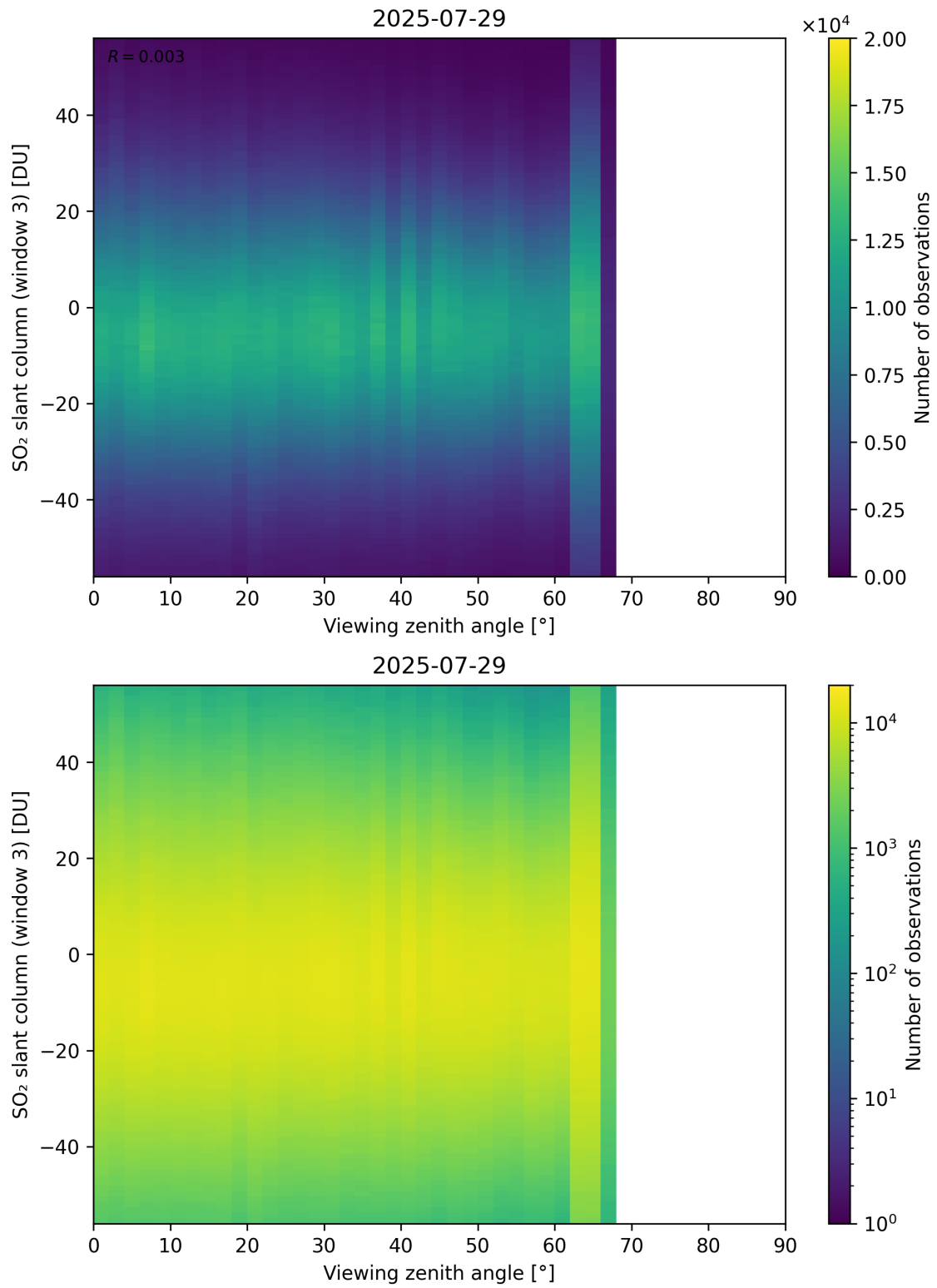
Figure 379: Scatter density plot of “Viewing zenith angle” against “SO 2 slant column (window 3)” for 2025-07-29 to 2025-07-30.
