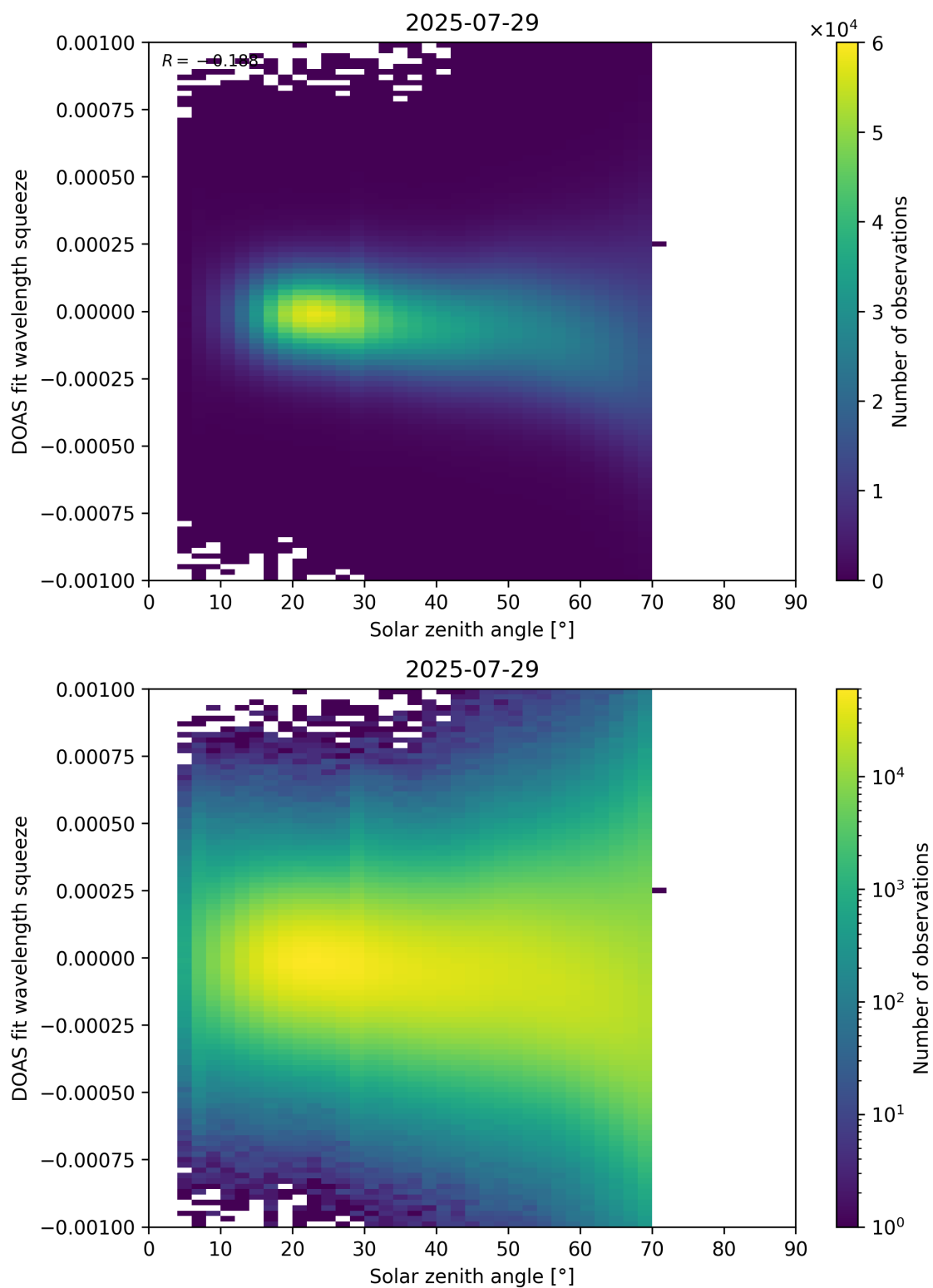
Figure 175: Scatter density plot of “Solar zenith angle” against “DOAS fit wavelength squeeze” for 2025-07-29 to 2025-07-30.
