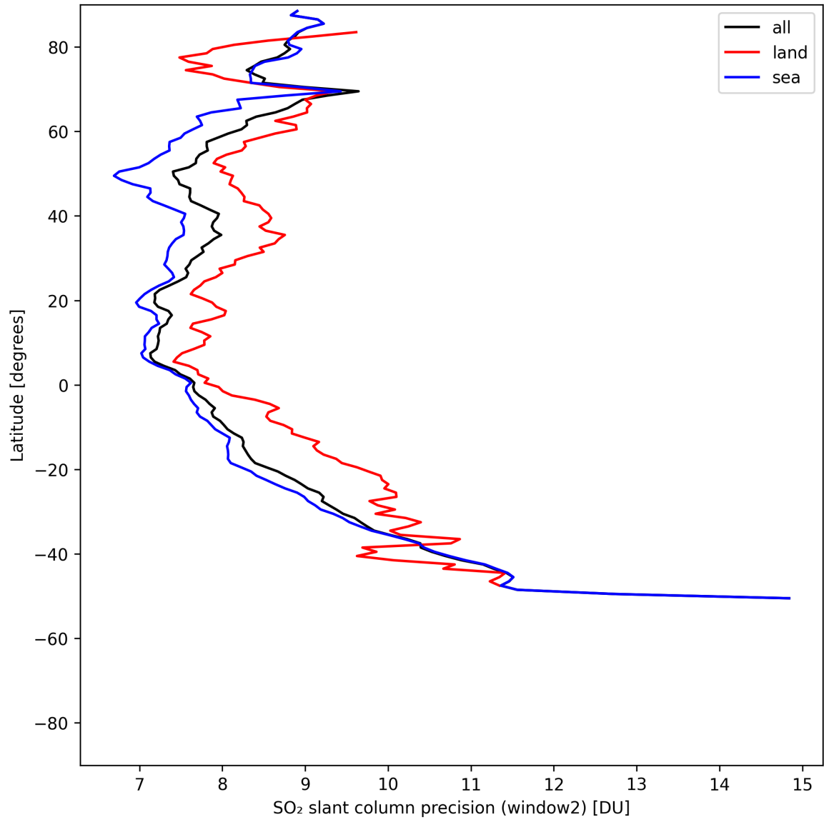
Figure 42: Zonal average of “SO 2 slant column precision (window2)” for 2025-07-29 to 2025-07-30.
