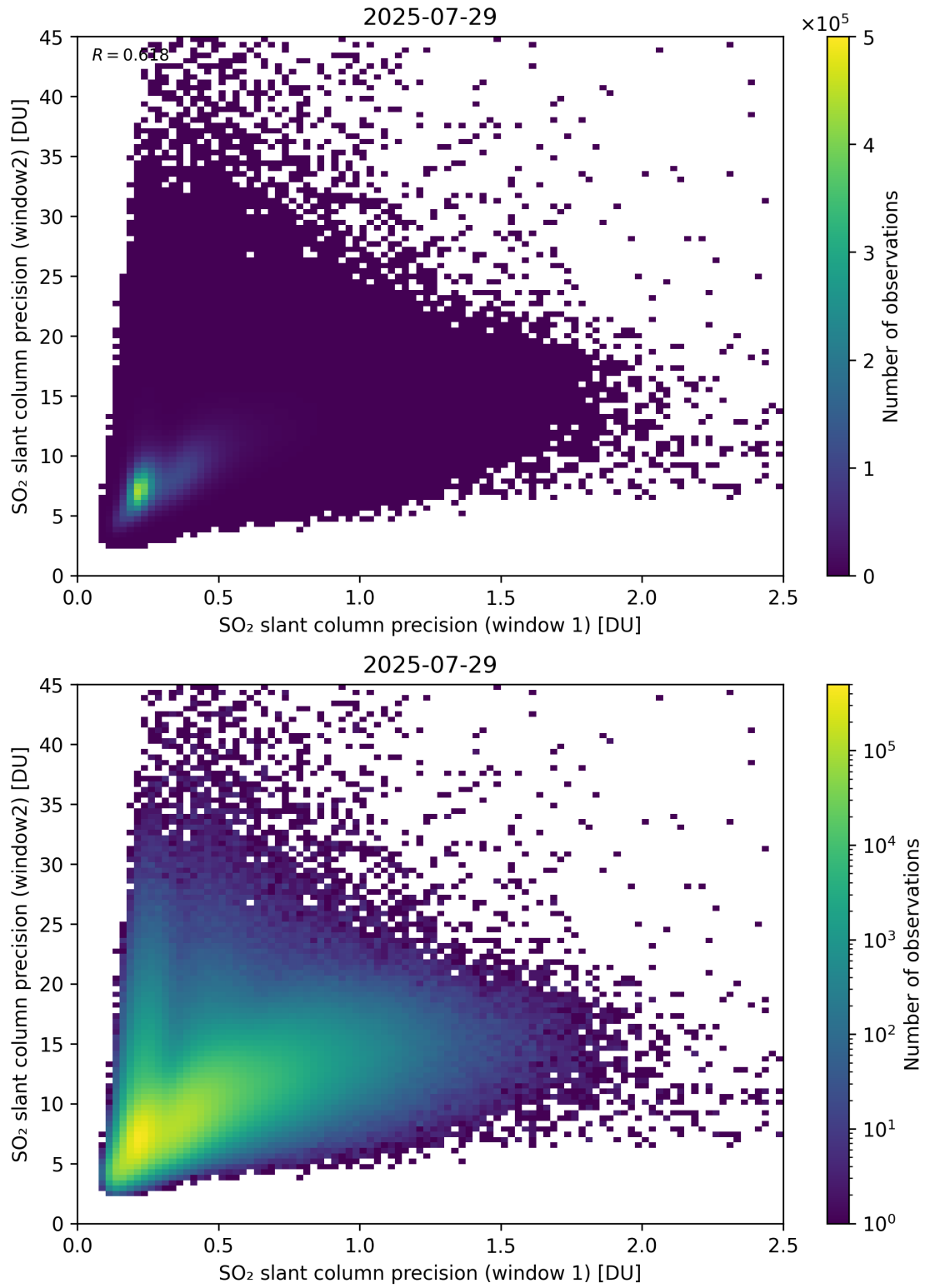
Figure 277: Scatter density plot of “SO 2 slant column precision (window 1)” against “SO 2 slant column precision (window2)” for 2025-07-29 to 2025-07-30.
