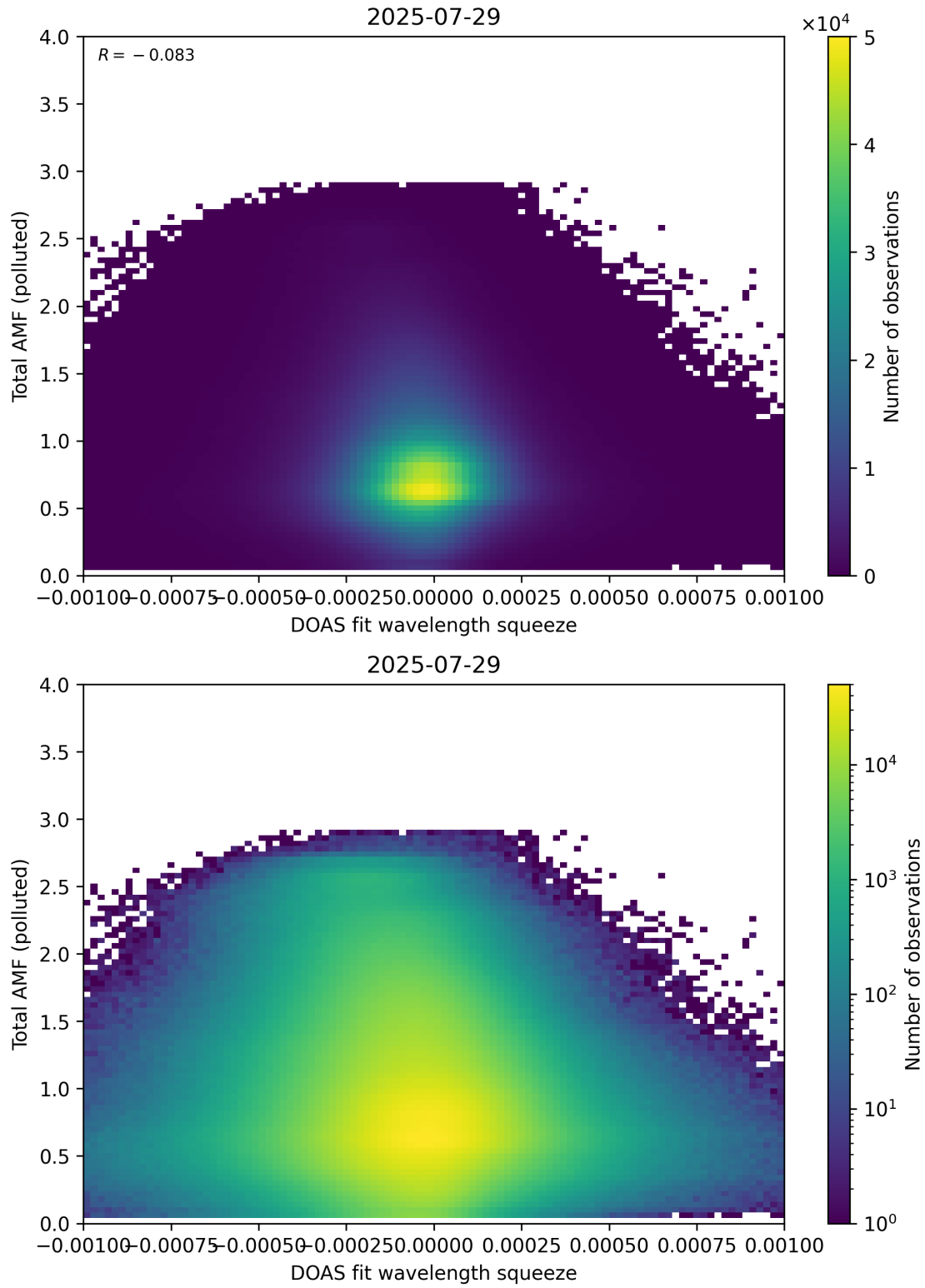
Figure 145: Scatter density plot of “DOAS fit wavelength squeeze” against “Total AMF (polluted)” for 2025-07-29 to 2025-07-30.
