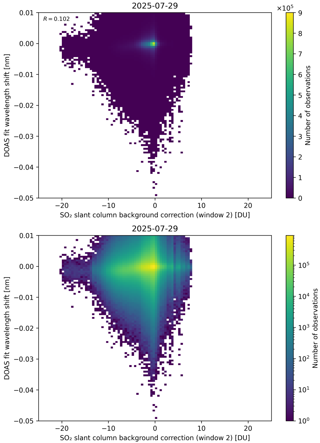
Figure 123: Scatter density plot of “SO 2 slant column background correction (window 2)” against “DOAS fit wavelength shift” for 2025-07-29 to 2025-07-30.
