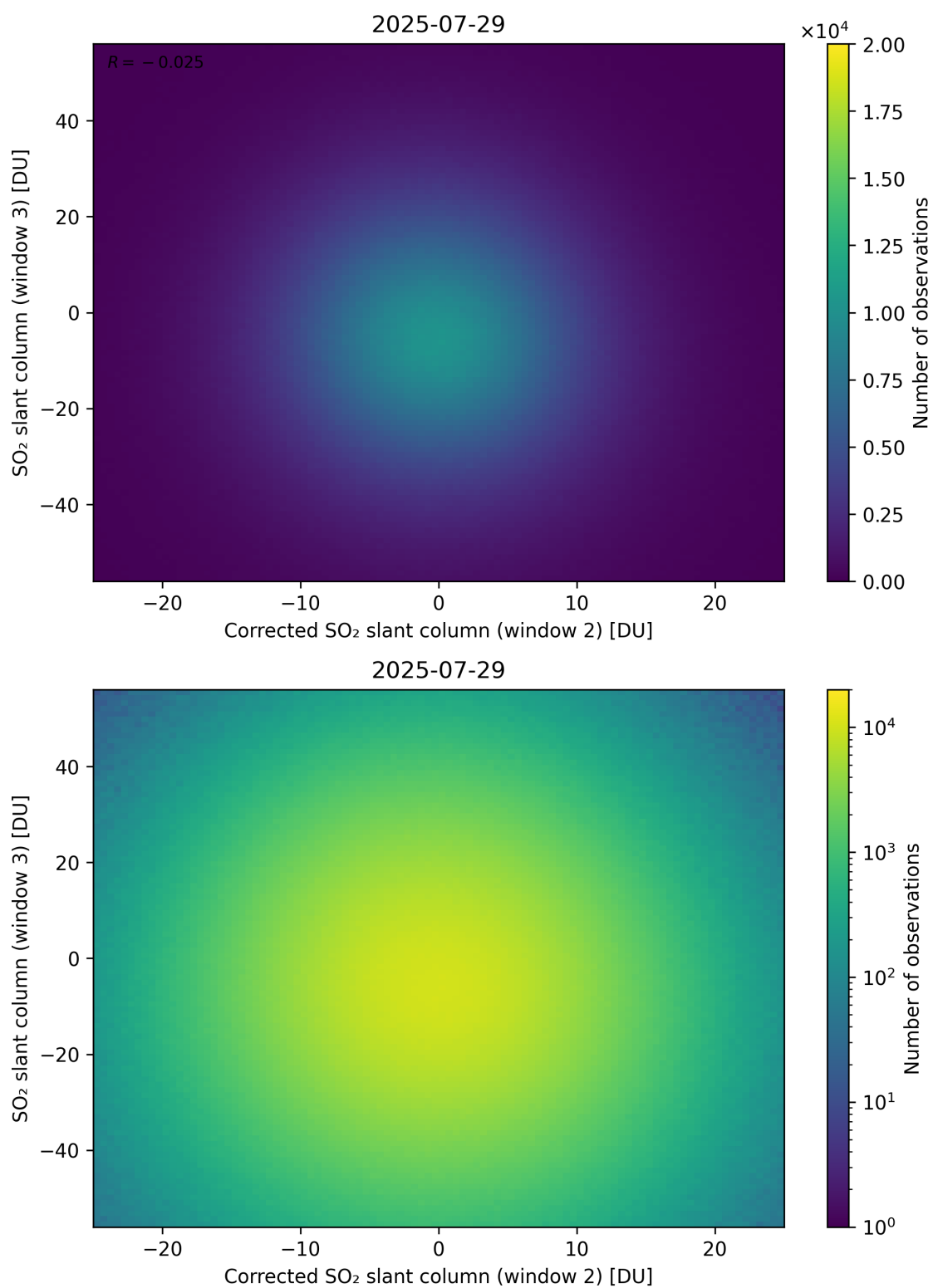
Figure 251: Scatter density plot of “Corrected SO 2 slant column (window 2)” against “SO 2 slant column (window 3)” for 2025-07-29 to 2025-07-30.
