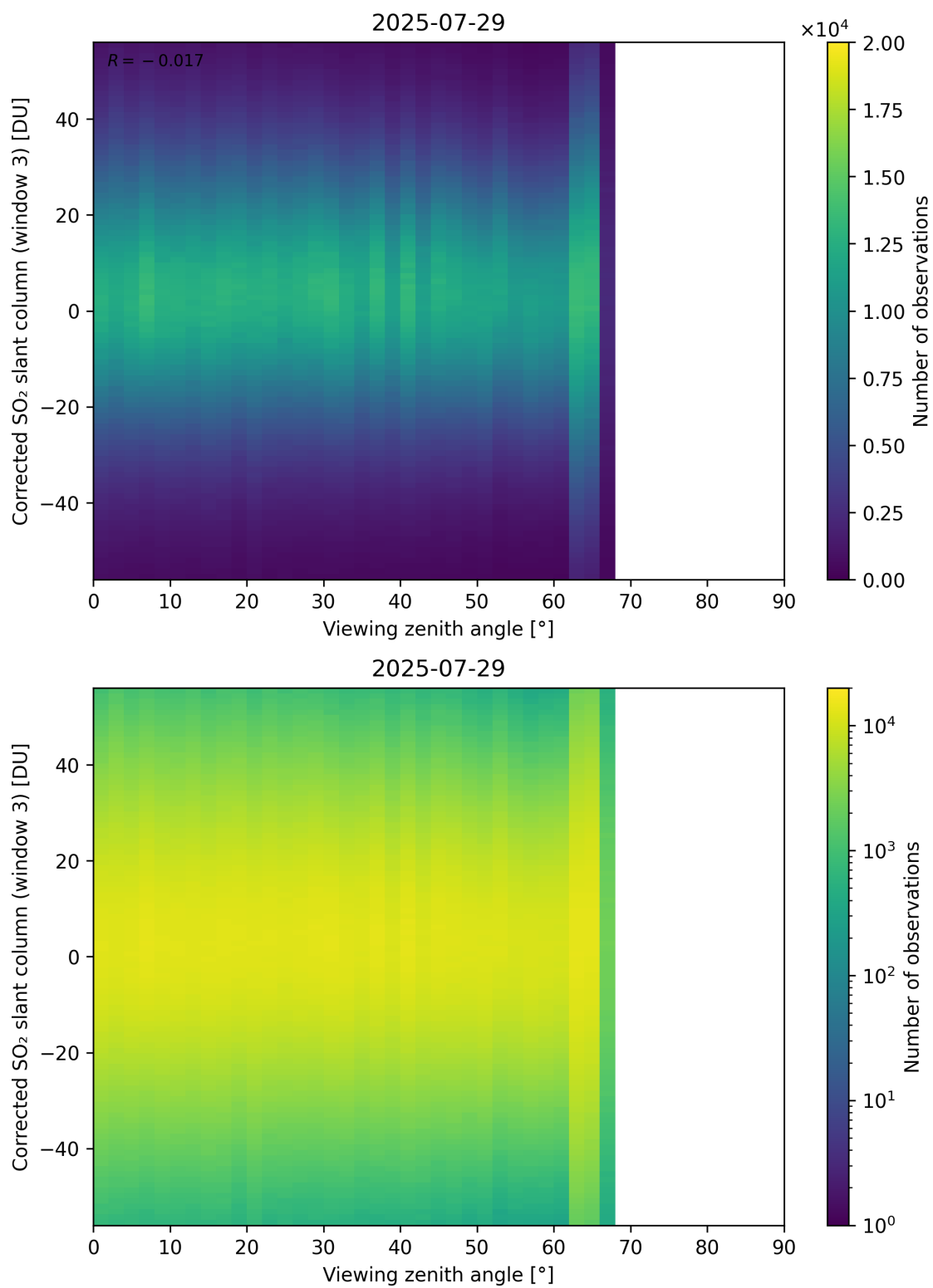
Figure 375: Scatter density plot of “Viewing zenith angle” against “Corrected SO 2 slant column (window 3)” for 2025-07-29 to 2025-07-30.
