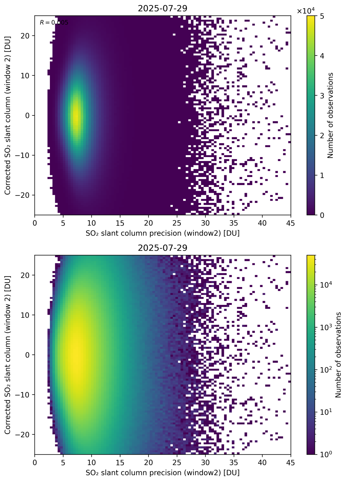
Figure 297: Scatter density plot of “SO 2 slant column precision (window2)” against “Corrected SO 2 slant column (window 2)” for 2025-07-29 to 2025-07-30.
