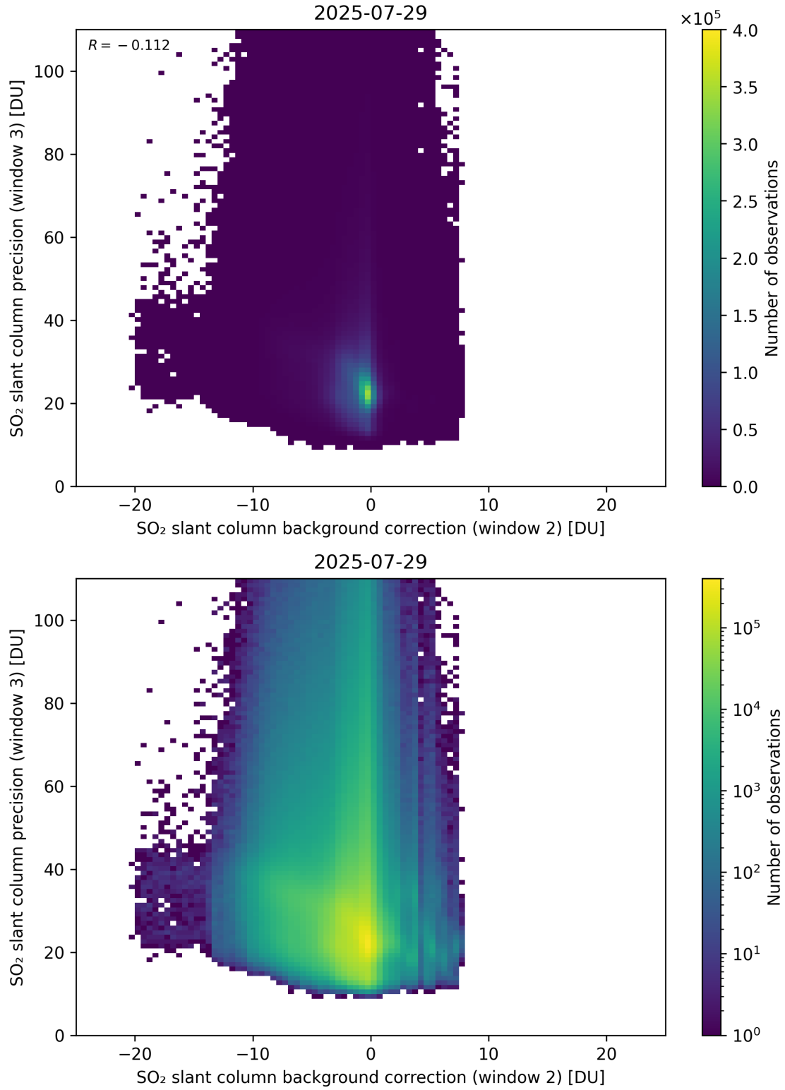
Figure 129: Scatter density plot of “SO 2 slant column background correction (window 2)” against “SO 2 slant column precision (window 3)” for 2025-07-29 to 2025-07-30.
