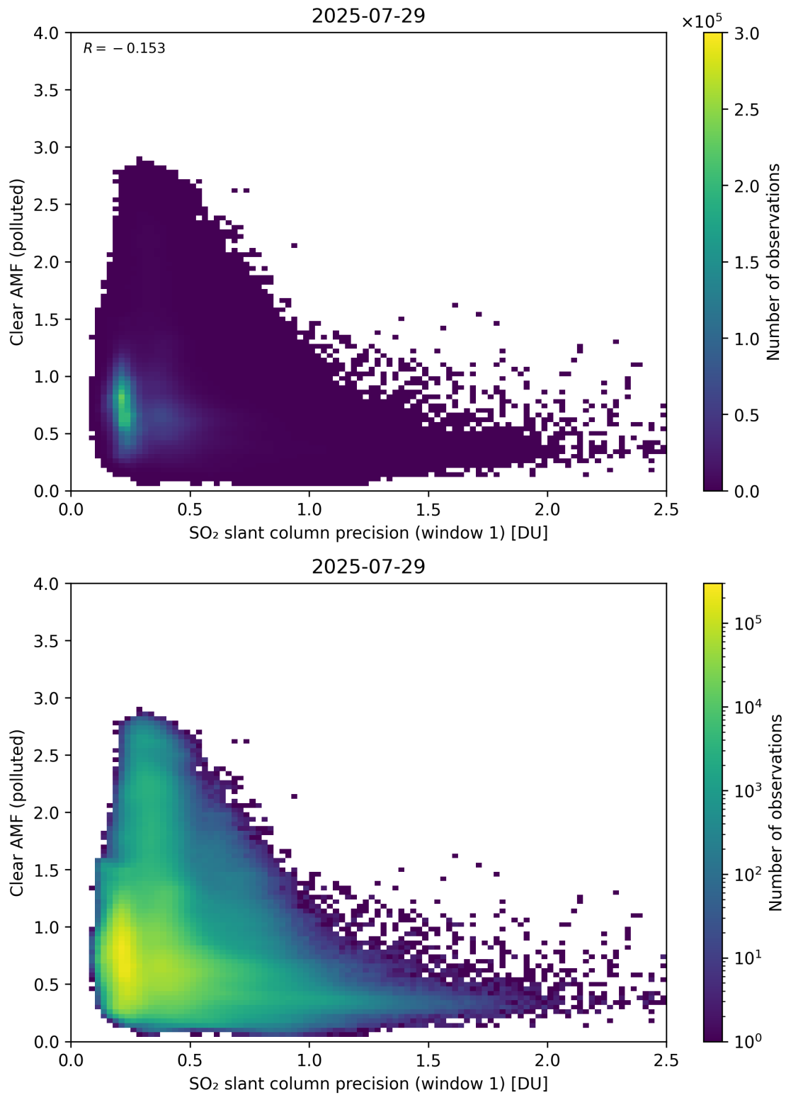
Figure 274: Scatter density plot of “SO 2 slant column precision (window 1)” against “Clear AMF (polluted)” for 2025-07-29 to 2025-07-30.
