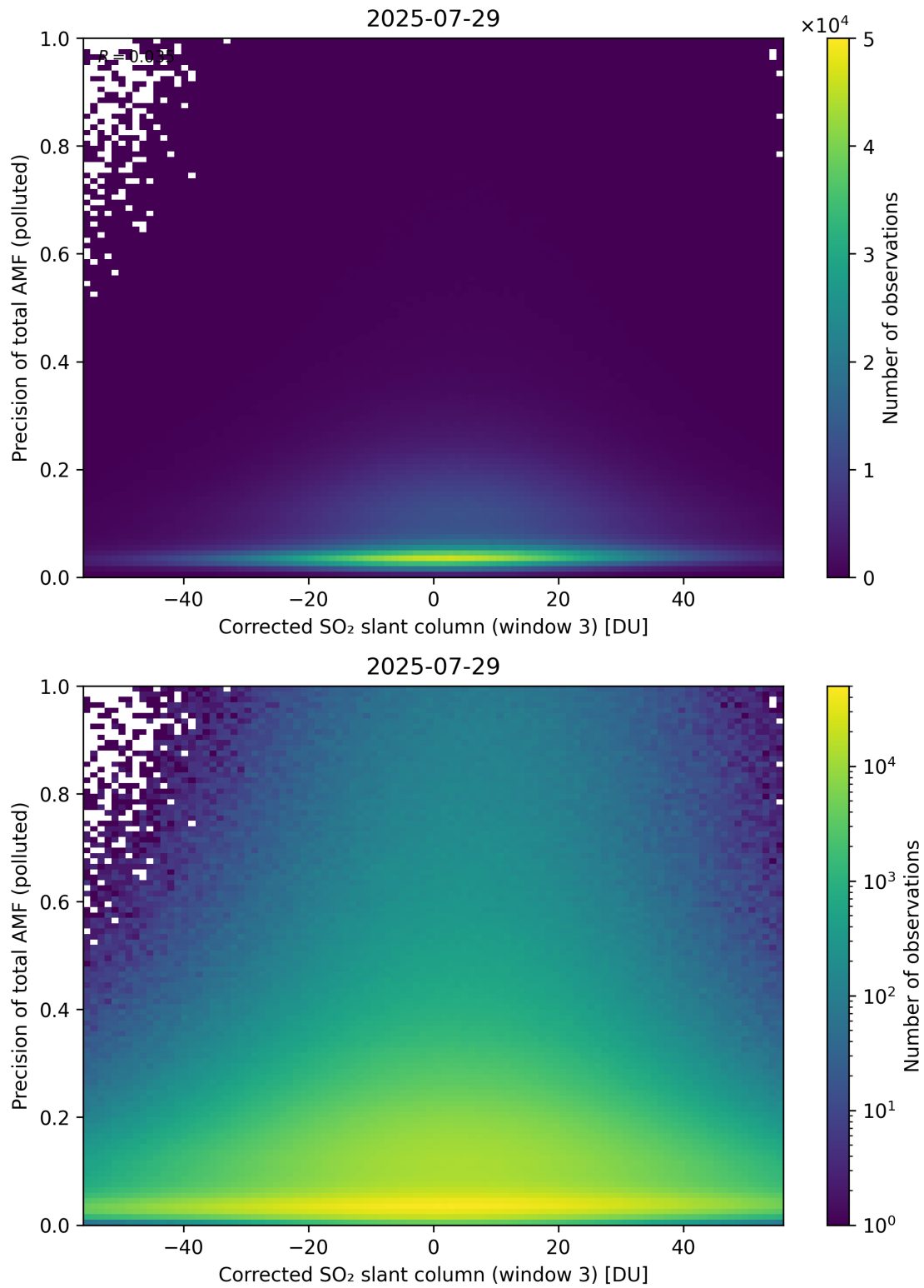
Figure 261: Scatter density plot of “Corrected SO 2 slant column (window 3)” against “Precision of total AMF (polluted)” for 2025-07-29 to 2025-07-30.
