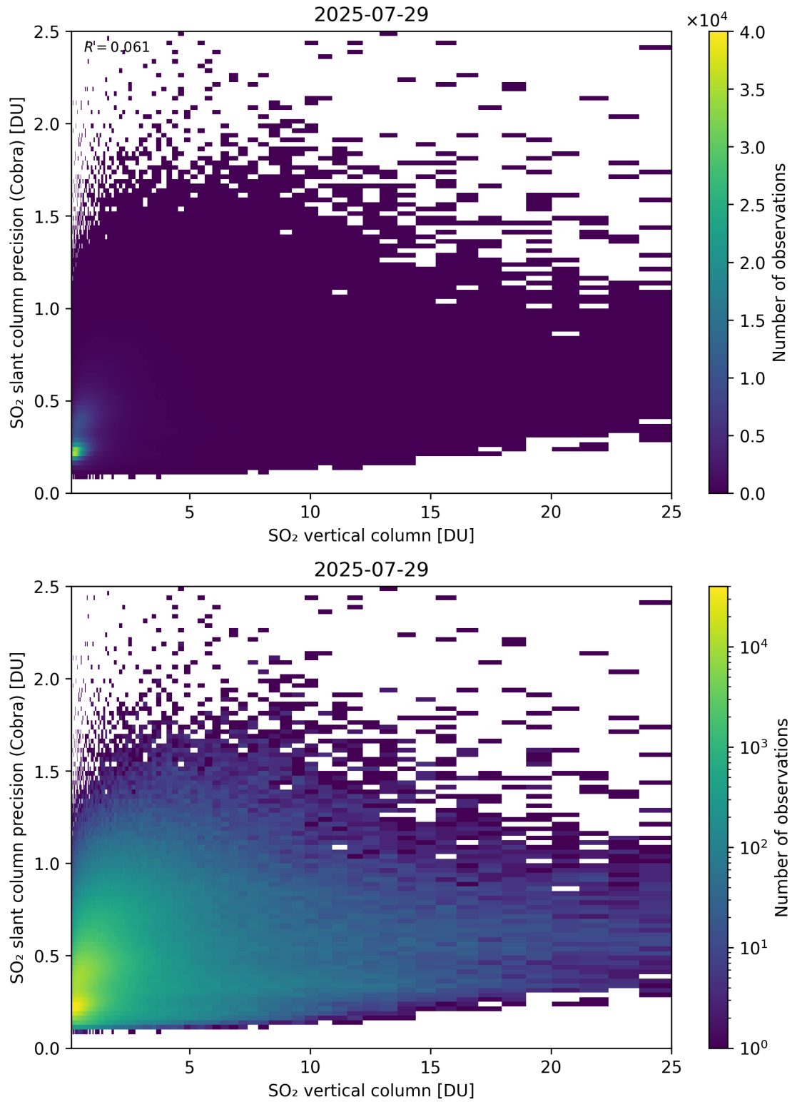
Figure 350: Scatter density plot of “SO 2 vertical column” against “SO 2 slant column precision (Cobra)” for 2025-07-29 to 2025-07-30.
