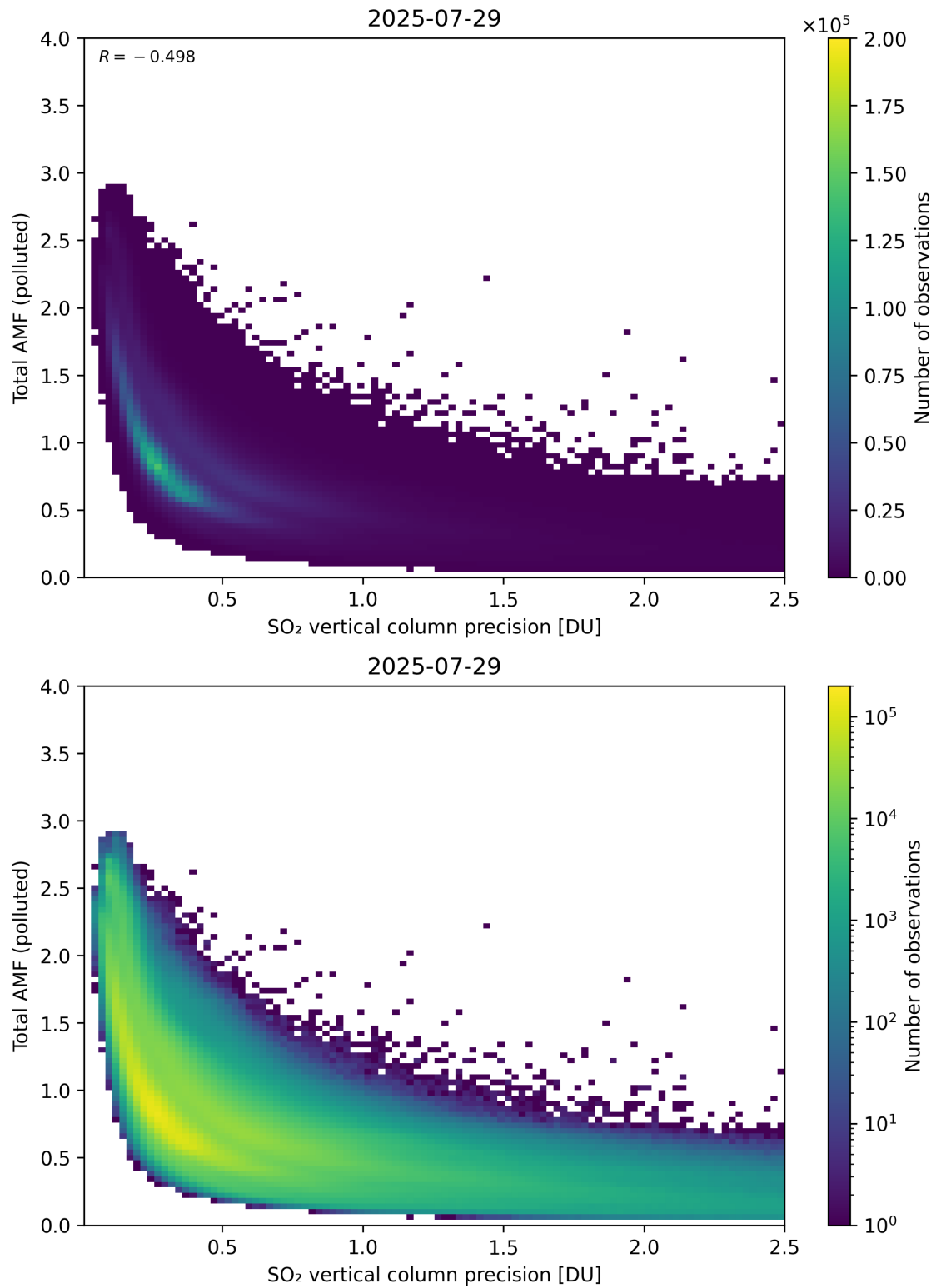
Figure 346: Scatter density plot of “SO 2 vertical column precision” against “Total AMF (polluted)” for 2025-07-29 to 2025-07-30.
