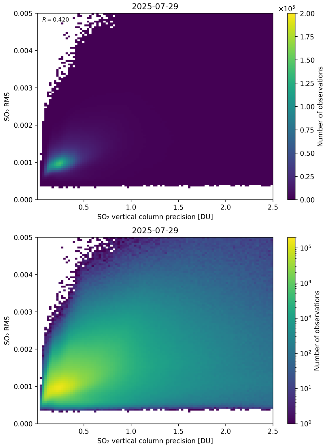
Figure 334: Scatter density plot of “SO 2 vertical column precision” against “SO 2 RMS” for 2025-07-29 to 2025-07-30.
