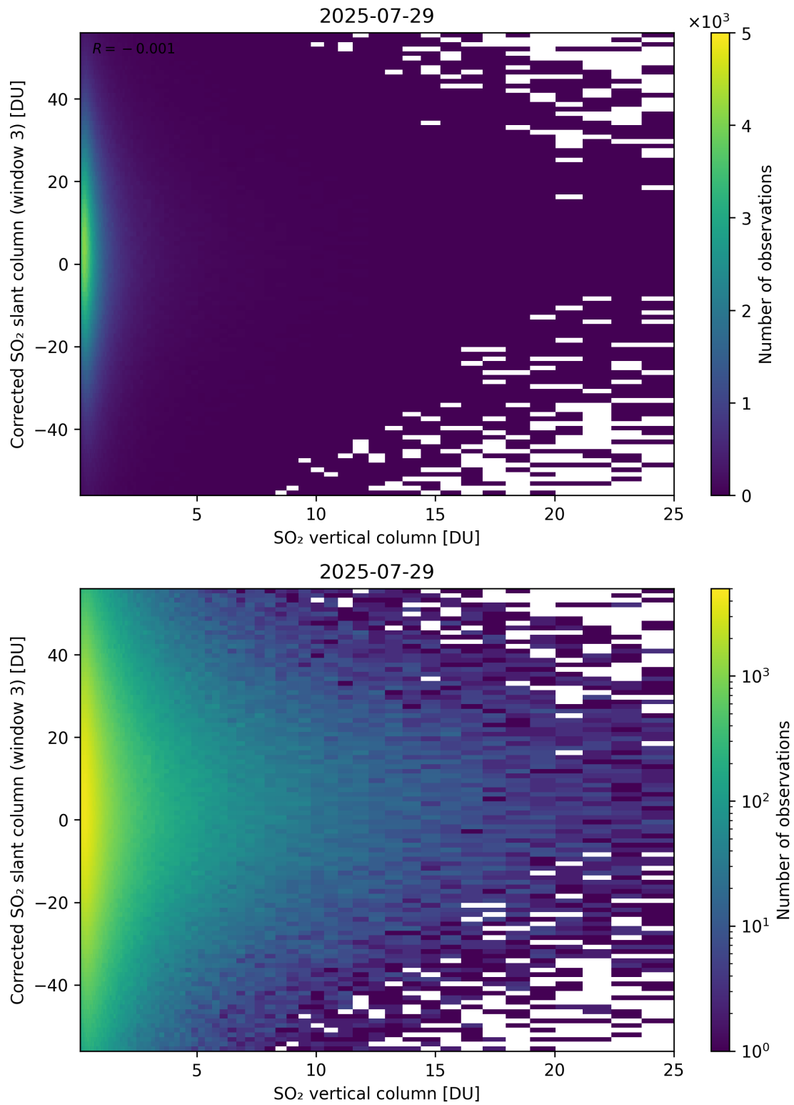
Figure 353: Scatter density plot of “SO 2 vertical column” against “Corrected SO 2 slant column (window 3)” for 2025-07-29 to 2025-07-30.
