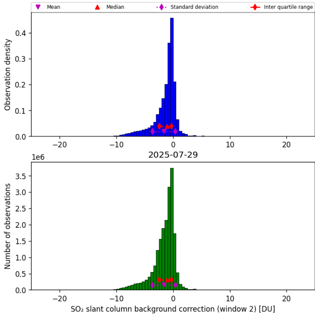
Figure 70: Histogram of “SO 2 slant column background correction (window 2)” for 2025-07-29 to 2025-07-30
