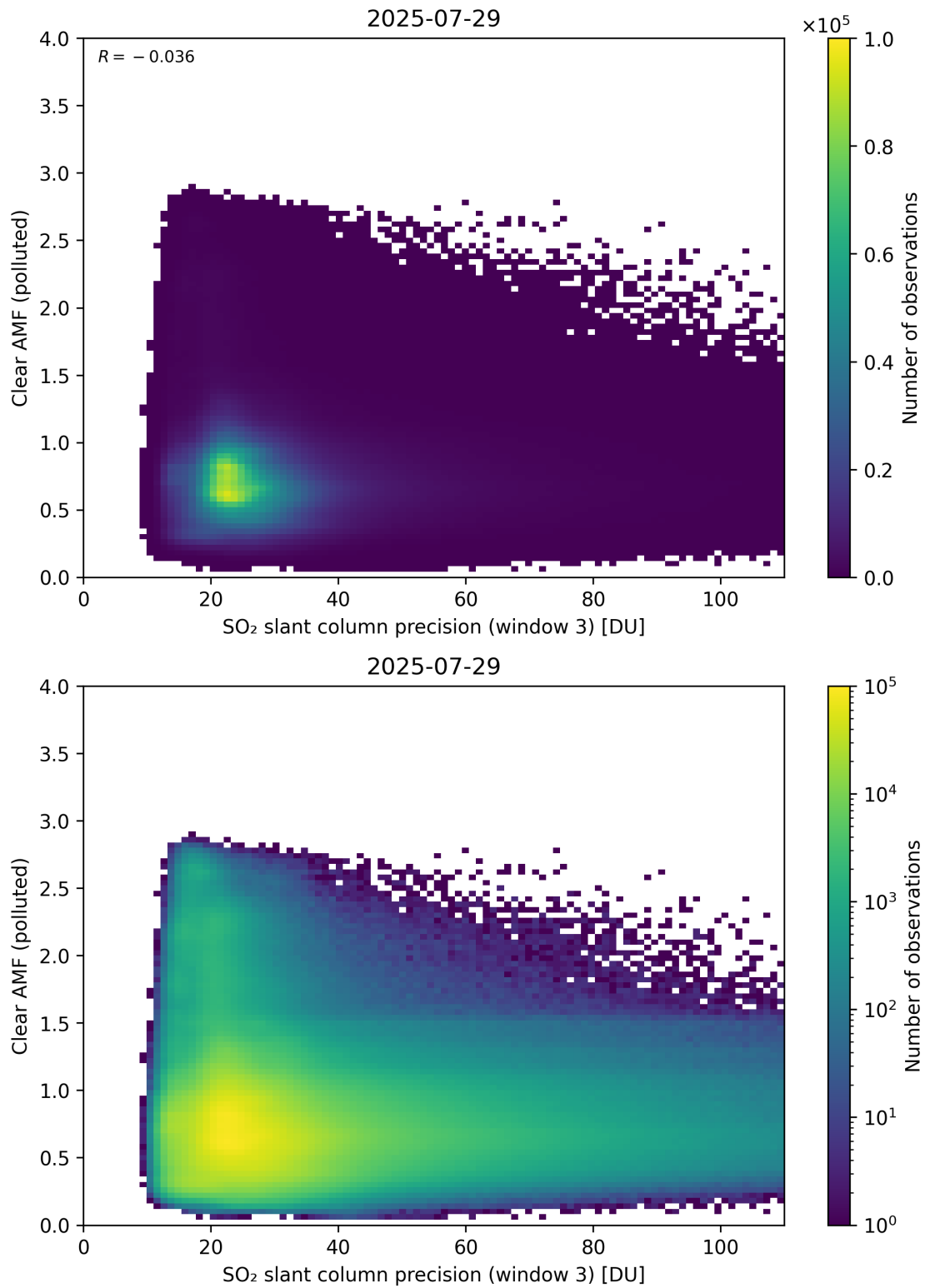
Figure 311: Scatter density plot of “SO 2 slant column precision (window 3)” against “Clear AMF (polluted)” for 2025-07-29 to 2025-07-30.
