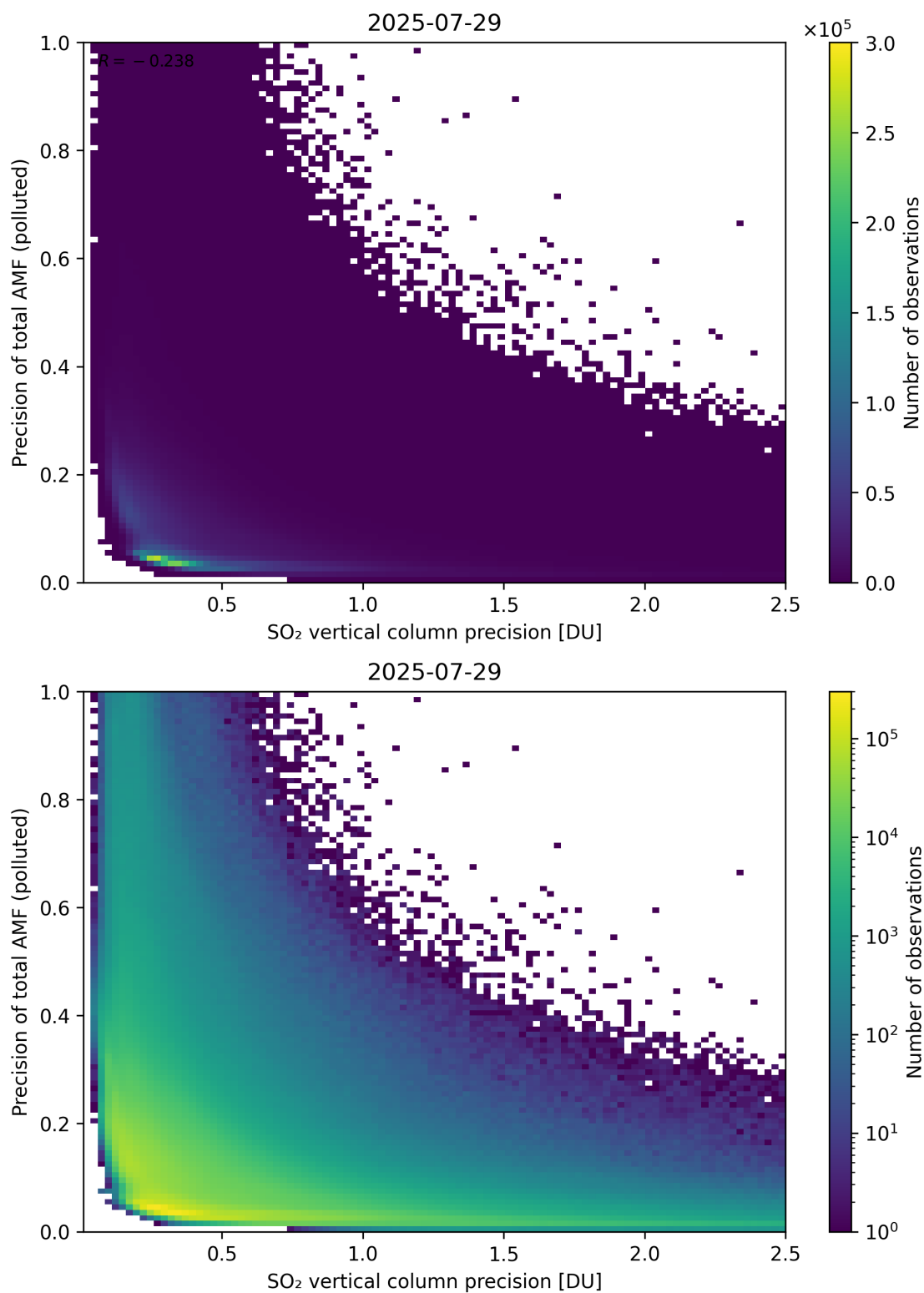
Figure 347: Scatter density plot of “SO 2 vertical column precision” against “Precision of total AMF (polluted)” for 2025-07-29 to 2025-07-30.
