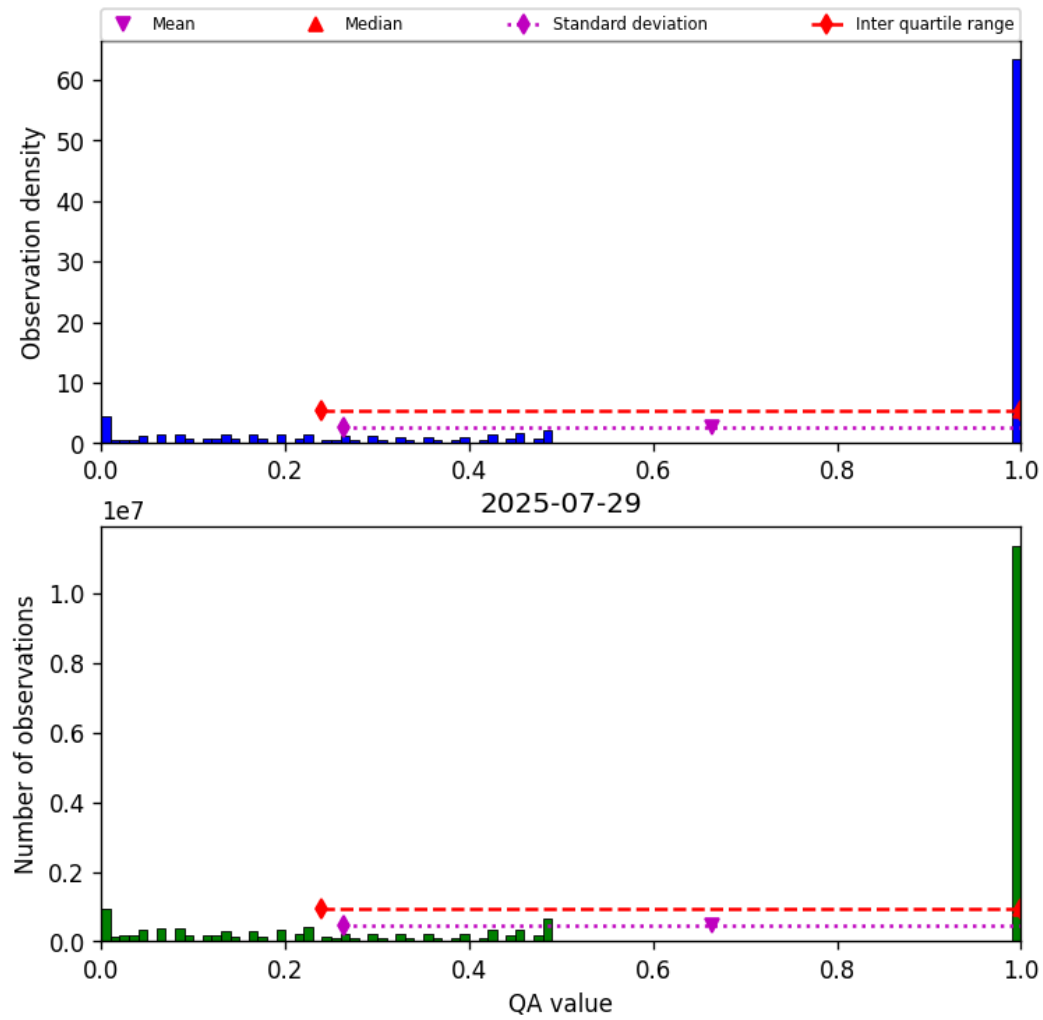
Figure 57: Histogram of “QA value” for 2025-07-29 to 2025-07-30
