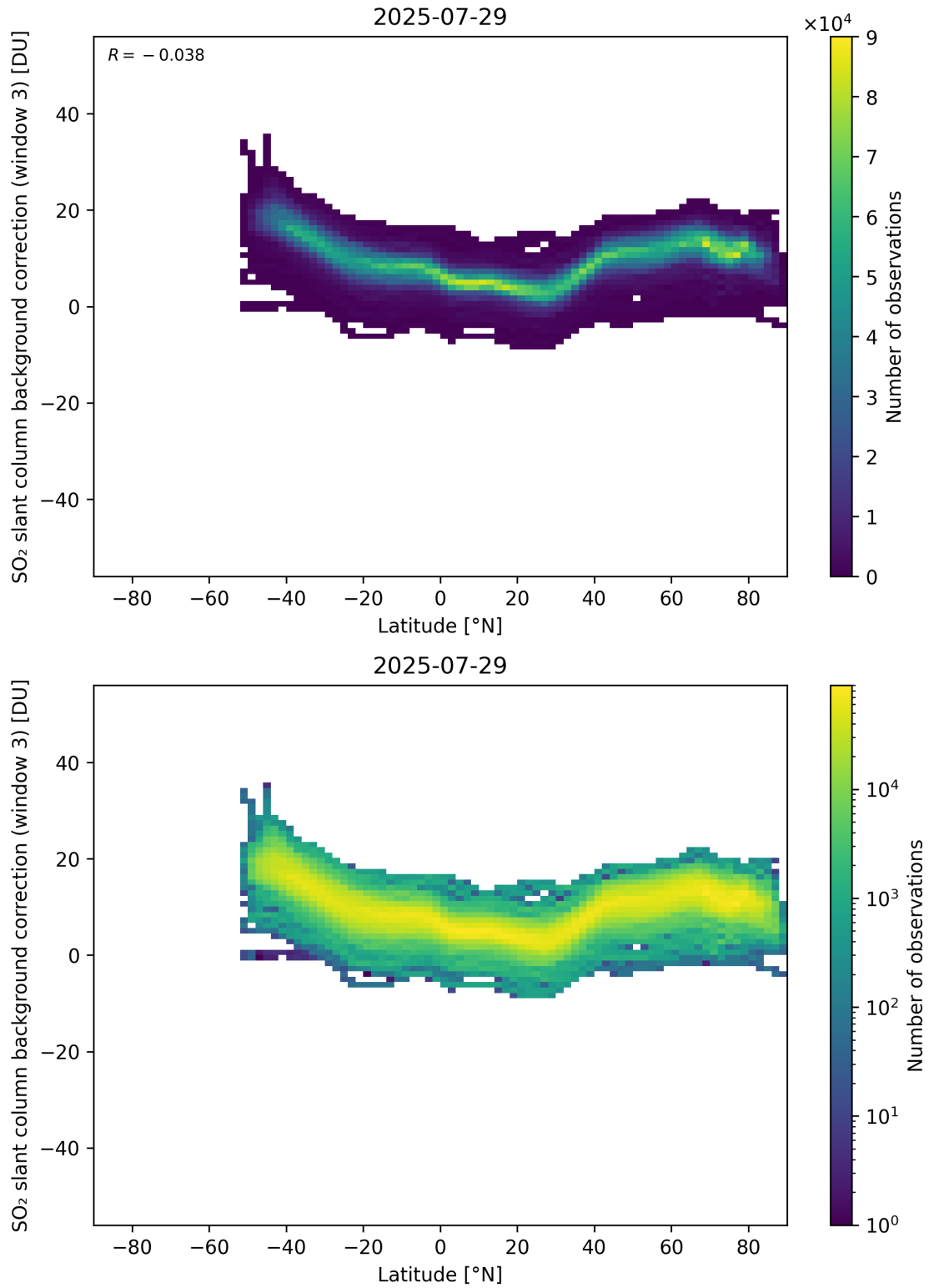
Figure 152: Scatter density plot of “Latitude” against “SO 2 slant column background correction (window 3)” for 2025-07-29 to 2025-07-30.
