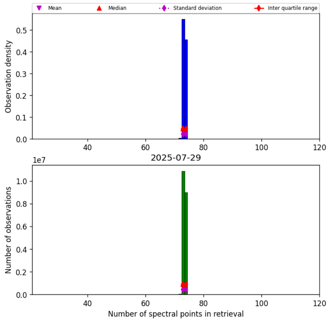
Figure 82: Histogram of “Number of spectral points in retrieval” for 2025-07-29 to 2025-07-30
