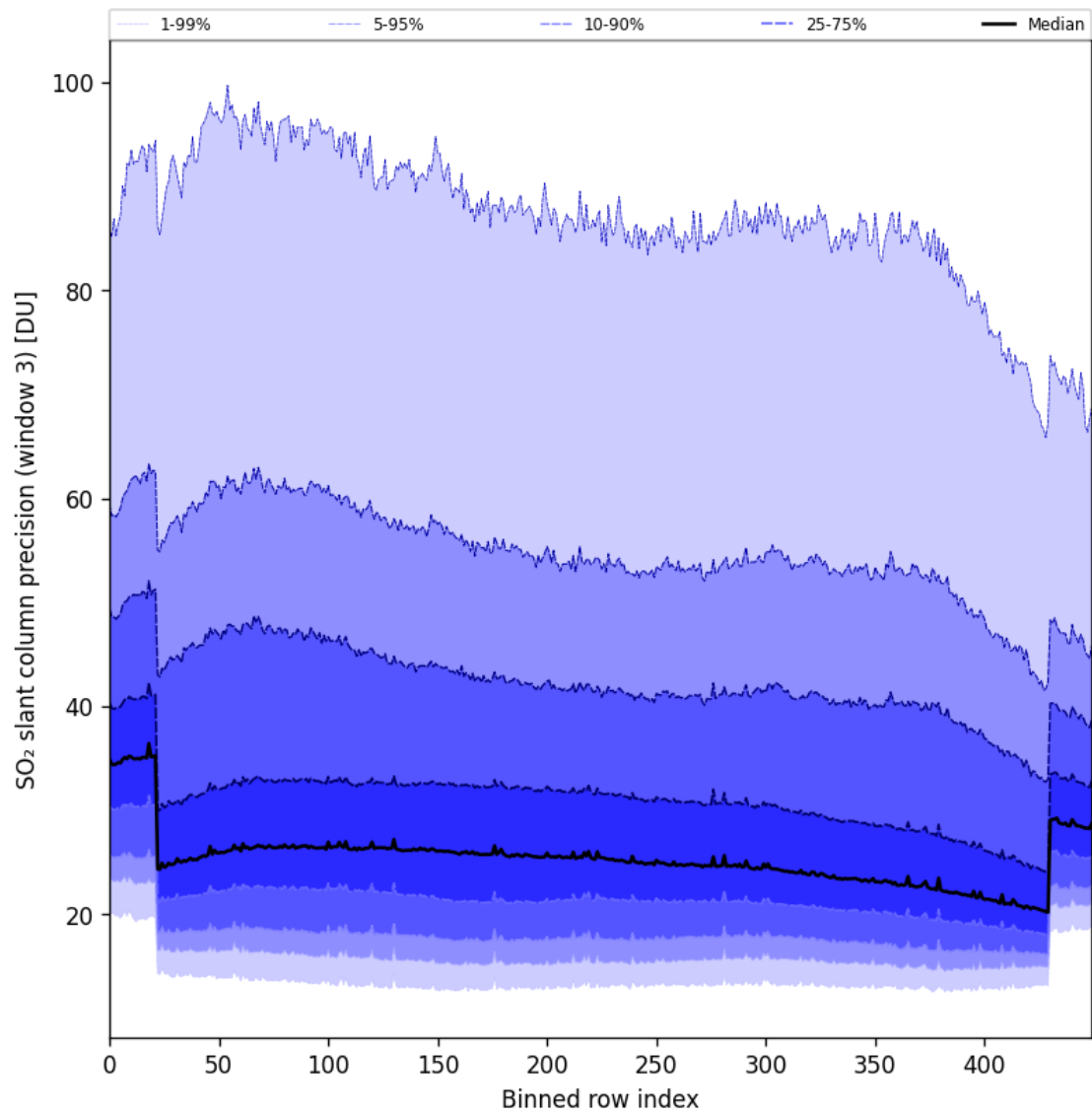
Figure 98: Along track statistics of “SO 2 slant column precision (window 3)” for 2025-07-29 to 2025-07-30
