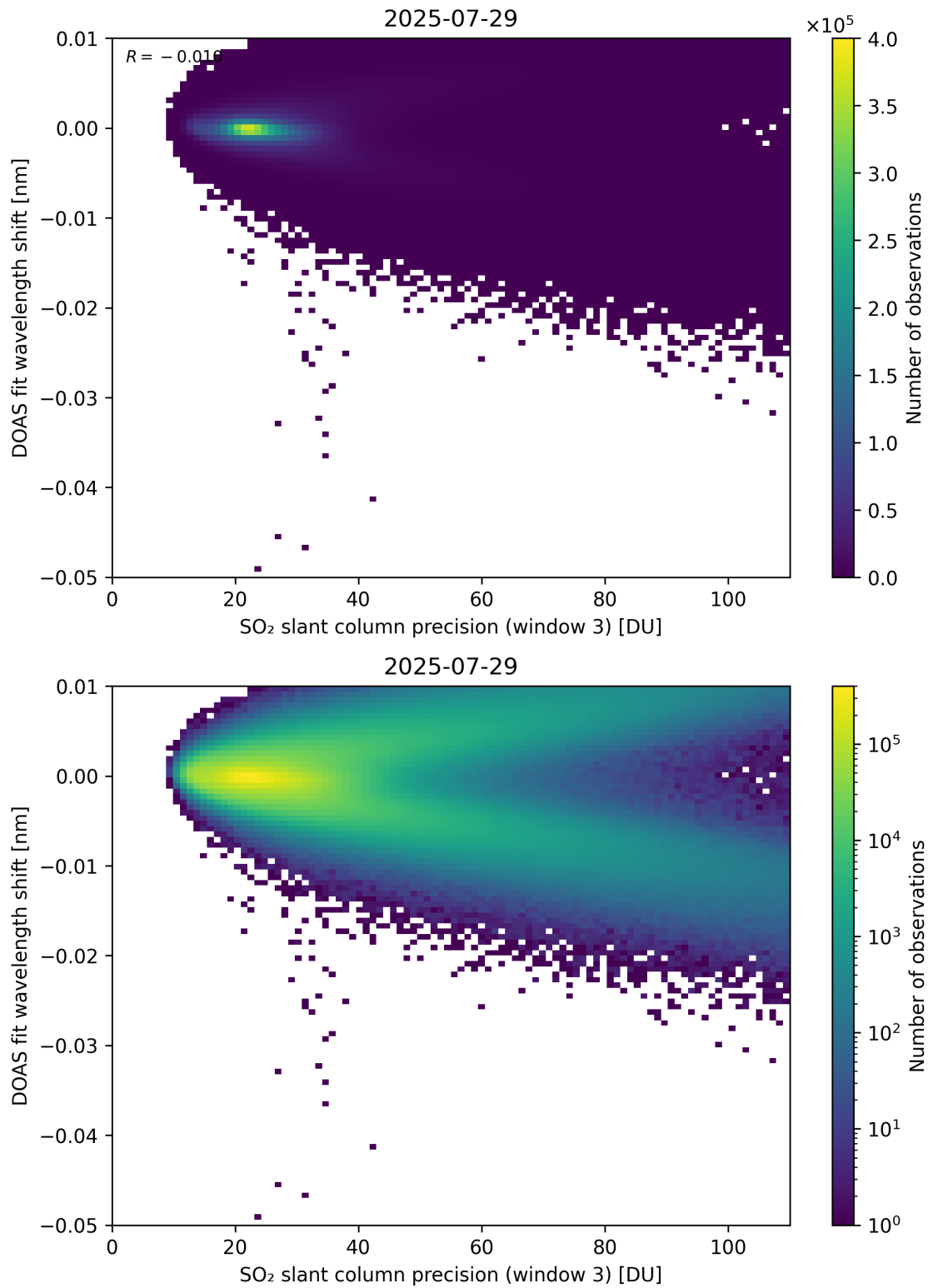
Figure 308: Scatter density plot of “SO 2 slant column precision (window 3)” against “DOAS fit wavelength shift” for 2025-07-29 to 2025-07-30.
