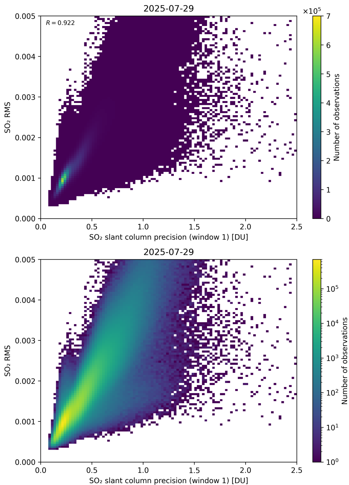
Figure 273: Scatter density plot of “SO 2 slant column precision (window 1)” against “SO 2 RMS” for 2025-07-29 to 2025-07-30.
