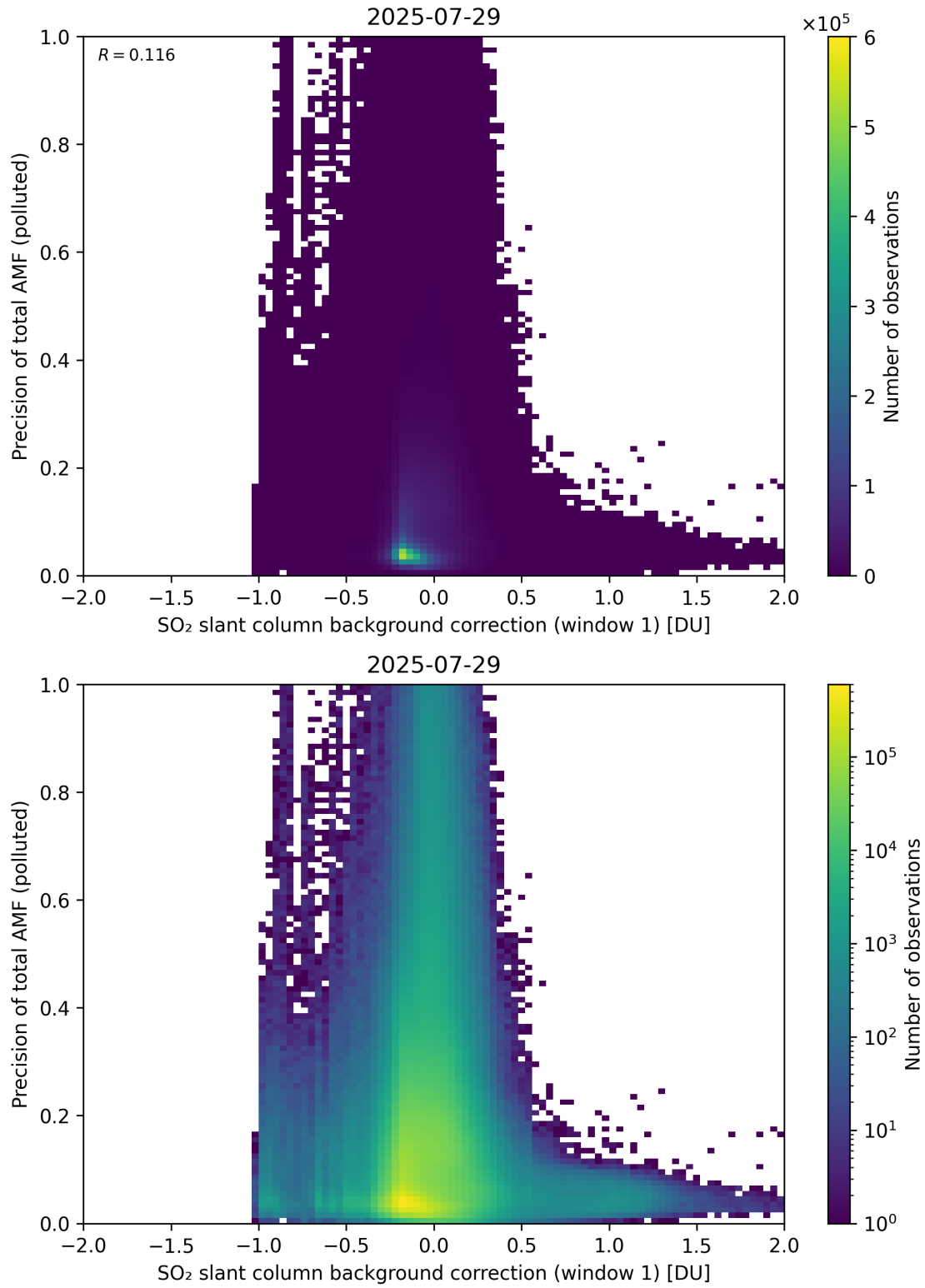
Figure 121: Scatter density plot of “SO 2 slant column background correction (window 1)” against “Precision of total AMF (polluted)” for 2025-07-29 to 2025-07-30.
