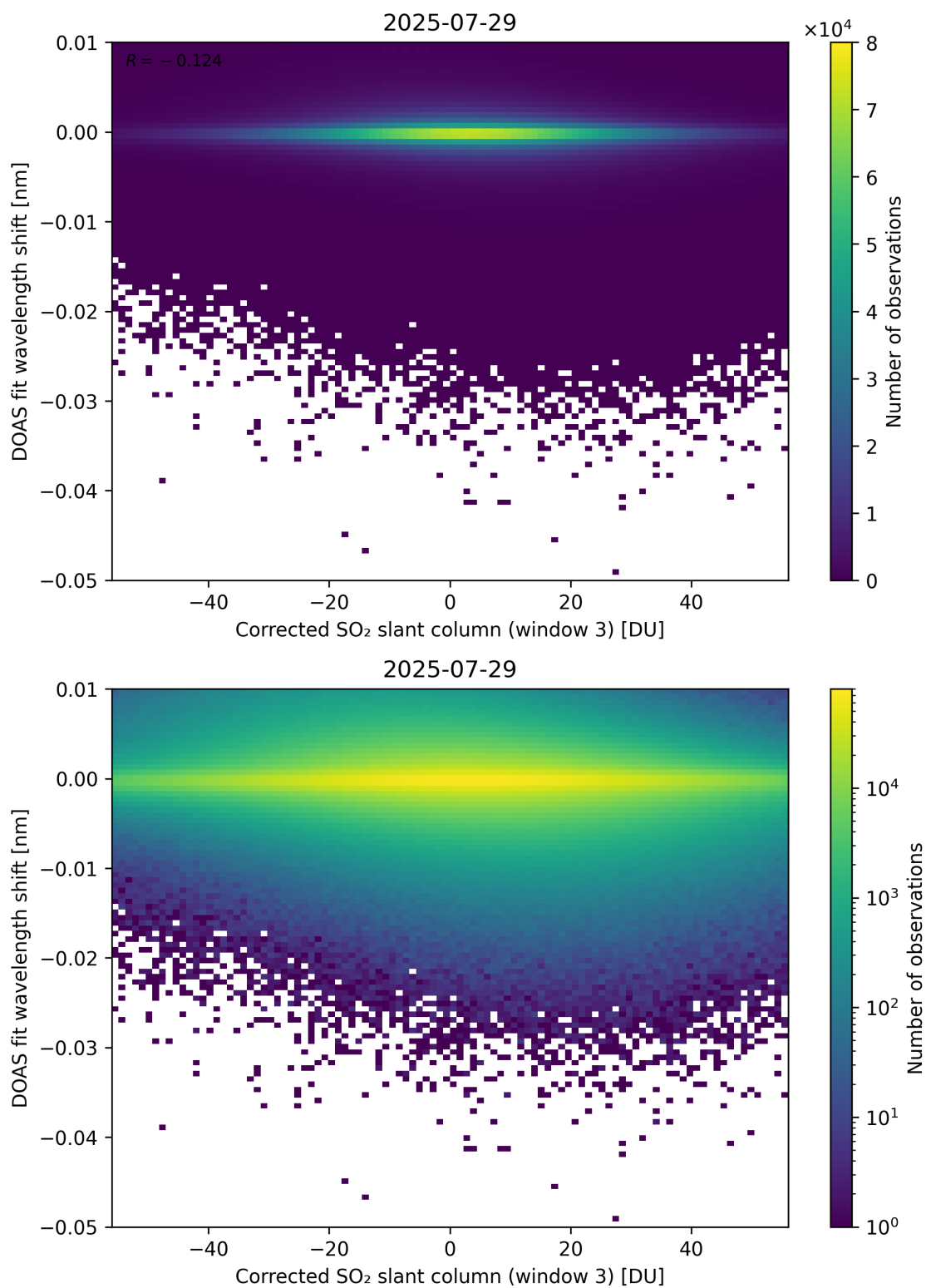
Figure 256: Scatter density plot of “Corrected SO 2 slant column (window 3)” against “DOAS fit wavelength shift” for 2025-07-29 to 2025-07-30.
