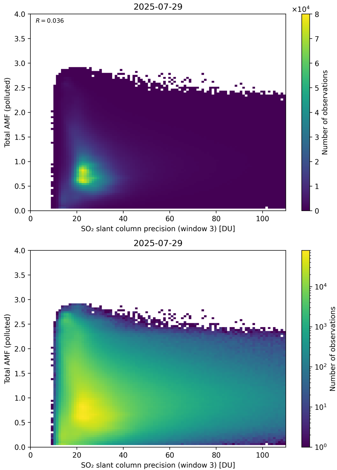
Figure 313: Scatter density plot of “SO 2 slant column precision (window 3)” against “Total AMF (polluted)” for 2025-07-29 to 2025-07-30.
