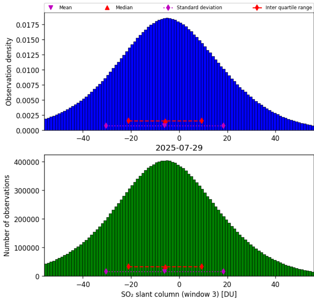
Figure 71: Histogram of “SO 2 slant column (window 3)” for 2025-07-29 to 2025-07-30
