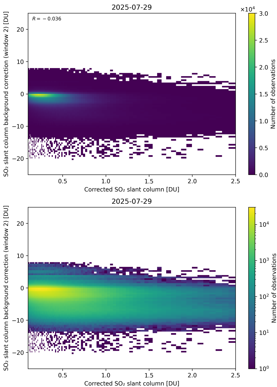
Figure 227: Scatter density plot of “Corrected SO 2 slant column” against “SO 2 slant column background correction (window 2)” for 2025-07-29 to 2025-07-30.
