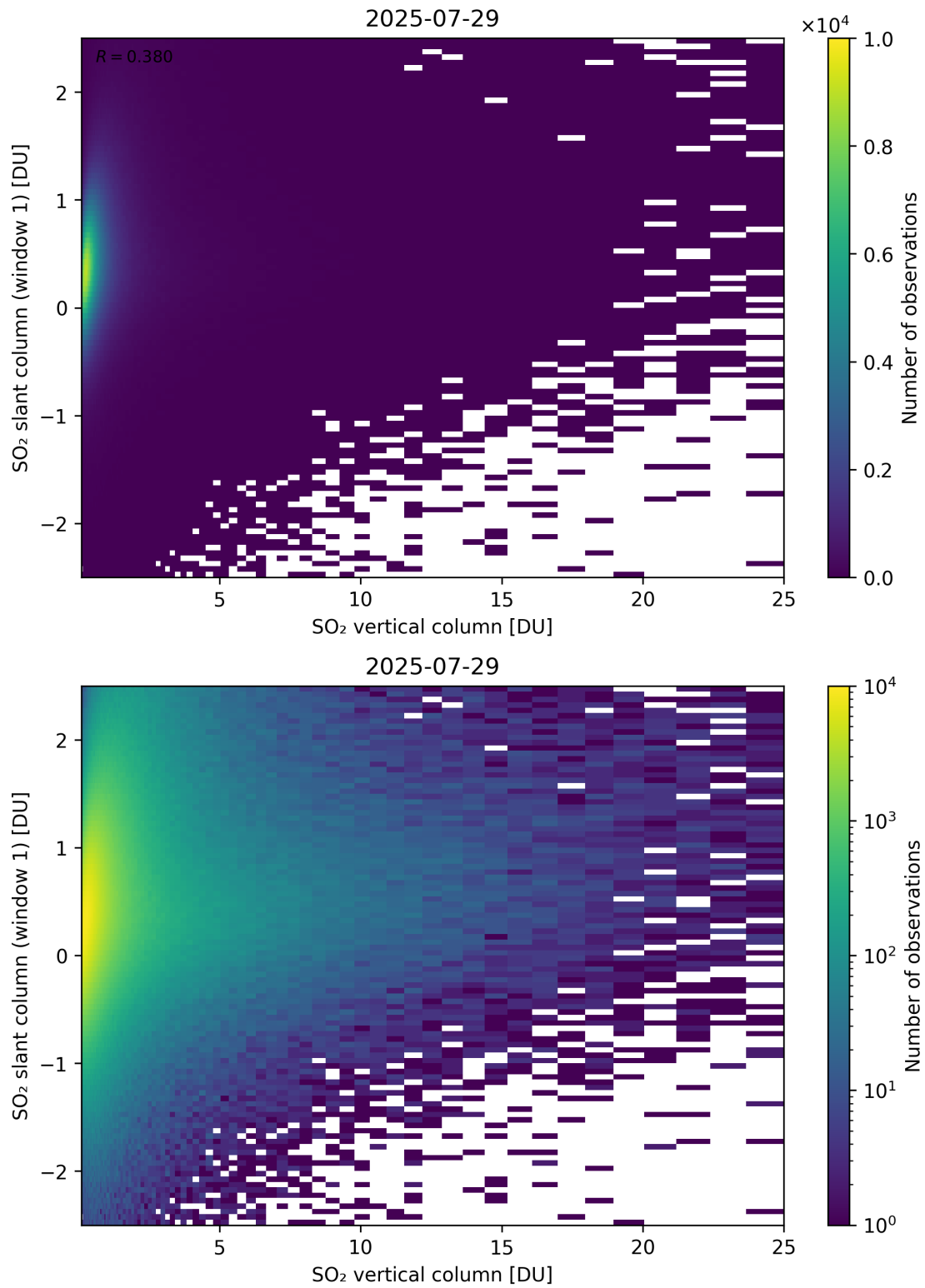
Figure 354: Scatter density plot of “SO 2 vertical column” against “SO 2 slant column (window 1)” for 2025-07-29 to 2025-07-30.
