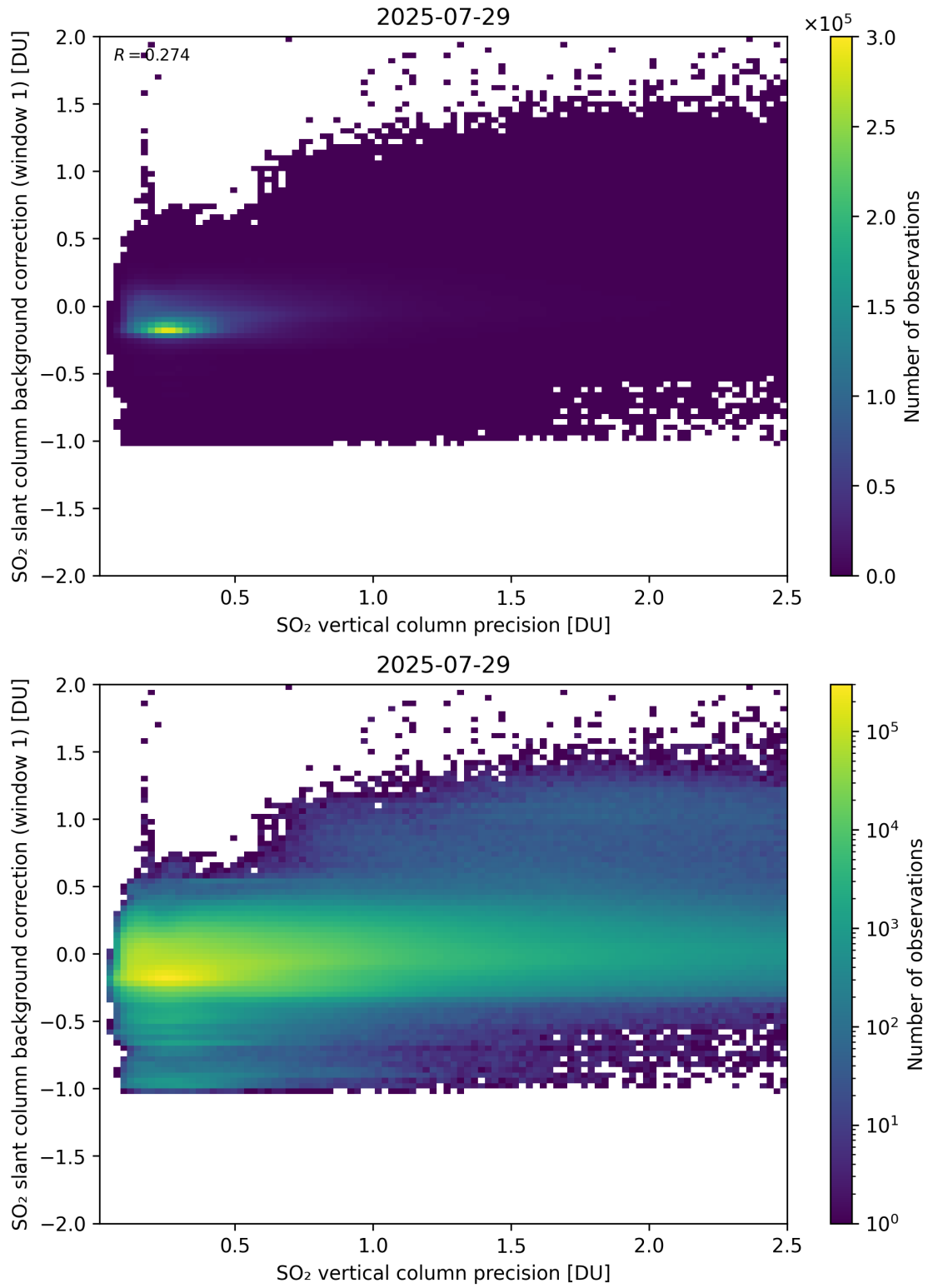
Figure 329: Scatter density plot of “SO 2 vertical column precision” against “SO 2 slant column background correction (window 1)” for 2025-07-29 to 2025-07-30.
