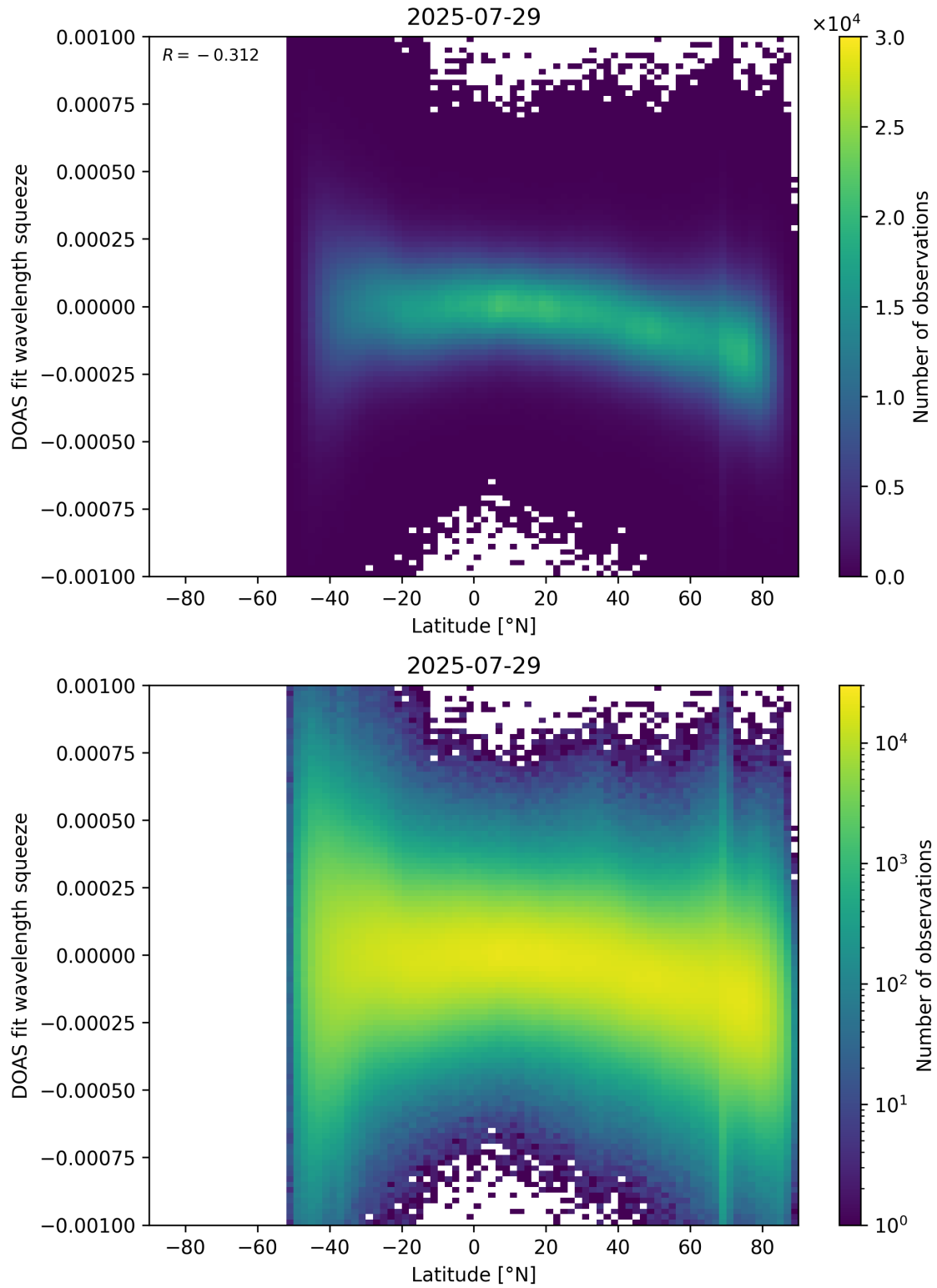
Figure 154: Scatter density plot of “Latitude” against “DOAS fit wavelength squeeze” for 2025-07-29 to 2025-07-30.
