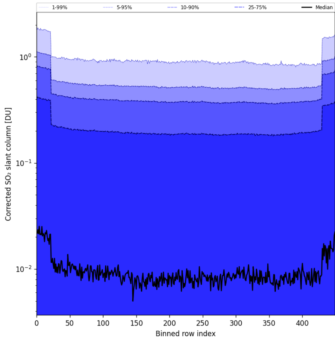
Figure 86: Along track statistics of “Corrected SO 2 slant column” for 2025-07-29 to 2025-07-30
