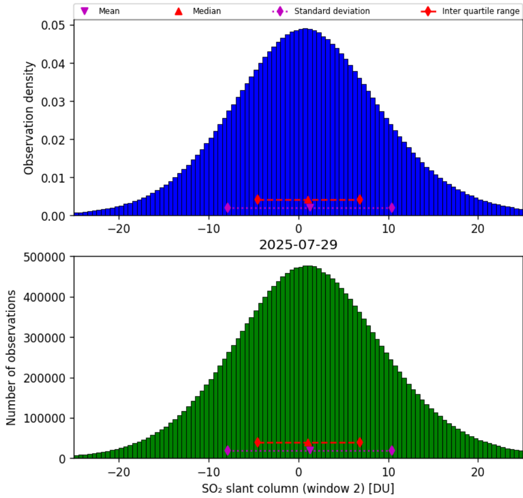
Figure 67: Histogram of “SO 2 slant column (window 2)” for 2025-07-29 to 2025-07-30
