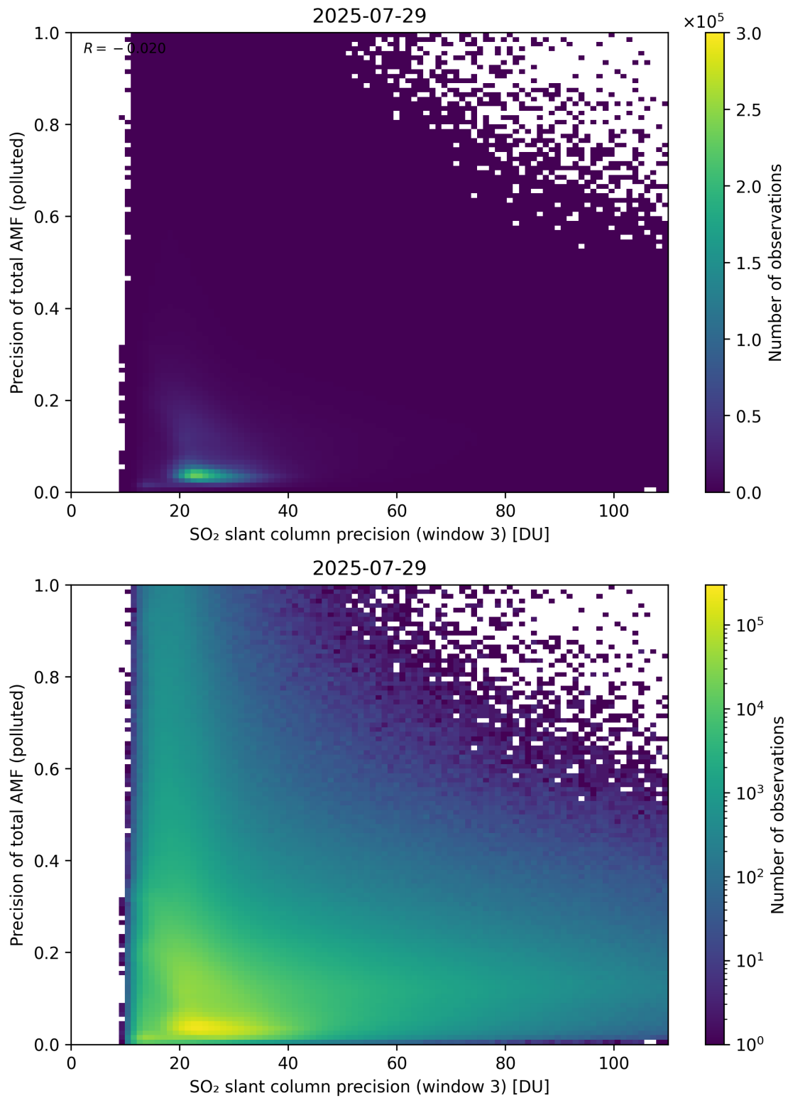
Figure 314: Scatter density plot of “SO 2 slant column precision (window 3)” against “Precision of total AMF (polluted)” for 2025-07-29 to 2025-07-30.
