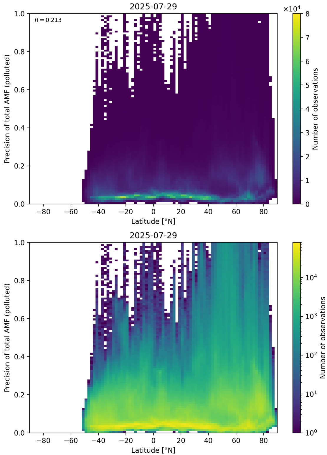
Figure 168: Scatter density plot of “Latitude” against “Precision of total AMF (polluted)” for 2025-07-29 to 2025-07-30.
