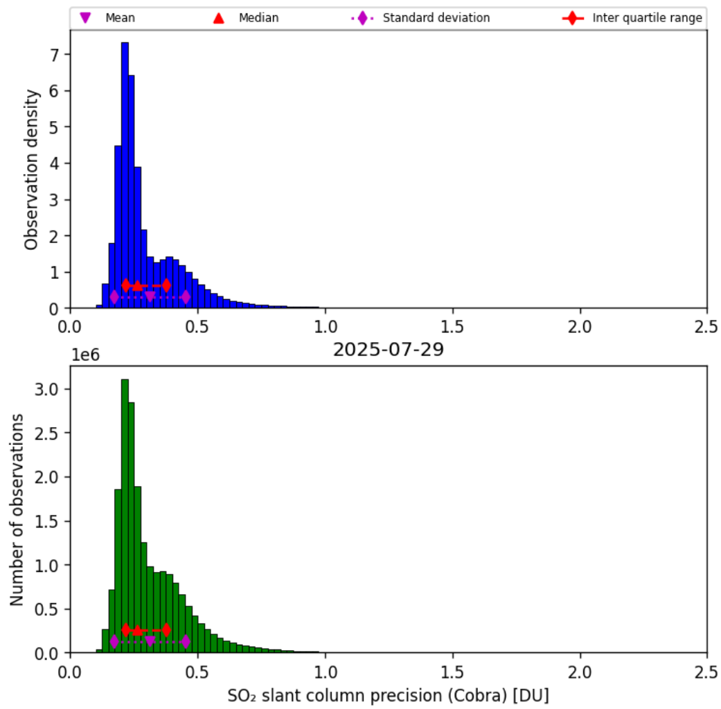
Figure 62: Histogram of “SO 2 slant column precision (Cobra)” for 2025-07-29 to 2025-07-30
