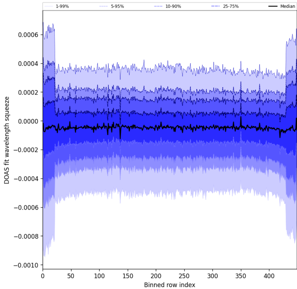
Figure 103: Along track statistics of “DOAS fit wavelength squeeze” for 2025-07-29 to 2025-07-30
