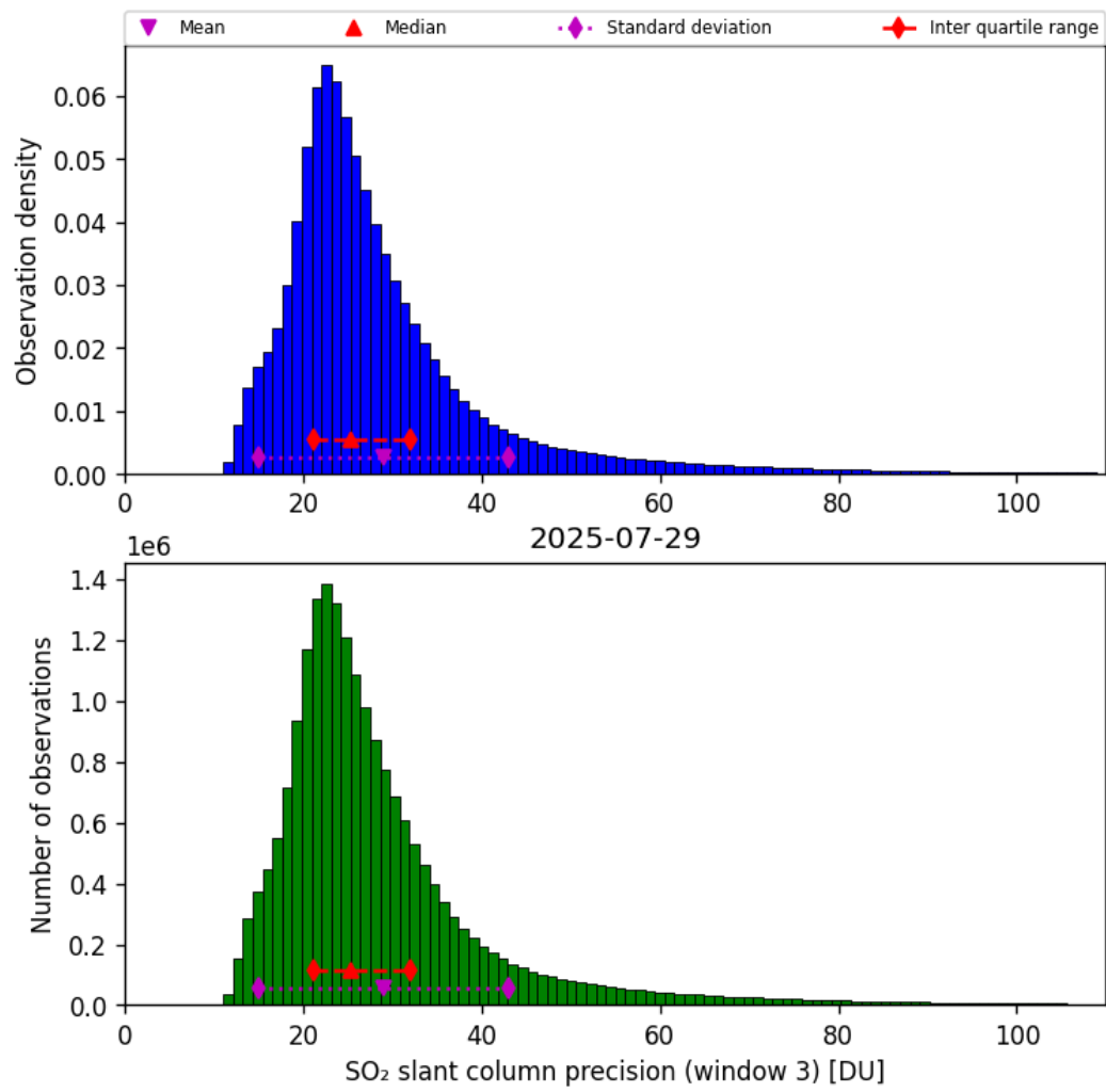
Figure 72: Histogram of “SO 2 slant column precision (window 3)” for 2025-07-29 to 2025-07-30
