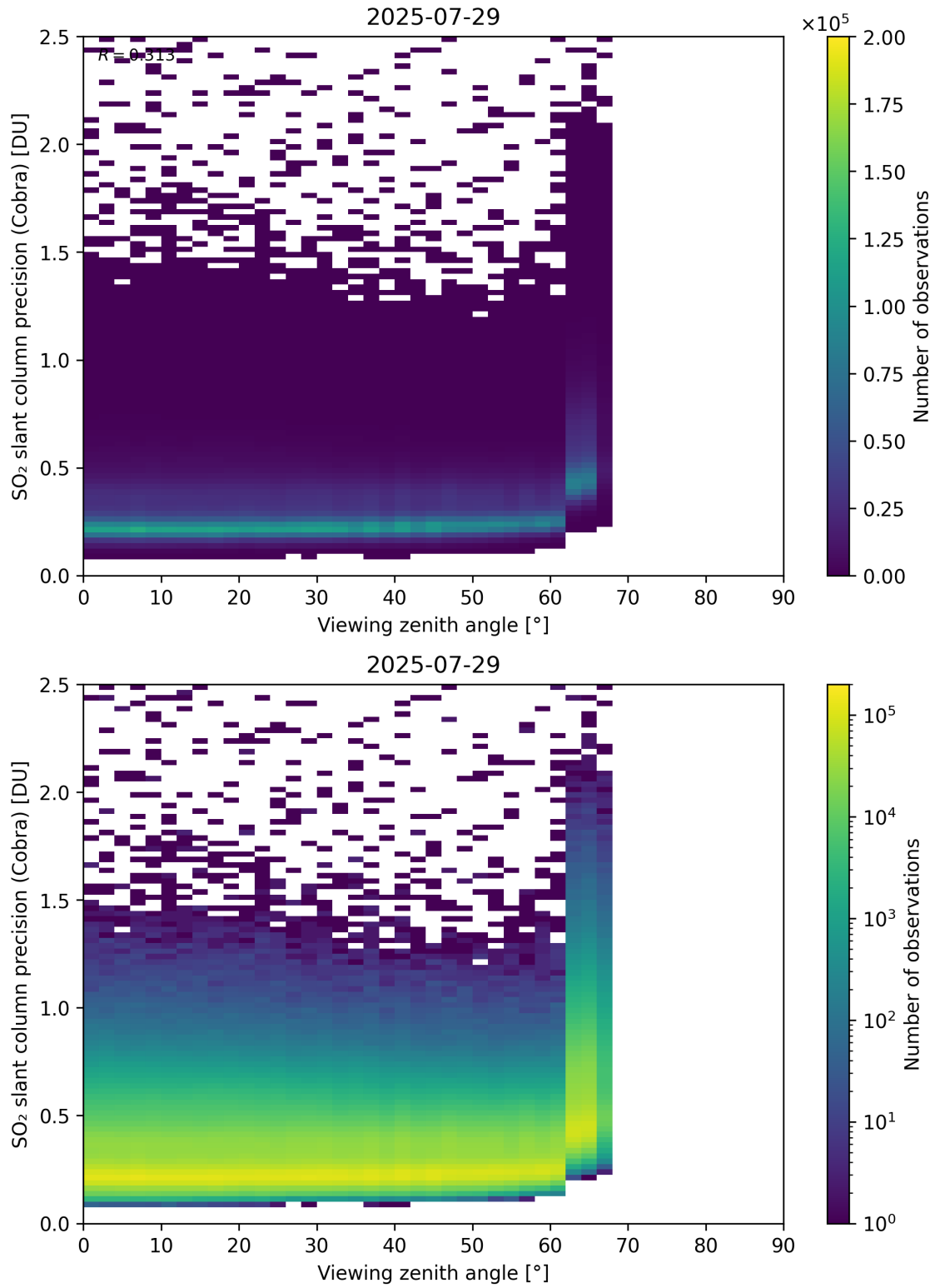
Figure 372: Scatter density plot of “Viewing zenith angle” against “SO 2 slant column precision (Cobra)” for 2025-07-29 to 2025-07-30.
