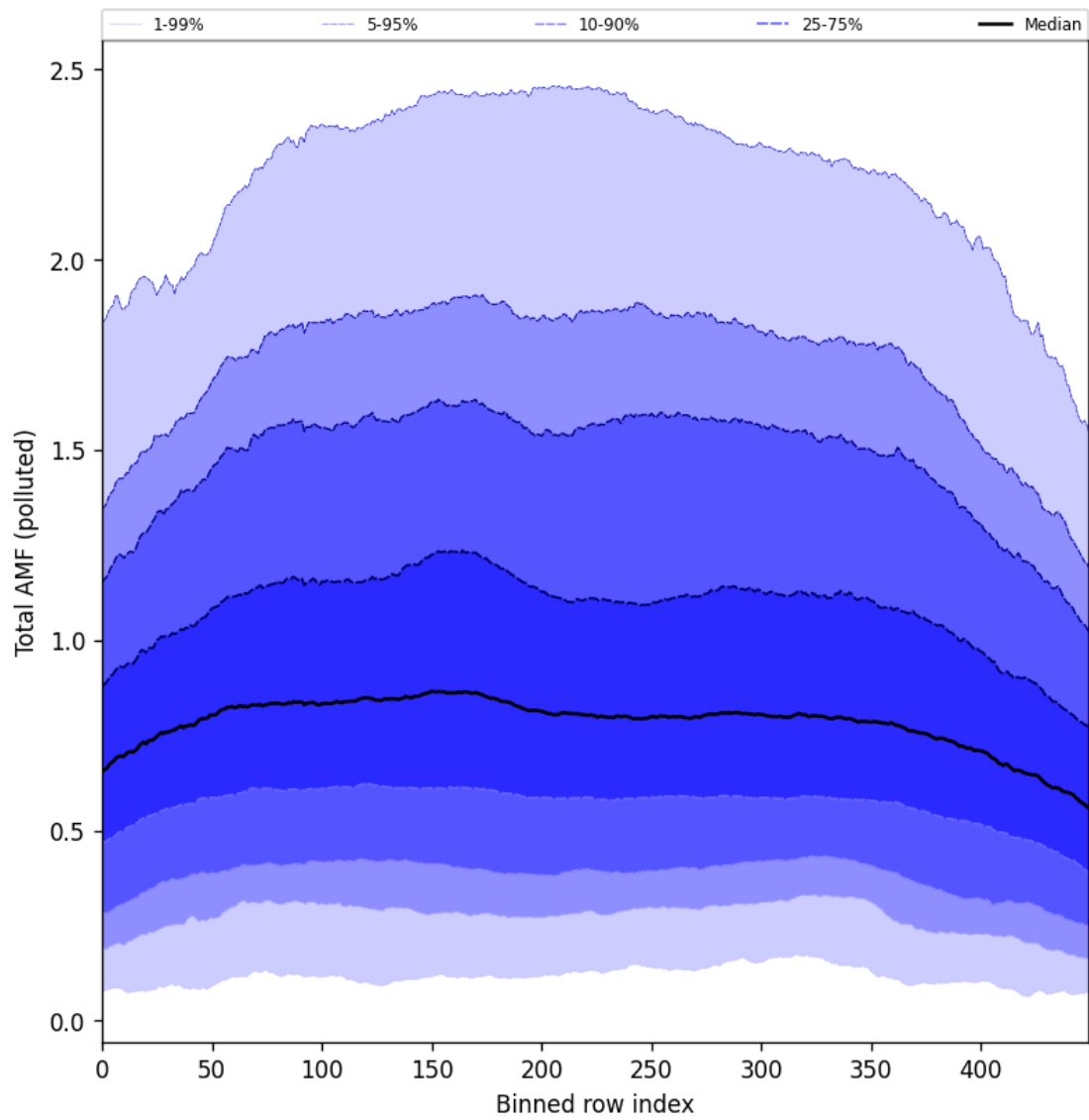
Figure 105: Along track statistics of “Total AMF (polluted)” for 2025-07-29 to 2025-07-30
