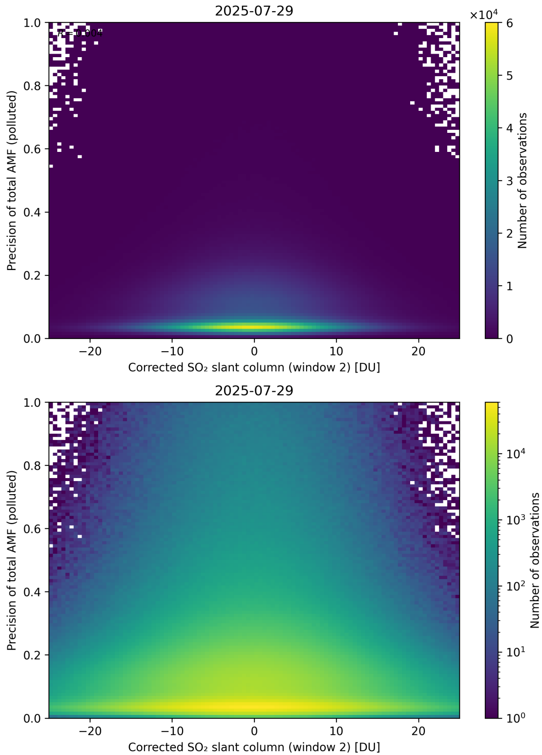
Figure 254: Scatter density plot of “Corrected SO 2 slant column (window 2)” against “Precision of total AMF (polluted)” for 2025-07-29 to 2025-07-30.
