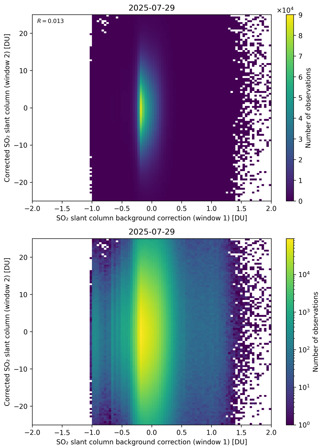
Figure 115: Scatter density plot of “SO 2 slant column background correction (window 1)” against “Corrected SO 2 slant column (window 2)” for 2025-07-29 to 2025-07-30.
