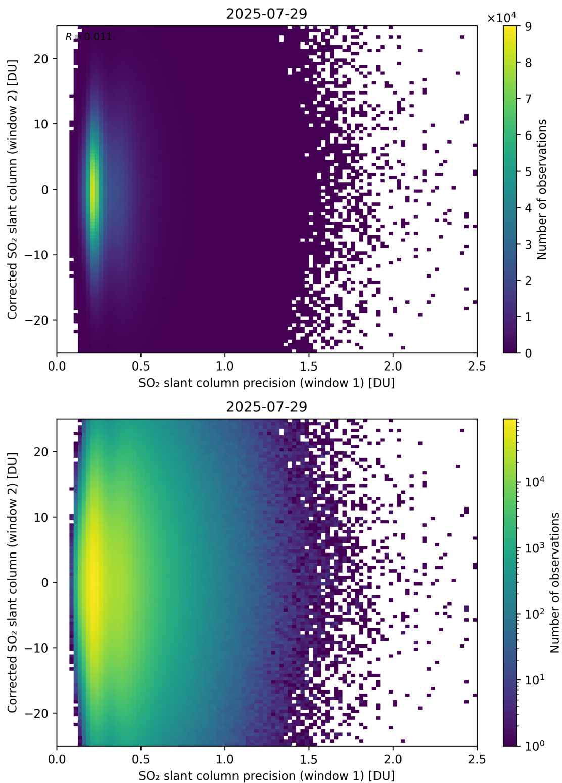
Figure 275: Scatter density plot of “SO 2 slant column precision (window 1)” against “Corrected SO 2 slant column (window 2)” for 2025-07-29 to 2025-07-30.
