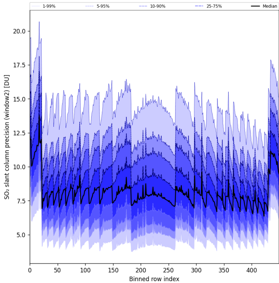
Figure 94: Along track statistics of “SO 2 slant column precision (window2)” for 2025-07-29 to 2025-07-30
