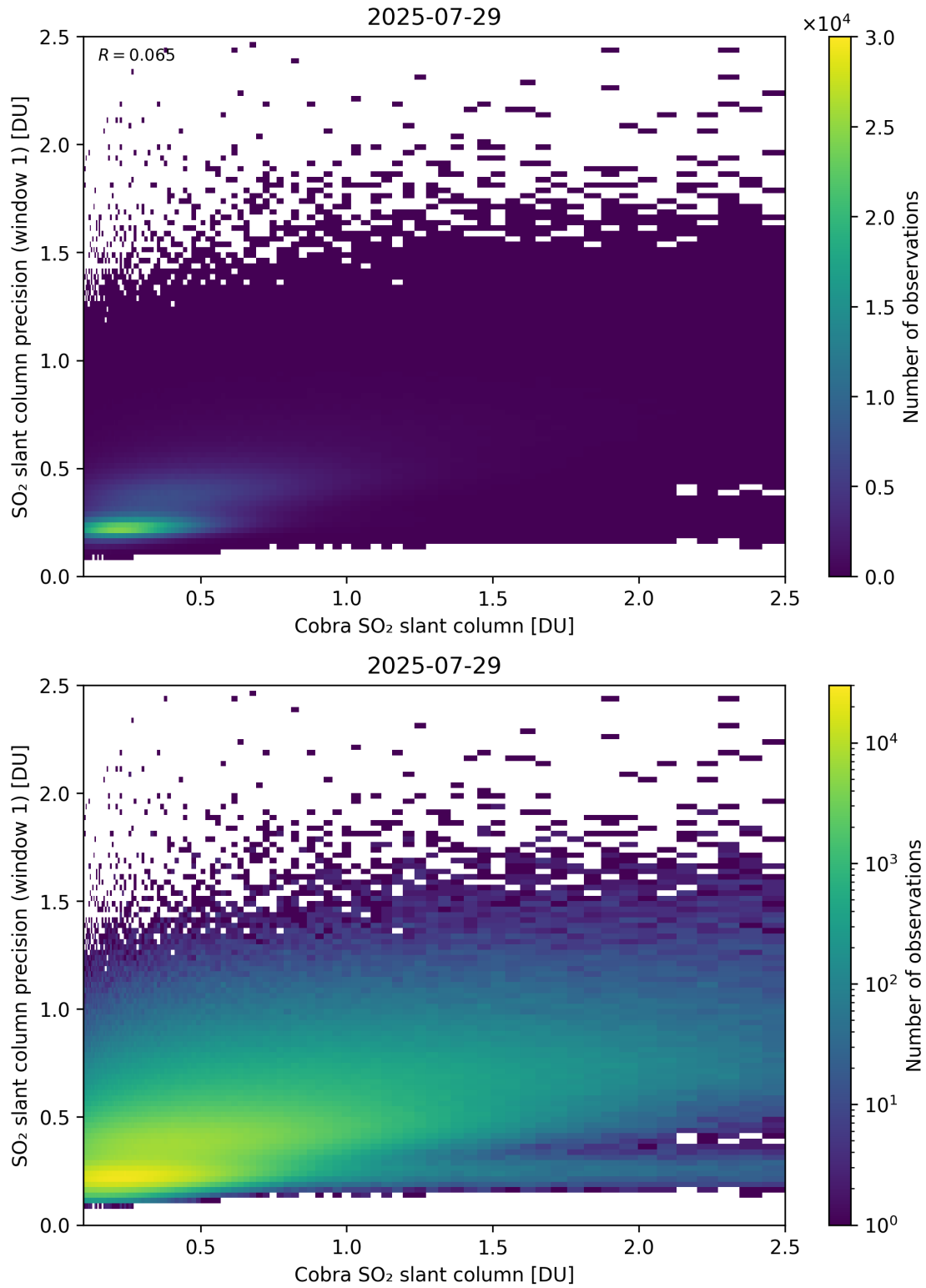
Figure 220: Scatter density plot of “Cobra SO 2 slant column” against “SO 2 slant column precision (window 1)” for 2025-07-29 to 2025-07-30.
