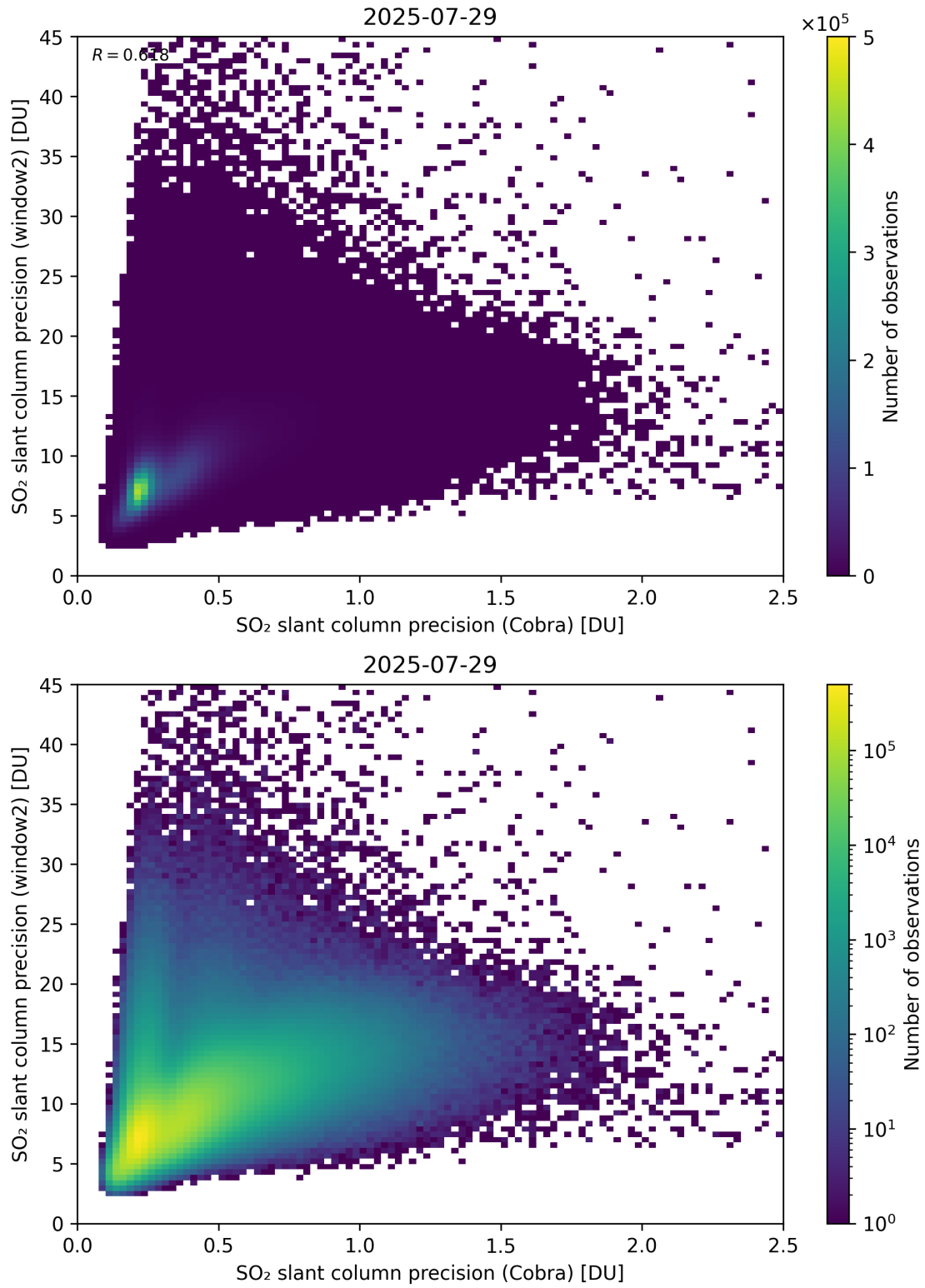
Figure 210: Scatter density plot of “SO 2 slant column precision (Cobra)” against “SO 2 slant column precision (window2)” for 2025-07-29 to 2025-07-30.
