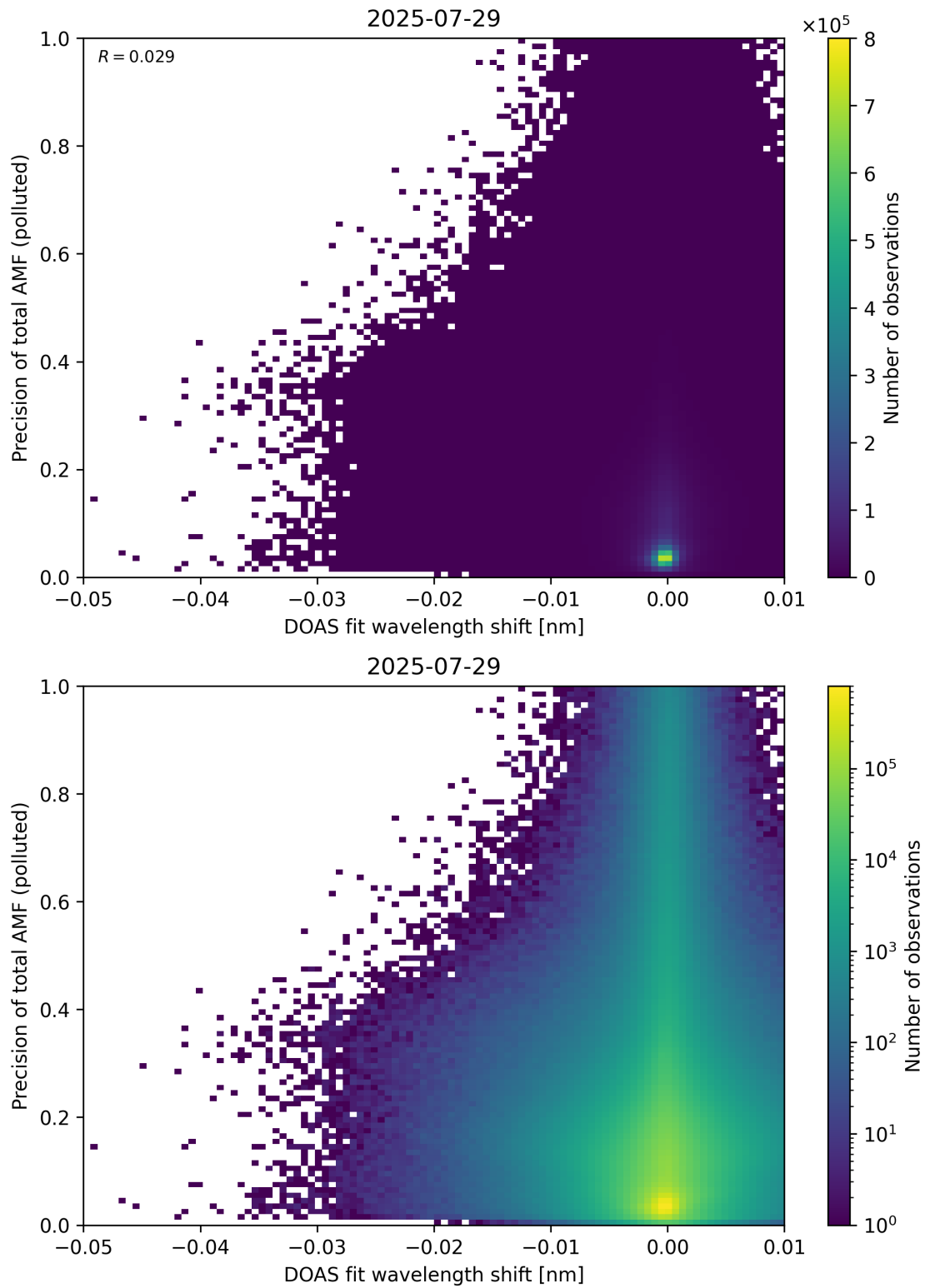
Figure 142: Scatter density plot of “DOAS fit wavelength shift” against “Precision of total AMF (polluted)” for 2025-07-29 to 2025-07-30.
