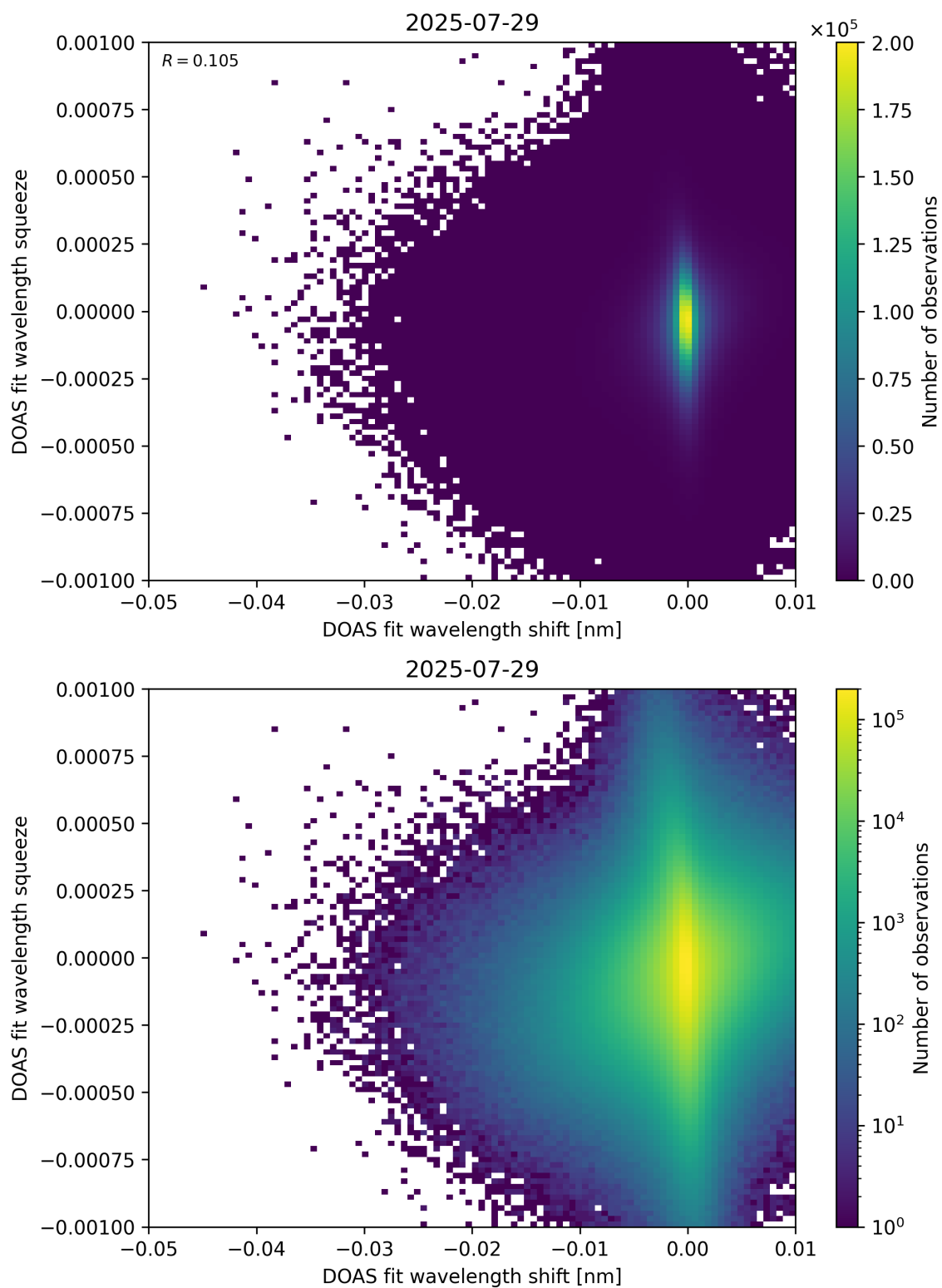
Figure 138: Scatter density plot of “DOAS fit wavelength shift” against “DOAS fit wavelength squeeze” for 2025-07-29 to 2025-07-30.
