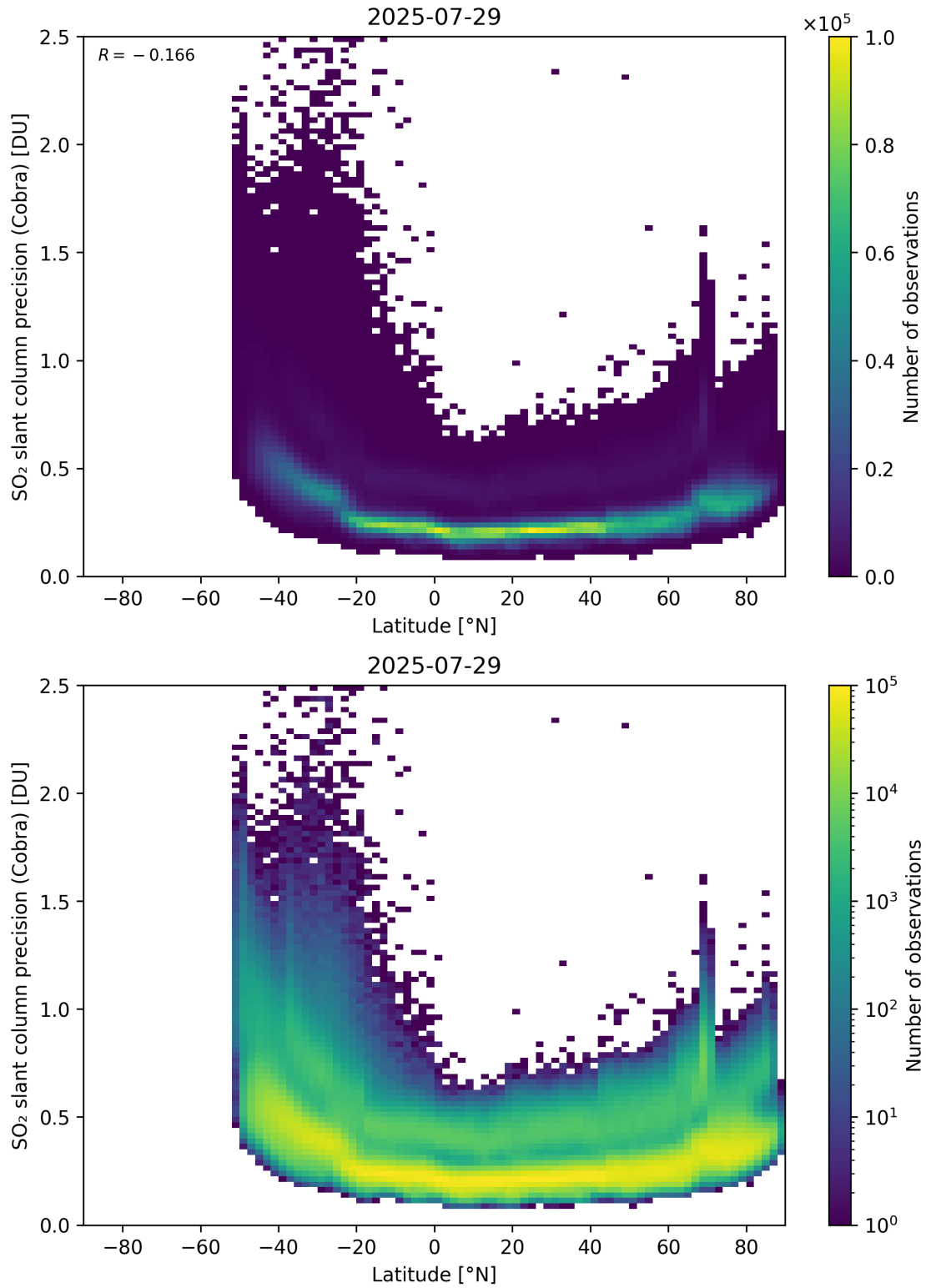
Figure 158: Scatter density plot of “Latitude” against “SO 2 slant column precision (Cobra)” for 2025-07-29 to 2025-07-30.
