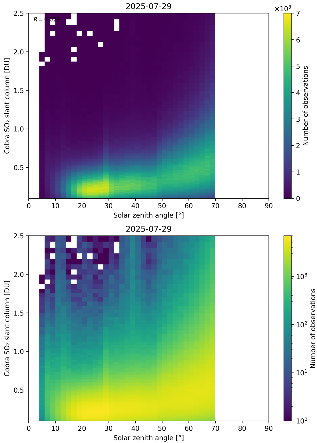
Figure 179: Scatter density plot of “Solar zenith angle” against “Cobra SO 2 slant column” for 2025-07-29 to 2025-07-30.
