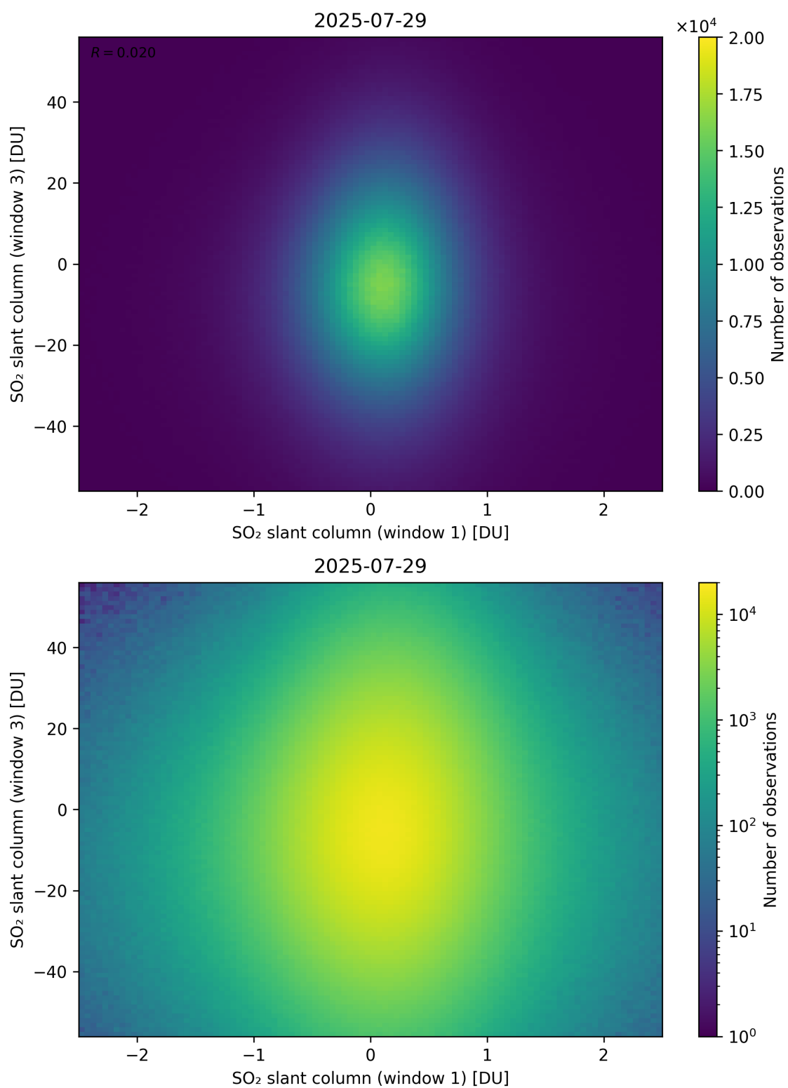
Figure 287: Scatter density plot of “SO 2 slant column (window 1)” against “SO 2 slant column (window 3)” for 2025-07-29 to 2025-07-30.
