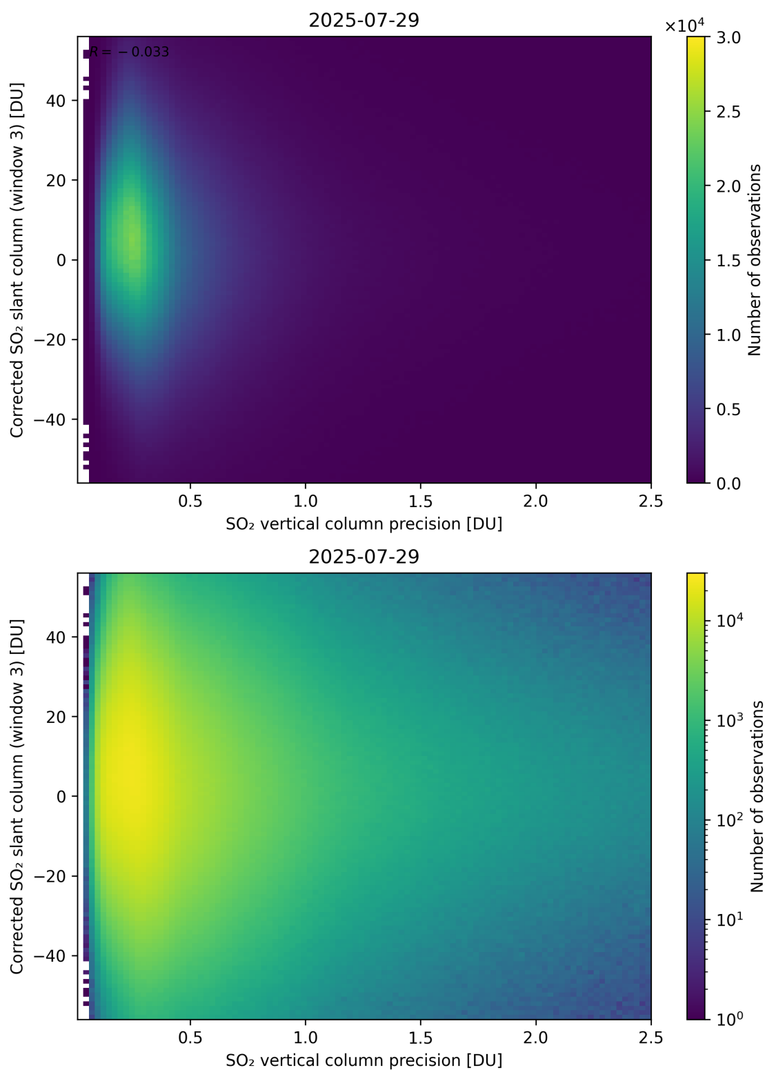
Figure 340: Scatter density plot of “SO 2 vertical column precision” against “Corrected SO 2 slant column (window 3)” for 2025-07-29 to 2025-07-30.
