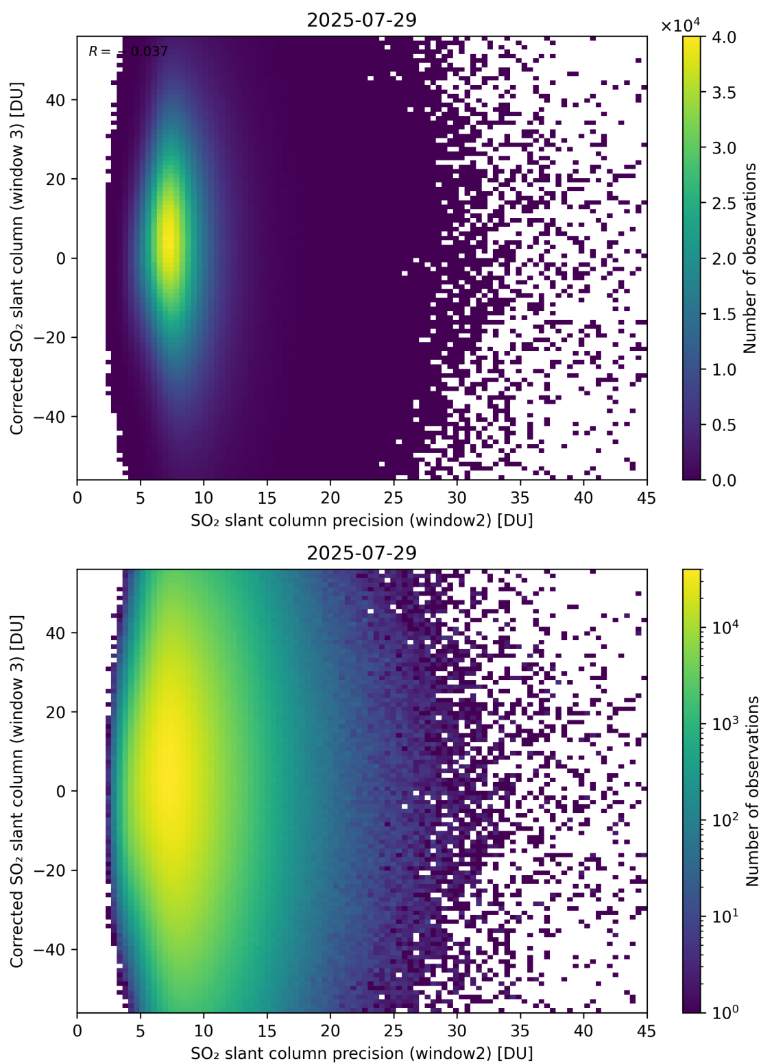
Figure 298: Scatter density plot of “SO 2 slant column precision (window2)” against “Corrected SO 2 slant column (window 3)” for 2025-07-29 to 2025-07-30.
