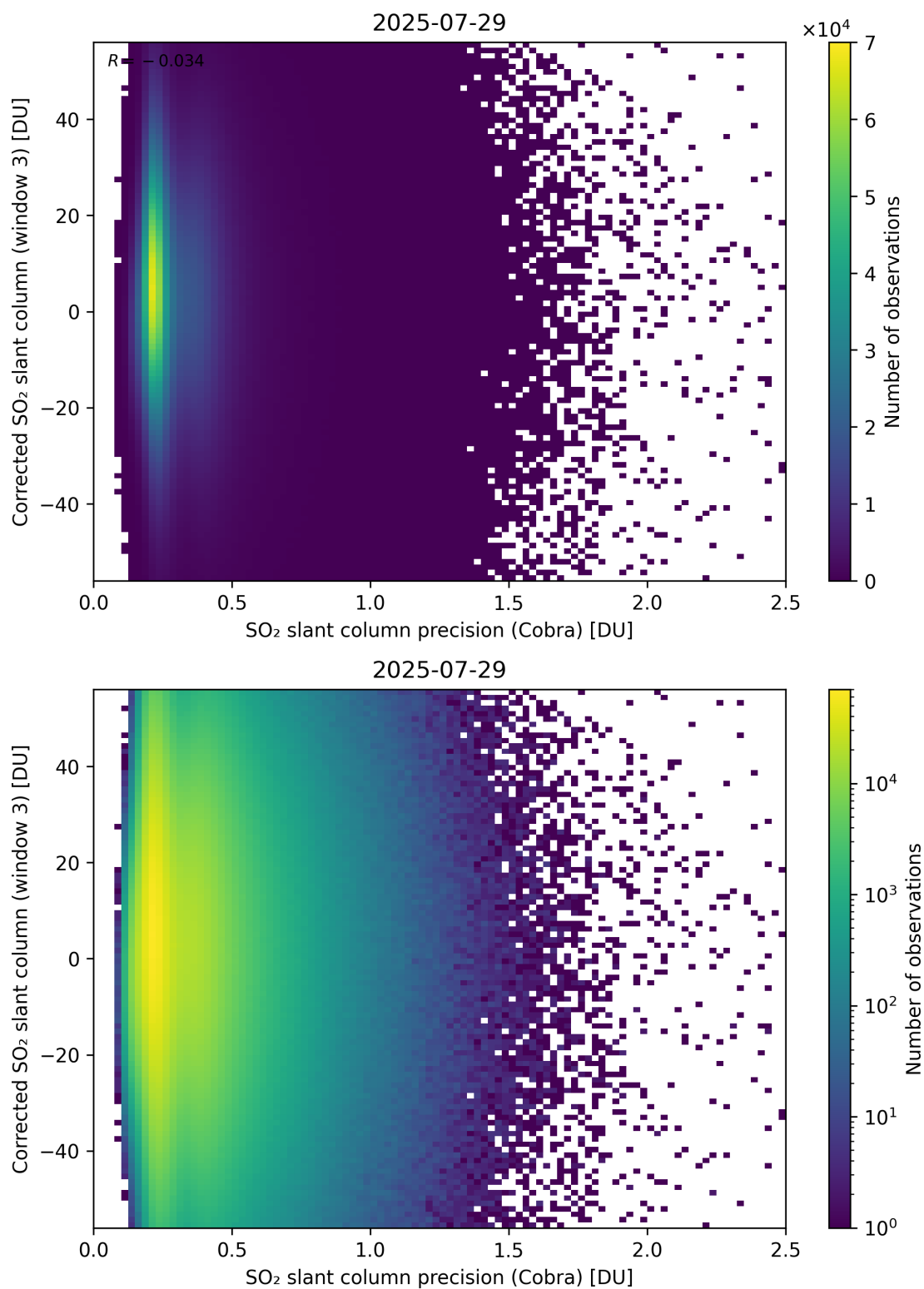
Figure 207: Scatter density plot of “SO 2 slant column precision (Cobra)” against “Corrected SO 2 slant column (window 3)” for 2025-07-29 to 2025-07-30.
