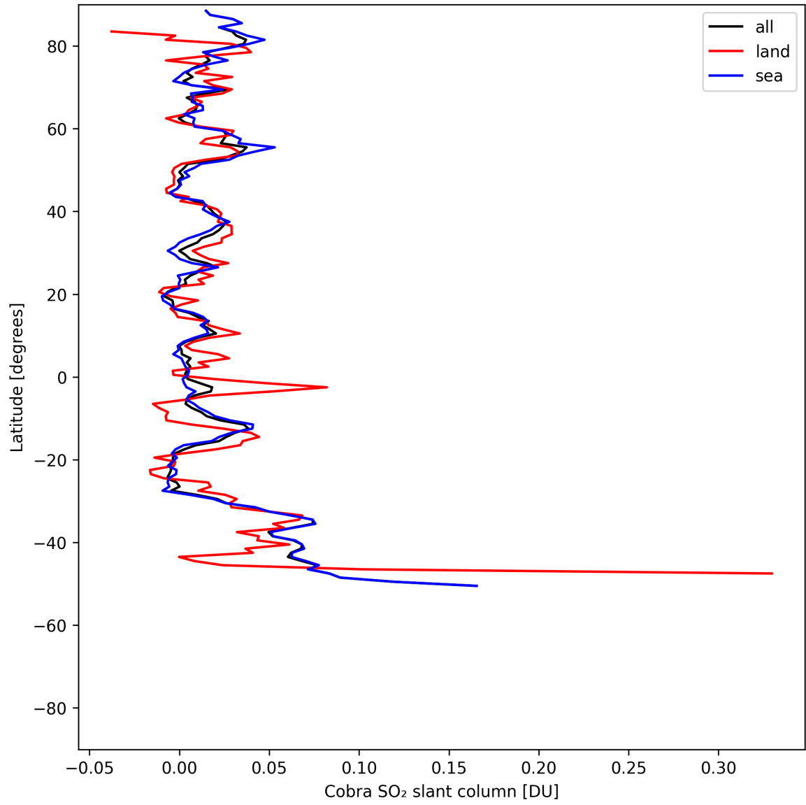
Figure 35: Zonal average of “Cobra SO 2 slant column” for 2025-07-29 to 2025-07-30.
