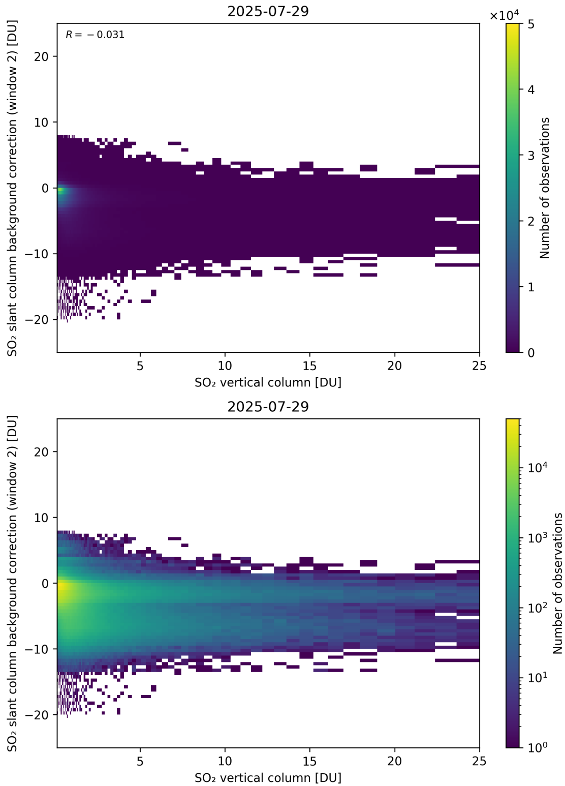
Figure 324: Scatter density plot of “SO 2 vertical column” against “SO 2 slant column background correction (window 2)” for 2025-07-29 to 2025-07-30.
