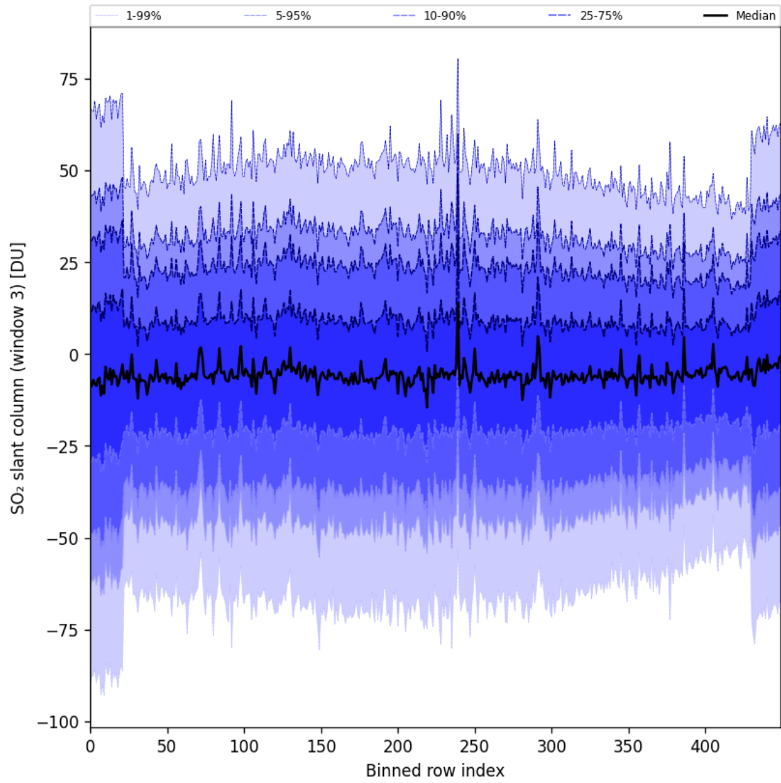
Figure 97: Along track statistics of “SO 2 slant column (window 3)” for 2025-07-29 to 2025-07-30
