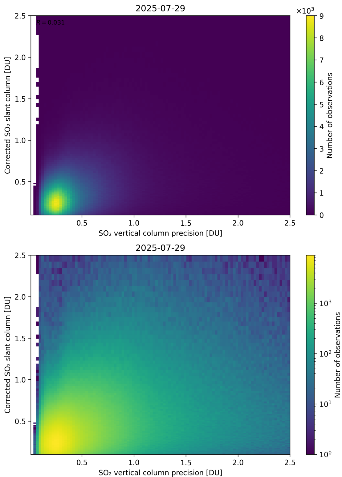
Figure 338: Scatter density plot of “SO 2 vertical column precision” against “Corrected SO 2 slant column” for 2025-07-29 to 2025-07-30.
