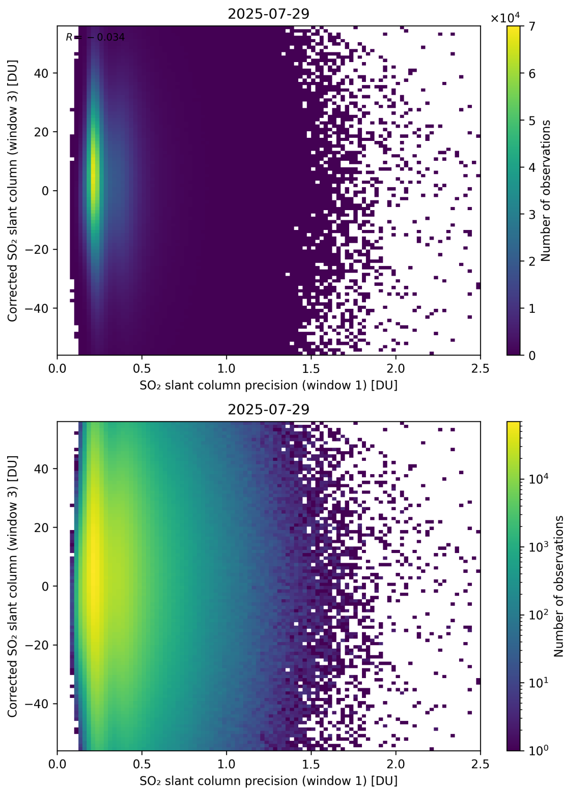
Figure 276: Scatter density plot of “SO 2 slant column precision (window 1)” against “Corrected SO 2 slant column (window 3)” for 2025-07-29 to 2025-07-30.
