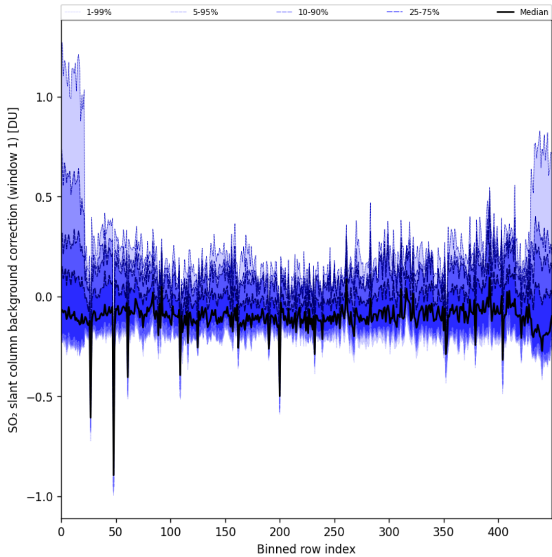
Figure 92: Along track statistics of “SO 2 slant column background correction (window 1)” for 2025-07-29 to 2025-07-30
