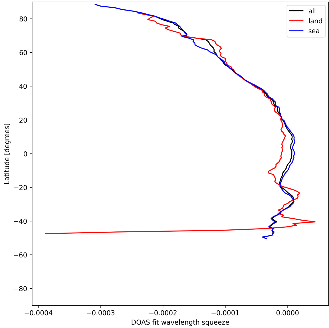
Figure 51: Zonal average of “DOAS fit wavelength squeeze” for 2025-07-29 to 2025-07-30.
