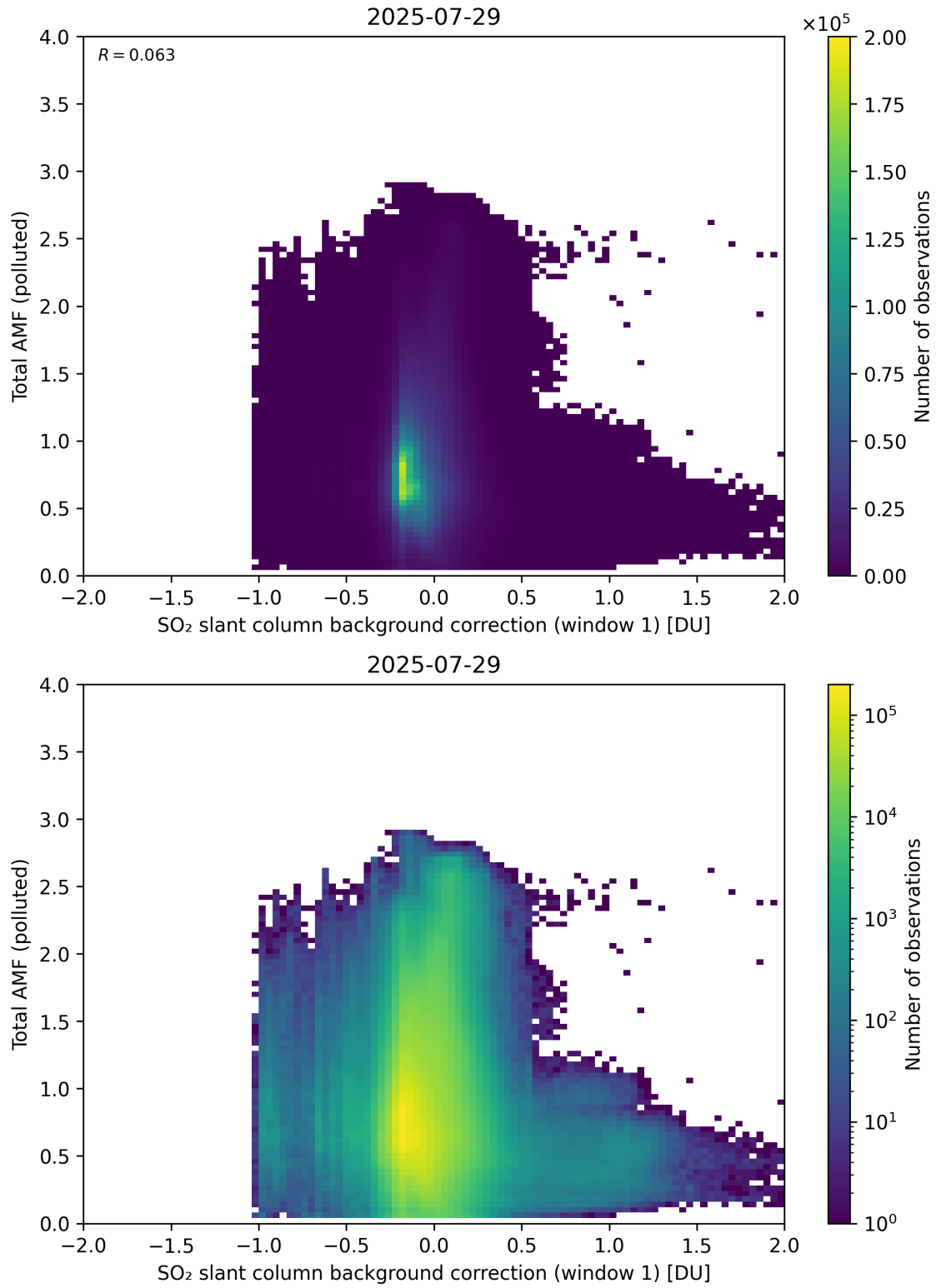
Figure 120: Scatter density plot of “SO 2 slant column background correction (window 1)” against “Total AMF (polluted)” for 2025-07-29 to 2025-07-30.
