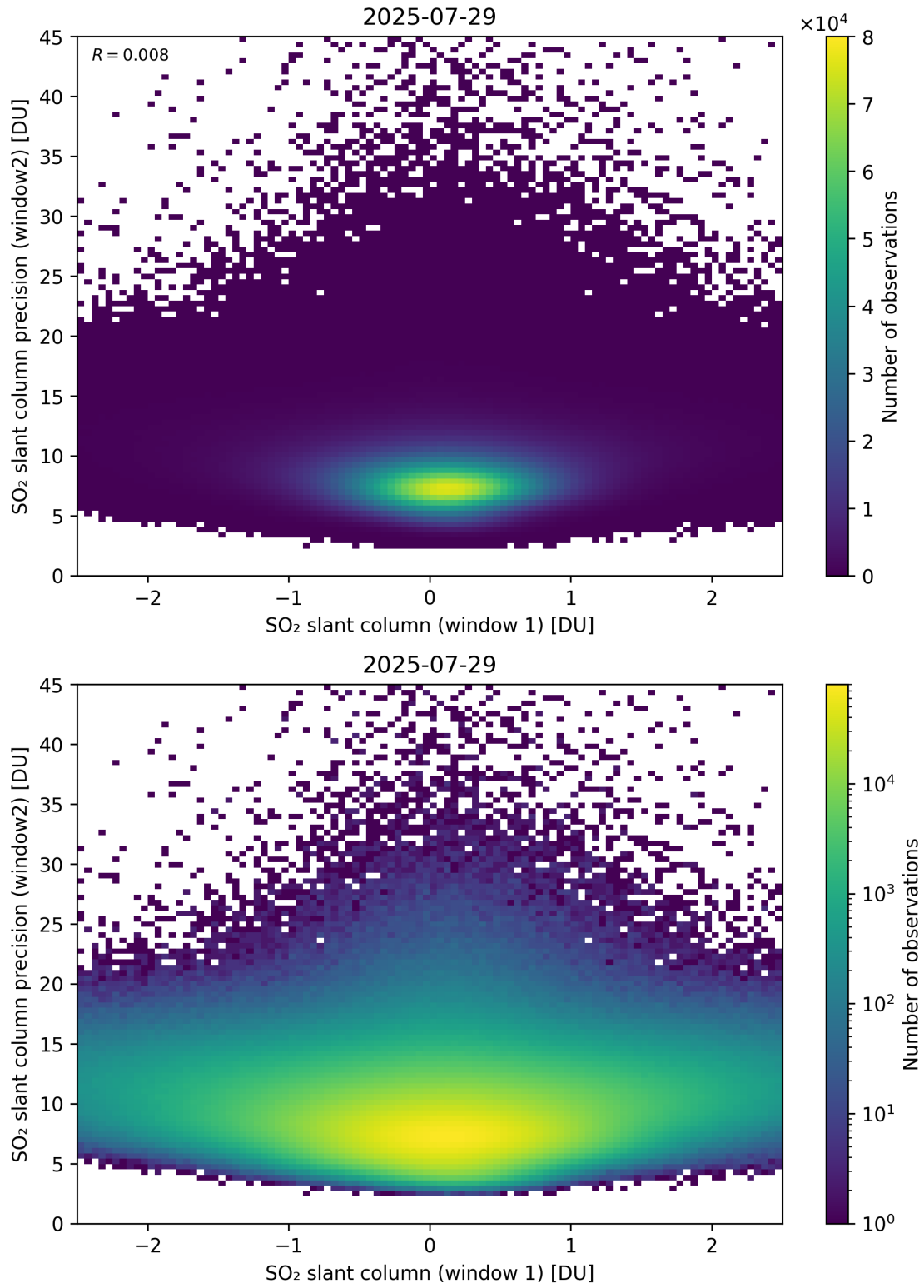
Figure 286: Scatter density plot of “SO 2 slant column (window 1)” against “SO 2 slant column precision (window2)” for 2025-07-29 to 2025-07-30.
