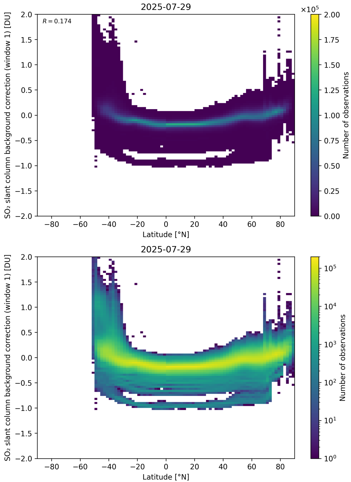
Figure 150: Scatter density plot of “Latitude” against “SO 2 slant column background correction (window 1)” for 2025-07-29 to 2025-07-30.
