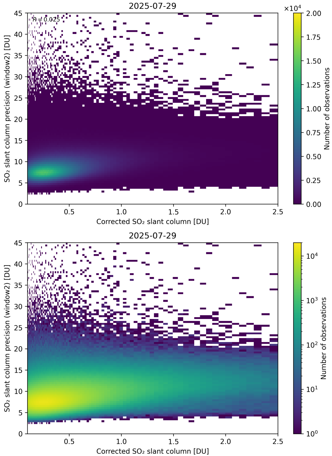
Figure 239: Scatter density plot of “Corrected SO 2 slant column” against “SO 2 slant column precision (window2)” for 2025-07-29 to 2025-07-30.
