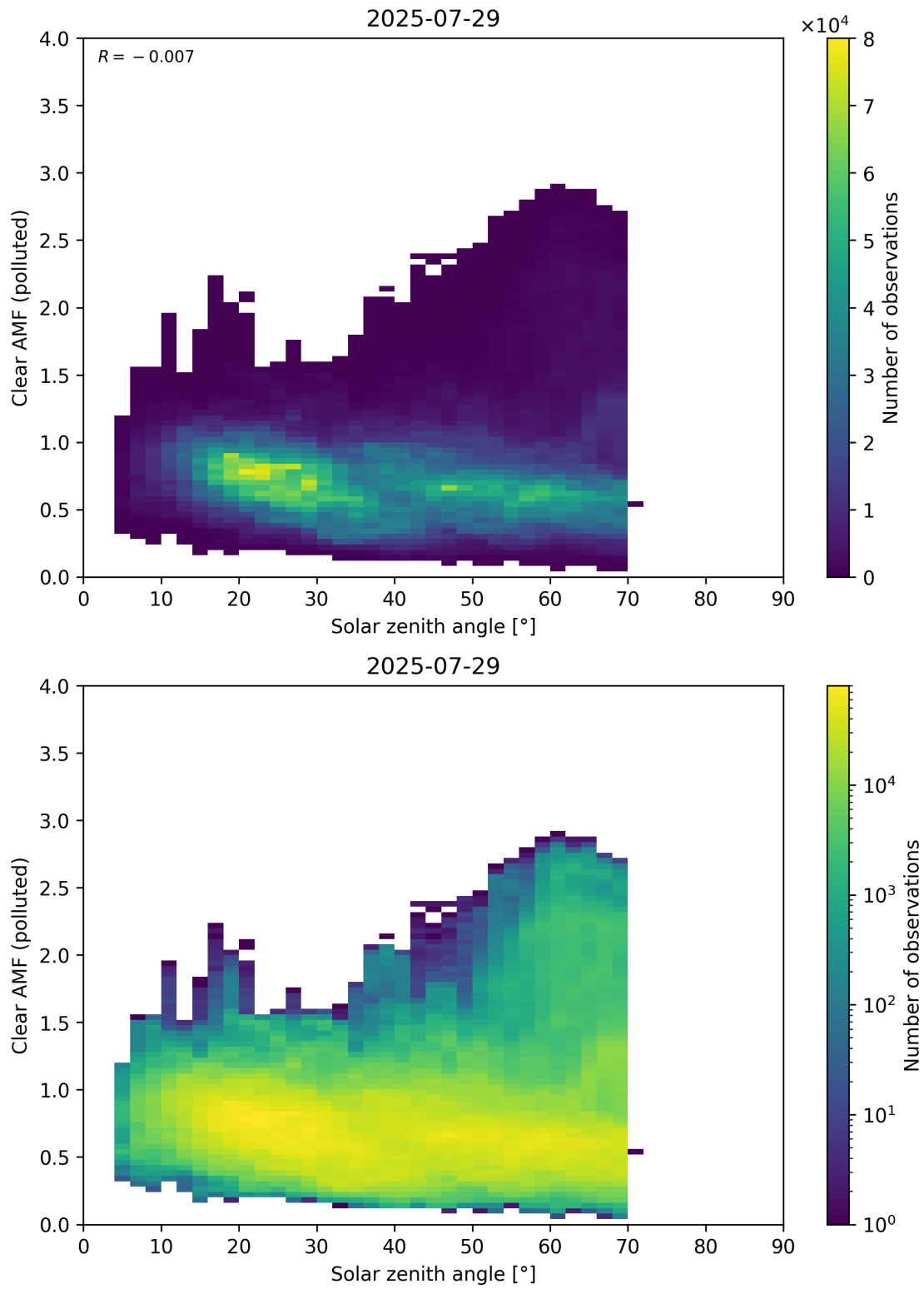
Figure 178: Scatter density plot of “Solar zenith angle” against “Clear AMF (polluted)” for 2025-07-29 to 2025-07-30.
