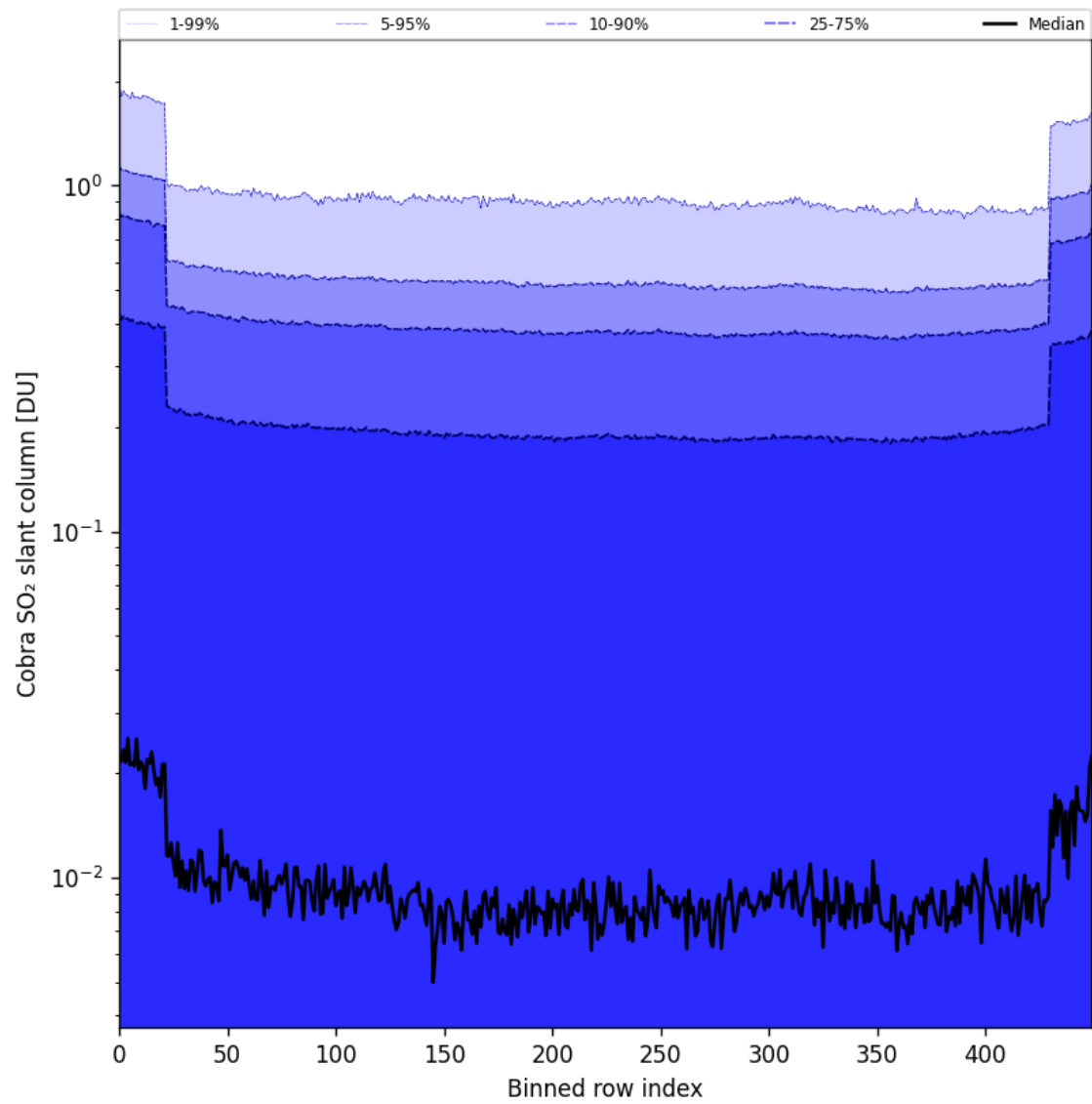
Figure 87: Along track statistics of “Cobra SO 2 slant column” for 2025-07-29 to 2025-07-30
