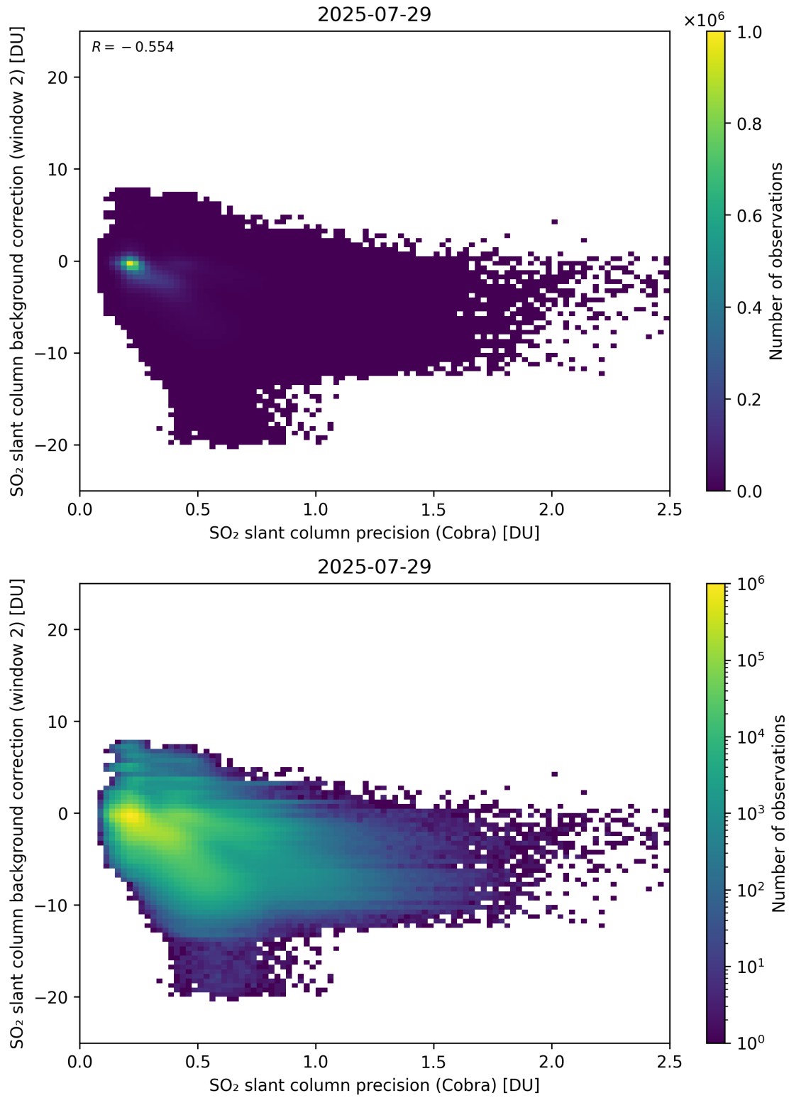
Figure 200: Scatter density plot of “SO 2 slant column precision (Cobra)” against “SO 2 slant column background correction (window 2)” for 2025-07-29 to 2025-07-30.
