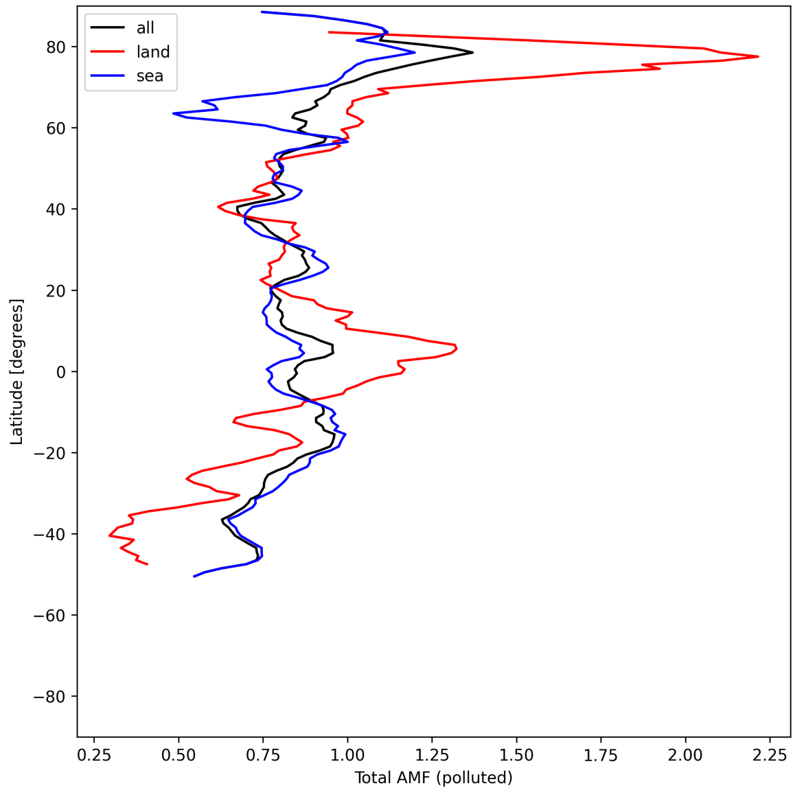
Figure 53: Zonal average of “Total AMF (polluted)” for 2025-07-29 to 2025-07-30.
