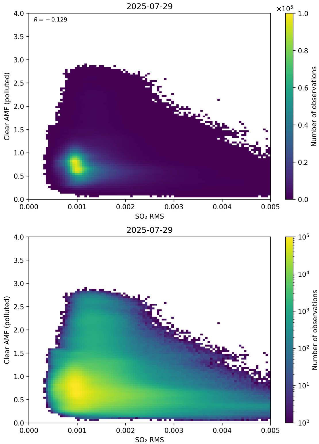
Figure 147: Scatter density plot of “SO 2 RMS” against “Clear AMF (polluted)” for 2025-07-29 to 2025-07-30.
