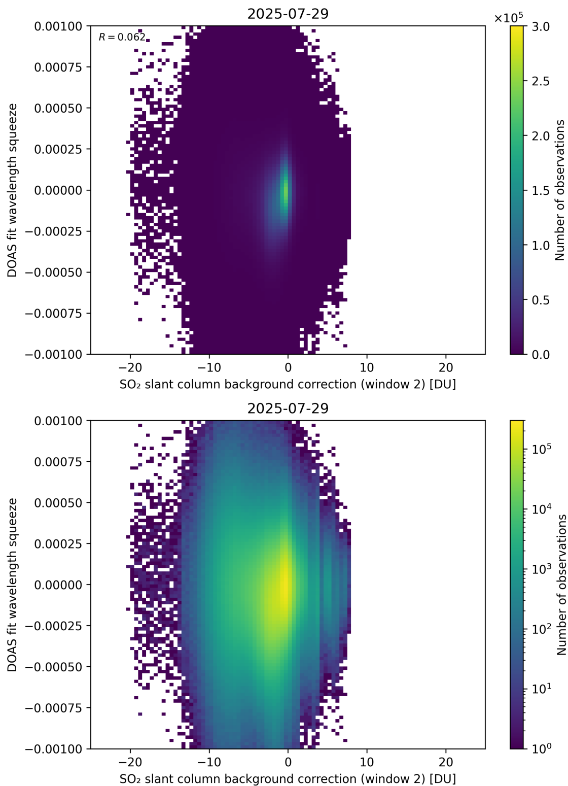
Figure 124: Scatter density plot of “SO 2 slant column background correction (window 2)” against “DOAS fit wavelength squeeze” for 2025-07-29 to 2025-07-30.
