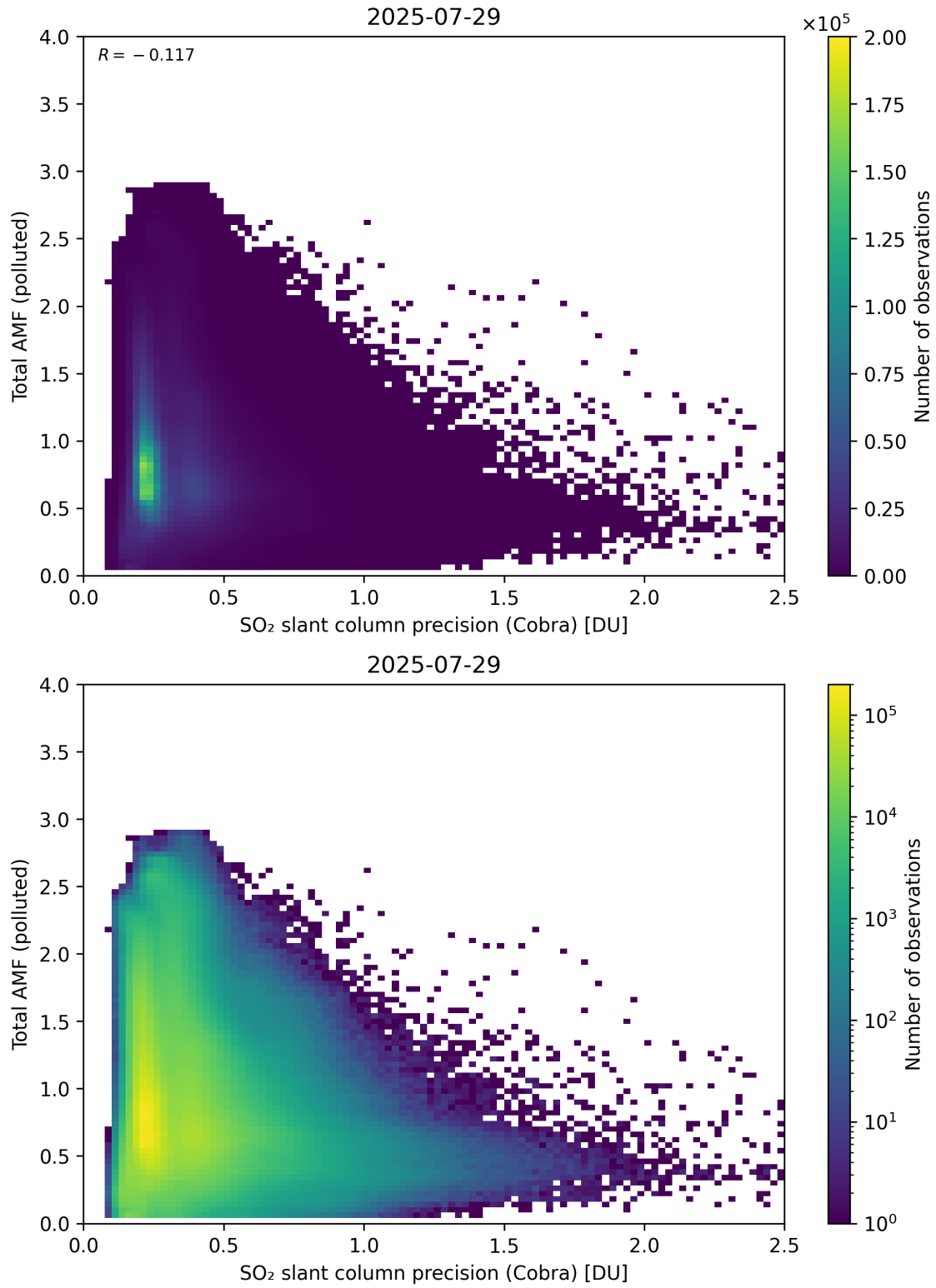
Figure 213: Scatter density plot of “SO 2 slant column precision (Cobra)” against “Total AMF (polluted)” for 2025-07-29 to 2025-07-30.
