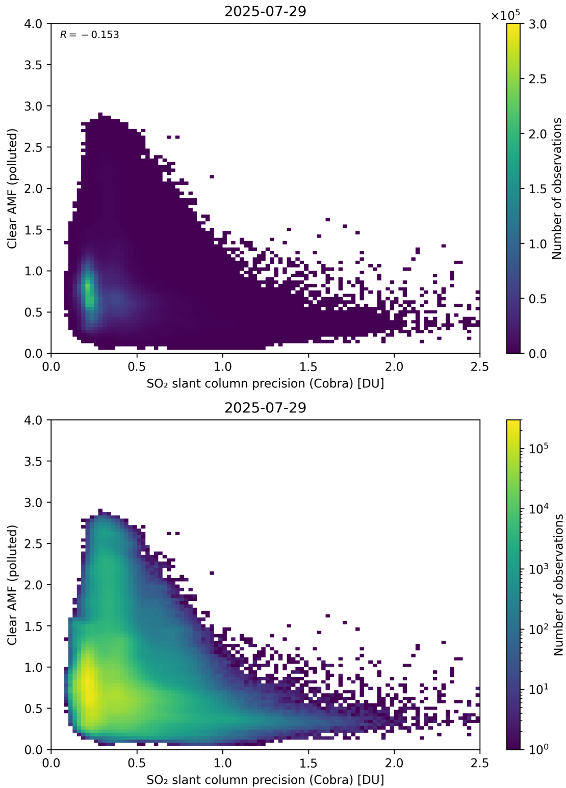
Figure 205: Scatter density plot of “SO 2 slant column precision (Cobra)” against “Clear AMF (polluted)” for 2025-07-29 to 2025-07-30.
