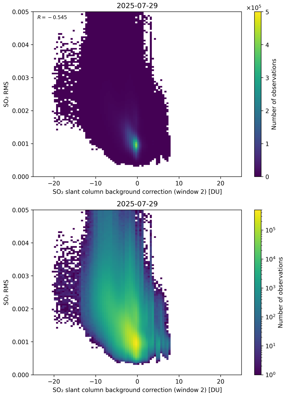
Figure 125: Scatter density plot of “SO 2 slant column background correction (window 2)” against “SO 2 RMS” for 2025-07-29 to 2025-07-30.
