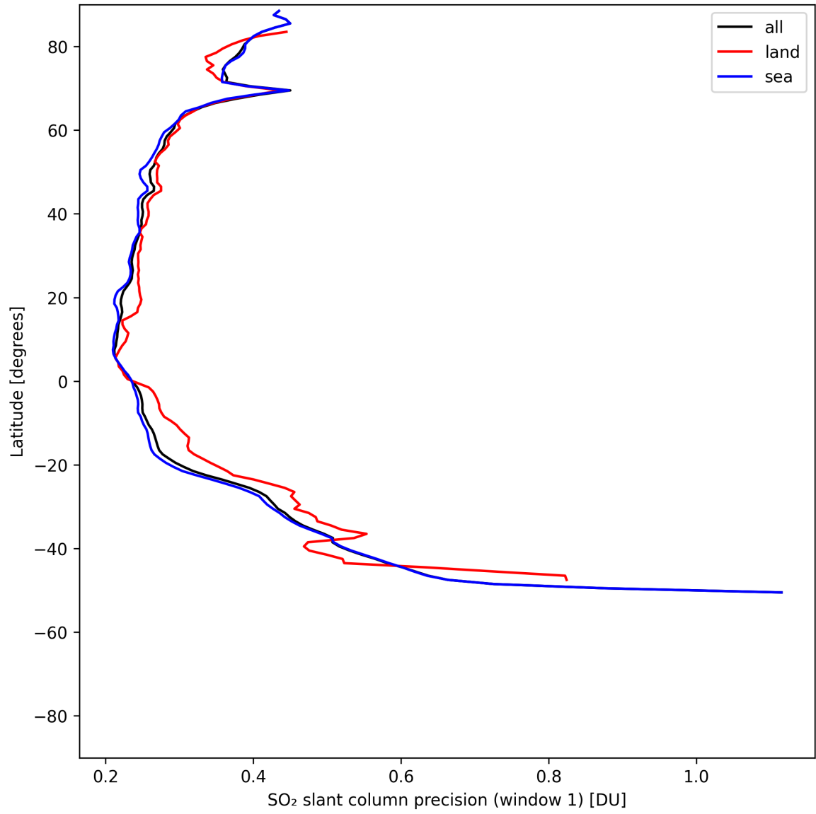
Figure 38: Zonal average of “SO 2 slant column precision (window 1)” for 2025-07-29 to 2025-07-30.
