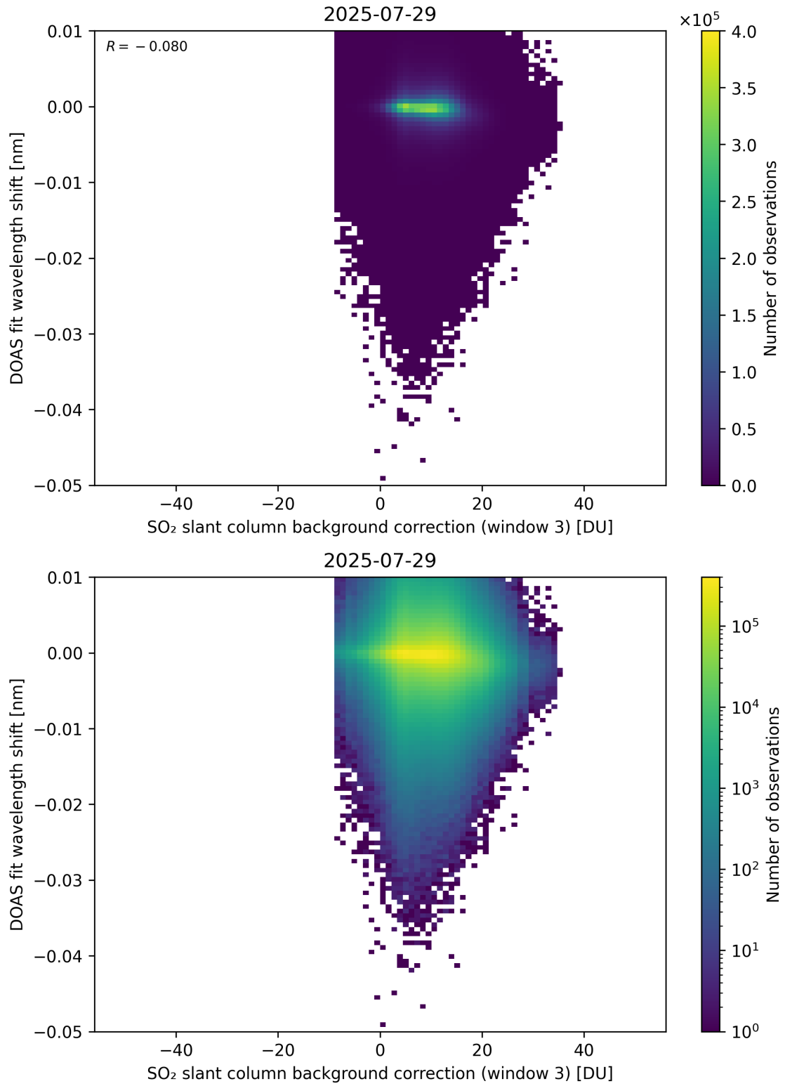
Figure 132: Scatter density plot of “SO 2 slant column background correction (window 3)” against “DOAS fit wavelength shift” for 2025-07-29 to 2025-07-30.
