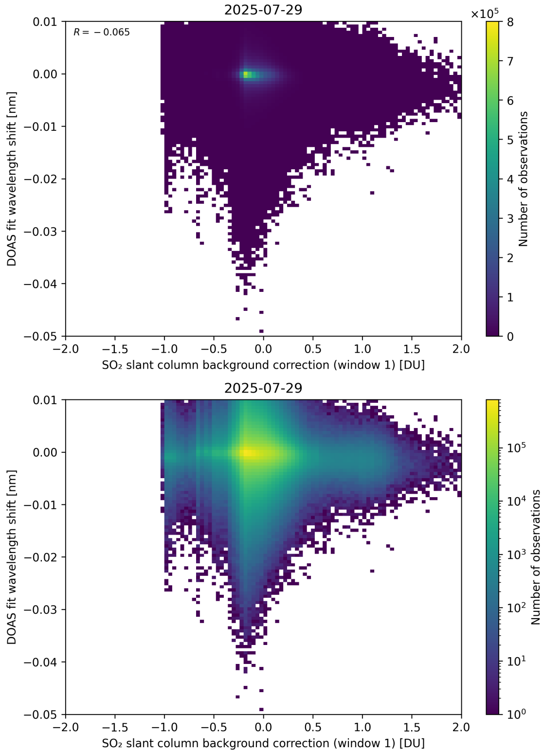
Figure 111: Scatter density plot of “SO 2 slant column background correction (window 1)” against “DOAS fit wavelength shift” for 2025-07-29 to 2025-07-30.
