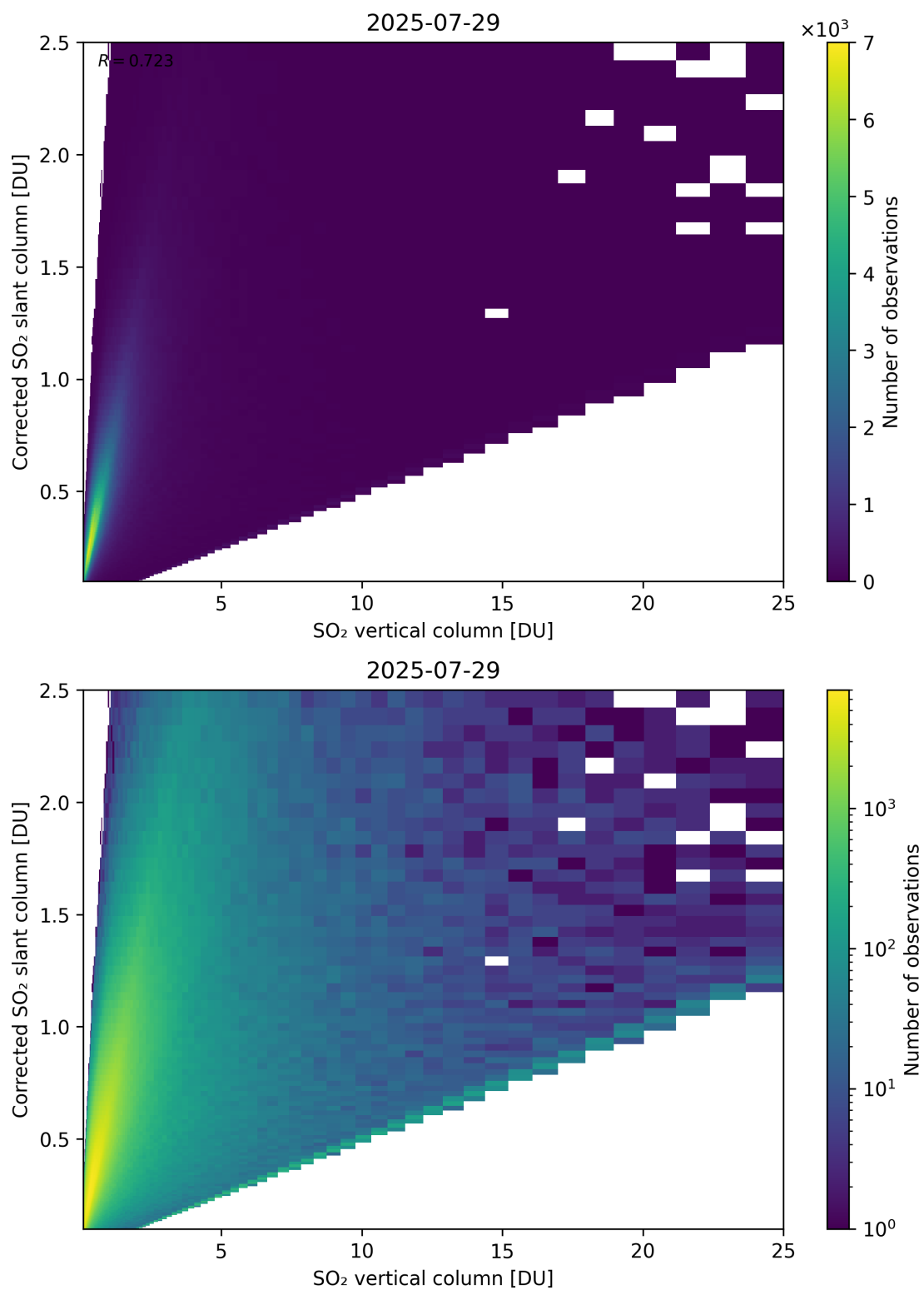
Figure 351: Scatter density plot of “SO 2 vertical column” against “Corrected SO 2 slant column” for 2025-07-29 to 2025-07-30.
