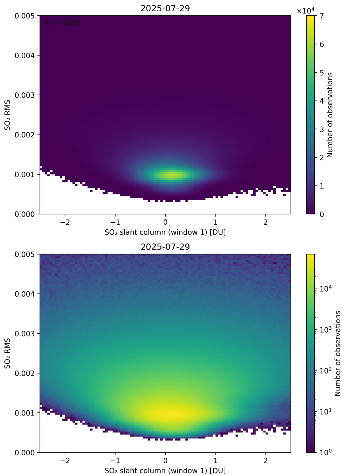
Figure 267: Scatter density plot of “SO 2 slant column (window 1)” against “SO 2 RMS” for 2025-07-29 to 2025-07-30.
