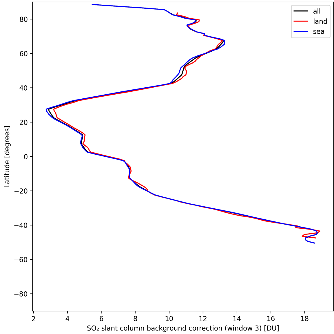
Figure 48: Zonal average of “SO 2 slant column background correction (window 3)” for 2025-07-29 to 2025-07-30.
