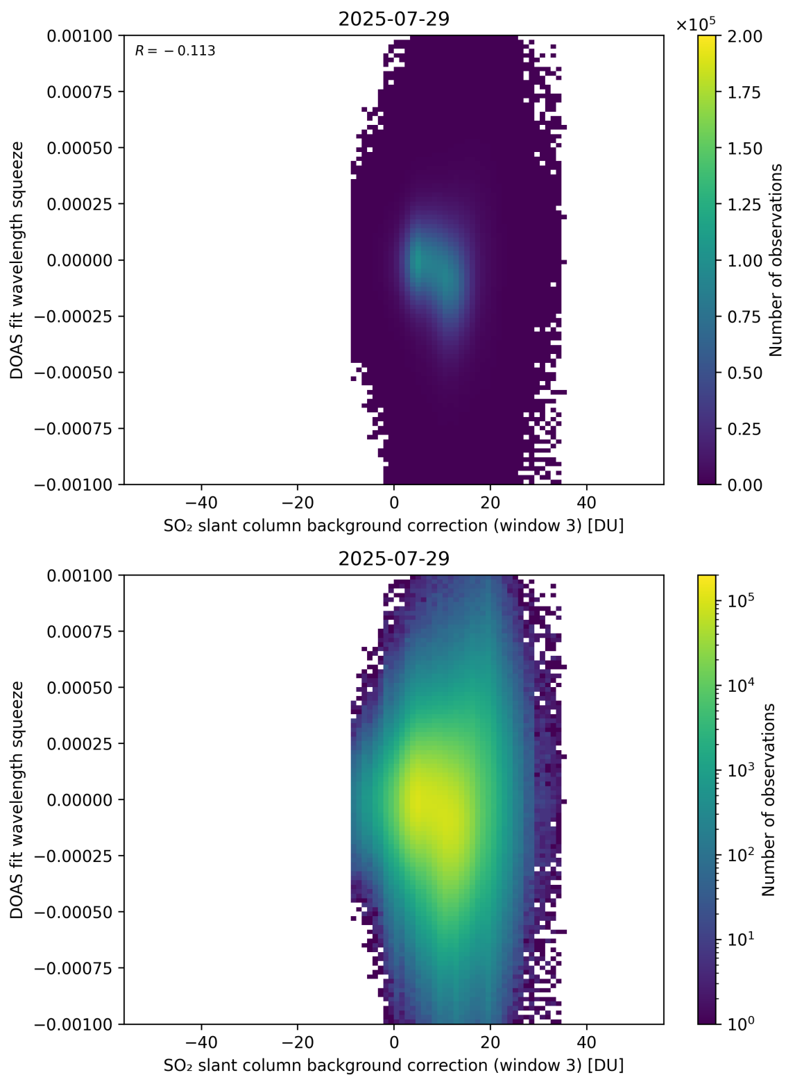
Figure 133: Scatter density plot of “SO 2 slant column background correction (window 3)” against “DOAS fit wavelength squeeze” for 2025-07-29 to 2025-07-30.
