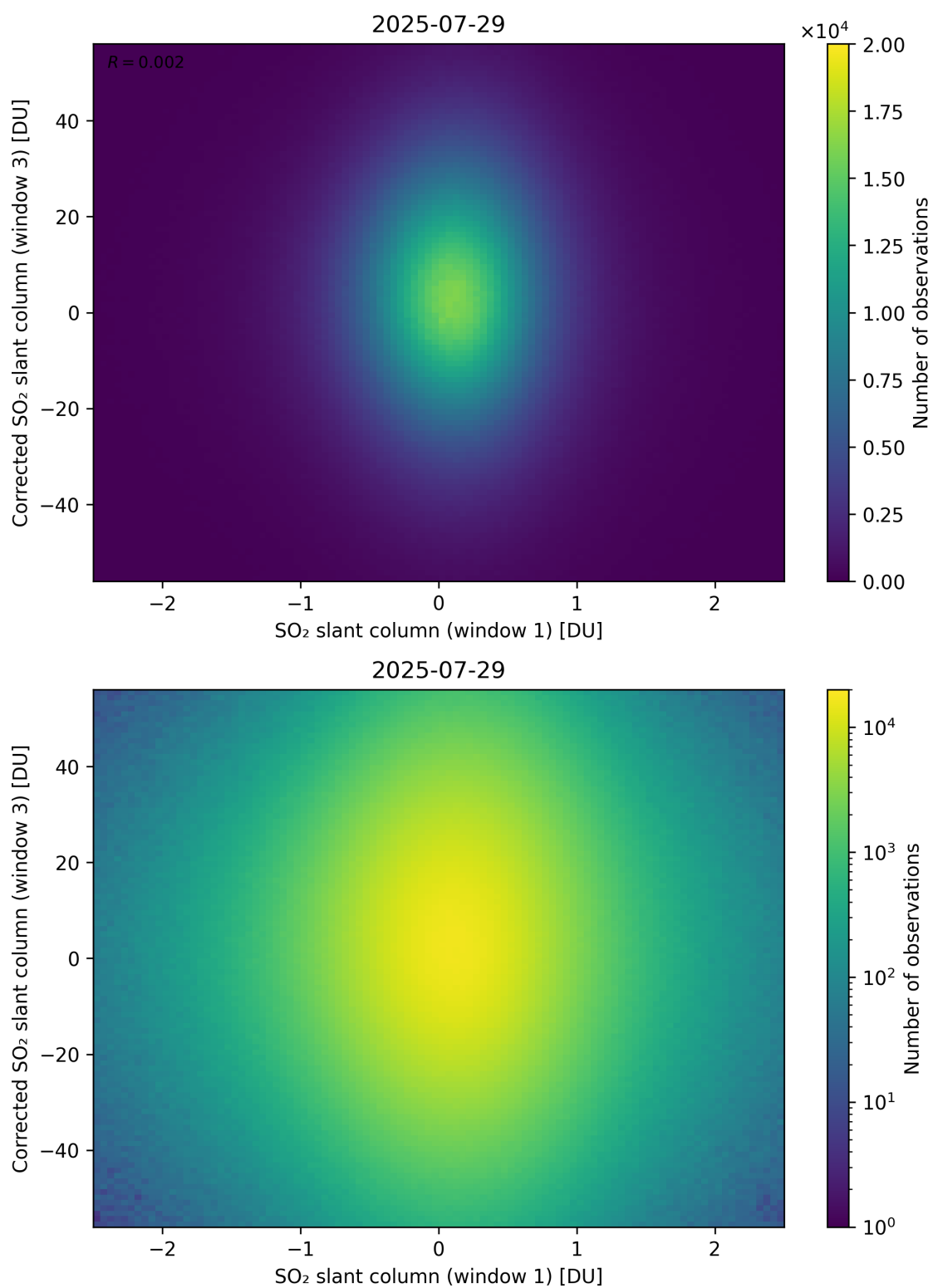
Figure 284: Scatter density plot of “SO 2 slant column (window 1)” against “Corrected SO 2 slant column (window 3)” for 2025-07-29 to 2025-07-30.
