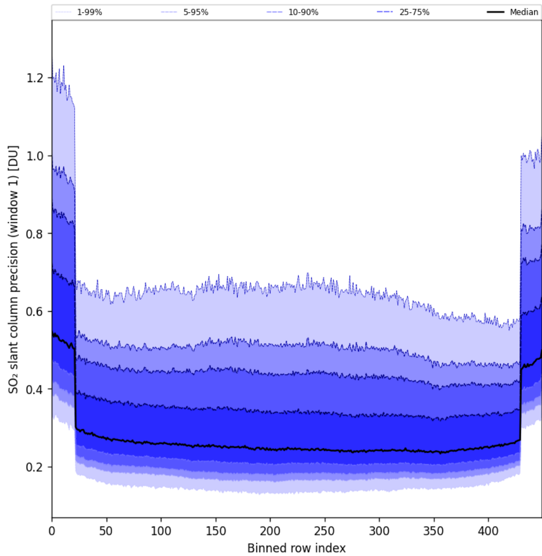
Figure 90: Along track statistics of “SO 2 slant column precision (window 1)” for 2025-07-29 to 2025-07-30
