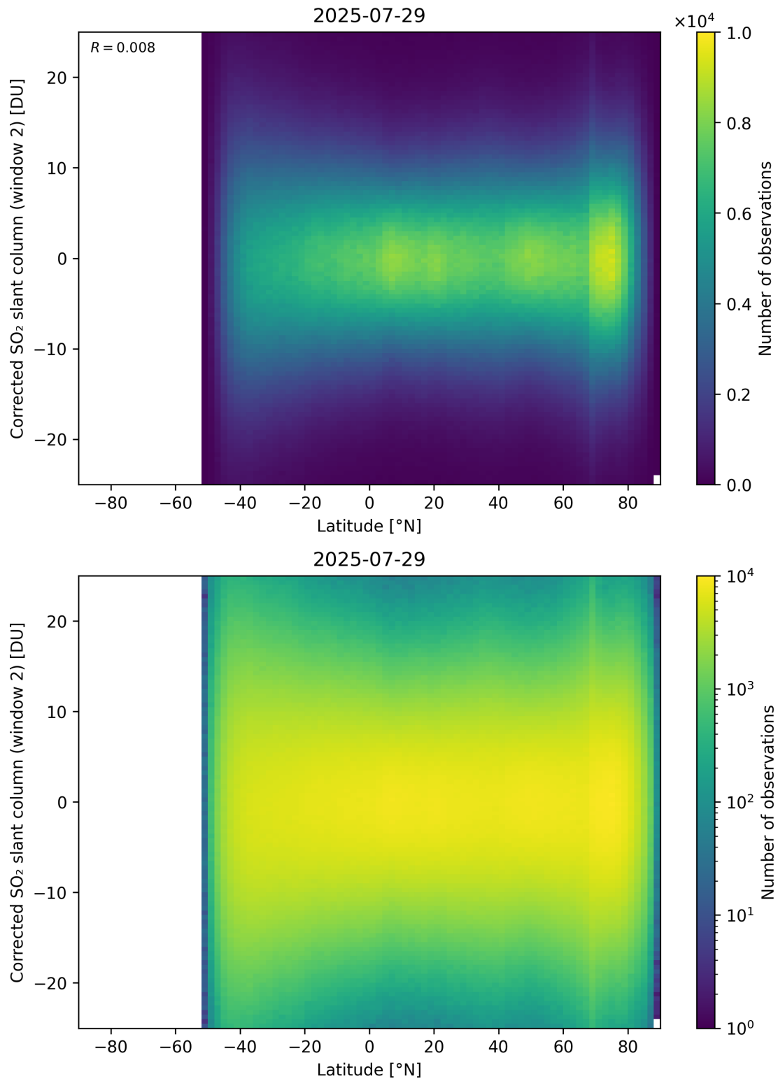
Figure 160: Scatter density plot of “Latitude” against “Corrected SO 2 slant column (window 2)” for 2025-07-29 to 2025-07-30.
