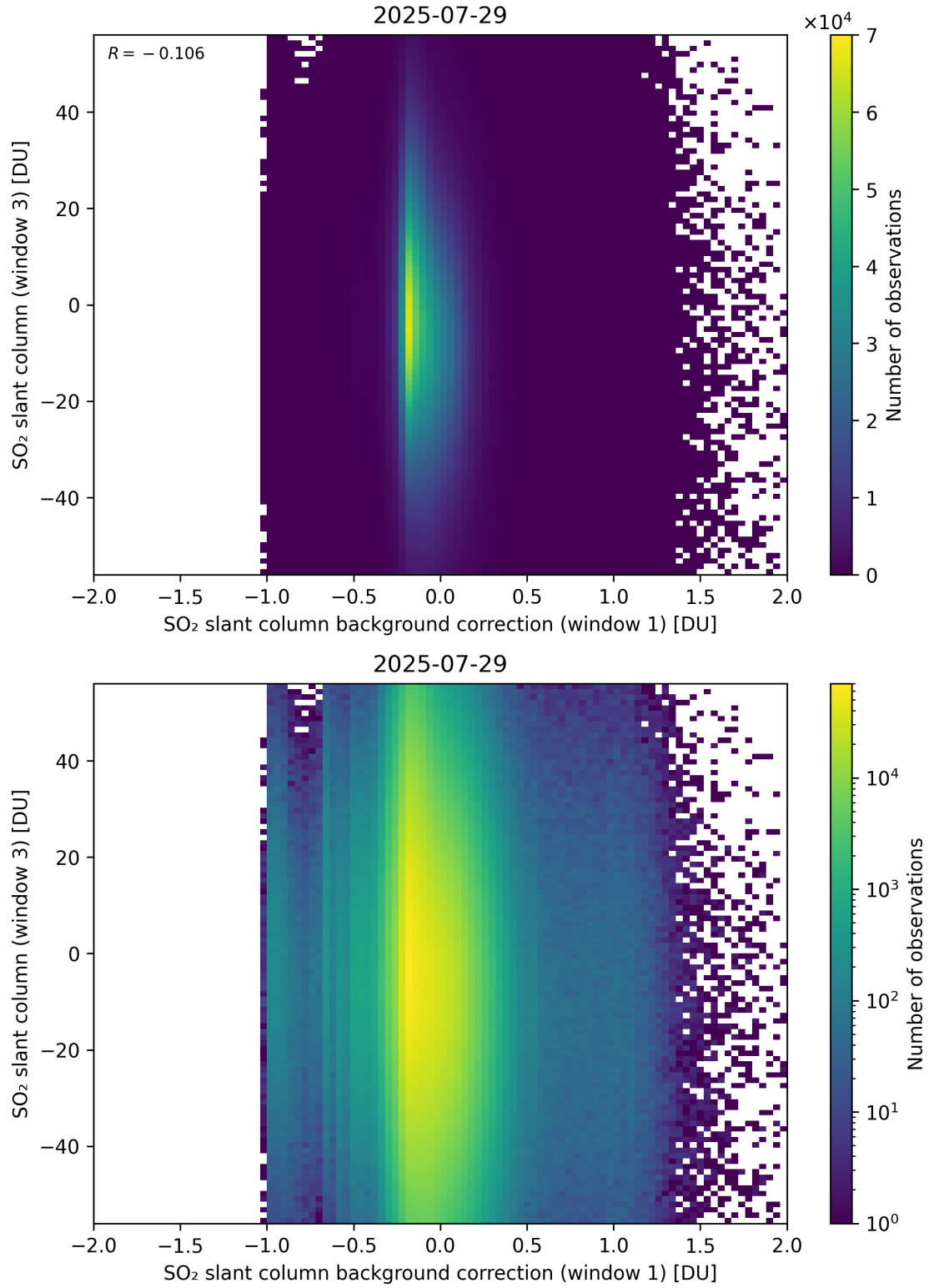
Figure 118: Scatter density plot of “SO 2 slant column background correction (window 1)” against “SO 2 slant column (window 3)” for 2025-07-29 to 2025-07-30.
