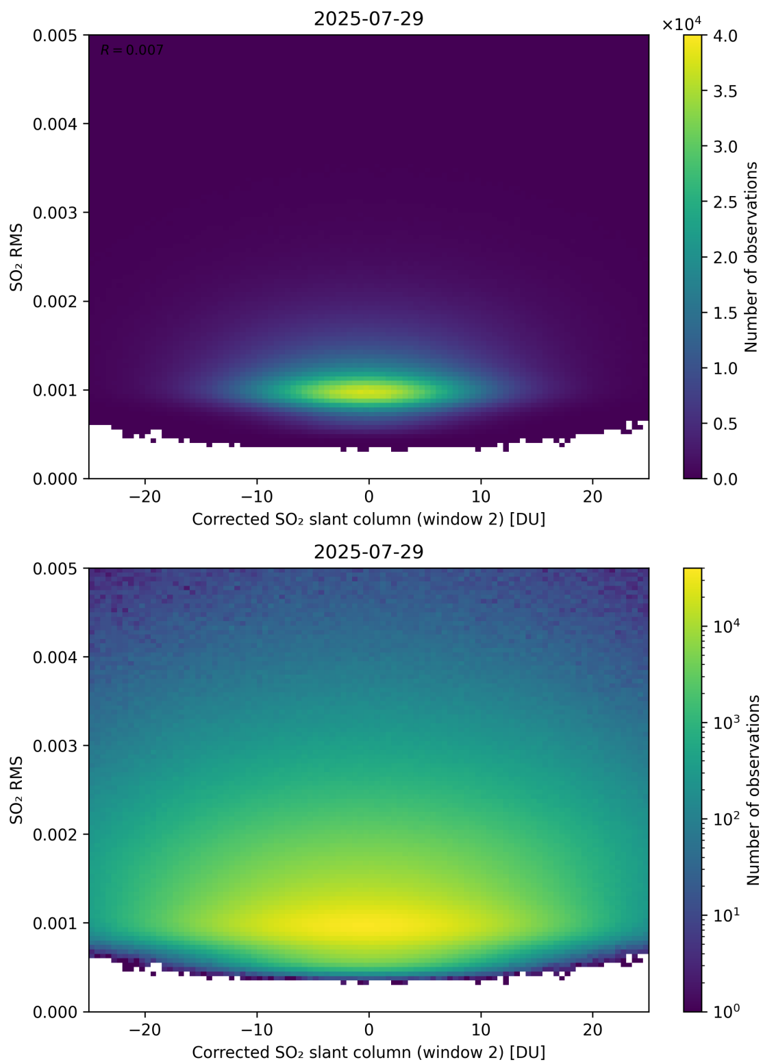
Figure 248: Scatter density plot of “Corrected SO 2 slant column (window 2)” against “SO 2 RMS” for 2025-07-29 to 2025-07-30.
