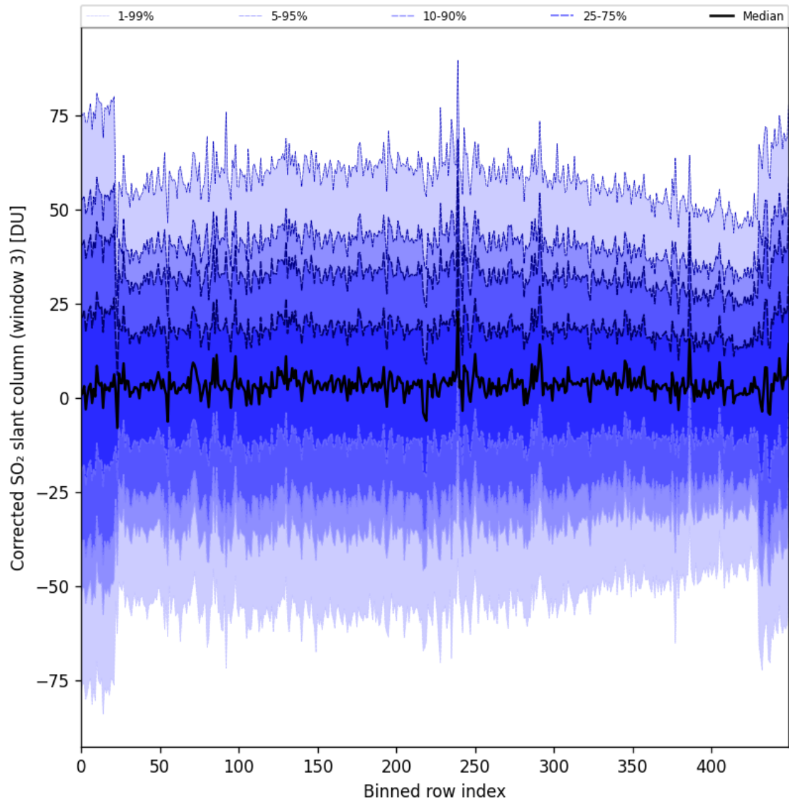
Figure 99: Along track statistics of “Corrected SO 2 slant column (window 3)” for 2025-07-29 to 2025-07-30
