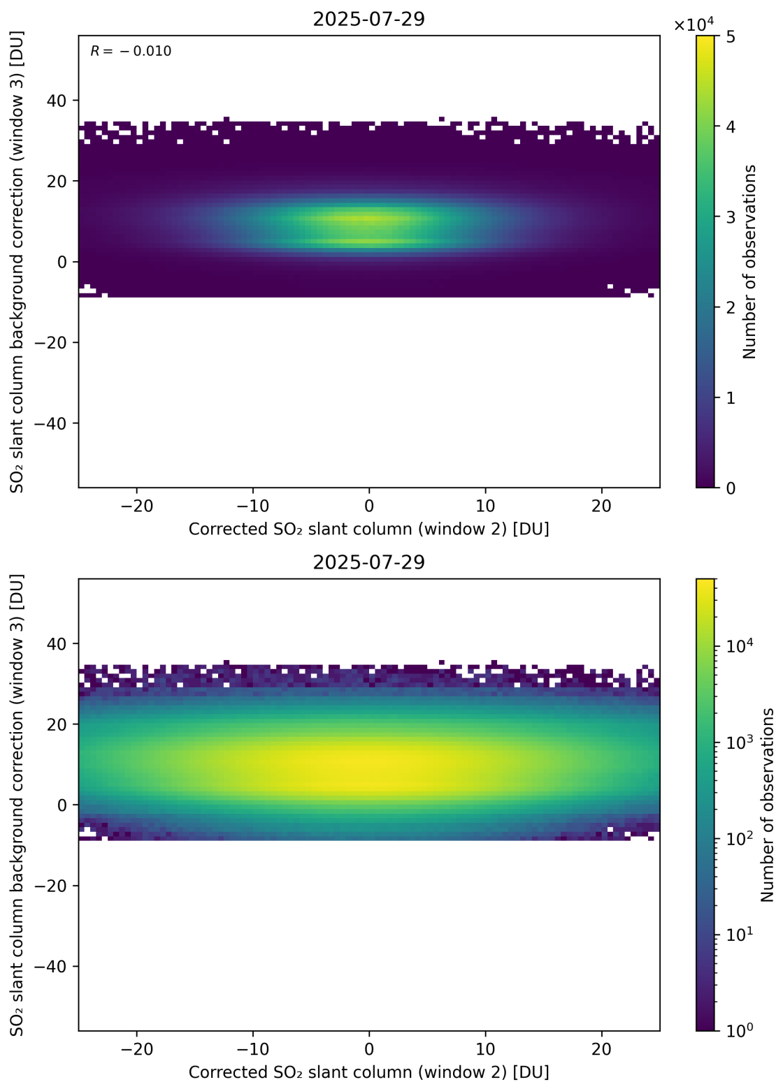
Figure 245: Scatter density plot of “Corrected SO 2 slant column (window 2)” against “SO 2 slant column background correction (window 3)” for 2025-07-29 to 2025-07-30.
