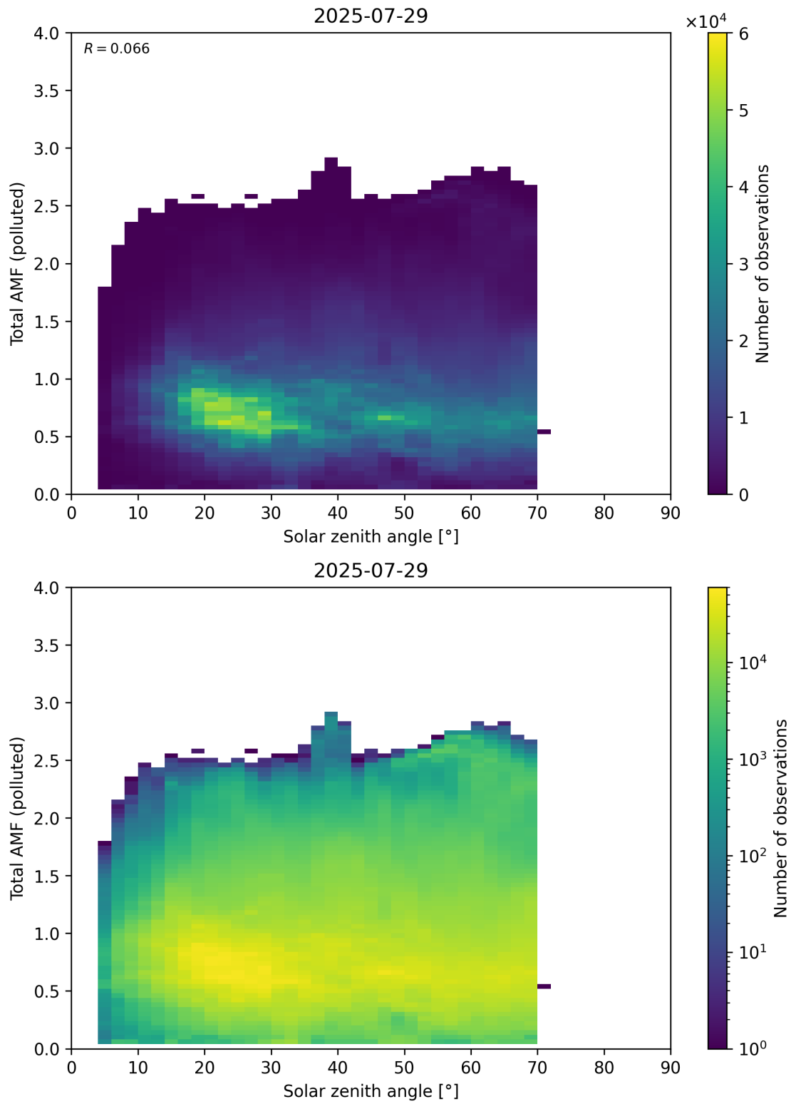
Figure 189: Scatter density plot of “Solar zenith angle” against “Total AMF (polluted)” for 2025-07-29 to 2025-07-30.
