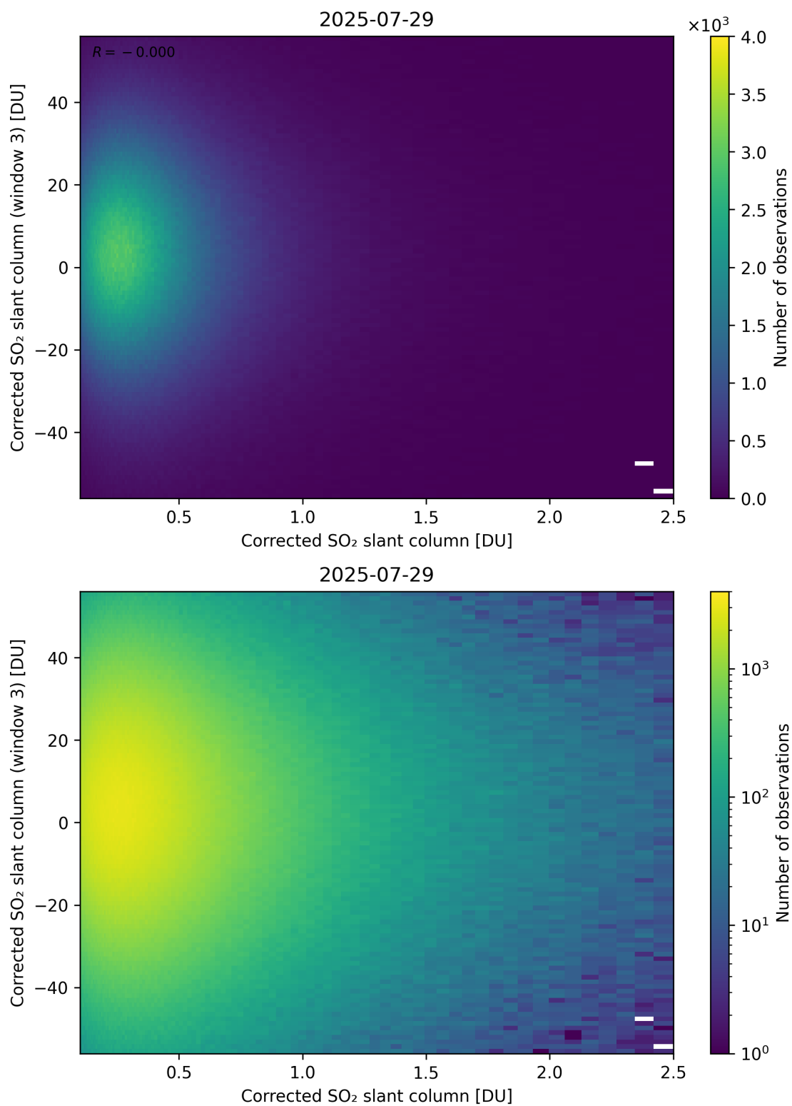
Figure 236: Scatter density plot of “Corrected SO 2 slant column” against “Corrected SO 2 slant column (window 3)” for 2025-07-29 to 2025-07-30.
