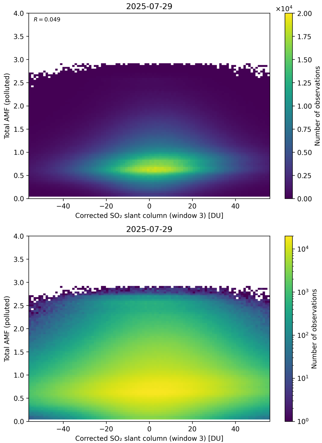
Figure 260: Scatter density plot of “Corrected SO 2 slant column (window 3)” against “Total AMF (polluted)” for 2025-07-29 to 2025-07-30.
