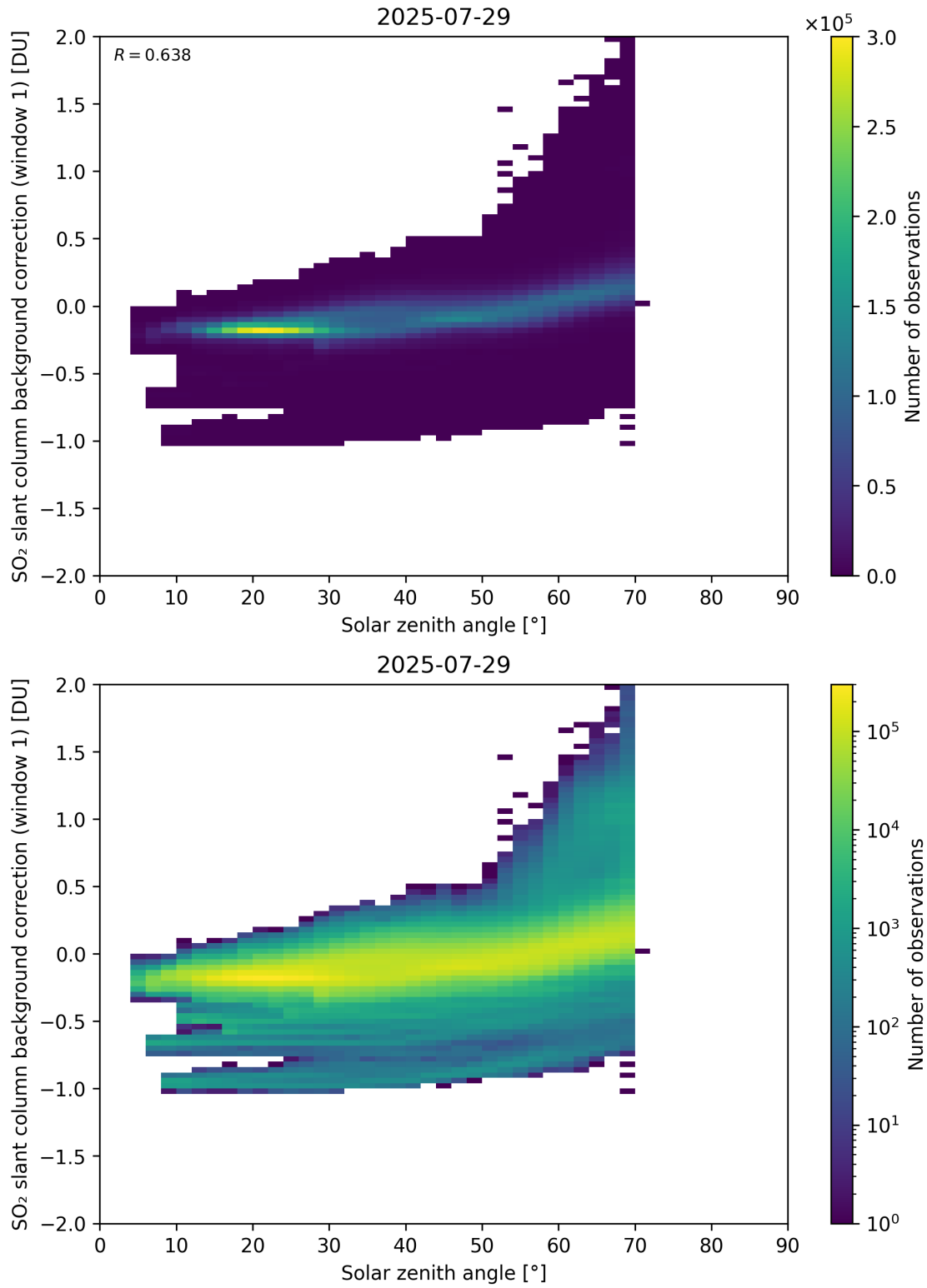
Figure 171: Scatter density plot of “Solar zenith angle” against “SO 2 slant column background correction (window 1)” for 2025-07-29 to 2025-07-30.
