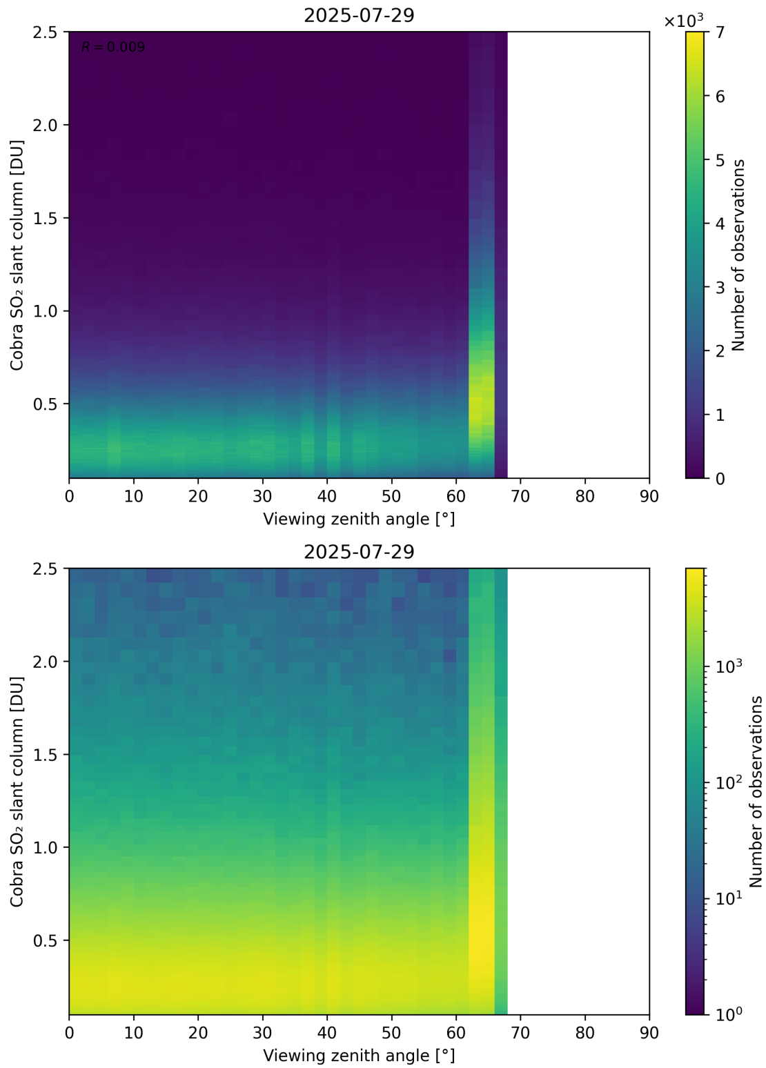
Figure 371: Scatter density plot of “Viewing zenith angle” against “Cobra SO 2 slant column” for 2025-07-29 to 2025-07-30.
