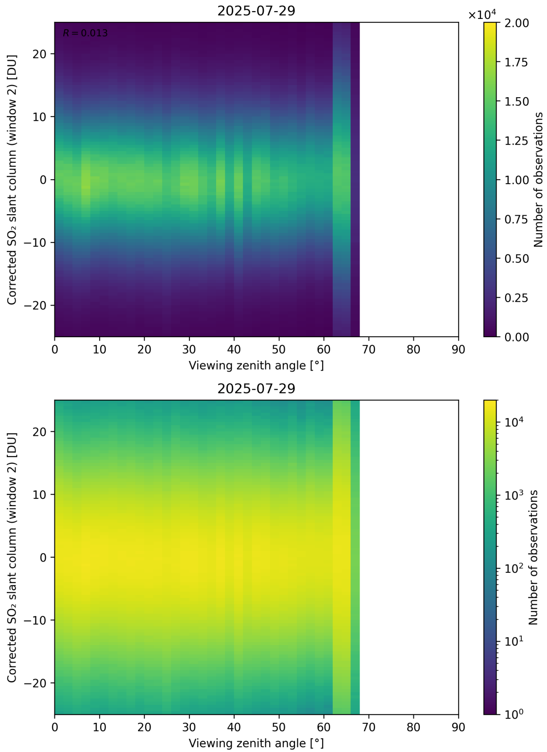
Figure 374: Scatter density plot of “Viewing zenith angle” against “Corrected SO 2 slant column (window 2)” for 2025-07-29 to 2025-07-30.
