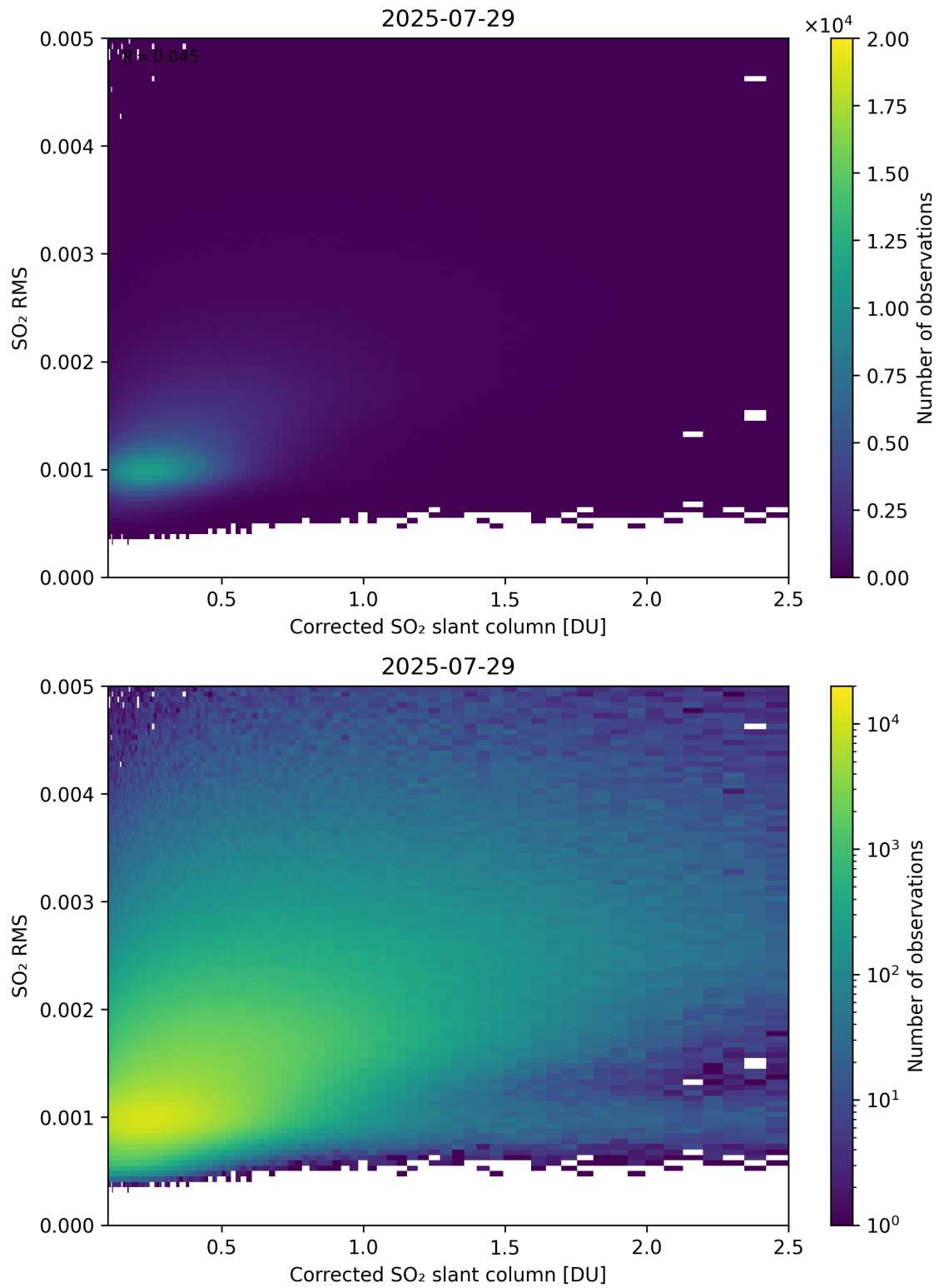
Figure 231: Scatter density plot of “Corrected SO 2 slant column” against “SO 2 RMS” for 2025-07-29 to 2025-07-30.
