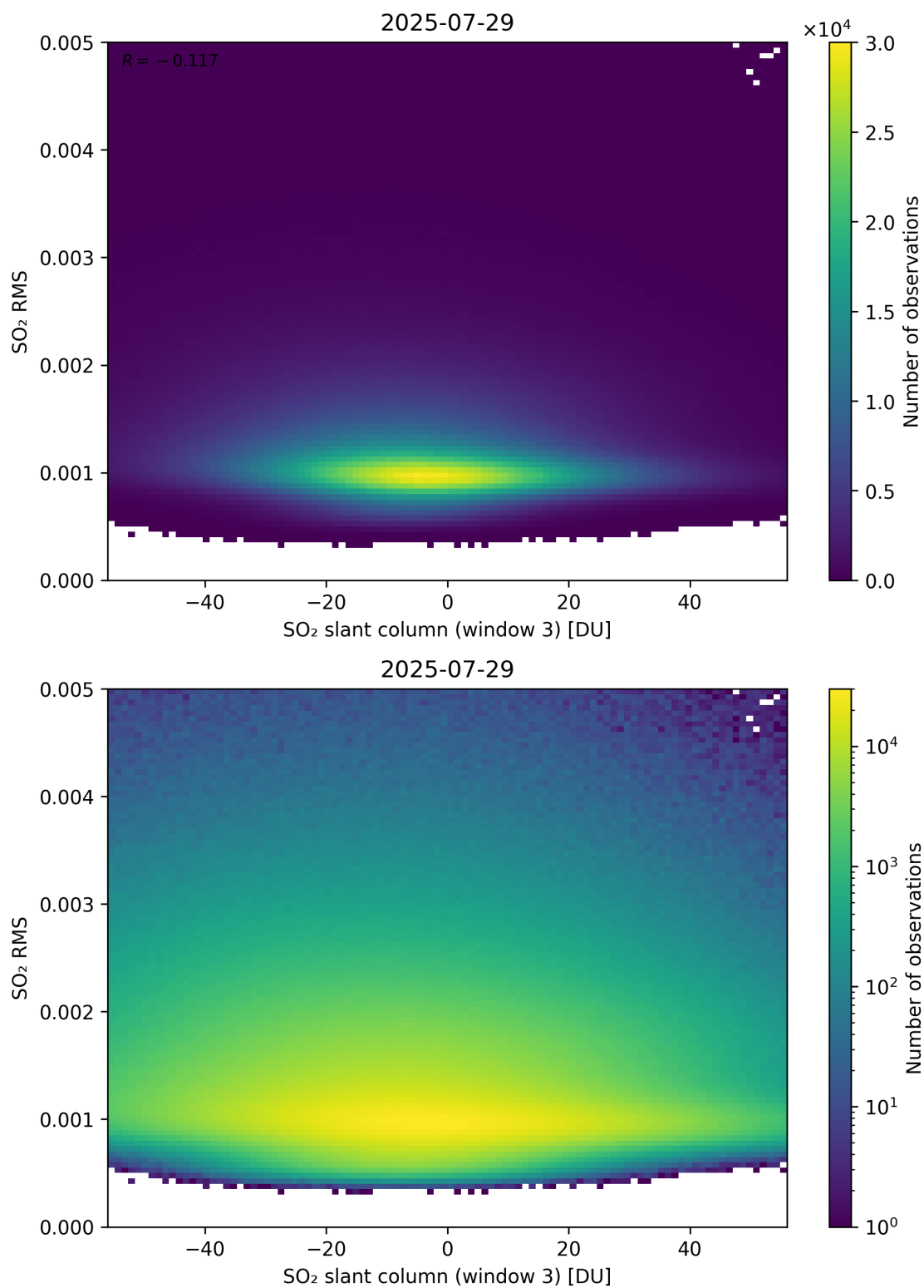
Figure 306: Scatter density plot of “SO 2 slant column (window 3)” against “SO 2 RMS” for 2025-07-29 to 2025-07-30.
