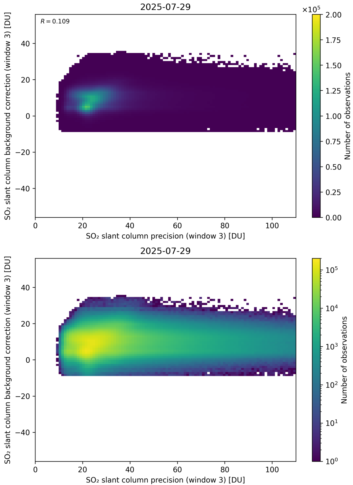
Figure 307: Scatter density plot of “SO 2 slant column precision (window 3)” against “SO 2 slant column background correction (window 3)” for 2025-07-29 to 2025-07-30.
