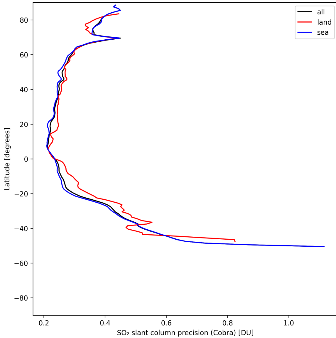
Figure 36: Zonal average of “SO 2 slant column precision (Cobra)” for 2025-07-29 to 2025-07-30.
