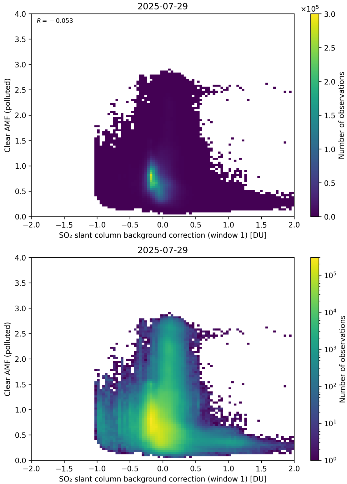
Figure 114: Scatter density plot of “SO 2 slant column background correction (window 1)” against “Clear AMF (polluted)” for 2025-07-29 to 2025-07-30.
