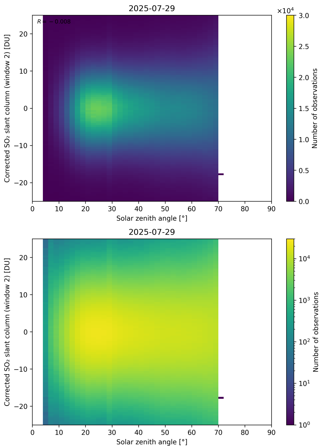
Figure 182: Scatter density plot of “Solar zenith angle” against “Corrected SO 2 slant column (window 2)” for 2025-07-29 to 2025-07-30.
