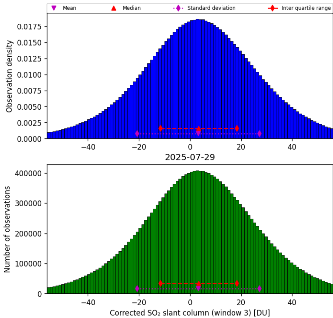
Figure 73: Histogram of “Corrected SO 2 slant column (window 3)” for 2025-07-29 to 2025-07-30
