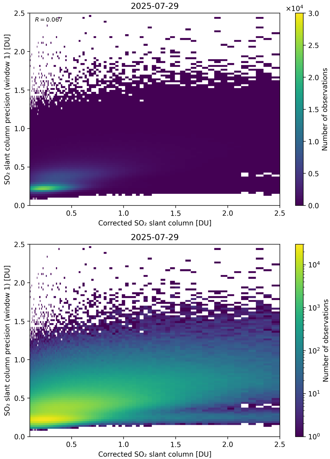
Figure 238: Scatter density plot of “Corrected SO 2 slant column” against “SO 2 slant column precision (window 1)” for 2025-07-29 to 2025-07-30.
