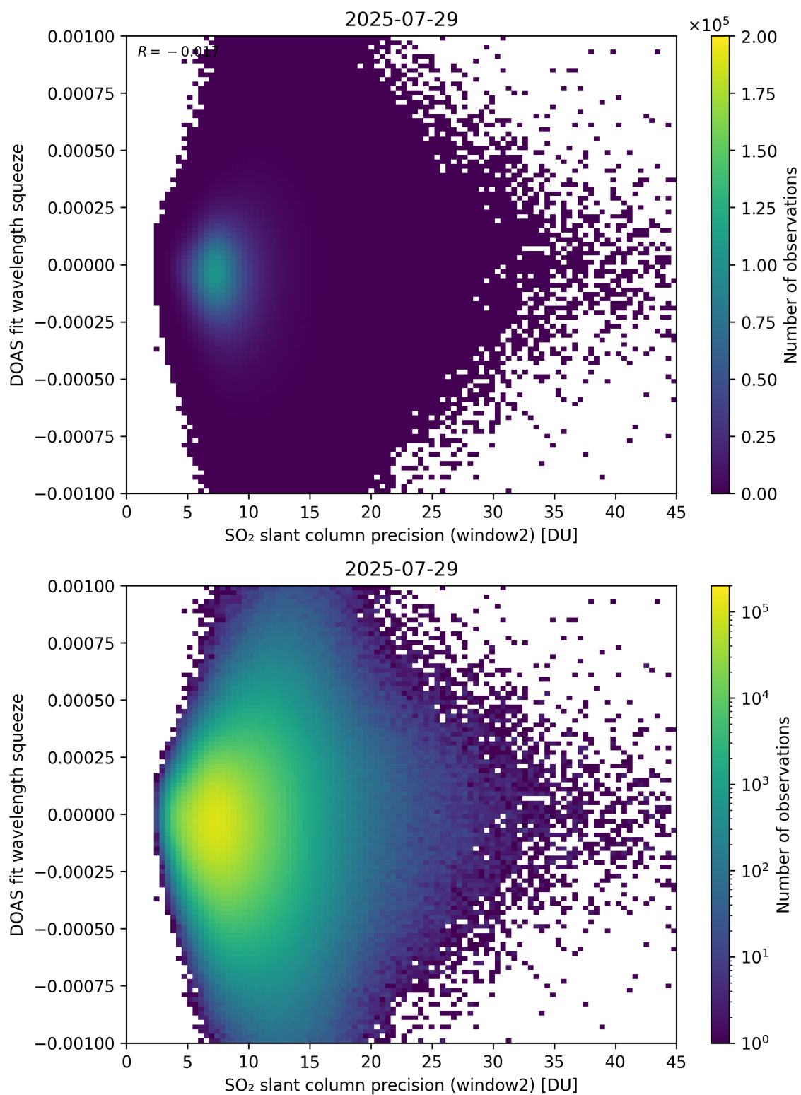
Figure 294: Scatter density plot of “SO 2 slant column precision (window2)” against “DOAS fit wavelength squeeze” for 2025-07-29 to 2025-07-30.
