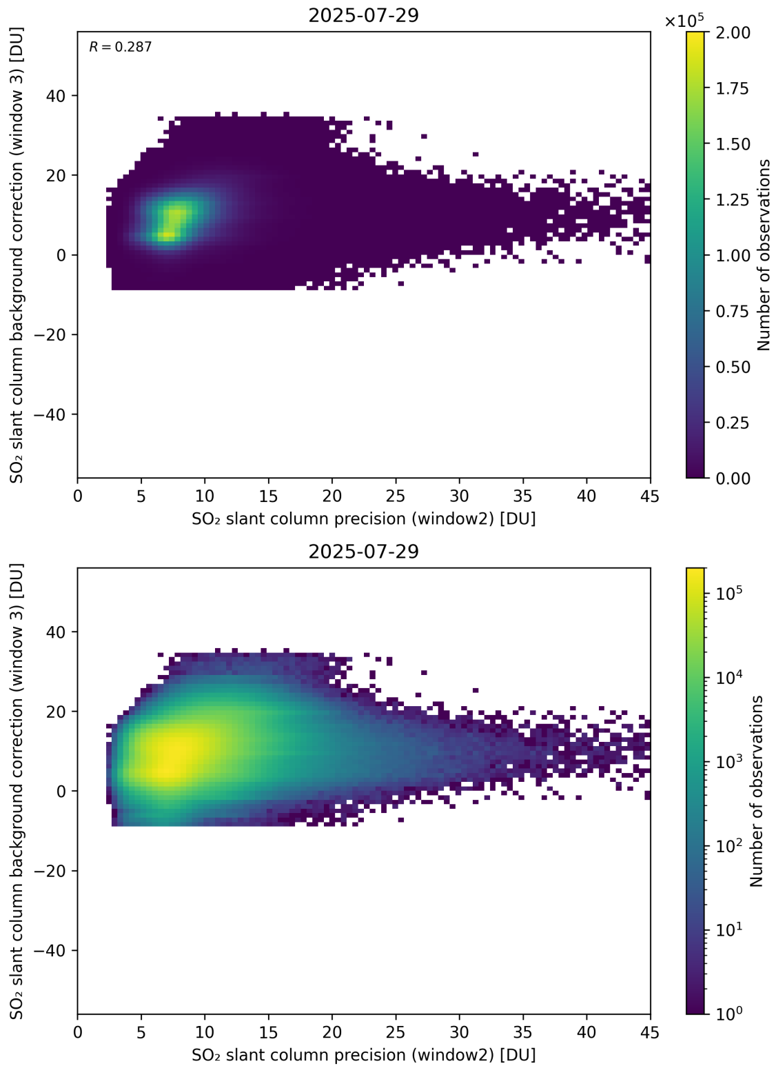
Figure 292: Scatter density plot of “SO 2 slant column precision (window2)” against “SO 2 slant column background correction (window 3)” for 2025-07-29 to 2025-07-30.
