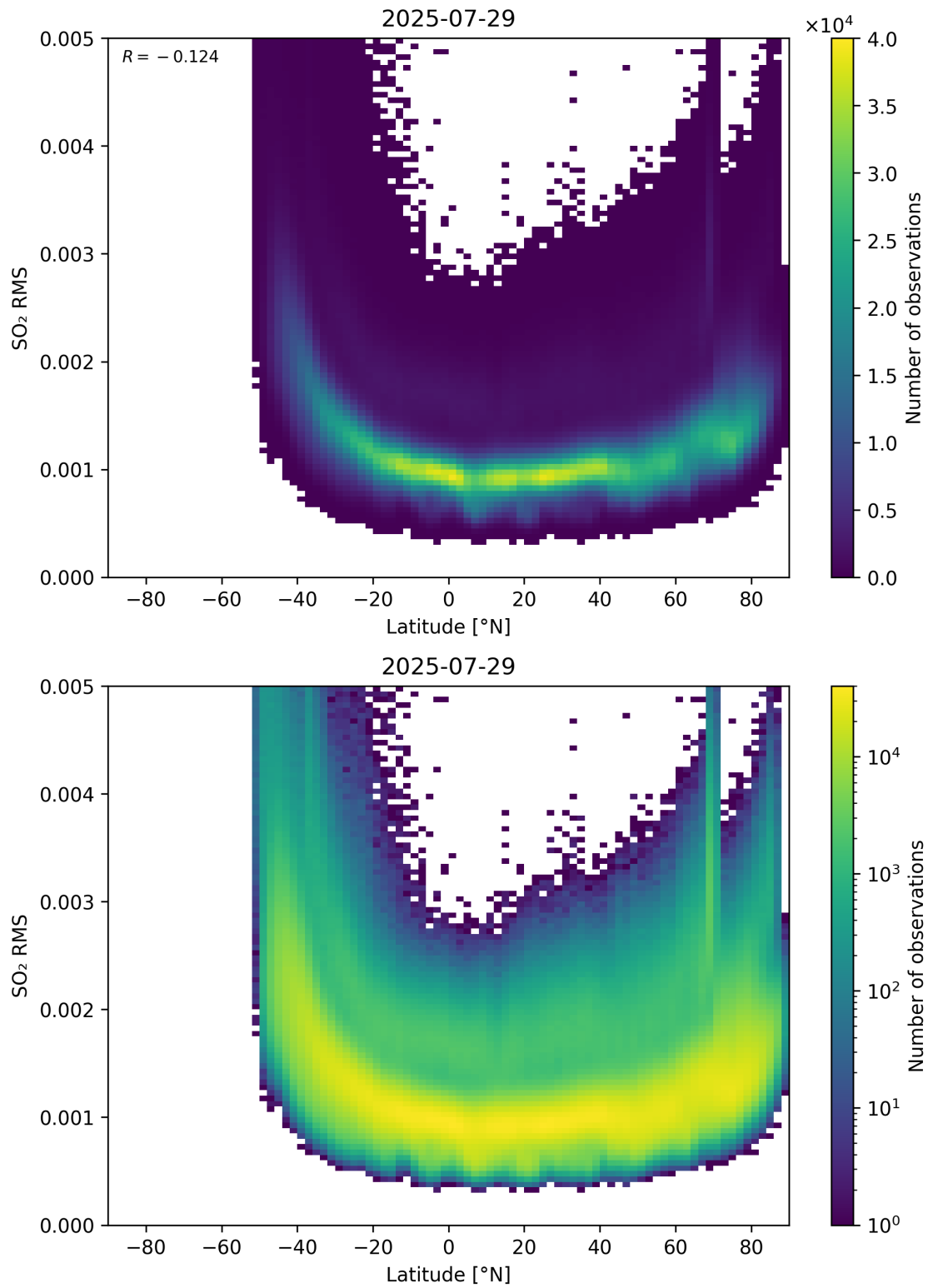
Figure 155: Scatter density plot of “Latitude” against “SO 2 RMS” for 2025-07-29 to 2025-07-30.
