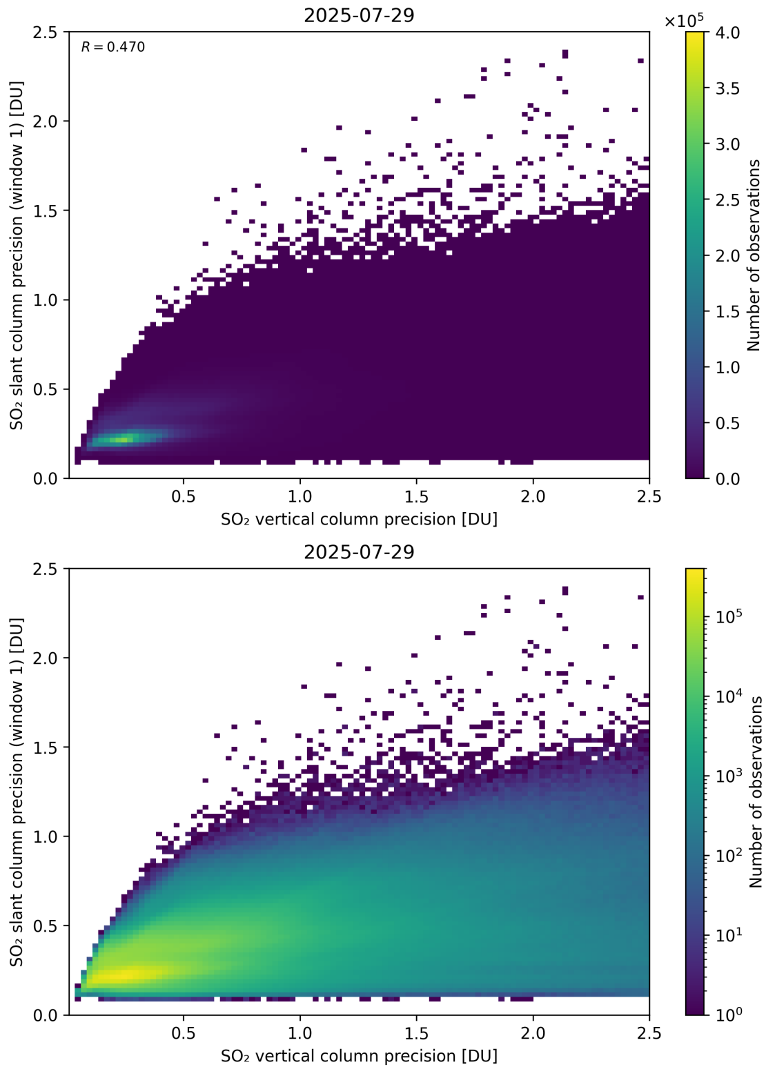
Figure 342: Scatter density plot of “SO 2 vertical column precision” against “SO 2 slant column precision (window 1)” for 2025-07-29 to 2025-07-30.
