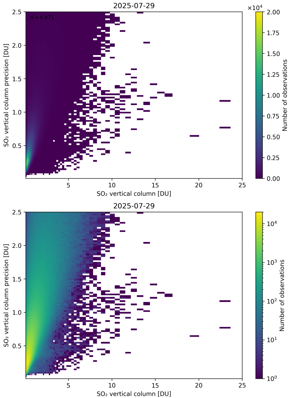
Figure 361: Scatter density plot of “SO 2 vertical column” against “SO 2 vertical column precision” for 2025-07-29 to 2025-07-30.
