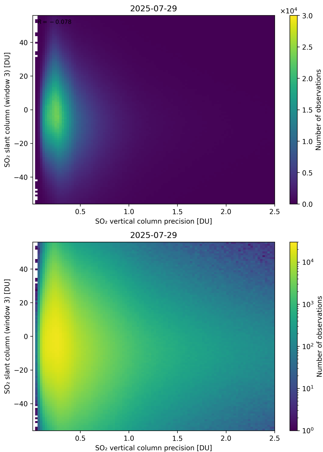
Figure 344: Scatter density plot of “SO 2 vertical column precision” against “SO 2 slant column (window 3)” for 2025-07-29 to 2025-07-30.
