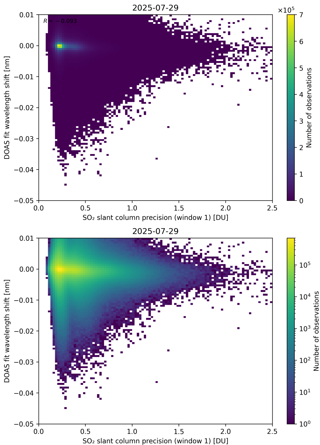
Figure 271: Scatter density plot of “SO 2 slant column precision (window 1)” against “DOAS fit wavelength shift” for 2025-07-29 to 2025-07-30.
