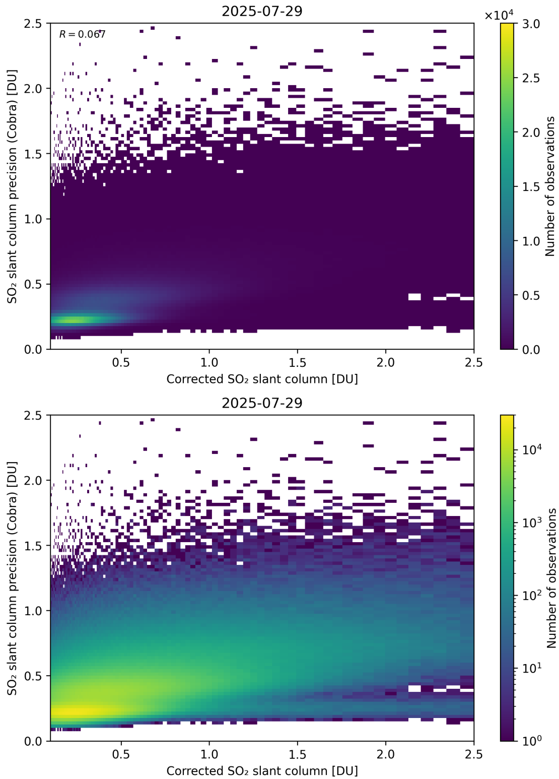
Figure 234: Scatter density plot of “Corrected SO 2 slant column” against “SO 2 slant column precision (Cobra)” for 2025-07-29 to 2025-07-30.
