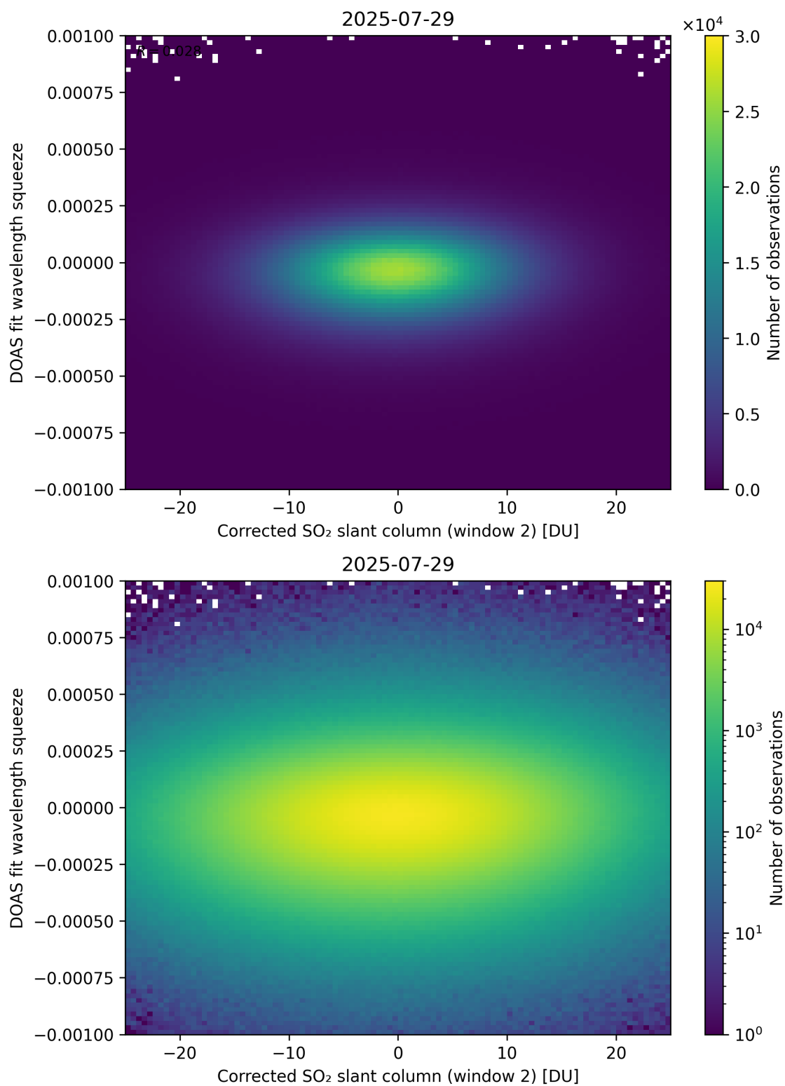
Figure 247: Scatter density plot of “Corrected SO 2 slant column (window 2)” against “DOAS fit wavelength squeeze” for 2025-07-29 to 2025-07-30.
