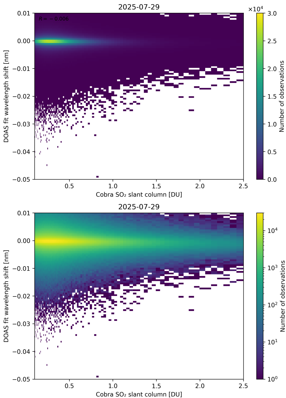
Figure 196: Scatter density plot of “Cobra SO 2 slant column” against “DOAS fit wavelength shift” for 2025-07-29 to 2025-07-30.
