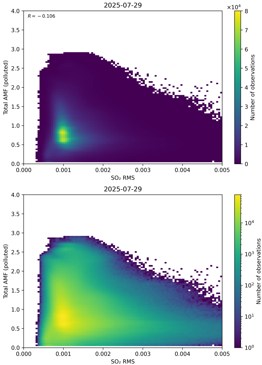
Figure 148: Scatter density plot of “SO 2 RMS” against “Total AMF (polluted)” for 2025-07-29 to 2025-07-30.
