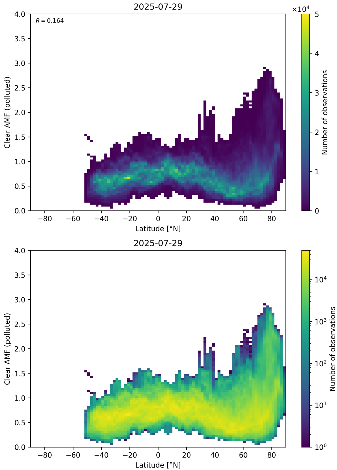
Figure 156: Scatter density plot of “Latitude” against “Clear AMF (polluted)” for 2025-07-29 to 2025-07-30.
