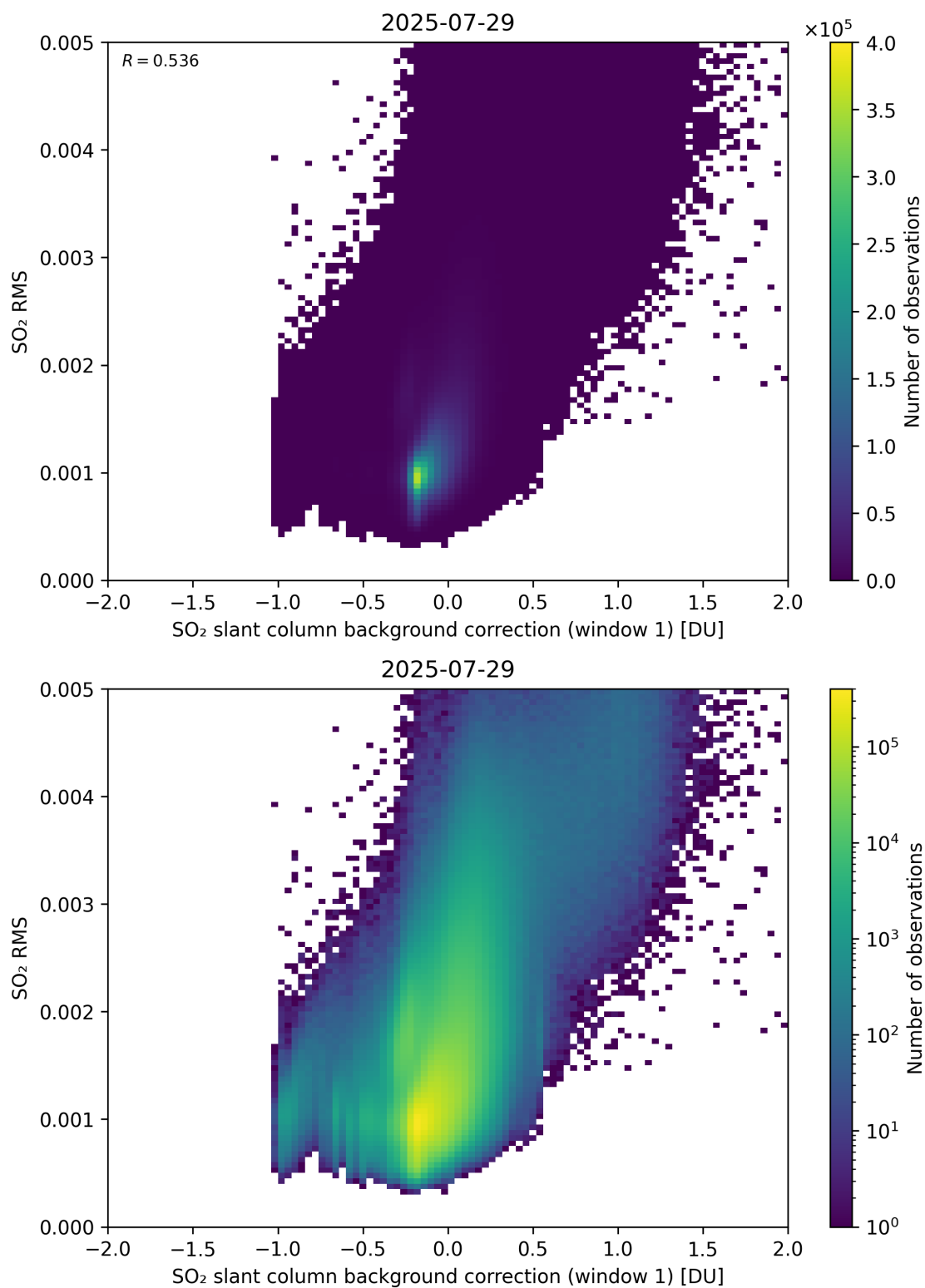
Figure 113: Scatter density plot of “SO 2 slant column background correction (window 1)” against “SO 2 RMS” for 2025-07-29 to 2025-07-30.
