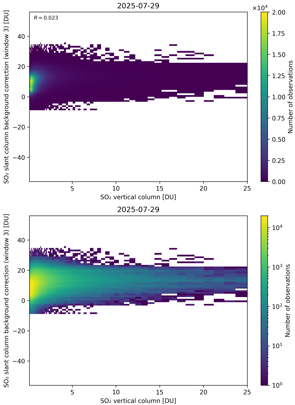
Figure 325: Scatter density plot of “SO 2 vertical column” against “SO 2 slant column background correction (window 3)” for 2025-07-29 to 2025-07-30.
