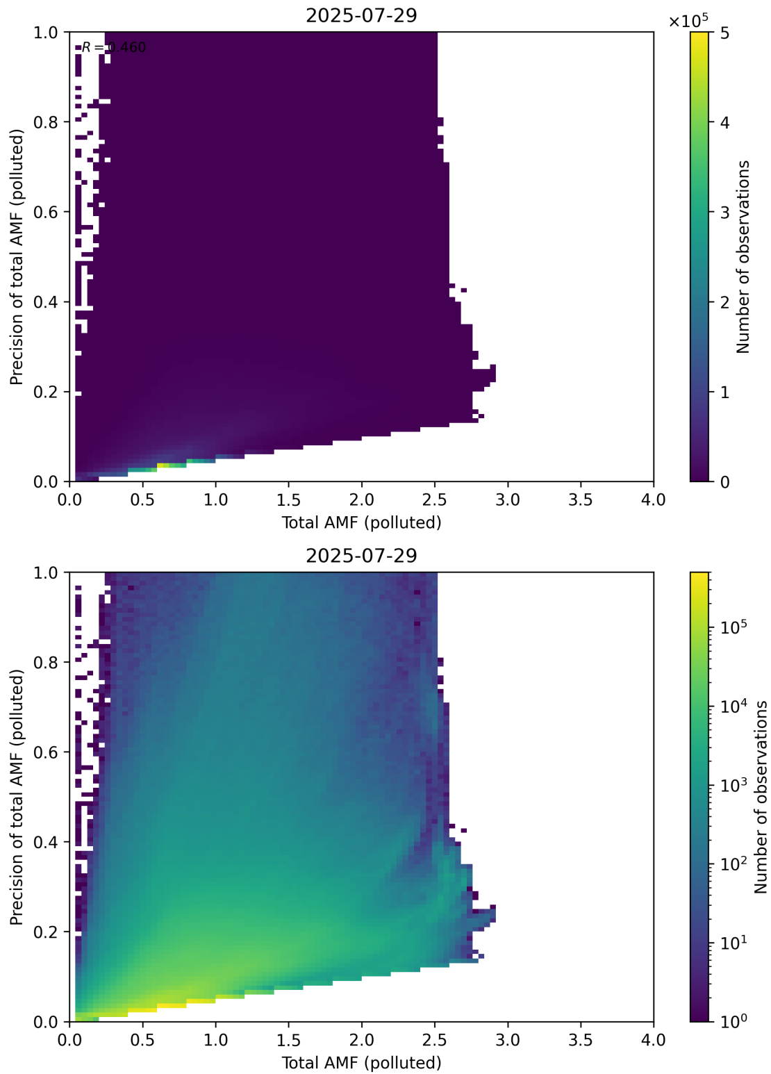
Figure 322: Scatter density plot of “Total AMF (polluted)” against “Precision of total AMF (polluted)” for 2025-07-29 to 2025-07-30.
