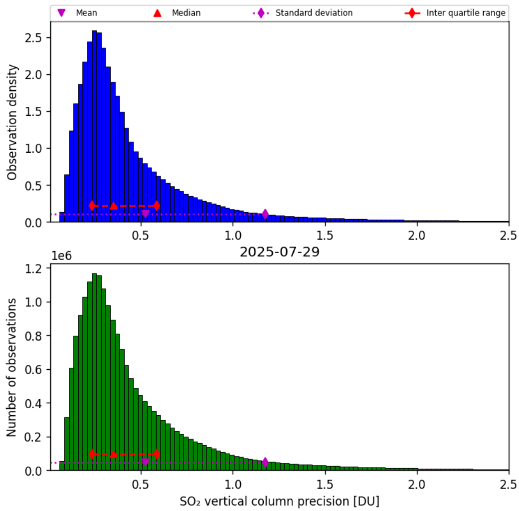
Figure 59: Histogram of “SO 2 vertical column precision” for 2025-07-29 to 2025-07-30
