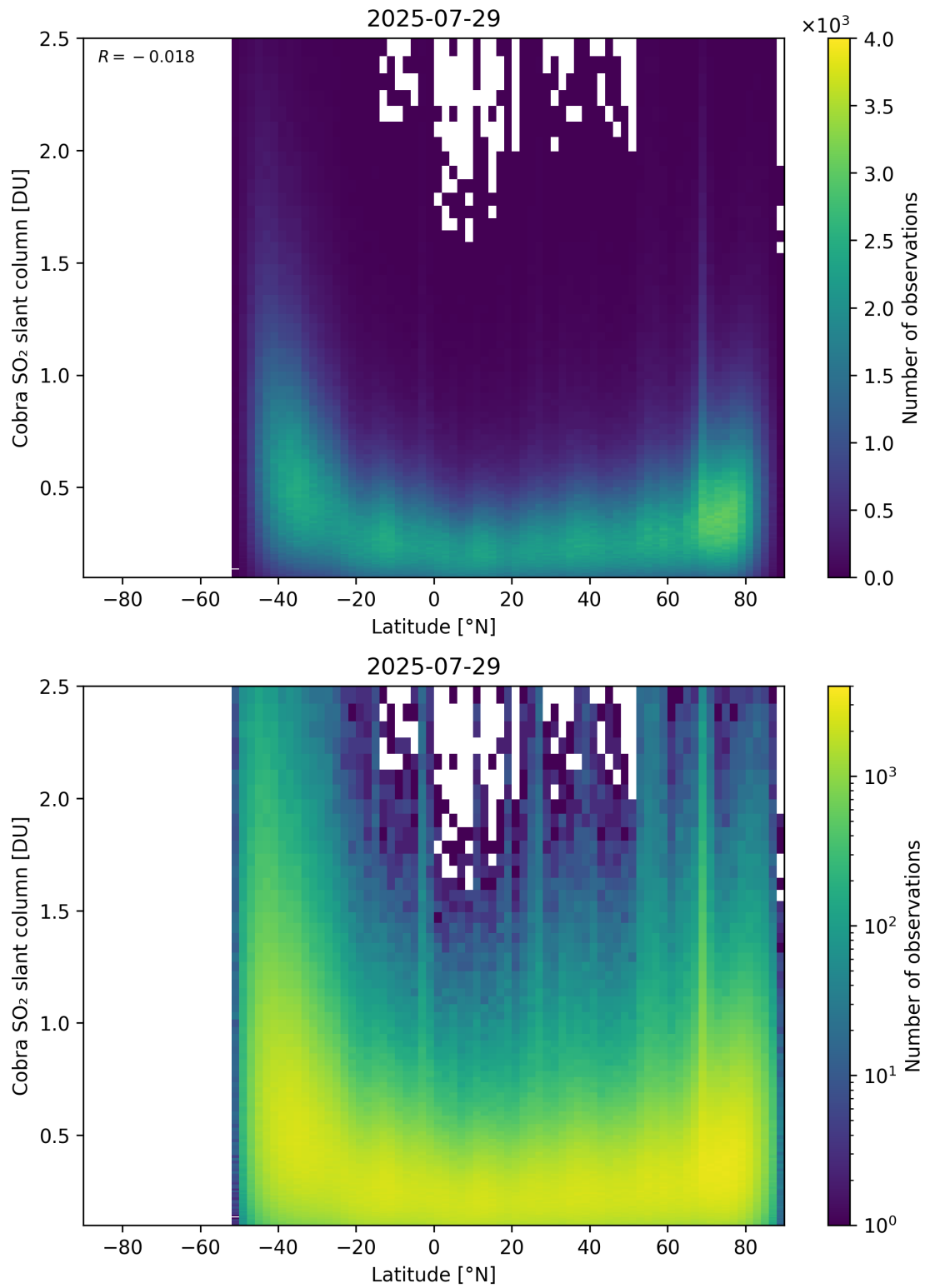
Figure 157: Scatter density plot of “Latitude” against “Cobra SO 2 slant column” for 2025-07-29 to 2025-07-30.
