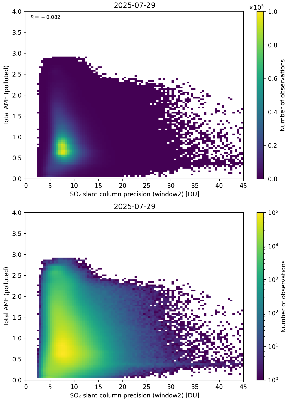
Figure 301: Scatter density plot of “SO 2 slant column precision (window2)” against “Total AMF (polluted)” for 2025-07-29 to 2025-07-30.
