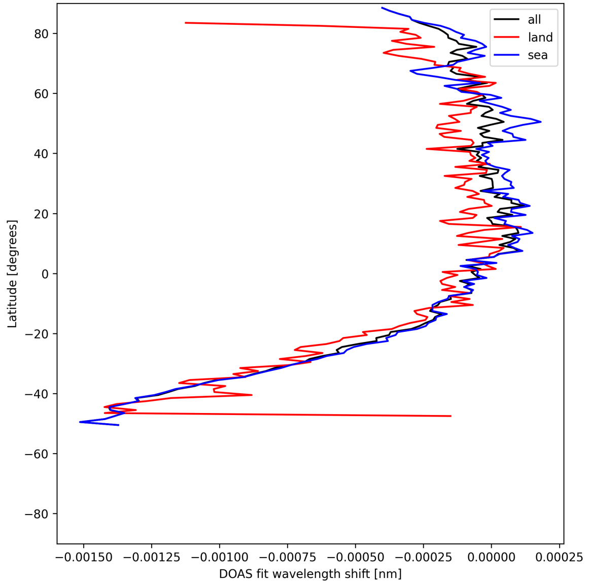
Figure 50: Zonal average of “DOAS fit wavelength shift” for 2025-07-29 to 2025-07-30.
