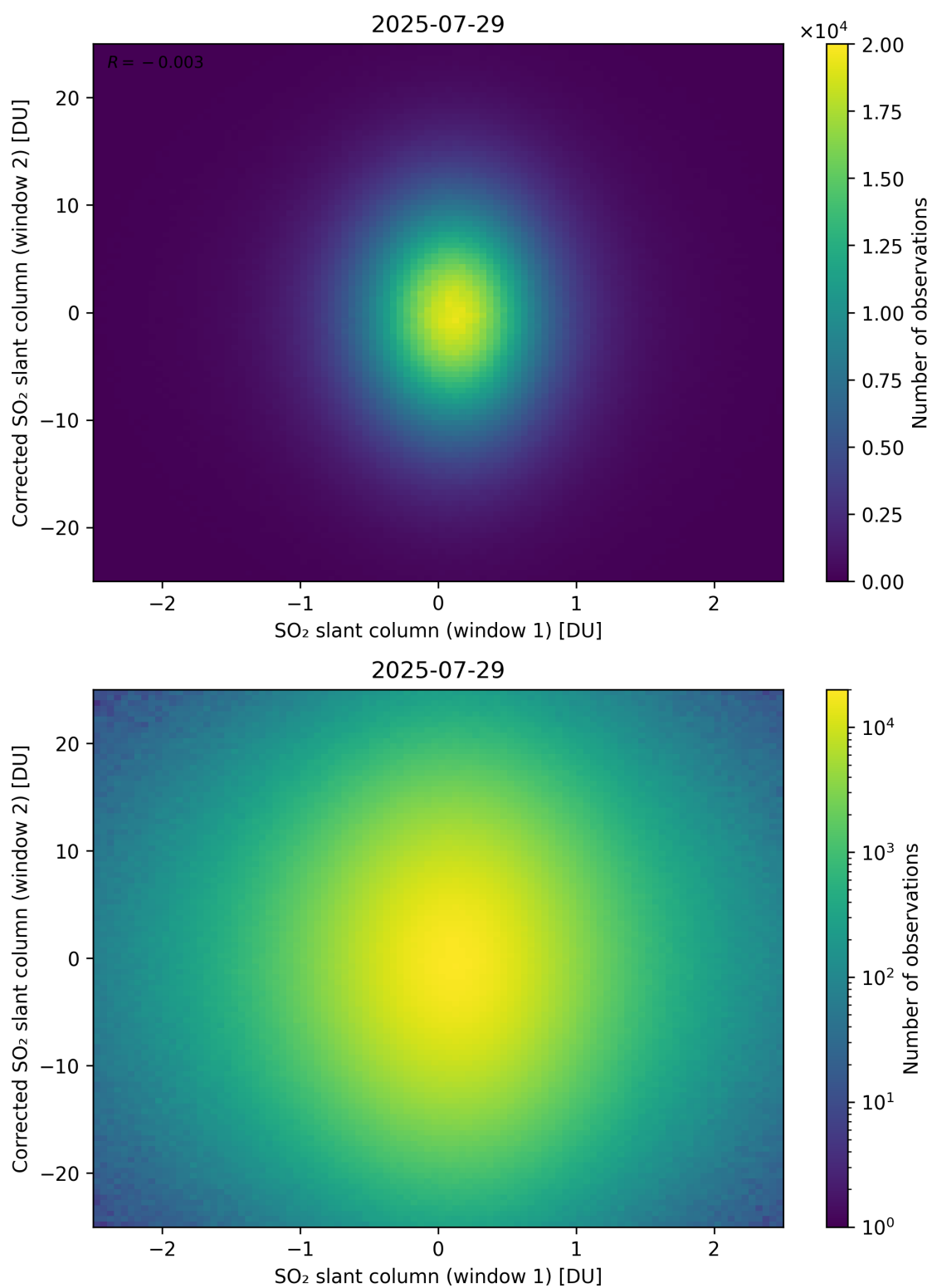
Figure 283: Scatter density plot of “SO 2 slant column (window 1)” against “Corrected SO 2 slant column (window 2)” for 2025-07-29 to 2025-07-30.
