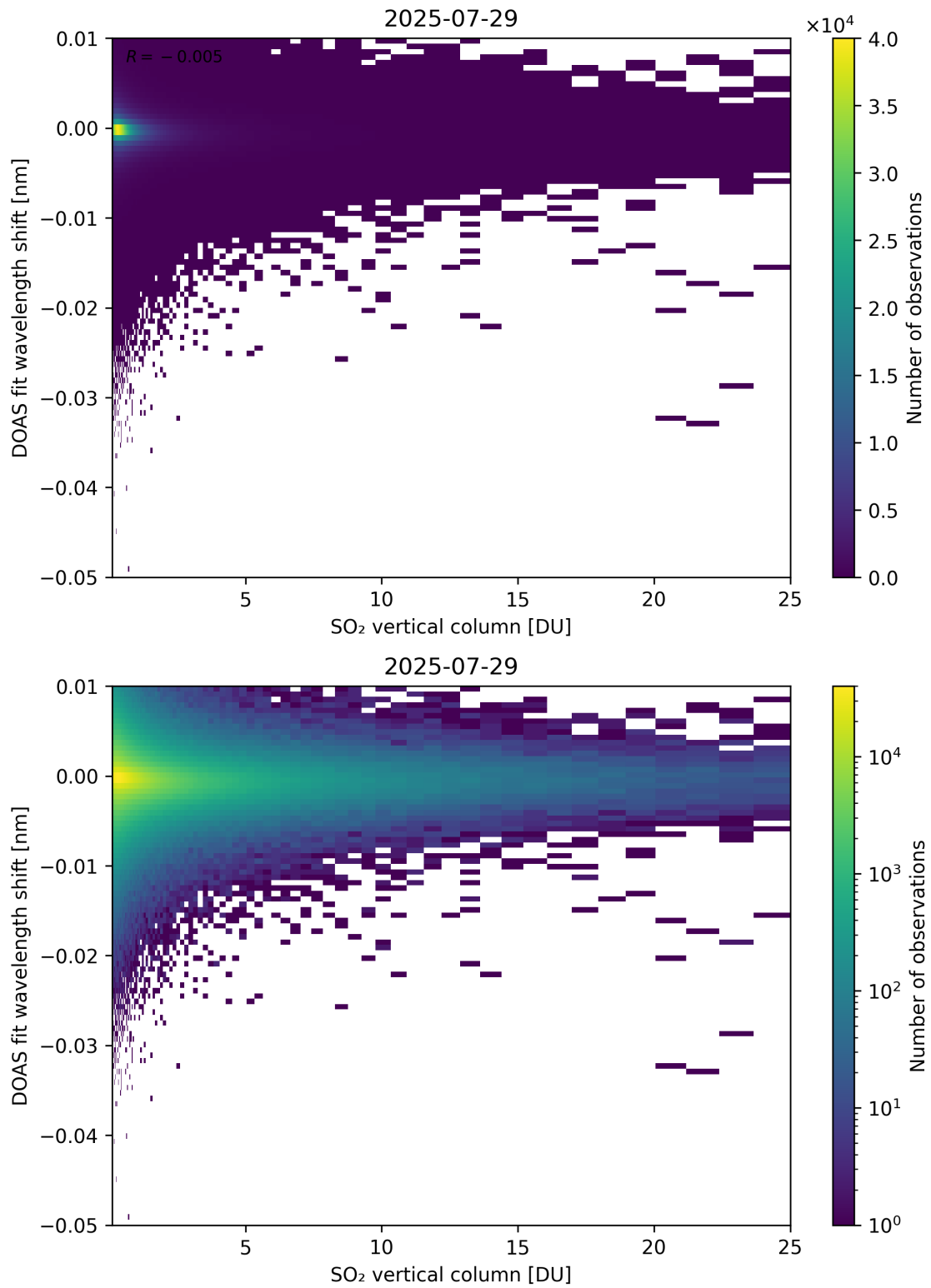
Figure 326: Scatter density plot of “SO 2 vertical column” against “DOAS fit wavelength shift” for 2025-07-29 to 2025-07-30.
