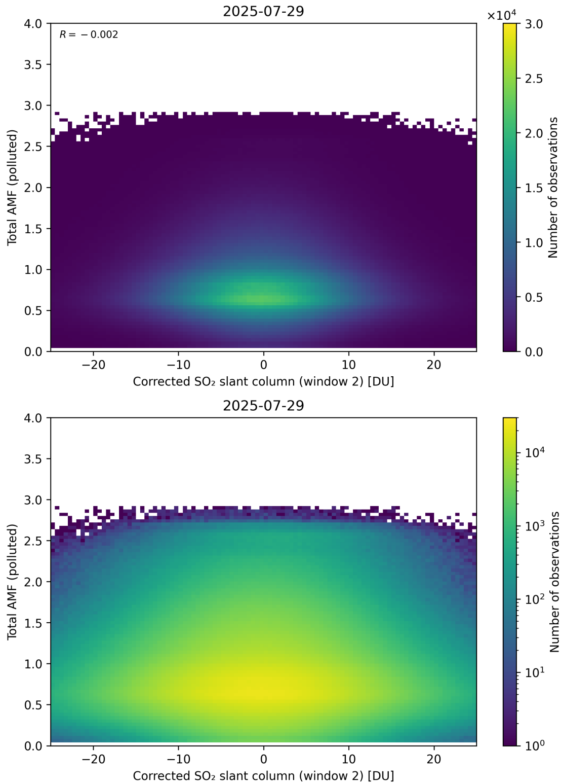
Figure 253: Scatter density plot of “Corrected SO 2 slant column (window 2)” against “Total AMF (polluted)” for 2025-07-29 to 2025-07-30.
