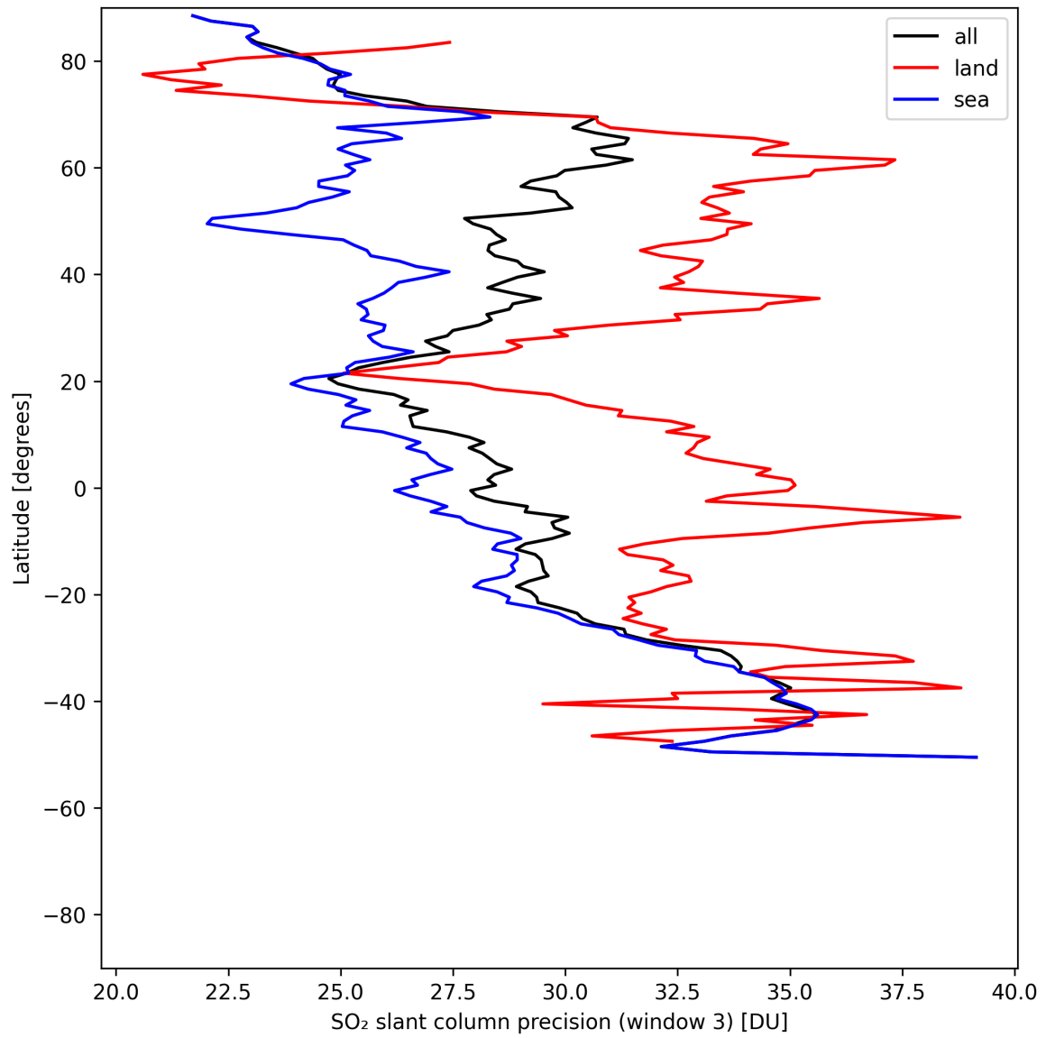
Figure 46: Zonal average of “SO 2 slant column precision (window 3)” for 2025-07-29 to 2025-07-30.
