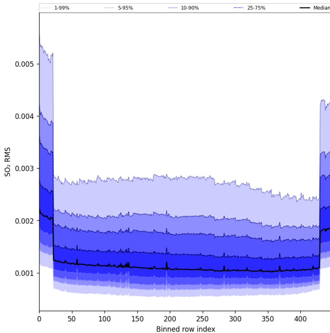
Figure 104: Along track statistics of “SO 2 RMS” for 2025-07-29 to 2025-07-30
