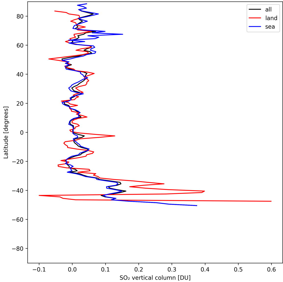
Figure 32: Zonal average of “SO 2 vertical column” for 2025-07-29 to 2025-07-30.
