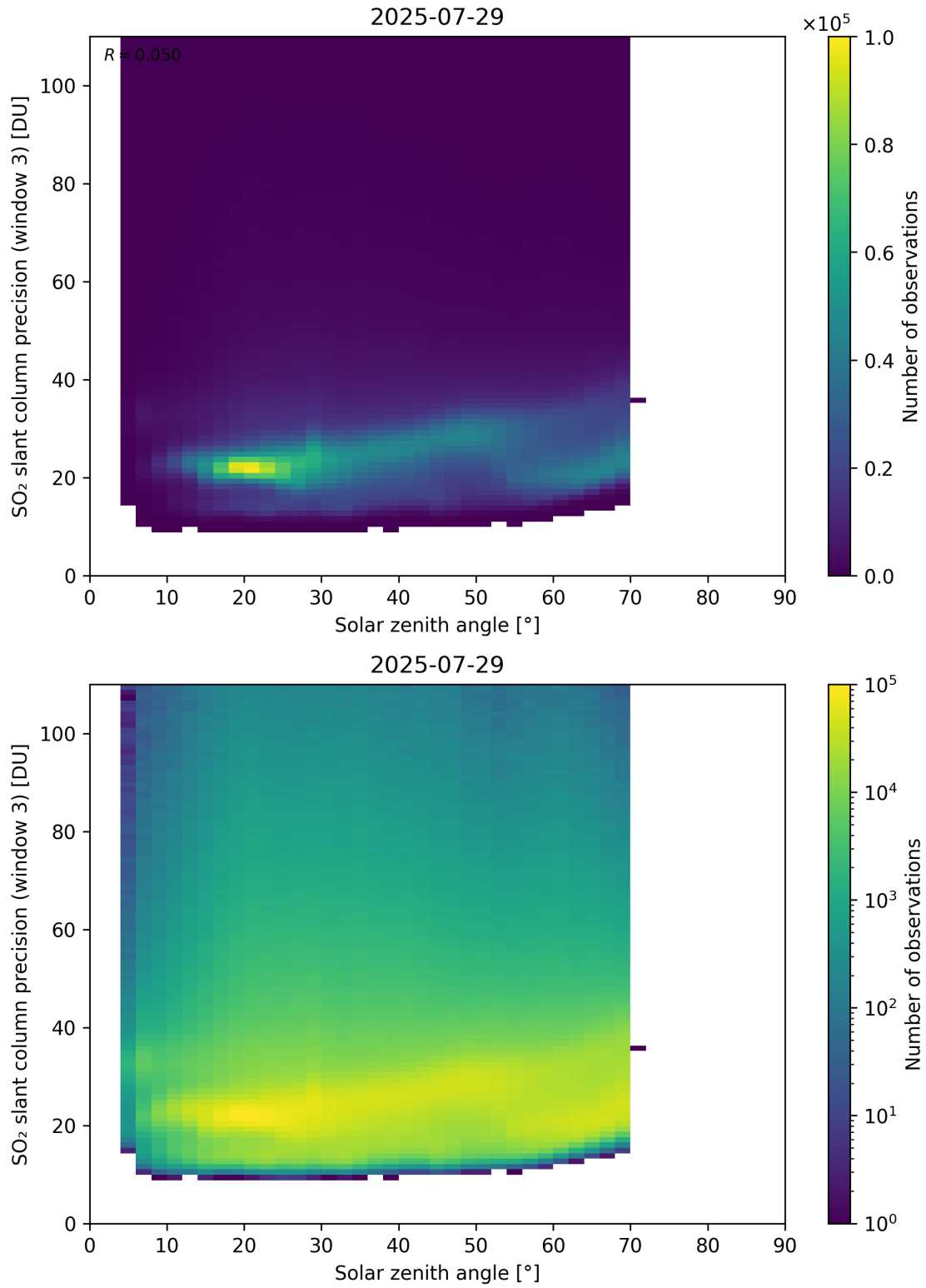
Figure 188: Scatter density plot of “Solar zenith angle” against “SO 2 slant column precision (window 3)” for 2025-07-29 to 2025-07-30.
