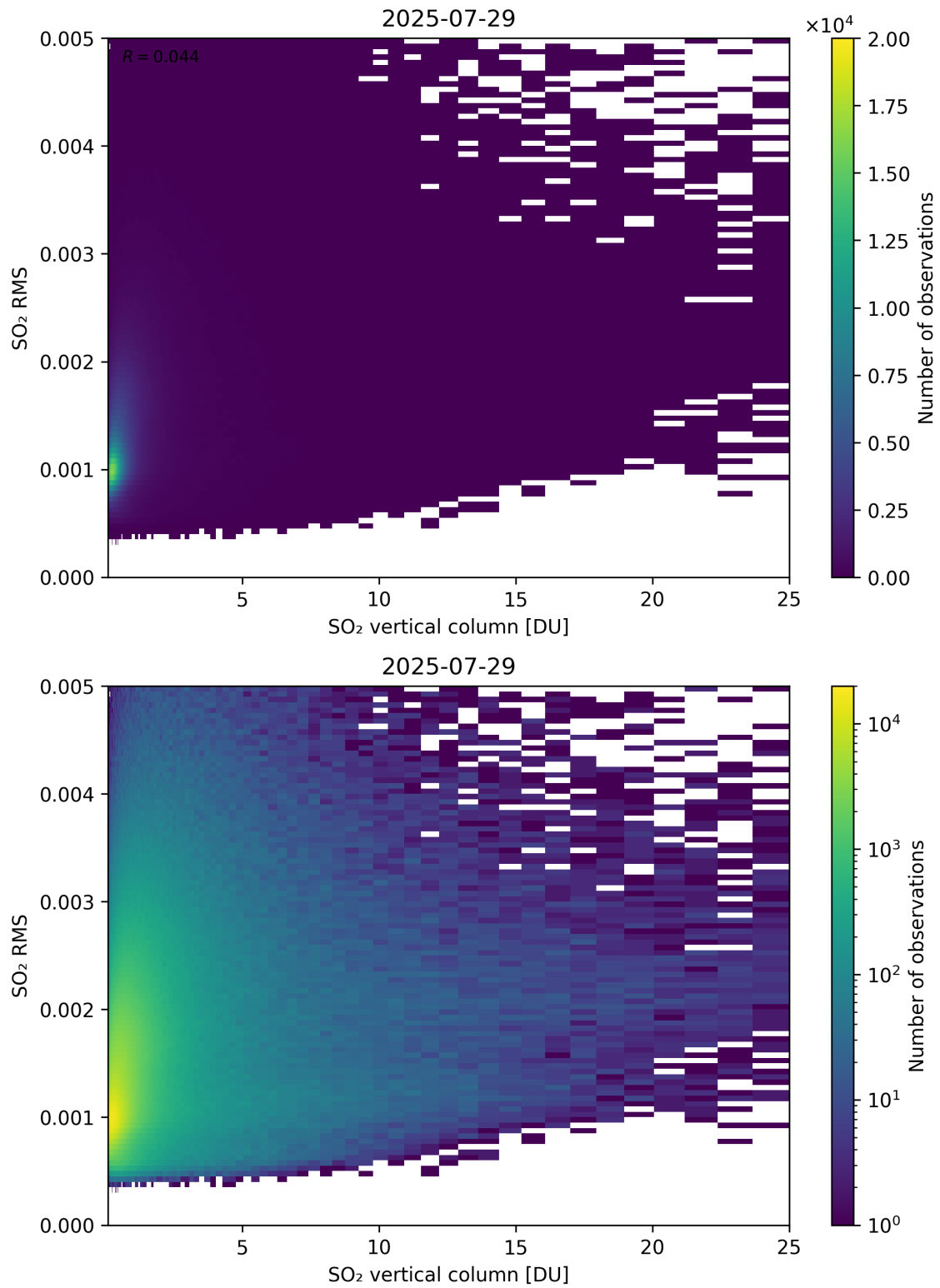
Figure 328: Scatter density plot of “SO 2 vertical column” against “SO 2 RMS” for 2025-07-29 to 2025-07-30.
