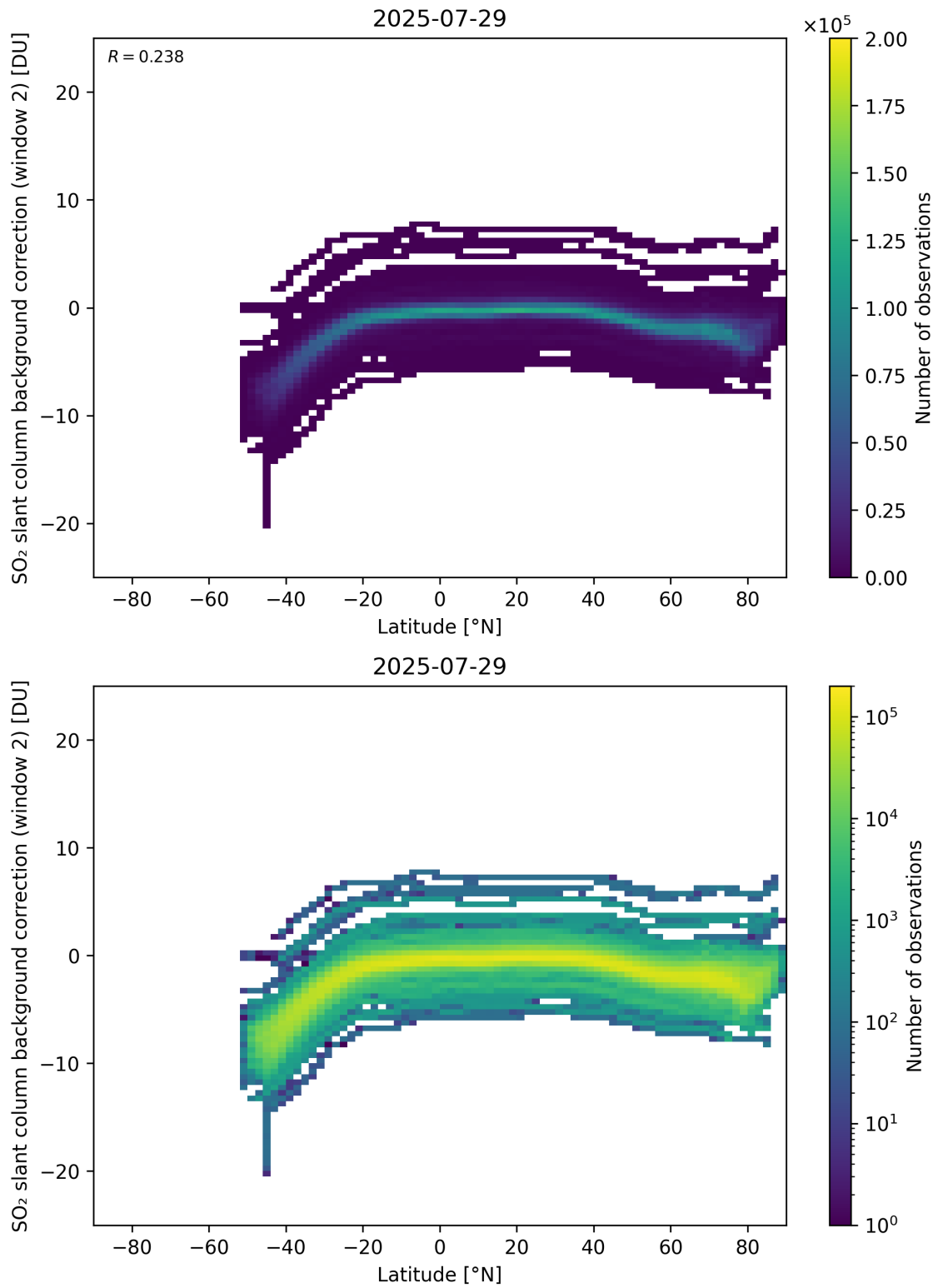
Figure 151: Scatter density plot of “Latitude” against “SO 2 slant column background correction (window 2)” for 2025-07-29 to 2025-07-30.
