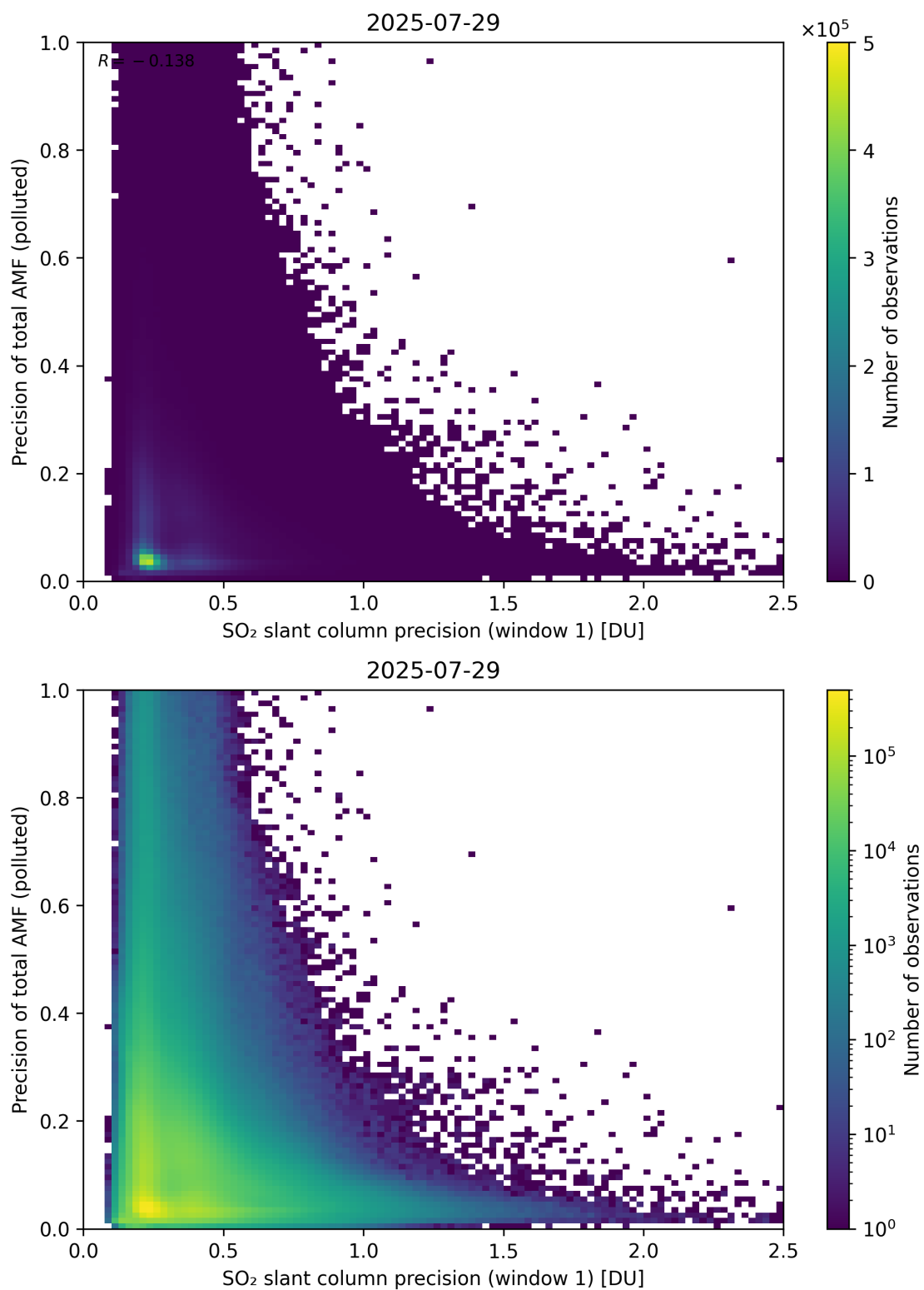
Figure 281: Scatter density plot of “SO 2 slant column precision (window 1)” against “Precision of total AMF (polluted)” for 2025-07-29 to 2025-07-30.
