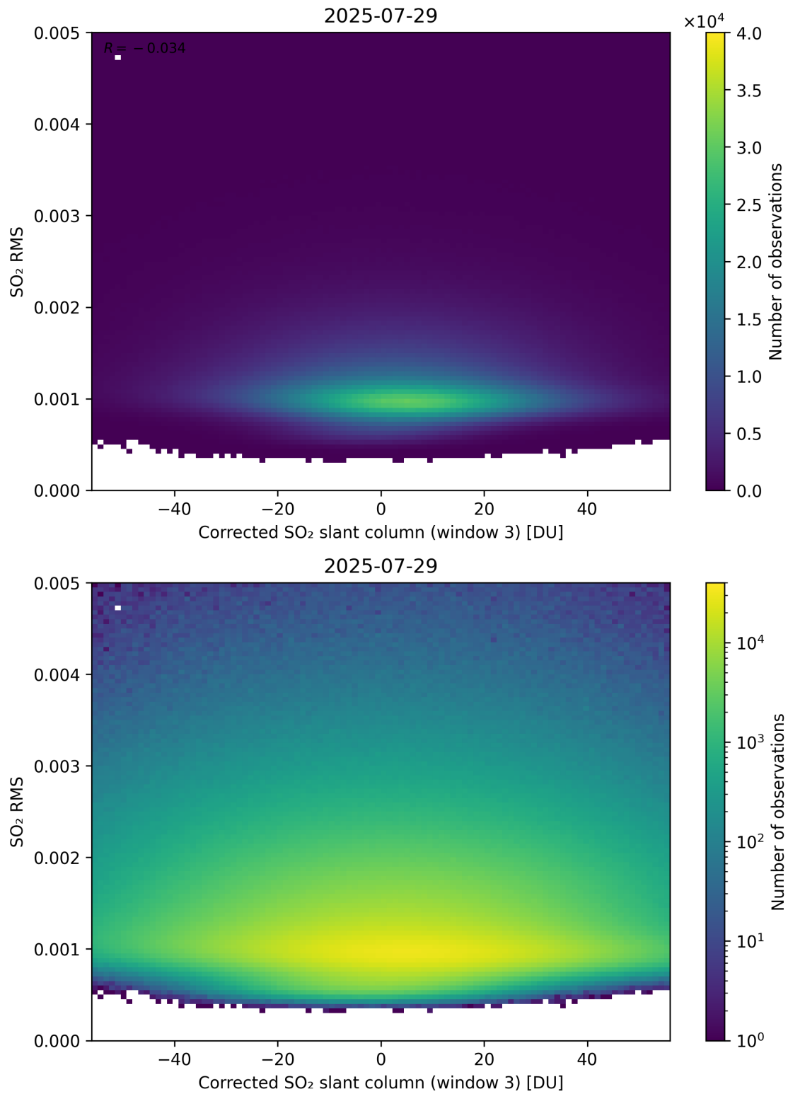
Figure 258: Scatter density plot of “Corrected SO 2 slant column (window 3)” against “SO 2 RMS” for 2025-07-29 to 2025-07-30.
