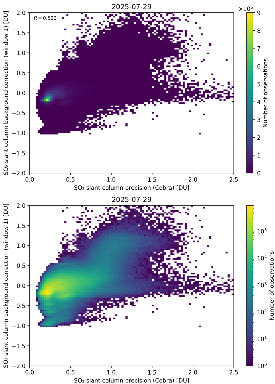
Figure 199: Scatter density plot of “SO 2 slant column precision (Cobra)” against “SO 2 slant column background correction (window 1)” for 2025-07-29 to 2025-07-30.
