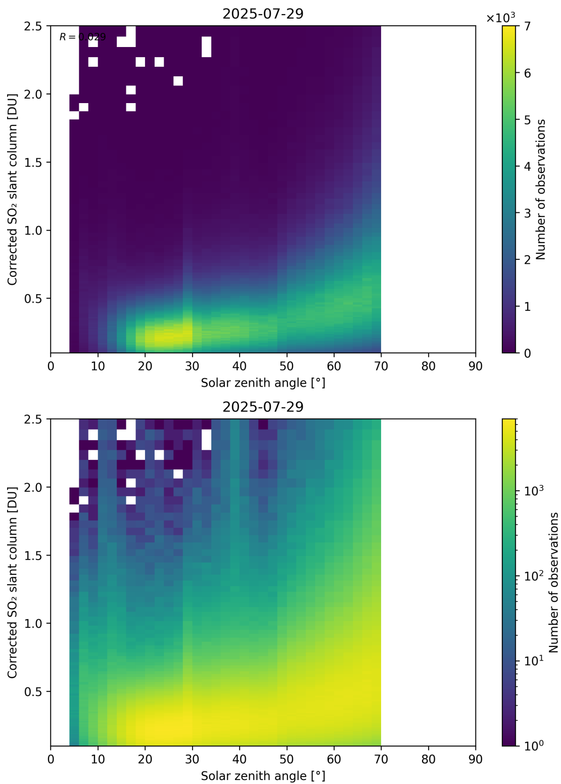
Figure 181: Scatter density plot of “Solar zenith angle” against “Corrected SO 2 slant column” for 2025-07-29 to 2025-07-30.
