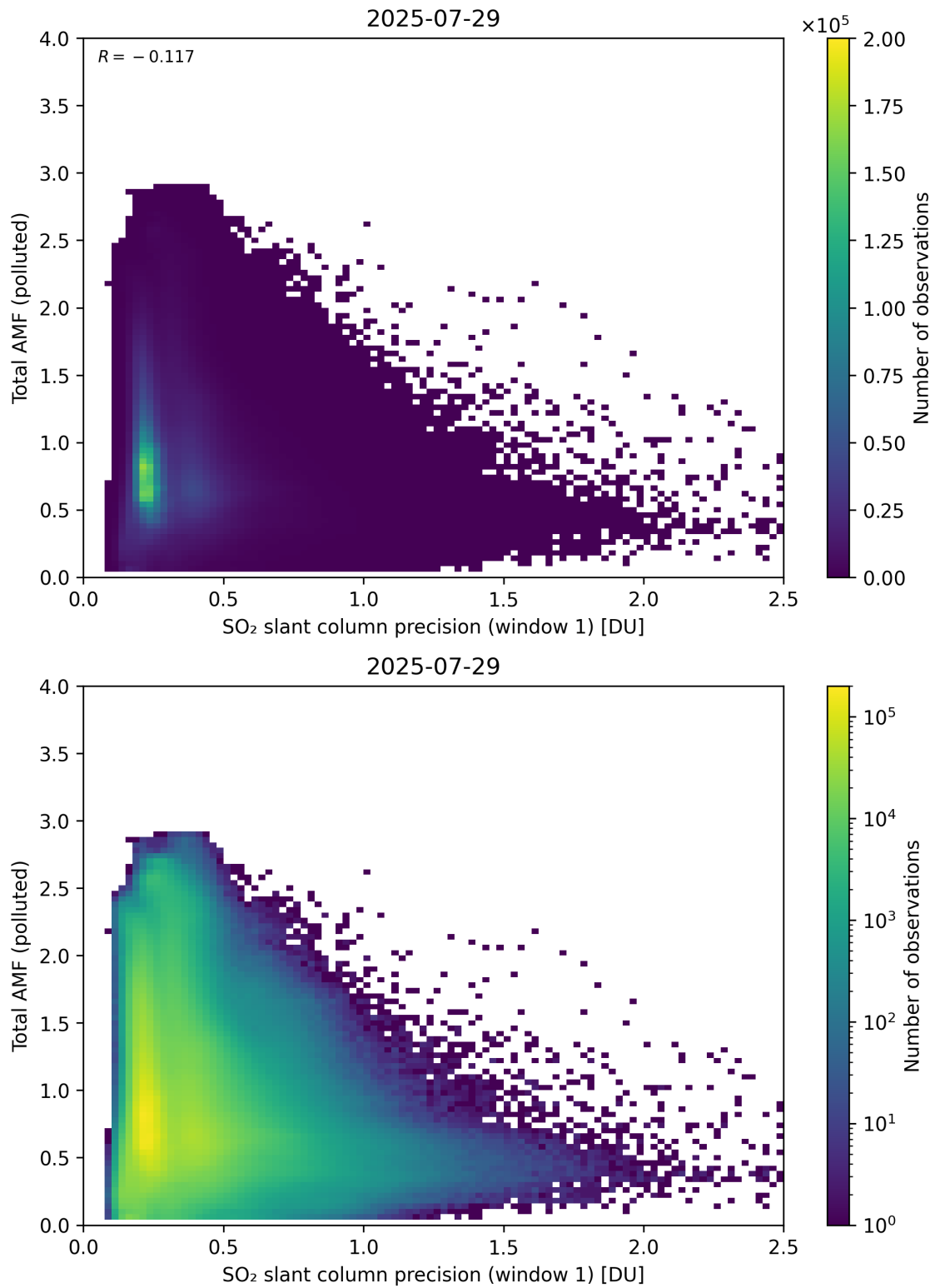
Figure 280: Scatter density plot of “SO 2 slant column precision (window 1)” against “Total AMF (polluted)” for 2025-07-29 to 2025-07-30.
