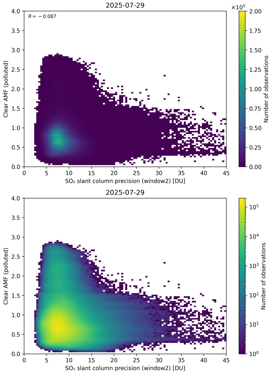
Figure 296: Scatter density plot of “SO 2 slant column precision (window2)” against “Clear AMF (polluted)” for 2025-07-29 to 2025-07-30.
