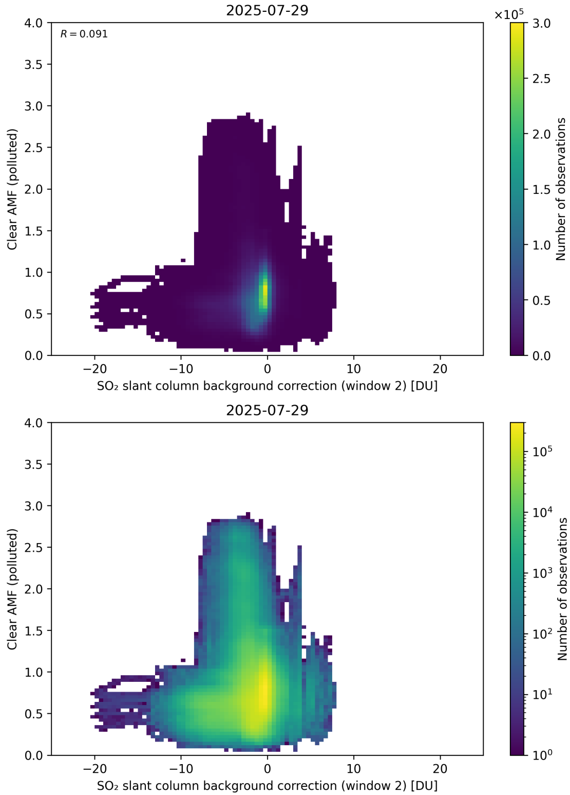
Figure 126: Scatter density plot of “SO 2 slant column background correction (window 2)” against “Clear AMF (polluted)” for 2025-07-29 to 2025-07-30.
