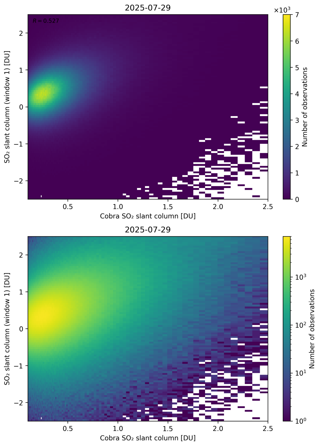
Figure 219: Scatter density plot of “Cobra SO 2 slant column” against “SO 2 slant column (window 1)” for 2025-07-29 to 2025-07-30.
