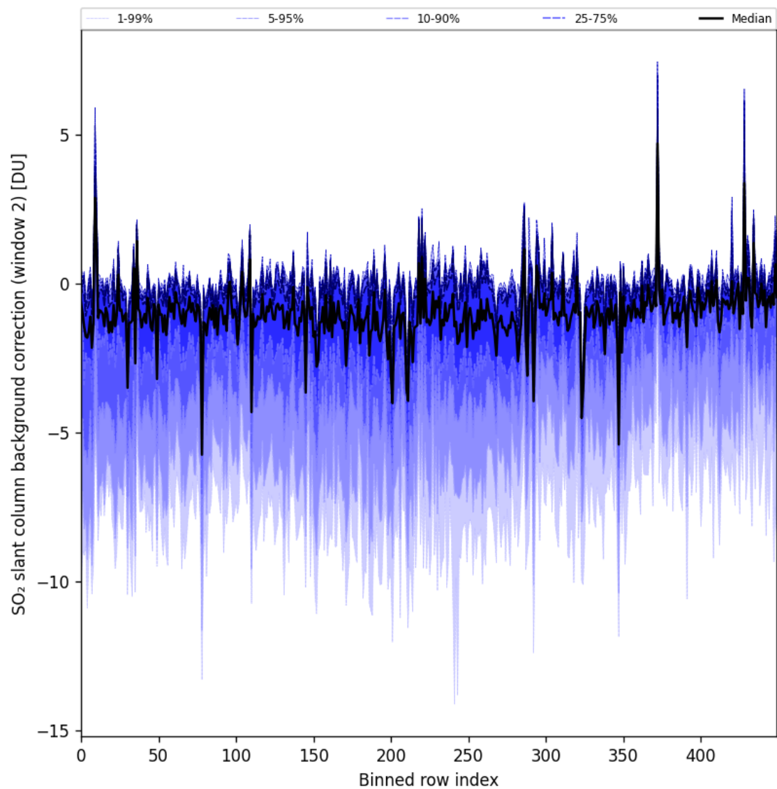
Figure 96: Along track statistics of “SO 2 slant column background correction (window 2)” for 2025-07-29 to 2025-07-30
