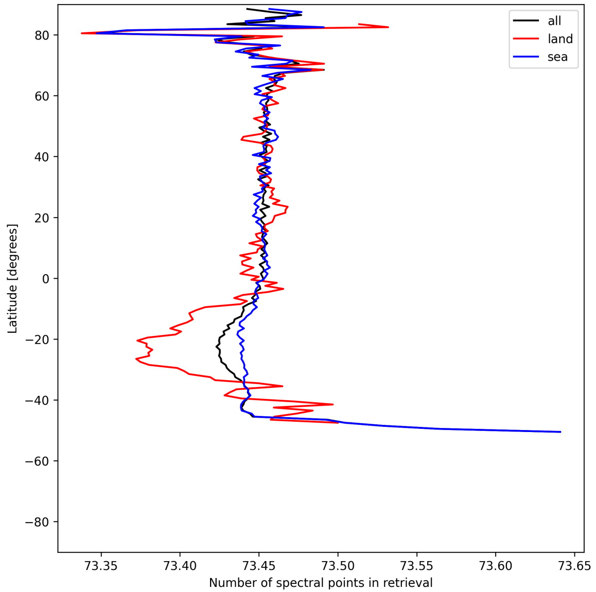
Figure 56: Zonal average of “Number of spectral points in retrieval” for 2025-07-29 to 2025-07-30.
