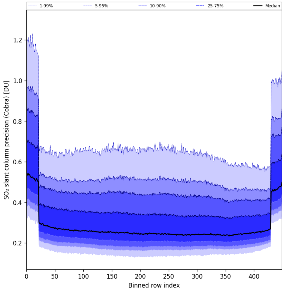
Figure 88: Along track statistics of “SO 2 slant column precision (Cobra)” for 2025-07-29 to 2025-07-30
