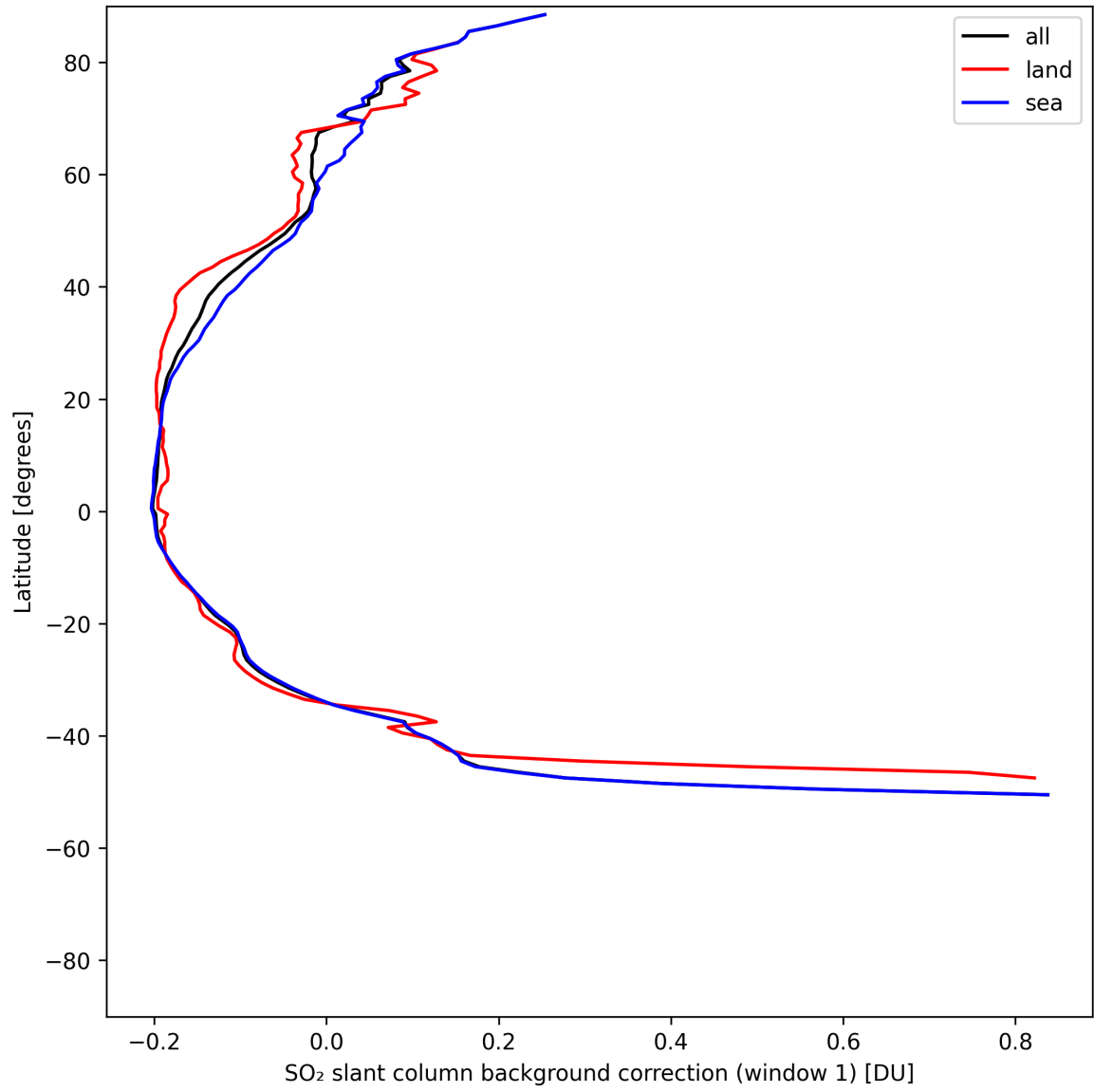
Figure 40: Zonal average of “SO 2 slant column background correction (window 1)” for 2025-07-29 to 2025-07-30.
