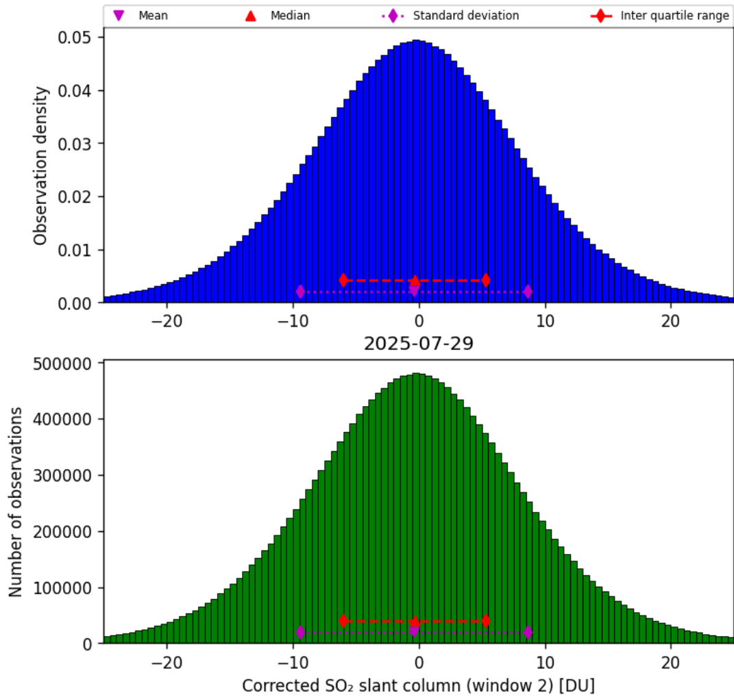
Figure 69: Histogram of “Corrected SO 2 slant column (window 2)” for 2025-07-29 to 2025-07-30
