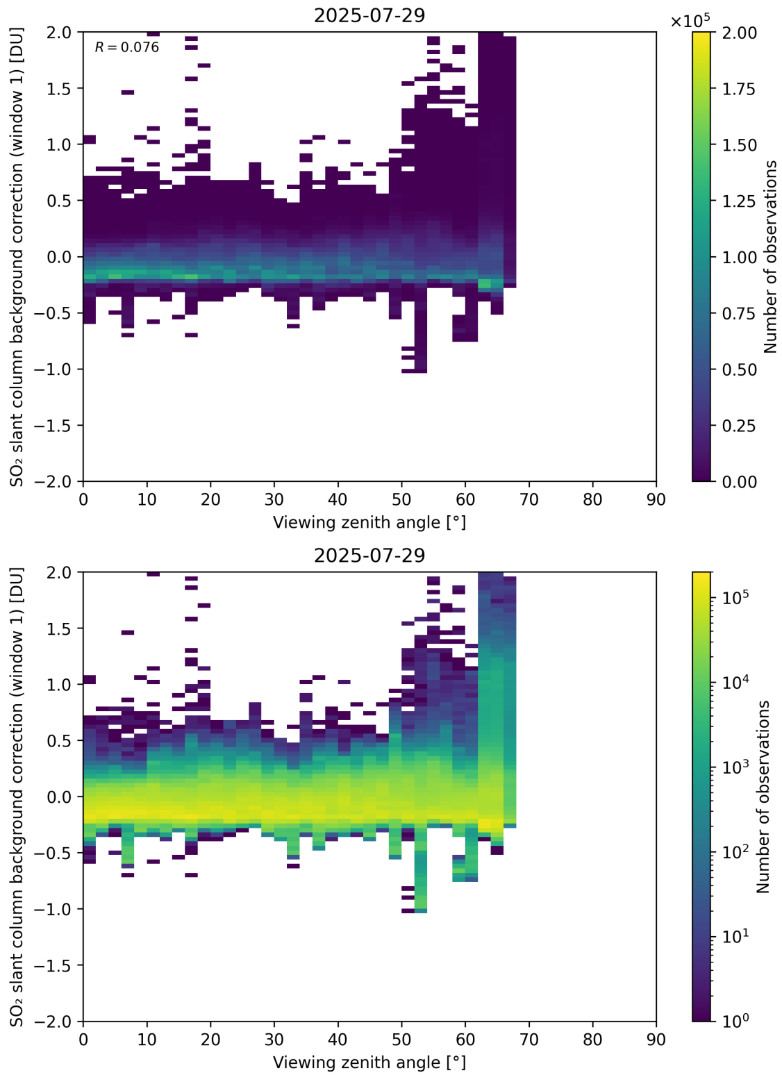
Figure 362: Scatter density plot of “Viewing zenith angle” against “SO 2 slant column background correction (window 1)” for 2025-07-29 to 2025-07-30.
