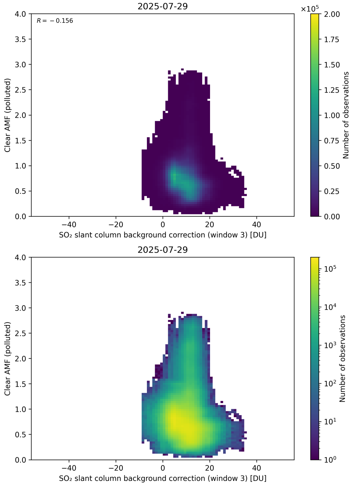
Figure 135: Scatter density plot of “SO 2 slant column background correction (window 3)” against “Clear AMF (polluted)” for 2025-07-29 to 2025-07-30.
