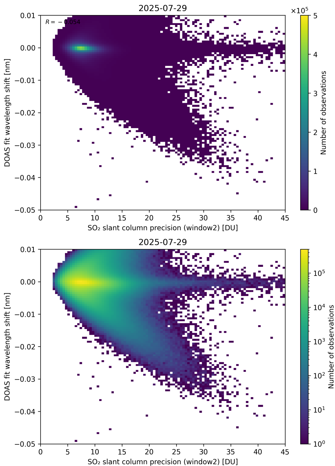
Figure 293: Scatter density plot of “SO 2 slant column precision (window2)” against “DOAS fit wavelength shift” for 2025-07-29 to 2025-07-30.
