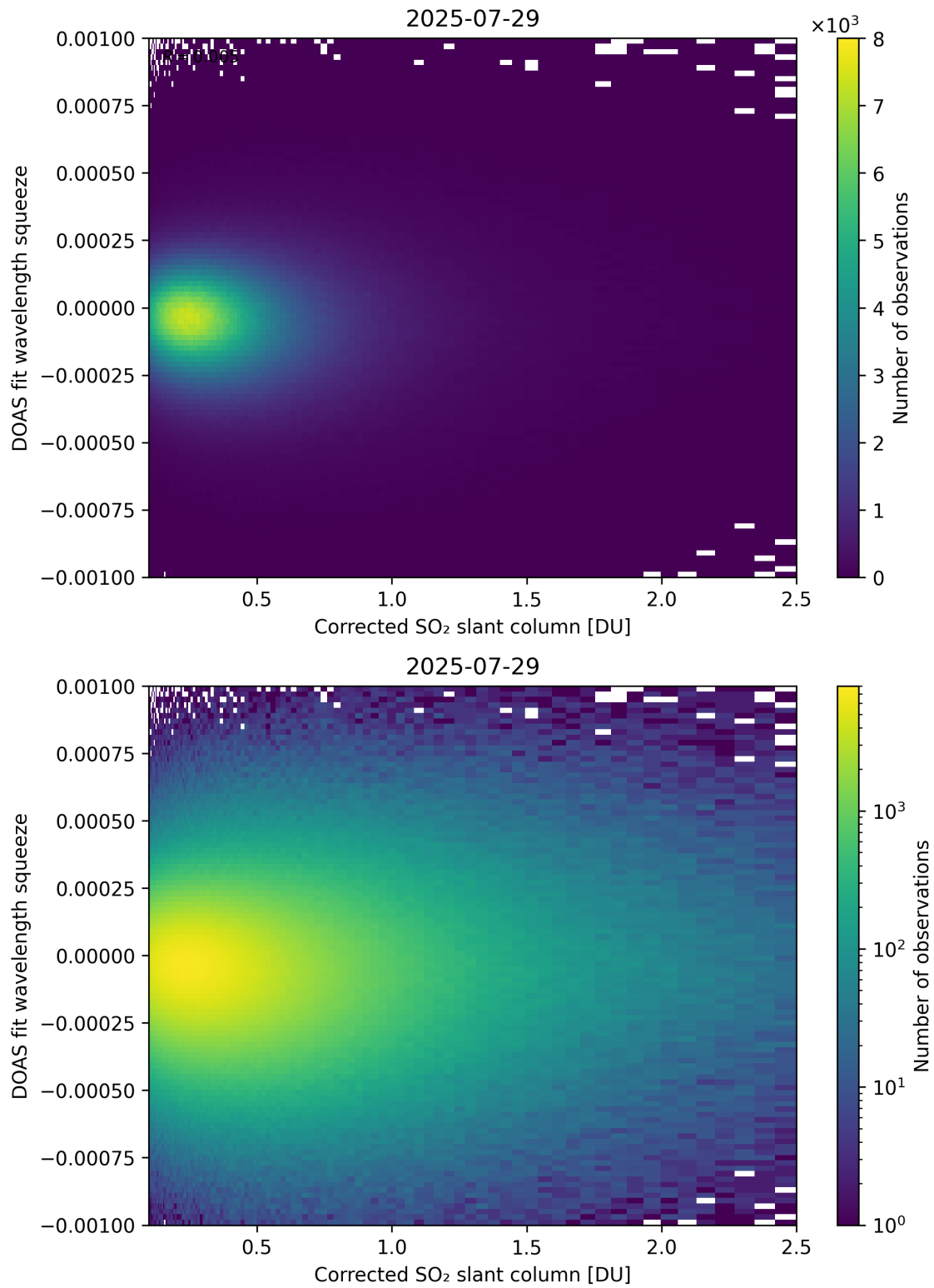
Figure 230: Scatter density plot of "Corrected SO 2 slant column" against "DOAS fit wavelength squeeze" for 2025-07-29 to 2025-07-30.
