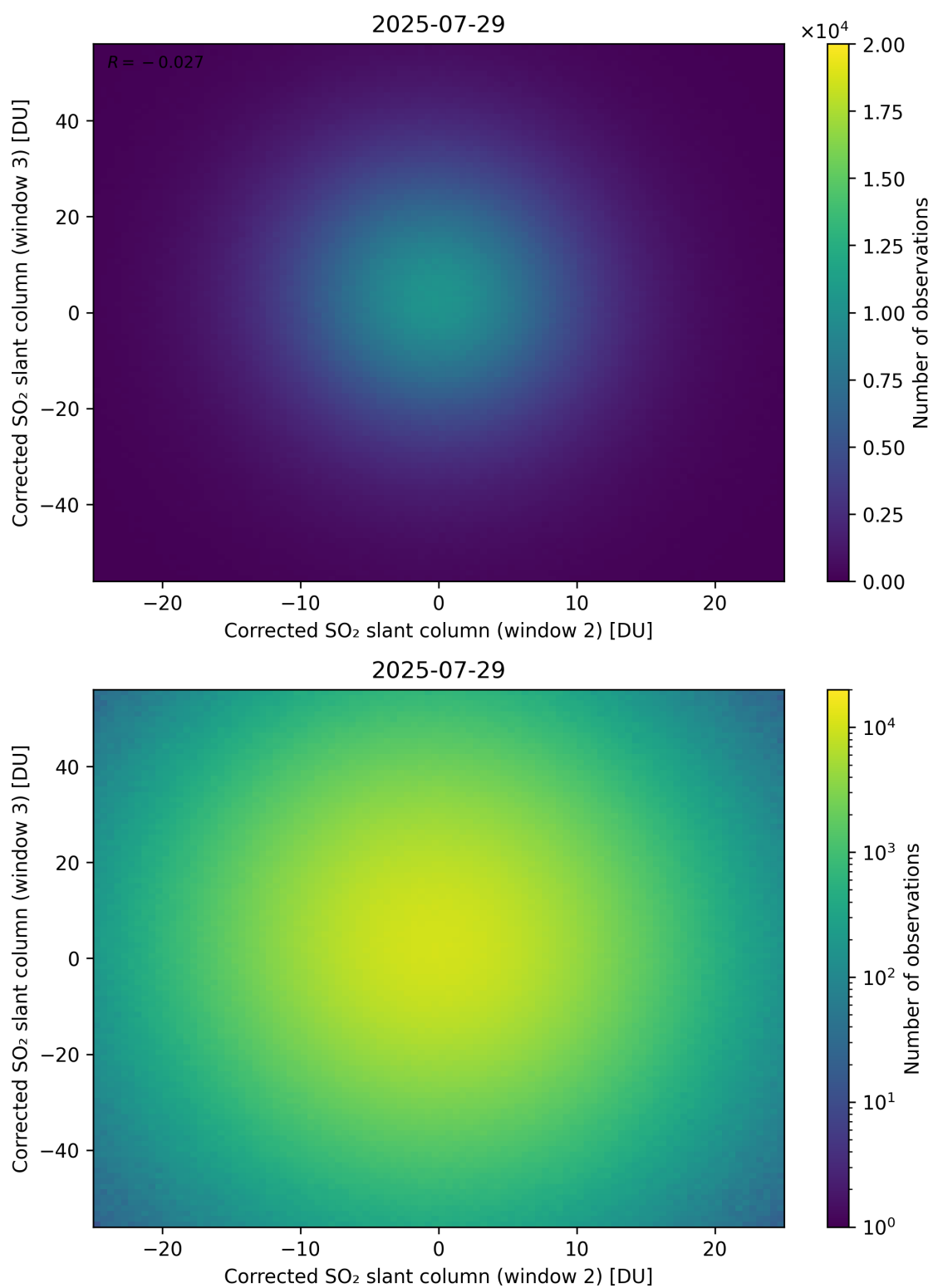
Figure 250: Scatter density plot of “Corrected SO 2 slant column (window 2)” against “Corrected SO 2 slant column (window 3)” for 2025-07-29 to 2025-07-30.
