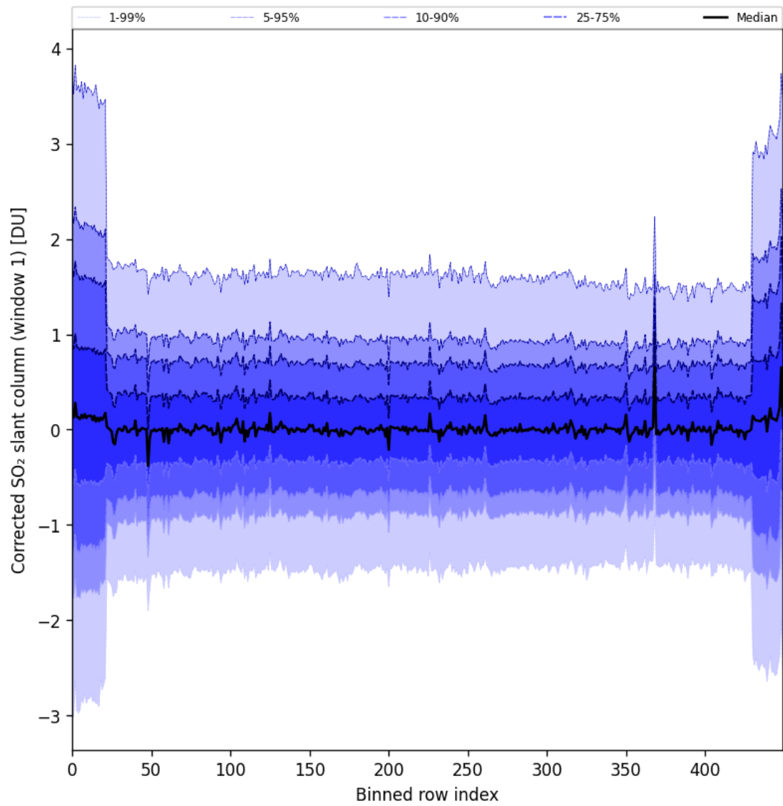
Figure 91: Along track statistics of “Corrected SO 2 slant column (window 1)” for 2025-07-29 to 2025-07-30
