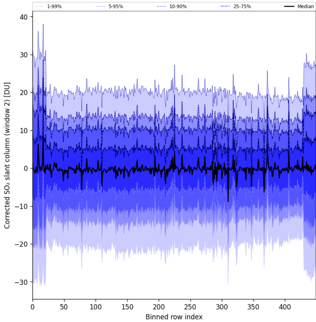
Figure 95: Along track statistics of “Corrected SO 2 slant column (window 2)” for 2025-07-29 to 2025-07-30
