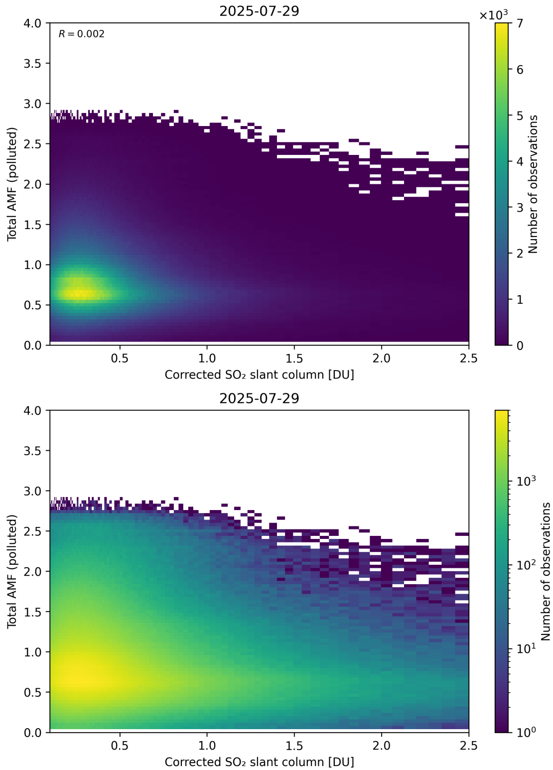
Figure 242: Scatter density plot of “Corrected SO 2 slant column” against “Total AMF (polluted)” for 2025-07-29 to 2025-07-30.
