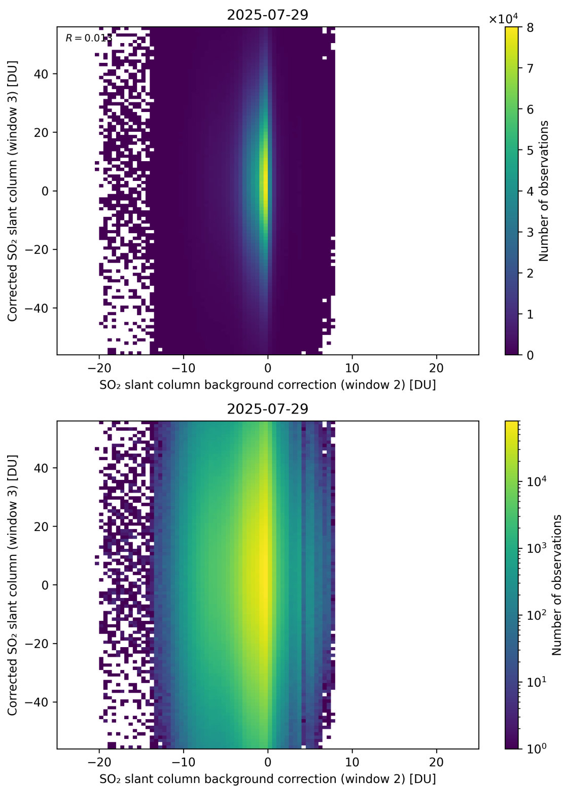
Figure 127: Scatter density plot of “SO 2 slant column background correction (window 2)” against “Corrected SO 2 slant column (window 3)” for 2025-07-29 to 2025-07-30.
