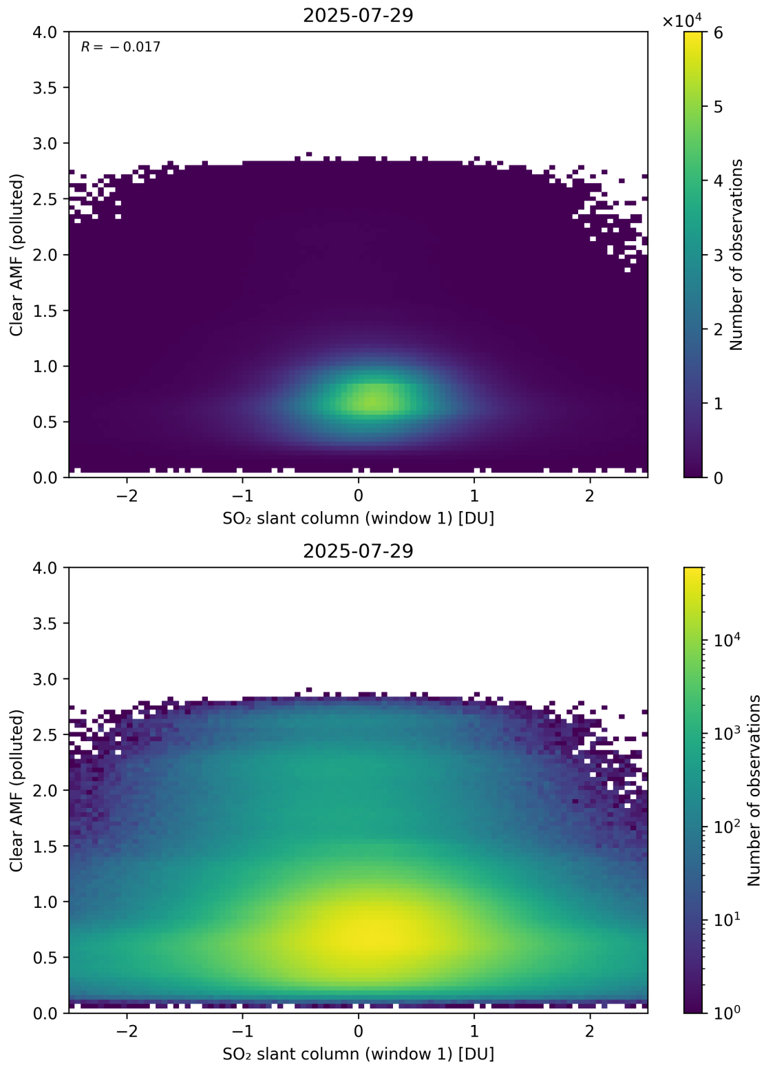
Figure 282: Scatter density plot of “SO 2 slant column (window 1)” against “Clear AMF (polluted)” for 2025-07-29 to 2025-07-30.
