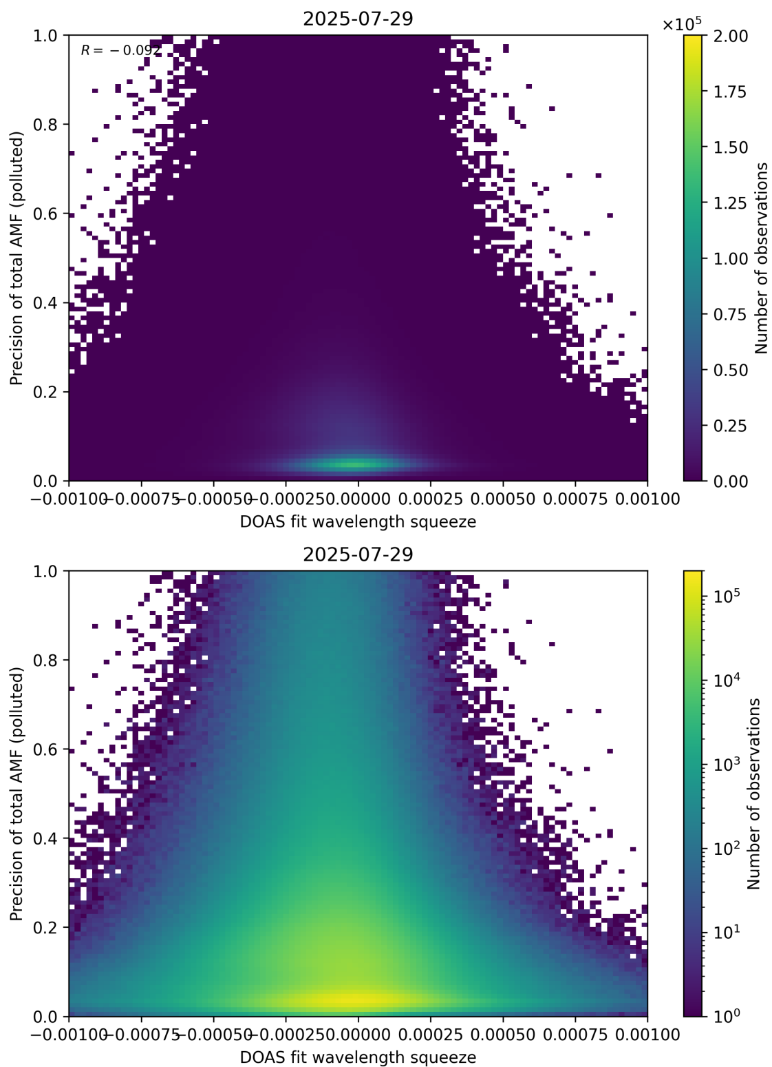
Figure 146: Scatter density plot of “DOAS fit wavelength squeeze” against “Precision of total AMF (polluted)” for 2025-07-29 to 2025-07-30.
