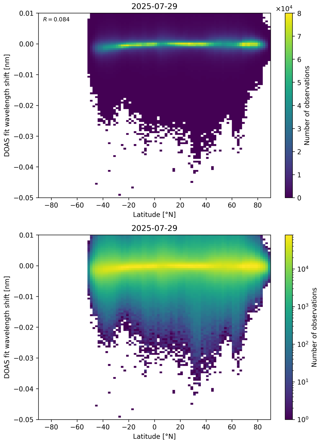
Figure 153: Scatter density plot of “Latitude” against “DOAS fit wavelength shift” for 2025-07-29 to 2025-07-30.
