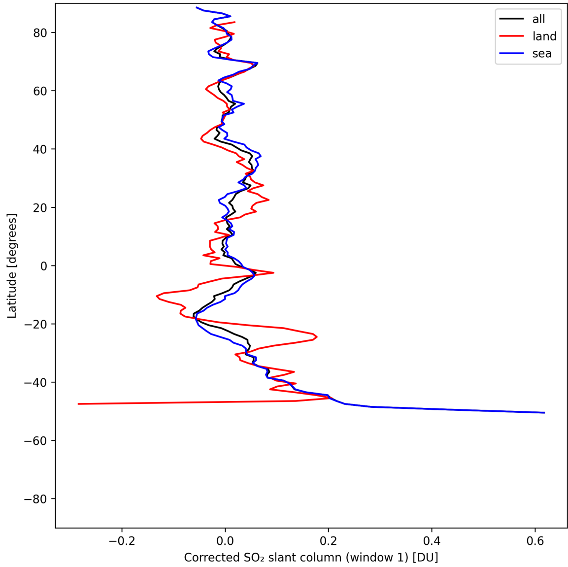
Figure 39: Zonal average of “Corrected SO 2 slant column (window 1)” for 2025-07-29 to 2025-07-30.
