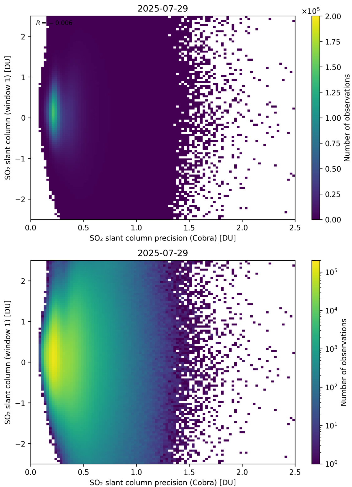
Figure 208: Scatter density plot of “SO 2 slant column precision (Cobra)” against “SO 2 slant column (window 1)” for 2025-07-29 to 2025-07-30.
