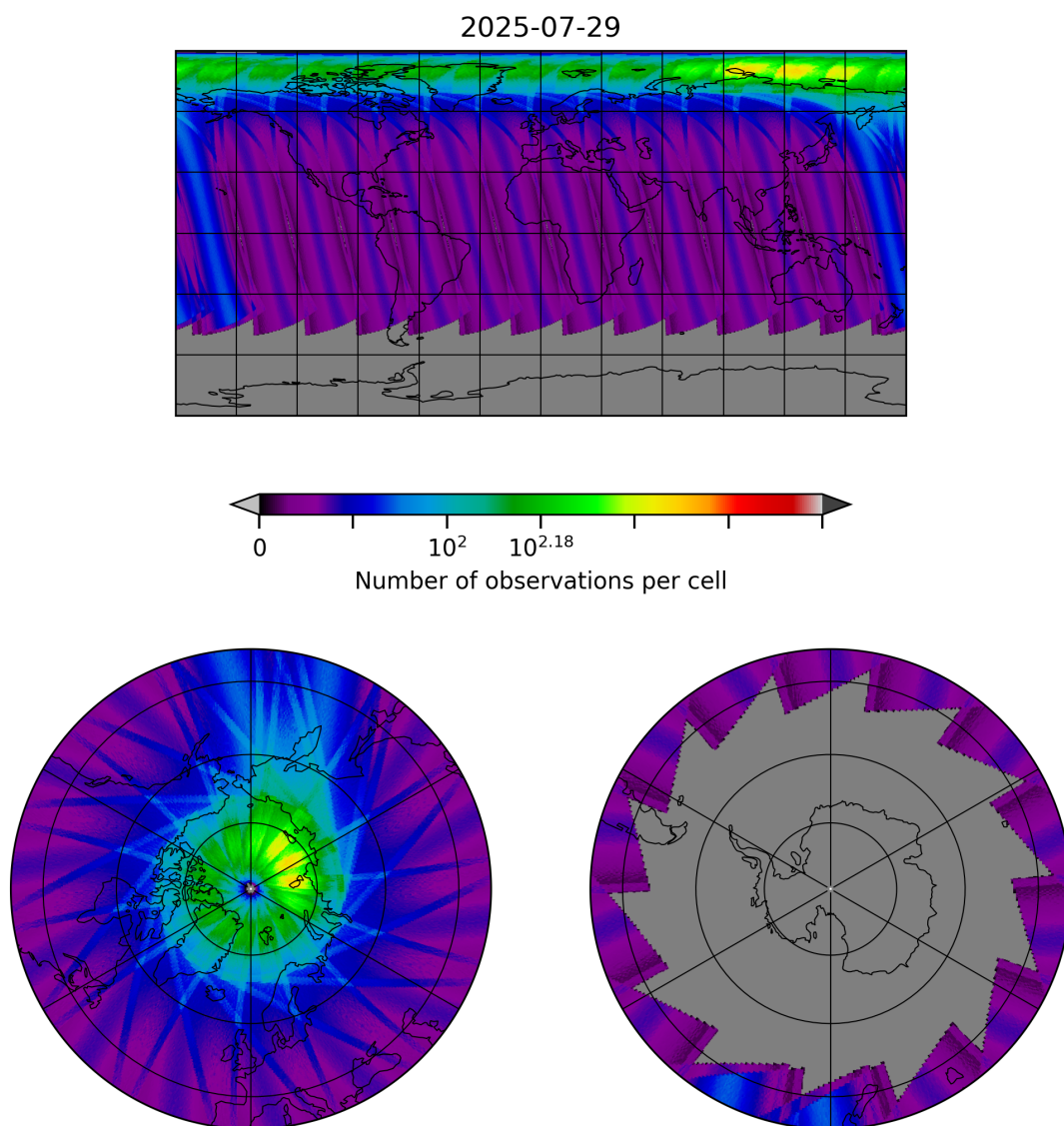
Figure 30: Map of the number of observations for 2025-07-29 to 2025-07-30
