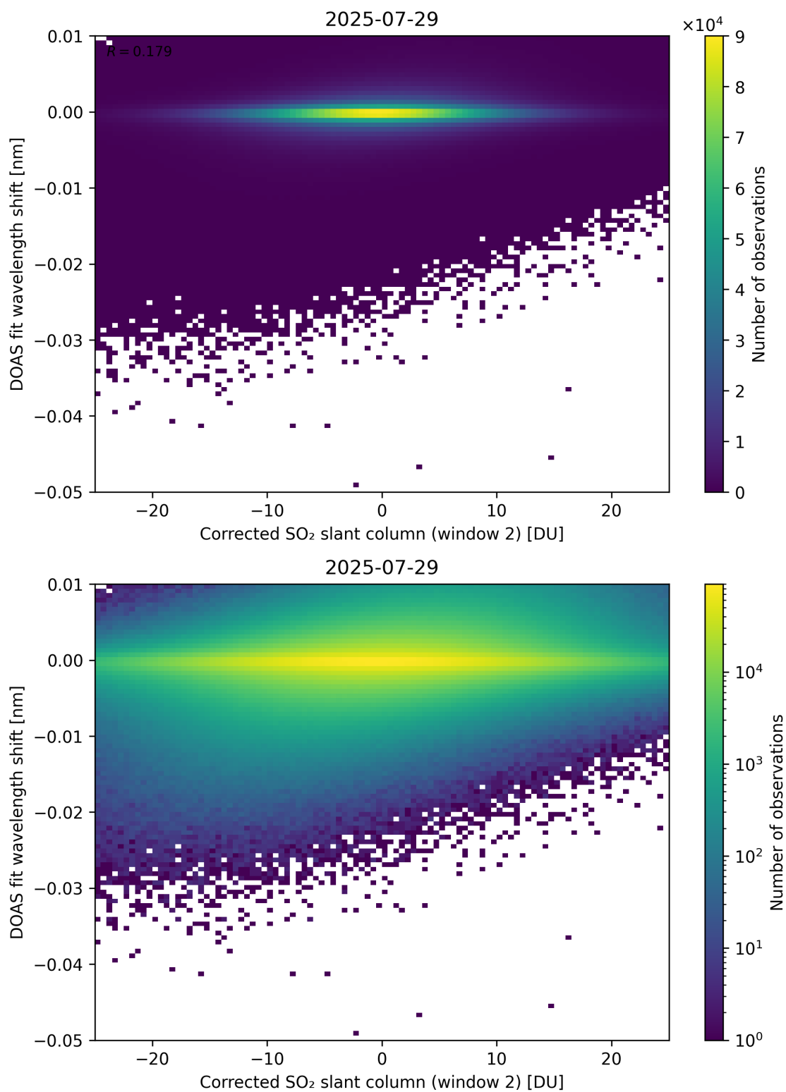
Figure 246: Scatter density plot of “Corrected SO 2 slant column (window 2)” against “DOAS fit wavelength shift” for 2025-07-29 to 2025-07-30.
