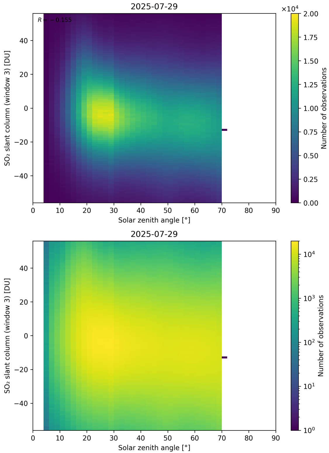
Figure 187: Scatter density plot of “Solar zenith angle” against “SO 2 slant column (window 3)” for 2025-07-29 to 2025-07-30.
