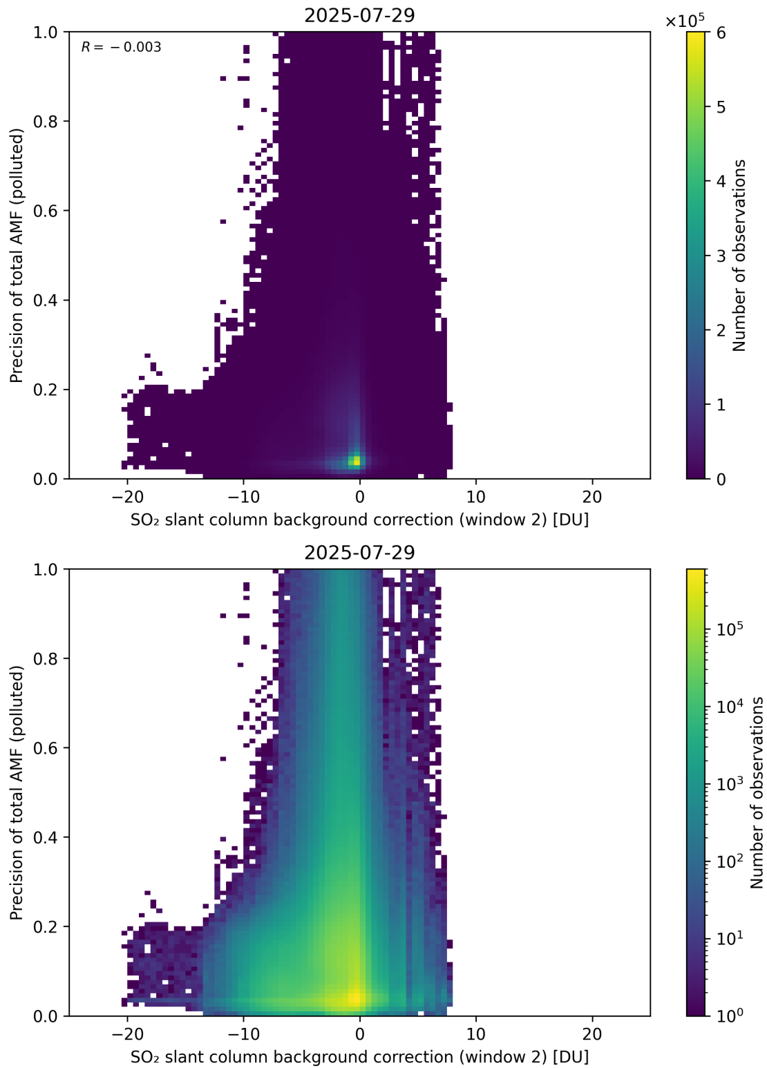
Figure 131: Scatter density plot of “SO 2 slant column background correction (window 2)” against “Precision of total AMF (polluted)” for 2025-07-29 to 2025-07-30.
