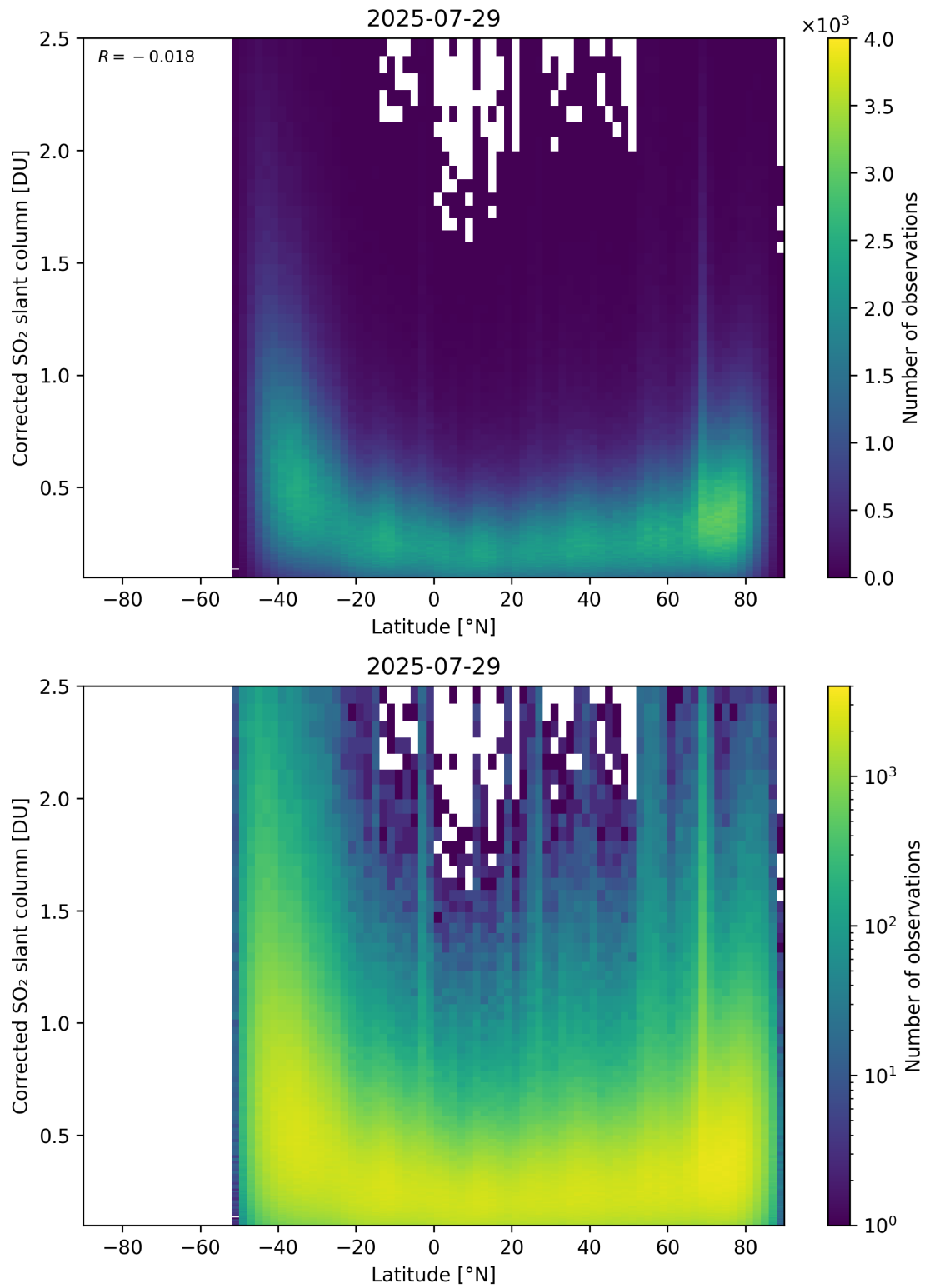
Figure 159: Scatter density plot of “Latitude” against “Corrected SO 2 slant column” for 2025-07-29 to 2025-07-30.
