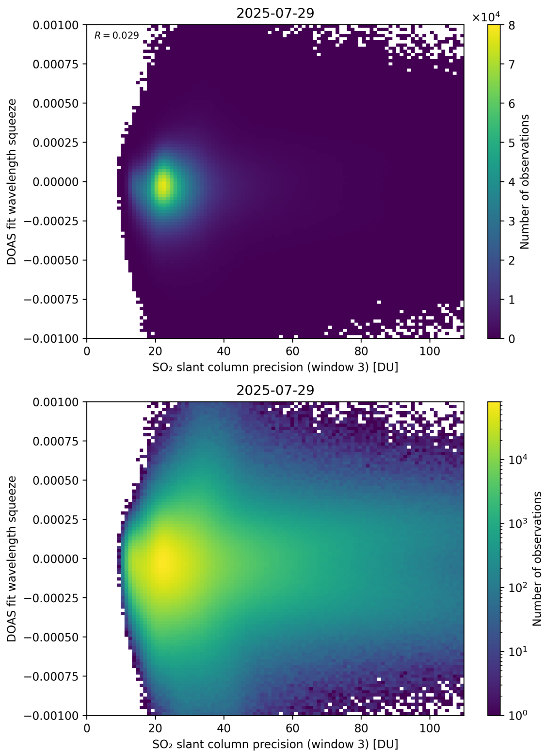
Figure 309: Scatter density plot of “SO 2 slant column precision (window 3)” against “DOAS fit wavelength squeeze” for 2025-07-29 to 2025-07-30.
