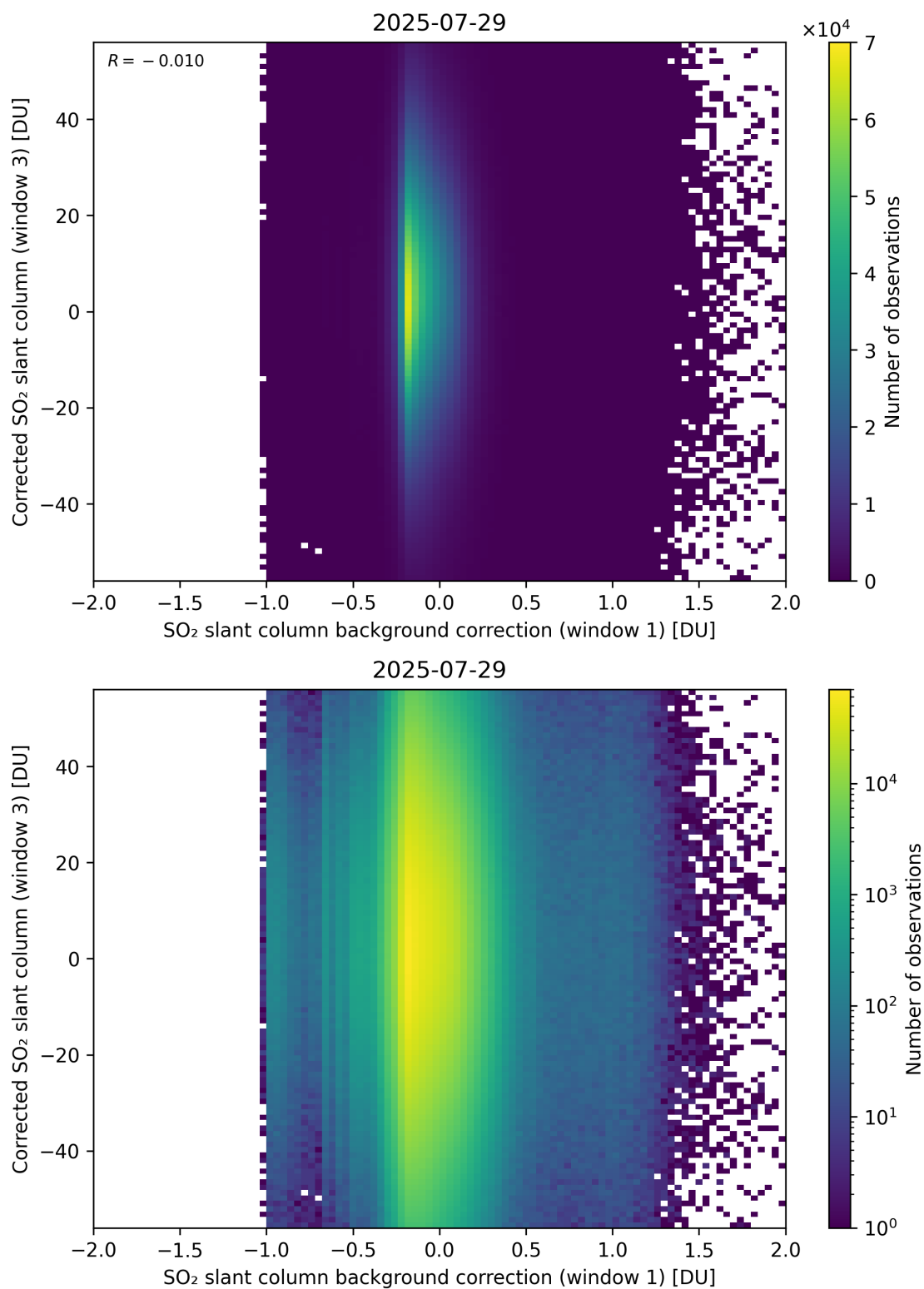
Figure 116: Scatter density plot of “SO 2 slant column background correction (window 1)” against “Corrected SO 2 slant column (window 3)” for 2025-07-29 to 2025-07-30.
