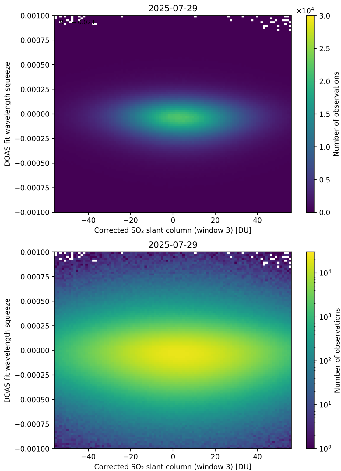
Figure 257: Scatter density plot of “Corrected SO 2 slant column (window 3)” against “DOAS fit wavelength squeeze” for 2025-07-29 to 2025-07-30.
