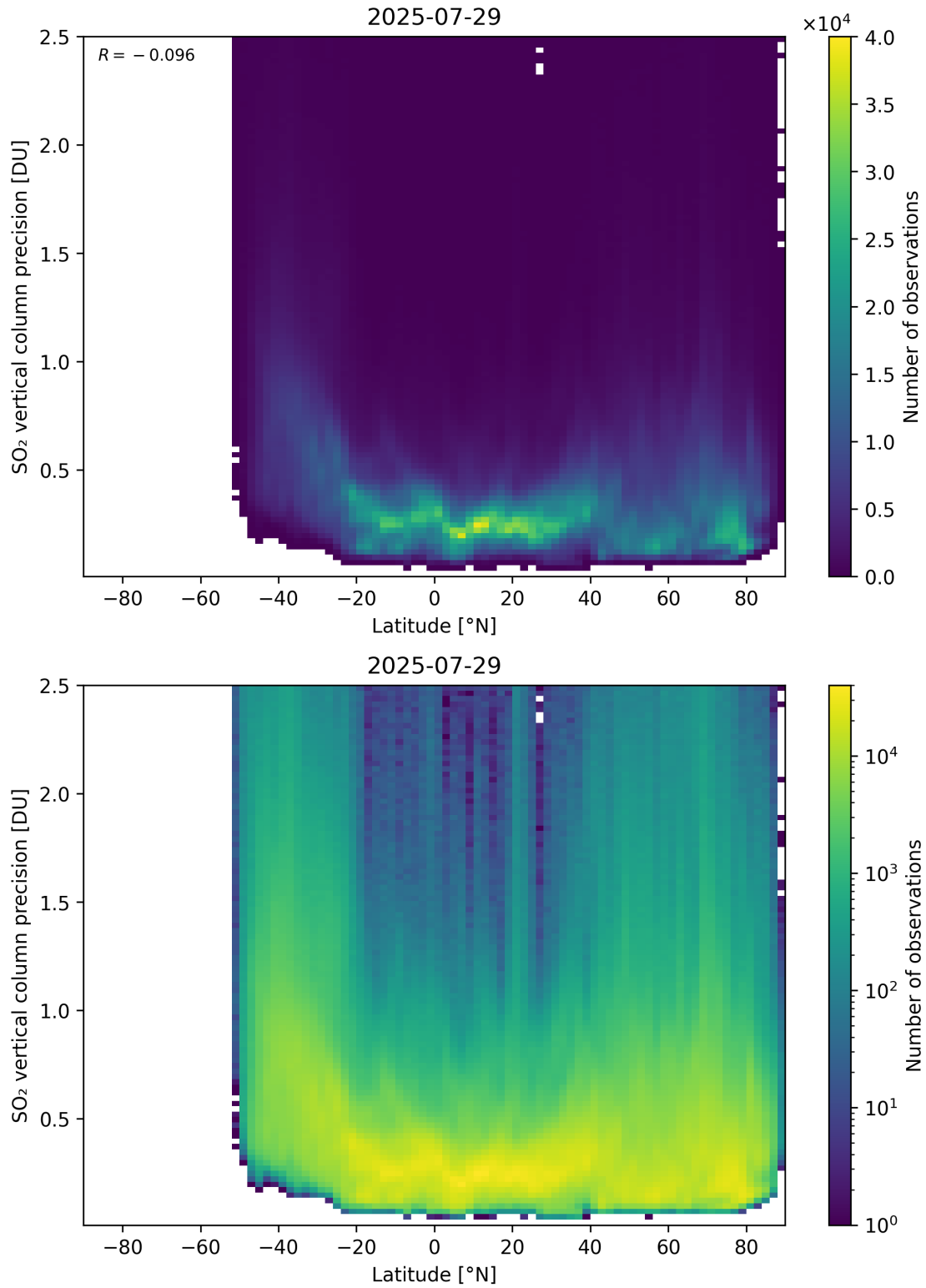
Figure 170: Scatter density plot of “Latitude” against “SO 2 vertical column precision” for 2025-07-29 to 2025-07-30.
