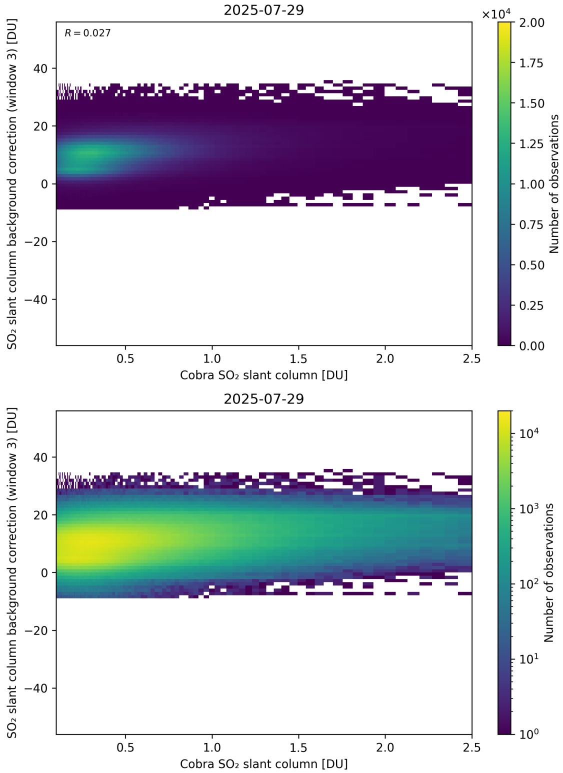
Figure 195: Scatter density plot of “Cobra SO 2 slant column” against “SO 2 slant column background correction (window 3)” for 2025-07-29 to 2025-07-30.
