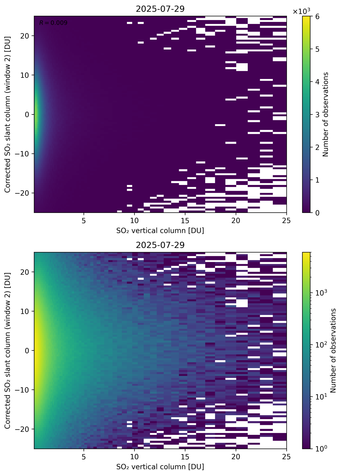
Figure 352: Scatter density plot of “SO 2 vertical column” against “Corrected SO 2 slant column (window 2)” for 2025-07-29 to 2025-07-30.
