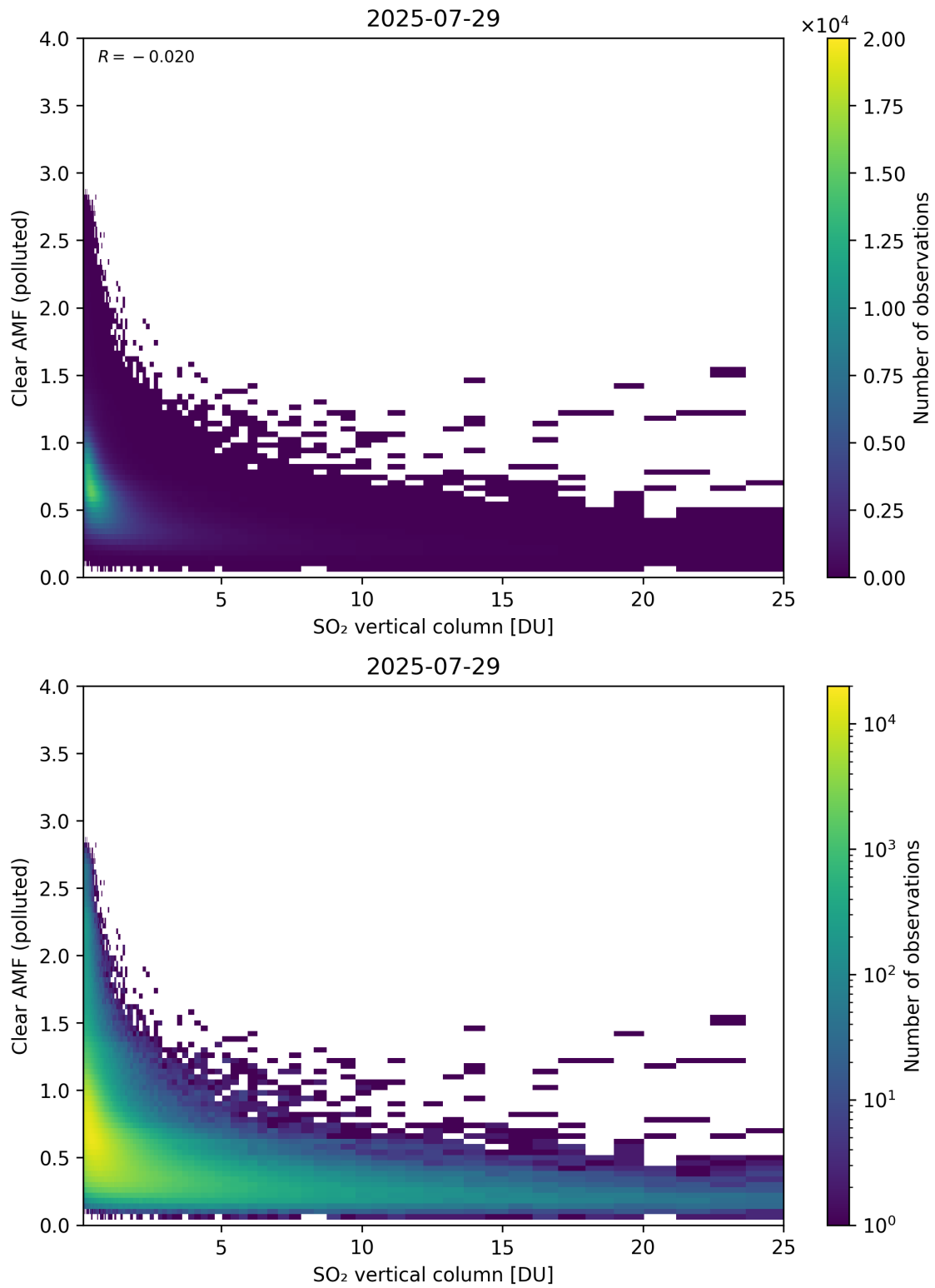
Figure 348: Scatter density plot of “SO 2 vertical column” against “Clear AMF (polluted)” for 2025-07-29 to 2025-07-30.
