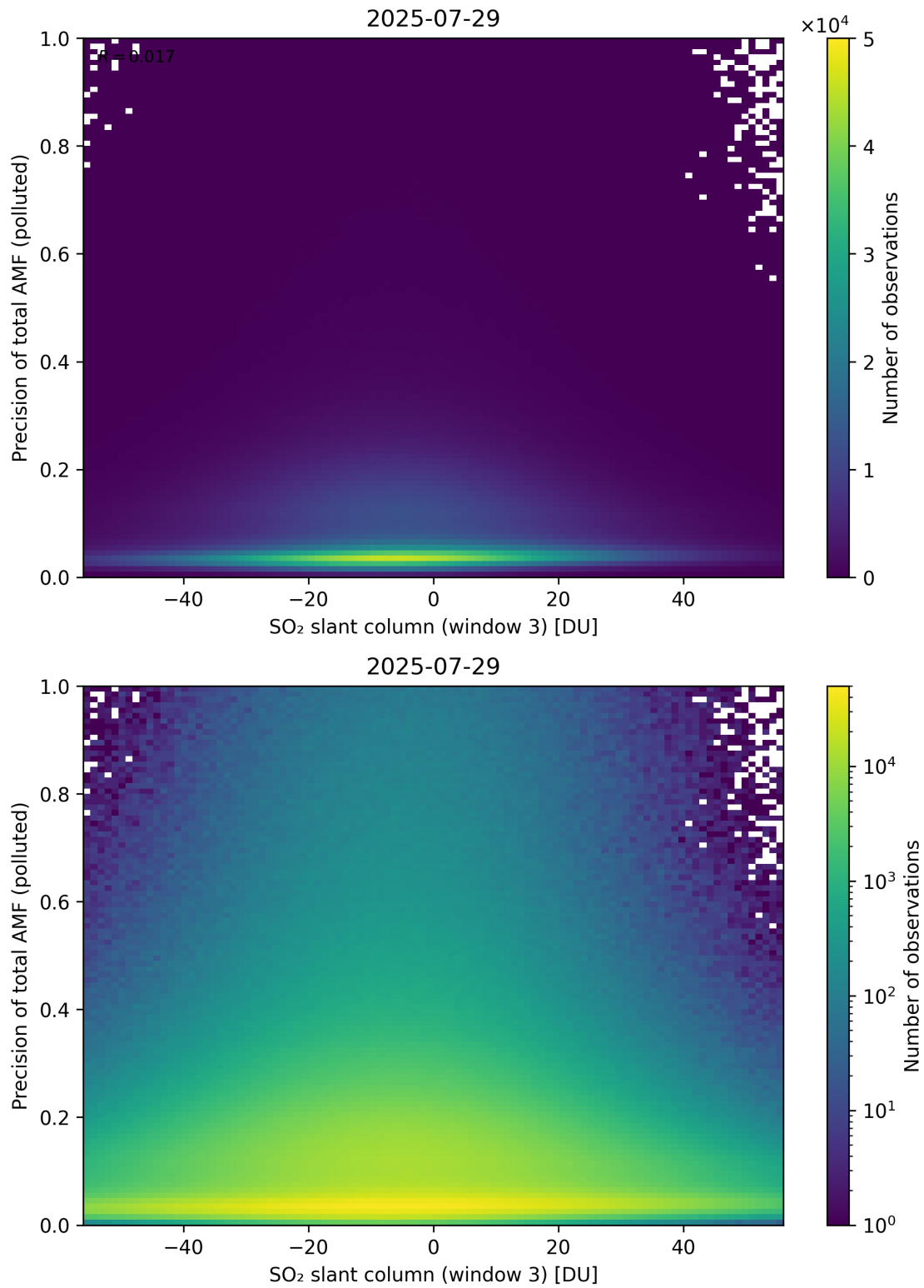
Figure 319: Scatter density plot of “SO 2 slant column (window 3)” against “Precision of total AMF (polluted)” for 2025-07-29 to 2025-07-30.
