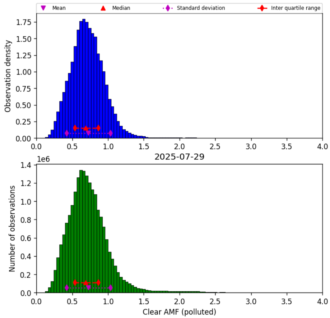
Figure 81: Histogram of “Clear AMF (polluted)” for 2025-07-29 to 2025-07-30
