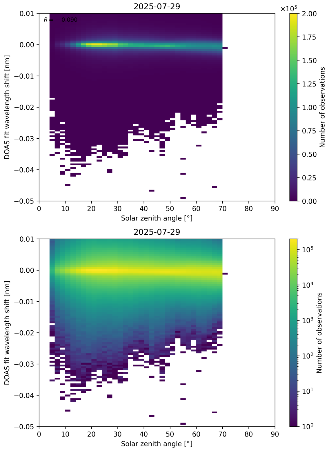
Figure 174: Scatter density plot of “Solar zenith angle” against “DOAS fit wavelength shift” for 2025-07-29 to 2025-07-30.
