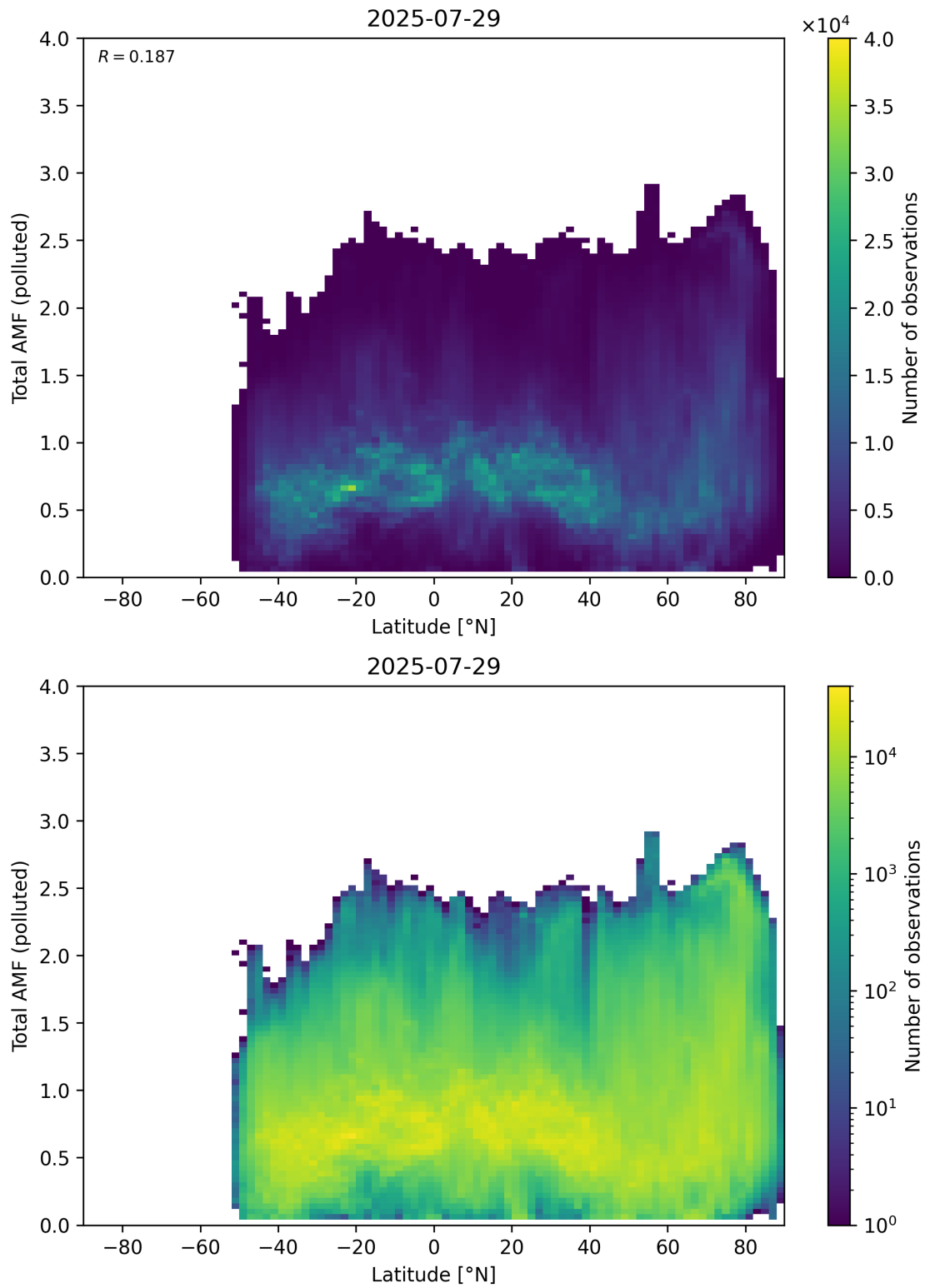
Figure 167: Scatter density plot of “Latitude” against “Total AMF (polluted)” for 2025-07-29 to 2025-07-30.
