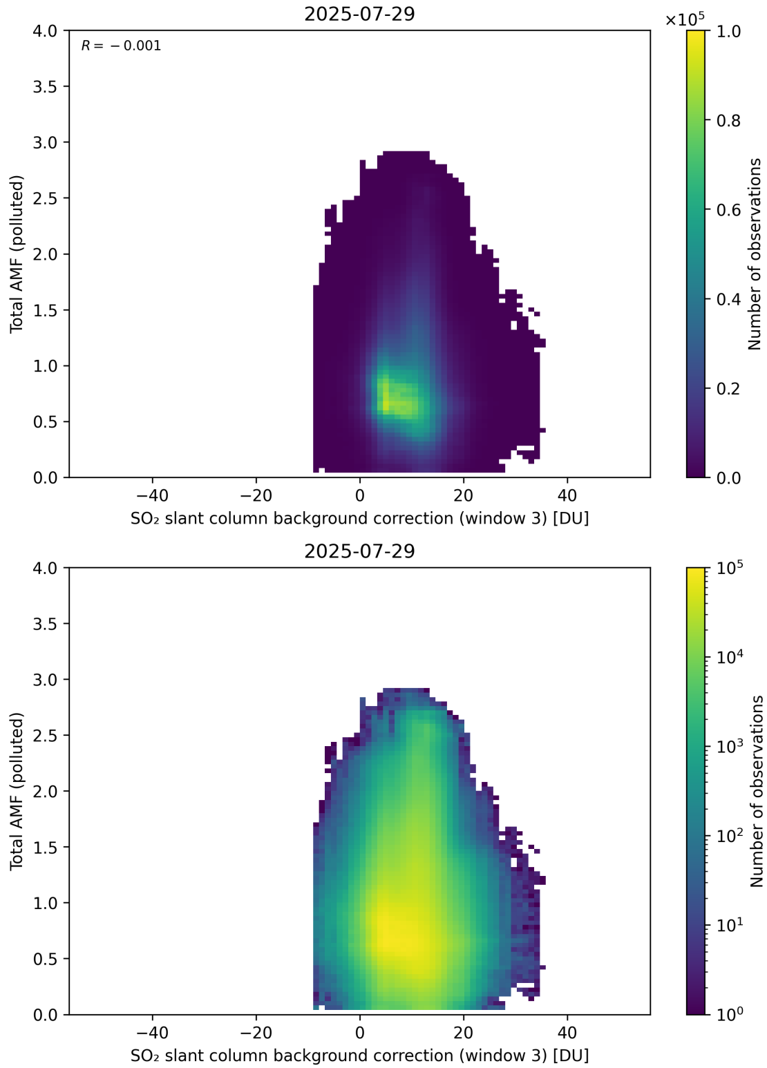
Figure 136: Scatter density plot of “SO 2 slant column background correction (window 3)” against “Total AMF (polluted)” for 2025-07-29 to 2025-07-30.
