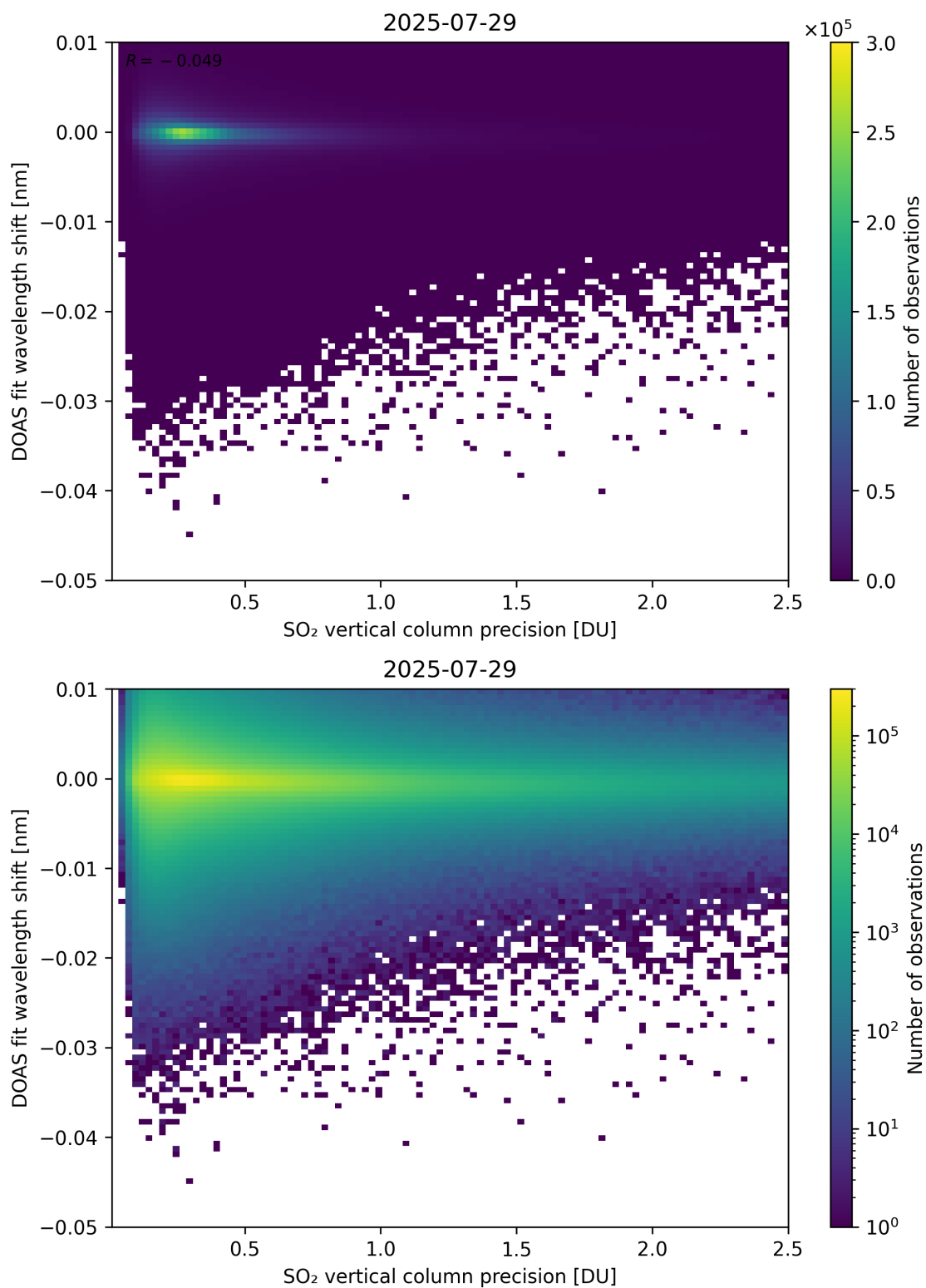
Figure 332: Scatter density plot of “SO 2 vertical column precision” against “DOAS fit wavelength shift” for 2025-07-29 to 2025-07-30.
