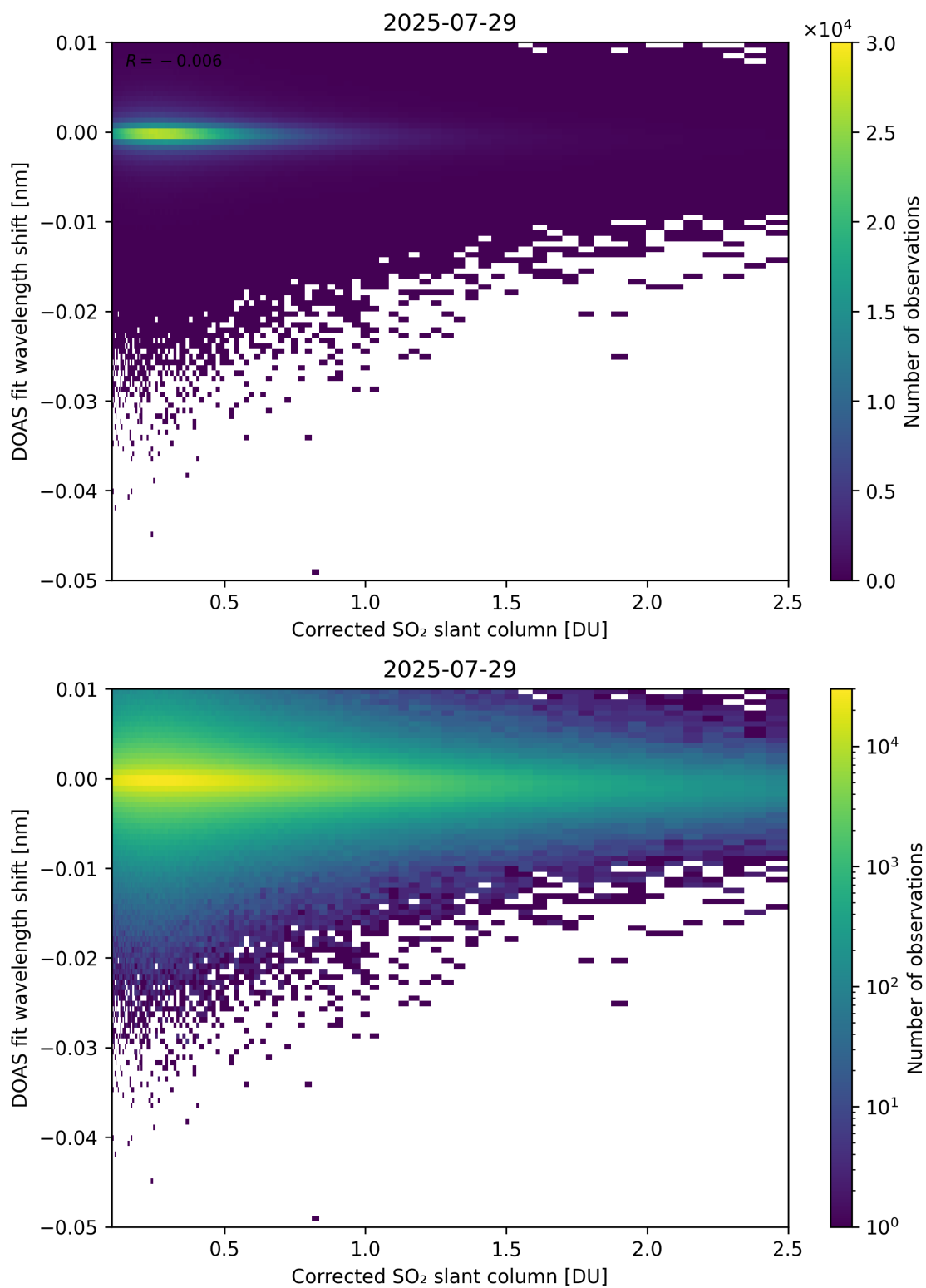
Figure 229: Scatter density plot of “Corrected SO 2 slant column” against “DOAS fit wavelength shift” for 2025-07-29 to 2025-07-30.
