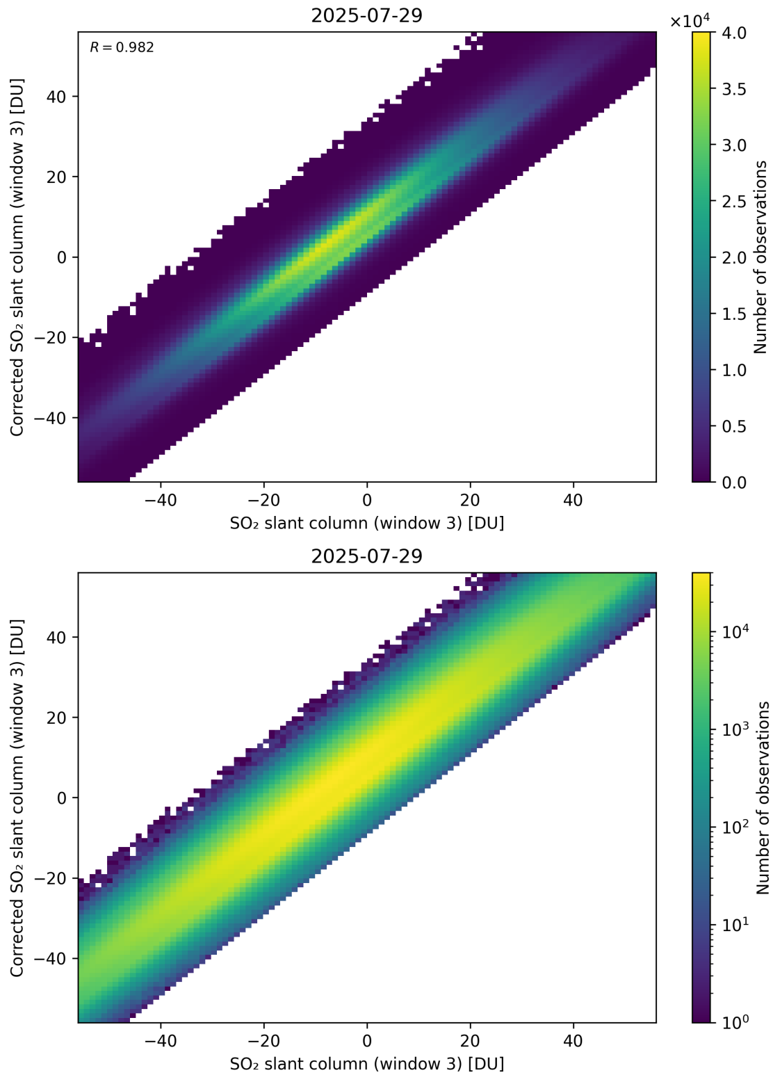
Figure 316: Scatter density plot of “SO 2 slant column (window 3)” against “Corrected SO 2 slant column (window 3)” for 2025-07-29 to 2025-07-30.
