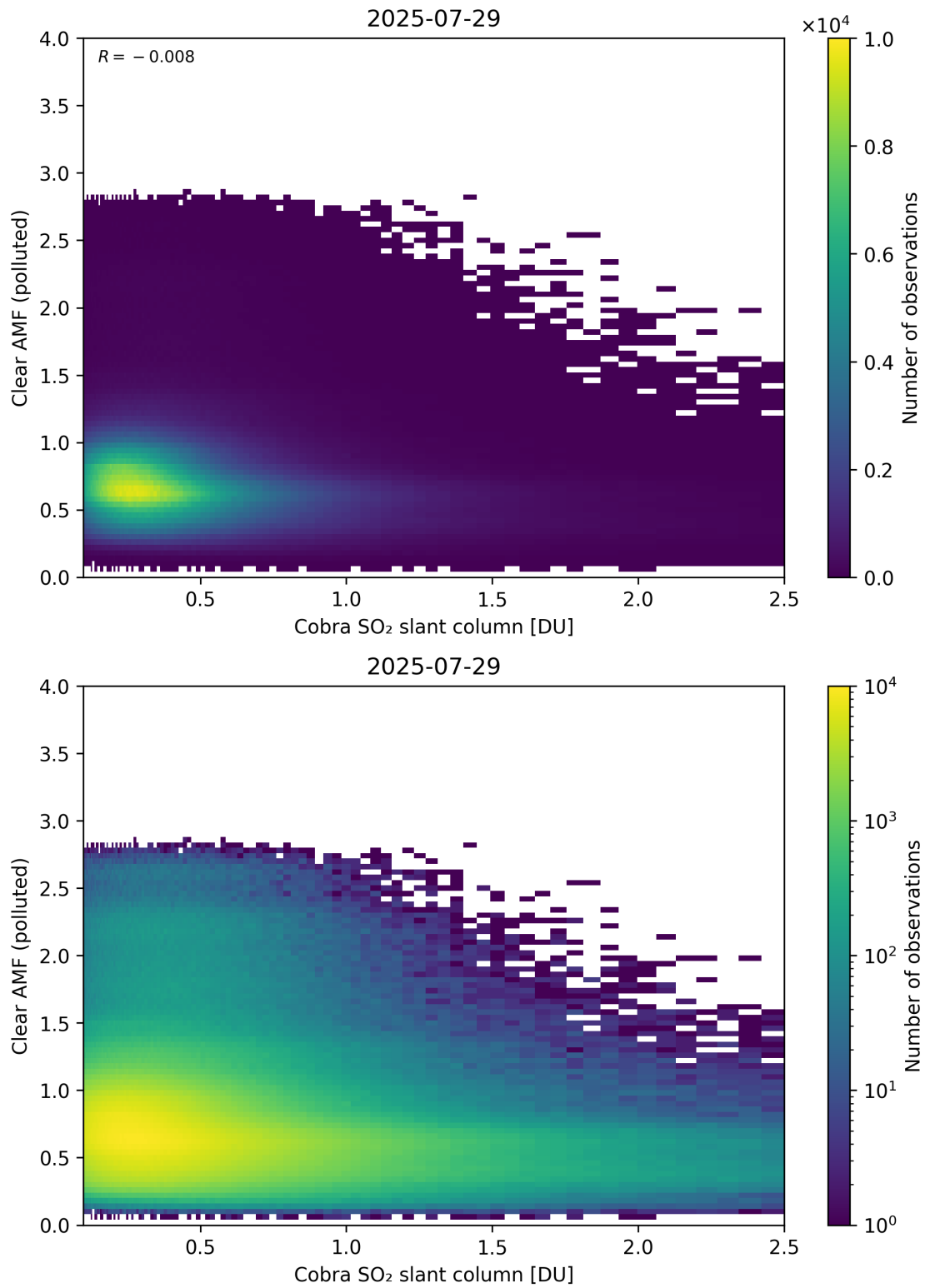
Figure 215: Scatter density plot of “Cobra SO 2 slant column” against “Clear AMF (polluted)” for 2025-07-29 to 2025-07-30.
