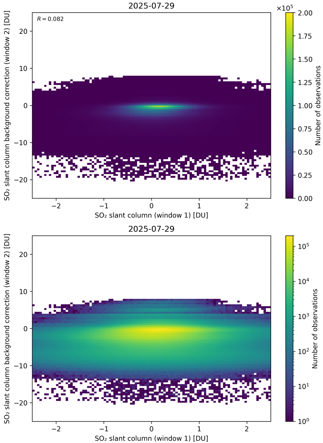
Figure 263: Scatter density plot of “SO 2 slant column (window 1)” against “SO 2 slant column background correction (window 2)” for 2025-07-29 to 2025-07-30.
