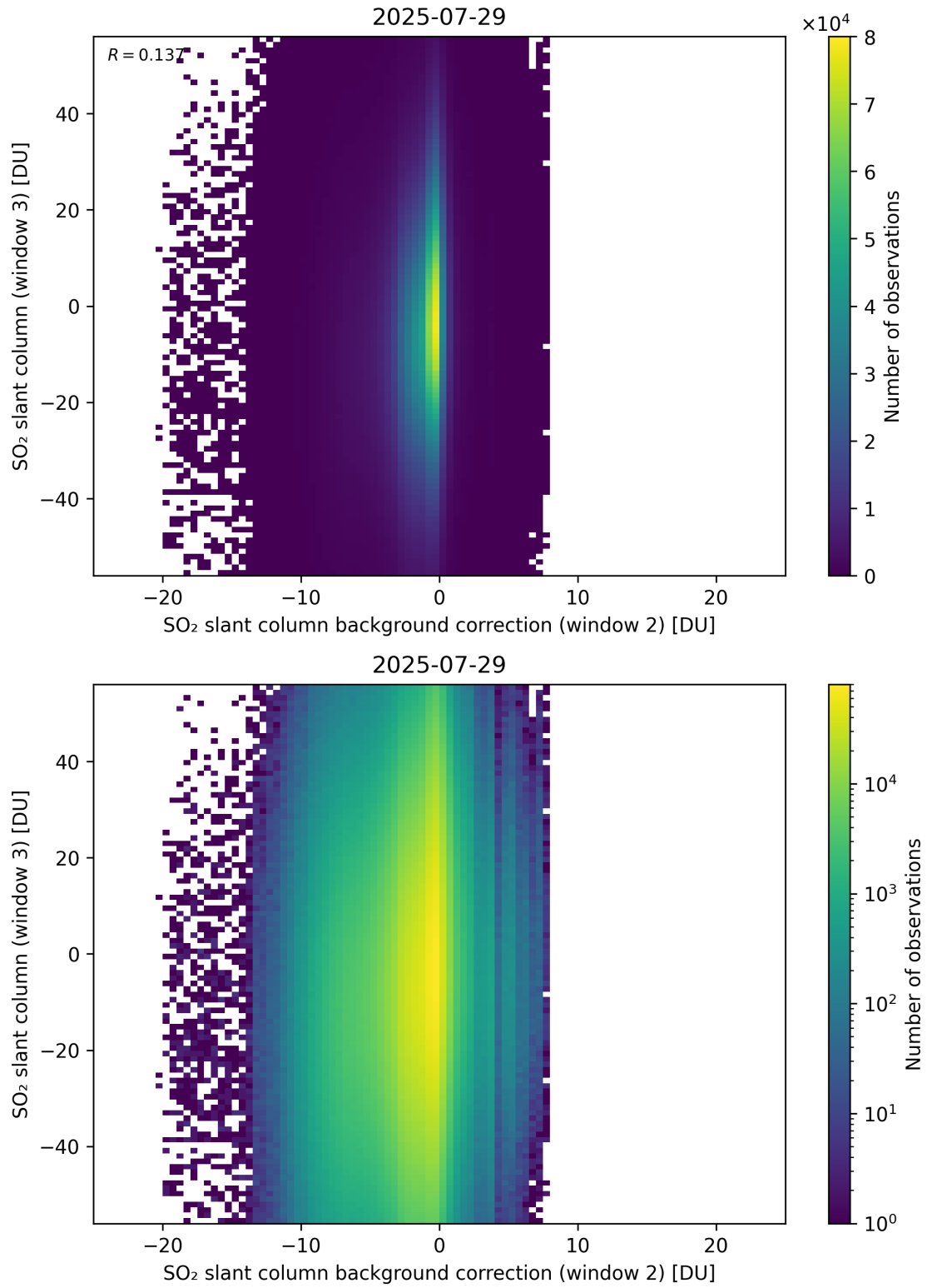
Figure 128: Scatter density plot of “SO 2 slant column background correction (window 2)” against “SO 2 slant column (window 3)” for 2025-07-29 to 2025-07-30.
