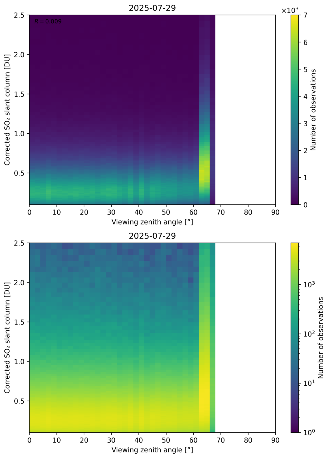
Figure 373: Scatter density plot of “Viewing zenith angle” against “Corrected SO 2 slant column” for 2025-07-29 to 2025-07-30.
