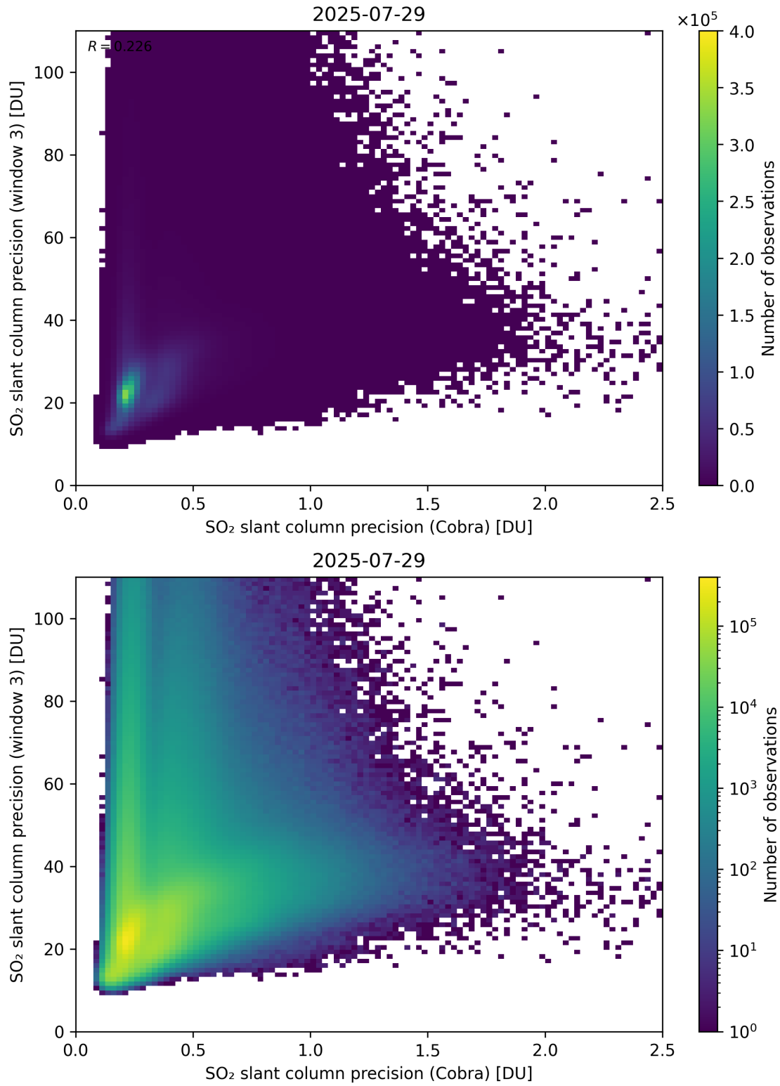
Figure 212: Scatter density plot of “SO 2 slant column precision (Cobra)” against “SO 2 slant column precision (window 3)” for 2025-07-29 to 2025-07-30.
