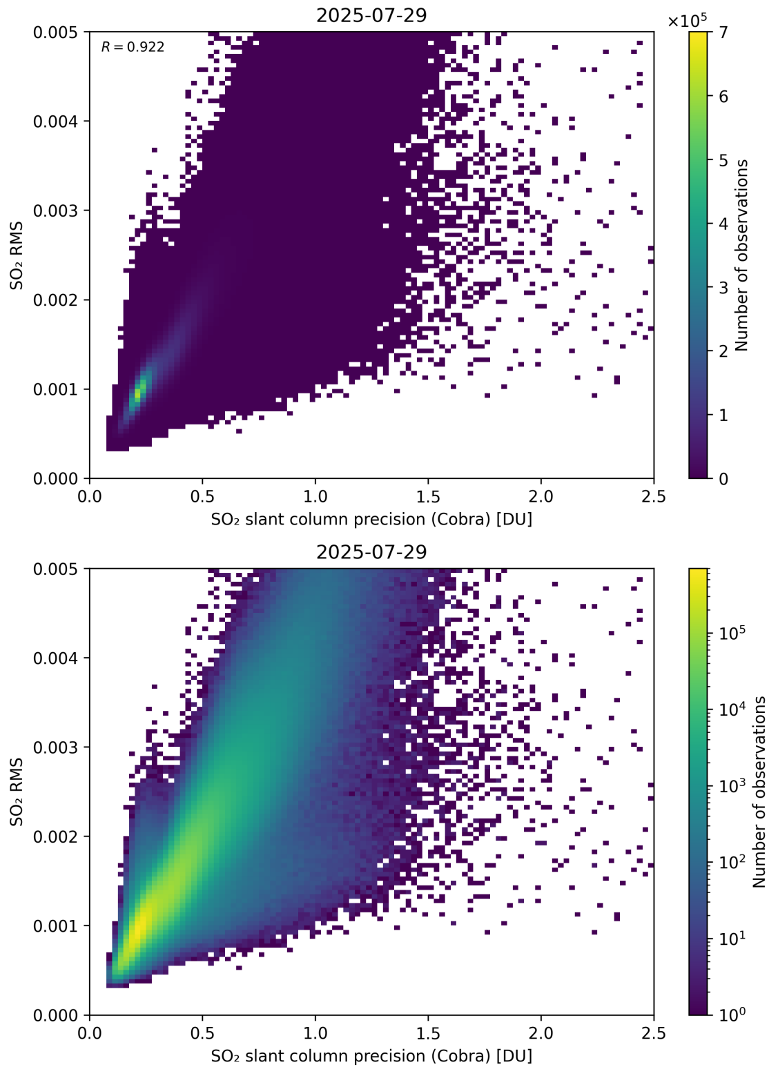
Figure 204: Scatter density plot of “SO 2 slant column precision (Cobra)” against “SO 2 RMS” for 2025-07-29 to 2025-07-30.
