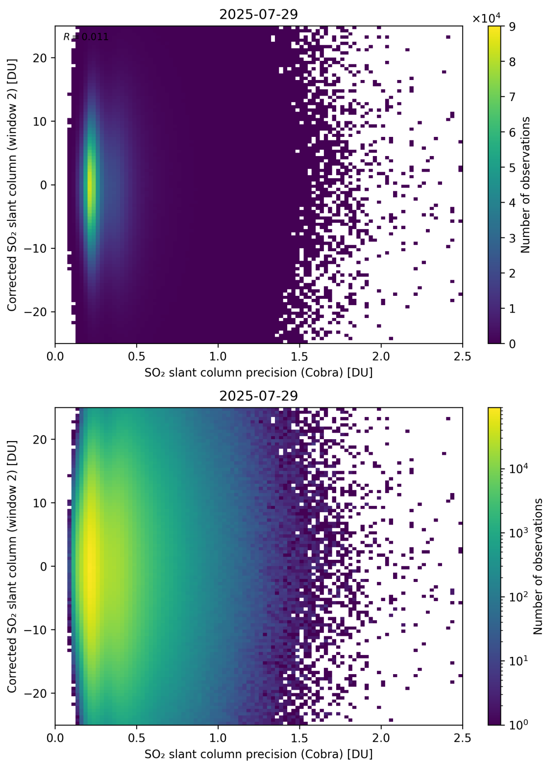
Figure 206: Scatter density plot of “SO 2 slant column precision (Cobra)” against “Corrected SO 2 slant column (window 2)” for 2025-07-29 to 2025-07-30.
