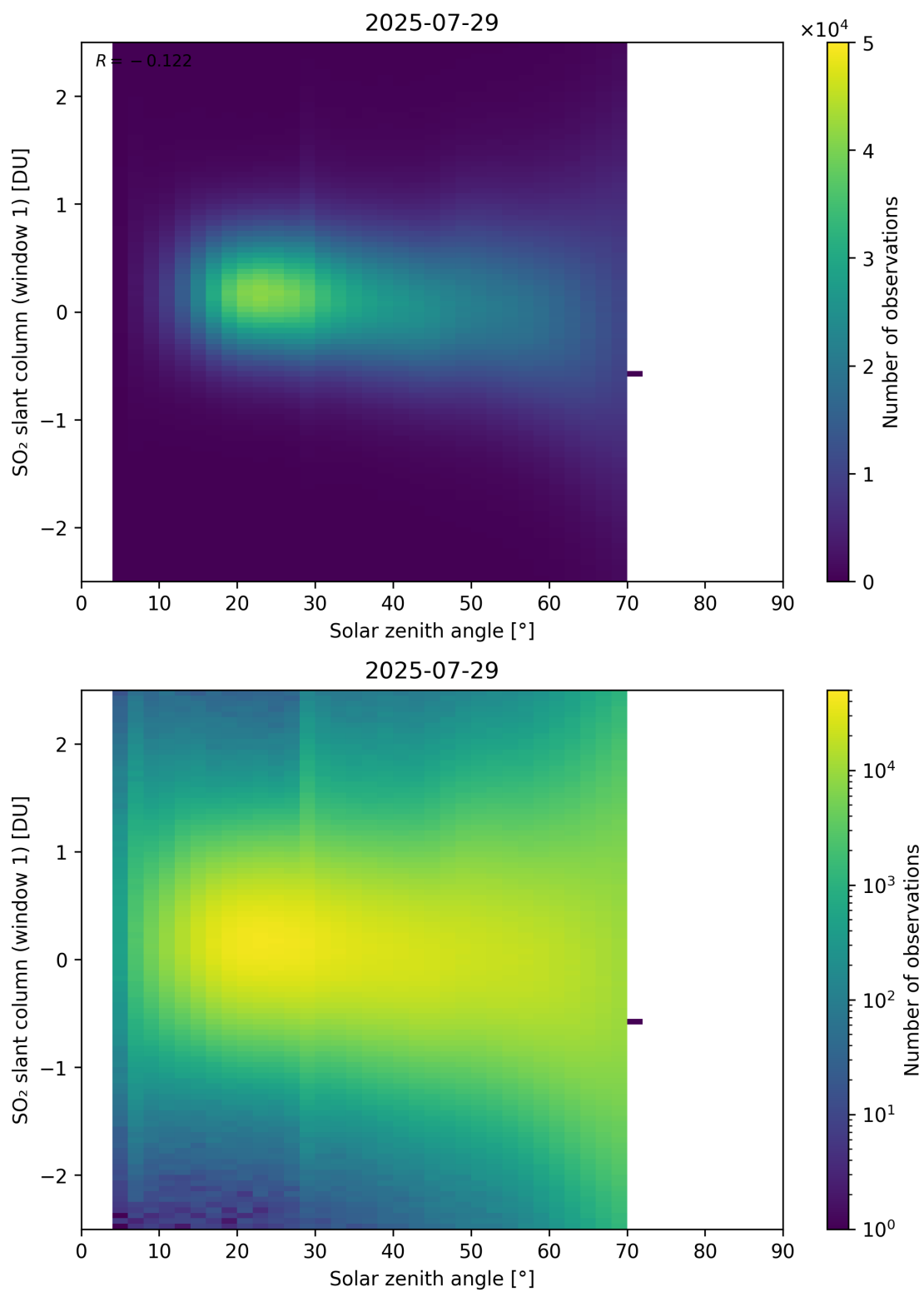
Figure 184: Scatter density plot of “Solar zenith angle” against “SO 2 slant column (window 1)” for 2025-07-29 to 2025-07-30.
