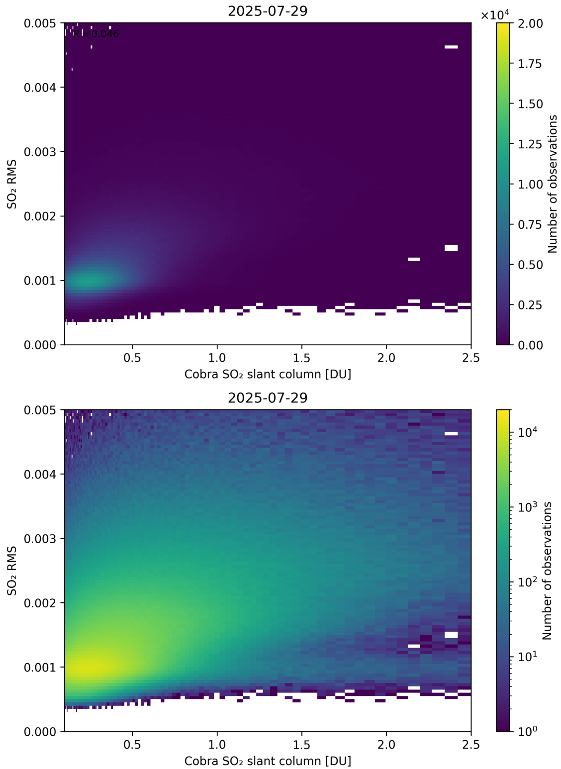
Figure 198: Scatter density plot of “Cobra SO 2 slant column” against “SO 2 RMS” for 2025-07-29 to 2025-07-30.
