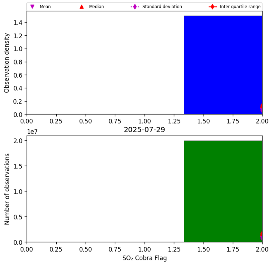
Figure 75: Histogram of “SO 2 Cobra Flag” for 2025-07-29 to 2025-07-30
