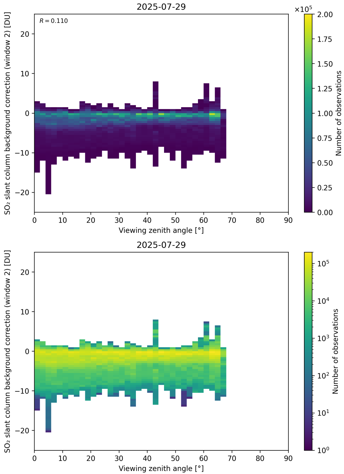
Figure 363: Scatter density plot of “Viewing zenith angle” against “SO 2 slant column background correction (window 2)” for 2025-07-29 to 2025-07-30.
