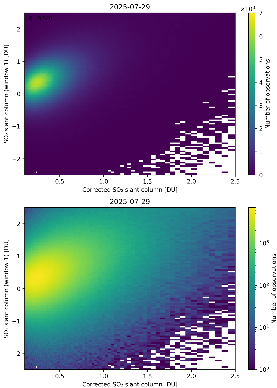
Figure 237: Scatter density plot of “Corrected SO 2 slant column” against “SO 2 slant column (window 1)” for 2025-07-29 to 2025-07-30.
