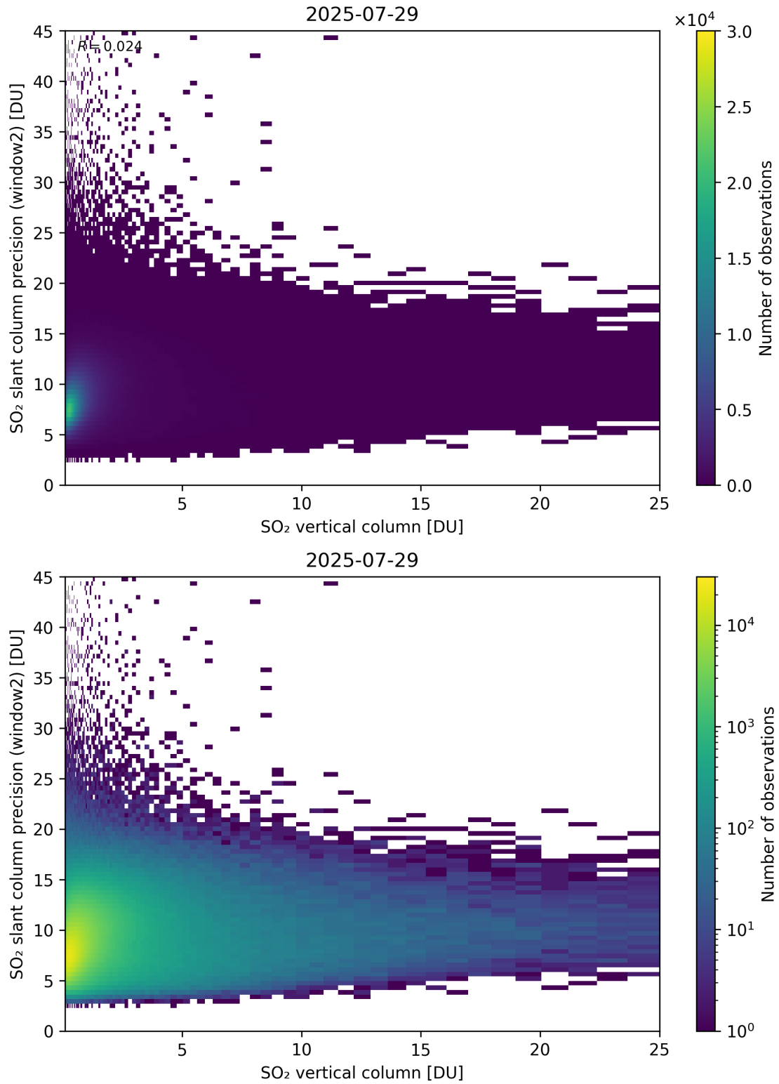
Figure 356: Scatter density plot of “SO 2 vertical column” against “SO 2 slant column precision (window2)” for 2025-07-29 to 2025-07-30.
