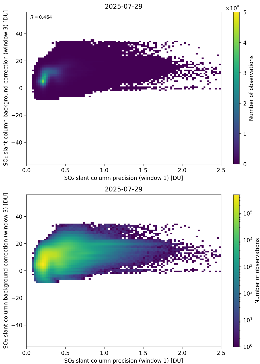
Figure 270: Scatter density plot of “SO 2 slant column precision (window 1)” against “SO 2 slant column background correction (window 3)” for 2025-07-29 to 2025-07-30.
