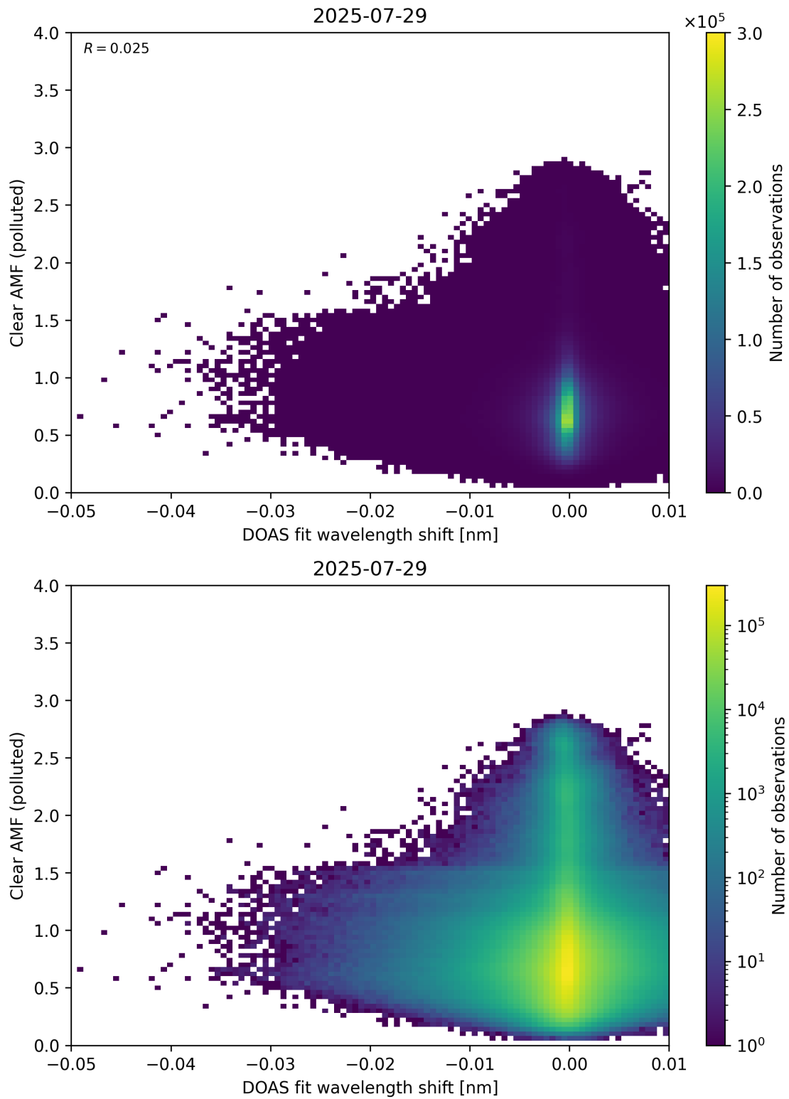
Figure 140: Scatter density plot of “DOAS fit wavelength shift” against “Clear AMF (polluted)” for 2025-07-29 to 2025-07-30.
