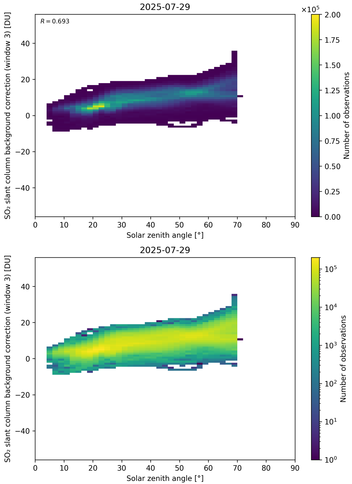
Figure 173: Scatter density plot of “Solar zenith angle” against “SO 2 slant column background correction (window 3)” for 2025-07-29 to 2025-07-30.
