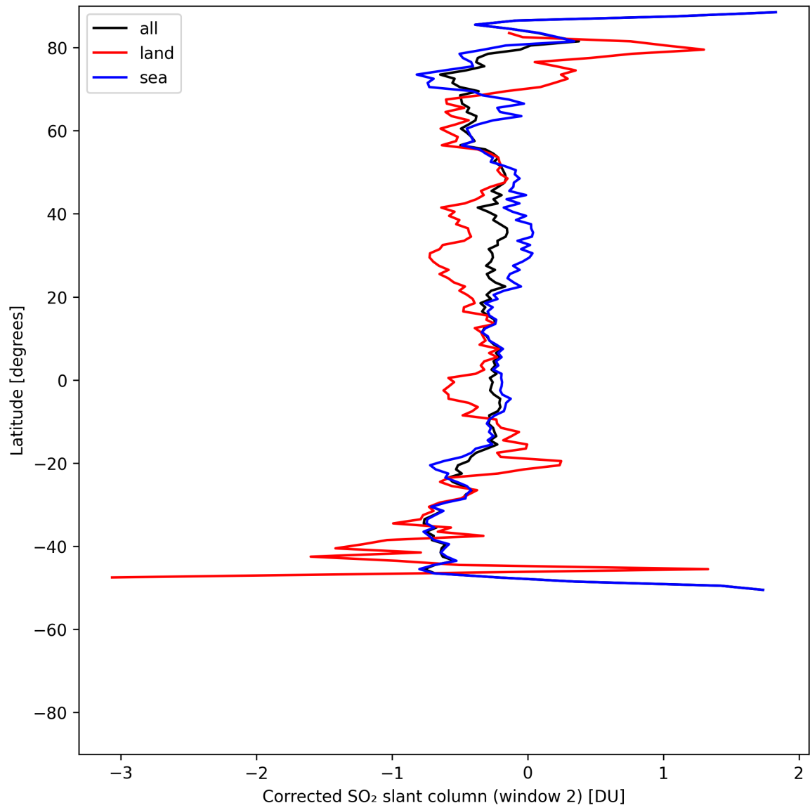
Figure 43: Zonal average of “Corrected SO 2 slant column (window 2)” for 2025-07-29 to 2025-07-30.
