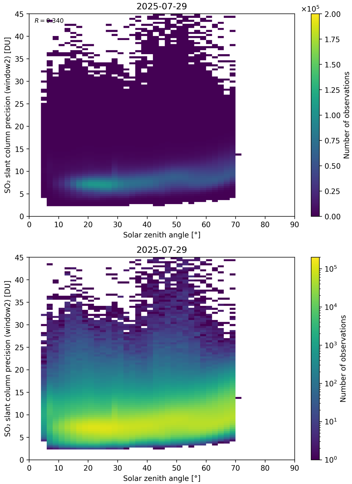
Figure 186: Scatter density plot of “Solar zenith angle” against “SO 2 slant column precision (window2)” for 2025-07-29 to 2025-07-30.
