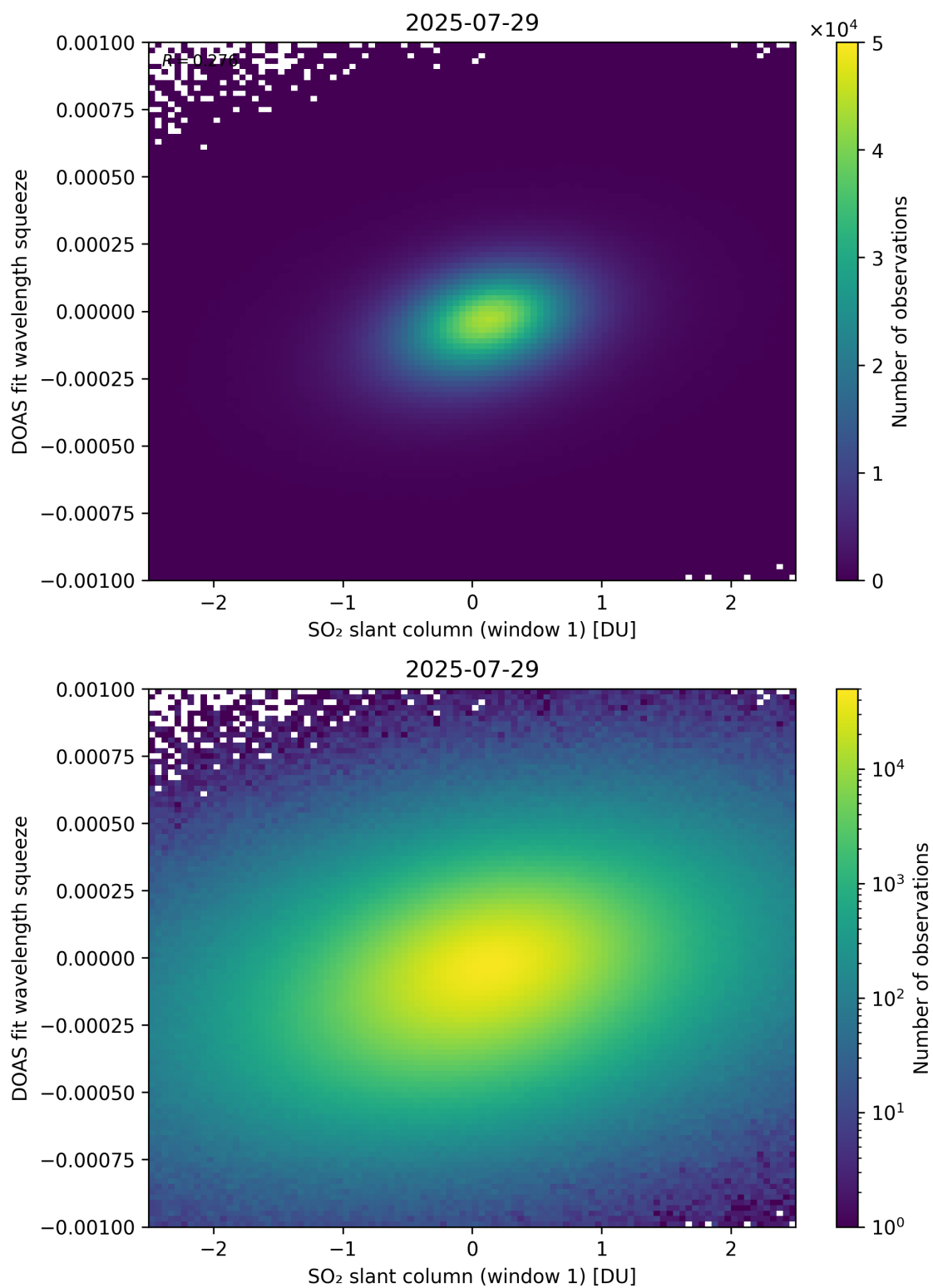
Figure 266: Scatter density plot of “SO 2 slant column (window 1)” against “DOAS fit wavelength squeeze” for 2025-07-29 to 2025-07-30.
