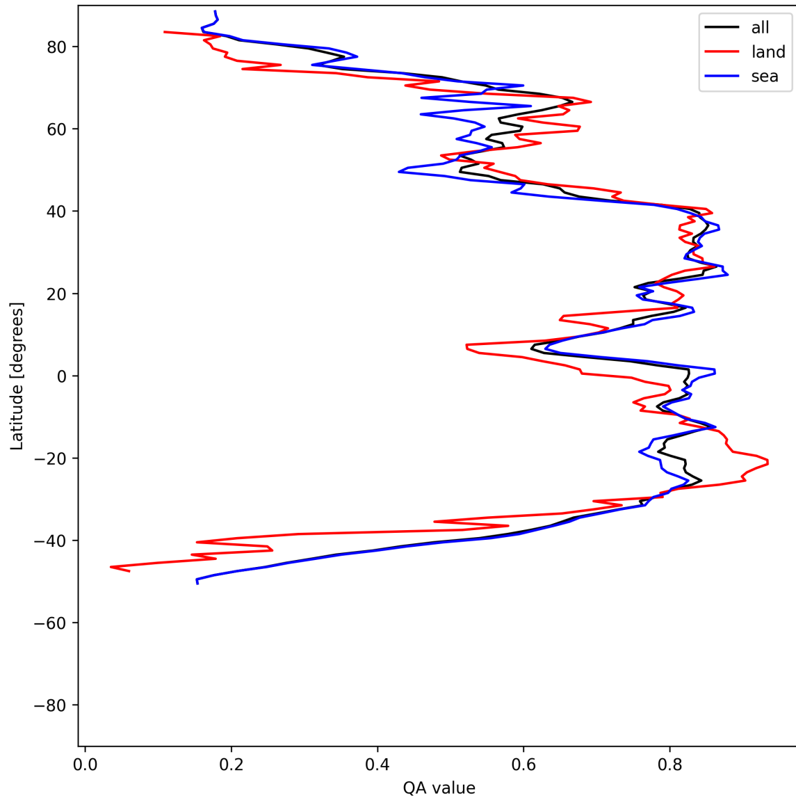
Figure 31: Zonal average of “QA value” for 2025-07-29 to 2025-07-30.
