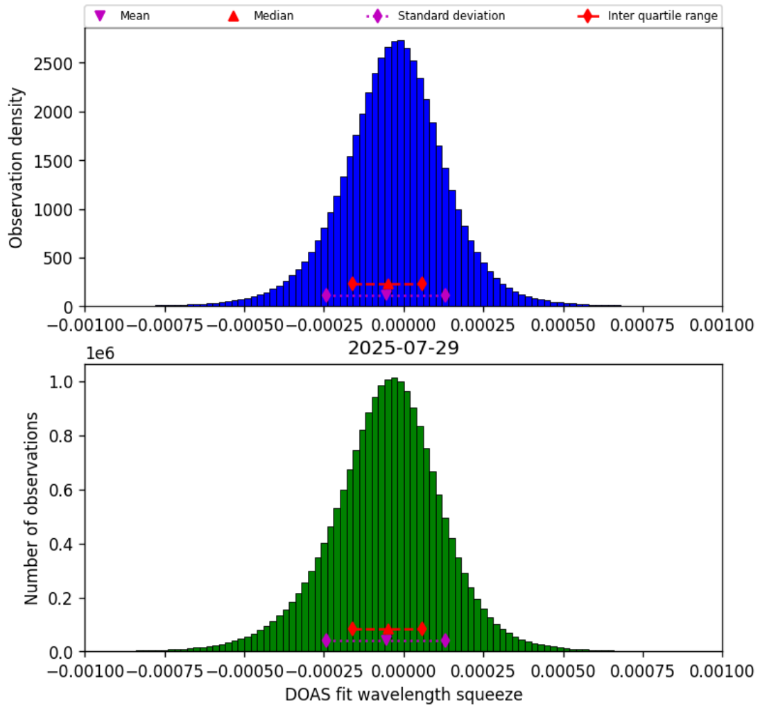
Figure 77: Histogram of “DOAS fit wavelength squeeze” for 2025-07-29 to 2025-07-30
