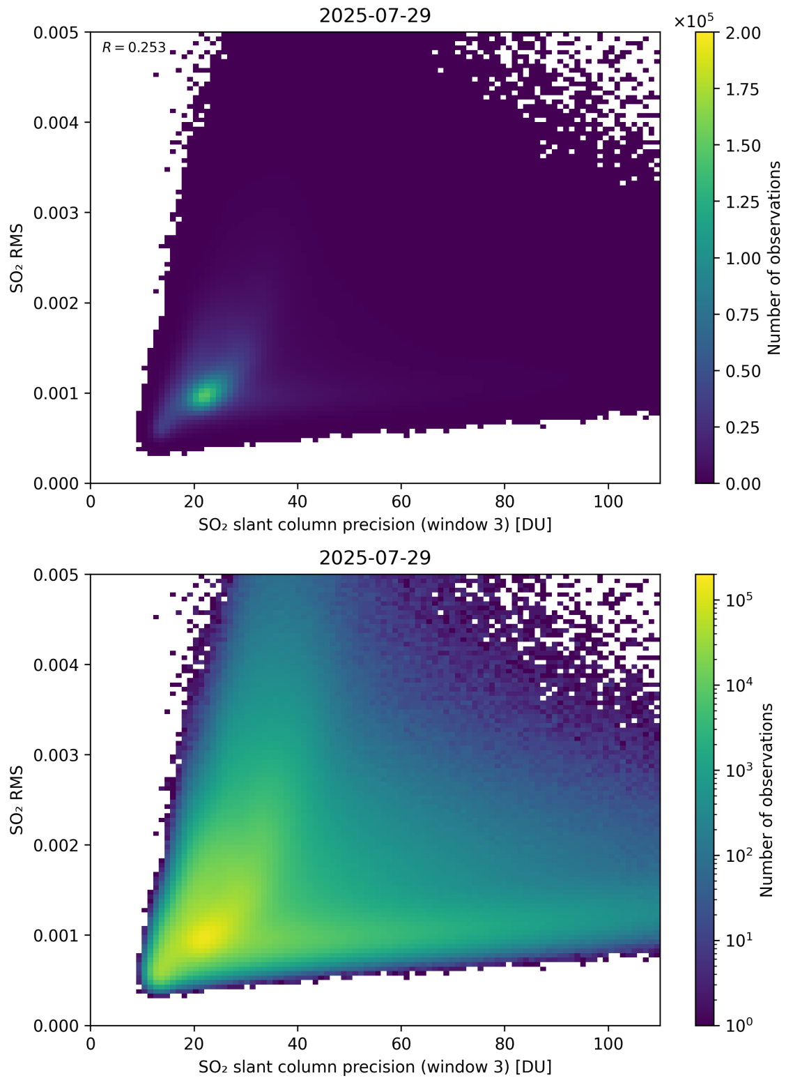
Figure 310: Scatter density plot of “SO 2 slant column precision (window 3)” against “SO 2 RMS” for 2025-07-29 to 2025-07-30.
