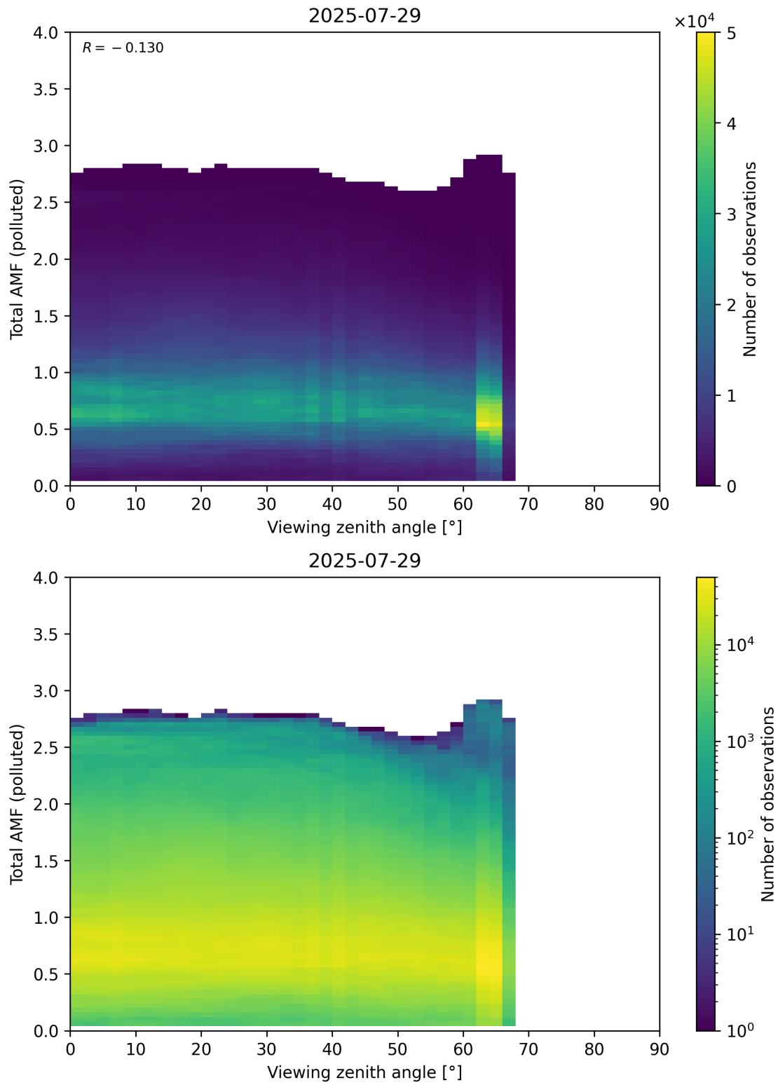
Figure 381: Scatter density plot of “Viewing zenith angle” against “Total AMF (polluted)” for 2025-07-29 to 2025-07-30.
