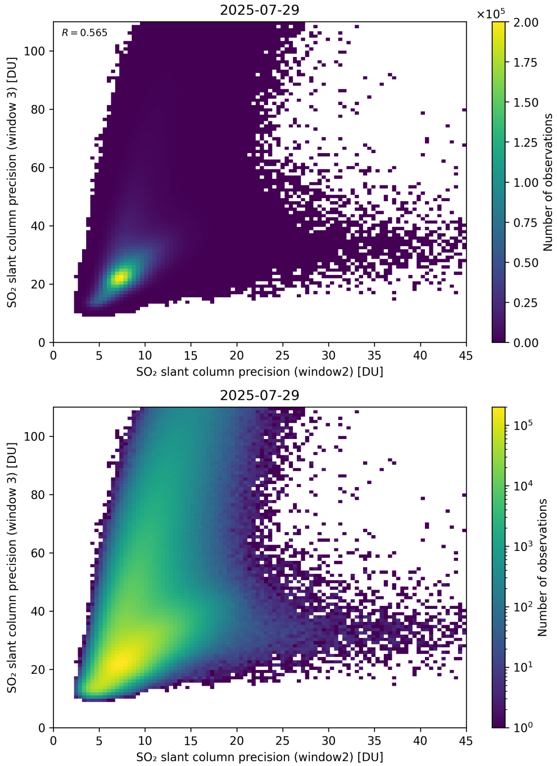
Figure 300: Scatter density plot of “SO 2 slant column precision (window2)” against “SO 2 slant column precision (window 3)” for 2025-07-29 to 2025-07-30.
