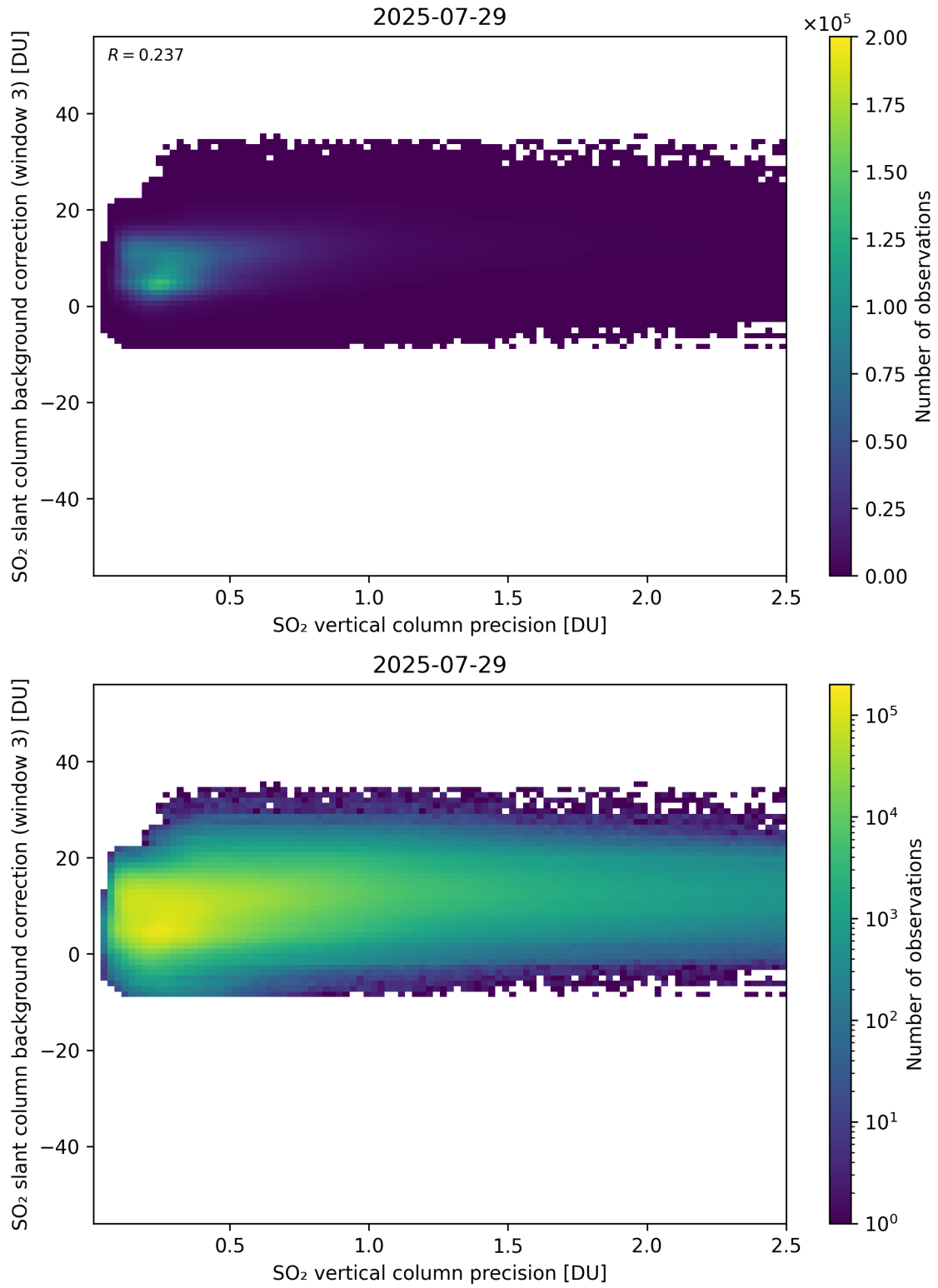
Figure 331: Scatter density plot of “SO 2 vertical column precision” against “SO 2 slant column background correction (window 3)” for 2025-07-29 to 2025-07-30.
