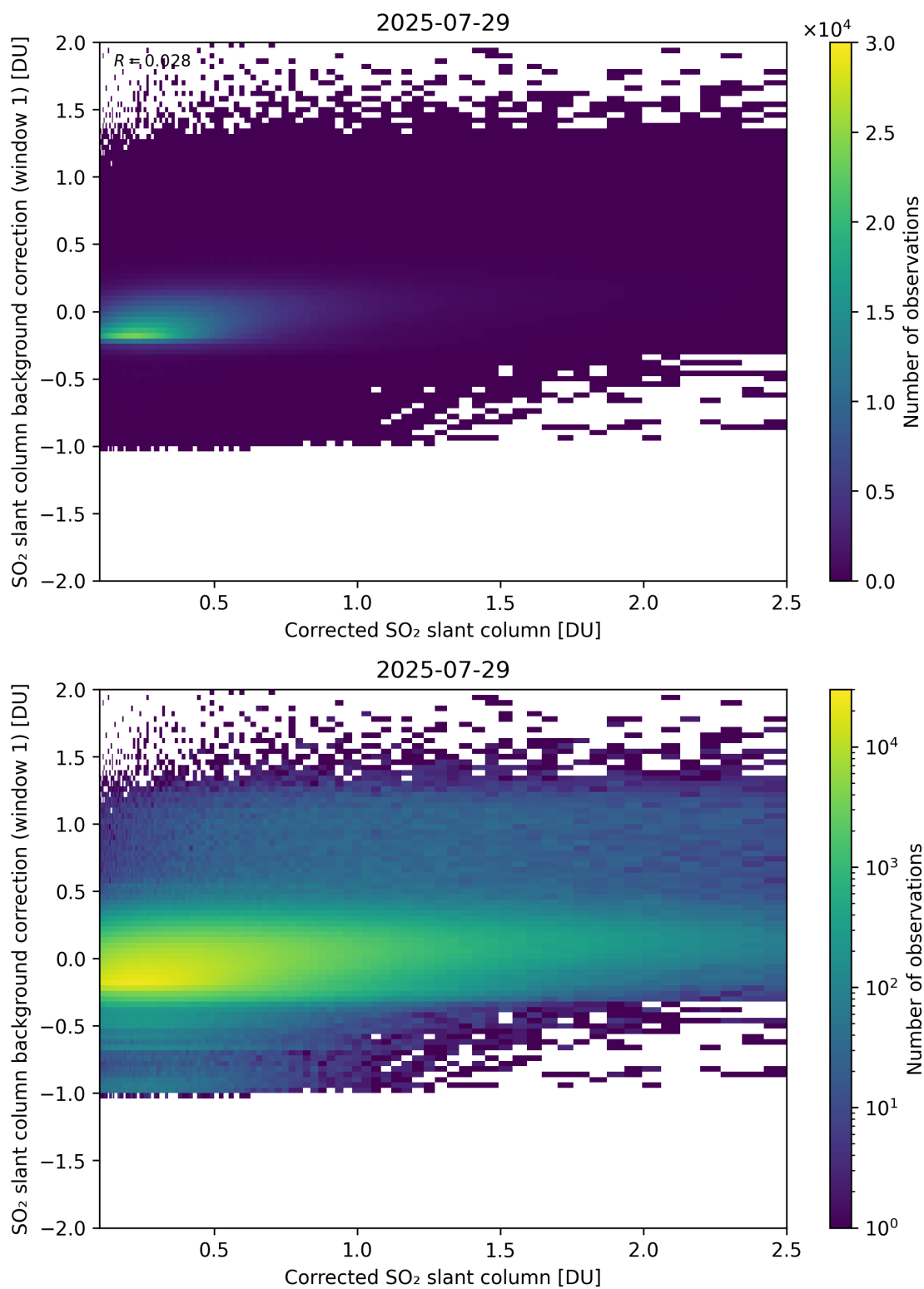
Figure 226: Scatter density plot of “Corrected SO 2 slant column” against “SO 2 slant column background correction (window 1)” for 2025-07-29 to 2025-07-30.
