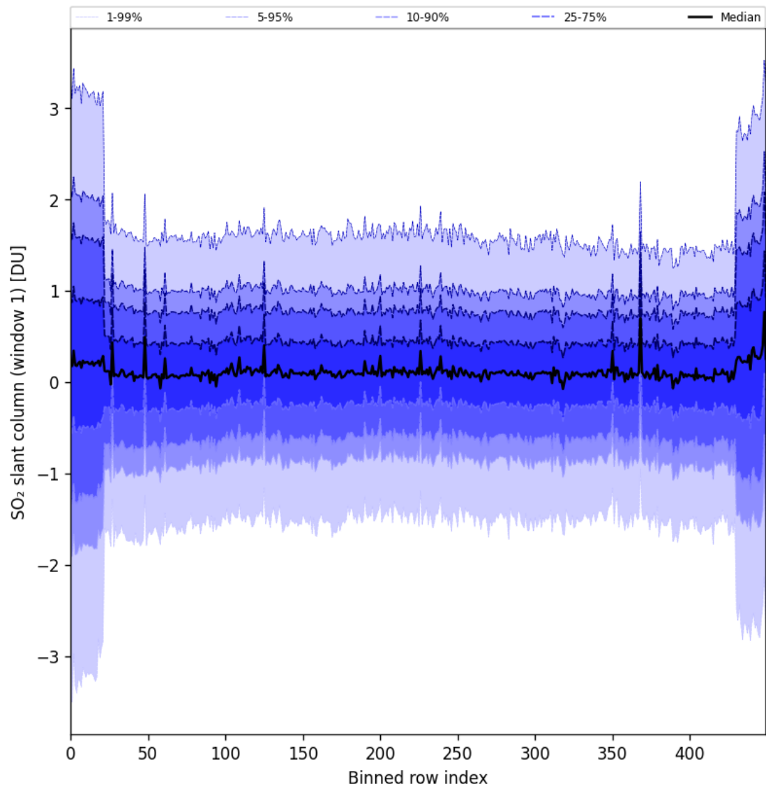
Figure 89: Along track statistics of “SO 2 slant column (window 1)” for 2025-07-29 to 2025-07-30
