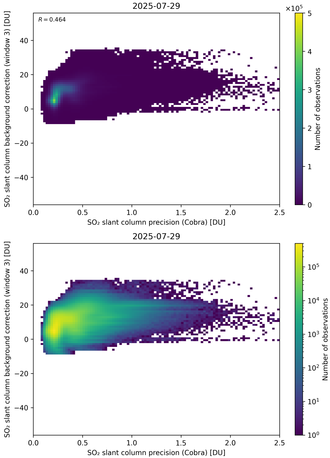
Figure 201: Scatter density plot of “SO 2 slant column precision (Cobra)” against “SO 2 slant column background correction (window 3)” for 2025-07-29 to 2025-07-30.
