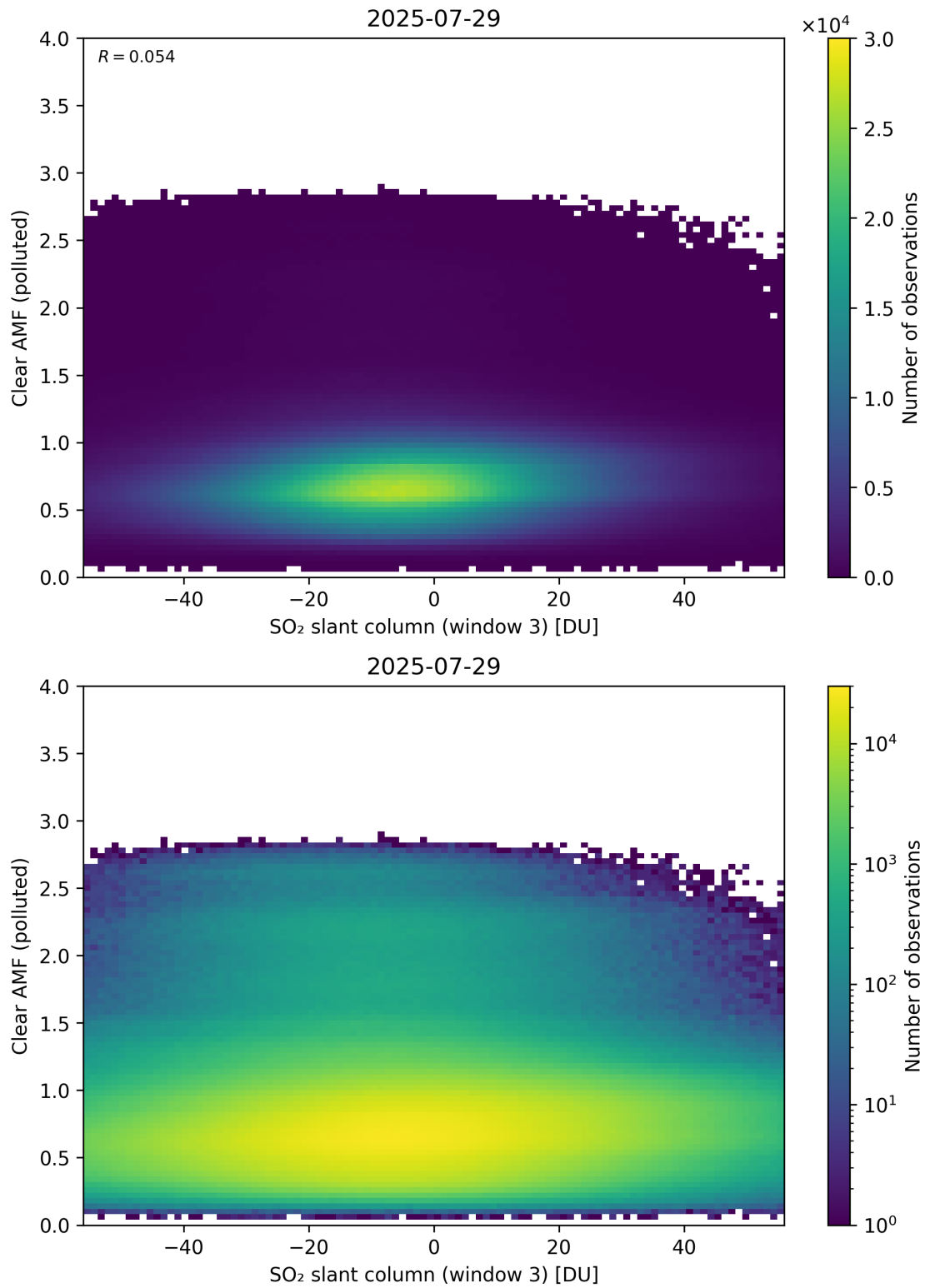
Figure 315: Scatter density plot of “SO 2 slant column (window 3)” against “Clear AMF (polluted)” for 2025-07-29 to 2025-07-30.
