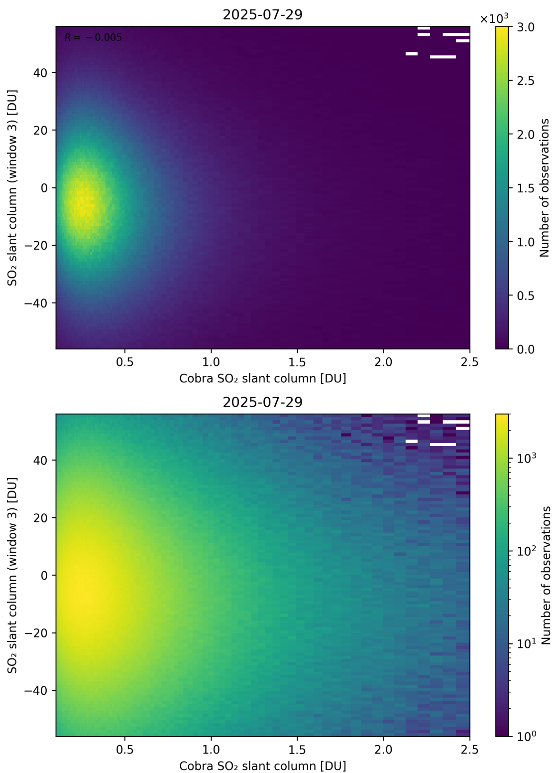
Figure 222: Scatter density plot of “Cobra SO 2 slant column” against “SO 2 slant column (window 3)” for 2025-07-29 to 2025-07-30.
