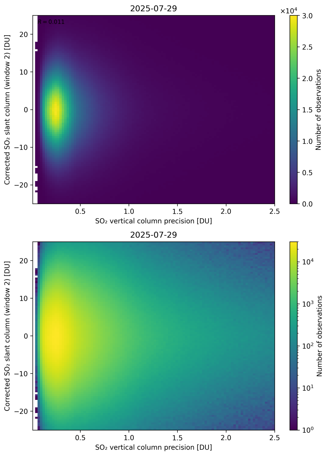
Figure 339: Scatter density plot of “SO 2 vertical column precision” against “Corrected SO 2 slant column (window 2)” for 2025-07-29 to 2025-07-30.
