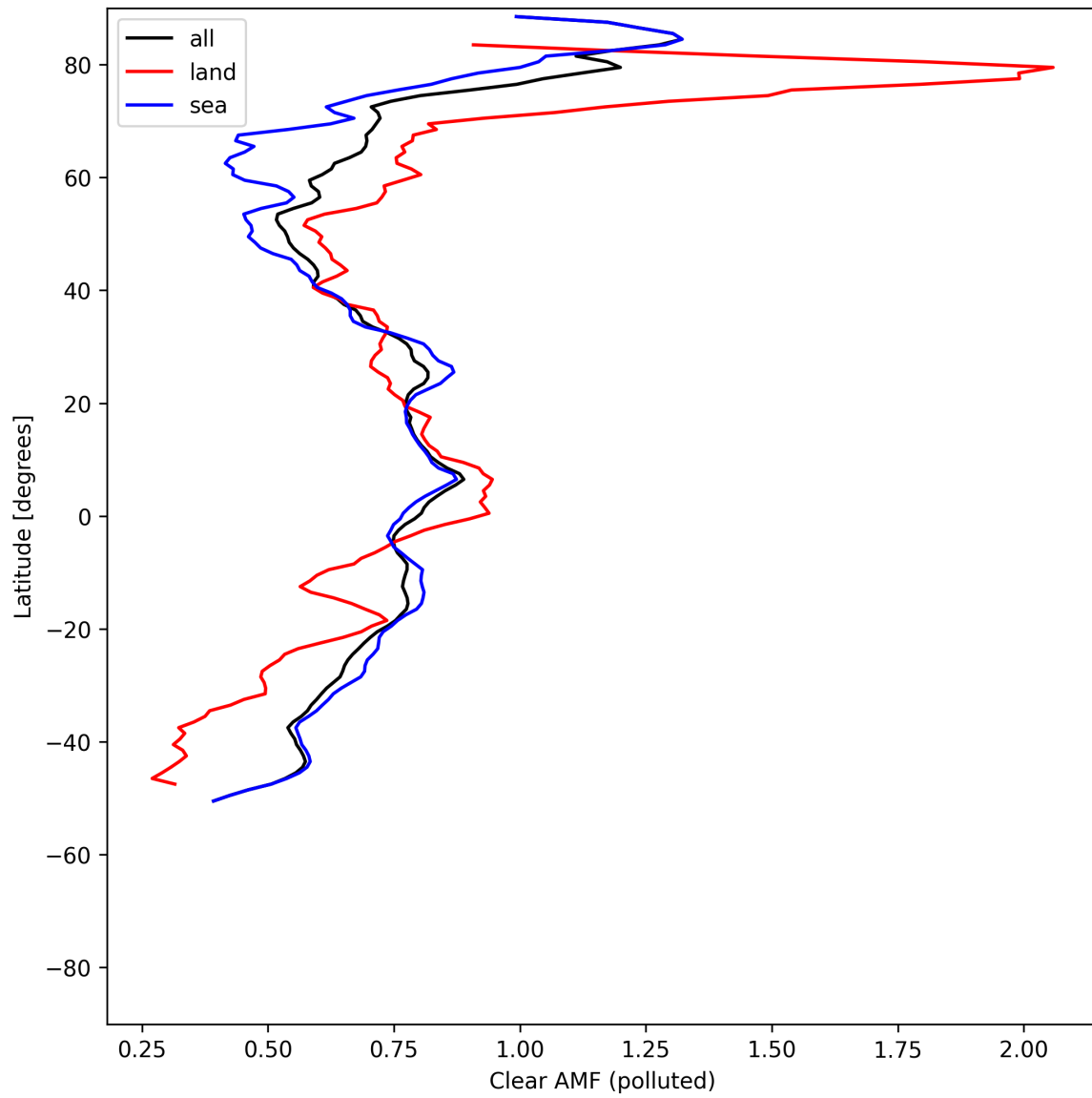
Figure 55: Zonal average of “Clear AMF (polluted)” for 2025-07-29 to 2025-07-30.
