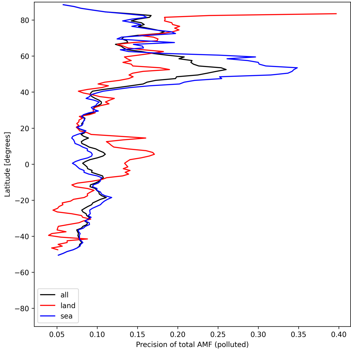
Figure 54: Zonal average of “Precision of total AMF (polluted)” for 2025-07-29 to 2025-07-30.
