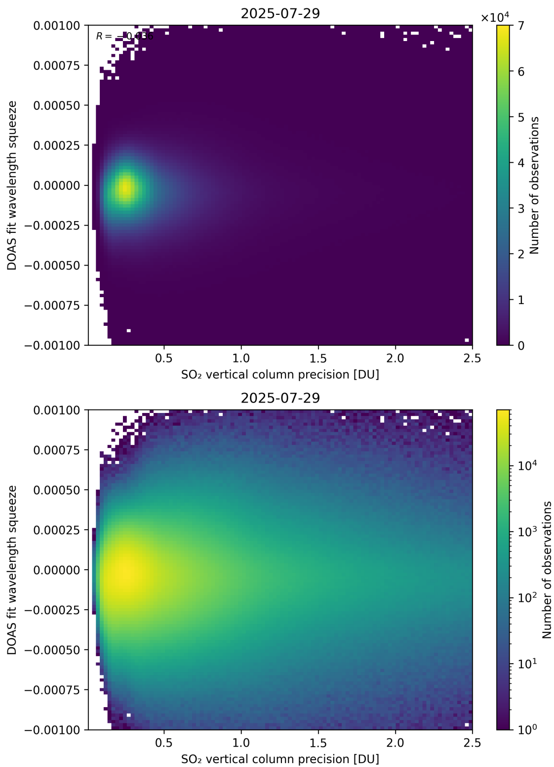
Figure 333: Scatter density plot of “SO 2 vertical column precision” against “DOAS fit wavelength squeeze” for 2025-07-29 to 2025-07-30.
