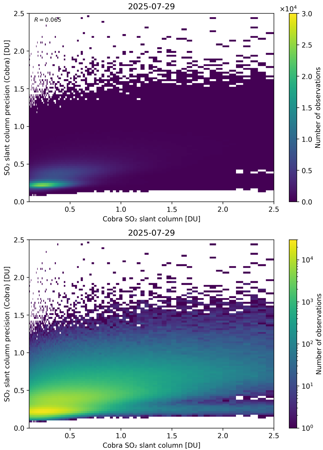
Figure 216: Scatter density plot of “Cobra SO 2 slant column” against “SO 2 slant column precision (Cobra)” for 2025-07-29 to 2025-07-30.
