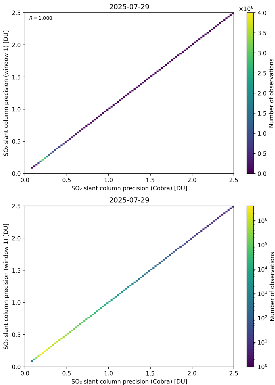
Figure 209: Scatter density plot of “SO 2 slant column precision (Cobra)” against “SO 2 slant column precision (window 1)” for 2025-07-29 to 2025-07-30.
