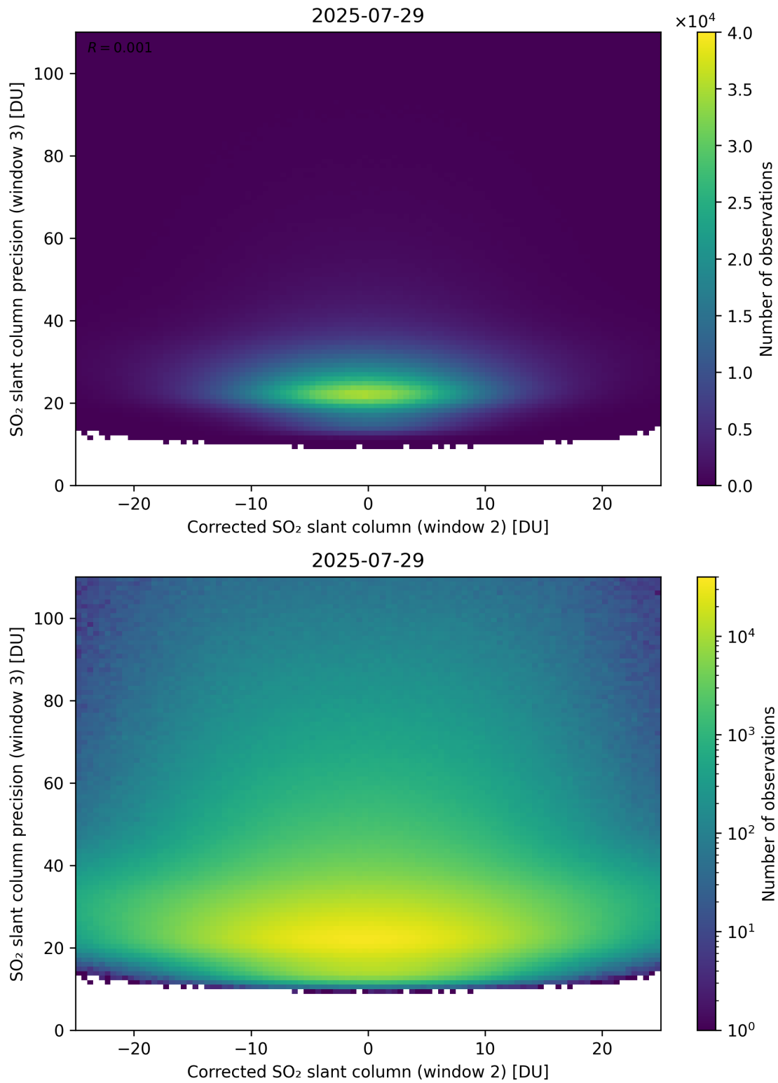
Figure 252: Scatter density plot of “Corrected SO 2 slant column (window 2)” against “SO 2 slant column precision (window 3)” for 2025-07-29 to 2025-07-30.
