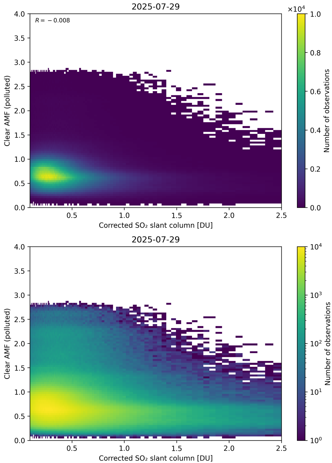
Figure 232: Scatter density plot of “Corrected SO 2 slant column” against “Clear AMF (polluted)” for 2025-07-29 to 2025-07-30.
