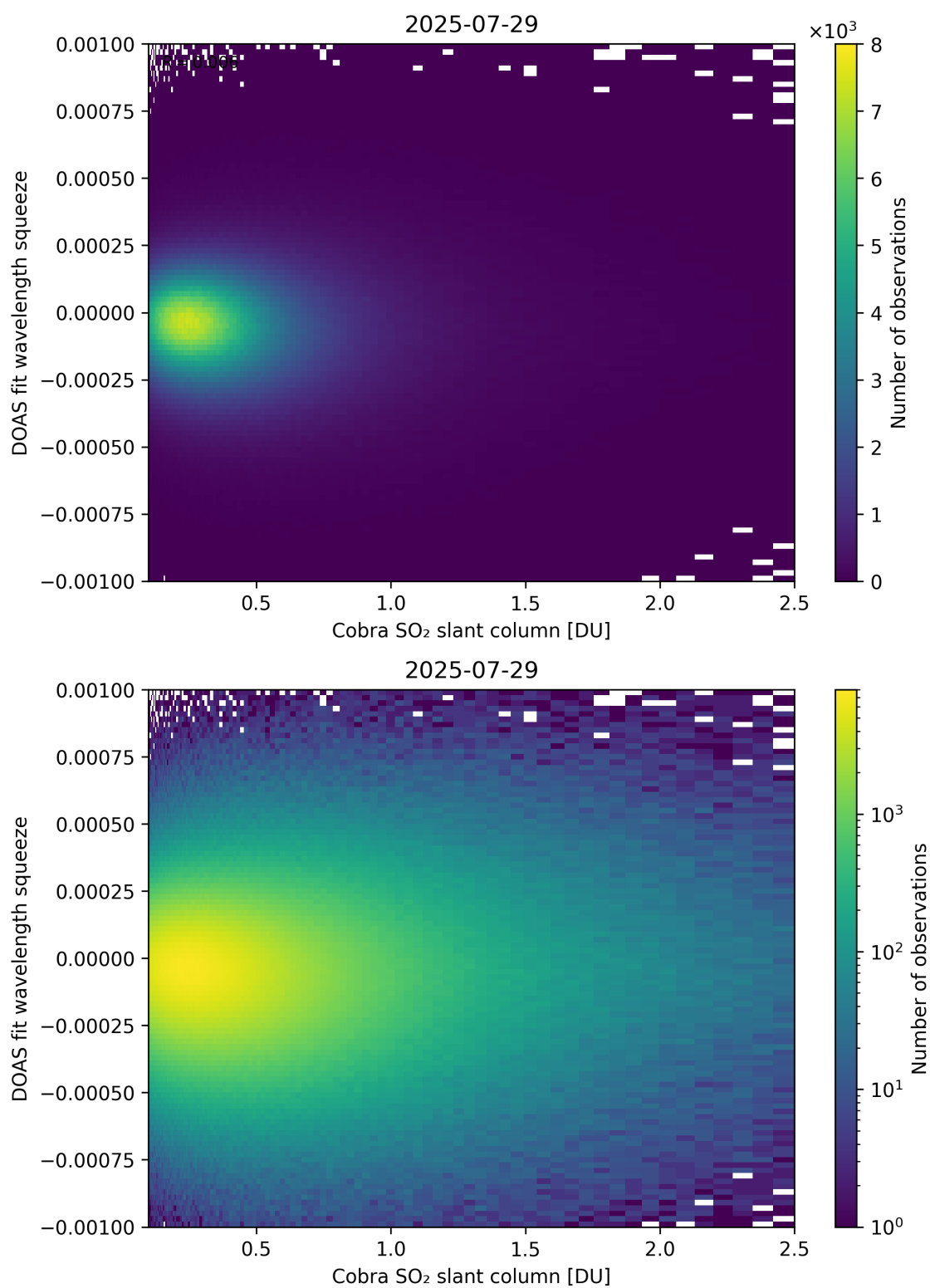
Figure 197: Scatter density plot of “Cobra SO 2 slant column” against “DOAS fit wavelength squeeze” for 2025-07-29 to 2025-07-30.
