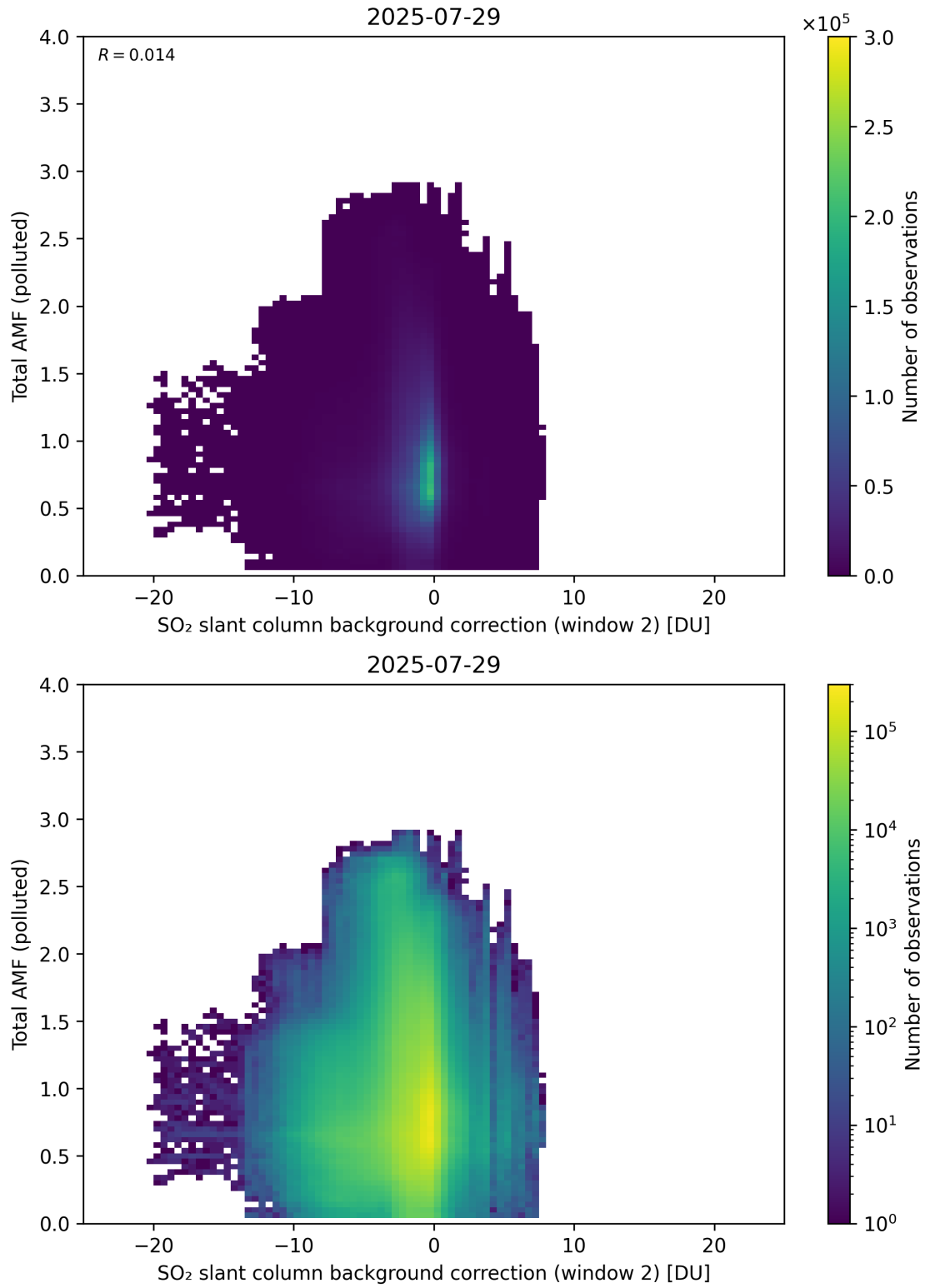
Figure 130: Scatter density plot of “SO 2 slant column background correction (window 2)” against “Total AMF (polluted)” for 2025-07-29 to 2025-07-30.
