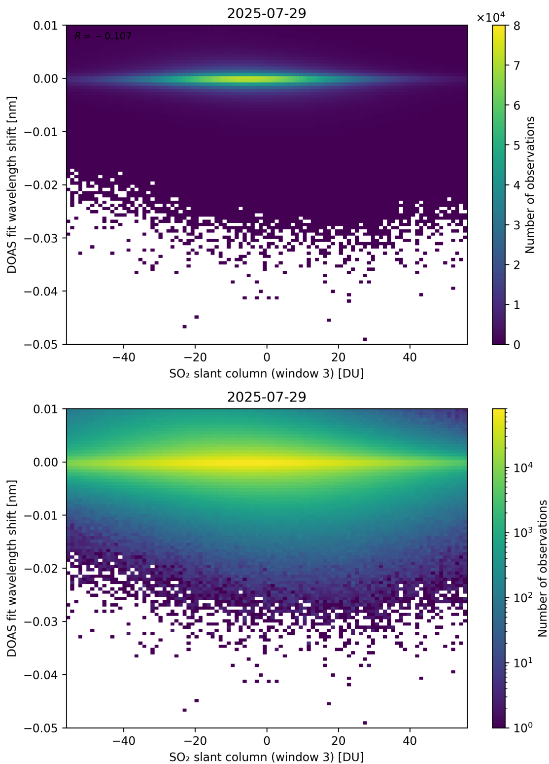
Figure 304: Scatter density plot of “SO 2 slant column (window 3)” against “DOAS fit wavelength shift” for 2025-07-29 to 2025-07-30.
