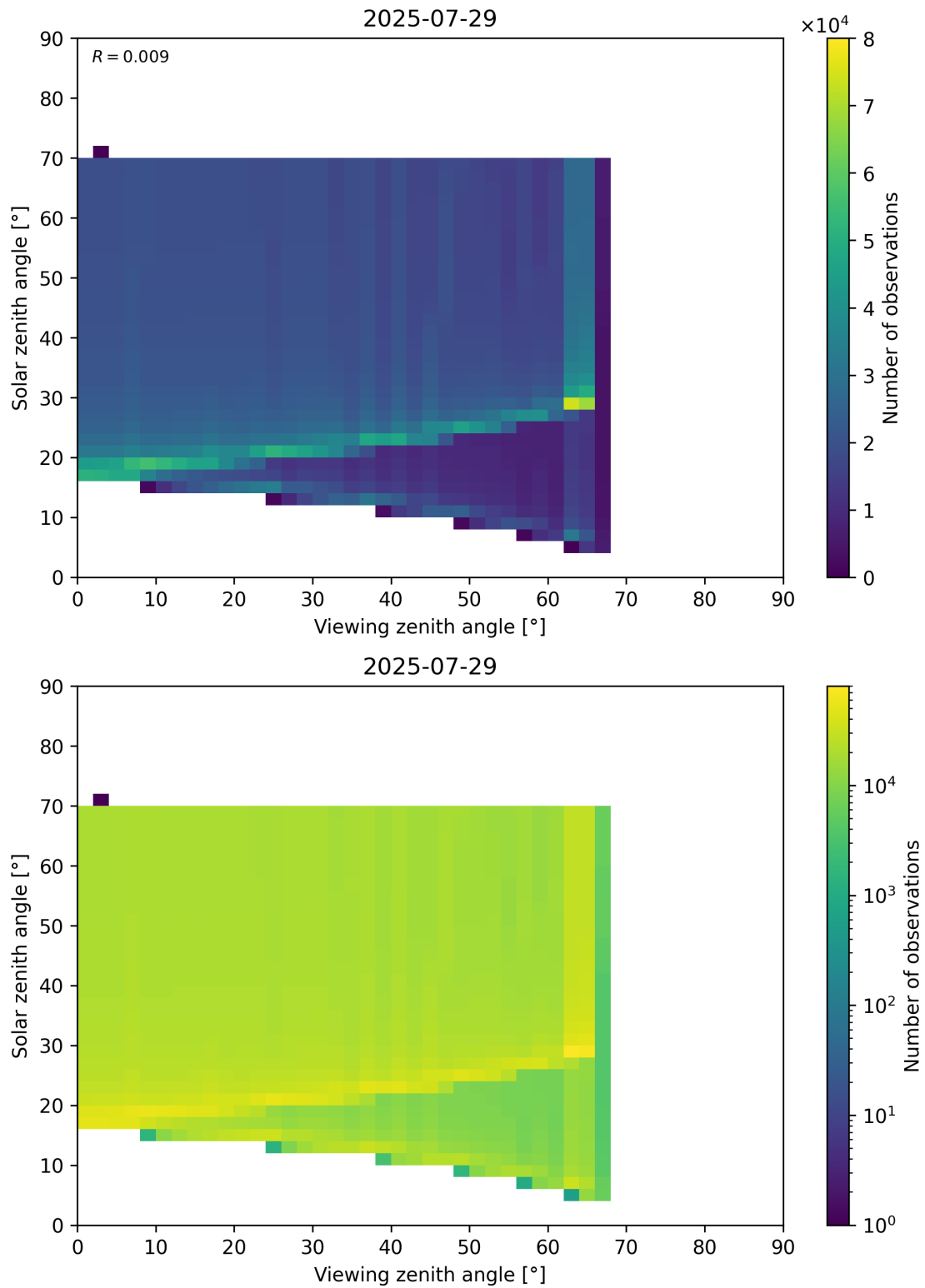
Figure 369: Scatter density plot of “Viewing zenith angle” against “Solar zenith angle” for 2025-07-29 to 2025-07-30.
