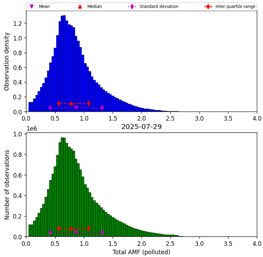
Figure 79: Histogram of “Total AMF (polluted)” for 2025-07-29 to 2025-07-30
