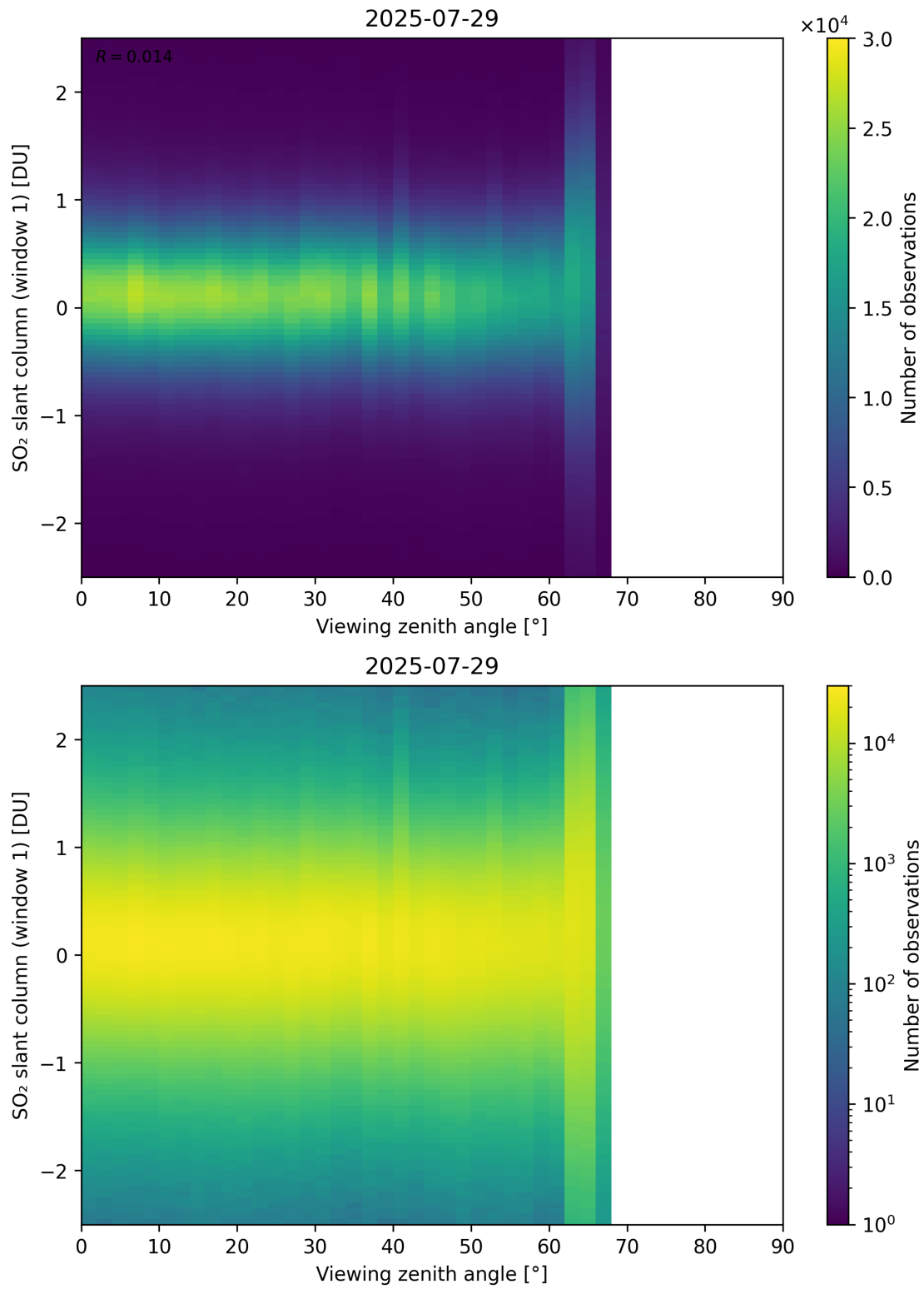
Figure 376: Scatter density plot of “Viewing zenith angle” against “SO 2 slant column (window 1)” for 2025-07-29 to 2025-07-30.
