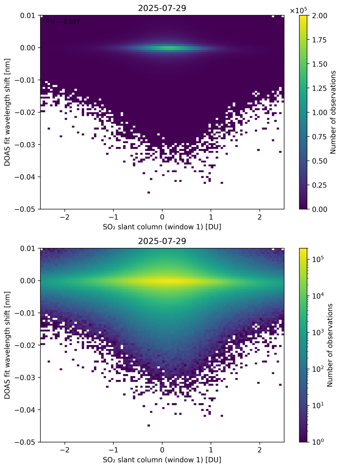
Figure 265: Scatter density plot of “SO 2 slant column (window 1)” against “DOAS fit wavelength shift” for 2025-07-29 to 2025-07-30.
