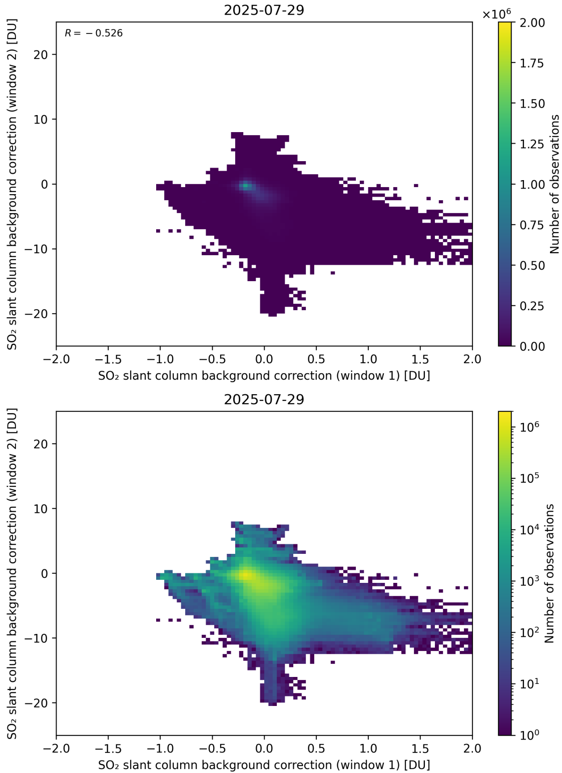
Figure 109: Scatter density plot of “SO 2 slant column background correction (window 1)” against “SO 2 slant column background correction (window 2)” for 2025-07-29 to 2025-07-30.
