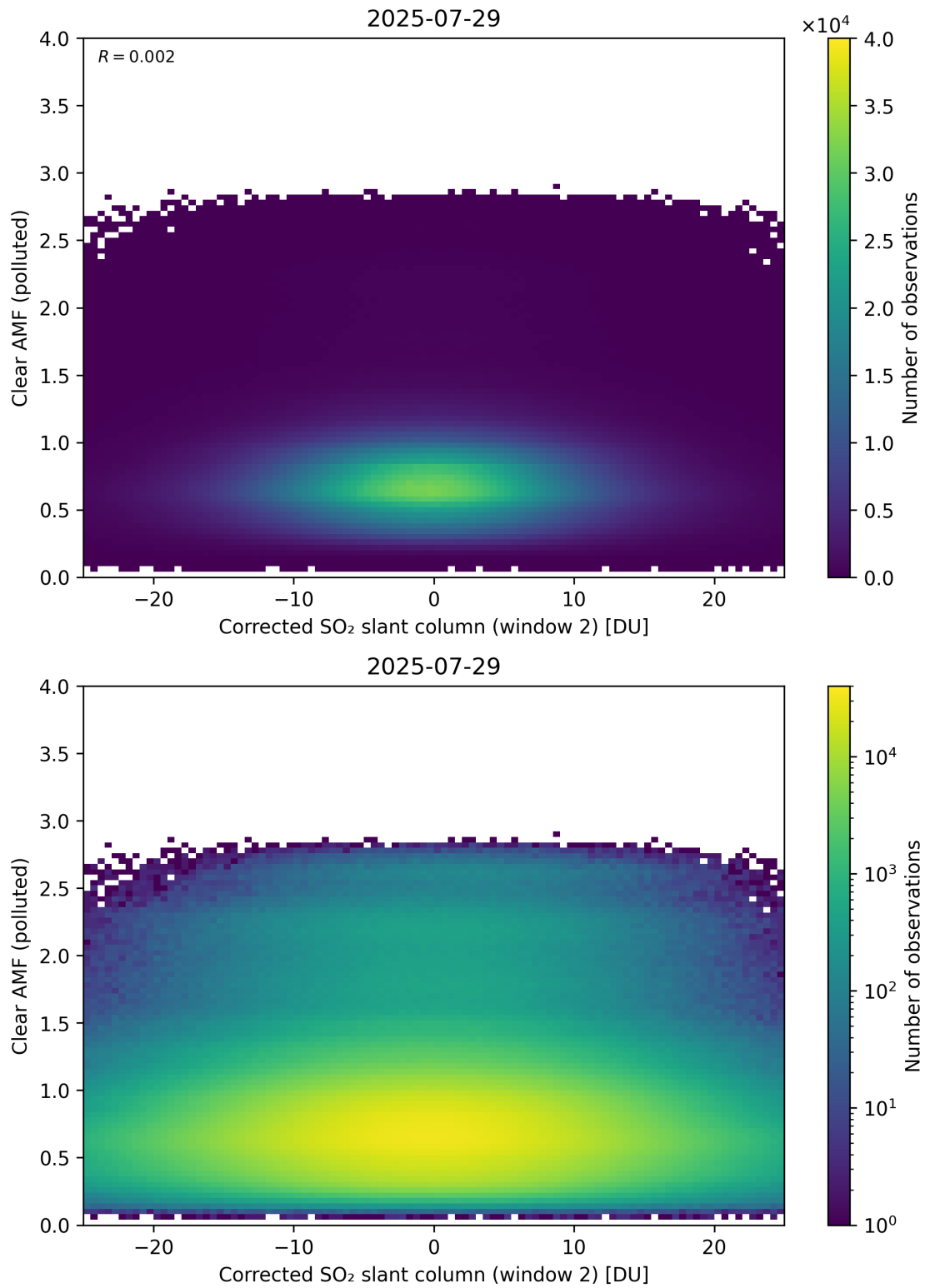
Figure 249: Scatter density plot of “Corrected SO 2 slant column (window 2)” against “Clear AMF (polluted)” for 2025-07-29 to 2025-07-30.
