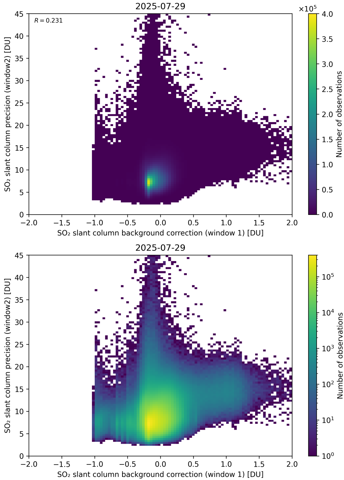
Figure 117: Scatter density plot of “SO 2 slant column background correction (window 1)” against “SO 2 slant column precision (window2)” for 2025-07-29 to 2025-07-30.
