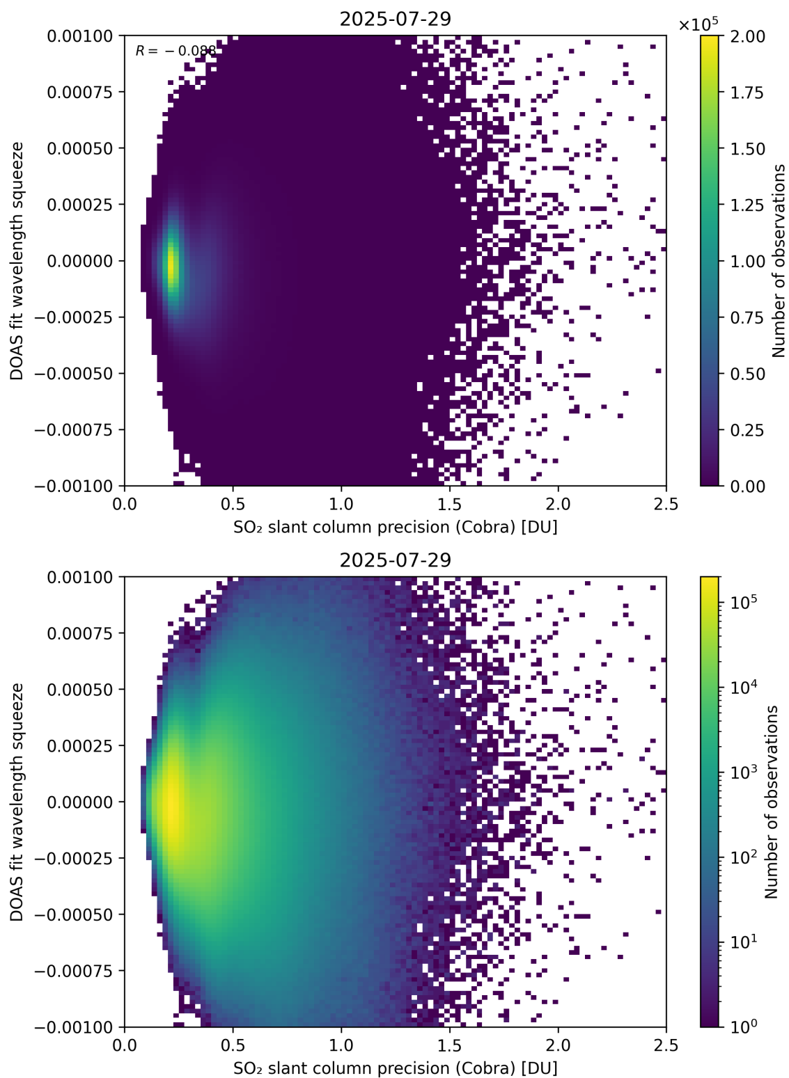
Figure 203: Scatter density plot of “SO 2 slant column precision (Cobra)” against “DOAS fit wavelength squeeze” for 2025-07-29 to 2025-07-30.
