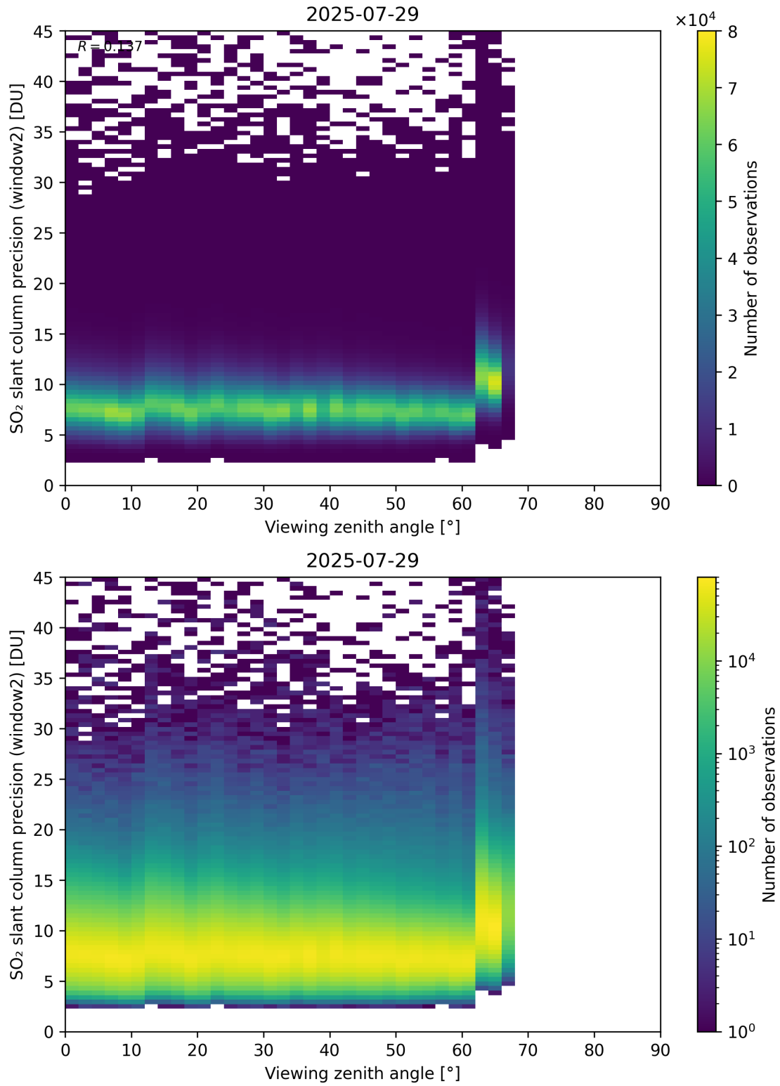
Figure 378: Scatter density plot of “Viewing zenith angle” against “SO 2 slant column precision (window2)” for 2025-07-29 to 2025-07-30.
