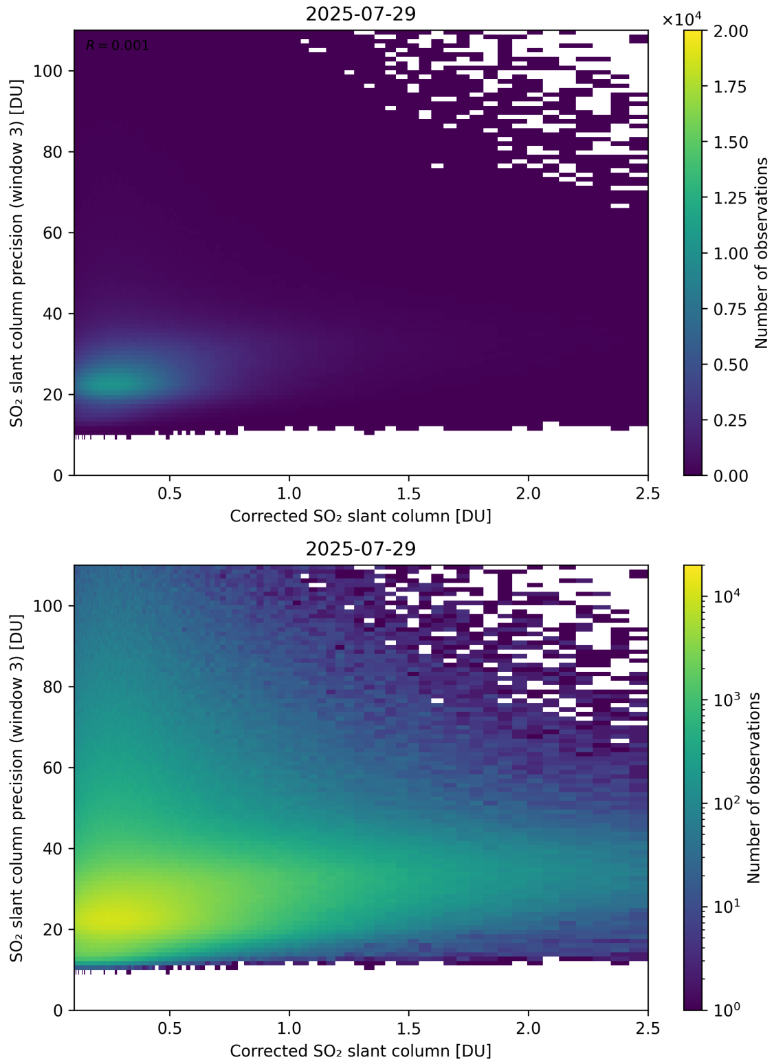
Figure 241: Scatter density plot of “Corrected SO 2 slant column” against “SO 2 slant column precision (window 3)” for 2025-07-29 to 2025-07-30.
