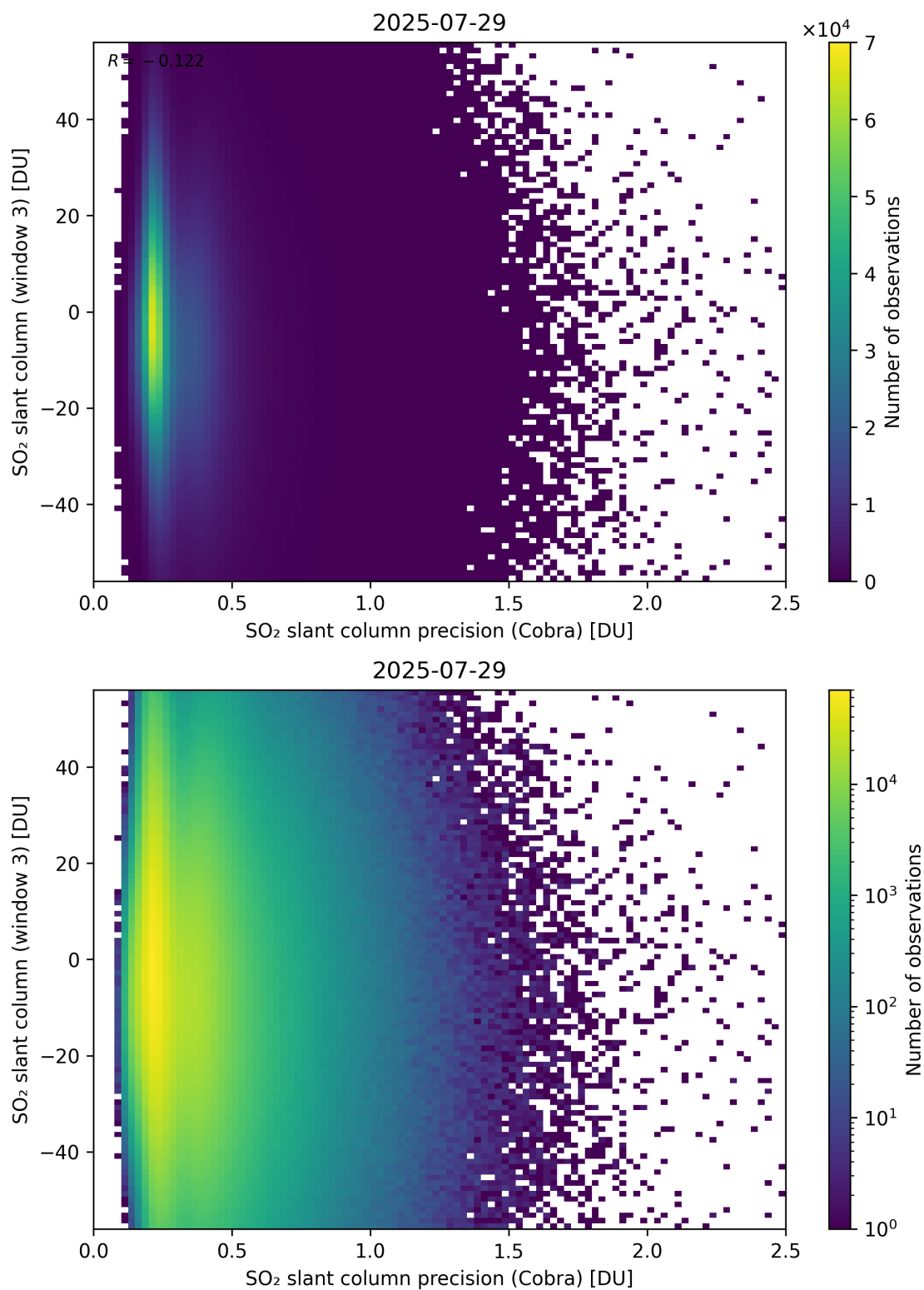
Figure 211: Scatter density plot of “SO 2 slant column precision (Cobra)” against “SO 2 slant column (window 3)” for 2025-07-29 to 2025-07-30.
