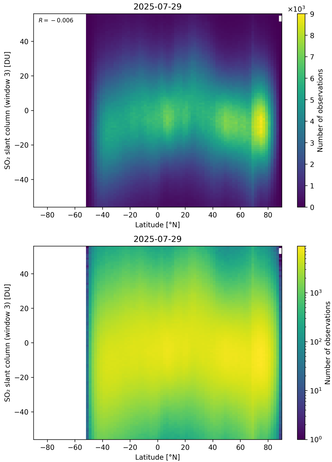
Figure 165: Scatter density plot of “Latitude” against “SO 2 slant column (window 3)” for 2025-07-29 to 2025-07-30.
