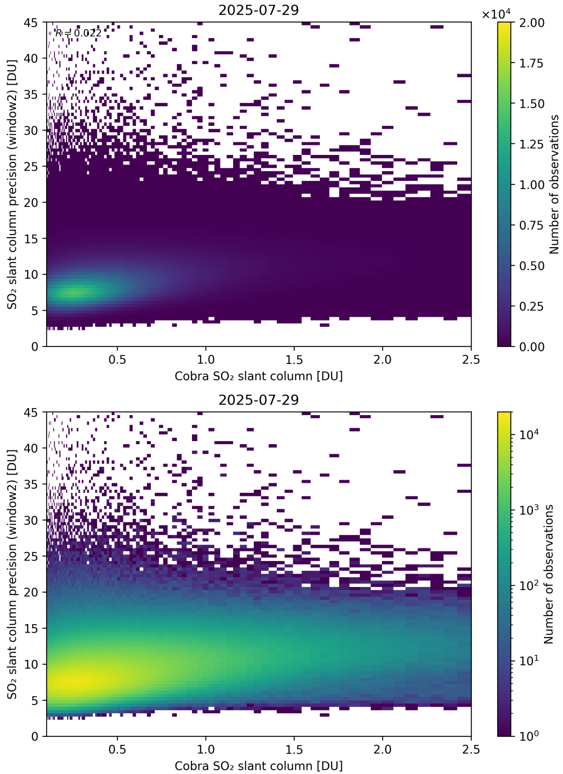
Figure 221: Scatter density plot of “Cobra SO 2 slant column” against “SO 2 slant column precision (window2)” for 2025-07-29 to 2025-07-30.
