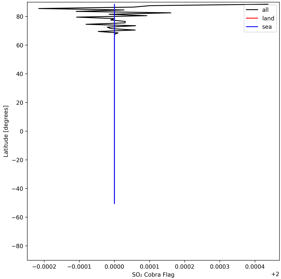
Figure 49: Zonal average of “SO 2 Cobra Flag” for 2025-07-29 to 2025-07-30.
