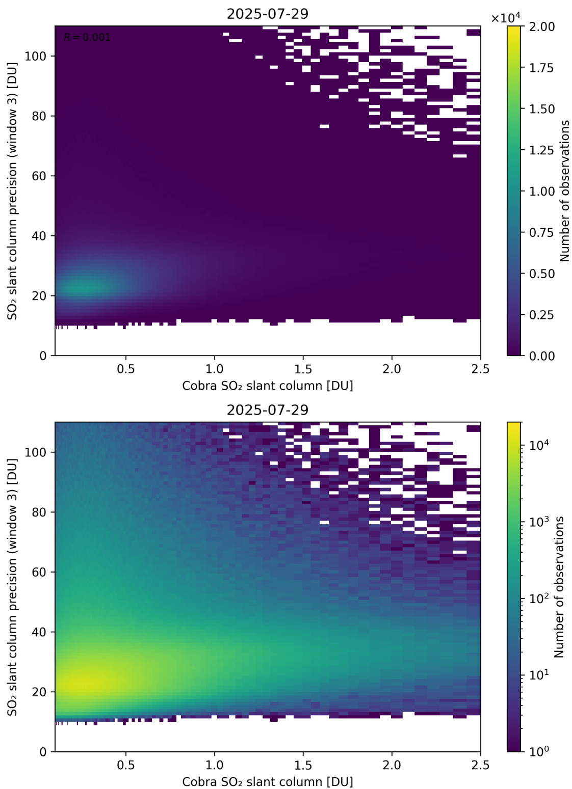
Figure 223: Scatter density plot of “Cobra SO 2 slant column” against “SO 2 slant column precision (window 3)” for 2025-07-29 to 2025-07-30.
