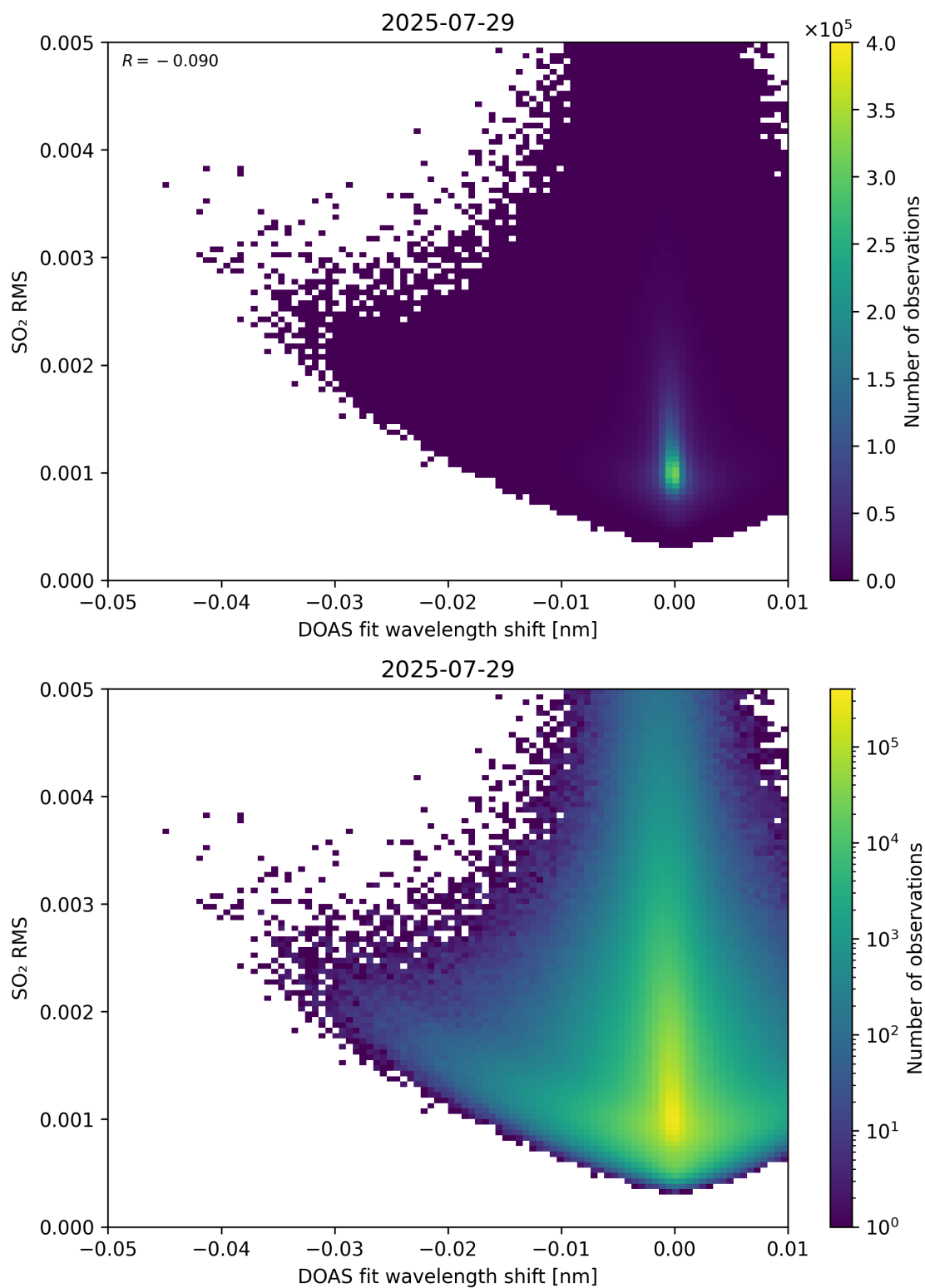
Figure 139: Scatter density plot of “DOAS fit wavelength shift” against “SO 2 RMS” for 2025-07-29 to 2025-07-30.
