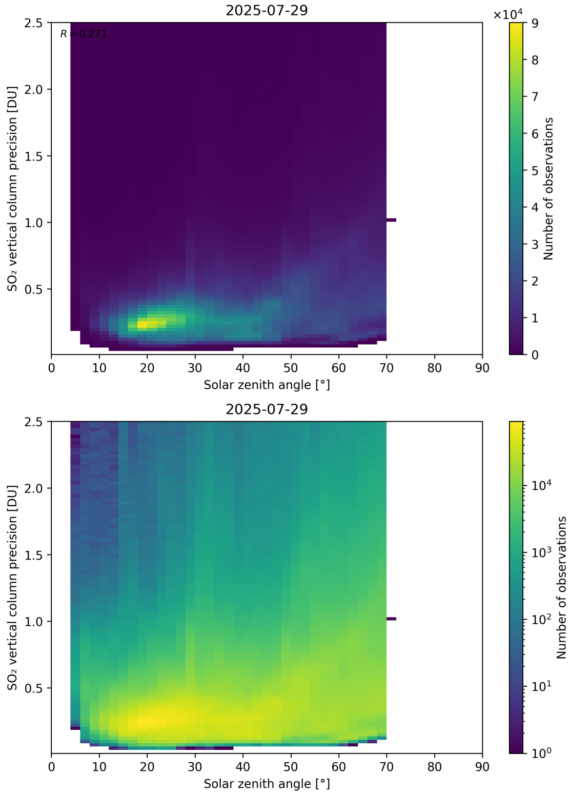
Figure 192: Scatter density plot of “Solar zenith angle” against “SO 2 vertical column precision” for 2025-07-29 to 2025-07-30.
