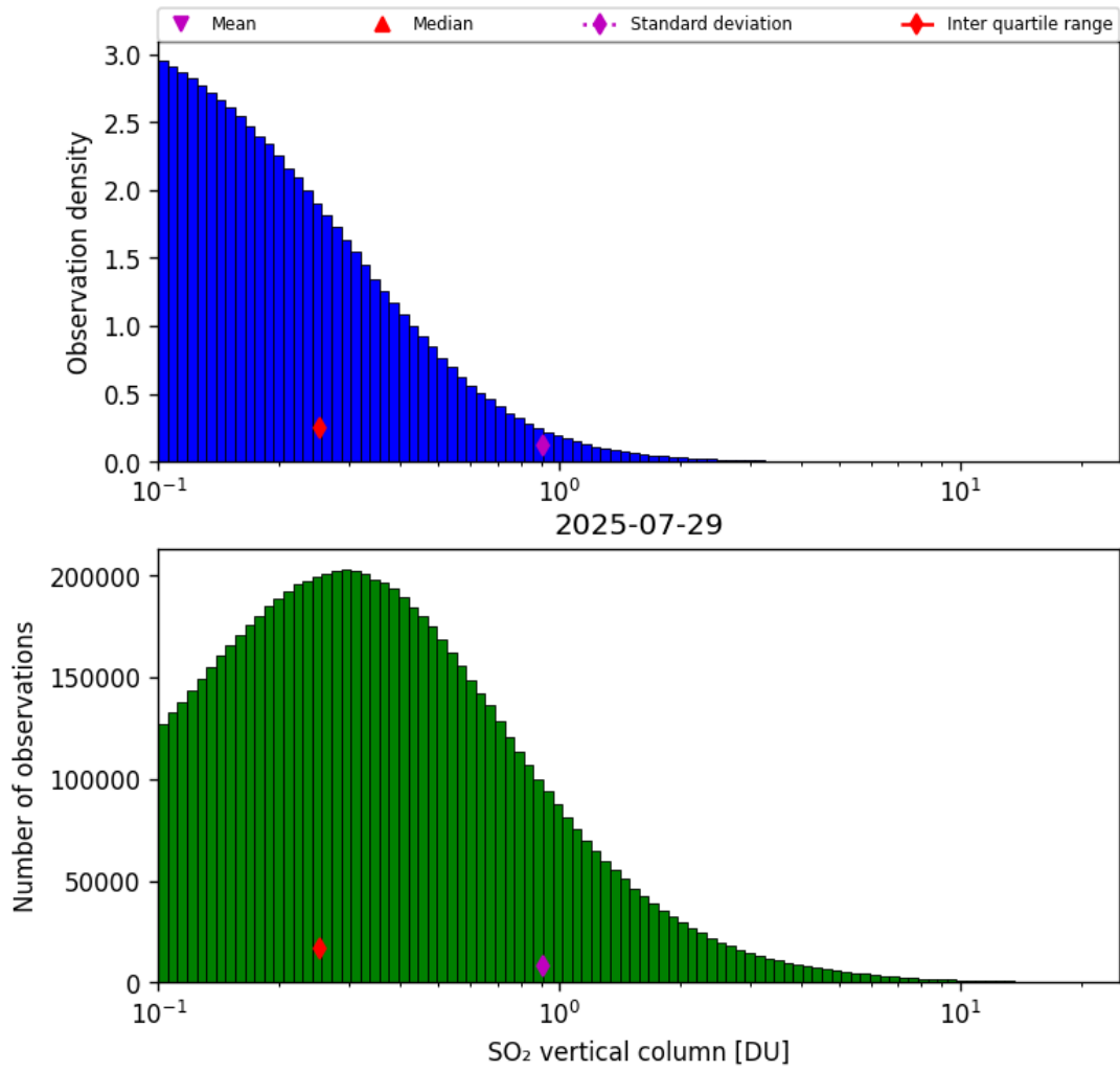
Figure 58: Histogram of “SO 2 vertical column” for 2025-07-29 to 2025-07-30
