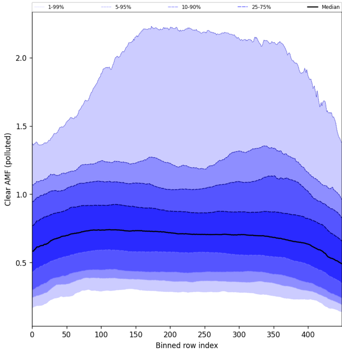
Figure 107: Along track statistics of “Clear AMF (polluted)” for 2025-07-29 to 2025-07-30
