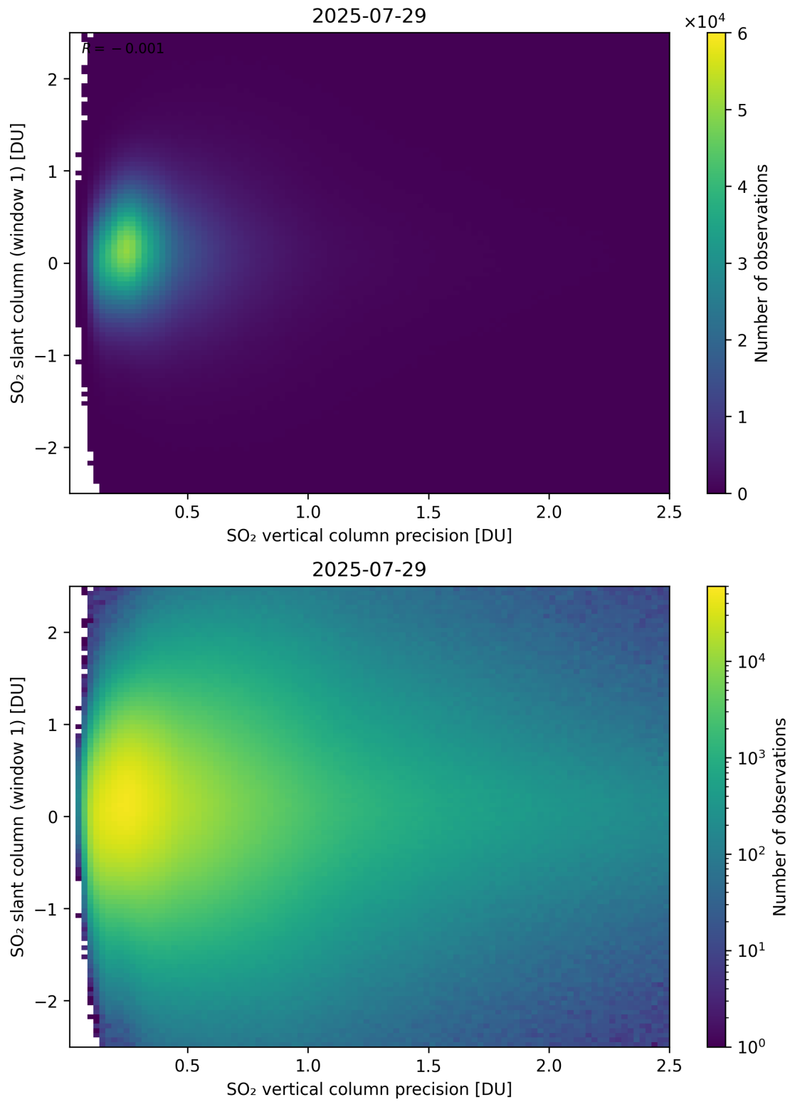
Figure 341: Scatter density plot of “SO 2 vertical column precision” against “SO 2 slant column (window 1)” for 2025-07-29 to 2025-07-30.
