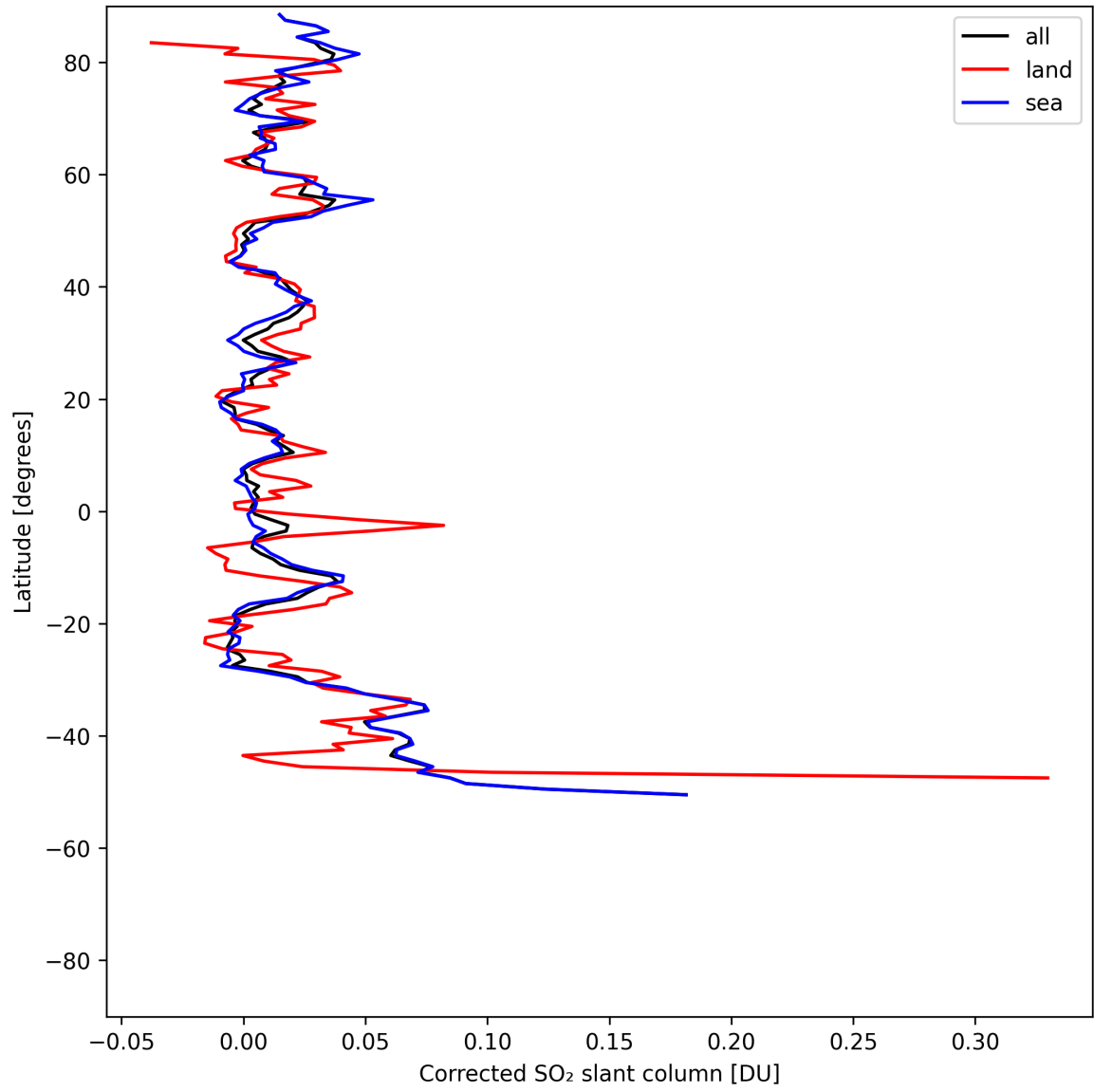
Figure 34: Zonal average of “Corrected SO 2 slant column” for 2025-07-29 to 2025-07-30.
