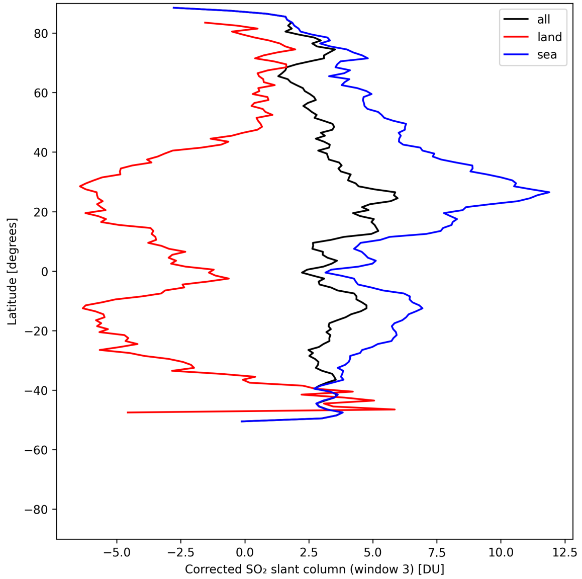
Figure 47: Zonal average of “Corrected SO 2 slant column (window 3)” for 2025-07-29 to 2025-07-30.
