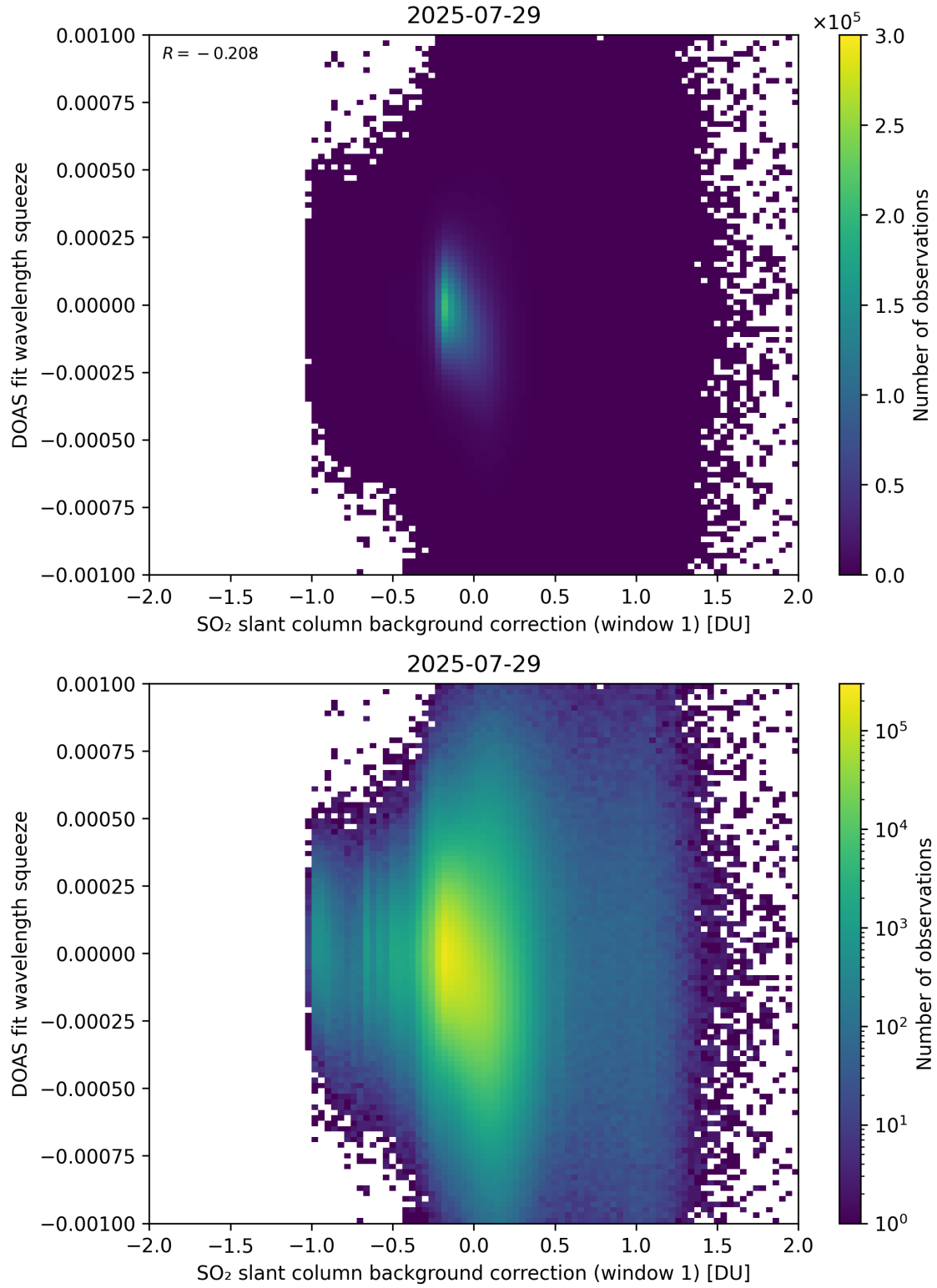
Figure 112: Scatter density plot of “SO 2 slant column background correction (window 1)” against “DOAS fit wavelength squeeze” for 2025-07-29 to 2025-07-30.
