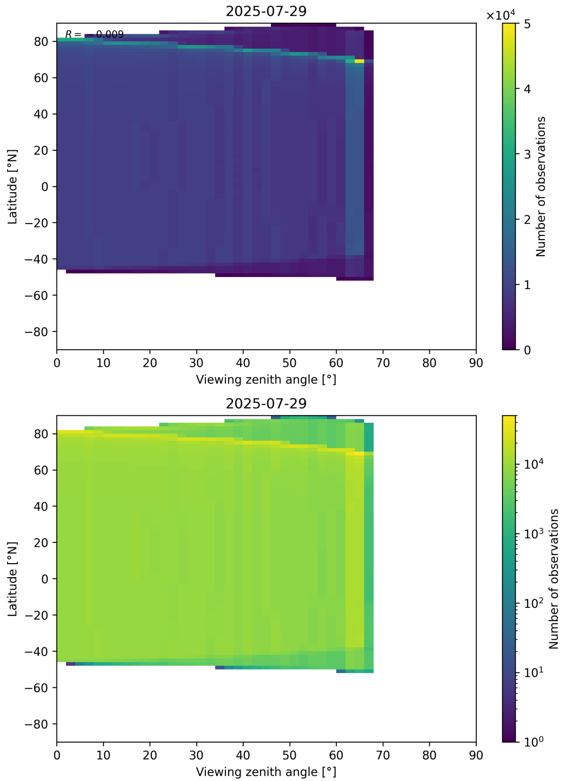
Figure 368: Scatter density plot of “Viewing zenith angle” against “Latitude” for 2025-07-29 to 2025-07-30.
