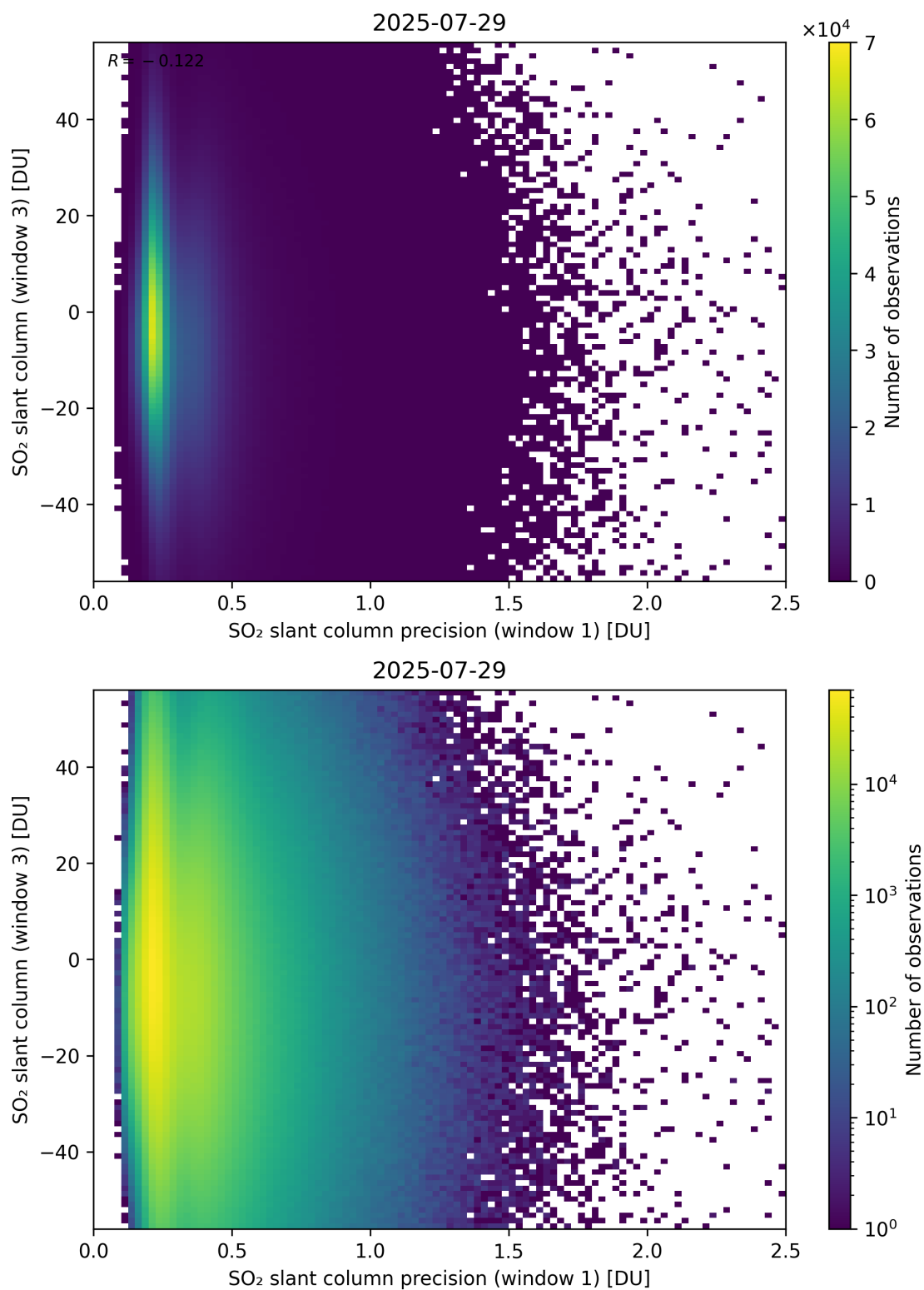
Figure 278: Scatter density plot of “SO 2 slant column precision (window 1)” against “SO 2 slant column (window 3)” for 2025-07-29 to 2025-07-30.
