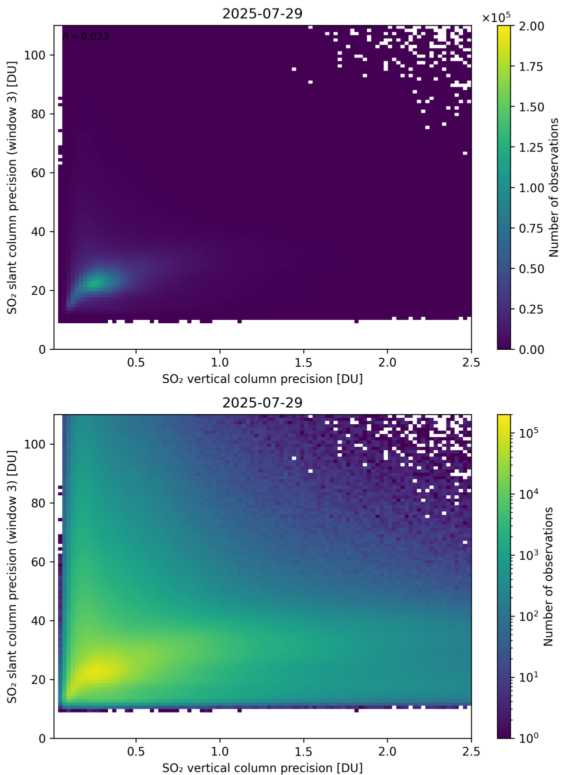
Figure 345: Scatter density plot of “SO 2 vertical column precision” against “SO 2 slant column precision (window 3)” for 2025-07-29 to 2025-07-30.
