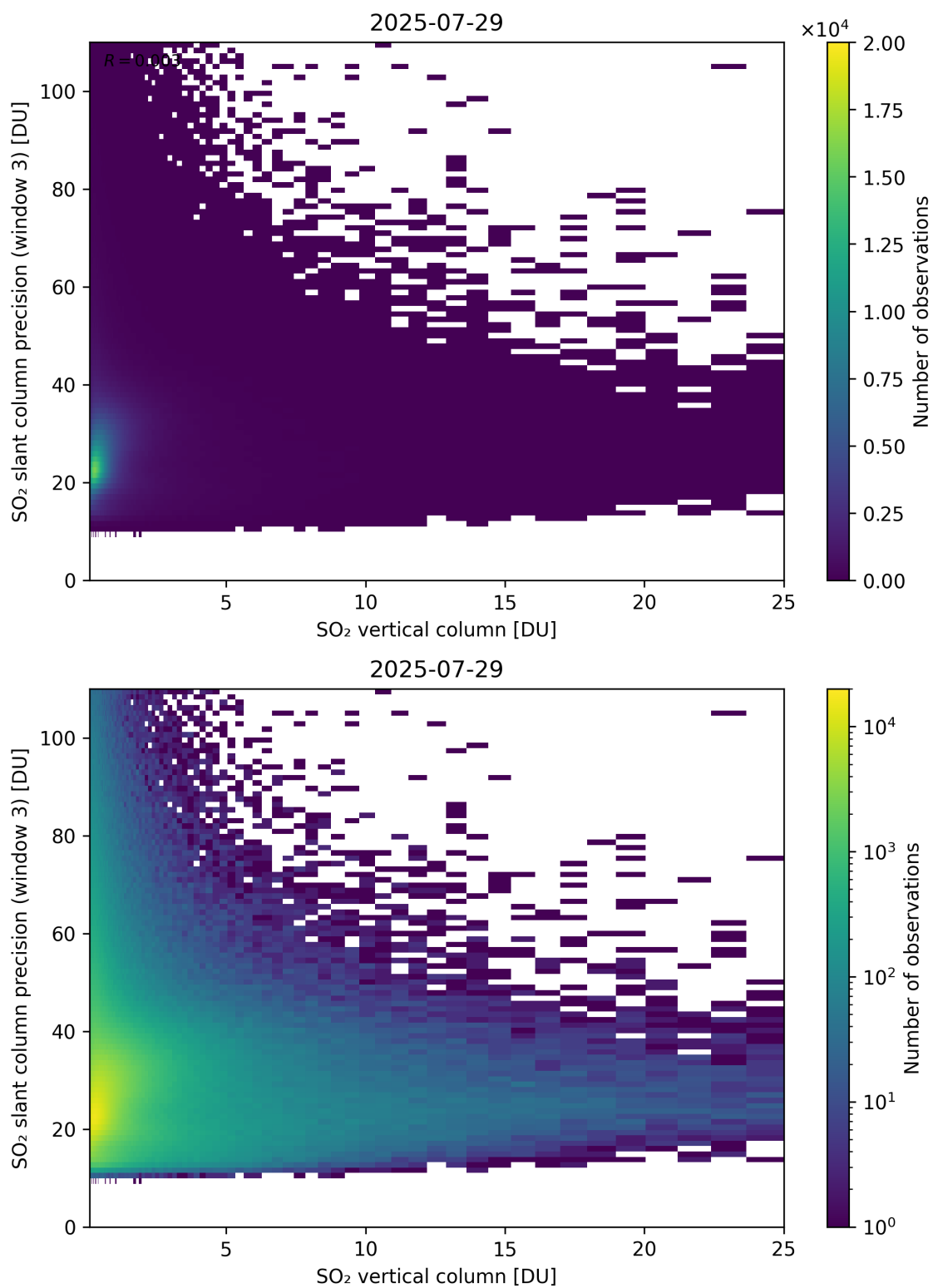
Figure 358: Scatter density plot of “SO 2 vertical column” against “SO 2 slant column precision (window 3)” for 2025-07-29 to 2025-07-30.
