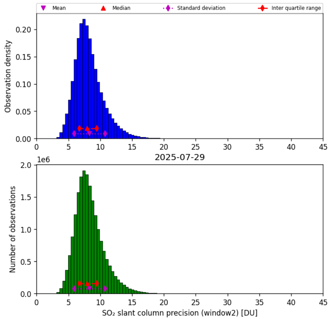
Figure 68: Histogram of “SO 2 slant column precision (window2)” for 2025-07-29 to 2025-07-30
