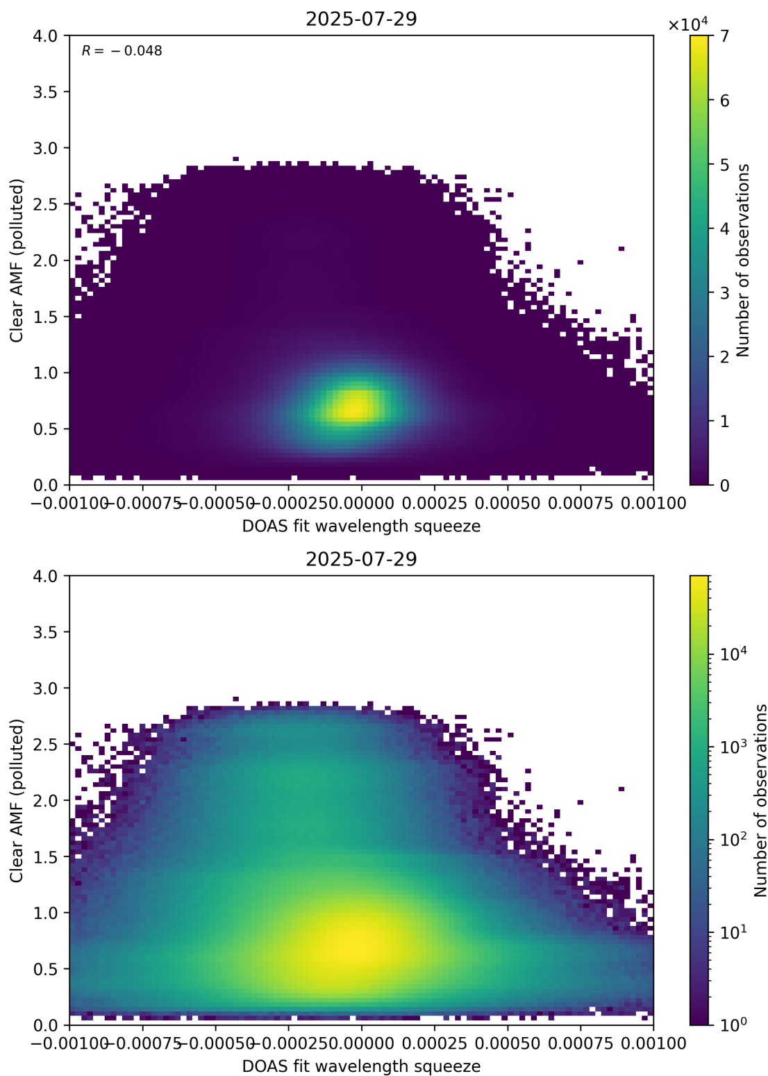
Figure 144: Scatter density plot of “DOAS fit wavelength squeeze” against “Clear AMF (polluted)” for 2025-07-29 to 2025-07-30.
