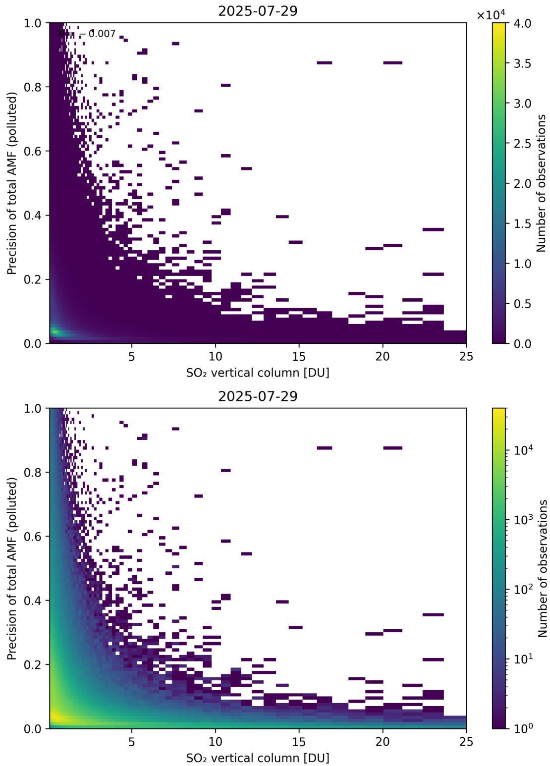
Figure 360: Scatter density plot of “SO 2 vertical column” against “Precision of total AMF (polluted)” for 2025-07-29 to 2025-07-30.
