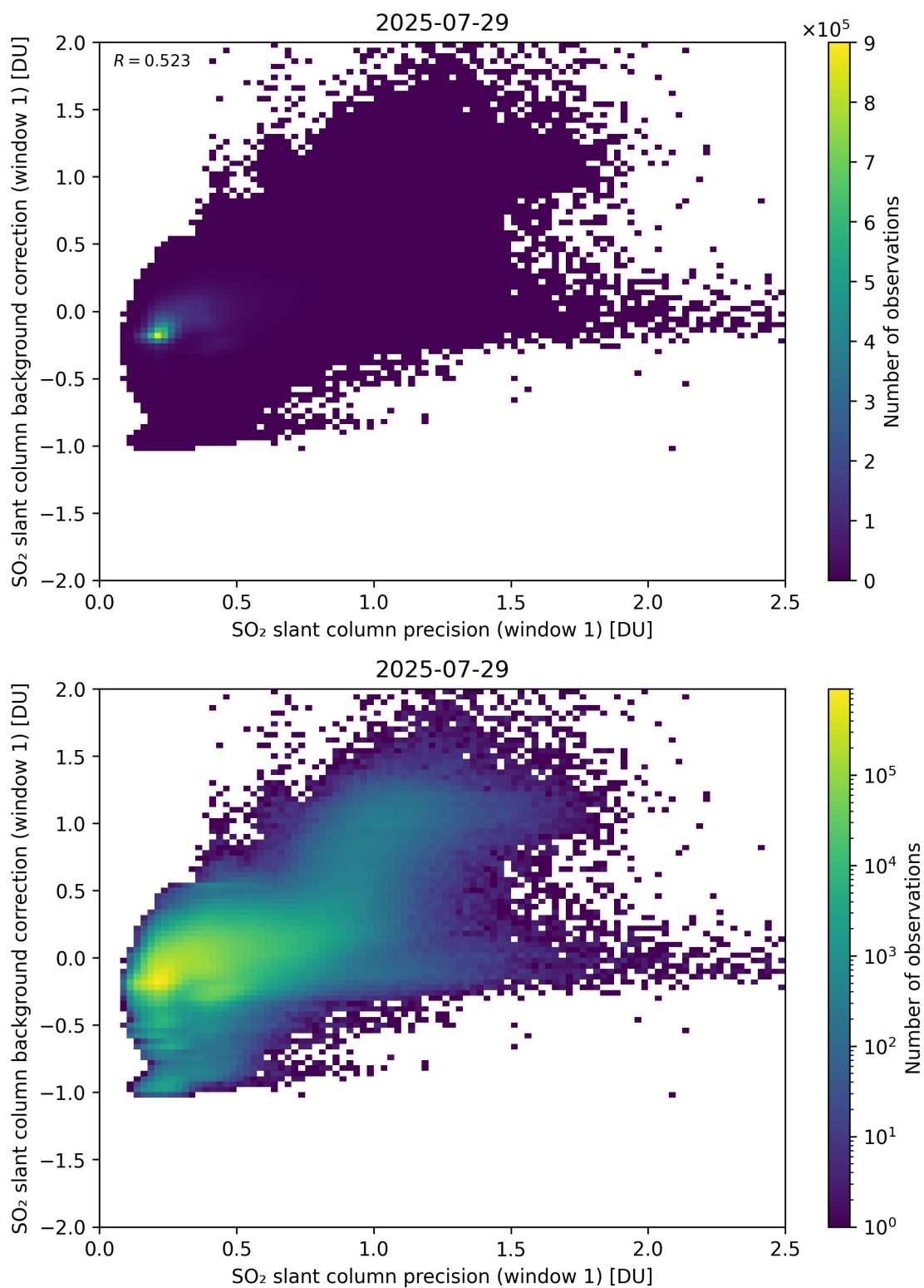
Figure 268: Scatter density plot of “SO 2 slant column precision (window 1)” against “SO 2 slant column background correction (window 1)” for 2025-07-29 to 2025-07-30.
