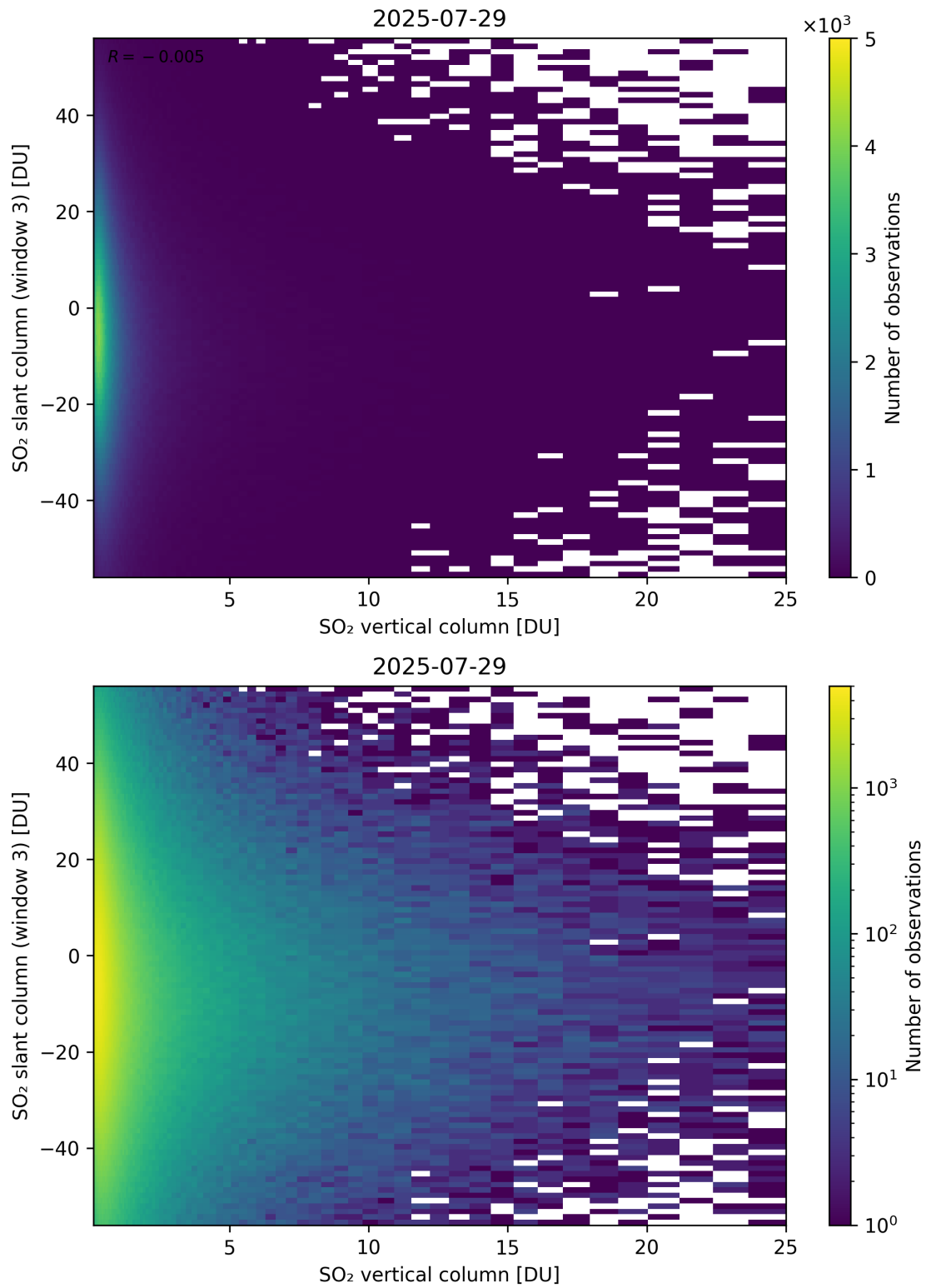
Figure 357: Scatter density plot of “SO 2 vertical column” against “SO 2 slant column (window 3)” for 2025-07-29 to 2025-07-30.
