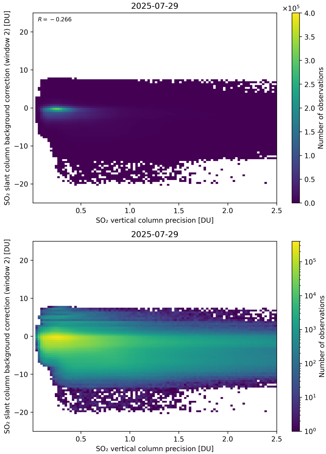
Figure 330: Scatter density plot of “SO 2 vertical column precision” against “SO 2 slant column background correction (window 2)” for 2025-07-29 to 2025-07-30.
