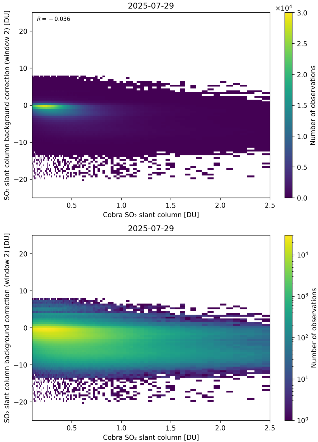
Figure 194: Scatter density plot of “Cobra SO 2 slant column” against “SO 2 slant column background correction (window 2)” for 2025-07-29 to 2025-07-30.
