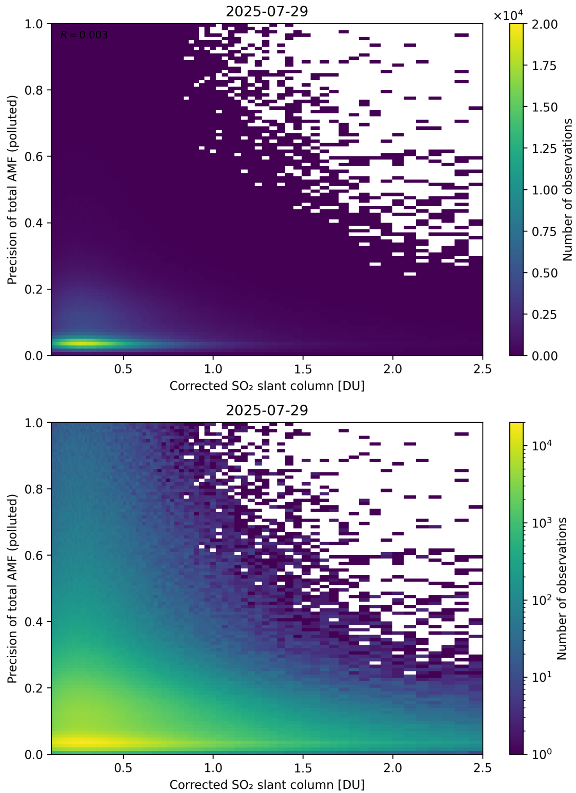
Figure 243: Scatter density plot of “Corrected SO 2 slant column” against “Precision of total AMF (polluted)” for 2025-07-29 to 2025-07-30.
