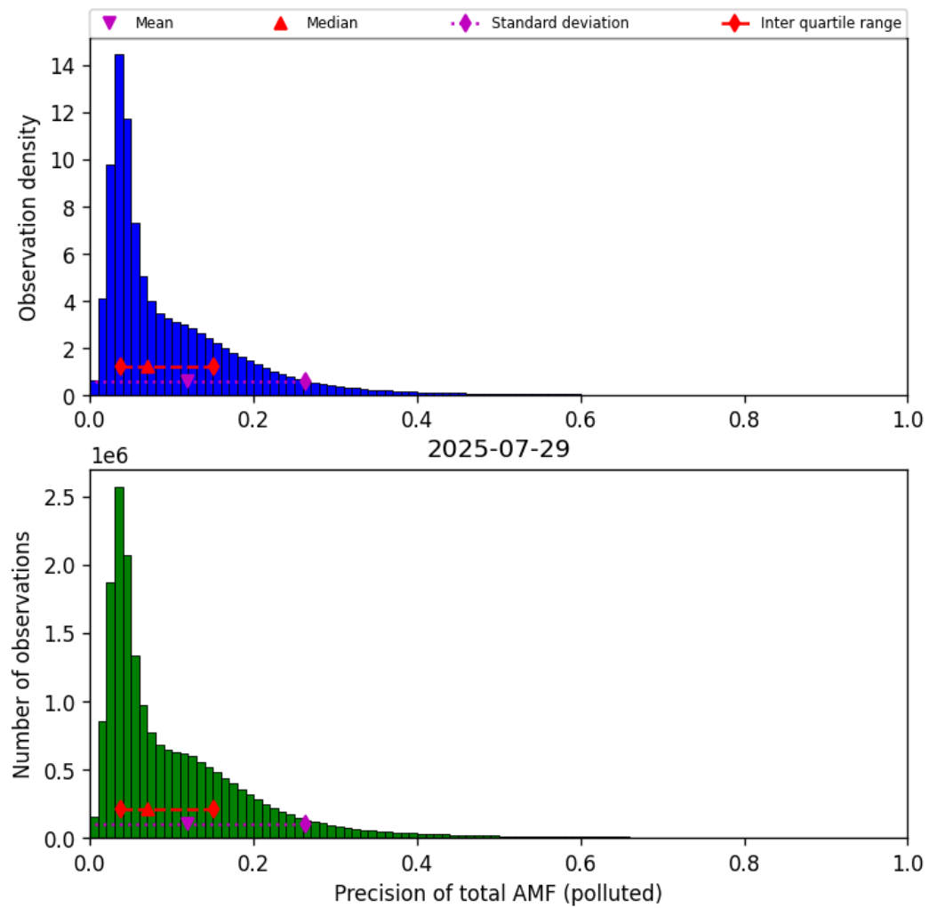
Figure 80: Histogram of “Precision of total AMF (polluted)” for 2025-07-29 to 2025-07-30
