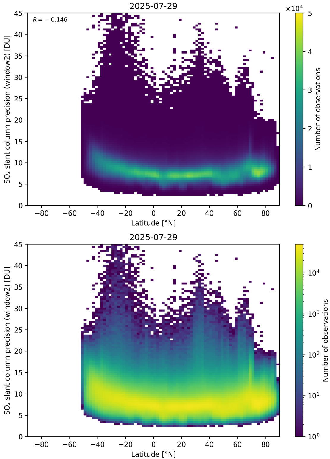
Figure 164: Scatter density plot of “Latitude” against “SO 2 slant column precision (window2)” for 2025-07-29 to 2025-07-30.
