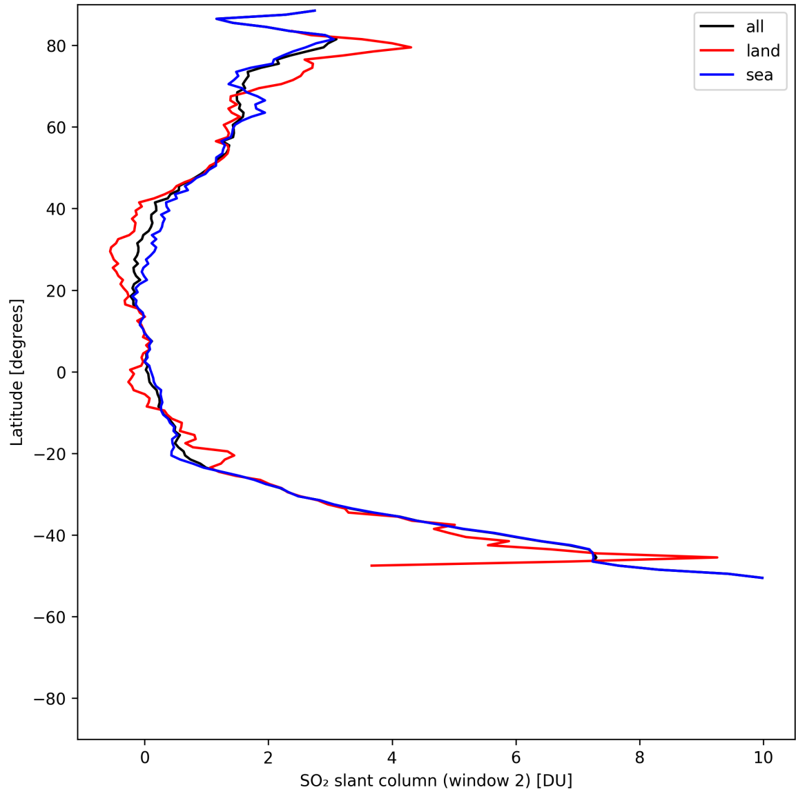
Figure 41: Zonal average of “SO 2 slant column (window 2)” for 2025-07-29 to 2025-07-30.
