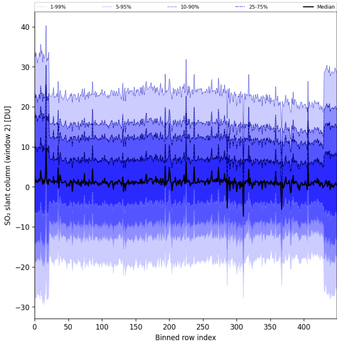
Figure 93: Along track statistics of “SO 2 slant column (window 2)” for 2025-07-29 to 2025-07-30
