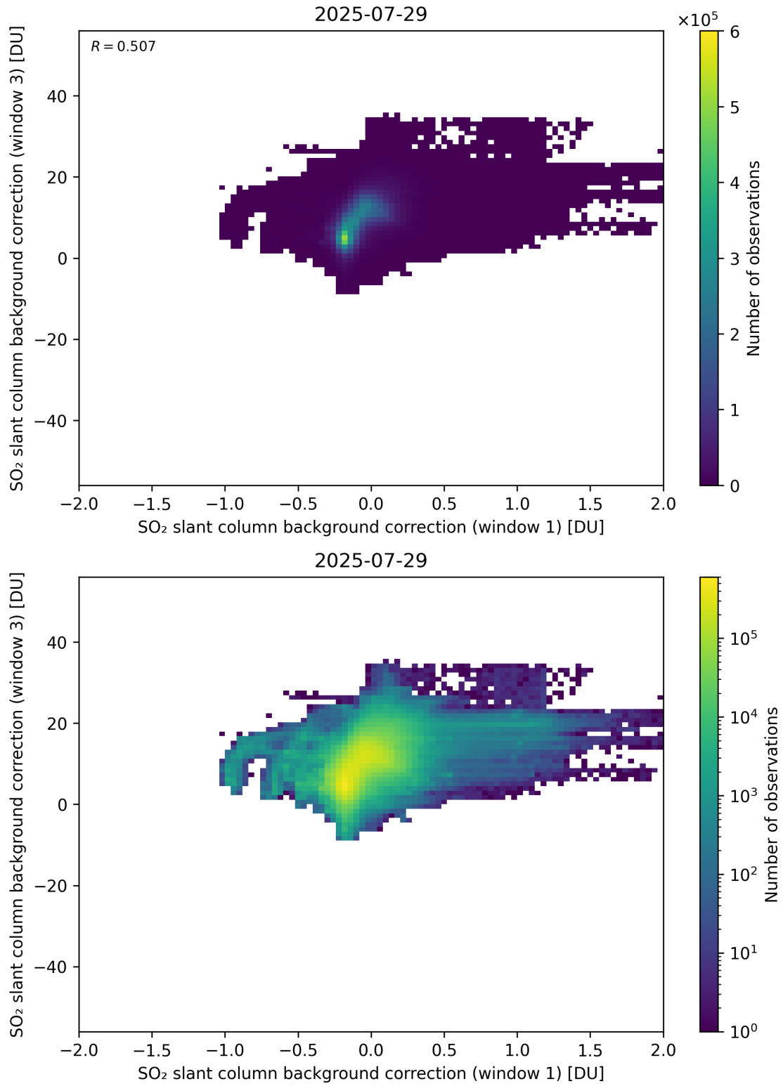
Figure 110: Scatter density plot of “SO 2 slant column background correction (window 1)” against “SO 2 slant column background correction (window 3)” for 2025-07-29 to 2025-07-30.
