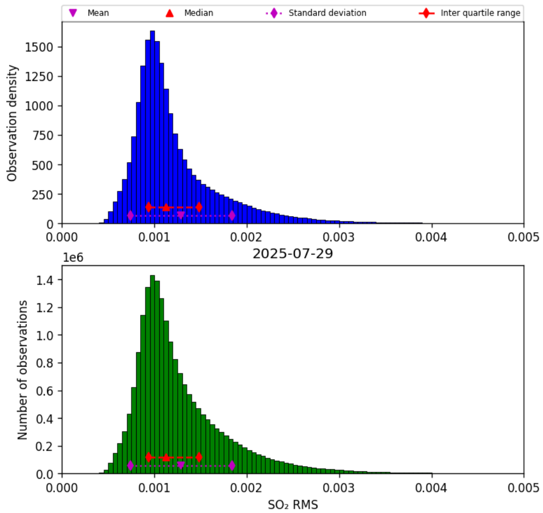
Figure 78: Histogram of “SO 2 RMS” for 2025-07-29 to 2025-07-30
