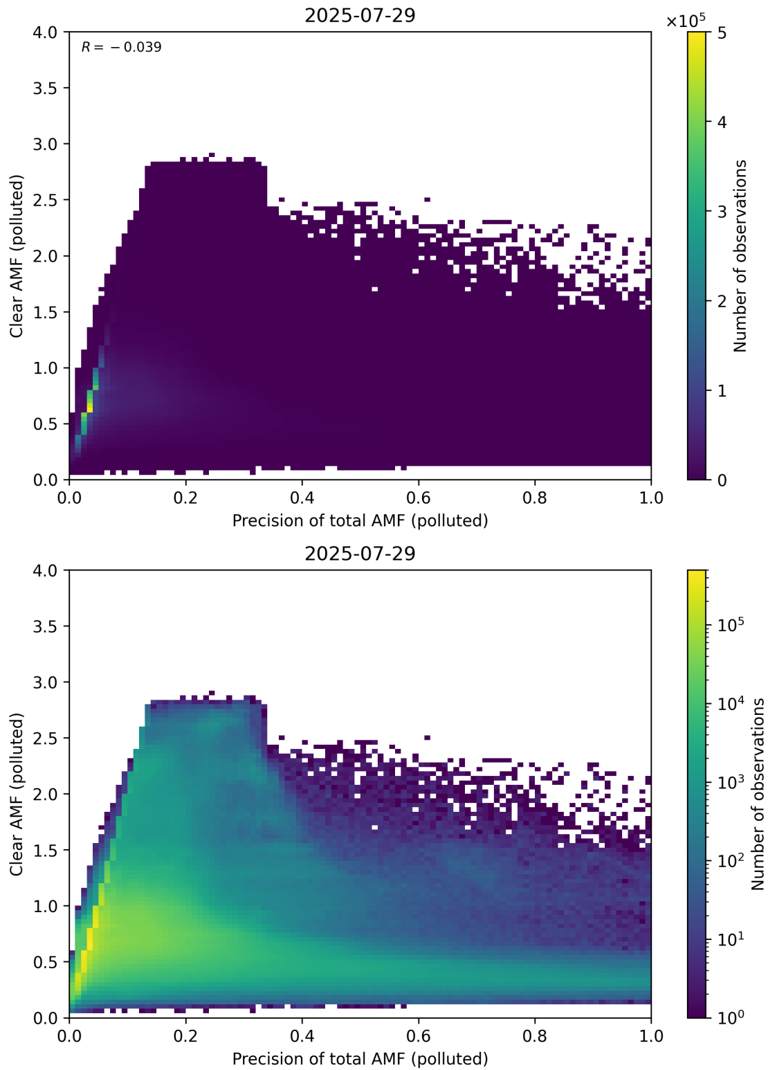
Figure 320: Scatter density plot of “Precision of total AMF (polluted)” against “Clear AMF (polluted)” for 2025-07-29 to 2025-07-30.
