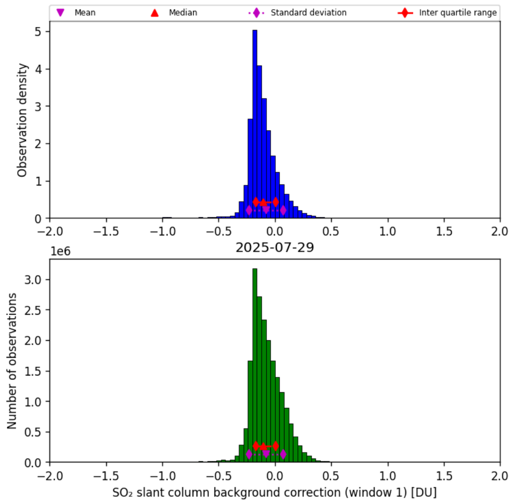
Figure 66: Histogram of “SO 2 slant column background correction (window 1)” for 2025-07-29 to 2025-07-30
