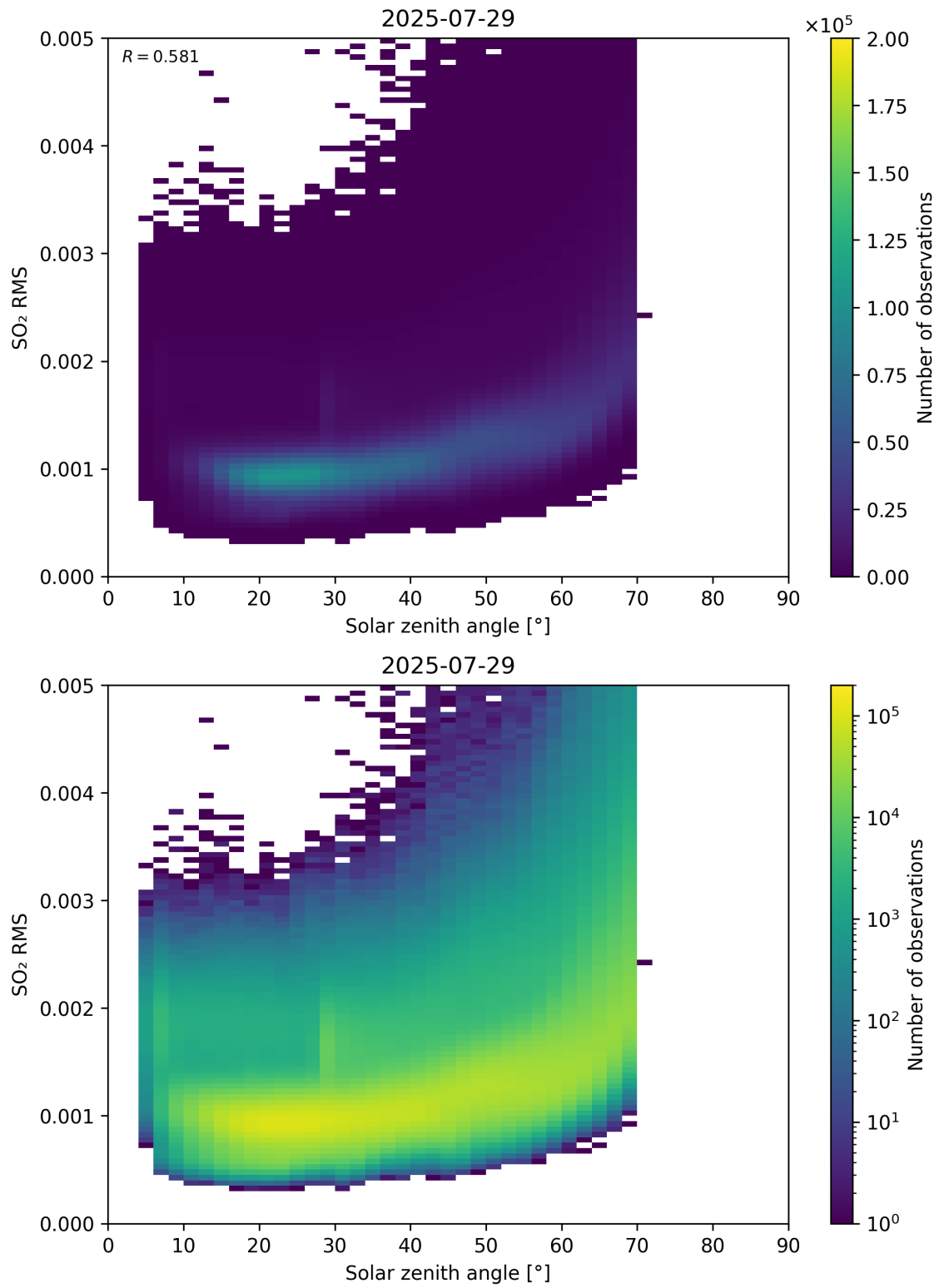
Figure 176: Scatter density plot of “Solar zenith angle” against “SO 2 RMS” for 2025-07-29 to 2025-07-30.
