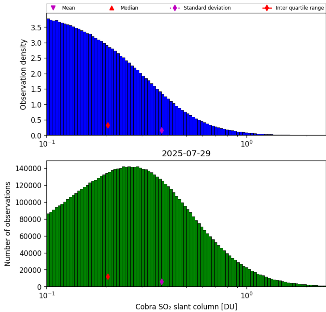
Figure 61: Histogram of “Cobra SO 2 slant column” for 2025-07-29 to 2025-07-30
