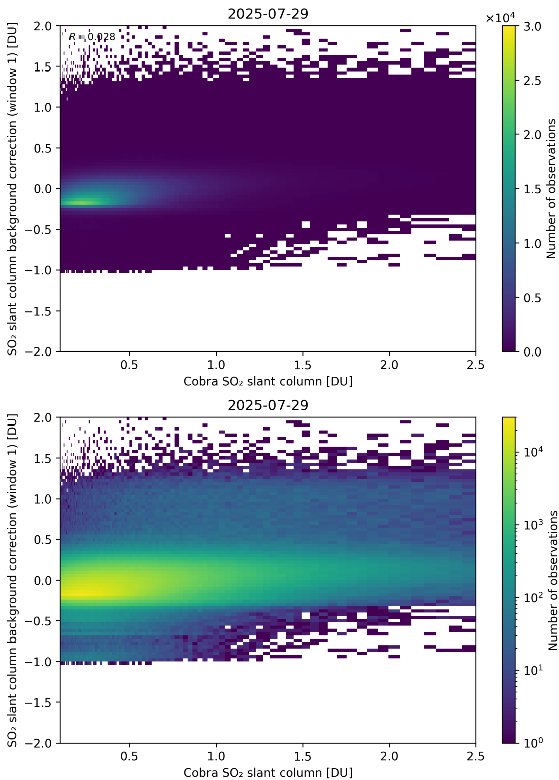
Figure 193: Scatter density plot of “Cobra SO 2 slant column” against “SO 2 slant column background correction (window 1)” for 2025-07-29 to 2025-07-30.
