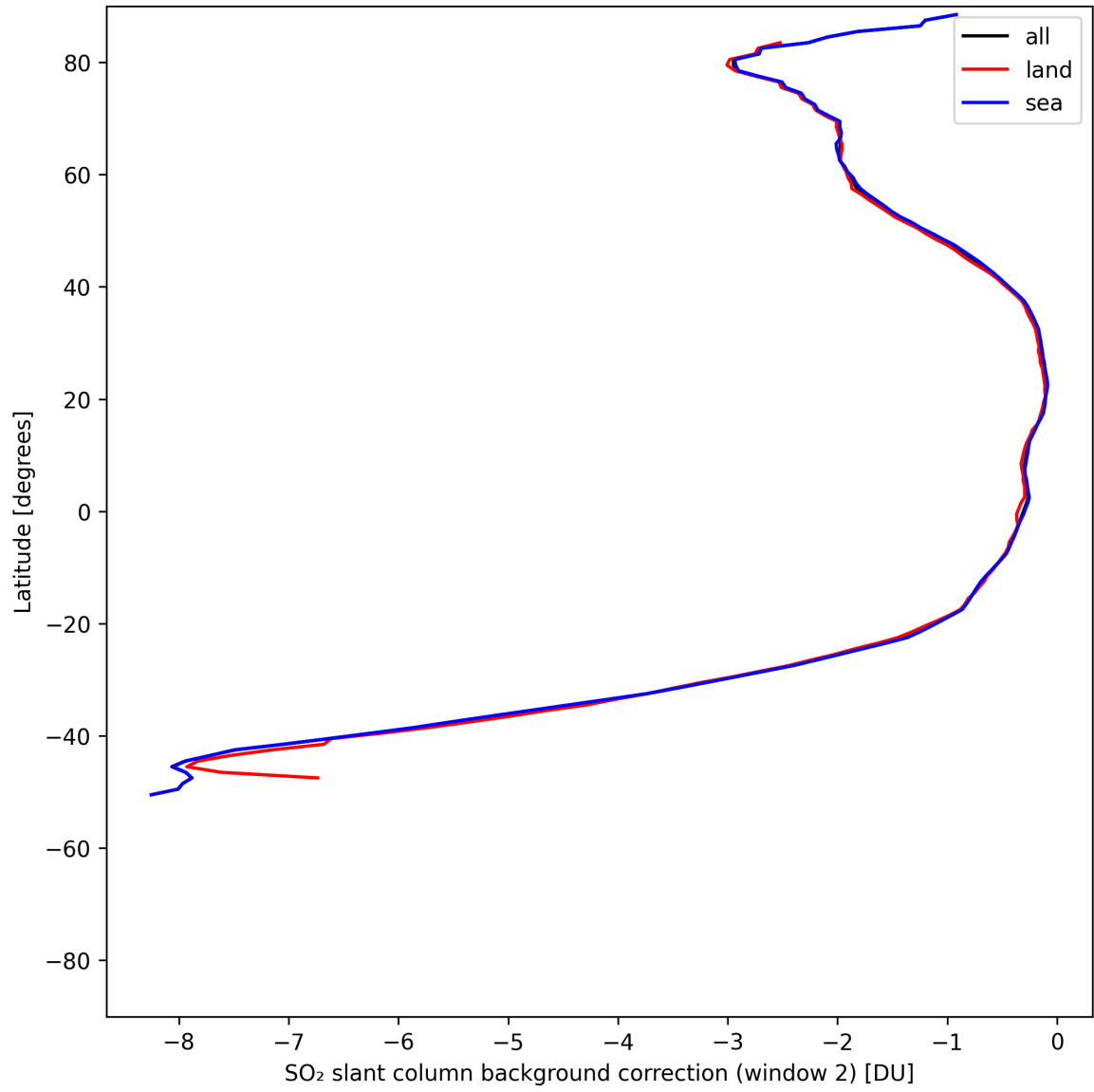
Figure 44: Zonal average of “SO 2 slant column background correction (window 2)” for 2025-07-29 to 2025-07-30.
