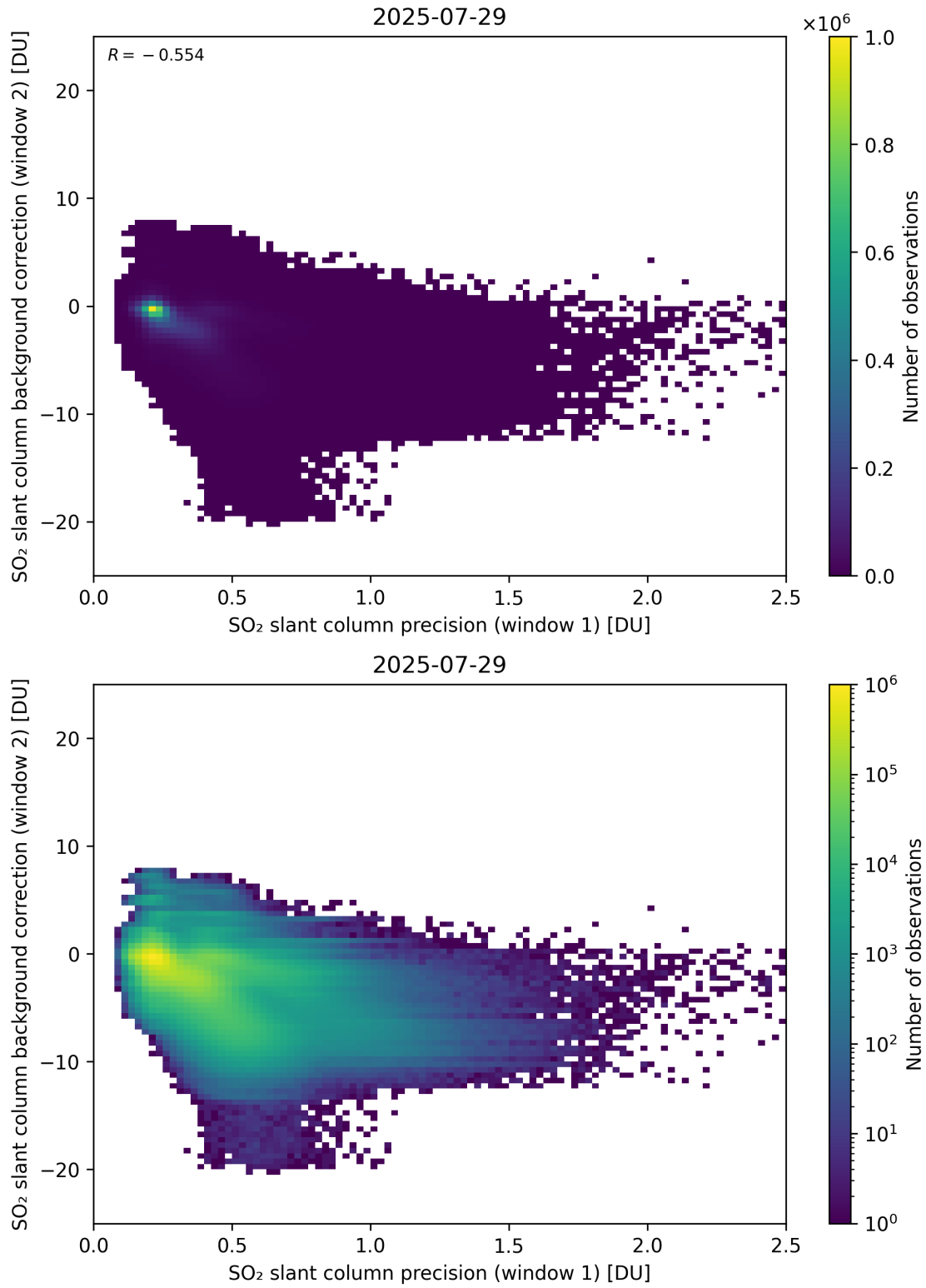
Figure 269: Scatter density plot of “SO 2 slant column precision (window 1)” against “SO 2 slant column background correction (window 2)” for 2025-07-29 to 2025-07-30.
