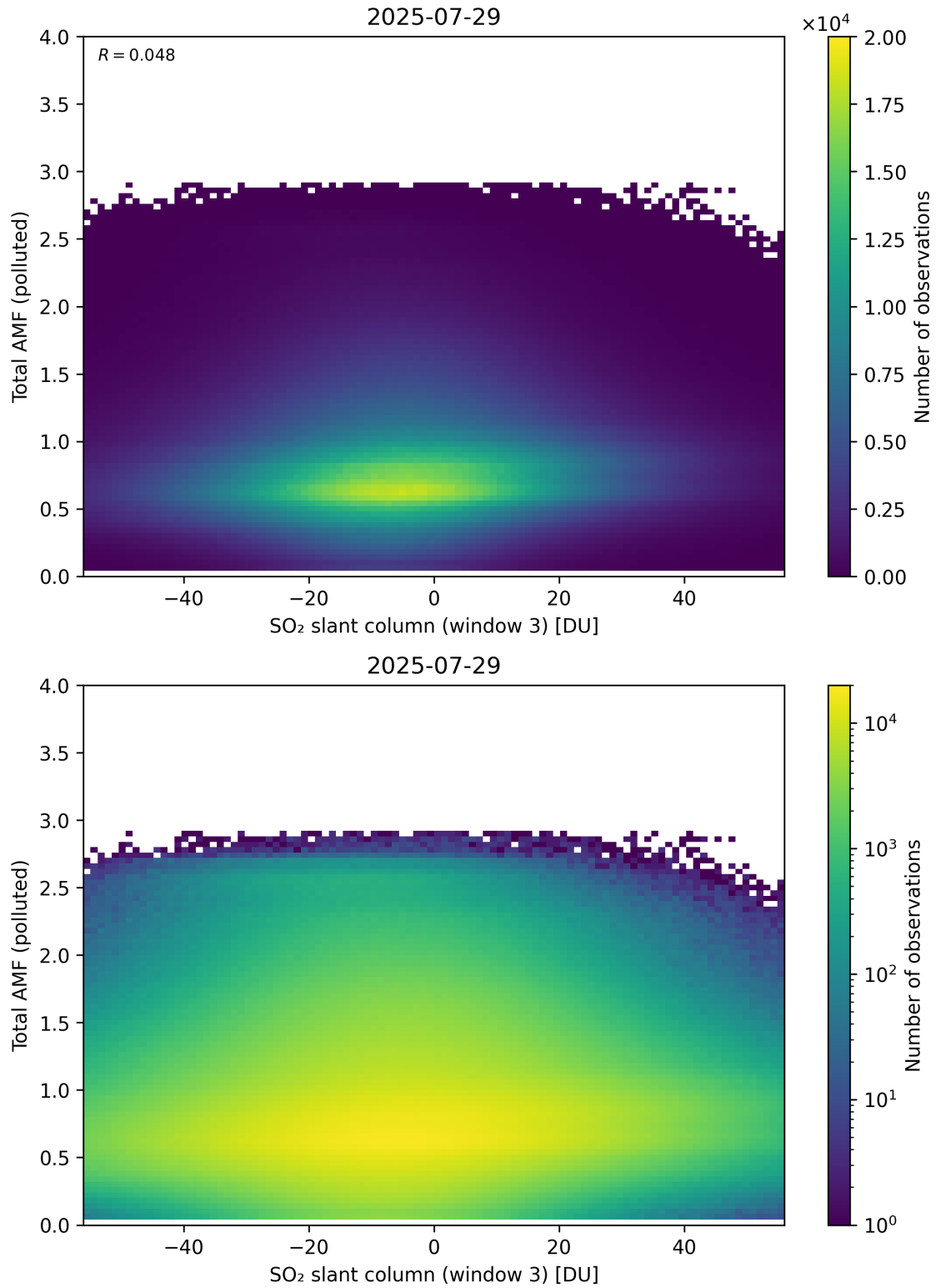
Figure 318: Scatter density plot of “SO 2 slant column (window 3)” against “Total AMF (polluted)” for 2025-07-29 to 2025-07-30.
