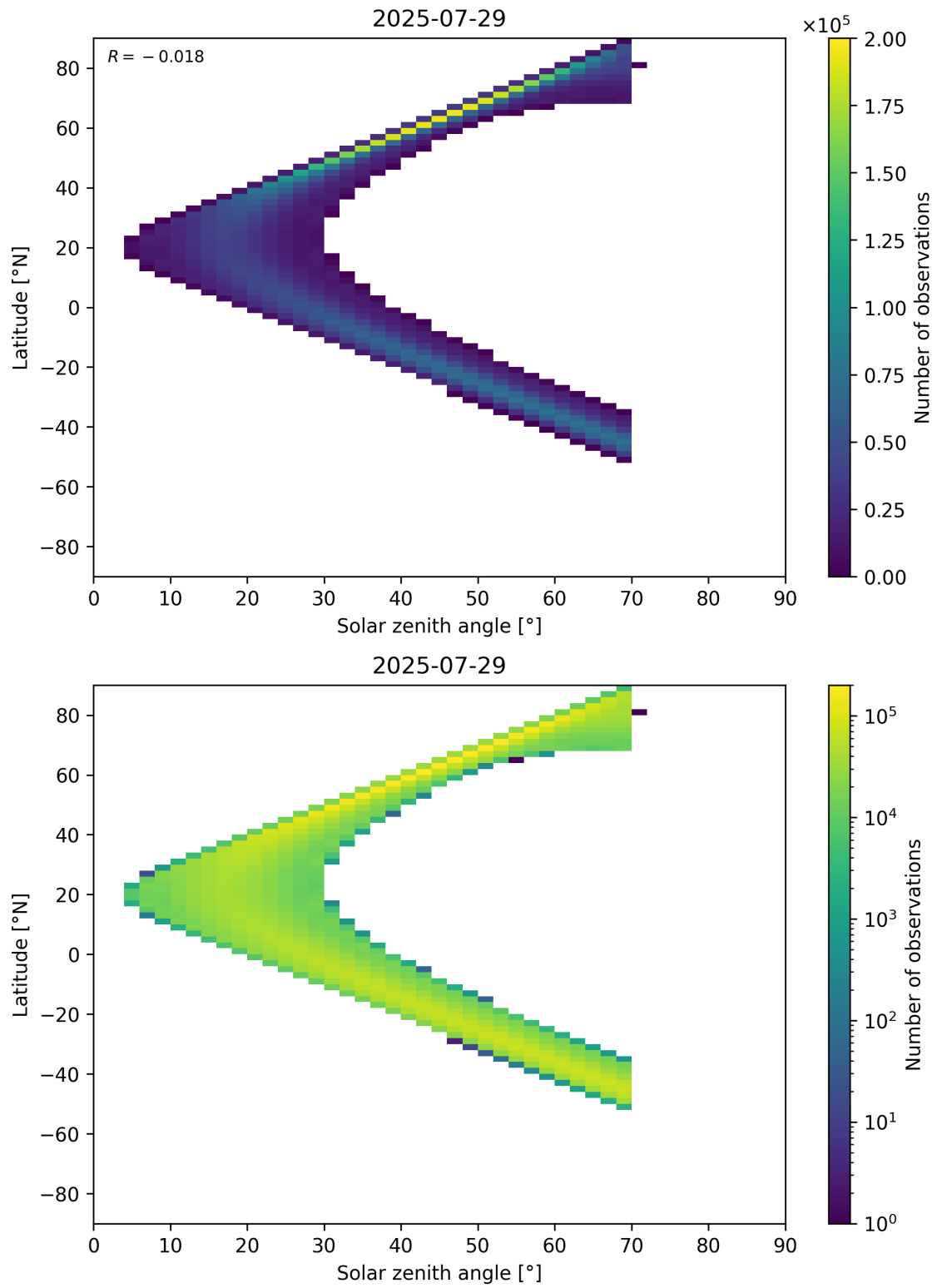
Figure 177: Scatter density plot of “Solar zenith angle” against “Latitude” for 2025-07-29 to 2025-07-30.
