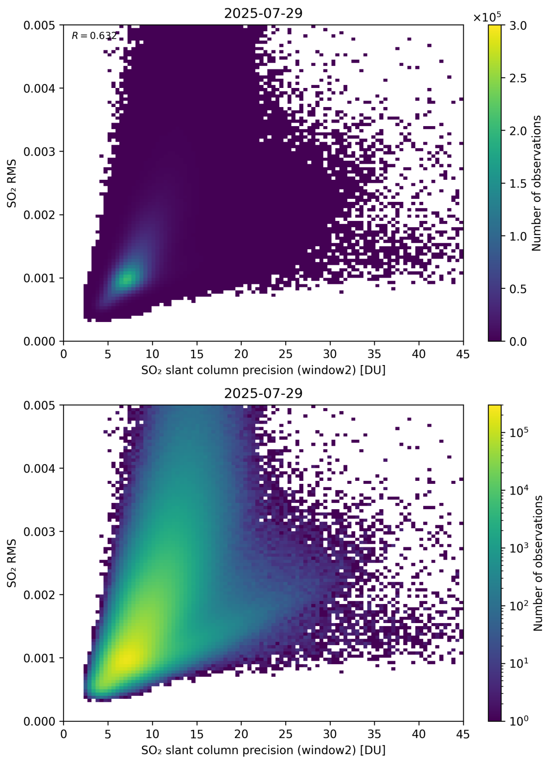
Figure 295: Scatter density plot of “SO 2 slant column precision (window2)” against “SO 2 RMS” for 2025-07-29 to 2025-07-30.
