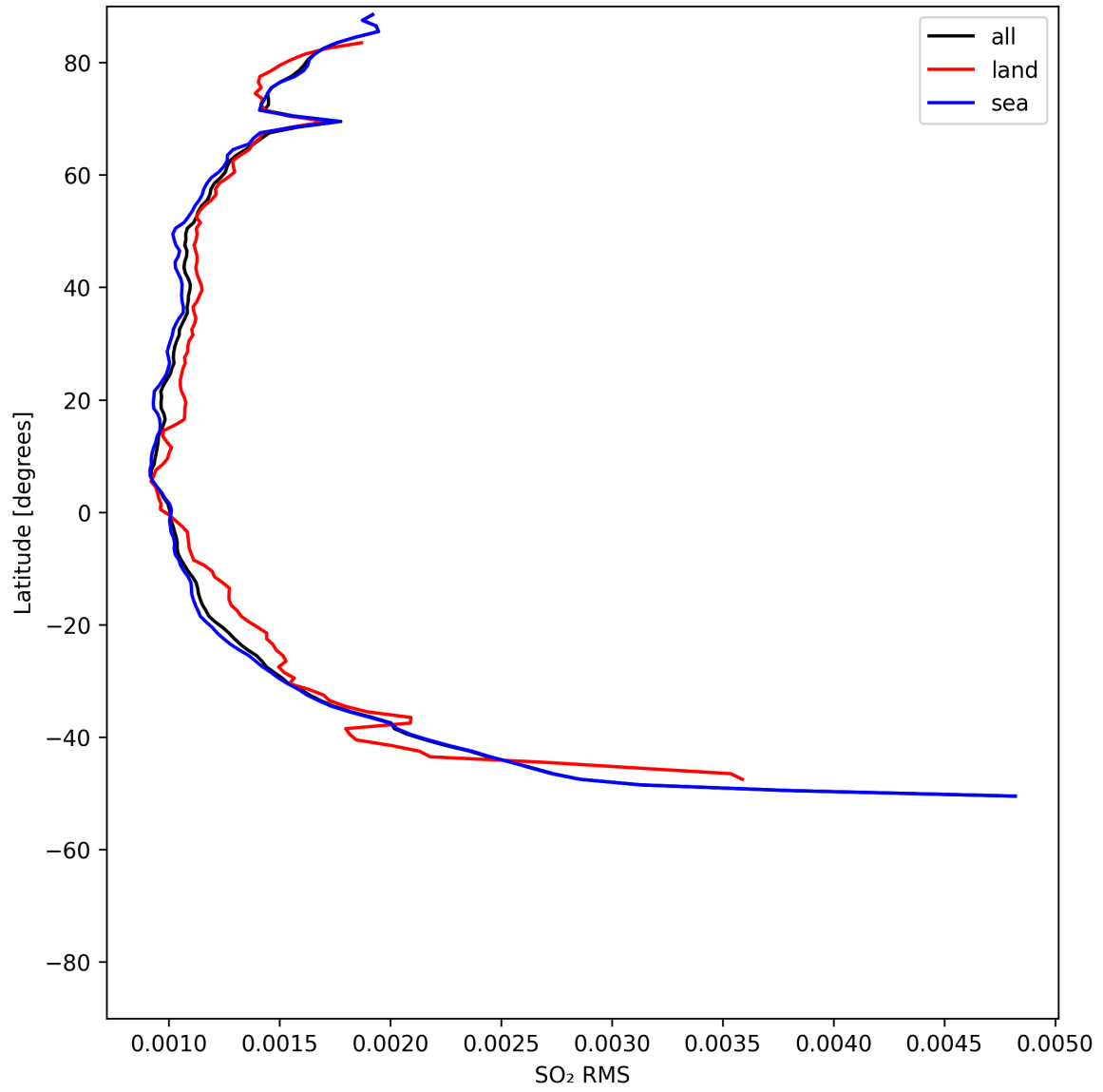
Figure 52: Zonal average of “SO 2 RMS” for 2025-07-29 to 2025-07-30.
