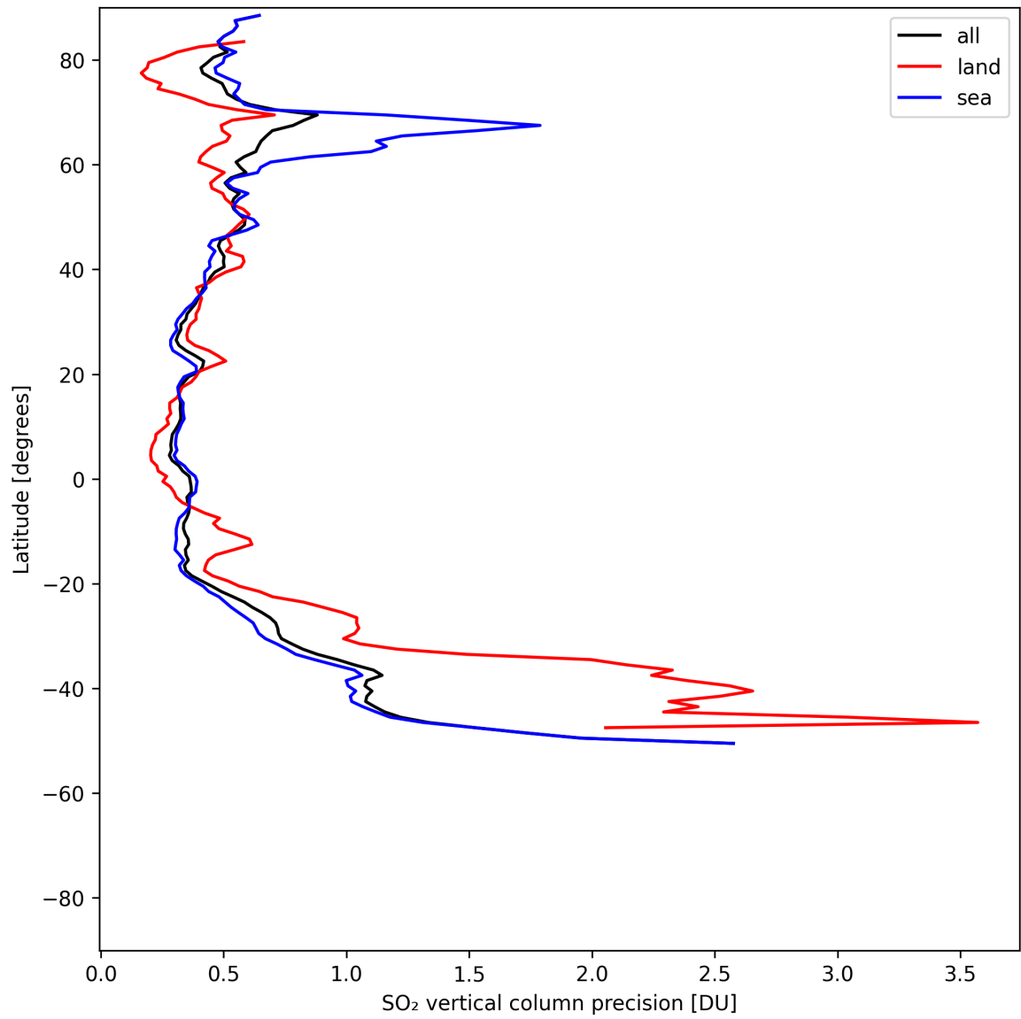
Figure 33: Zonal average of “SO 2 vertical column precision” for 2025-07-29 to 2025-07-30.
