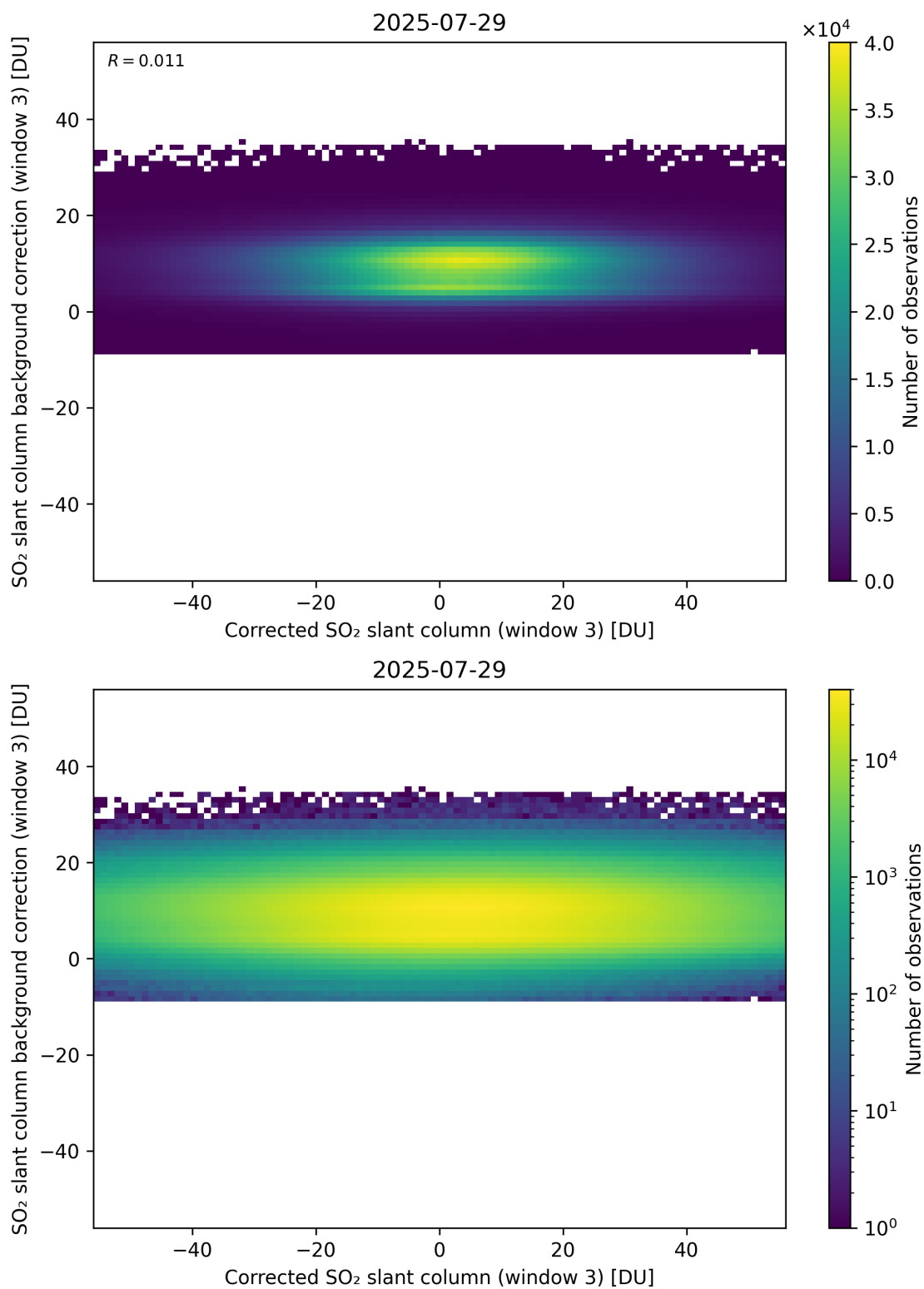
Figure 255: Scatter density plot of “Corrected SO 2 slant column (window 3)” against “SO 2 slant column background correction (window 3)” for 2025-07-29 to 2025-07-30.
