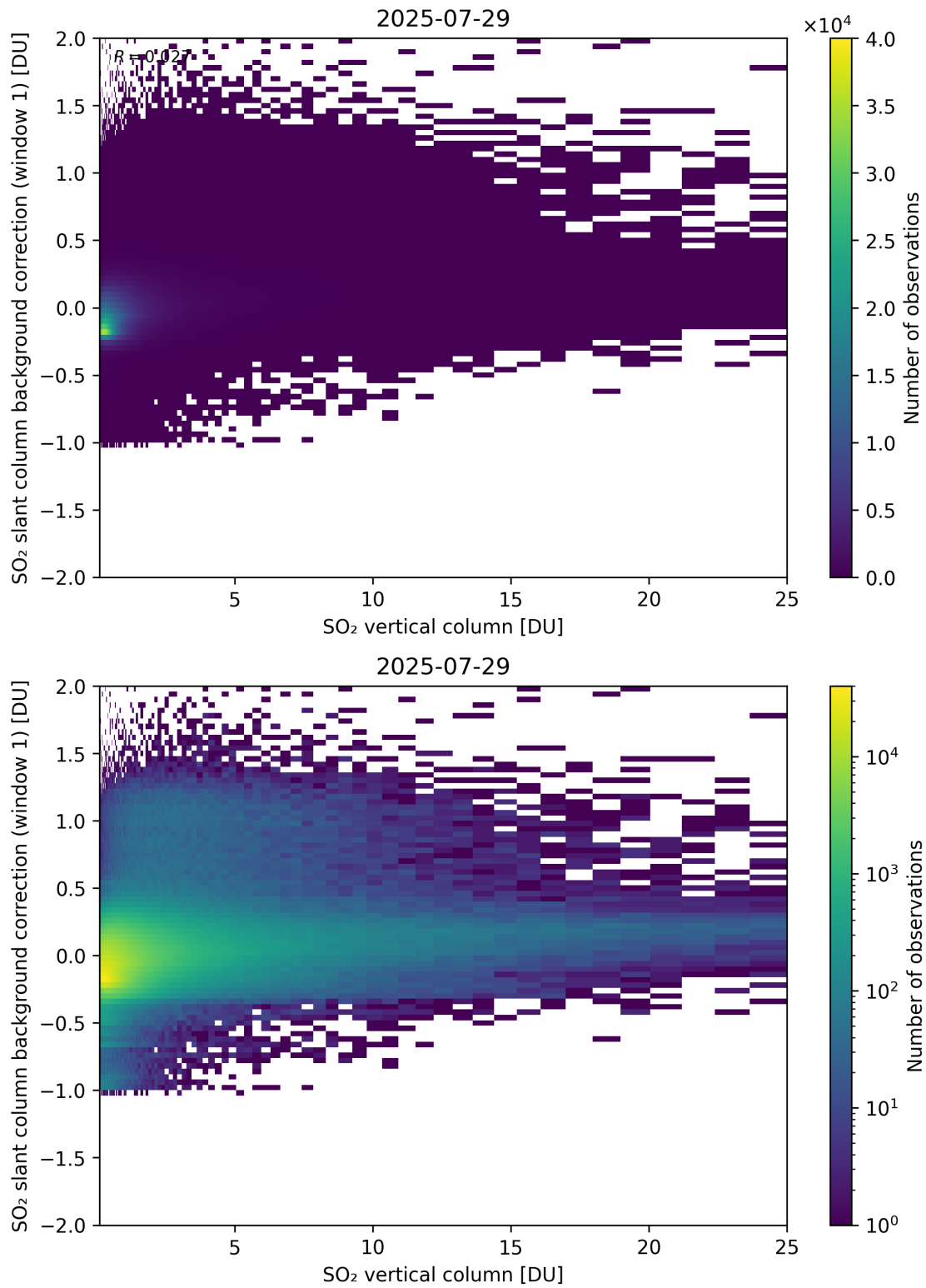
Figure 323: Scatter density plot of “SO 2 vertical column” against “SO 2 slant column background correction (window 1)” for 2025-07-29 to 2025-07-30.
