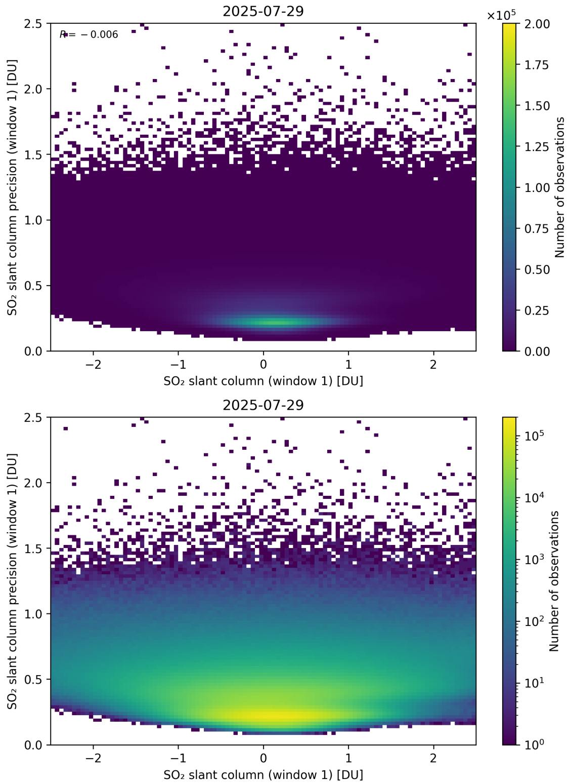
Figure 285: Scatter density plot of “SO 2 slant column (window 1)” against “SO 2 slant column precision (window 1)” for 2025-07-29 to 2025-07-30.
