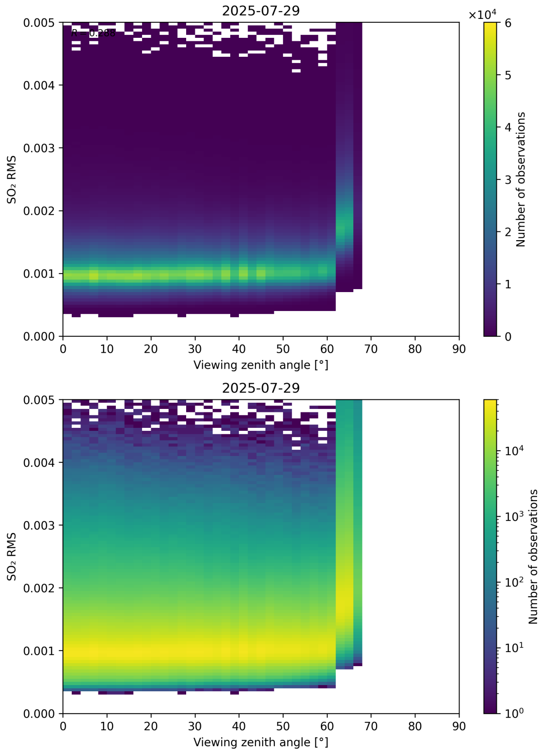
Figure 367: Scatter density plot of “Viewing zenith angle” against “SO 2 RMS” for 2025-07-29 to 2025-07-30.
