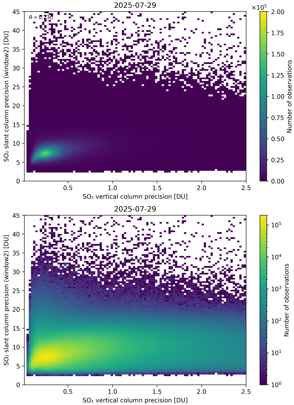
Figure 343: Scatter density plot of “SO 2 vertical column precision” against “SO 2 slant column precision (window2)” for 2025-07-29 to 2025-07-30.
