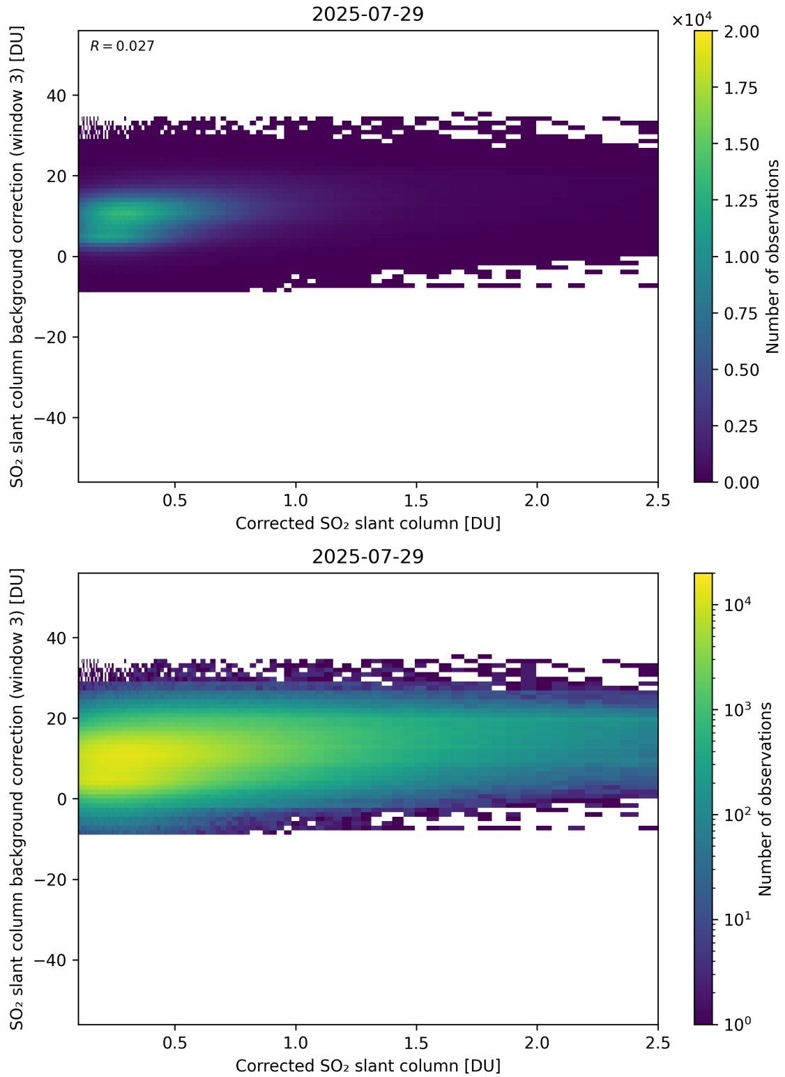
Figure 228: Scatter density plot of “Corrected SO 2 slant column” against “SO 2 slant column background correction (window 3)” for 2025-07-29 to 2025-07-30.
