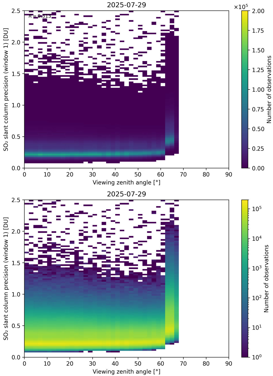
Figure 377: Scatter density plot of “Viewing zenith angle” against “SO 2 slant column precision (window 1)” for 2025-07-29 to 2025-07-30.
