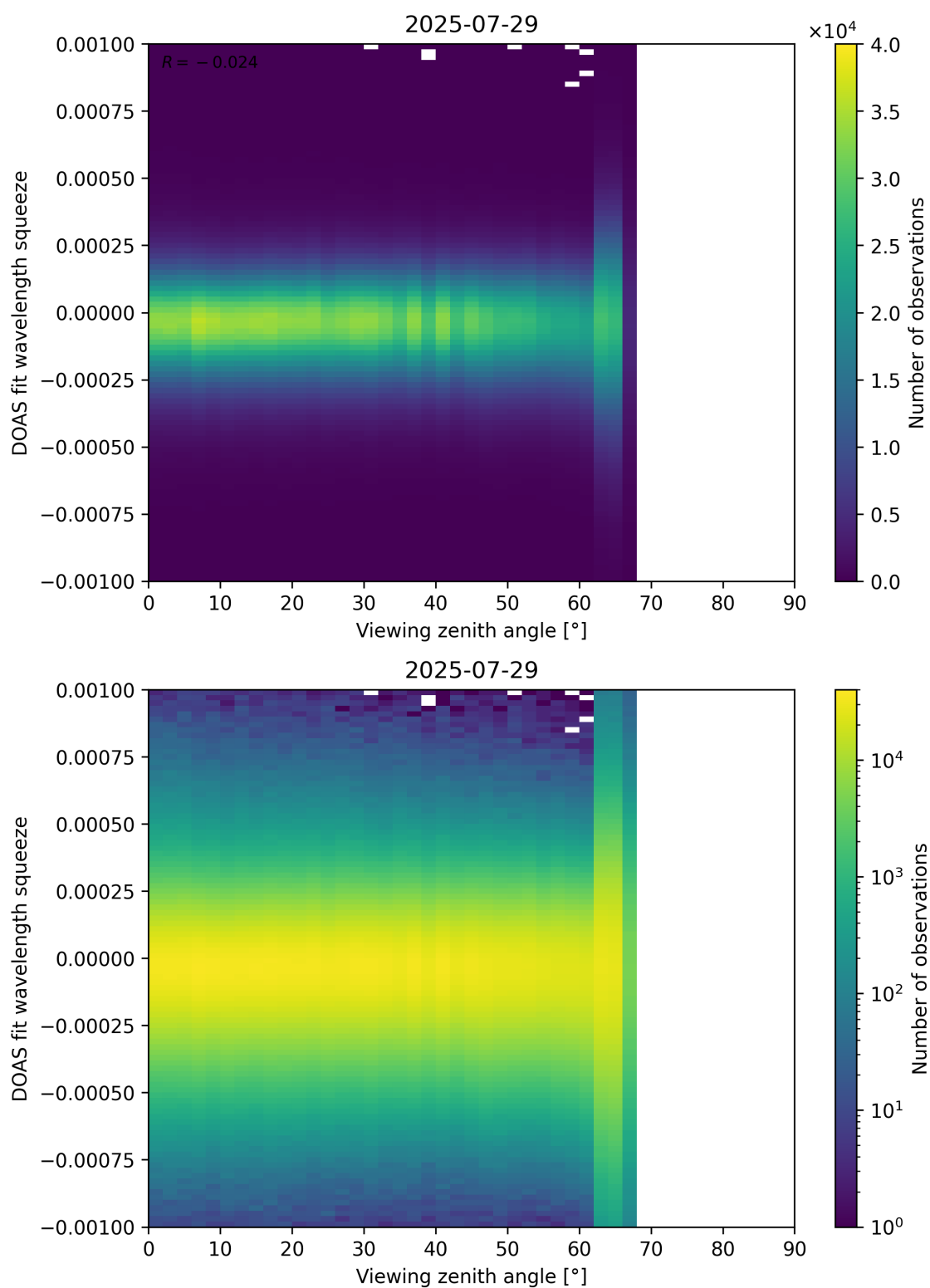
Figure 366: Scatter density plot of “Viewing zenith angle” against “DOAS fit wavelength squeeze” for 2025-07-29 to 2025-07-30.
