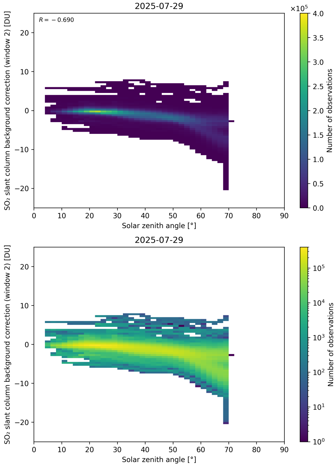
Figure 172: Scatter density plot of “Solar zenith angle” against “SO 2 slant column background correction (window 2)” for 2025-07-29 to 2025-07-30.
