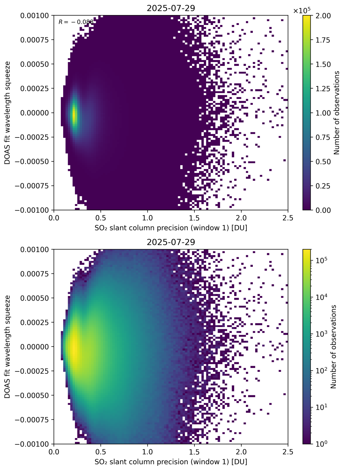
Figure 272: Scatter density plot of “SO 2 slant column precision (window 1)” against “DOAS fit wavelength squeeze” for 2025-07-29 to 2025-07-30.
