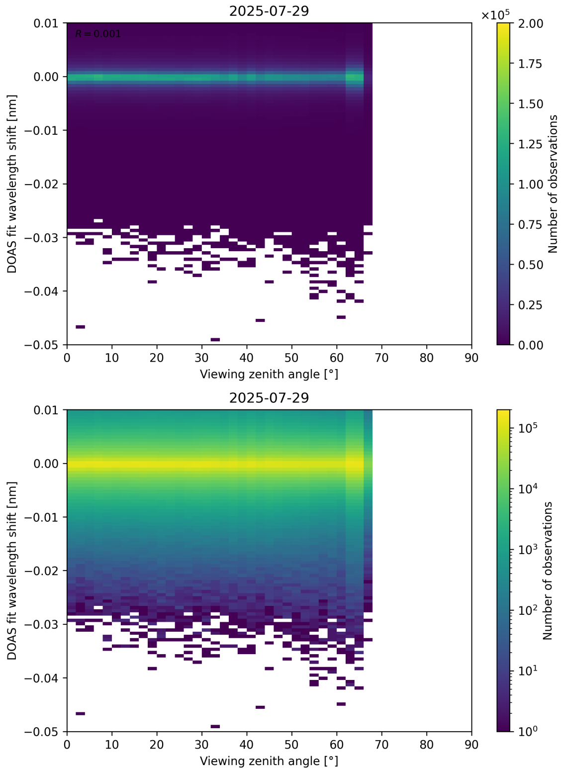
Figure 365: Scatter density plot of “Viewing zenith angle” against “DOAS fit wavelength shift” for 2025-07-29 to 2025-07-30.
