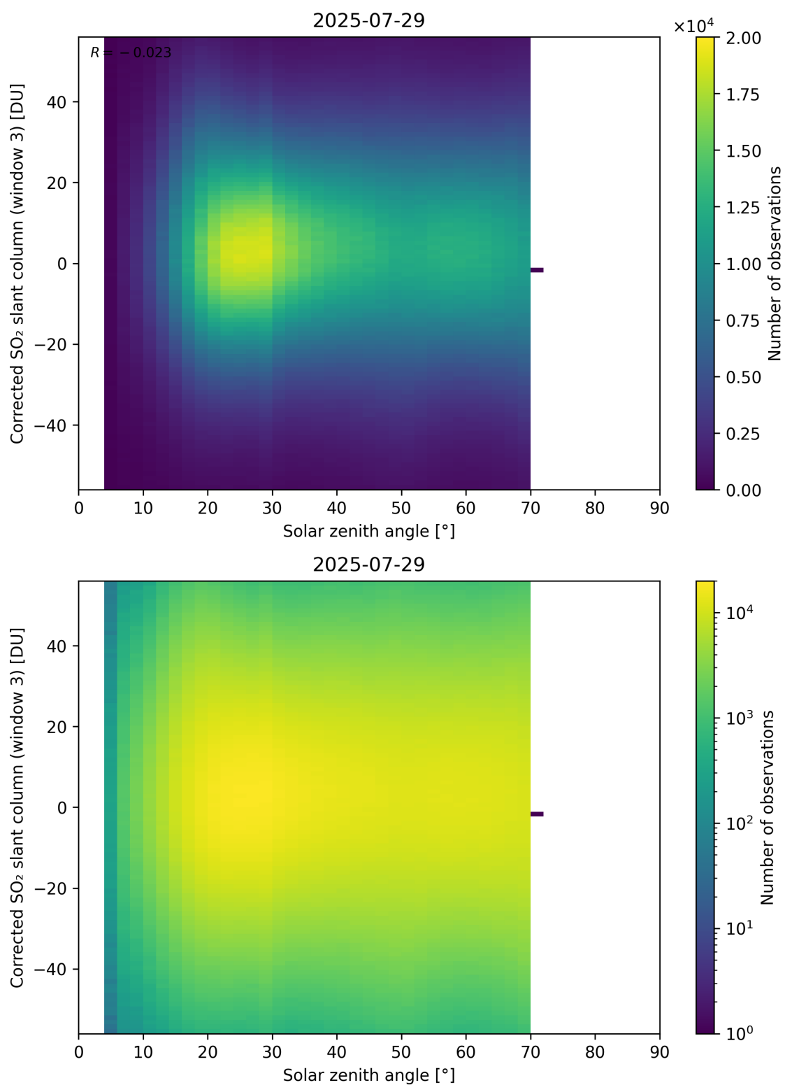
Figure 183: Scatter density plot of “Solar zenith angle” against “Corrected SO 2 slant column (window 3)” for 2025-07-29 to 2025-07-30.
