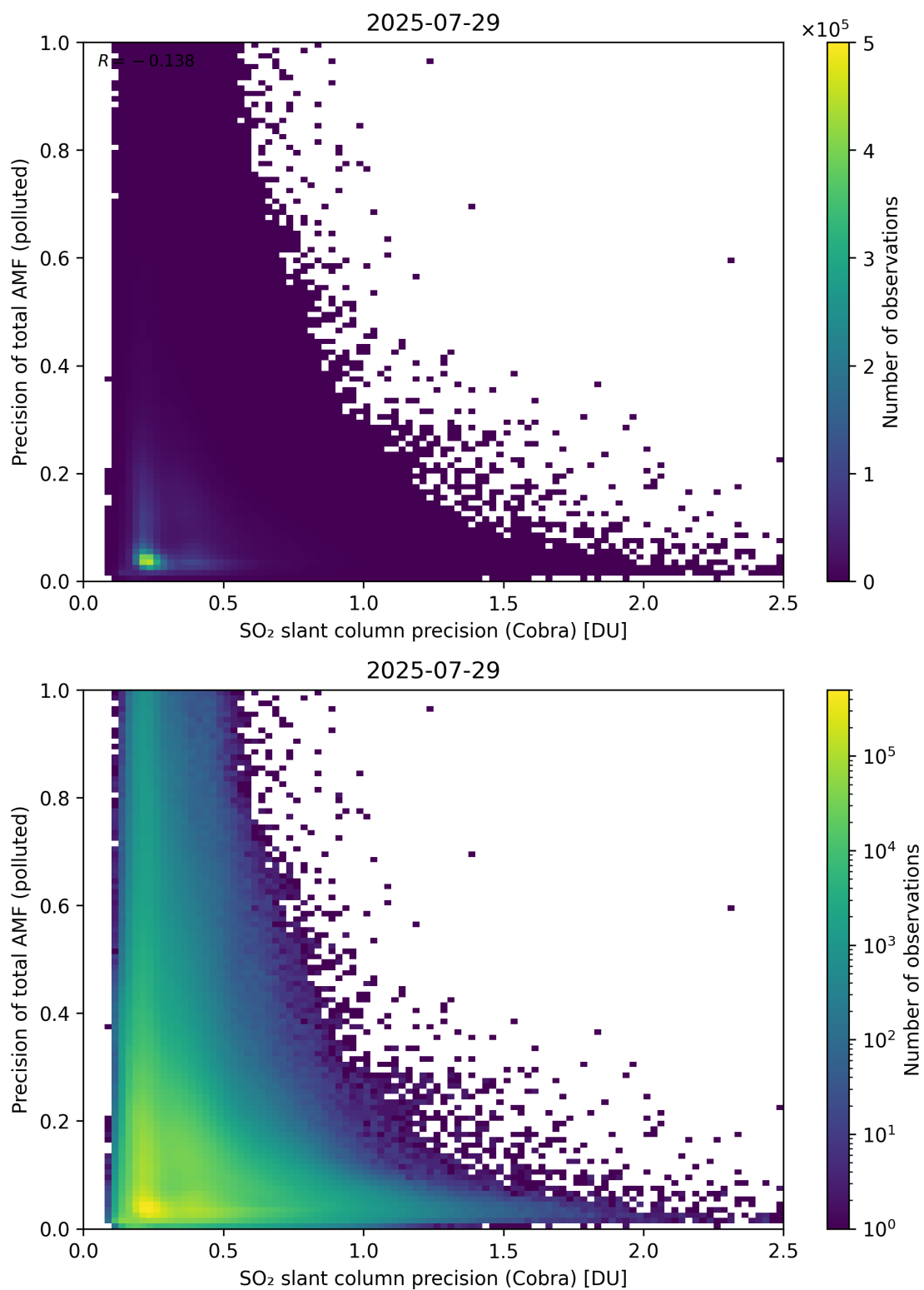
Figure 214: Scatter density plot of “SO 2 slant column precision (Cobra)” against “Precision of total AMF (polluted)” for 2025-07-29 to 2025-07-30.
