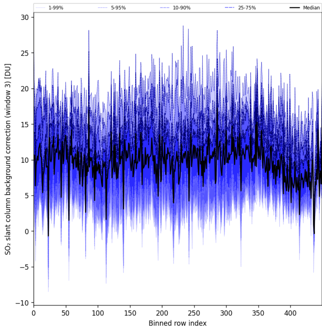
Figure 100: Along track statistics of “SO 2 slant column background correction (window 3)” for 2025-07-29 to 2025-07-30
