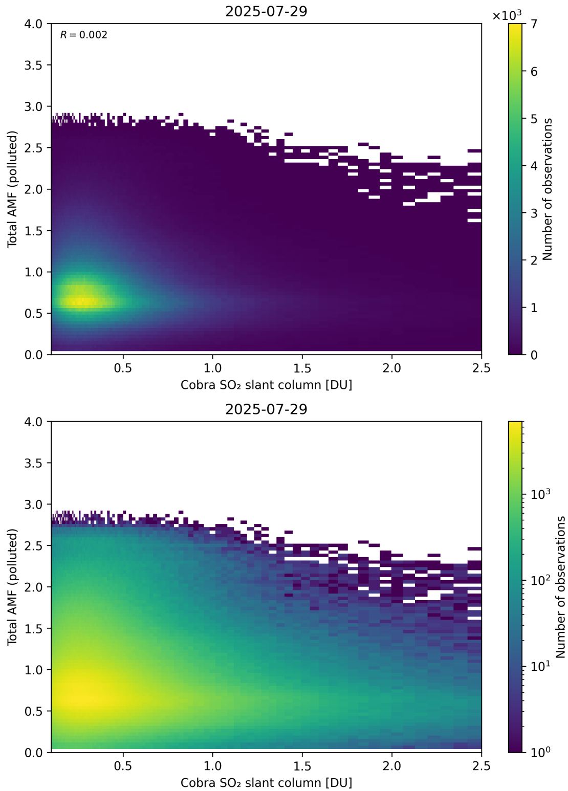
Figure 224: Scatter density plot of “Cobra SO 2 slant column” against “Total AMF (polluted)” for 2025-07-29 to 2025-07-30.
