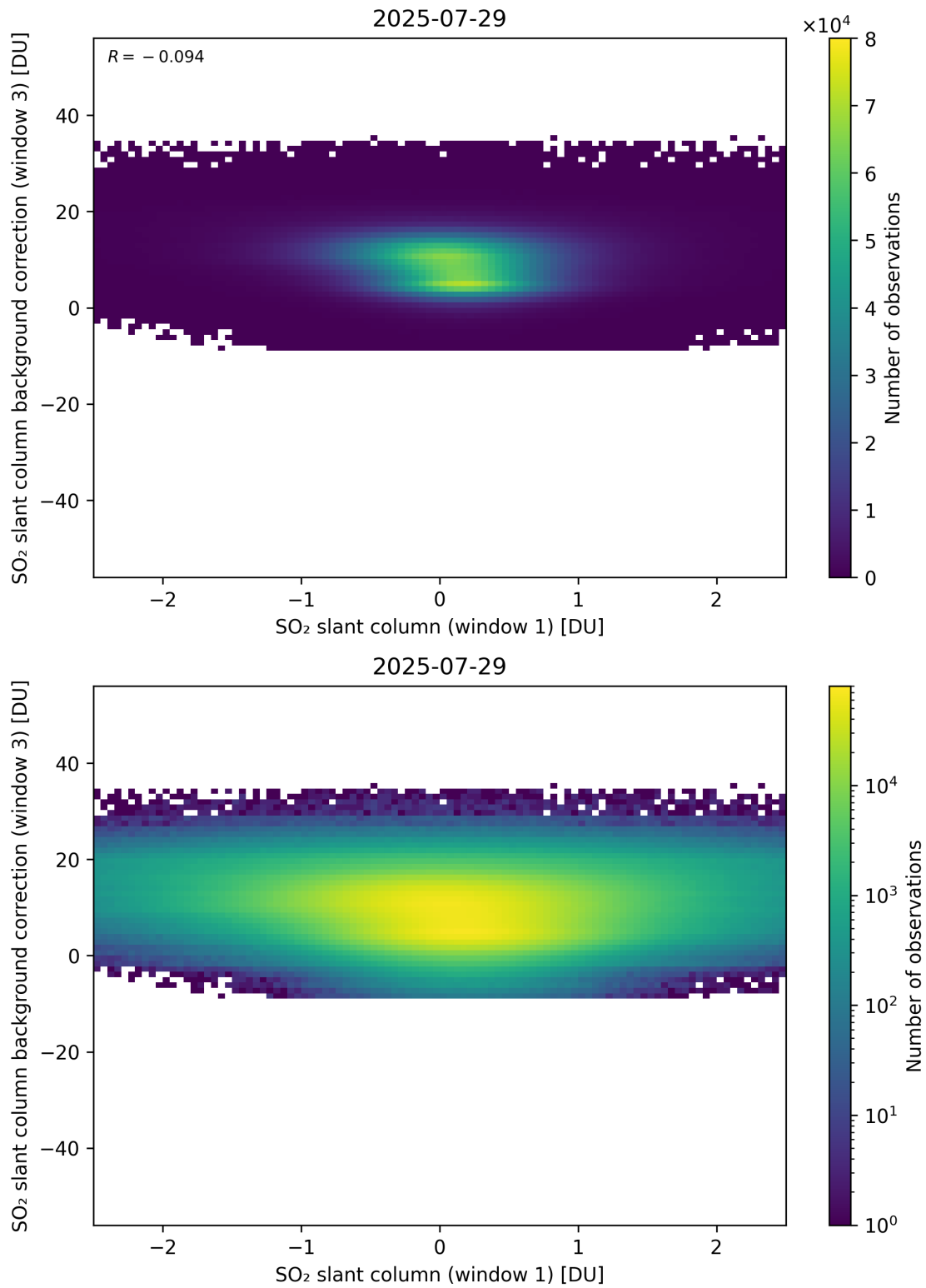
Figure 264: Scatter density plot of “SO 2 slant column (window 1)” against “SO 2 slant column background correction (window 3)” for 2025-07-29 to 2025-07-30.
