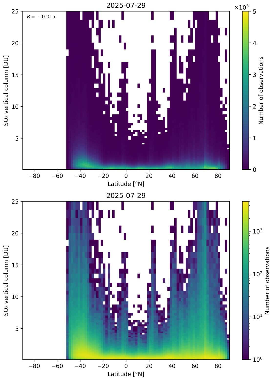
Figure 169: Scatter density plot of “Latitude” against “SO 2 vertical column” for 2025-07-29 to 2025-07-30.
