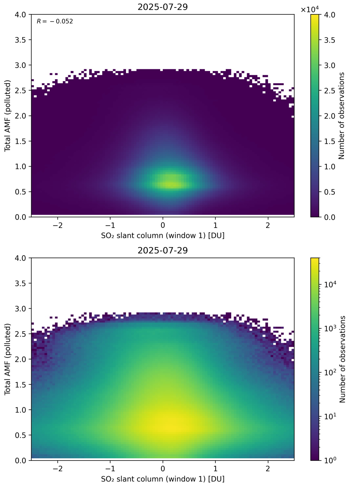
Figure 289: Scatter density plot of “SO 2 slant column (window 1)” against “Total AMF (polluted)” for 2025-07-29 to 2025-07-30.
