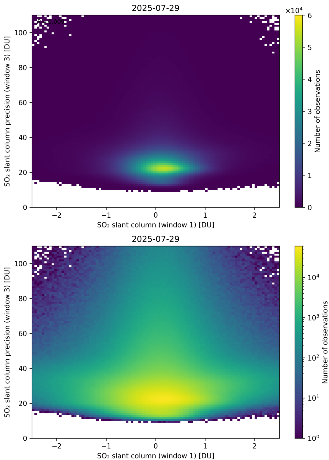
Figure 288: Scatter density plot of “SO 2 slant column (window 1)” against “SO 2 slant column precision (window 3)” for 2025-07-29 to 2025-07-30.
