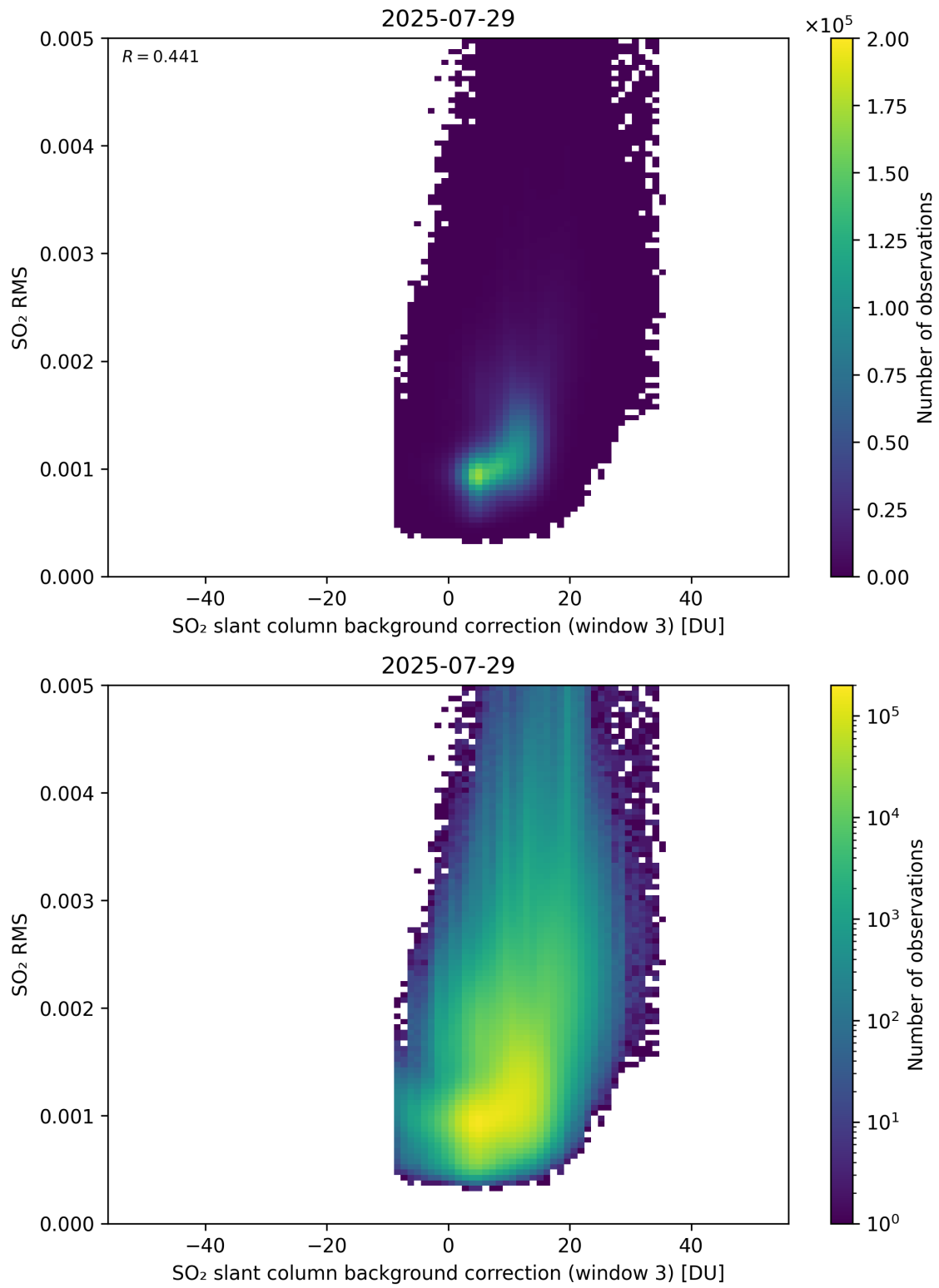
Figure 134: Scatter density plot of “SO 2 slant column background correction (window 3)” against “SO 2 RMS” for 2025-07-29 to 2025-07-30.
