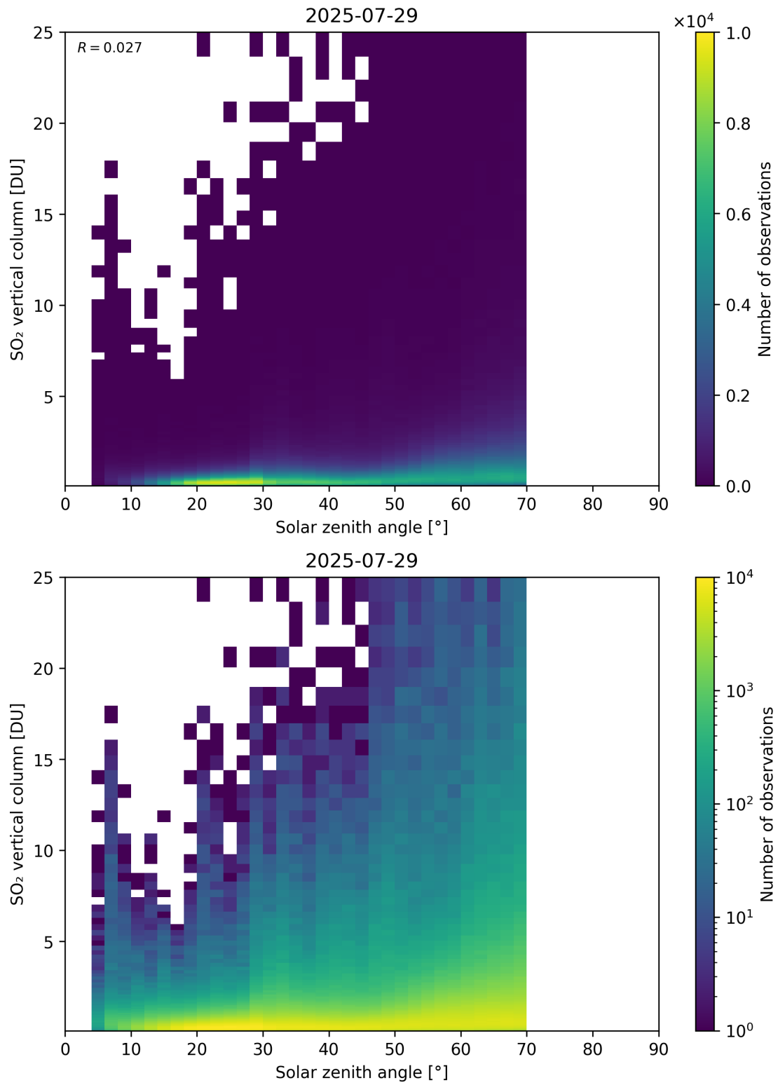
Figure 191: Scatter density plot of “Solar zenith angle” against “SO 2 vertical column” for 2025-07-29 to 2025-07-30.
