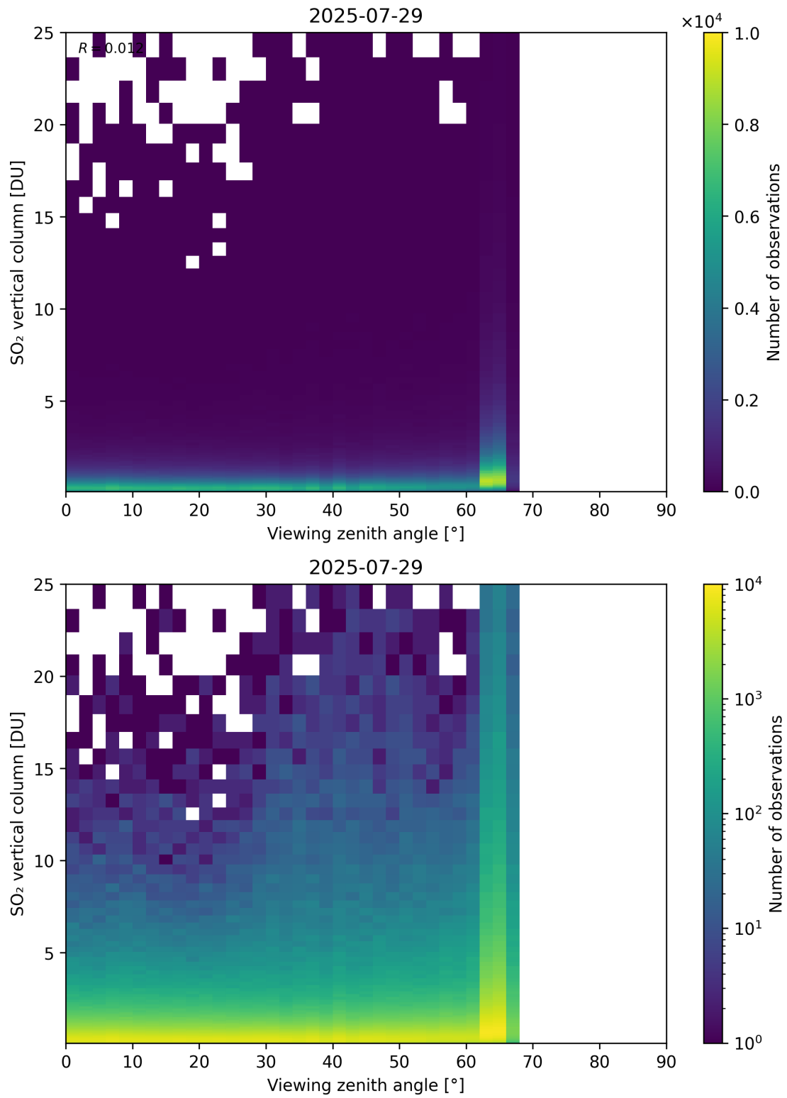
Figure 383: Scatter density plot of “Viewing zenith angle” against “SO 2 vertical column” for 2025-07-29 to 2025-07-30.
