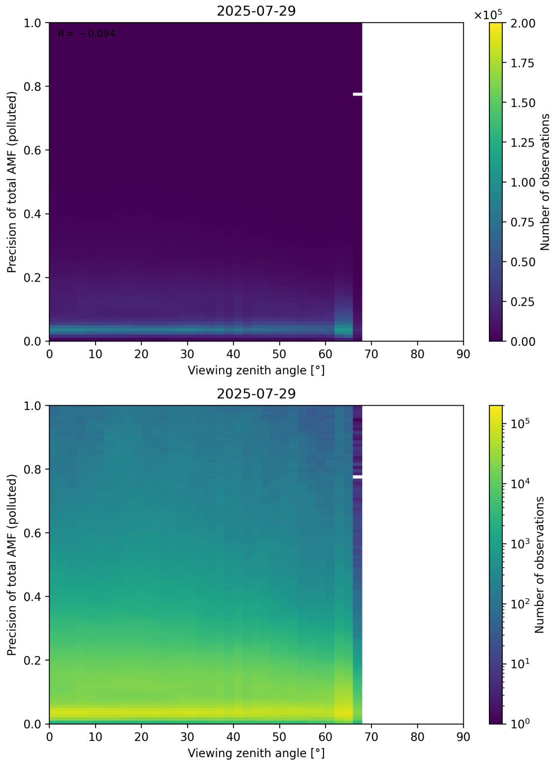
Figure 382: Scatter density plot of “Viewing zenith angle” against “Precision of total AMF (polluted)” for 2025-07-29 to 2025-07-30.
