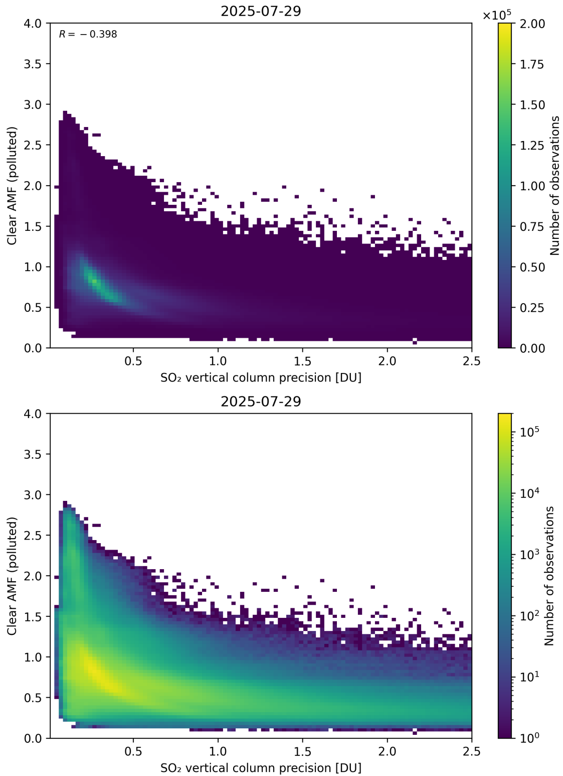
Figure 335: Scatter density plot of “SO 2 vertical column precision” against “Clear AMF (polluted)” for 2025-07-29 to 2025-07-30.
