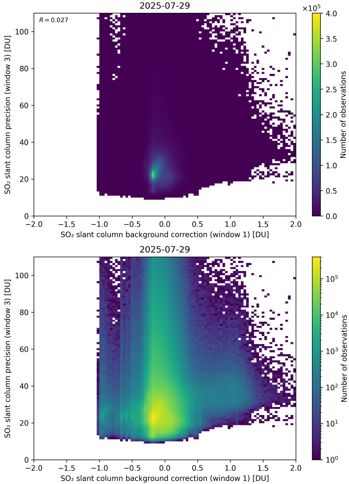
Figure 119: Scatter density plot of “SO 2 slant column background correction (window 1)” against “SO 2 slant column precision (window 3)” for 2025-07-29 to 2025-07-30.
