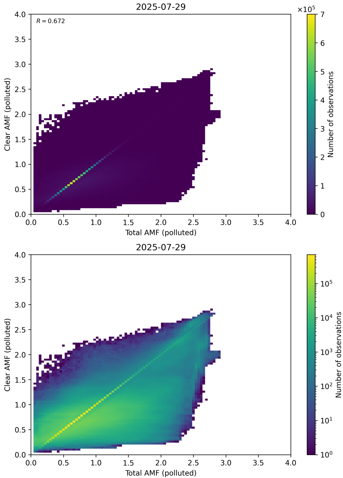
Figure 321: Scatter density plot of “Total AMF (polluted)” against “Clear AMF (polluted)” for 2025-07-29 to 2025-07-30.
