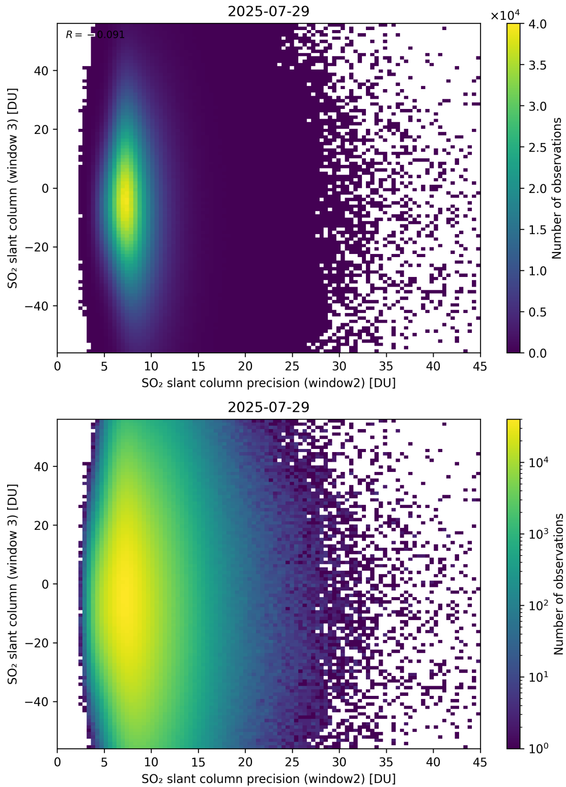
Figure 299: Scatter density plot of “SO 2 slant column precision (window2)” against “SO 2 slant column (window 3)” for 2025-07-29 to 2025-07-30.
