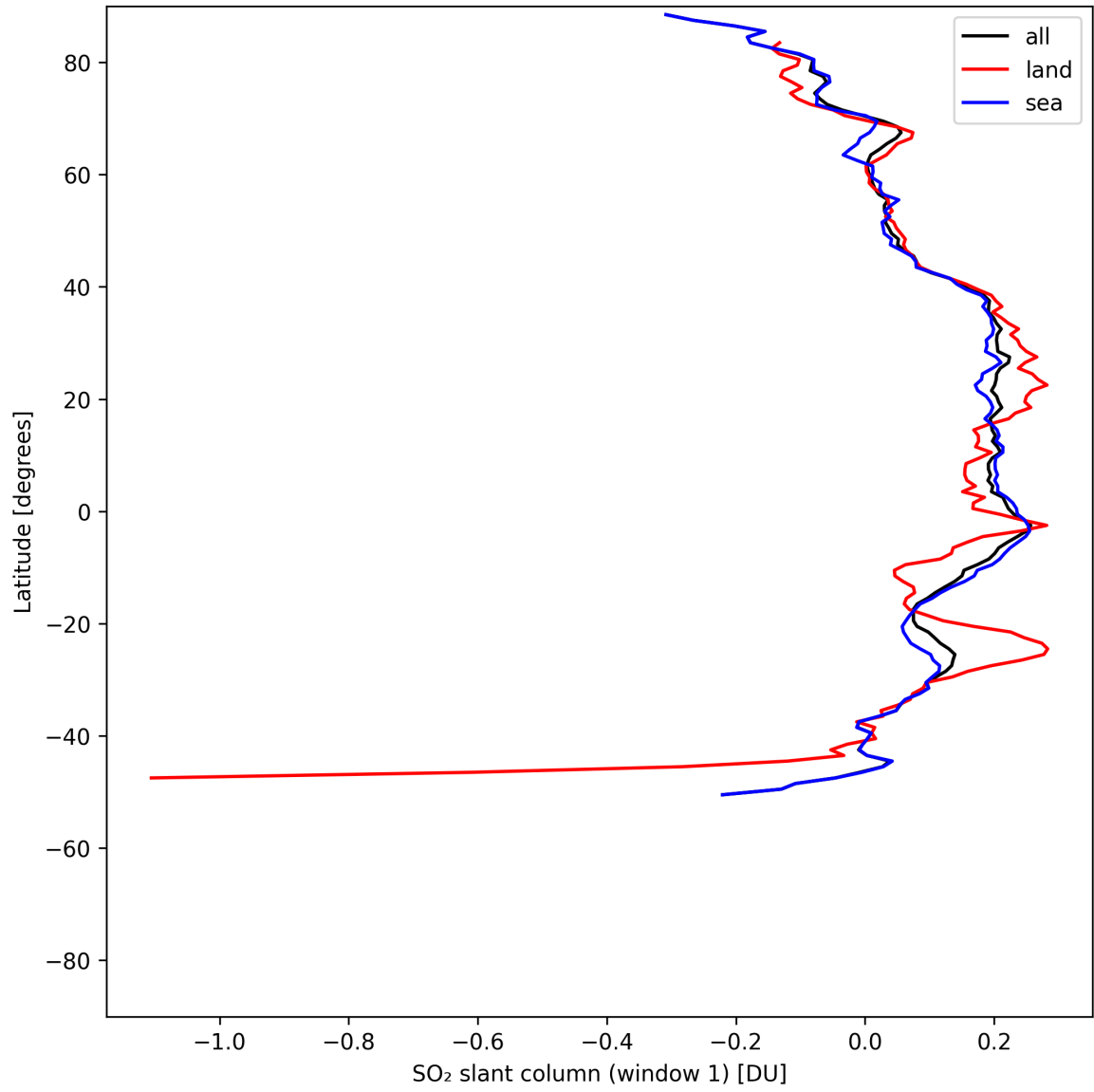
Figure 37: Zonal average of “SO 2 slant column (window 1)” for 2025-07-29 to 2025-07-30.
