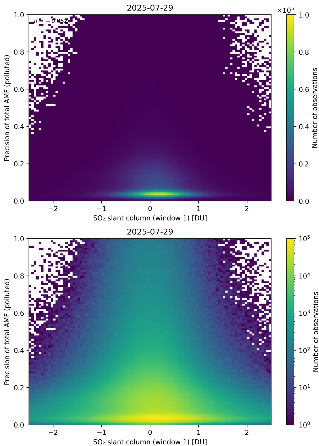
Figure 290: Scatter density plot of “SO 2 slant column (window 1)” against “Precision of total AMF (polluted)” for 2025-07-29 to 2025-07-30.
