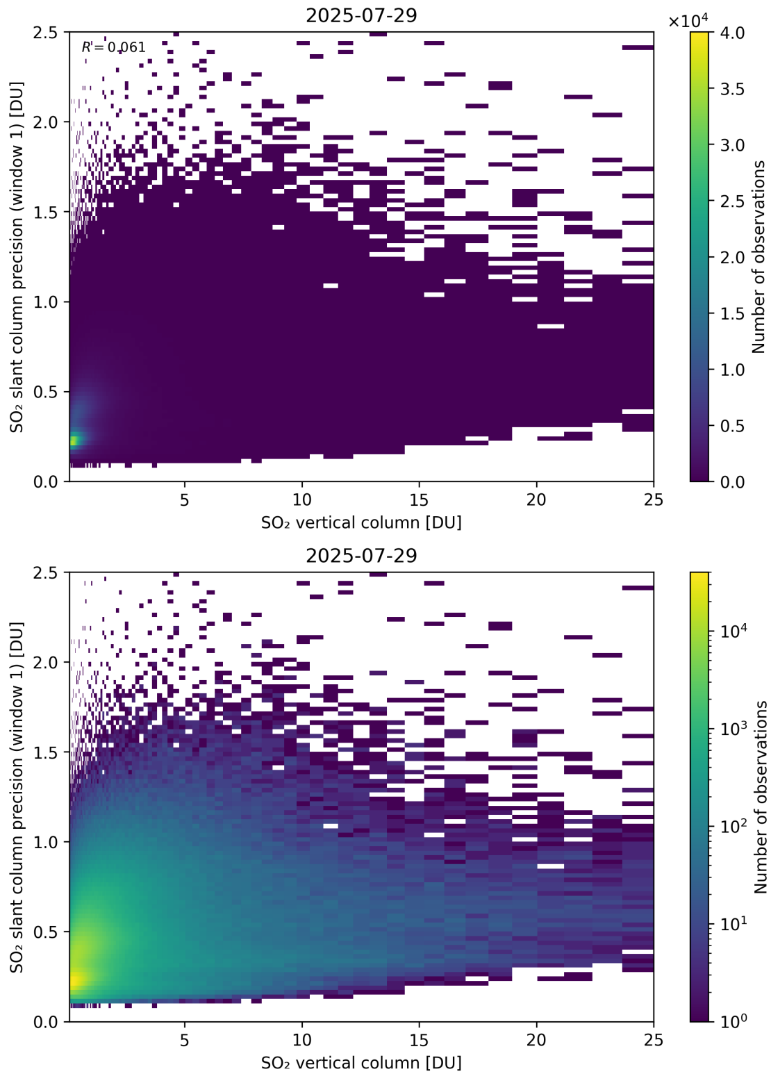
Figure 355: Scatter density plot of “SO 2 vertical column” against “SO 2 slant column precision (window 1)” for 2025-07-29 to 2025-07-30.
