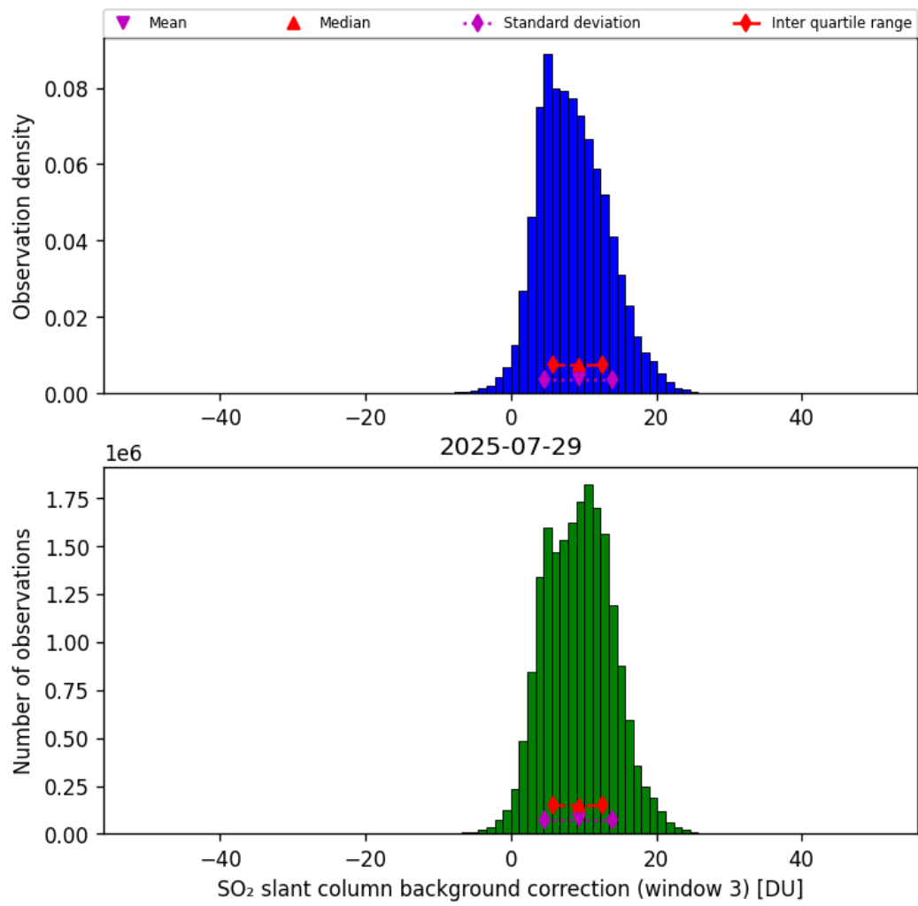
Figure 74: Histogram of “SO 2 slant column background correction (window 3)” for 2025-07-29 to 2025-07-30
