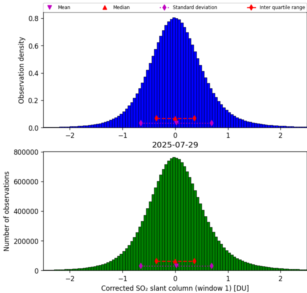
Figure 65: Histogram of “Corrected SO 2 slant column (window 1)” for 2025-07-29 to 2025-07-30
