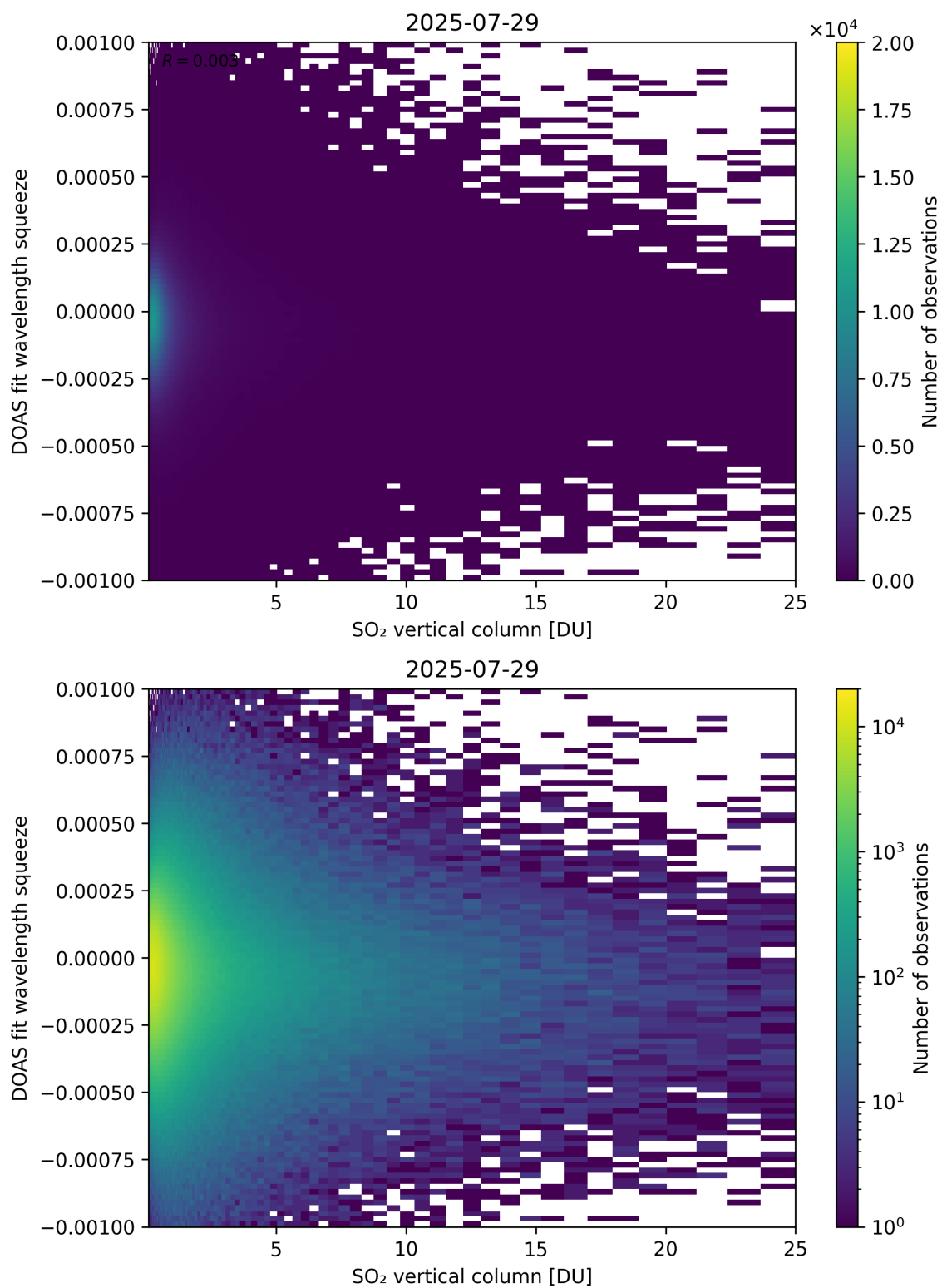
Figure 327: Scatter density plot of “SO 2 vertical column” against “DOAS fit wavelength squeeze” for 2025-07-29 to 2025-07-30.
