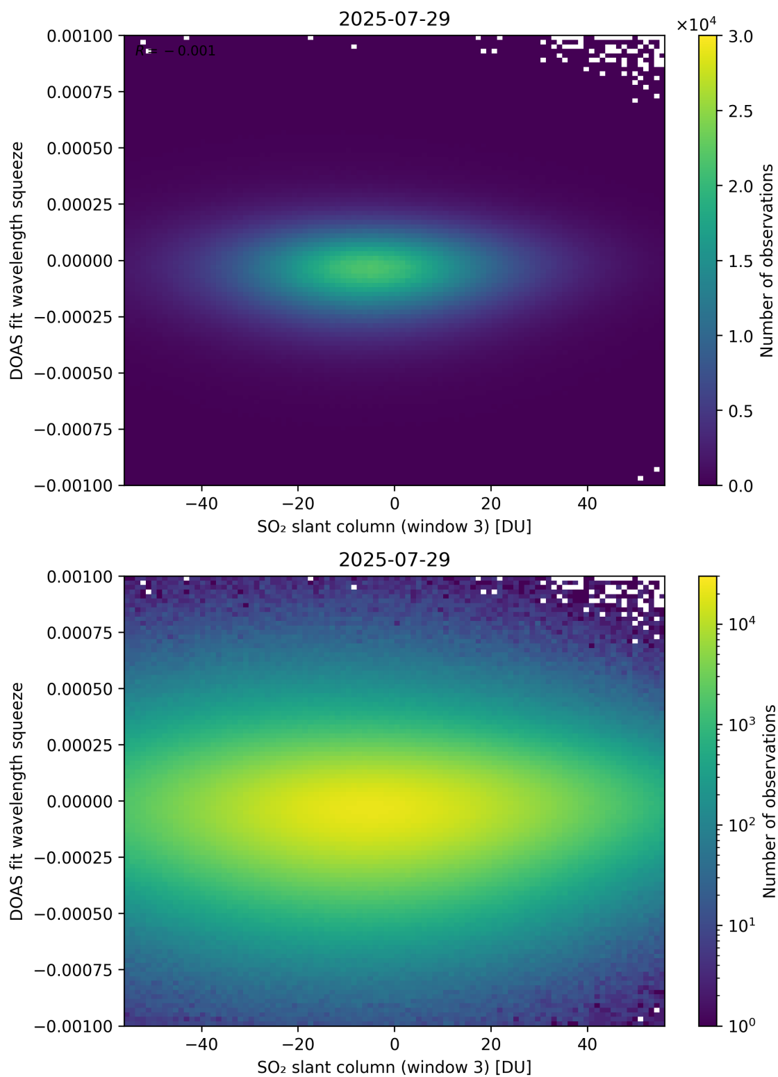
Figure 305: Scatter density plot of “SO 2 slant column (window 3)” against “DOAS fit wavelength squeeze” for 2025-07-29 to 2025-07-30.
