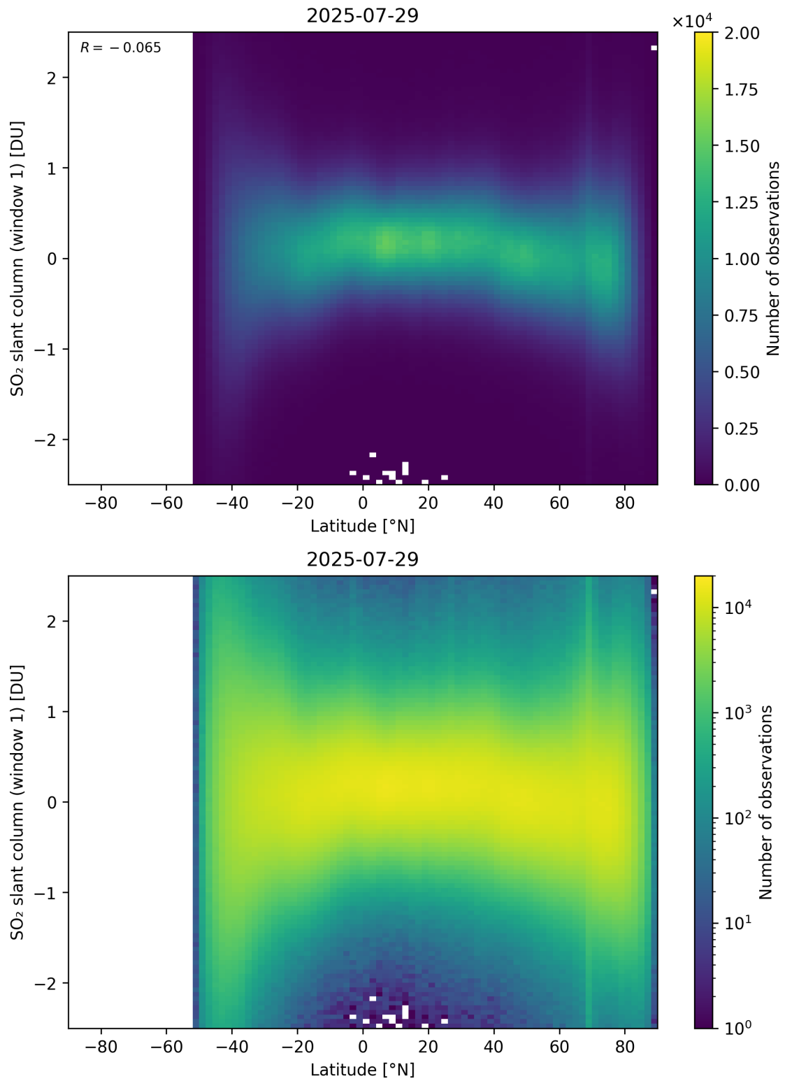
Figure 162: Scatter density plot of “Latitude” against “SO 2 slant column (window 1)” for 2025-07-29 to 2025-07-30.
