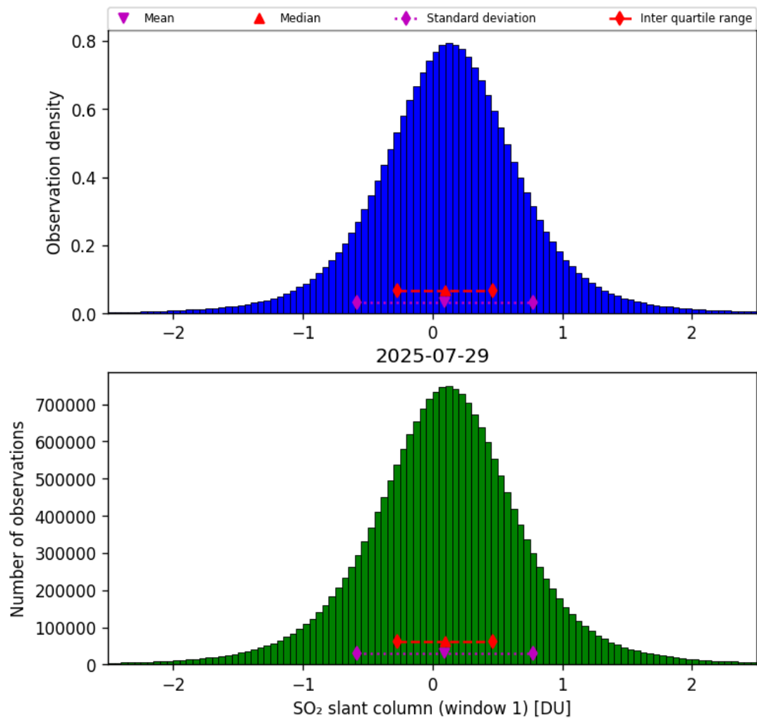
Figure 63: Histogram of “SO 2 slant column (window 1)” for 2025-07-29 to 2025-07-30
