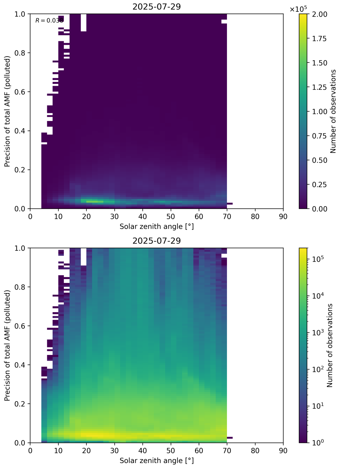
Figure 190: Scatter density plot of “Solar zenith angle” against “Precision of total AMF (polluted)” for 2025-07-29 to 2025-07-30.
