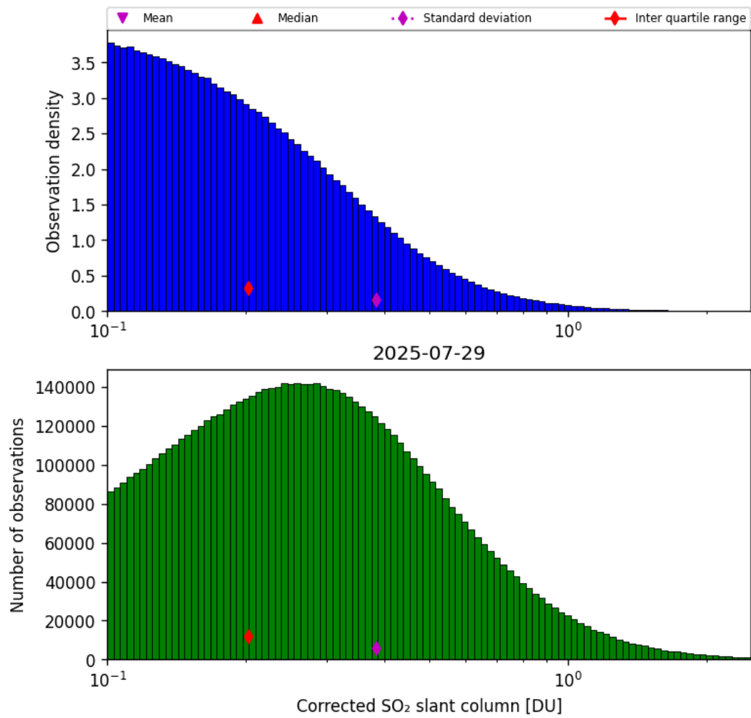
Figure 60: Histogram of “Corrected SO 2 slant column” for 2025-07-29 to 2025-07-30
