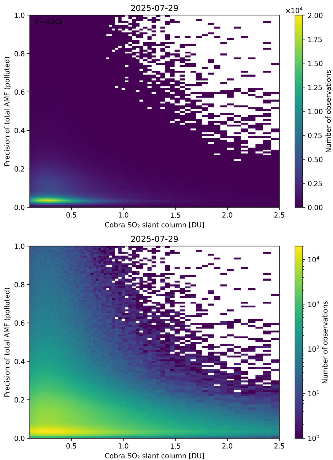
Figure 225: Scatter density plot of “Cobra SO 2 slant column” against “Precision of total AMF (polluted)” for 2025-07-29 to 2025-07-30.
