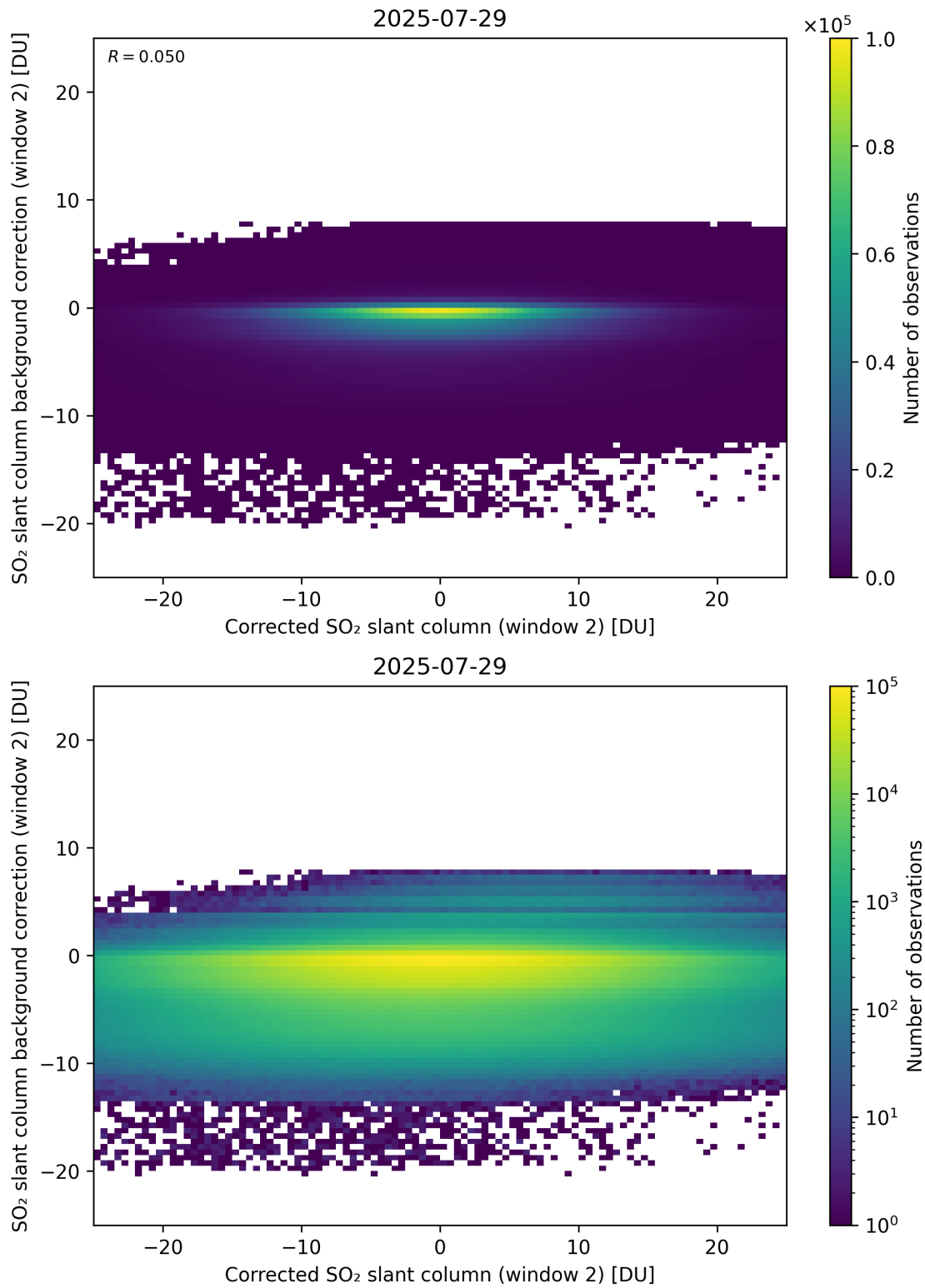
Figure 244: Scatter density plot of “Corrected SO 2 slant column (window 2)” against “SO 2 slant column background correction (window 2)” for 2025-07-29 to 2025-07-30.
