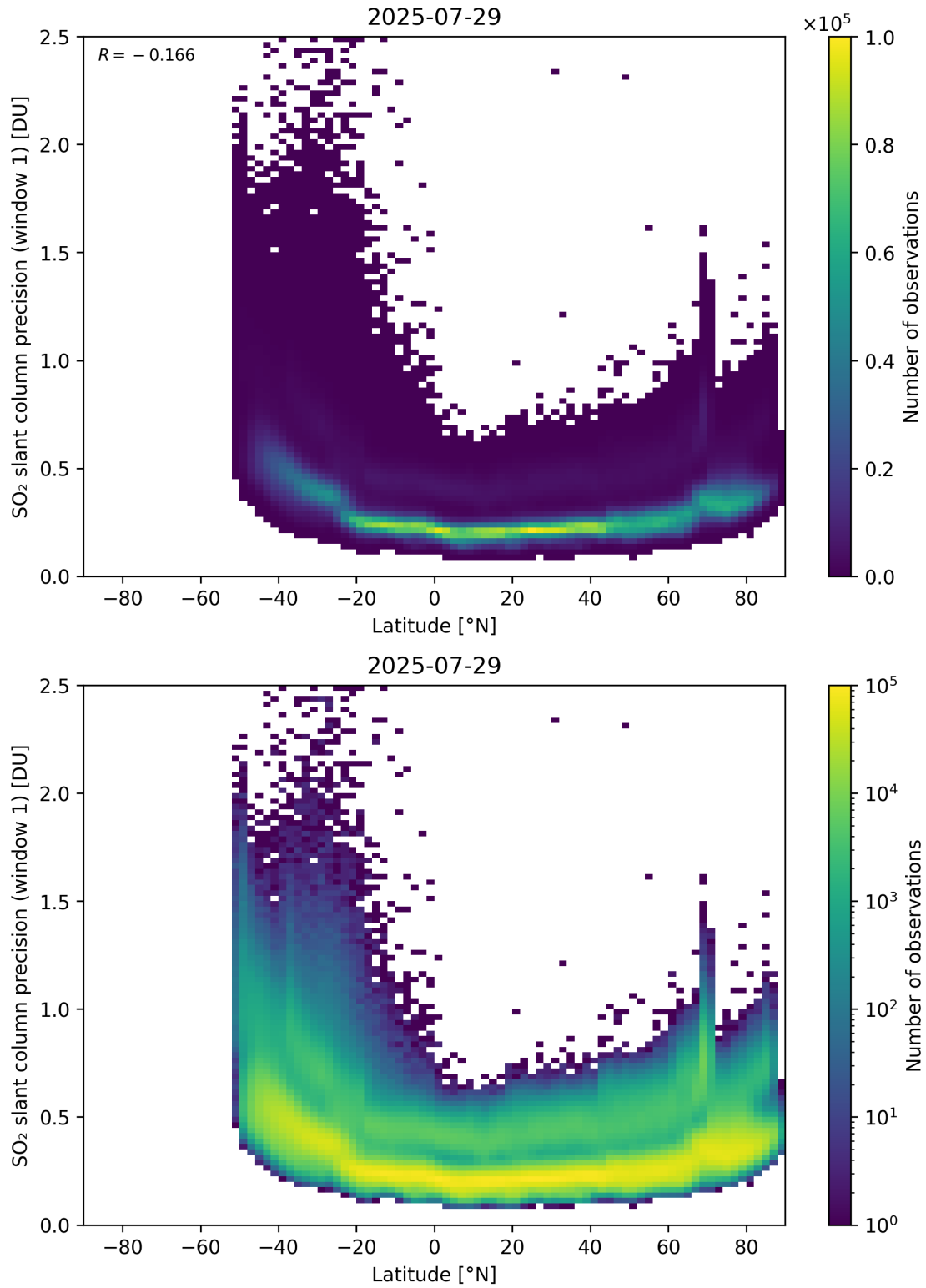
Figure 163: Scatter density plot of “Latitude” against “SO 2 slant column precision (window 1)” for 2025-07-29 to 2025-07-30.
