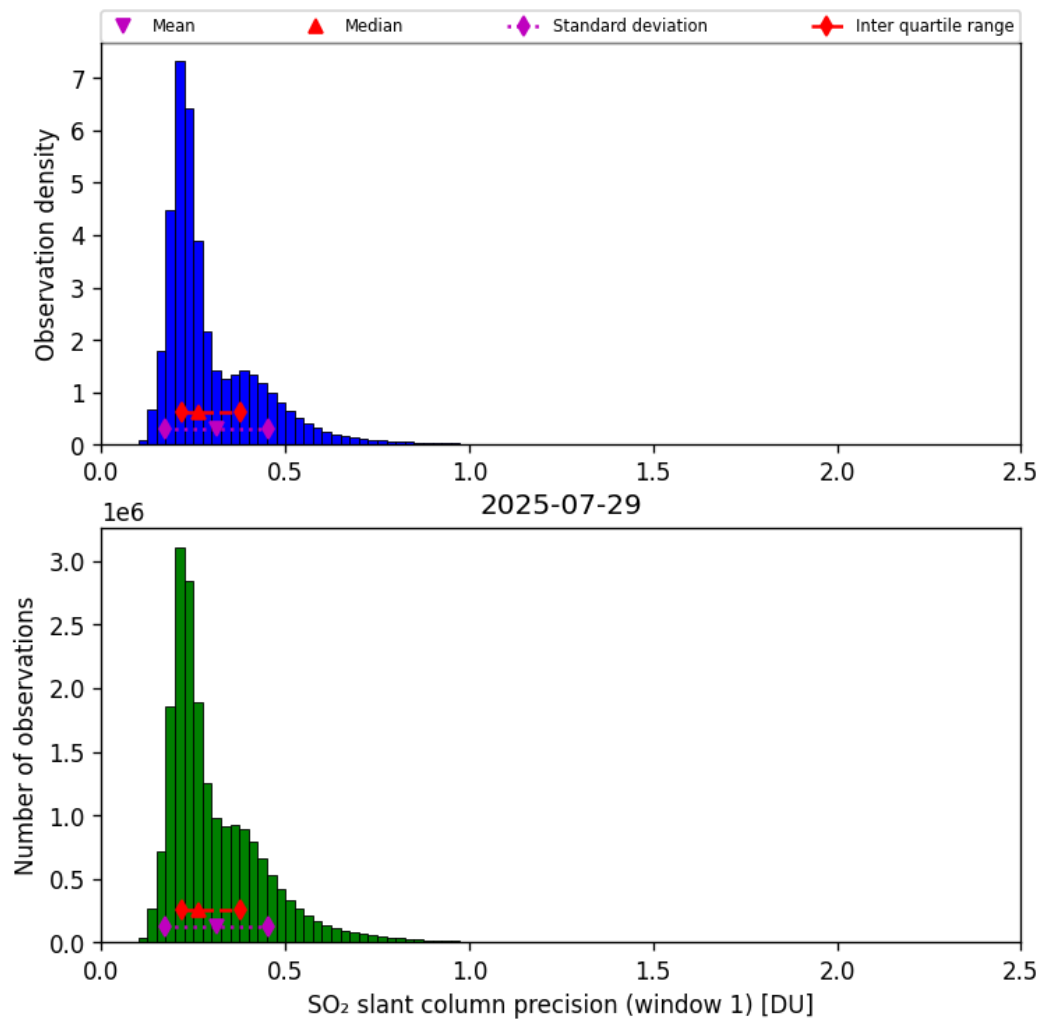
Figure 64: Histogram of “SO 2 slant column precision (window 1)” for 2025-07-29 to 2025-07-30
