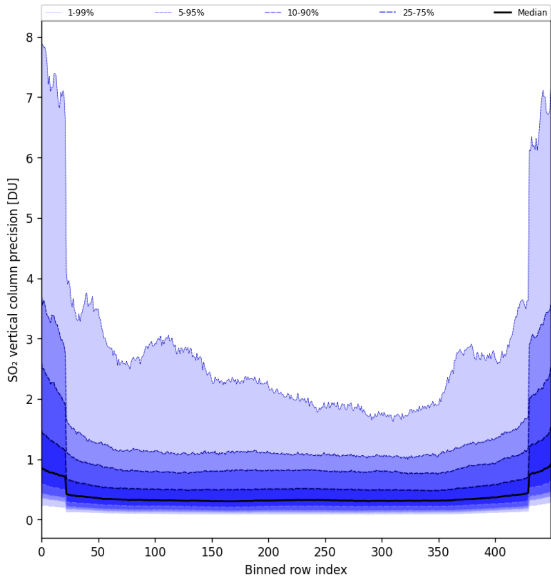
Figure 85: Along track statistics of “SO 2 vertical column precision” for 2025-07-29 to 2025-07-30
