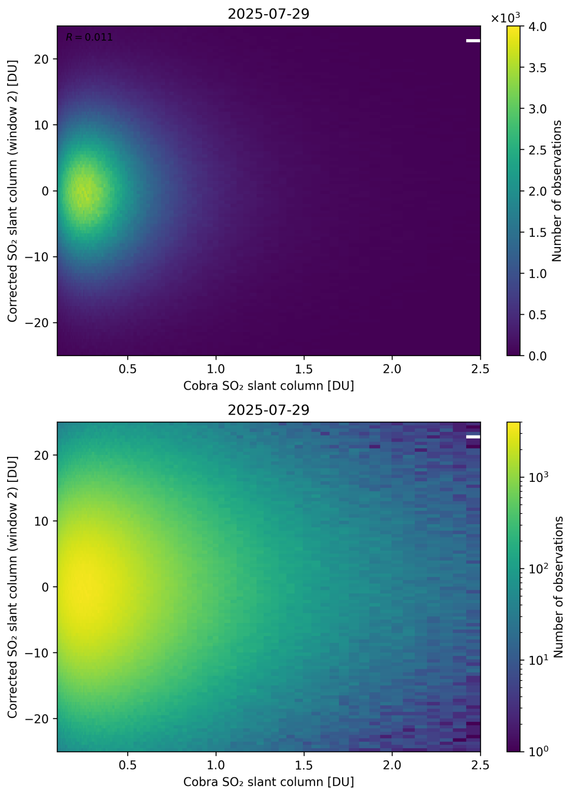
Figure 217: Scatter density plot of “Cobra SO 2 slant column” against “Corrected SO 2 slant column (window 2)” for 2025-07-29 to 2025-07-30.
