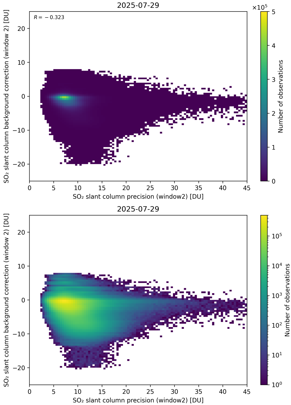
Figure 291: Scatter density plot of “SO 2 slant column precision (window2)” against “SO 2 slant column background correction (window 2)” for 2025-07-29 to 2025-07-30.
