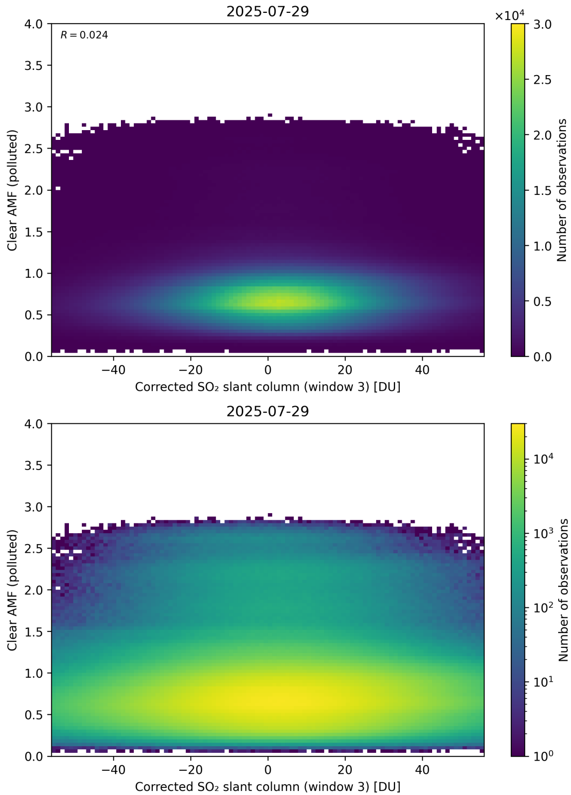
Figure 259: Scatter density plot of “Corrected SO 2 slant column (window 3)” against “Clear AMF (polluted)” for 2025-07-29 to 2025-07-30.
