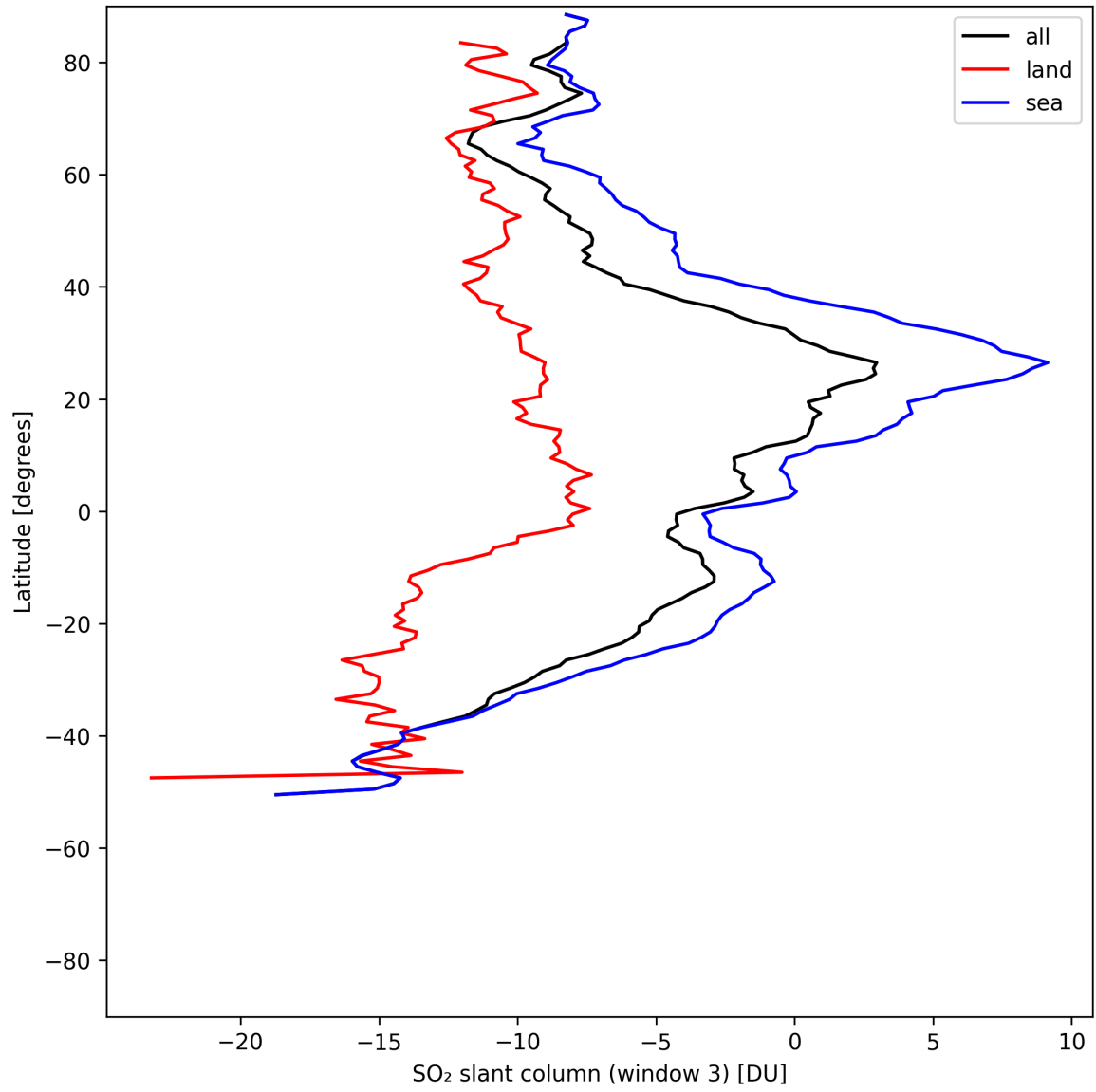
Figure 45: Zonal average of “SO 2 slant column (window 3)” for 2025-07-29 to 2025-07-30.
