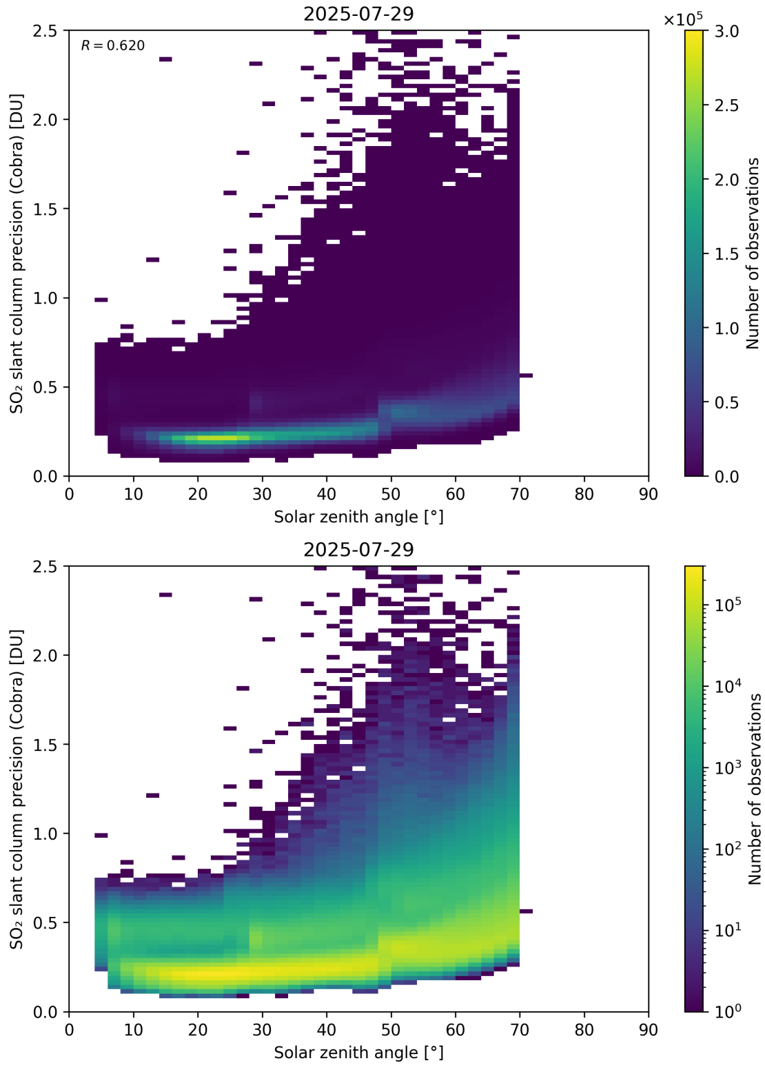
Figure 180: Scatter density plot of “Solar zenith angle” against “SO 2 slant column precision (Cobra)” for 2025-07-29 to 2025-07-30.
