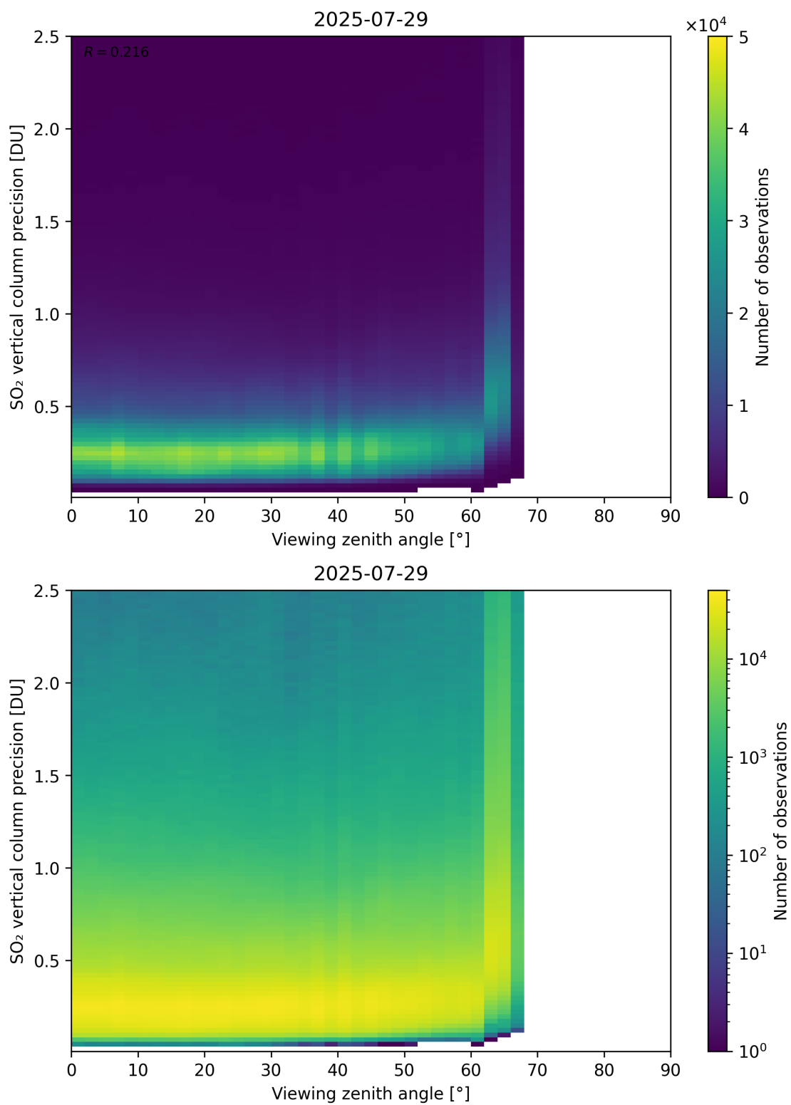
Figure 384: Scatter density plot of “Viewing zenith angle” against “SO 2 vertical column precision” for 2025-07-29 to 2025-07-30.
