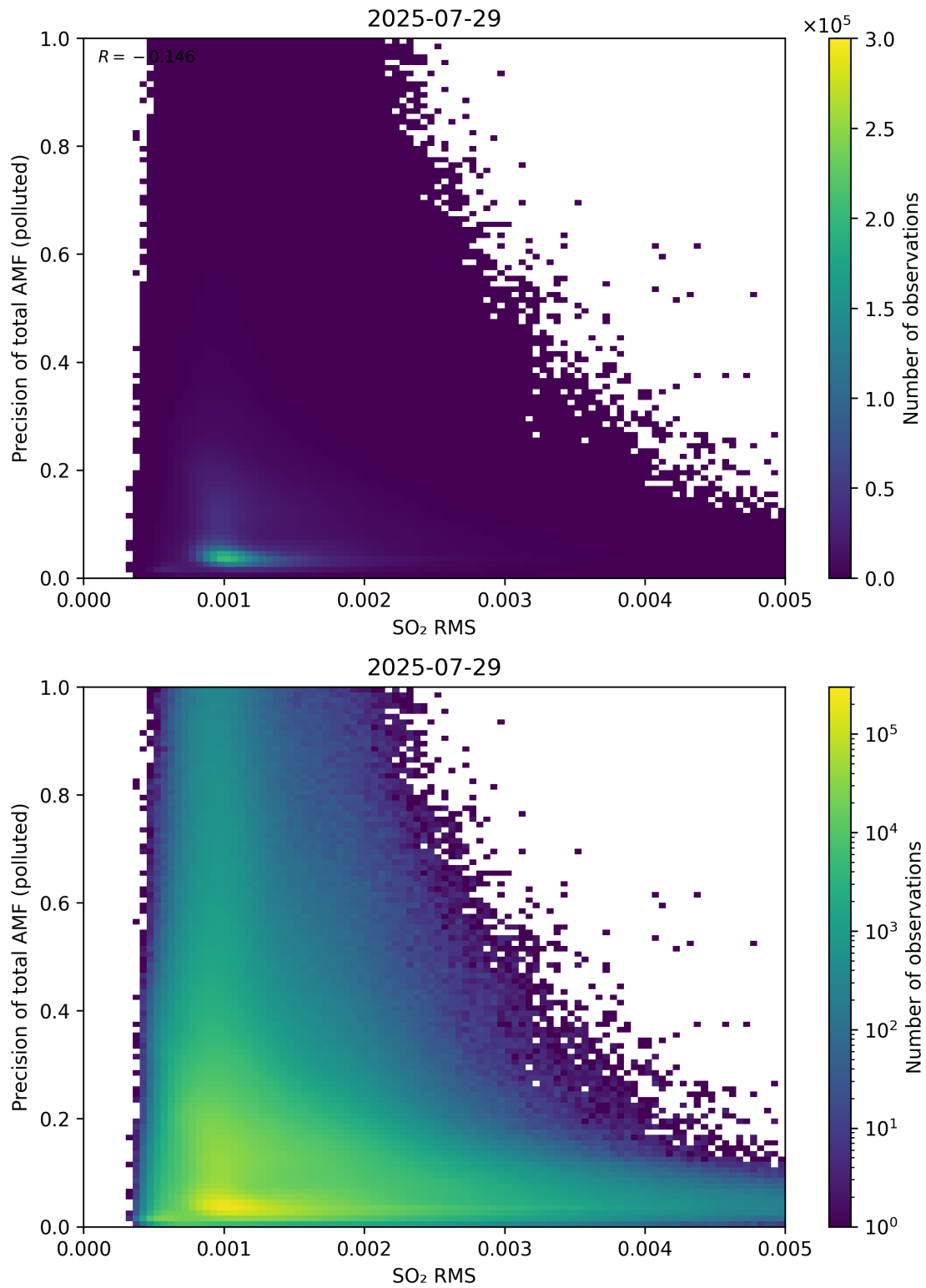
Figure 149: Scatter density plot of “SO 2 RMS” against “Precision of total AMF (polluted)” for 2025-07-29 to 2025-07-30.
