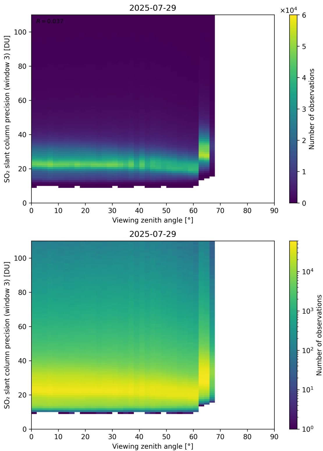
Figure 380: Scatter density plot of “Viewing zenith angle” against “SO 2 slant column precision (window 3)” for 2025-07-29 to 2025-07-30.
