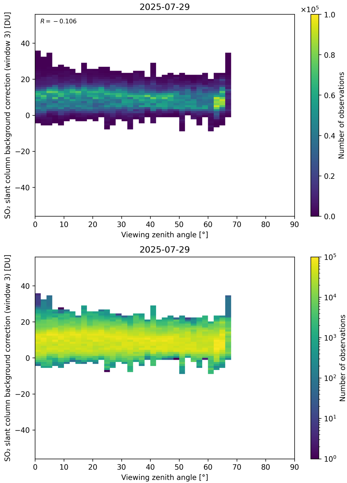
Figure 364: Scatter density plot of “Viewing zenith angle” against “SO 2 slant column background correction (window 3)” for 2025-07-29 to 2025-07-30.
