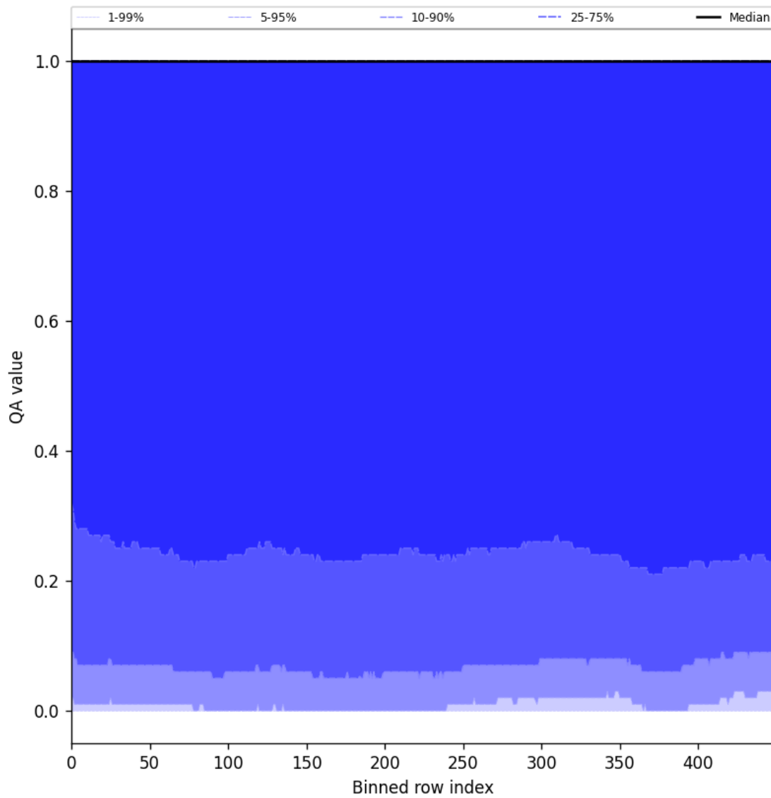
Figure 83: Along track statistics of “QA value” for 2025-07-29 to 2025-07-30
