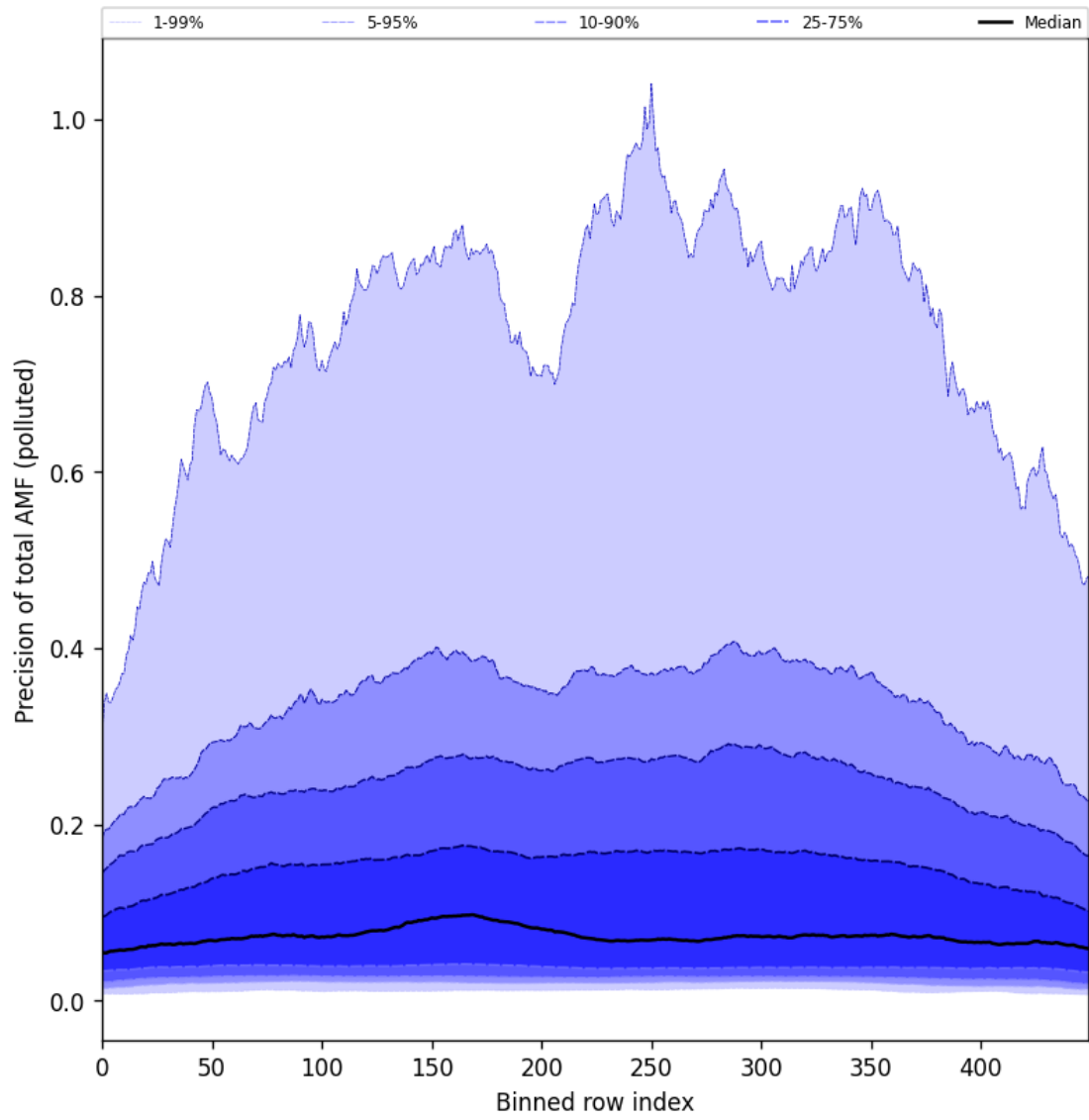
Figure 106: Along track statistics of “Precision of total AMF (polluted)” for 2025-07-29 to 2025-07-30
