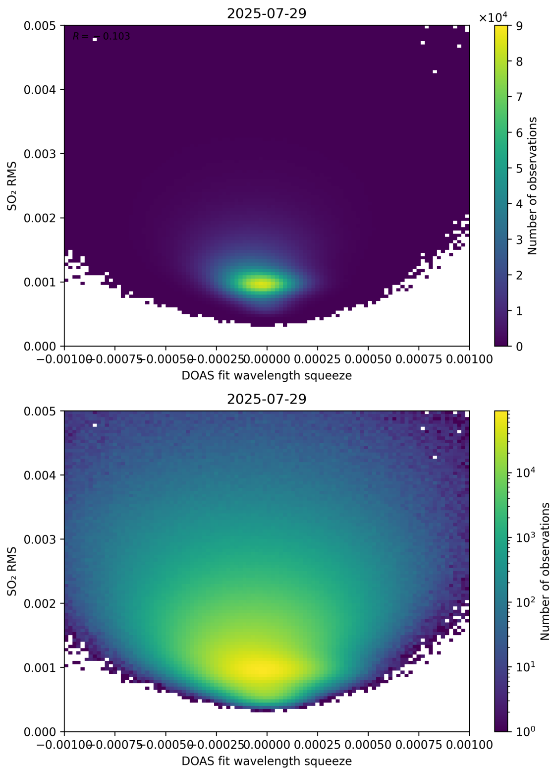
Figure 143: Scatter density plot of “DOAS fit wavelength squeeze” against “SO 2 RMS” for 2025-07-29 to 2025-07-30.
