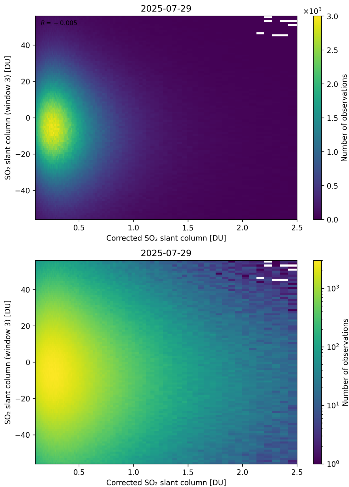
Figure 240: Scatter density plot of “Corrected SO 2 slant column” against “SO 2 slant column (window 3)” for 2025-07-29 to 2025-07-30.
