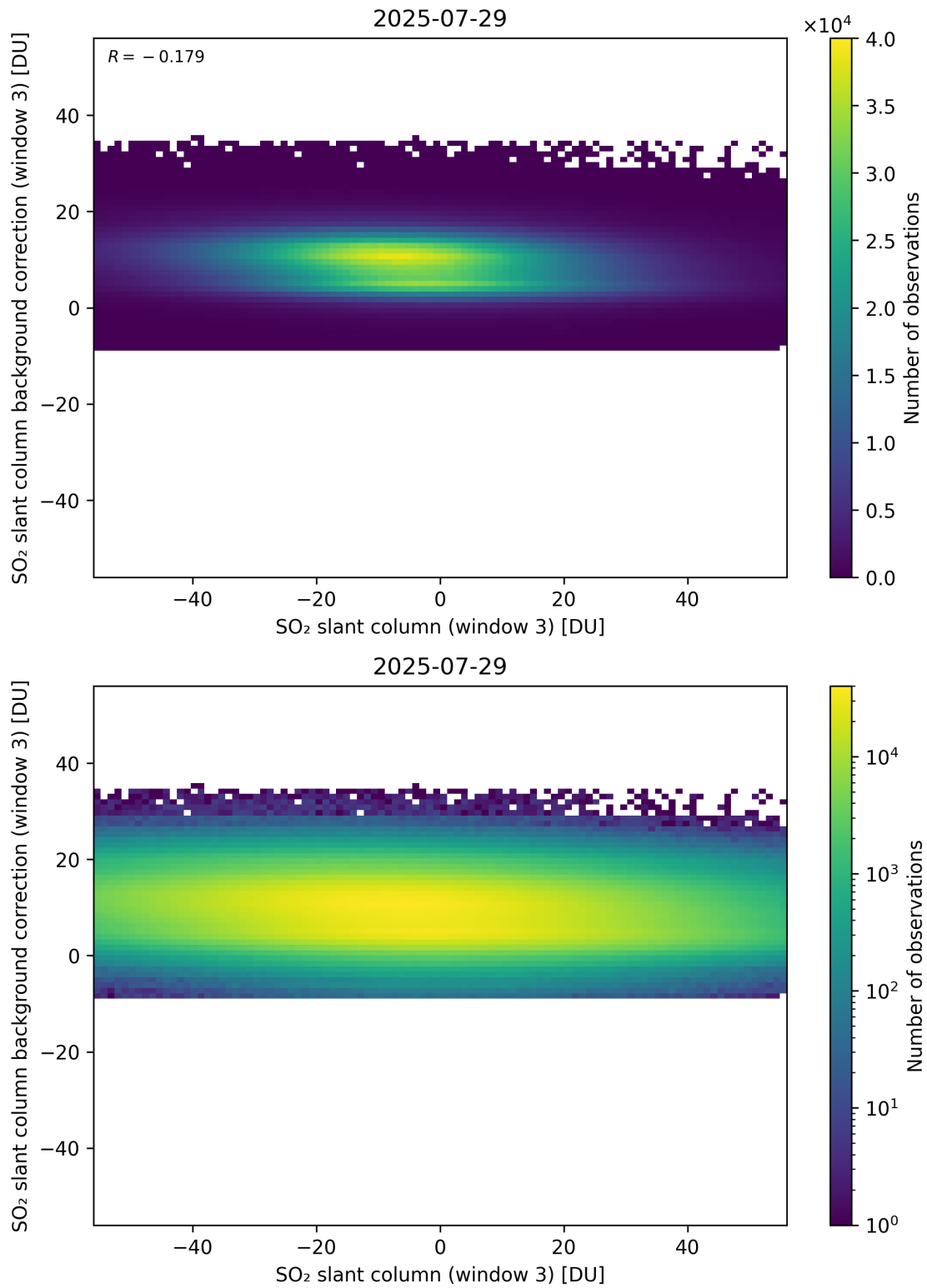
Figure 303: Scatter density plot of “SO 2 slant column (window 3)” against “SO 2 slant column background correction (window 3)” for 2025-07-29 to 2025-07-30.
