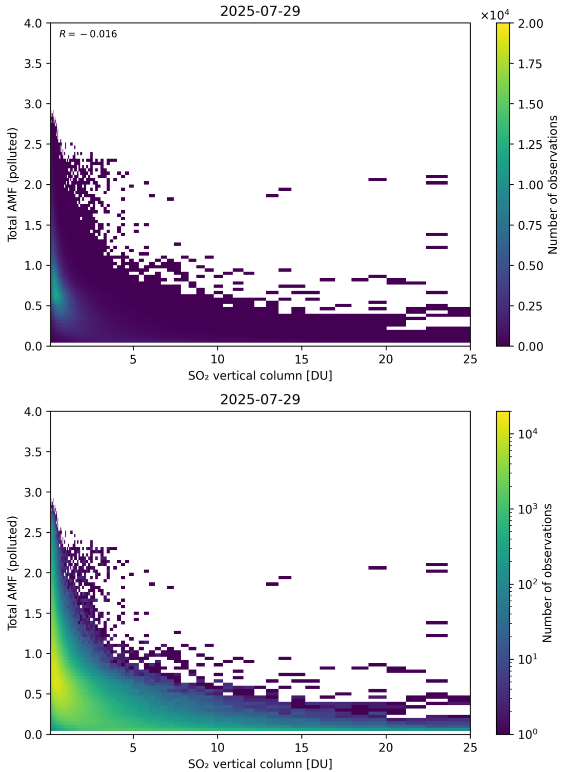
Figure 359: Scatter density plot of “SO 2 vertical column” against “Total AMF (polluted)” for 2025-07-29 to 2025-07-30.
