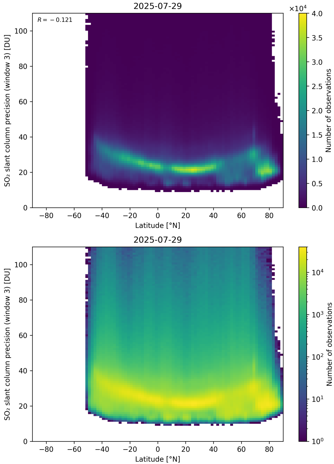
Figure 166: Scatter density plot of “Latitude” against “SO 2 slant column precision (window 3)” for 2025-07-29 to 2025-07-30.
