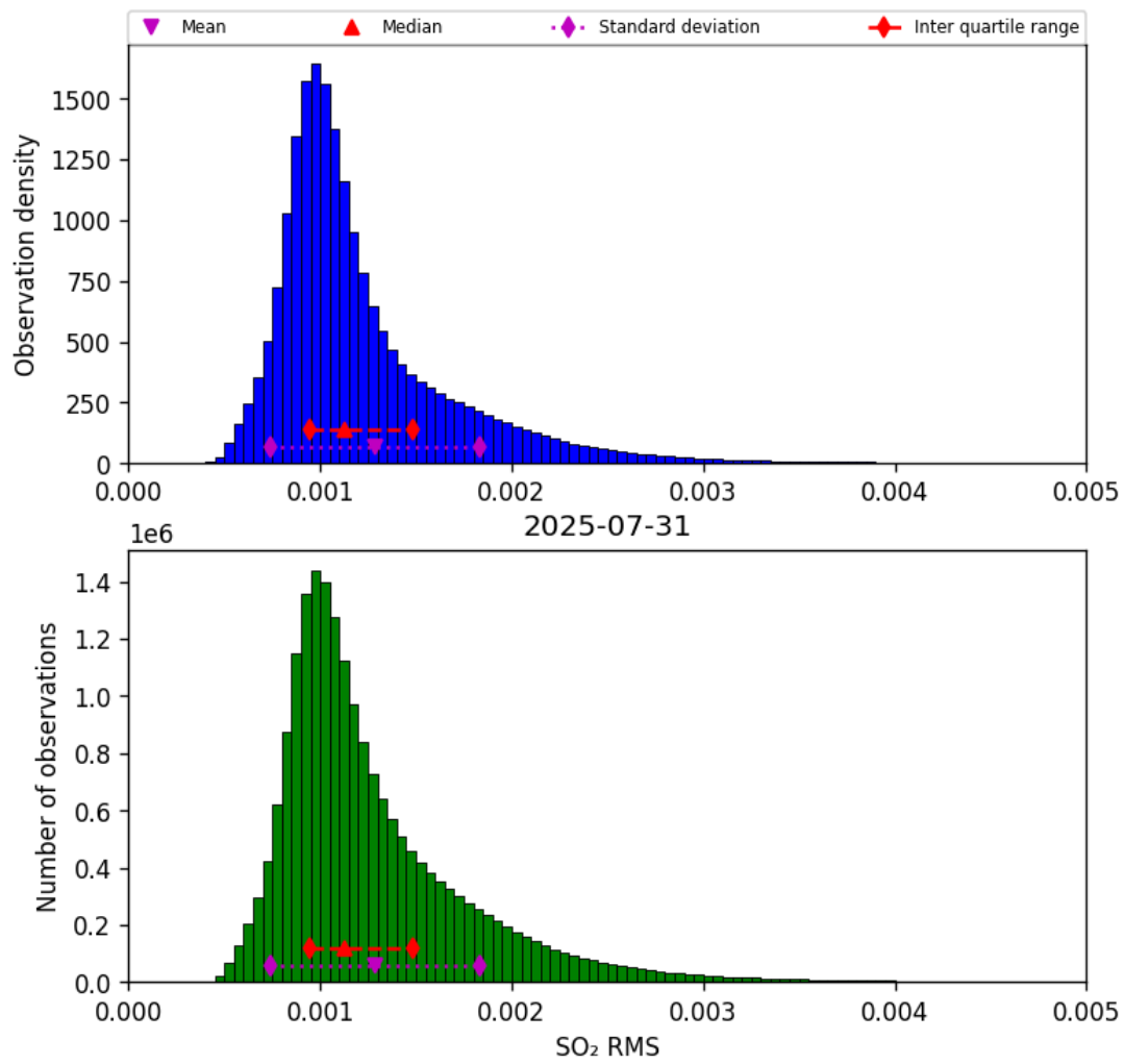
Figure 78: Histogram of “SO 2 RMS” for 2025-07-30 to 2025-08-01
