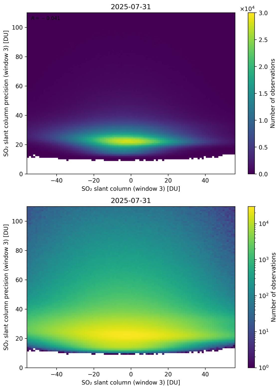
Figure 317: Scatter density plot of “SO 2 slant column (window 3)” against “SO 2 slant column precision (window 3)” for 2025-07-30 to 2025-08-01.
