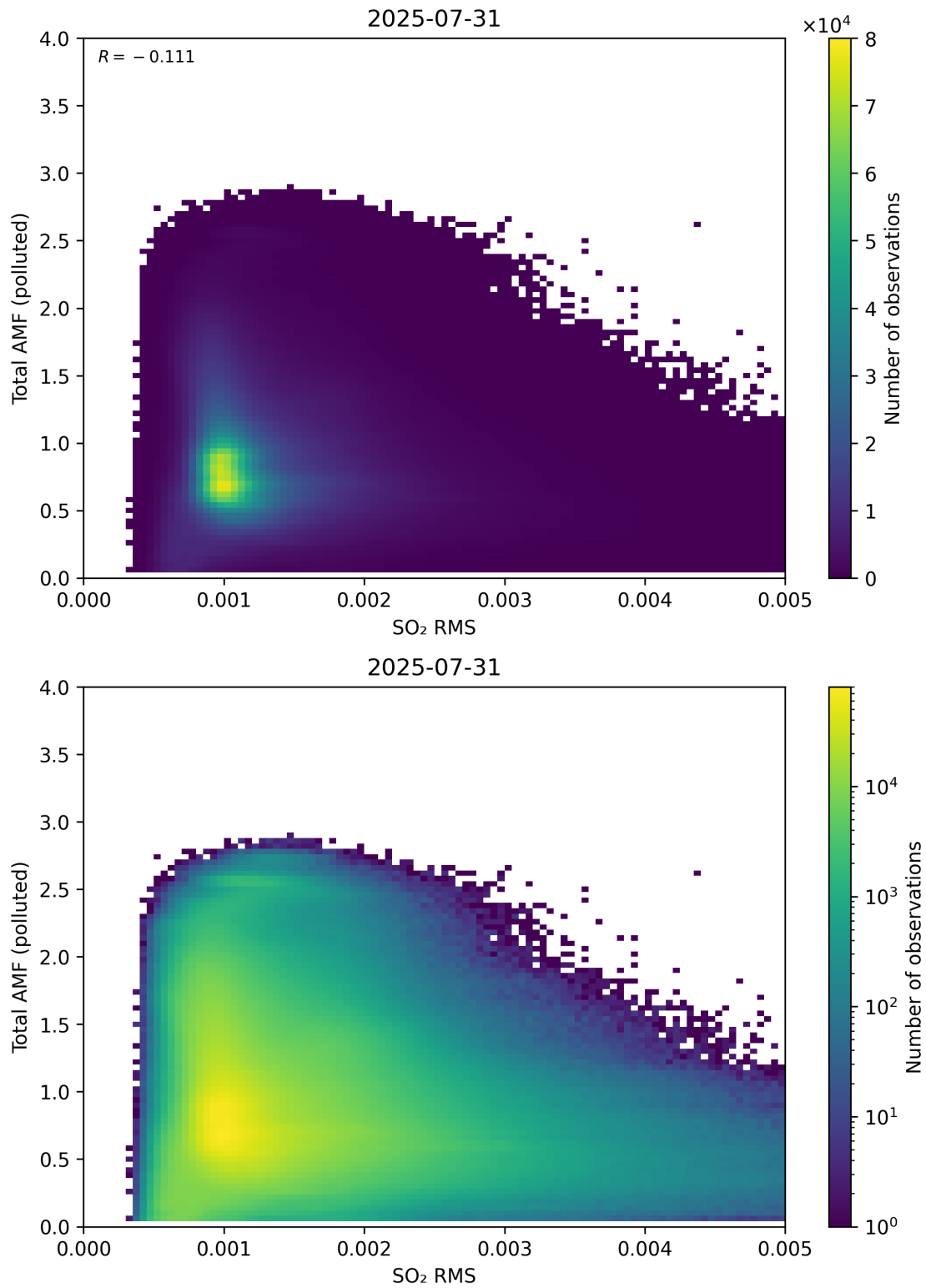
Figure 148: Scatter density plot of “SO 2 RMS” against “Total AMF (polluted)” for 2025-07-30 to 2025-08-01.
