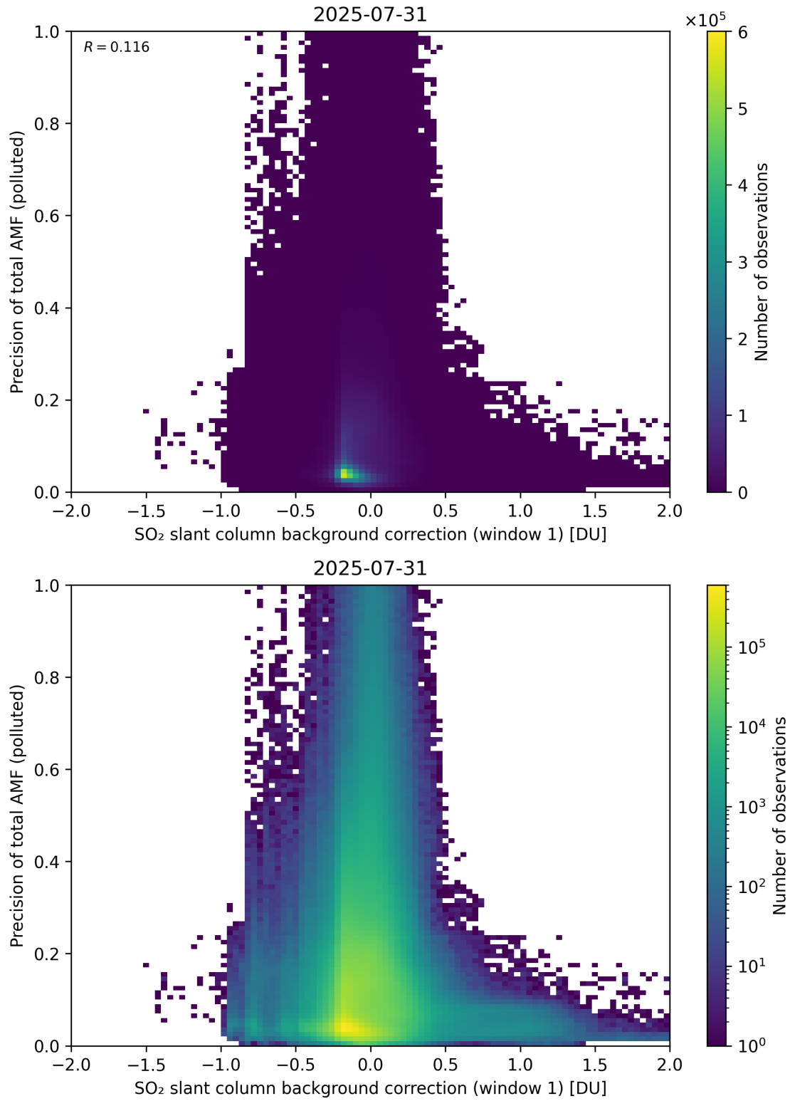
Figure 121: Scatter density plot of “SO 2 slant column background correction (window 1)” against “Precision of total AMF (polluted)” for 2025-07-30 to 2025-08-01.
