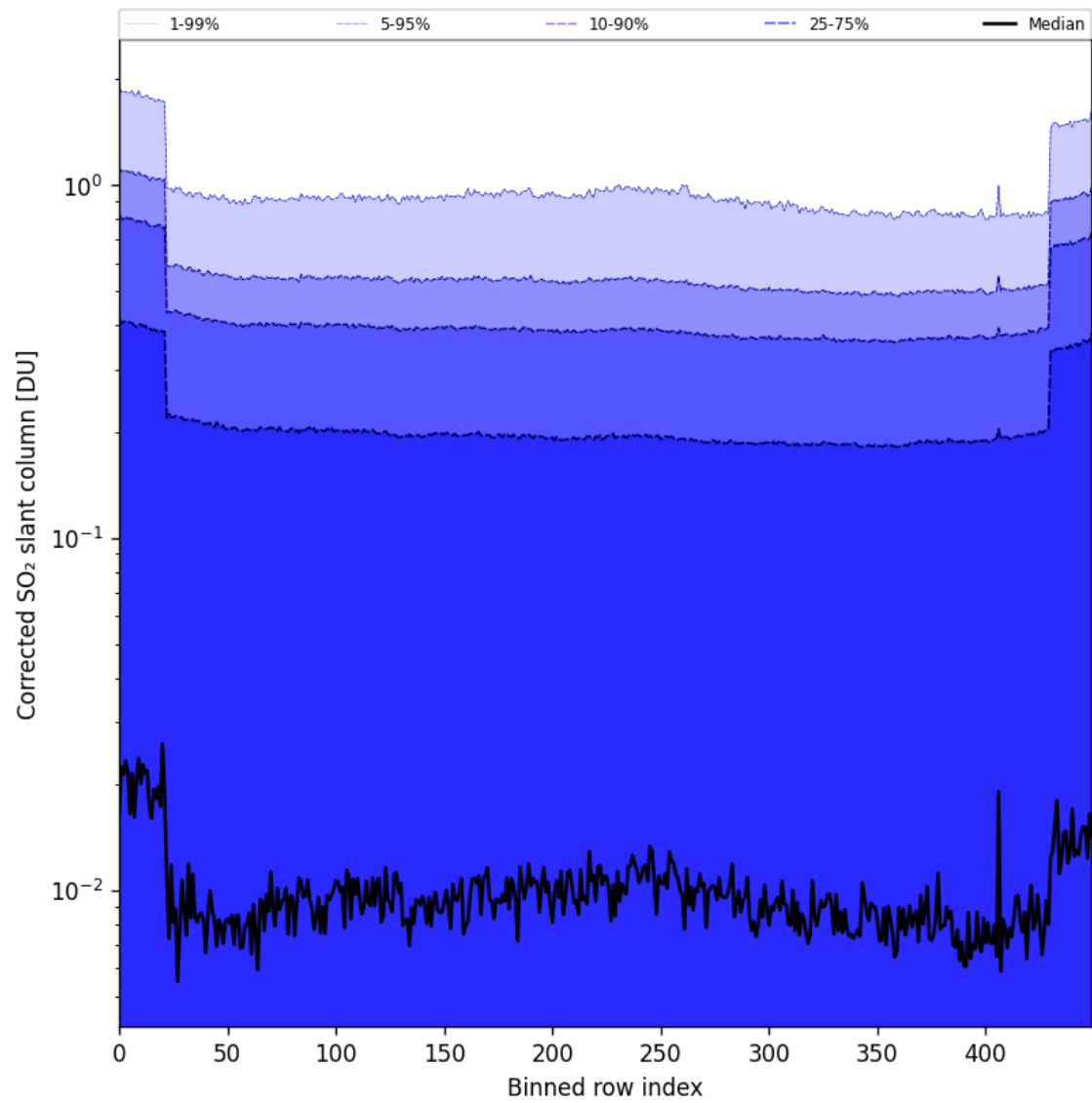
Figure 86: Along track statistics of "Corrected SO 2 slant column" for 2025-07-30 to 2025-08-01
