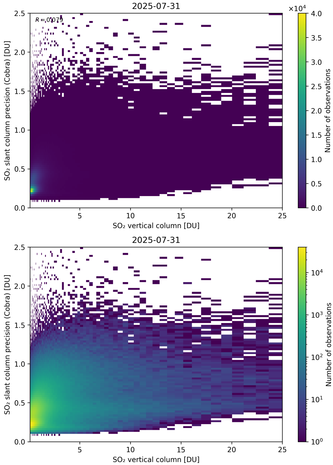
Figure 350: Scatter density plot of “SO 2 vertical column” against “SO 2 slant column precision (Cobra)” for 2025-07-30 to 2025-08-01.
