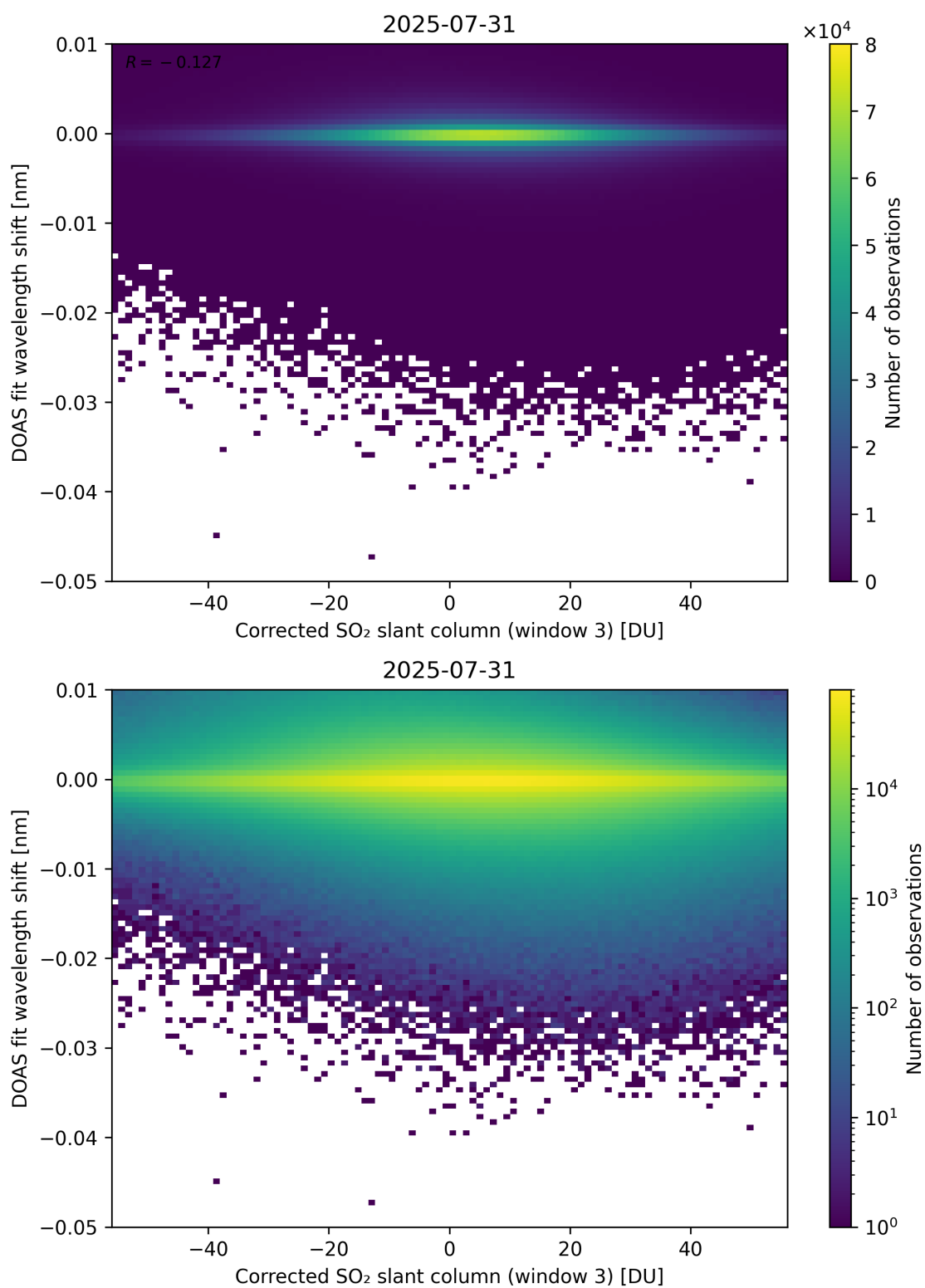
Figure 256: Scatter density plot of “Corrected SO 2 slant column (window 3)” against “DOAS fit wavelength shift” for 2025-07-30 to 2025-08-01.
