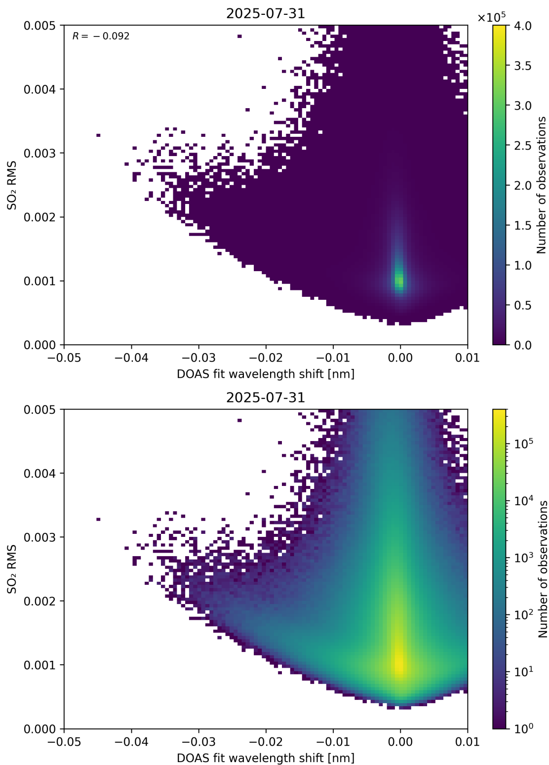
Figure 139: Scatter density plot of “DOAS fit wavelength shift” against “SO 2 RMS” for 2025-07-30 to 2025-08-01.
