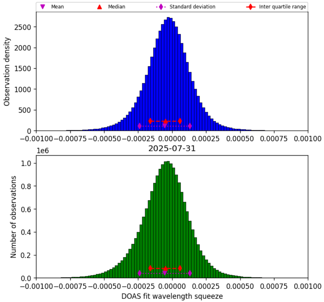
Figure 77: Histogram of “DOAS fit wavelength squeeze” for 2025-07-30 to 2025-08-01
