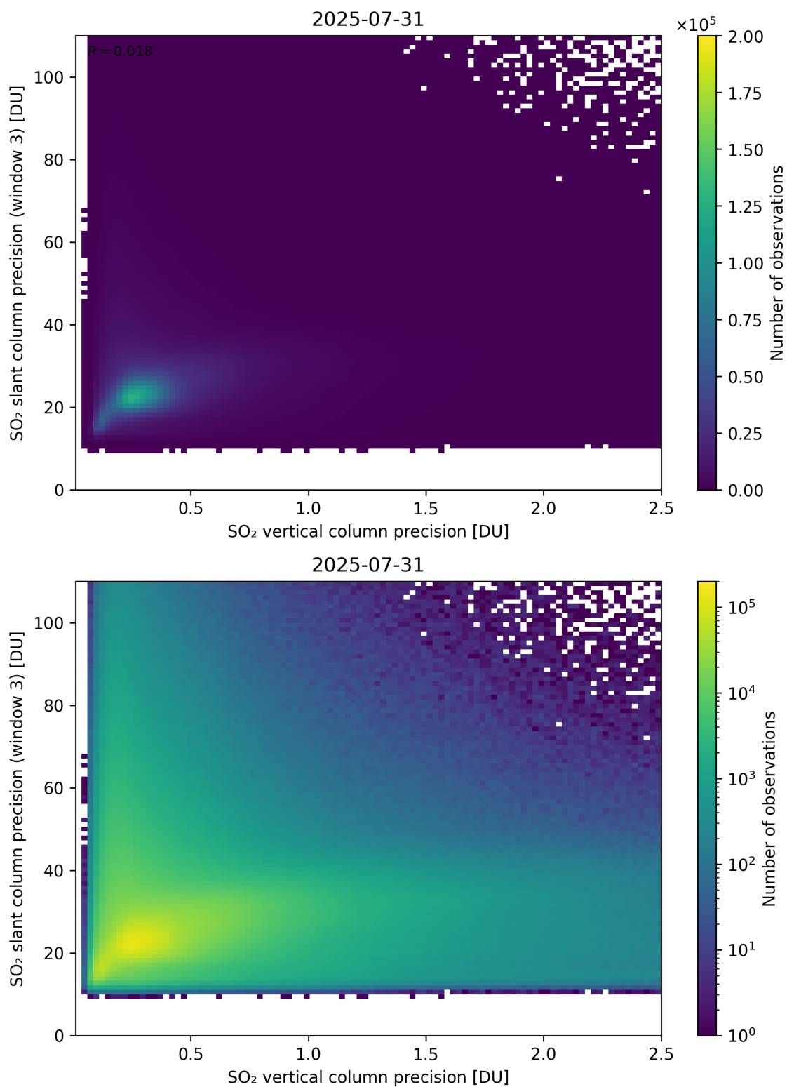
Figure 345: Scatter density plot of “SO 2 vertical column precision” against “SO 2 slant column precision (window 3)” for 2025-07-30 to 2025-08-01.
