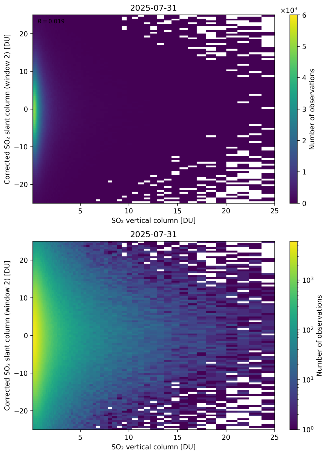
Figure 352: Scatter density plot of “SO 2 vertical column” against “Corrected SO 2 slant column (window 2)” for 2025-07-30 to 2025-08-01.
