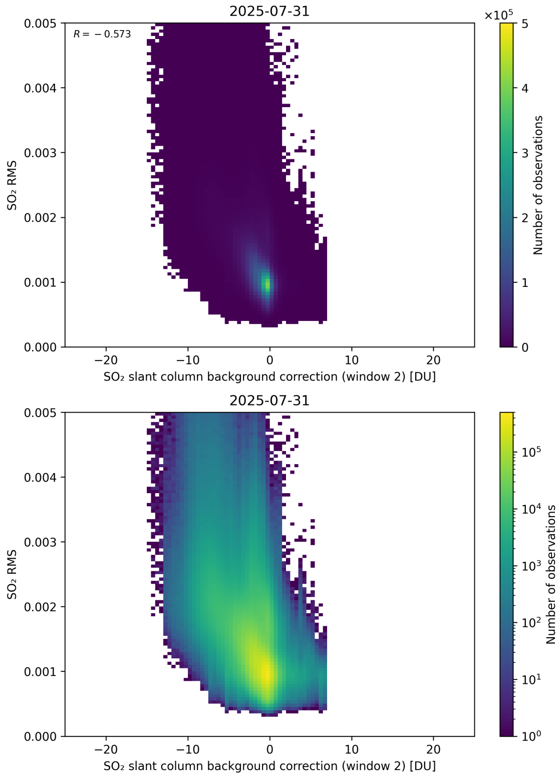
Figure 125: Scatter density plot of “SO 2 slant column background correction (window 2)” against “SO 2 RMS” for 2025-07-30 to 2025-08-01.
