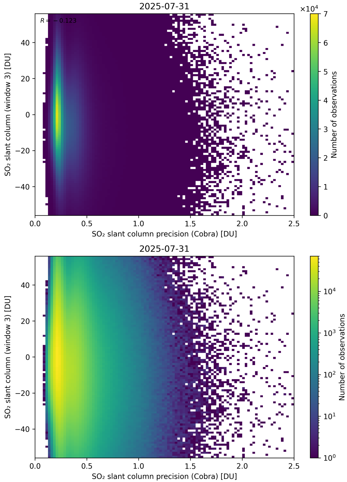
Figure 211: Scatter density plot of “SO 2 slant column precision (Cobra)” against “SO 2 slant column (window 3)” for 2025-07-30 to 2025-08-01.
