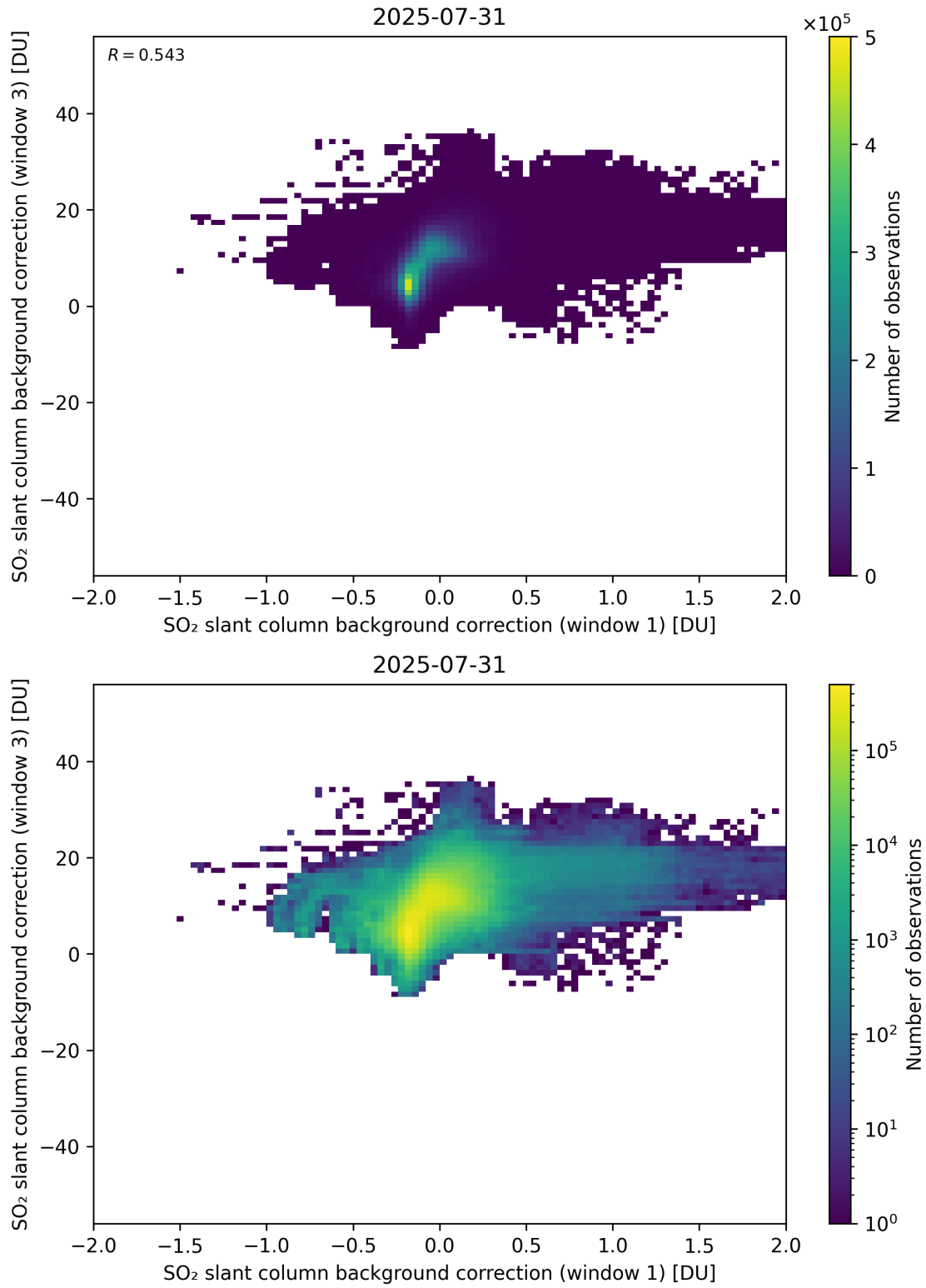
Figure 110: Scatter density plot of “SO 2 slant column background correction (window 1)” against “SO 2 slant column background correction (window 3)” for 2025-07-30 to 2025-08-01.
