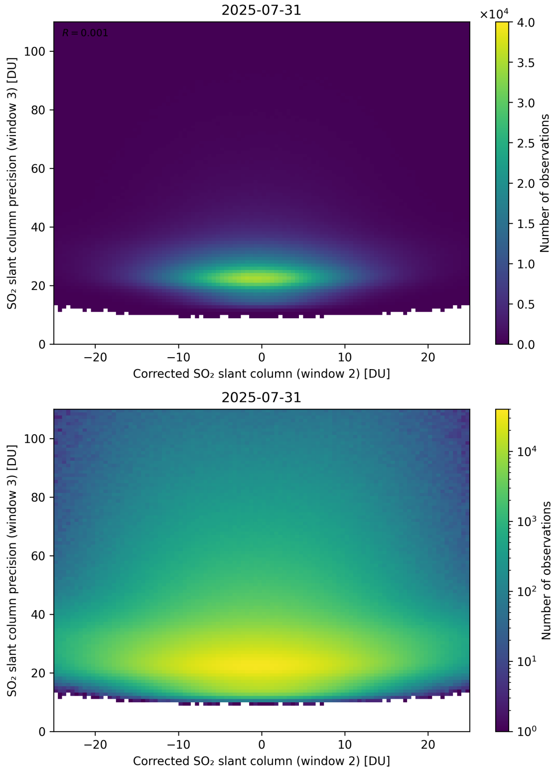
Figure 252: Scatter density plot of “Corrected SO 2 slant column (window 2)” against “SO 2 slant column precision (window 3)” for 2025-07-30 to 2025-08-01.
