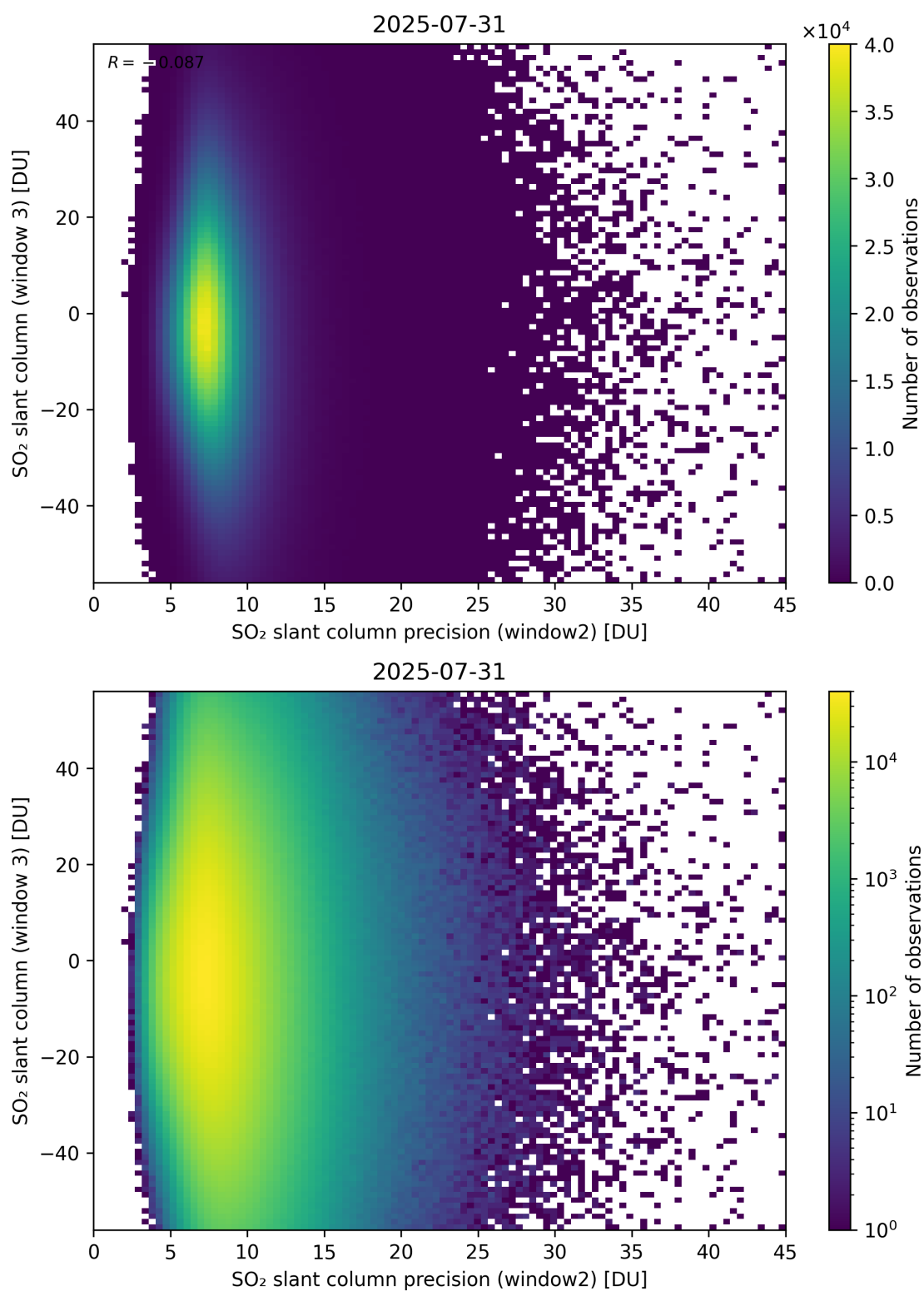
Figure 299: Scatter density plot of “SO 2 slant column precision (window2)” against “SO 2 slant column (window 3)” for 2025-07-30 to 2025-08-01.
