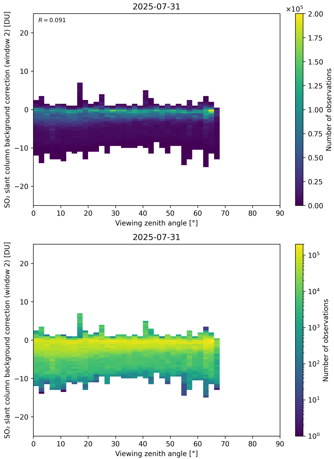
Figure 363: Scatter density plot of “Viewing zenith angle” against “SO 2 slant column background correction (window 2)” for 2025-07-30 to 2025-08-01.
