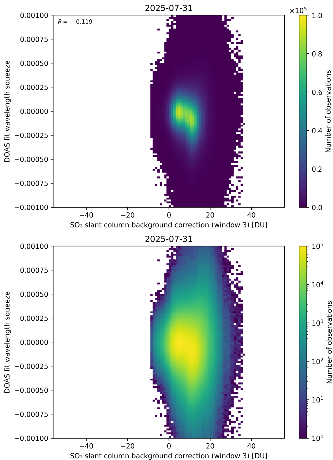
Figure 133: Scatter density plot of “SO 2 slant column background correction (window 3)” against “DOAS fit wavelength squeeze” for 2025-07-30 to 2025-08-01.
