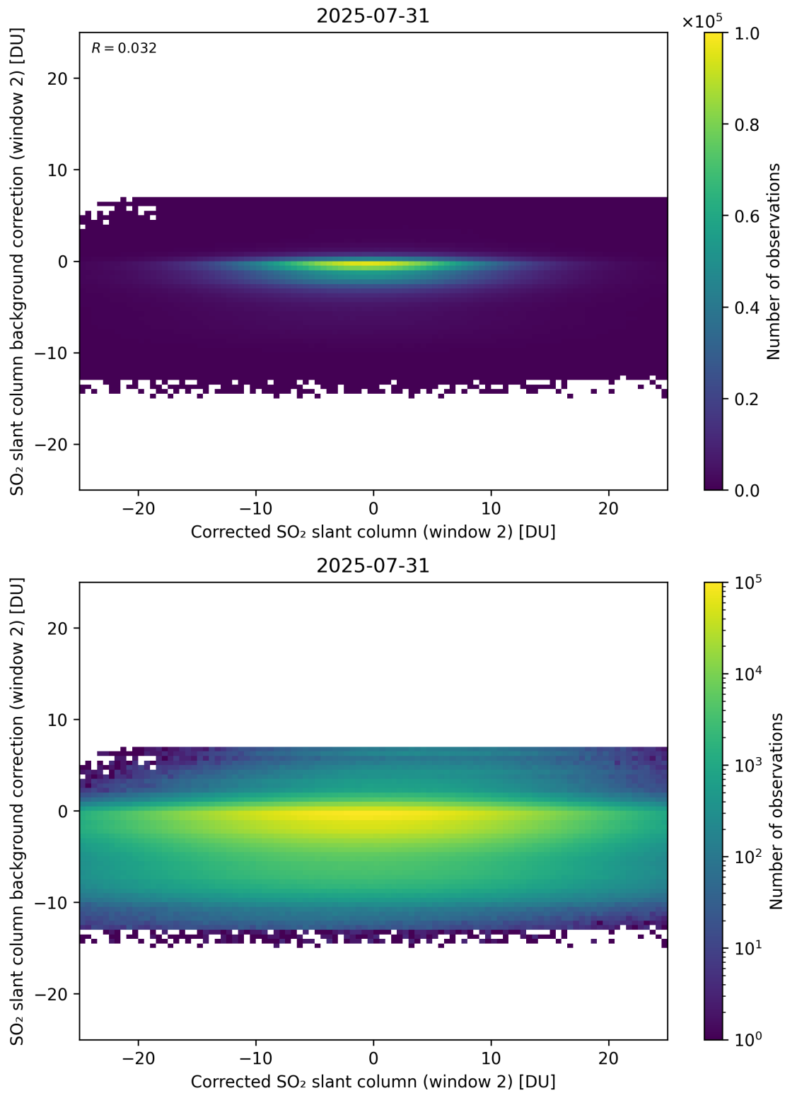
Figure 244: Scatter density plot of “Corrected SO 2 slant column (window 2)” against “SO 2 slant column background correction (window 2)” for 2025-07-30 to 2025-08-01.
