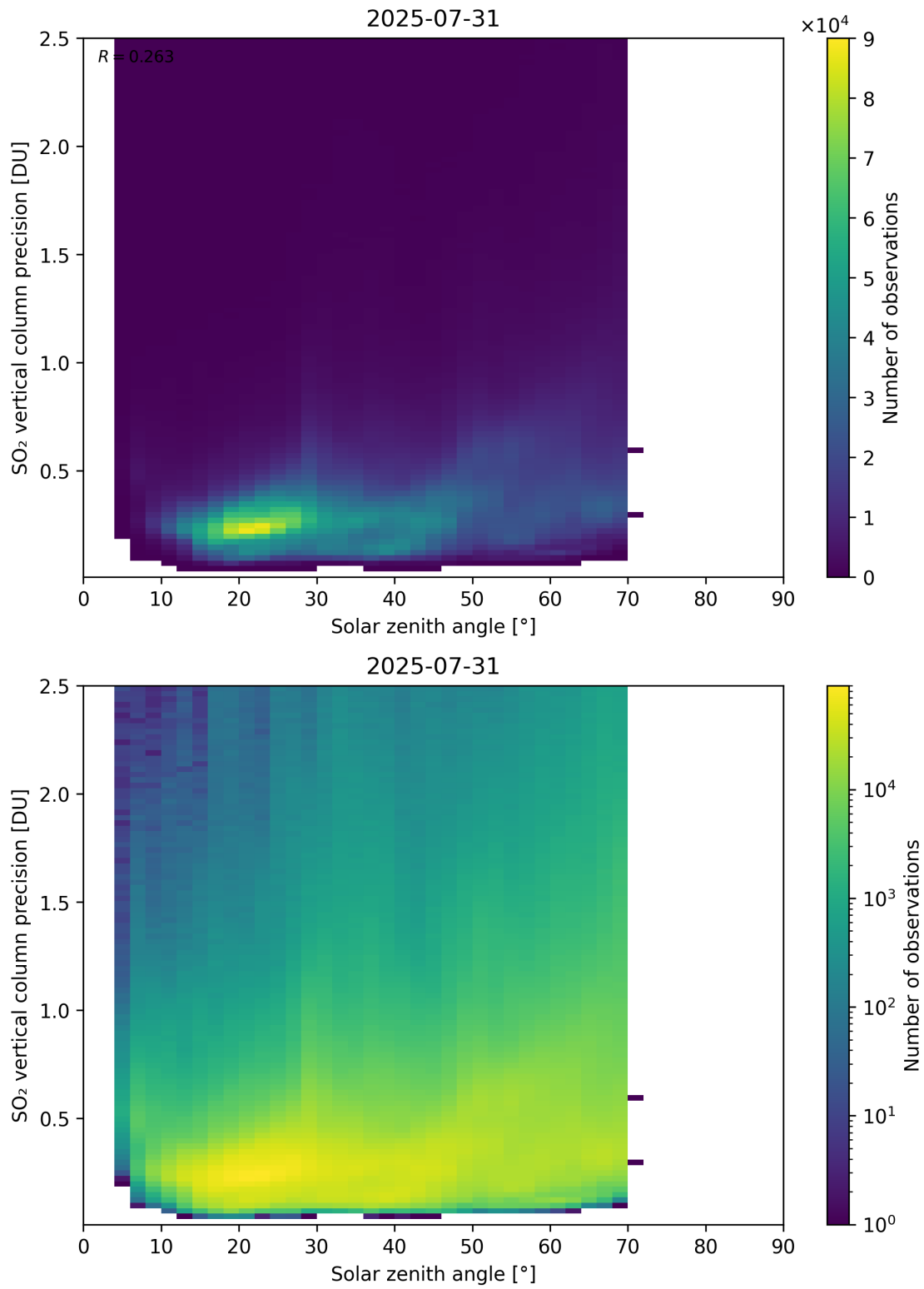
Figure 192: Scatter density plot of “Solar zenith angle” against “SO 2 vertical column precision” for 2025-07-30 to 2025-08-01.
