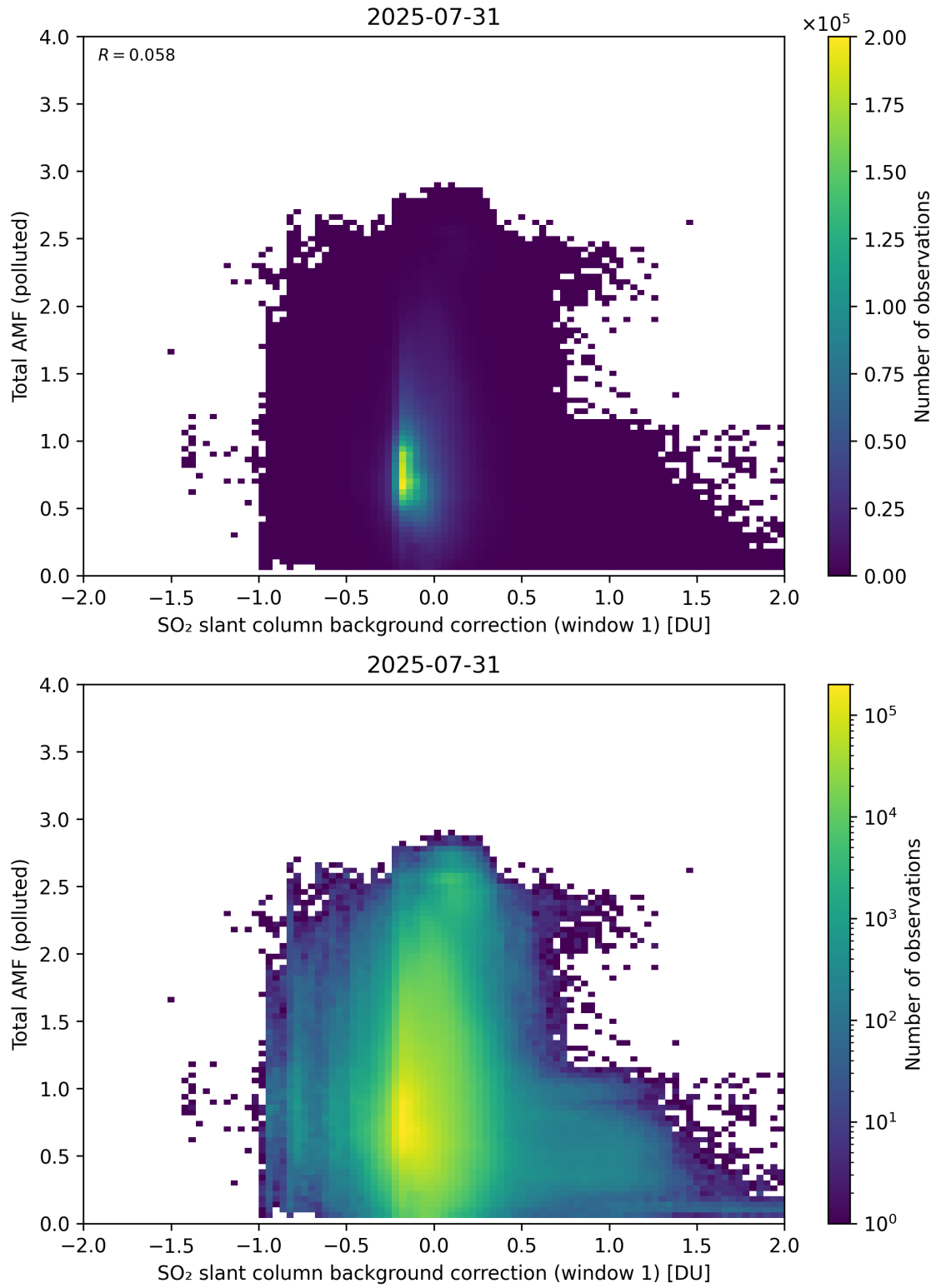
Figure 120: Scatter density plot of “SO 2 slant column background correction (window 1)” against “Total AMF (polluted)” for 2025-07-30 to 2025-08-01.
