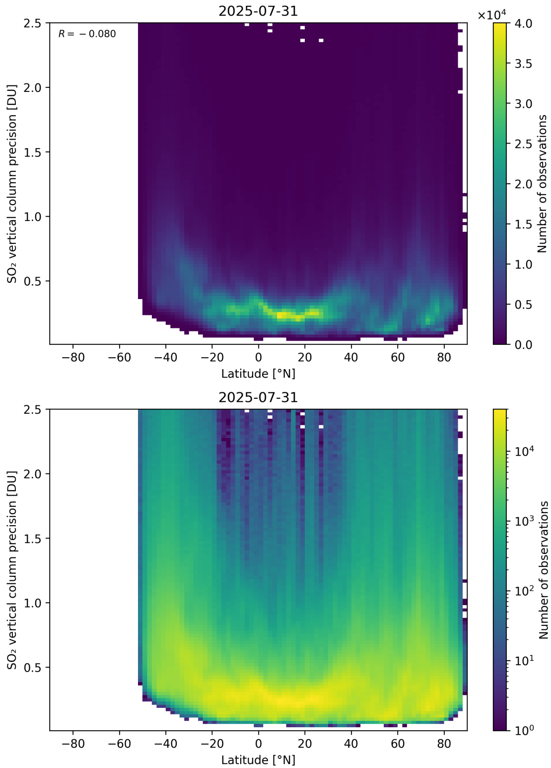
Figure 170: Scatter density plot of “Latitude” against “SO 2 vertical column precision” for 2025-07-30 to 2025-08-01.
