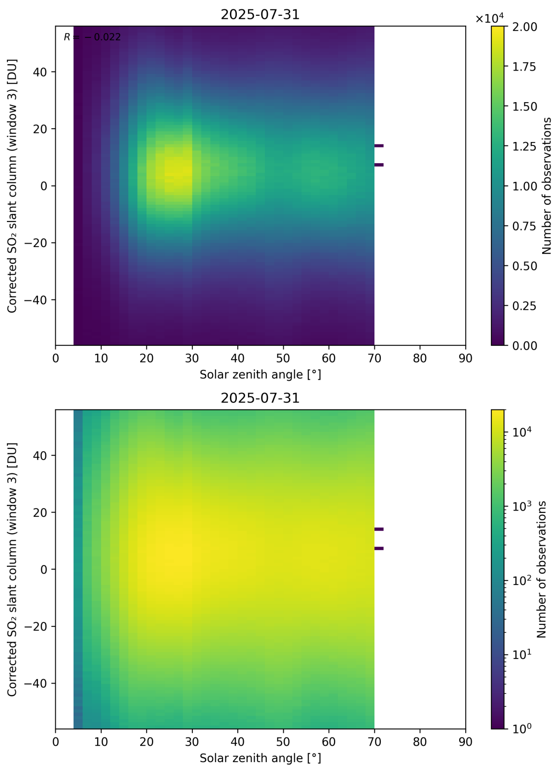
Figure 183: Scatter density plot of “Solar zenith angle” against “Corrected SO 2 slant column (window 3)” for 2025-07-30 to 2025-08-01.
