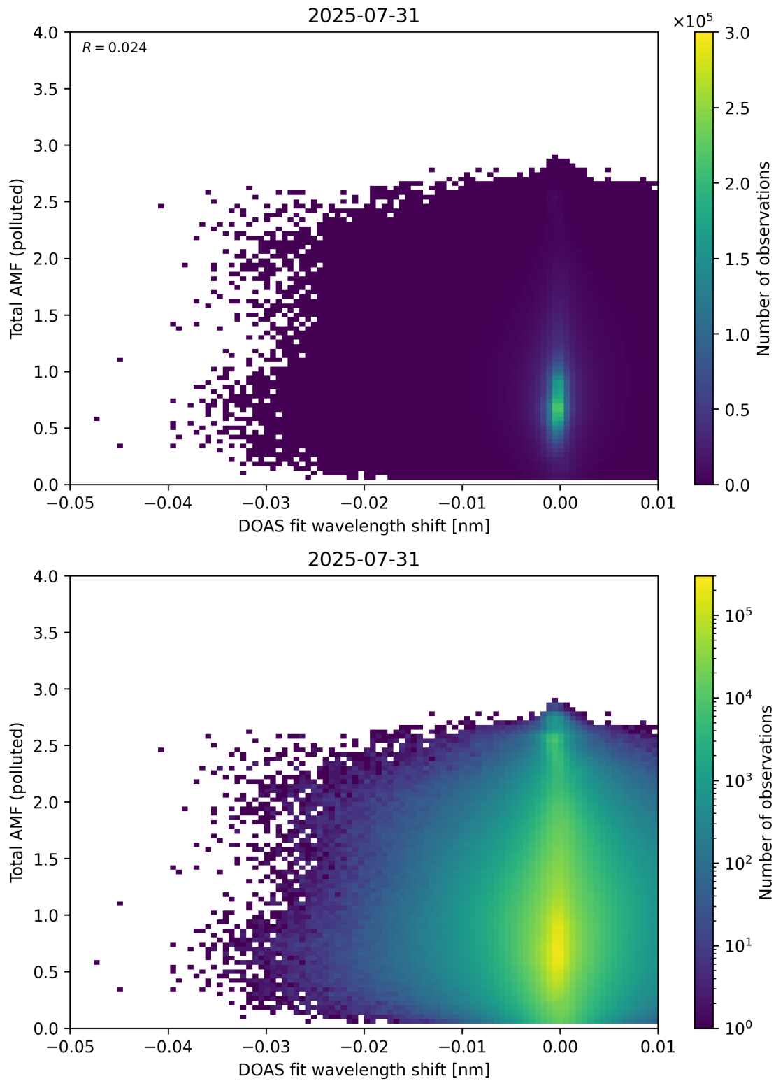
Figure 141: Scatter density plot of “DOAS fit wavelength shift” against “Total AMF (polluted)” for 2025-07-30 to 2025-08-01.
