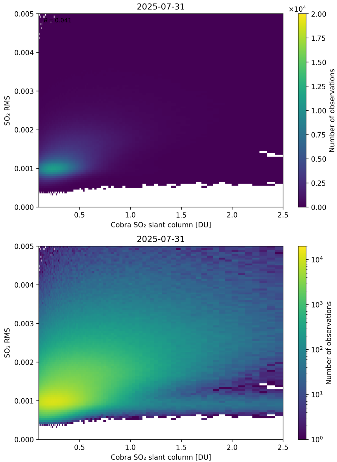
Figure 198: Scatter density plot of “Cobra SO 2 slant column” against “SO 2 RMS” for 2025-07-30 to 2025-08-01.
