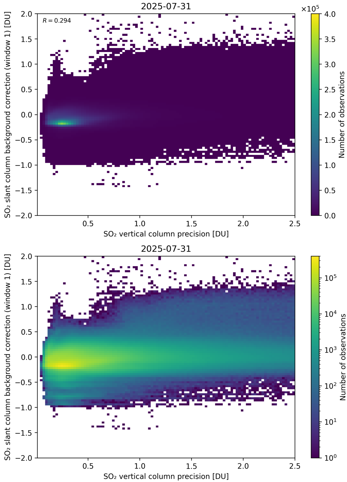
Figure 329: Scatter density plot of “SO 2 vertical column precision” against “SO 2 slant column background correction (window 1)” for 2025-07-30 to 2025-08-01.
