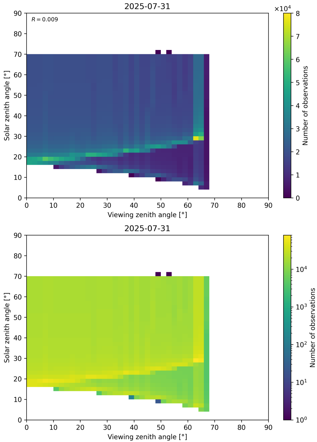
Figure 369: Scatter density plot of “Viewing zenith angle” against “Solar zenith angle” for 2025-07-30 to 2025-08-01.
