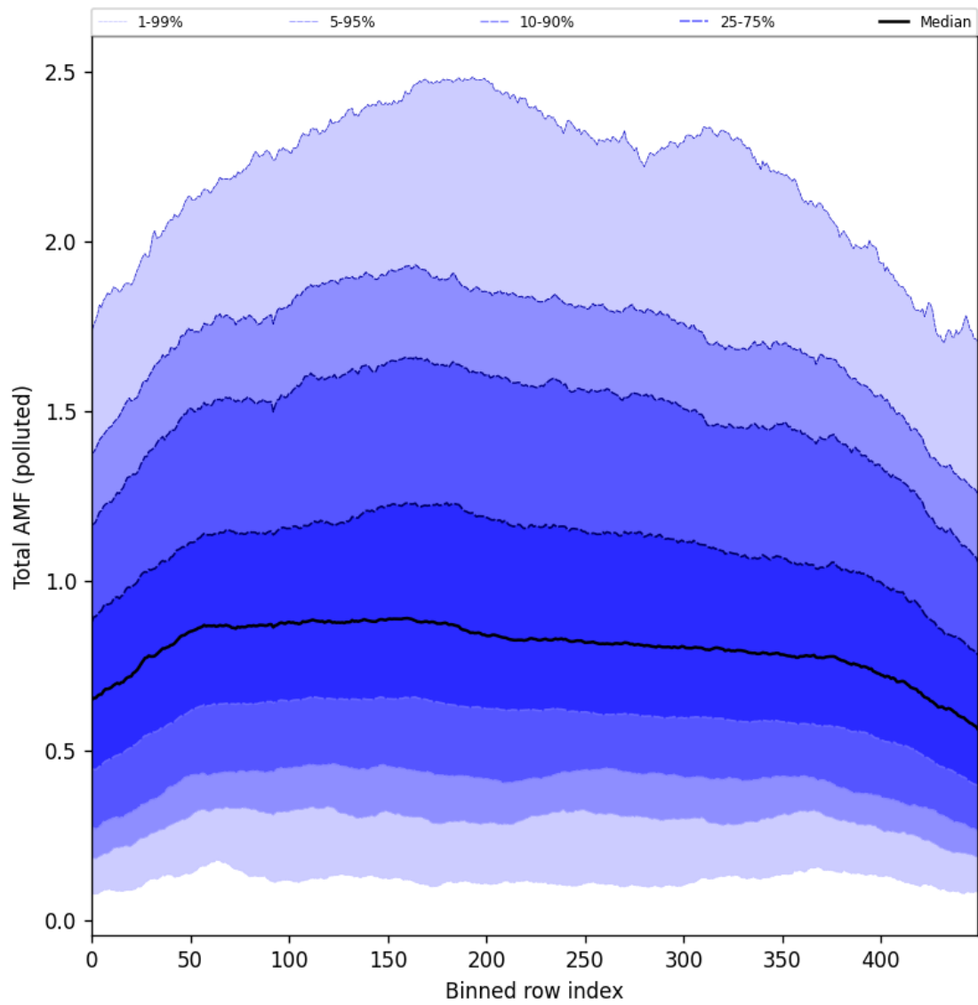
Figure 105: Along track statistics of “Total AMF (polluted)” for 2025-07-30 to 2025-08-01
