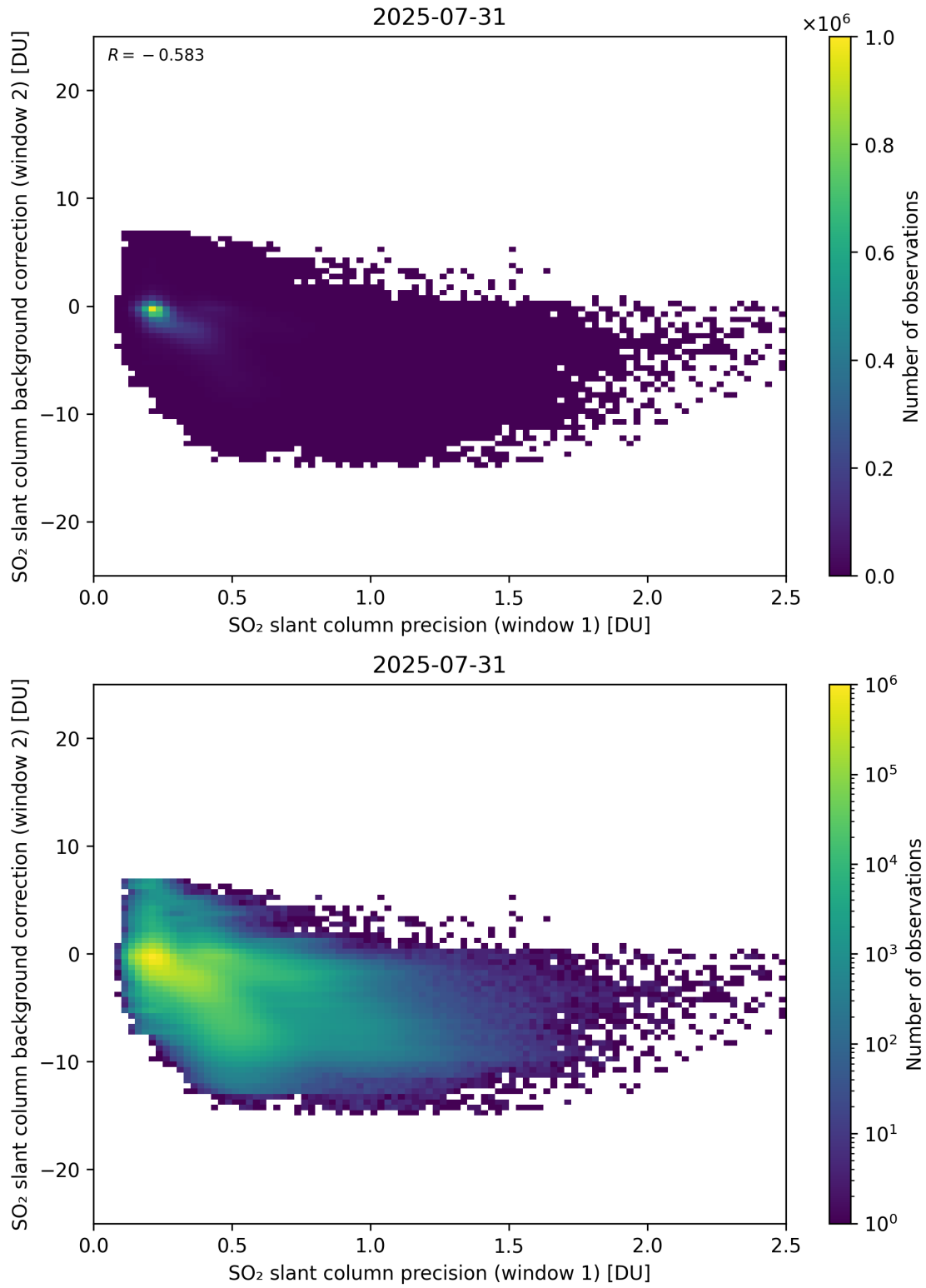
Figure 269: Scatter density plot of “SO 2 slant column precision (window 1)” against “SO 2 slant column background correction (window 2)” for 2025-07-30 to 2025-08-01.
