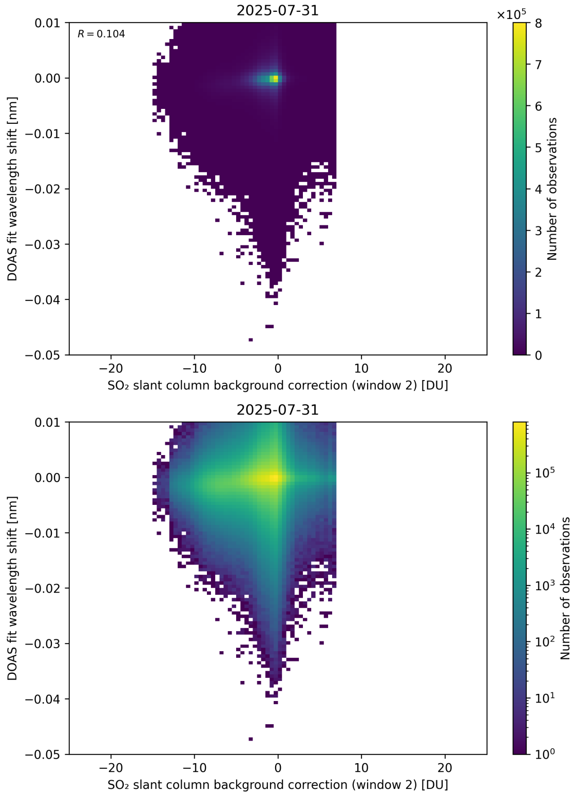
Figure 123: Scatter density plot of “SO 2 slant column background correction (window 2)” against “DOAS fit wavelength shift” for 2025-07-30 to 2025-08-01.
