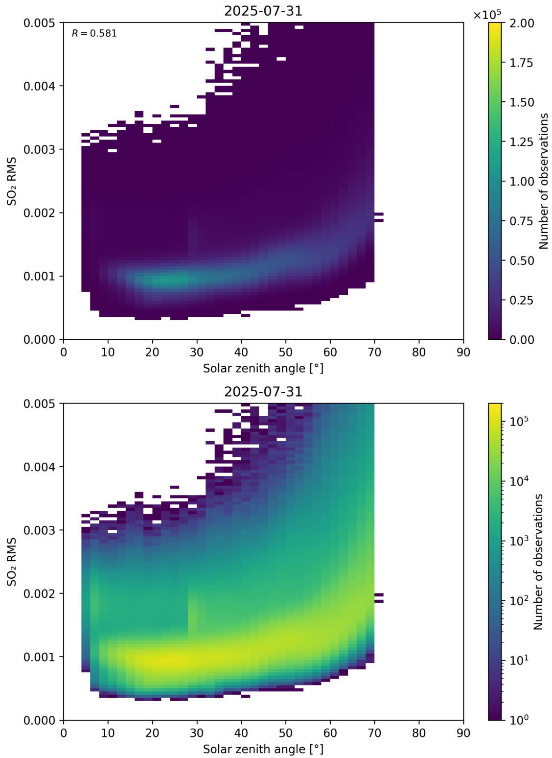
Figure 176: Scatter density plot of “Solar zenith angle” against “SO 2 RMS” for 2025-07-30 to 2025-08-01.
