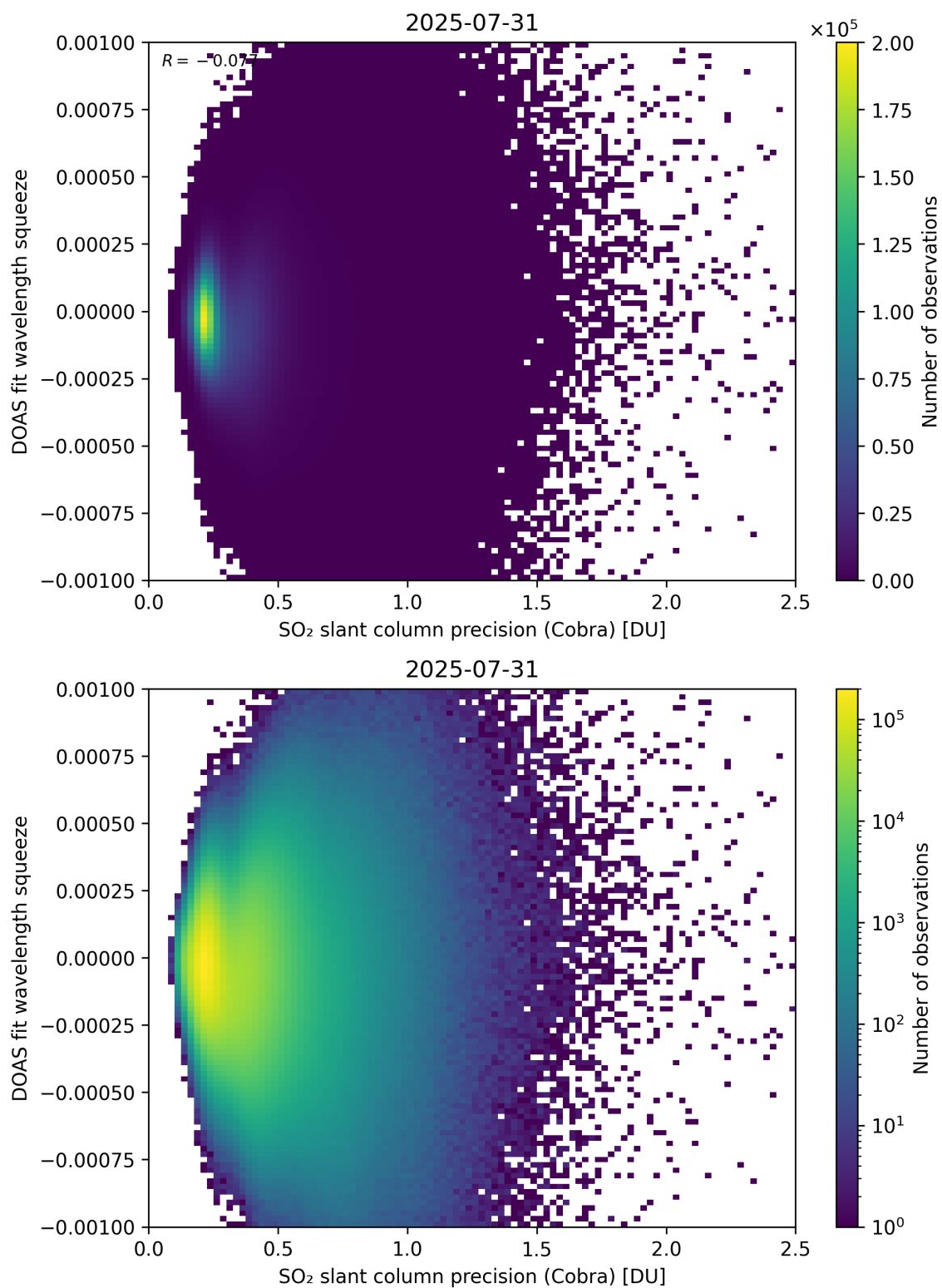
Figure 203: Scatter density plot of “SO 2 slant column precision (Cobra)” against “DOAS fit wavelength squeeze” for 2025-07-30 to 2025-08-01.
