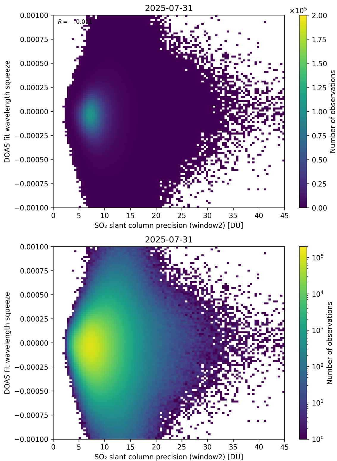
Figure 294: Scatter density plot of “SO 2 slant column precision (window2)” against “DOAS fit wavelength squeeze” for 2025-07-30 to 2025-08-01.
