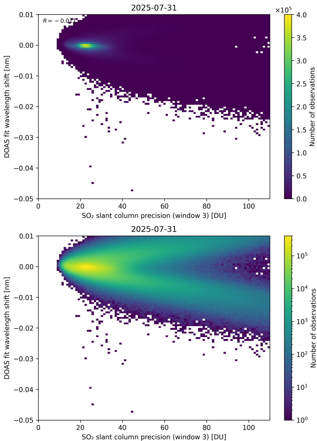
Figure 308: Scatter density plot of “SO 2 slant column precision (window 3)” against “DOAS fit wavelength shift” for 2025-07-30 to 2025-08-01.
