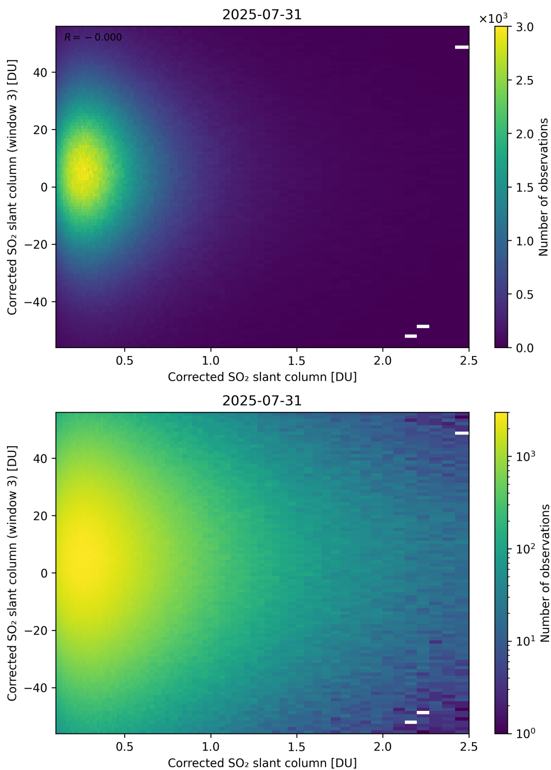
Figure 236: Scatter density plot of “Corrected SO 2 slant column” against “Corrected SO 2 slant column (window 3)” for 2025-07-30 to 2025-08-01.
