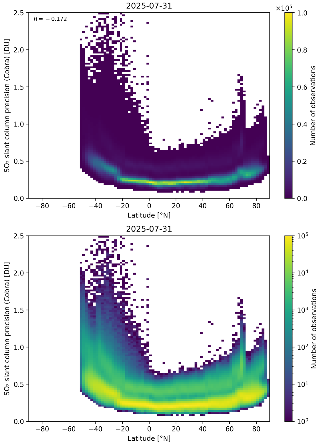
Figure 158: Scatter density plot of “Latitude” against “SO 2 slant column precision (Cobra)” for 2025-07-30 to 2025-08-01.
