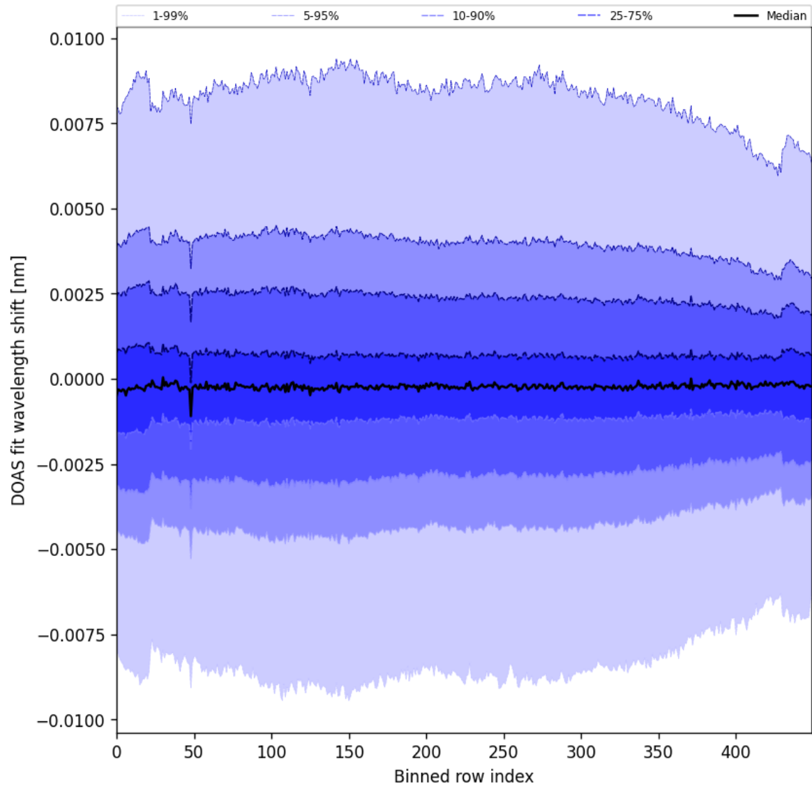
Figure 102: Along track statistics of “DOAS fit wavelength shift” for 2025-07-30 to 2025-08-01
