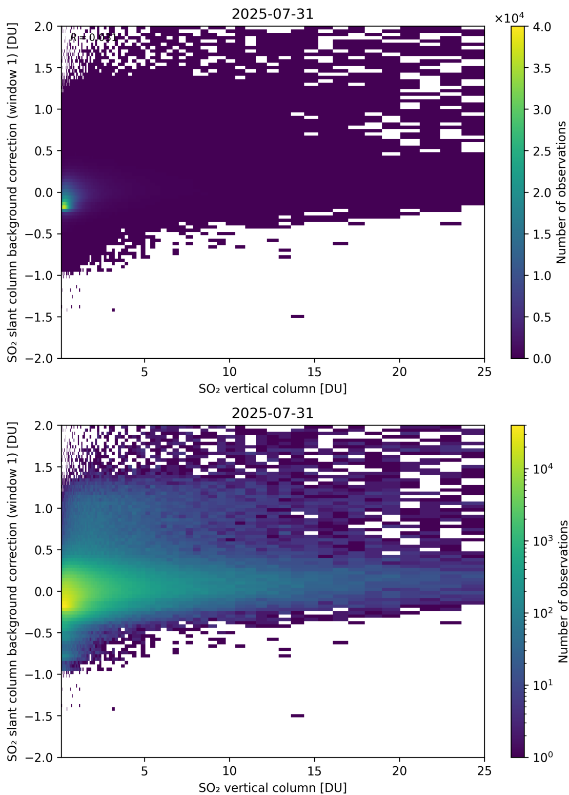
Figure 323: Scatter density plot of “SO 2 vertical column” against “SO 2 slant column background correction (window 1)” for 2025-07-30 to 2025-08-01.
