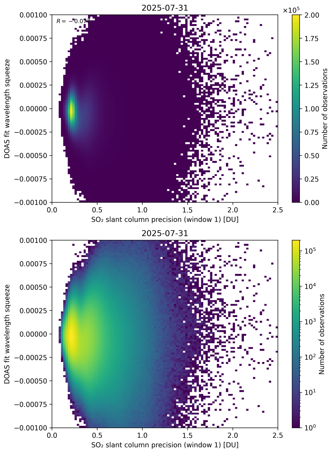
Figure 272: Scatter density plot of “SO 2 slant column precision (window 1)” against “DOAS fit wavelength squeeze” for 2025-07-30 to 2025-08-01.
