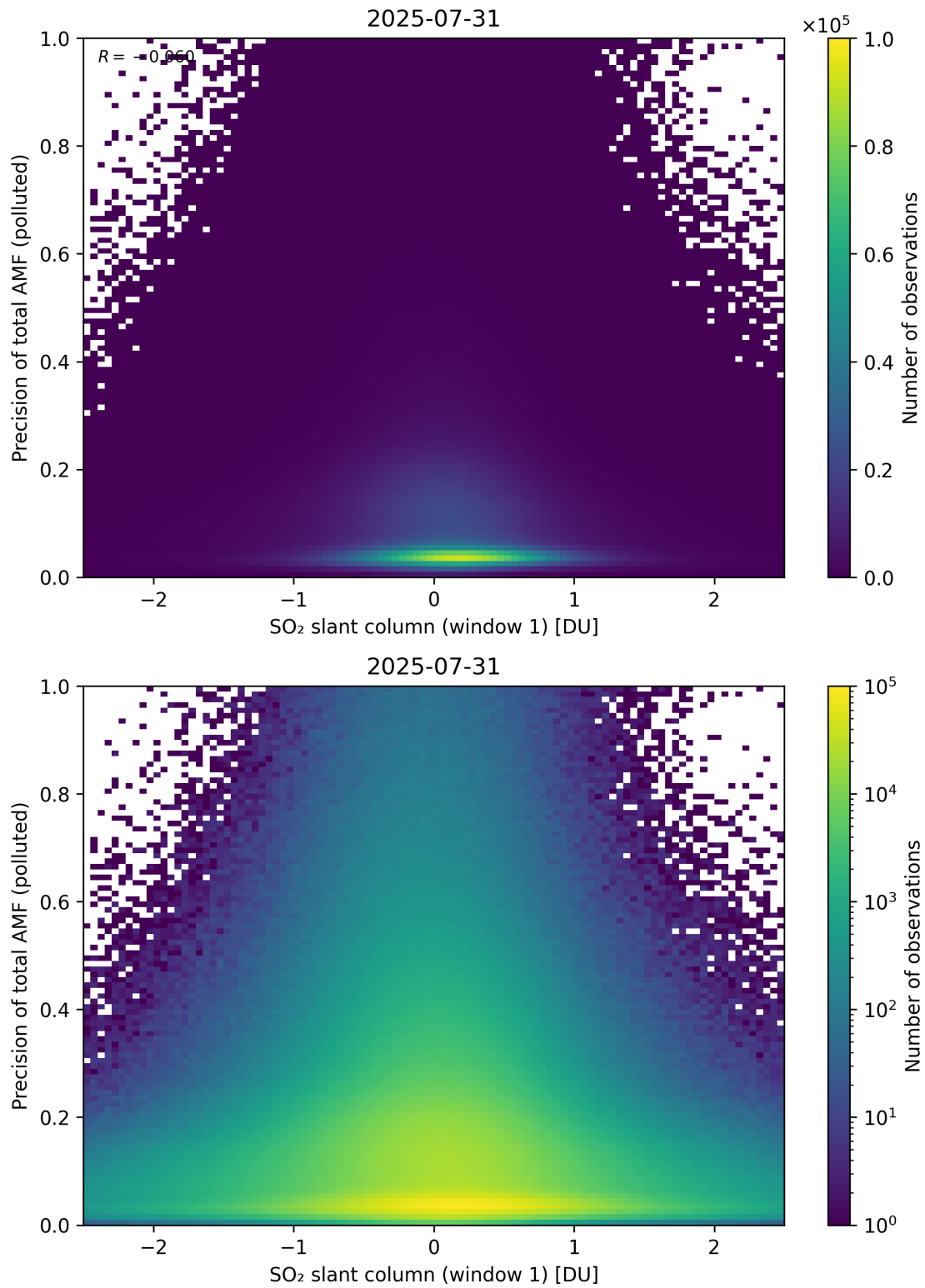
Figure 290: Scatter density plot of “SO 2 slant column (window 1)” against “Precision of total AMF (polluted)” for 2025-07-30 to 2025-08-01.
