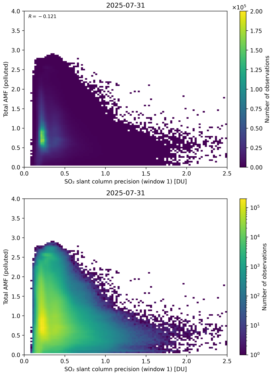
Figure 280: Scatter density plot of “SO 2 slant column precision (window 1)” against “Total AMF (polluted)” for 2025-07-30 to 2025-08-01.
