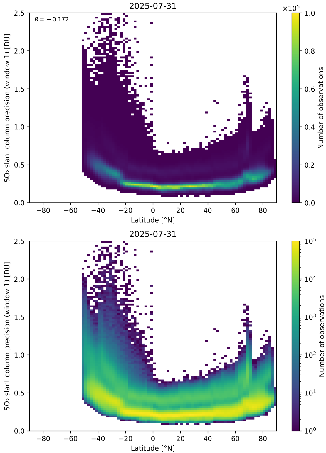
Figure 163: Scatter density plot of “Latitude” against “SO 2 slant column precision (window 1)” for 2025-07-30 to 2025-08-01.
