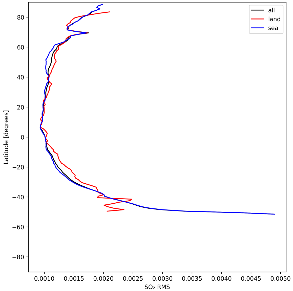
Figure 52: Zonal average of “SO 2 RMS” for 2025-07-30 to 2025-08-01.
