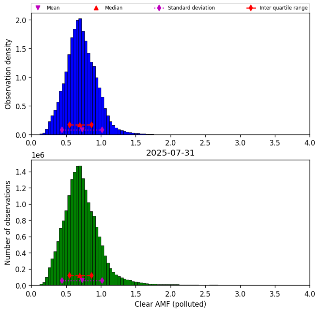
Figure 81: Histogram of “Clear AMF (polluted)” for 2025-07-30 to 2025-08-01
