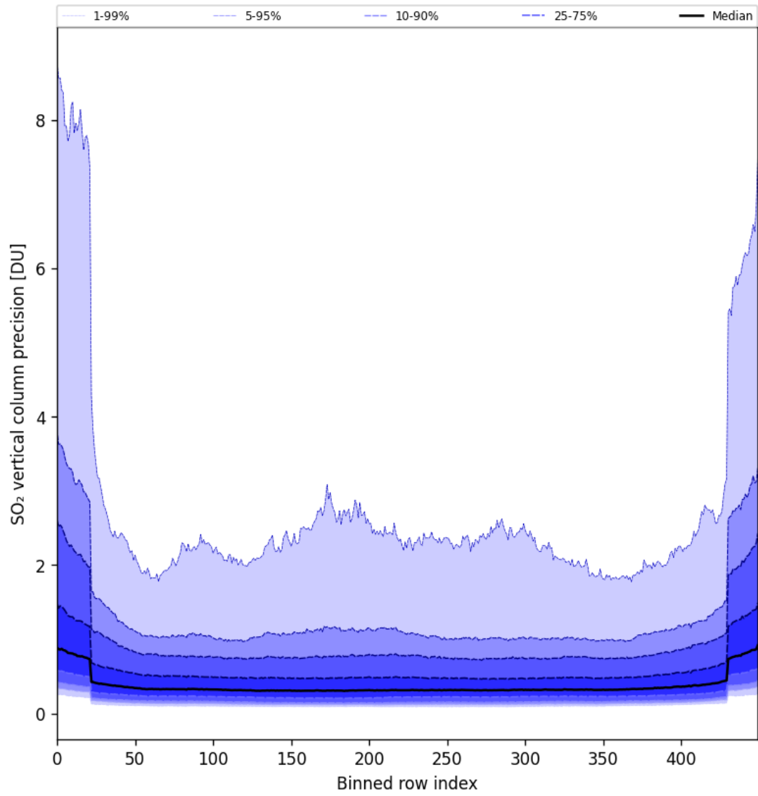
Figure 85: Along track statistics of “SO 2 vertical column precision” for 2025-07-30 to 2025-08-01
