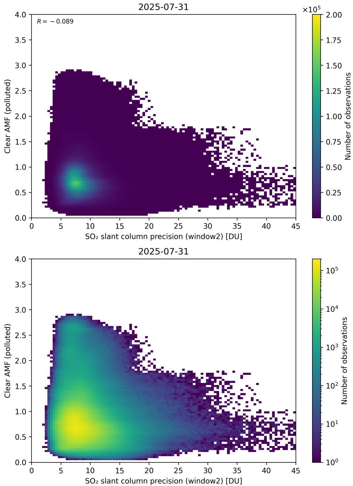
Figure 296: Scatter density plot of “SO 2 slant column precision (window2)” against “Clear AMF (polluted)” for 2025-07-30 to 2025-08-01.
