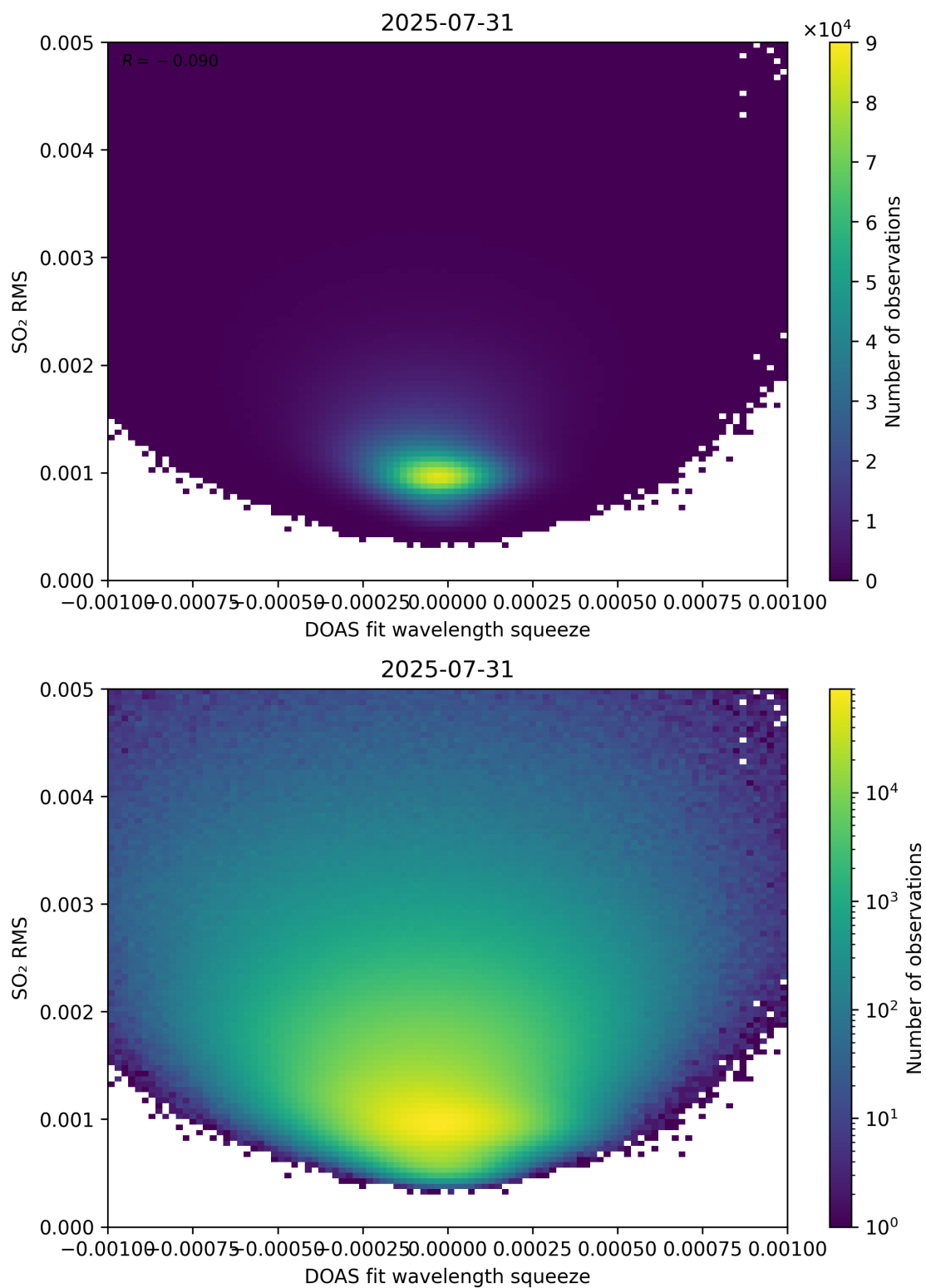
Figure 143: Scatter density plot of “DOAS fit wavelength squeeze” against “SO 2 RMS” for 2025-07-30 to 2025-08-01.
