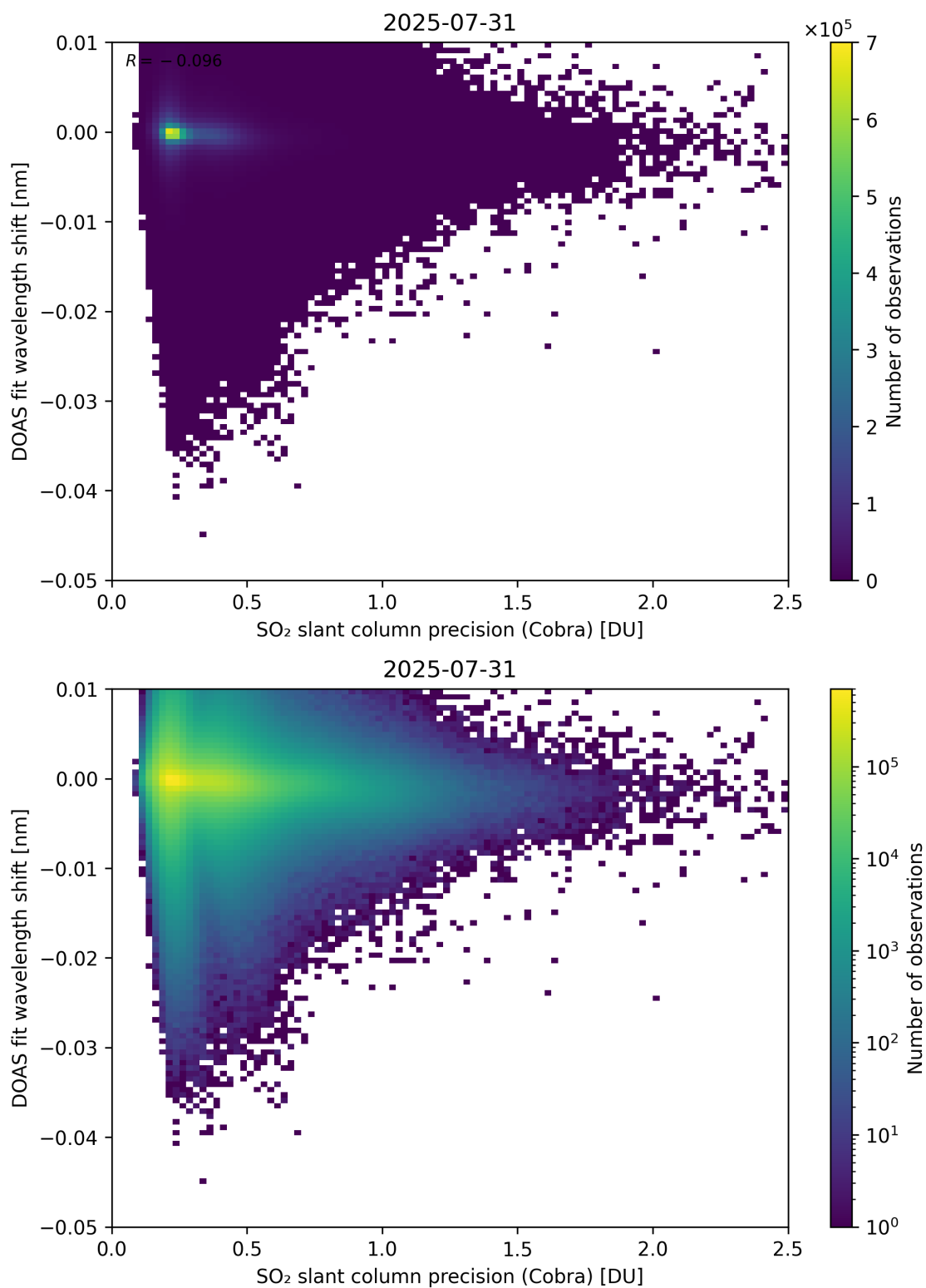
Figure 202: Scatter density plot of “SO 2 slant column precision (Cobra)” against “DOAS fit wavelength shift” for 2025-07-30 to 2025-08-01.
