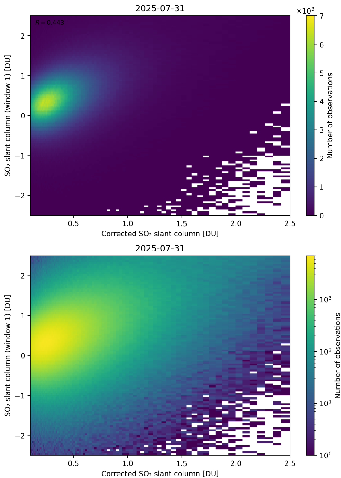
Figure 237: Scatter density plot of “Corrected SO 2 slant column” against “SO 2 slant column (window 1)” for 2025-07-30 to 2025-08-01.
