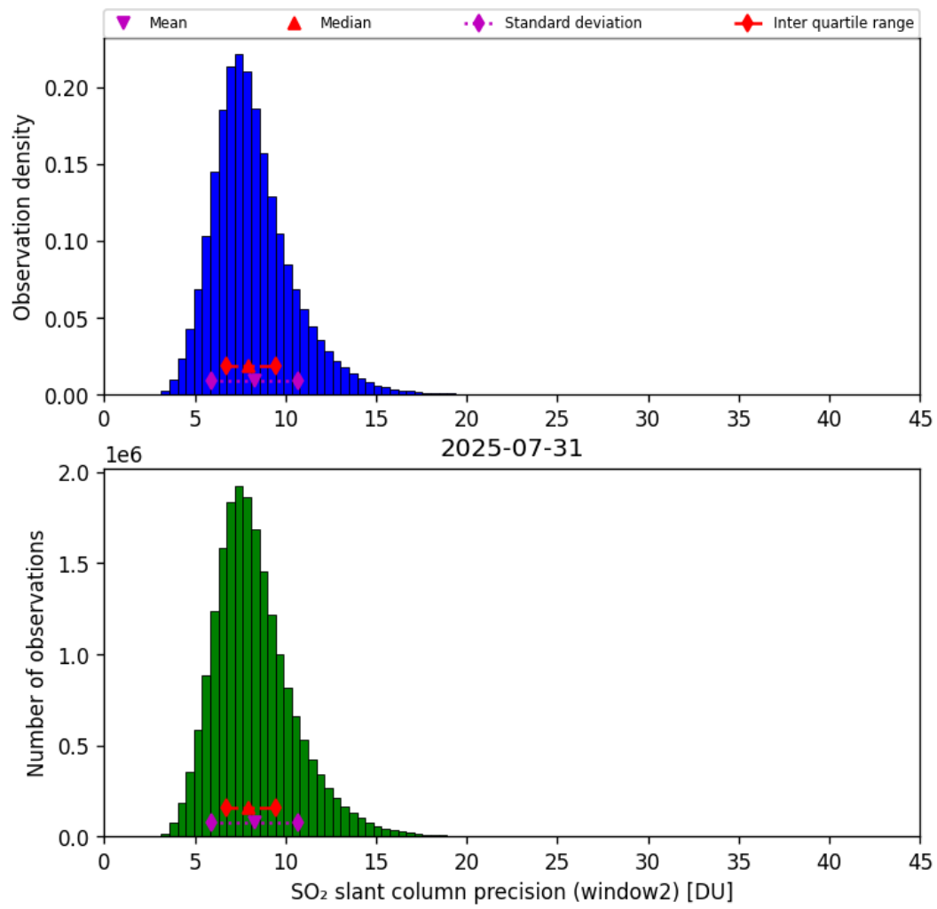
Figure 68: Histogram of “SO 2 slant column precision (window2)” for 2025-07-30 to 2025-08-01
