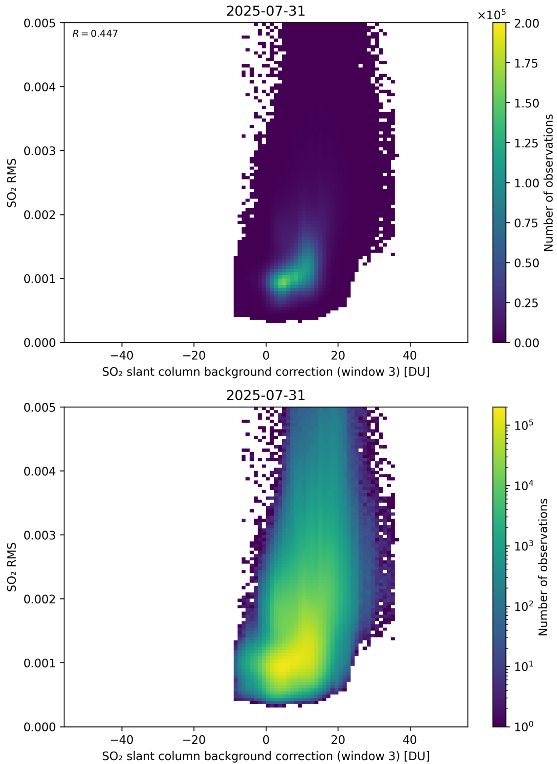
Figure 134: Scatter density plot of “SO 2 slant column background correction (window 3)” against “SO 2 RMS” for 2025-07-30 to 2025-08-01.
