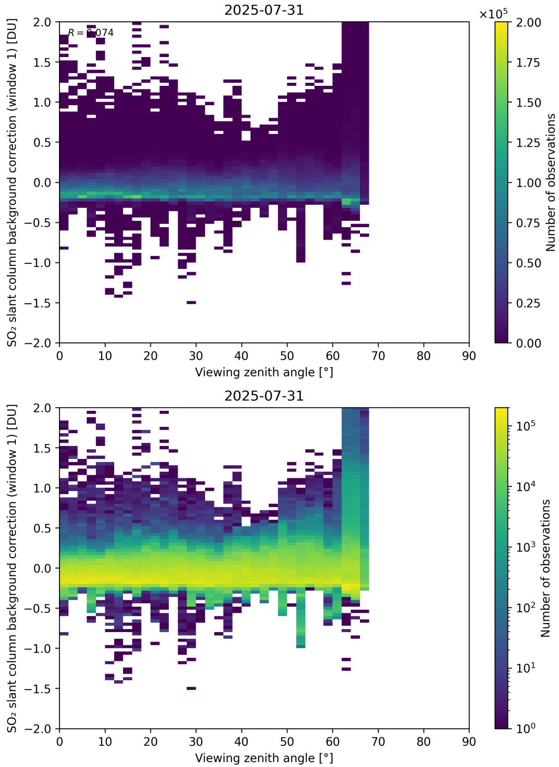
Figure 362: Scatter density plot of “Viewing zenith angle” against “SO 2 slant column background correction (window 1)” for 2025-07-30 to 2025-08-01.
