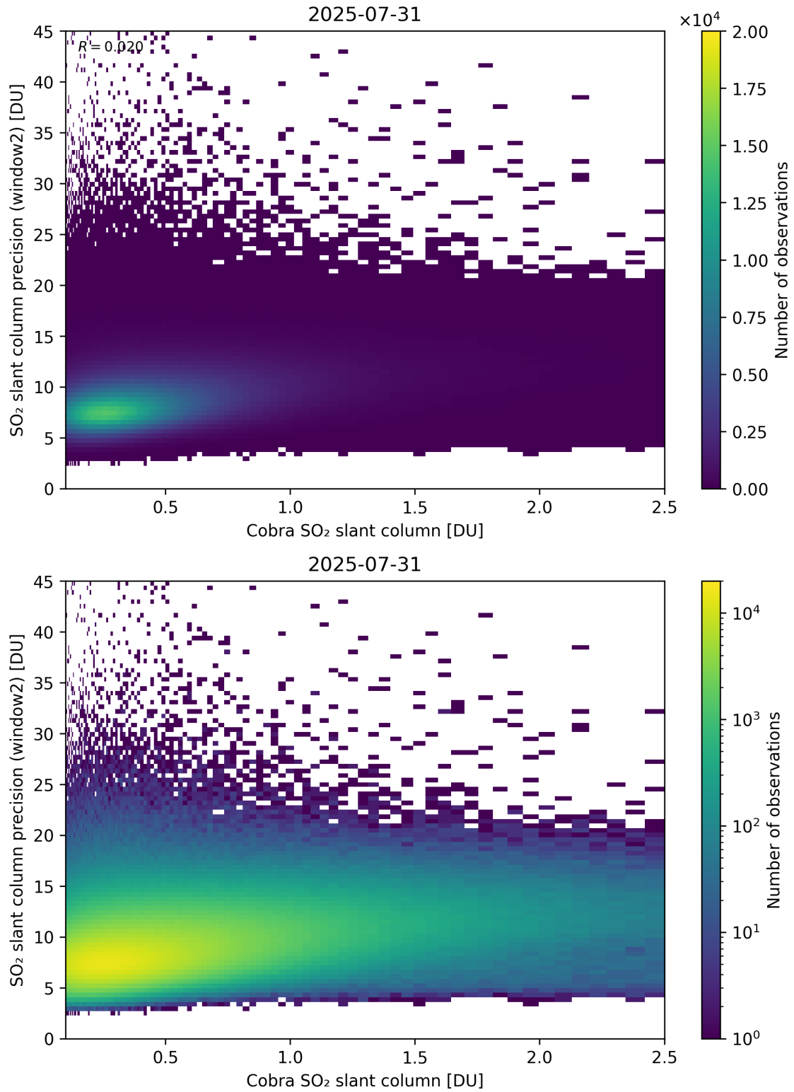
Figure 221: Scatter density plot of “Cobra SO 2 slant column” against “SO 2 slant column precision (window2)” for 2025-07-30 to 2025-08-01.
