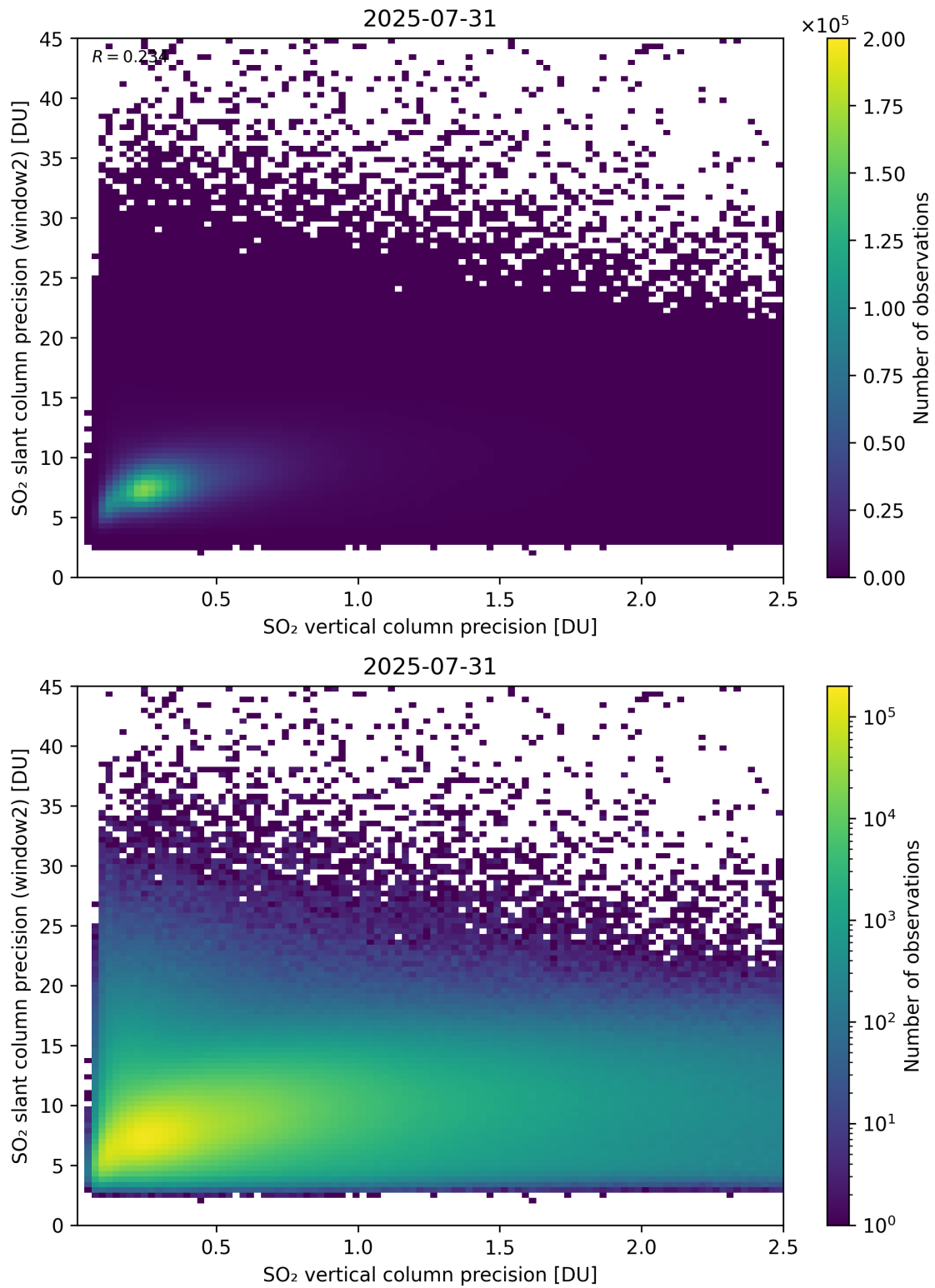
Figure 343: Scatter density plot of “SO 2 vertical column precision” against “SO 2 slant column precision (window2)” for 2025-07-30 to 2025-08-01.
