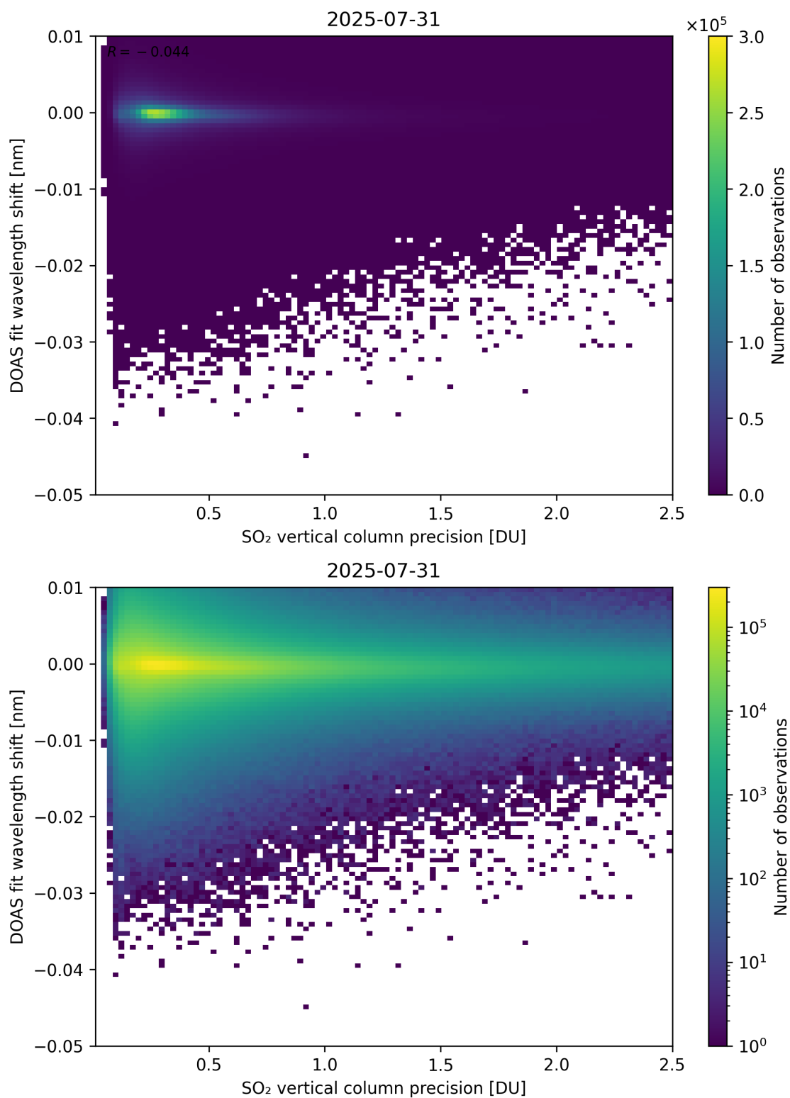
Figure 332: Scatter density plot of “SO 2 vertical column precision” against “DOAS fit wavelength shift” for 2025-07-30 to 2025-08-01.
