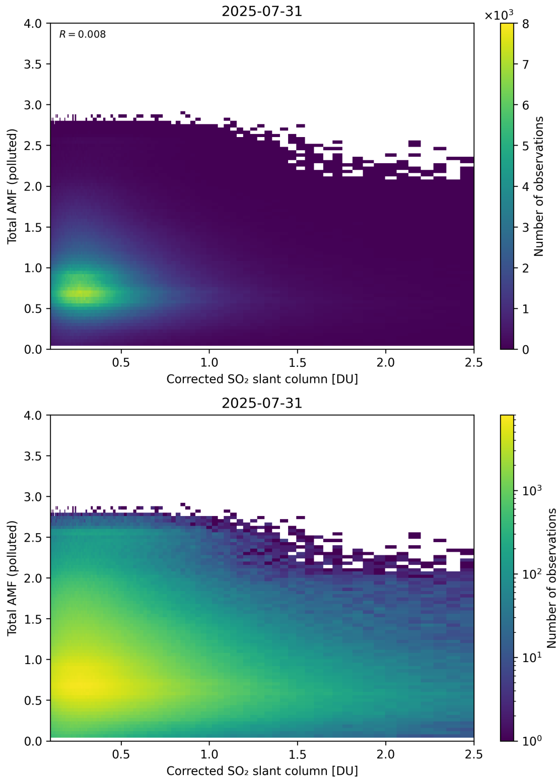
Figure 242: Scatter density plot of “Corrected SO 2 slant column” against “Total AMF (polluted)” for 2025-07-30 to 2025-08-01.
