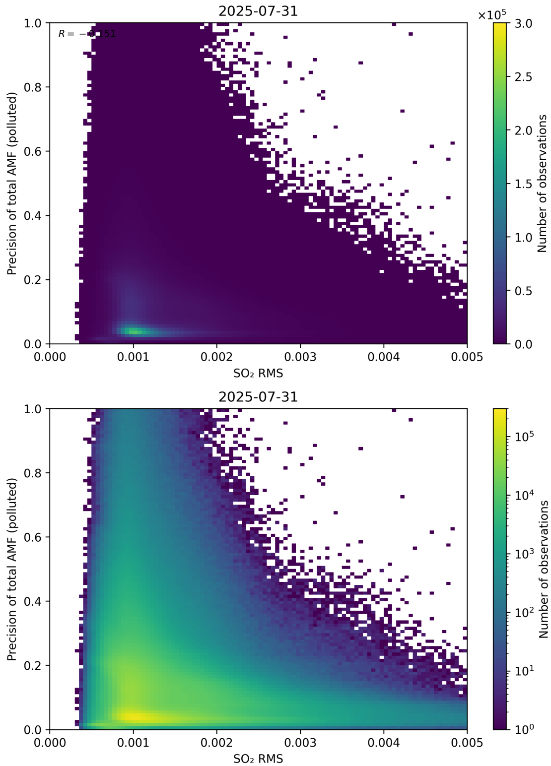
Figure 149: Scatter density plot of “SO 2 RMS” against “Precision of total AMF (polluted)” for 2025-07-30 to 2025-08-01.
