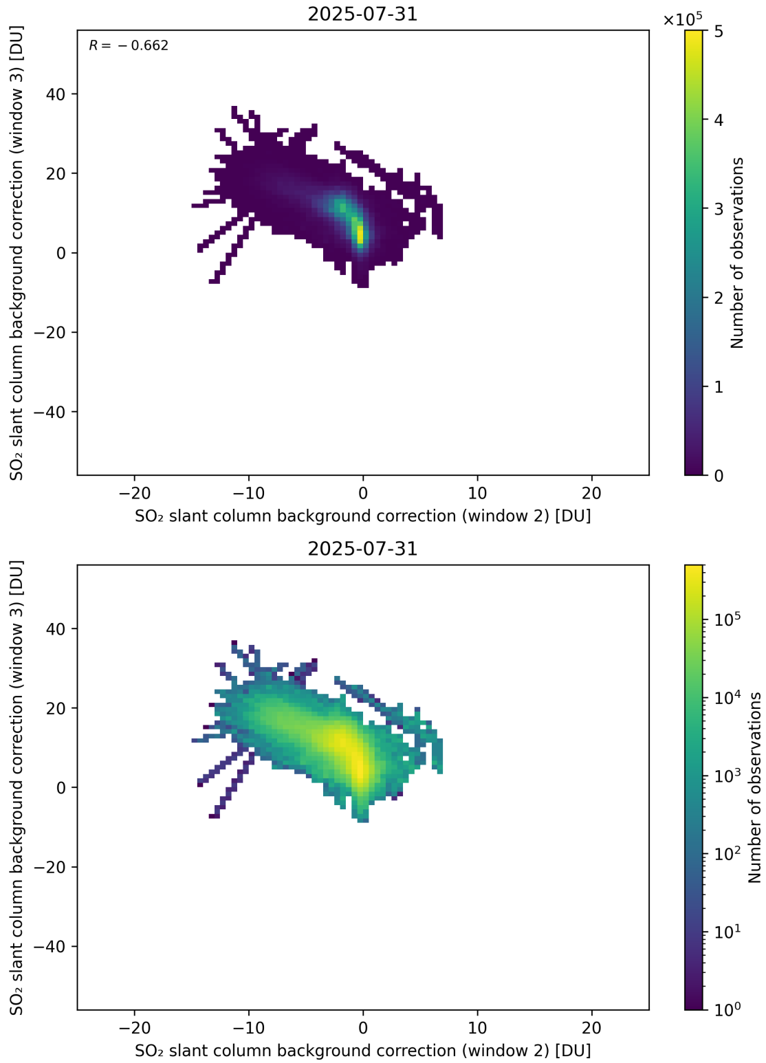
Figure 122: Scatter density plot of “SO 2 slant column background correction (window 2)” against “SO 2 slant column background correction (window 3)” for 2025-07-30 to 2025-08-01.
