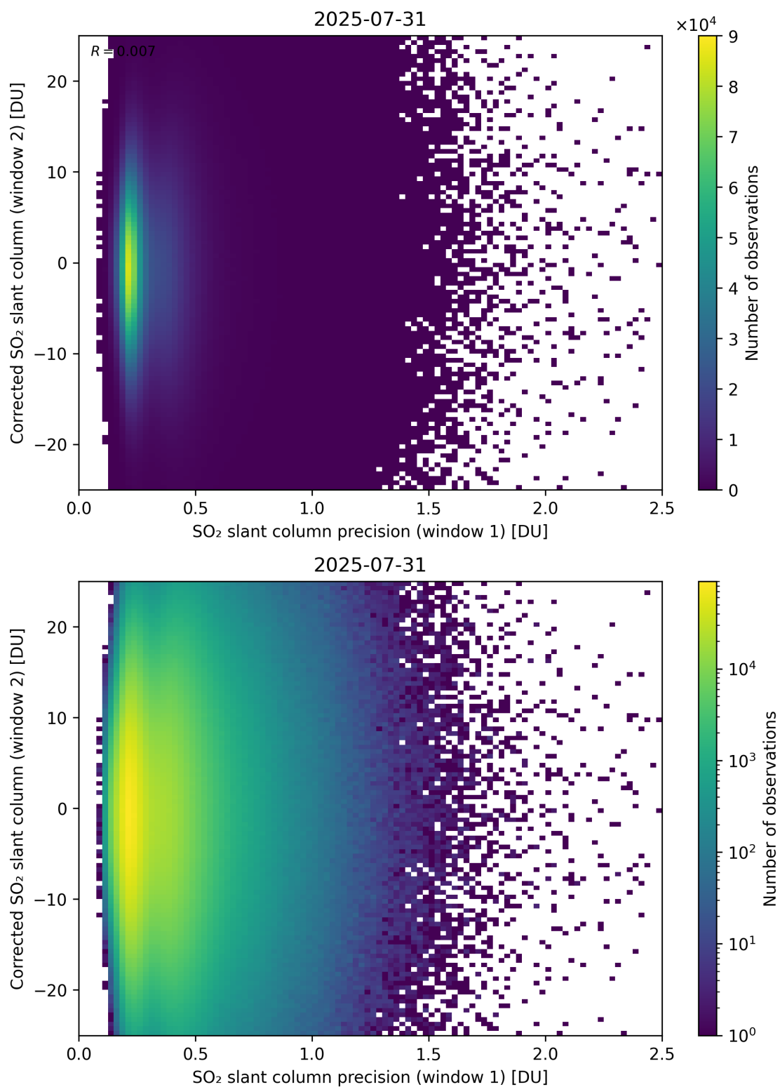
Figure 275: Scatter density plot of “SO 2 slant column precision (window 1)” against “Corrected SO 2 slant column (window 2)” for 2025-07-30 to 2025-08-01.
