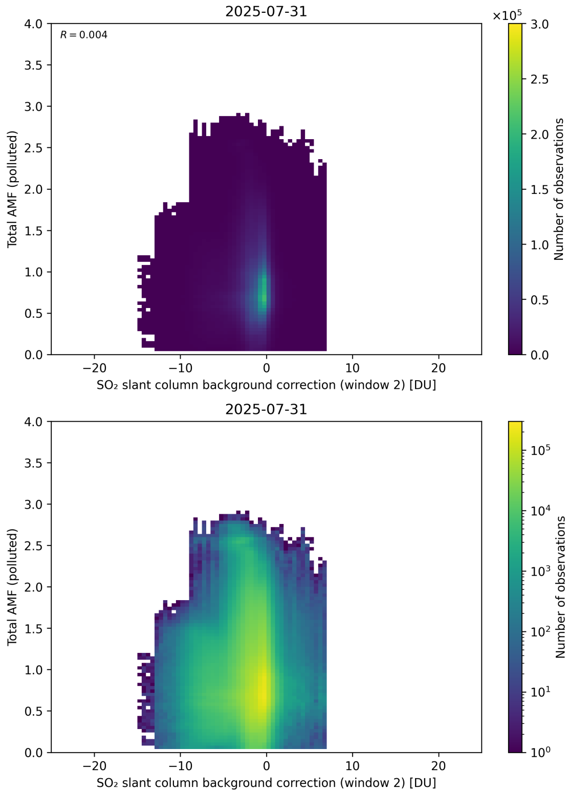
Figure 130: Scatter density plot of “SO 2 slant column background correction (window 2)” against “Total AMF (polluted)” for 2025-07-30 to 2025-08-01.
