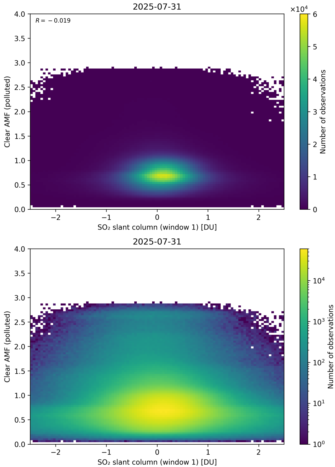
Figure 282: Scatter density plot of “SO 2 slant column (window 1)” against “Clear AMF (polluted)” for 2025-07-30 to 2025-08-01.
