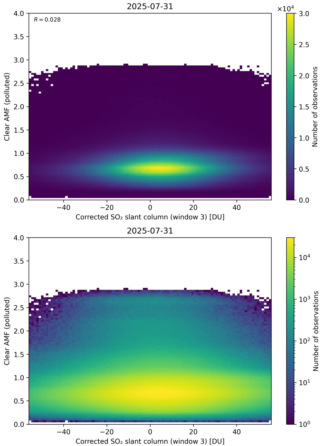
Figure 259: Scatter density plot of “Corrected SO 2 slant column (window 3)” against “Clear AMF (polluted)” for 2025-07-30 to 2025-08-01.
