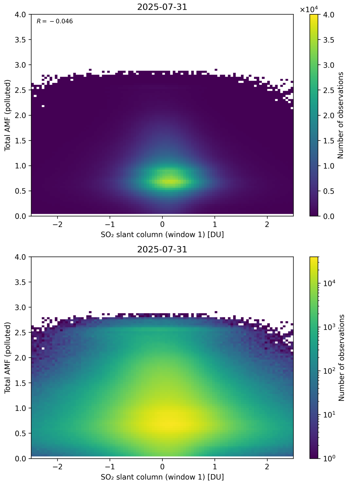
Figure 289: Scatter density plot of “SO 2 slant column (window 1)” against “Total AMF (polluted)” for 2025-07-30 to 2025-08-01.
