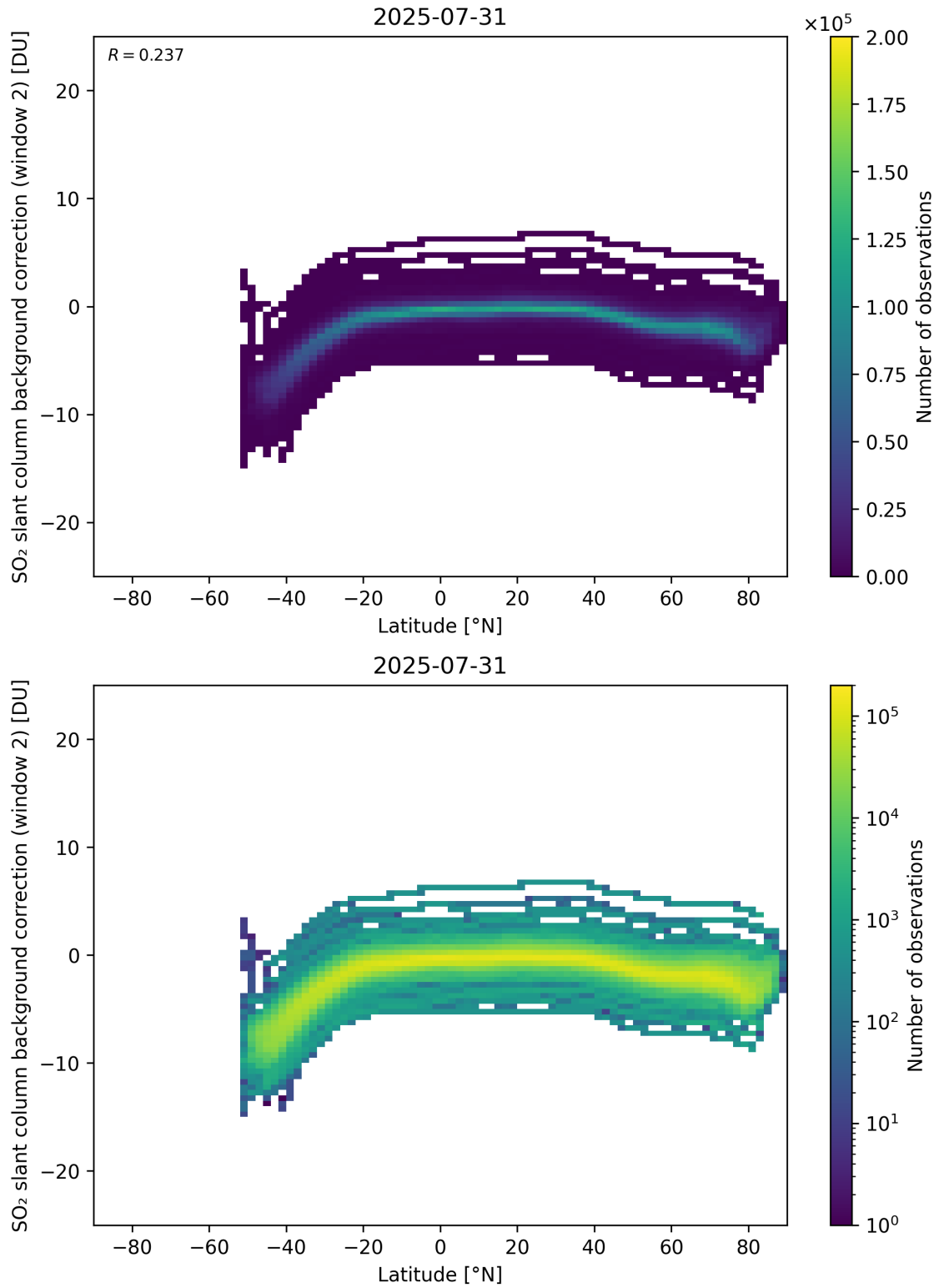
Figure 151: Scatter density plot of “Latitude” against “SO 2 slant column background correction (window 2)” for 2025-07-30 to 2025-08-01.
