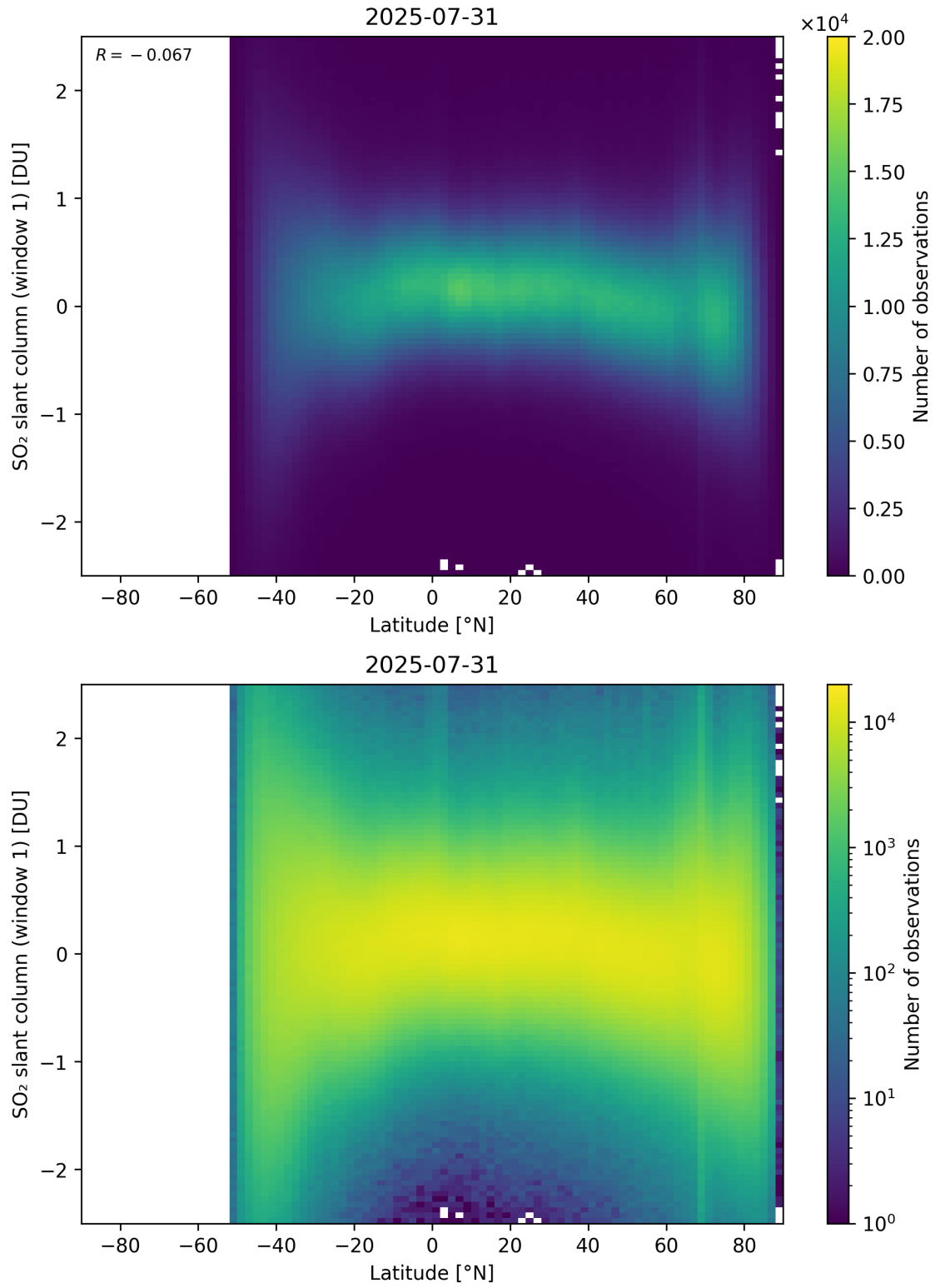
Figure 162: Scatter density plot of “Latitude” against “SO 2 slant column (window 1)” for 2025-07-30 to 2025-08-01.
