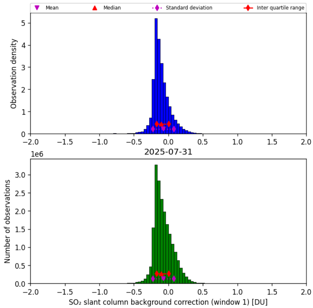
Figure 66: Histogram of “SO 2 slant column background correction (window 1)” for 2025-07-30 to 2025-08-01
