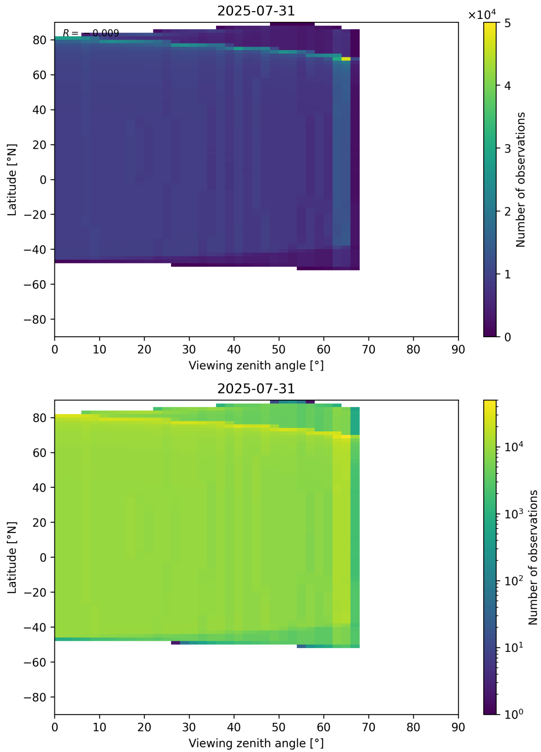
Figure 368: Scatter density plot of “Viewing zenith angle” against “Latitude” for 2025-07-30 to 2025-08-01.
