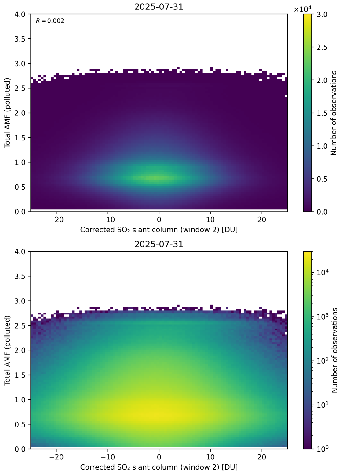
Figure 253: Scatter density plot of “Corrected SO 2 slant column (window 2)” against “Total AMF (polluted)” for 2025-07-30 to 2025-08-01.
