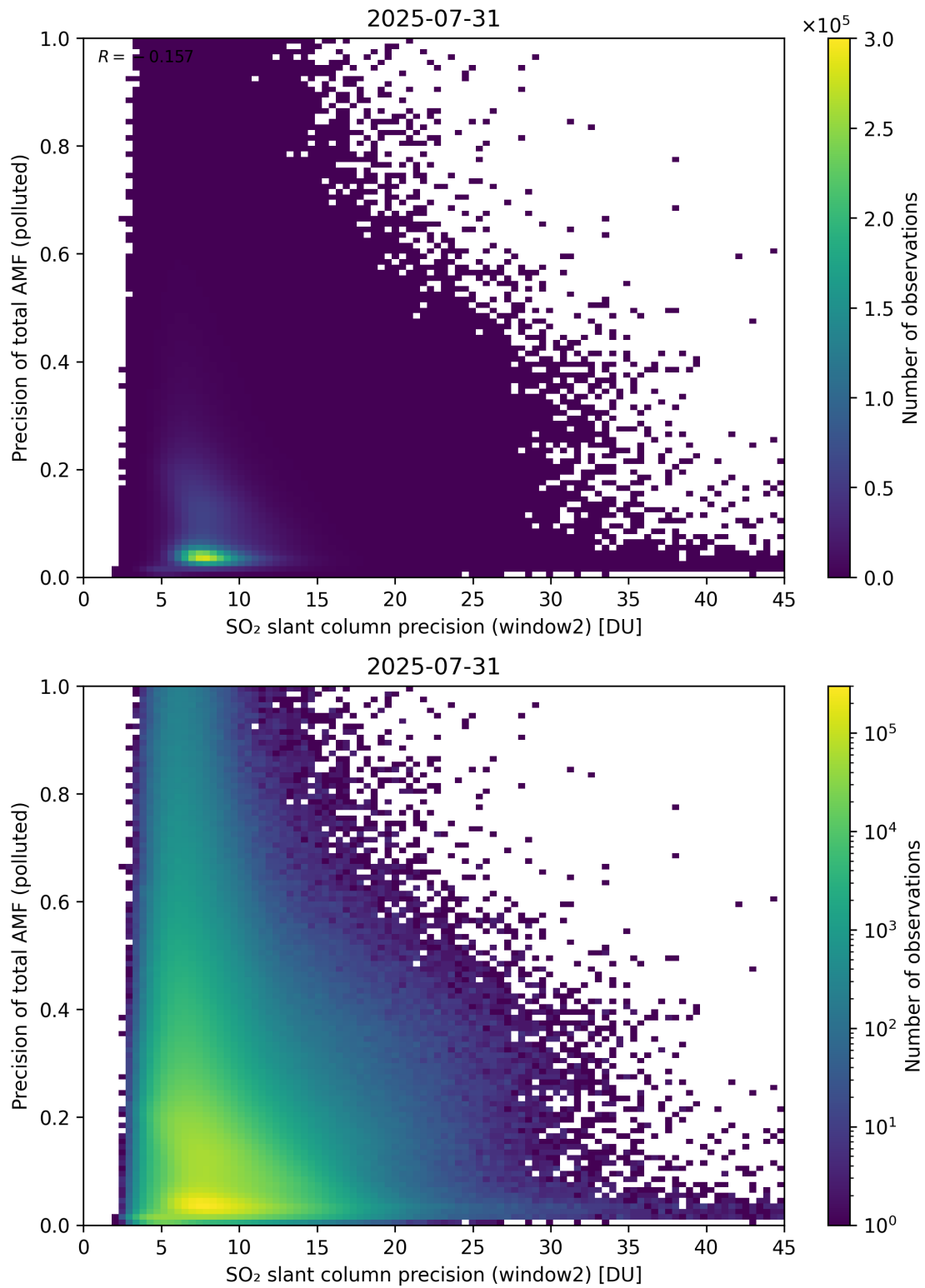
Figure 302: Scatter density plot of “SO 2 slant column precision (window2)” against “Precision of total AMF (polluted)” for 2025-07-30 to 2025-08-01.
