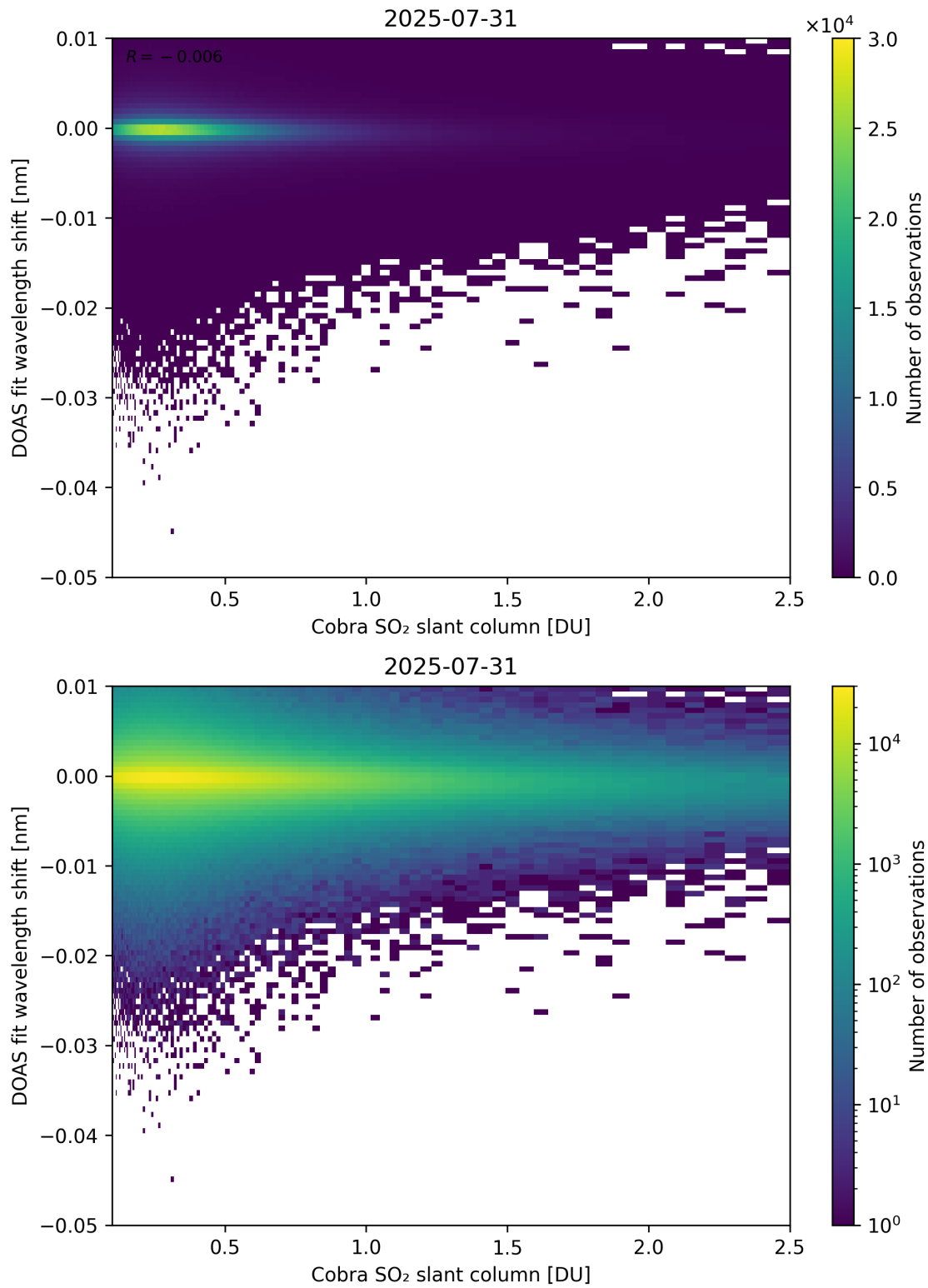
Figure 196: Scatter density plot of “Cobra SO 2 slant column” against “DOAS fit wavelength shift” for 2025-07-30 to 2025-08-01.
