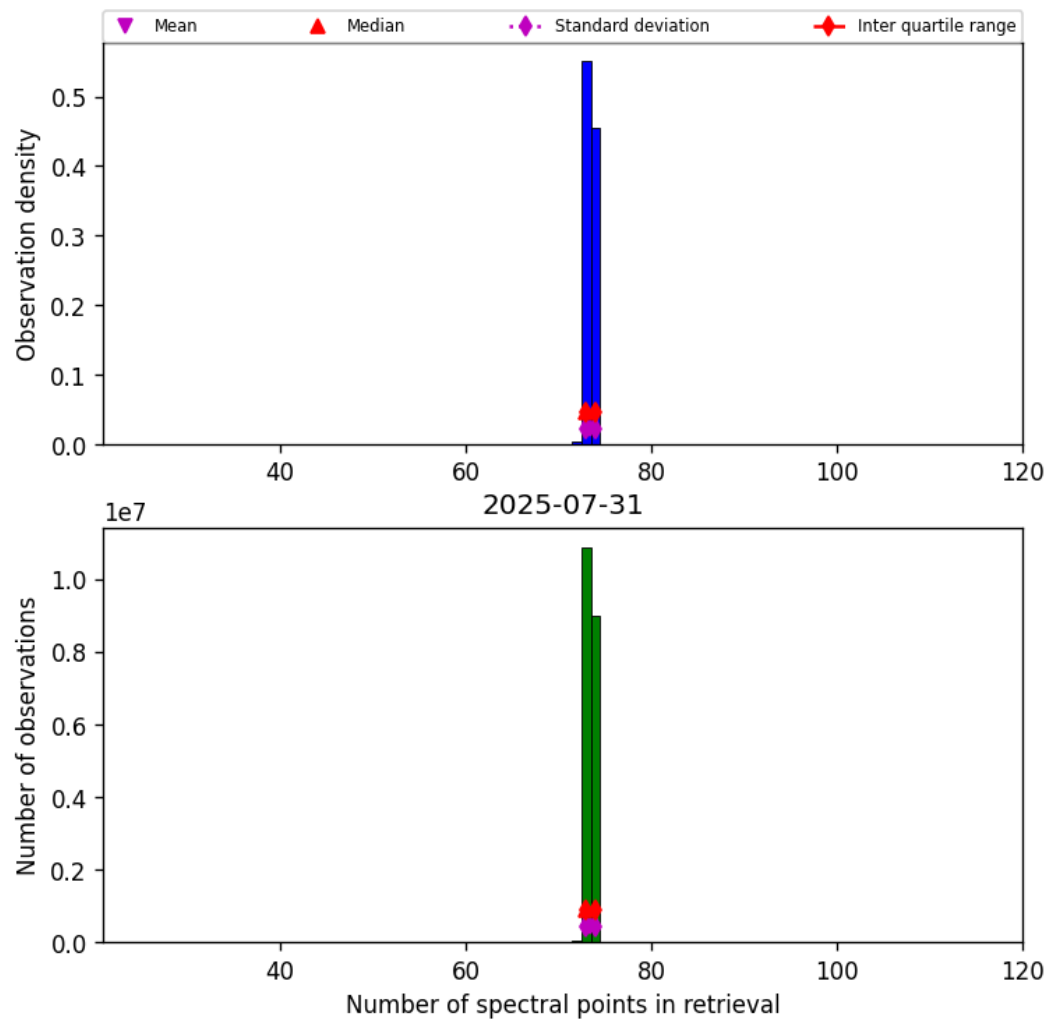
Figure 82: Histogram of “Number of spectral points in retrieval” for 2025-07-30 to 2025-08-01
