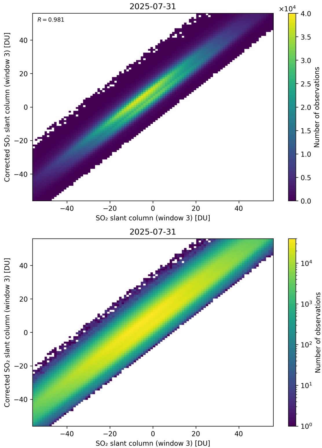
Figure 316: Scatter density plot of “SO 2 slant column (window 3)” against “Corrected SO 2 slant column (window 3)” for 2025-07-30 to 2025-08-01.
