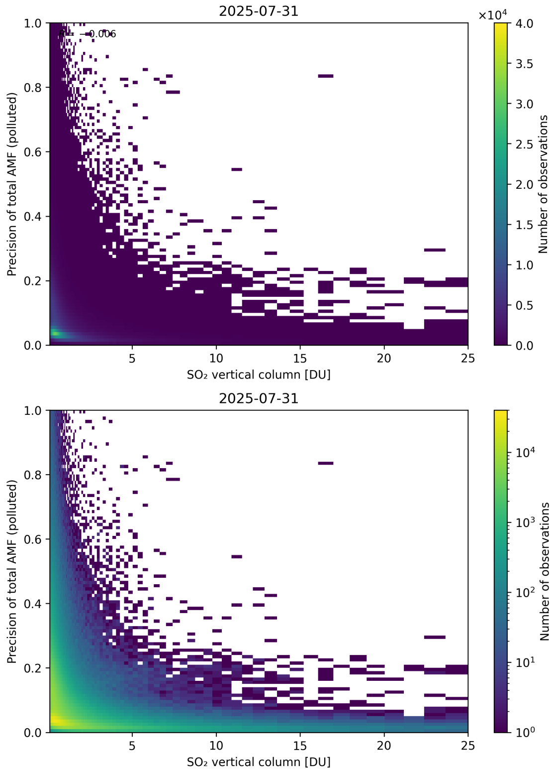
Figure 360: Scatter density plot of “SO 2 vertical column” against “Precision of total AMF (polluted)” for 2025-07-30 to 2025-08-01.
