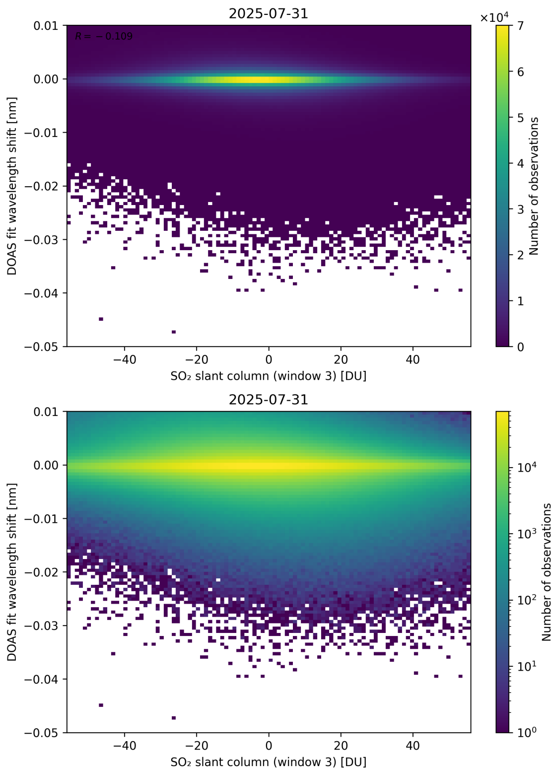
Figure 304: Scatter density plot of “SO 2 slant column (window 3)” against “DOAS fit wavelength shift” for 2025-07-30 to 2025-08-01.
