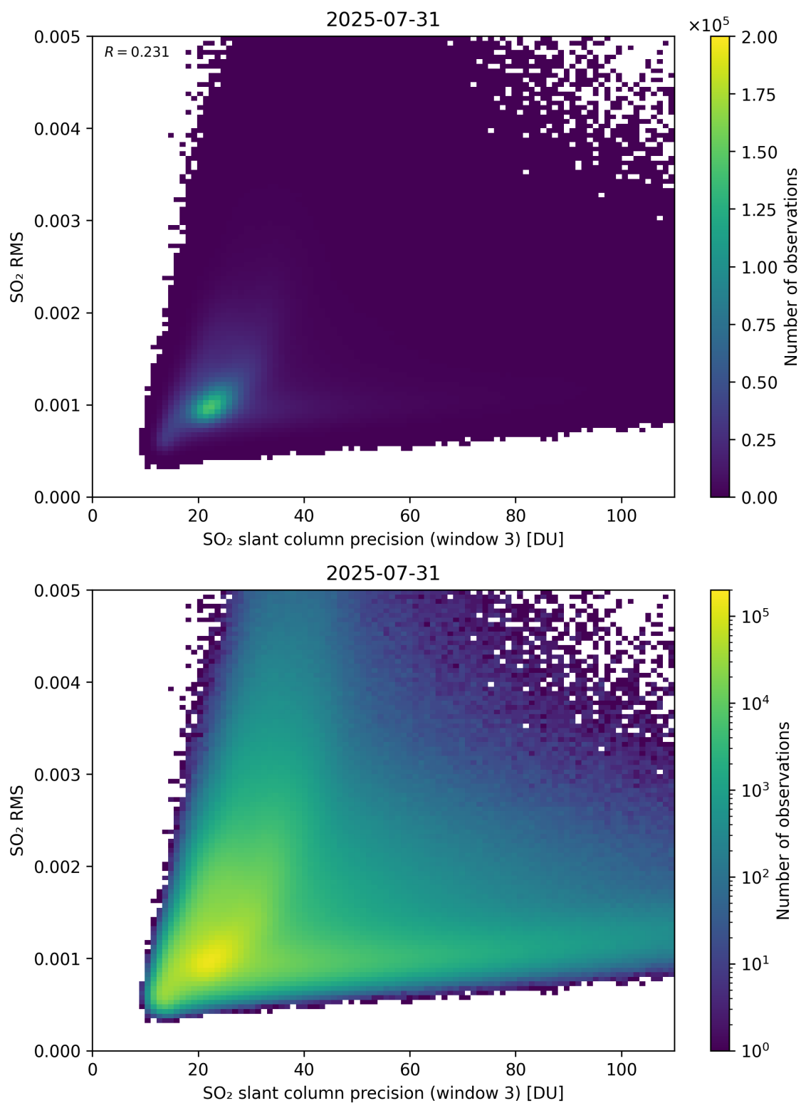
Figure 310: Scatter density plot of “SO 2 slant column precision (window 3)” against “SO 2 RMS” for 2025-07-30 to 2025-08-01.
