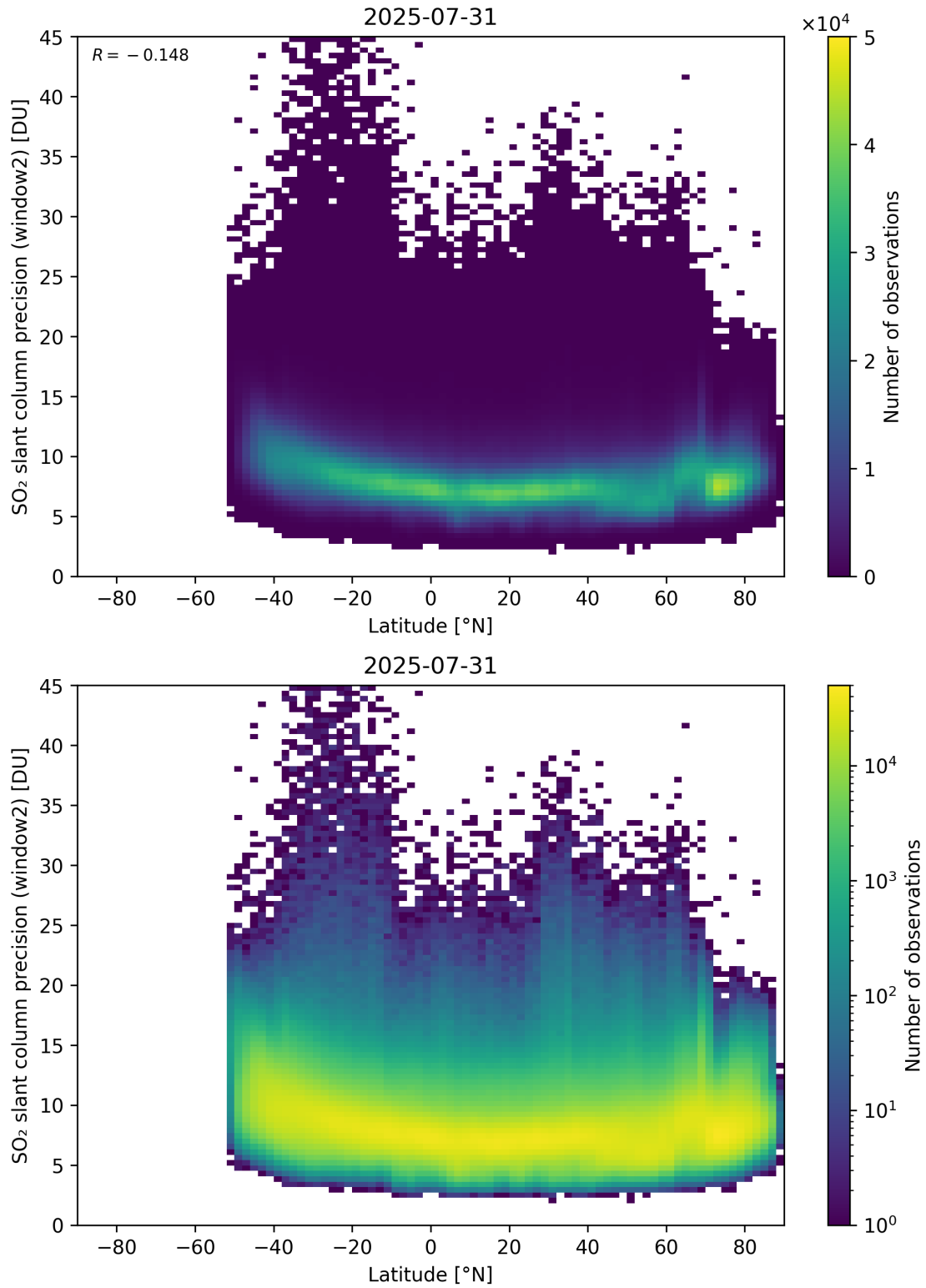
Figure 164: Scatter density plot of “Latitude” against “SO 2 slant column precision (window2)” for 2025-07-30 to 2025-08-01.
