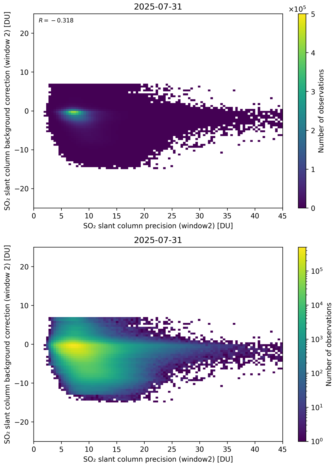
Figure 291: Scatter density plot of “SO 2 slant column precision (window2)” against “SO 2 slant column background correction (window 2)” for 2025-07-30 to 2025-08-01.
