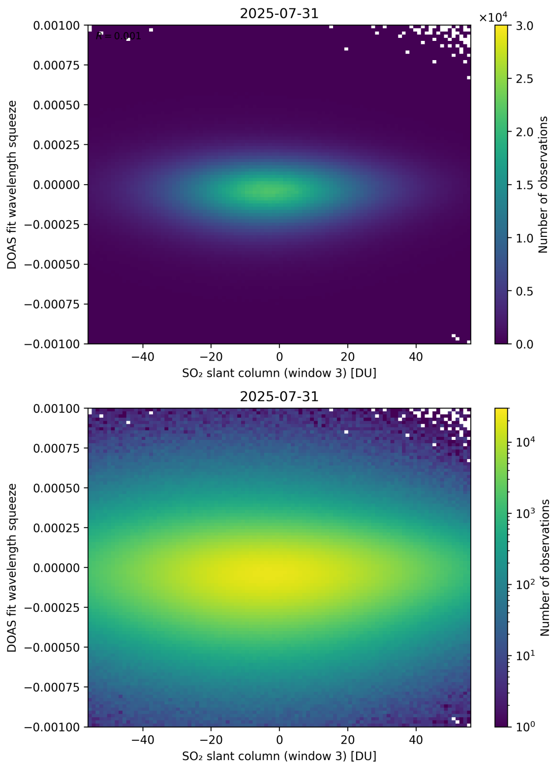
Figure 305: Scatter density plot of “SO 2 slant column (window 3)” against “DOAS fit wavelength squeeze” for 2025-07-30 to 2025-08-01.
