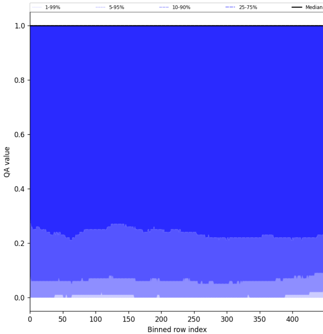
Figure 83: Along track statistics of “QA value” for 2025-07-30 to 2025-08-01
