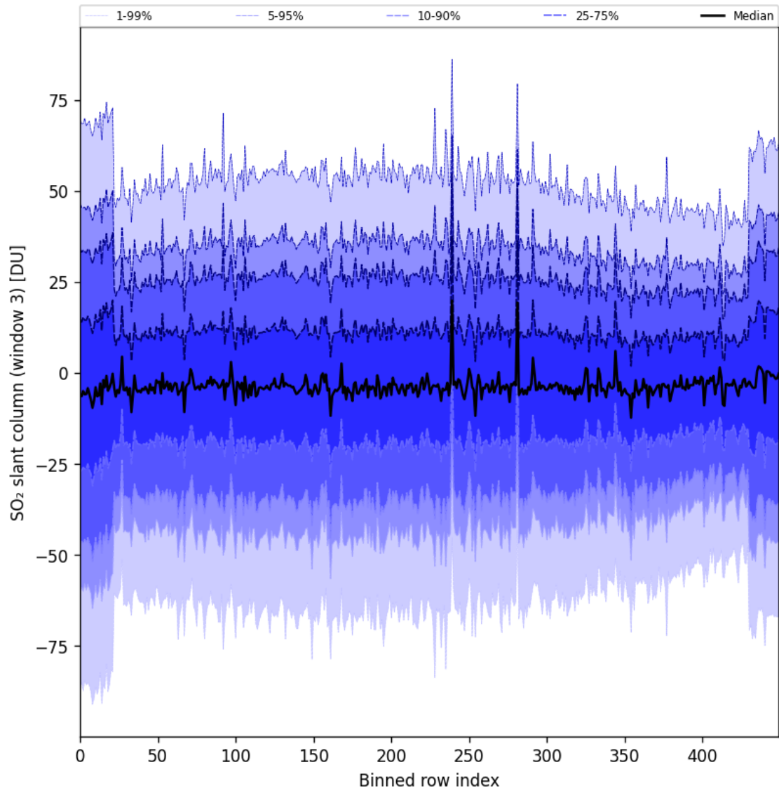
Figure 97: Along track statistics of “SO 2 slant column (window 3)” for 2025-07-30 to 2025-08-01
