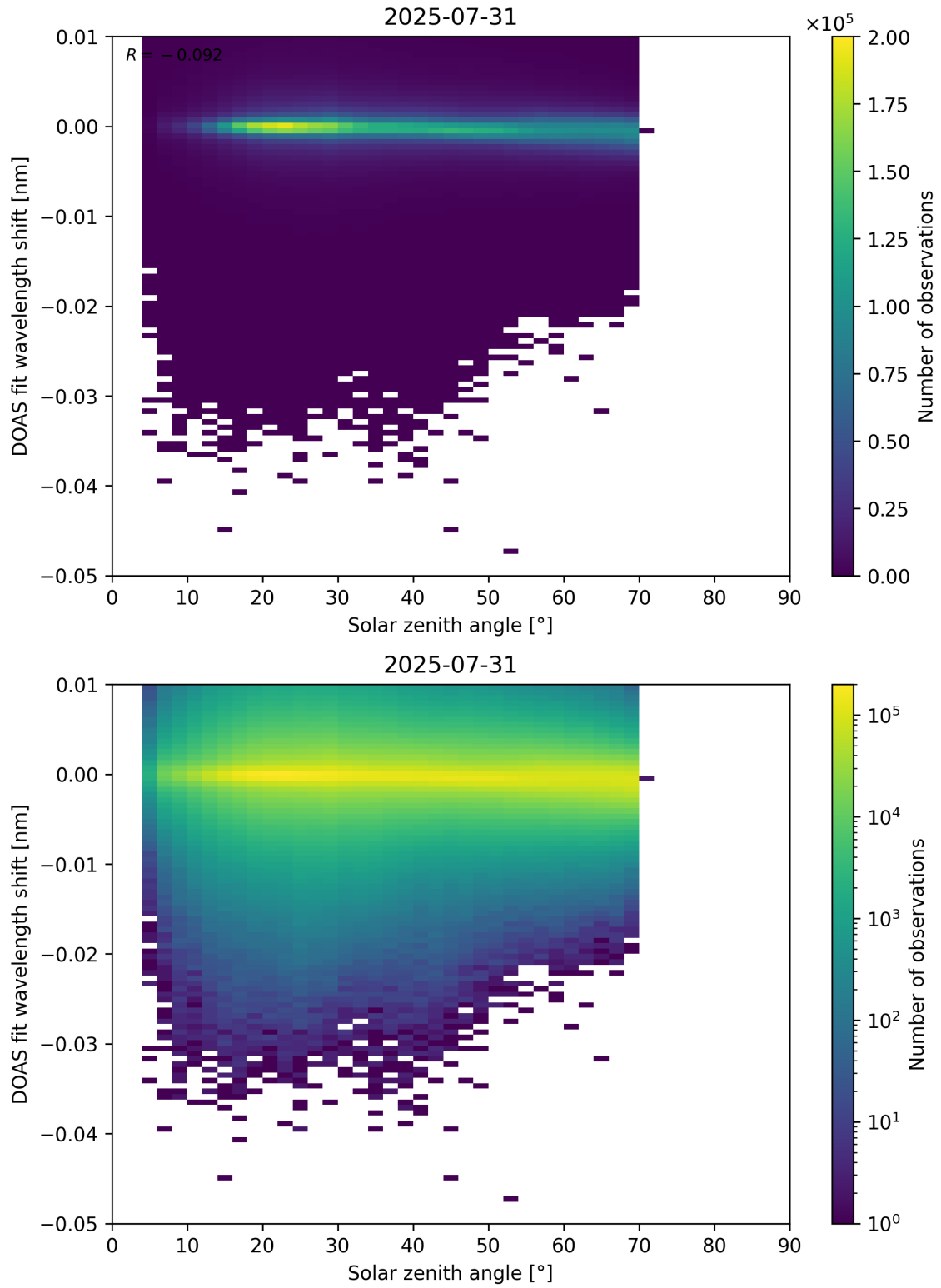
Figure 174: Scatter density plot of “Solar zenith angle” against “DOAS fit wavelength shift” for 2025-07-30 to 2025-08-01.
