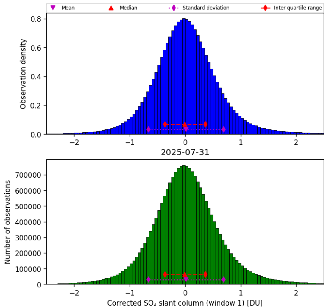
Figure 65: Histogram of “Corrected SO 2 slant column (window 1)” for 2025-07-30 to 2025-08-01
