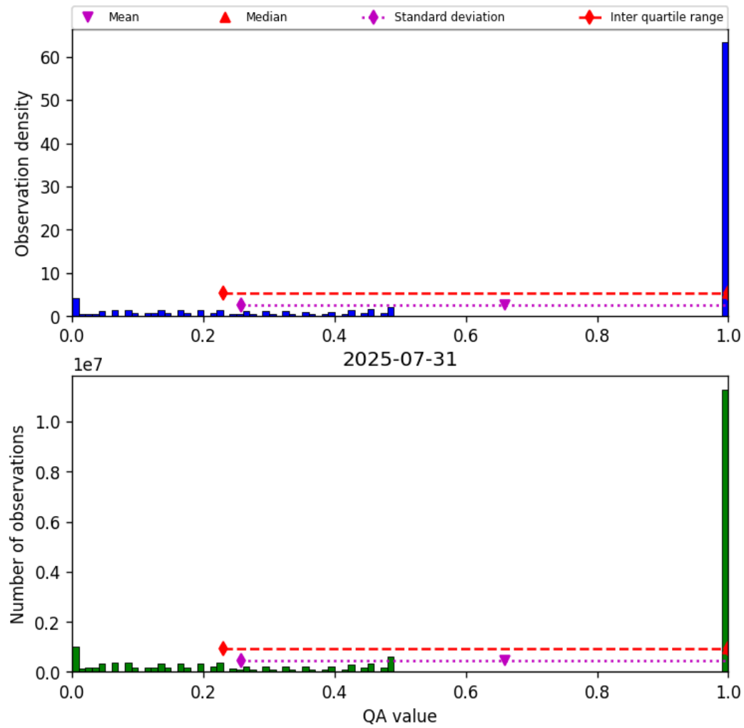
Figure 57: Histogram of “QA value” for 2025-07-30 to 2025-08-01
