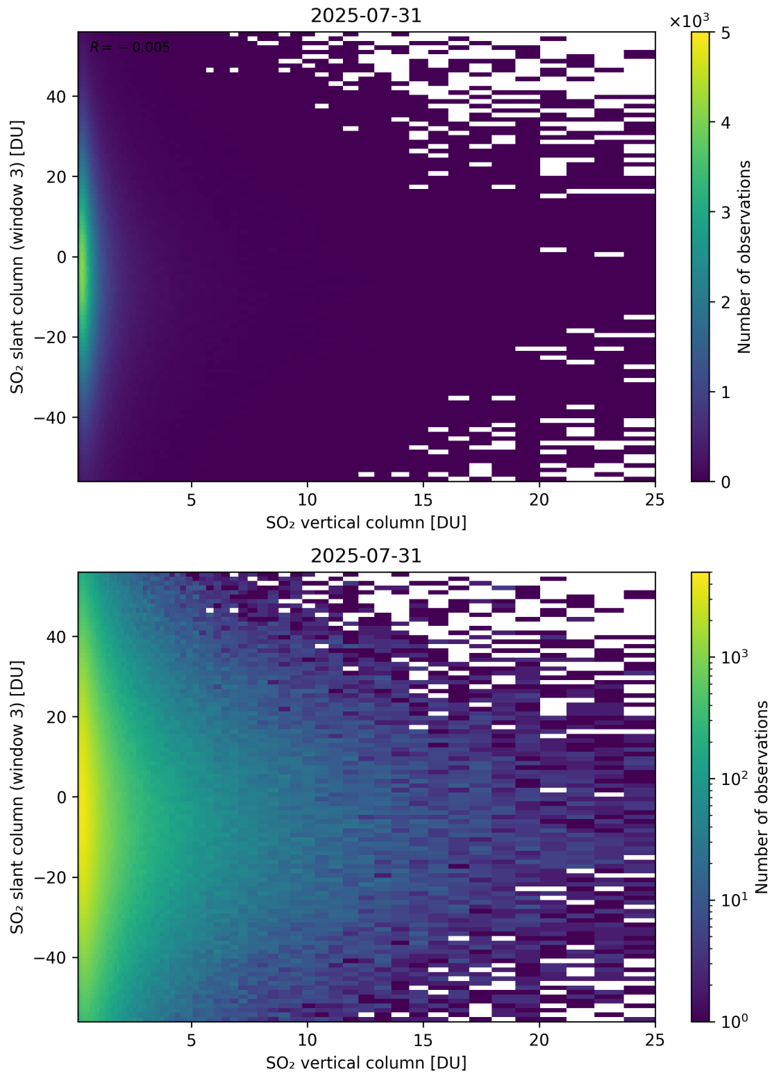
Figure 357: Scatter density plot of “SO 2 vertical column” against “SO 2 slant column (window 3)” for 2025-07-30 to 2025-08-01.
