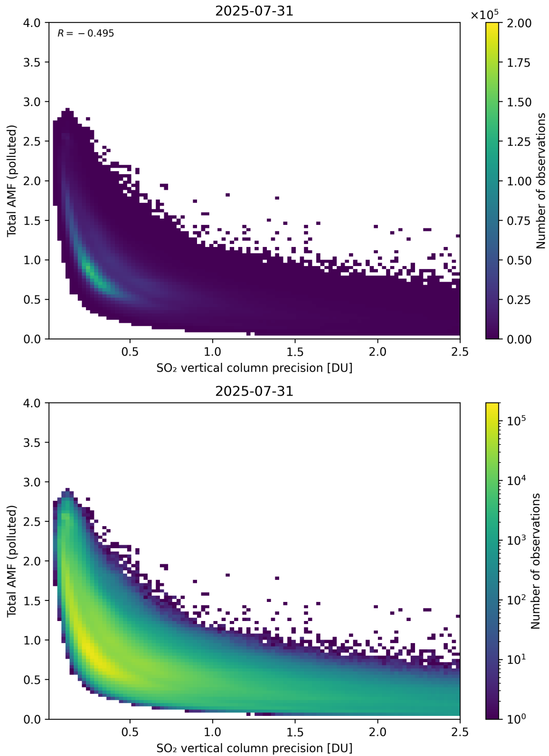
Figure 346: Scatter density plot of “SO 2 vertical column precision” against “Total AMF (polluted)” for 2025-07-30 to 2025-08-01.
