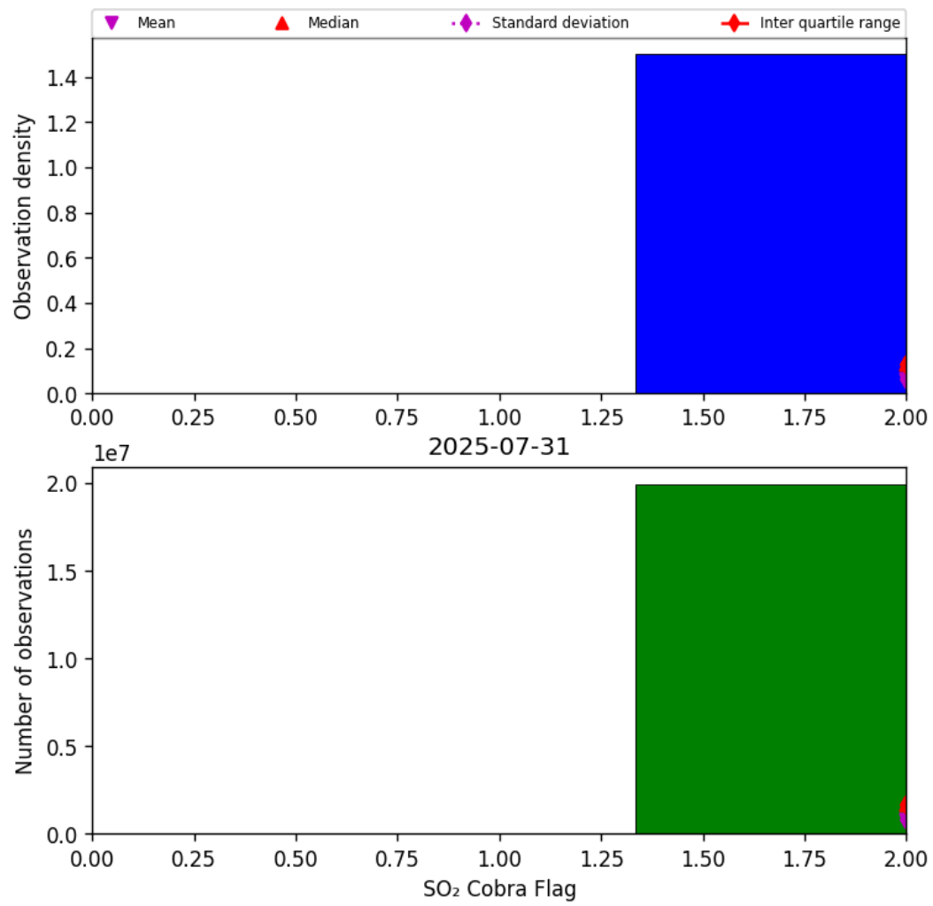
Figure 75: Histogram of “SO 2 Cobra Flag” for 2025-07-30 to 2025-08-01
