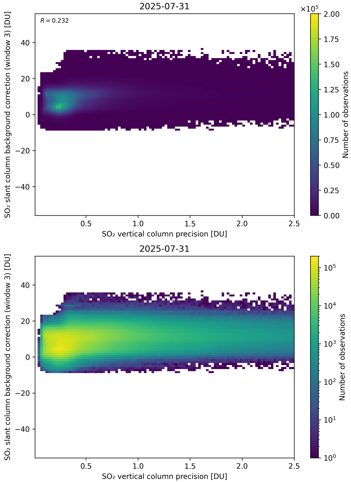
Figure 331: Scatter density plot of “SO 2 vertical column precision” against “SO 2 slant column background correction (window 3)” for 2025-07-30 to 2025-08-01.
