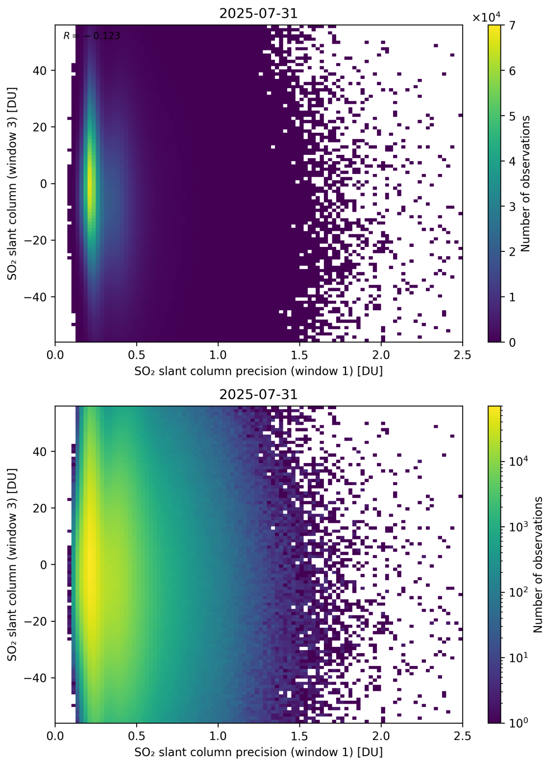
Figure 278: Scatter density plot of “SO 2 slant column precision (window 1)” against “SO 2 slant column (window 3)” for 2025-07-30 to 2025-08-01.
