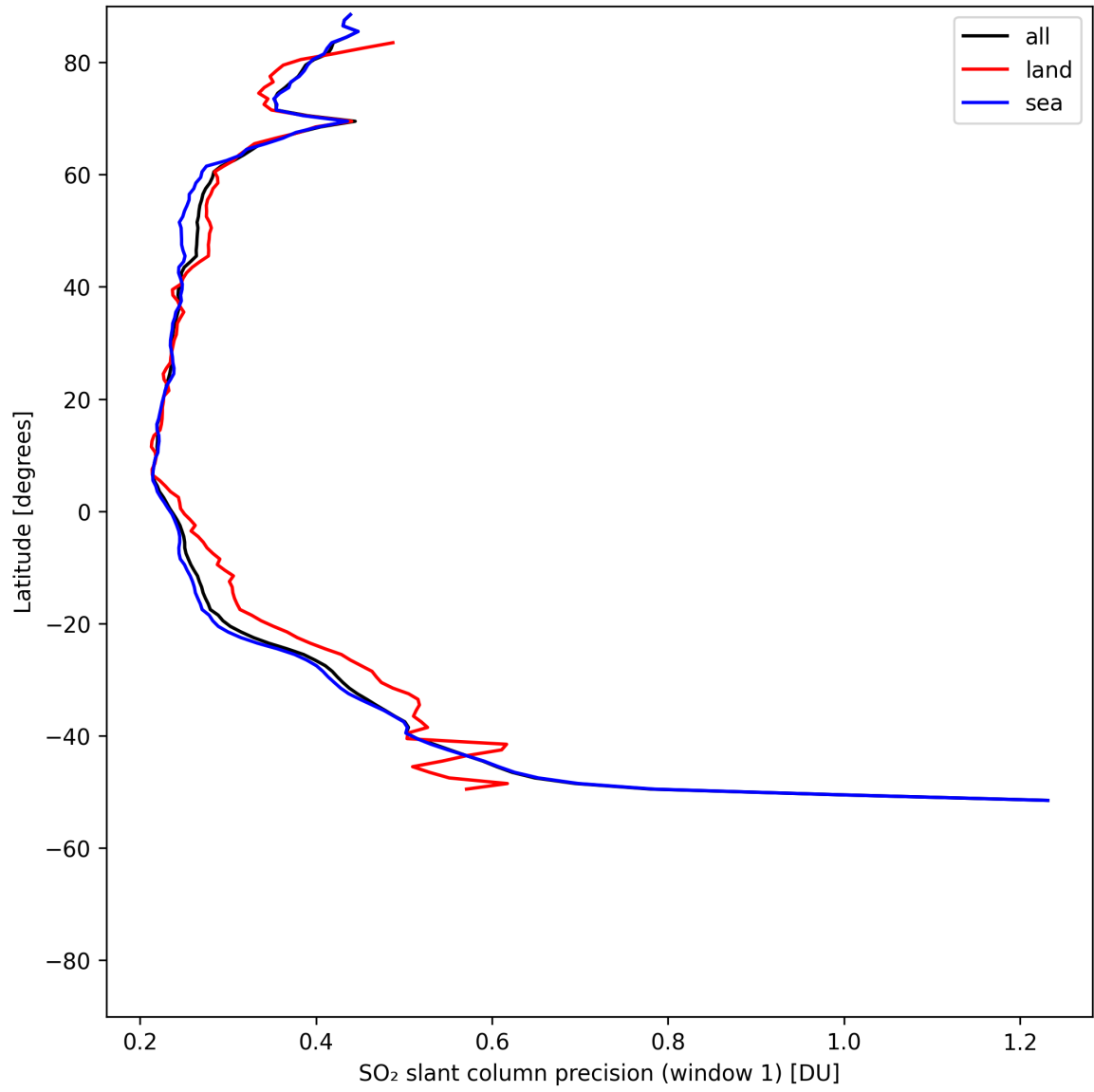
Figure 38: Zonal average of "SO 2 slant column precision (window 1)" for 2025-07-30 to 2025-08-01.
