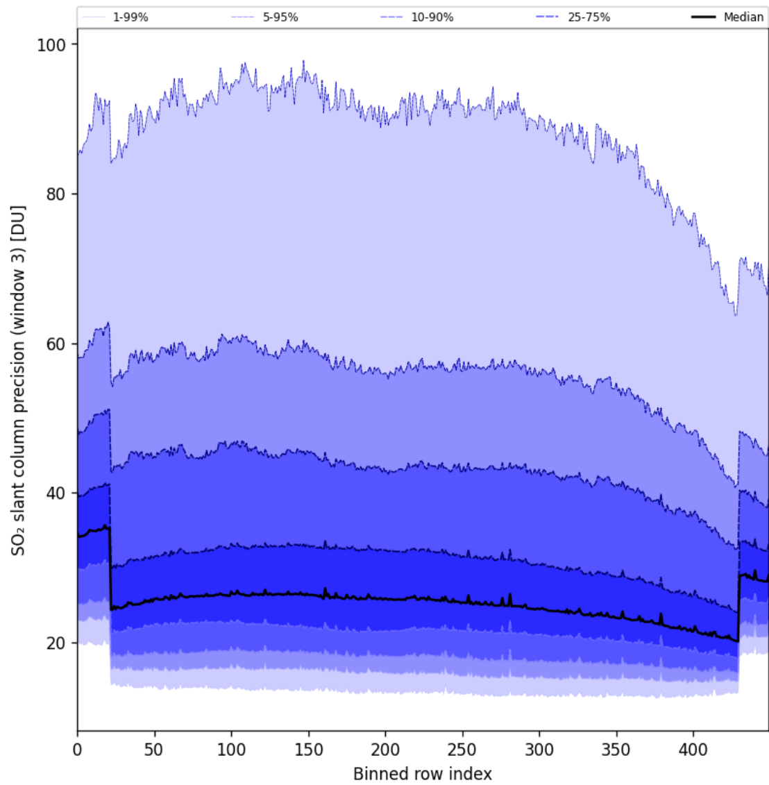
Figure 98: Along track statistics of “SO 2 slant column precision (window 3)” for 2025-07-30 to 2025-08-01
