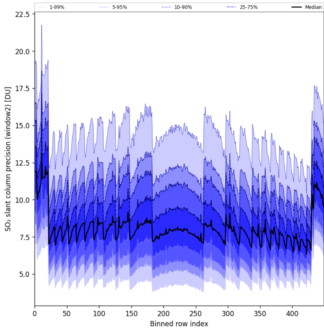
Figure 94: Along track statistics of “SO 2 slant column precision (window2)” for 2025-07-30 to 2025-08-01
