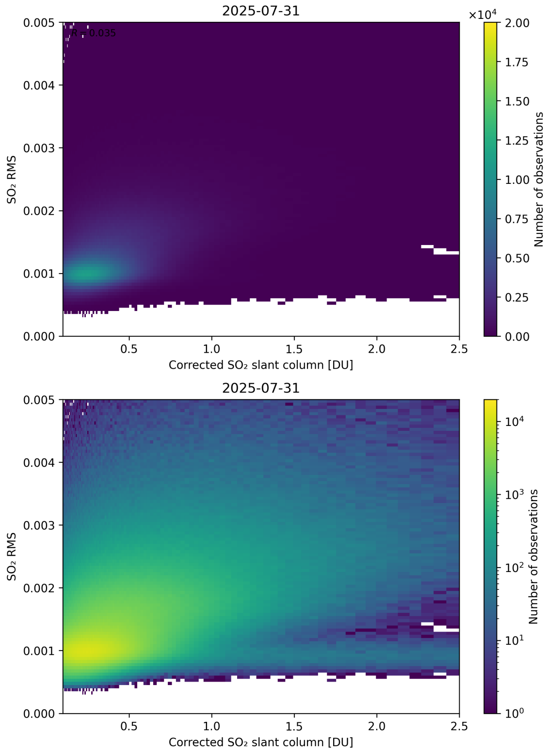
Figure 231: Scatter density plot of “Corrected SO 2 slant column” against “SO 2 RMS” for 2025-07-30 to 2025-08-01.
