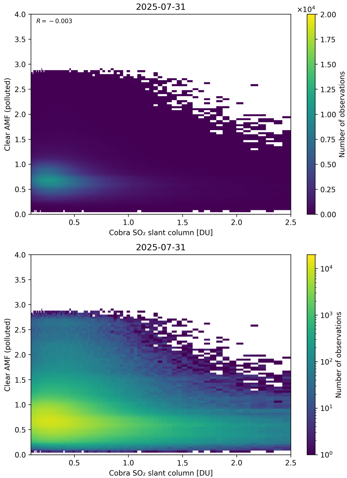
Figure 215: Scatter density plot of “Cobra SO 2 slant column” against “Clear AMF (polluted)” for 2025-07-30 to 2025-08-01.
