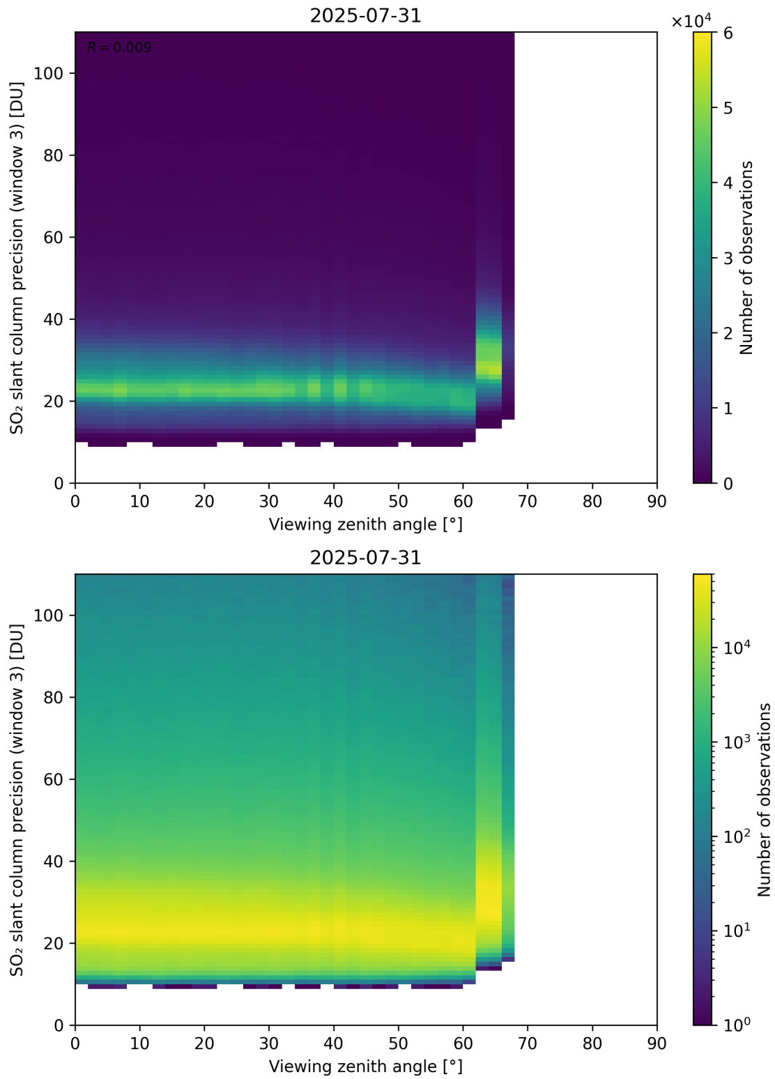
Figure 380: Scatter density plot of “Viewing zenith angle” against “SO 2 slant column precision (window 3)” for 2025-07-30 to 2025-08-01.
