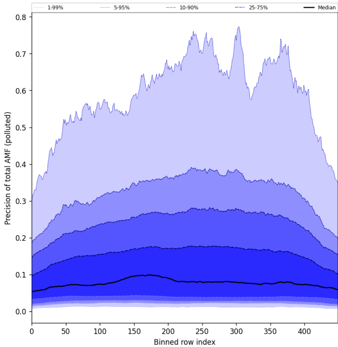
Figure 106: Along track statistics of “Precision of total AMF (polluted)” for 2025-07-30 to 2025-08-01
