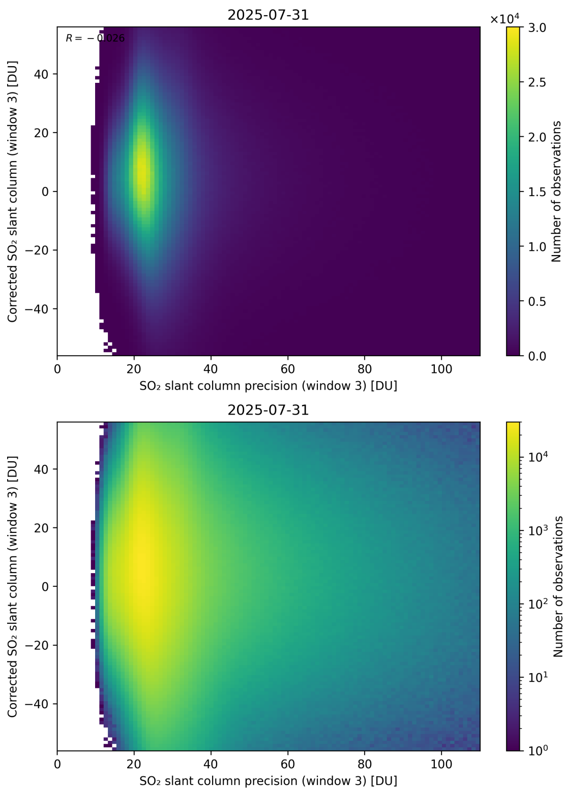
Figure 312: Scatter density plot of “SO 2 slant column precision (window 3)” against “Corrected SO 2 slant column (window 3)” for 2025-07-30 to 2025-08-01.
