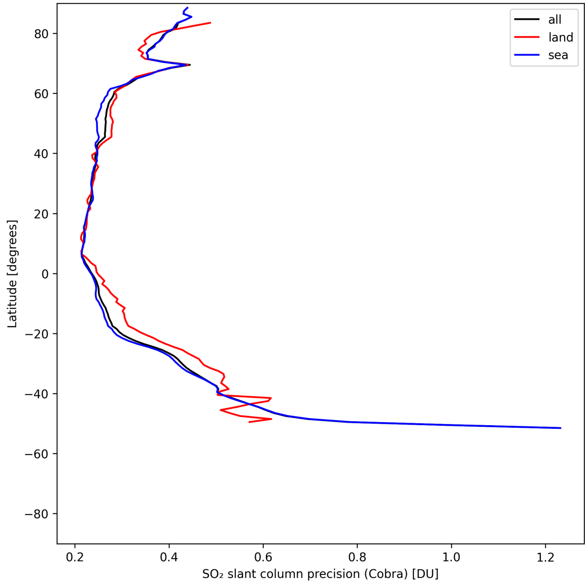
Figure 36: Zonal average of “SO 2 slant column precision (Cobra)” for 2025-07-30 to 2025-08-01.
