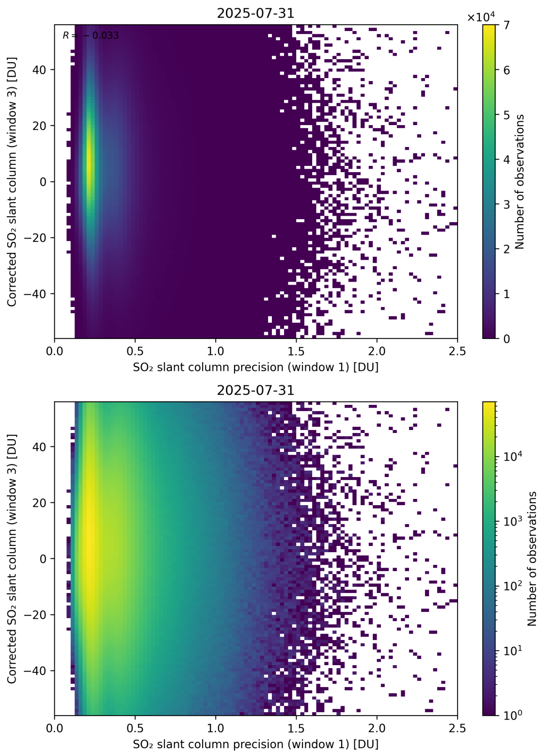
Figure 276: Scatter density plot of “SO 2 slant column precision (window 1)” against “Corrected SO 2 slant column (window 3)” for 2025-07-30 to 2025-08-01.
