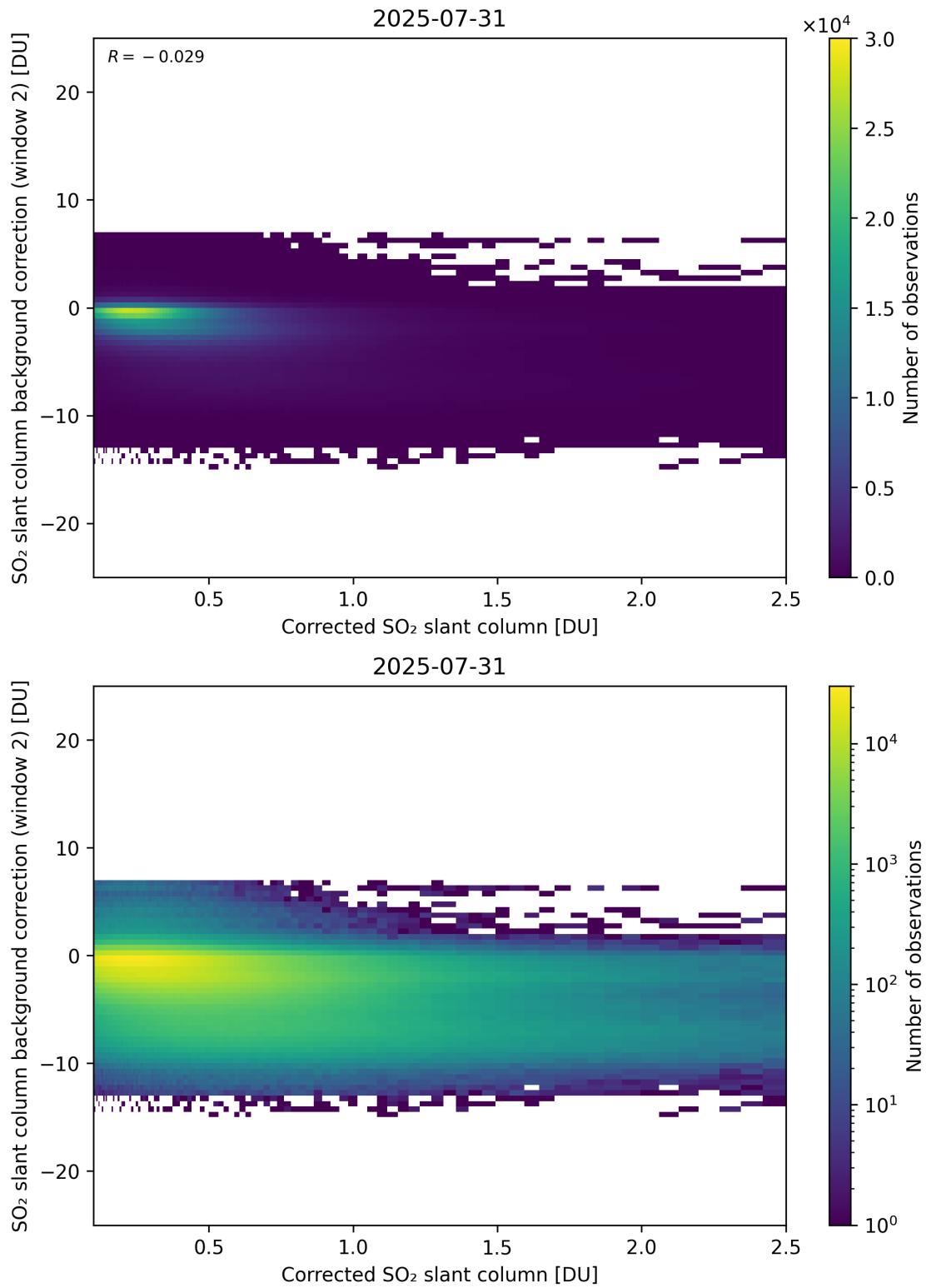
Figure 227: Scatter density plot of “Corrected SO 2 slant column” against “SO 2 slant column background correction (window 2)” for 2025-07-30 to 2025-08-01.
