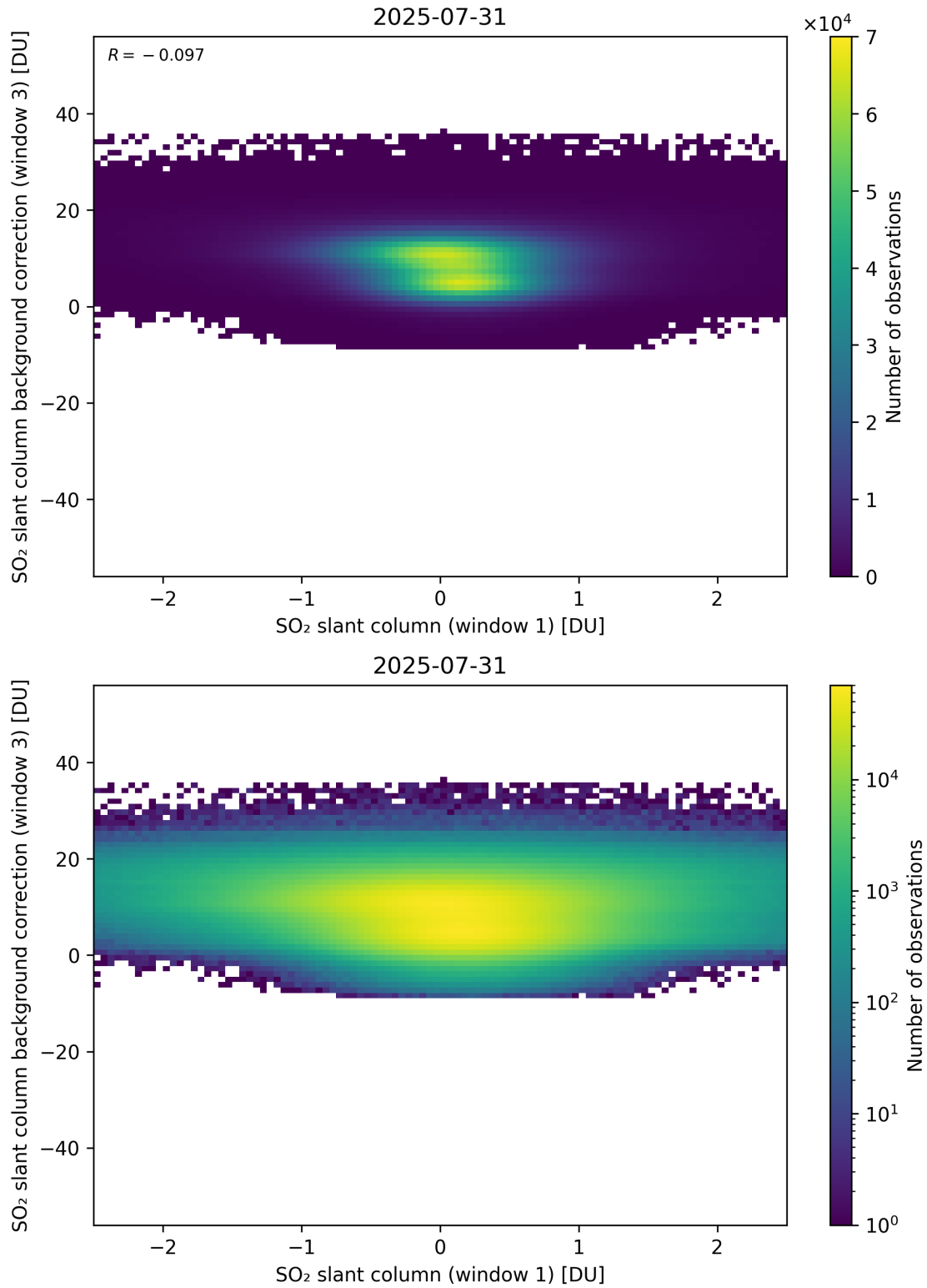
Figure 264: Scatter density plot of “SO 2 slant column (window 1)” against “SO 2 slant column background correction (window 3)” for 2025-07-30 to 2025-08-01.
