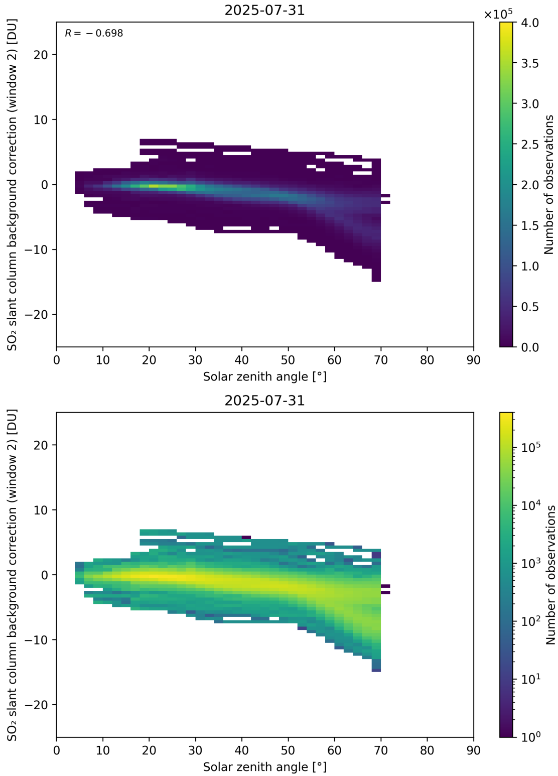
Figure 172: Scatter density plot of “Solar zenith angle” against “SO 2 slant column background correction (window 2)” for 2025-07-30 to 2025-08-01.
