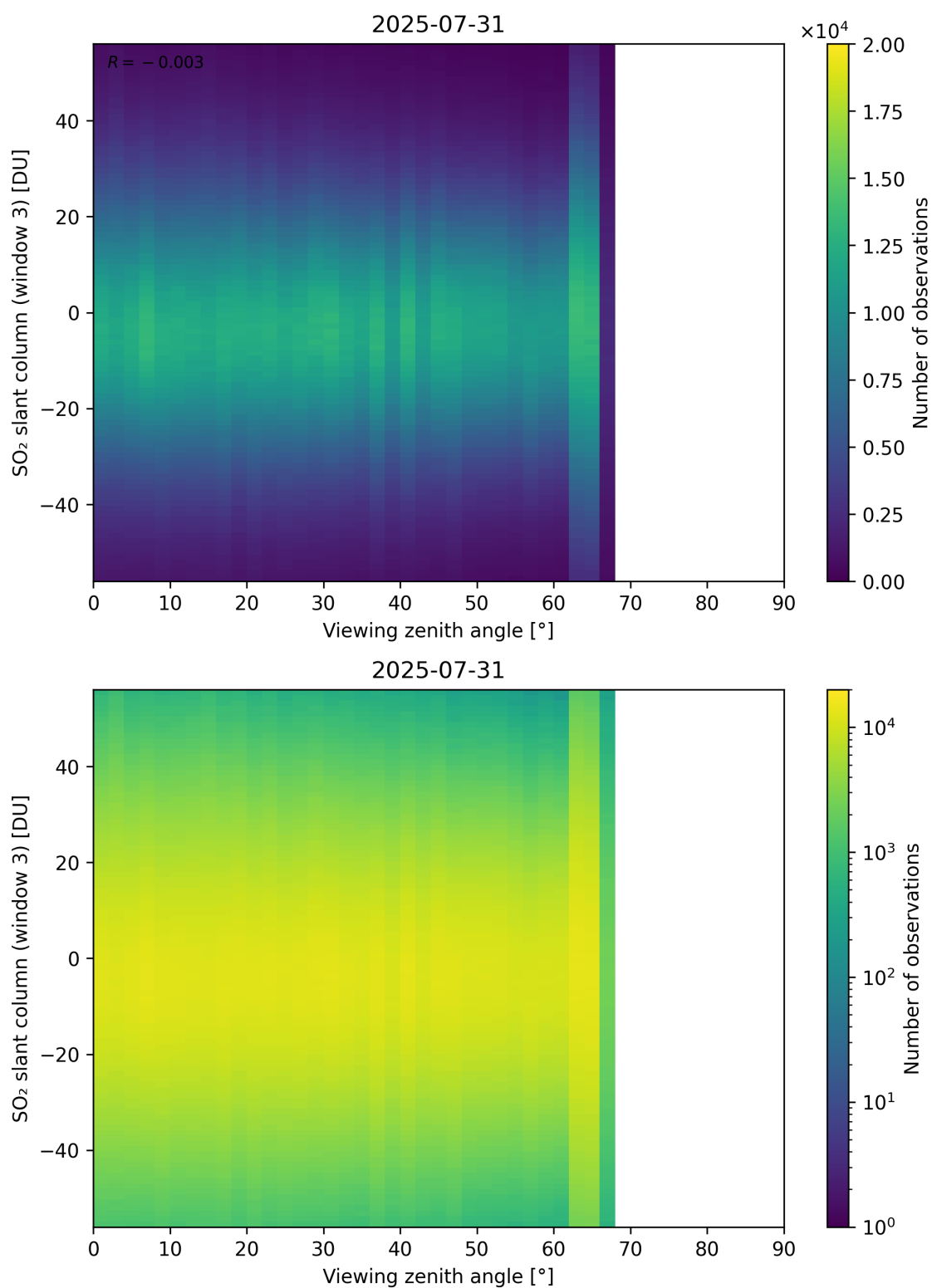
Figure 379: Scatter density plot of “Viewing zenith angle” against “SO 2 slant column (window 3)” for 2025-07-30 to 2025-08-01.
