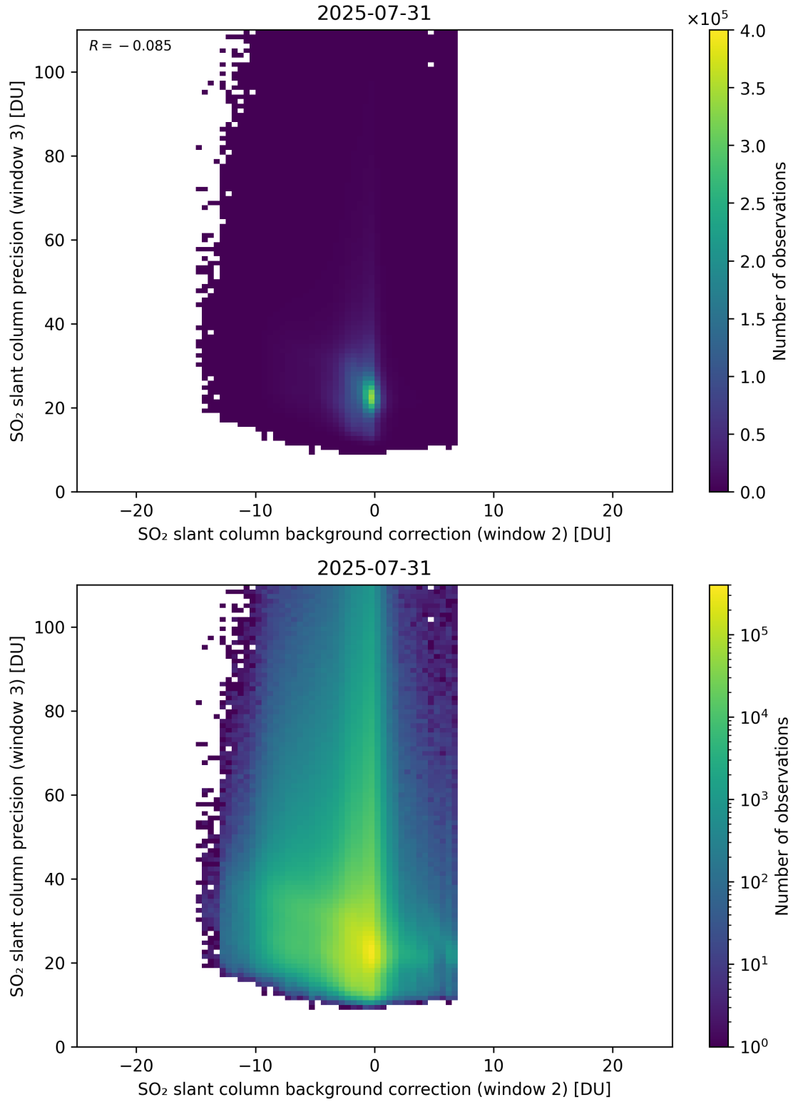
Figure 129: Scatter density plot of “SO 2 slant column background correction (window 2)” against “SO 2 slant column precision (window 3)” for 2025-07-30 to 2025-08-01.
