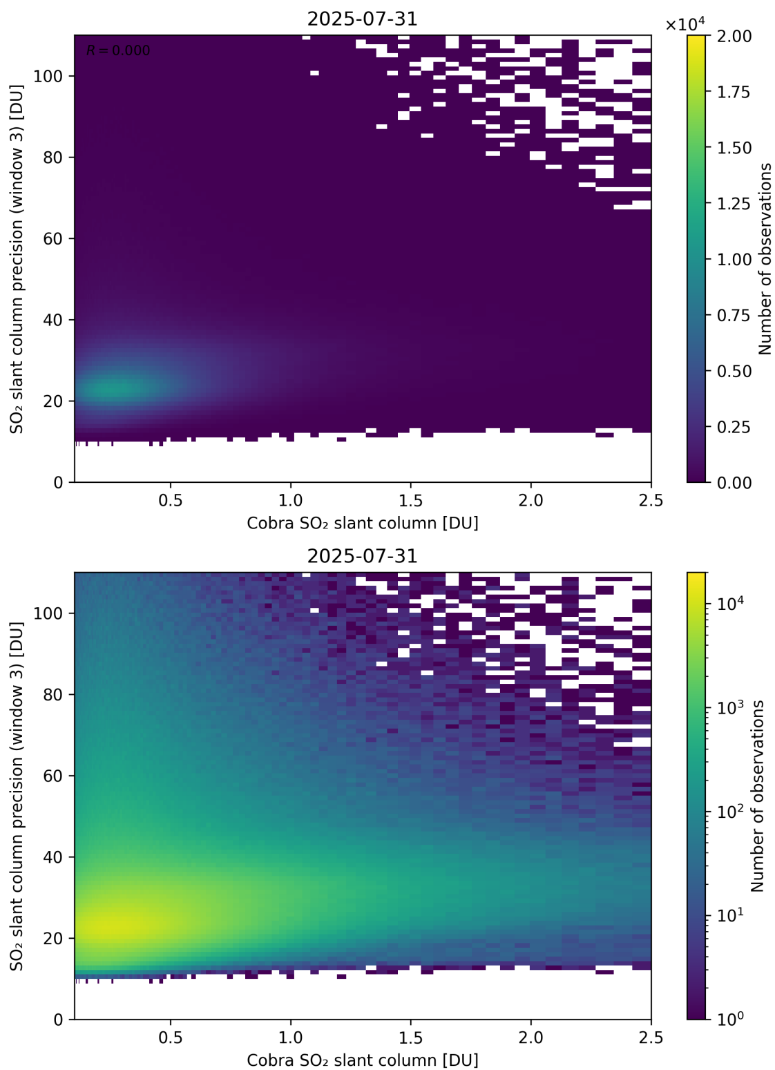
Figure 223: Scatter density plot of “Cobra SO 2 slant column” against “SO 2 slant column precision (window 3)” for 2025-07-30 to 2025-08-01.
