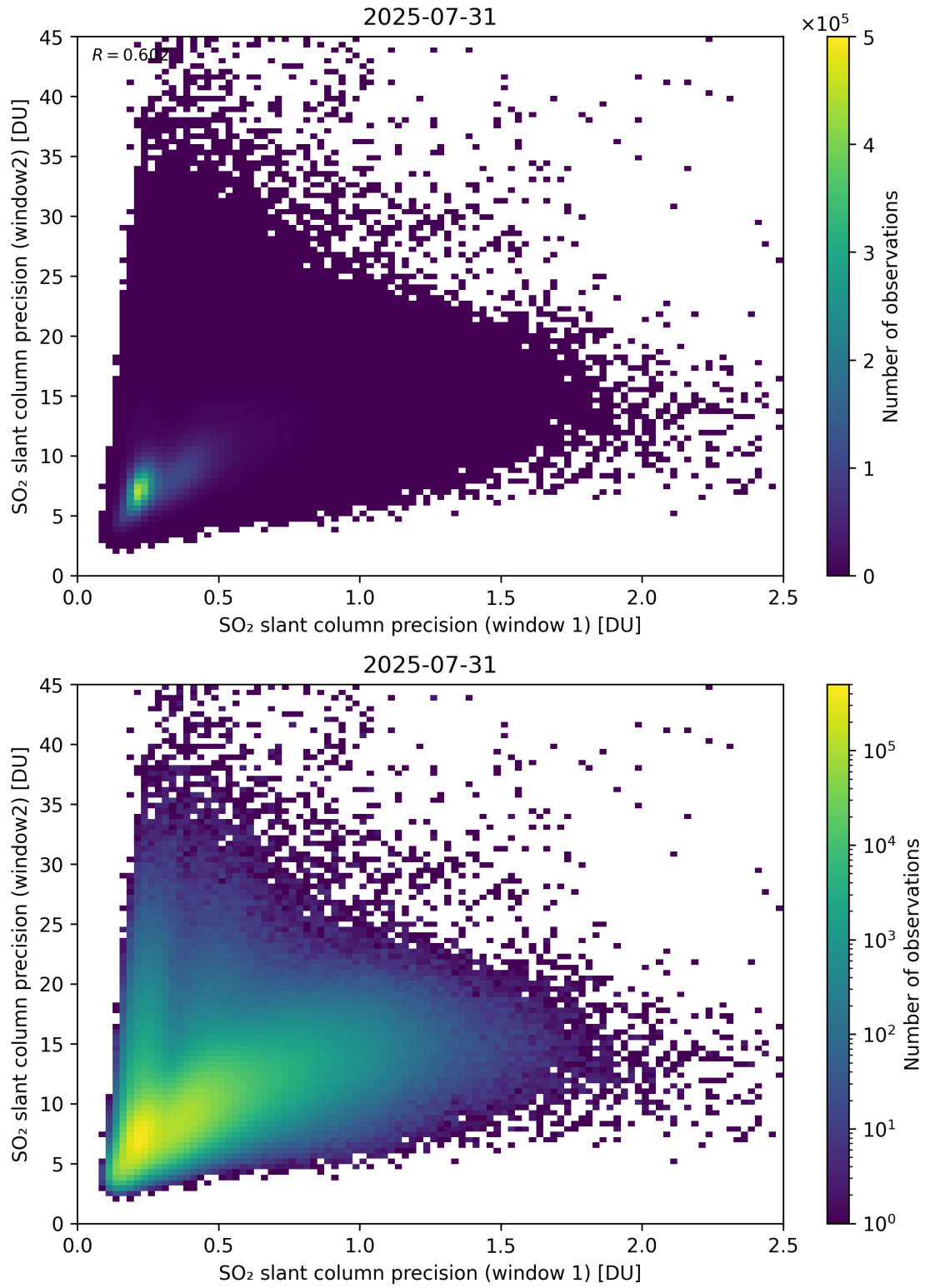
Figure 277: Scatter density plot of “SO 2 slant column precision (window 1)” against “SO 2 slant column precision (window2)” for 2025-07-30 to 2025-08-01.
