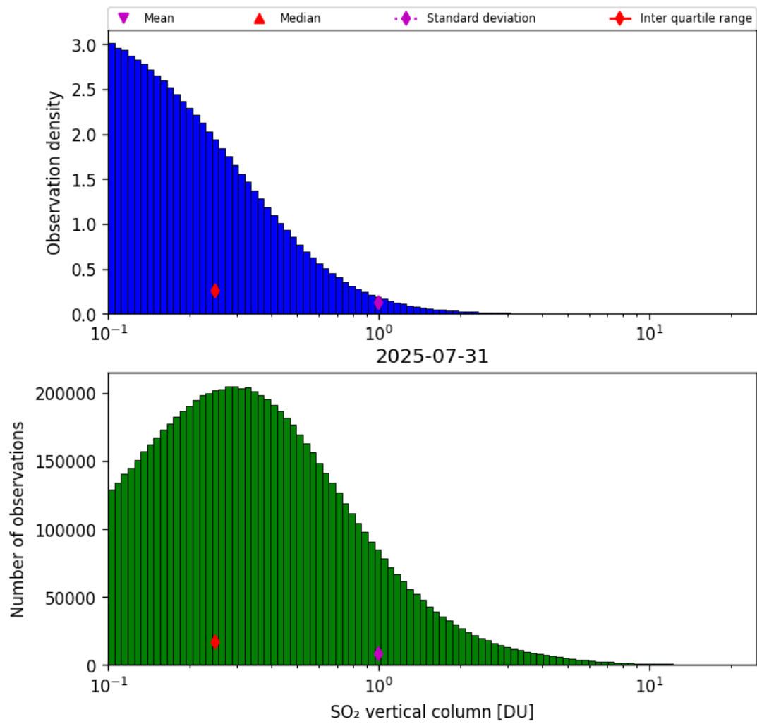
Figure 58: Histogram of “SO 2 vertical column” for 2025-07-30 to 2025-08-01
