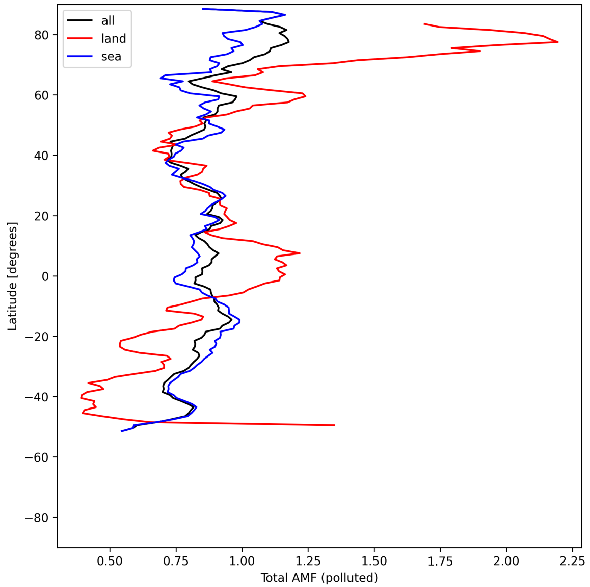
Figure 53: Zonal average of “Total AMF (polluted)” for 2025-07-30 to 2025-08-01.
