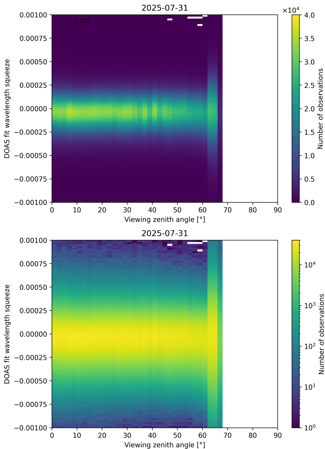
Figure 366: Scatter density plot of “Viewing zenith angle” against “DOAS fit wavelength squeeze” for 2025-07-30 to 2025-08-01.
