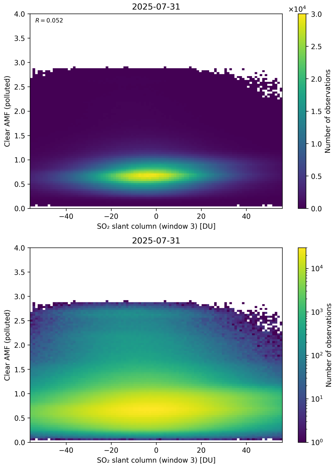
Figure 315: Scatter density plot of “SO 2 slant column (window 3)” against “Clear AMF (polluted)” for 2025-07-30 to 2025-08-01.
