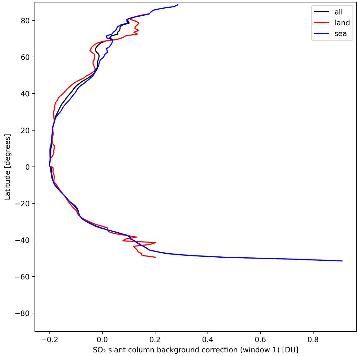
Figure 40: Zonal average of “SO 2 slant column background correction (window 1)” for 2025-07-30 to 2025-08-01.
