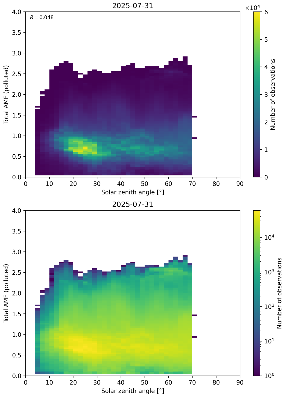
Figure 189: Scatter density plot of “Solar zenith angle” against “Total AMF (polluted)” for 2025-07-30 to 2025-08-01.
