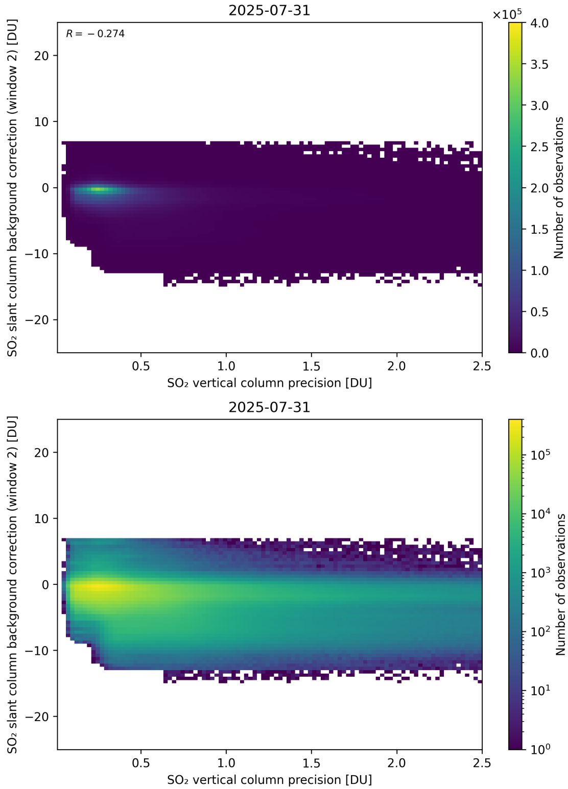
Figure 330: Scatter density plot of “SO 2 vertical column precision” against “SO 2 slant column background correction (window 2)” for 2025-07-30 to 2025-08-01.
