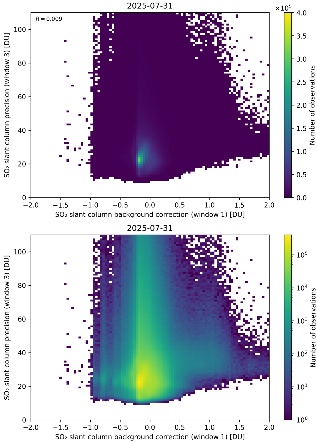
Figure 119: Scatter density plot of “SO 2 slant column background correction (window 1)” against “SO 2 slant column precision (window 3)” for 2025-07-30 to 2025-08-01.
