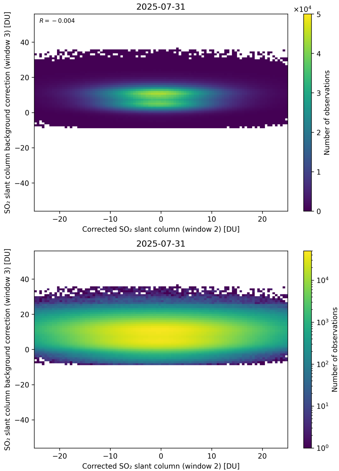
Figure 245: Scatter density plot of “Corrected SO 2 slant column (window 2)” against “SO 2 slant column background correction (window 3)” for 2025-07-30 to 2025-08-01.
