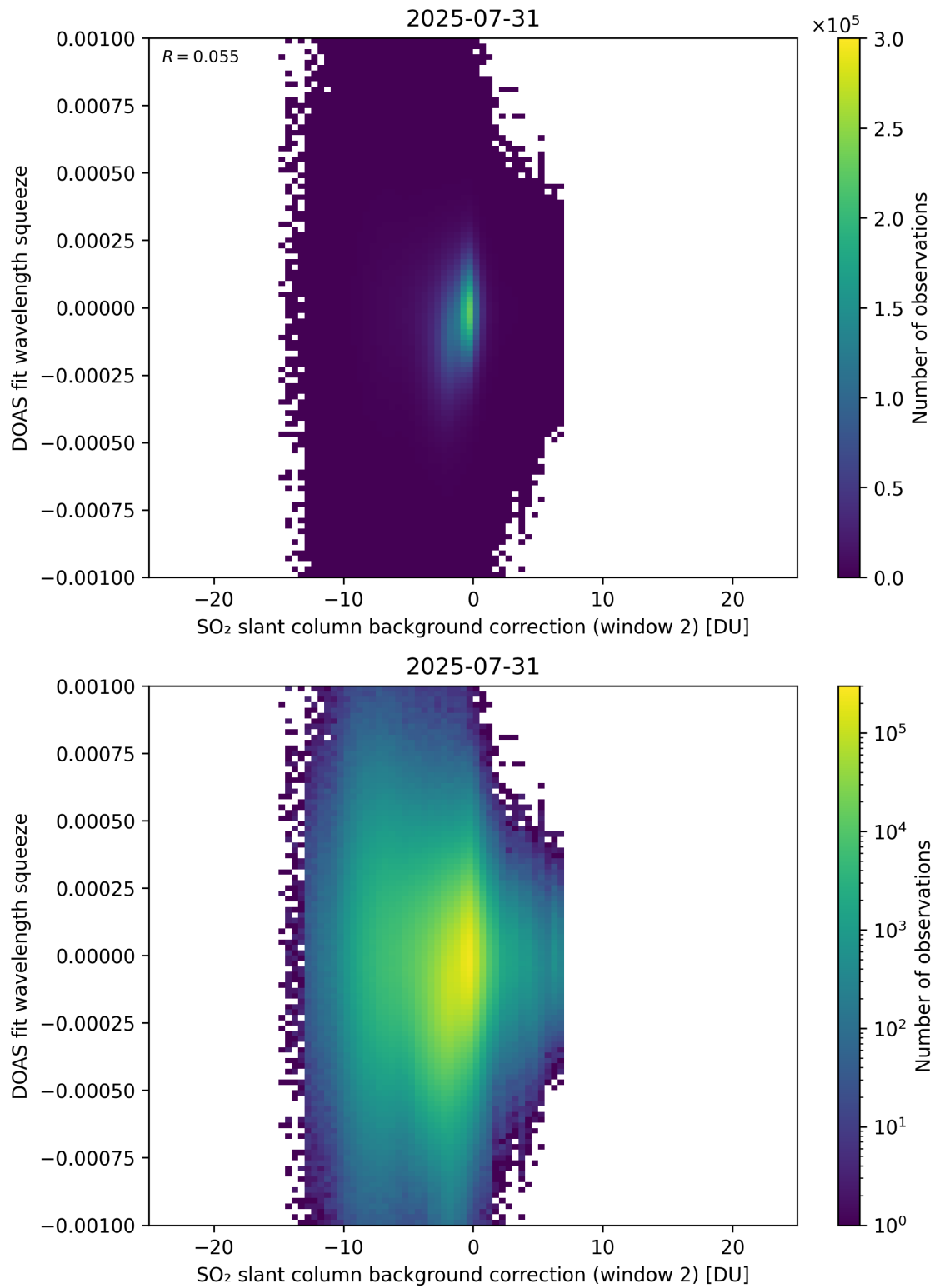
Figure 124: Scatter density plot of “SO 2 slant column background correction (window 2)” against “DOAS fit wavelength squeeze” for 2025-07-30 to 2025-08-01.
