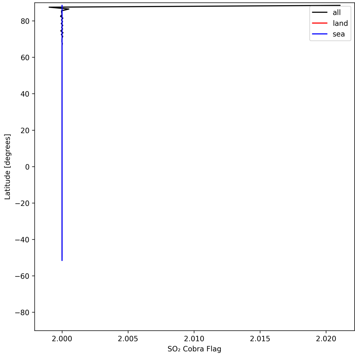
Figure 49: Zonal average of “SO 2 Cobra Flag” for 2025-07-30 to 2025-08-01.
