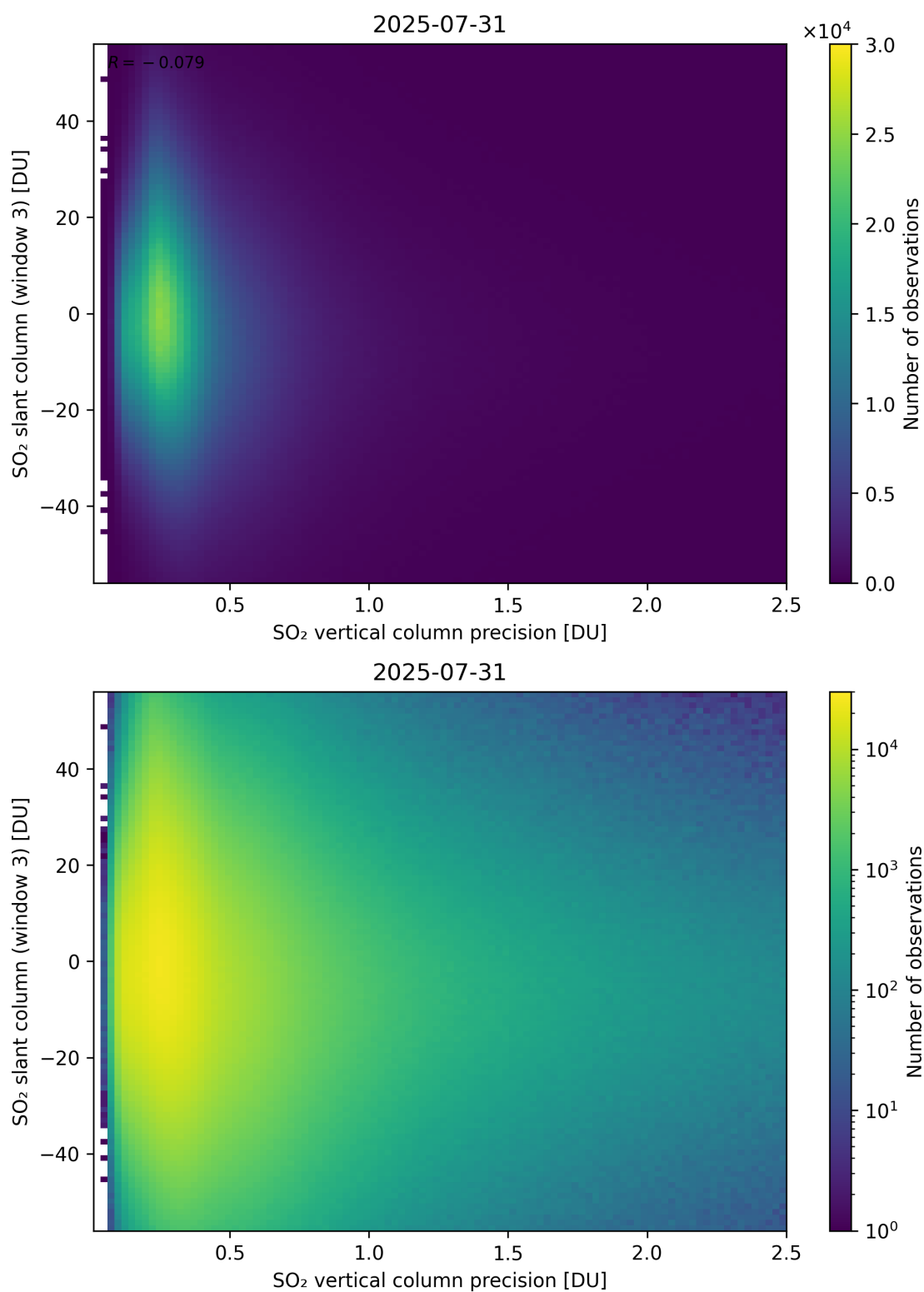
Figure 344: Scatter density plot of “SO 2 vertical column precision” against “SO 2 slant column (window 3)” for 2025-07-30 to 2025-08-01.
