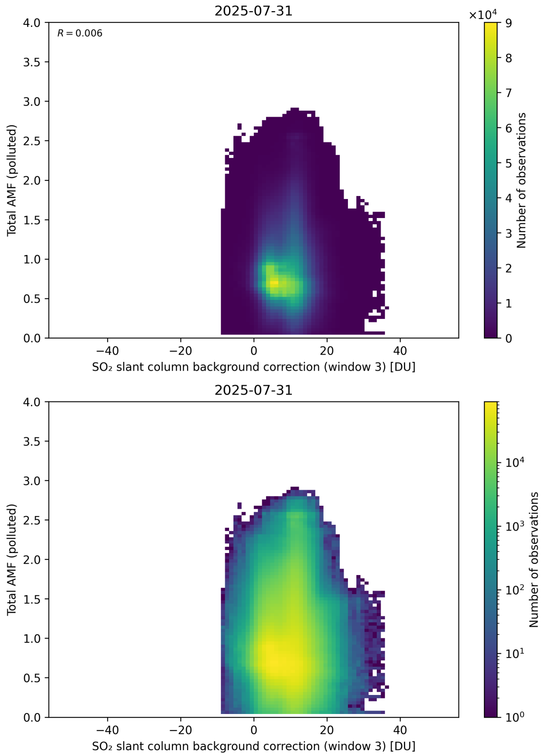
Figure 136: Scatter density plot of “SO 2 slant column background correction (window 3)” against “Total AMF (polluted)” for 2025-07-30 to 2025-08-01.
