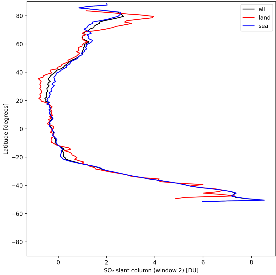
Figure 41: Zonal average of “SO 2 slant column (window 2)” for 2025-07-30 to 2025-08-01.
