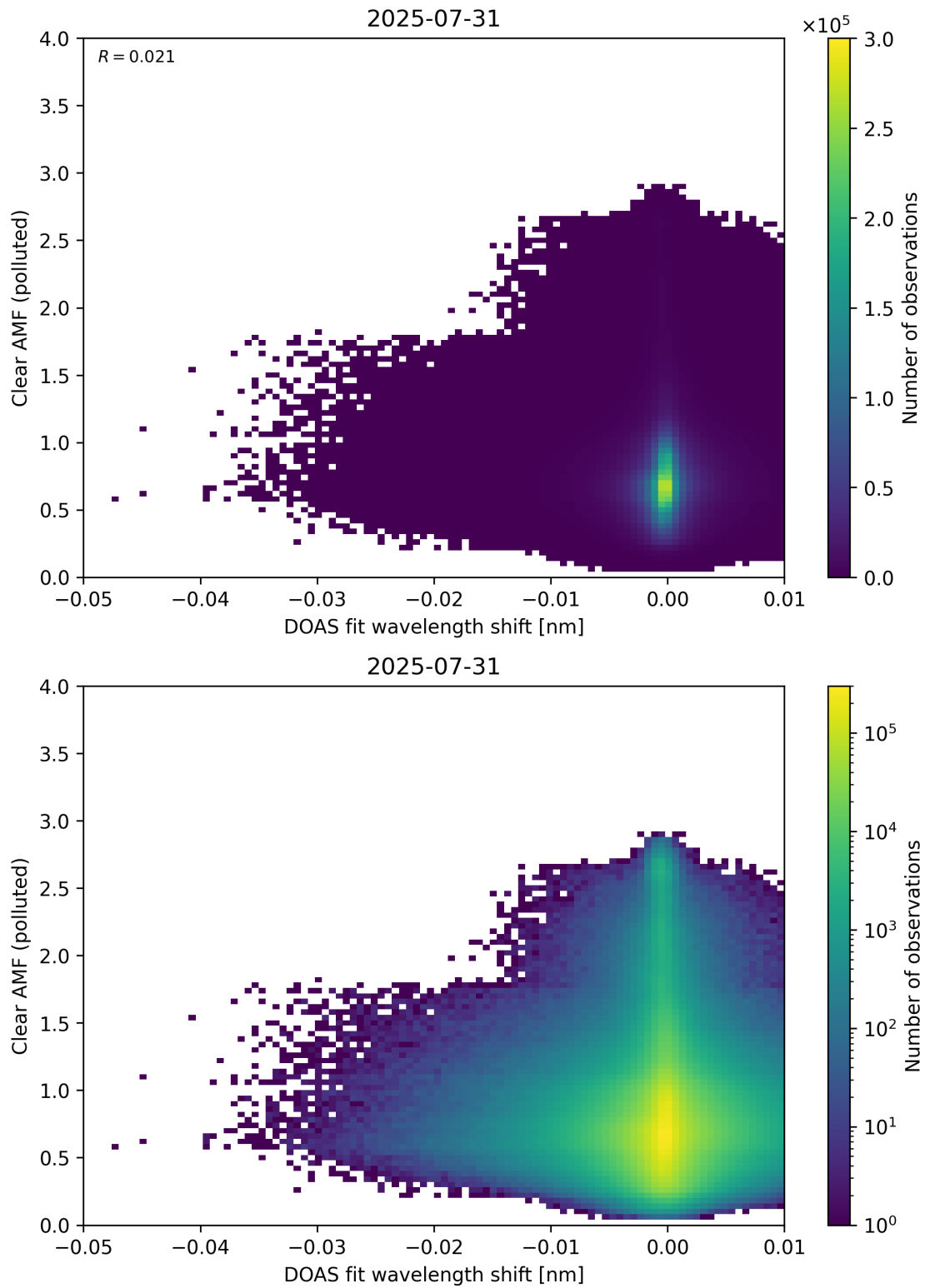
Figure 140: Scatter density plot of “DOAS fit wavelength shift” against “Clear AMF (polluted)” for 2025-07-30 to 2025-08-01.
