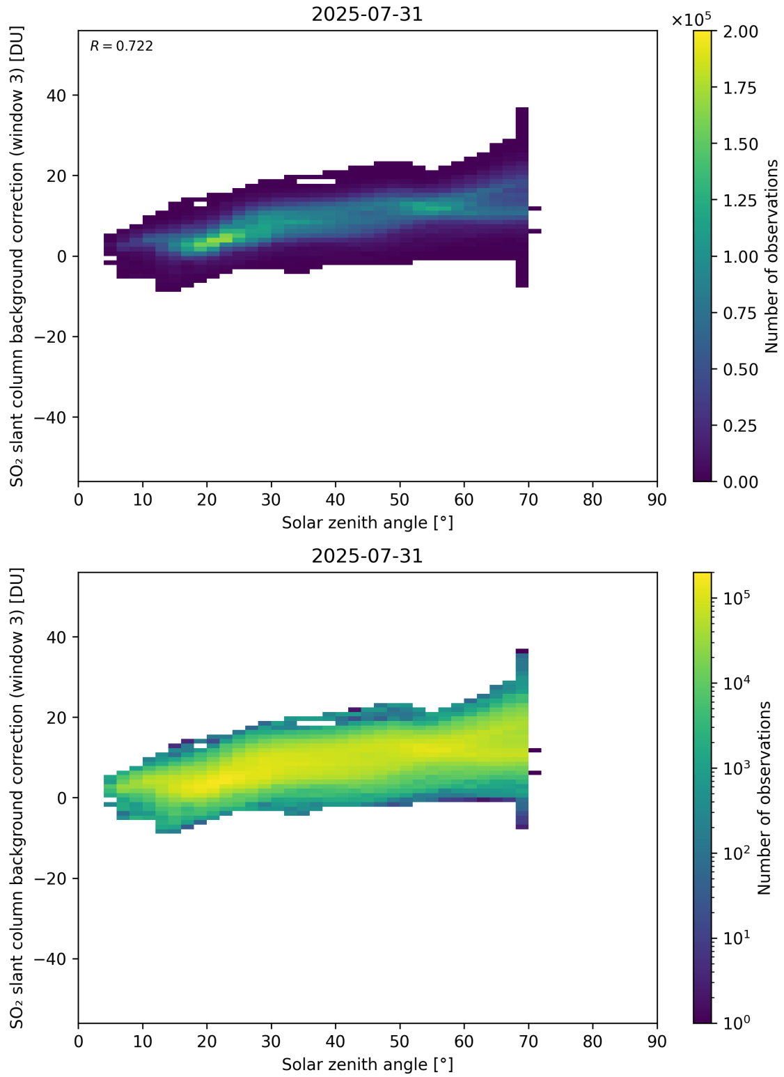
Figure 173: Scatter density plot of “Solar zenith angle” against “SO 2 slant column background correction (window 3)” for 2025-07-30 to 2025-08-01.
