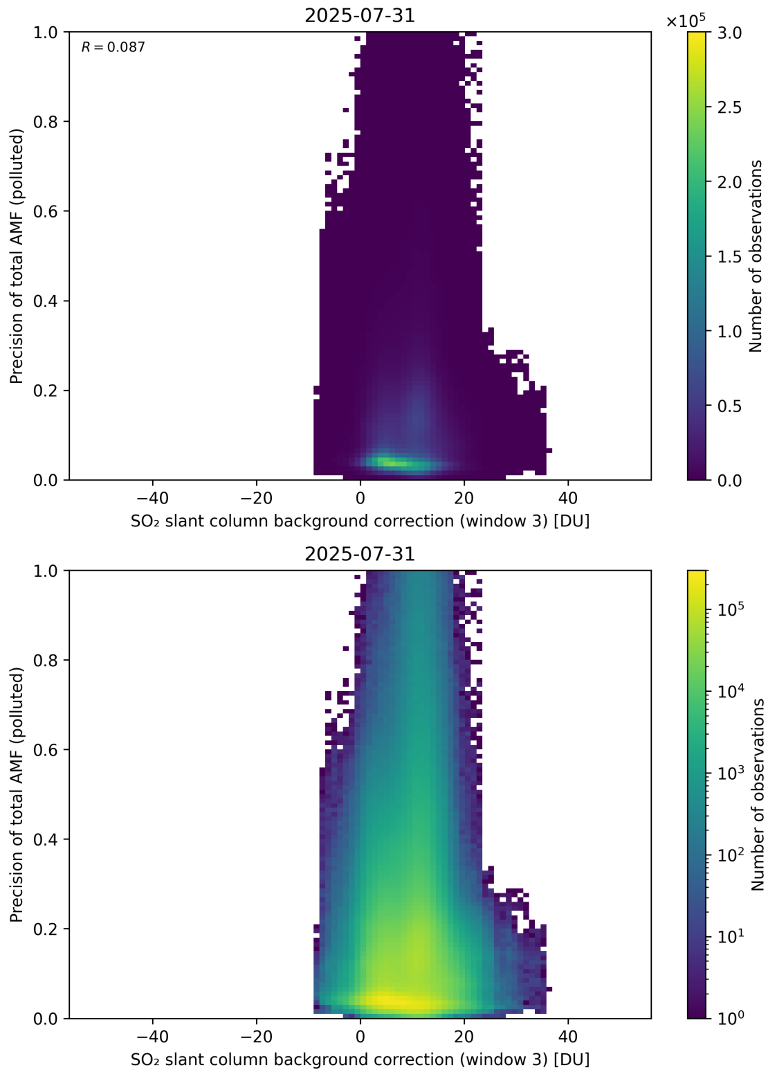
Figure 137: Scatter density plot of “SO 2 slant column background correction (window 3)” against “Precision of total AMF (polluted)” for 2025-07-30 to 2025-08-01.
