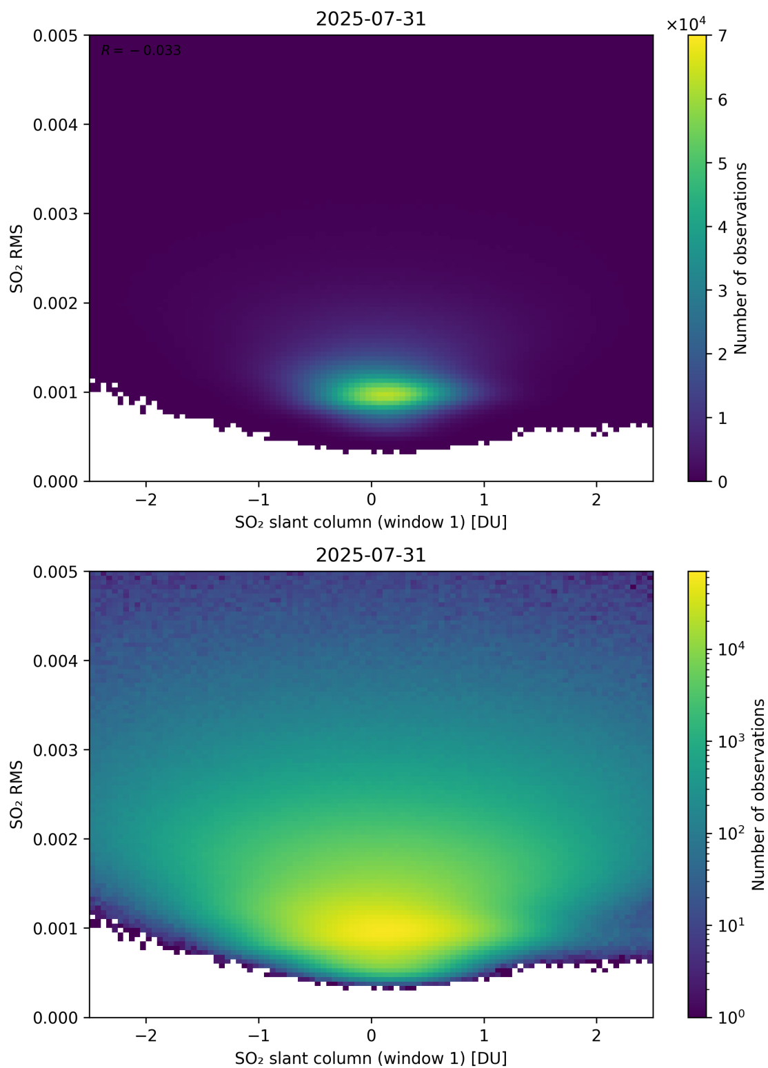
Figure 267: Scatter density plot of “SO 2 slant column (window 1)” against “SO 2 RMS” for 2025-07-30 to 2025-08-01.
