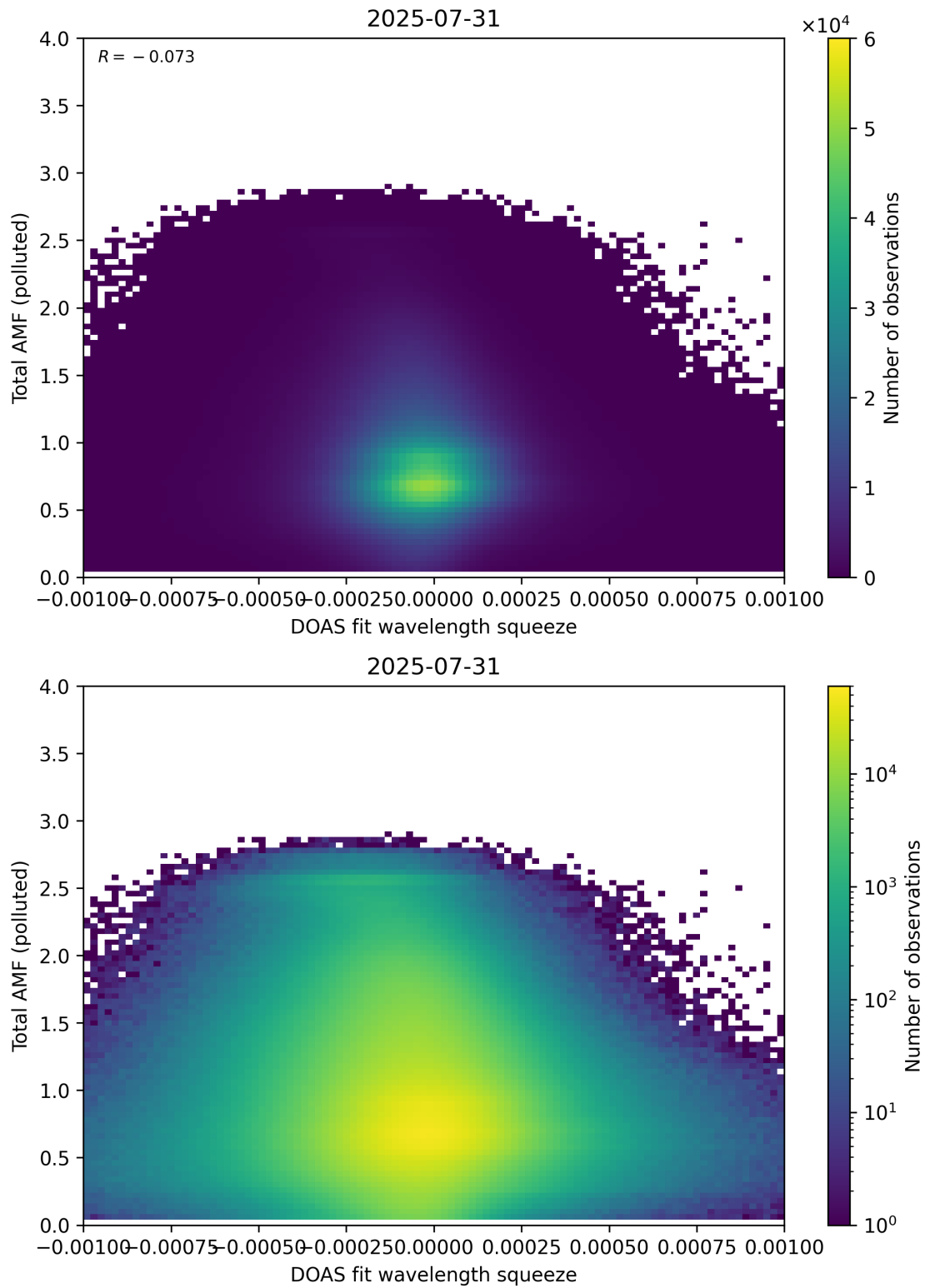
Figure 145: Scatter density plot of “DOAS fit wavelength squeeze” against “Total AMF (polluted)” for 2025-07-30 to 2025-08-01.
