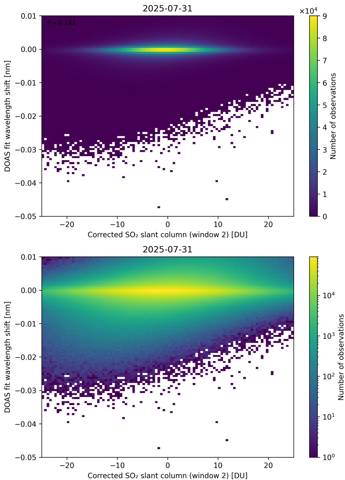
Figure 246: Scatter density plot of “Corrected SO 2 slant column (window 2)” against “DOAS fit wavelength shift” for 2025-07-30 to 2025-08-01.
