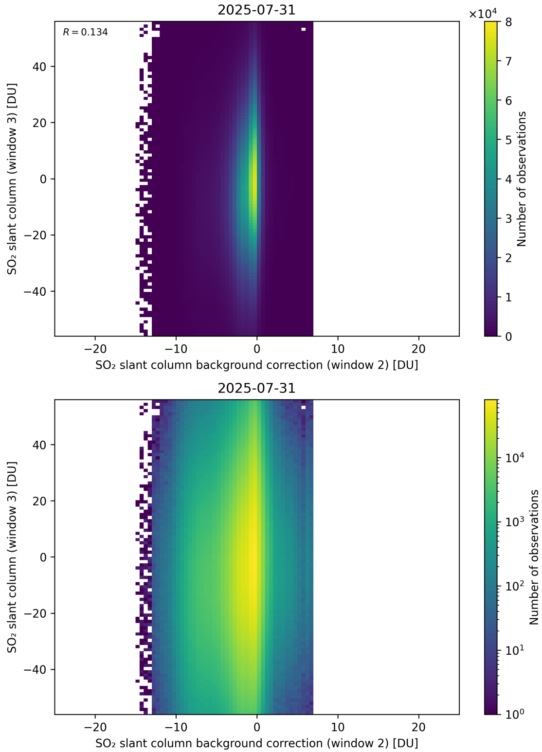
Figure 128: Scatter density plot of “SO 2 slant column background correction (window 2)” against “SO 2 slant column (window 3)” for 2025-07-30 to 2025-08-01.
