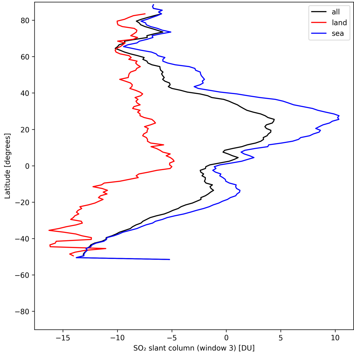
Figure 45: Zonal average of “SO 2 slant column (window 3)” for 2025-07-30 to 2025-08-01.
