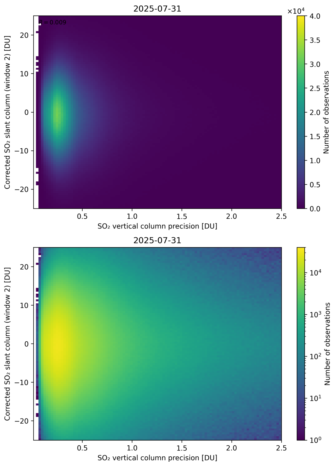
Figure 339: Scatter density plot of “SO 2 vertical column precision” against “Corrected SO 2 slant column (window 2)” for 2025-07-30 to 2025-08-01.
