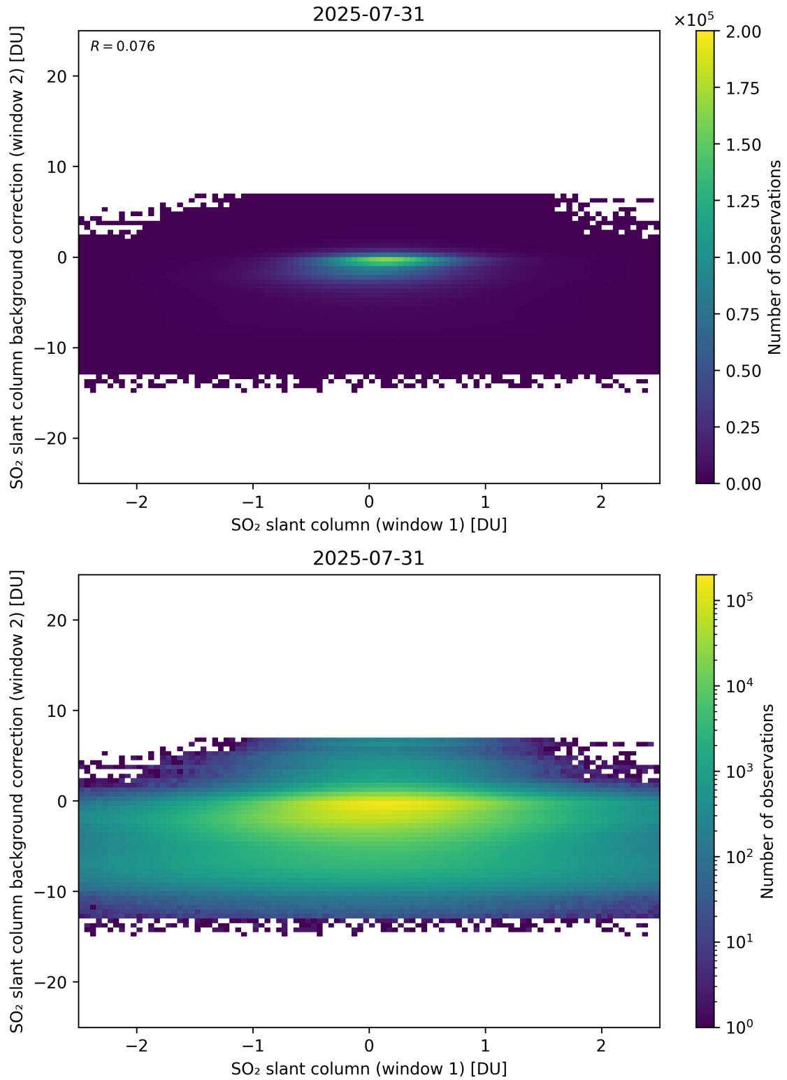
Figure 263: Scatter density plot of “SO 2 slant column (window 1)” against “SO 2 slant column background correction (window 2)” for 2025-07-30 to 2025-08-01.
