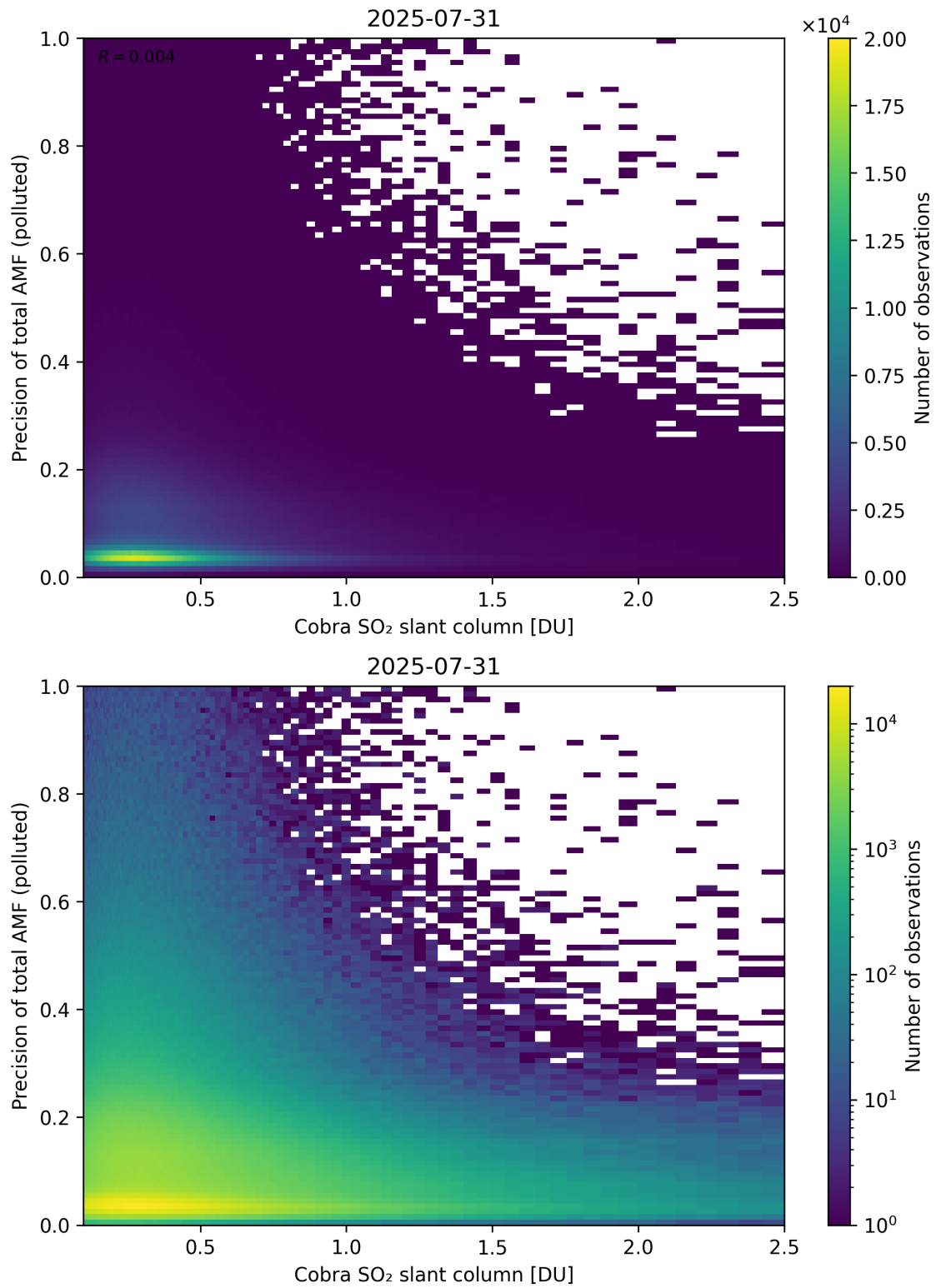
Figure 225: Scatter density plot of “Cobra SO 2 slant column” against “Precision of total AMF (polluted)” for 2025-07-30 to 2025-08-01.
