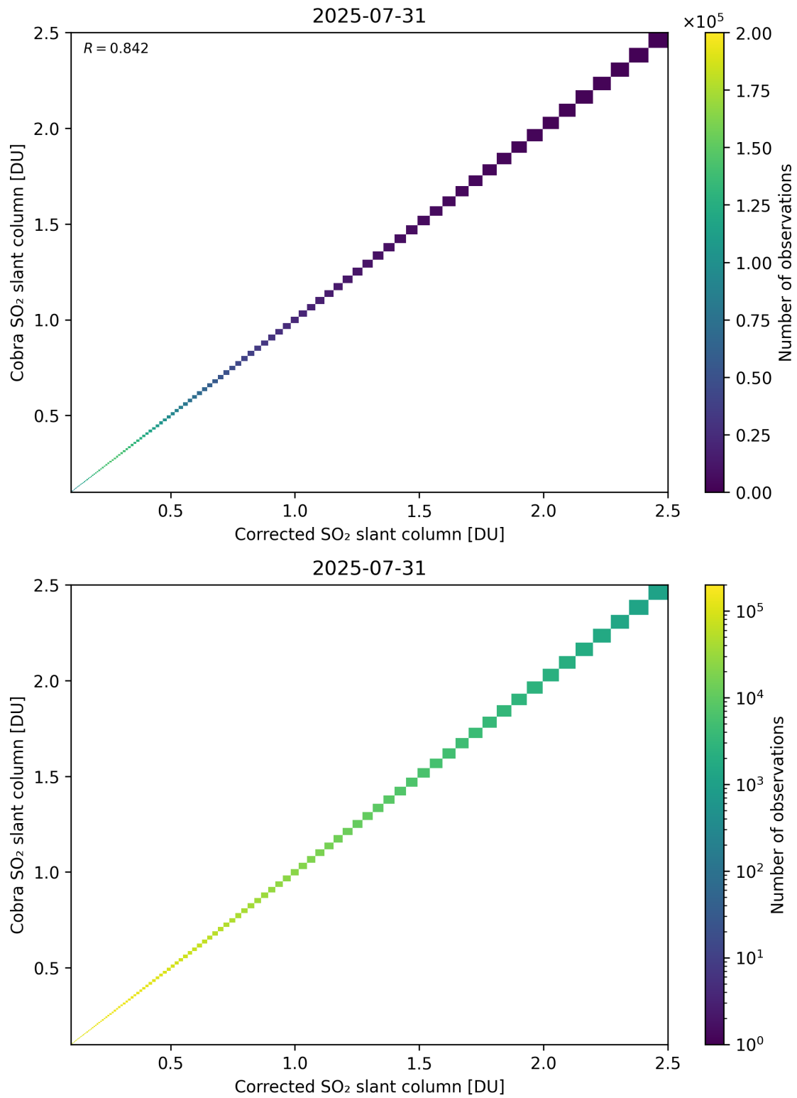
Figure 233: Scatter density plot of “Corrected SO 2 slant column” against “Cobra SO 2 slant column” for 2025-07-30 to 2025-08-01.
