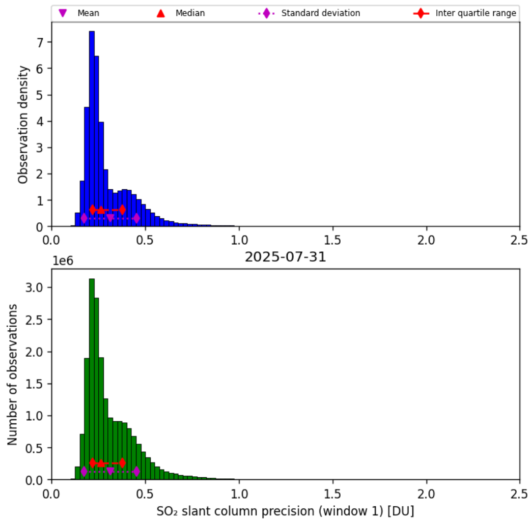
Figure 64: Histogram of “SO 2 slant column precision (window 1)” for 2025-07-30 to 2025-08-01
