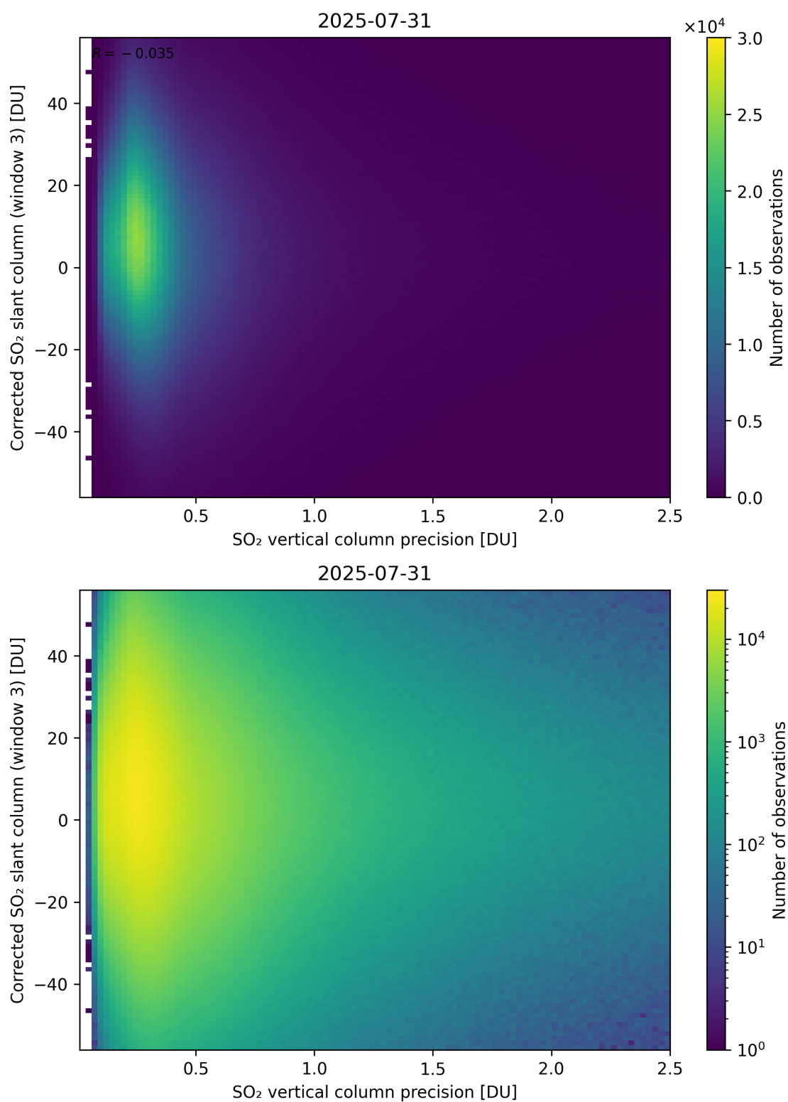
Figure 340: Scatter density plot of “SO 2 vertical column precision” against “Corrected SO 2 slant column (window 3)” for 2025-07-30 to 2025-08-01.
