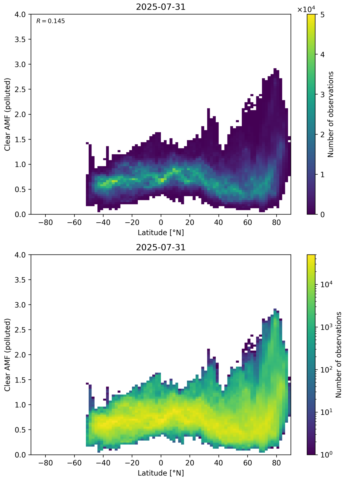
Figure 156: Scatter density plot of “Latitude” against “Clear AMF (polluted)” for 2025-07-30 to 2025-08-01.
