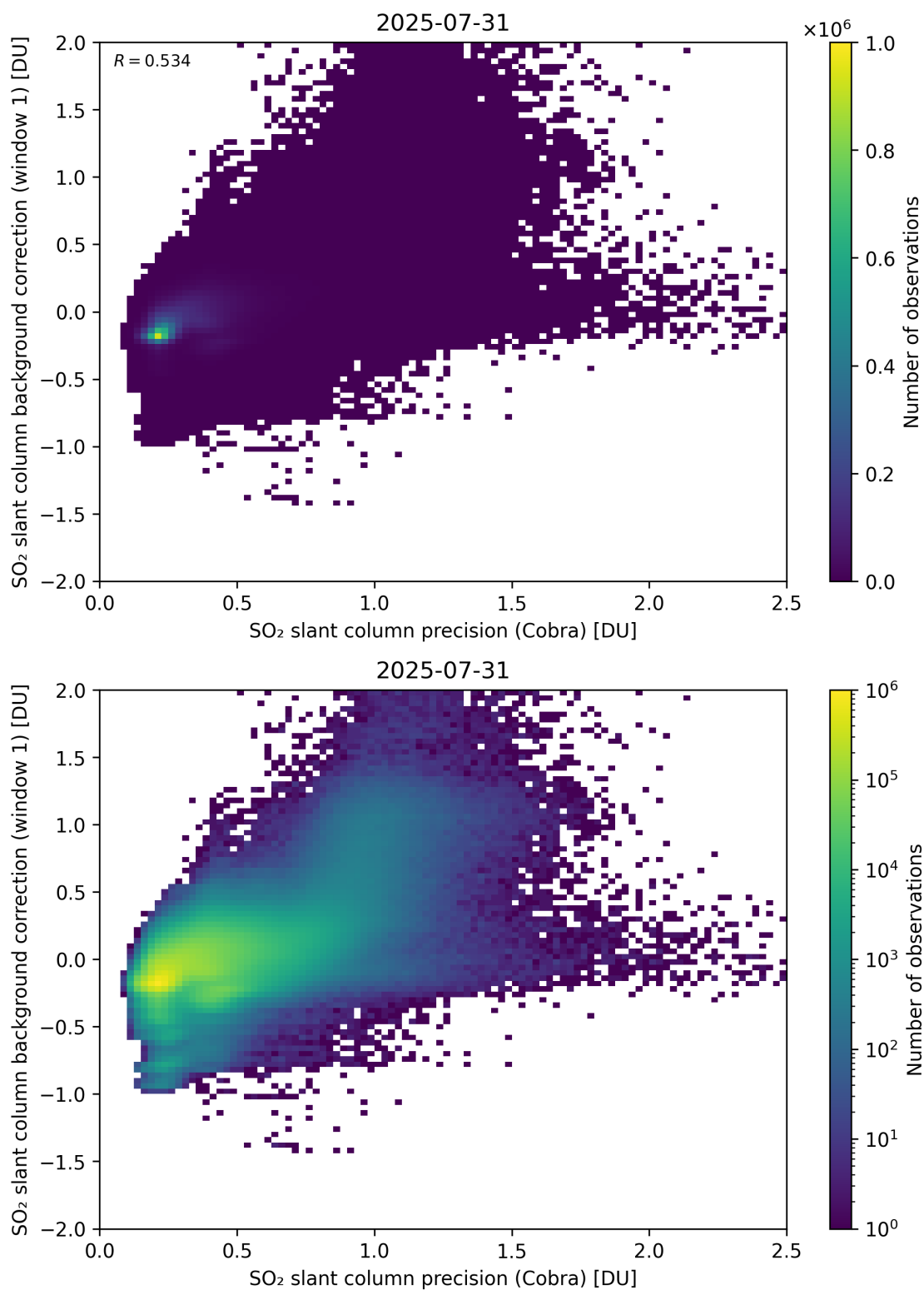
Figure 199: Scatter density plot of “SO 2 slant column precision (Cobra)” against “SO 2 slant column background correction (window 1)” for 2025-07-30 to 2025-08-01.
