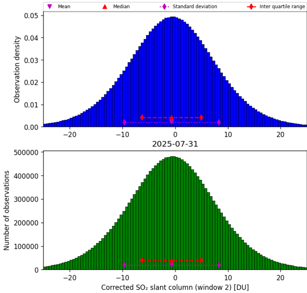
Figure 69: Histogram of “Corrected SO 2 slant column (window 2)” for 2025-07-30 to 2025-08-01
