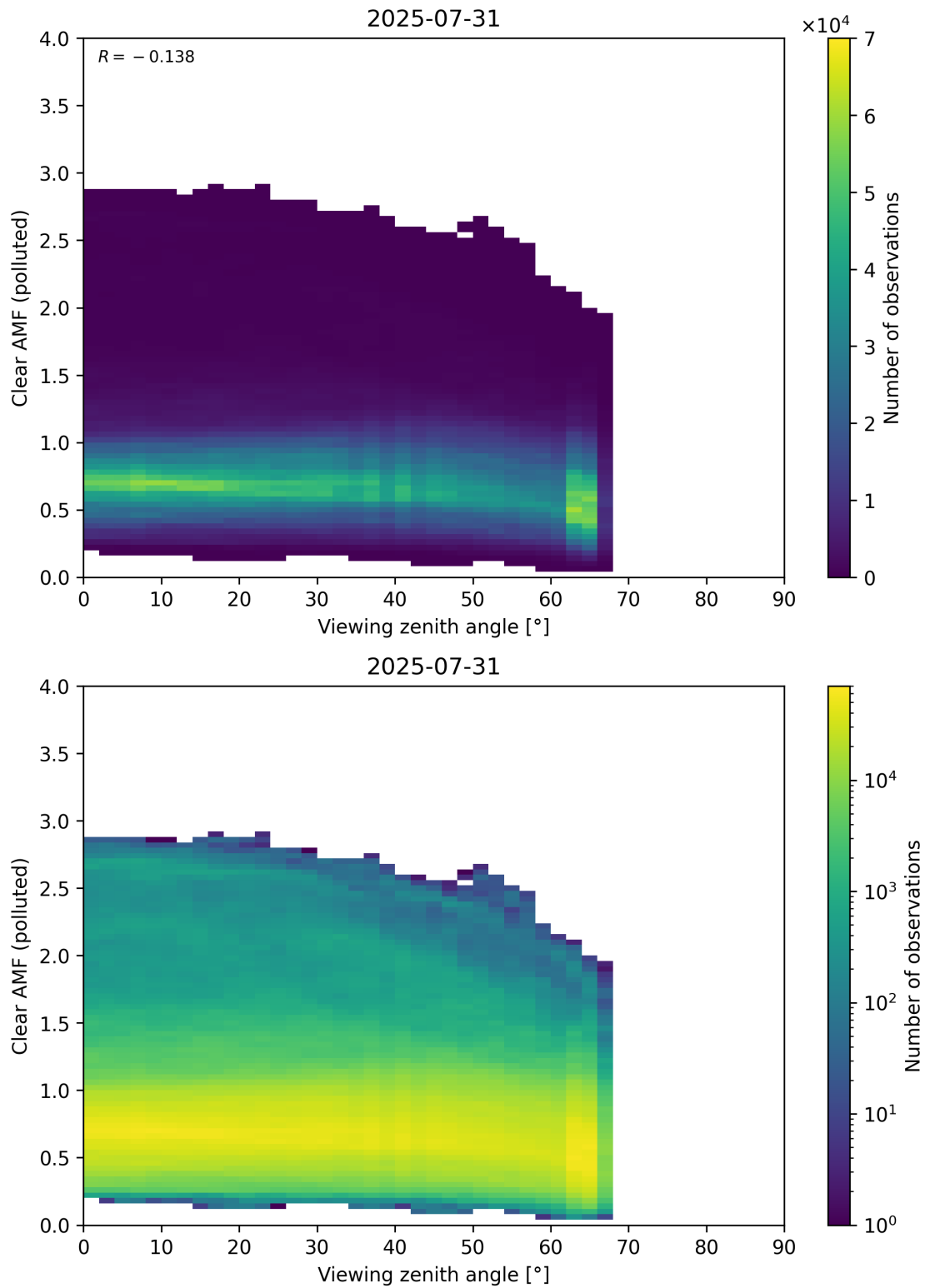
Figure 370: Scatter density plot of “Viewing zenith angle” against “Clear AMF (polluted)” for 2025-07-30 to 2025-08-01.
