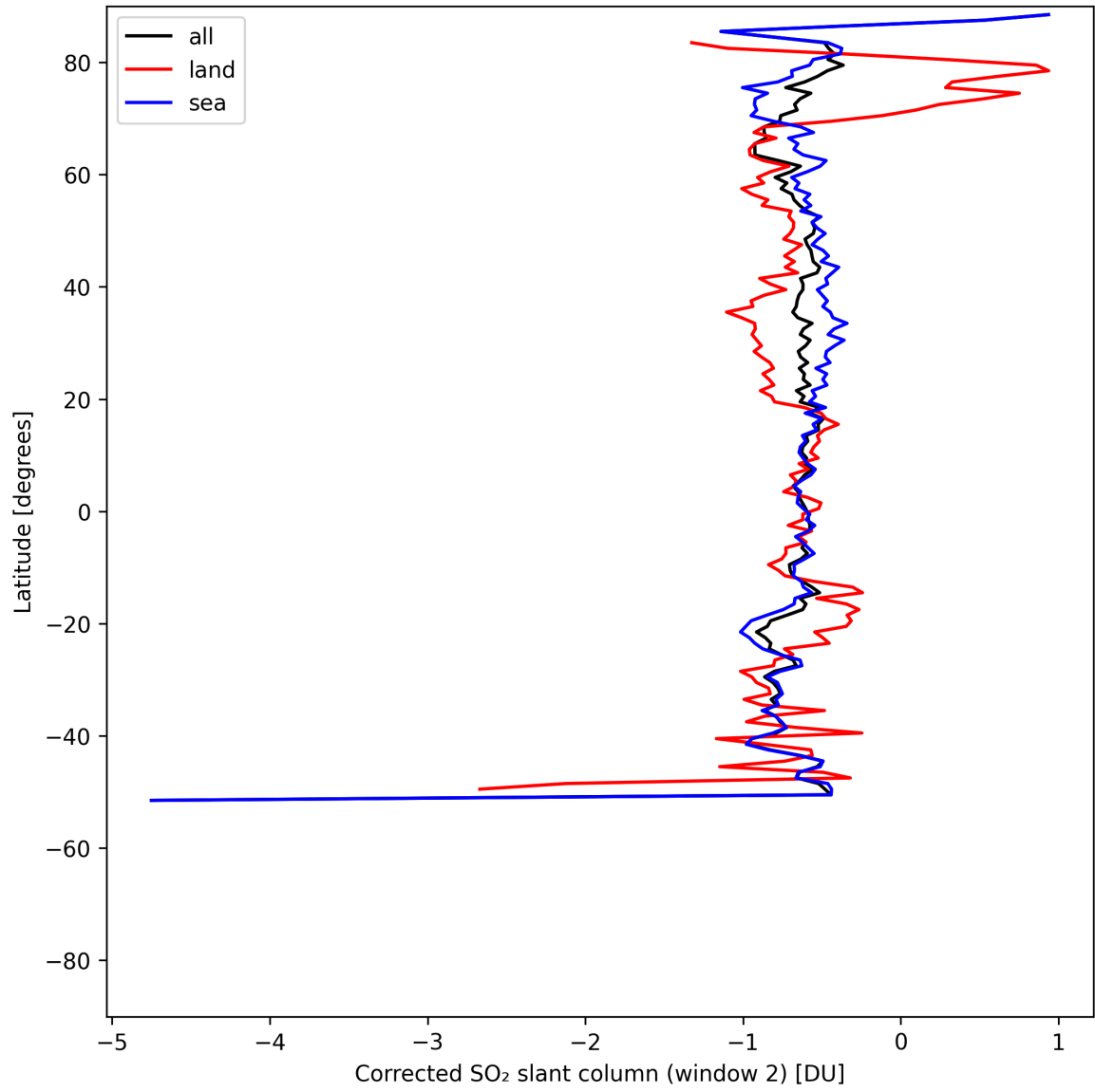
Figure 43: Zonal average of “Corrected SO 2 slant column (window 2)” for 2025-07-30 to 2025-08-01.
