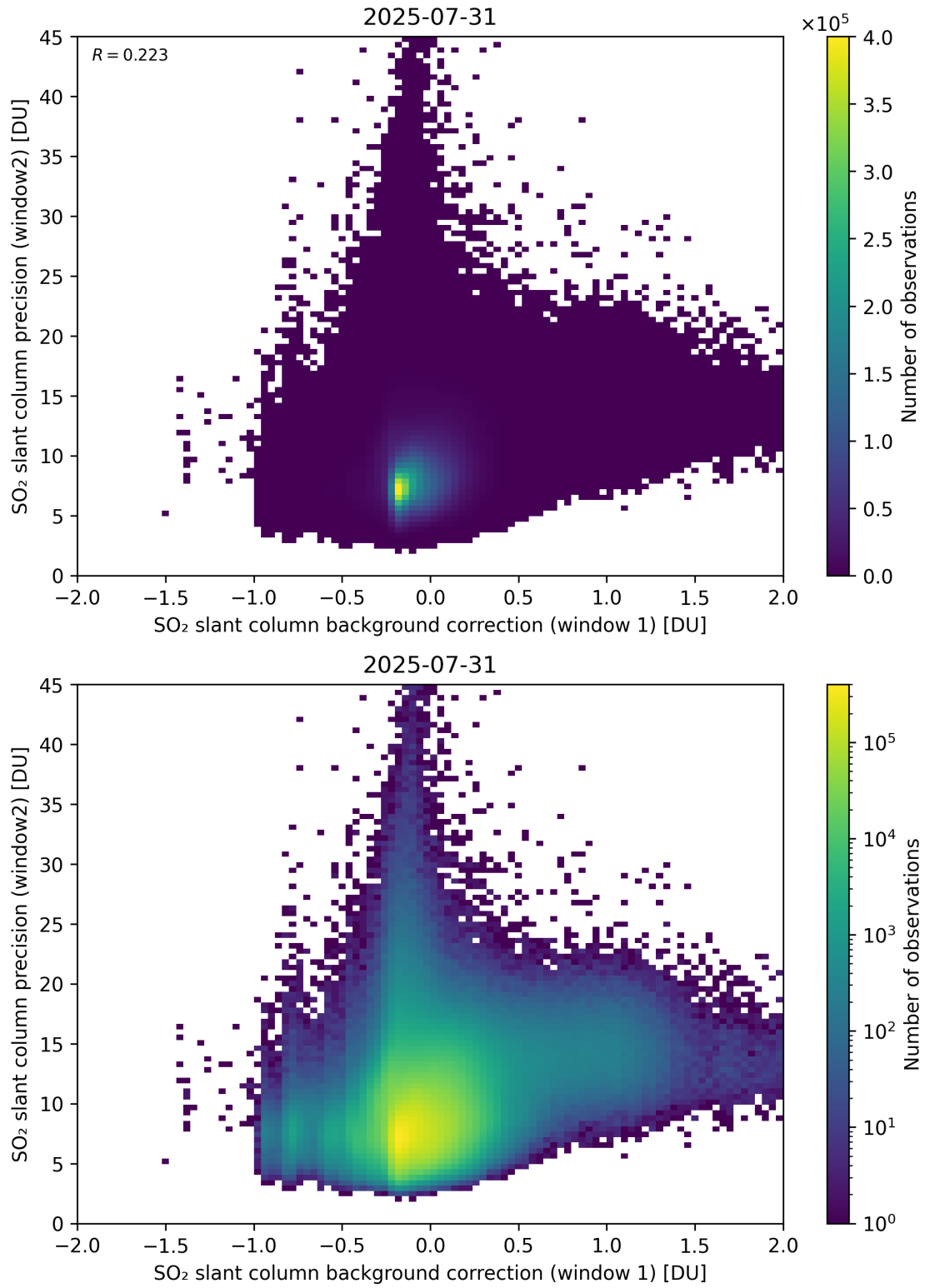
Figure 117: Scatter density plot of “SO 2 slant column background correction (window 1)” against “SO 2 slant column precision (window2)” for 2025-07-30 to 2025-08-01.
