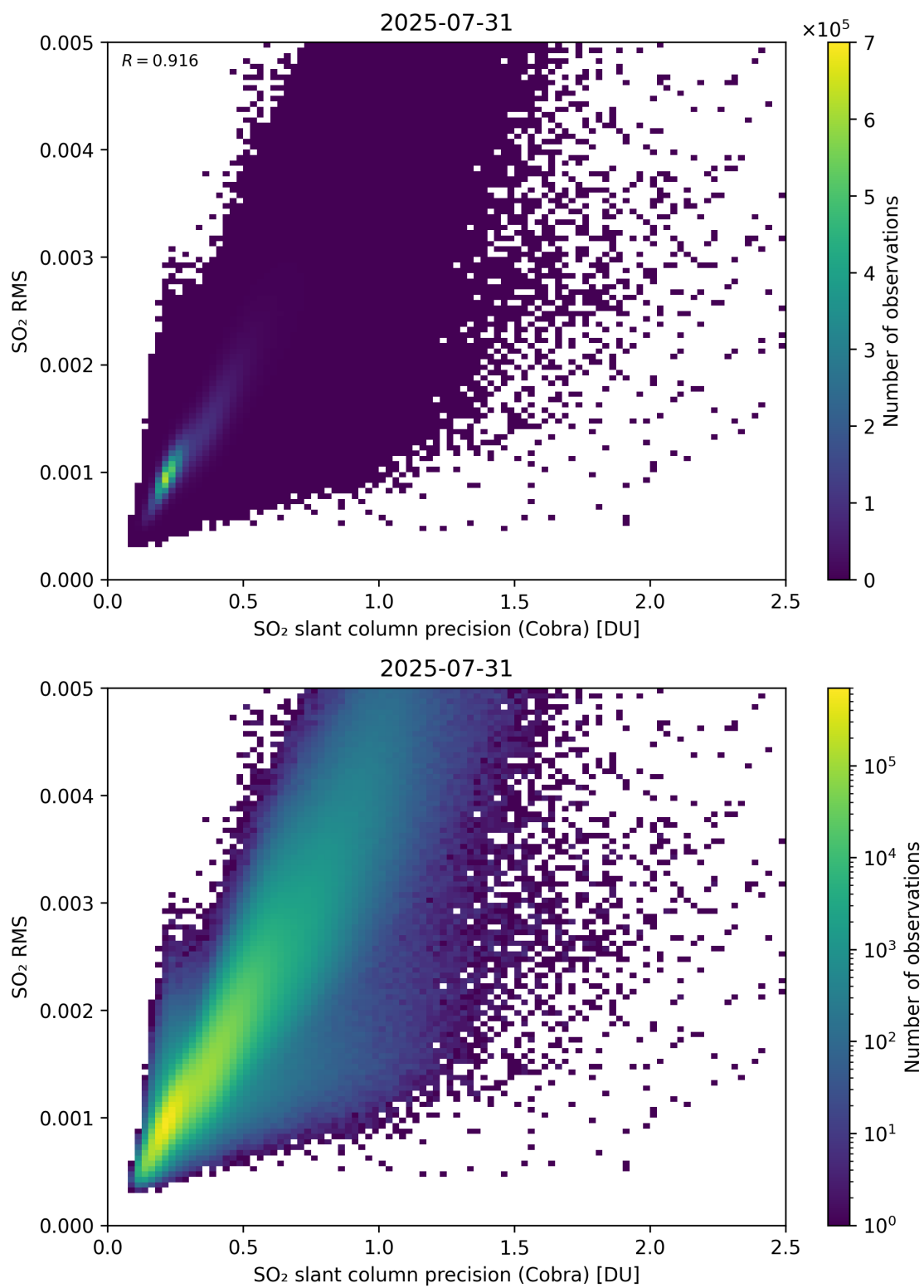
Figure 204: Scatter density plot of “SO 2 slant column precision (Cobra)” against “SO 2 RMS” for 2025-07-30 to 2025-08-01.
