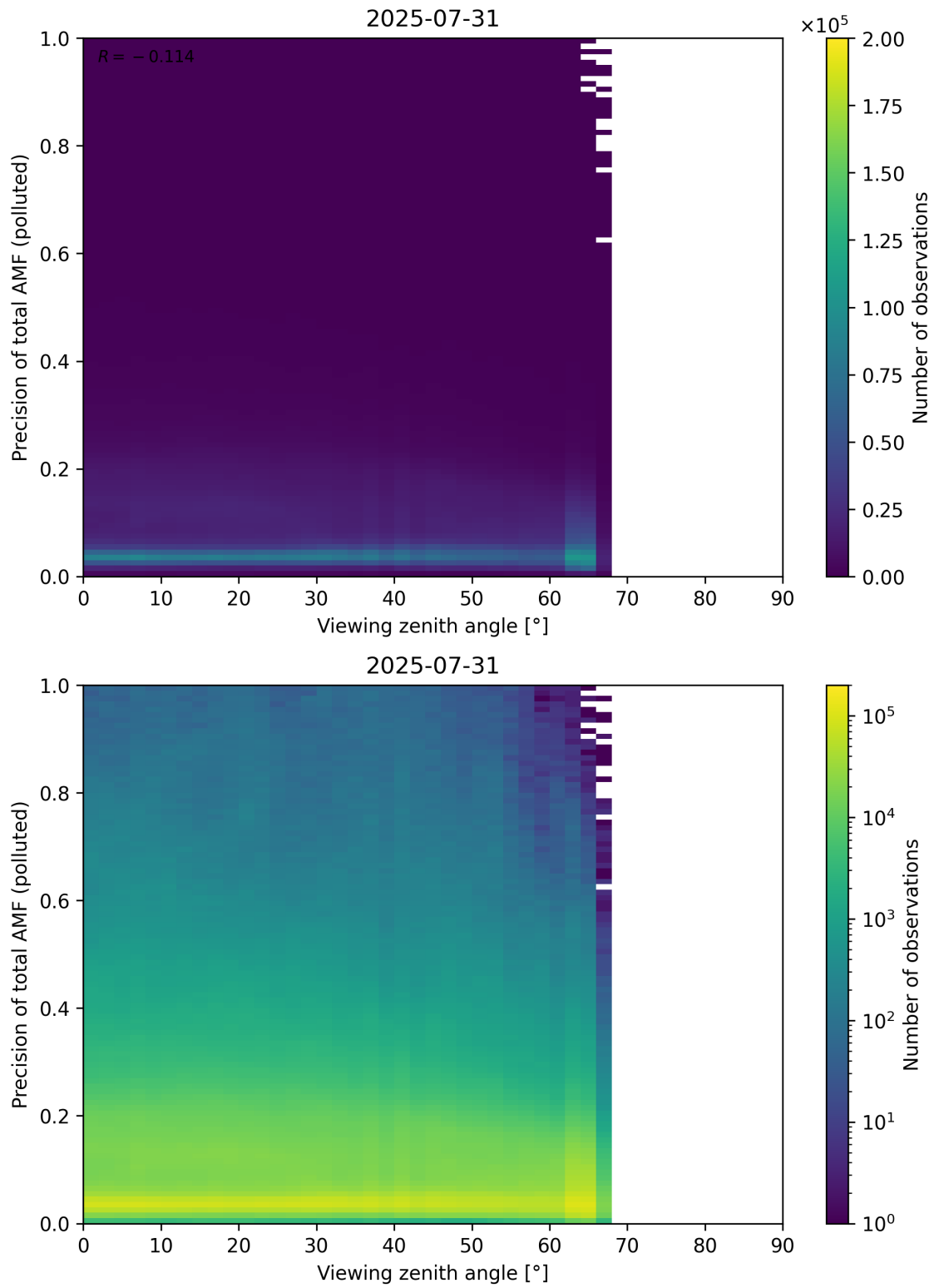
Figure 382: Scatter density plot of “Viewing zenith angle” against “Precision of total AMF (polluted)” for 2025-07-30 to 2025-08-01.
