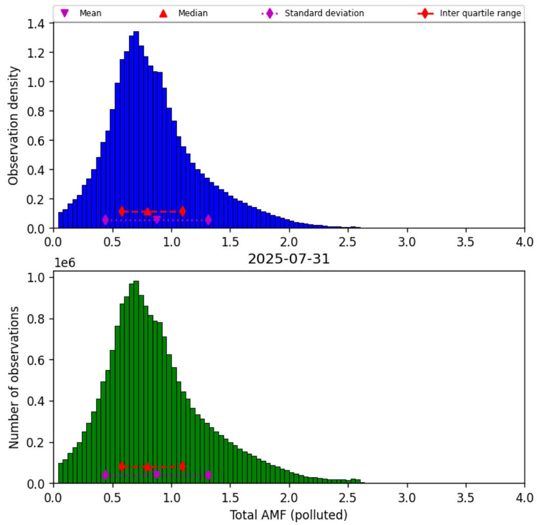
Figure 79: Histogram of “Total AMF (polluted)” for 2025-07-30 to 2025-08-01
