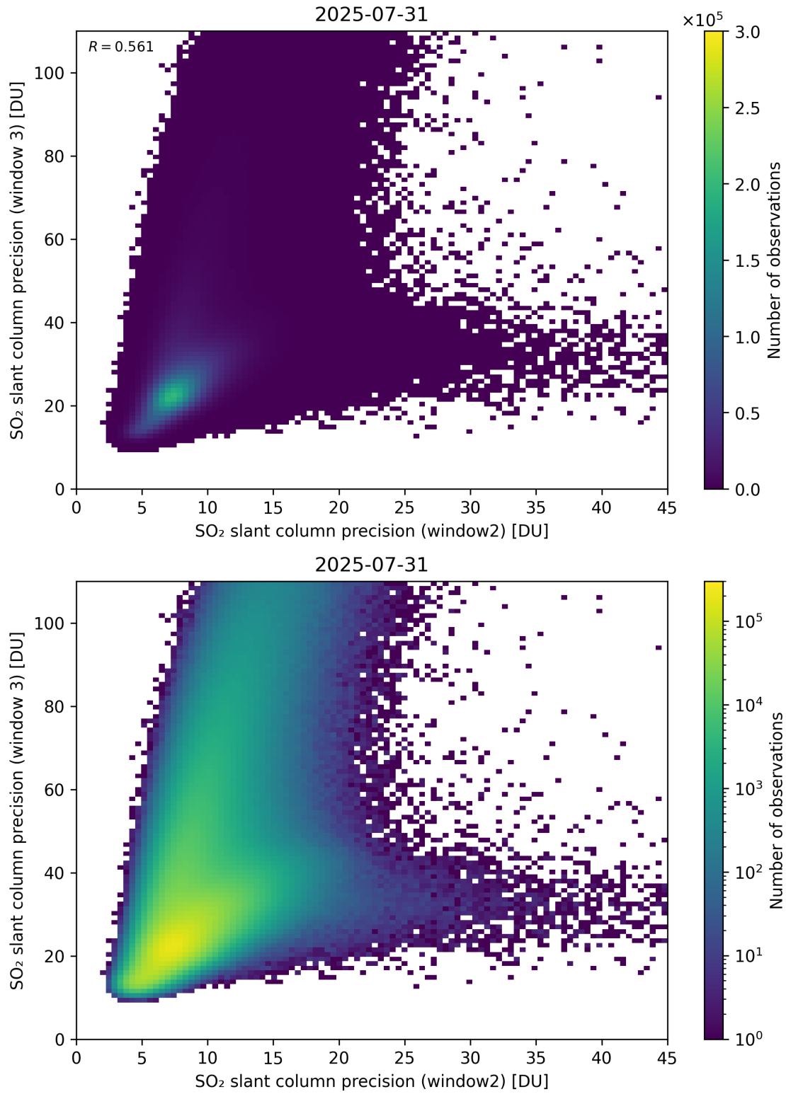
Figure 300: Scatter density plot of “SO 2 slant column precision (window2)” against “SO 2 slant column precision (window 3)” for 2025-07-30 to 2025-08-01.
