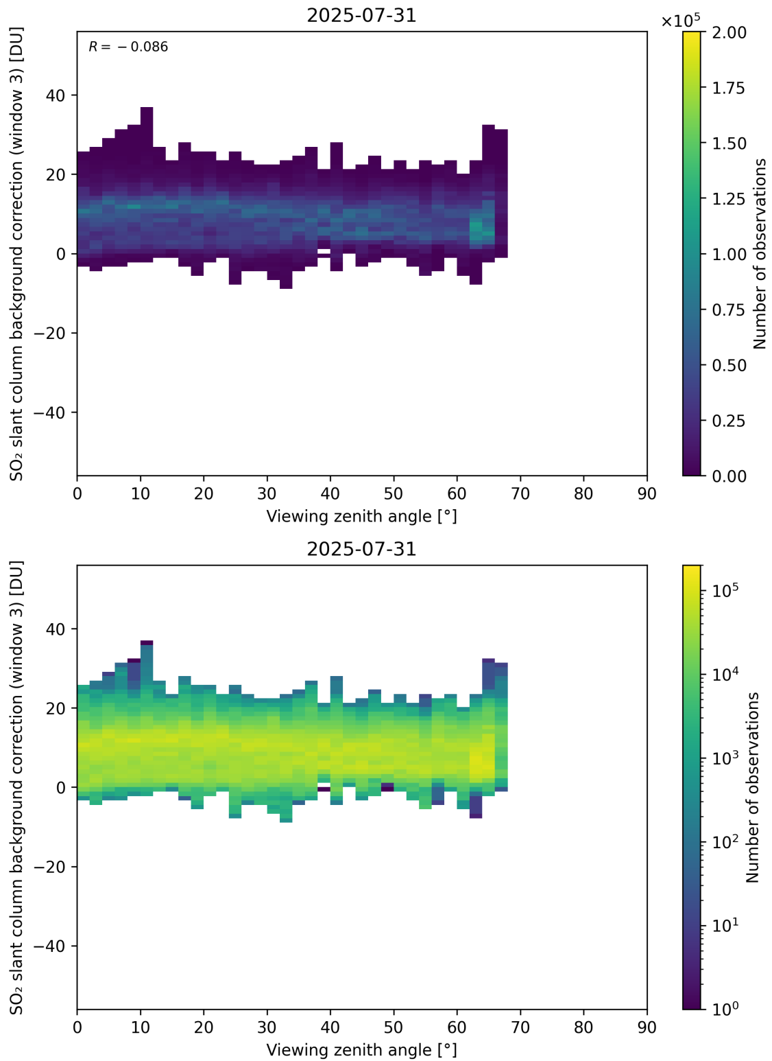
Figure 364: Scatter density plot of “Viewing zenith angle” against “SO 2 slant column background correction (window 3)” for 2025-07-30 to 2025-08-01.
