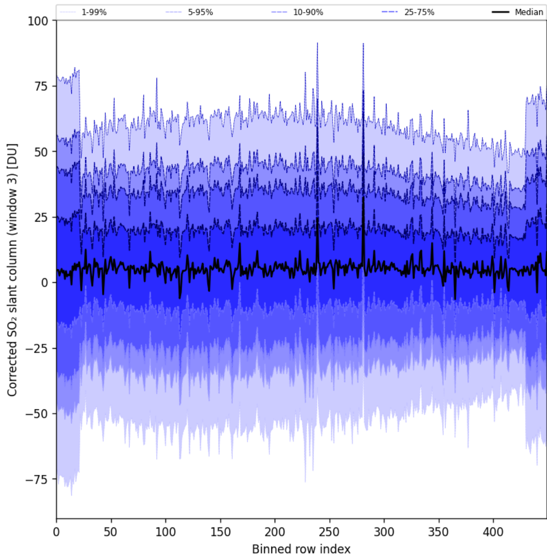
Figure 99: Along track statistics of “Corrected SO 2 slant column (window 3)” for 2025-07-30 to 2025-08-01
