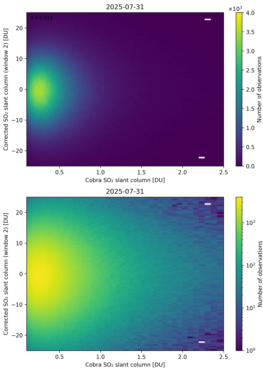
Figure 217: Scatter density plot of “Cobra SO 2 slant column” against “Corrected SO 2 slant column (window 2)” for 2025-07-30 to 2025-08-01.
