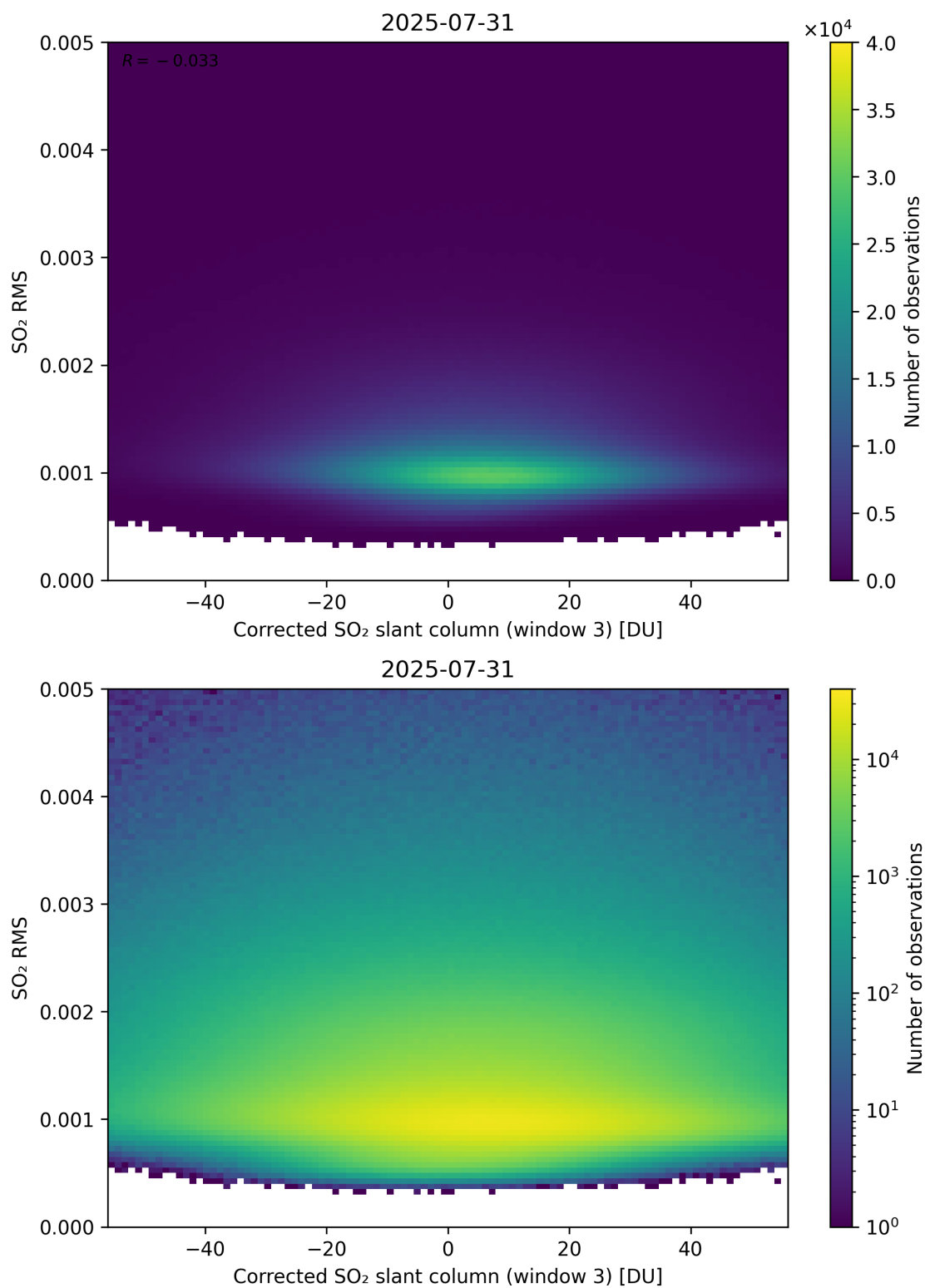
Figure 258: Scatter density plot of “Corrected SO 2 slant column (window 3)” against “SO 2 RMS” for 2025-07-30 to 2025-08-01.
