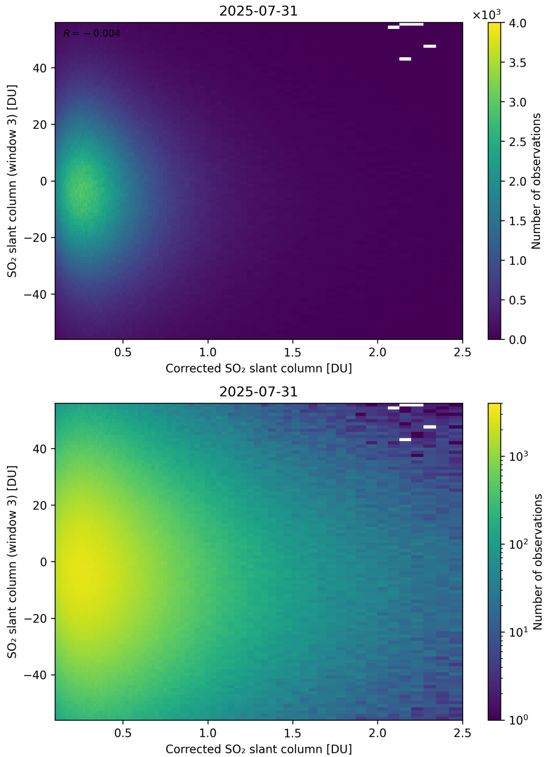
Figure 240: Scatter density plot of “Corrected SO 2 slant column” against “SO 2 slant column (window 3)” for 2025-07-30 to 2025-08-01.
