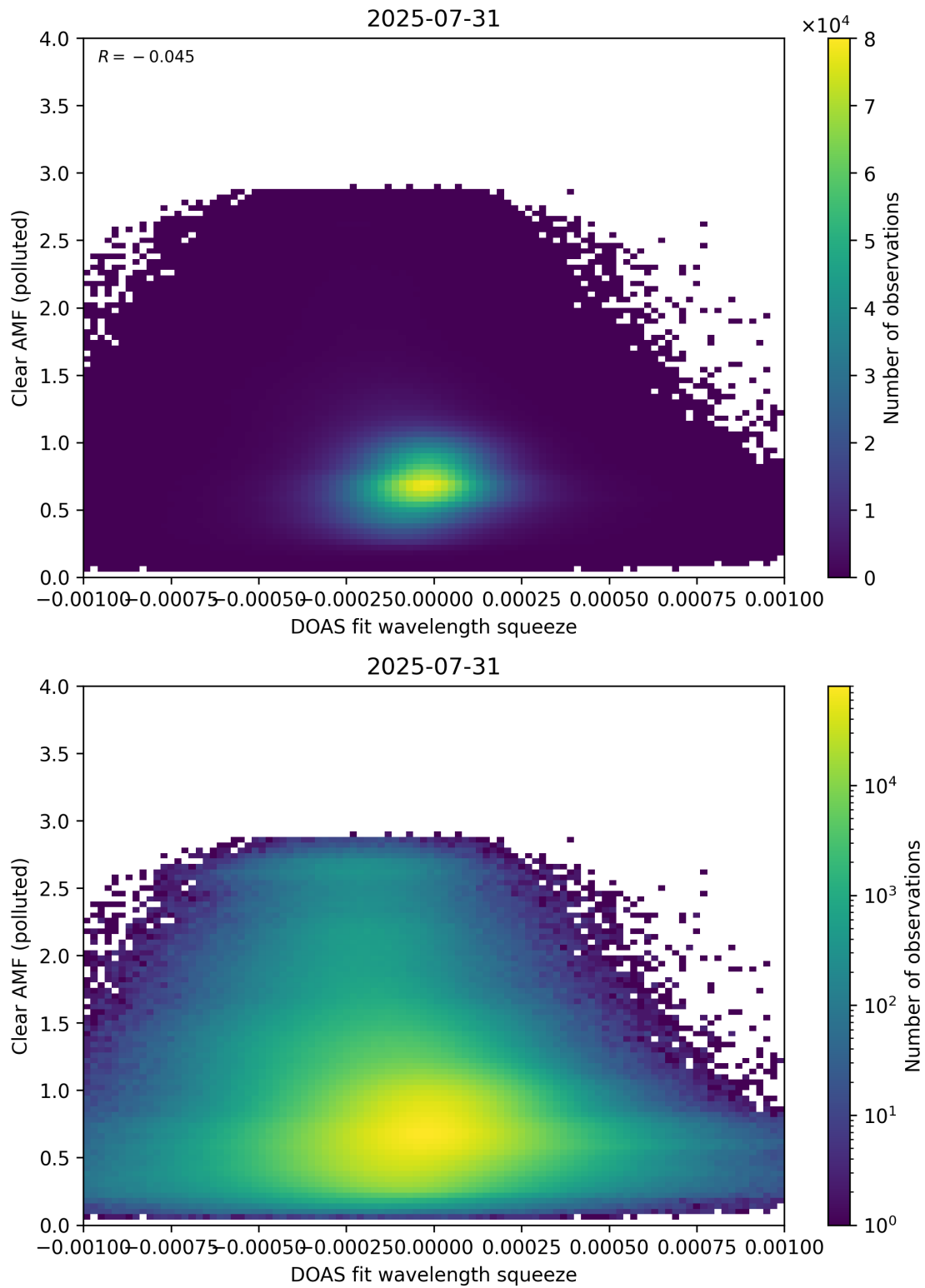
Figure 144: Scatter density plot of “DOAS fit wavelength squeeze” against “Clear AMF (polluted)” for 2025-07-30 to 2025-08-01.
