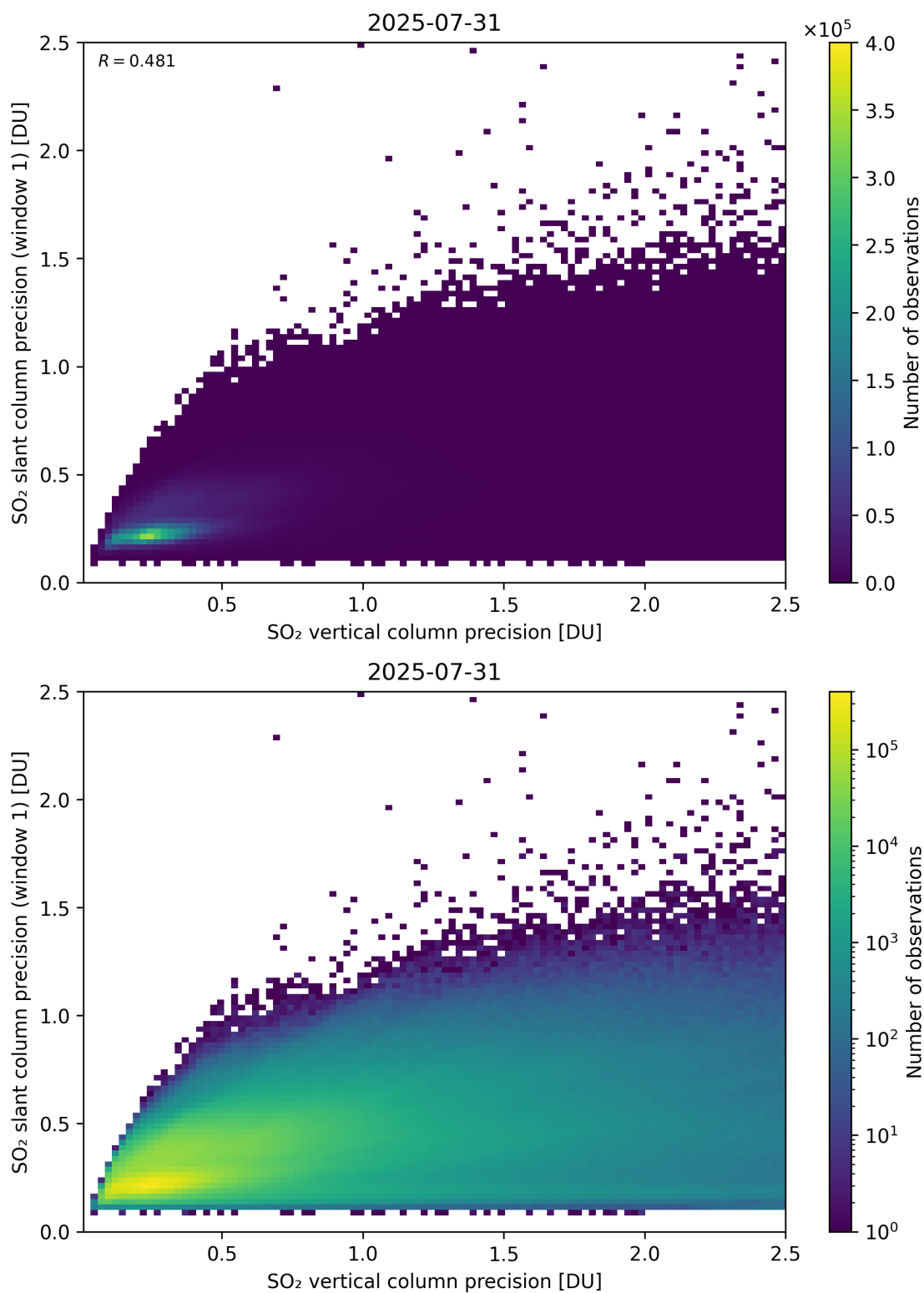
Figure 342: Scatter density plot of “SO 2 vertical column precision” against “SO 2 slant column precision (window 1)” for 2025-07-30 to 2025-08-01.
