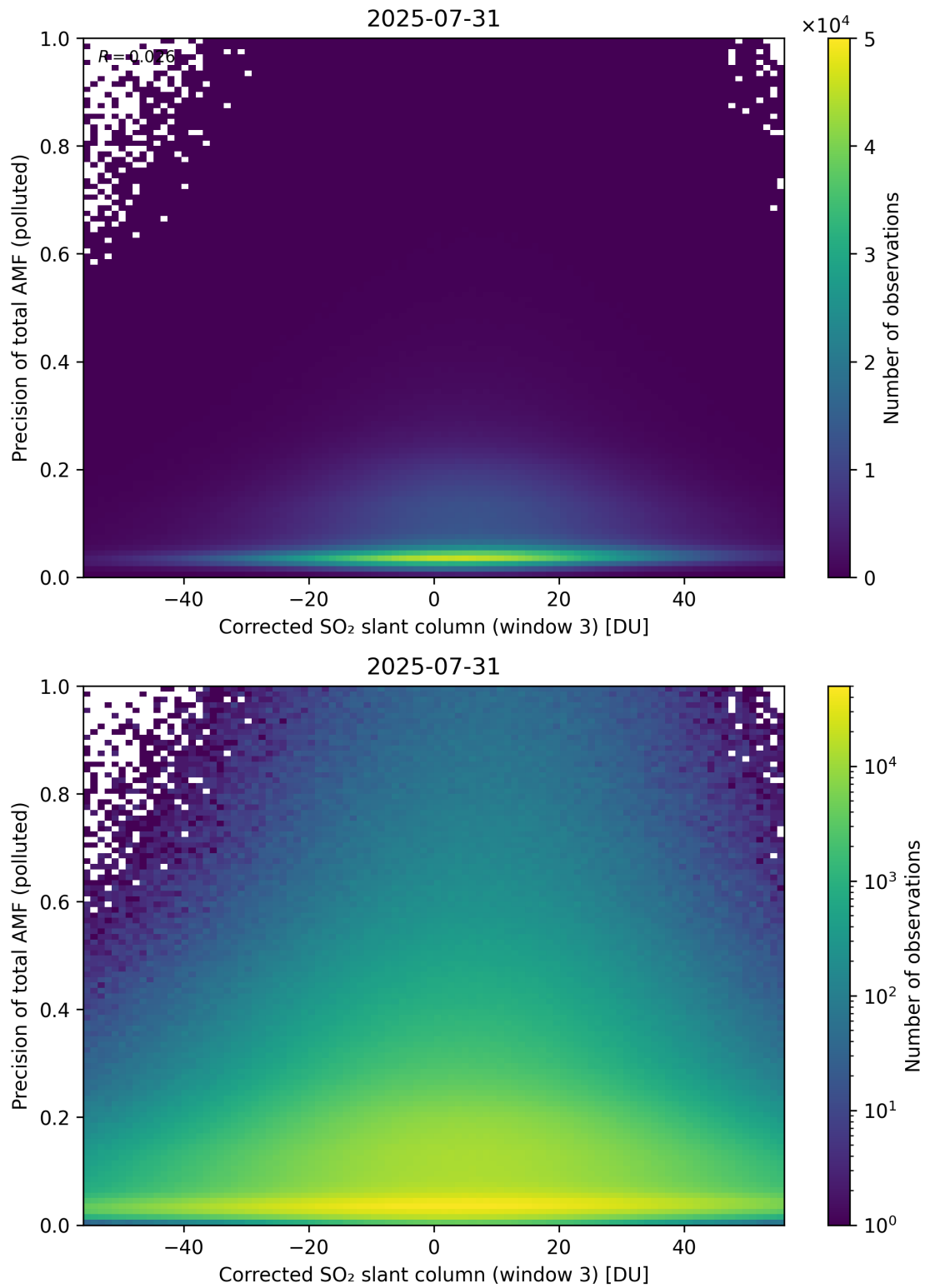
Figure 261: Scatter density plot of “Corrected SO 2 slant column (window 3)” against “Precision of total AMF (polluted)” for 2025-07-30 to 2025-08-01.
