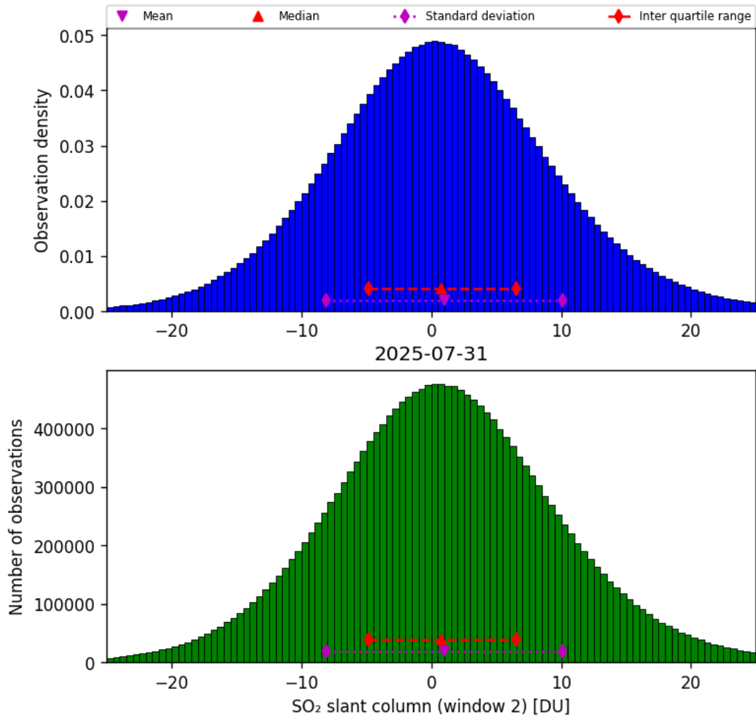
Figure 67: Histogram of “SO 2 slant column (window 2)” for 2025-07-30 to 2025-08-01
