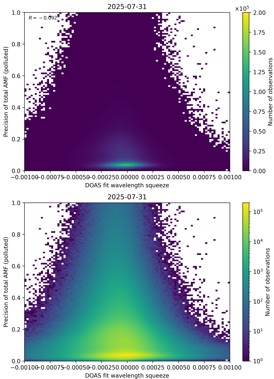
Figure 146: Scatter density plot of “DOAS fit wavelength squeeze” against “Precision of total AMF (polluted)” for 2025-07-30 to 2025-08-01.
