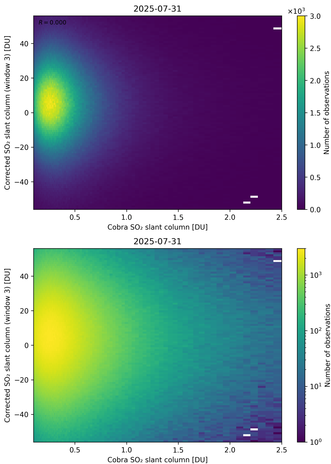
Figure 218: Scatter density plot of “Cobra SO 2 slant column” against “Corrected SO 2 slant column (window 3)” for 2025-07-30 to 2025-08-01.
