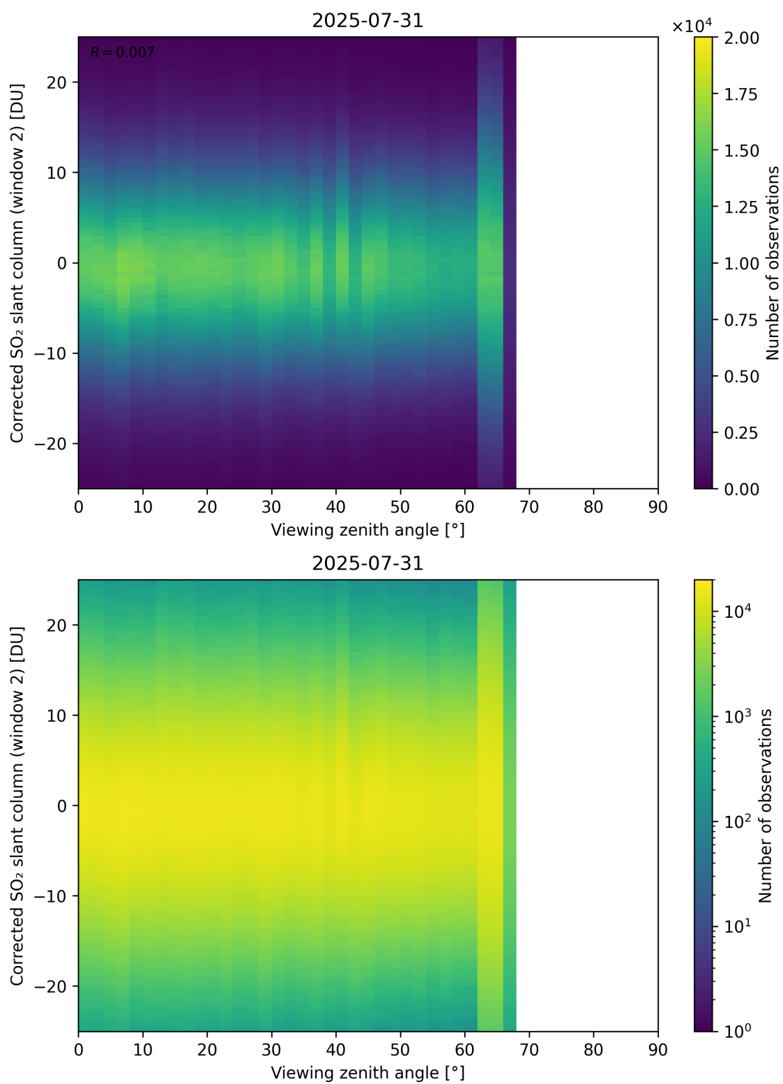
Figure 374: Scatter density plot of “Viewing zenith angle” against “Corrected SO 2 slant column (window 2)” for 2025-07-30 to 2025-08-01.
