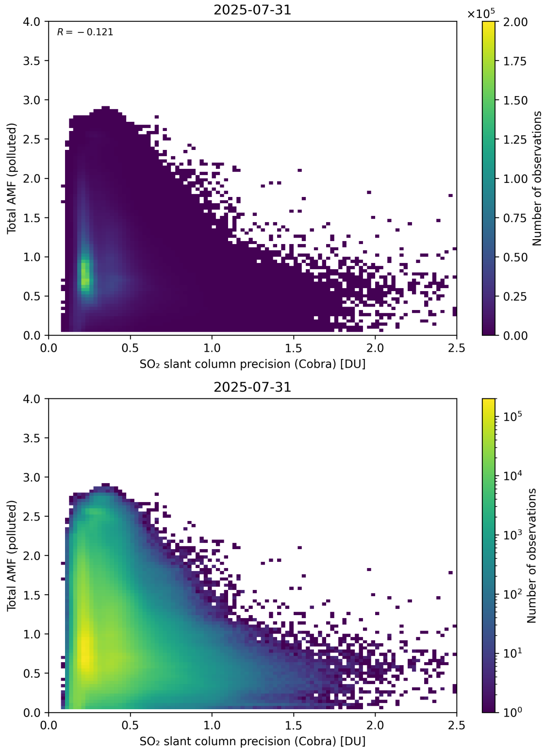
Figure 213: Scatter density plot of “SO 2 slant column precision (Cobra)” against “Total AMF (polluted)” for 2025-07-30 to 2025-08-01.
