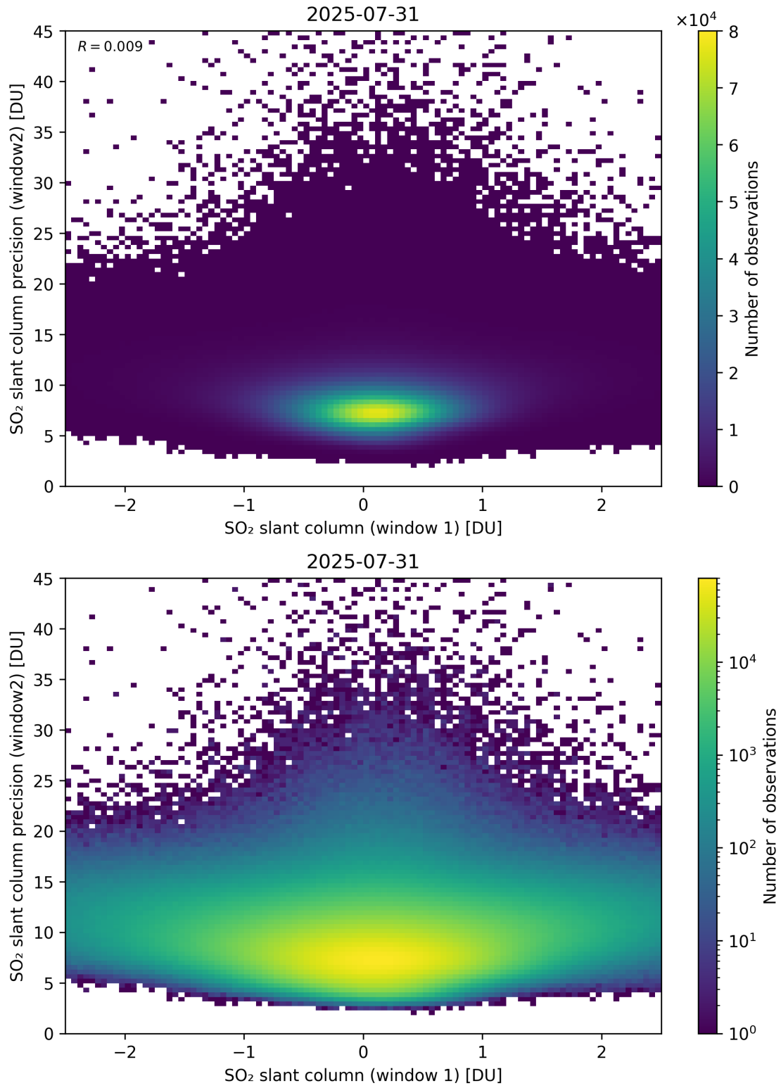
Figure 286: Scatter density plot of “SO 2 slant column (window 1)” against “SO 2 slant column precision (window2)” for 2025-07-30 to 2025-08-01.
