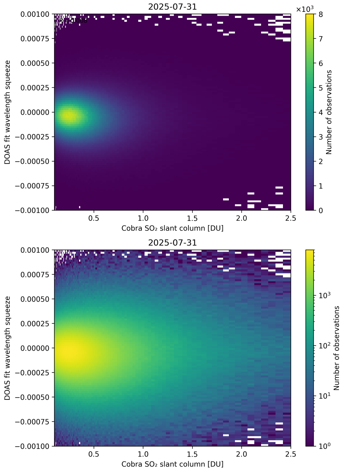
Figure 197: Scatter density plot of “Cobra SO 2 slant column” against “DOAS fit wavelength squeeze” for 2025-07-30 to 2025-08-01.
