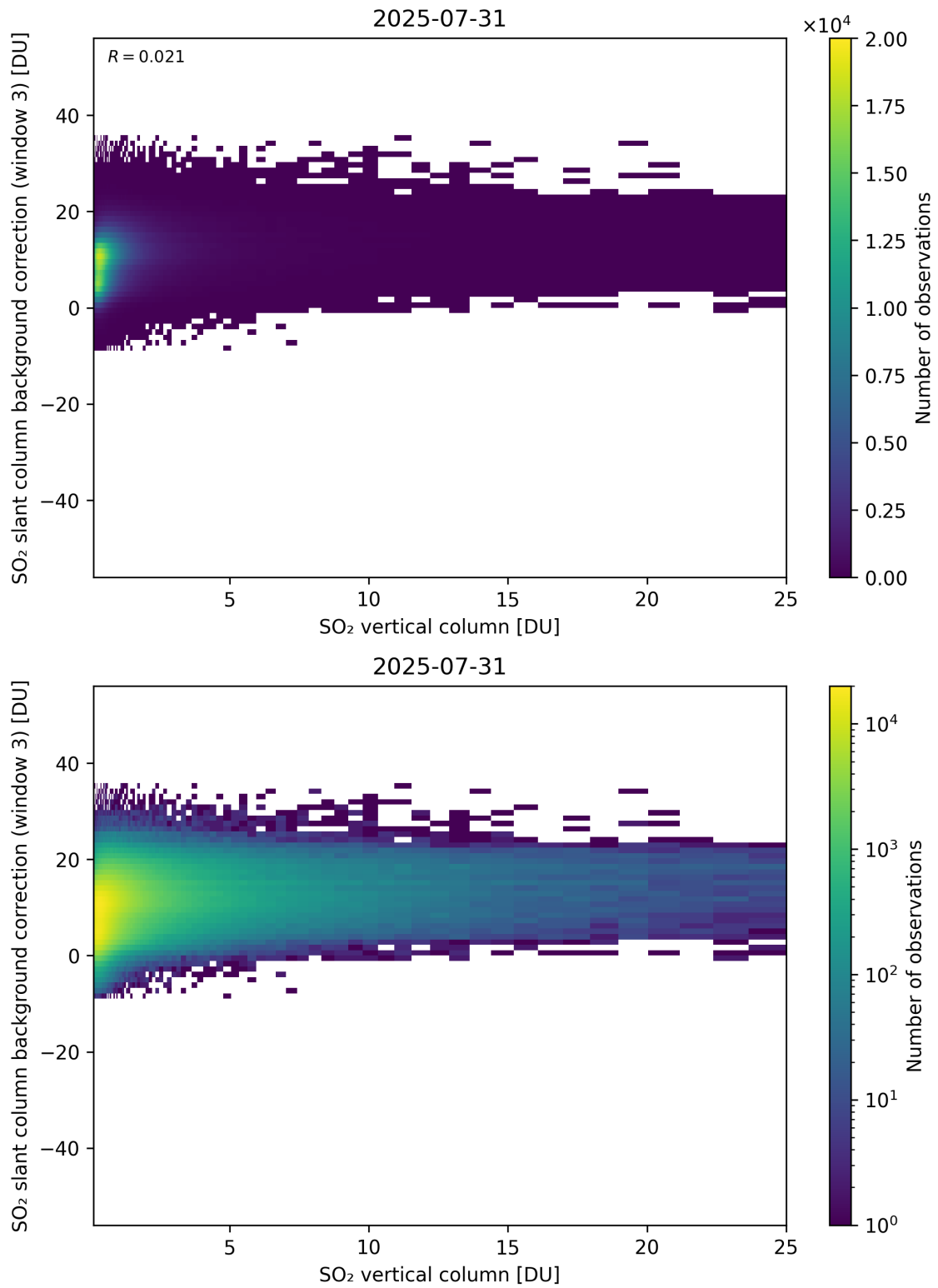
Figure 325: Scatter density plot of “SO 2 vertical column” against “SO 2 slant column background correction (window 3)” for 2025-07-30 to 2025-08-01.
