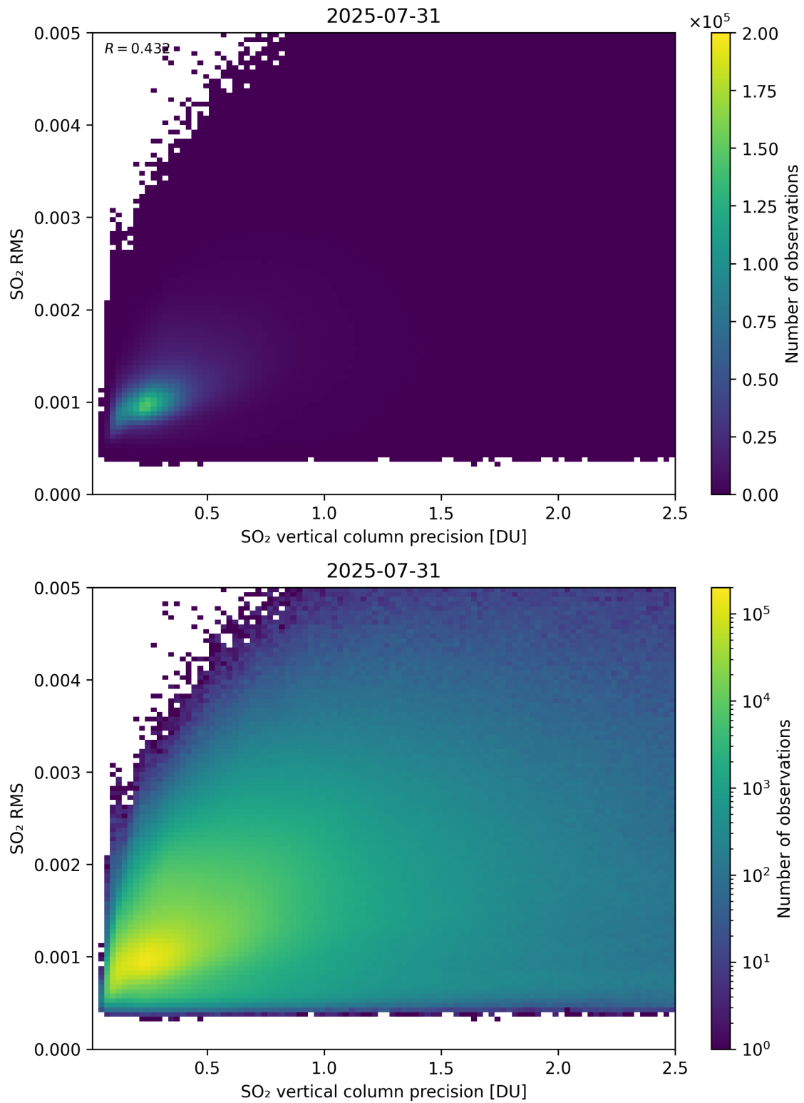
Figure 334: Scatter density plot of “SO 2 vertical column precision” against “SO 2 RMS” for 2025-07-30 to 2025-08-01.
