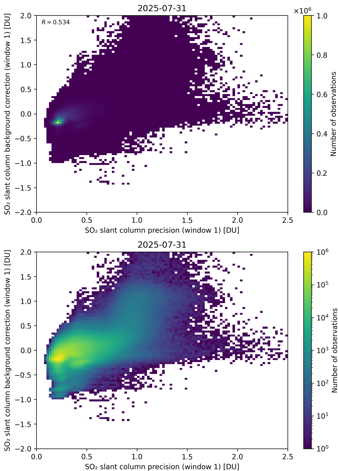
Figure 268: Scatter density plot of “SO 2 slant column precision (window 1)” against “SO 2 slant column background correction (window 1)” for 2025-07-30 to 2025-08-01.
