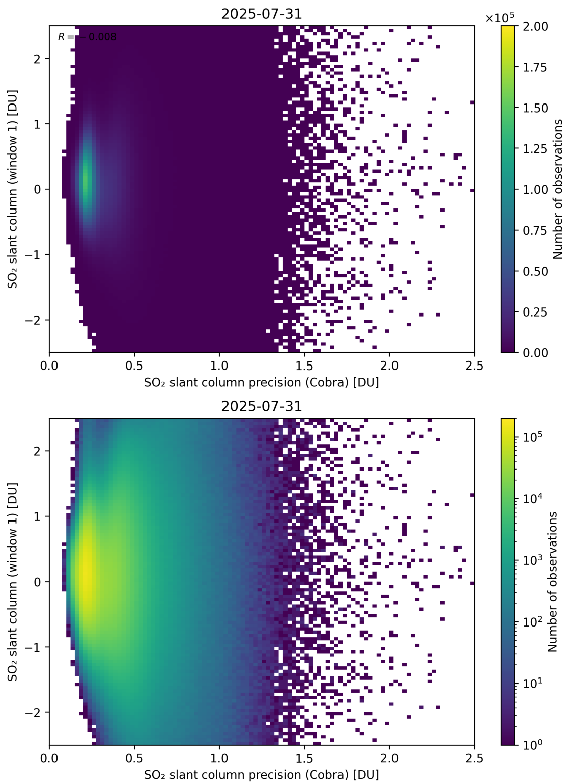
Figure 208: Scatter density plot of “SO 2 slant column precision (Cobra)” against “SO 2 slant column (window 1)” for 2025-07-30 to 2025-08-01.
