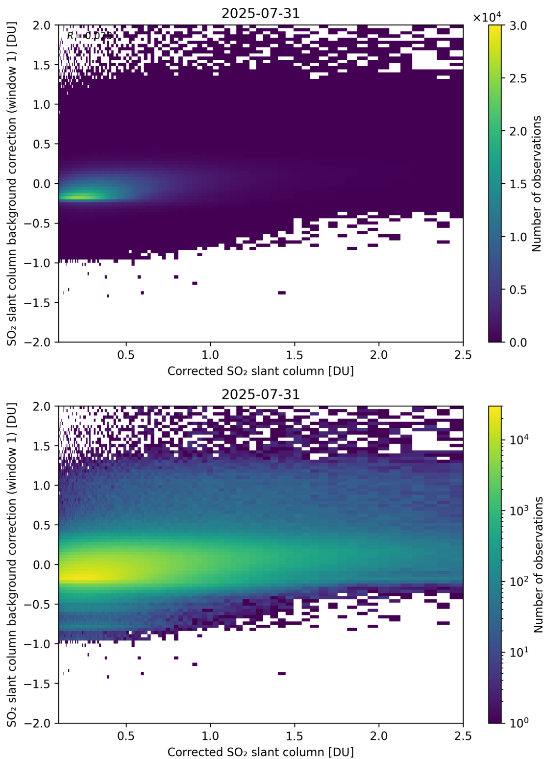
Figure 226: Scatter density plot of “Corrected SO 2 slant column” against “SO 2 slant column background correction (window 1)” for 2025-07-30 to 2025-08-01.
