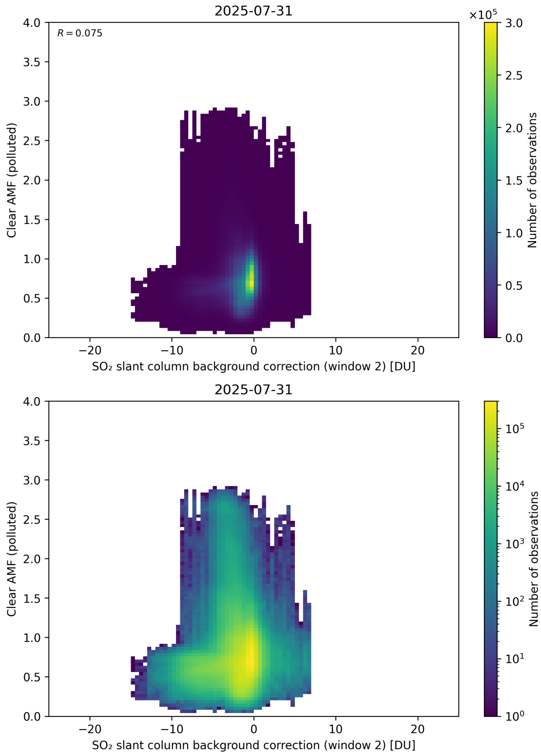
Figure 126: Scatter density plot of “SO 2 slant column background correction (window 2)” against “Clear AMF (polluted)” for 2025-07-30 to 2025-08-01.
