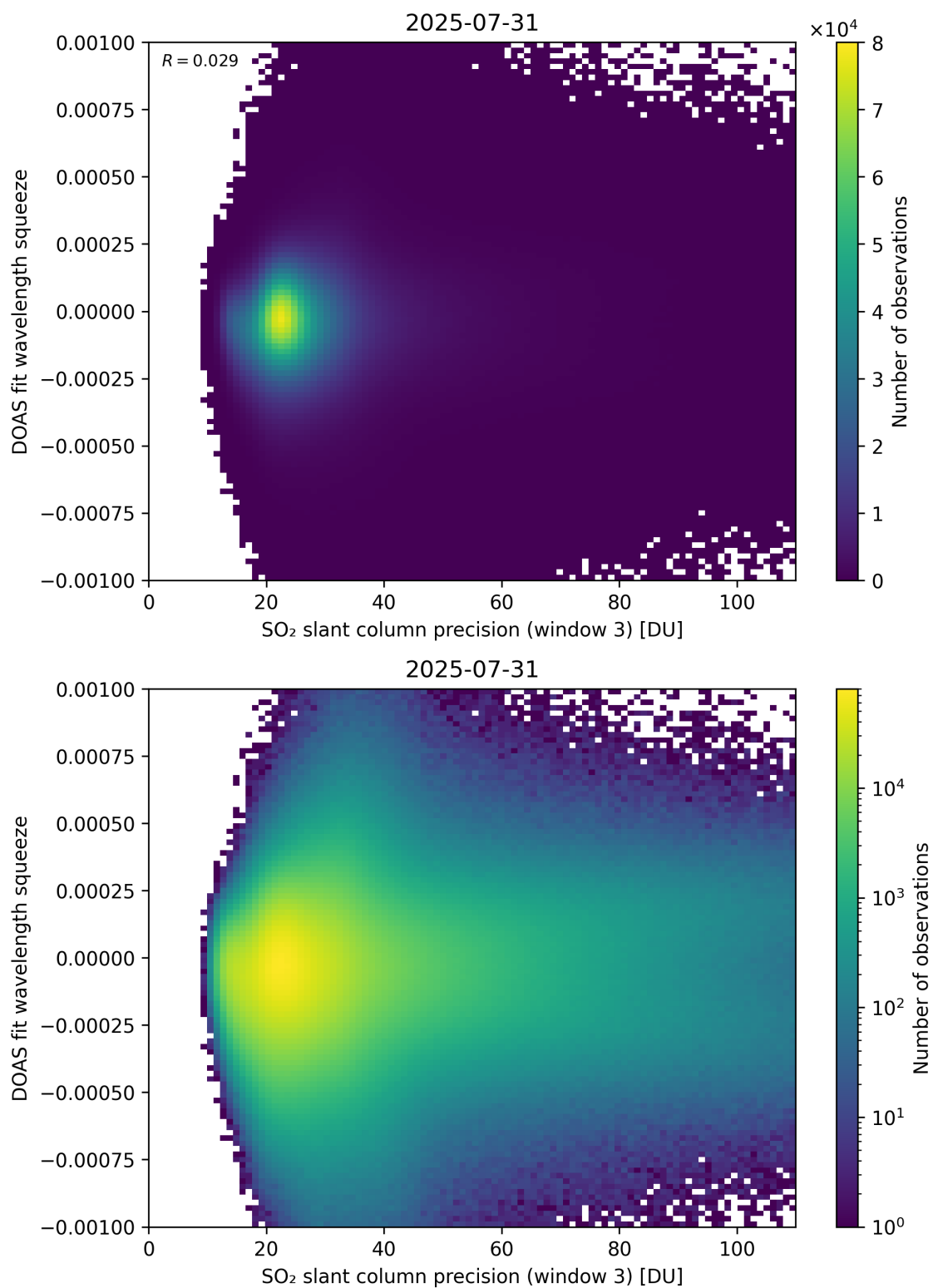
Figure 309: Scatter density plot of “SO 2 slant column precision (window 3)” against “DOAS fit wavelength squeeze” for 2025-07-30 to 2025-08-01.
