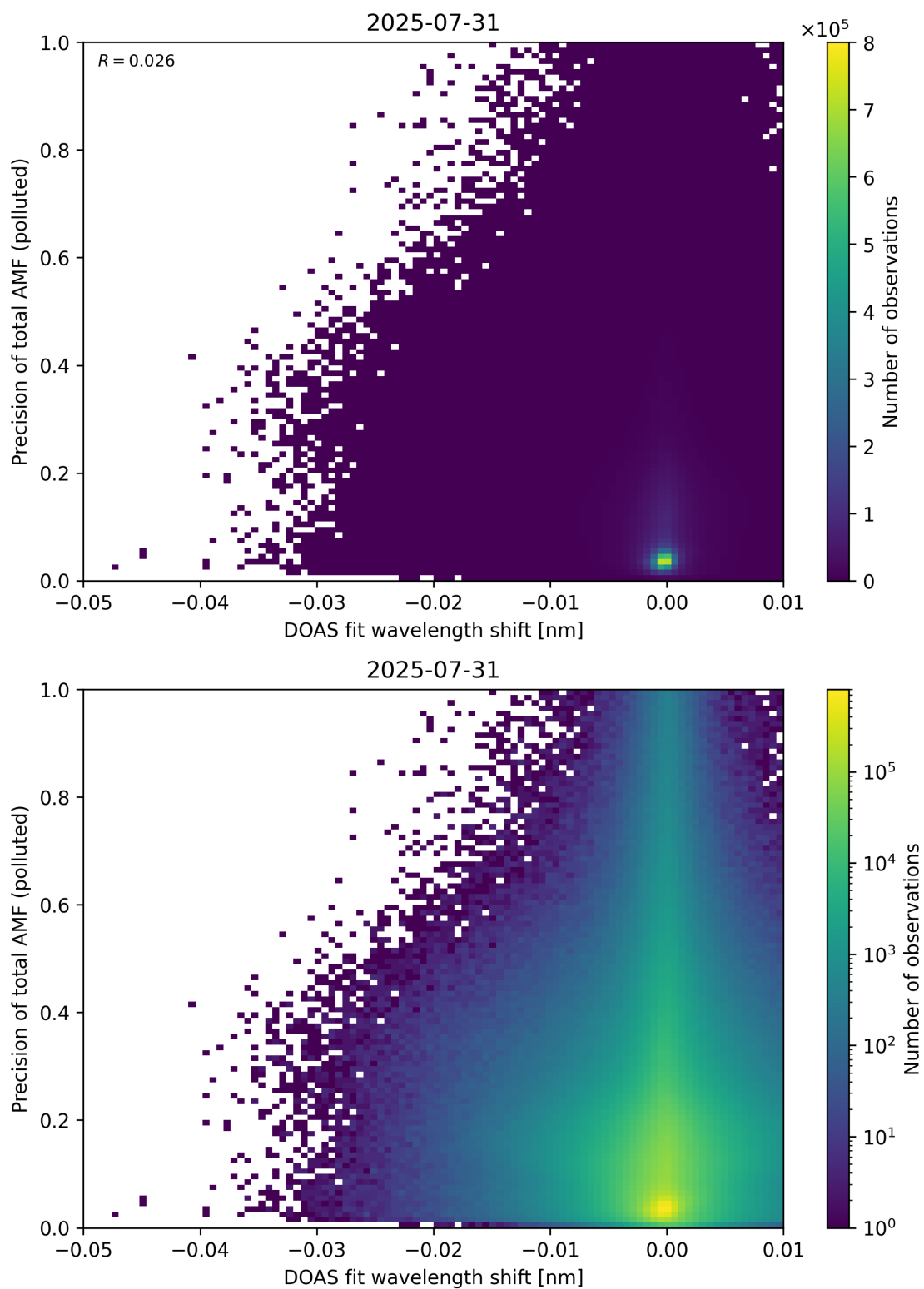
Figure 142: Scatter density plot of “DOAS fit wavelength shift” against “Precision of total AMF (polluted)” for 2025-07-30 to 2025-08-01.
