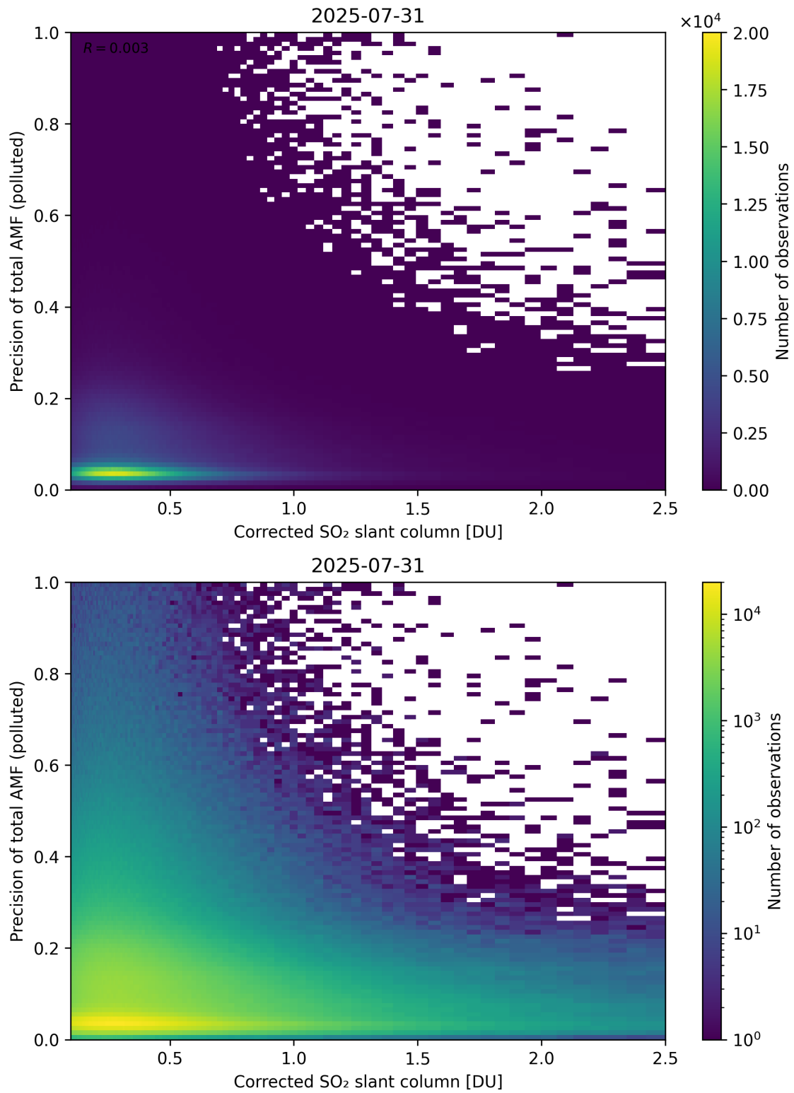
Figure 243: Scatter density plot of “Corrected SO 2 slant column” against “Precision of total AMF (polluted)” for 2025-07-30 to 2025-08-01.
