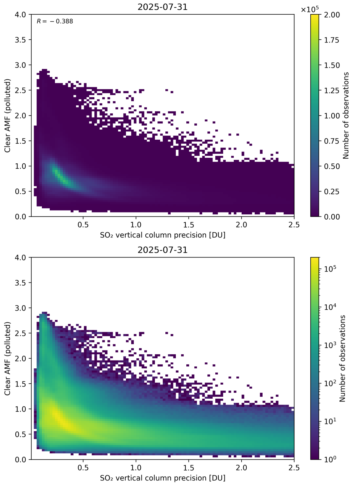
Figure 335: Scatter density plot of “SO 2 vertical column precision” against “Clear AMF (polluted)” for 2025-07-30 to 2025-08-01.
