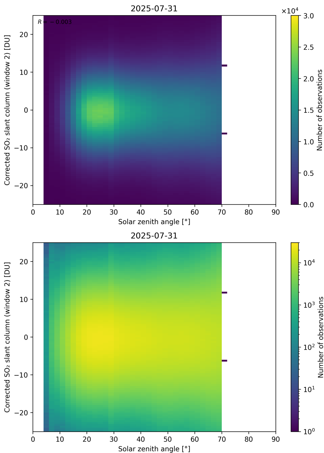
Figure 182: Scatter density plot of “Solar zenith angle” against “Corrected SO 2 slant column (window 2)” for 2025-07-30 to 2025-08-01.
