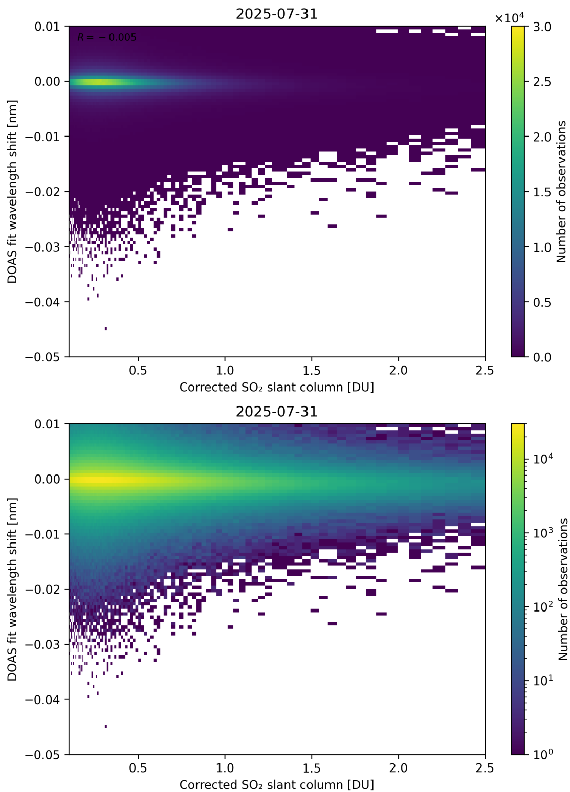
Figure 229: Scatter density plot of “Corrected SO 2 slant column” against “DOAS fit wavelength shift” for 2025-07-30 to 2025-08-01.
