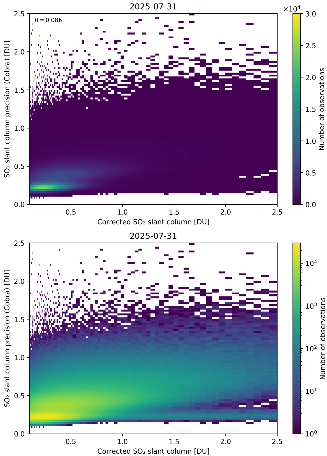
Figure 234: Scatter density plot of “Corrected SO 2 slant column” against “SO 2 slant column precision (Cobra)” for 2025-07-30 to 2025-08-01.
