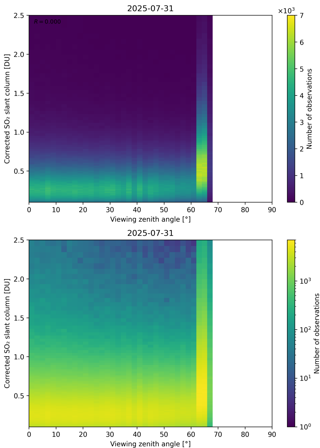
Figure 373: Scatter density plot of “Viewing zenith angle” against “Corrected SO 2 slant column” for 2025-07-30 to 2025-08-01.
