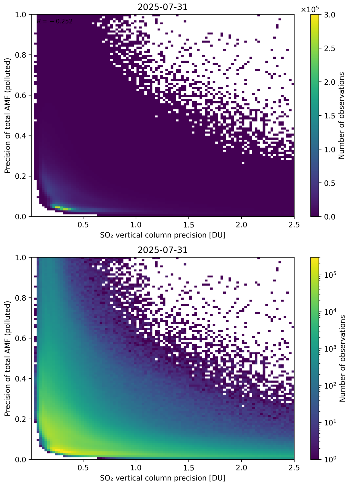
Figure 347: Scatter density plot of “SO 2 vertical column precision” against “Precision of total AMF (polluted)” for 2025-07-30 to 2025-08-01.
