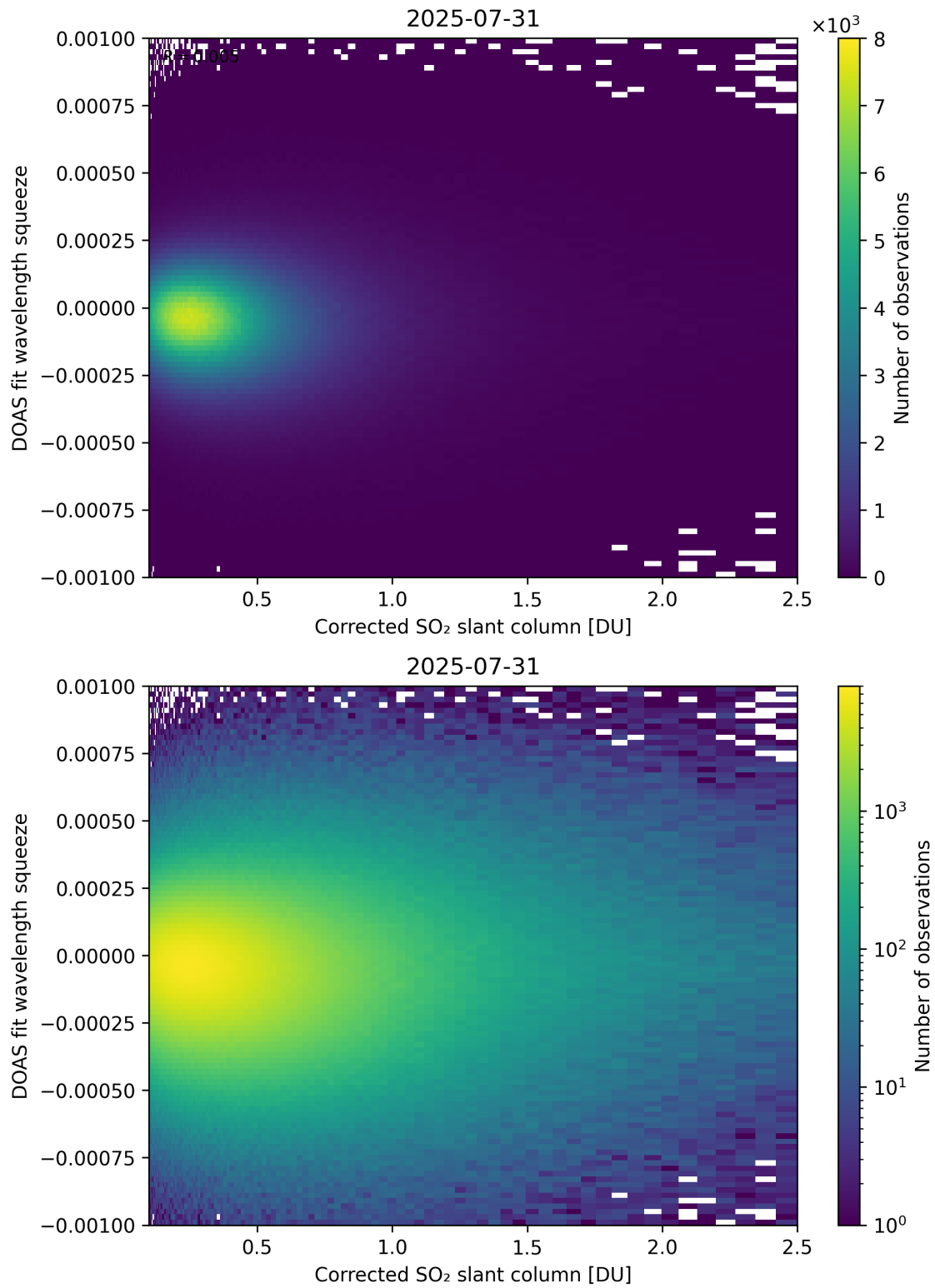
Figure 230: Scatter density plot of “Corrected SO 2 slant column” against “DOAS fit wavelength squeeze” for 2025-07-30 to 2025-08-01.
