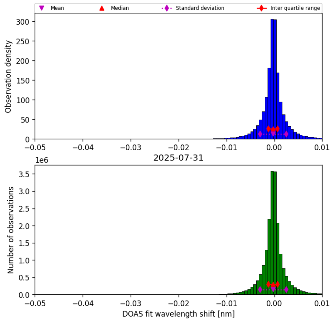
Figure 76: Histogram of “DOAS fit wavelength shift” for 2025-07-30 to 2025-08-01
