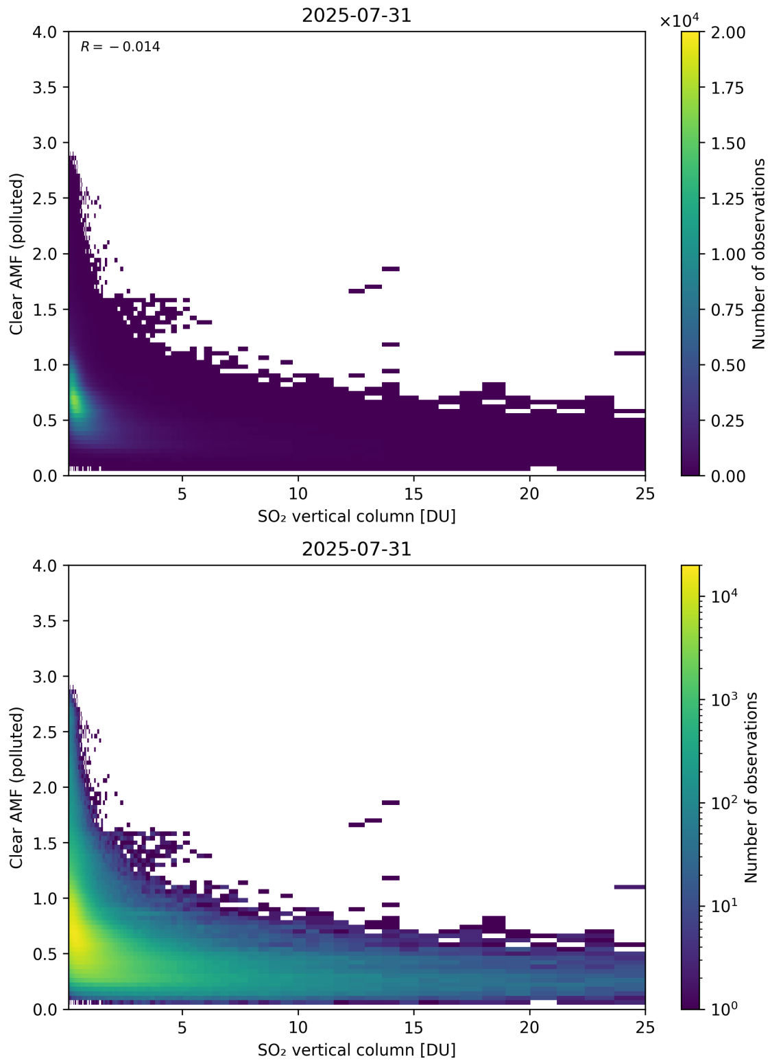
Figure 348: Scatter density plot of “SO 2 vertical column” against “Clear AMF (polluted)” for 2025-07-30 to 2025-08-01.
