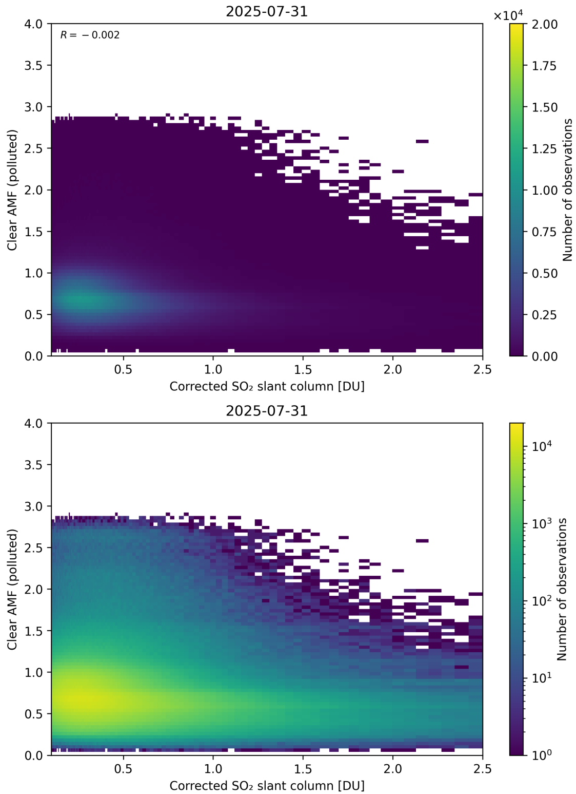
Figure 232: Scatter density plot of “Corrected SO 2 slant column” against “Clear AMF (polluted)” for 2025-07-30 to 2025-08-01.
