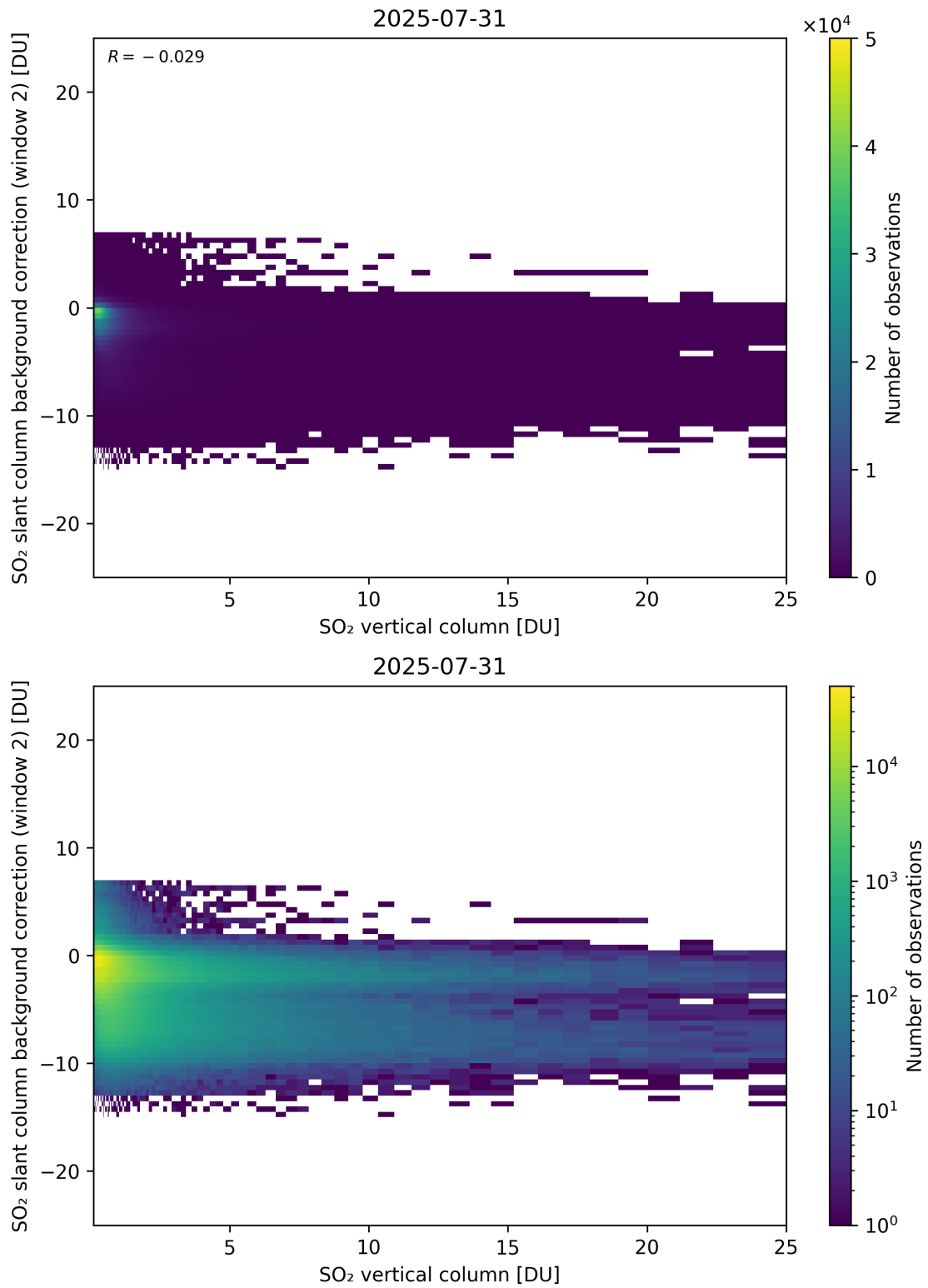
Figure 324: Scatter density plot of “SO 2 vertical column” against “SO 2 slant column background correction (window 2)” for 2025-07-30 to 2025-08-01.
