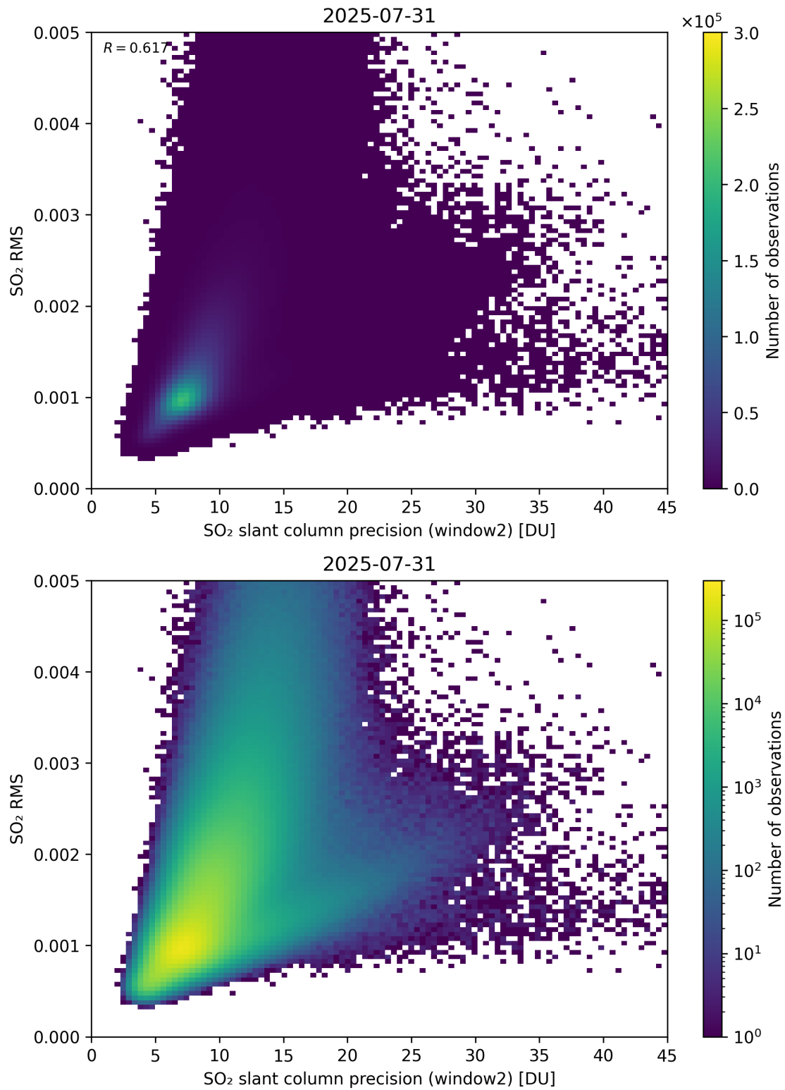
Figure 295: Scatter density plot of “SO 2 slant column precision (window2)” against “SO 2 RMS” for 2025-07-30 to 2025-08-01.
