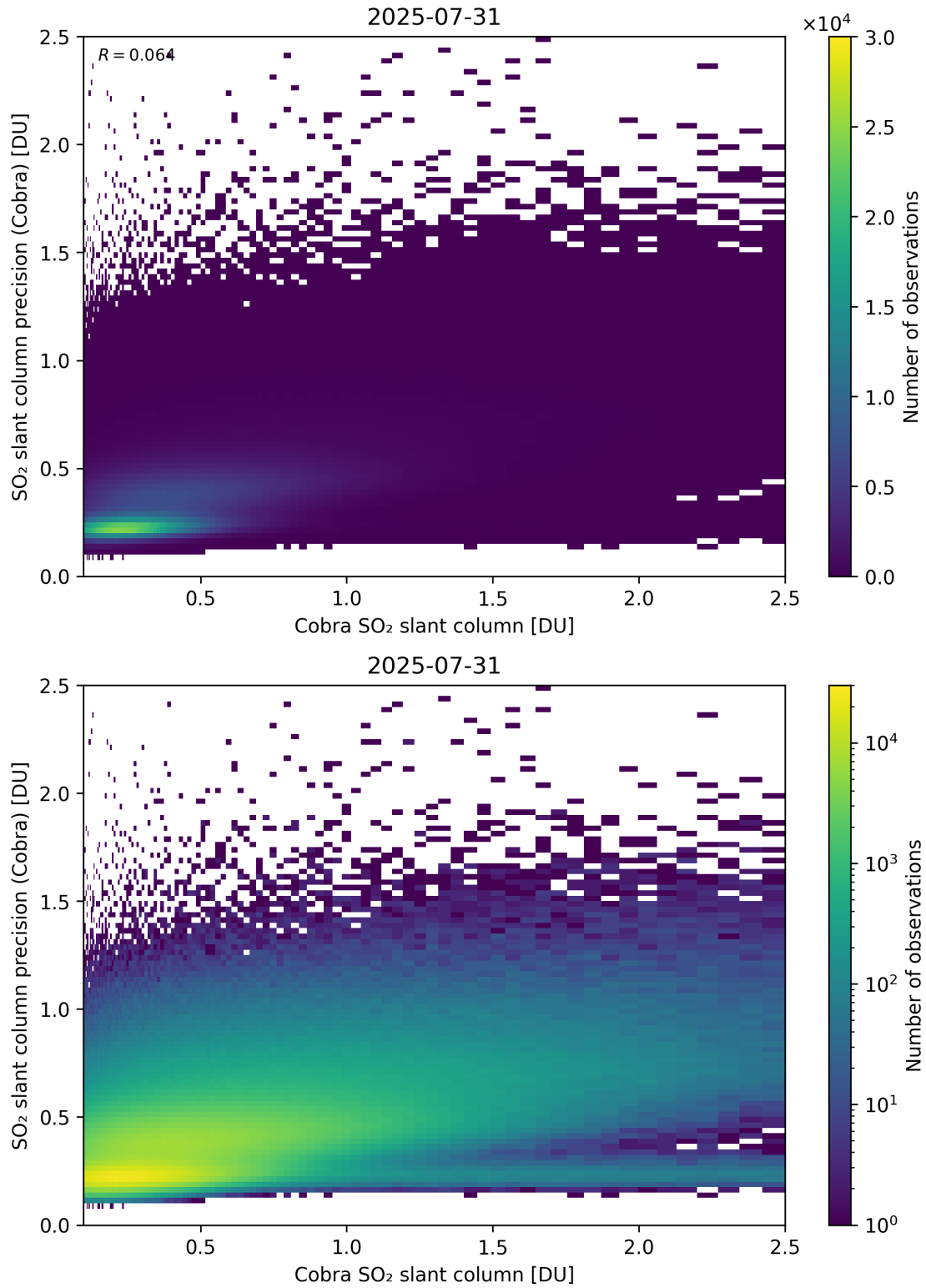
Figure 216: Scatter density plot of “Cobra SO 2 slant column” against “SO 2 slant column precision (Cobra)” for 2025-07-30 to 2025-08-01.
