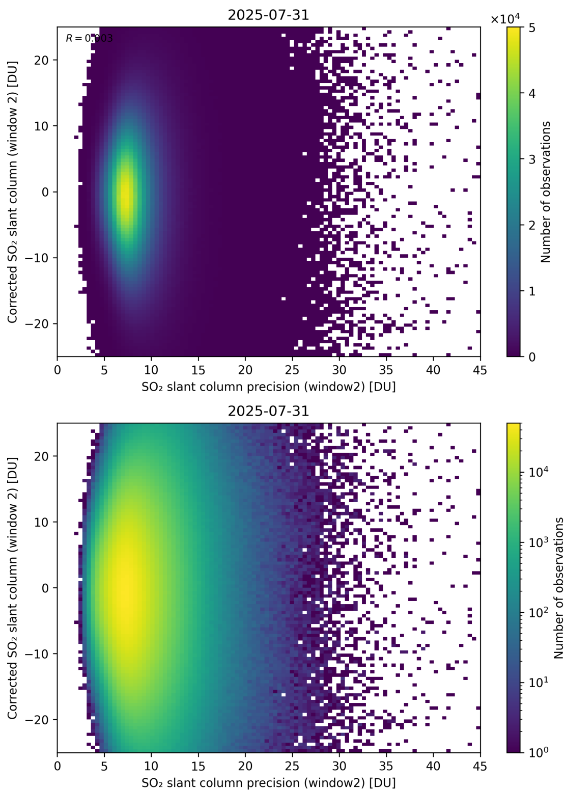
Figure 297: Scatter density plot of “SO 2 slant column precision (window2)” against “Corrected SO 2 slant column (window 2)” for 2025-07-30 to 2025-08-01.
