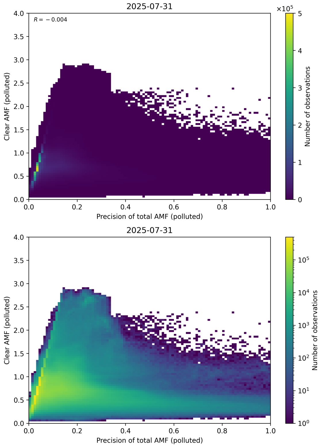
Figure 320: Scatter density plot of “Precision of total AMF (polluted)” against “Clear AMF (polluted)” for 2025-07-30 to 2025-08-01.
