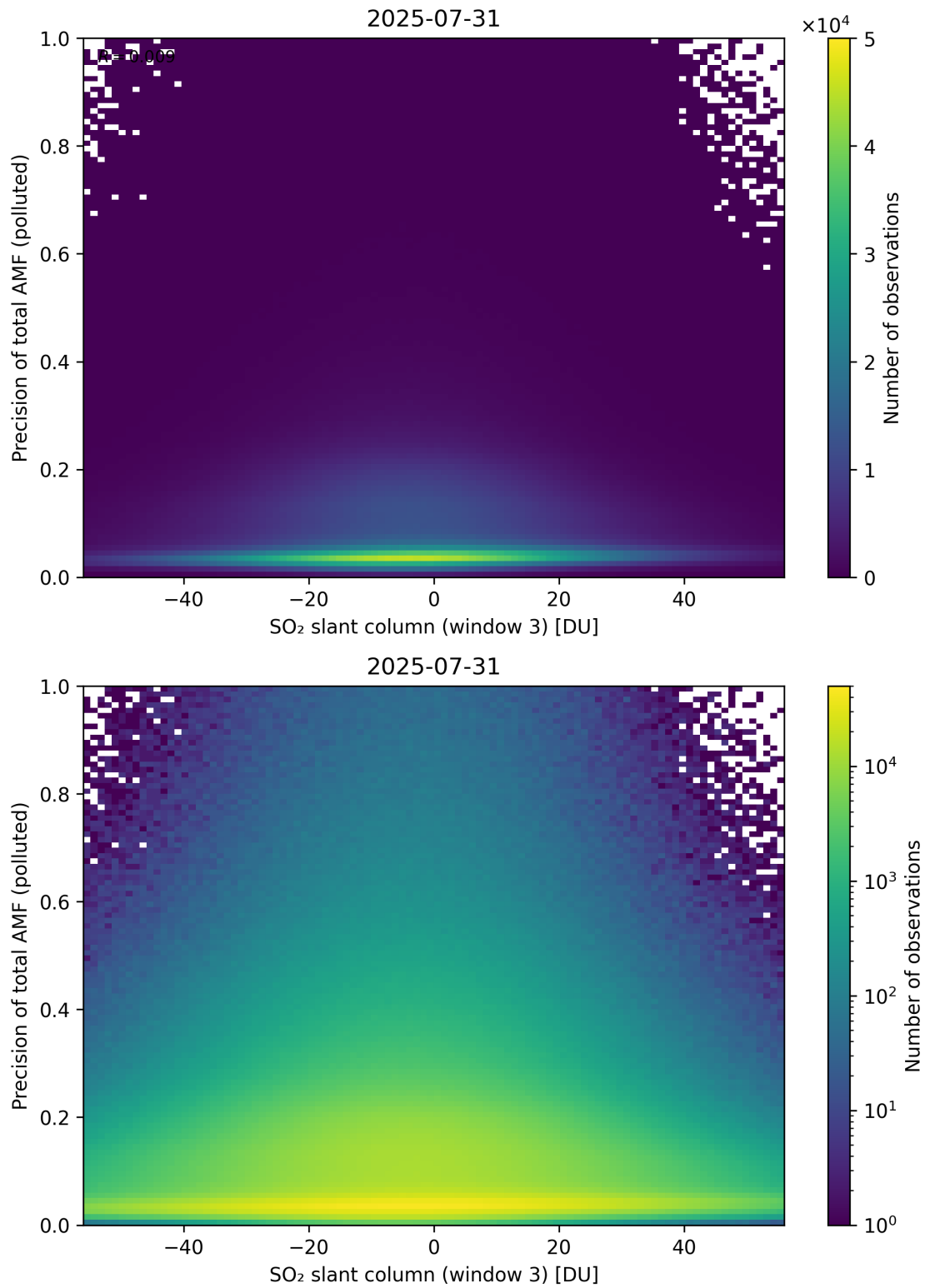
Figure 319: Scatter density plot of “SO 2 slant column (window 3)” against “Precision of total AMF (polluted)” for 2025-07-30 to 2025-08-01.
