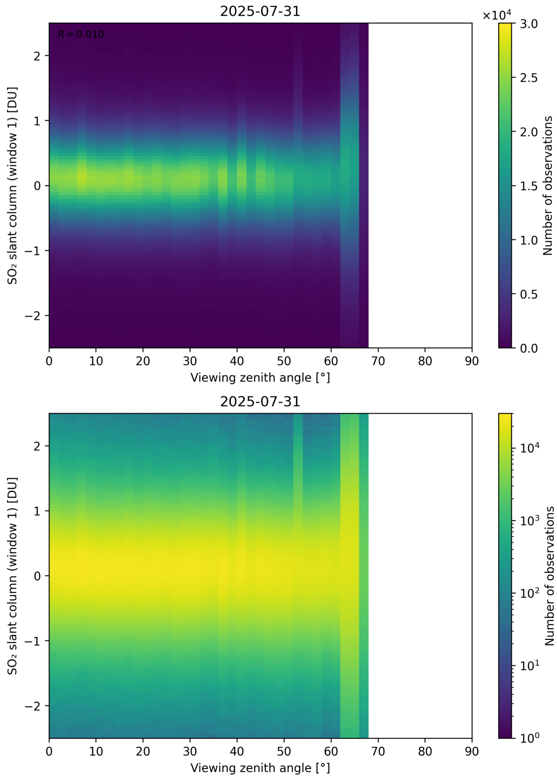
Figure 376: Scatter density plot of “Viewing zenith angle” against “SO 2 slant column (window 1)” for 2025-07-30 to 2025-08-01.
