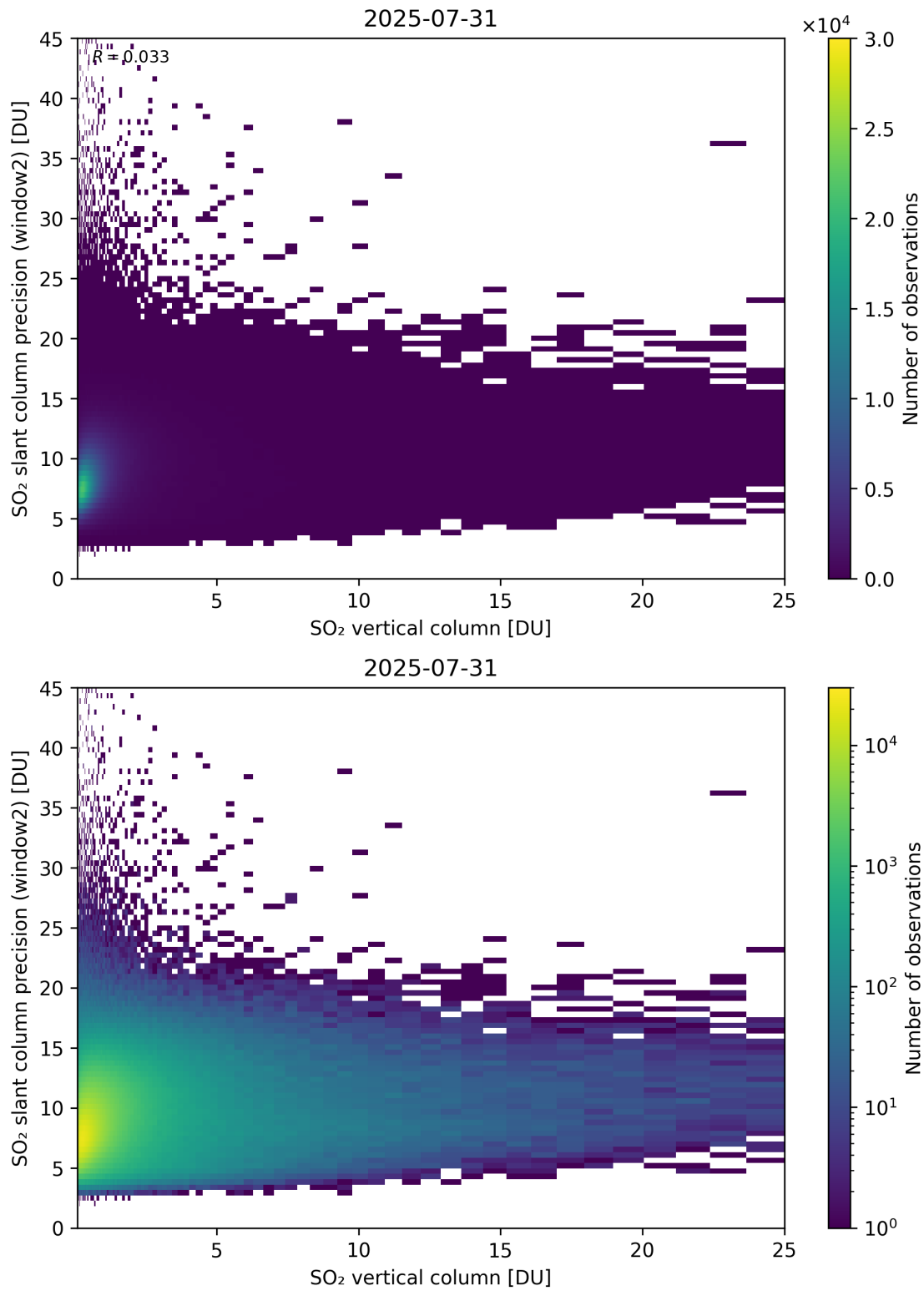
Figure 356: Scatter density plot of “SO 2 vertical column” against “SO 2 slant column precision (window2)” for 2025-07-30 to 2025-08-01.
