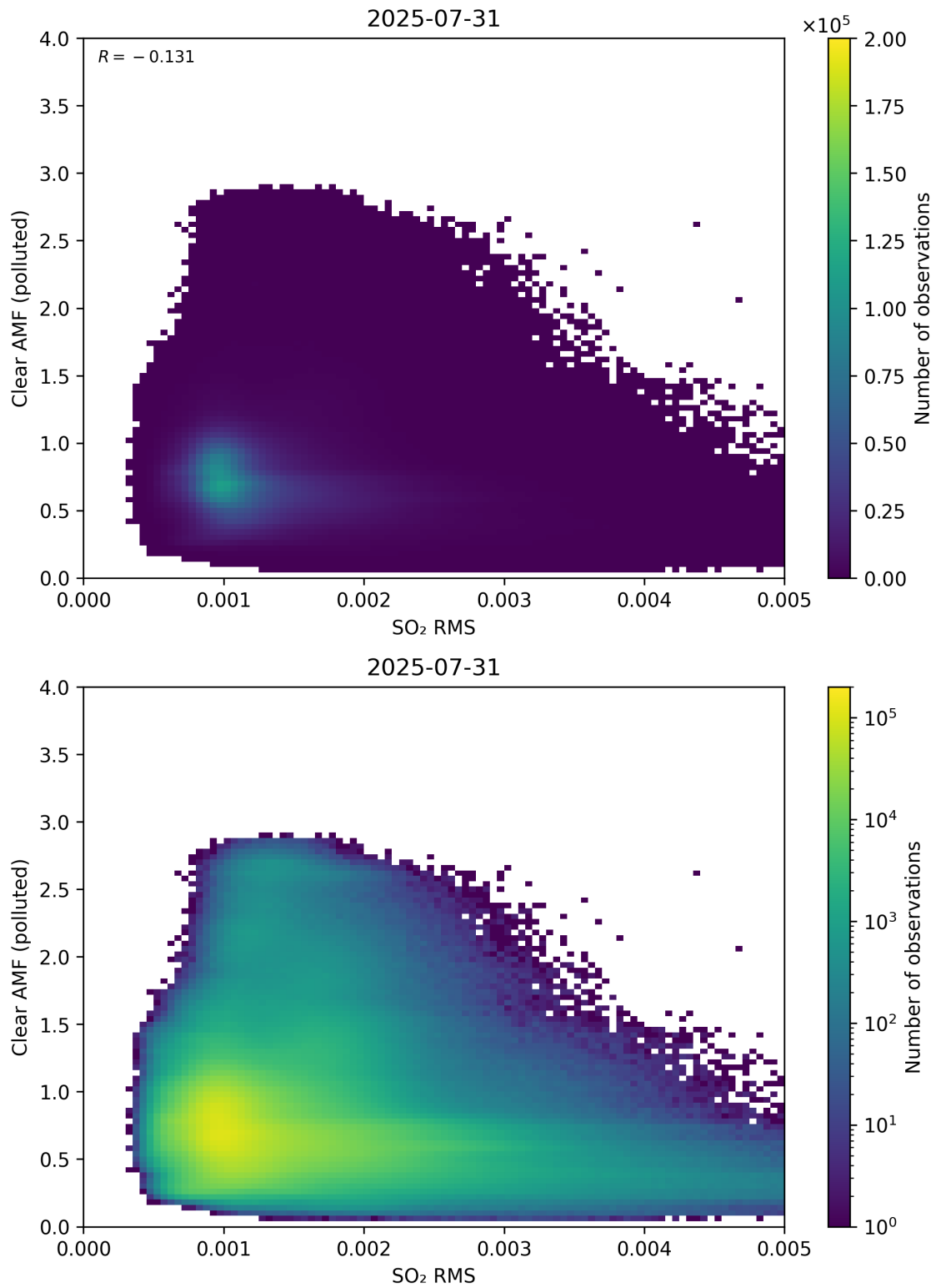
Figure 147: Scatter density plot of “SO 2 RMS” against “Clear AMF (polluted)” for 2025-07-30 to 2025-08-01.
