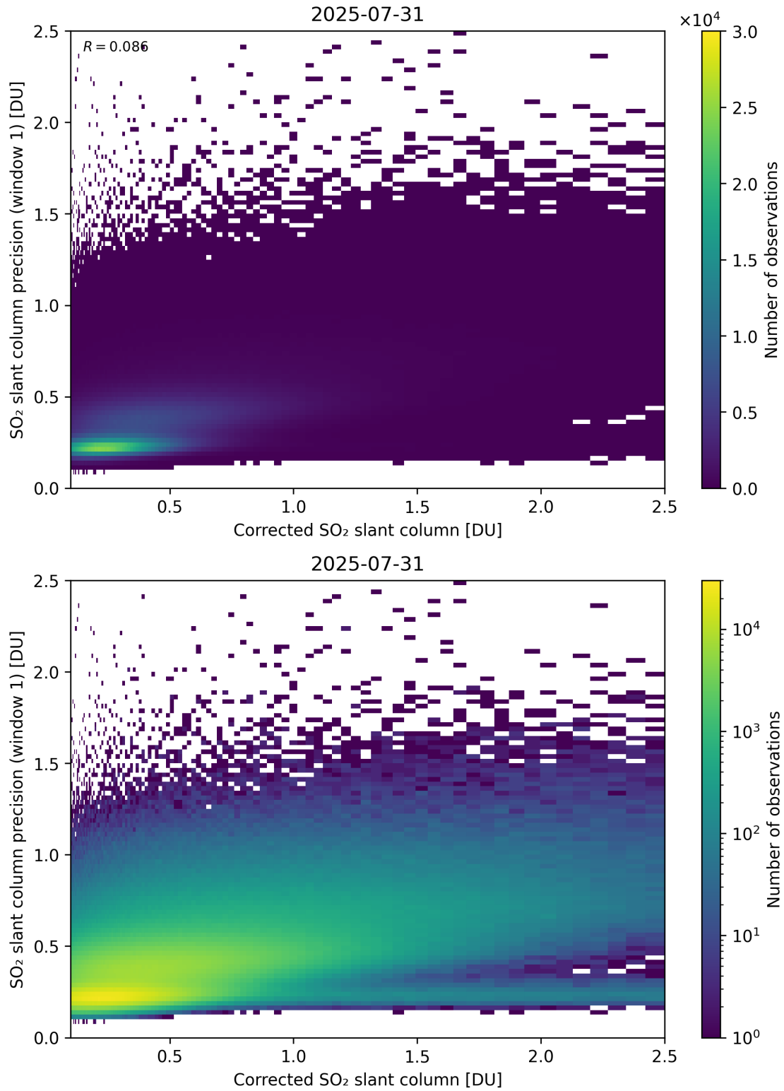
Figure 238: Scatter density plot of “Corrected SO 2 slant column” against “SO 2 slant column precision (window 1)” for 2025-07-30 to 2025-08-01.
