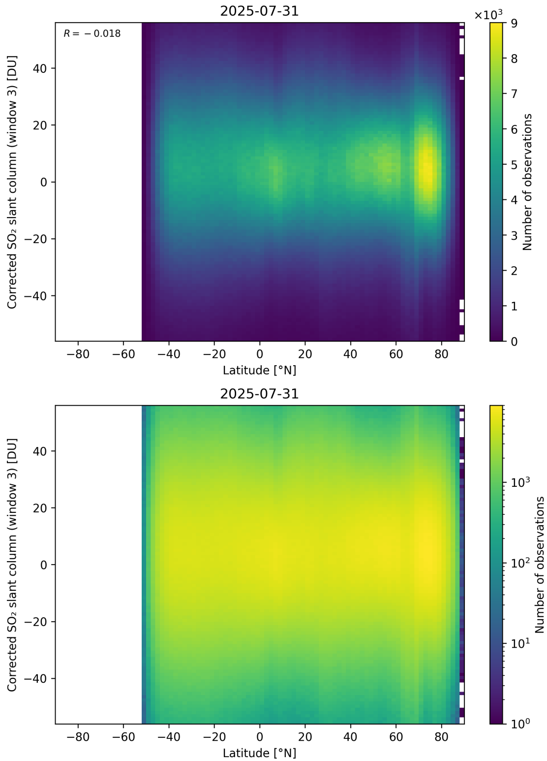
Figure 161: Scatter density plot of “Latitude” against “Corrected SO 2 slant column (window 3)” for 2025-07-30 to 2025-08-01.
