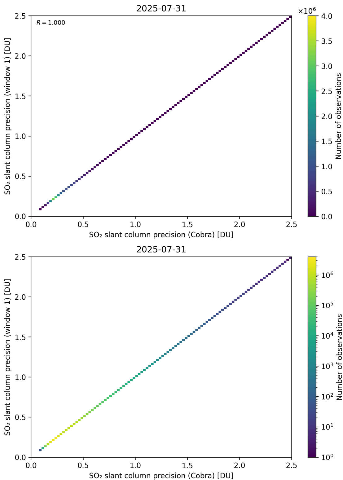
Figure 209: Scatter density plot of “SO 2 slant column precision (Cobra)” against “SO 2 slant column precision (window 1)” for 2025-07-30 to 2025-08-01.
