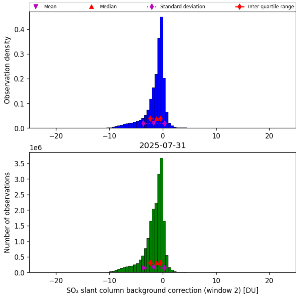
Figure 70: Histogram of “SO 2 slant column background correction (window 2)” for 2025-07-30 to 2025-08-01
