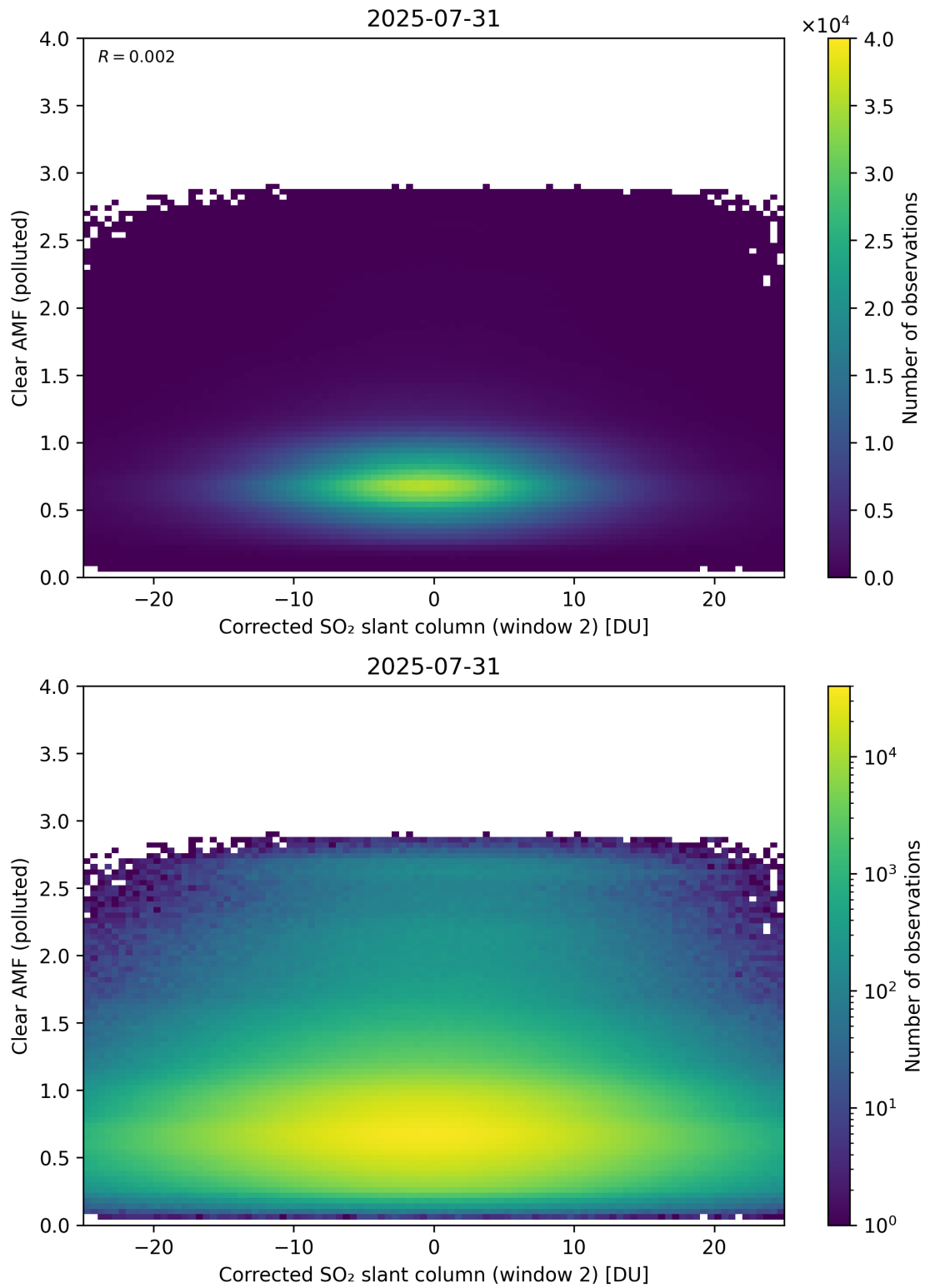
Figure 249: Scatter density plot of “Corrected SO 2 slant column (window 2)” against “Clear AMF (polluted)” for 2025-07-30 to 2025-08-01.
