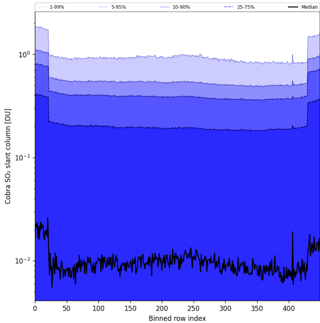
Figure 87: Along track statistics of “Cobra SO 2 slant column” for 2025-07-30 to 2025-08-01
