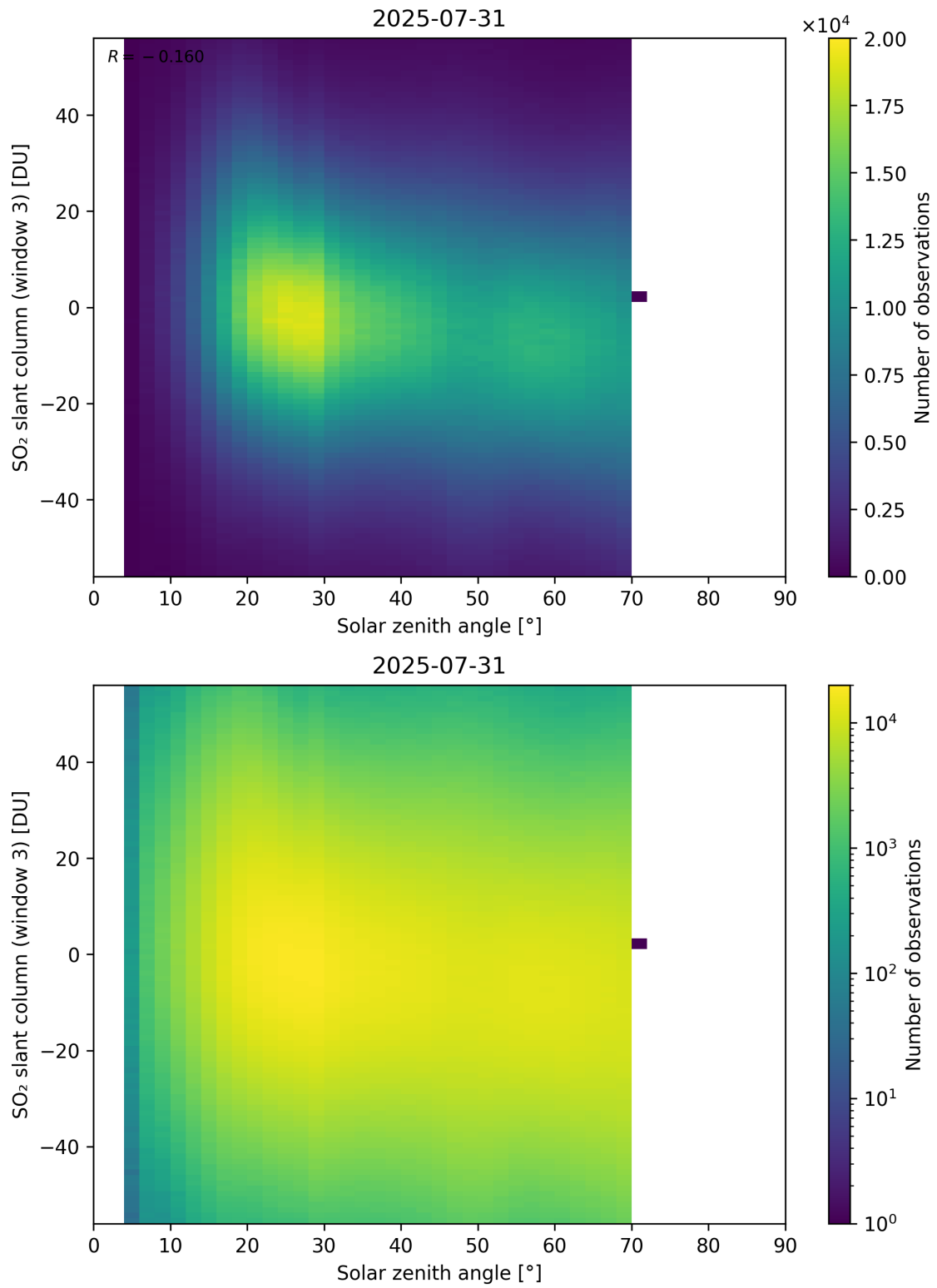
Figure 187: Scatter density plot of “Solar zenith angle” against “SO 2 slant column (window 3)” for 2025-07-30 to 2025-08-01.
