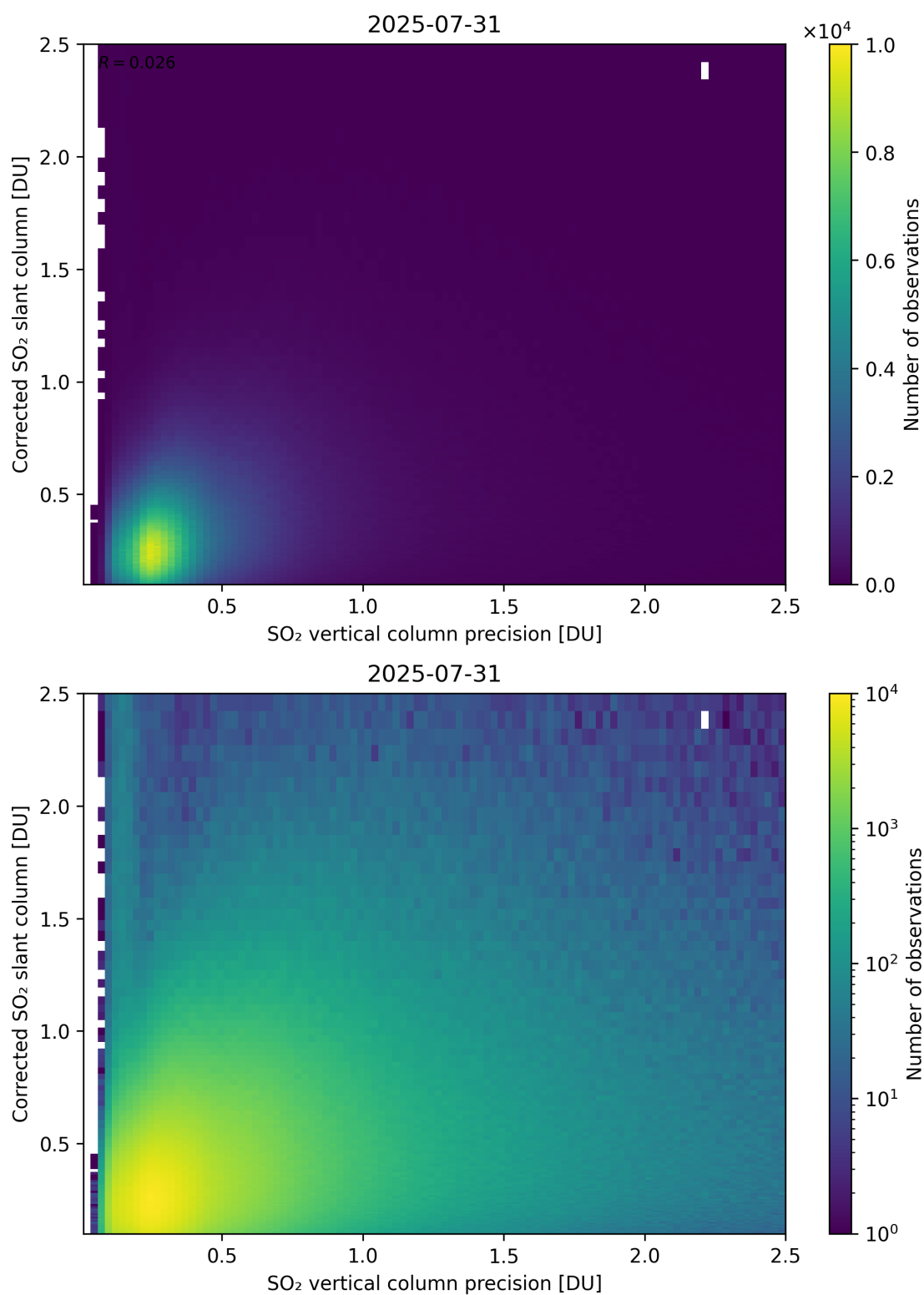
Figure 338: Scatter density plot of “SO 2 vertical column precision” against “Corrected SO 2 slant column” for 2025-07-30 to 2025-08-01.
