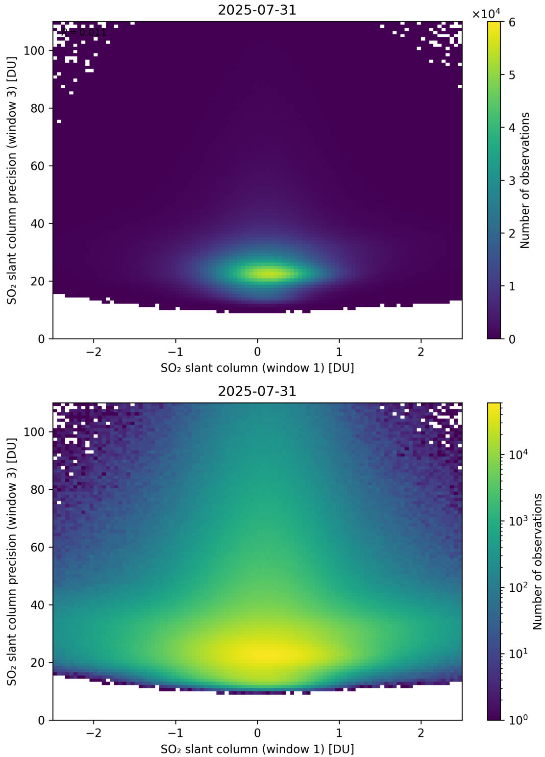
Figure 288: Scatter density plot of “SO 2 slant column (window 1)” against “SO 2 slant column precision (window 3)” for 2025-07-30 to 2025-08-01.
