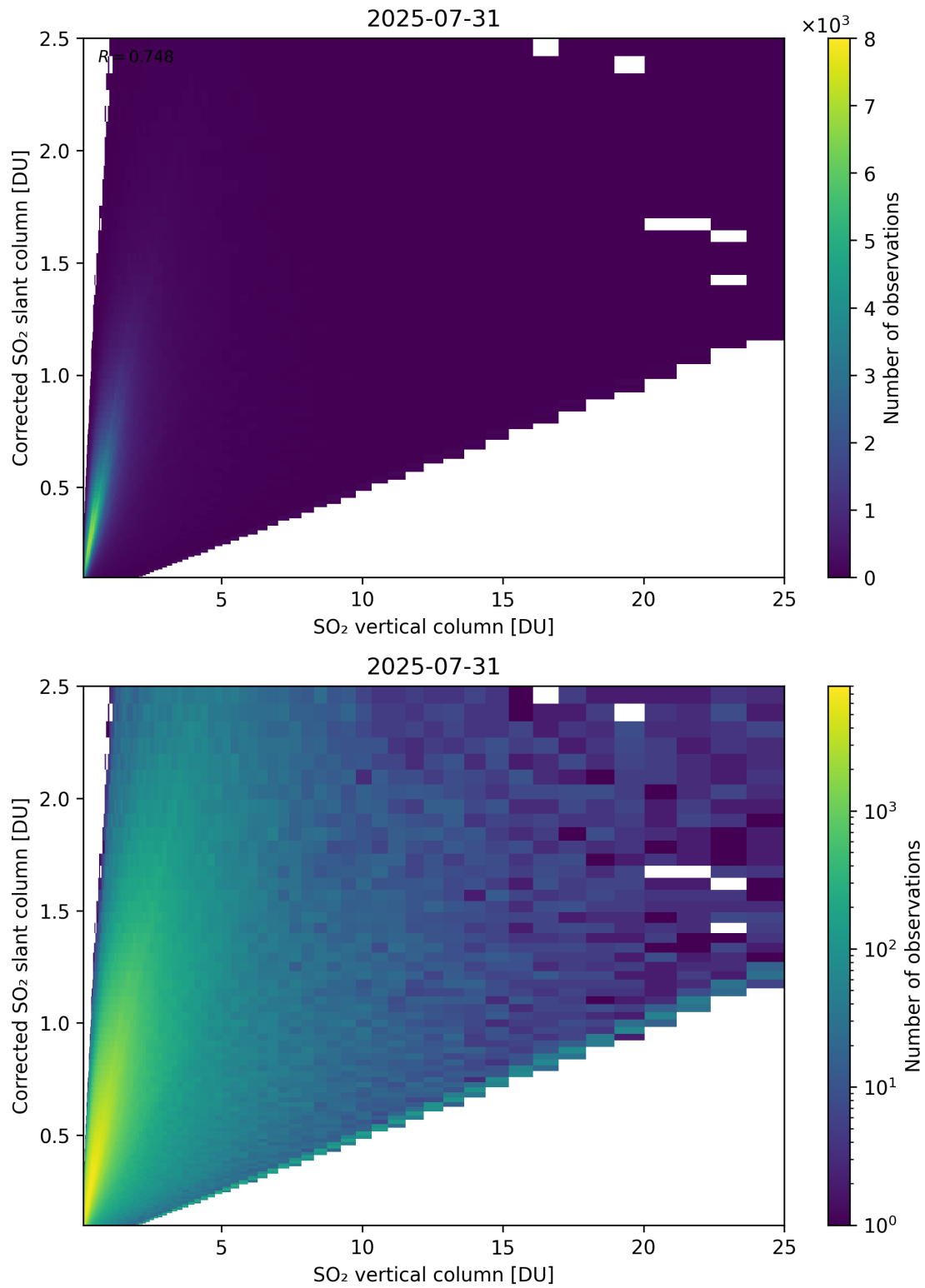
Figure 351: Scatter density plot of “SO 2 vertical column” against “Corrected SO 2 slant column” for 2025-07-30 to 2025-08-01.
