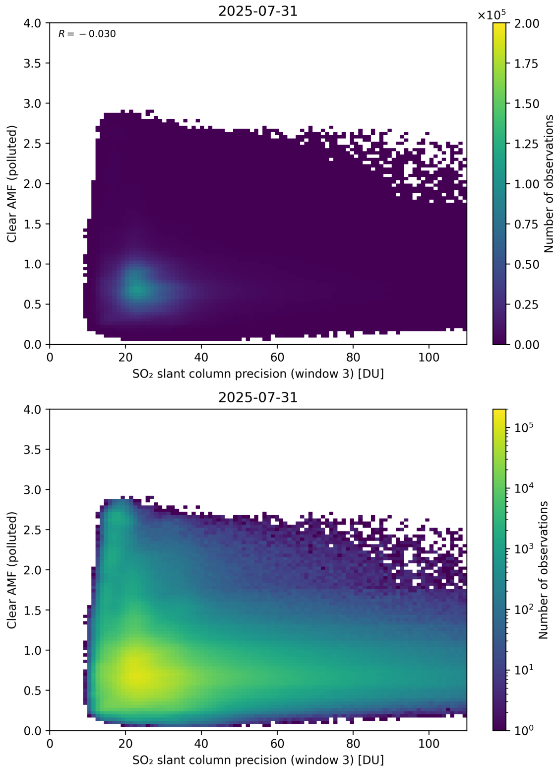
Figure 311: Scatter density plot of “SO 2 slant column precision (window 3)” against “Clear AMF (polluted)” for 2025-07-30 to 2025-08-01.
