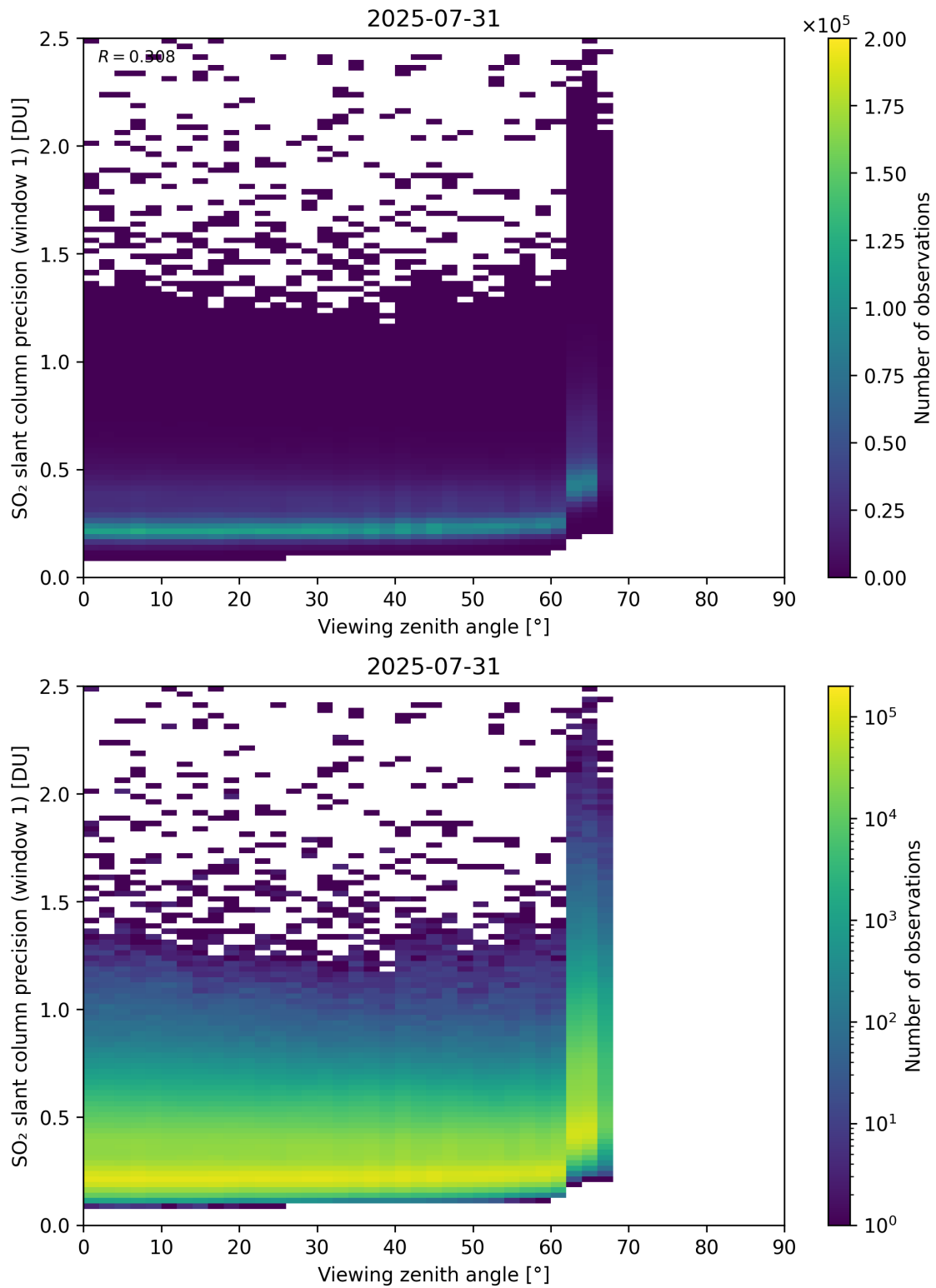
Figure 377: Scatter density plot of “Viewing zenith angle” against “SO 2 slant column precision (window 1)” for 2025-07-30 to 2025-08-01.
