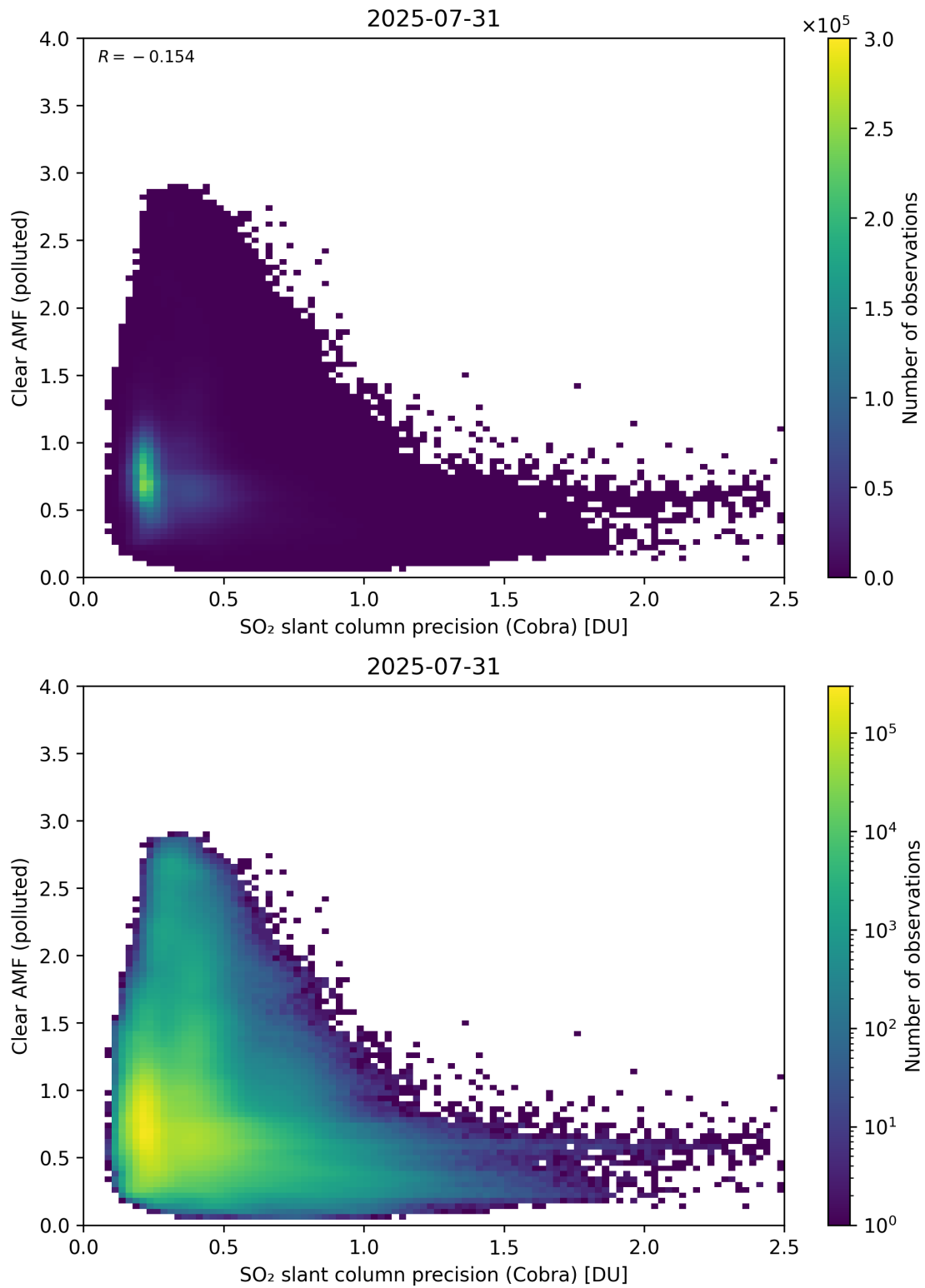
Figure 205: Scatter density plot of “SO 2 slant column precision (Cobra)” against “Clear AMF (polluted)” for 2025-07-30 to 2025-08-01.
