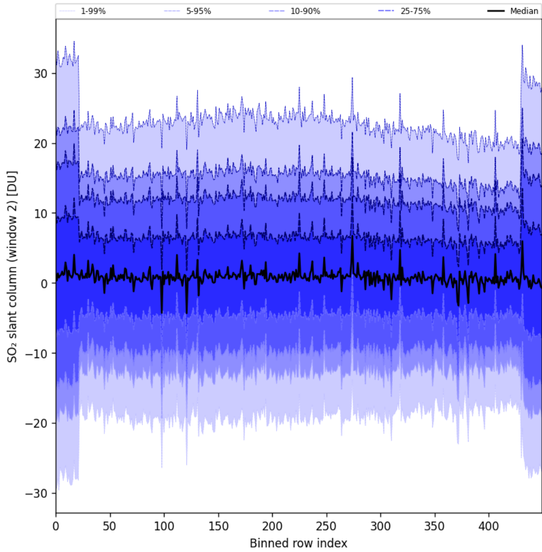
Figure 93: Along track statistics of “SO 2 slant column (window 2)” for 2025-07-30 to 2025-08-01
