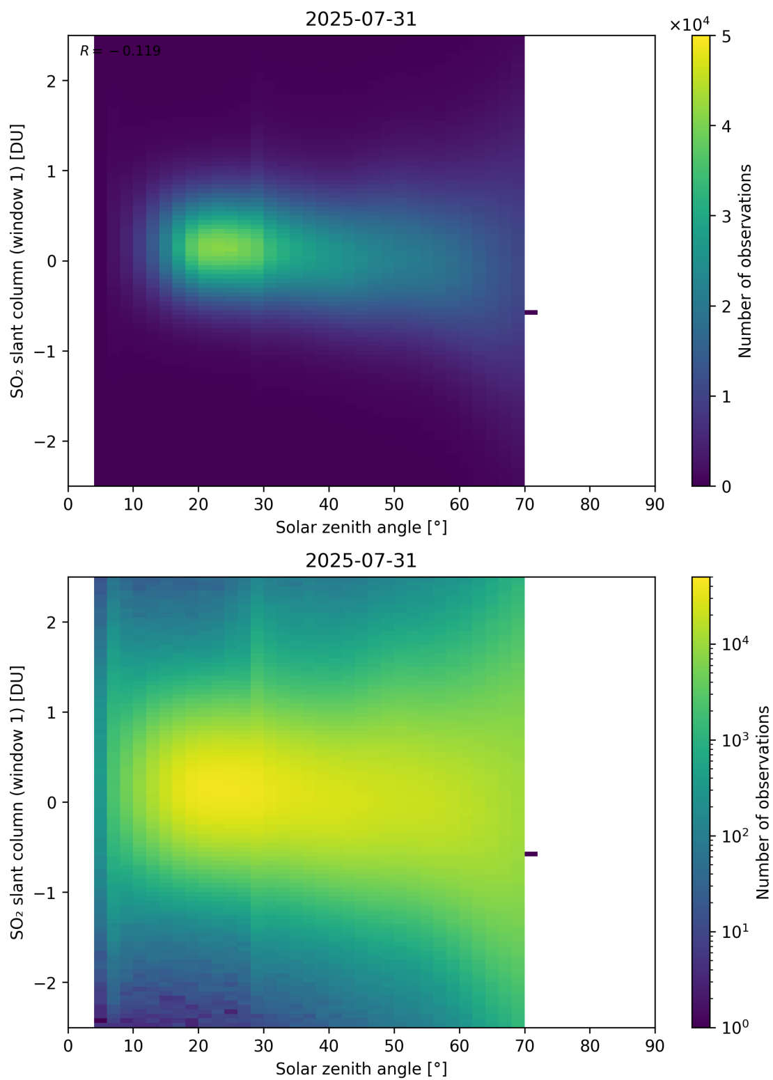
Figure 184: Scatter density plot of “Solar zenith angle” against “SO 2 slant column (window 1)” for 2025-07-30 to 2025-08-01.
