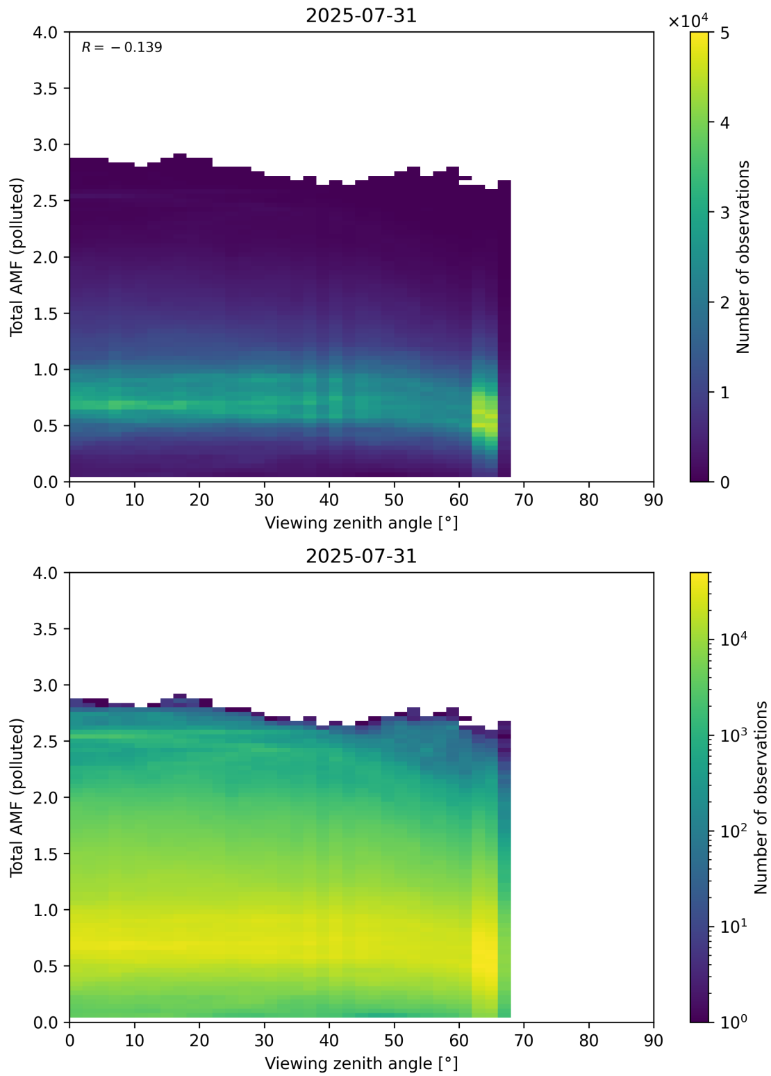
Figure 381: Scatter density plot of “Viewing zenith angle” against “Total AMF (polluted)” for 2025-07-30 to 2025-08-01.
