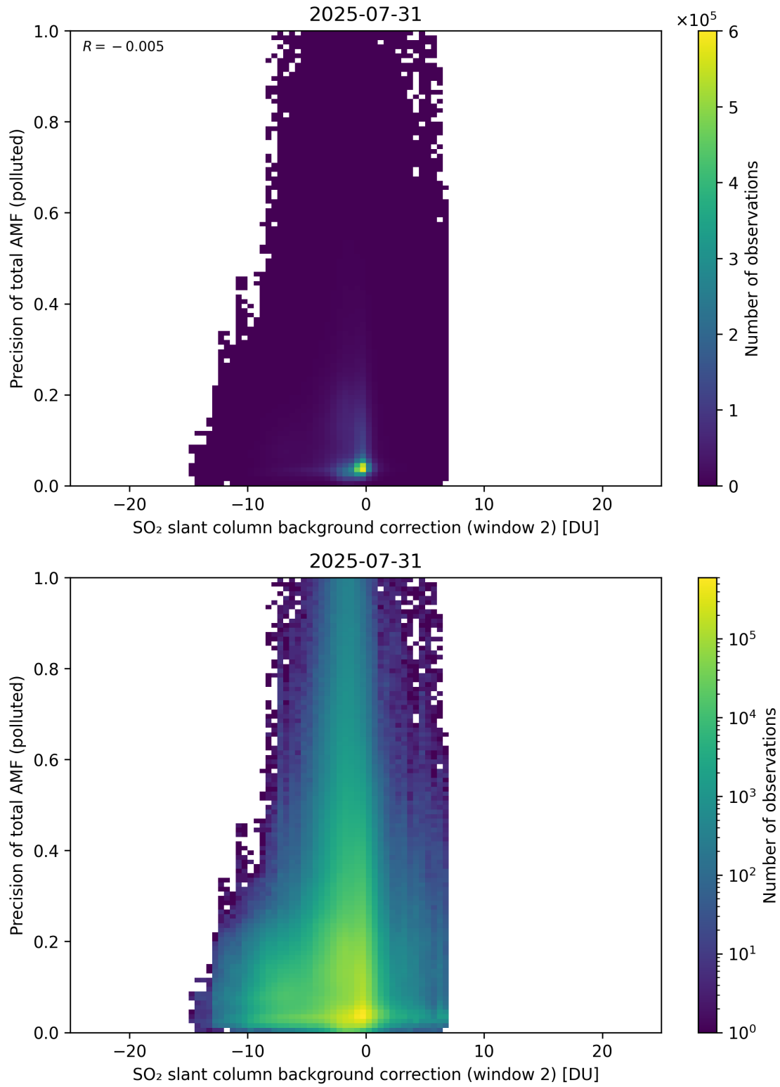
Figure 131: Scatter density plot of “SO 2 slant column background correction (window 2)” against “Precision of total AMF (polluted)” for 2025-07-30 to 2025-08-01.
