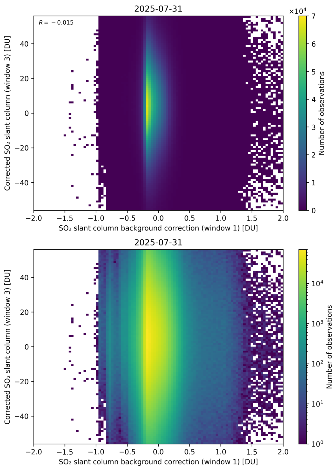
Figure 116: Scatter density plot of “SO 2 slant column background correction (window 1)” against “Corrected SO 2 slant column (window 3)” for 2025-07-30 to 2025-08-01.
