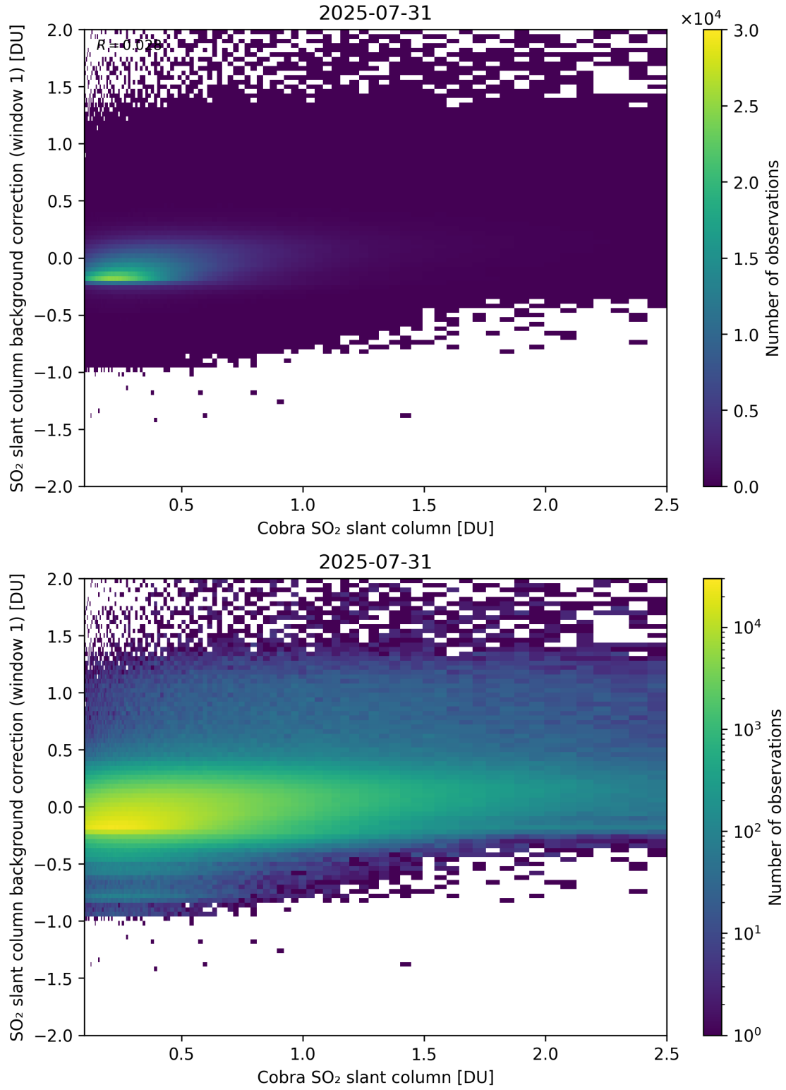
Figure 193: Scatter density plot of “Cobra SO 2 slant column” against “SO 2 slant column background correction (window 1)” for 2025-07-30 to 2025-08-01.
