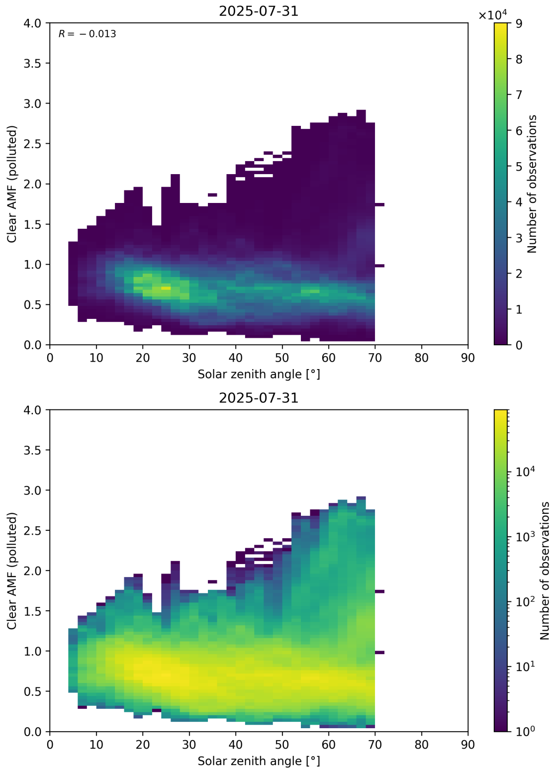
Figure 178: Scatter density plot of “Solar zenith angle” against “Clear AMF (polluted)” for 2025-07-30 to 2025-08-01.
