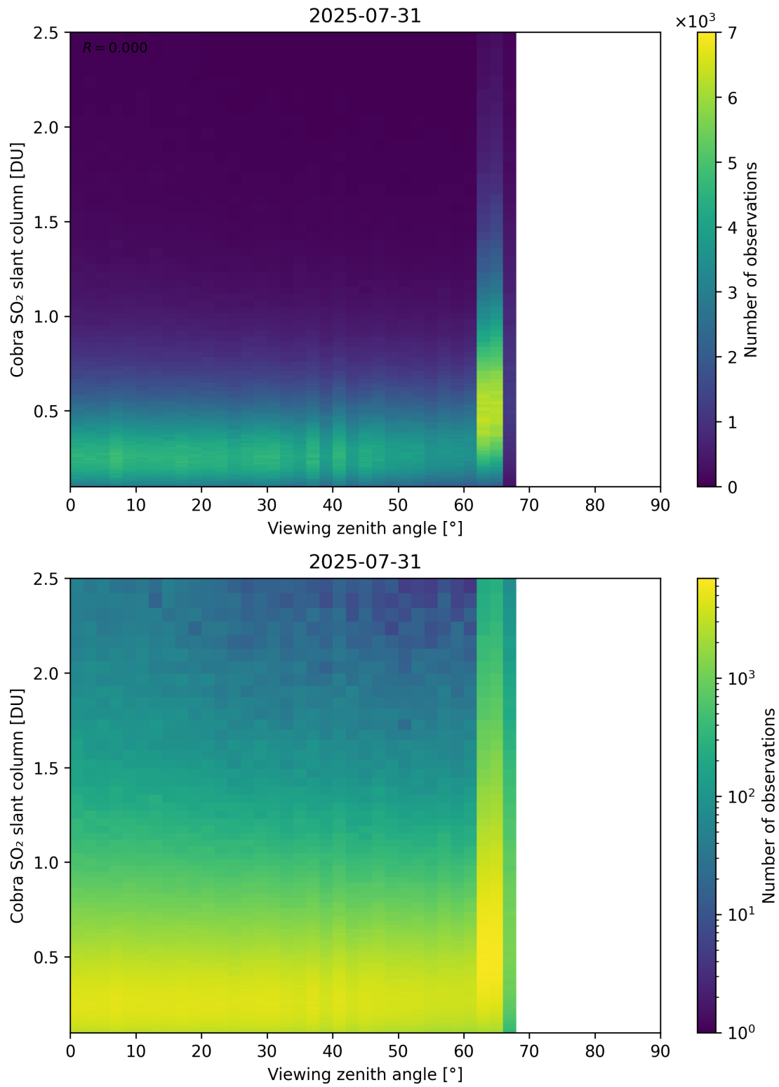
Figure 371: Scatter density plot of “Viewing zenith angle” against “Cobra SO 2 slant column” for 2025-07-30 to 2025-08-01.
