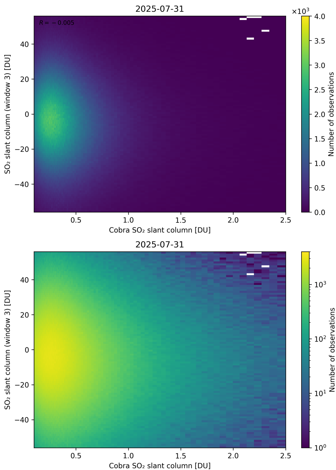
Figure 222: Scatter density plot of “Cobra SO 2 slant column” against “SO 2 slant column (window 3)” for 2025-07-30 to 2025-08-01.
