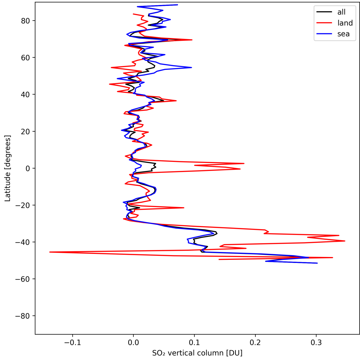
Figure 32: Zonal average of “SO 2 vertical column” for 2025-07-30 to 2025-08-01.
