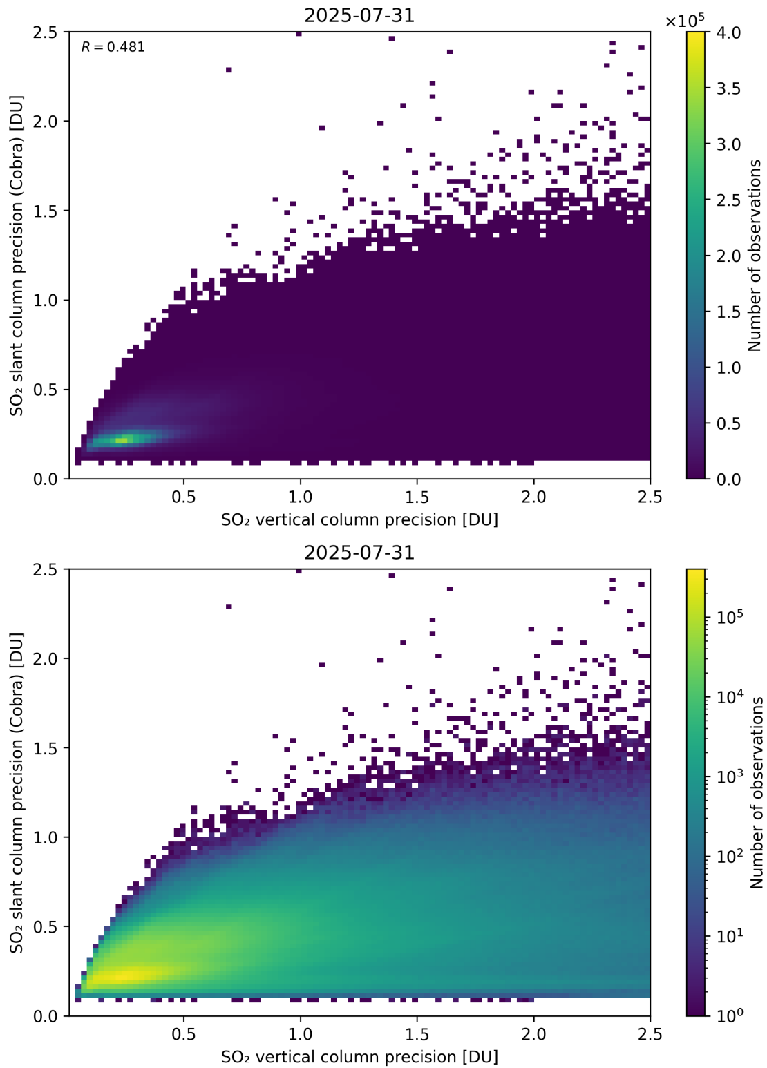
Figure 337: Scatter density plot of “SO 2 vertical column precision” against “SO 2 slant column precision (Cobra)” for 2025-07-30 to 2025-08-01.
