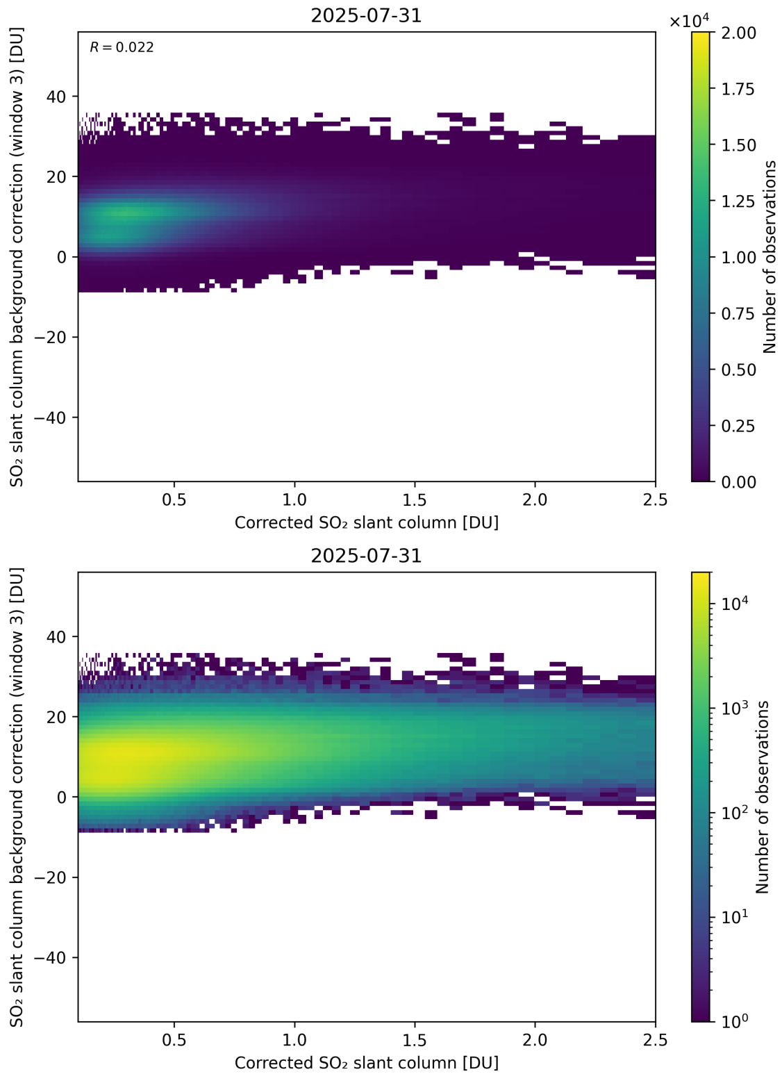
Figure 228: Scatter density plot of “Corrected SO 2 slant column” against “SO 2 slant column background correction (window 3)” for 2025-07-30 to 2025-08-01.
