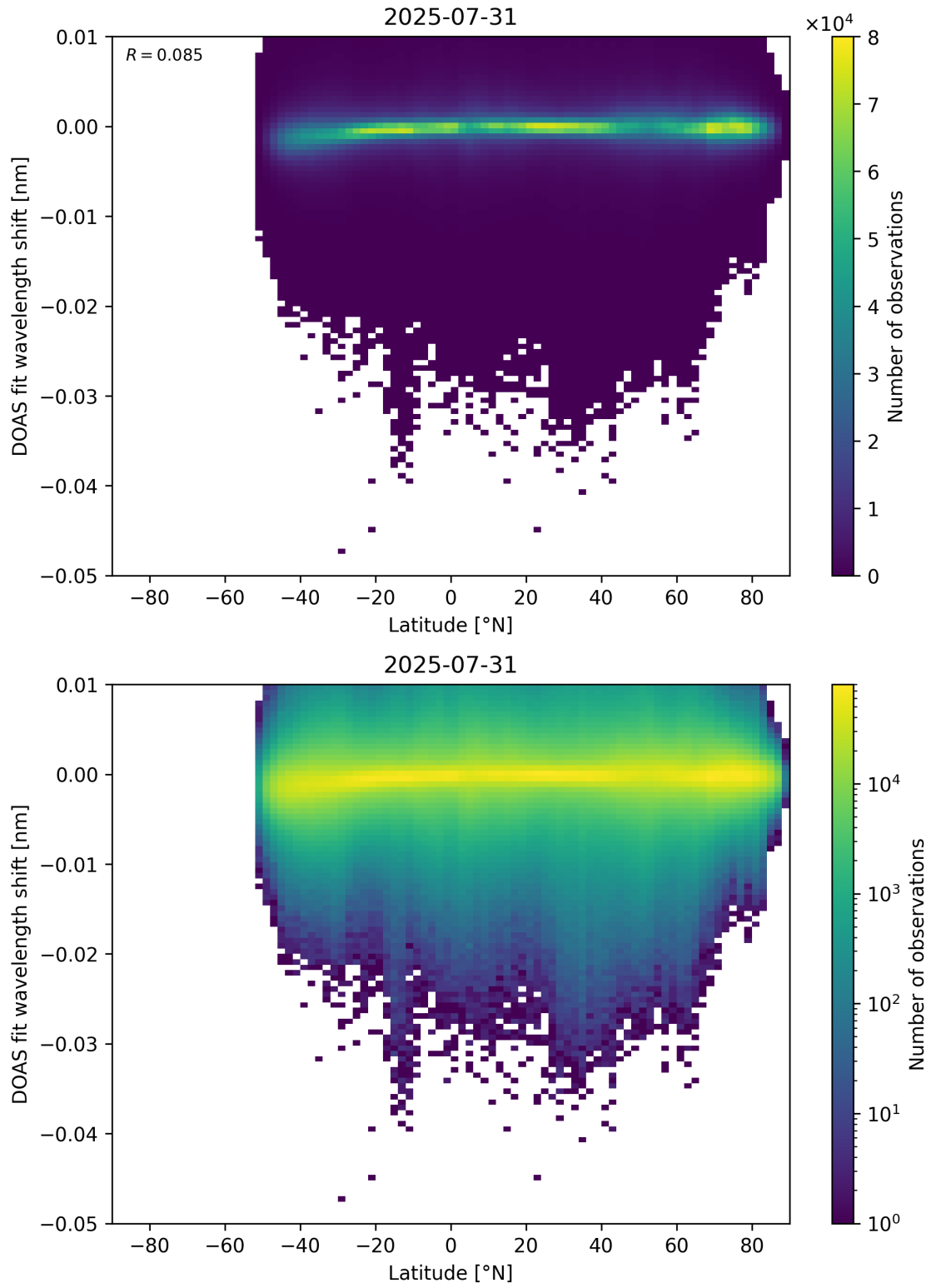
Figure 153: Scatter density plot of “Latitude” against “DOAS fit wavelength shift” for 2025-07-30 to 2025-08-01.
