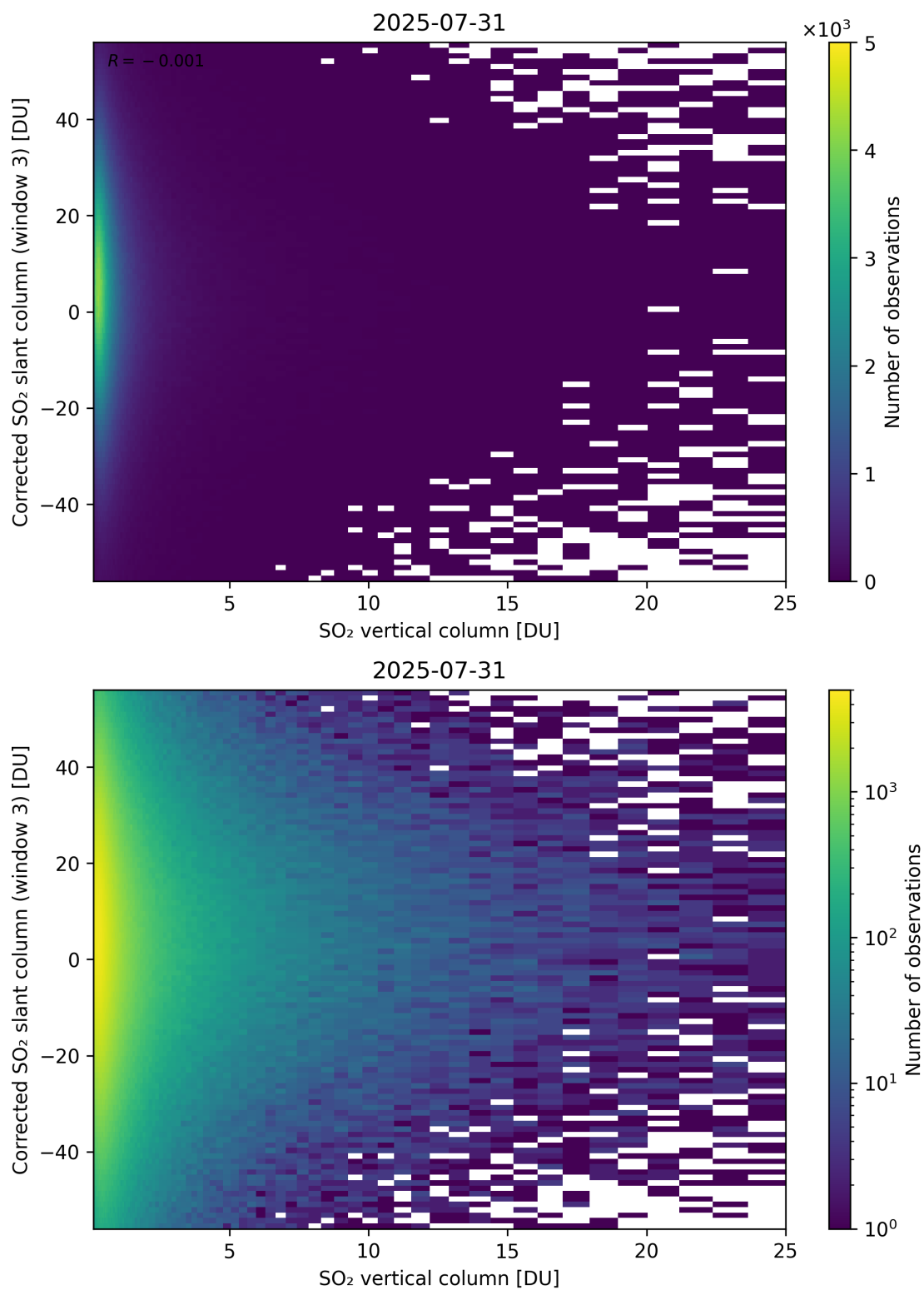
Figure 353: Scatter density plot of “SO 2 vertical column” against “Corrected SO 2 slant column (window 3)” for 2025-07-30 to 2025-08-01.
