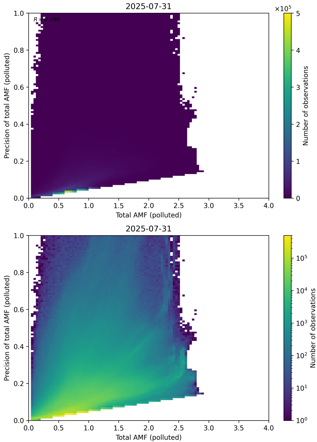
Figure 322: Scatter density plot of “Total AMF (polluted)” against “Precision of total AMF (polluted)” for 2025-07-30 to 2025-08-01.
