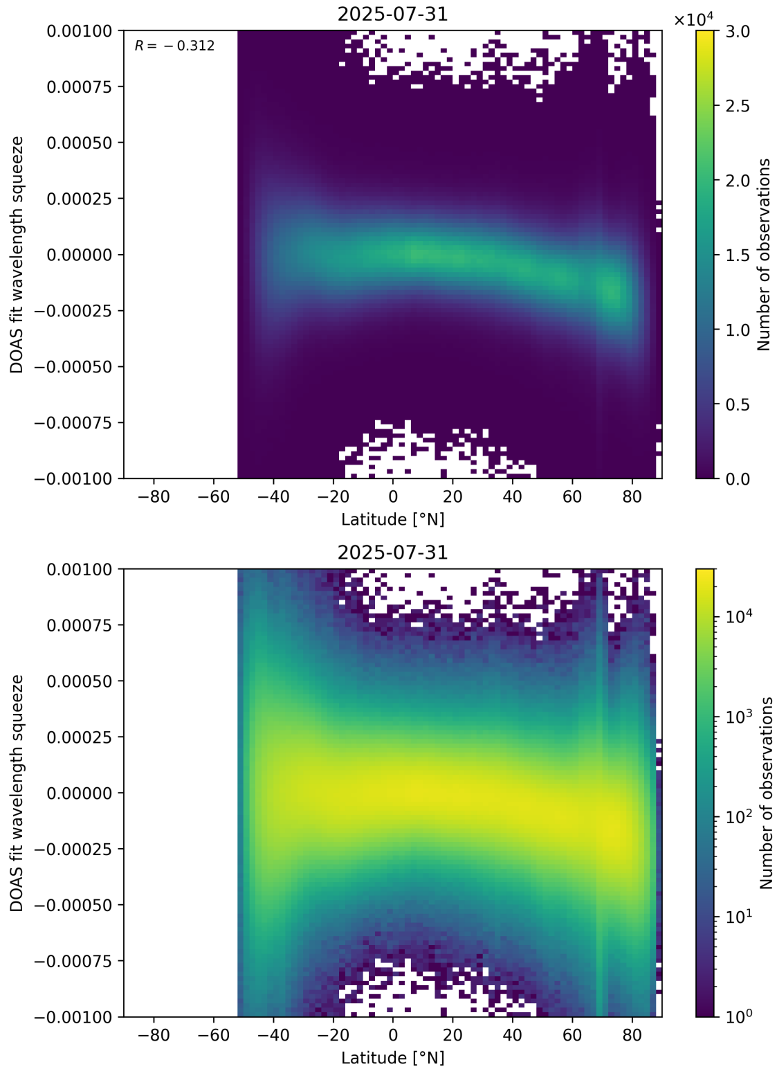
Figure 154: Scatter density plot of “Latitude” against “DOAS fit wavelength squeeze” for 2025-07-30 to 2025-08-01.
