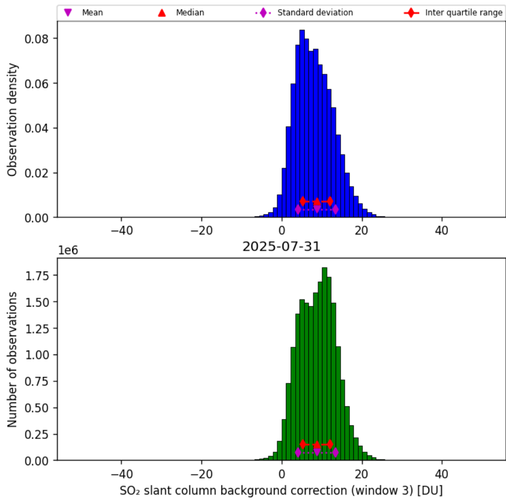
Figure 74: Histogram of “SO 2 slant column background correction (window 3)” for 2025-07-30 to 2025-08-01
