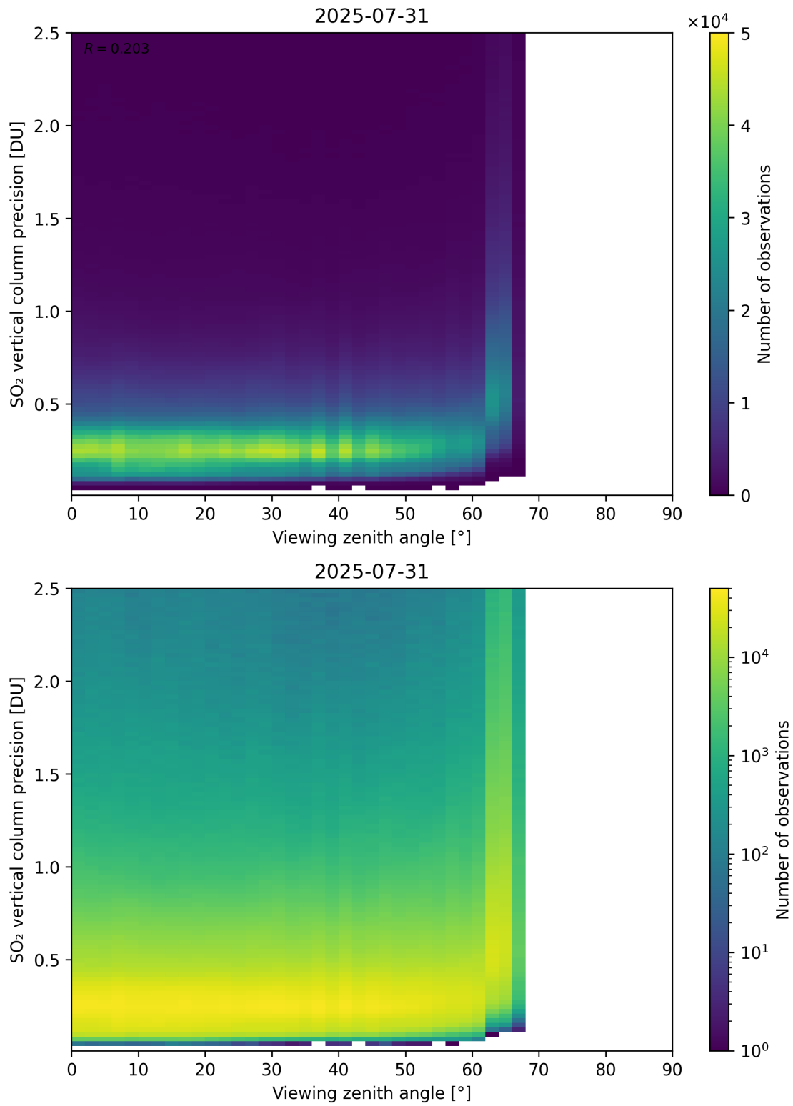
Figure 384: Scatter density plot of “Viewing zenith angle” against “SO 2 vertical column precision” for 2025-07-30 to 2025-08-01.
