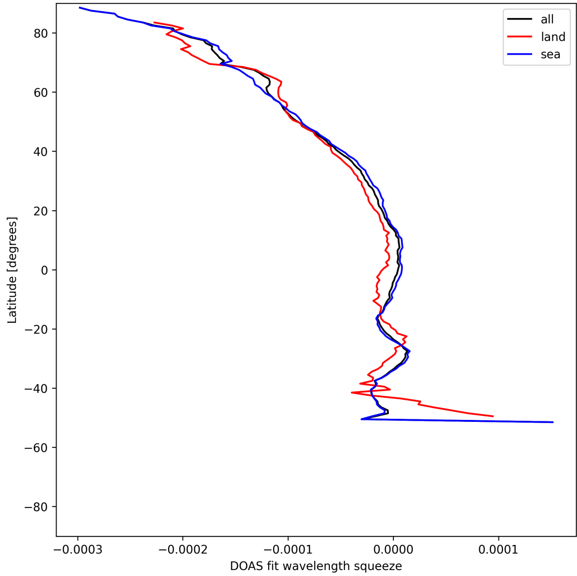
Figure 51: Zonal average of “DOAS fit wavelength squeeze” for 2025-07-30 to 2025-08-01.
