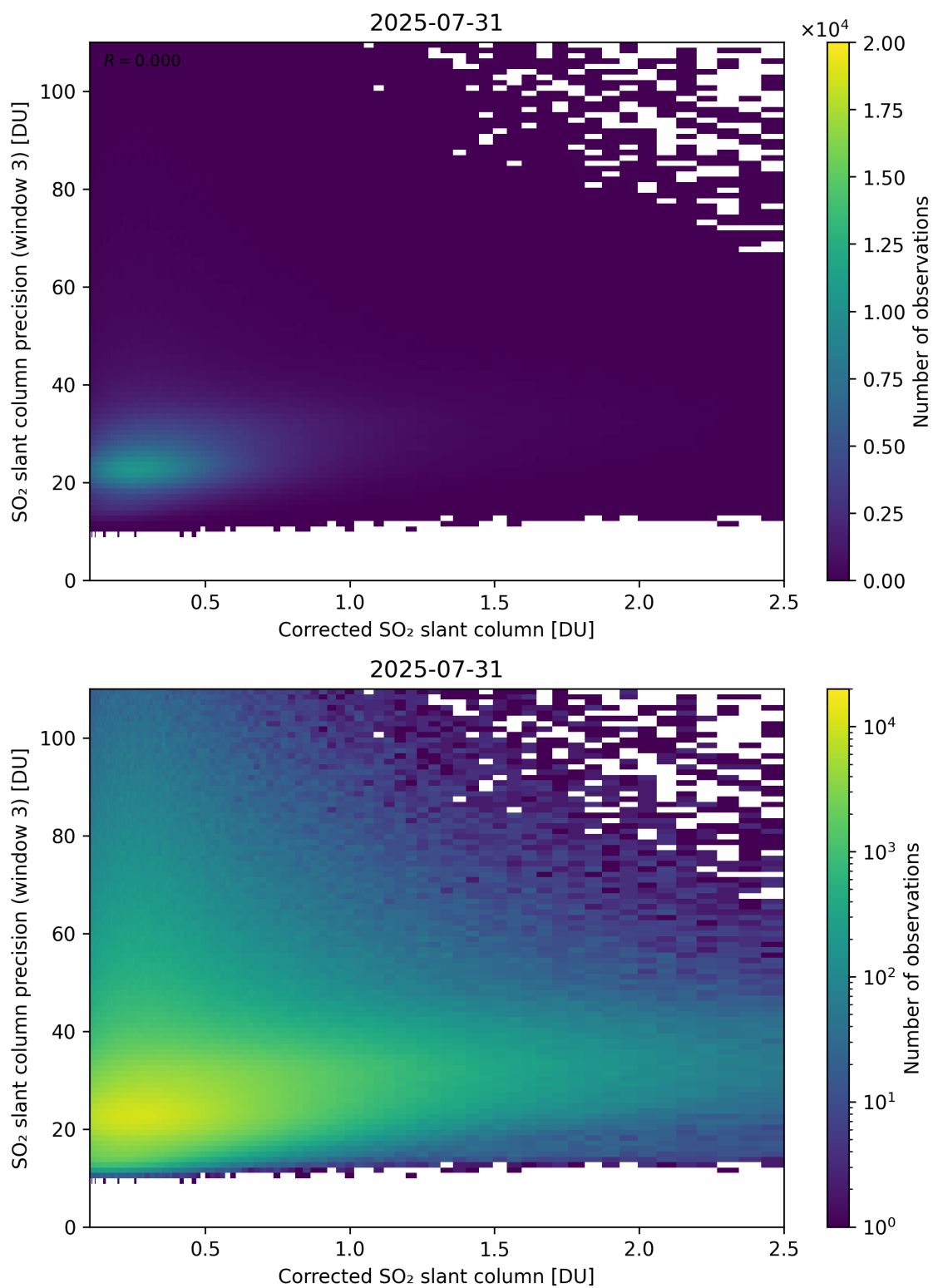
Figure 241: Scatter density plot of “Corrected SO 2 slant column” against “SO 2 slant column precision (window 3)” for 2025-07-30 to 2025-08-01.
