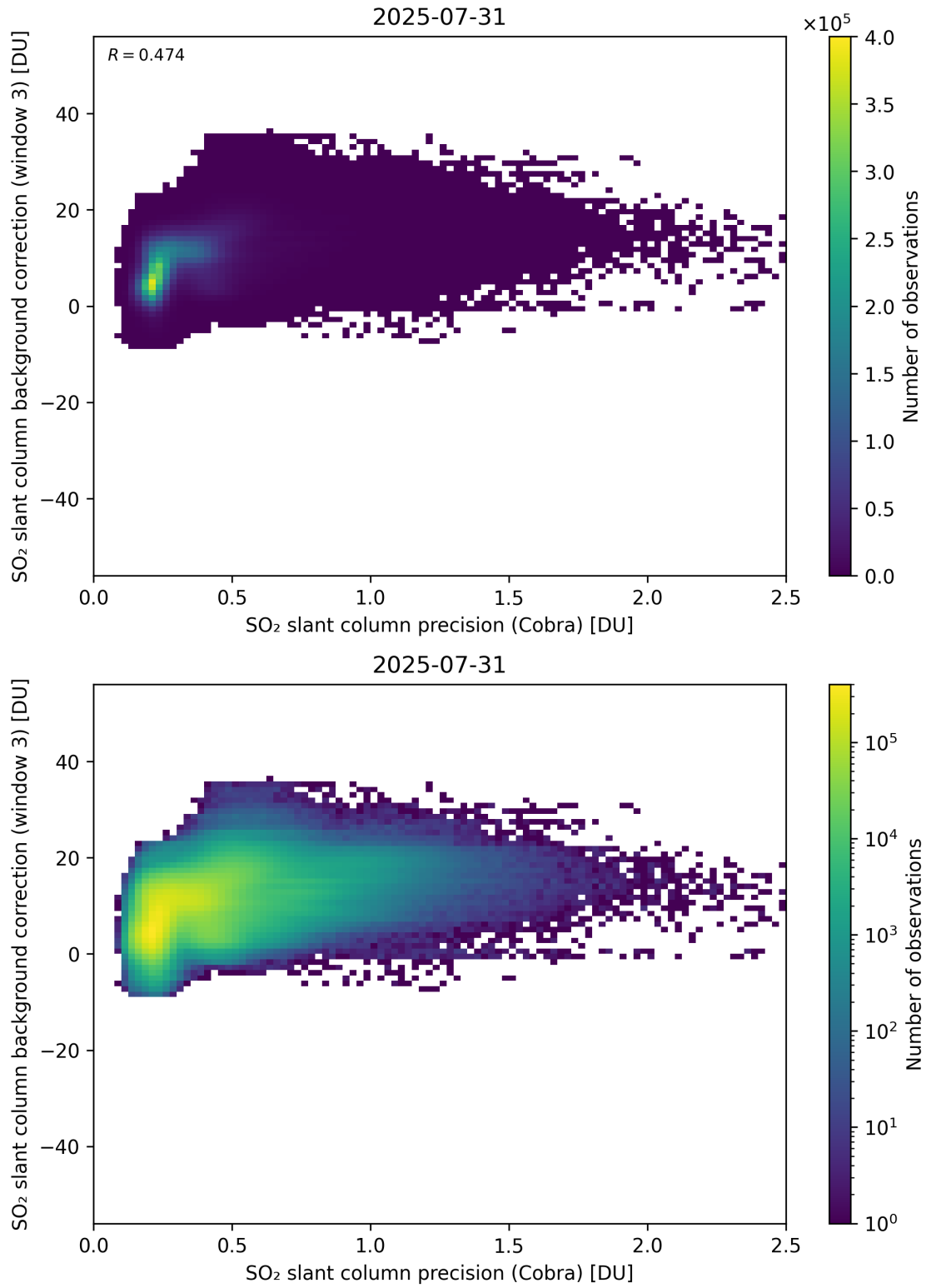
Figure 201: Scatter density plot of “SO 2 slant column precision (Cobra)” against “SO 2 slant column background correction (window 3)” for 2025-07-30 to 2025-08-01.
