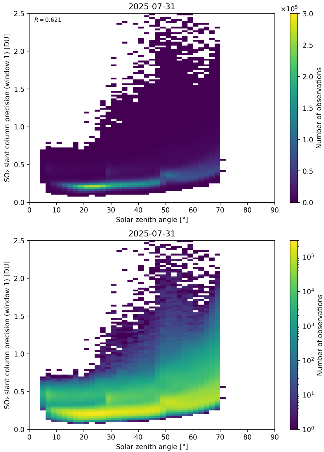
Figure 185: Scatter density plot of “Solar zenith angle” against “SO 2 slant column precision (window 1)” for 2025-07-30 to 2025-08-01.
