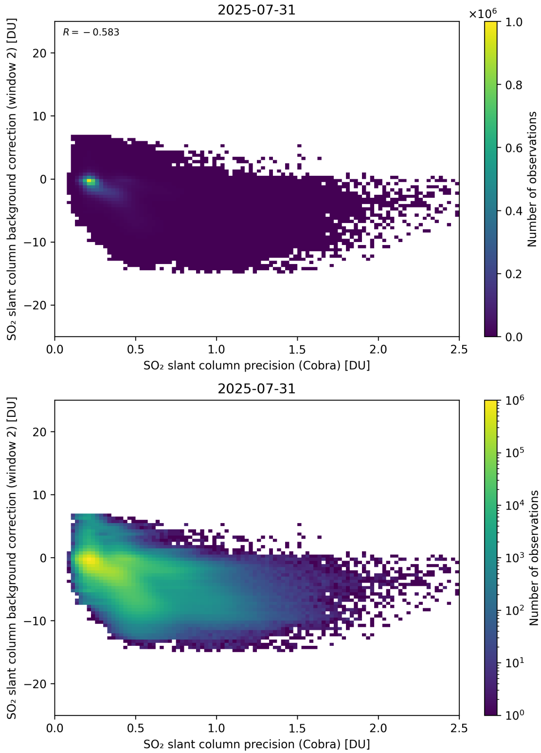
Figure 200: Scatter density plot of “SO 2 slant column precision (Cobra)” against “SO 2 slant column background correction (window 2)” for 2025-07-30 to 2025-08-01.
