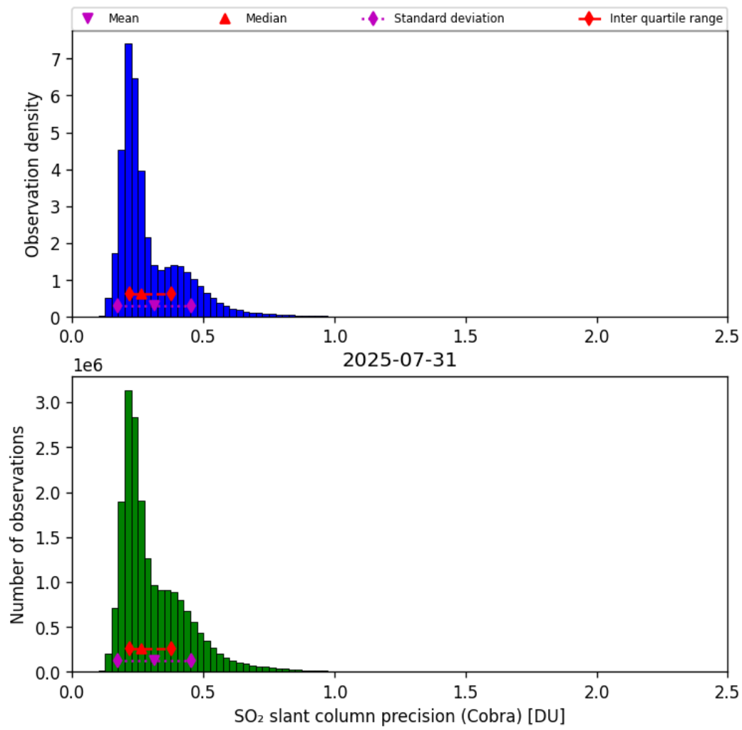
Figure 62: Histogram of “SO 2 slant column precision (Cobra)” for 2025-07-30 to 2025-08-01
