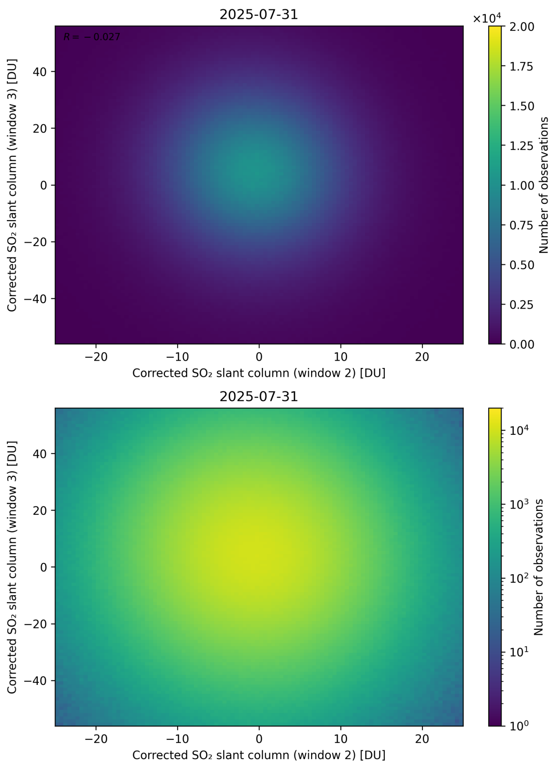
Figure 250: Scatter density plot of “Corrected SO 2 slant column (window 2)” against “Corrected SO 2 slant column (window 3)” for 2025-07-30 to 2025-08-01.
