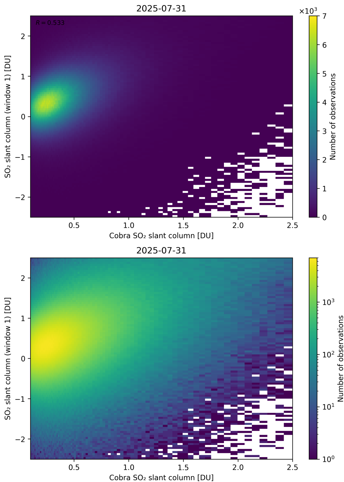
Figure 219: Scatter density plot of “Cobra SO 2 slant column” against “SO 2 slant column (window 1)” for 2025-07-30 to 2025-08-01.
