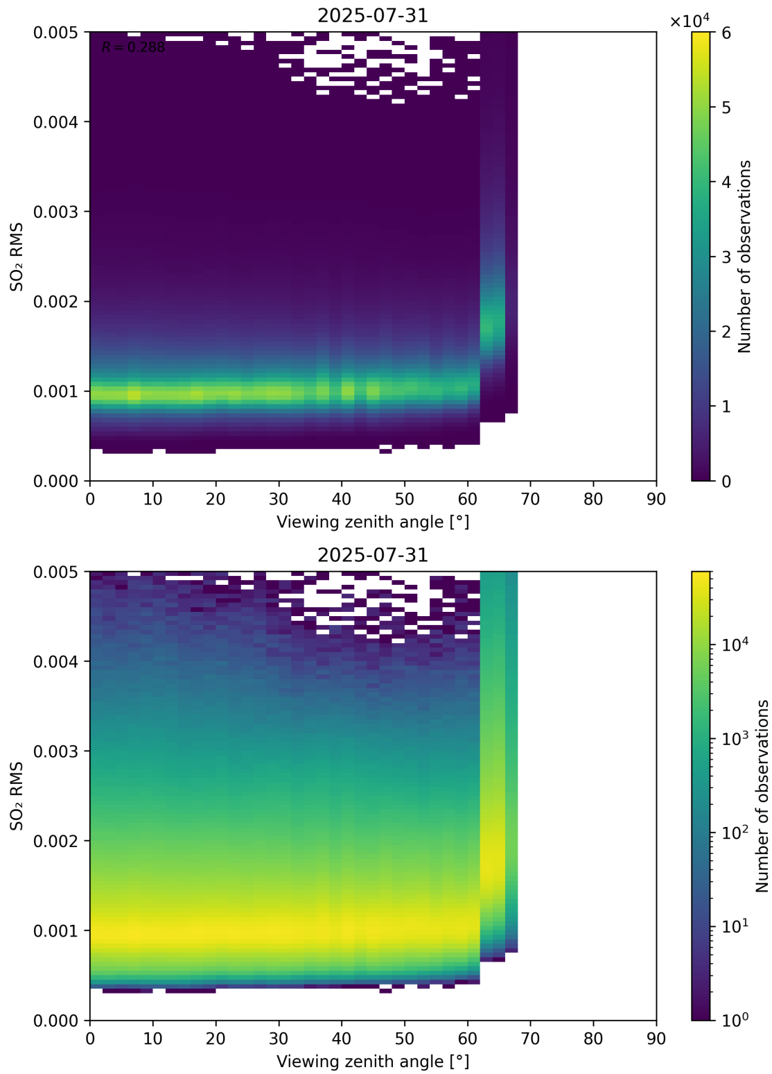
Figure 367: Scatter density plot of “Viewing zenith angle” against “SO 2 RMS” for 2025-07-30 to 2025-08-01.
