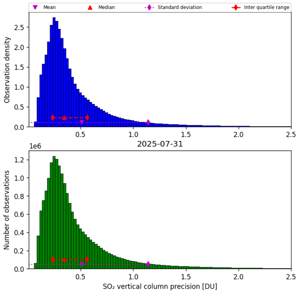
Figure 59: Histogram of “SO 2 vertical column precision” for 2025-07-30 to 2025-08-01
