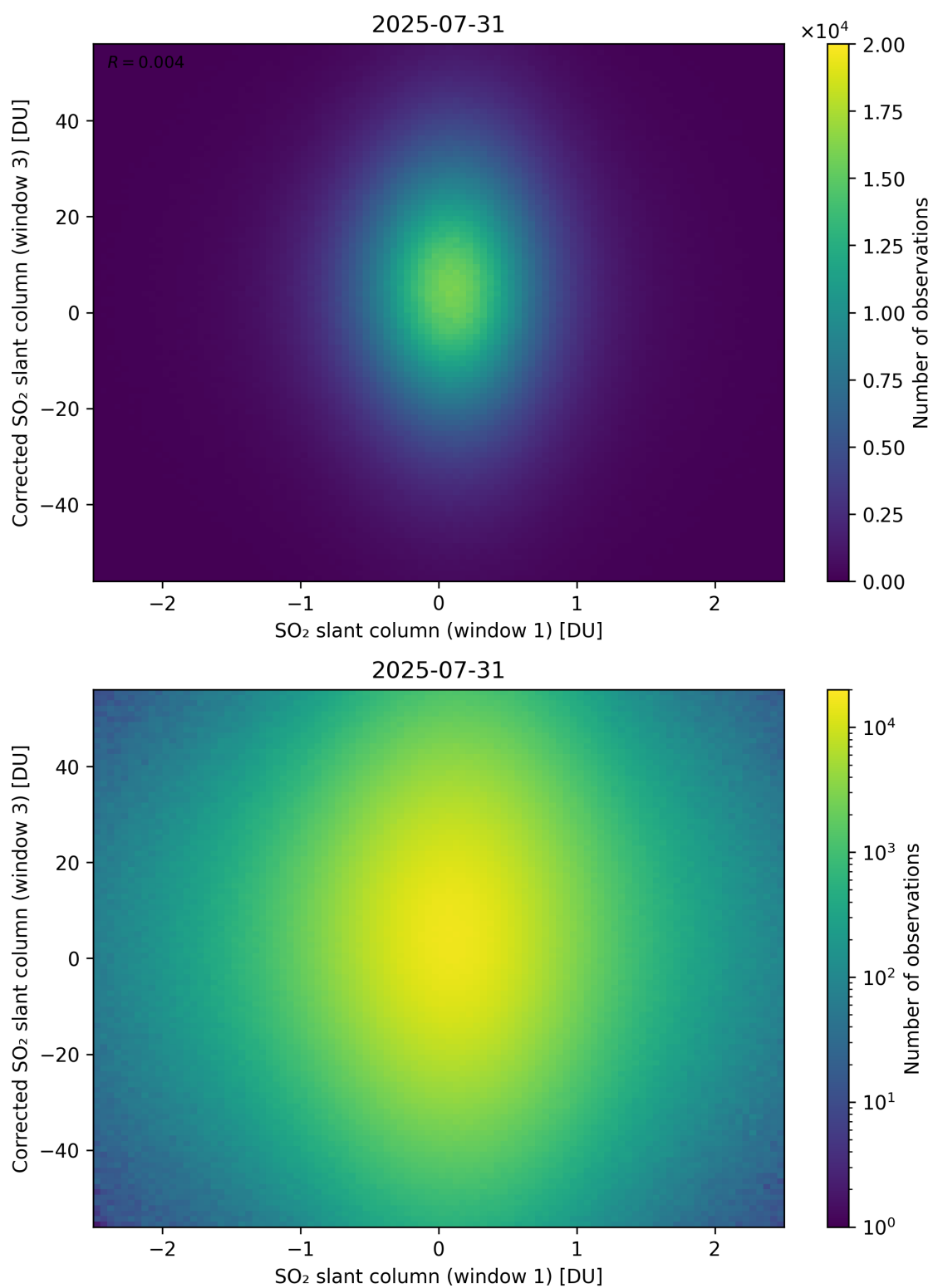
Figure 284: Scatter density plot of “SO 2 slant column (window 1)” against “Corrected SO 2 slant column (window 3)” for 2025-07-30 to 2025-08-01.
