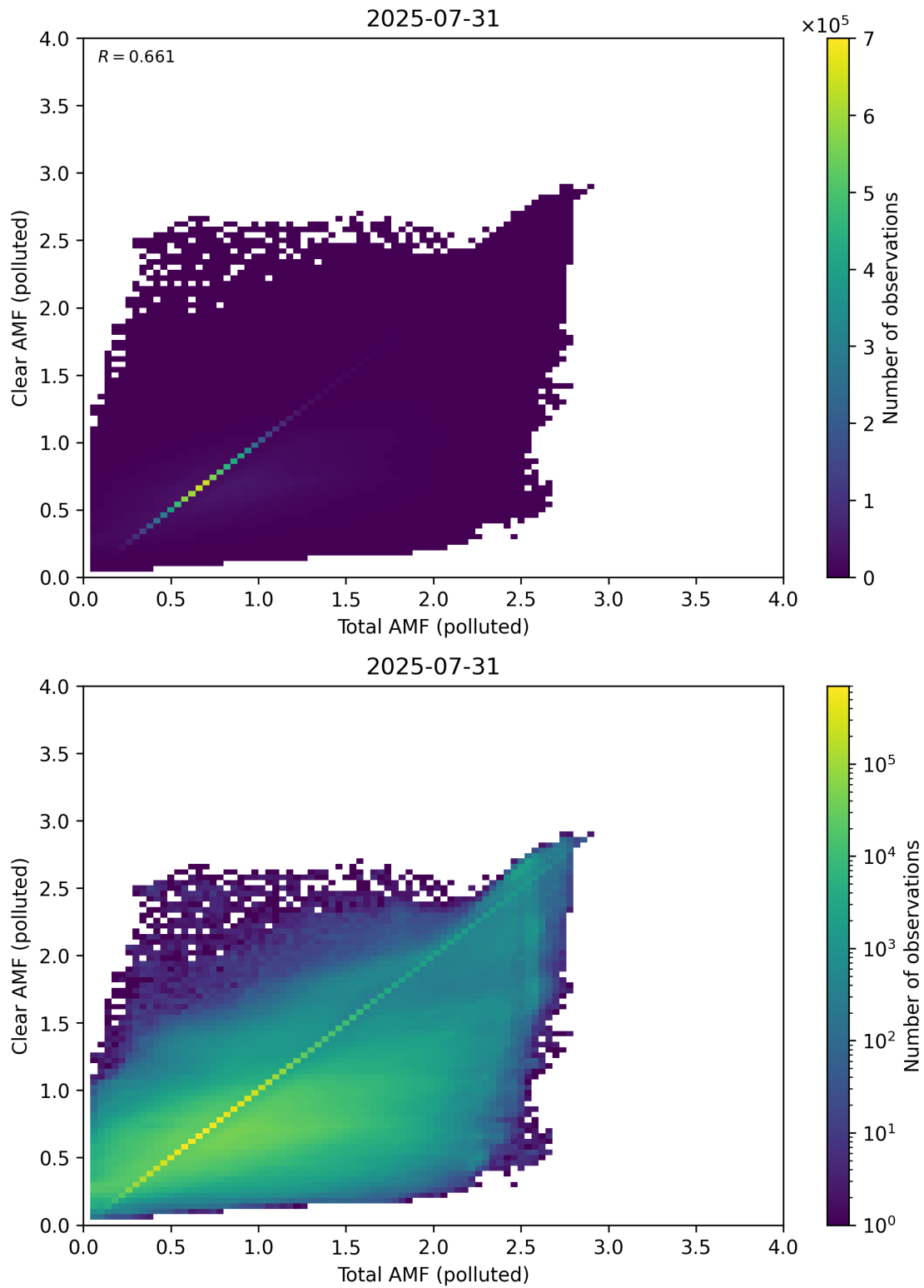
Figure 321: Scatter density plot of “Total AMF (polluted)” against “Clear AMF (polluted)” for 2025-07-30 to 2025-08-01.
