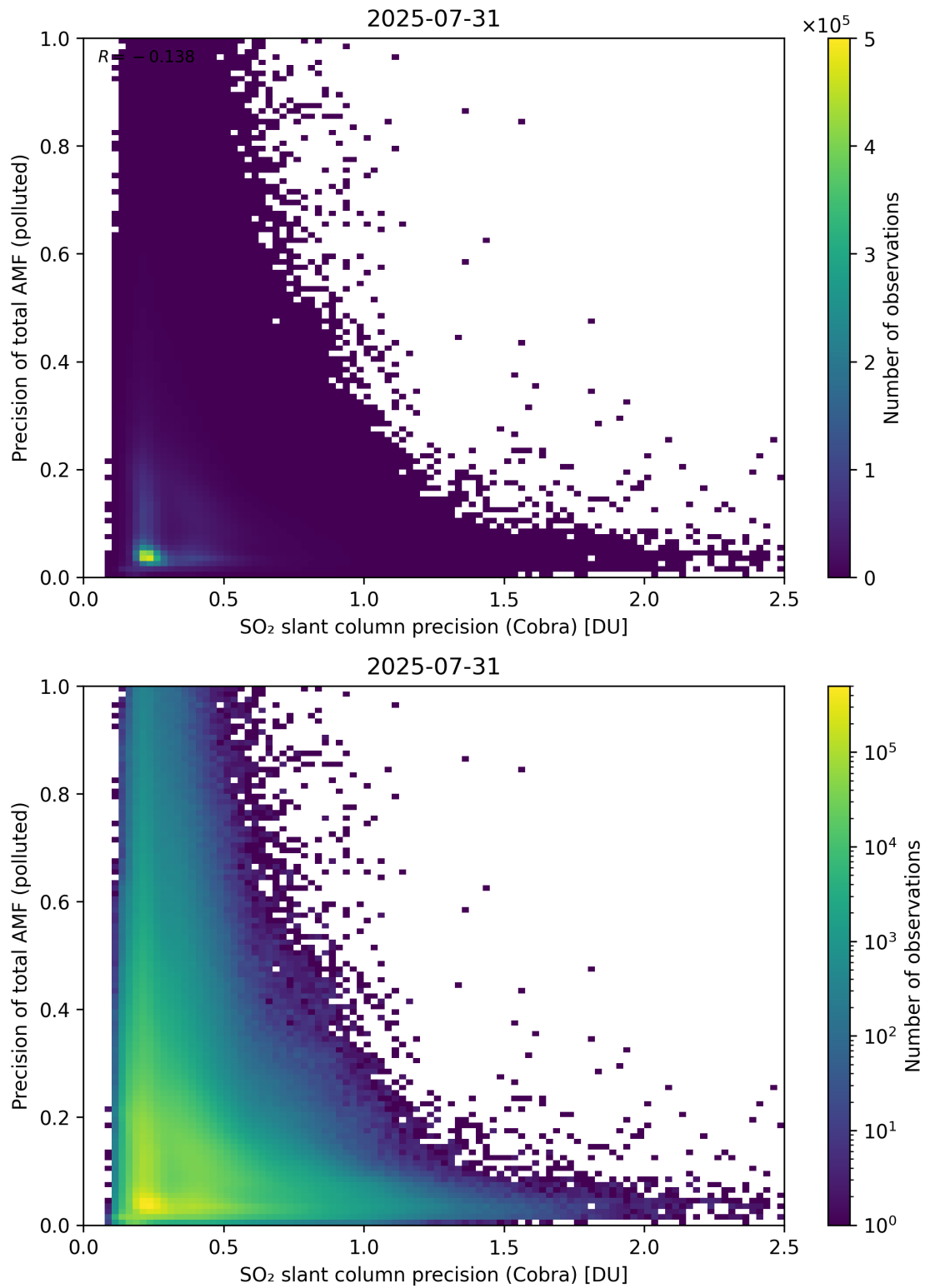
Figure 214: Scatter density plot of “SO 2 slant column precision (Cobra)” against “Precision of total AMF (polluted)” for 2025-07-30 to 2025-08-01.
