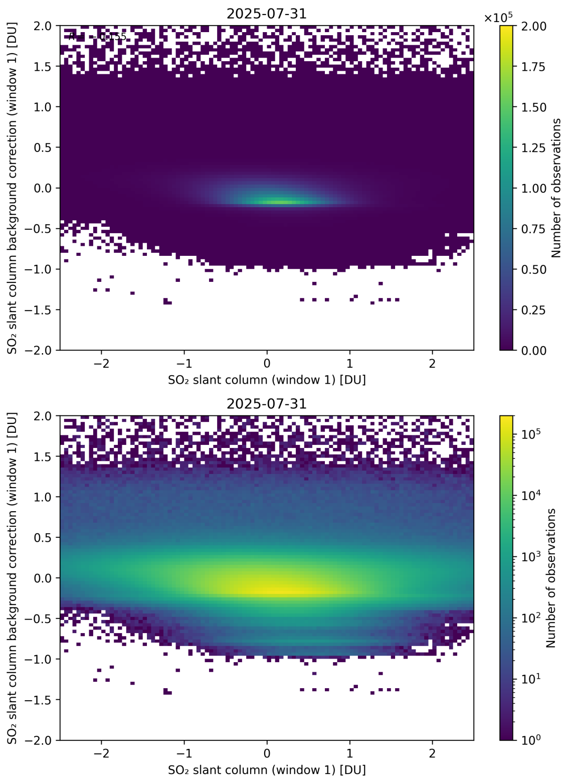
Figure 262: Scatter density plot of “SO 2 slant column (window 1)” against “SO 2 slant column background correction (window 1)” for 2025-07-30 to 2025-08-01.
