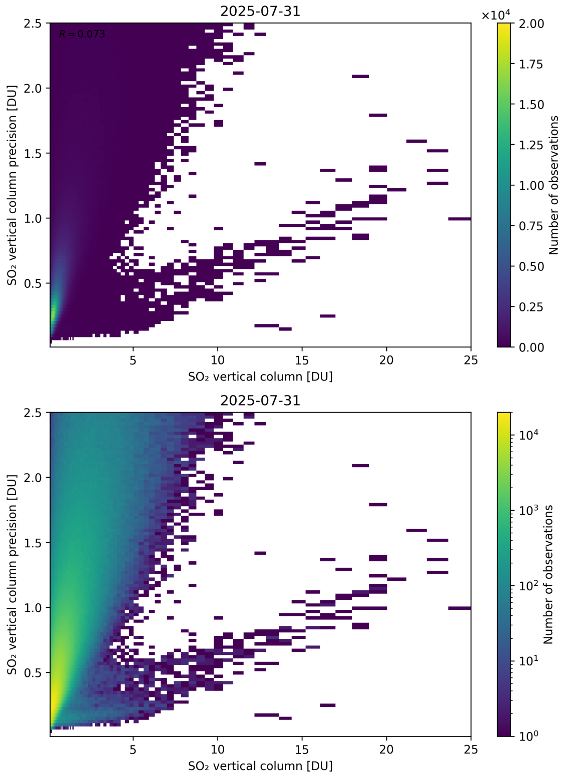
Figure 361: Scatter density plot of “SO 2 vertical column” against “SO 2 vertical column precision” for 2025-07-30 to 2025-08-01.
