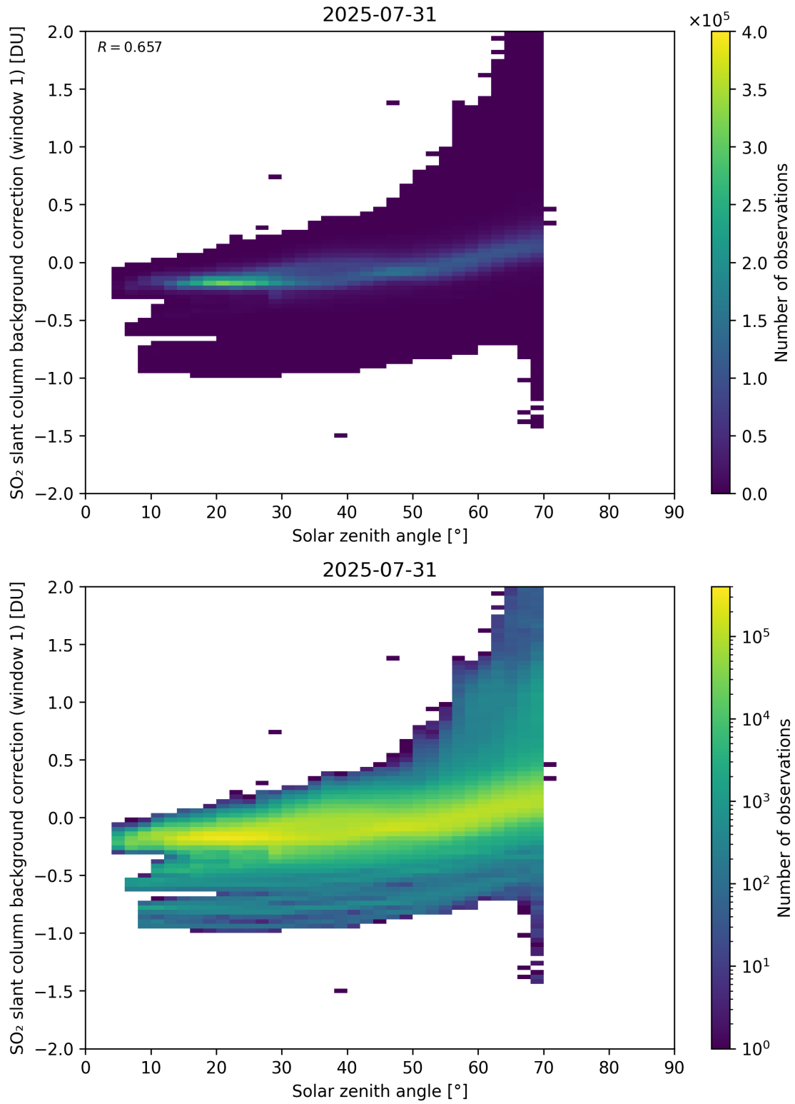
Figure 171: Scatter density plot of “Solar zenith angle” against “SO 2 slant column background correction (window 1)” for 2025-07-30 to 2025-08-01.
