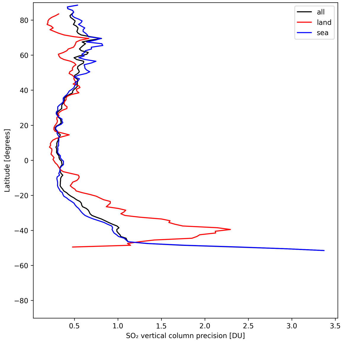
Figure 33: Zonal average of “SO 2 vertical column precision” for 2025-07-30 to 2025-08-01.
