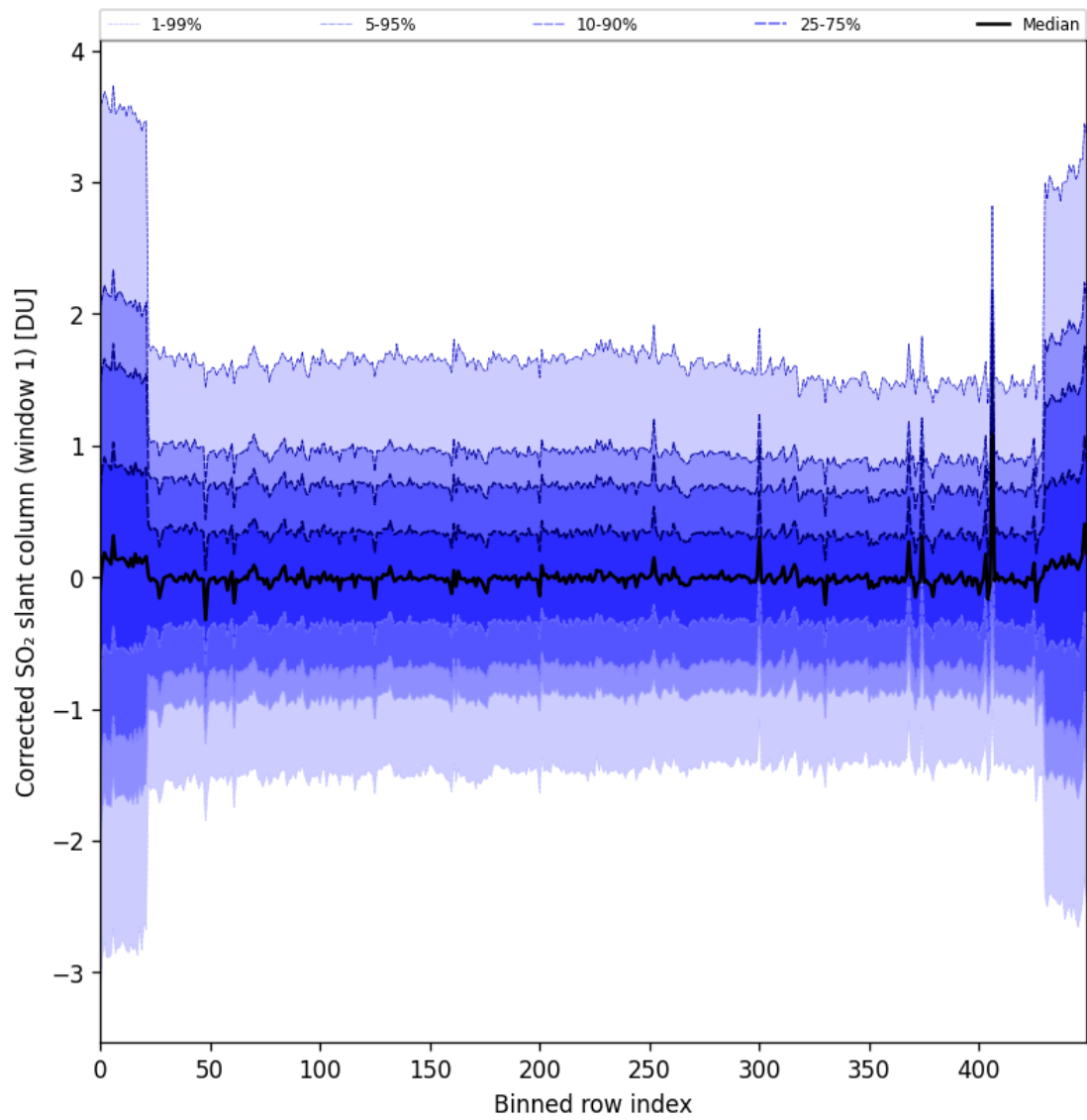
Figure 91: Along track statistics of “Corrected SO 2 slant column (window 1)” for 2025-07-30 to 2025-08-01
