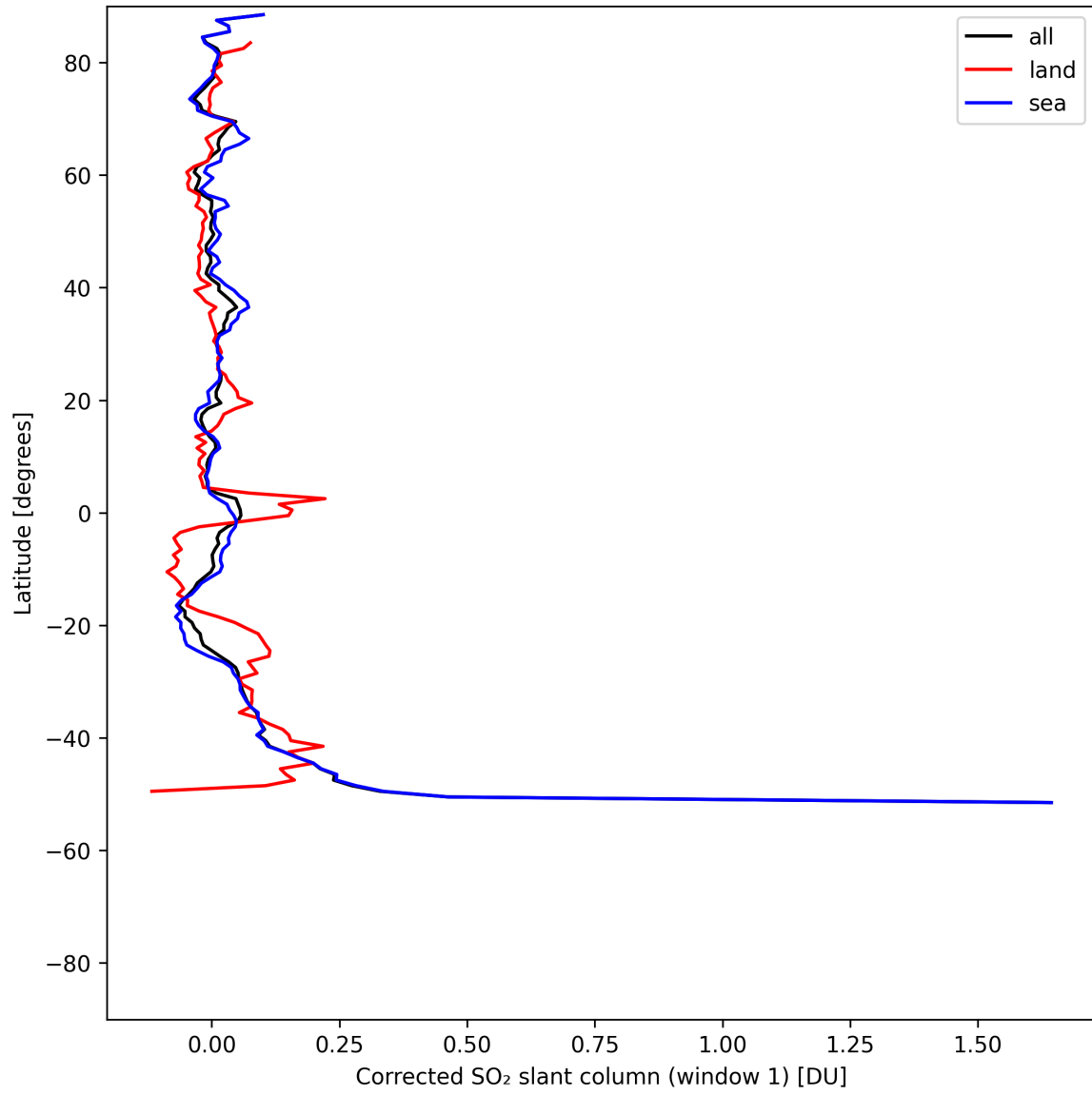
Figure 39: Zonal average of “Corrected SO 2 slant column (window 1)” for 2025-07-30 to 2025-08-01.
