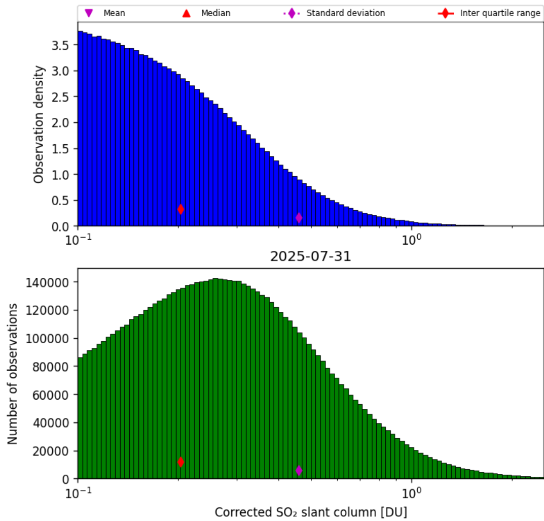
Figure 60: Histogram of "Corrected SO 2 slant column" for 2025-07-30 to 2025-08-01
