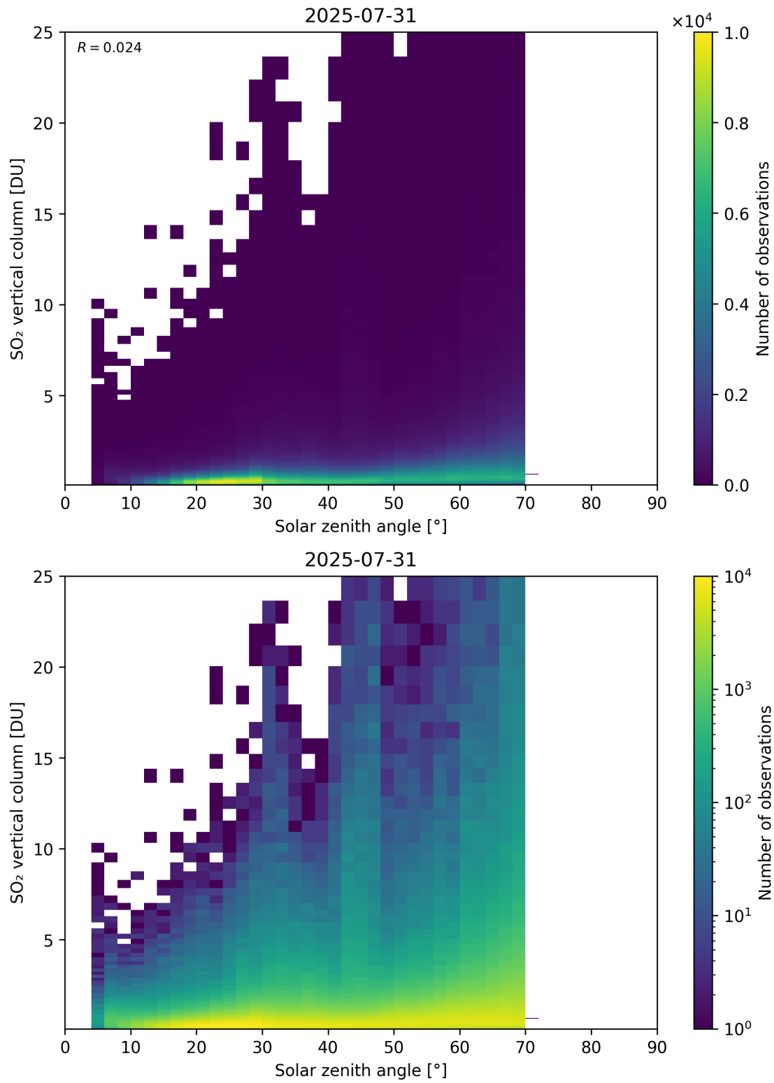
Figure 191: Scatter density plot of “Solar zenith angle” against “SO 2 vertical column” for 2025-07-30 to 2025-08-01.
