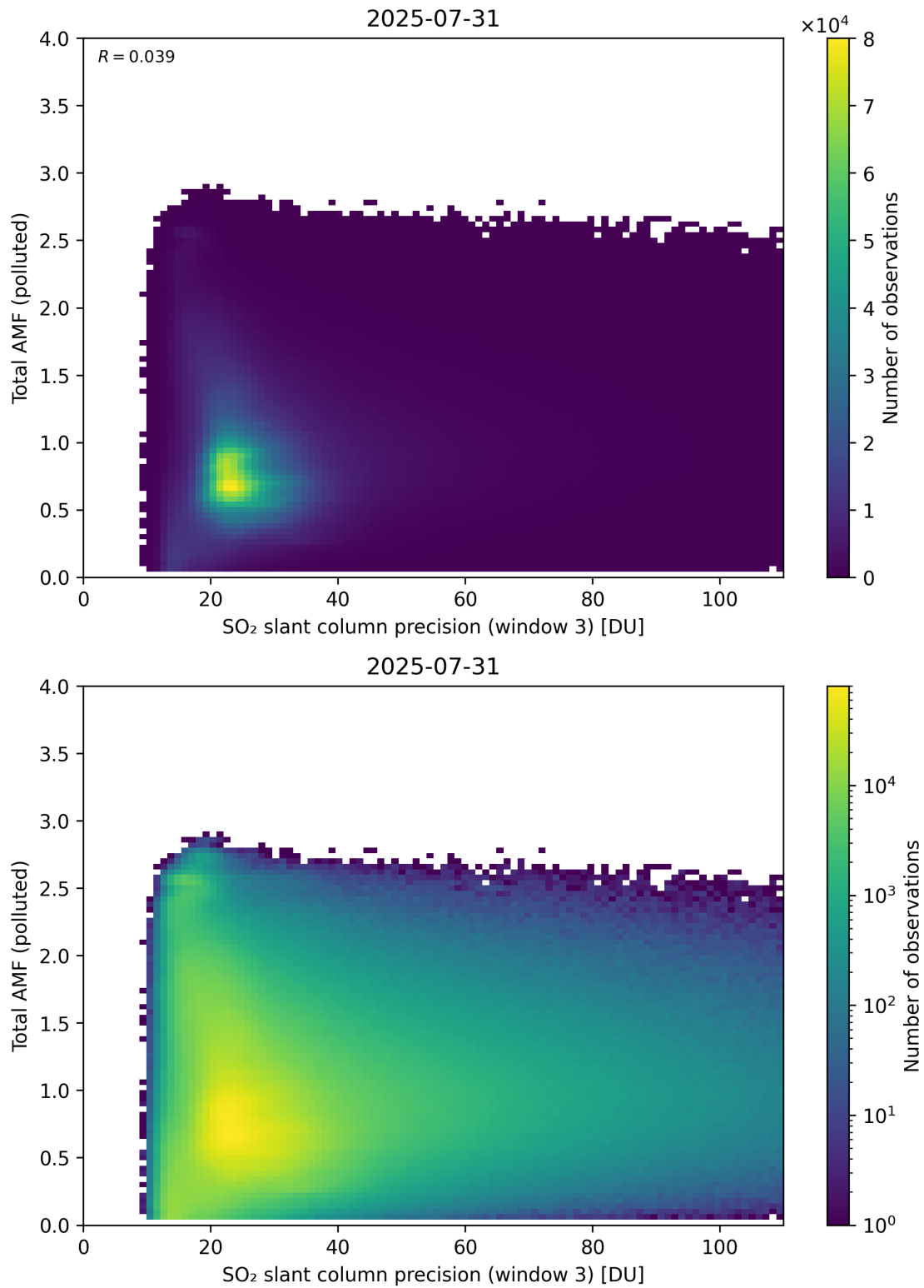
Figure 313: Scatter density plot of “SO 2 slant column precision (window 3)” against “Total AMF (polluted)” for 2025-07-30 to 2025-08-01.
