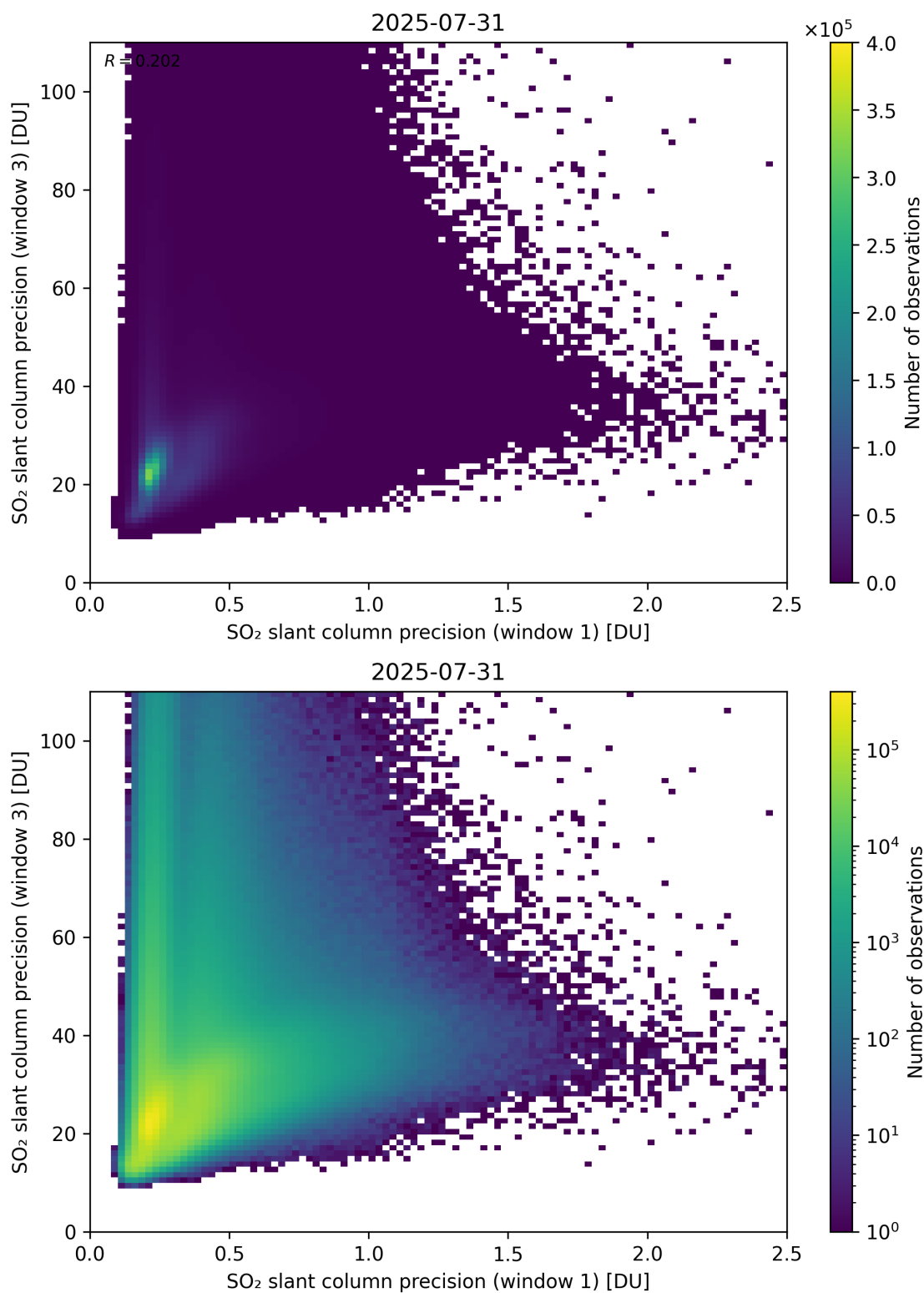
Figure 279: Scatter density plot of “SO 2 slant column precision (window 1)” against “SO 2 slant column precision (window 3)” for 2025-07-30 to 2025-08-01.
