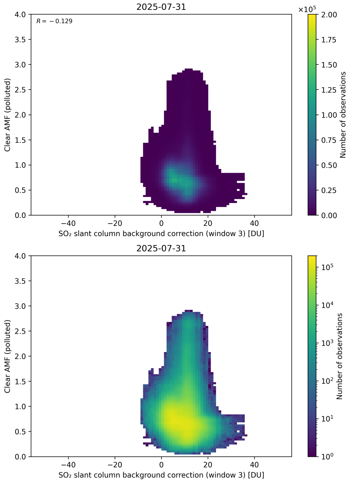
Figure 135: Scatter density plot of “SO 2 slant column background correction (window 3)” against “Clear AMF (polluted)” for 2025-07-30 to 2025-08-01.
