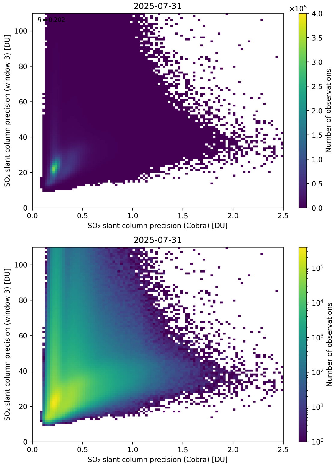
Figure 212: Scatter density plot of “SO 2 slant column precision (Cobra)” against “SO 2 slant column precision (window 3)” for 2025-07-30 to 2025-08-01.
