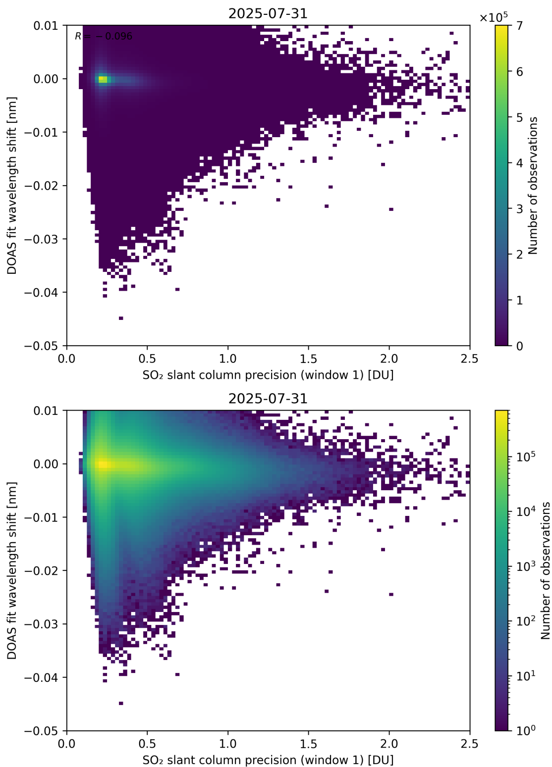
Figure 271: Scatter density plot of “SO 2 slant column precision (window 1)” against “DOAS fit wavelength shift” for 2025-07-30 to 2025-08-01.
