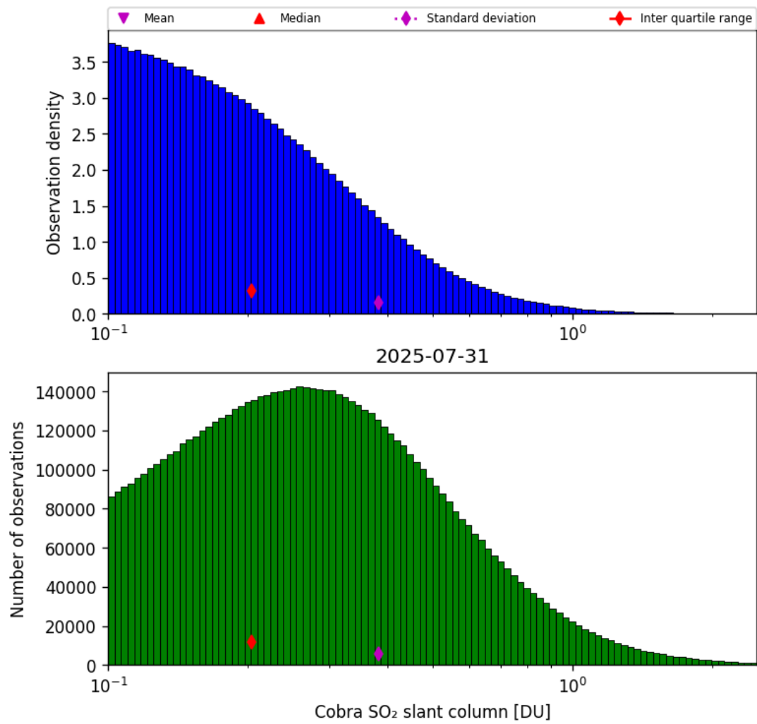
Figure 61: Histogram of “Cobra SO 2 slant column” for 2025-07-30 to 2025-08-01
