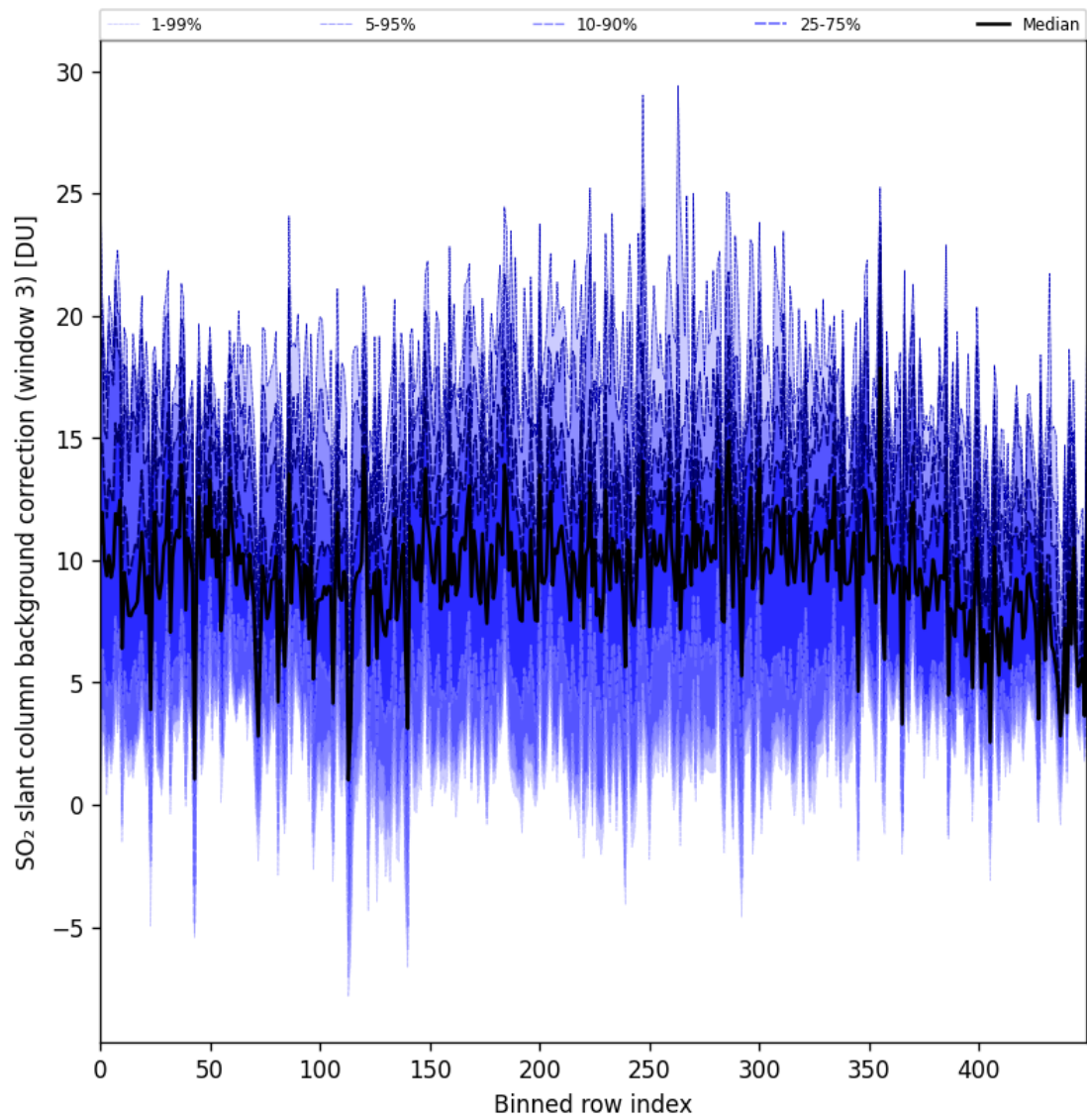
Figure 100: Along track statistics of “SO 2 slant column background correction (window 3)” for 2025-07-30 to 2025-08-01
