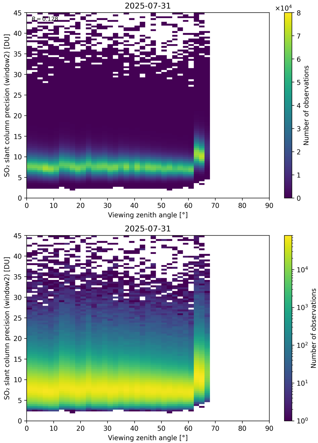
Figure 378: Scatter density plot of “Viewing zenith angle” against “SO 2 slant column precision (window2)” for 2025-07-30 to 2025-08-01.
