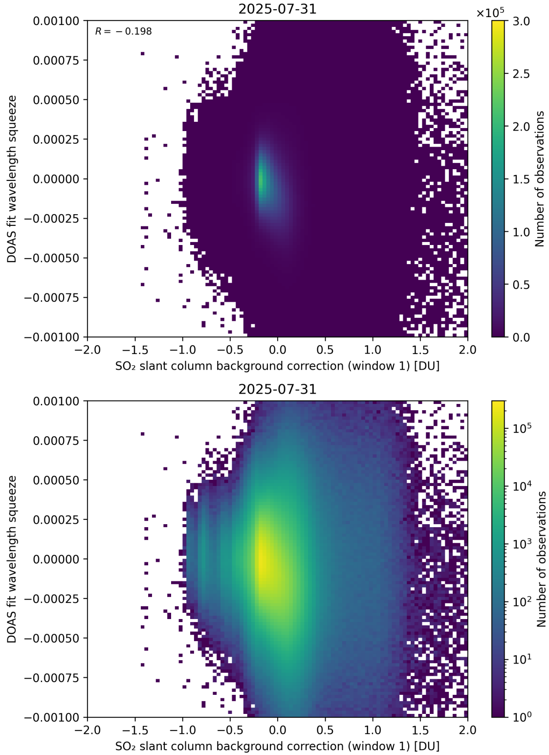
Figure 112: Scatter density plot of “SO 2 slant column background correction (window 1)” against “DOAS fit wavelength squeeze” for 2025-07-30 to 2025-08-01.
