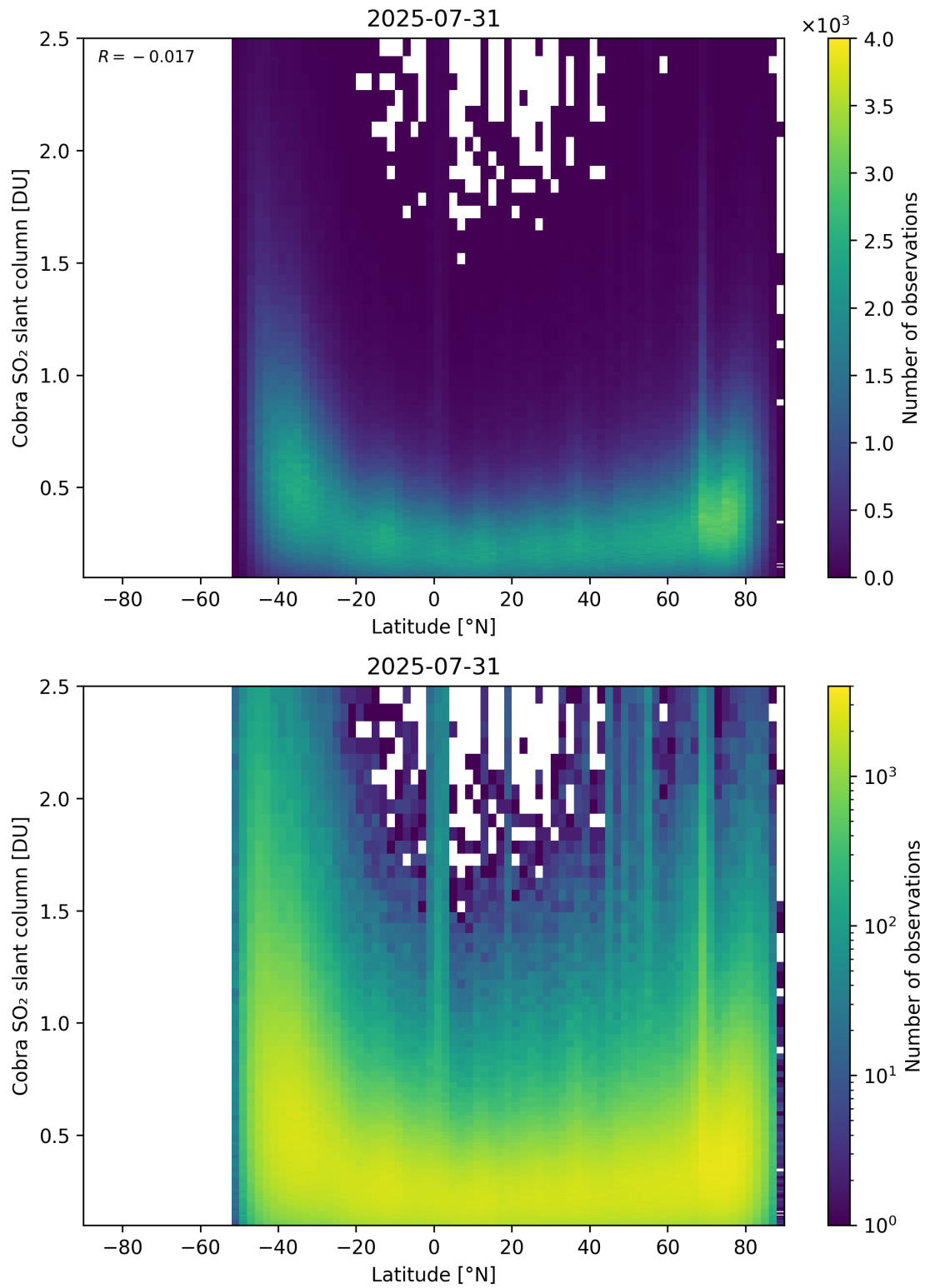
Figure 157: Scatter density plot of “Latitude” against “Cobra SO 2 slant column” for 2025-07-30 to 2025-08-01.
