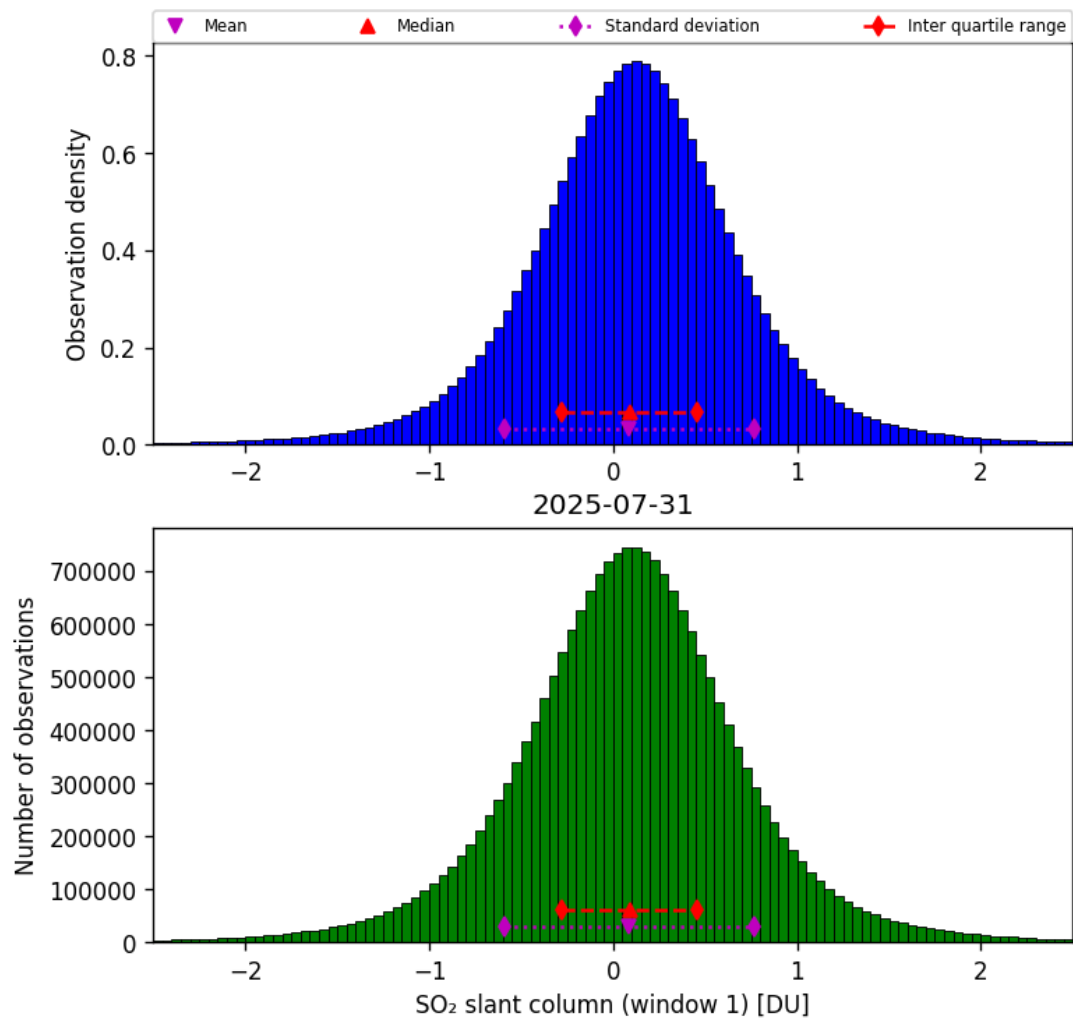
Figure 63: Histogram of “SO 2 slant column (window 1)” for 2025-07-30 to 2025-08-01
