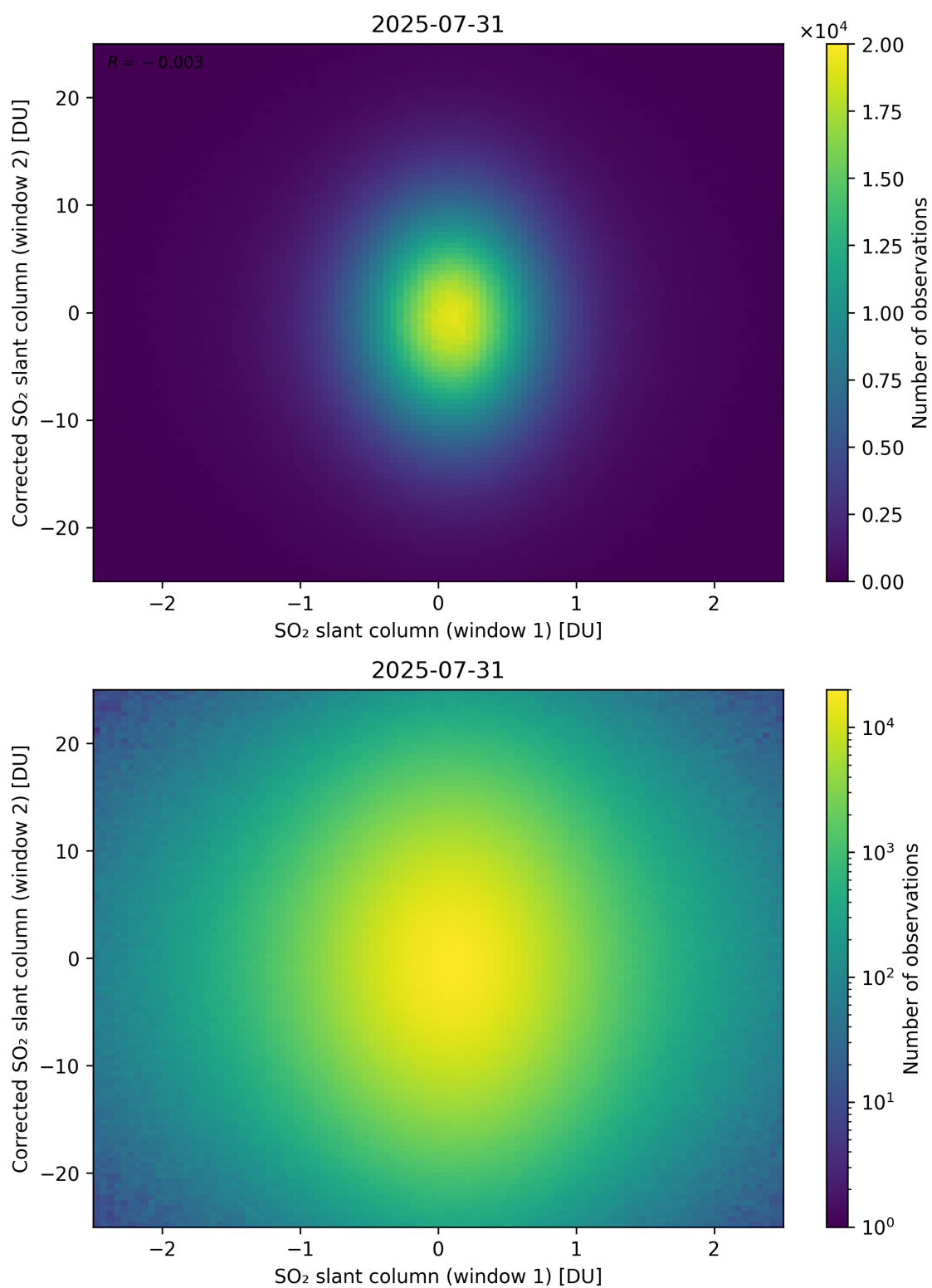
Figure 283: Scatter density plot of “SO 2 slant column (window 1)” against “Corrected SO 2 slant column (window 2)” for 2025-07-30 to 2025-08-01.
