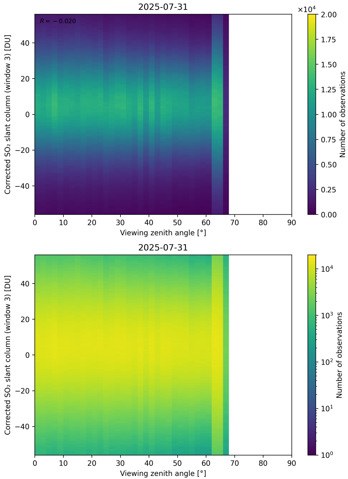
Figure 375: Scatter density plot of “Viewing zenith angle” against “Corrected SO 2 slant column (window 3)” for 2025-07-30 to 2025-08-01.
