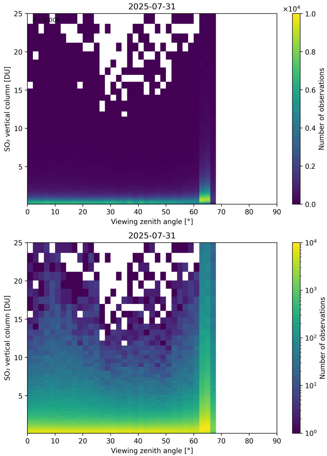
Figure 383: Scatter density plot of “Viewing zenith angle” against “SO 2 vertical column” for 2025-07-30 to 2025-08-01.
