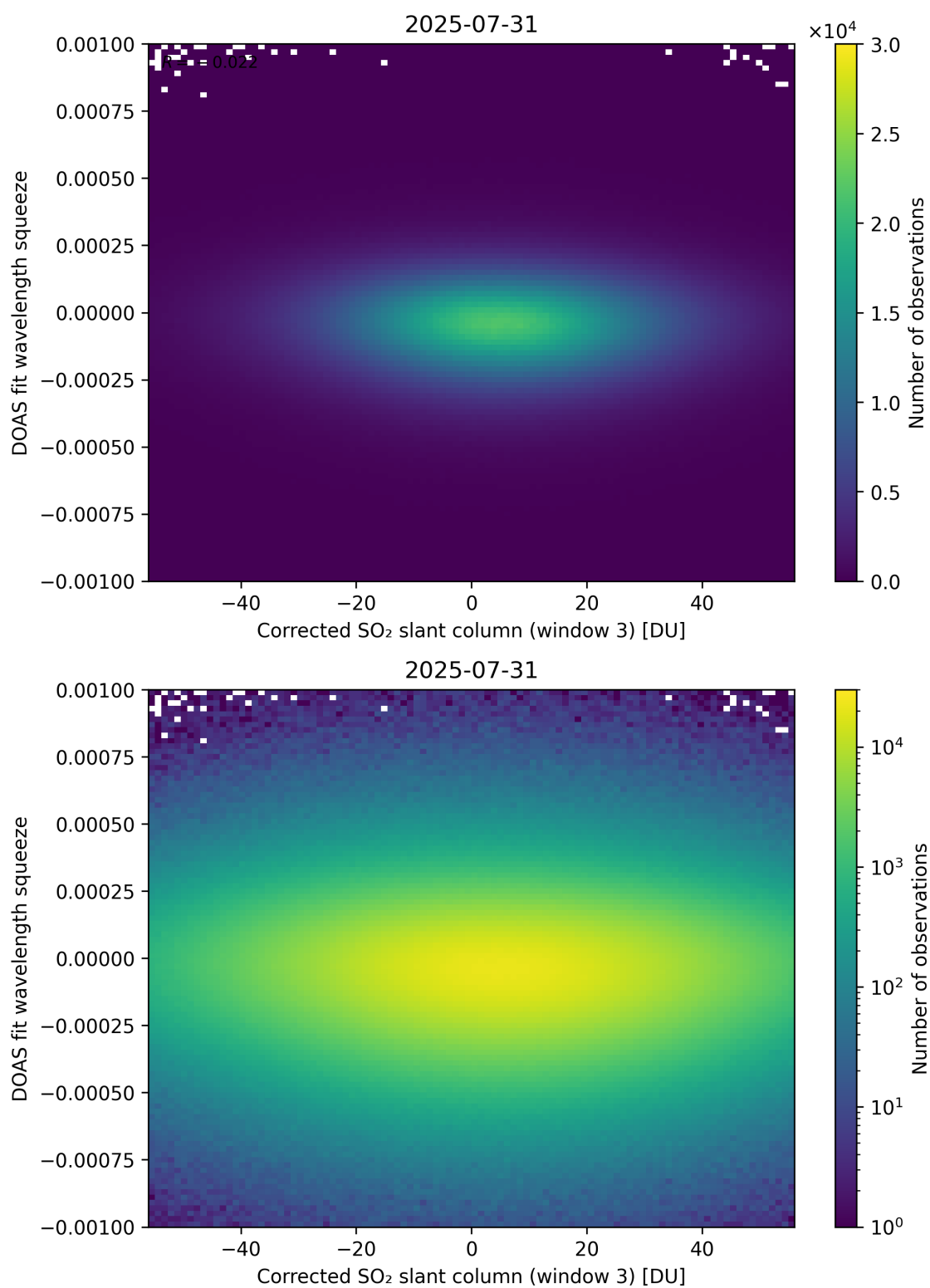
Figure 257: Scatter density plot of “Corrected SO 2 slant column (window 3)” against “DOAS fit wavelength squeeze” for 2025-07-30 to 2025-08-01.
