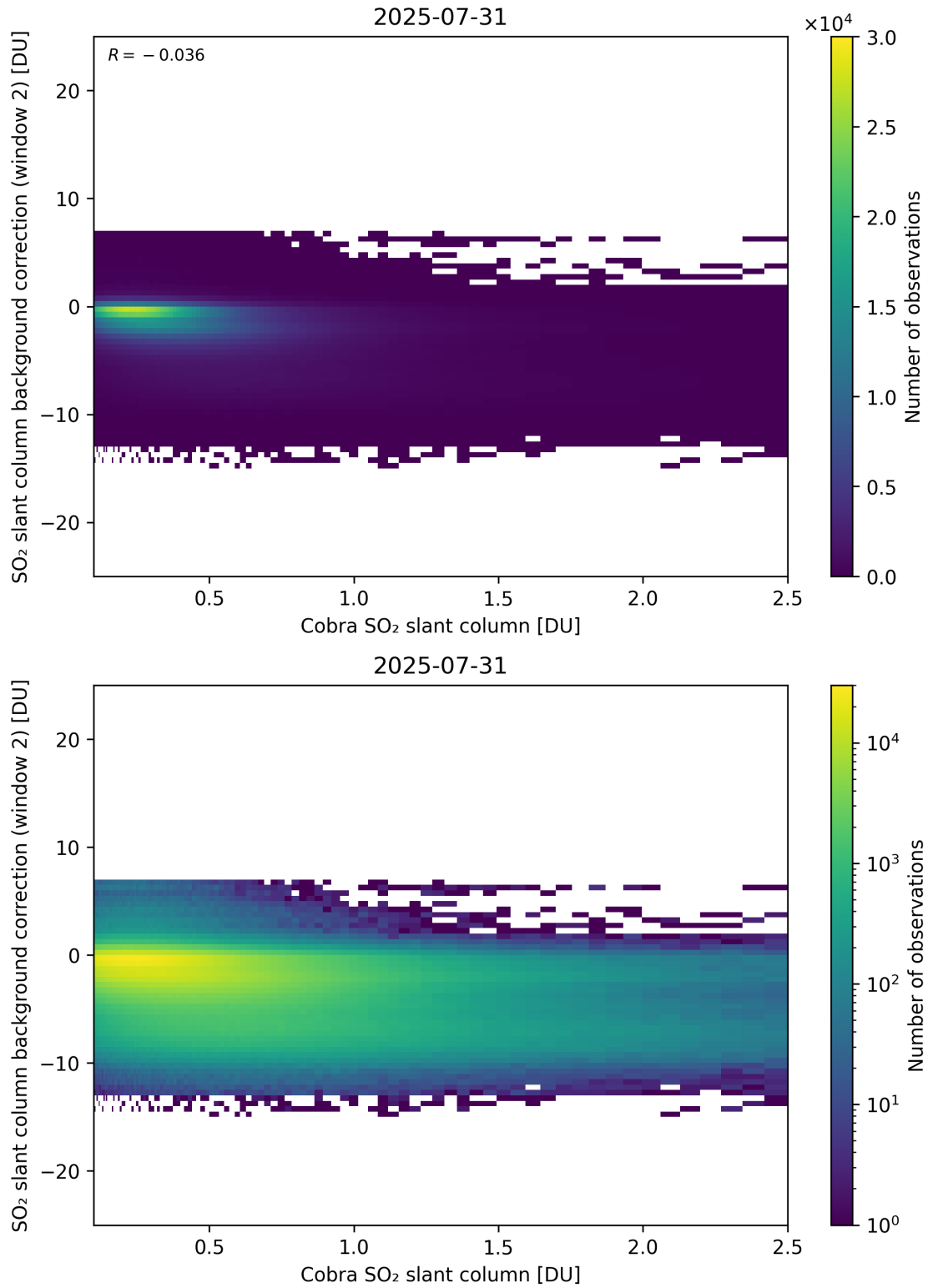
Figure 194: Scatter density plot of “Cobra SO 2 slant column” against “SO 2 slant column background correction (window 2)” for 2025-07-30 to 2025-08-01.
