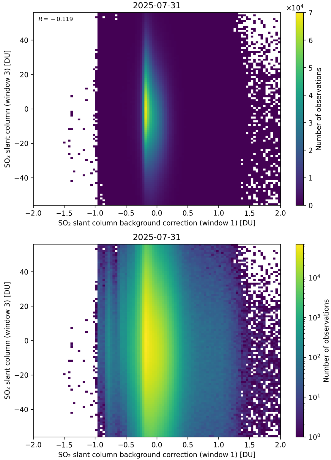
Figure 118: Scatter density plot of “SO 2 slant column background correction (window 1)” against “SO 2 slant column (window 3)” for 2025-07-30 to 2025-08-01.
