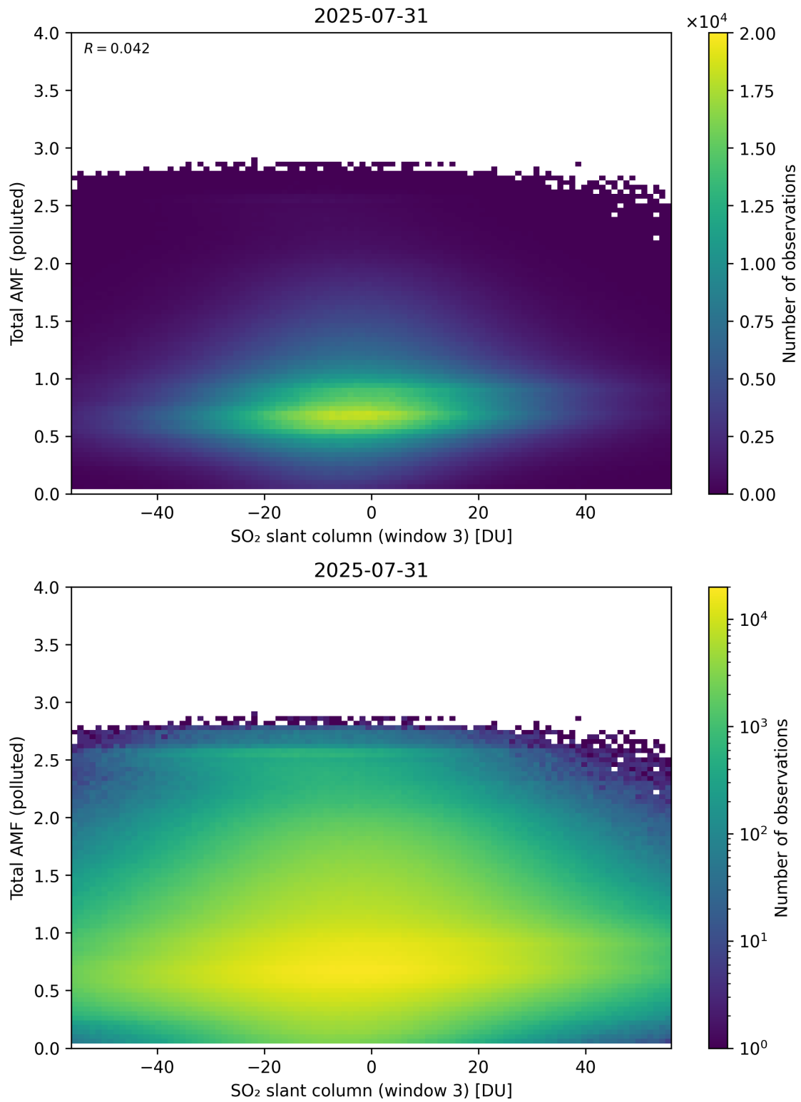
Figure 318: Scatter density plot of “SO 2 slant column (window 3)” against “Total AMF (polluted)” for 2025-07-30 to 2025-08-01.
