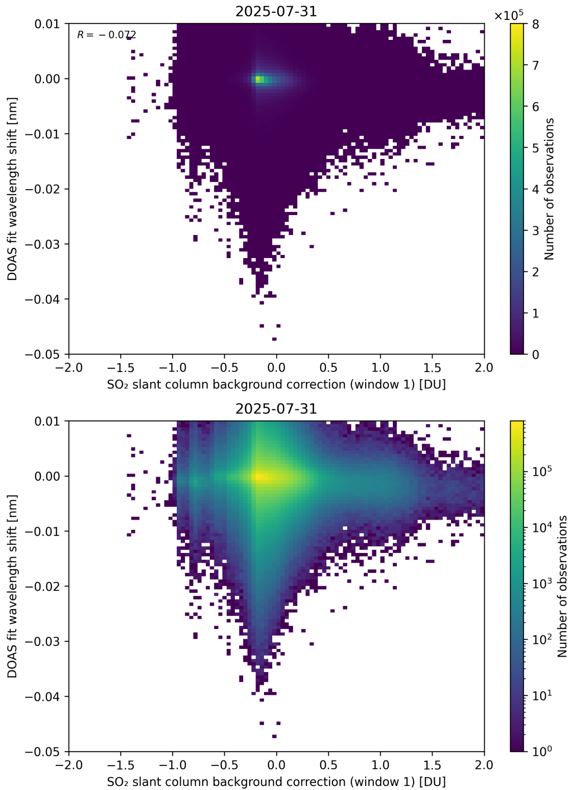
Figure 111: Scatter density plot of “SO 2 slant column background correction (window 1)” against “DOAS fit wavelength shift” for 2025-07-30 to 2025-08-01.
