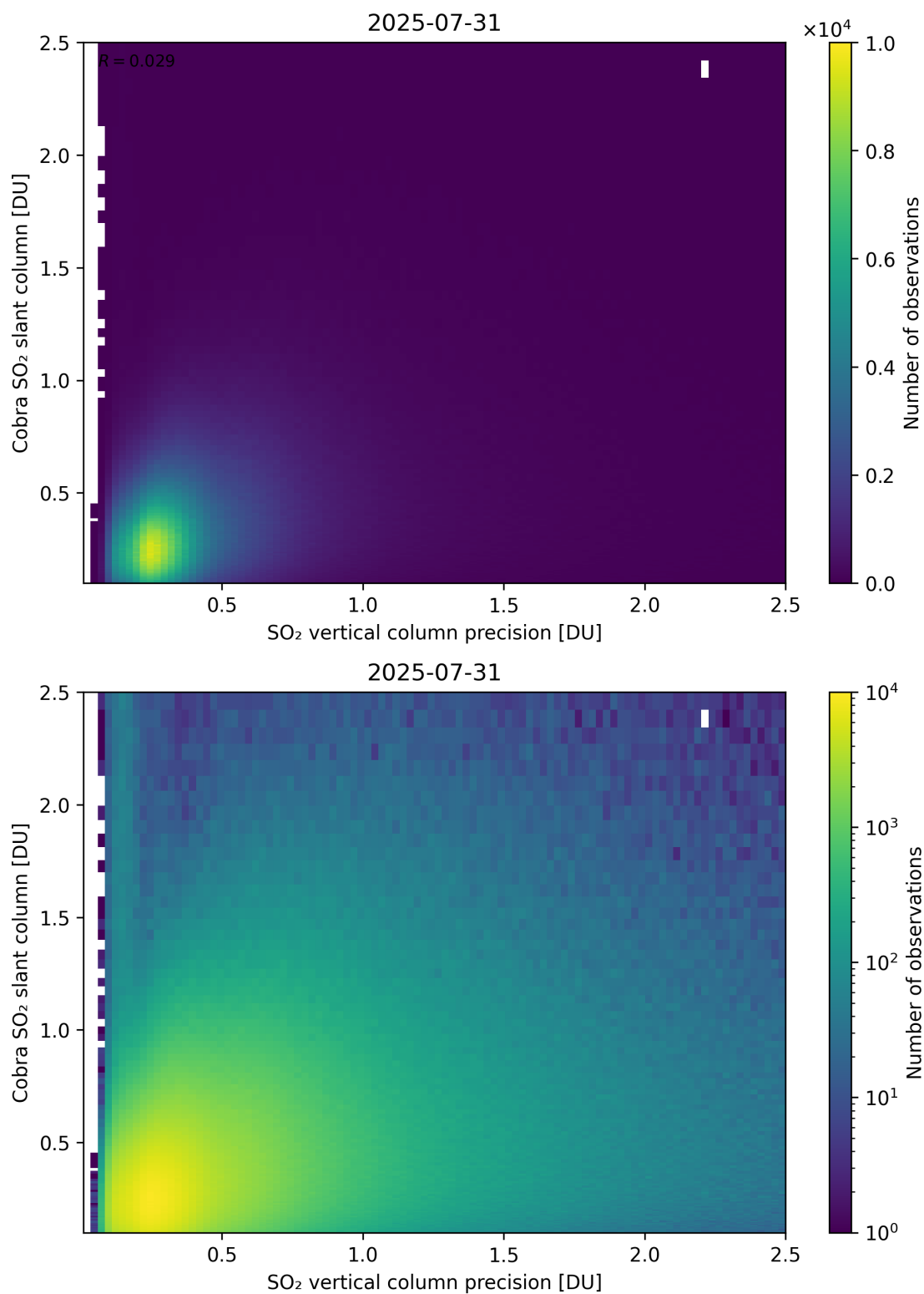
Figure 336: Scatter density plot of “SO 2 vertical column precision” against “Cobra SO 2 slant column” for 2025-07-30 to 2025-08-01.
