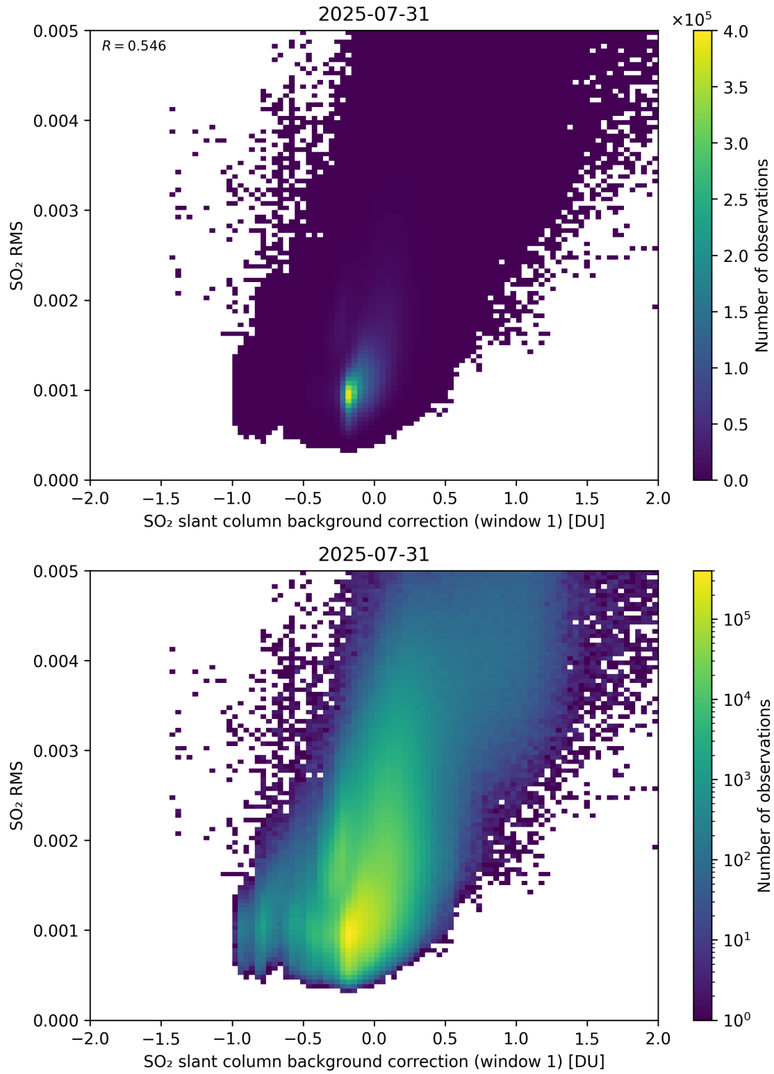
Figure 113: Scatter density plot of “SO 2 slant column background correction (window 1)” against “SO 2 RMS” for 2025-07-30 to 2025-08-01.
