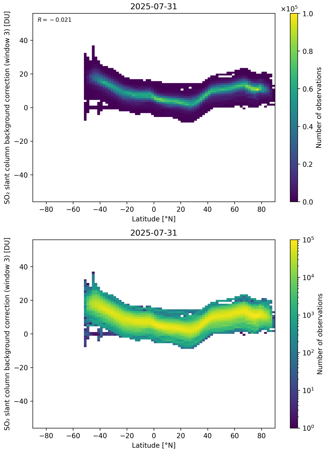
Figure 152: Scatter density plot of “Latitude” against “SO 2 slant column background correction (window 3)” for 2025-07-30 to 2025-08-01.
