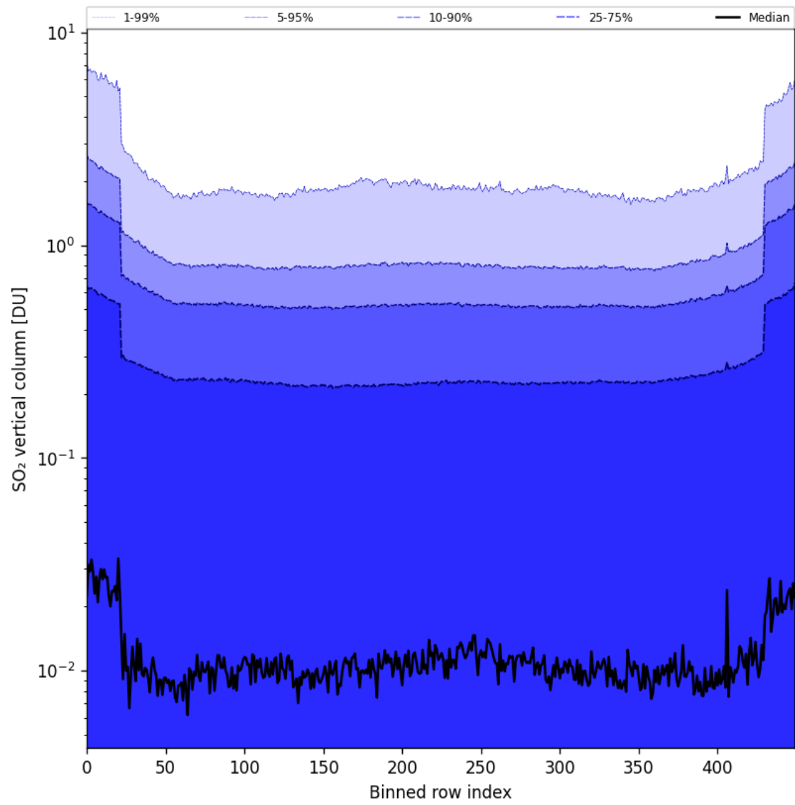
Figure 84: Along track statistics of “SO 2 vertical column” for 2025-07-30 to 2025-08-01
