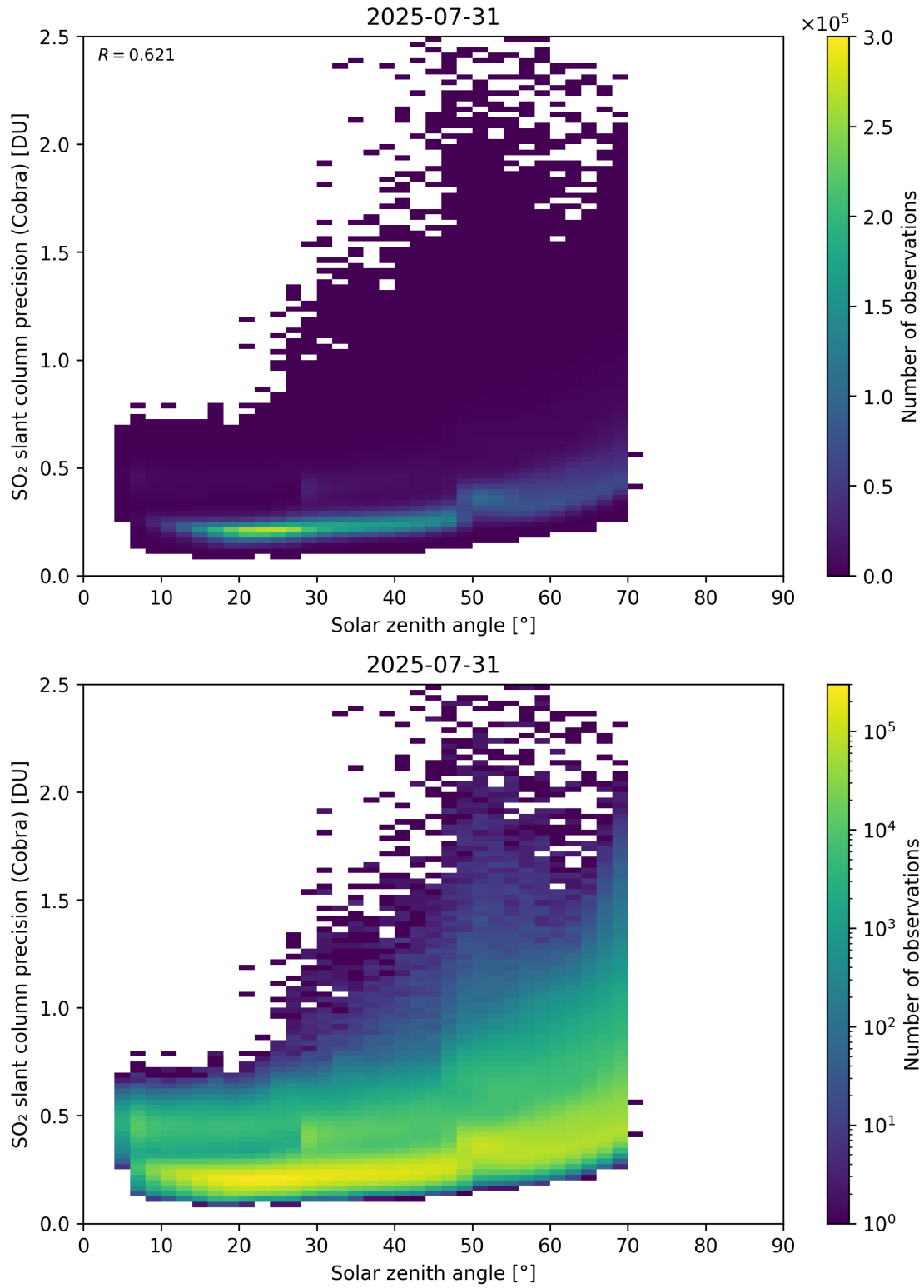
Figure 180: Scatter density plot of “Solar zenith angle” against “SO 2 slant column precision (Cobra)” for 2025-07-30 to 2025-08-01.
