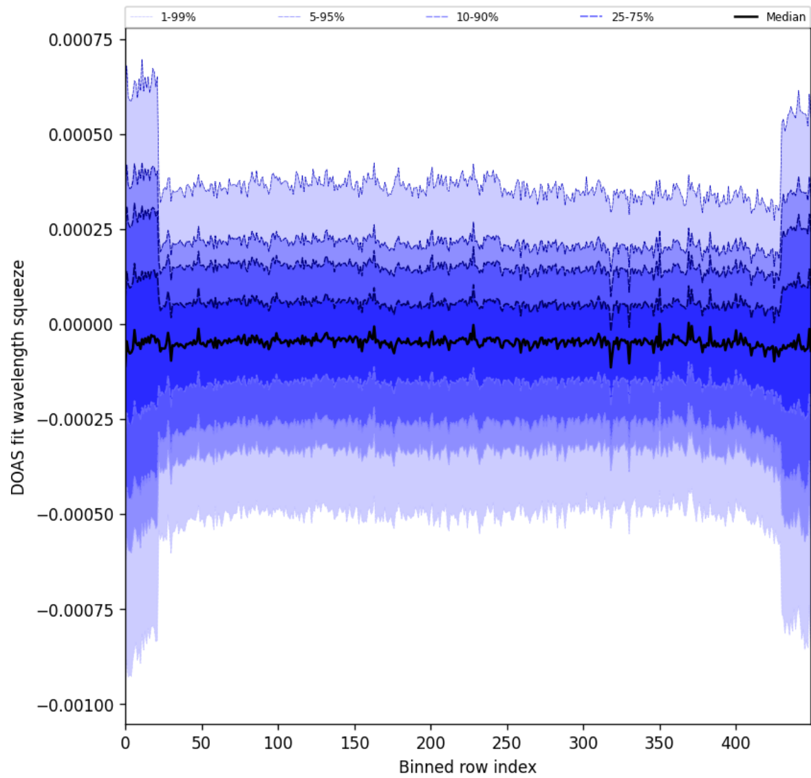
Figure 103: Along track statistics of “DOAS fit wavelength squeeze” for 2025-07-30 to 2025-08-01
