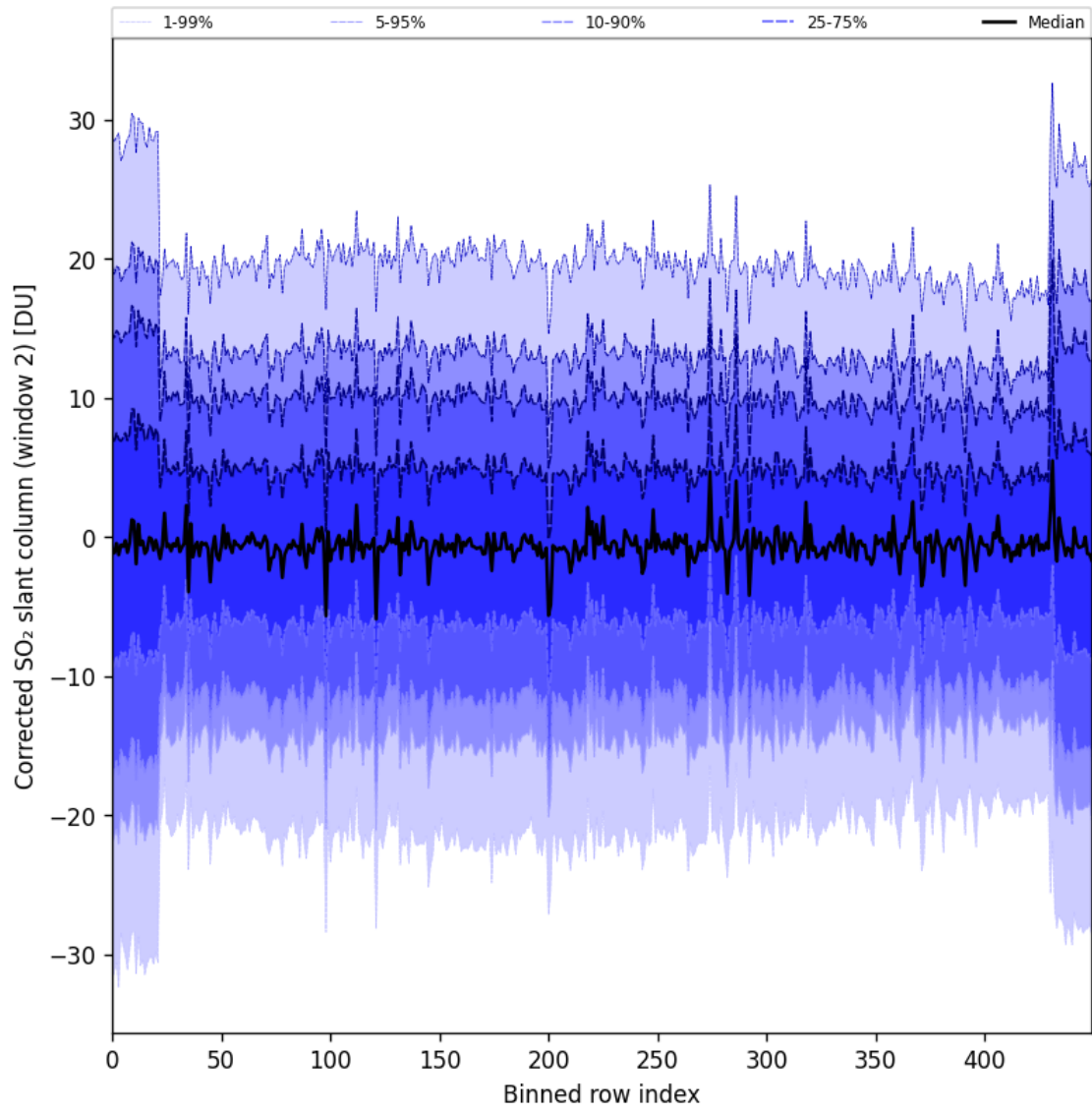
Figure 95: Along track statistics of “Corrected SO 2 slant column (window 2)” for 2025-07-30 to 2025-08-01
