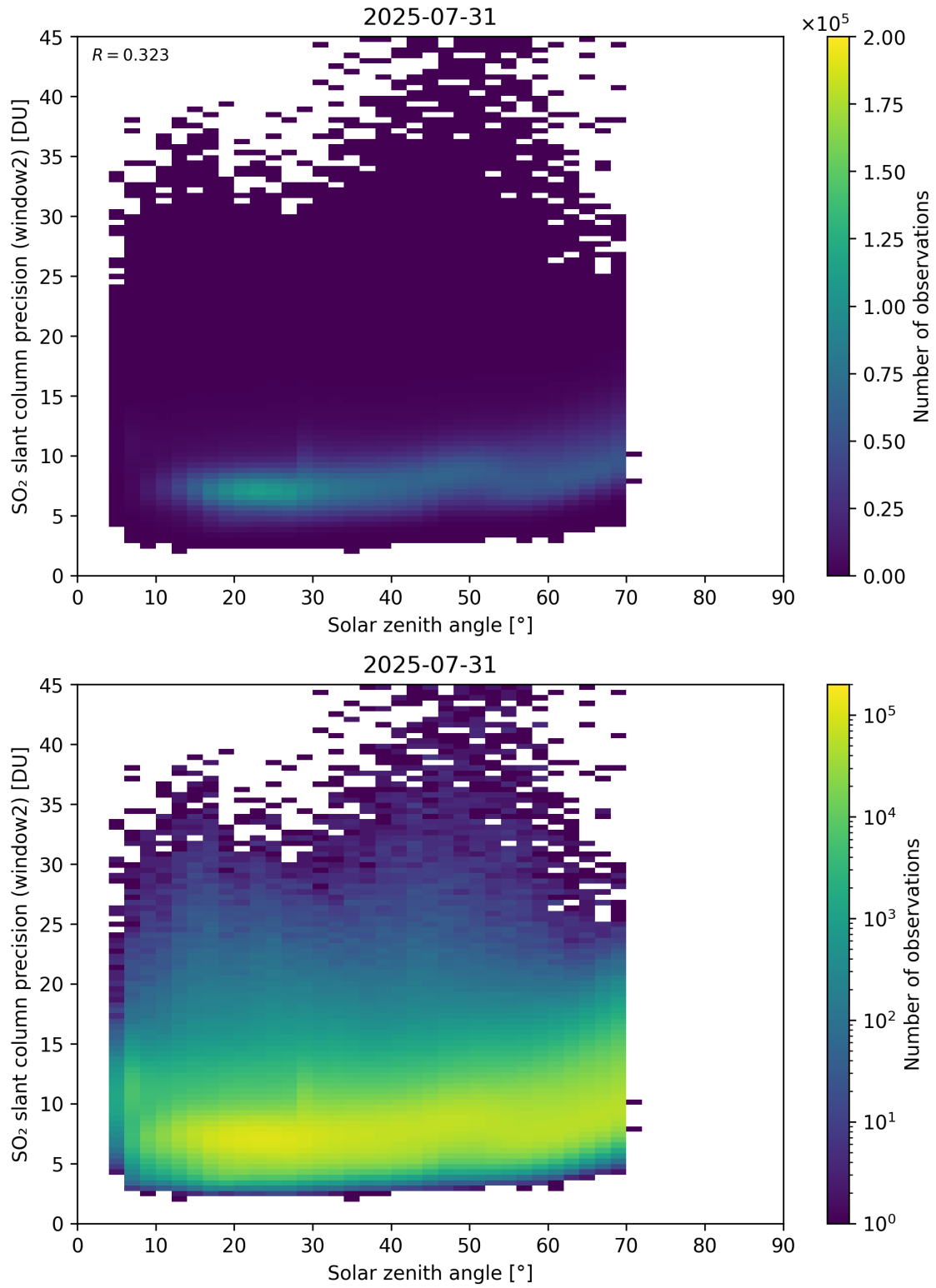
Figure 186: Scatter density plot of “Solar zenith angle” against “SO 2 slant column precision (window2)” for 2025-07-30 to 2025-08-01.
