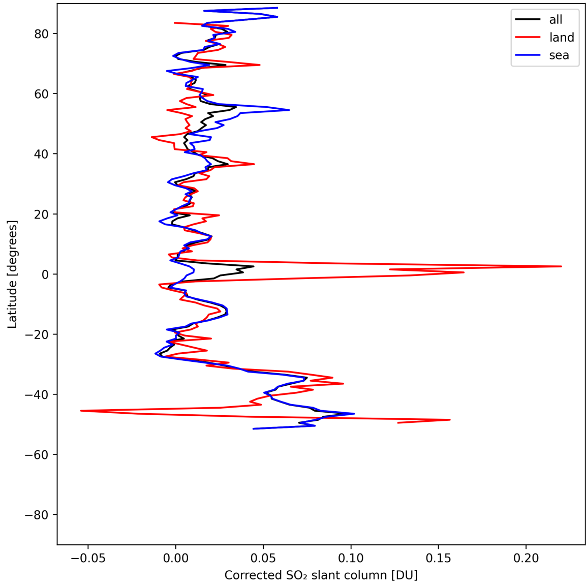
Figure 34: Zonal average of “Corrected SO 2 slant column” for 2025-07-30 to 2025-08-01.
