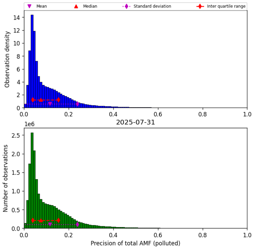
Figure 80: Histogram of “Precision of total AMF (polluted)” for 2025-07-30 to 2025-08-01
