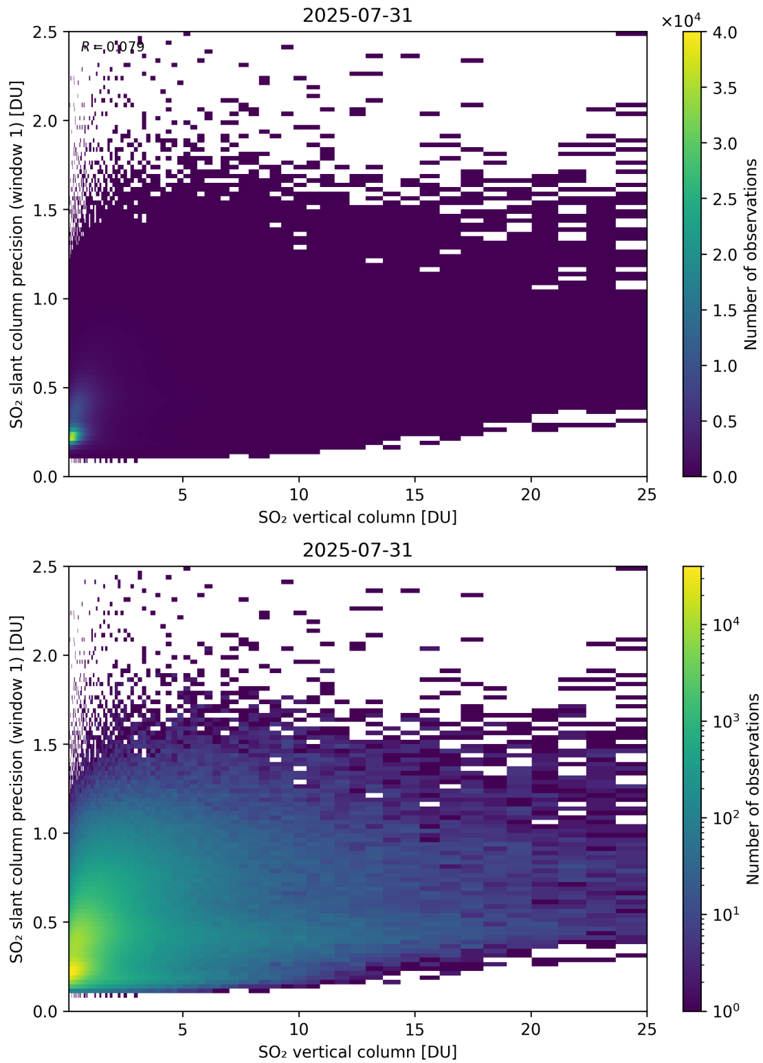
Figure 355: Scatter density plot of “SO 2 vertical column” against “SO 2 slant column precision (window 1)” for 2025-07-30 to 2025-08-01.
