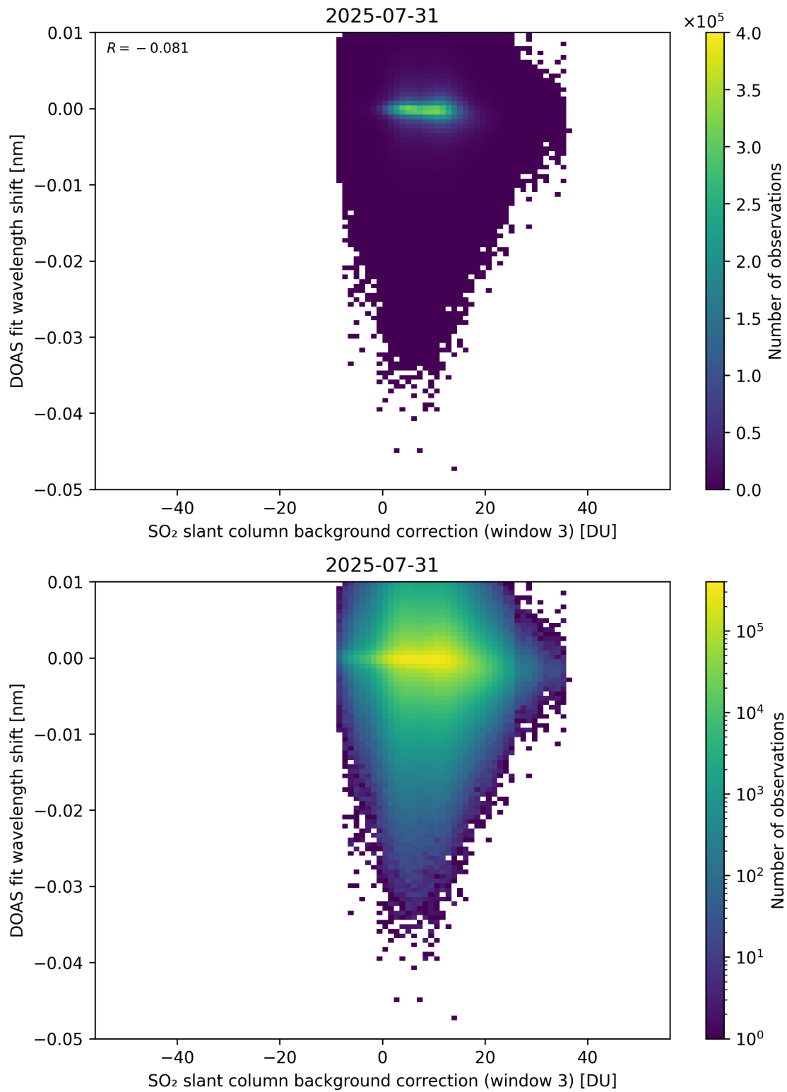
Figure 132: Scatter density plot of “SO 2 slant column background correction (window 3)” against “DOAS fit wavelength shift” for 2025-07-30 to 2025-08-01.
