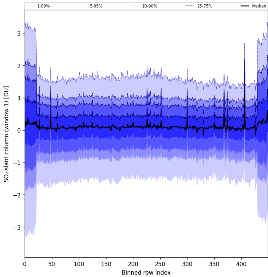
Figure 89: Along track statistics of “SO 2 slant column (window 1)” for 2025-07-30 to 2025-08-01
