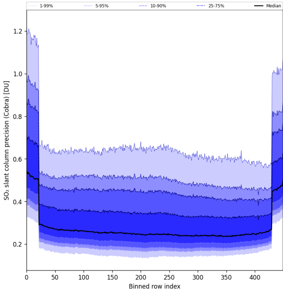
Figure 88: Along track statistics of “SO 2 slant column precision (Cobra)” for 2025-07-30 to 2025-08-01
