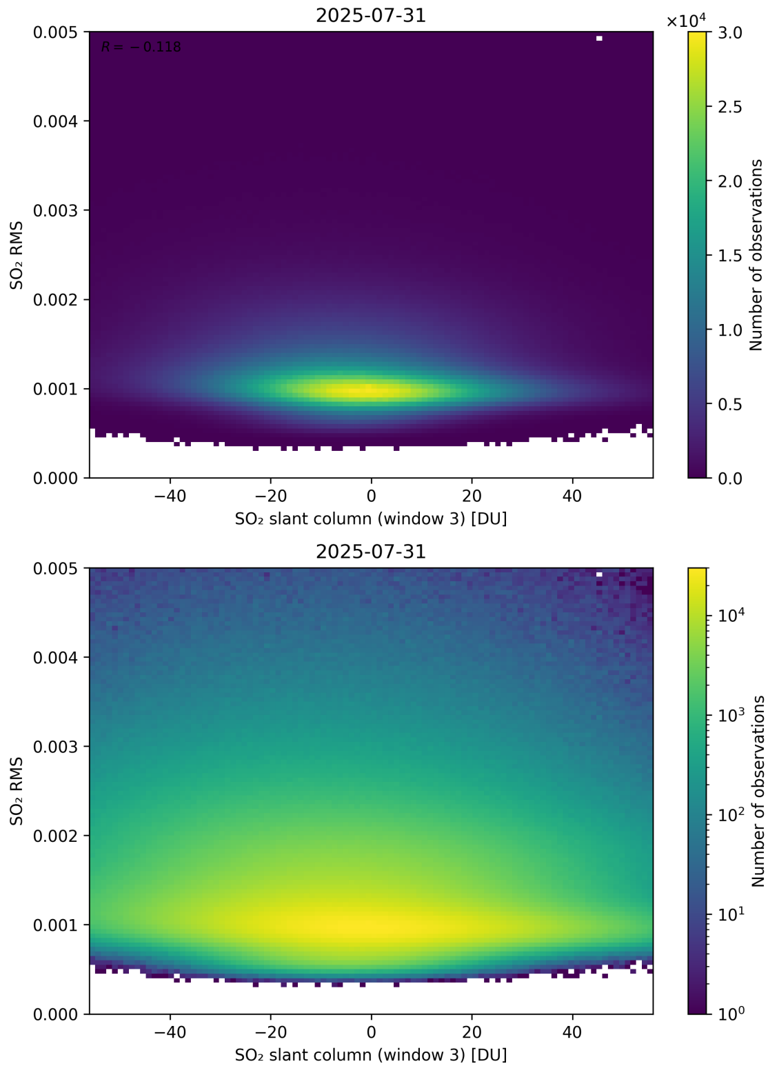
Figure 306: Scatter density plot of “SO 2 slant column (window 3)” against “SO 2 RMS” for 2025-07-30 to 2025-08-01.
