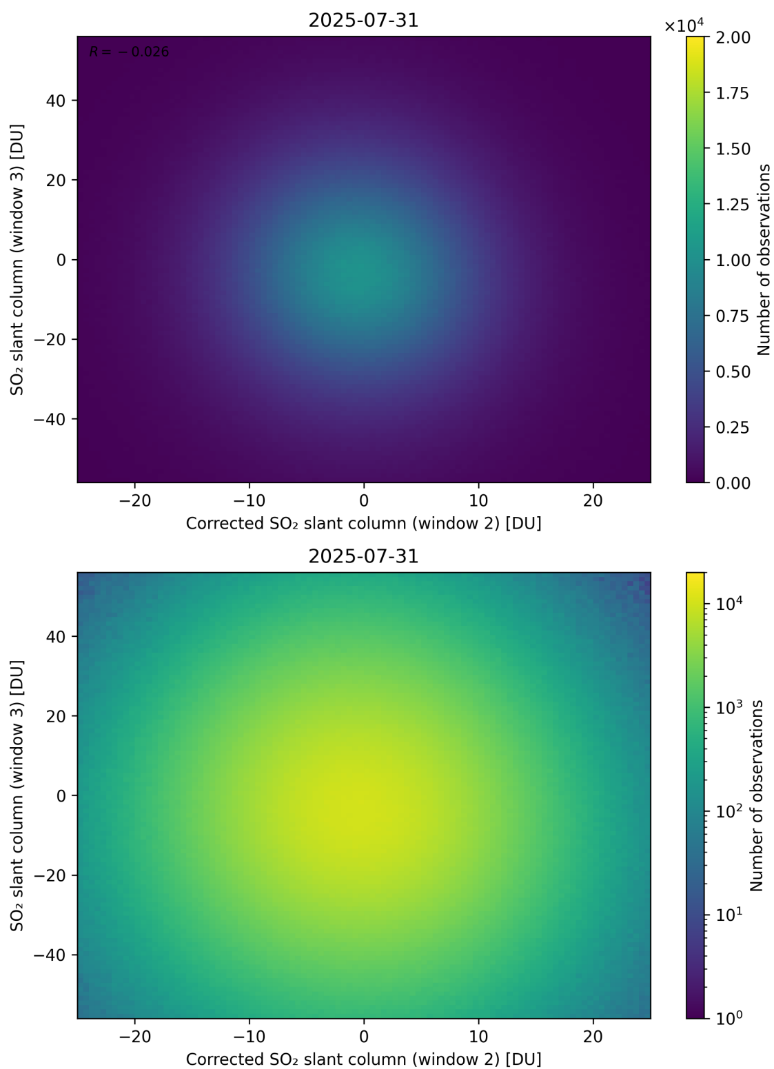
Figure 251: Scatter density plot of “Corrected SO 2 slant column (window 2)” against “SO 2 slant column (window 3)” for 2025-07-30 to 2025-08-01.
