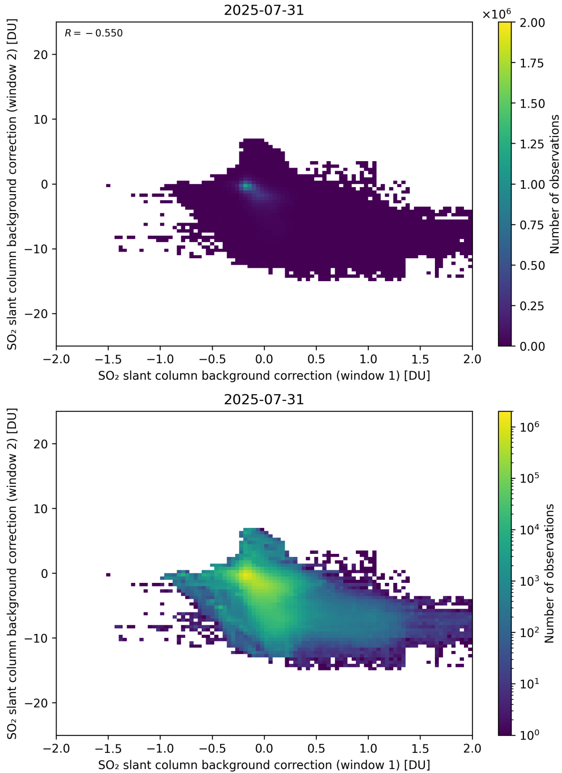
Figure 109: Scatter density plot of “SO 2 slant column background correction (window 1)” against “SO 2 slant column background correction (window 2)” for 2025-07-30 to 2025-08-01.
