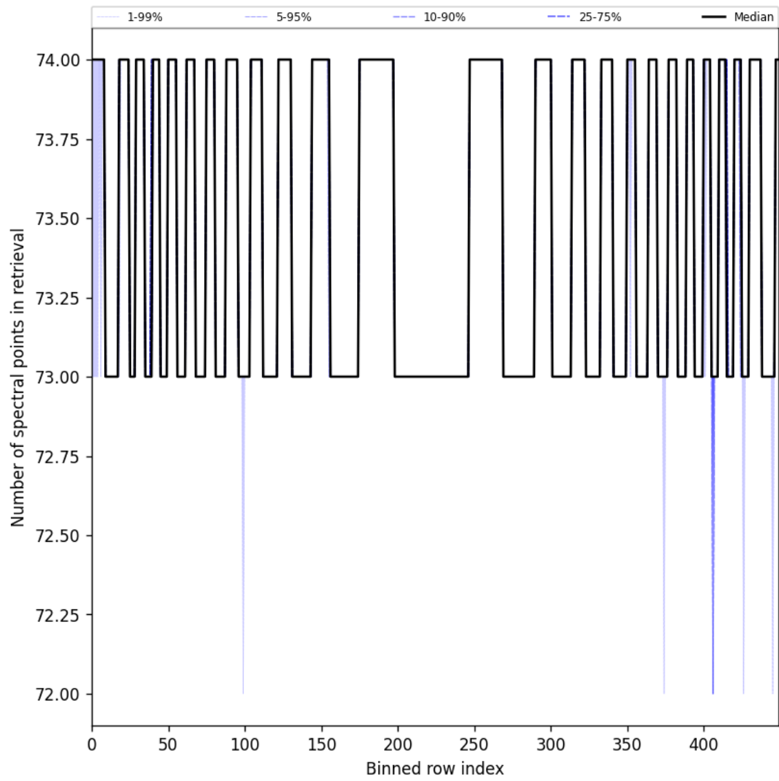
Figure 108: Along track statistics of “Number of spectral points in retrieval” for 2025-07-30 to 2025-08-01
