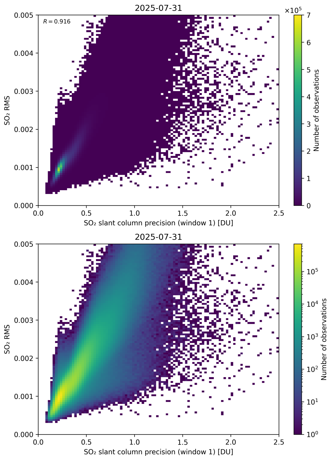
Figure 273: Scatter density plot of “SO 2 slant column precision (window 1)” against “SO 2 RMS” for 2025-07-30 to 2025-08-01.
