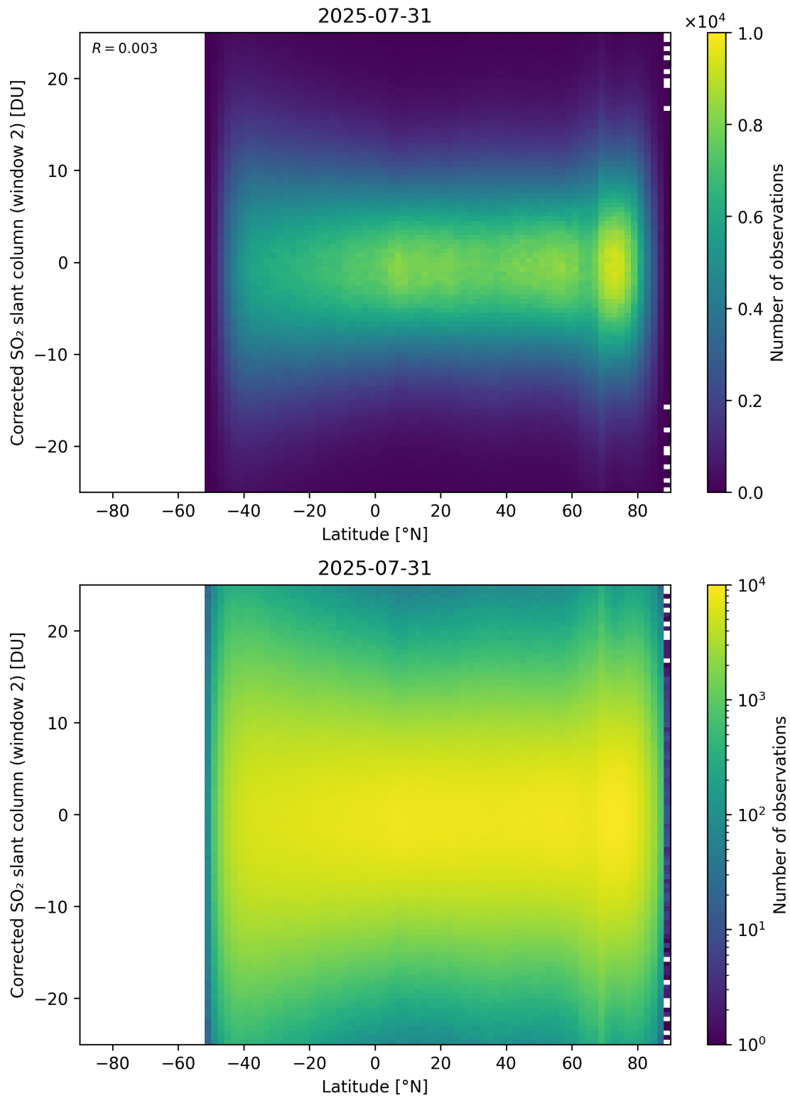
Figure 160: Scatter density plot of “Latitude” against “Corrected SO 2 slant column (window 2)” for 2025-07-30 to 2025-08-01.
