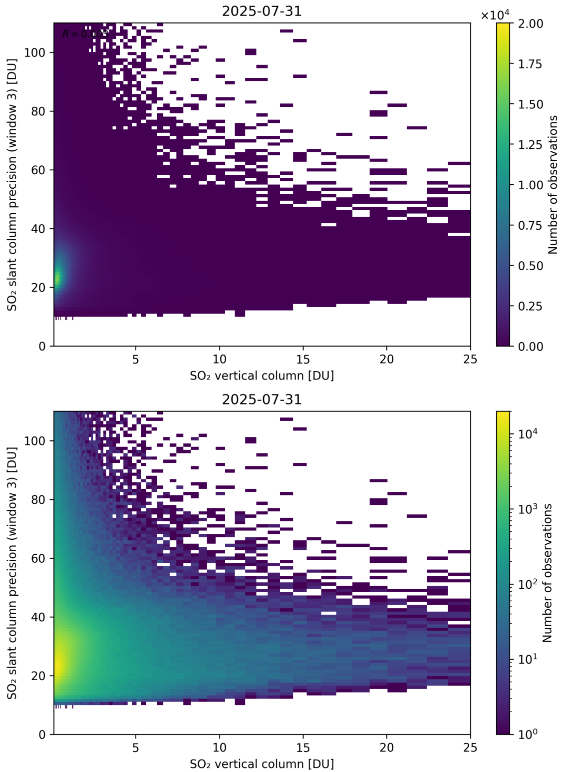
Figure 358: Scatter density plot of “SO 2 vertical column” against “SO 2 slant column precision (window 3)” for 2025-07-30 to 2025-08-01.
