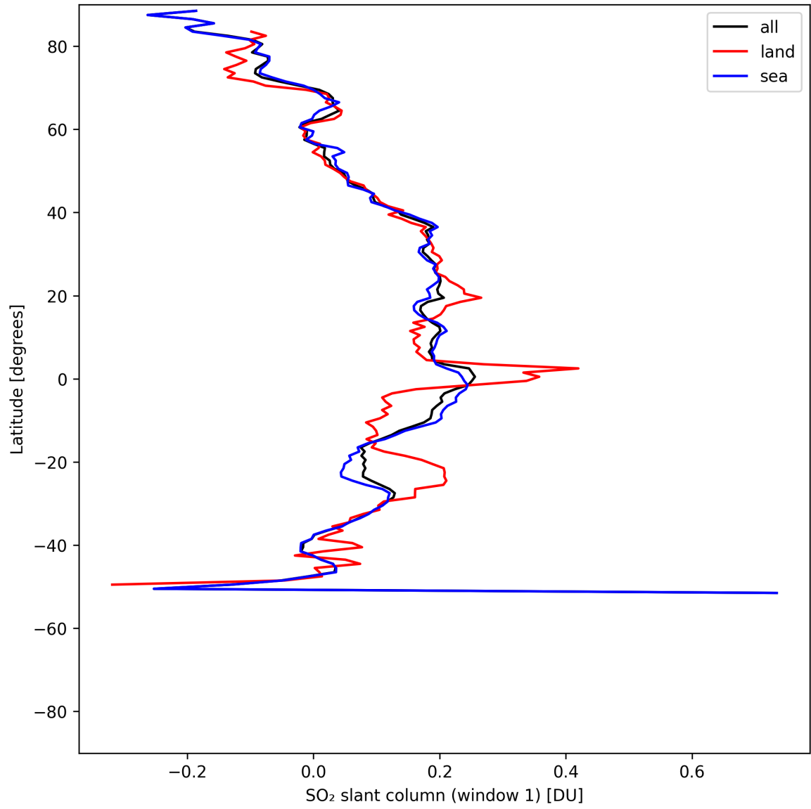
Figure 37: Zonal average of “SO 2 slant column (window 1)” for 2025-07-30 to 2025-08-01.
