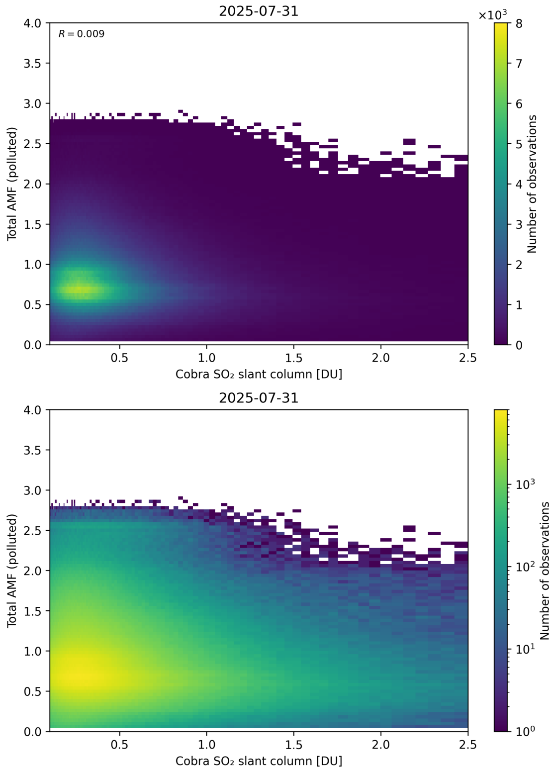
Figure 224: Scatter density plot of “Cobra SO 2 slant column” against “Total AMF (polluted)” for 2025-07-30 to 2025-08-01.
