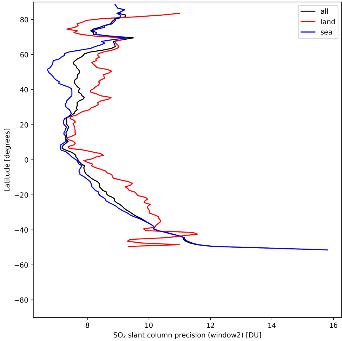
Figure 42: Zonal average of “SO 2 slant column precision (window2)” for 2025-07-30 to 2025-08-01.
