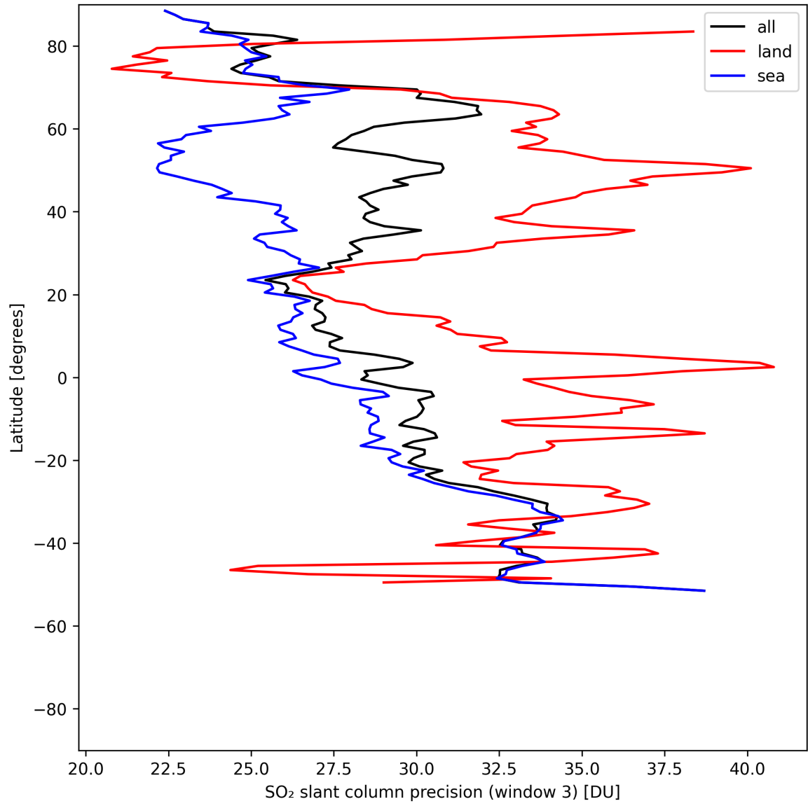
Figure 46: Zonal average of “SO 2 slant column precision (window 3)” for 2025-07-30 to 2025-08-01.
