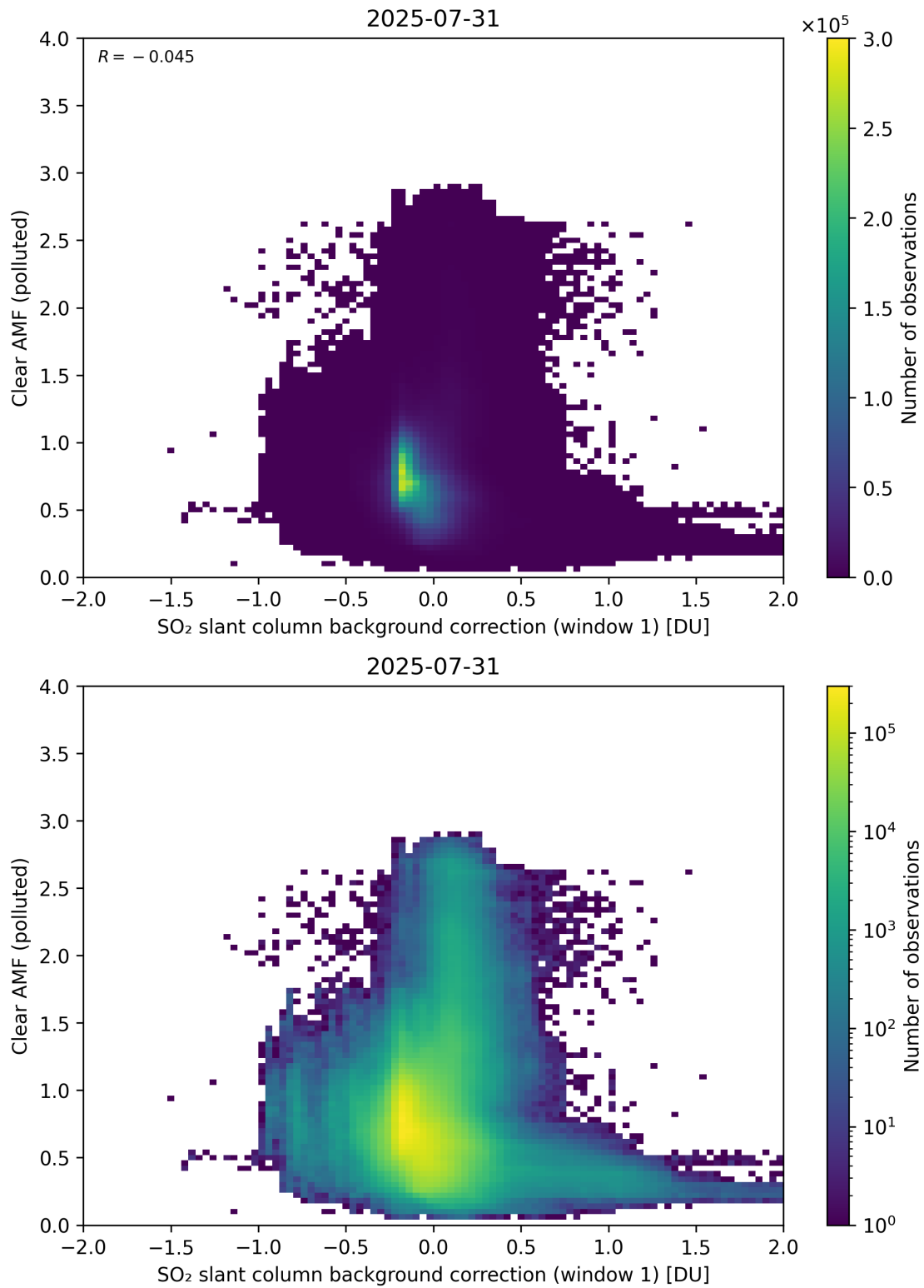
Figure 114: Scatter density plot of “SO 2 slant column background correction (window 1)” against “Clear AMF (polluted)” for 2025-07-30 to 2025-08-01.
