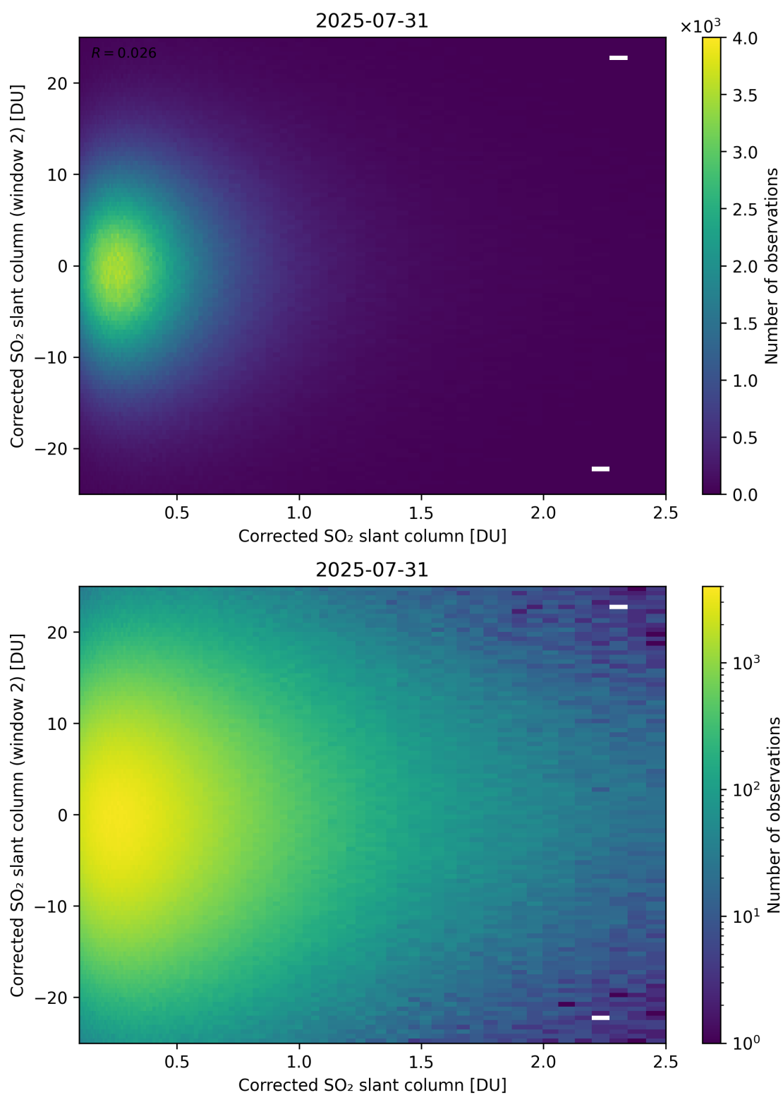
Figure 235: Scatter density plot of “Corrected SO 2 slant column” against “Corrected SO 2 slant column (window 2)” for 2025-07-30 to 2025-08-01.
