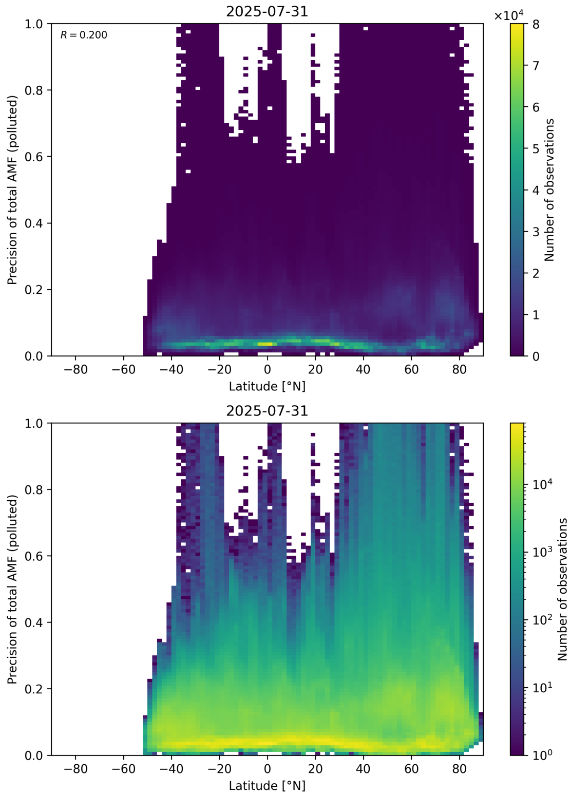
Figure 168: Scatter density plot of “Latitude” against “Precision of total AMF (polluted)” for 2025-07-30 to 2025-08-01.
