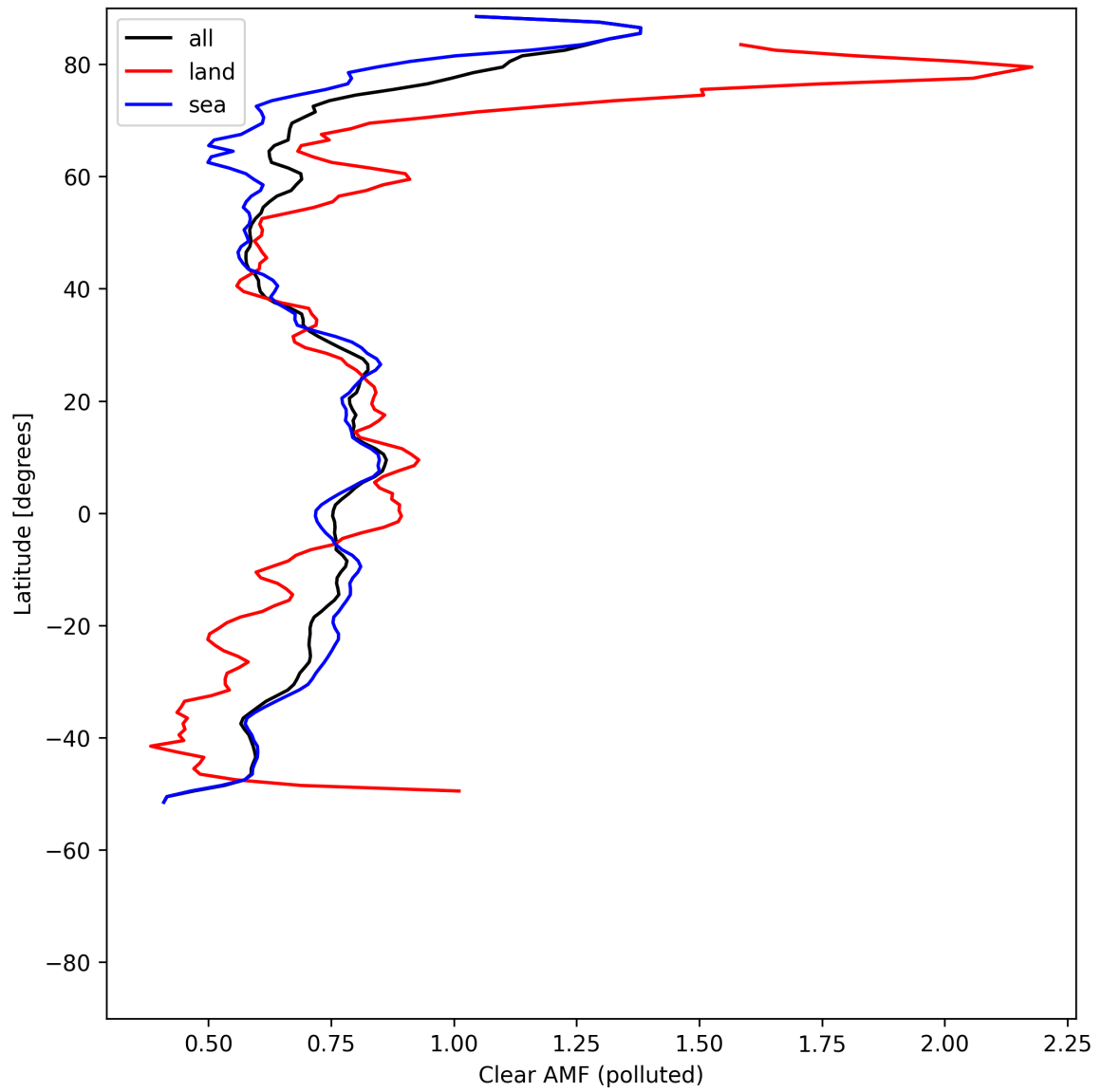
Figure 55: Zonal average of “Clear AMF (polluted)” for 2025-07-30 to 2025-08-01.
