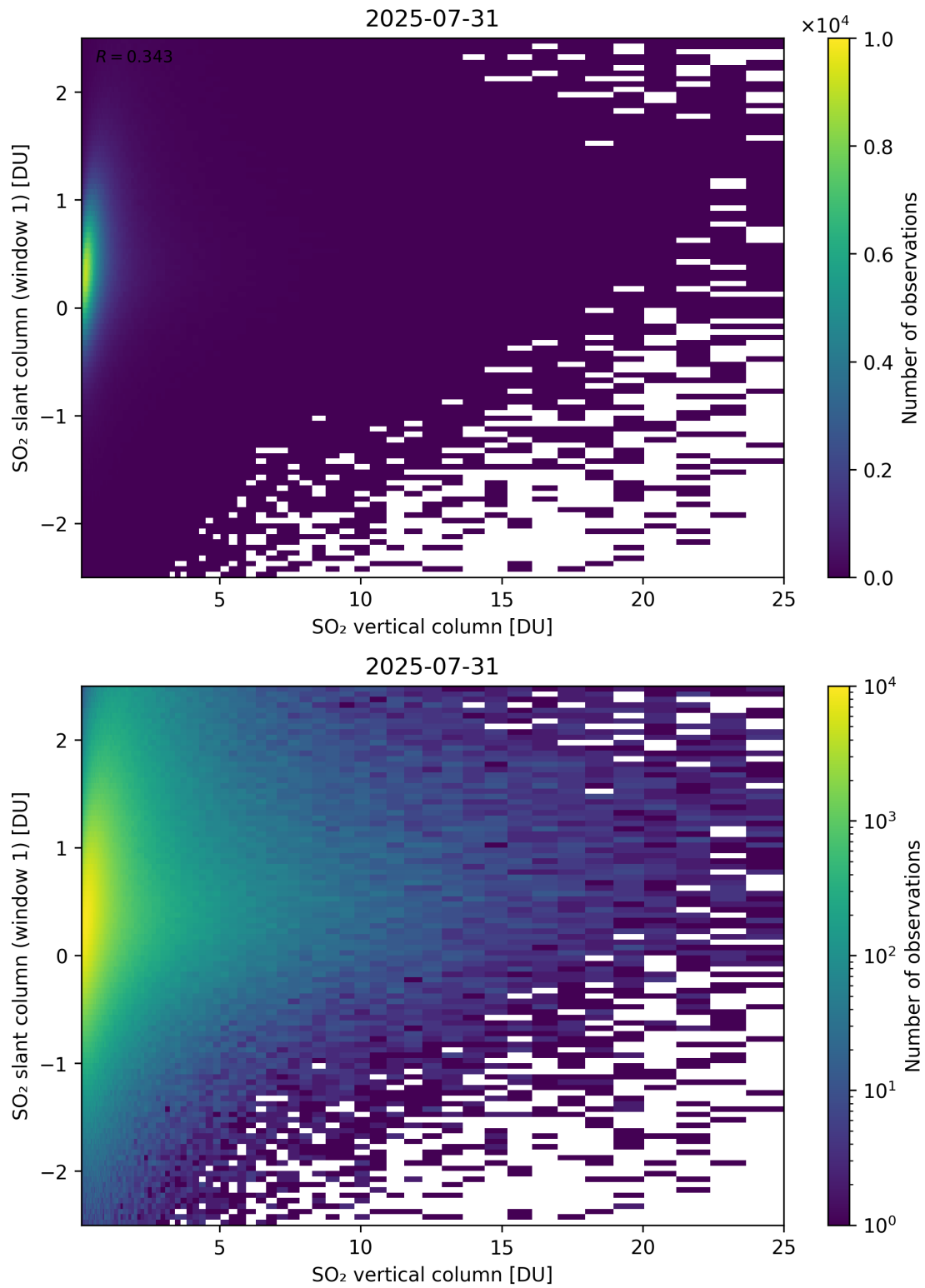
Figure 354: Scatter density plot of “SO 2 vertical column” against “SO 2 slant column (window 1)” for 2025-07-30 to 2025-08-01.
