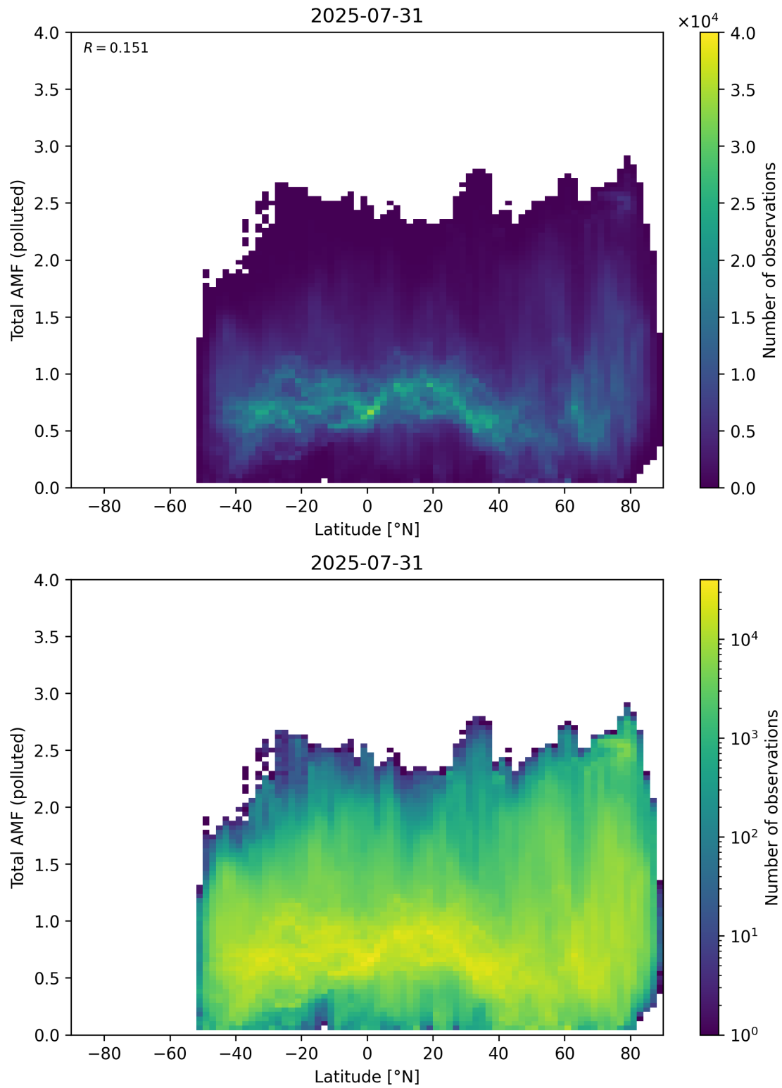
Figure 167: Scatter density plot of “Latitude” against “Total AMF (polluted)” for 2025-07-30 to 2025-08-01.
