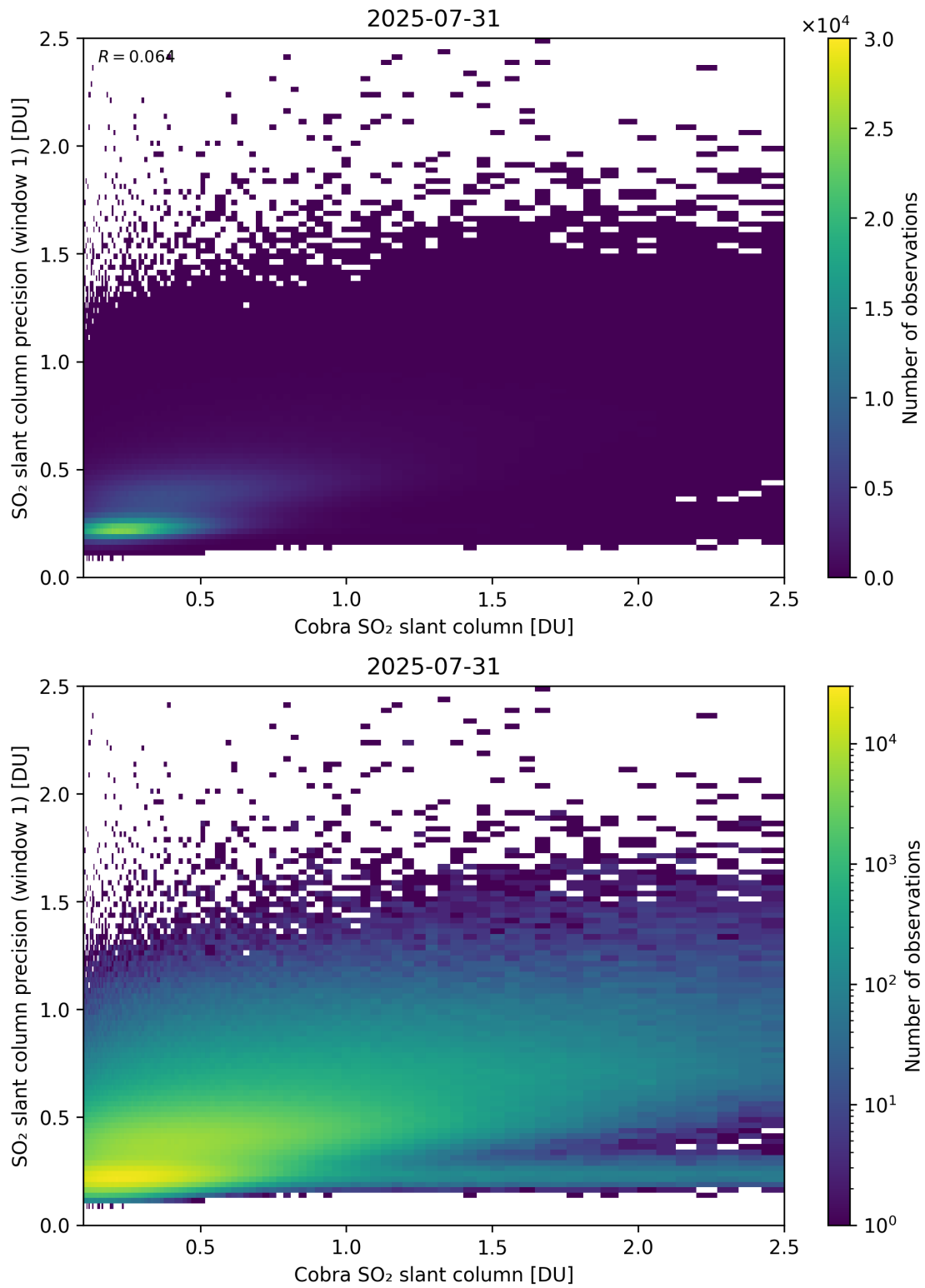
Figure 220: Scatter density plot of “Cobra SO 2 slant column” against “SO 2 slant column precision (window 1)” for 2025-07-30 to 2025-08-01.
