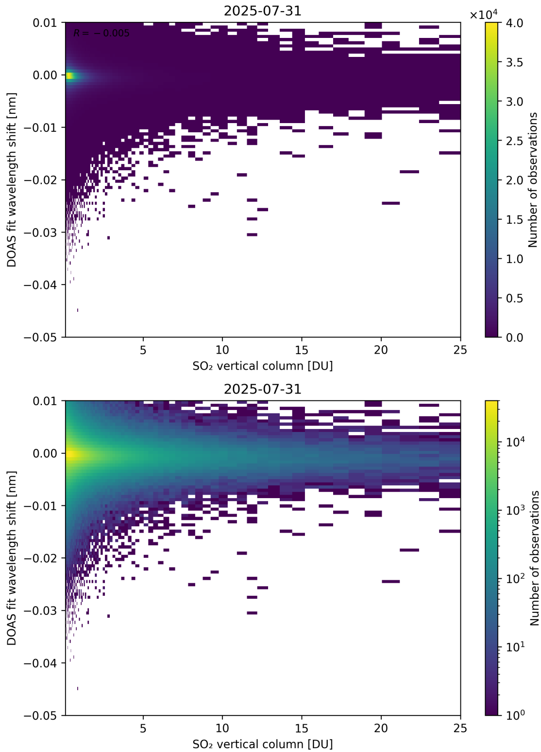
Figure 326: Scatter density plot of “SO 2 vertical column” against “DOAS fit wavelength shift” for 2025-07-30 to 2025-08-01.
