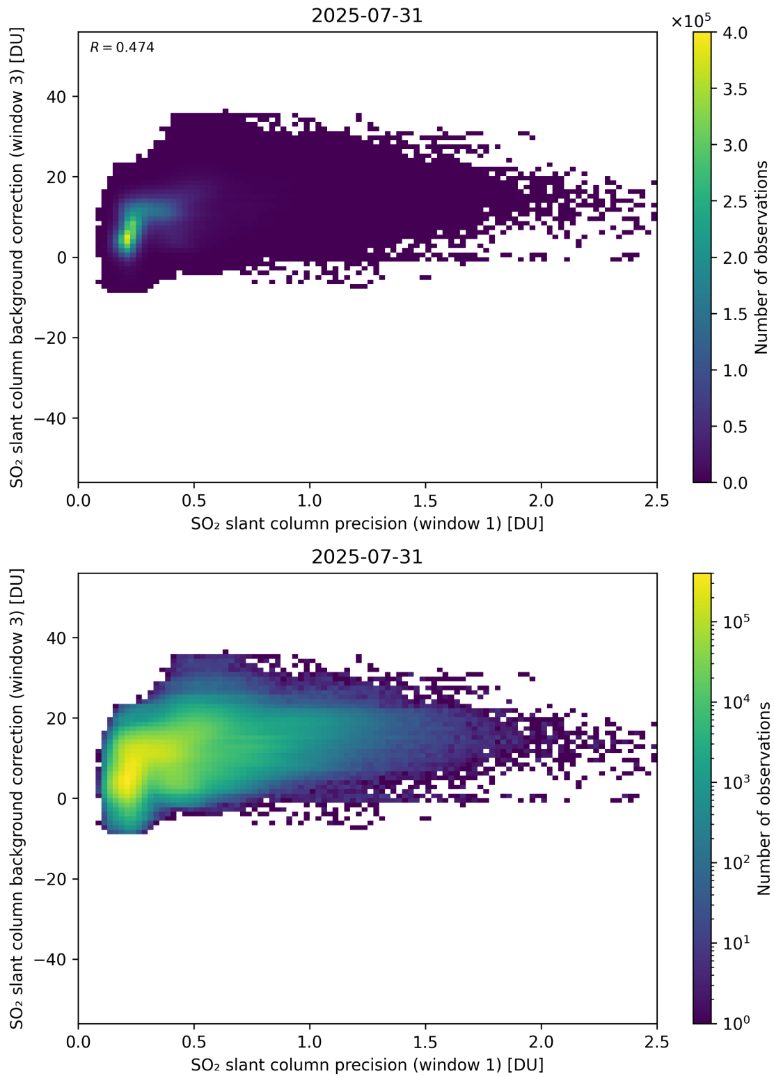
Figure 270: Scatter density plot of “SO 2 slant column precision (window 1)” against “SO 2 slant column background correction (window 3)” for 2025-07-30 to 2025-08-01.
