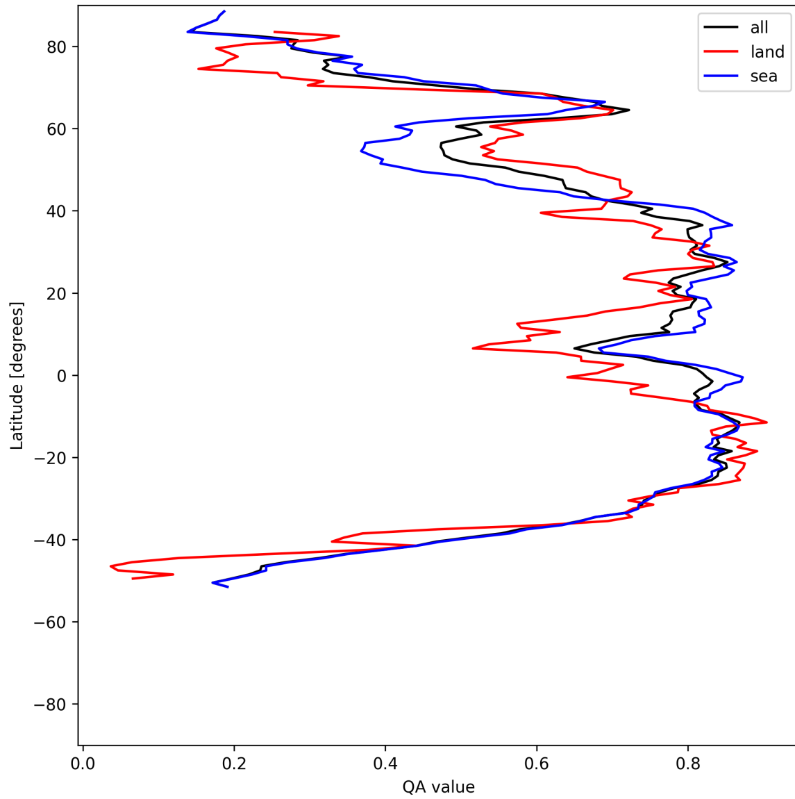
Figure 31: Zonal average of “QA value” for 2025-07-30 to 2025-08-01.
