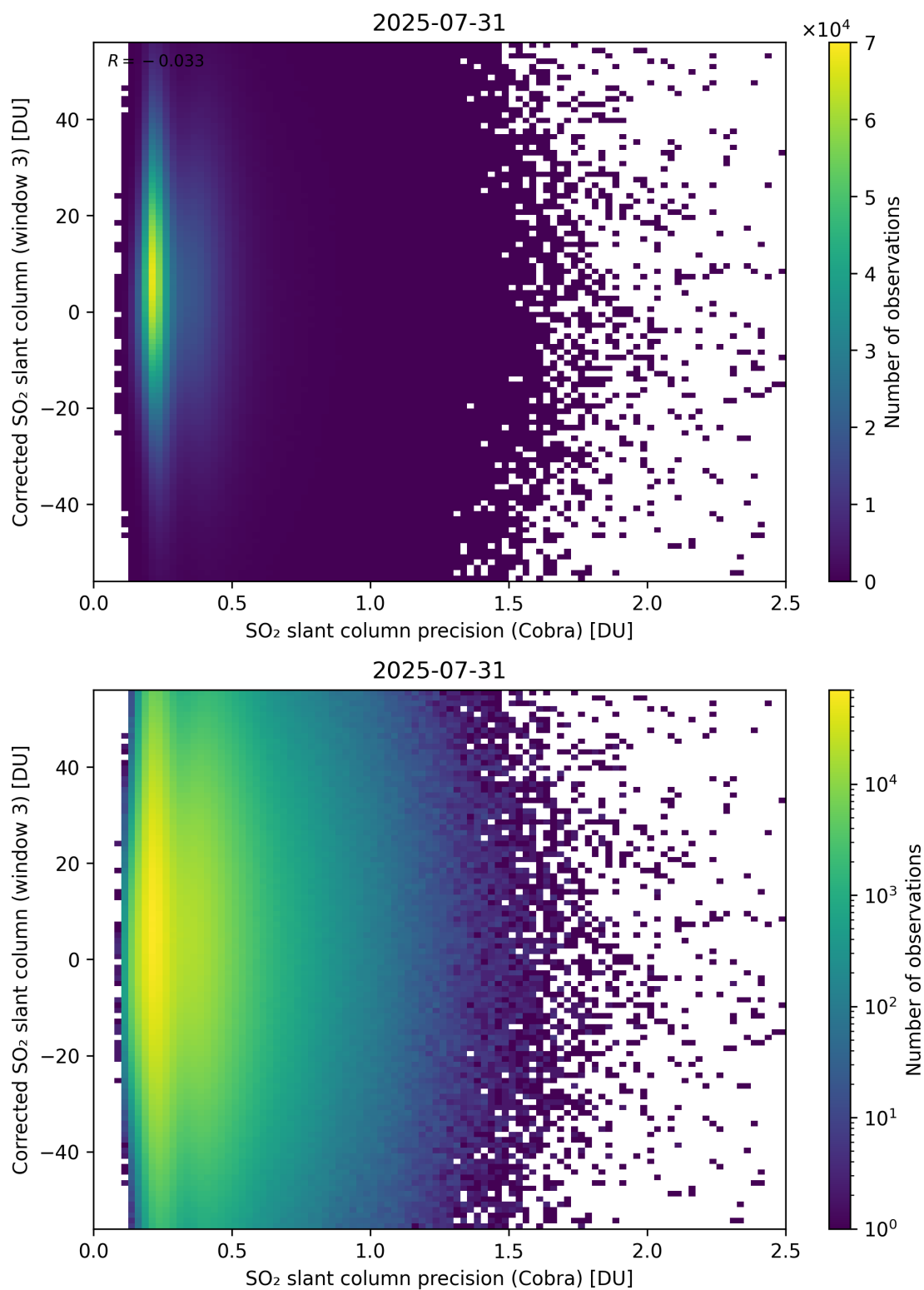
Figure 207: Scatter density plot of “SO 2 slant column precision (Cobra)” against “Corrected SO 2 slant column (window 3)” for 2025-07-30 to 2025-08-01.
