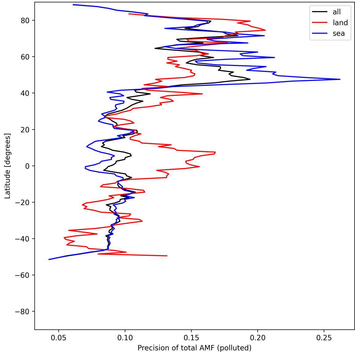
Figure 54: Zonal average of “Precision of total AMF (polluted)” for 2025-07-30 to 2025-08-01.
