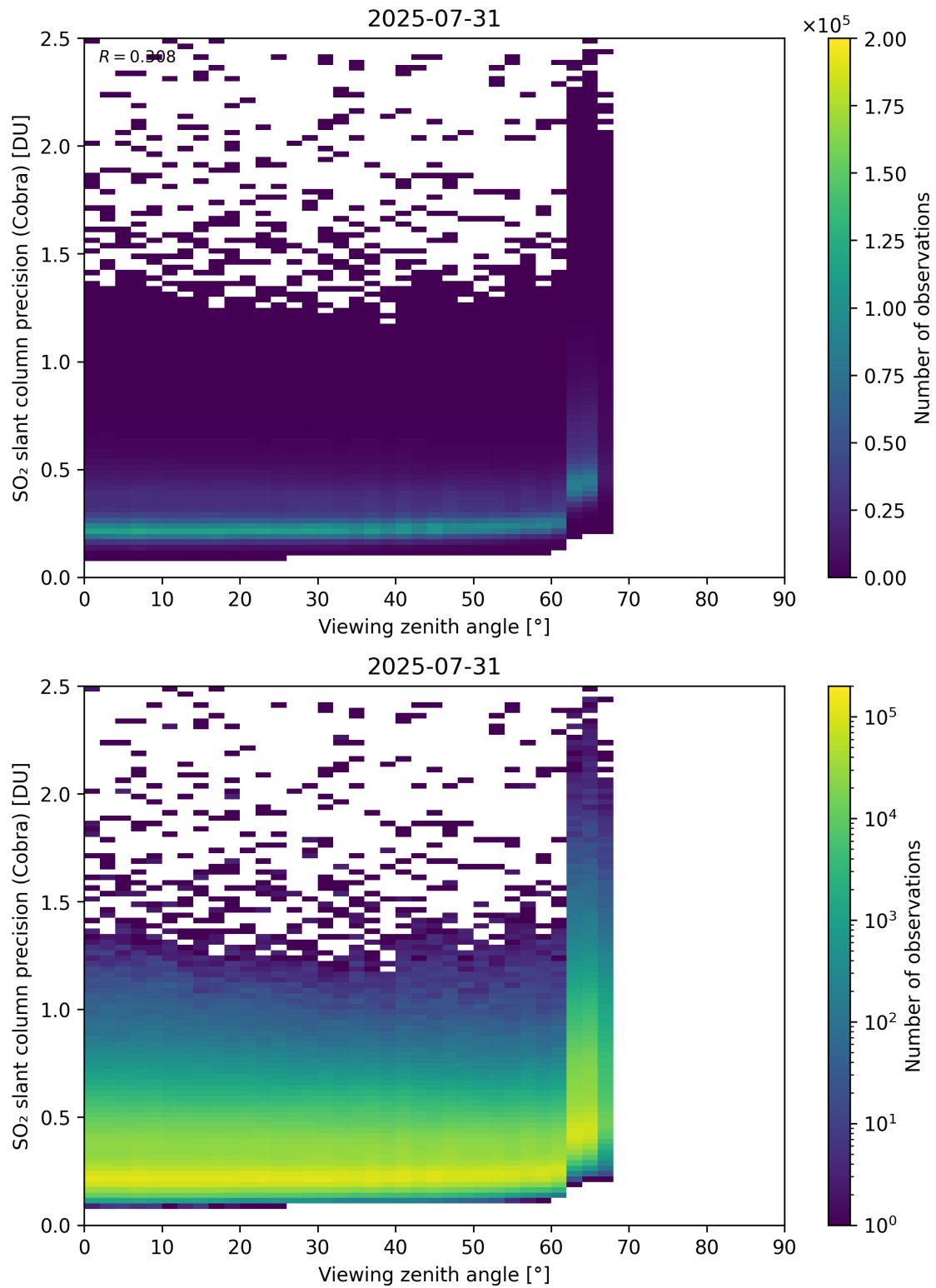
Figure 372: Scatter density plot of “Viewing zenith angle” against “SO 2 slant column precision (Cobra)” for 2025-07-30 to 2025-08-01.
