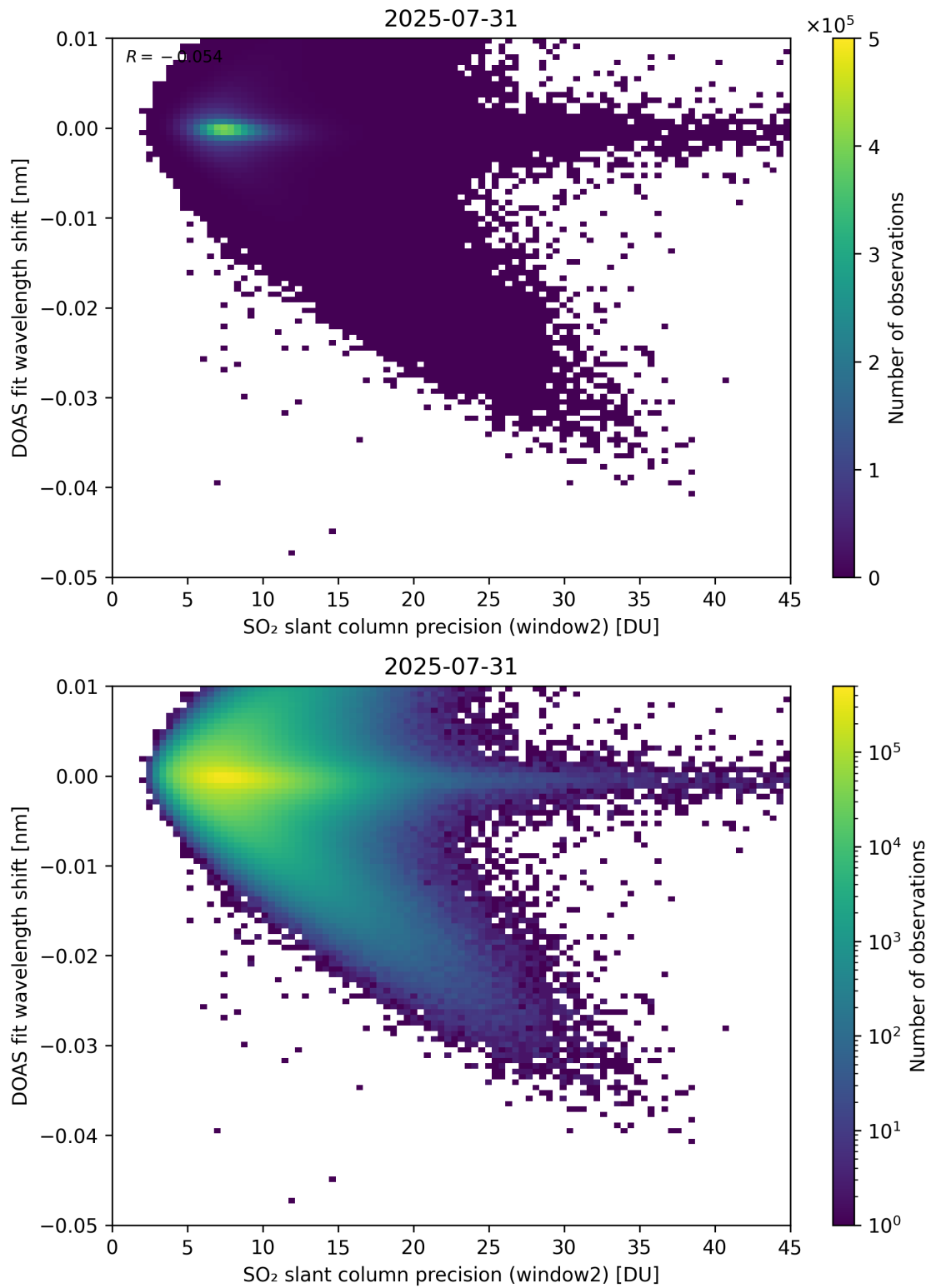
Figure 293: Scatter density plot of “SO 2 slant column precision (window2)” against “DOAS fit wavelength shift” for 2025-07-30 to 2025-08-01.
