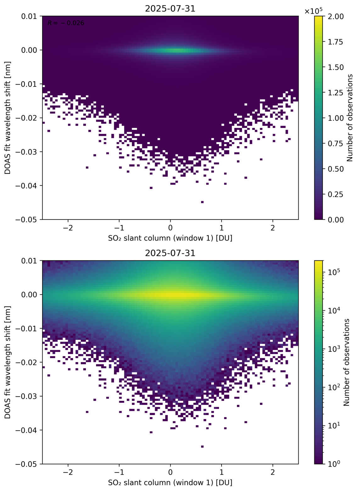
Figure 265: Scatter density plot of “SO 2 slant column (window 1)” against “DOAS fit wavelength shift” for 2025-07-30 to 2025-08-01.
