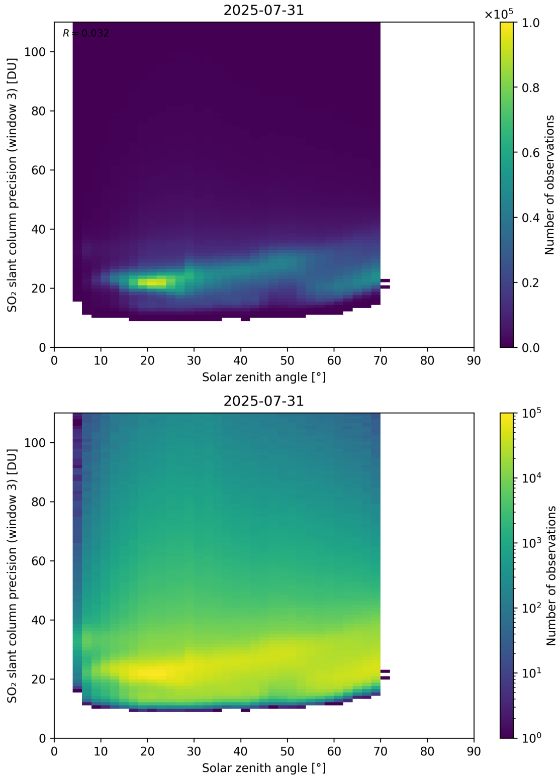
Figure 188: Scatter density plot of “Solar zenith angle” against “SO 2 slant column precision (window 3)” for 2025-07-30 to 2025-08-01.
