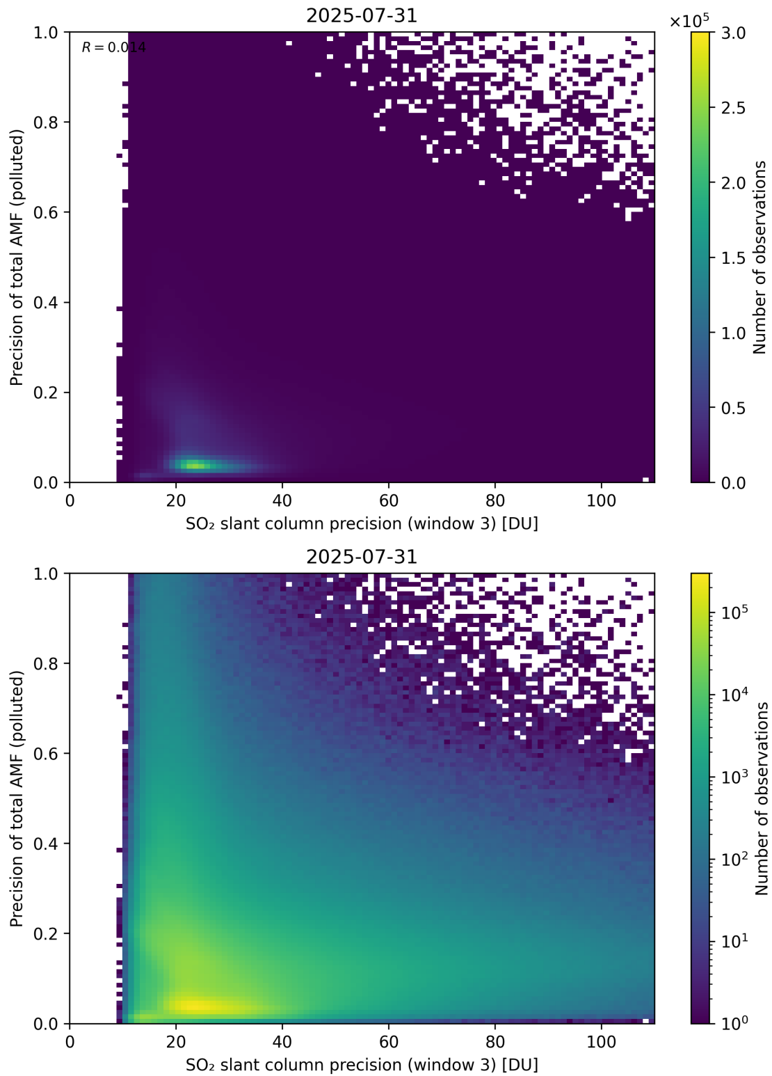
Figure 314: Scatter density plot of “SO 2 slant column precision (window 3)” against “Precision of total AMF (polluted)” for 2025-07-30 to 2025-08-01.
