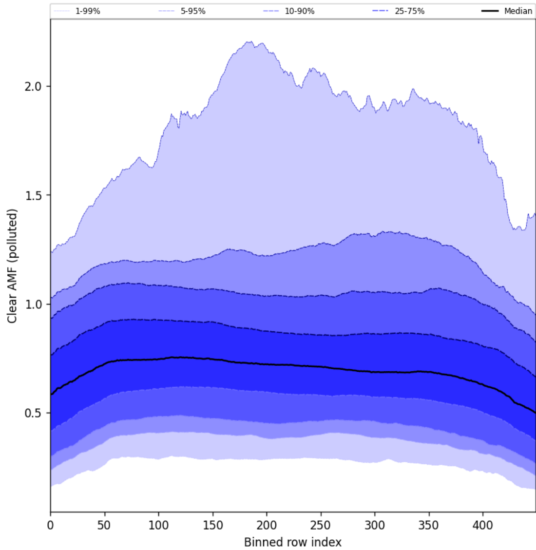
Figure 107: Along track statistics of “Clear AMF (polluted)” for 2025-07-30 to 2025-08-01
