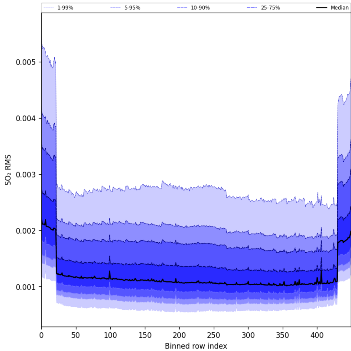
Figure 104: Along track statistics of “SO 2 RMS” for 2025-07-30 to 2025-08-01
