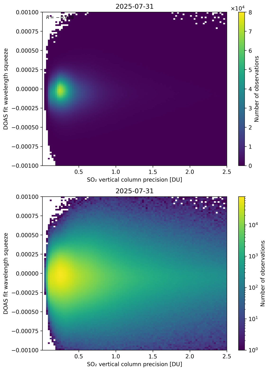
Figure 333: Scatter density plot of “SO 2 vertical column precision” against “DOAS fit wavelength squeeze” for 2025-07-30 to 2025-08-01.
