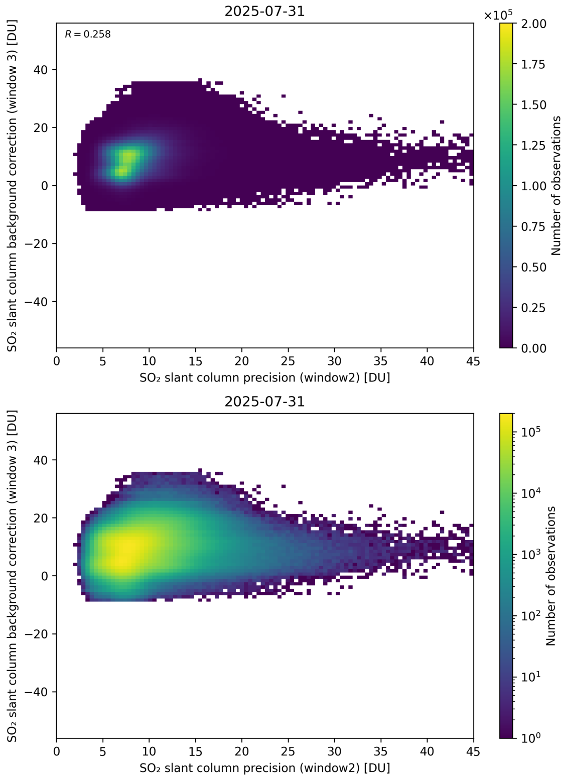
Figure 292: Scatter density plot of “SO 2 slant column precision (window2)” against “SO 2 slant column background correction (window 3)” for 2025-07-30 to 2025-08-01.
