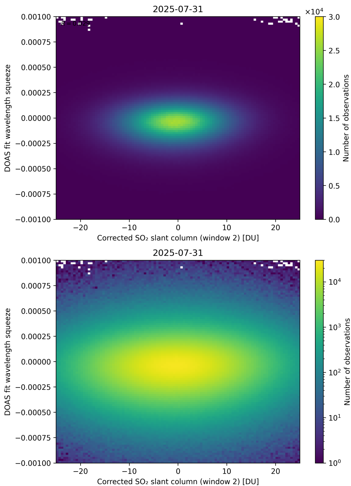
Figure 247: Scatter density plot of “Corrected SO 2 slant column (window 2)” against “DOAS fit wavelength squeeze” for 2025-07-30 to 2025-08-01.
