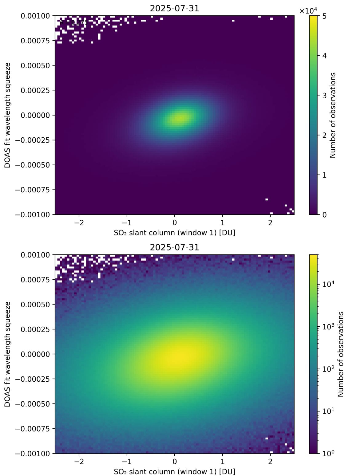
Figure 266: Scatter density plot of “SO 2 slant column (window 1)” against “DOAS fit wavelength squeeze” for 2025-07-30 to 2025-08-01.
