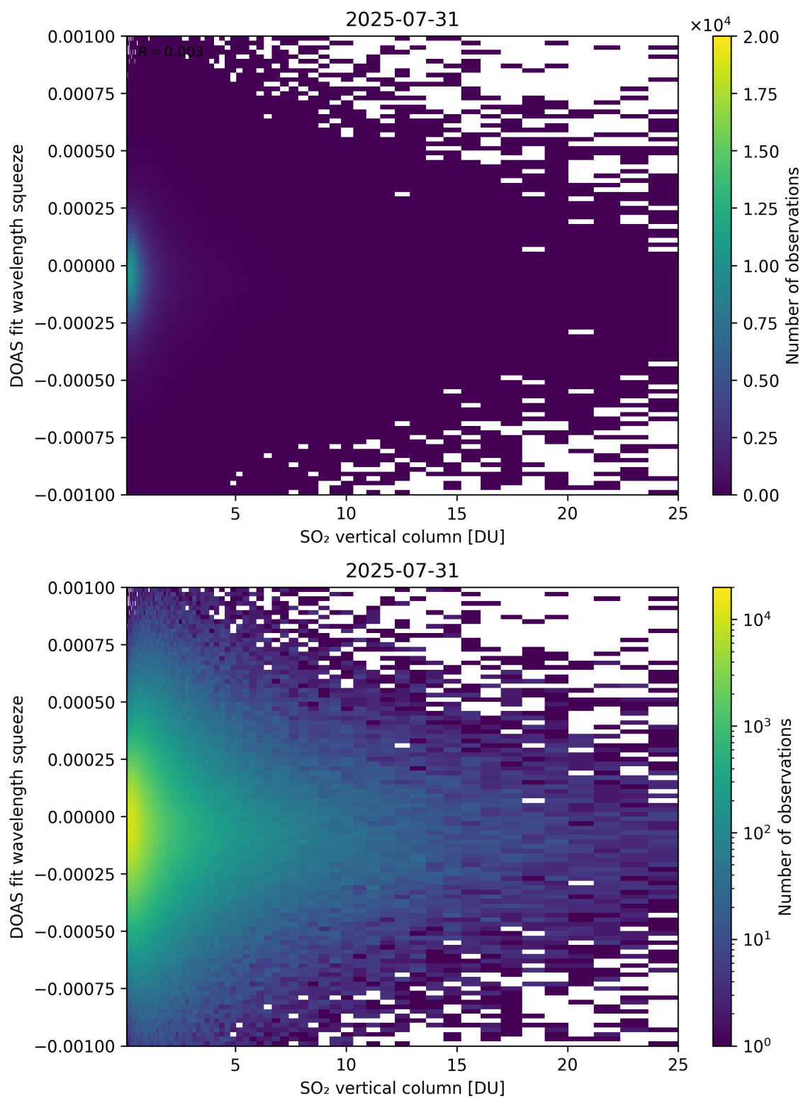
Figure 327: Scatter density plot of “SO 2 vertical column” against “DOAS fit wavelength squeeze” for 2025-07-30 to 2025-08-01.
