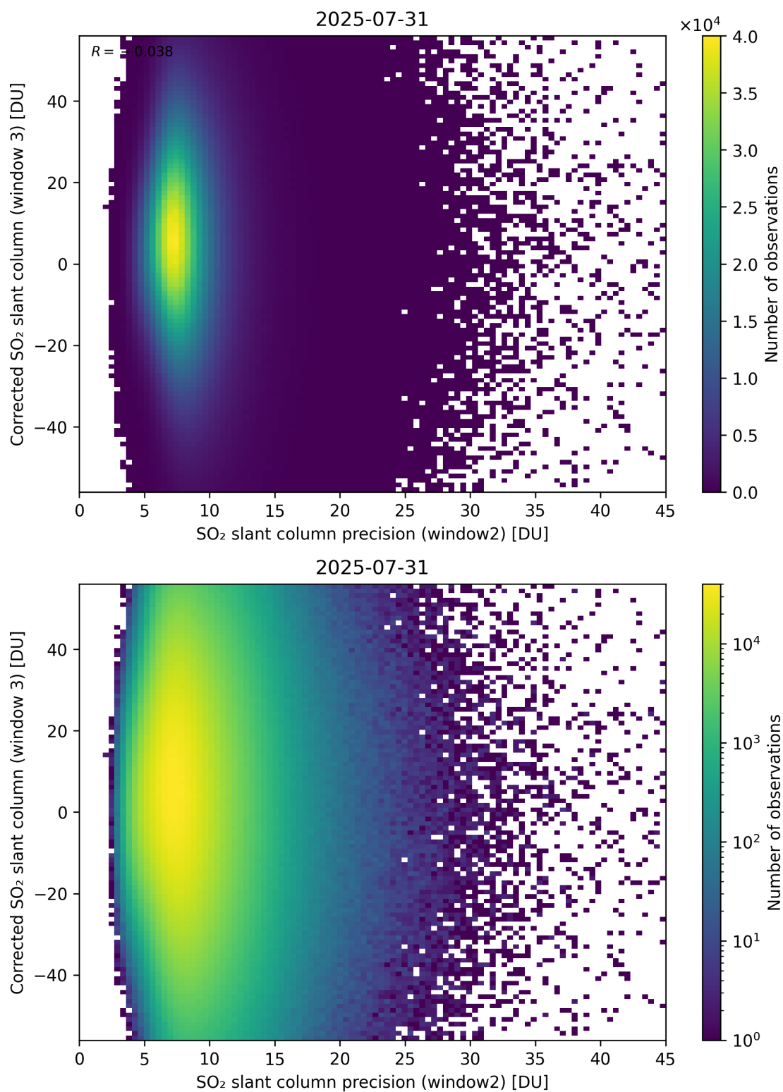
Figure 298: Scatter density plot of “SO 2 slant column precision (window2)” against “Corrected SO 2 slant column (window 3)” for 2025-07-30 to 2025-08-01.
