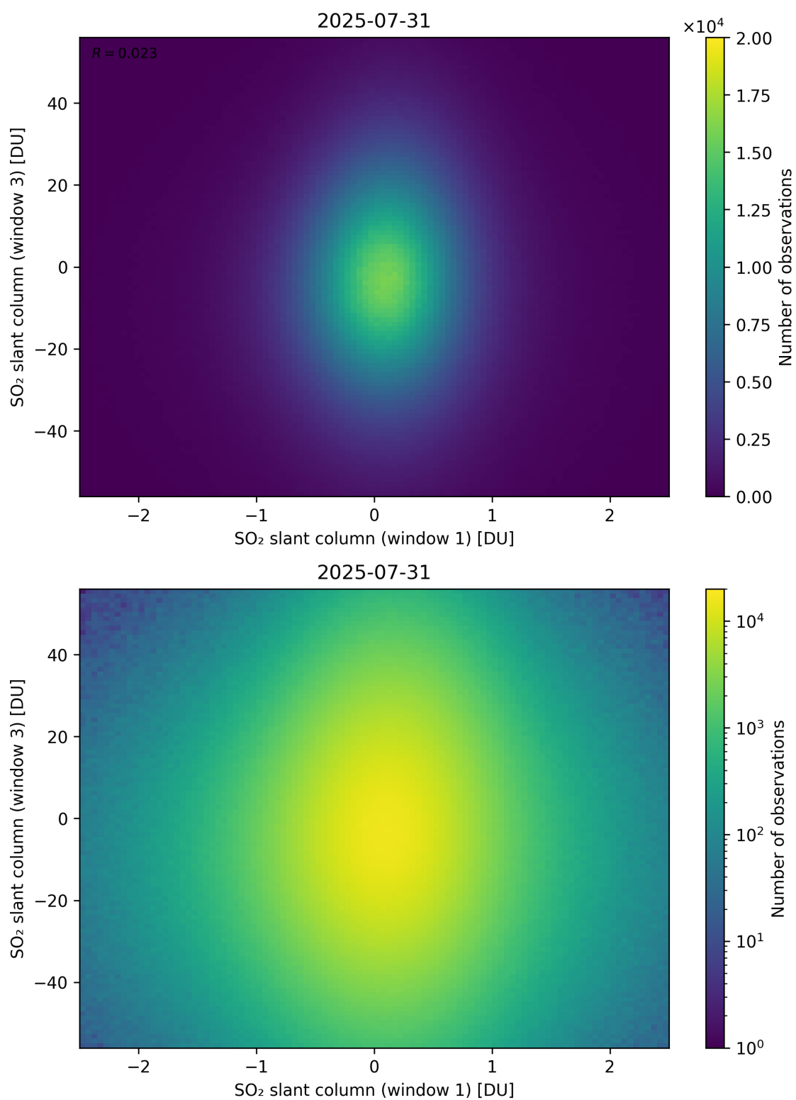
Figure 287: Scatter density plot of “SO 2 slant column (window 1)” against “SO 2 slant column (window 3)” for 2025-07-30 to 2025-08-01.
