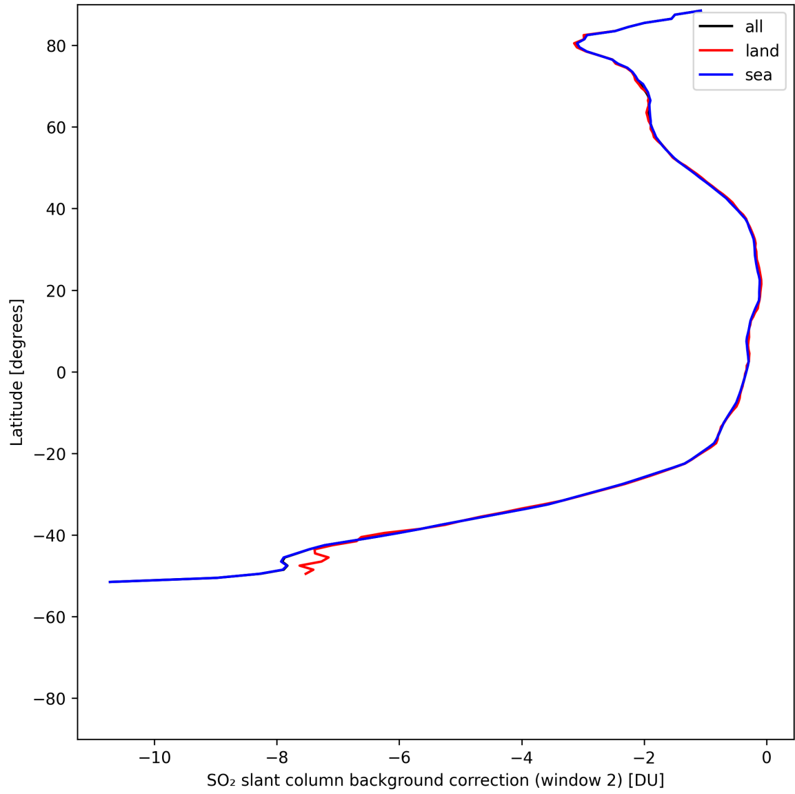
Figure 44: Zonal average of “SO 2 slant column background correction (window 2)” for 2025-07-30 to 2025-08-01.
