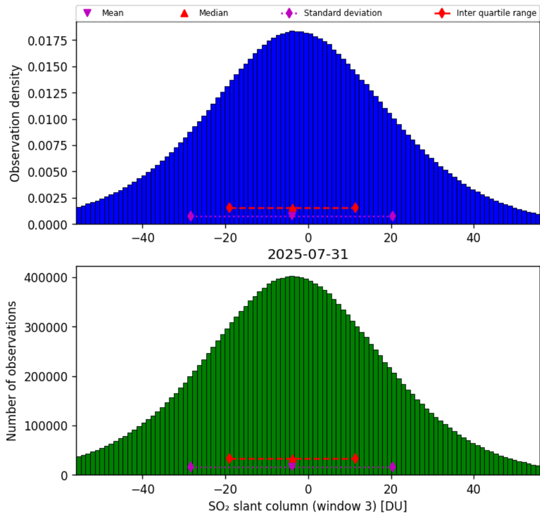
Figure 71: Histogram of “SO 2 slant column (window 3)” for 2025-07-30 to 2025-08-01
