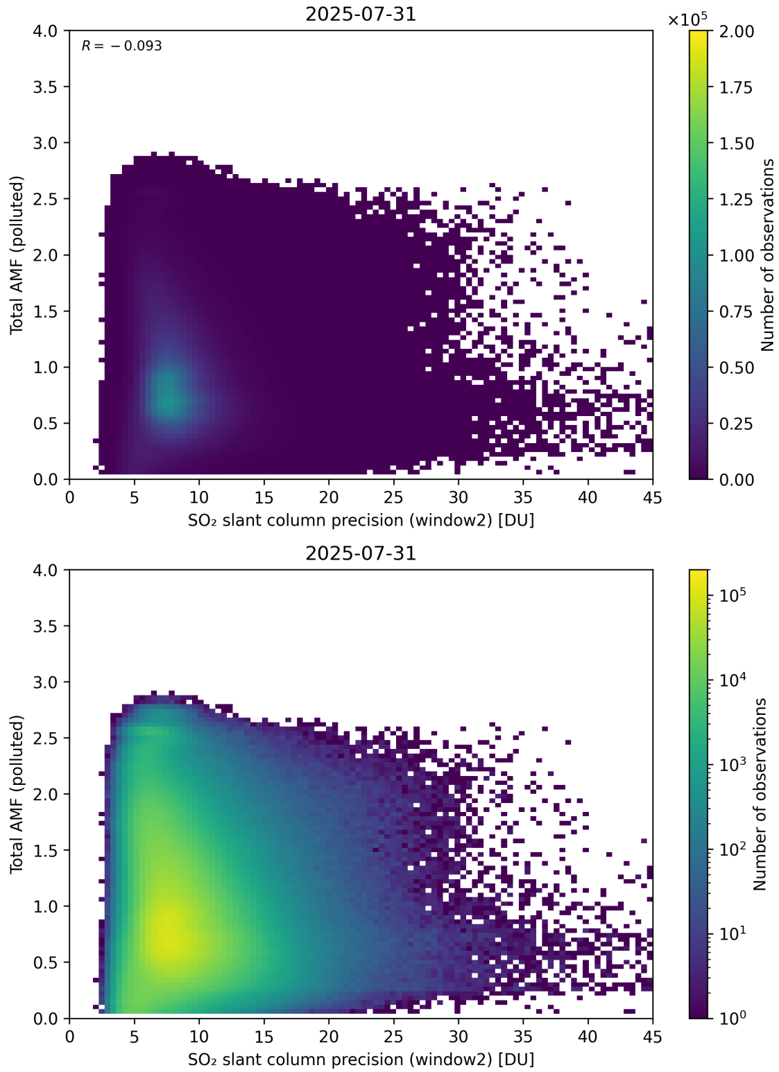
Figure 301: Scatter density plot of “SO 2 slant column precision (window2)” against “Total AMF (polluted)” for 2025-07-30 to 2025-08-01.
