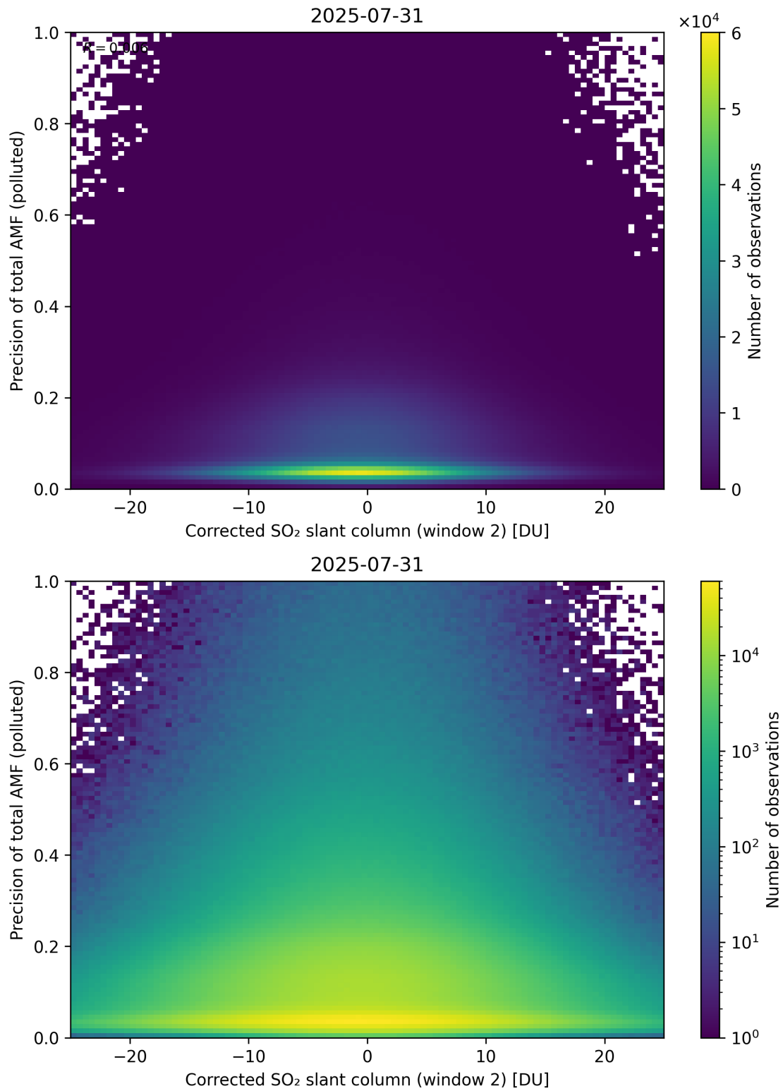
Figure 254: Scatter density plot of “Corrected SO 2 slant column (window 2)” against “Precision of total AMF (polluted)” for 2025-07-30 to 2025-08-01.
