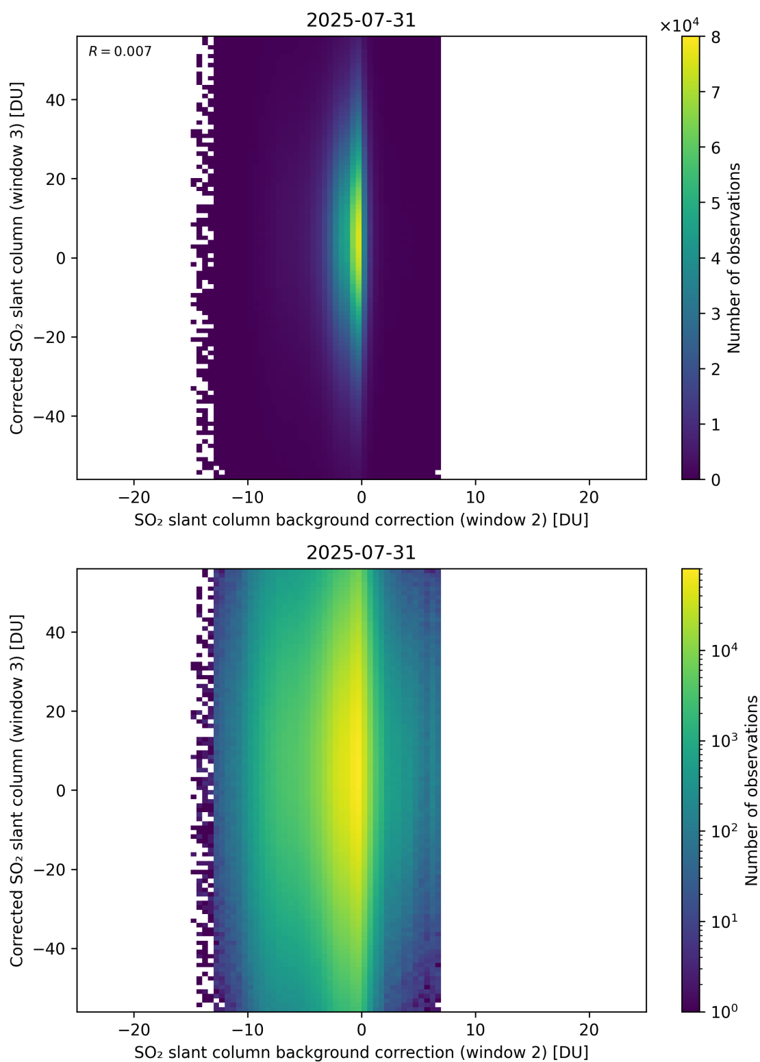
Figure 127: Scatter density plot of “SO 2 slant column background correction (window 2)” against “Corrected SO 2 slant column (window 3)” for 2025-07-30 to 2025-08-01.
