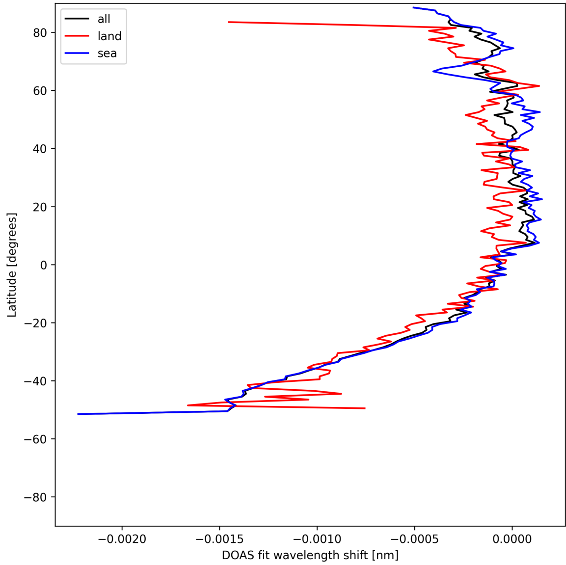
Figure 50: Zonal average of “DOAS fit wavelength shift” for 2025-07-30 to 2025-08-01.
