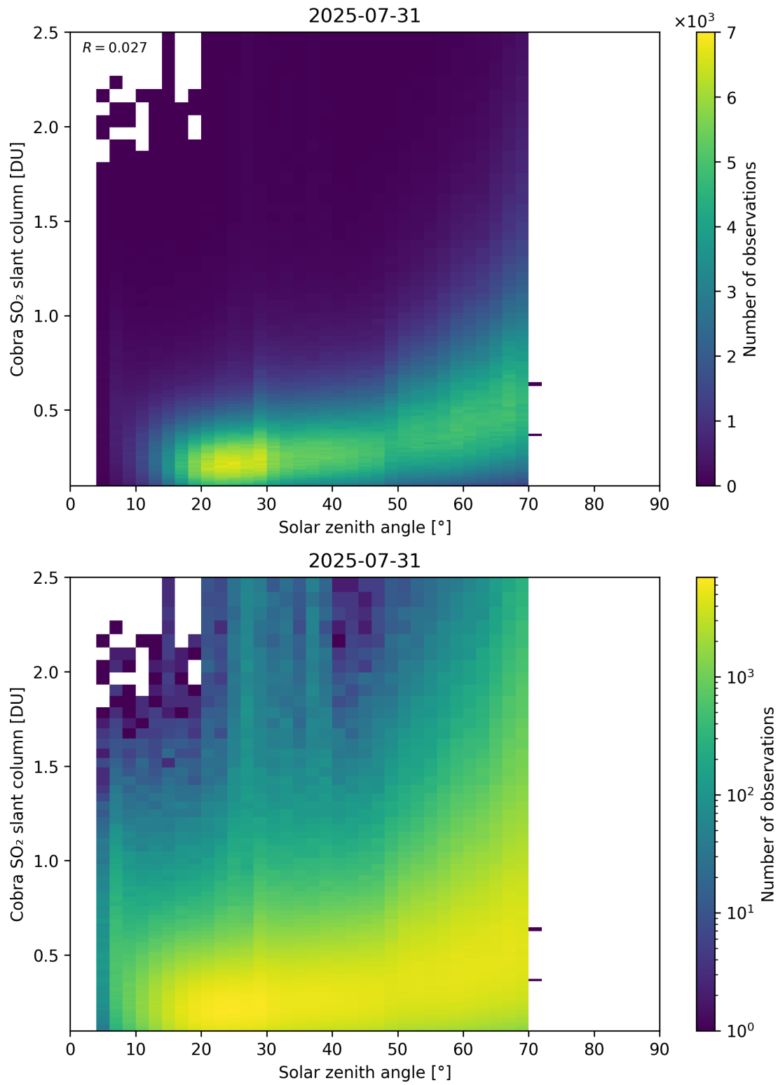
Figure 179: Scatter density plot of “Solar zenith angle” against “Cobra SO 2 slant column” for 2025-07-30 to 2025-08-01.
