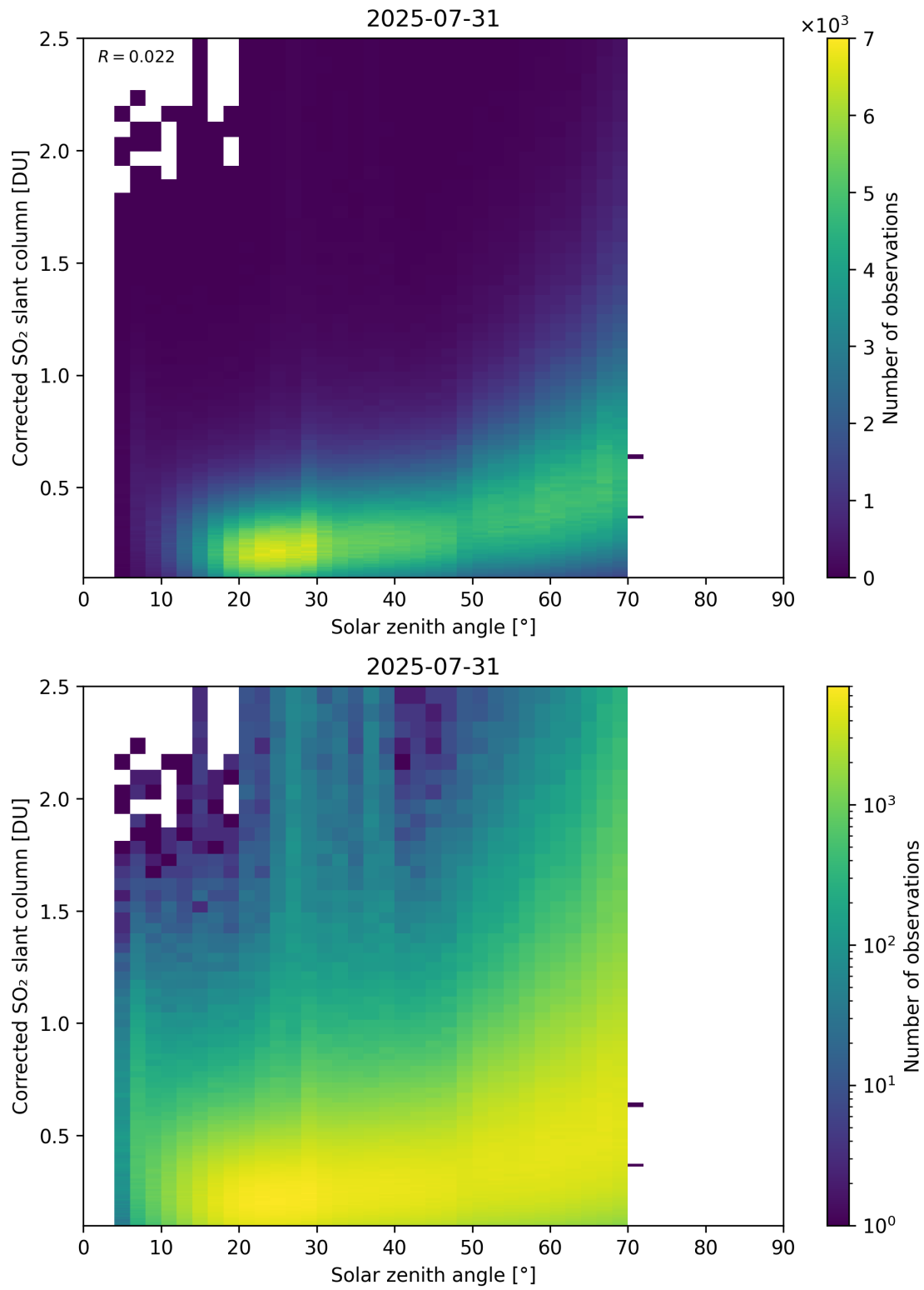
Figure 181: Scatter density plot of “Solar zenith angle” against “Corrected SO 2 slant column” for 2025-07-30 to 2025-08-01.
