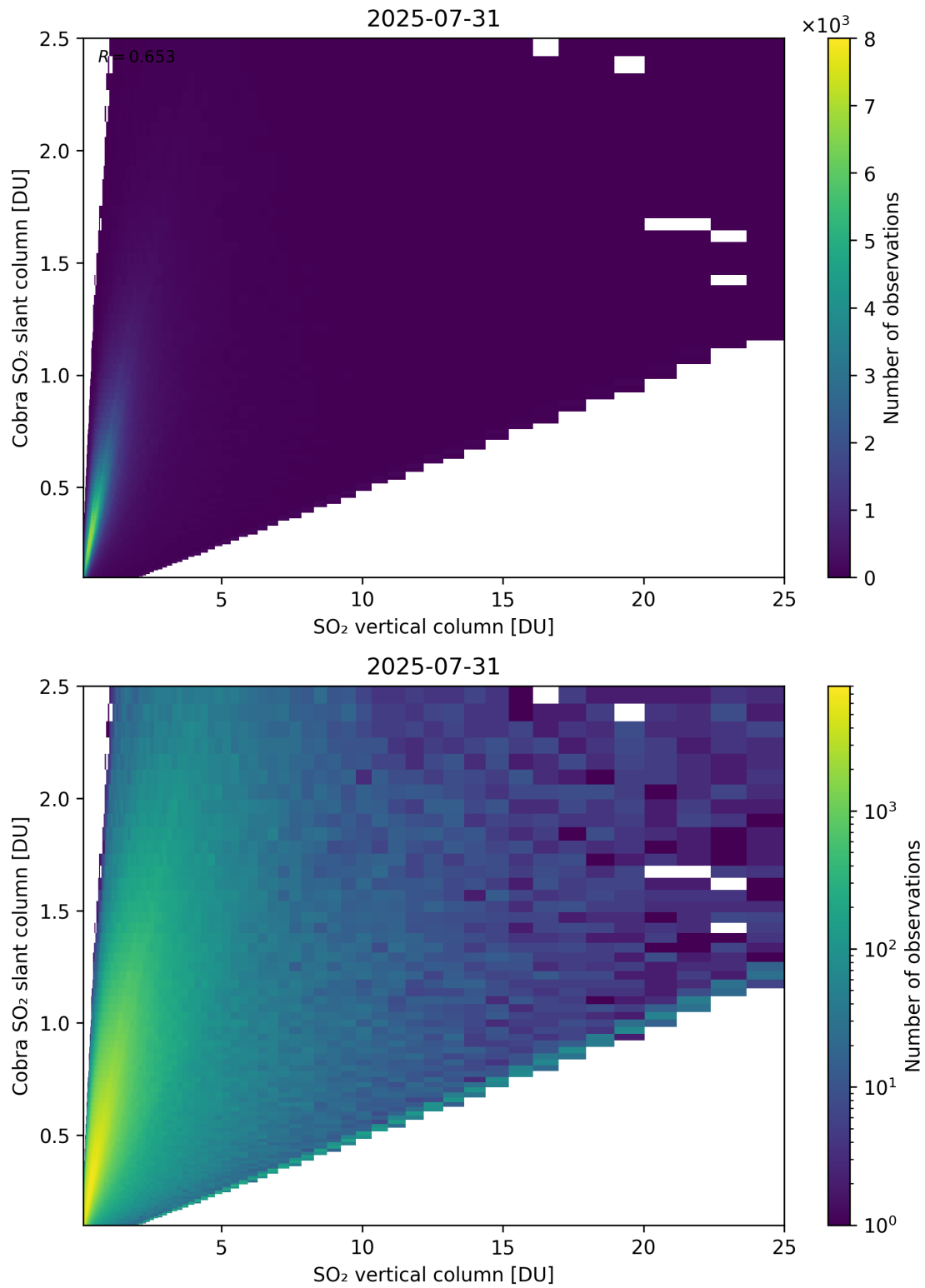
Figure 349: Scatter density plot of “SO 2 vertical column” against “Cobra SO 2 slant column” for 2025-07-30 to 2025-08-01.
