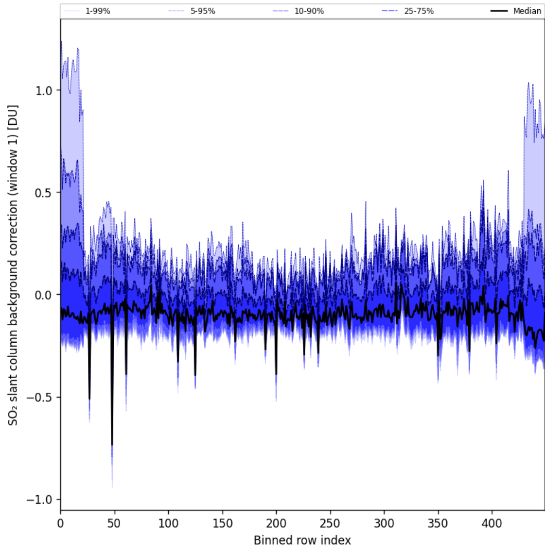
Figure 92: Along track statistics of “SO 2 slant column background correction (window 1)” for 2025-07-30 to 2025-08-01
