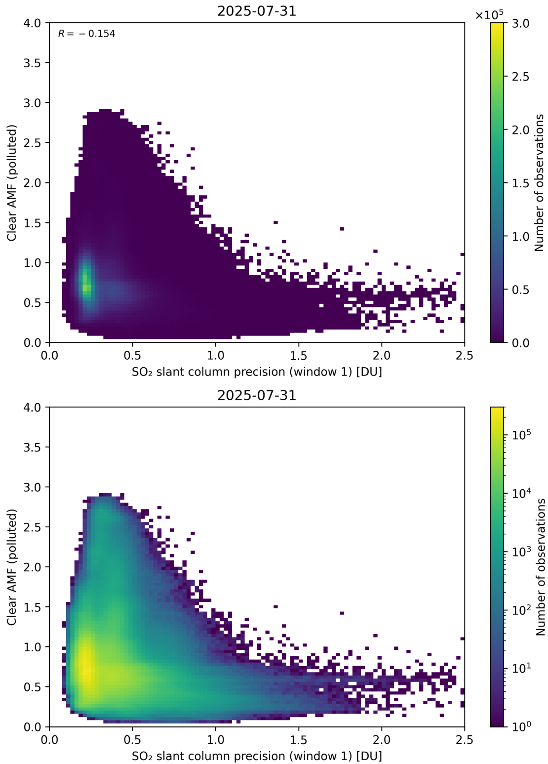
Figure 274: Scatter density plot of “SO 2 slant column precision (window 1)” against “Clear AMF (polluted)” for 2025-07-30 to 2025-08-01.
