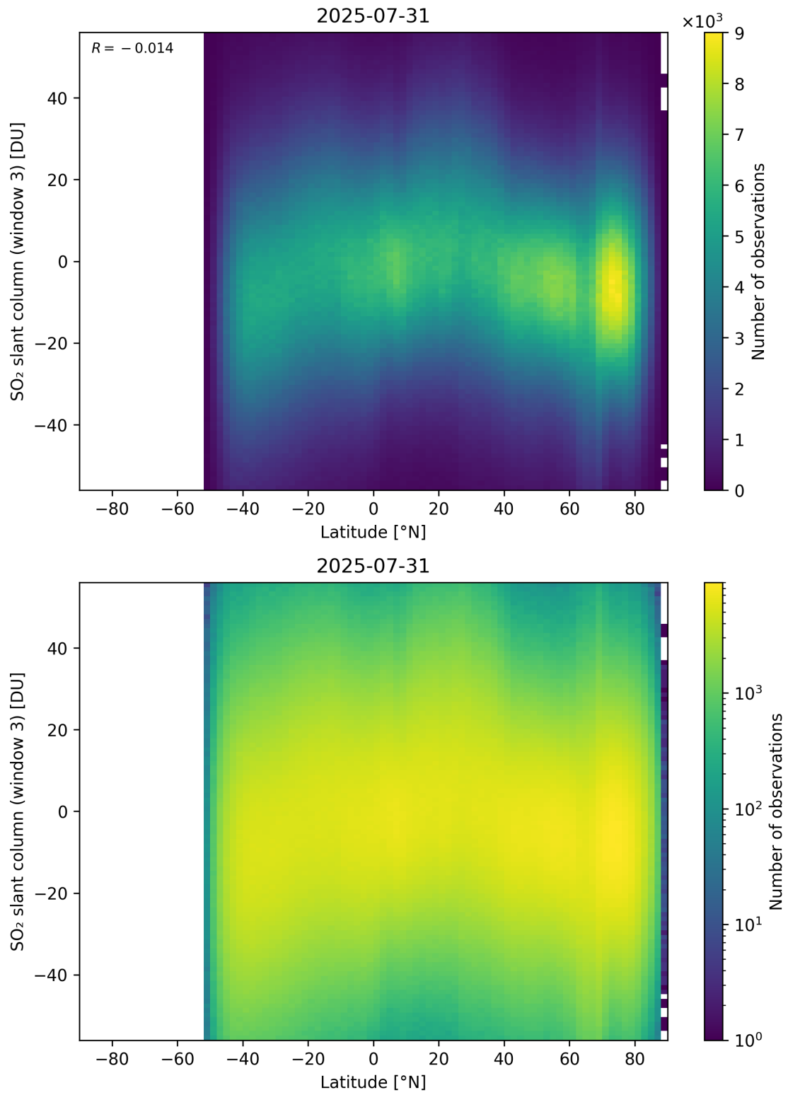
Figure 165: Scatter density plot of “Latitude” against “SO 2 slant column (window 3)” for 2025-07-30 to 2025-08-01.
