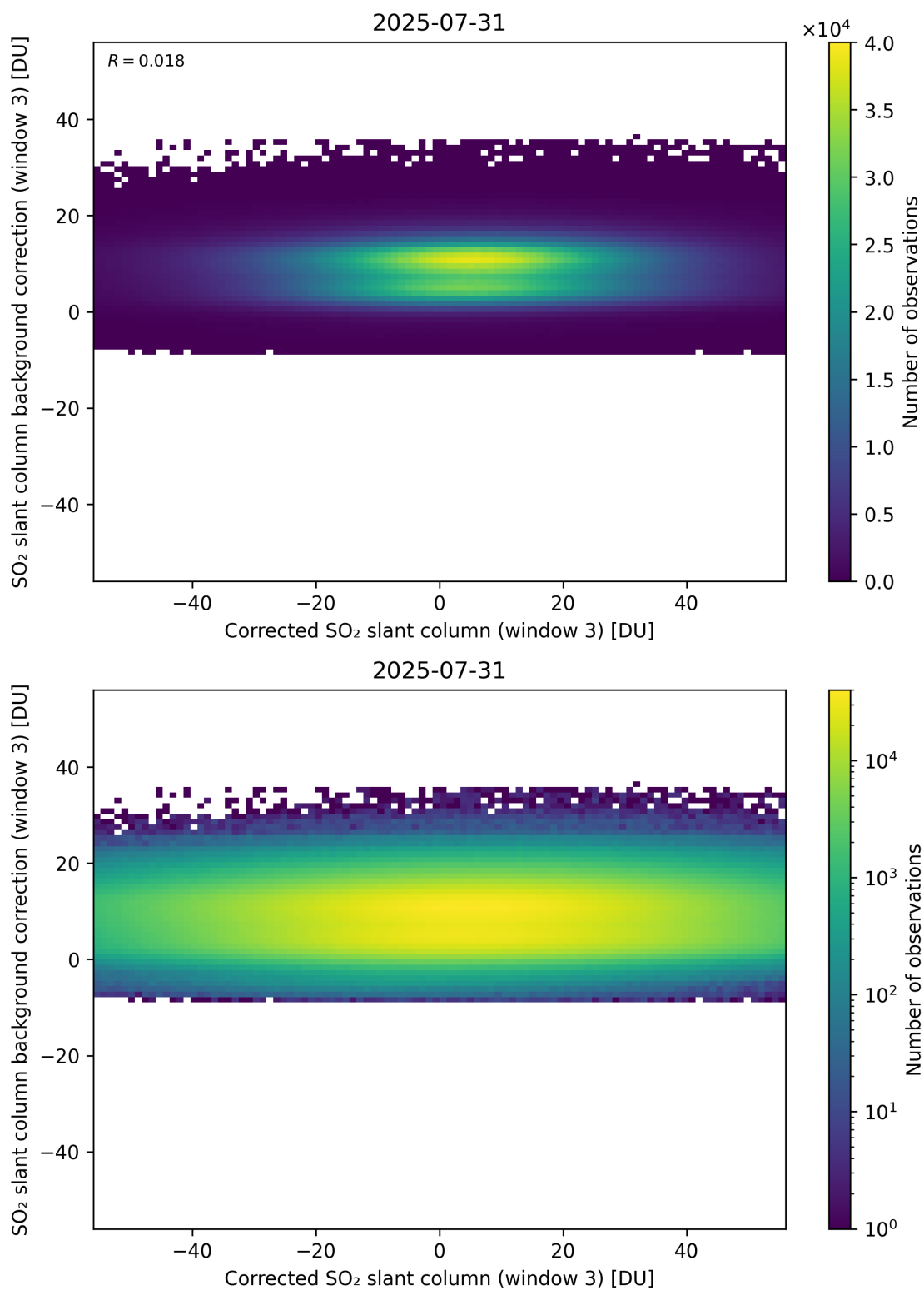
Figure 255: Scatter density plot of “Corrected SO 2 slant column (window 3)” against “SO 2 slant column background correction (window 3)” for 2025-07-30 to 2025-08-01.
