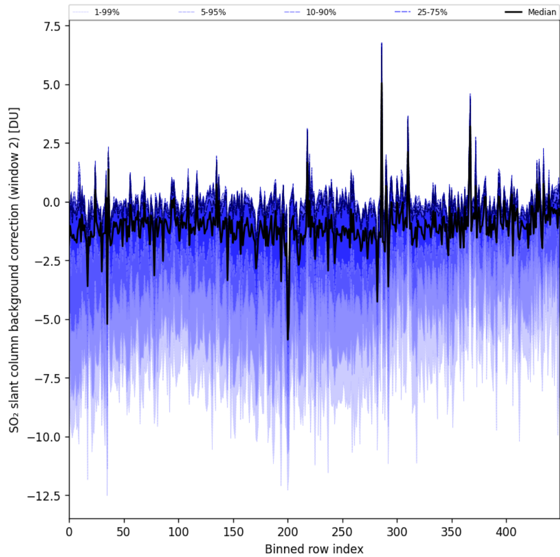
Figure 96: Along track statistics of “SO 2 slant column background correction (window 2)” for 2025-07-30 to 2025-08-01
