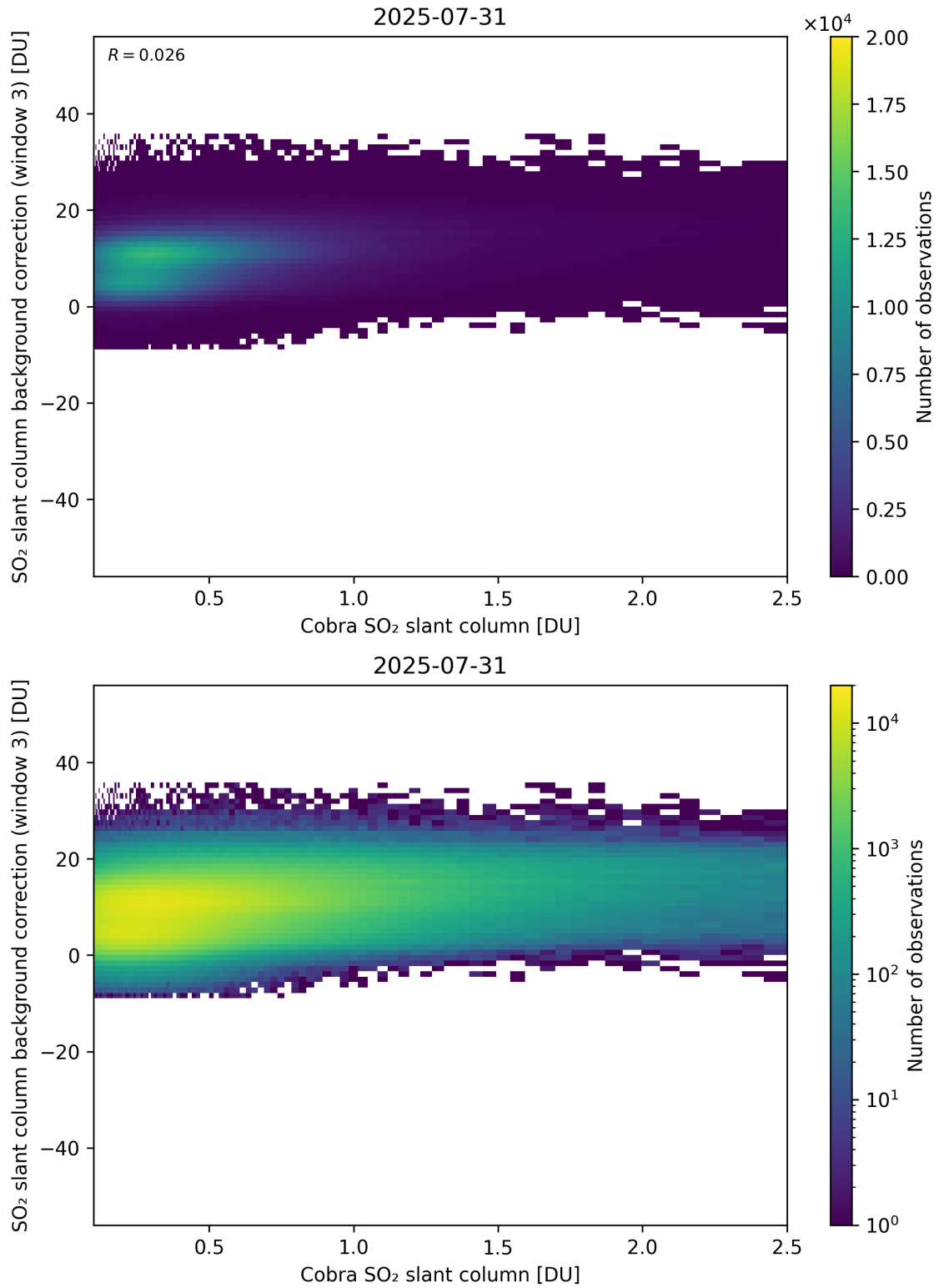
Figure 195: Scatter density plot of “Cobra SO 2 slant column” against “SO 2 slant column background correction (window 3)” for 2025-07-30 to 2025-08-01.
