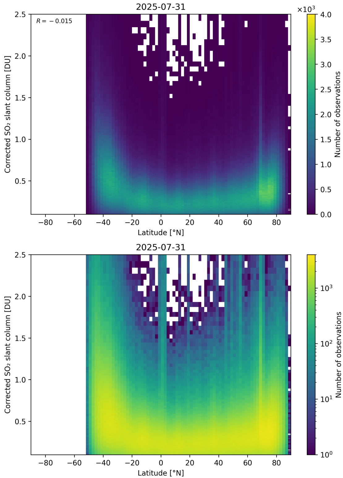
Figure 159: Scatter density plot of “Latitude” against “Corrected SO 2 slant column” for 2025-07-30 to 2025-08-01.
