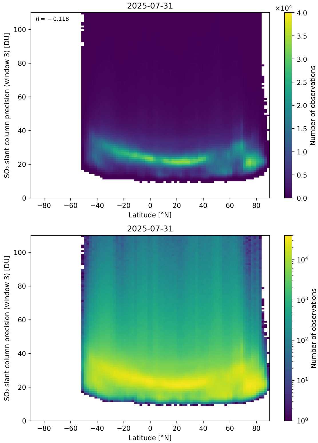
Figure 166: Scatter density plot of “Latitude” against “SO 2 slant column precision (window 3)” for 2025-07-30 to 2025-08-01.
