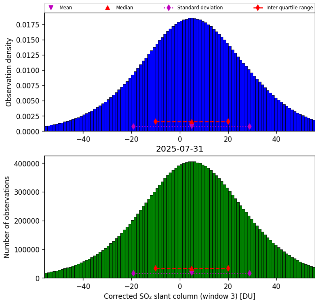
Figure 73: Histogram of “Corrected SO 2 slant column (window 3)” for 2025-07-30 to 2025-08-01
