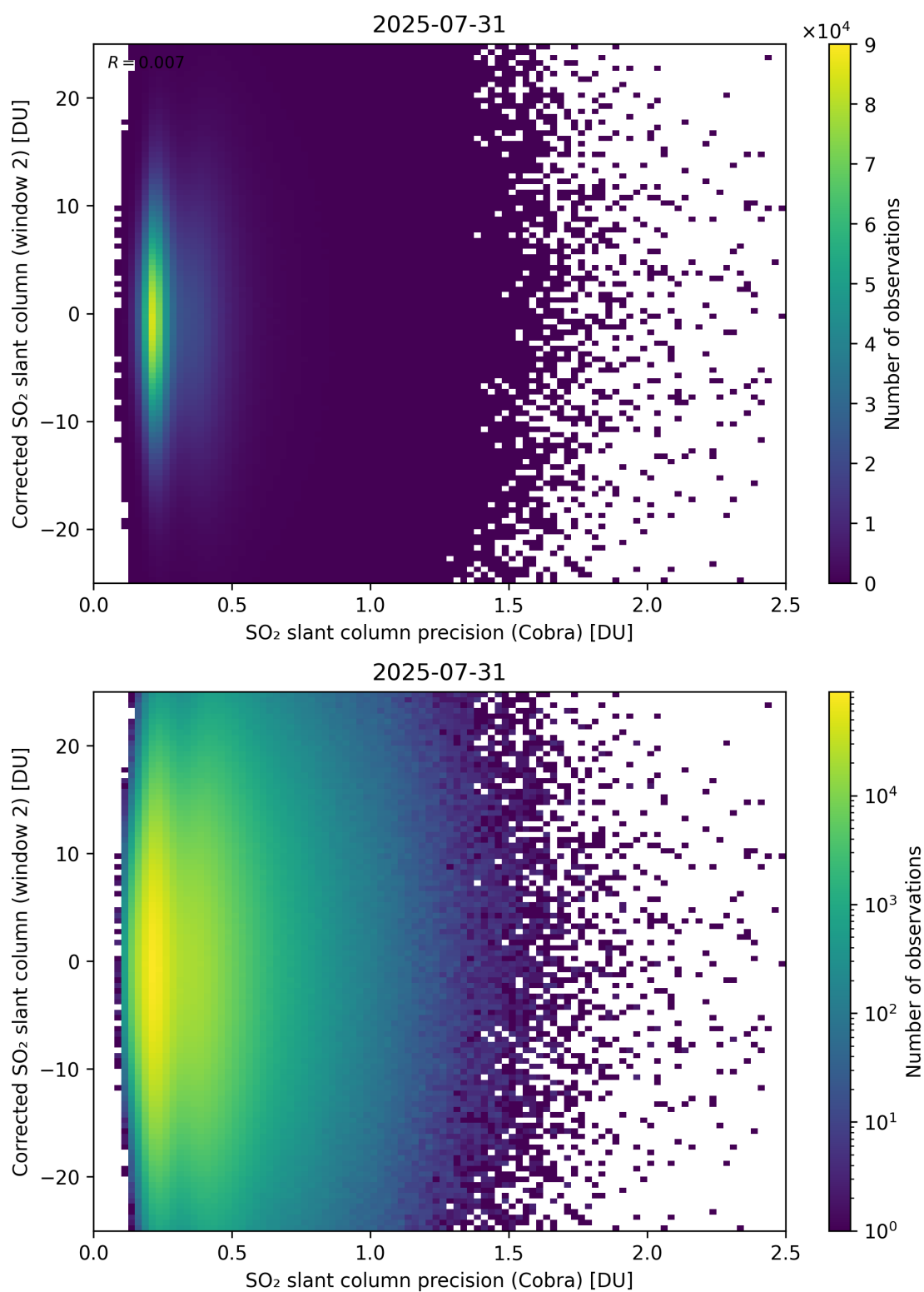
Figure 206: Scatter density plot of “SO 2 slant column precision (Cobra)” against “Corrected SO 2 slant column (window 2)” for 2025-07-30 to 2025-08-01.
