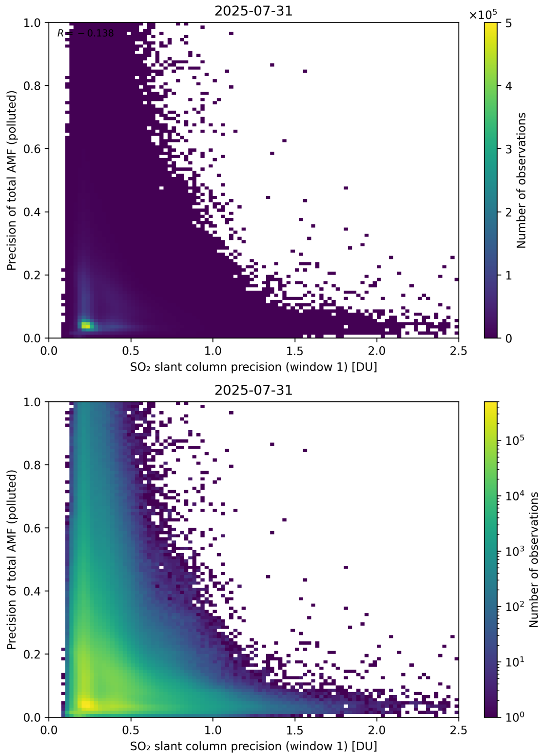
Figure 281: Scatter density plot of “SO 2 slant column precision (window 1)” against “Precision of total AMF (polluted)” for 2025-07-30 to 2025-08-01.
