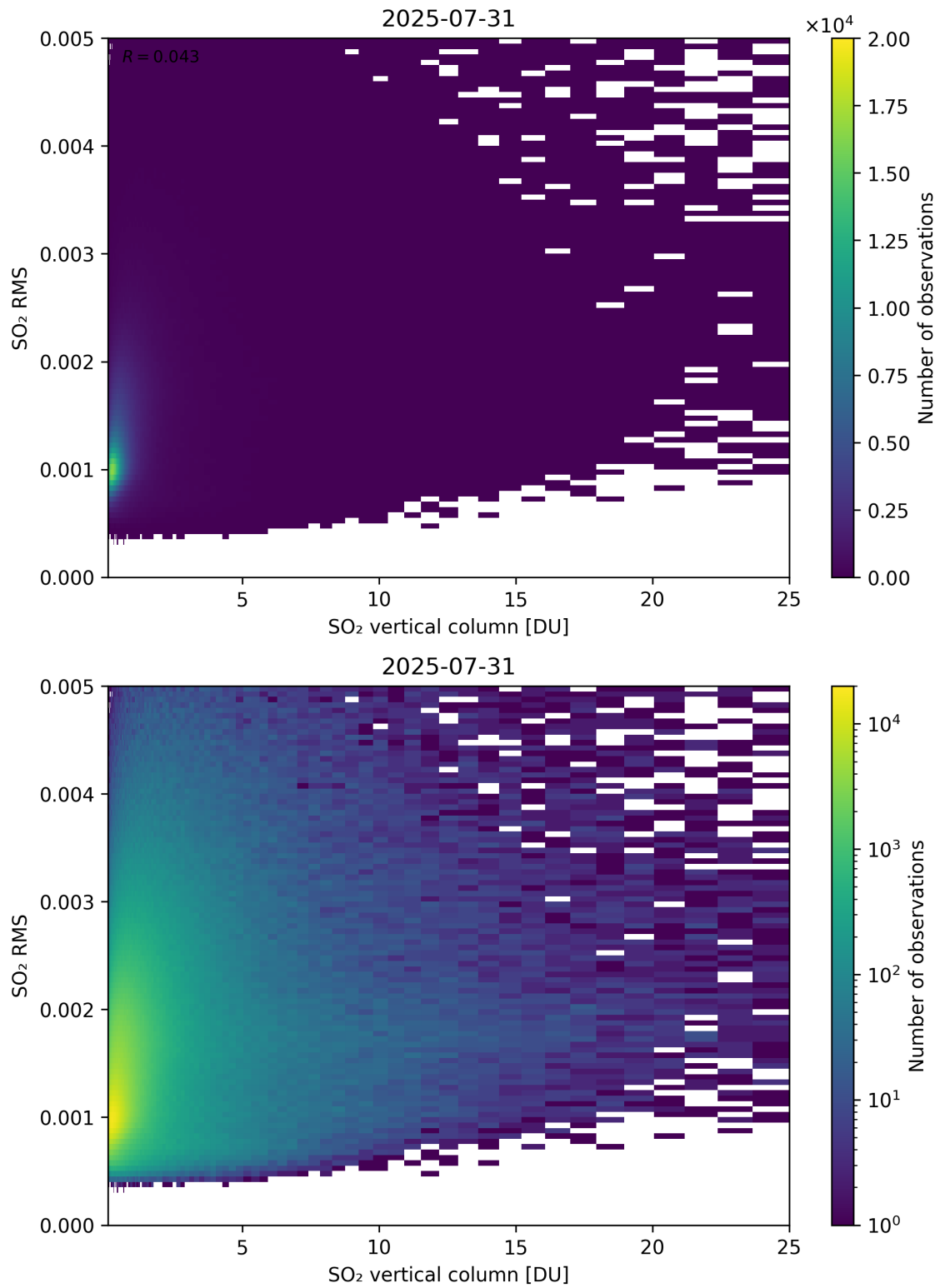
Figure 328: Scatter density plot of “SO 2 vertical column” against “SO 2 RMS” for 2025-07-30 to 2025-08-01.
