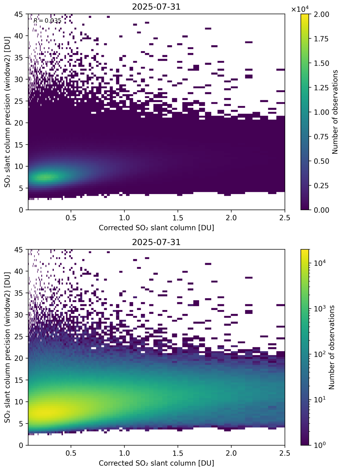
Figure 239: Scatter density plot of “Corrected SO 2 slant column” against “SO 2 slant column precision (window2)” for 2025-07-30 to 2025-08-01.
