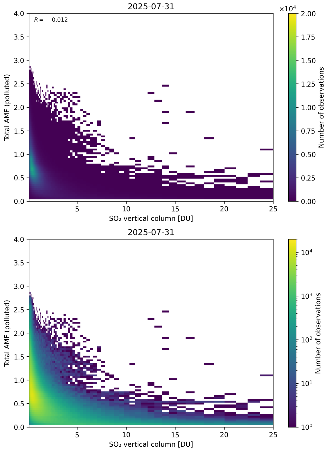
Figure 359: Scatter density plot of “SO 2 vertical column” against “Total AMF (polluted)” for 2025-07-30 to 2025-08-01.
