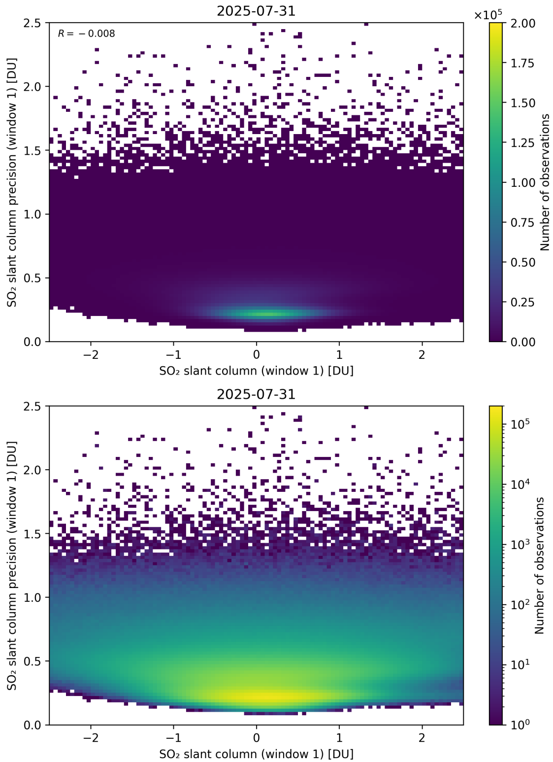
Figure 285: Scatter density plot of “SO 2 slant column (window 1)” against “SO 2 slant column precision (window 1)” for 2025-07-30 to 2025-08-01.
