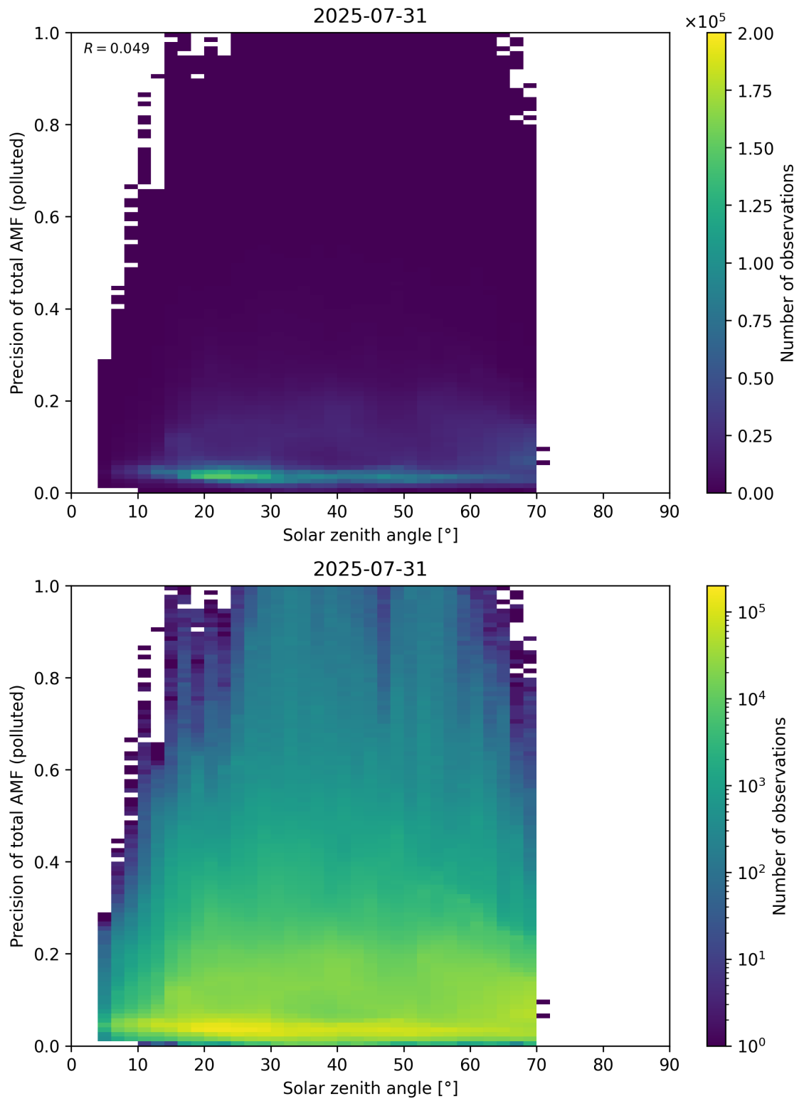
Figure 190: Scatter density plot of “Solar zenith angle” against “Precision of total AMF (polluted)” for 2025-07-30 to 2025-08-01.
