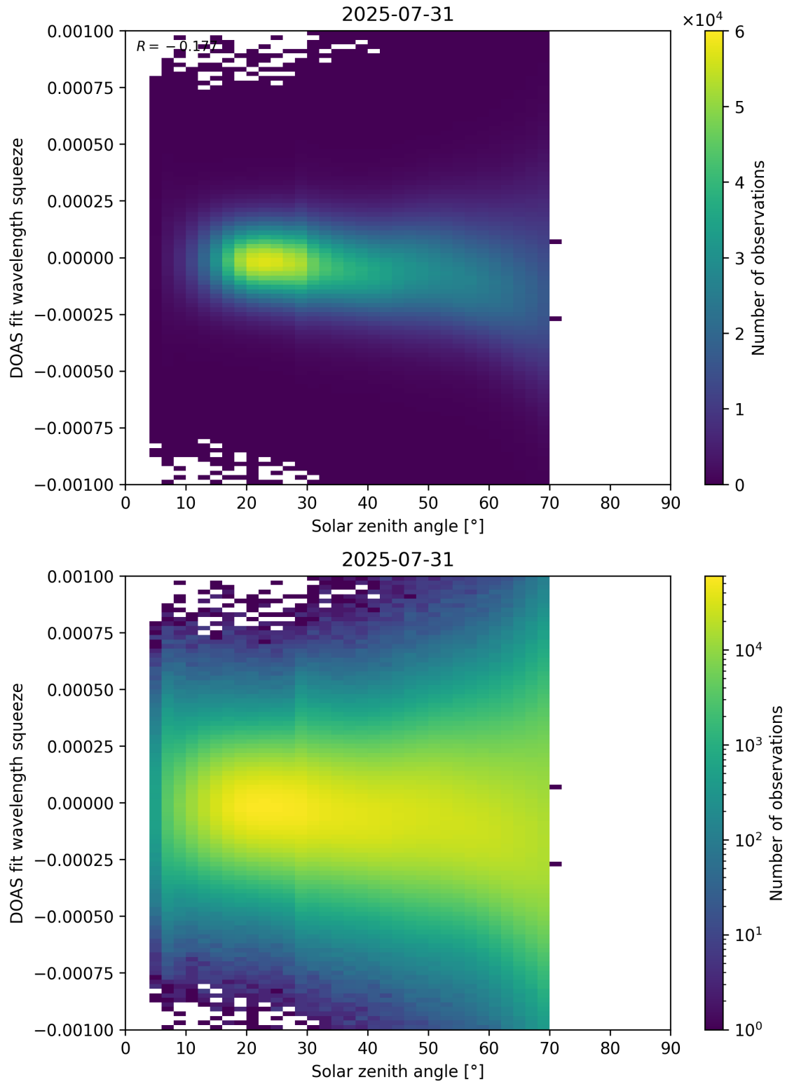
Figure 175: Scatter density plot of “Solar zenith angle” against “DOAS fit wavelength squeeze” for 2025-07-30 to 2025-08-01.
