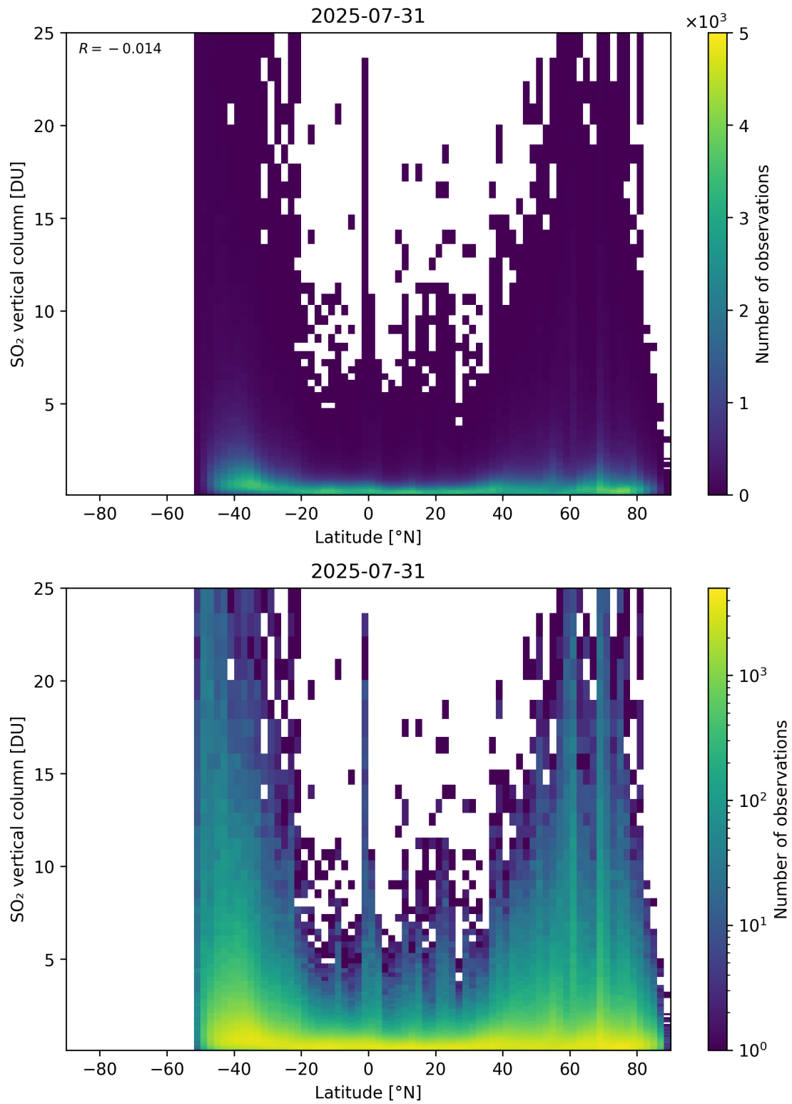
Figure 169: Scatter density plot of “Latitude” against “SO 2 vertical column” for 2025-07-30 to 2025-08-01.
