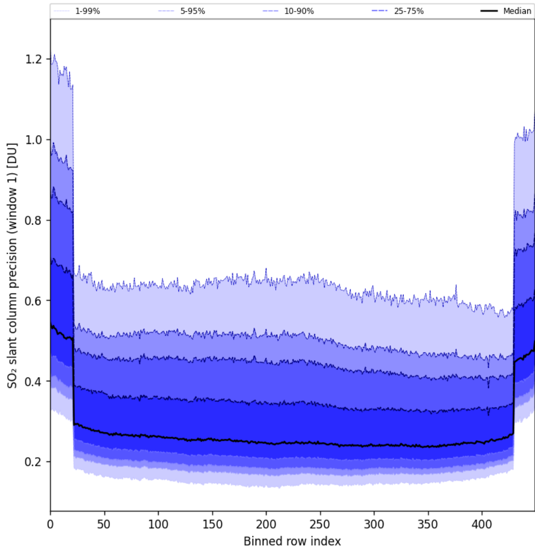
Figure 90: Along track statistics of “SO 2 slant column precision (window 1)” for 2025-07-30 to 2025-08-01
