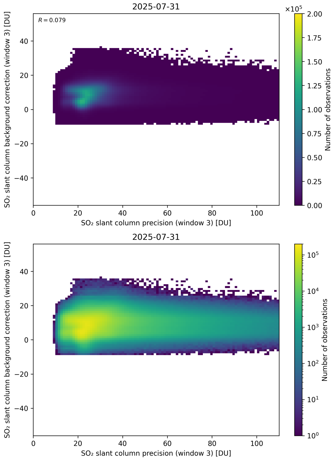
Figure 307: Scatter density plot of “SO 2 slant column precision (window 3)” against “SO 2 slant column background correction (window 3)” for 2025-07-30 to 2025-08-01.
