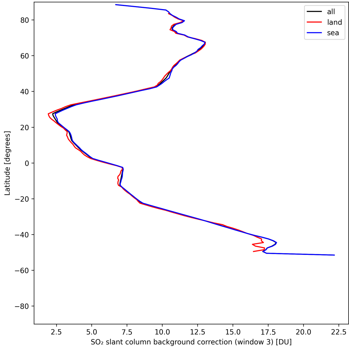
Figure 48: Zonal average of “SO 2 slant column background correction (window 3)” for 2025-07-30 to 2025-08-01.
