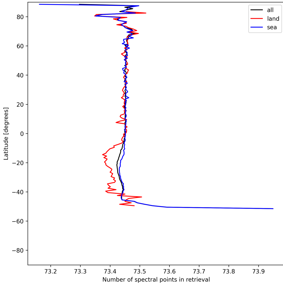
Figure 56: Zonal average of “Number of spectral points in retrieval” for 2025-07-30 to 2025-08-01.
