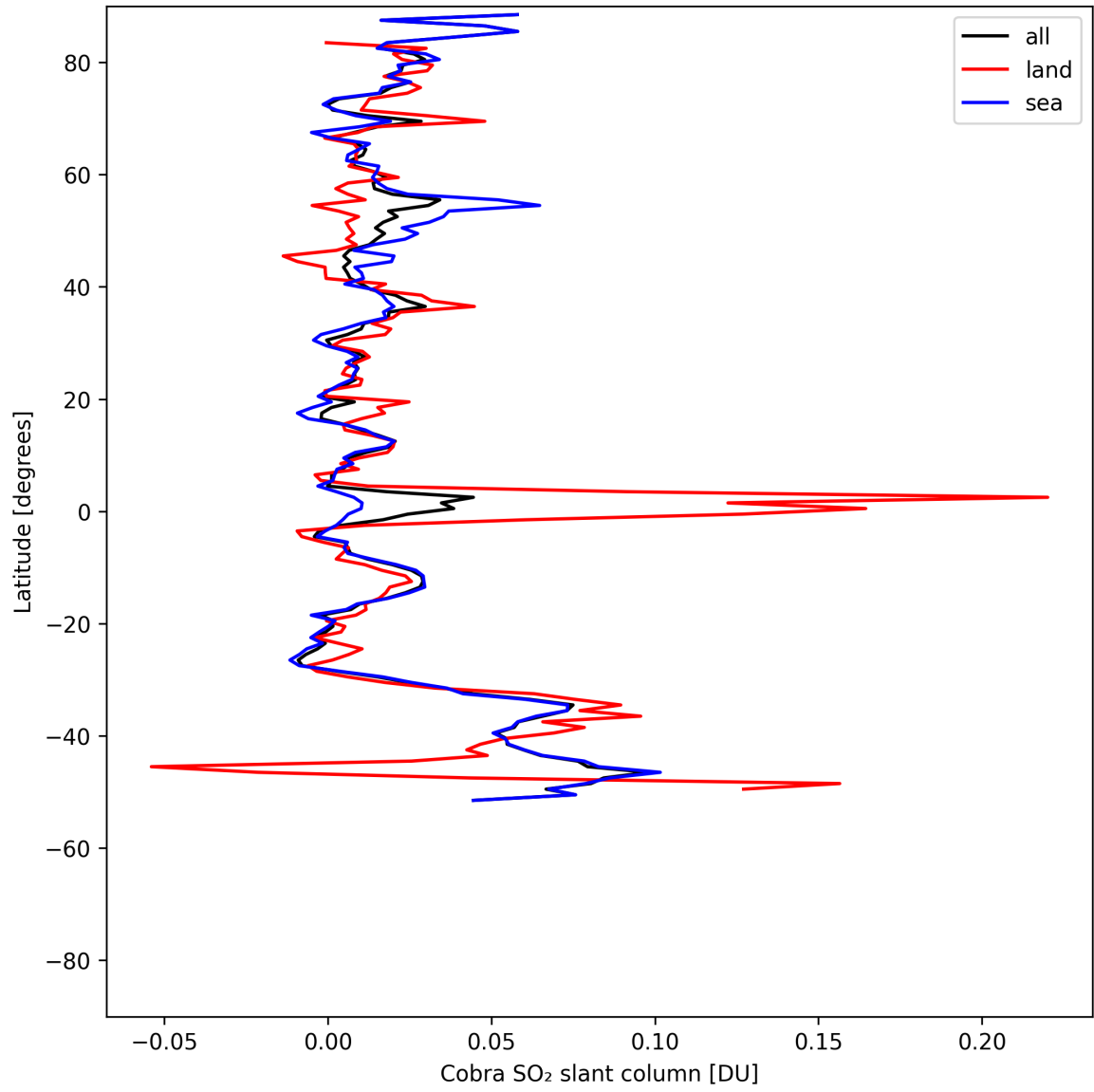
Figure 35: Zonal average of “Cobra SO 2 slant column” for 2025-07-30 to 2025-08-01.
