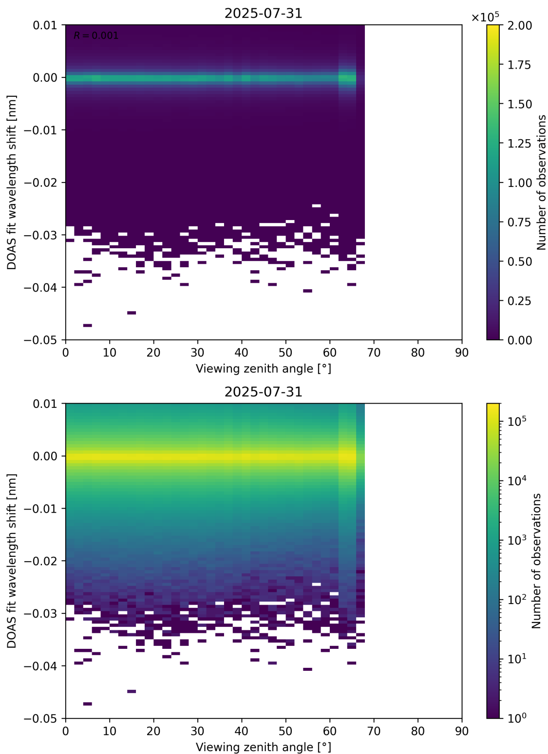
Figure 365: Scatter density plot of “Viewing zenith angle” against “DOAS fit wavelength shift” for 2025-07-30 to 2025-08-01.
