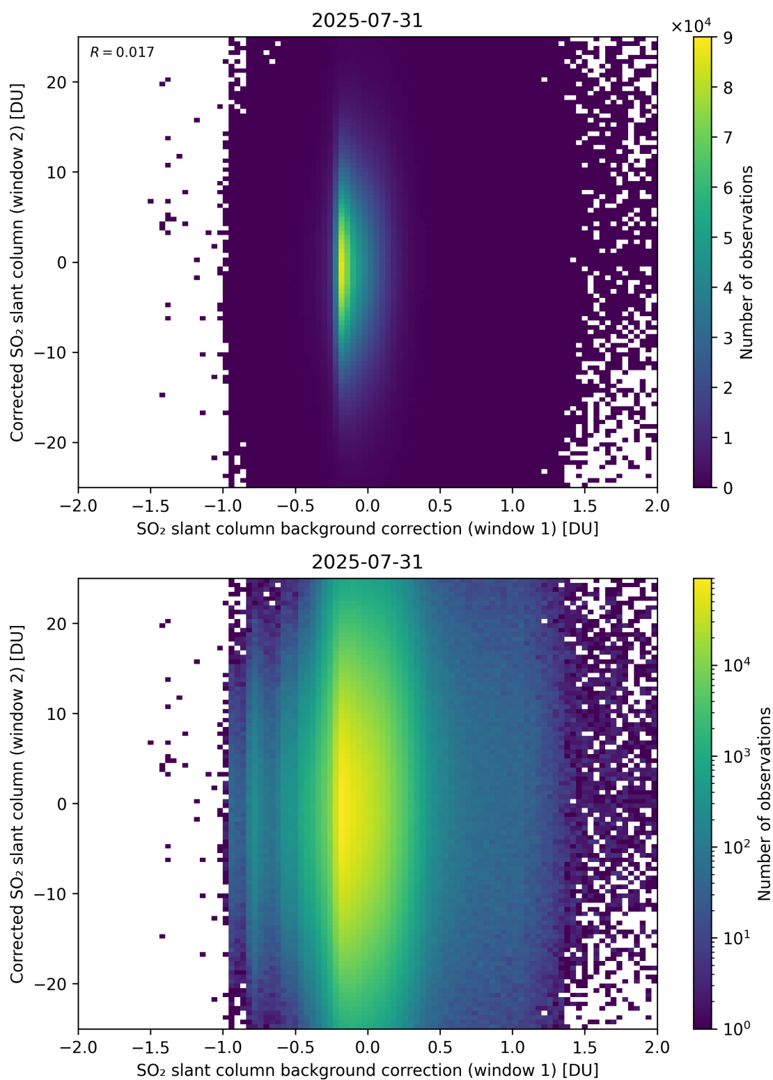
Figure 115: Scatter density plot of “SO 2 slant column background correction (window 1)” against “Corrected SO 2 slant column (window 2)” for 2025-07-30 to 2025-08-01.
