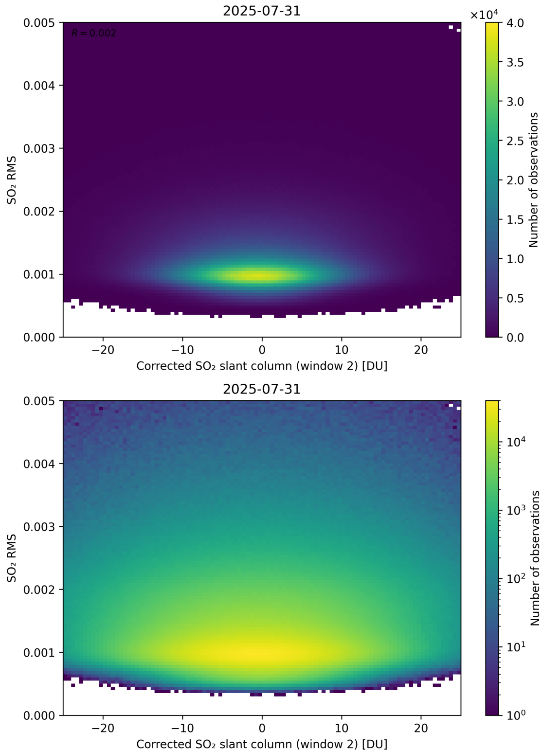
Figure 248: Scatter density plot of “Corrected SO 2 slant column (window 2)” against “SO 2 RMS” for 2025-07-30 to 2025-08-01.
