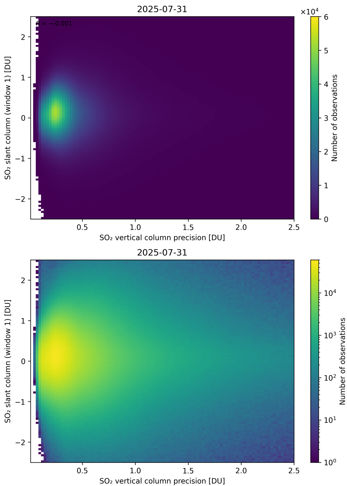
Figure 341: Scatter density plot of “SO 2 vertical column precision” against “SO 2 slant column (window 1)” for 2025-07-30 to 2025-08-01.
