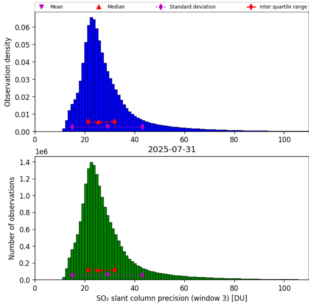
Figure 72: Histogram of “SO 2 slant column precision (window 3)” for 2025-07-30 to 2025-08-01
