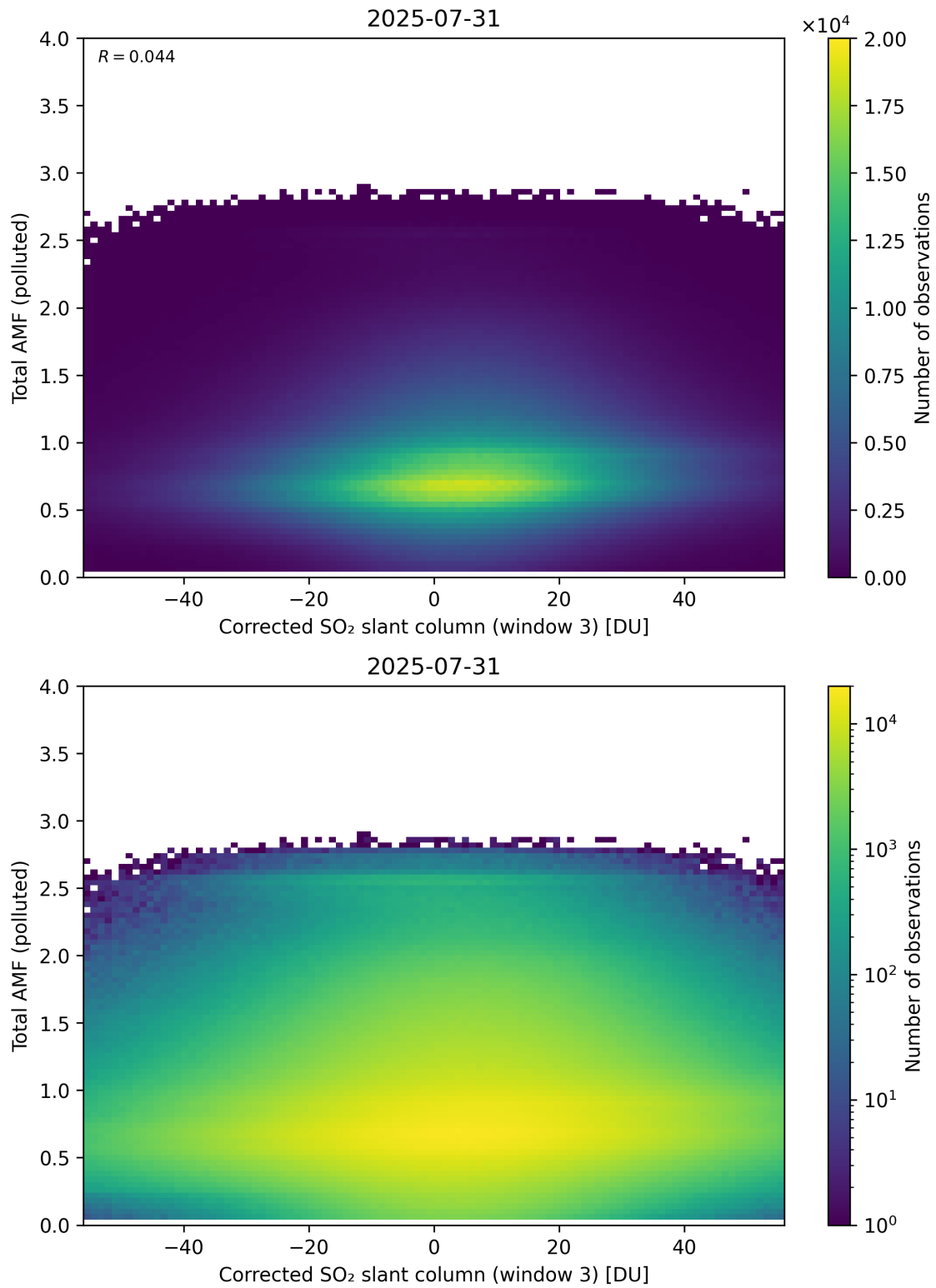
Figure 260: Scatter density plot of “Corrected SO 2 slant column (window 3)” against “Total AMF (polluted)” for 2025-07-30 to 2025-08-01.
