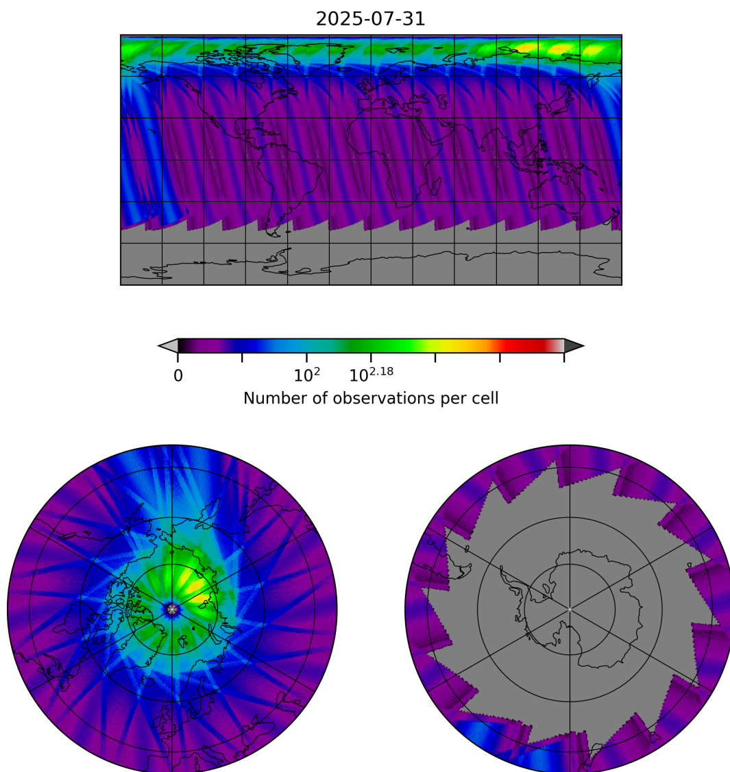
Figure 30: Map of the number of observations for 2025-07-30 to 2025-08-01
