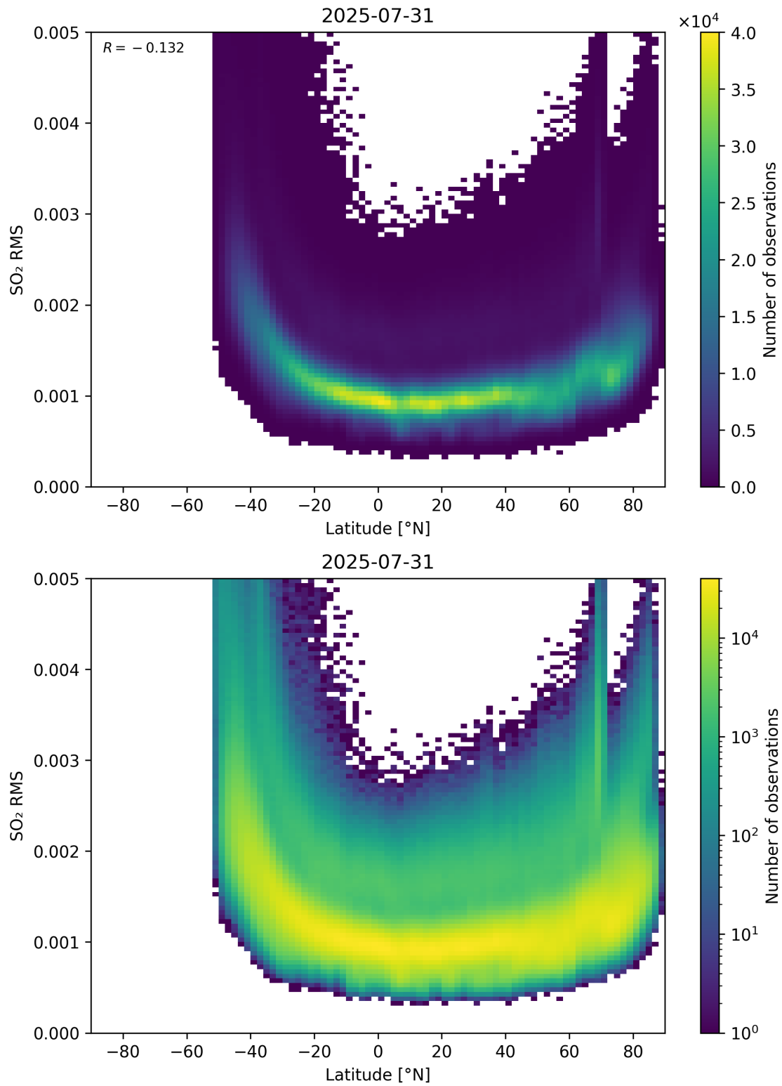
Figure 155: Scatter density plot of “Latitude” against “SO 2 RMS” for 2025-07-30 to 2025-08-01.
