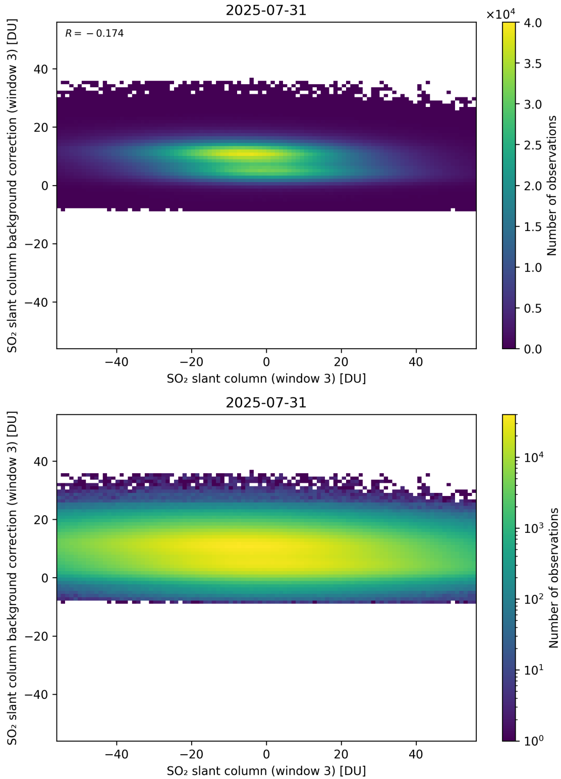
Figure 303: Scatter density plot of “SO 2 slant column (window 3)” against “SO 2 slant column background correction (window 3)” for 2025-07-30 to 2025-08-01.
