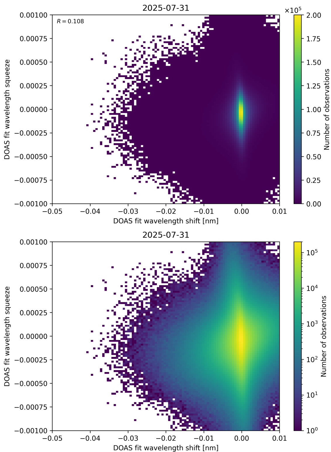
Figure 138: Scatter density plot of “DOAS fit wavelength shift” against “DOAS fit wavelength squeeze” for 2025-07-30 to 2025-08-01.
