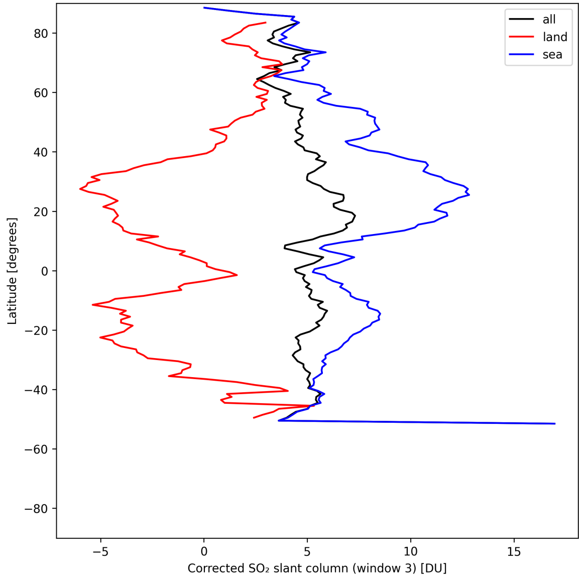
Figure 47: Zonal average of “Corrected SO 2 slant column (window 3)” for 2025-07-30 to 2025-08-01.
