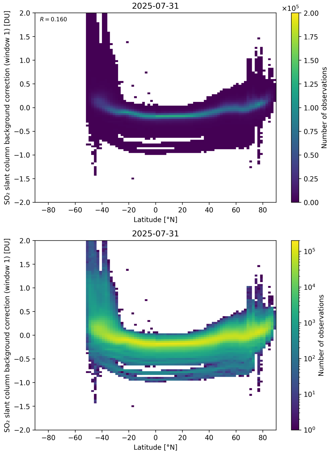
Figure 150: Scatter density plot of “Latitude” against “SO 2 slant column background correction (window 1)” for 2025-07-30 to 2025-08-01.
