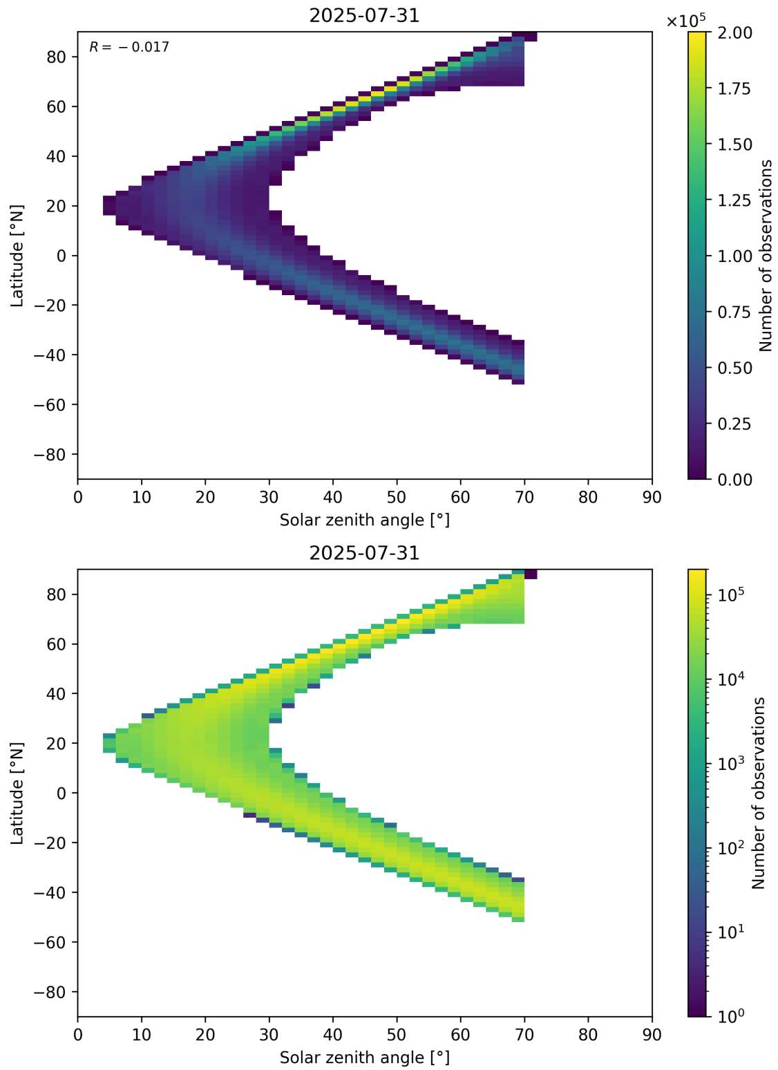
Figure 177: Scatter density plot of “Solar zenith angle” against “Latitude” for 2025-07-30 to 2025-08-01.
