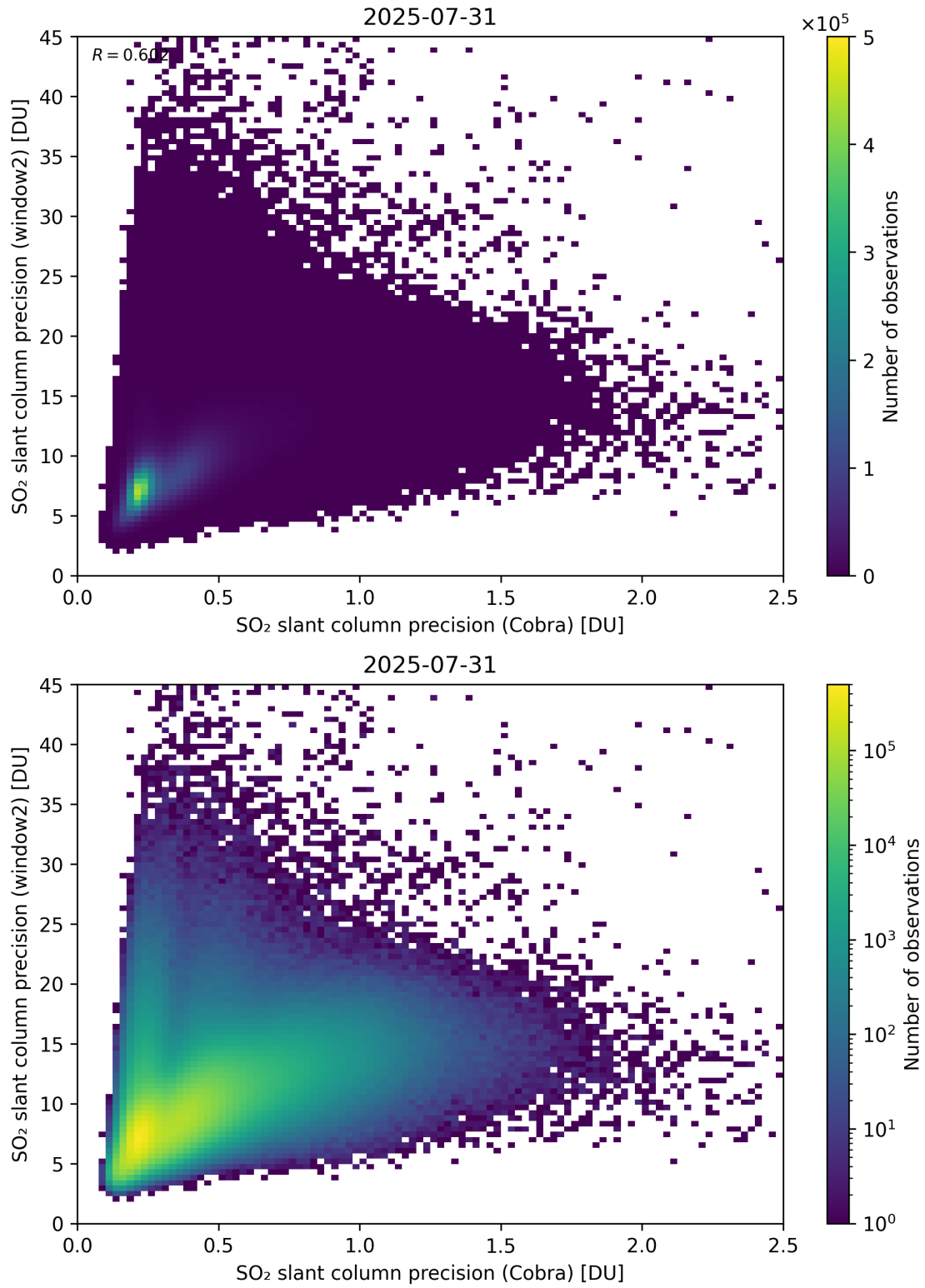
Figure 210: Scatter density plot of “SO 2 slant column precision (Cobra)” against “SO 2 slant column precision (window2)” for 2025-07-30 to 2025-08-01.
