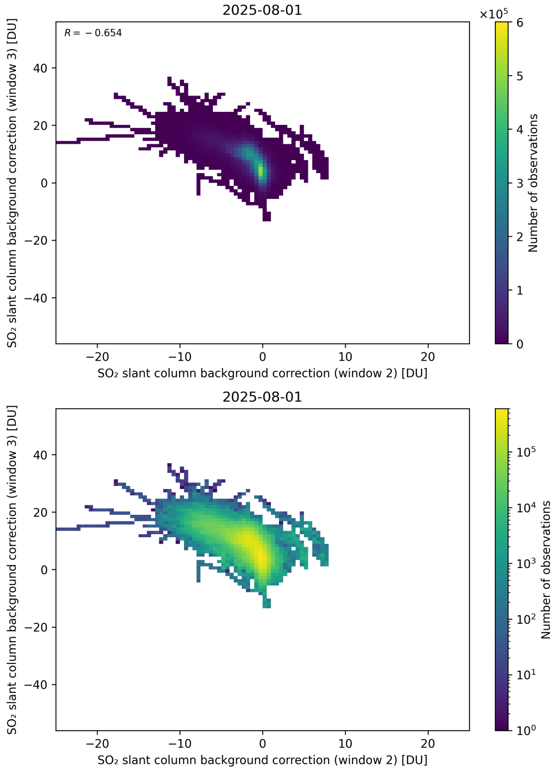
Figure 122: Scatter density plot of “SO 2 slant column background correction (window 2)” against “SO 2 slant column background correction (window 3)” for 2025-07-31 to 2025-08-02.
