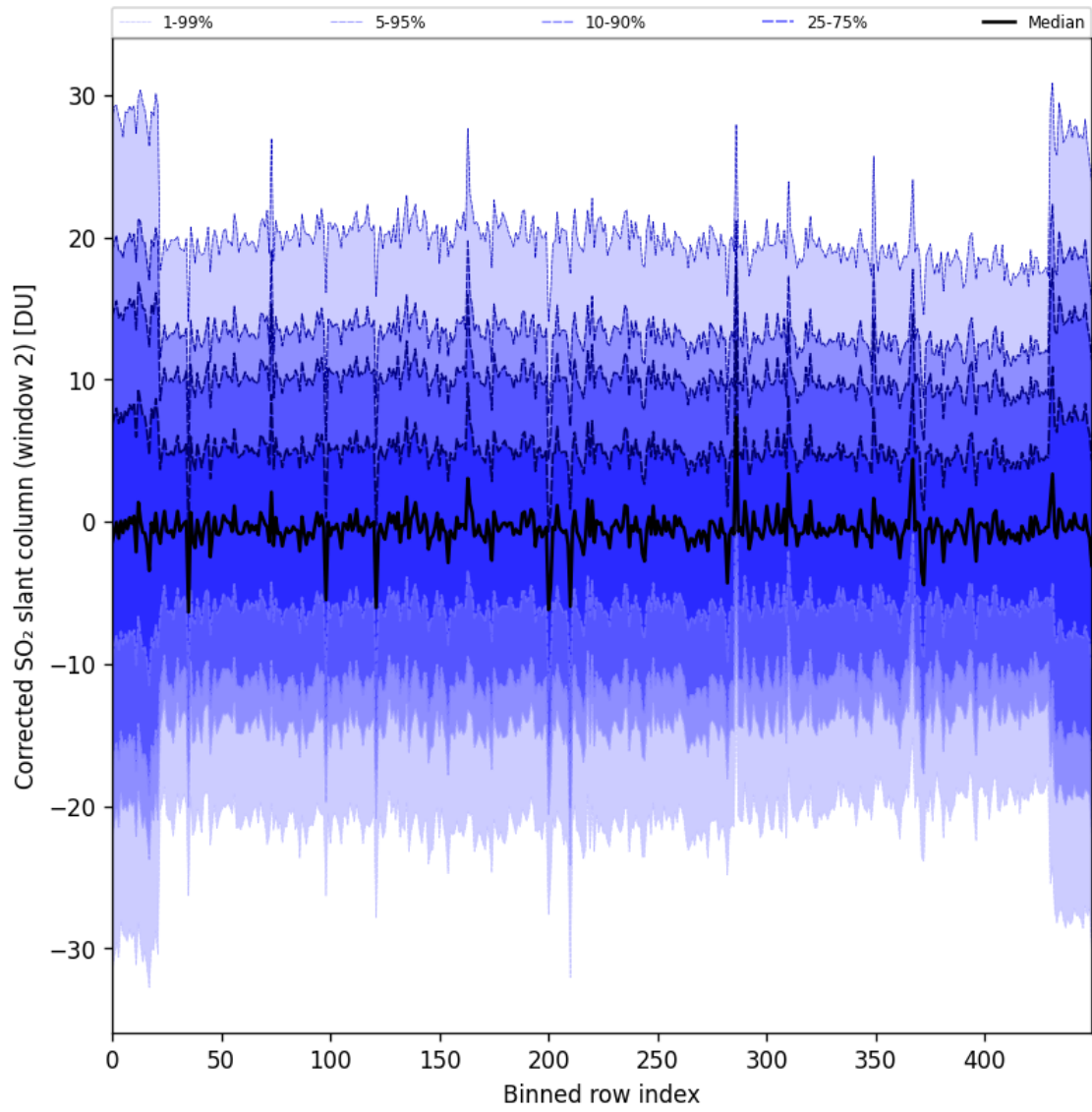
Figure 95: Along track statistics of “Corrected SO 2 slant column (window 2)” for 2025-07-31 to 2025-08-02
