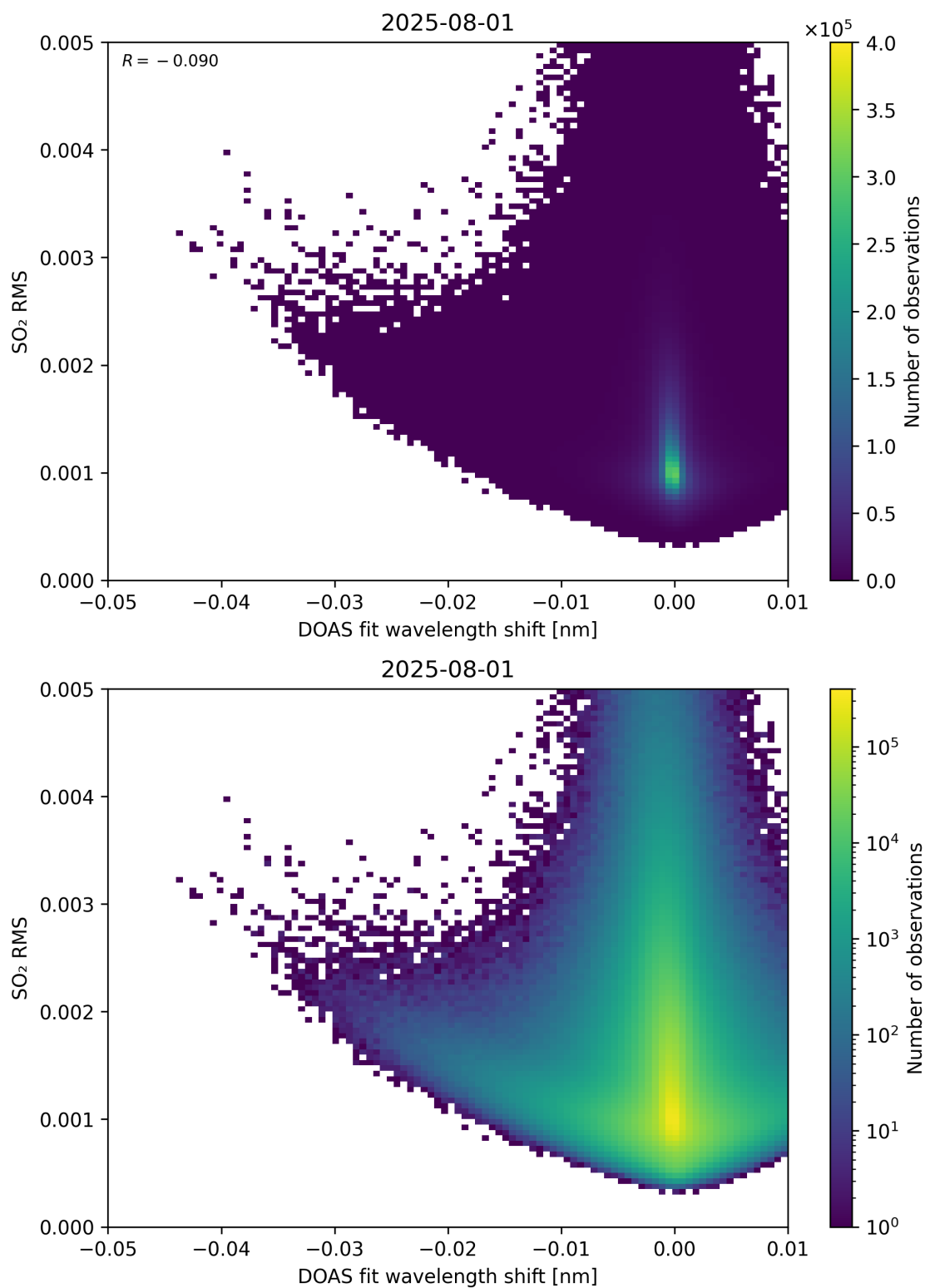
Figure 139: Scatter density plot of “DOAS fit wavelength shift” against “SO 2 RMS” for 2025-07-31 to 2025-08-02.
