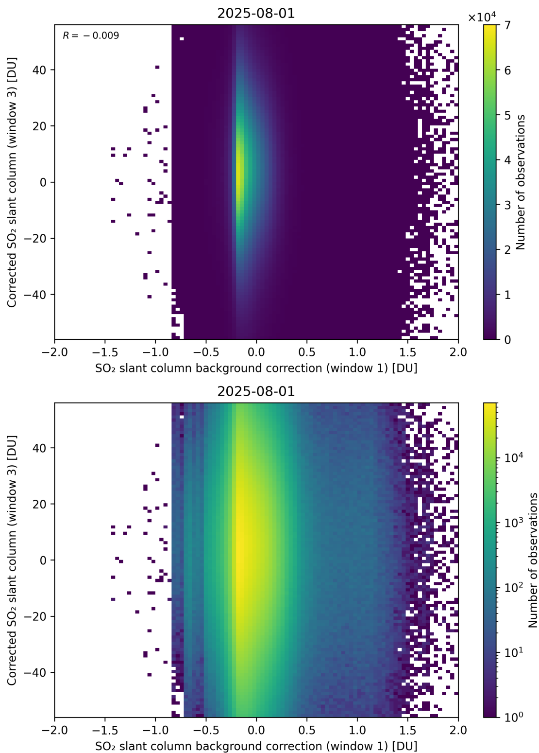
Figure 116: Scatter density plot of “SO 2 slant column background correction (window 1)” against “Corrected SO 2 slant column (window 3)” for 2025-07-31 to 2025-08-02.
