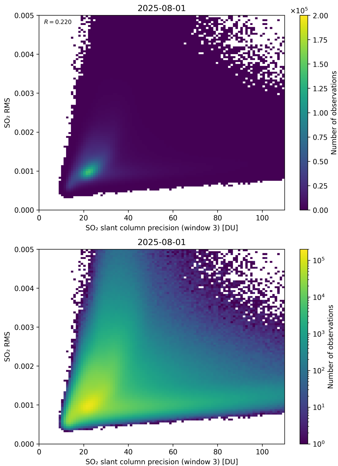
Figure 310: Scatter density plot of “SO 2 slant column precision (window 3)” against “SO 2 RMS” for 2025-07-31 to 2025-08-02.
