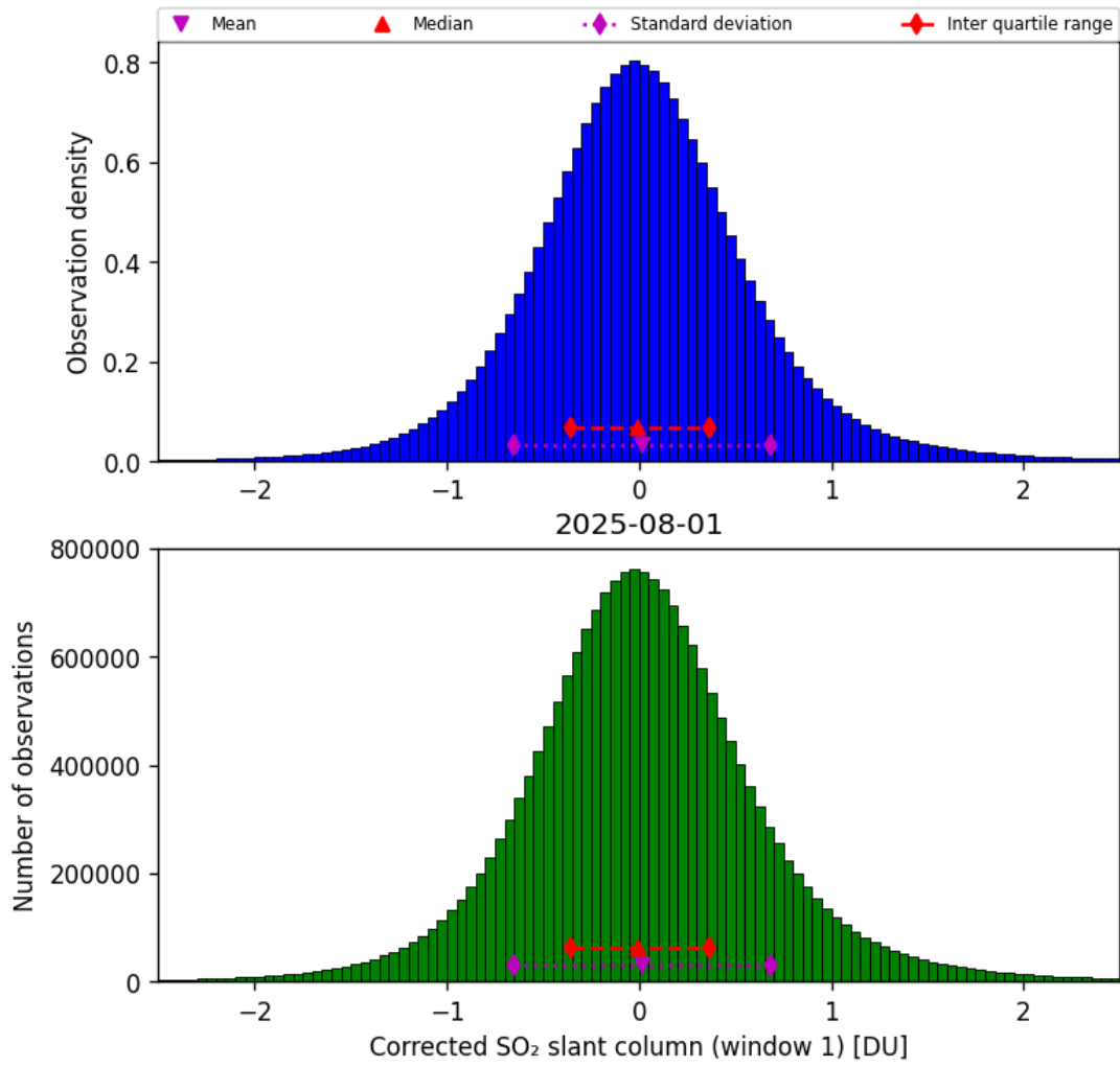
Figure 65: Histogram of “Corrected SO 2 slant column (window 1)” for 2025-07-31 to 2025-08-02
