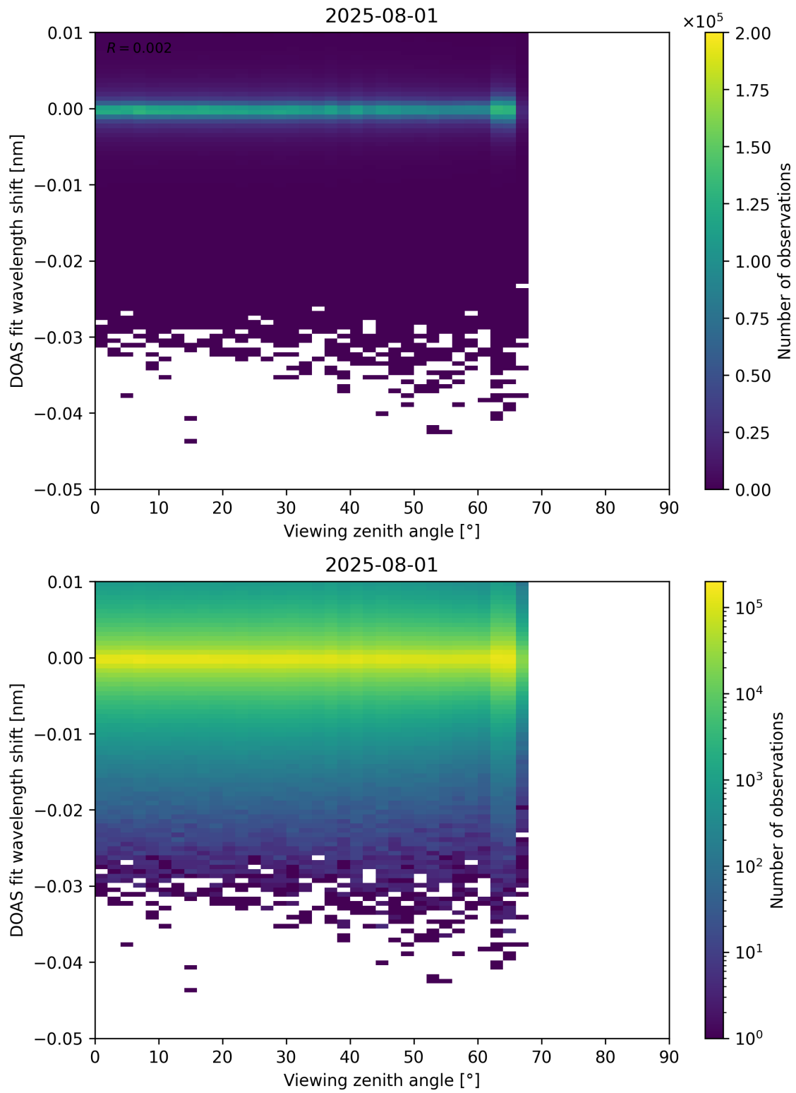
Figure 365: Scatter density plot of “Viewing zenith angle” against “DOAS fit wavelength shift” for 2025-07-31 to 2025-08-02.
