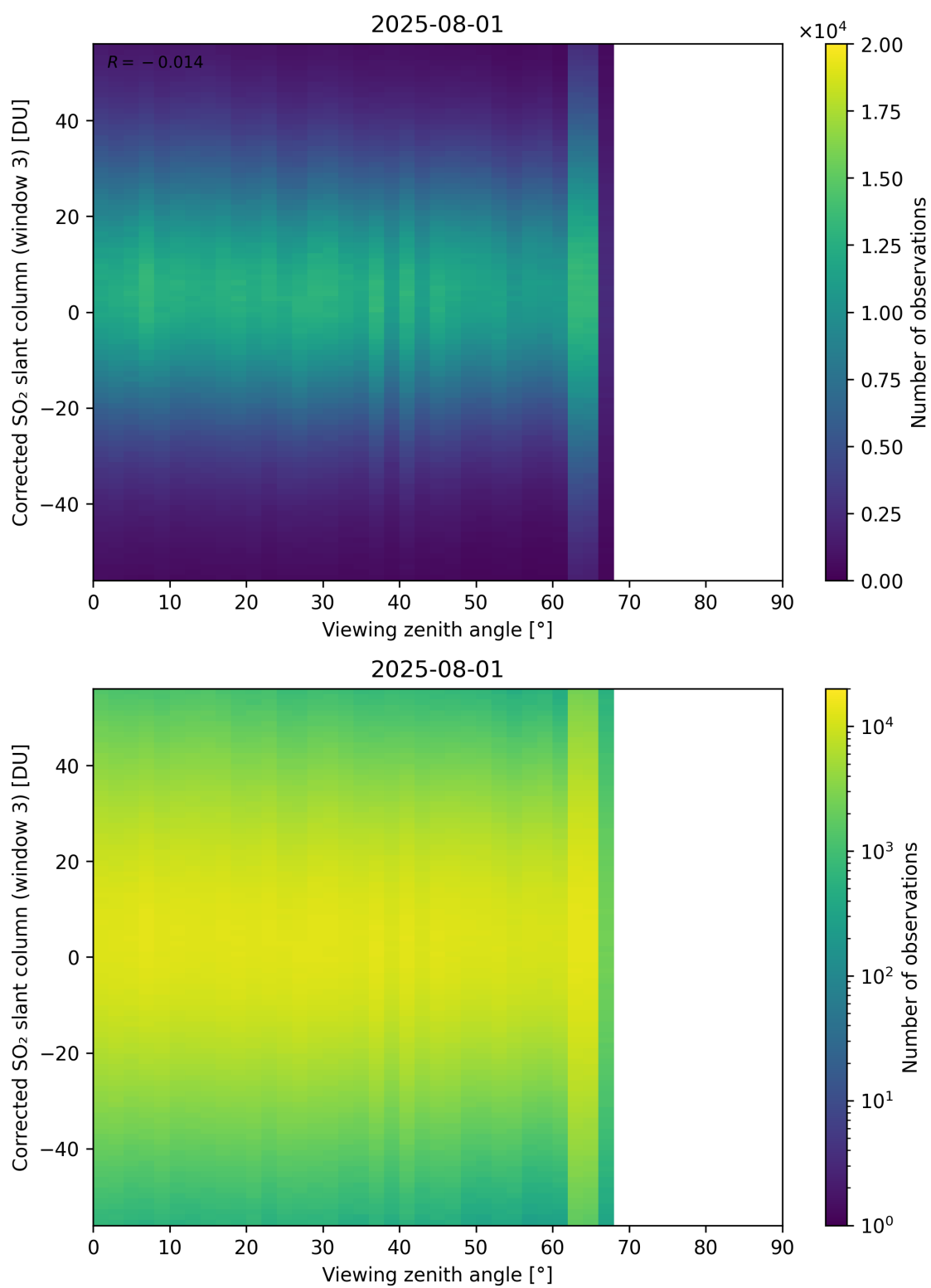
Figure 375: Scatter density plot of “Viewing zenith angle” against “Corrected SO 2 slant column (window 3)” for 2025-07-31 to 2025-08-02.
