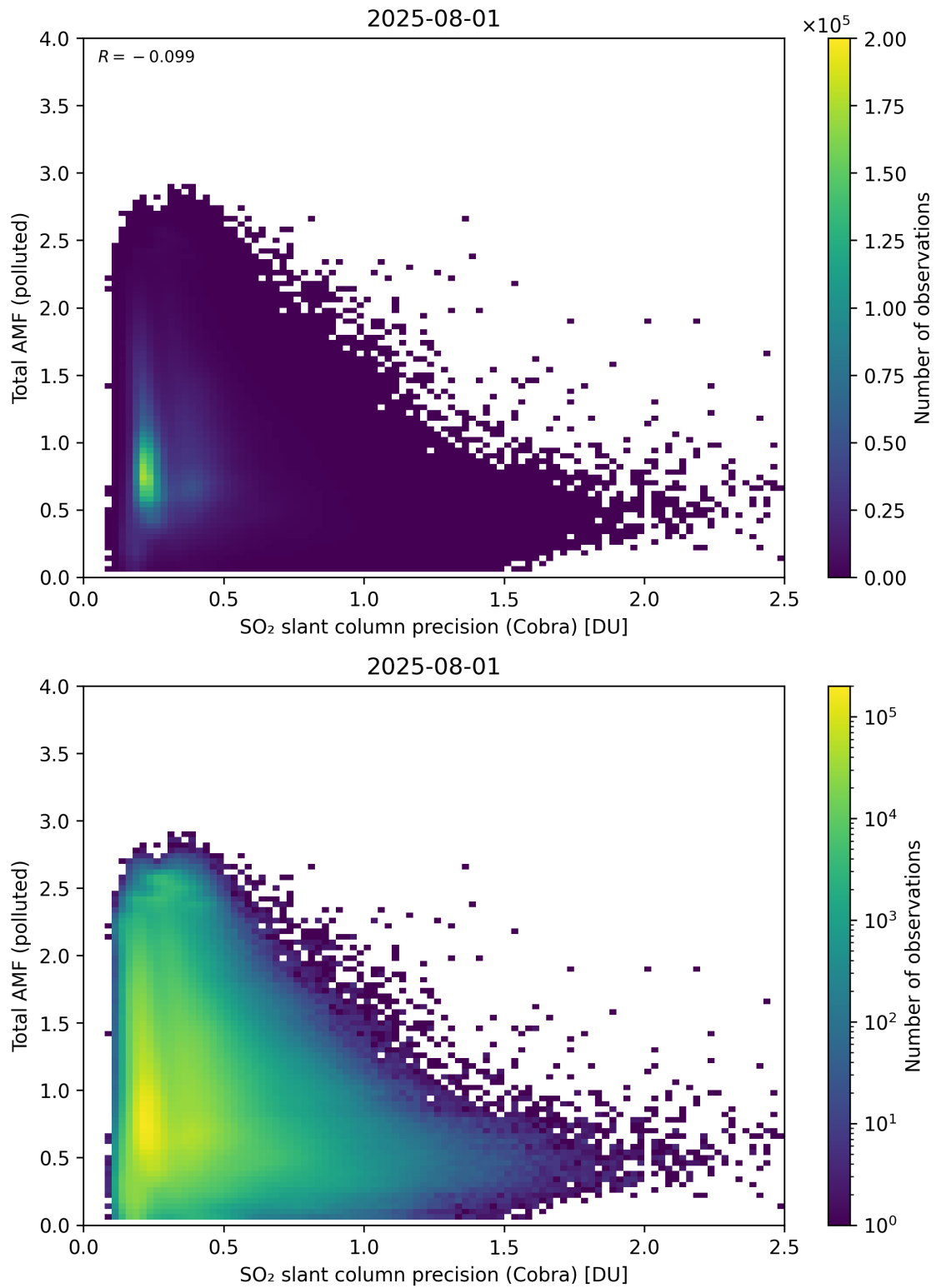
Figure 213: Scatter density plot of “SO 2 slant column precision (Cobra)” against “Total AMF (polluted)” for 2025-07-31 to 2025-08-02.
