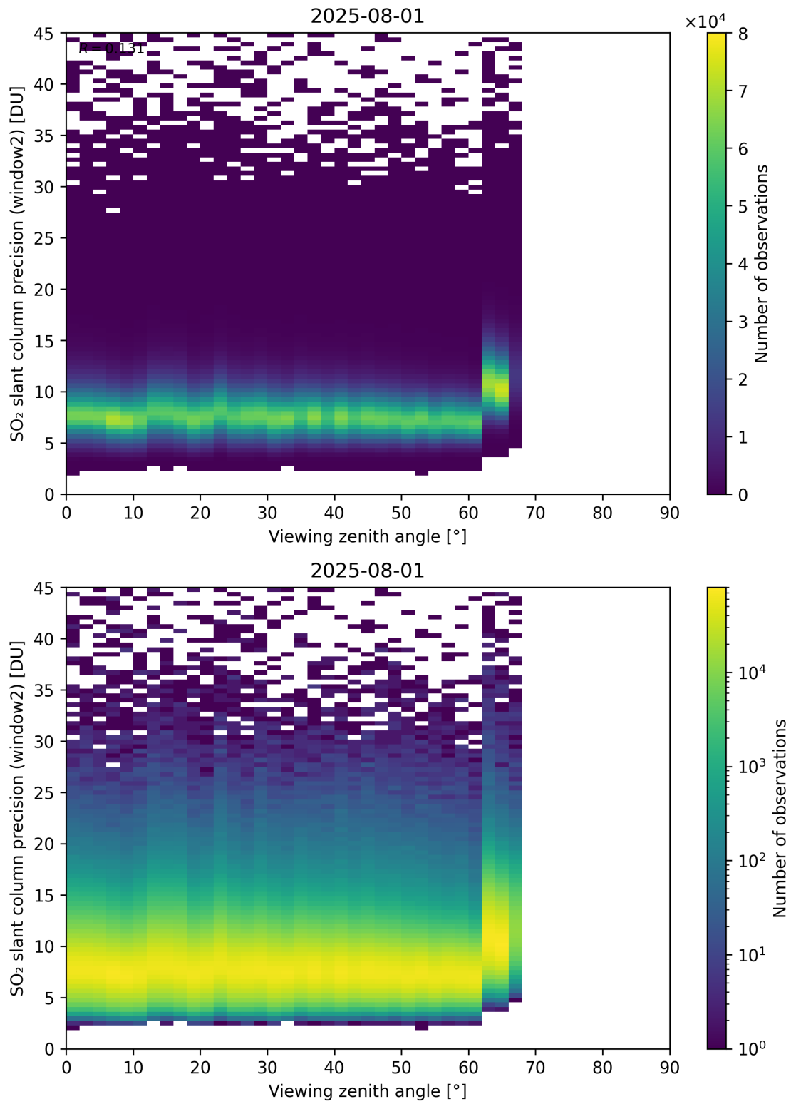
Figure 378: Scatter density plot of “Viewing zenith angle” against “SO 2 slant column precision (window2)” for 2025-07-31 to 2025-08-02.
