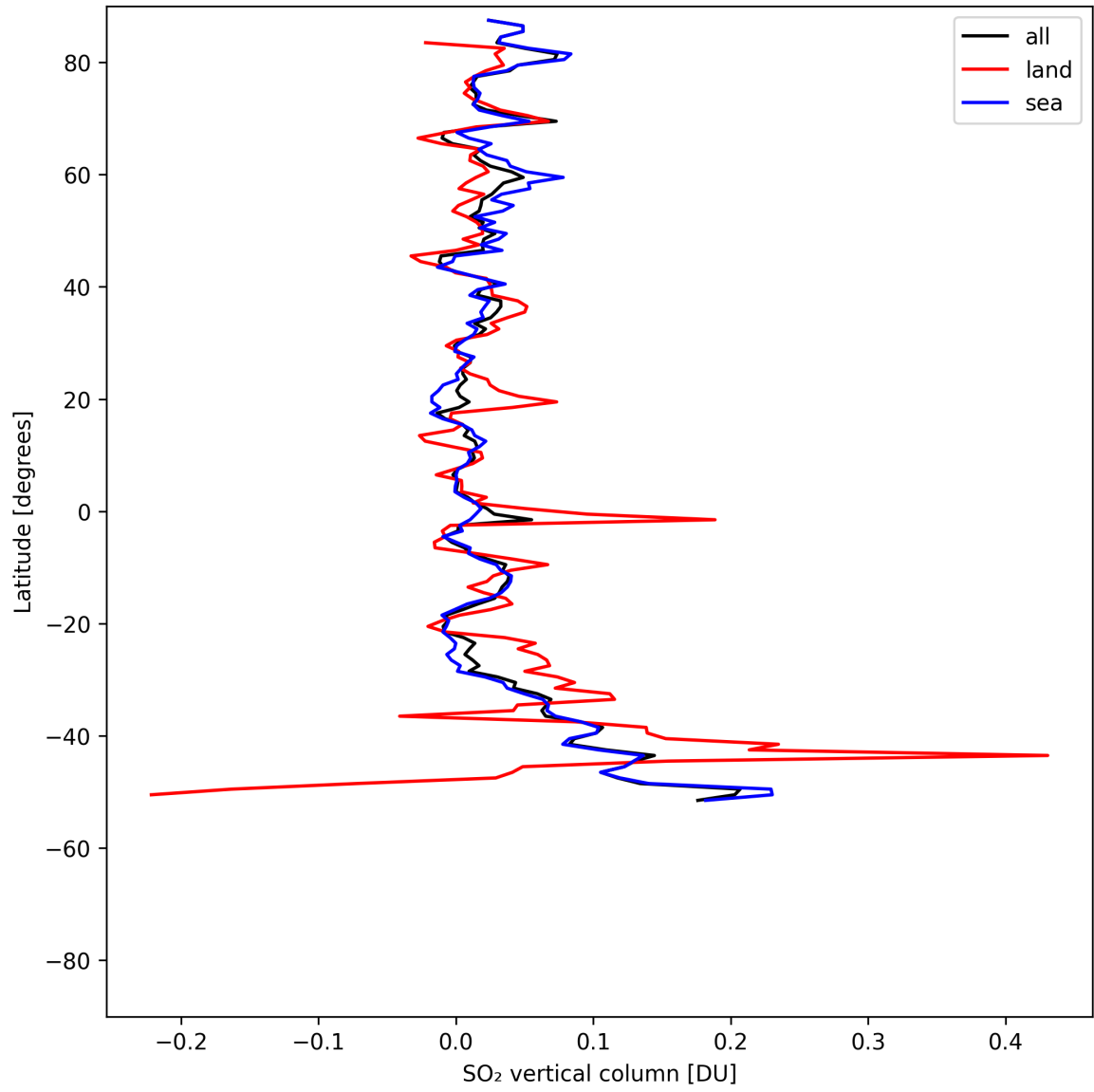
Figure 32: Zonal average of “SO 2 vertical column” for 2025-07-31 to 2025-08-02.
