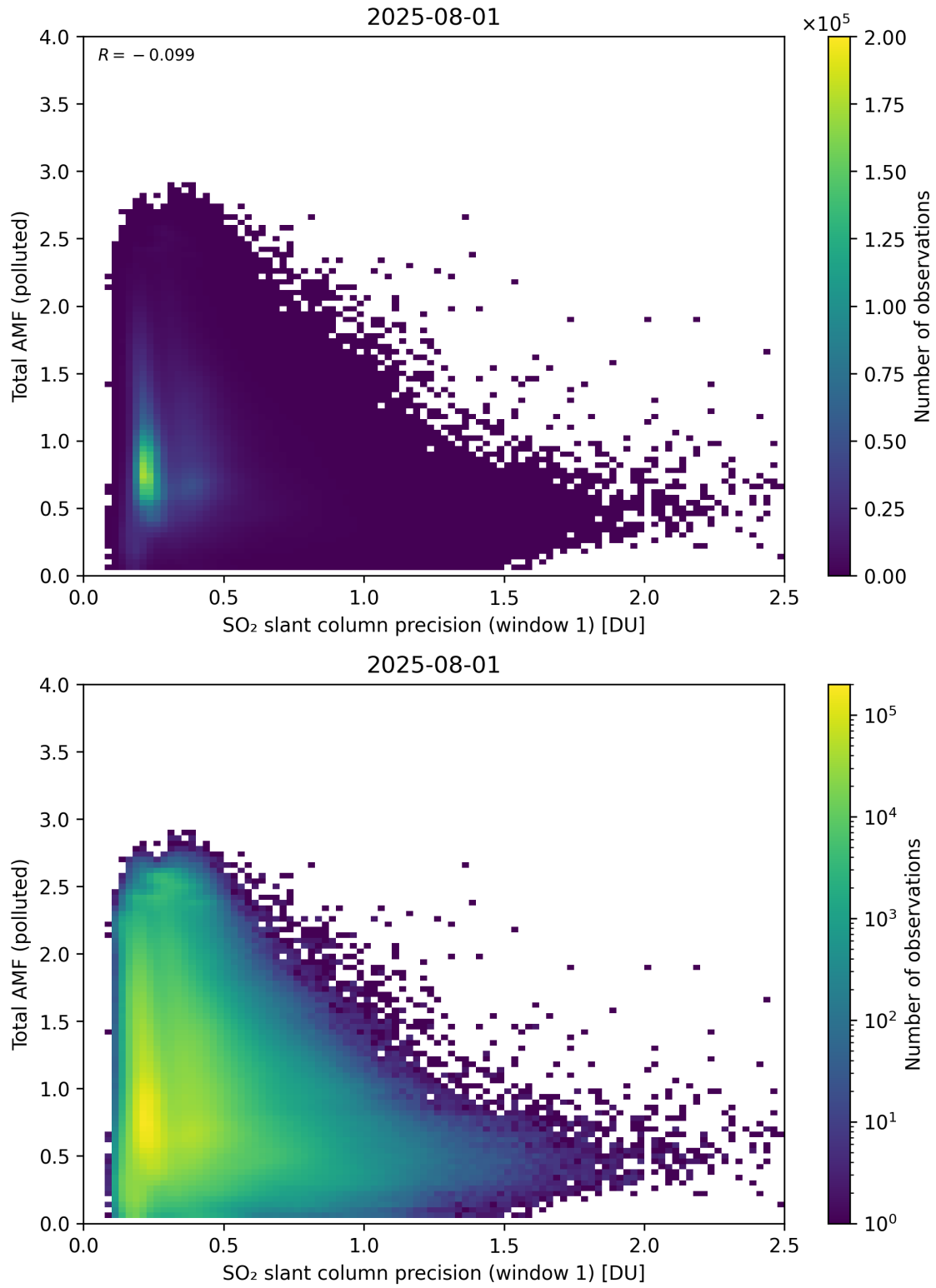
Figure 280: Scatter density plot of “SO 2 slant column precision (window 1)” against “Total AMF (polluted)” for 2025-07-31 to 2025-08-02.
