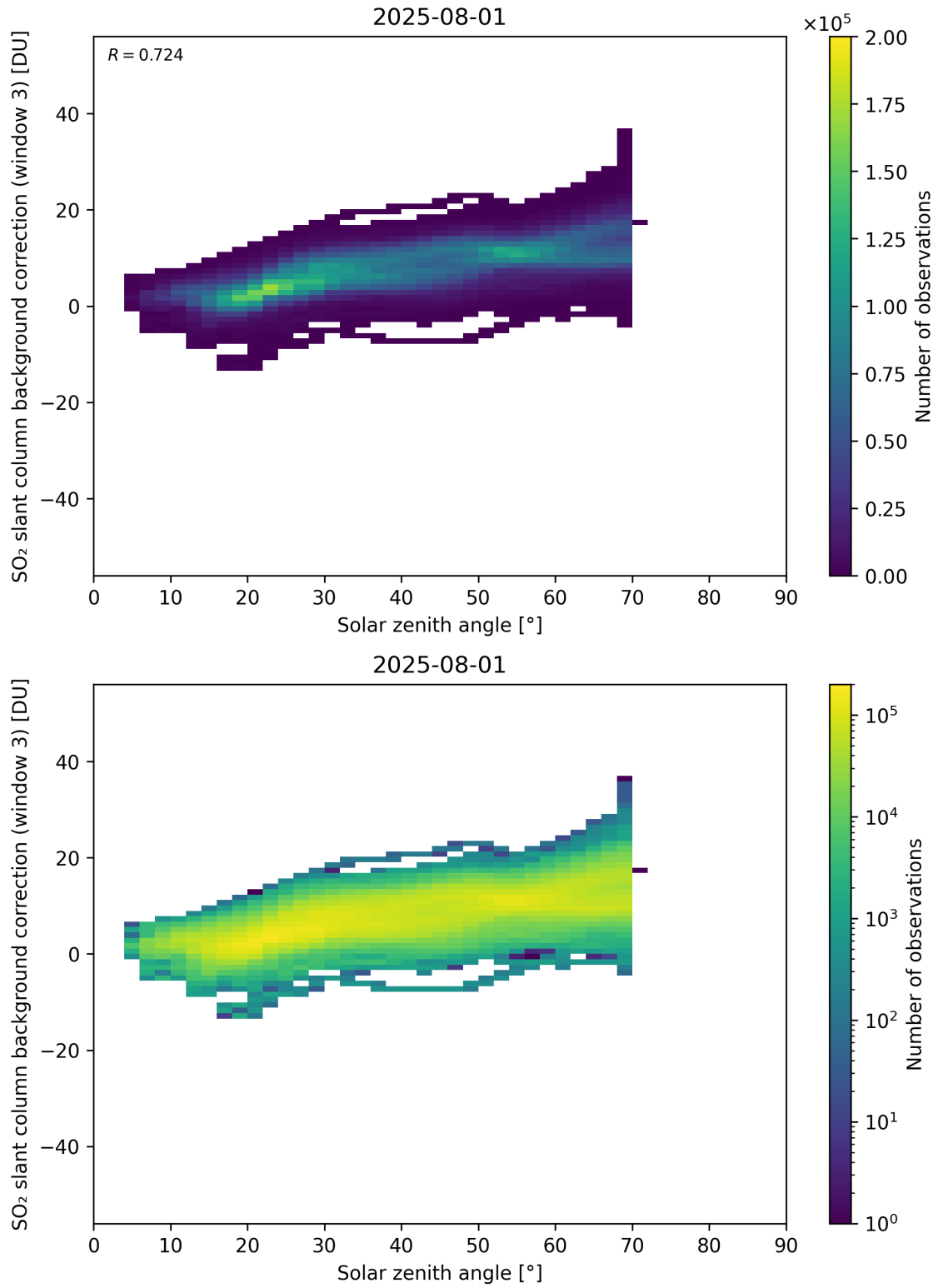
Figure 173: Scatter density plot of “Solar zenith angle” against “SO 2 slant column background correction (window 3)” for 2025-07-31 to 2025-08-02.
