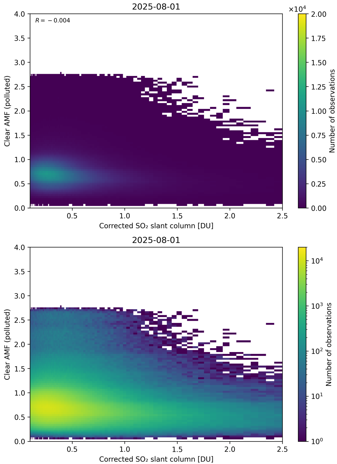
Figure 232: Scatter density plot of “Corrected SO 2 slant column” against “Clear AMF (polluted)” for 2025-07-31 to 2025-08-02.
