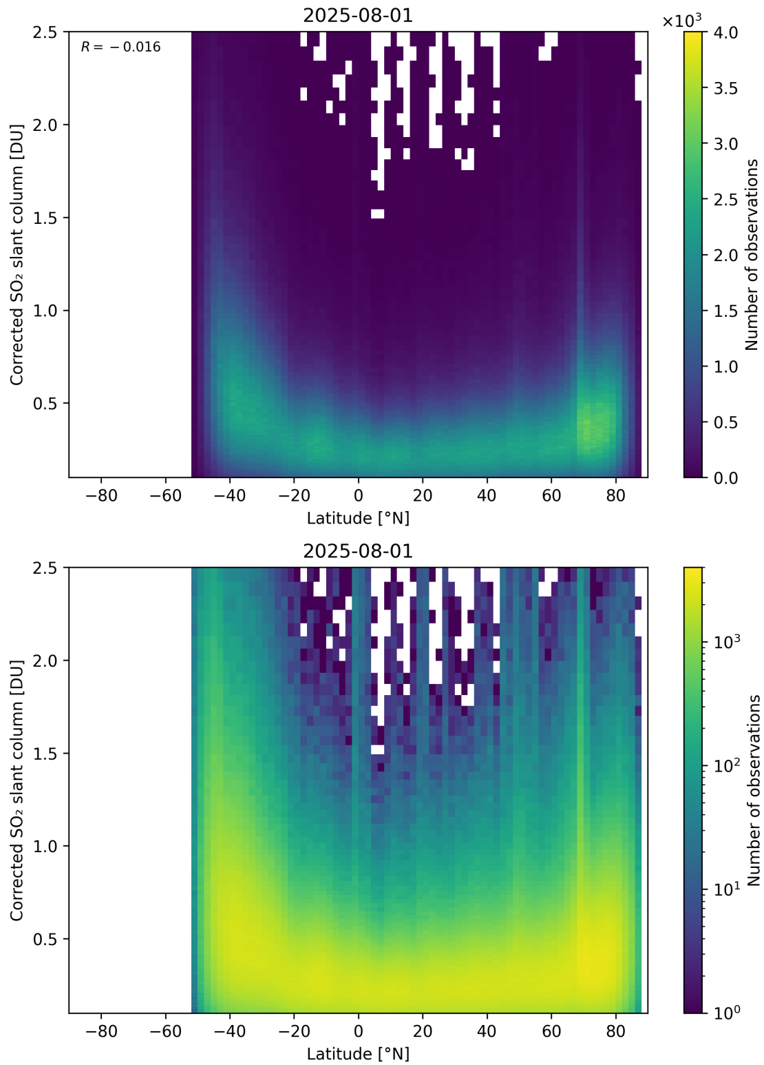
Figure 159: Scatter density plot of “Latitude” against “Corrected SO 2 slant column” for 2025-07-31 to 2025-08-02.
