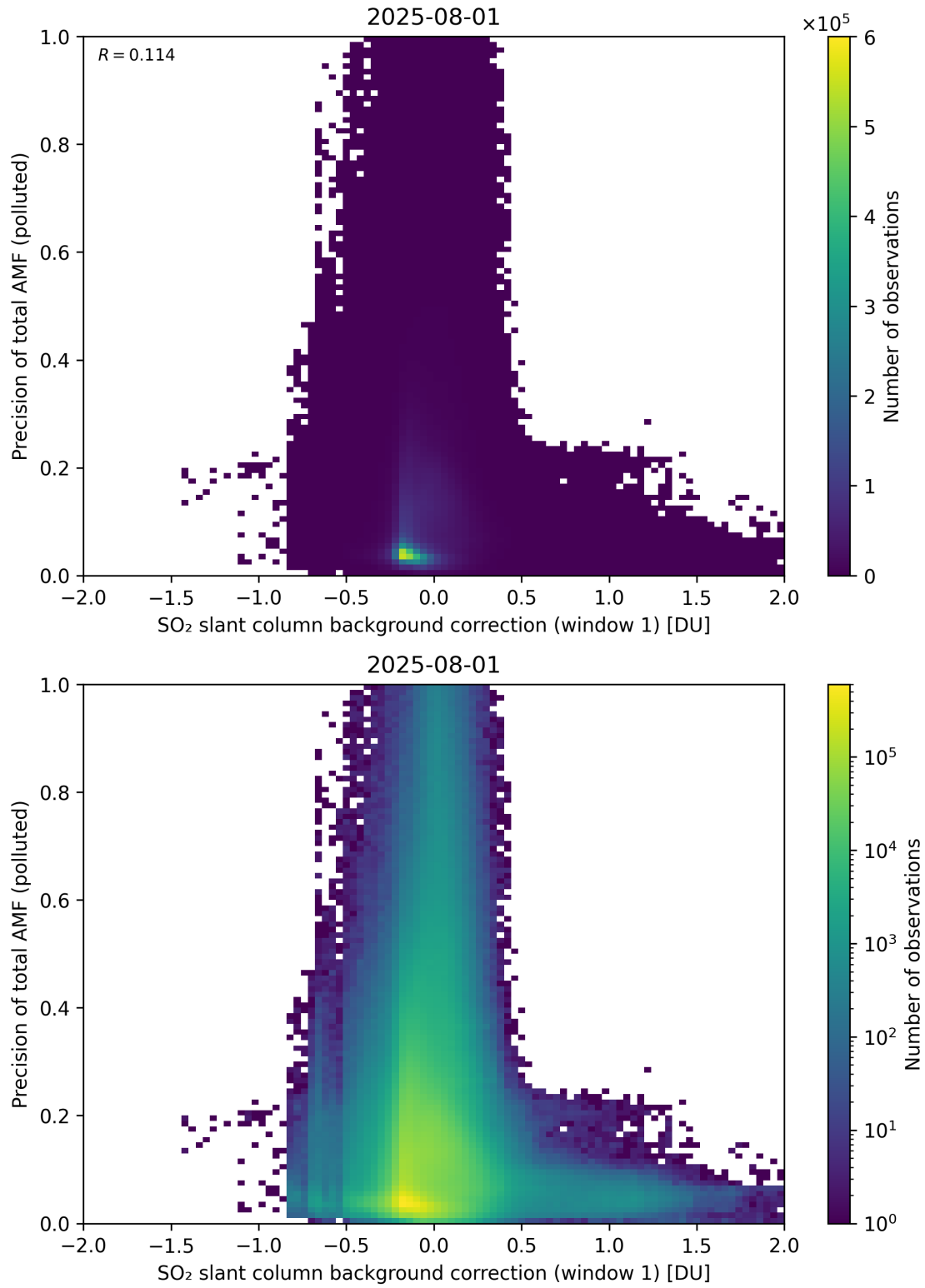
Figure 121: Scatter density plot of “SO 2 slant column background correction (window 1)” against “Precision of total AMF (polluted)” for 2025-07-31 to 2025-08-02.
