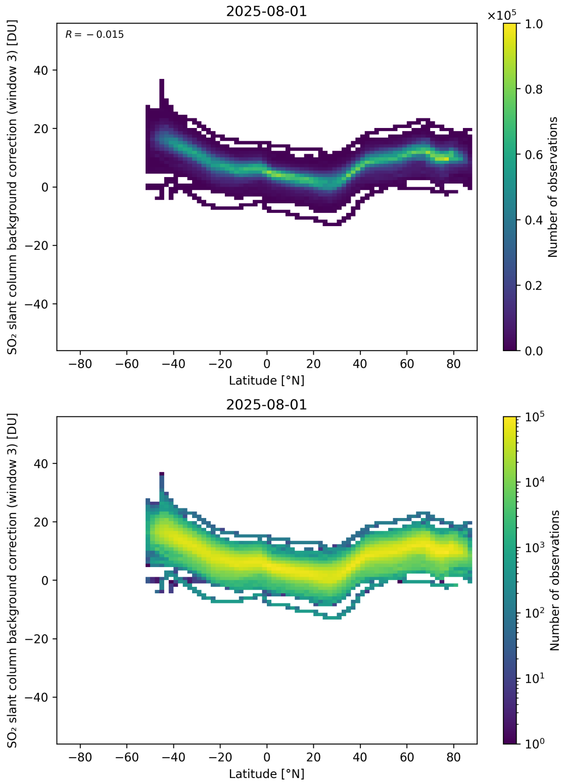
Figure 152: Scatter density plot of “Latitude” against “SO 2 slant column background correction (window 3)” for 2025-07-31 to 2025-08-02.
