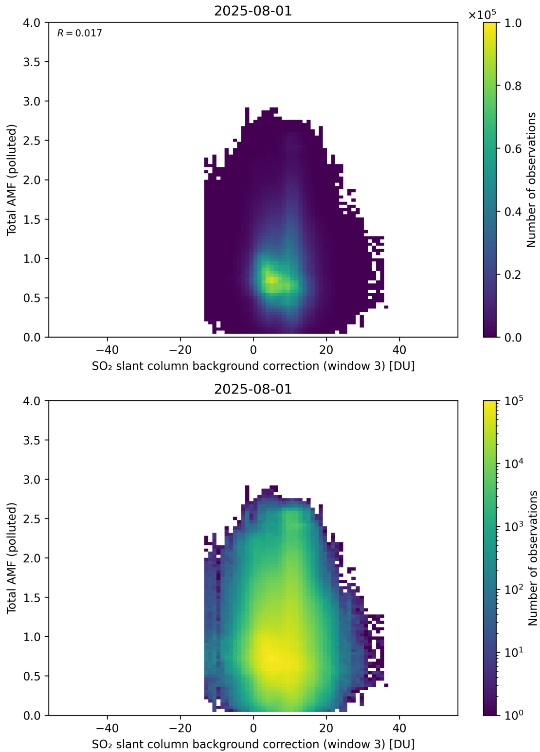
Figure 136: Scatter density plot of “SO 2 slant column background correction (window 3)” against “Total AMF (polluted)” for 2025-07-31 to 2025-08-02.
