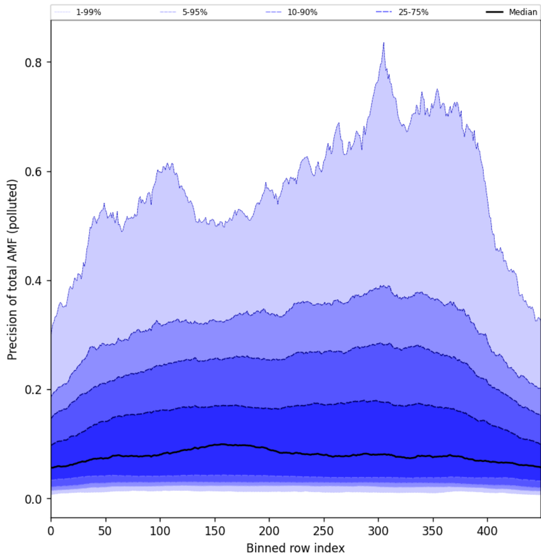
Figure 106: Along track statistics of “Precision of total AMF (polluted)” for 2025-07-31 to 2025-08-02
