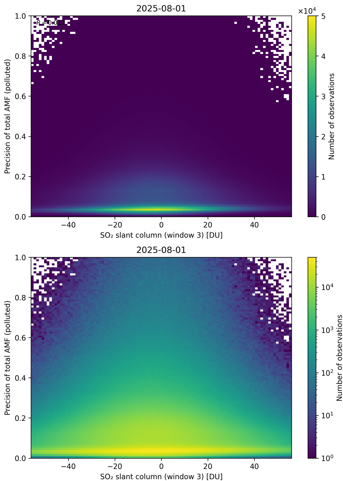
Figure 319: Scatter density plot of “SO 2 slant column (window 3)” against “Precision of total AMF (polluted)” for 2025-07-31 to 2025-08-02.
