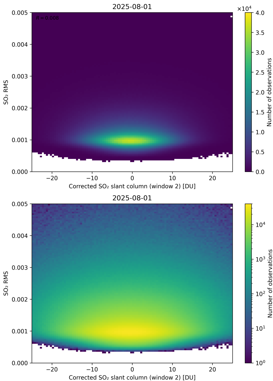
Figure 248: Scatter density plot of “Corrected SO 2 slant column (window 2)” against “SO 2 RMS” for 2025-07-31 to 2025-08-02.
