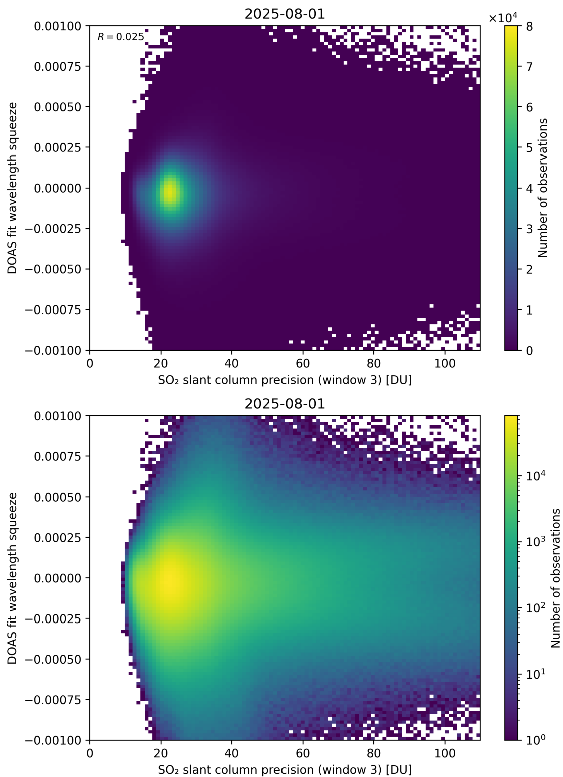
Figure 309: Scatter density plot of “SO 2 slant column precision (window 3)” against “DOAS fit wavelength squeeze” for 2025-07-31 to 2025-08-02.
