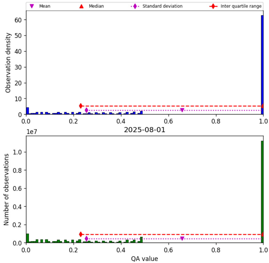
Figure 57: Histogram of “QA value” for 2025-07-31 to 2025-08-02
