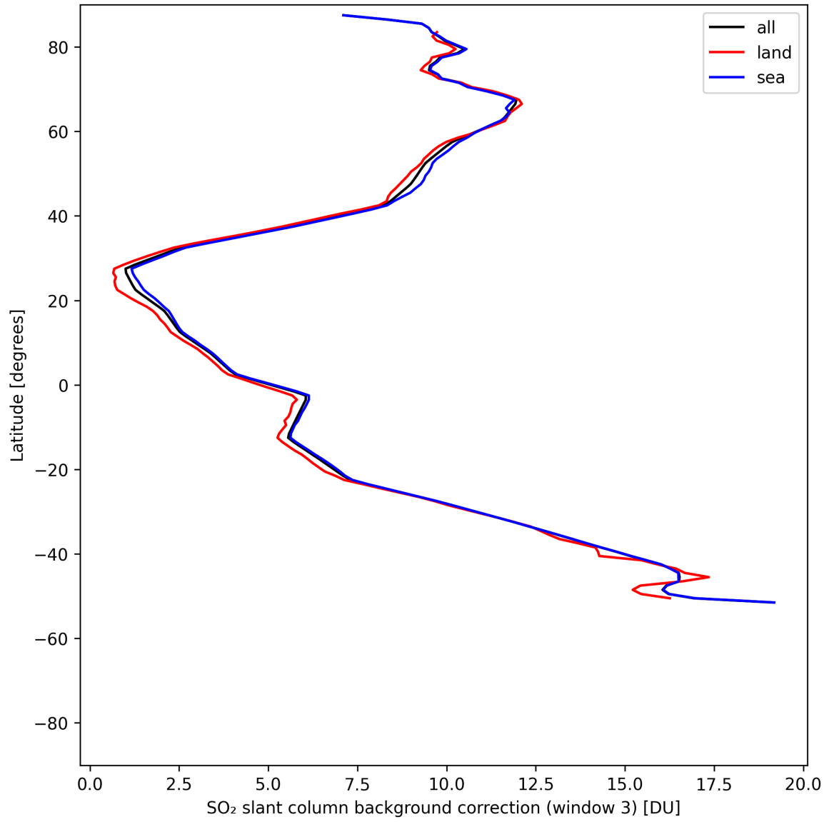
Figure 48: Zonal average of “SO 2 slant column background correction (window 3)” for 2025-07-31 to 2025-08-02.
