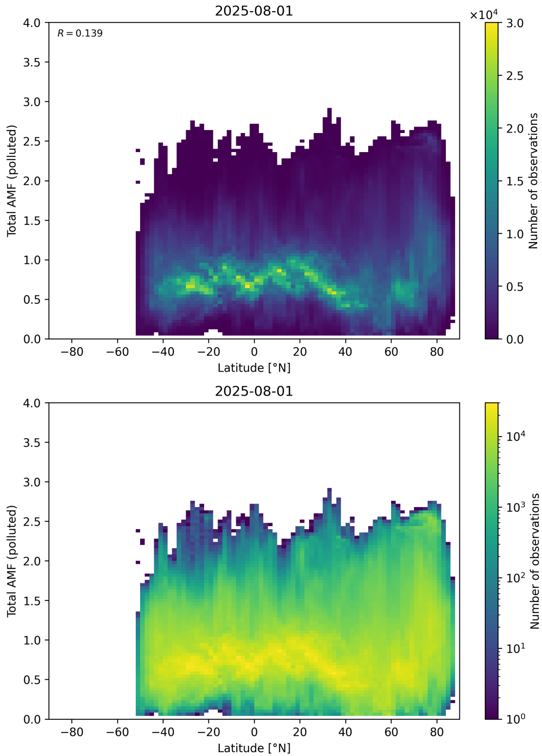
Figure 167: Scatter density plot of “Latitude” against “Total AMF (polluted)” for 2025-07-31 to 2025-08-02.
