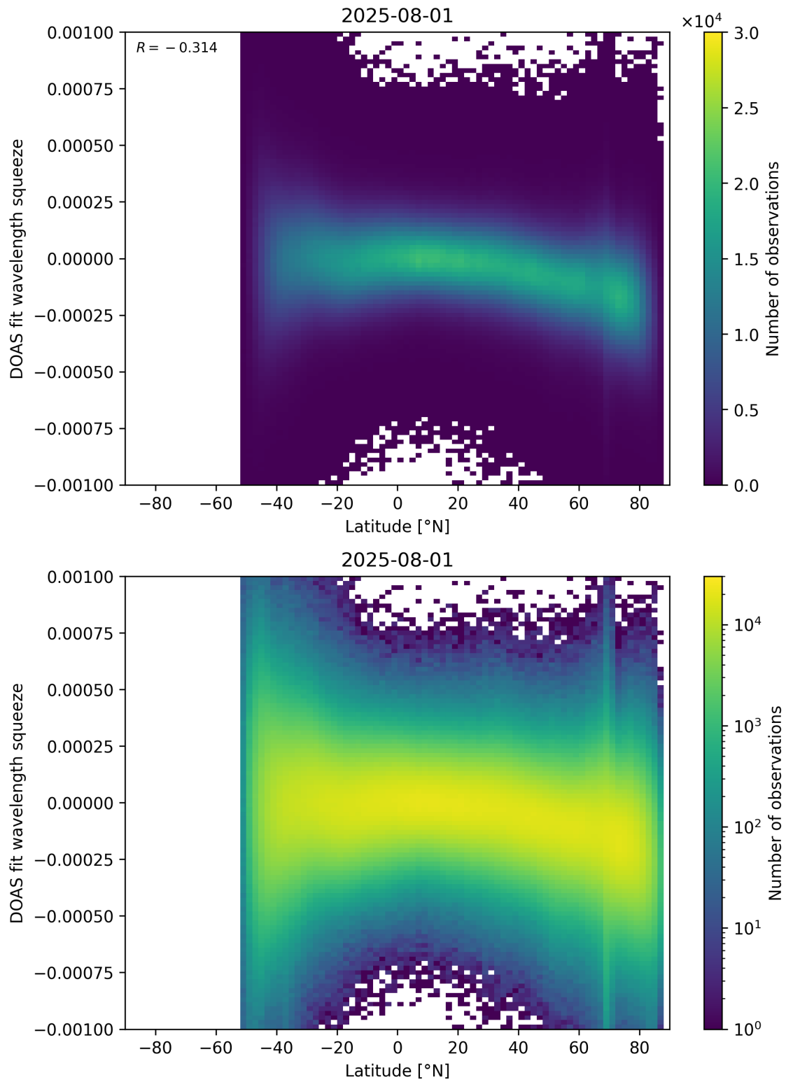
Figure 154: Scatter density plot of “Latitude” against “DOAS fit wavelength squeeze” for 2025-07-31 to 2025-08-02.
