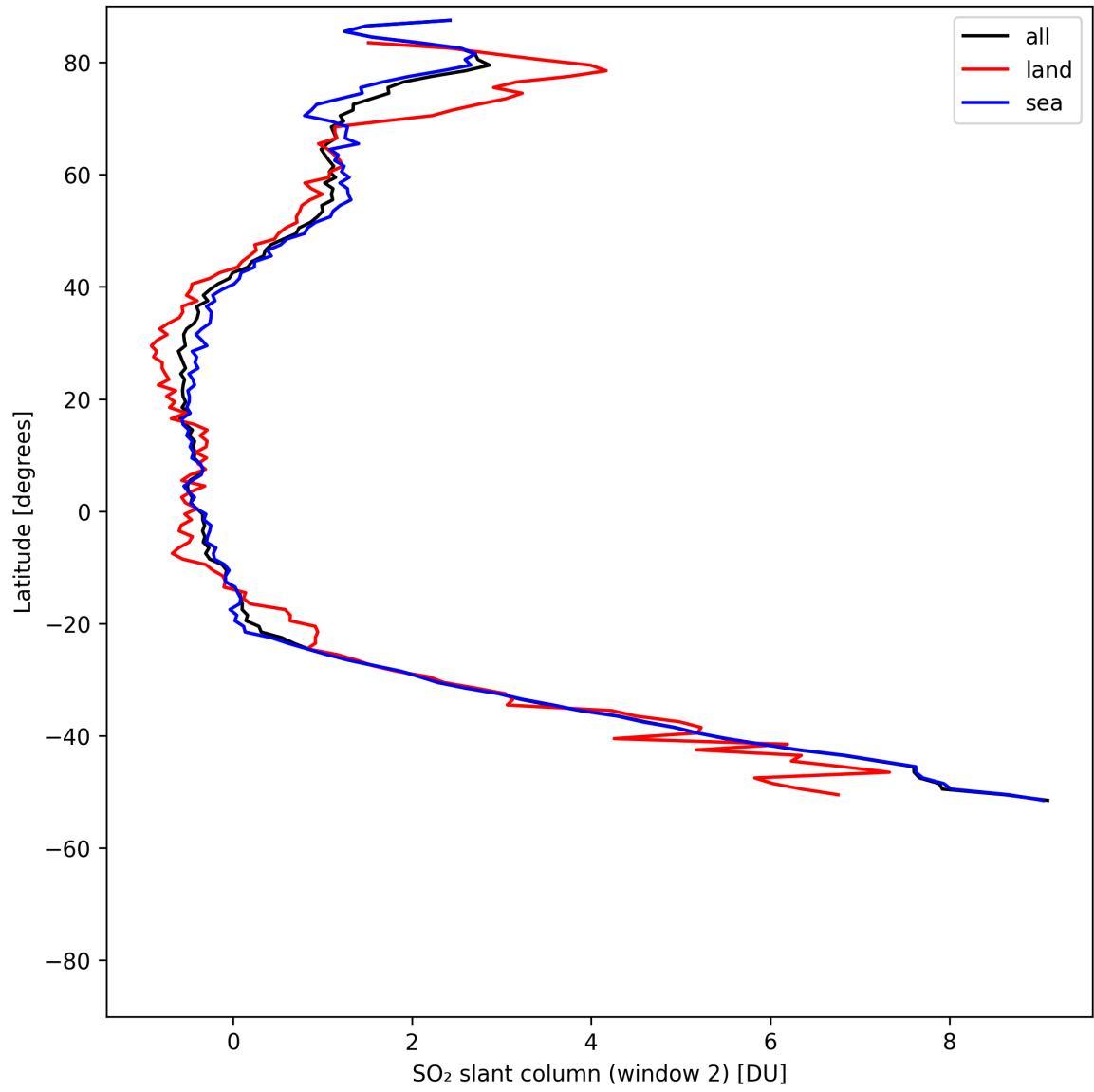
Figure 41: Zonal average of “SO 2 slant column (window 2)” for 2025-07-31 to 2025-08-02.
