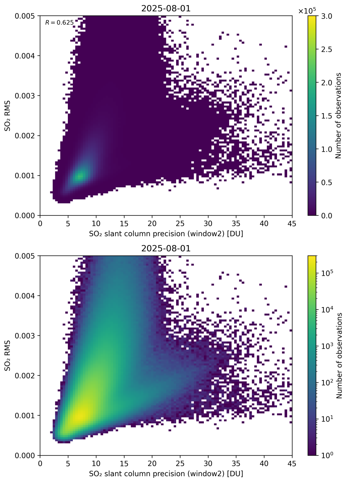
Figure 295: Scatter density plot of “SO 2 slant column precision (window2)” against “SO 2 RMS” for 2025-07-31 to 2025-08-02.
