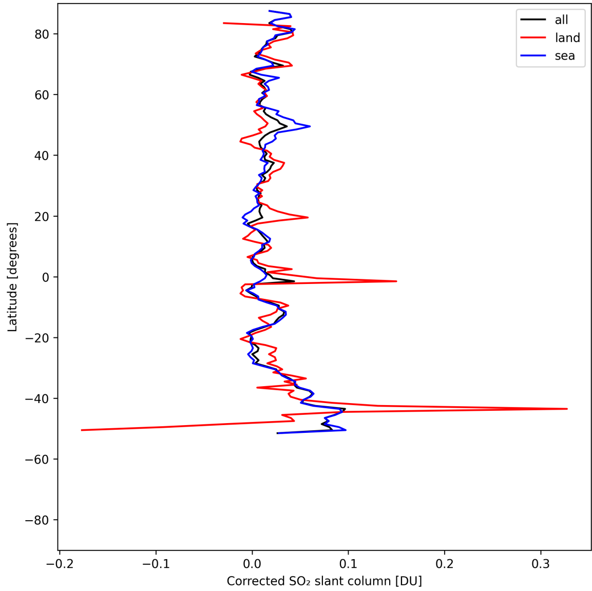
Figure 34: Zonal average of “Corrected SO 2 slant column” for 2025-07-31 to 2025-08-02.
