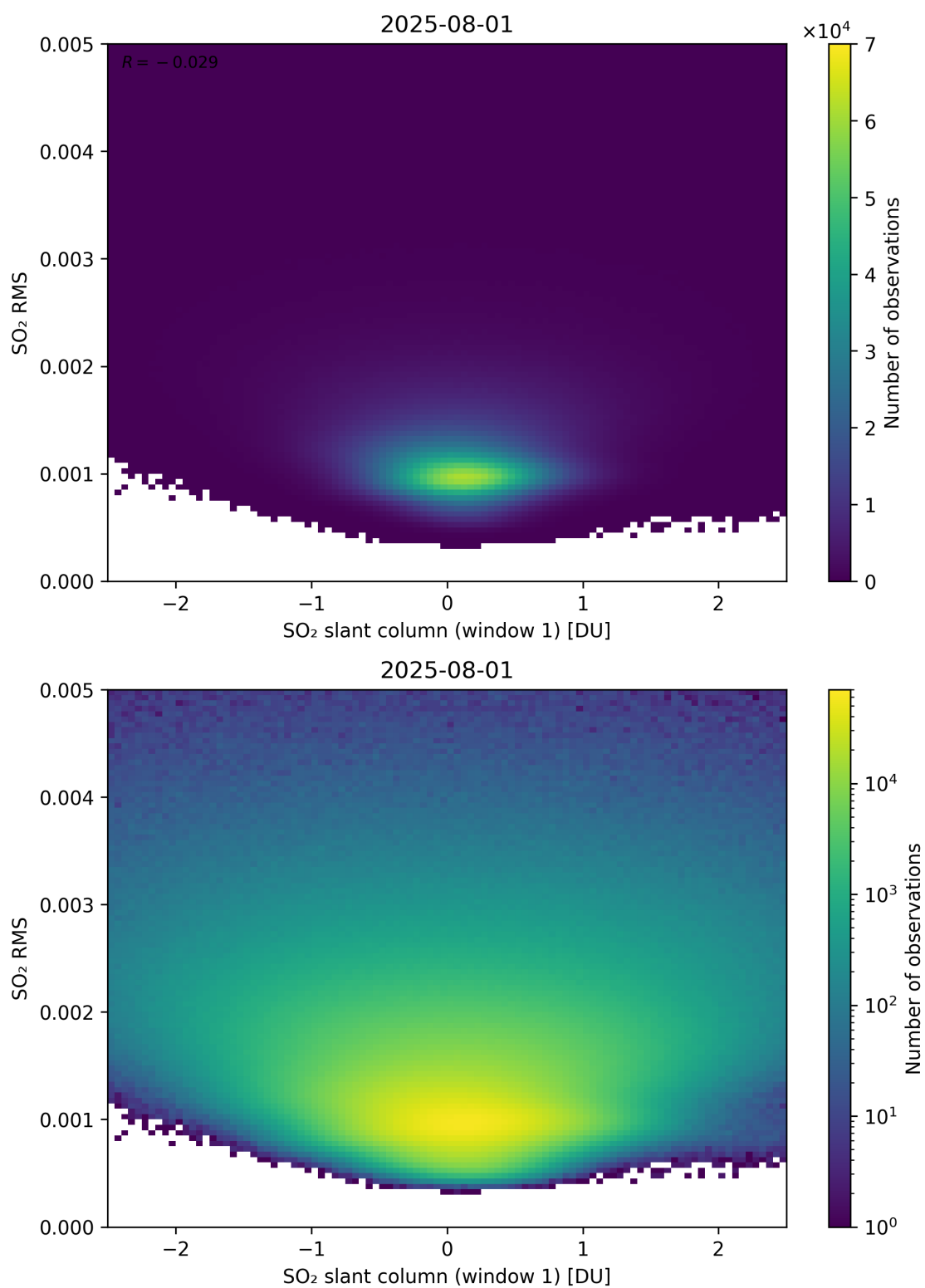
Figure 267: Scatter density plot of “SO 2 slant column (window 1)” against “SO 2 RMS” for 2025-07-31 to 2025-08-02.
