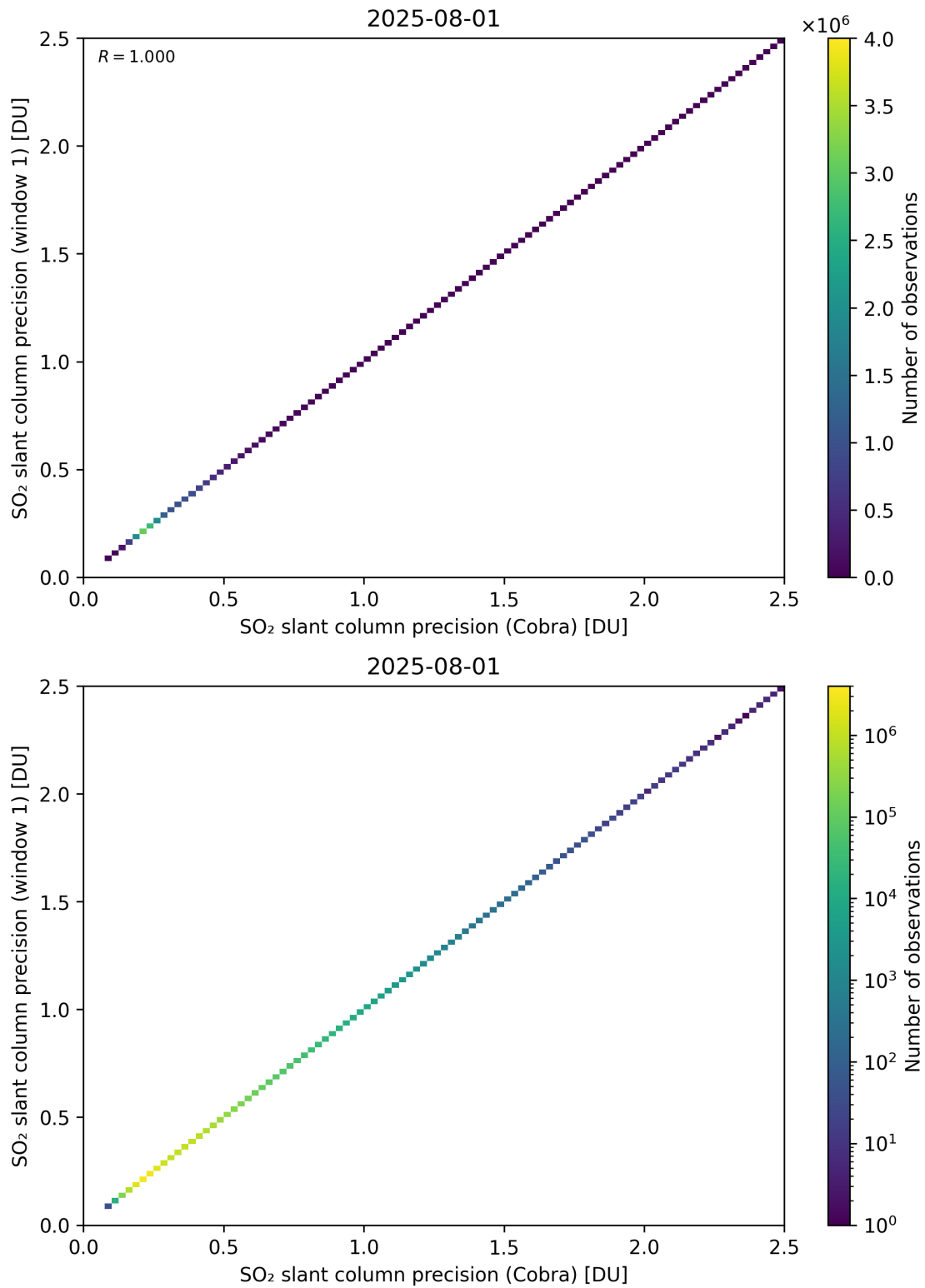
Figure 209: Scatter density plot of “SO 2 slant column precision (Cobra)” against “SO 2 slant column precision (window 1)” for 2025-07-31 to 2025-08-02.
