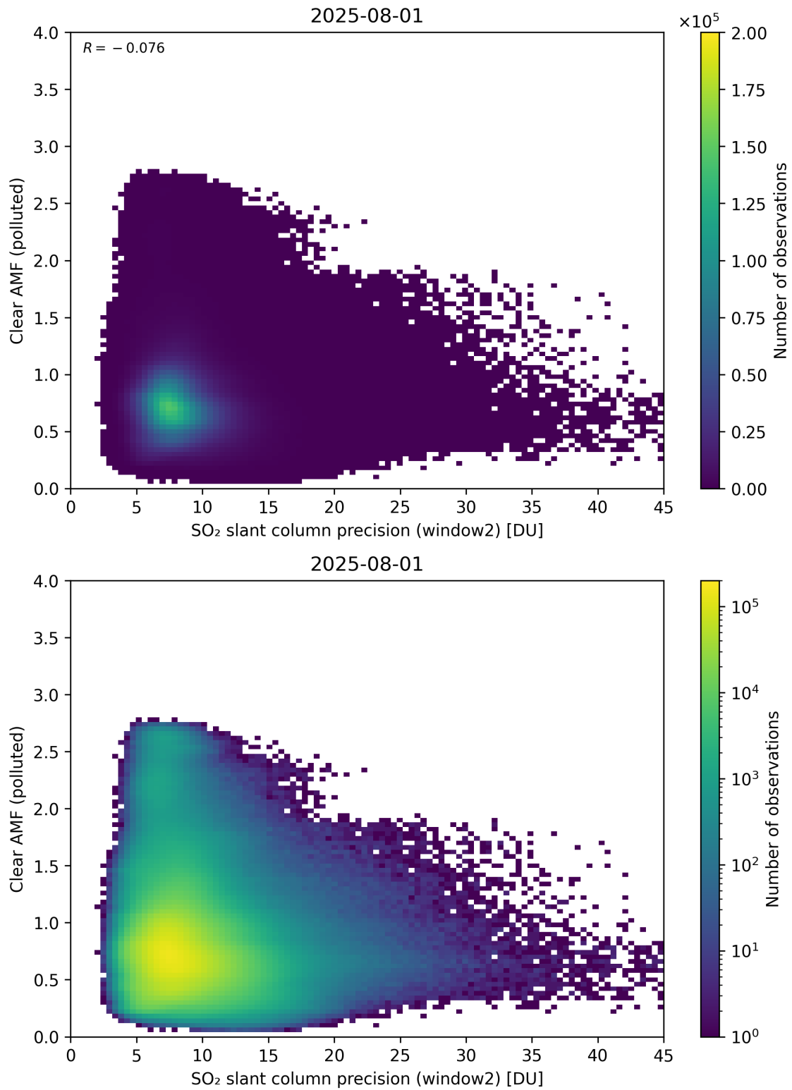
Figure 296: Scatter density plot of “SO 2 slant column precision (window2)” against “Clear AMF (polluted)” for 2025-07-31 to 2025-08-02.
