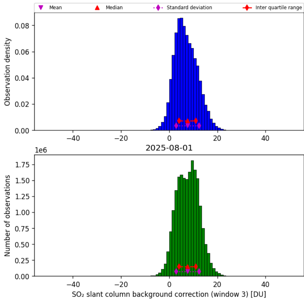
Figure 74: Histogram of “SO 2 slant column background correction (window 3)” for 2025-07-31 to 2025-08-02
