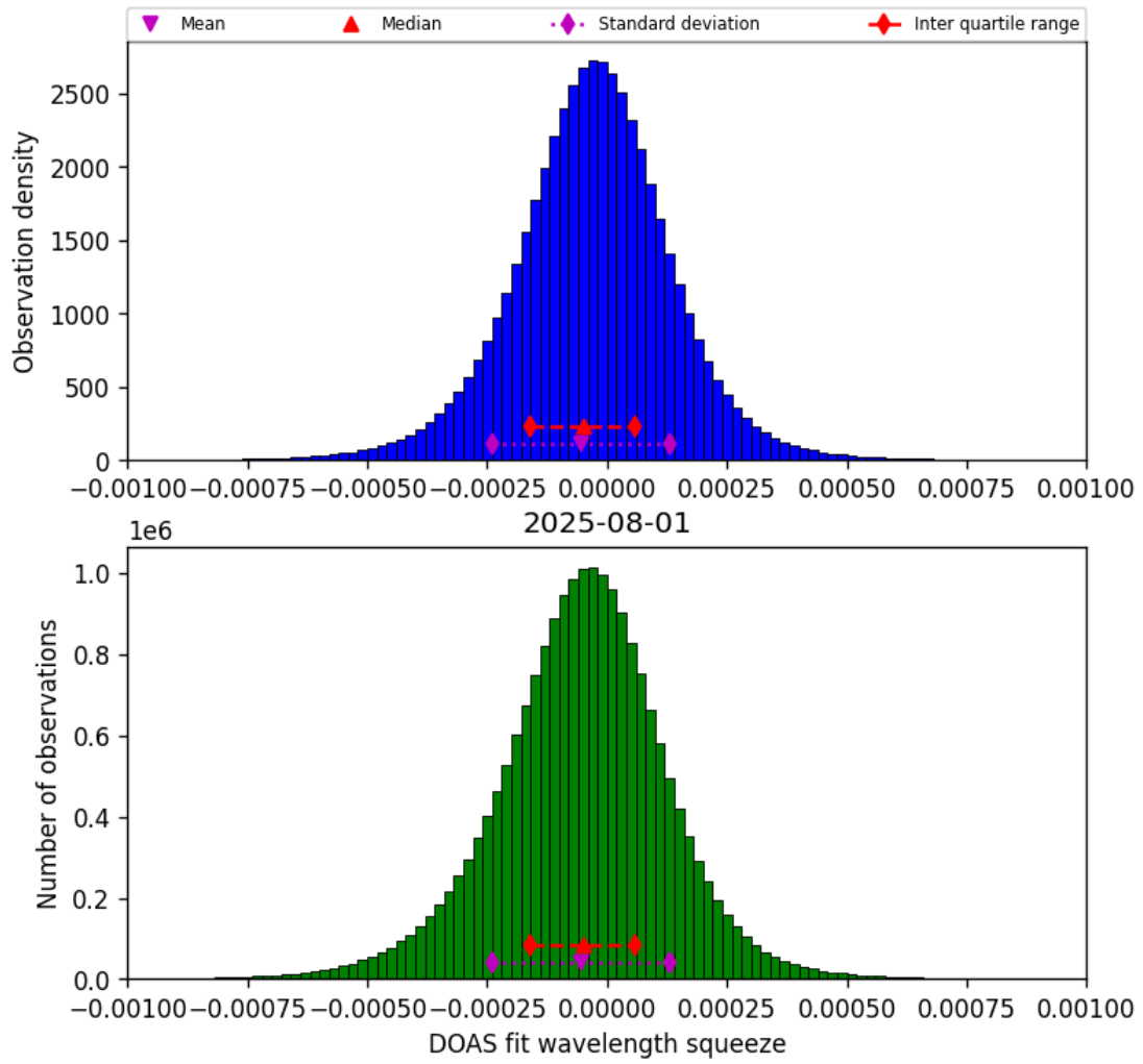
Figure 77: Histogram of “DOAS fit wavelength squeeze” for 2025-07-31 to 2025-08-02
