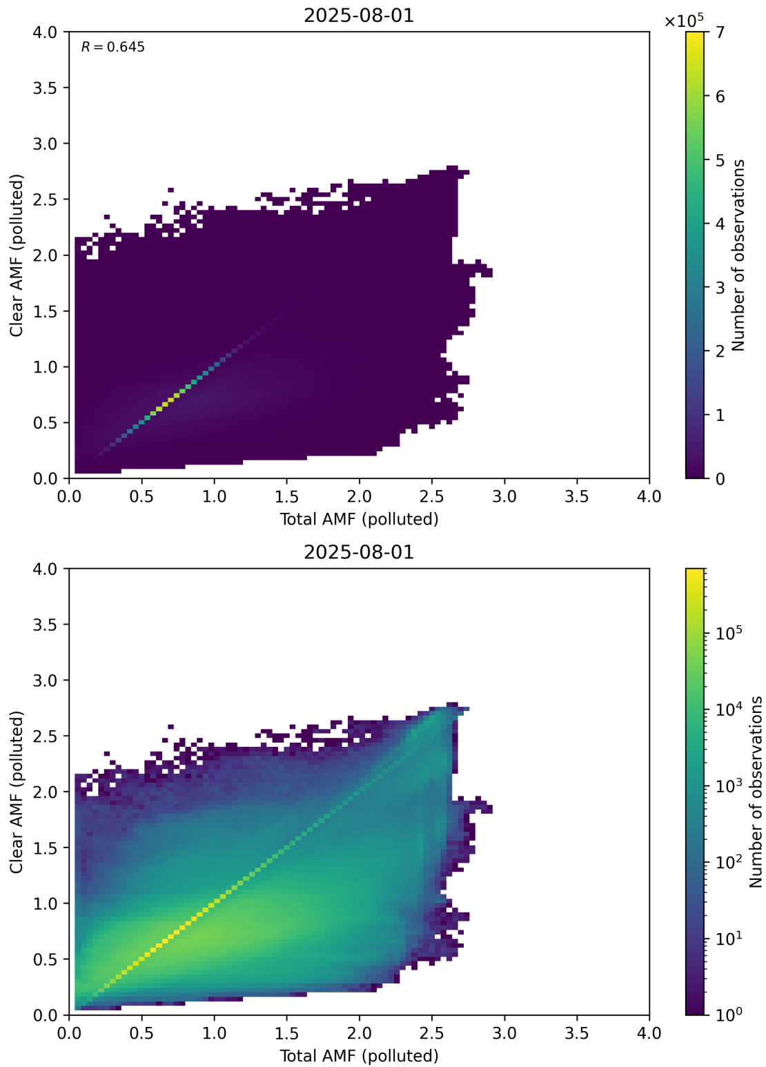
Figure 321: Scatter density plot of “Total AMF (polluted)” against “Clear AMF (polluted)” for 2025-07-31 to 2025-08-02.
