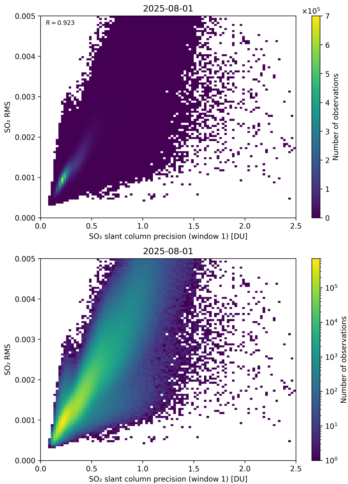
Figure 273: Scatter density plot of “SO 2 slant column precision (window 1)” against “SO 2 RMS” for 2025-07-31 to 2025-08-02.
