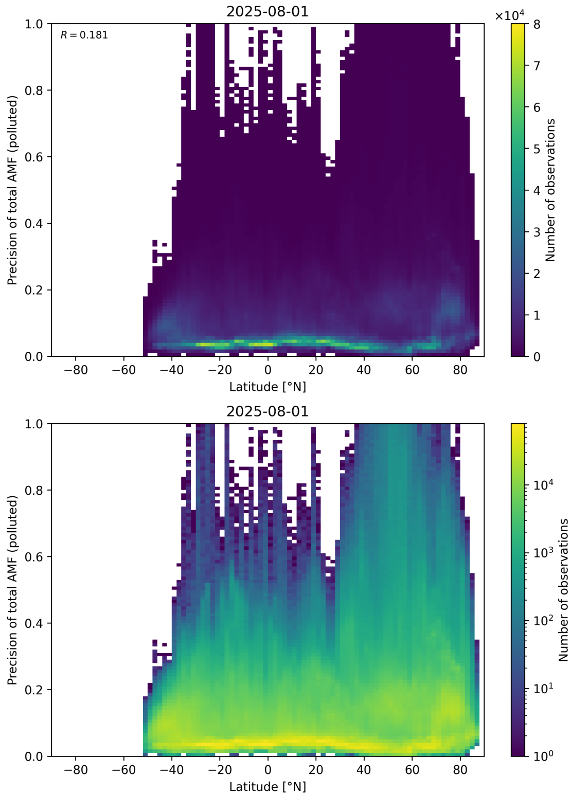
Figure 168: Scatter density plot of “Latitude” against “Precision of total AMF (polluted)” for 2025-07-31 to 2025-08-02.
