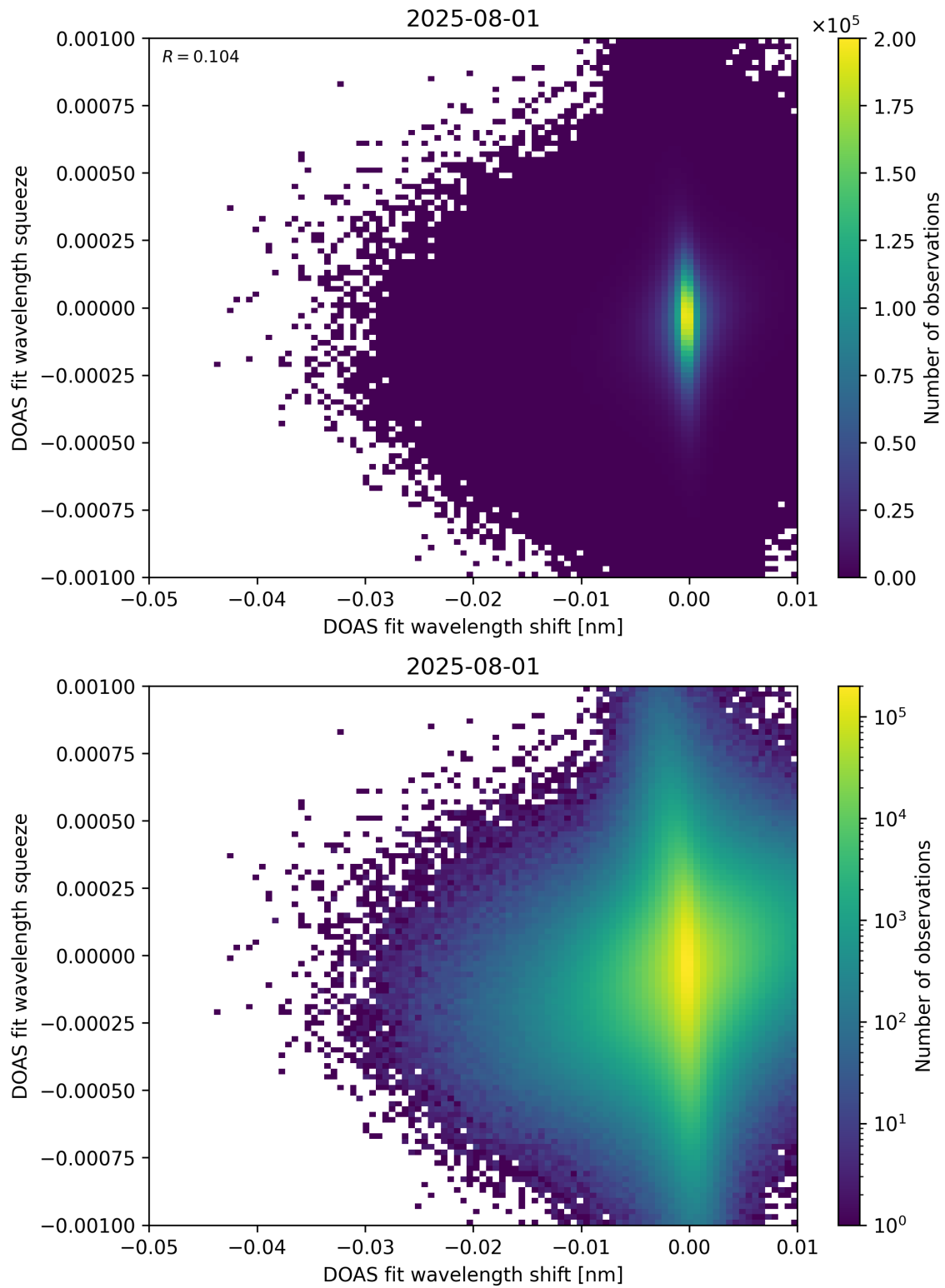
Figure 138: Scatter density plot of “DOAS fit wavelength shift” against “DOAS fit wavelength squeeze” for 2025-07-31 to 2025-08-02.
