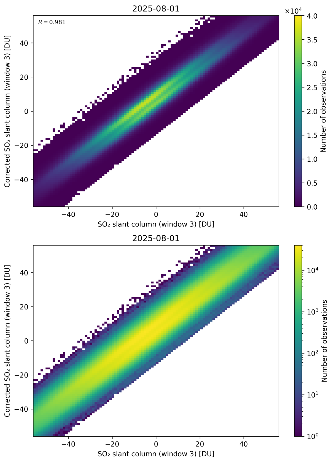
Figure 316: Scatter density plot of “SO 2 slant column (window 3)” against “Corrected SO 2 slant column (window 3)” for 2025-07-31 to 2025-08-02.
