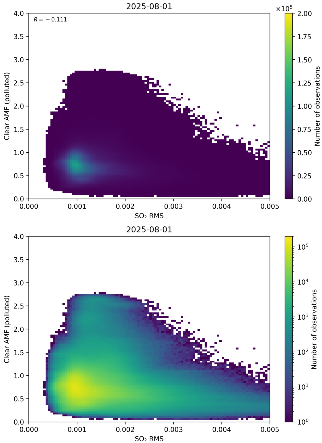
Figure 147: Scatter density plot of “SO 2 RMS” against “Clear AMF (polluted)” for 2025-07-31 to 2025-08-02.
