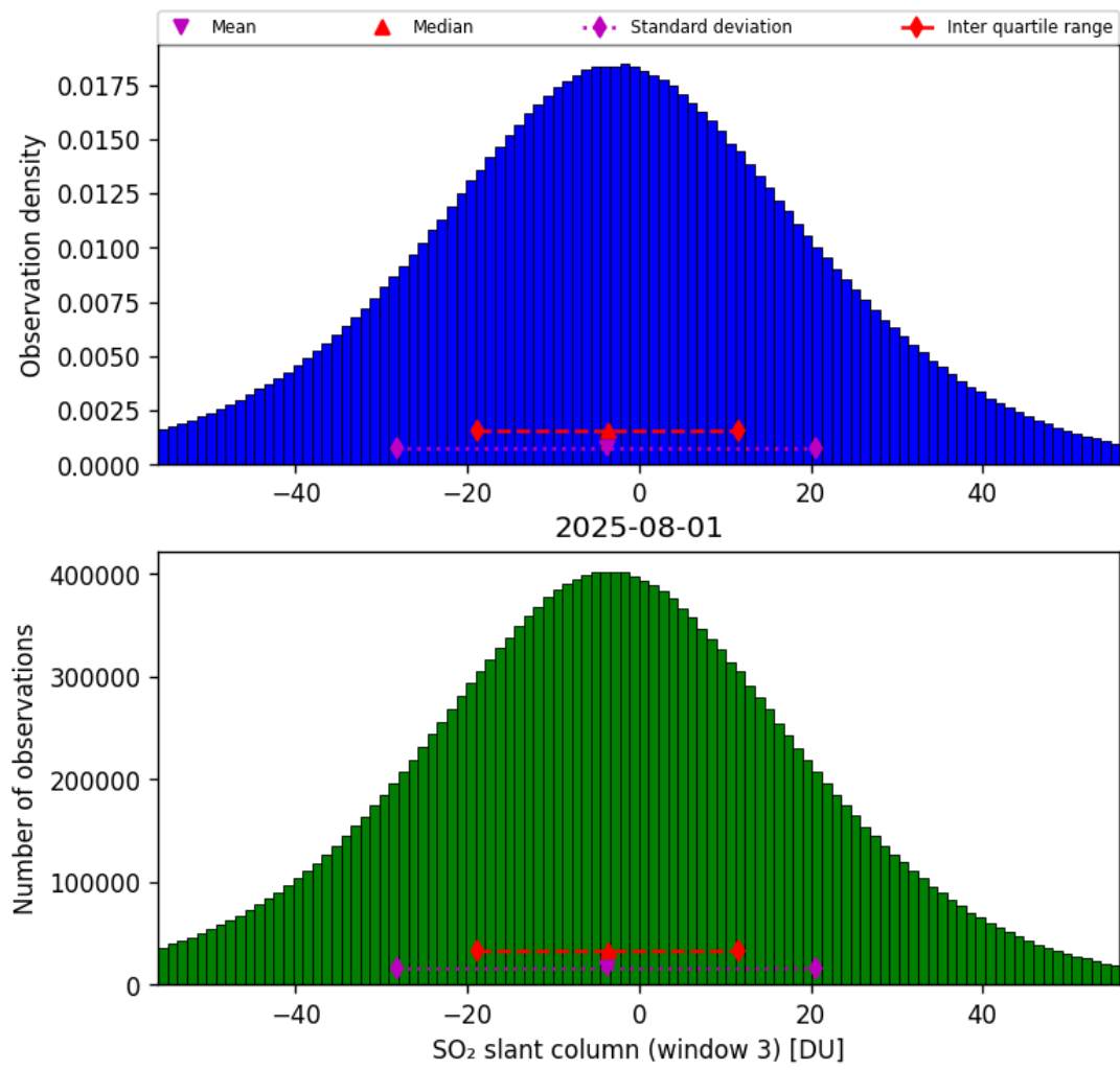
Figure 71: Histogram of “SO 2 slant column (window 3)” for 2025-07-31 to 2025-08-02
