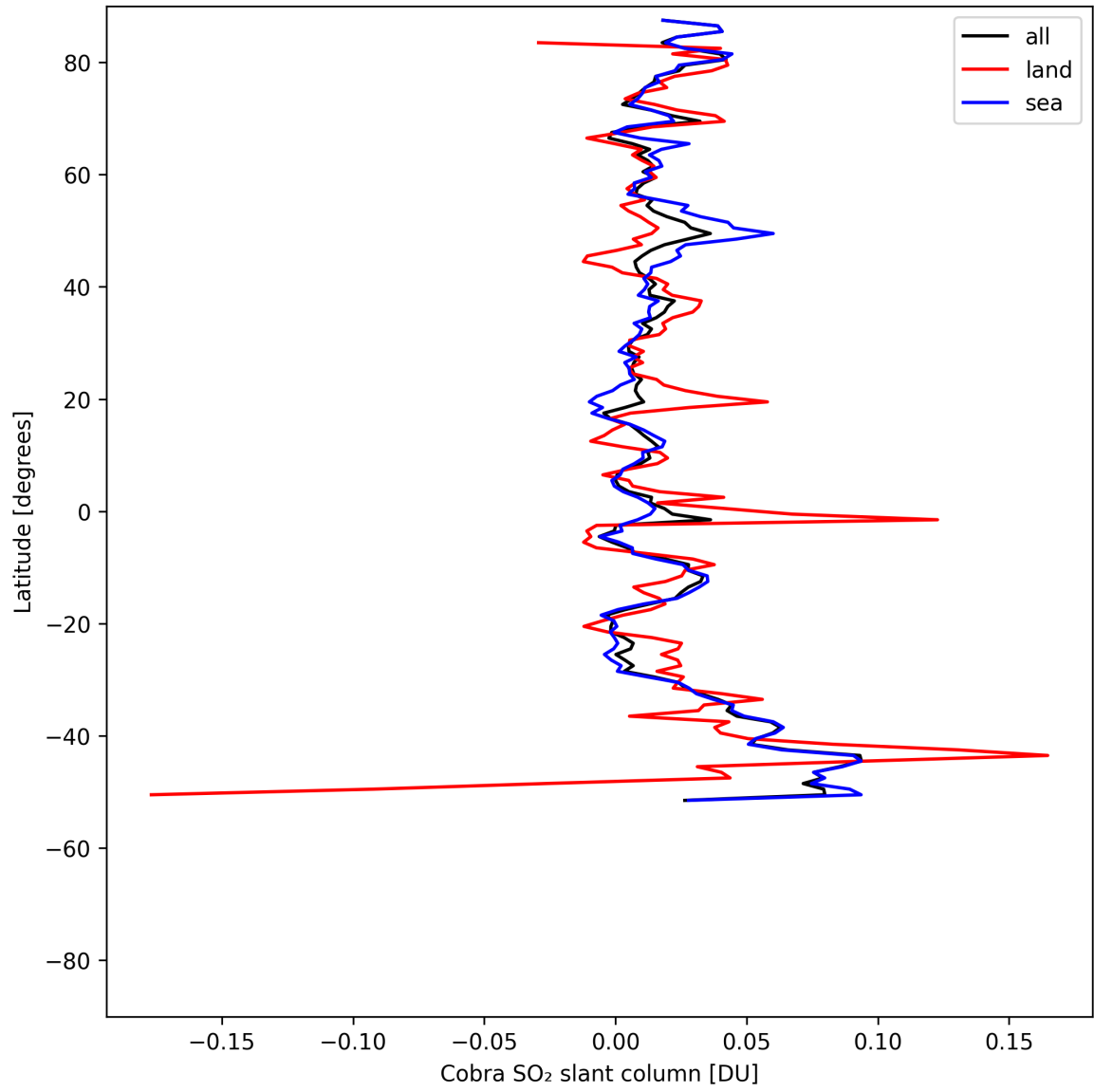
Figure 35: Zonal average of “Cobra SO 2 slant column” for 2025-07-31 to 2025-08-02.
