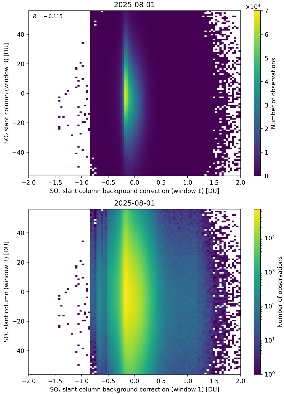
Figure 118: Scatter density plot of “SO 2 slant column background correction (window 1)” against “SO 2 slant column (window 3)” for 2025-07-31 to 2025-08-02.
