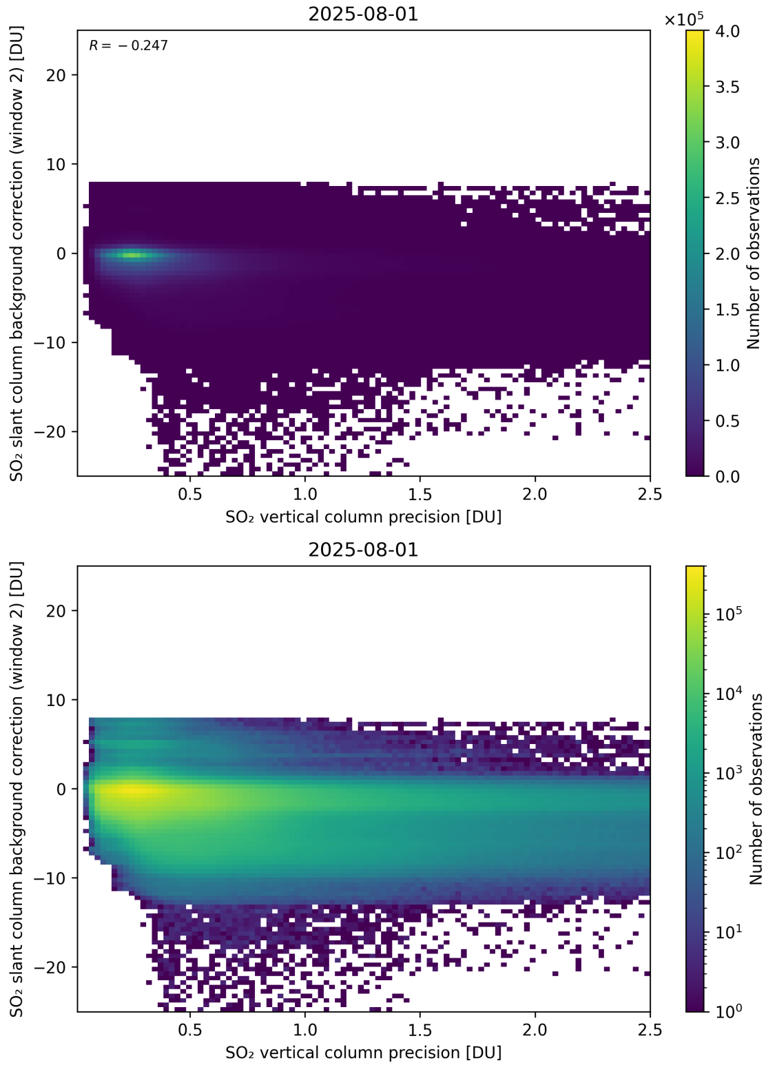
Figure 330: Scatter density plot of “SO 2 vertical column precision” against “SO 2 slant column background correction (window 2)” for 2025-07-31 to 2025-08-02.
