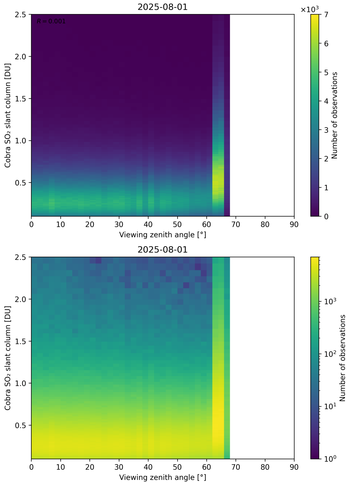
Figure 371: Scatter density plot of “Viewing zenith angle” against “Cobra SO 2 slant column” for 2025-07-31 to 2025-08-02.
