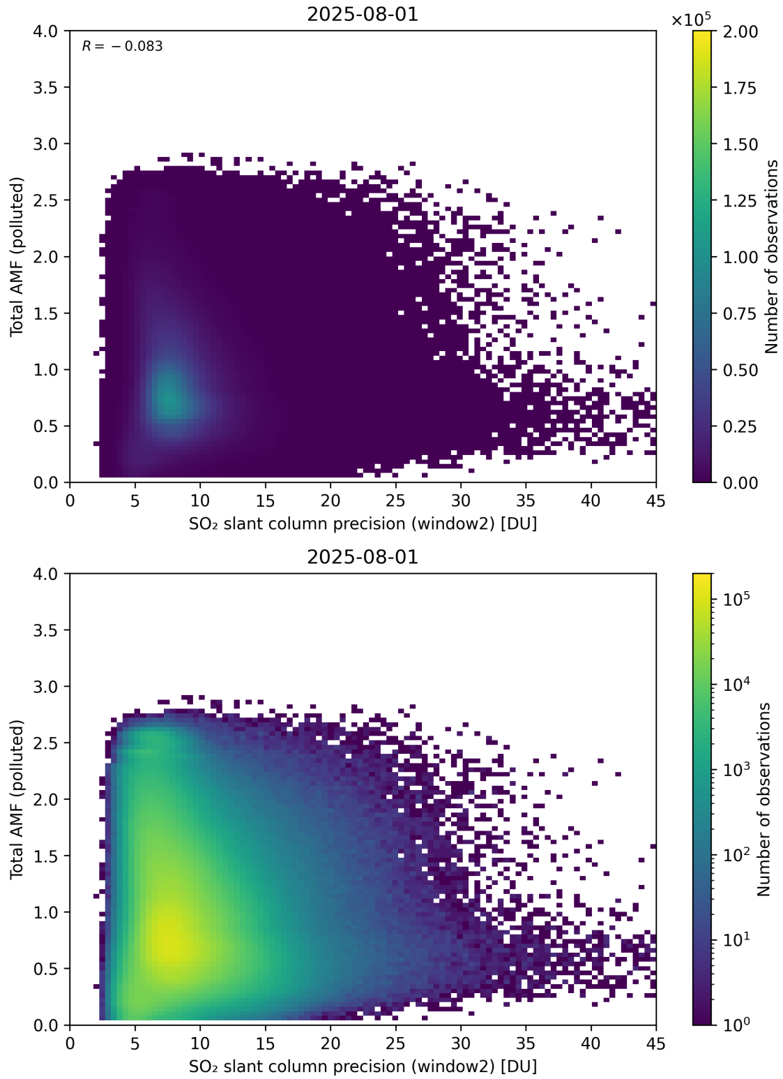
Figure 301: Scatter density plot of “SO 2 slant column precision (window2)” against “Total AMF (polluted)” for 2025-07-31 to 2025-08-02.
