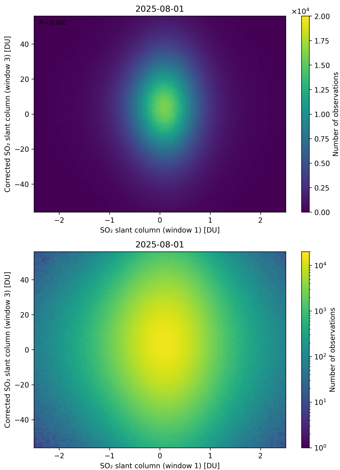
Figure 284: Scatter density plot of “SO 2 slant column (window 1)” against “Corrected SO 2 slant column (window 3)” for 2025-07-31 to 2025-08-02.
