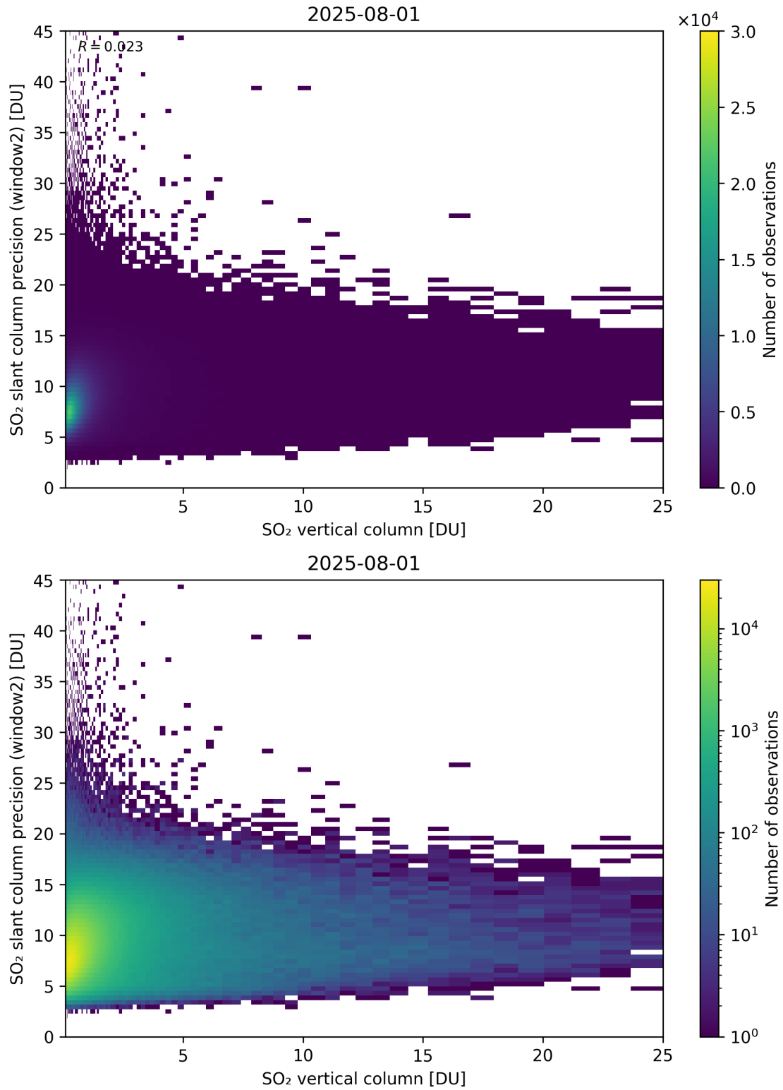
Figure 356: Scatter density plot of “SO 2 vertical column” against “SO 2 slant column precision (window2)” for 2025-07-31 to 2025-08-02.
