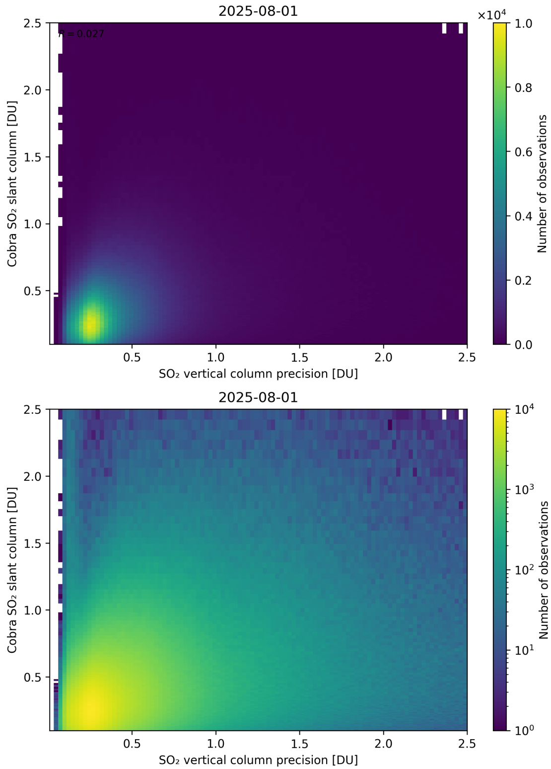
Figure 336: Scatter density plot of “SO 2 vertical column precision” against “Cobra SO 2 slant column” for 2025-07-31 to 2025-08-02.
