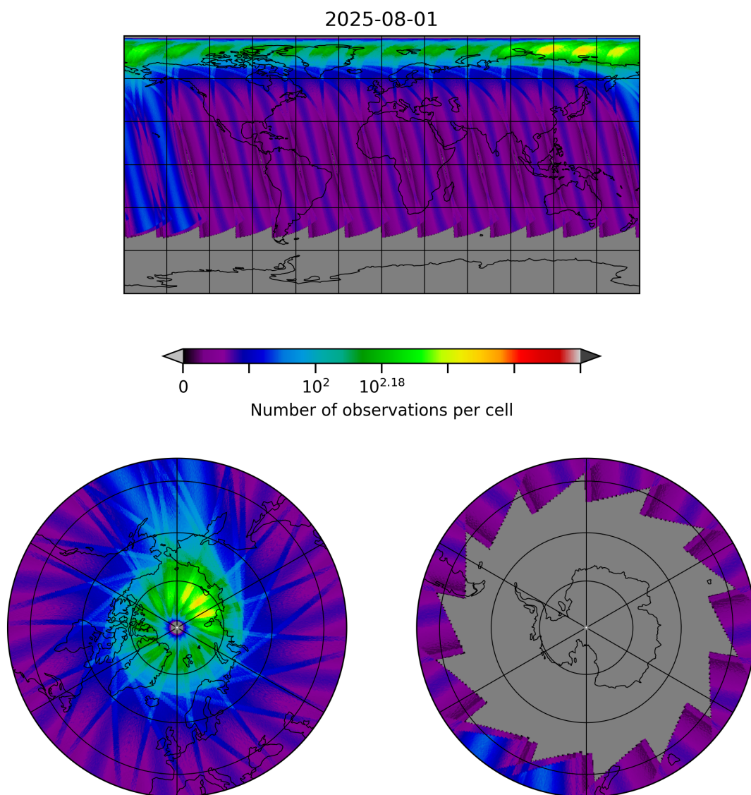
Figure 30: Map of the number of observations for 2025-07-31 to 2025-08-02
