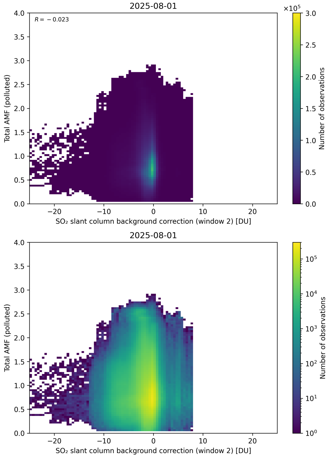
Figure 130: Scatter density plot of “SO 2 slant column background correction (window 2)” against “Total AMF (polluted)” for 2025-07-31 to 2025-08-02.
