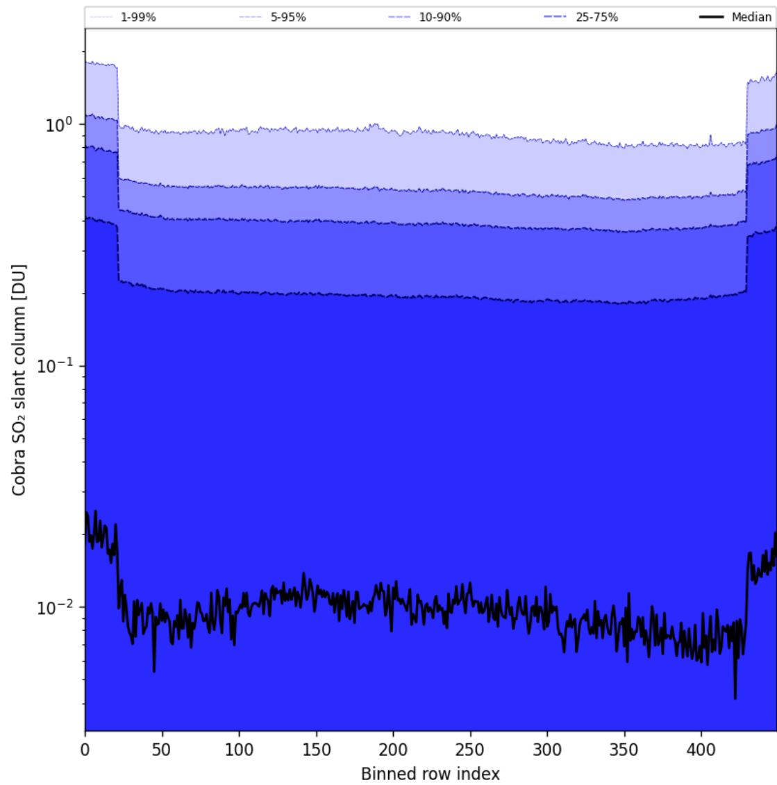
Figure 87: Along track statistics of “Cobra SO 2 slant column” for 2025-07-31 to 2025-08-02
