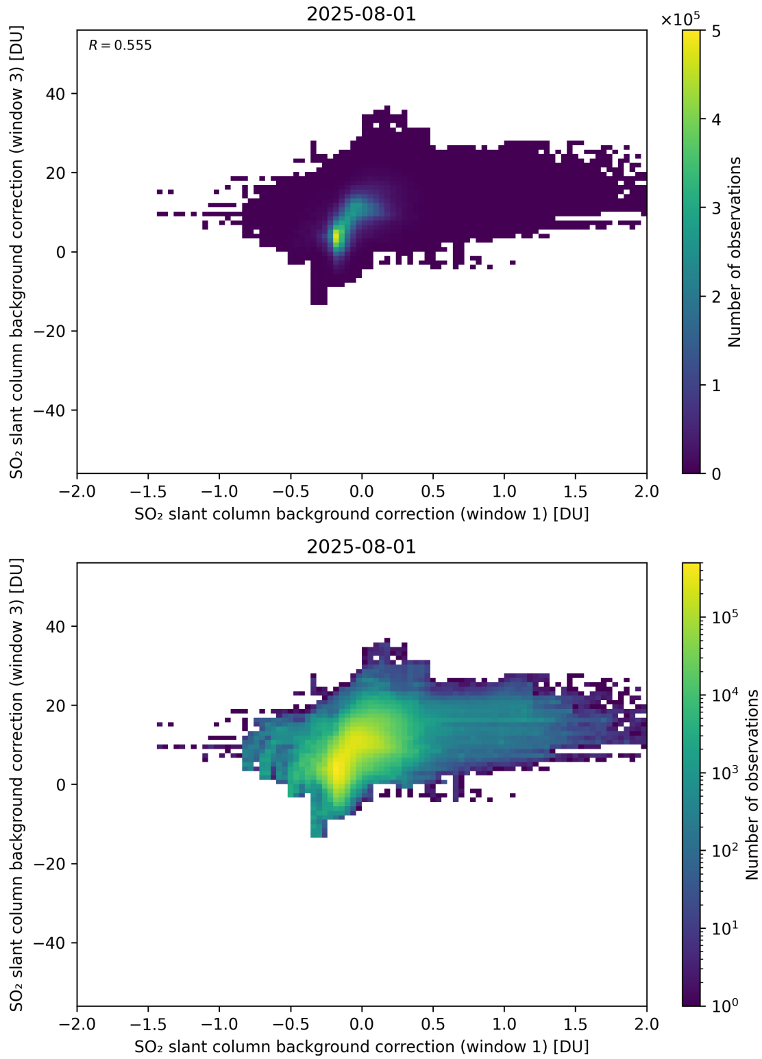
Figure 110: Scatter density plot of “SO 2 slant column background correction (window 1)” against “SO 2 slant column background correction (window 3)” for 2025-07-31 to 2025-08-02.
