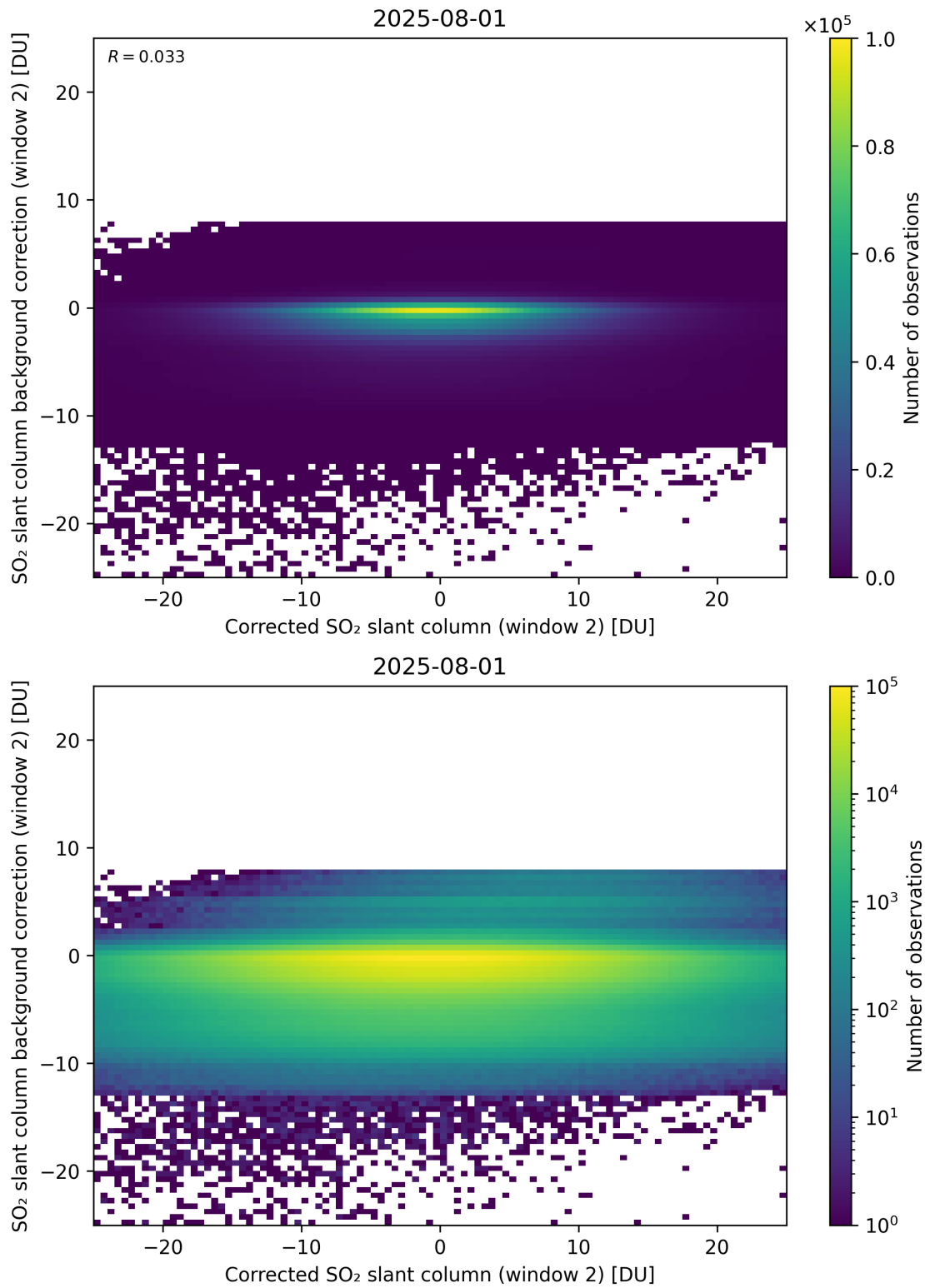
Figure 244: Scatter density plot of “Corrected SO 2 slant column (window 2)” against “SO 2 slant column background correction (window 2)” for 2025-07-31 to 2025-08-02.
