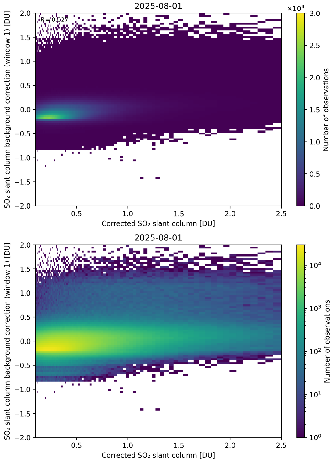
Figure 226: Scatter density plot of “Corrected SO 2 slant column” against “SO 2 slant column background correction (window 1)” for 2025-07-31 to 2025-08-02.
