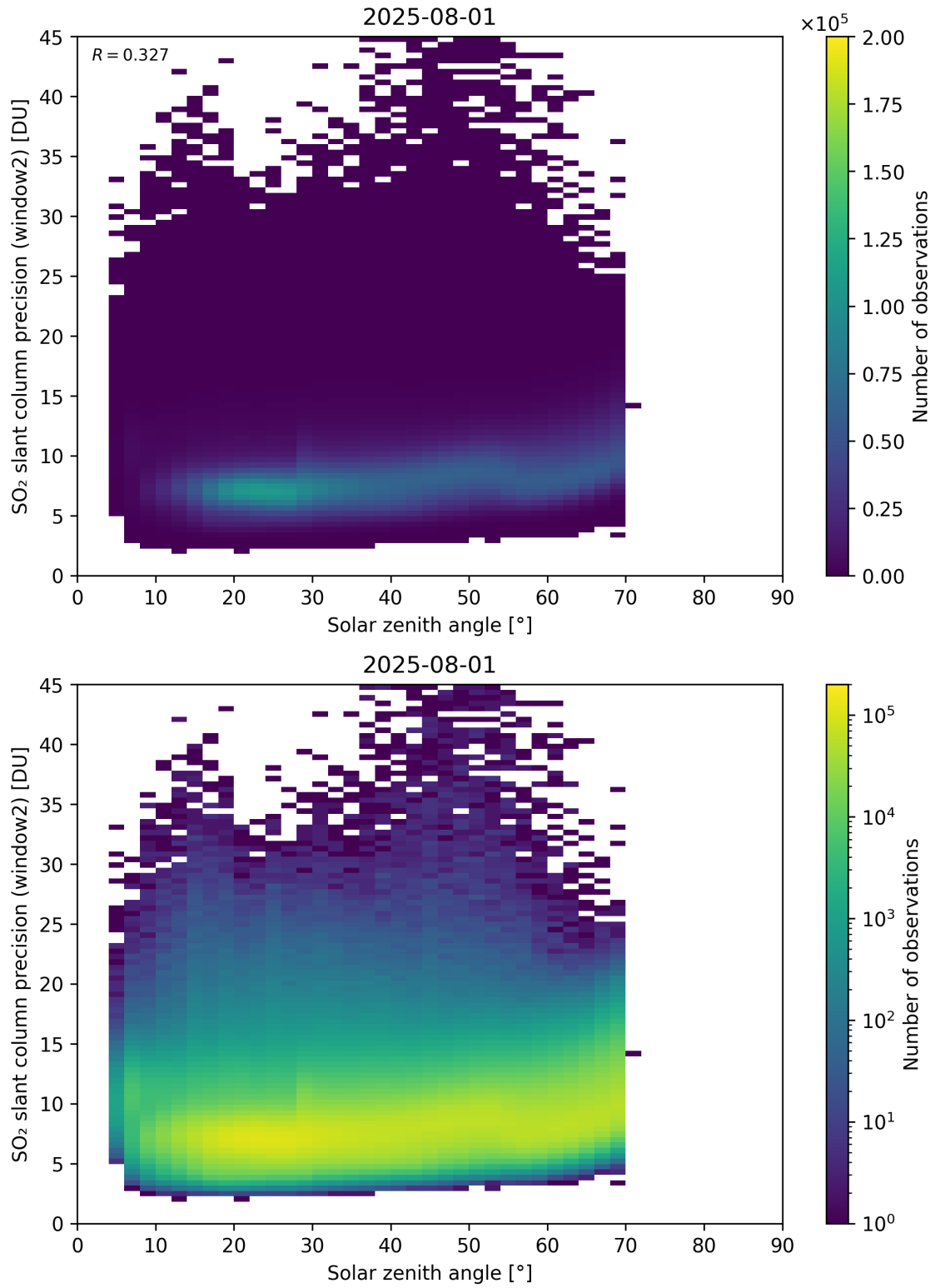
Figure 186: Scatter density plot of “Solar zenith angle” against “SO 2 slant column precision (window2)” for 2025-07-31 to 2025-08-02.
