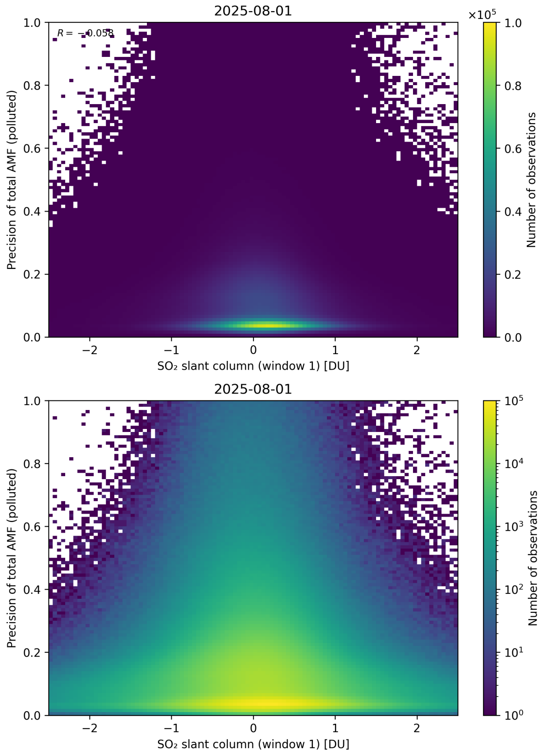
Figure 290: Scatter density plot of “SO 2 slant column (window 1)” against “Precision of total AMF (polluted)” for 2025-07-31 to 2025-08-02.
