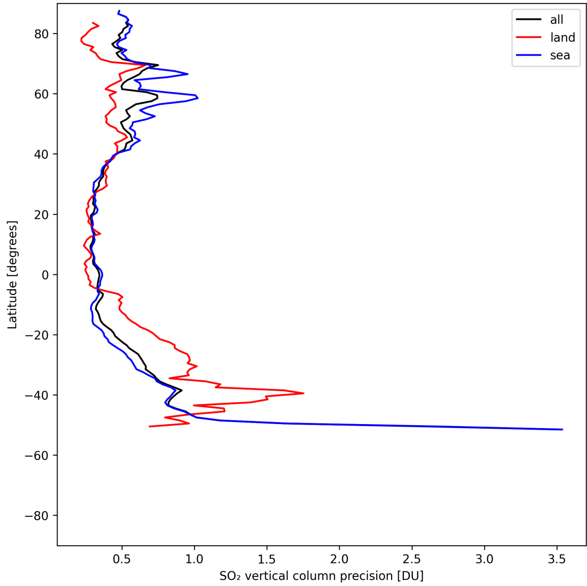
Figure 33: Zonal average of “SO 2 vertical column precision” for 2025-07-31 to 2025-08-02.
