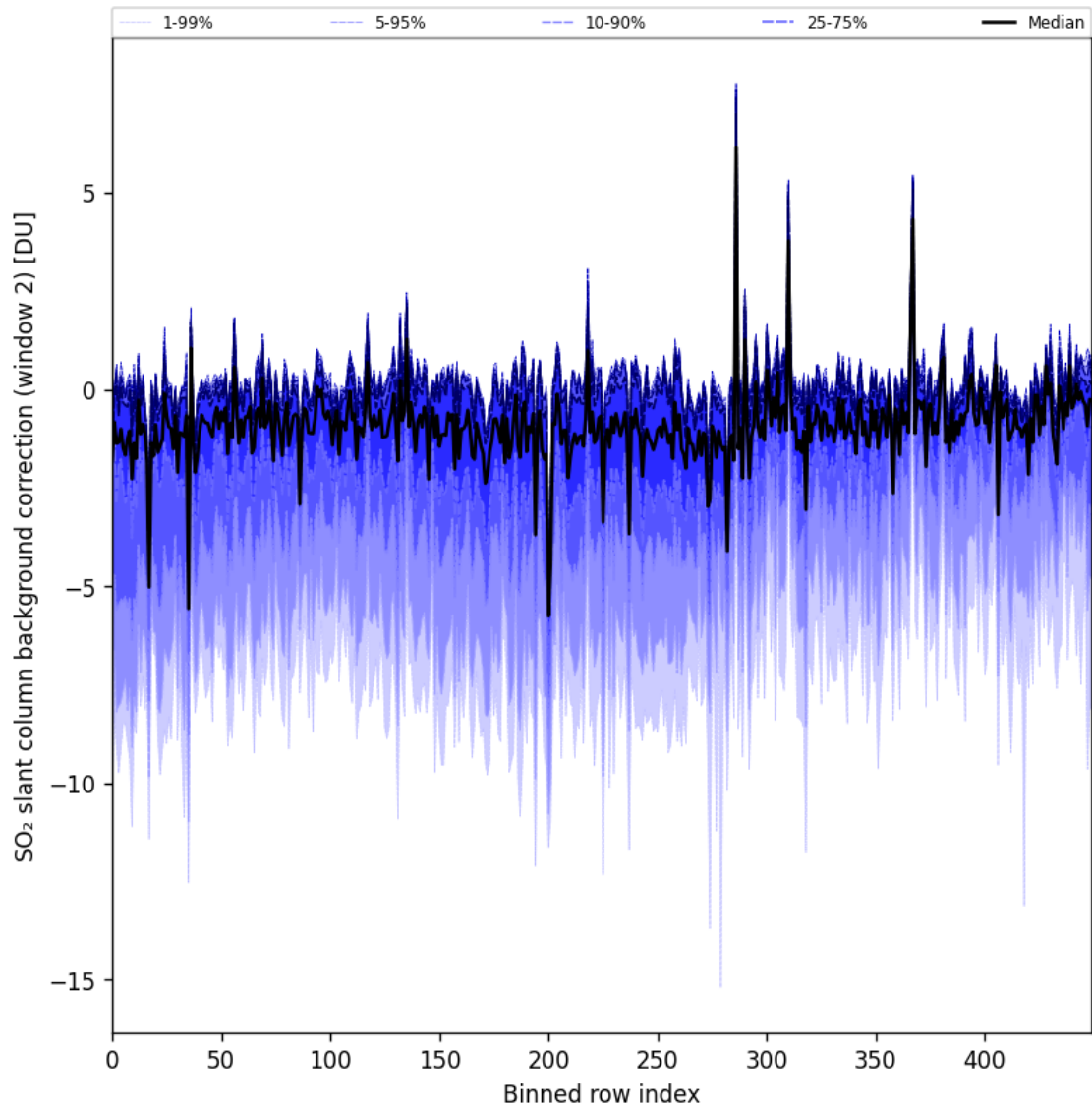
Figure 96: Along track statistics of “SO 2 slant column background correction (window 2)” for 2025-07-31 to 2025-08-02
