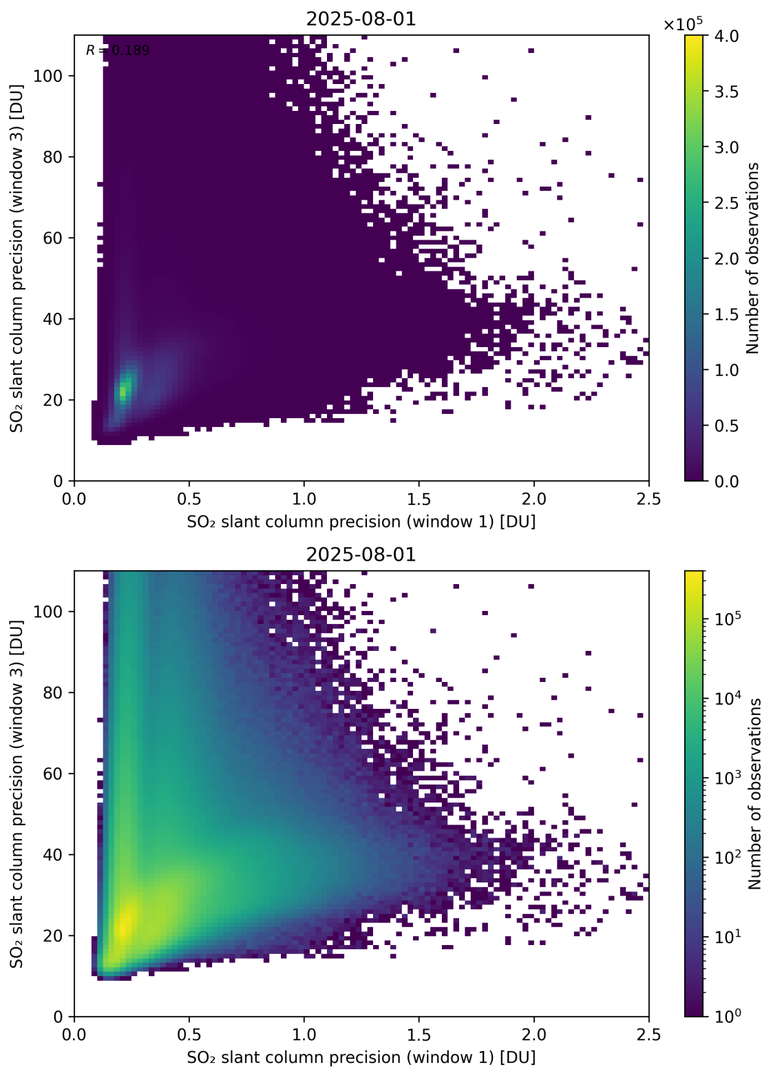
Figure 279: Scatter density plot of “SO 2 slant column precision (window 1)” against “SO 2 slant column precision (window 3)” for 2025-07-31 to 2025-08-02.
