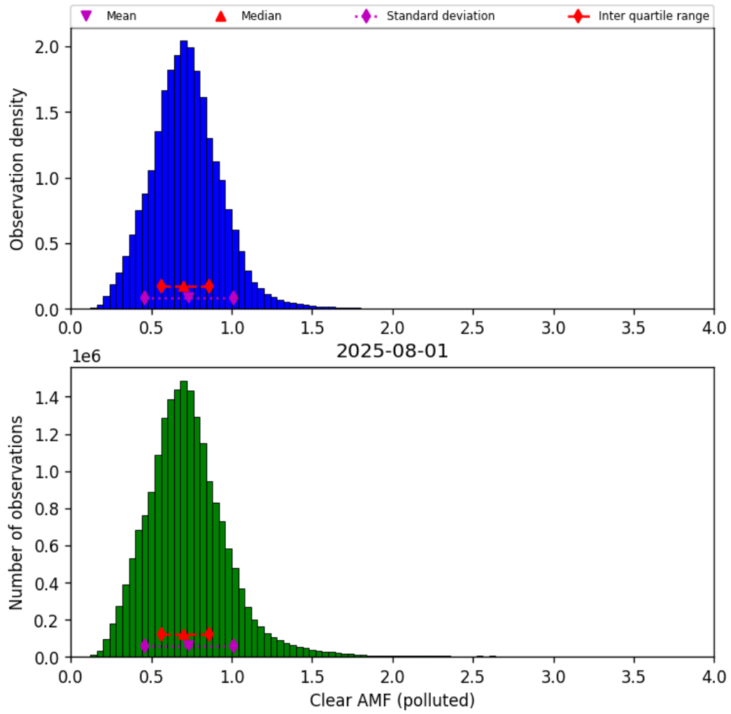
Figure 81: Histogram of “Clear AMF (polluted)” for 2025-07-31 to 2025-08-02
