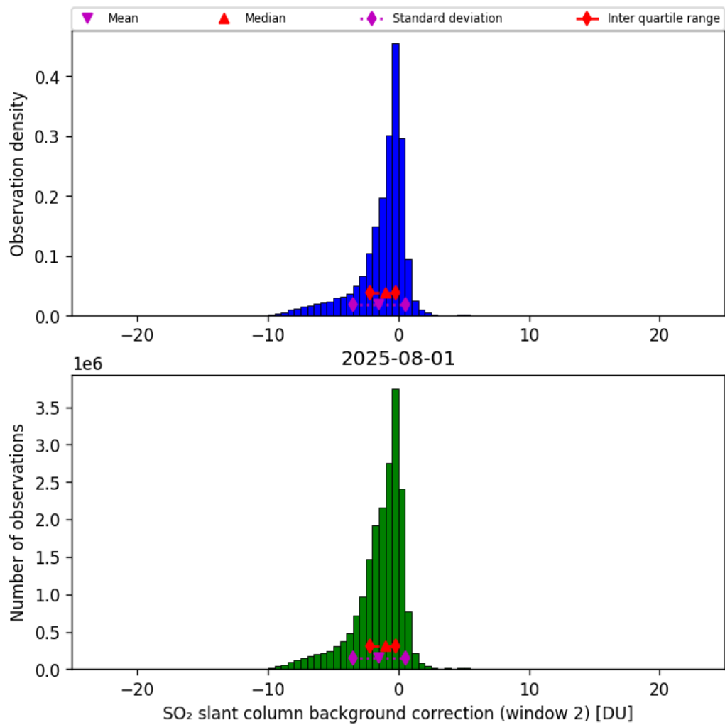
Figure 70: Histogram of “SO 2 slant column background correction (window 2)” for 2025-07-31 to 2025-08-02
