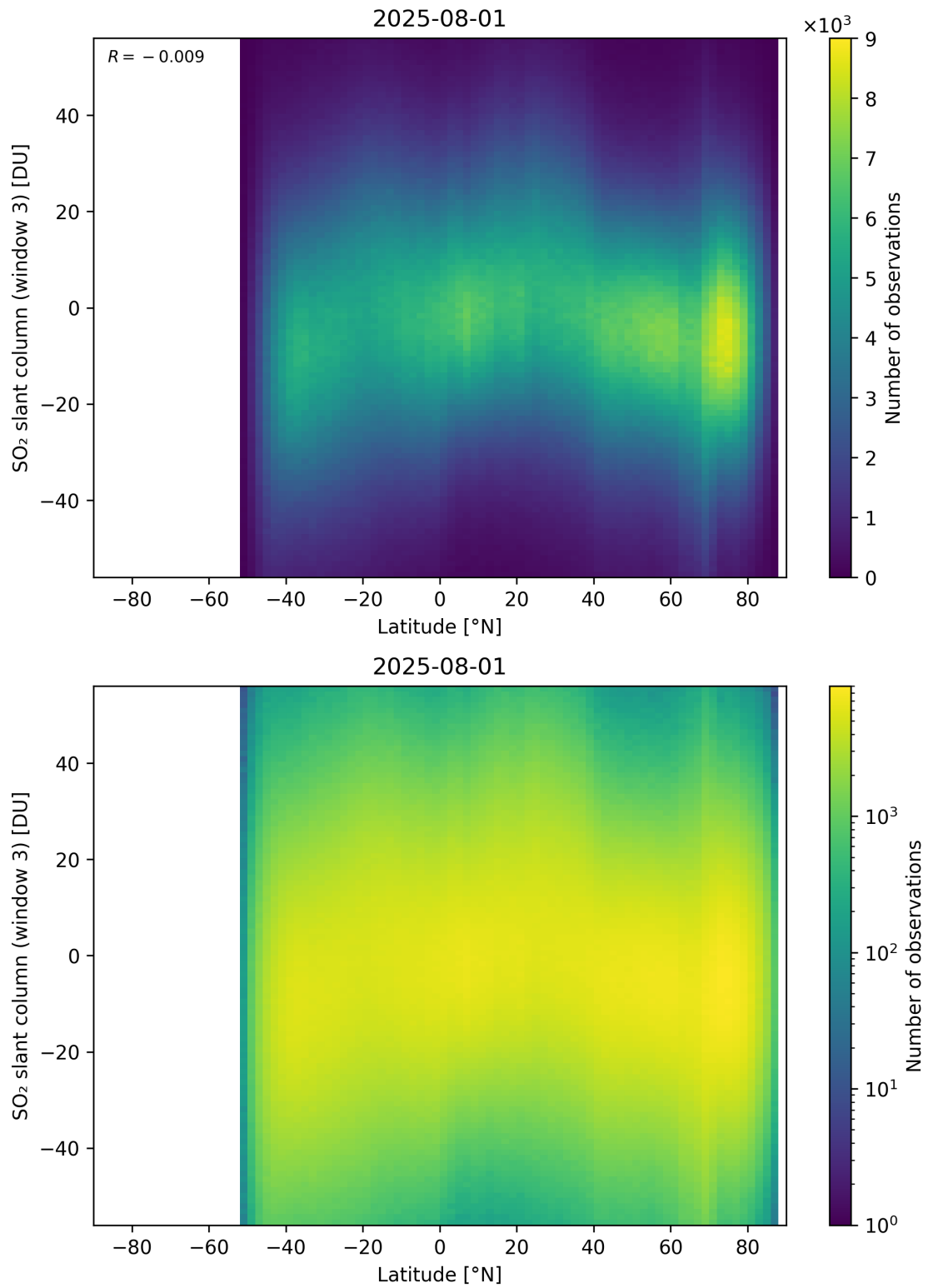
Figure 165: Scatter density plot of “Latitude” against “SO 2 slant column (window 3)” for 2025-07-31 to 2025-08-02.
