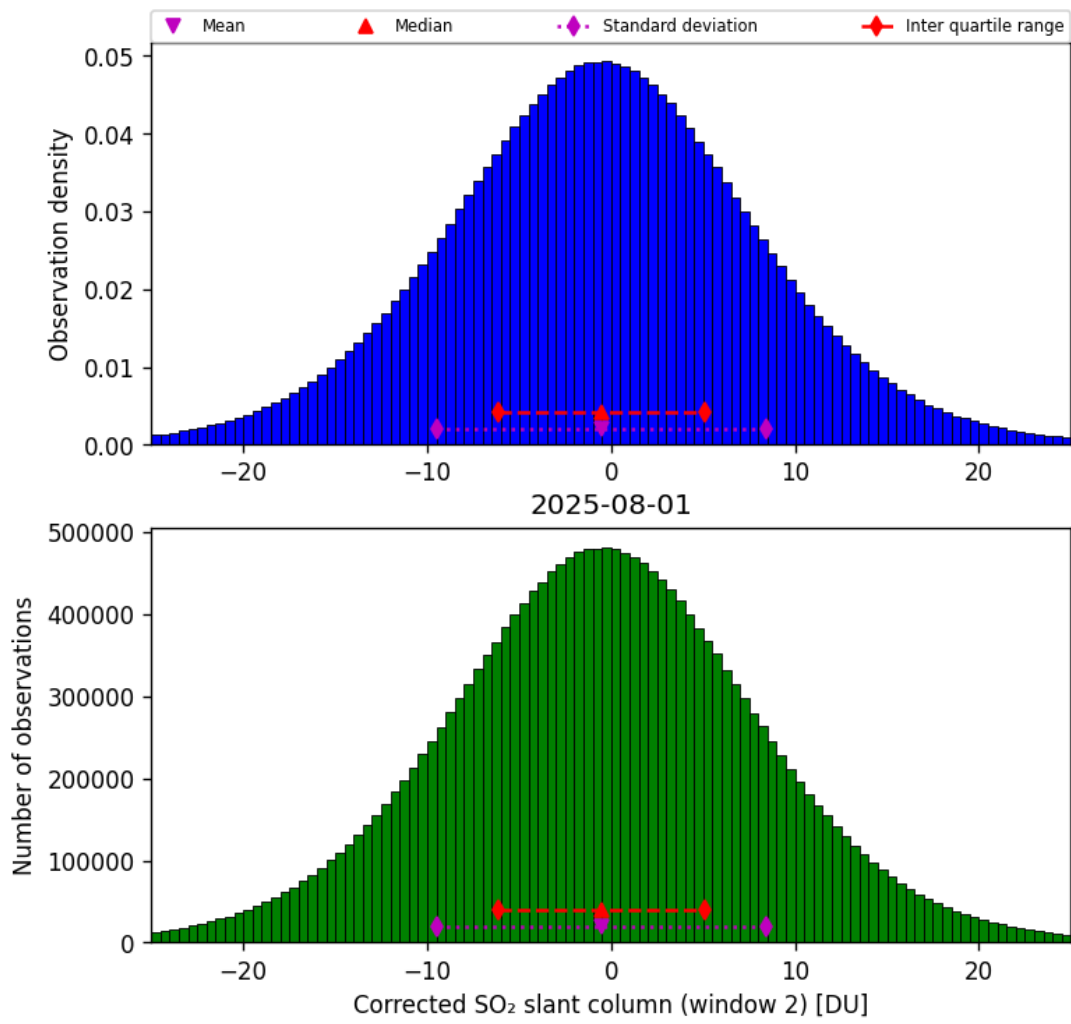
Figure 69: Histogram of “Corrected SO 2 slant column (window 2)” for 2025-07-31 to 2025-08-02
