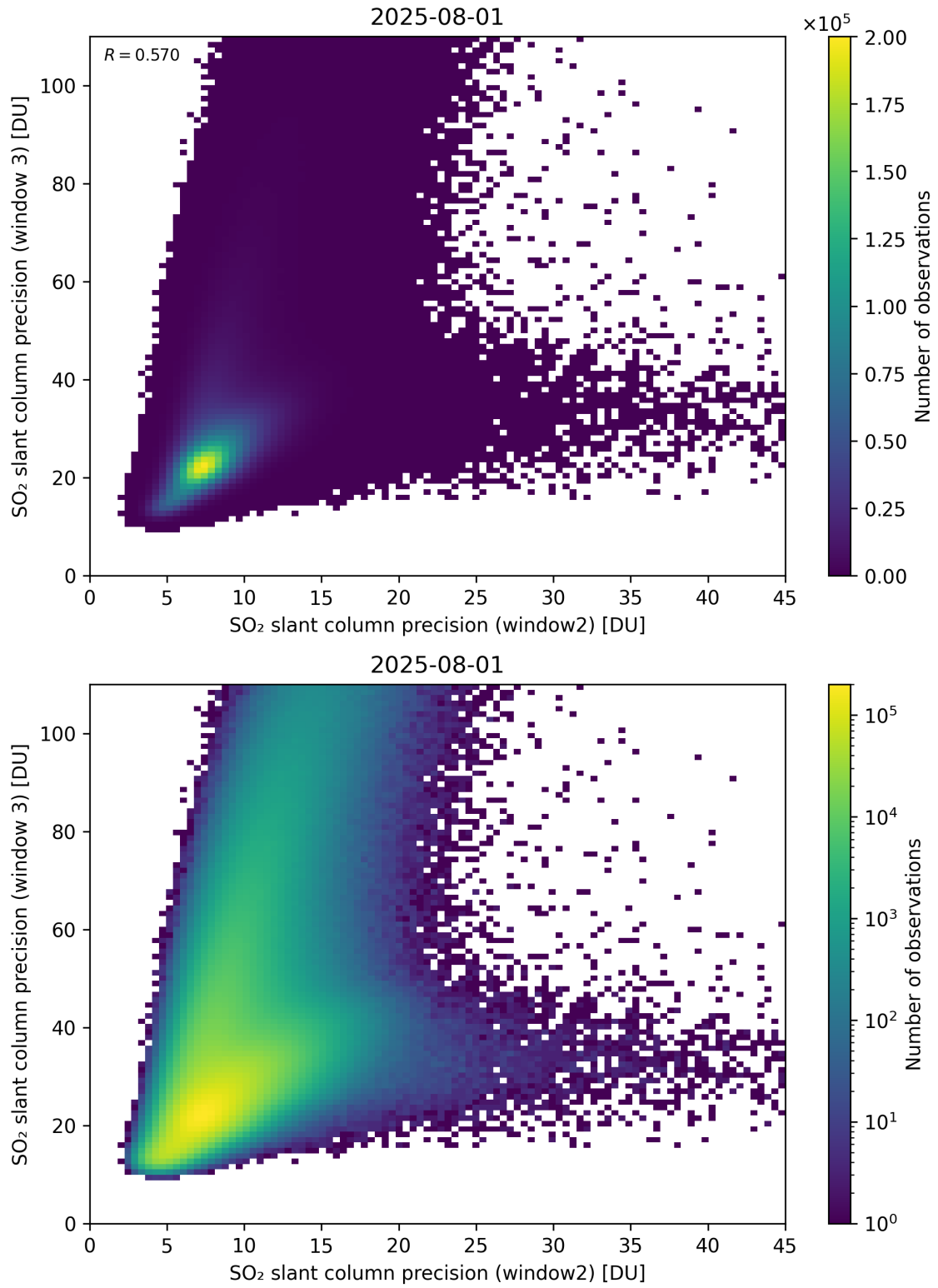
Figure 300: Scatter density plot of “SO 2 slant column precision (window2)” against “SO 2 slant column precision (window 3)” for 2025-07-31 to 2025-08-02.
