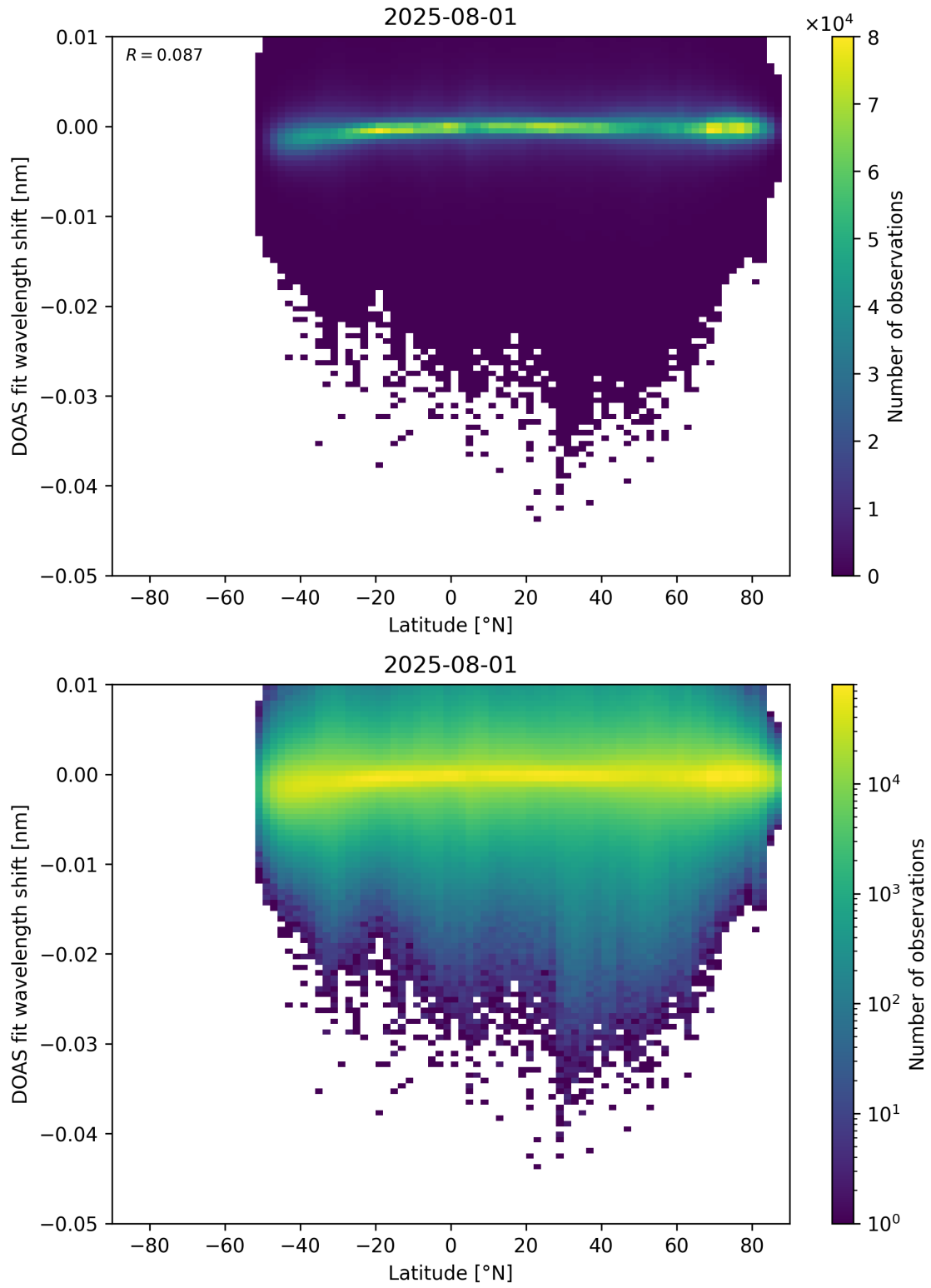
Figure 153: Scatter density plot of “Latitude” against “DOAS fit wavelength shift” for 2025-07-31 to 2025-08-02.
