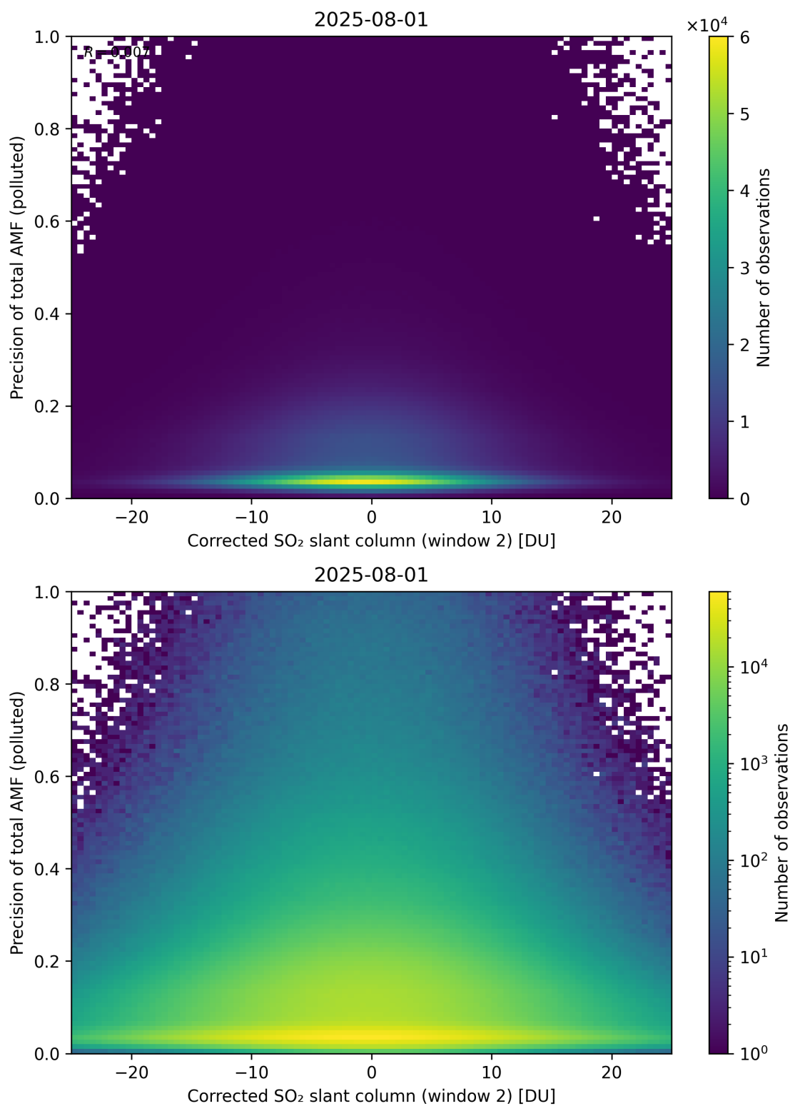
Figure 254: Scatter density plot of “Corrected SO 2 slant column (window 2)” against “Precision of total AMF (polluted)” for 2025-07-31 to 2025-08-02.
