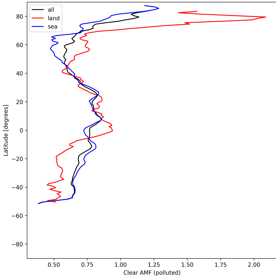
Figure 55: Zonal average of “Clear AMF (polluted)” for 2025-07-31 to 2025-08-02.
