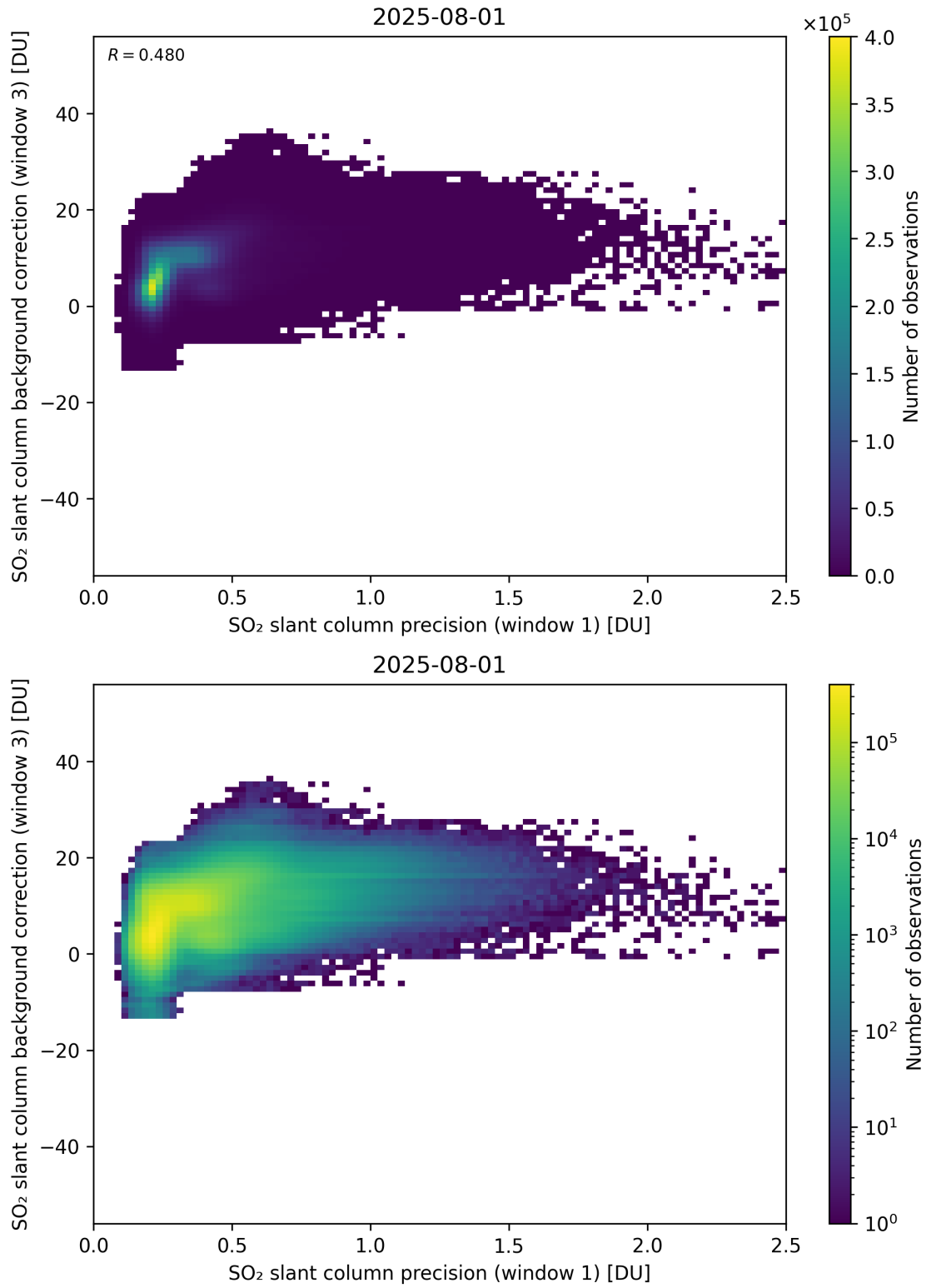
Figure 270: Scatter density plot of “SO 2 slant column precision (window 1)” against “SO 2 slant column background correction (window 3)” for 2025-07-31 to 2025-08-02.
