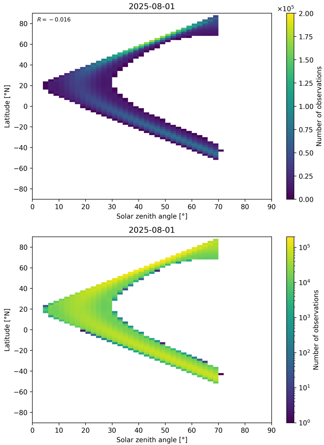
Figure 177: Scatter density plot of “Solar zenith angle” against “Latitude” for 2025-07-31 to 2025-08-02.
