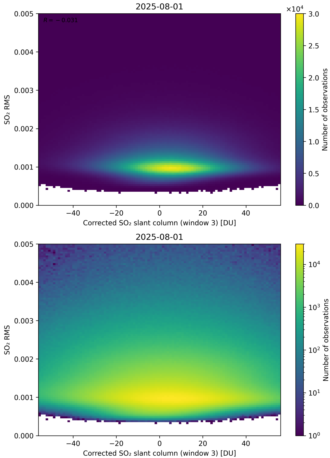
Figure 258: Scatter density plot of “Corrected SO 2 slant column (window 3)” against “SO 2 RMS” for 2025-07-31 to 2025-08-02.
