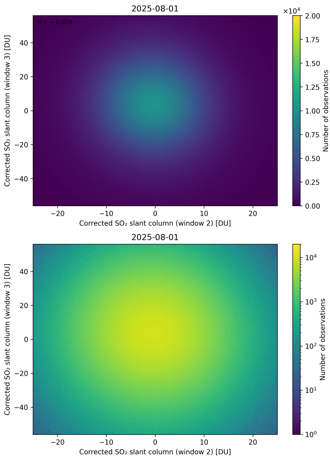
Figure 250: Scatter density plot of “Corrected SO 2 slant column (window 2)” against “Corrected SO 2 slant column (window 3)” for 2025-07-31 to 2025-08-02.
