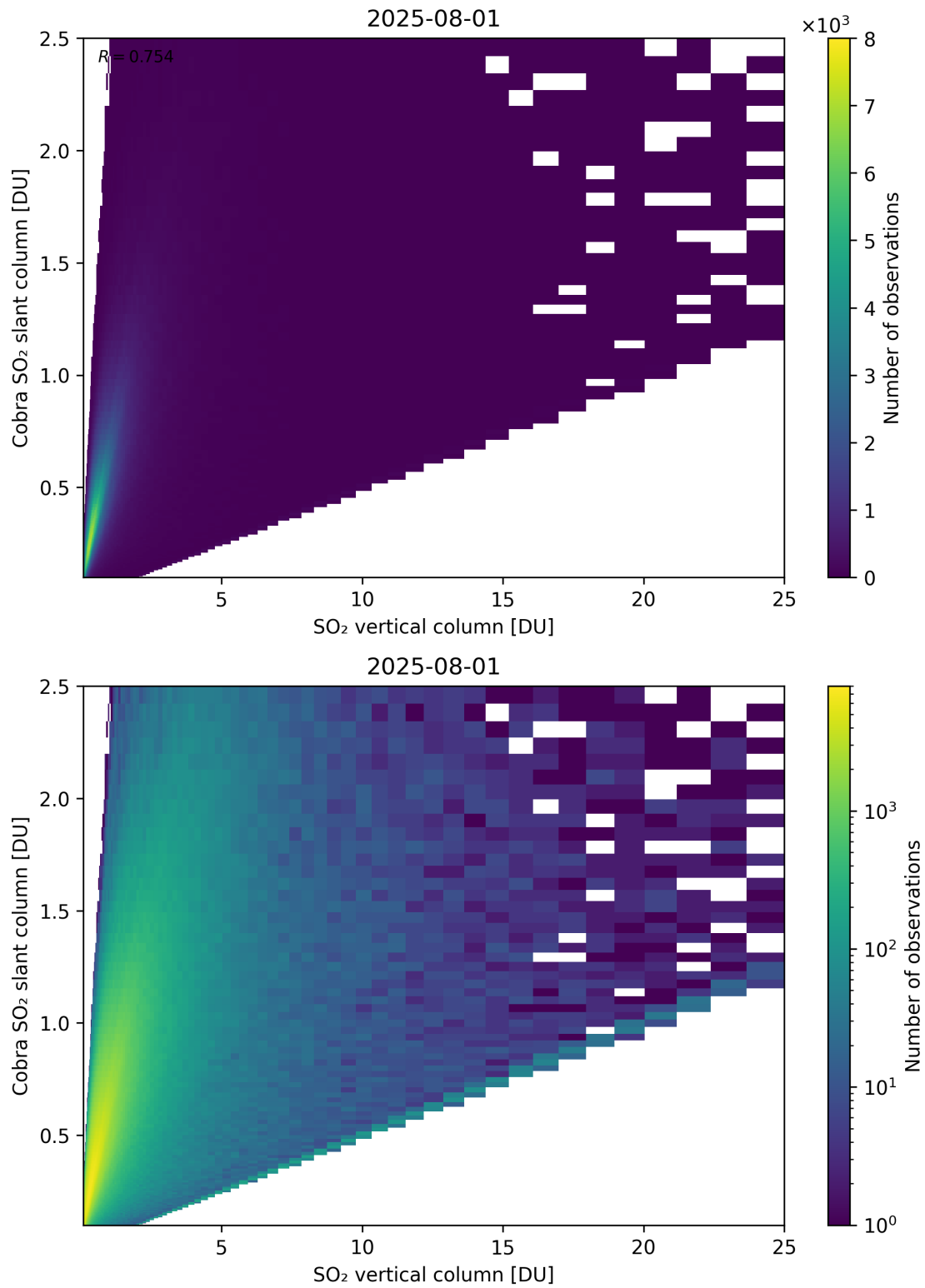
Figure 349: Scatter density plot of “SO 2 vertical column” against “Cobra SO 2 slant column” for 2025-07-31 to 2025-08-02.
