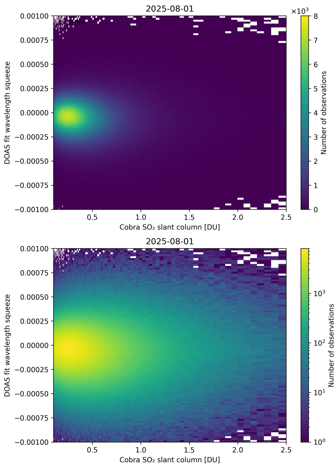
Figure 197: Scatter density plot of “Cobra SO 2 slant column” against “DOAS fit wavelength squeeze” for 2025-07-31 to 2025-08-02.
