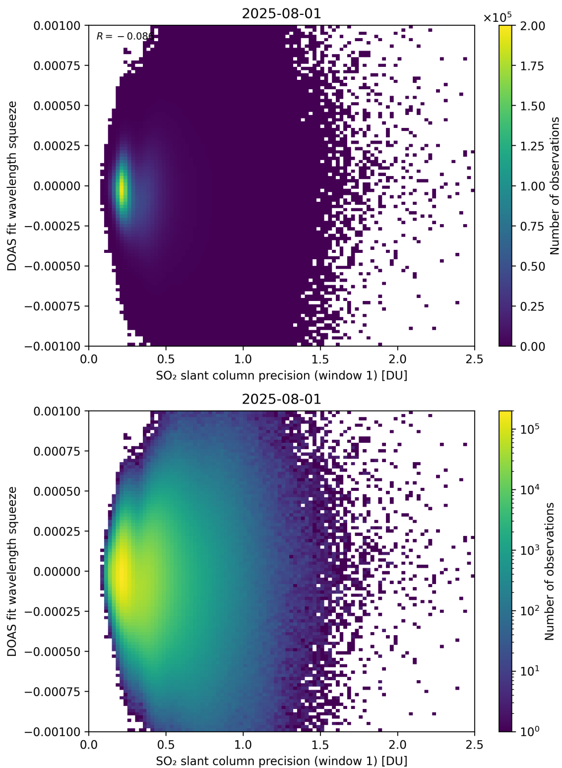
Figure 272: Scatter density plot of “SO 2 slant column precision (window 1)” against “DOAS fit wavelength squeeze” for 2025-07-31 to 2025-08-02.
