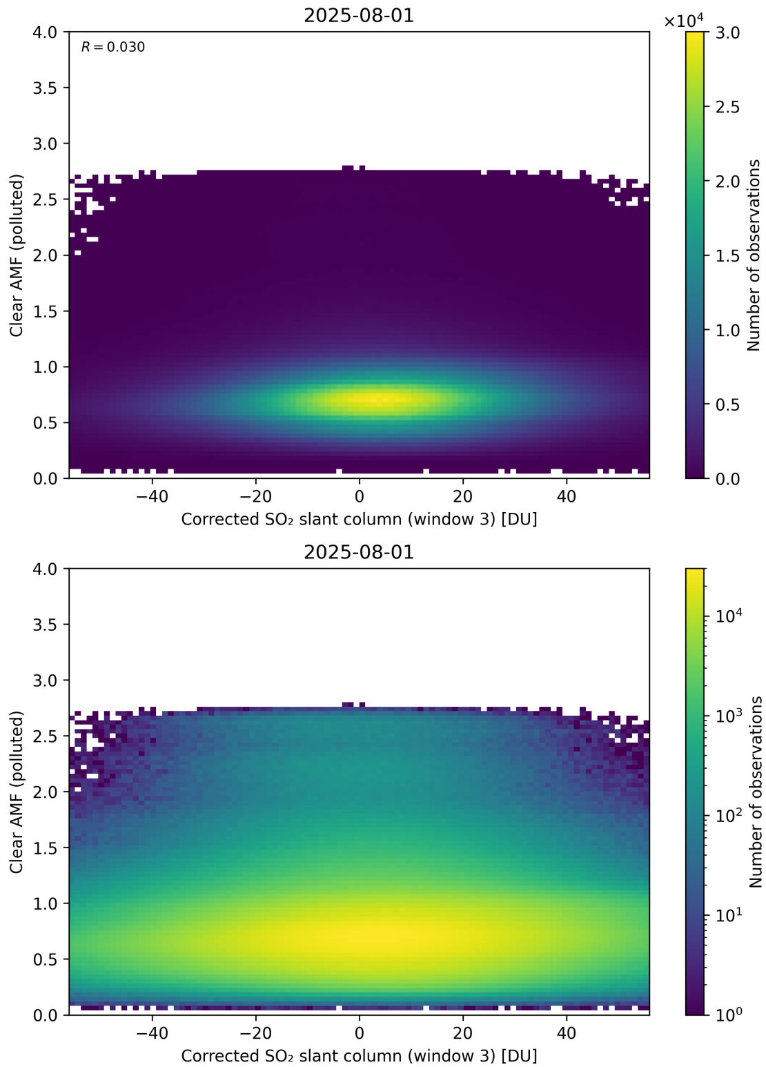
Figure 259: Scatter density plot of “Corrected SO 2 slant column (window 3)” against “Clear AMF (polluted)” for 2025-07-31 to 2025-08-02.
