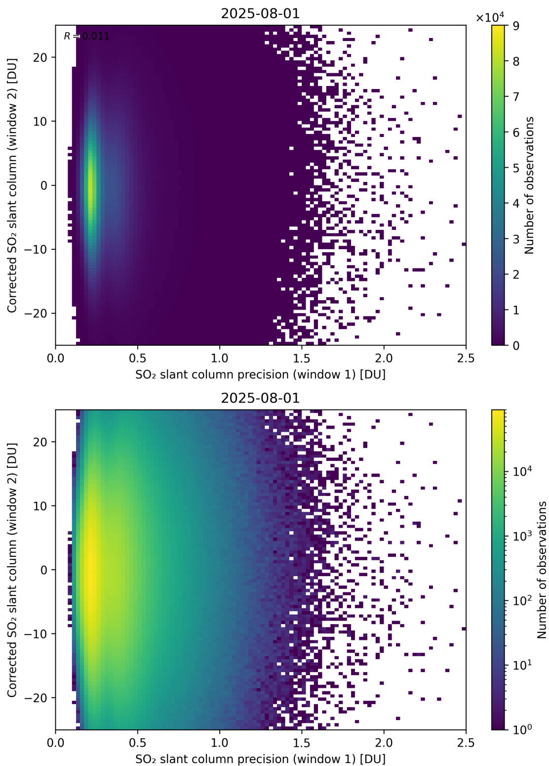
Figure 275: Scatter density plot of “SO 2 slant column precision (window 1)” against “Corrected SO 2 slant column (window 2)” for 2025-07-31 to 2025-08-02.
