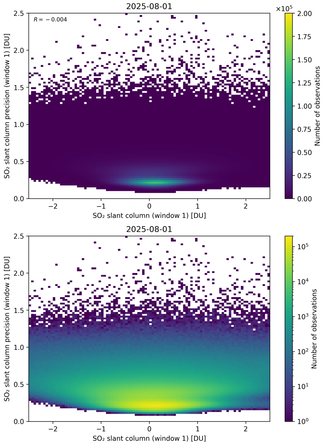
Figure 285: Scatter density plot of “SO 2 slant column (window 1)” against “SO 2 slant column precision (window 1)” for 2025-07-31 to 2025-08-02.
