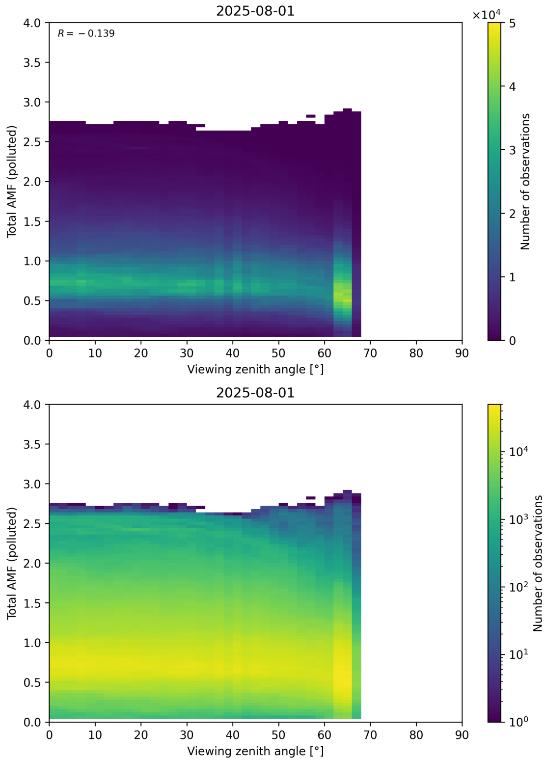
Figure 381: Scatter density plot of “Viewing zenith angle” against “Total AMF (polluted)” for 2025-07-31 to 2025-08-02.
