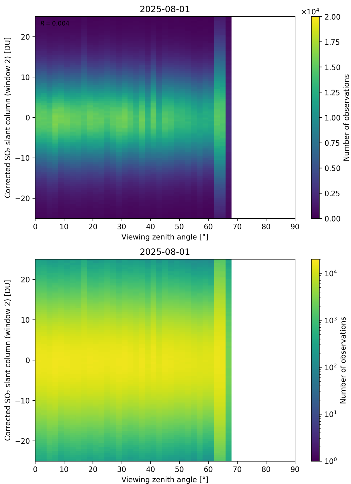
Figure 374: Scatter density plot of “Viewing zenith angle” against “Corrected SO 2 slant column (window 2)” for 2025-07-31 to 2025-08-02.
