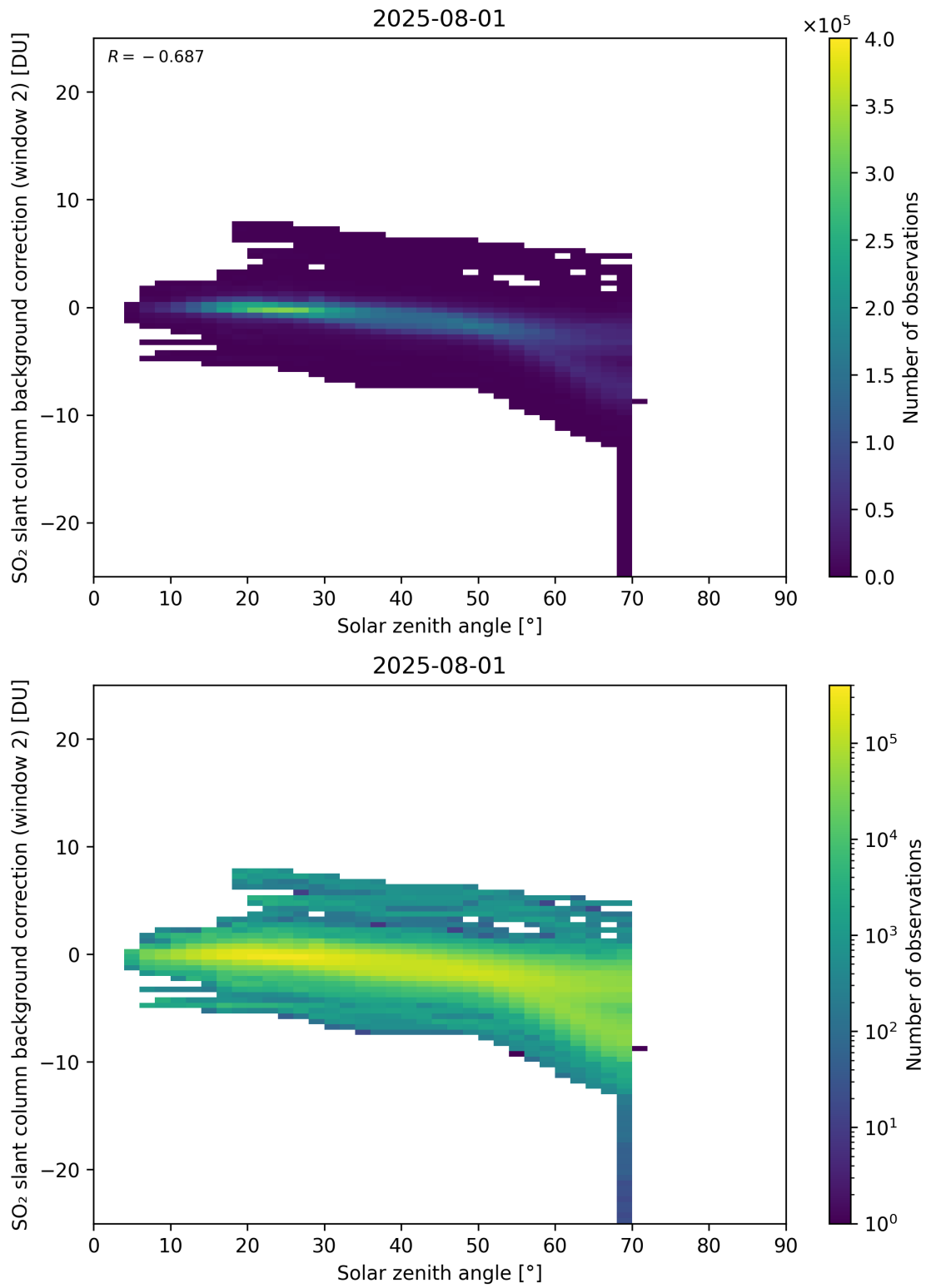
Figure 172: Scatter density plot of “Solar zenith angle” against “SO 2 slant column background correction (window 2)” for 2025-07-31 to 2025-08-02.
