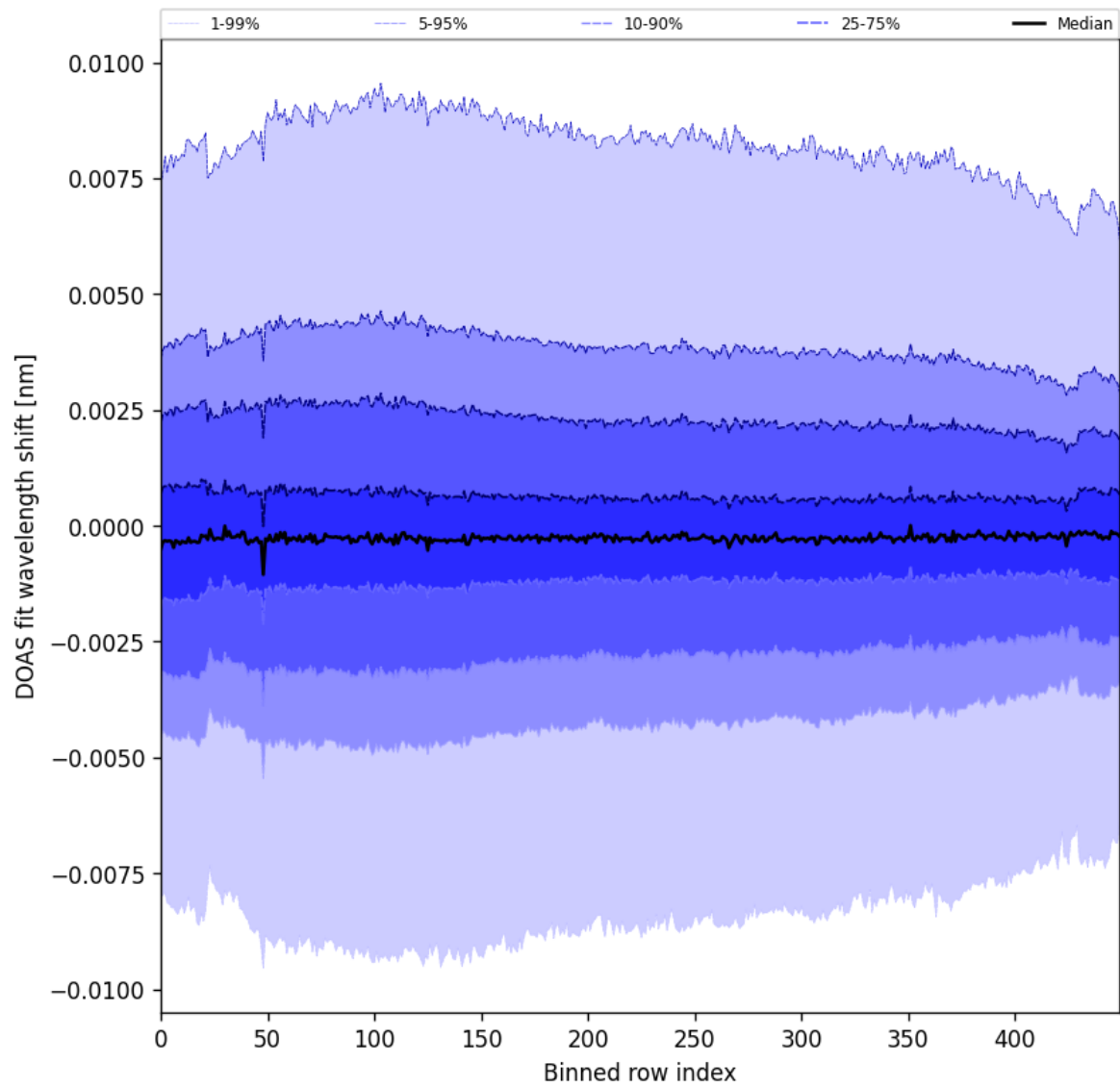
Figure 102: Along track statistics of “DOAS fit wavelength shift” for 2025-07-31 to 2025-08-02
