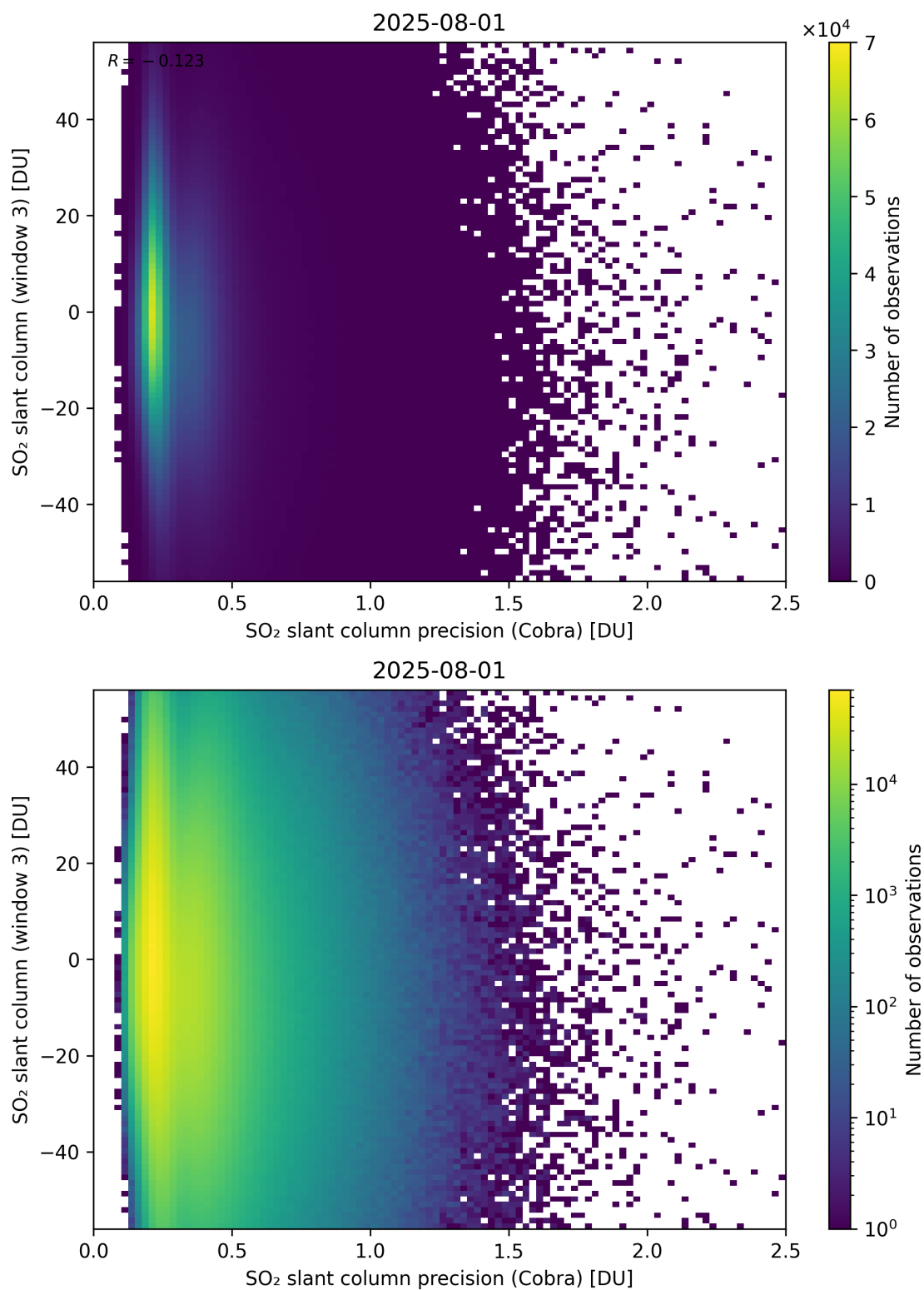
Figure 211: Scatter density plot of “SO 2 slant column precision (Cobra)” against “SO 2 slant column (window 3)” for 2025-07-31 to 2025-08-02.
