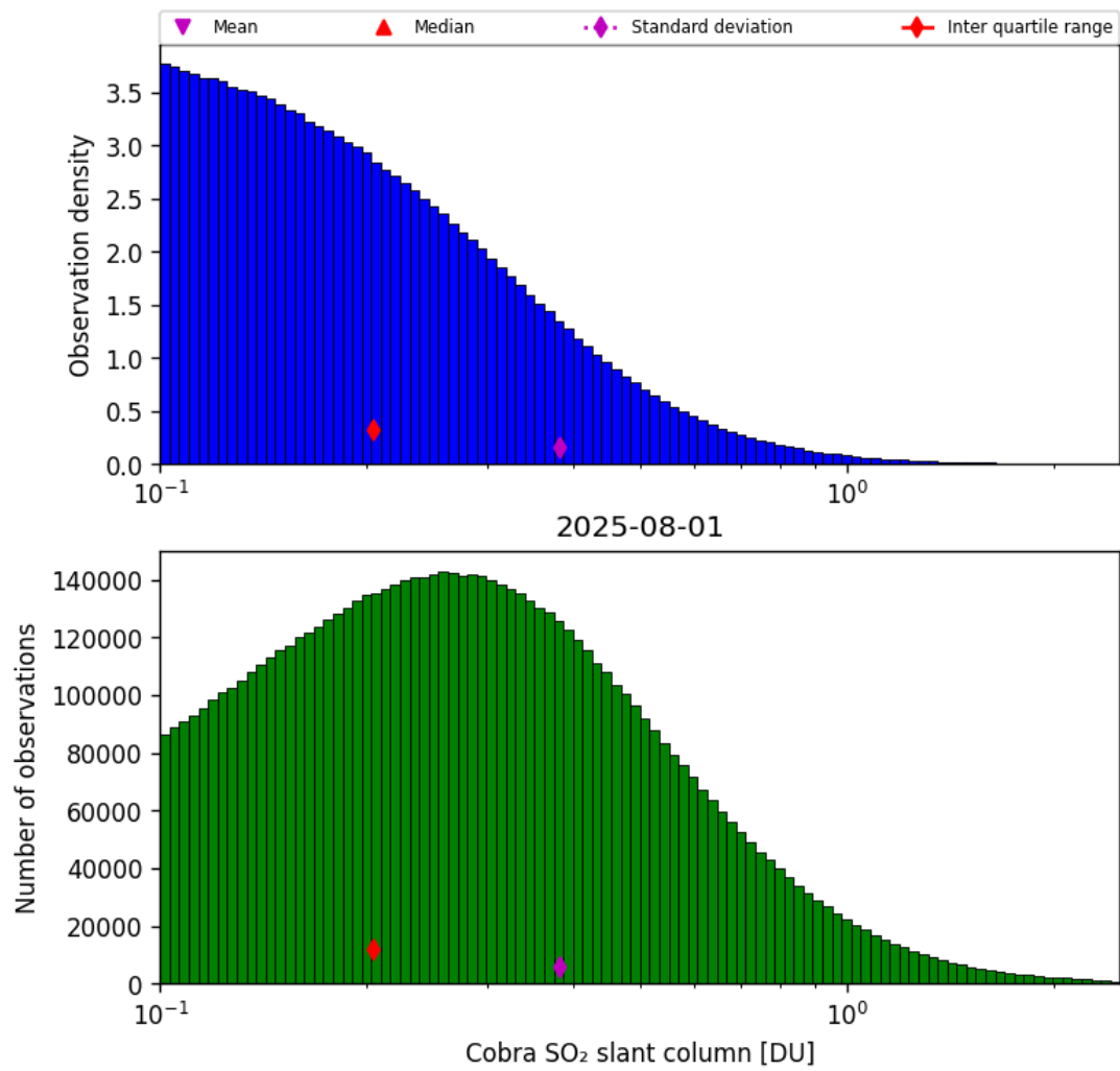
Figure 61: Histogram of “Cobra SO 2 slant column” for 2025-07-31 to 2025-08-02
