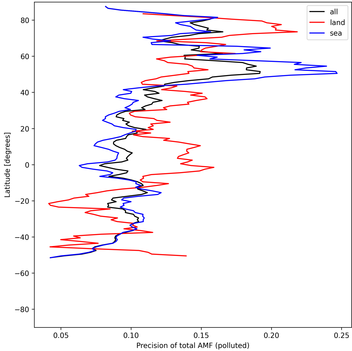
Figure 54: Zonal average of “Precision of total AMF (polluted)” for 2025-07-31 to 2025-08-02.
