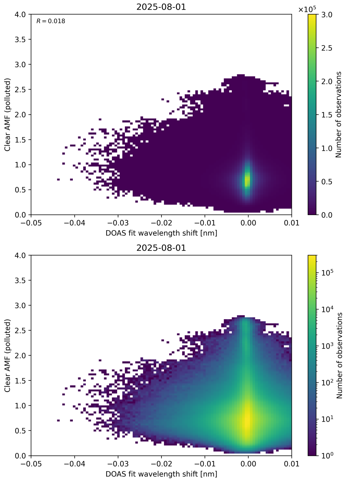
Figure 140: Scatter density plot of “DOAS fit wavelength shift” against “Clear AMF (polluted)” for 2025-07-31 to 2025-08-02.
