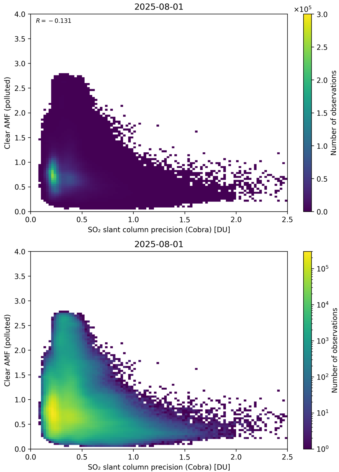
Figure 205: Scatter density plot of “SO 2 slant column precision (Cobra)” against “Clear AMF (polluted)” for 2025-07-31 to 2025-08-02.
