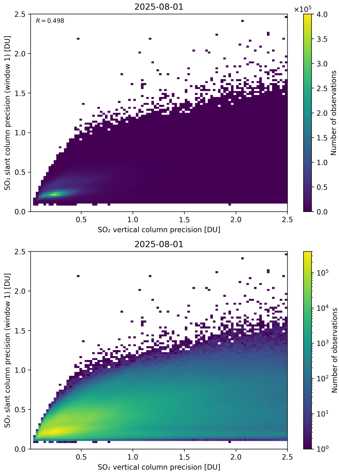
Figure 342: Scatter density plot of “SO 2 vertical column precision” against “SO 2 slant column precision (window 1)” for 2025-07-31 to 2025-08-02.
