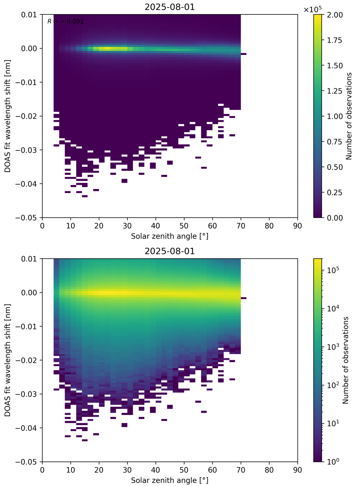
Figure 174: Scatter density plot of “Solar zenith angle” against “DOAS fit wavelength shift” for 2025-07-31 to 2025-08-02.
