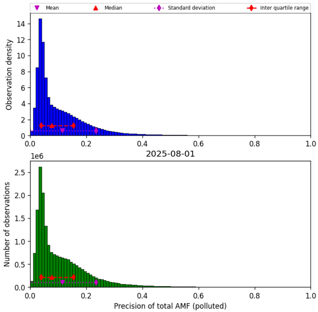
Figure 80: Histogram of “Precision of total AMF (polluted)” for 2025-07-31 to 2025-08-02
