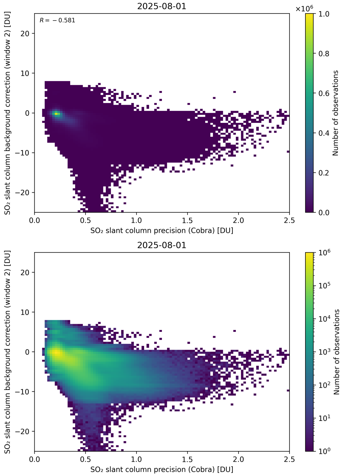
Figure 200: Scatter density plot of “SO 2 slant column precision (Cobra)” against “SO 2 slant column background correction (window 2)” for 2025-07-31 to 2025-08-02.
