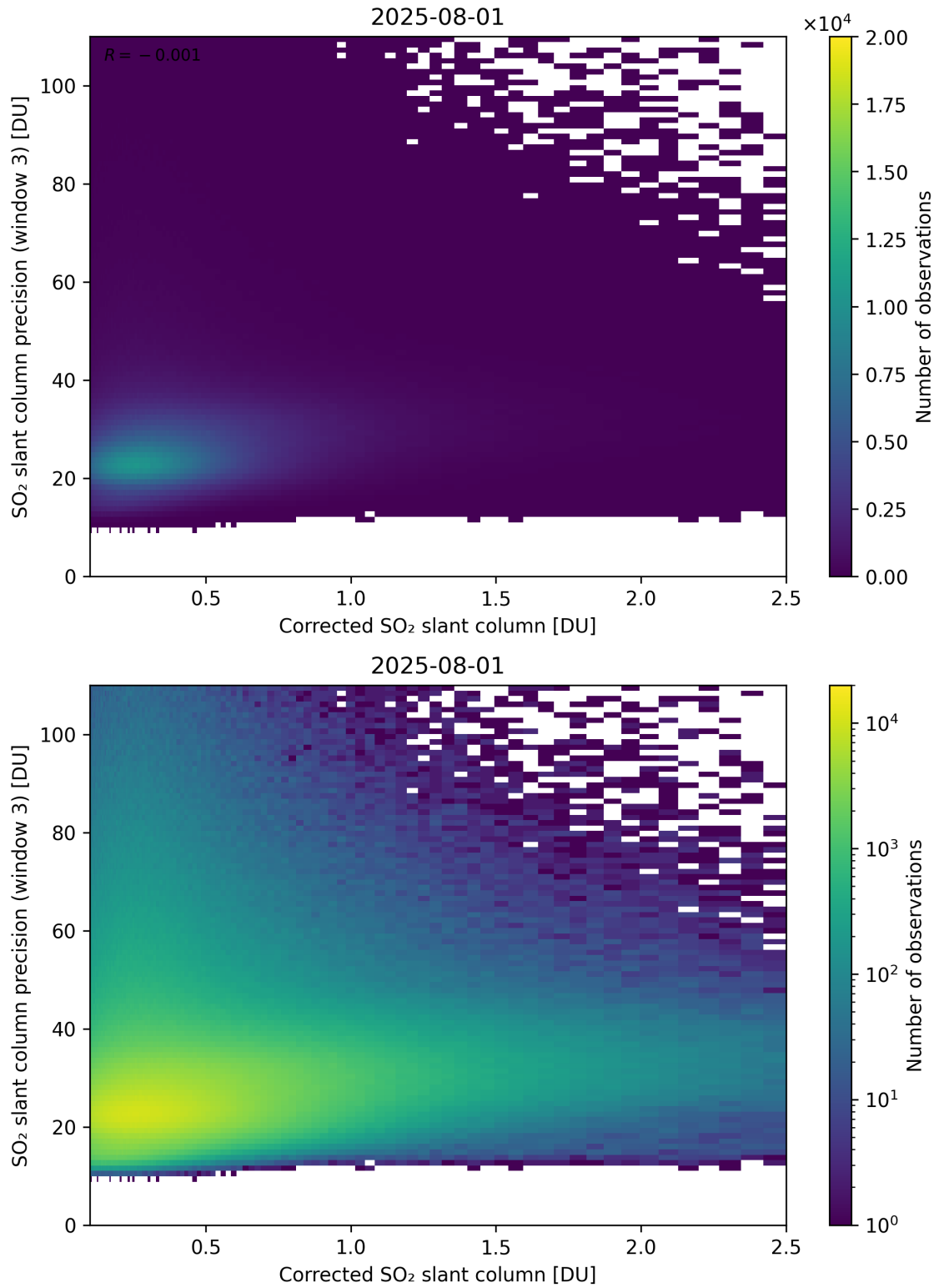
Figure 241: Scatter density plot of “Corrected SO 2 slant column” against “SO 2 slant column precision (window 3)” for 2025-07-31 to 2025-08-02.
