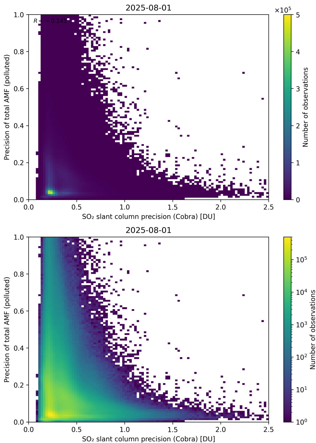
Figure 214: Scatter density plot of “SO 2 slant column precision (Cobra)” against “Precision of total AMF (polluted)” for 2025-07-31 to 2025-08-02.
