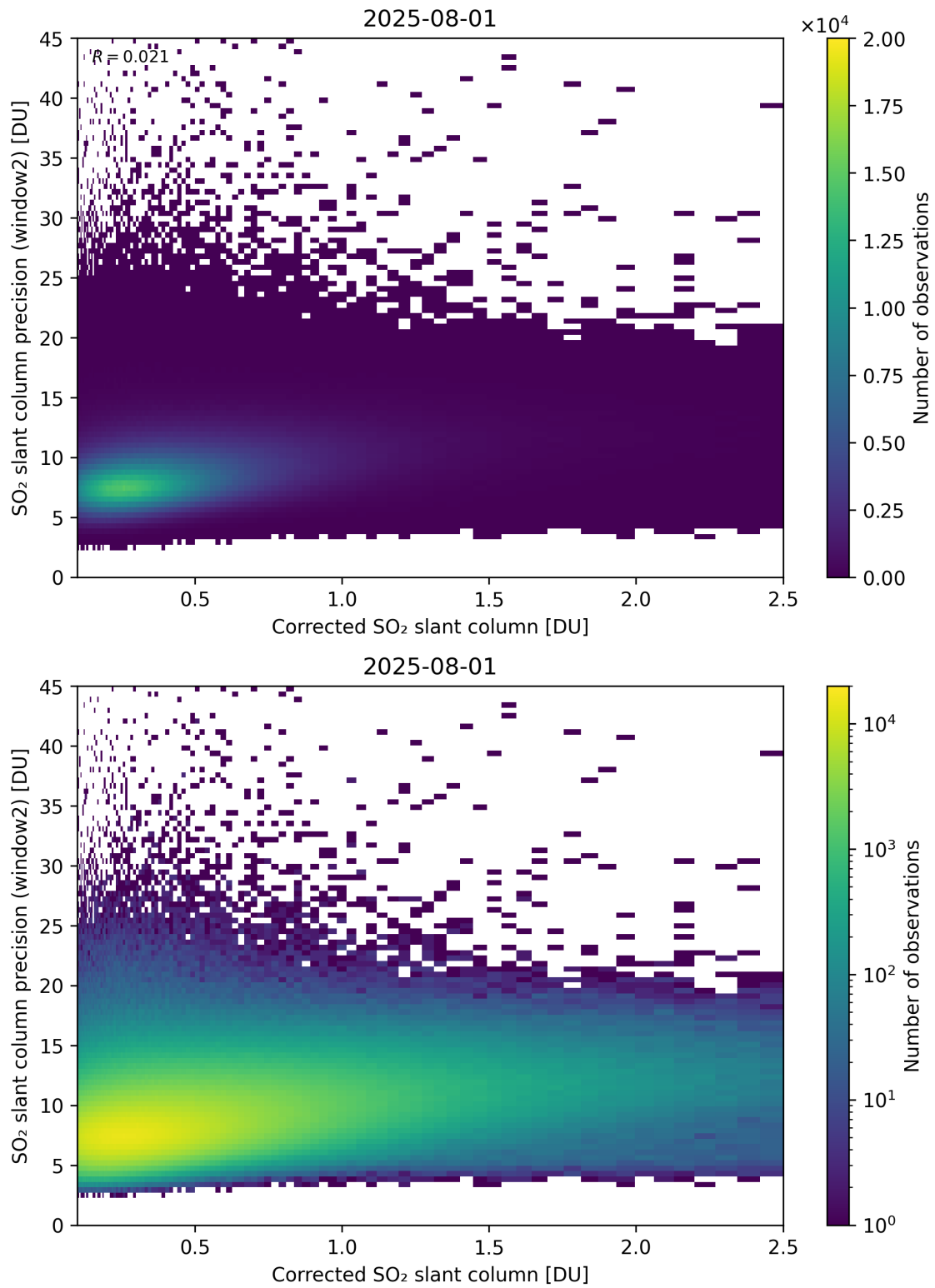
Figure 239: Scatter density plot of “Corrected SO 2 slant column” against “SO 2 slant column precision (window2)” for 2025-07-31 to 2025-08-02.
