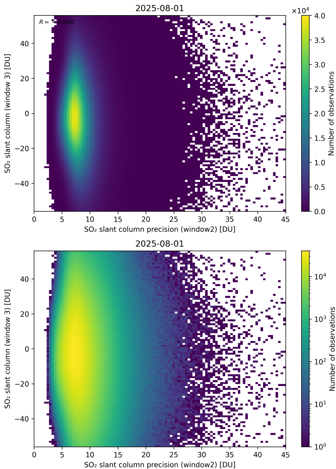
Figure 299: Scatter density plot of “SO 2 slant column precision (window2)” against “SO 2 slant column (window 3)” for 2025-07-31 to 2025-08-02.
