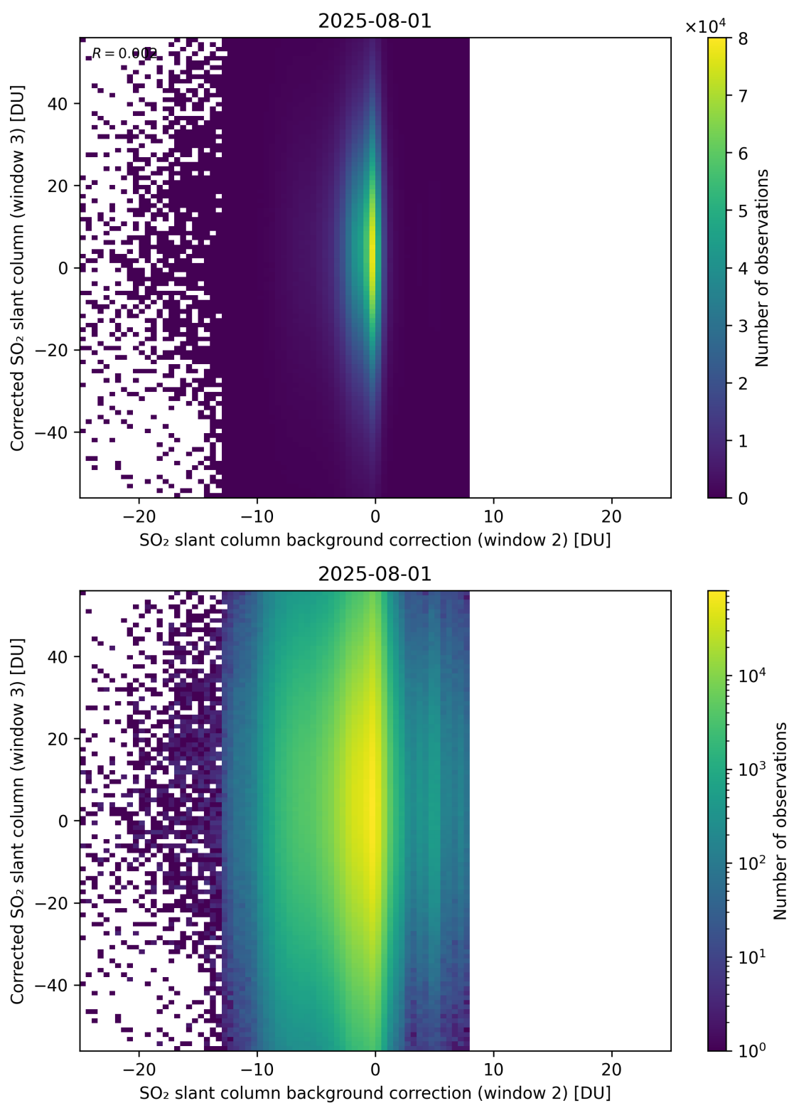
Figure 127: Scatter density plot of “SO 2 slant column background correction (window 2)” against “Corrected SO 2 slant column (window 3)” for 2025-07-31 to 2025-08-02.
