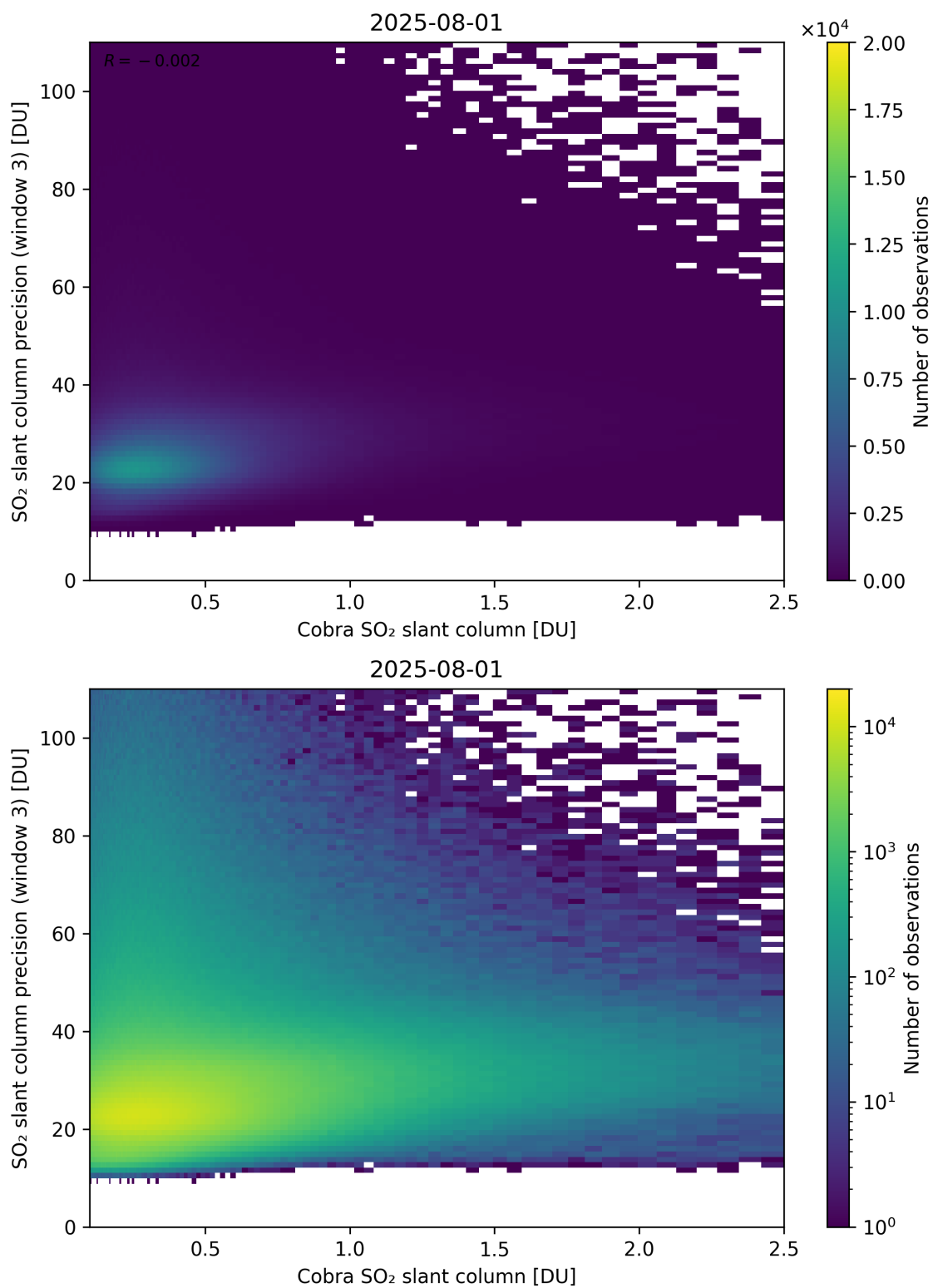
Figure 223: Scatter density plot of “Cobra SO 2 slant column” against “SO 2 slant column precision (window 3)” for 2025-07-31 to 2025-08-02.
