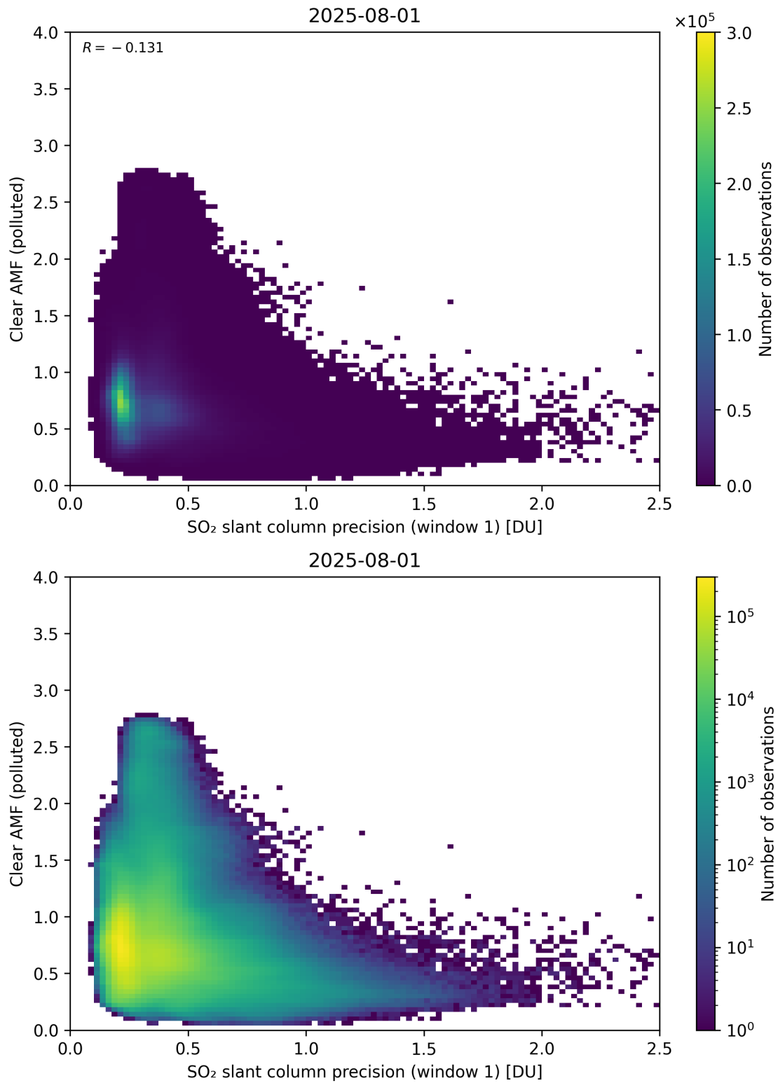
Figure 274: Scatter density plot of “SO 2 slant column precision (window 1)” against “Clear AMF (polluted)” for 2025-07-31 to 2025-08-02.
