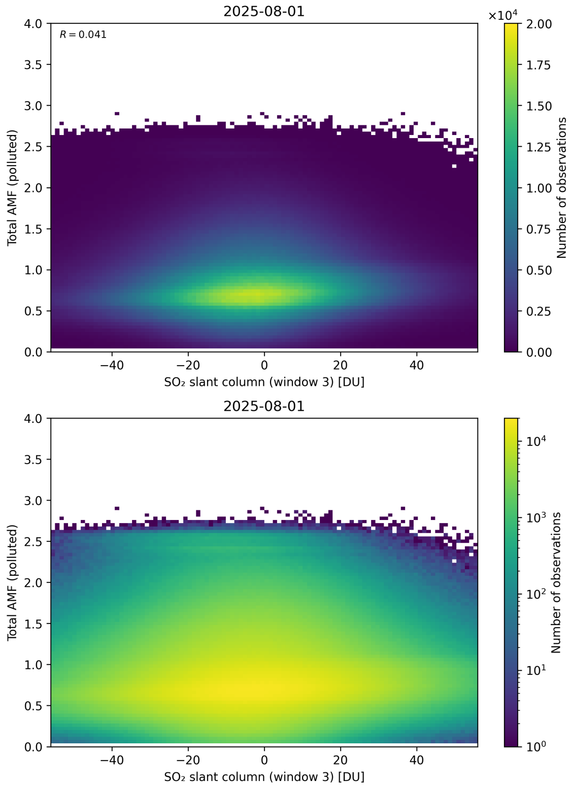
Figure 318: Scatter density plot of “SO 2 slant column (window 3)” against “Total AMF (polluted)” for 2025-07-31 to 2025-08-02.
