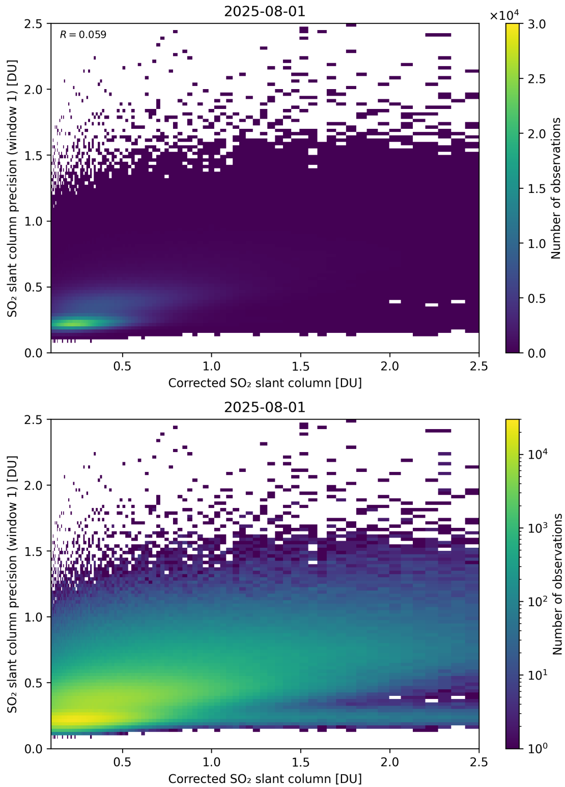
Figure 238: Scatter density plot of “Corrected SO 2 slant column” against “SO 2 slant column precision (window 1)” for 2025-07-31 to 2025-08-02.
