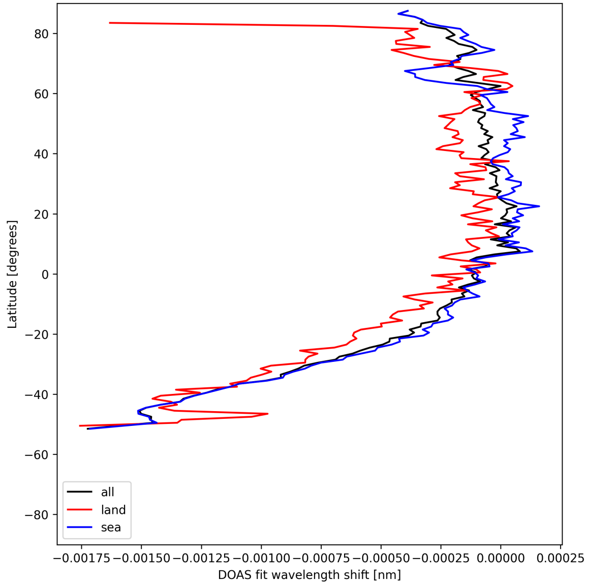
Figure 50: Zonal average of “DOAS fit wavelength shift” for 2025-07-31 to 2025-08-02.
