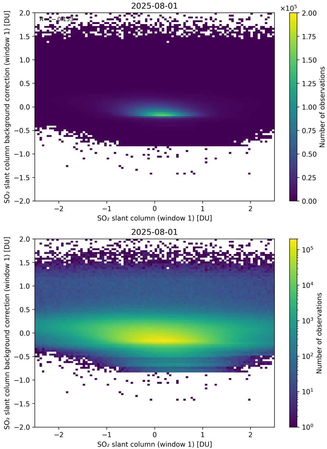
Figure 262: Scatter density plot of “SO 2 slant column (window 1)” against “SO 2 slant column background correction (window 1)” for 2025-07-31 to 2025-08-02.
