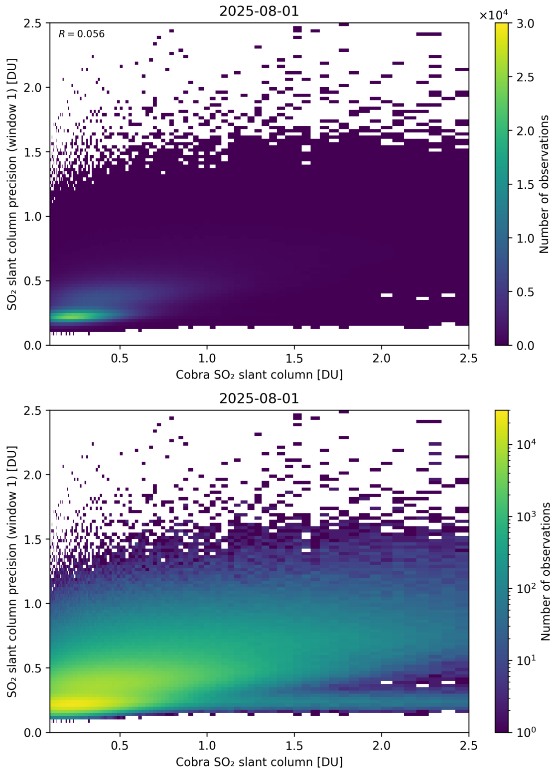
Figure 220: Scatter density plot of “Cobra SO 2 slant column” against “SO 2 slant column precision (window 1)” for 2025-07-31 to 2025-08-02.
