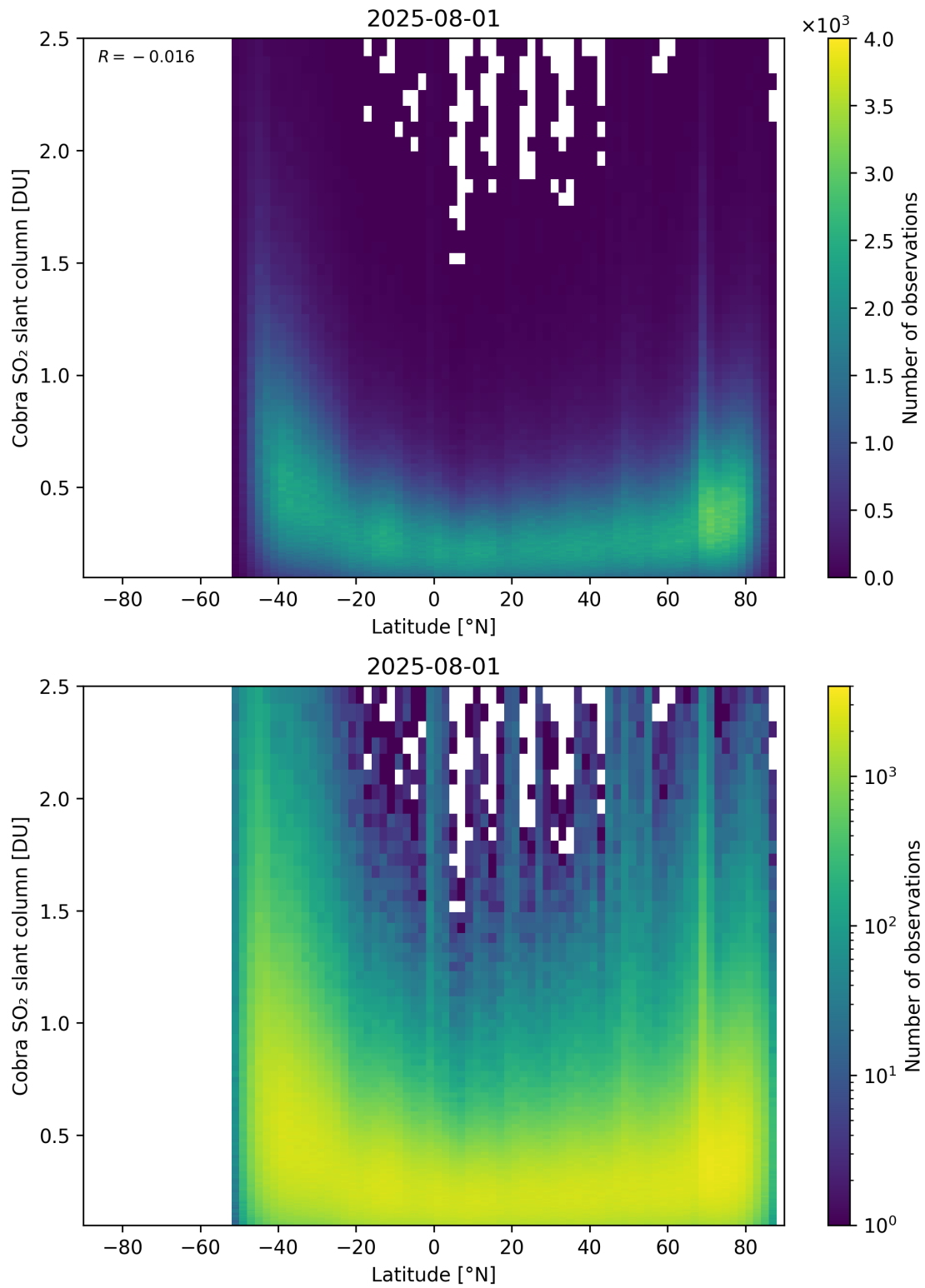
Figure 157: Scatter density plot of “Latitude” against “Cobra SO 2 slant column” for 2025-07-31 to 2025-08-02.
