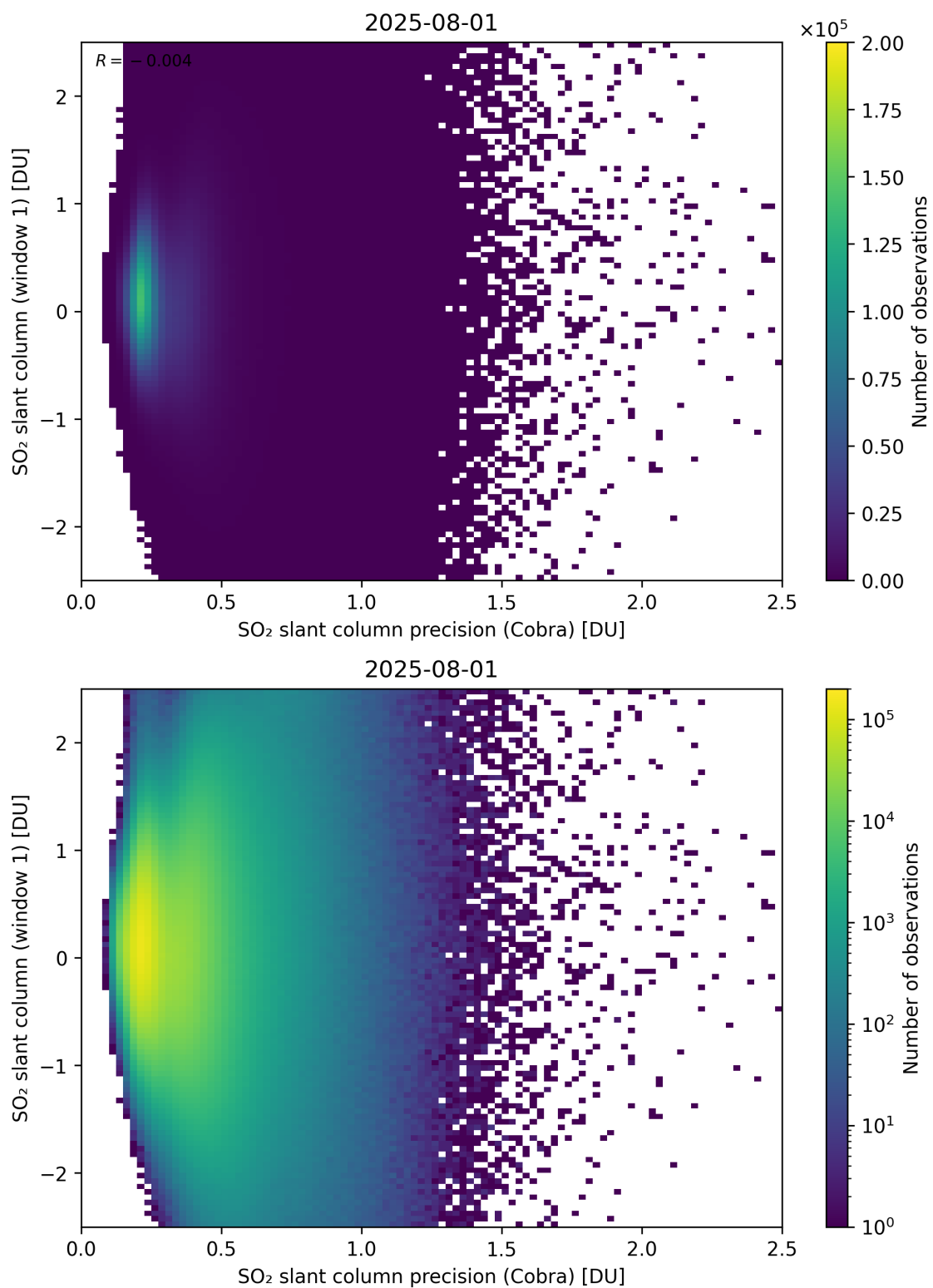
Figure 208: Scatter density plot of “SO 2 slant column precision (Cobra)” against “SO 2 slant column (window 1)” for 2025-07-31 to 2025-08-02.
