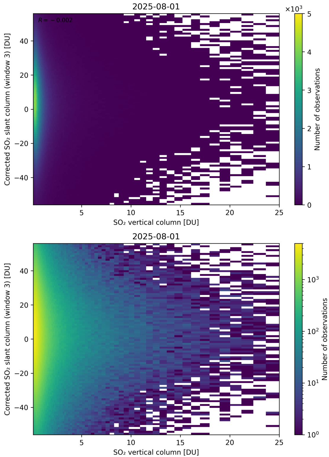
Figure 353: Scatter density plot of “SO 2 vertical column” against “Corrected SO 2 slant column (window 3)” for 2025-07-31 to 2025-08-02.
