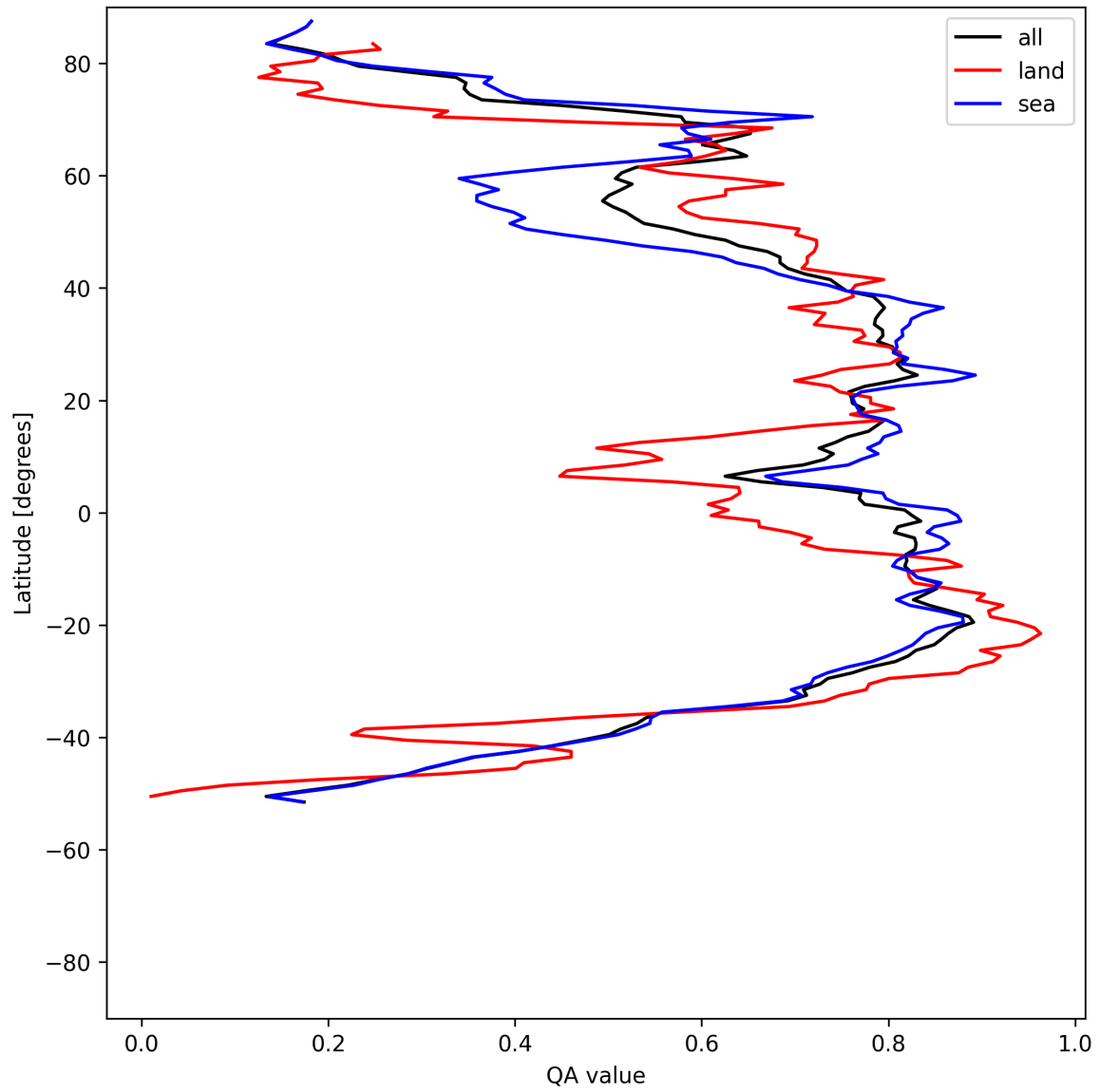
Figure 31: Zonal average of “QA value” for 2025-07-31 to 2025-08-02.
