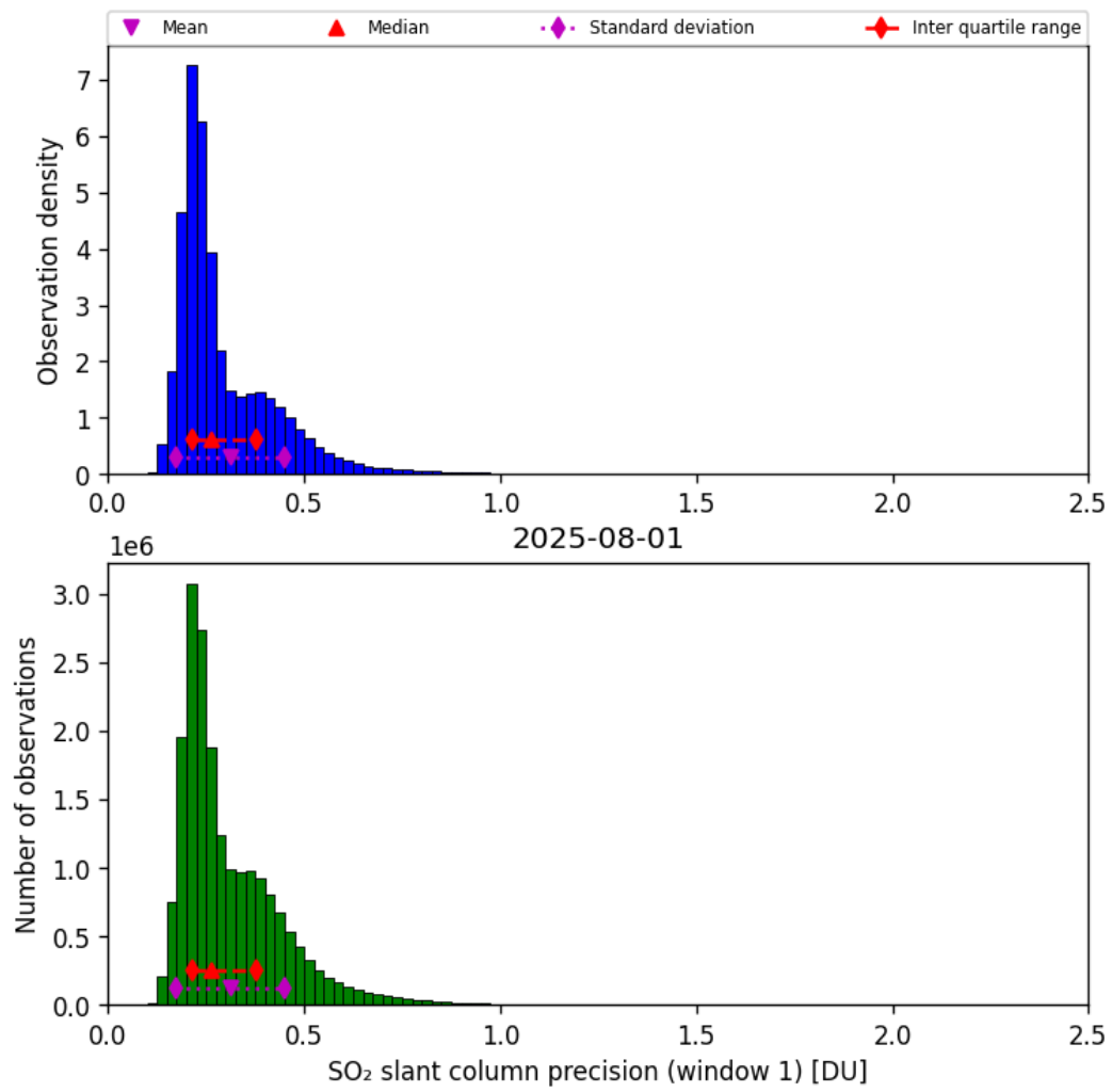
Figure 64: Histogram of “SO 2 slant column precision (window 1)” for 2025-07-31 to 2025-08-02
