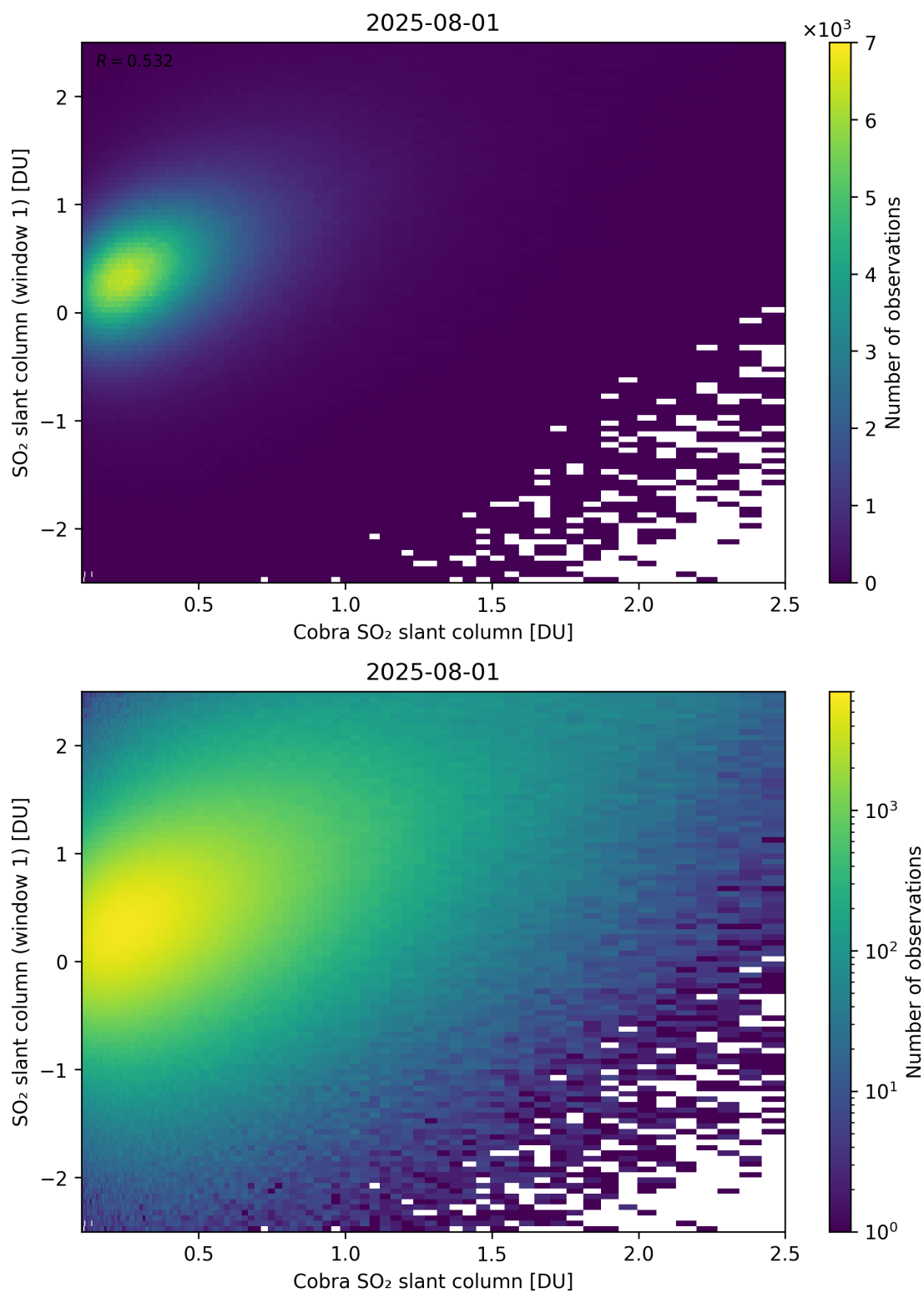
Figure 219: Scatter density plot of “Cobra SO 2 slant column” against “SO 2 slant column (window 1)” for 2025-07-31 to 2025-08-02.
