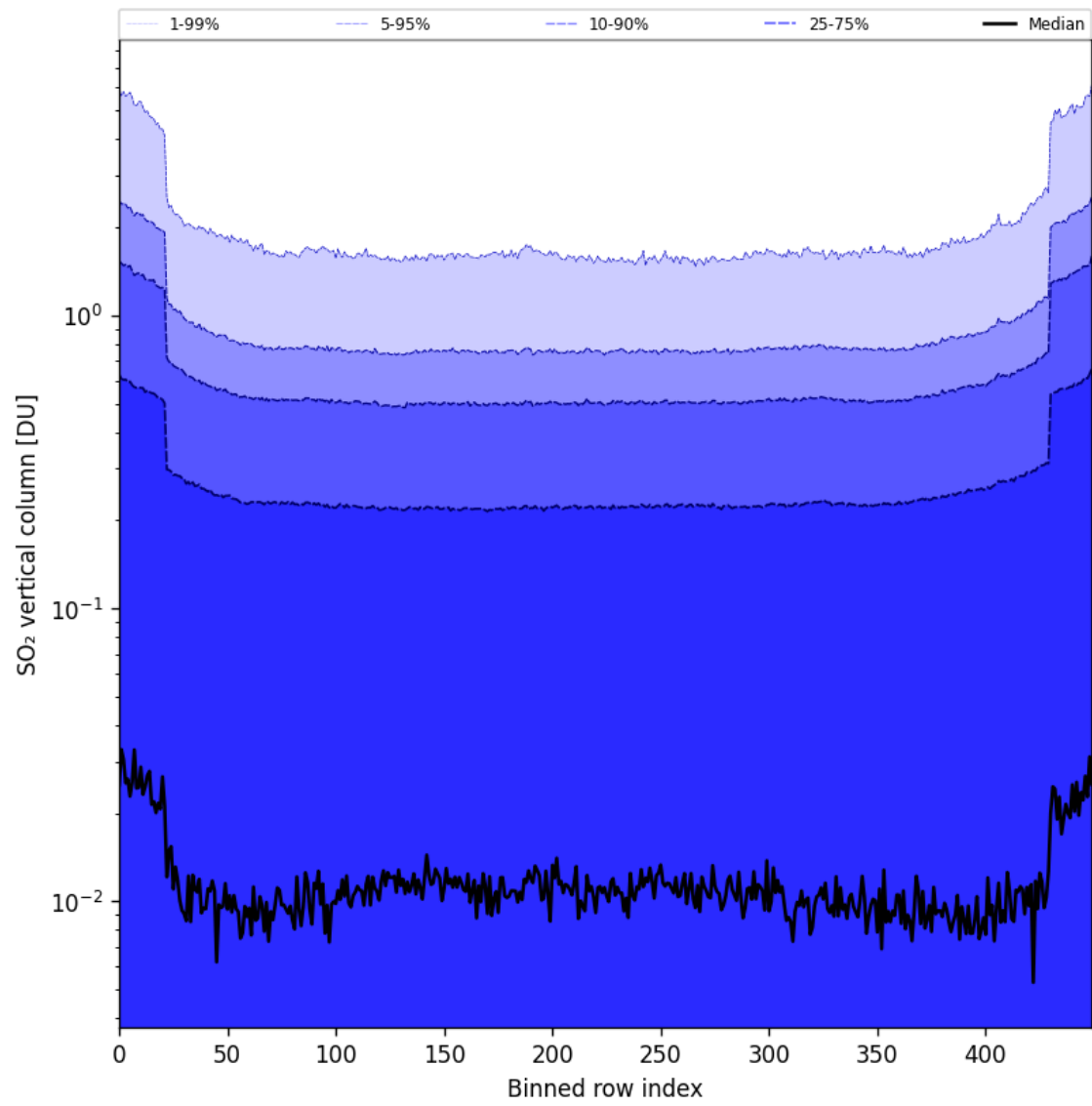
Figure 84: Along track statistics of “SO 2 vertical column” for 2025-07-31 to 2025-08-02
