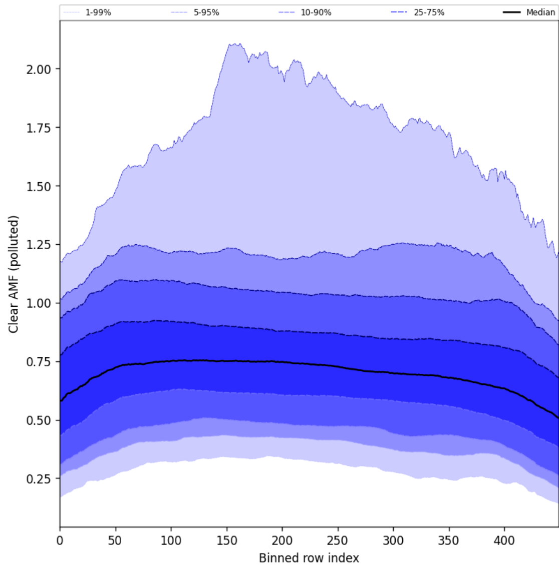
Figure 107: Along track statistics of “Clear AMF (polluted)” for 2025-07-31 to 2025-08-02
