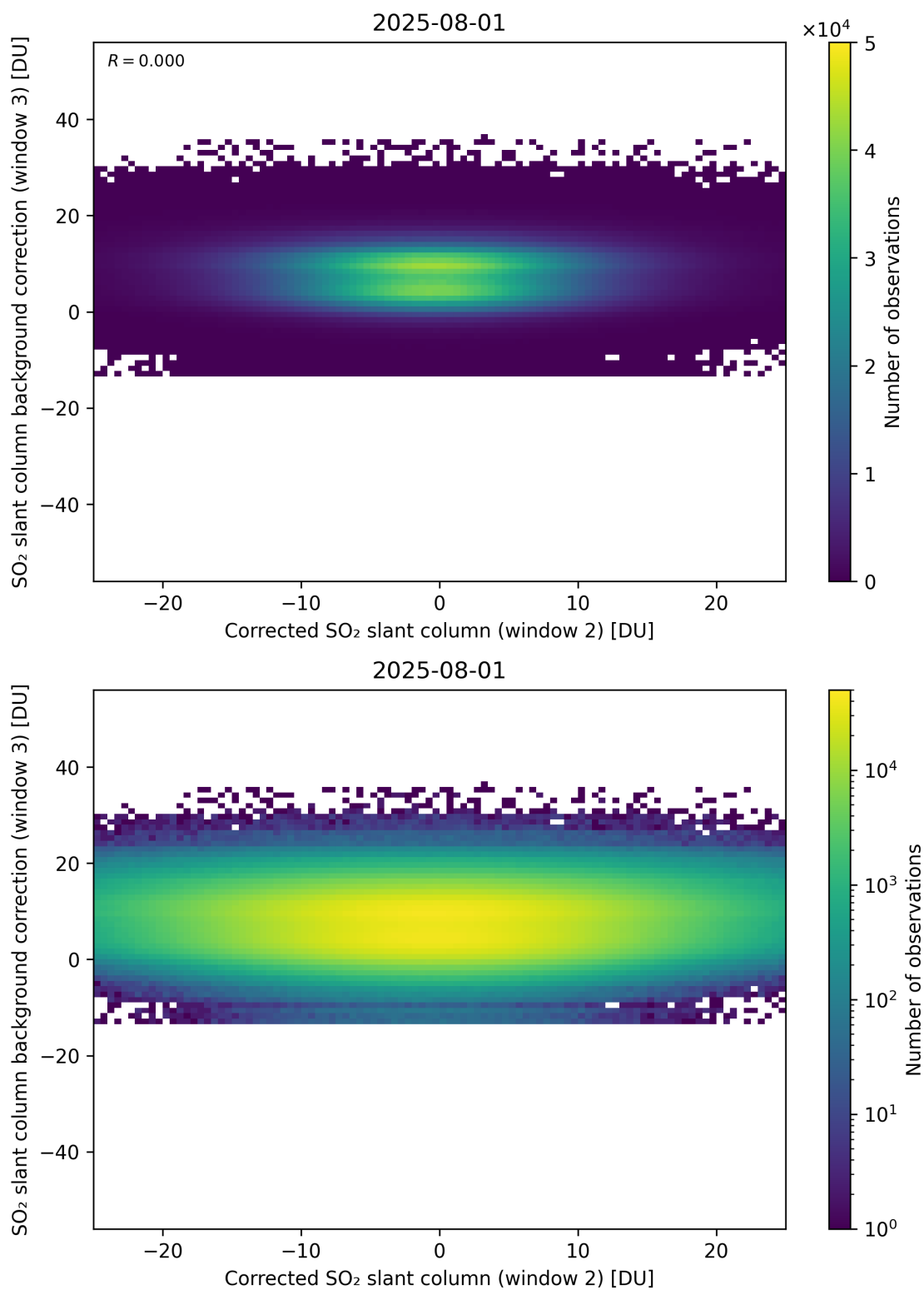
Figure 245: Scatter density plot of “Corrected SO 2 slant column (window 2)” against “SO 2 slant column background correction (window 3)” for 2025-07-31 to 2025-08-02.
