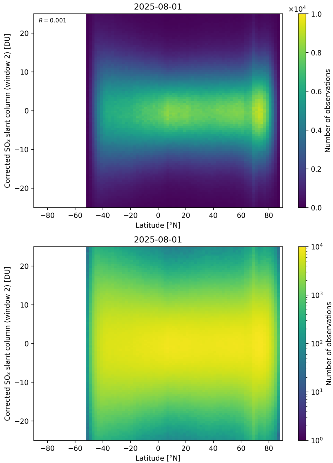
Figure 160: Scatter density plot of “Latitude” against “Corrected SO 2 slant column (window 2)” for 2025-07-31 to 2025-08-02.
