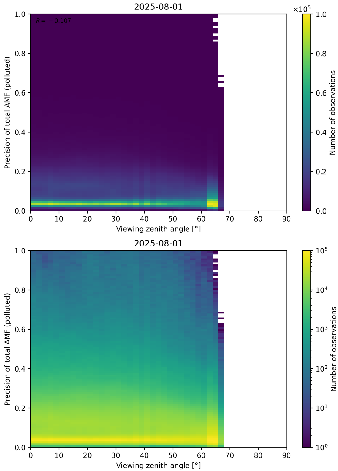
Figure 382: Scatter density plot of “Viewing zenith angle” against “Precision of total AMF (polluted)” for 2025-07-31 to 2025-08-02.
