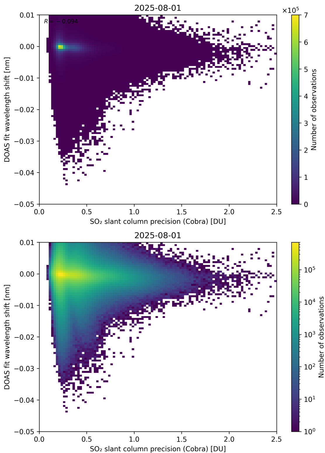
Figure 202: Scatter density plot of “SO 2 slant column precision (Cobra)” against “DOAS fit wavelength shift” for 2025-07-31 to 2025-08-02.
