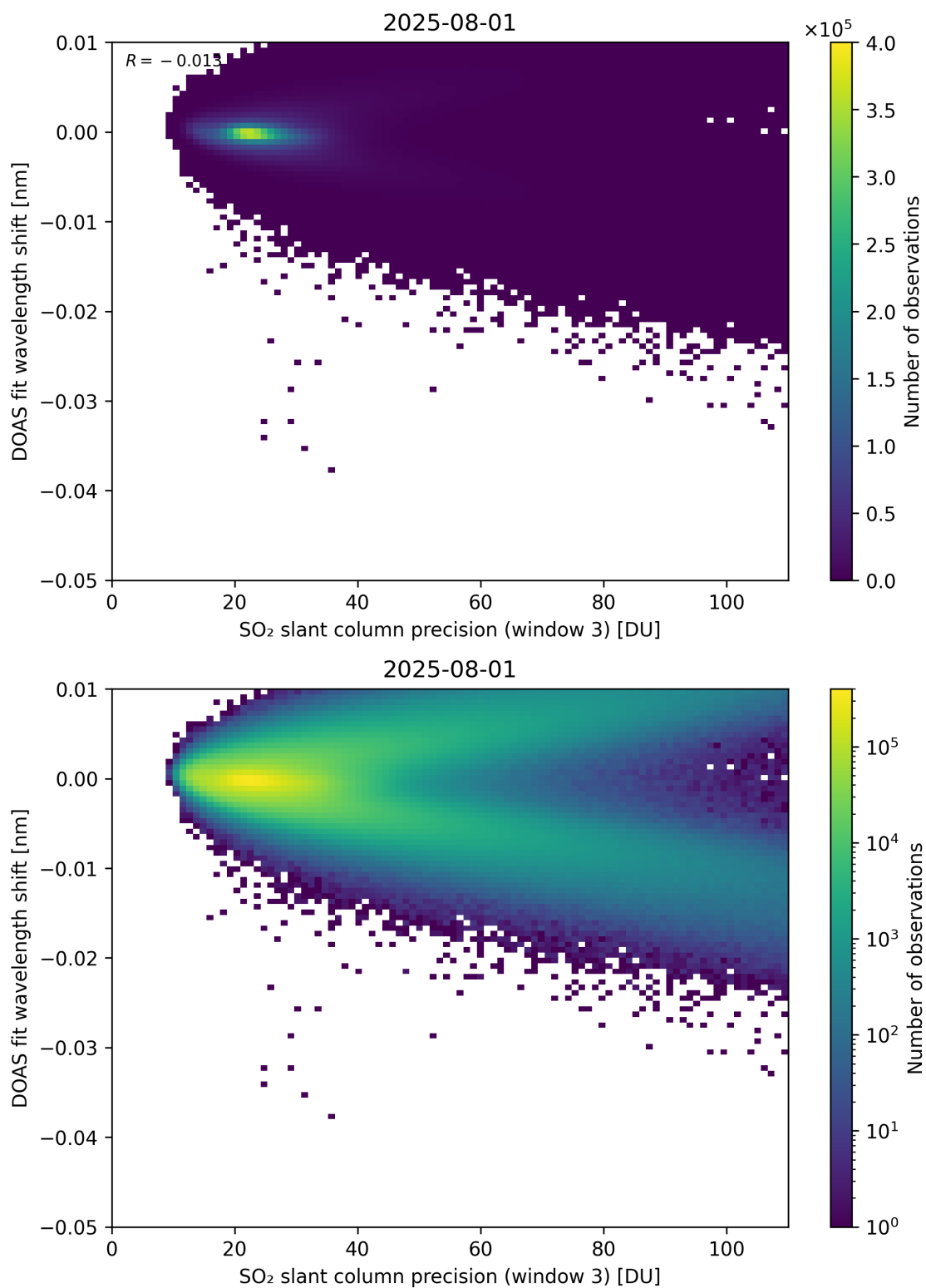
Figure 308: Scatter density plot of “SO 2 slant column precision (window 3)” against “DOAS fit wavelength shift” for 2025-07-31 to 2025-08-02.
