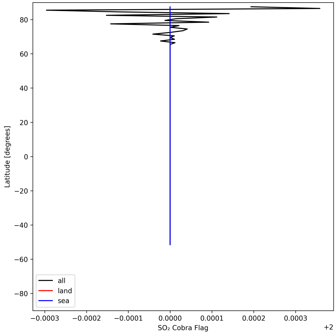
Figure 49: Zonal average of “SO 2 Cobra Flag” for 2025-07-31 to 2025-08-02.
