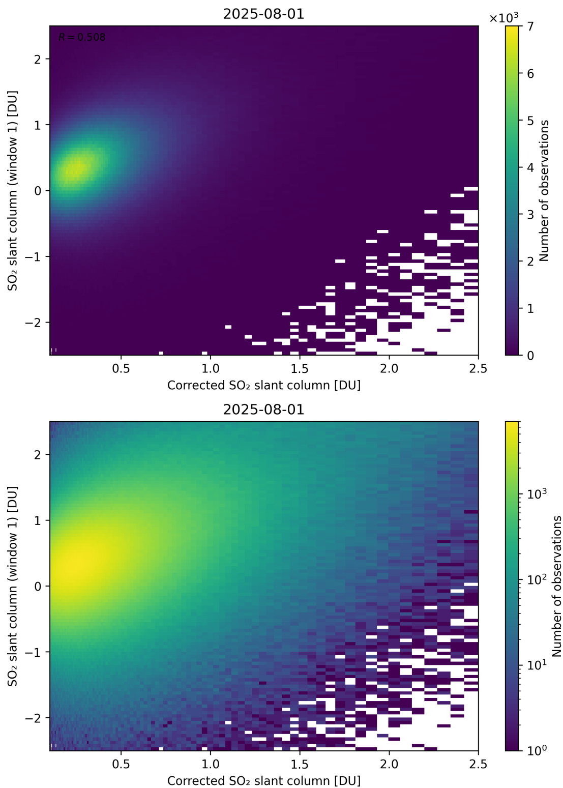
Figure 237: Scatter density plot of “Corrected SO 2 slant column” against “SO 2 slant column (window 1)” for 2025-07-31 to 2025-08-02.
