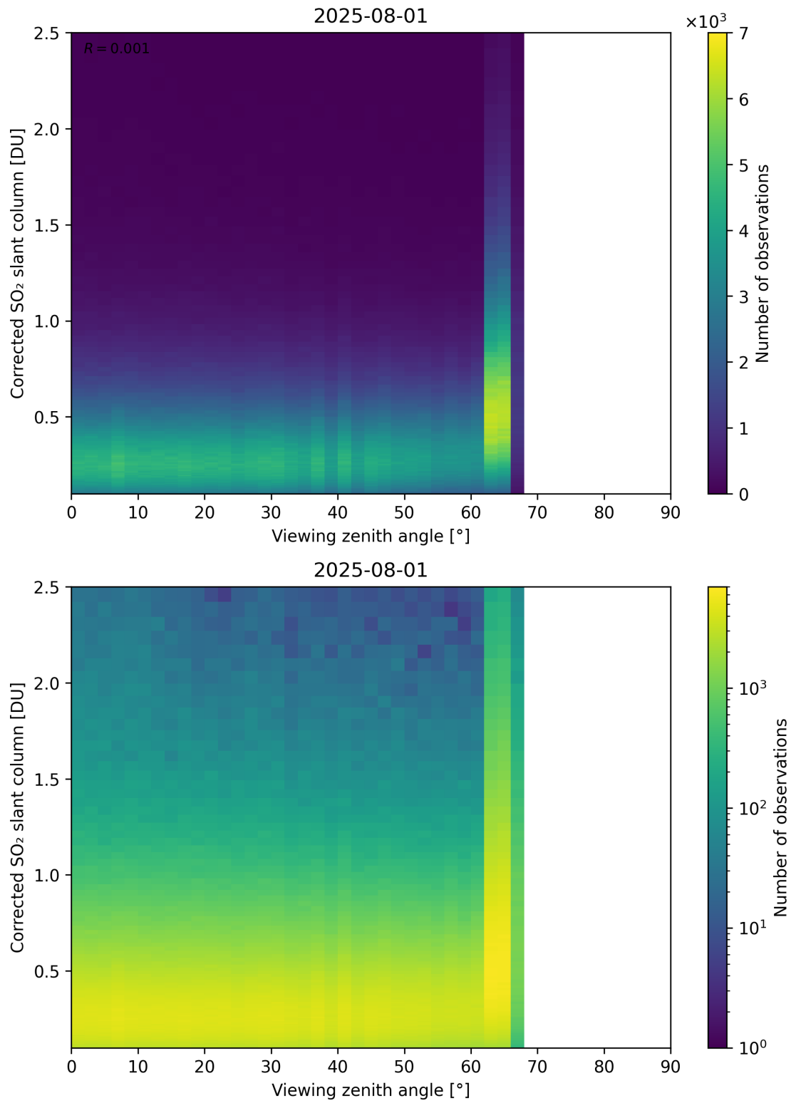
Figure 373: Scatter density plot of “Viewing zenith angle” against “Corrected SO 2 slant column” for 2025-07-31 to 2025-08-02.
