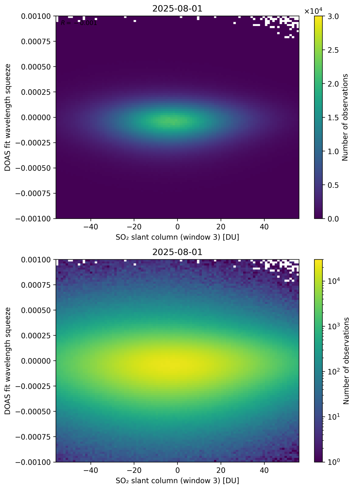
Figure 305: Scatter density plot of “SO 2 slant column (window 3)” against “DOAS fit wavelength squeeze” for 2025-07-31 to 2025-08-02.
