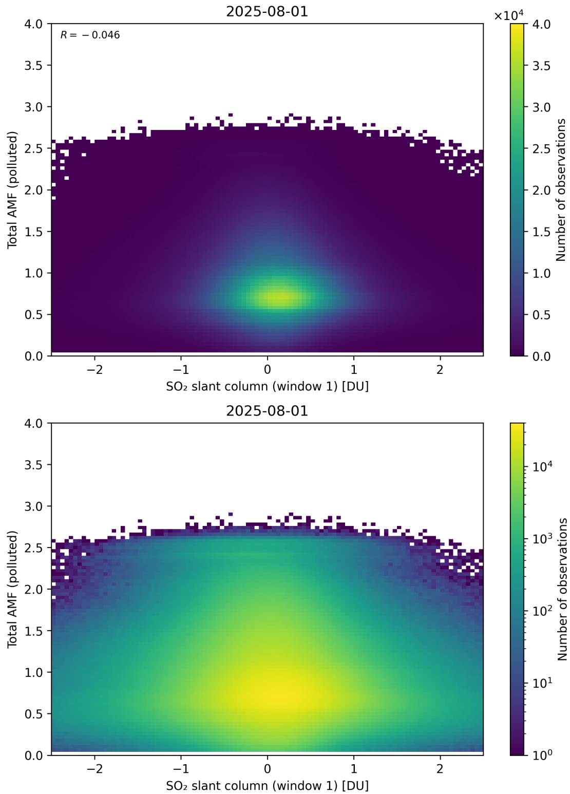
Figure 289: Scatter density plot of “SO 2 slant column (window 1)” against “Total AMF (polluted)” for 2025-07-31 to 2025-08-02.
