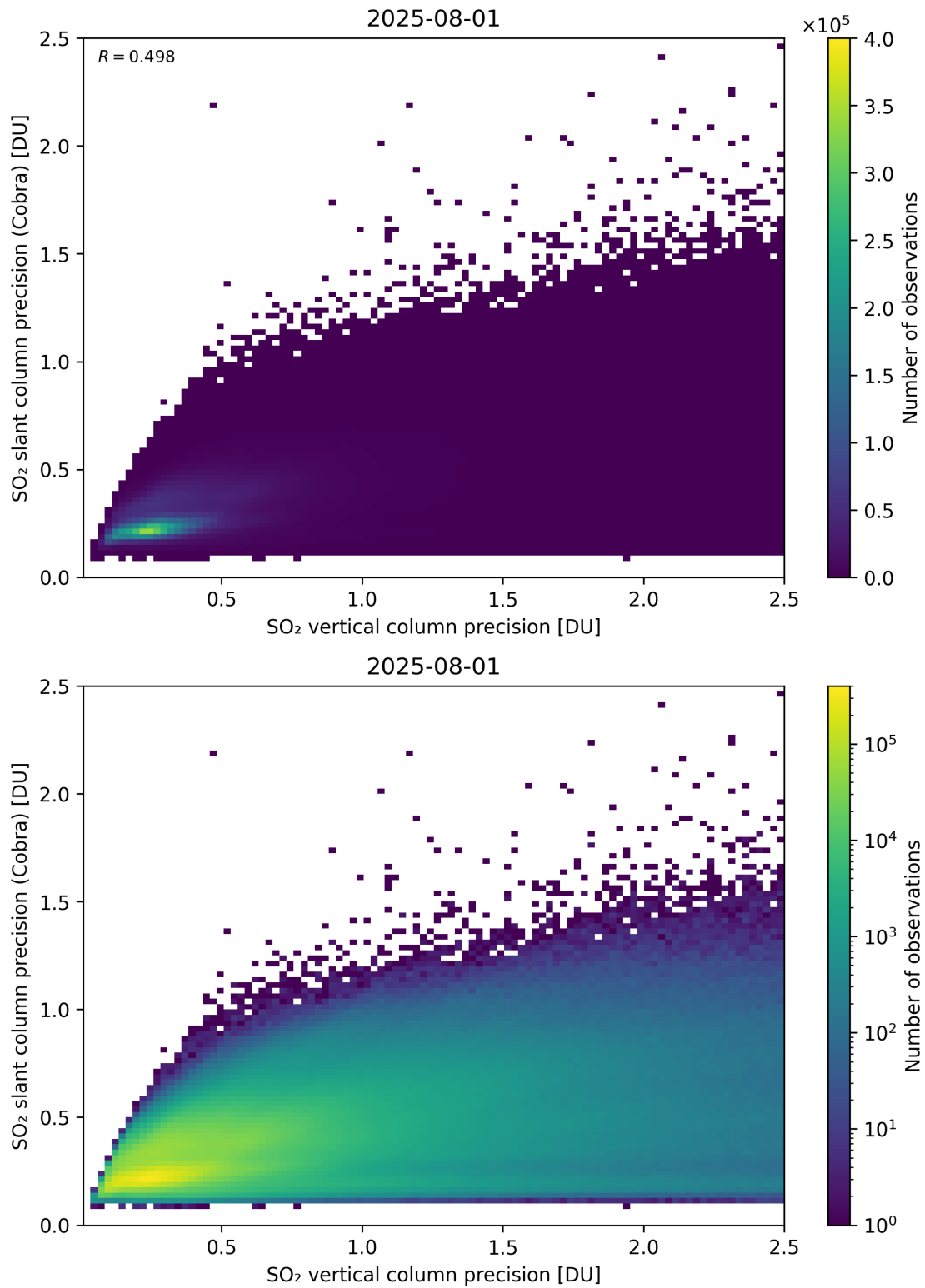
Figure 337: Scatter density plot of “SO 2 vertical column precision” against “SO 2 slant column precision (Cobra)” for 2025-07-31 to 2025-08-02.
