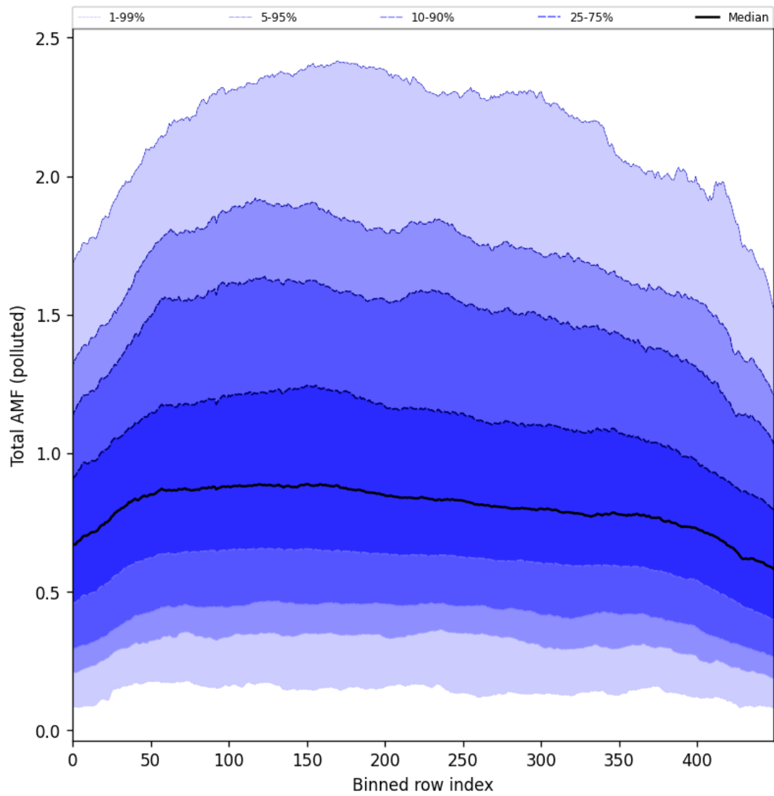
Figure 105: Along track statistics of “Total AMF (polluted)” for 2025-07-31 to 2025-08-02
