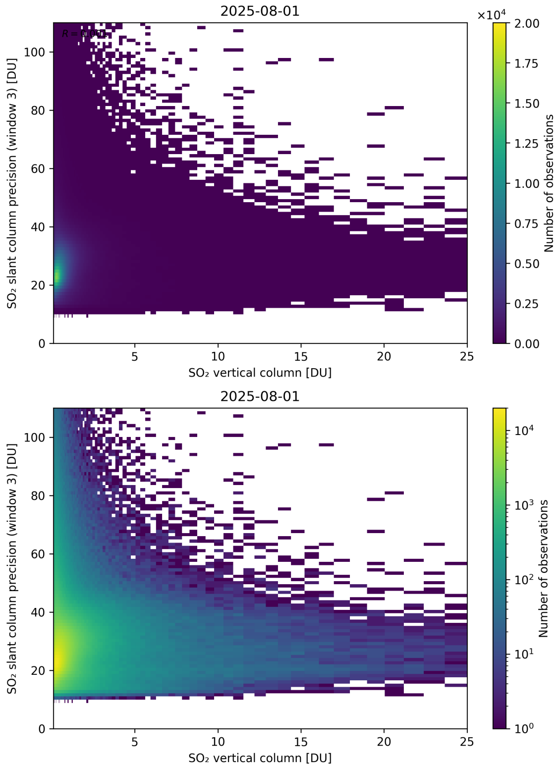
Figure 358: Scatter density plot of “SO 2 vertical column” against “SO 2 slant column precision (window 3)” for 2025-07-31 to 2025-08-02.
