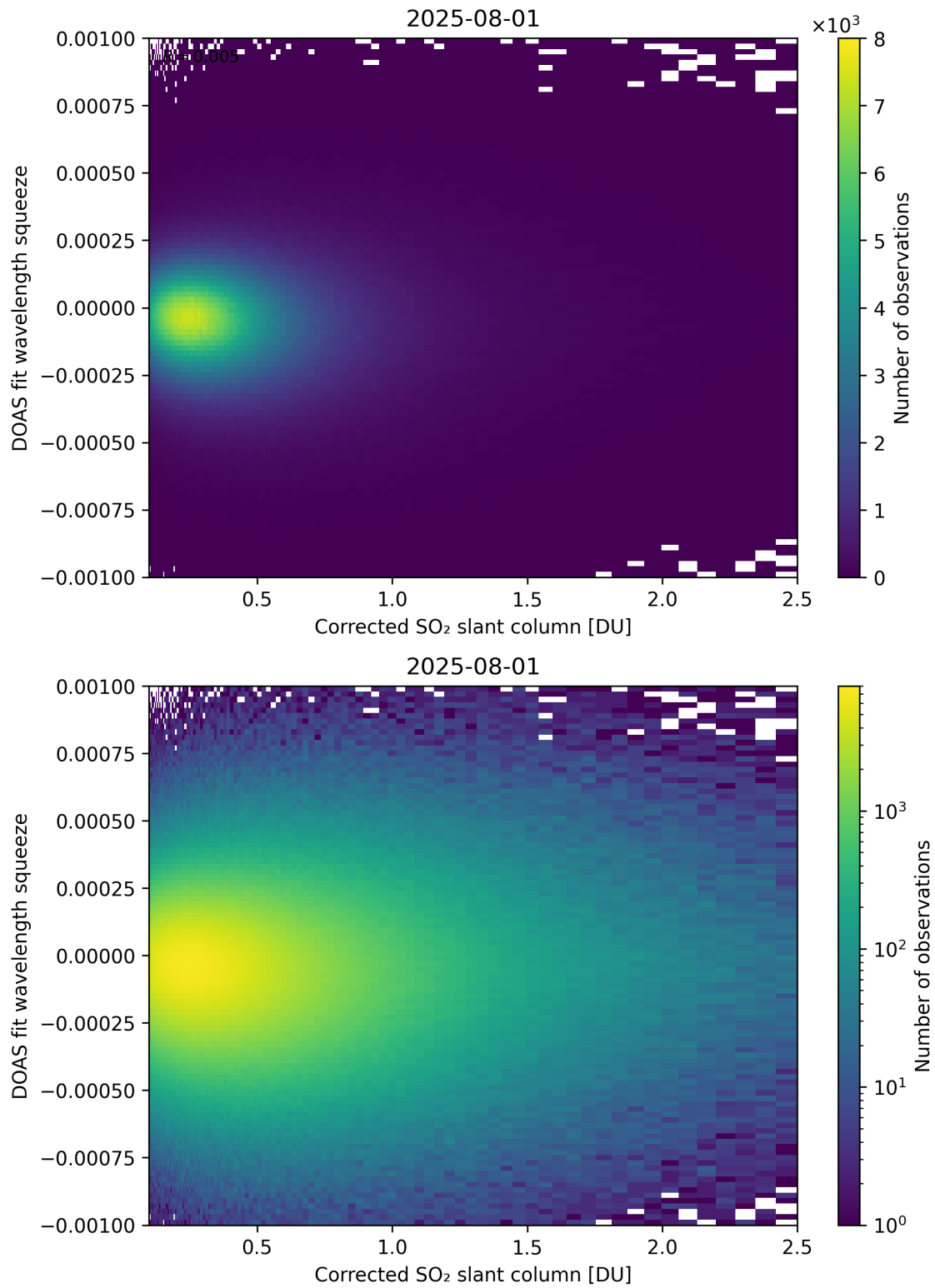
Figure 230: Scatter density plot of "Corrected SO 2 slant column" against "DOAS fit wavelength squeeze" for 2025-07-31 to 2025-08-02.
