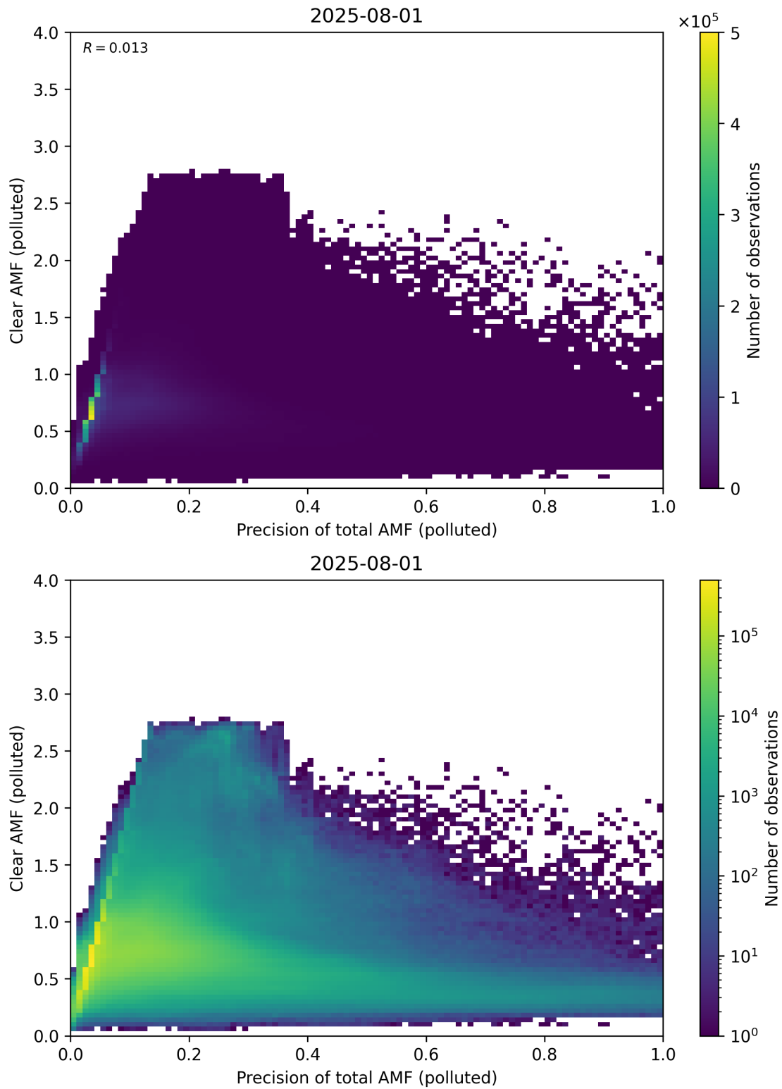
Figure 320: Scatter density plot of “Precision of total AMF (polluted)” against “Clear AMF (polluted)” for 2025-07-31 to 2025-08-02.
