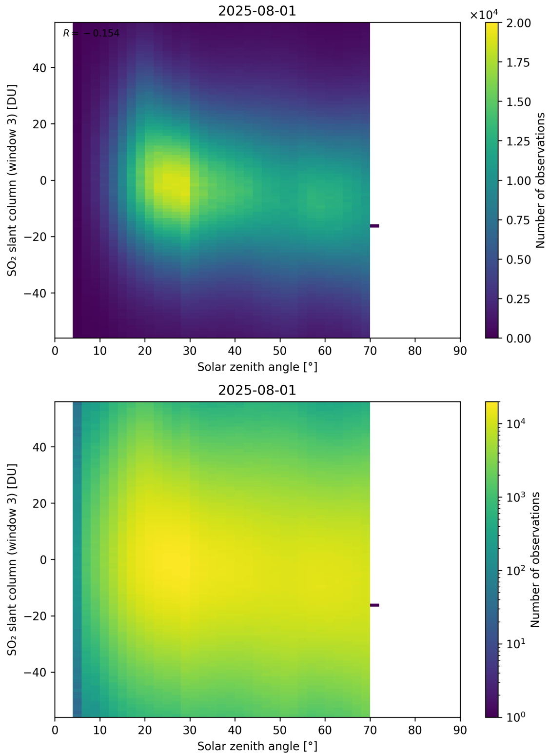
Figure 187: Scatter density plot of “Solar zenith angle” against “SO 2 slant column (window 3)” for 2025-07-31 to 2025-08-02.
