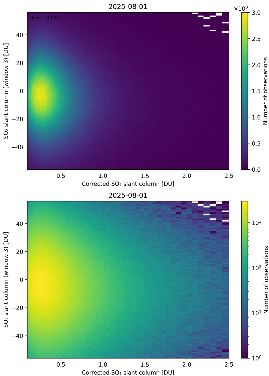
Figure 240: Scatter density plot of “Corrected SO 2 slant column” against “SO 2 slant column (window 3)” for 2025-07-31 to 2025-08-02.
