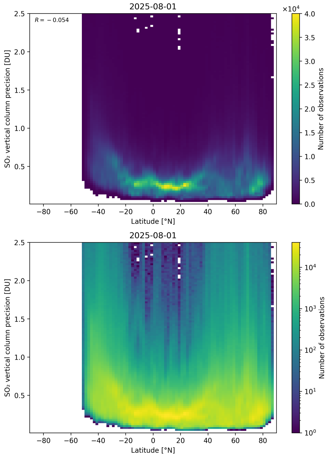
Figure 170: Scatter density plot of “Latitude” against “SO 2 vertical column precision” for 2025-07-31 to 2025-08-02.
