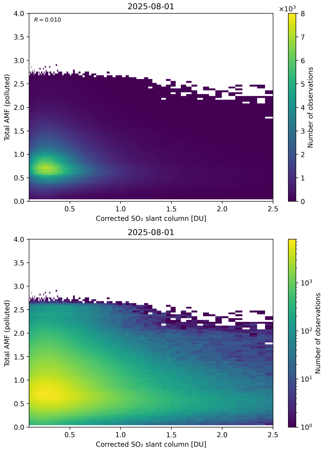
Figure 242: Scatter density plot of “Corrected SO 2 slant column” against “Total AMF (polluted)” for 2025-07-31 to 2025-08-02.
