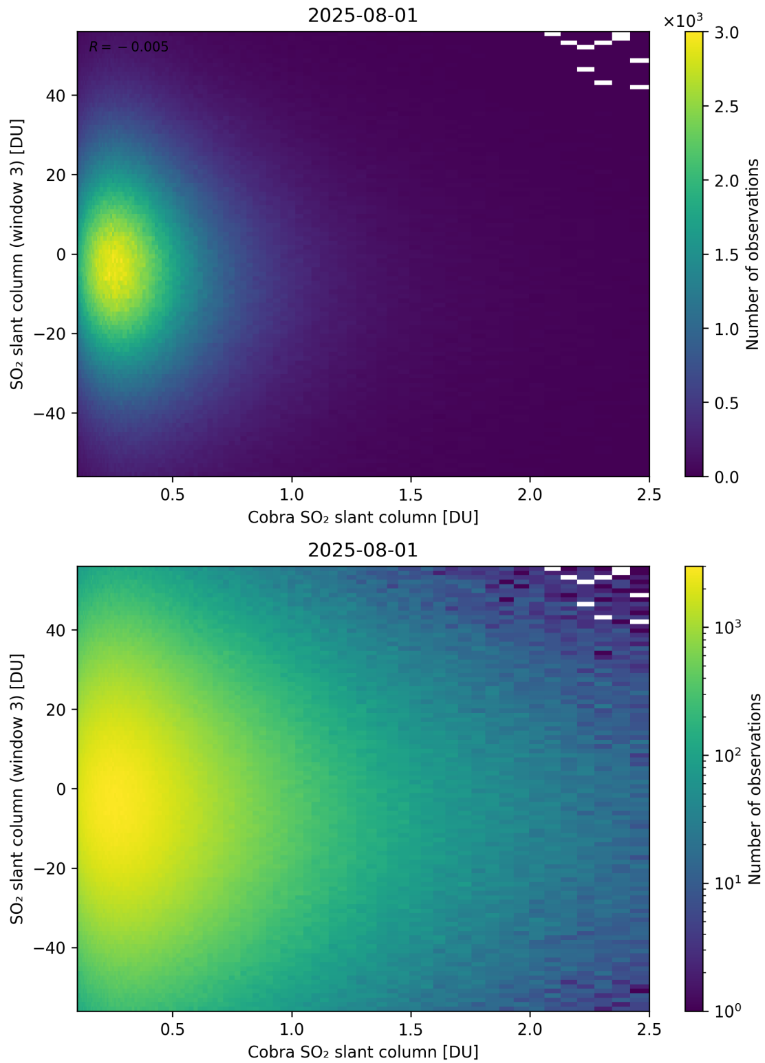
Figure 222: Scatter density plot of “Cobra SO 2 slant column” against “SO 2 slant column (window 3)” for 2025-07-31 to 2025-08-02.
