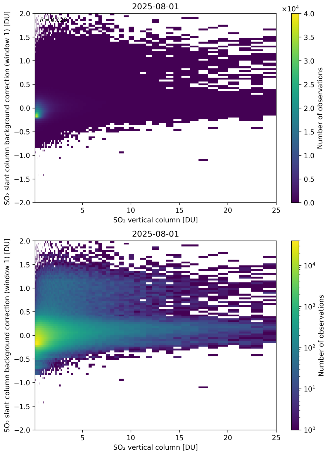
Figure 323: Scatter density plot of “SO 2 vertical column” against “SO 2 slant column background correction (window 1)” for 2025-07-31 to 2025-08-02.
