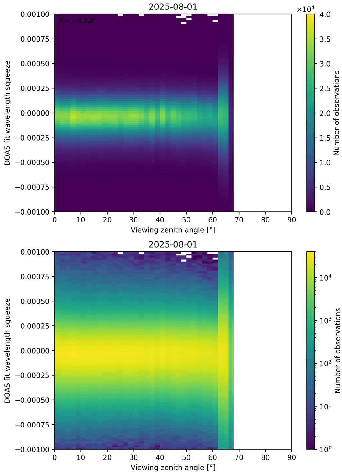
Figure 366: Scatter density plot of “Viewing zenith angle” against “DOAS fit wavelength squeeze” for 2025-07-31 to 2025-08-02.
