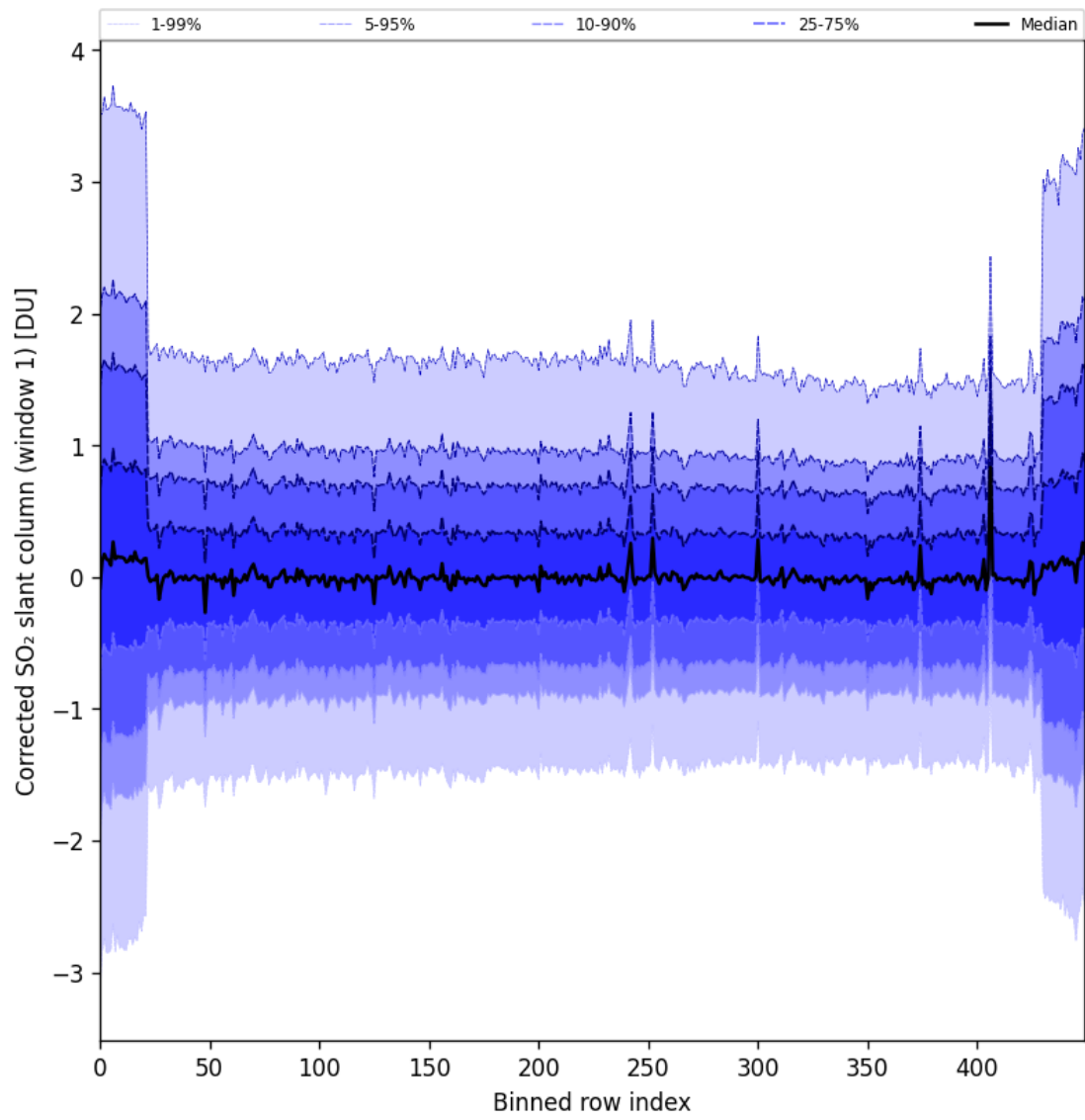
Figure 91: Along track statistics of “Corrected SO 2 slant column (window 1)” for 2025-07-31 to 2025-08-02
