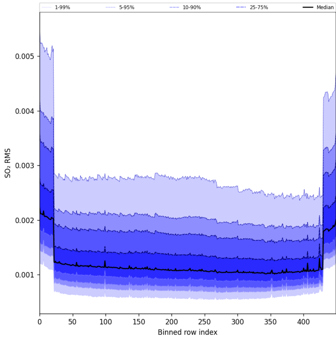
Figure 104: Along track statistics of “SO 2 RMS” for 2025-07-31 to 2025-08-02
