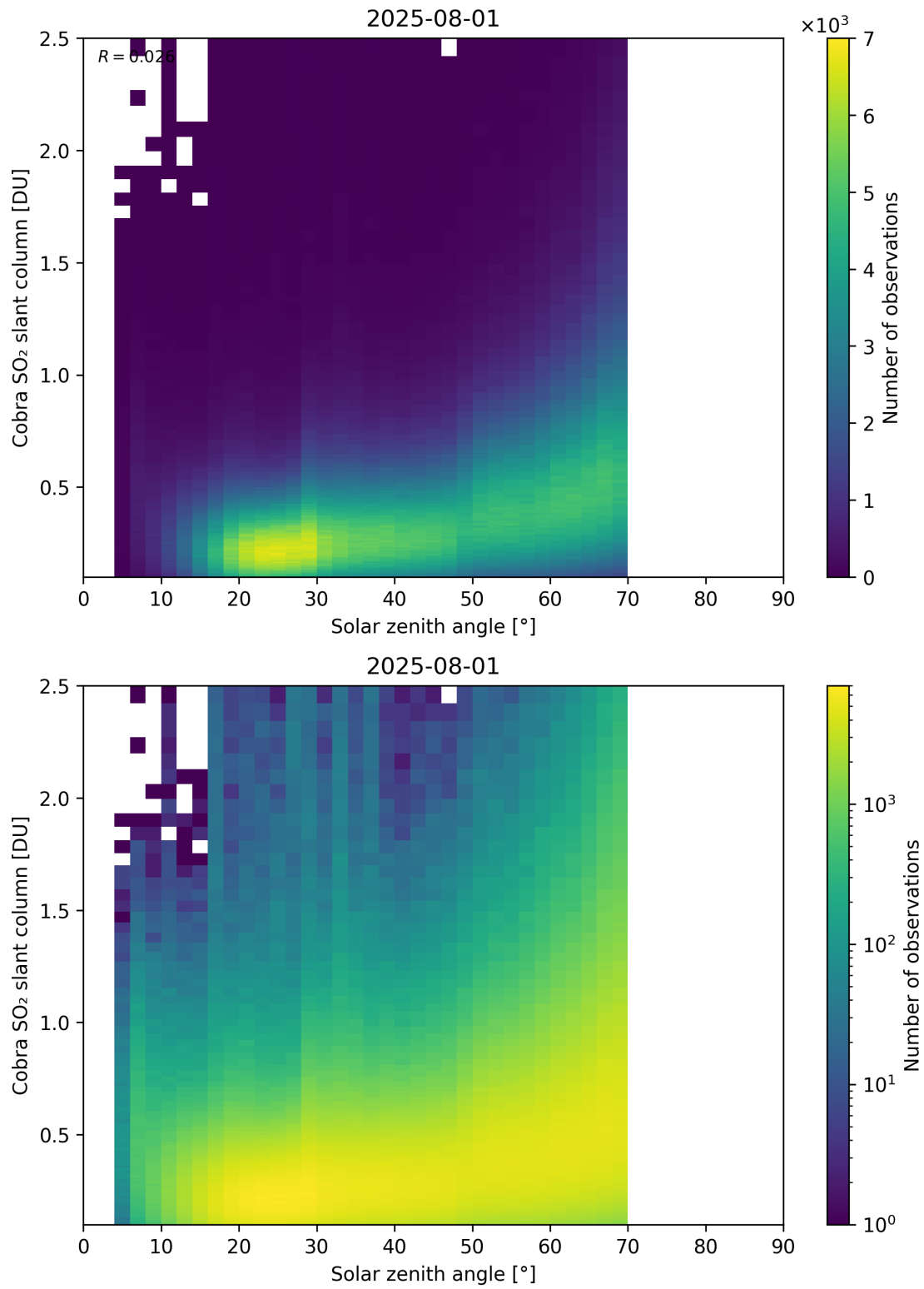
Figure 179: Scatter density plot of “Solar zenith angle” against “Cobra SO 2 slant column” for 2025-07-31 to 2025-08-02.
