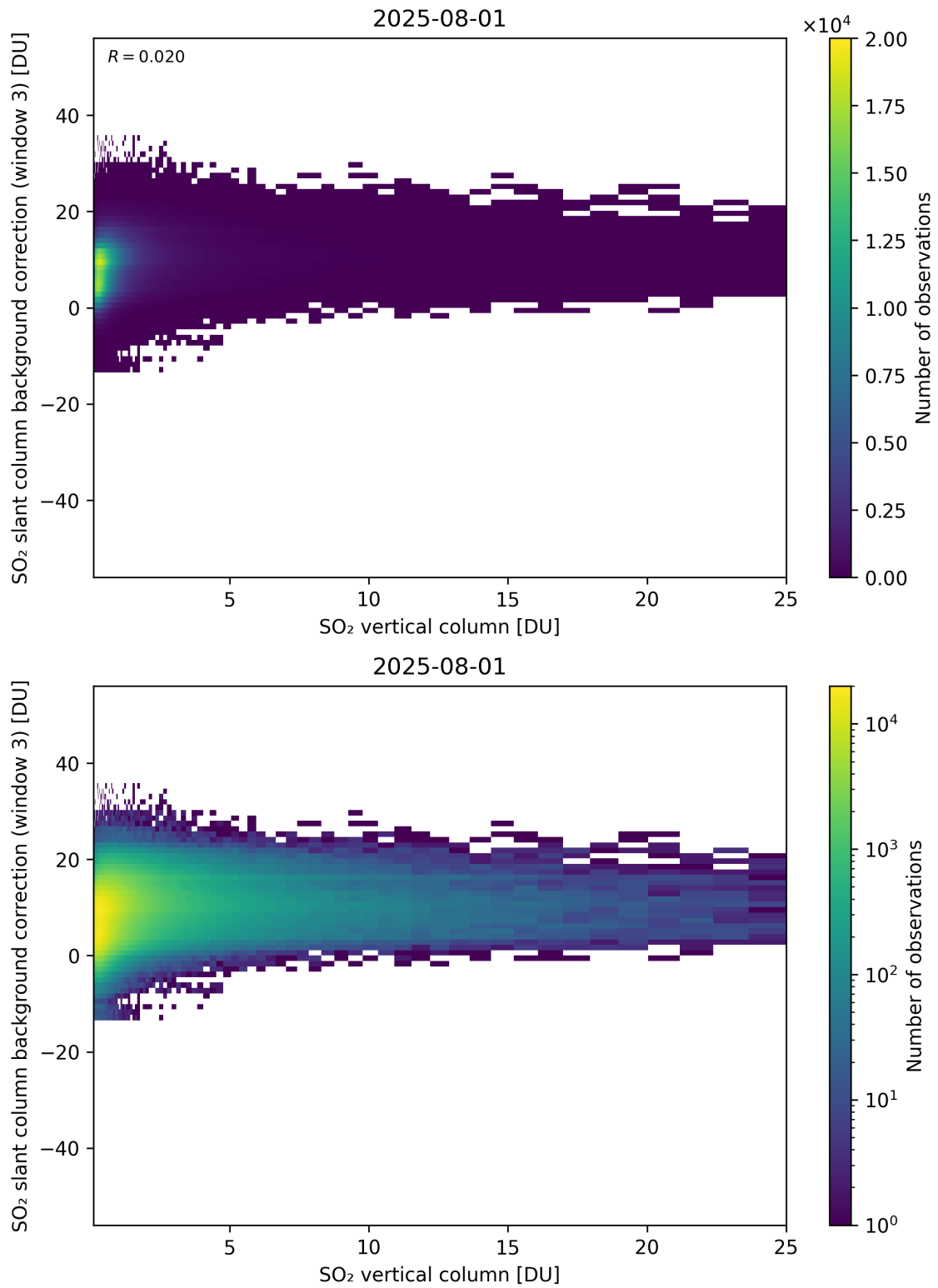
Figure 325: Scatter density plot of “SO 2 vertical column” against “SO 2 slant column background correction (window 3)” for 2025-07-31 to 2025-08-02.
