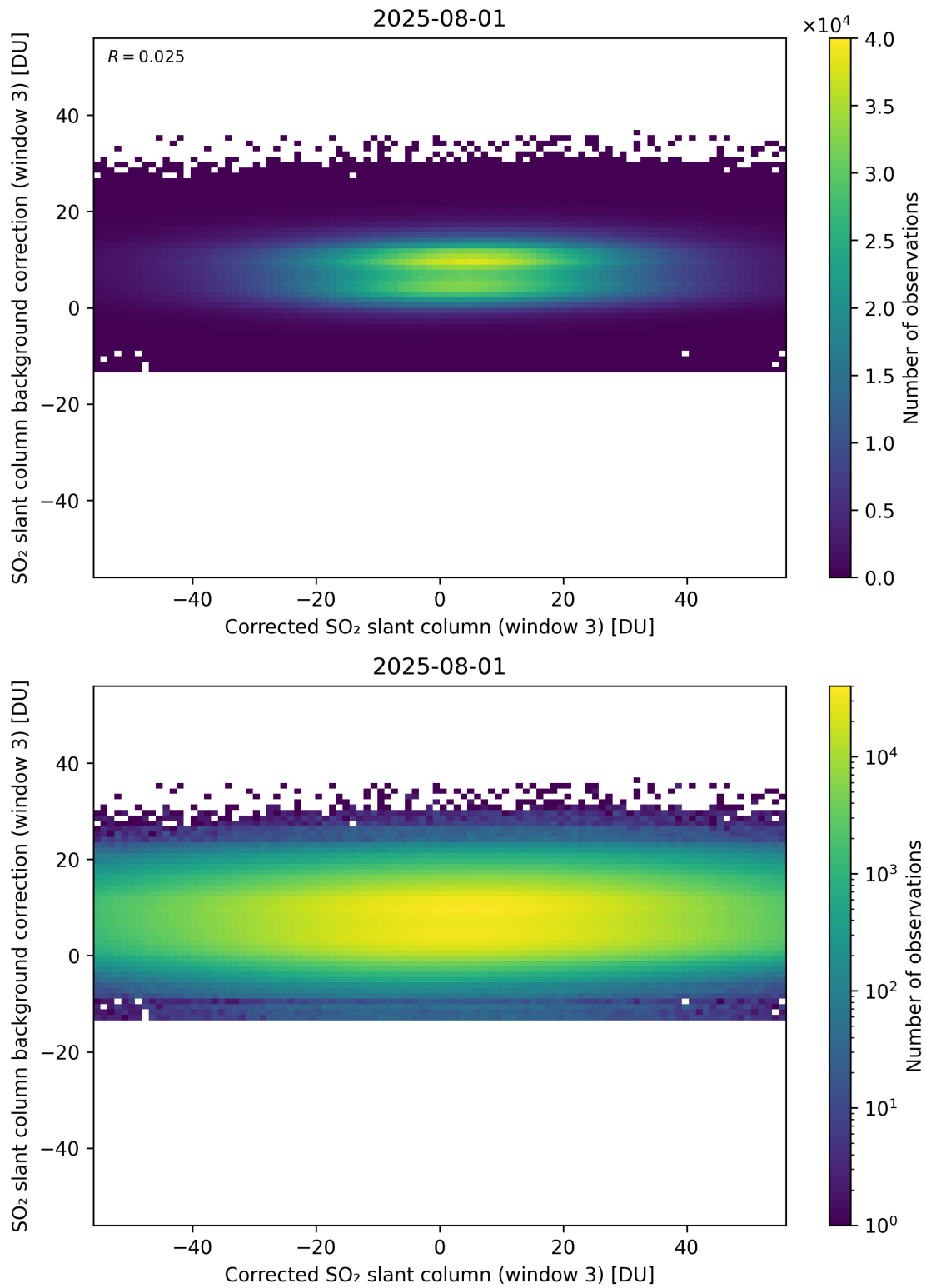
Figure 255: Scatter density plot of “Corrected SO 2 slant column (window 3)” against “SO 2 slant column background correction (window 3)” for 2025-07-31 to 2025-08-02.
