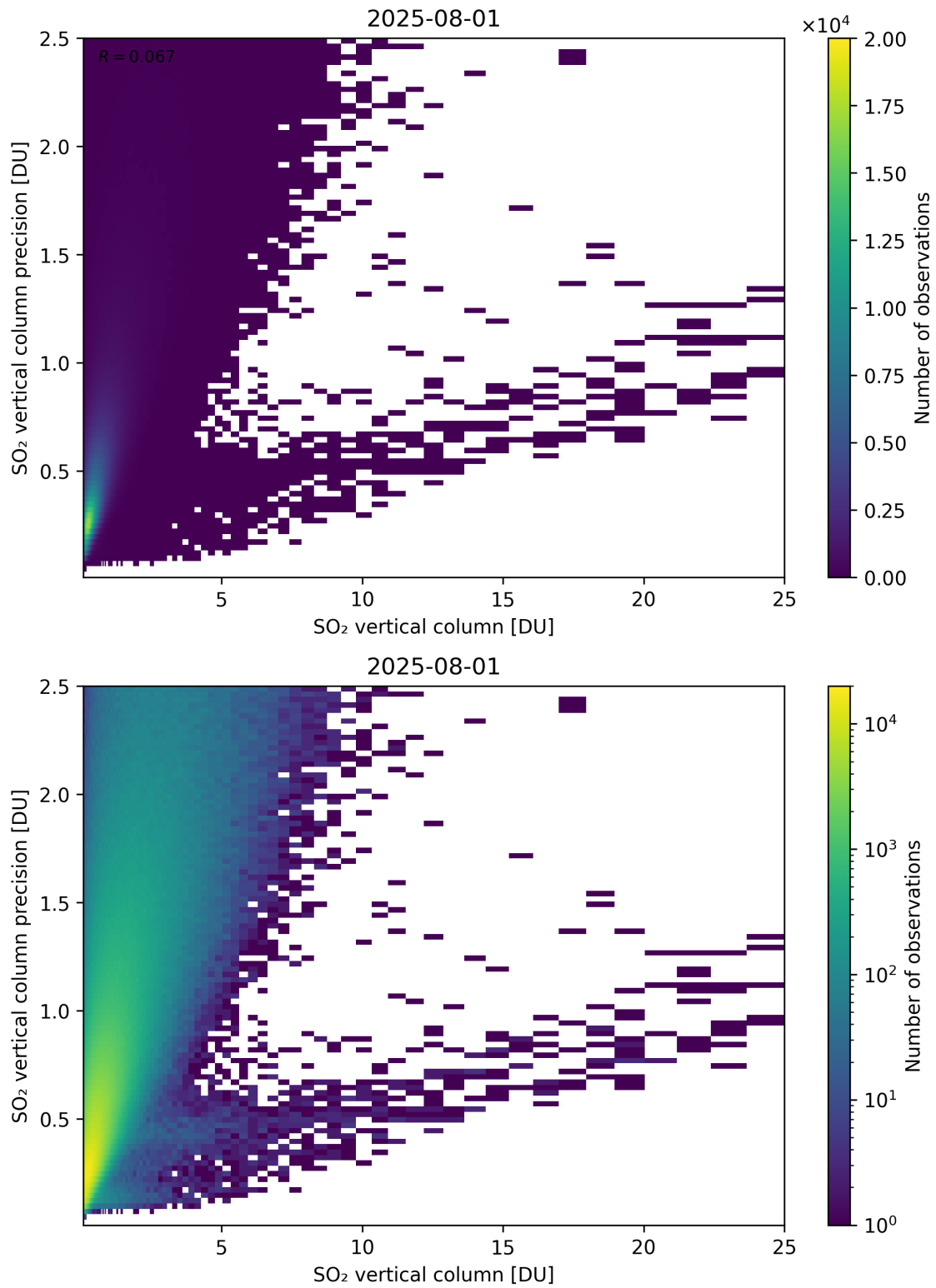
Figure 361: Scatter density plot of “SO 2 vertical column” against “SO 2 vertical column precision” for 2025-07-31 to 2025-08-02.
