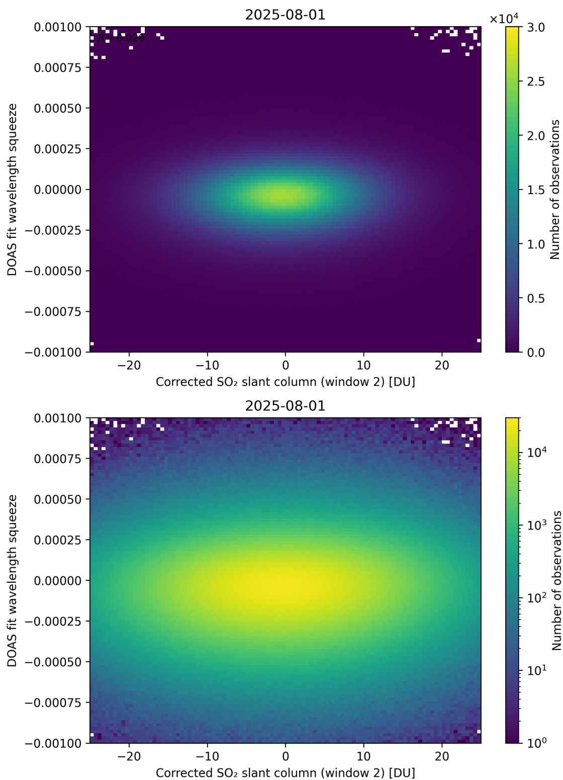
Figure 247: Scatter density plot of “Corrected SO 2 slant column (window 2)” against “DOAS fit wavelength squeeze” for 2025-07-31 to 2025-08-02.
