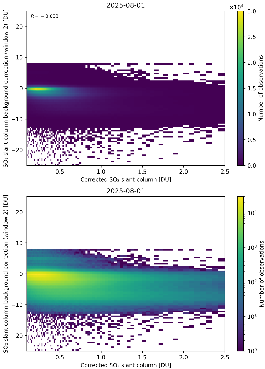
Figure 227: Scatter density plot of “Corrected SO 2 slant column” against “SO 2 slant column background correction (window 2)” for 2025-07-31 to 2025-08-02.
