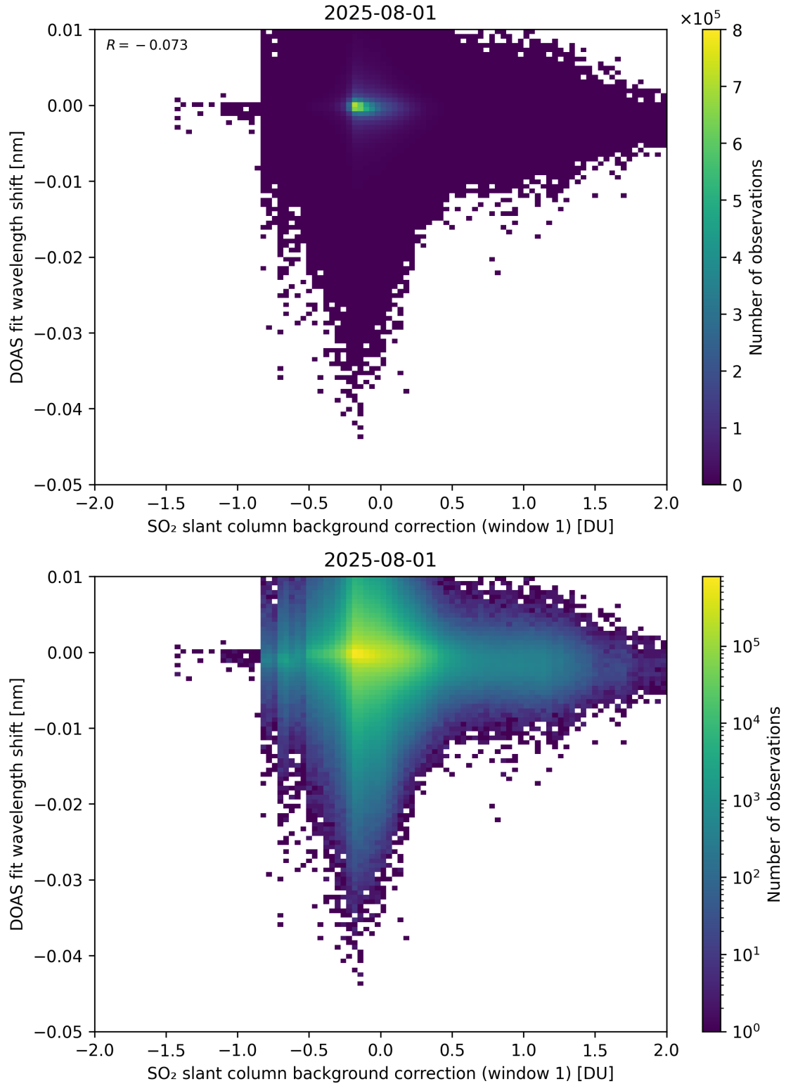
Figure 111: Scatter density plot of “SO 2 slant column background correction (window 1)” against “DOAS fit wavelength shift” for 2025-07-31 to 2025-08-02.
