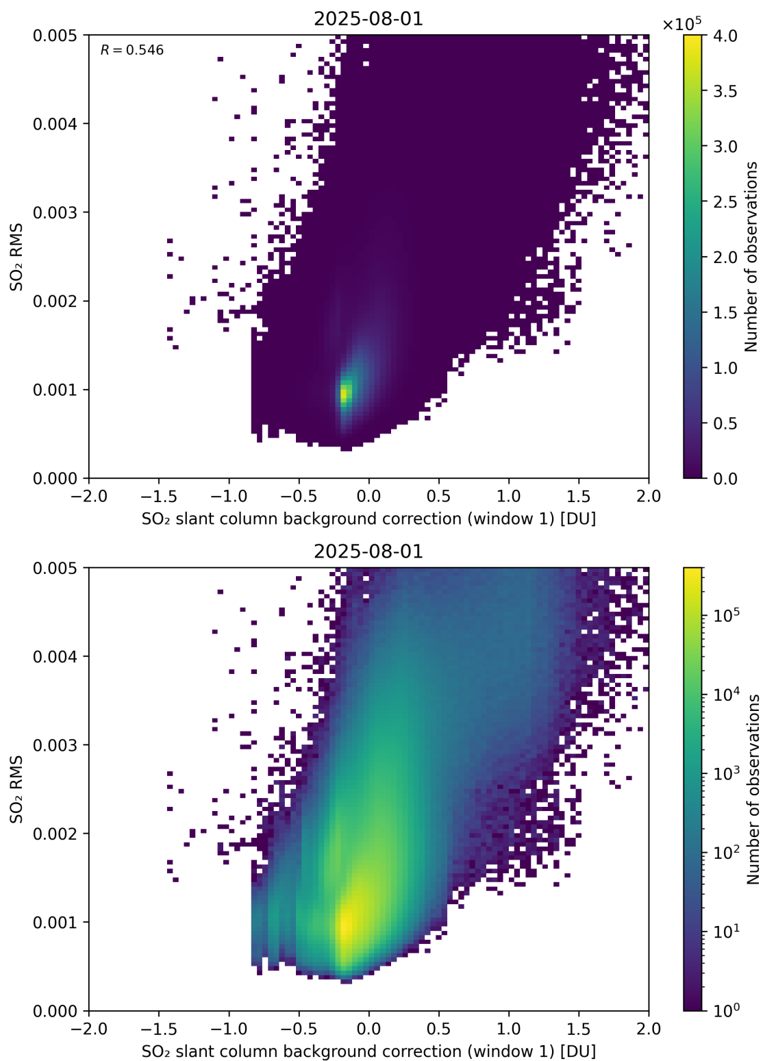
Figure 113: Scatter density plot of “SO 2 slant column background correction (window 1)” against “SO 2 RMS” for 2025-07-31 to 2025-08-02.
