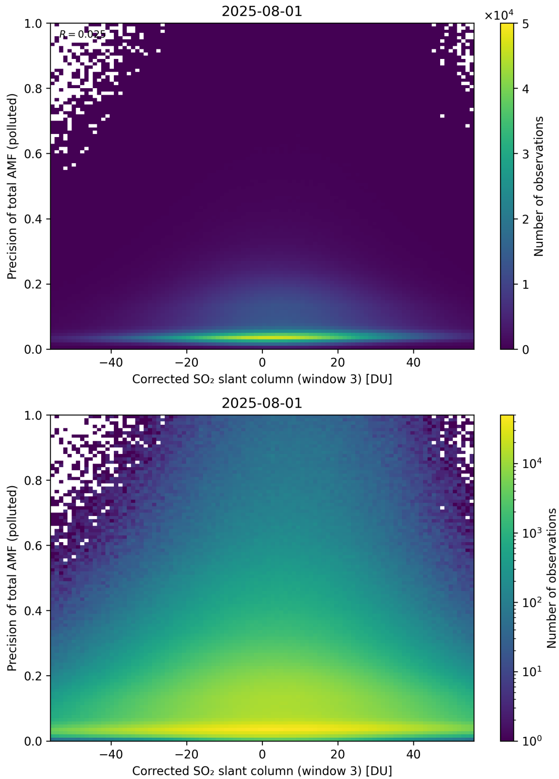
Figure 261: Scatter density plot of “Corrected SO 2 slant column (window 3)” against “Precision of total AMF (polluted)” for 2025-07-31 to 2025-08-02.
