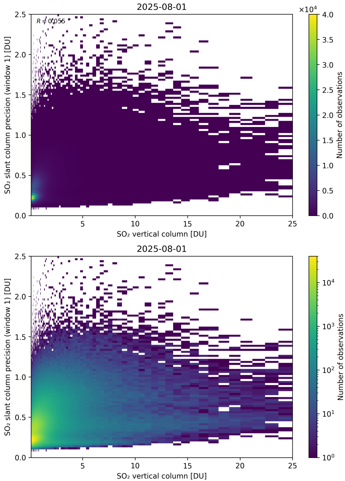
Figure 355: Scatter density plot of “SO 2 vertical column” against “SO 2 slant column precision (window 1)” for 2025-07-31 to 2025-08-02.
