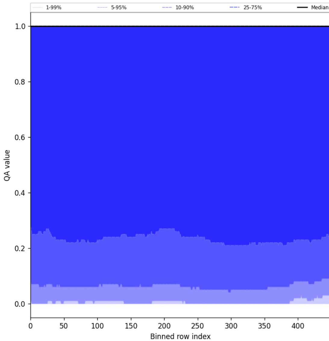
Figure 83: Along track statistics of “QA value” for 2025-07-31 to 2025-08-02
