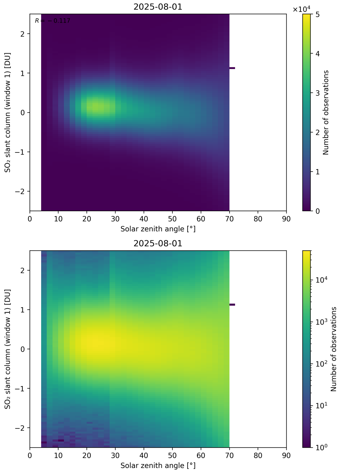
Figure 184: Scatter density plot of “Solar zenith angle” against “SO 2 slant column (window 1)” for 2025-07-31 to 2025-08-02.
