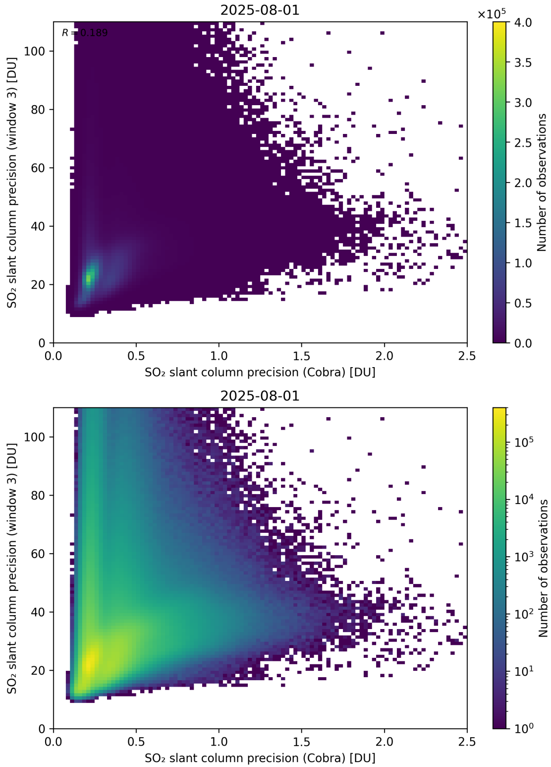
Figure 212: Scatter density plot of “SO 2 slant column precision (Cobra)” against “SO 2 slant column precision (window 3)” for 2025-07-31 to 2025-08-02.
