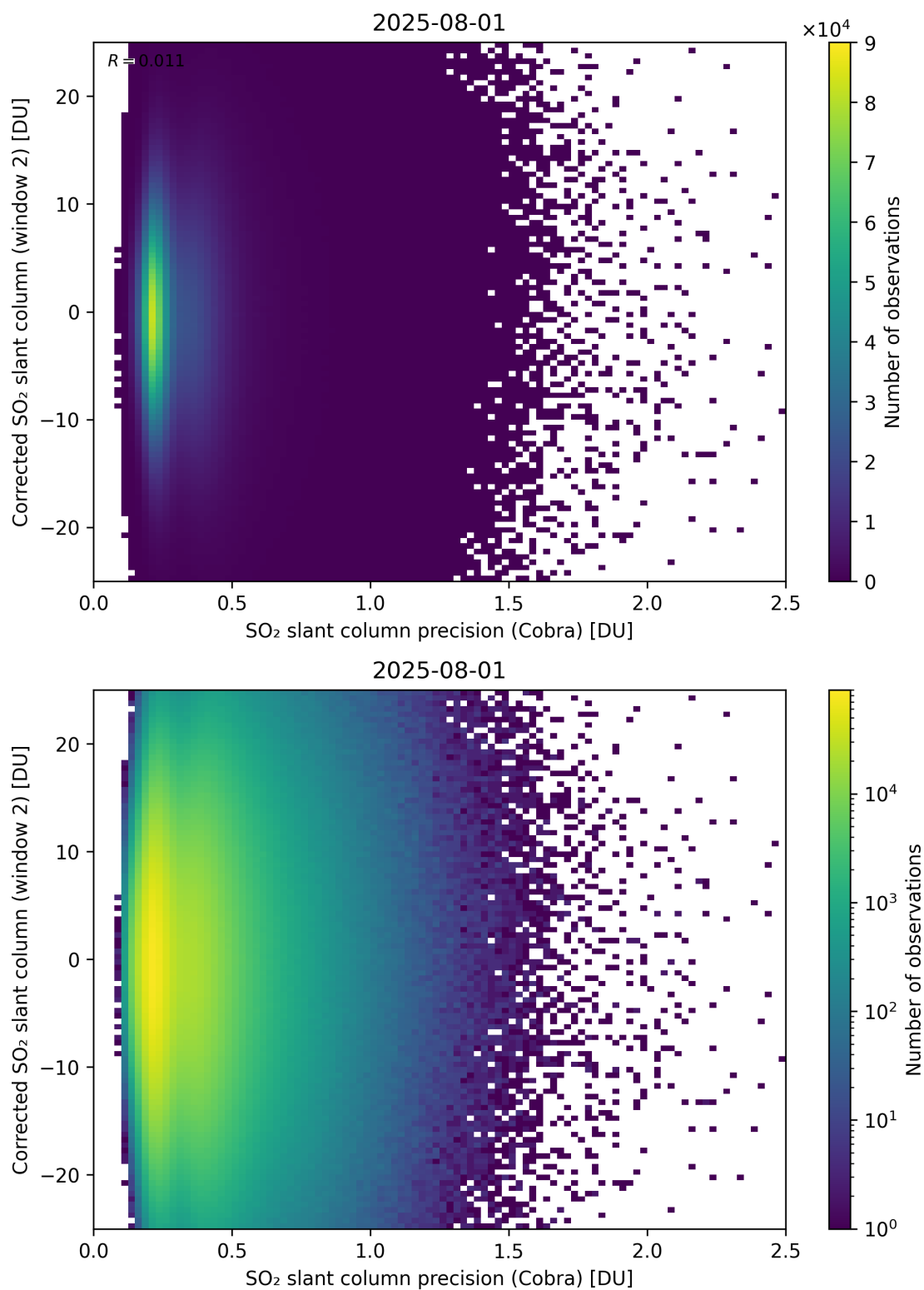
Figure 206: Scatter density plot of “SO 2 slant column precision (Cobra)” against “Corrected SO 2 slant column (window 2)” for 2025-07-31 to 2025-08-02.
