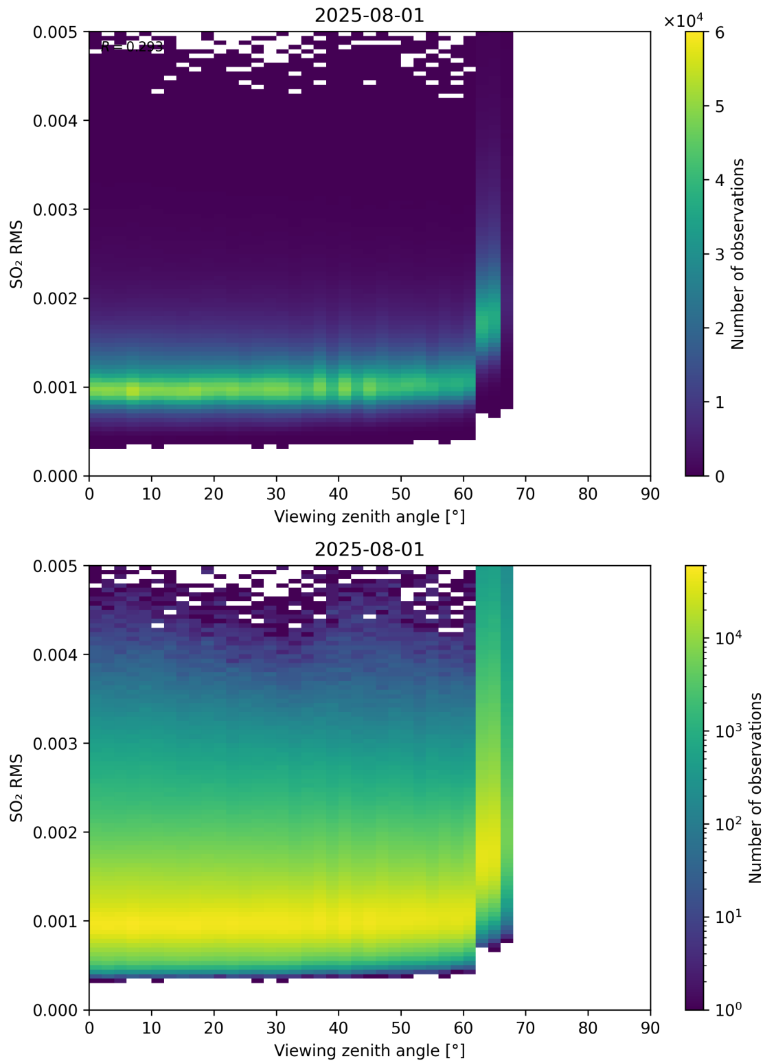
Figure 367: Scatter density plot of “Viewing zenith angle” against “SO 2 RMS” for 2025-07-31 to 2025-08-02.
