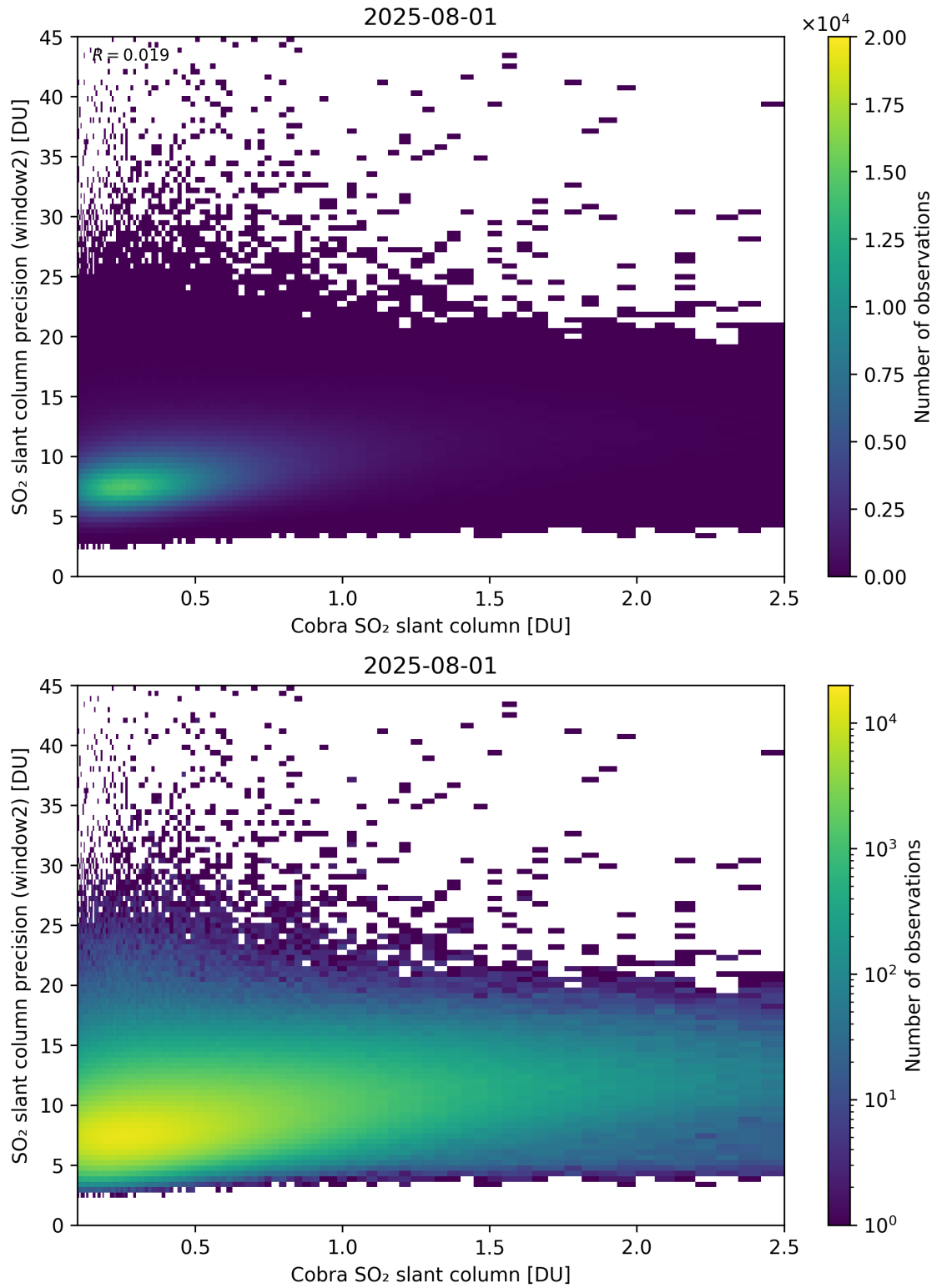
Figure 221: Scatter density plot of “Cobra SO 2 slant column” against “SO 2 slant column precision (window2)” for 2025-07-31 to 2025-08-02.
