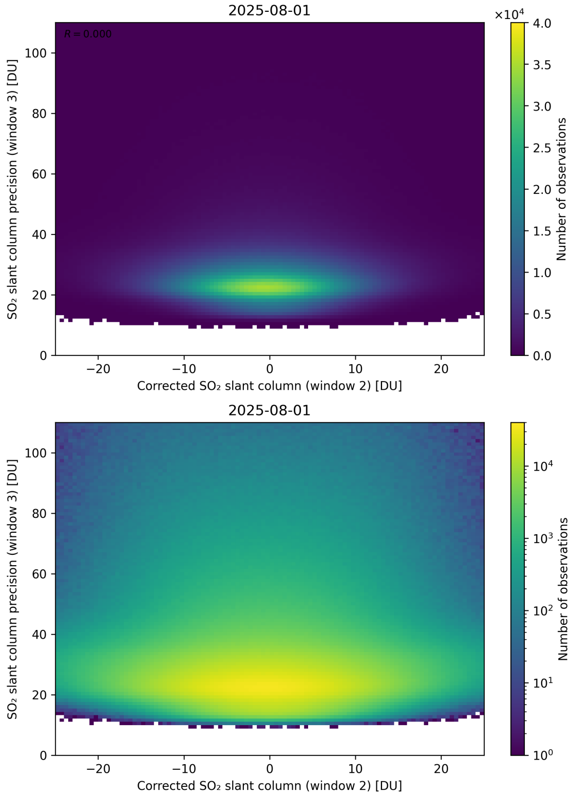
Figure 252: Scatter density plot of “Corrected SO 2 slant column (window 2)” against “SO 2 slant column precision (window 3)” for 2025-07-31 to 2025-08-02.
