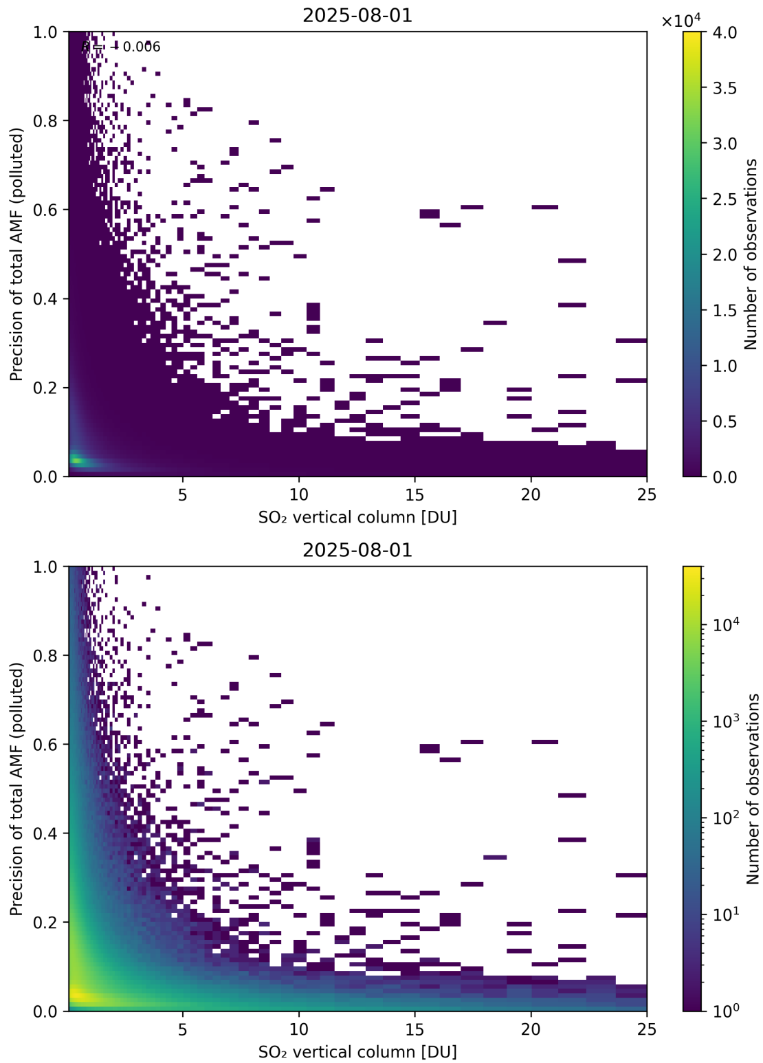
Figure 360: Scatter density plot of “SO 2 vertical column” against “Precision of total AMF (polluted)” for 2025-07-31 to 2025-08-02.
