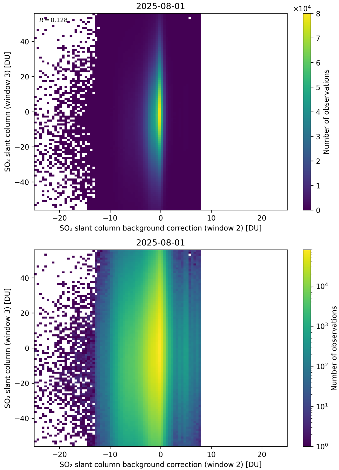
Figure 128: Scatter density plot of “SO 2 slant column background correction (window 2)” against “SO 2 slant column (window 3)” for 2025-07-31 to 2025-08-02.
