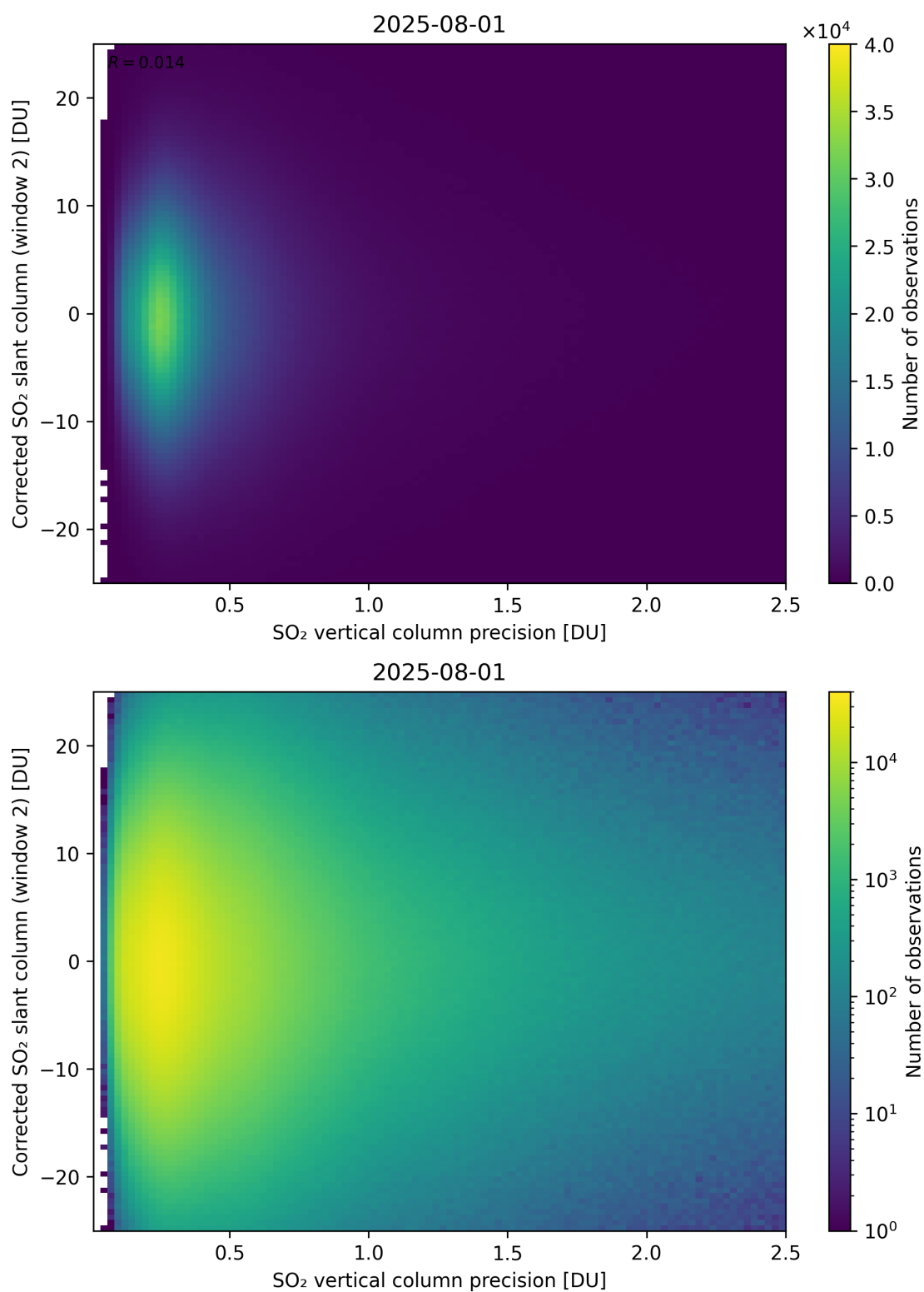
Figure 339: Scatter density plot of “SO 2 vertical column precision” against “Corrected SO 2 slant column (window 2)” for 2025-07-31 to 2025-08-02.
