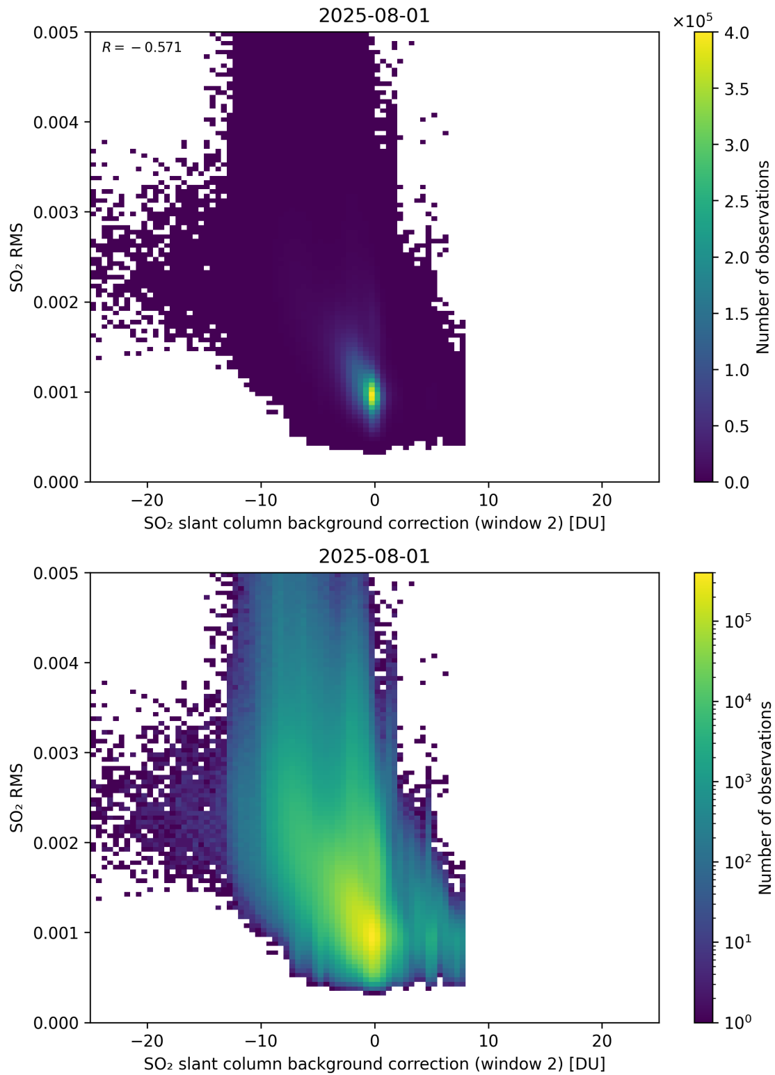
Figure 125: Scatter density plot of “SO 2 slant column background correction (window 2)” against “SO 2 RMS” for 2025-07-31 to 2025-08-02.
