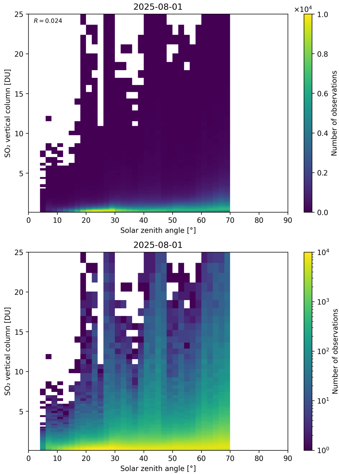
Figure 191: Scatter density plot of “Solar zenith angle” against “SO 2 vertical column” for 2025-07-31 to 2025-08-02.
