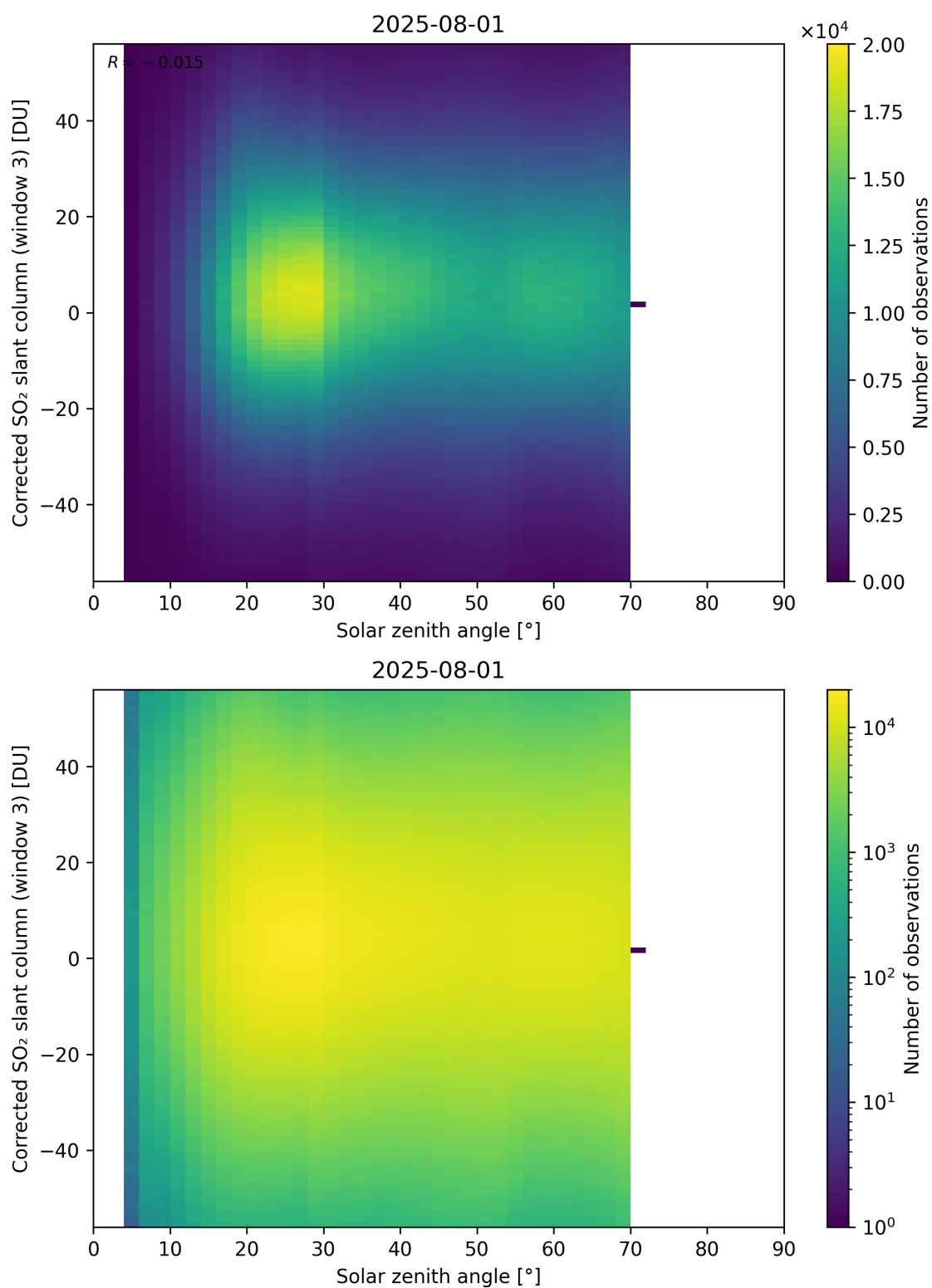
Figure 183: Scatter density plot of “Solar zenith angle” against “Corrected SO 2 slant column (window 3)” for 2025-07-31 to 2025-08-02.
