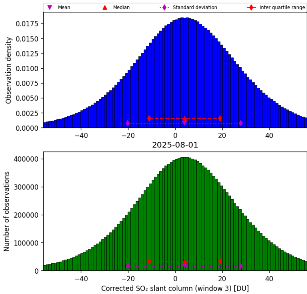
Figure 73: Histogram of “Corrected SO 2 slant column (window 3)” for 2025-07-31 to 2025-08-02
