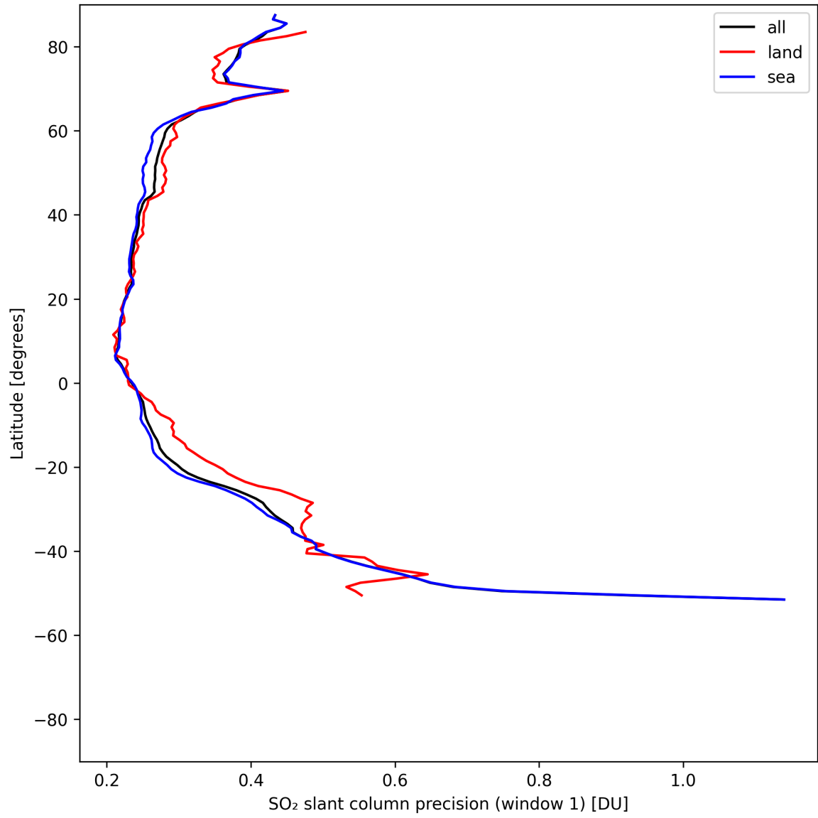
Figure 38: Zonal average of “SO 2 slant column precision (window 1)” for 2025-07-31 to 2025-08-02.
