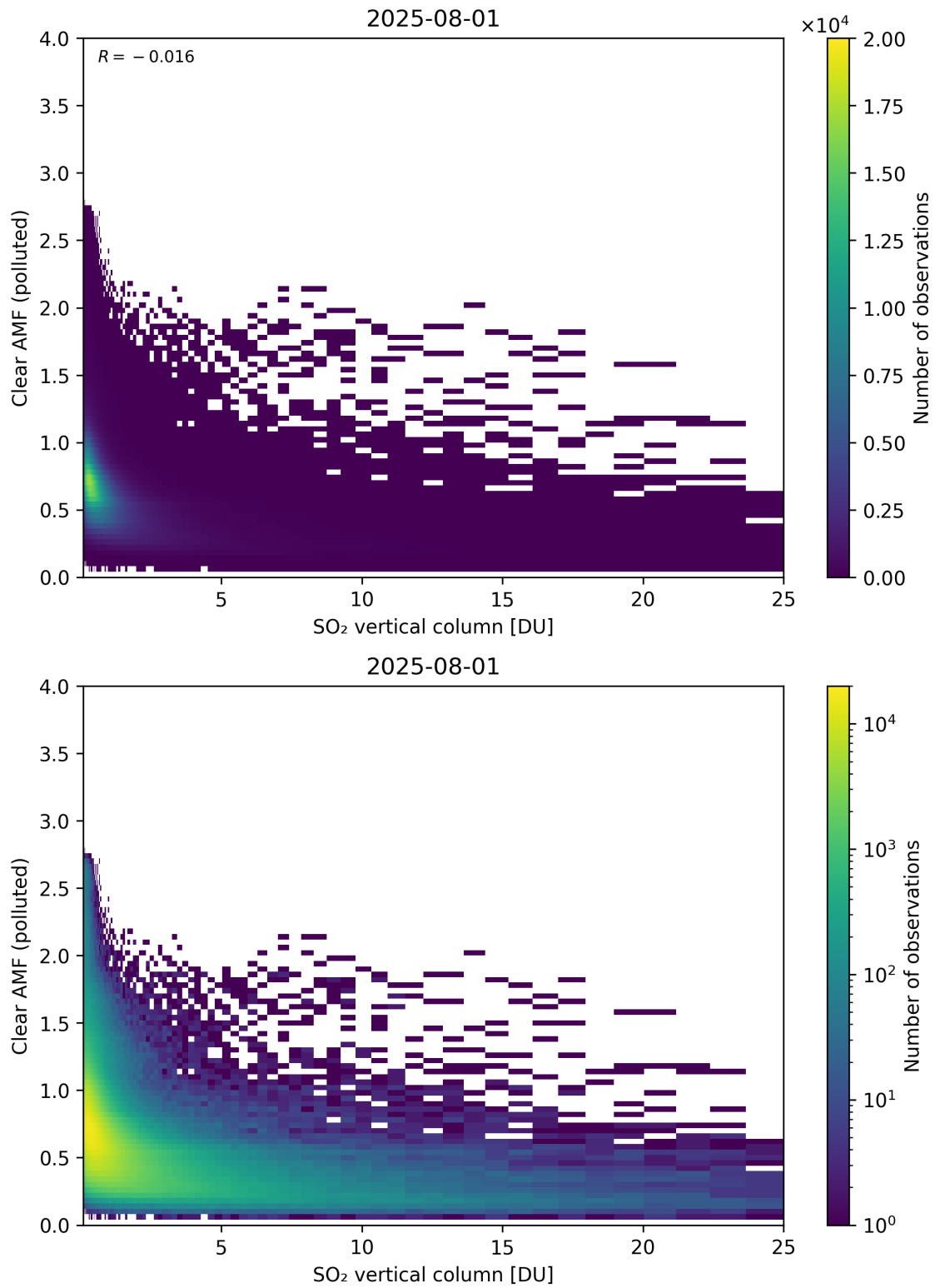
Figure 348: Scatter density plot of “SO 2 vertical column” against “Clear AMF (polluted)” for 2025-07-31 to 2025-08-02.
