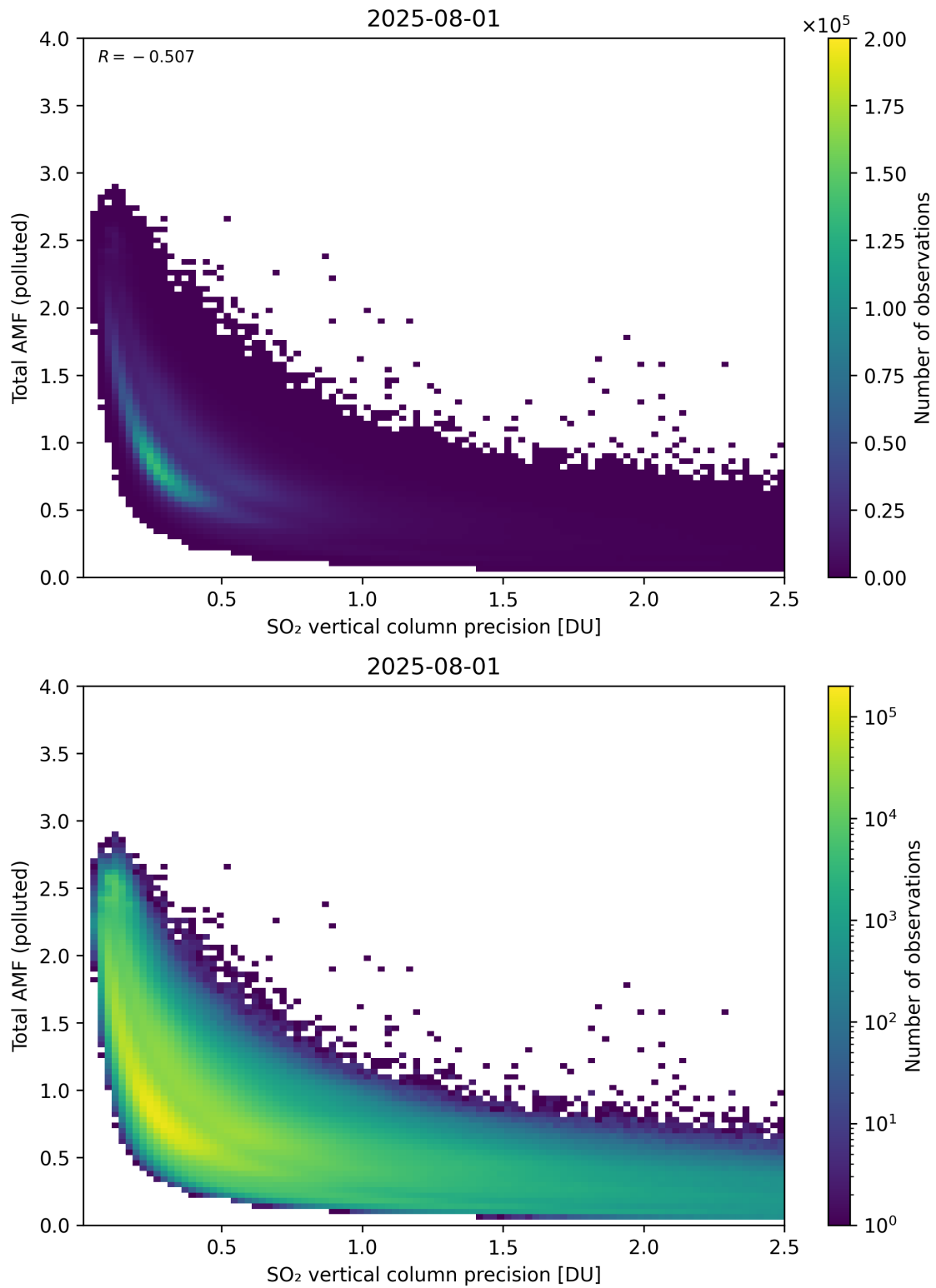
Figure 346: Scatter density plot of “SO 2 vertical column precision” against “Total AMF (polluted)” for 2025-07-31 to 2025-08-02.
