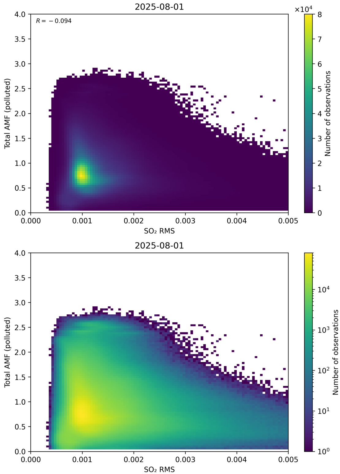
Figure 148: Scatter density plot of “SO 2 RMS” against “Total AMF (polluted)” for 2025-07-31 to 2025-08-02.
