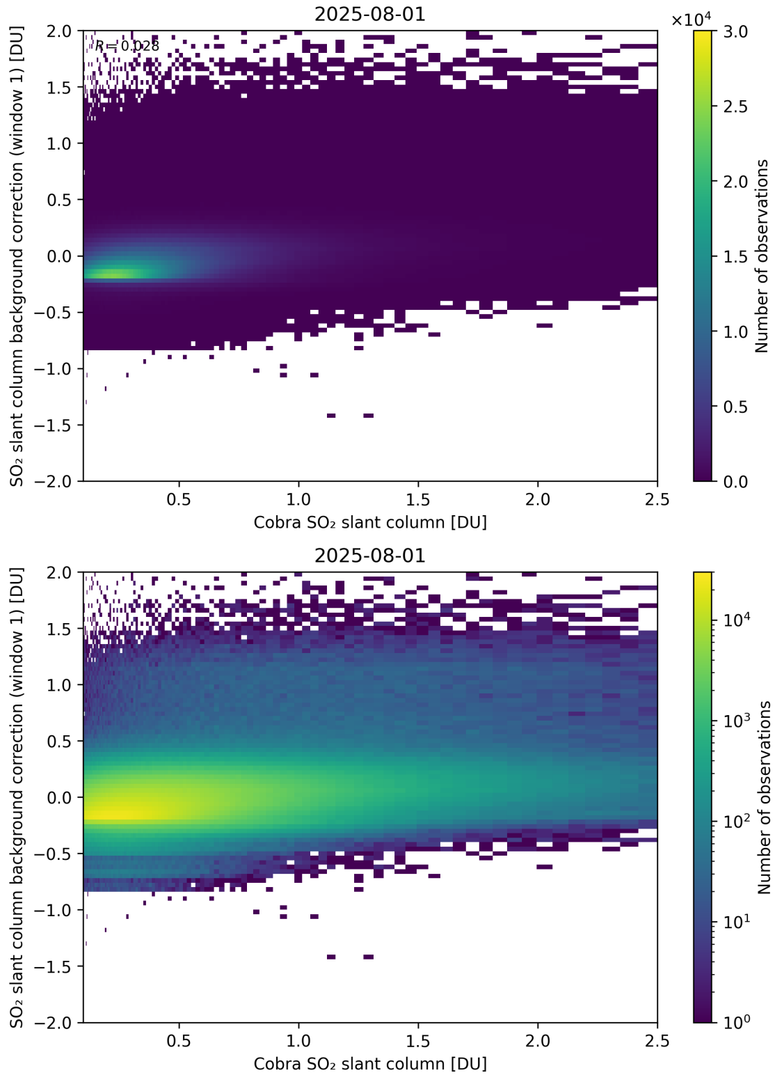
Figure 193: Scatter density plot of “Cobra SO 2 slant column” against “SO 2 slant column background correction (window 1)” for 2025-07-31 to 2025-08-02.
