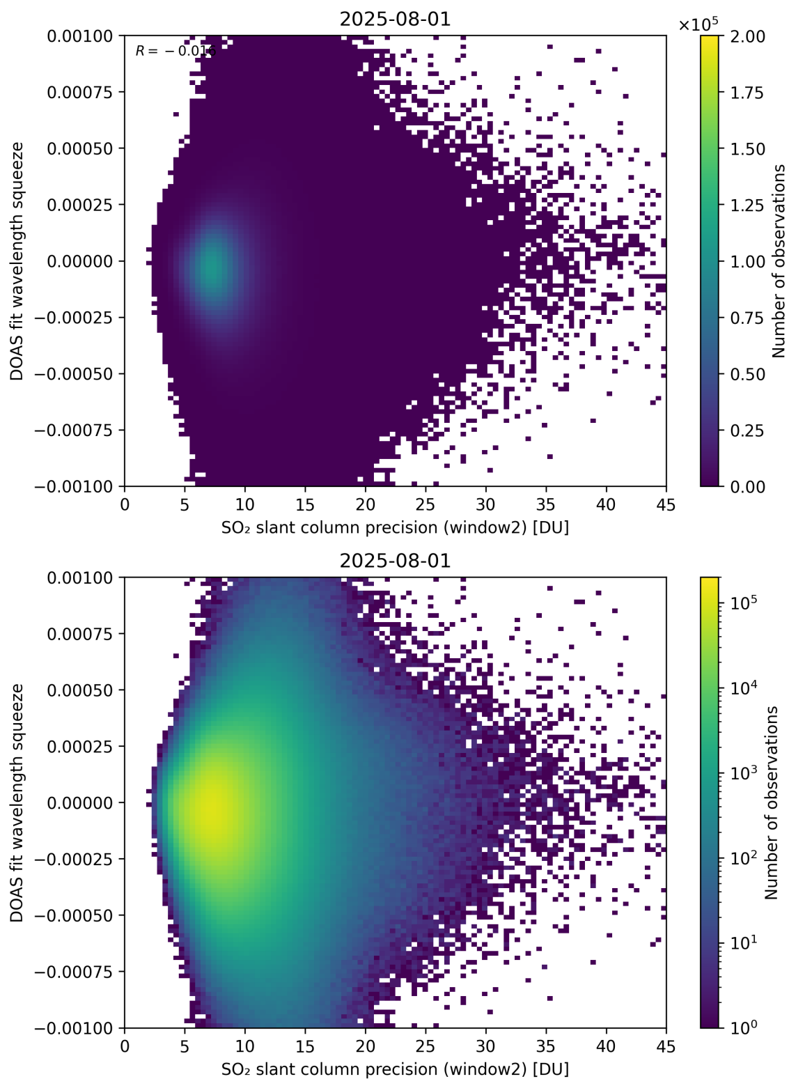
Figure 294: Scatter density plot of “SO 2 slant column precision (window2)” against “DOAS fit wavelength squeeze” for 2025-07-31 to 2025-08-02.
