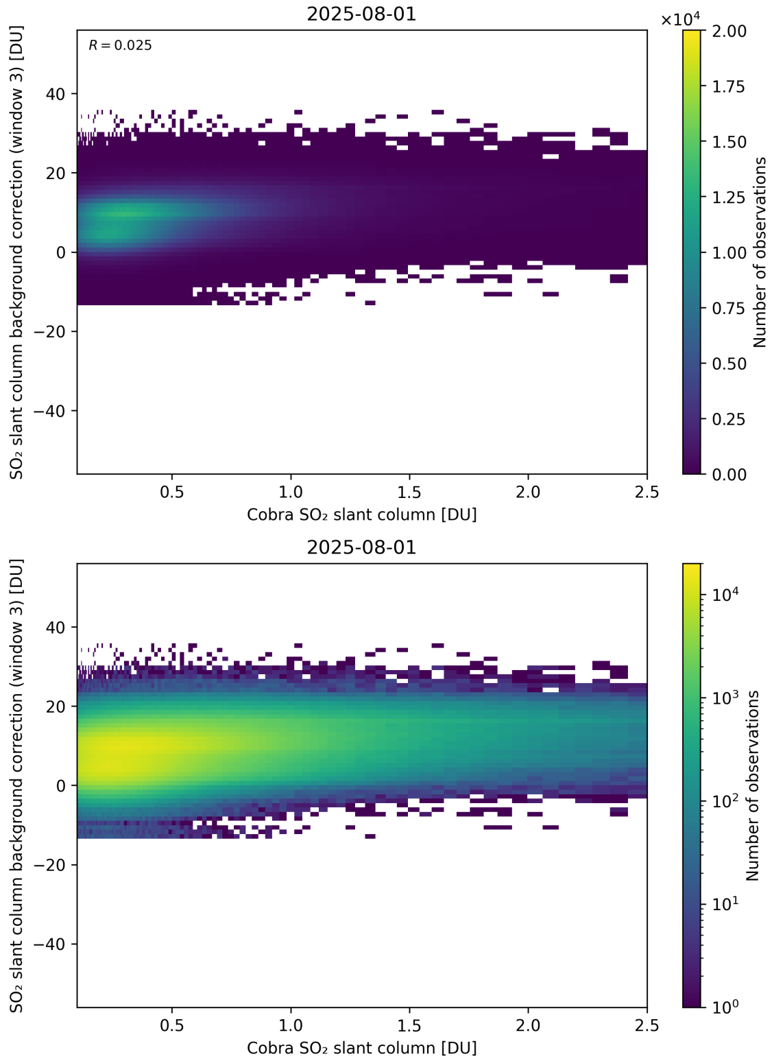
Figure 195: Scatter density plot of “Cobra SO 2 slant column” against “SO 2 slant column background correction (window 3)” for 2025-07-31 to 2025-08-02.
