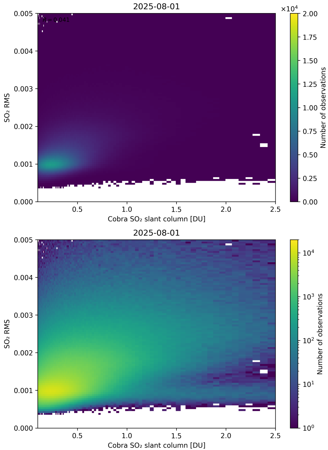
Figure 198: Scatter density plot of “Cobra SO 2 slant column” against “SO 2 RMS” for 2025-07-31 to 2025-08-02.
