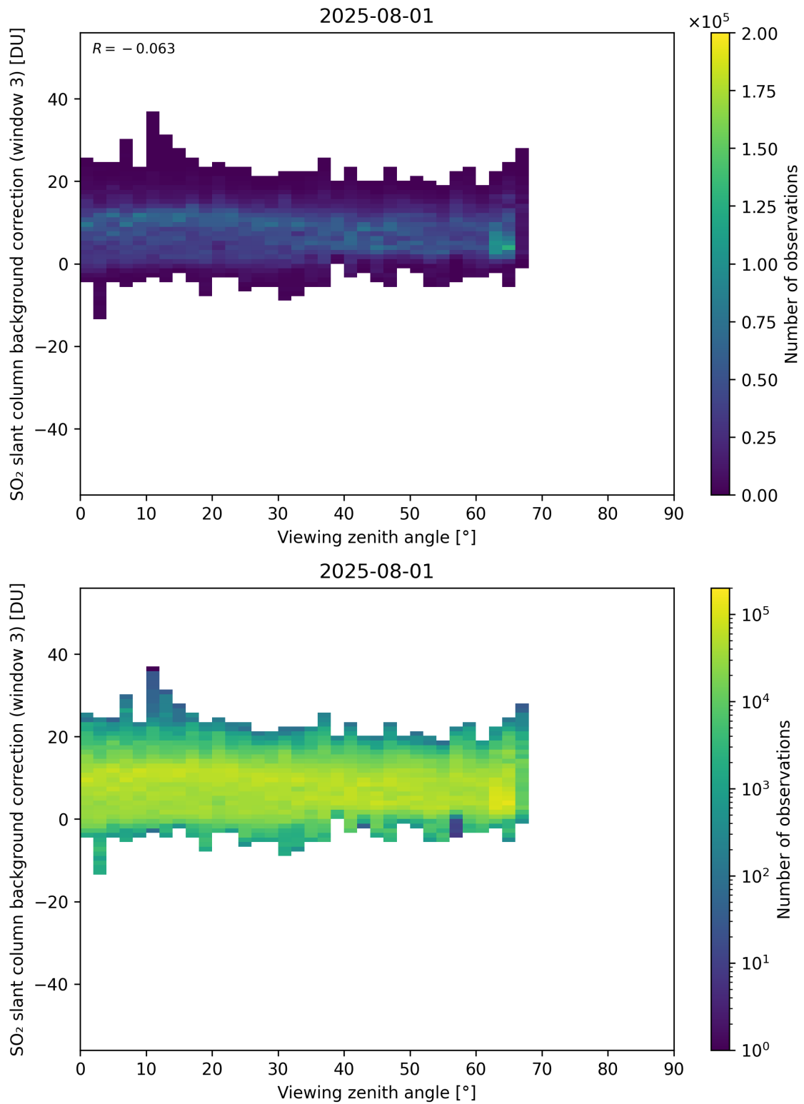
Figure 364: Scatter density plot of “Viewing zenith angle” against “SO 2 slant column background correction (window 3)” for 2025-07-31 to 2025-08-02.
