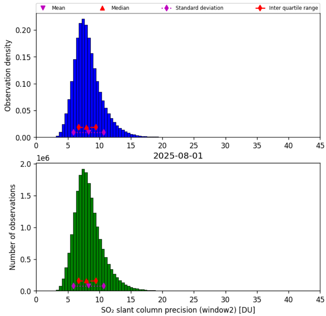
Figure 68: Histogram of “SO 2 slant column precision (window2)” for 2025-07-31 to 2025-08-02
