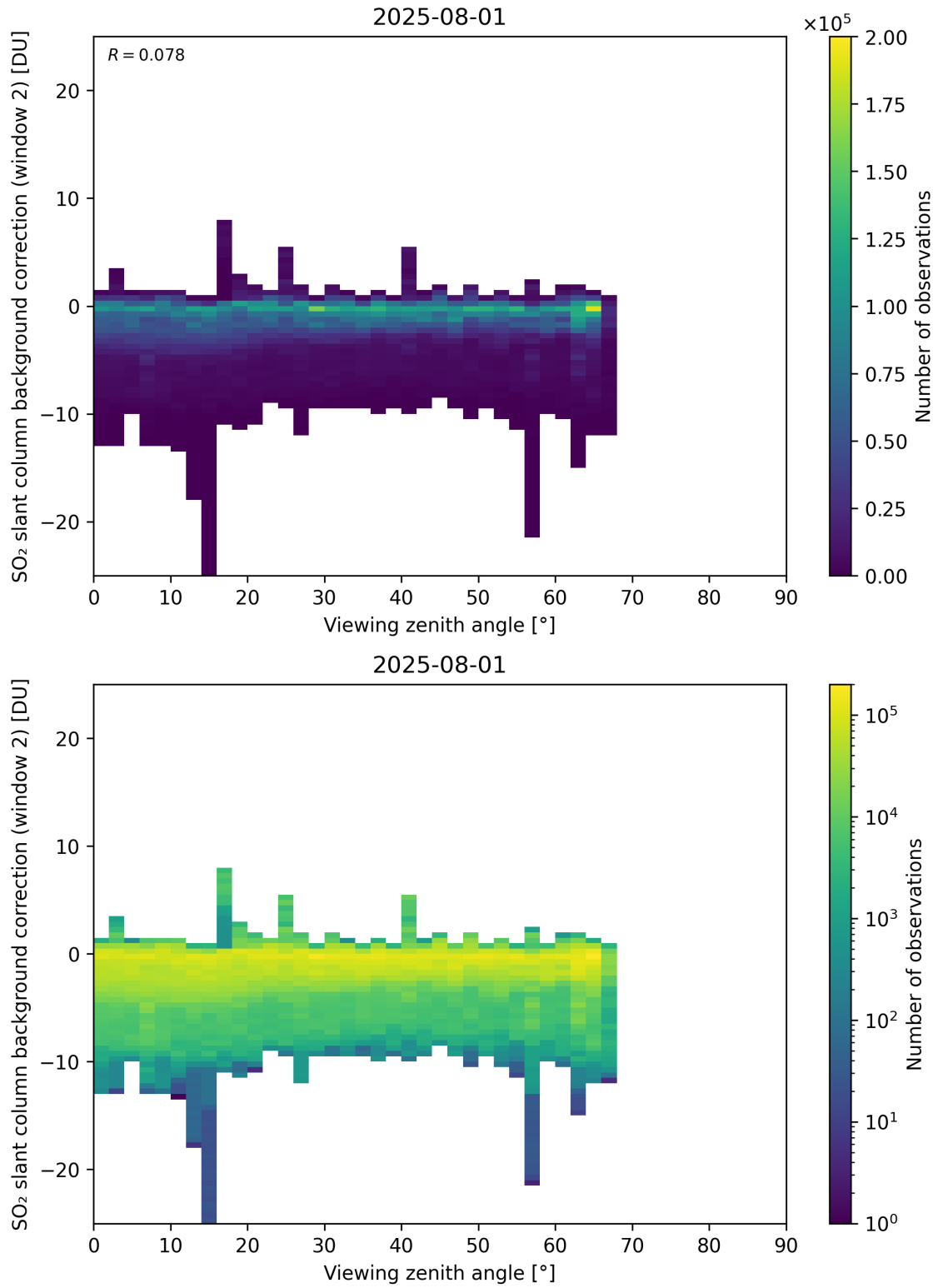
Figure 363: Scatter density plot of “Viewing zenith angle” against “SO 2 slant column background correction (window 2)” for 2025-07-31 to 2025-08-02.
