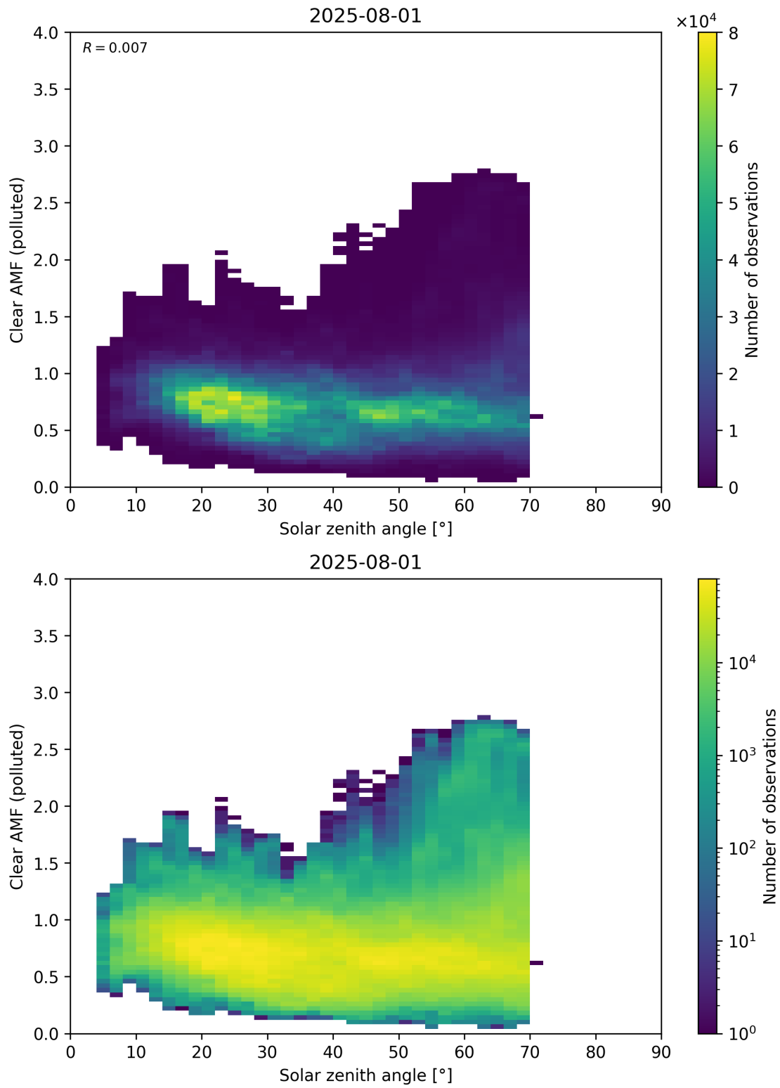
Figure 178: Scatter density plot of “Solar zenith angle” against “Clear AMF (polluted)” for 2025-07-31 to 2025-08-02.
