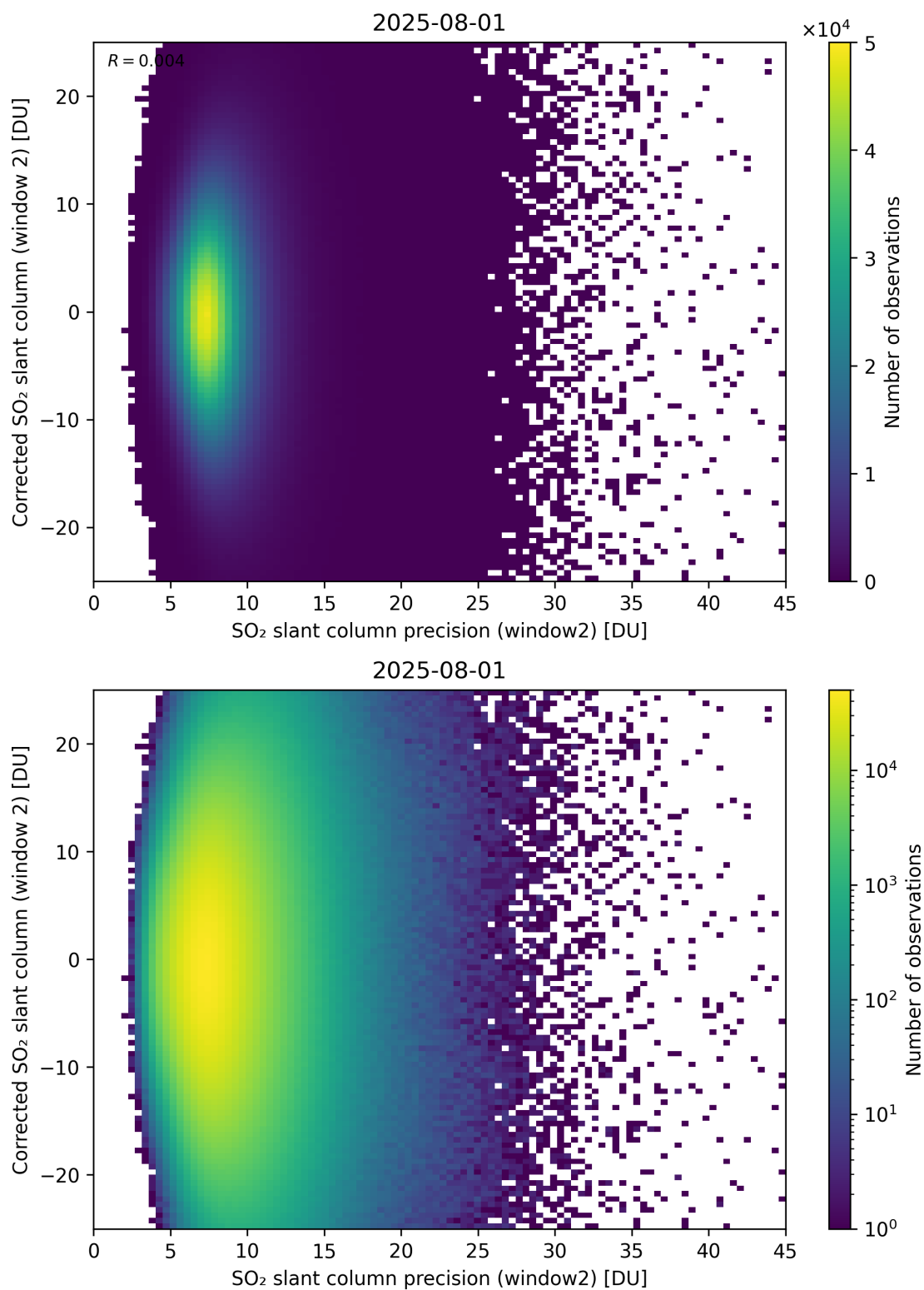
Figure 297: Scatter density plot of “SO 2 slant column precision (window2)” against “Corrected SO 2 slant column (window 2)” for 2025-07-31 to 2025-08-02.
