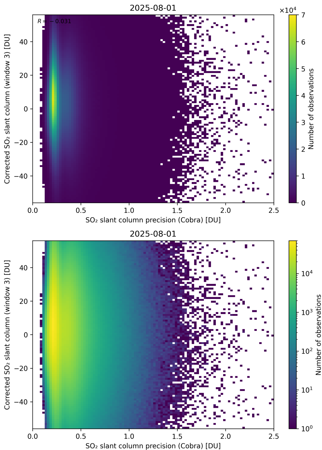
Figure 207: Scatter density plot of “SO 2 slant column precision (Cobra)” against “Corrected SO 2 slant column (window 3)” for 2025-07-31 to 2025-08-02.
