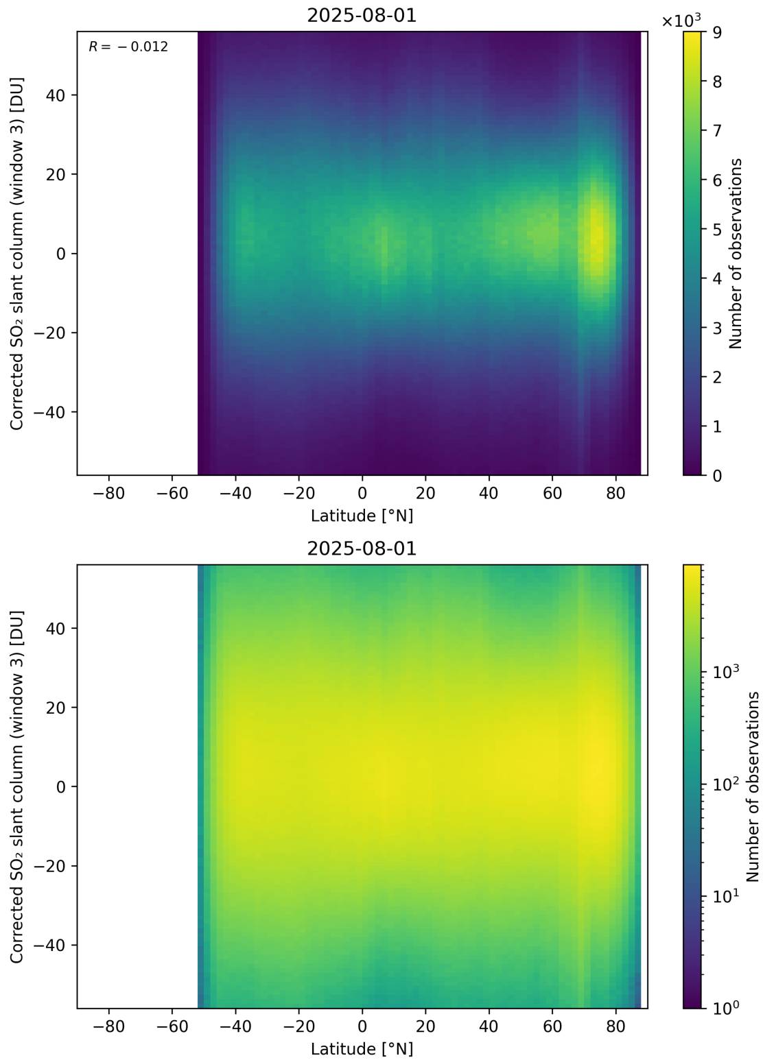
Figure 161: Scatter density plot of “Latitude” against “Corrected SO 2 slant column (window 3)” for 2025-07-31 to 2025-08-02.
