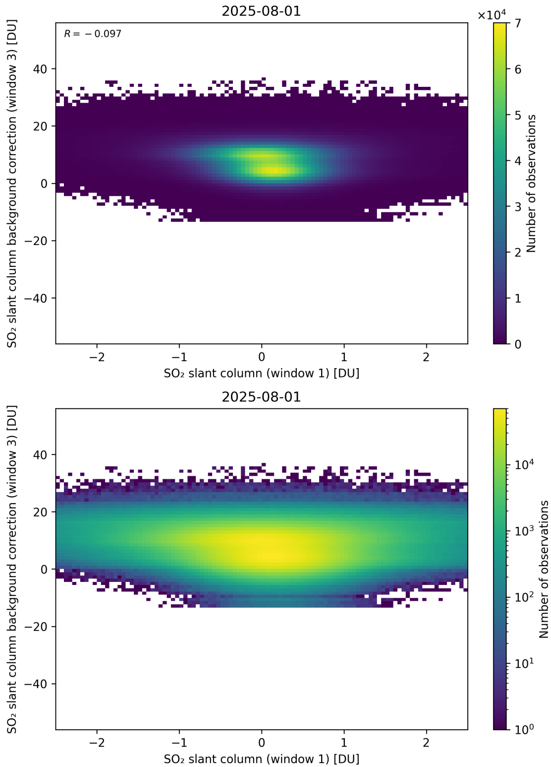
Figure 264: Scatter density plot of “SO 2 slant column (window 1)” against “SO 2 slant column background correction (window 3)” for 2025-07-31 to 2025-08-02.
