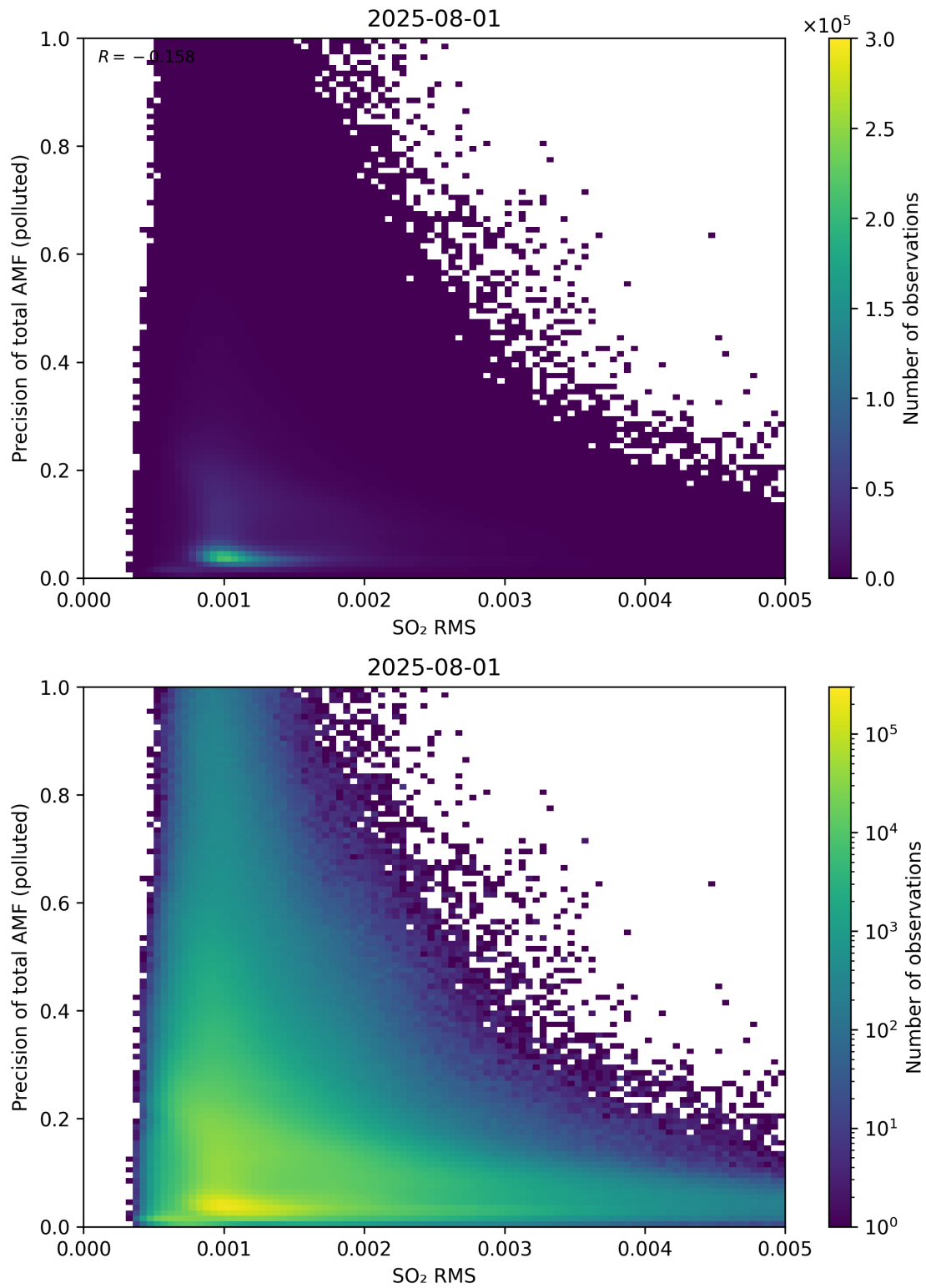
Figure 149: Scatter density plot of “SO 2 RMS” against “Precision of total AMF (polluted)” for 2025-07-31 to 2025-08-02.
