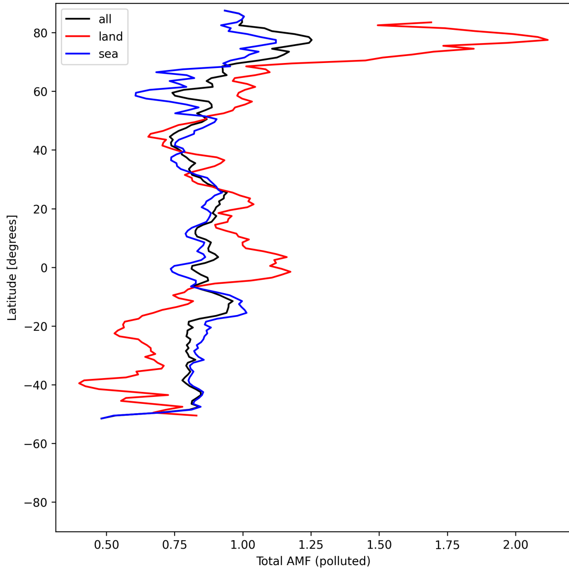
Figure 53: Zonal average of “Total AMF (polluted)” for 2025-07-31 to 2025-08-02.
