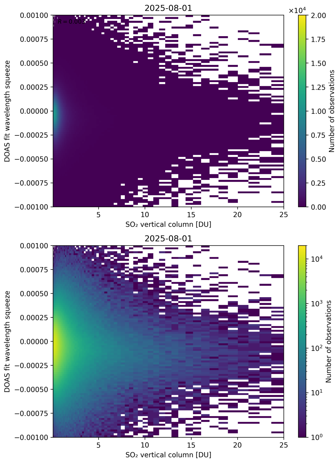
Figure 327: Scatter density plot of “SO 2 vertical column” against “DOAS fit wavelength squeeze” for 2025-07-31 to 2025-08-02.
