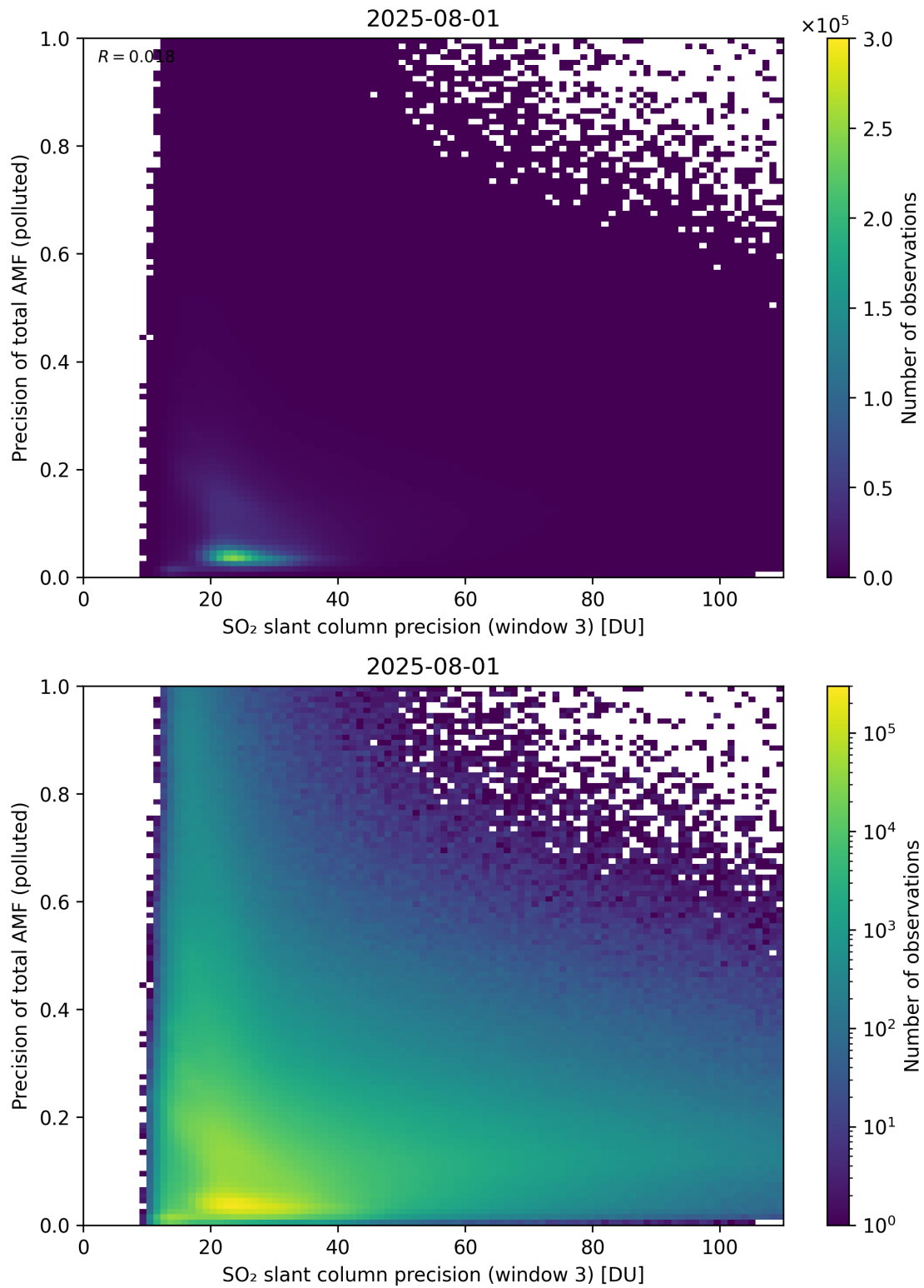
Figure 314: Scatter density plot of “SO 2 slant column precision (window 3)” against “Precision of total AMF (polluted)” for 2025-07-31 to 2025-08-02.
