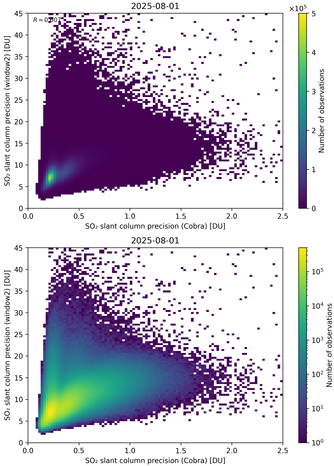
Figure 210: Scatter density plot of “SO 2 slant column precision (Cobra)” against “SO 2 slant column precision (window2)” for 2025-07-31 to 2025-08-02.
