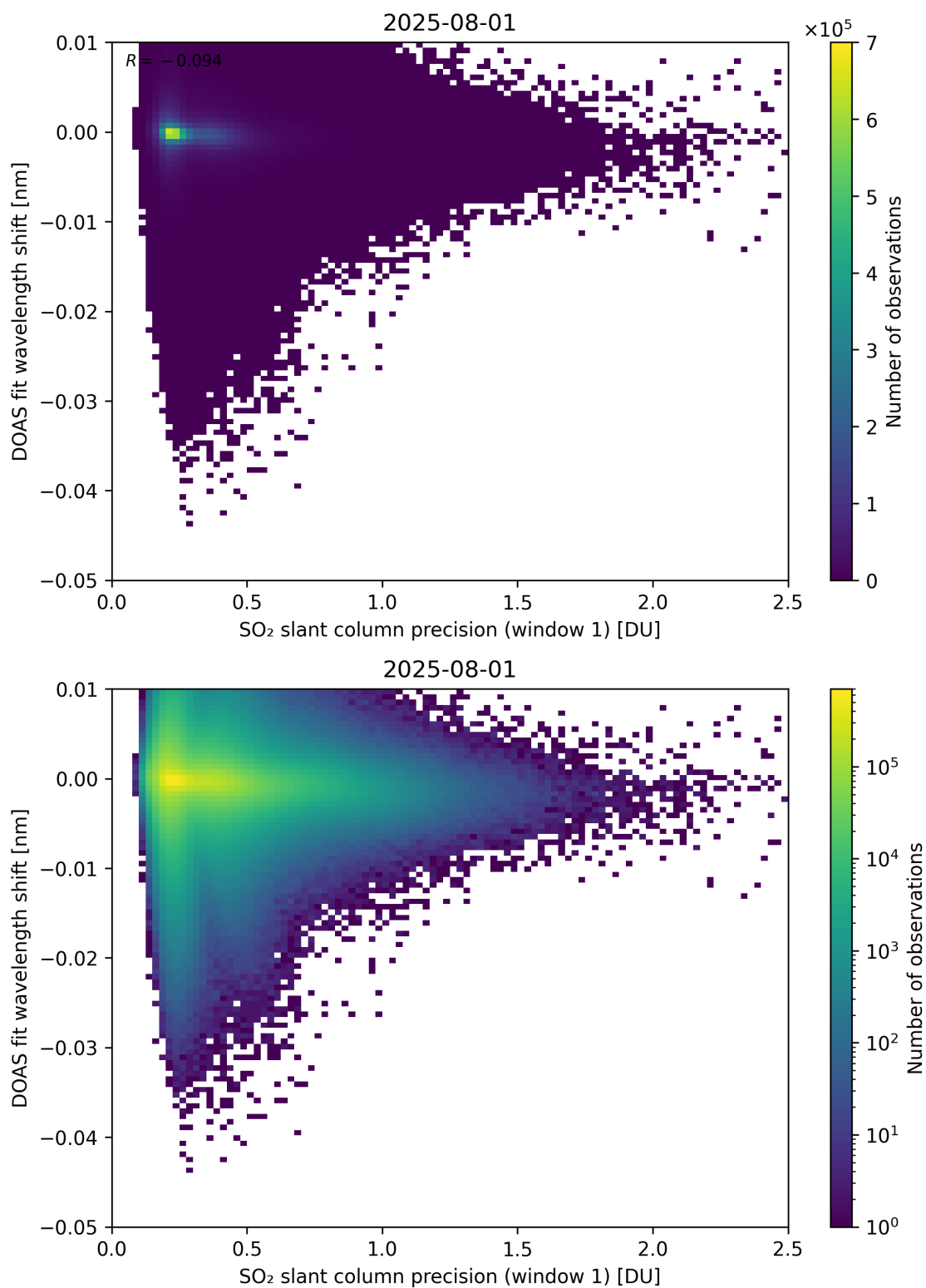
Figure 271: Scatter density plot of “SO 2 slant column precision (window 1)” against “DOAS fit wavelength shift” for 2025-07-31 to 2025-08-02.
