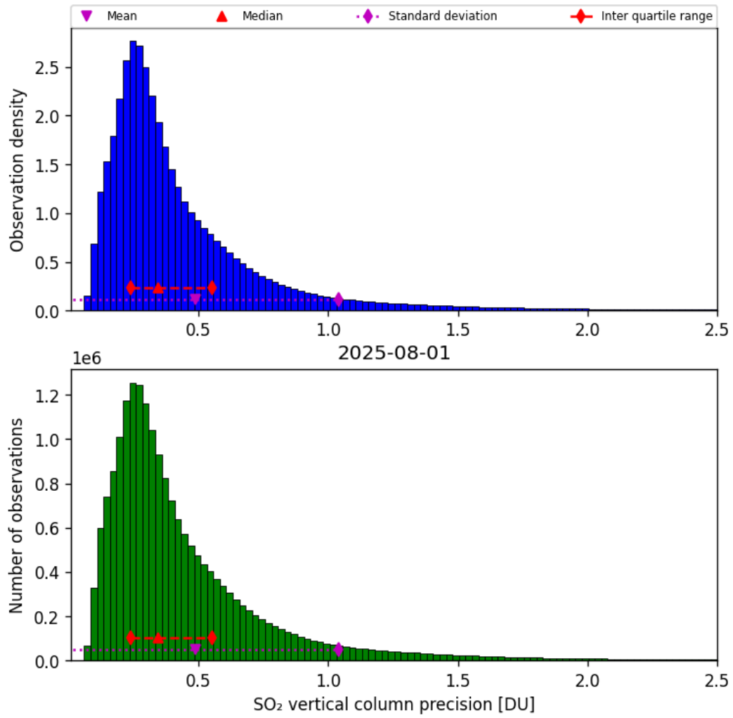
Figure 59: Histogram of “SO 2 vertical column precision” for 2025-07-31 to 2025-08-02
