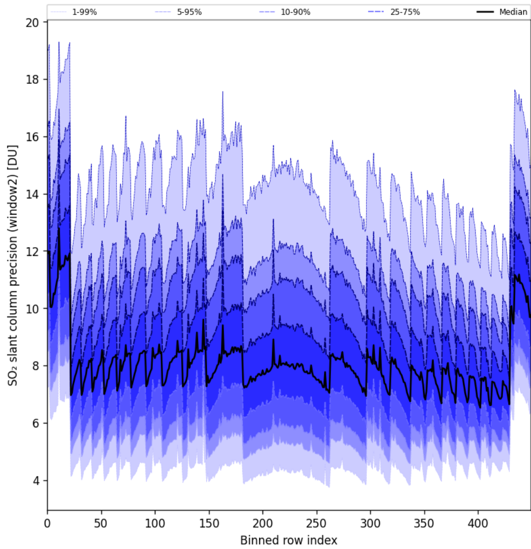
Figure 94: Along track statistics of “SO 2 slant column precision (window2)” for 2025-07-31 to 2025-08-02
