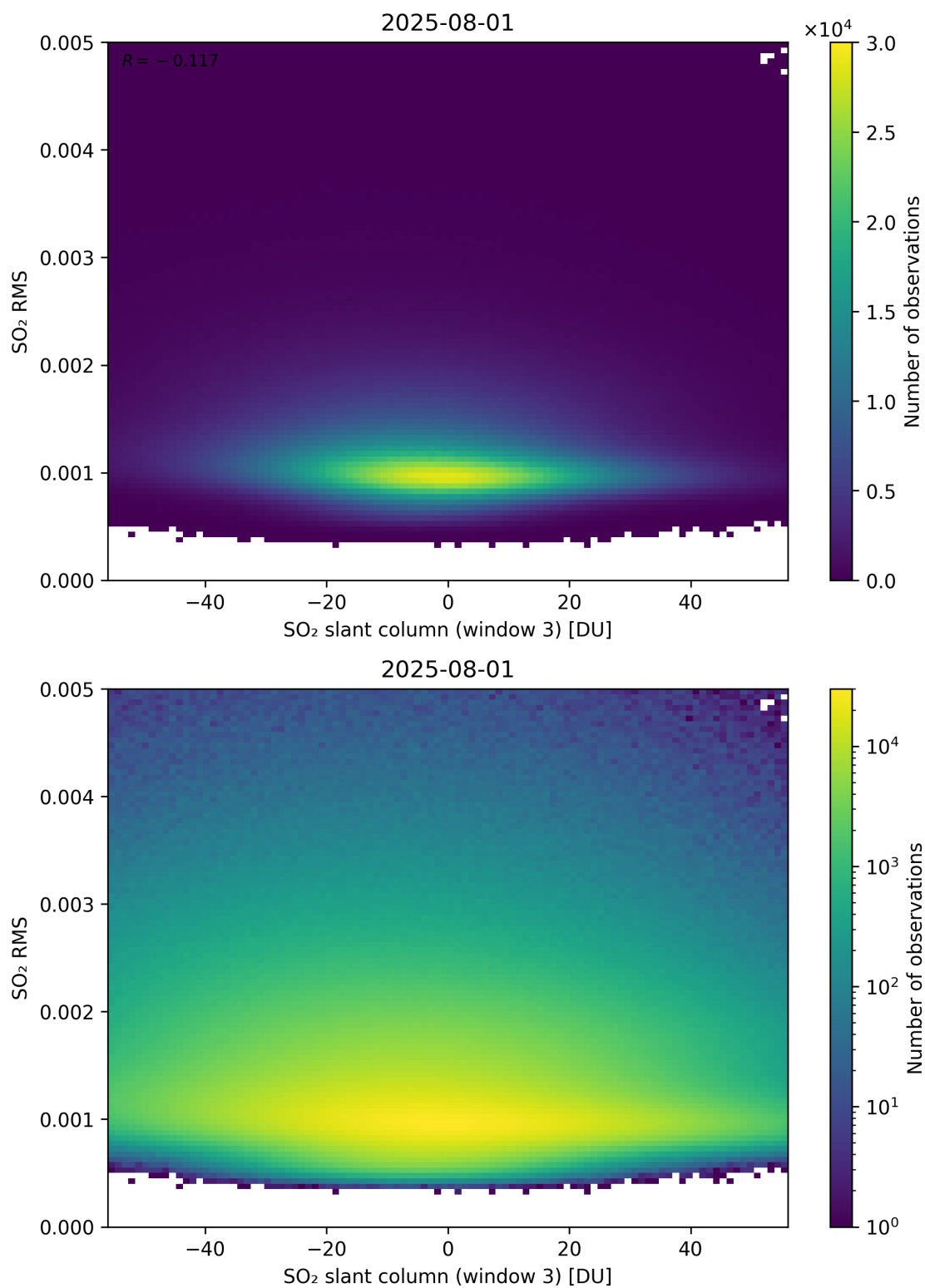
Figure 306: Scatter density plot of “SO 2 slant column (window 3)” against “SO 2 RMS” for 2025-07-31 to 2025-08-02.
