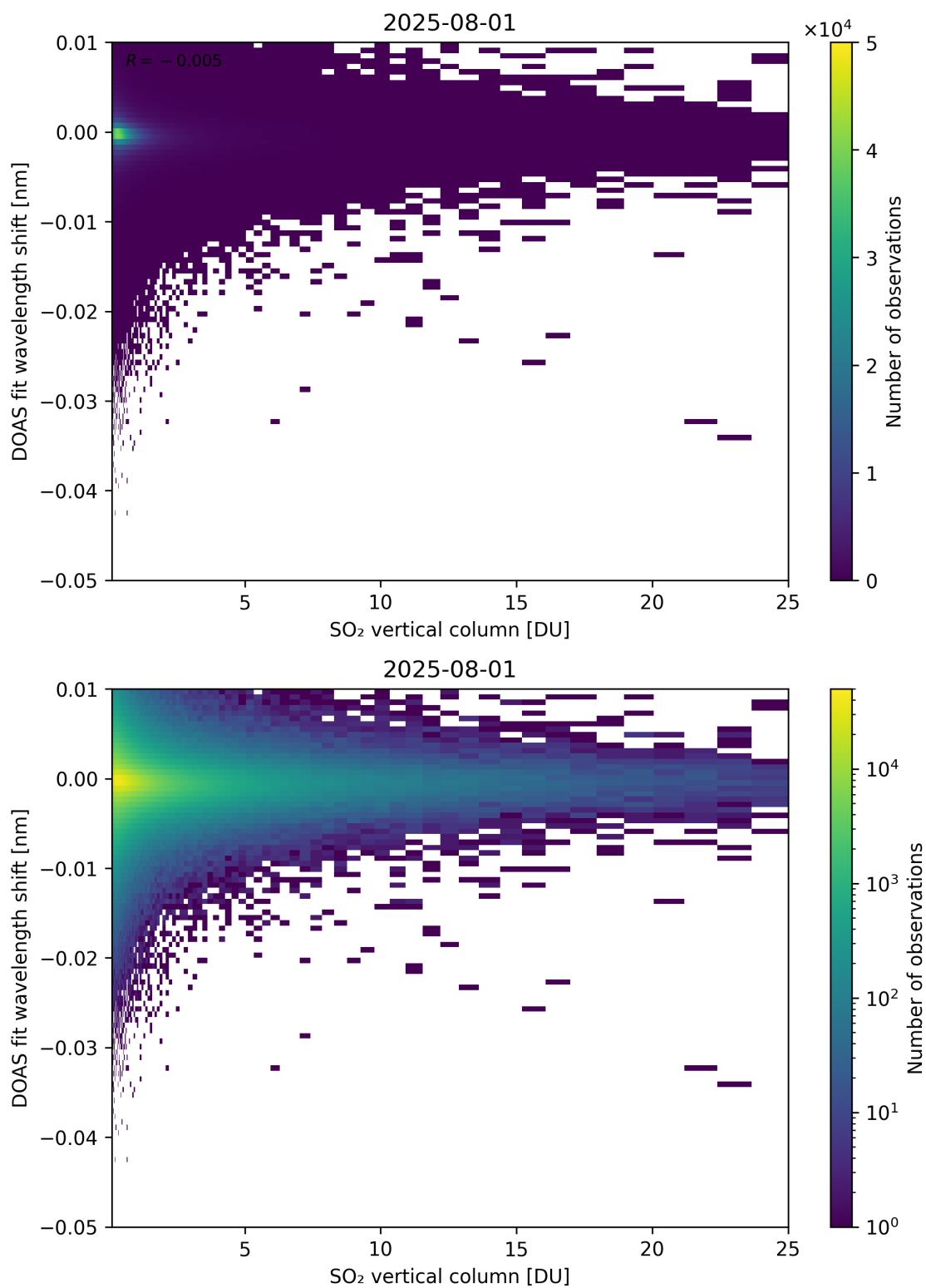
Figure 326: Scatter density plot of “SO 2 vertical column” against “DOAS fit wavelength shift” for 2025-07-31 to 2025-08-02.
