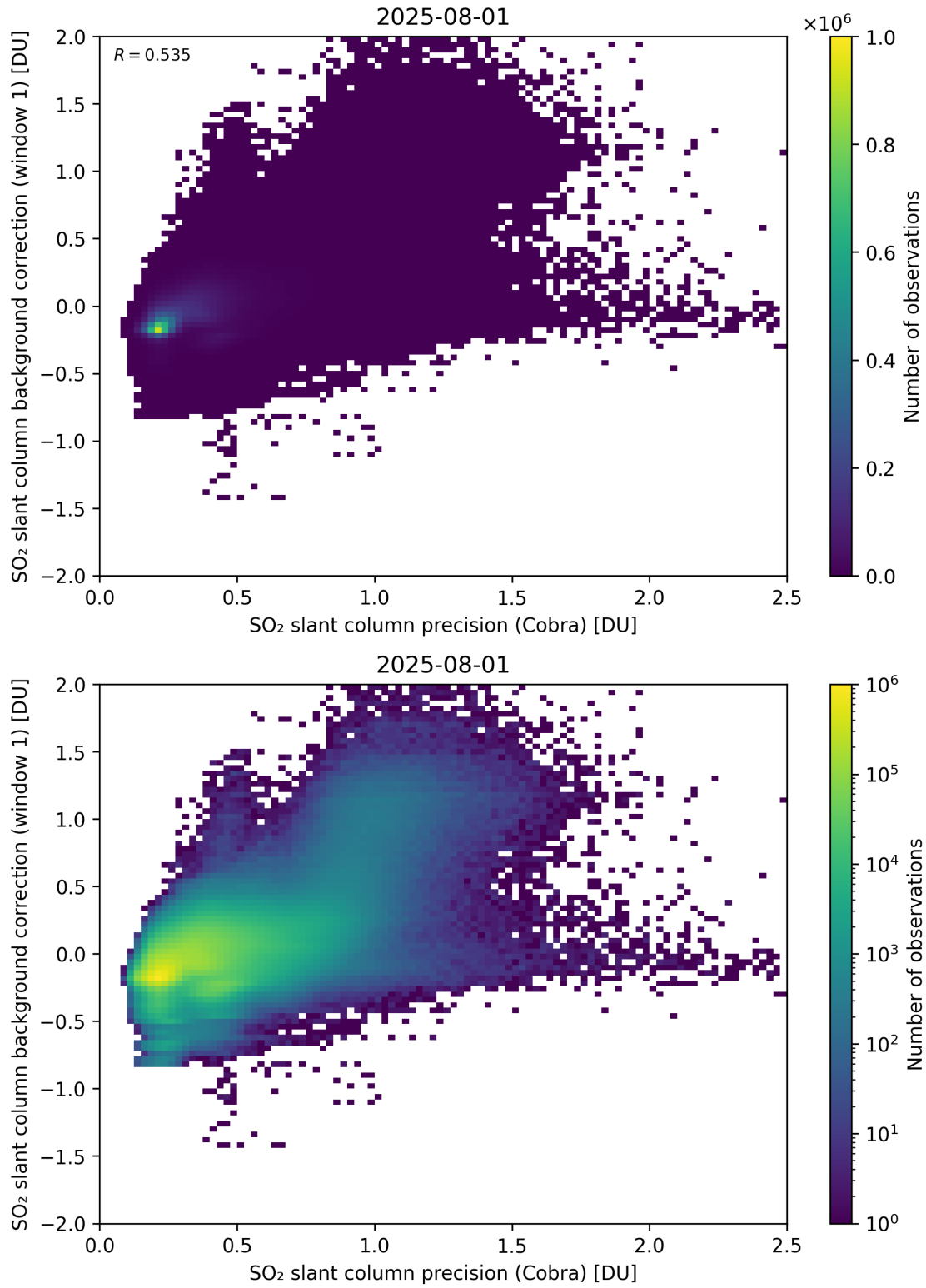
Figure 199: Scatter density plot of “SO 2 slant column precision (Cobra)” against “SO 2 slant column background correction (window 1)” for 2025-07-31 to 2025-08-02.
