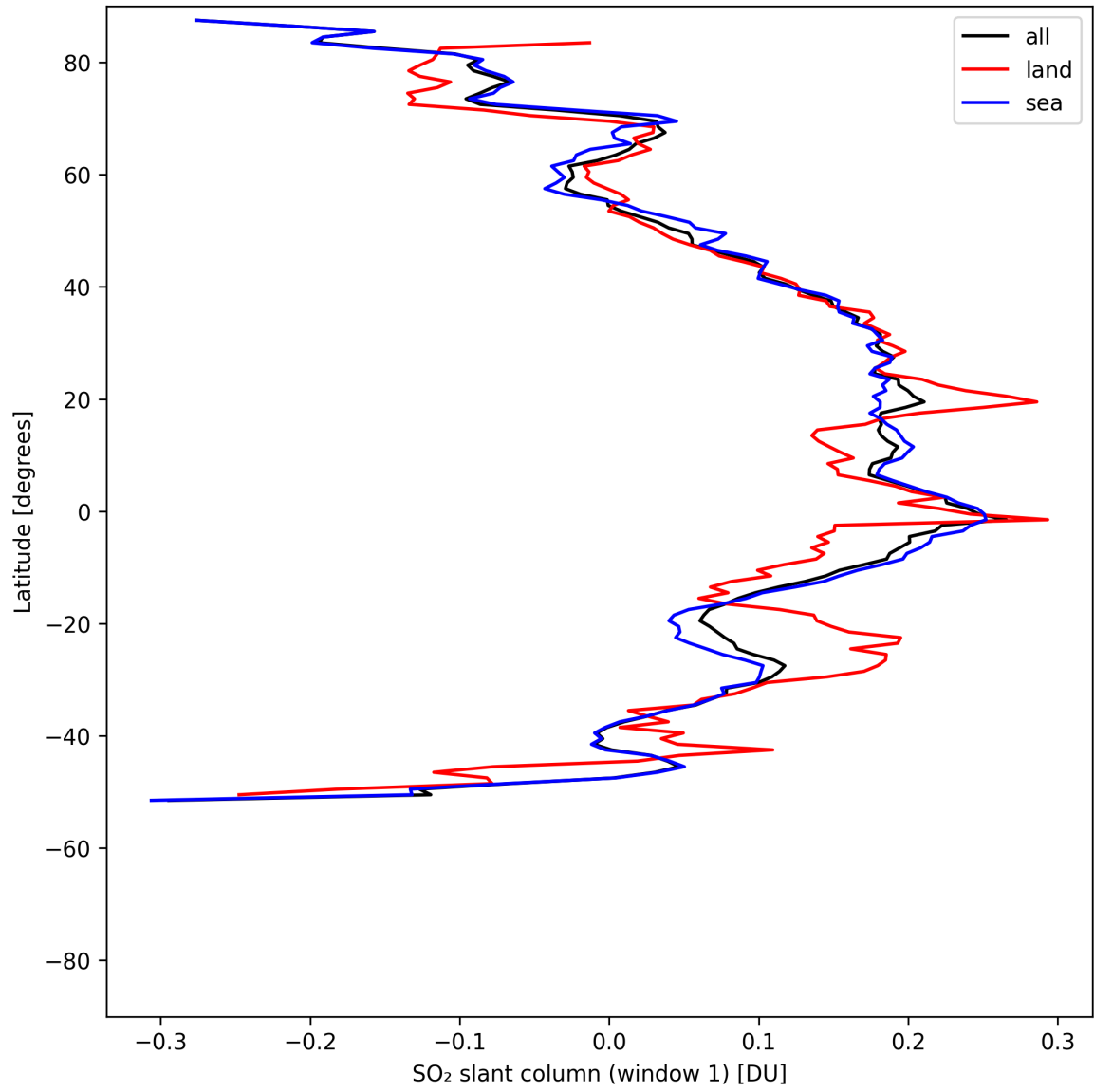
Figure 37: Zonal average of “SO 2 slant column (window 1)” for 2025-07-31 to 2025-08-02.
