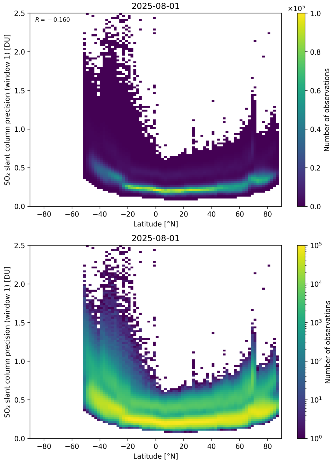
Figure 163: Scatter density plot of “Latitude” against “SO 2 slant column precision (window 1)” for 2025-07-31 to 2025-08-02.
