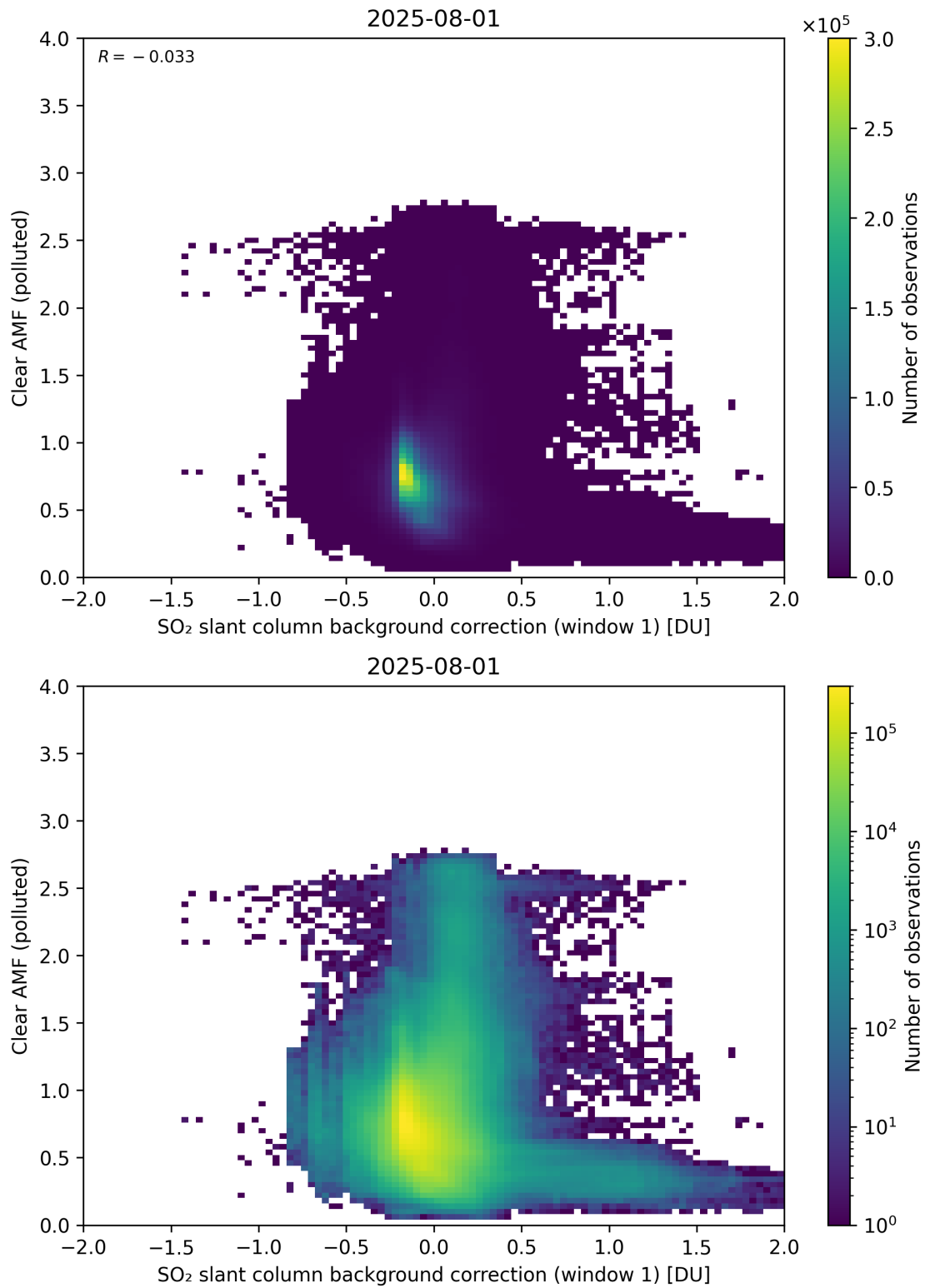
Figure 114: Scatter density plot of “SO 2 slant column background correction (window 1)” against “Clear AMF (polluted)” for 2025-07-31 to 2025-08-02.
