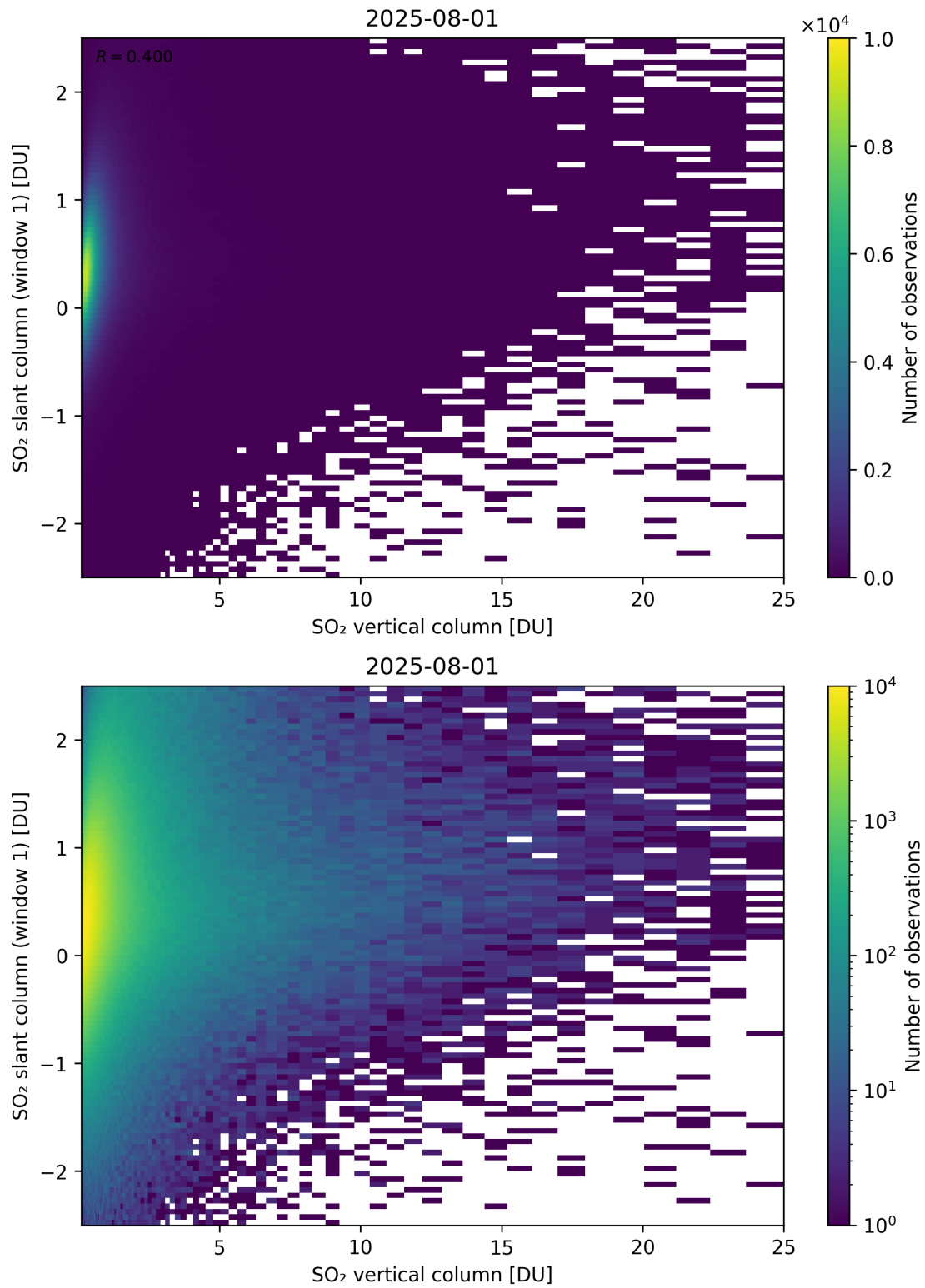
Figure 354: Scatter density plot of “SO 2 vertical column” against “SO 2 slant column (window 1)” for 2025-07-31 to 2025-08-02.
