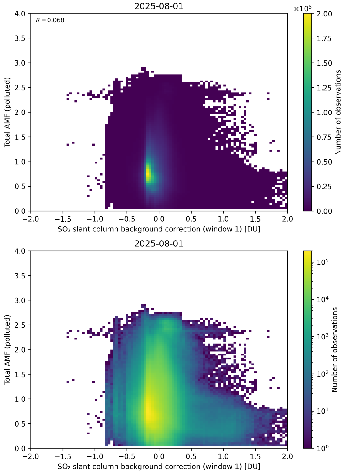
Figure 120: Scatter density plot of “SO 2 slant column background correction (window 1)” against “Total AMF (polluted)” for 2025-07-31 to 2025-08-02.
