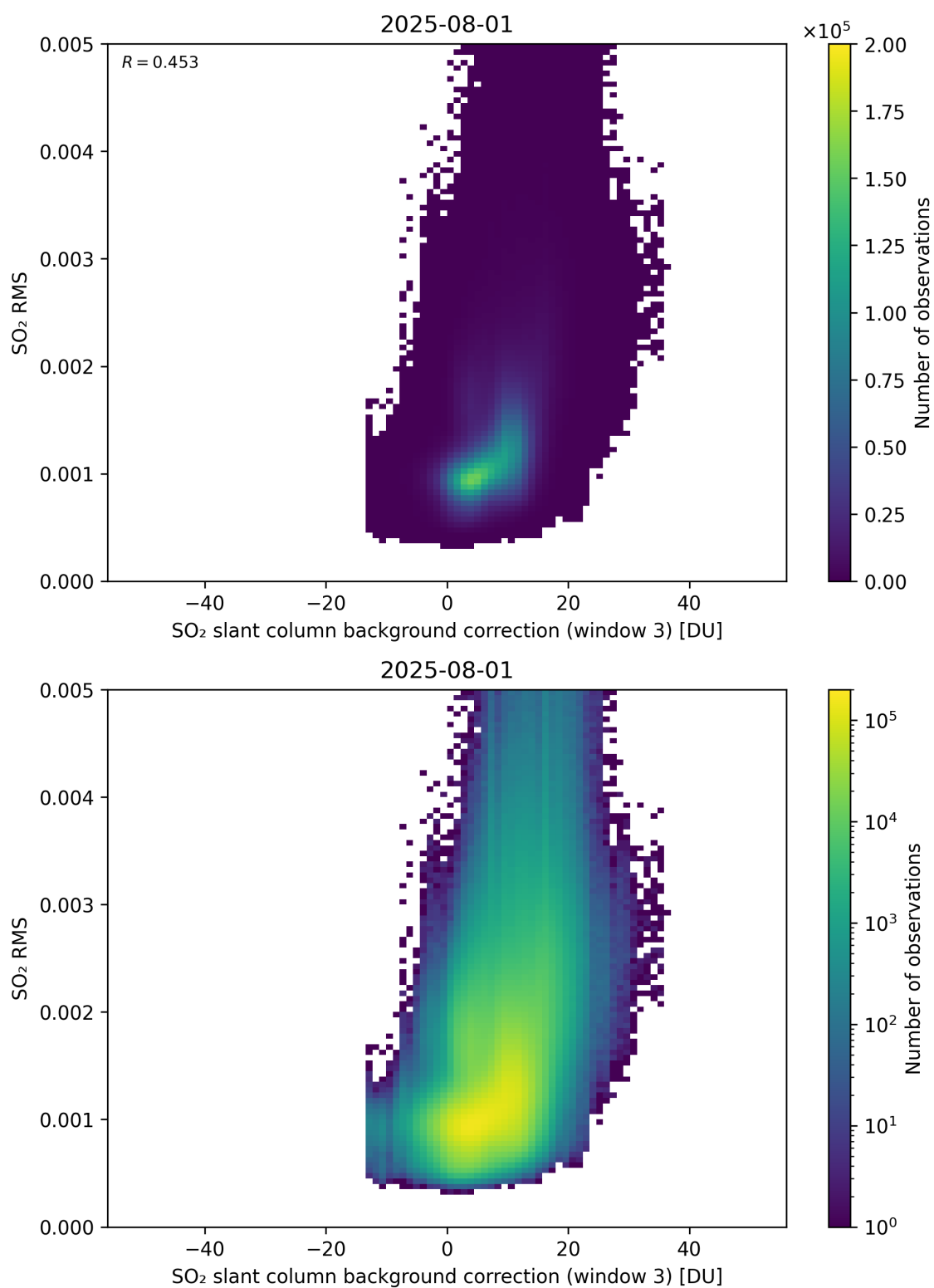
Figure 134: Scatter density plot of “SO 2 slant column background correction (window 3)” against “SO 2 RMS” for 2025-07-31 to 2025-08-02.
