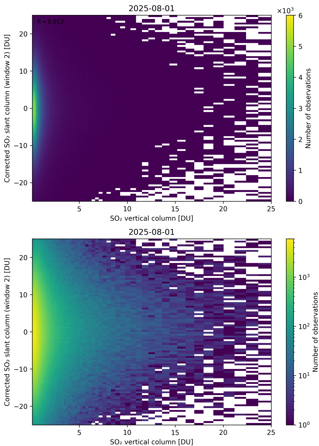
Figure 352: Scatter density plot of “SO 2 vertical column” against “Corrected SO 2 slant column (window 2)” for 2025-07-31 to 2025-08-02.
