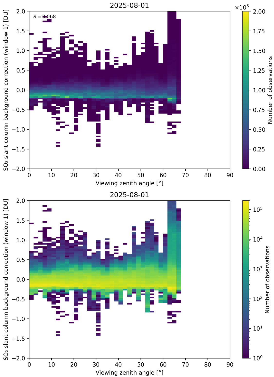
Figure 362: Scatter density plot of “Viewing zenith angle” against “SO 2 slant column background correction (window 1)” for 2025-07-31 to 2025-08-02.
