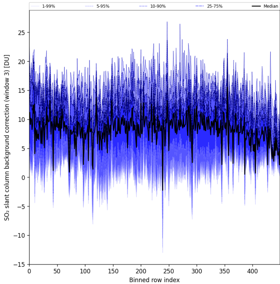
Figure 100: Along track statistics of “SO 2 slant column background correction (window 3)” for 2025-07-31 to 2025-08-02
