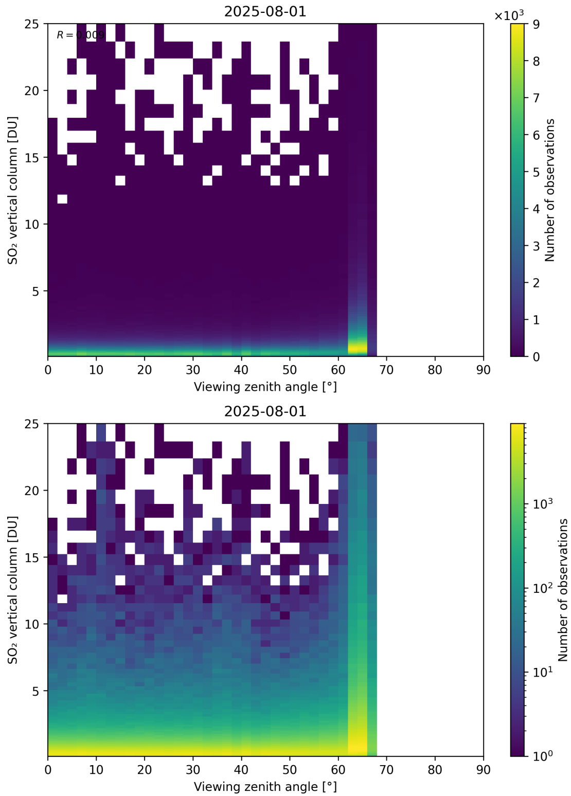
Figure 383: Scatter density plot of “Viewing zenith angle” against “SO 2 vertical column” for 2025-07-31 to 2025-08-02.
