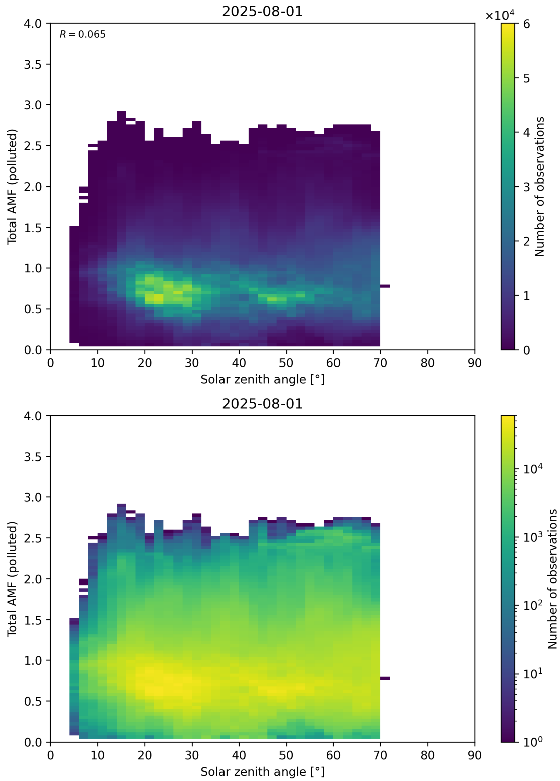
Figure 189: Scatter density plot of “Solar zenith angle” against “Total AMF (polluted)” for 2025-07-31 to 2025-08-02.
