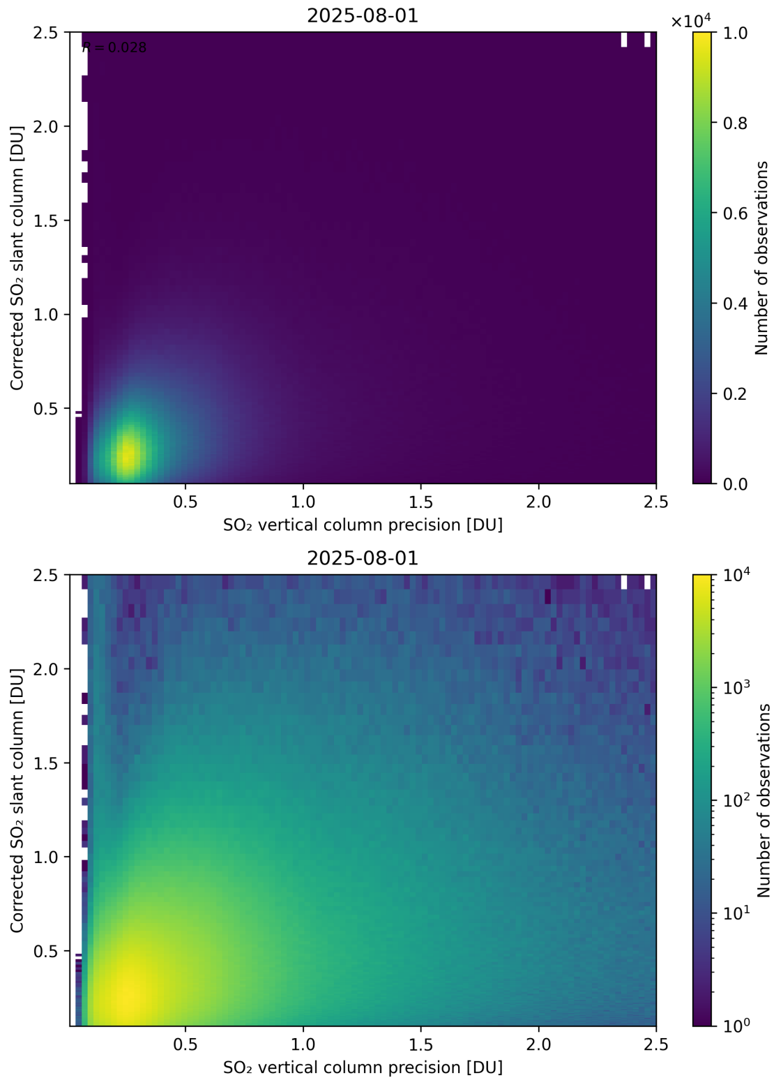
Figure 338: Scatter density plot of “SO 2 vertical column precision” against “Corrected SO 2 slant column” for 2025-07-31 to 2025-08-02.
