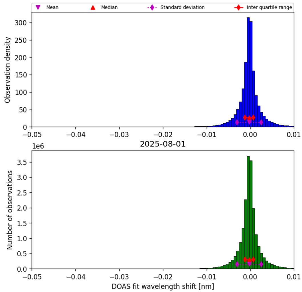
Figure 76: Histogram of “DOAS fit wavelength shift” for 2025-07-31 to 2025-08-02
