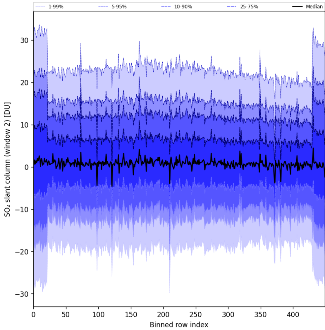
Figure 93: Along track statistics of “SO 2 slant column (window 2)” for 2025-07-31 to 2025-08-02
