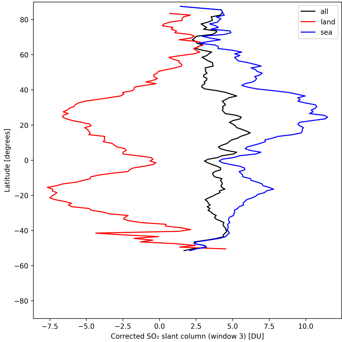
Figure 47: Zonal average of “Corrected SO 2 slant column (window 3)” for 2025-07-31 to 2025-08-02.
