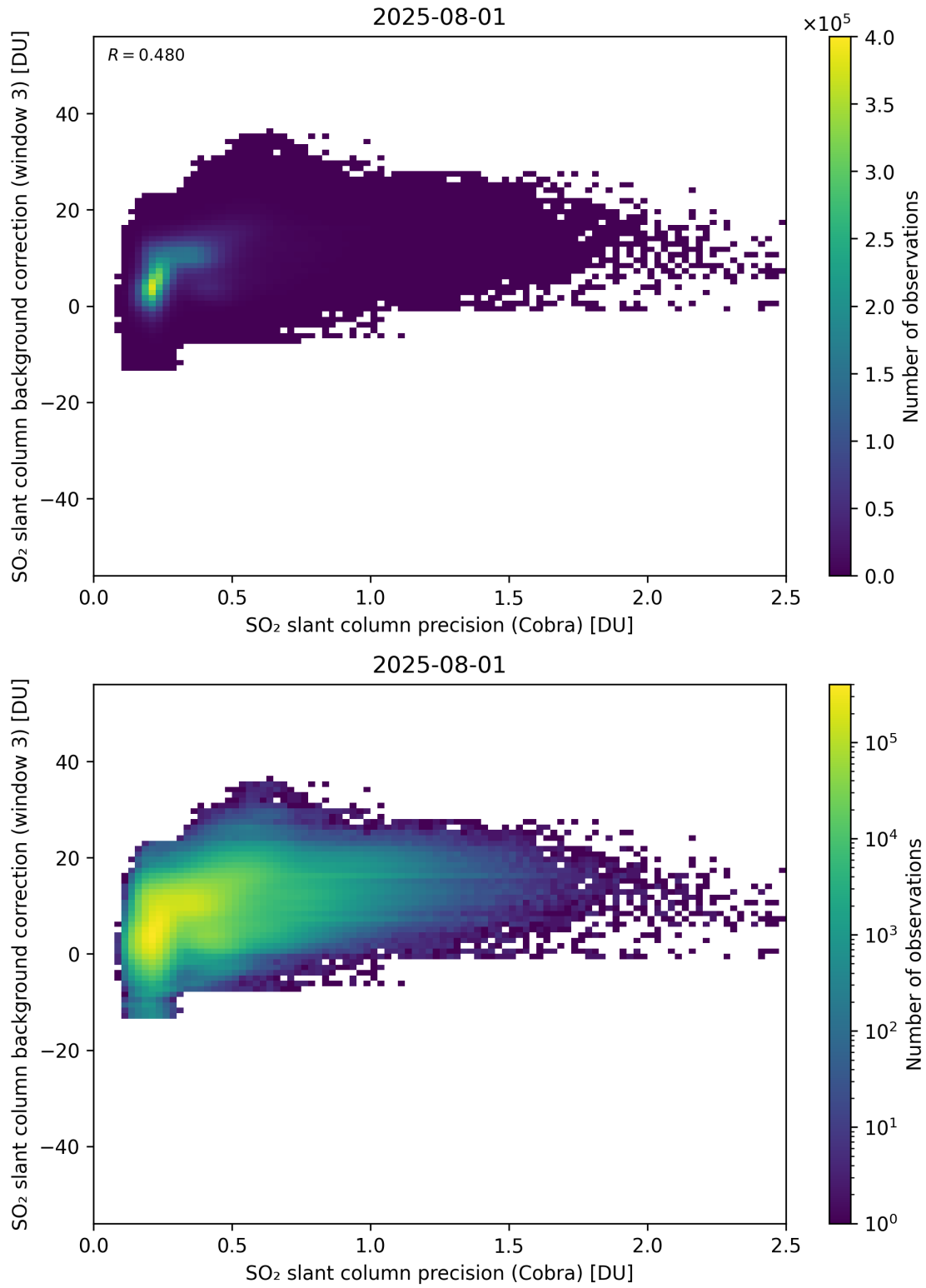
Figure 201: Scatter density plot of “SO 2 slant column precision (Cobra)” against “SO 2 slant column background correction (window 3)” for 2025-07-31 to 2025-08-02.
