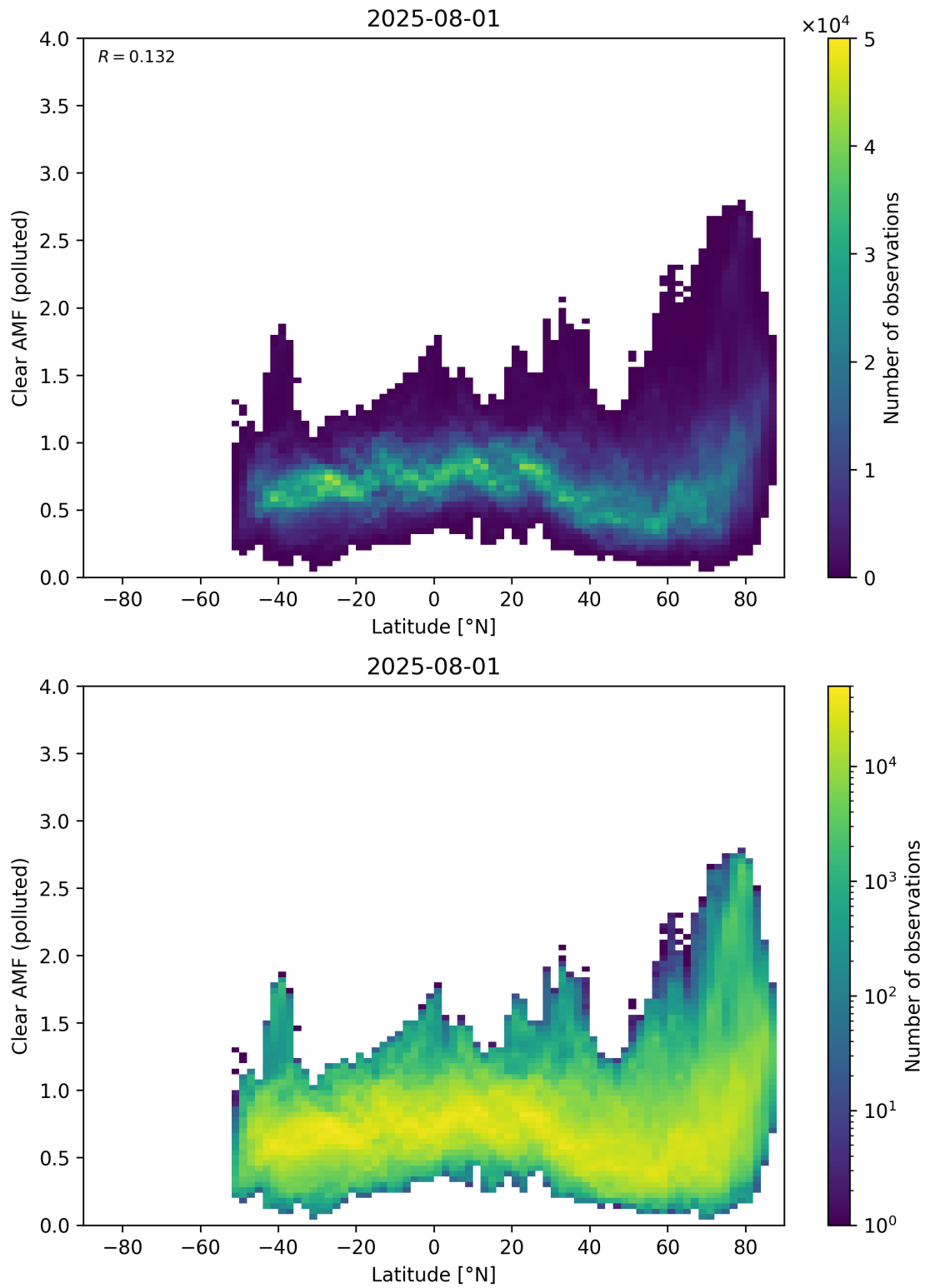
Figure 156: Scatter density plot of “Latitude” against “Clear AMF (polluted)” for 2025-07-31 to 2025-08-02.
