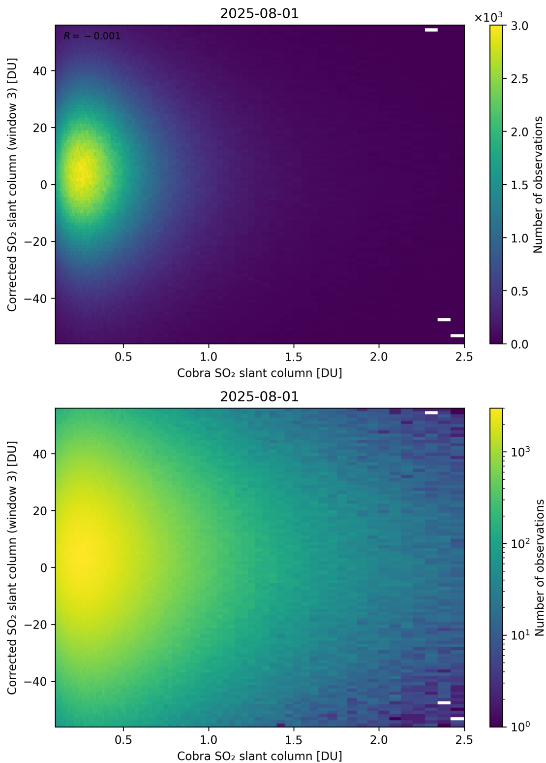
Figure 218: Scatter density plot of “Cobra SO 2 slant column” against “Corrected SO 2 slant column (window 3)” for 2025-07-31 to 2025-08-02.
