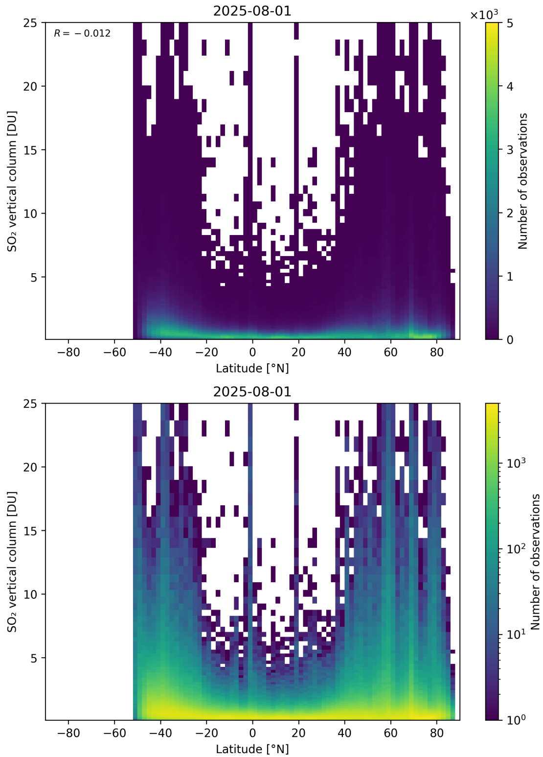
Figure 169: Scatter density plot of “Latitude” against “SO 2 vertical column” for 2025-07-31 to 2025-08-02.
