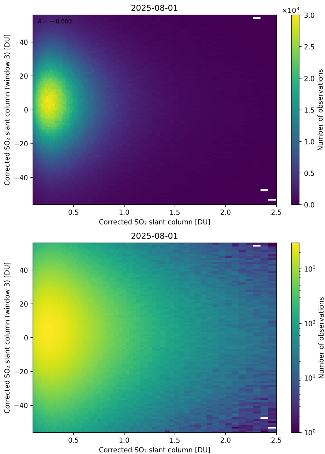
Figure 236: Scatter density plot of “Corrected SO 2 slant column” against “Corrected SO 2 slant column (window 3)” for 2025-07-31 to 2025-08-02.
