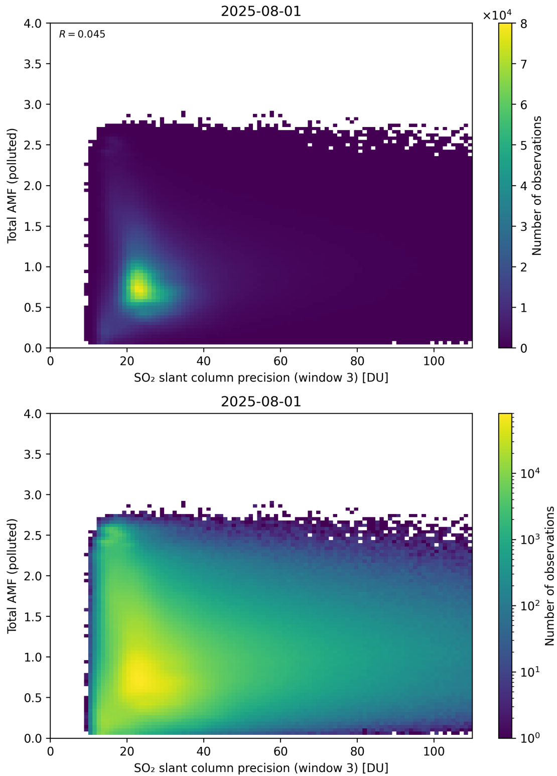
Figure 313: Scatter density plot of “SO 2 slant column precision (window 3)” against “Total AMF (polluted)” for 2025-07-31 to 2025-08-02.
