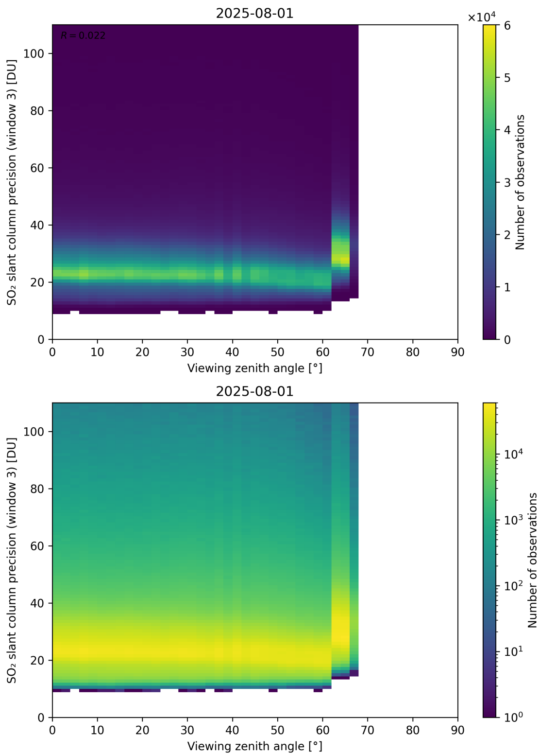
Figure 380: Scatter density plot of “Viewing zenith angle” against “SO 2 slant column precision (window 3)” for 2025-07-31 to 2025-08-02.
