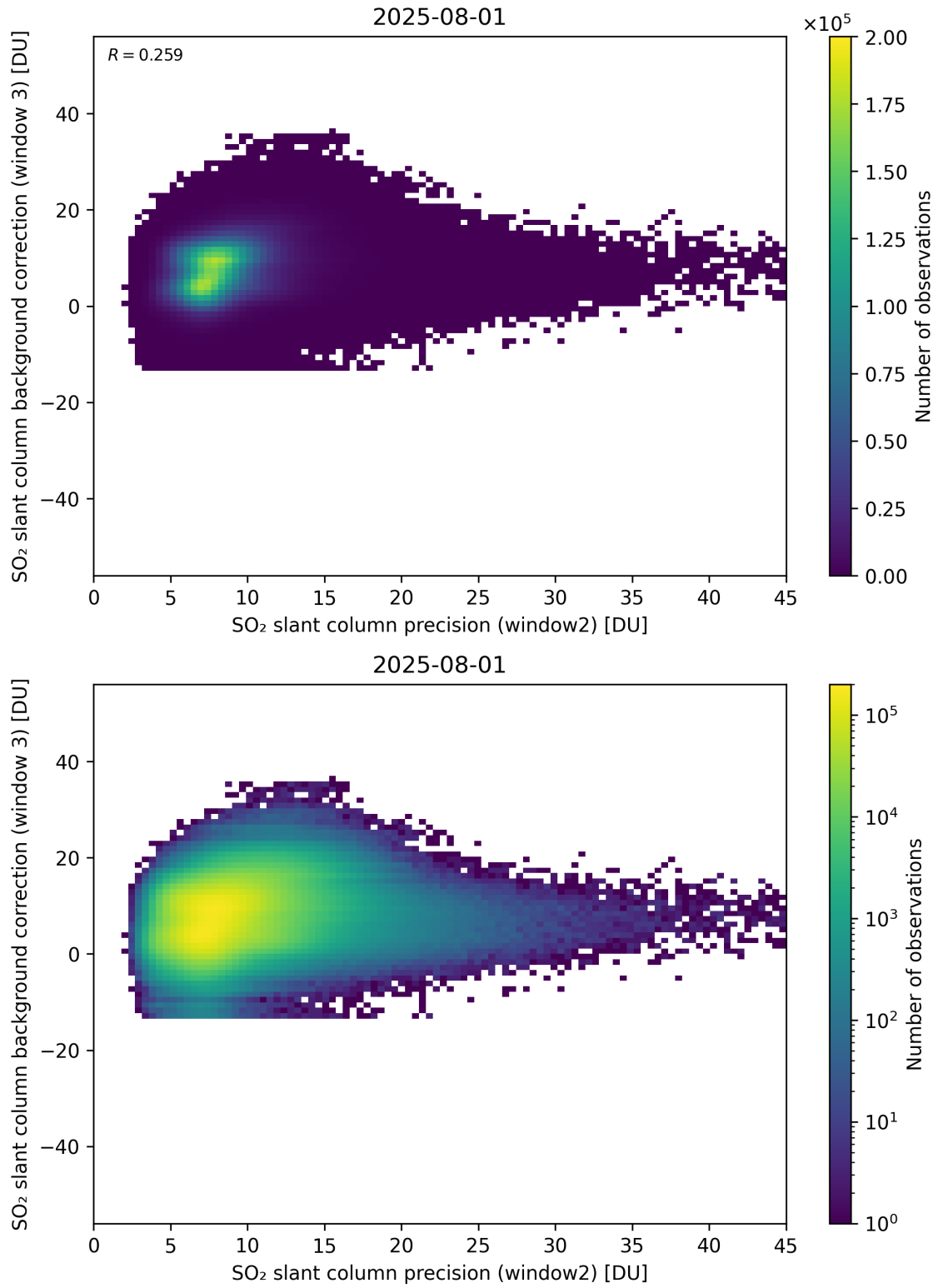
Figure 292: Scatter density plot of “SO 2 slant column precision (window2)” against “SO 2 slant column background correction (window 3)” for 2025-07-31 to 2025-08-02.
