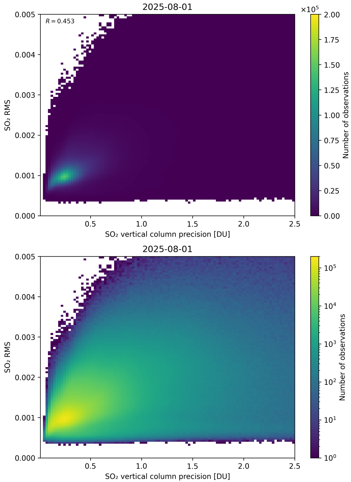
Figure 334: Scatter density plot of “SO 2 vertical column precision” against “SO 2 RMS” for 2025-07-31 to 2025-08-02.
