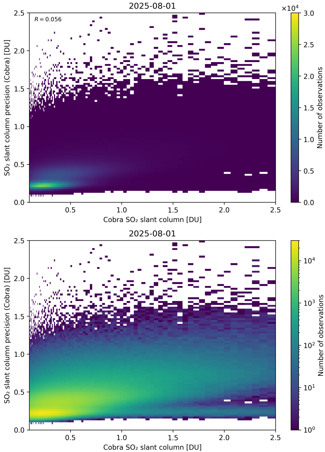
Figure 216: Scatter density plot of “Cobra SO 2 slant column” against “SO 2 slant column precision (Cobra)” for 2025-07-31 to 2025-08-02.
