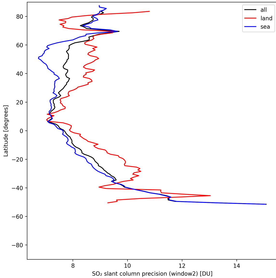
Figure 42: Zonal average of “SO 2 slant column precision (window2)” for 2025-07-31 to 2025-08-02.
