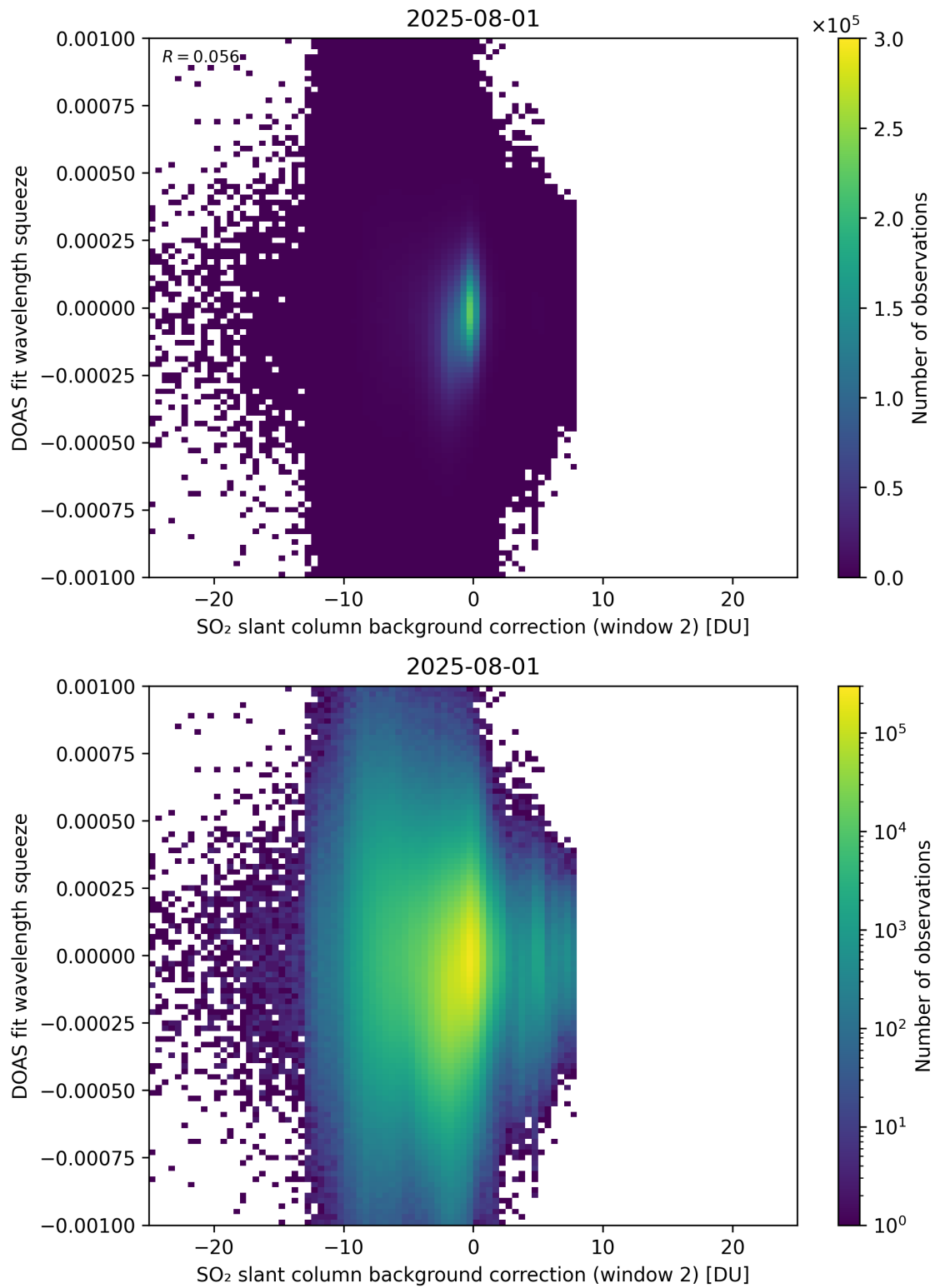
Figure 124: Scatter density plot of “SO 2 slant column background correction (window 2)” against “DOAS fit wavelength squeeze” for 2025-07-31 to 2025-08-02.
