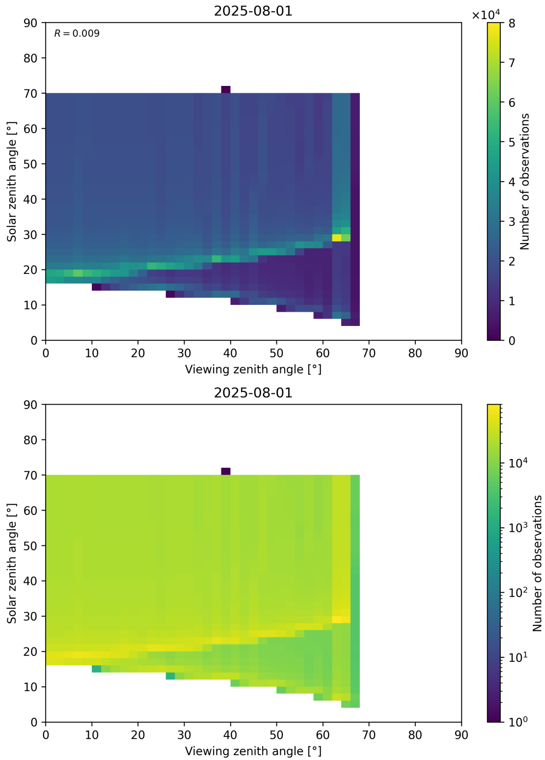
Figure 369: Scatter density plot of “Viewing zenith angle” against “Solar zenith angle” for 2025-07-31 to 2025-08-02.
