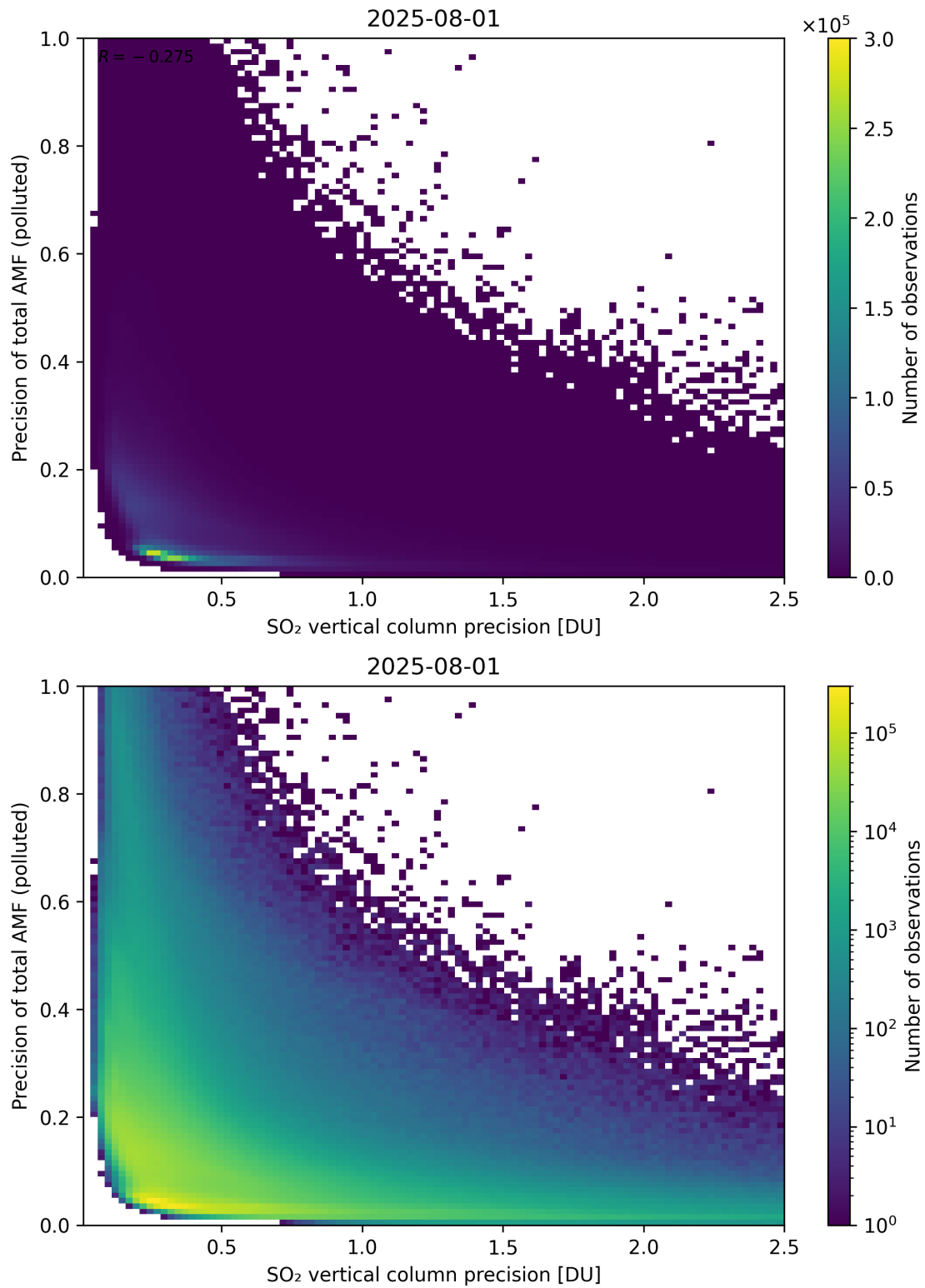
Figure 347: Scatter density plot of “SO 2 vertical column precision” against “Precision of total AMF (polluted)” for 2025-07-31 to 2025-08-02.
