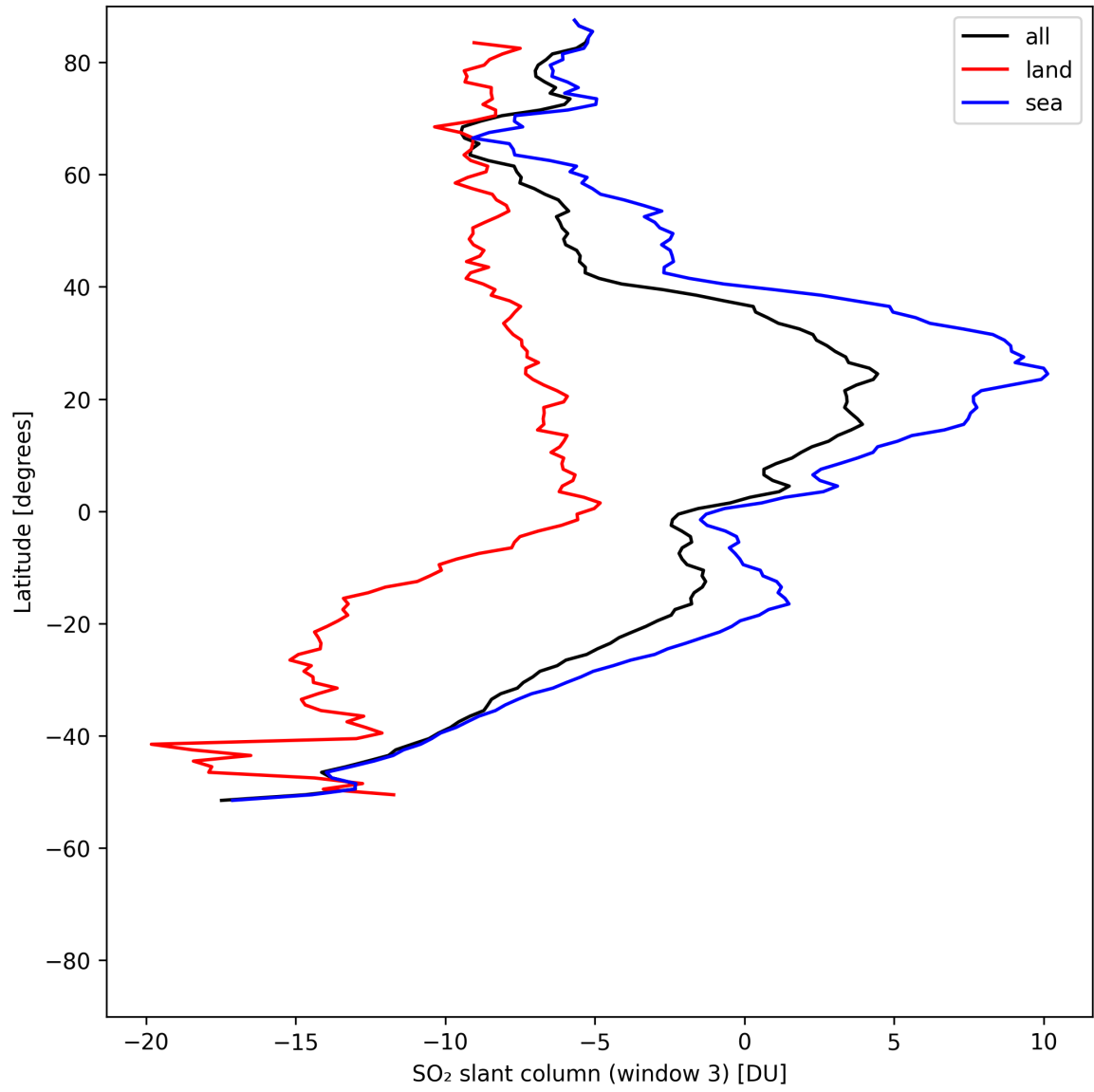
Figure 45: Zonal average of “SO 2 slant column (window 3)” for 2025-07-31 to 2025-08-02.
