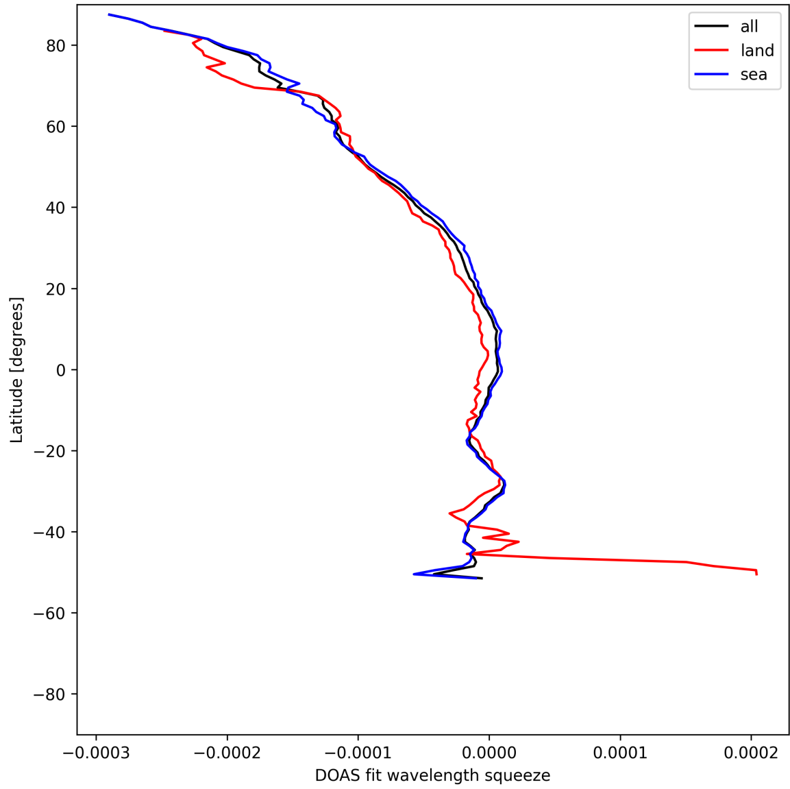
Figure 51: Zonal average of “DOAS fit wavelength squeeze” for 2025-07-31 to 2025-08-02.
