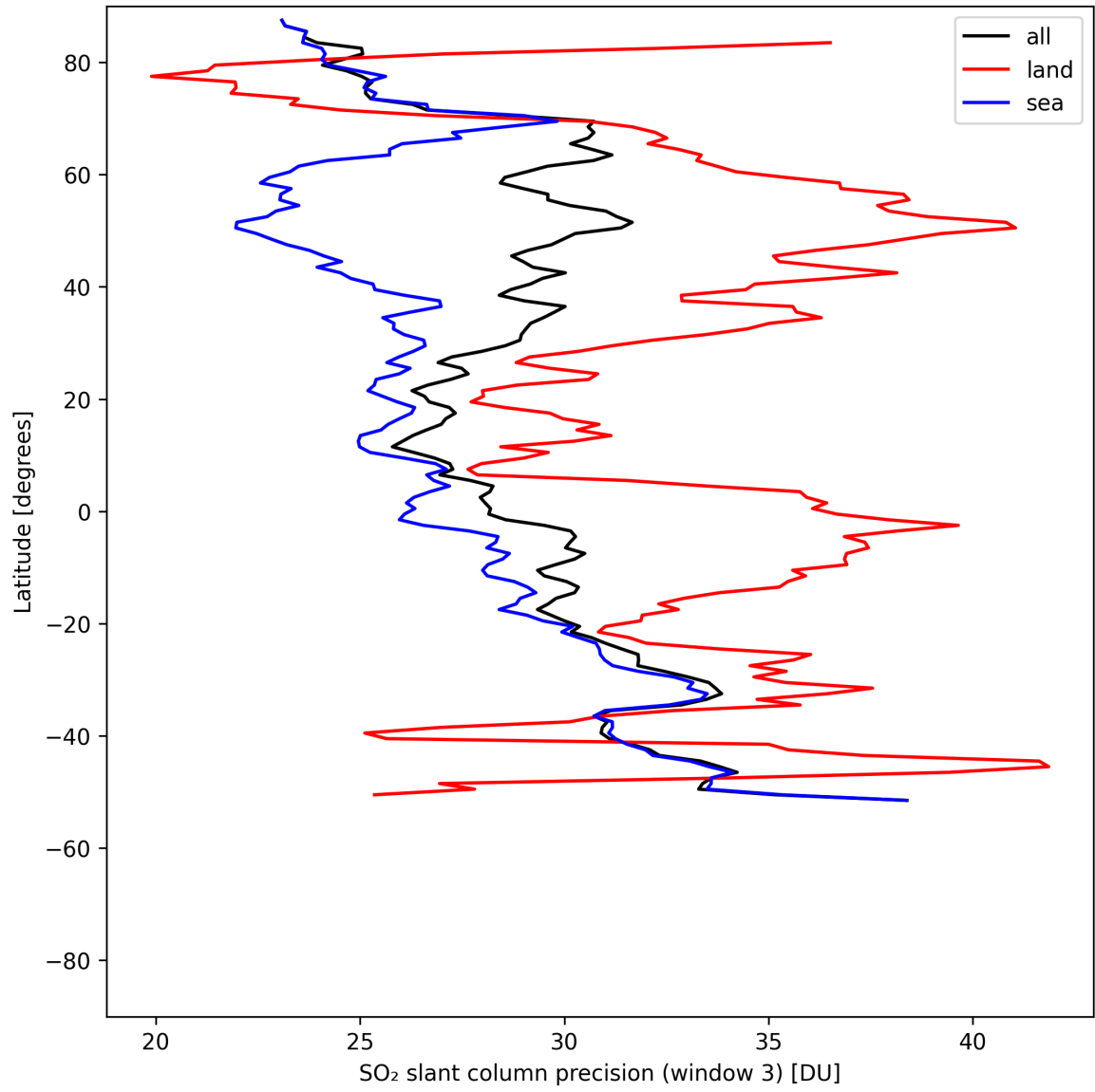
Figure 46: Zonal average of “SO 2 slant column precision (window 3)” for 2025-07-31 to 2025-08-02.
