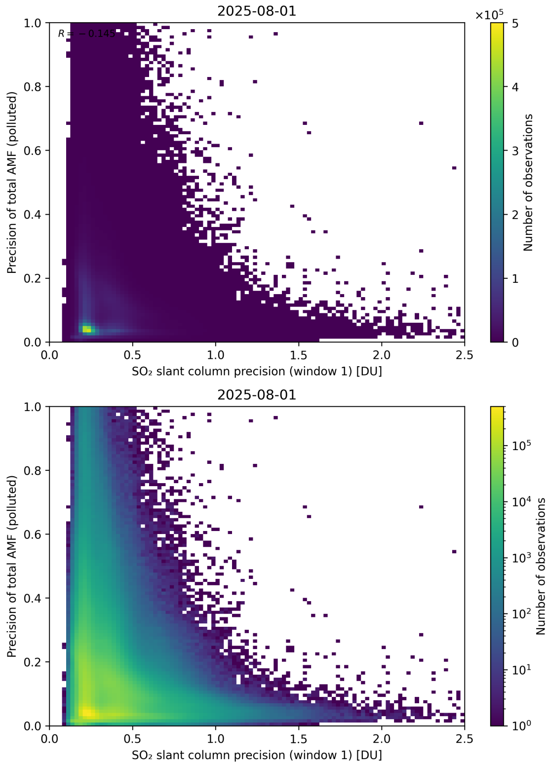
Figure 281: Scatter density plot of “SO 2 slant column precision (window 1)” against “Precision of total AMF (polluted)” for 2025-07-31 to 2025-08-02.
