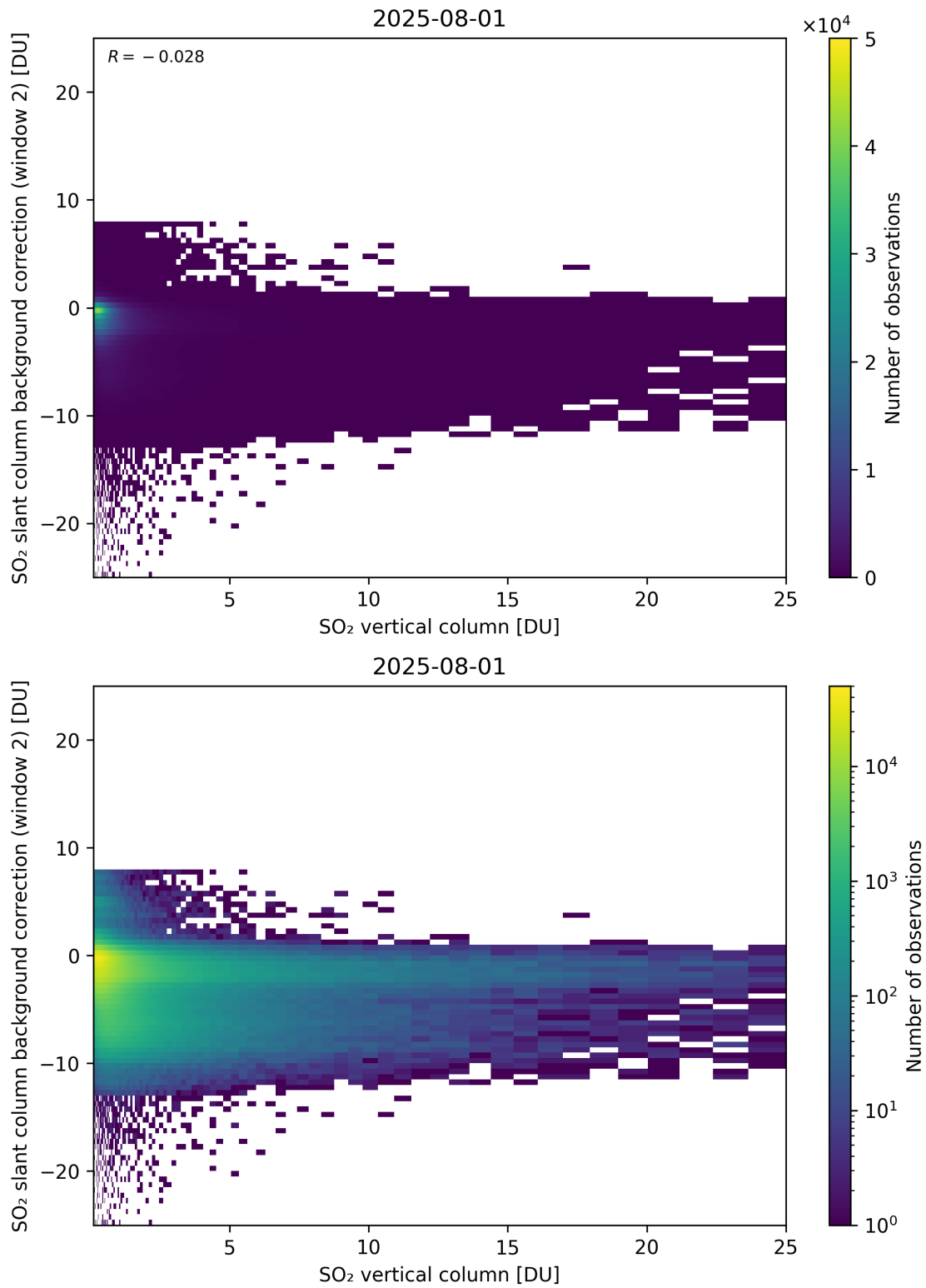
Figure 324: Scatter density plot of “SO 2 vertical column” against “SO 2 slant column background correction (window 2)” for 2025-07-31 to 2025-08-02.
