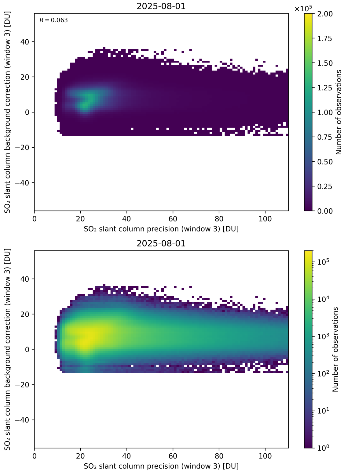
Figure 307: Scatter density plot of “SO 2 slant column precision (window 3)” against “SO 2 slant column background correction (window 3)” for 2025-07-31 to 2025-08-02.
