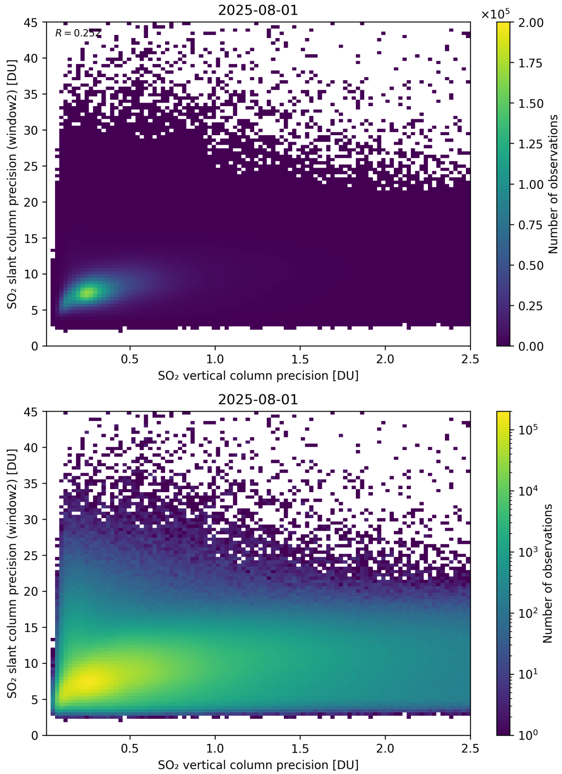
Figure 343: Scatter density plot of “SO 2 vertical column precision” against “SO 2 slant column precision (window2)” for 2025-07-31 to 2025-08-02.
