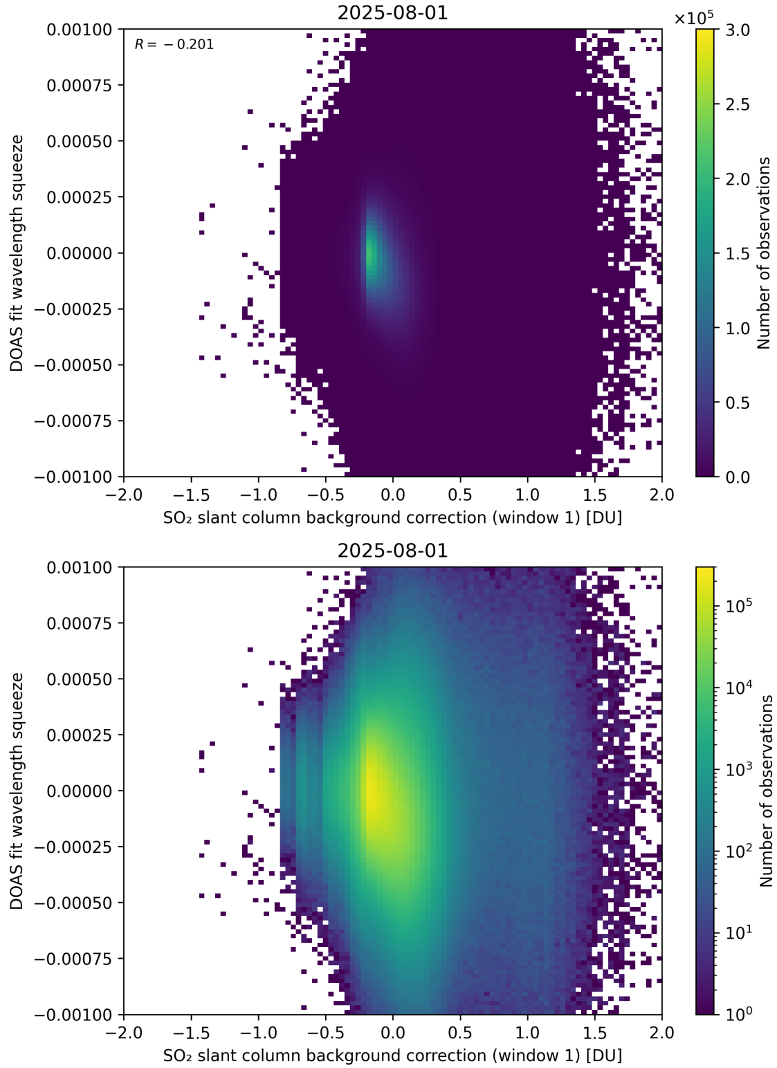
Figure 112: Scatter density plot of “SO 2 slant column background correction (window 1)” against “DOAS fit wavelength squeeze” for 2025-07-31 to 2025-08-02.
