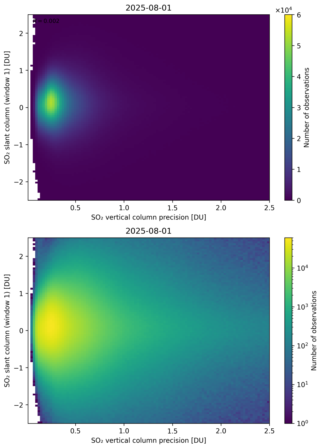
Figure 341: Scatter density plot of “SO 2 vertical column precision” against “SO 2 slant column (window 1)” for 2025-07-31 to 2025-08-02.
