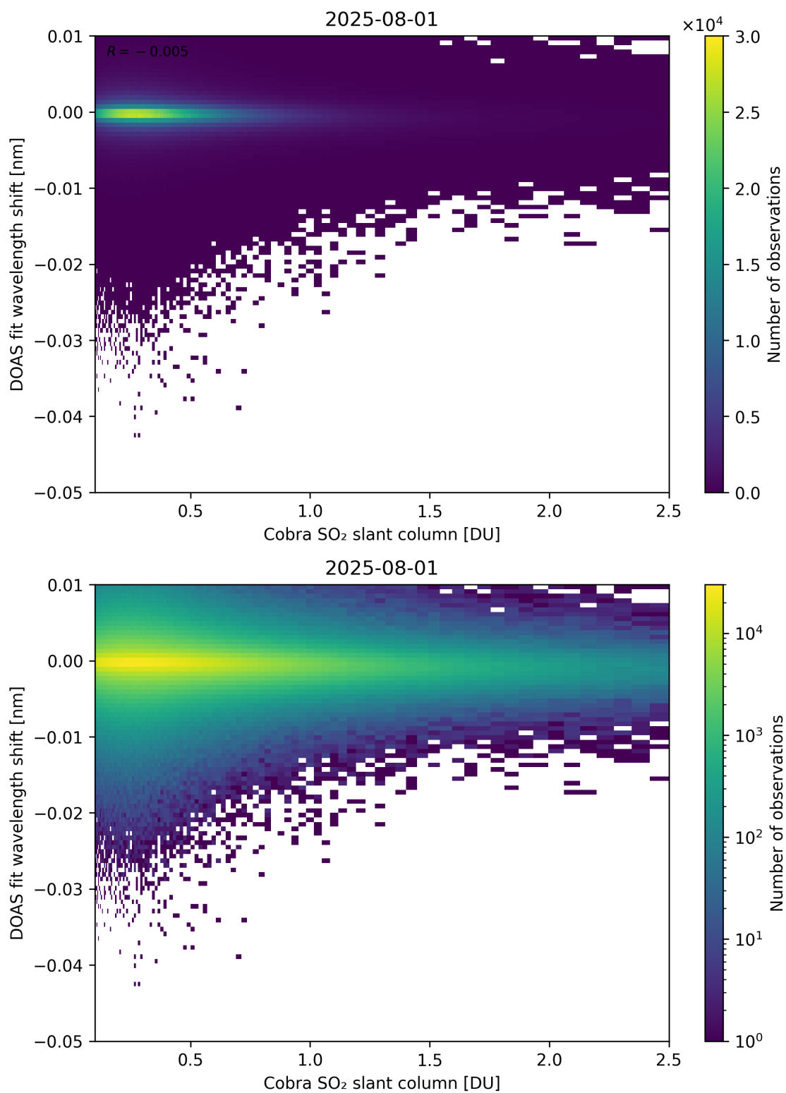
Figure 196: Scatter density plot of “Cobra SO 2 slant column” against “DOAS fit wavelength shift” for 2025-07-31 to 2025-08-02.
