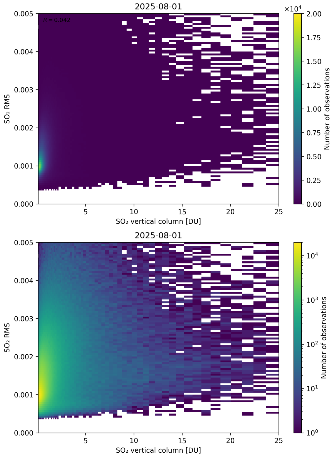
Figure 328: Scatter density plot of “SO 2 vertical column” against “SO 2 RMS” for 2025-07-31 to 2025-08-02.
