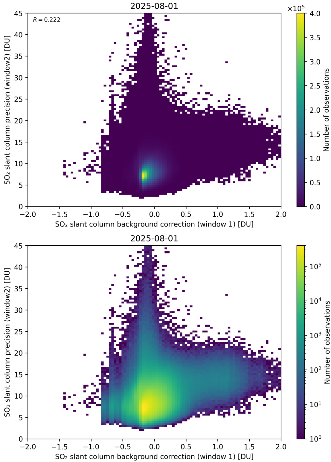
Figure 117: Scatter density plot of “SO 2 slant column background correction (window 1)” against “SO 2 slant column precision (window2)” for 2025-07-31 to 2025-08-02.
