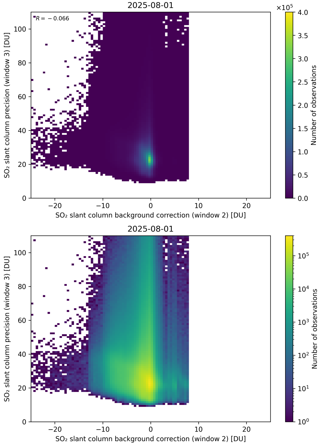
Figure 129: Scatter density plot of “SO 2 slant column background correction (window 2)” against “SO 2 slant column precision (window 3)” for 2025-07-31 to 2025-08-02.
