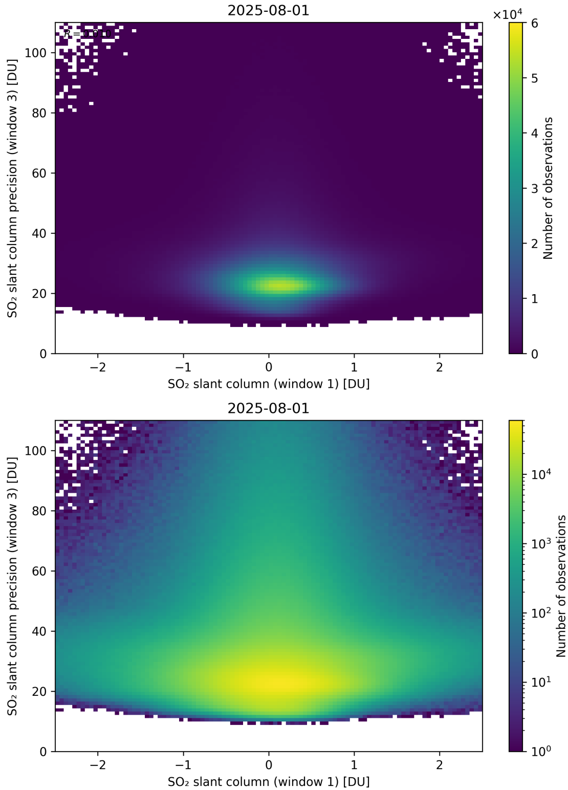
Figure 288: Scatter density plot of “SO 2 slant column (window 1)” against “SO 2 slant column precision (window 3)” for 2025-07-31 to 2025-08-02.
