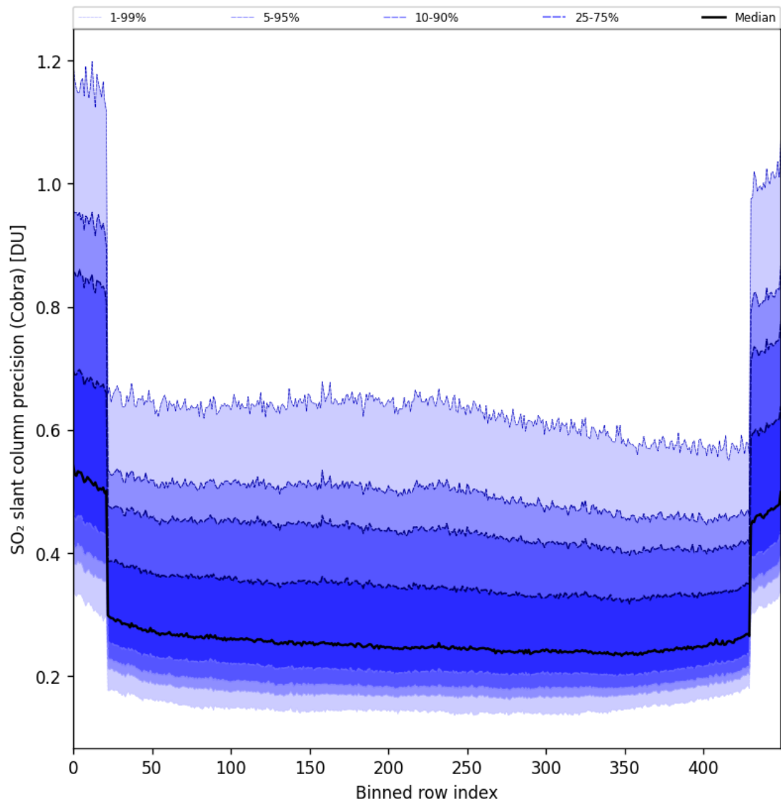
Figure 88: Along track statistics of “SO 2 slant column precision (Cobra)” for 2025-07-31 to 2025-08-02
