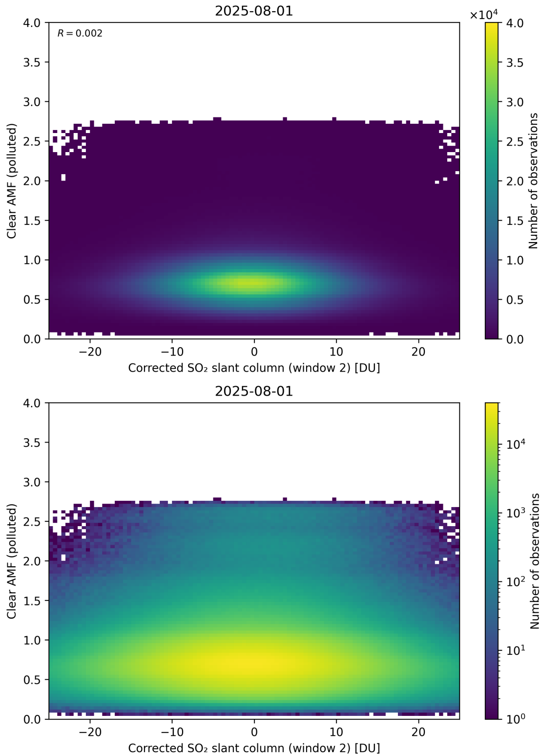
Figure 249: Scatter density plot of “Corrected SO 2 slant column (window 2)” against “Clear AMF (polluted)” for 2025-07-31 to 2025-08-02.
