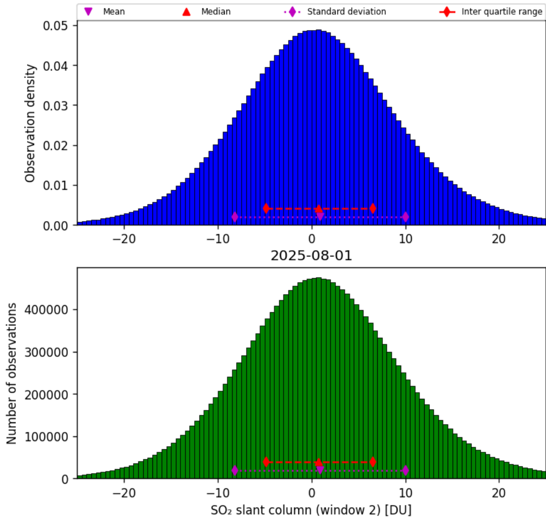
Figure 67: Histogram of “SO 2 slant column (window 2)” for 2025-07-31 to 2025-08-02
