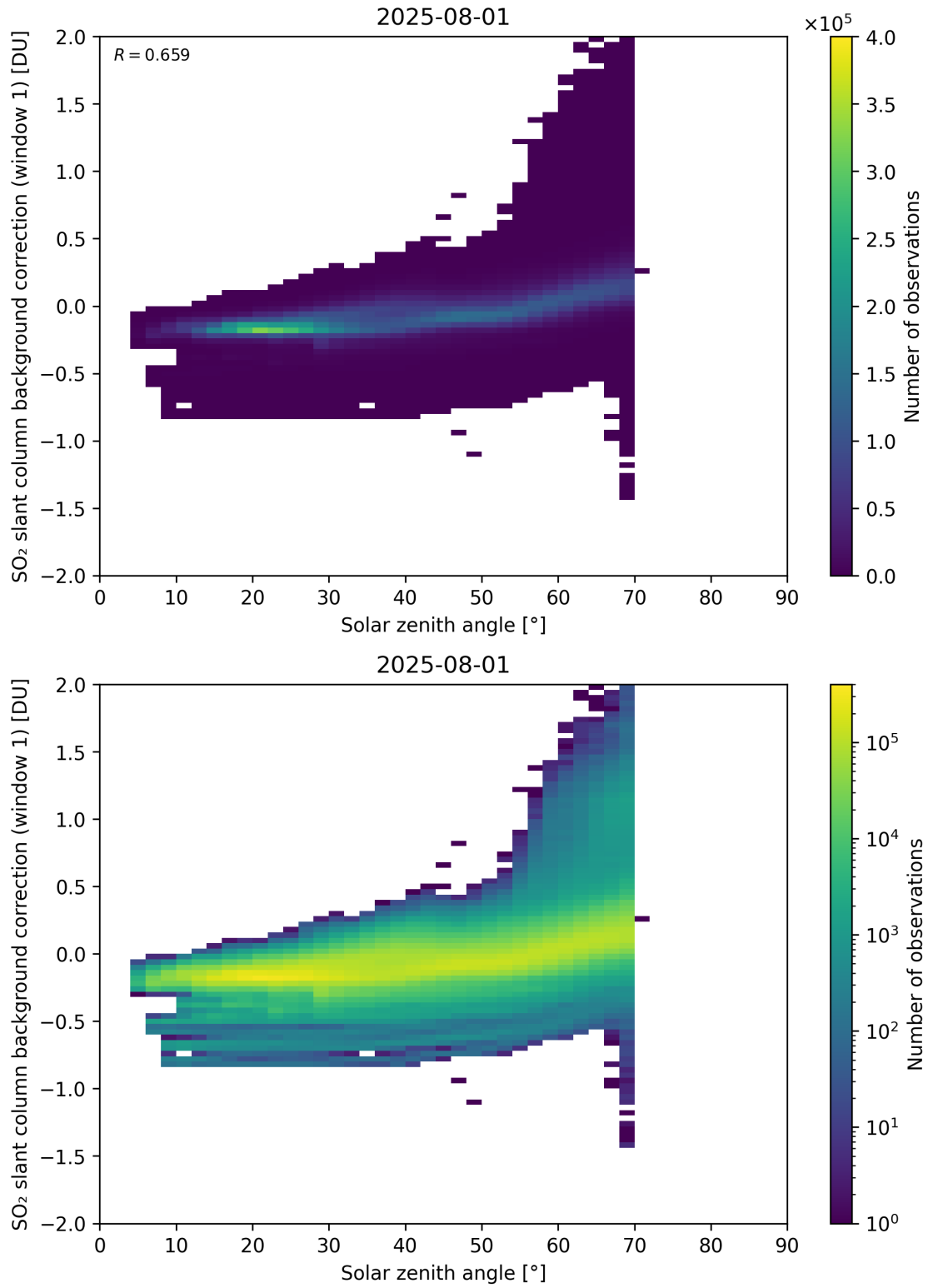
Figure 171: Scatter density plot of “Solar zenith angle” against “SO 2 slant column background correction (window 1)” for 2025-07-31 to 2025-08-02.
