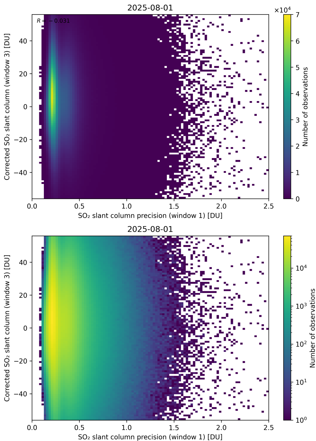
Figure 276: Scatter density plot of “SO 2 slant column precision (window 1)” against “Corrected SO 2 slant column (window 3)” for 2025-07-31 to 2025-08-02.
