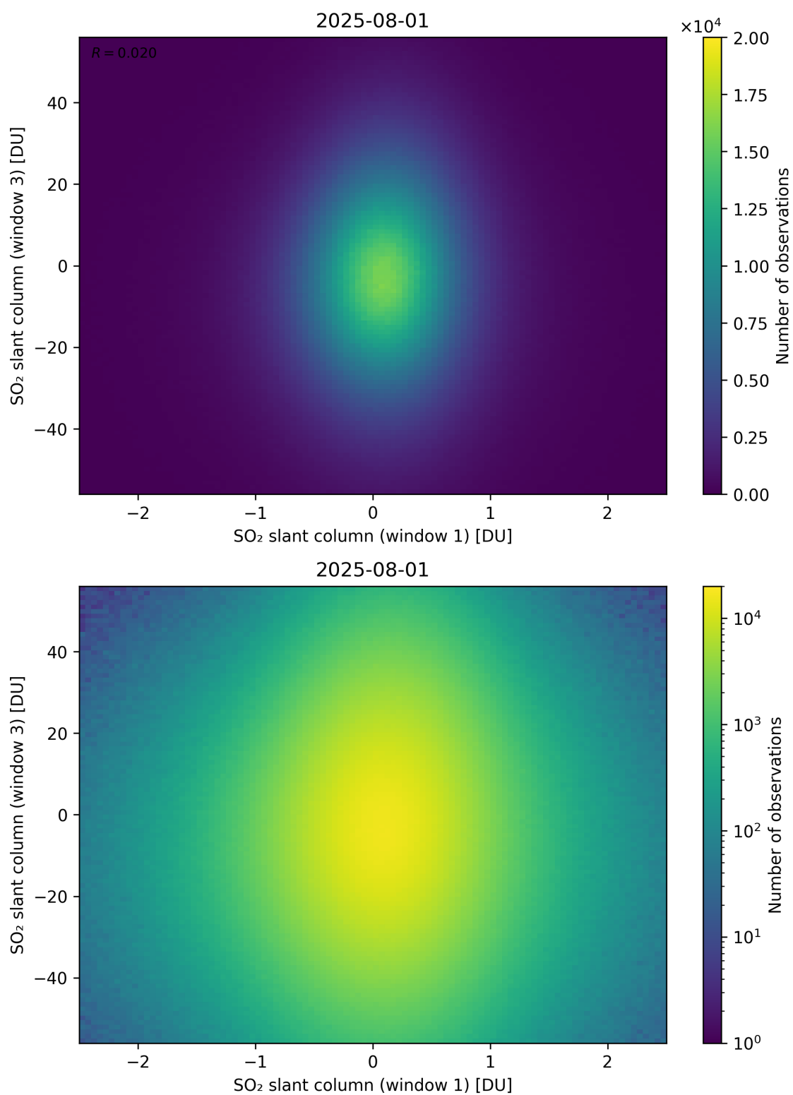
Figure 287: Scatter density plot of “SO 2 slant column (window 1)” against “SO 2 slant column (window 3)” for 2025-07-31 to 2025-08-02.
