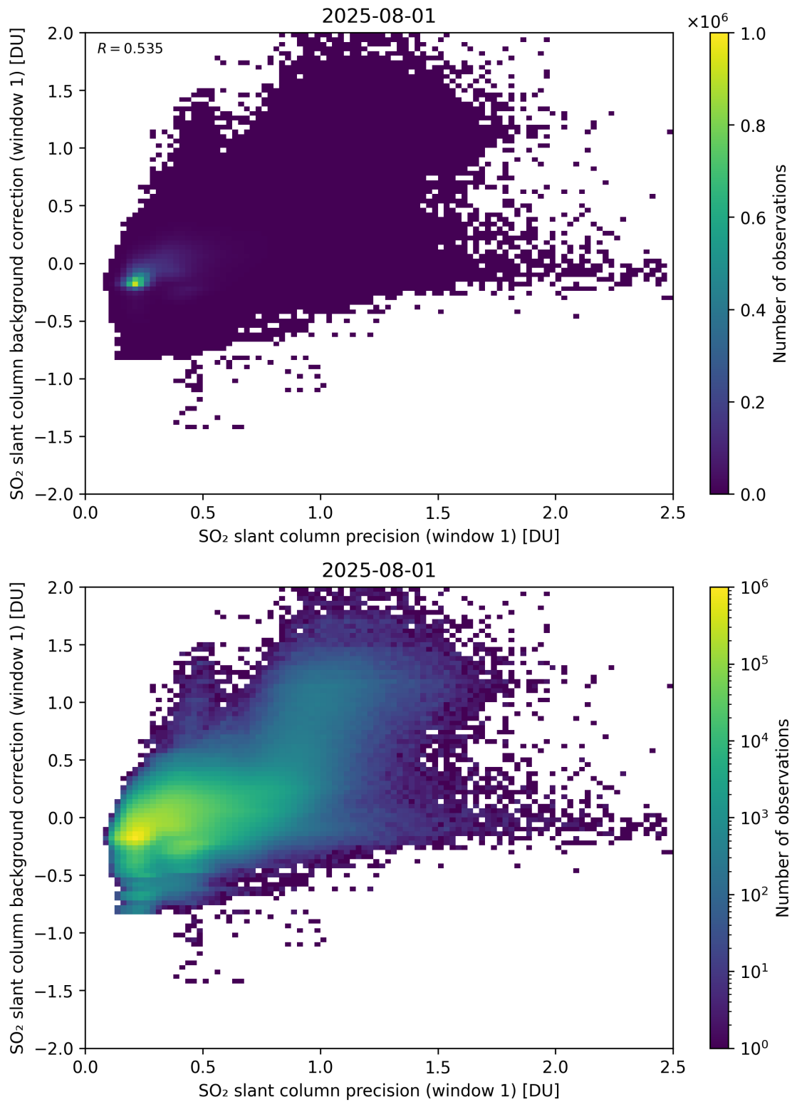
Figure 268: Scatter density plot of “SO 2 slant column precision (window 1)” against “SO 2 slant column background correction (window 1)” for 2025-07-31 to 2025-08-02.
