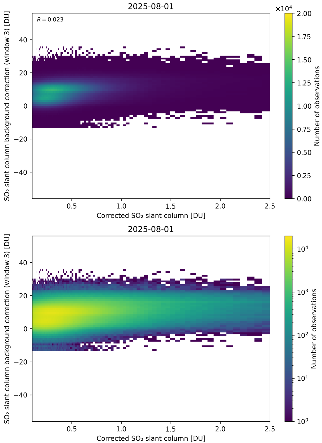
Figure 228: Scatter density plot of “Corrected SO 2 slant column” against “SO 2 slant column background correction (window 3)” for 2025-07-31 to 2025-08-02.
