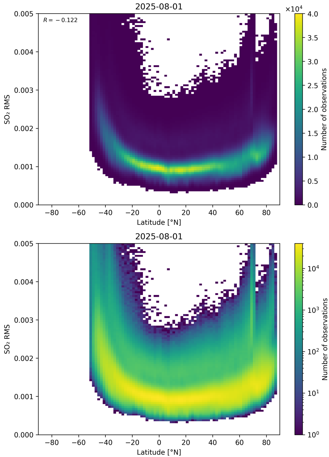
Figure 155: Scatter density plot of “Latitude” against “SO 2 RMS” for 2025-07-31 to 2025-08-02.
