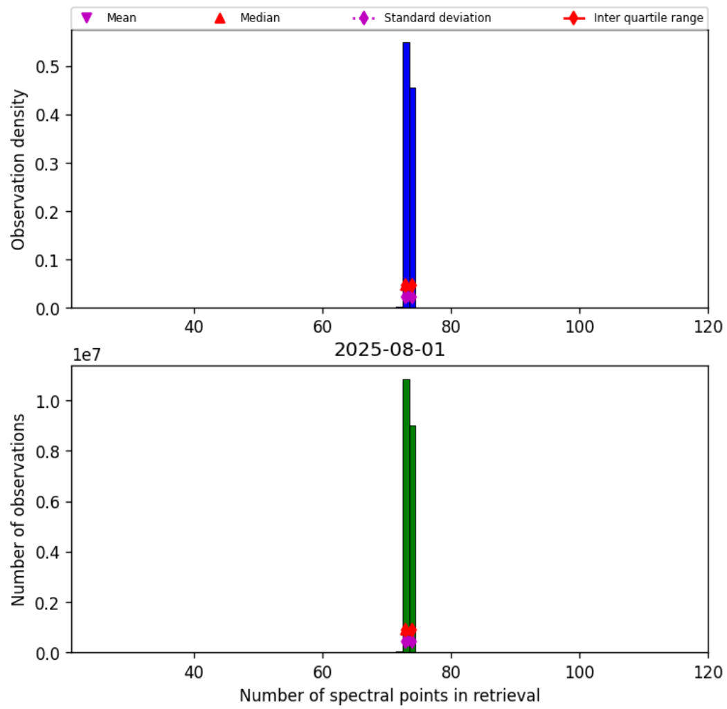
Figure 82: Histogram of “Number of spectral points in retrieval” for 2025-07-31 to 2025-08-02
