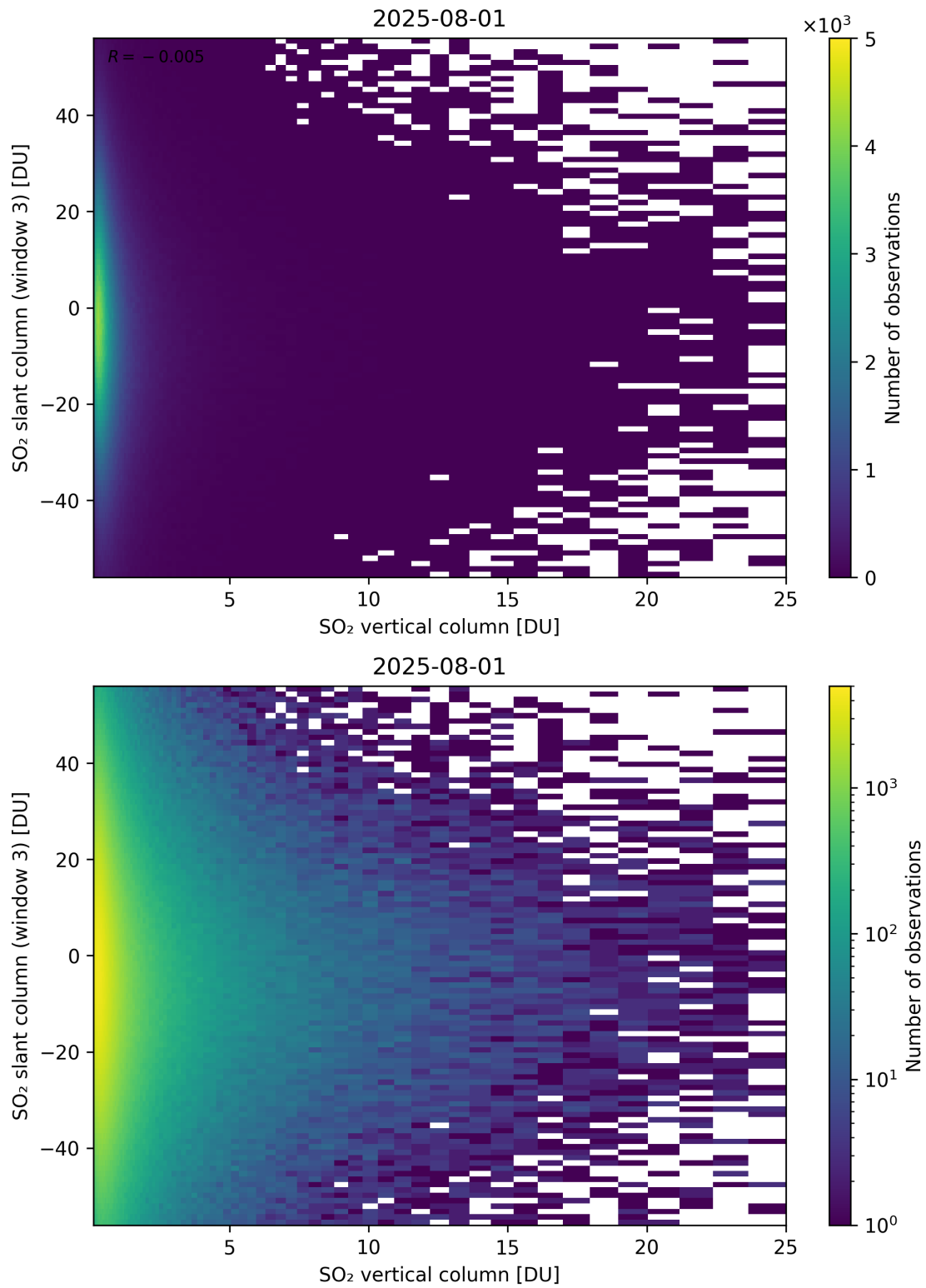
Figure 357: Scatter density plot of “SO 2 vertical column” against “SO 2 slant column (window 3)” for 2025-07-31 to 2025-08-02.
