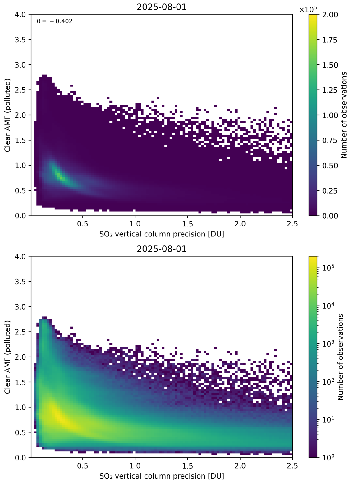
Figure 335: Scatter density plot of “SO 2 vertical column precision” against “Clear AMF (polluted)” for 2025-07-31 to 2025-08-02.
