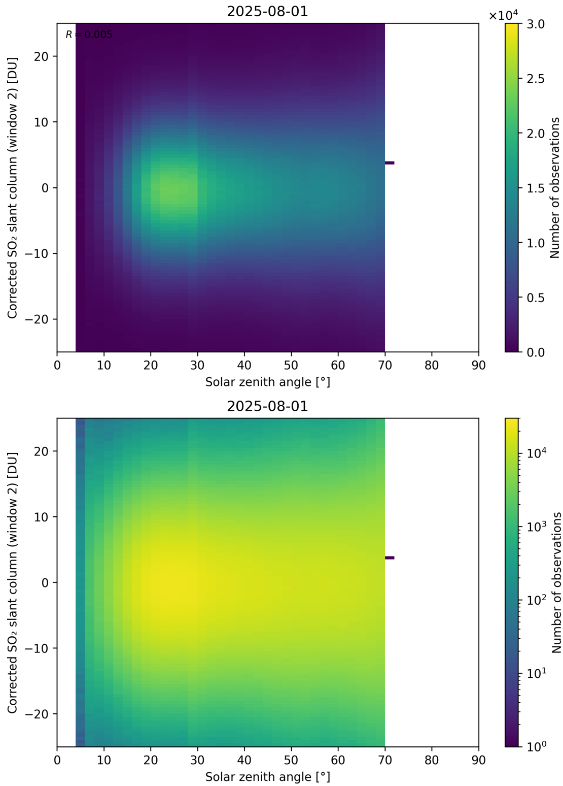
Figure 182: Scatter density plot of “Solar zenith angle” against “Corrected SO 2 slant column (window 2)” for 2025-07-31 to 2025-08-02.
