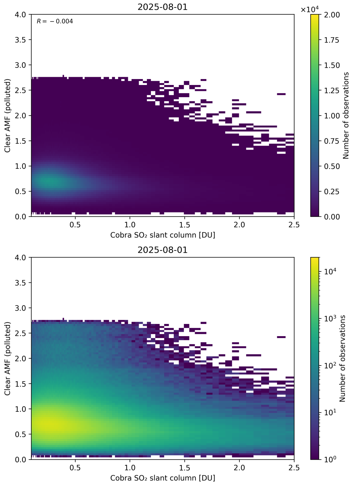
Figure 215: Scatter density plot of “Cobra SO 2 slant column” against “Clear AMF (polluted)” for 2025-07-31 to 2025-08-02.
