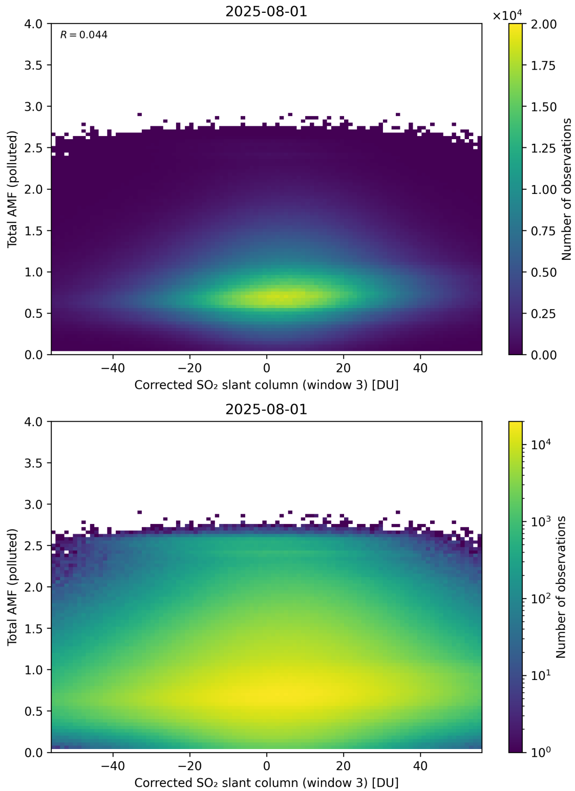
Figure 260: Scatter density plot of “Corrected SO 2 slant column (window 3)” against “Total AMF (polluted)” for 2025-07-31 to 2025-08-02.
