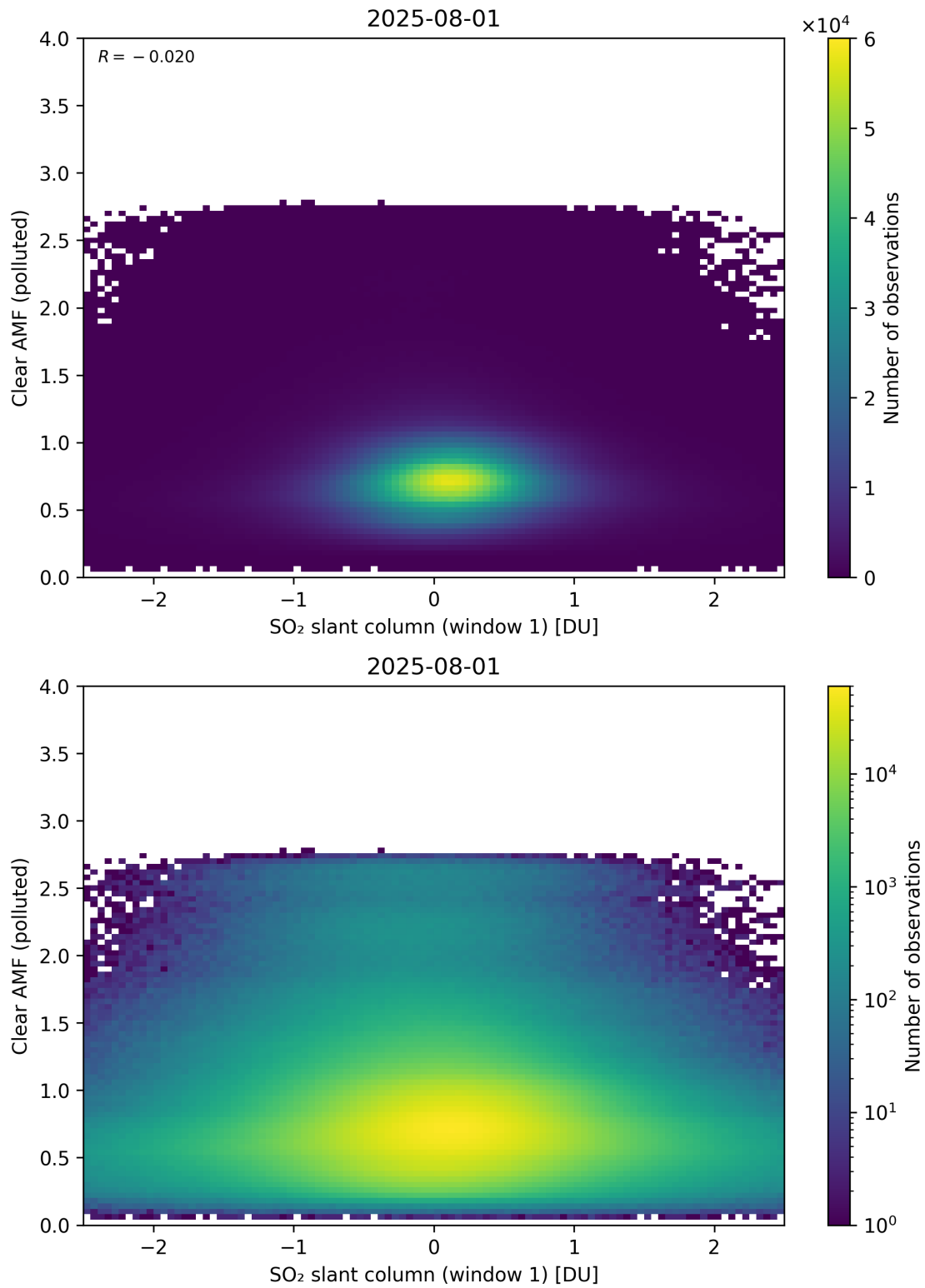
Figure 282: Scatter density plot of “SO 2 slant column (window 1)” against “Clear AMF (polluted)” for 2025-07-31 to 2025-08-02.
