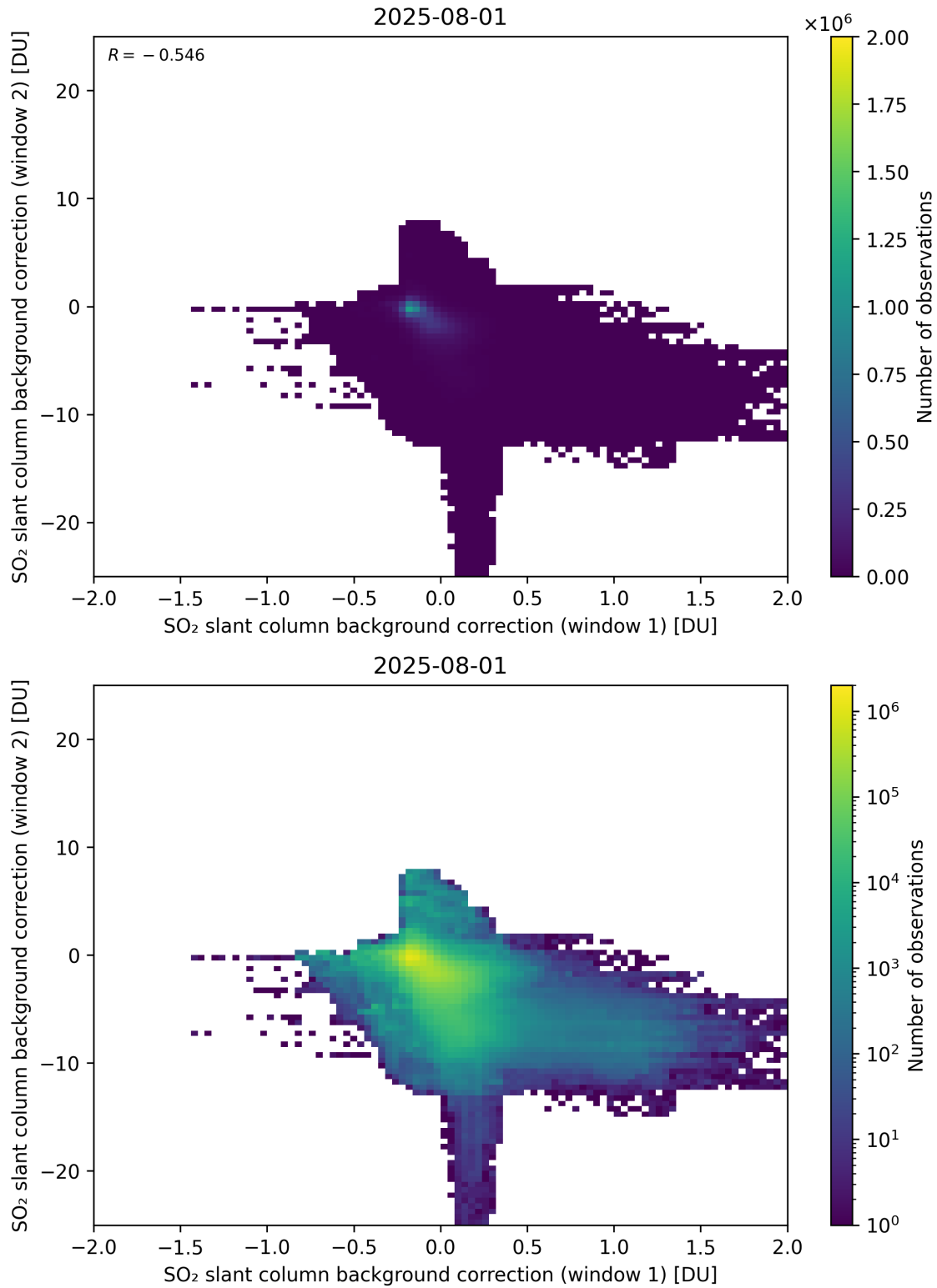
Figure 109: Scatter density plot of “SO 2 slant column background correction (window 1)” against “SO 2 slant column background correction (window 2)” for 2025-07-31 to 2025-08-02.
