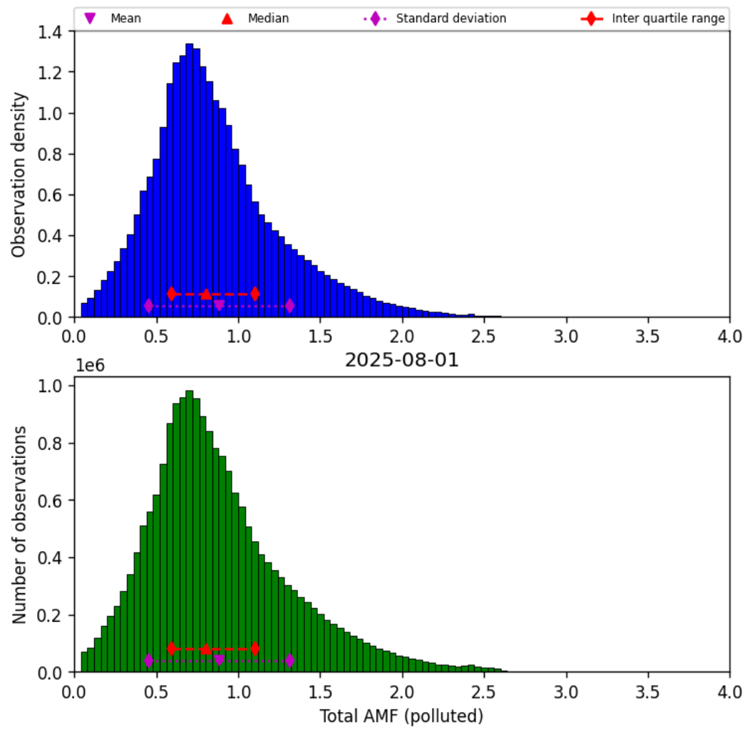
Figure 79: Histogram of “Total AMF (polluted)” for 2025-07-31 to 2025-08-02
