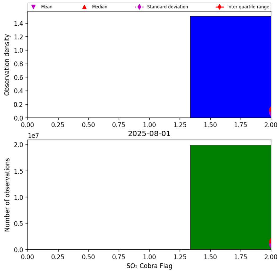
Figure 75: Histogram of “SO 2 Cobra Flag” for 2025-07-31 to 2025-08-02
