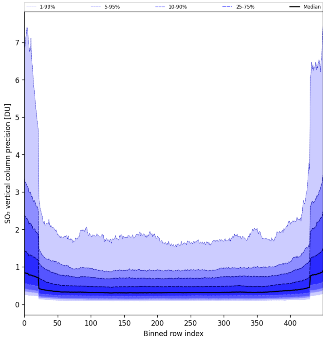
Figure 85: Along track statistics of “SO 2 vertical column precision” for 2025-07-31 to 2025-08-02
