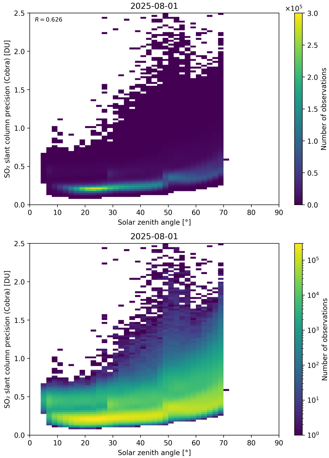
Figure 180: Scatter density plot of “Solar zenith angle” against “SO 2 slant column precision (Cobra)” for 2025-07-31 to 2025-08-02.
