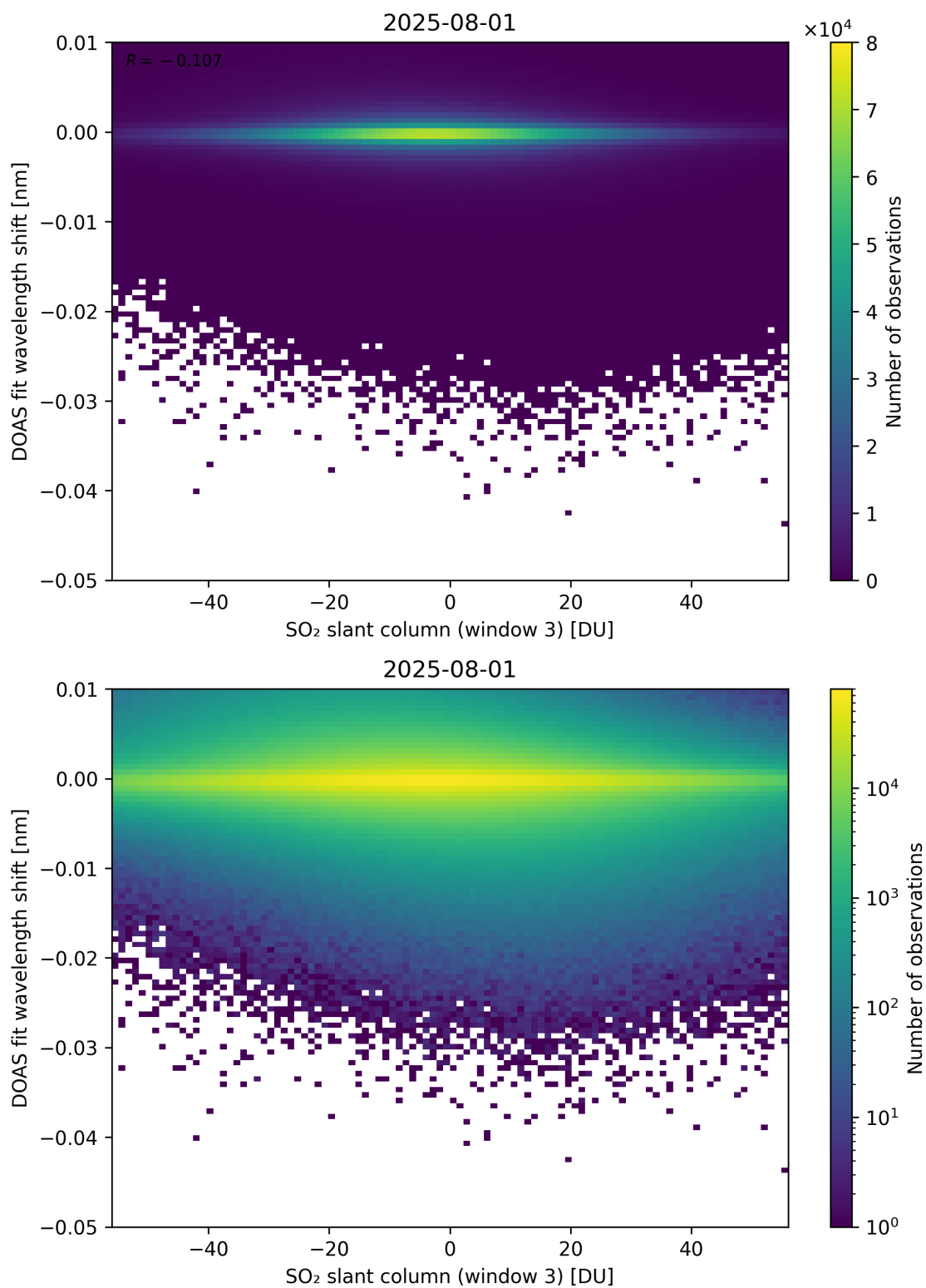
Figure 304: Scatter density plot of “SO 2 slant column (window 3)” against “DOAS fit wavelength shift” for 2025-07-31 to 2025-08-02.
