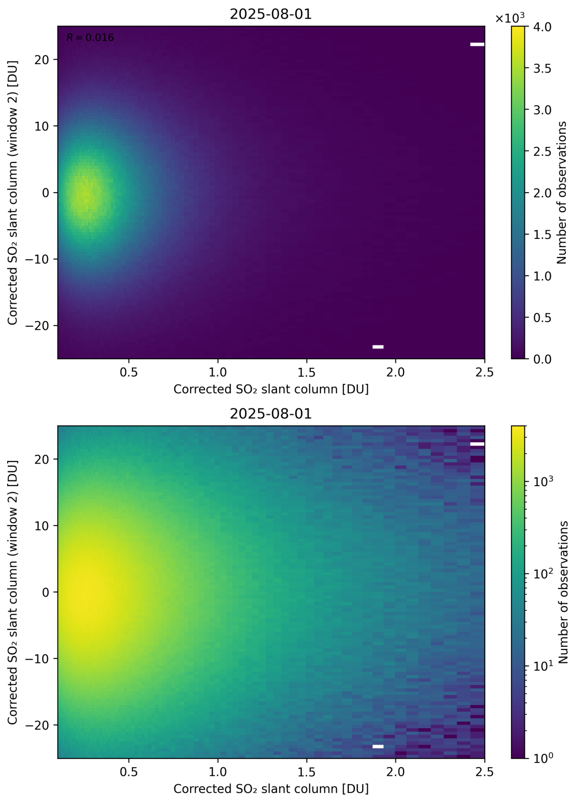
Figure 235: Scatter density plot of “Corrected SO 2 slant column” against “Corrected SO 2 slant column (window 2)” for 2025-07-31 to 2025-08-02.
