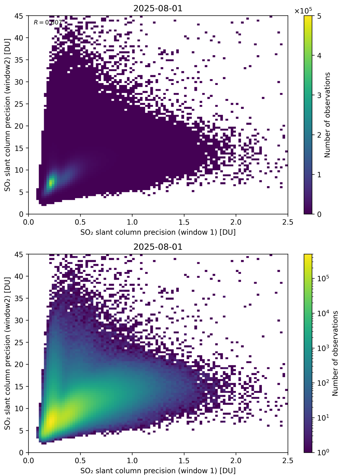
Figure 277: Scatter density plot of “SO 2 slant column precision (window 1)” against “SO 2 slant column precision (window2)” for 2025-07-31 to 2025-08-02.
