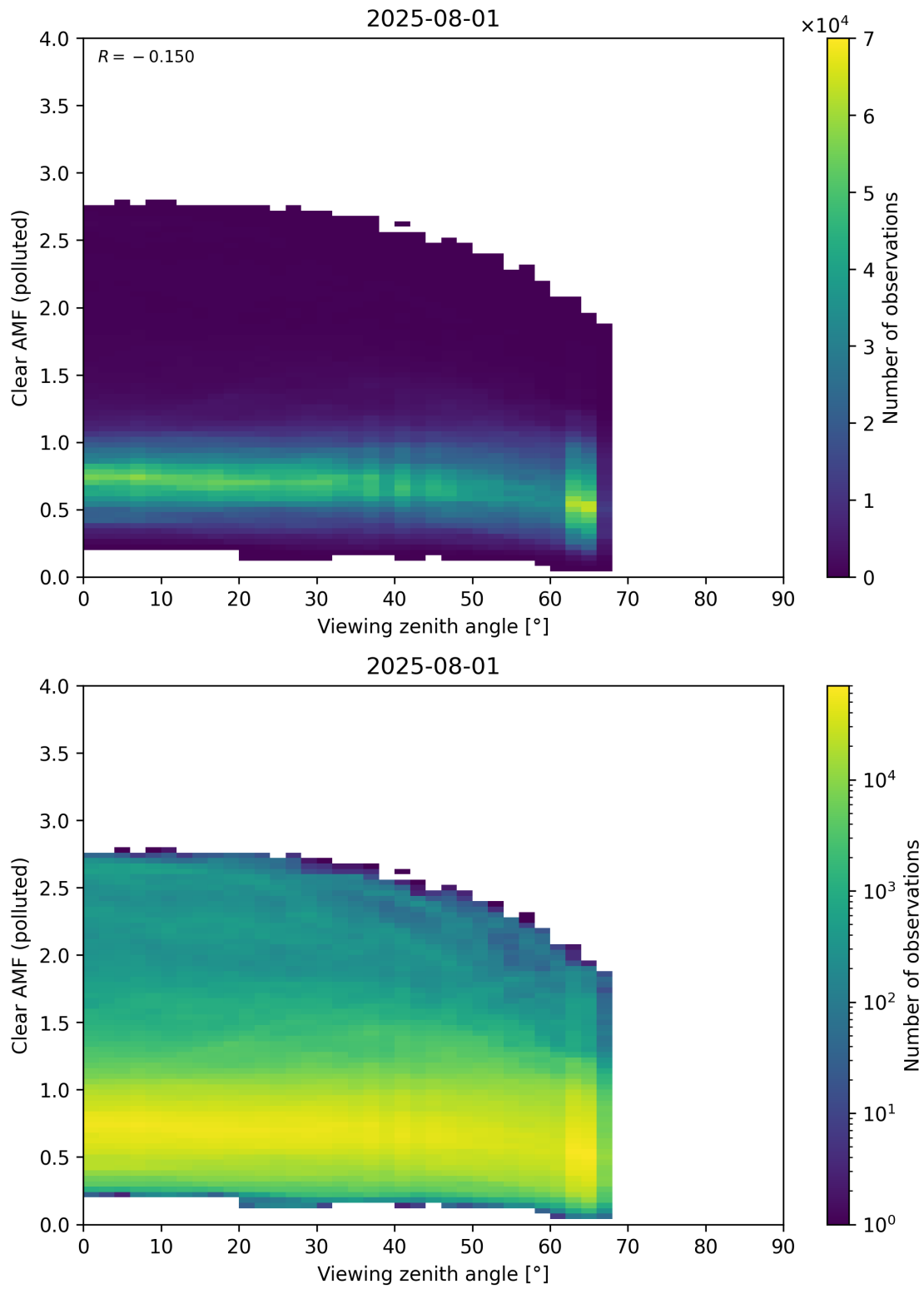
Figure 370: Scatter density plot of “Viewing zenith angle” against “Clear AMF (polluted)” for 2025-07-31 to 2025-08-02.
