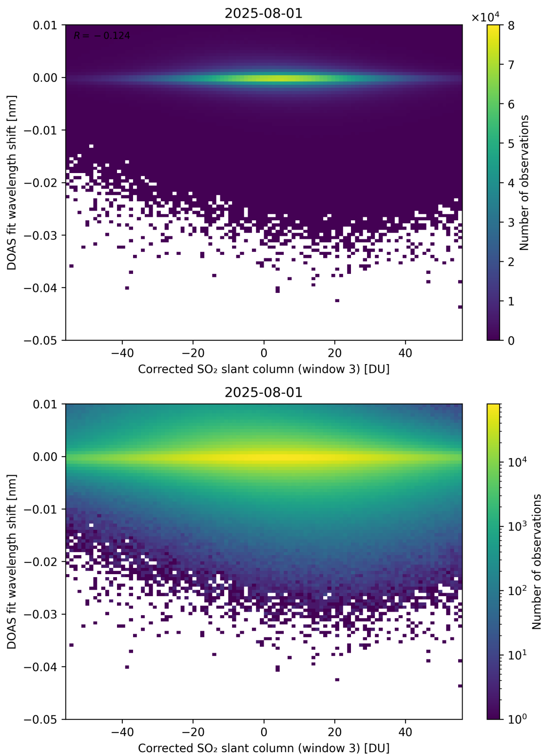
Figure 256: Scatter density plot of “Corrected SO 2 slant column (window 3)” against “DOAS fit wavelength shift” for 2025-07-31 to 2025-08-02.
