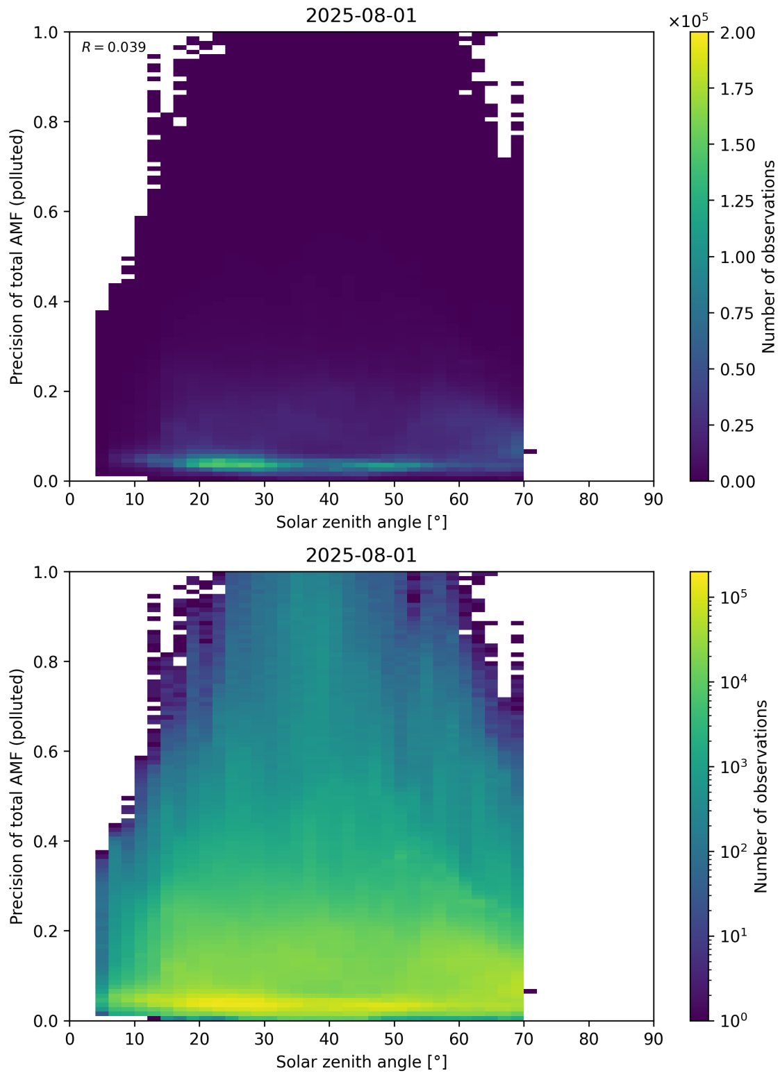
Figure 190: Scatter density plot of “Solar zenith angle” against “Precision of total AMF (polluted)” for 2025-07-31 to 2025-08-02.
