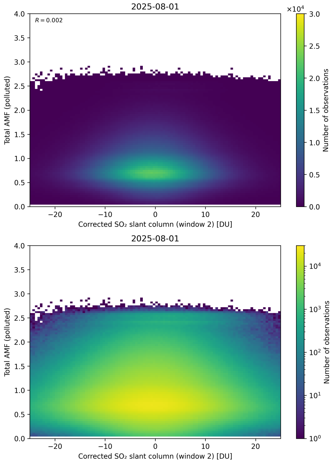
Figure 253: Scatter density plot of “Corrected SO 2 slant column (window 2)” against “Total AMF (polluted)” for 2025-07-31 to 2025-08-02.
