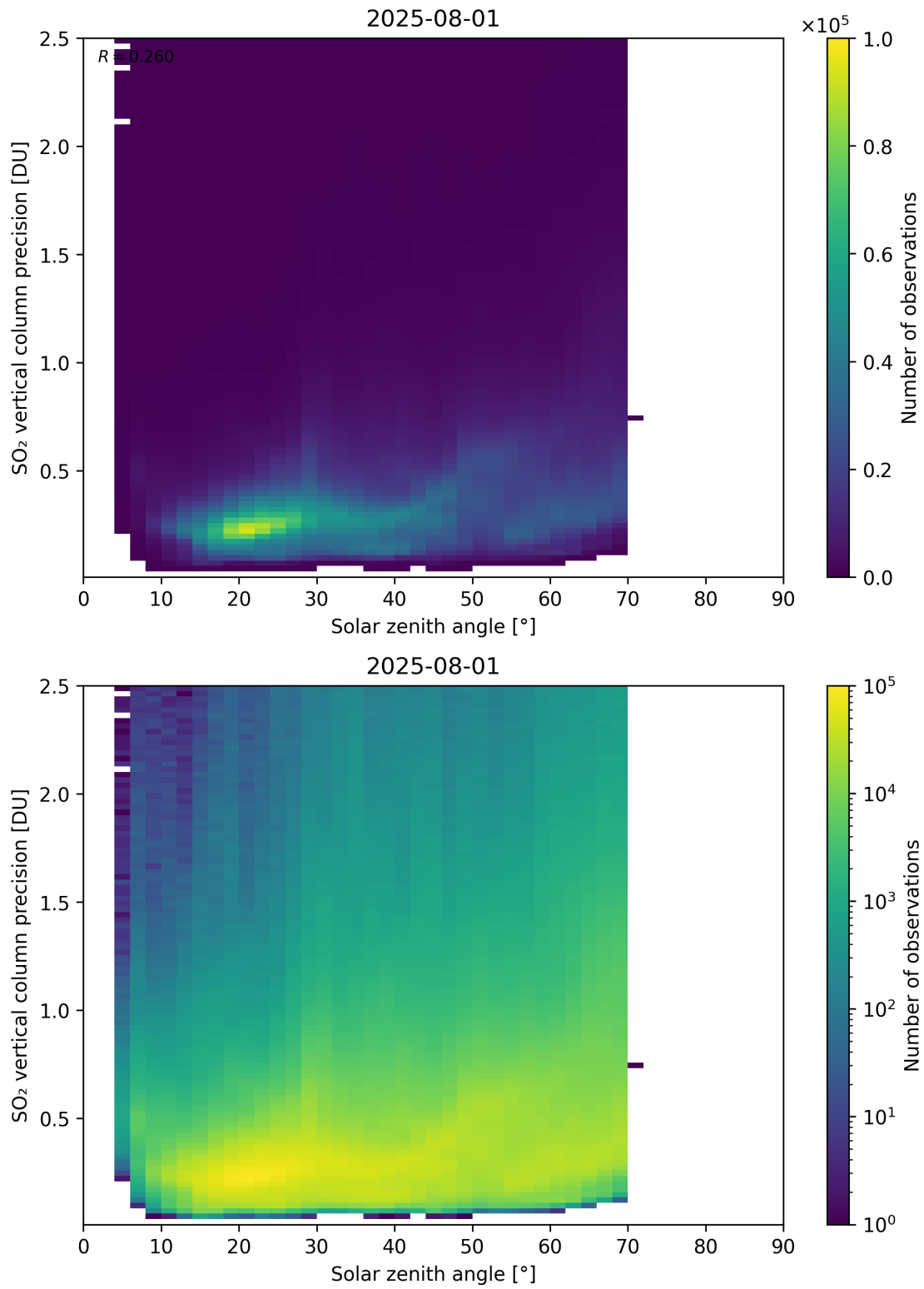
Figure 192: Scatter density plot of “Solar zenith angle” against “SO 2 vertical column precision” for 2025-07-31 to 2025-08-02.
