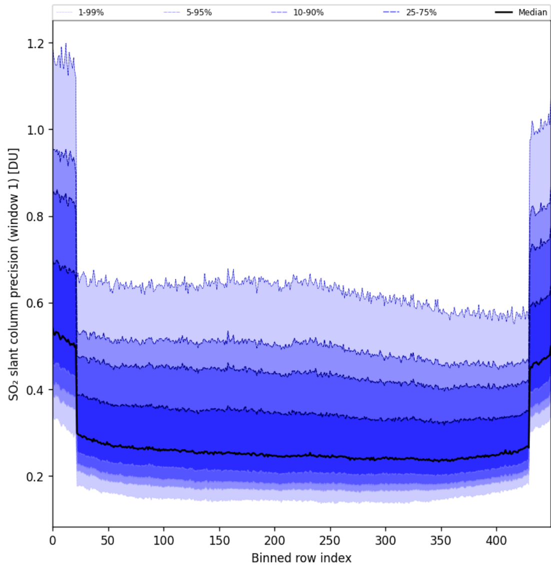
Figure 90: Along track statistics of “SO 2 slant column precision (window 1)” for 2025-07-31 to 2025-08-02
