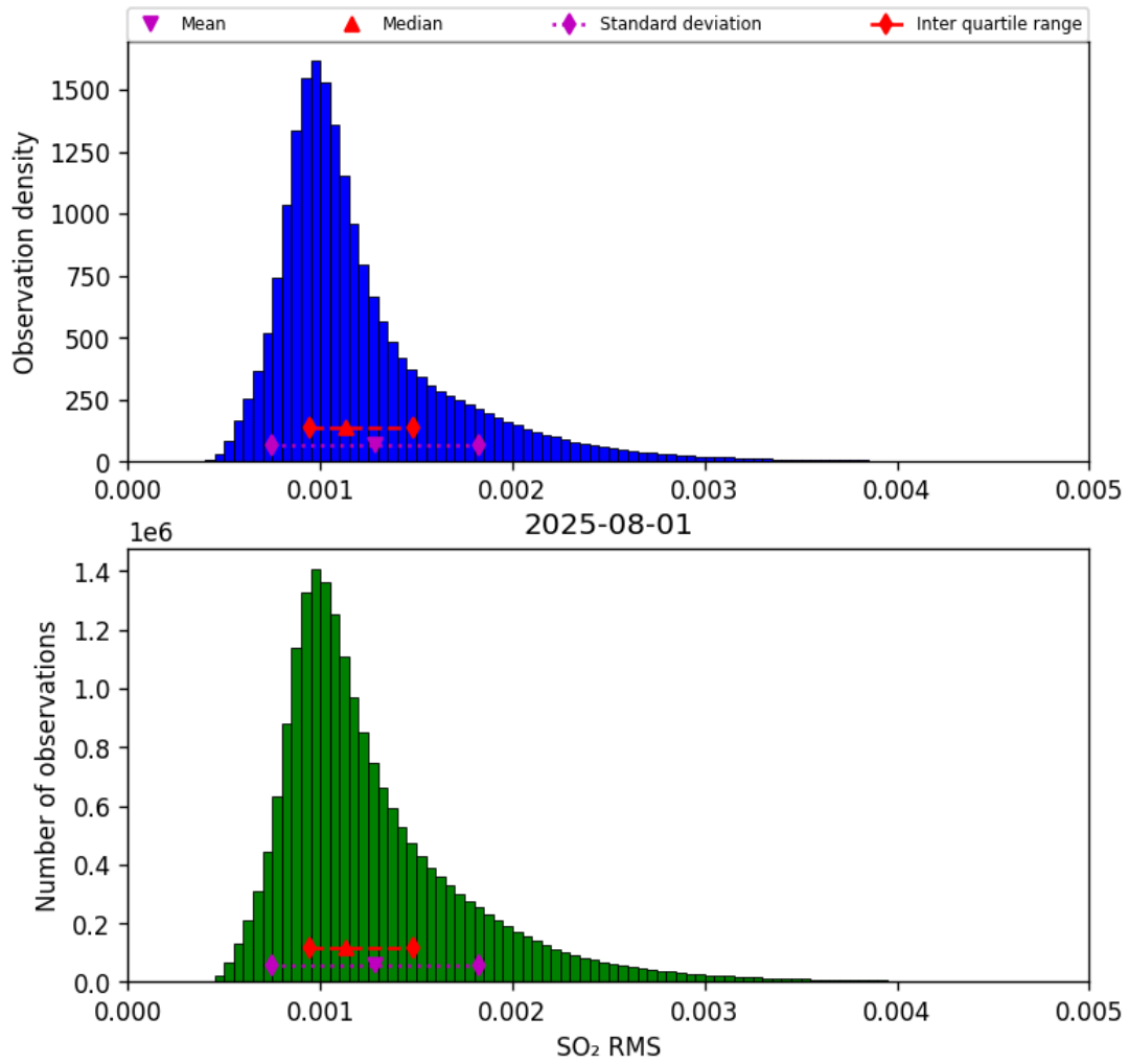
Figure 78: Histogram of “SO 2 RMS” for 2025-07-31 to 2025-08-02
