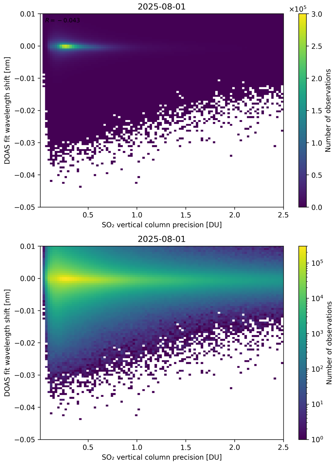
Figure 332: Scatter density plot of “SO 2 vertical column precision” against “DOAS fit wavelength shift” for 2025-07-31 to 2025-08-02.
