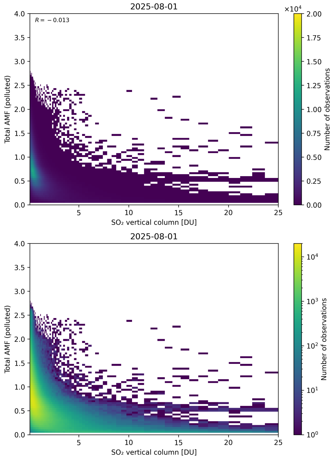
Figure 359: Scatter density plot of “SO 2 vertical column” against “Total AMF (polluted)” for 2025-07-31 to 2025-08-02.
