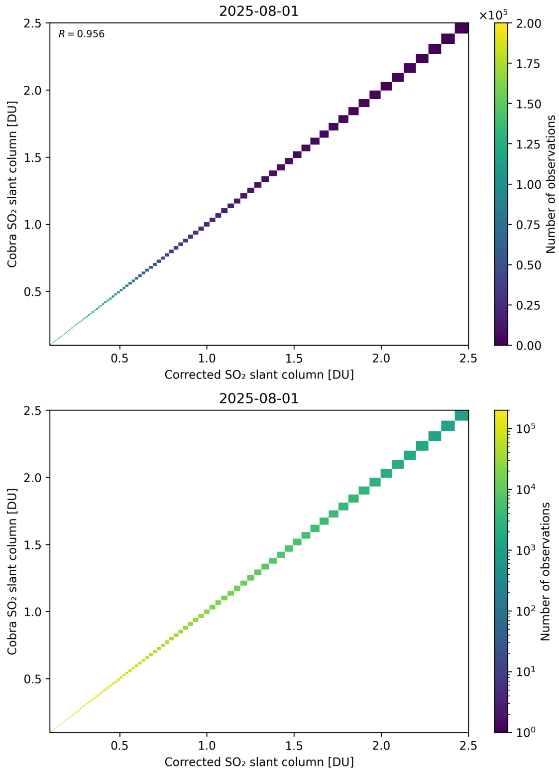
Figure 233: Scatter density plot of “Corrected SO 2 slant column” against “Cobra SO 2 slant column” for 2025-07-31 to 2025-08-02.
