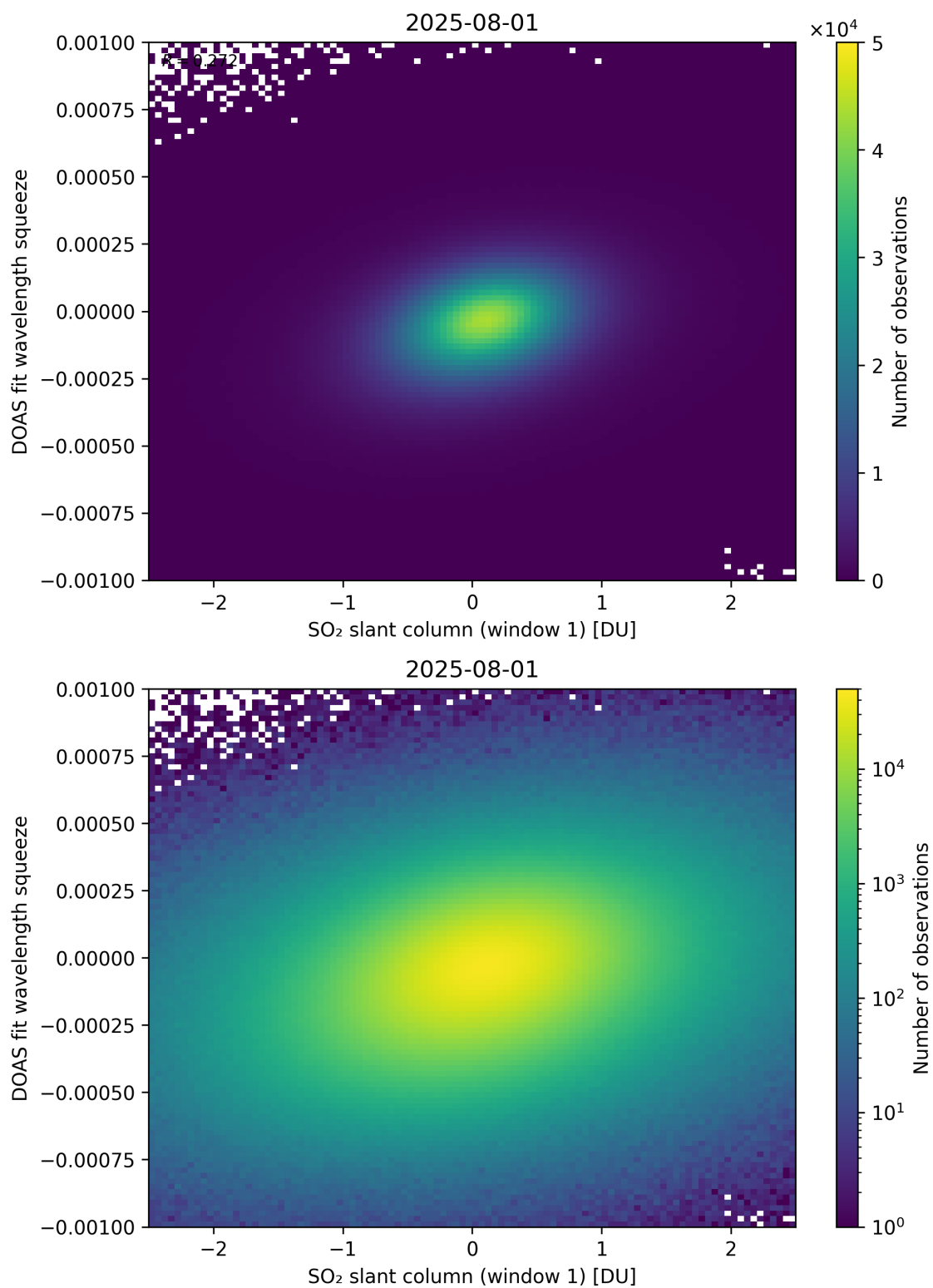
Figure 266: Scatter density plot of “SO 2 slant column (window 1)” against “DOAS fit wavelength squeeze” for 2025-07-31 to 2025-08-02.
