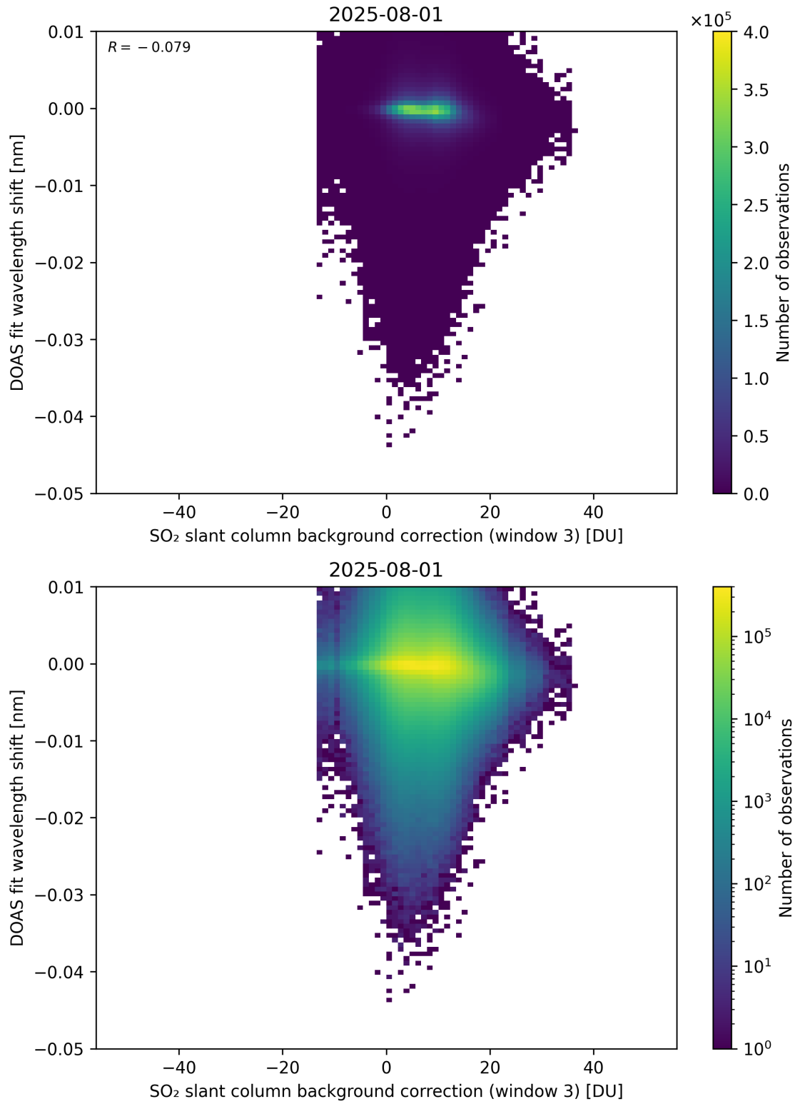
Figure 132: Scatter density plot of “SO 2 slant column background correction (window 3)” against “DOAS fit wavelength shift” for 2025-07-31 to 2025-08-02.
