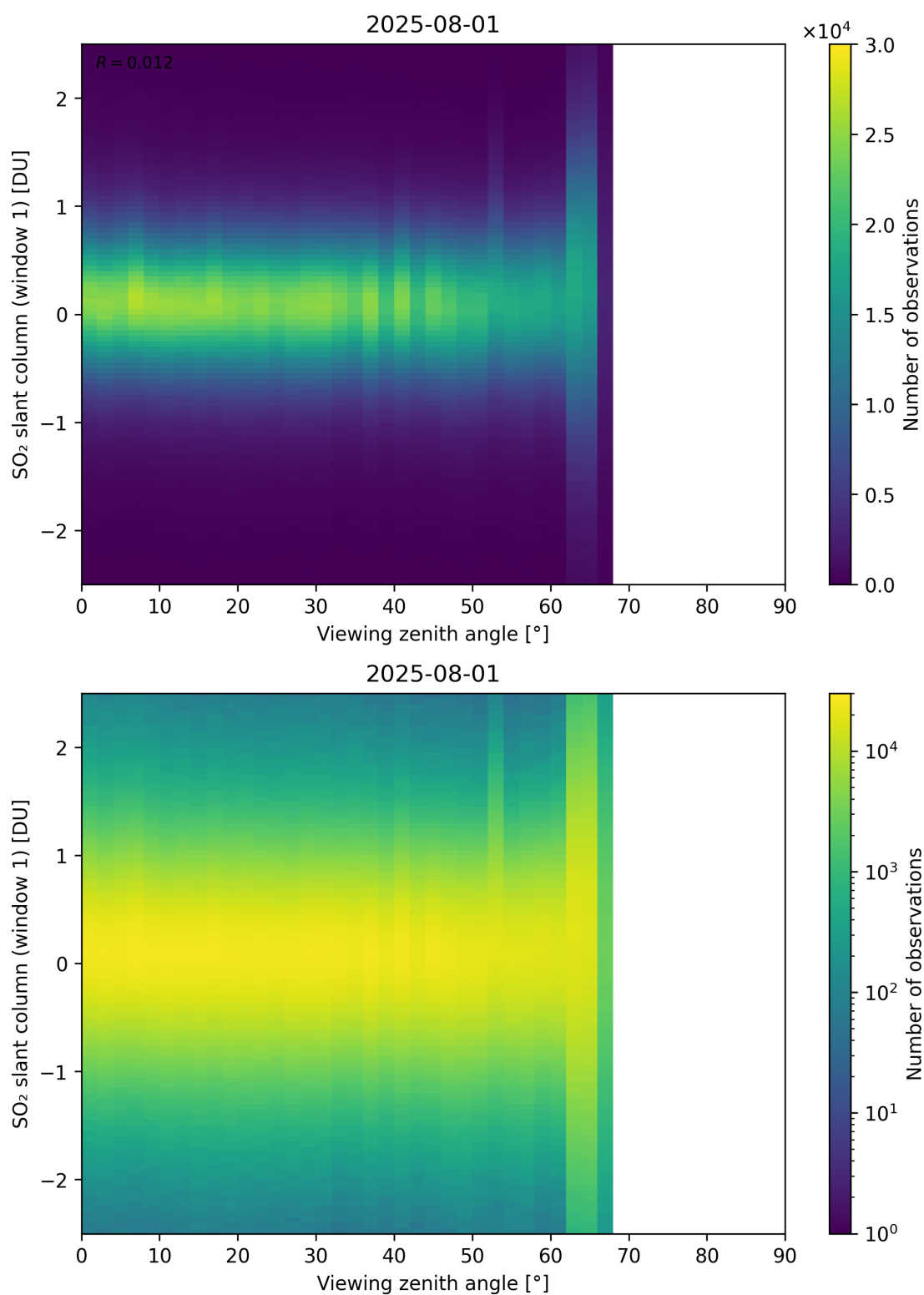
Figure 376: Scatter density plot of “Viewing zenith angle” against “SO 2 slant column (window 1)” for 2025-07-31 to 2025-08-02.
