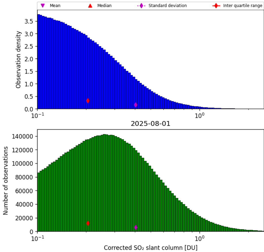
Figure 60: Histogram of "Corrected SO 2 slant column" for 2025-07-31 to 2025-08-02
