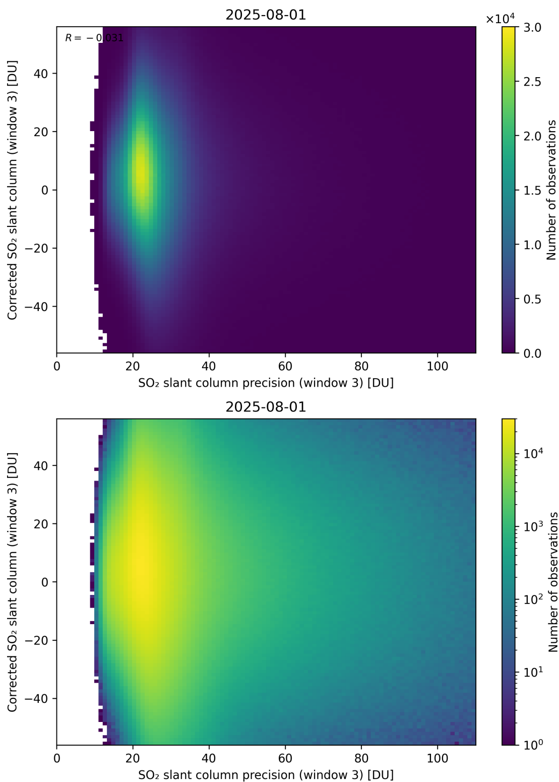
Figure 312: Scatter density plot of “SO 2 slant column precision (window 3)” against “Corrected SO 2 slant column (window 3)” for 2025-07-31 to 2025-08-02.
