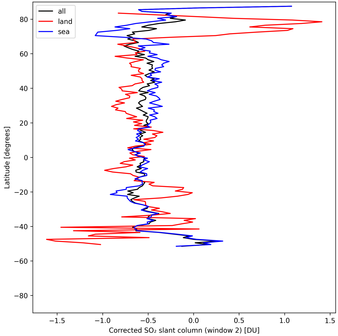
Figure 43: Zonal average of “Corrected SO 2 slant column (window 2)” for 2025-07-31 to 2025-08-02.
