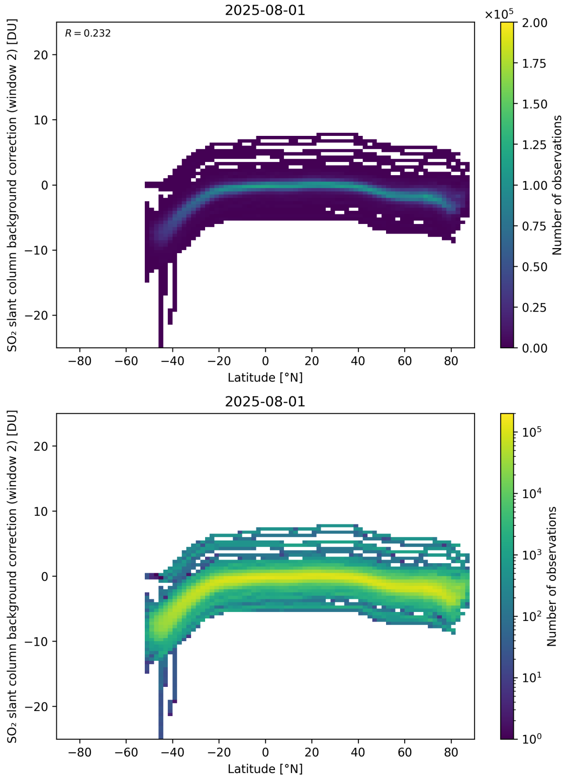
Figure 151: Scatter density plot of “Latitude” against “SO 2 slant column background correction (window 2)” for 2025-07-31 to 2025-08-02.
