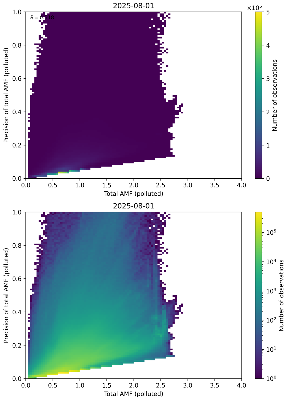
Figure 322: Scatter density plot of “Total AMF (polluted)” against “Precision of total AMF (polluted)” for 2025-07-31 to 2025-08-02.
