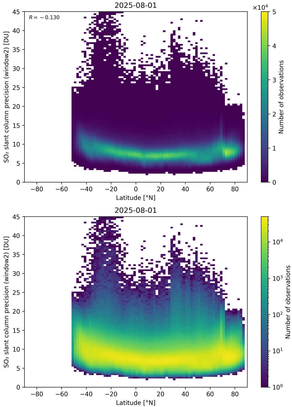
Figure 164: Scatter density plot of “Latitude” against “SO 2 slant column precision (window2)” for 2025-07-31 to 2025-08-02.
