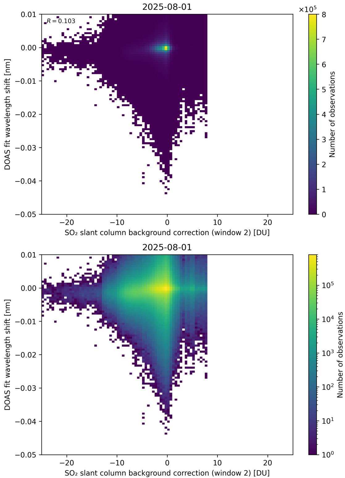
Figure 123: Scatter density plot of “SO 2 slant column background correction (window 2)” against “DOAS fit wavelength shift” for 2025-07-31 to 2025-08-02.
