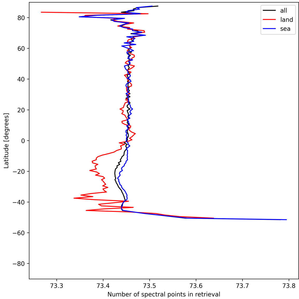
Figure 56: Zonal average of “Number of spectral points in retrieval” for 2025-07-31 to 2025-08-02.
