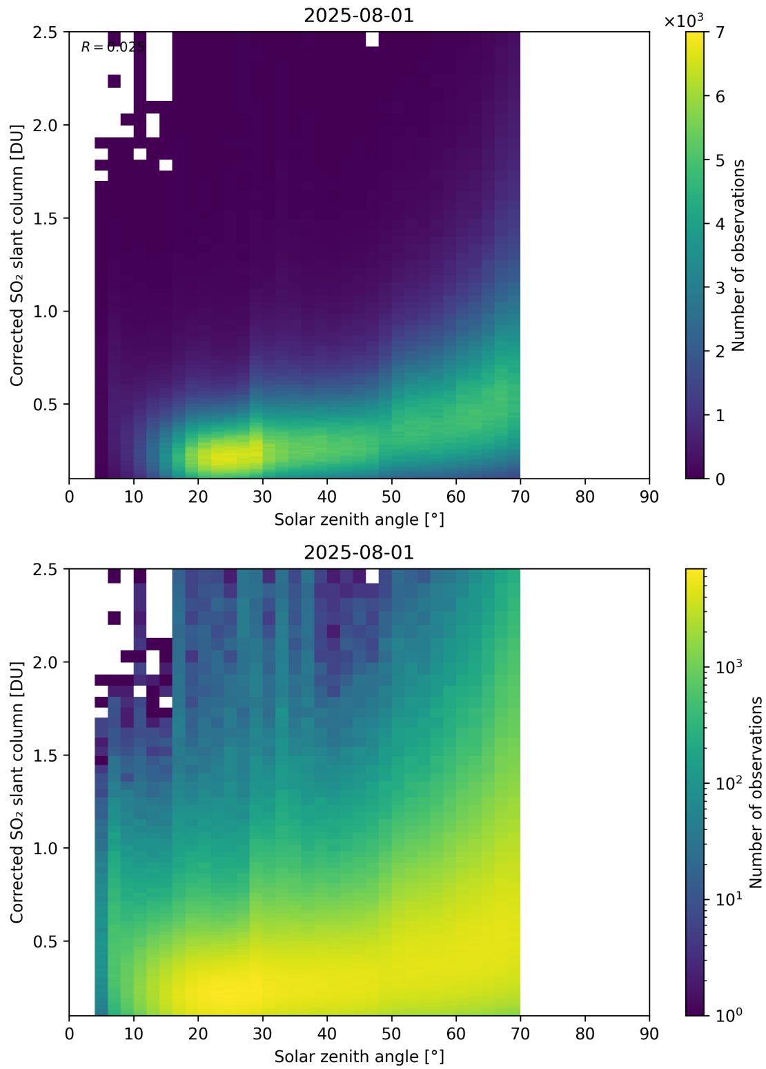
Figure 181: Scatter density plot of “Solar zenith angle” against “Corrected SO 2 slant column” for 2025-07-31 to 2025-08-02.
