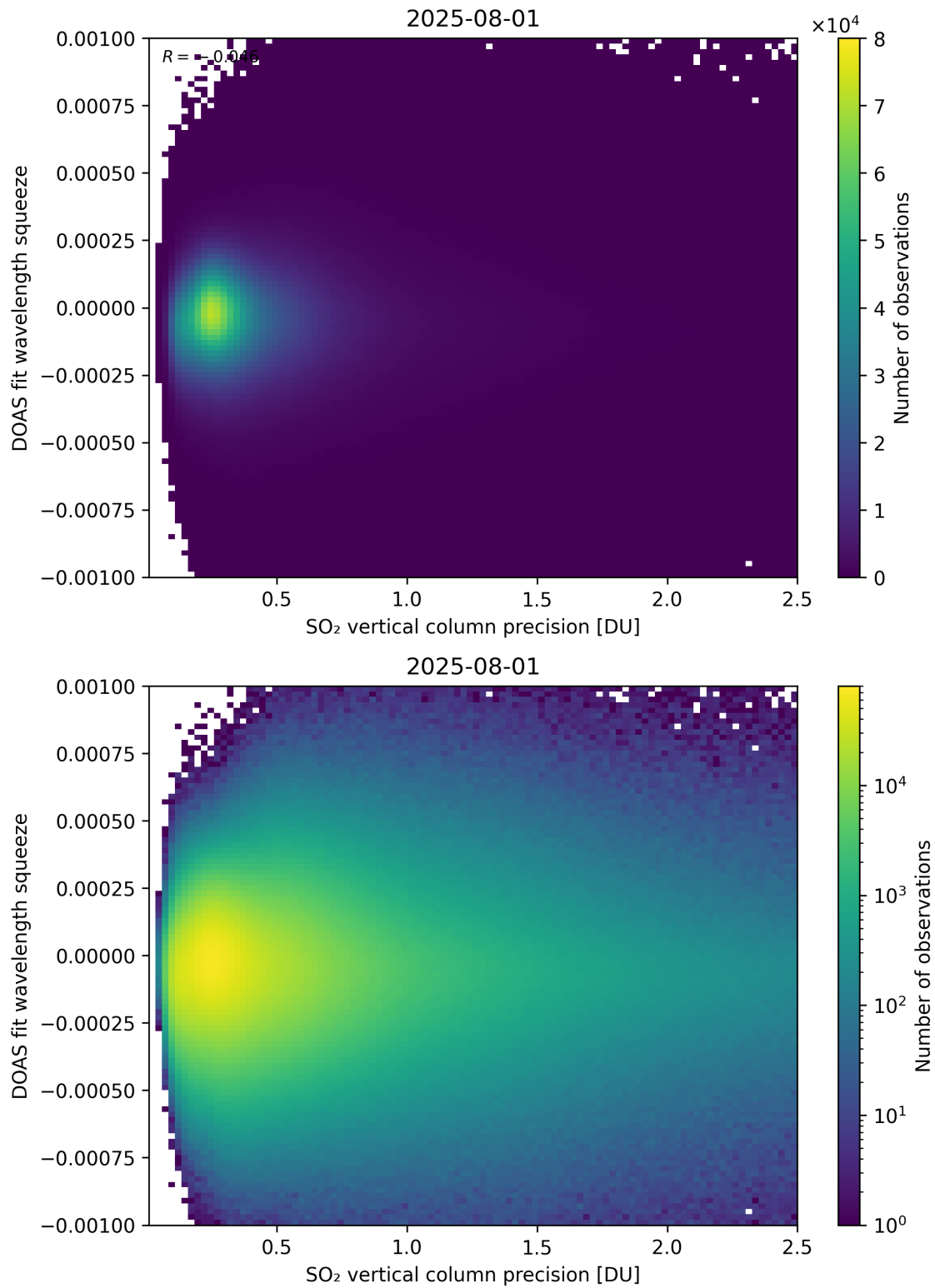
Figure 333: Scatter density plot of “SO 2 vertical column precision” against “DOAS fit wavelength squeeze” for 2025-07-31 to 2025-08-02.
