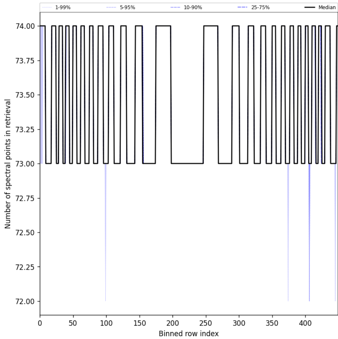
Figure 108: Along track statistics of “Number of spectral points in retrieval” for 2025-07-31 to 2025-08-02
