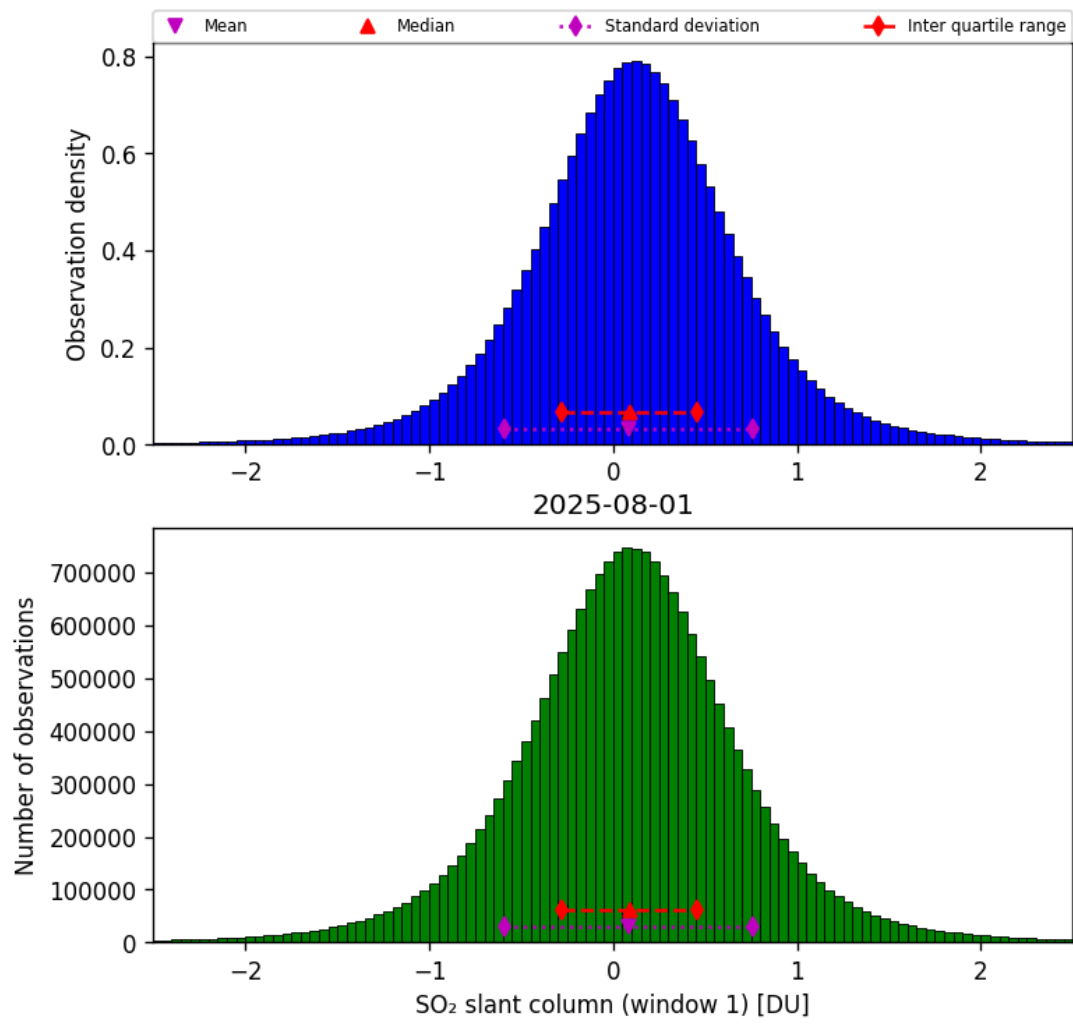
Figure 63: Histogram of “SO 2 slant column (window 1)” for 2025-07-31 to 2025-08-02
