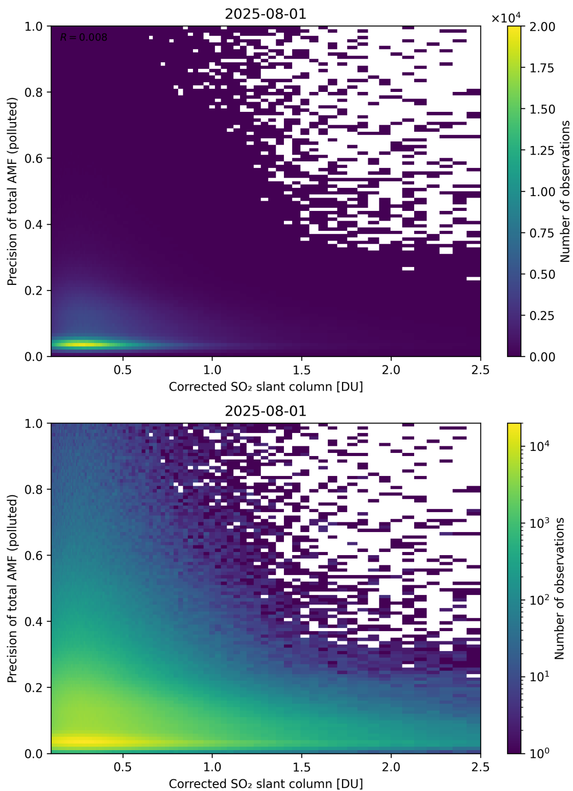
Figure 243: Scatter density plot of “Corrected SO 2 slant column” against “Precision of total AMF (polluted)” for 2025-07-31 to 2025-08-02.
