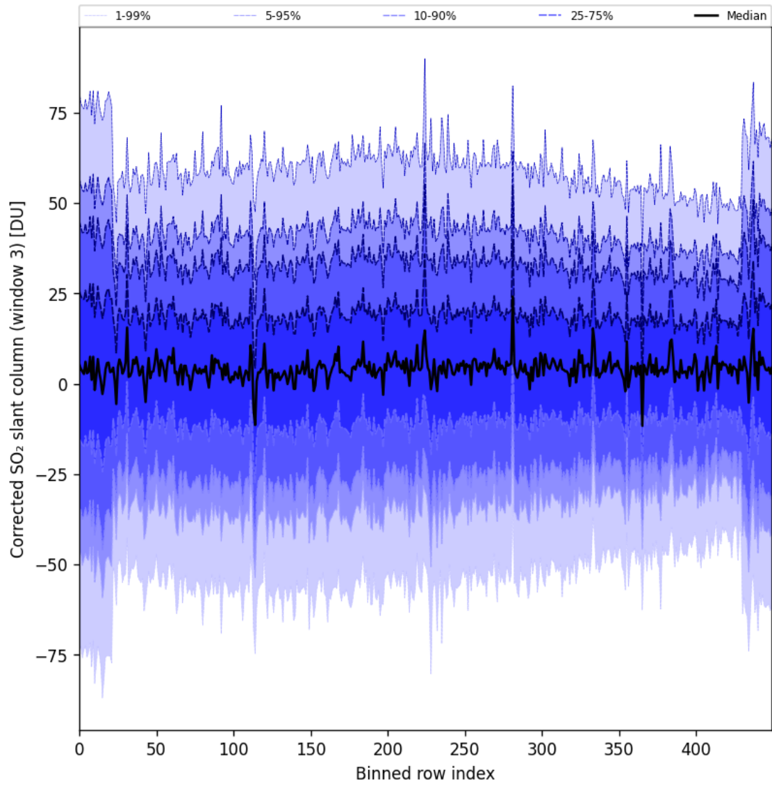
Figure 99: Along track statistics of "Corrected SO 2 slant column (window 3)" for 2025-07-31 to 2025-08-02
