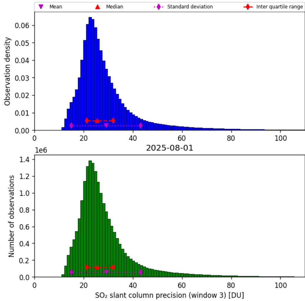
Figure 72: Histogram of “SO 2 slant column precision (window 3)” for 2025-07-31 to 2025-08-02
