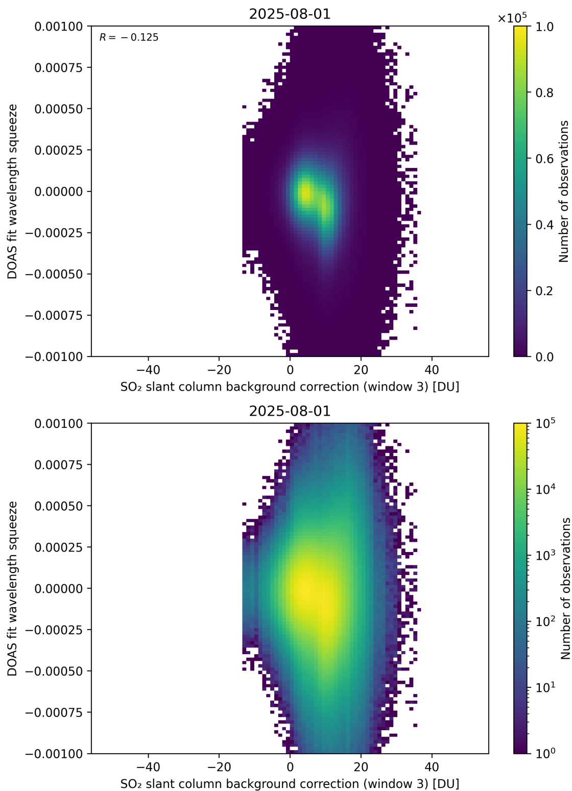
Figure 133: Scatter density plot of “SO 2 slant column background correction (window 3)” against “DOAS fit wavelength squeeze” for 2025-07-31 to 2025-08-02.
