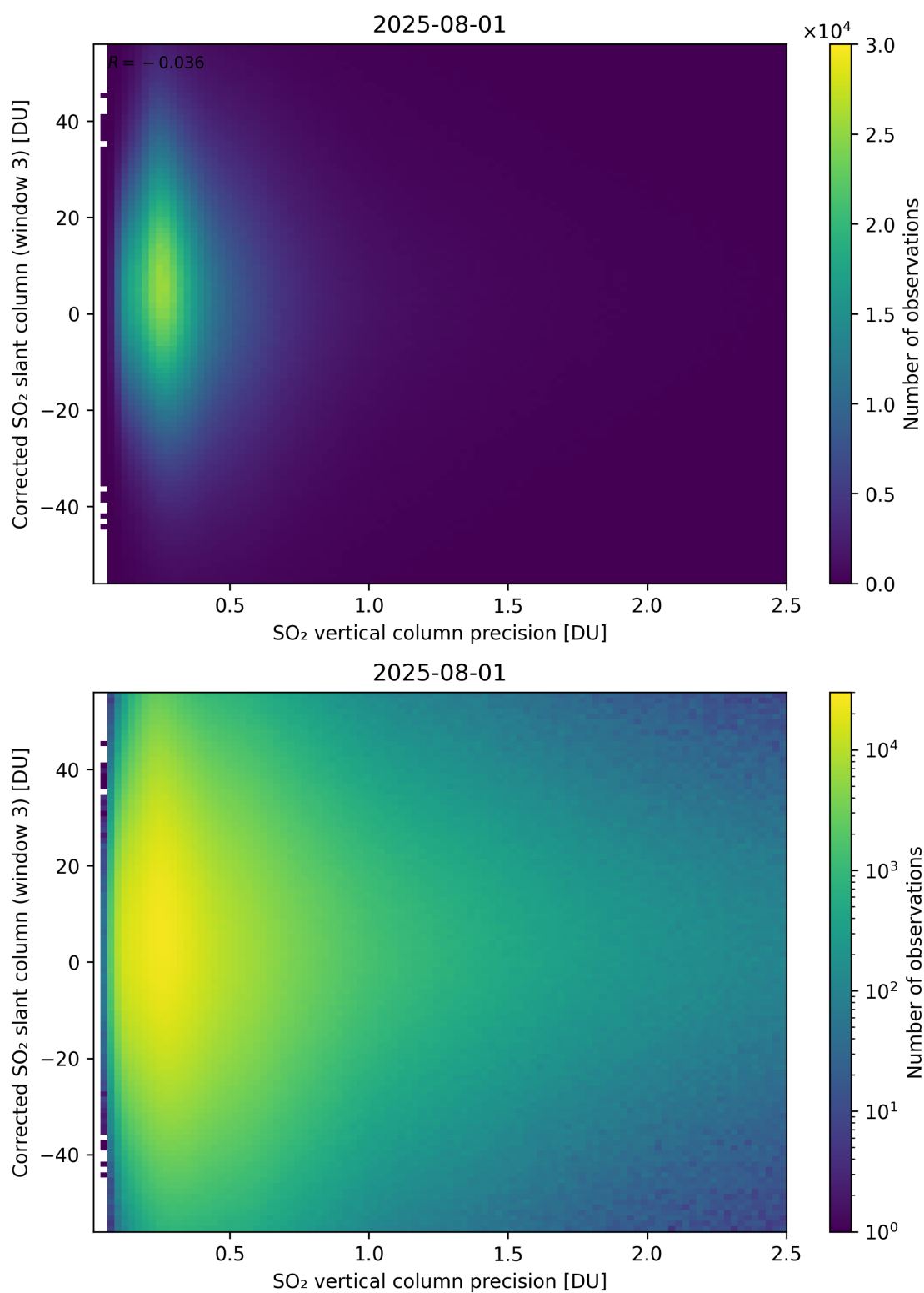
Figure 340: Scatter density plot of “SO 2 vertical column precision” against “Corrected SO 2 slant column (window 3)” for 2025-07-31 to 2025-08-02.
