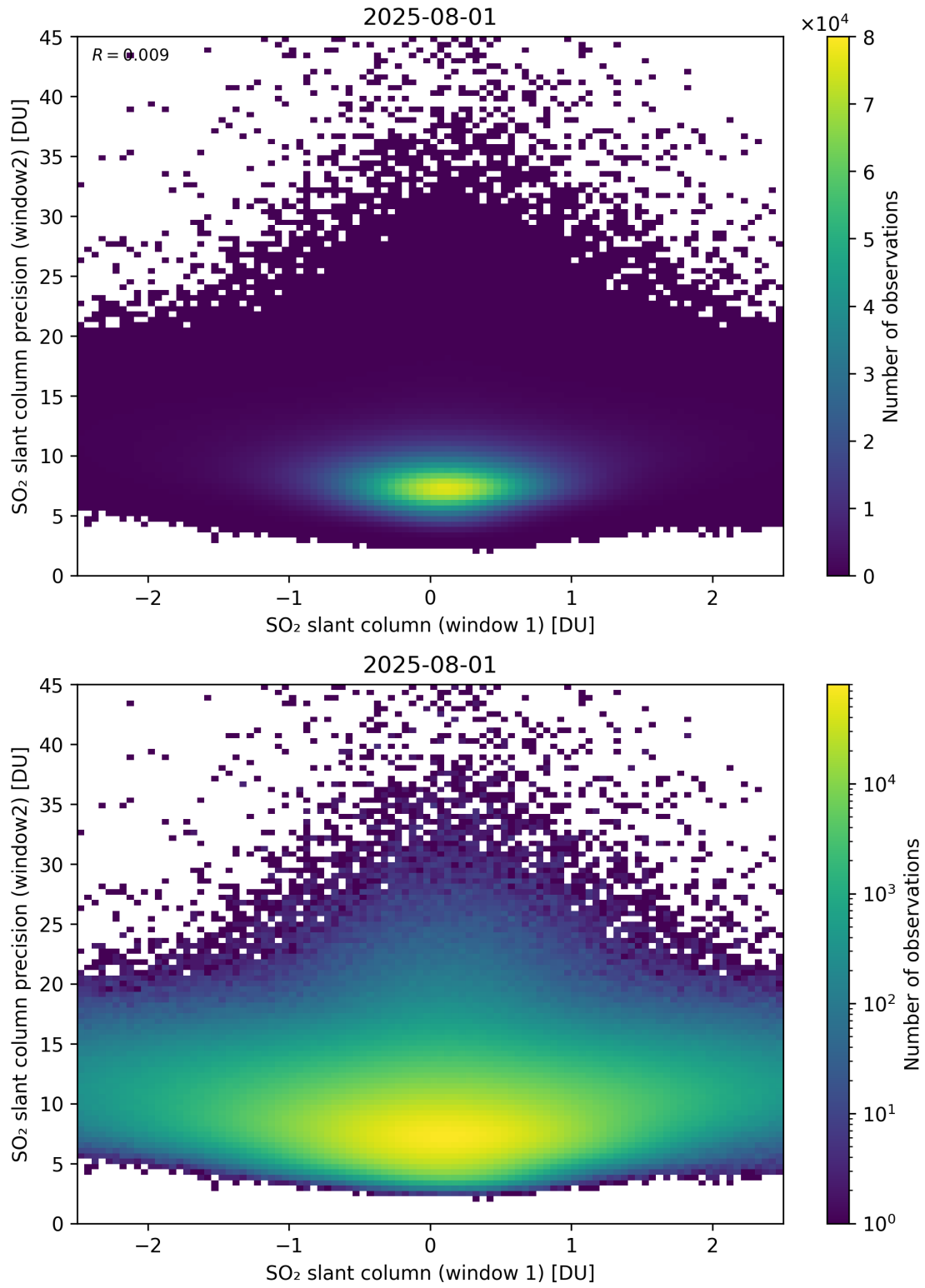
Figure 286: Scatter density plot of “SO 2 slant column (window 1)” against “SO 2 slant column precision (window2)” for 2025-07-31 to 2025-08-02.
