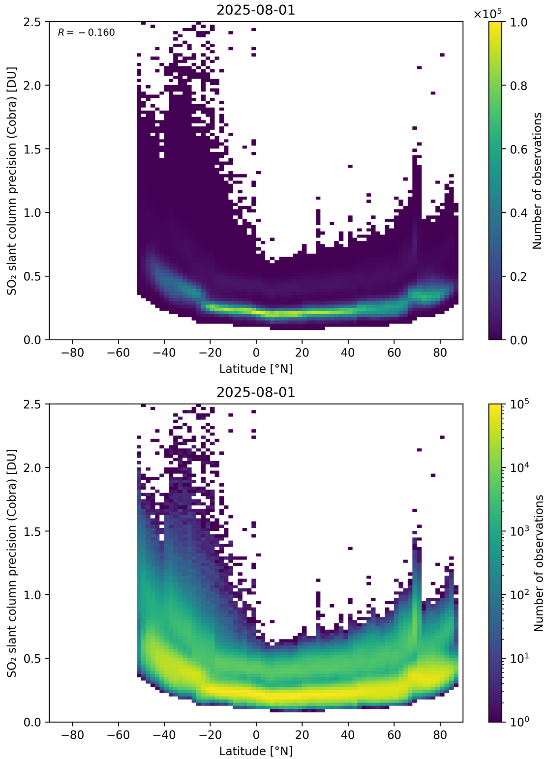
Figure 158: Scatter density plot of “Latitude” against “SO 2 slant column precision (Cobra)” for 2025-07-31 to 2025-08-02.
