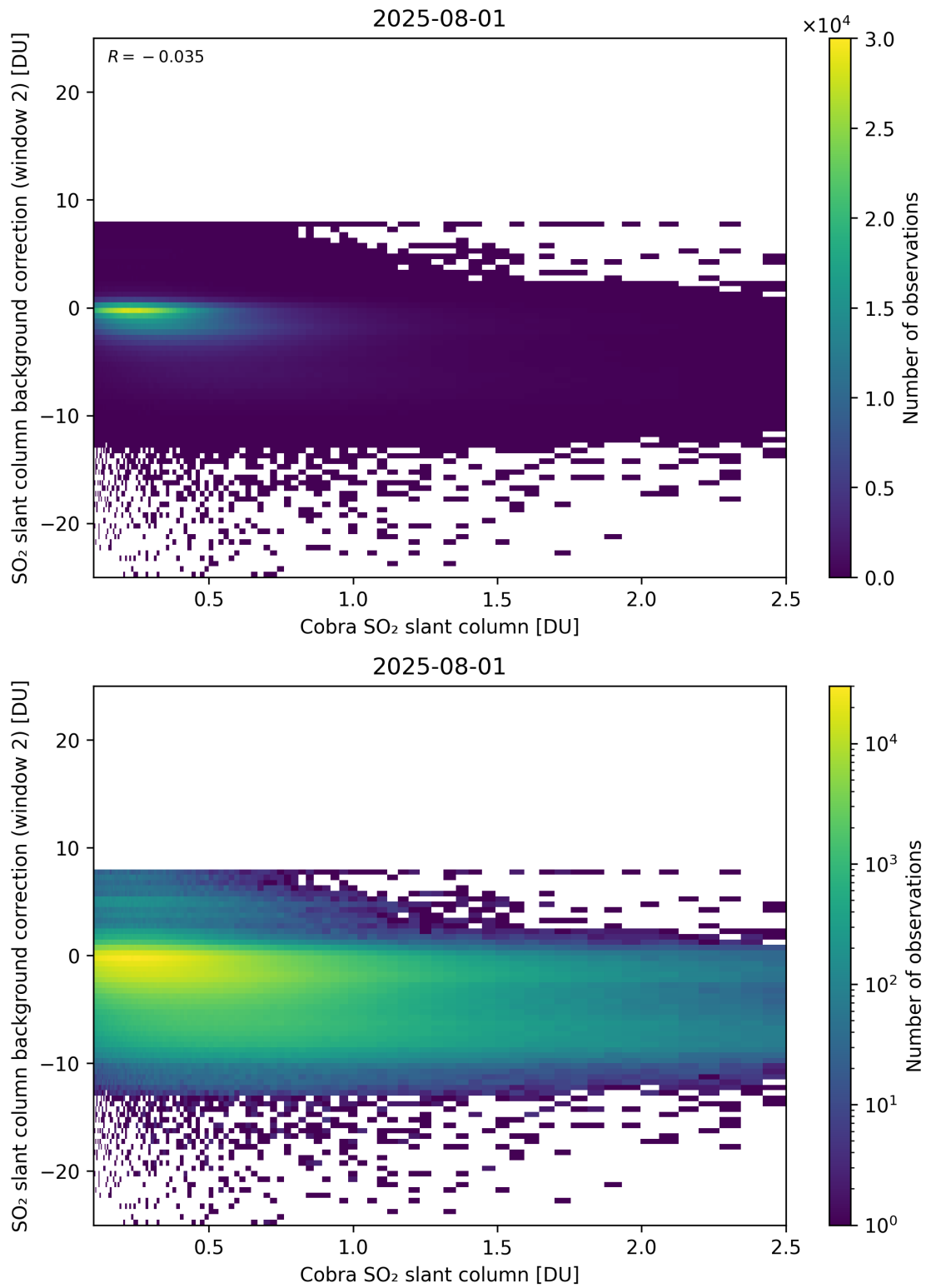
Figure 194: Scatter density plot of “Cobra SO 2 slant column” against “SO 2 slant column background correction (window 2)” for 2025-07-31 to 2025-08-02.
