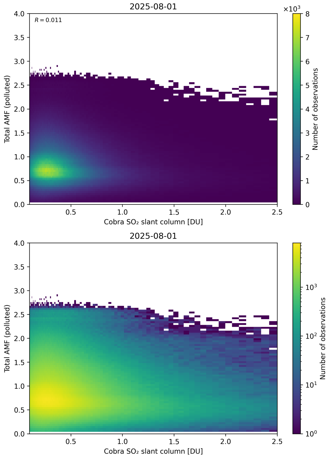
Figure 224: Scatter density plot of “Cobra SO 2 slant column” against “Total AMF (polluted)” for 2025-07-31 to 2025-08-02.
