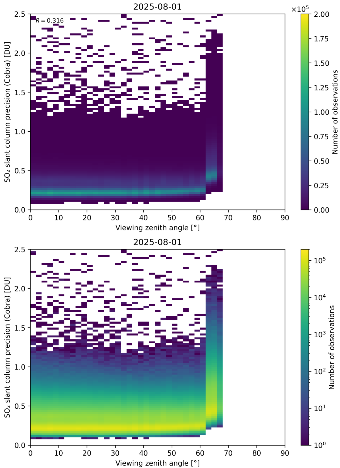
Figure 372: Scatter density plot of “Viewing zenith angle” against “SO 2 slant column precision (Cobra)” for 2025-07-31 to 2025-08-02.
