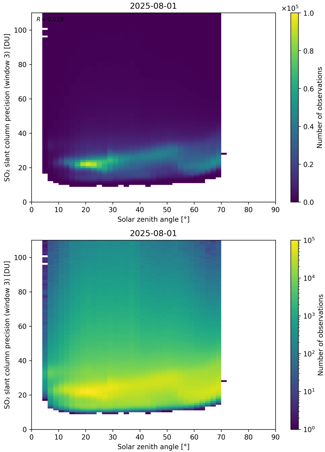
Figure 188: Scatter density plot of “Solar zenith angle” against “SO 2 slant column precision (window 3)” for 2025-07-31 to 2025-08-02.
