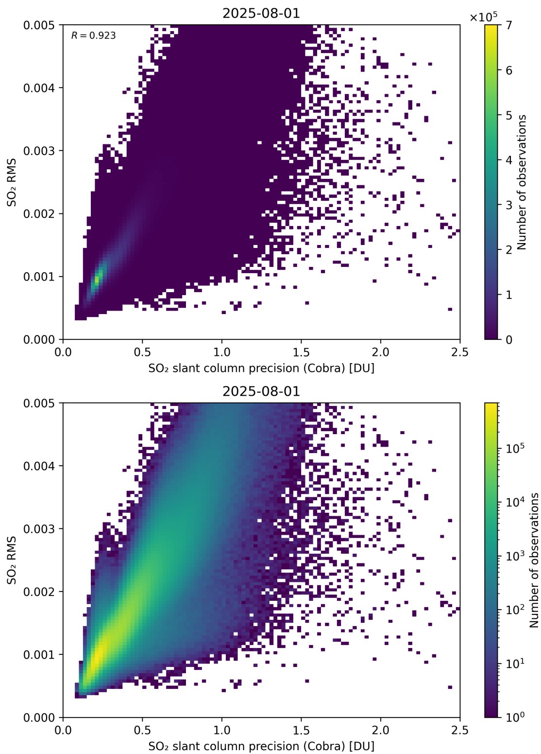
Figure 204: Scatter density plot of “SO 2 slant column precision (Cobra)” against “SO 2 RMS” for 2025-07-31 to 2025-08-02.
