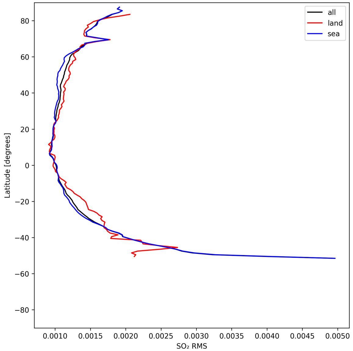
Figure 52: Zonal average of “SO 2 RMS” for 2025-07-31 to 2025-08-02.
