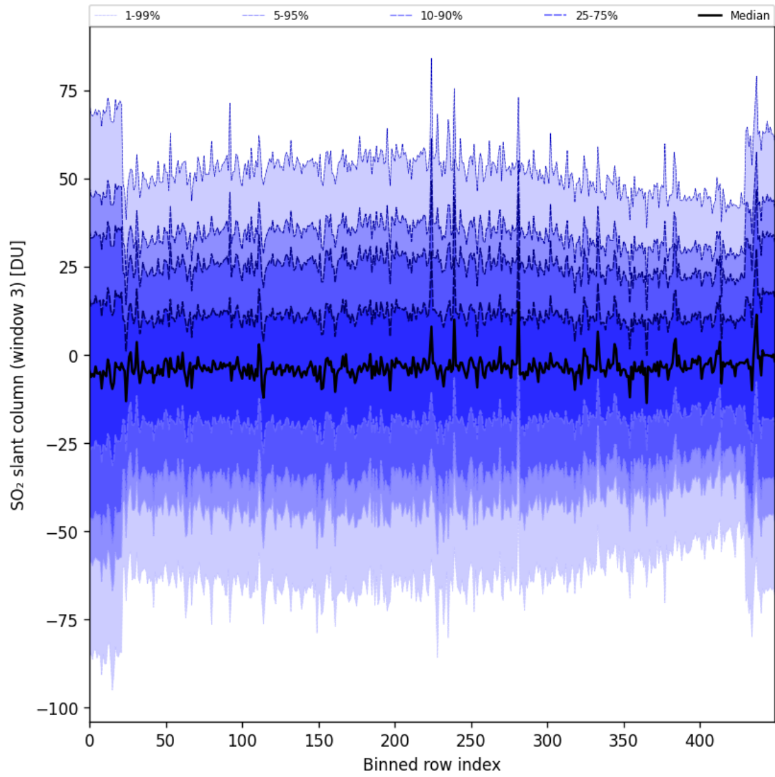
Figure 97: Along track statistics of “SO 2 slant column (window 3)” for 2025-07-31 to 2025-08-02
