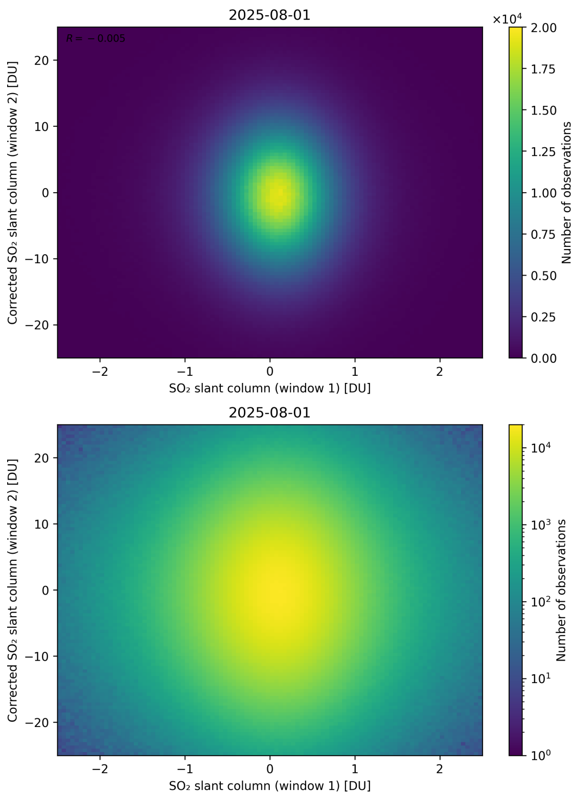
Figure 283: Scatter density plot of “SO 2 slant column (window 1)” against “Corrected SO 2 slant column (window 2)” for 2025-07-31 to 2025-08-02.
