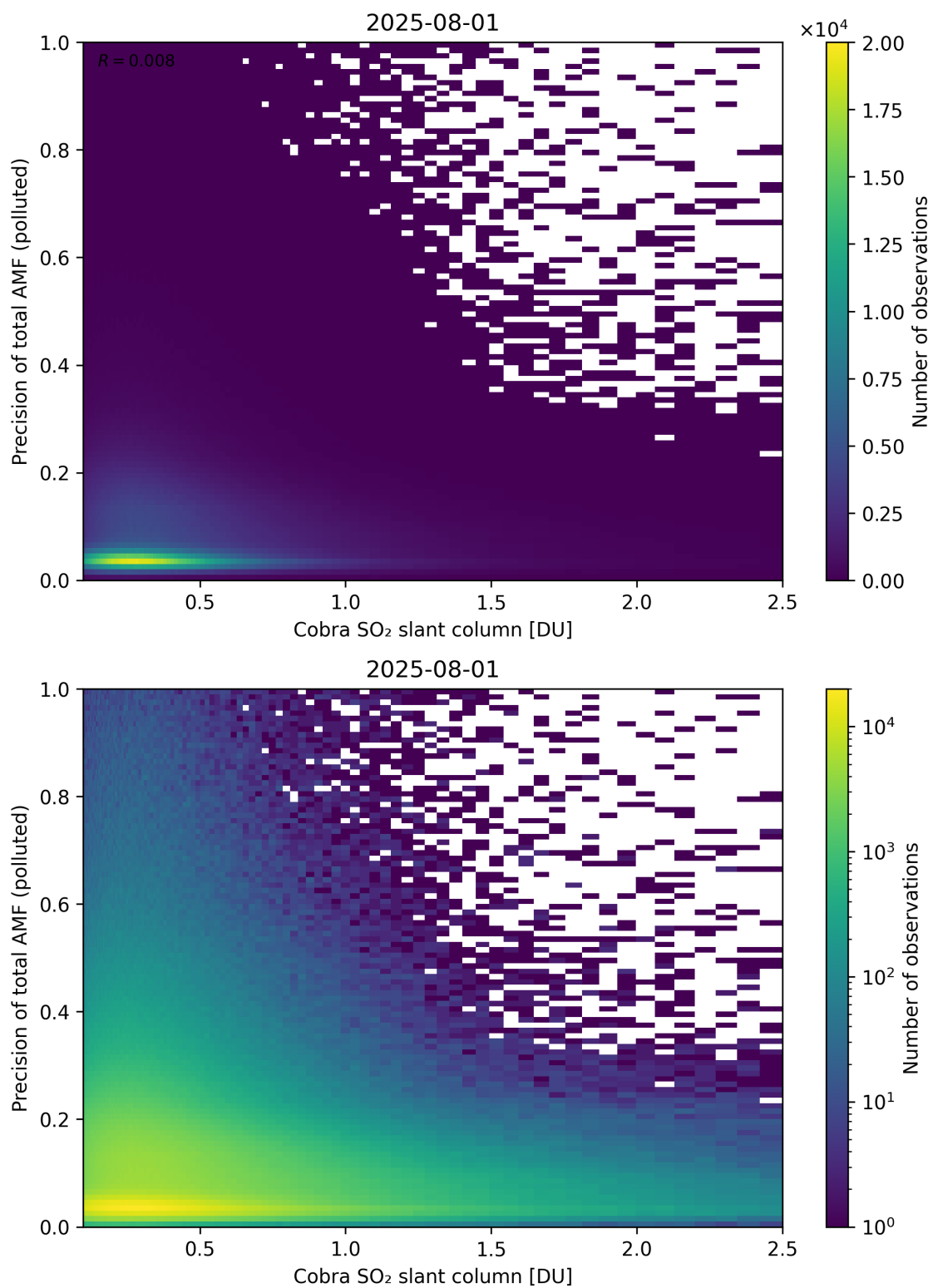
Figure 225: Scatter density plot of “Cobra SO 2 slant column” against “Precision of total AMF (polluted)” for 2025-07-31 to 2025-08-02.
