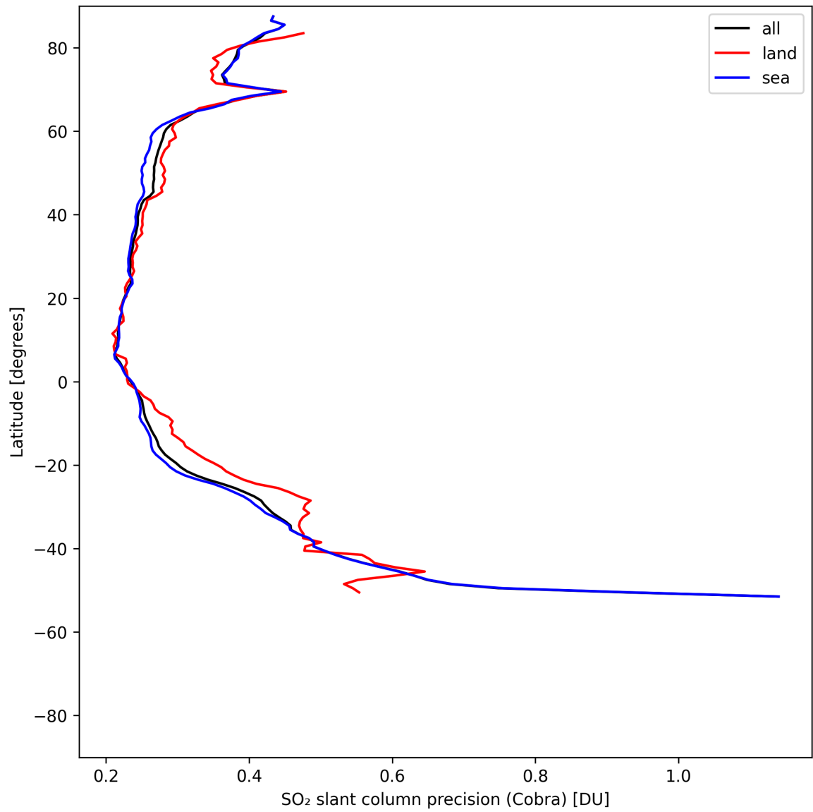
Figure 36: Zonal average of “SO 2 slant column precision (Cobra)” for 2025-07-31 to 2025-08-02.
