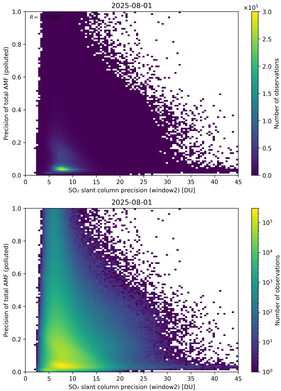
Figure 302: Scatter density plot of “SO 2 slant column precision (window2)” against “Precision of total AMF (polluted)” for 2025-07-31 to 2025-08-02.
