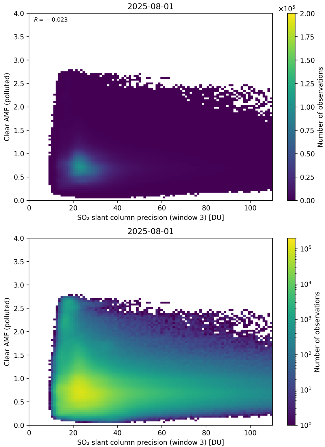
Figure 311: Scatter density plot of “SO 2 slant column precision (window 3)” against “Clear AMF (polluted)” for 2025-07-31 to 2025-08-02.
