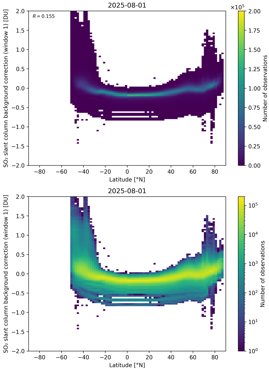
Figure 150: Scatter density plot of “Latitude” against “SO 2 slant column background correction (window 1)” for 2025-07-31 to 2025-08-02.
