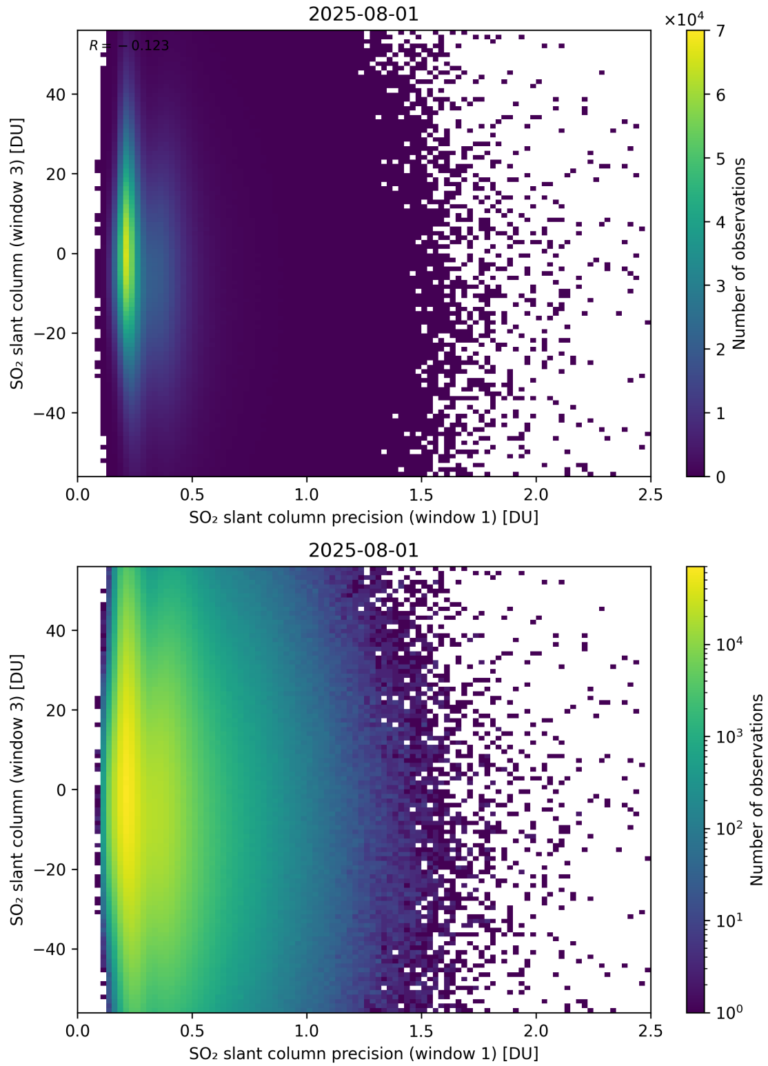
Figure 278: Scatter density plot of “SO 2 slant column precision (window 1)” against “SO 2 slant column (window 3)” for 2025-07-31 to 2025-08-02.
