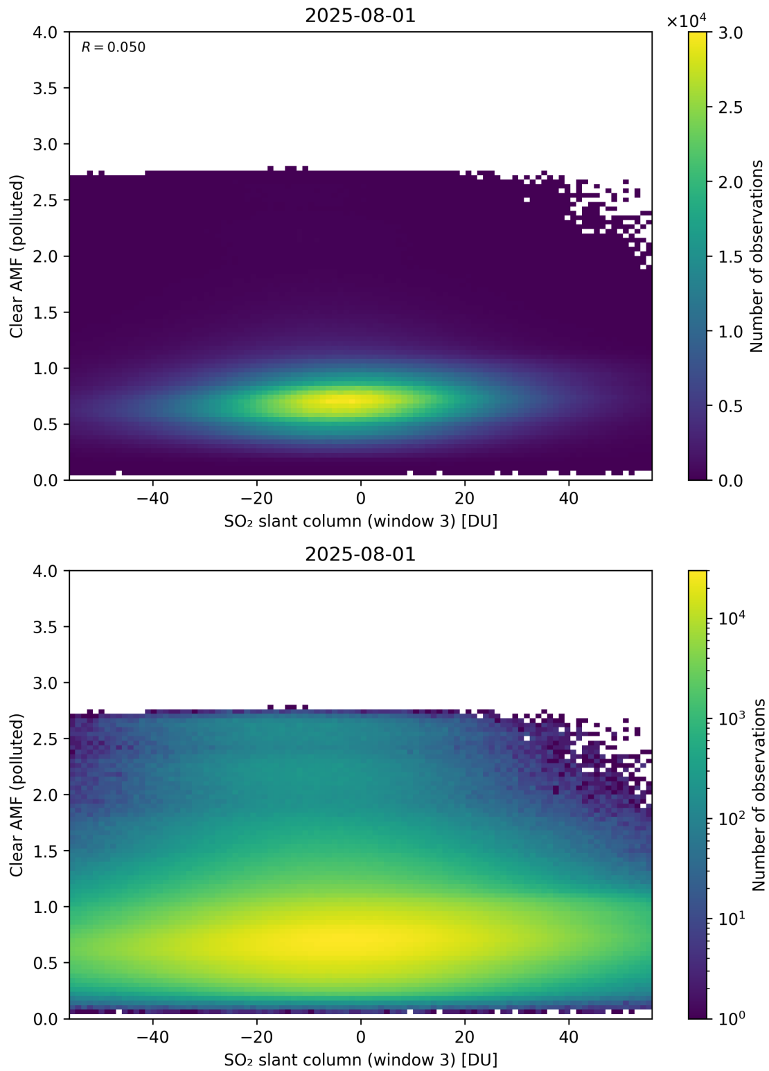
Figure 315: Scatter density plot of “SO 2 slant column (window 3)” against “Clear AMF (polluted)” for 2025-07-31 to 2025-08-02.
