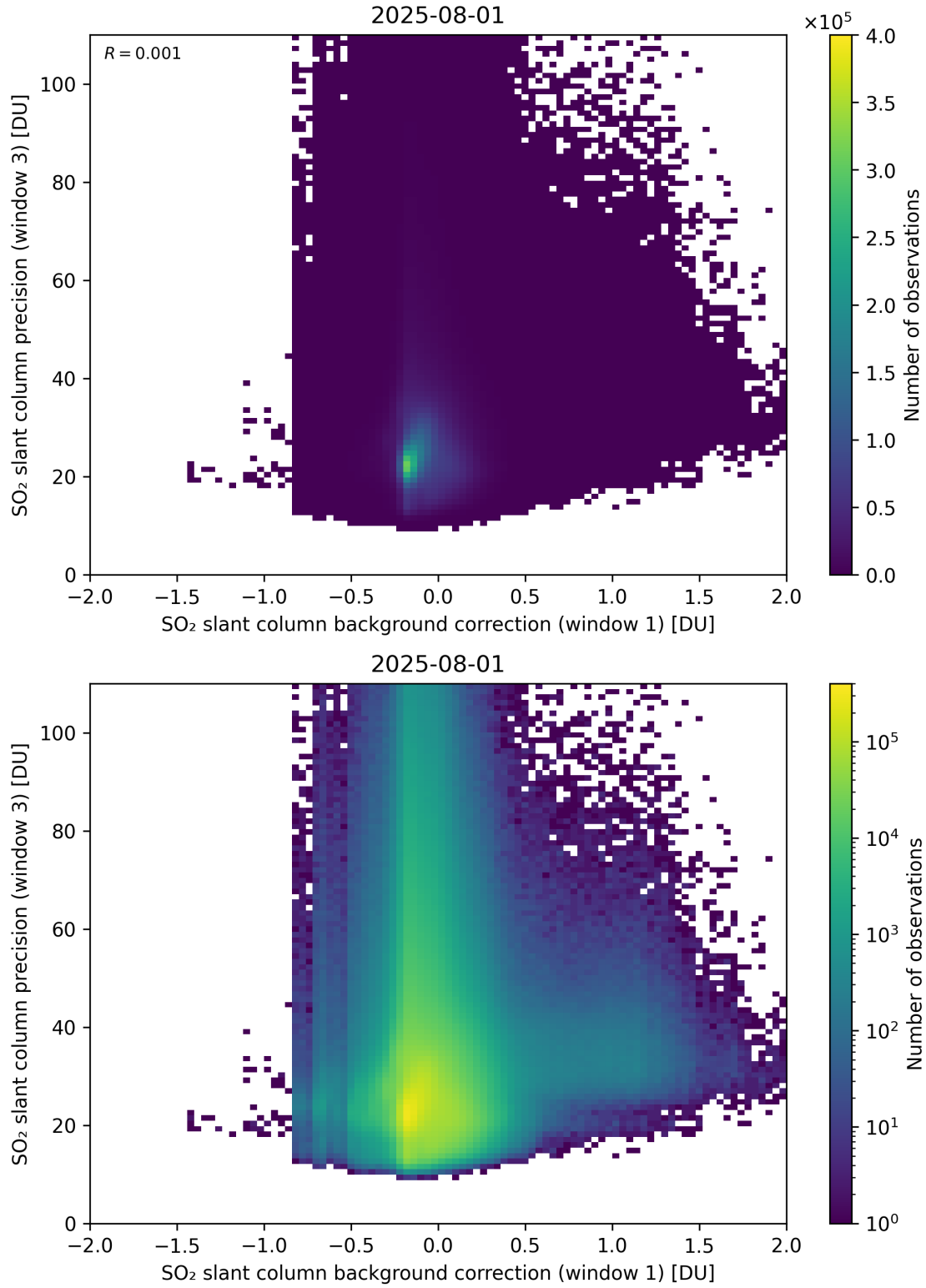
Figure 119: Scatter density plot of “SO 2 slant column background correction (window 1)” against “SO 2 slant column precision (window 3)” for 2025-07-31 to 2025-08-02.
