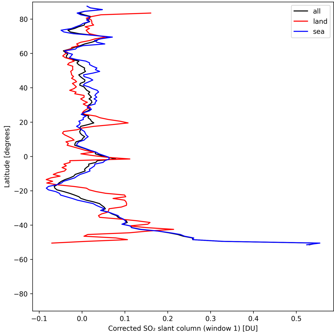
Figure 39: Zonal average of “Corrected SO 2 slant column (window 1)” for 2025-07-31 to 2025-08-02.
