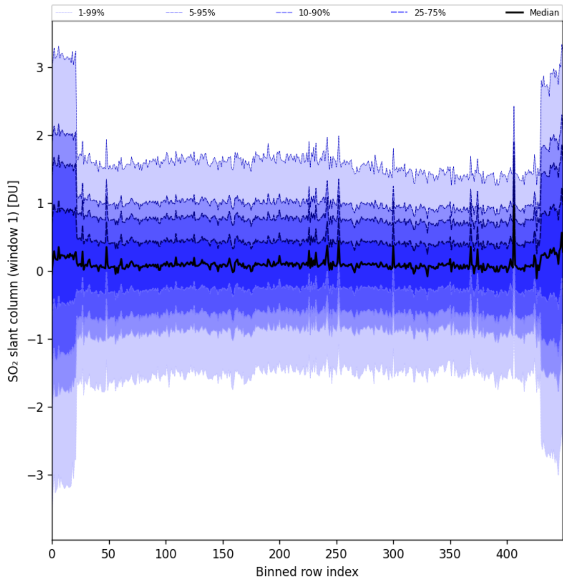
Figure 89: Along track statistics of “SO 2 slant column (window 1)” for 2025-07-31 to 2025-08-02
