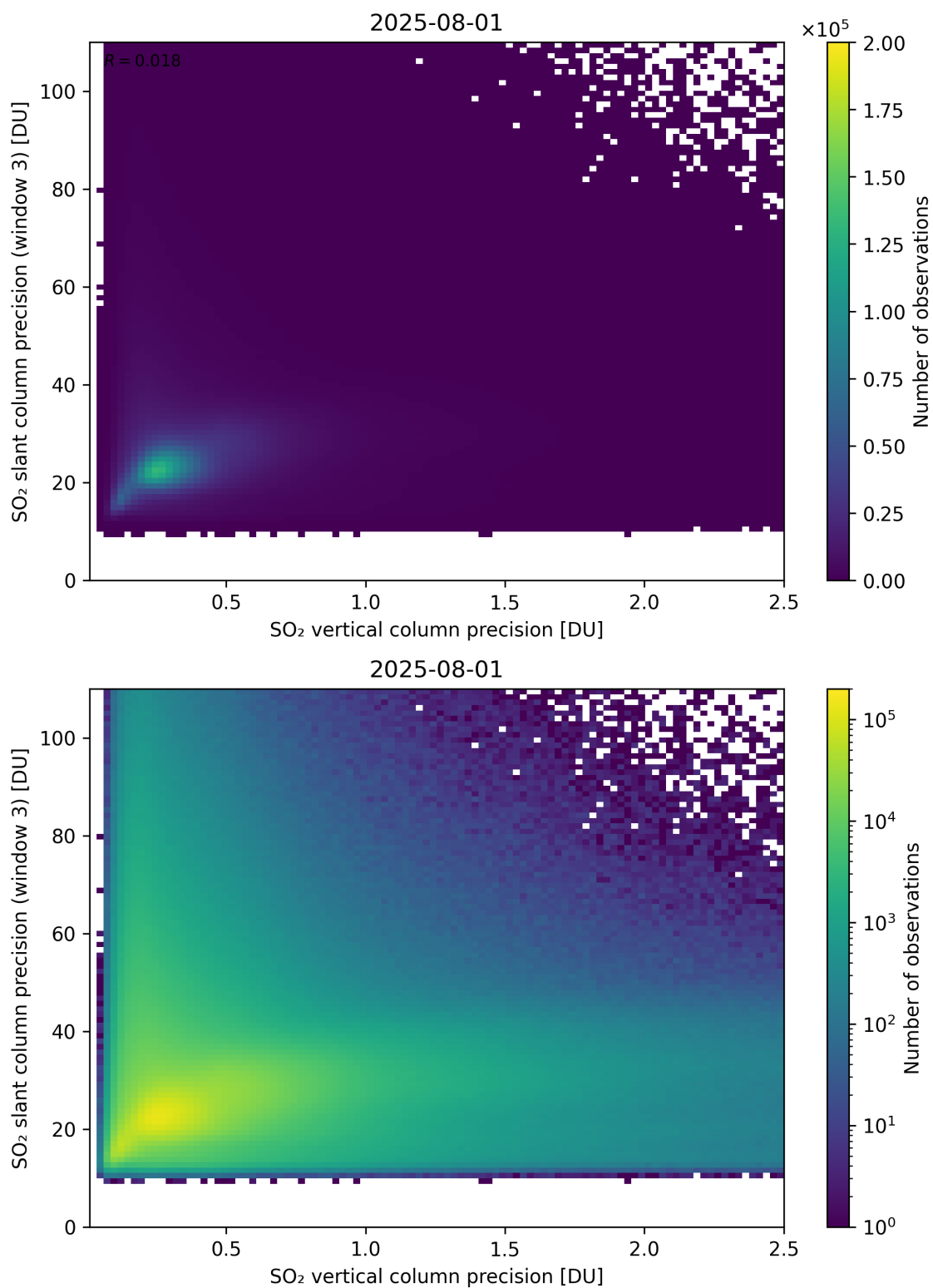
Figure 345: Scatter density plot of “SO 2 vertical column precision” against “SO 2 slant column precision (window 3)” for 2025-07-31 to 2025-08-02.
