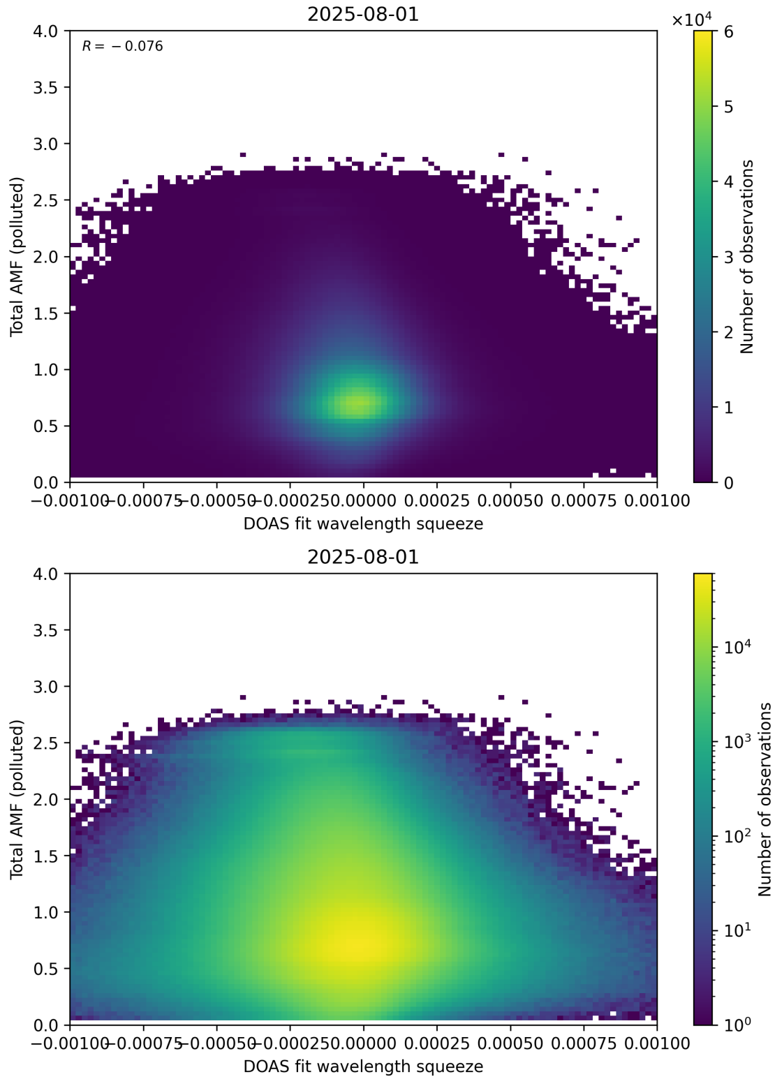
Figure 145: Scatter density plot of “DOAS fit wavelength squeeze” against “Total AMF (polluted)” for 2025-07-31 to 2025-08-02.
