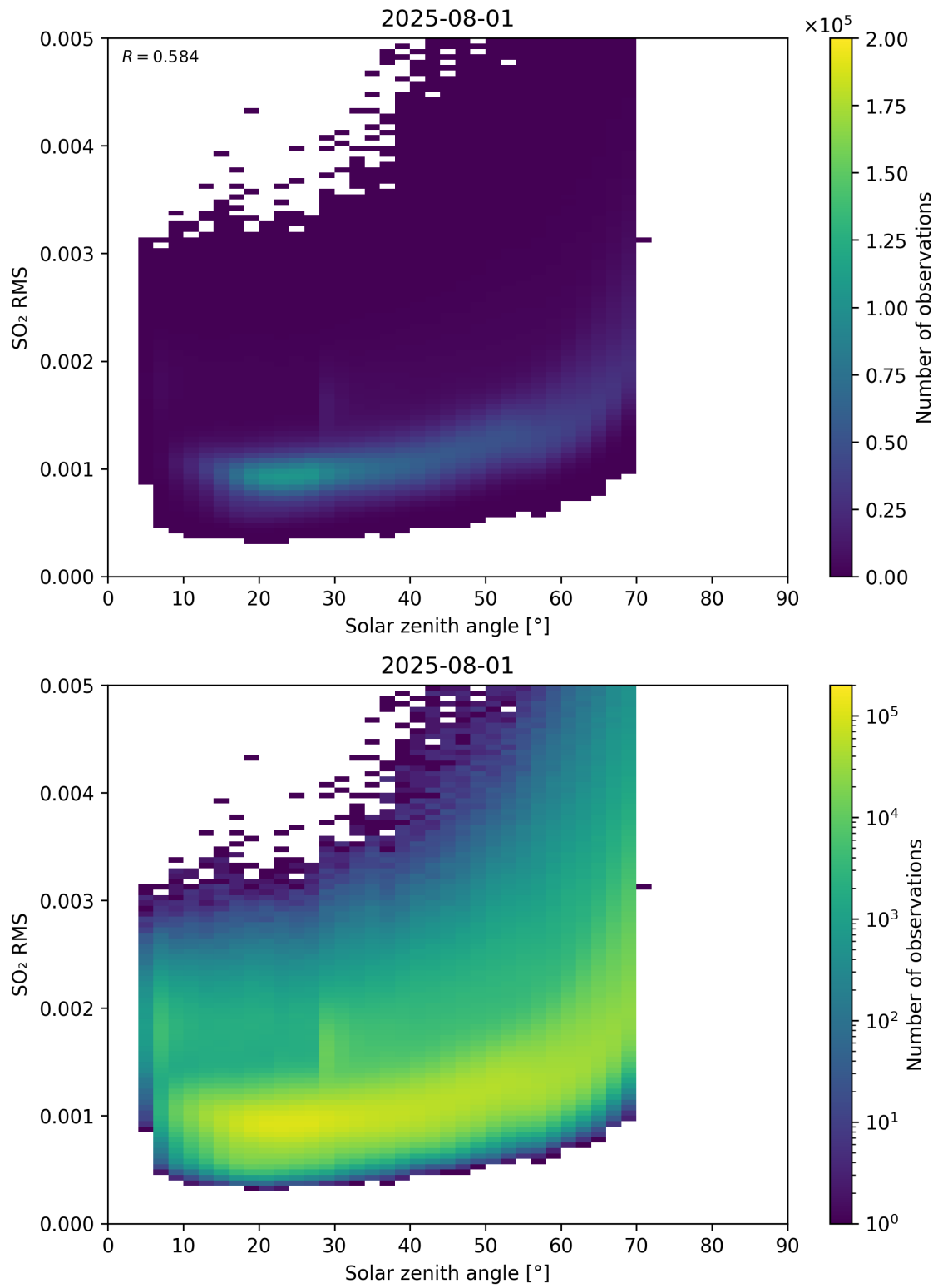
Figure 176: Scatter density plot of “Solar zenith angle” against “SO 2 RMS” for 2025-07-31 to 2025-08-02.
