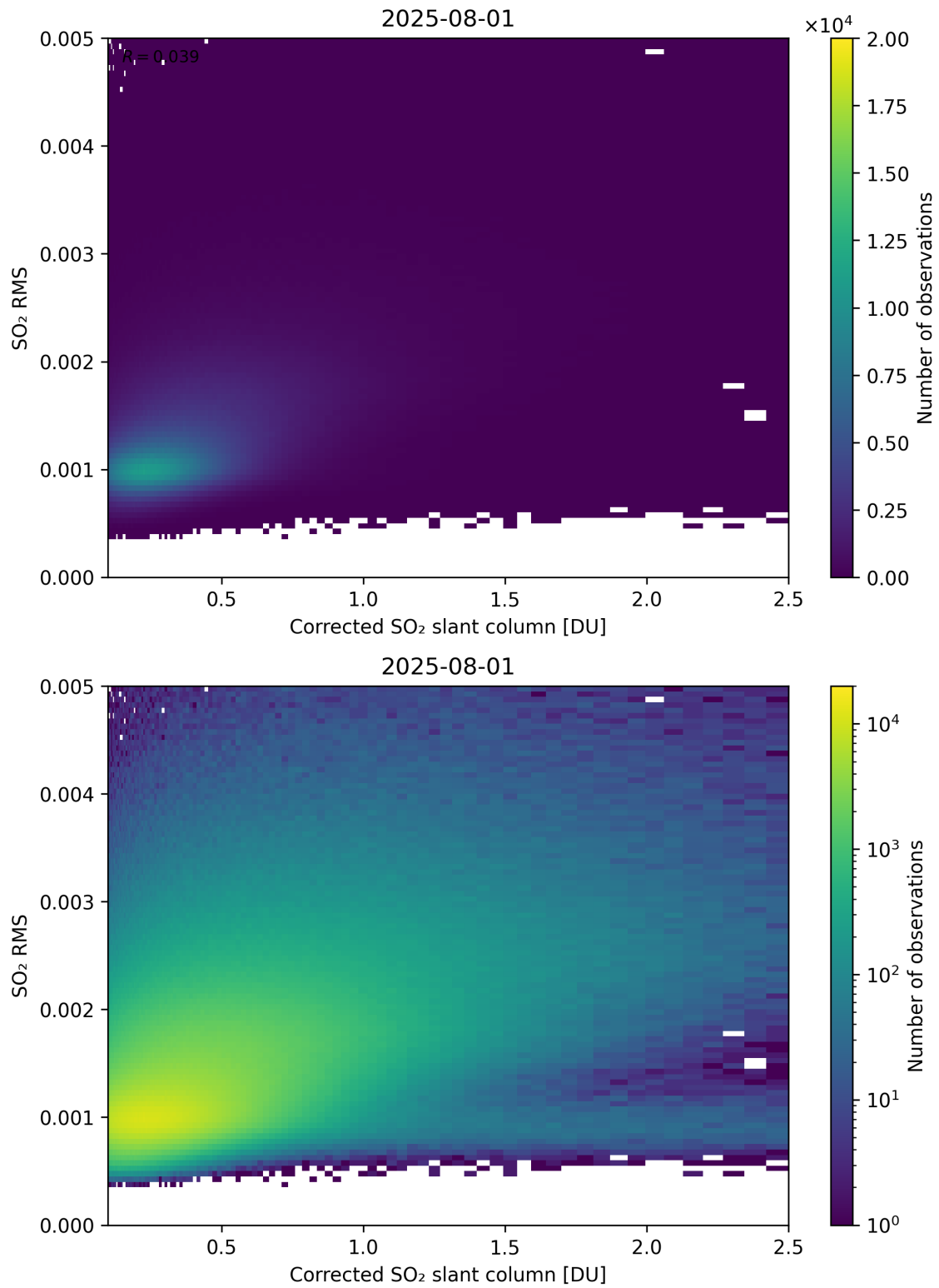
Figure 231: Scatter density plot of “Corrected SO 2 slant column” against “SO 2 RMS” for 2025-07-31 to 2025-08-02.
