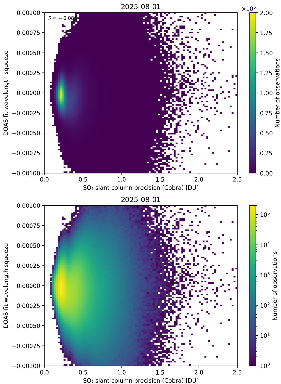
Figure 203: Scatter density plot of “SO 2 slant column precision (Cobra)” against “DOAS fit wavelength squeeze” for 2025-07-31 to 2025-08-02.
