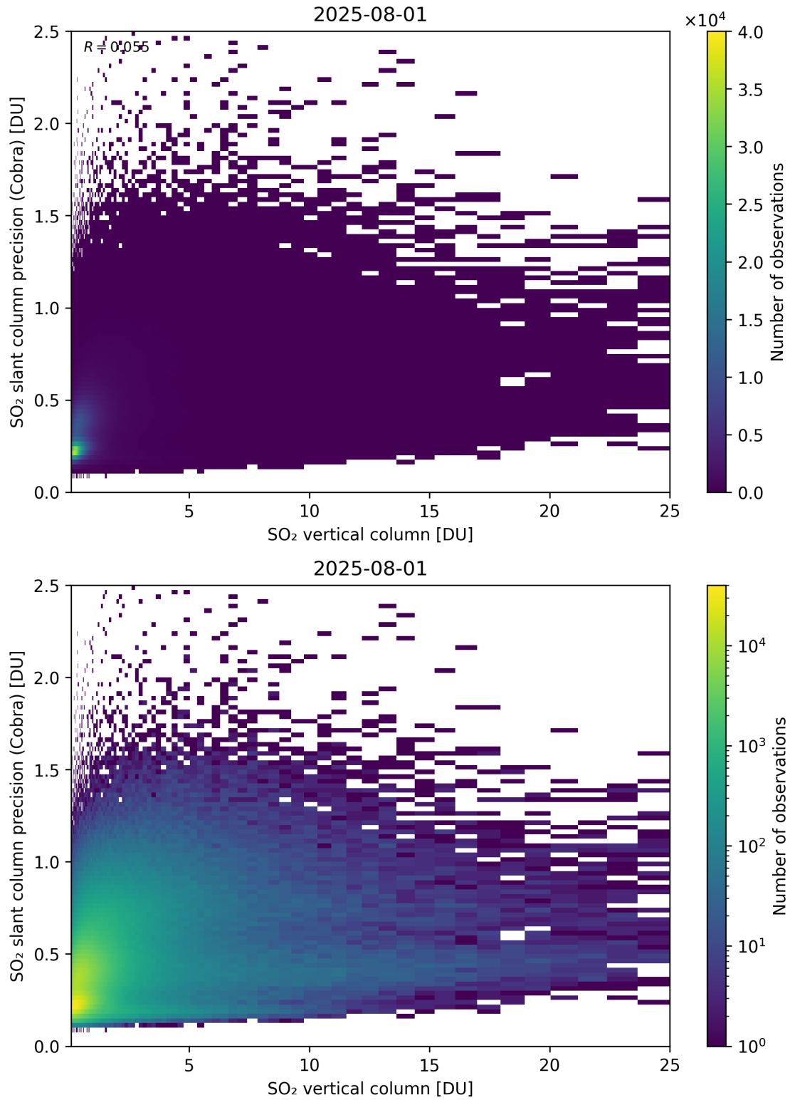
Figure 350: Scatter density plot of “SO 2 vertical column” against “SO 2 slant column precision (Cobra)” for 2025-07-31 to 2025-08-02.
