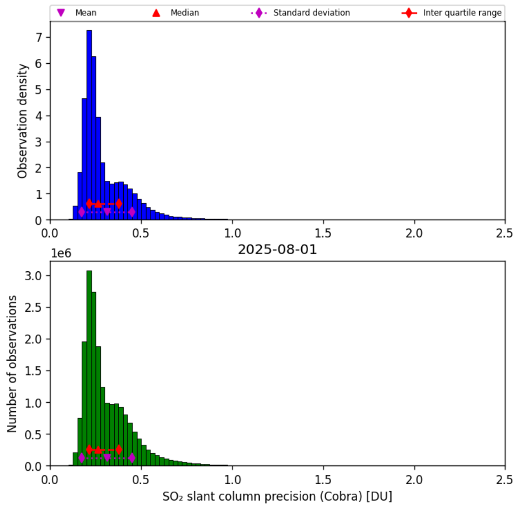
Figure 62: Histogram of “SO 2 slant column precision (Cobra)” for 2025-07-31 to 2025-08-02
