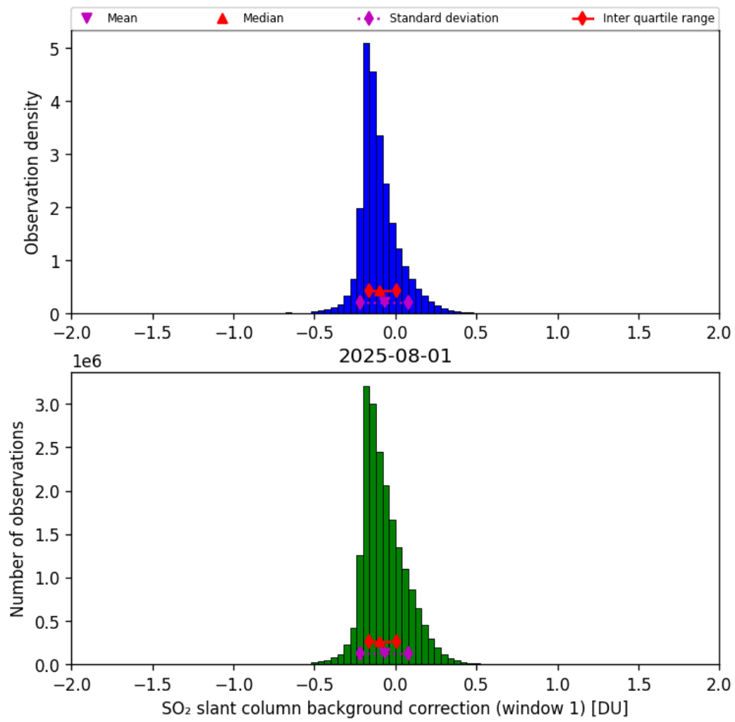
Figure 66: Histogram of “SO 2 slant column background correction (window 1)” for 2025-07-31 to 2025-08-02
