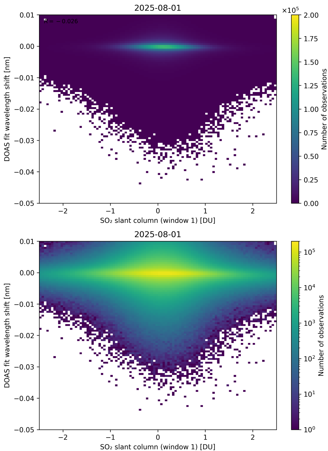
Figure 265: Scatter density plot of “SO 2 slant column (window 1)” against “DOAS fit wavelength shift” for 2025-07-31 to 2025-08-02.
