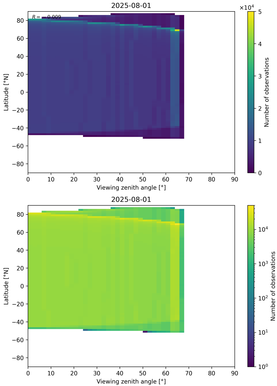
Figure 368: Scatter density plot of “Viewing zenith angle” against “Latitude” for 2025-07-31 to 2025-08-02.
