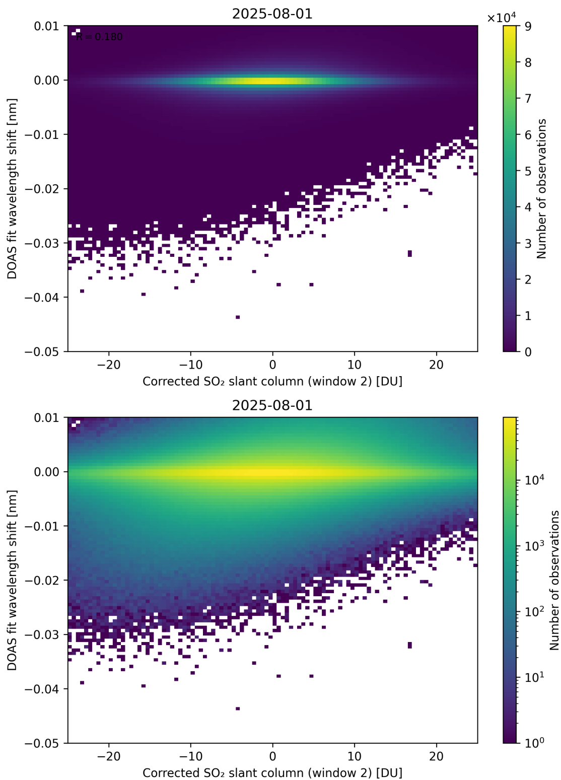
Figure 246: Scatter density plot of “Corrected SO 2 slant column (window 2)” against “DOAS fit wavelength shift” for 2025-07-31 to 2025-08-02.
