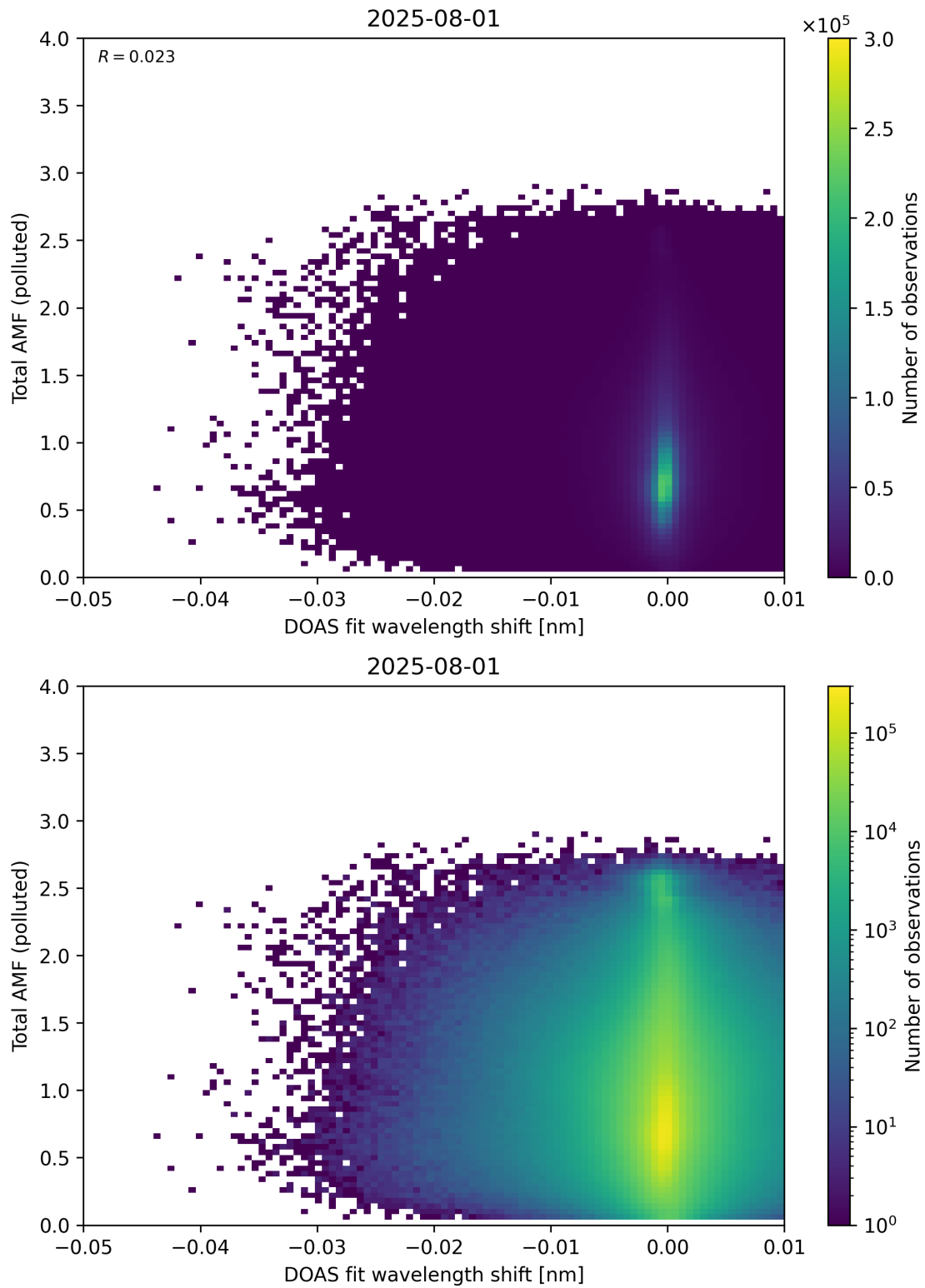
Figure 141: Scatter density plot of “DOAS fit wavelength shift” against “Total AMF (polluted)” for 2025-07-31 to 2025-08-02.
