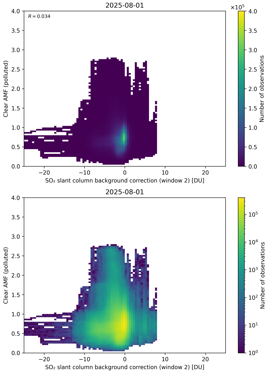
Figure 126: Scatter density plot of “SO 2 slant column background correction (window 2)” against “Clear AMF (polluted)” for 2025-07-31 to 2025-08-02.
