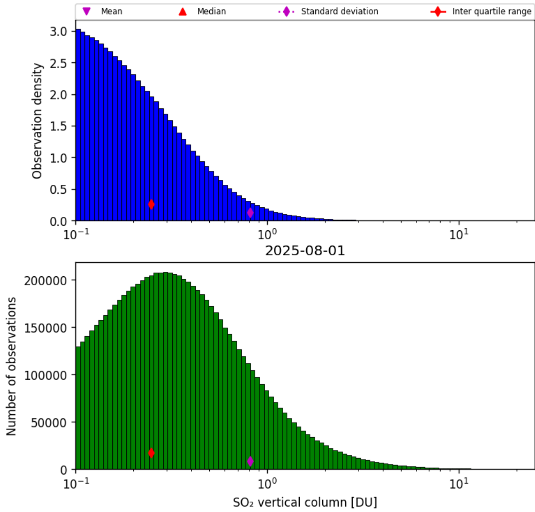
Figure 58: Histogram of “SO 2 vertical column” for 2025-07-31 to 2025-08-02
