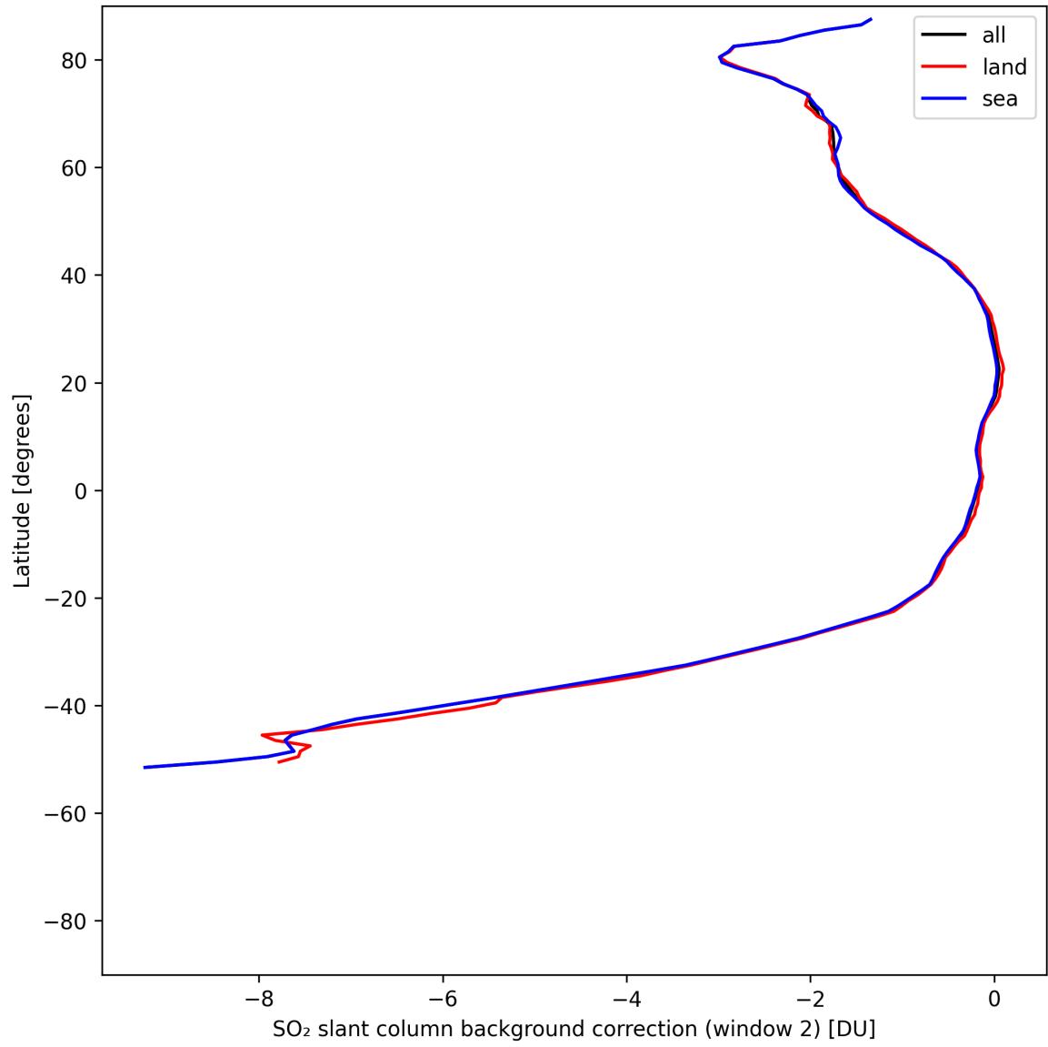
Figure 44: Zonal average of “SO 2 slant column background correction (window 2)” for 2025-07-31 to 2025-08-02.
