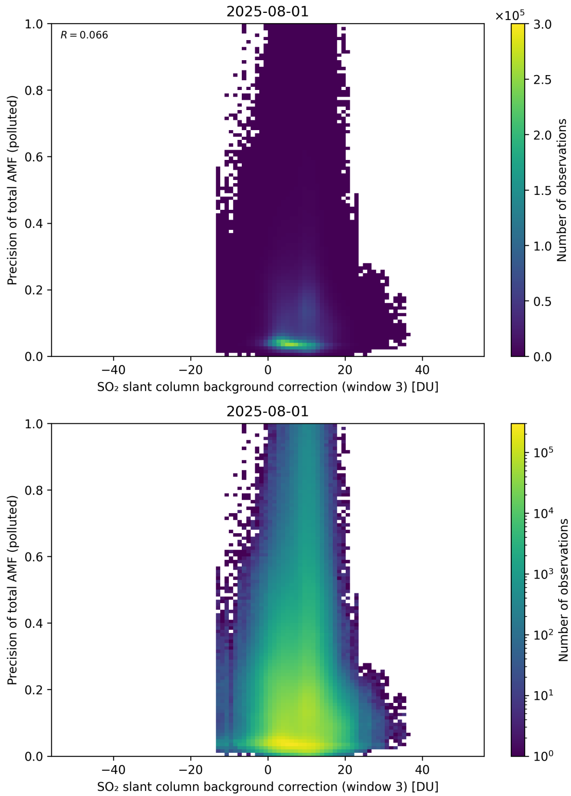
Figure 137: Scatter density plot of “SO 2 slant column background correction (window 3)” against “Precision of total AMF (polluted)” for 2025-07-31 to 2025-08-02.
