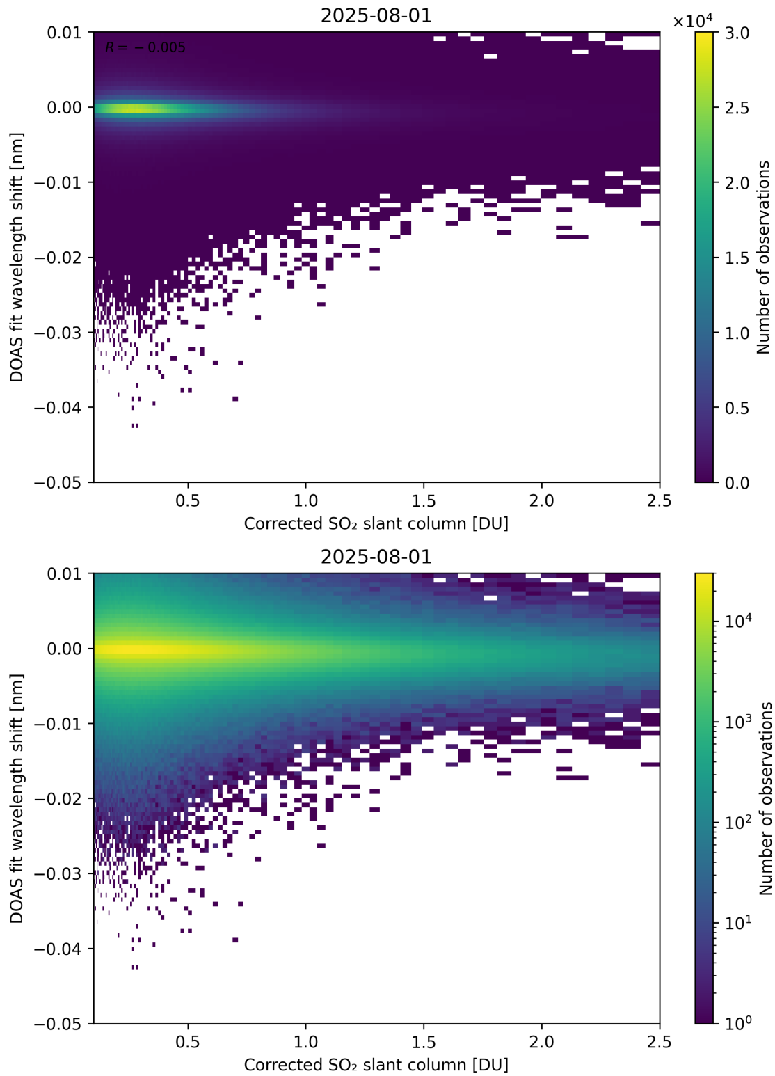
Figure 229: Scatter density plot of “Corrected SO 2 slant column” against “DOAS fit wavelength shift” for 2025-07-31 to 2025-08-02.
