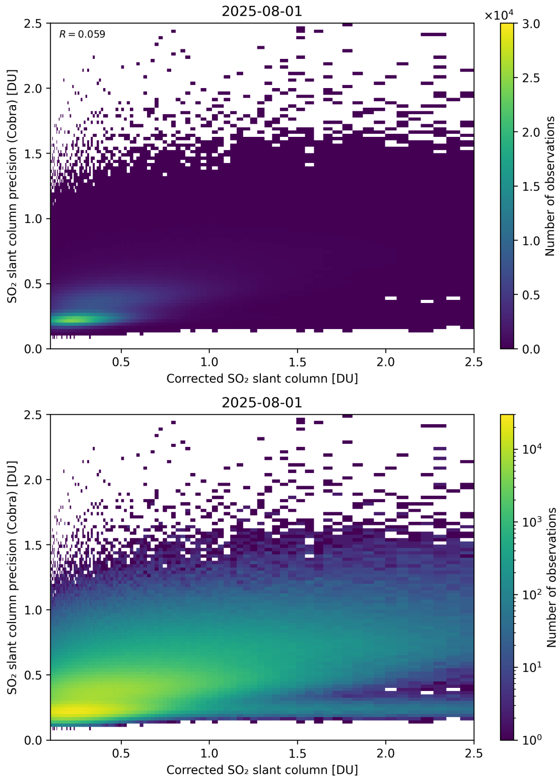
Figure 234: Scatter density plot of “Corrected SO 2 slant column” against “SO 2 slant column precision (Cobra)” for 2025-07-31 to 2025-08-02.
