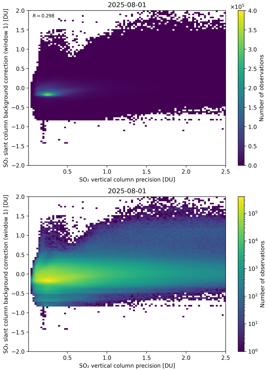
Figure 329: Scatter density plot of “SO 2 vertical column precision” against “SO 2 slant column background correction (window 1)” for 2025-07-31 to 2025-08-02.
