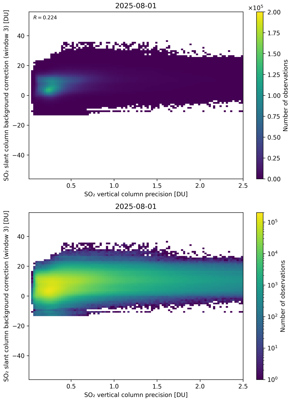
Figure 331: Scatter density plot of “SO 2 vertical column precision” against “SO 2 slant column background correction (window 3)” for 2025-07-31 to 2025-08-02.
