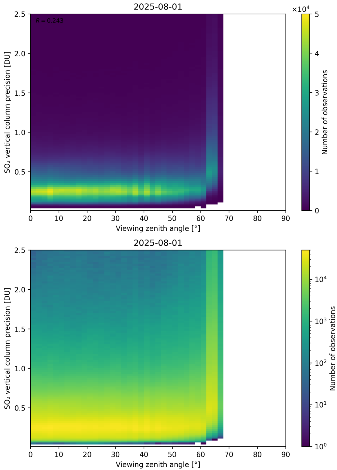
Figure 384: Scatter density plot of “Viewing zenith angle” against “SO 2 vertical column precision” for 2025-07-31 to 2025-08-02.
