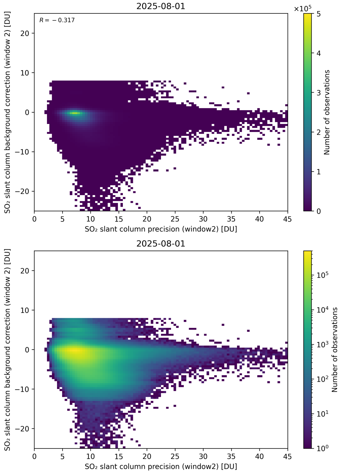
Figure 291: Scatter density plot of “SO 2 slant column precision (window2)” against “SO 2 slant column background correction (window 2)” for 2025-07-31 to 2025-08-02.
