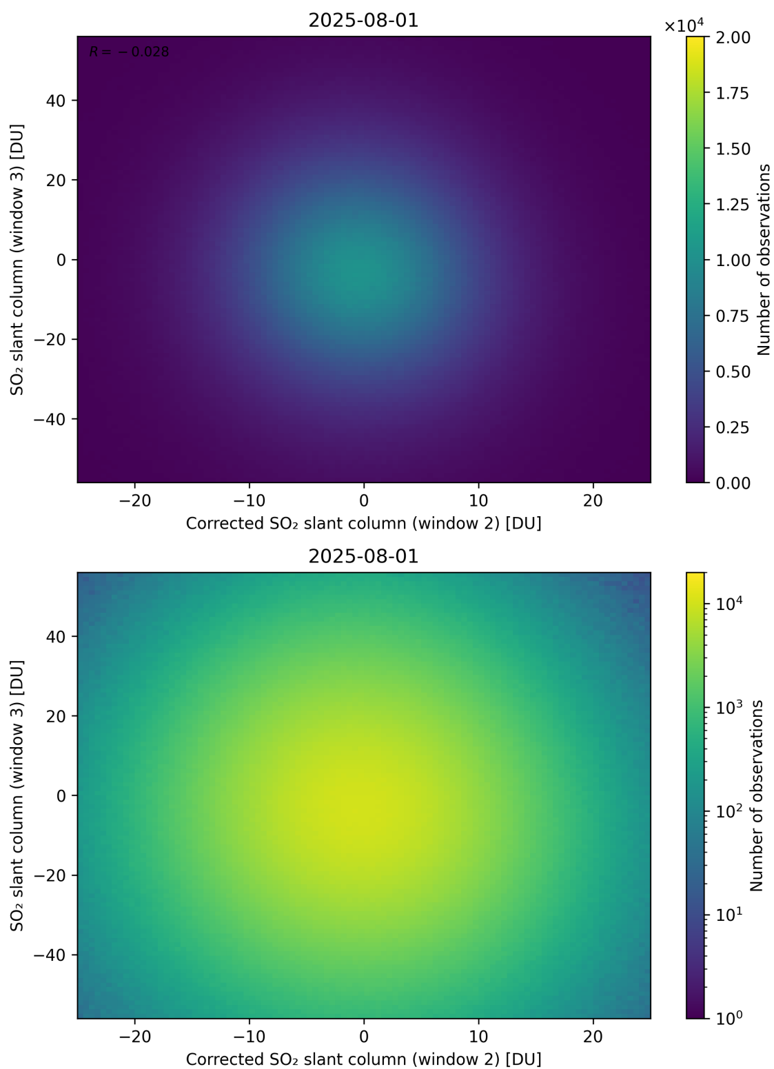
Figure 251: Scatter density plot of “Corrected SO 2 slant column (window 2)” against “SO 2 slant column (window 3)” for 2025-07-31 to 2025-08-02.
