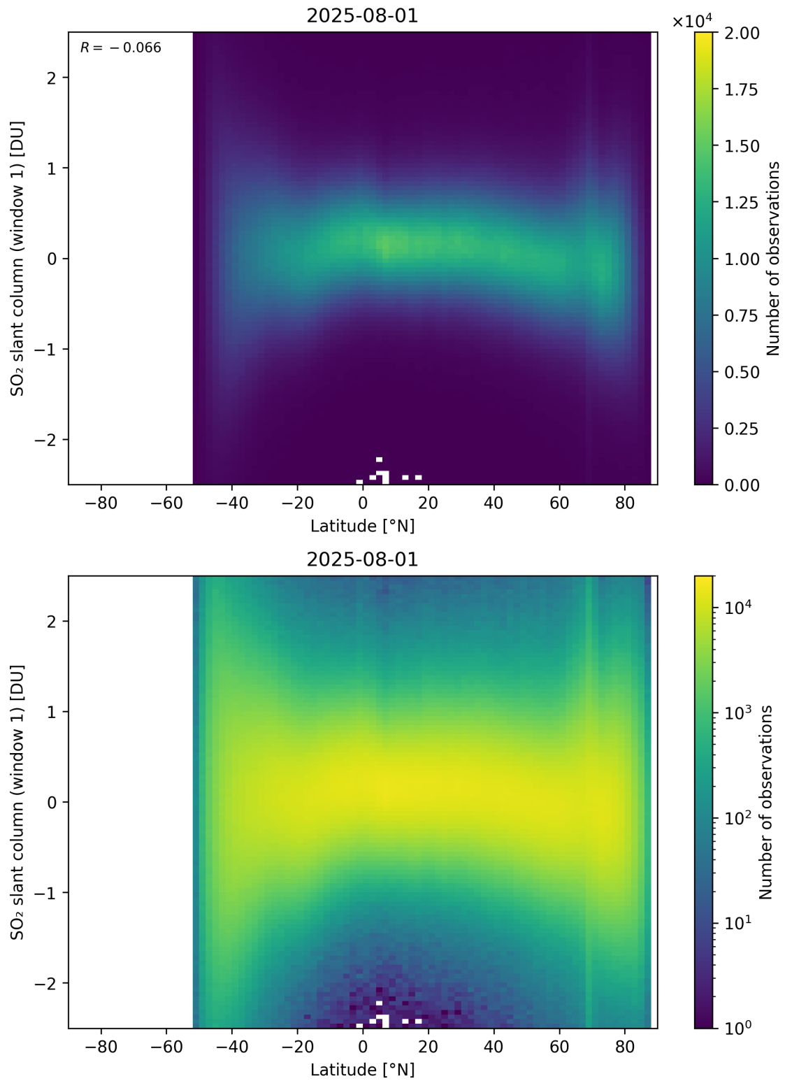
Figure 162: Scatter density plot of “Latitude” against “SO 2 slant column (window 1)” for 2025-07-31 to 2025-08-02.
