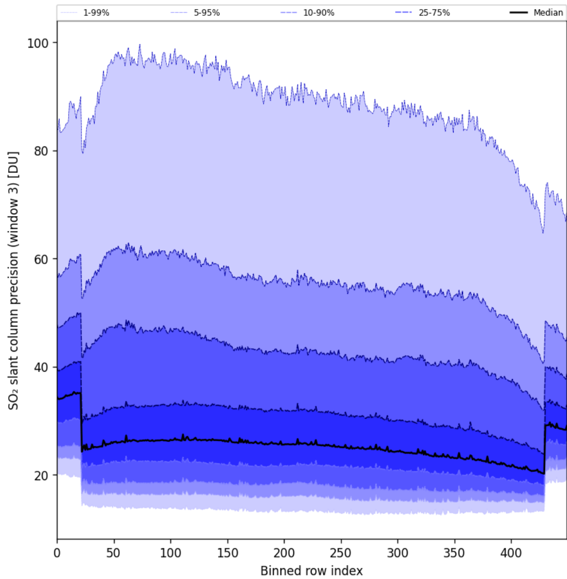
Figure 98: Along track statistics of “SO 2 slant column precision (window 3)” for 2025-07-31 to 2025-08-02
