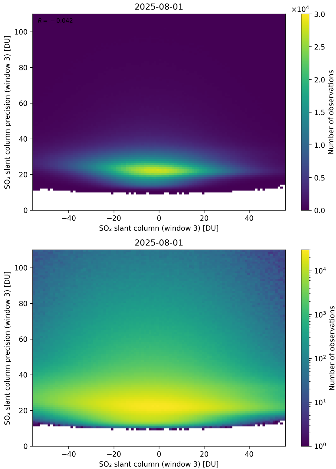
Figure 317: Scatter density plot of “SO 2 slant column (window 3)” against “SO 2 slant column precision (window 3)” for 2025-07-31 to 2025-08-02.
