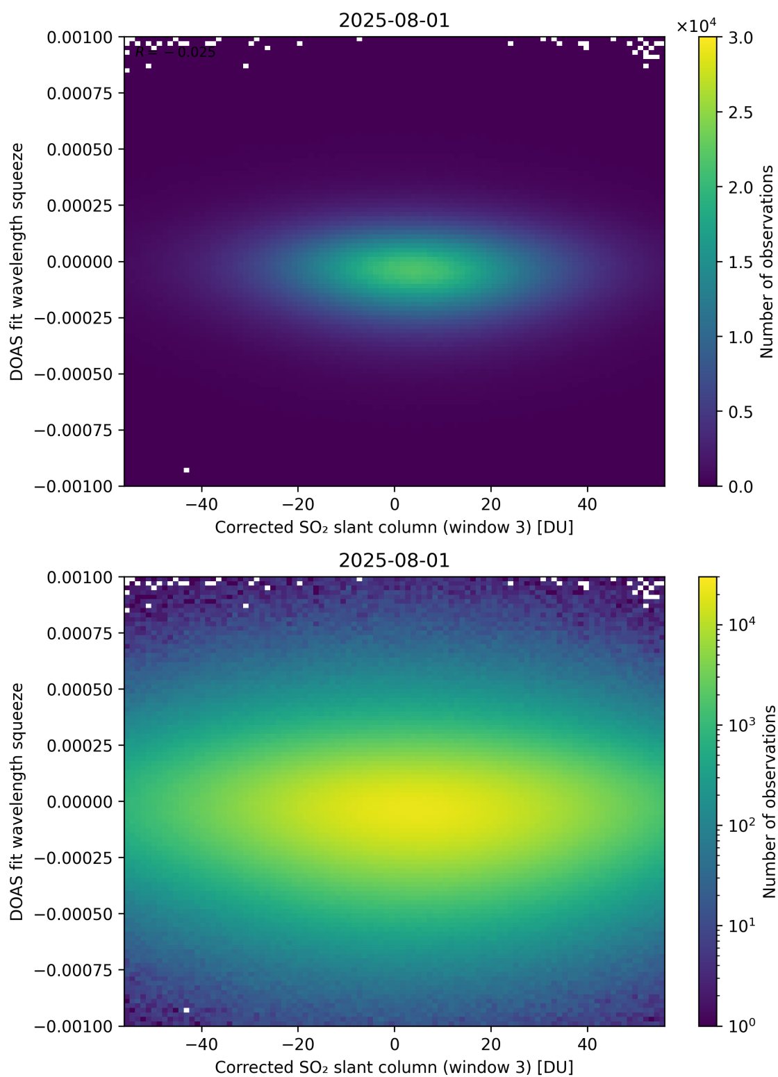
Figure 257: Scatter density plot of “Corrected SO 2 slant column (window 3)” against “DOAS fit wavelength squeeze” for 2025-07-31 to 2025-08-02.
