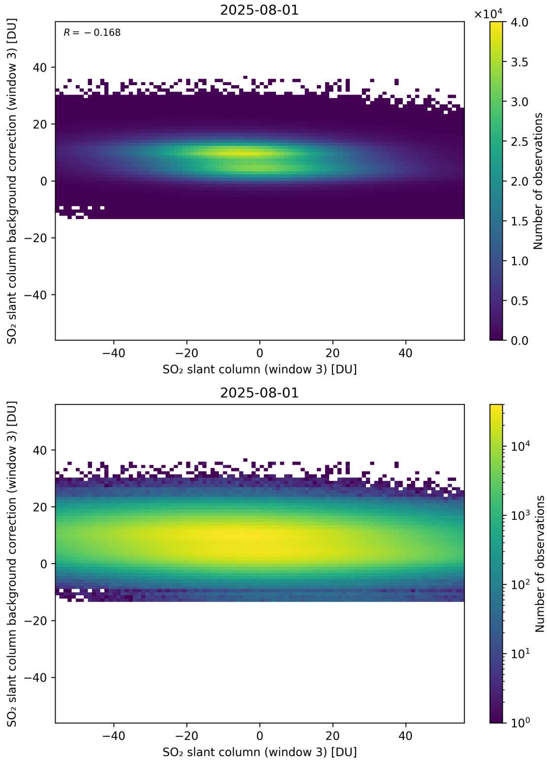
Figure 303: Scatter density plot of “SO 2 slant column (window 3)” against “SO 2 slant column background correction (window 3)” for 2025-07-31 to 2025-08-02.
