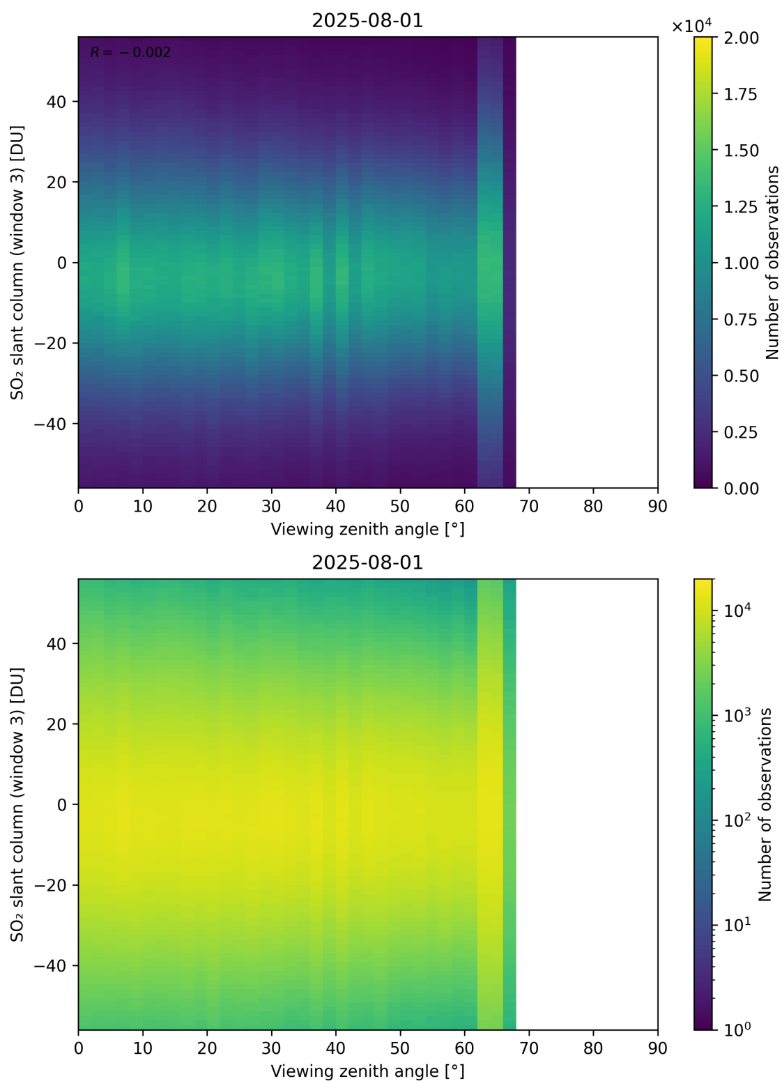
Figure 379: Scatter density plot of “Viewing zenith angle” against “SO 2 slant column (window 3)” for 2025-07-31 to 2025-08-02.
