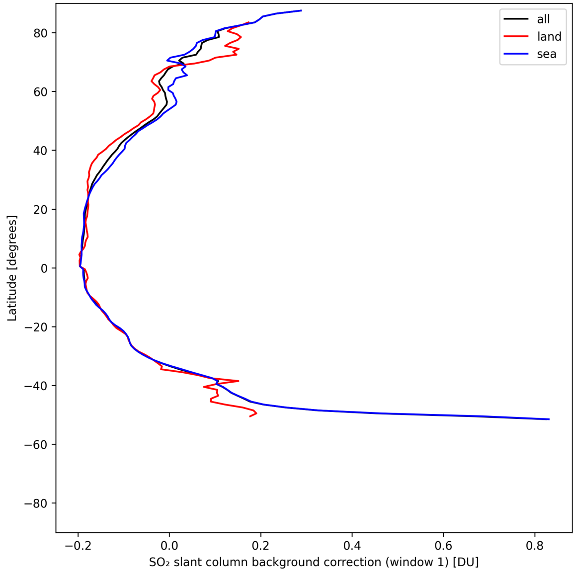
Figure 40: Zonal average of “SO 2 slant column background correction (window 1)” for 2025-07-31 to 2025-08-02.
