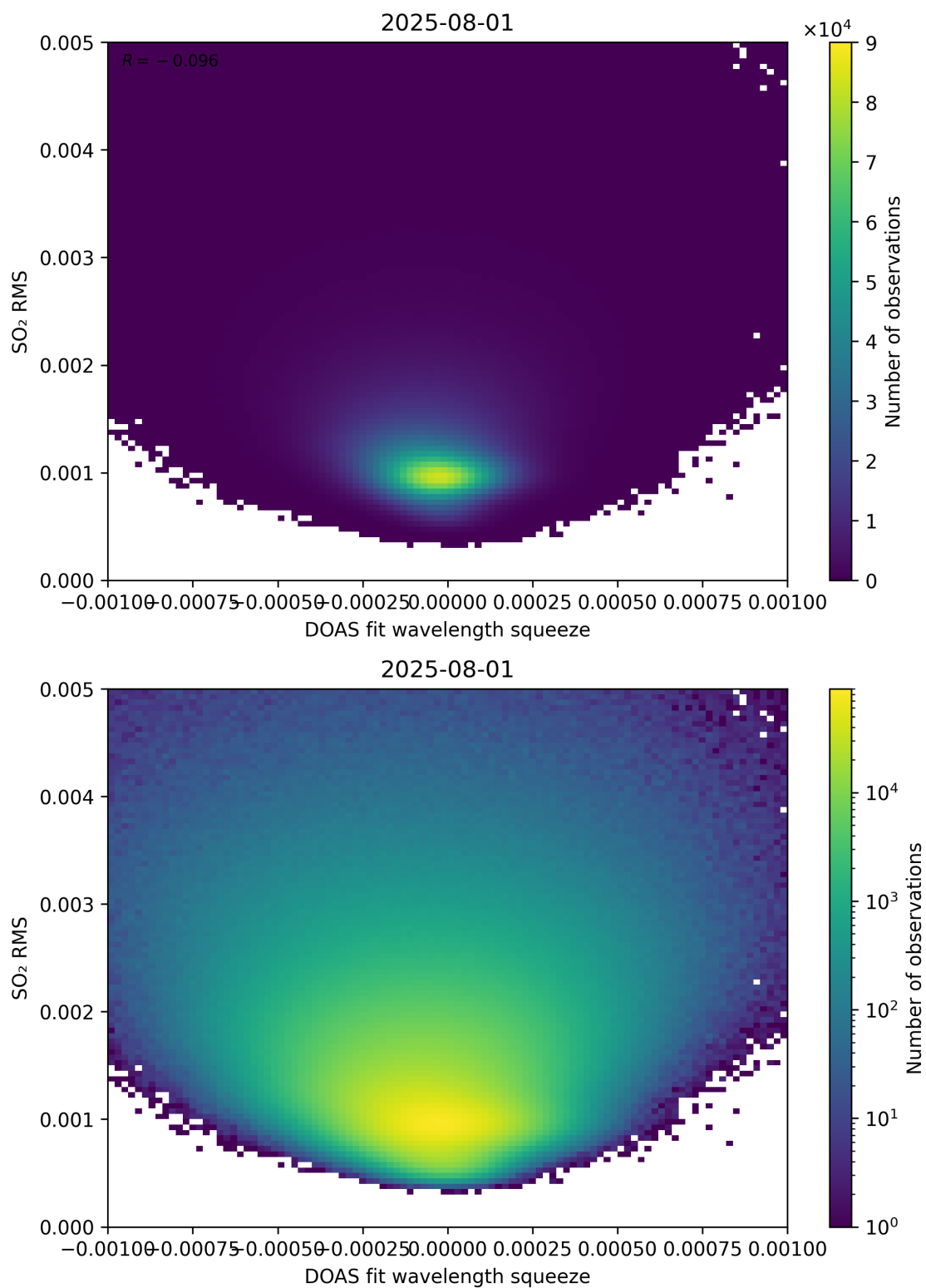
Figure 143: Scatter density plot of “DOAS fit wavelength squeeze” against “SO 2 RMS” for 2025-07-31 to 2025-08-02.
