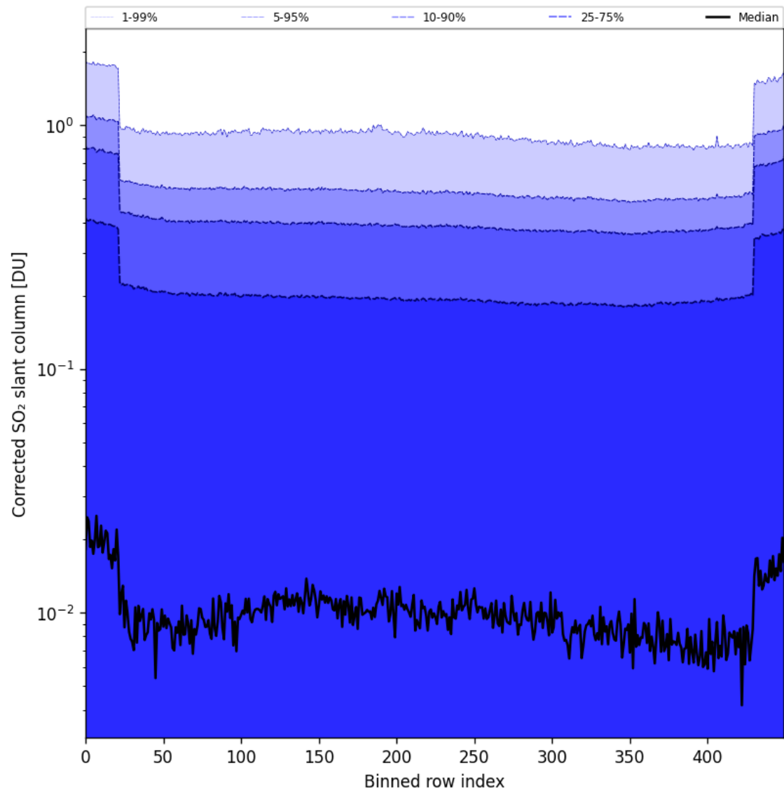
Figure 86: Along track statistics of “Corrected SO 2 slant column” for 2025-07-31 to 2025-08-02
