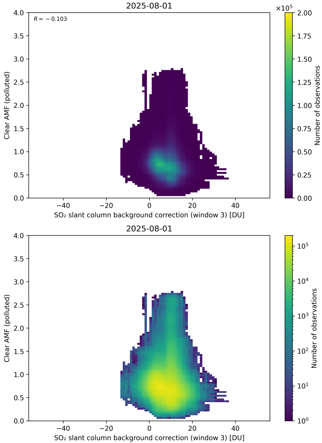
Figure 135: Scatter density plot of “SO 2 slant column background correction (window 3)” against “Clear AMF (polluted)” for 2025-07-31 to 2025-08-02.
