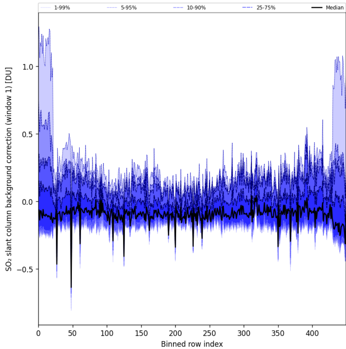
Figure 92: Along track statistics of “SO 2 slant column background correction (window 1)” for 2025-07-31 to 2025-08-02
