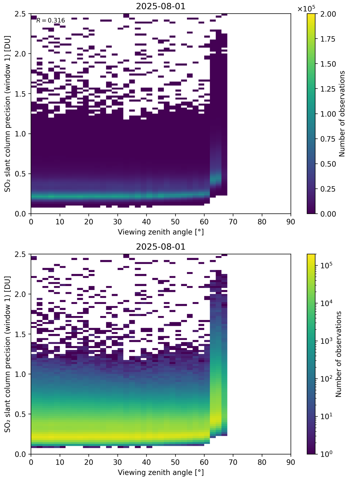
Figure 377: Scatter density plot of “Viewing zenith angle” against “SO 2 slant column precision (window 1)” for 2025-07-31 to 2025-08-02.
