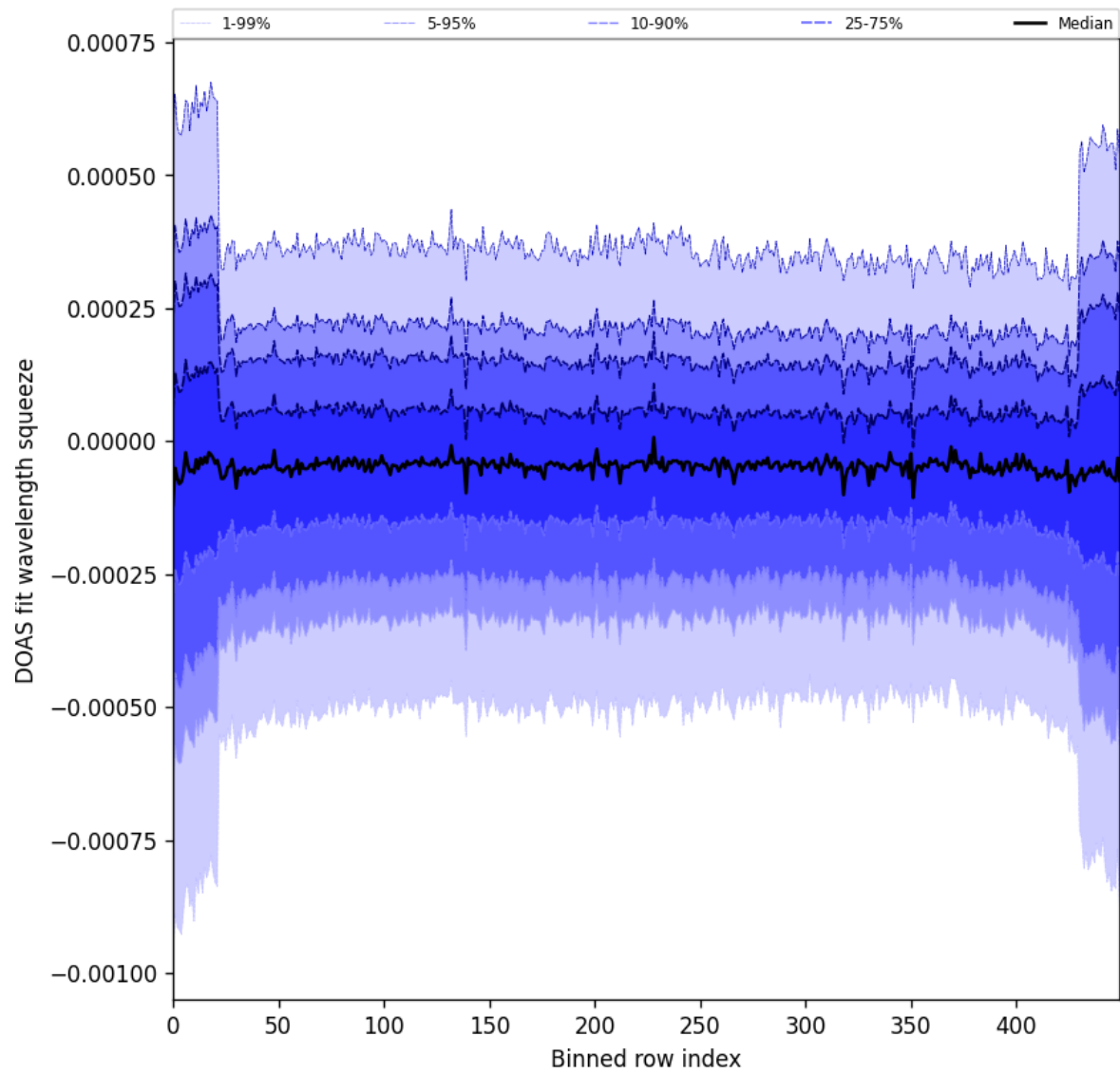
Figure 103: Along track statistics of “DOAS fit wavelength squeeze” for 2025-07-31 to 2025-08-02
