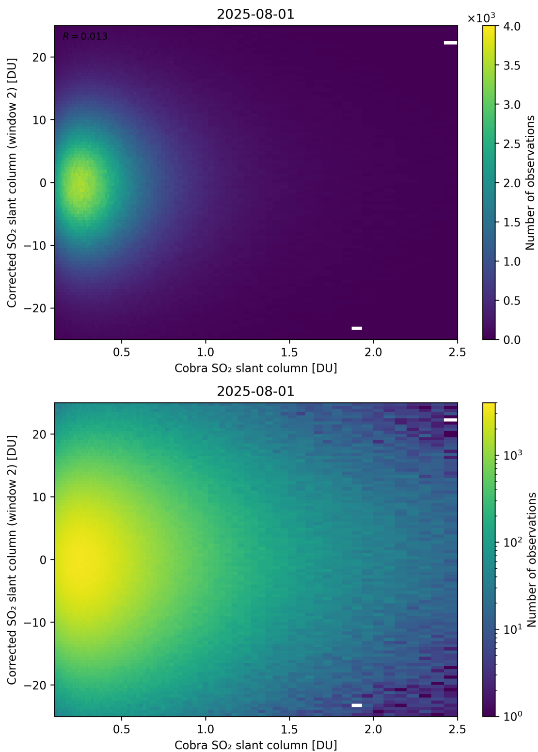
Figure 217: Scatter density plot of “Cobra SO 2 slant column” against “Corrected SO 2 slant column (window 2)” for 2025-07-31 to 2025-08-02.
