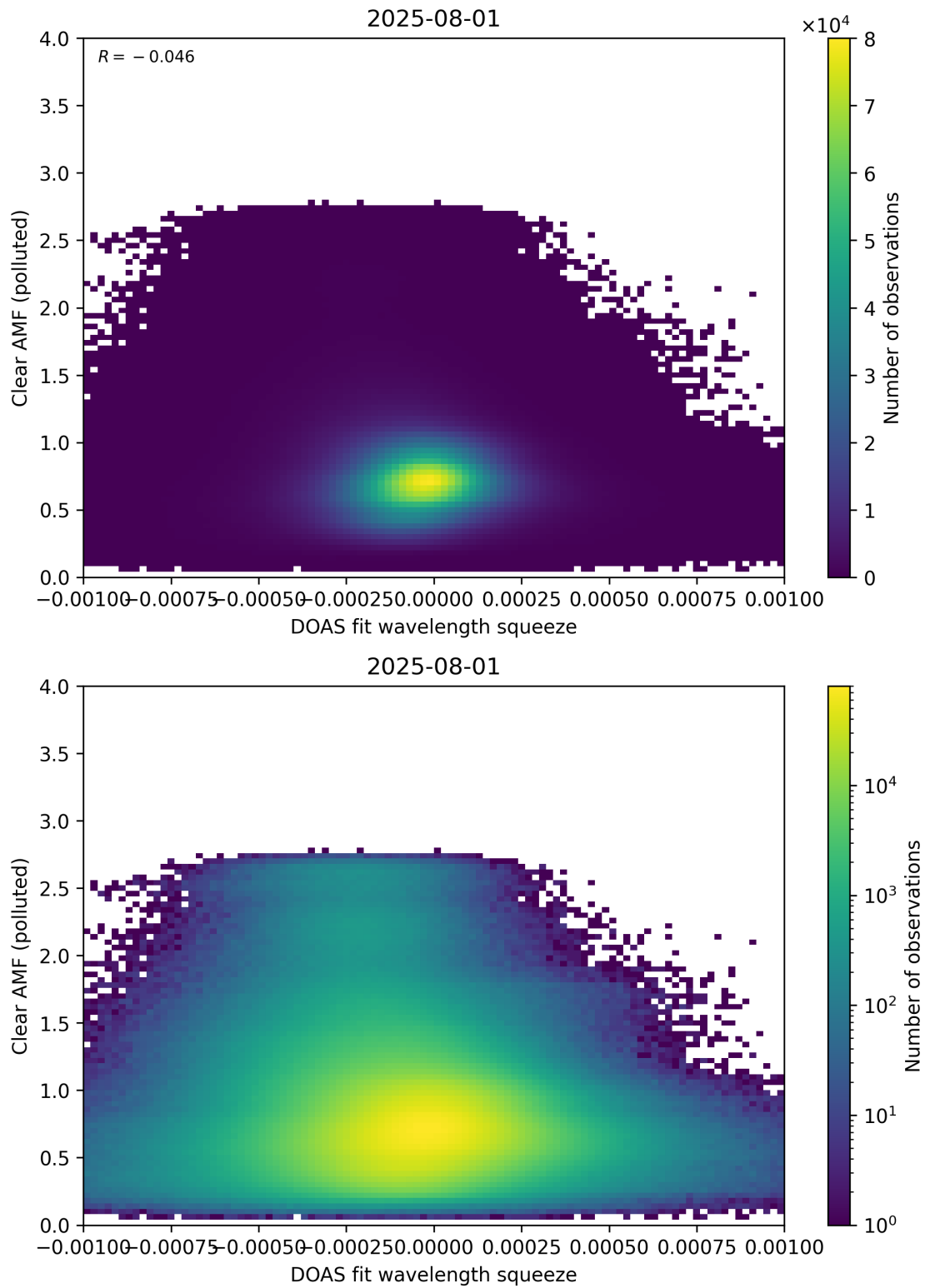
Figure 144: Scatter density plot of “DOAS fit wavelength squeeze” against “Clear AMF (polluted)” for 2025-07-31 to 2025-08-02.
