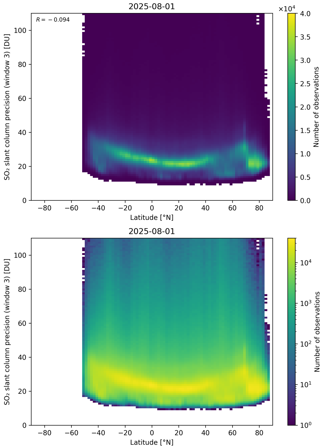
Figure 166: Scatter density plot of “Latitude” against “SO 2 slant column precision (window 3)” for 2025-07-31 to 2025-08-02.
