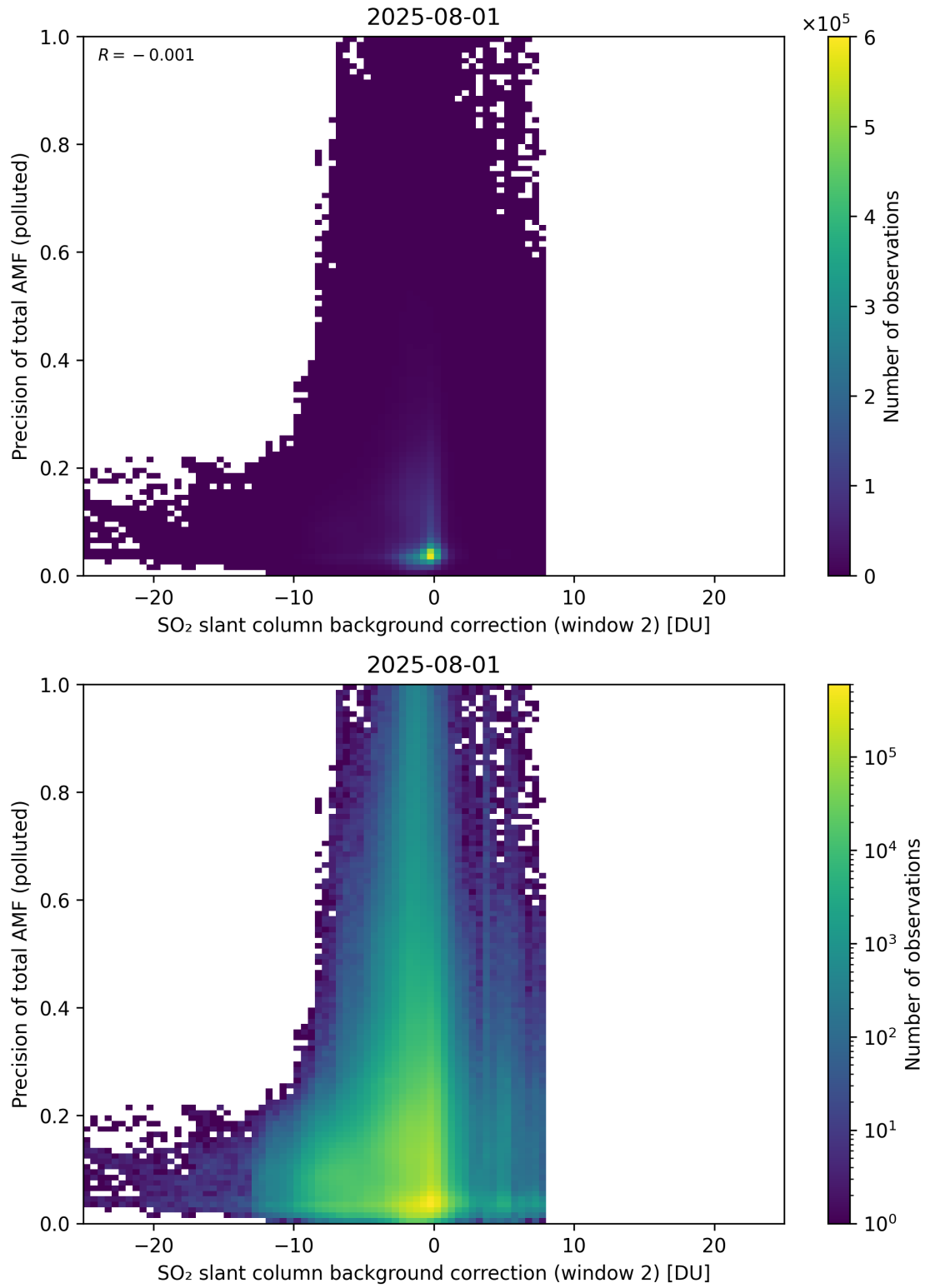
Figure 131: Scatter density plot of “SO 2 slant column background correction (window 2)” against “Precision of total AMF (polluted)” for 2025-07-31 to 2025-08-02.
