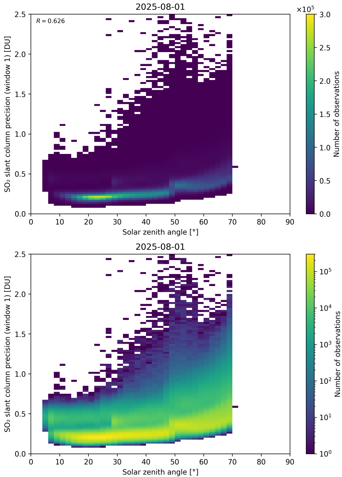
Figure 185: Scatter density plot of “Solar zenith angle” against “SO 2 slant column precision (window 1)” for 2025-07-31 to 2025-08-02.
