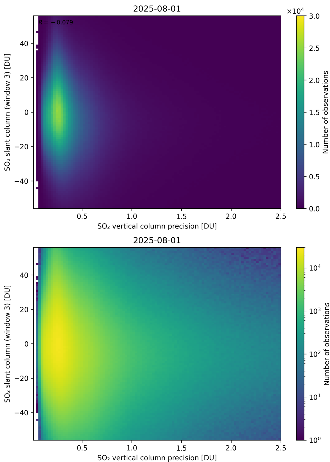
Figure 344: Scatter density plot of “SO 2 vertical column precision” against “SO 2 slant column (window 3)” for 2025-07-31 to 2025-08-02.
