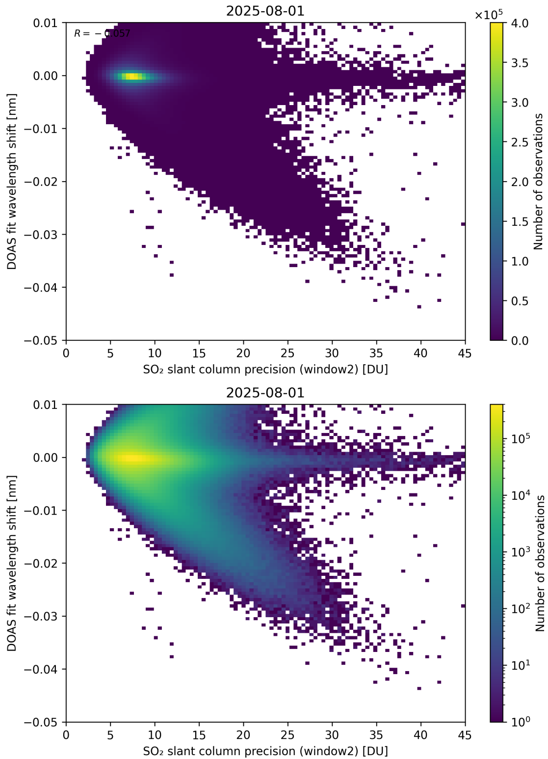
Figure 293: Scatter density plot of “SO 2 slant column precision (window2)” against “DOAS fit wavelength shift” for 2025-07-31 to 2025-08-02.
