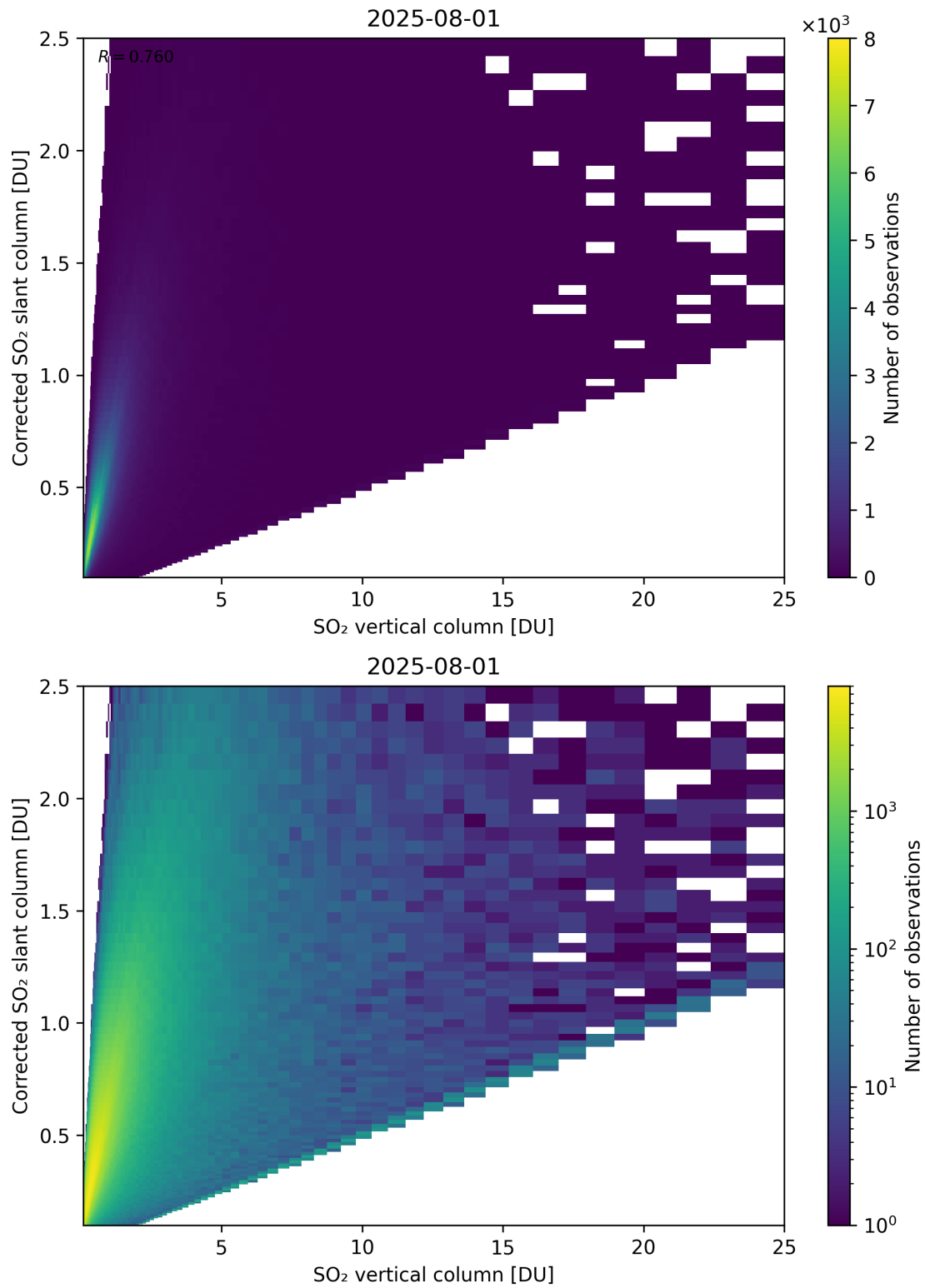
Figure 351: Scatter density plot of “SO 2 vertical column” against “Corrected SO 2 slant column” for 2025-07-31 to 2025-08-02.
