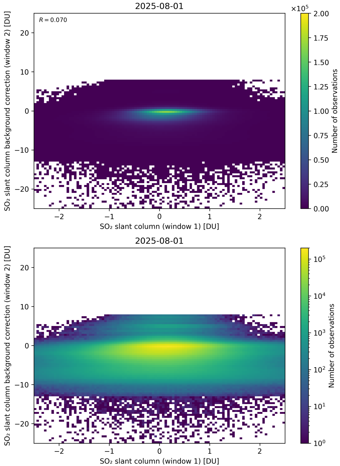
Figure 263: Scatter density plot of “SO 2 slant column (window 1)” against “SO 2 slant column background correction (window 2)” for 2025-07-31 to 2025-08-02.
