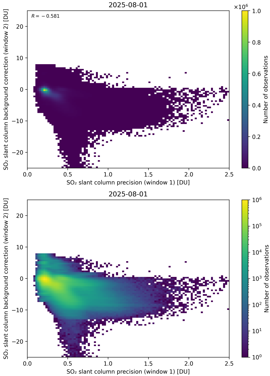
Figure 269: Scatter density plot of “SO 2 slant column precision (window 1)” against “SO 2 slant column background correction (window 2)” for 2025-07-31 to 2025-08-02.
