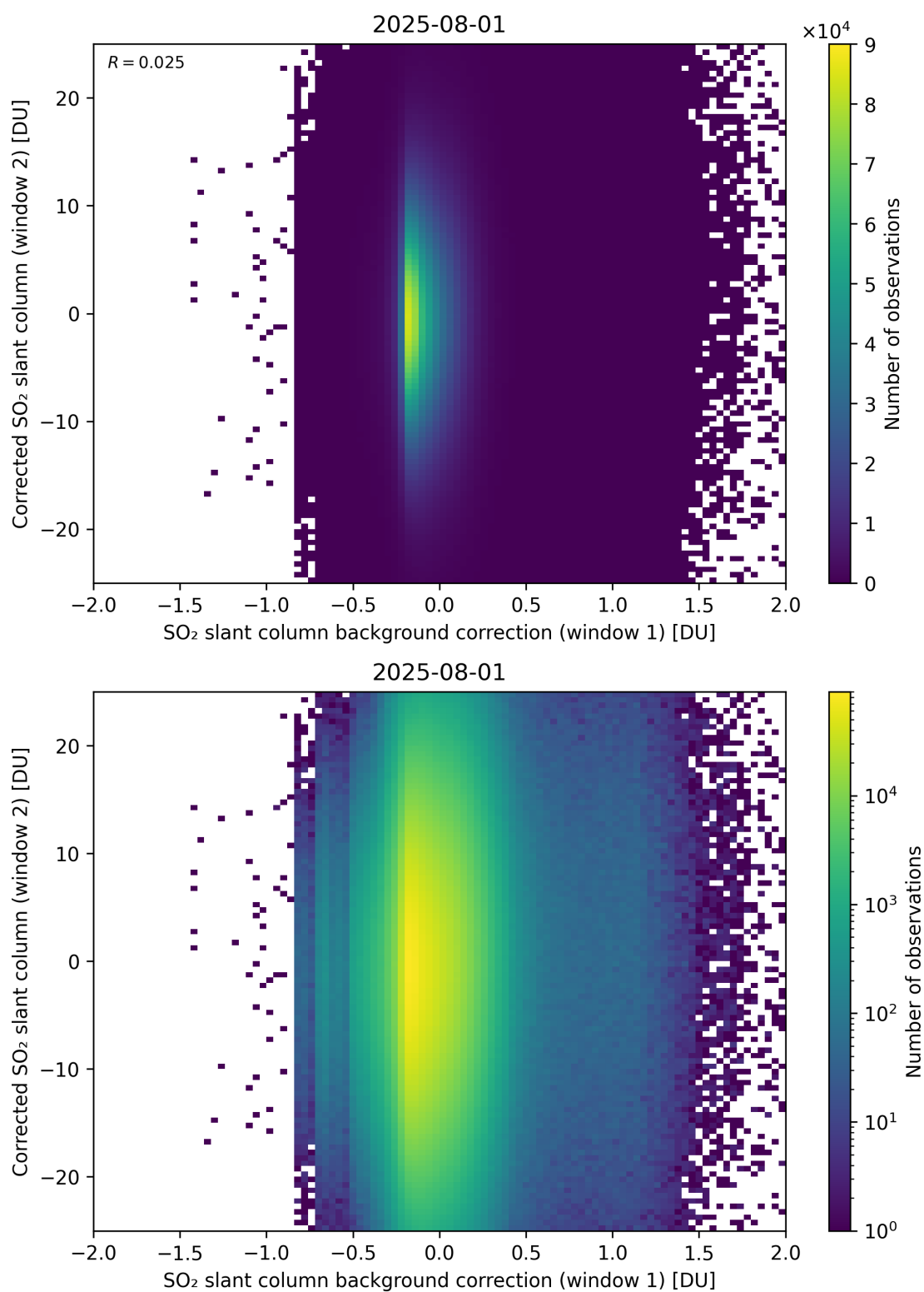
Figure 115: Scatter density plot of “SO 2 slant column background correction (window 1)” against “Corrected SO 2 slant column (window 2)” for 2025-07-31 to 2025-08-02.
