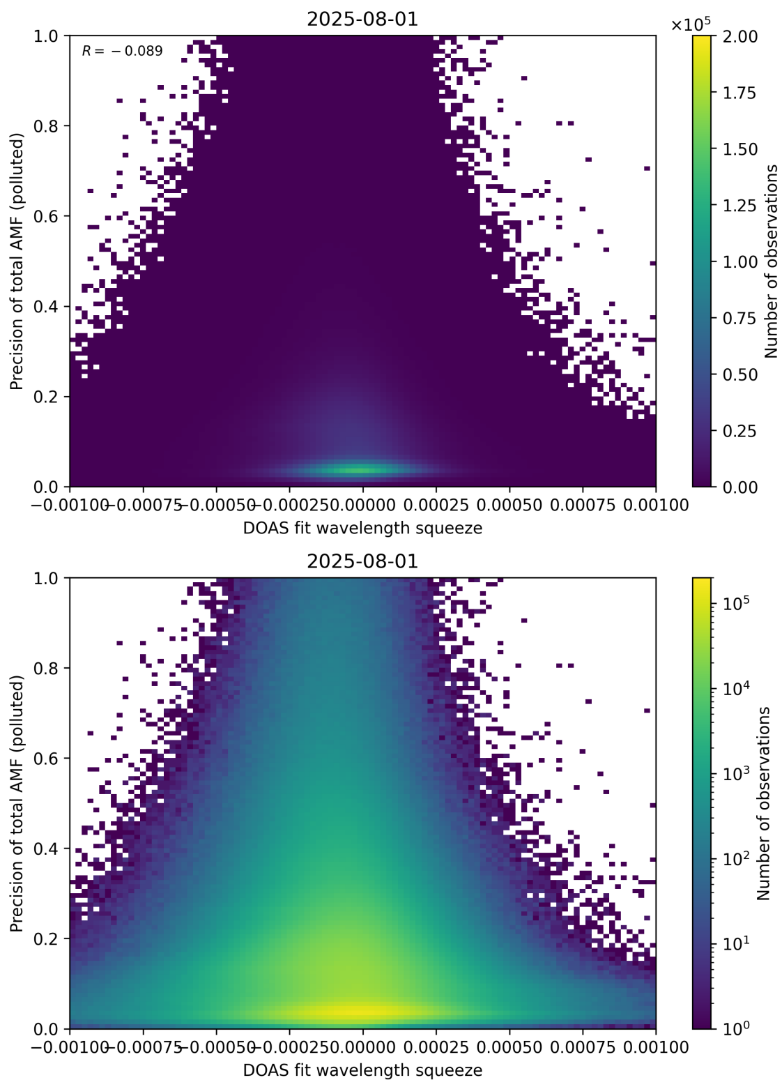
Figure 146: Scatter density plot of “DOAS fit wavelength squeeze” against “Precision of total AMF (polluted)” for 2025-07-31 to 2025-08-02.
