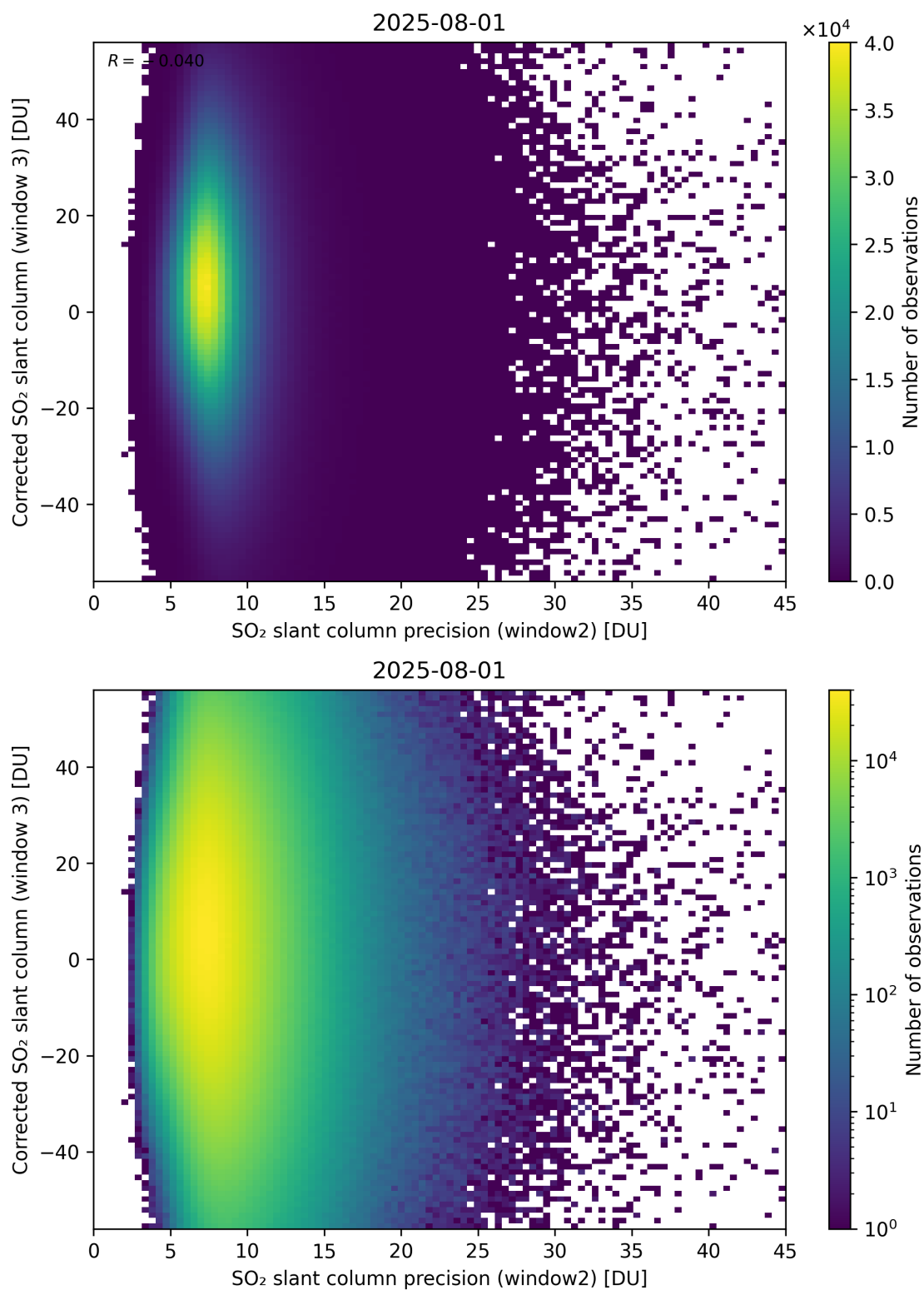
Figure 298: Scatter density plot of “SO 2 slant column precision (window2)” against “Corrected SO 2 slant column (window 3)” for 2025-07-31 to 2025-08-02.
