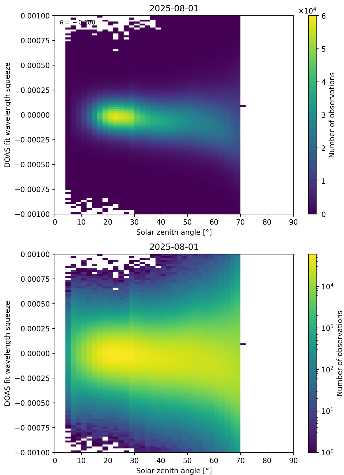
Figure 175: Scatter density plot of “Solar zenith angle” against “DOAS fit wavelength squeeze” for 2025-07-31 to 2025-08-02.
