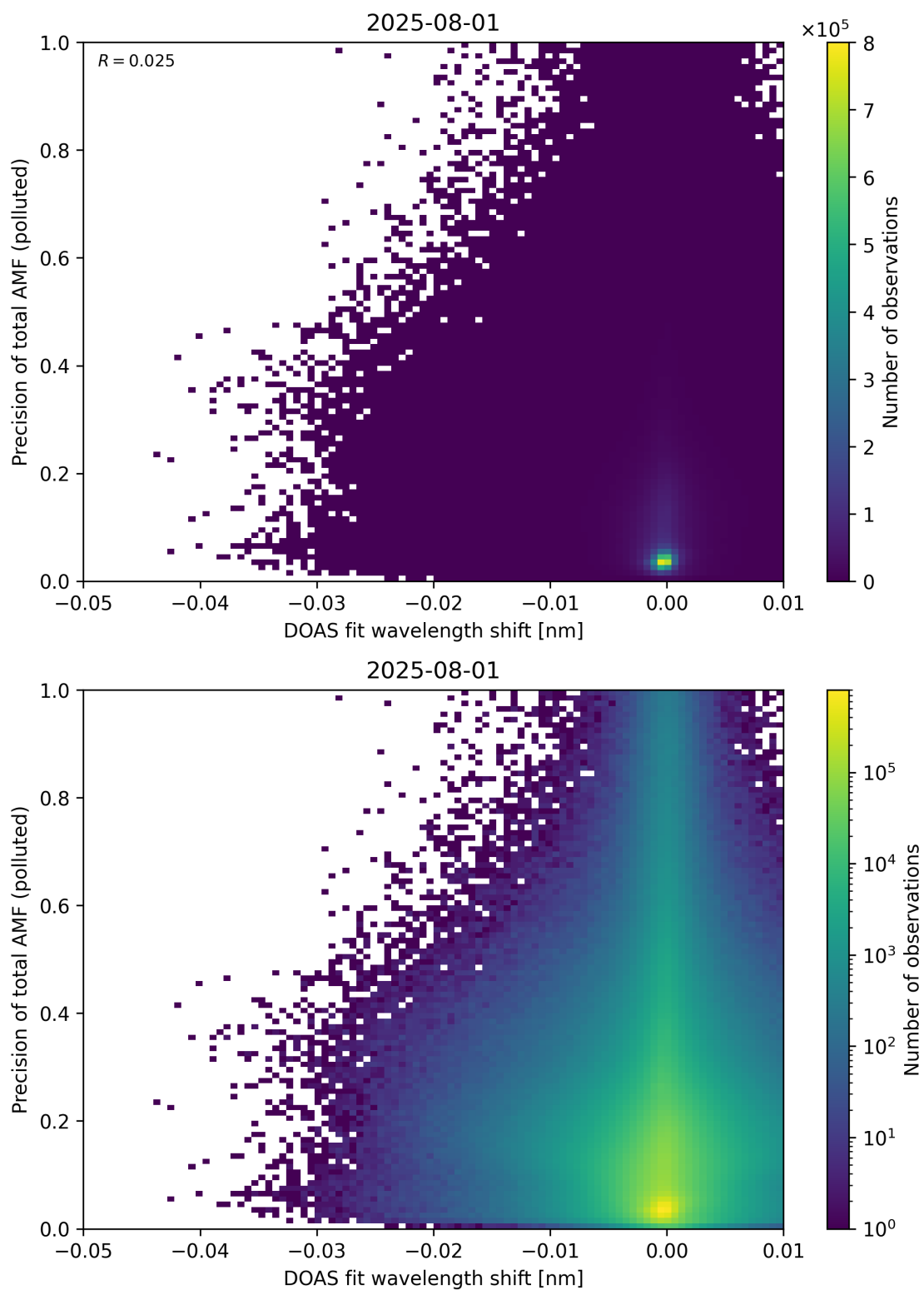
Figure 142: Scatter density plot of “DOAS fit wavelength shift” against “Precision of total AMF (polluted)” for 2025-07-31 to 2025-08-02.
