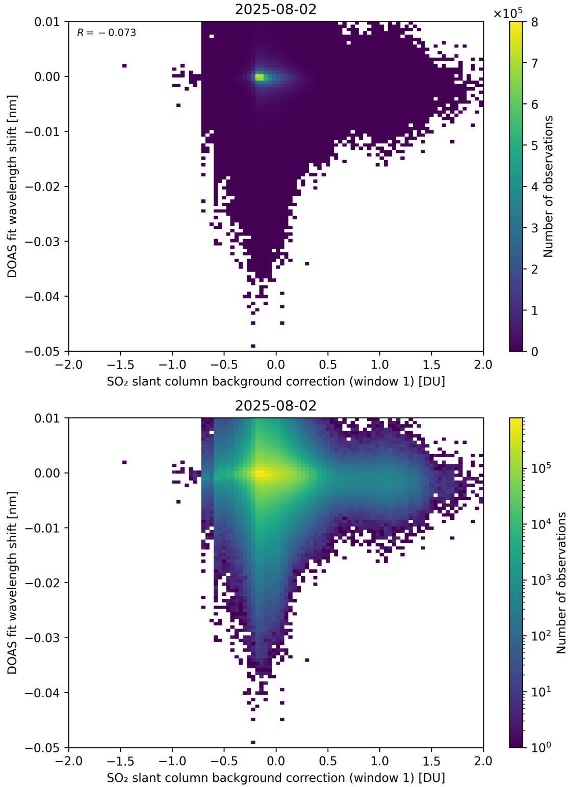
Figure 111: Scatter density plot of “SO 2 slant column background correction (window 1)” against “DOAS fit wavelength shift” for 2025-08-01 to 2025-08-03.
