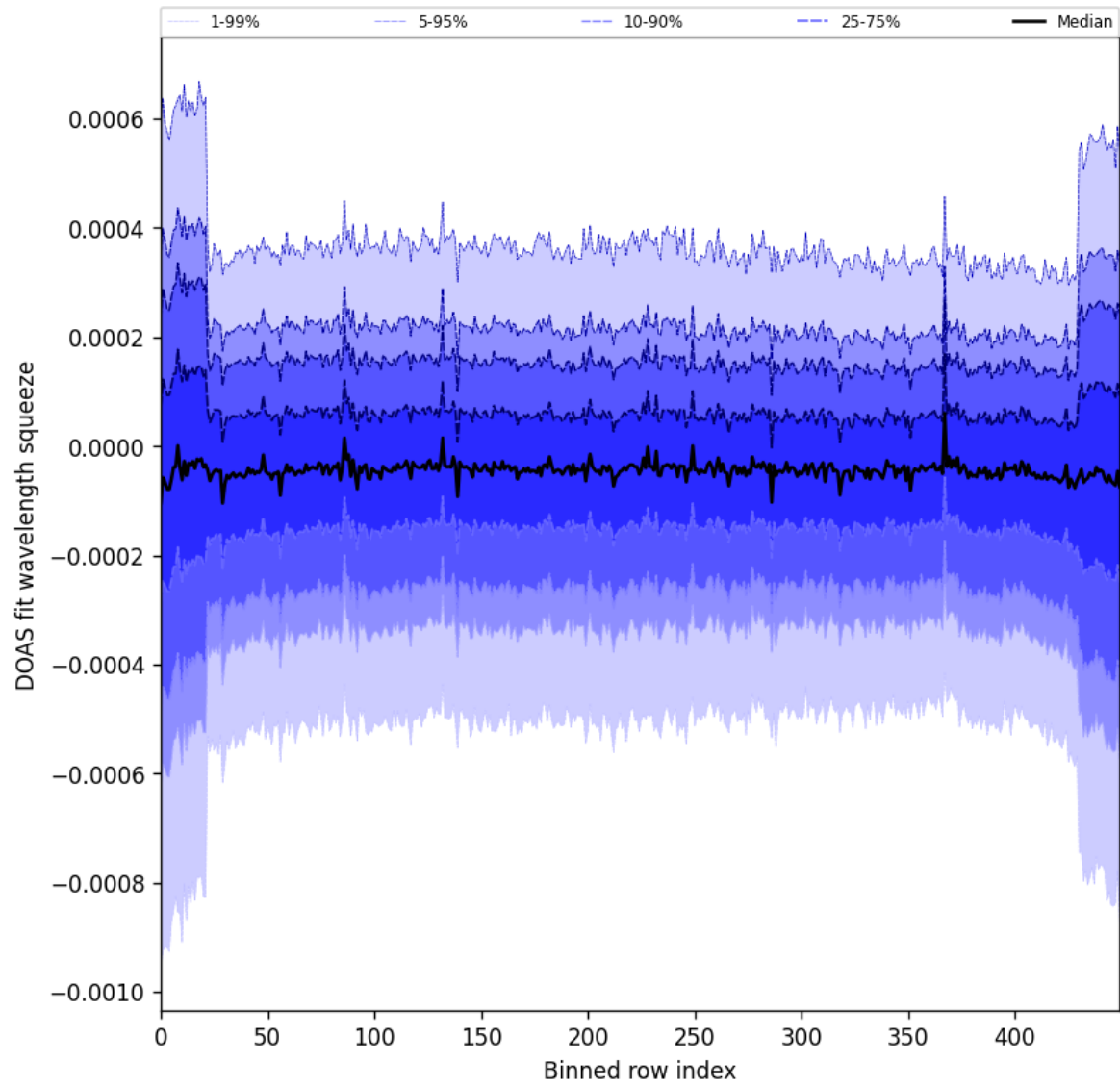
Figure 103: Along track statistics of “DOAS fit wavelength squeeze” for 2025-08-01 to 2025-08-03
