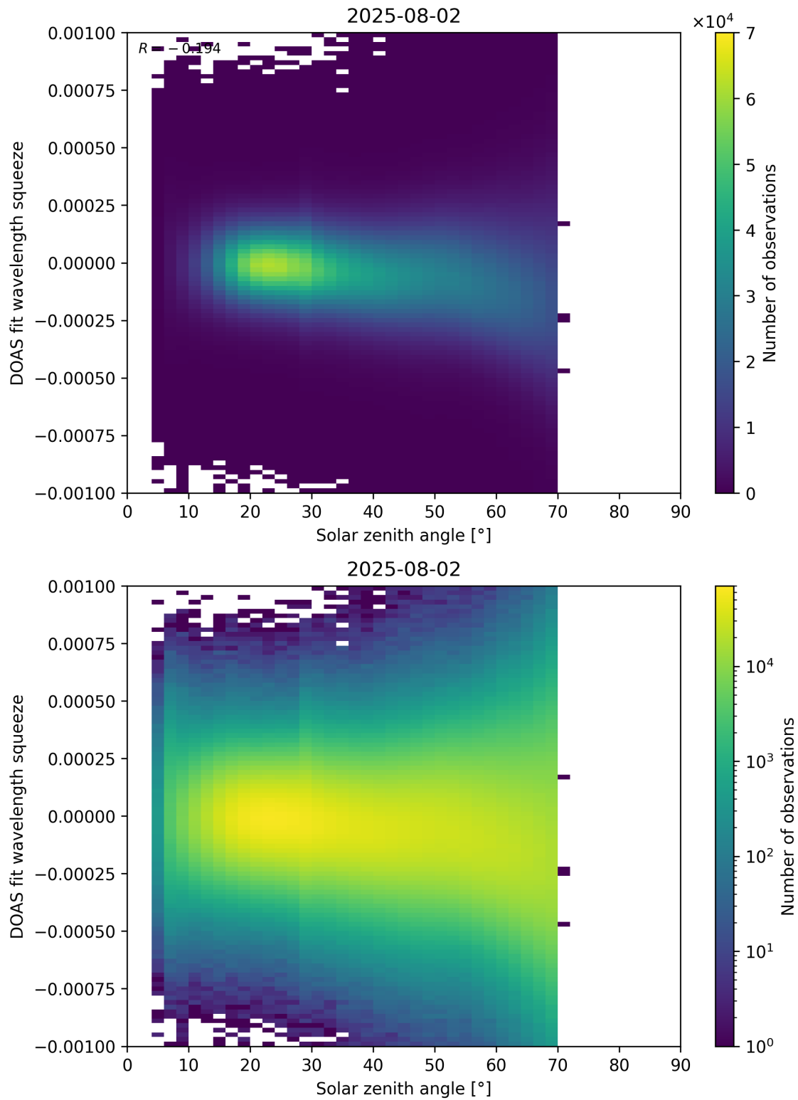
Figure 175: Scatter density plot of “Solar zenith angle” against “DOAS fit wavelength squeeze” for 2025-08-01 to 2025-08-03.
