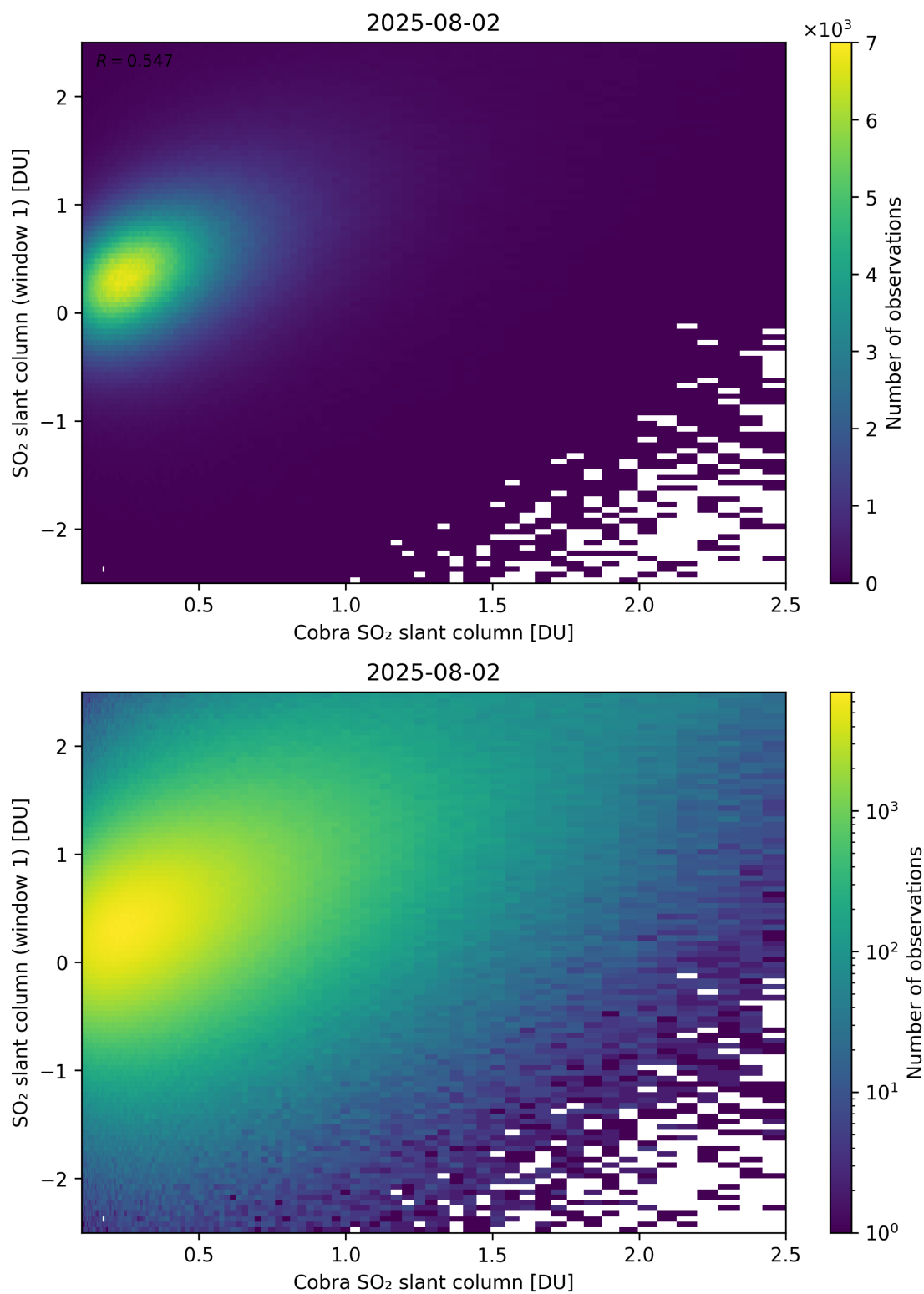
Figure 219: Scatter density plot of “Cobra SO 2 slant column” against “SO 2 slant column (window 1)” for 2025-08-01 to 2025-08-03.
