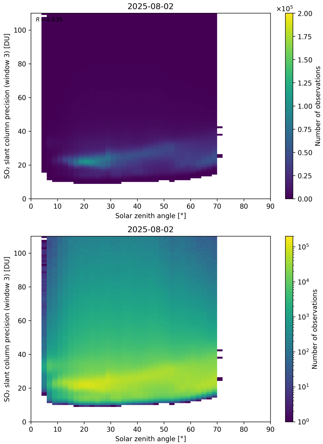
Figure 188: Scatter density plot of “Solar zenith angle” against “SO 2 slant column precision (window 3)” for 2025-08-01 to 2025-08-03.
