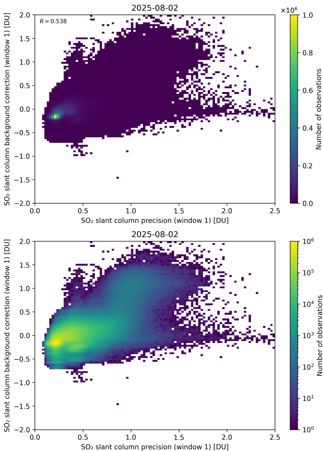
Figure 268: Scatter density plot of “SO 2 slant column precision (window 1)” against “SO 2 slant column background correction (window 1)” for 2025-08-01 to 2025-08-03.
