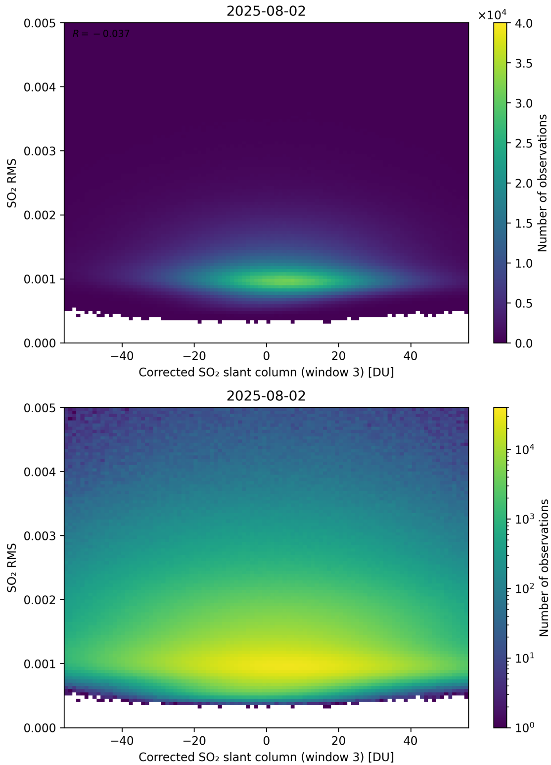
Figure 258: Scatter density plot of “Corrected SO 2 slant column (window 3)” against “SO 2 RMS” for 2025-08-01 to 2025-08-03.
