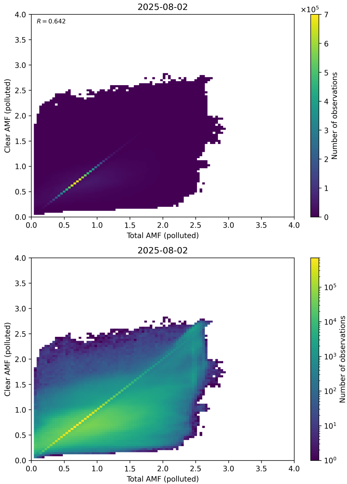
Figure 321: Scatter density plot of “Total AMF (polluted)” against “Clear AMF (polluted)” for 2025-08-01 to 2025-08-03.
