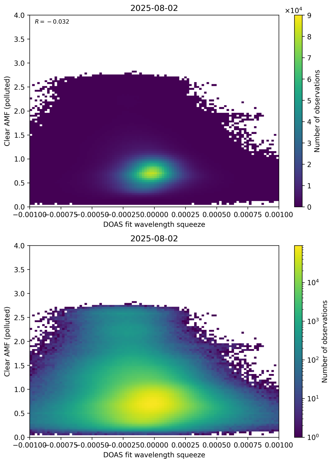
Figure 144: Scatter density plot of “DOAS fit wavelength squeeze” against “Clear AMF (polluted)” for 2025-08-01 to 2025-08-03.
