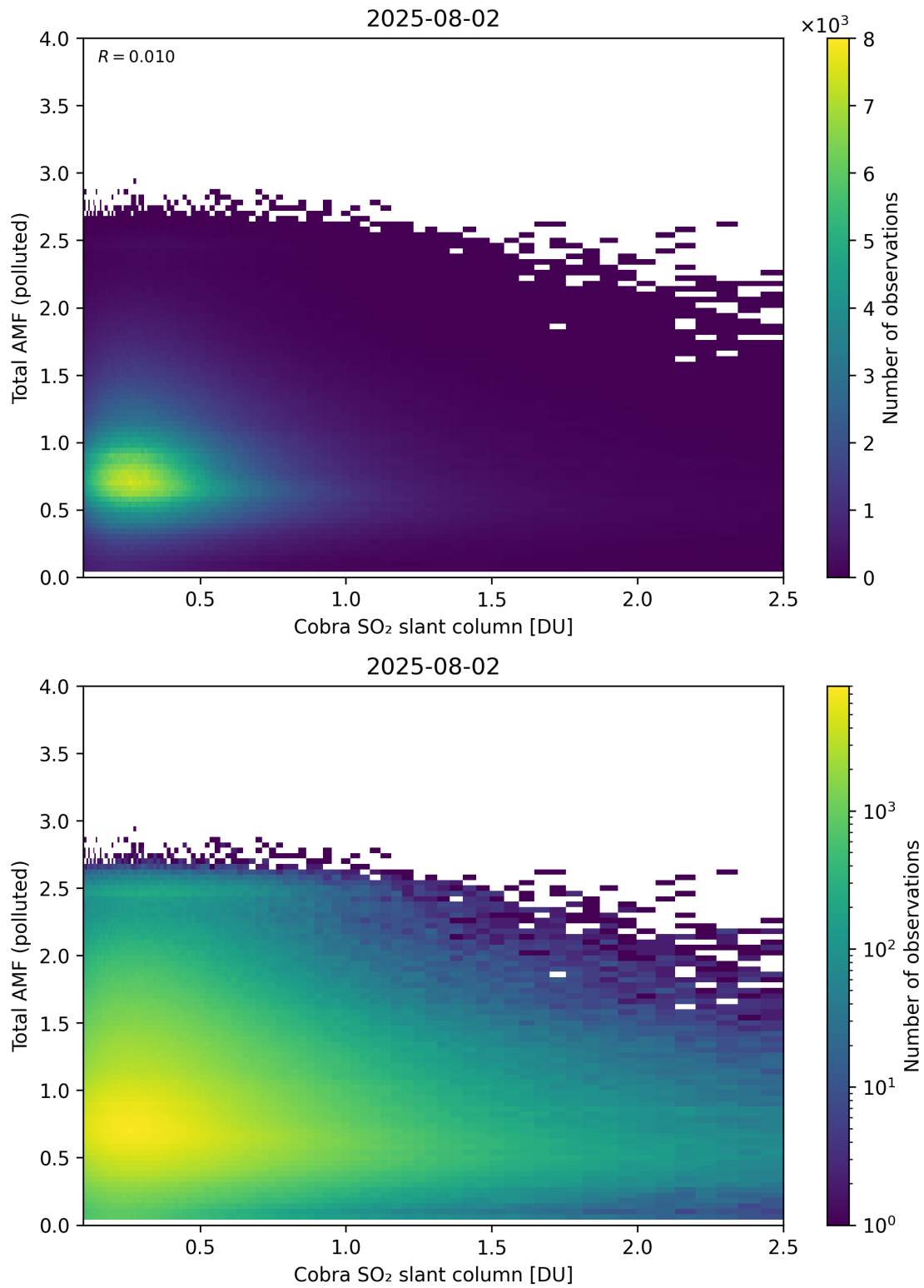
Figure 224: Scatter density plot of “Cobra SO 2 slant column” against “Total AMF (polluted)” for 2025-08-01 to 2025-08-03.
