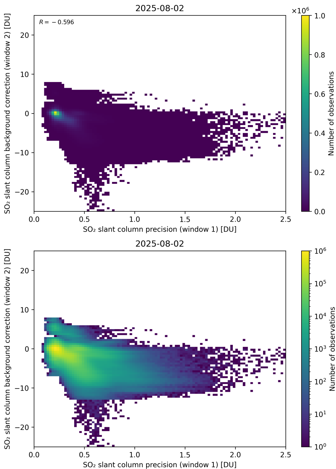
Figure 269: Scatter density plot of “SO 2 slant column precision (window 1)” against “SO 2 slant column background correction (window 2)” for 2025-08-01 to 2025-08-03.
