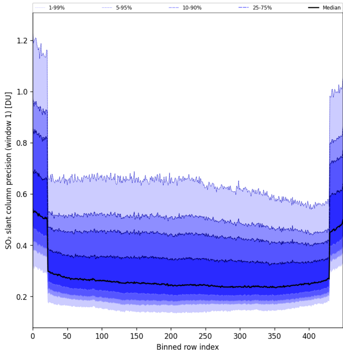
Figure 90: Along track statistics of “SO 2 slant column precision (window 1)” for 2025-08-01 to 2025-08-03
