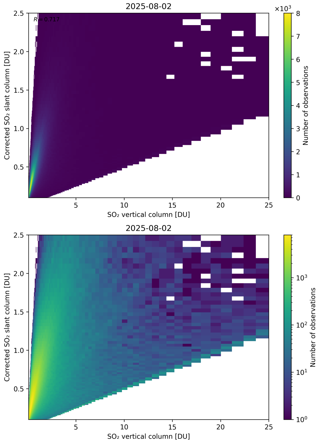
Figure 351: Scatter density plot of “SO 2 vertical column” against “Corrected SO 2 slant column” for 2025-08-01 to 2025-08-03.
