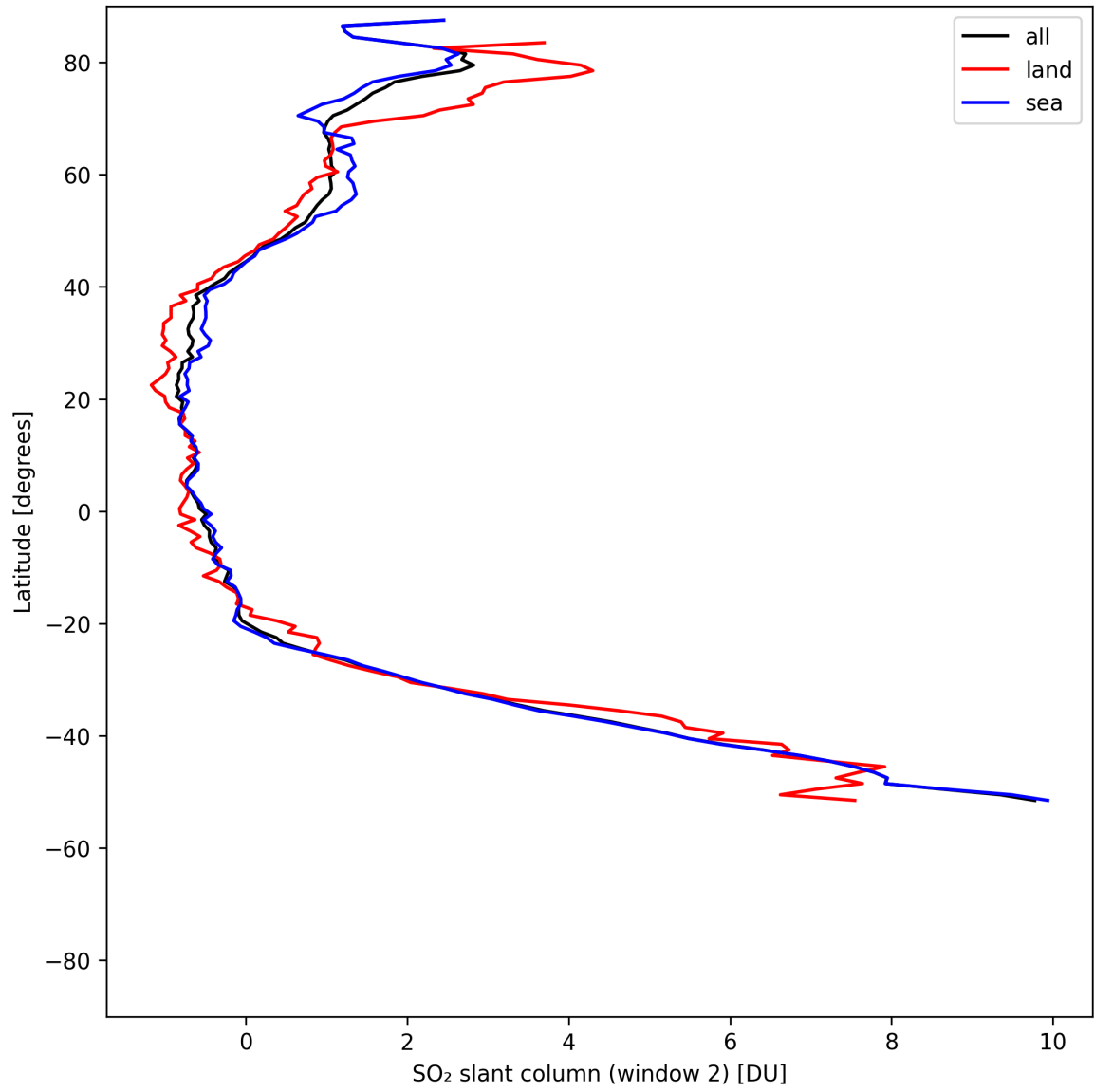
Figure 41: Zonal average of “SO 2 slant column (window 2)” for 2025-08-01 to 2025-08-03.
