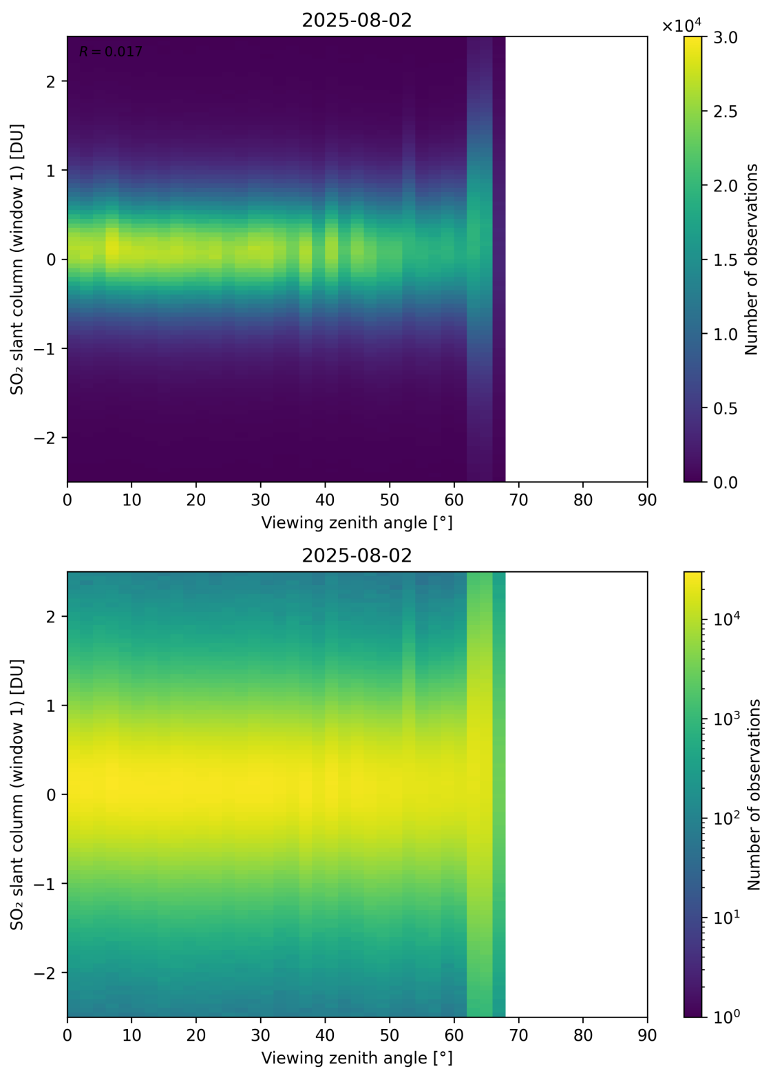
Figure 376: Scatter density plot of “Viewing zenith angle” against “SO 2 slant column (window 1)” for 2025-08-01 to 2025-08-03.
