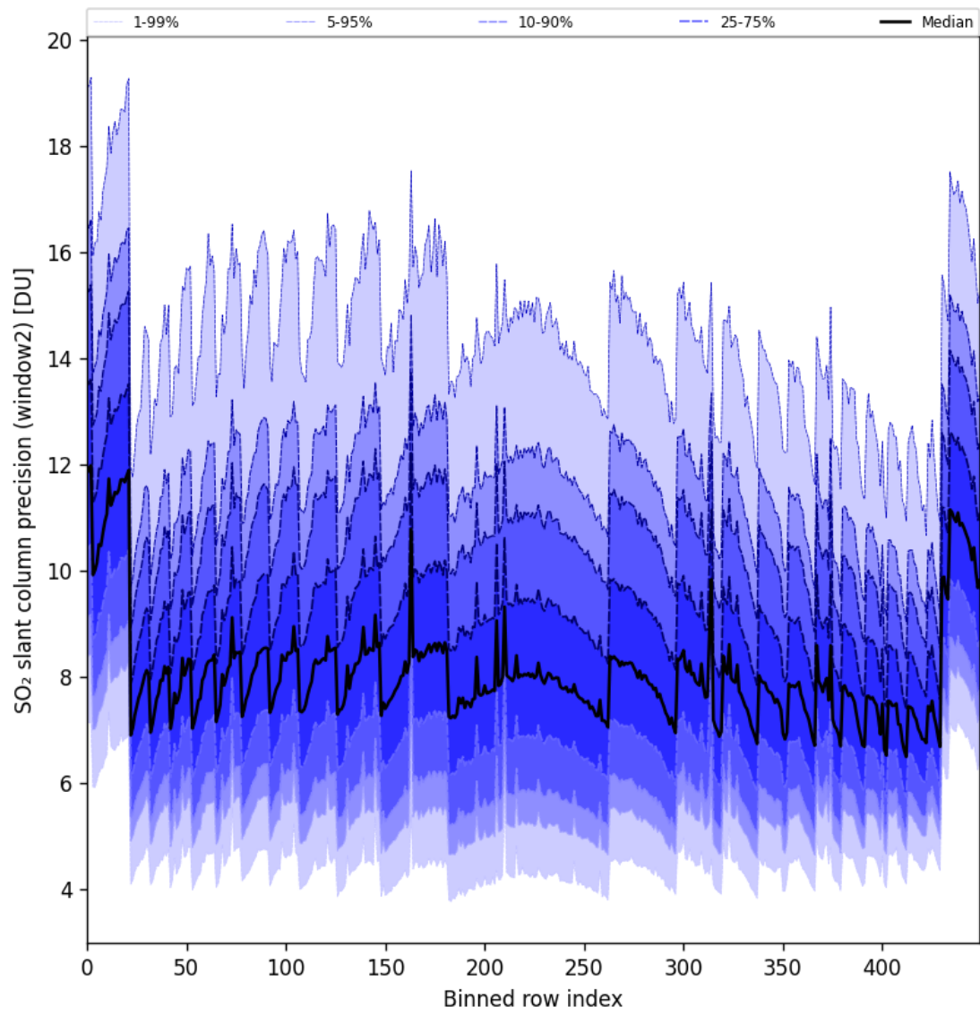
Figure 94: Along track statistics of “SO 2 slant column precision (window2)” for 2025-08-01 to 2025-08-03
