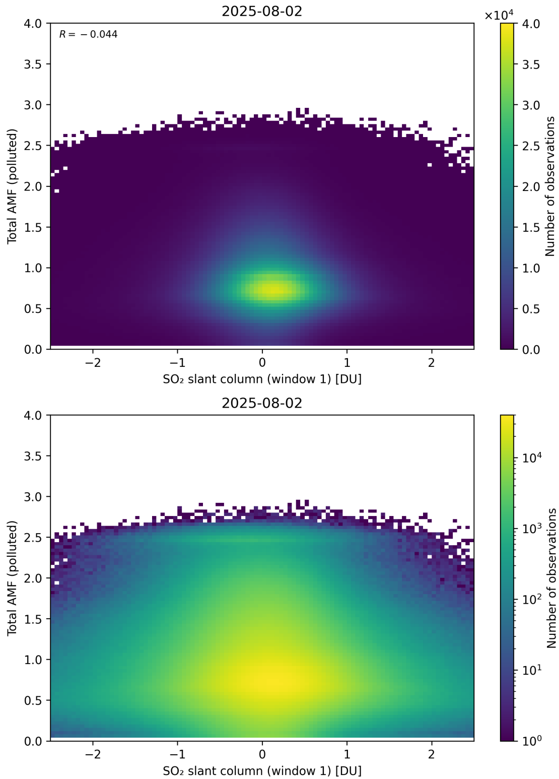
Figure 289: Scatter density plot of “SO 2 slant column (window 1)” against “Total AMF (polluted)” for 2025-08-01 to 2025-08-03.
