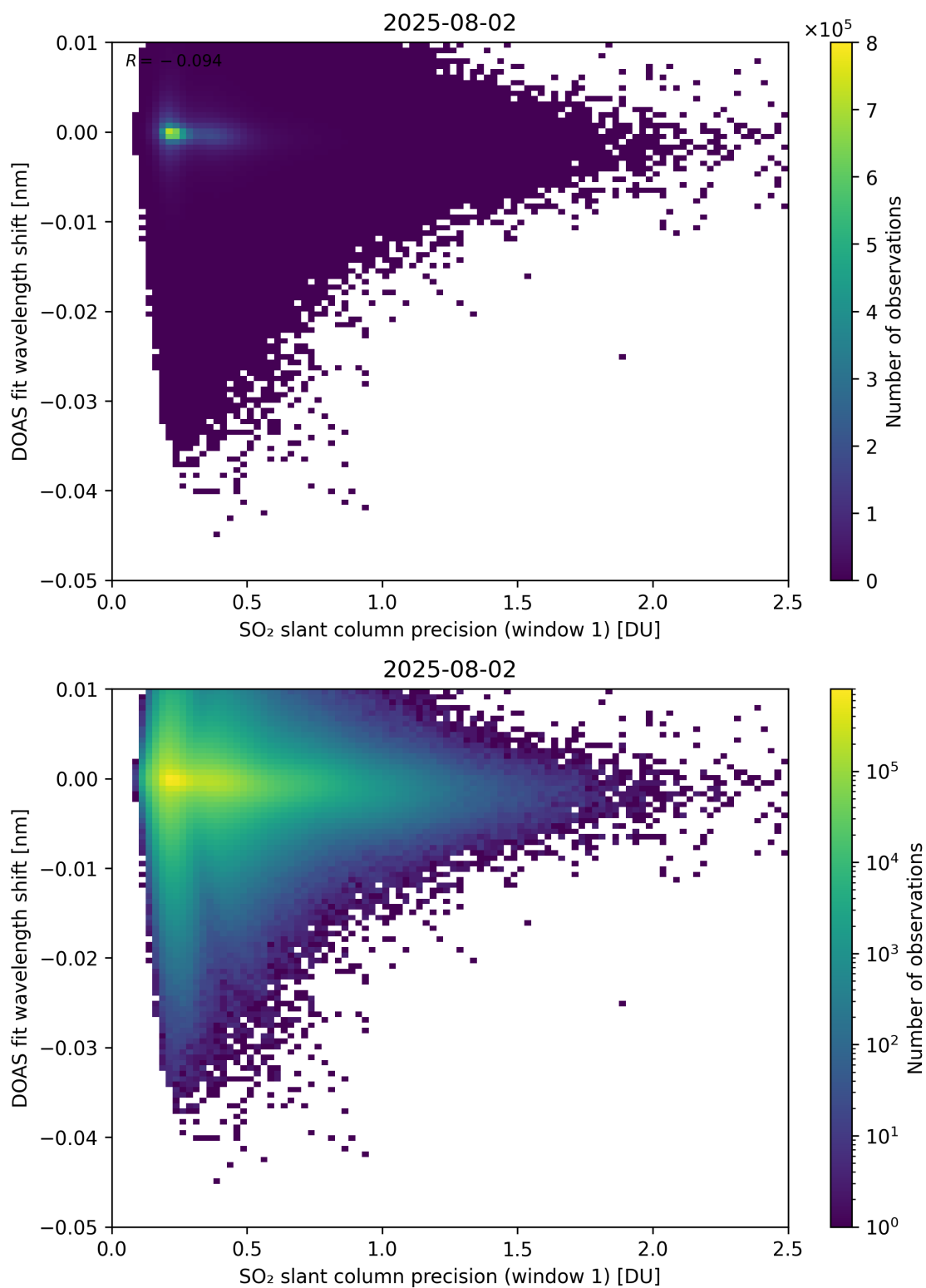
Figure 271: Scatter density plot of “SO 2 slant column precision (window 1)” against “DOAS fit wavelength shift” for 2025-08-01 to 2025-08-03.
