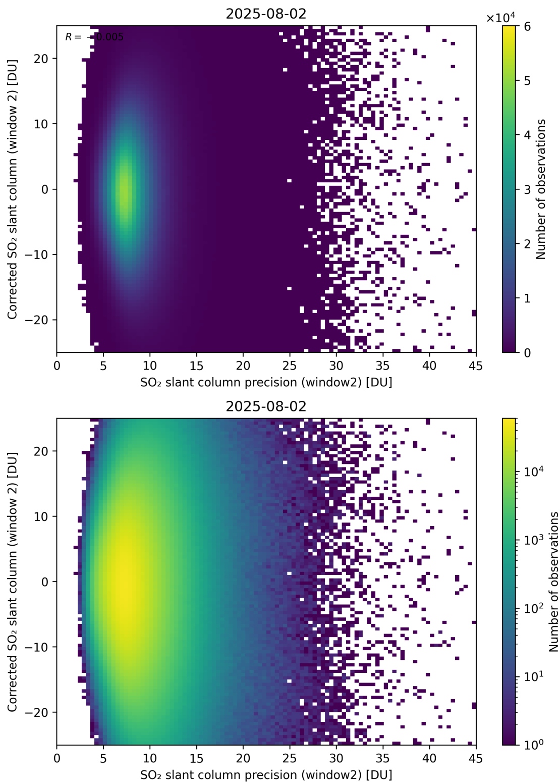
Figure 297: Scatter density plot of “SO 2 slant column precision (window2)” against “Corrected SO 2 slant column (window 2)” for 2025-08-01 to 2025-08-03.
