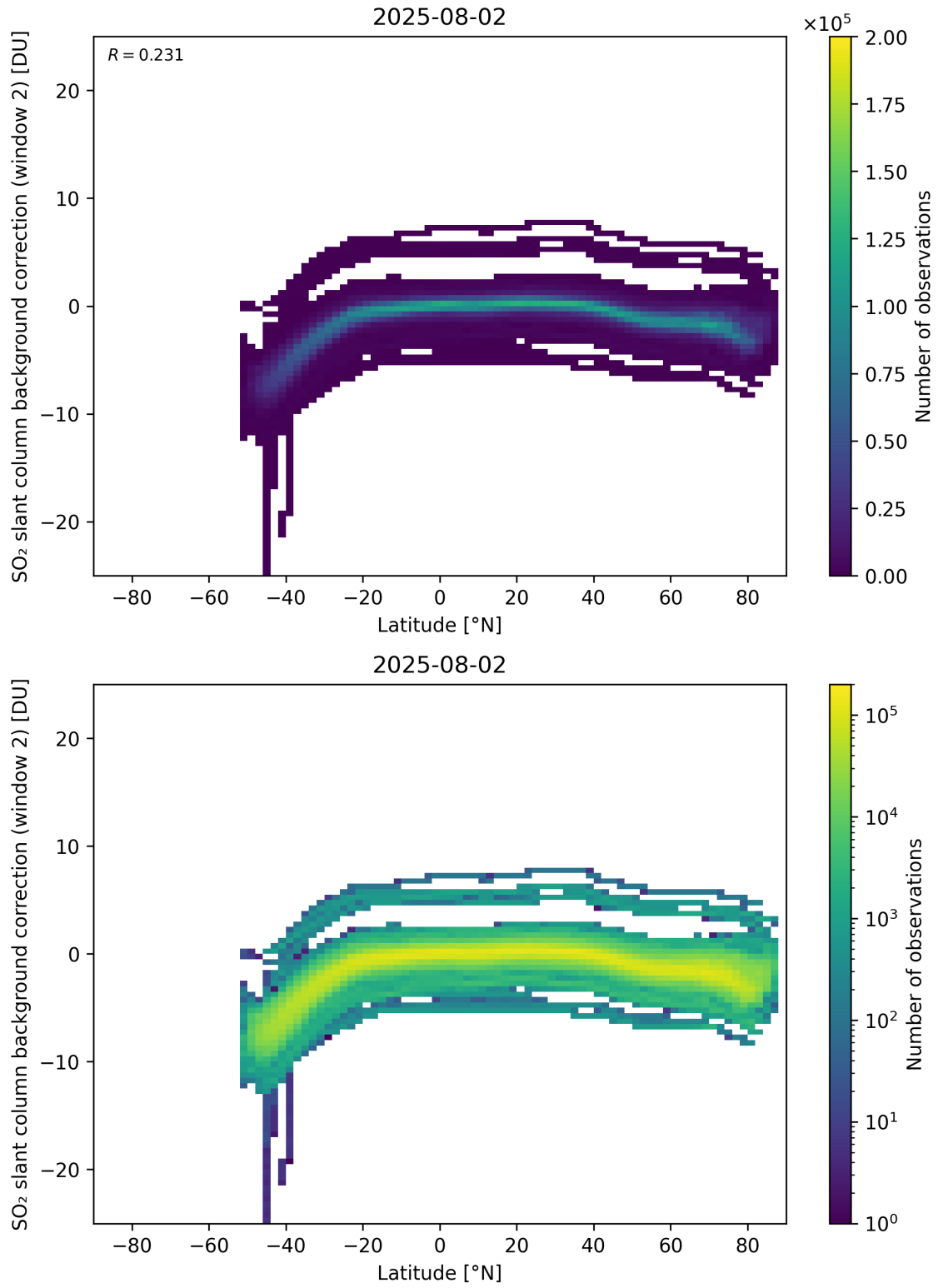
Figure 151: Scatter density plot of “Latitude” against “SO 2 slant column background correction (window 2)” for 2025-08-01 to 2025-08-03.
