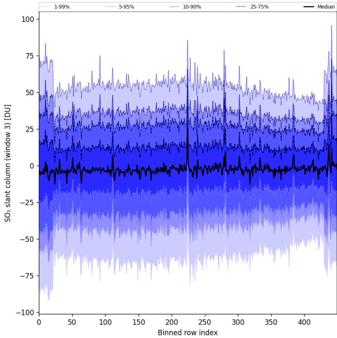
Figure 97: Along track statistics of “SO 2 slant column (window 3)” for 2025-08-01 to 2025-08-03
