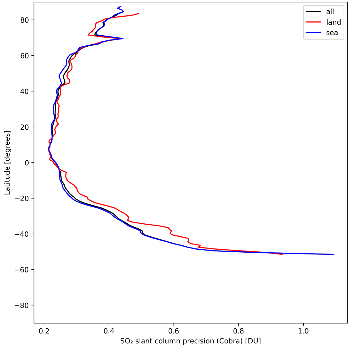
Figure 36: Zonal average of “SO 2 slant column precision (Cobra)” for 2025-08-01 to 2025-08-03.
