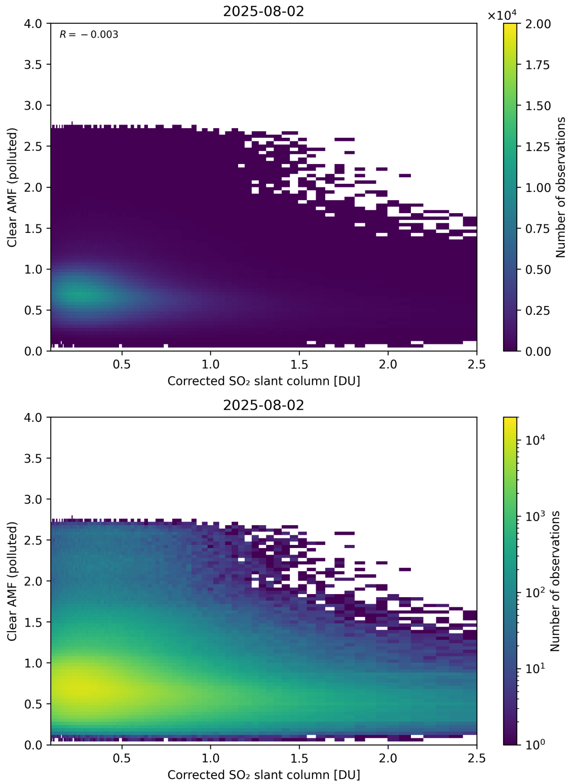
Figure 232: Scatter density plot of “Corrected SO 2 slant column” against “Clear AMF (polluted)” for 2025-08-01 to 2025-08-03.
