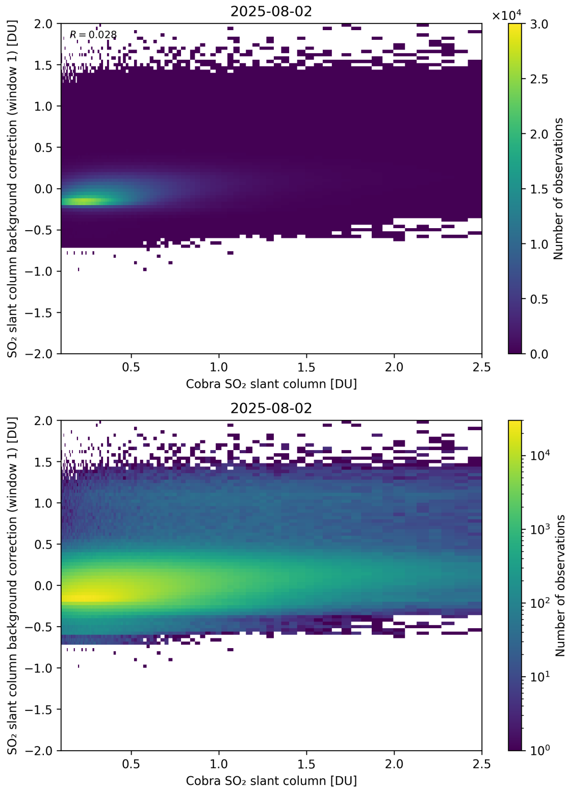
Figure 193: Scatter density plot of “Cobra SO 2 slant column” against “SO 2 slant column background correction (window 1)” for 2025-08-01 to 2025-08-03.
