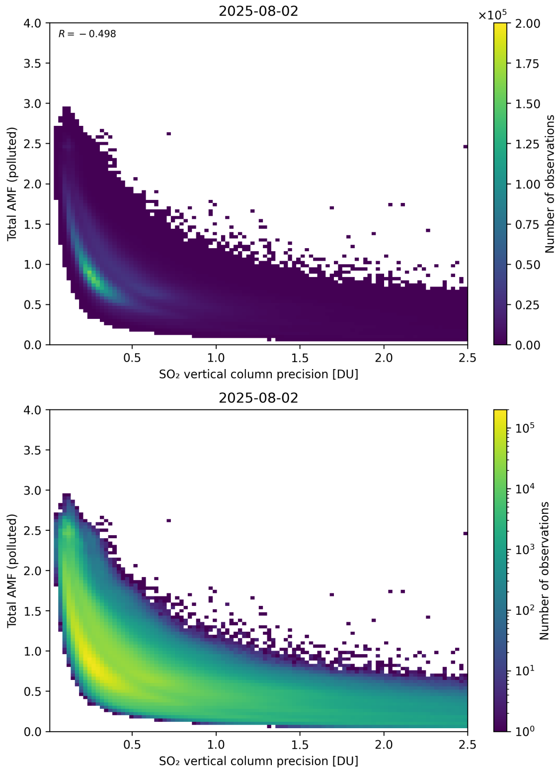
Figure 346: Scatter density plot of “SO 2 vertical column precision” against “Total AMF (polluted)” for 2025-08-01 to 2025-08-03.
