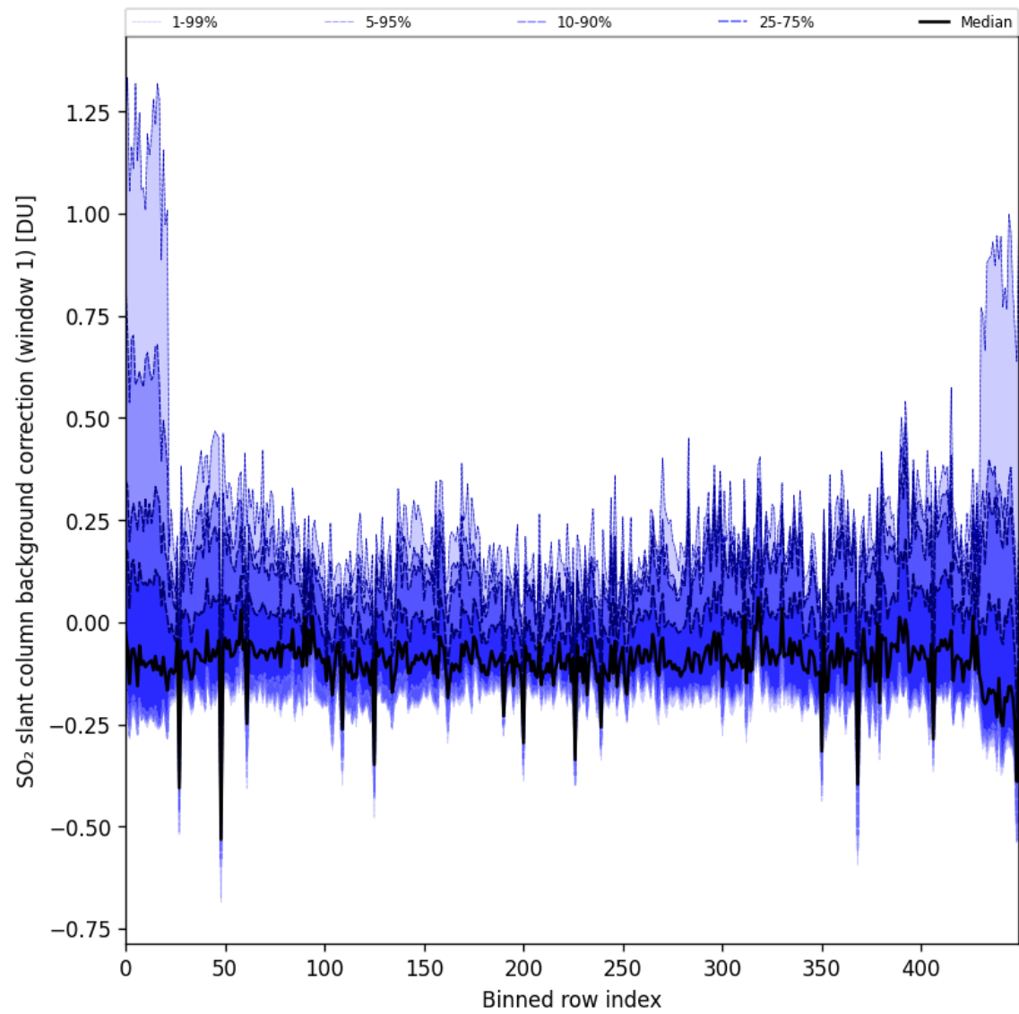
Figure 92: Along track statistics of “SO 2 slant column background correction (window 1)” for 2025-08-01 to 2025-08-03
