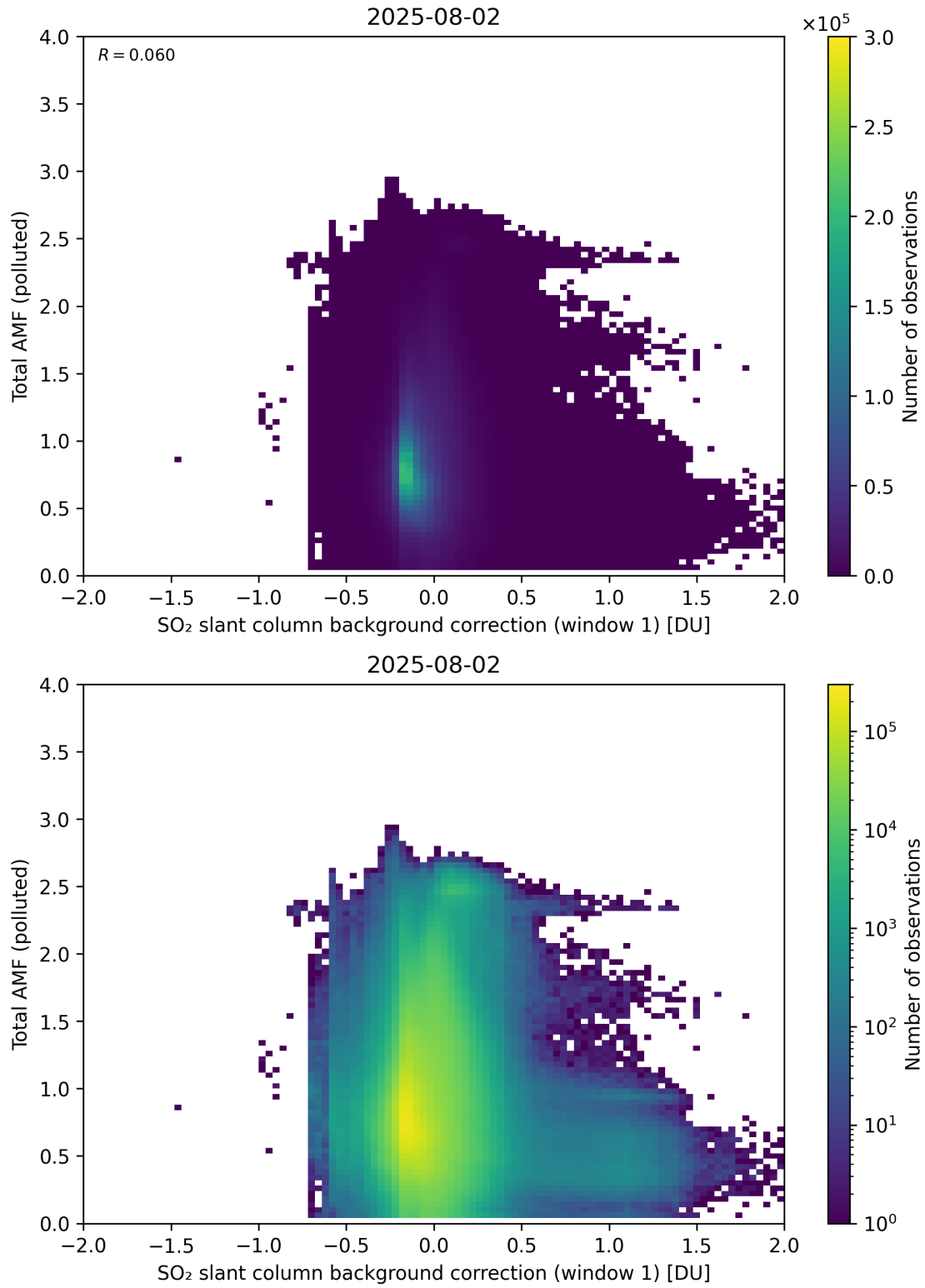
Figure 120: Scatter density plot of “SO 2 slant column background correction (window 1)” against “Total AMF (polluted)” for 2025-08-01 to 2025-08-03.
