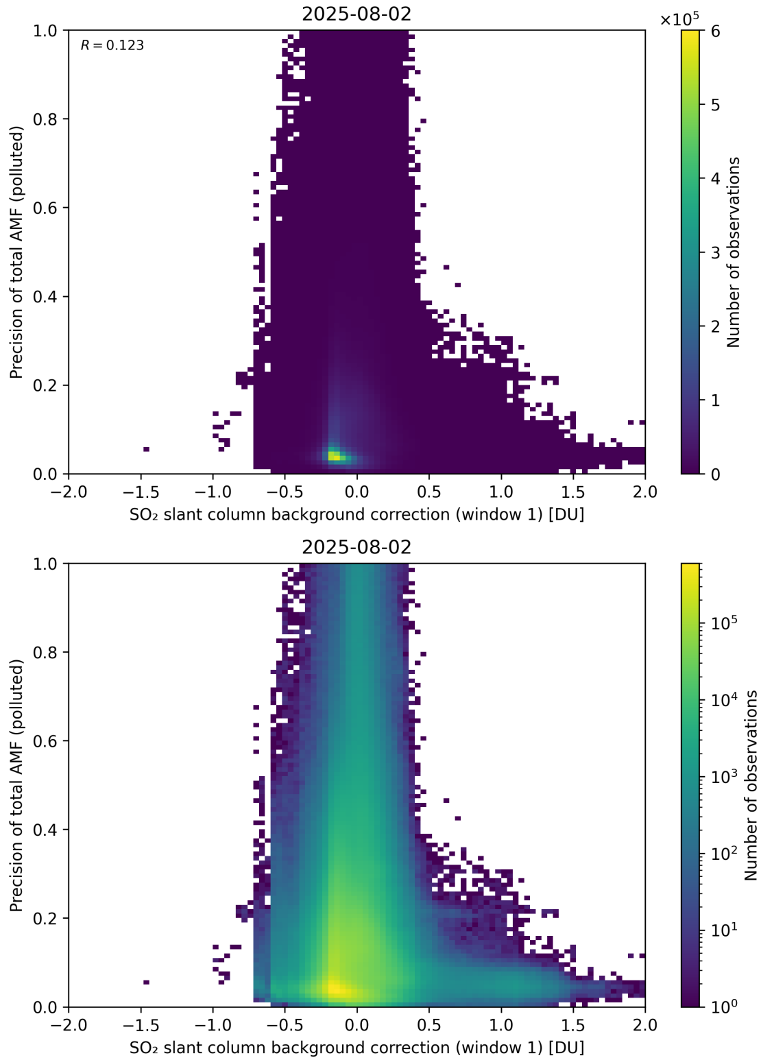
Figure 121: Scatter density plot of “SO 2 slant column background correction (window 1)” against “Precision of total AMF (polluted)” for 2025-08-01 to 2025-08-03.
