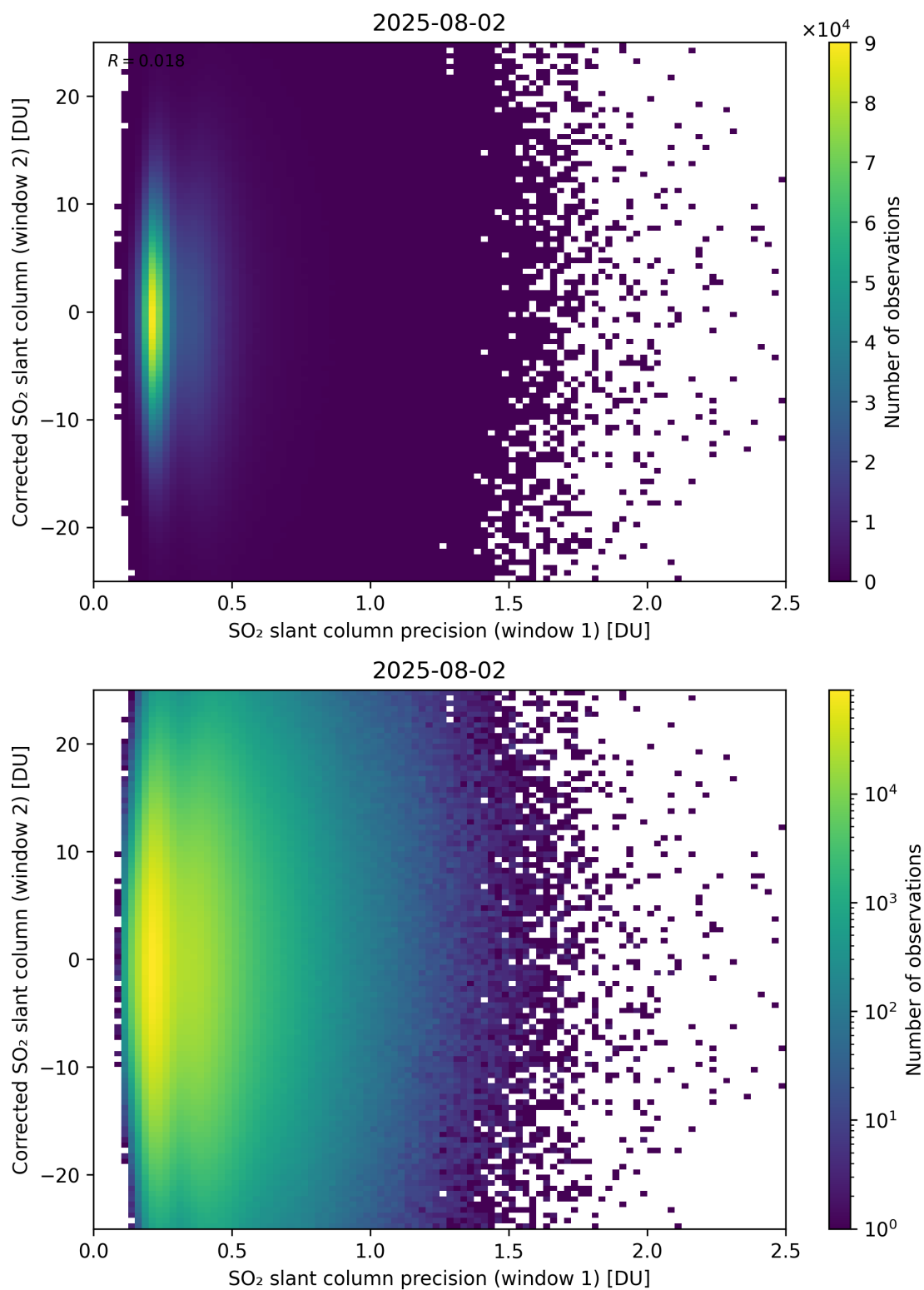
Figure 275: Scatter density plot of “SO 2 slant column precision (window 1)” against “Corrected SO 2 slant column (window 2)” for 2025-08-01 to 2025-08-03.
