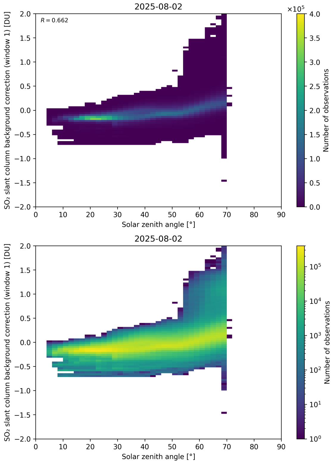
Figure 171: Scatter density plot of “Solar zenith angle” against “SO 2 slant column background correction (window 1)” for 2025-08-01 to 2025-08-03.
