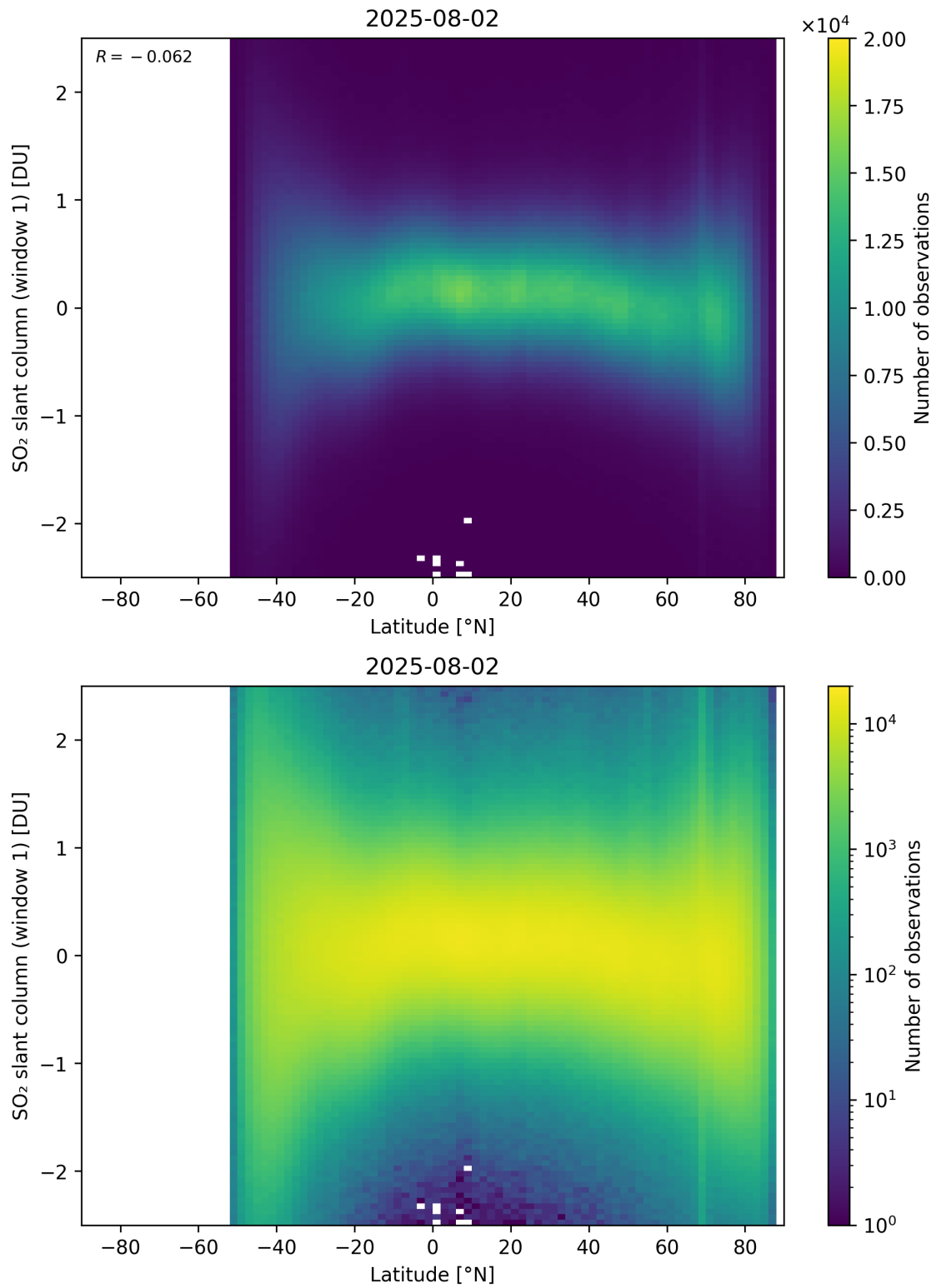
Figure 162: Scatter density plot of “Latitude” against “SO 2 slant column (window 1)” for 2025-08-01 to 2025-08-03.
