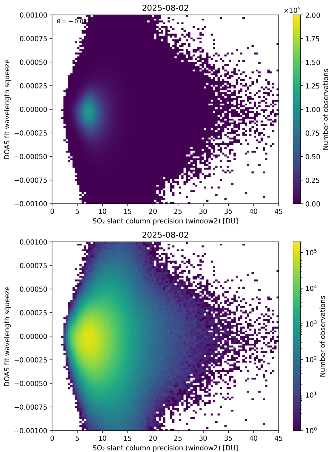
Figure 294: Scatter density plot of “SO 2 slant column precision (window2)” against “DOAS fit wavelength squeeze” for 2025-08-01 to 2025-08-03.
