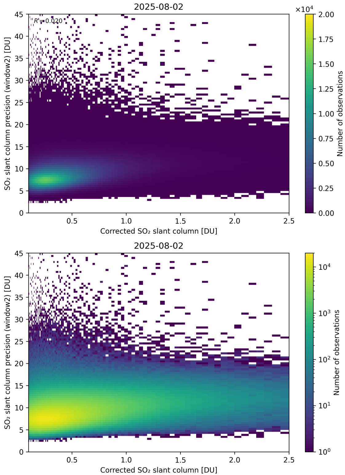
Figure 239: Scatter density plot of “Corrected SO 2 slant column” against “SO 2 slant column precision (window2)” for 2025-08-01 to 2025-08-03.
