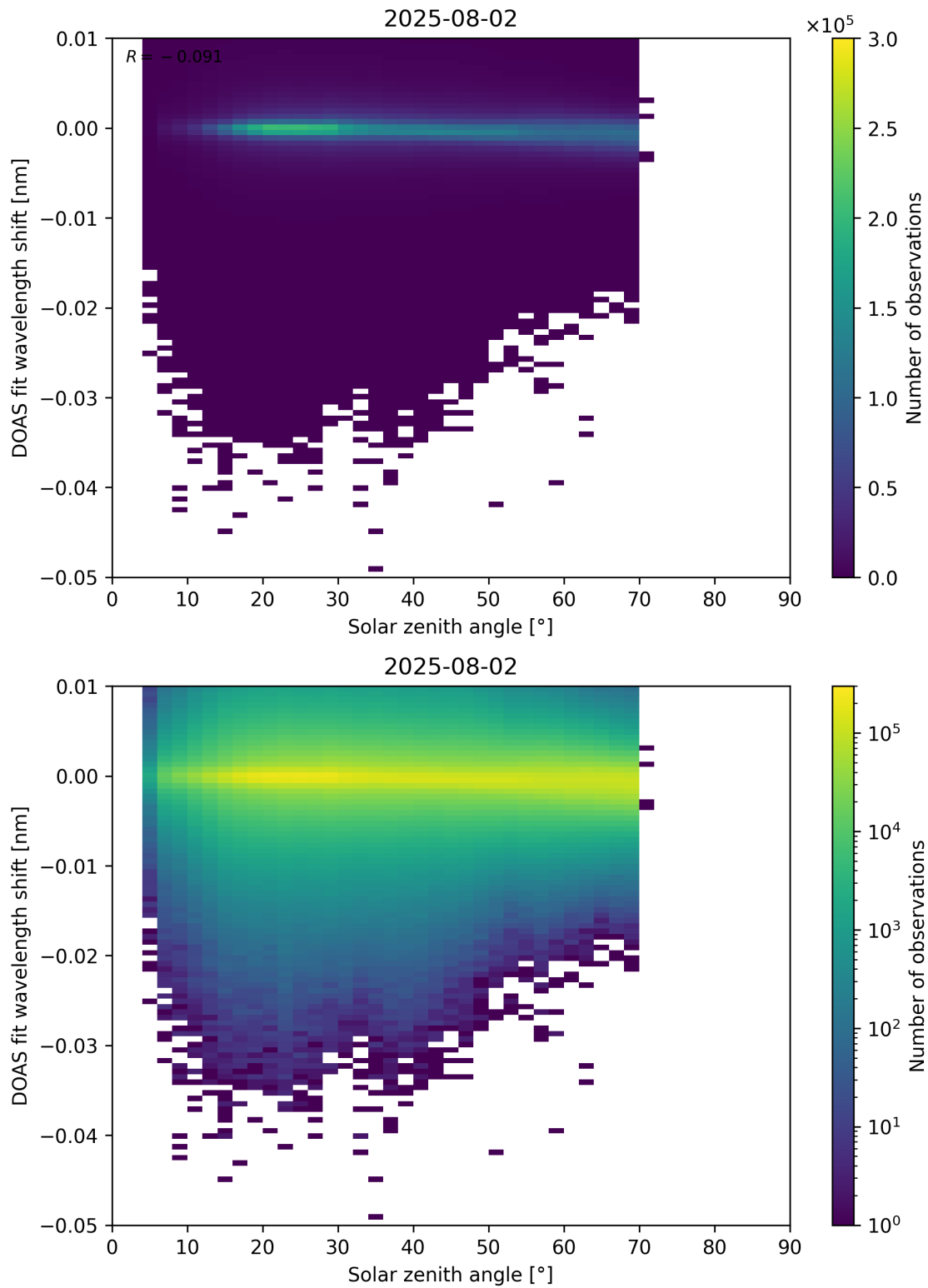
Figure 174: Scatter density plot of “Solar zenith angle” against “DOAS fit wavelength shift” for 2025-08-01 to 2025-08-03.
