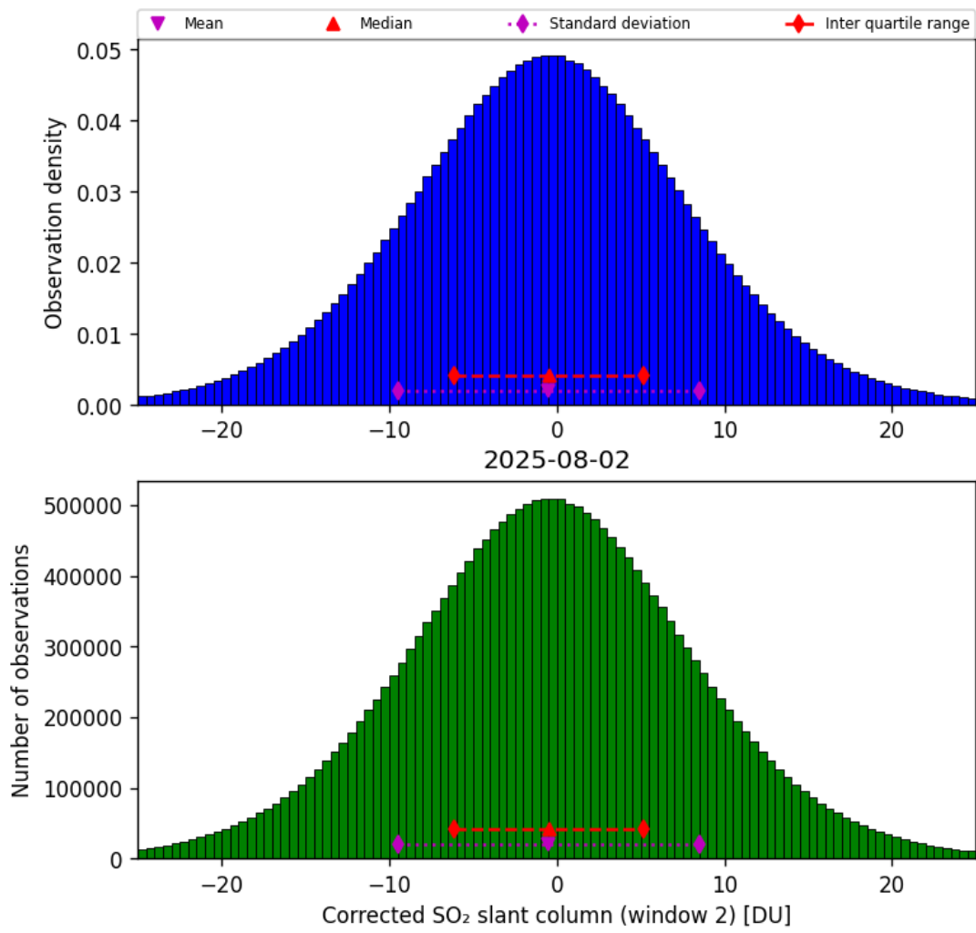
Figure 69: Histogram of “Corrected SO 2 slant column (window 2)” for 2025-08-01 to 2025-08-03
