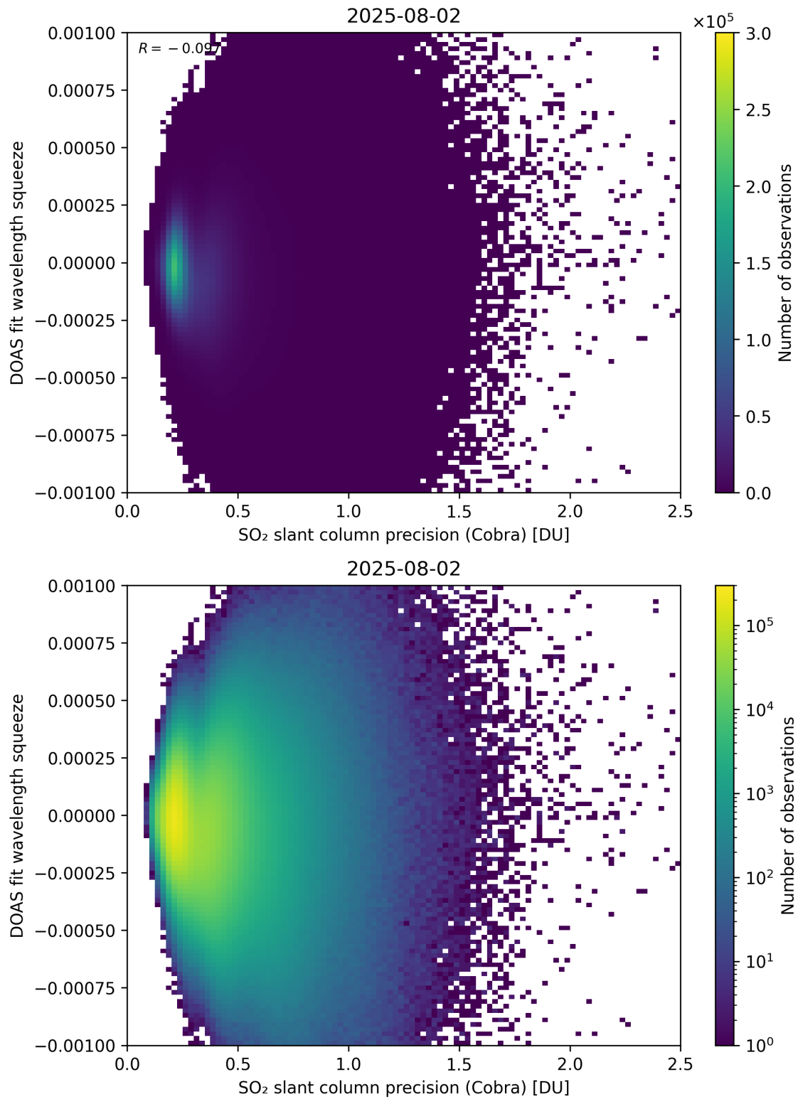
Figure 203: Scatter density plot of “SO 2 slant column precision (Cobra)” against “DOAS fit wavelength squeeze” for 2025-08-01 to 2025-08-03.
