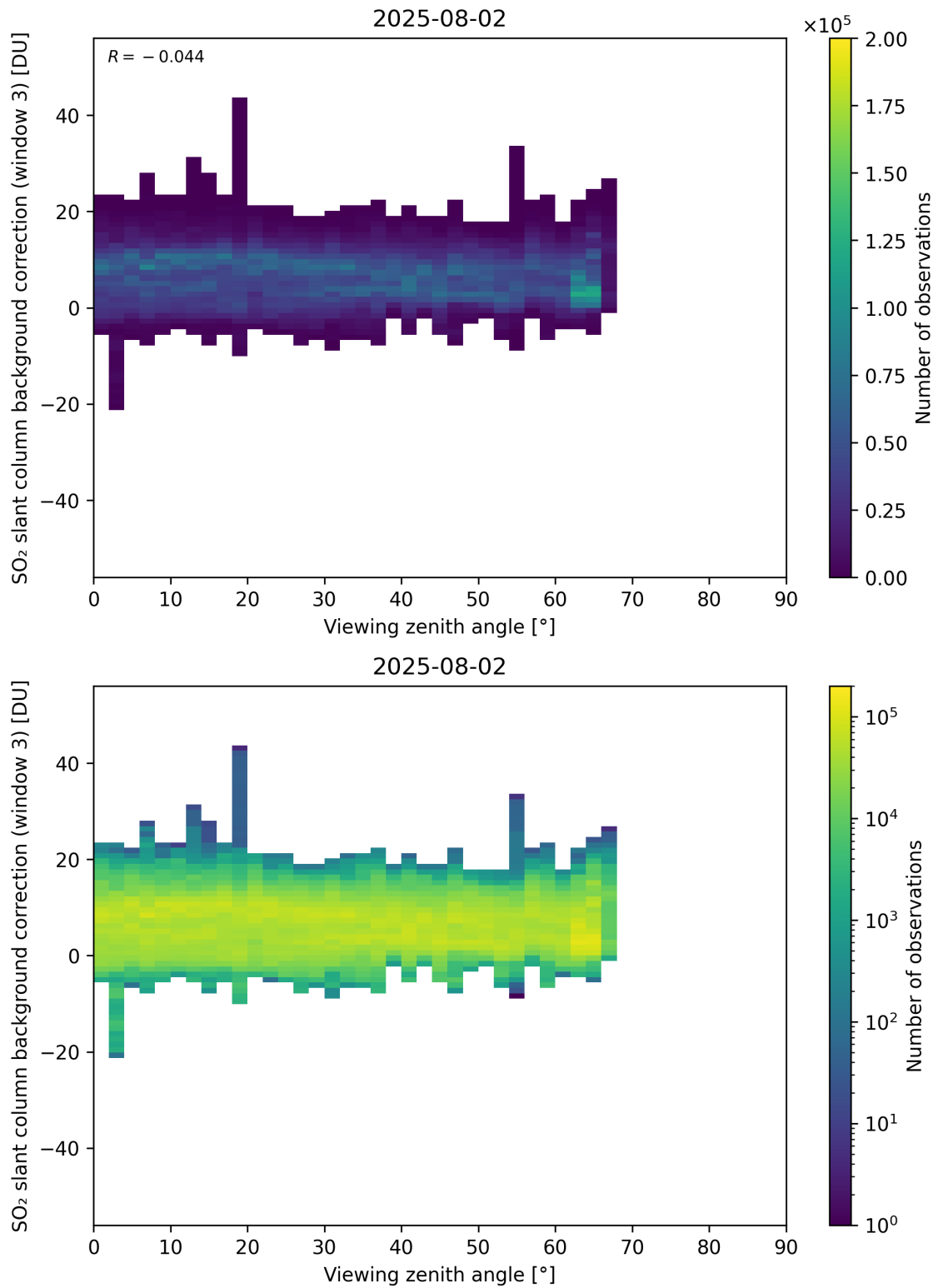
Figure 364: Scatter density plot of “Viewing zenith angle” against “SO 2 slant column background correction (window 3)” for 2025-08-01 to 2025-08-03.
