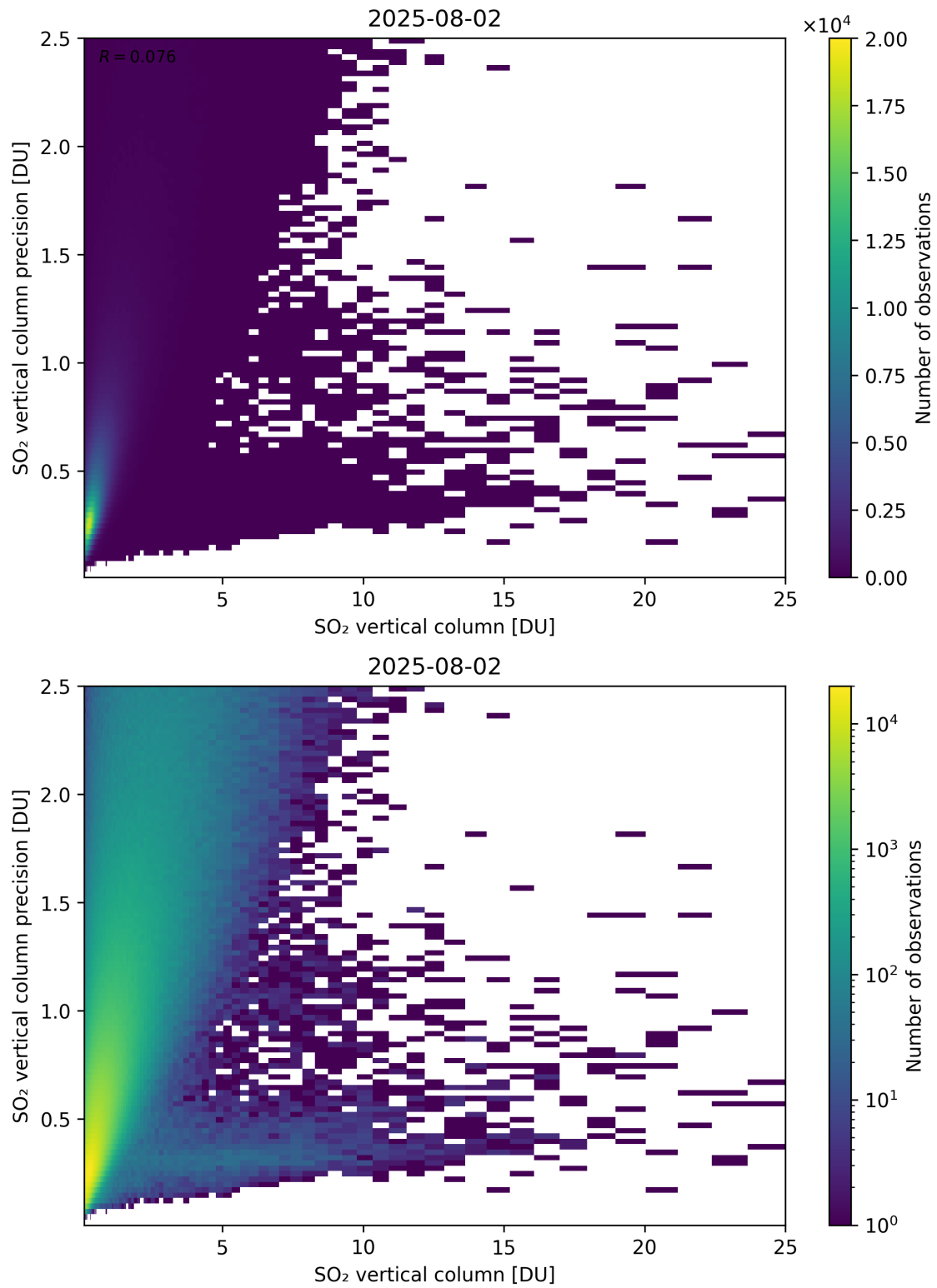
Figure 361: Scatter density plot of “SO 2 vertical column” against “SO 2 vertical column precision” for 2025-08-01 to 2025-08-03.
