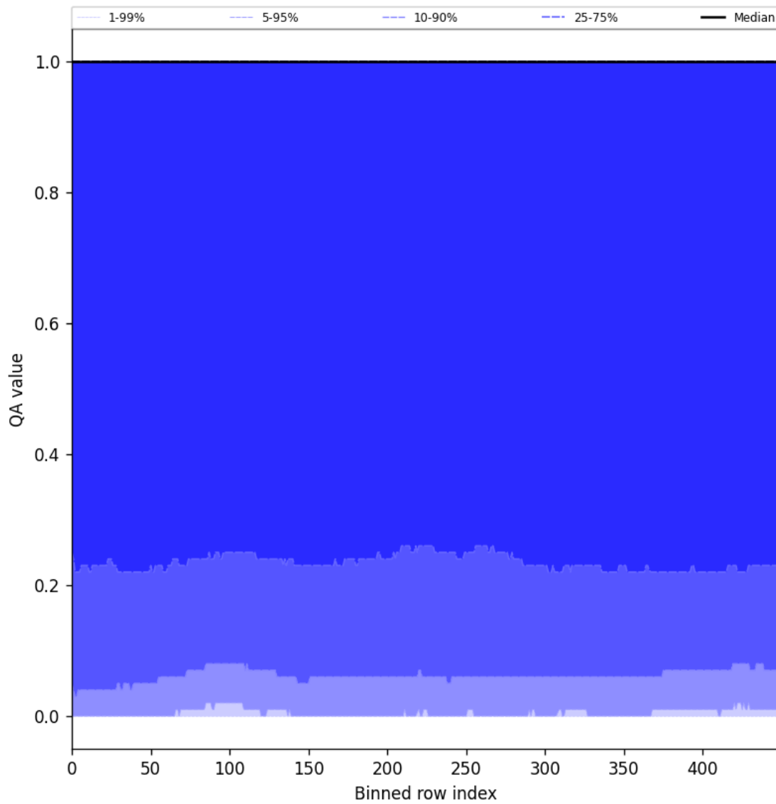
Figure 83: Along track statistics of “QA value” for 2025-08-01 to 2025-08-03
