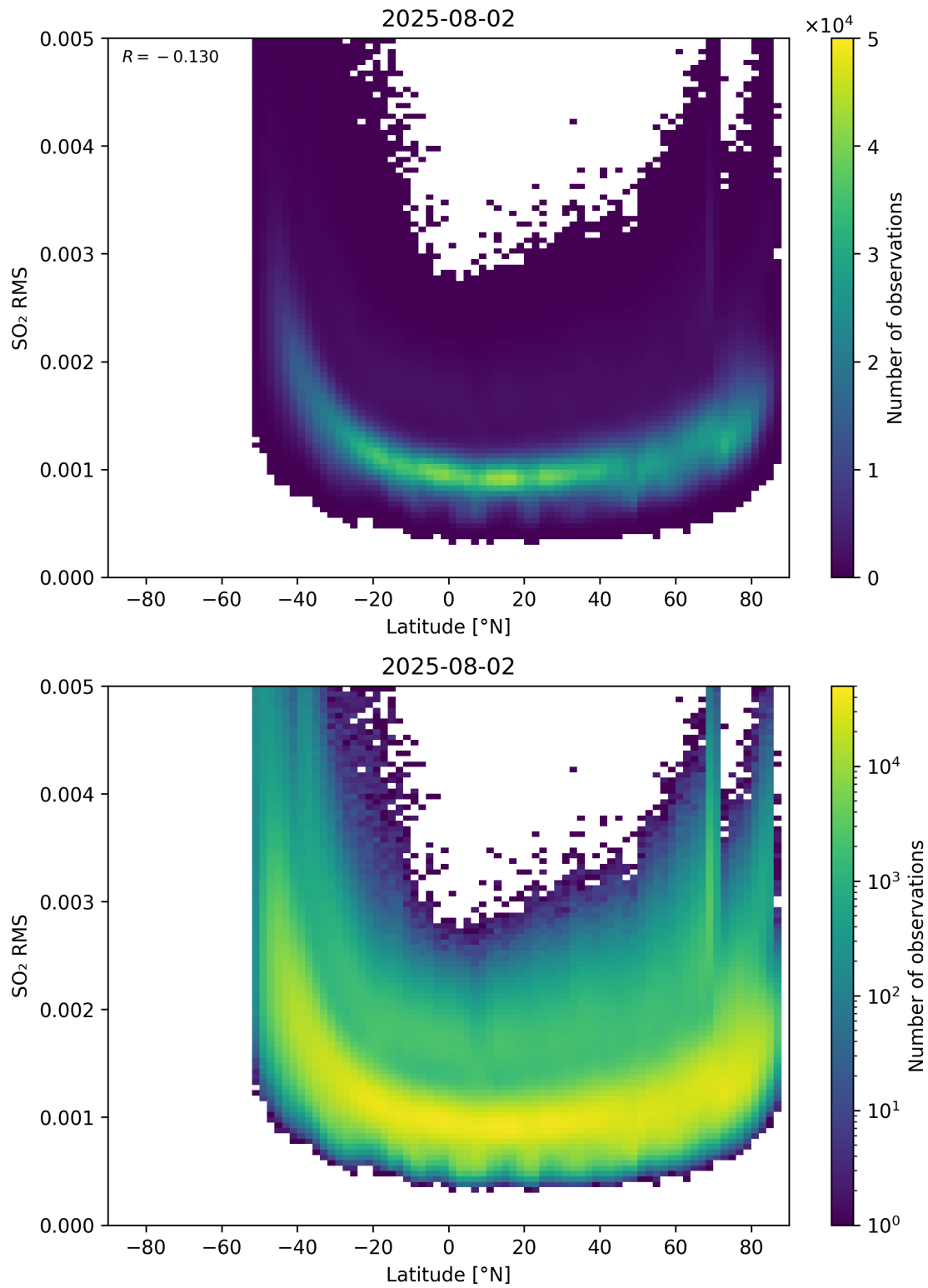
Figure 155: Scatter density plot of “Latitude” against “SO 2 RMS” for 2025-08-01 to 2025-08-03.
