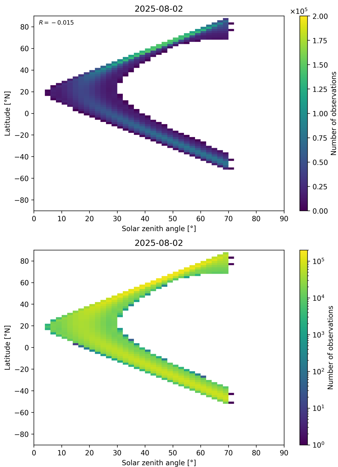
Figure 177: Scatter density plot of “Solar zenith angle” against “Latitude” for 2025-08-01 to 2025-08-03.
