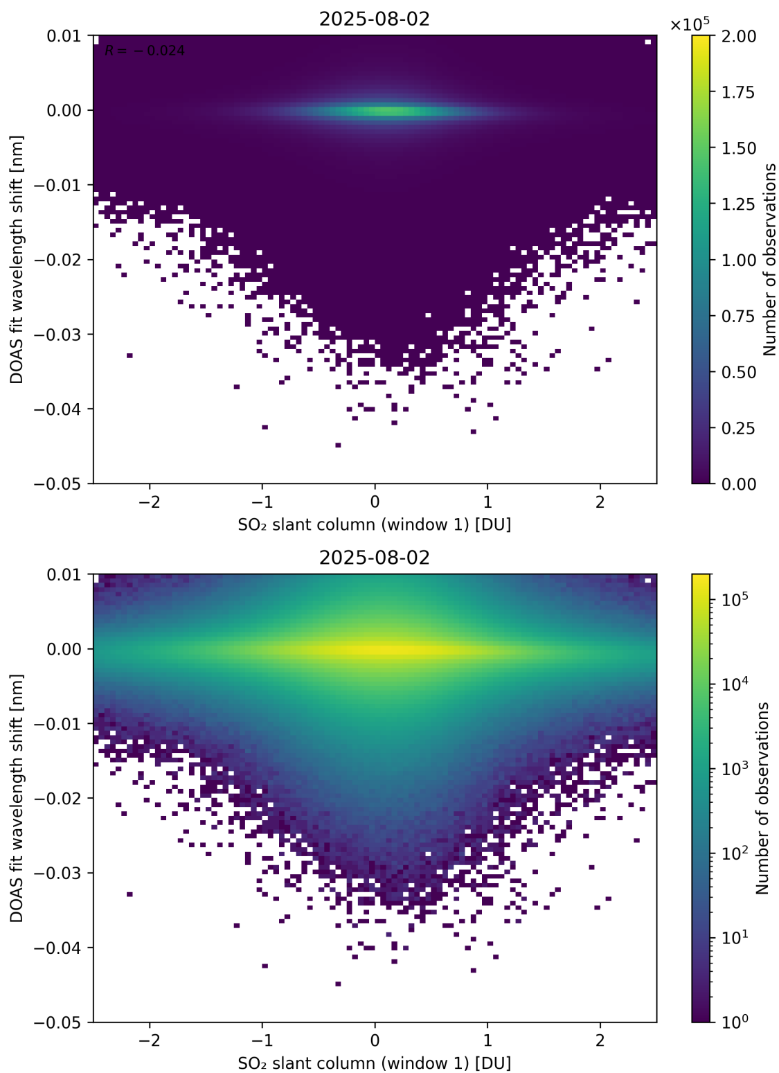
Figure 265: Scatter density plot of “SO 2 slant column (window 1)” against “DOAS fit wavelength shift” for 2025-08-01 to 2025-08-03.
