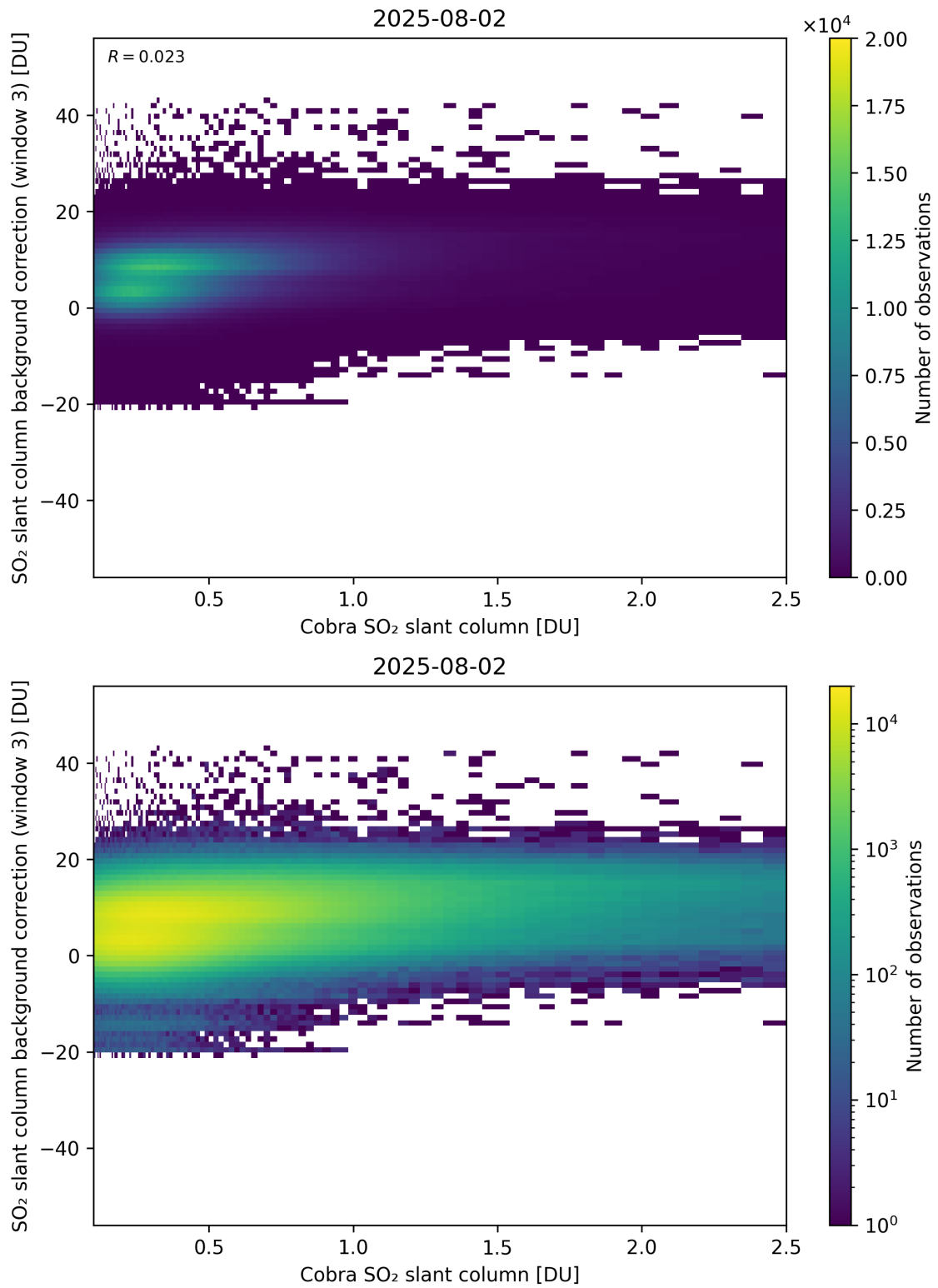
Figure 195: Scatter density plot of “Cobra SO 2 slant column” against “SO 2 slant column background correction (window 3)” for 2025-08-01 to 2025-08-03.
