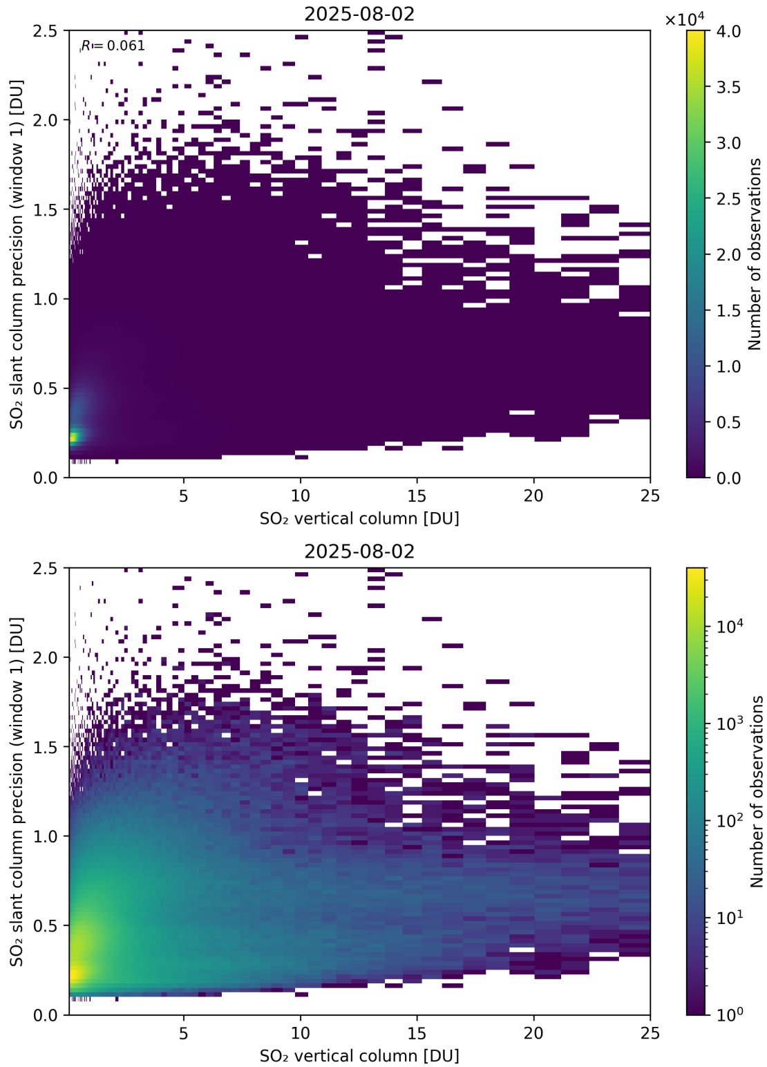
Figure 355: Scatter density plot of “SO 2 vertical column” against “SO 2 slant column precision (window 1)” for 2025-08-01 to 2025-08-03.
