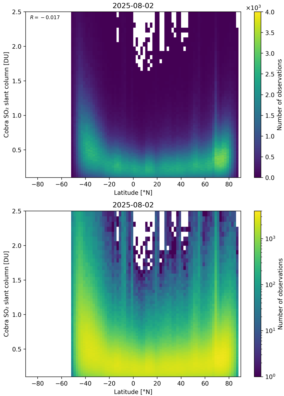
Figure 157: Scatter density plot of “Latitude” against “Cobra SO 2 slant column” for 2025-08-01 to 2025-08-03.
