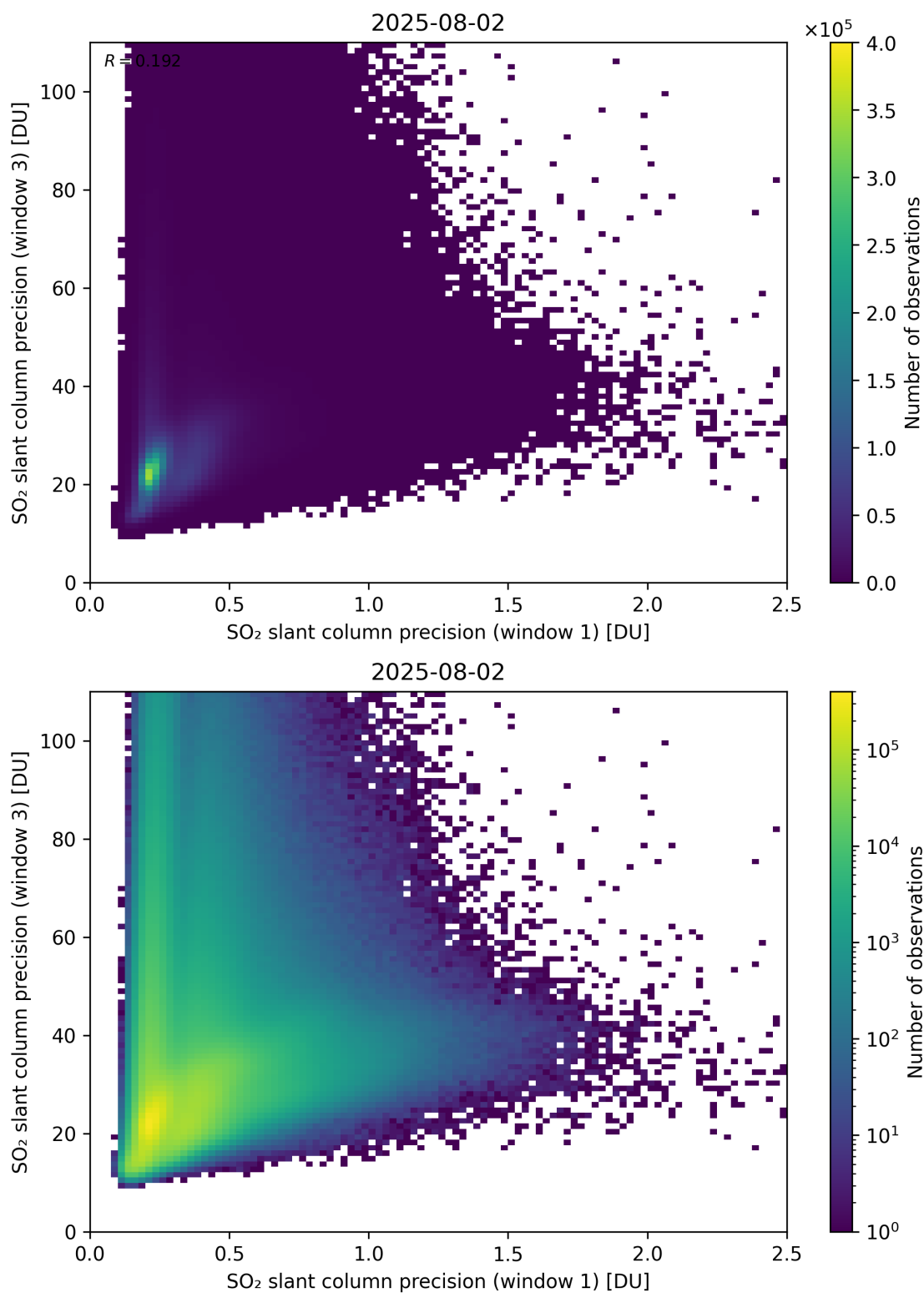
Figure 279: Scatter density plot of “SO 2 slant column precision (window 1)” against “SO 2 slant column precision (window 3)” for 2025-08-01 to 2025-08-03.
