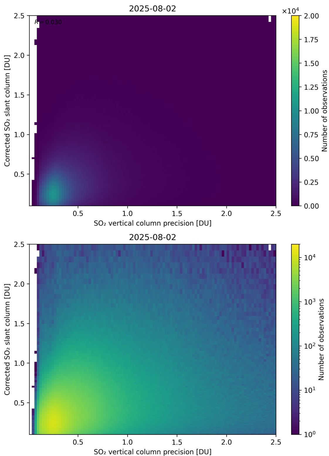
Figure 338: Scatter density plot of “SO 2 vertical column precision” against “Corrected SO 2 slant column” for 2025-08-01 to 2025-08-03.
