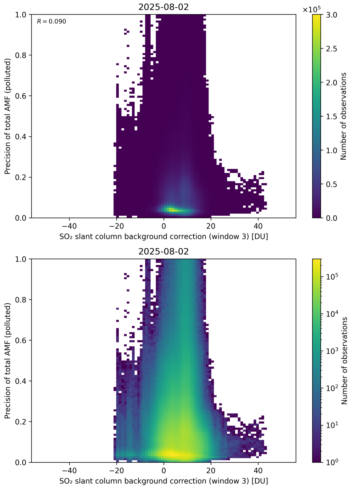
Figure 137: Scatter density plot of “SO 2 slant column background correction (window 3)” against “Precision of total AMF (polluted)” for 2025-08-01 to 2025-08-03.
