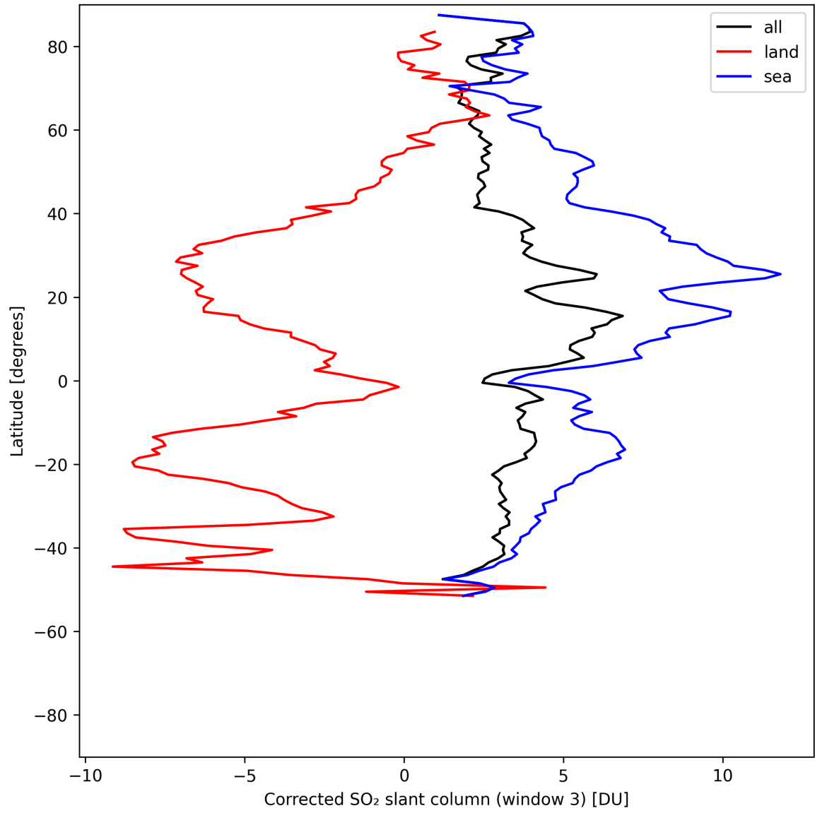
Figure 47: Zonal average of “Corrected SO 2 slant column (window 3)” for 2025-08-01 to 2025-08-03.
