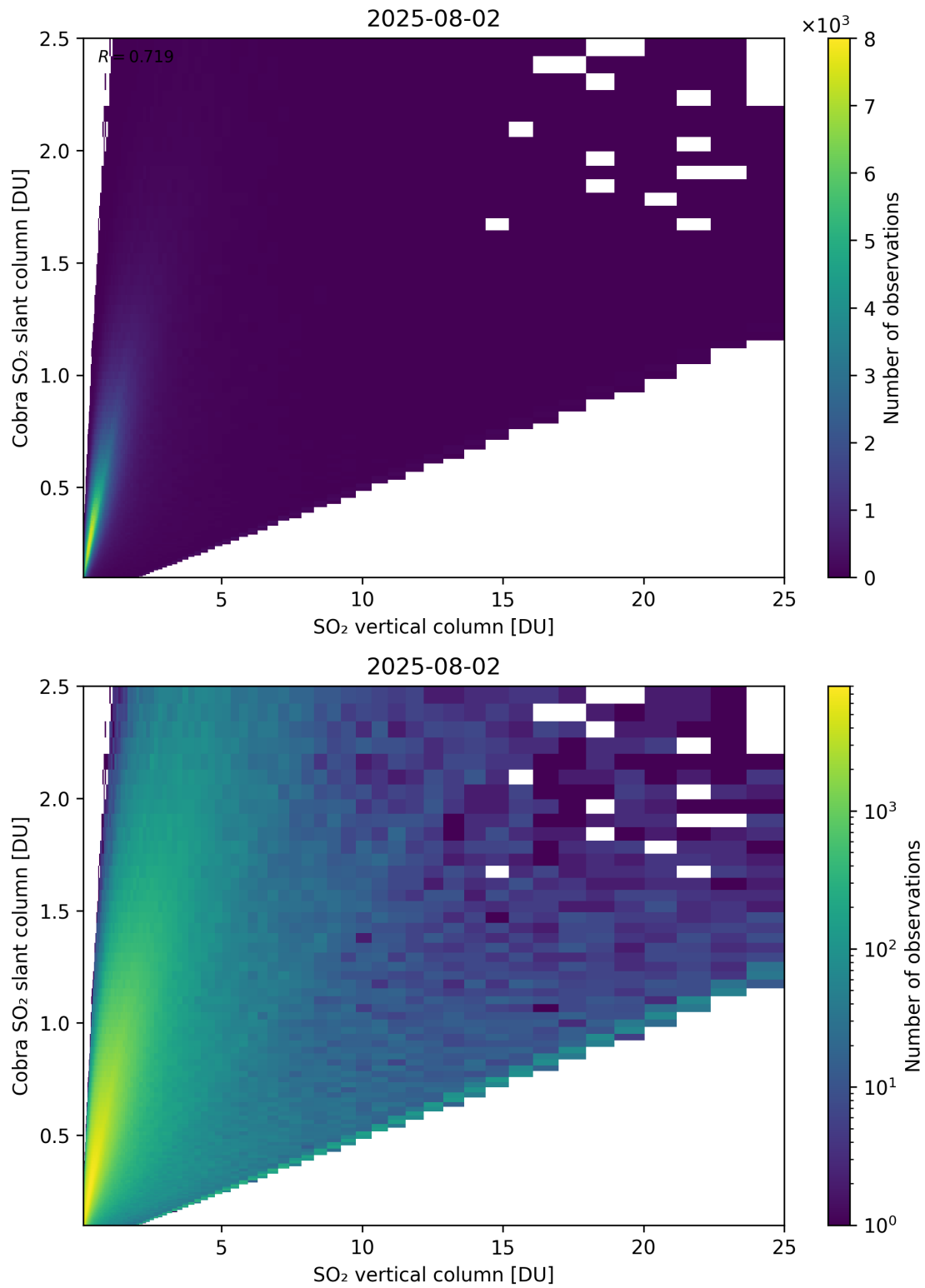
Figure 349: Scatter density plot of “SO 2 vertical column” against “Cobra SO 2 slant column” for 2025-08-01 to 2025-08-03.
