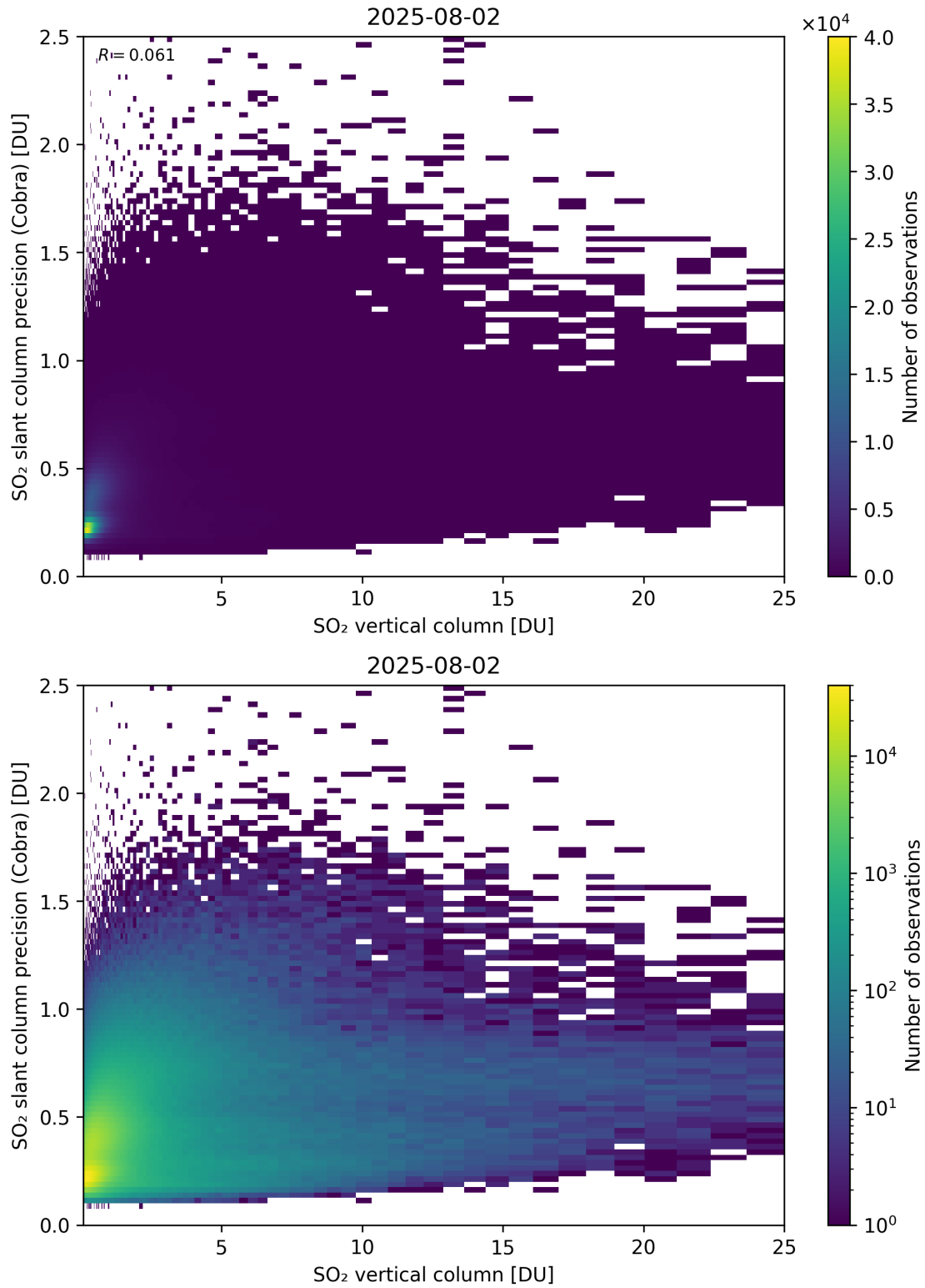
Figure 350: Scatter density plot of “SO 2 vertical column” against “SO 2 slant column precision (Cobra)” for 2025-08-01 to 2025-08-03.
