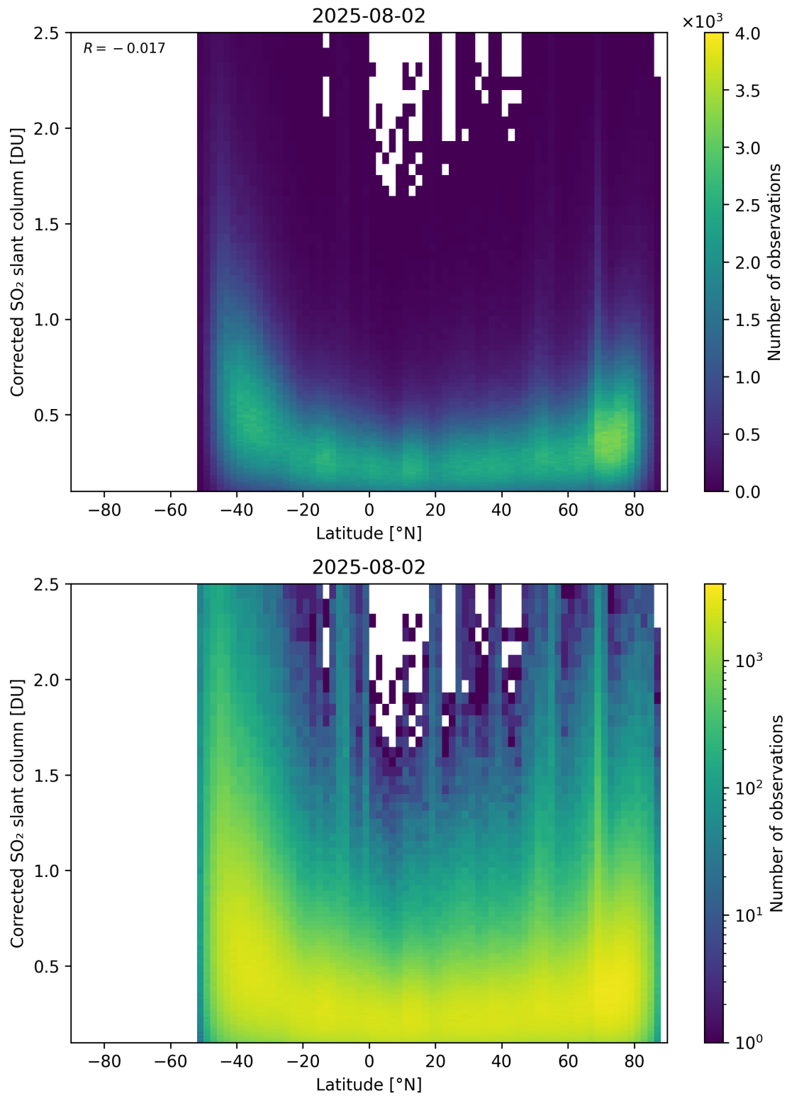
Figure 159: Scatter density plot of “Latitude” against “Corrected SO 2 slant column” for 2025-08-01 to 2025-08-03.
