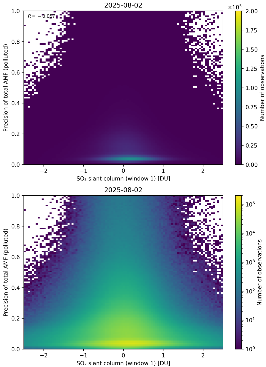
Figure 290: Scatter density plot of “SO 2 slant column (window 1)” against “Precision of total AMF (polluted)” for 2025-08-01 to 2025-08-03.
