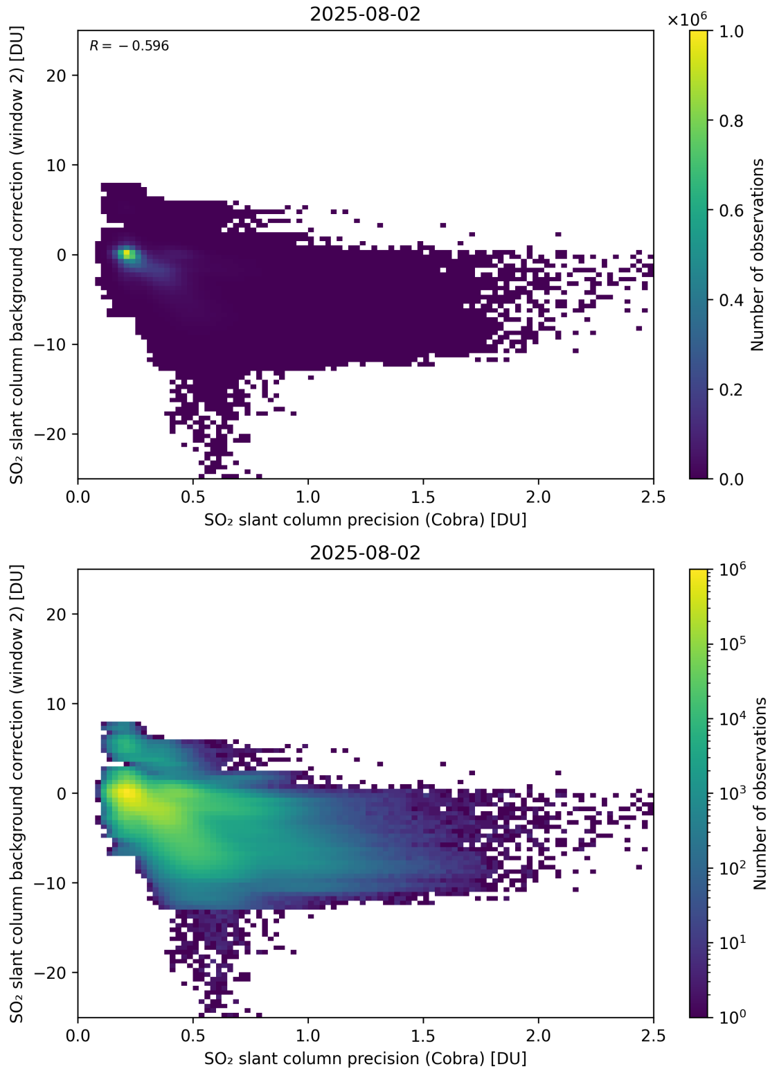
Figure 200: Scatter density plot of “SO 2 slant column precision (Cobra)” against “SO 2 slant column background correction (window 2)” for 2025-08-01 to 2025-08-03.
