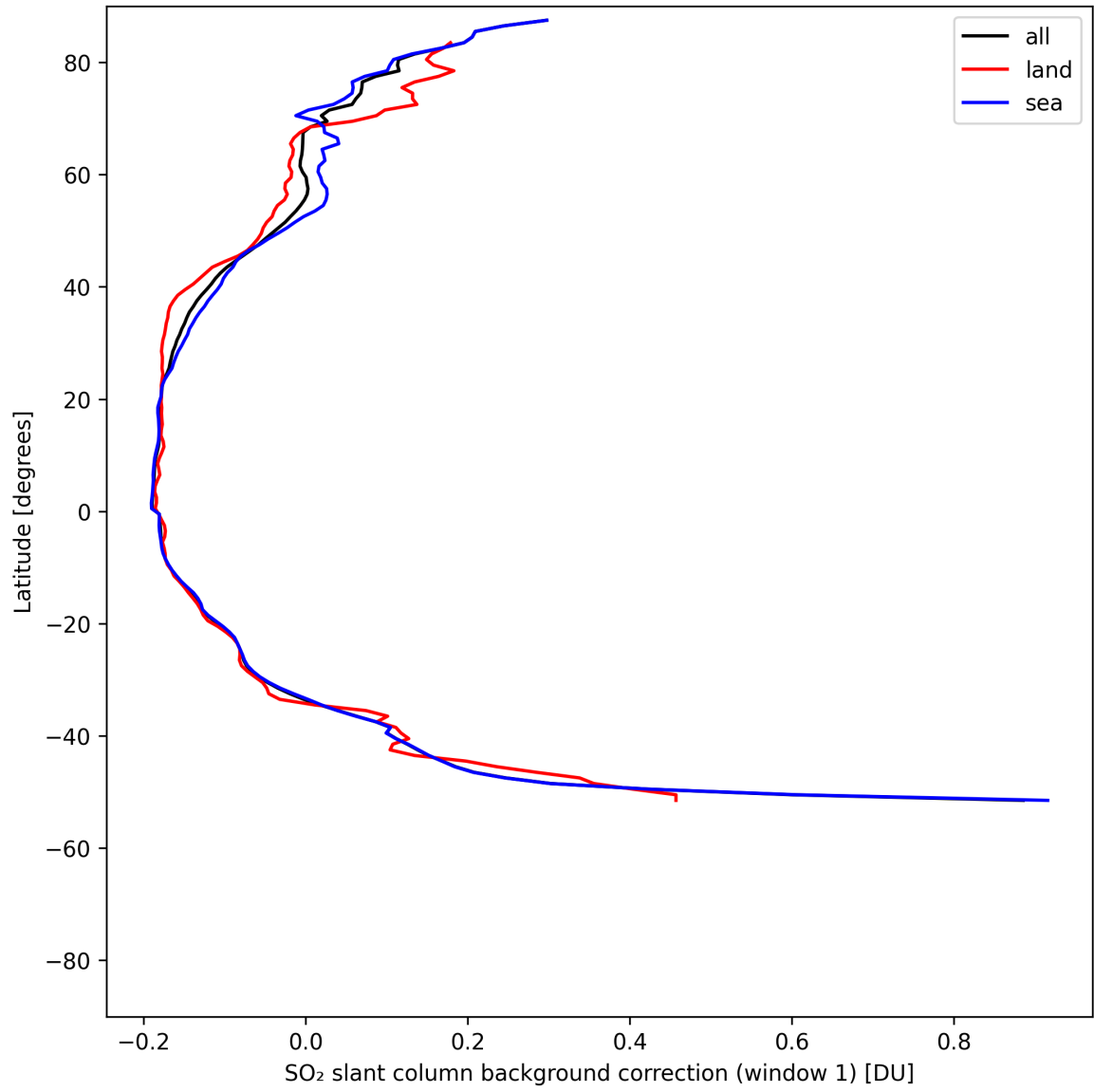
Figure 40: Zonal average of “SO 2 slant column background correction (window 1)” for 2025-08-01 to 2025-08-03.
