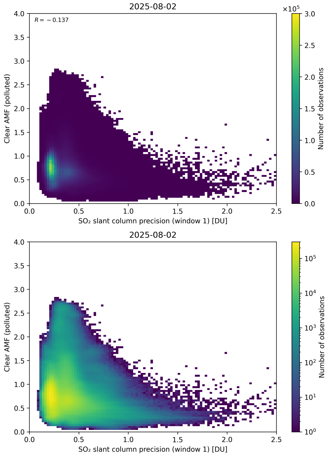
Figure 274: Scatter density plot of “SO 2 slant column precision (window 1)” against “Clear AMF (polluted)” for 2025-08-01 to 2025-08-03.
