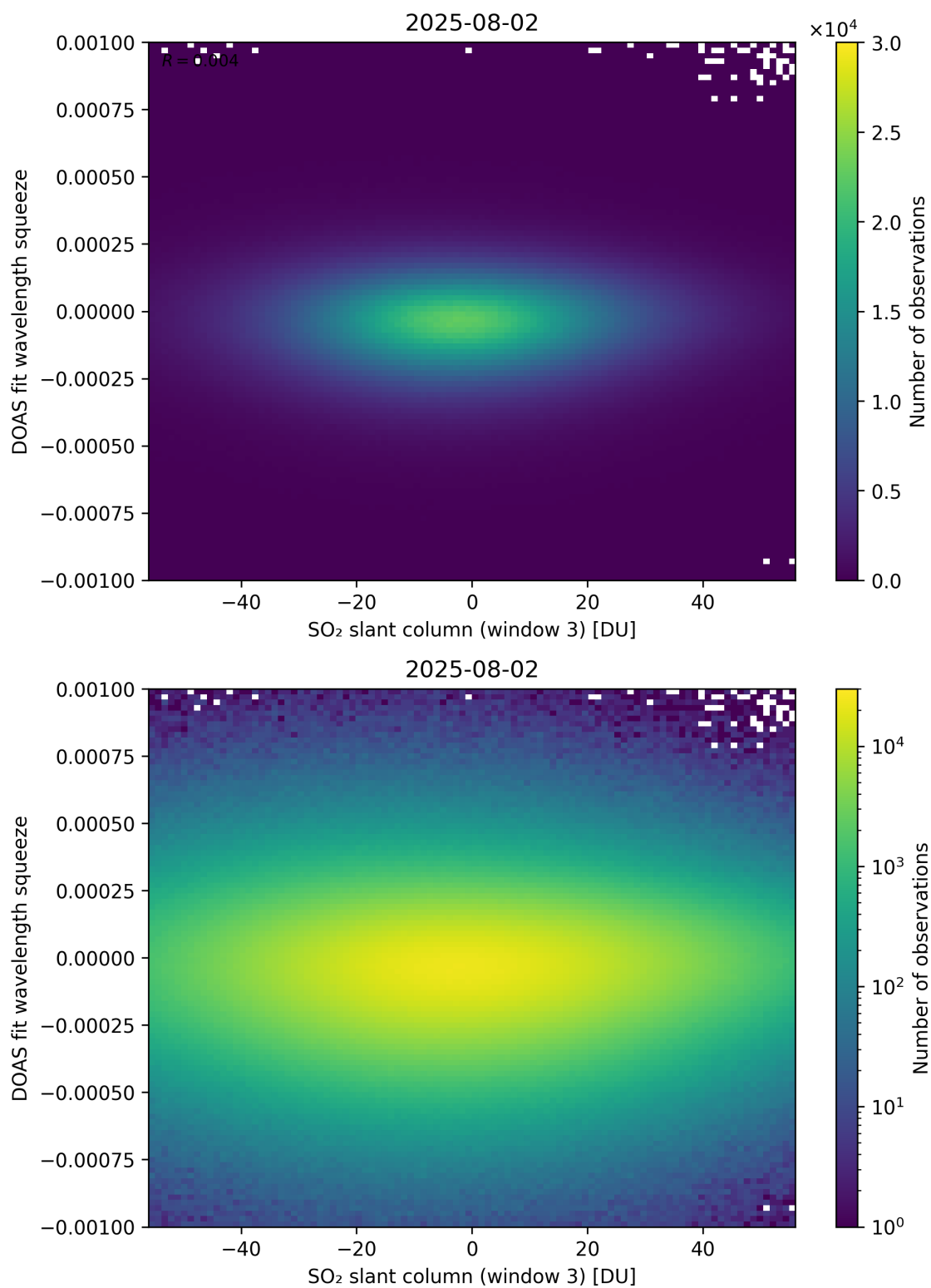
Figure 305: Scatter density plot of “SO 2 slant column (window 3)” against “DOAS fit wavelength squeeze” for 2025-08-01 to 2025-08-03.
