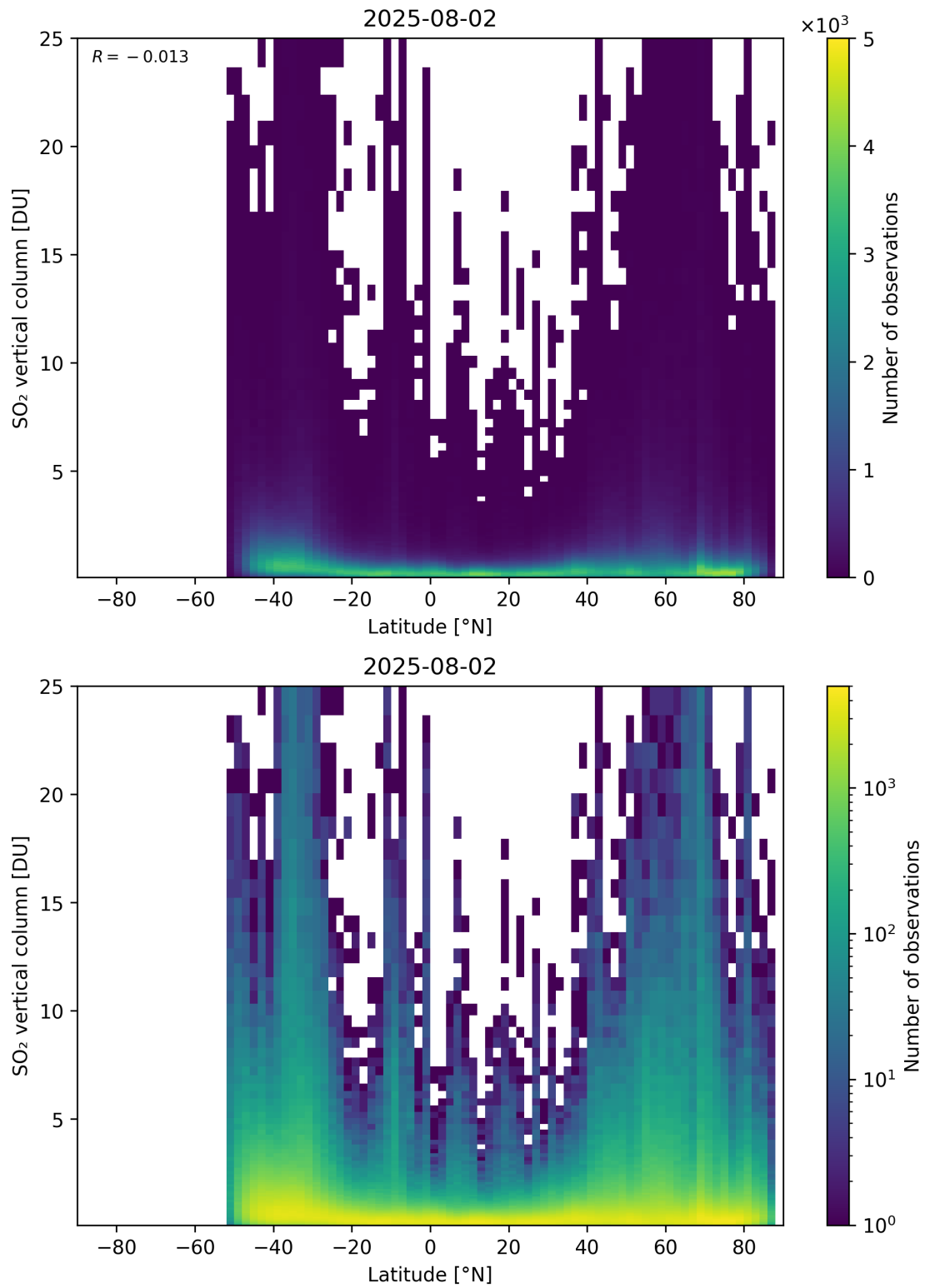
Figure 169: Scatter density plot of “Latitude” against “SO 2 vertical column” for 2025-08-01 to 2025-08-03.
