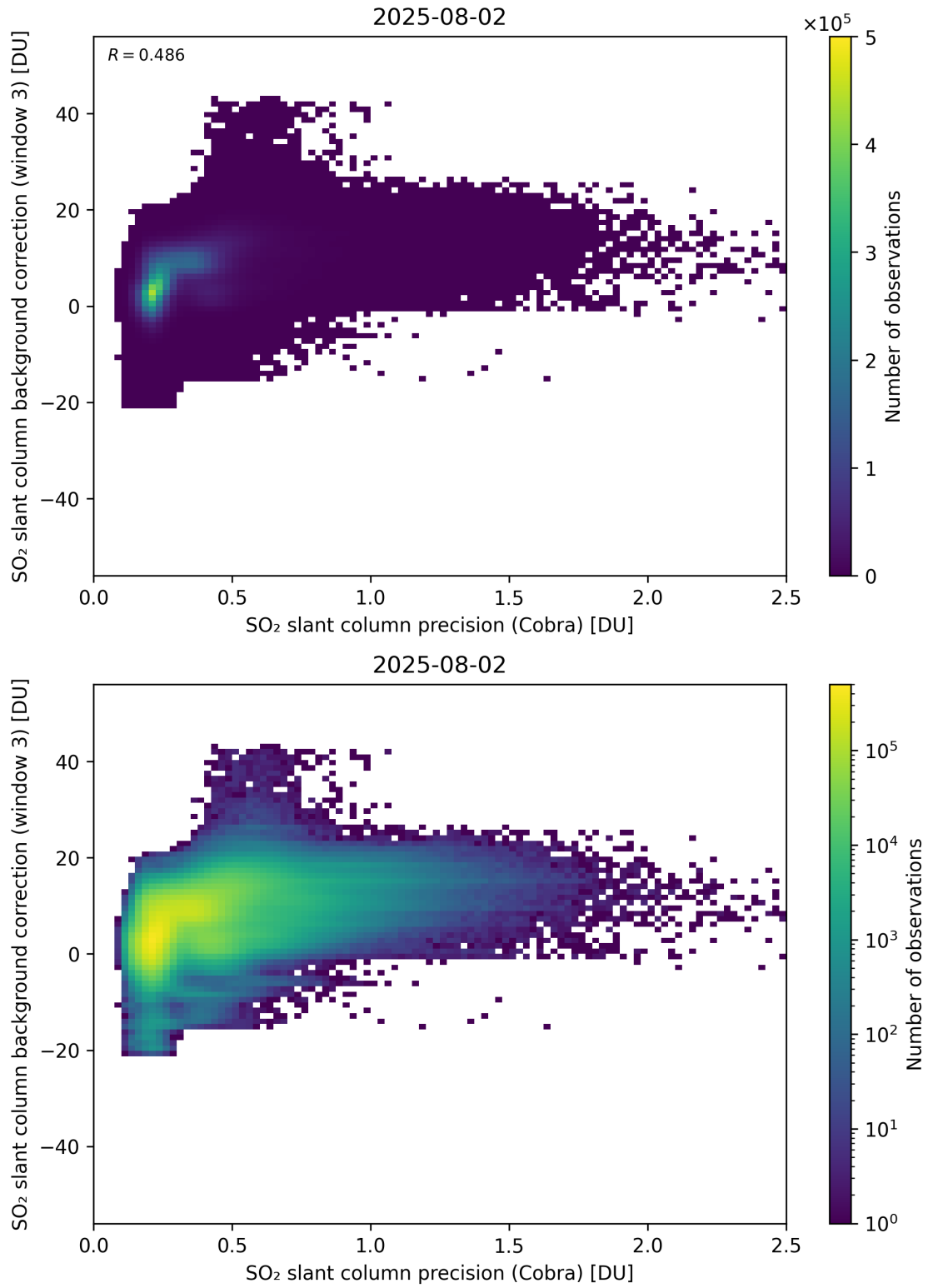
Figure 201: Scatter density plot of “SO 2 slant column precision (Cobra)” against “SO 2 slant column background correction (window 3)” for 2025-08-01 to 2025-08-03.
