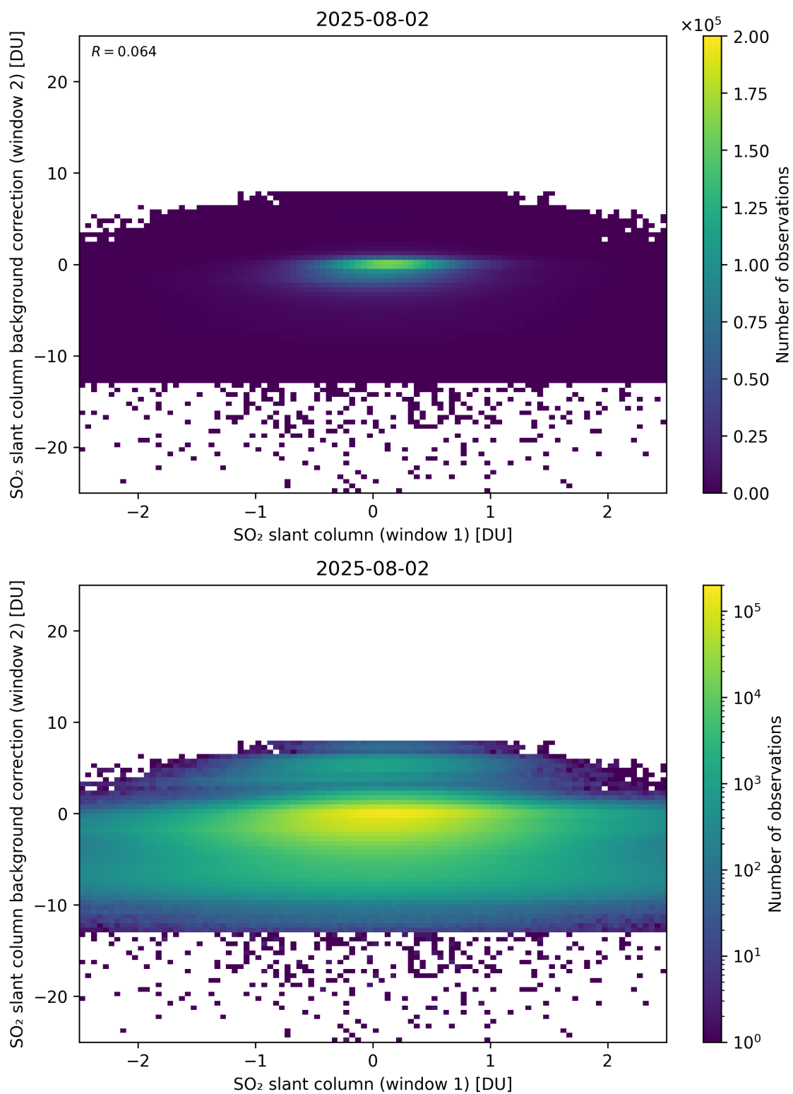
Figure 263: Scatter density plot of “SO 2 slant column (window 1)” against “SO 2 slant column background correction (window 2)” for 2025-08-01 to 2025-08-03.
