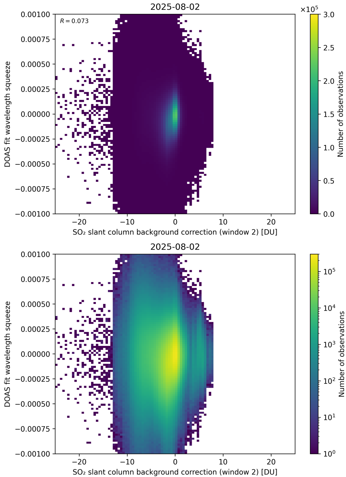
Figure 124: Scatter density plot of “SO 2 slant column background correction (window 2)” against “DOAS fit wavelength squeeze” for 2025-08-01 to 2025-08-03.
