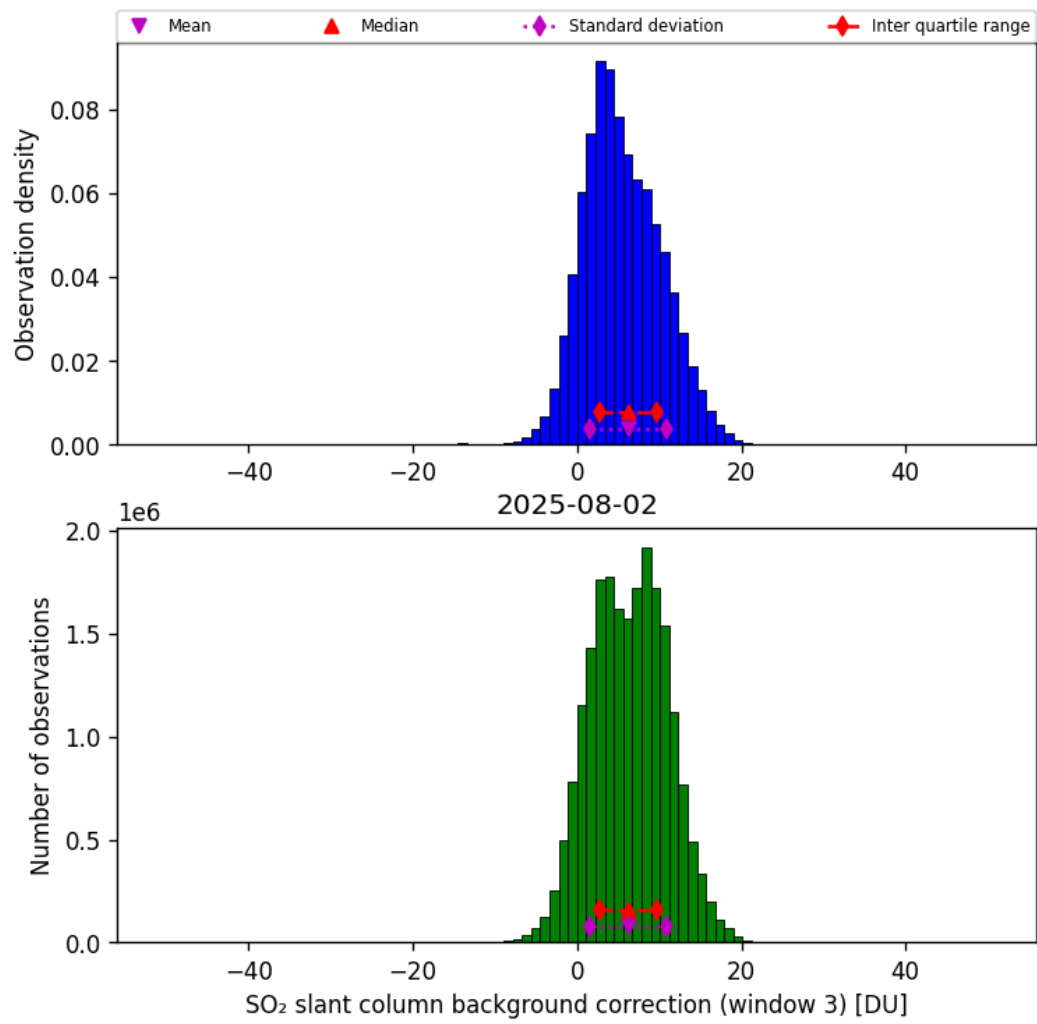
Figure 74: Histogram of “SO 2 slant column background correction (window 3)” for 2025-08-01 to 2025-08-03
