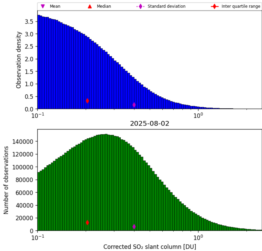
Figure 60: Histogram of “Corrected SO 2 slant column” for 2025-08-01 to 2025-08-03
