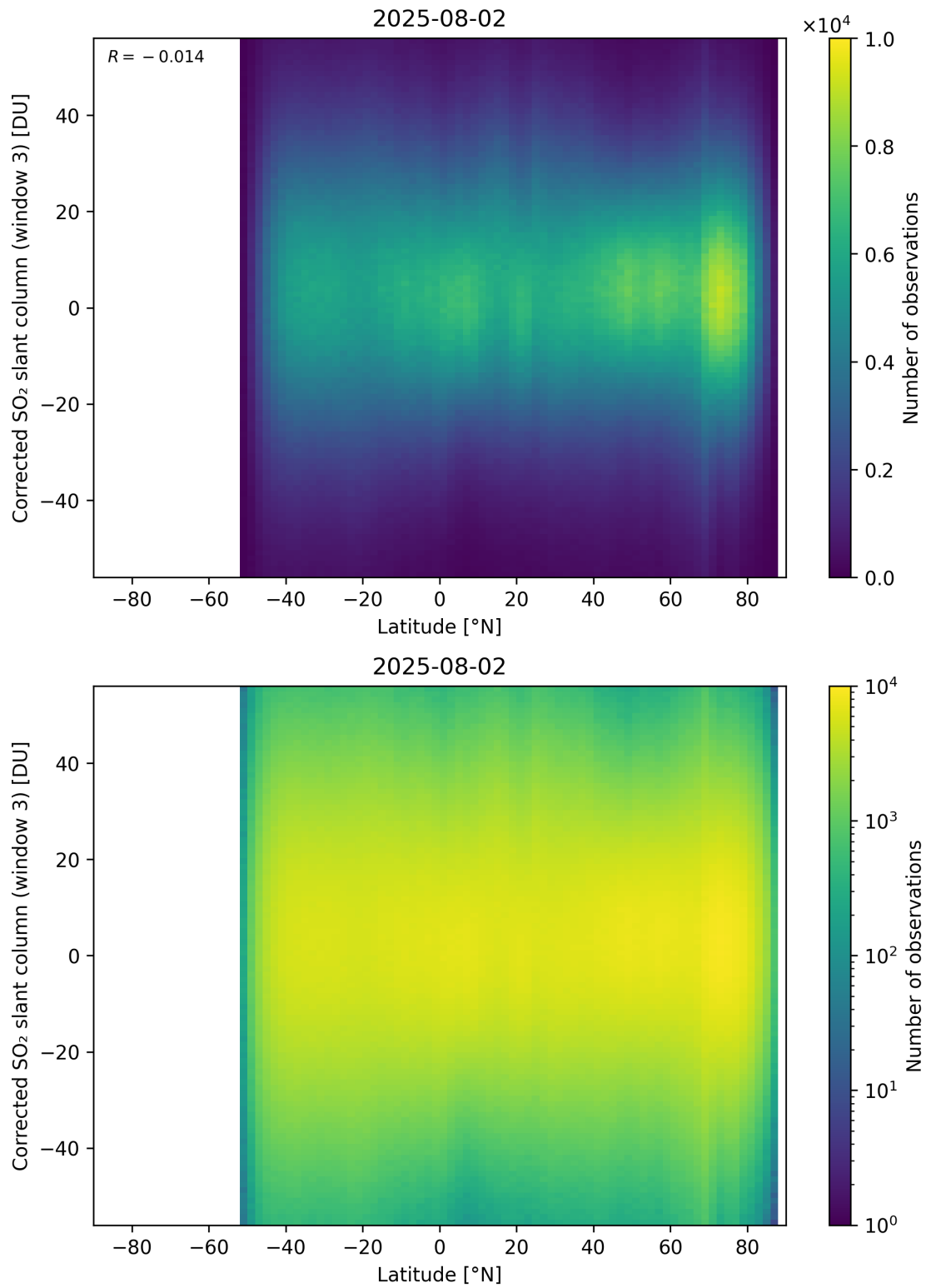
Figure 161: Scatter density plot of “Latitude” against “Corrected SO 2 slant column (window 3)” for 2025-08-01 to 2025-08-03.
