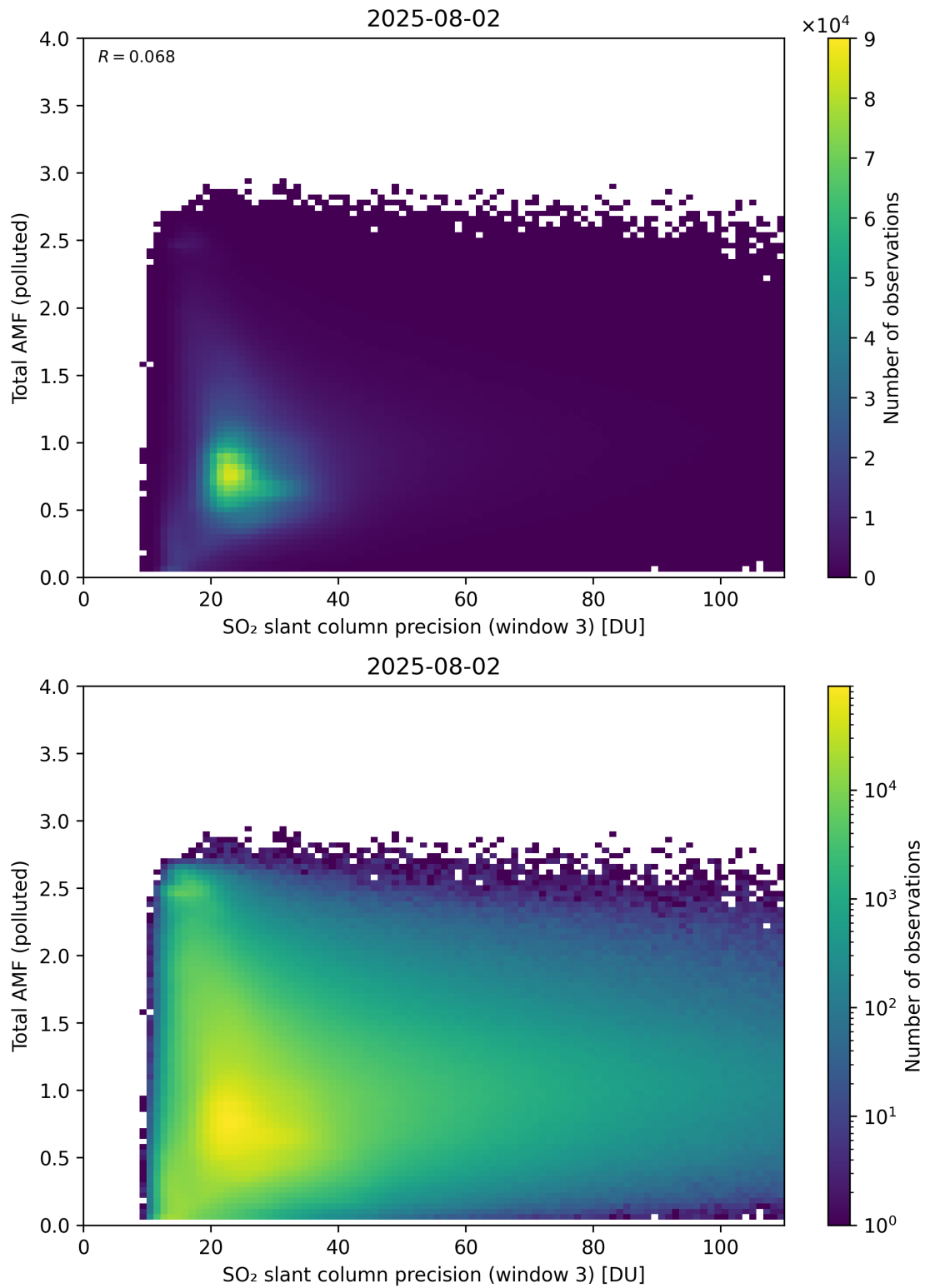
Figure 313: Scatter density plot of “SO 2 slant column precision (window 3)” against “Total AMF (polluted)” for 2025-08-01 to 2025-08-03.
