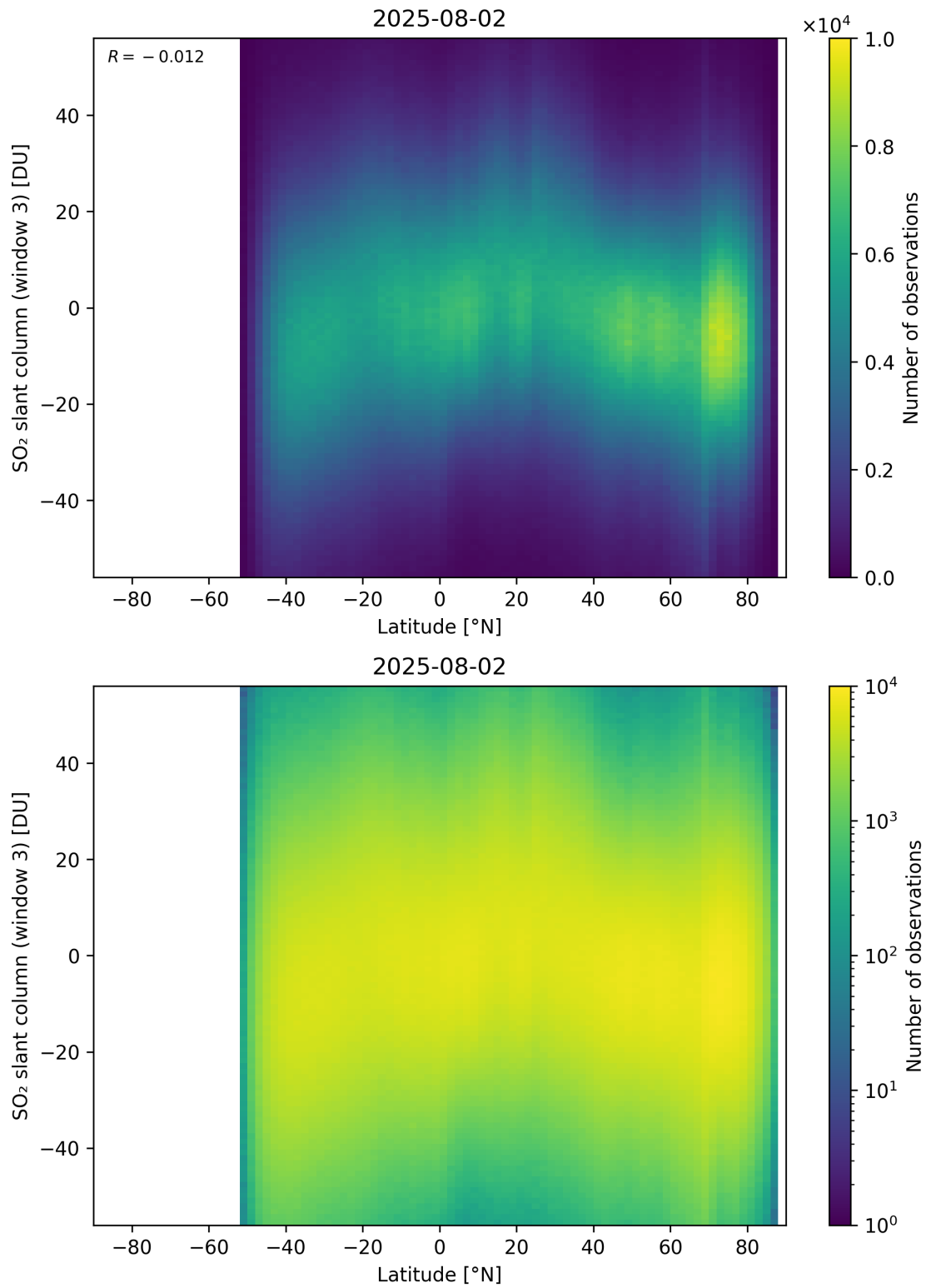
Figure 165: Scatter density plot of “Latitude” against “SO 2 slant column (window 3)” for 2025-08-01 to 2025-08-03.
