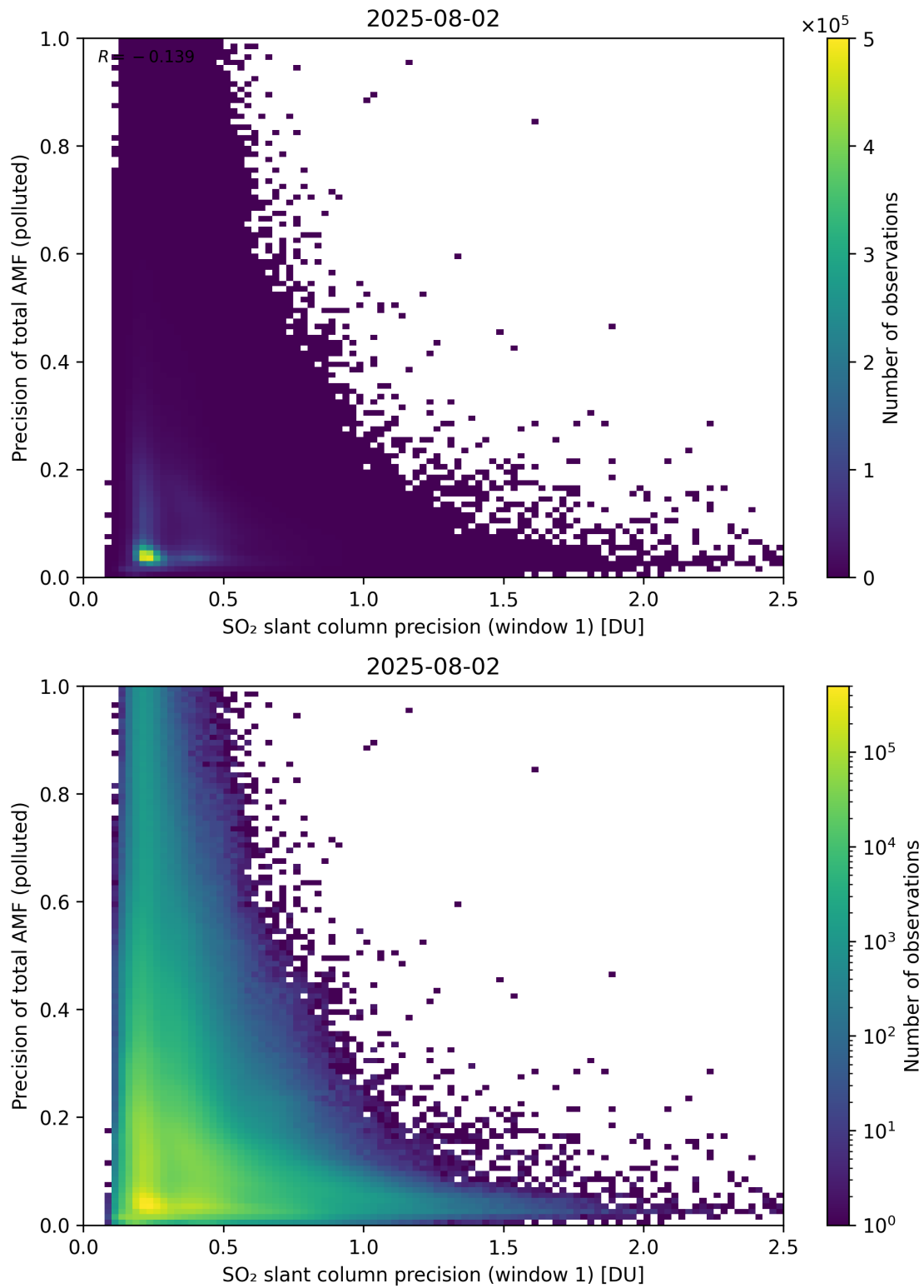
Figure 281: Scatter density plot of “SO 2 slant column precision (window 1)” against “Precision of total AMF (polluted)” for 2025-08-01 to 2025-08-03.
