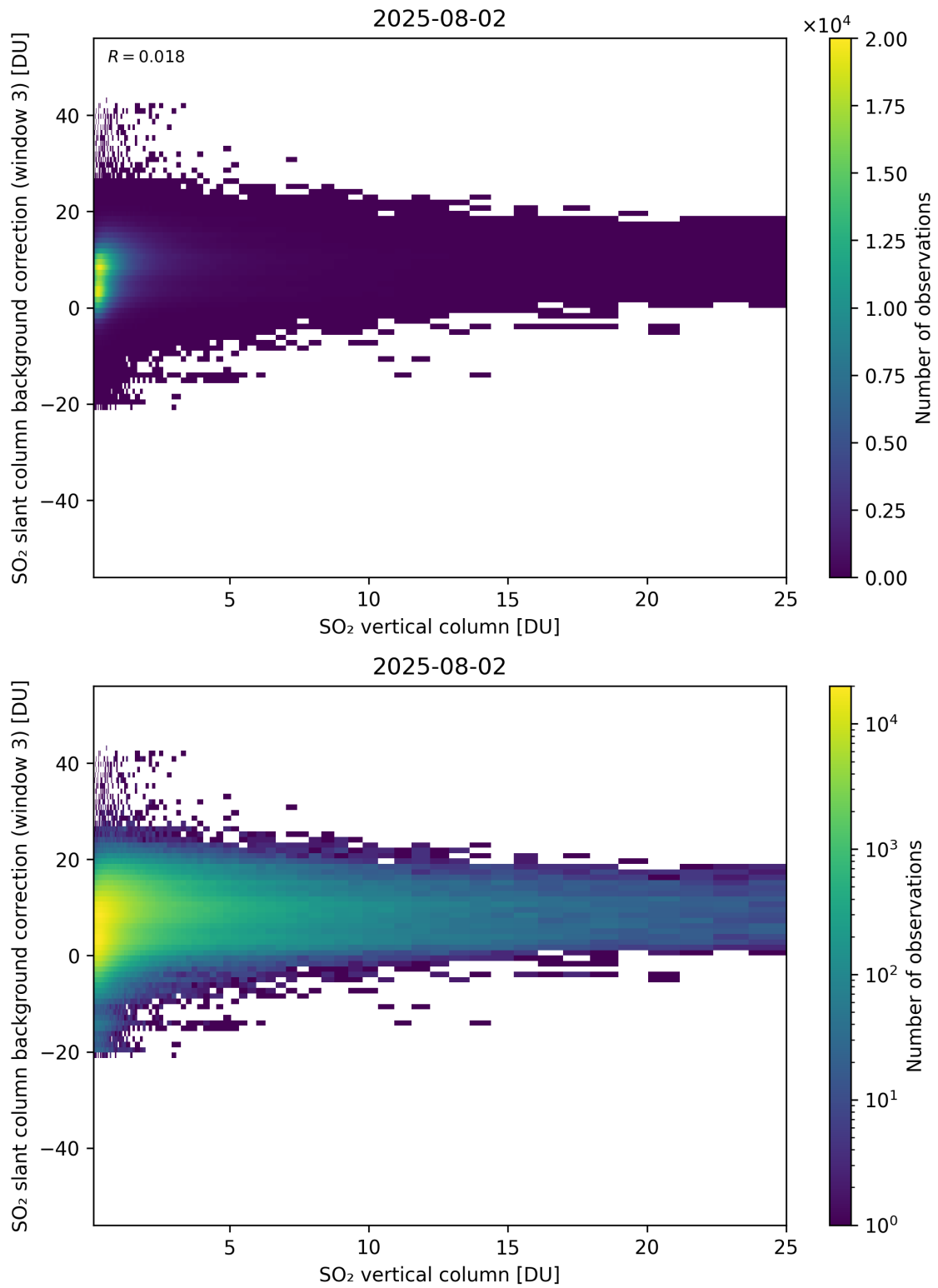
Figure 325: Scatter density plot of “SO 2 vertical column” against “SO 2 slant column background correction (window 3)” for 2025-08-01 to 2025-08-03.
