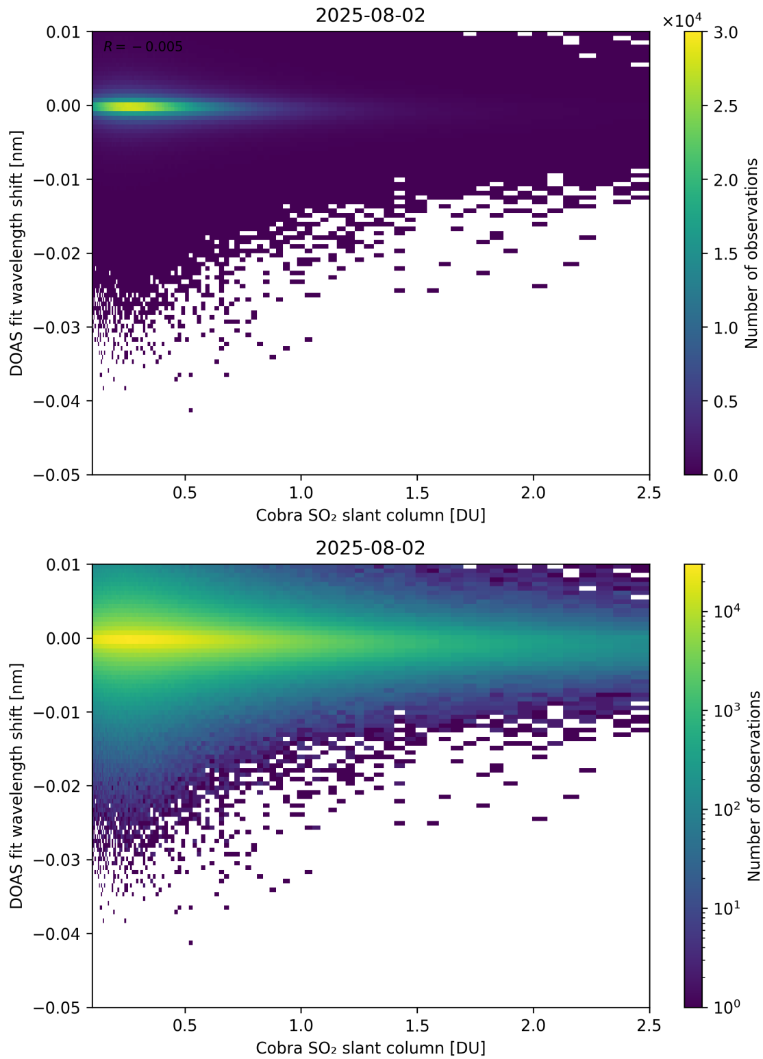
Figure 196: Scatter density plot of “Cobra SO 2 slant column” against “DOAS fit wavelength shift” for 2025-08-01 to 2025-08-03.
