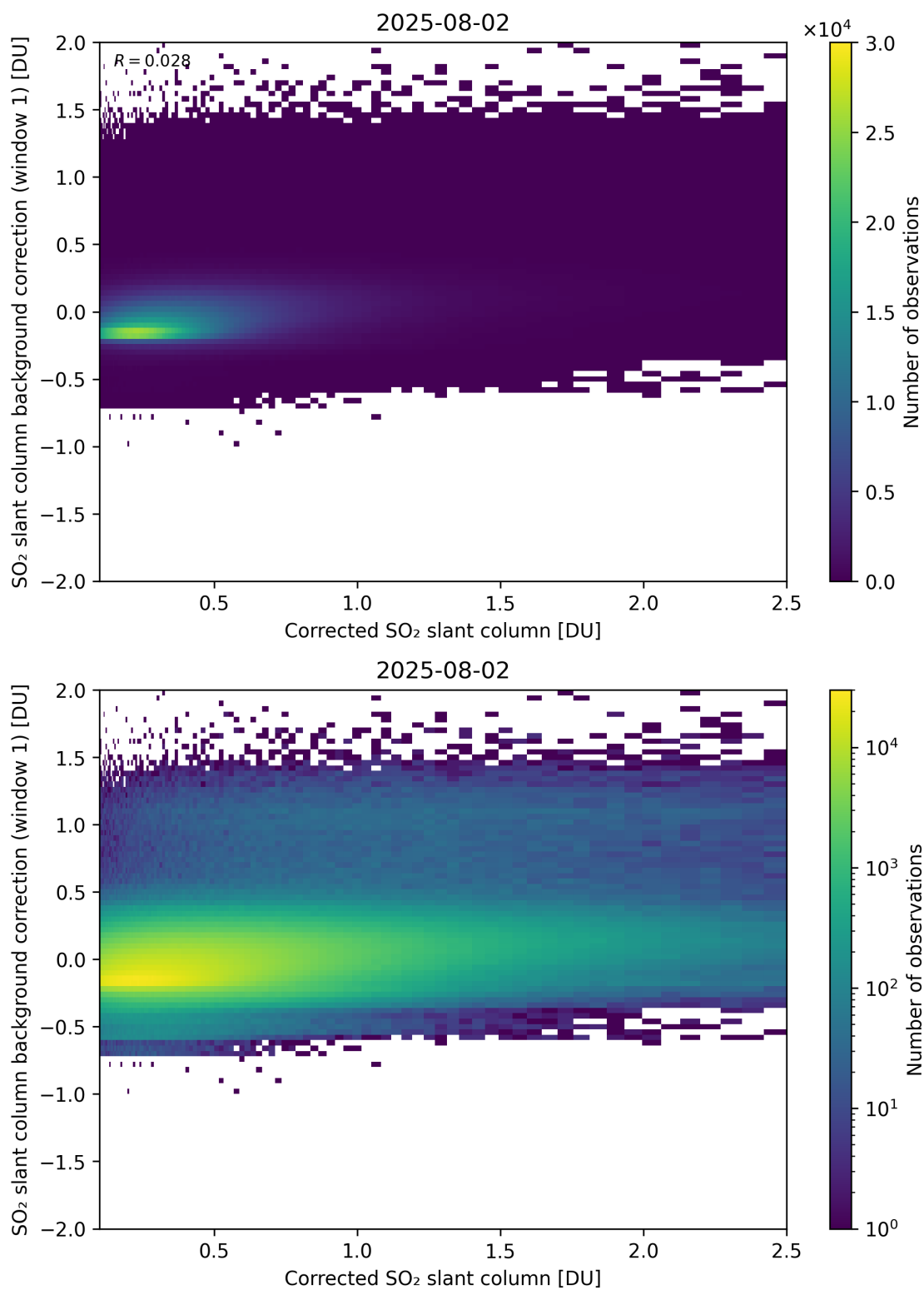
Figure 226: Scatter density plot of “Corrected SO 2 slant column” against “SO 2 slant column background correction (window 1)” for 2025-08-01 to 2025-08-03.
