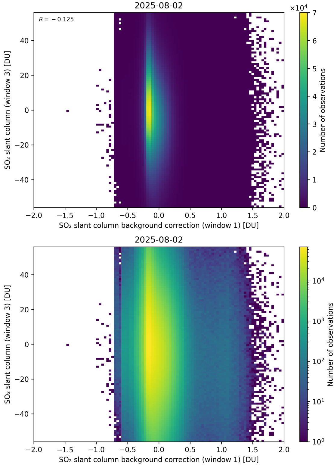
Figure 118: Scatter density plot of “SO 2 slant column background correction (window 1)” against “SO 2 slant column (window 3)” for 2025-08-01 to 2025-08-03.
