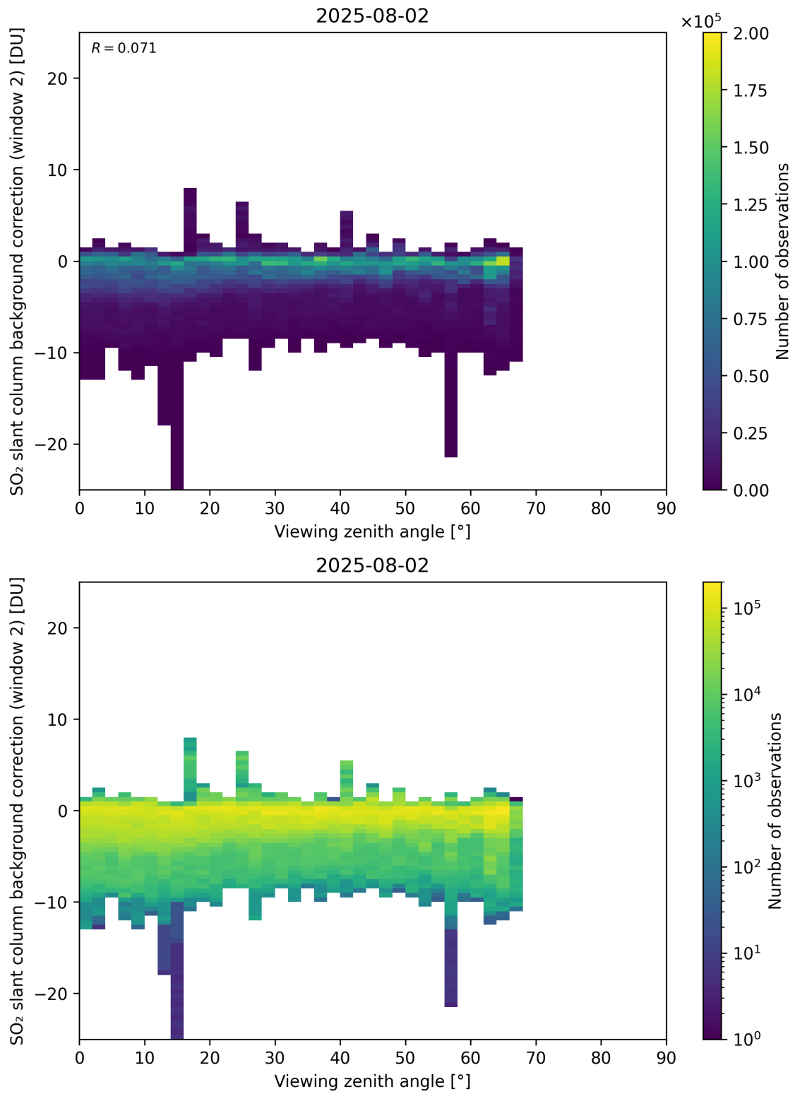
Figure 363: Scatter density plot of “Viewing zenith angle” against “SO 2 slant column background correction (window 2)” for 2025-08-01 to 2025-08-03.
