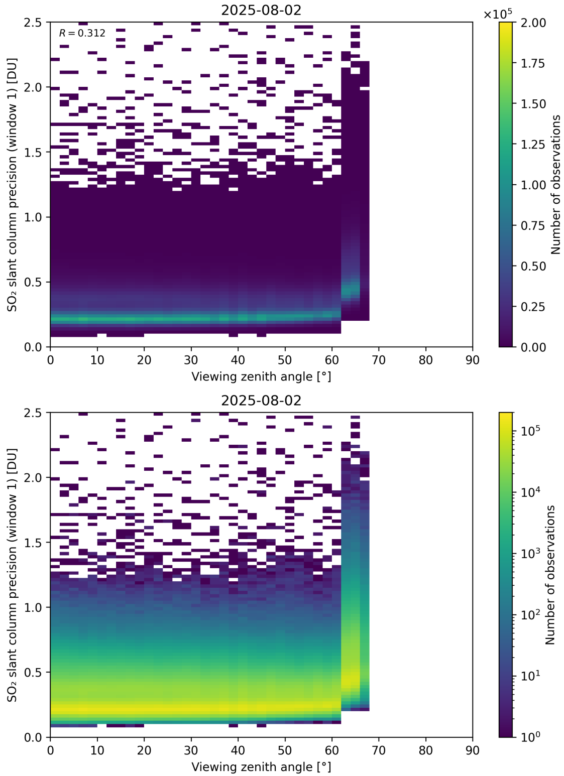
Figure 377: Scatter density plot of “Viewing zenith angle” against “SO 2 slant column precision (window 1)” for 2025-08-01 to 2025-08-03.
