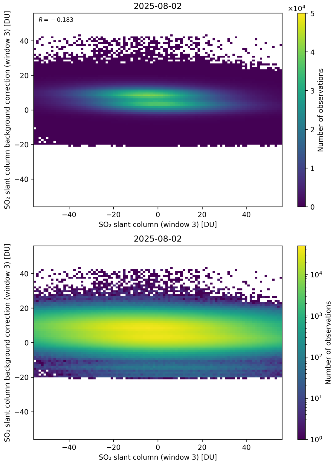
Figure 303: Scatter density plot of “SO 2 slant column (window 3)” against “SO 2 slant column background correction (window 3)” for 2025-08-01 to 2025-08-03.
