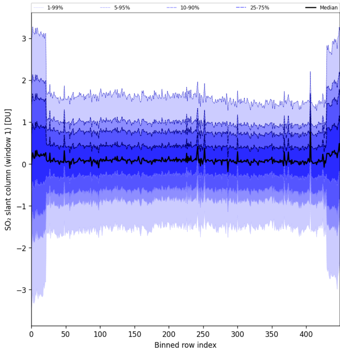
Figure 89: Along track statistics of “SO 2 slant column (window 1)” for 2025-08-01 to 2025-08-03
