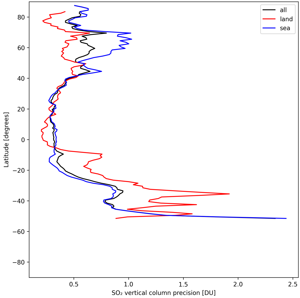
Figure 33: Zonal average of “SO 2 vertical column precision” for 2025-08-01 to 2025-08-03.
