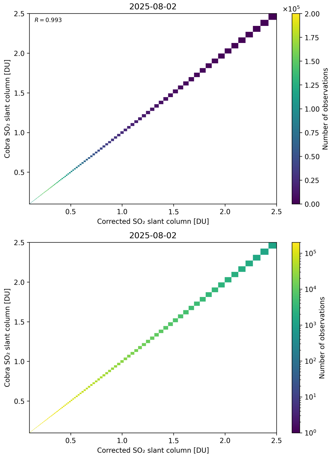
Figure 233: Scatter density plot of “Corrected SO 2 slant column” against “Cobra SO 2 slant column” for 2025-08-01 to 2025-08-03.
