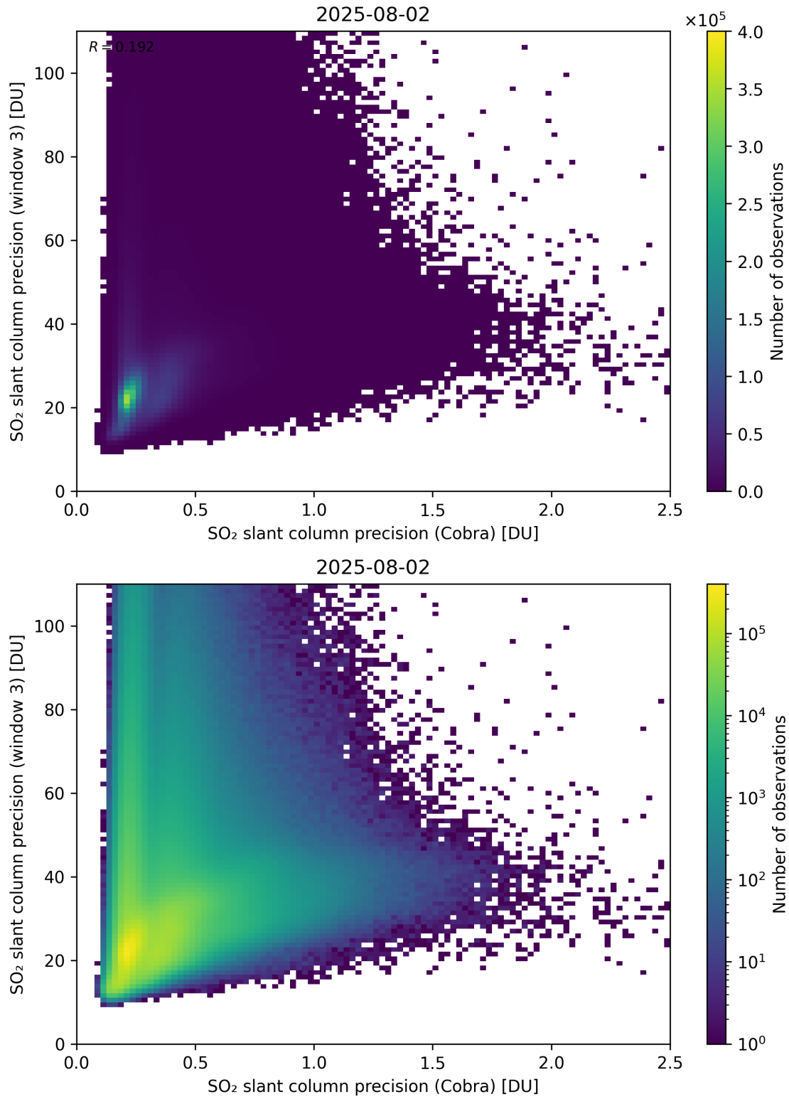
Figure 212: Scatter density plot of “SO 2 slant column precision (Cobra)” against “SO 2 slant column precision (window 3)” for 2025-08-01 to 2025-08-03.
