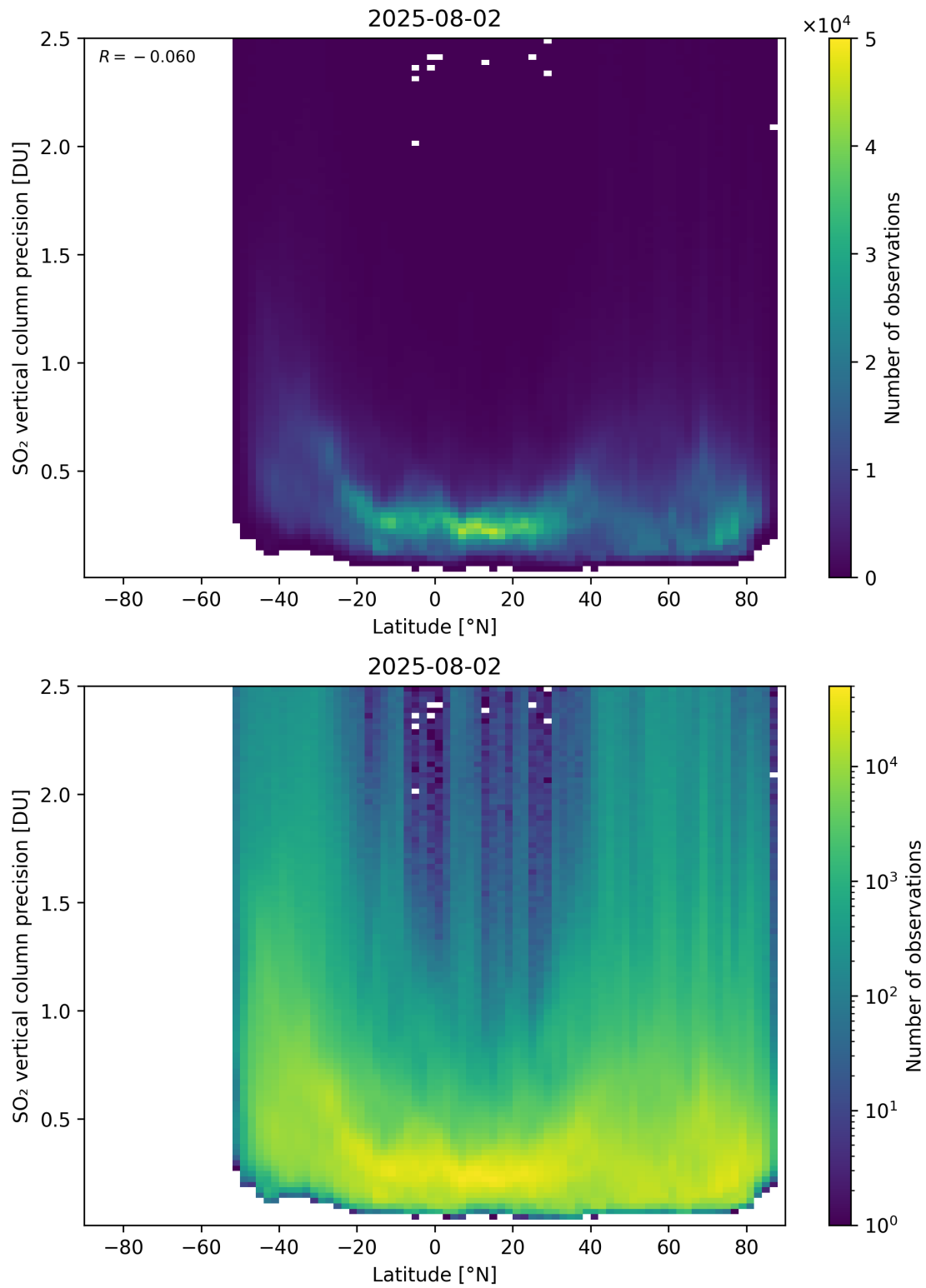
Figure 170: Scatter density plot of “Latitude” against “SO 2 vertical column precision” for 2025-08-01 to 2025-08-03.
