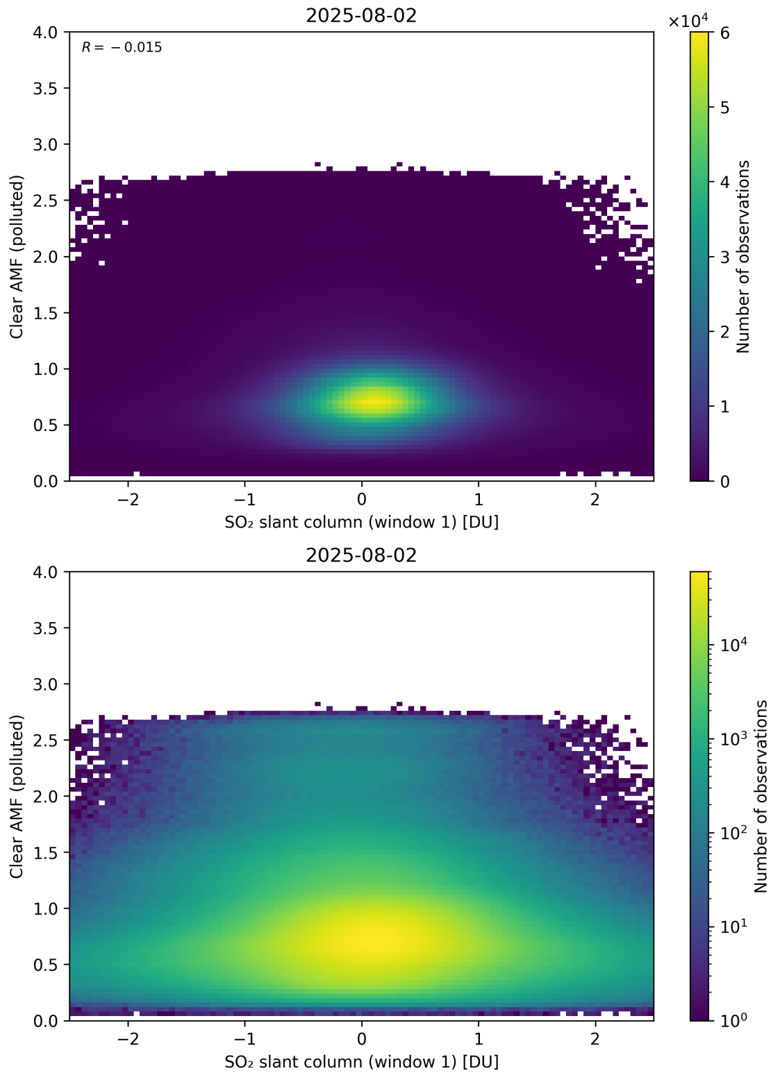
Figure 282: Scatter density plot of “SO 2 slant column (window 1)” against “Clear AMF (polluted)” for 2025-08-01 to 2025-08-03.
