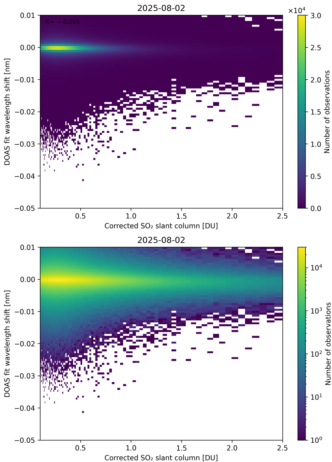
Figure 229: Scatter density plot of “Corrected SO 2 slant column” against “DOAS fit wavelength shift” for 2025-08-01 to 2025-08-03.
