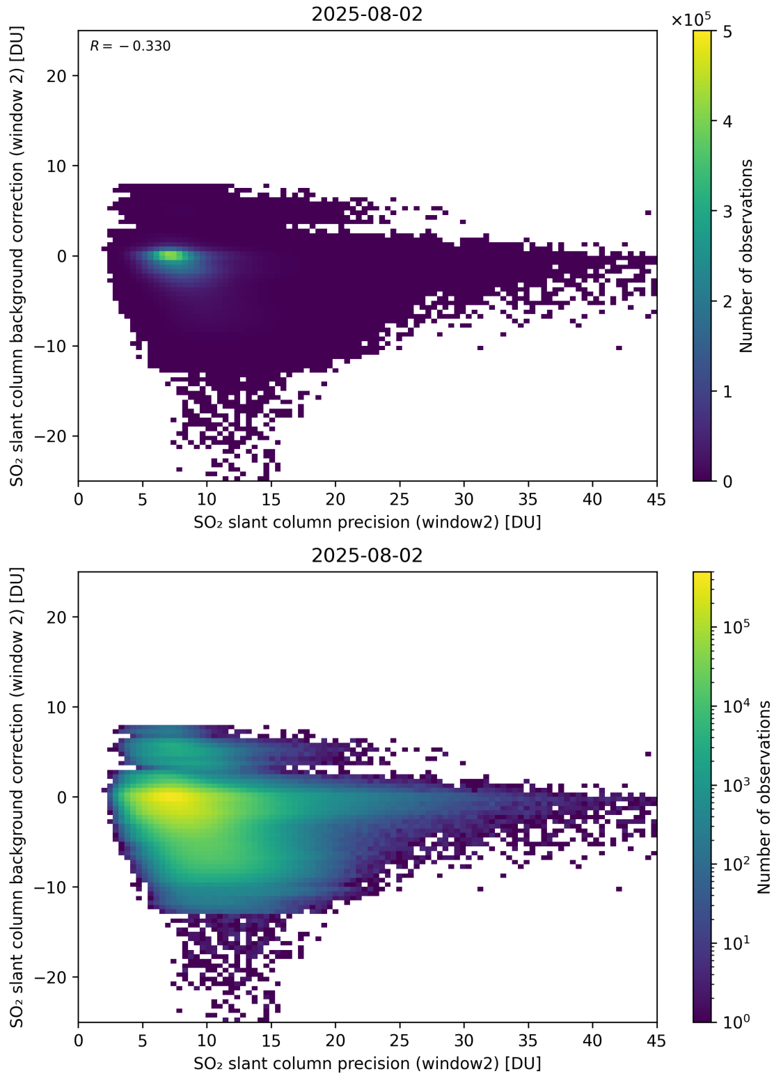
Figure 291: Scatter density plot of “SO 2 slant column precision (window2)” against “SO 2 slant column background correction (window 2)” for 2025-08-01 to 2025-08-03.
