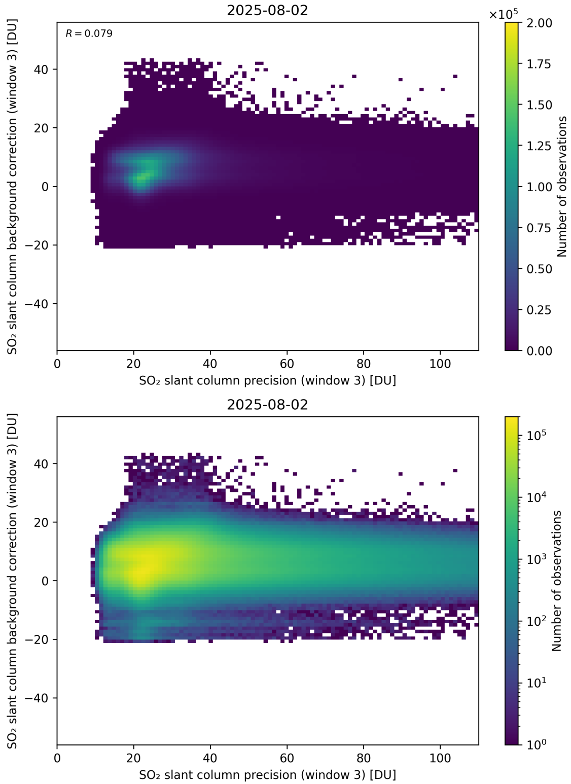
Figure 307: Scatter density plot of “SO 2 slant column precision (window 3)” against “SO 2 slant column background correction (window 3)” for 2025-08-01 to 2025-08-03.
