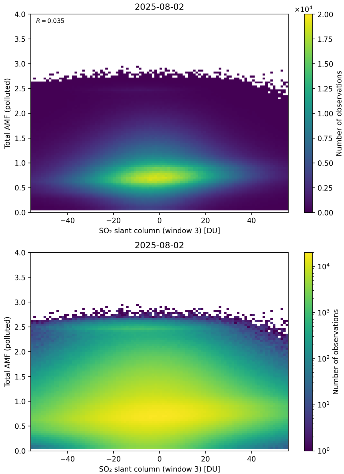
Figure 318: Scatter density plot of “SO 2 slant column (window 3)” against “Total AMF (polluted)” for 2025-08-01 to 2025-08-03.
