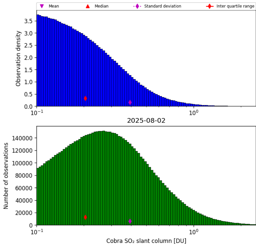
Figure 61: Histogram of “Cobra SO 2 slant column” for 2025-08-01 to 2025-08-03
