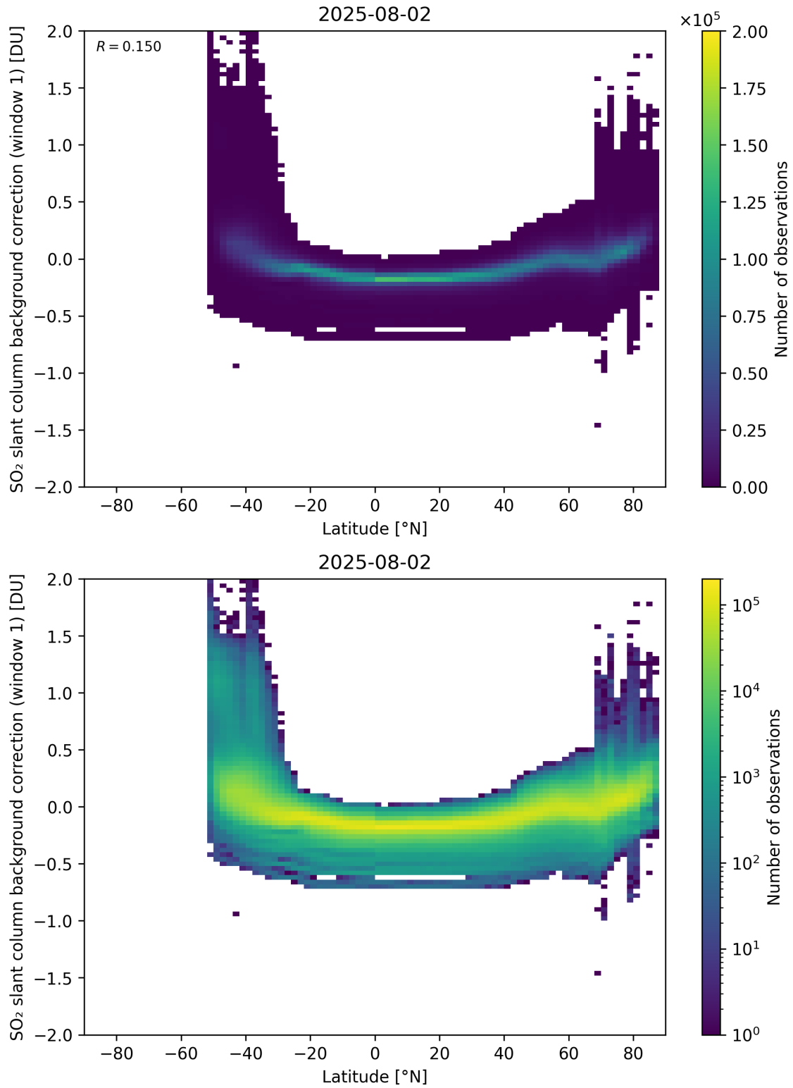
Figure 150: Scatter density plot of “Latitude” against “SO 2 slant column background correction (window 1)” for 2025-08-01 to 2025-08-03.
