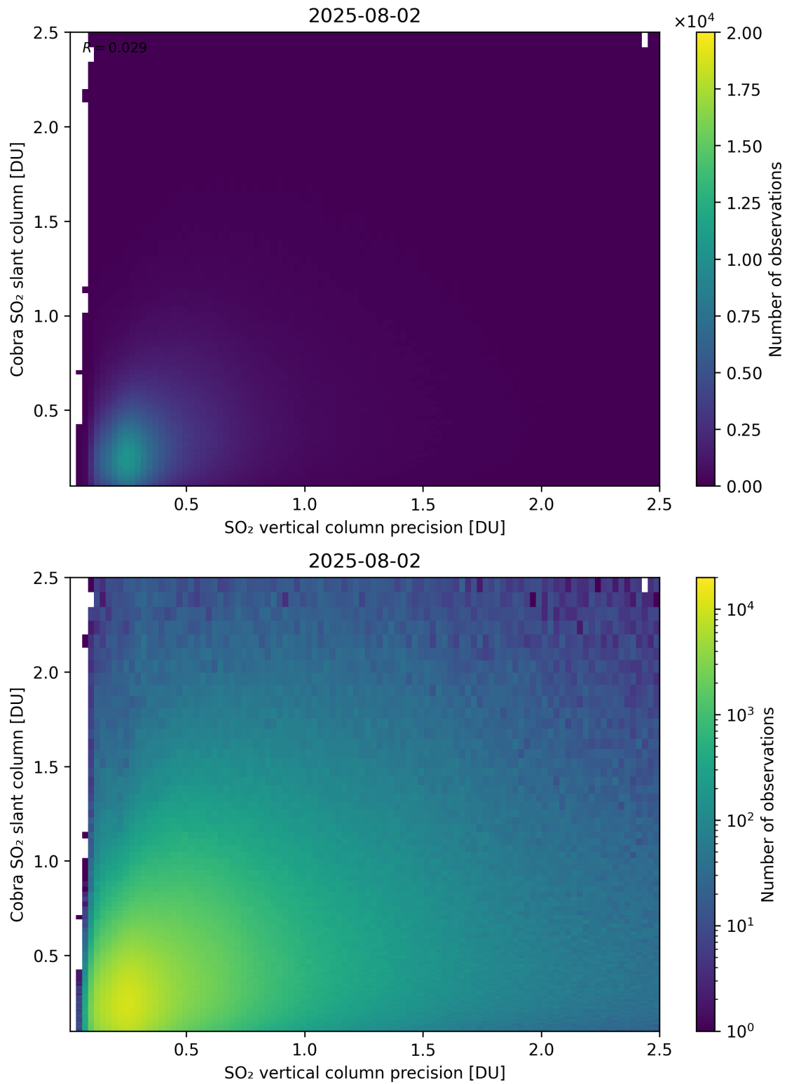
Figure 336: Scatter density plot of “SO 2 vertical column precision” against “Cobra SO 2 slant column” for 2025-08-01 to 2025-08-03.
