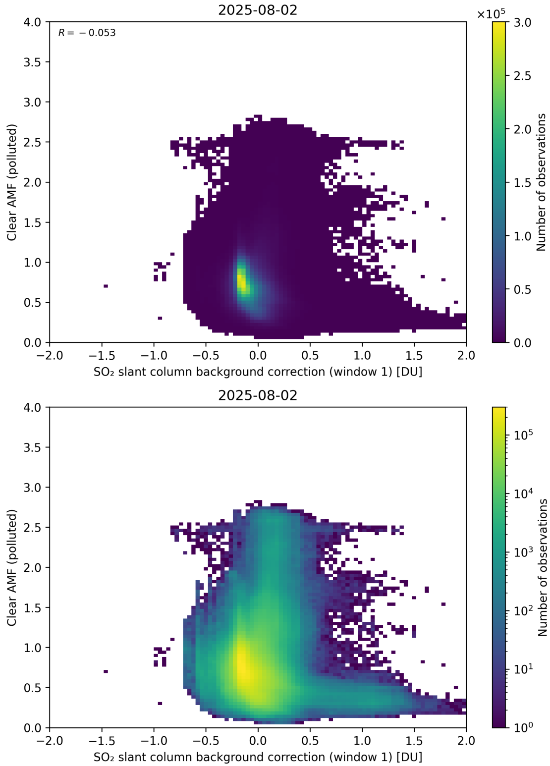
Figure 114: Scatter density plot of “SO 2 slant column background correction (window 1)” against “Clear AMF (polluted)” for 2025-08-01 to 2025-08-03.
