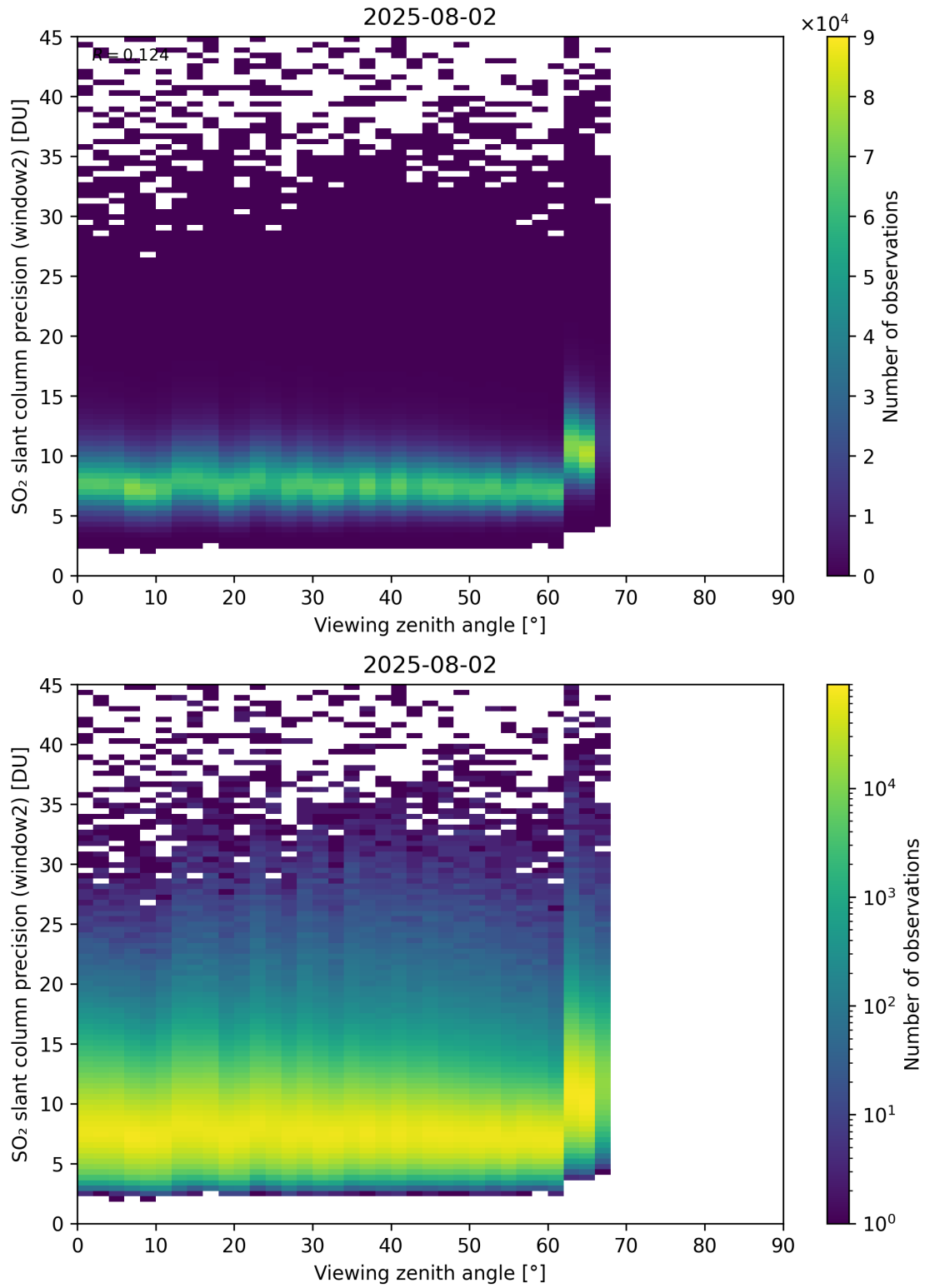
Figure 378: Scatter density plot of “Viewing zenith angle” against “SO 2 slant column precision (window2)” for 2025-08-01 to 2025-08-03.
