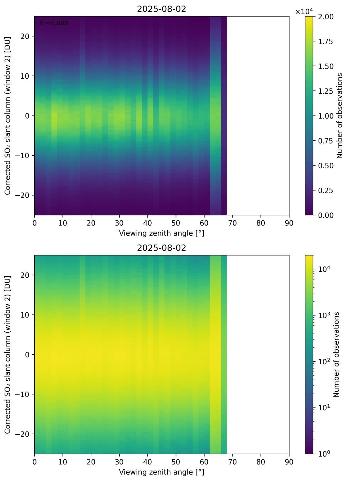
Figure 374: Scatter density plot of “Viewing zenith angle” against “Corrected SO 2 slant column (window 2)” for 2025-08-01 to 2025-08-03.
