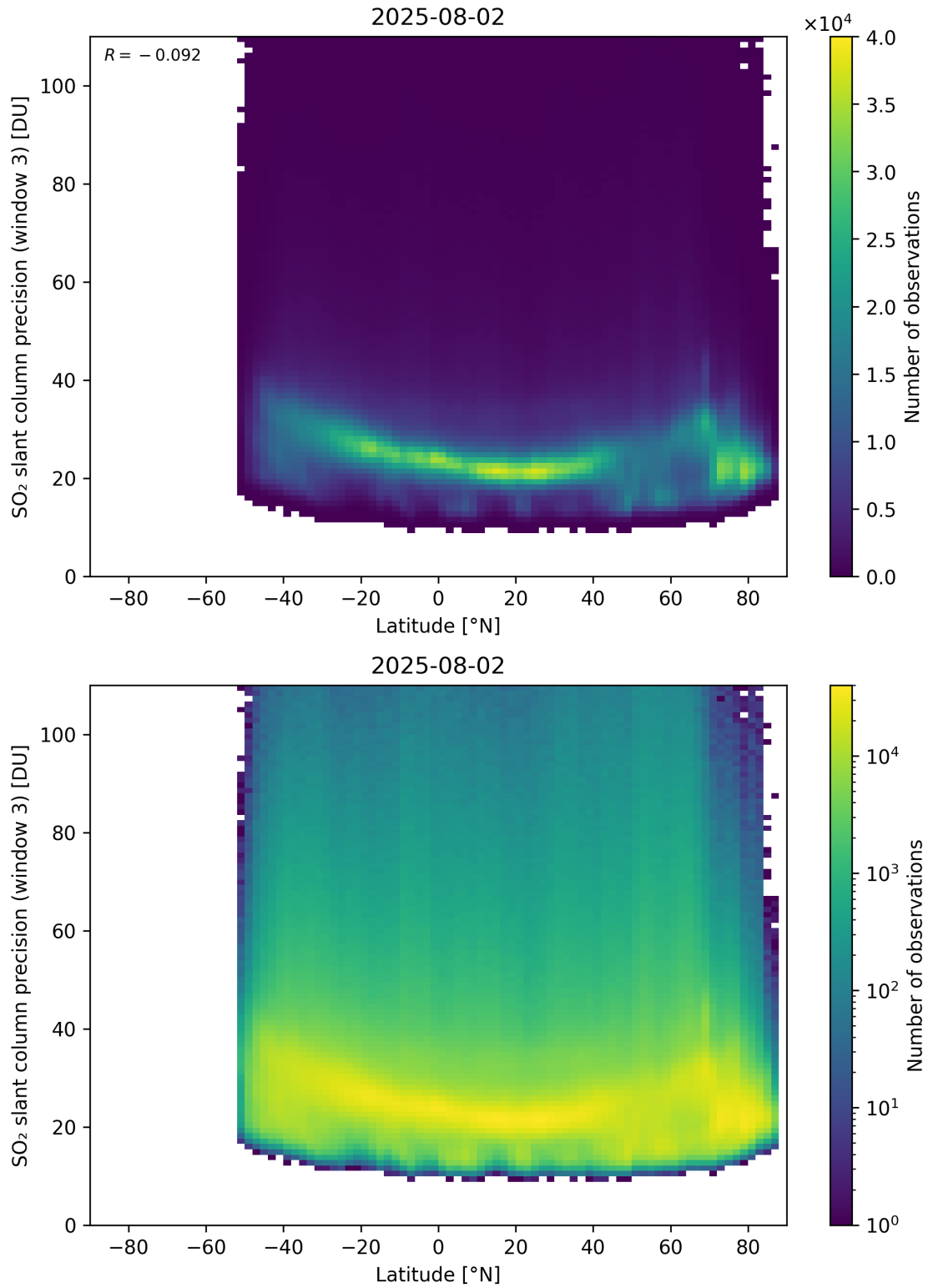
Figure 166: Scatter density plot of “Latitude” against “SO 2 slant column precision (window 3)” for 2025-08-01 to 2025-08-03.
