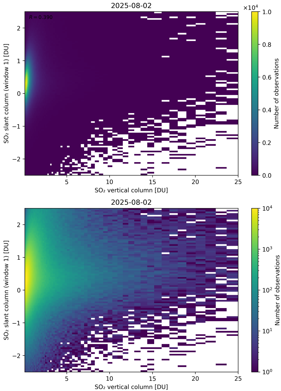
Figure 354: Scatter density plot of “SO 2 vertical column” against “SO 2 slant column (window 1)” for 2025-08-01 to 2025-08-03.
