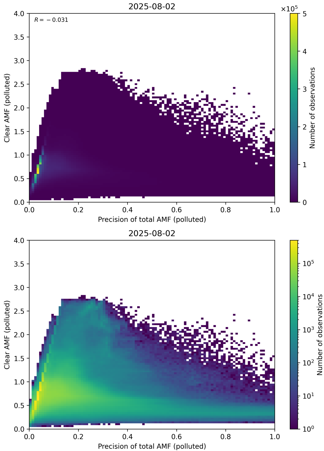
Figure 320: Scatter density plot of “Precision of total AMF (polluted)” against “Clear AMF (polluted)” for 2025-08-01 to 2025-08-03.
