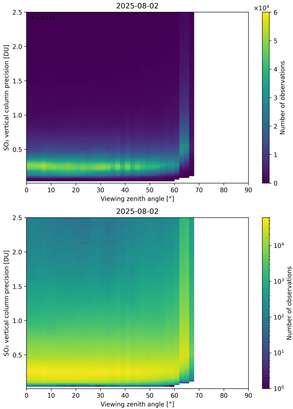
Figure 384: Scatter density plot of “Viewing zenith angle” against “SO 2 vertical column precision” for 2025-08-01 to 2025-08-03.
