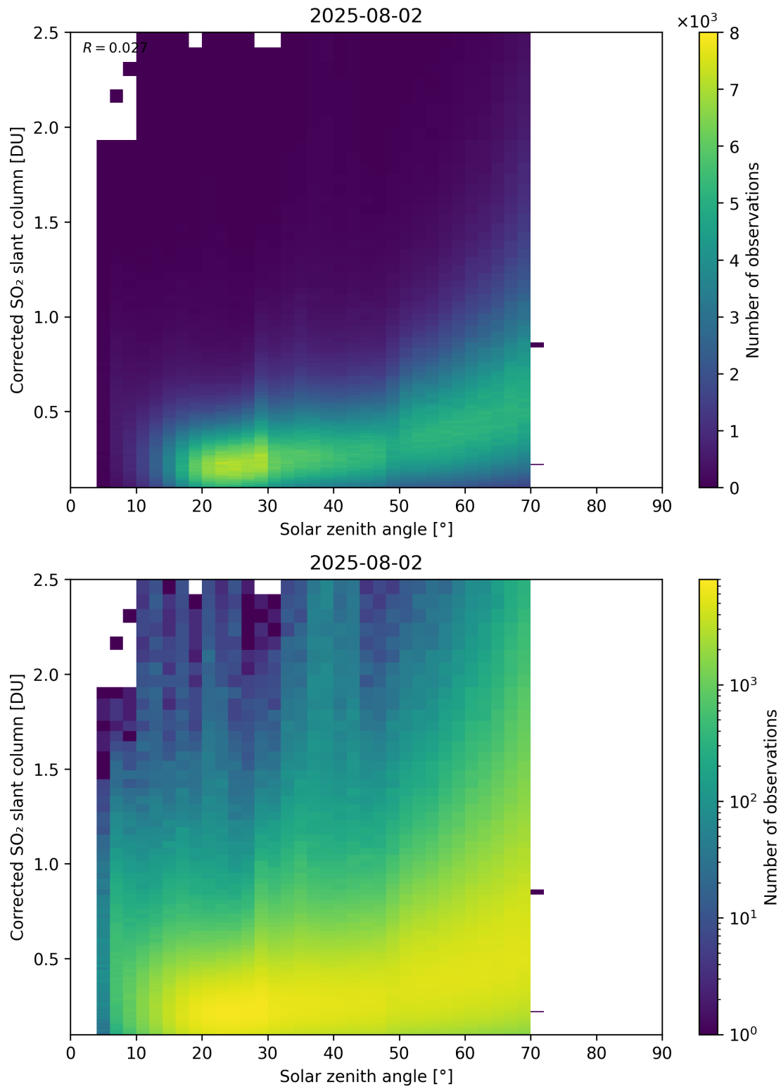
Figure 181: Scatter density plot of “Solar zenith angle” against “Corrected SO 2 slant column” for 2025-08-01 to 2025-08-03.
