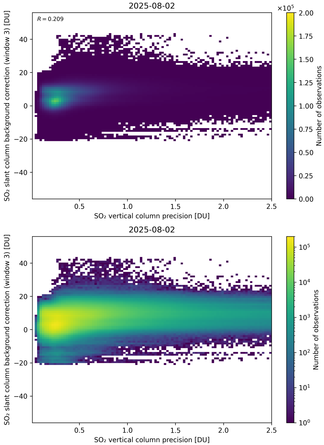
Figure 331: Scatter density plot of “SO 2 vertical column precision” against “SO 2 slant column background correction (window 3)” for 2025-08-01 to 2025-08-03.
