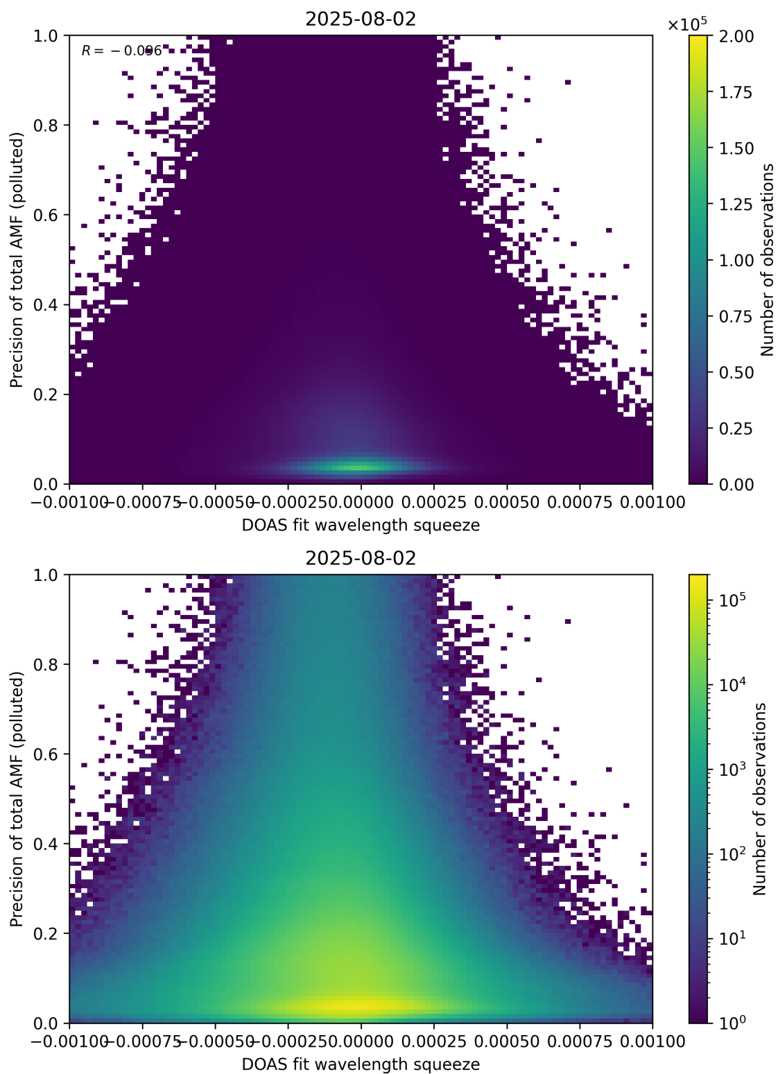
Figure 146: Scatter density plot of “DOAS fit wavelength squeeze” against “Precision of total AMF (polluted)” for 2025-08-01 to 2025-08-03.
