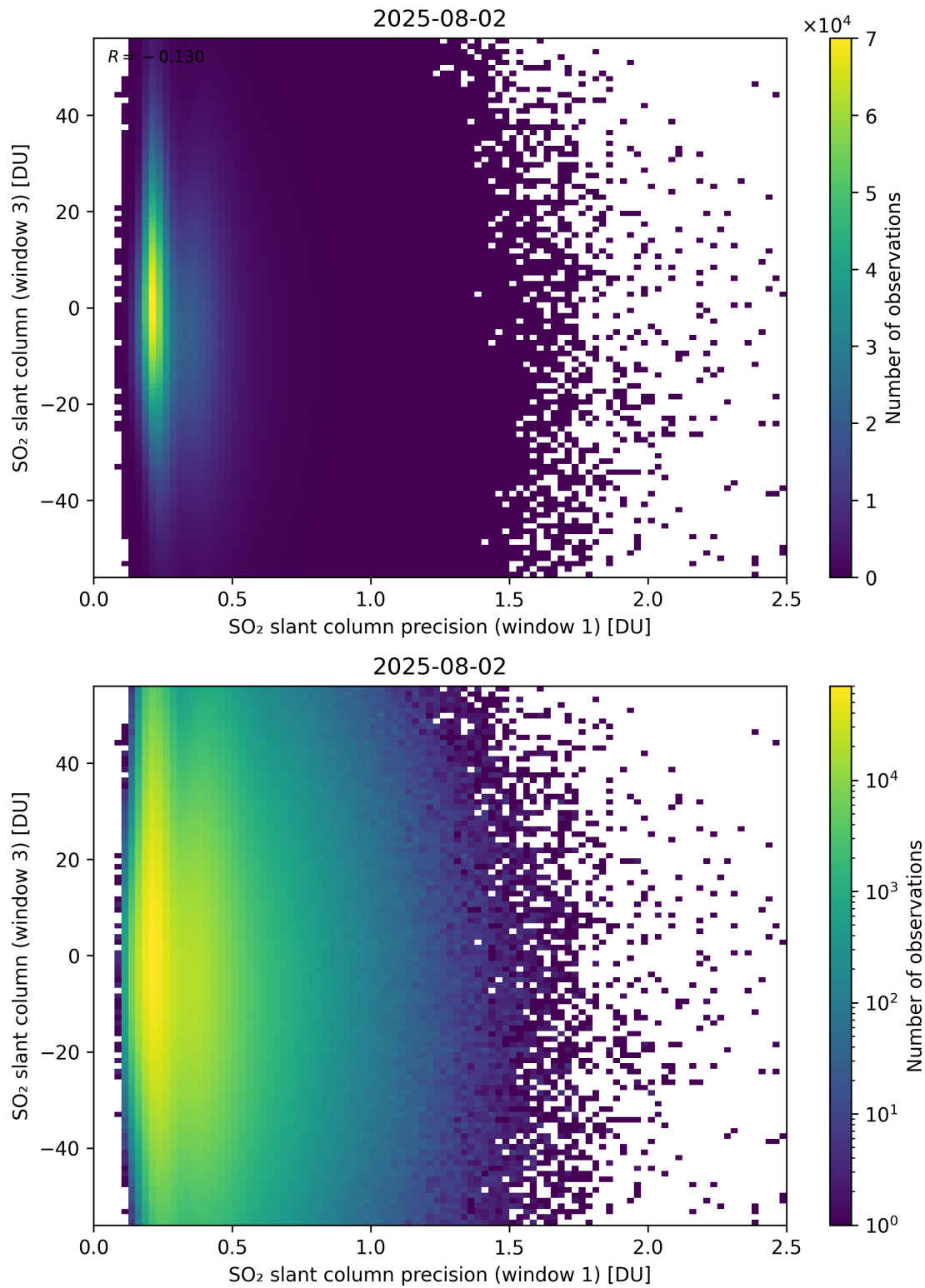
Figure 278: Scatter density plot of “SO 2 slant column precision (window 1)” against “SO 2 slant column (window 3)” for 2025-08-01 to 2025-08-03.
