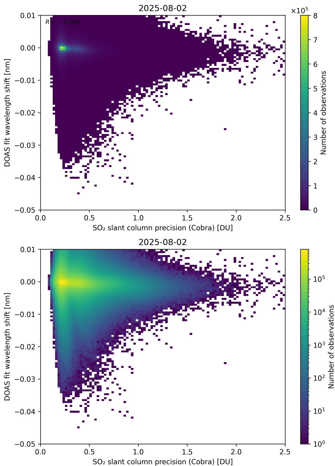
Figure 202: Scatter density plot of “SO 2 slant column precision (Cobra)” against “DOAS fit wavelength shift” for 2025-08-01 to 2025-08-03.
