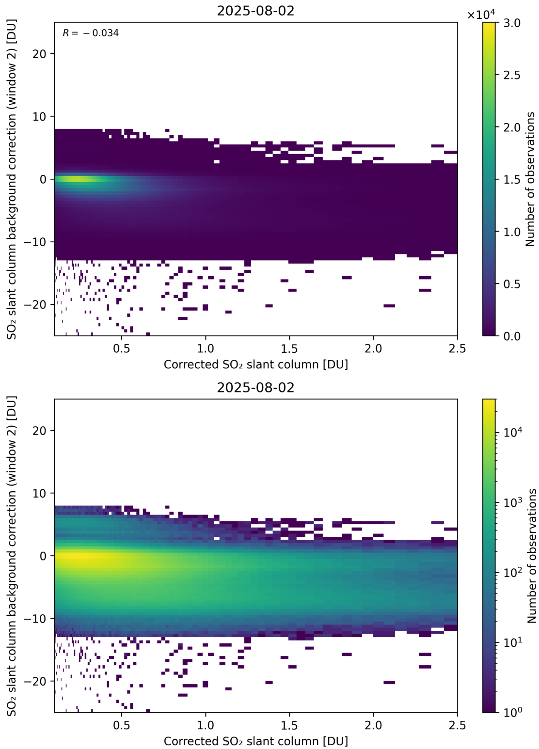
Figure 227: Scatter density plot of “Corrected SO 2 slant column” against “SO 2 slant column background correction (window 2)” for 2025-08-01 to 2025-08-03.
