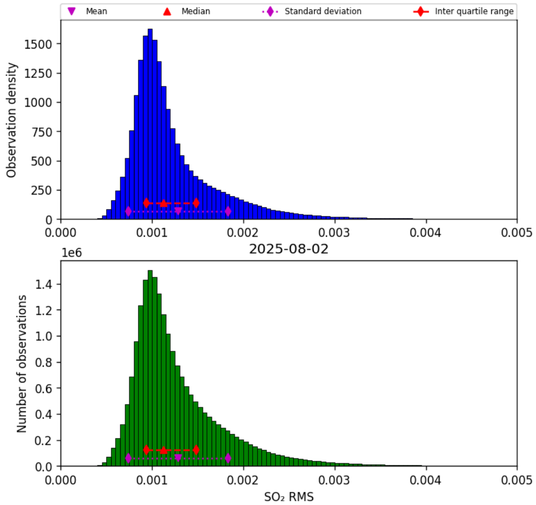
Figure 78: Histogram of “SO 2 RMS” for 2025-08-01 to 2025-08-03
