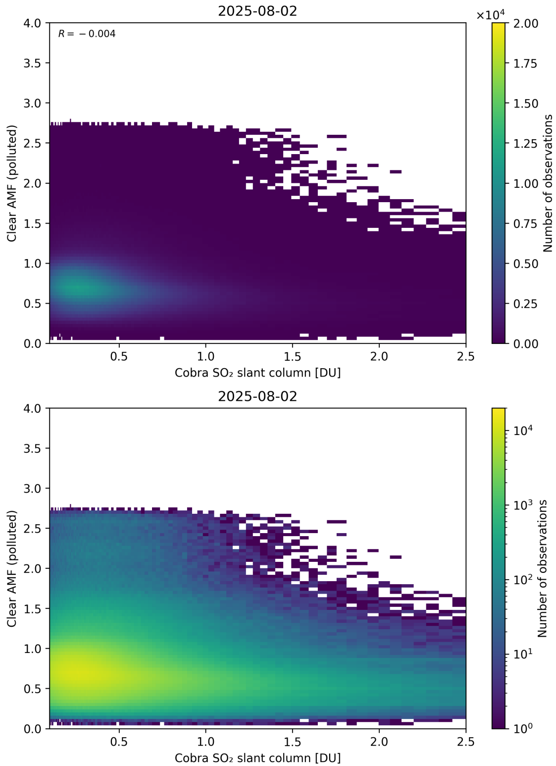
Figure 215: Scatter density plot of “Cobra SO 2 slant column” against “Clear AMF (polluted)” for 2025-08-01 to 2025-08-03.
