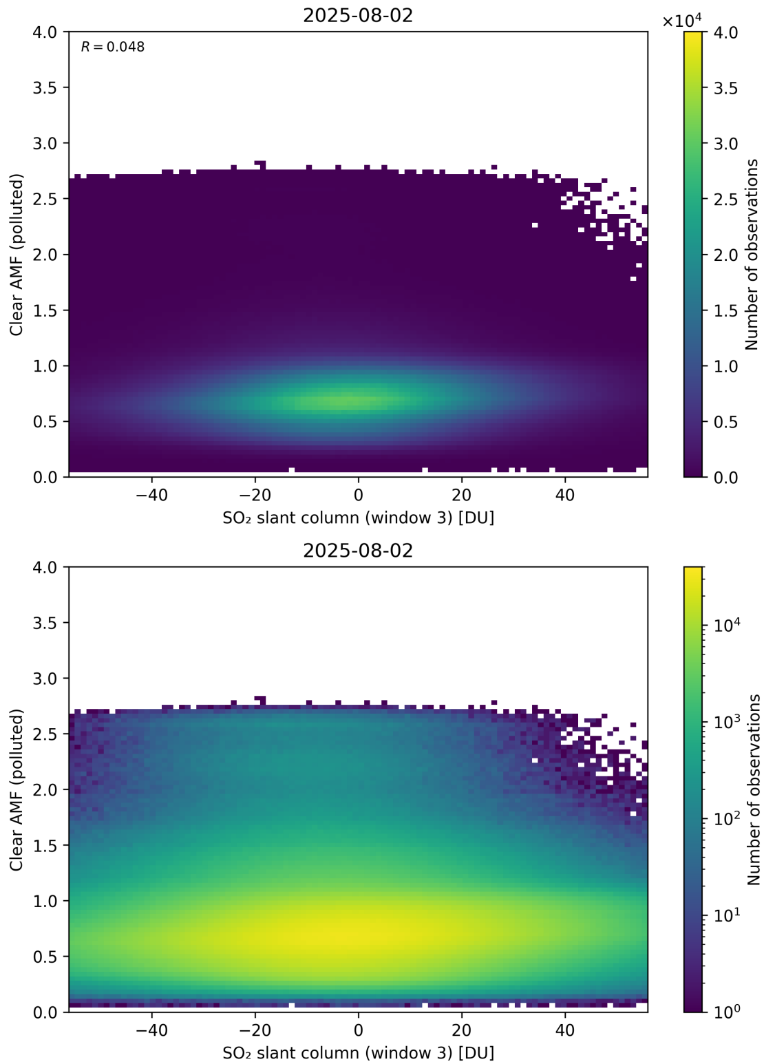
Figure 315: Scatter density plot of “SO 2 slant column (window 3)” against “Clear AMF (polluted)” for 2025-08-01 to 2025-08-03.
