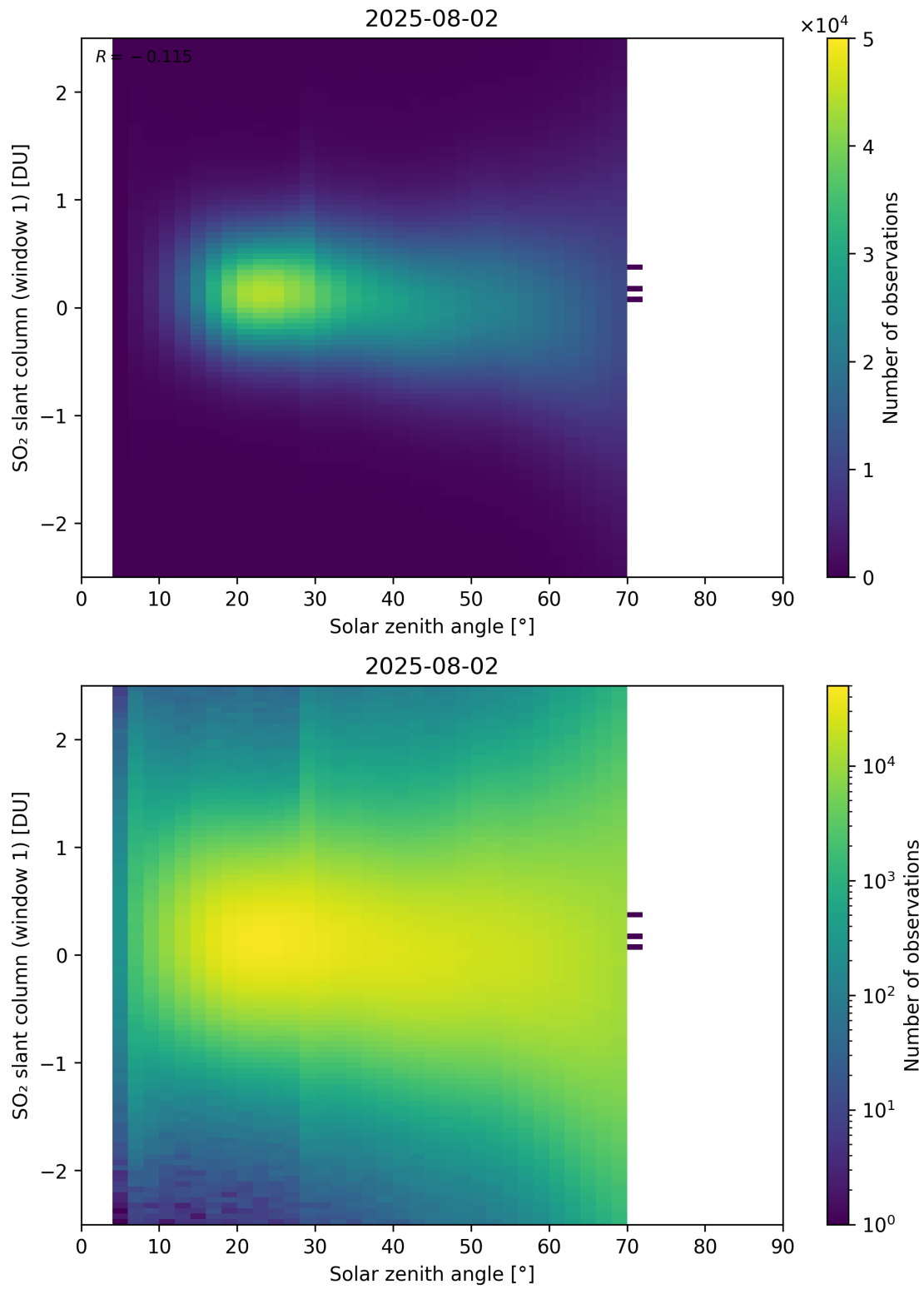
Figure 184: Scatter density plot of “Solar zenith angle” against “SO 2 slant column (window 1)” for 2025-08-01 to 2025-08-03.
