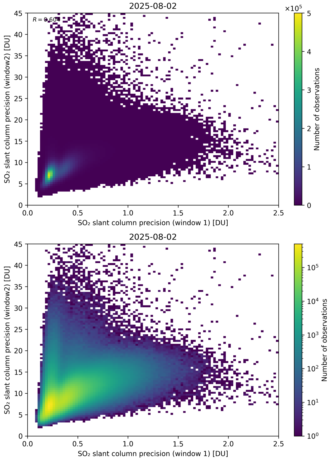
Figure 277: Scatter density plot of “SO 2 slant column precision (window 1)” against “SO 2 slant column precision (window2)” for 2025-08-01 to 2025-08-03.
