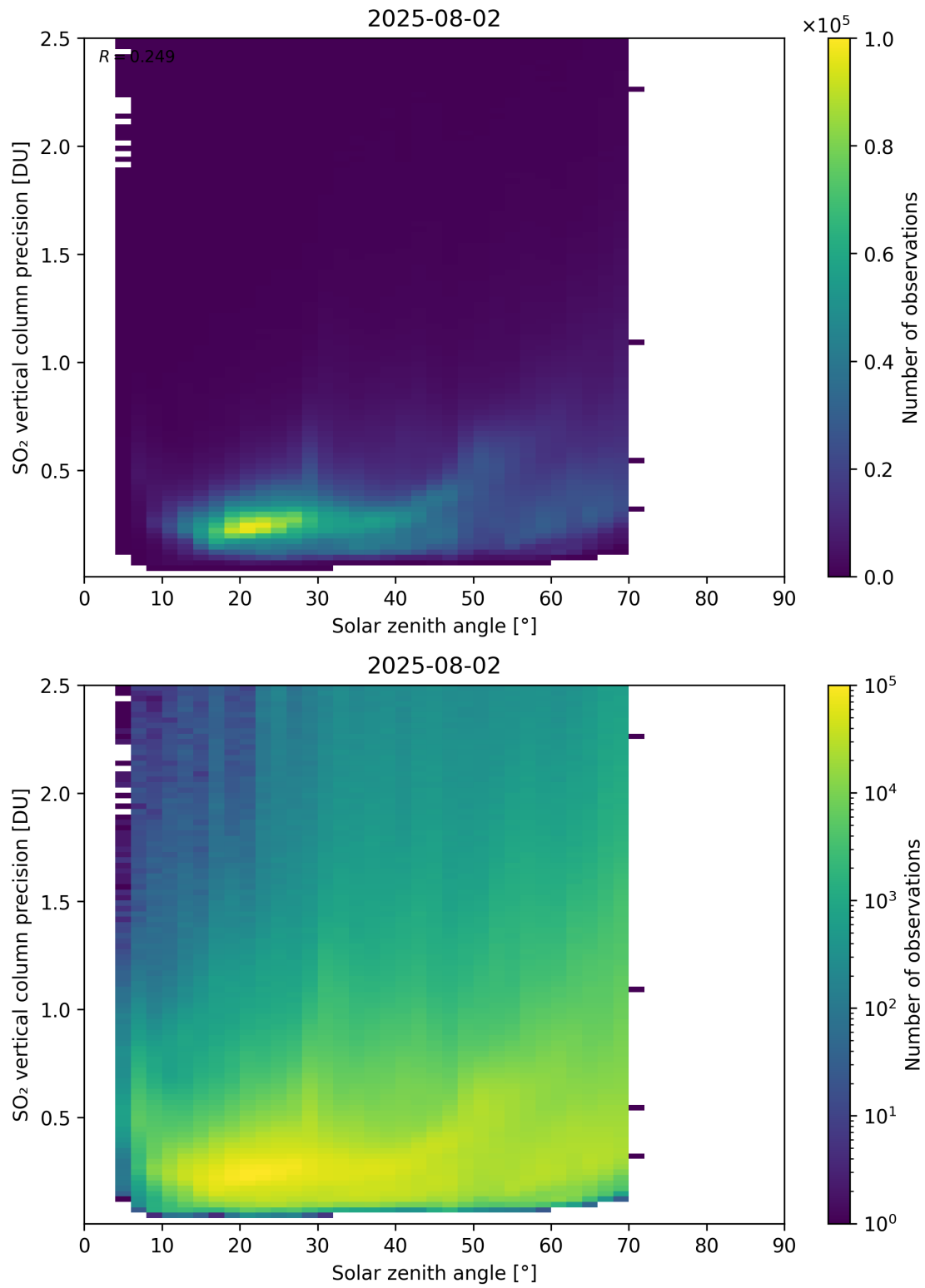
Figure 192: Scatter density plot of “Solar zenith angle” against “SO 2 vertical column precision” for 2025-08-01 to 2025-08-03.
