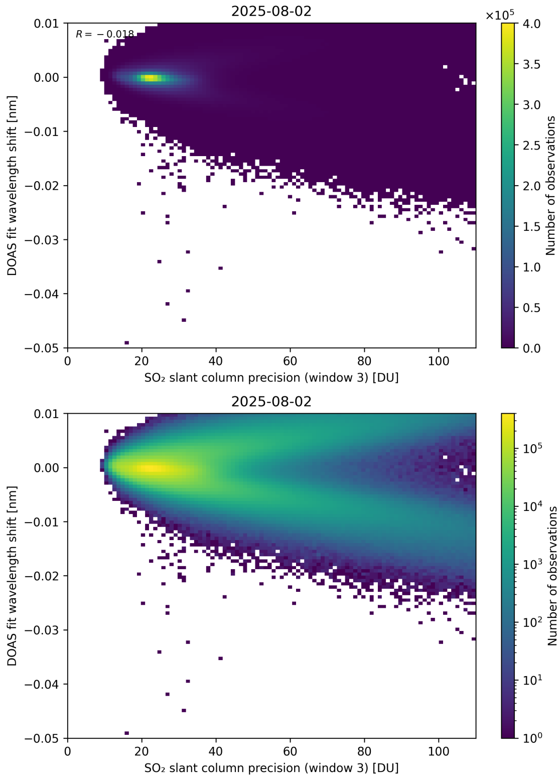
Figure 308: Scatter density plot of “SO 2 slant column precision (window 3)” against “DOAS fit wavelength shift” for 2025-08-01 to 2025-08-03.
