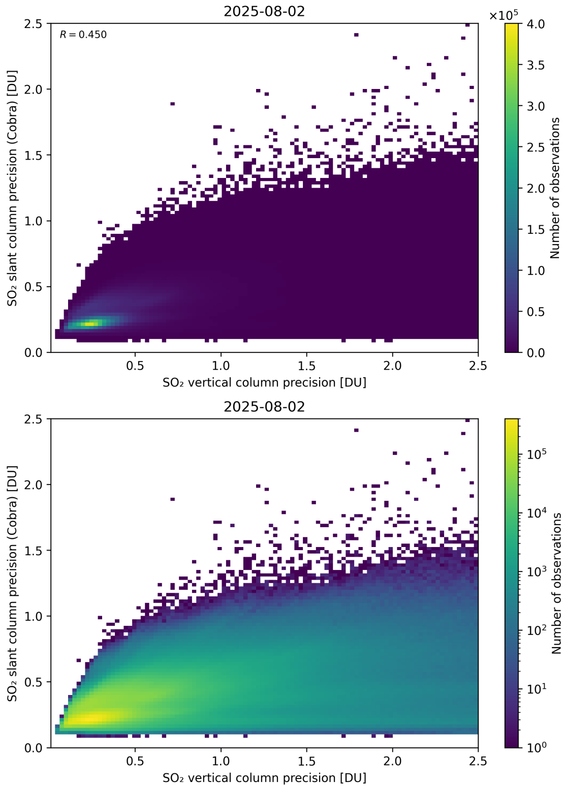
Figure 337: Scatter density plot of “SO 2 vertical column precision” against “SO 2 slant column precision (Cobra)” for 2025-08-01 to 2025-08-03.
