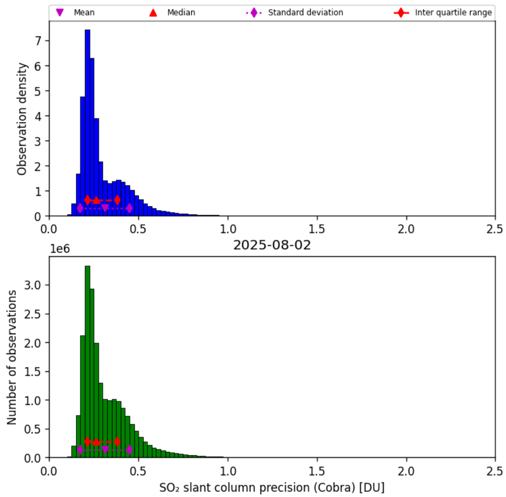
Figure 62: Histogram of “SO 2 slant column precision (Cobra)” for 2025-08-01 to 2025-08-03
