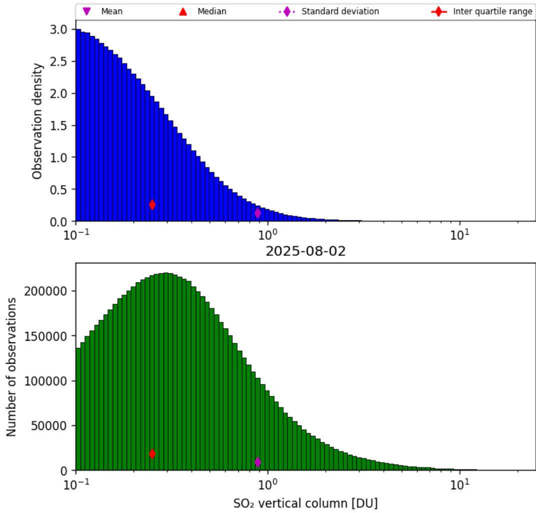
Figure 58: Histogram of “SO 2 vertical column” for 2025-08-01 to 2025-08-03
