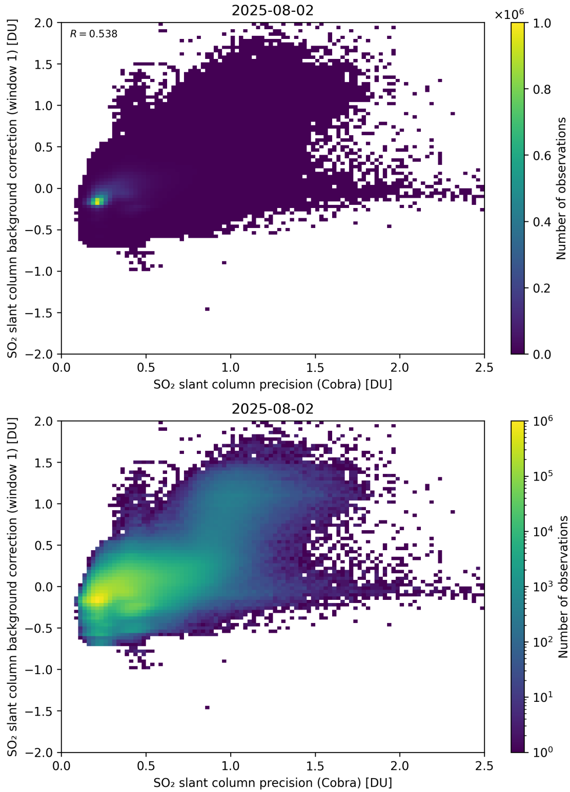
Figure 199: Scatter density plot of “SO 2 slant column precision (Cobra)” against “SO 2 slant column background correction (window 1)” for 2025-08-01 to 2025-08-03.
