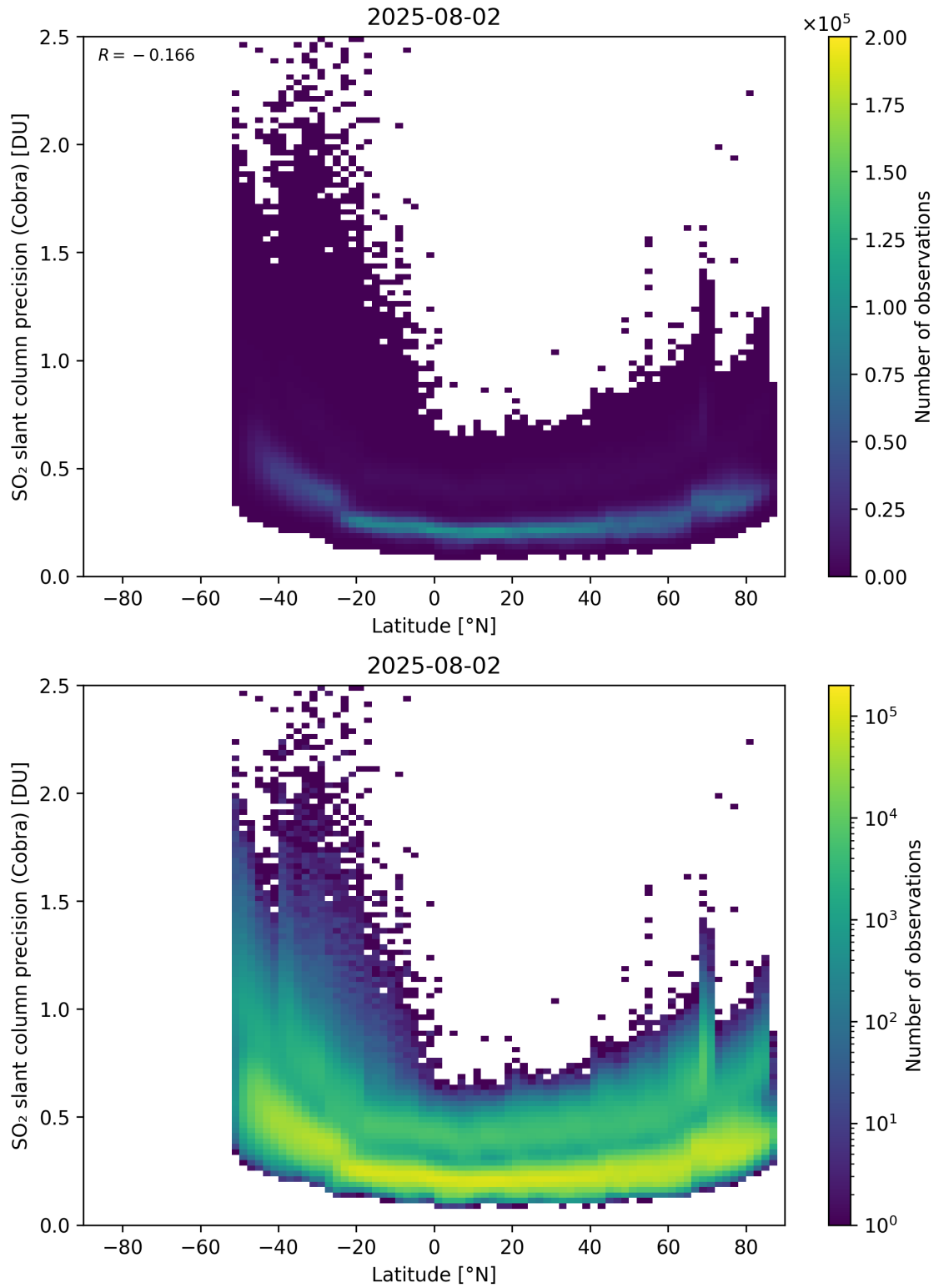
Figure 158: Scatter density plot of “Latitude” against “SO 2 slant column precision (Cobra)” for 2025-08-01 to 2025-08-03.
