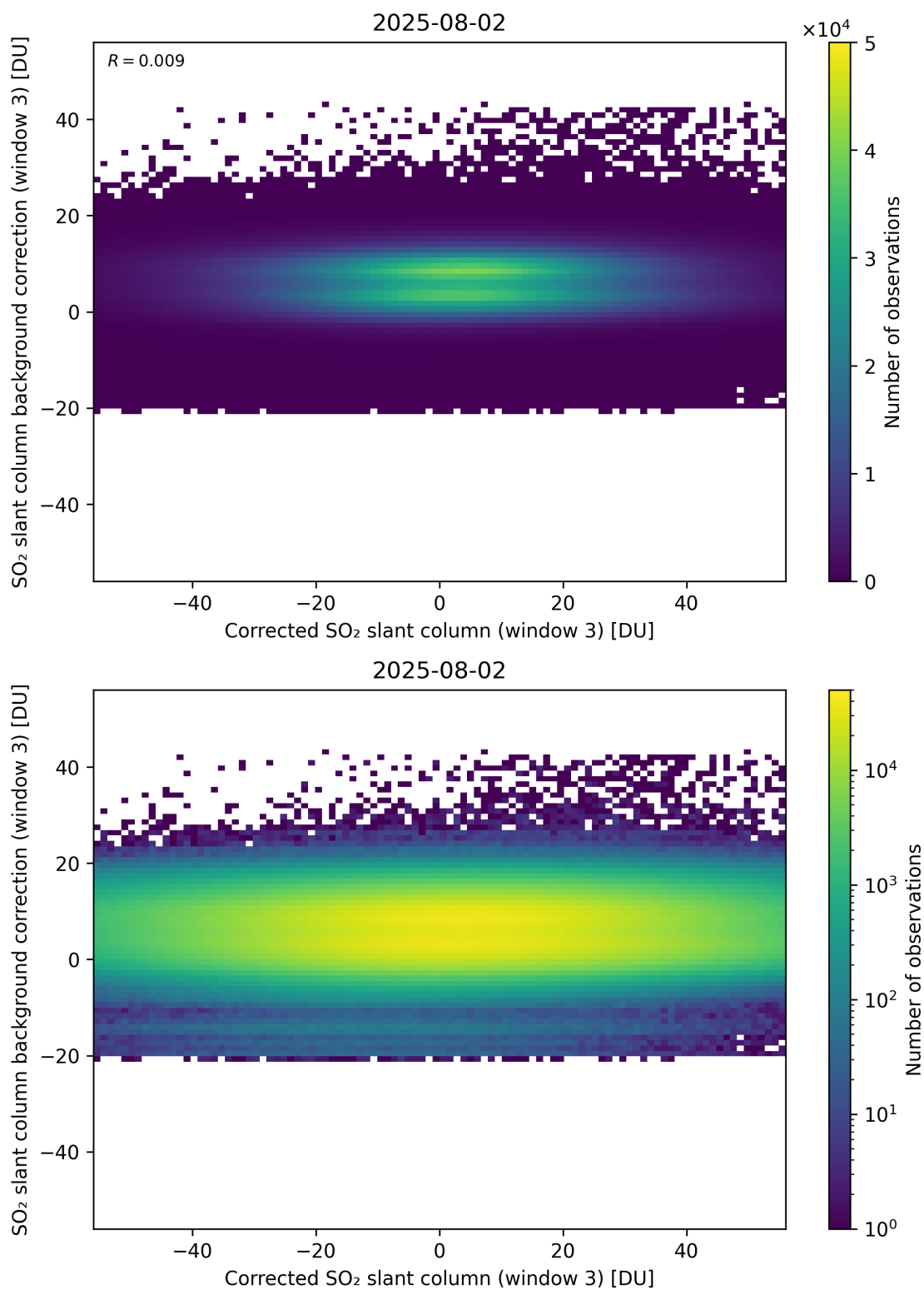
Figure 255: Scatter density plot of “Corrected SO 2 slant column (window 3)” against “SO 2 slant column background correction (window 3)” for 2025-08-01 to 2025-08-03.
