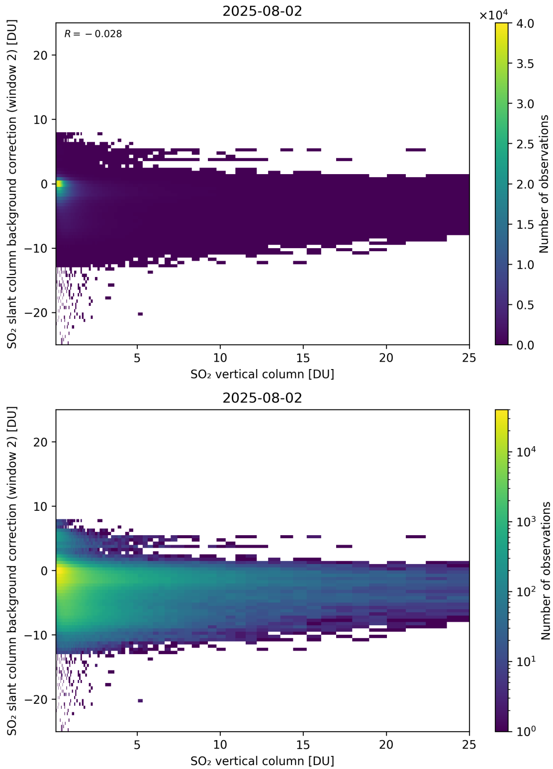
Figure 324: Scatter density plot of “SO 2 vertical column” against “SO 2 slant column background correction (window 2)” for 2025-08-01 to 2025-08-03.
