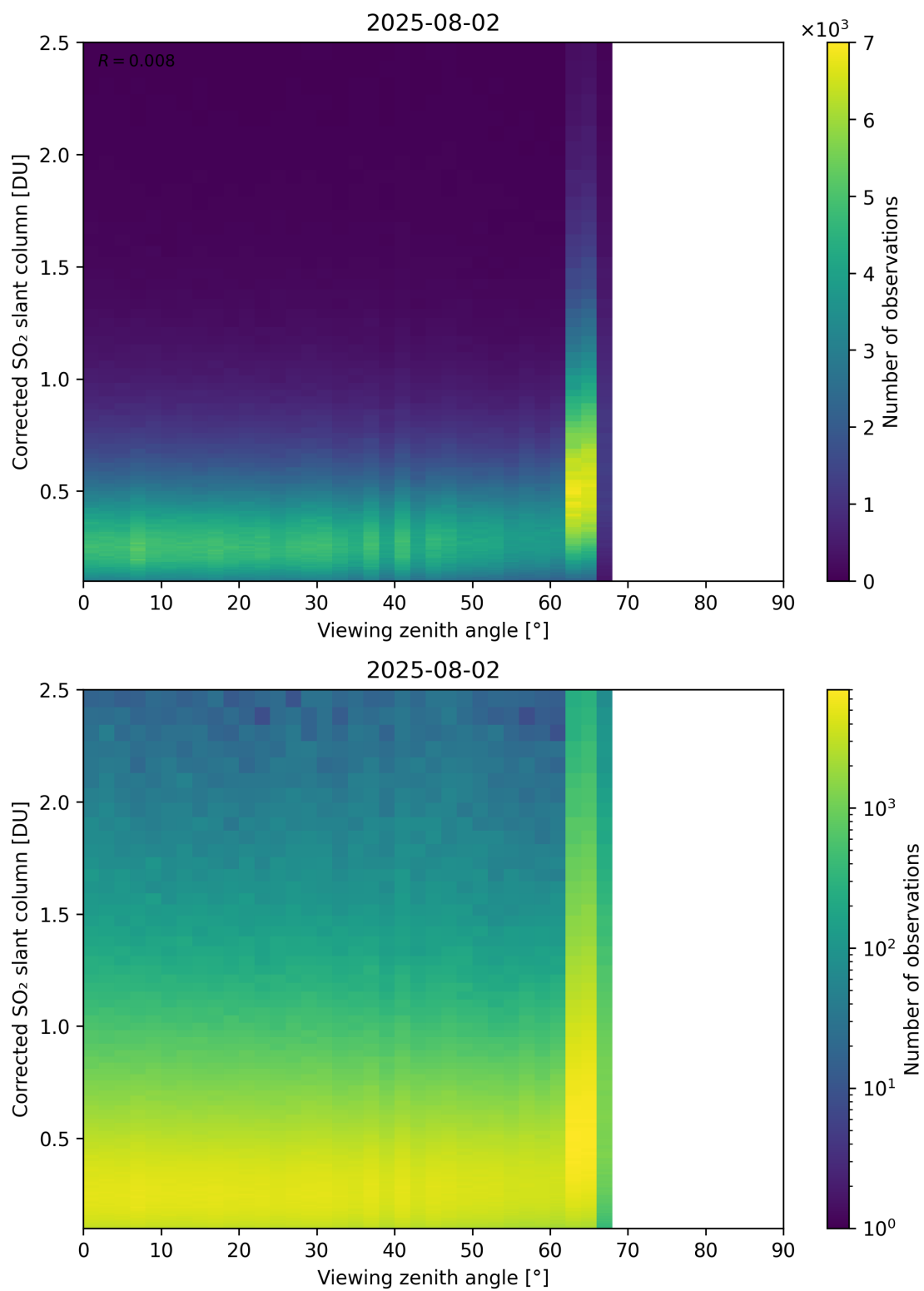
Figure 373: Scatter density plot of “Viewing zenith angle” against “Corrected SO 2 slant column” for 2025-08-01 to 2025-08-03.
