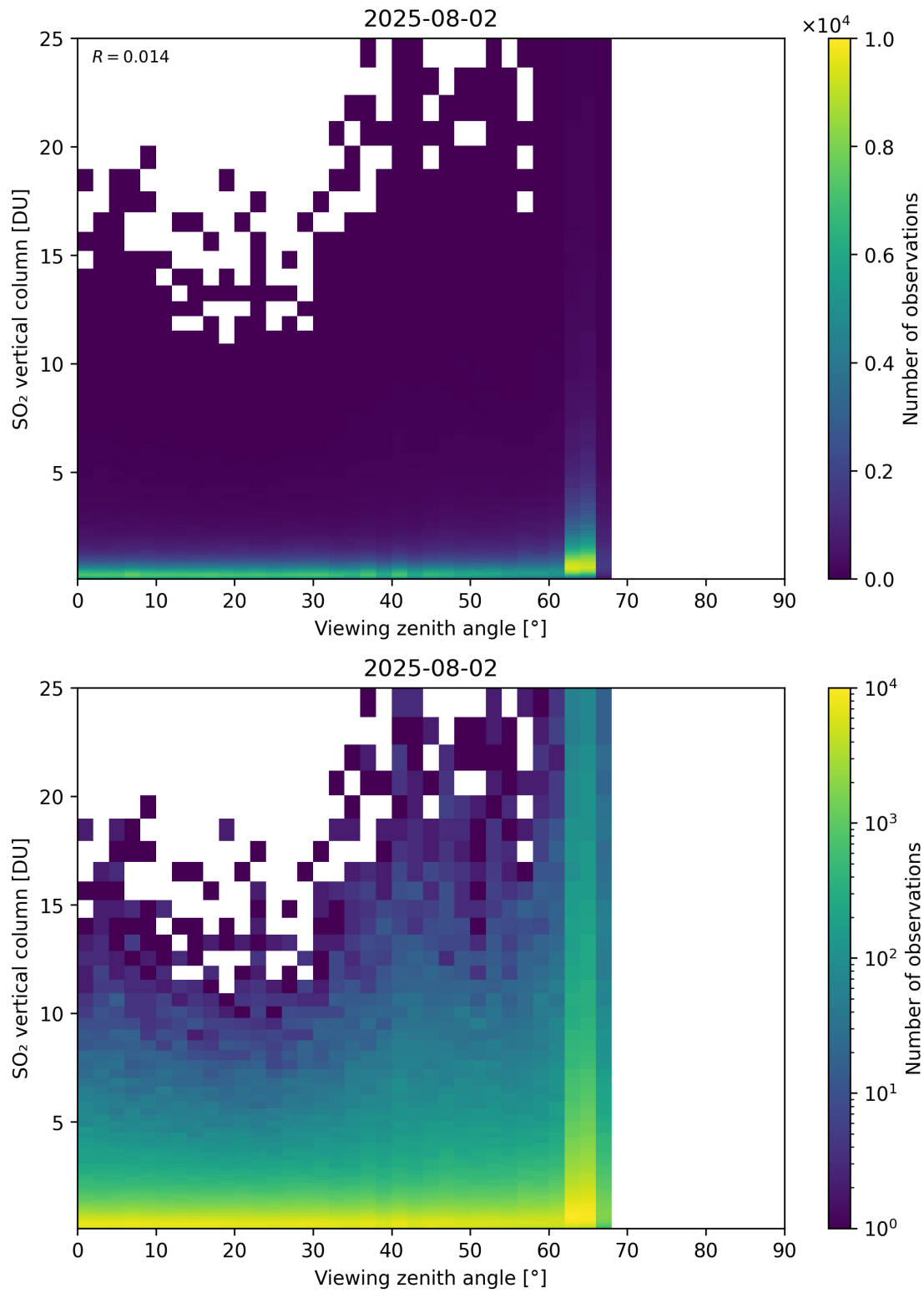
Figure 383: Scatter density plot of “Viewing zenith angle” against “SO 2 vertical column” for 2025-08-01 to 2025-08-03.
