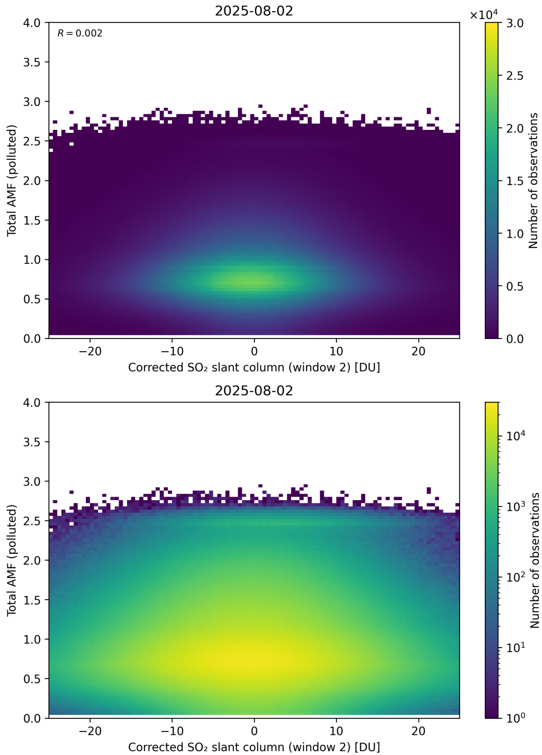
Figure 253: Scatter density plot of “Corrected SO 2 slant column (window 2)” against “Total AMF (polluted)” for 2025-08-01 to 2025-08-03.
