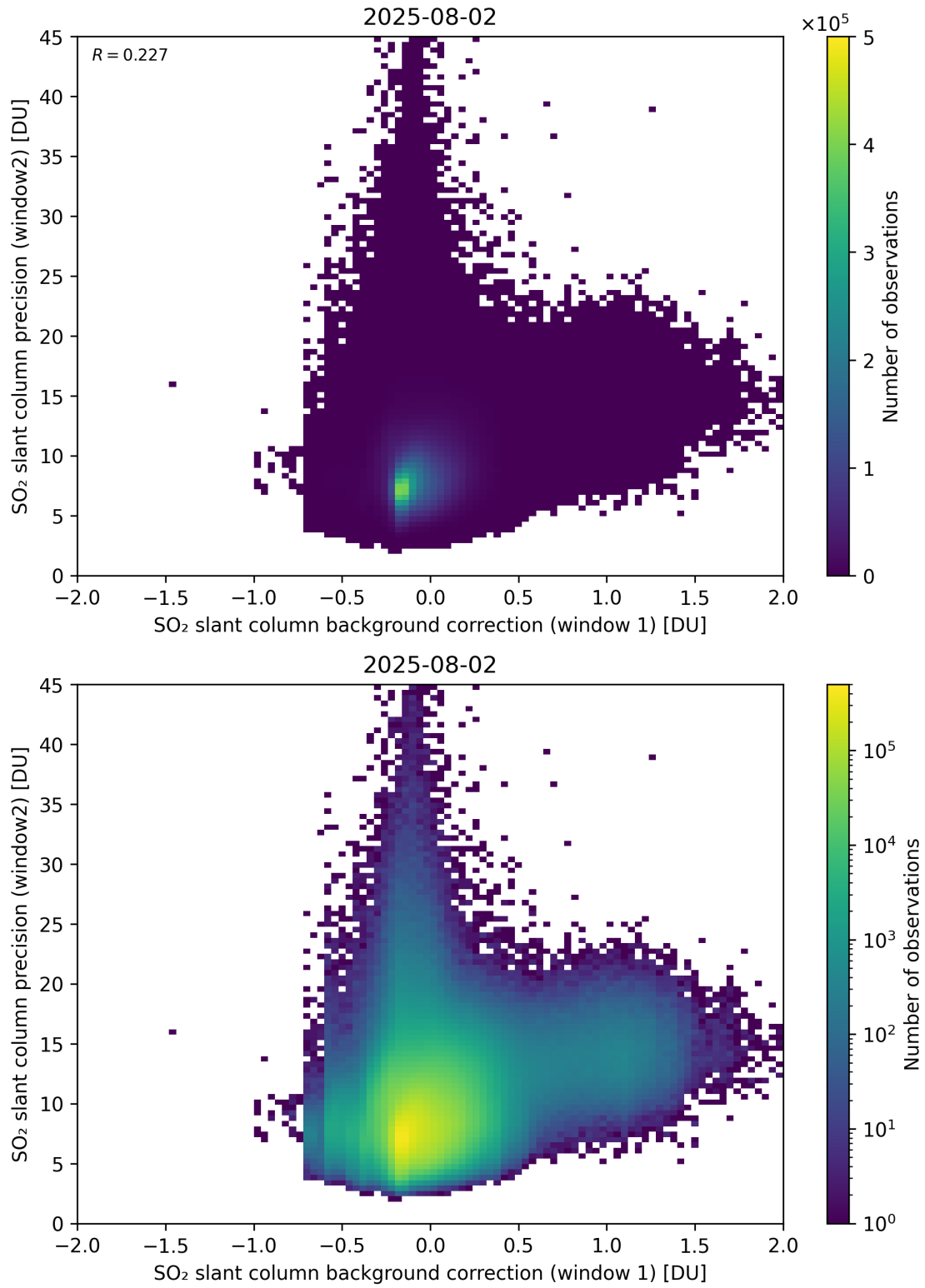
Figure 117: Scatter density plot of “SO 2 slant column background correction (window 1)” against “SO 2 slant column precision (window2)” for 2025-08-01 to 2025-08-03.
