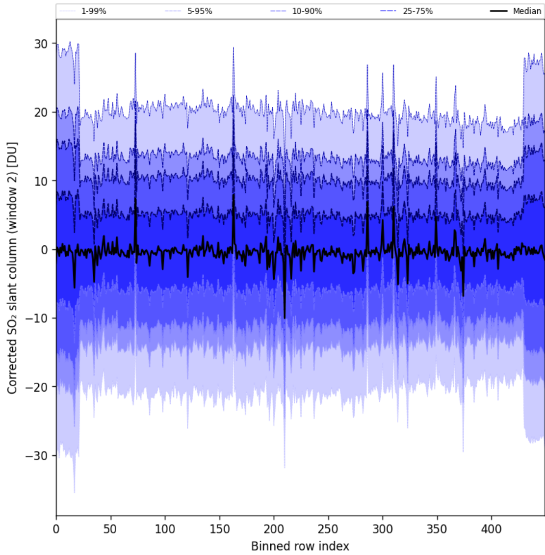
Figure 95: Along track statistics of “Corrected SO 2 slant column (window 2)” for 2025-08-01 to 2025-08-03
