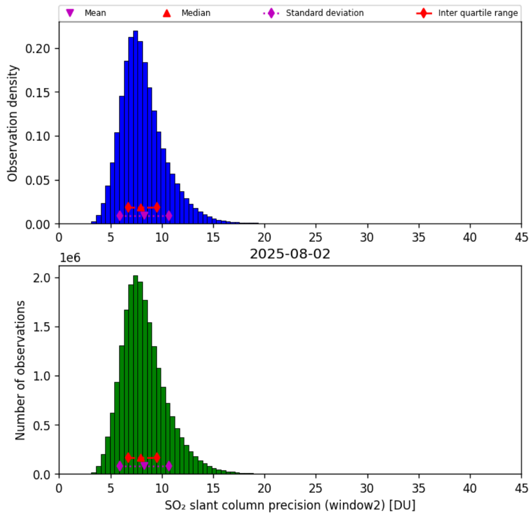
Figure 68: Histogram of “SO 2 slant column precision (window2)” for 2025-08-01 to 2025-08-03
