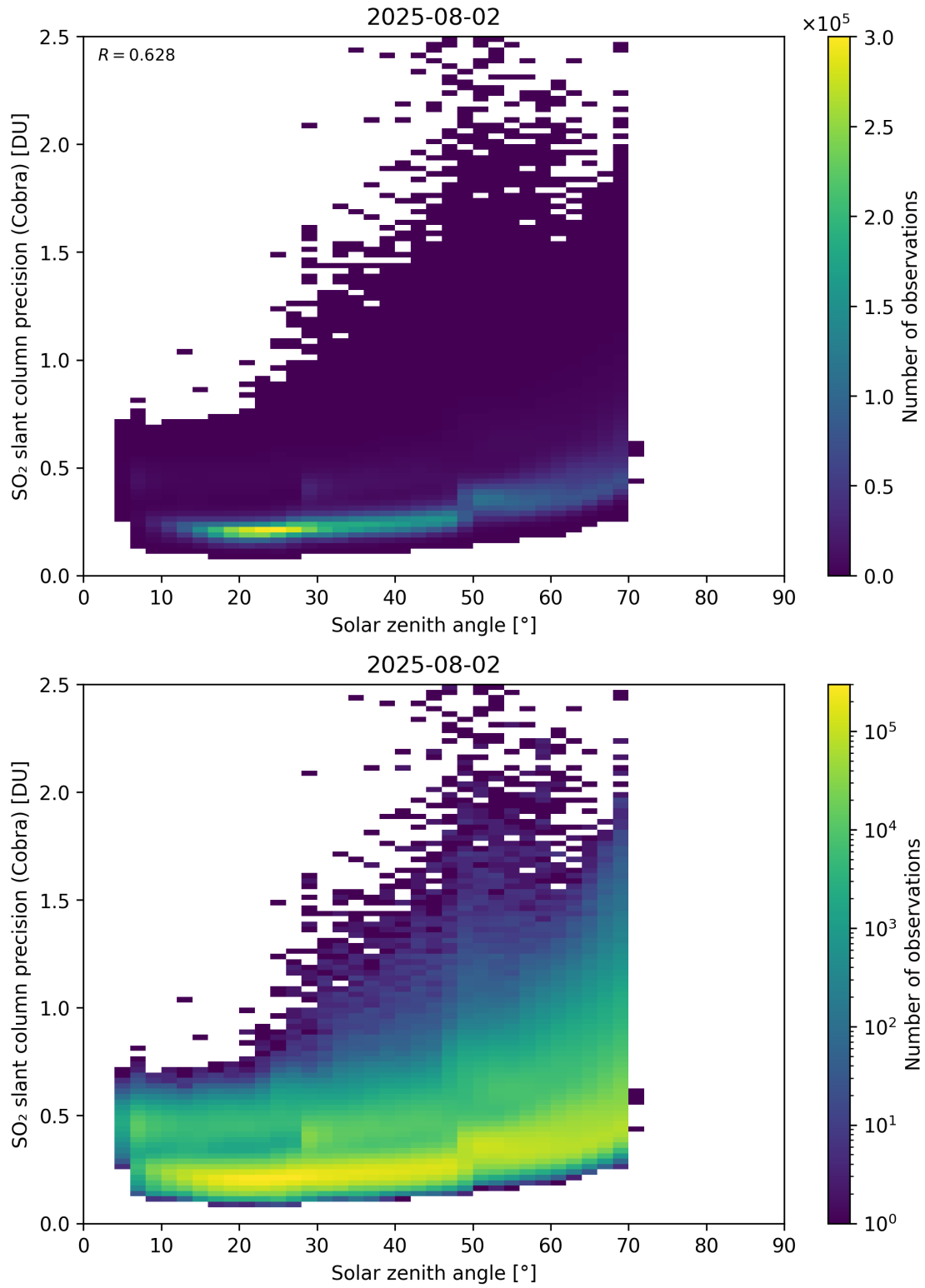
Figure 180: Scatter density plot of “Solar zenith angle” against “SO 2 slant column precision (Cobra)” for 2025-08-01 to 2025-08-03.
