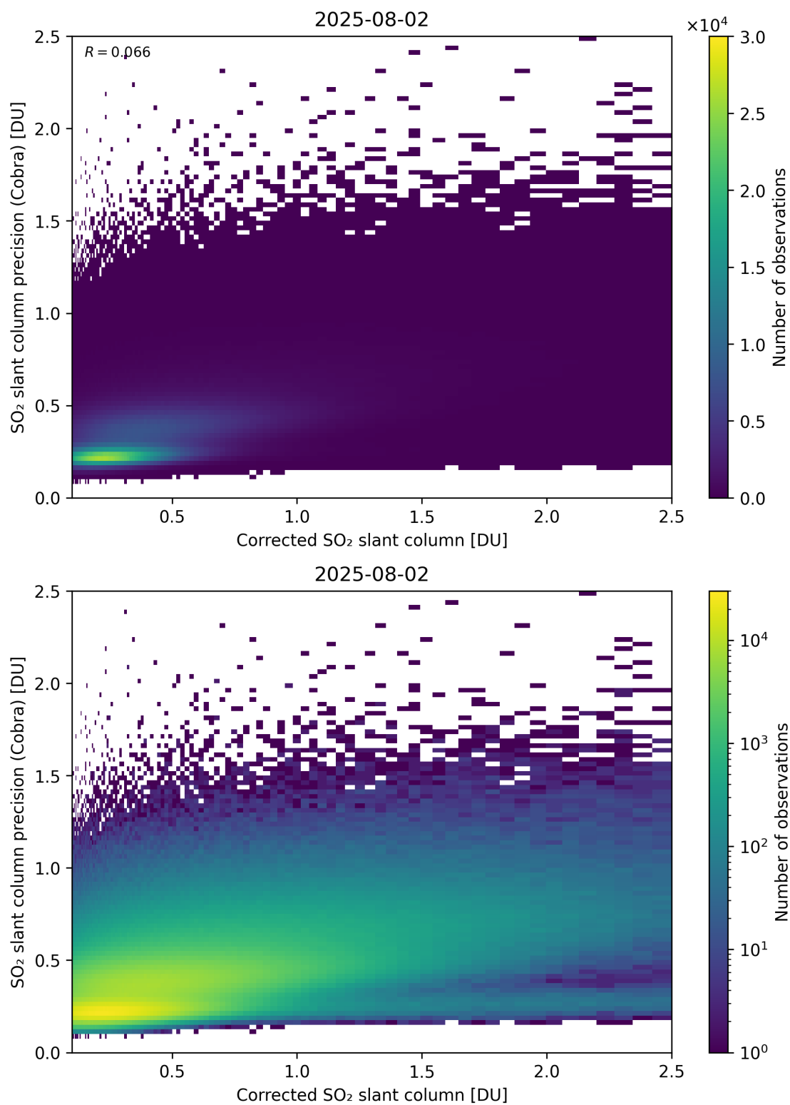
Figure 234: Scatter density plot of “Corrected SO 2 slant column” against “SO 2 slant column precision (Cobra)” for 2025-08-01 to 2025-08-03.
