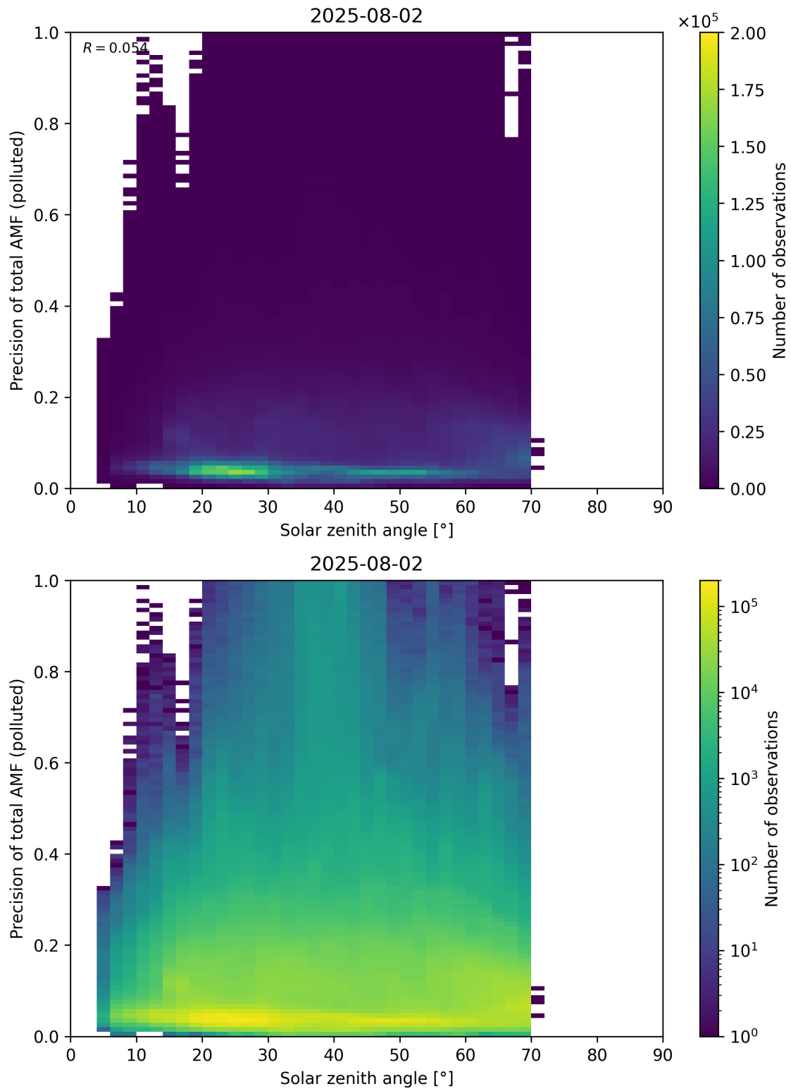
Figure 190: Scatter density plot of “Solar zenith angle” against “Precision of total AMF (polluted)” for 2025-08-01 to 2025-08-03.
