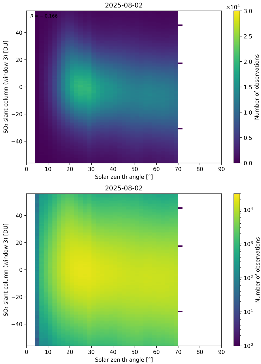
Figure 187: Scatter density plot of “Solar zenith angle” against “SO 2 slant column (window 3)” for 2025-08-01 to 2025-08-03.
