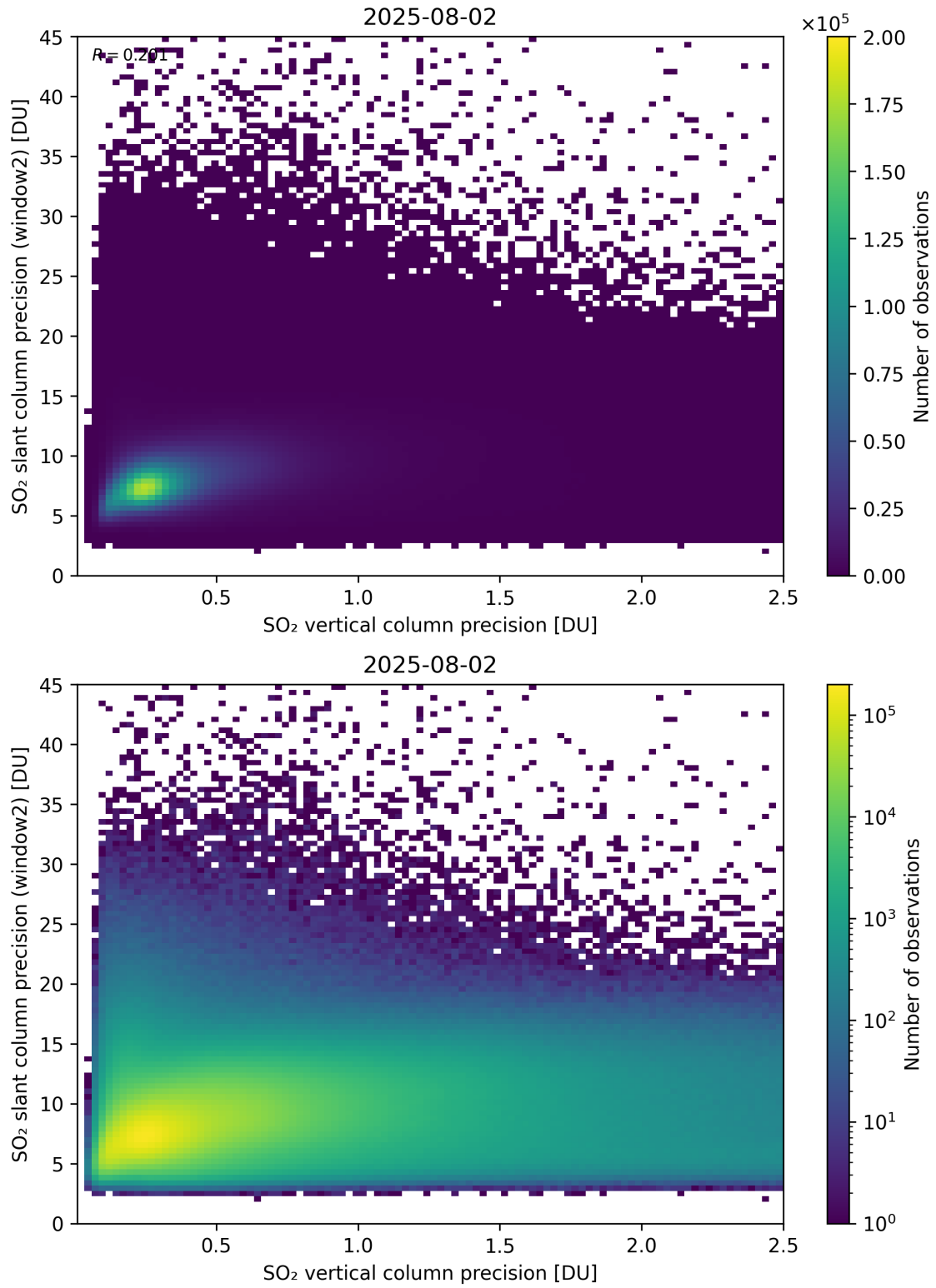
Figure 343: Scatter density plot of “SO 2 vertical column precision” against “SO 2 slant column precision (window2)” for 2025-08-01 to 2025-08-03.
