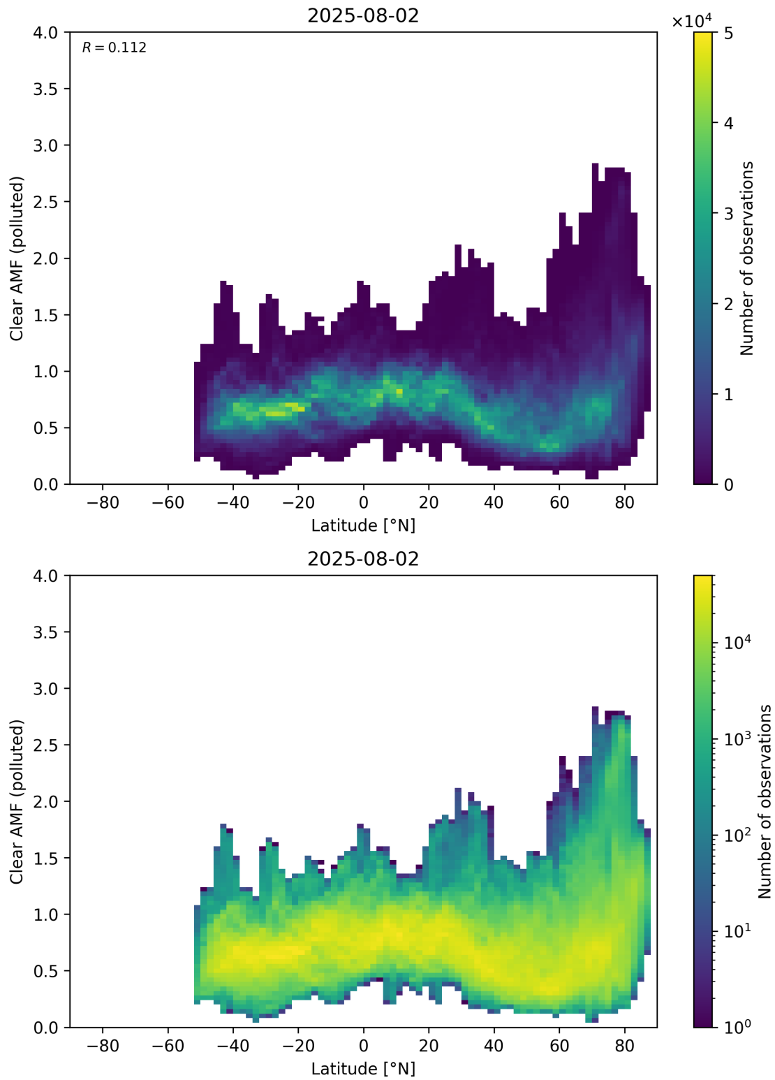
Figure 156: Scatter density plot of “Latitude” against “Clear AMF (polluted)” for 2025-08-01 to 2025-08-03.
