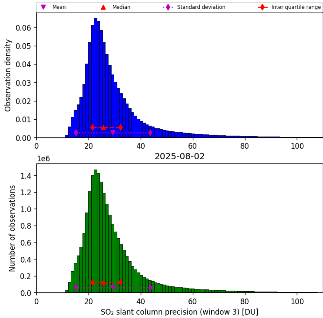
Figure 72: Histogram of “SO 2 slant column precision (window 3)” for 2025-08-01 to 2025-08-03
