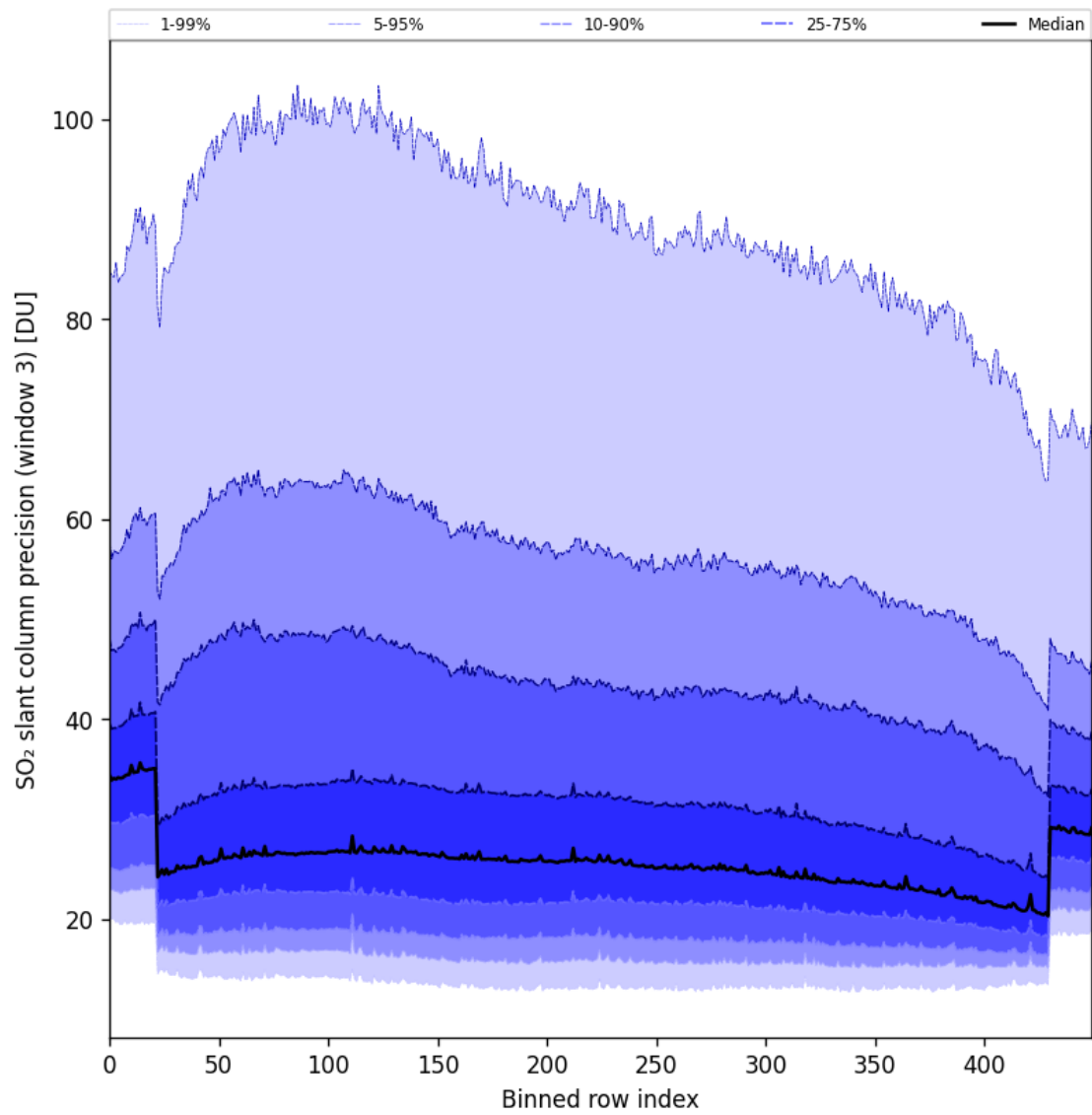
Figure 98: Along track statistics of “SO 2 slant column precision (window 3)” for 2025-08-01 to 2025-08-03
