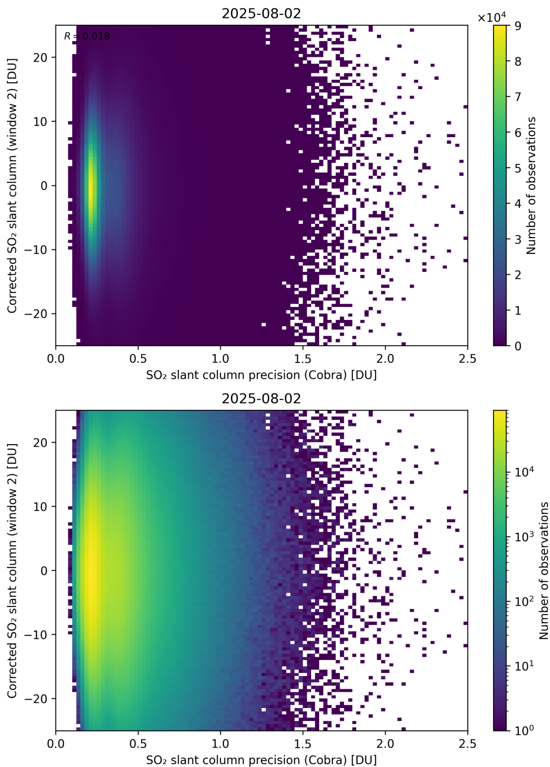
Figure 206: Scatter density plot of “SO 2 slant column precision (Cobra)” against “Corrected SO 2 slant column (window 2)” for 2025-08-01 to 2025-08-03.
