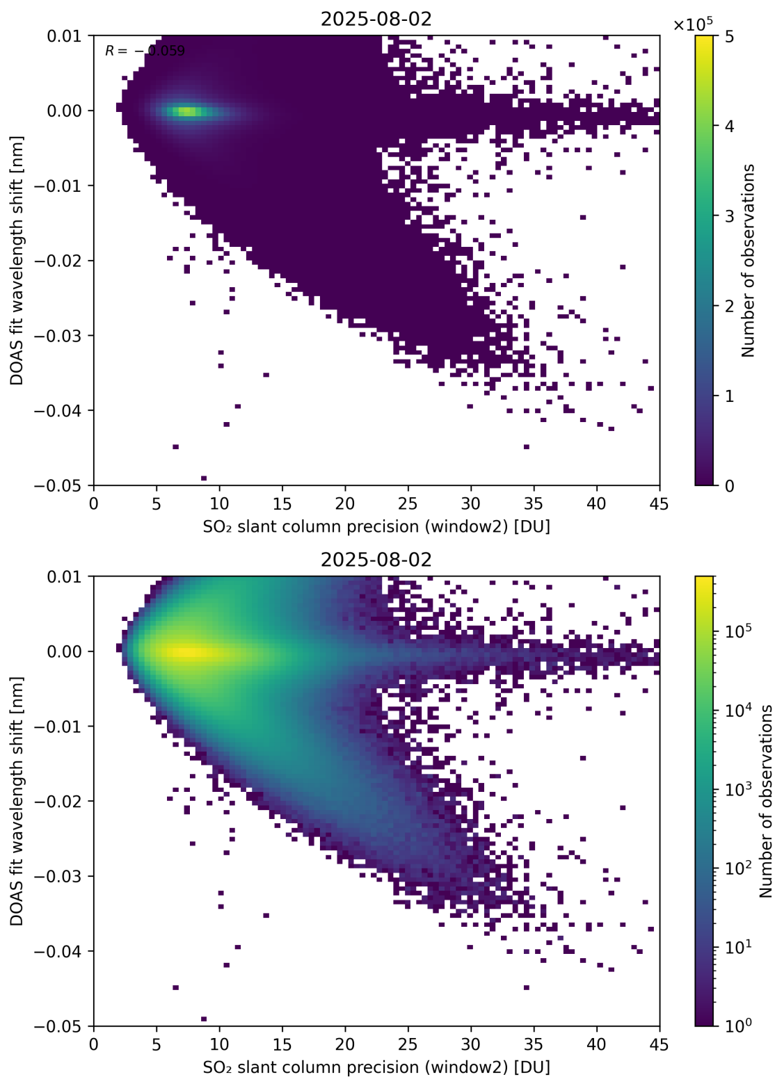
Figure 293: Scatter density plot of “SO 2 slant column precision (window2)” against “DOAS fit wavelength shift” for 2025-08-01 to 2025-08-03.
