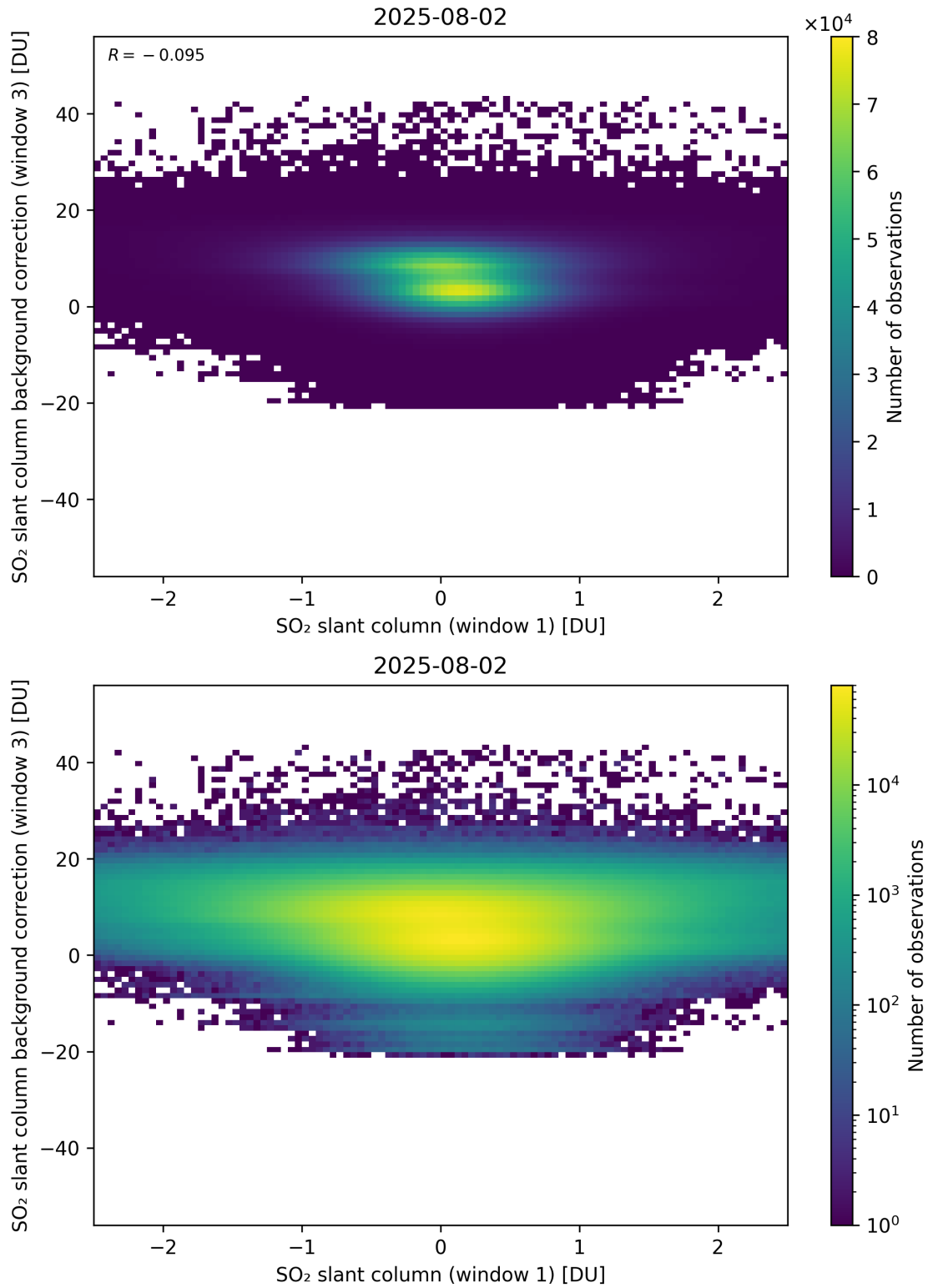
Figure 264: Scatter density plot of “SO 2 slant column (window 1)” against “SO 2 slant column background correction (window 3)” for 2025-08-01 to 2025-08-03.
