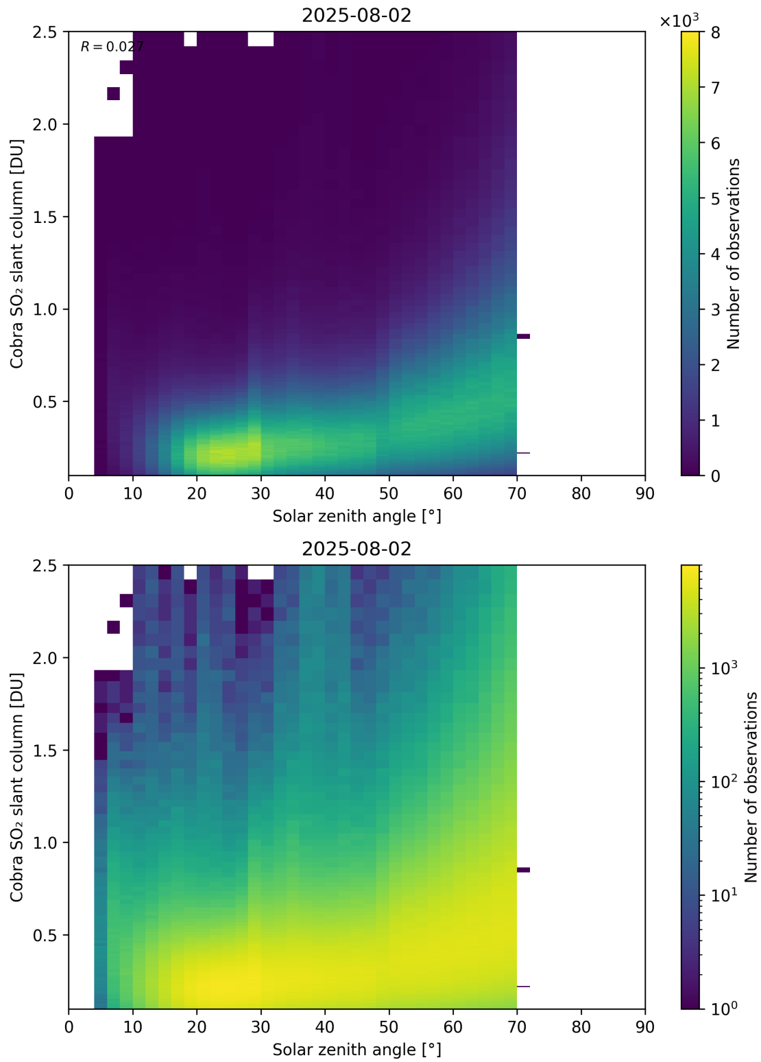
Figure 179: Scatter density plot of “Solar zenith angle” against “Cobra SO 2 slant column” for 2025-08-01 to 2025-08-03.
