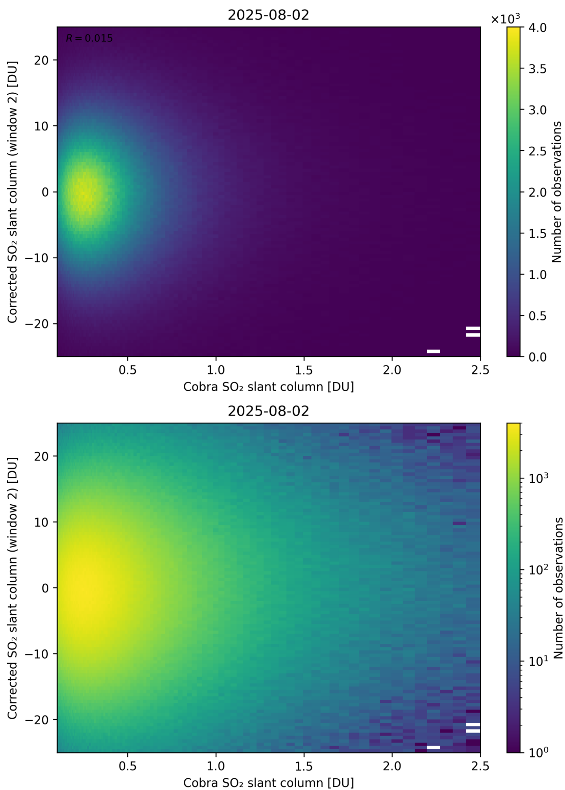
Figure 217: Scatter density plot of “Cobra SO 2 slant column” against “Corrected SO 2 slant column (window 2)” for 2025-08-01 to 2025-08-03.
