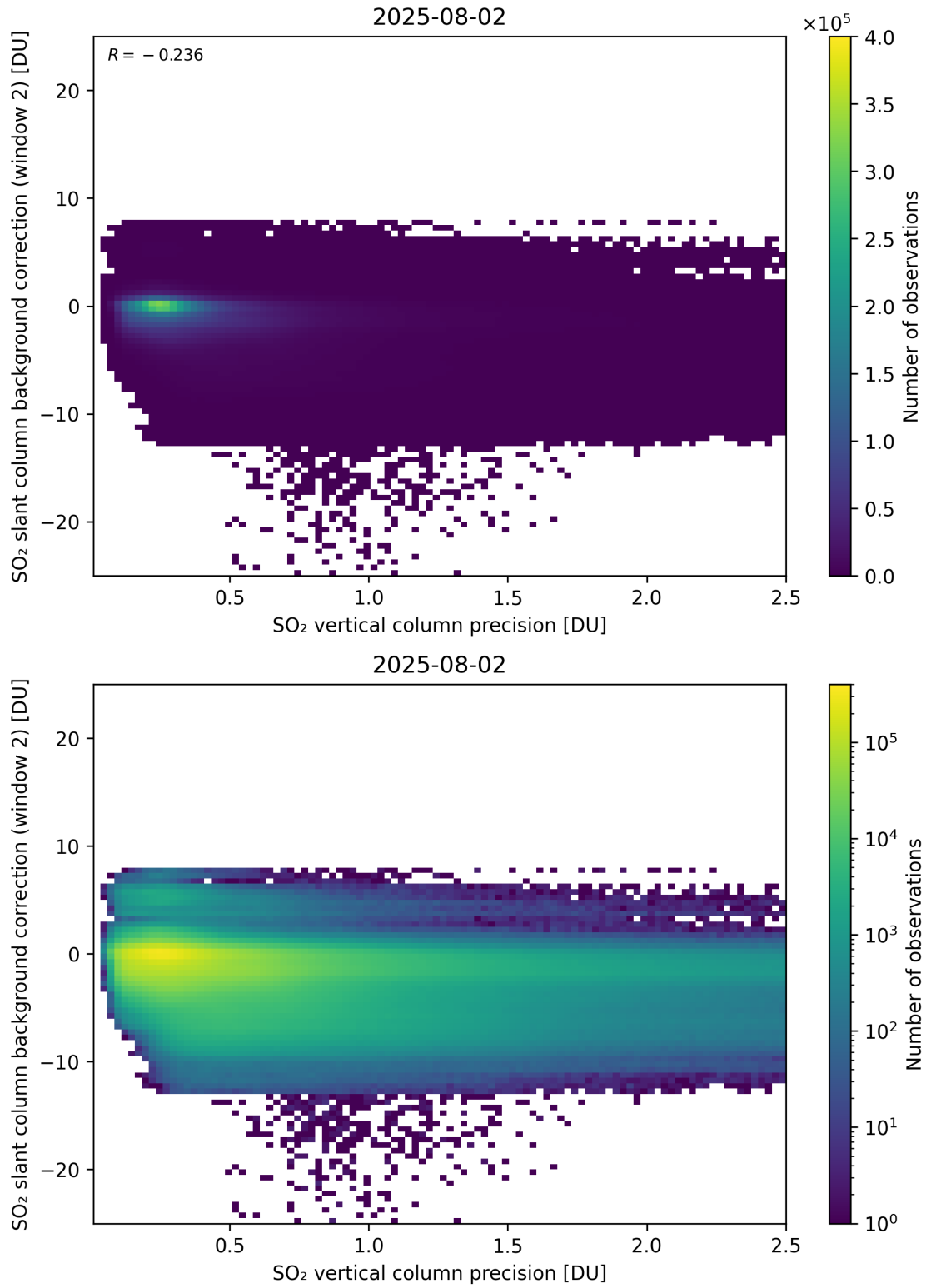
Figure 330: Scatter density plot of “SO 2 vertical column precision” against “SO 2 slant column background correction (window 2)” for 2025-08-01 to 2025-08-03.
