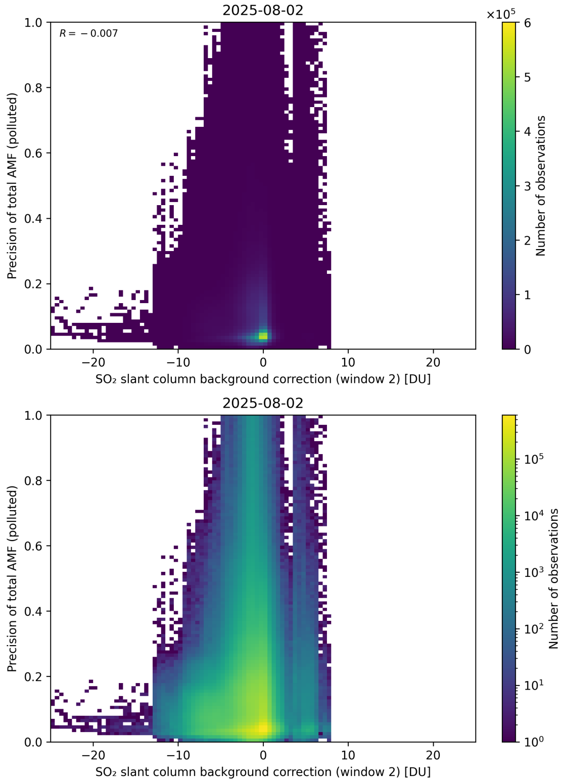
Figure 131: Scatter density plot of “SO 2 slant column background correction (window 2)” against “Precision of total AMF (polluted)” for 2025-08-01 to 2025-08-03.
