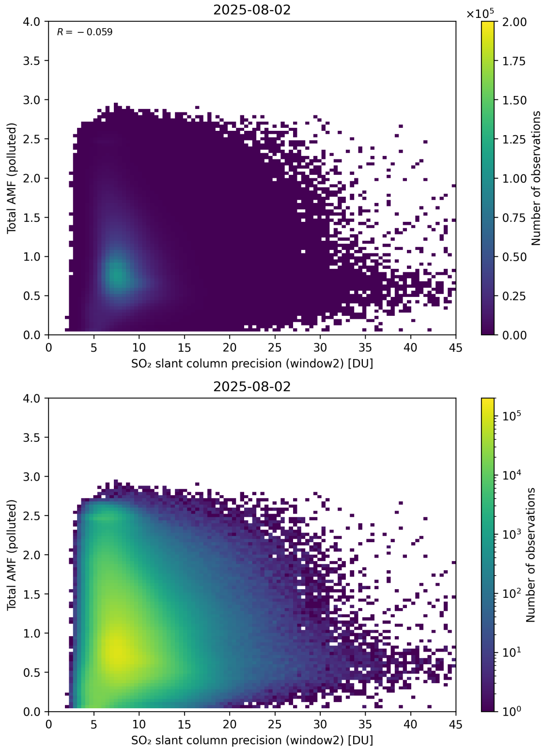
Figure 301: Scatter density plot of “SO 2 slant column precision (window2)” against “Total AMF (polluted)” for 2025-08-01 to 2025-08-03.
