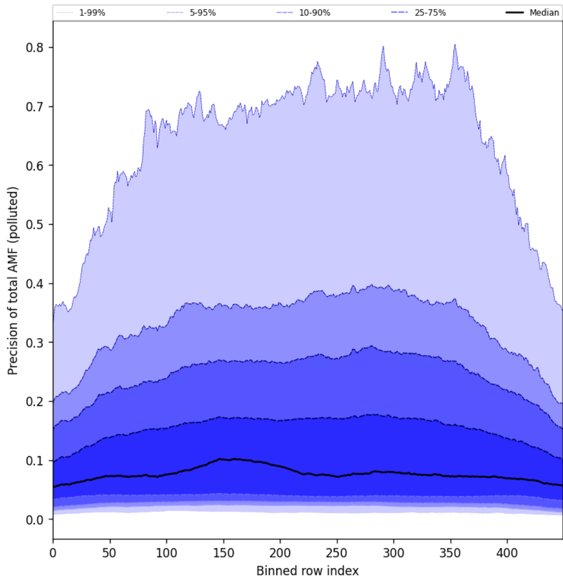
Figure 106: Along track statistics of “Precision of total AMF (polluted)” for 2025-08-01 to 2025-08-03
