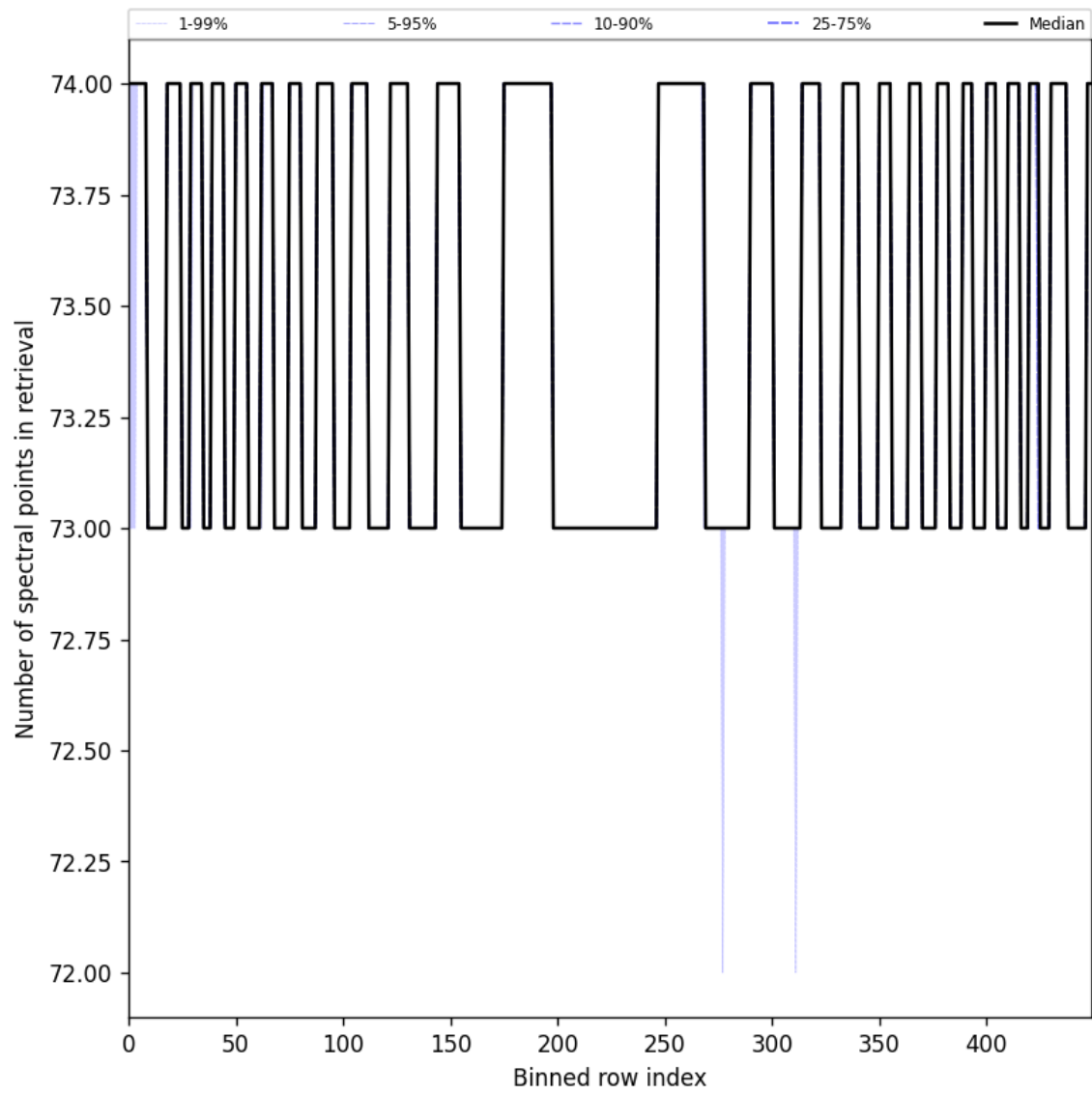
Figure 108: Along track statistics of “Number of spectral points in retrieval” for 2025-08-01 to 2025-08-03
