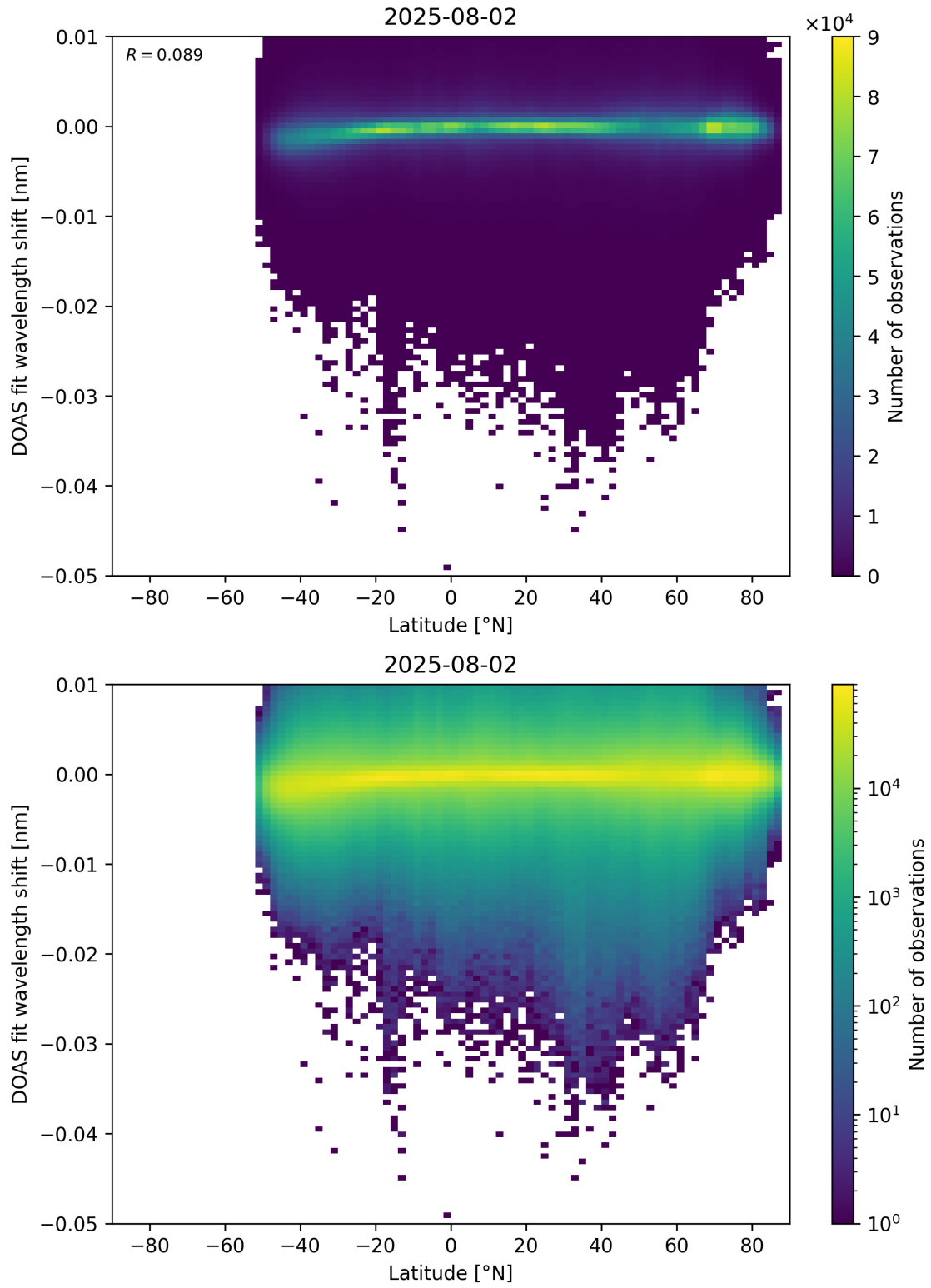
Figure 153: Scatter density plot of “Latitude” against “DOAS fit wavelength shift” for 2025-08-01 to 2025-08-03.
