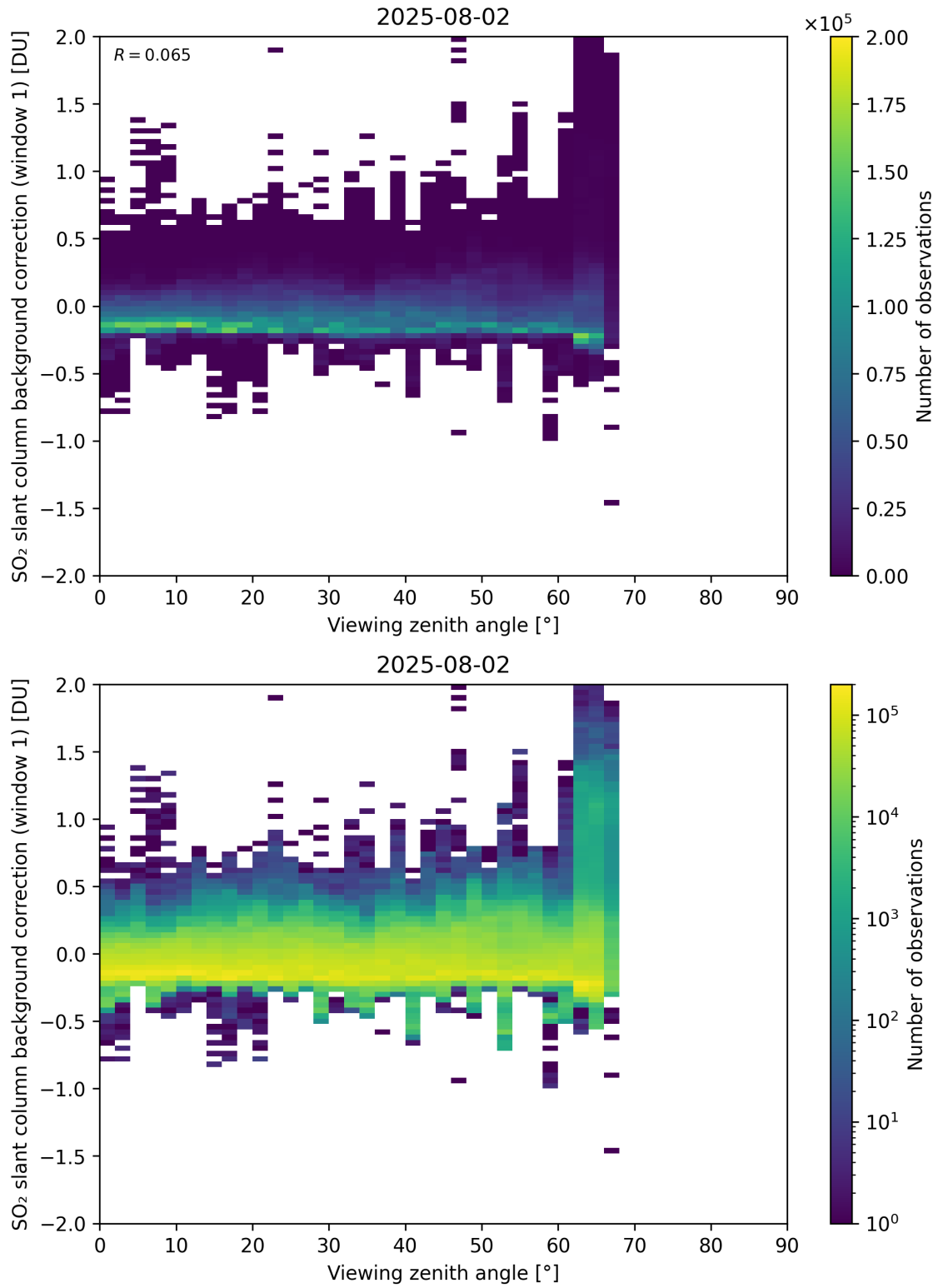
Figure 362: Scatter density plot of “Viewing zenith angle” against “SO 2 slant column background correction (window 1)” for 2025-08-01 to 2025-08-03.
