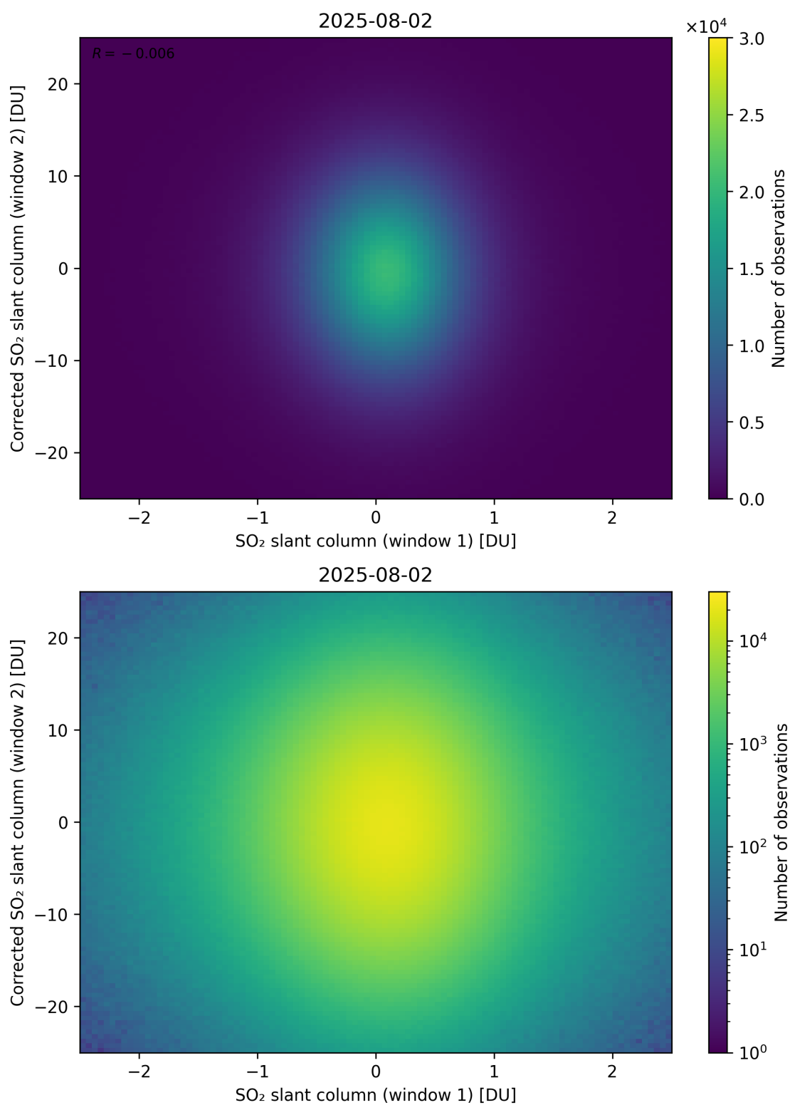
Figure 283: Scatter density plot of “SO 2 slant column (window 1)” against “Corrected SO 2 slant column (window 2)” for 2025-08-01 to 2025-08-03.
