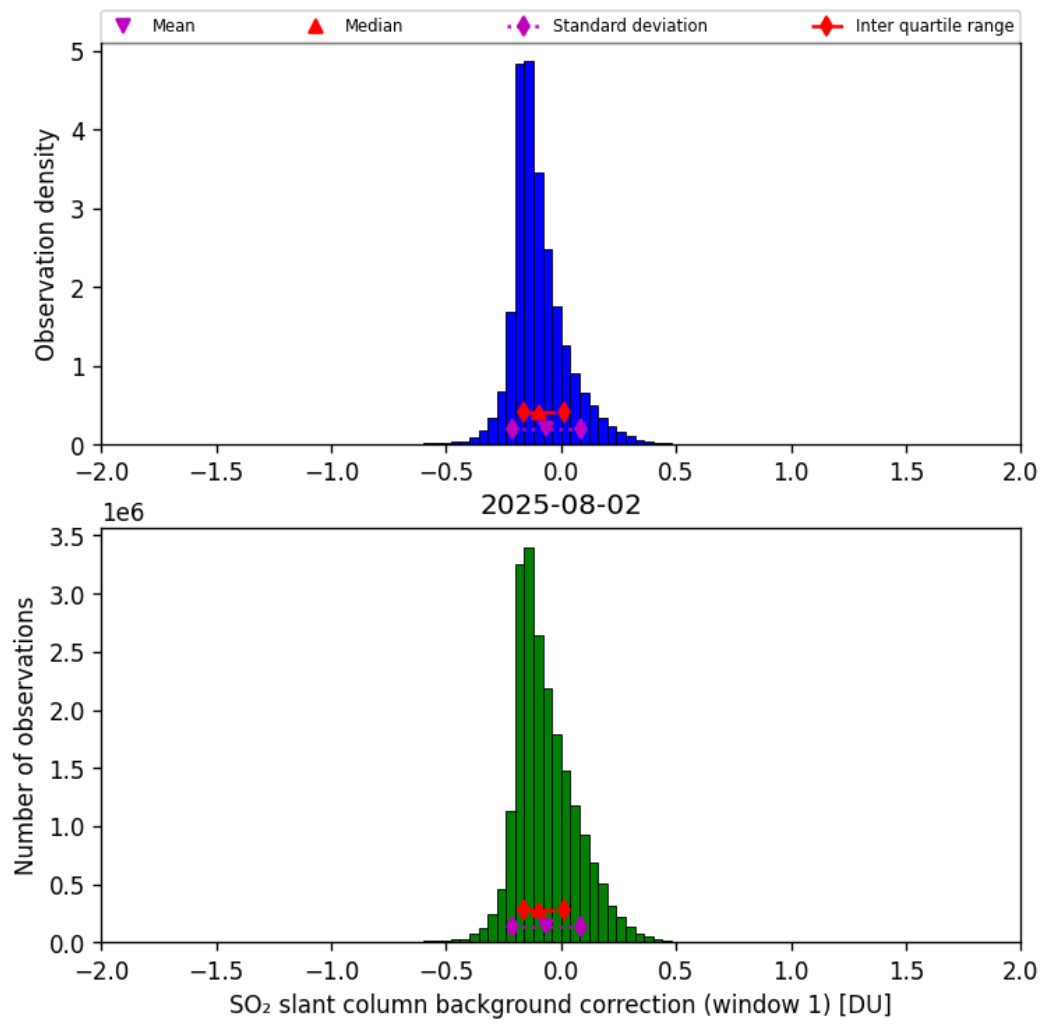
Figure 66: Histogram of “SO 2 slant column background correction (window 1)” for 2025-08-01 to 2025-08-03
