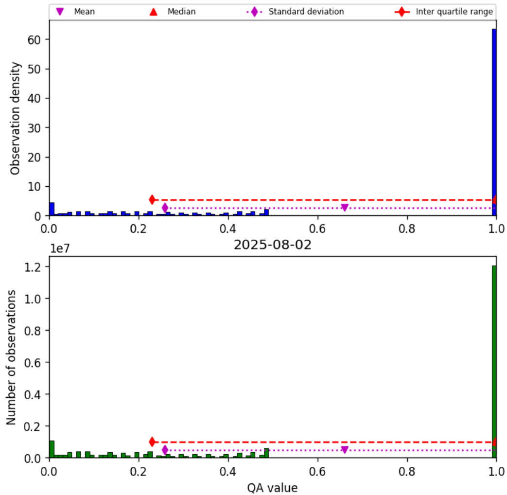
Figure 57: Histogram of “QA value” for 2025-08-01 to 2025-08-03
