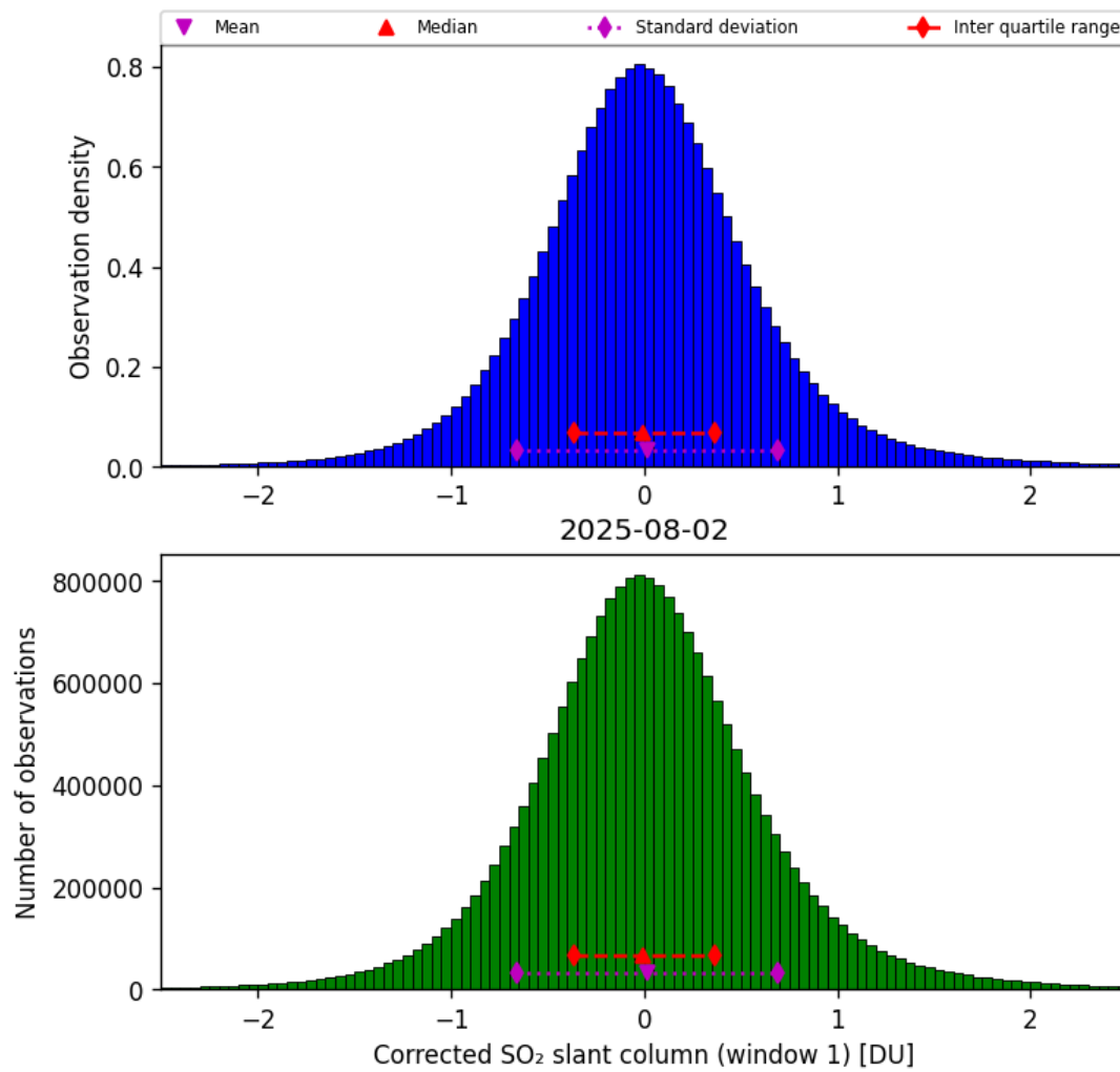
Figure 65: Histogram of “Corrected SO 2 slant column (window 1)” for 2025-08-01 to 2025-08-03
