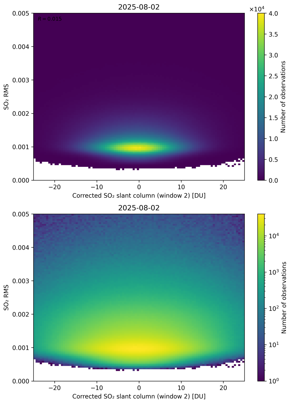
Figure 248: Scatter density plot of “Corrected SO 2 slant column (window 2)” against “SO 2 RMS” for 2025-08-01 to 2025-08-03.
