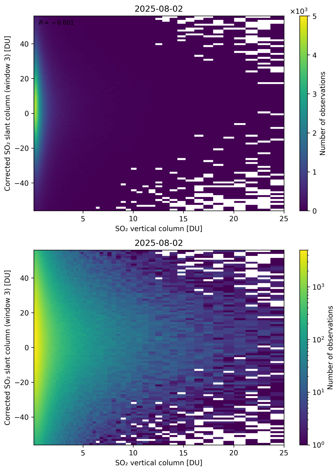
Figure 353: Scatter density plot of “SO 2 vertical column” against “Corrected SO 2 slant column (window 3)” for 2025-08-01 to 2025-08-03.
