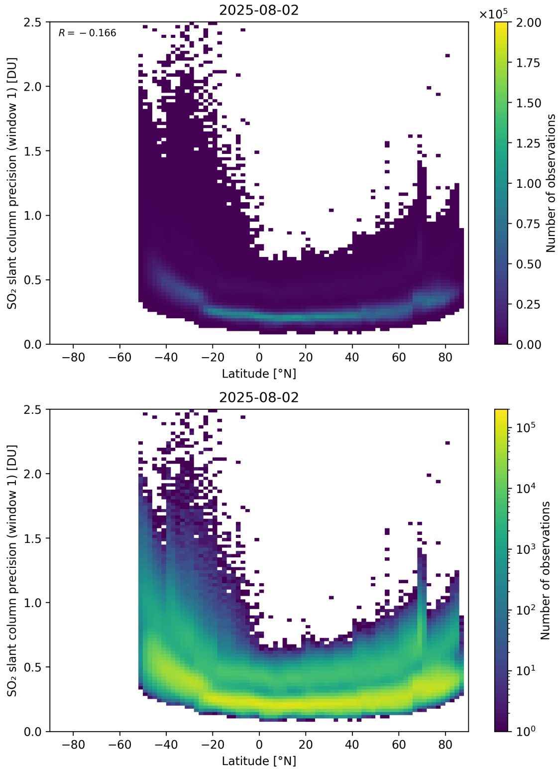
Figure 163: Scatter density plot of “Latitude” against “SO 2 slant column precision (window 1)” for 2025-08-01 to 2025-08-03.
