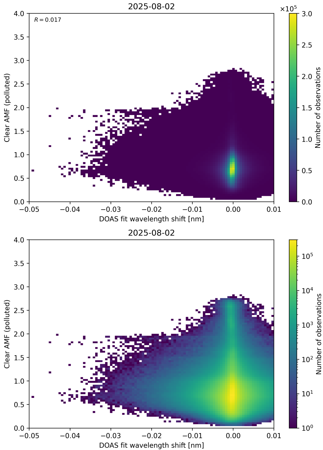
Figure 140: Scatter density plot of “DOAS fit wavelength shift” against “Clear AMF (polluted)” for 2025-08-01 to 2025-08-03.
