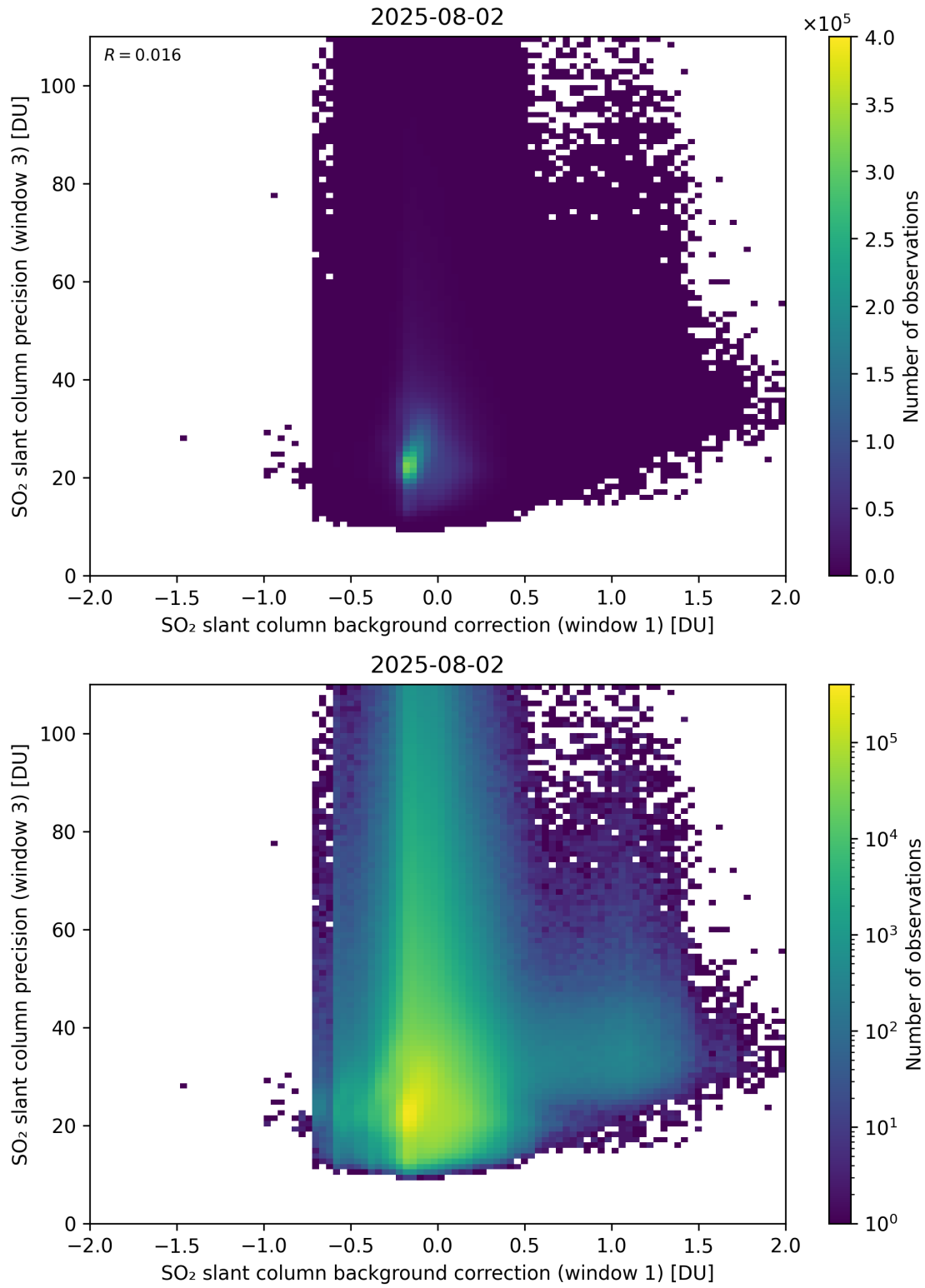
Figure 119: Scatter density plot of “SO 2 slant column background correction (window 1)” against “SO 2 slant column precision (window 3)” for 2025-08-01 to 2025-08-03.
