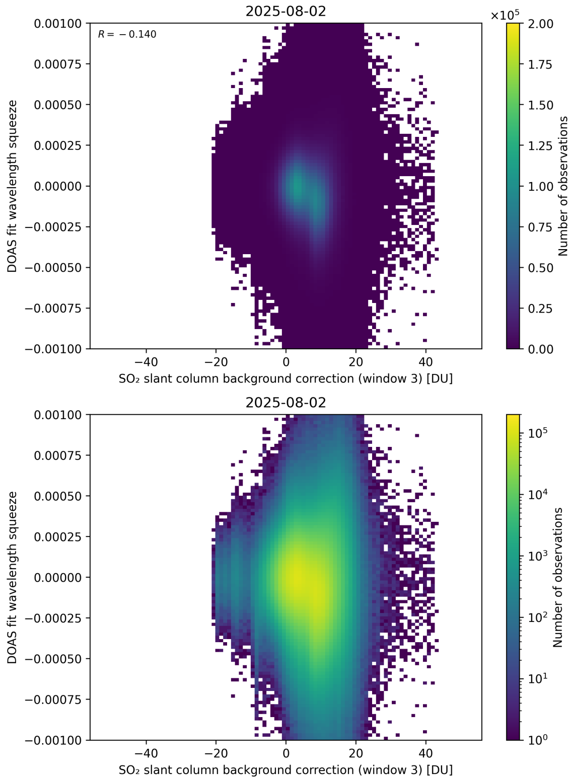
Figure 133: Scatter density plot of “SO 2 slant column background correction (window 3)” against “DOAS fit wavelength squeeze” for 2025-08-01 to 2025-08-03.
