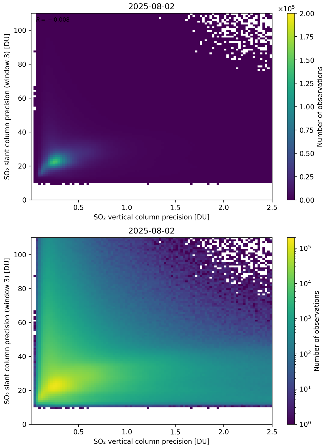
Figure 345: Scatter density plot of “SO 2 vertical column precision” against “SO 2 slant column precision (window 3)” for 2025-08-01 to 2025-08-03.
