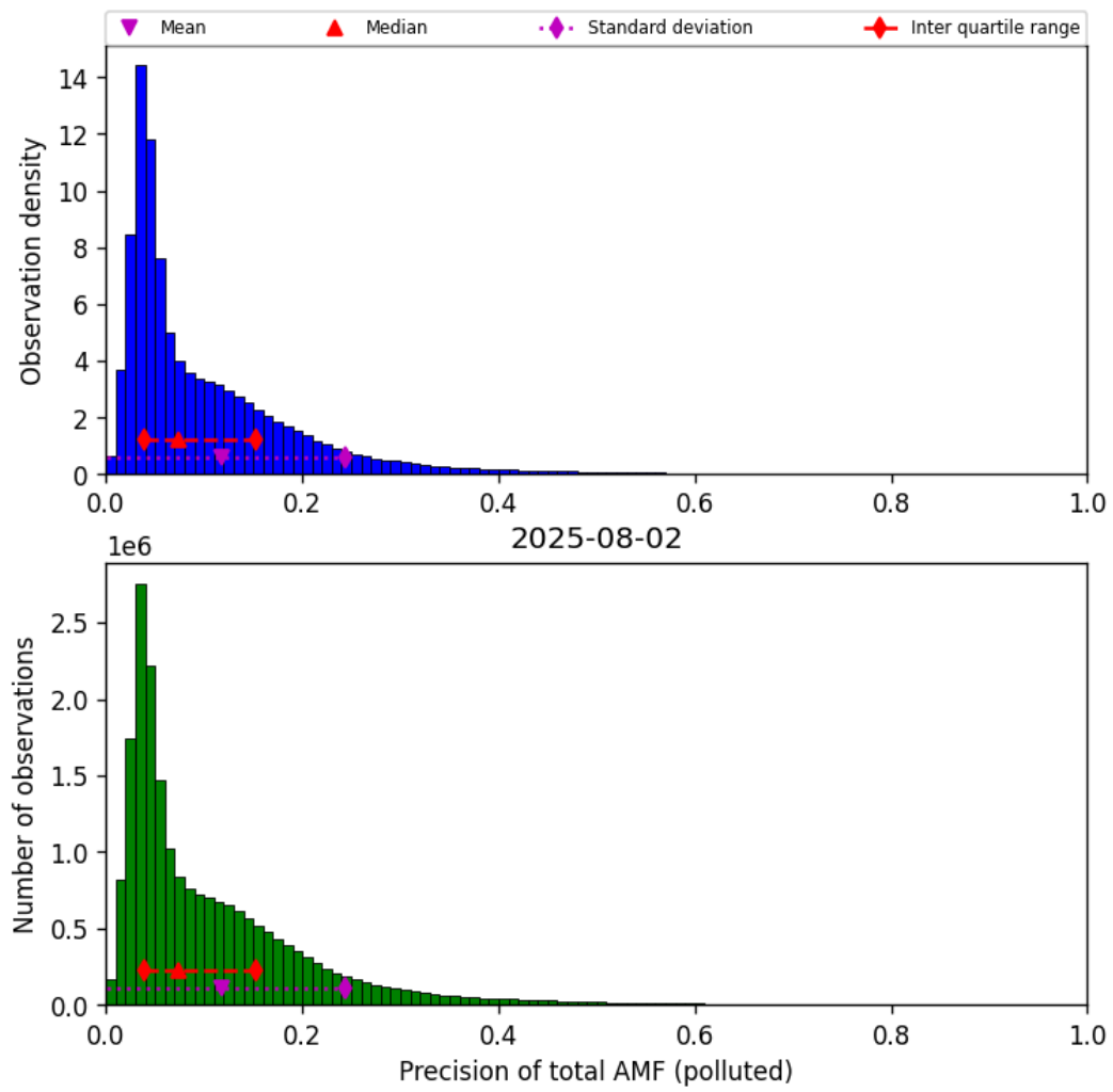
Figure 80: Histogram of “Precision of total AMF (polluted)” for 2025-08-01 to 2025-08-03
