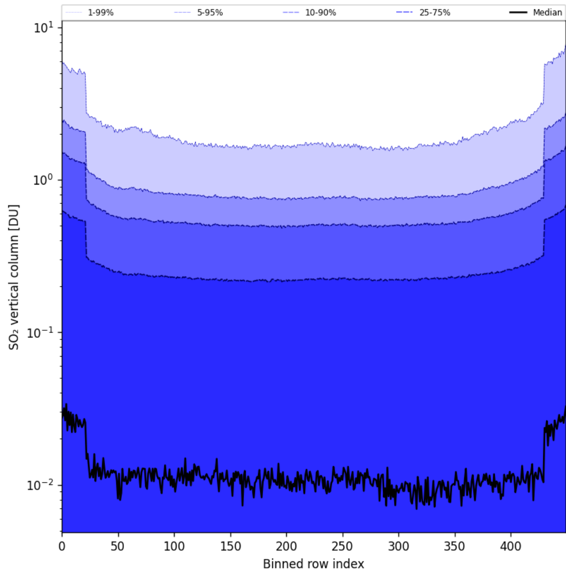
Figure 84: Along track statistics of “SO 2 vertical column” for 2025-08-01 to 2025-08-03
