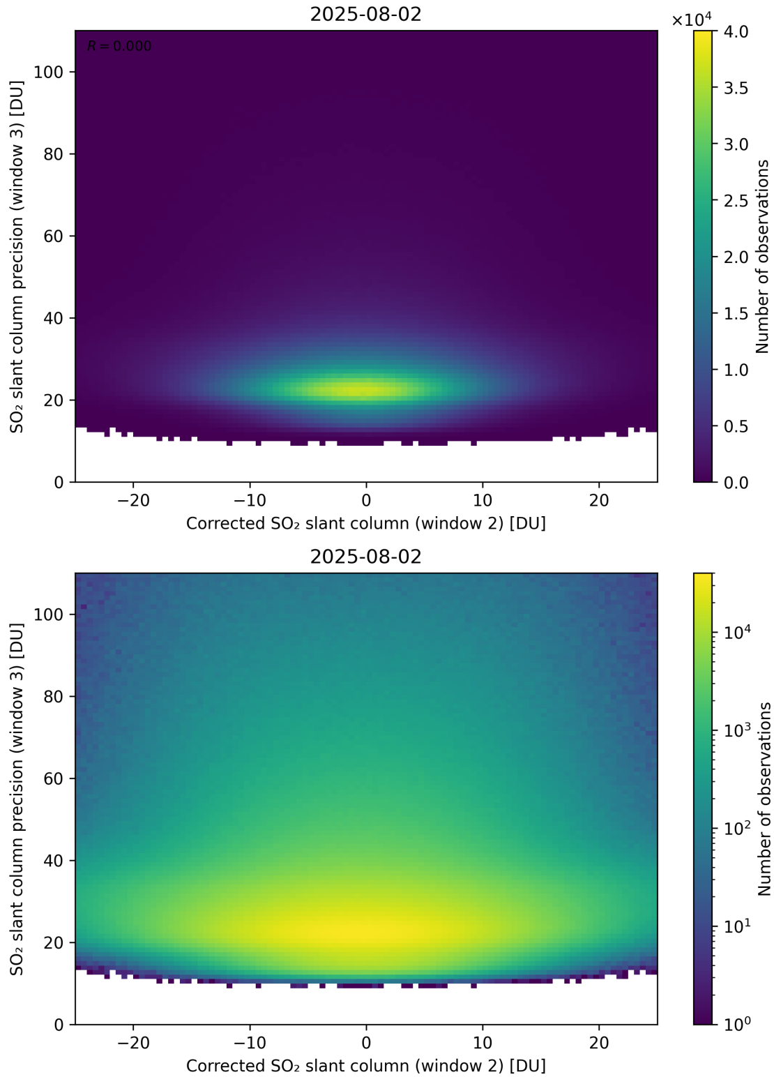
Figure 252: Scatter density plot of “Corrected SO 2 slant column (window 2)” against “SO 2 slant column precision (window 3)” for 2025-08-01 to 2025-08-03.
