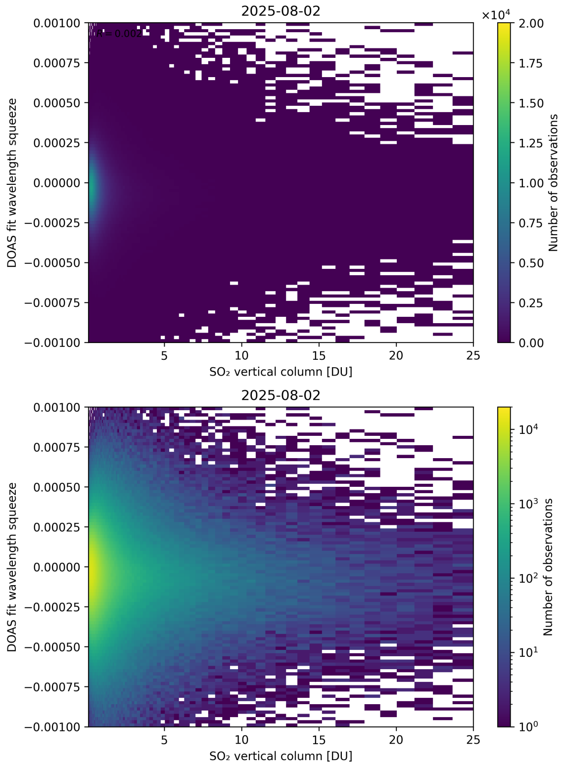
Figure 327: Scatter density plot of “SO 2 vertical column” against “DOAS fit wavelength squeeze” for 2025-08-01 to 2025-08-03.
