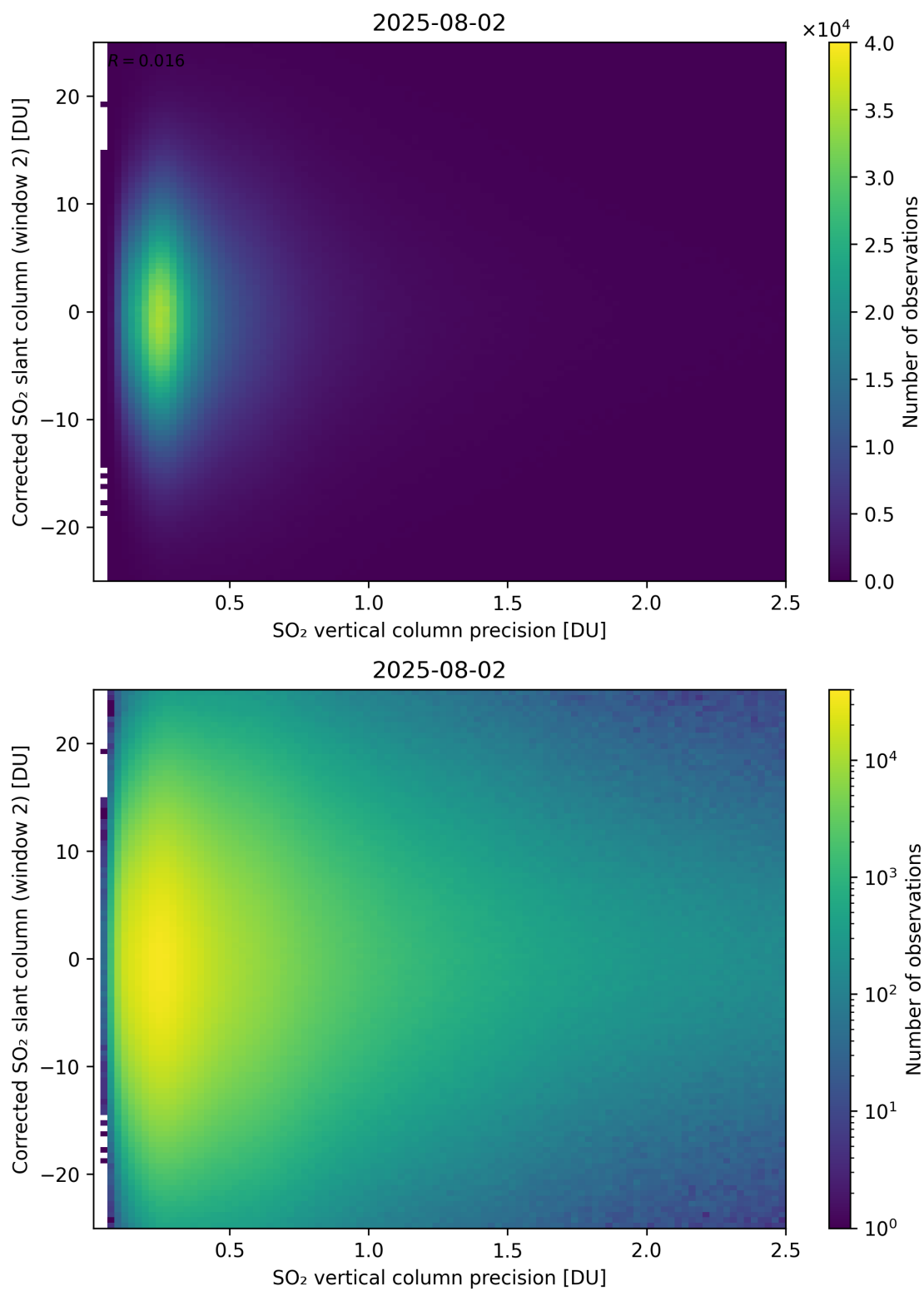
Figure 339: Scatter density plot of “SO 2 vertical column precision” against “Corrected SO 2 slant column (window 2)” for 2025-08-01 to 2025-08-03.
