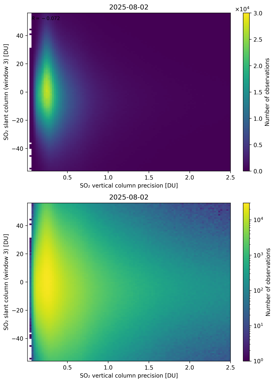
Figure 344: Scatter density plot of “SO 2 vertical column precision” against “SO 2 slant column (window 3)” for 2025-08-01 to 2025-08-03.
