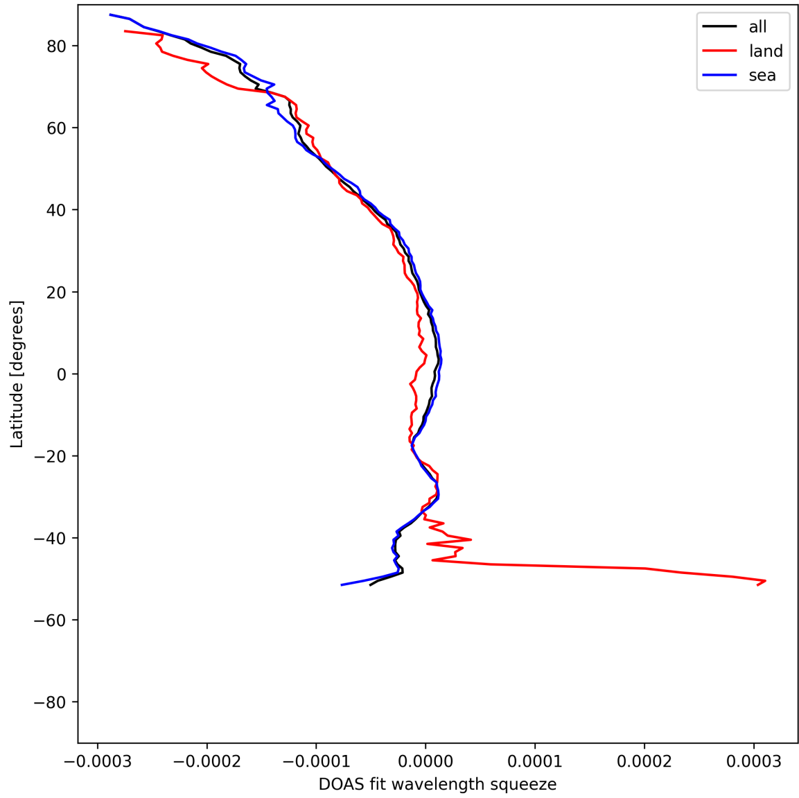
Figure 51: Zonal average of "DOAS fit wavelength squeeze" for 2025-08-01 to 2025-08-03.
