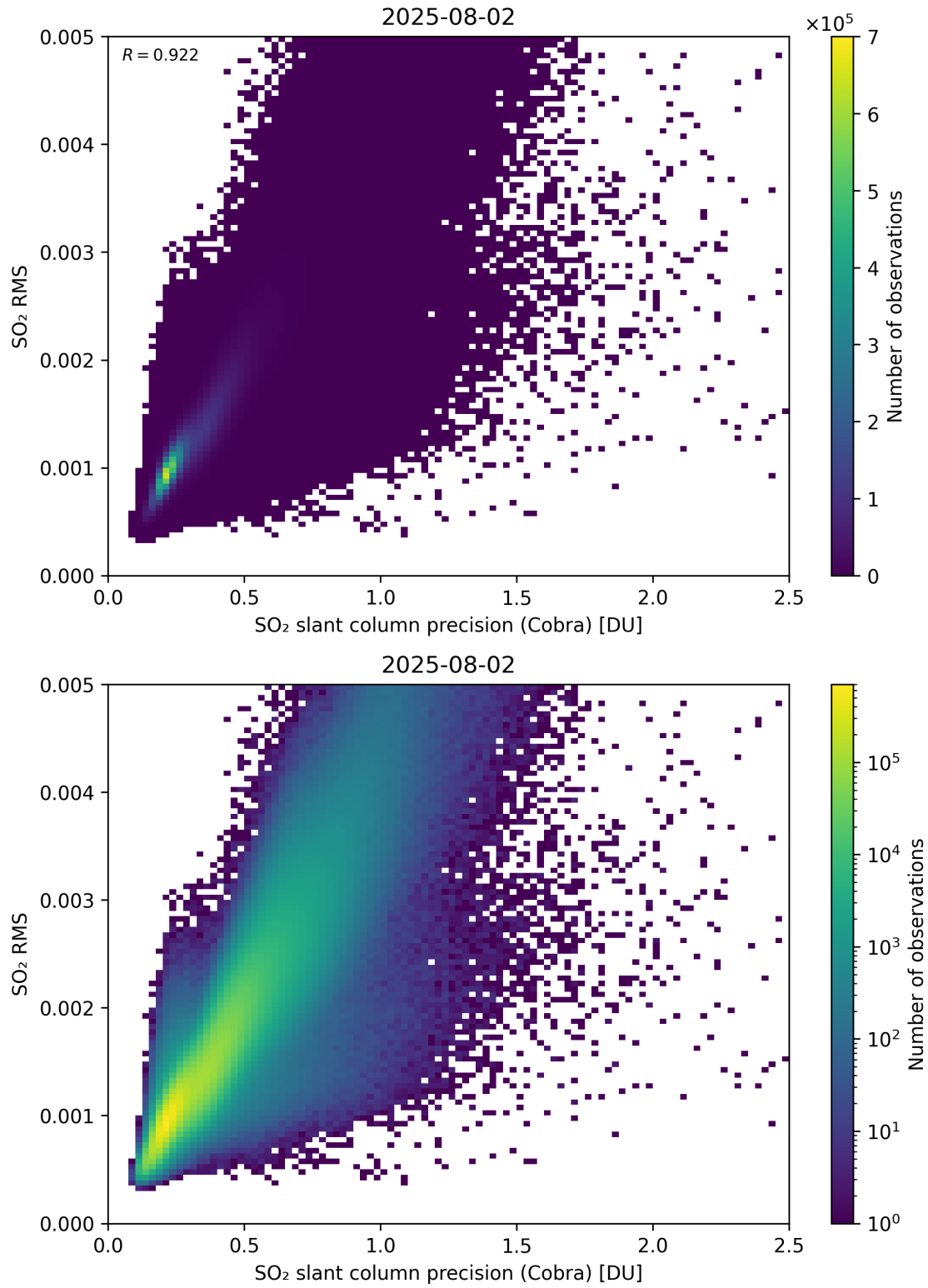
Figure 204: Scatter density plot of “SO 2 slant column precision (Cobra)” against “SO 2 RMS” for 2025-08-01 to 2025-08-03.
