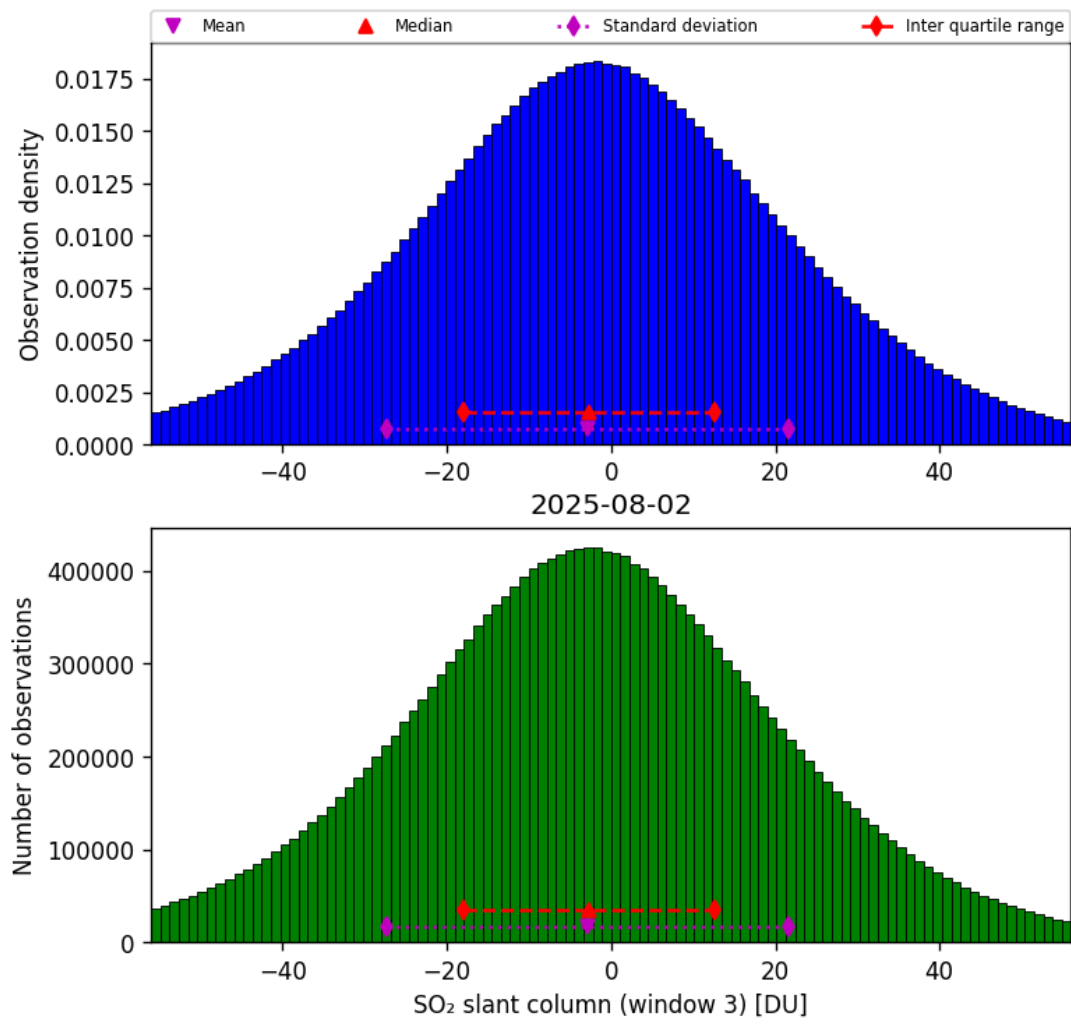
Figure 71: Histogram of “SO 2 slant column (window 3)” for 2025-08-01 to 2025-08-03
