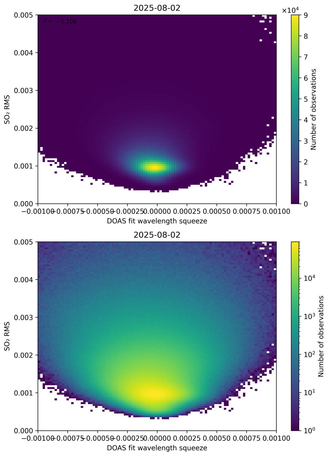
Figure 143: Scatter density plot of “DOAS fit wavelength squeeze” against “SO 2 RMS” for 2025-08-01 to 2025-08-03.
