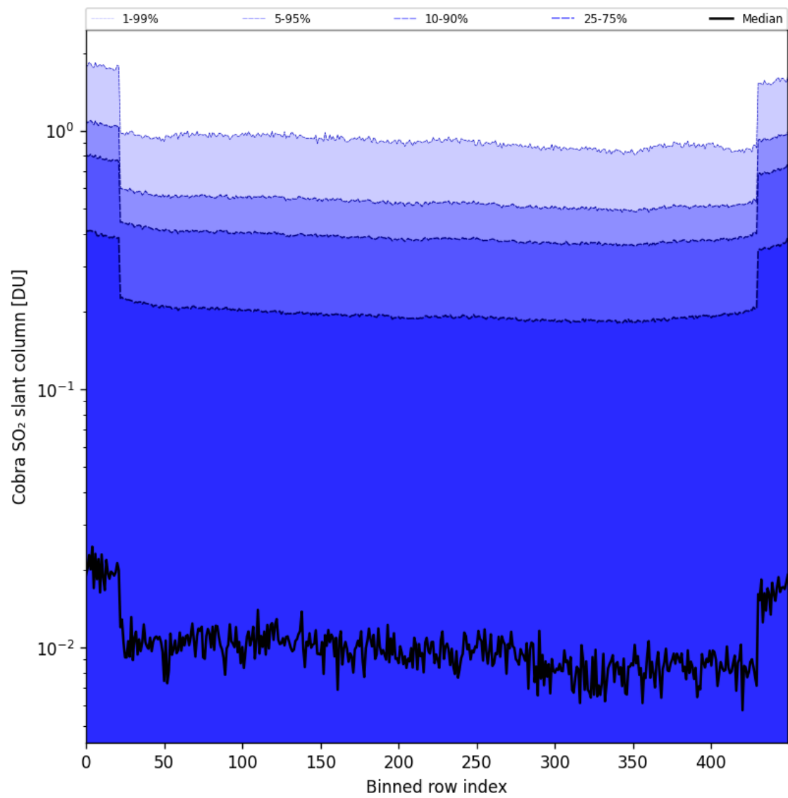
Figure 87: Along track statistics of “Cobra SO 2 slant column” for 2025-08-01 to 2025-08-03
