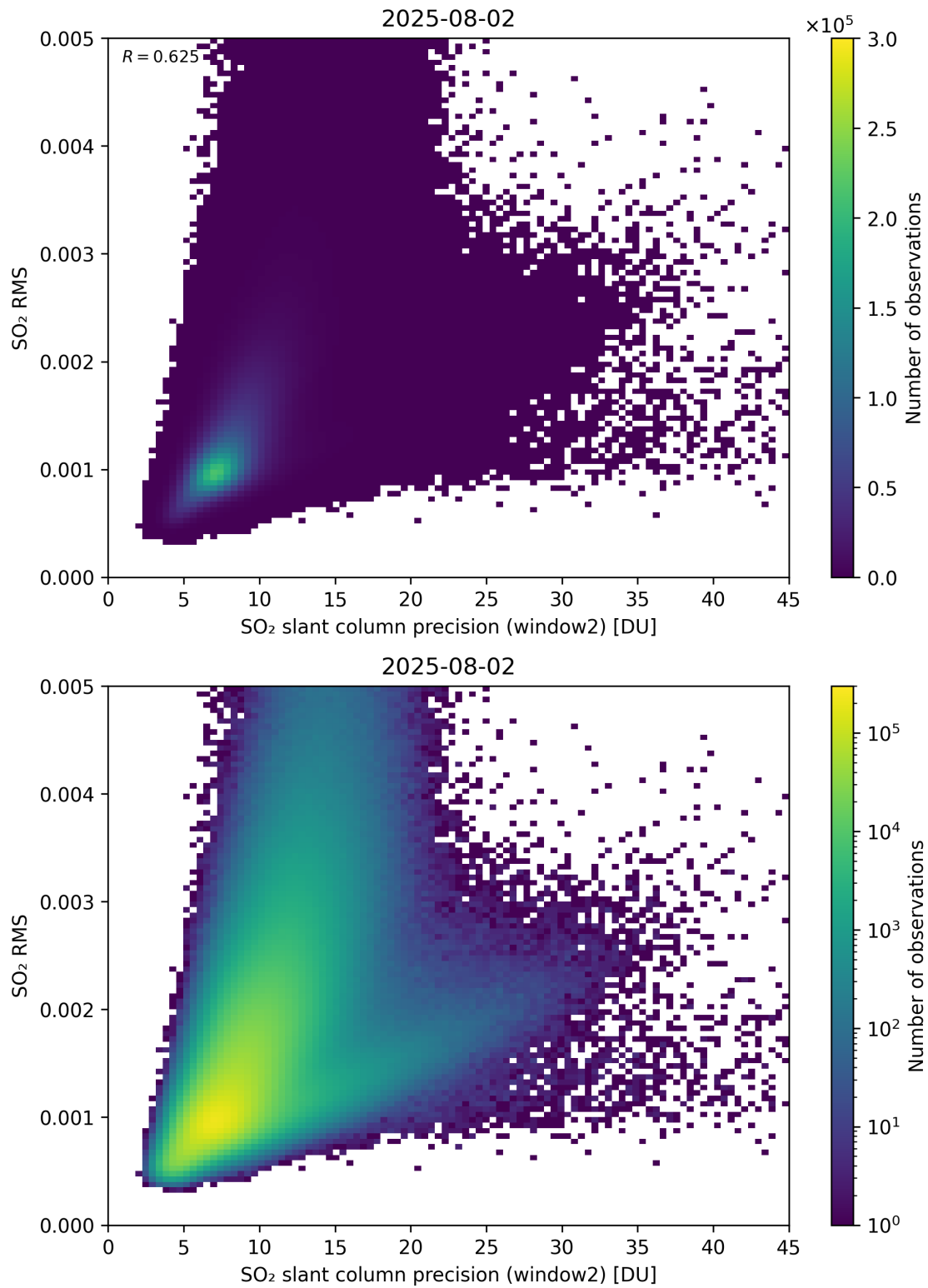
Figure 295: Scatter density plot of “SO 2 slant column precision (window2)” against “SO 2 RMS” for 2025-08-01 to 2025-08-03.
