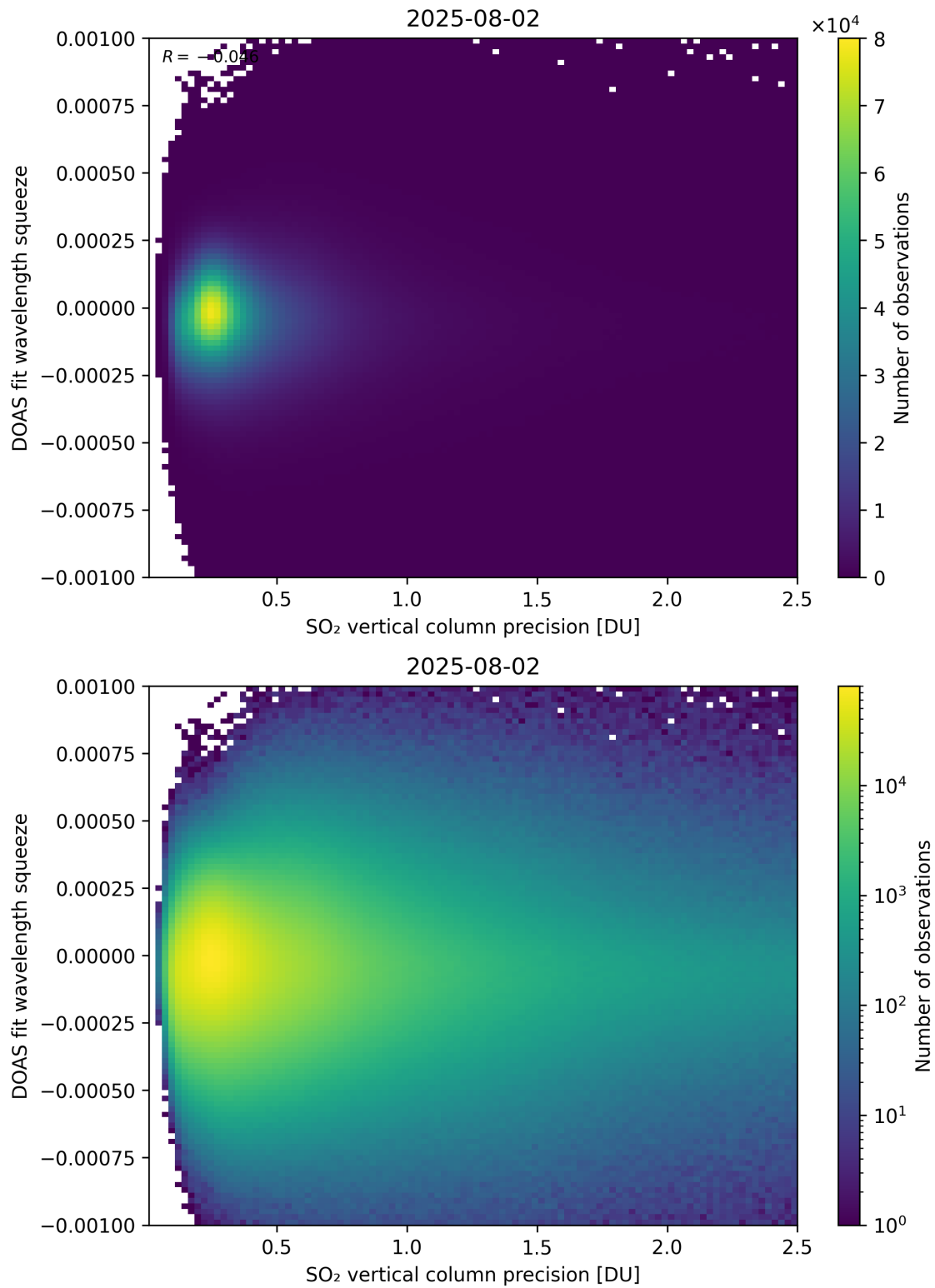
Figure 333: Scatter density plot of “SO 2 vertical column precision” against “DOAS fit wavelength squeeze” for 2025-08-01 to 2025-08-03.
