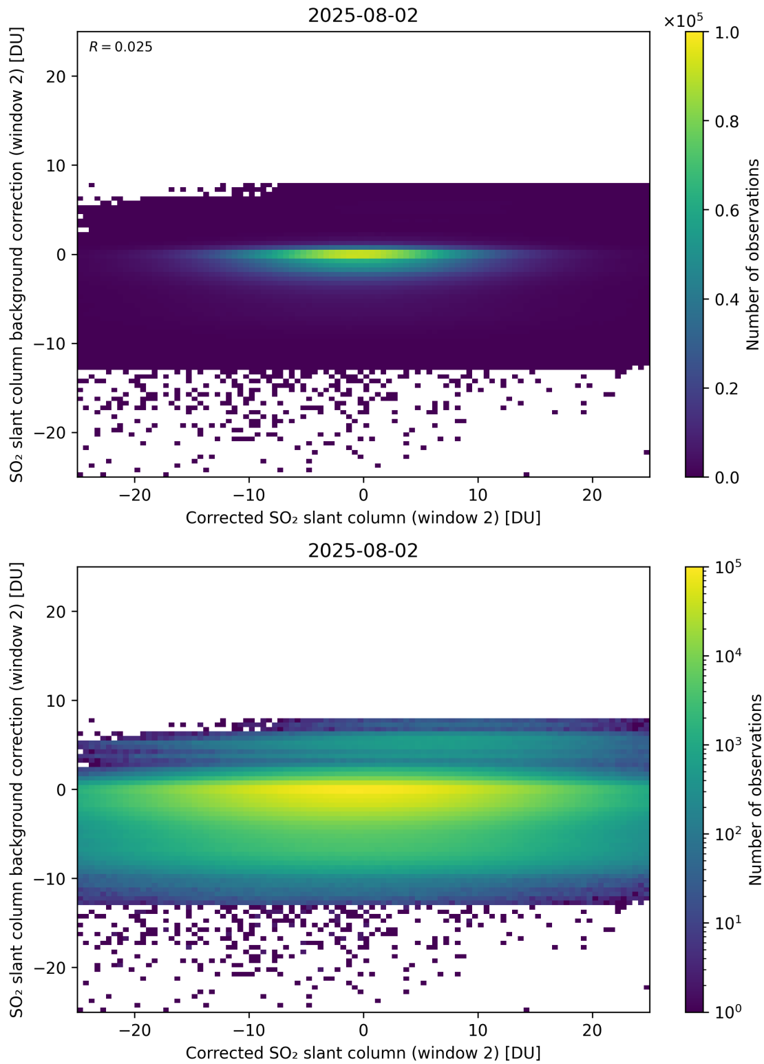
Figure 244: Scatter density plot of “Corrected SO 2 slant column (window 2)” against “SO 2 slant column background correction (window 2)” for 2025-08-01 to 2025-08-03.
