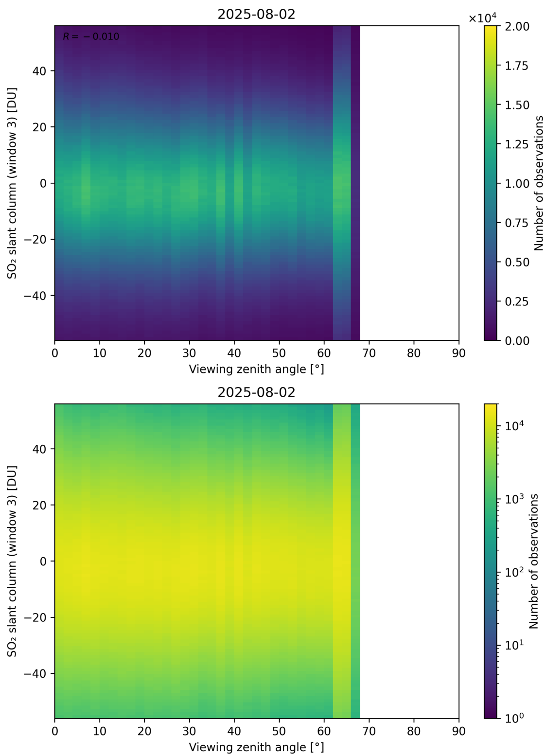
Figure 379: Scatter density plot of “Viewing zenith angle” against “SO 2 slant column (window 3)” for 2025-08-01 to 2025-08-03.
