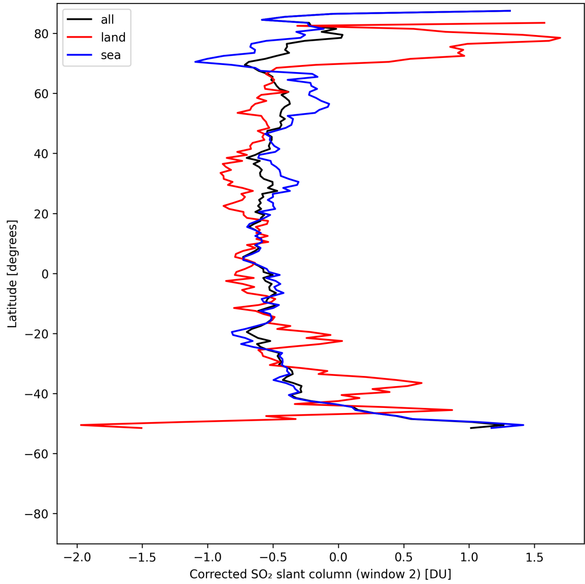
Figure 43: Zonal average of “Corrected SO 2 slant column (window 2)” for 2025-08-01 to 2025-08-03.
