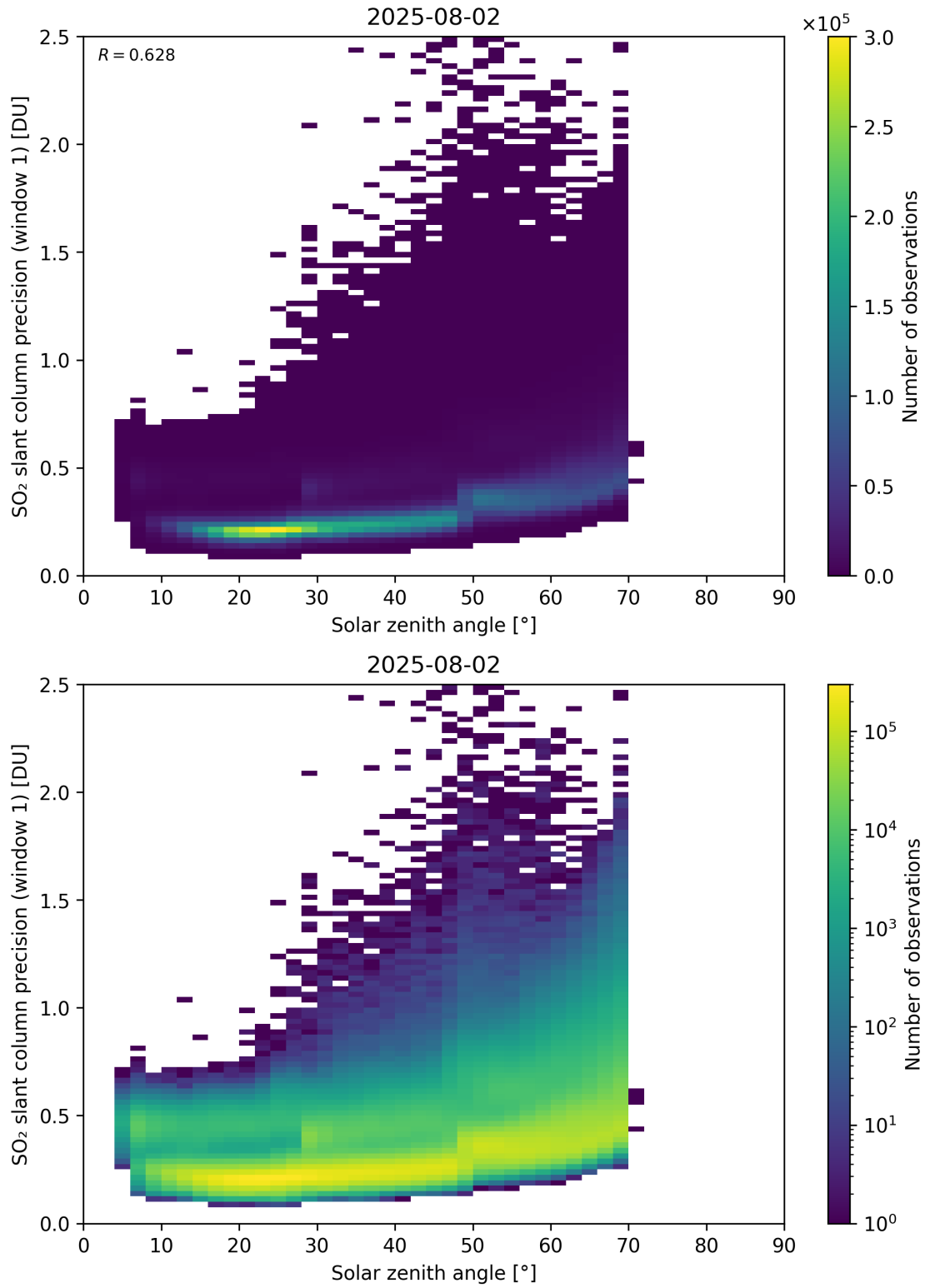
Figure 185: Scatter density plot of “Solar zenith angle” against “SO 2 slant column precision (window 1)” for 2025-08-01 to 2025-08-03.
