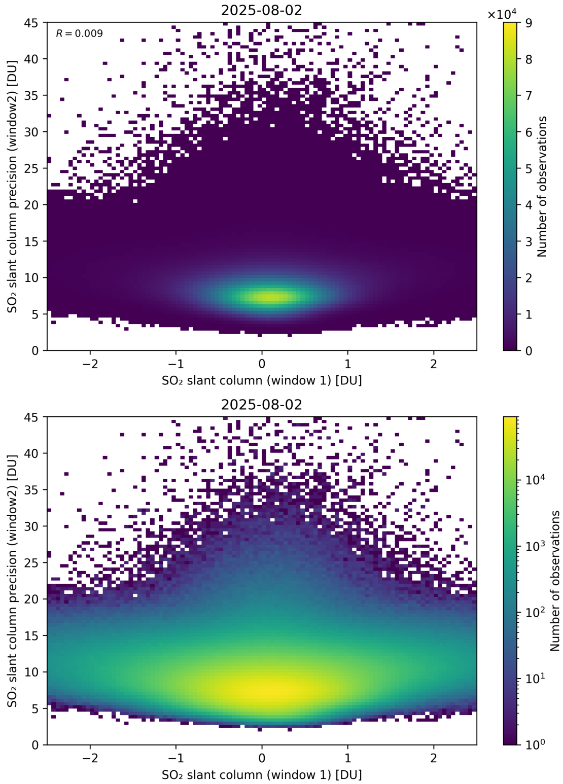
Figure 286: Scatter density plot of “SO 2 slant column (window 1)” against “SO 2 slant column precision (window2)” for 2025-08-01 to 2025-08-03.
