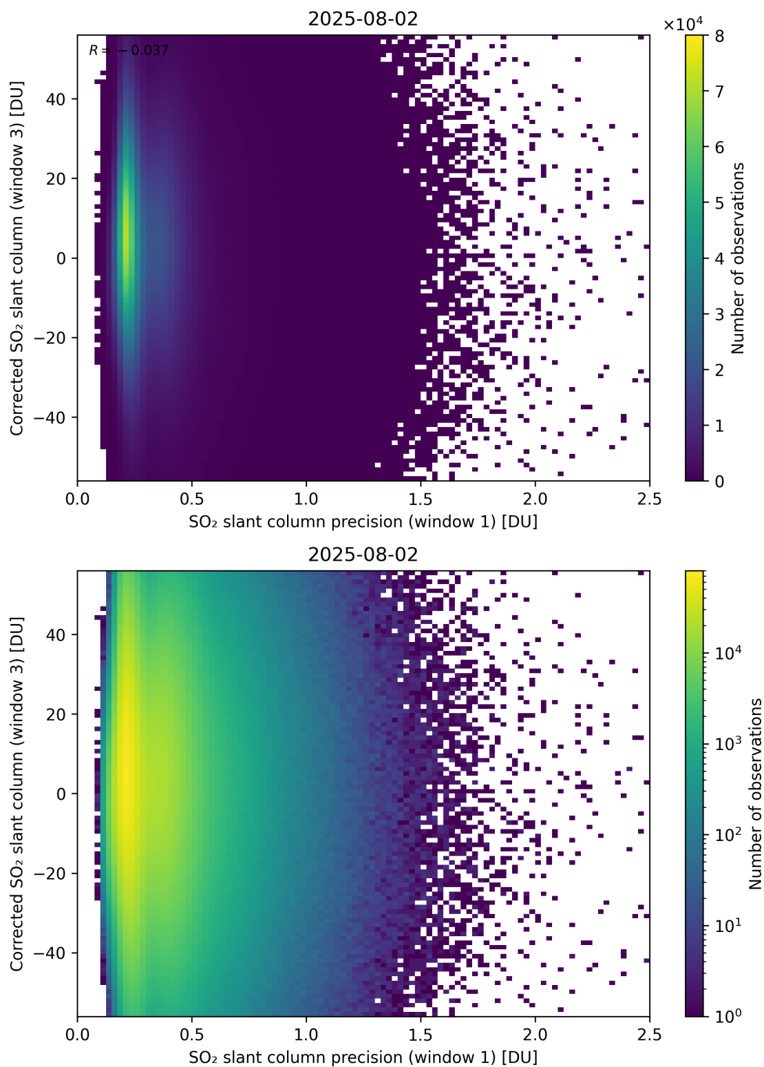
Figure 276: Scatter density plot of “SO 2 slant column precision (window 1)” against “Corrected SO 2 slant column (window 3)” for 2025-08-01 to 2025-08-03.
