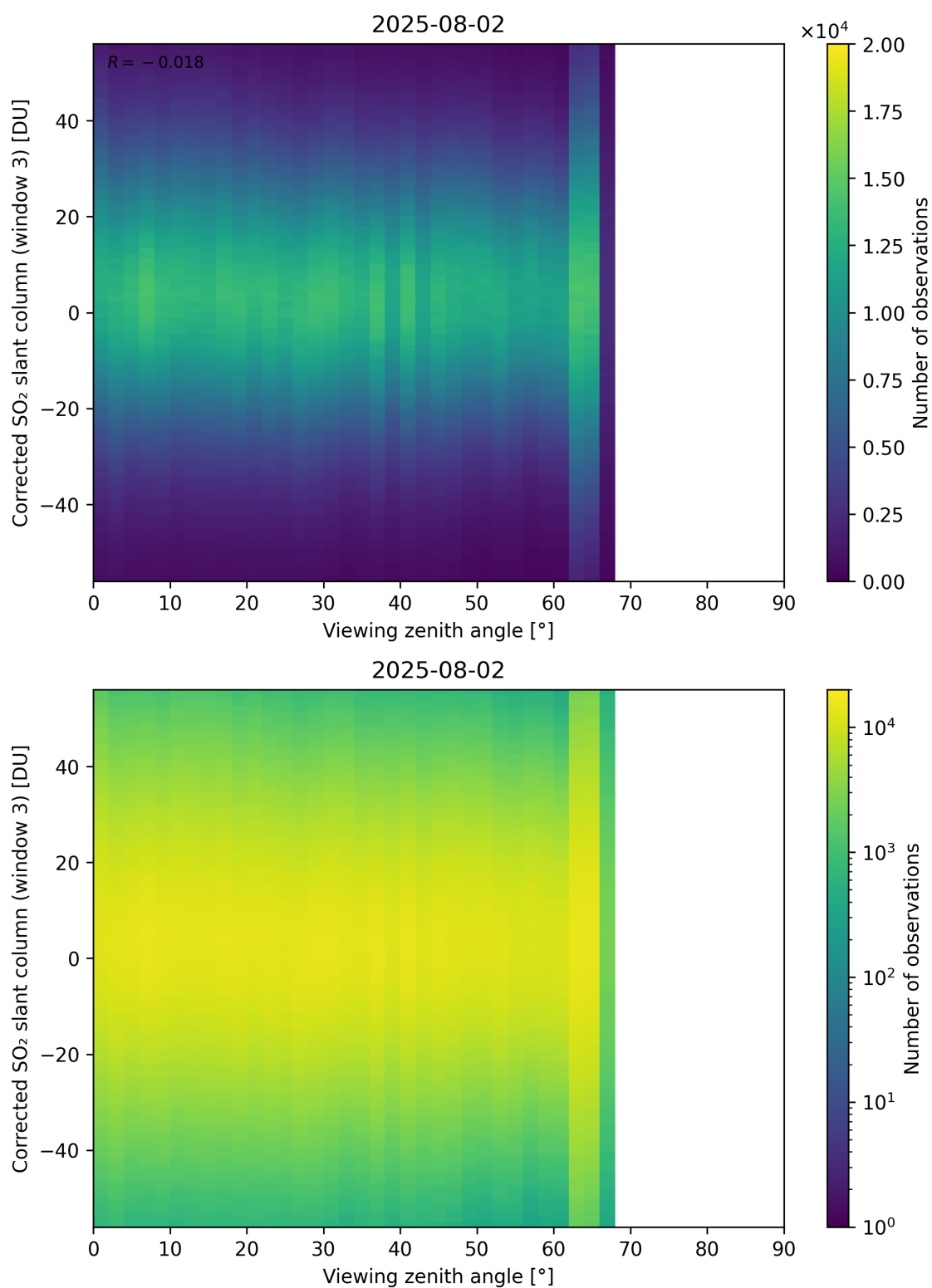
Figure 375: Scatter density plot of “Viewing zenith angle” against “Corrected SO 2 slant column (window 3)” for 2025-08-01 to 2025-08-03.
