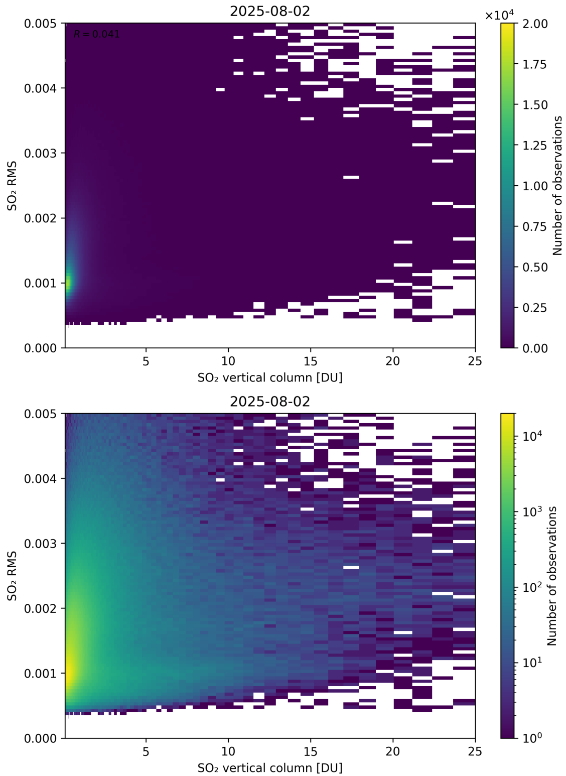
Figure 328: Scatter density plot of “SO 2 vertical column” against “SO 2 RMS” for 2025-08-01 to 2025-08-03.
