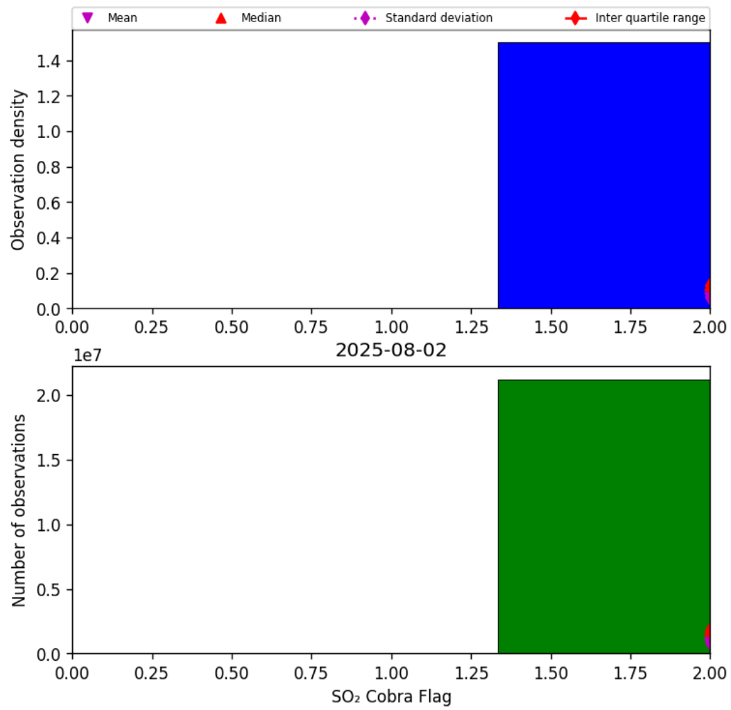
Figure 75: Histogram of “SO 2 Cobra Flag” for 2025-08-01 to 2025-08-03
