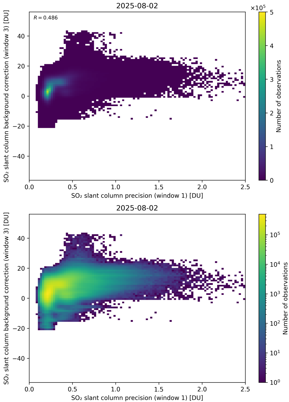
Figure 270: Scatter density plot of “SO 2 slant column precision (window 1)” against “SO 2 slant column background correction (window 3)” for 2025-08-01 to 2025-08-03.
