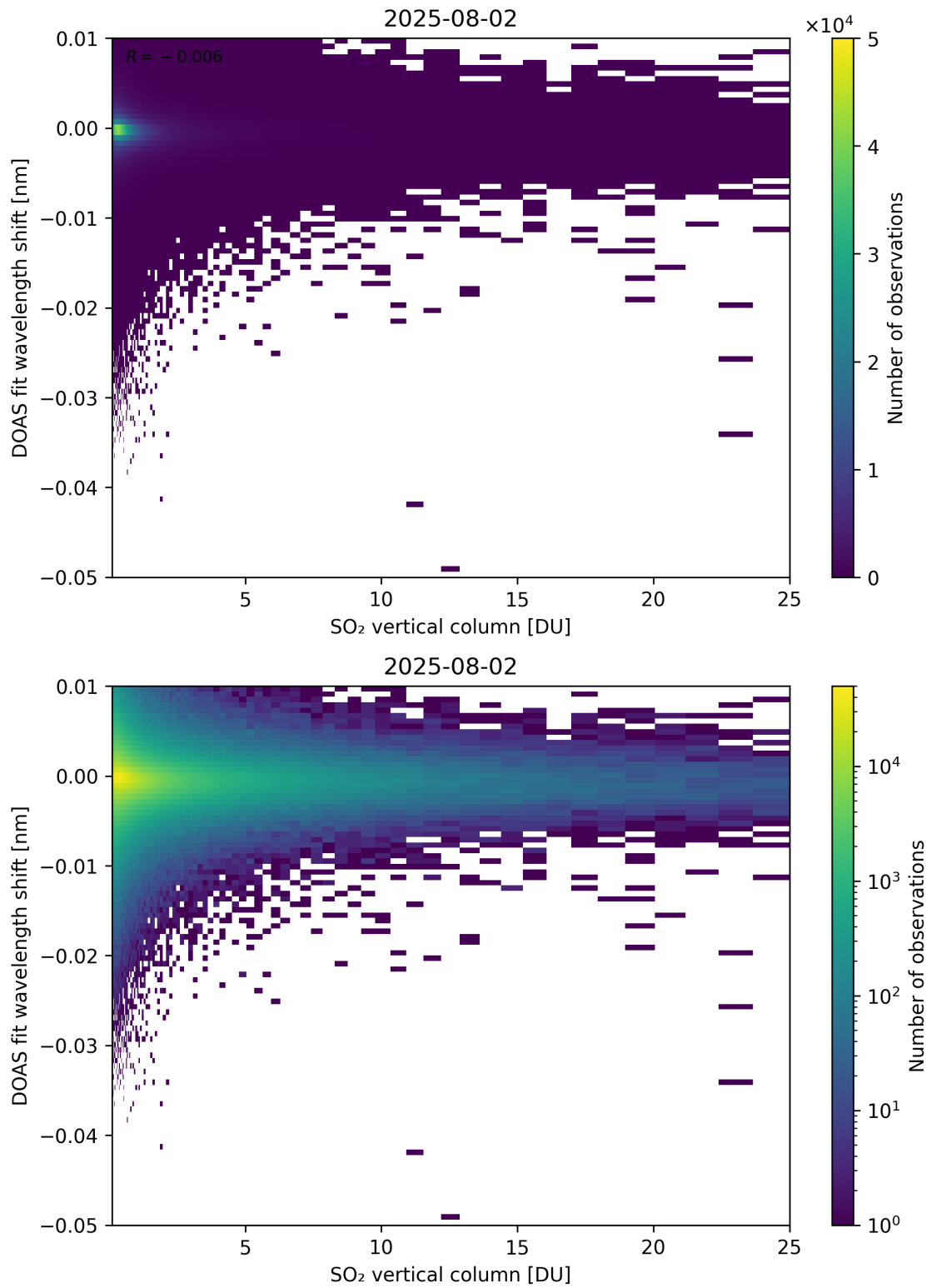
Figure 326: Scatter density plot of “SO 2 vertical column” against “DOAS fit wavelength shift” for 2025-08-01 to 2025-08-03.
