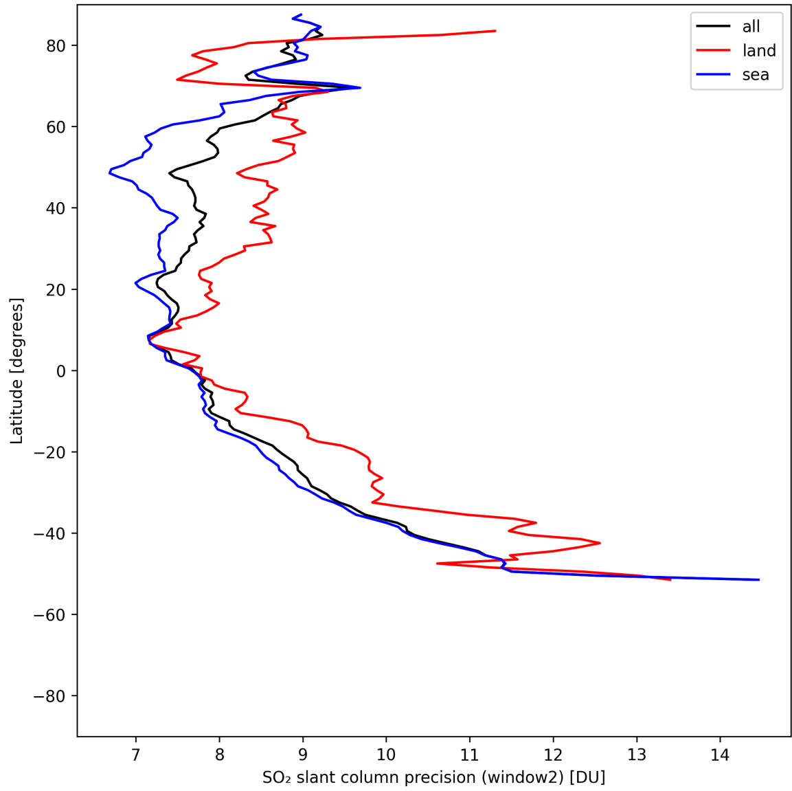
Figure 42: Zonal average of “SO 2 slant column precision (window2)” for 2025-08-01 to 2025-08-03.
