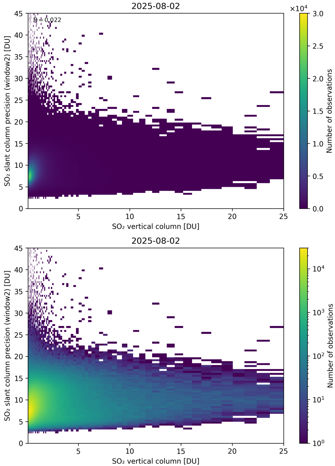
Figure 356: Scatter density plot of “SO 2 vertical column” against “SO 2 slant column precision (window2)” for 2025-08-01 to 2025-08-03.
