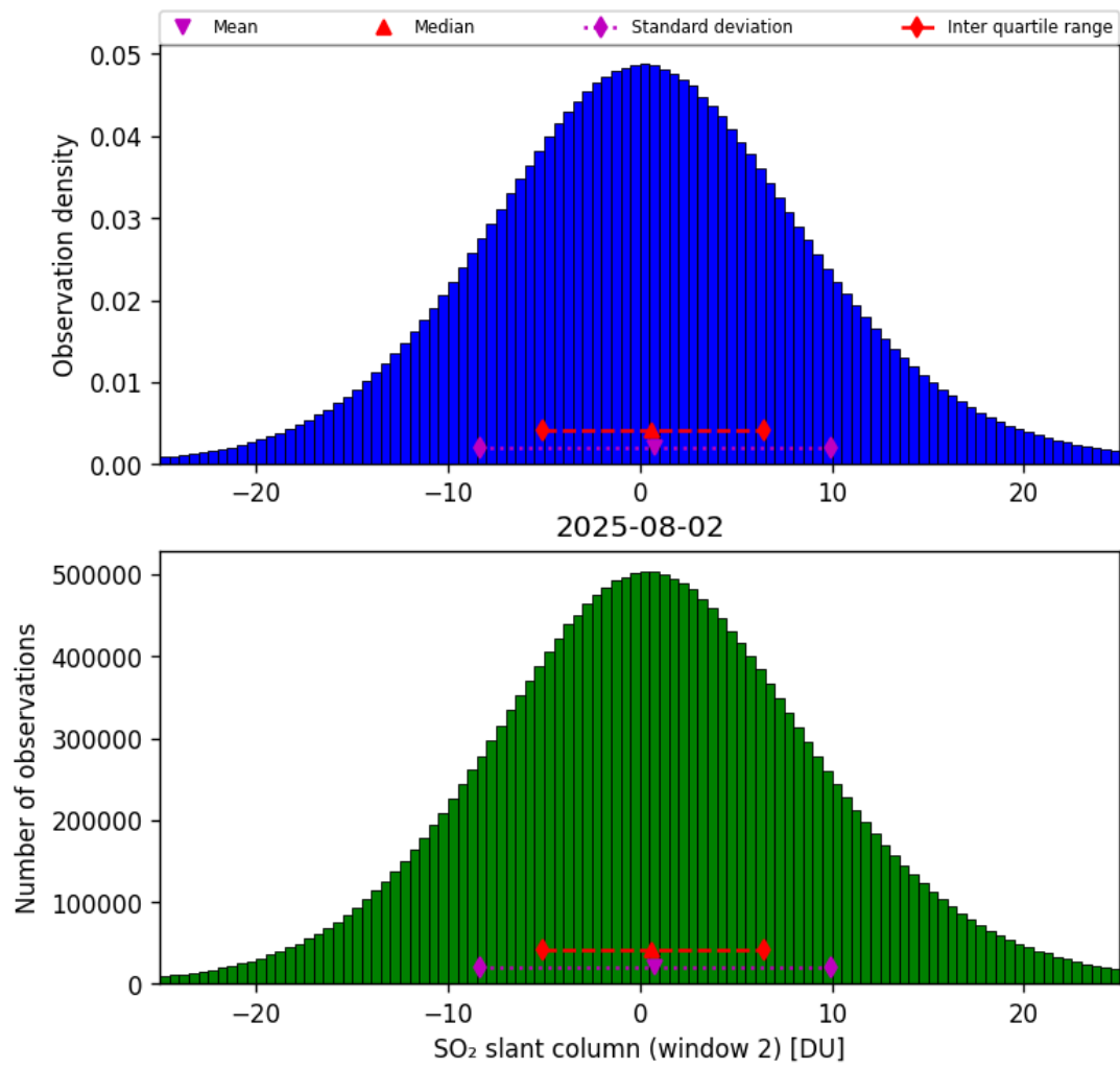
Figure 67: Histogram of “SO 2 slant column (window 2)” for 2025-08-01 to 2025-08-03
