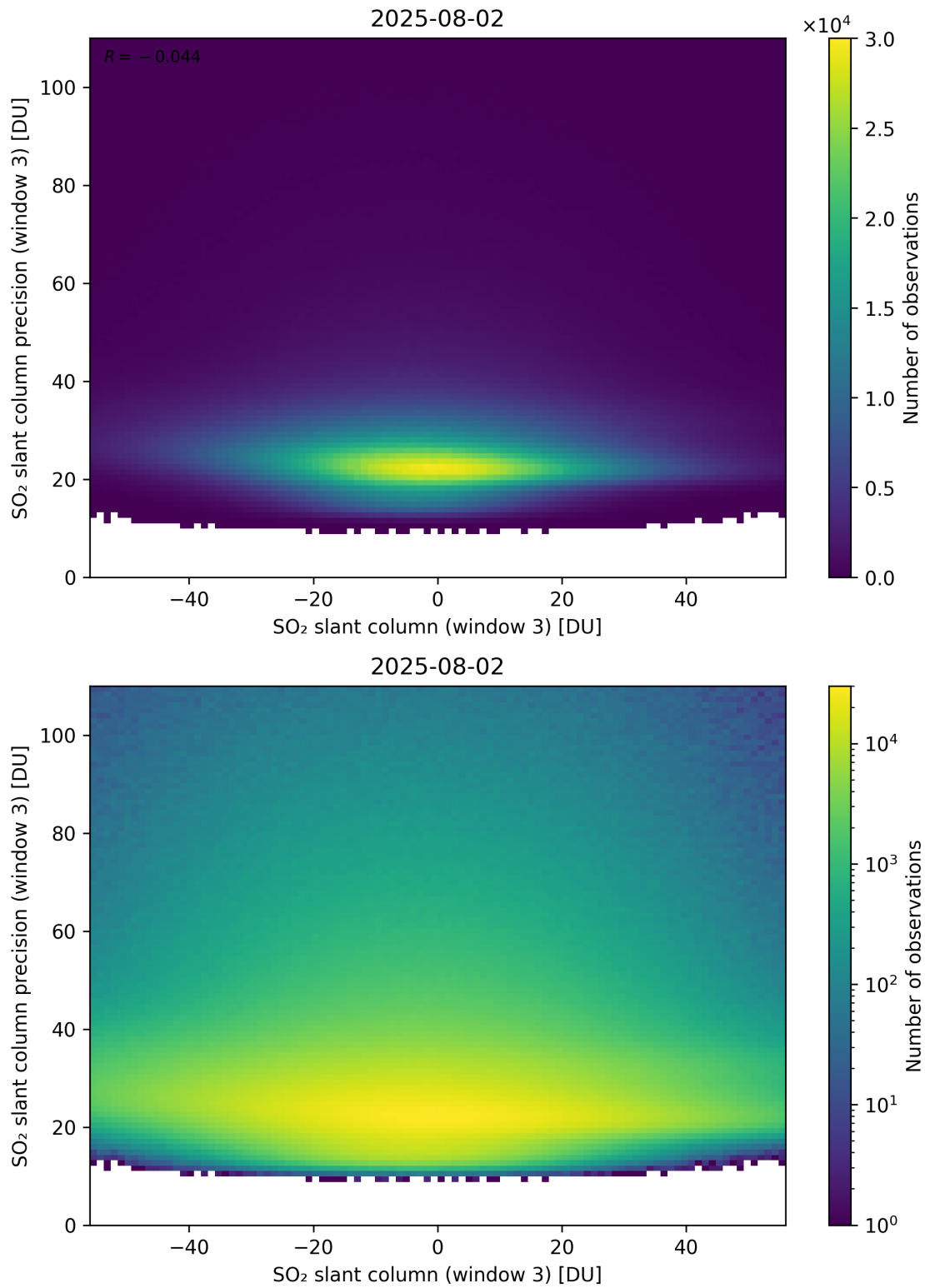
Figure 317: Scatter density plot of “SO 2 slant column (window 3)” against “SO 2 slant column precision (window 3)” for 2025-08-01 to 2025-08-03.
