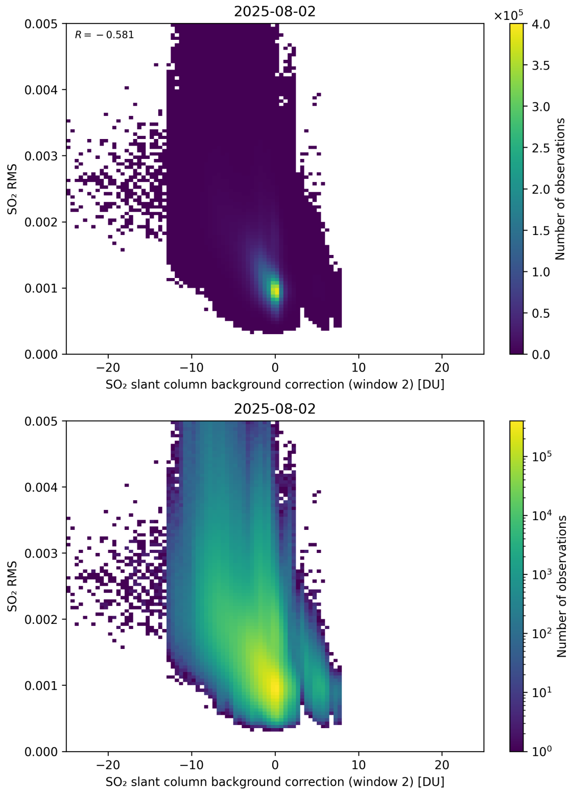
Figure 125: Scatter density plot of “SO 2 slant column background correction (window 2)” against “SO 2 RMS” for 2025-08-01 to 2025-08-03.
