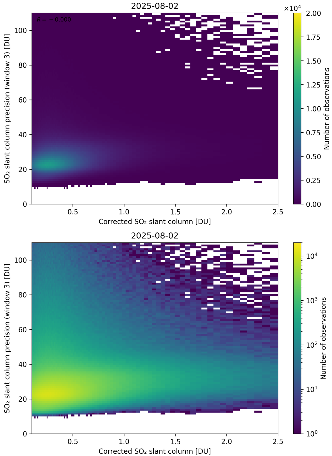
Figure 241: Scatter density plot of “Corrected SO 2 slant column” against “SO 2 slant column precision (window 3)” for 2025-08-01 to 2025-08-03.
