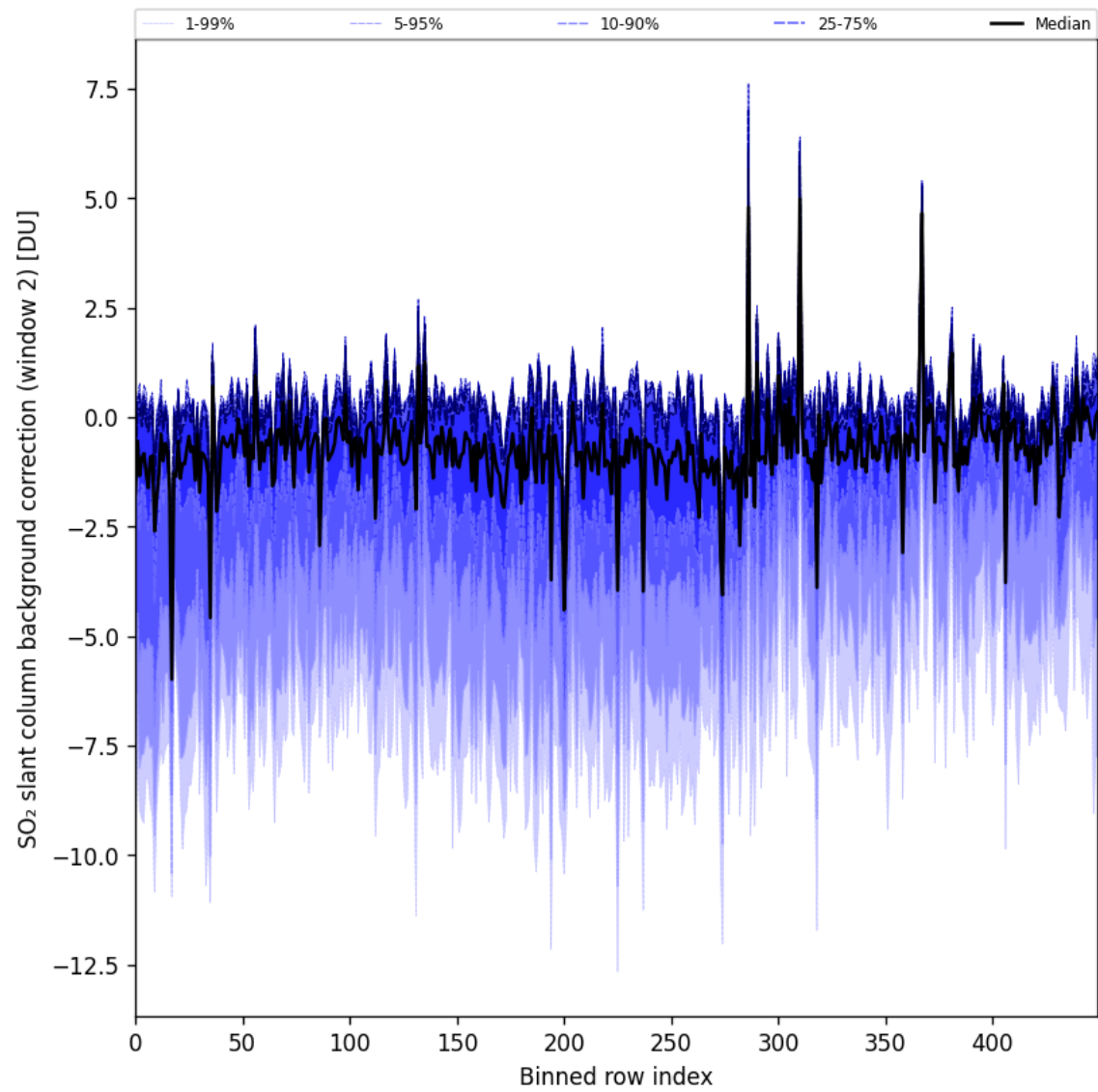
Figure 96: Along track statistics of “SO 2 slant column background correction (window 2)” for 2025-08-01 to 2025-08-03
