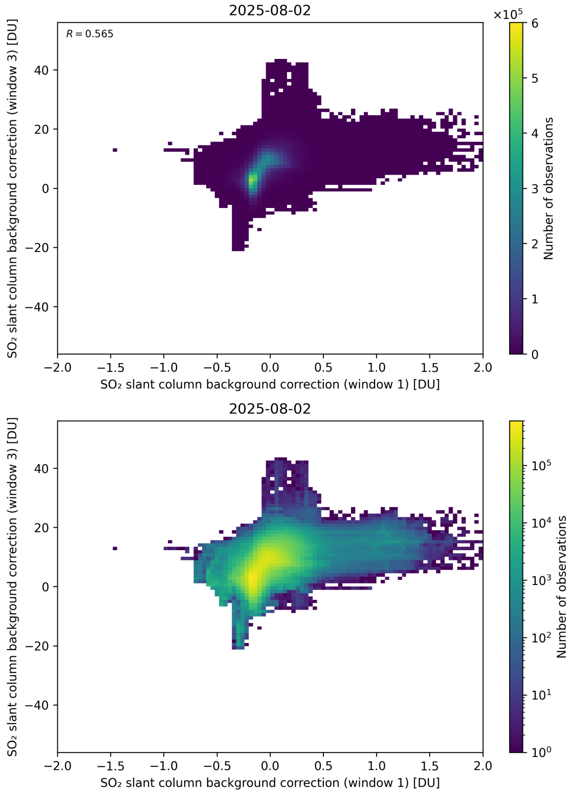
Figure 110: Scatter density plot of “SO 2 slant column background correction (window 1)” against “SO 2 slant column background correction (window 3)” for 2025-08-01 to 2025-08-03.
