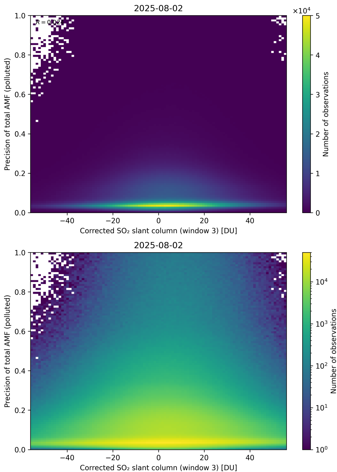
Figure 261: Scatter density plot of “Corrected SO 2 slant column (window 3)” against “Precision of total AMF (polluted)” for 2025-08-01 to 2025-08-03.
