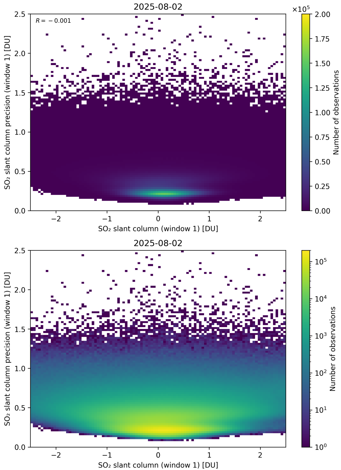
Figure 285: Scatter density plot of “SO 2 slant column (window 1)” against “SO 2 slant column precision (window 1)” for 2025-08-01 to 2025-08-03.
