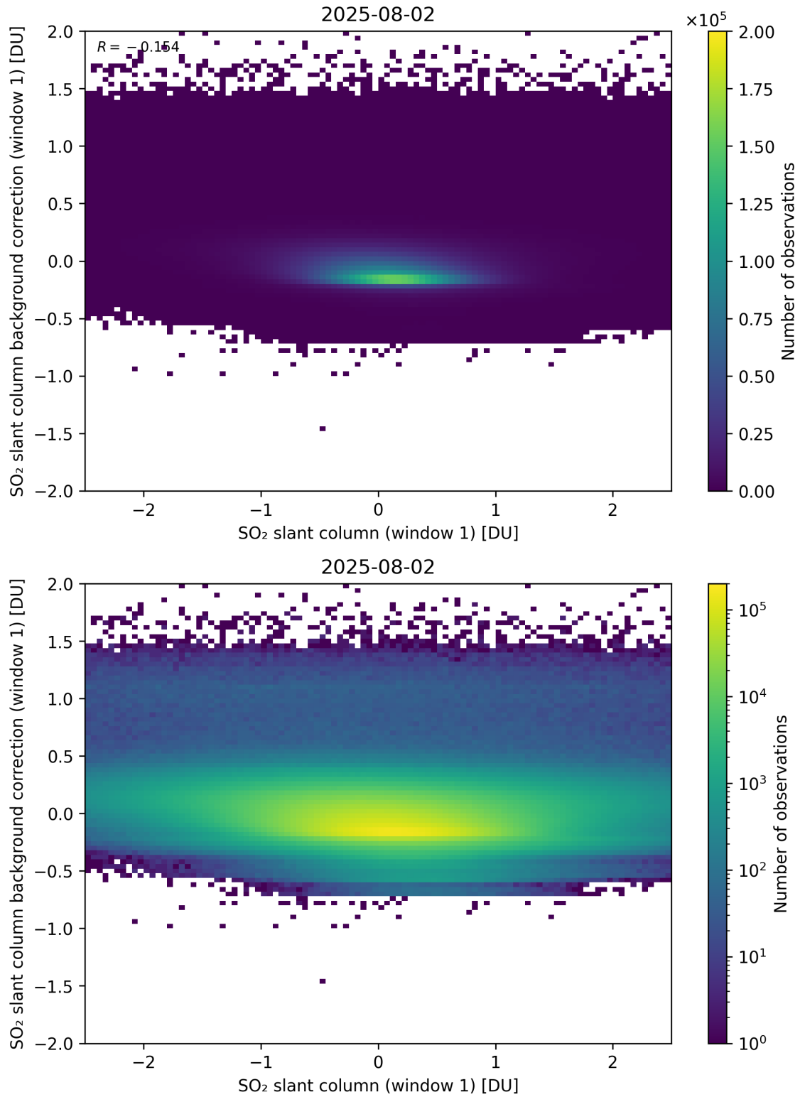
Figure 262: Scatter density plot of “SO 2 slant column (window 1)” against “SO 2 slant column background correction (window 1)” for 2025-08-01 to 2025-08-03.
