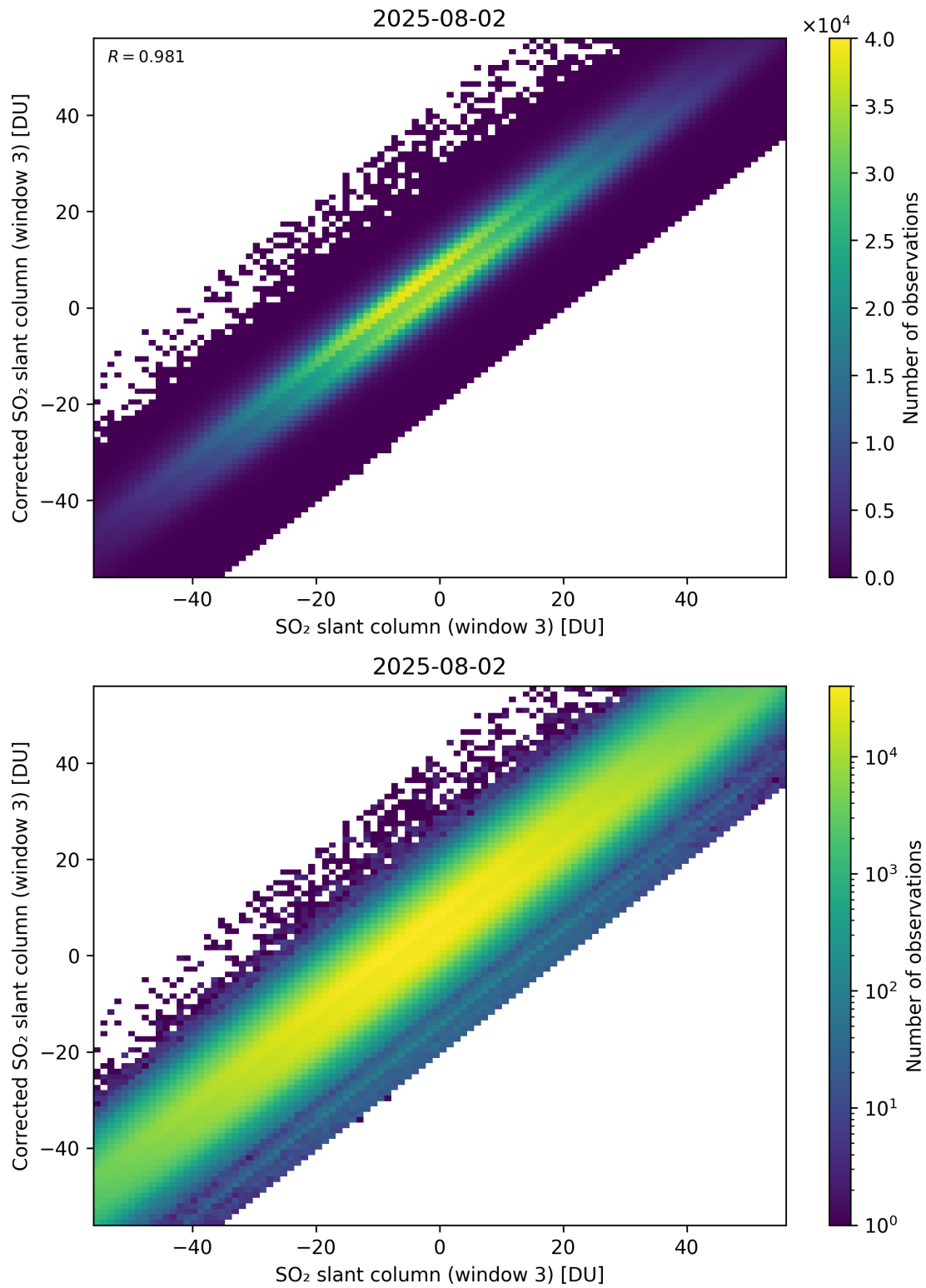
Figure 316: Scatter density plot of “SO 2 slant column (window 3)” against “Corrected SO 2 slant column (window 3)” for 2025-08-01 to 2025-08-03.
