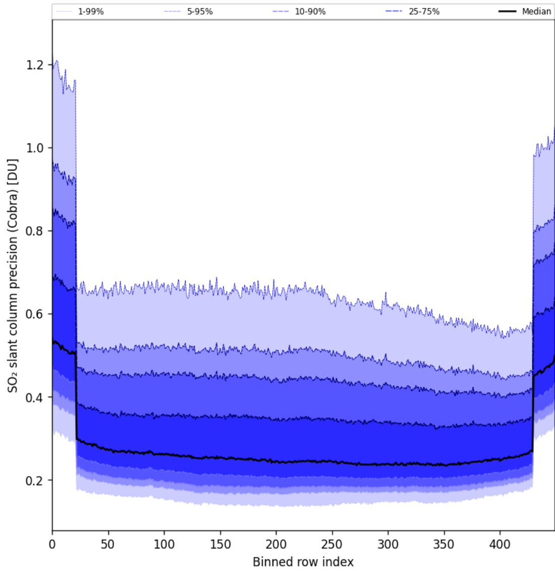
Figure 88: Along track statistics of “SO 2 slant column precision (Cobra)” for 2025-08-01 to 2025-08-03
