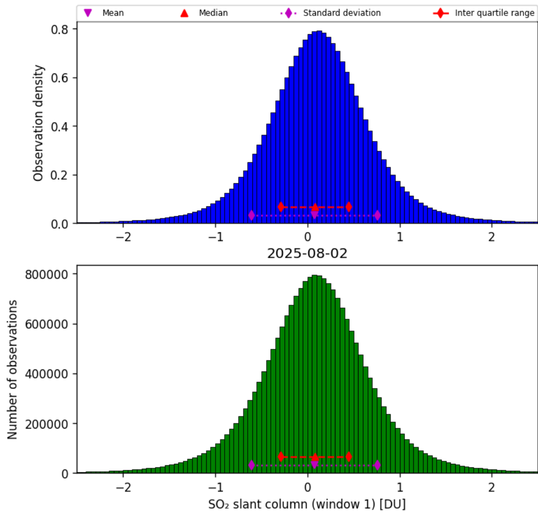
Figure 63: Histogram of “SO 2 slant column (window 1)” for 2025-08-01 to 2025-08-03
