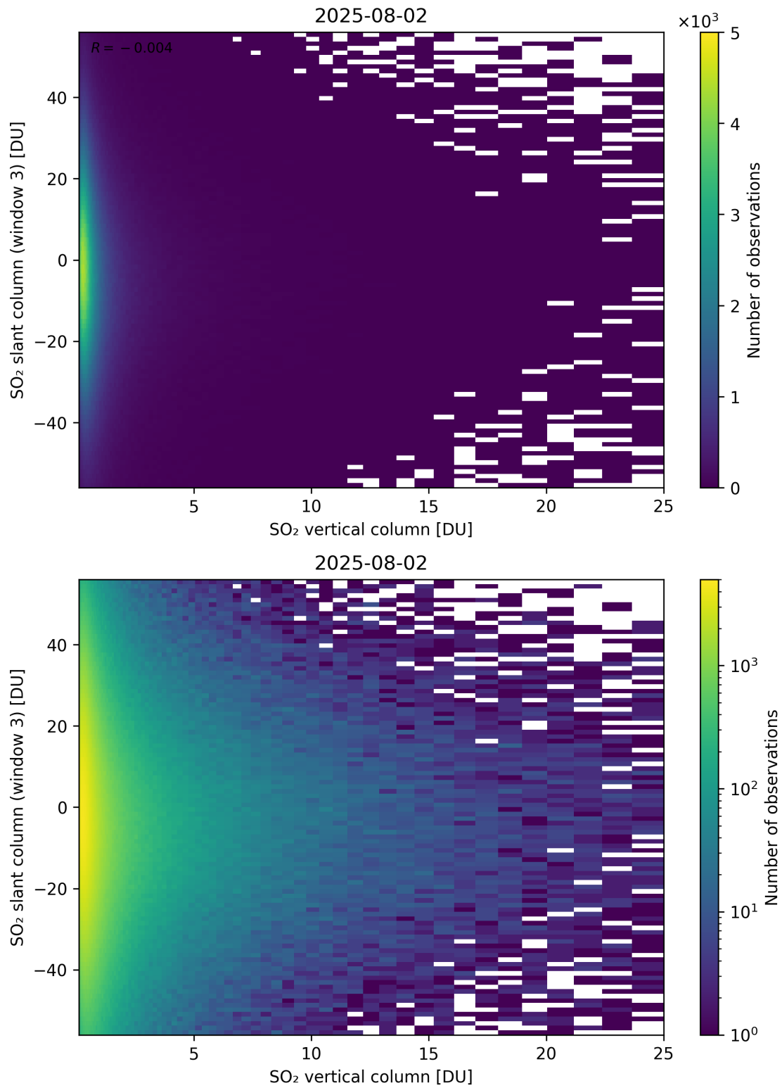
Figure 357: Scatter density plot of “SO 2 vertical column” against “SO 2 slant column (window 3)” for 2025-08-01 to 2025-08-03.
