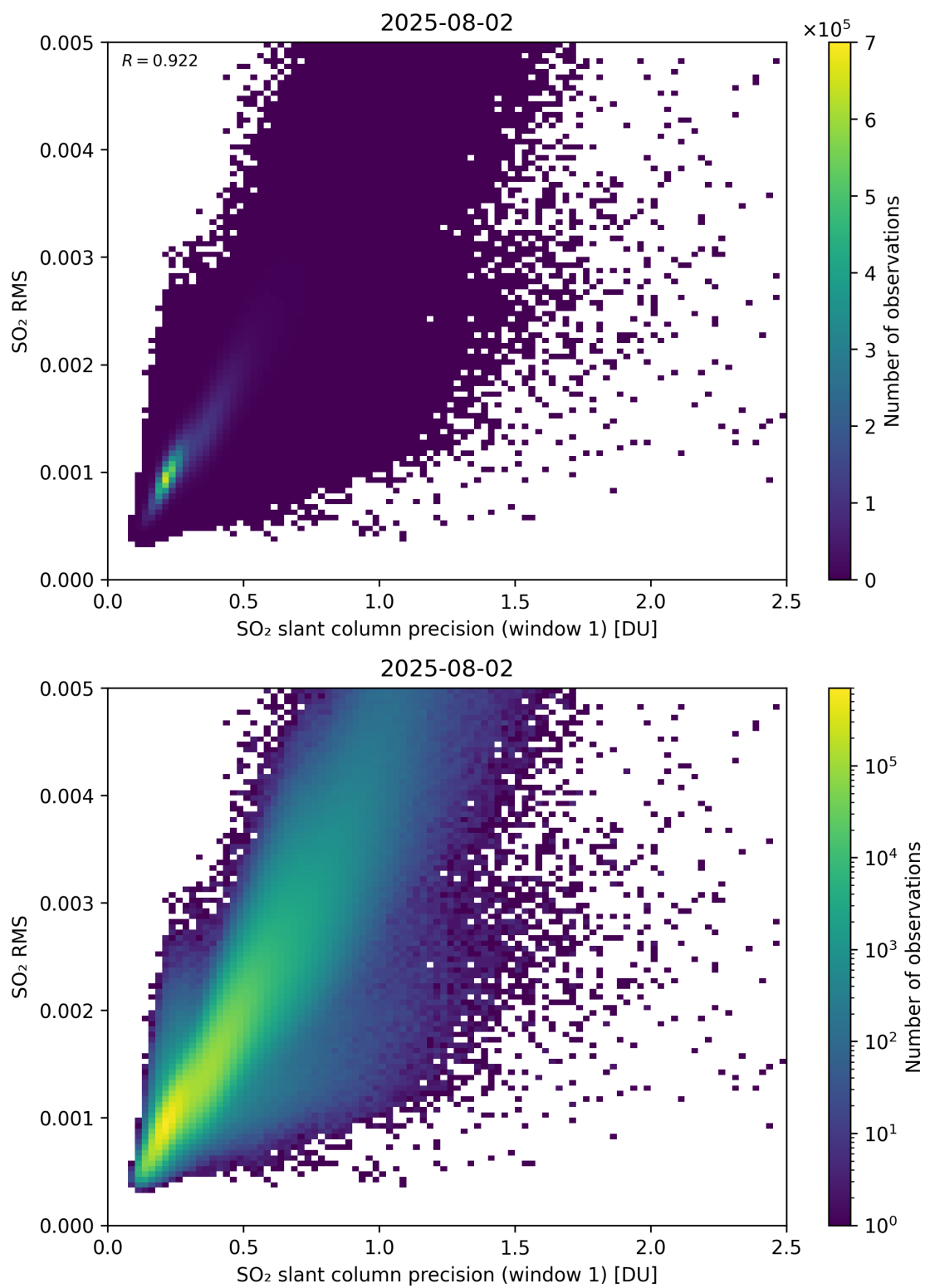
Figure 273: Scatter density plot of “SO 2 slant column precision (window 1)” against “SO 2 RMS” for 2025-08-01 to 2025-08-03.
