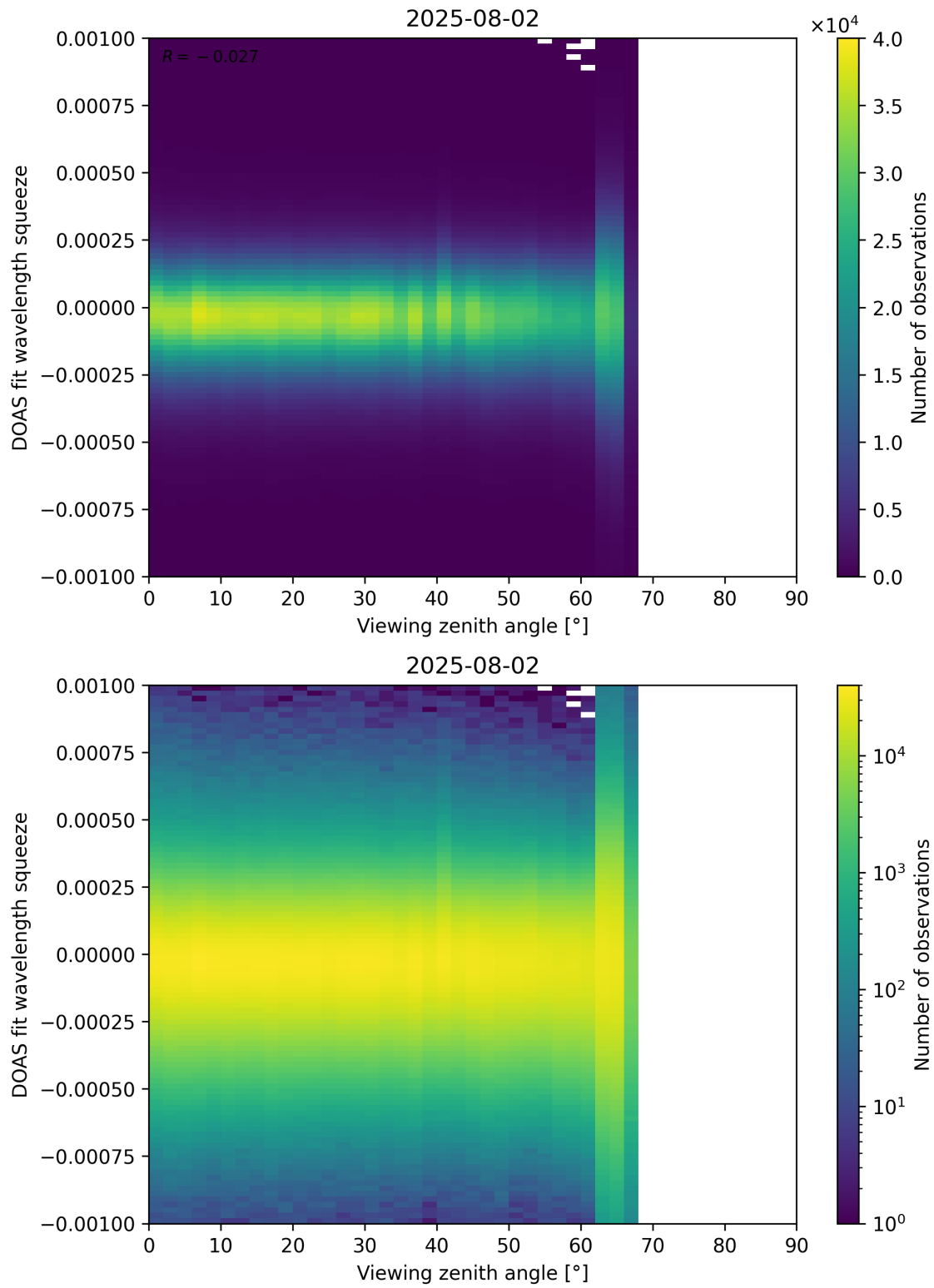
Figure 366: Scatter density plot of “Viewing zenith angle” against “DOAS fit wavelength squeeze” for 2025-08-01 to 2025-08-03.
