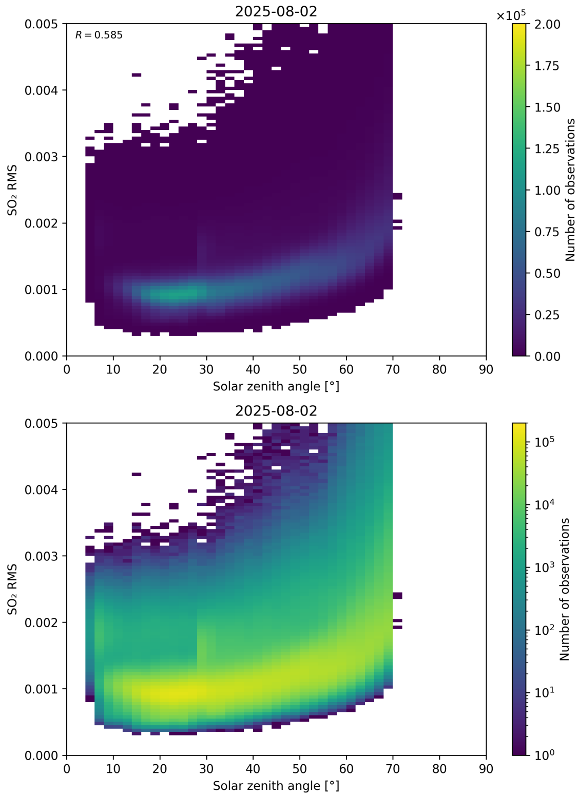
Figure 176: Scatter density plot of “Solar zenith angle” against “SO 2 RMS” for 2025-08-01 to 2025-08-03.
