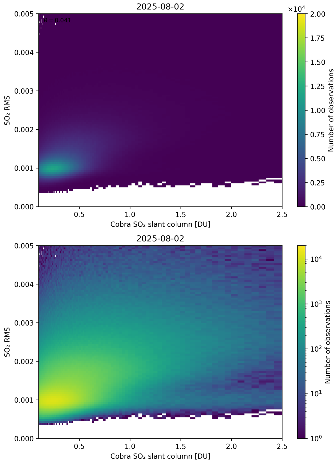
Figure 198: Scatter density plot of “Cobra SO 2 slant column” against “SO 2 RMS” for 2025-08-01 to 2025-08-03.
