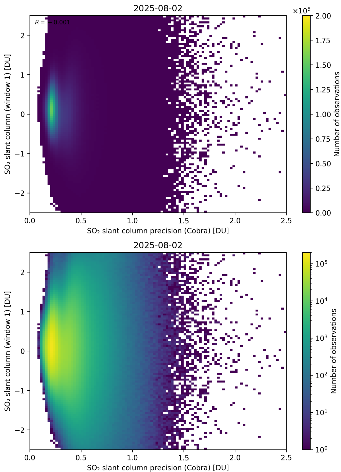
Figure 208: Scatter density plot of “SO 2 slant column precision (Cobra)” against “SO 2 slant column (window 1)” for 2025-08-01 to 2025-08-03.
