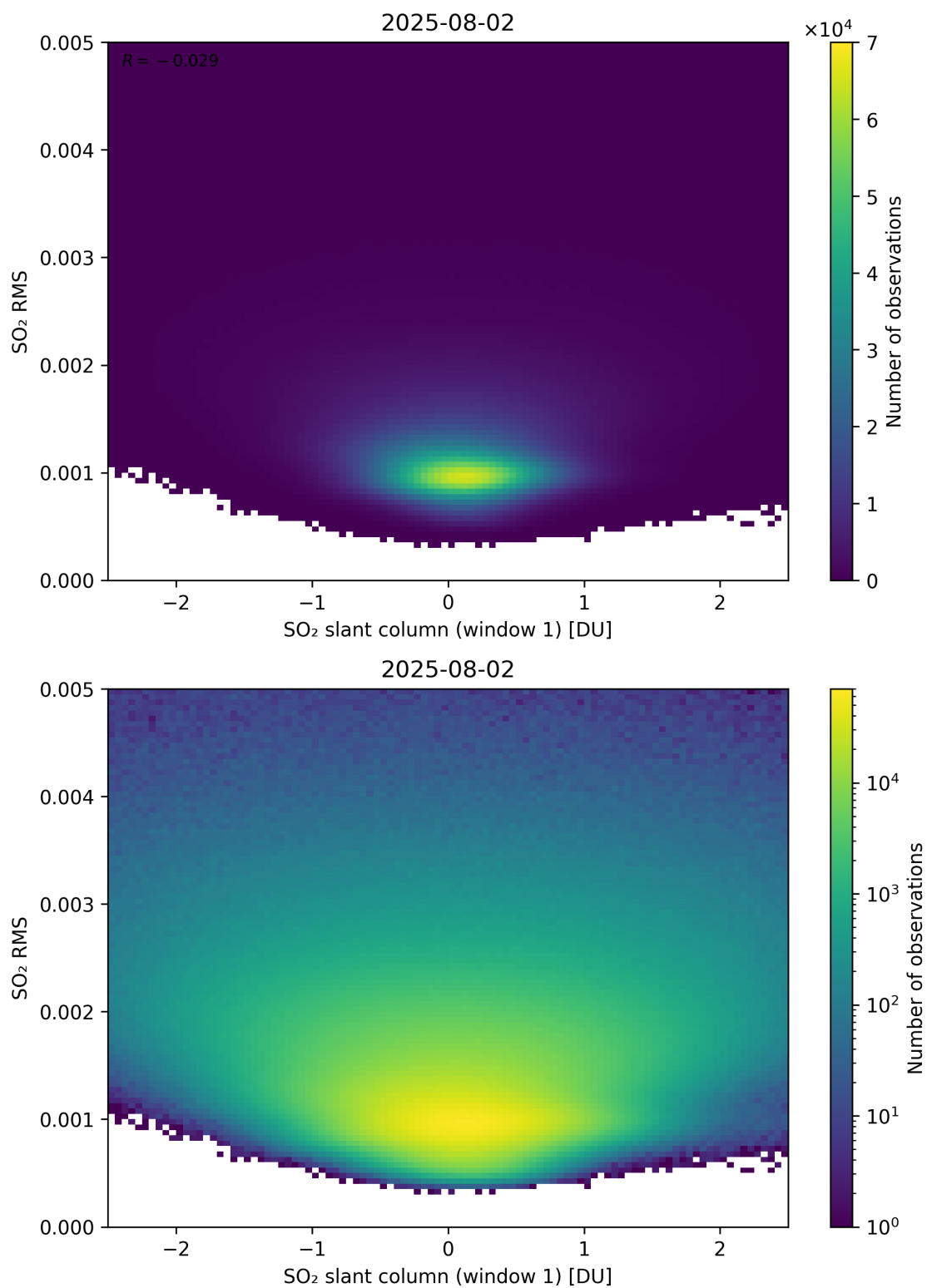
Figure 267: Scatter density plot of “SO 2 slant column (window 1)” against “SO 2 RMS” for 2025-08-01 to 2025-08-03.
