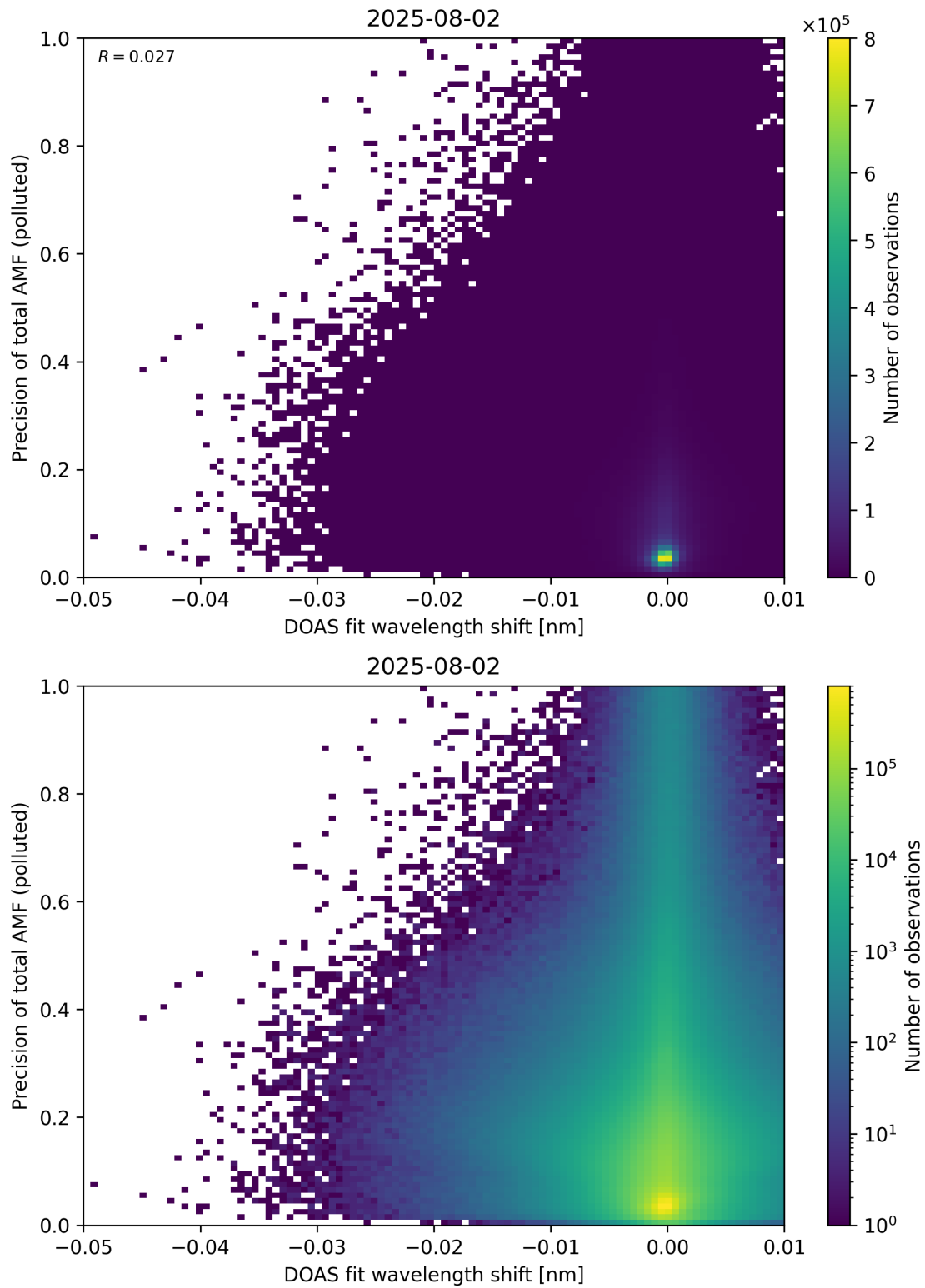
Figure 142: Scatter density plot of “DOAS fit wavelength shift” against “Precision of total AMF (polluted)” for 2025-08-01 to 2025-08-03.
