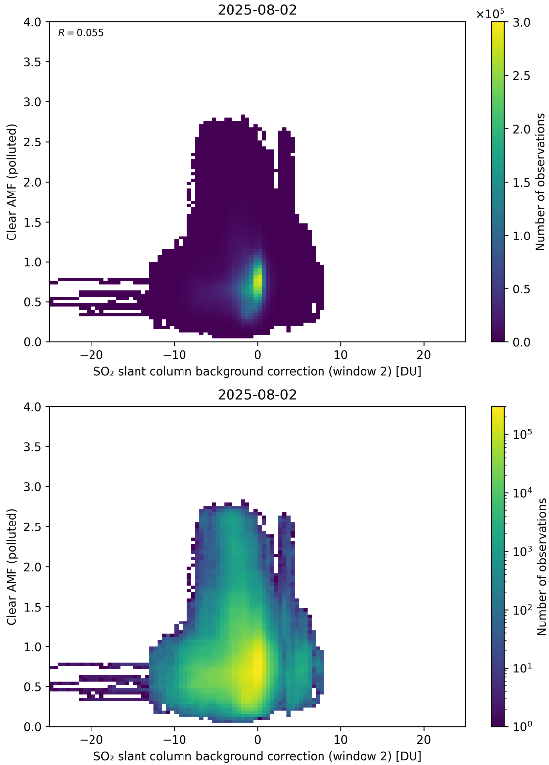
Figure 126: Scatter density plot of “SO 2 slant column background correction (window 2)” against “Clear AMF (polluted)” for 2025-08-01 to 2025-08-03.
