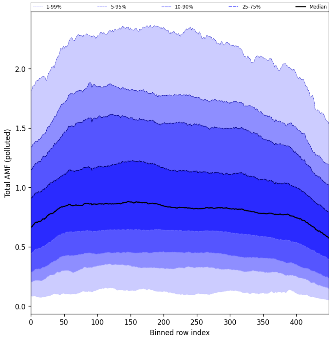
Figure 105: Along track statistics of “Total AMF (polluted)” for 2025-08-01 to 2025-08-03
