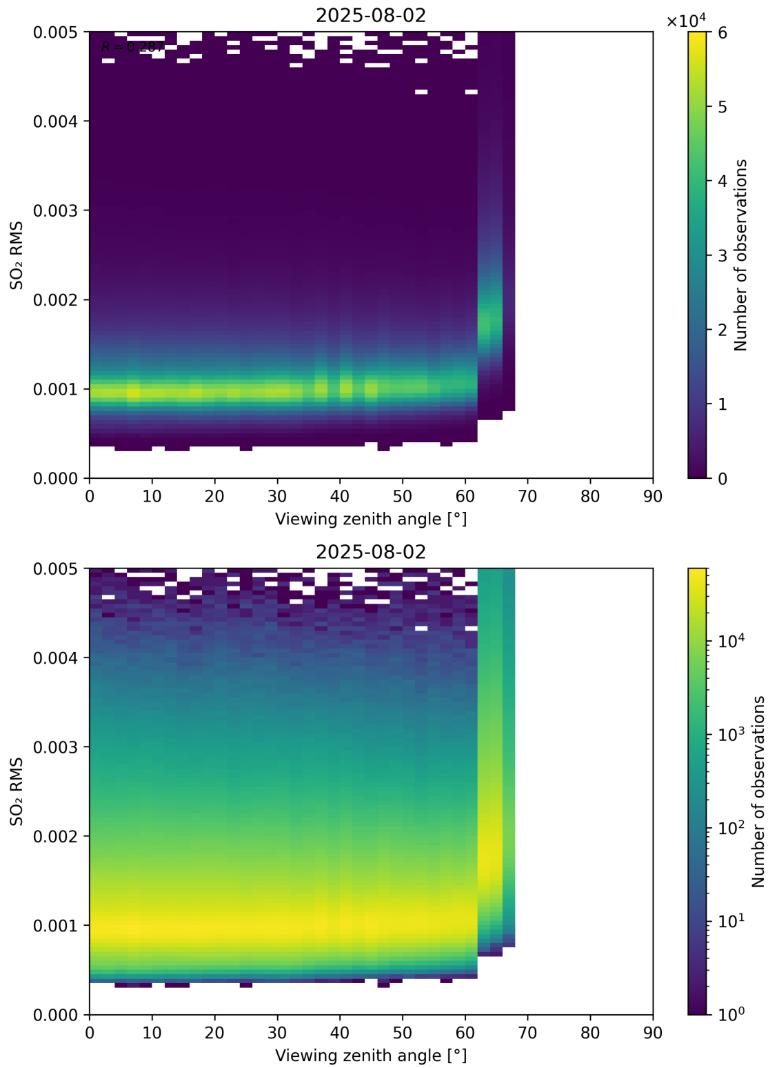
Figure 367: Scatter density plot of “Viewing zenith angle” against “SO 2 RMS” for 2025-08-01 to 2025-08-03.
