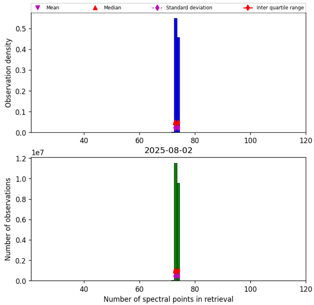
Figure 82: Histogram of “Number of spectral points in retrieval” for 2025-08-01 to 2025-08-03
