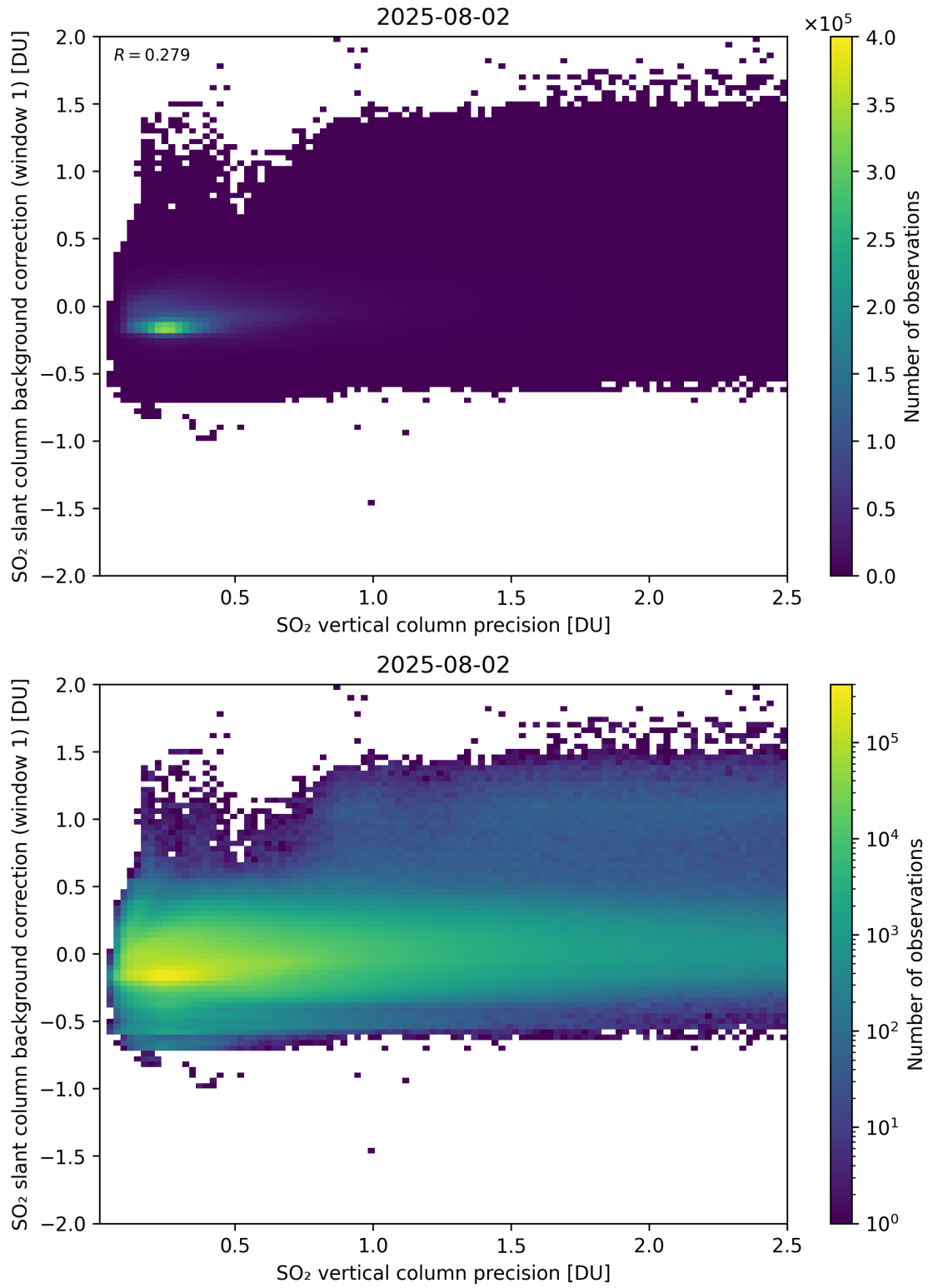
Figure 329: Scatter density plot of “SO 2 vertical column precision” against “SO 2 slant column background correction (window 1)” for 2025-08-01 to 2025-08-03.
