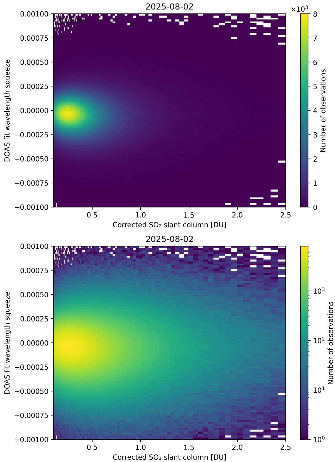
Figure 230: Scatter density plot of “Corrected SO 2 slant column” against “DOAS fit wavelength squeeze” for 2025-08-01 to 2025-08-03.
