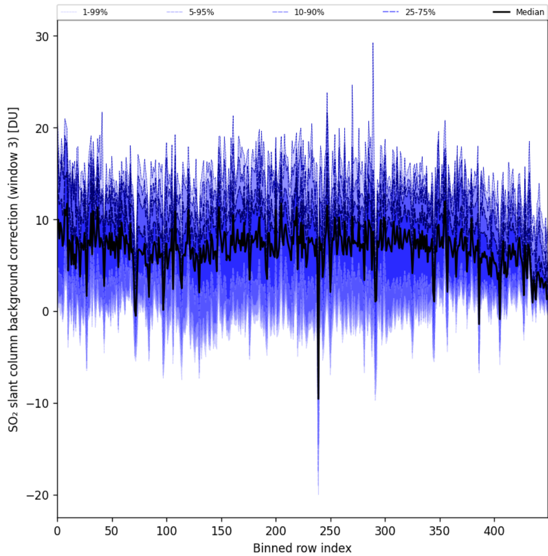
Figure 100: Along track statistics of “SO 2 slant column background correction (window 3)” for 2025-08-01 to 2025-08-03
