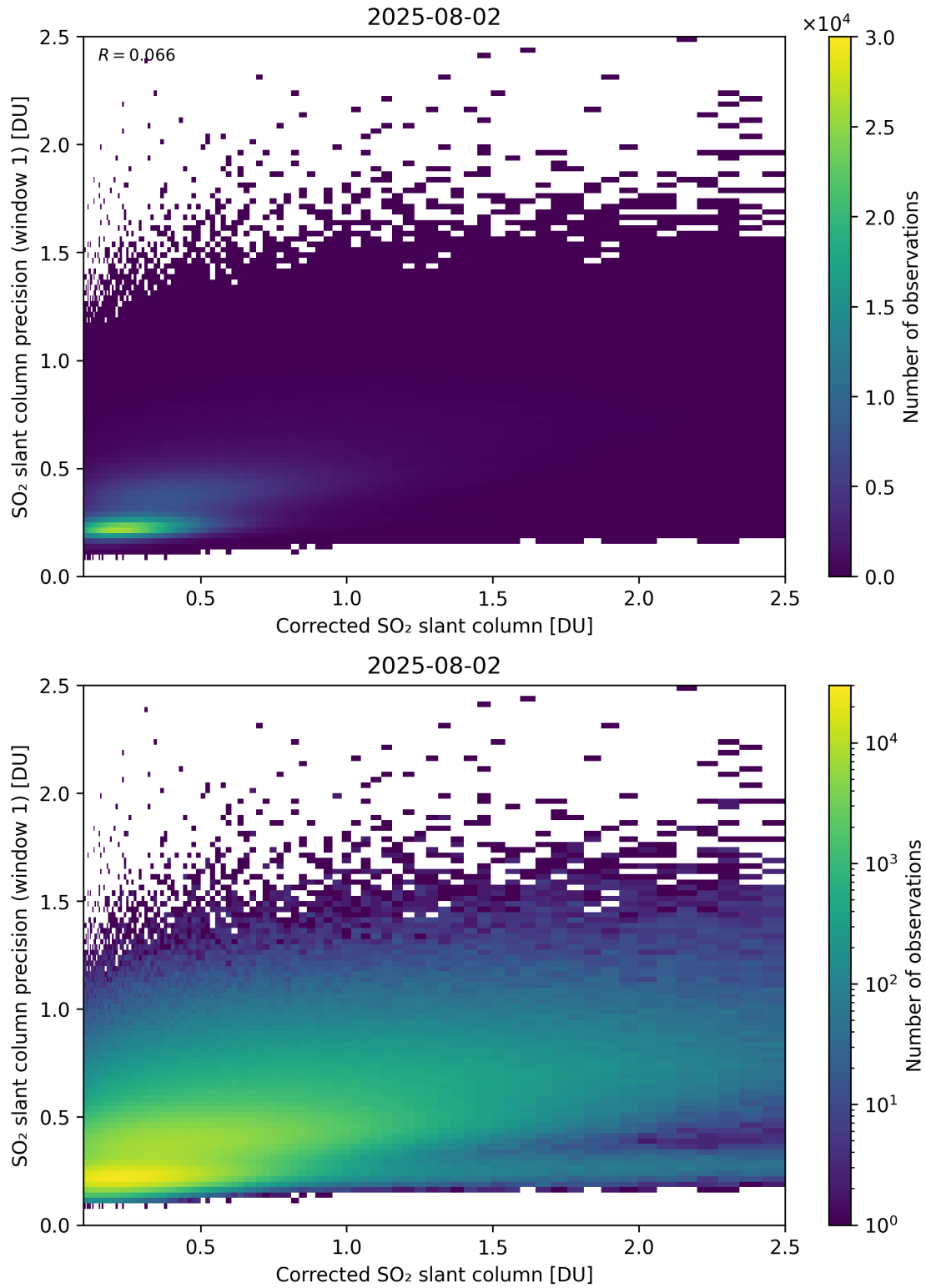
Figure 238: Scatter density plot of “Corrected SO 2 slant column” against “SO 2 slant column precision (window 1)” for 2025-08-01 to 2025-08-03.
