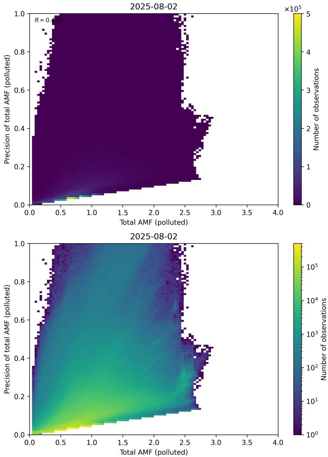
Figure 322: Scatter density plot of “Total AMF (polluted)” against “Precision of total AMF (polluted)” for 2025-08-01 to 2025-08-03.
