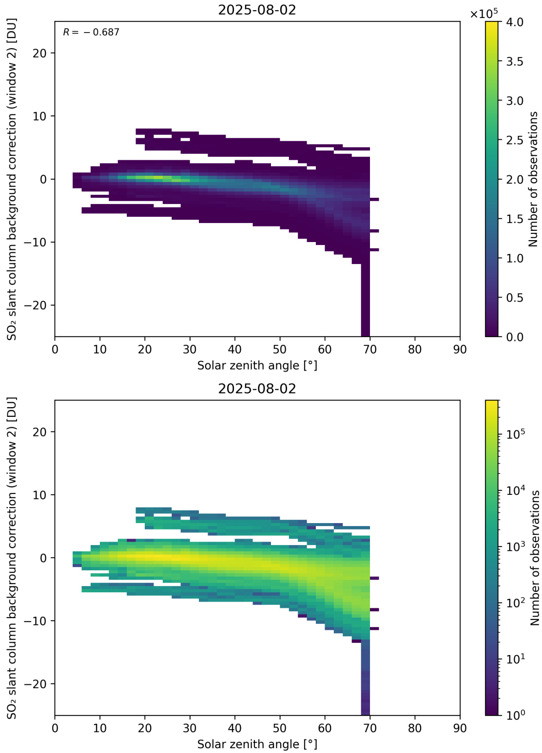
Figure 172: Scatter density plot of “Solar zenith angle” against “SO 2 slant column background correction (window 2)” for 2025-08-01 to 2025-08-03.
