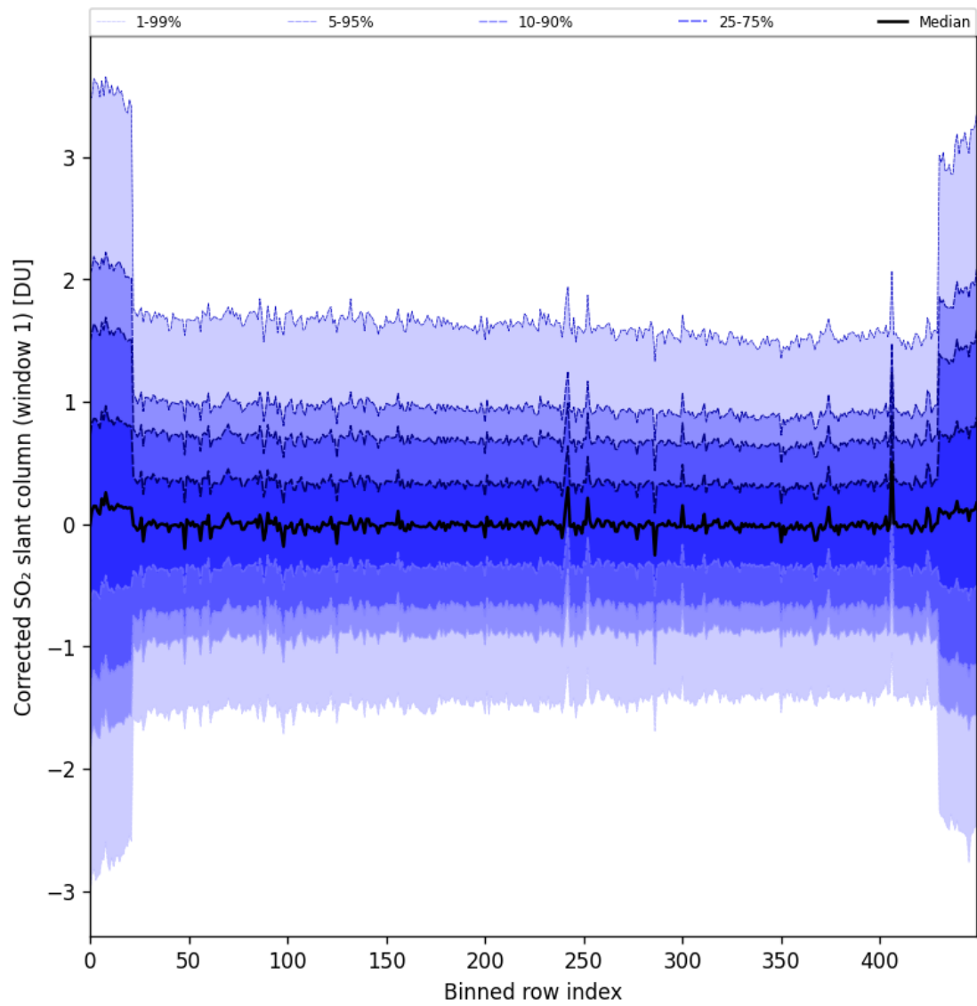
Figure 91: Along track statistics of “Corrected SO 2 slant column (window 1)” for 2025-08-01 to 2025-08-03
