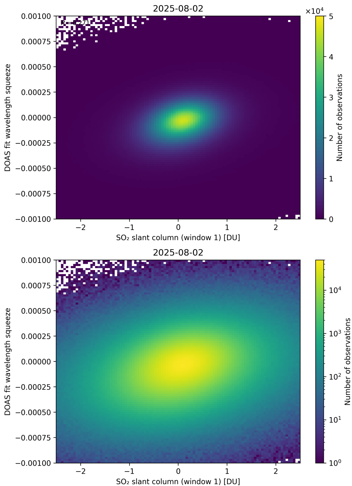
Figure 266: Scatter density plot of “SO 2 slant column (window 1)” against “DOAS fit wavelength squeeze” for 2025-08-01 to 2025-08-03.
