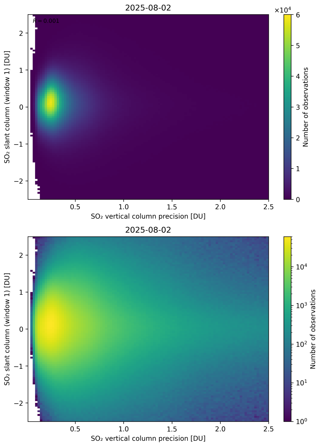
Figure 341: Scatter density plot of “SO 2 vertical column precision” against “SO 2 slant column (window 1)” for 2025-08-01 to 2025-08-03.
