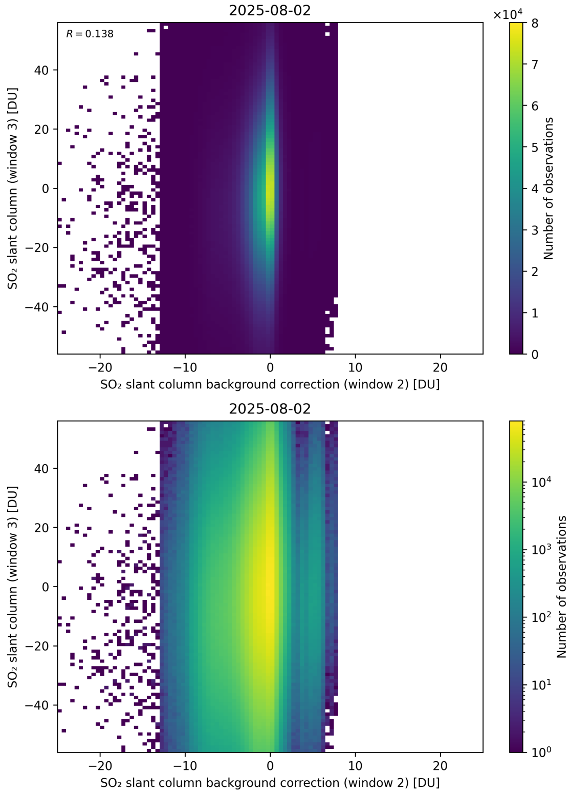
Figure 128: Scatter density plot of “SO 2 slant column background correction (window 2)” against “SO 2 slant column (window 3)” for 2025-08-01 to 2025-08-03.
