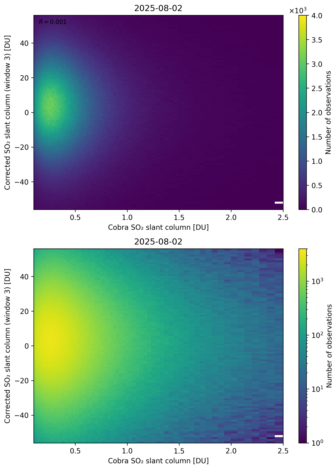
Figure 218: Scatter density plot of “Cobra SO 2 slant column” against “Corrected SO 2 slant column (window 3)” for 2025-08-01 to 2025-08-03.
