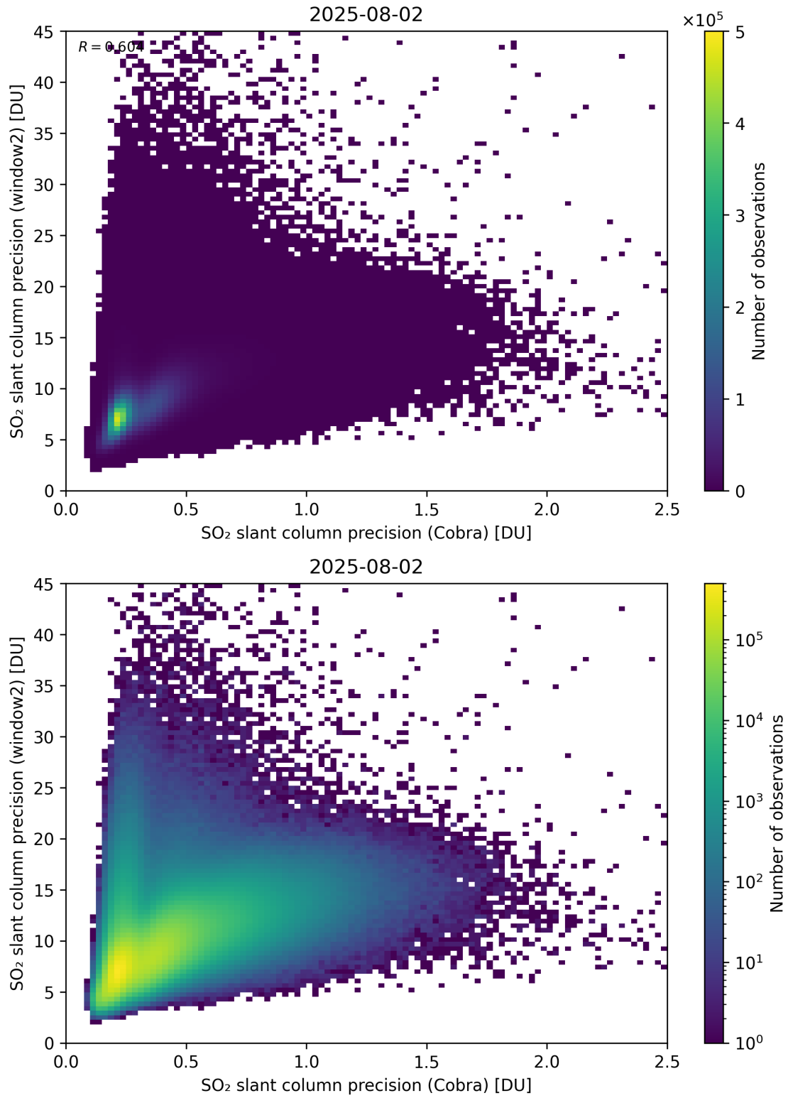
Figure 210: Scatter density plot of “SO 2 slant column precision (Cobra)” against “SO 2 slant column precision (window2)” for 2025-08-01 to 2025-08-03.
