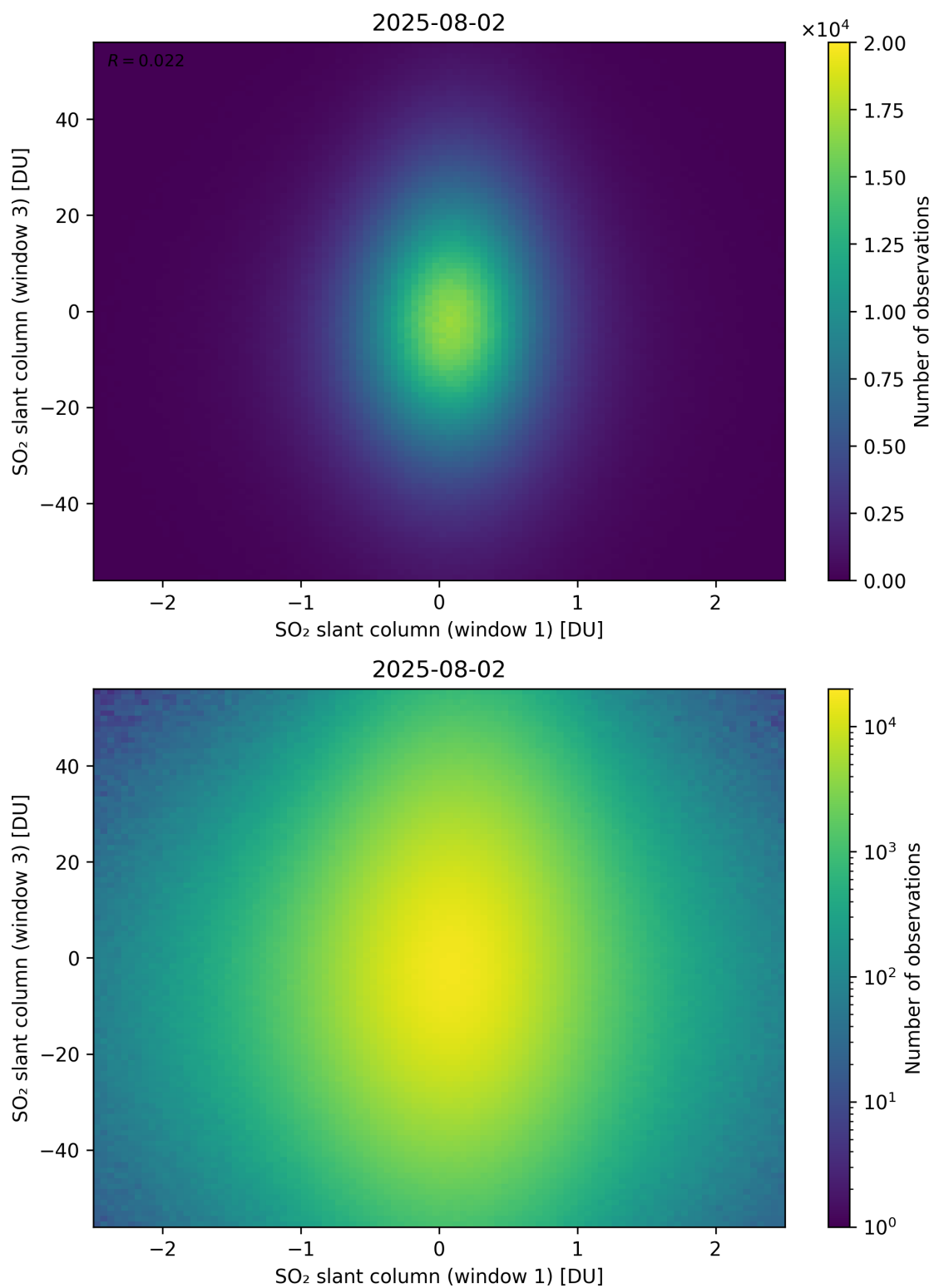
Figure 287: Scatter density plot of “SO 2 slant column (window 1)” against “SO 2 slant column (window 3)” for 2025-08-01 to 2025-08-03.
