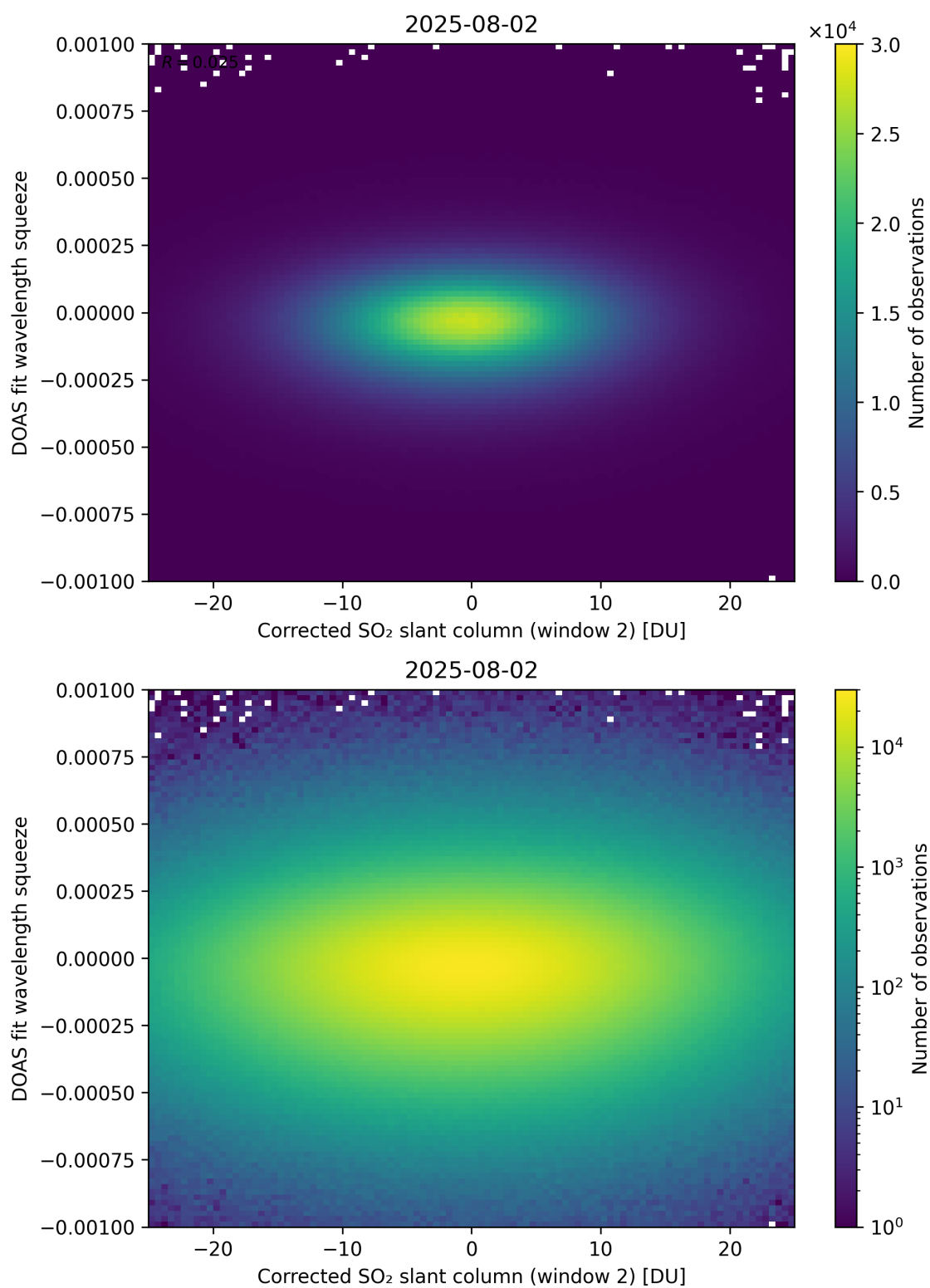
Figure 247: Scatter density plot of “Corrected SO 2 slant column (window 2)” against “DOAS fit wavelength squeeze” for 2025-08-01 to 2025-08-03.
