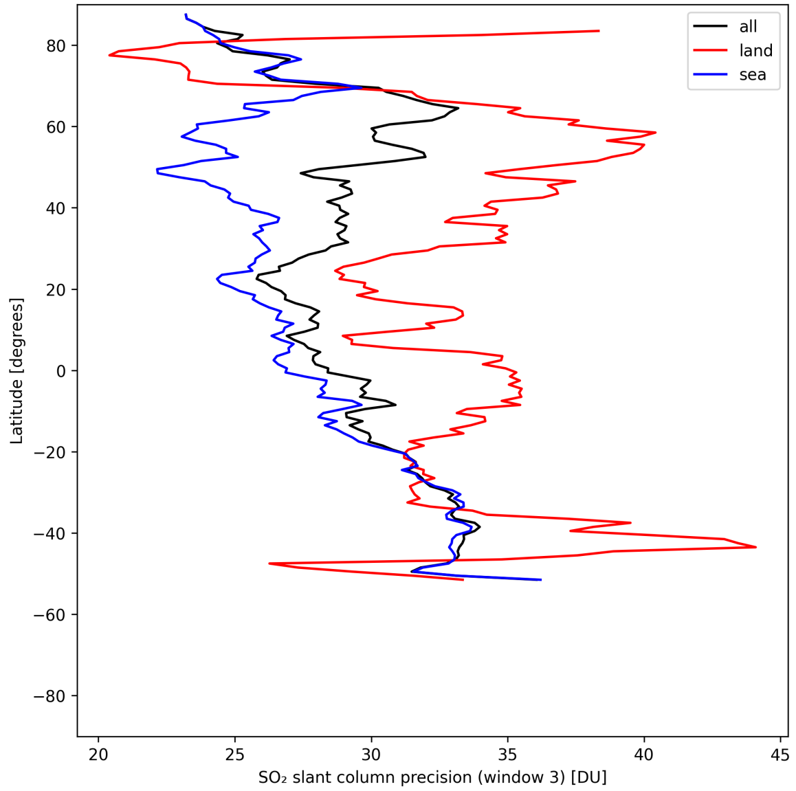
Figure 46: Zonal average of “SO 2 slant column precision (window 3)” for 2025-08-01 to 2025-08-03.
