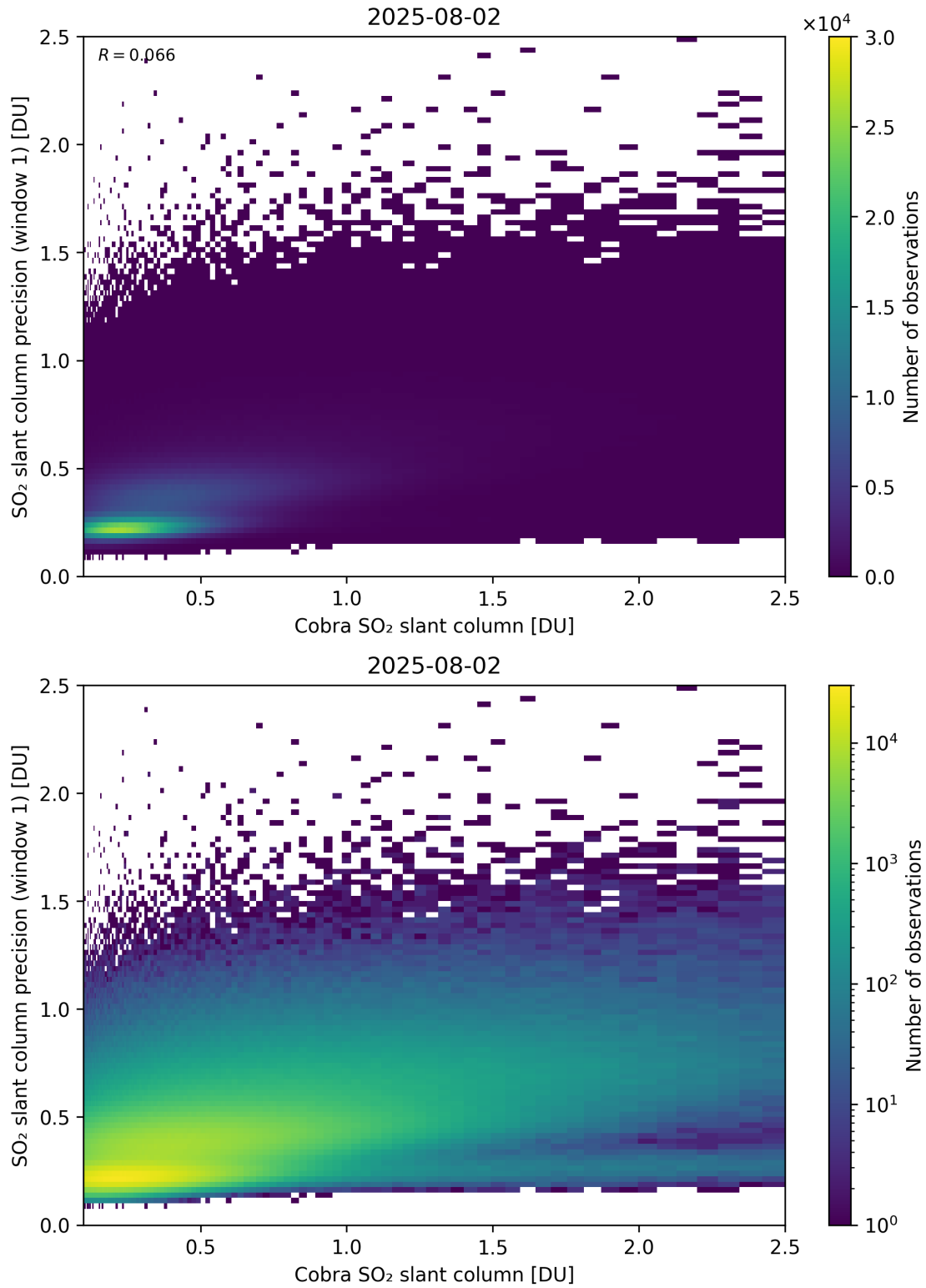
Figure 220: Scatter density plot of “Cobra SO 2 slant column” against “SO 2 slant column precision (window 1)” for 2025-08-01 to 2025-08-03.
