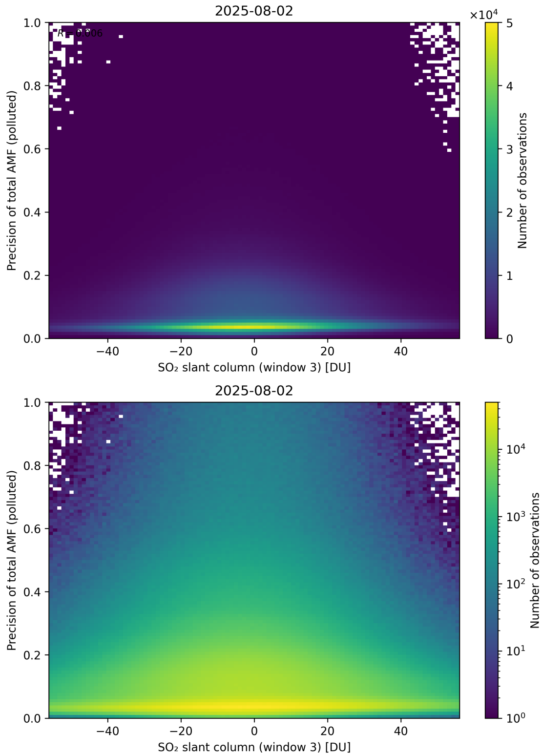
Figure 319: Scatter density plot of “SO 2 slant column (window 3)” against “Precision of total AMF (polluted)” for 2025-08-01 to 2025-08-03.
