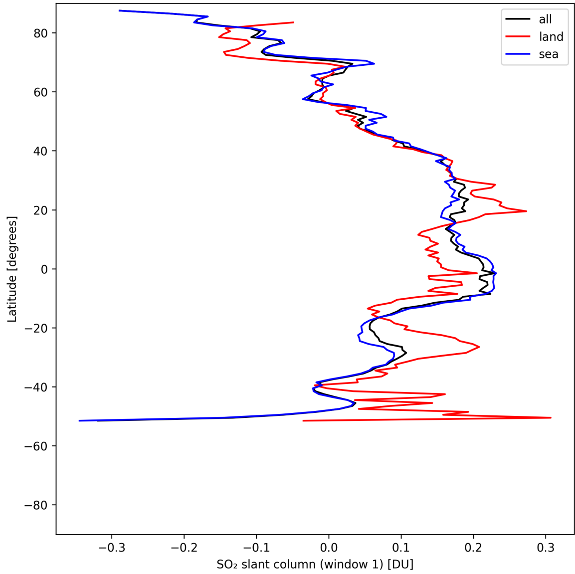
Figure 37: Zonal average of “SO 2 slant column (window 1)” for 2025-08-01 to 2025-08-03.
