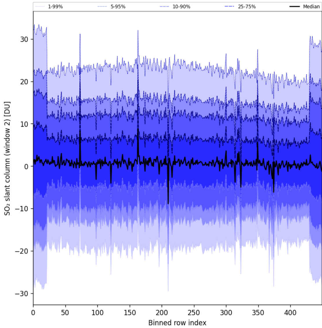
Figure 93: Along track statistics of “SO 2 slant column (window 2)” for 2025-08-01 to 2025-08-03
