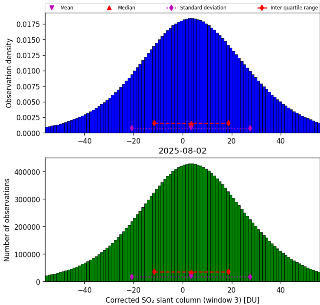
Figure 73: Histogram of “Corrected SO 2 slant column (window 3)” for 2025-08-01 to 2025-08-03
