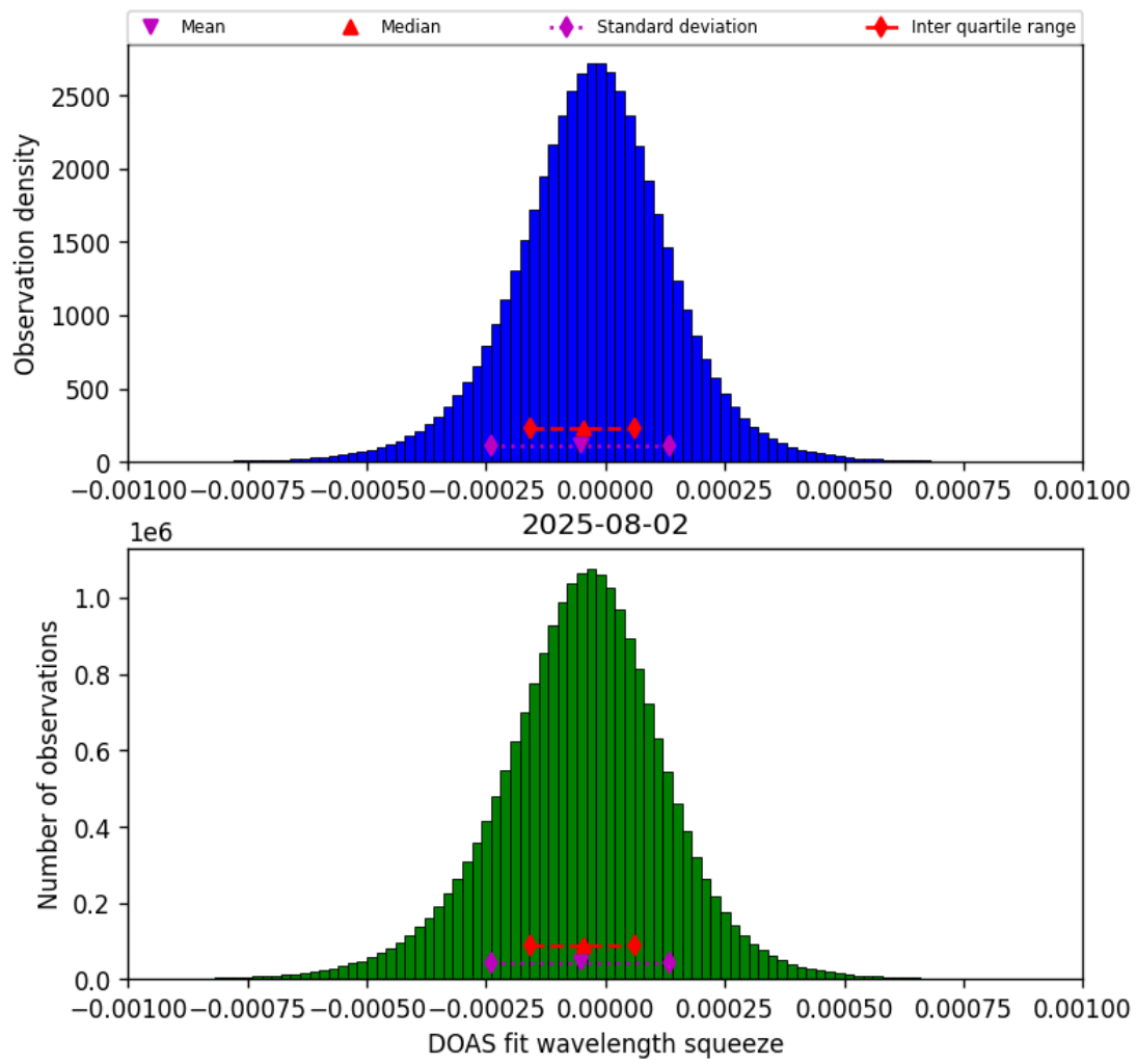
Figure 77: Histogram of “DOAS fit wavelength squeeze” for 2025-08-01 to 2025-08-03
