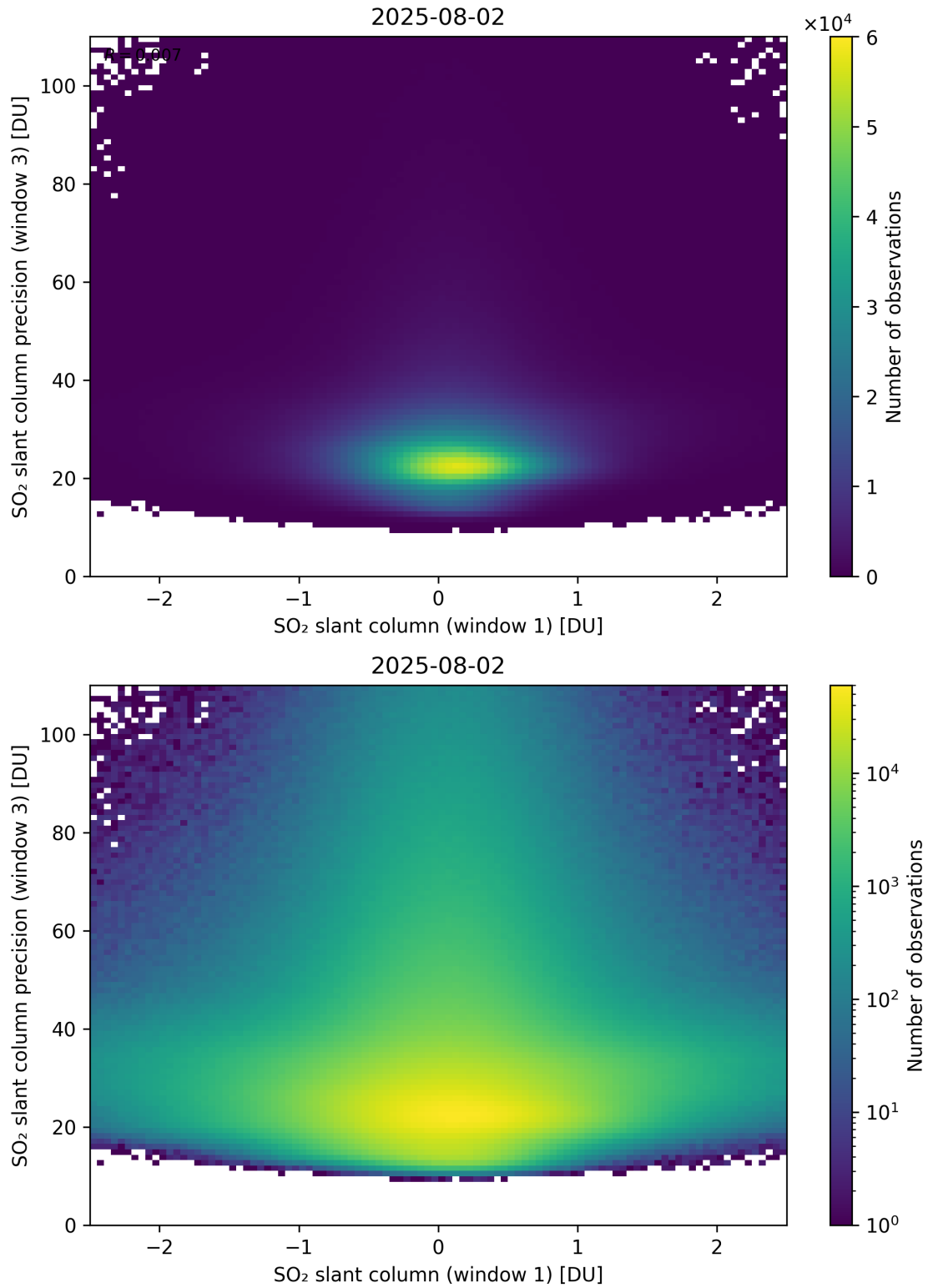
Figure 288: Scatter density plot of “SO 2 slant column (window 1)” against “SO 2 slant column precision (window 3)” for 2025-08-01 to 2025-08-03.
