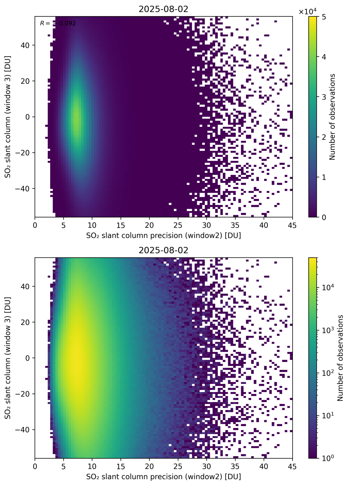
Figure 299: Scatter density plot of “SO 2 slant column precision (window2)” against “SO 2 slant column (window 3)” for 2025-08-01 to 2025-08-03.
