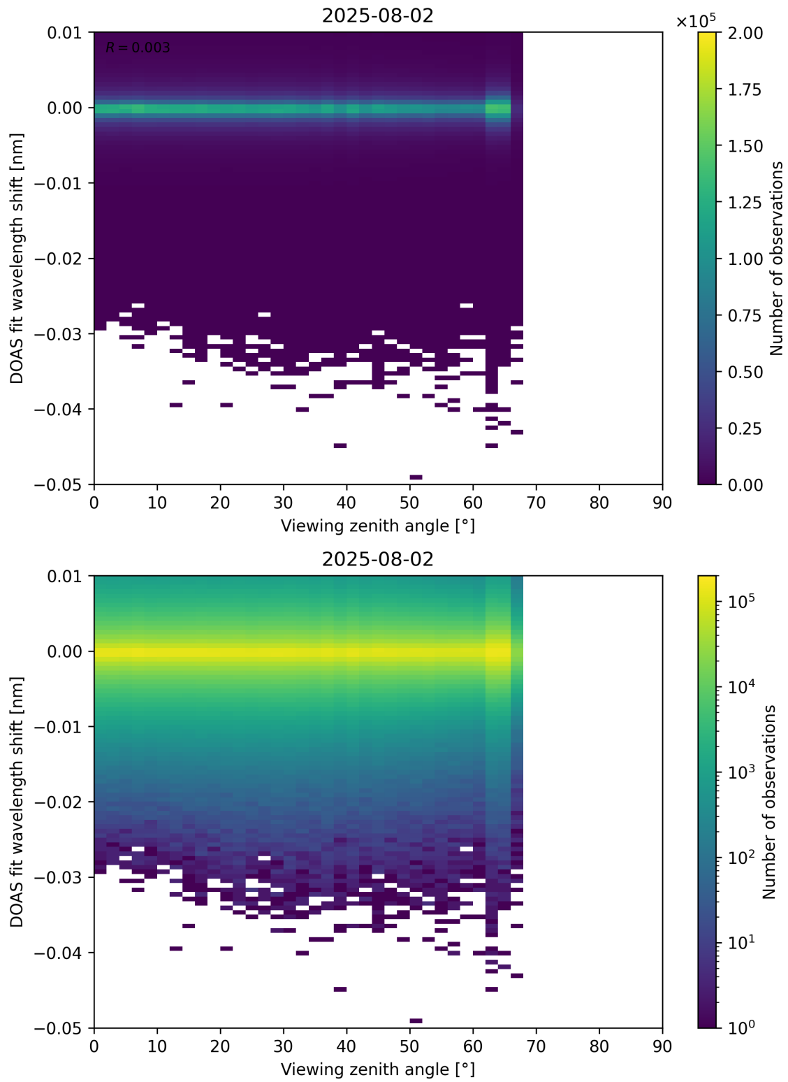
Figure 365: Scatter density plot of “Viewing zenith angle” against “DOAS fit wavelength shift” for 2025-08-01 to 2025-08-03.
