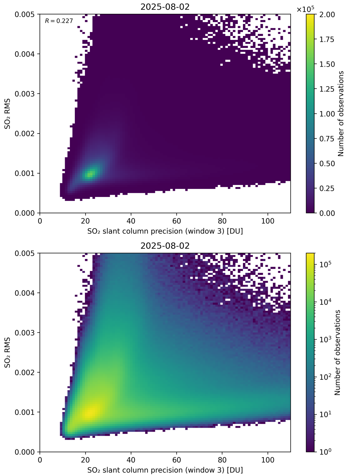
Figure 310: Scatter density plot of “SO 2 slant column precision (window 3)” against “SO 2 RMS” for 2025-08-01 to 2025-08-03.
