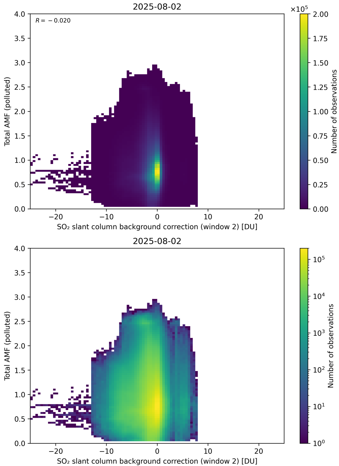
Figure 130: Scatter density plot of “SO 2 slant column background correction (window 2)” against “Total AMF (polluted)” for 2025-08-01 to 2025-08-03.
