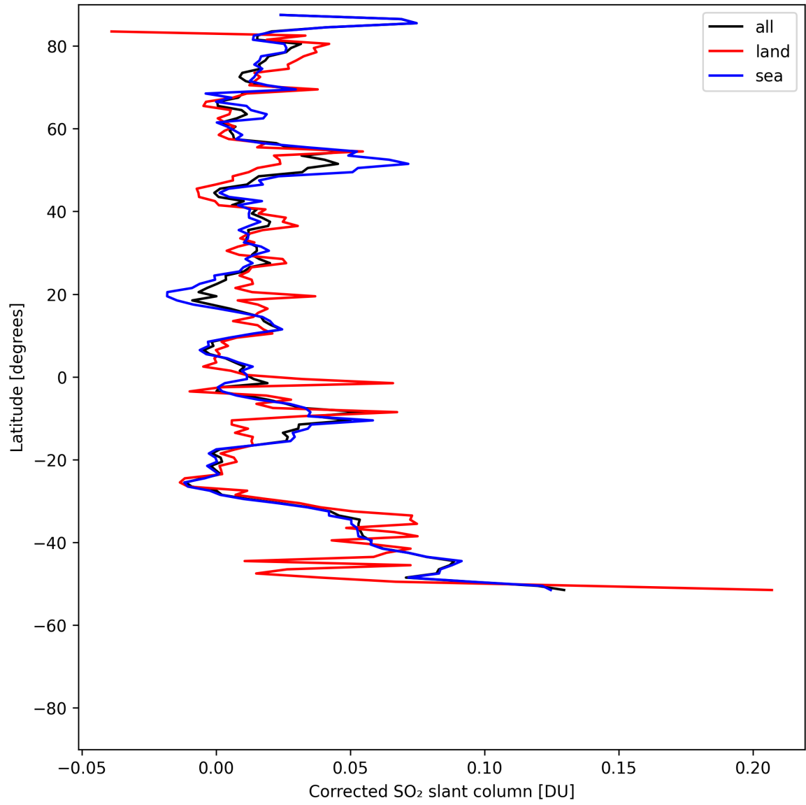
Figure 34: Zonal average of “Corrected SO 2 slant column” for 2025-08-01 to 2025-08-03.
