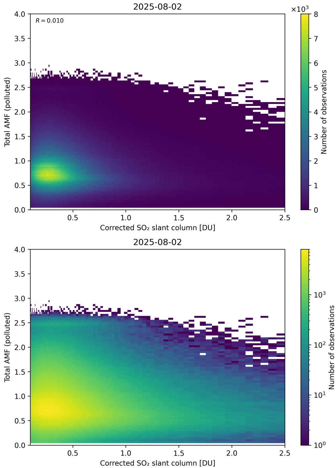
Figure 242: Scatter density plot of “Corrected SO 2 slant column” against “Total AMF (polluted)” for 2025-08-01 to 2025-08-03.
