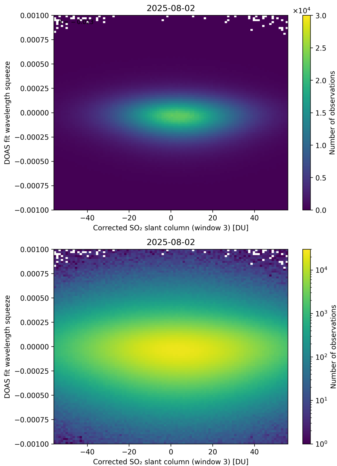
Figure 257: Scatter density plot of “Corrected SO 2 slant column (window 3)” against “DOAS fit wavelength squeeze” for 2025-08-01 to 2025-08-03.
