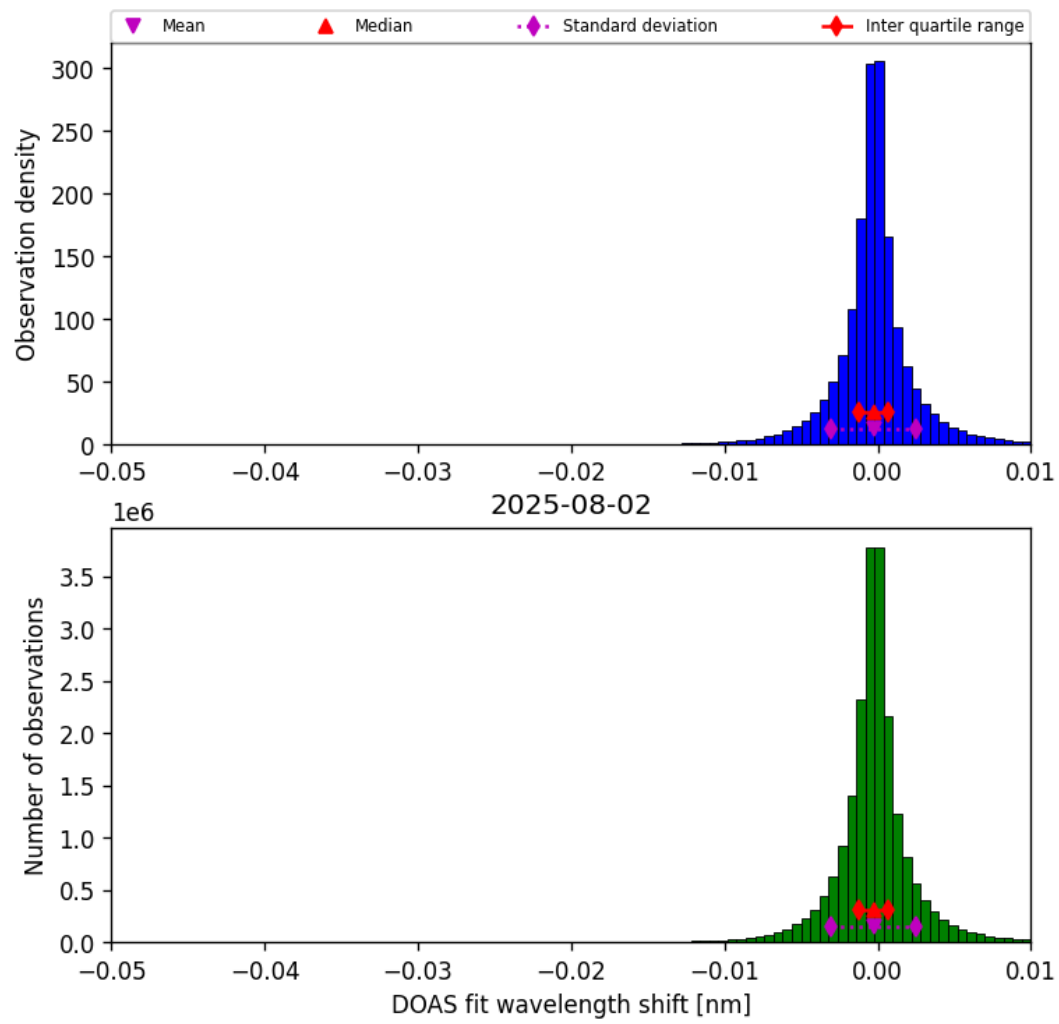
Figure 76: Histogram of “DOAS fit wavelength shift” for 2025-08-01 to 2025-08-03
