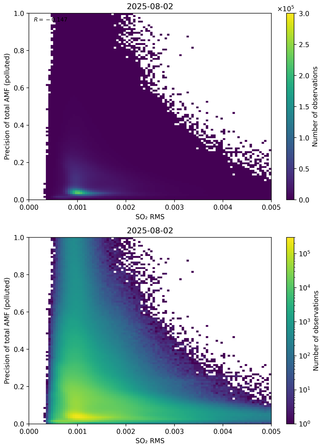
Figure 149: Scatter density plot of “SO 2 RMS” against “Precision of total AMF (polluted)” for 2025-08-01 to 2025-08-03.
