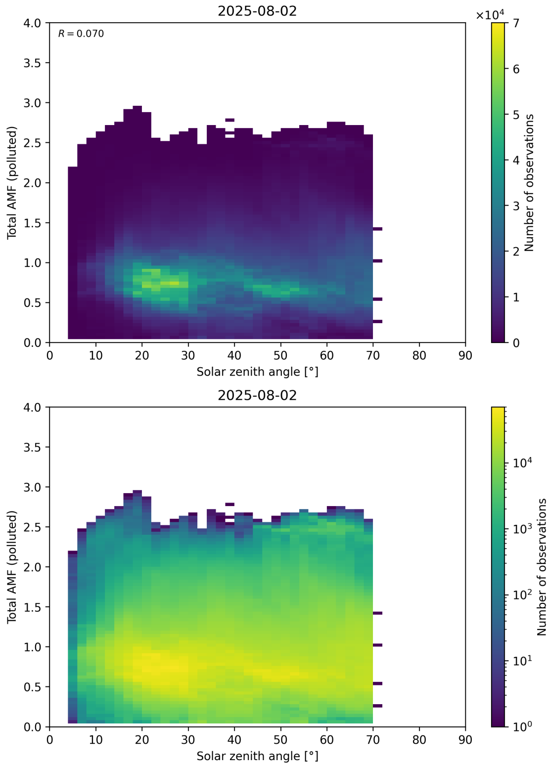
Figure 189: Scatter density plot of “Solar zenith angle” against “Total AMF (polluted)” for 2025-08-01 to 2025-08-03.
