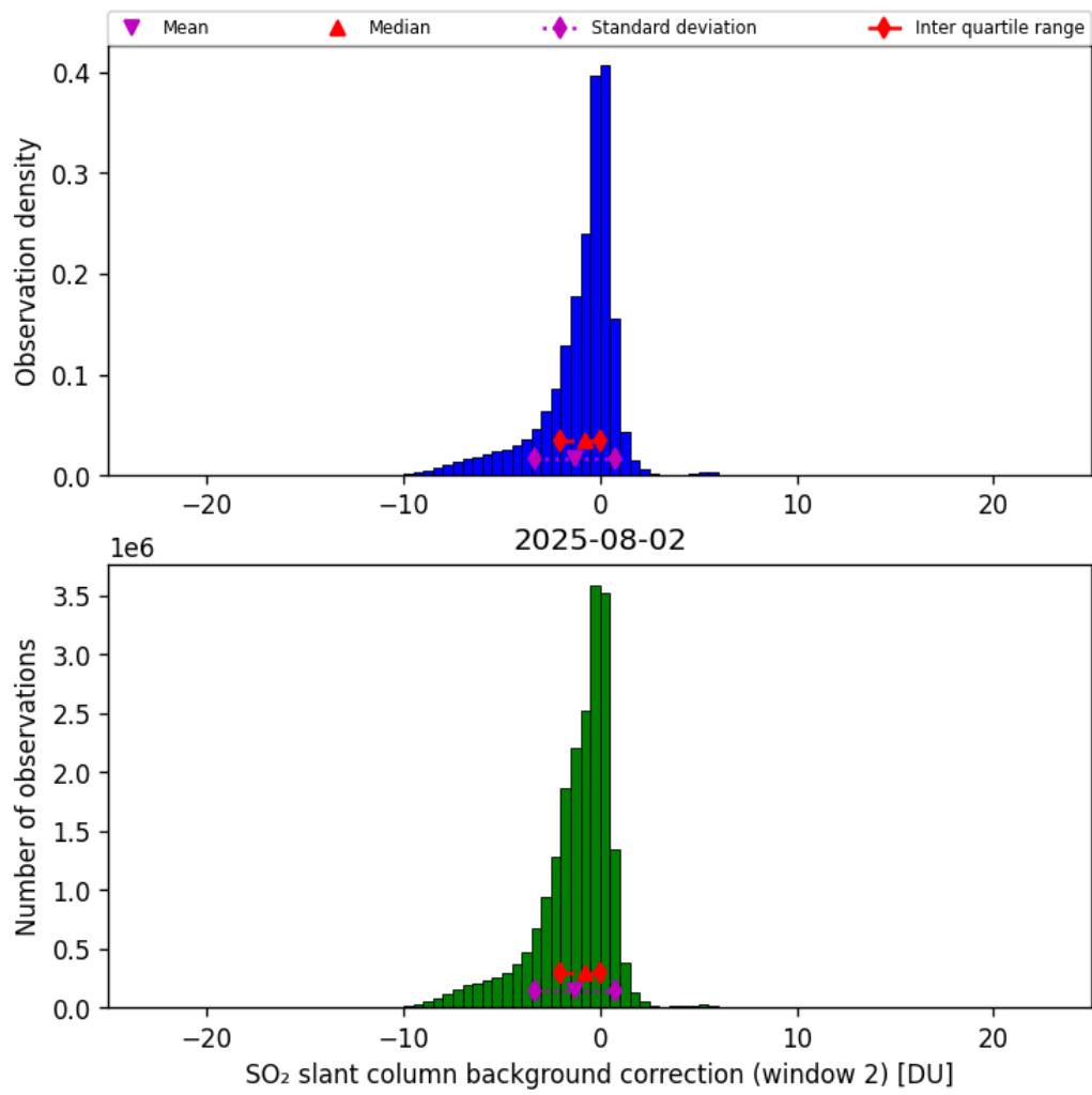
Figure 70: Histogram of “SO 2 slant column background correction (window 2)” for 2025-08-01 to 2025-08-03
