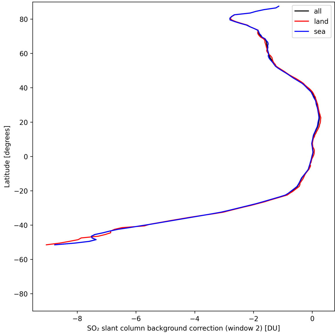
Figure 44: Zonal average of “SO 2 slant column background correction (window 2)” for 2025-08-01 to 2025-08-03.
