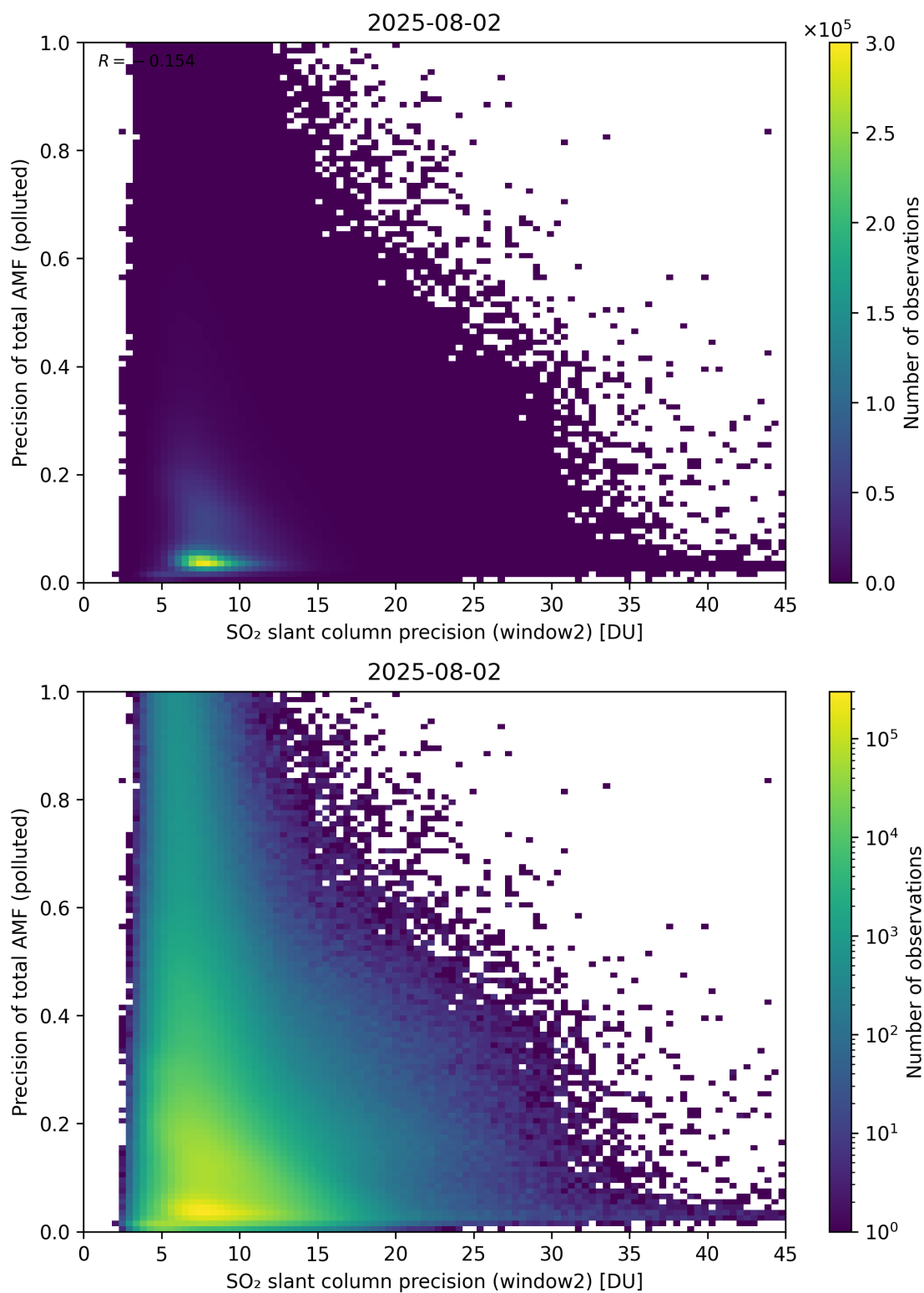
Figure 302: Scatter density plot of “SO 2 slant column precision (window2)” against “Precision of total AMF (polluted)” for 2025-08-01 to 2025-08-03.
