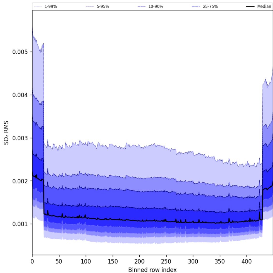
Figure 104: Along track statistics of “SO 2 RMS” for 2025-08-01 to 2025-08-03
