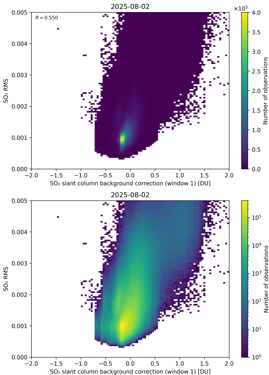
Figure 113: Scatter density plot of “SO 2 slant column background correction (window 1)” against “SO 2 RMS” for 2025-08-01 to 2025-08-03.
