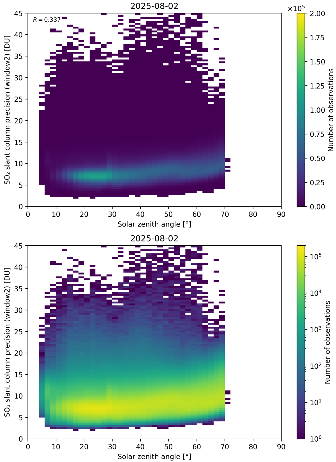
Figure 186: Scatter density plot of “Solar zenith angle” against “SO 2 slant column precision (window2)” for 2025-08-01 to 2025-08-03.
