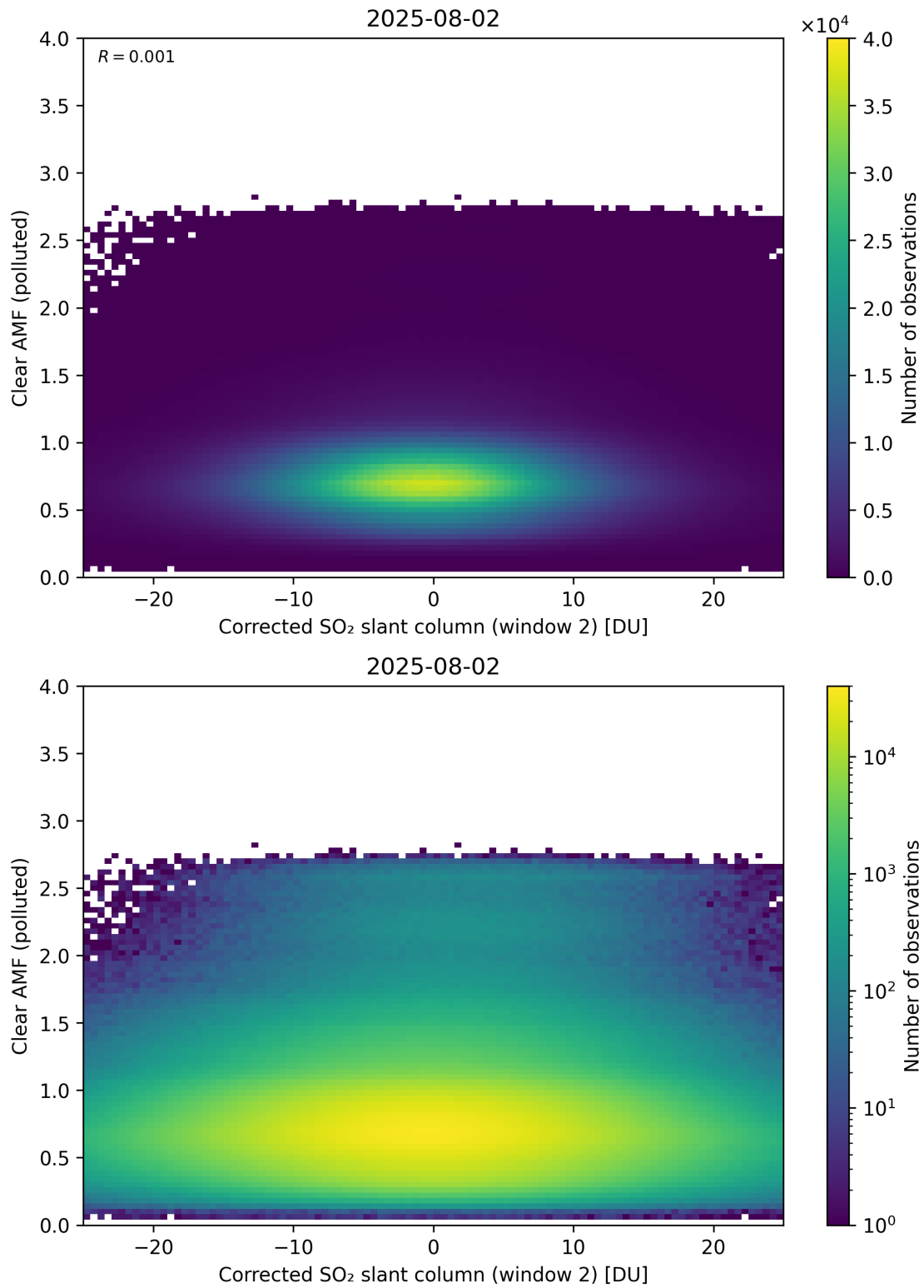
Figure 249: Scatter density plot of “Corrected SO 2 slant column (window 2)” against “Clear AMF (polluted)” for 2025-08-01 to 2025-08-03.
