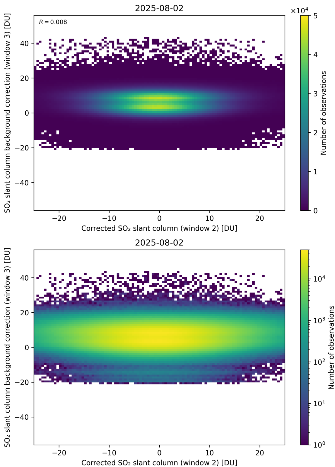
Figure 245: Scatter density plot of “Corrected SO 2 slant column (window 2)” against “SO 2 slant column background correction (window 3)” for 2025-08-01 to 2025-08-03.
