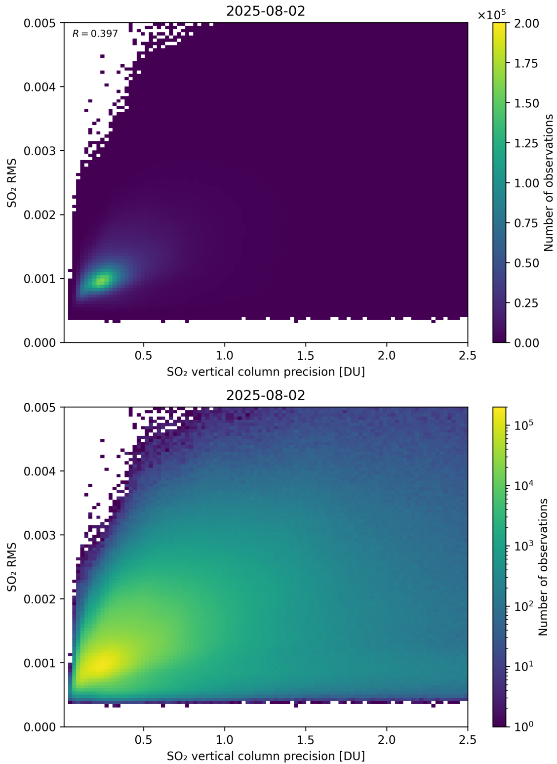
Figure 334: Scatter density plot of “SO 2 vertical column precision” against “SO 2 RMS” for 2025-08-01 to 2025-08-03.
