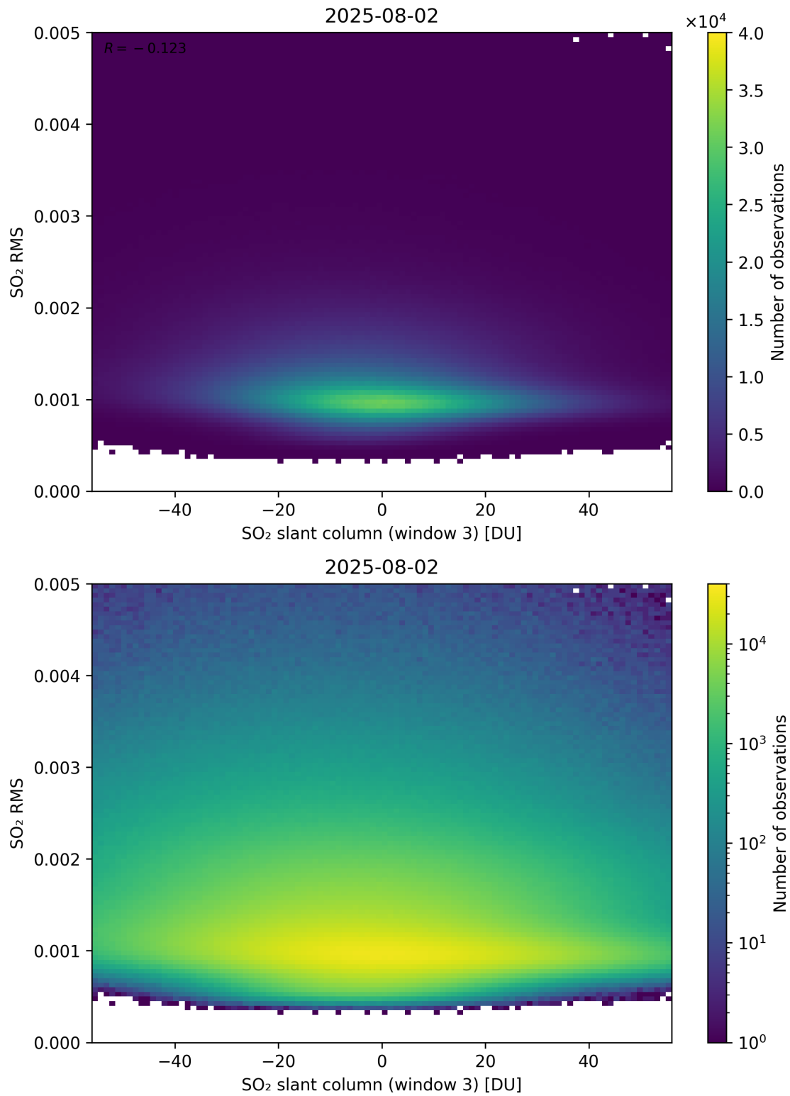
Figure 306: Scatter density plot of “SO 2 slant column (window 3)” against “SO 2 RMS” for 2025-08-01 to 2025-08-03.
