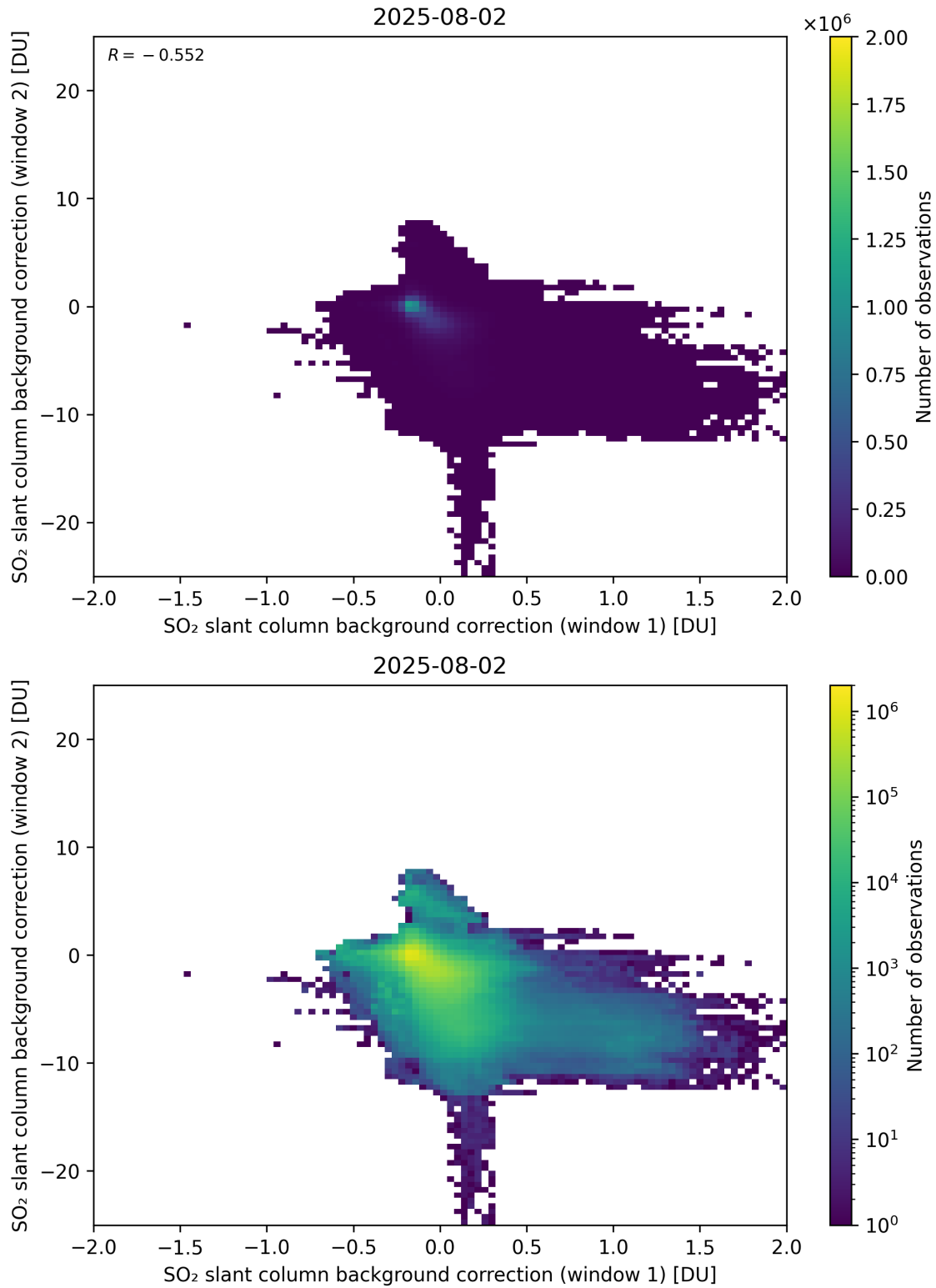
Figure 109: Scatter density plot of “SO 2 slant column background correction (window 1)” against “SO 2 slant column background correction (window 2)” for 2025-08-01 to 2025-08-03.
