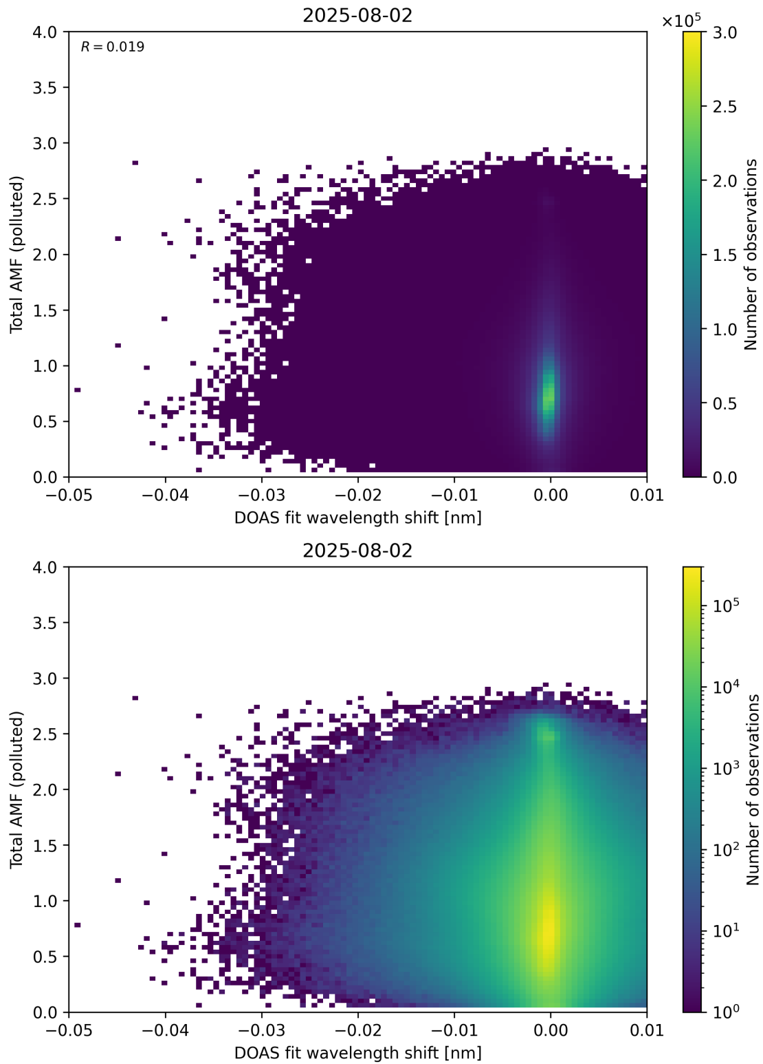
Figure 141: Scatter density plot of “DOAS fit wavelength shift” against “Total AMF (polluted)” for 2025-08-01 to 2025-08-03.
