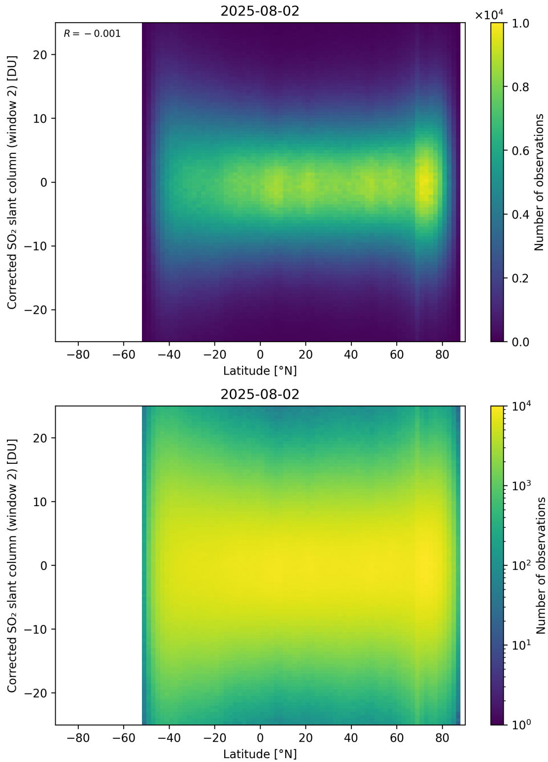
Figure 160: Scatter density plot of “Latitude” against “Corrected SO 2 slant column (window 2)” for 2025-08-01 to 2025-08-03.
