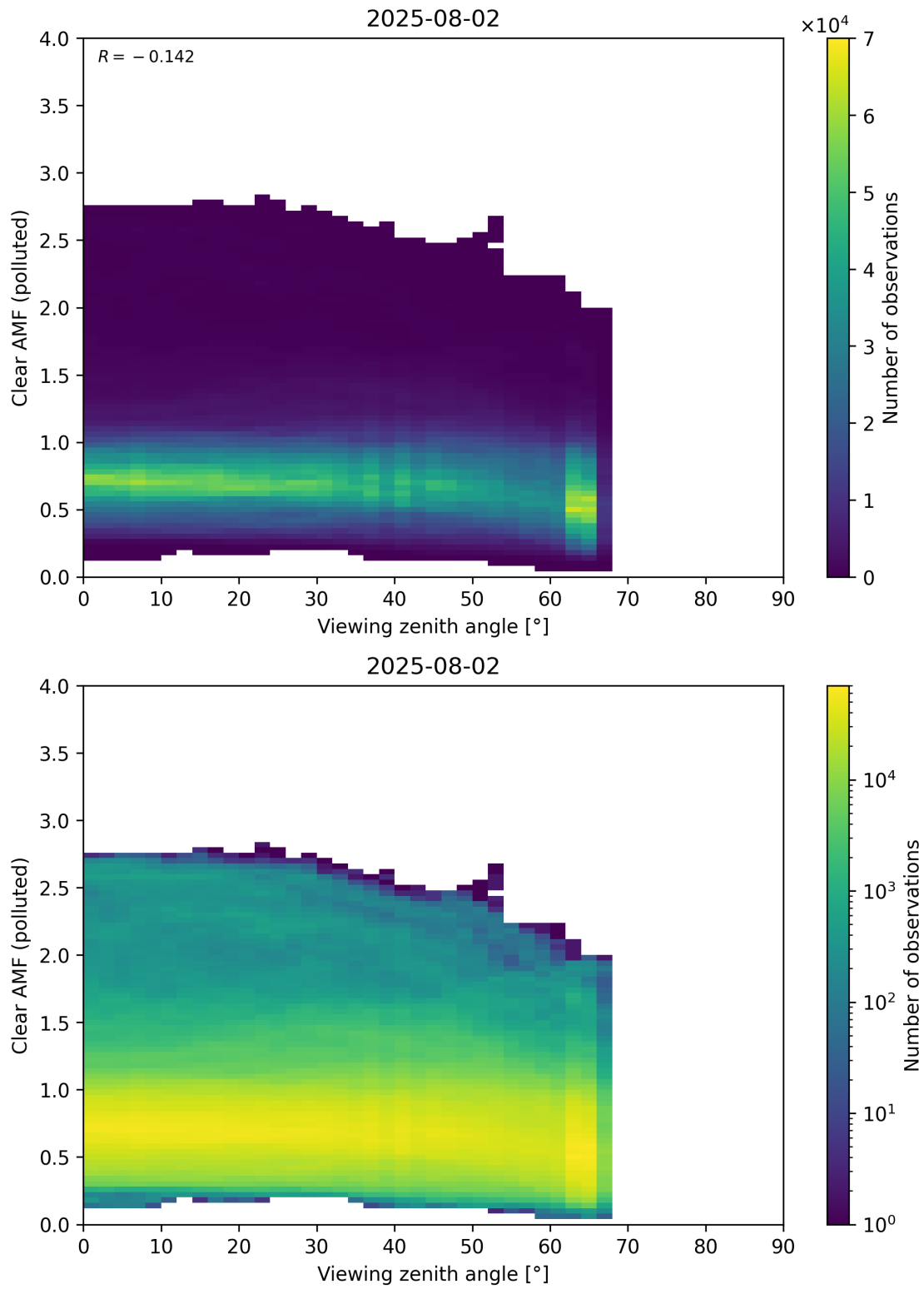
Figure 370: Scatter density plot of “Viewing zenith angle” against “Clear AMF (polluted)” for 2025-08-01 to 2025-08-03.
