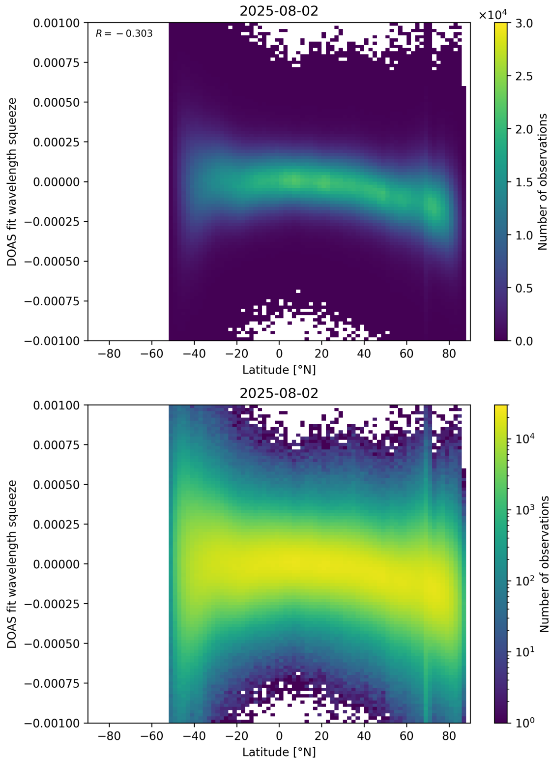
Figure 154: Scatter density plot of “Latitude” against “DOAS fit wavelength squeeze” for 2025-08-01 to 2025-08-03.
