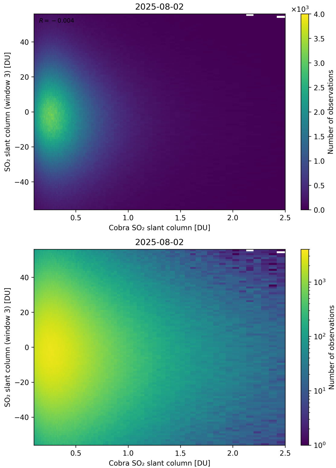
Figure 222: Scatter density plot of “Cobra SO 2 slant column” against “SO 2 slant column (window 3)” for 2025-08-01 to 2025-08-03.
