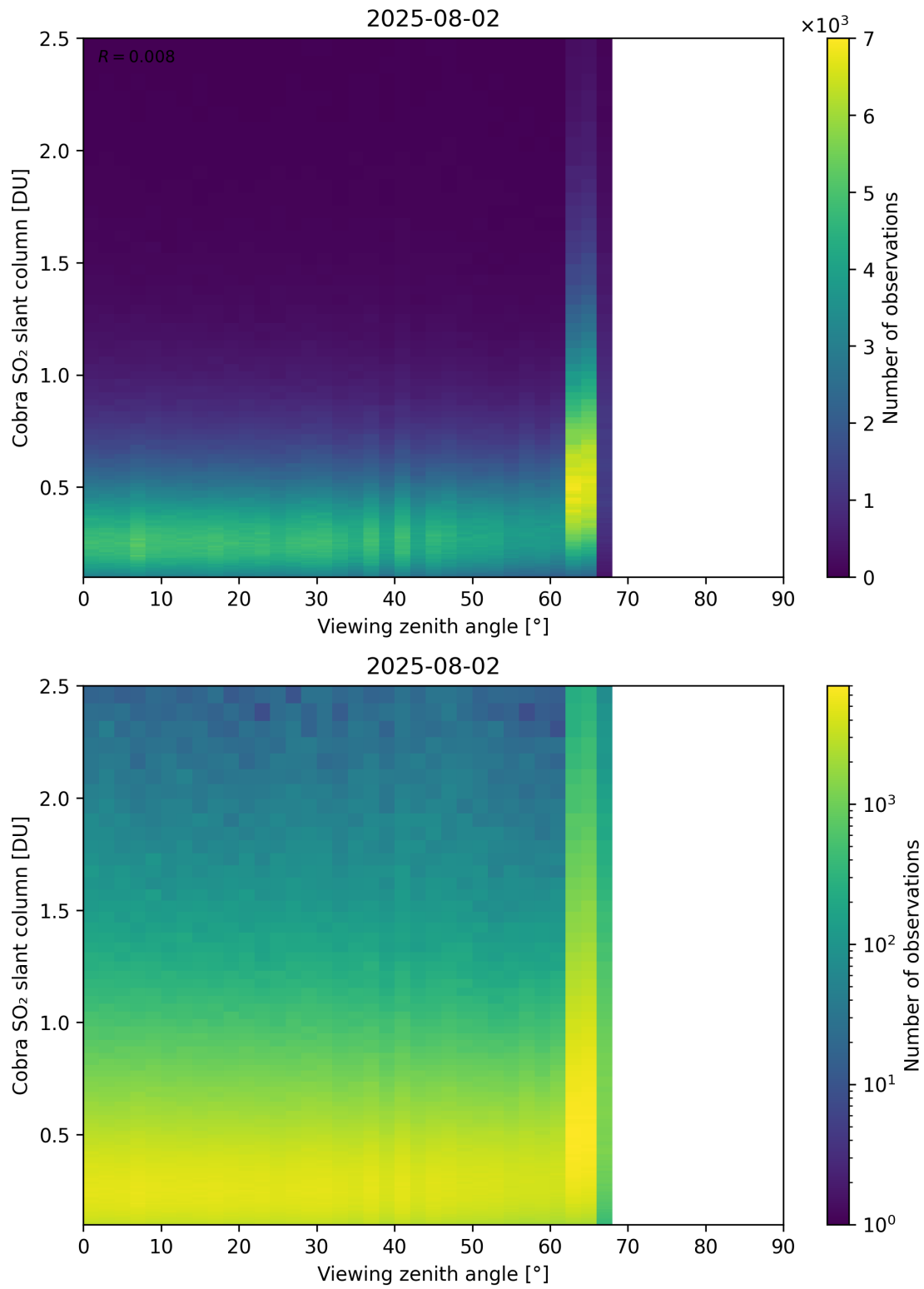
Figure 371: Scatter density plot of “Viewing zenith angle” against “Cobra SO 2 slant column” for 2025-08-01 to 2025-08-03.
