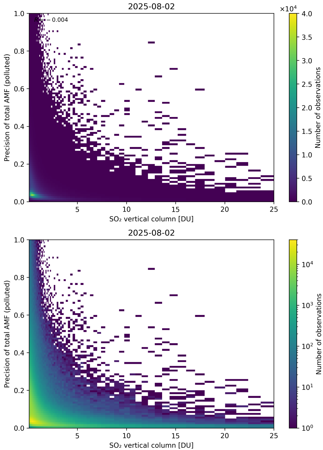
Figure 360: Scatter density plot of “SO 2 vertical column” against “Precision of total AMF (polluted)” for 2025-08-01 to 2025-08-03.
