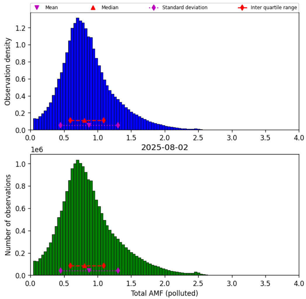
Figure 79: Histogram of “Total AMF (polluted)” for 2025-08-01 to 2025-08-03
