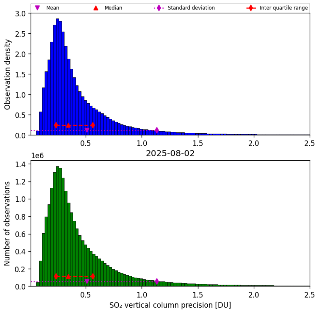
Figure 59: Histogram of “SO 2 vertical column precision” for 2025-08-01 to 2025-08-03
