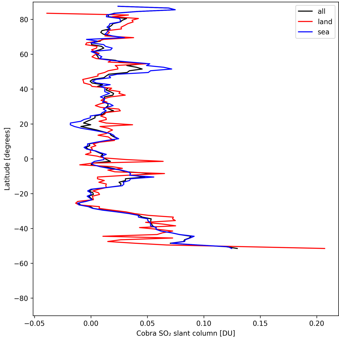
Figure 35: Zonal average of “Cobra SO 2 slant column” for 2025-08-01 to 2025-08-03.
