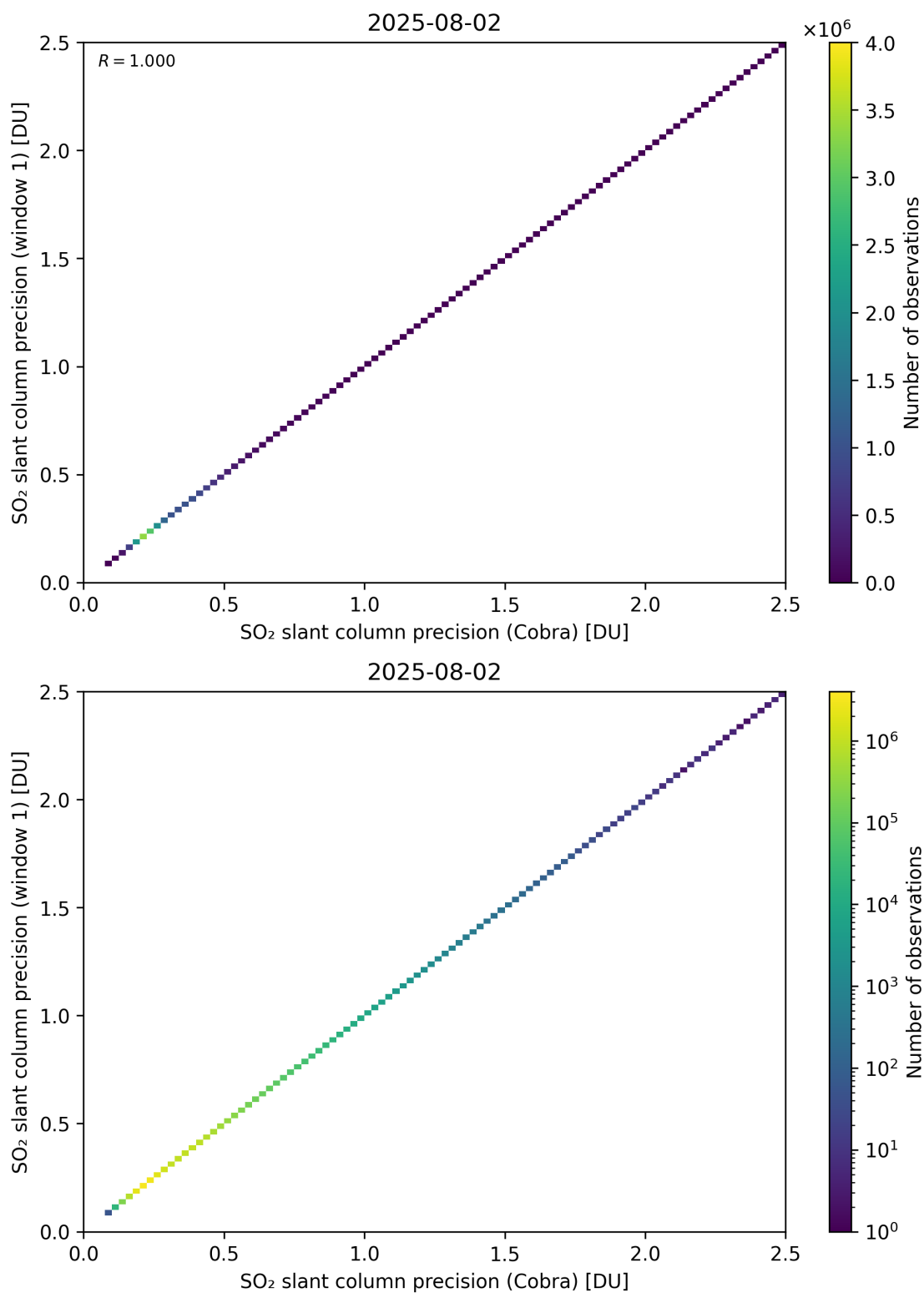
Figure 209: Scatter density plot of “SO 2 slant column precision (Cobra)” against “SO 2 slant column precision (window 1)” for 2025-08-01 to 2025-08-03.
