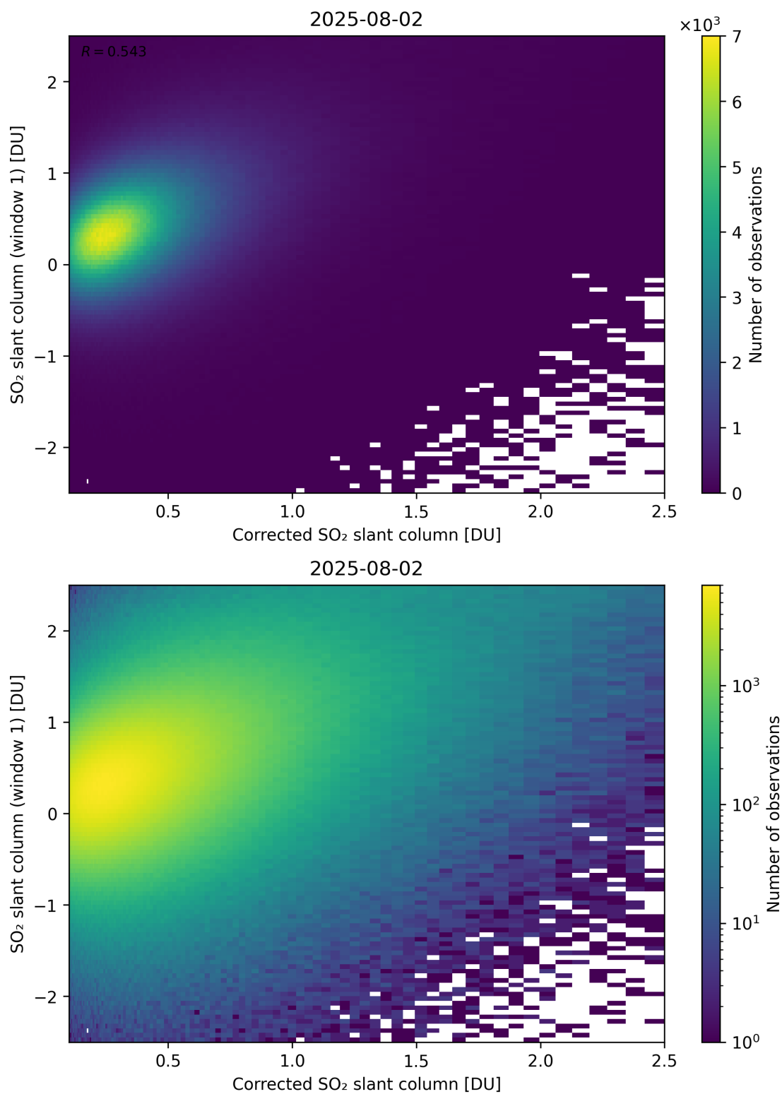
Figure 237: Scatter density plot of “Corrected SO 2 slant column” against “SO 2 slant column (window 1)” for 2025-08-01 to 2025-08-03.
