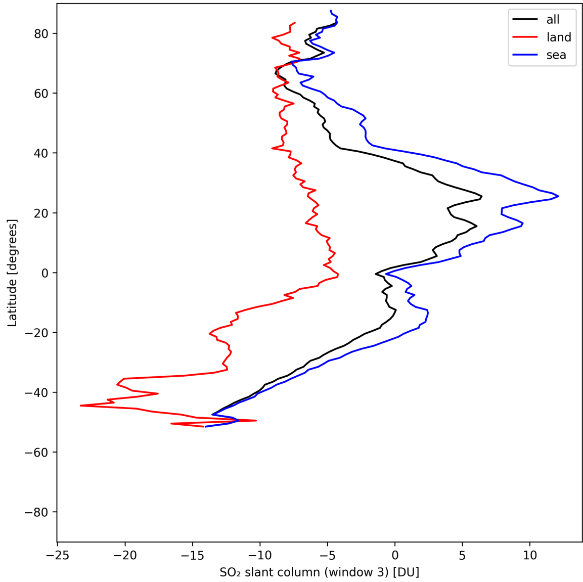
Figure 45: Zonal average of “SO 2 slant column (window 3)” for 2025-08-01 to 2025-08-03.
