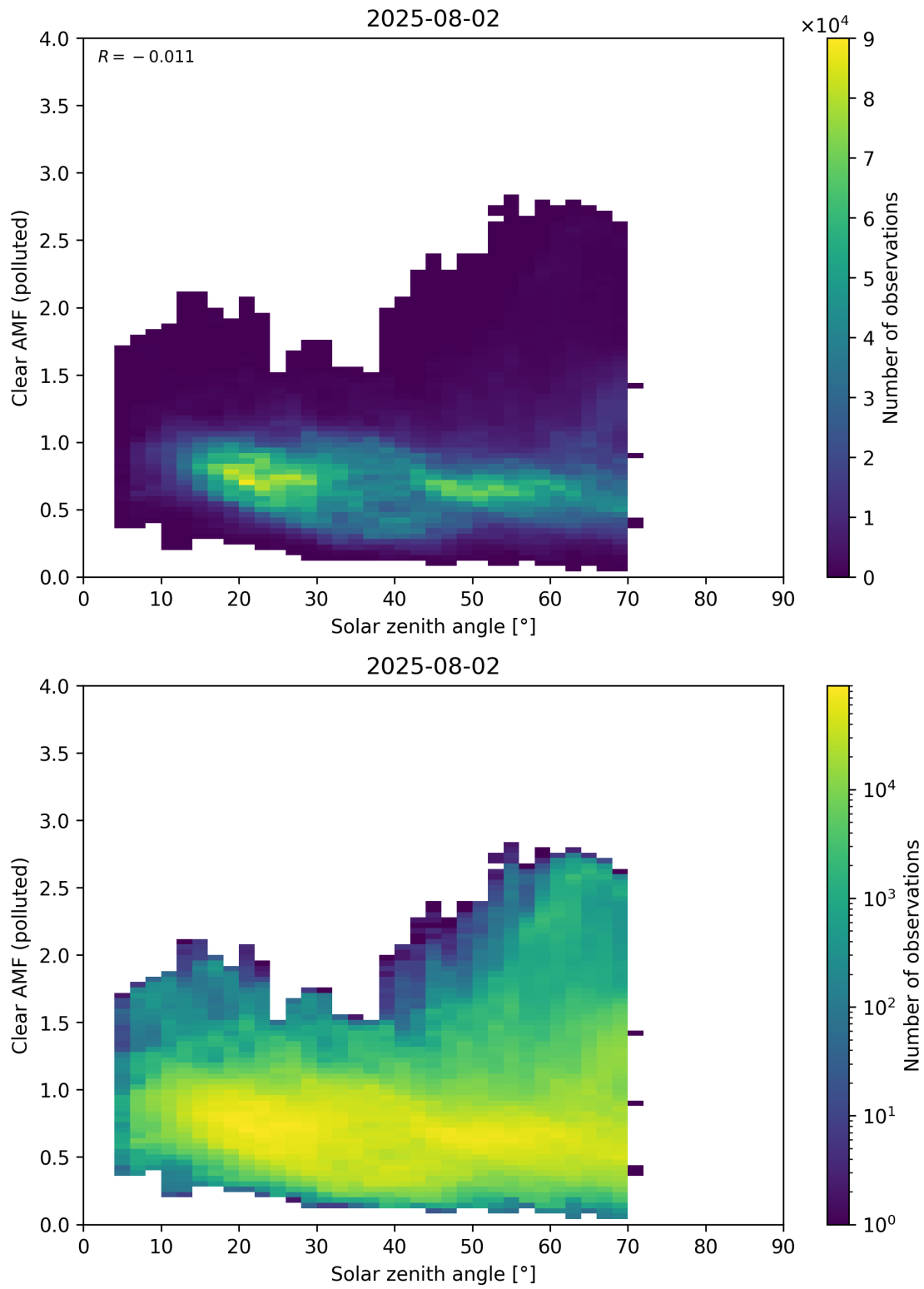
Figure 178: Scatter density plot of “Solar zenith angle” against “Clear AMF (polluted)” for 2025-08-01 to 2025-08-03.
