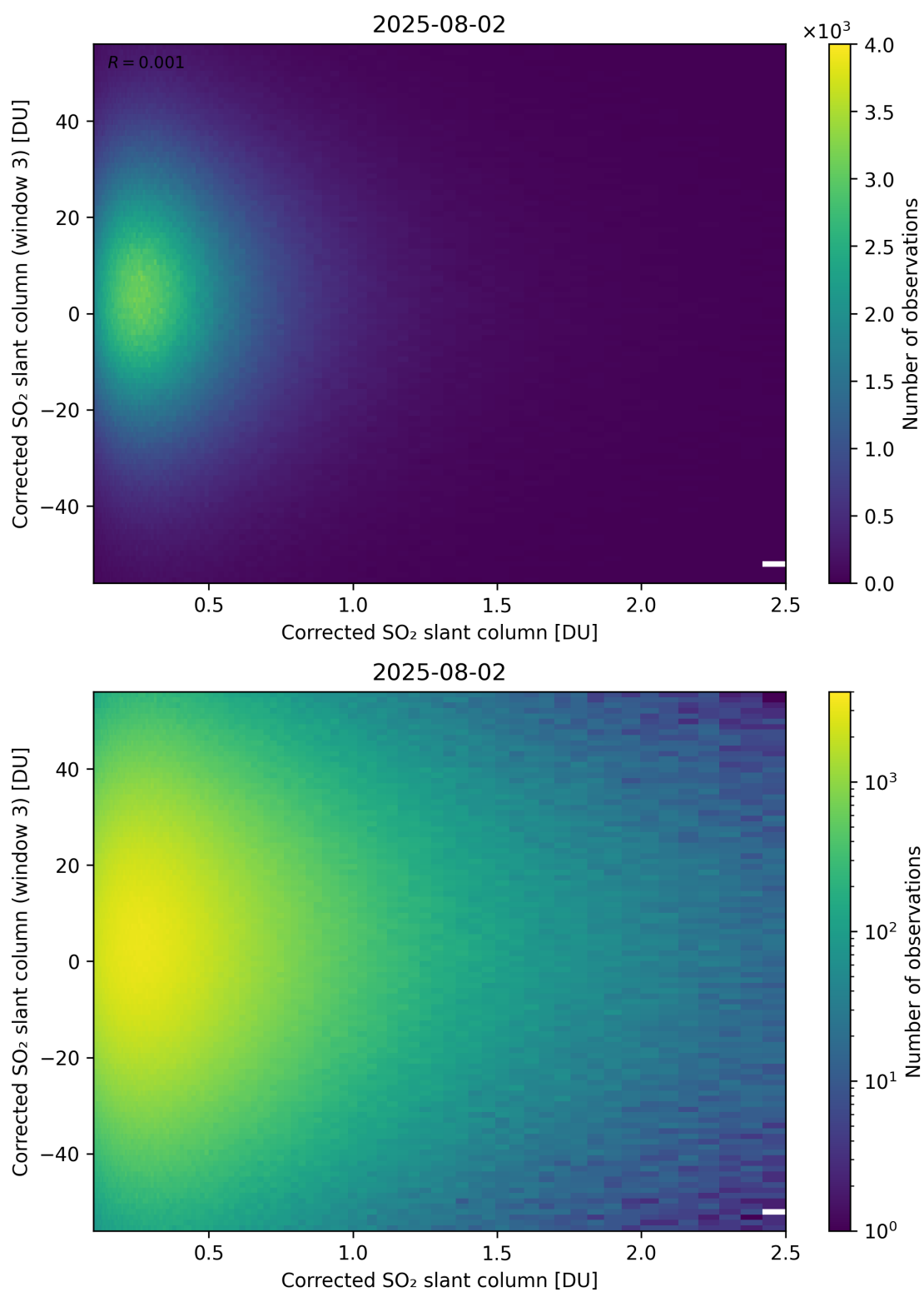
Figure 236: Scatter density plot of “Corrected SO 2 slant column” against “Corrected SO 2 slant column (window 3)” for 2025-08-01 to 2025-08-03.
