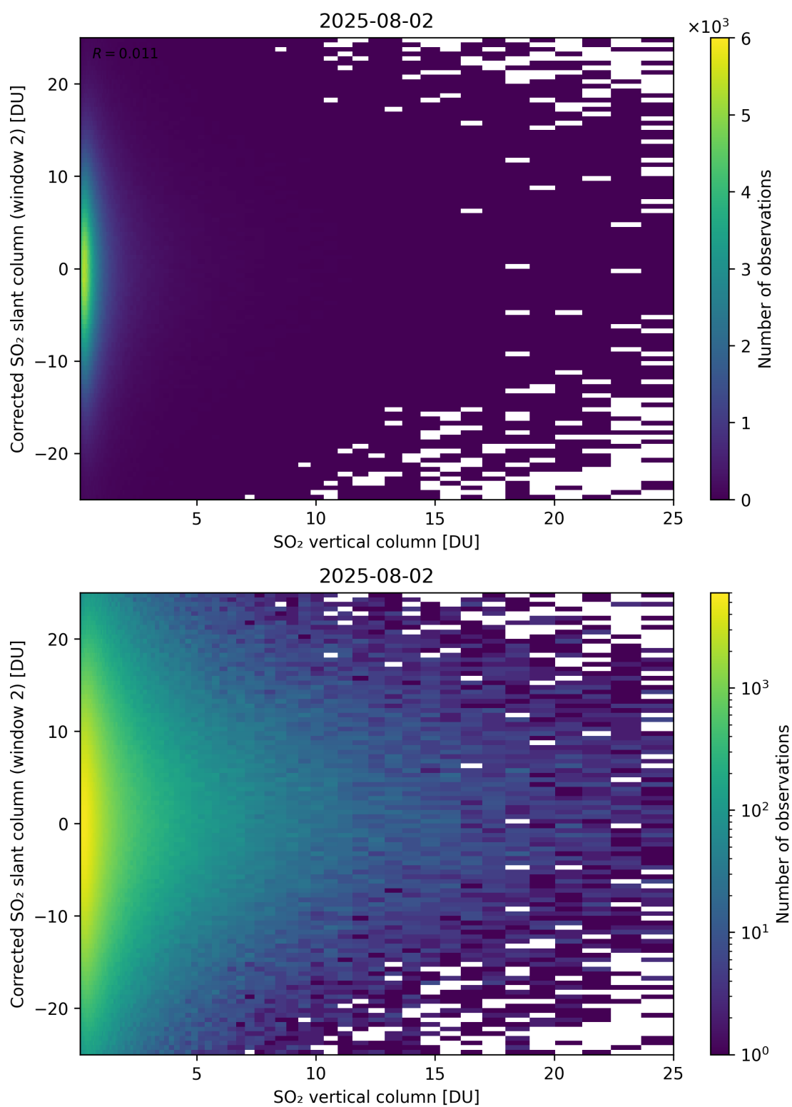
Figure 352: Scatter density plot of “SO 2 vertical column” against “Corrected SO 2 slant column (window 2)” for 2025-08-01 to 2025-08-03.
