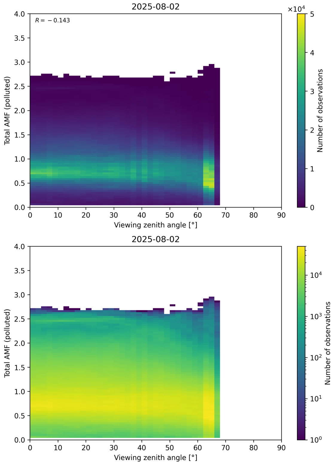
Figure 381: Scatter density plot of “Viewing zenith angle” against “Total AMF (polluted)” for 2025-08-01 to 2025-08-03.
