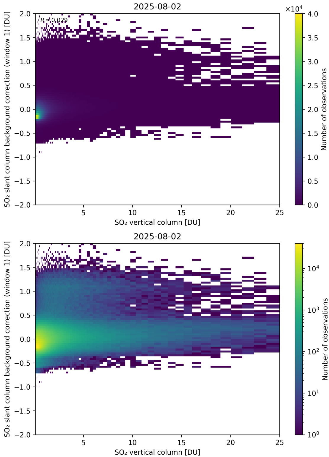
Figure 323: Scatter density plot of “SO 2 vertical column” against “SO 2 slant column background correction (window 1)” for 2025-08-01 to 2025-08-03.
