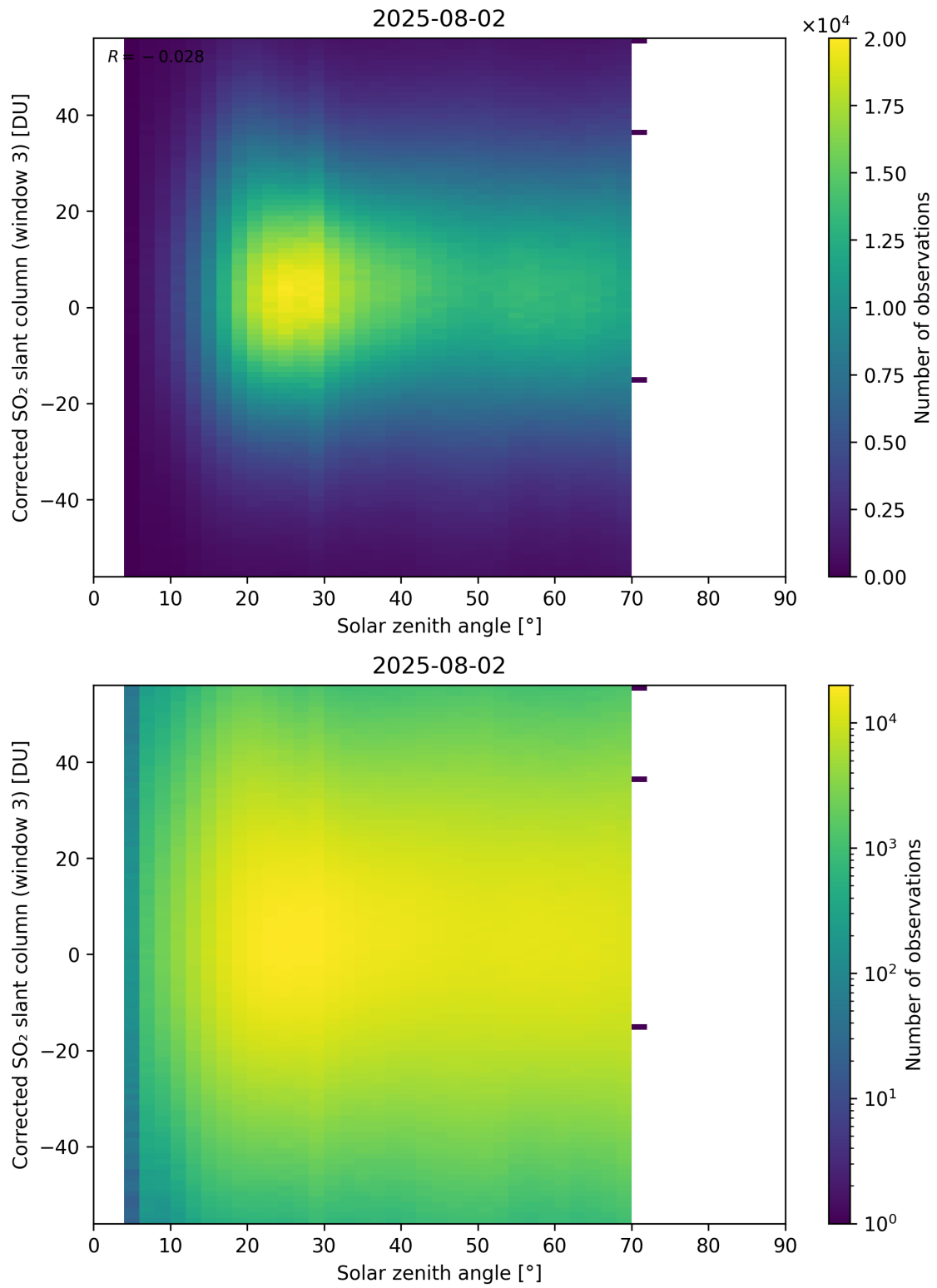
Figure 183: Scatter density plot of “Solar zenith angle” against “Corrected SO 2 slant column (window 3)” for 2025-08-01 to 2025-08-03.
