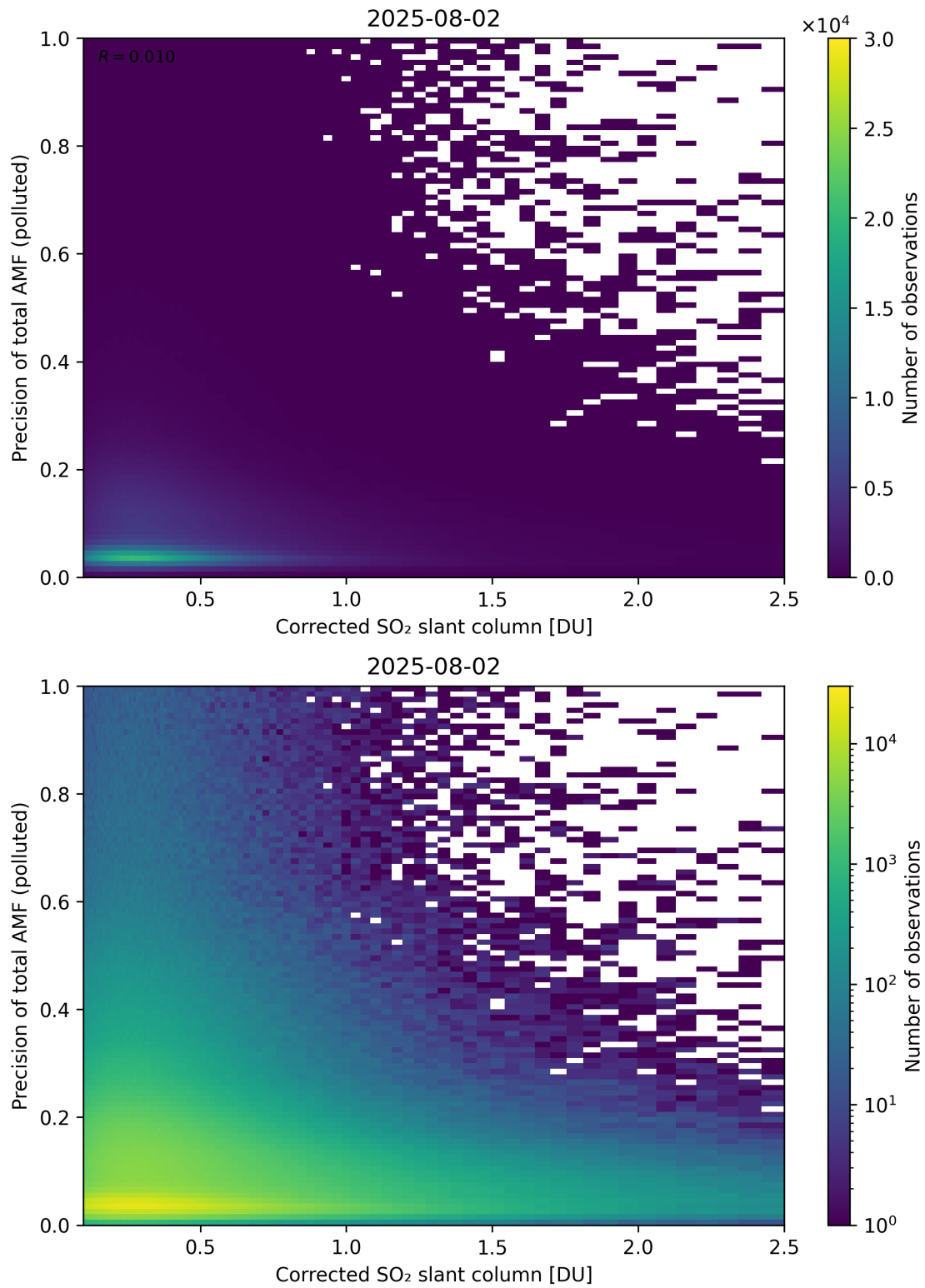
Figure 243: Scatter density plot of “Corrected SO 2 slant column” against “Precision of total AMF (polluted)” for 2025-08-01 to 2025-08-03.
