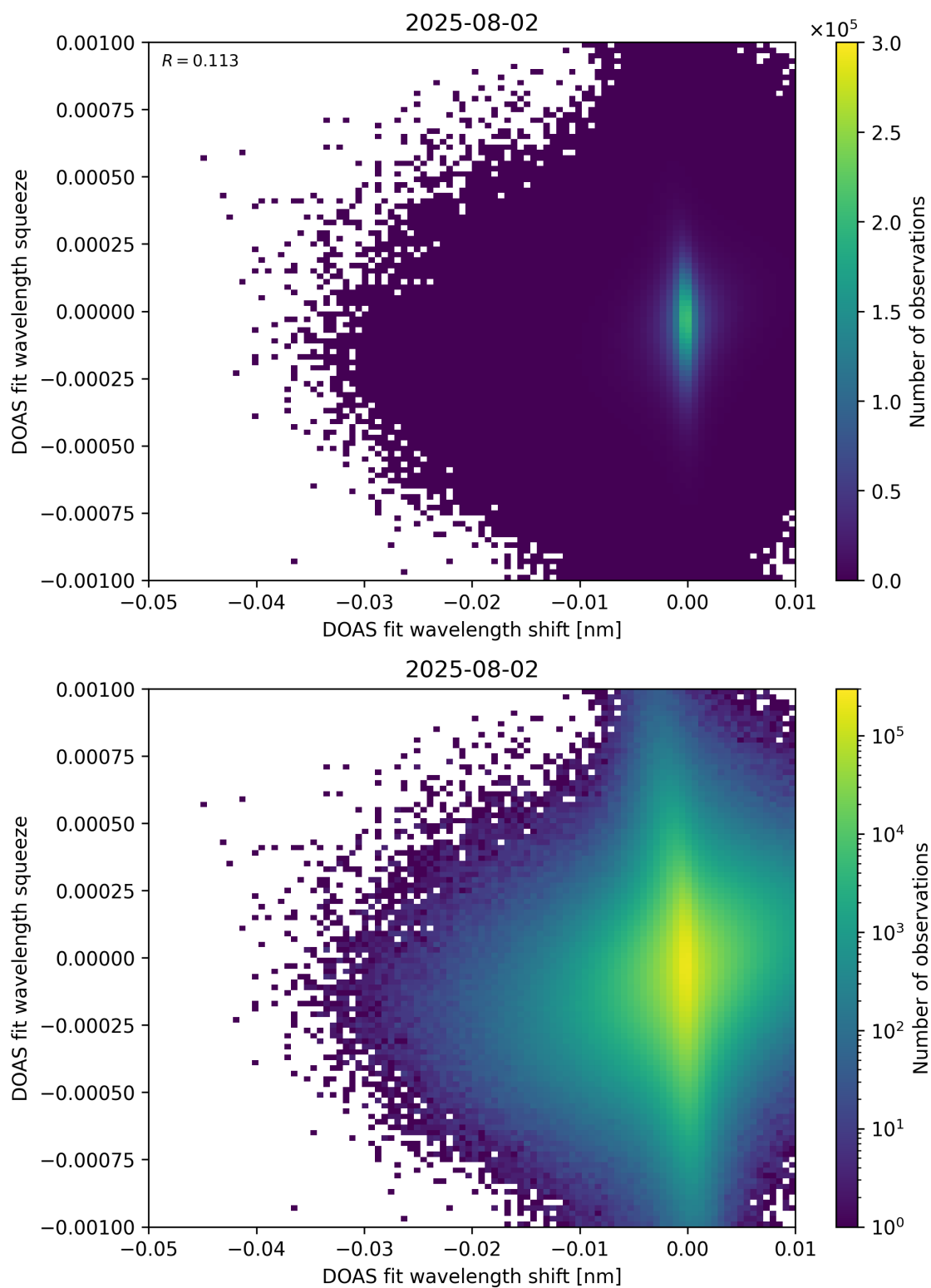
Figure 138: Scatter density plot of “DOAS fit wavelength shift” against “DOAS fit wavelength squeeze” for 2025-08-01 to 2025-08-03.
