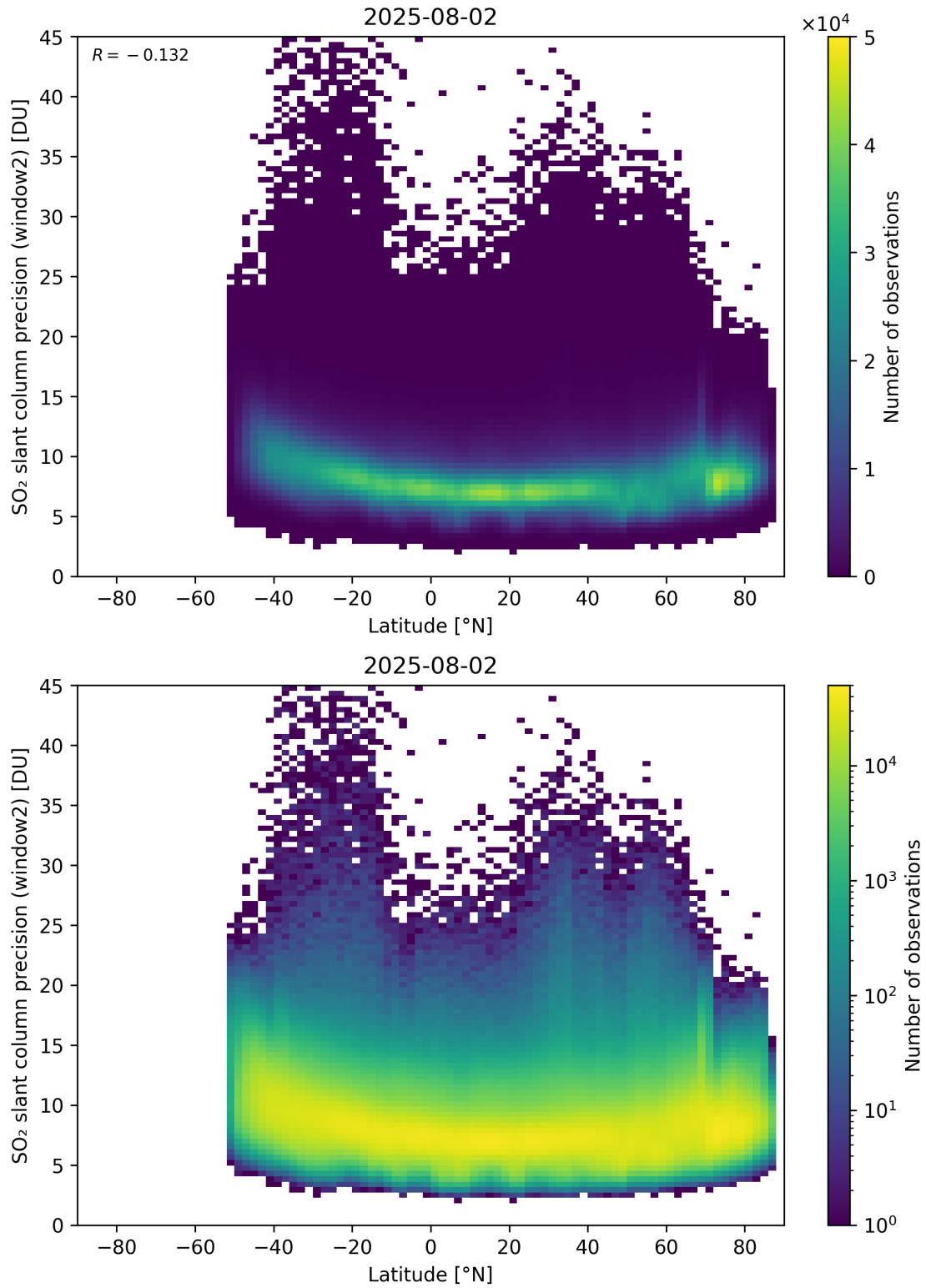
Figure 164: Scatter density plot of “Latitude” against “SO 2 slant column precision (window2)” for 2025-08-01 to 2025-08-03.
