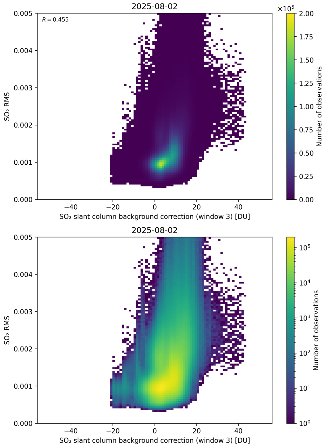
Figure 134: Scatter density plot of “SO 2 slant column background correction (window 3)” against “SO 2 RMS” for 2025-08-01 to 2025-08-03.
