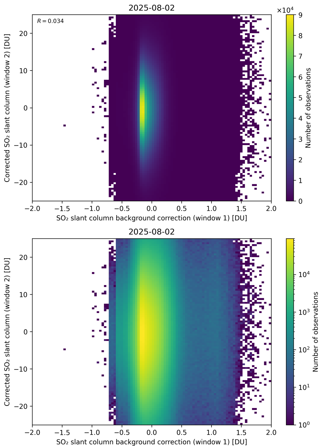
Figure 115: Scatter density plot of “SO 2 slant column background correction (window 1)” against “Corrected SO 2 slant column (window 2)” for 2025-08-01 to 2025-08-03.
