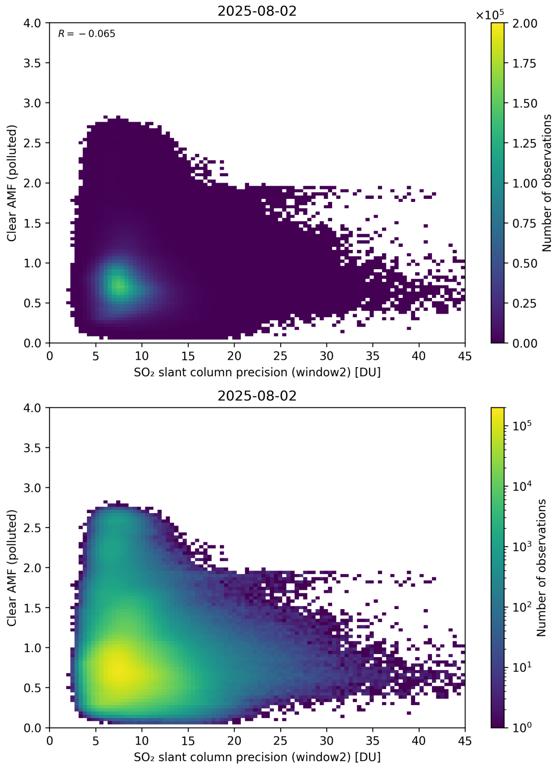
Figure 296: Scatter density plot of “SO 2 slant column precision (window2)” against “Clear AMF (polluted)” for 2025-08-01 to 2025-08-03.
