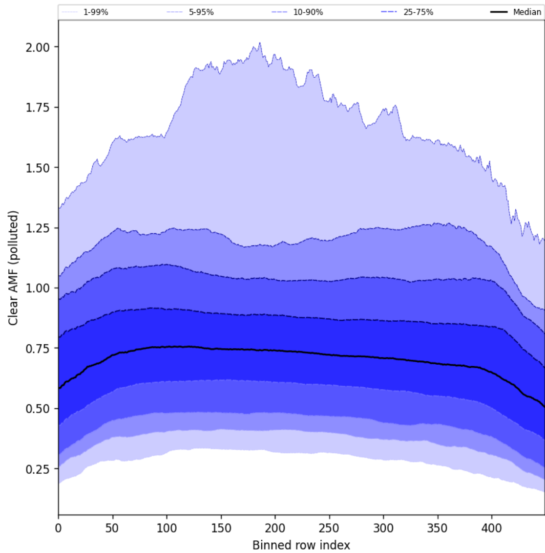
Figure 107: Along track statistics of “Clear AMF (polluted)” for 2025-08-01 to 2025-08-03
