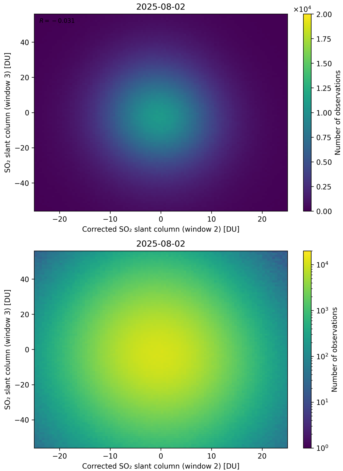
Figure 251: Scatter density plot of “Corrected SO 2 slant column (window 2)” against “SO 2 slant column (window 3)” for 2025-08-01 to 2025-08-03.
