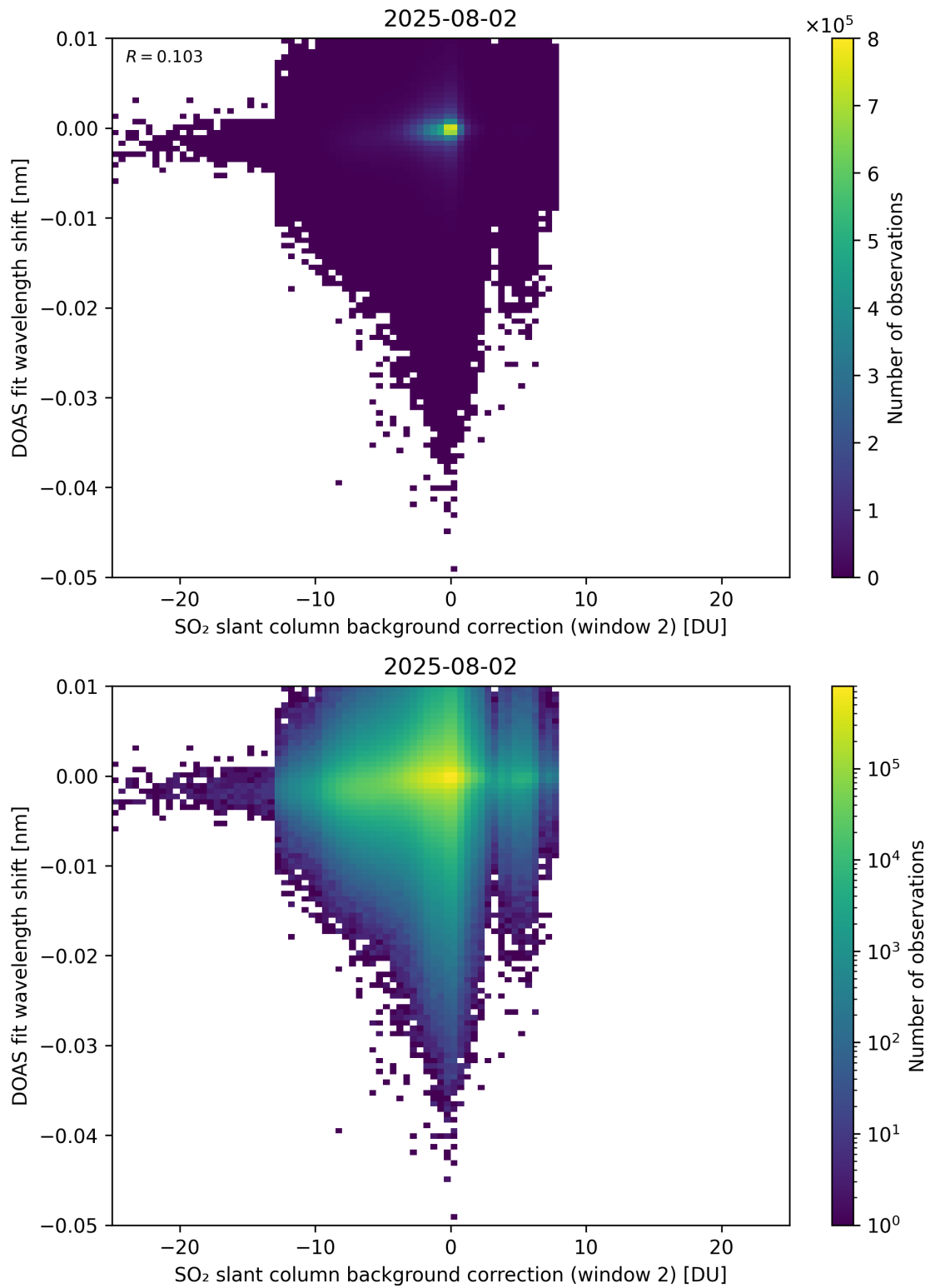
Figure 123: Scatter density plot of “SO 2 slant column background correction (window 2)” against “DOAS fit wavelength shift” for 2025-08-01 to 2025-08-03.
