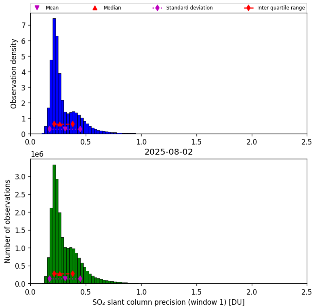
Figure 64: Histogram of “SO 2 slant column precision (window 1)” for 2025-08-01 to 2025-08-03
