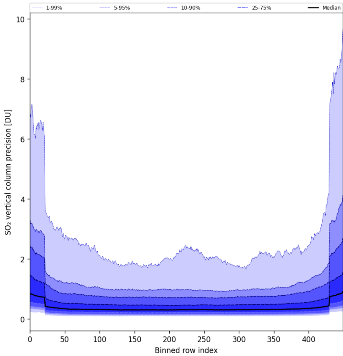
Figure 85: Along track statistics of “SO 2 vertical column precision” for 2025-08-01 to 2025-08-03
