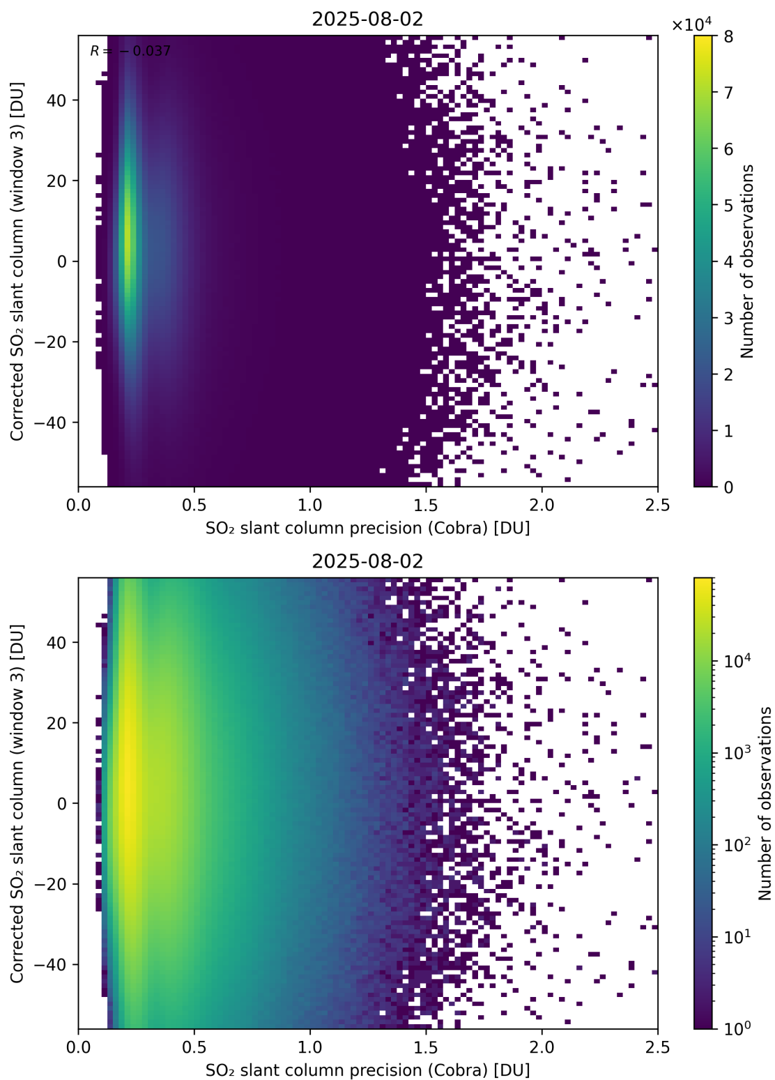
Figure 207: Scatter density plot of “SO 2 slant column precision (Cobra)” against “Corrected SO 2 slant column (window 3)” for 2025-08-01 to 2025-08-03.
