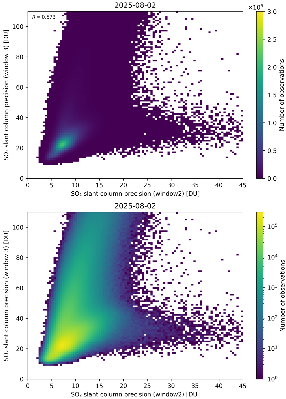
Figure 300: Scatter density plot of “SO 2 slant column precision (window2)” against “SO 2 slant column precision (window 3)” for 2025-08-01 to 2025-08-03.
