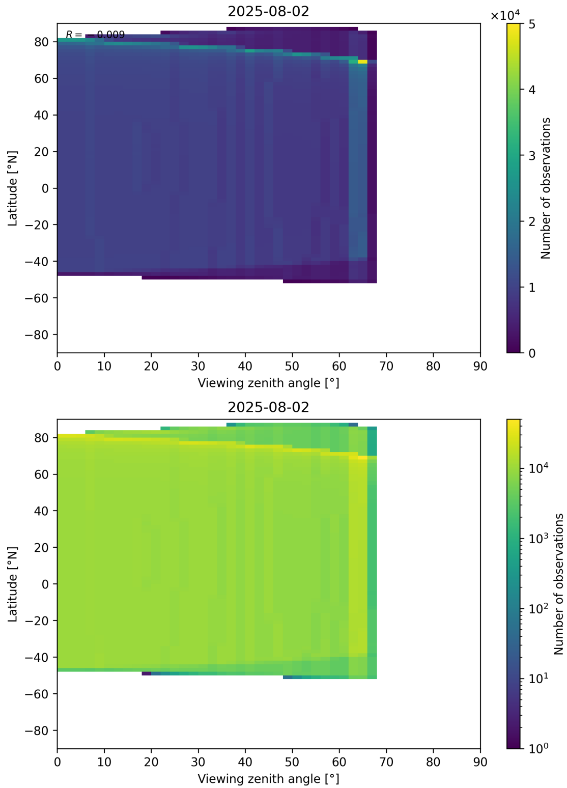
Figure 368: Scatter density plot of “Viewing zenith angle” against “Latitude” for 2025-08-01 to 2025-08-03.
