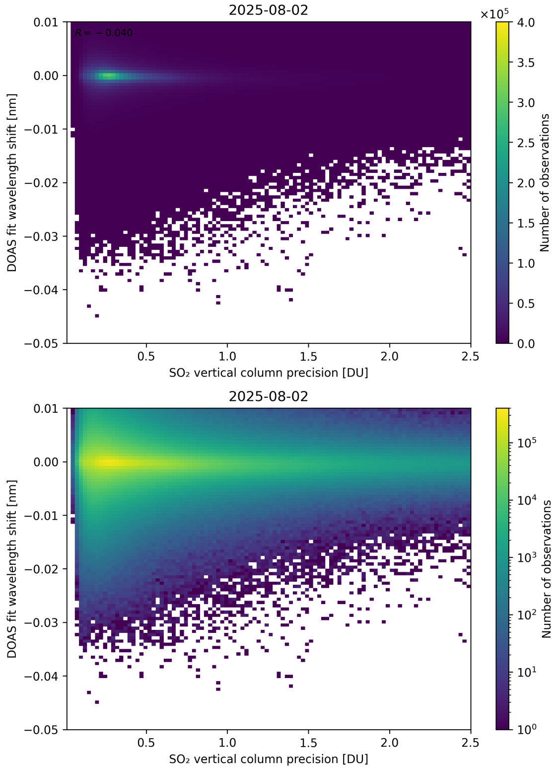
Figure 332: Scatter density plot of “SO 2 vertical column precision” against “DOAS fit wavelength shift” for 2025-08-01 to 2025-08-03.
