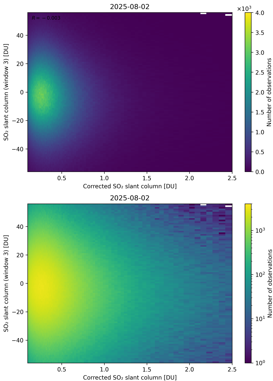
Figure 240: Scatter density plot of “Corrected SO 2 slant column” against “SO 2 slant column (window 3)” for 2025-08-01 to 2025-08-03.
