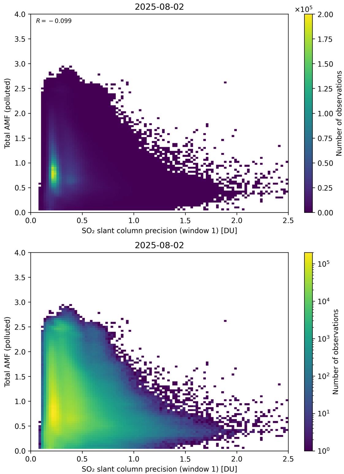
Figure 280: Scatter density plot of “SO 2 slant column precision (window 1)” against “Total AMF (polluted)” for 2025-08-01 to 2025-08-03.
