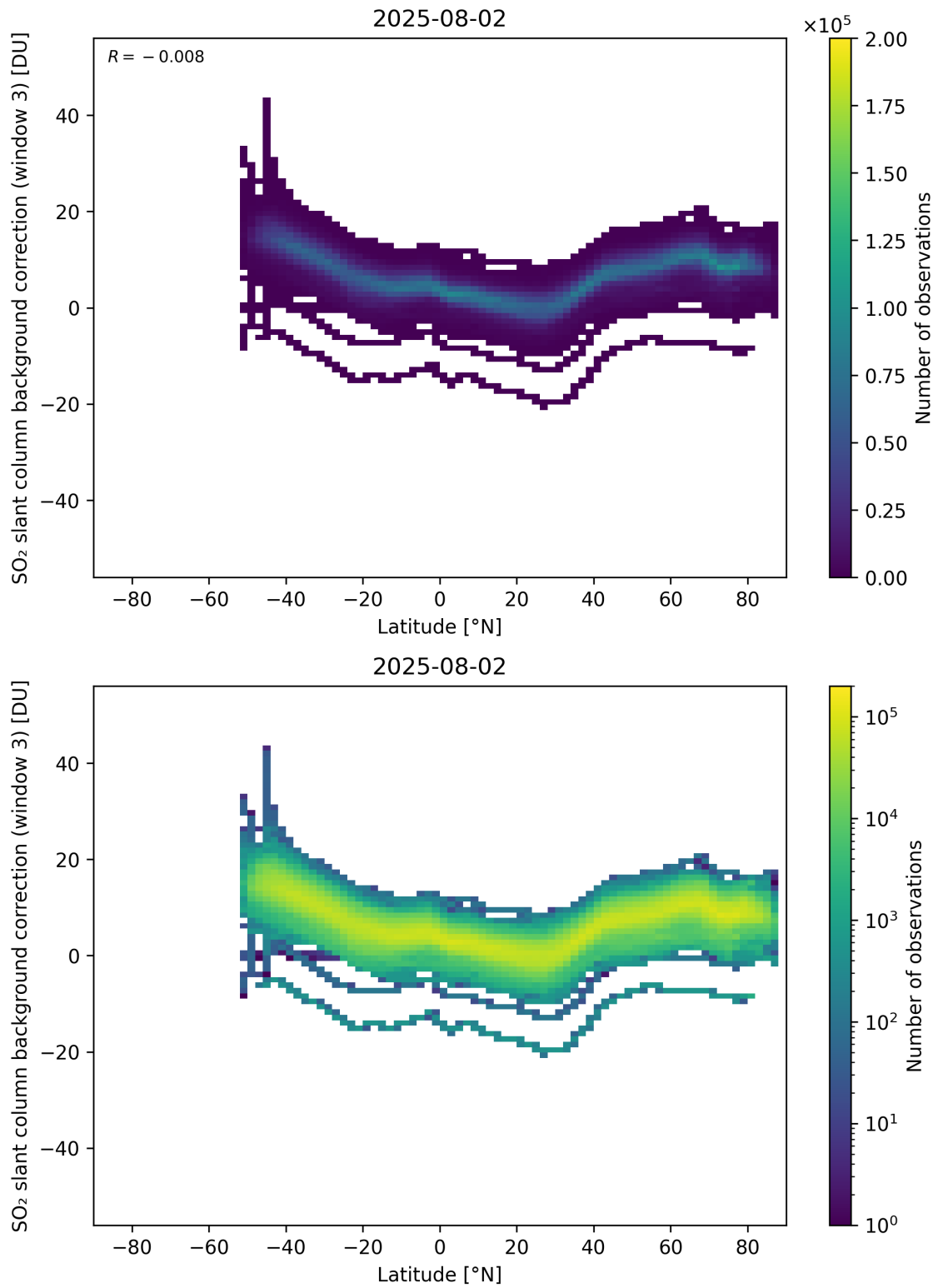
Figure 152: Scatter density plot of “Latitude” against “SO 2 slant column background correction (window 3)” for 2025-08-01 to 2025-08-03.
