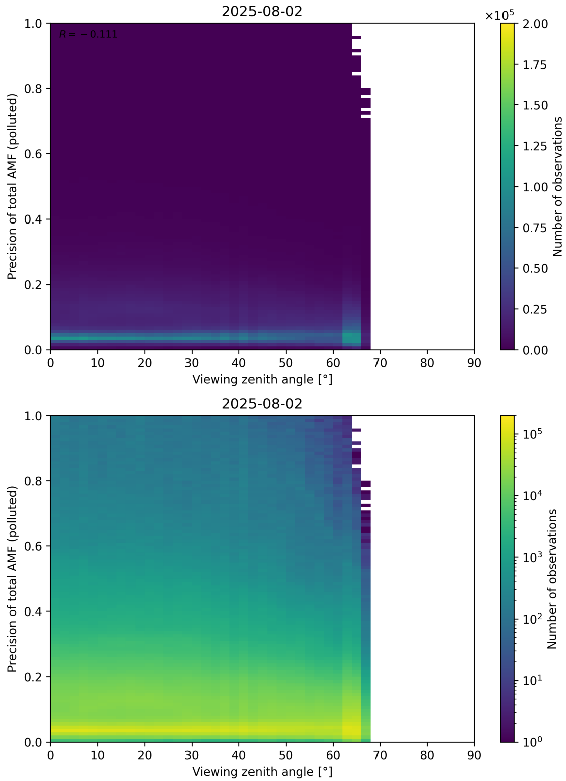
Figure 382: Scatter density plot of “Viewing zenith angle” against “Precision of total AMF (polluted)” for 2025-08-01 to 2025-08-03.
