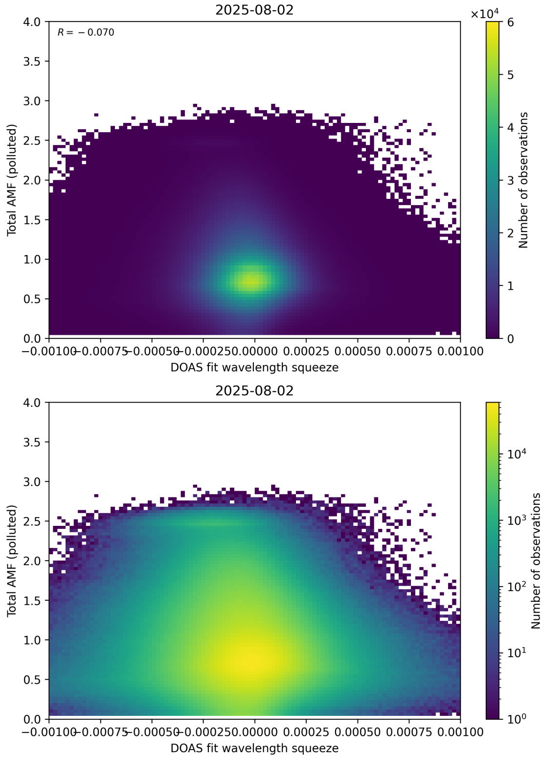
Figure 145: Scatter density plot of “DOAS fit wavelength squeeze” against “Total AMF (polluted)” for 2025-08-01 to 2025-08-03.
