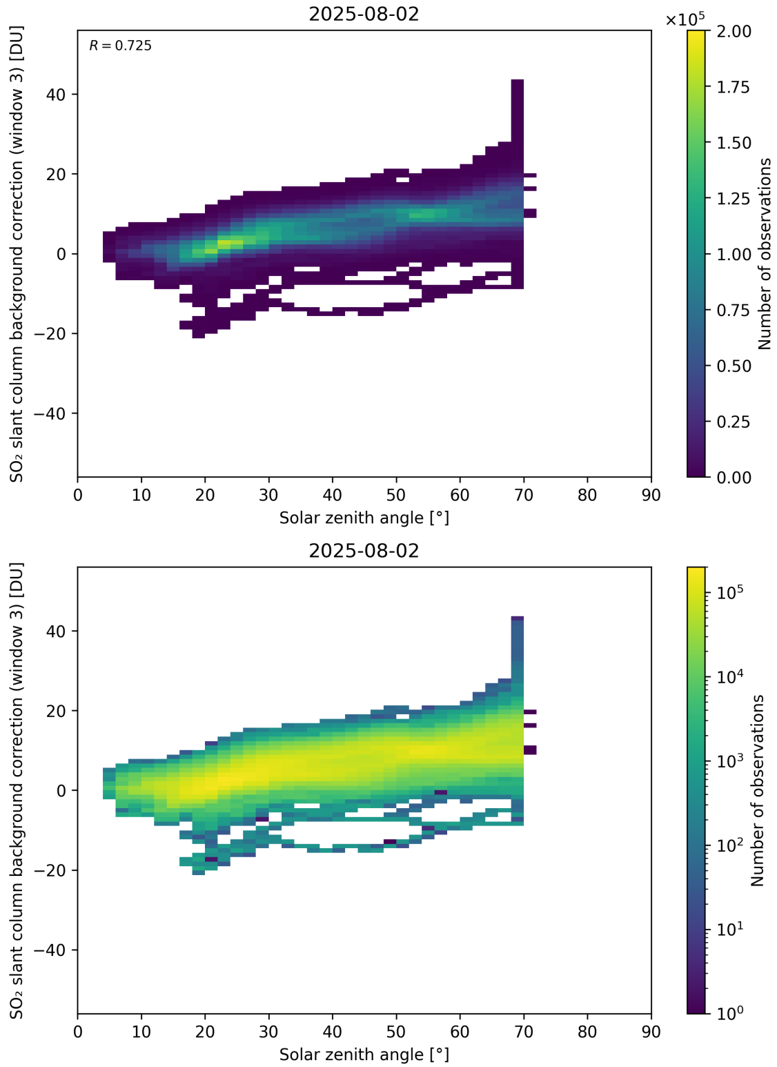
Figure 173: Scatter density plot of “Solar zenith angle” against “SO 2 slant column background correction (window 3)” for 2025-08-01 to 2025-08-03.
