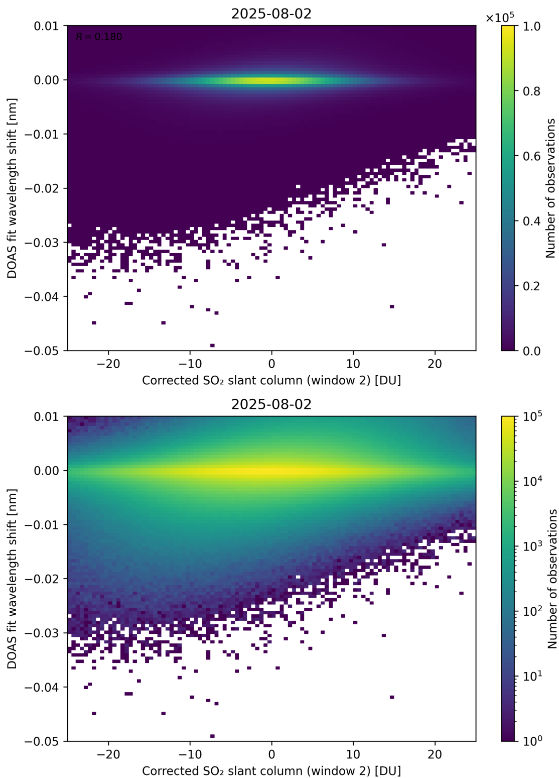
Figure 246: Scatter density plot of “Corrected SO 2 slant column (window 2)” against “DOAS fit wavelength shift” for 2025-08-01 to 2025-08-03.
