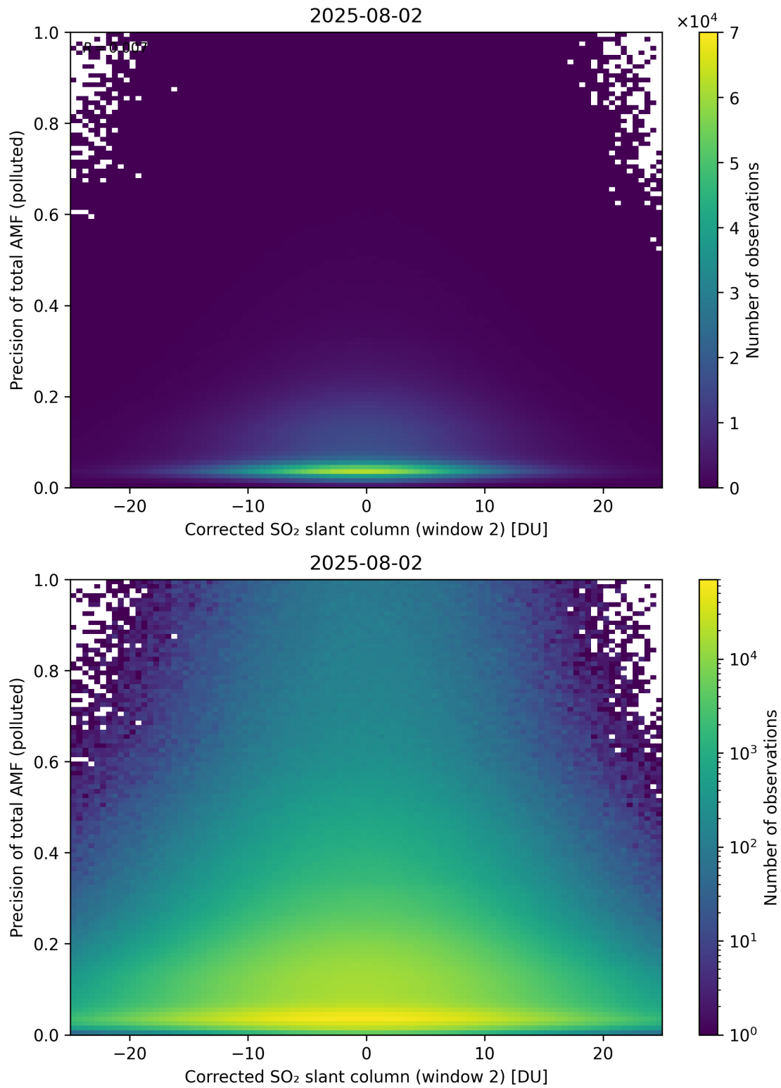
Figure 254: Scatter density plot of “Corrected SO 2 slant column (window 2)” against “Precision of total AMF (polluted)” for 2025-08-01 to 2025-08-03.
