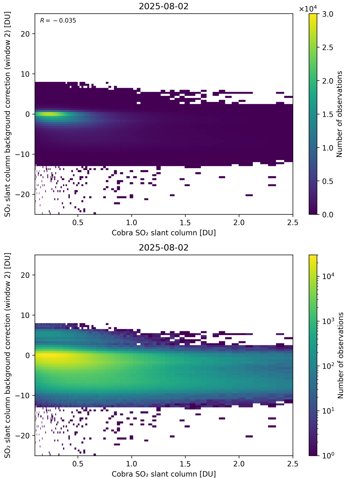
Figure 194: Scatter density plot of “Cobra SO 2 slant column” against “SO 2 slant column background correction (window 2)” for 2025-08-01 to 2025-08-03.
