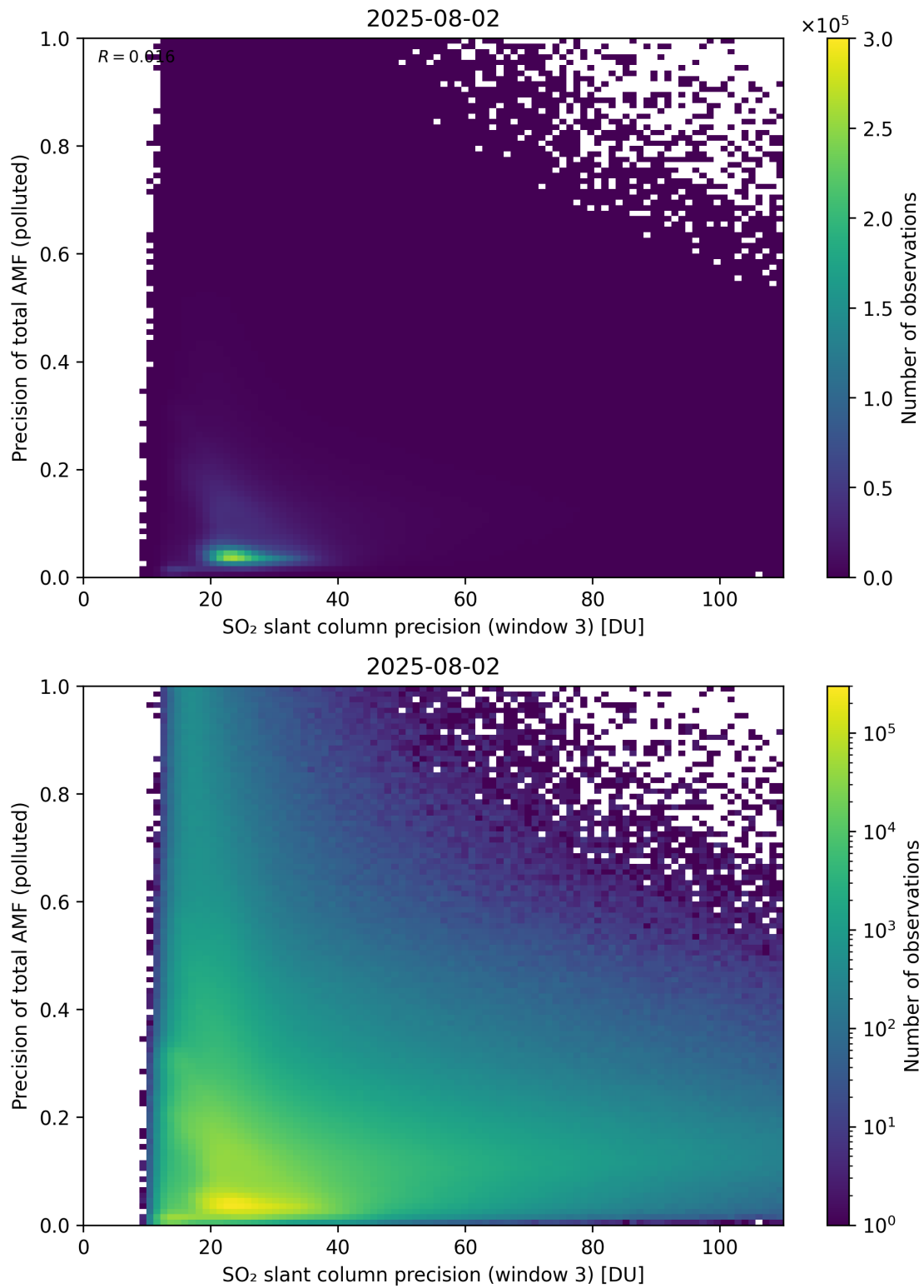
Figure 314: Scatter density plot of “SO 2 slant column precision (window 3)” against “Precision of total AMF (polluted)” for 2025-08-01 to 2025-08-03.
