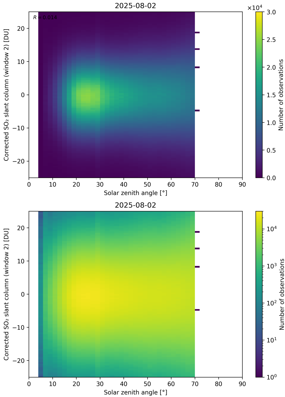
Figure 182: Scatter density plot of “Solar zenith angle” against “Corrected SO 2 slant column (window 2)” for 2025-08-01 to 2025-08-03.
