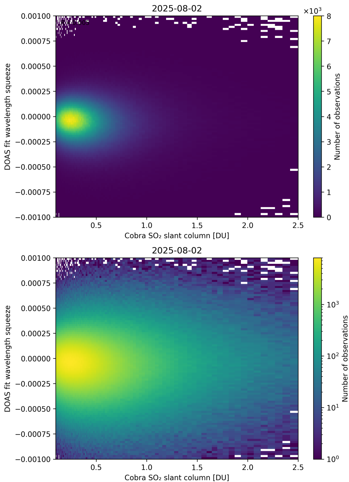
Figure 197: Scatter density plot of “Cobra SO 2 slant column” against “DOAS fit wavelength squeeze” for 2025-08-01 to 2025-08-03.
