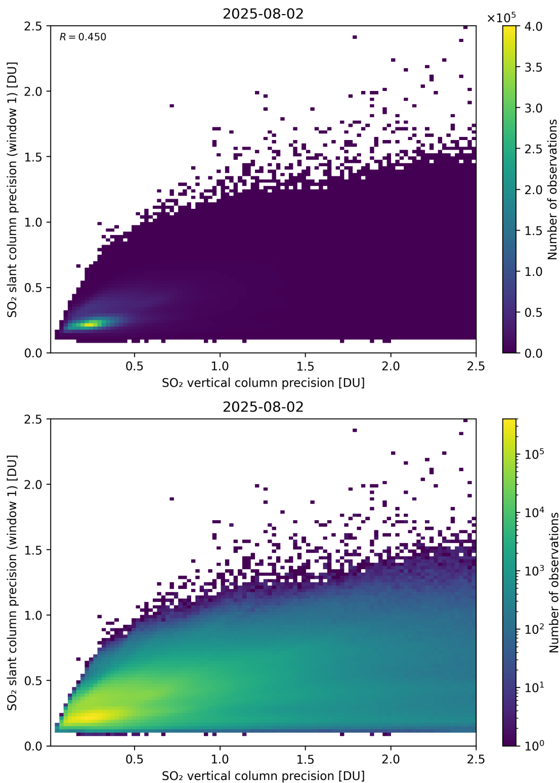
Figure 342: Scatter density plot of “SO 2 vertical column precision” against “SO 2 slant column precision (window 1)” for 2025-08-01 to 2025-08-03.
