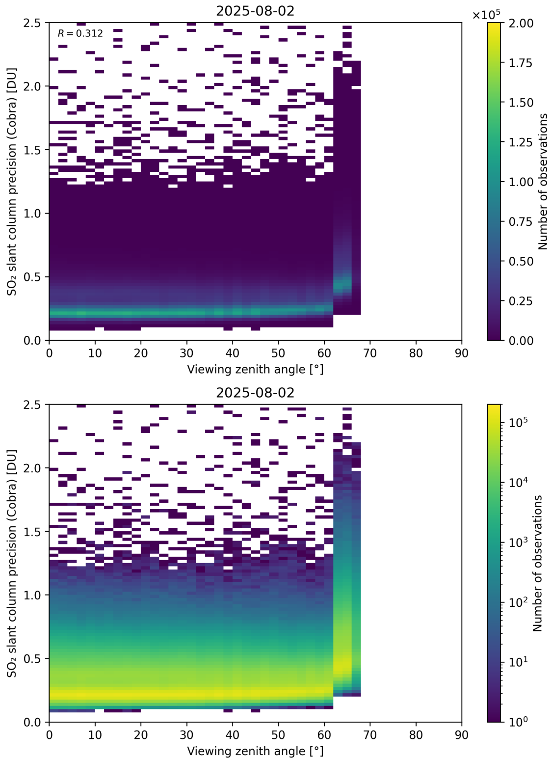
Figure 372: Scatter density plot of “Viewing zenith angle” against “SO 2 slant column precision (Cobra)” for 2025-08-01 to 2025-08-03.
