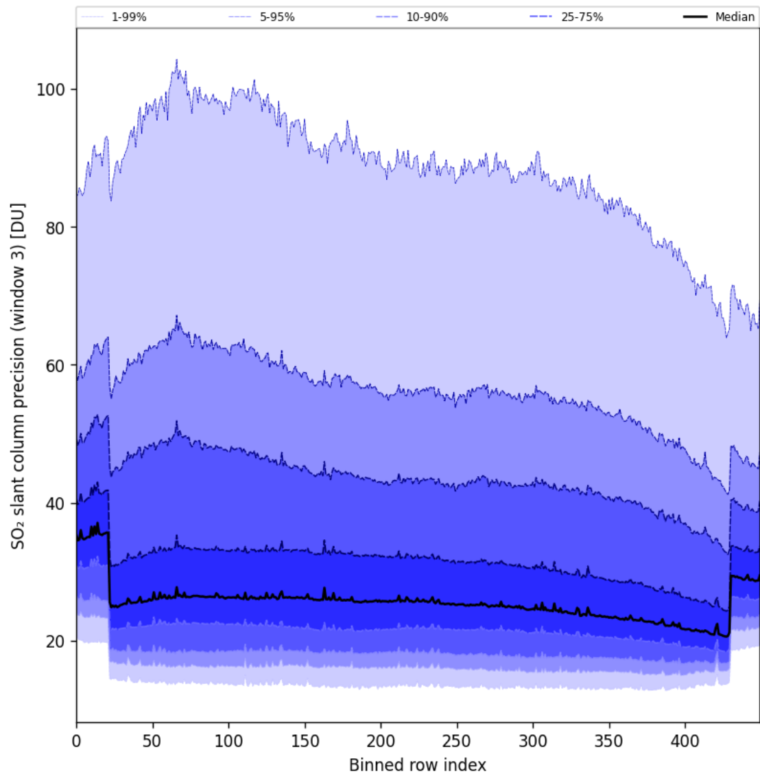
Figure 98: Along track statistics of “SO 2 slant column precision (window 3)” for 2025-08-03 to 2025-08-04
