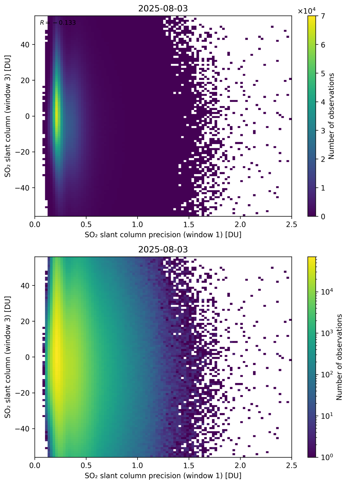
Figure 278: Scatter density plot of “SO 2 slant column precision (window 1)” against “SO 2 slant column (window 3)” for 2025-08-03 to 2025-08-04.
