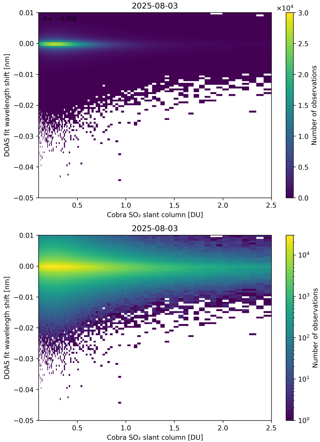
Figure 196: Scatter density plot of “Cobra SO 2 slant column” against “DOAS fit wavelength shift” for 2025-08-03 to 2025-08-04.
