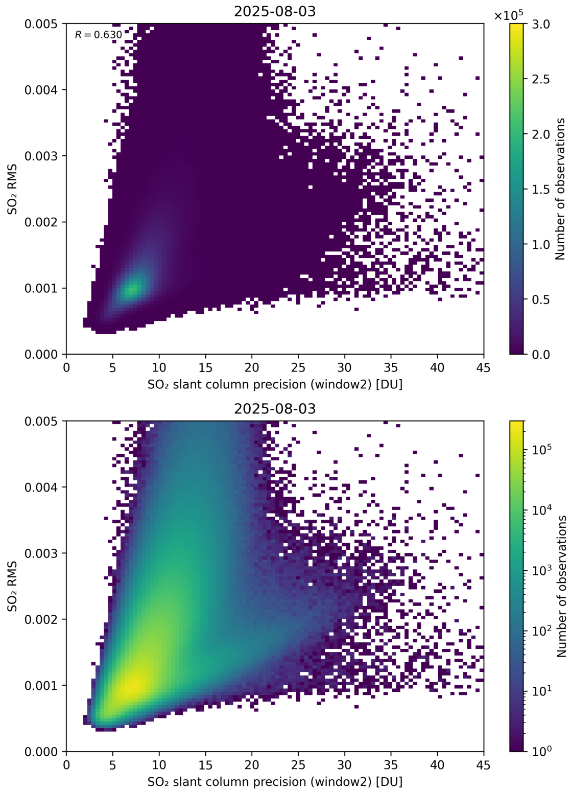
Figure 295: Scatter density plot of “SO 2 slant column precision (window2)” against “SO 2 RMS” for 2025-08-03 to 2025-08-04.
