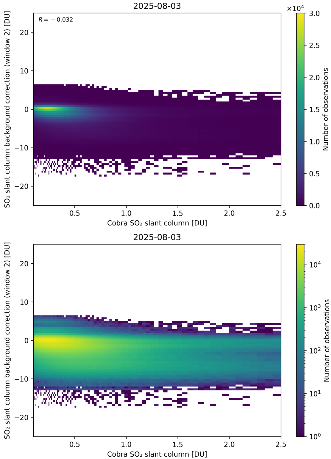
Figure 194: Scatter density plot of “Cobra SO 2 slant column” against “SO 2 slant column background correction (window 2)” for 2025-08-03 to 2025-08-04.
