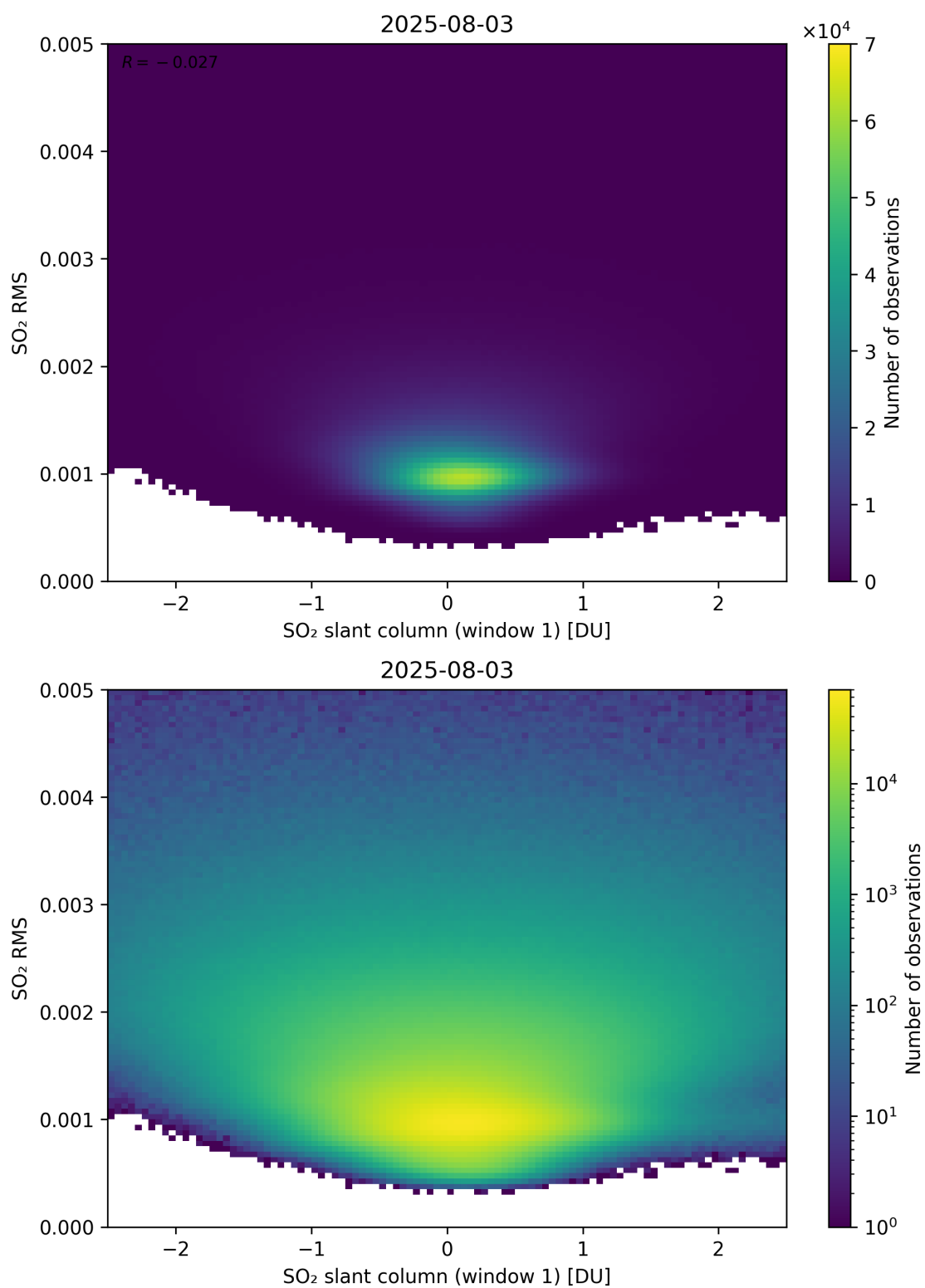
Figure 267: Scatter density plot of “SO 2 slant column (window 1)” against “SO 2 RMS” for 2025-08-03 to 2025-08-04.
