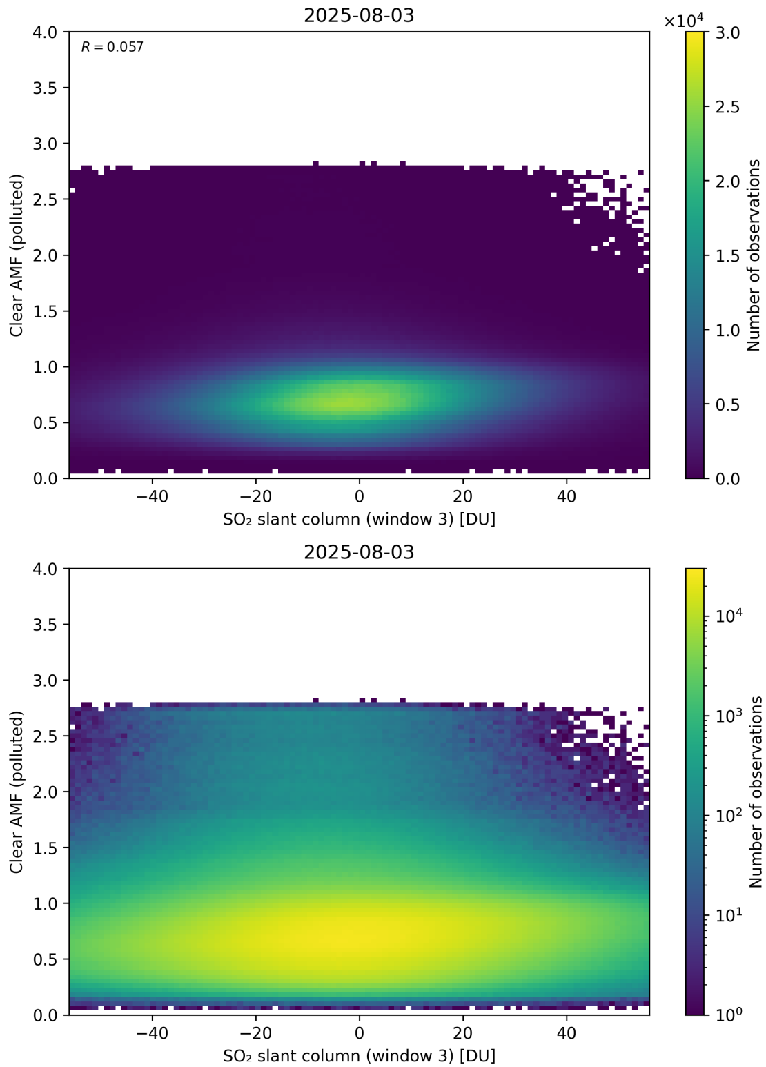
Figure 315: Scatter density plot of “SO 2 slant column (window 3)” against “Clear AMF (polluted)” for 2025-08-03 to 2025-08-04.
