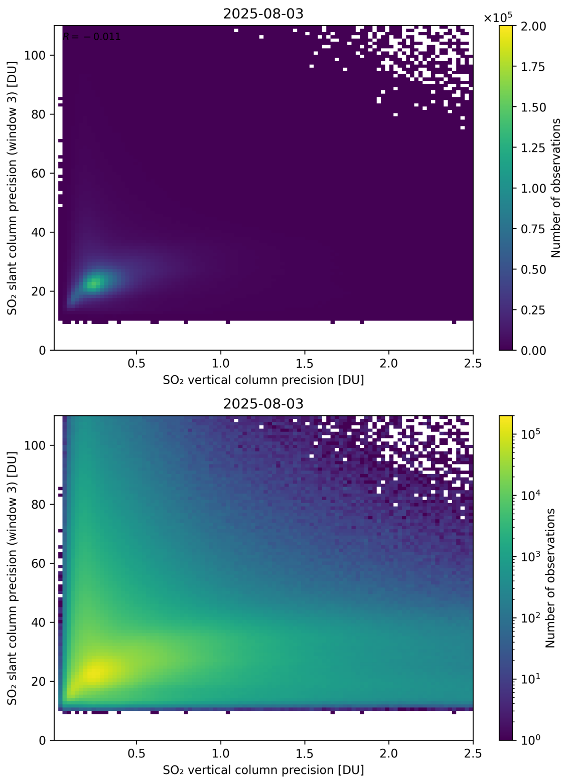
Figure 345: Scatter density plot of “SO 2 vertical column precision” against “SO 2 slant column precision (window 3)” for 2025-08-03 to 2025-08-04.
