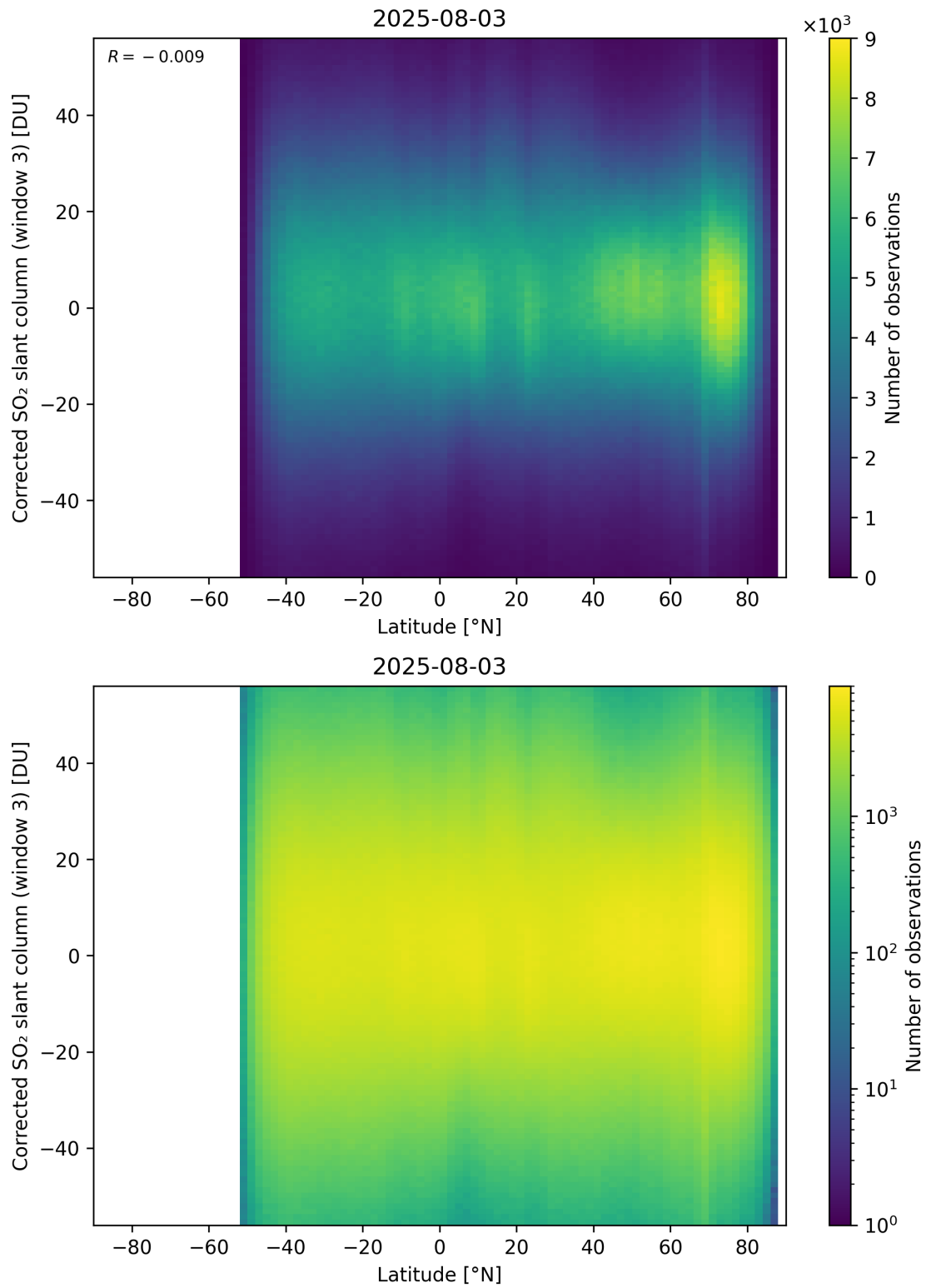
Figure 161: Scatter density plot of “Latitude” against “Corrected SO 2 slant column (window 3)” for 2025-08-03 to 2025-08-04.
