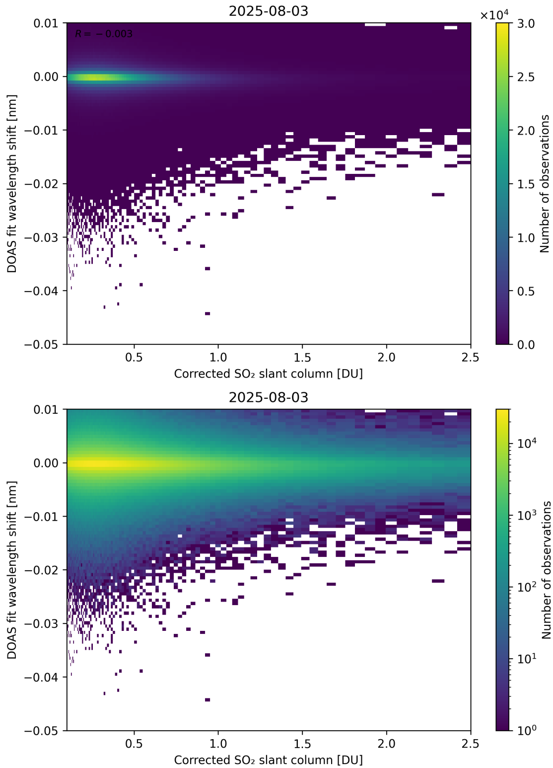
Figure 229: Scatter density plot of “Corrected SO 2 slant column” against “DOAS fit wavelength shift” for 2025-08-03 to 2025-08-04.
