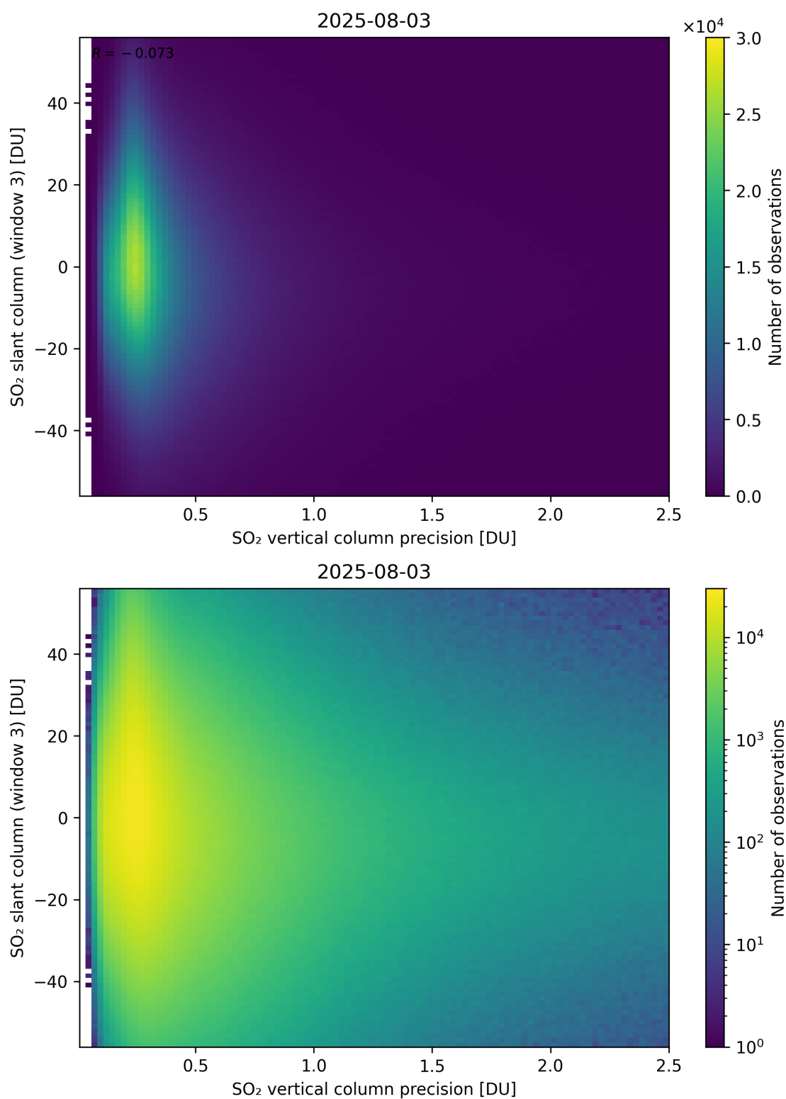
Figure 344: Scatter density plot of “SO 2 vertical column precision” against “SO 2 slant column (window 3)” for 2025-08-03 to 2025-08-04.
