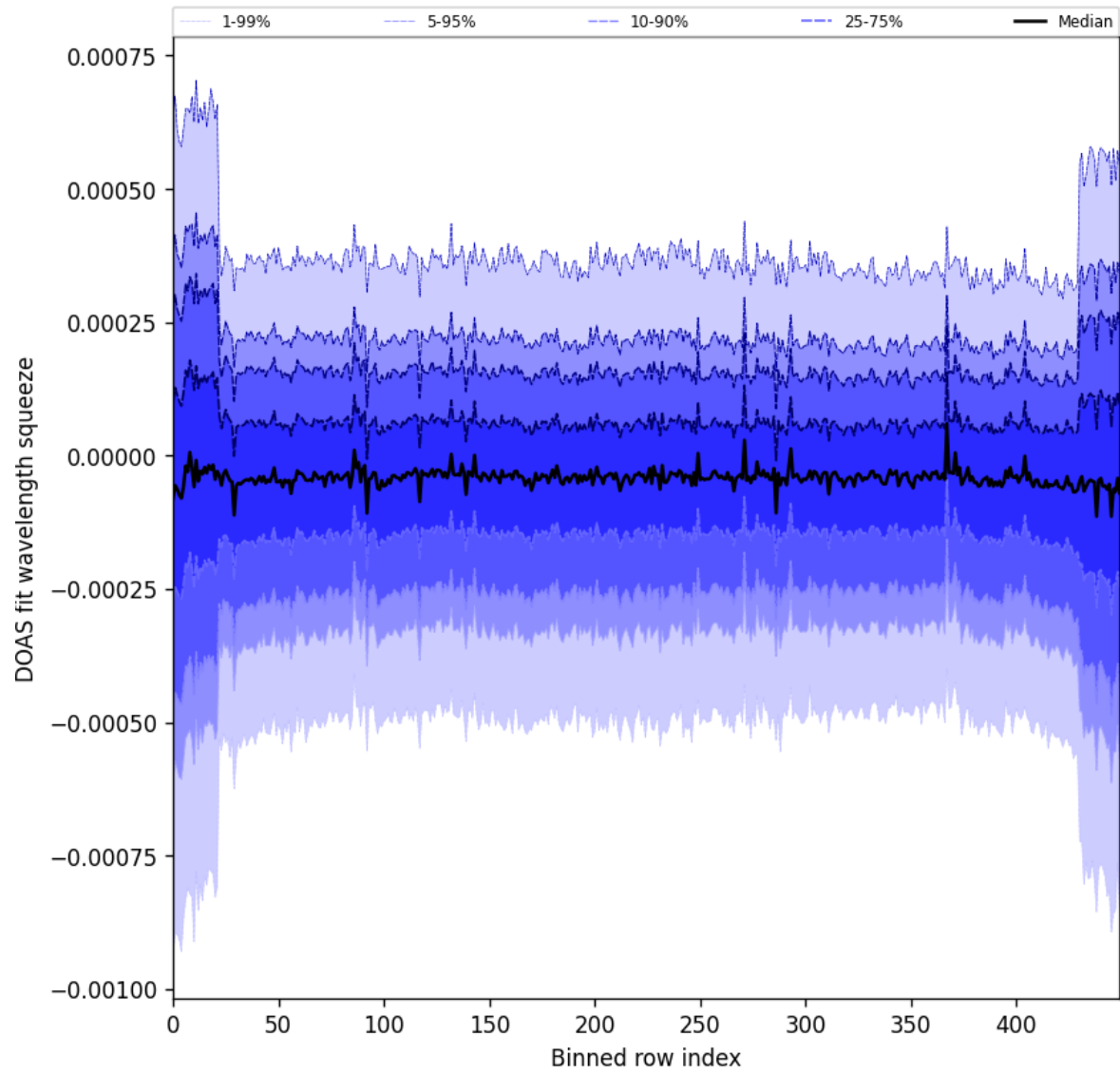
Figure 103: Along track statistics of “DOAS fit wavelength squeeze” for 2025-08-03 to 2025-08-04
