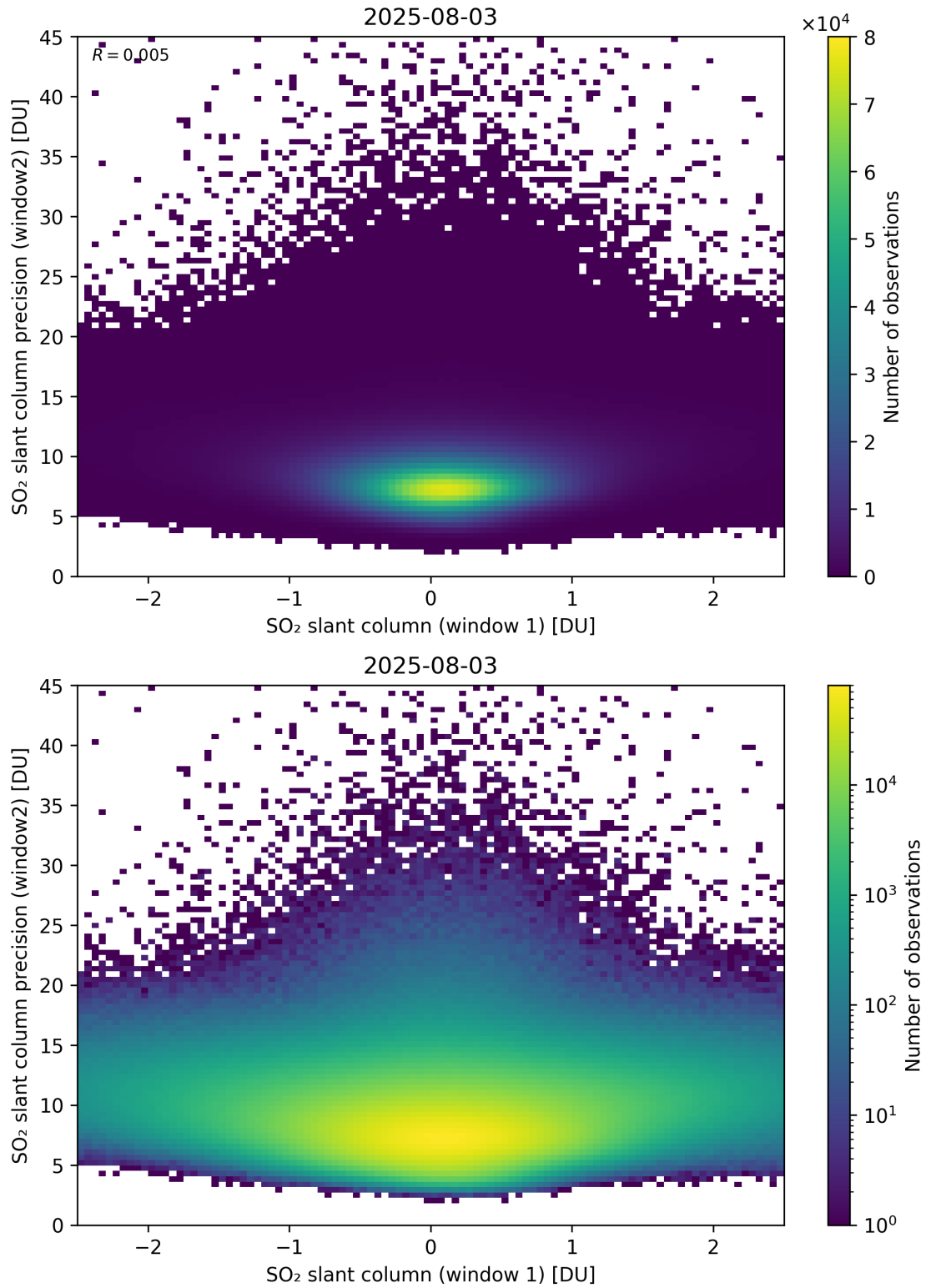
Figure 286: Scatter density plot of “SO 2 slant column (window 1)” against “SO 2 slant column precision (window2)” for 2025-08-03 to 2025-08-04.
