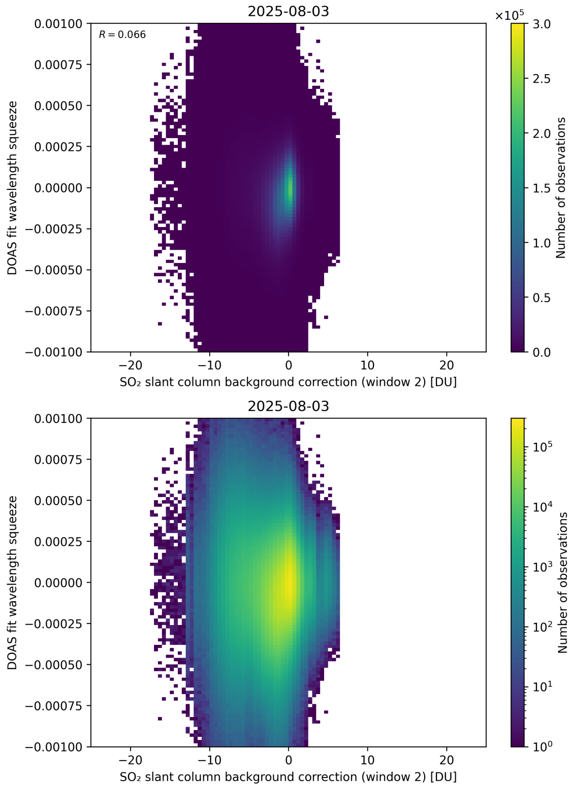
Figure 124: Scatter density plot of “SO 2 slant column background correction (window 2)” against “DOAS fit wavelength squeeze” for 2025-08-03 to 2025-08-04.
