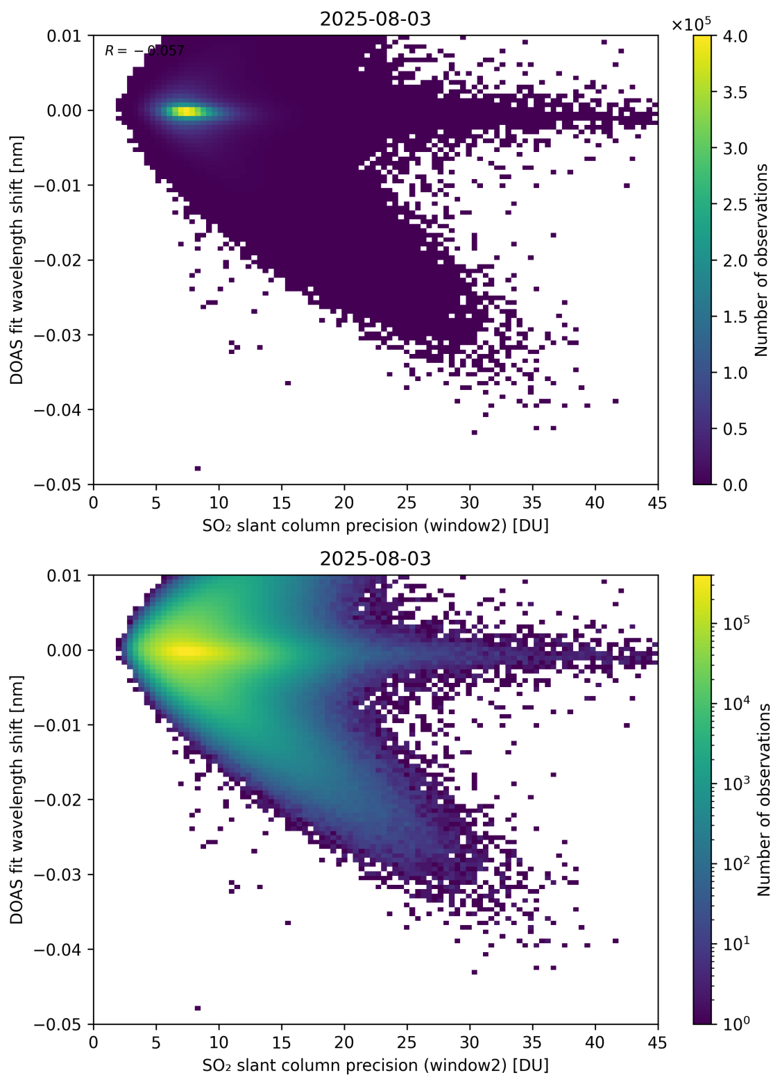
Figure 293: Scatter density plot of “SO 2 slant column precision (window2)” against “DOAS fit wavelength shift” for 2025-08-03 to 2025-08-04.
