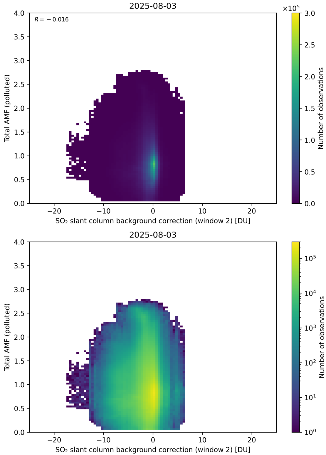
Figure 130: Scatter density plot of “SO 2 slant column background correction (window 2)” against “Total AMF (polluted)” for 2025-08-03 to 2025-08-04.
