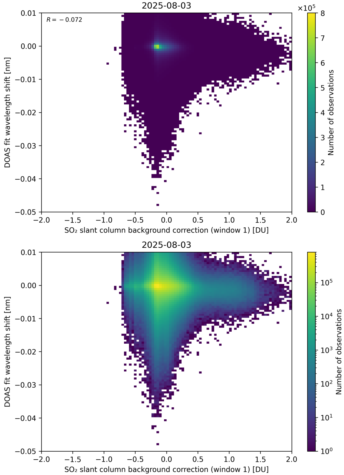
Figure 111: Scatter density plot of “SO 2 slant column background correction (window 1)” against “DOAS fit wavelength shift” for 2025-08-03 to 2025-08-04.
