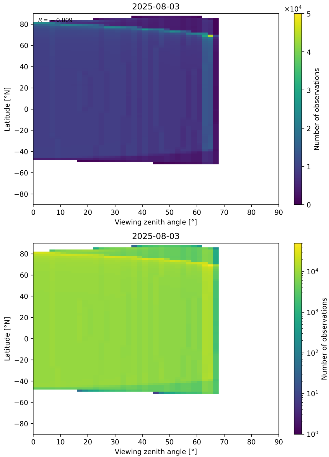
Figure 368: Scatter density plot of “Viewing zenith angle” against “Latitude” for 2025-08-03 to 2025-08-04.
