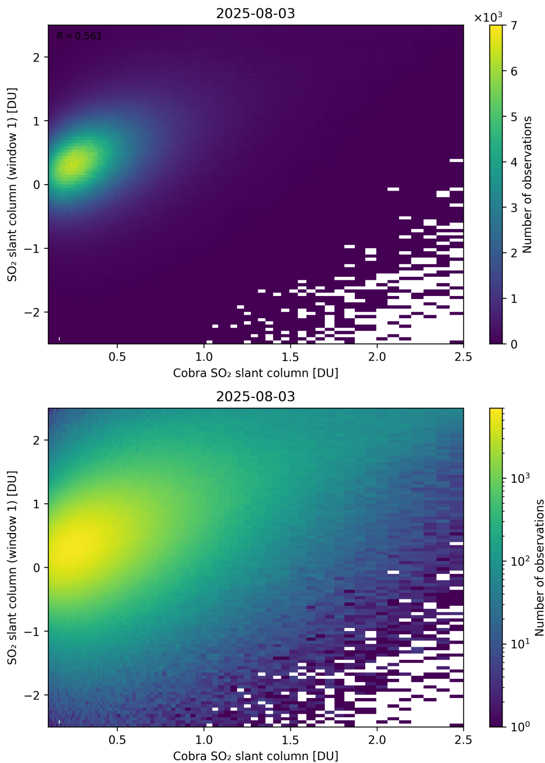
Figure 219: Scatter density plot of “Cobra SO 2 slant column” against “SO 2 slant column (window 1)” for 2025-08-03 to 2025-08-04.
