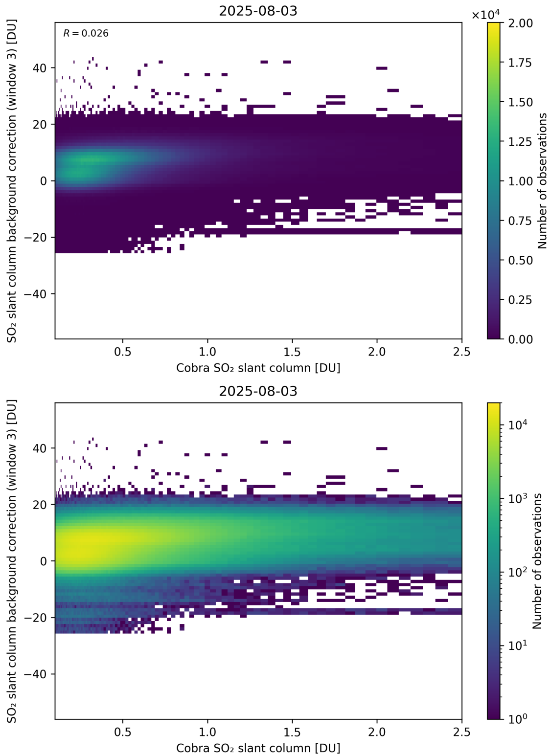
Figure 195: Scatter density plot of “Cobra SO 2 slant column” against “SO 2 slant column background correction (window 3)” for 2025-08-03 to 2025-08-04.
