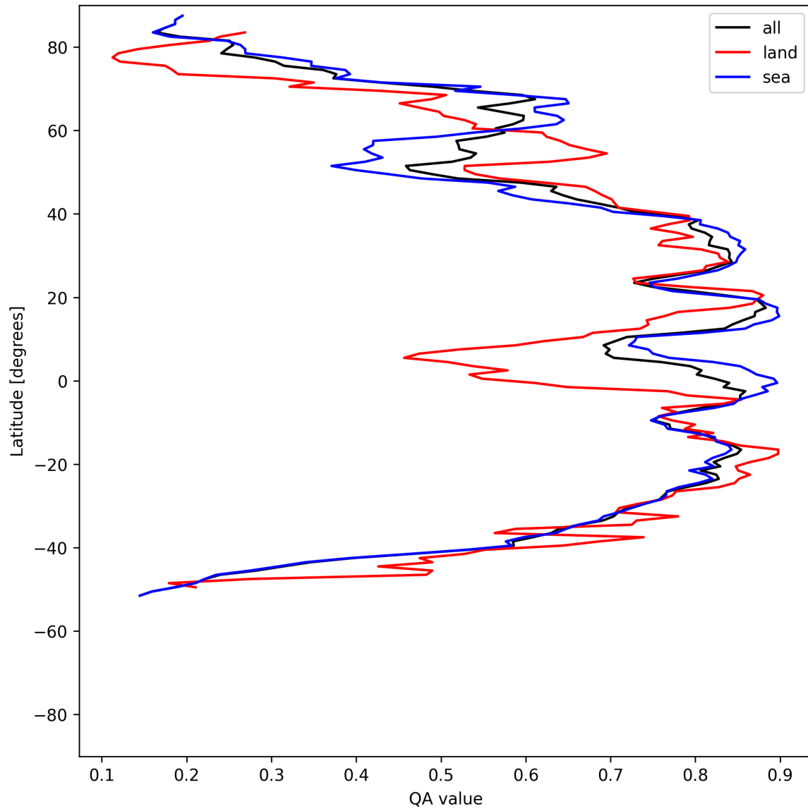
Figure 31: Zonal average of “QA value” for 2025-08-03 to 2025-08-04.
