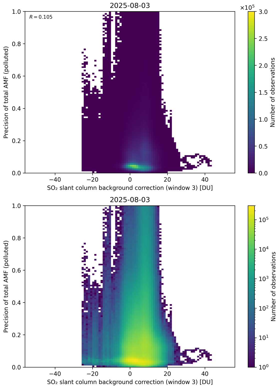
Figure 137: Scatter density plot of “SO 2 slant column background correction (window 3)” against “Precision of total AMF (polluted)” for 2025-08-03 to 2025-08-04.
