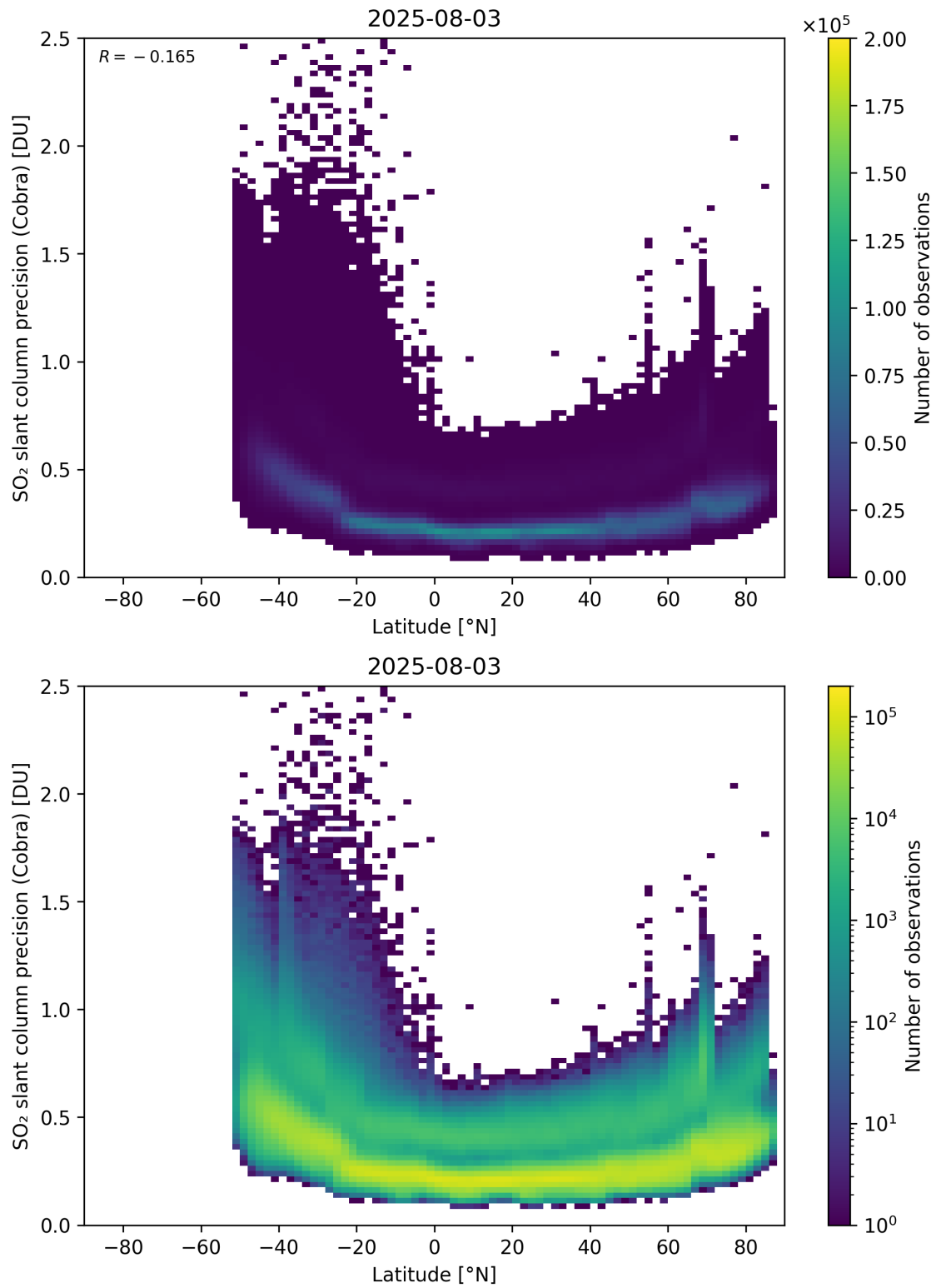
Figure 158: Scatter density plot of “Latitude” against “SO 2 slant column precision (Cobra)” for 2025-08-03 to 2025-08-04.
