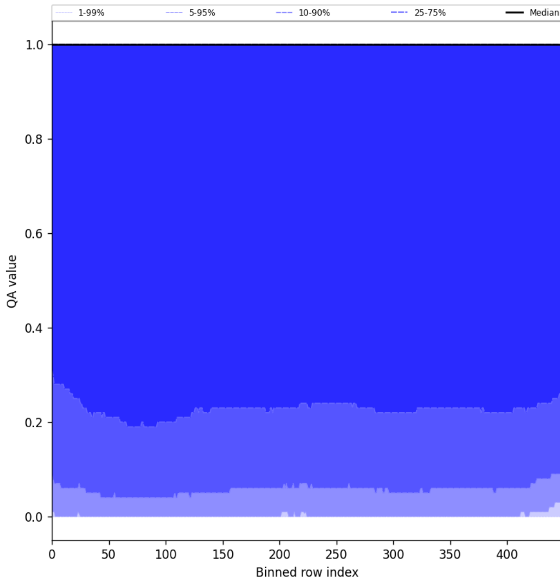
Figure 83: Along track statistics of “QA value” for 2025-08-03 to 2025-08-04
