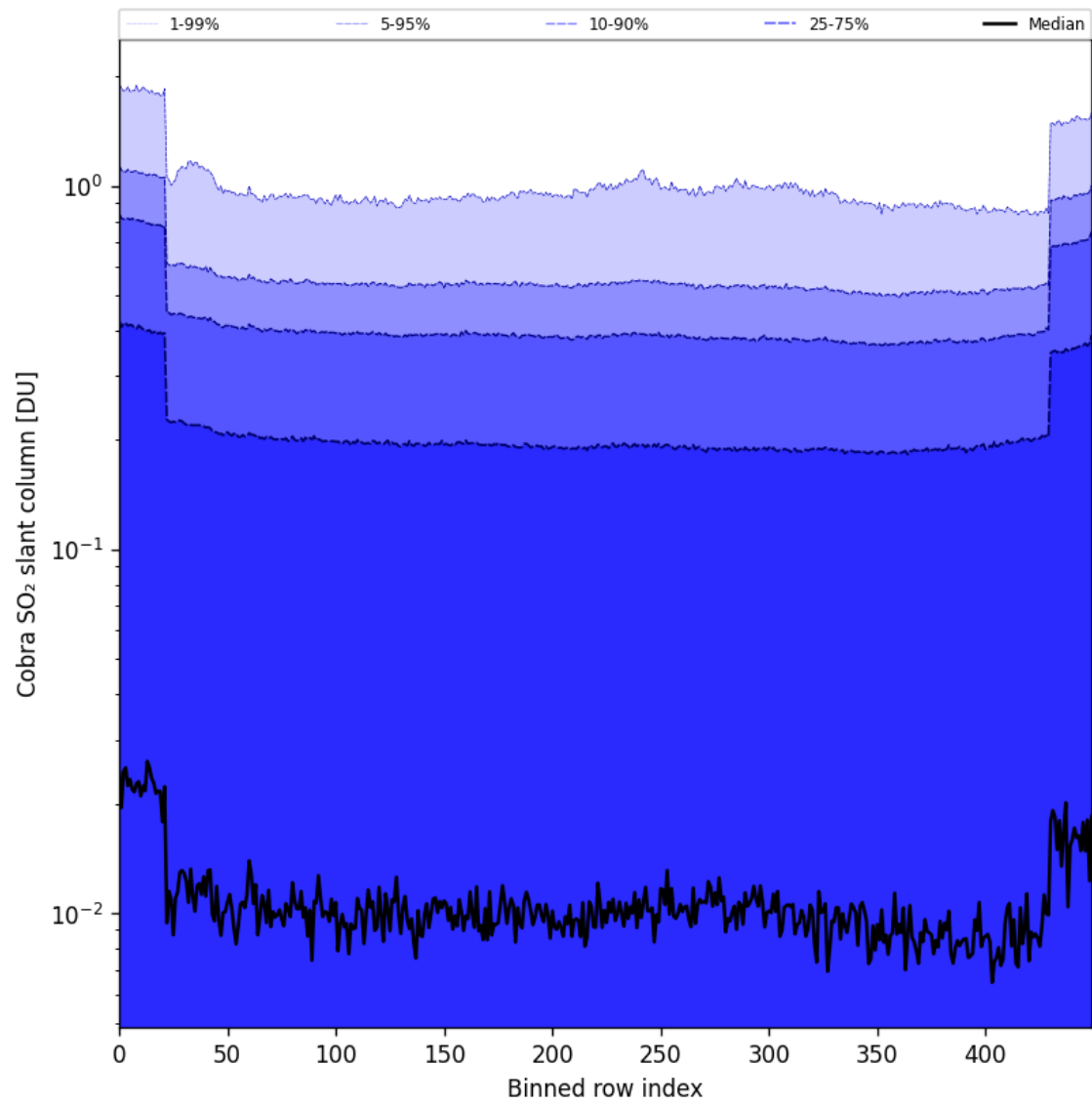
Figure 87: Along track statistics of “Cobra SO 2 slant column” for 2025-08-03 to 2025-08-04
