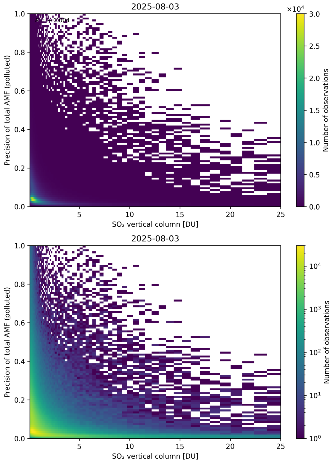
Figure 360: Scatter density plot of “SO 2 vertical column” against “Precision of total AMF (polluted)” for 2025-08-03 to 2025-08-04.
