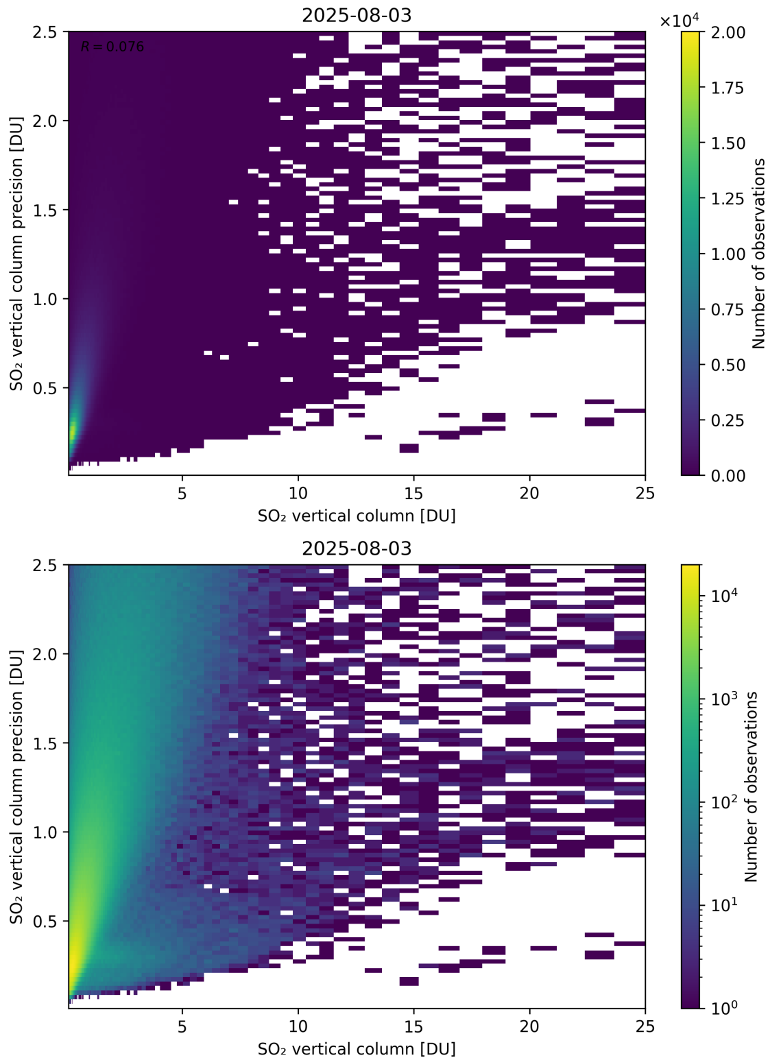
Figure 361: Scatter density plot of “SO 2 vertical column” against “SO 2 vertical column precision” for 2025-08-03 to 2025-08-04.
