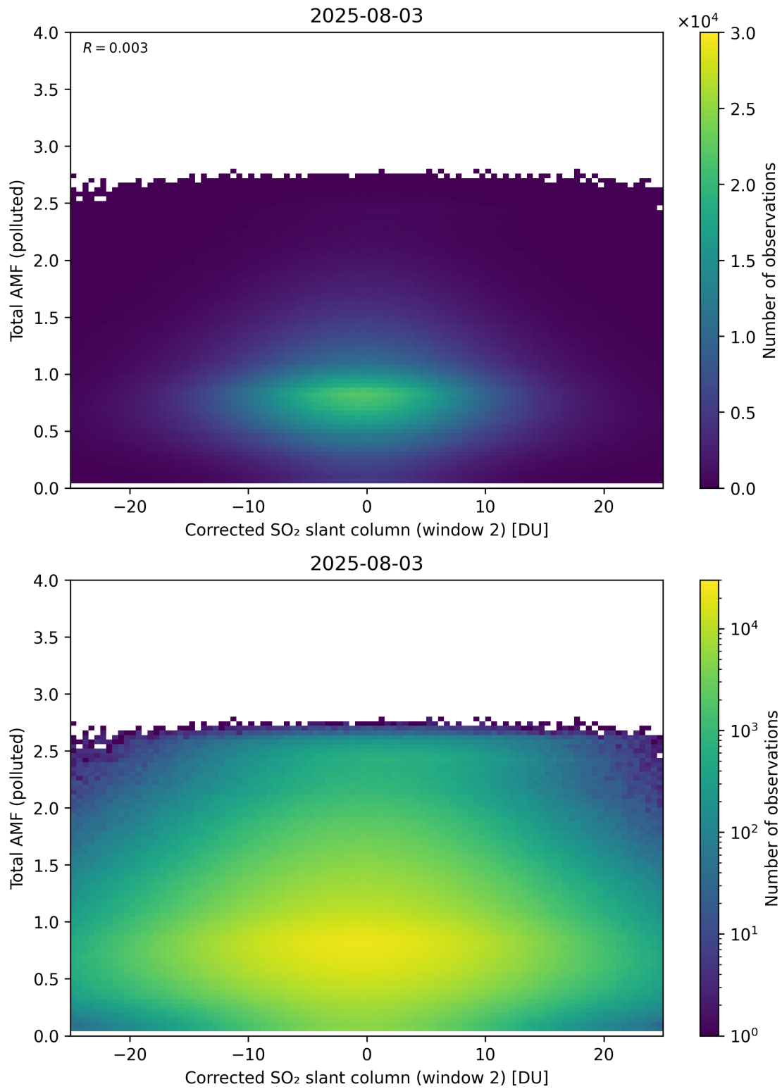
Figure 253: Scatter density plot of “Corrected SO 2 slant column (window 2)” against “Total AMF (polluted)” for 2025-08-03 to 2025-08-04.
