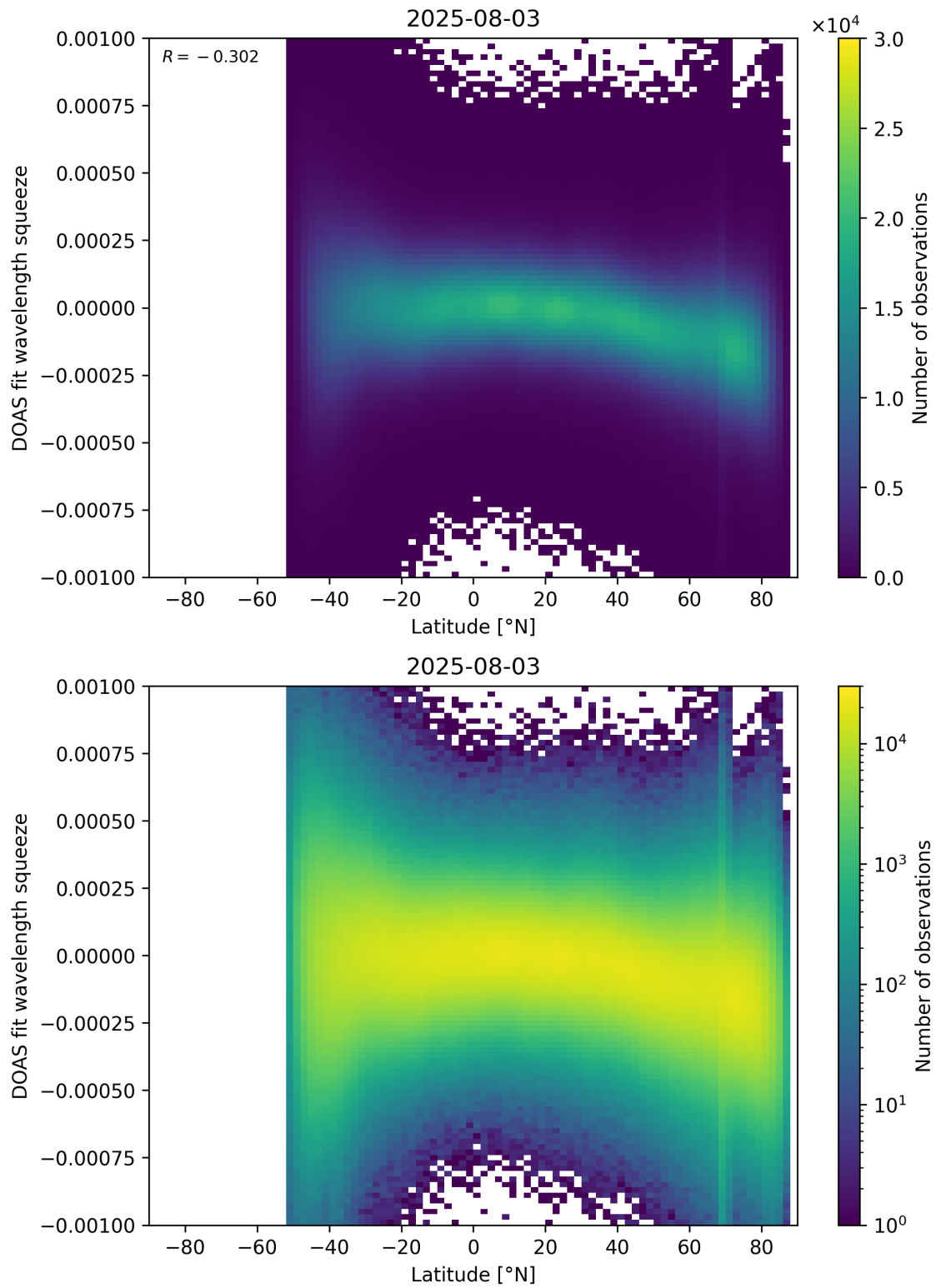
Figure 154: Scatter density plot of “Latitude” against “DOAS fit wavelength squeeze” for 2025-08-03 to 2025-08-04.
