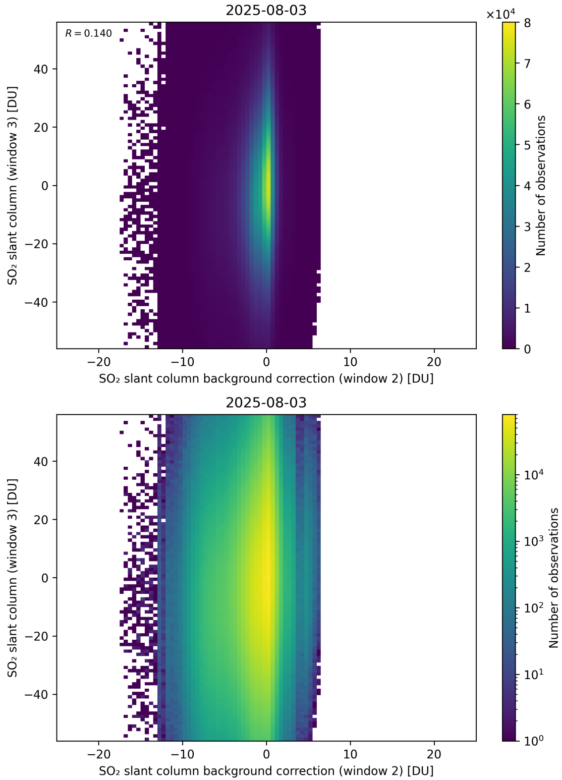
Figure 128: Scatter density plot of “SO 2 slant column background correction (window 2)” against “SO 2 slant column (window 3)” for 2025-08-03 to 2025-08-04.
