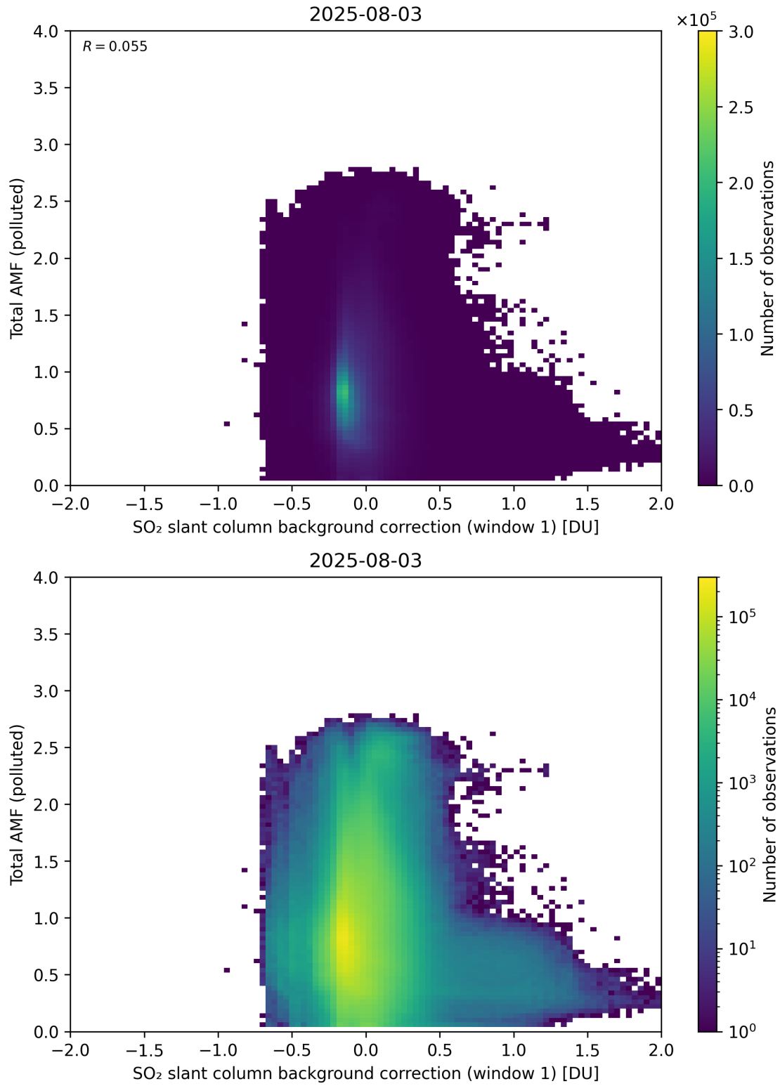
Figure 120: Scatter density plot of “SO 2 slant column background correction (window 1)” against “Total AMF (polluted)” for 2025-08-03 to 2025-08-04.
