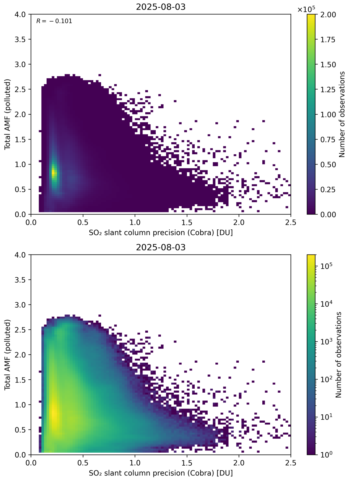
Figure 213: Scatter density plot of “SO 2 slant column precision (Cobra)” against “Total AMF (polluted)” for 2025-08-03 to 2025-08-04.
