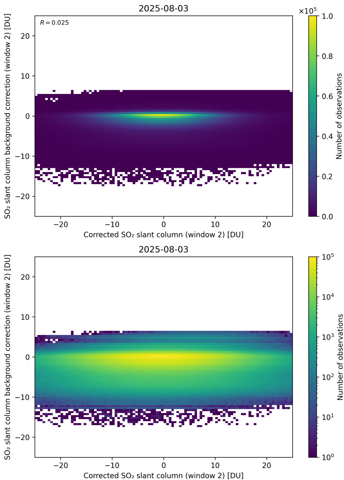
Figure 244: Scatter density plot of “Corrected SO 2 slant column (window 2)” against “SO 2 slant column background correction (window 2)” for 2025-08-03 to 2025-08-04.
