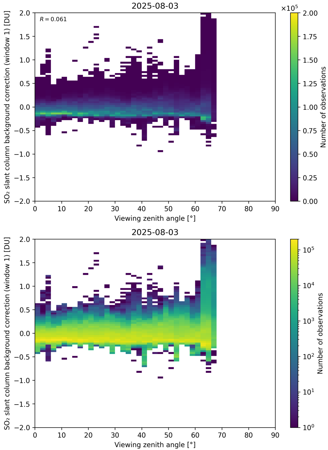
Figure 362: Scatter density plot of “Viewing zenith angle” against “SO 2 slant column background correction (window 1)” for 2025-08-03 to 2025-08-04.
