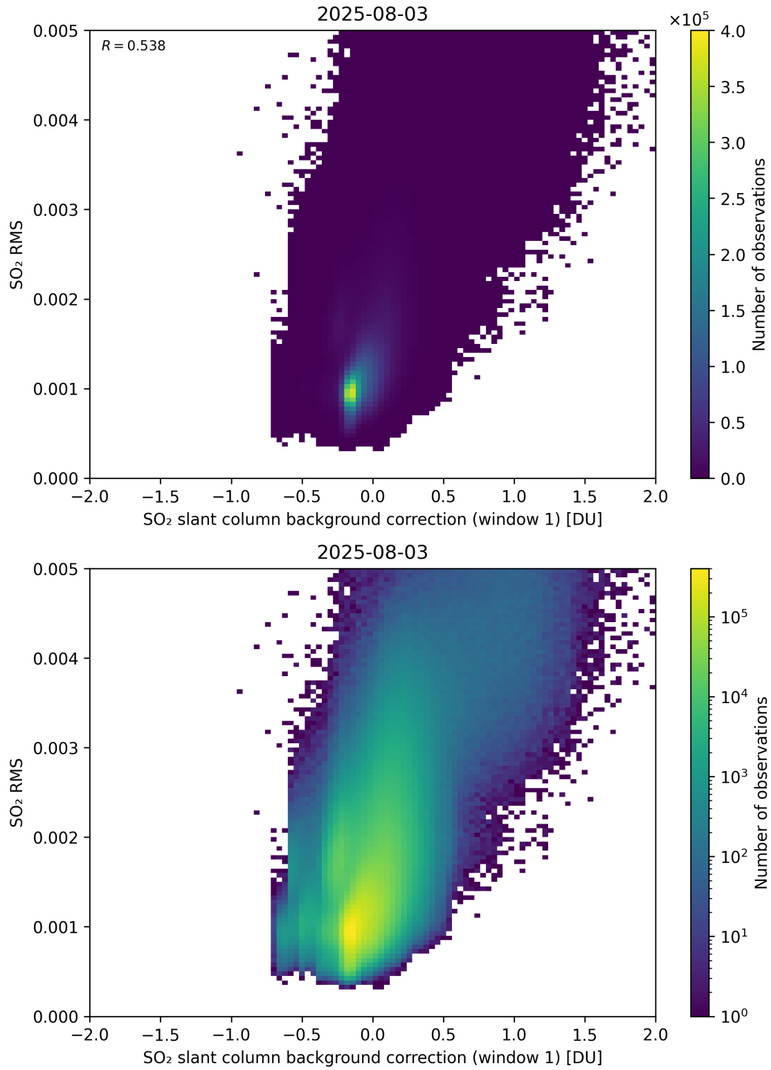
Figure 113: Scatter density plot of “SO 2 slant column background correction (window 1)” against “SO 2 RMS” for 2025-08-03 to 2025-08-04.
