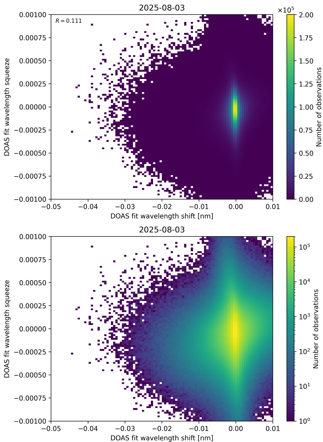
Figure 138: Scatter density plot of “DOAS fit wavelength shift” against “DOAS fit wavelength squeeze” for 2025-08-03 to 2025-08-04.
