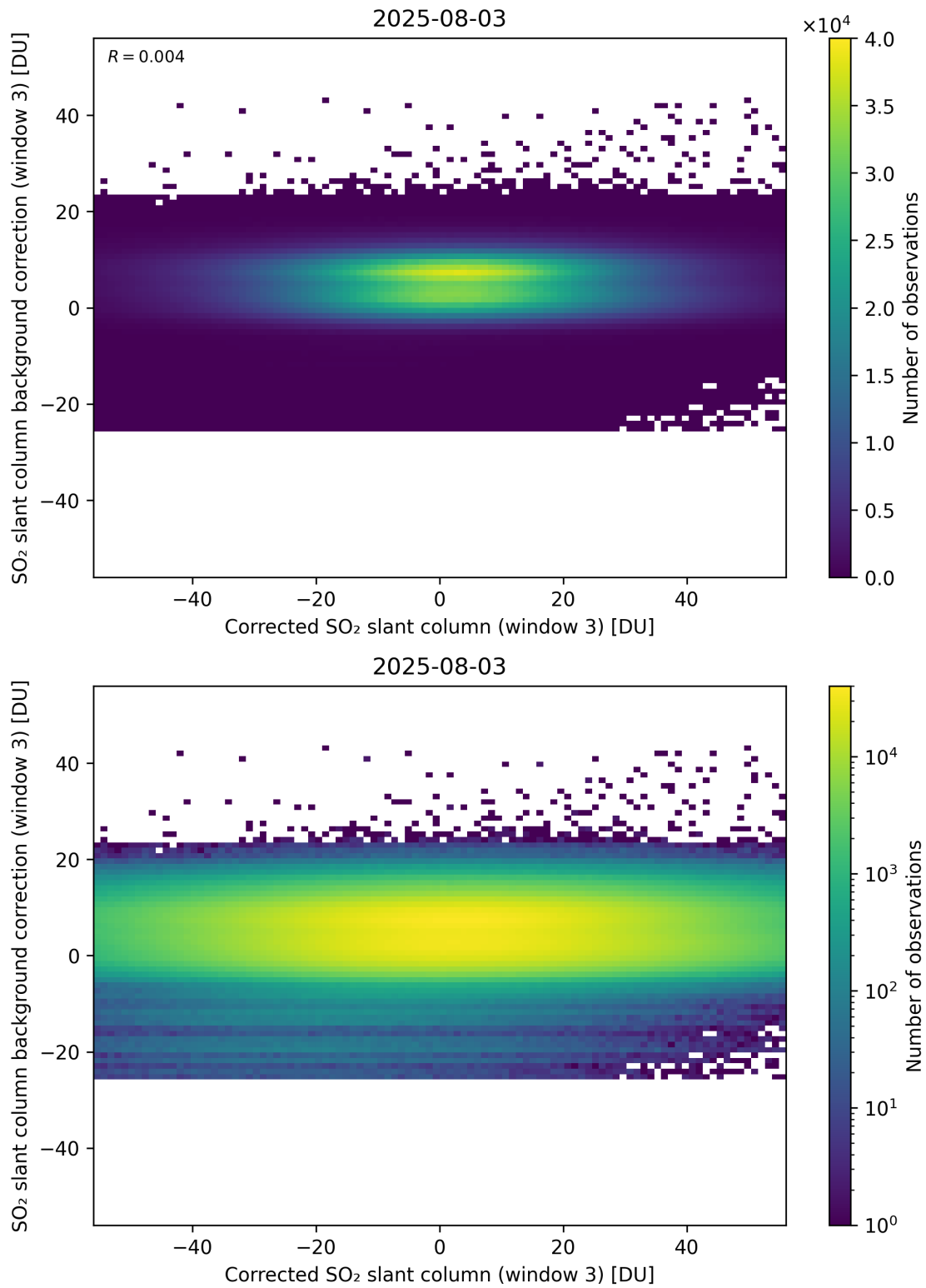
Figure 255: Scatter density plot of “Corrected SO 2 slant column (window 3)” against “SO 2 slant column background correction (window 3)” for 2025-08-03 to 2025-08-04.
