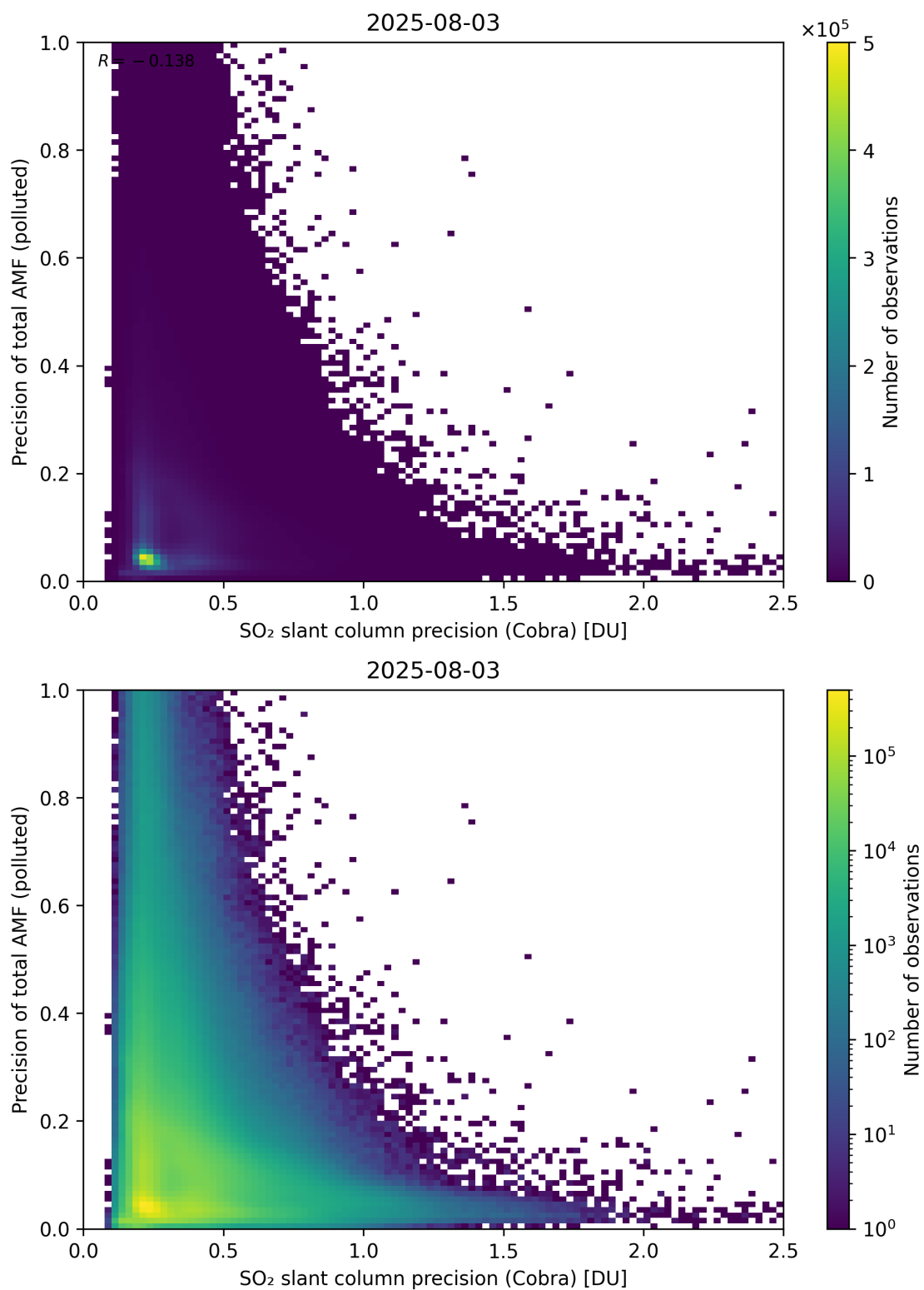
Figure 214: Scatter density plot of “SO 2 slant column precision (Cobra)” against “Precision of total AMF (polluted)” for 2025-08-03 to 2025-08-04.
