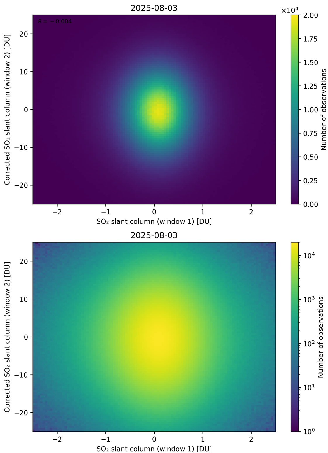
Figure 283: Scatter density plot of “SO 2 slant column (window 1)” against “Corrected SO 2 slant column (window 2)” for 2025-08-03 to 2025-08-04.
