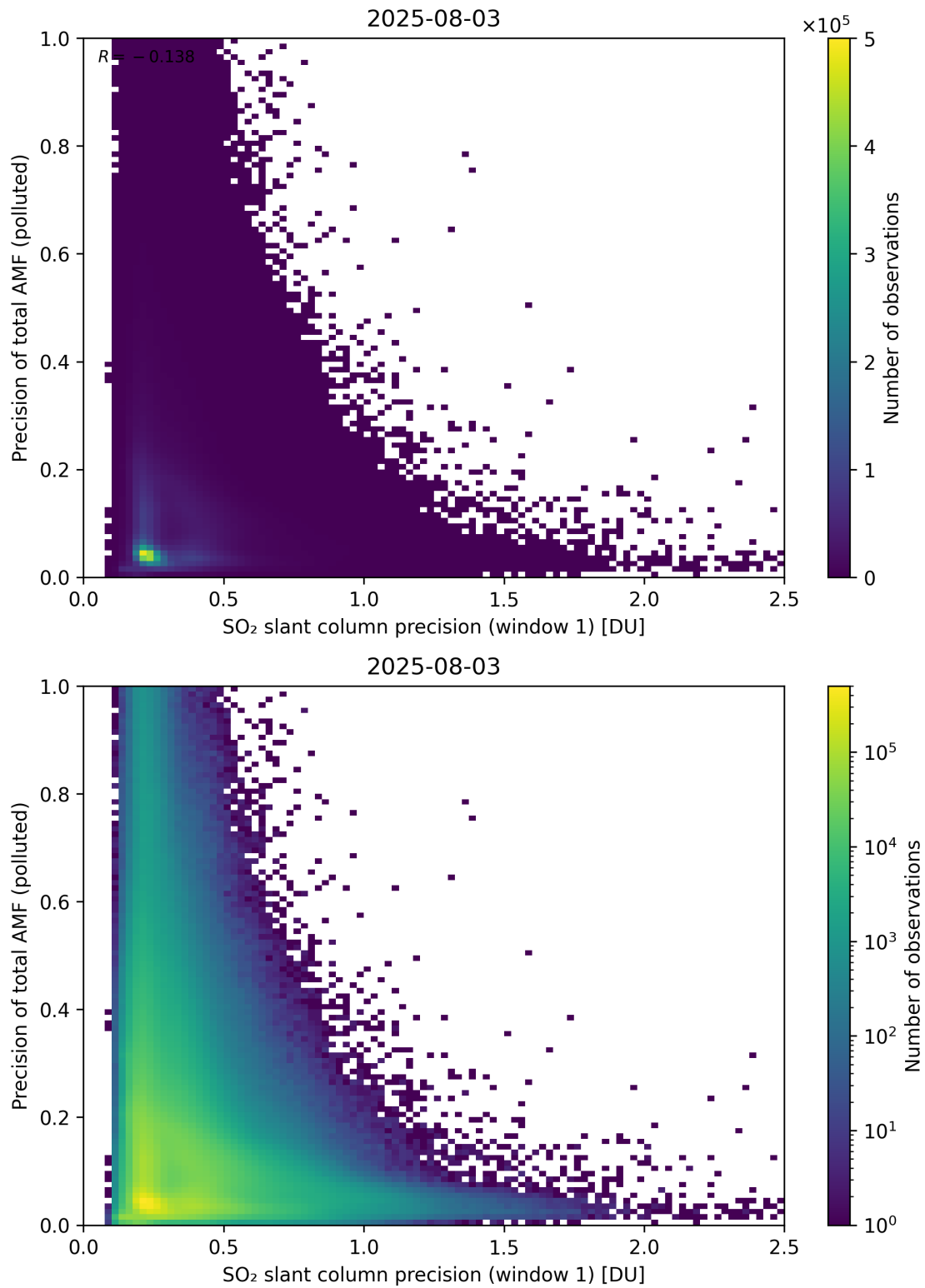
Figure 281: Scatter density plot of “SO 2 slant column precision (window 1)” against “Precision of total AMF (polluted)” for 2025-08-03 to 2025-08-04.
