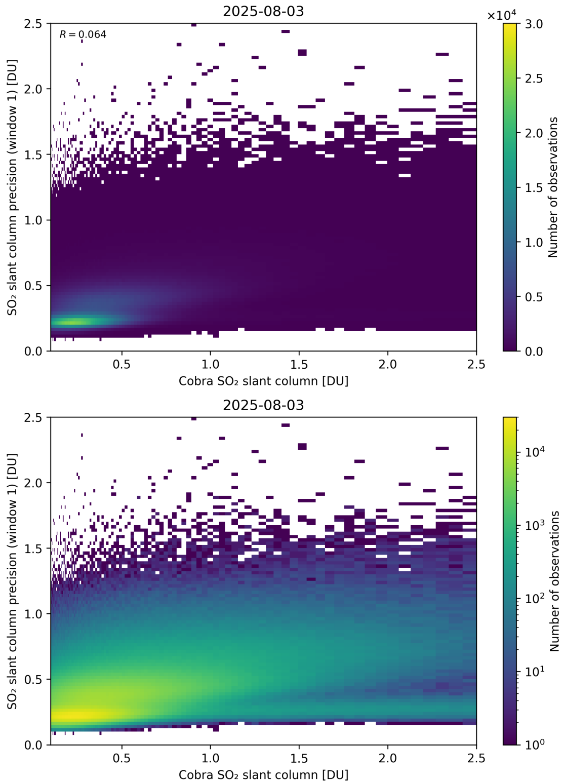
Figure 220: Scatter density plot of “Cobra SO 2 slant column” against “SO 2 slant column precision (window 1)” for 2025-08-03 to 2025-08-04.
