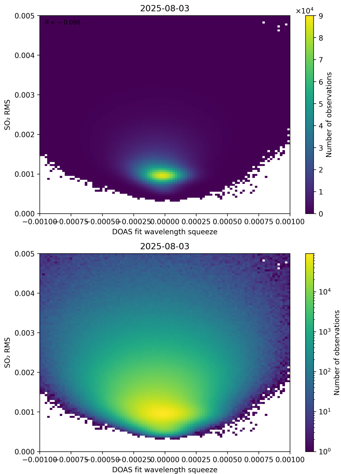
Figure 143: Scatter density plot of “DOAS fit wavelength squeeze” against “SO 2 RMS” for 2025-08-03 to 2025-08-04.
