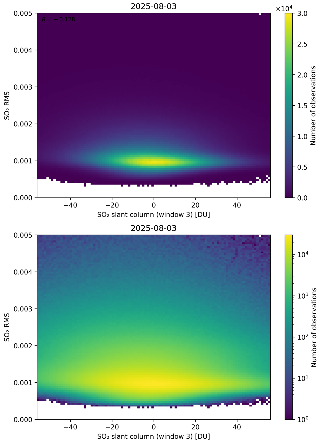
Figure 306: Scatter density plot of “SO 2 slant column (window 3)” against “SO 2 RMS” for 2025-08-03 to 2025-08-04.
