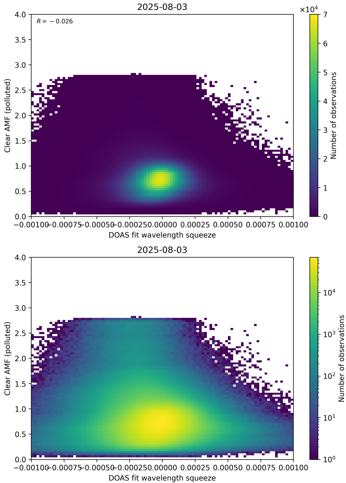
Figure 144: Scatter density plot of “DOAS fit wavelength squeeze” against “Clear AMF (polluted)” for 2025-08-03 to 2025-08-04.
