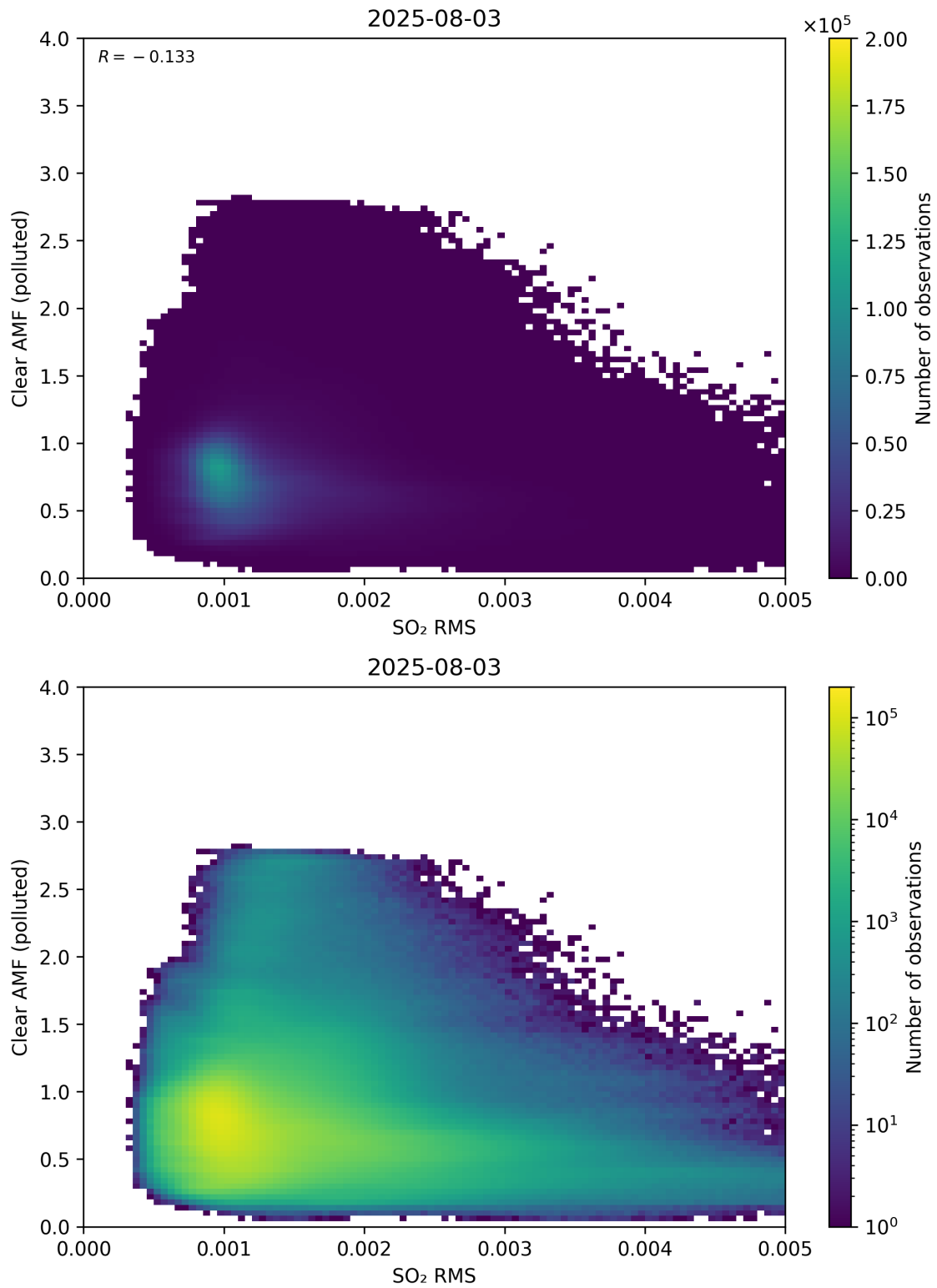
Figure 147: Scatter density plot of “SO 2 RMS” against “Clear AMF (polluted)” for 2025-08-03 to 2025-08-04.
