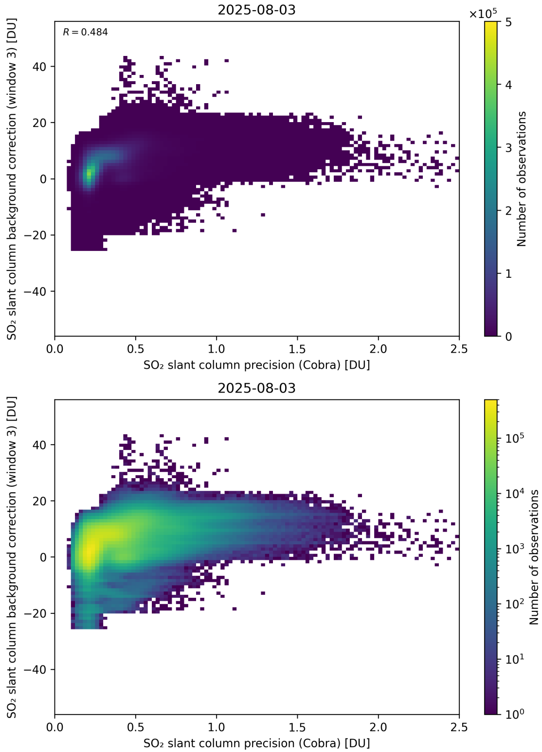
Figure 201: Scatter density plot of “SO 2 slant column precision (Cobra)” against “SO 2 slant column background correction (window 3)” for 2025-08-03 to 2025-08-04.
