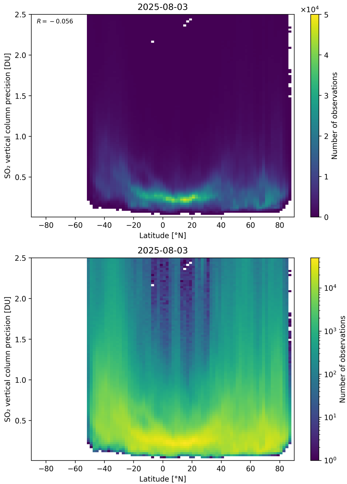
Figure 170: Scatter density plot of “Latitude” against “SO 2 vertical column precision” for 2025-08-03 to 2025-08-04.
