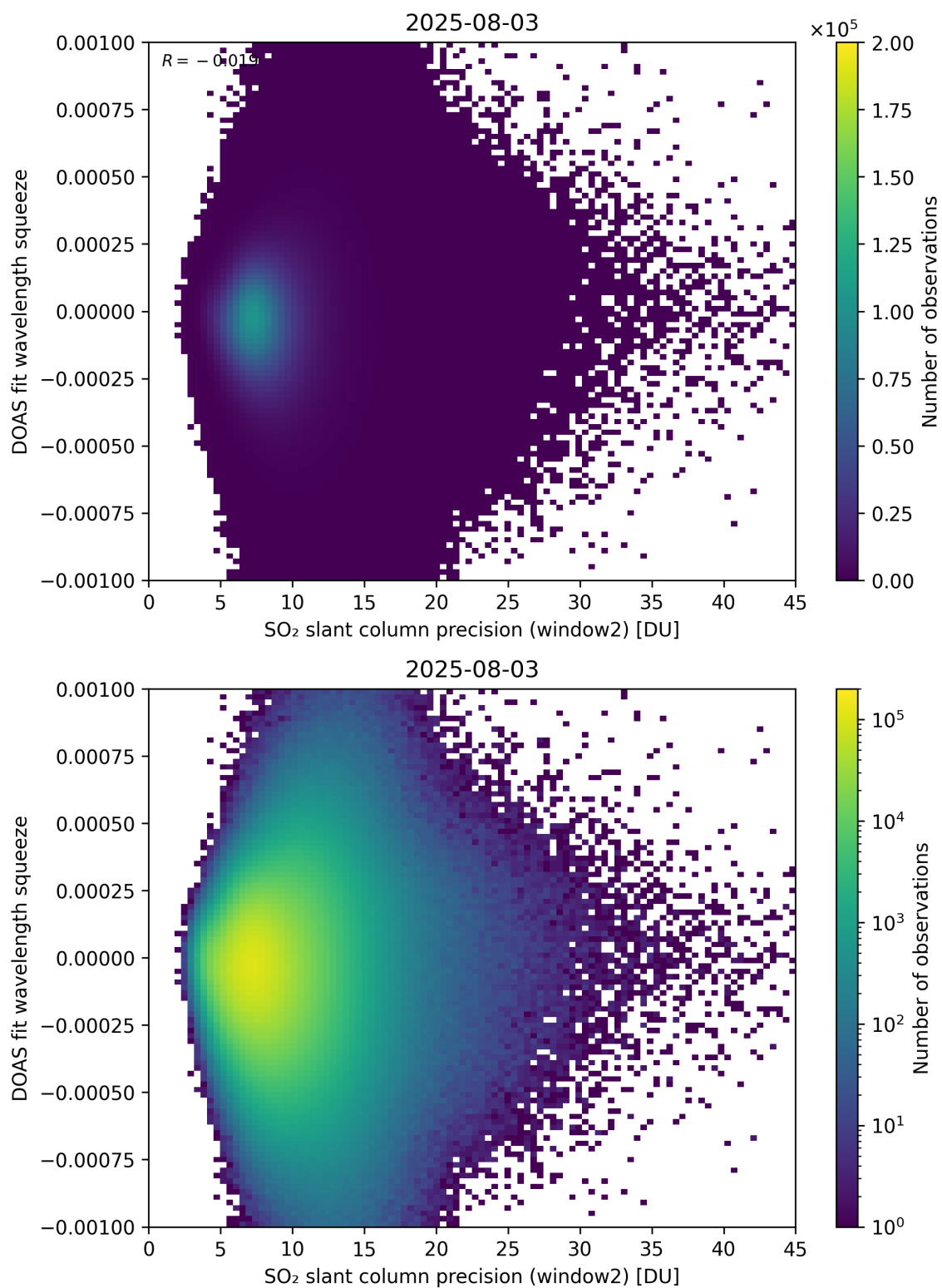
Figure 294: Scatter density plot of “SO 2 slant column precision (window2)” against “DOAS fit wavelength squeeze” for 2025-08-03 to 2025-08-04.
