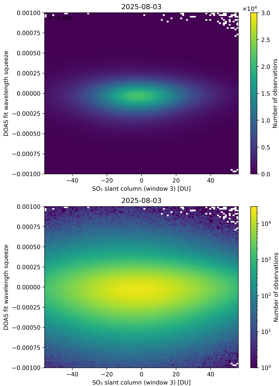
Figure 305: Scatter density plot of “SO 2 slant column (window 3)” against “DOAS fit wavelength squeeze” for 2025-08-03 to 2025-08-04.
