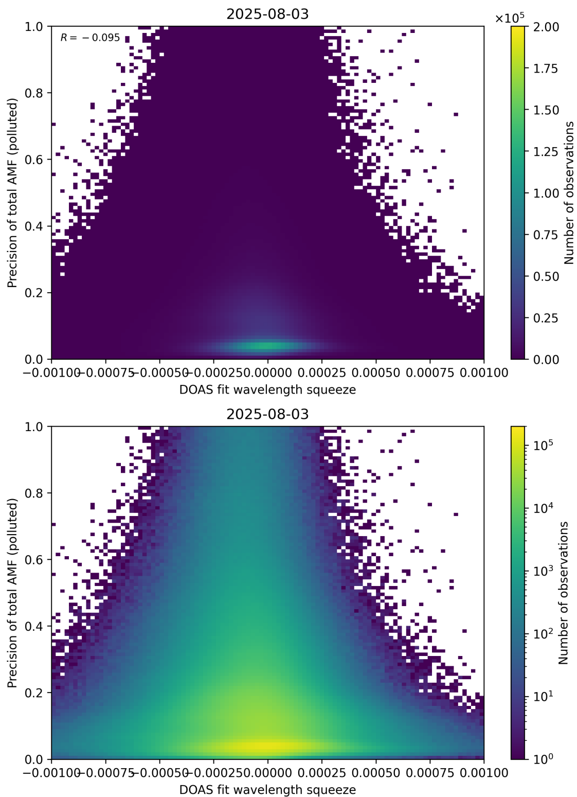
Figure 146: Scatter density plot of “DOAS fit wavelength squeeze” against “Precision of total AMF (polluted)” for 2025-08-03 to 2025-08-04.
