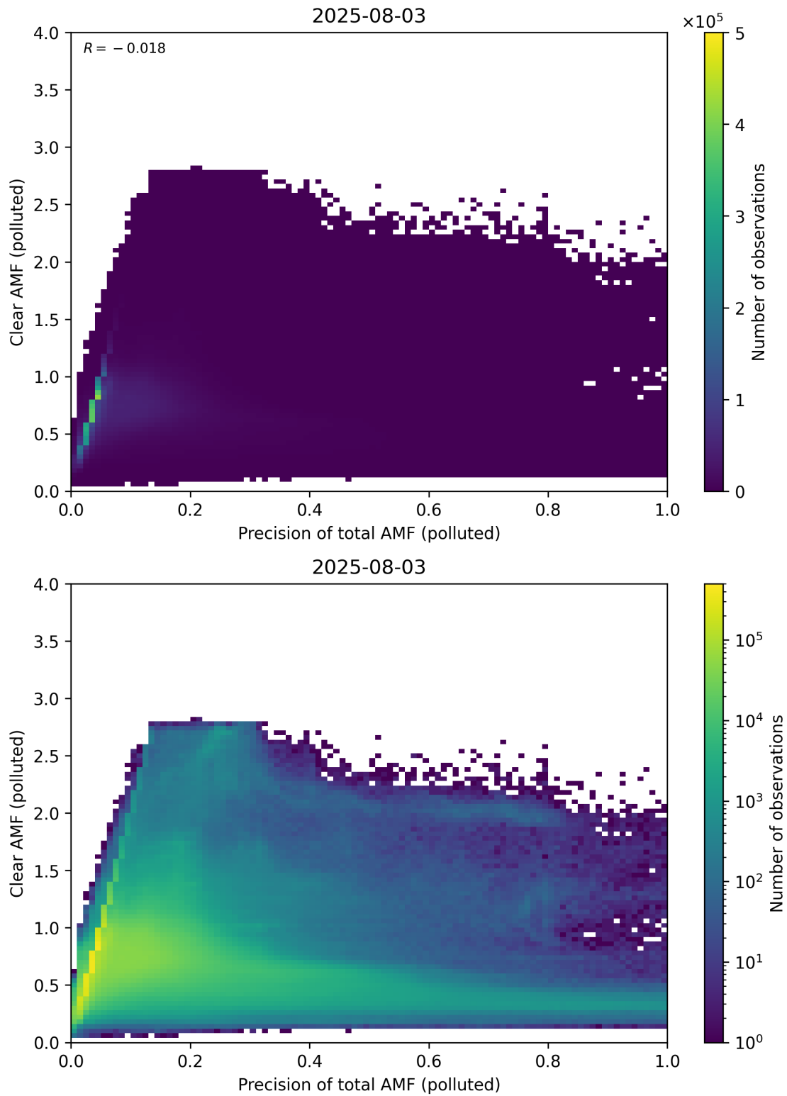
Figure 320: Scatter density plot of “Precision of total AMF (polluted)” against “Clear AMF (polluted)” for 2025-08-03 to 2025-08-04.
