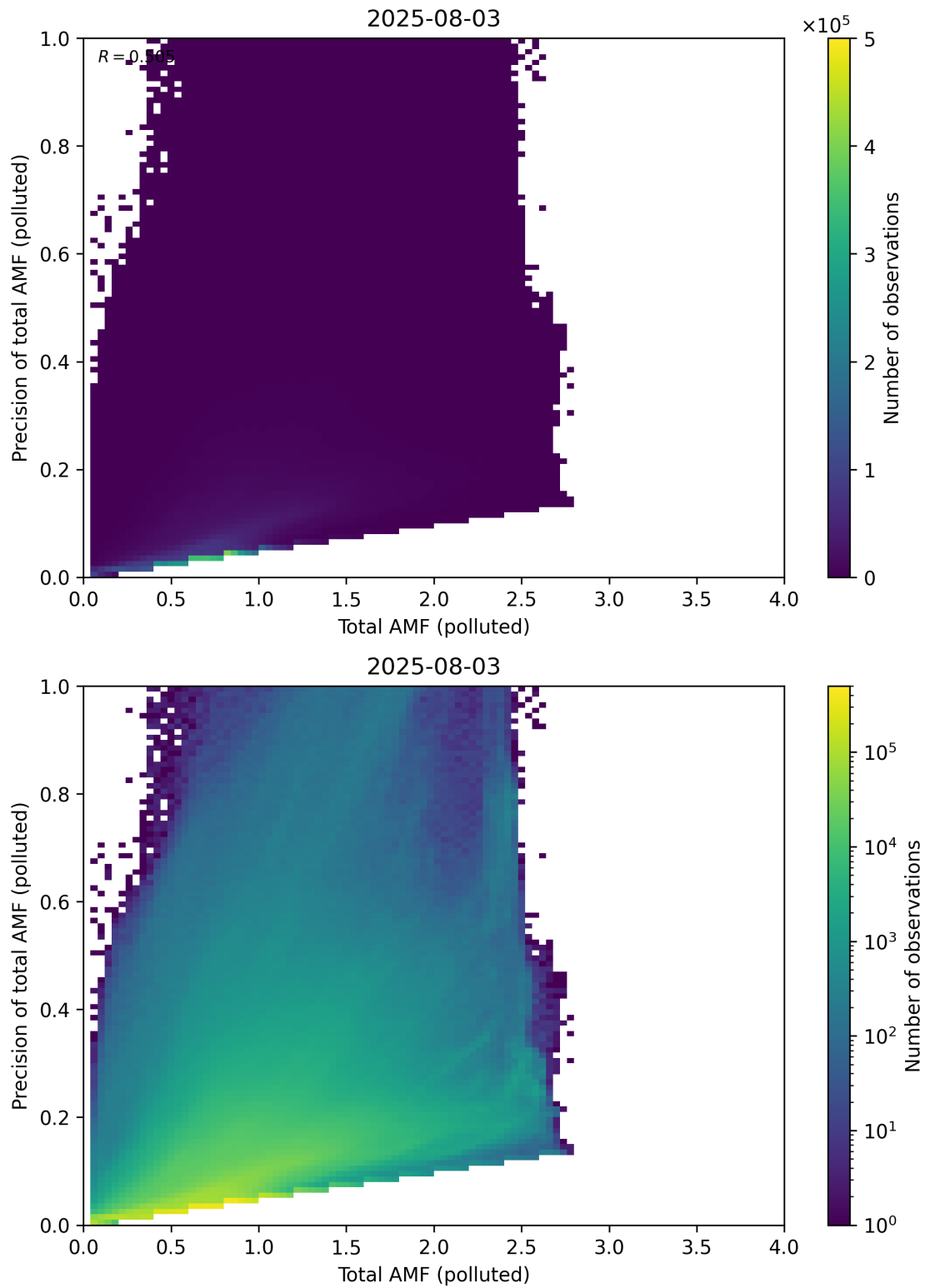
Figure 322: Scatter density plot of “Total AMF (polluted)” against “Precision of total AMF (polluted)” for 2025-08-03 to 2025-08-04.
