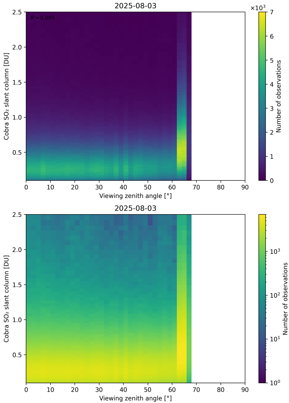
Figure 371: Scatter density plot of “Viewing zenith angle” against “Cobra SO 2 slant column” for 2025-08-03 to 2025-08-04.
