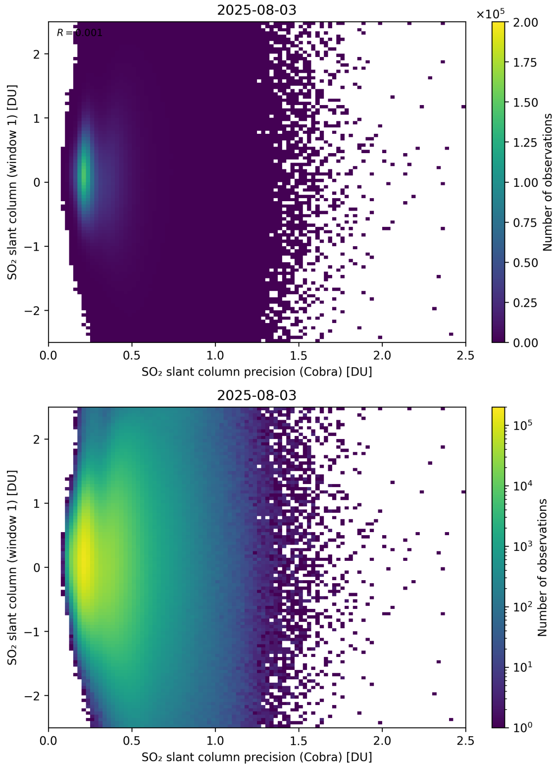
Figure 208: Scatter density plot of “SO 2 slant column precision (Cobra)” against “SO 2 slant column (window 1)” for 2025-08-03 to 2025-08-04.
