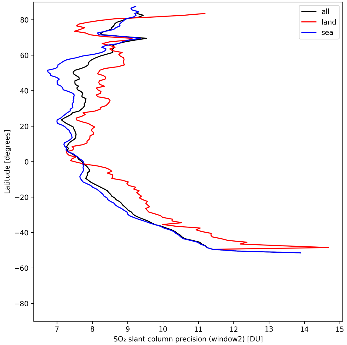
Figure 42: Zonal average of “SO 2 slant column precision (window2)” for 2025-08-03 to 2025-08-04.
