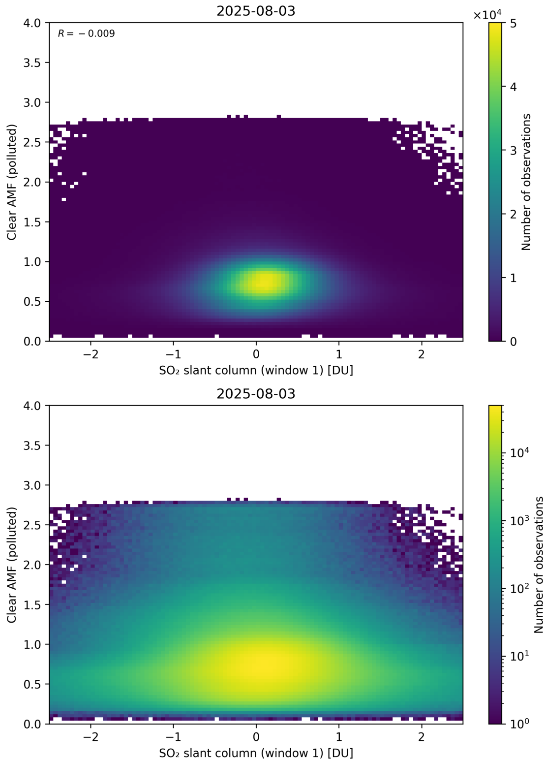
Figure 282: Scatter density plot of “SO 2 slant column (window 1)” against “Clear AMF (polluted)” for 2025-08-03 to 2025-08-04.
