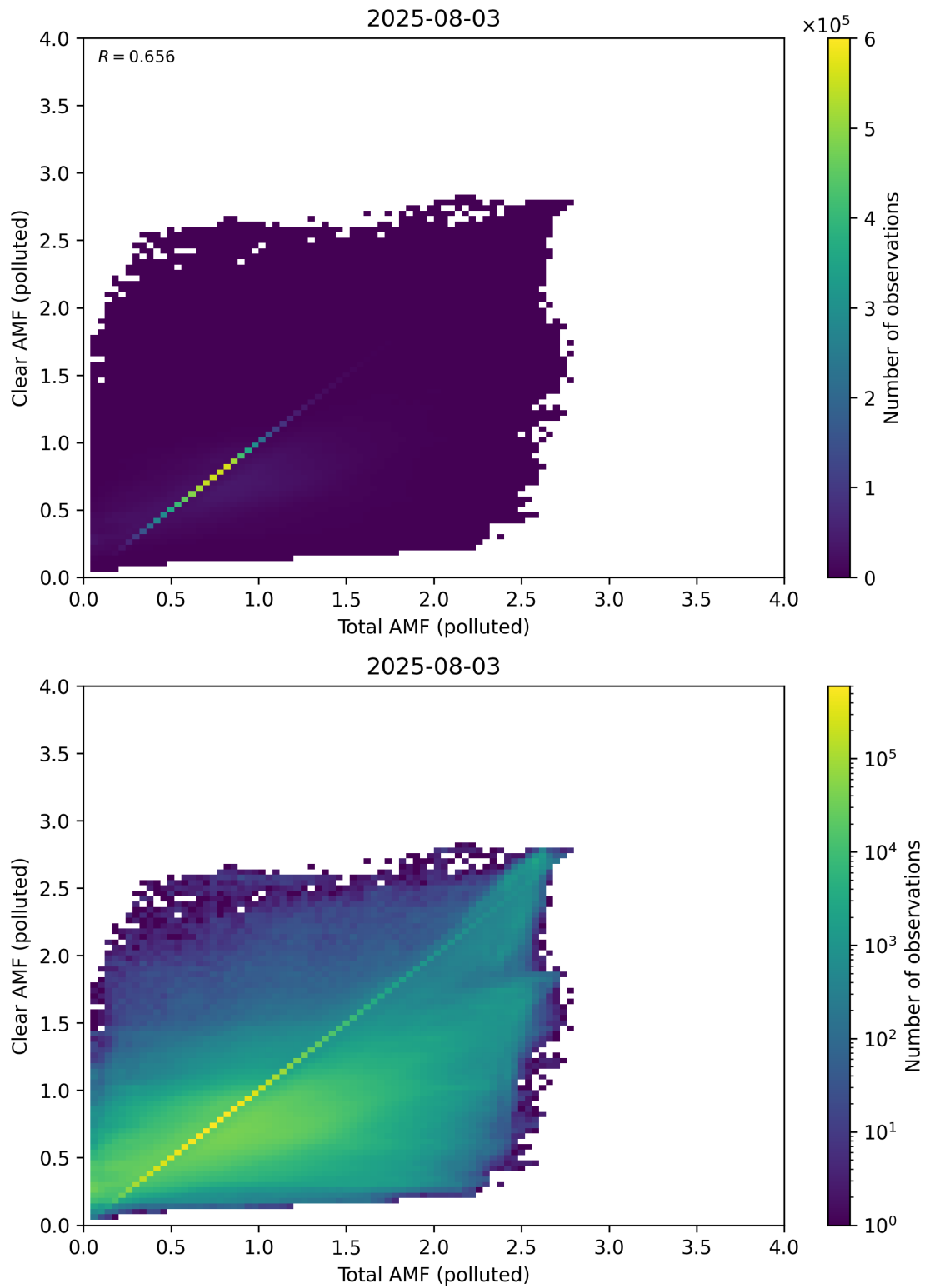
Figure 321: Scatter density plot of “Total AMF (polluted)” against “Clear AMF (polluted)” for 2025-08-03 to 2025-08-04.
