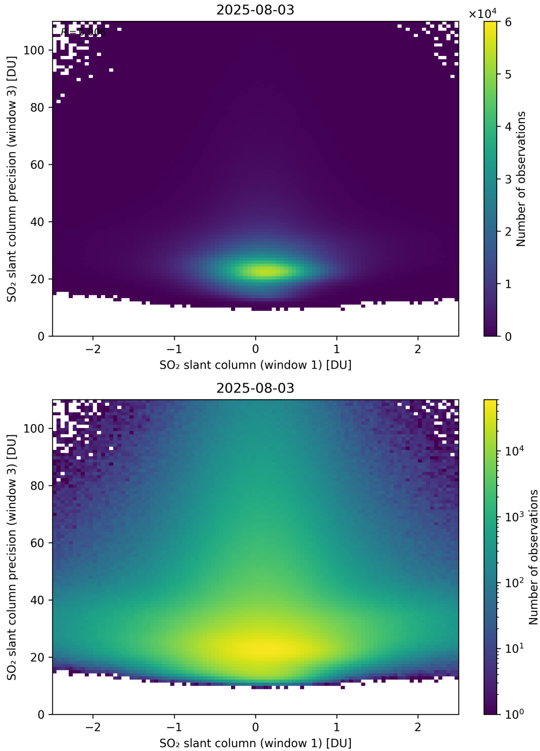
Figure 288: Scatter density plot of “SO 2 slant column (window 1)” against “SO 2 slant column precision (window 3)” for 2025-08-03 to 2025-08-04.
