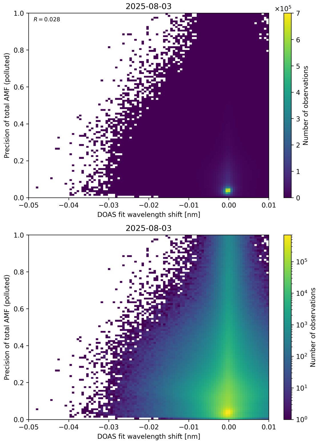
Figure 142: Scatter density plot of “DOAS fit wavelength shift” against “Precision of total AMF (polluted)” for 2025-08-03 to 2025-08-04.
