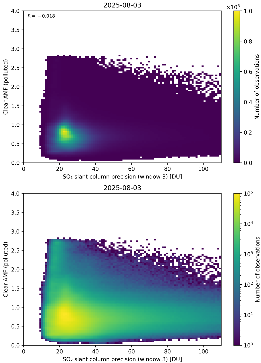
Figure 311: Scatter density plot of “SO 2 slant column precision (window 3)” against “Clear AMF (polluted)” for 2025-08-03 to 2025-08-04.
