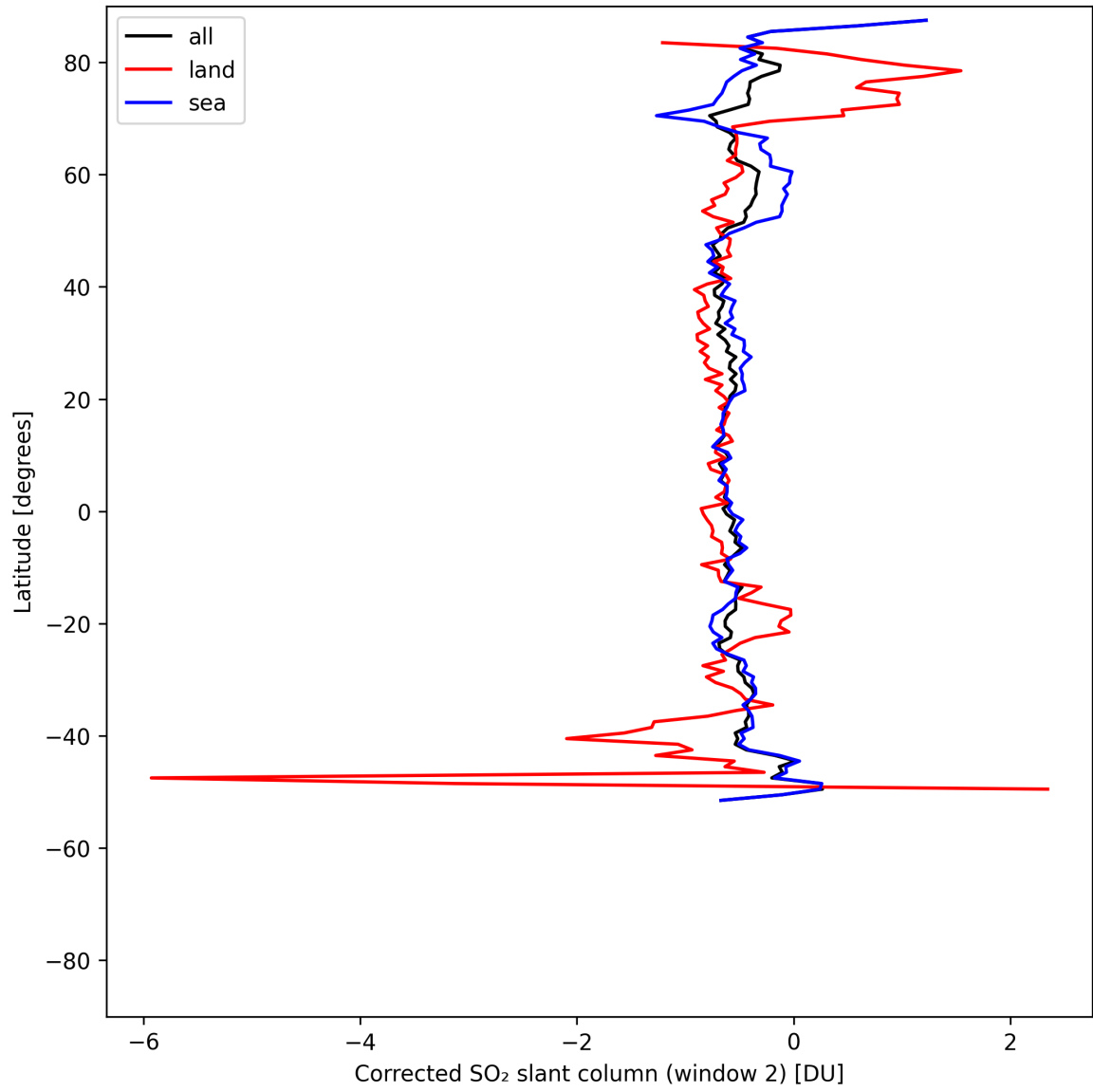
Figure 43: Zonal average of “Corrected SO 2 slant column (window 2)” for 2025-08-03 to 2025-08-04.
