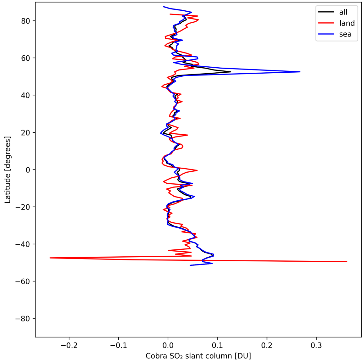
Figure 35: Zonal average of “Cobra SO 2 slant column” for 2025-08-03 to 2025-08-04.
