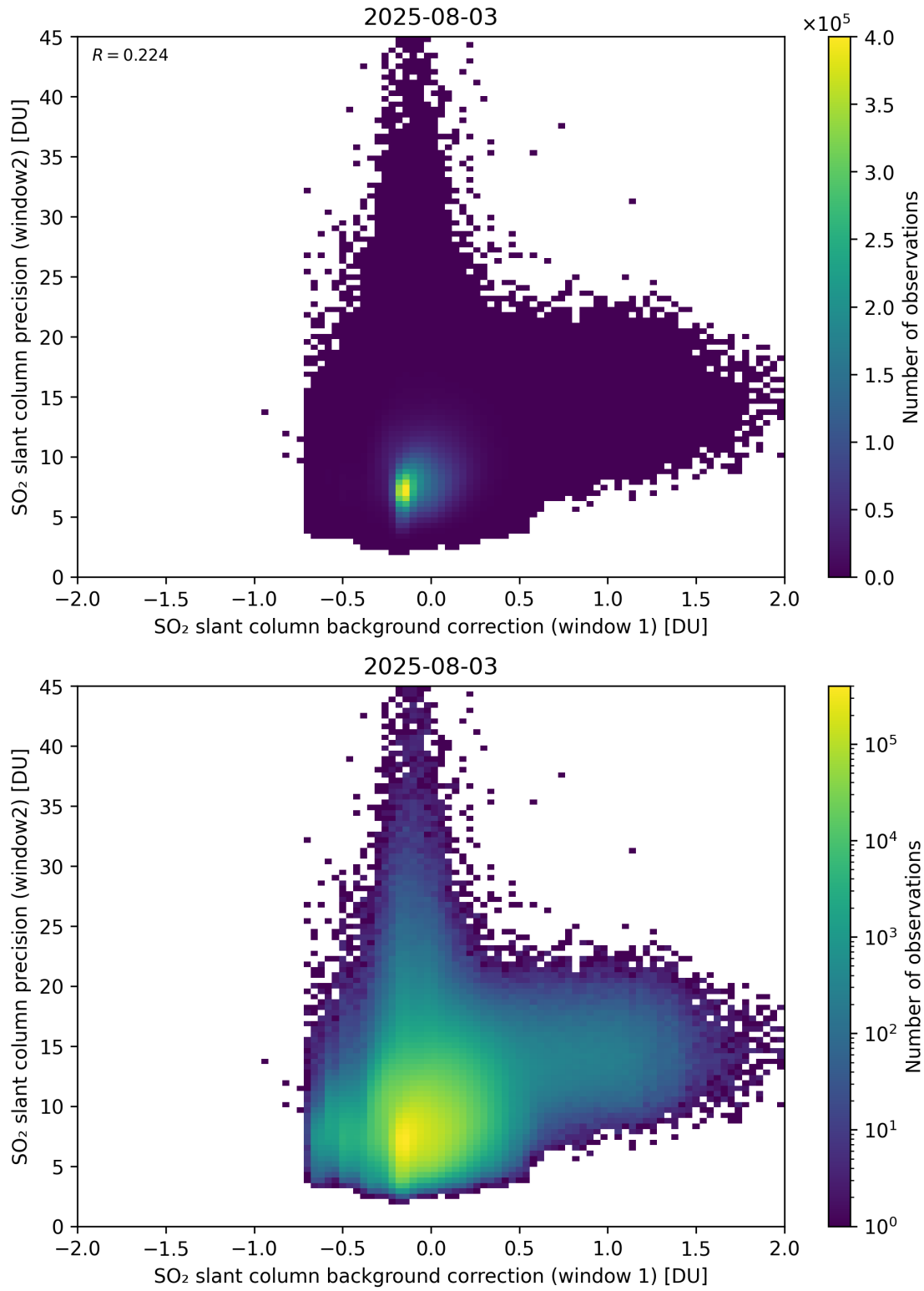
Figure 117: Scatter density plot of “SO 2 slant column background correction (window 1)” against “SO 2 slant column precision (window2)” for 2025-08-03 to 2025-08-04.
