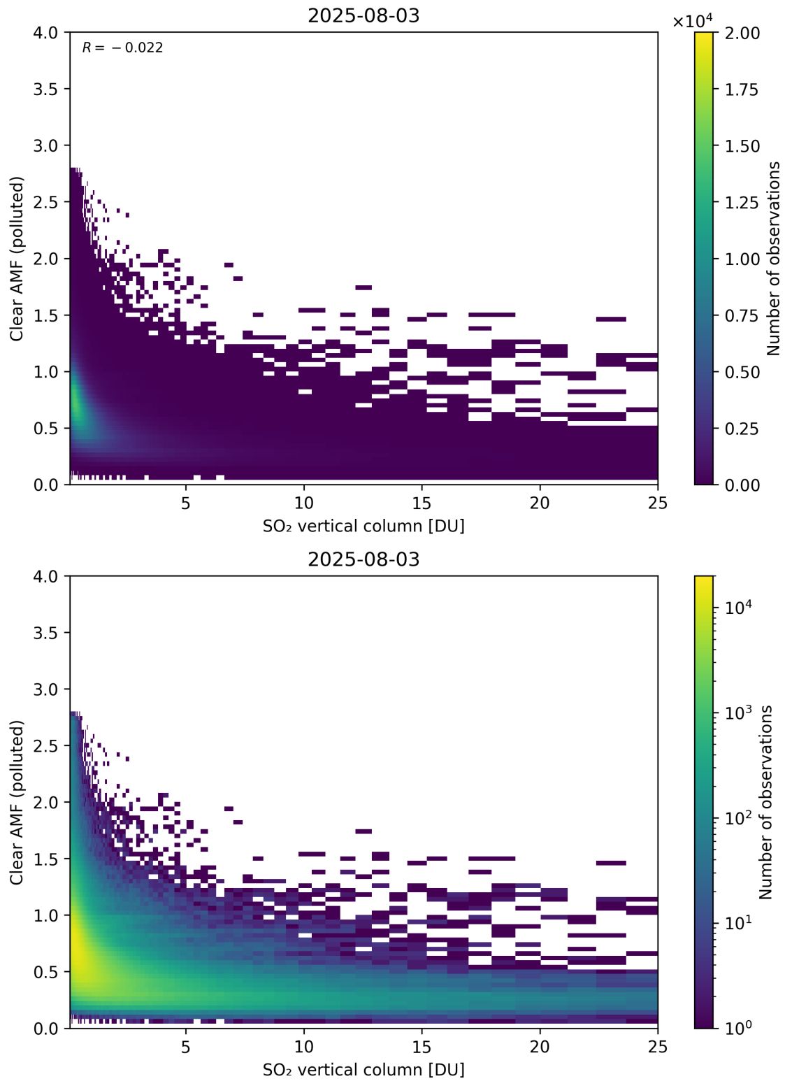
Figure 348: Scatter density plot of “SO 2 vertical column” against “Clear AMF (polluted)” for 2025-08-03 to 2025-08-04.
