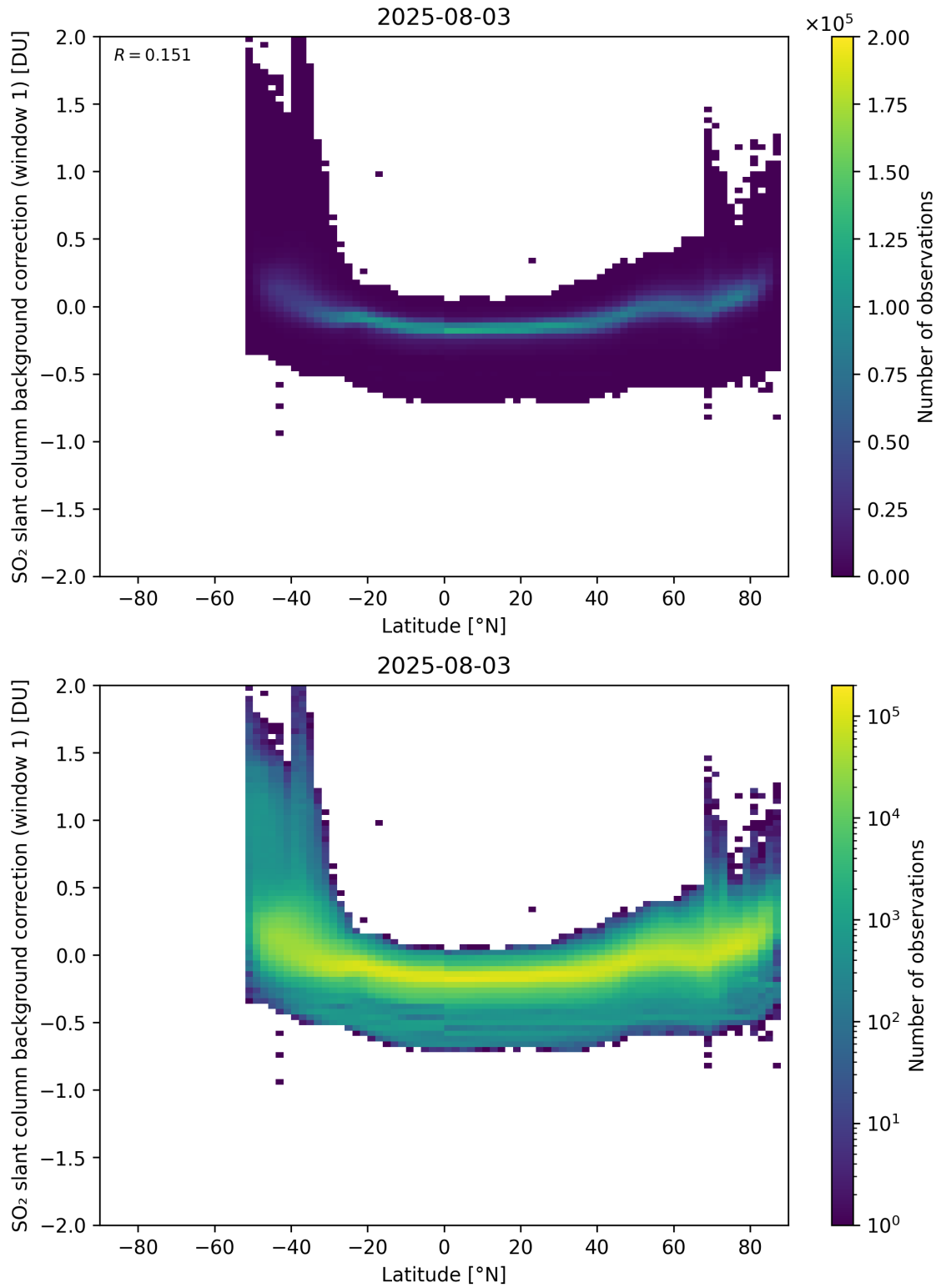
Figure 150: Scatter density plot of “Latitude” against “SO 2 slant column background correction (window 1)” for 2025-08-03 to 2025-08-04.
