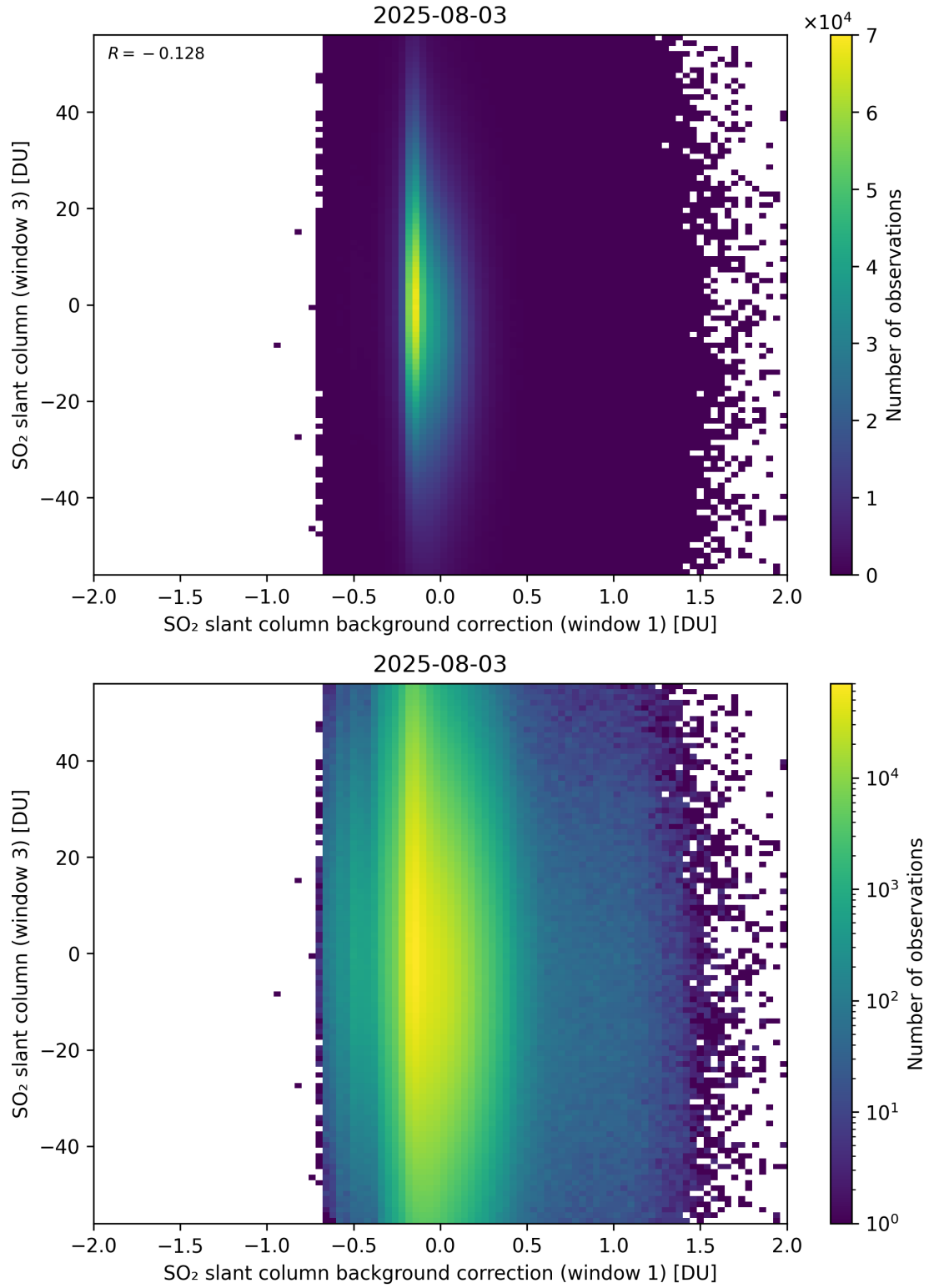
Figure 118: Scatter density plot of “SO 2 slant column background correction (window 1)” against “SO 2 slant column (window 3)” for 2025-08-03 to 2025-08-04.
