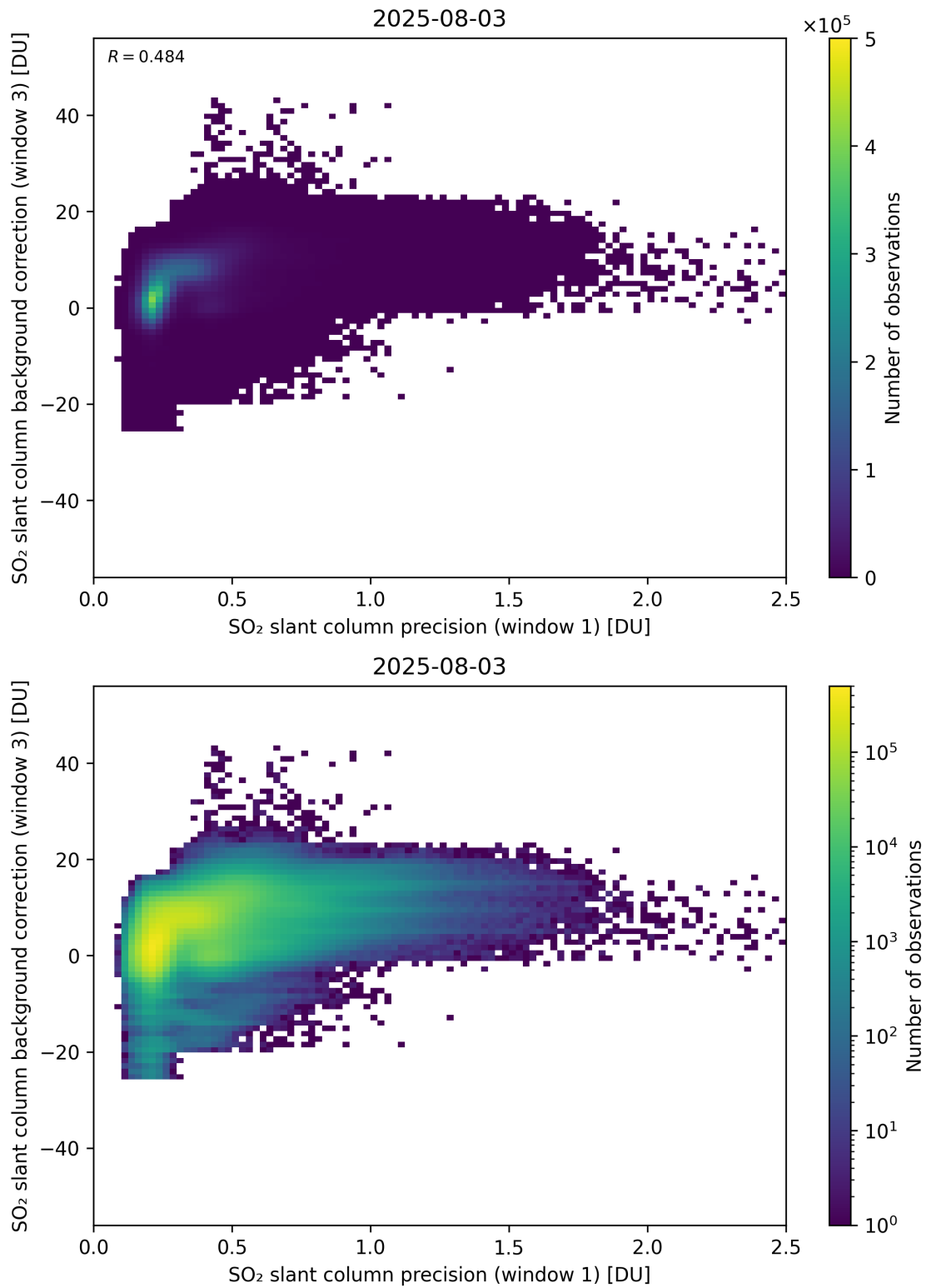
Figure 270: Scatter density plot of “SO 2 slant column precision (window 1)” against “SO 2 slant column background correction (window 3)” for 2025-08-03 to 2025-08-04.
