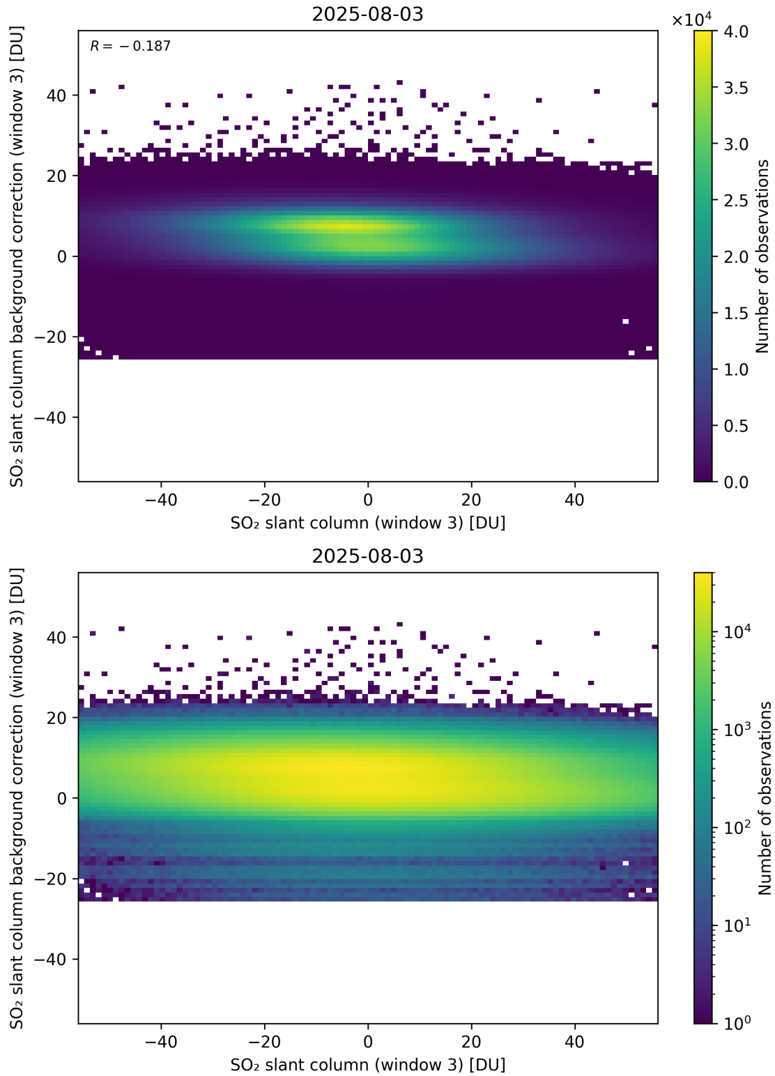
Figure 303: Scatter density plot of “SO 2 slant column (window 3)” against “SO 2 slant column background correction (window 3)” for 2025-08-03 to 2025-08-04.
