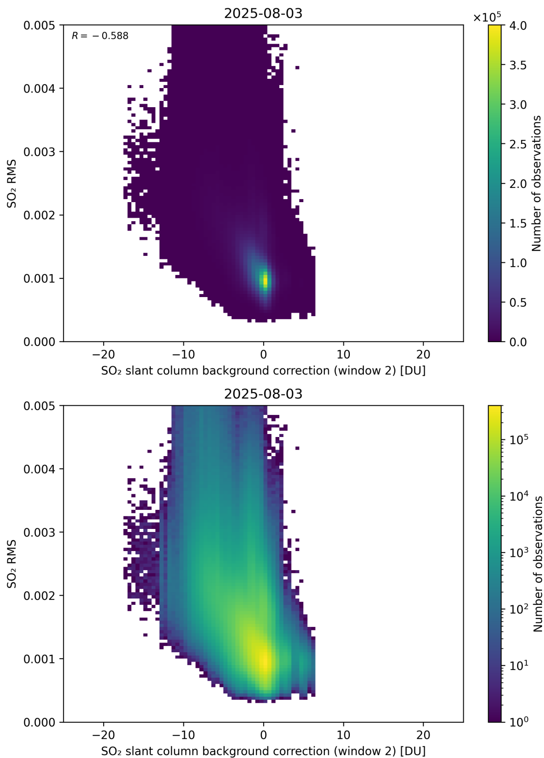
Figure 125: Scatter density plot of “SO 2 slant column background correction (window 2)” against “SO 2 RMS” for 2025-08-03 to 2025-08-04.
