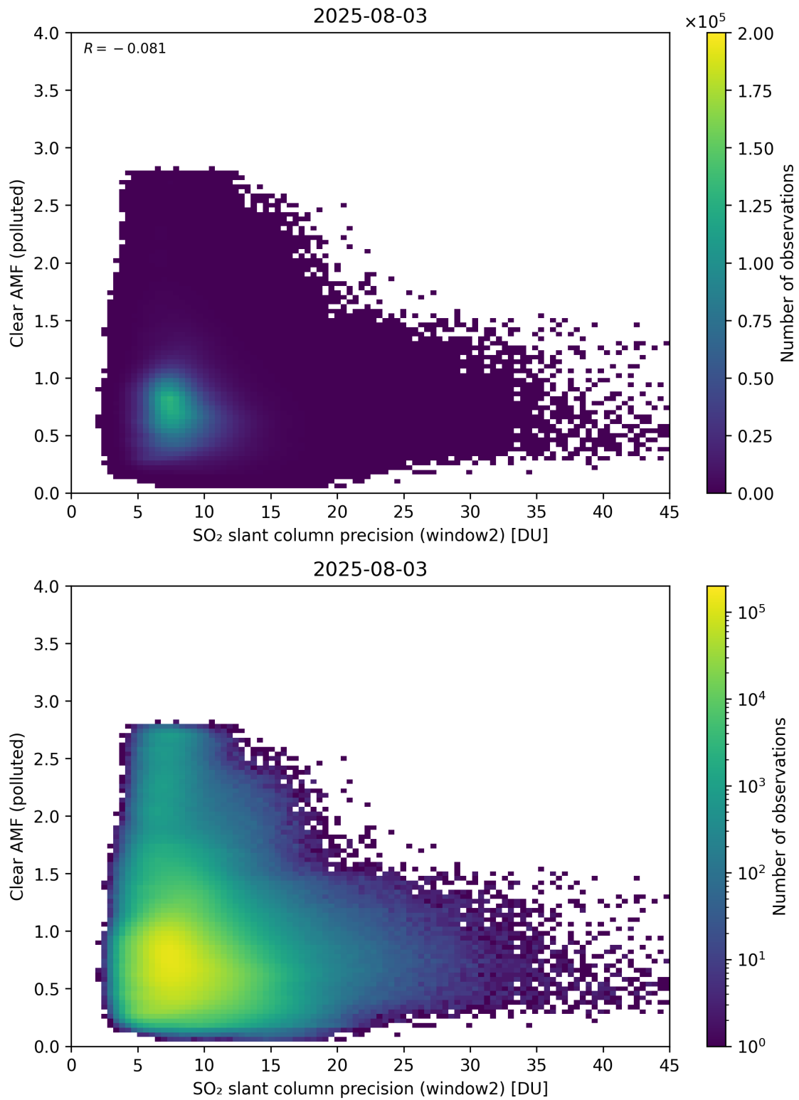
Figure 296: Scatter density plot of “SO 2 slant column precision (window2)” against “Clear AMF (polluted)” for 2025-08-03 to 2025-08-04.
