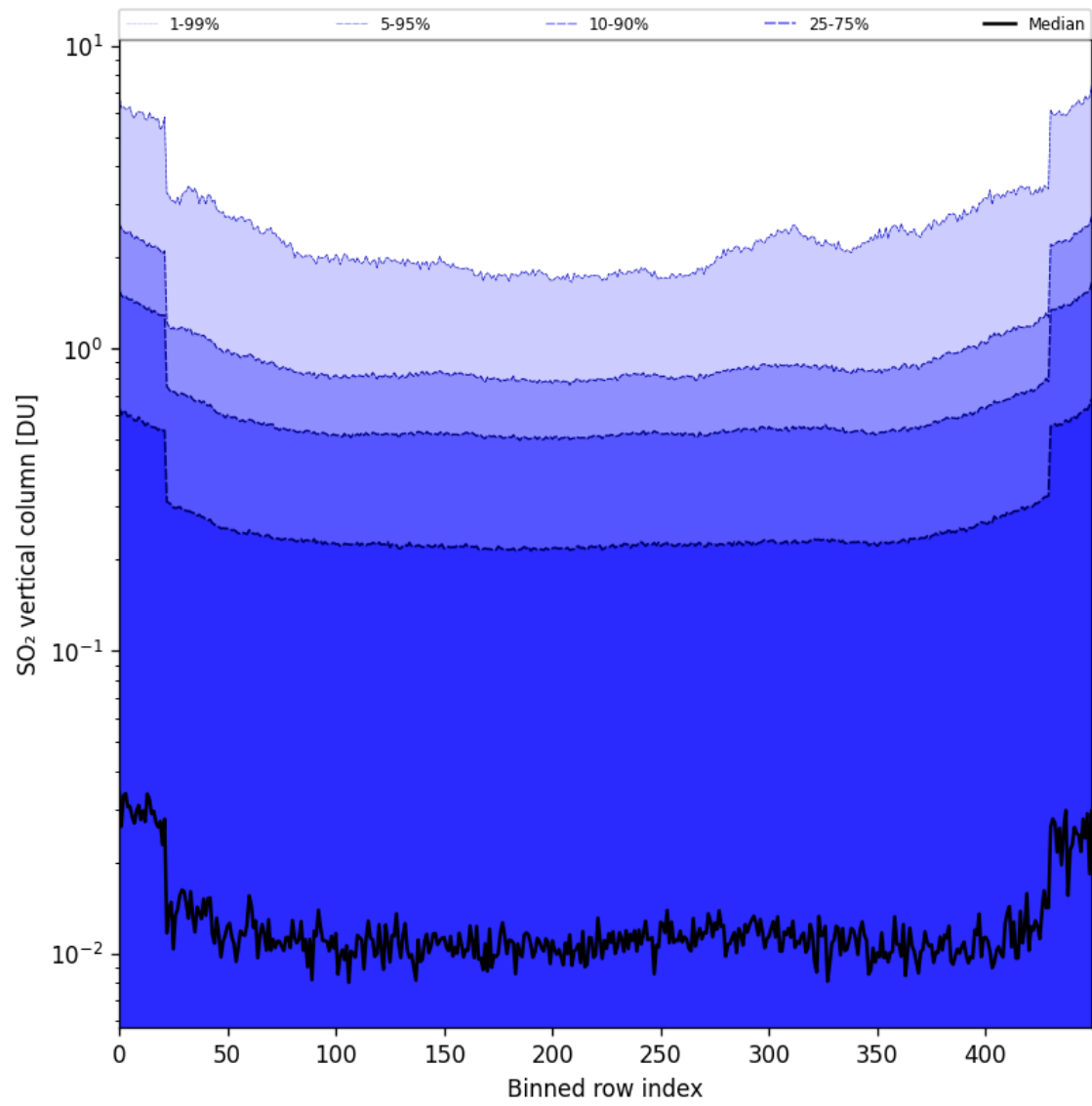
Figure 84: Along track statistics of “SO 2 vertical column” for 2025-08-03 to 2025-08-04
