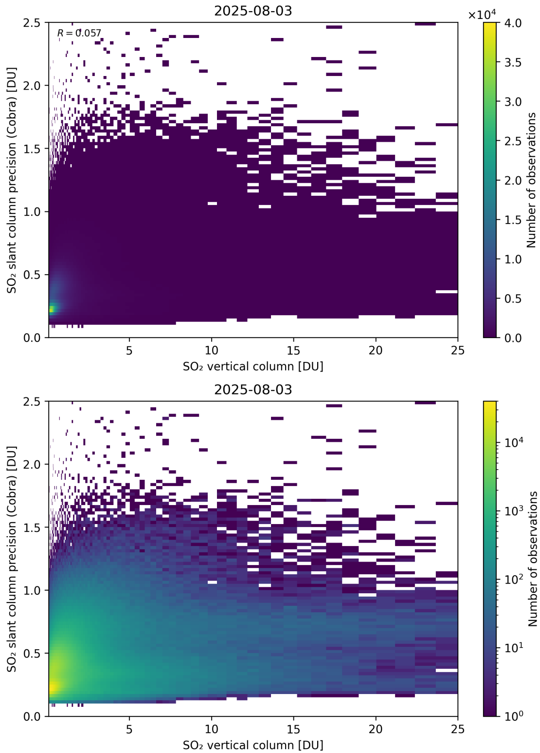
Figure 350: Scatter density plot of “SO 2 vertical column” against “SO 2 slant column precision (Cobra)” for 2025-08-03 to 2025-08-04.
