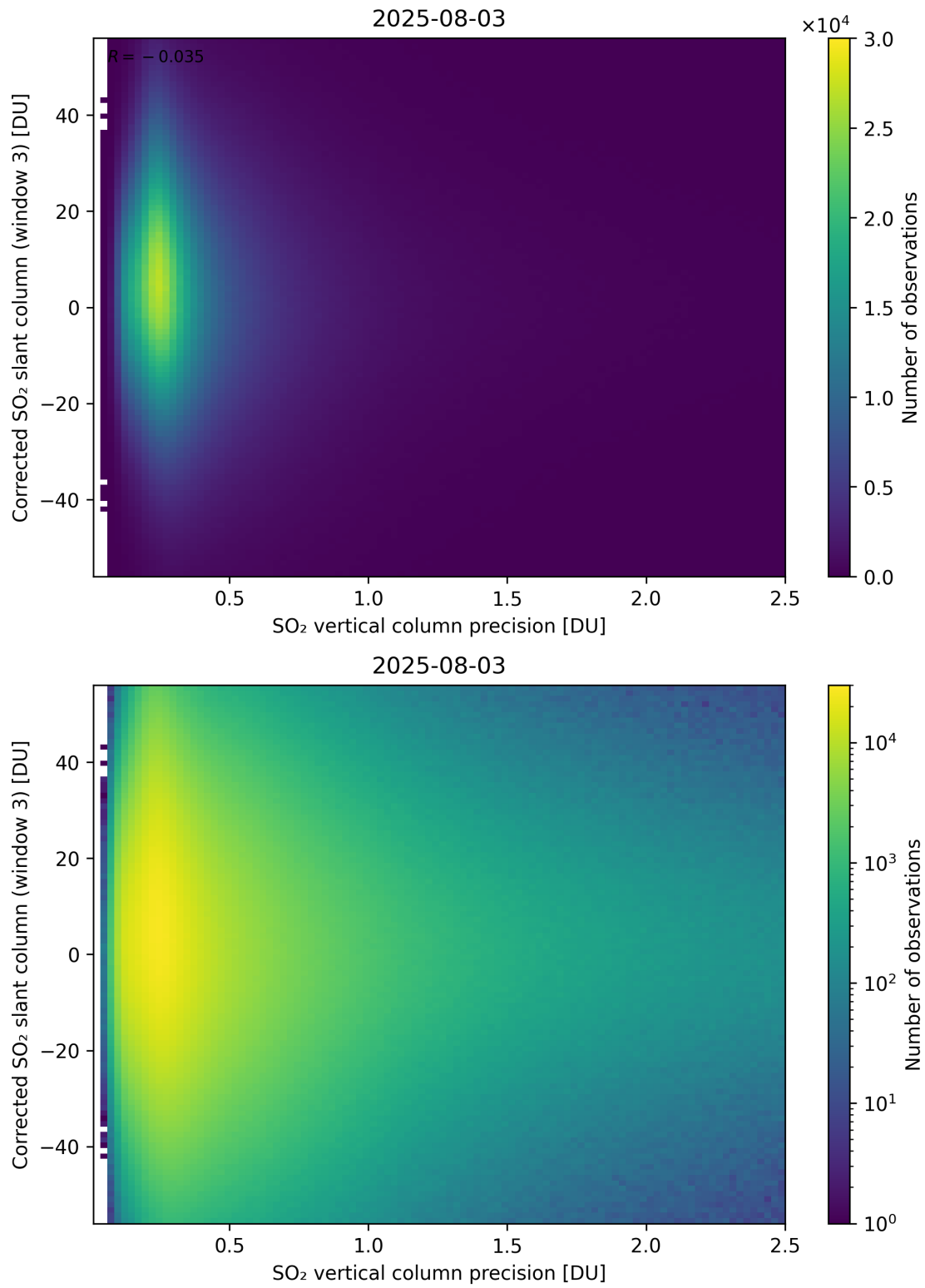
Figure 340: Scatter density plot of “SO 2 vertical column precision” against “Corrected SO 2 slant column (window 3)” for 2025-08-03 to 2025-08-04.
