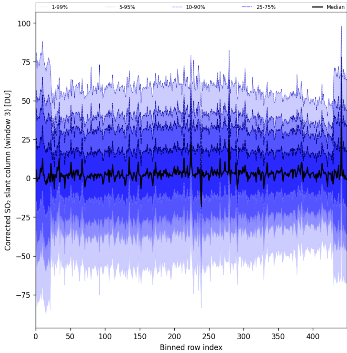
Figure 99: Along track statistics of “Corrected SO 2 slant column (window 3)” for 2025-08-03 to 2025-08-04
