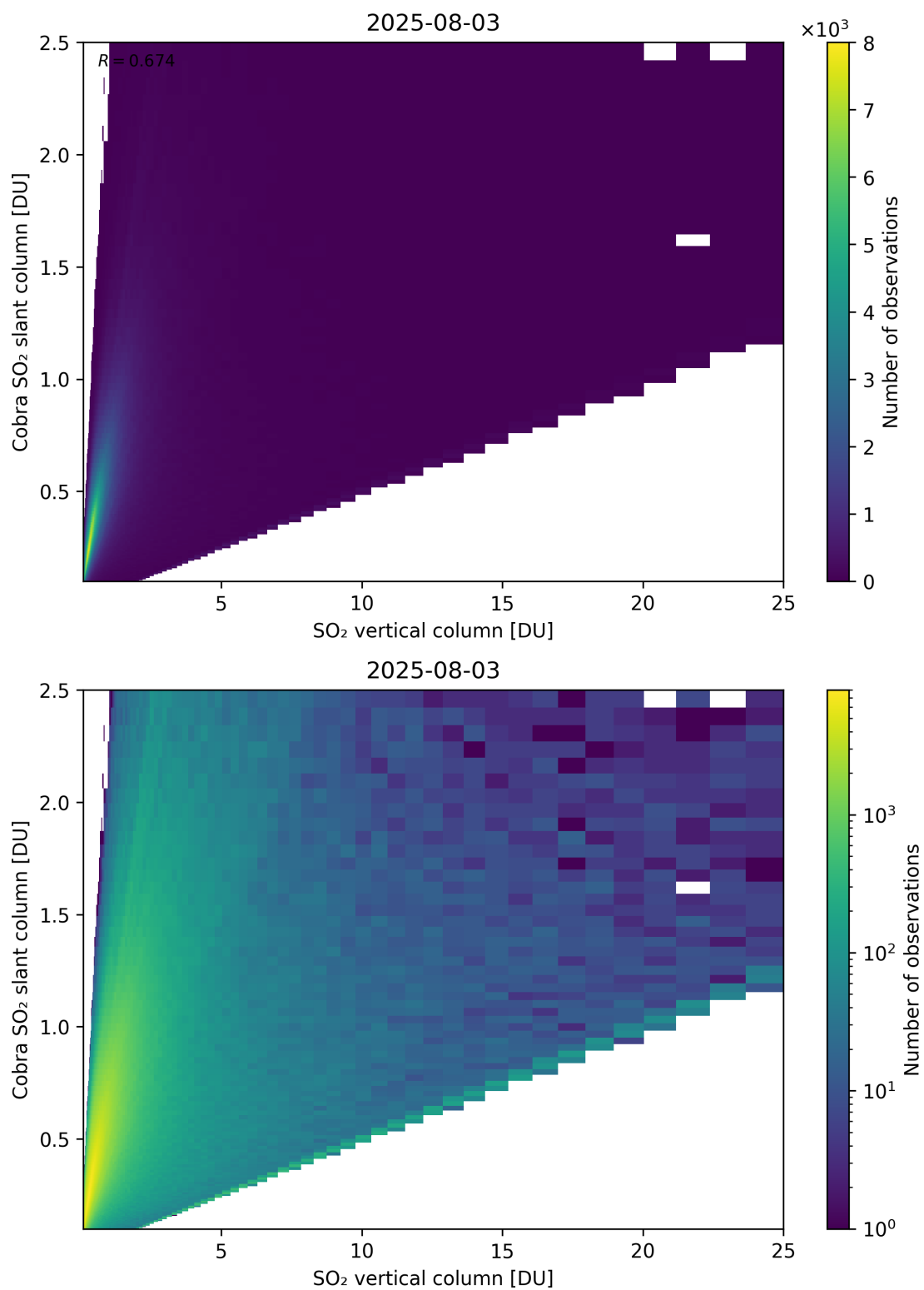
Figure 349: Scatter density plot of “SO 2 vertical column” against “Cobra SO 2 slant column” for 2025-08-03 to 2025-08-04.
