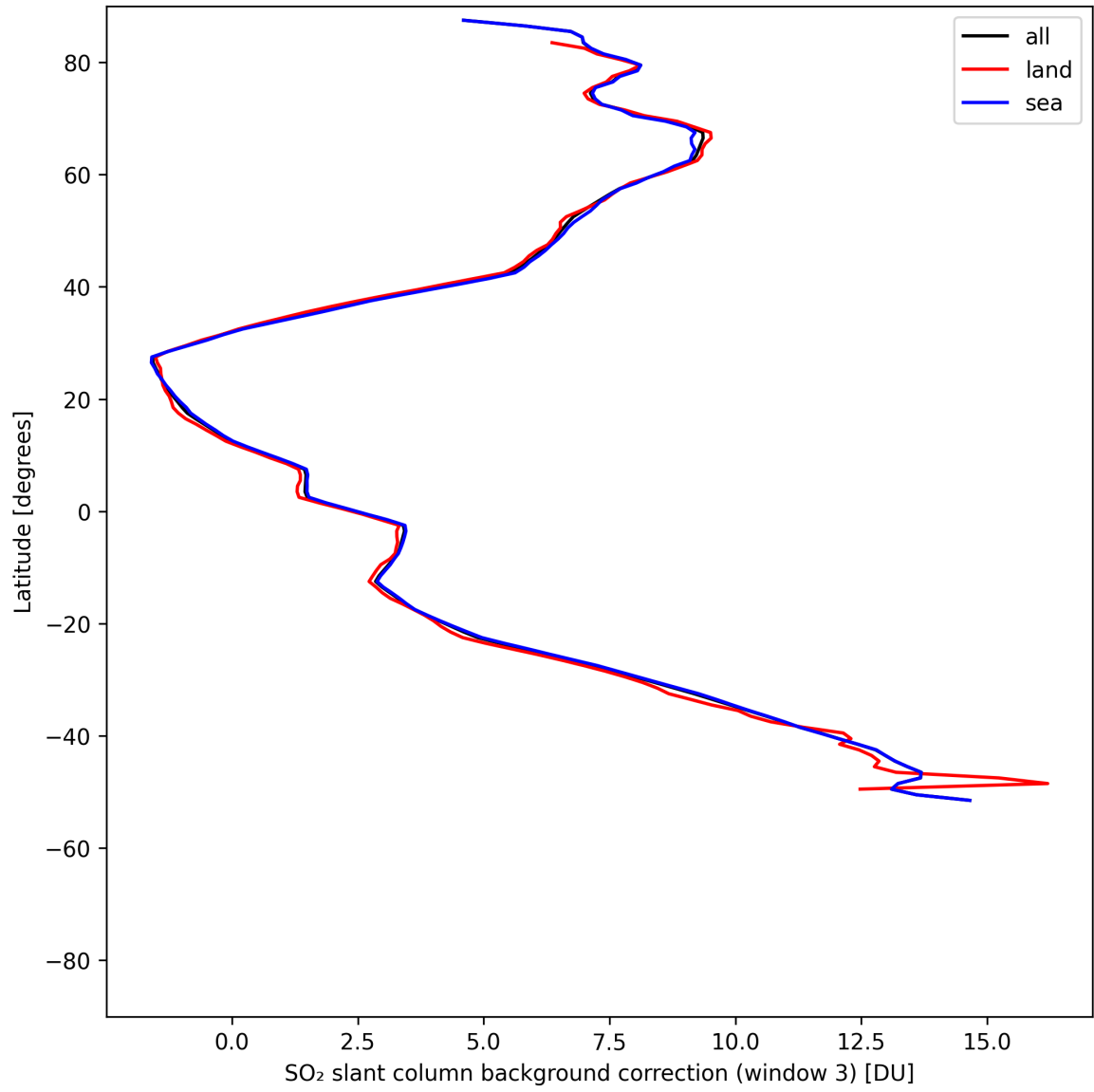
Figure 48: Zonal average of “SO 2 slant column background correction (window 3)” for 2025-08-03 to 2025-08-04.
