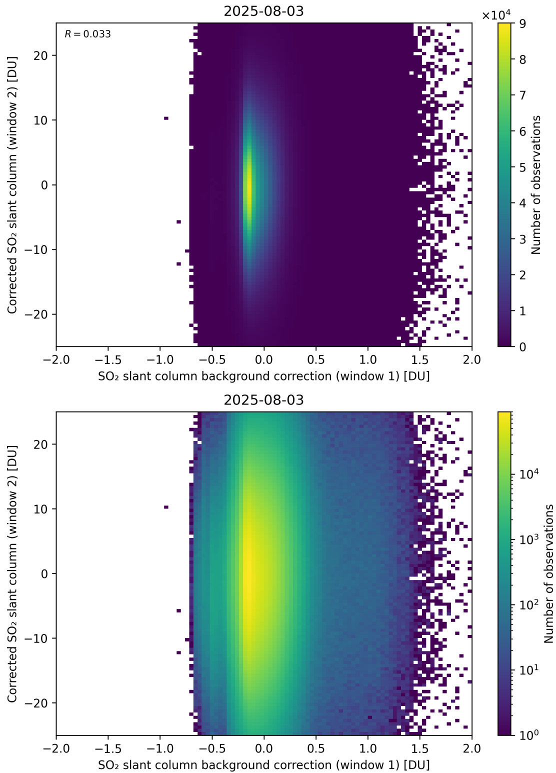
Figure 115: Scatter density plot of “SO 2 slant column background correction (window 1)” against “Corrected SO 2 slant column (window 2)” for 2025-08-03 to 2025-08-04.
