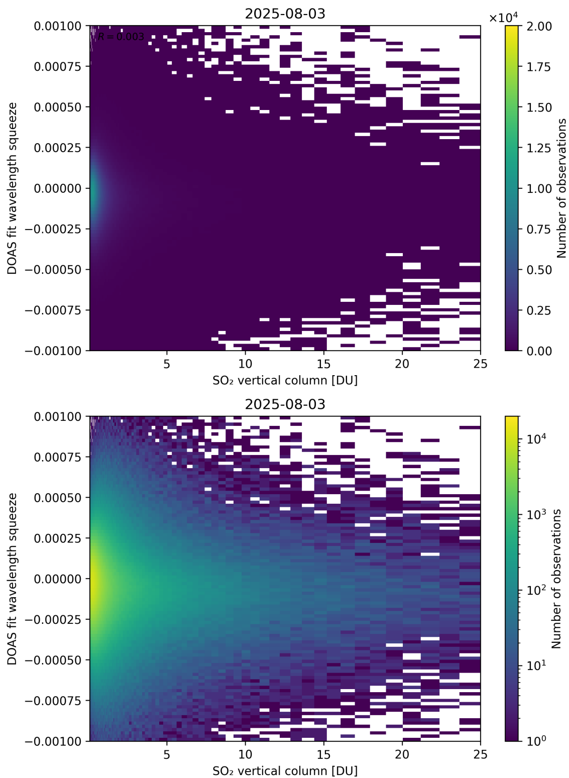
Figure 327: Scatter density plot of “SO 2 vertical column” against “DOAS fit wavelength squeeze” for 2025-08-03 to 2025-08-04.
