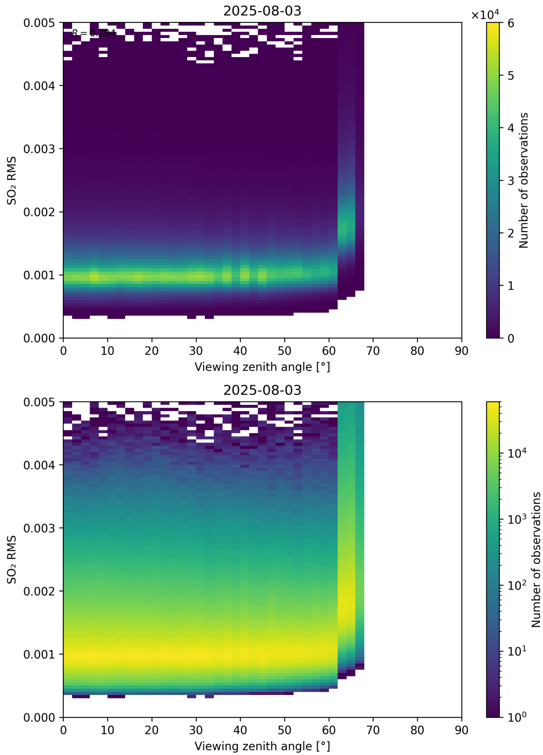
Figure 367: Scatter density plot of “Viewing zenith angle” against “SO 2 RMS” for 2025-08-03 to 2025-08-04.
