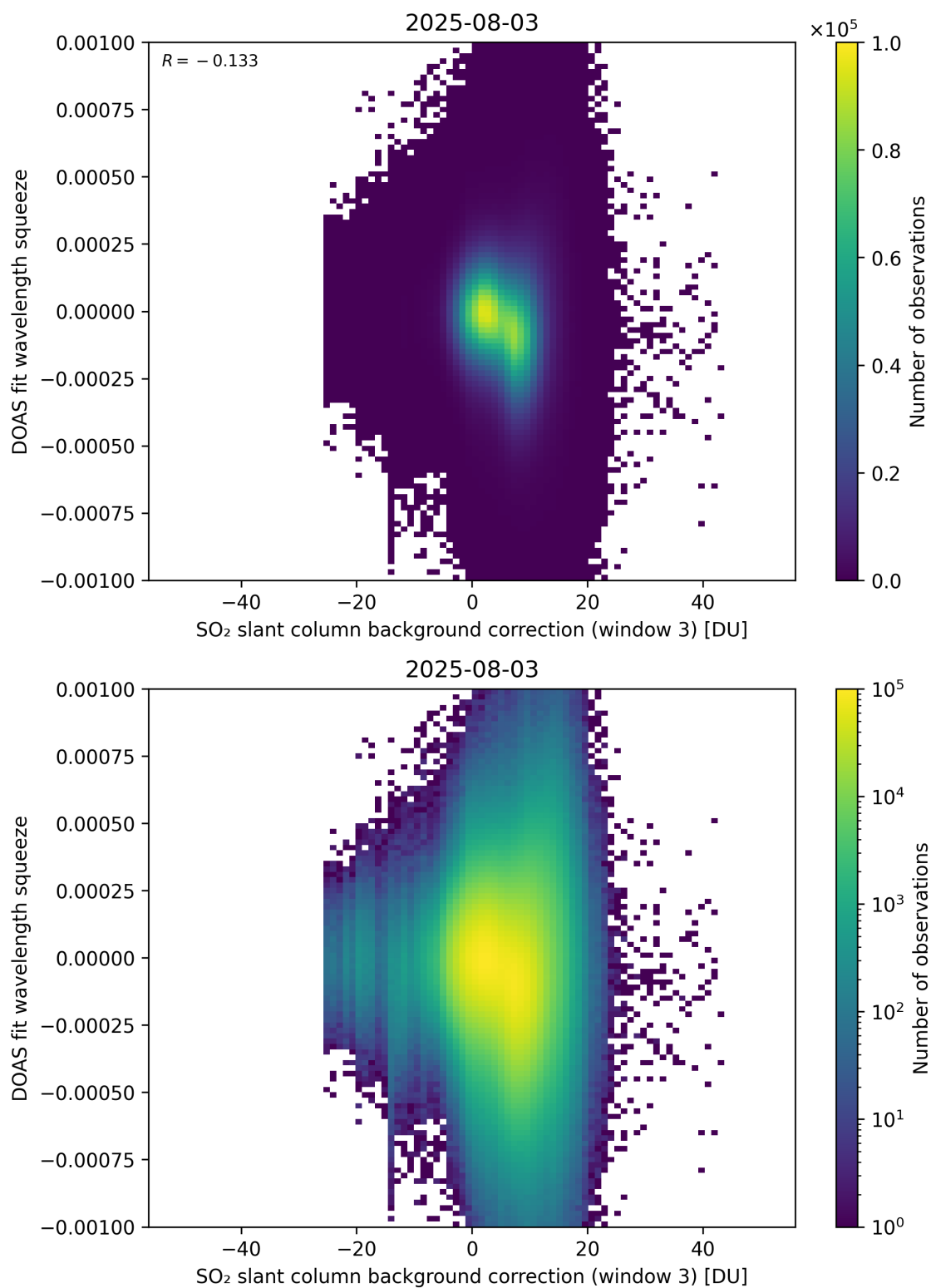
Figure 133: Scatter density plot of “SO 2 slant column background correction (window 3)” against “DOAS fit wavelength squeeze” for 2025-08-03 to 2025-08-04.
