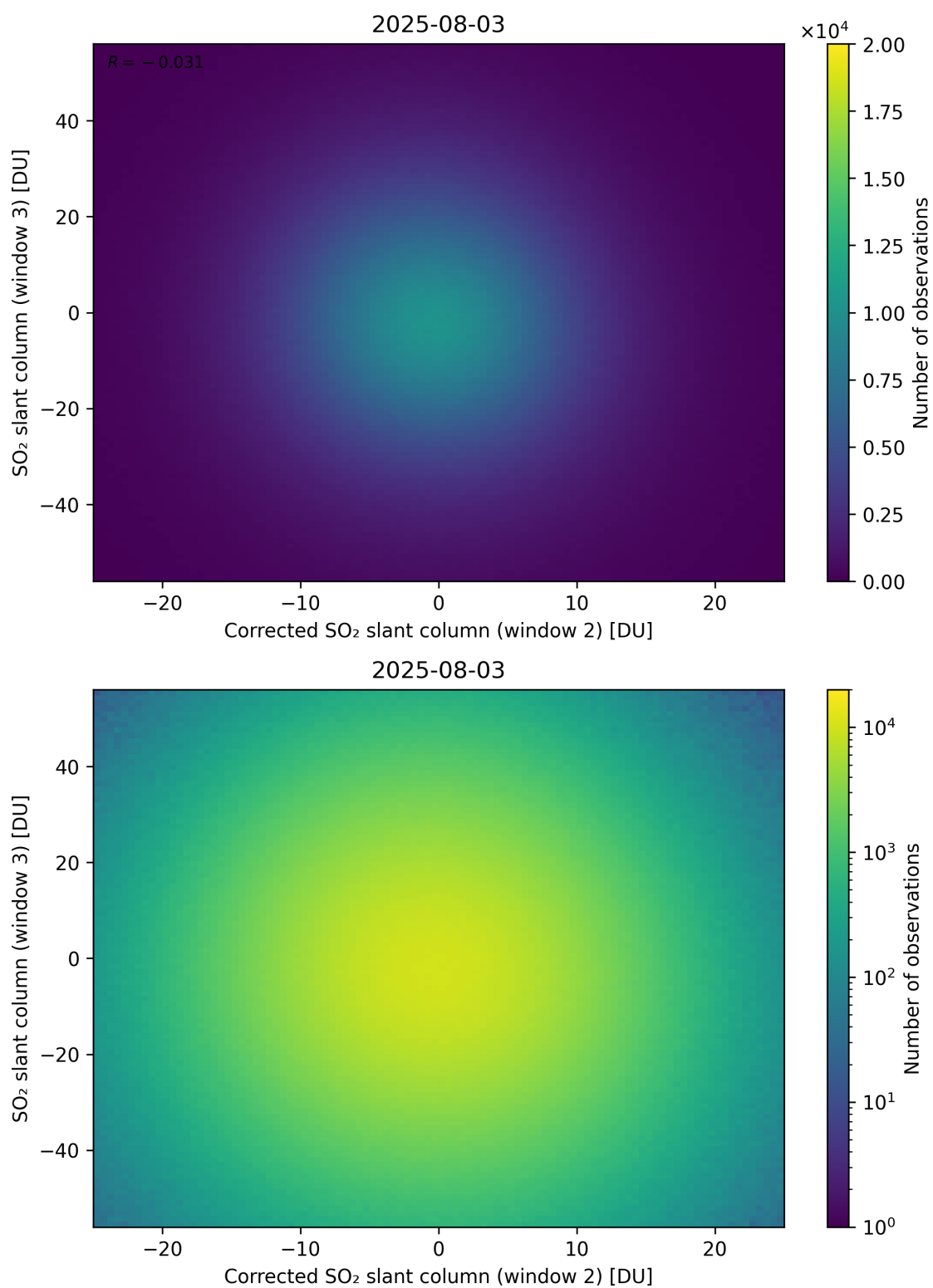
Figure 251: Scatter density plot of “Corrected SO 2 slant column (window 2)” against “SO 2 slant column (window 3)” for 2025-08-03 to 2025-08-04.
