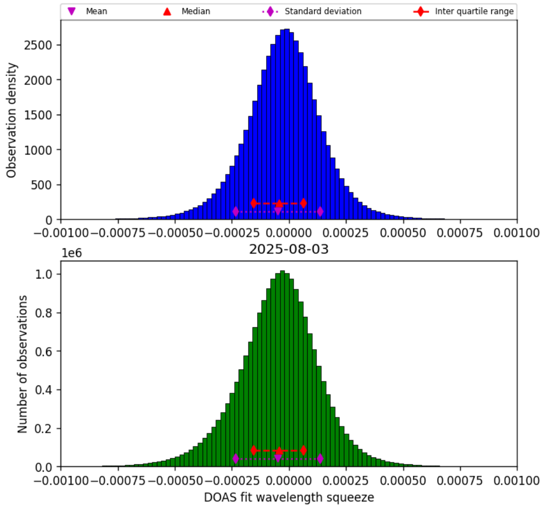
Figure 77: Histogram of “DOAS fit wavelength squeeze” for 2025-08-03 to 2025-08-04
