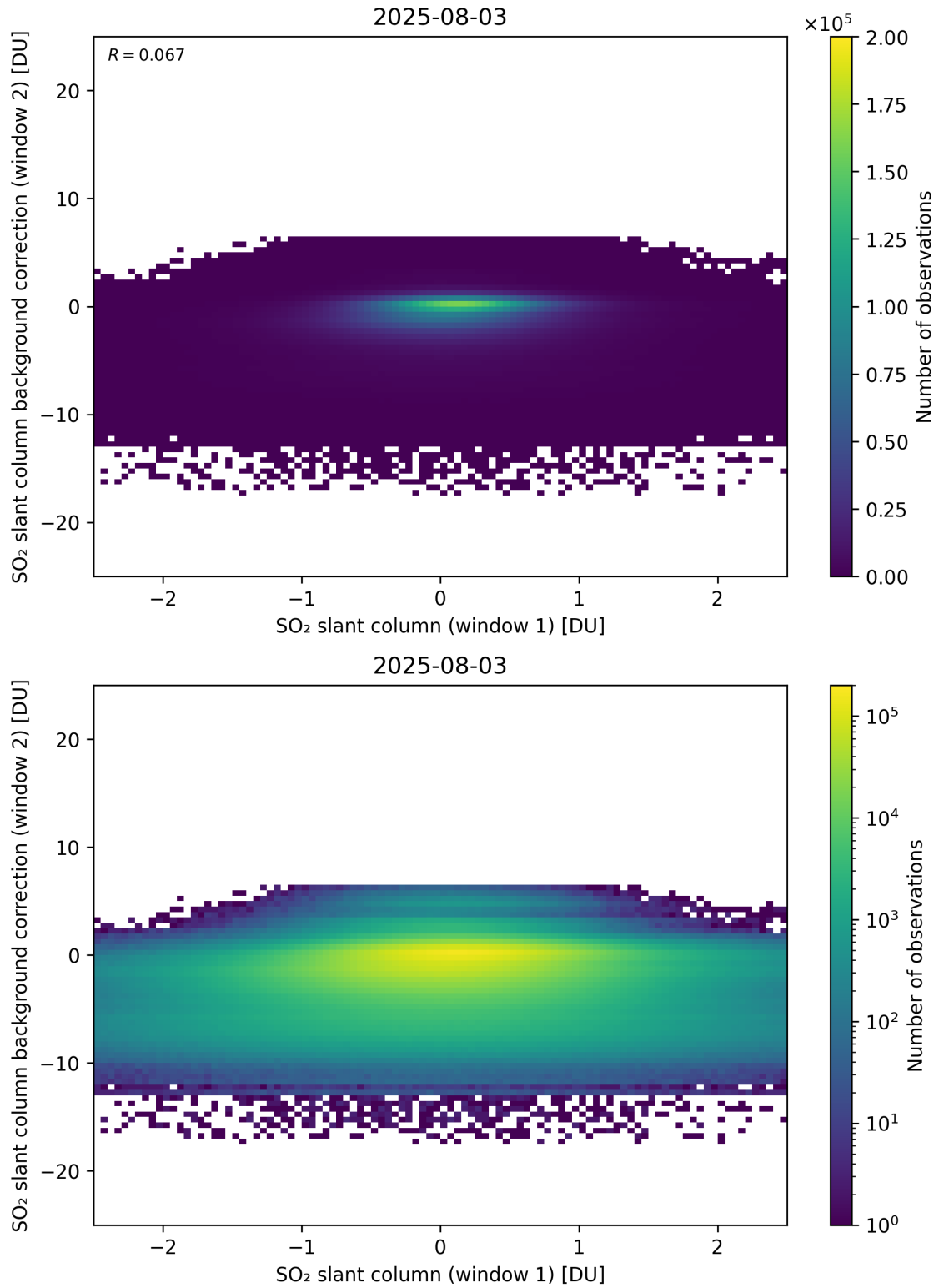
Figure 263: Scatter density plot of “SO 2 slant column (window 1)” against “SO 2 slant column background correction (window 2)” for 2025-08-03 to 2025-08-04.
