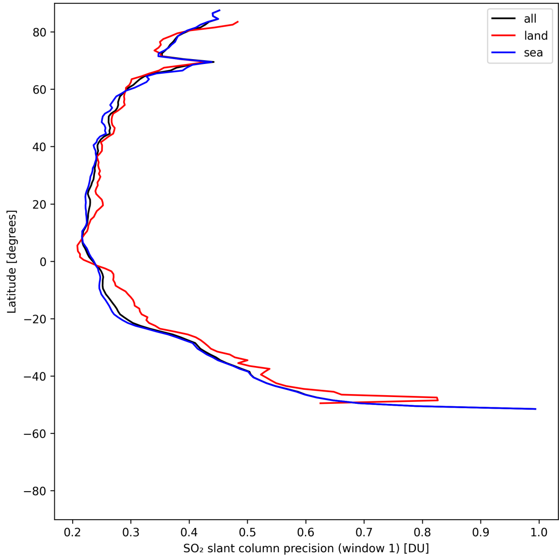
Figure 38: Zonal average of “SO 2 slant column precision (window 1)” for 2025-08-03 to 2025-08-04.
