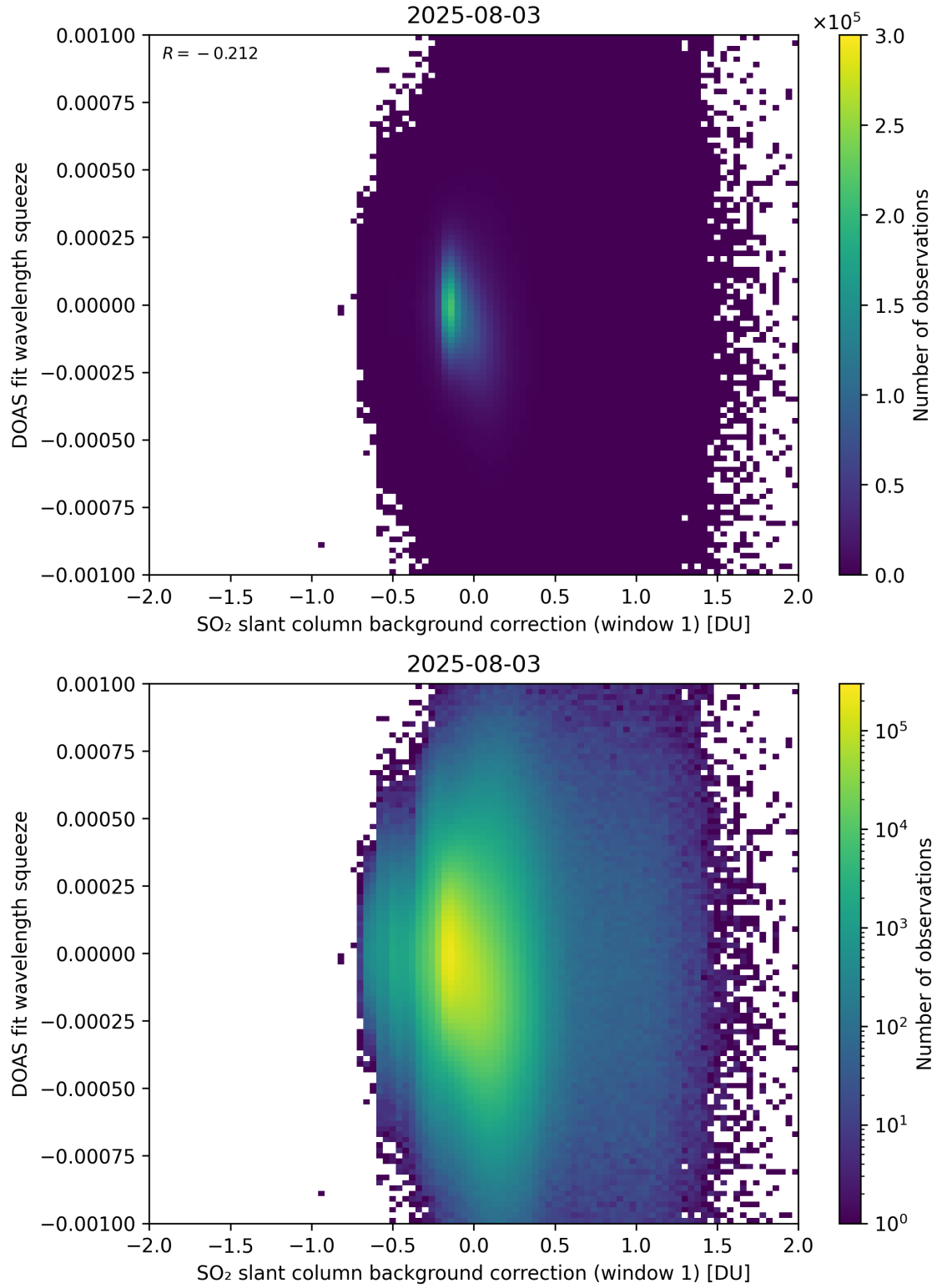
Figure 112: Scatter density plot of “SO 2 slant column background correction (window 1)” against “DOAS fit wavelength squeeze” for 2025-08-03 to 2025-08-04.
