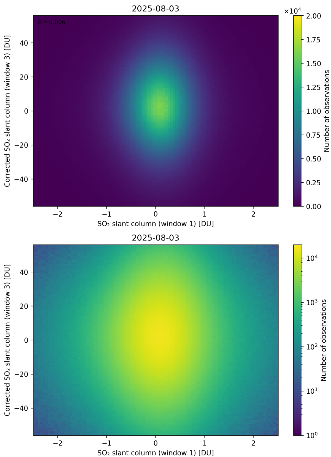
Figure 284: Scatter density plot of “SO 2 slant column (window 1)” against “Corrected SO 2 slant column (window 3)” for 2025-08-03 to 2025-08-04.
