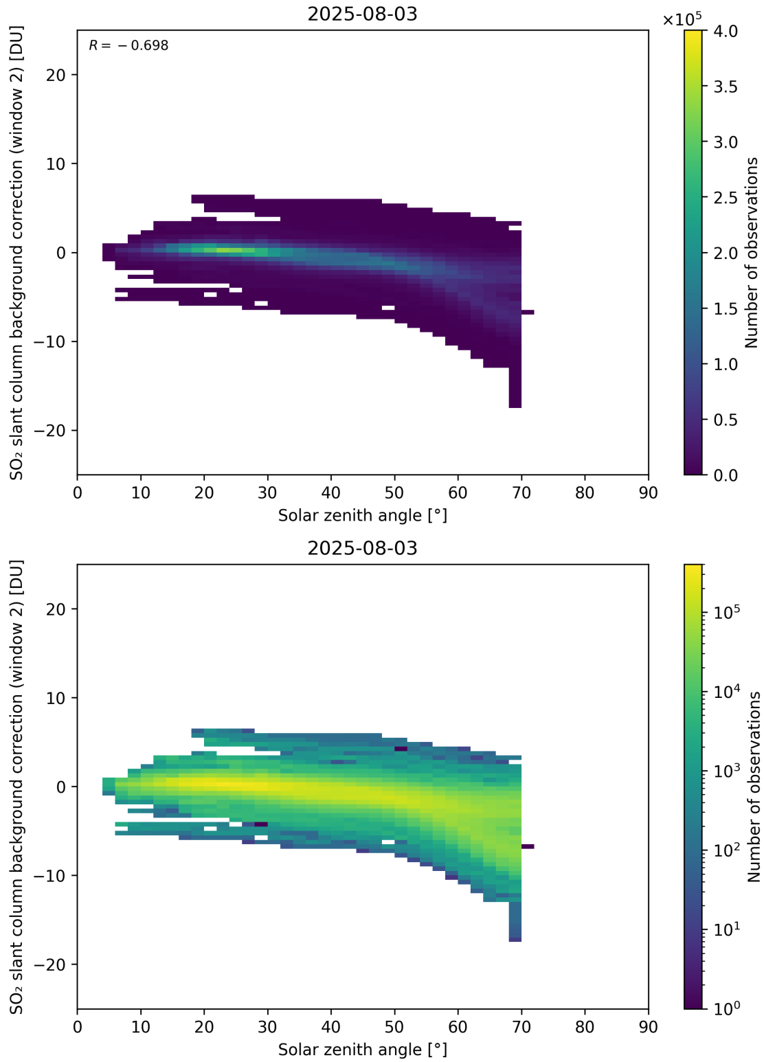
Figure 172: Scatter density plot of “Solar zenith angle” against “SO 2 slant column background correction (window 2)” for 2025-08-03 to 2025-08-04.
