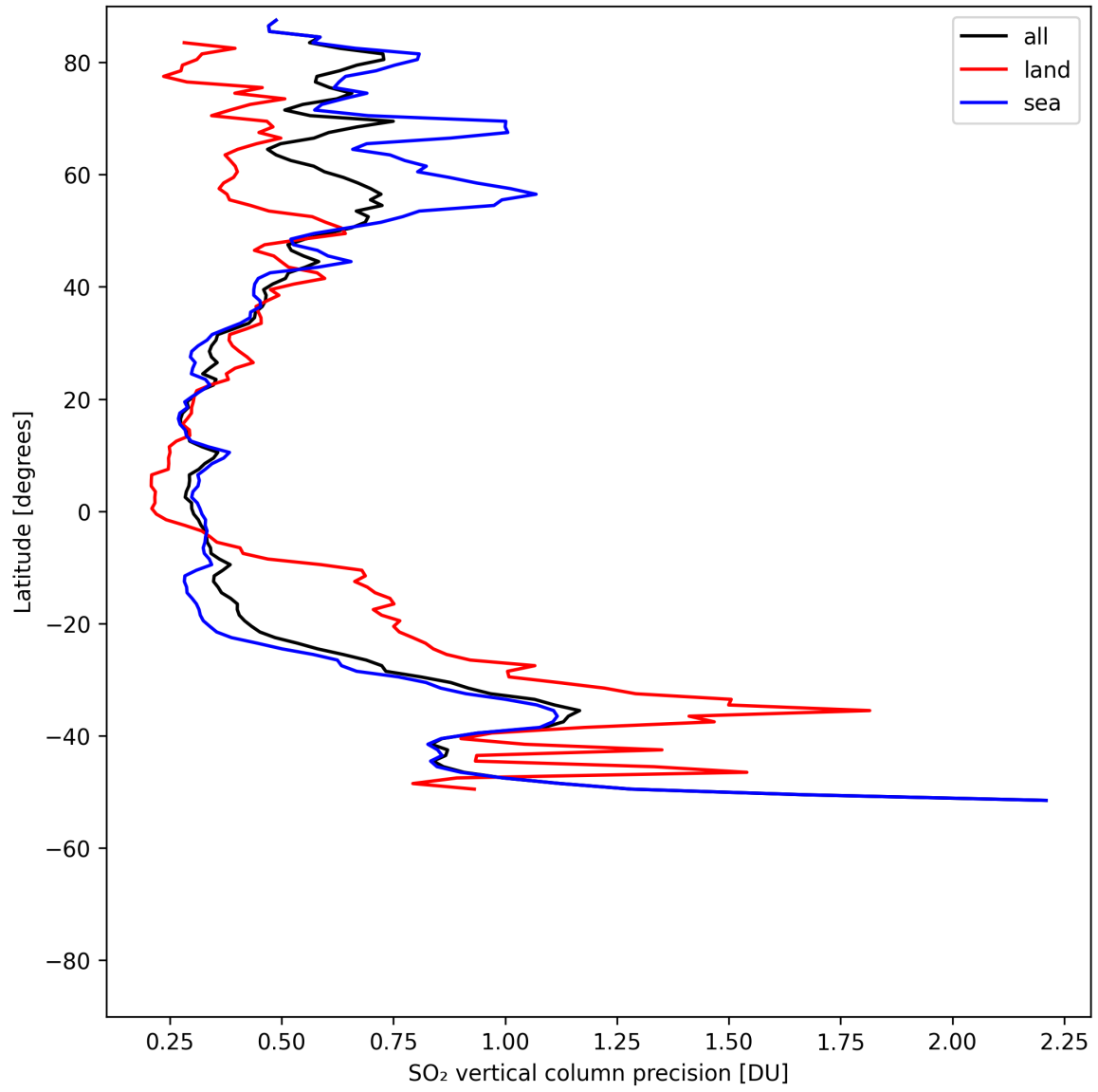
Figure 33: Zonal average of “SO 2 vertical column precision” for 2025-08-03 to 2025-08-04.
