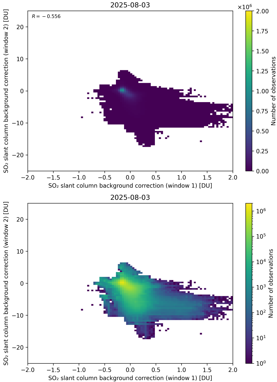
Figure 109: Scatter density plot of “SO 2 slant column background correction (window 1)” against “SO 2 slant column background correction (window 2)” for 2025-08-03 to 2025-08-04.
