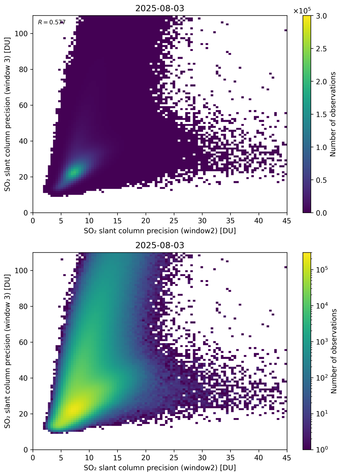
Figure 300: Scatter density plot of “SO 2 slant column precision (window2)” against “SO 2 slant column precision (window 3)” for 2025-08-03 to 2025-08-04.
