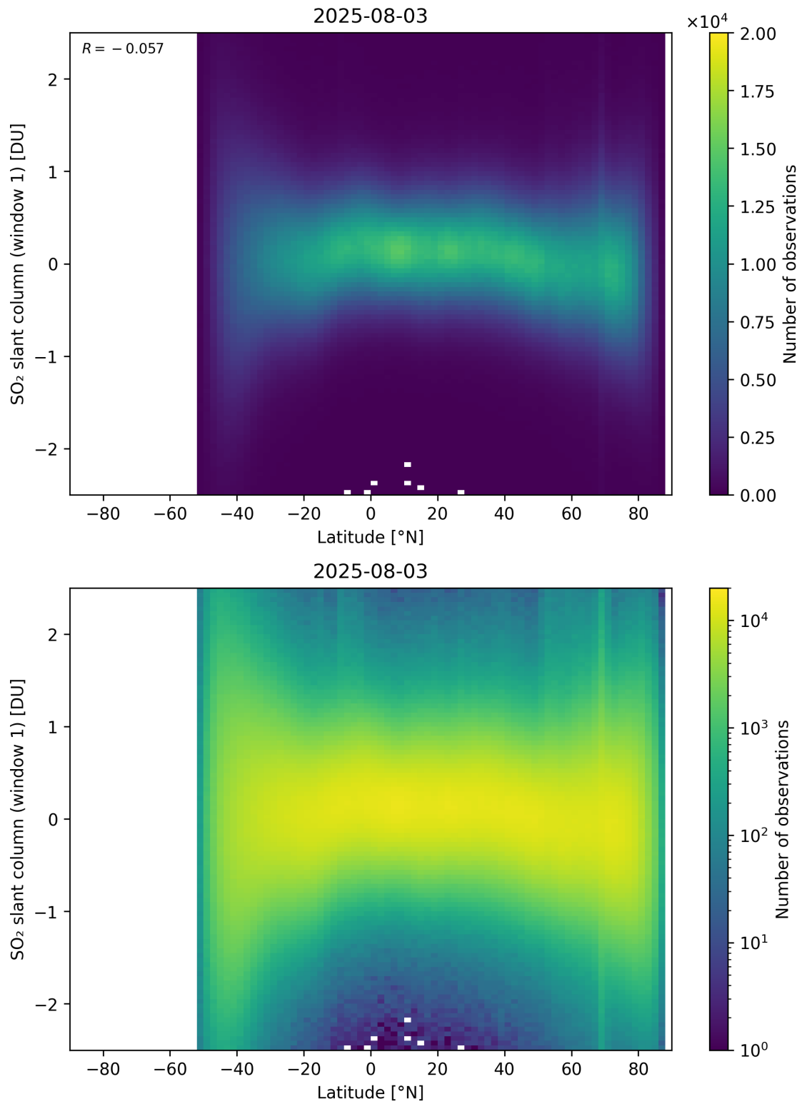
Figure 162: Scatter density plot of “Latitude” against “SO 2 slant column (window 1)” for 2025-08-03 to 2025-08-04.
