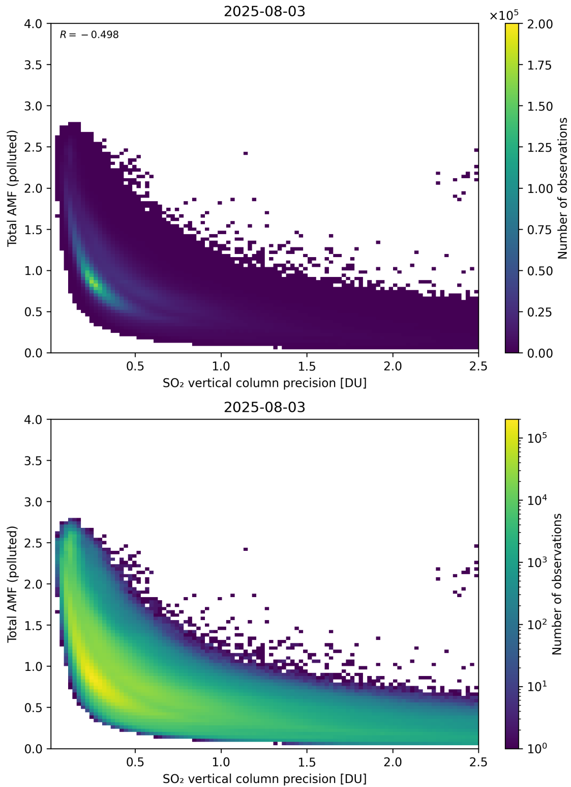
Figure 346: Scatter density plot of “SO 2 vertical column precision” against “Total AMF (polluted)” for 2025-08-03 to 2025-08-04.
