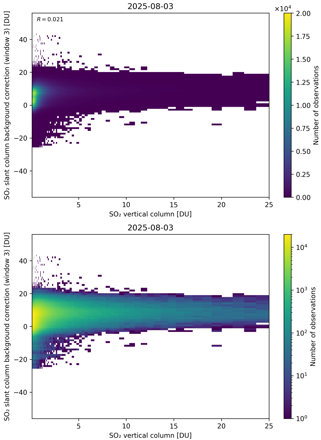
Figure 325: Scatter density plot of “SO 2 vertical column” against “SO 2 slant column background correction (window 3)” for 2025-08-03 to 2025-08-04.
