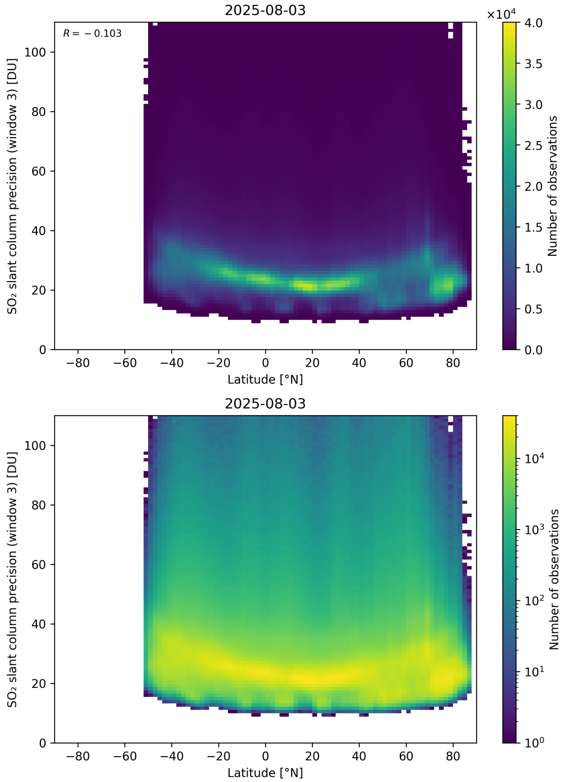
Figure 166: Scatter density plot of “Latitude” against “SO 2 slant column precision (window 3)” for 2025-08-03 to 2025-08-04.
