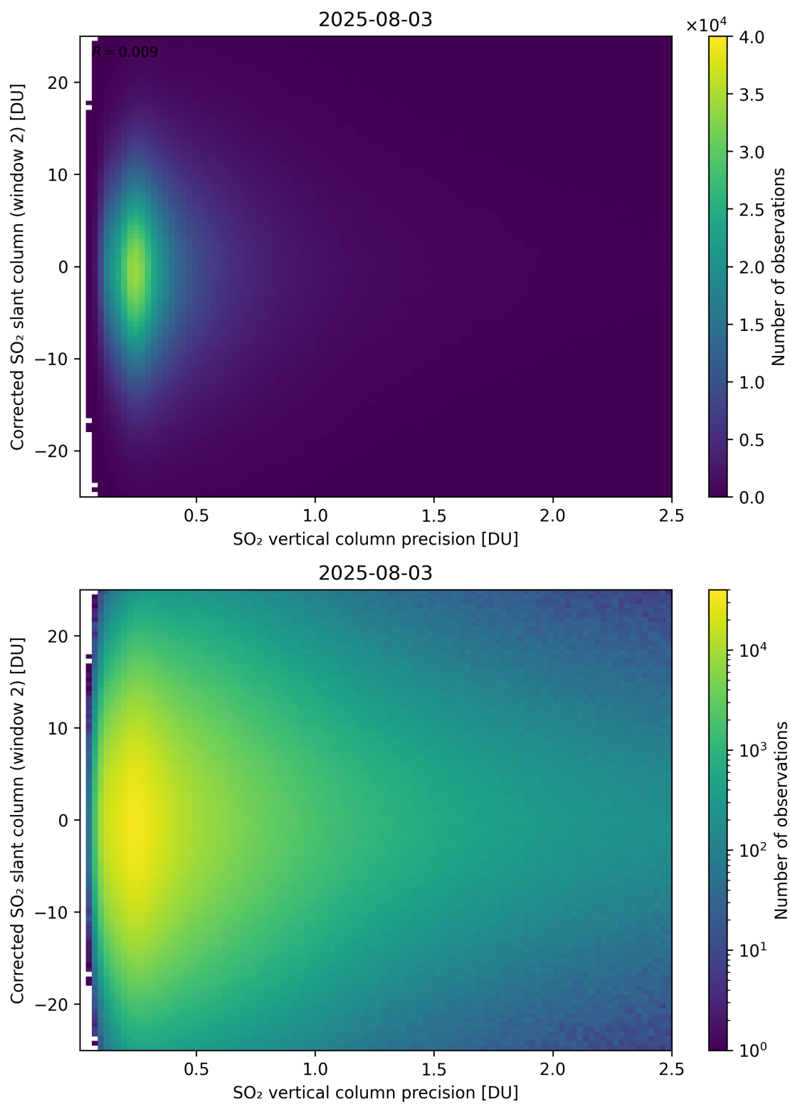
Figure 339: Scatter density plot of “SO 2 vertical column precision” against “Corrected SO 2 slant column (window 2)” for 2025-08-03 to 2025-08-04.
