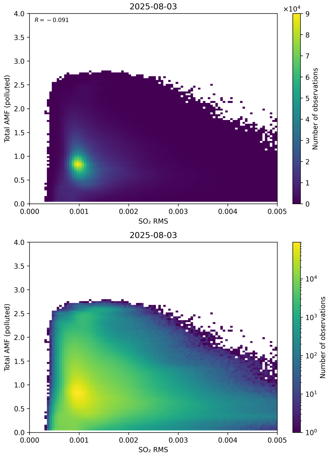
Figure 148: Scatter density plot of “SO 2 RMS” against “Total AMF (polluted)” for 2025-08-03 to 2025-08-04.
