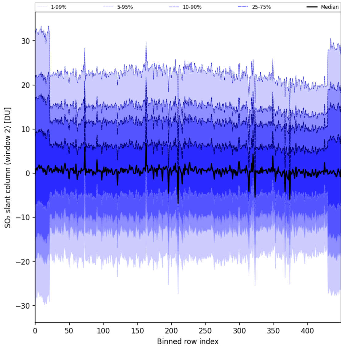
Figure 93: Along track statistics of “SO 2 slant column (window 2)” for 2025-08-03 to 2025-08-04
