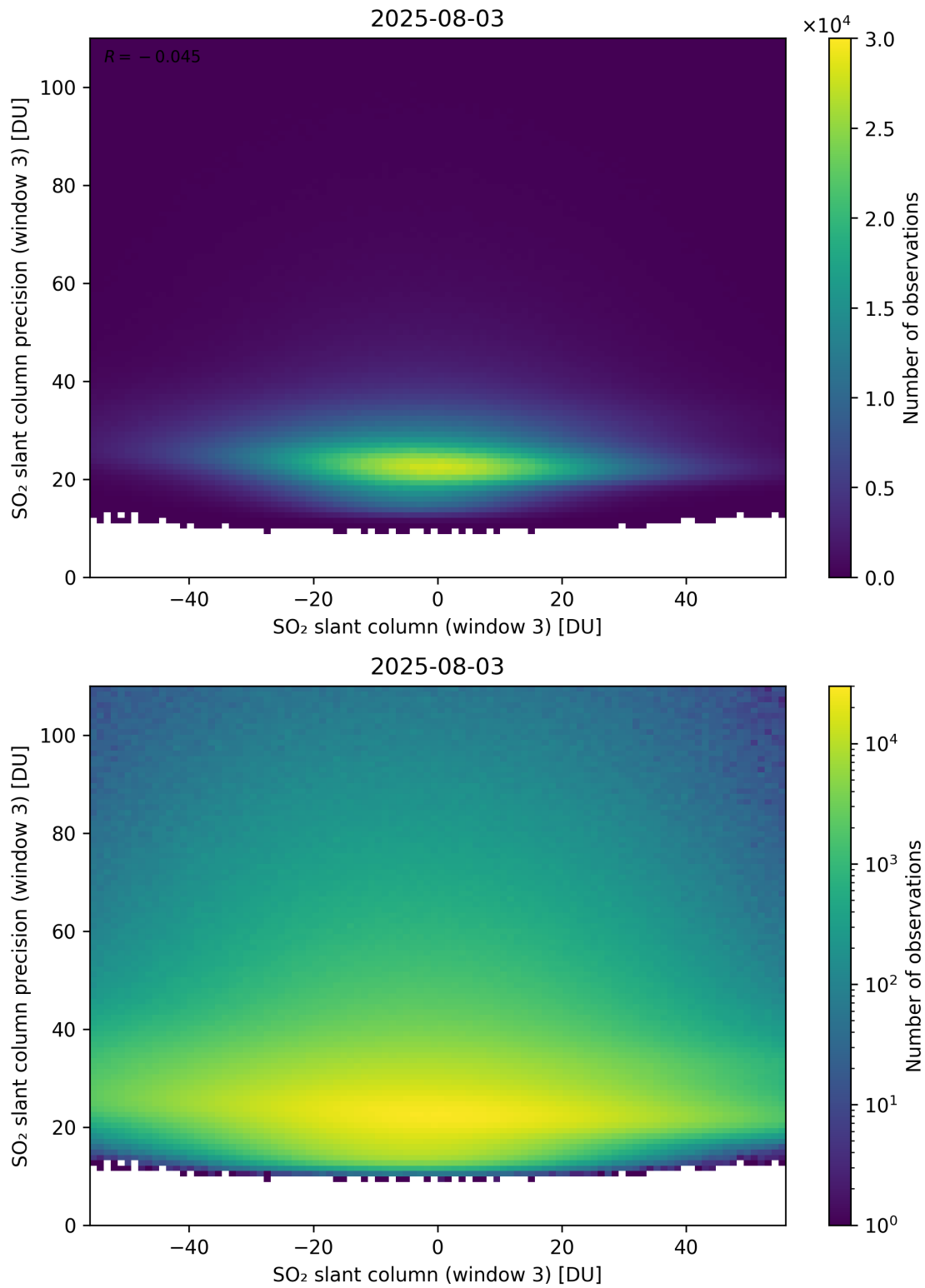
Figure 317: Scatter density plot of “SO 2 slant column (window 3)” against “SO 2 slant column precision (window 3)” for 2025-08-03 to 2025-08-04.
