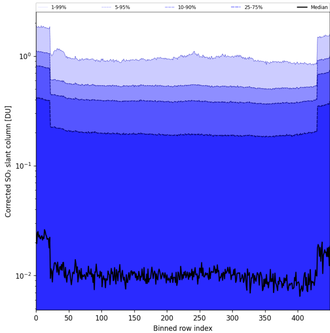
Figure 86: Along track statistics of “Corrected SO 2 slant column” for 2025-08-03 to 2025-08-04
