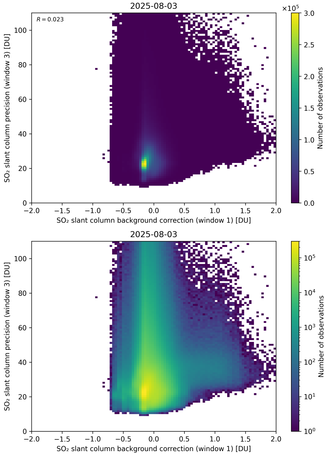
Figure 119: Scatter density plot of “SO 2 slant column background correction (window 1)” against “SO 2 slant column precision (window 3)” for 2025-08-03 to 2025-08-04.
