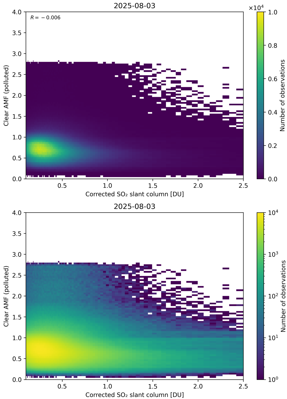
Figure 232: Scatter density plot of “Corrected SO 2 slant column” against “Clear AMF (polluted)” for 2025-08-03 to 2025-08-04.
