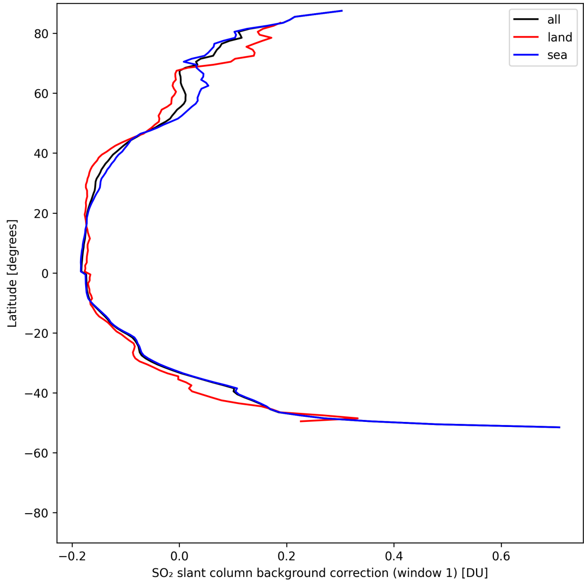
Figure 40: Zonal average of “SO 2 slant column background correction (window 1)” for 2025-08-03 to 2025-08-04.
