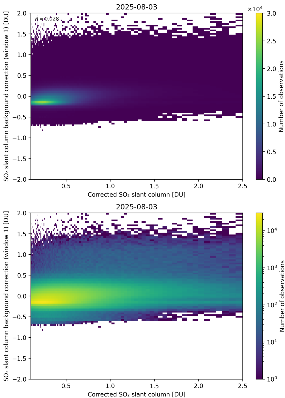
Figure 226: Scatter density plot of “Corrected SO 2 slant column” against “SO 2 slant column background correction (window 1)” for 2025-08-03 to 2025-08-04.
