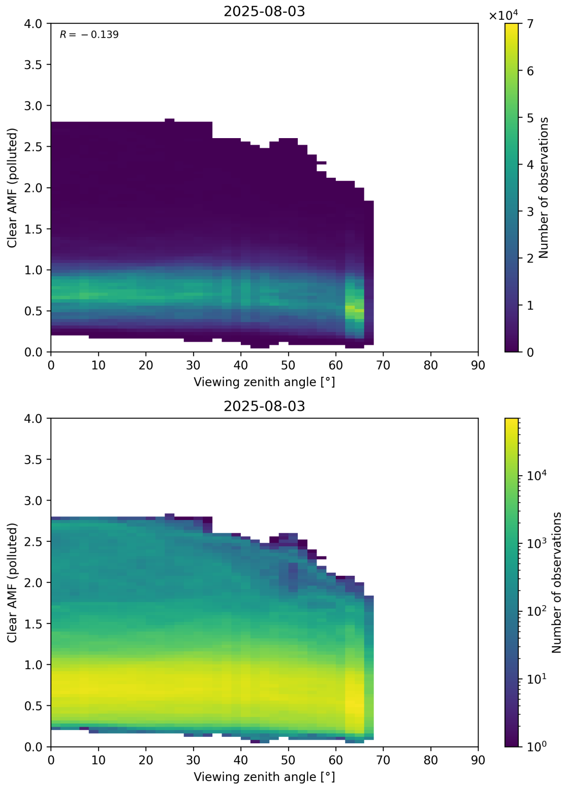
Figure 370: Scatter density plot of “Viewing zenith angle” against “Clear AMF (polluted)” for 2025-08-03 to 2025-08-04.
