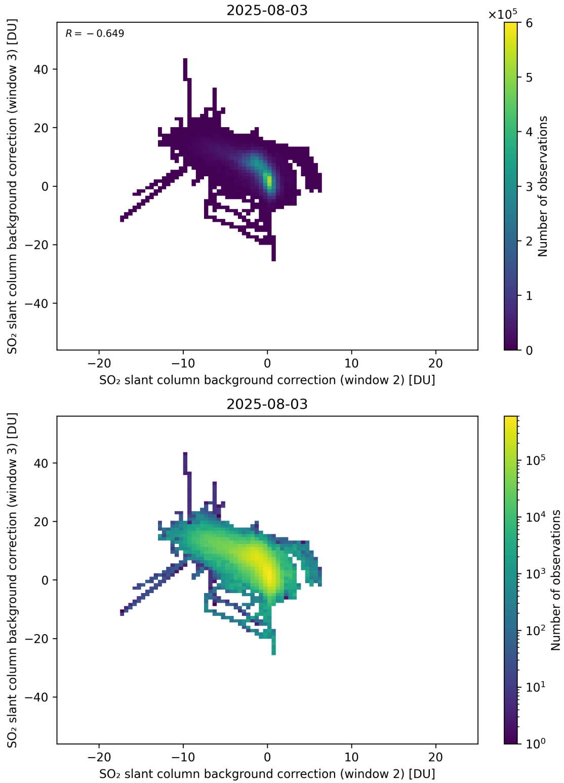
Figure 122: Scatter density plot of “SO 2 slant column background correction (window 2)” against “SO 2 slant column background correction (window 3)” for 2025-08-03 to 2025-08-04.
