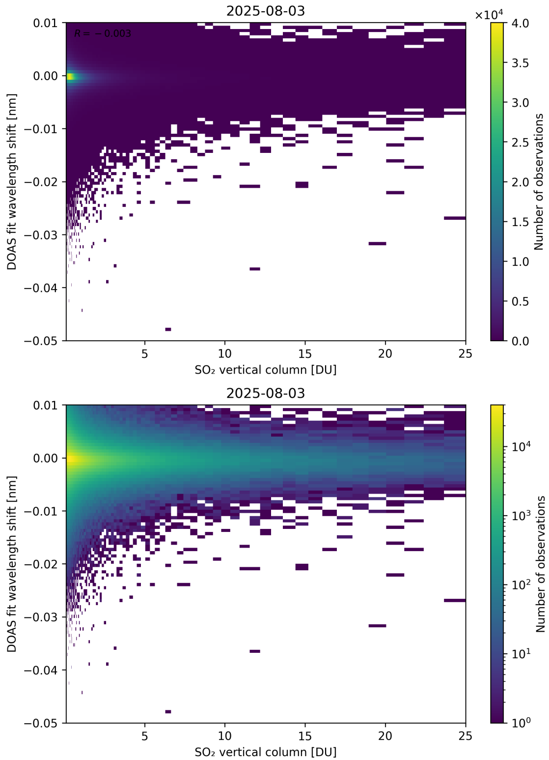
Figure 326: Scatter density plot of “SO 2 vertical column” against “DOAS fit wavelength shift” for 2025-08-03 to 2025-08-04.
