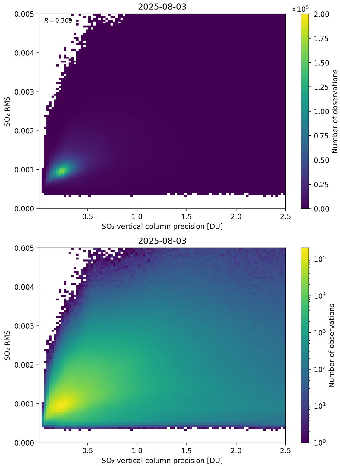
Figure 334: Scatter density plot of “SO 2 vertical column precision” against “SO 2 RMS” for 2025-08-03 to 2025-08-04.
