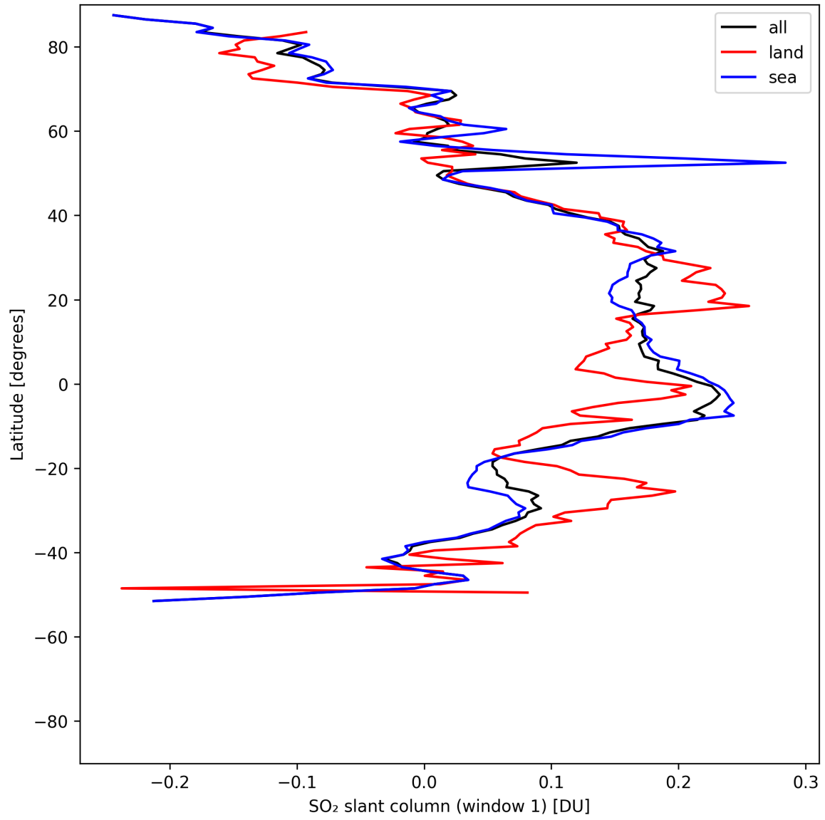
Figure 37: Zonal average of “SO 2 slant column (window 1)” for 2025-08-03 to 2025-08-04.
