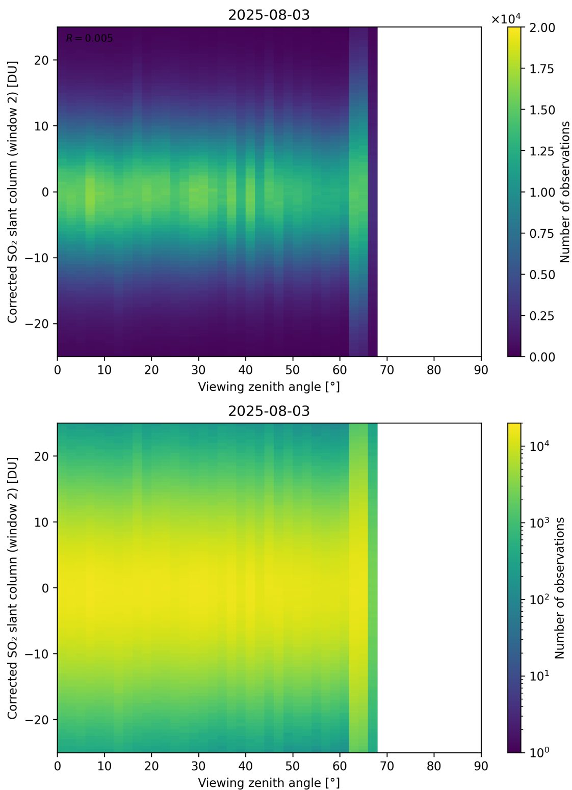
Figure 374: Scatter density plot of “Viewing zenith angle” against “Corrected SO 2 slant column (window 2)” for 2025-08-03 to 2025-08-04.
