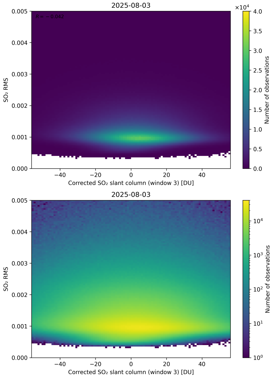
Figure 258: Scatter density plot of “Corrected SO 2 slant column (window 3)” against “SO 2 RMS” for 2025-08-03 to 2025-08-04.
