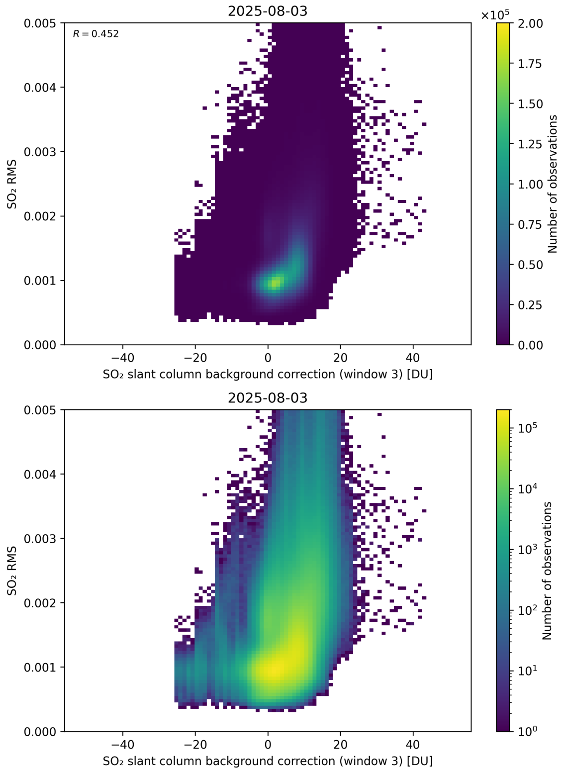
Figure 134: Scatter density plot of “SO 2 slant column background correction (window 3)” against “SO 2 RMS” for 2025-08-03 to 2025-08-04.
