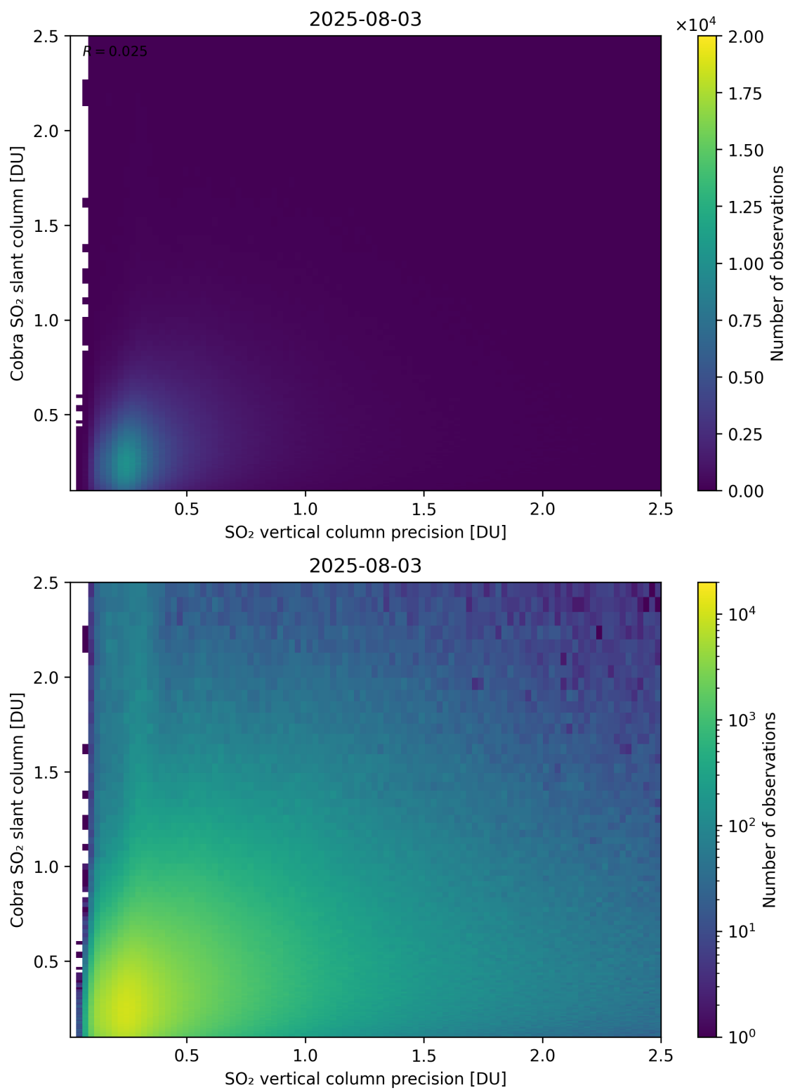
Figure 336: Scatter density plot of “SO 2 vertical column precision” against “Cobra SO 2 slant column” for 2025-08-03 to 2025-08-04.
