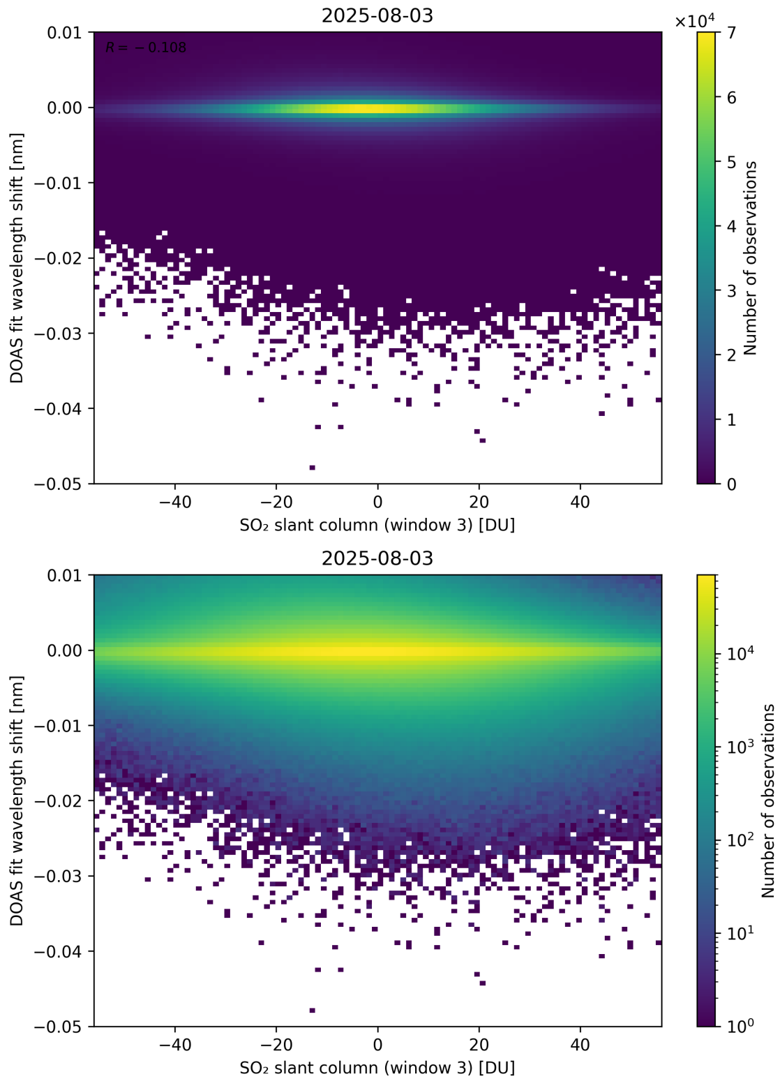
Figure 304: Scatter density plot of “SO 2 slant column (window 3)” against “DOAS fit wavelength shift” for 2025-08-03 to 2025-08-04.
