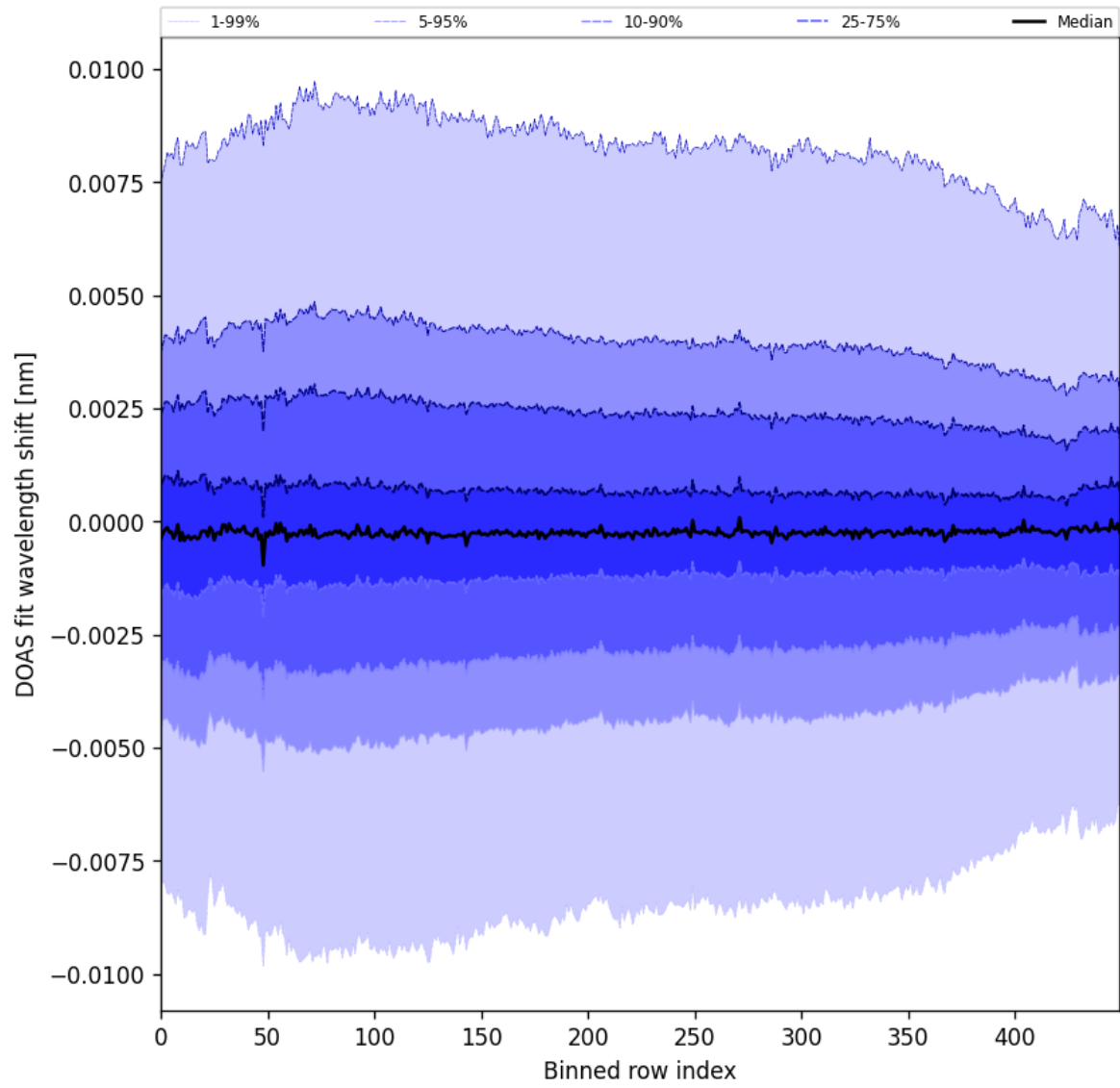
Figure 102: Along track statistics of “DOAS fit wavelength shift” for 2025-08-03 to 2025-08-04
