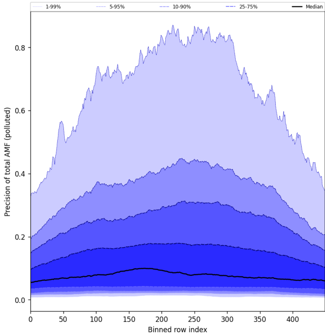
Figure 106: Along track statistics of “Precision of total AMF (polluted)” for 2025-08-03 to 2025-08-04
