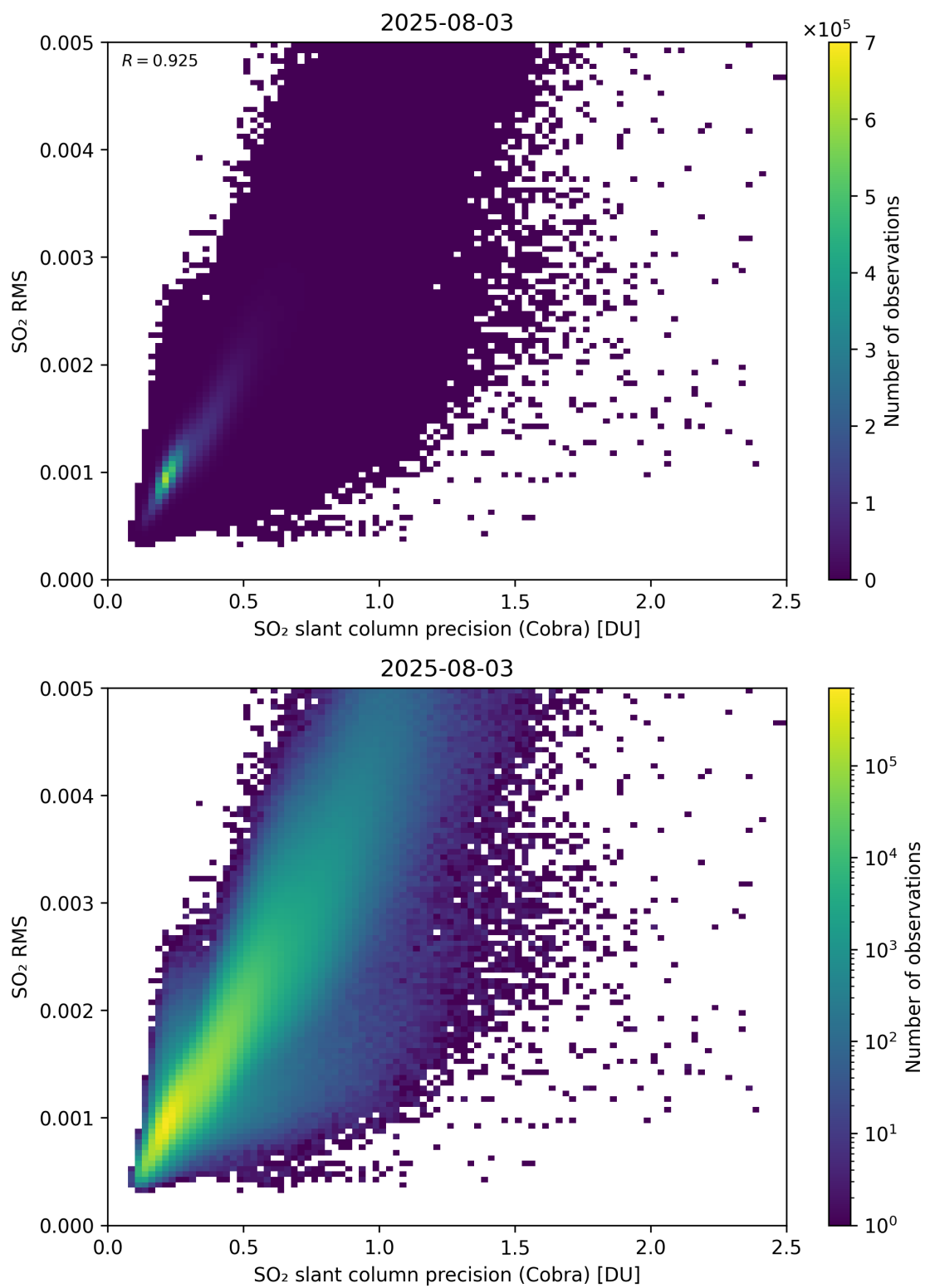
Figure 204: Scatter density plot of “SO 2 slant column precision (Cobra)” against “SO 2 RMS” for 2025-08-03 to 2025-08-04.
