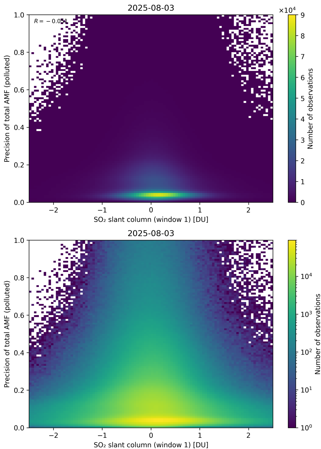
Figure 290: Scatter density plot of “SO 2 slant column (window 1)” against “Precision of total AMF (polluted)” for 2025-08-03 to 2025-08-04.
