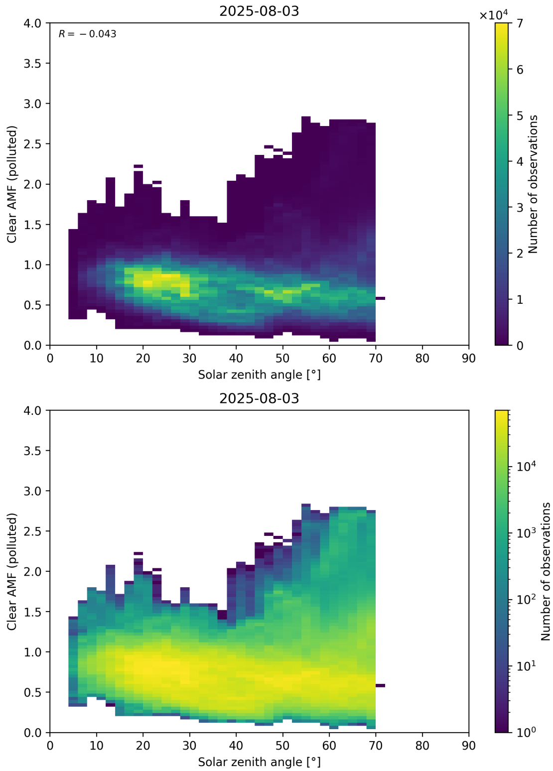
Figure 178: Scatter density plot of “Solar zenith angle” against “Clear AMF (polluted)” for 2025-08-03 to 2025-08-04.
