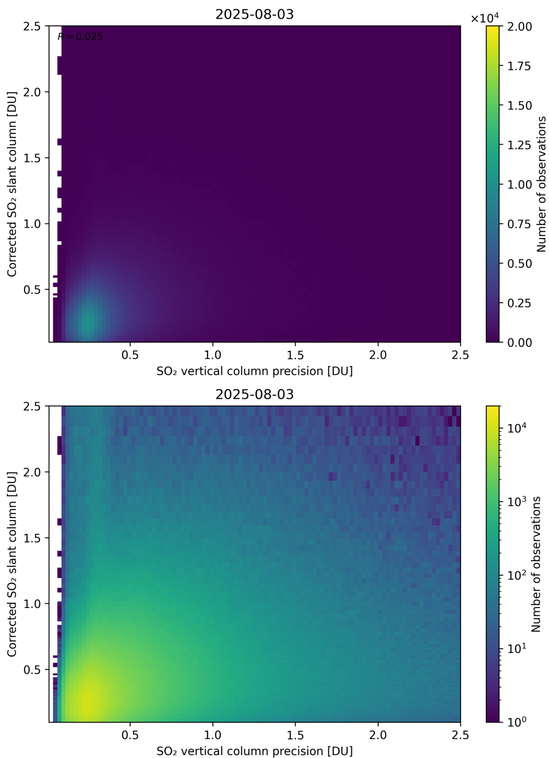
Figure 338: Scatter density plot of “SO 2 vertical column precision” against “Corrected SO 2 slant column” for 2025-08-03 to 2025-08-04.
