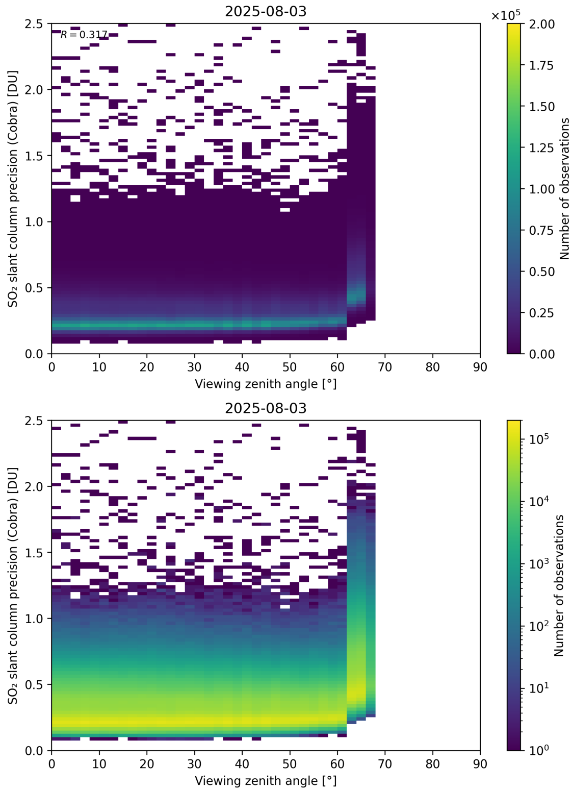
Figure 372: Scatter density plot of “Viewing zenith angle” against “SO 2 slant column precision (Cobra)” for 2025-08-03 to 2025-08-04.
