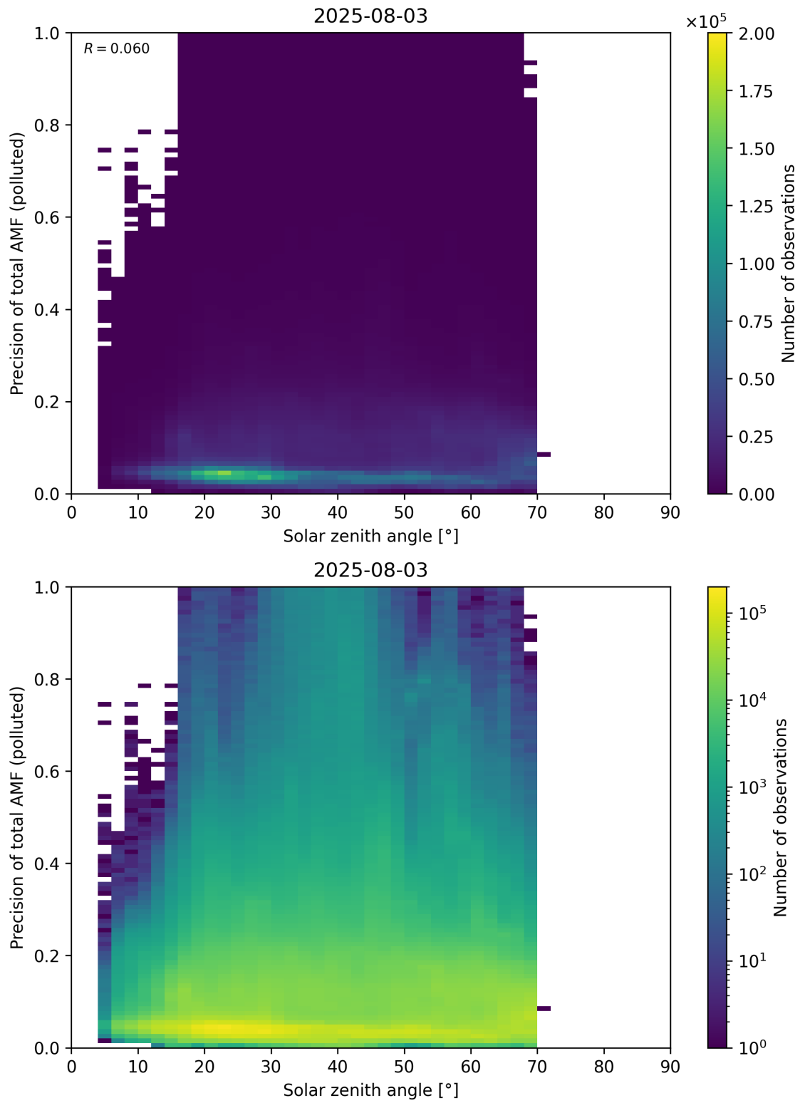
Figure 190: Scatter density plot of “Solar zenith angle” against “Precision of total AMF (polluted)” for 2025-08-03 to 2025-08-04.
