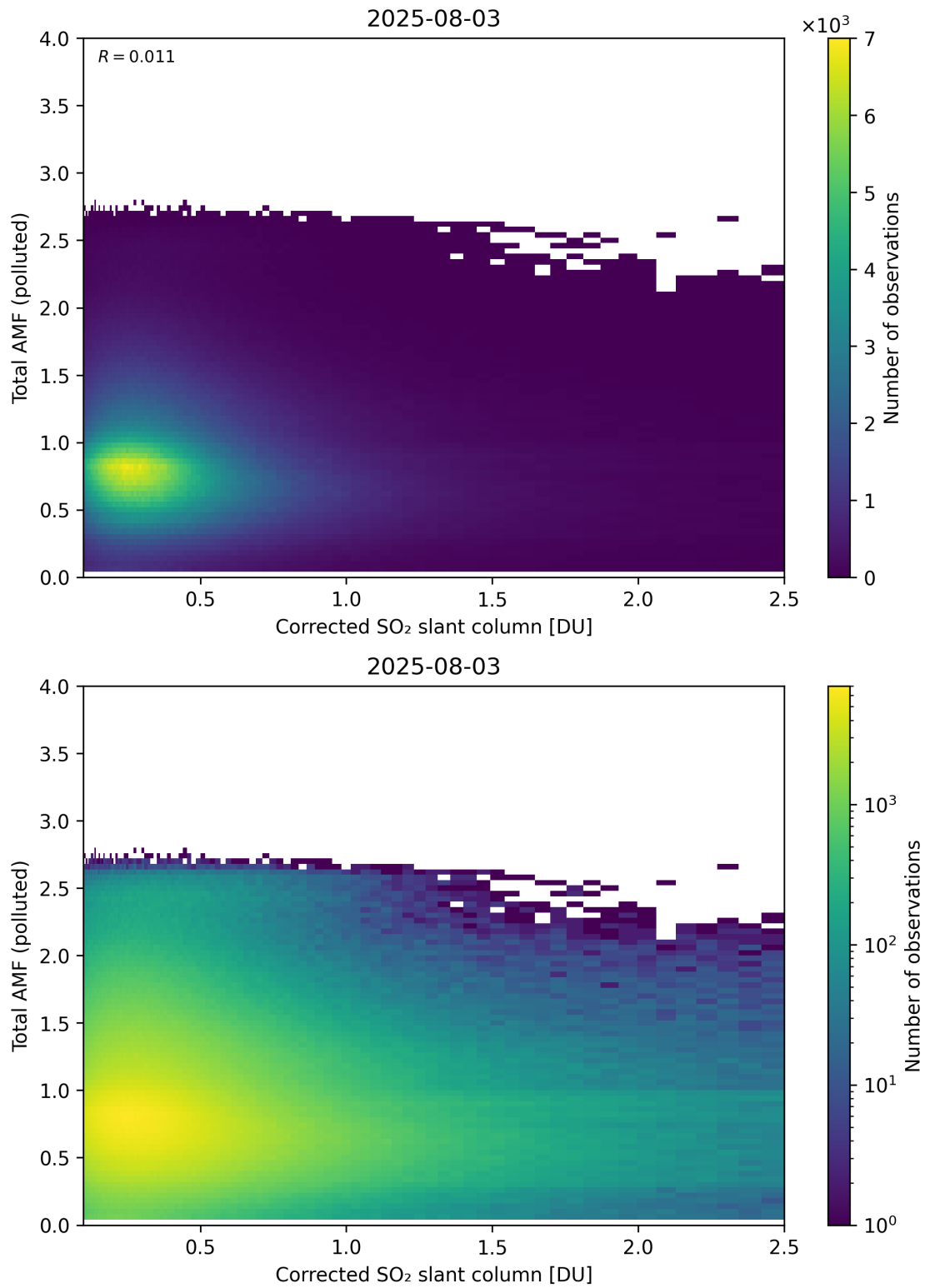
Figure 242: Scatter density plot of “Corrected SO 2 slant column” against “Total AMF (polluted)” for 2025-08-03 to 2025-08-04.
