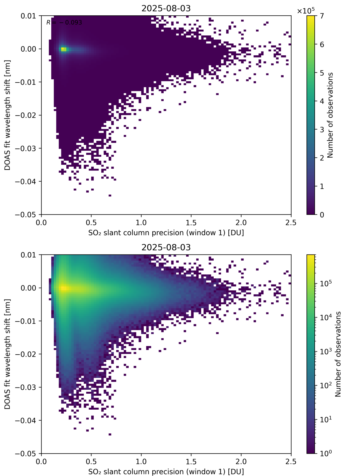
Figure 271: Scatter density plot of “SO 2 slant column precision (window 1)” against “DOAS fit wavelength shift” for 2025-08-03 to 2025-08-04.
