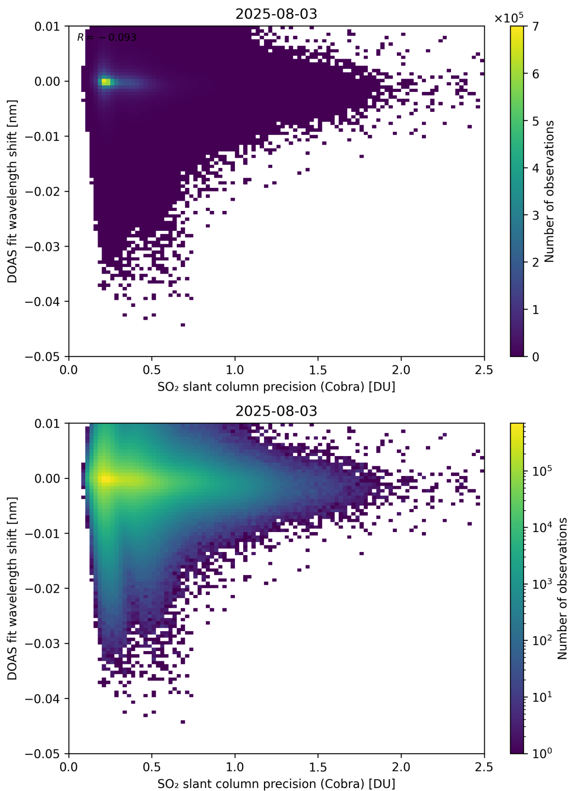
Figure 202: Scatter density plot of “SO 2 slant column precision (Cobra)” against “DOAS fit wavelength shift” for 2025-08-03 to 2025-08-04.
