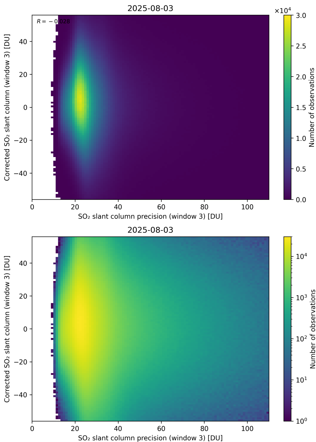
Figure 312: Scatter density plot of “SO 2 slant column precision (window 3)” against “Corrected SO 2 slant column (window 3)” for 2025-08-03 to 2025-08-04.
