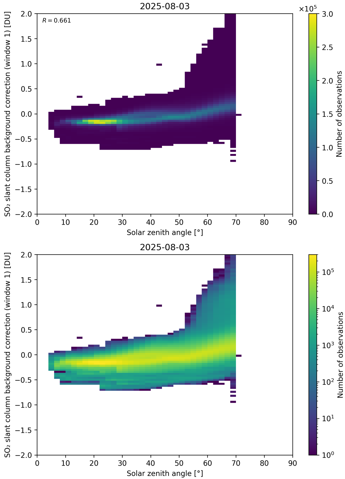
Figure 171: Scatter density plot of “Solar zenith angle” against “SO 2 slant column background correction (window 1)” for 2025-08-03 to 2025-08-04.
