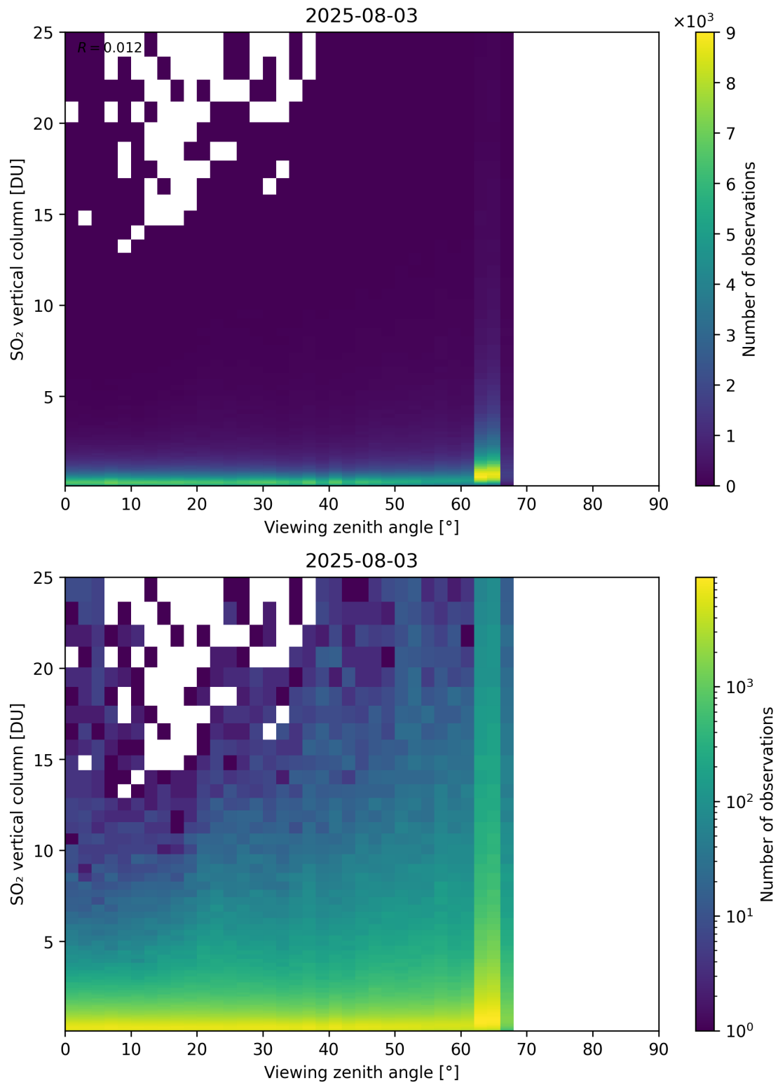
Figure 383: Scatter density plot of “Viewing zenith angle” against “SO 2 vertical column” for 2025-08-03 to 2025-08-04.
