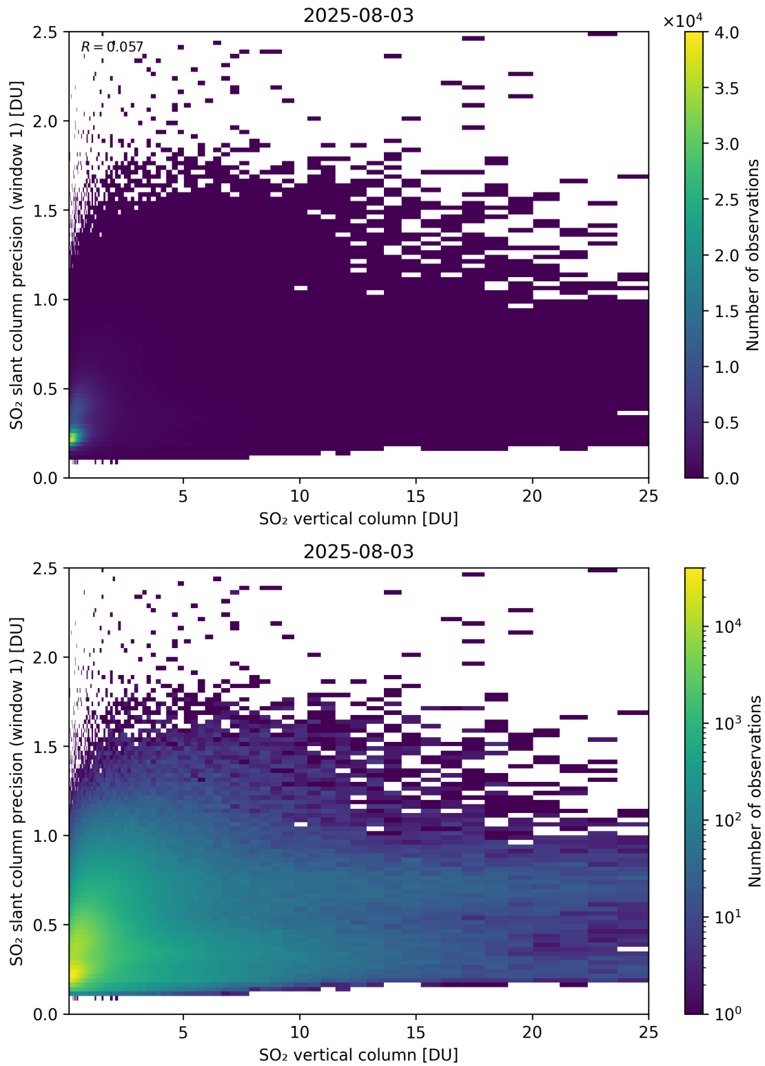
Figure 355: Scatter density plot of “SO 2 vertical column” against “SO 2 slant column precision (window 1)” for 2025-08-03 to 2025-08-04.
