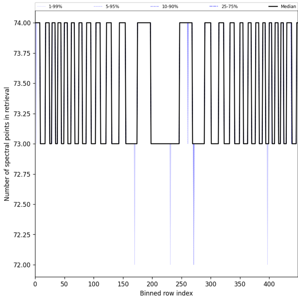
Figure 108: Along track statistics of “Number of spectral points in retrieval” for 2025-08-03 to 2025-08-04
