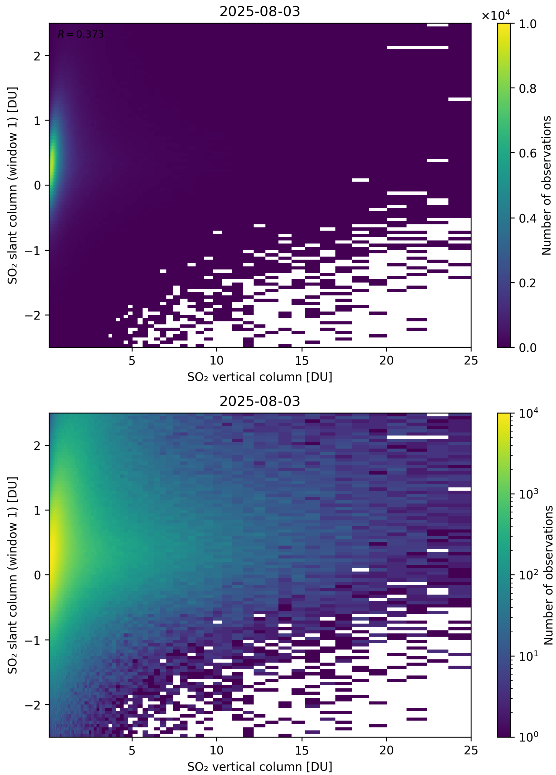
Figure 354: Scatter density plot of “SO 2 vertical column” against “SO 2 slant column (window 1)” for 2025-08-03 to 2025-08-04.
