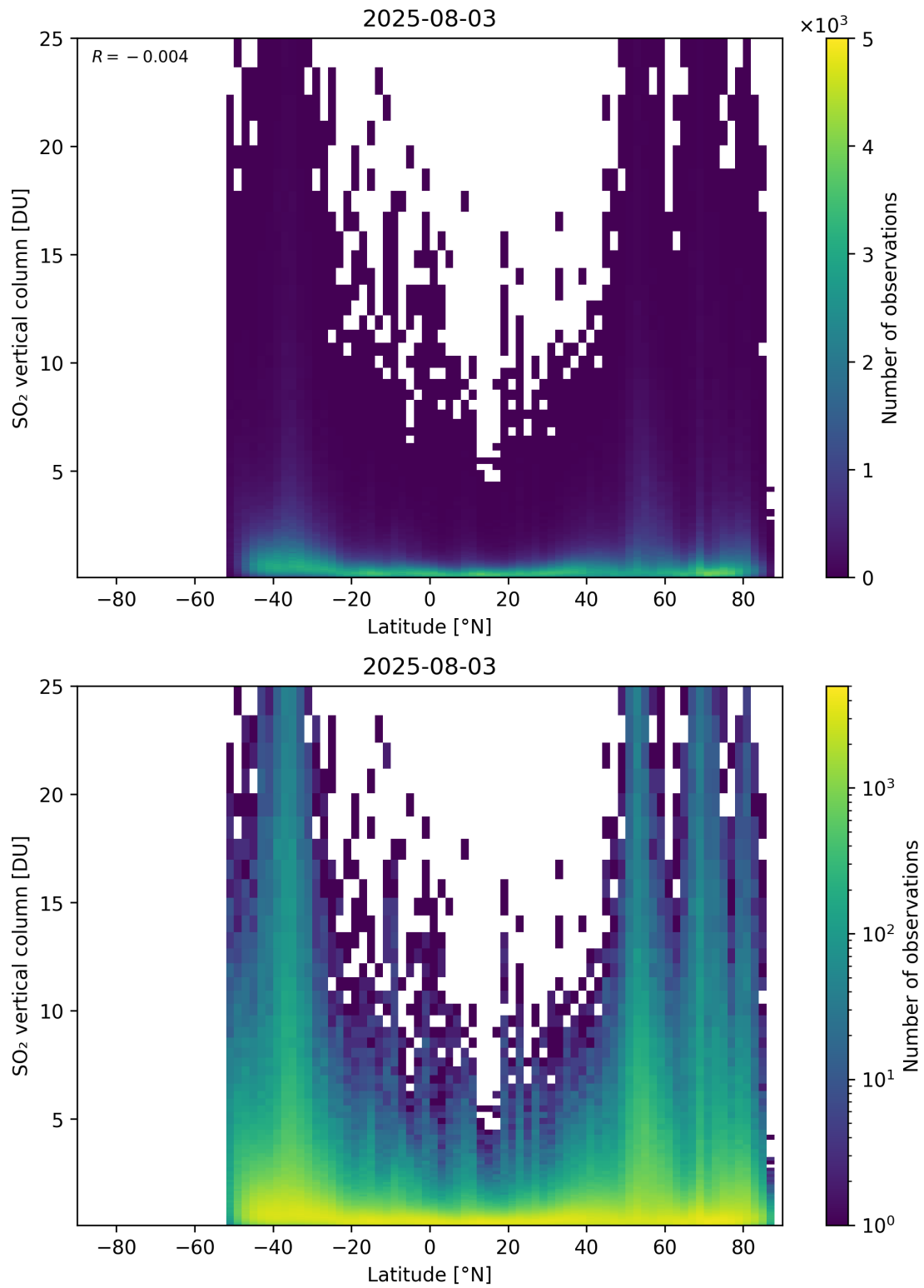
Figure 169: Scatter density plot of “Latitude” against “SO 2 vertical column” for 2025-08-03 to 2025-08-04.
