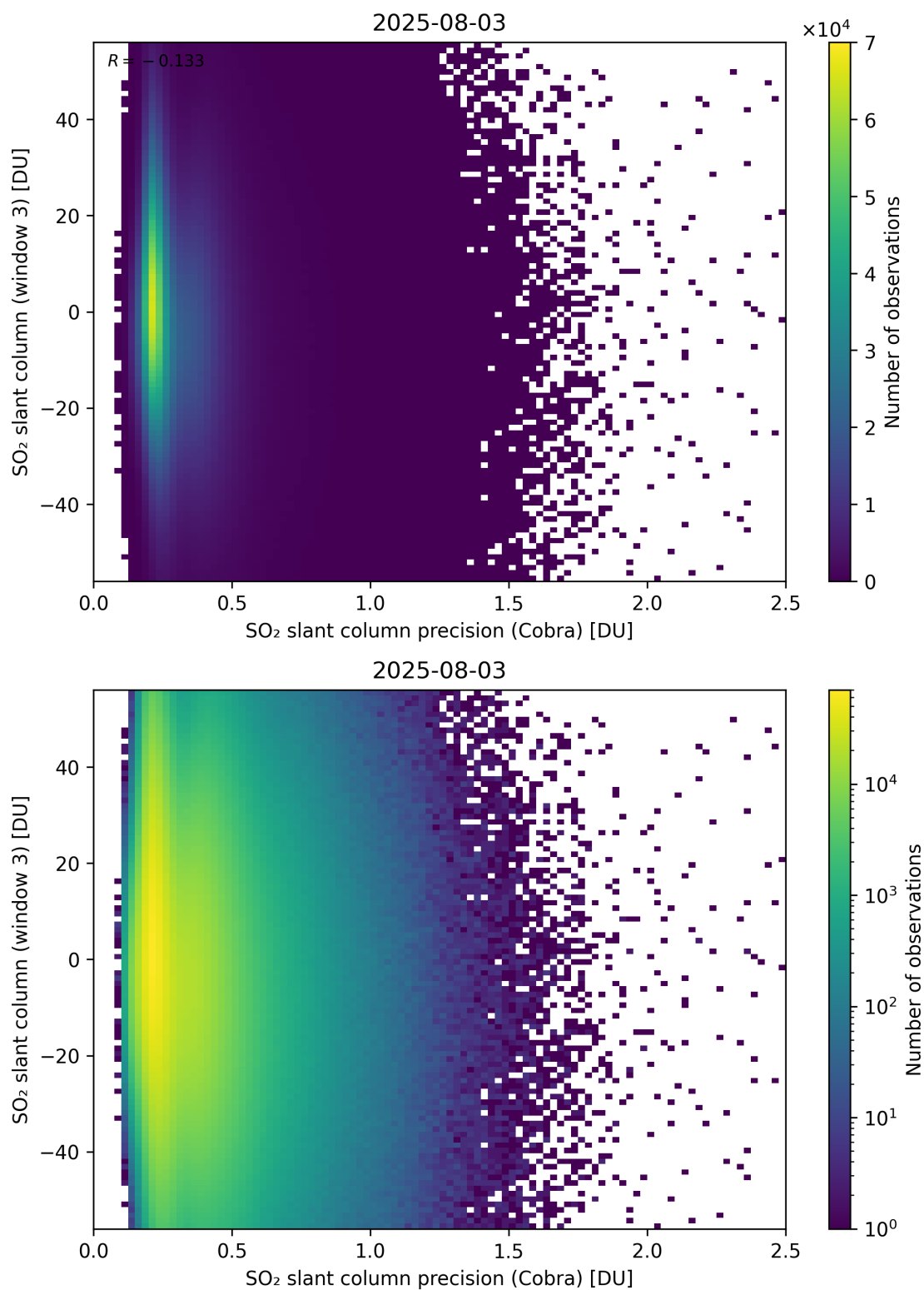
Figure 211: Scatter density plot of “SO 2 slant column precision (Cobra)” against “SO 2 slant column (window 3)” for 2025-08-03 to 2025-08-04.
