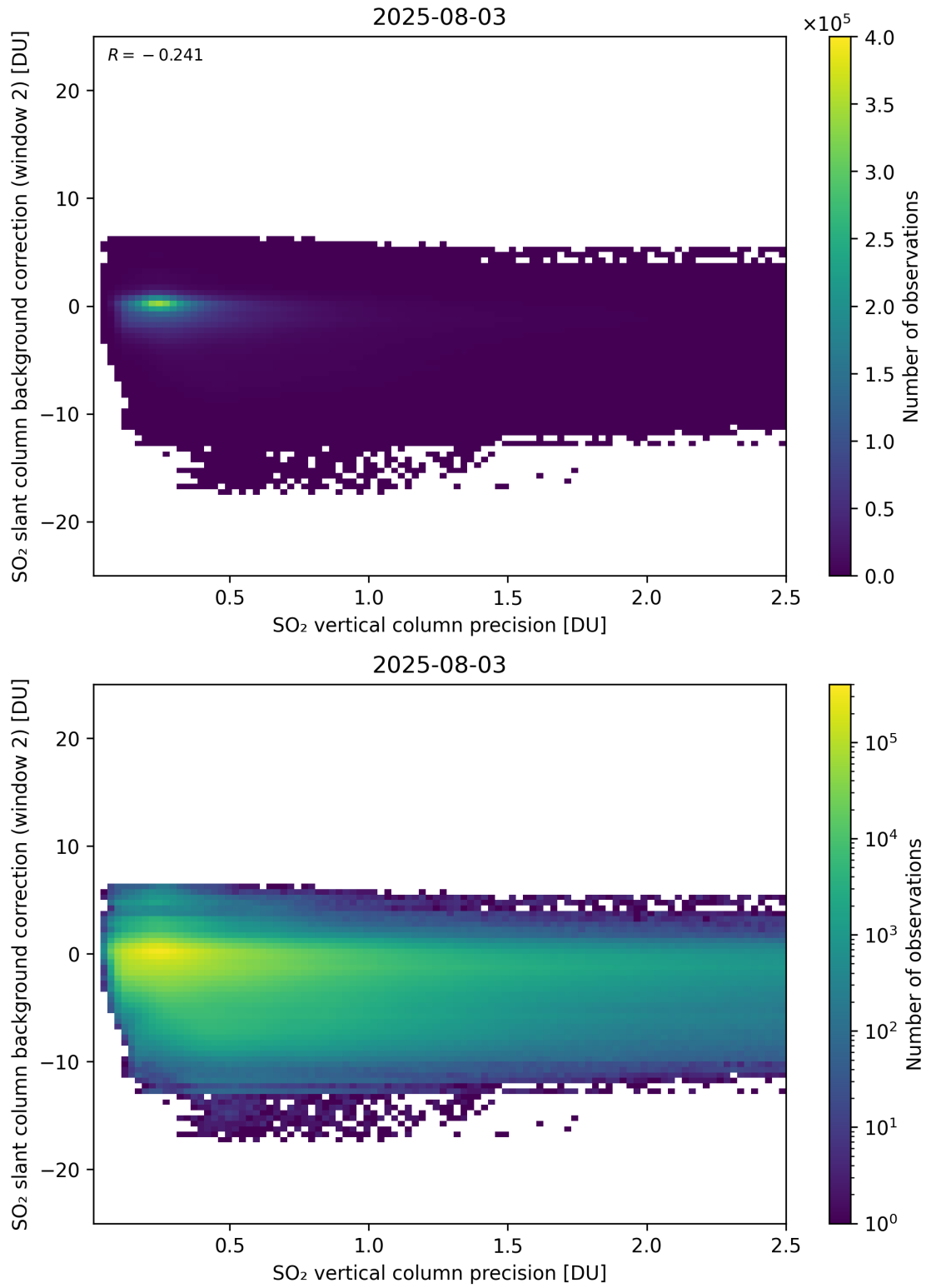
Figure 330: Scatter density plot of “SO 2 vertical column precision” against “SO 2 slant column background correction (window 2)” for 2025-08-03 to 2025-08-04.
