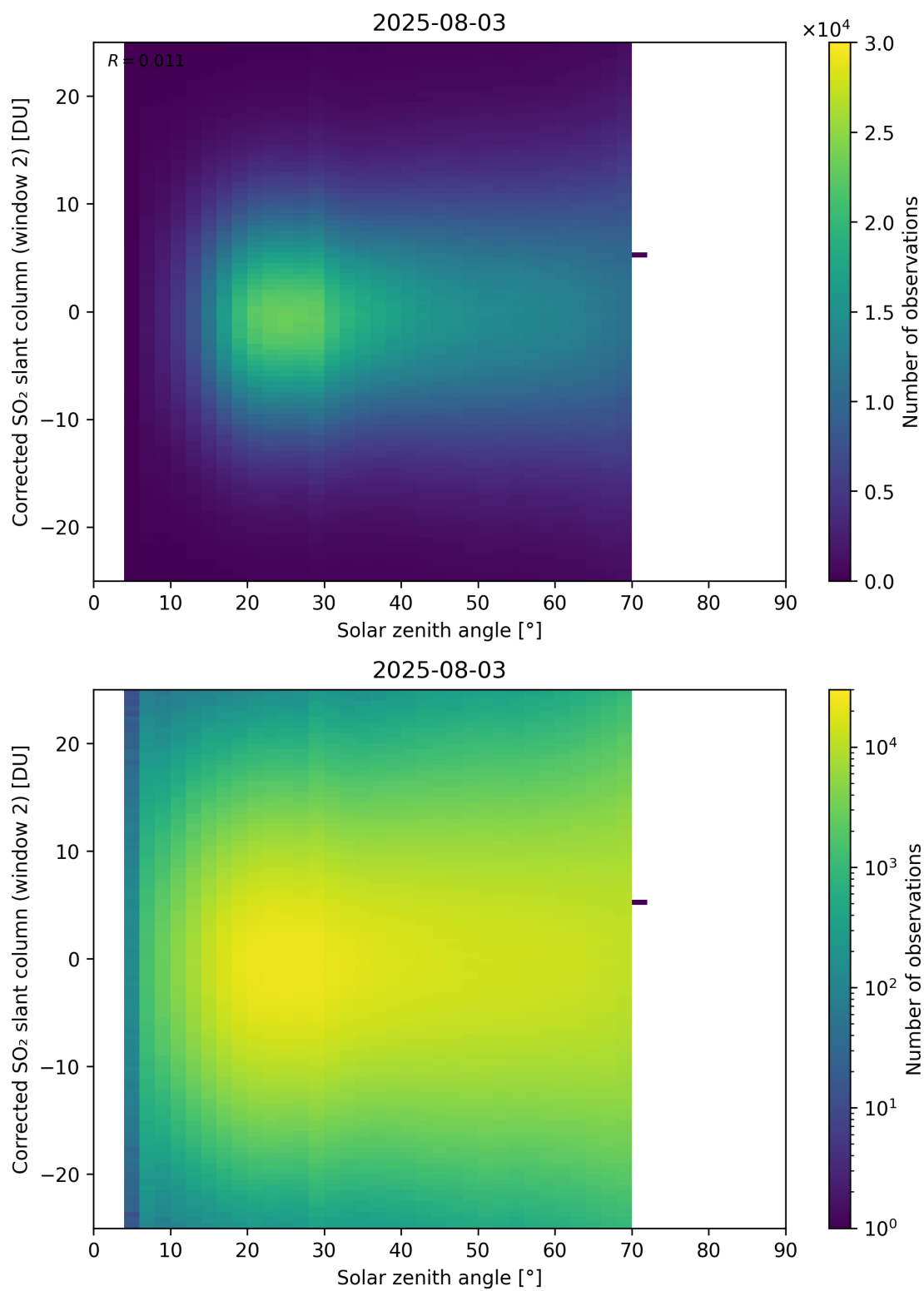
Figure 182: Scatter density plot of “Solar zenith angle” against “Corrected SO 2 slant column (window 2)” for 2025-08-03 to 2025-08-04.
