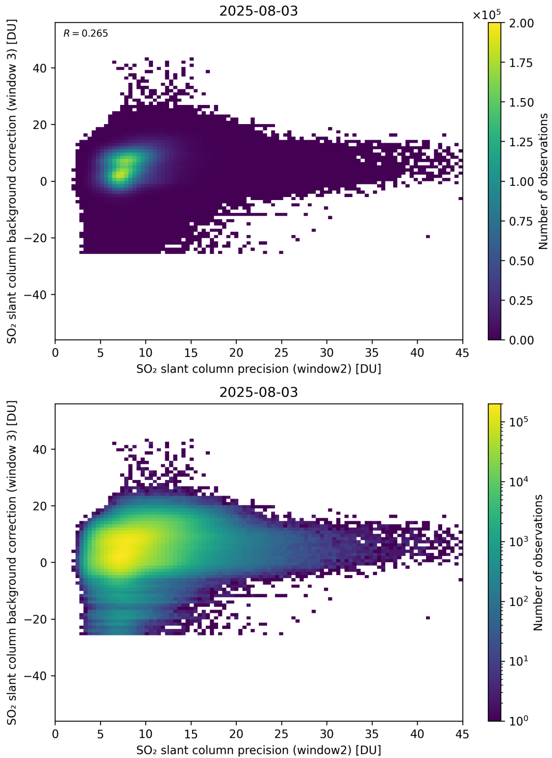
Figure 292: Scatter density plot of “SO 2 slant column precision (window2)” against “SO 2 slant column background correction (window 3)” for 2025-08-03 to 2025-08-04.
