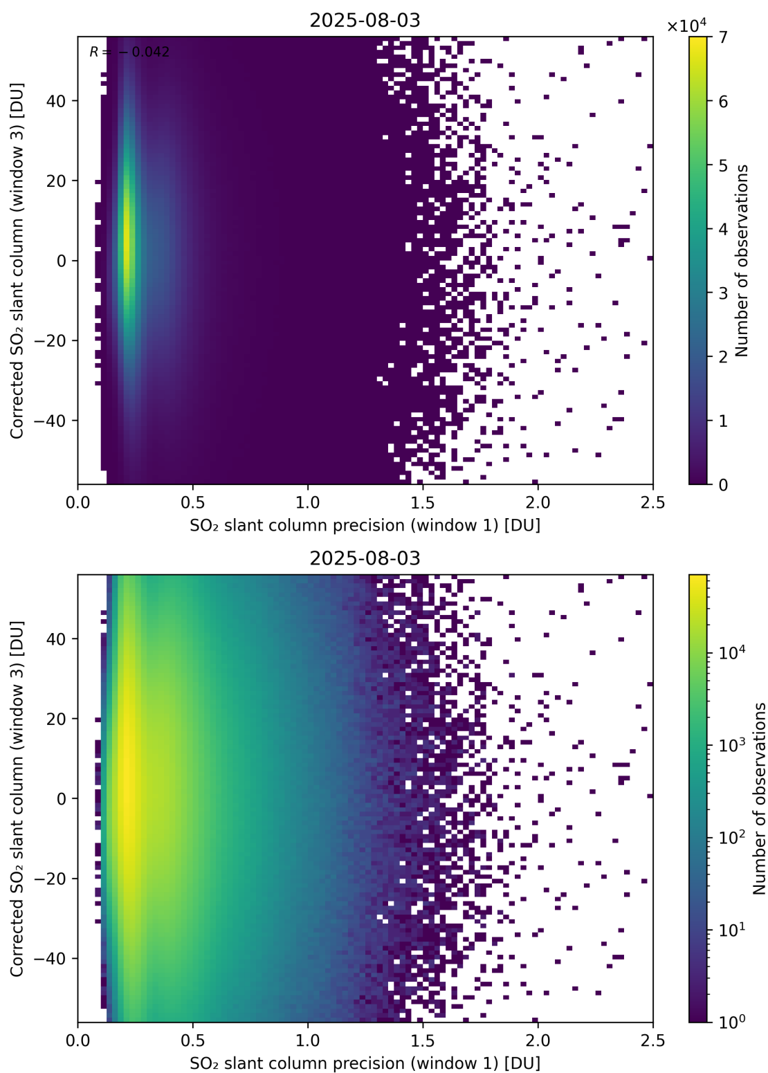
Figure 276: Scatter density plot of “SO 2 slant column precision (window 1)” against “Corrected SO 2 slant column (window 3)” for 2025-08-03 to 2025-08-04.
