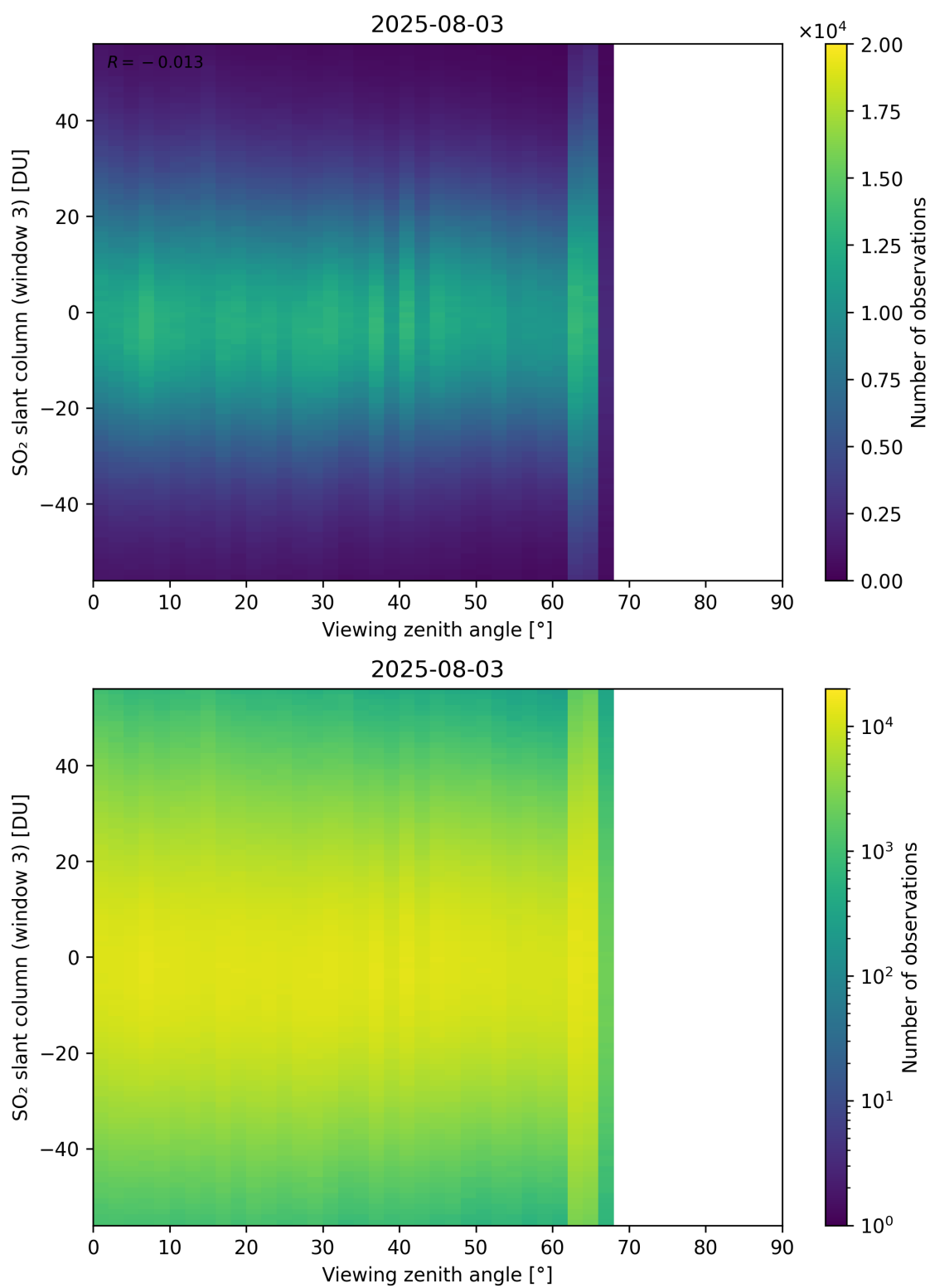
Figure 379: Scatter density plot of “Viewing zenith angle” against “SO 2 slant column (window 3)” for 2025-08-03 to 2025-08-04.
