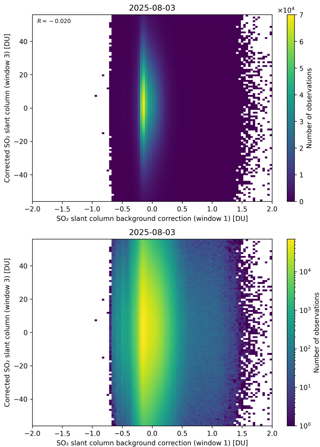
Figure 116: Scatter density plot of “SO 2 slant column background correction (window 1)” against “Corrected SO 2 slant column (window 3)” for 2025-08-03 to 2025-08-04.
