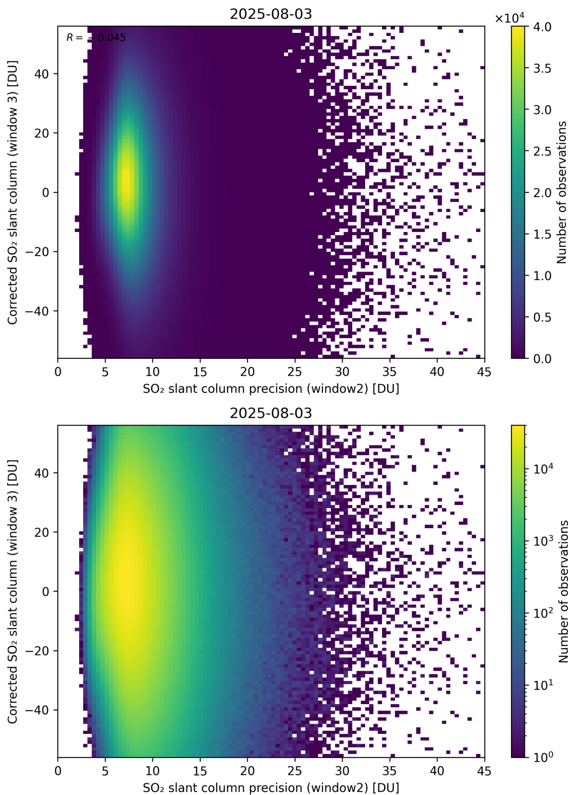
Figure 298: Scatter density plot of “SO 2 slant column precision (window2)” against “Corrected SO 2 slant column (window 3)” for 2025-08-03 to 2025-08-04.
