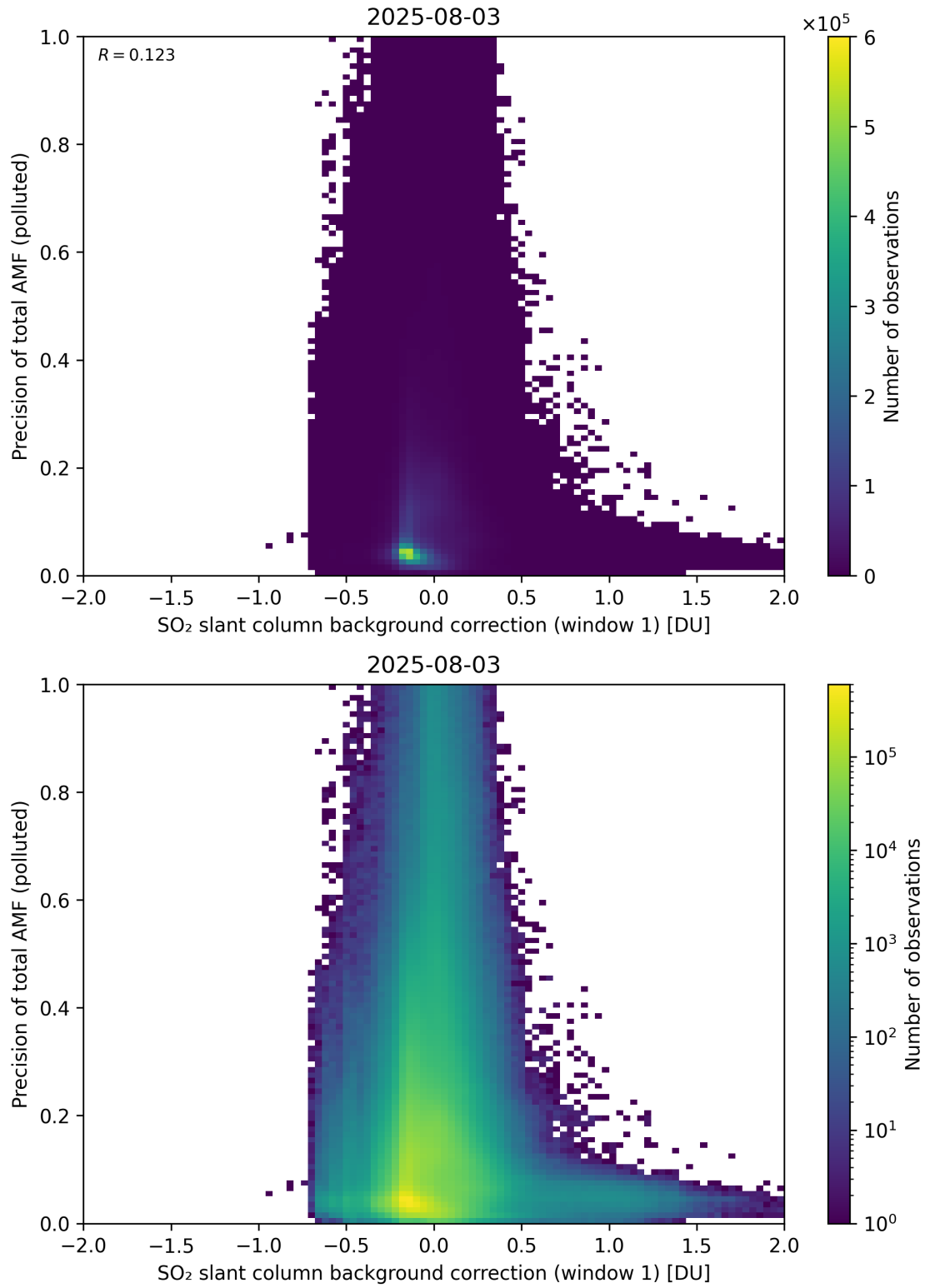
Figure 121: Scatter density plot of “SO 2 slant column background correction (window 1)” against “Precision of total AMF (polluted)” for 2025-08-03 to 2025-08-04.
