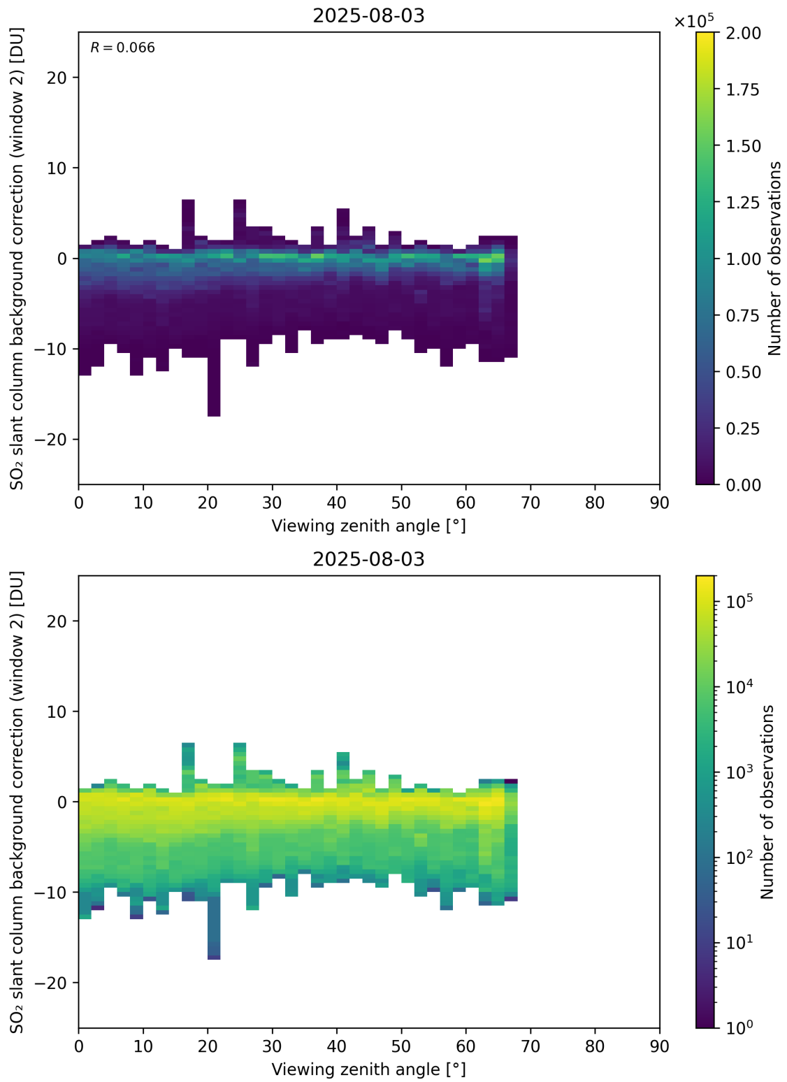
Figure 363: Scatter density plot of “Viewing zenith angle” against “SO 2 slant column background correction (window 2)” for 2025-08-03 to 2025-08-04.
