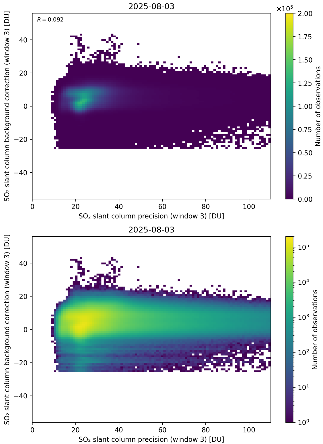
Figure 307: Scatter density plot of “SO 2 slant column precision (window 3)” against “SO 2 slant column background correction (window 3)” for 2025-08-03 to 2025-08-04.
