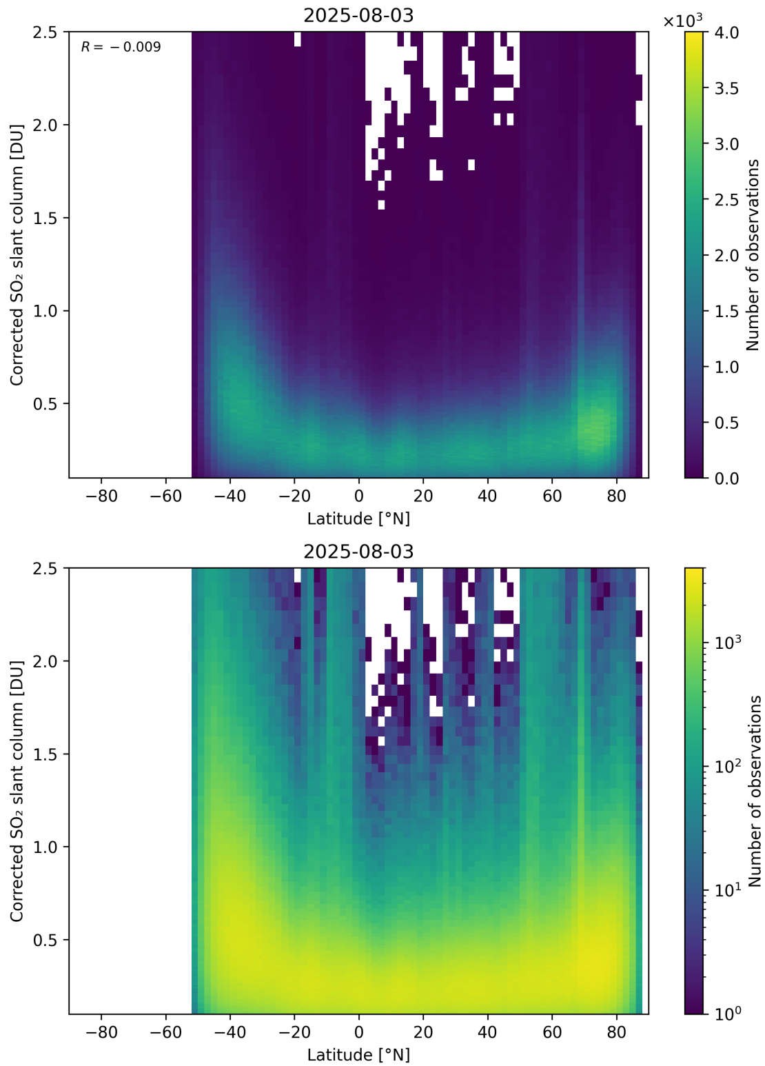
Figure 159: Scatter density plot of “Latitude” against “Corrected SO 2 slant column” for 2025-08-03 to 2025-08-04.
