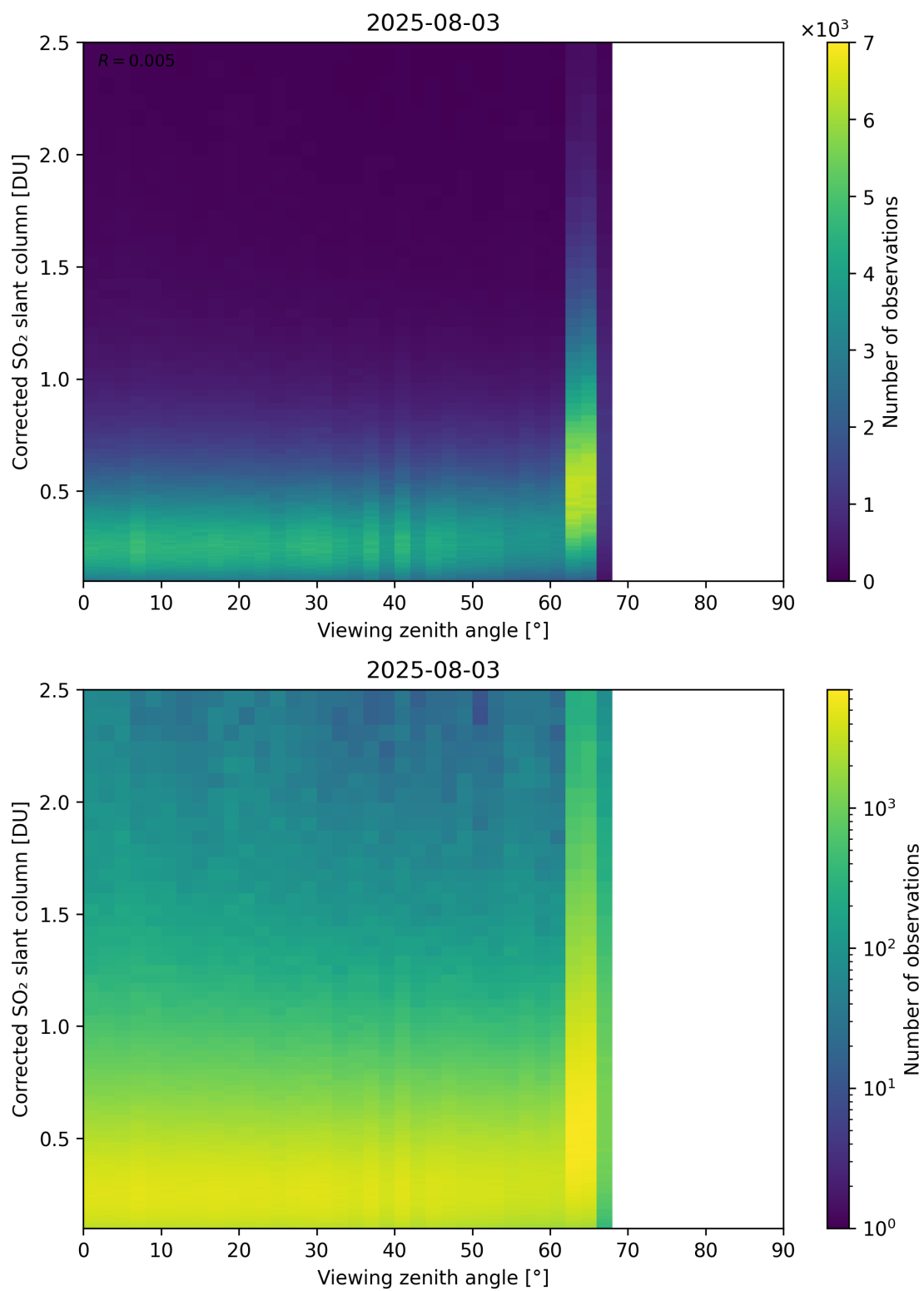
Figure 373: Scatter density plot of “Viewing zenith angle” against “Corrected SO 2 slant column” for 2025-08-03 to 2025-08-04.
