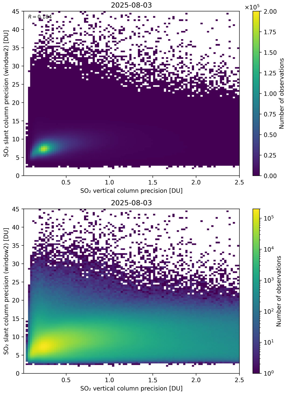
Figure 343: Scatter density plot of “SO 2 vertical column precision” against “SO 2 slant column precision (window2)” for 2025-08-03 to 2025-08-04.
