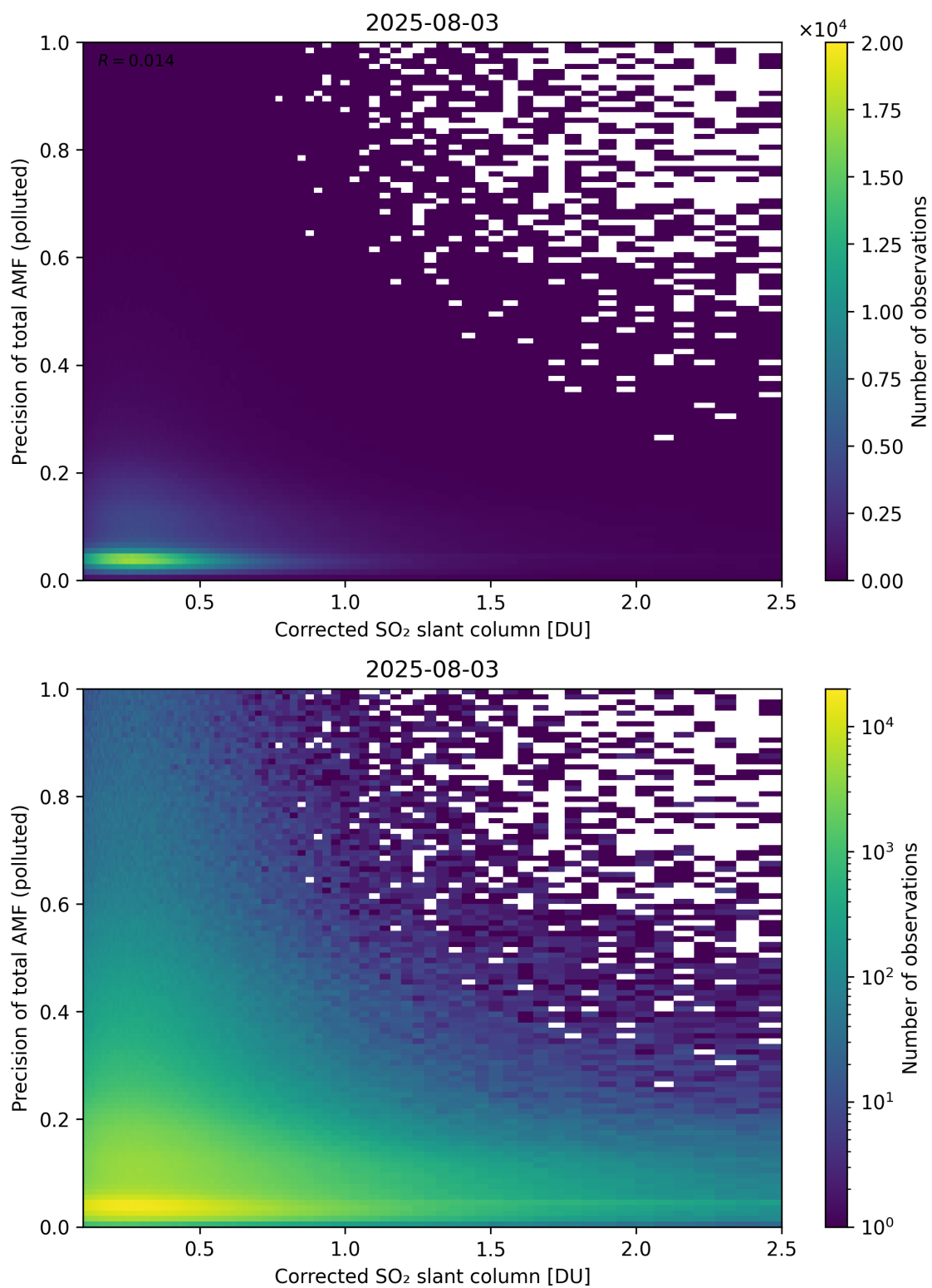
Figure 243: Scatter density plot of “Corrected SO 2 slant column” against “Precision of total AMF (polluted)” for 2025-08-03 to 2025-08-04.
