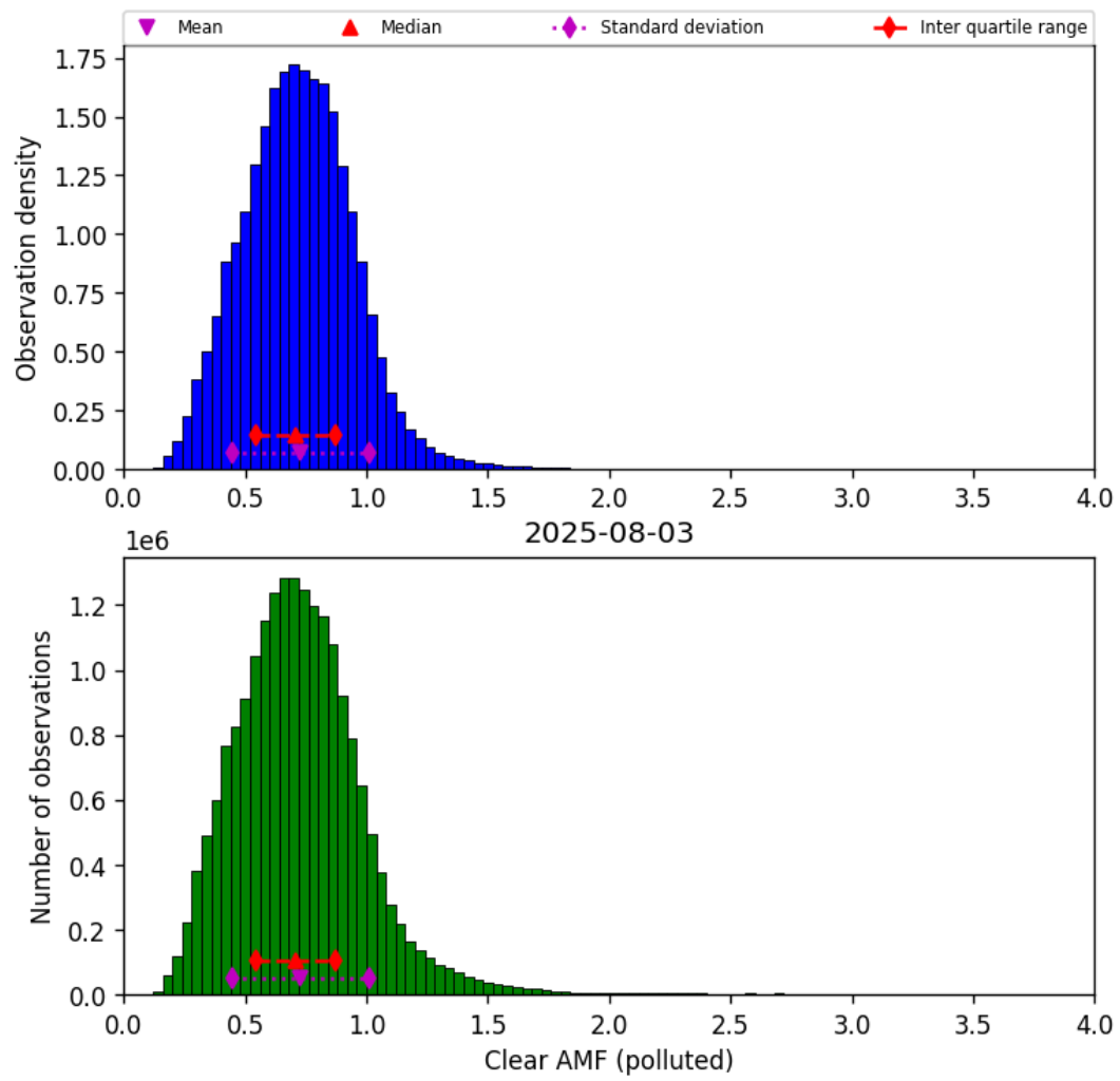
Figure 81: Histogram of “Clear AMF (polluted)” for 2025-08-03 to 2025-08-04
