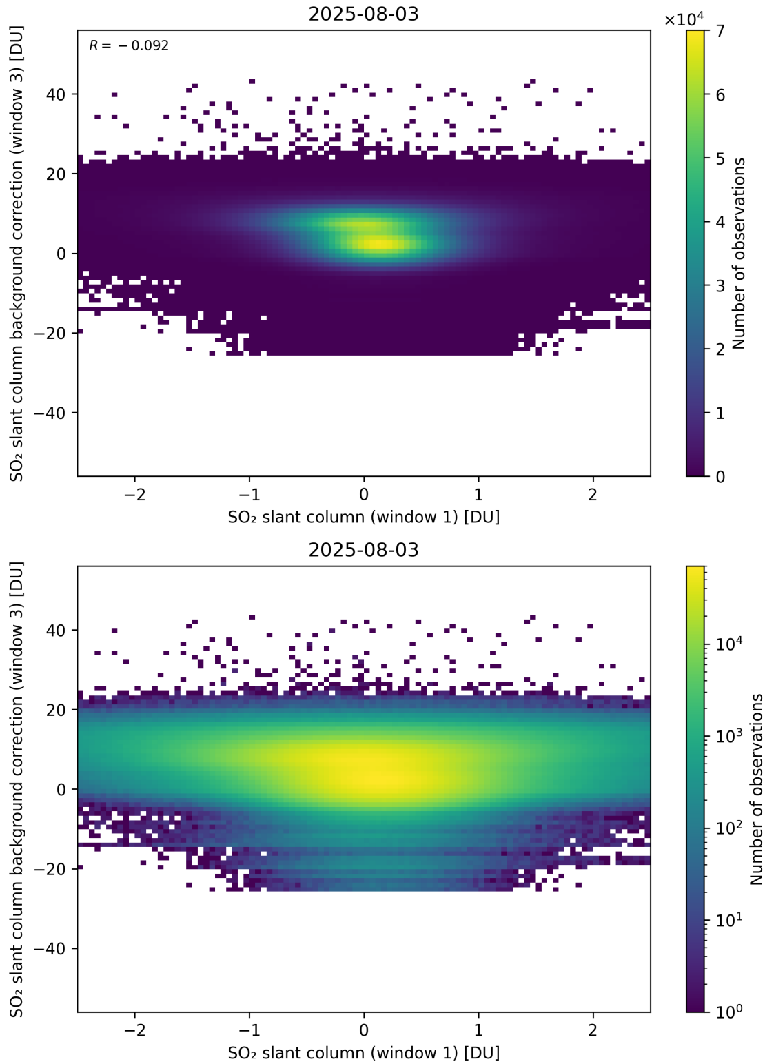
Figure 264: Scatter density plot of “SO 2 slant column (window 1)” against “SO 2 slant column background correction (window 3)” for 2025-08-03 to 2025-08-04.
