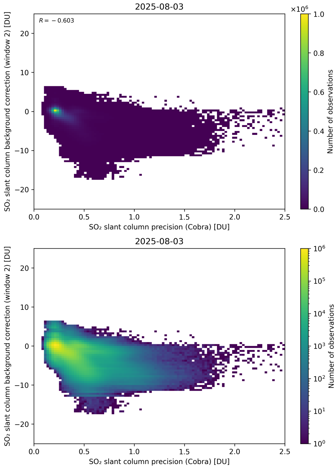
Figure 200: Scatter density plot of “SO 2 slant column precision (Cobra)” against “SO 2 slant column background correction (window 2)” for 2025-08-03 to 2025-08-04.
