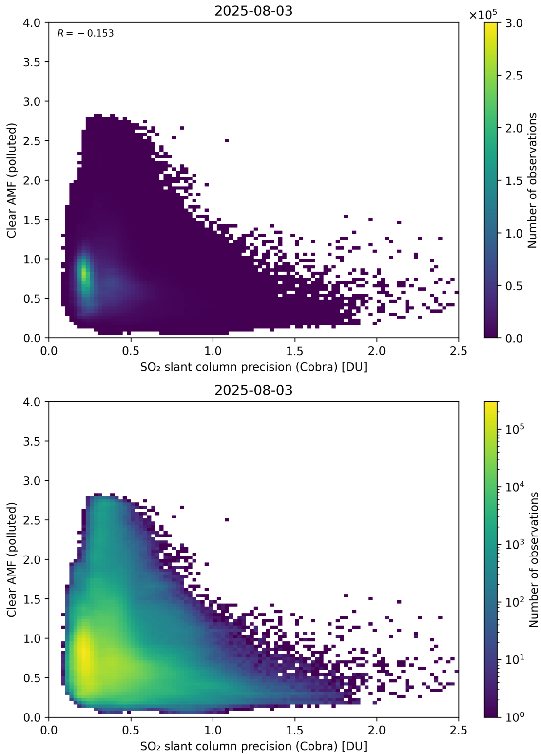
Figure 205: Scatter density plot of “SO 2 slant column precision (Cobra)” against “Clear AMF (polluted)” for 2025-08-03 to 2025-08-04.
