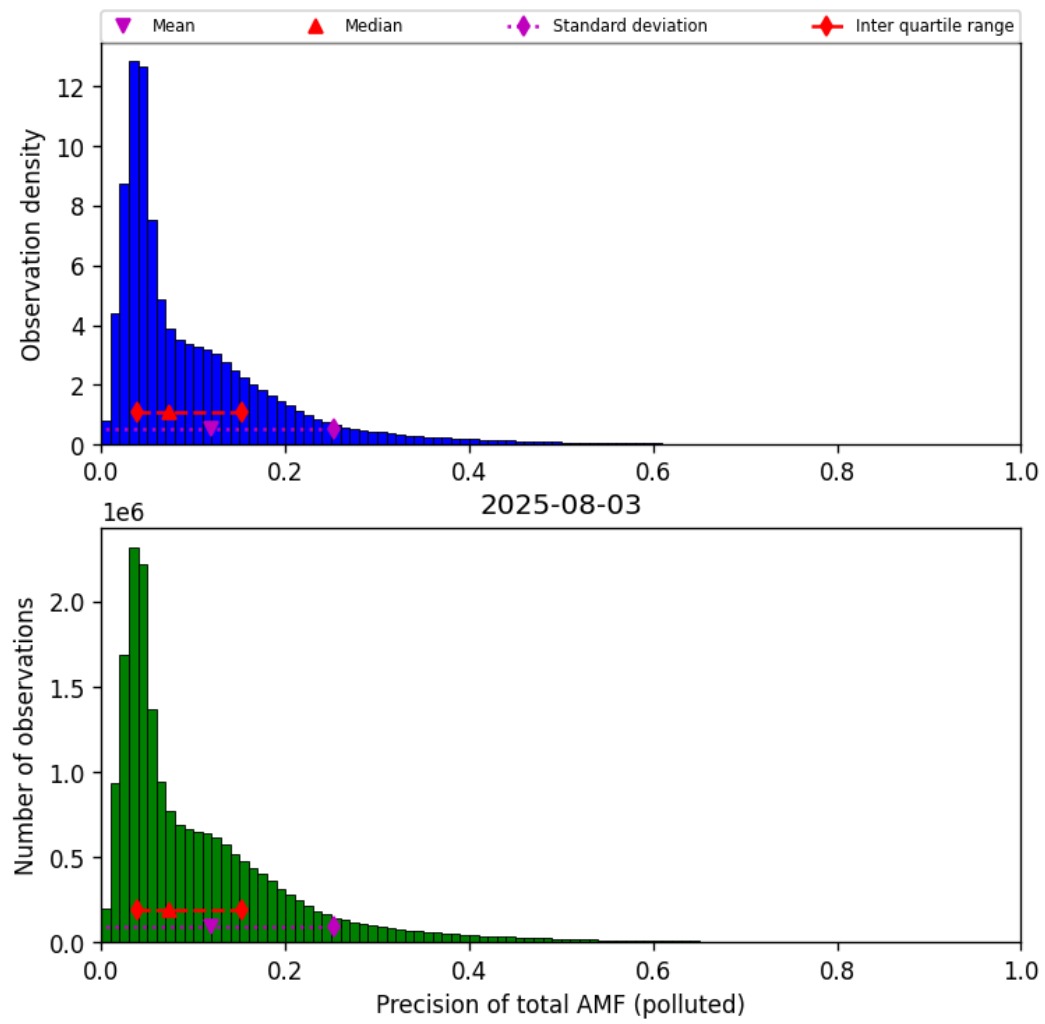
Figure 80: Histogram of “Precision of total AMF (polluted)” for 2025-08-03 to 2025-08-04
