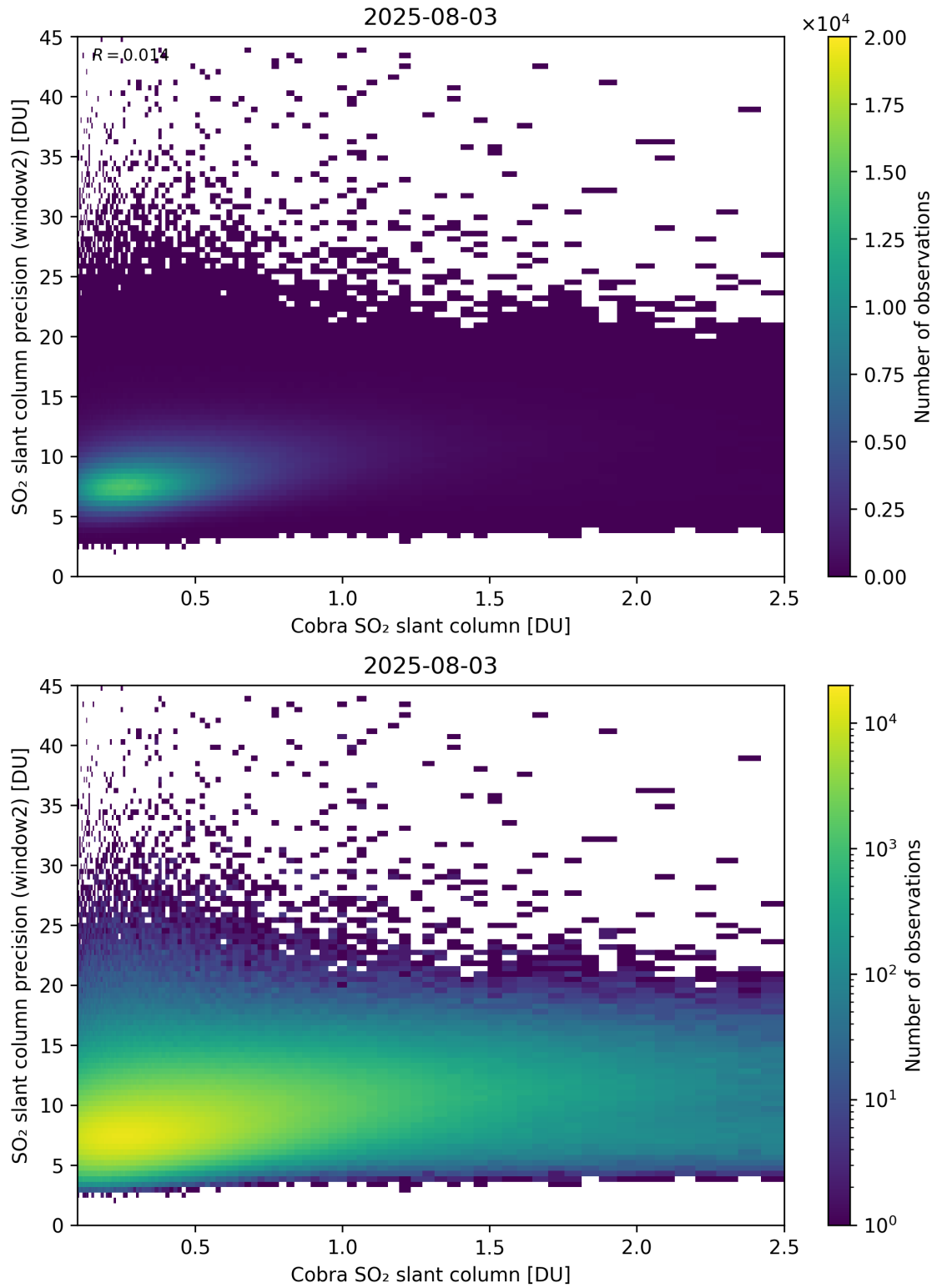
Figure 221: Scatter density plot of “Cobra SO 2 slant column” against “SO 2 slant column precision (window2)” for 2025-08-03 to 2025-08-04.
