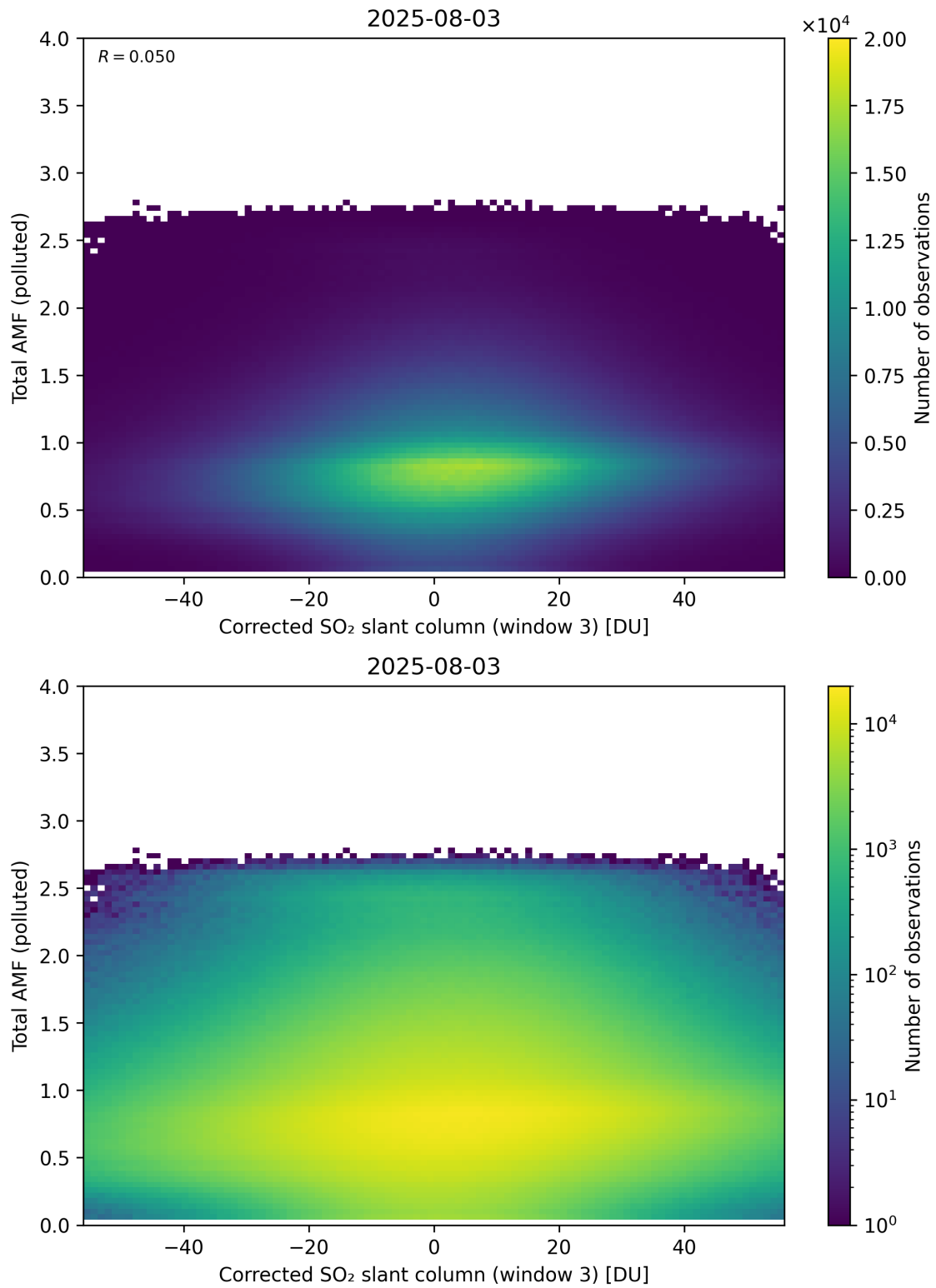
Figure 260: Scatter density plot of “Corrected SO 2 slant column (window 3)” against “Total AMF (polluted)” for 2025-08-03 to 2025-08-04.
