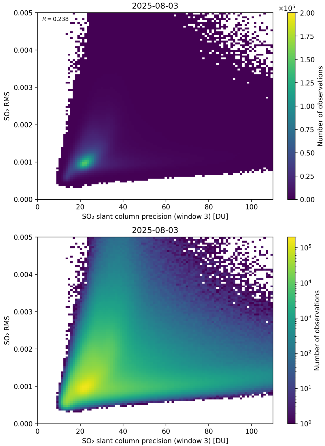
Figure 310: Scatter density plot of “SO 2 slant column precision (window 3)” against “SO 2 RMS” for 2025-08-03 to 2025-08-04.
