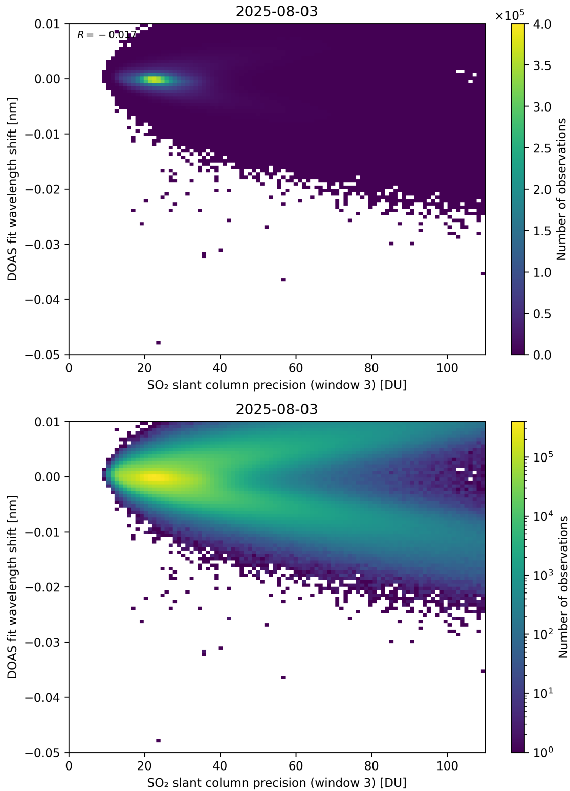
Figure 308: Scatter density plot of “SO 2 slant column precision (window 3)” against “DOAS fit wavelength shift” for 2025-08-03 to 2025-08-04.
