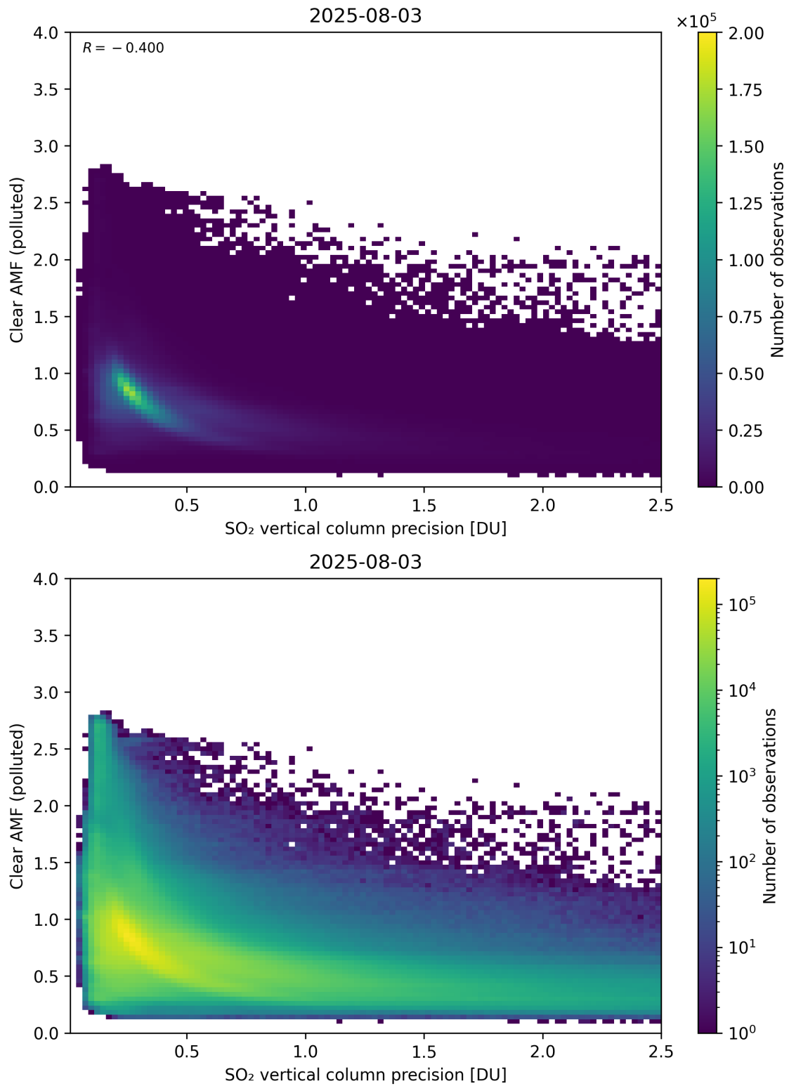
Figure 335: Scatter density plot of “SO 2 vertical column precision” against “Clear AMF (polluted)” for 2025-08-03 to 2025-08-04.
