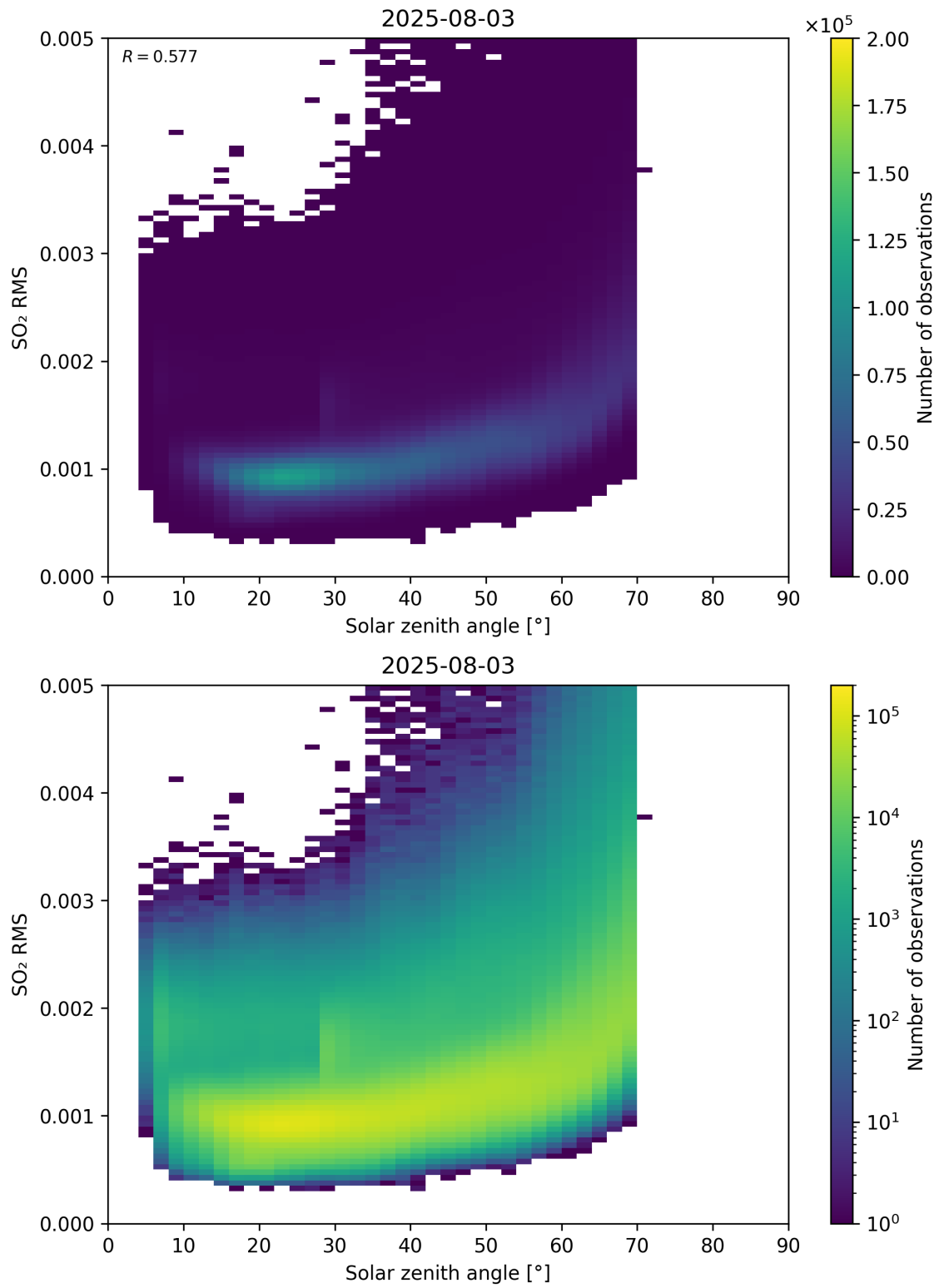
Figure 176: Scatter density plot of “Solar zenith angle” against “SO 2 RMS” for 2025-08-03 to 2025-08-04.
