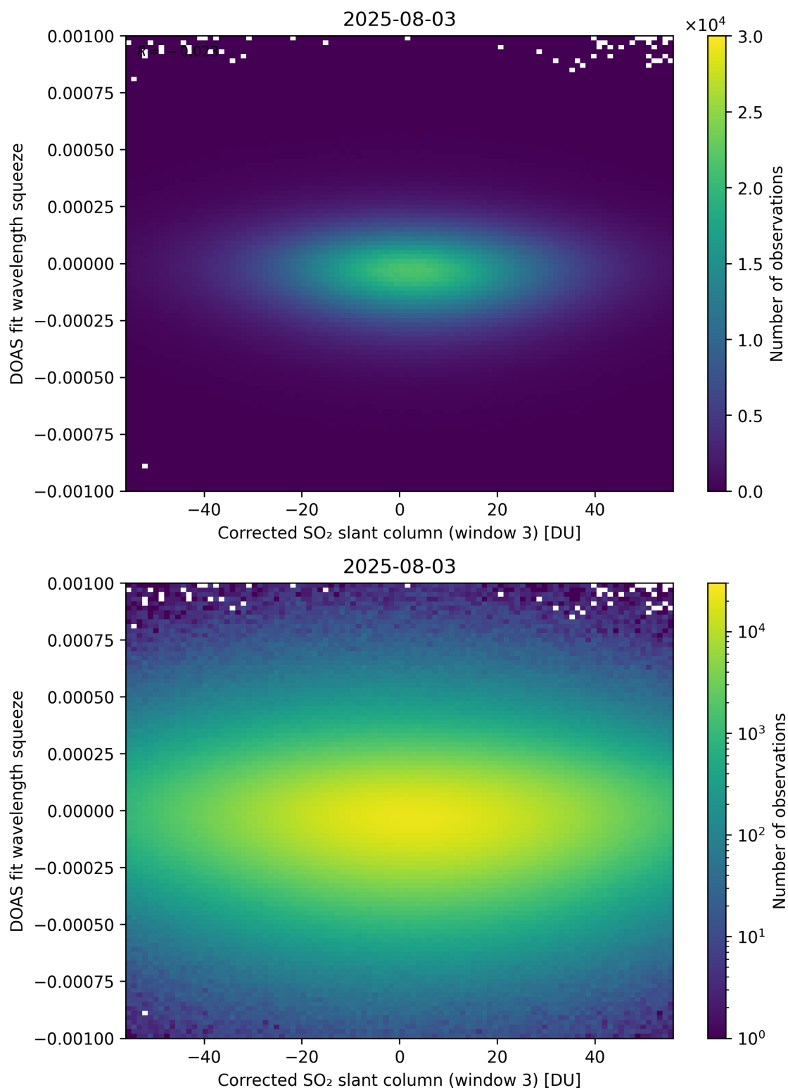
Figure 257: Scatter density plot of “Corrected SO 2 slant column (window 3)” against “DOAS fit wavelength squeeze” for 2025-08-03 to 2025-08-04.
