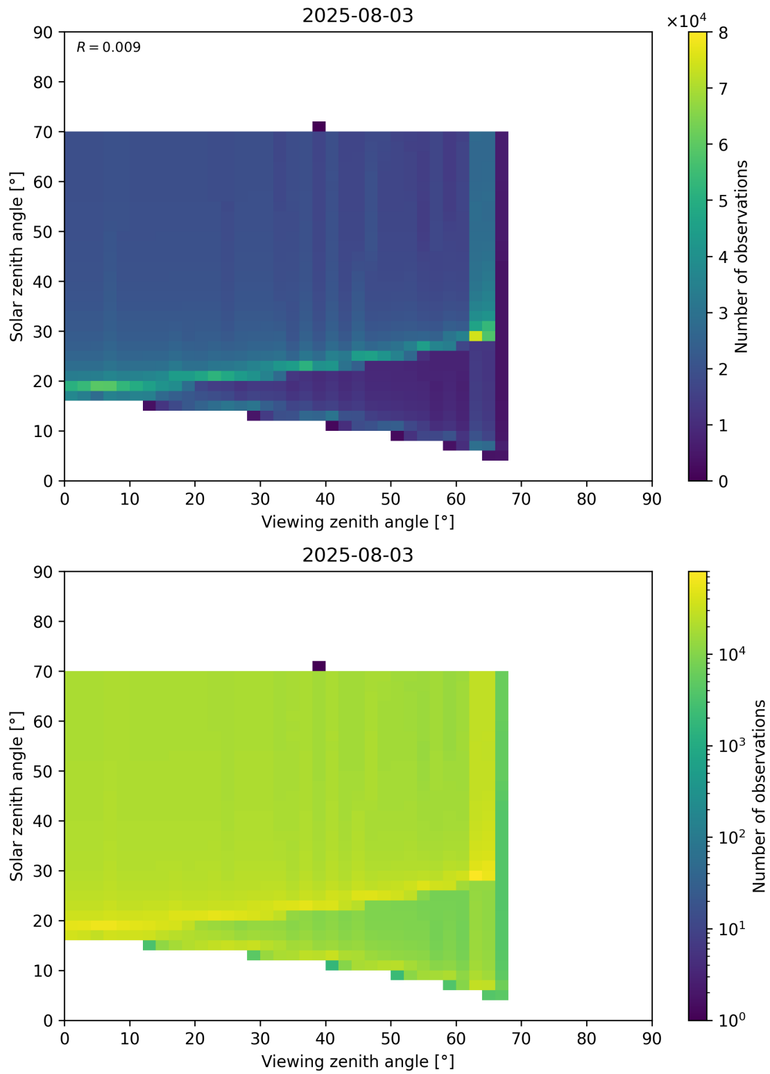
Figure 369: Scatter density plot of “Viewing zenith angle” against “Solar zenith angle” for 2025-08-03 to 2025-08-04.
