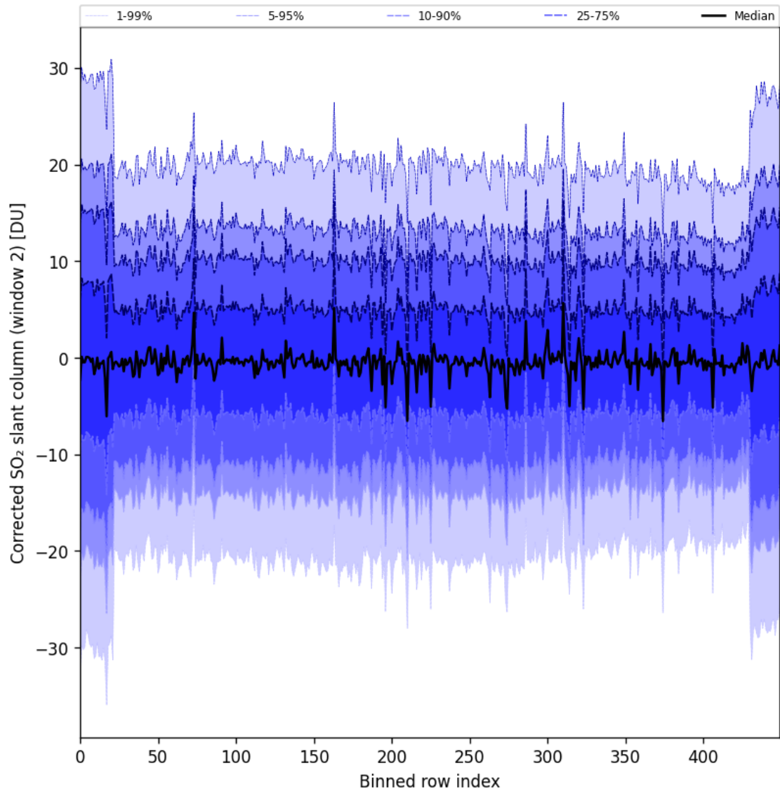
Figure 95: Along track statistics of “Corrected SO 2 slant column (window 2)” for 2025-08-03 to 2025-08-04
