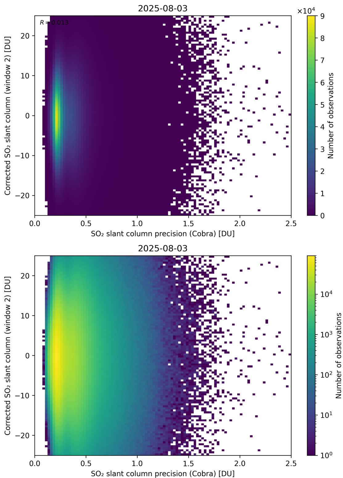
Figure 206: Scatter density plot of “SO 2 slant column precision (Cobra)” against “Corrected SO 2 slant column (window 2)” for 2025-08-03 to 2025-08-04.
