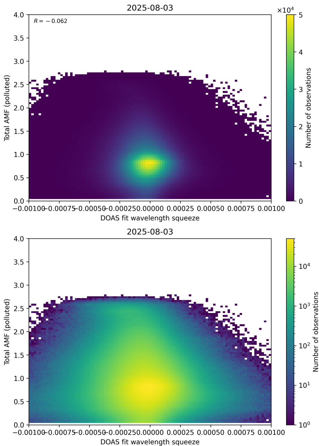
Figure 145: Scatter density plot of “DOAS fit wavelength squeeze” against “Total AMF (polluted)” for 2025-08-03 to 2025-08-04.
