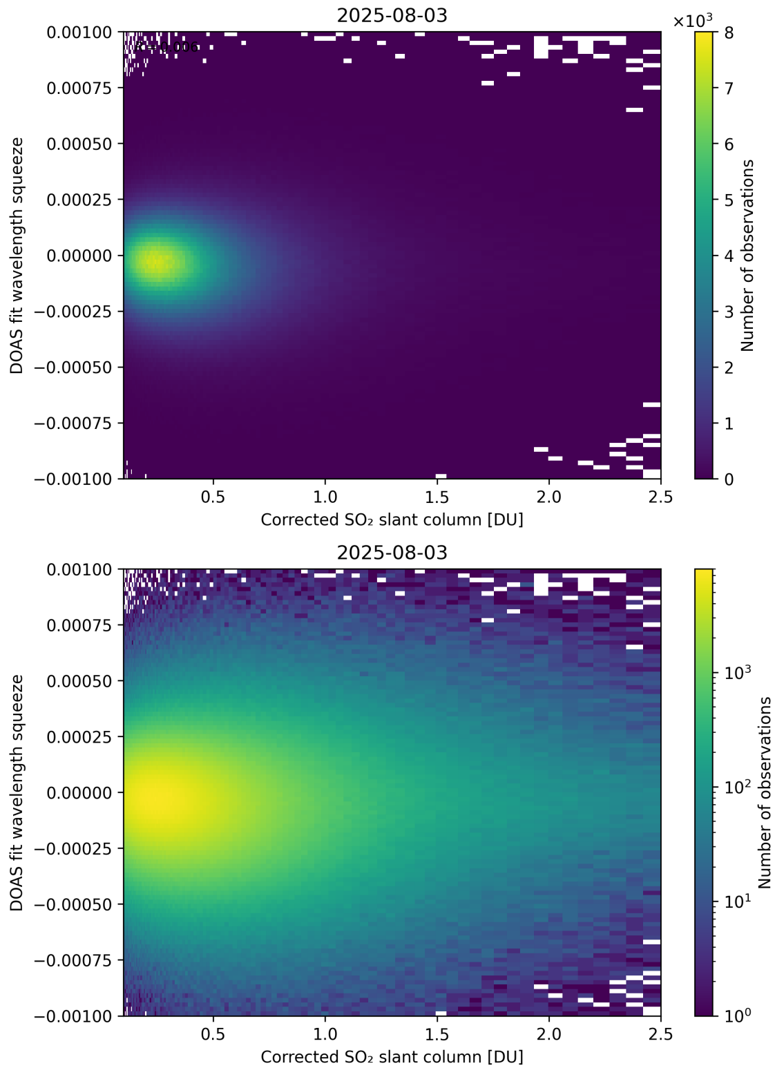
Figure 230: Scatter density plot of “Corrected SO 2 slant column” against “DOAS fit wavelength squeeze” for 2025-08-03 to 2025-08-04.
