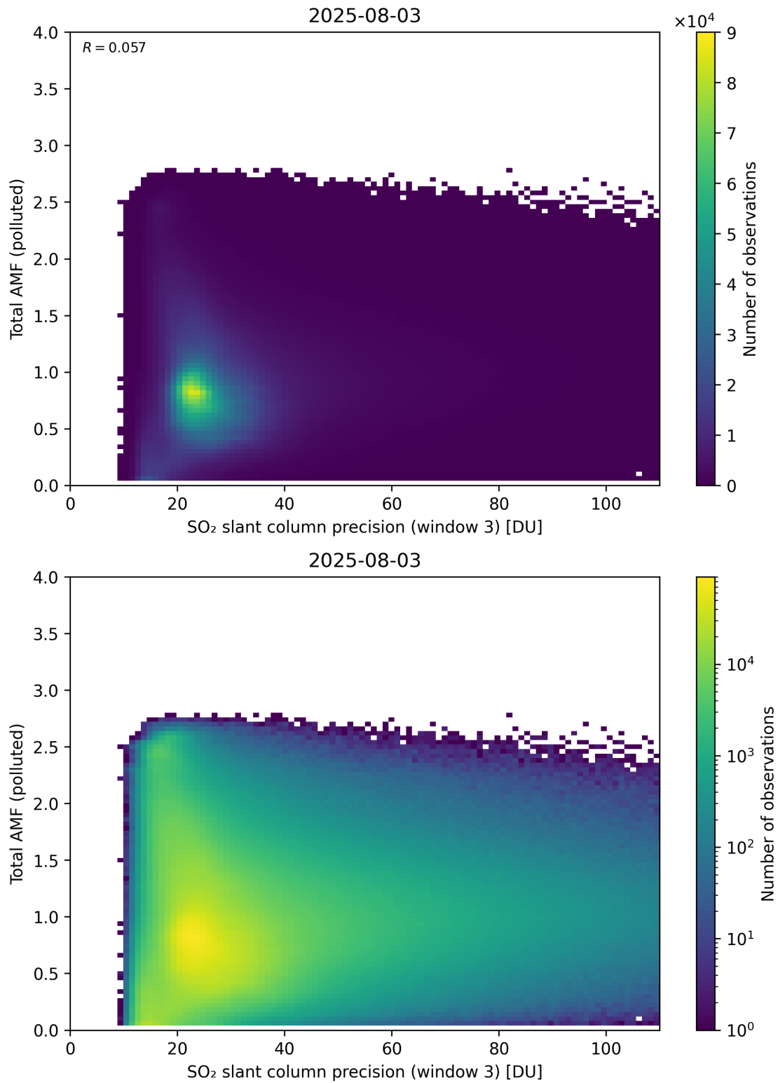
Figure 313: Scatter density plot of “SO 2 slant column precision (window 3)” against “Total AMF (polluted)” for 2025-08-03 to 2025-08-04.
