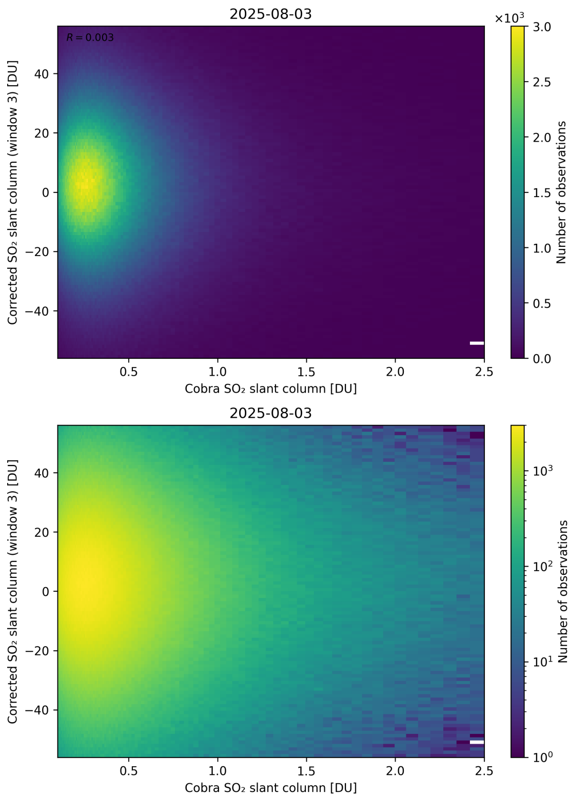
Figure 218: Scatter density plot of “Cobra SO 2 slant column” against “Corrected SO 2 slant column (window 3)” for 2025-08-03 to 2025-08-04.
