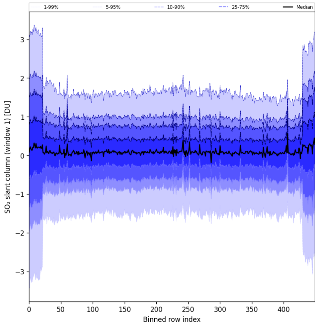
Figure 89: Along track statistics of “SO 2 slant column (window 1)” for 2025-08-03 to 2025-08-04
