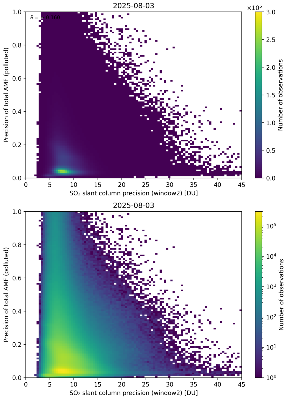
Figure 302: Scatter density plot of “SO 2 slant column precision (window2)” against “Precision of total AMF (polluted)” for 2025-08-03 to 2025-08-04.
