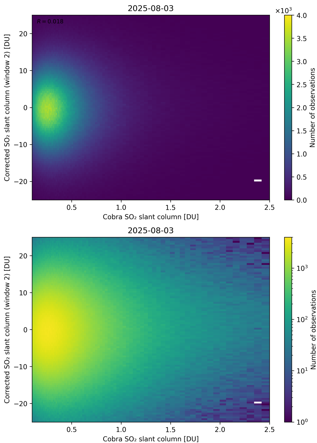
Figure 217: Scatter density plot of “Cobra SO 2 slant column” against “Corrected SO 2 slant column (window 2)” for 2025-08-03 to 2025-08-04.
