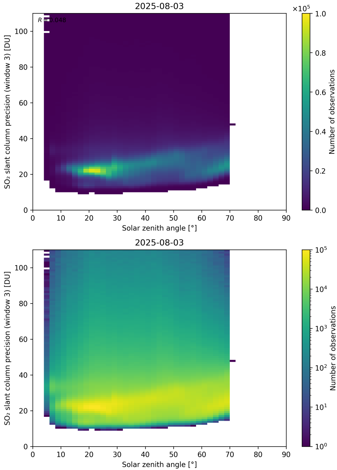
Figure 188: Scatter density plot of “Solar zenith angle” against “SO 2 slant column precision (window 3)” for 2025-08-03 to 2025-08-04.
