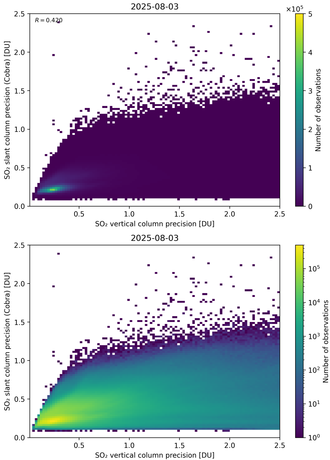
Figure 337: Scatter density plot of “SO 2 vertical column precision” against “SO 2 slant column precision (Cobra)” for 2025-08-03 to 2025-08-04.
