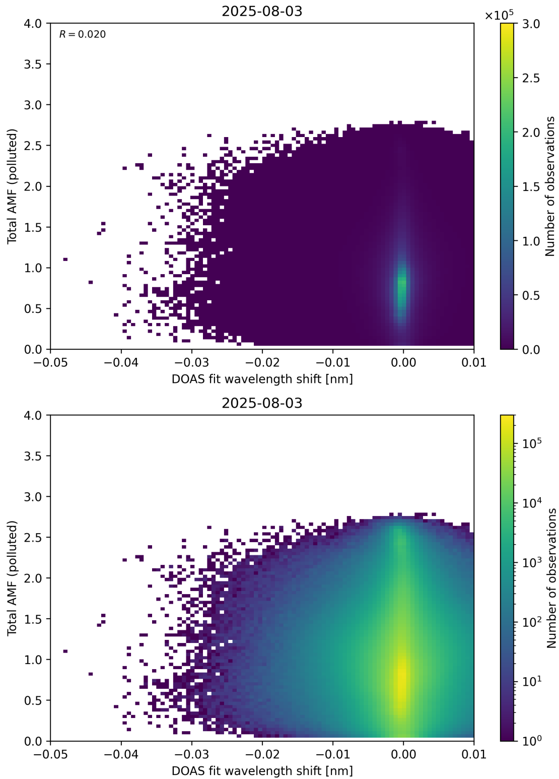
Figure 141: Scatter density plot of “DOAS fit wavelength shift” against “Total AMF (polluted)” for 2025-08-03 to 2025-08-04.
