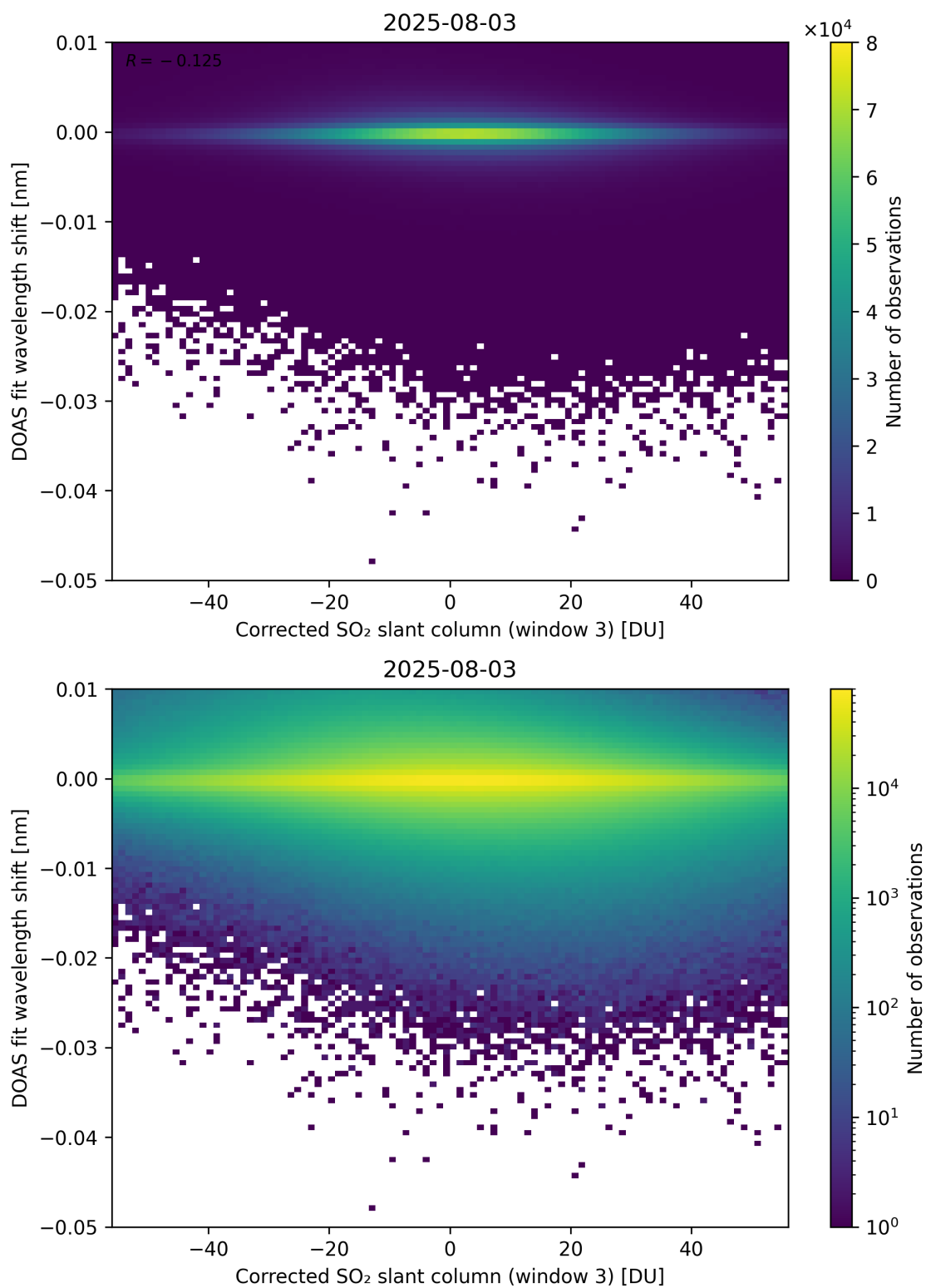
Figure 256: Scatter density plot of “Corrected SO 2 slant column (window 3)” against “DOAS fit wavelength shift” for 2025-08-03 to 2025-08-04.
