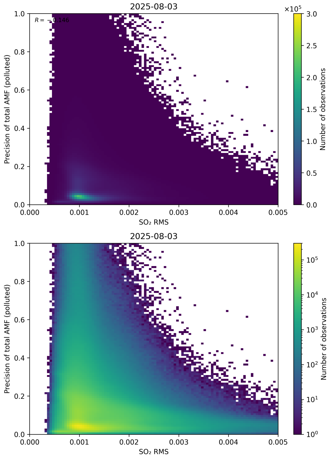
Figure 149: Scatter density plot of “SO 2 RMS” against “Precision of total AMF (polluted)” for 2025-08-03 to 2025-08-04.
