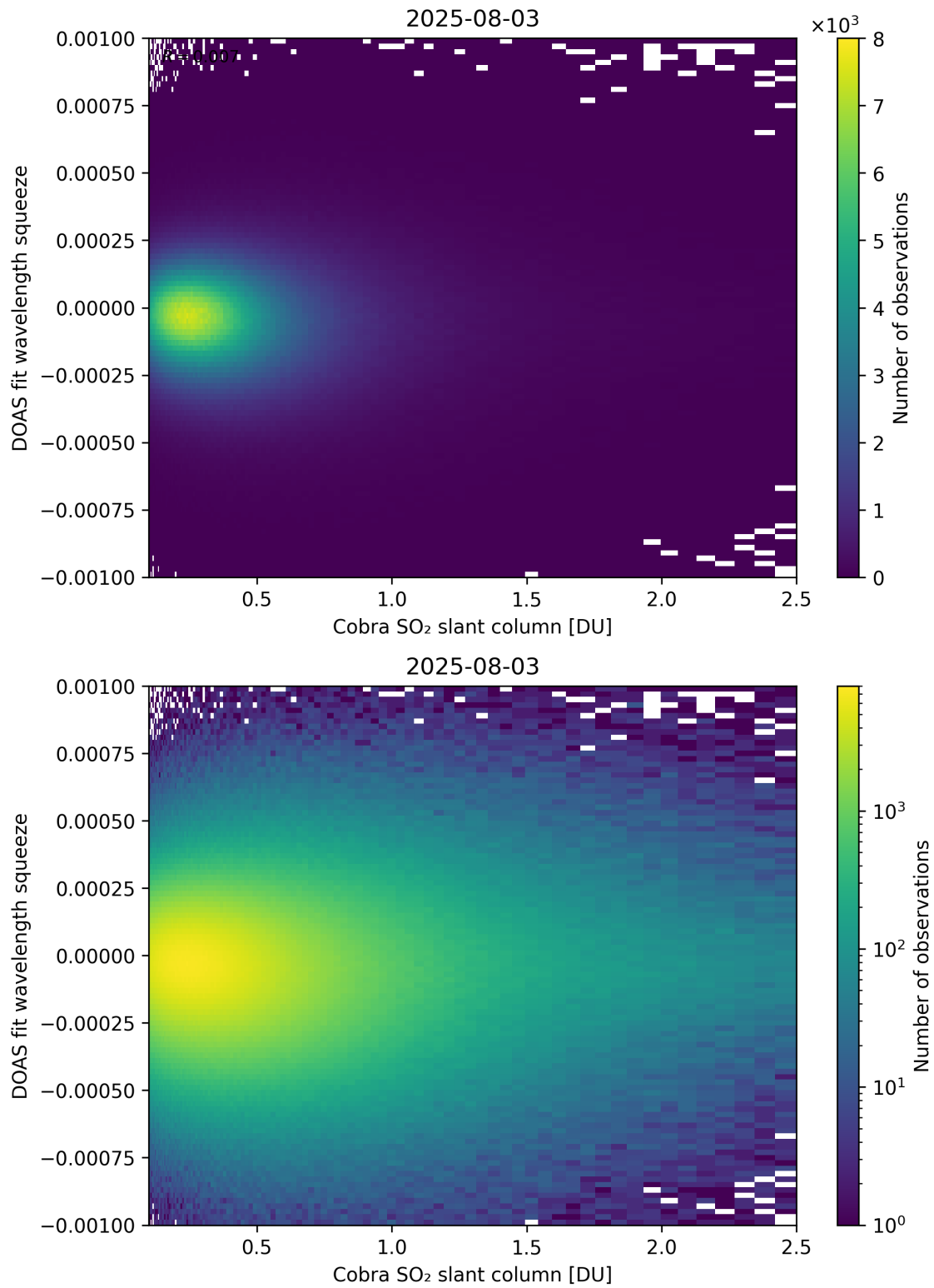
Figure 197: Scatter density plot of “Cobra SO 2 slant column” against “DOAS fit wavelength squeeze” for 2025-08-03 to 2025-08-04.
