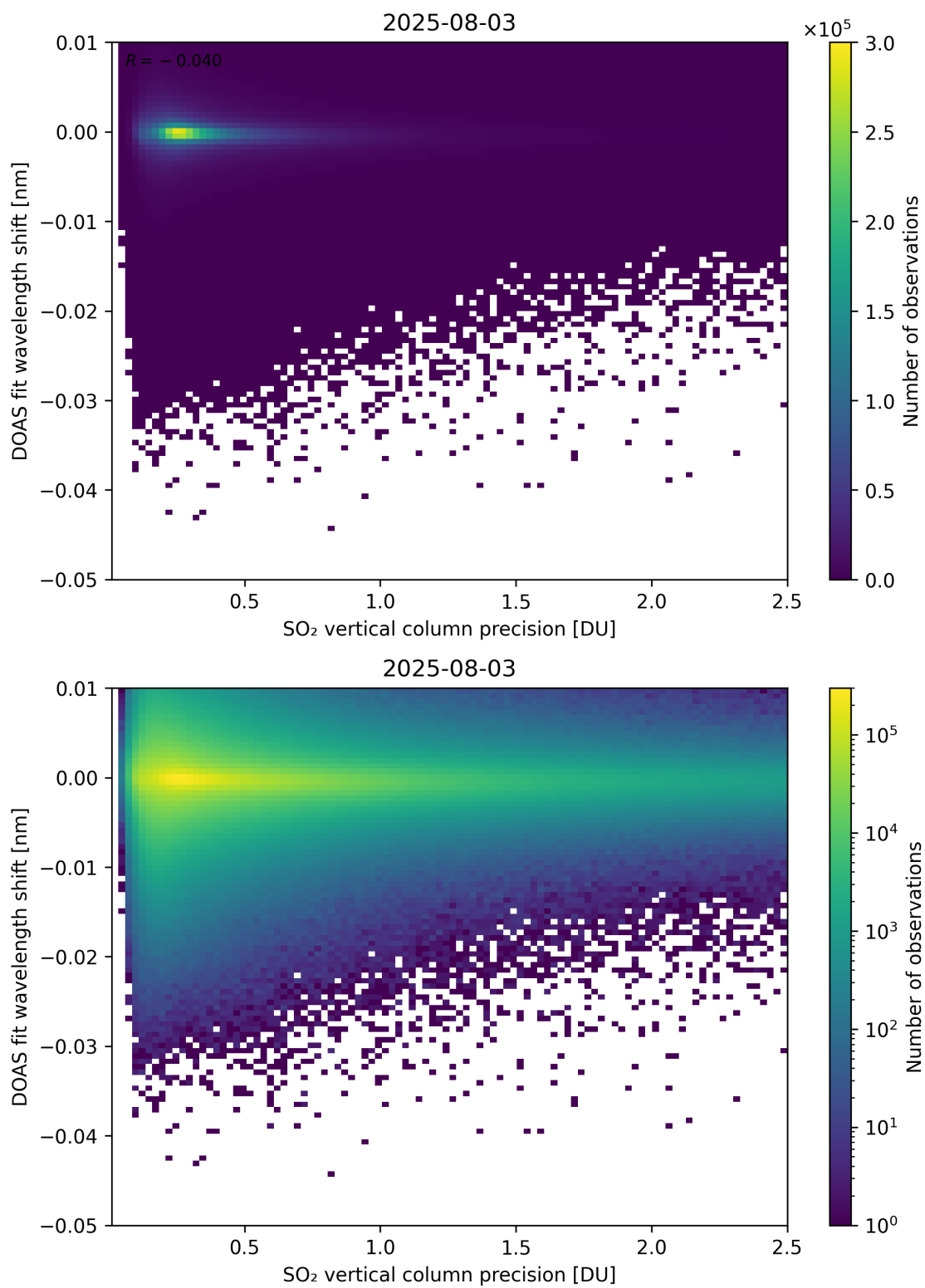
Figure 332: Scatter density plot of “SO 2 vertical column precision” against “DOAS fit wavelength shift” for 2025-08-03 to 2025-08-04.
