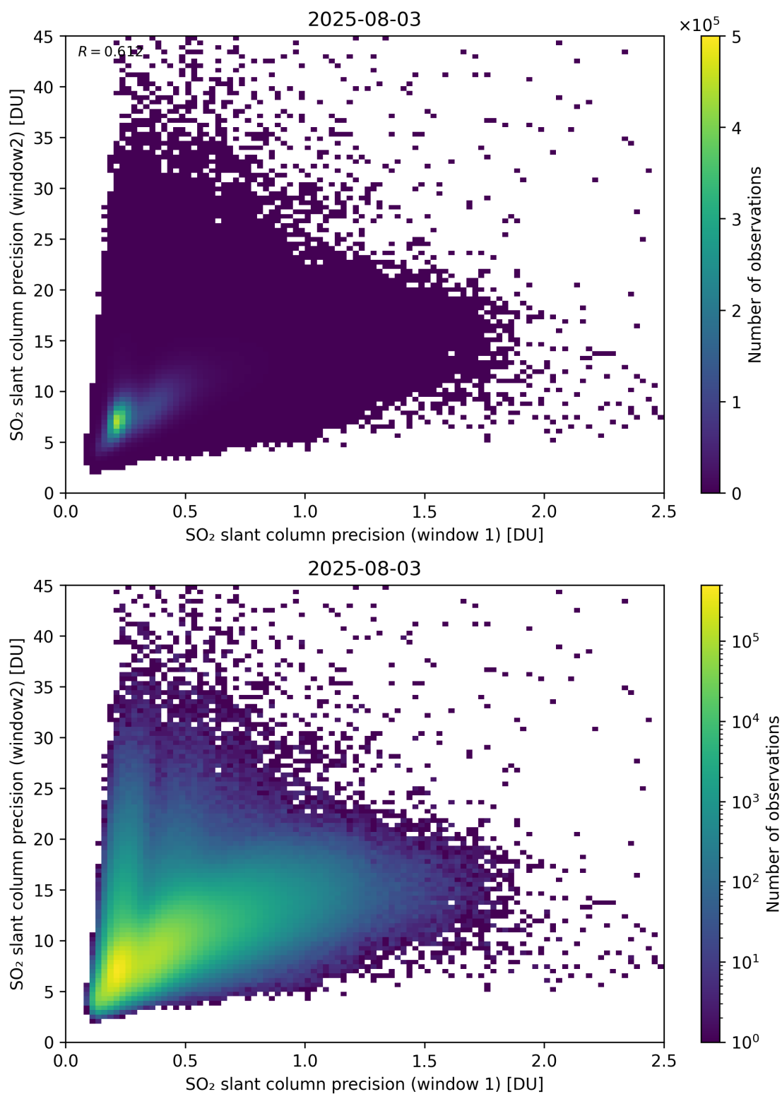
Figure 277: Scatter density plot of “SO 2 slant column precision (window 1)” against “SO 2 slant column precision (window2)” for 2025-08-03 to 2025-08-04.
