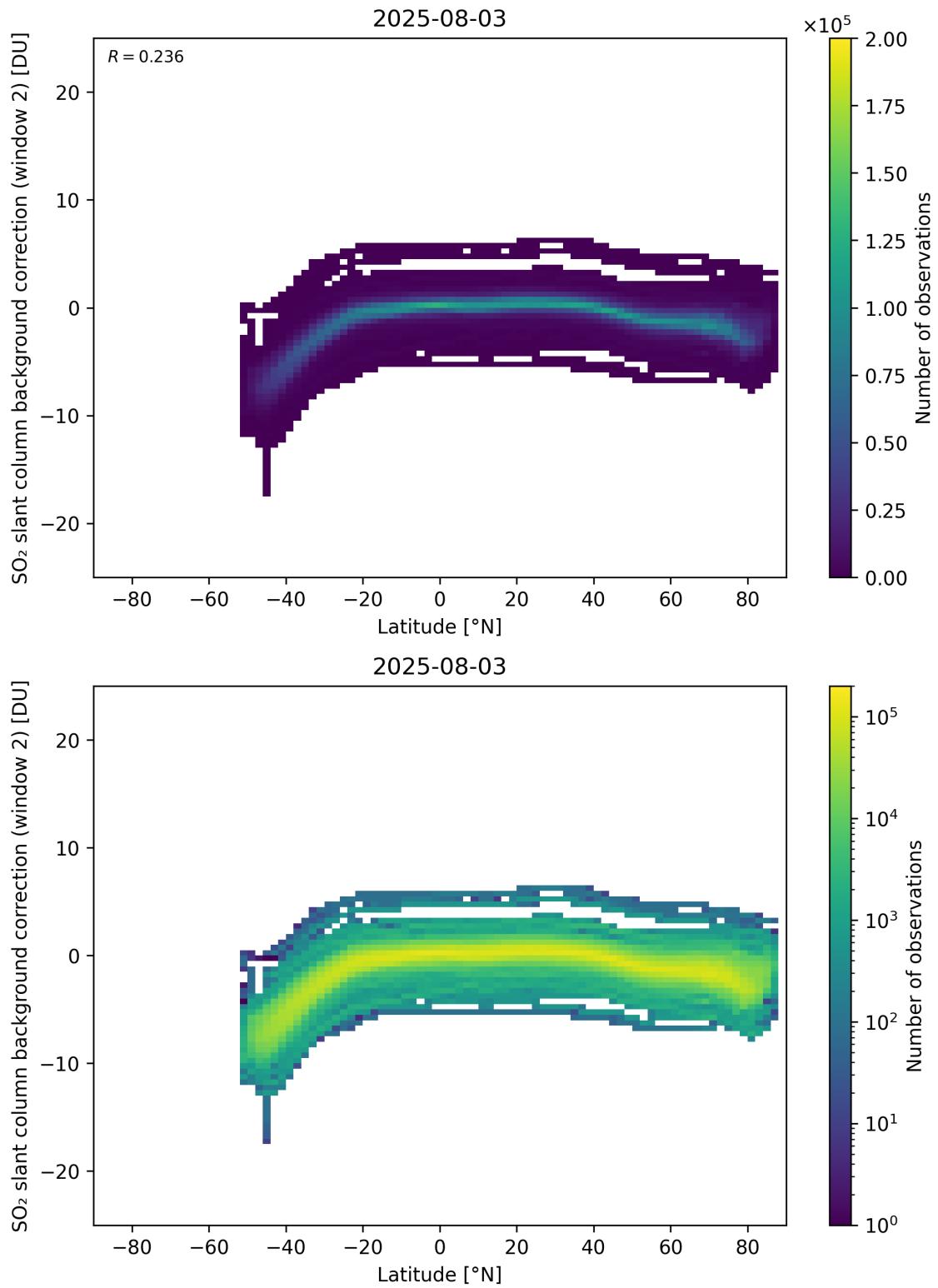
Figure 151: Scatter density plot of “Latitude” against “SO 2 slant column background correction (window 2)” for 2025-08-03 to 2025-08-04.
