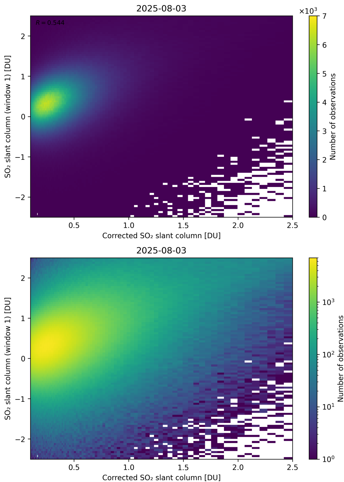
Figure 237: Scatter density plot of “Corrected SO 2 slant column” against “SO 2 slant column (window 1)” for 2025-08-03 to 2025-08-04.
