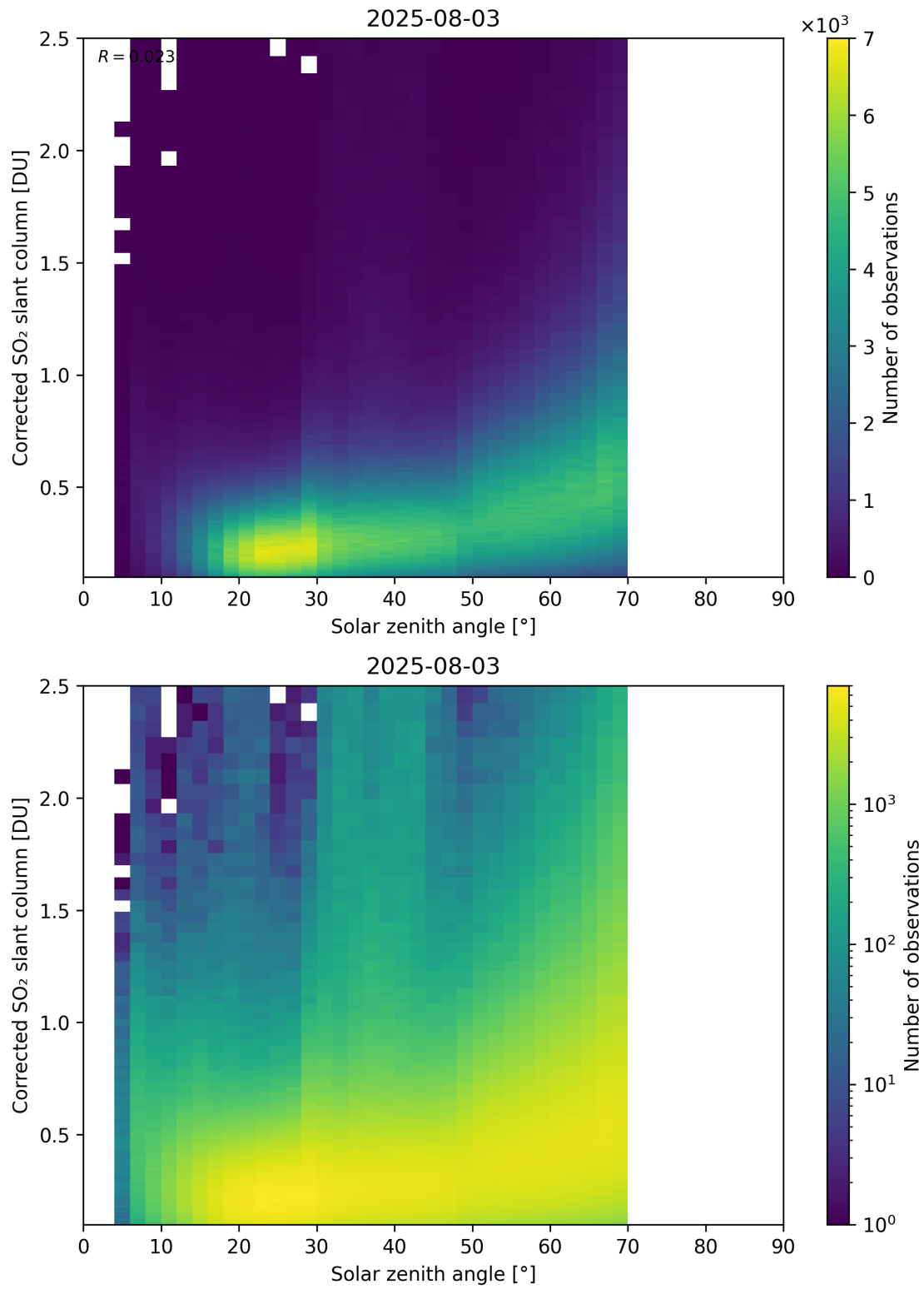
Figure 181: Scatter density plot of “Solar zenith angle” against “Corrected SO 2 slant column” for 2025-08-03 to 2025-08-04.
