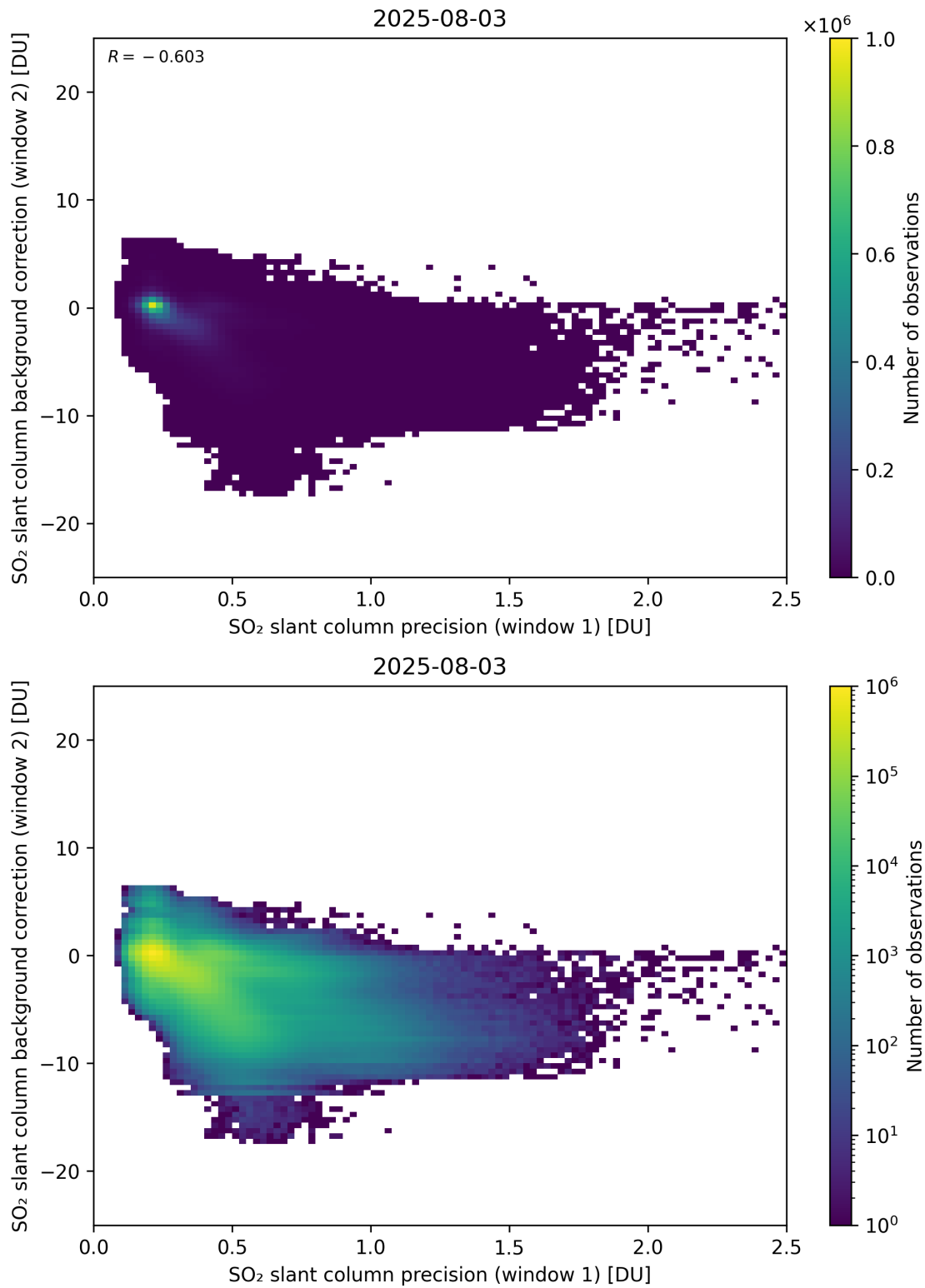
Figure 269: Scatter density plot of “SO 2 slant column precision (window 1)” against “SO 2 slant column background correction (window 2)” for 2025-08-03 to 2025-08-04.
