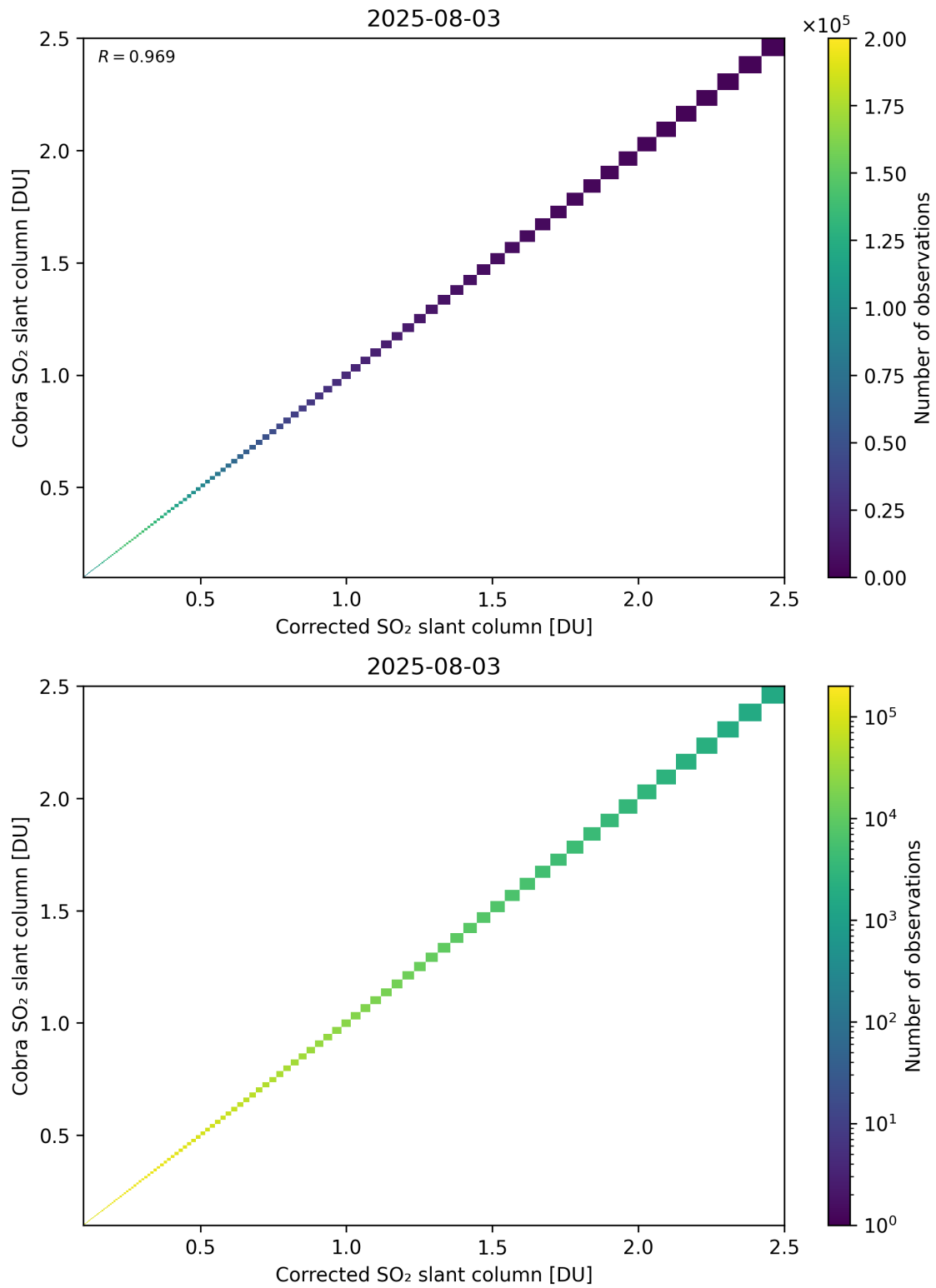
Figure 233: Scatter density plot of “Corrected SO 2 slant column” against “Cobra SO 2 slant column” for 2025-08-03 to 2025-08-04.
