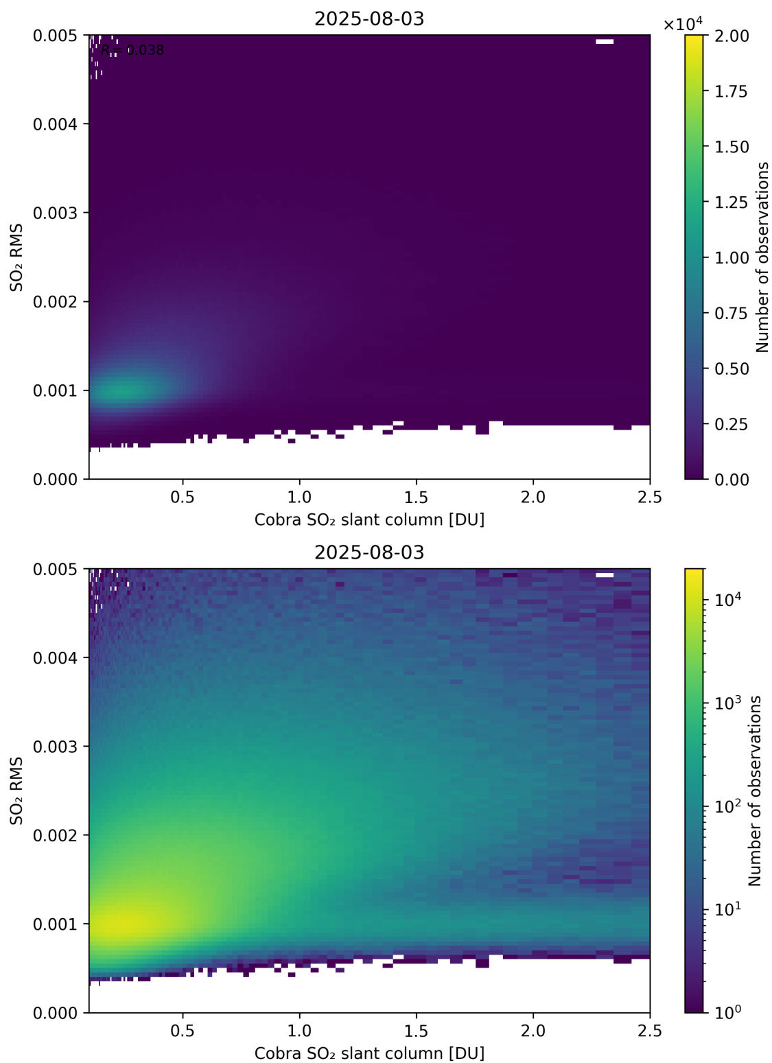
Figure 198: Scatter density plot of “Cobra SO 2 slant column” against “SO 2 RMS” for 2025-08-03 to 2025-08-04.
