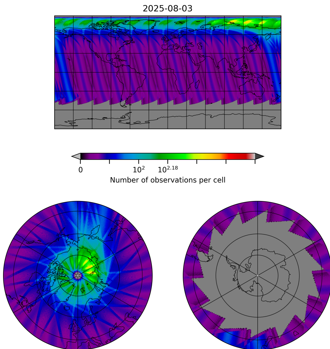
Figure 30: Map of the number of observations for 2025-08-03 to 2025-08-04
