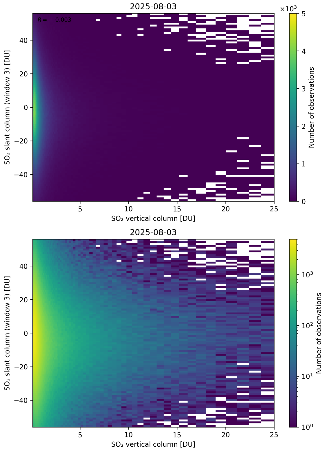
Figure 357: Scatter density plot of “SO 2 vertical column” against “SO 2 slant column (window 3)” for 2025-08-03 to 2025-08-04.
