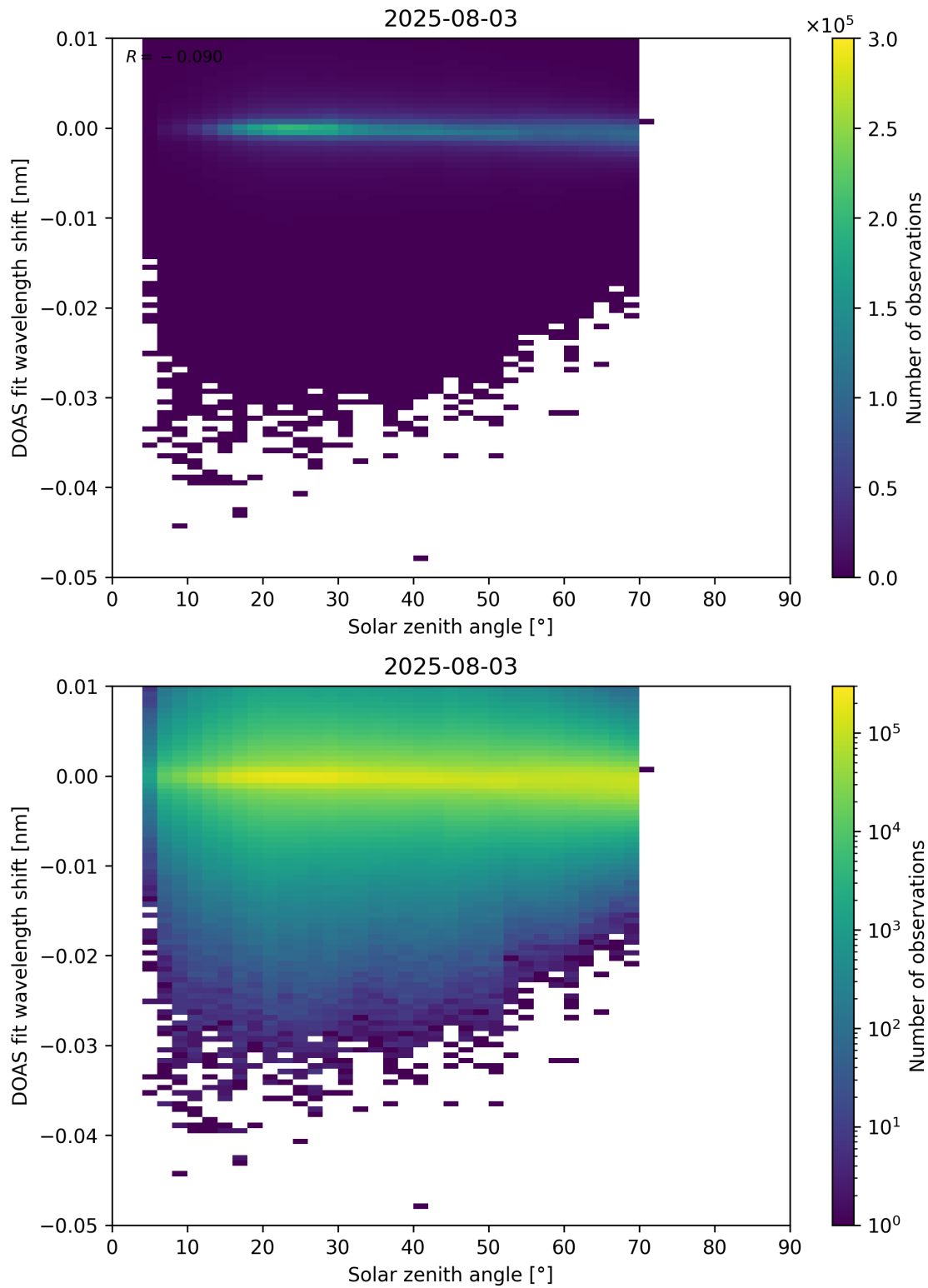
Figure 174: Scatter density plot of “Solar zenith angle” against “DOAS fit wavelength shift” for 2025-08-03 to 2025-08-04.
