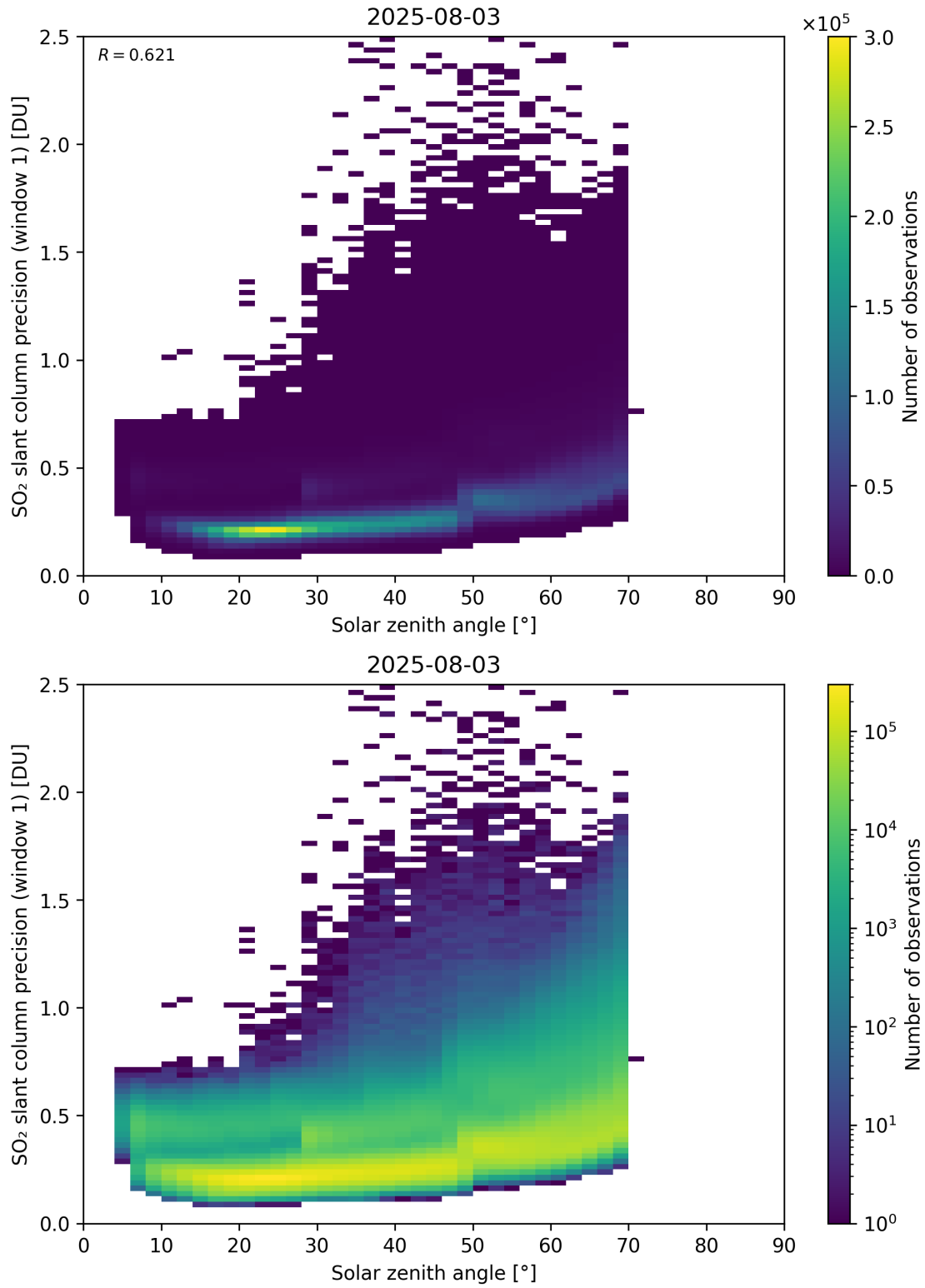
Figure 185: Scatter density plot of “Solar zenith angle” against “SO 2 slant column precision (window 1)” for 2025-08-03 to 2025-08-04.
