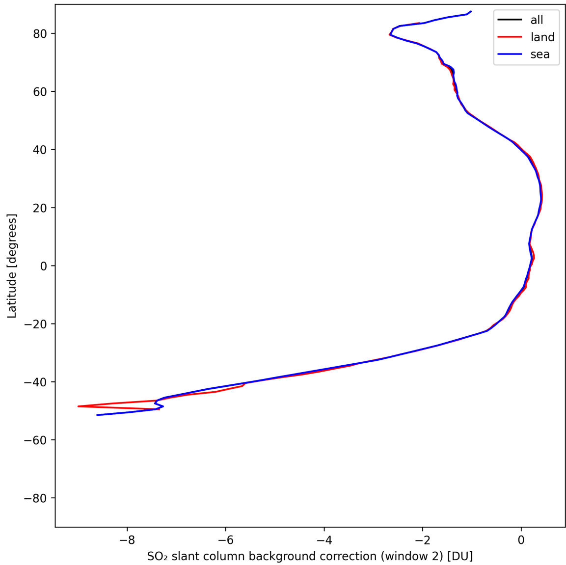
Figure 44: Zonal average of “SO 2 slant column background correction (window 2)” for 2025-08-03 to 2025-08-04.
