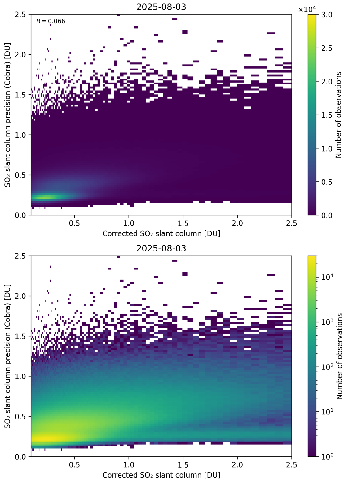
Figure 234: Scatter density plot of “Corrected SO 2 slant column” against “SO 2 slant column precision (Cobra)” for 2025-08-03 to 2025-08-04.
