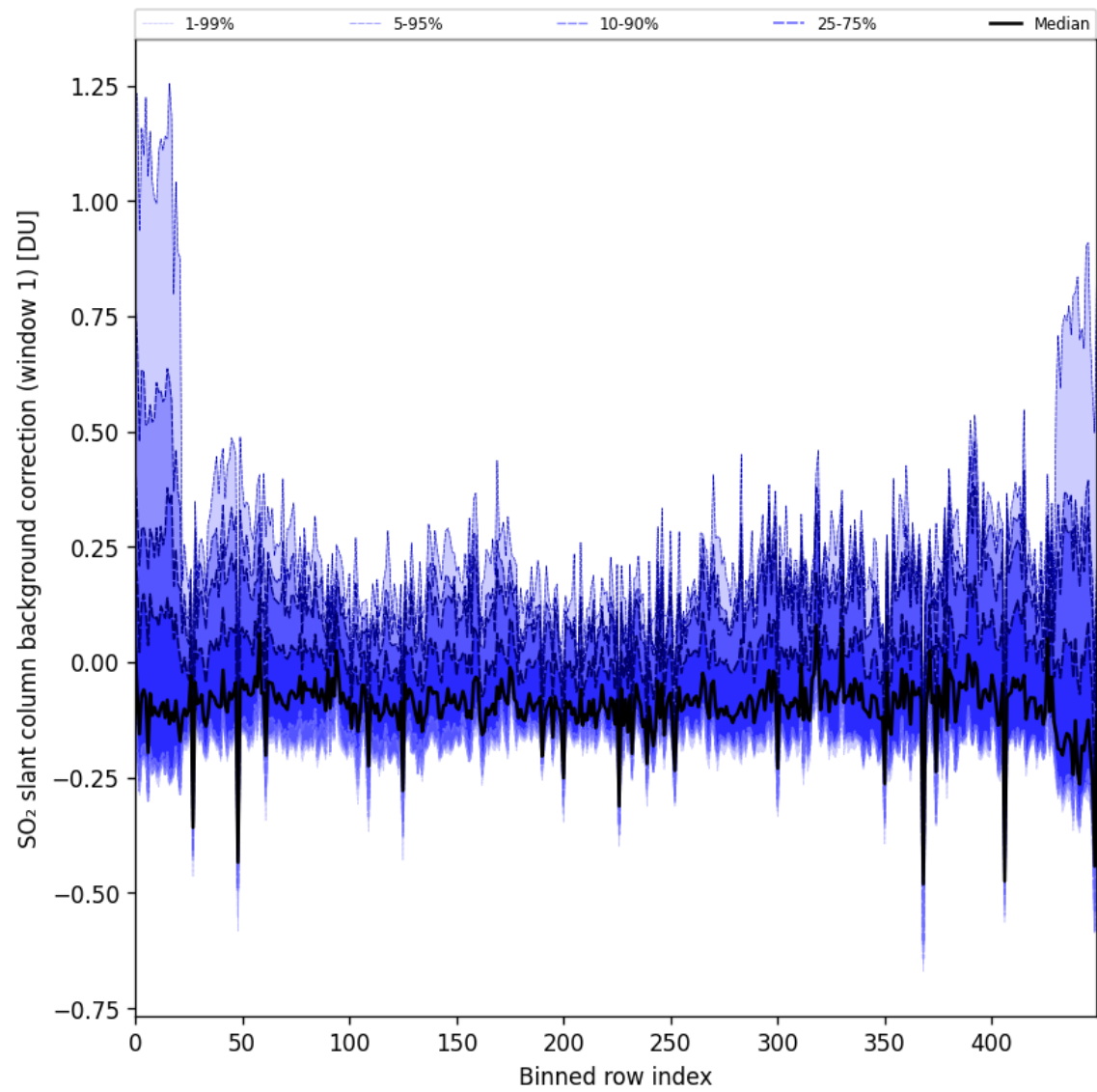
Figure 92: Along track statistics of “SO 2 slant column background correction (window 1)” for 2025-08-03 to 2025-08-04
