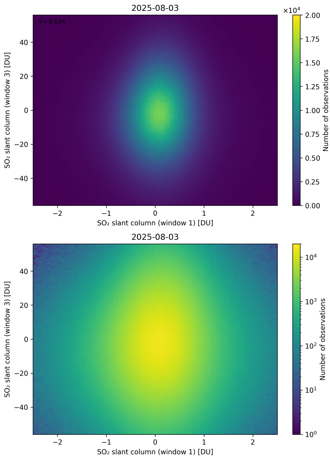
Figure 287: Scatter density plot of “SO 2 slant column (window 1)” against “SO 2 slant column (window 3)” for 2025-08-03 to 2025-08-04.
