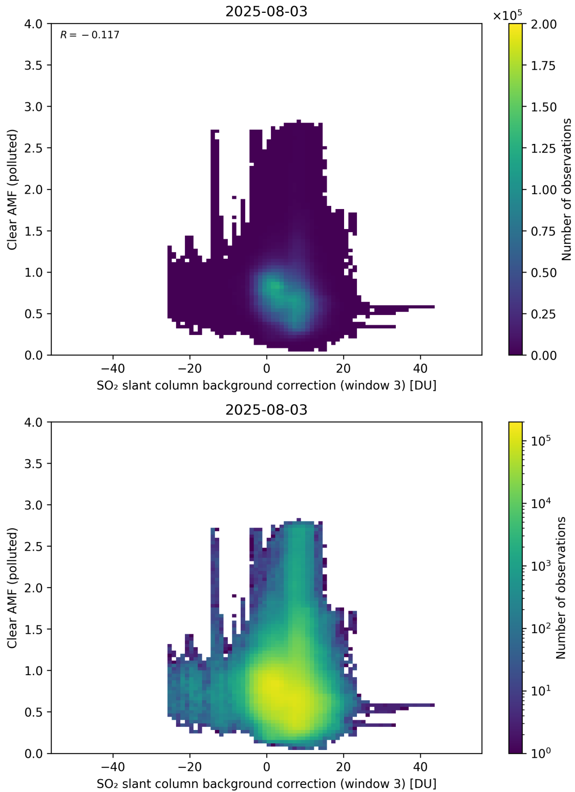
Figure 135: Scatter density plot of “SO 2 slant column background correction (window 3)” against “Clear AMF (polluted)” for 2025-08-03 to 2025-08-04.
