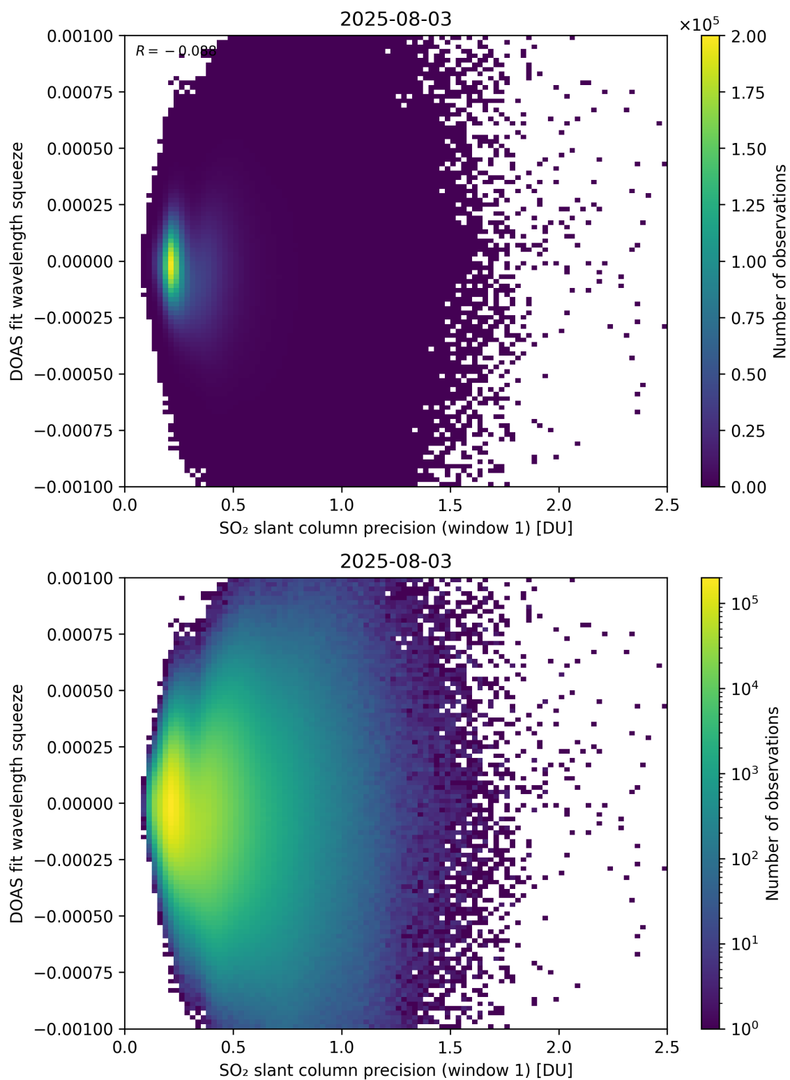
Figure 272: Scatter density plot of “SO 2 slant column precision (window 1)” against “DOAS fit wavelength squeeze” for 2025-08-03 to 2025-08-04.
