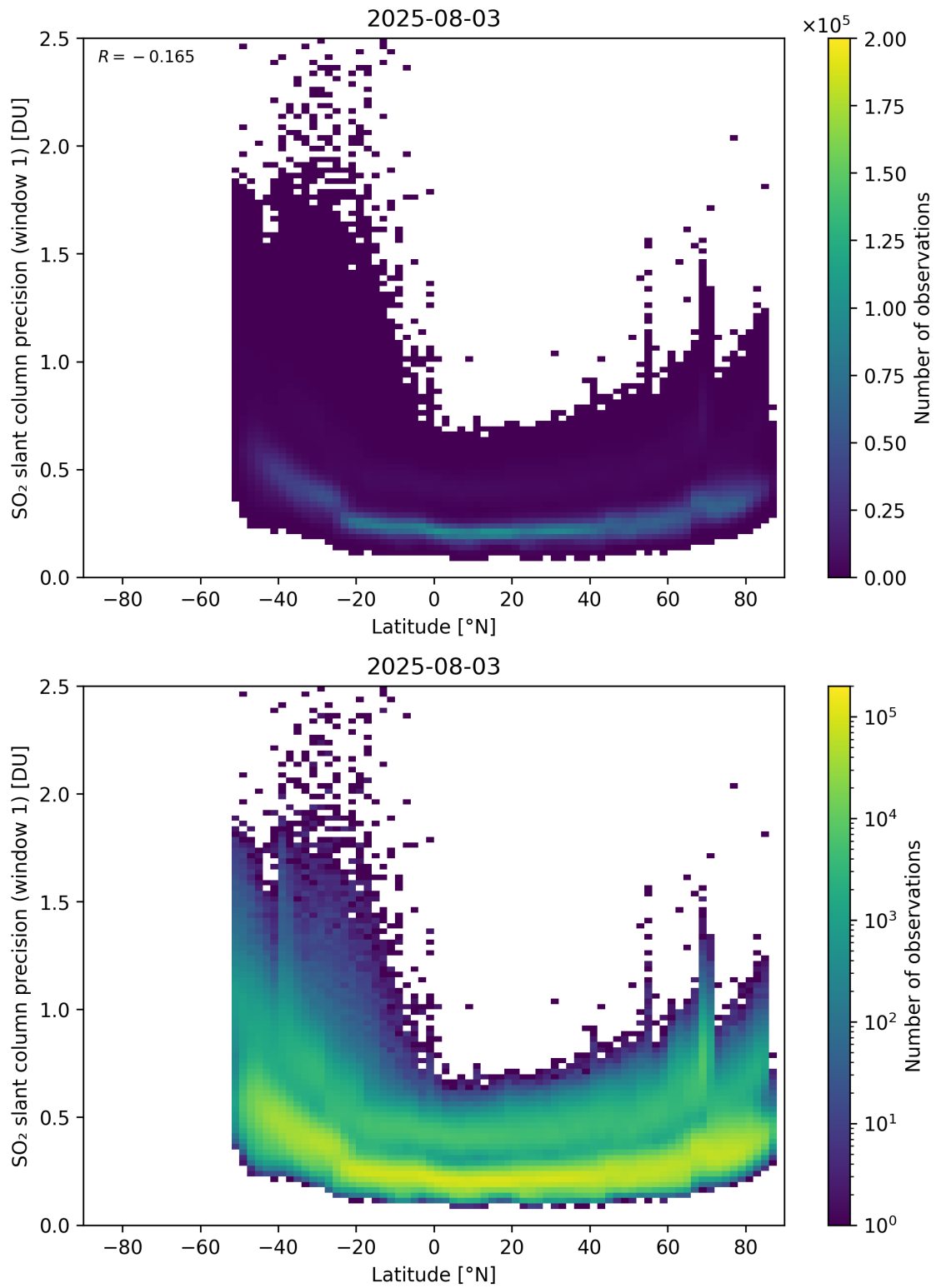
Figure 163: Scatter density plot of “Latitude” against “SO 2 slant column precision (window 1)” for 2025-08-03 to 2025-08-04.
