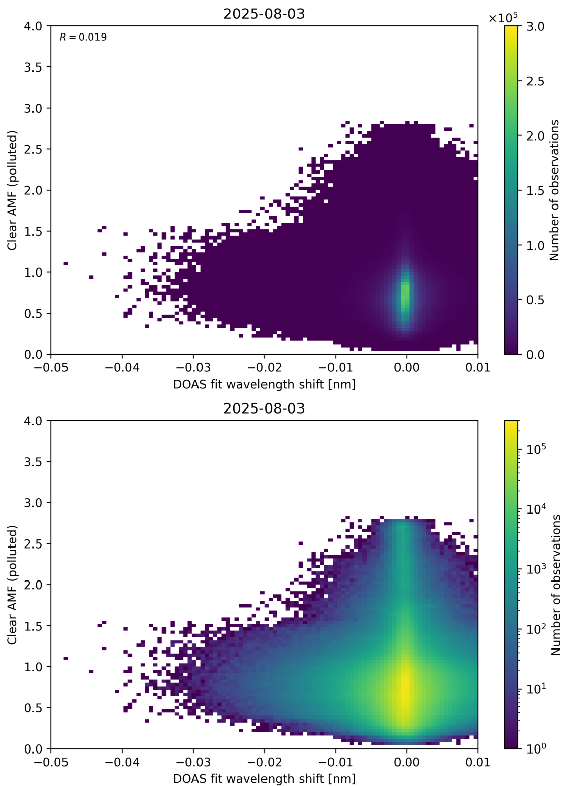
Figure 140: Scatter density plot of “DOAS fit wavelength shift” against “Clear AMF (polluted)” for 2025-08-03 to 2025-08-04.
