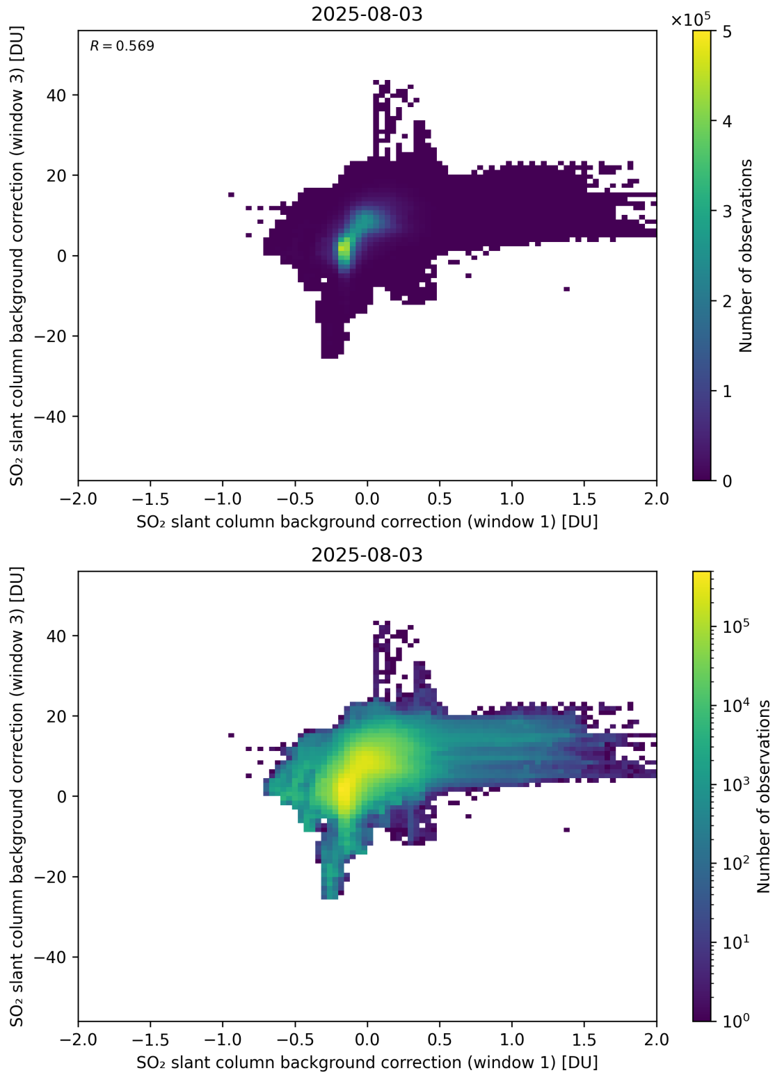
Figure 110: Scatter density plot of “SO 2 slant column background correction (window 1)” against “SO 2 slant column background correction (window 3)” for 2025-08-03 to 2025-08-04.
