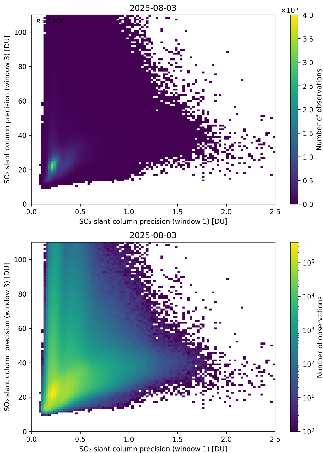
Figure 279: Scatter density plot of “SO 2 slant column precision (window 1)” against “SO 2 slant column precision (window 3)” for 2025-08-03 to 2025-08-04.
