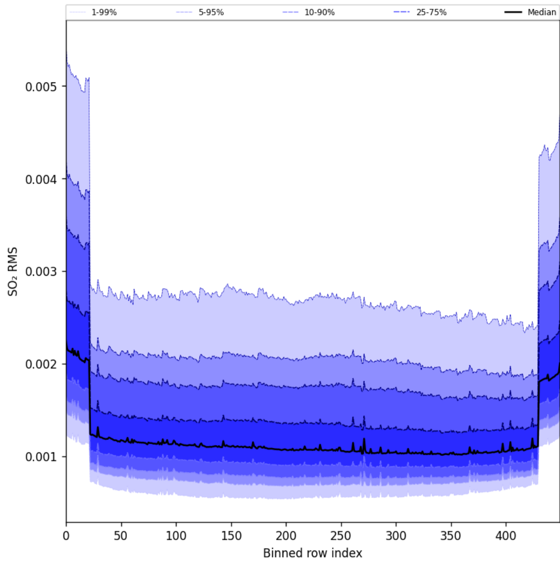
Figure 104: Along track statistics of “SO 2 RMS” for 2025-08-03 to 2025-08-04
