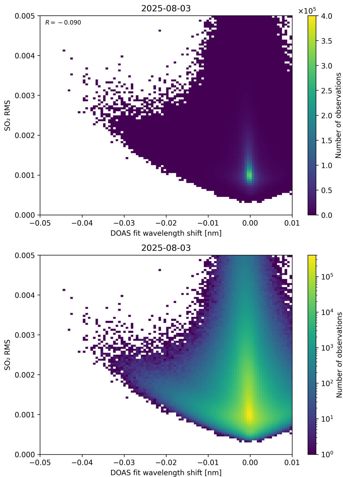
Figure 139: Scatter density plot of “DOAS fit wavelength shift” against “SO 2 RMS” for 2025-08-03 to 2025-08-04.
