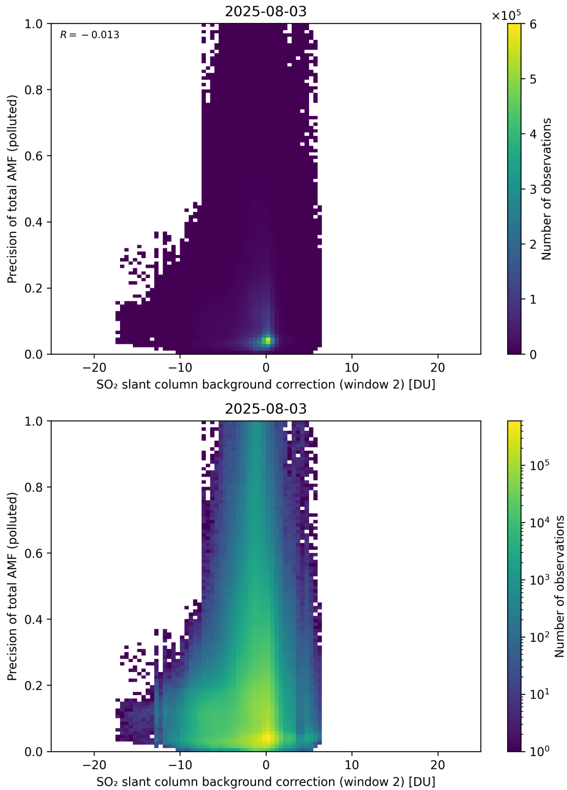
Figure 131: Scatter density plot of “SO 2 slant column background correction (window 2)” against “Precision of total AMF (polluted)” for 2025-08-03 to 2025-08-04.
