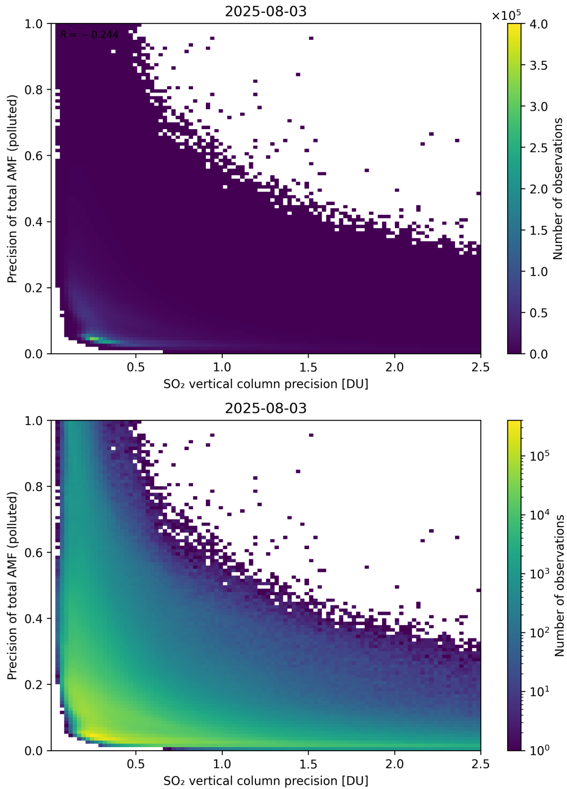
Figure 347: Scatter density plot of “SO 2 vertical column precision” against “Precision of total AMF (polluted)” for 2025-08-03 to 2025-08-04.
