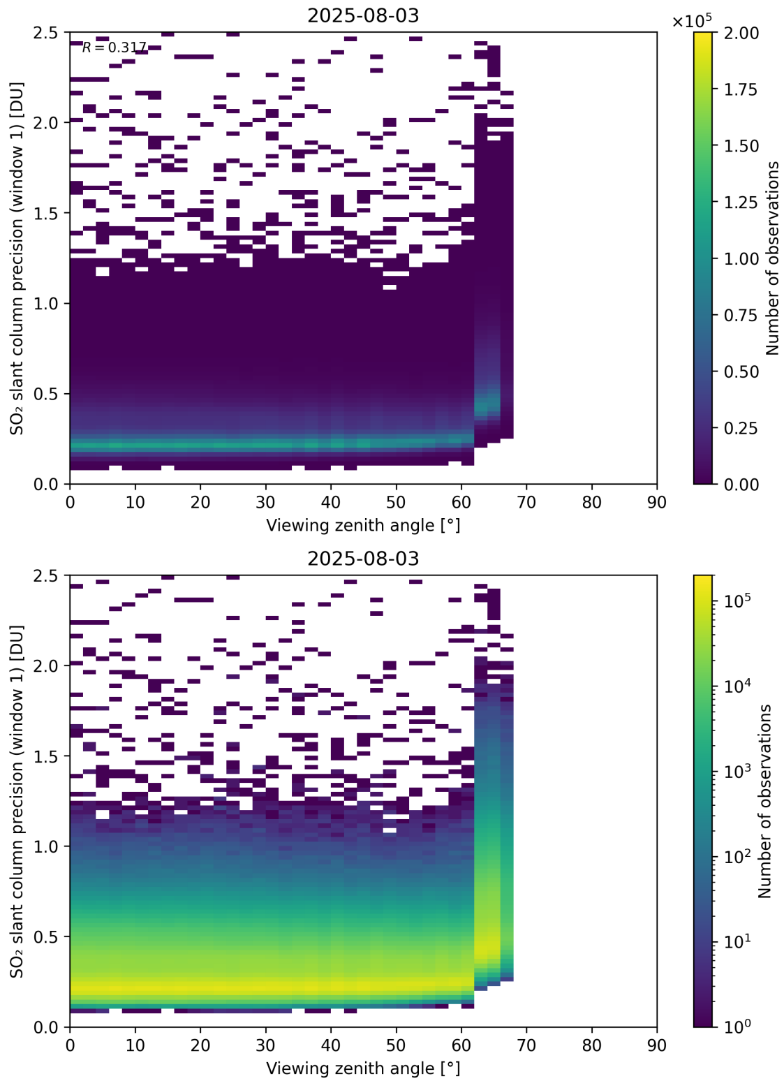
Figure 377: Scatter density plot of “Viewing zenith angle” against “SO 2 slant column precision (window 1)” for 2025-08-03 to 2025-08-04.
