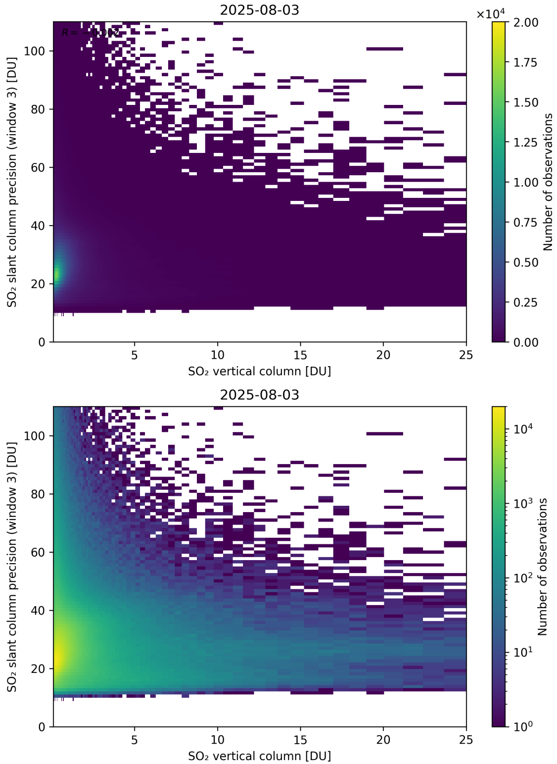
Figure 358: Scatter density plot of “SO 2 vertical column” against “SO 2 slant column precision (window 3)” for 2025-08-03 to 2025-08-04.
