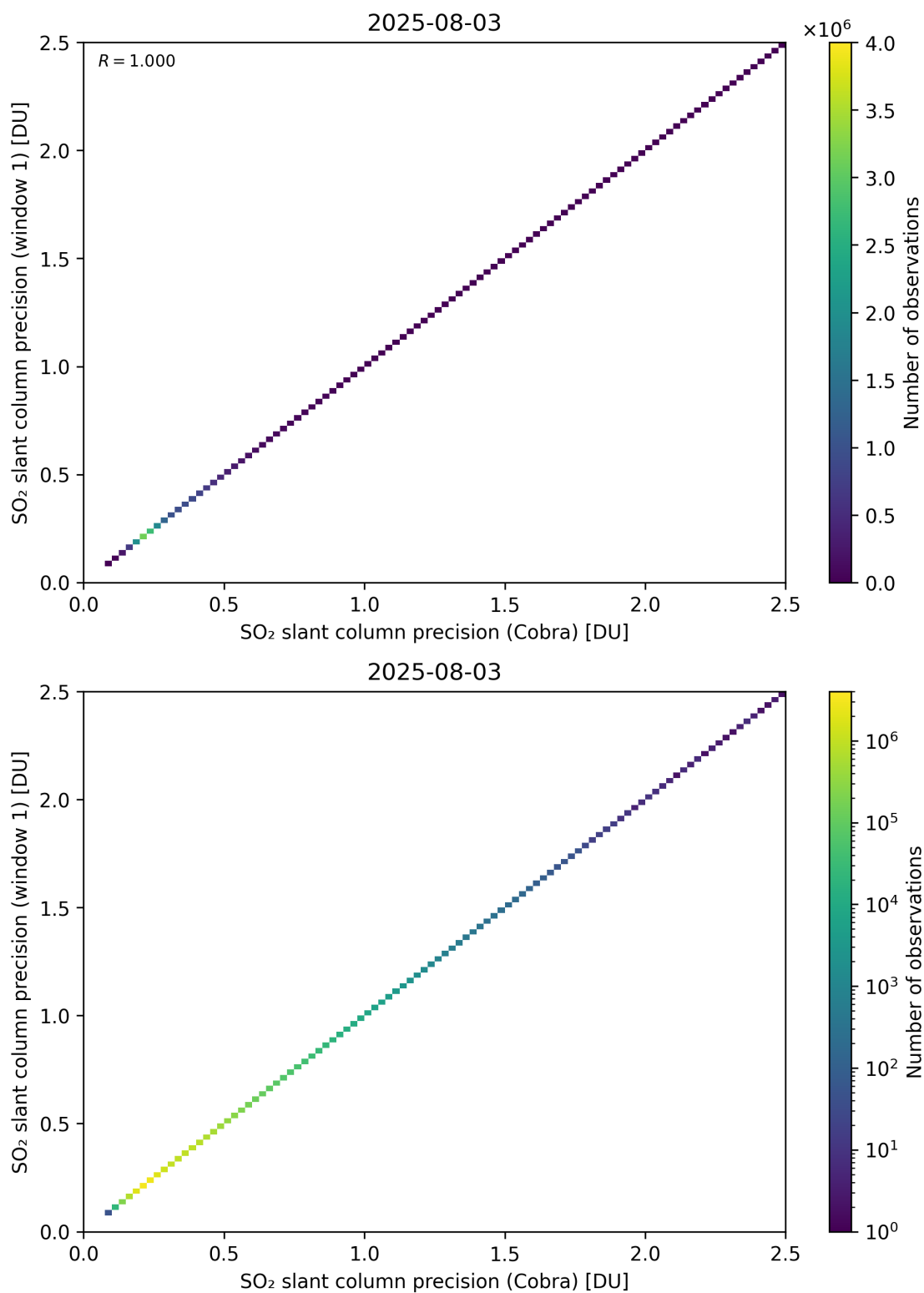
Figure 209: Scatter density plot of “SO 2 slant column precision (Cobra)” against “SO 2 slant column precision (window 1)” for 2025-08-03 to 2025-08-04.
