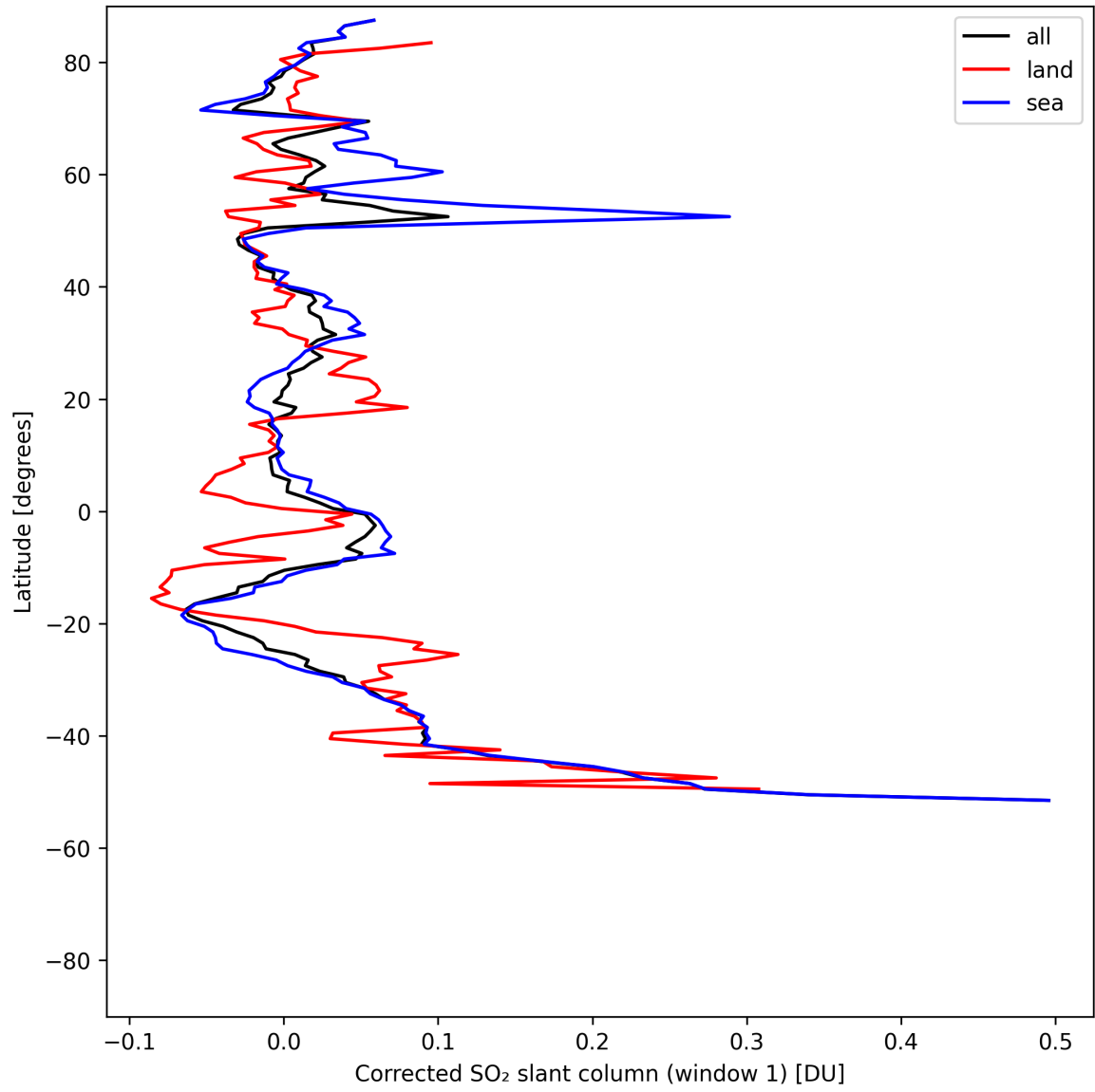
Figure 39: Zonal average of “Corrected SO 2 slant column (window 1)” for 2025-08-03 to 2025-08-04.
