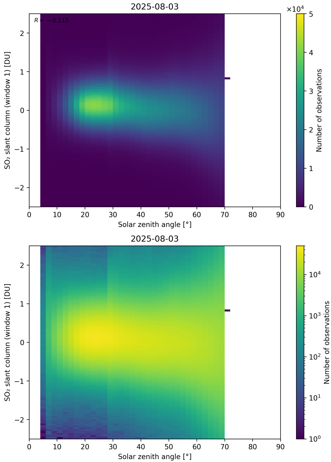
Figure 184: Scatter density plot of “Solar zenith angle” against “SO 2 slant column (window 1)” for 2025-08-03 to 2025-08-04.
