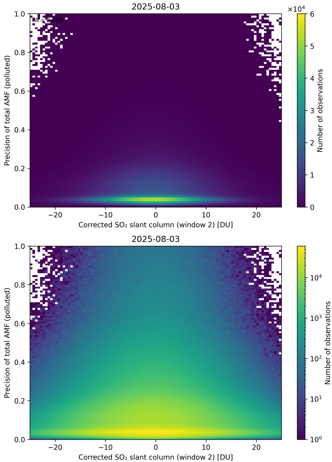
Figure 254: Scatter density plot of “Corrected SO 2 slant column (window 2)” against “Precision of total AMF (polluted)” for 2025-08-03 to 2025-08-04.
