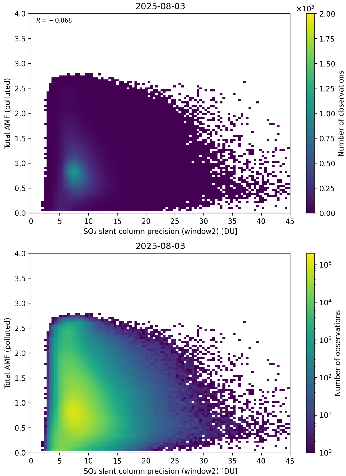
Figure 301: Scatter density plot of “SO 2 slant column precision (window2)” against “Total AMF (polluted)” for 2025-08-03 to 2025-08-04.
