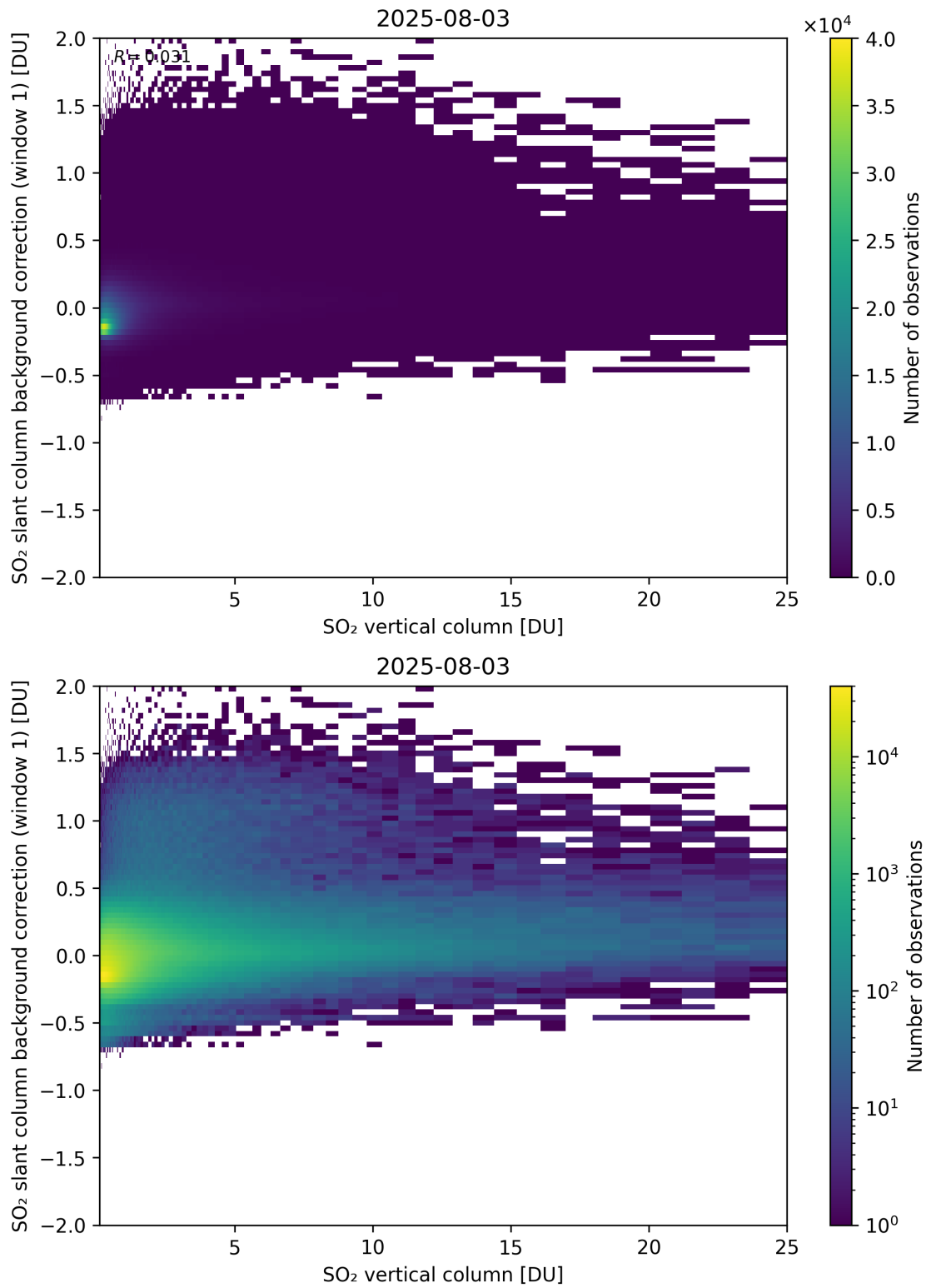
Figure 323: Scatter density plot of “SO 2 vertical column” against “SO 2 slant column background correction (window 1)” for 2025-08-03 to 2025-08-04.
