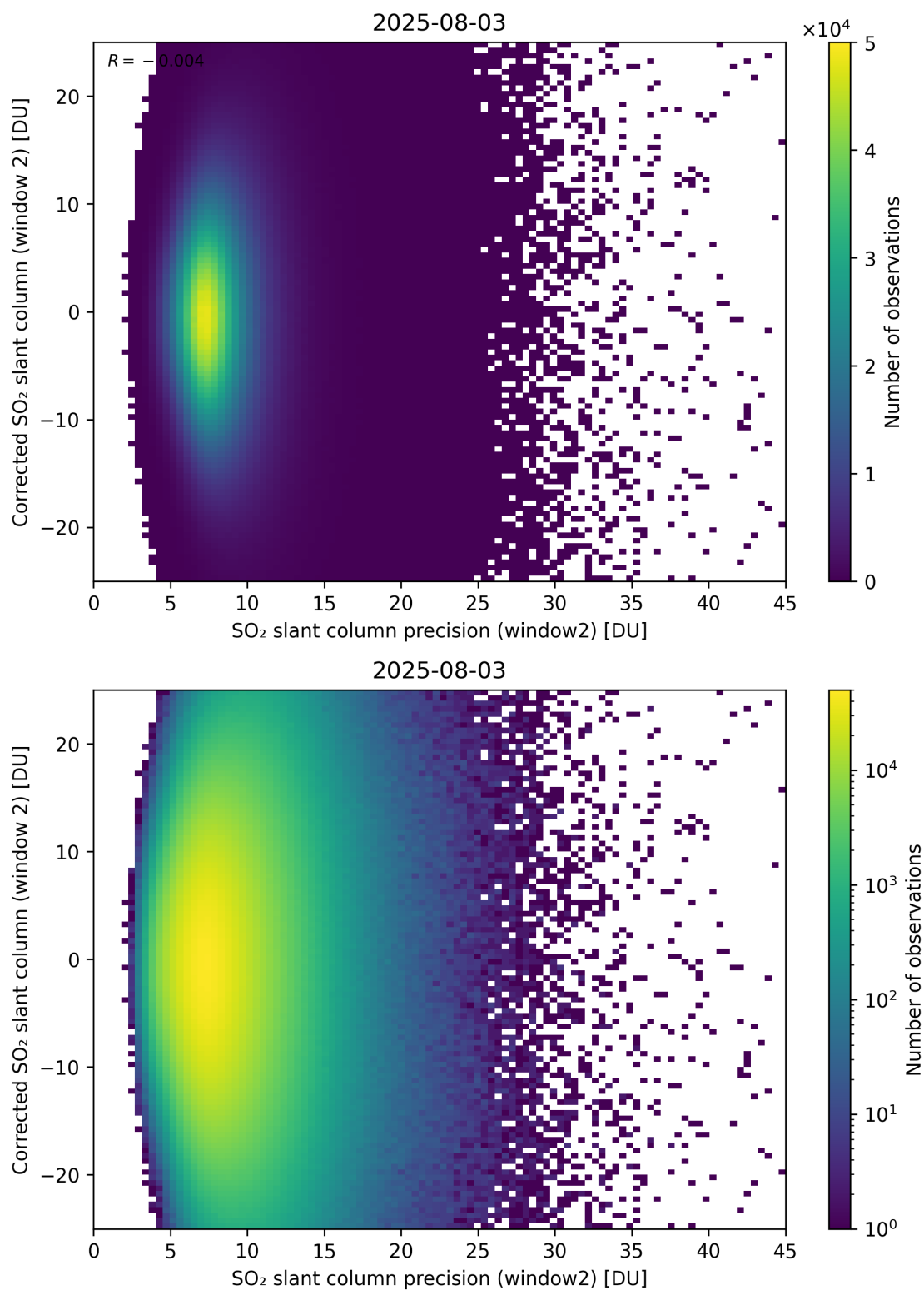
Figure 297: Scatter density plot of “SO 2 slant column precision (window2)” against “Corrected SO 2 slant column (window 2)” for 2025-08-03 to 2025-08-04.
