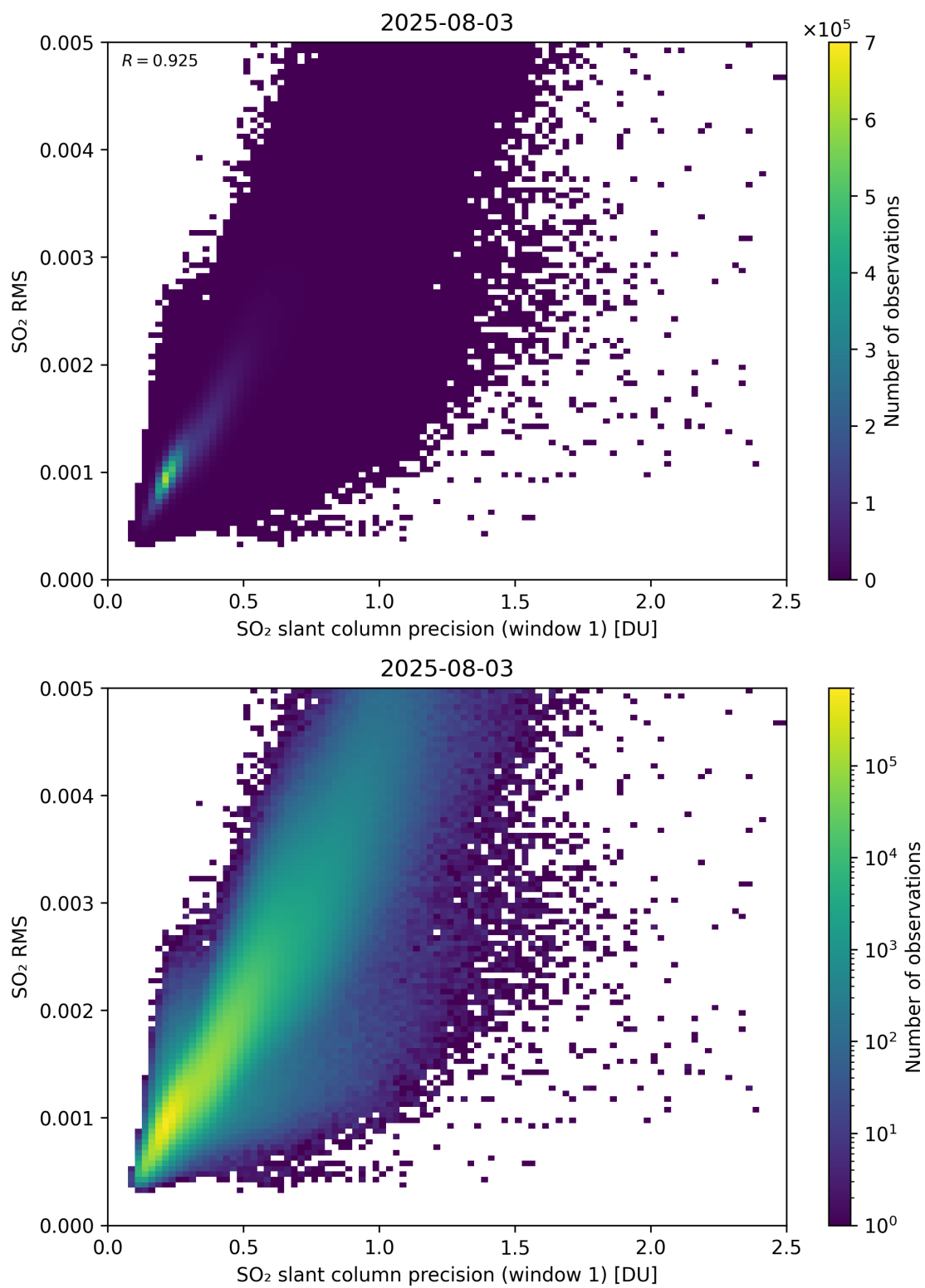
Figure 273: Scatter density plot of “SO 2 slant column precision (window 1)” against “SO 2 RMS” for 2025-08-03 to 2025-08-04.
