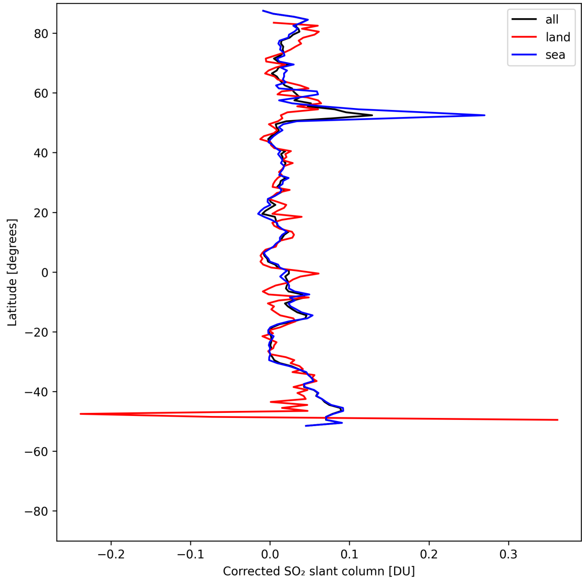
Figure 34: Zonal average of "Corrected SO 2 slant column" for 2025-08-03 to 2025-08-04.
