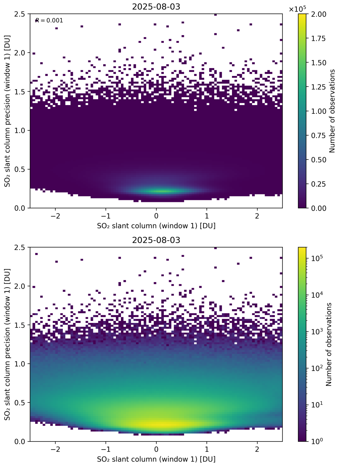
Figure 285: Scatter density plot of “SO 2 slant column (window 1)” against “SO 2 slant column precision (window 1)” for 2025-08-03 to 2025-08-04.
