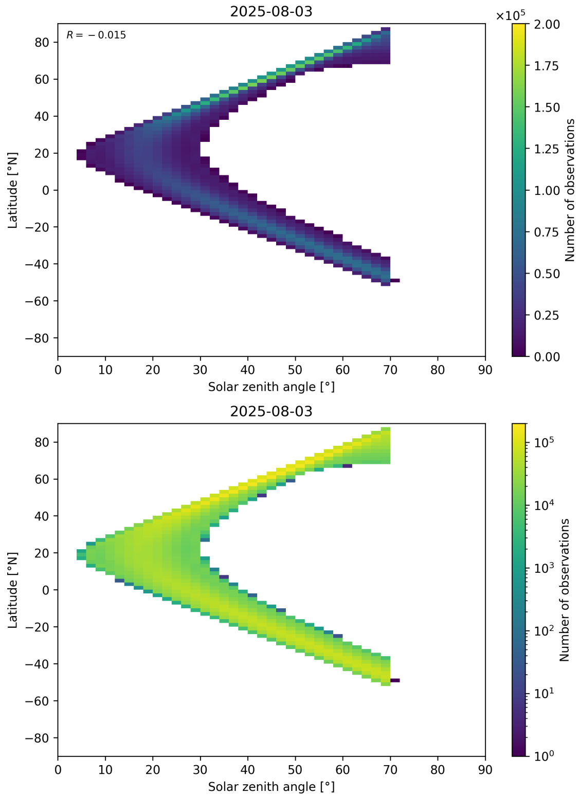
Figure 177: Scatter density plot of “Solar zenith angle” against “Latitude” for 2025-08-03 to 2025-08-04.
