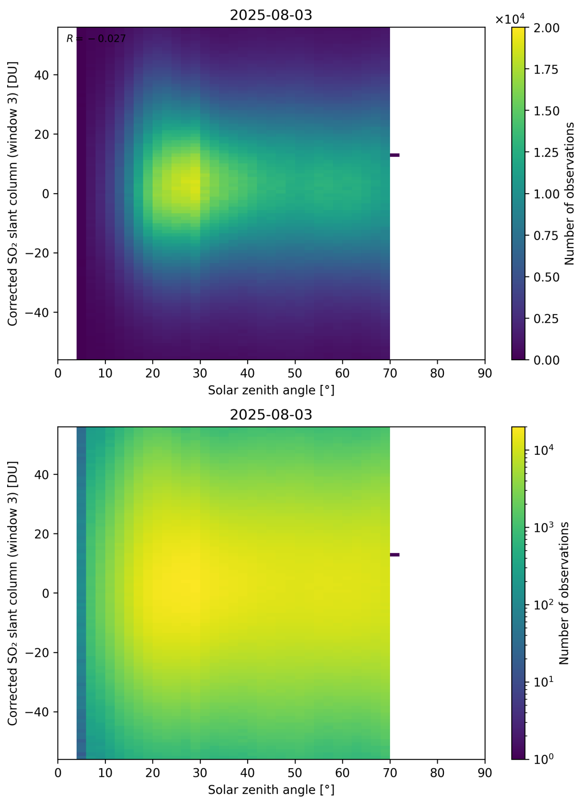
Figure 183: Scatter density plot of “Solar zenith angle” against “Corrected SO 2 slant column (window 3)” for 2025-08-03 to 2025-08-04.
