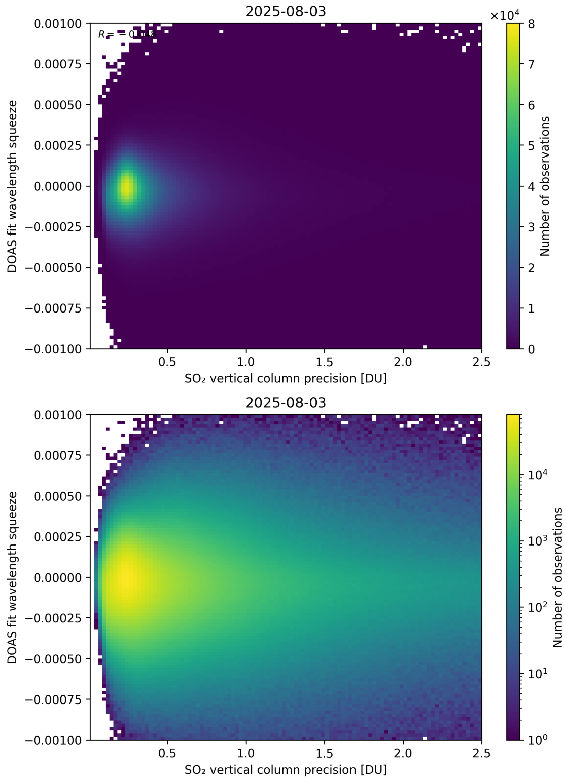
Figure 333: Scatter density plot of “SO 2 vertical column precision” against “DOAS fit wavelength squeeze” for 2025-08-03 to 2025-08-04.
