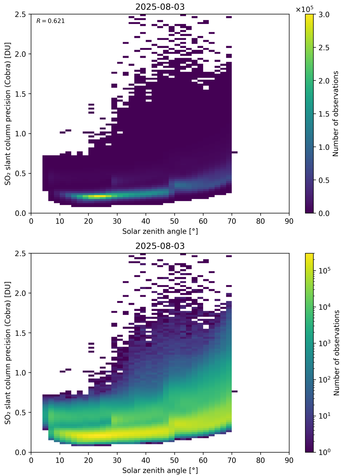
Figure 180: Scatter density plot of “Solar zenith angle” against “SO 2 slant column precision (Cobra)” for 2025-08-03 to 2025-08-04.
