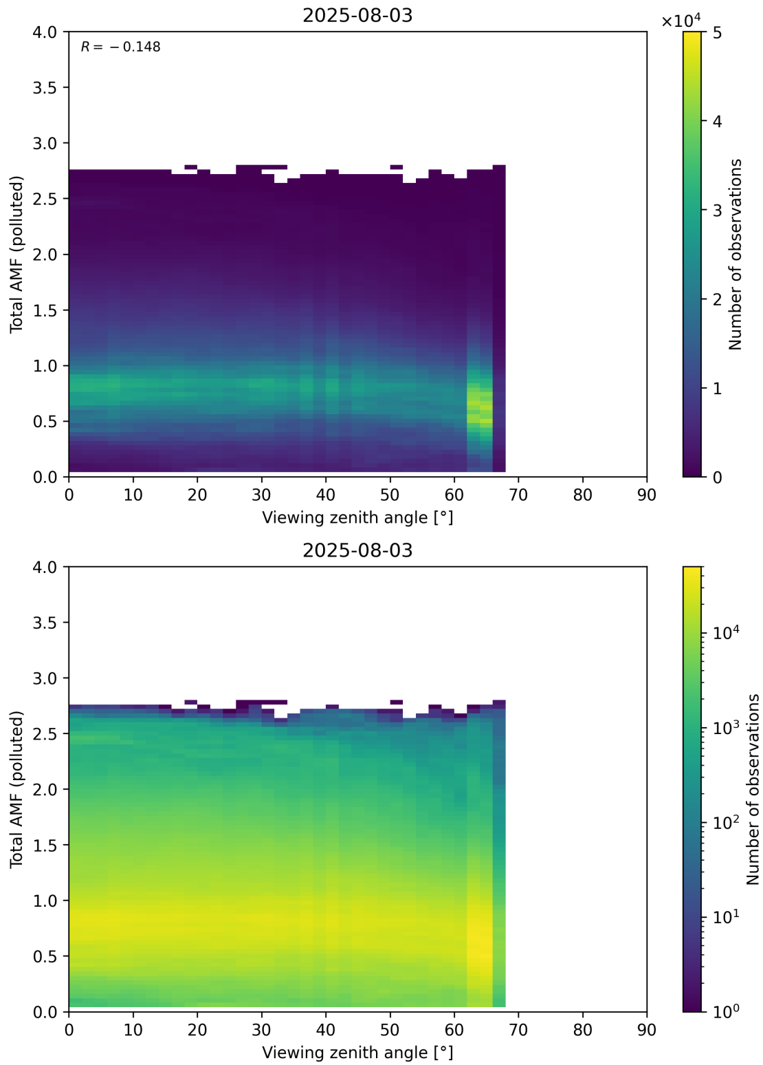
Figure 381: Scatter density plot of “Viewing zenith angle” against “Total AMF (polluted)” for 2025-08-03 to 2025-08-04.
