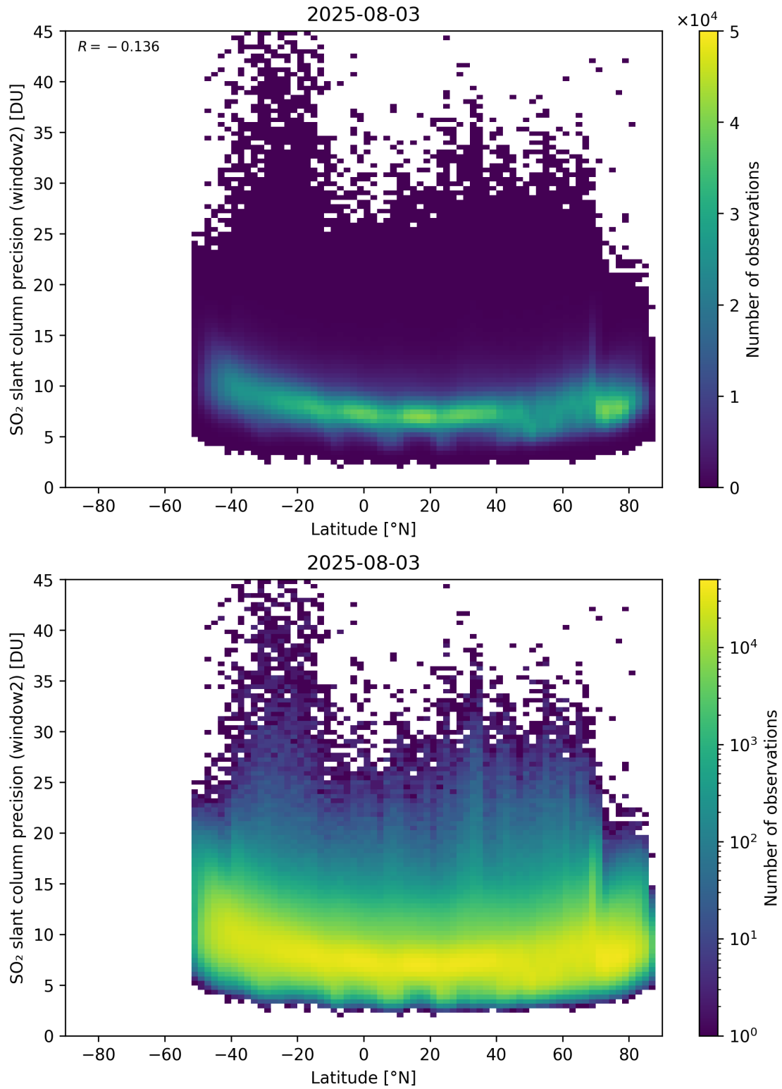
Figure 164: Scatter density plot of “Latitude” against “SO 2 slant column precision (window2)” for 2025-08-03 to 2025-08-04.
