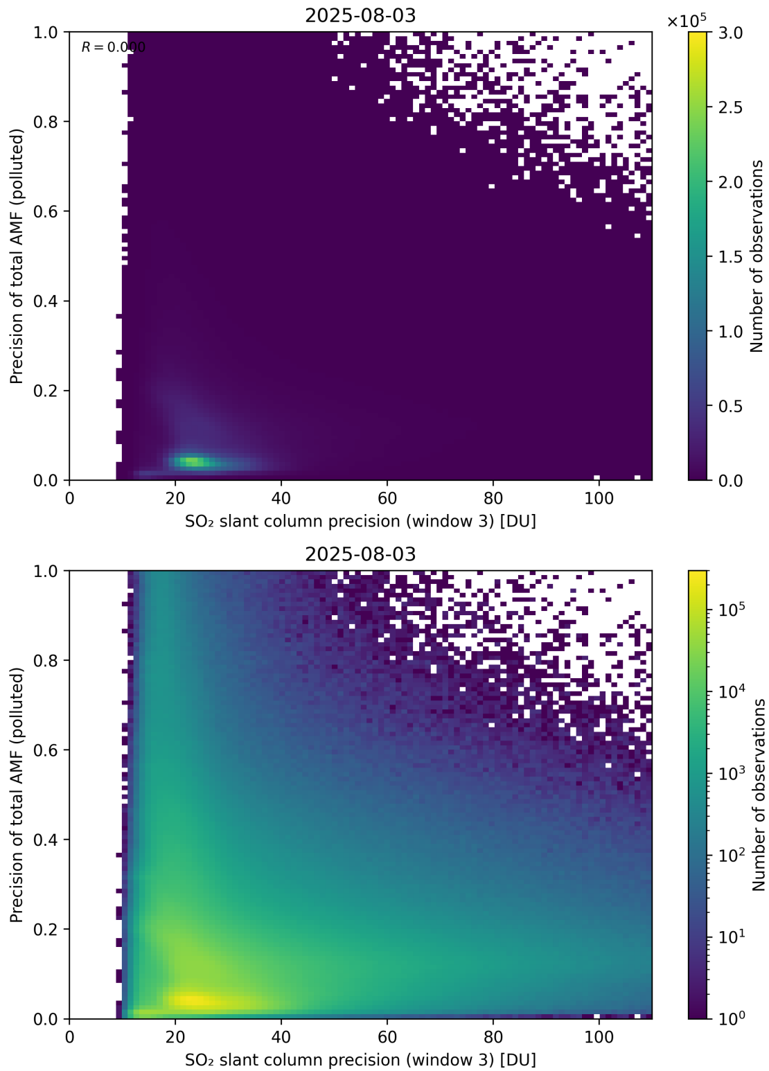
Figure 314: Scatter density plot of “SO 2 slant column precision (window 3)” against “Precision of total AMF (polluted)” for 2025-08-03 to 2025-08-04.
