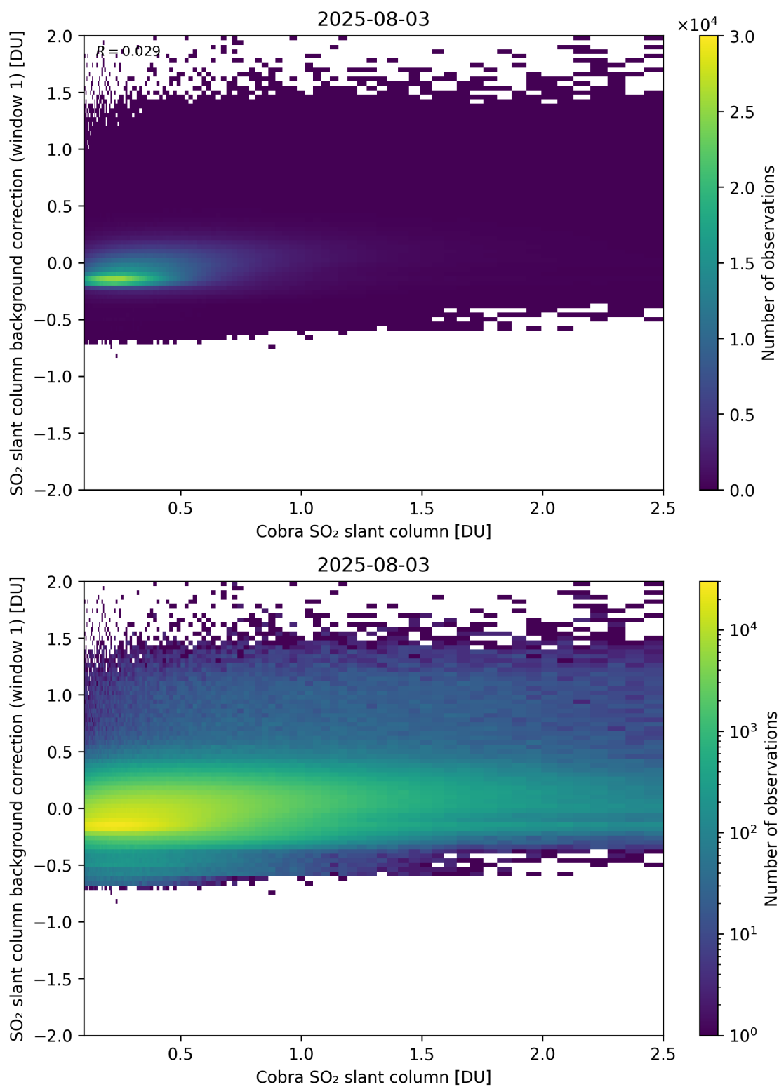
Figure 193: Scatter density plot of “Cobra SO 2 slant column” against “SO 2 slant column background correction (window 1)” for 2025-08-03 to 2025-08-04.
