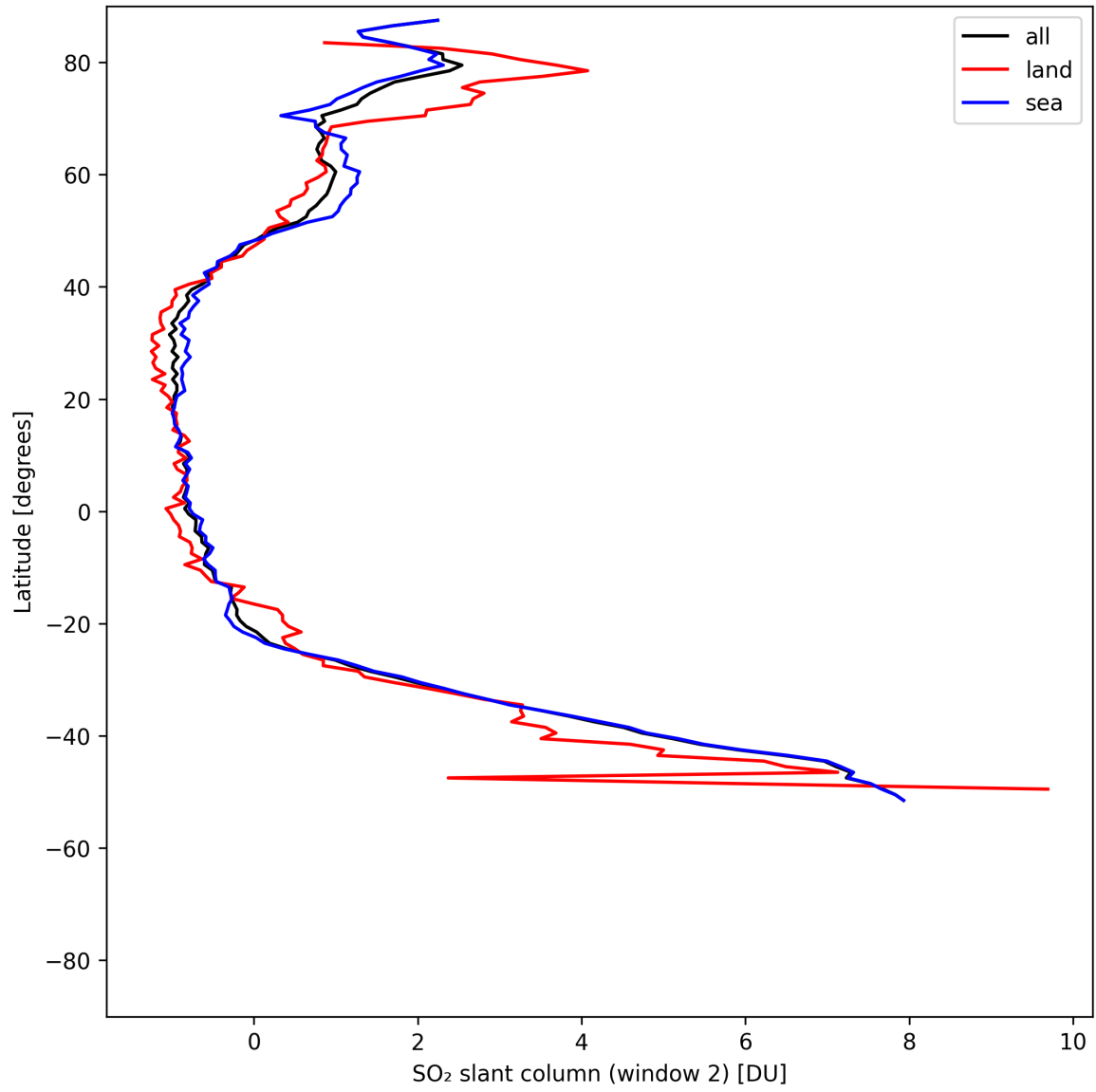
Figure 41: Zonal average of “SO 2 slant column (window 2)” for 2025-08-03 to 2025-08-04.
