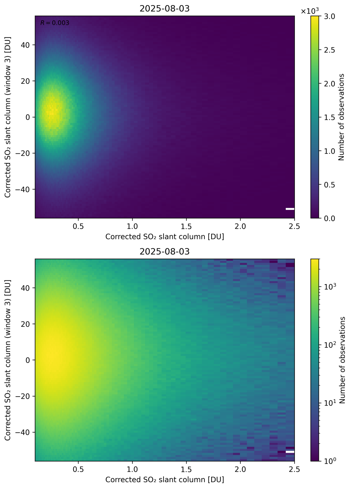
Figure 236: Scatter density plot of “Corrected SO 2 slant column” against “Corrected SO 2 slant column (window 3)” for 2025-08-03 to 2025-08-04.
