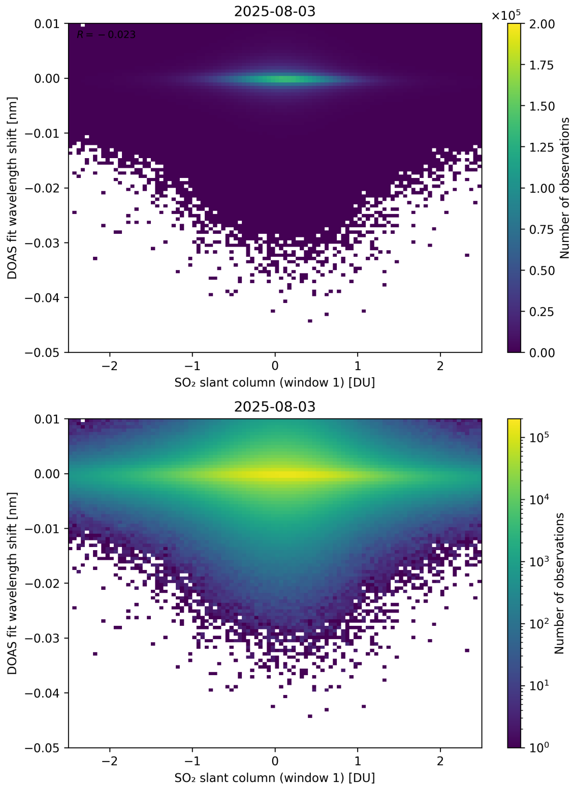
Figure 265: Scatter density plot of “SO 2 slant column (window 1)” against “DOAS fit wavelength shift” for 2025-08-03 to 2025-08-04.
