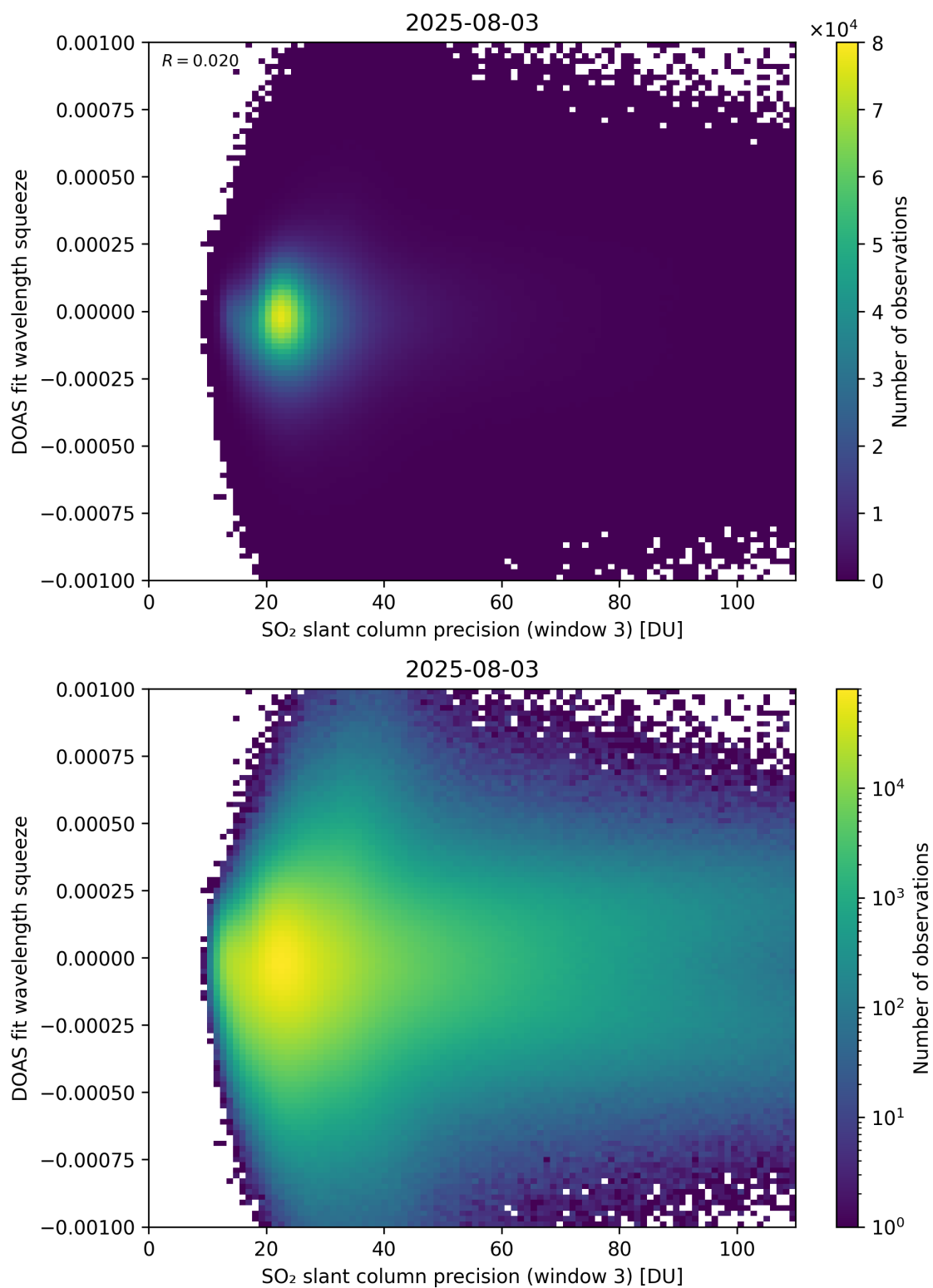
Figure 309: Scatter density plot of “SO 2 slant column precision (window 3)” against “DOAS fit wavelength squeeze” for 2025-08-03 to 2025-08-04.
