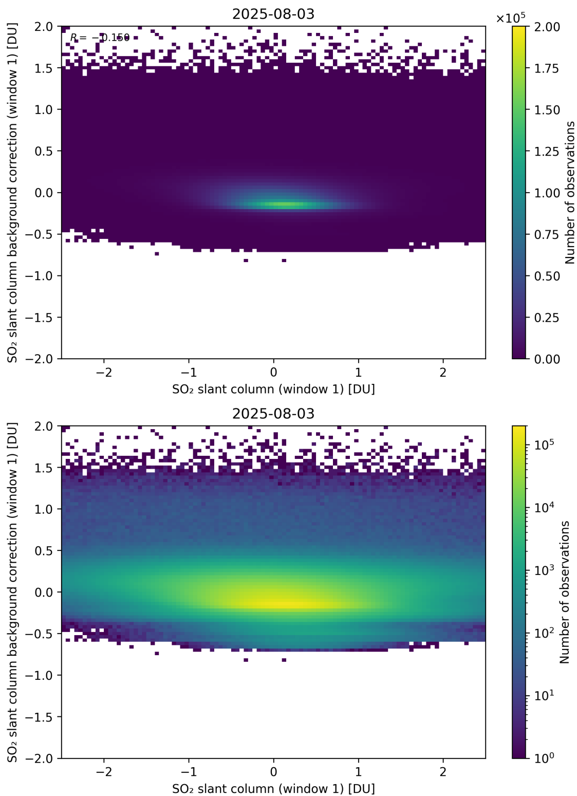
Figure 262: Scatter density plot of “SO 2 slant column (window 1)” against “SO 2 slant column background correction (window 1)” for 2025-08-03 to 2025-08-04.
