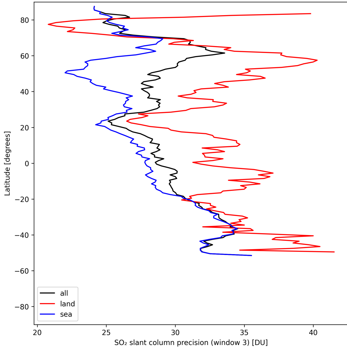
Figure 46: Zonal average of “SO 2 slant column precision (window 3)” for 2025-08-03 to 2025-08-04.
