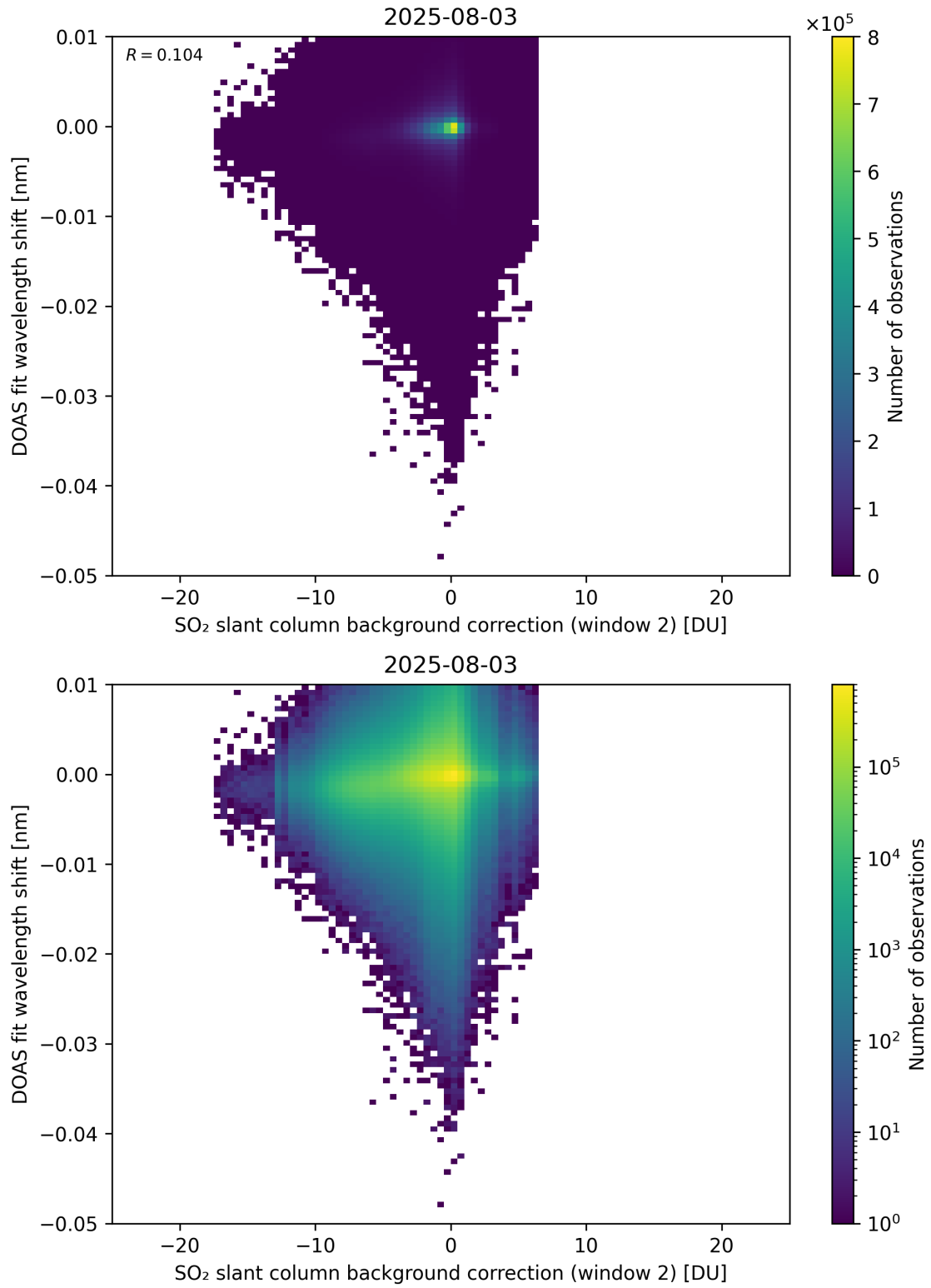
Figure 123: Scatter density plot of “SO 2 slant column background correction (window 2)” against “DOAS fit wavelength shift” for 2025-08-03 to 2025-08-04.
