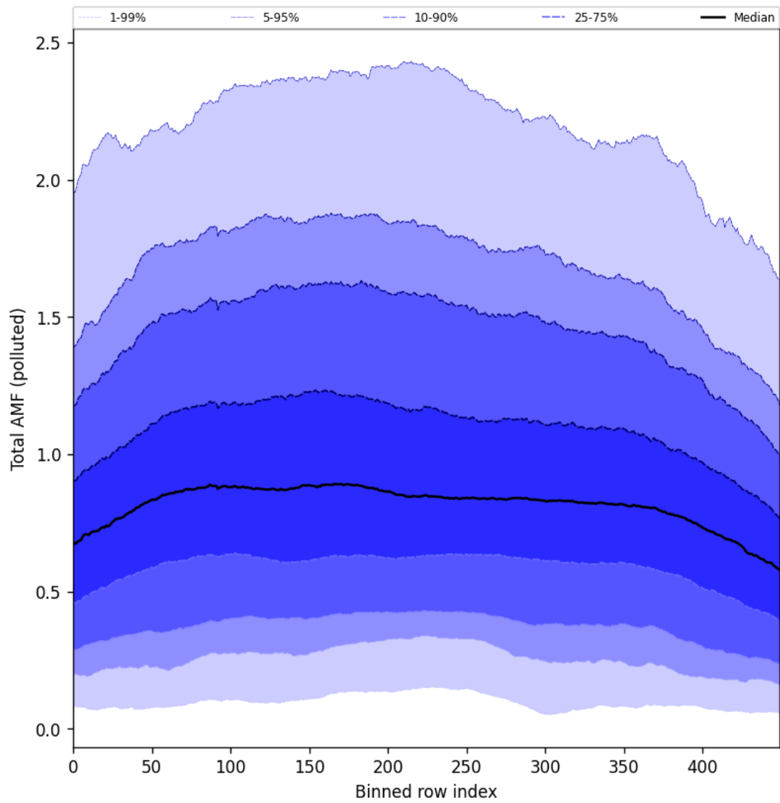
Figure 105: Along track statistics of “Total AMF (polluted)” for 2025-08-03 to 2025-08-04
