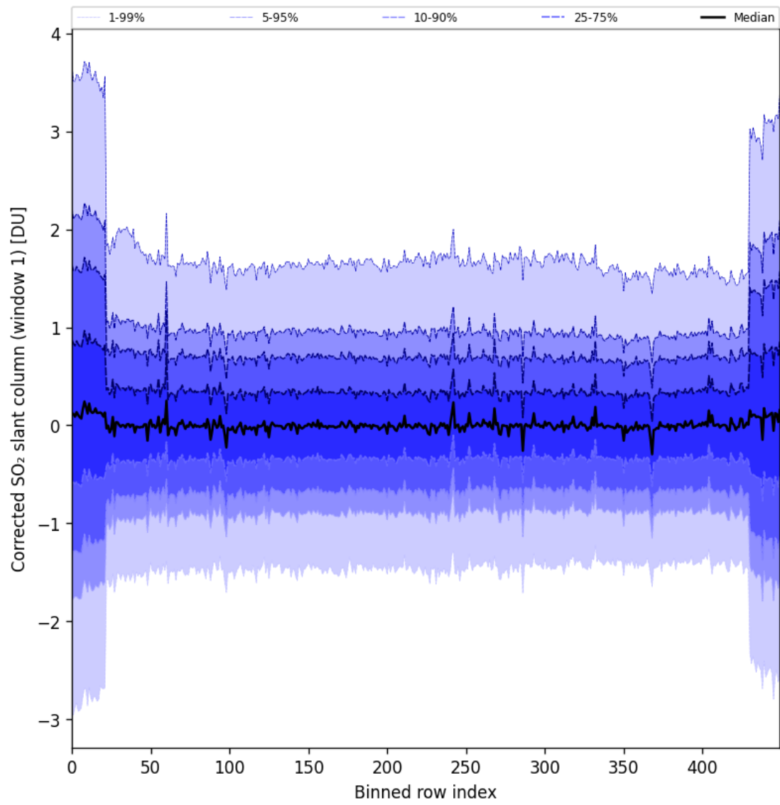
Figure 91: Along track statistics of “Corrected SO 2 slant column (window 1)” for 2025-08-03 to 2025-08-04
