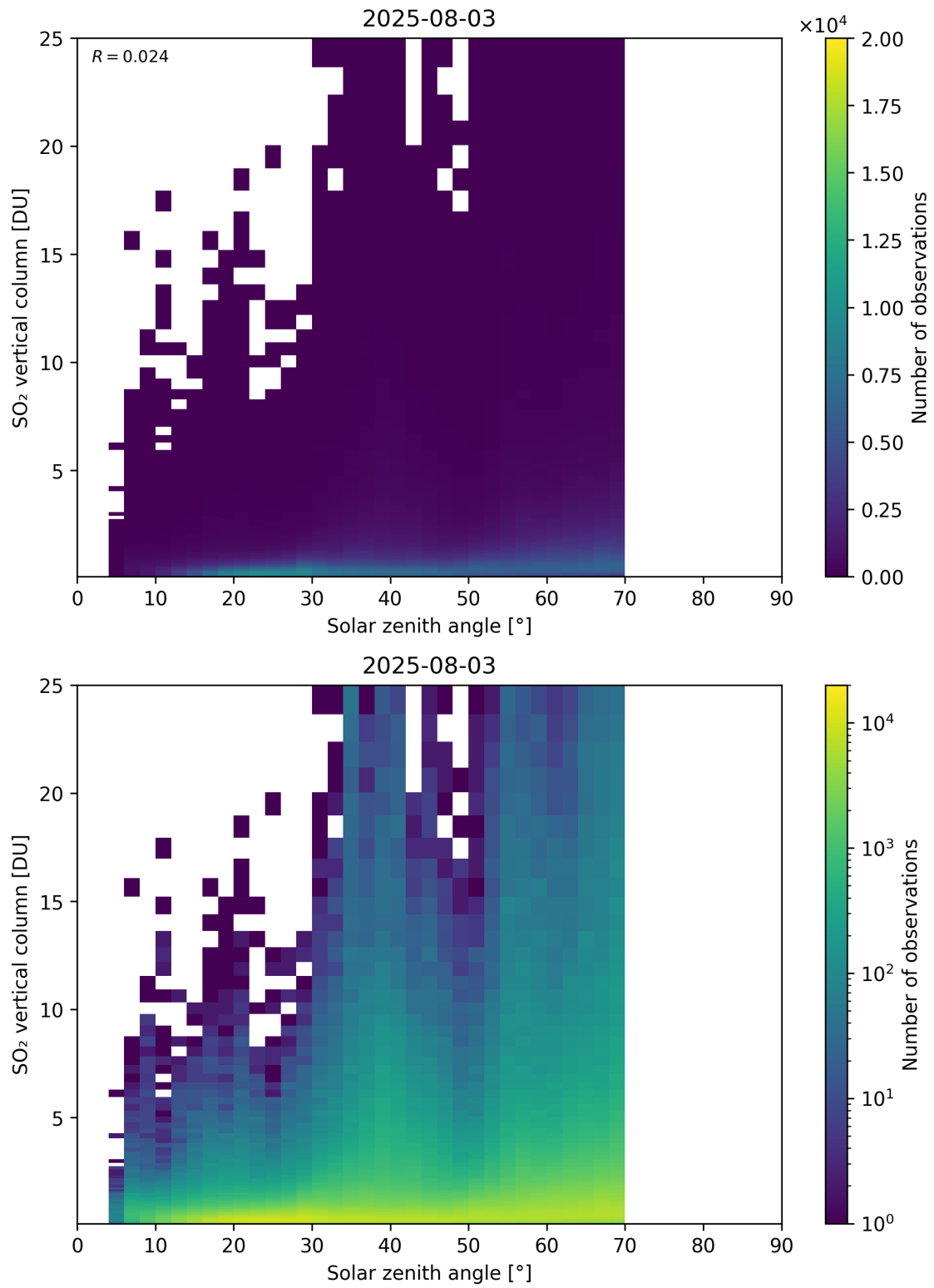
Figure 191: Scatter density plot of “Solar zenith angle” against “SO 2 vertical column” for 2025-08-03 to 2025-08-04.
