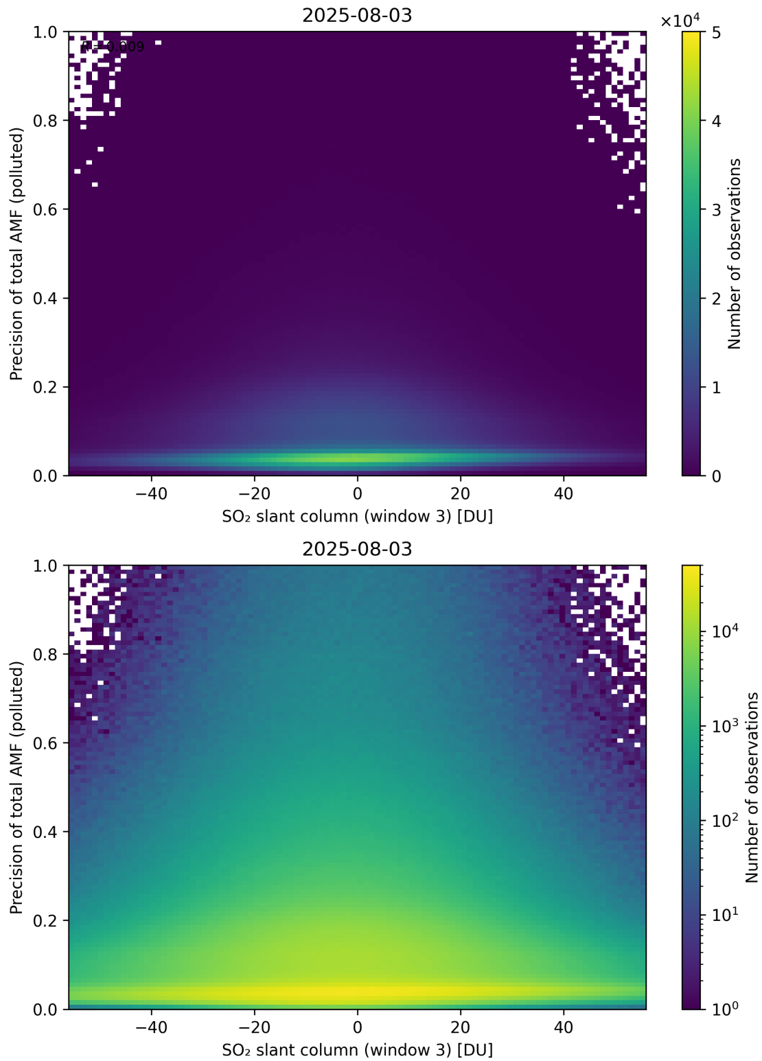
Figure 319: Scatter density plot of “SO 2 slant column (window 3)” against “Precision of total AMF (polluted)” for 2025-08-03 to 2025-08-04.
