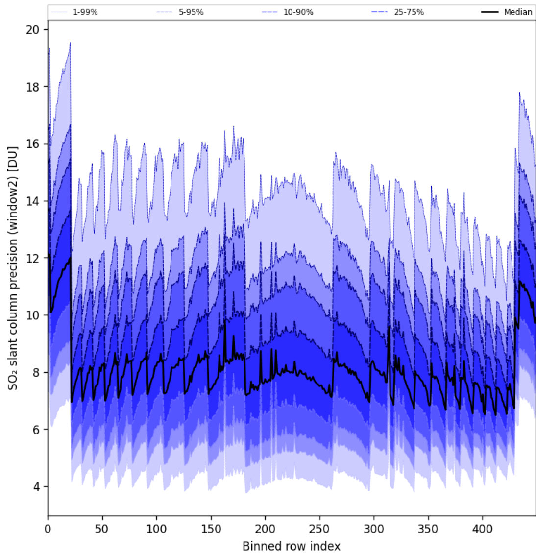
Figure 94: Along track statistics of “SO 2 slant column precision (window2)” for 2025-08-03 to 2025-08-04
