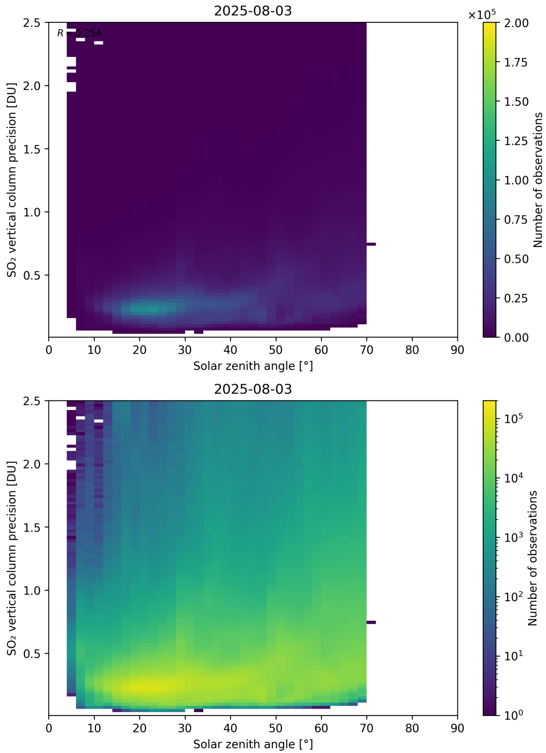
Figure 192: Scatter density plot of “Solar zenith angle” against “SO 2 vertical column precision” for 2025-08-03 to 2025-08-04.
