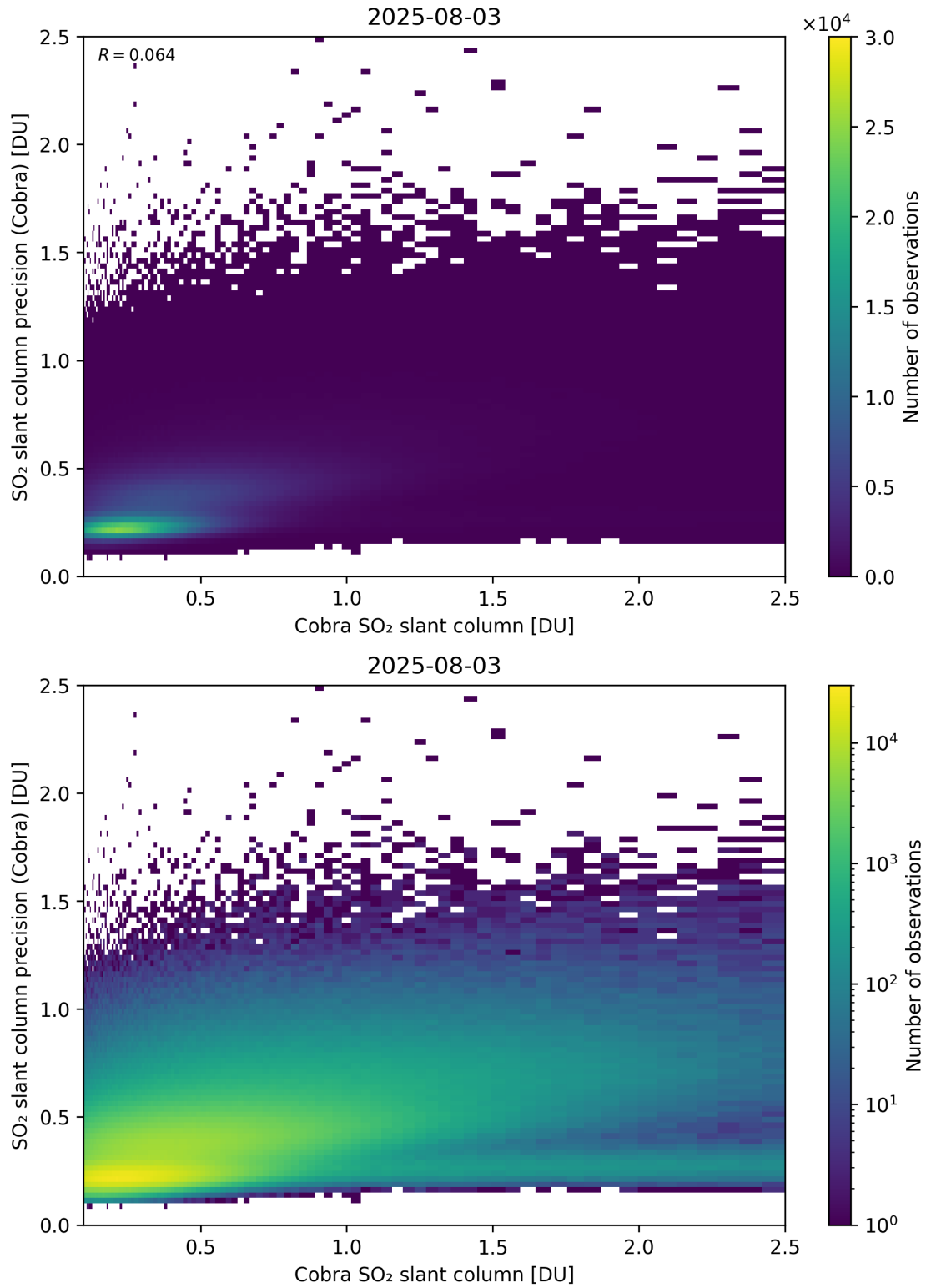
Figure 216: Scatter density plot of “Cobra SO 2 slant column” against “SO 2 slant column precision (Cobra)” for 2025-08-03 to 2025-08-04.
