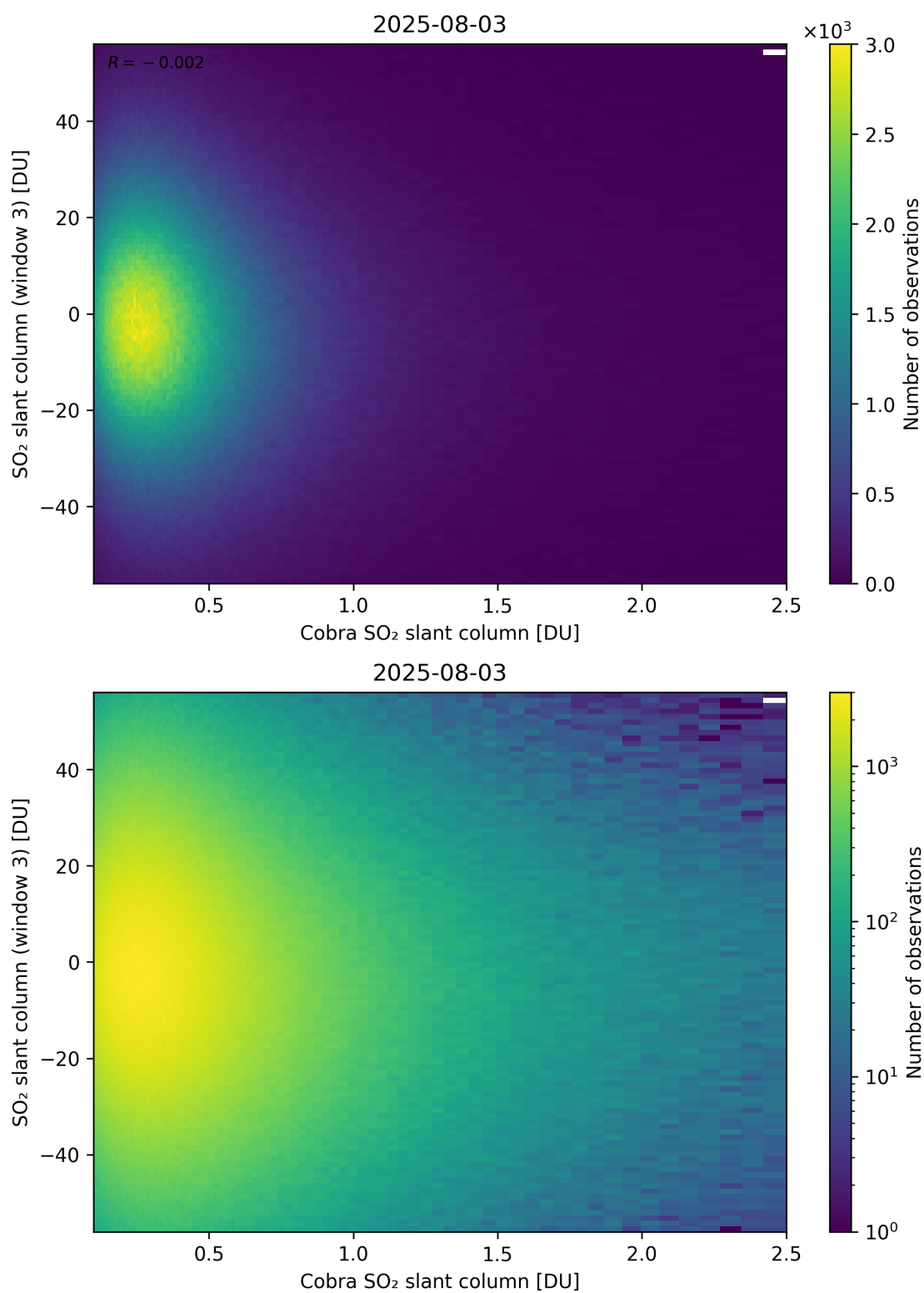
Figure 222: Scatter density plot of “Cobra SO 2 slant column” against “SO 2 slant column (window 3)” for 2025-08-03 to 2025-08-04.
