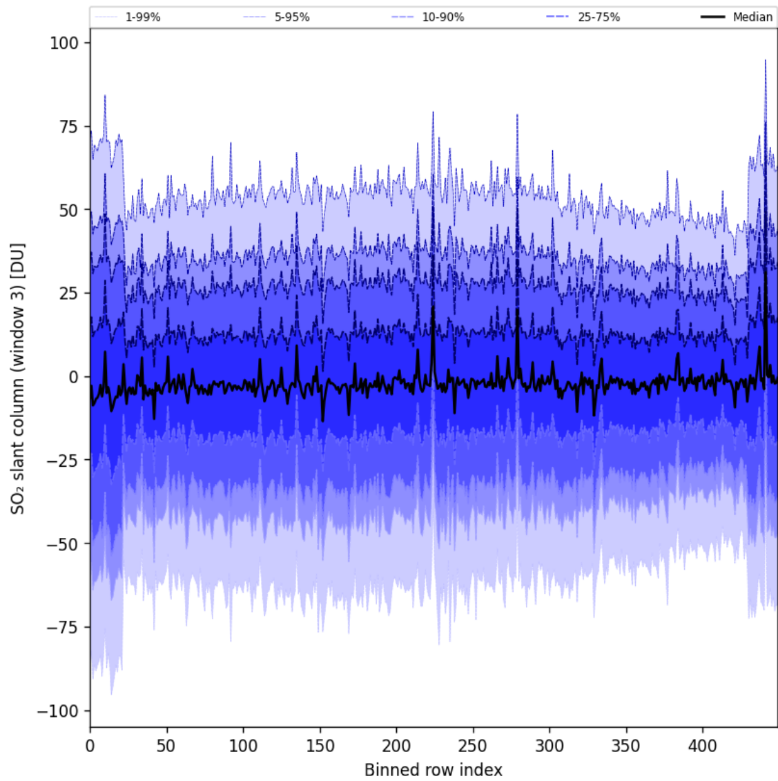
Figure 97: Along track statistics of “SO 2 slant column (window 3)” for 2025-08-03 to 2025-08-04
