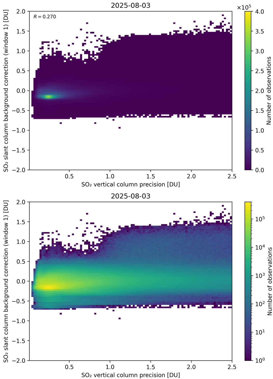
Figure 329: Scatter density plot of “SO 2 vertical column precision” against “SO 2 slant column background correction (window 1)” for 2025-08-03 to 2025-08-04.
