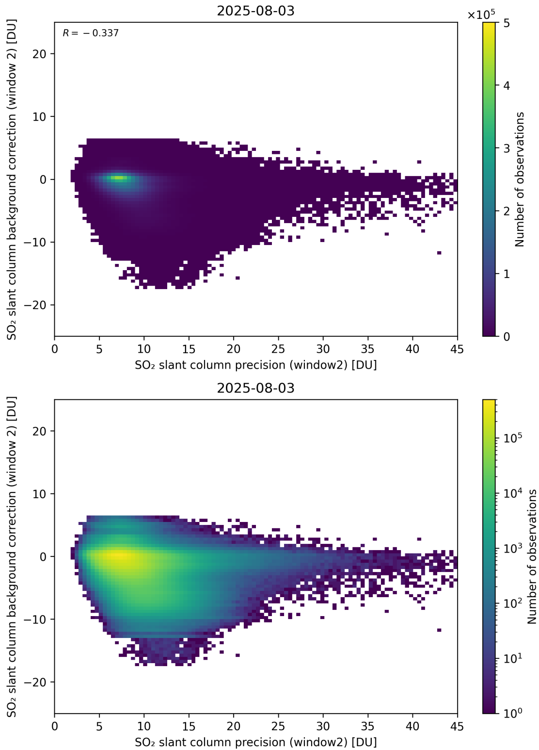
Figure 291: Scatter density plot of “SO 2 slant column precision (window2)” against “SO 2 slant column background correction (window 2)” for 2025-08-03 to 2025-08-04.
