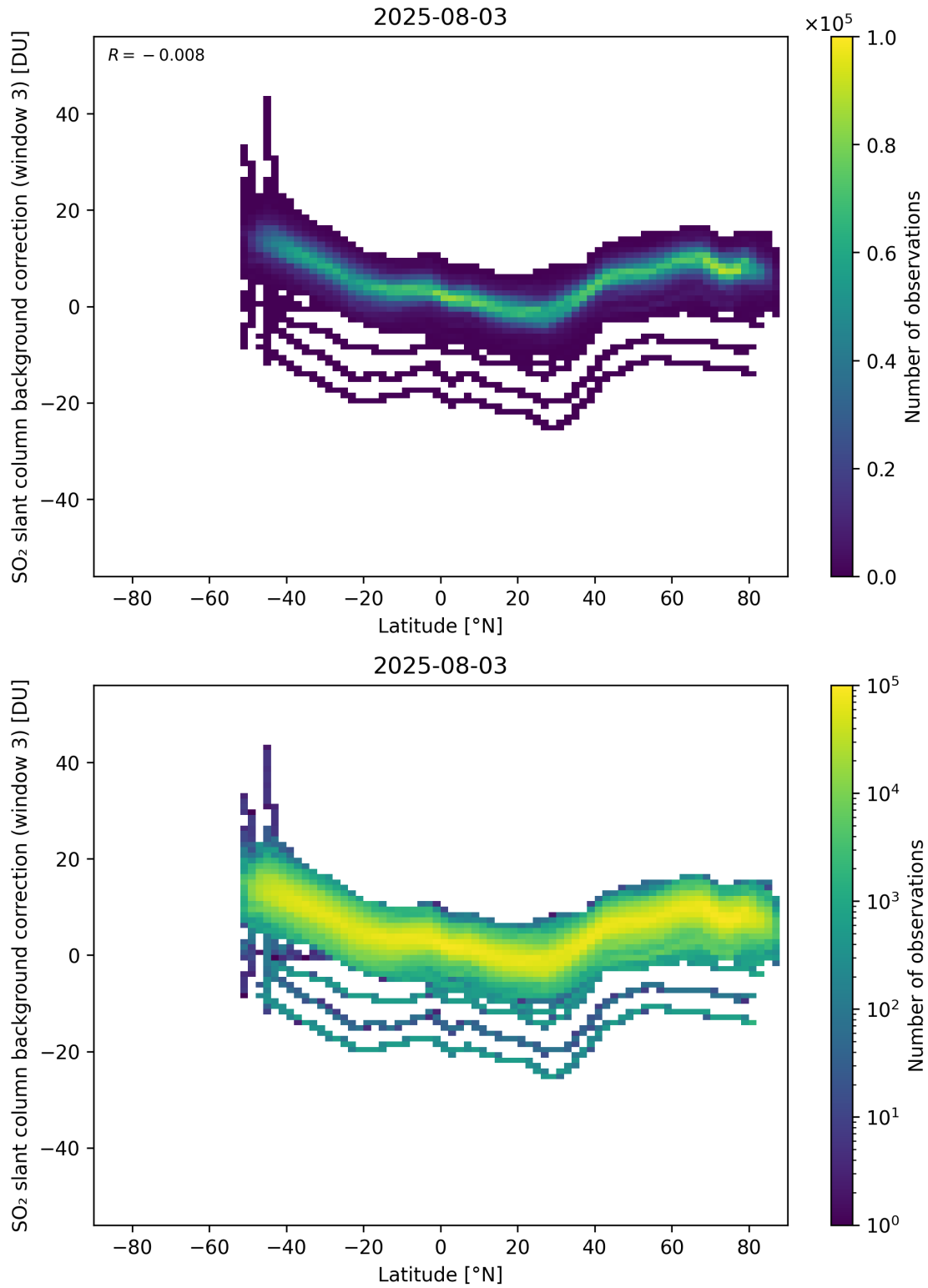
Figure 152: Scatter density plot of “Latitude” against “SO 2 slant column background correction (window 3)” for 2025-08-03 to 2025-08-04.
