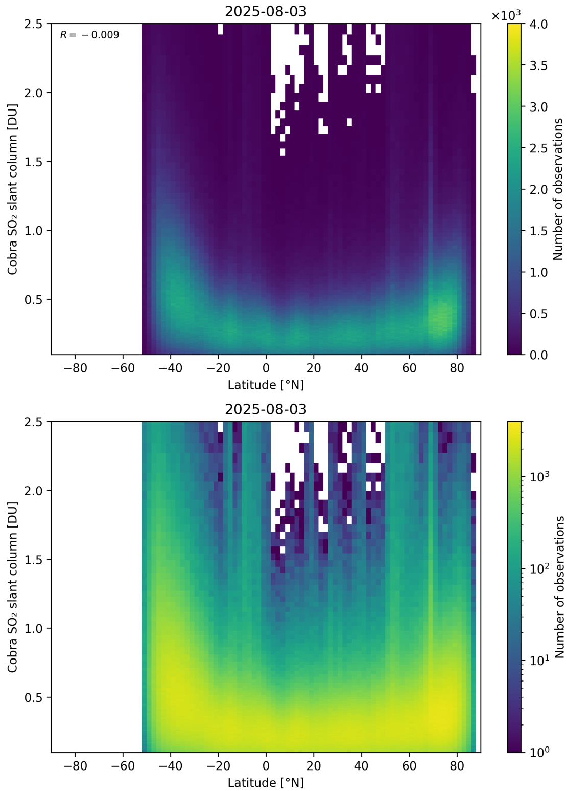
Figure 157: Scatter density plot of “Latitude” against “Cobra SO 2 slant column” for 2025-08-03 to 2025-08-04.
