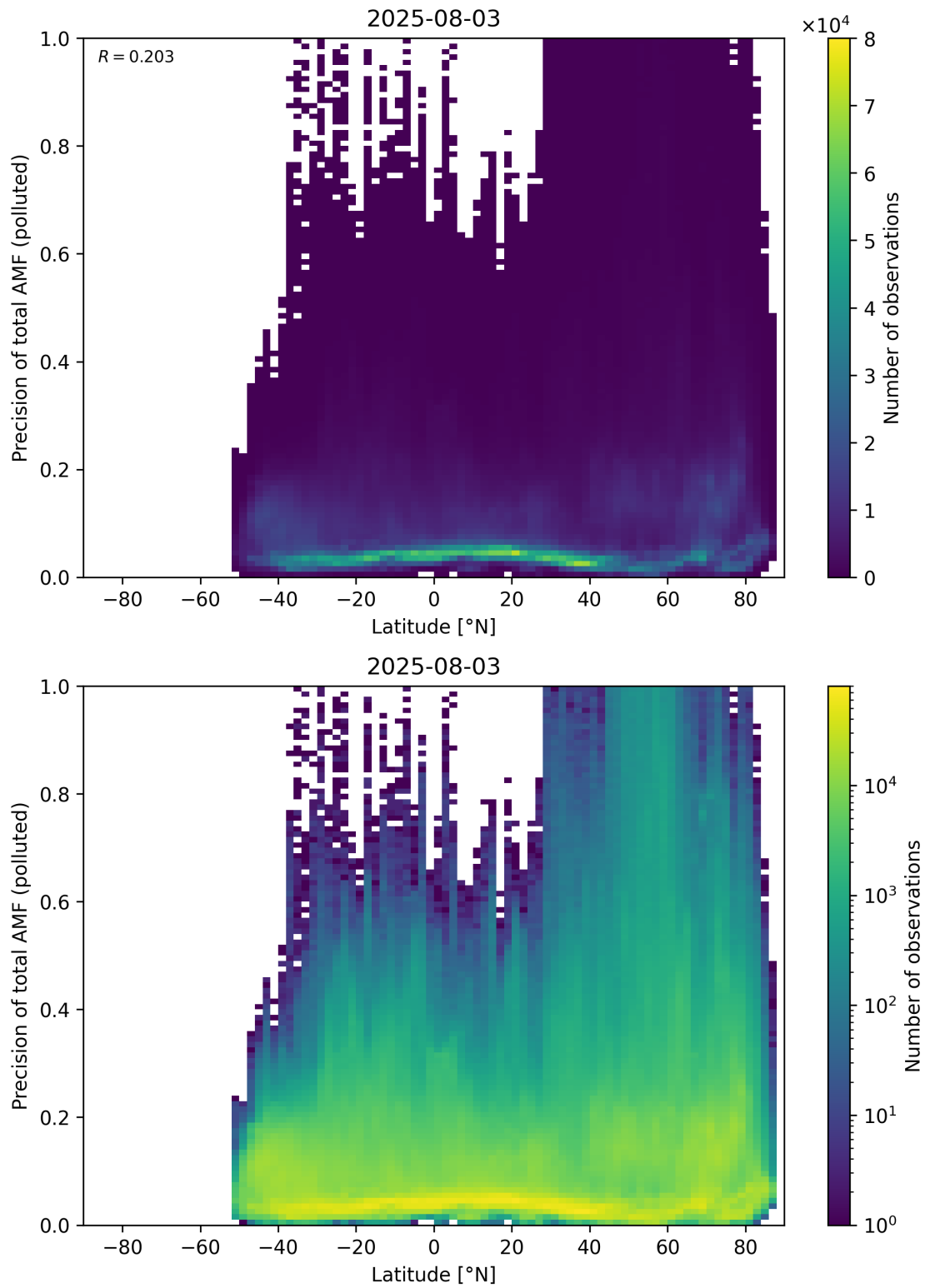
Figure 168: Scatter density plot of “Latitude” against “Precision of total AMF (polluted)” for 2025-08-03 to 2025-08-04.
