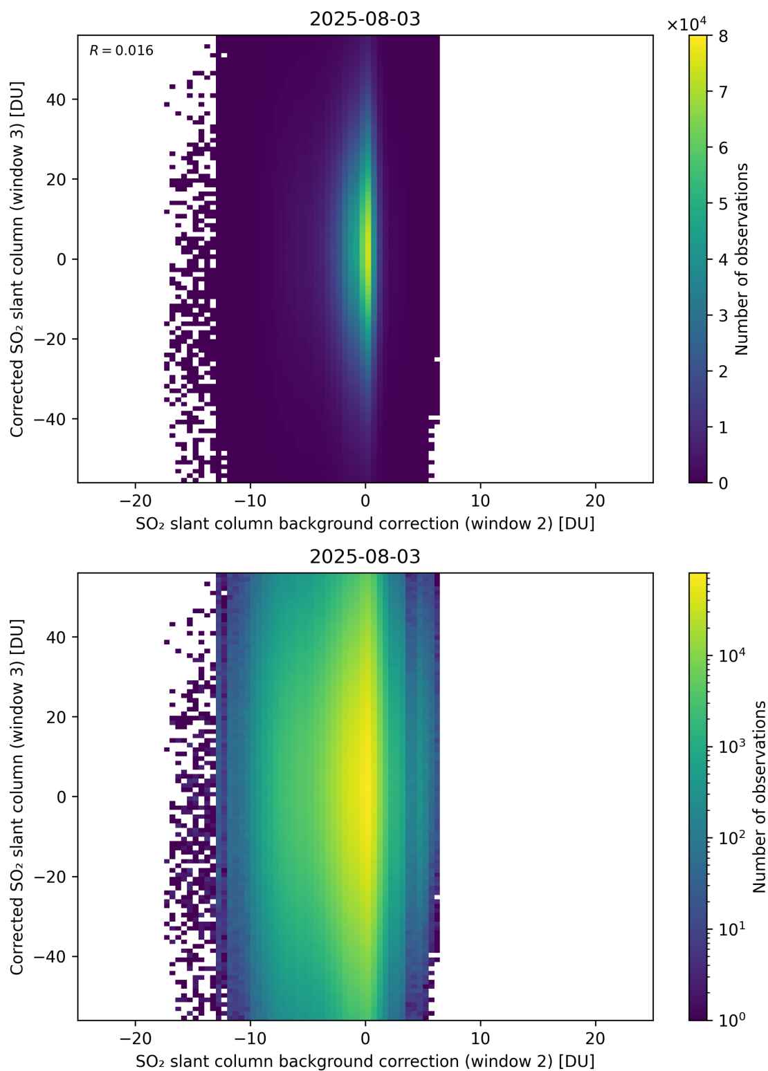
Figure 127: Scatter density plot of “SO 2 slant column background correction (window 2)” against “Corrected SO 2 slant column (window 3)” for 2025-08-03 to 2025-08-04.
