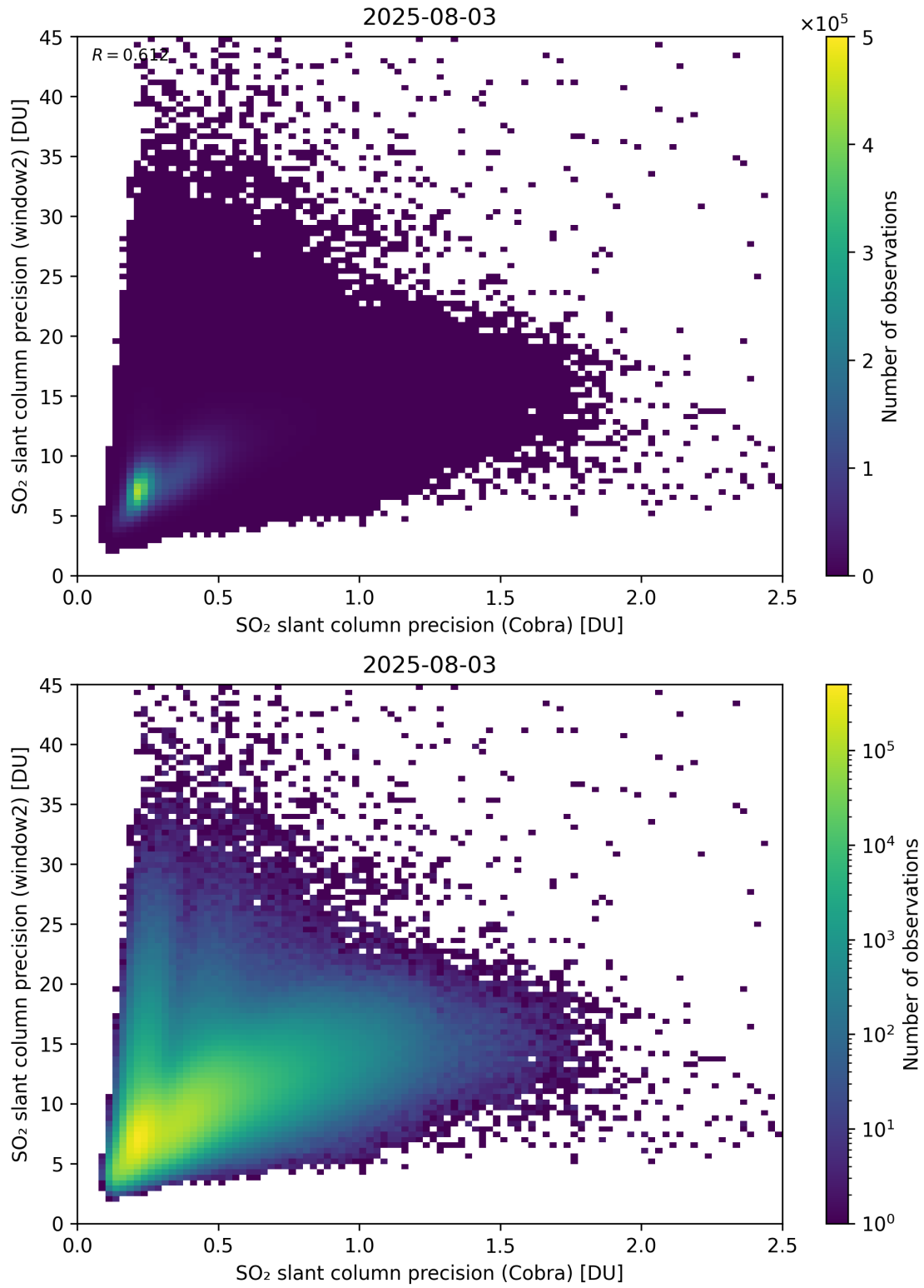
Figure 210: Scatter density plot of “SO 2 slant column precision (Cobra)” against “SO 2 slant column precision (window2)” for 2025-08-03 to 2025-08-04.
