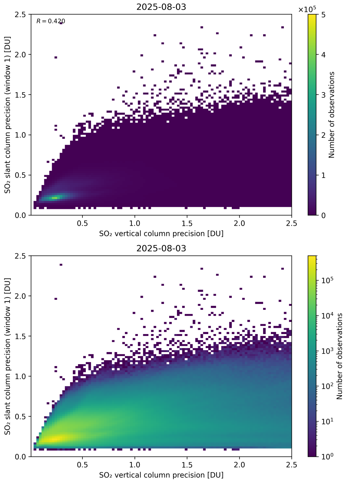
Figure 342: Scatter density plot of “SO 2 vertical column precision” against “SO 2 slant column precision (window 1)” for 2025-08-03 to 2025-08-04.
