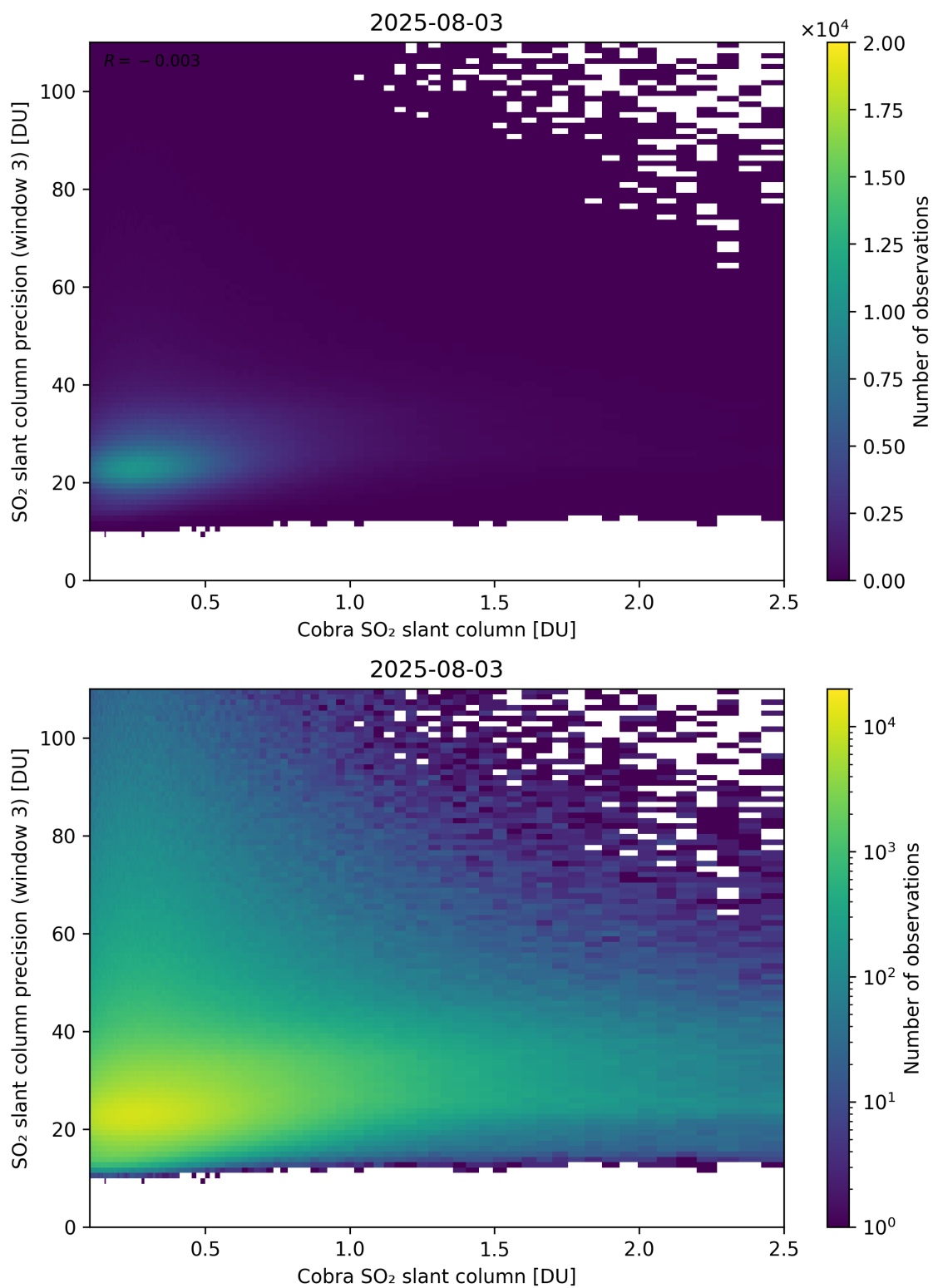
Figure 223: Scatter density plot of “Cobra SO 2 slant column” against “SO 2 slant column precision (window 3)” for 2025-08-03 to 2025-08-04.
