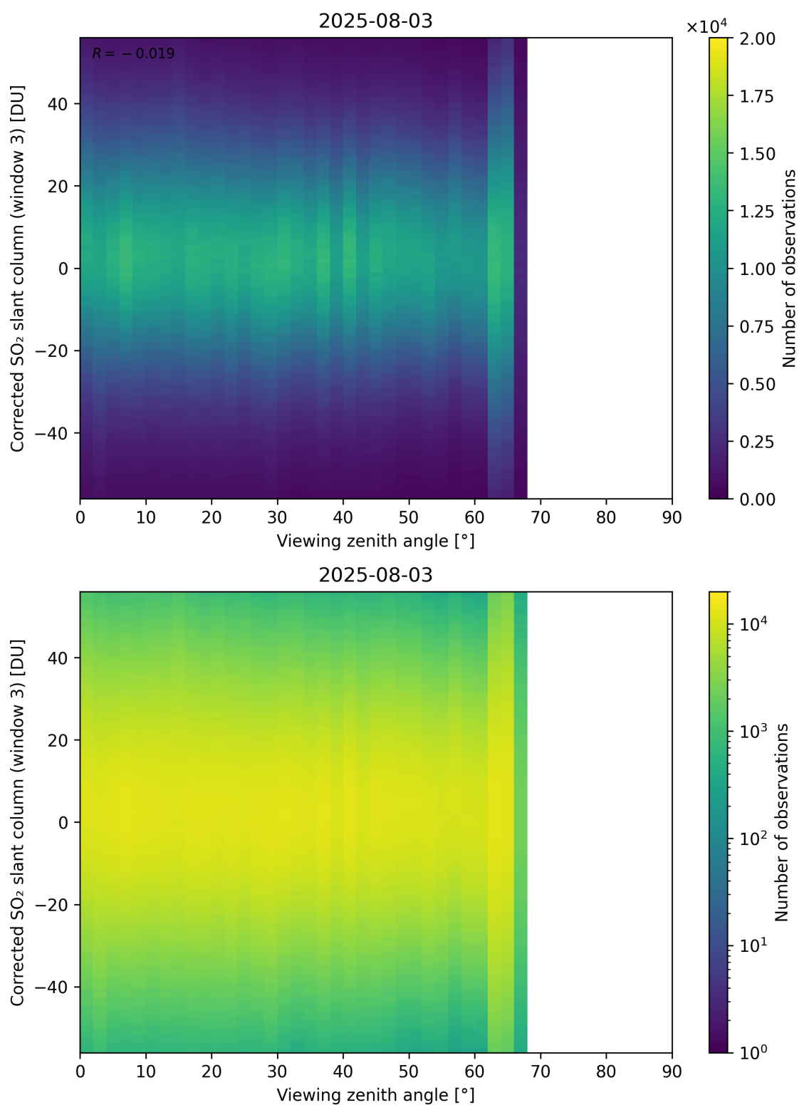
Figure 375: Scatter density plot of “Viewing zenith angle” against “Corrected SO 2 slant column (window 3)” for 2025-08-03 to 2025-08-04.
