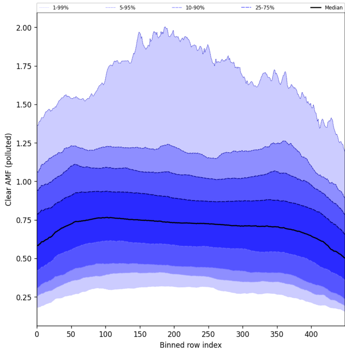
Figure 107: Along track statistics of “Clear AMF (polluted)” for 2025-08-03 to 2025-08-04
