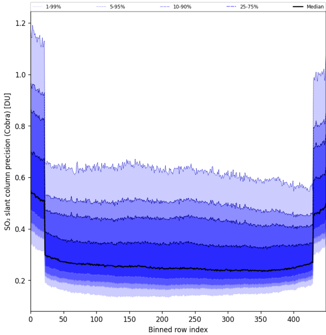
Figure 88: Along track statistics of “SO 2 slant column precision (Cobra)” for 2025-08-03 to 2025-08-04
