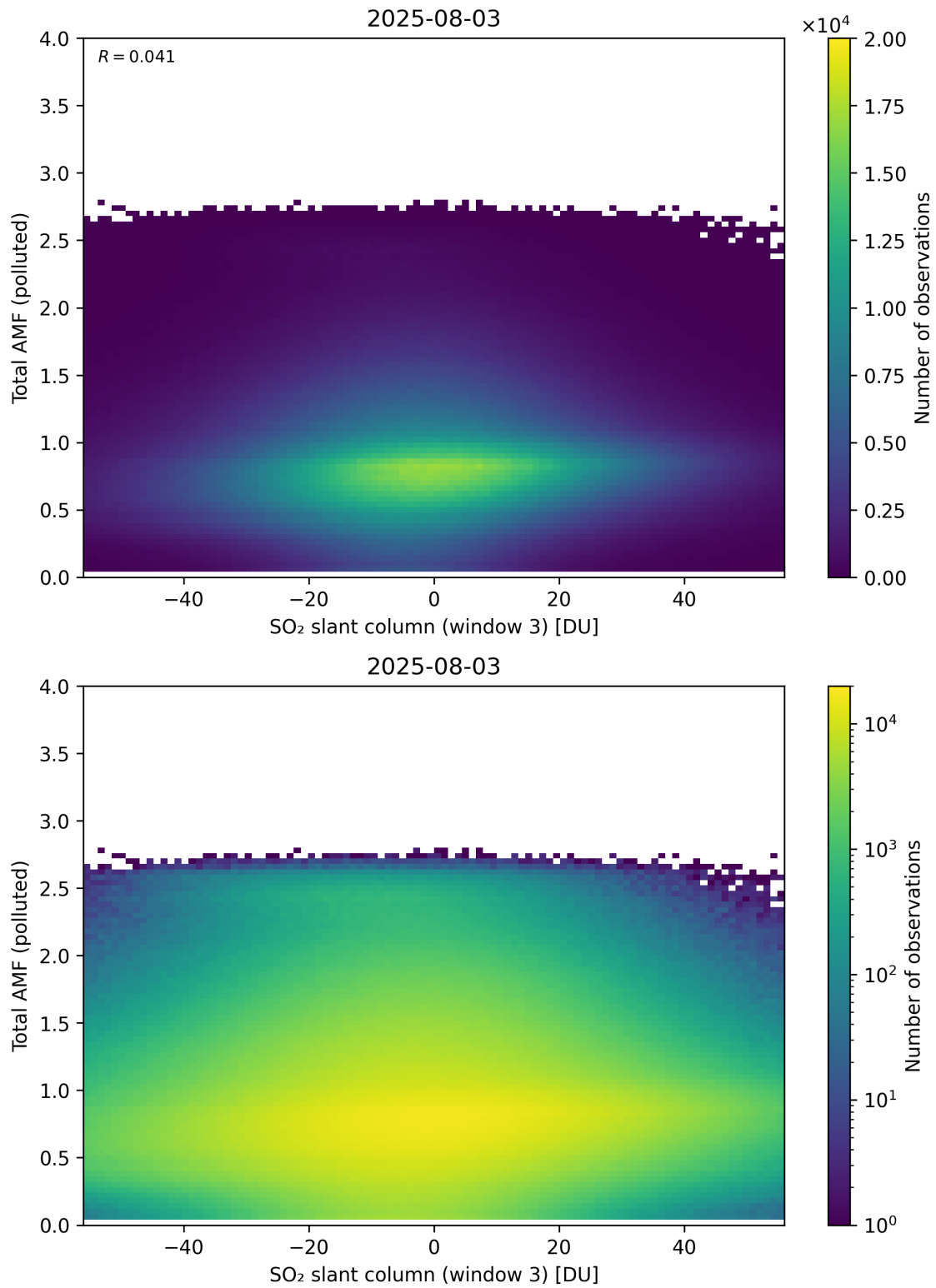
Figure 318: Scatter density plot of “SO 2 slant column (window 3)” against “Total AMF (polluted)” for 2025-08-03 to 2025-08-04.
