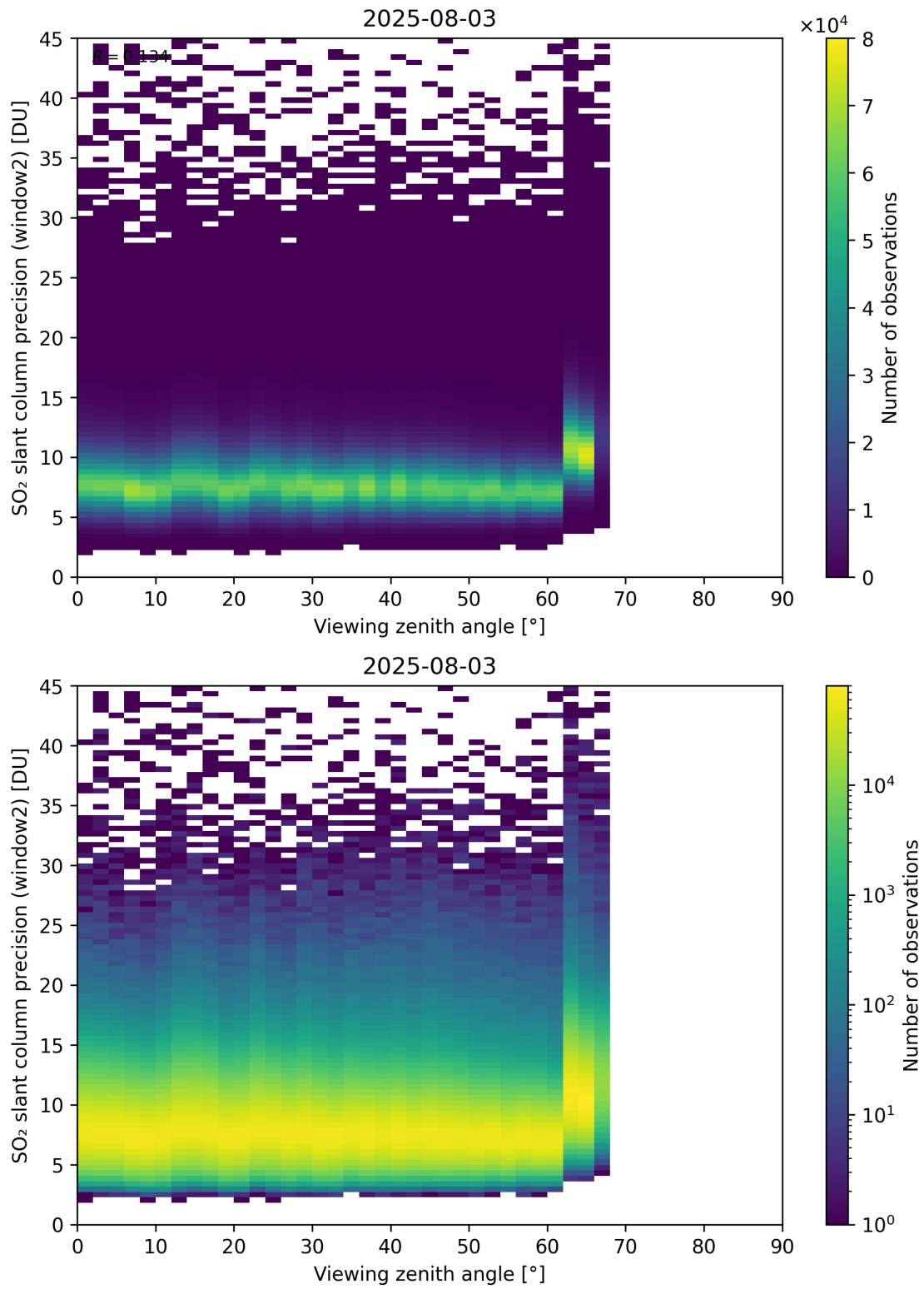
Figure 378: Scatter density plot of “Viewing zenith angle” against “SO 2 slant column precision (window2)” for 2025-08-03 to 2025-08-04.
