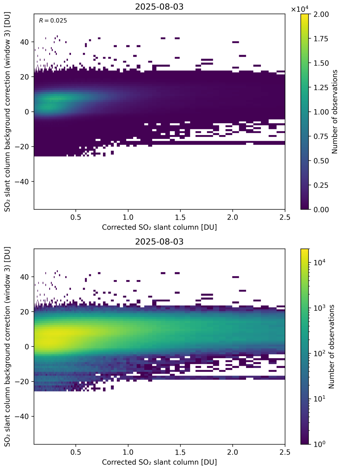
Figure 228: Scatter density plot of “Corrected SO 2 slant column” against “SO 2 slant column background correction (window 3)” for 2025-08-03 to 2025-08-04.
