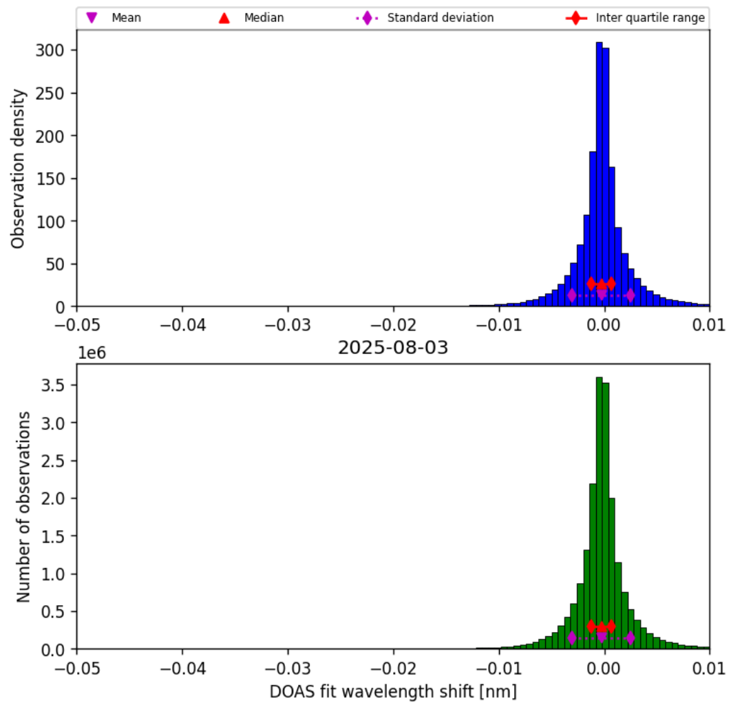
Figure 76: Histogram of “DOAS fit wavelength shift” for 2025-08-03 to 2025-08-04
